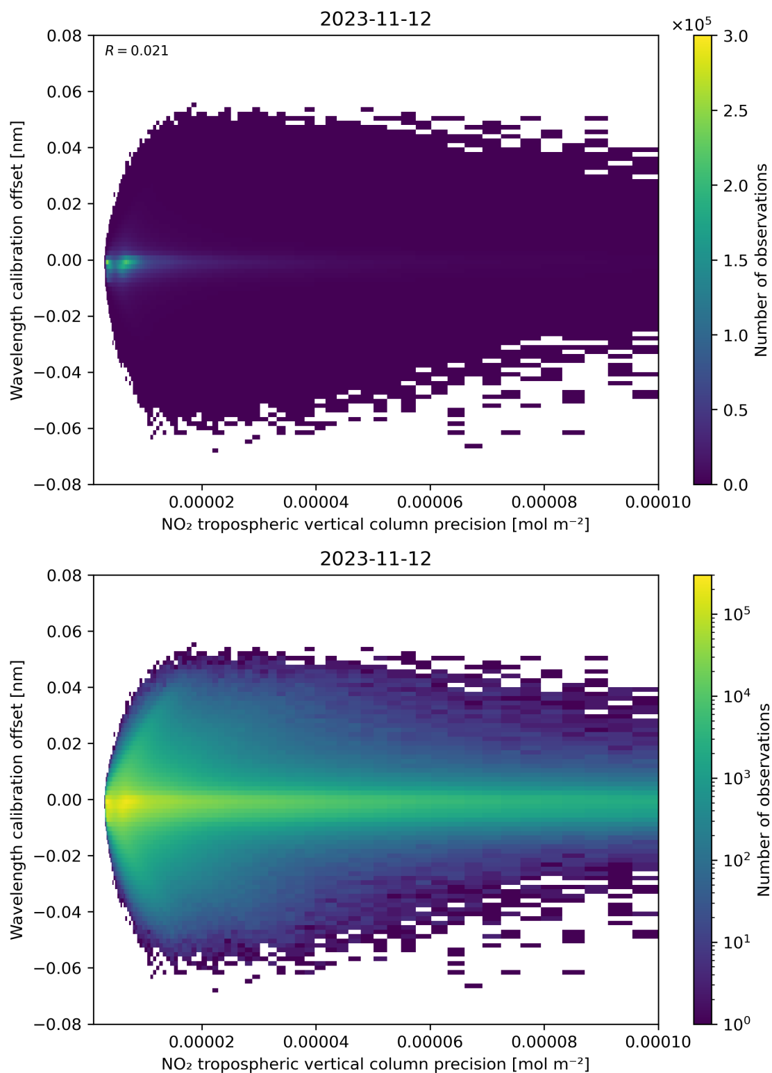
Figure 141: Scatter density plot of “NO 2 tropospheric vertical column precision” against “Wavelength calibration offset” for 2023-11-12 to 2023-11-13.
