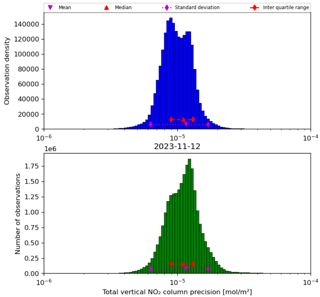
Figure 39: Histogram of “Total vertical NO 2 column precision” for 2023-11-12 to 2023-11-13
