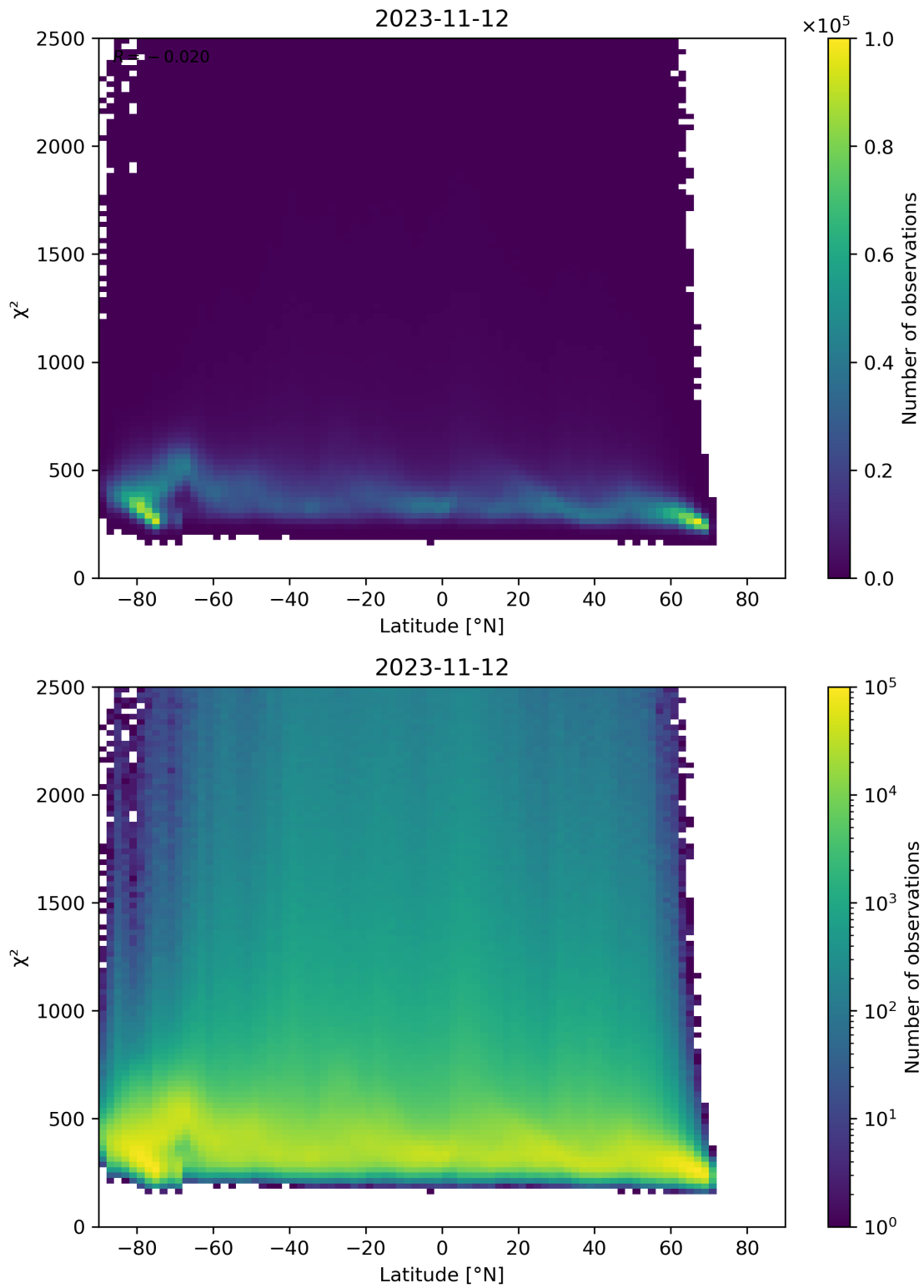
Figure 86: Scatter density plot of “Latitude” against “ \chi^2 ” for 2023-11-12 to 2023-11-13.
