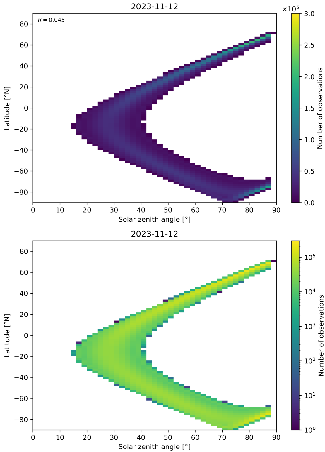
Figure 149: Scatter density plot of “Solar zenith angle” against “Latitude” for 2023-11-12 to 2023-11-13.
