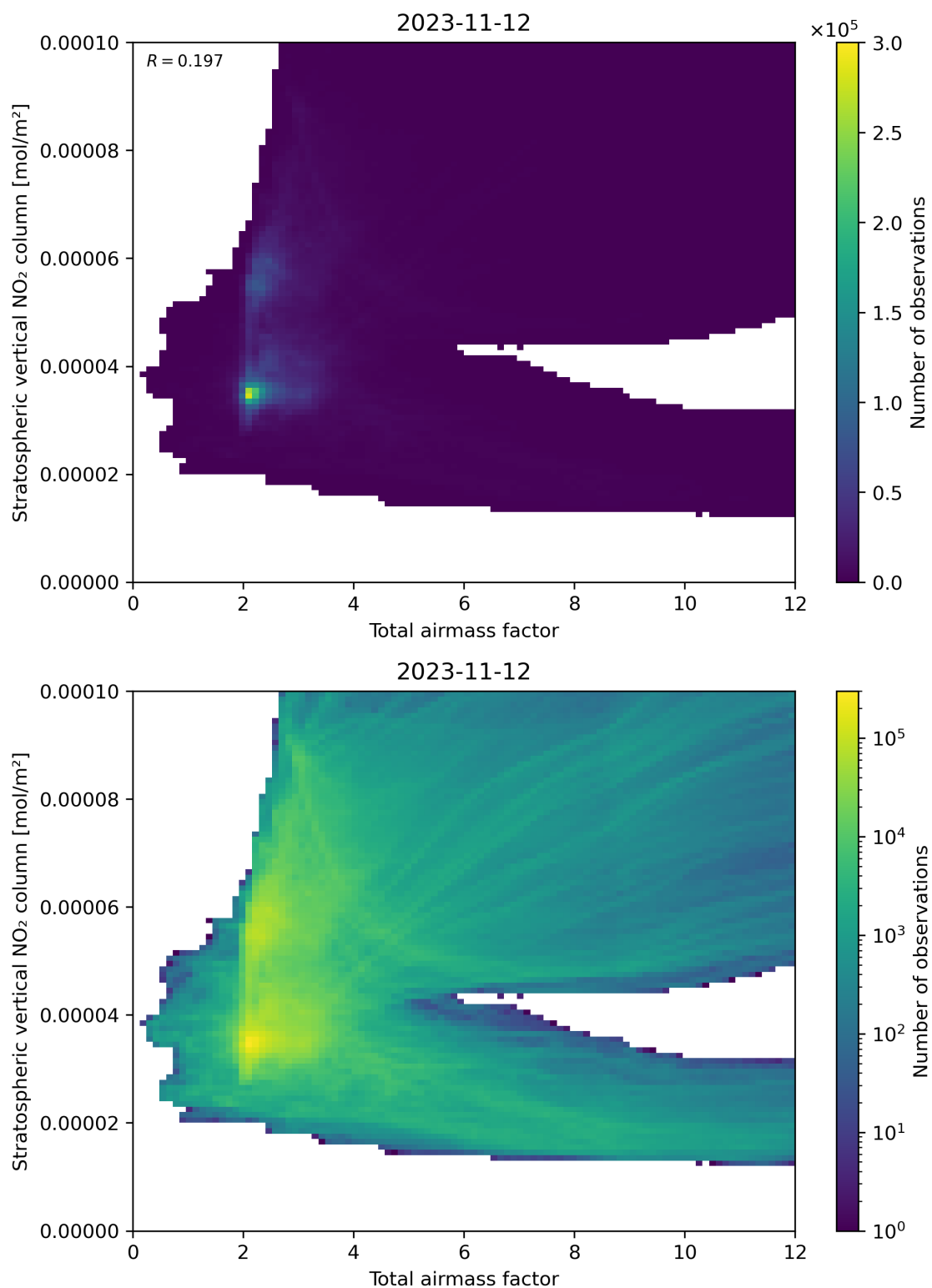
Figure 64: Scatter density plot of “Total airmass factor” against “Stratospheric vertical NO 2 column” for 2023-11-12 to 2023-11-13.
