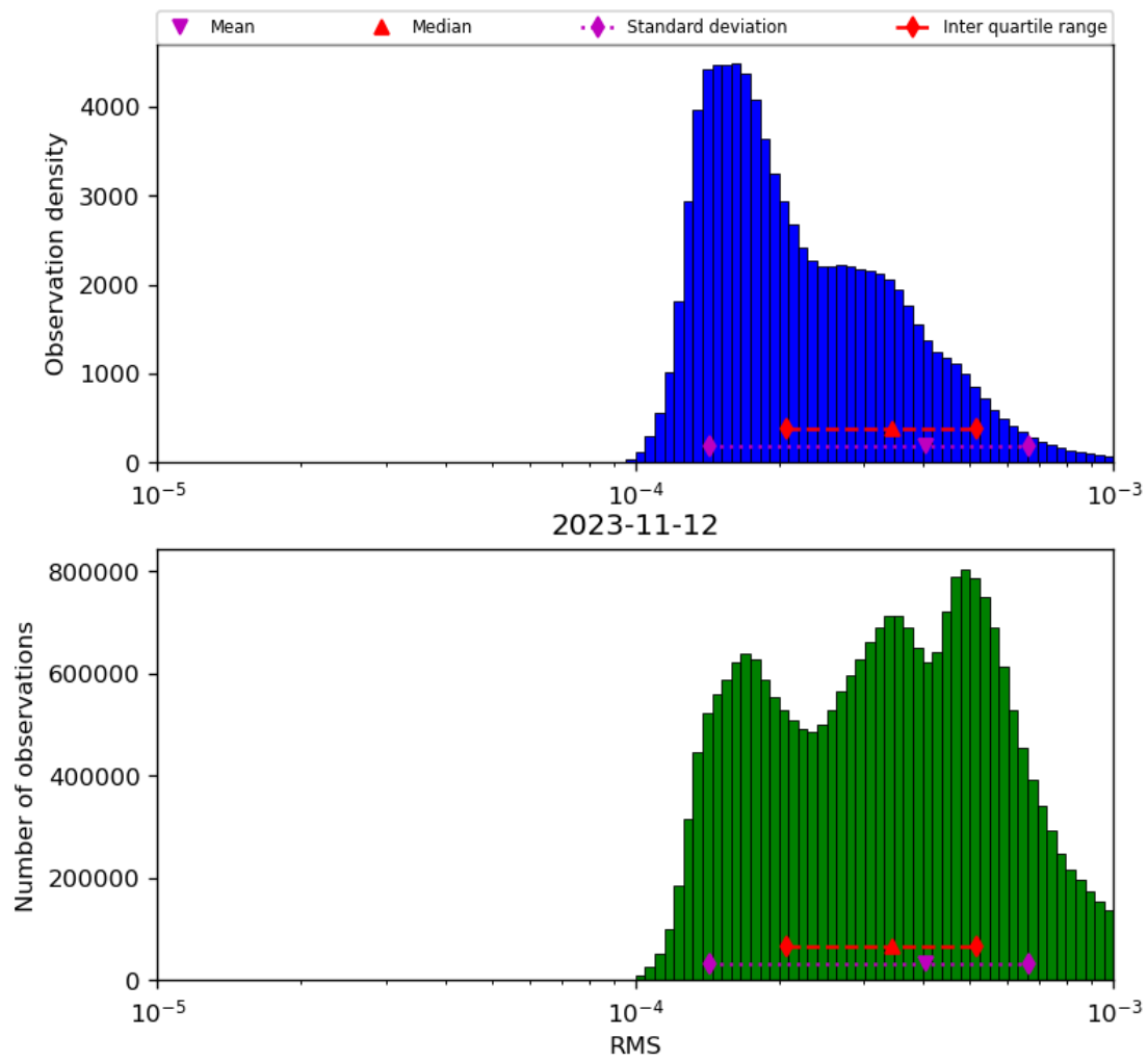
Figure 43: Histogram of “RMS” for 2023-11-12 to 2023-11-13
