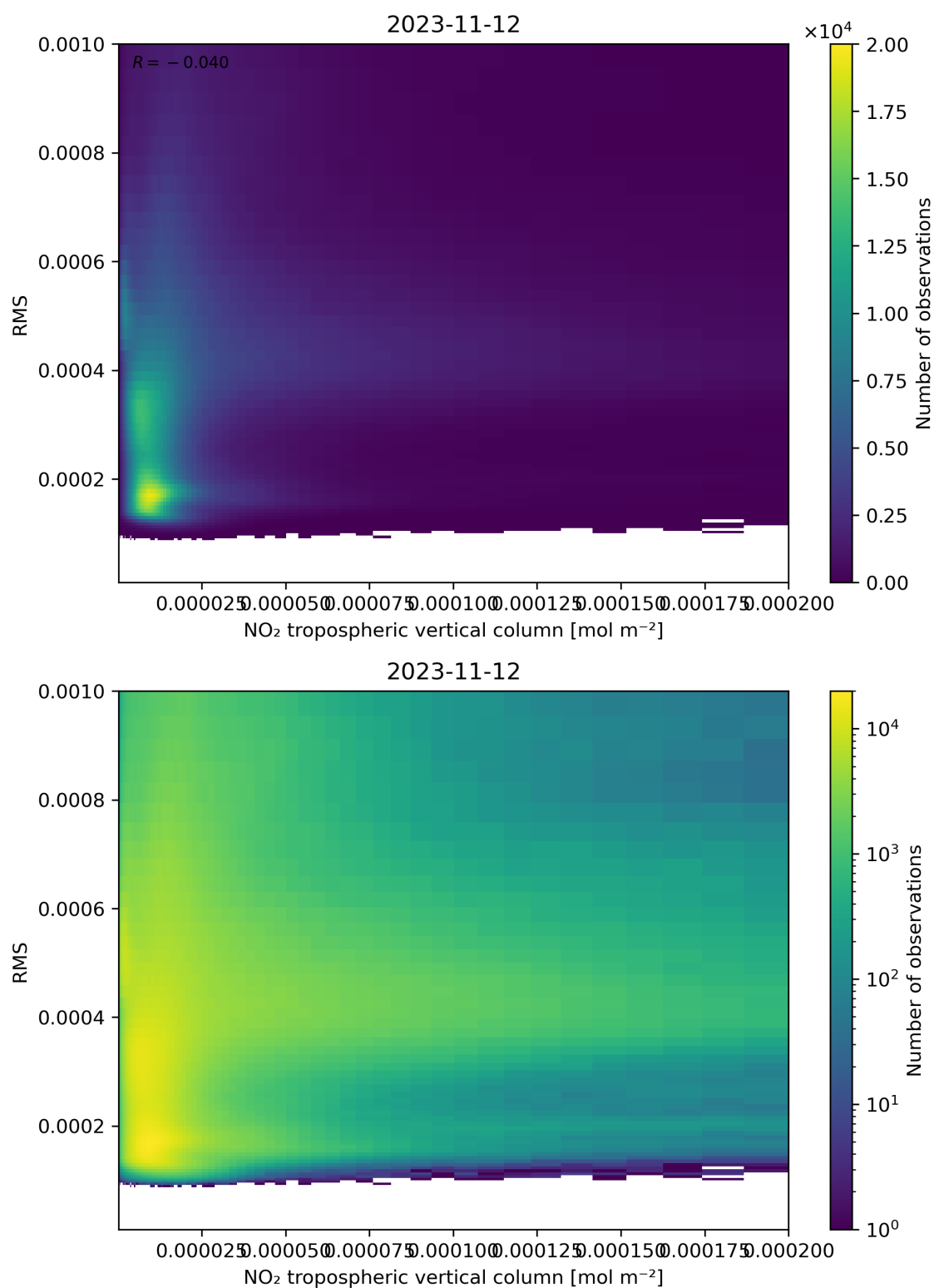
Figure 142: Scatter density plot of “NO 2 tropospheric vertical column” against “RMS” for 2023-11-12 to 2023-11-13.
