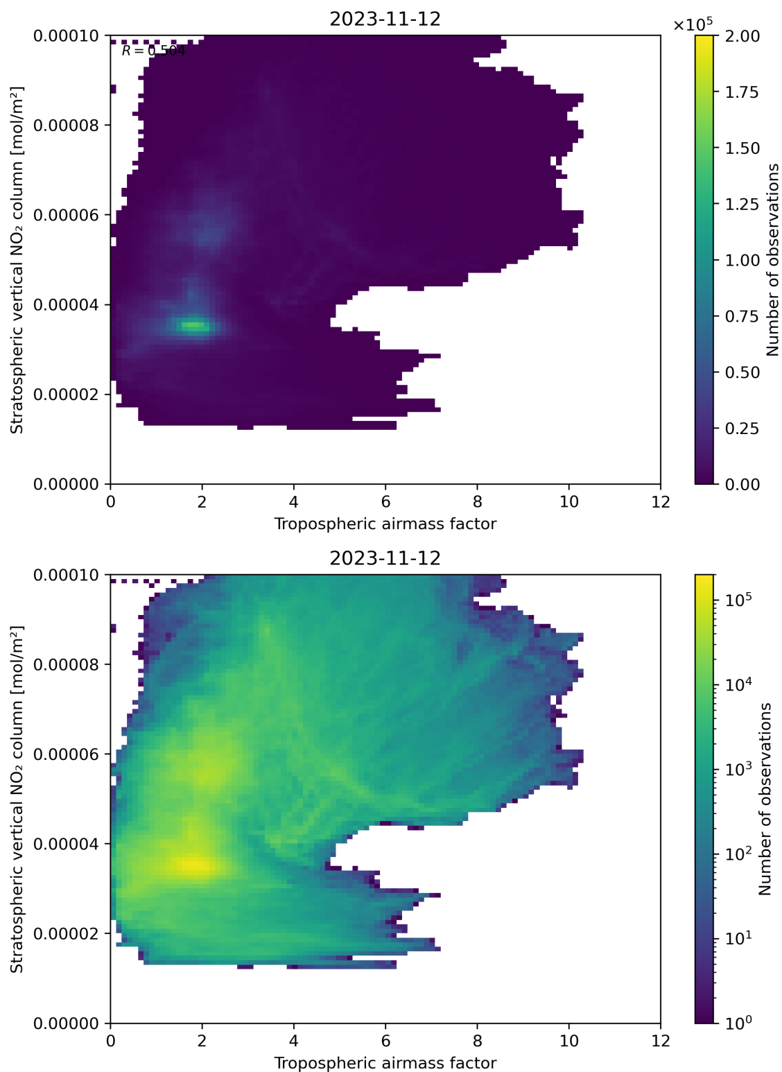
Figure 74: Scatter density plot of “Tropospheric air mass factor” against “Stratospheric vertical NO 2 column” for 2023-11-12 to 2023-11-13.
