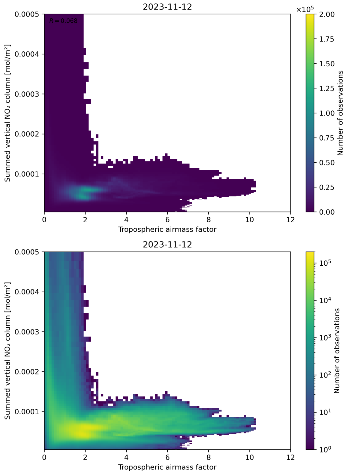
Figure 75: Scatter density plot of “Tropospheric airmass factor” against “Summed vertical NO 2 column” for 2023-11-12 to 2023-11-13.
