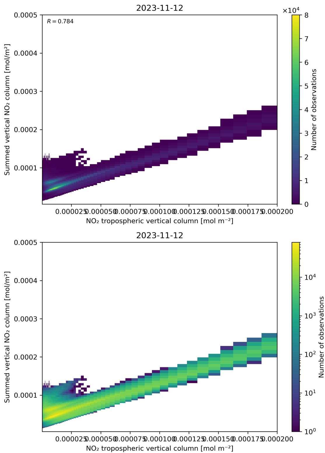
Figure 126: Scatter density plot of “NO 2 tropospheric vertical column” against “Summed vertical NO 2 column” for 2023-11-12 to 2023-11-13.
