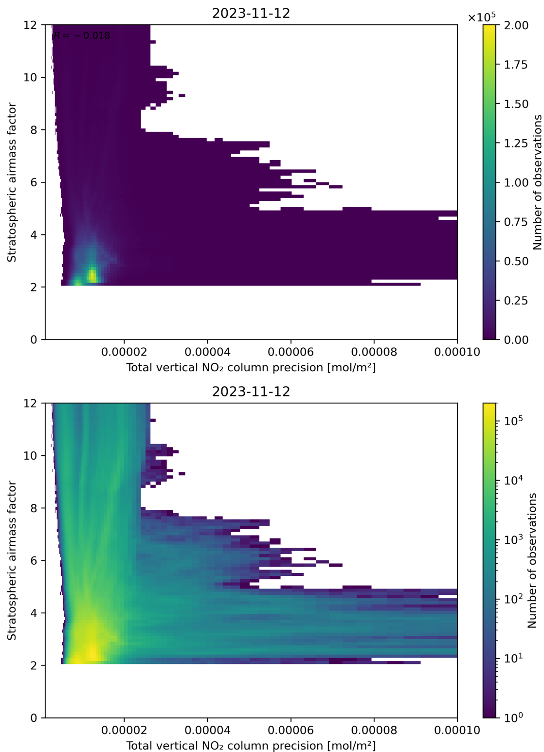
Figure 115: Scatter density plot of “Total vertical NO 2 column precision” against “Stratospheric air mass factor” for 2023-11-12 to 2023-11-13.
