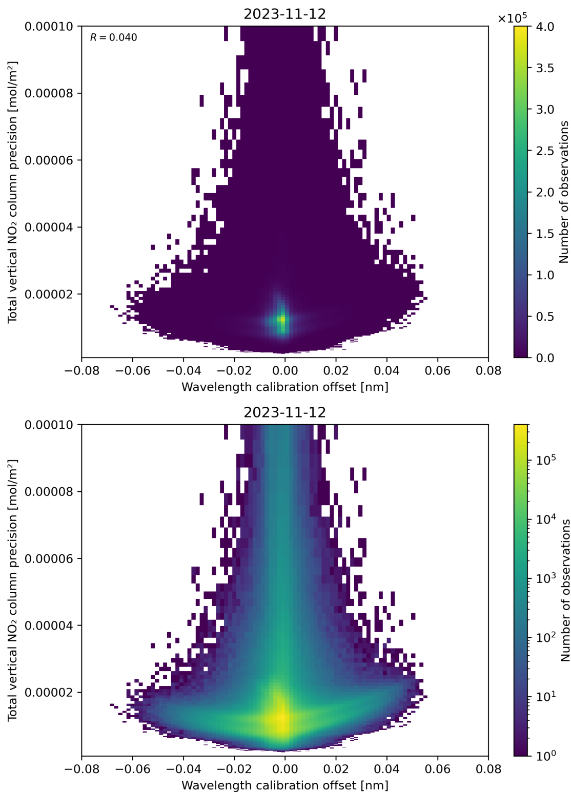
Figure 180: Scatter density plot of “Wavelength calibration offset” against “Total vertical NO 2 column precision” for 2023-11-12 to 2023-11-13.
