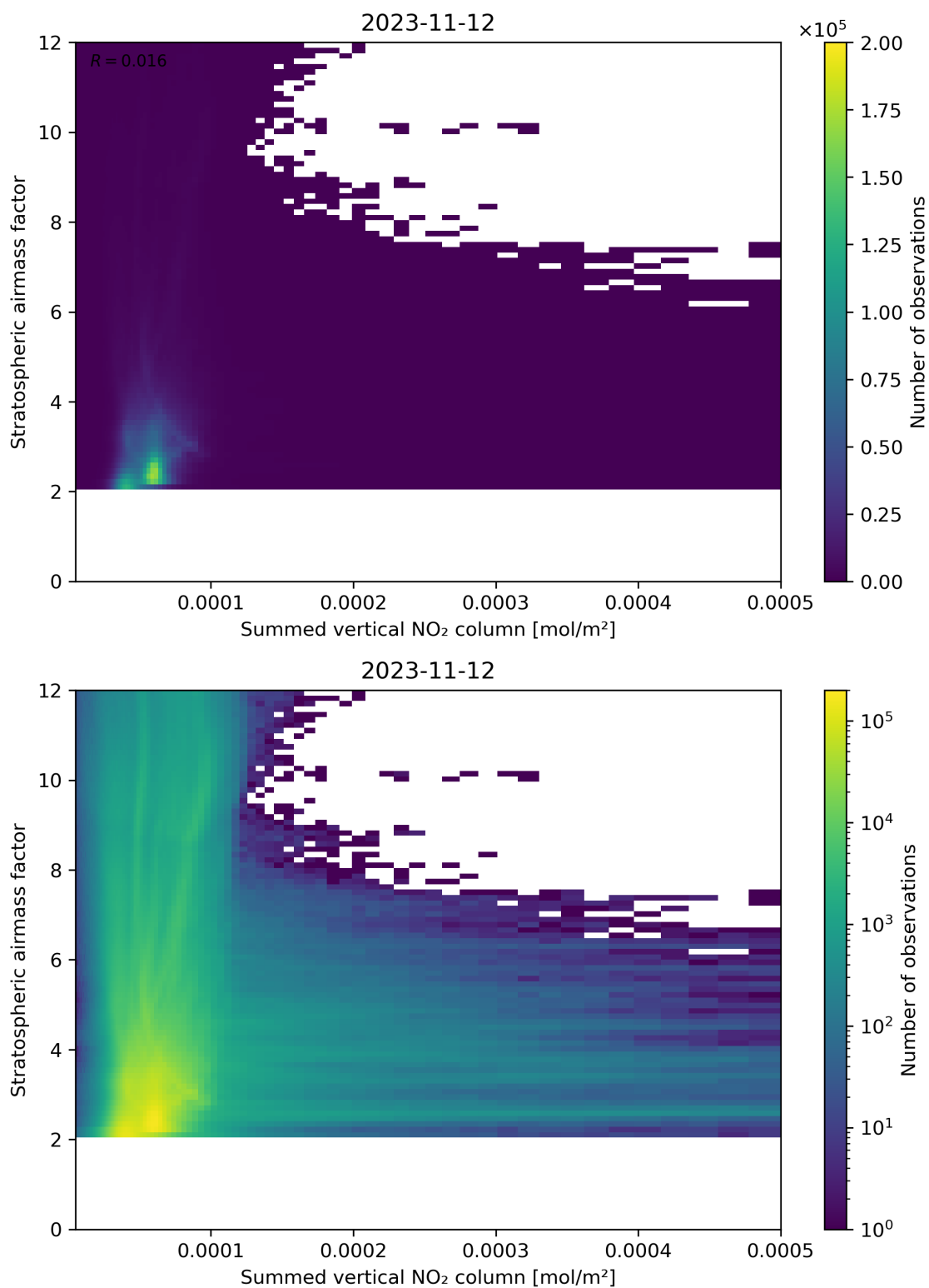
Figure 103: Scatter density plot of “Summed vertical NO 2 column” against “Stratospheric air mass factor” for 2023-11-12 to 2023-11-13.
