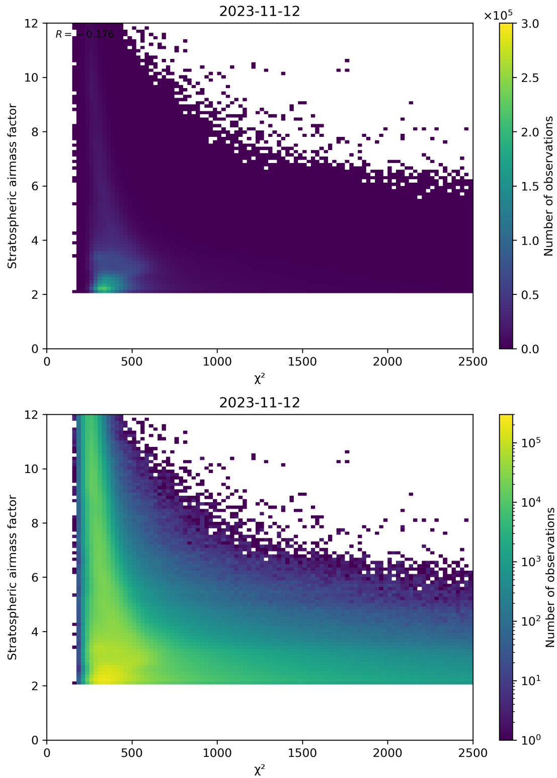
Figure 81: Scatter density plot of " \chi^2 " against "Stratospheric airmass factor" for 2023-11-12 to 2023-11-13.
