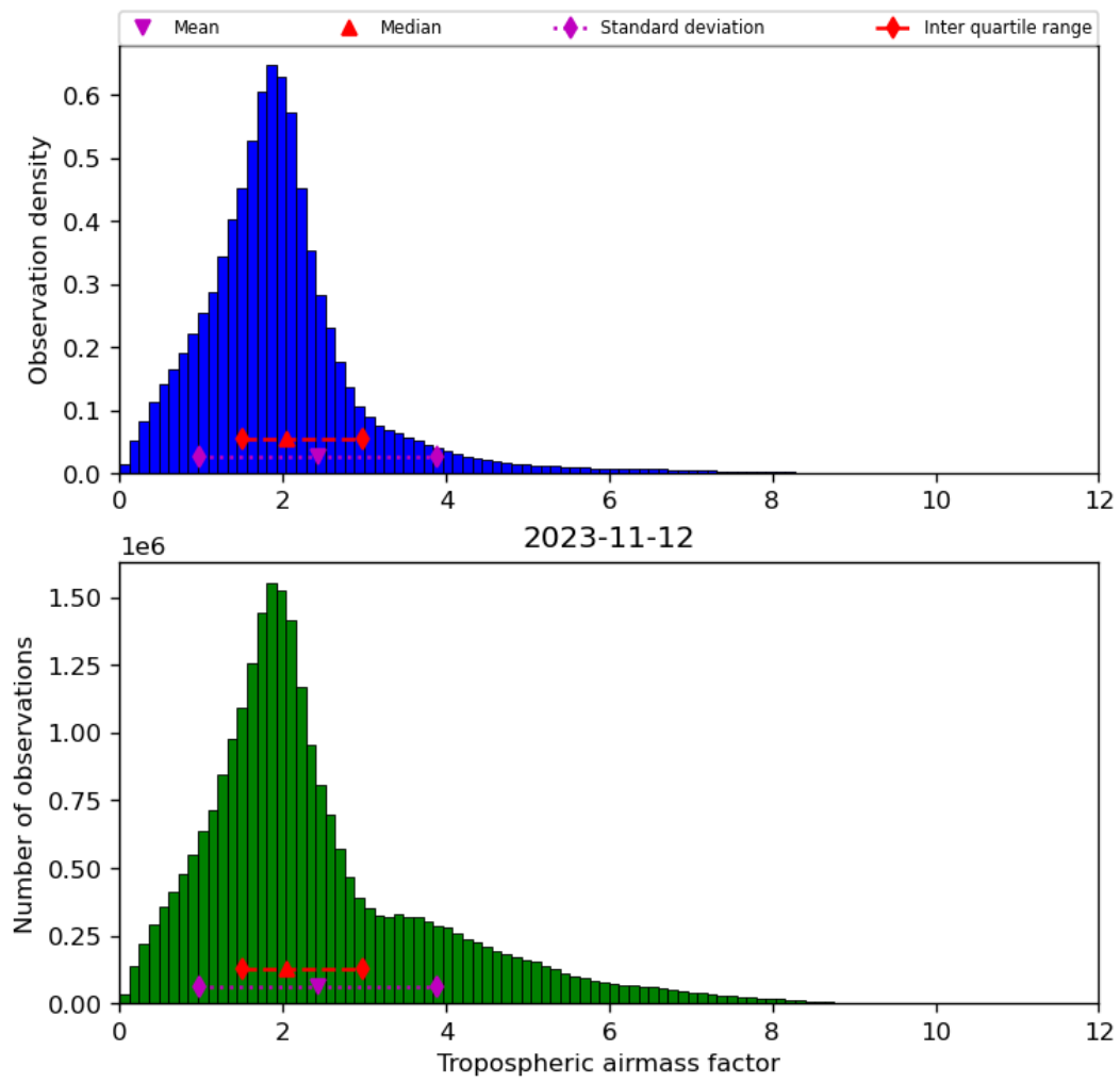
Figure 31: Histogram of “Tropospheric airmass factor” for 2023-11-12 to 2023-11-13
