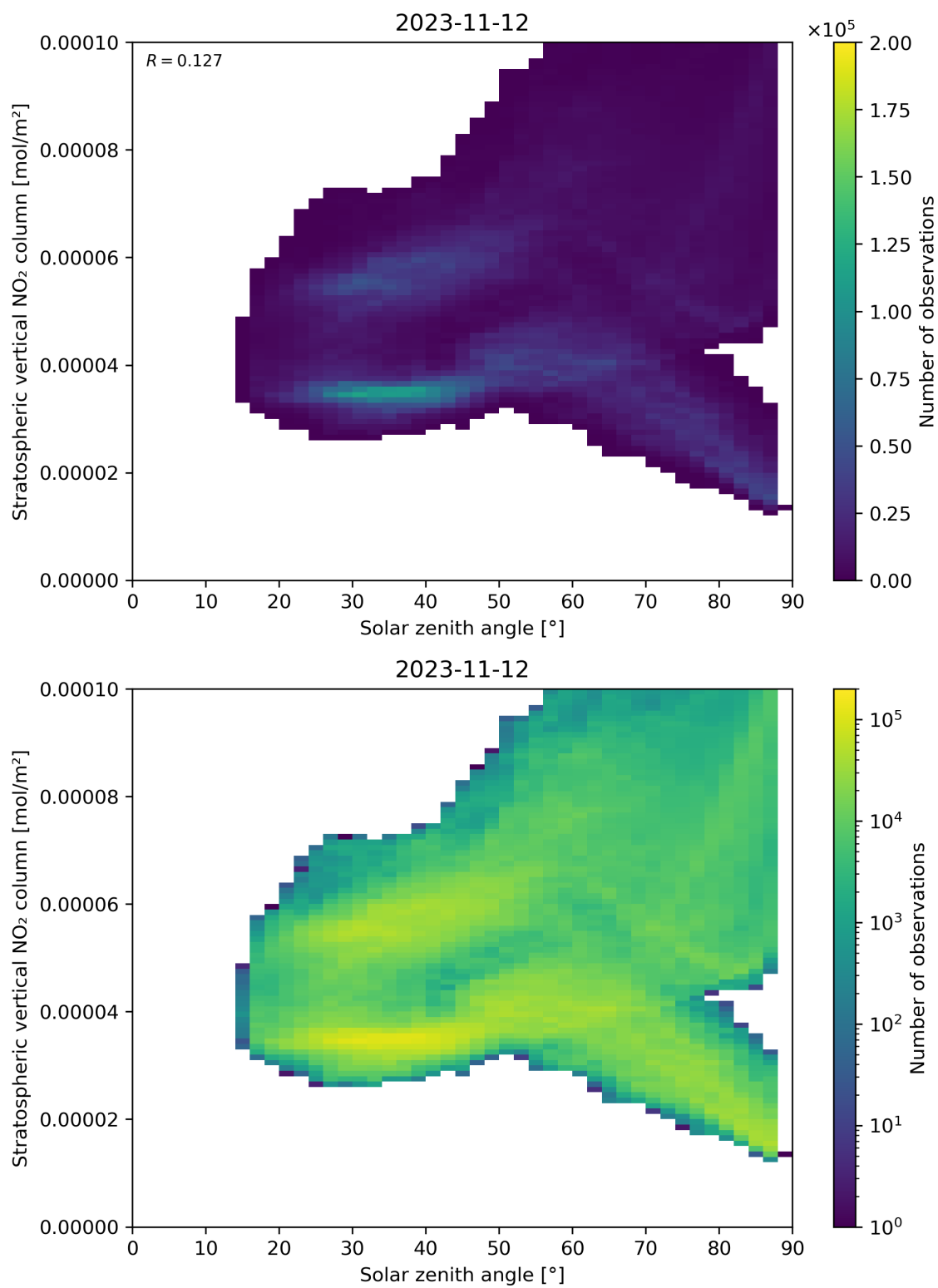
Figure 150: Scatter density plot of “Solar zenith angle” against “Stratospheric vertical NO 2 column” for 2023-11-12 to 2023-11-13.
