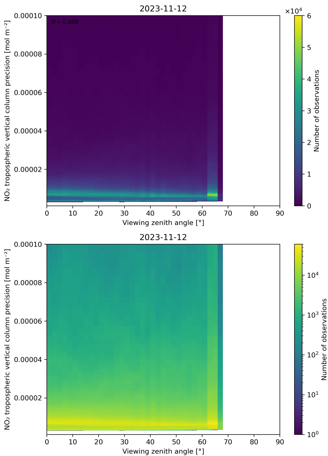
Figure 170: Scatter density plot of “Viewing zenith angle” against “NO 2 tropospheric vertical column precision” for 2023-11-12 to 2023-11-13.
