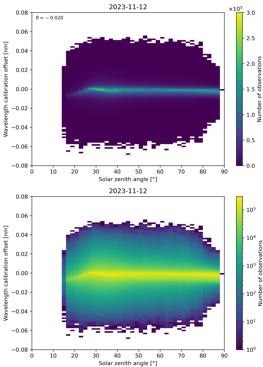
Figure 158: Scatter density plot of “Solar zenith angle” against “Wavelength calibration offset” for 2023-11-12 to 2023-11-13.
