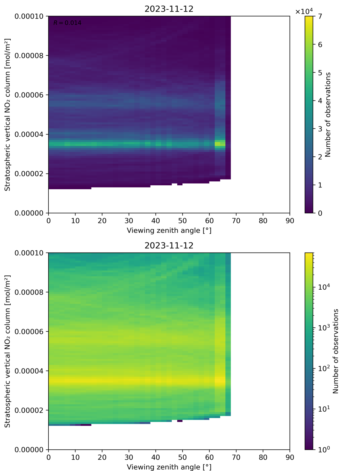
Figure 164: Scatter density plot of “Viewing zenith angle” against “Stratospheric vertical NO 2 column” for 2023-11-12 to 2023-11-13.
