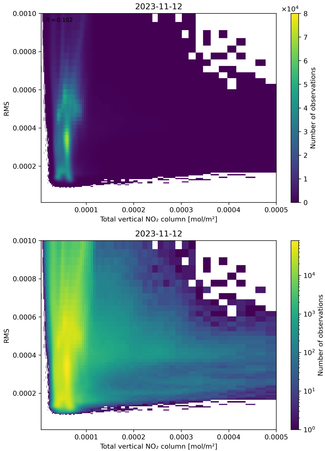
Figure 120: Scatter density plot of “Total vertical NO 2 column” against “RMS” for 2023-11-12 to 2023-11-13.
