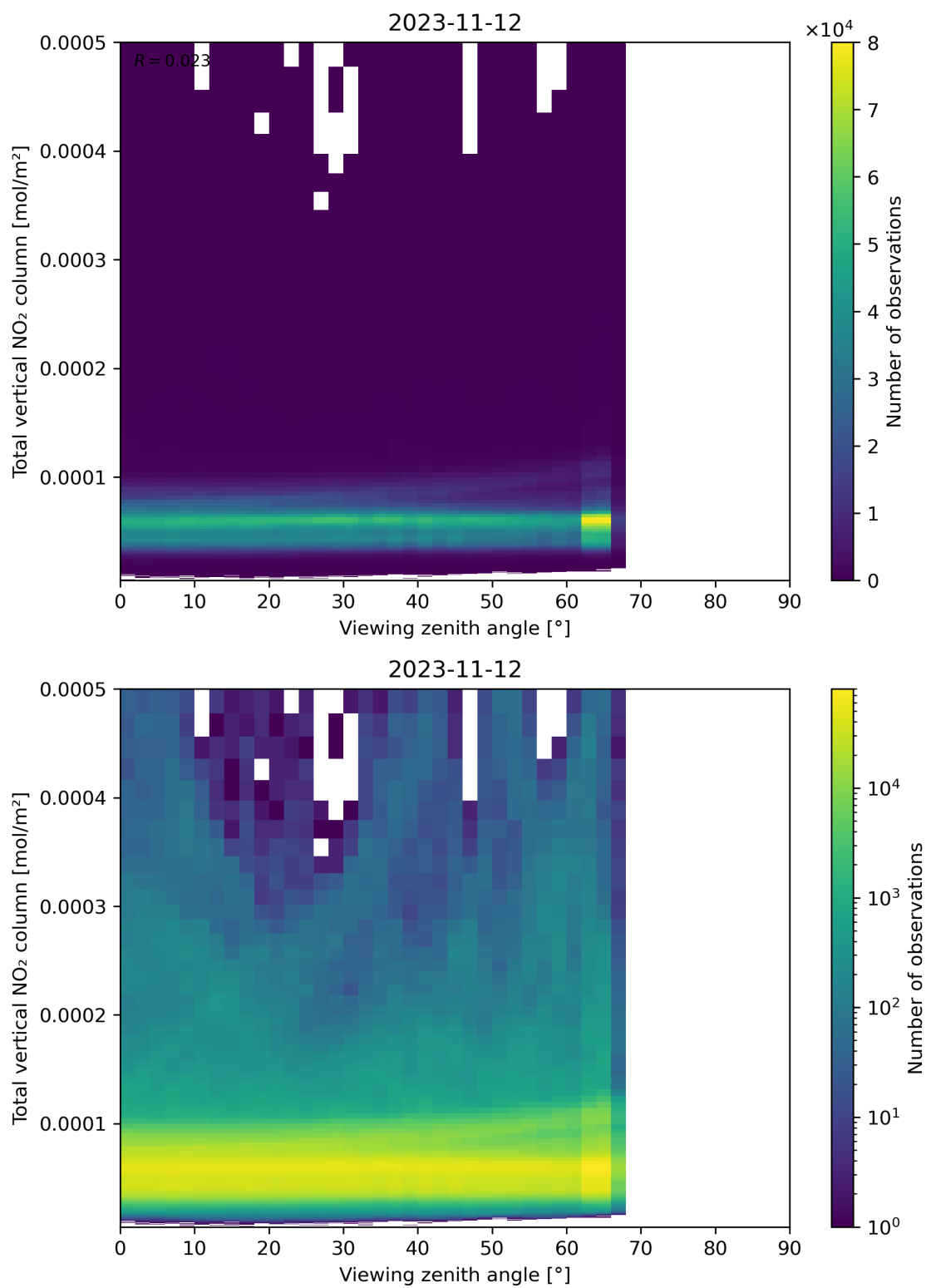
Figure 167: Scatter density plot of “Viewing zenith angle” against “Total vertical NO 2 column” for 2023-11-12 to 2023-11-13.
