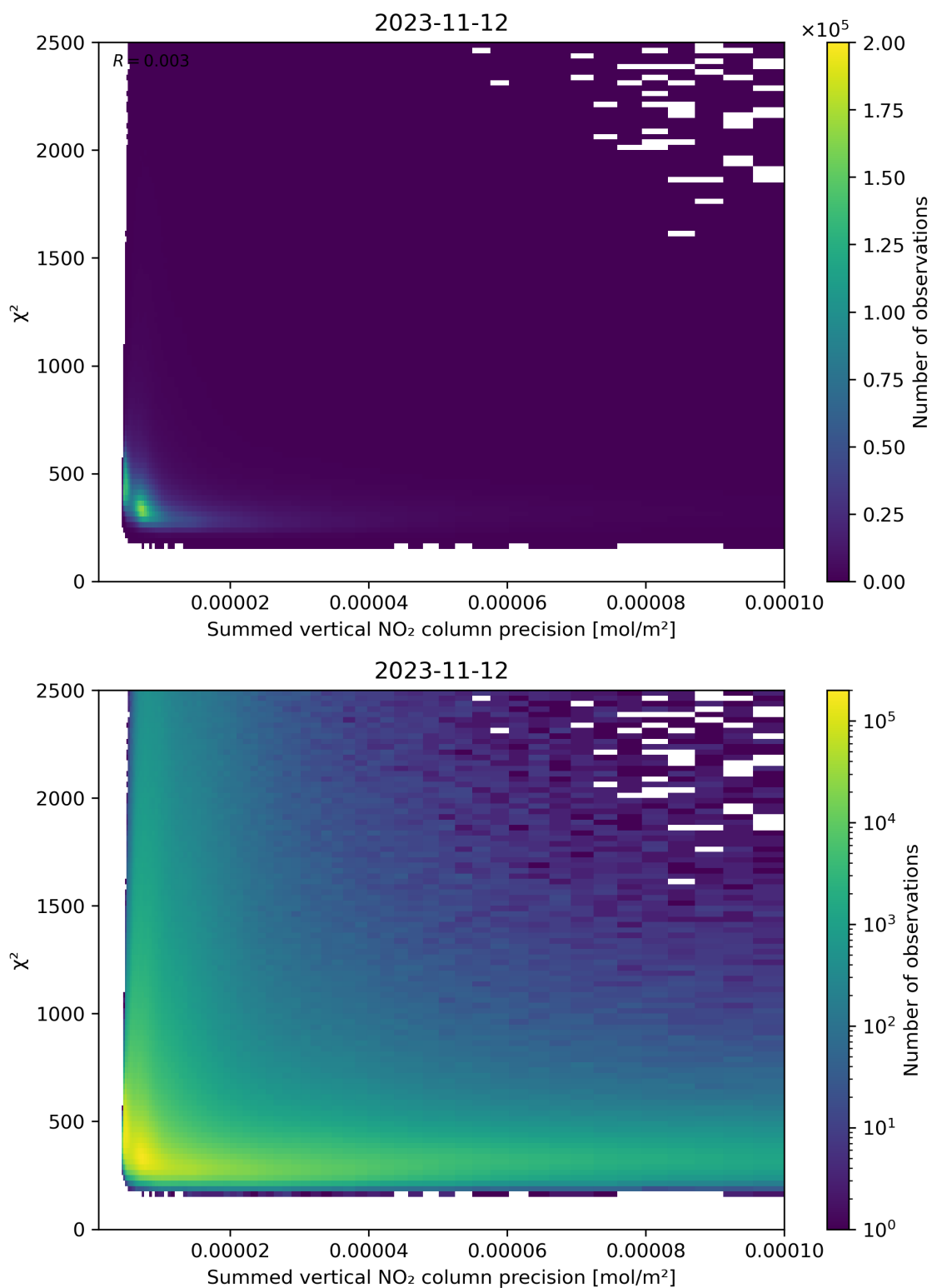
Figure 107: Scatter density plot of “Summed vertical NO 2 column precision” against “ \chi^2 ” for 2023-11-12 to 2023-11-13.
