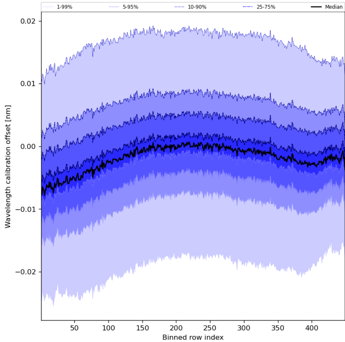
Figure 52: Along track statistics of “Wavelength calibration offset” for 2023-11-12 to 2023-11-13
