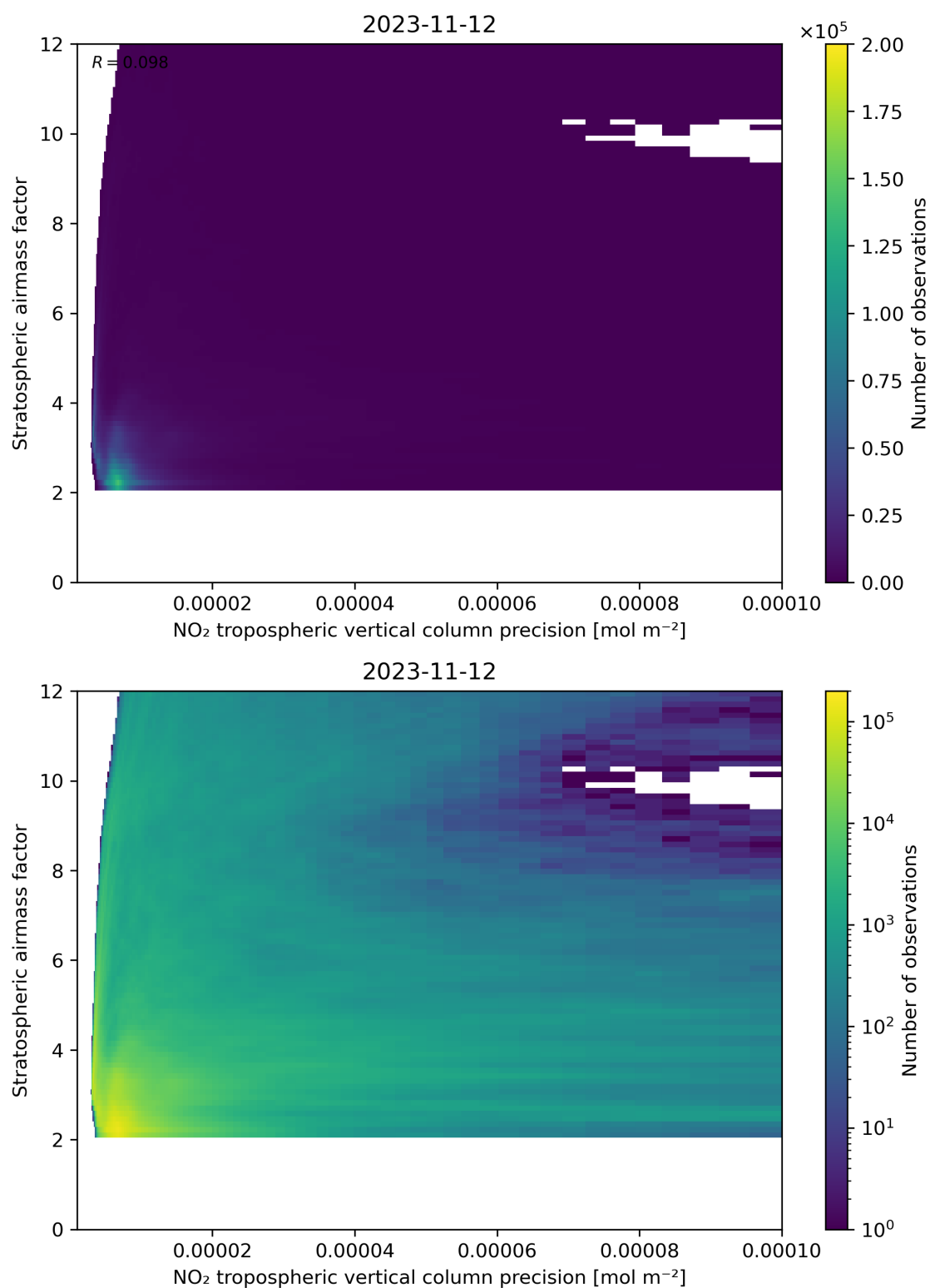
Figure 131: Scatter density plot of “NO 2 tropospheric vertical column precision” against “Stratospheric airmass factor” for 2023-11-12 to 2023-11-13.
