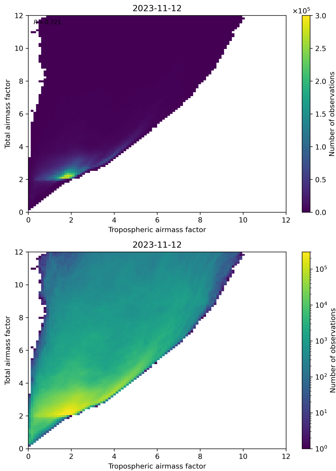
Figure 72: Scatter density plot of “Tropospheric airmass factor” against “Total airmass factor” for 2023-11-12 to 2023-11-13.
