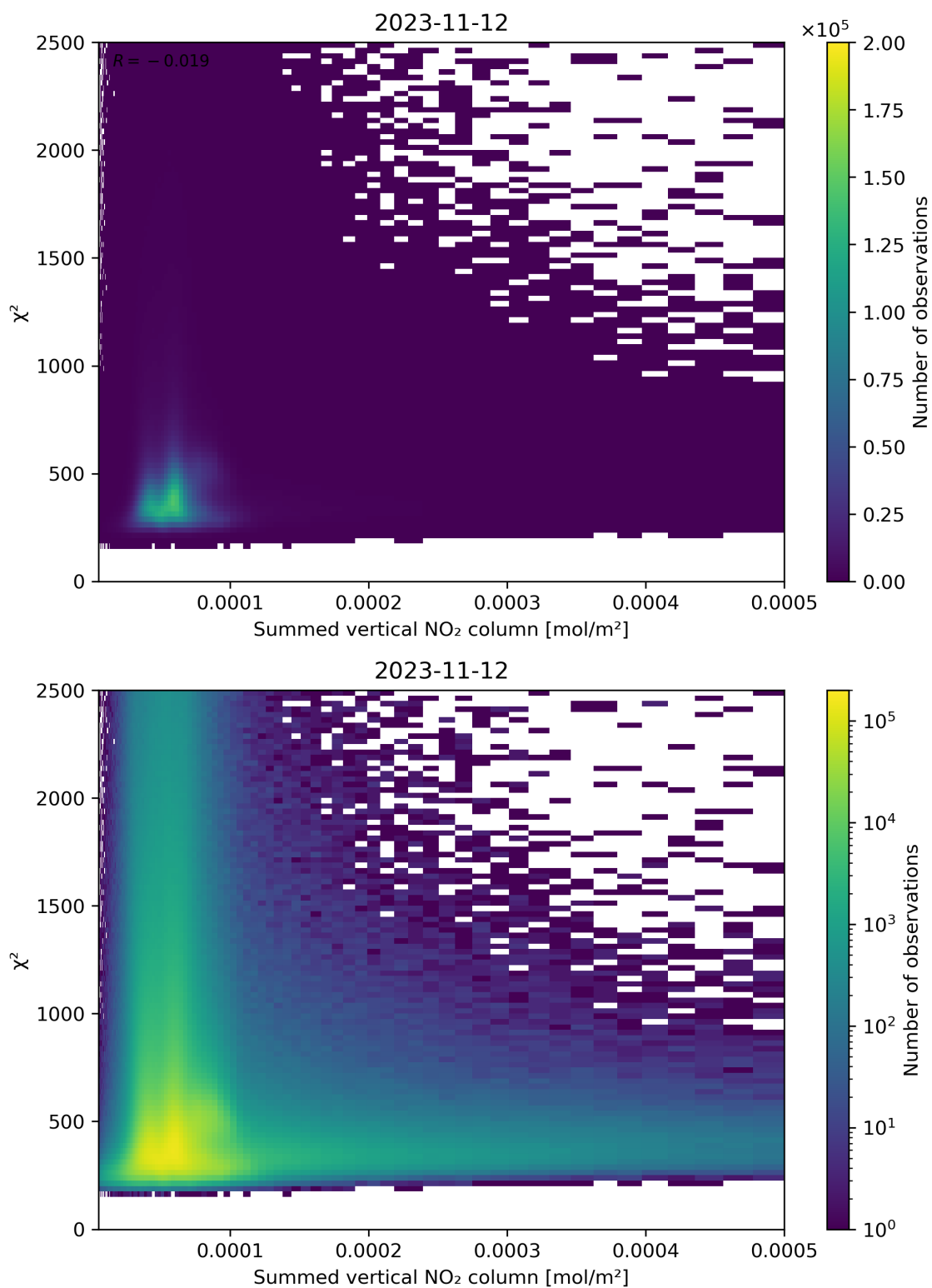
Figure 104: Scatter density plot of “Summed vertical NO 2 column” against “ \chi^2 ” for 2023-11-12 to 2023-11-13.
