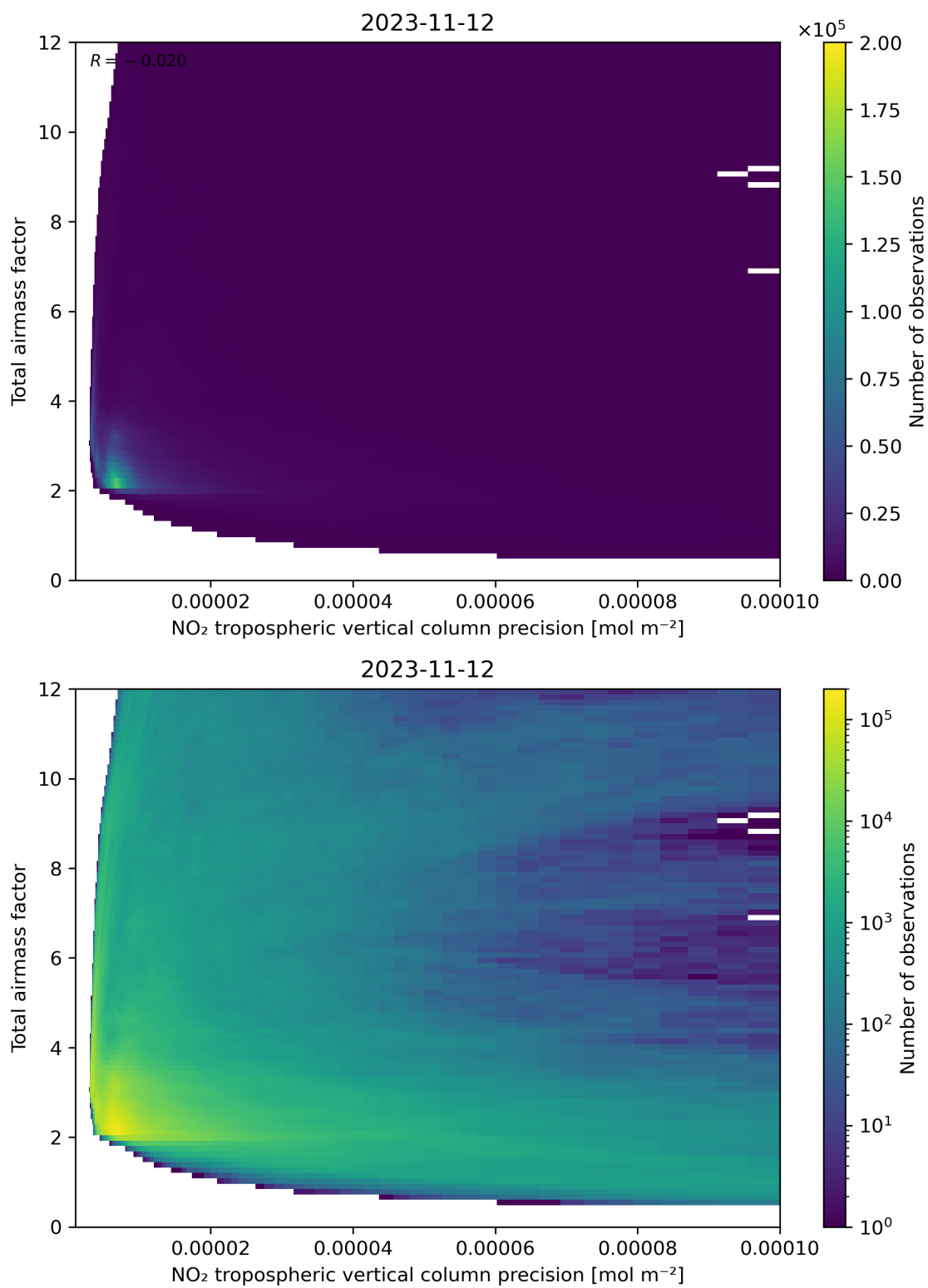
Figure 132: Scatter density plot of “NO 2 tropospheric vertical column precision” against “Total air mass factor” for 2023-11-12 to 2023-11-13.
