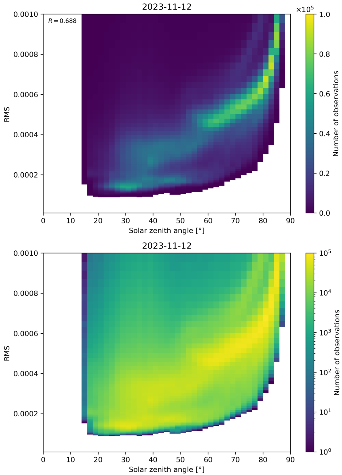
Figure 157: Scatter density plot of “Solar zenith angle” against “RMS” for 2023-11-12 to 2023-11-13.
