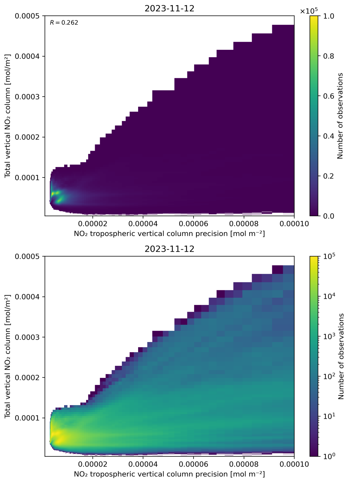
Figure 138: Scatter density plot of “NO 2 tropospheric vertical column precision” against “Total vertical NO 2 column” for 2023-11-12 to 2023-11-13.
