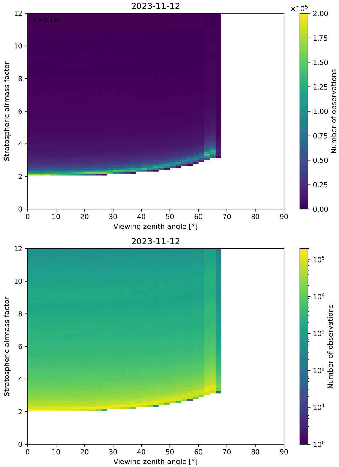
Figure 159: Scatter density plot of “Viewing zenith angle” against “Stratospheric airmass factor” for 2023-11-12 to 2023-11-13.
