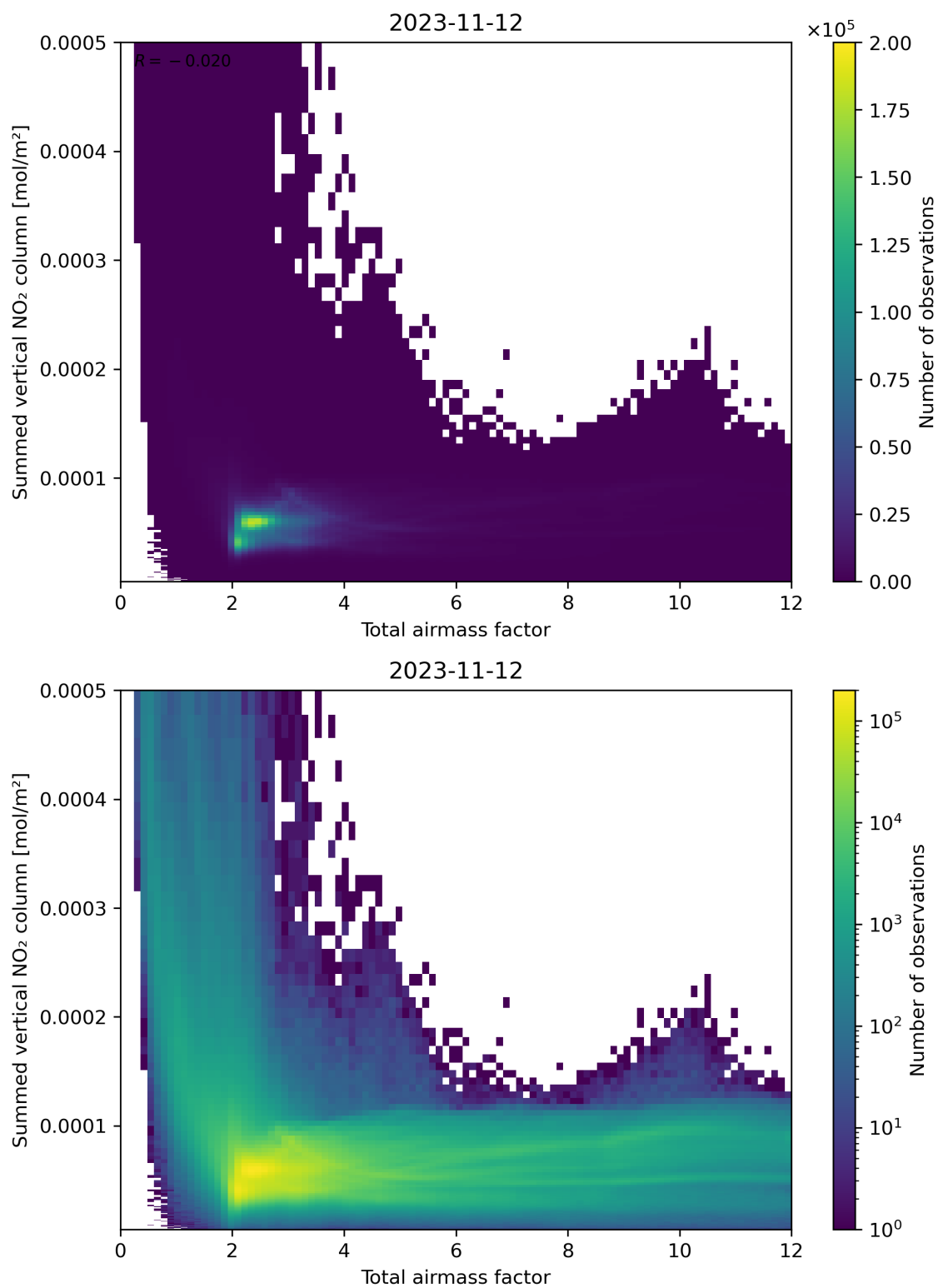
Figure 65: Scatter density plot of “Total airmass factor” against “Summed vertical NO 2 column” for 2023-11-12 to 2023-11-13.
