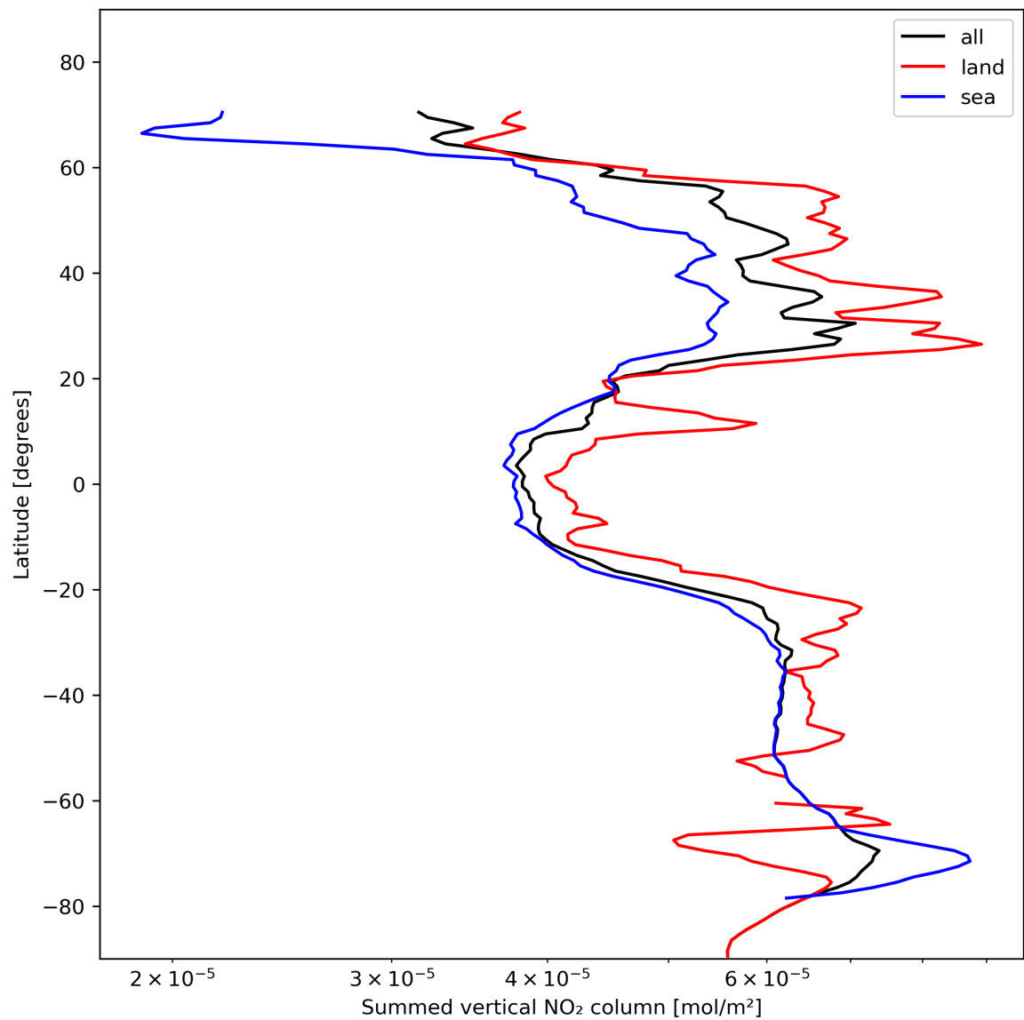
Figure 23: Zonal average of “Summed vertical NO 2 column” for 2023-11-12 to 2023-11-13.
