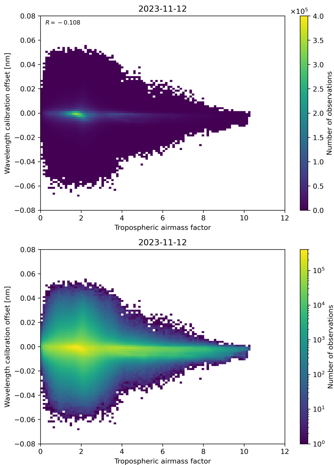
Figure 80: Scatter density plot of “Tropospheric air mass factor” against “Wavelength calibration offset” for 2023-11-12 to 2023-11-13.
