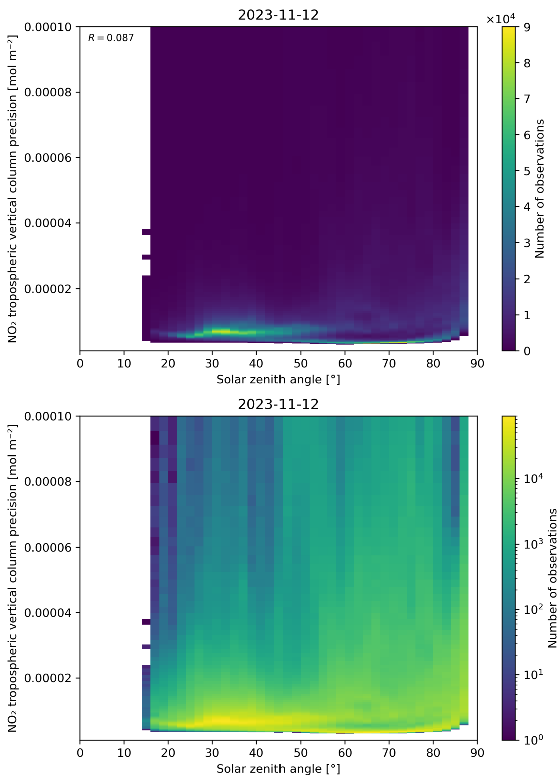
Figure 156: Scatter density plot of “Solar zenith angle” against “NO 2 tropospheric vertical column precision” for 2023-11-12 to 2023-11-13.
