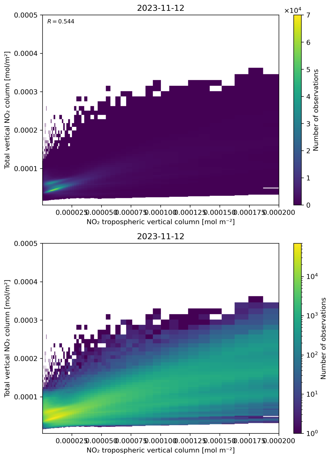
Figure 128: Scatter density plot of “NO 2 tropospheric vertical column” against “Total vertical NO 2 column” for 2023-11-12 to 2023-11-13.
