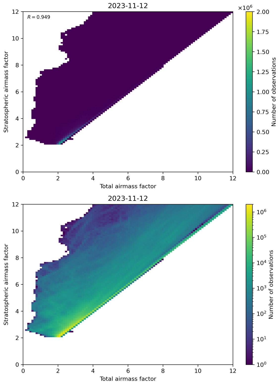
Figure 62: Scatter density plot of “Total air mass factor” against “Stratospheric air mass factor” for 2023-11-12 to 2023-11-13.
