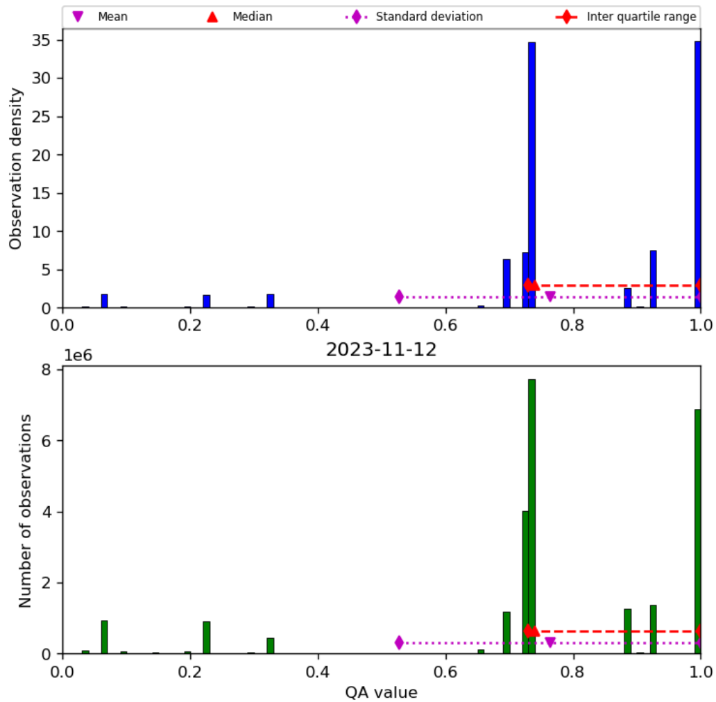
Figure 28: Histogram of “QA value” for 2023-11-12 to 2023-11-13
