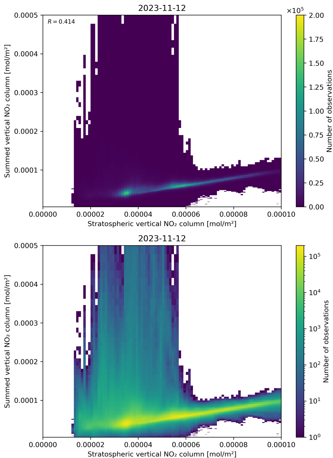
Figure 98: Scatter density plot of “Stratospheric vertical NO 2 column” against “Summed vertical NO 2 column” for 2023-11-12 to 2023-11-13.
