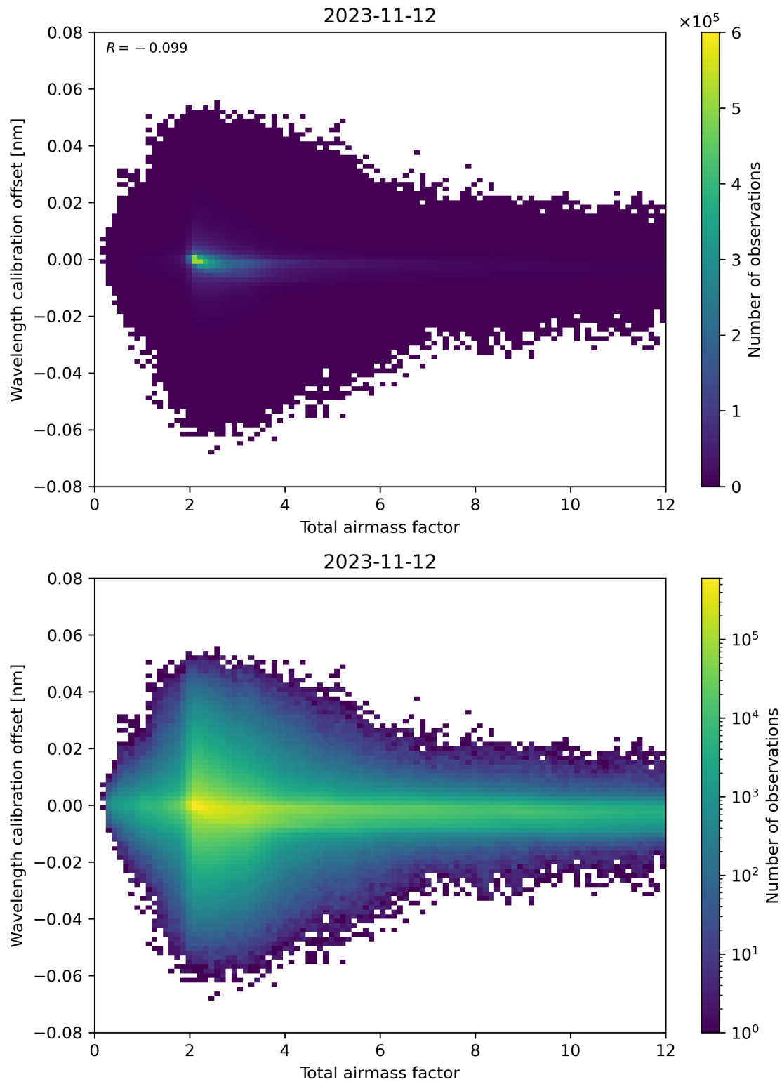
Figure 70: Scatter density plot of “Total airmass factor” against “Wavelength calibration offset” for 2023-11-12 to 2023-11-13.
