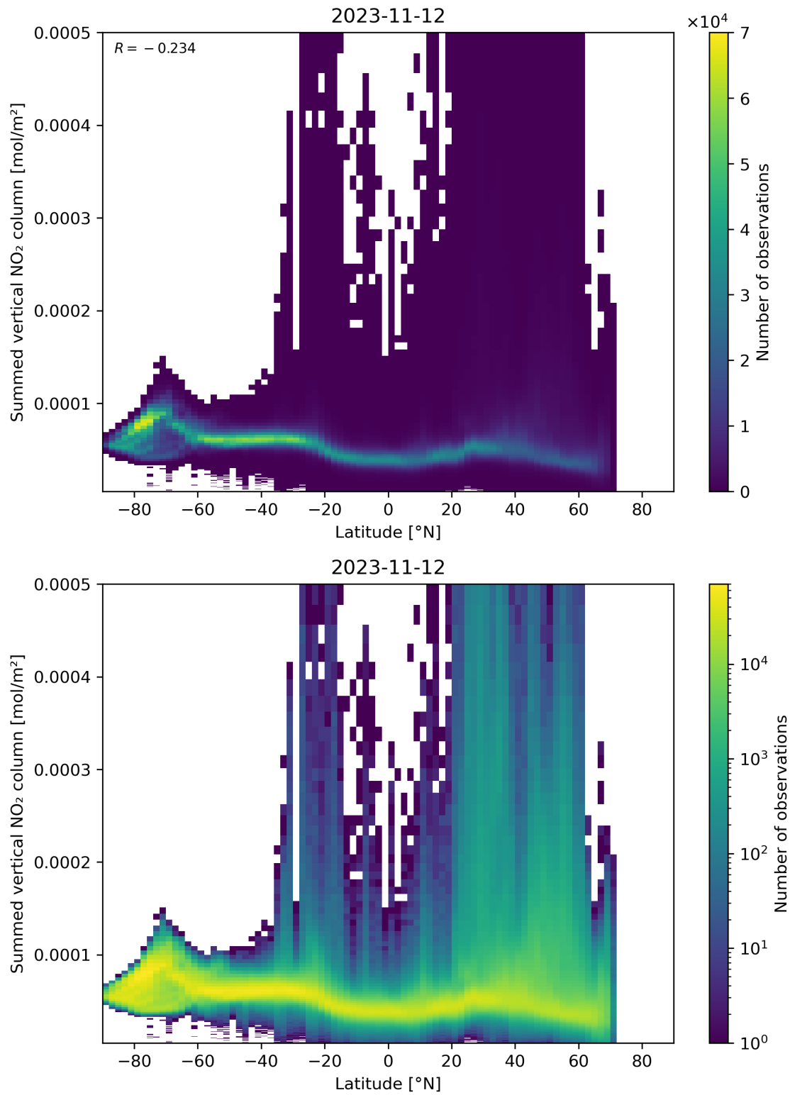
Figure 88: Scatter density plot of “Latitude” against “Summed vertical NO 2 column” for 2023-11-12 to 2023-11-13.
