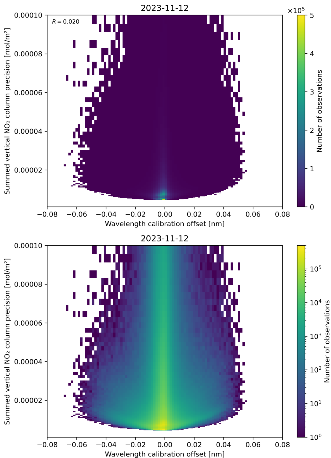
Figure 178: Scatter density plot of “Wavelength calibration offset” against “Summed vertical NO 2 column precision” for 2023-11-12 to 2023-11-13.
