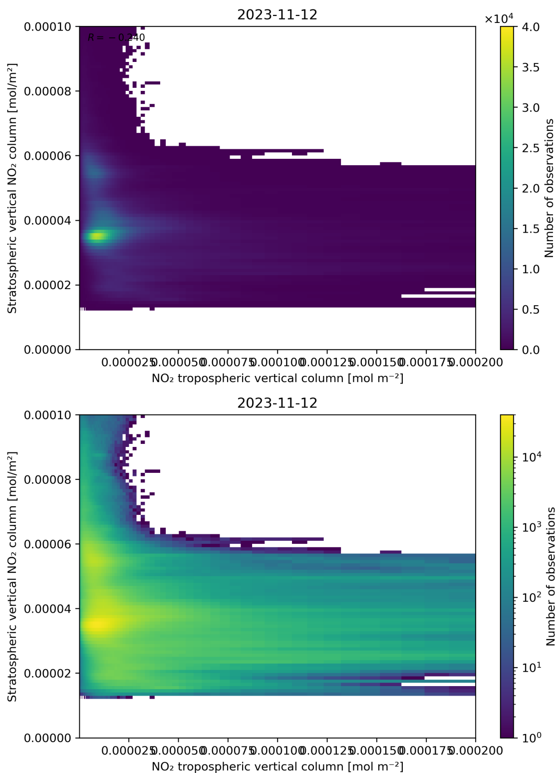
Figure 125: Scatter density plot of “NO 2 tropospheric vertical column” against “Stratospheric vertical NO 2 column” for 2023-11-12 to 2023-11-13.
