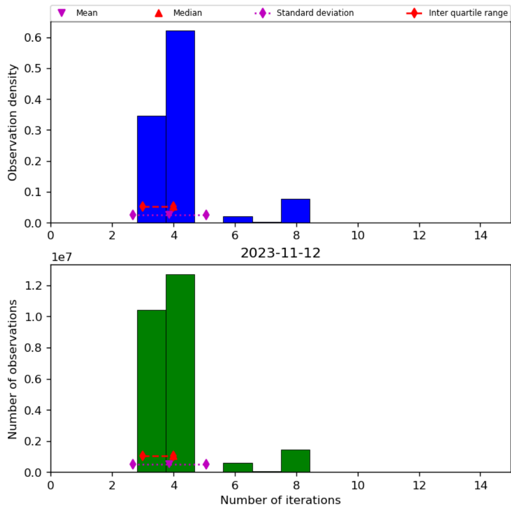
Figure 34: Histogram of “Number of iterations” for 2023-11-12 to 2023-11-13
