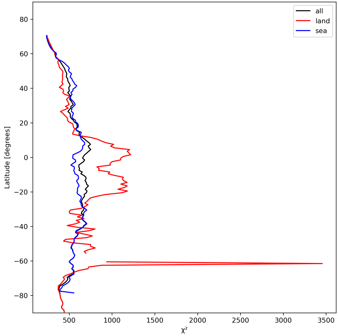
Figure 25: Zonal average of “ \chi^2 ” for 2023-11-12 to 2023-11-13.
