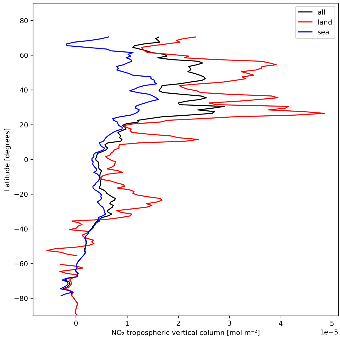
Figure 12: Zonal average of “NO 2 tropospheric vertical column” for 2023-11-12 to 2023-11-13.
