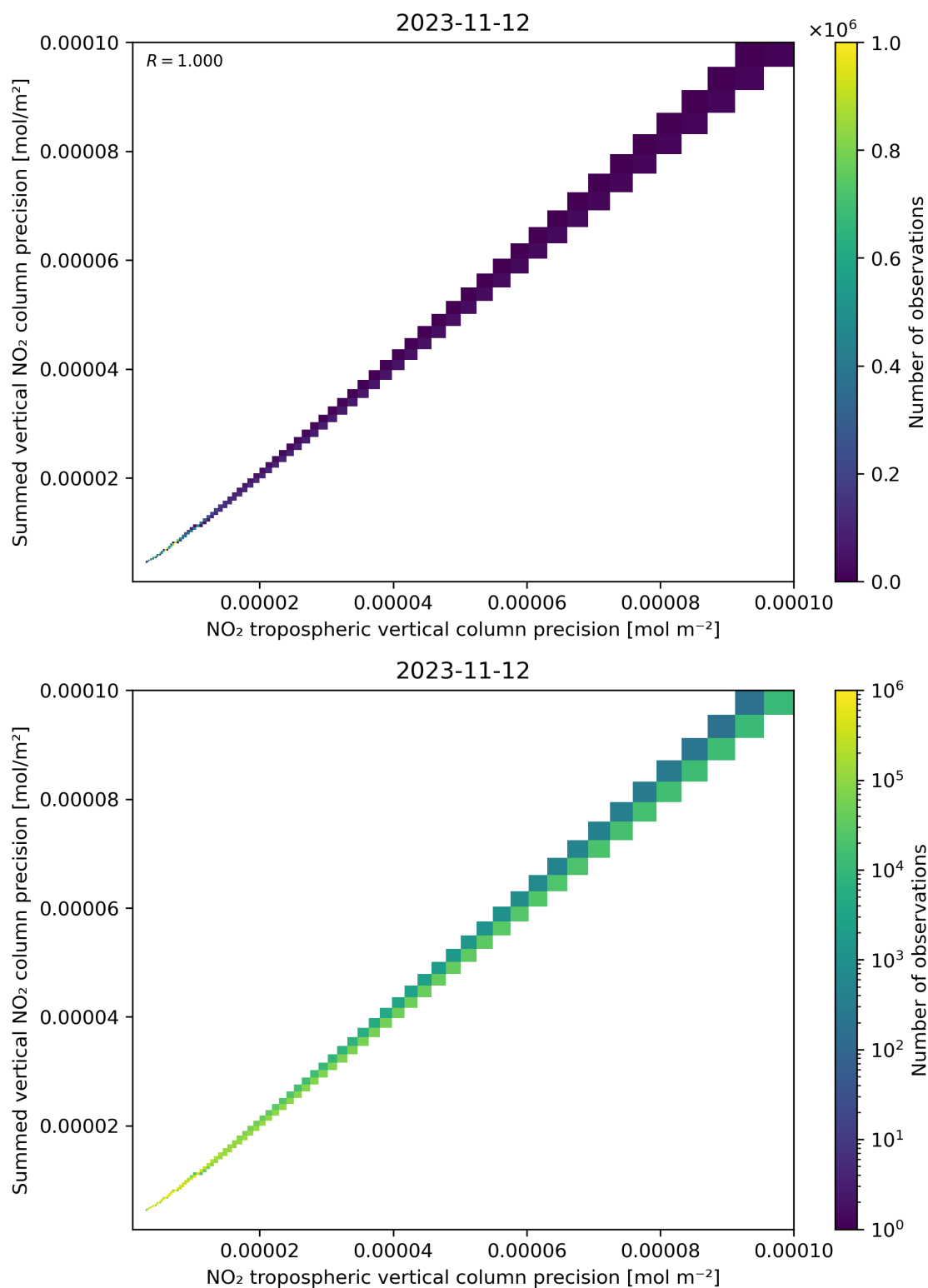
Figure 137: Scatter density plot of “NO 2 tropospheric vertical column precision” against “Summed vertical NO 2 column precision” for 2023-11-12 to 2023-11-13.
