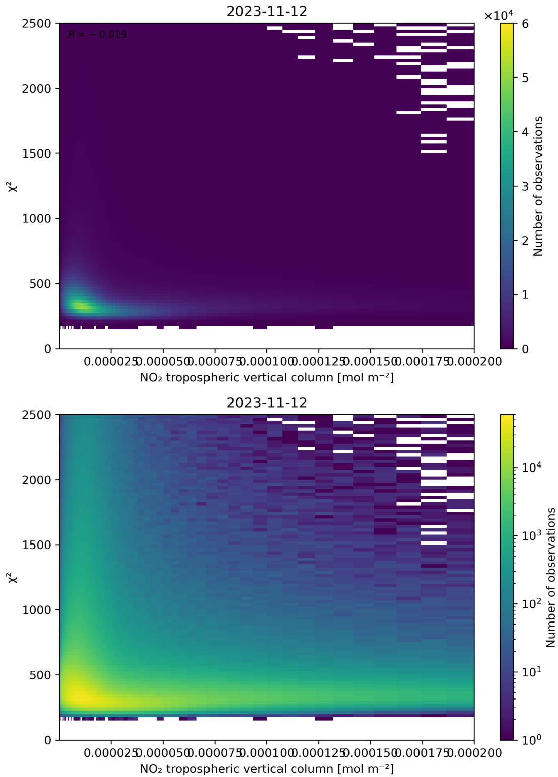
Figure 124: Scatter density plot of “NO 2 tropospheric vertical column” against “ \chi^2 ” for 2023-11-12 to 2023-11-13.
