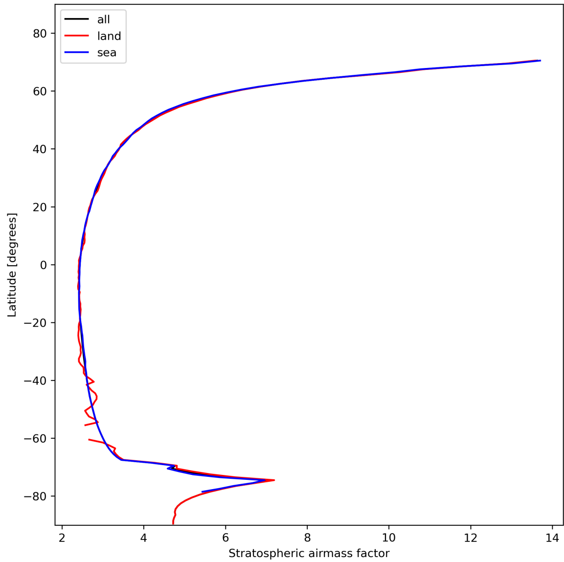
Figure 27: Zonal average of “Stratospheric air mass factor” for 2023-11-12 to 2023-11-13.
