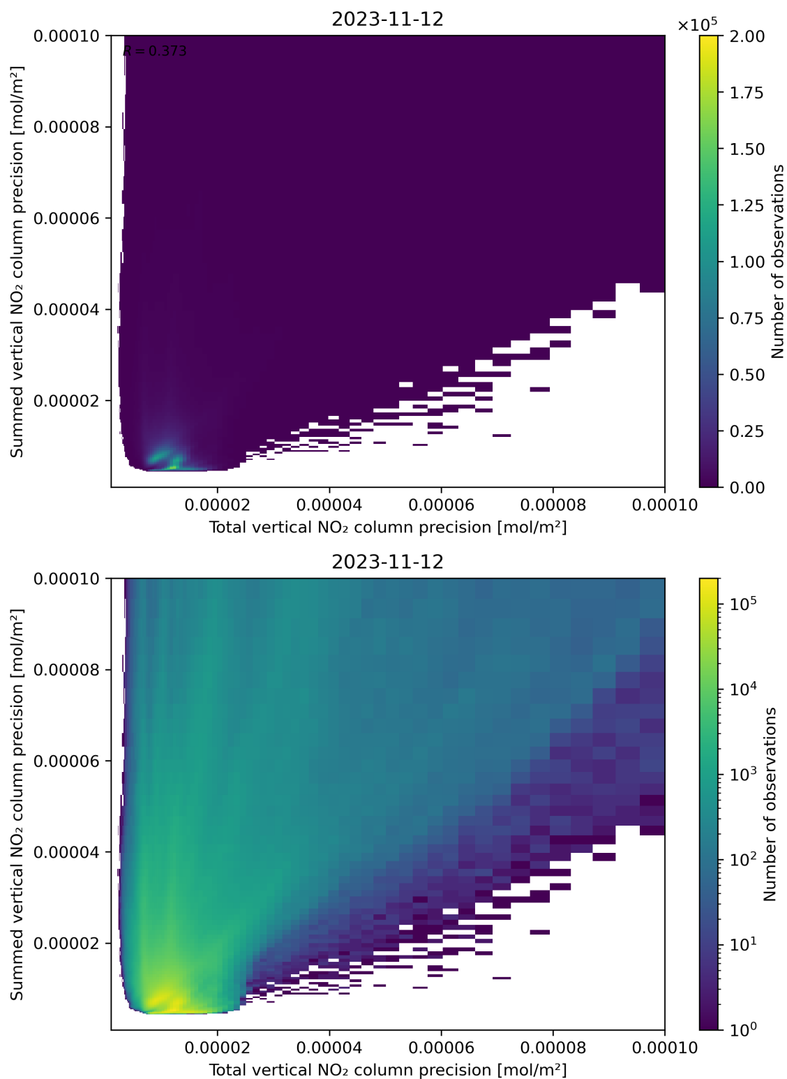
Figure 118: Scatter density plot of “Total vertical NO 2 column precision” against “Summed vertical NO 2 column precision” for 2023-11-12 to 2023-11-13.
