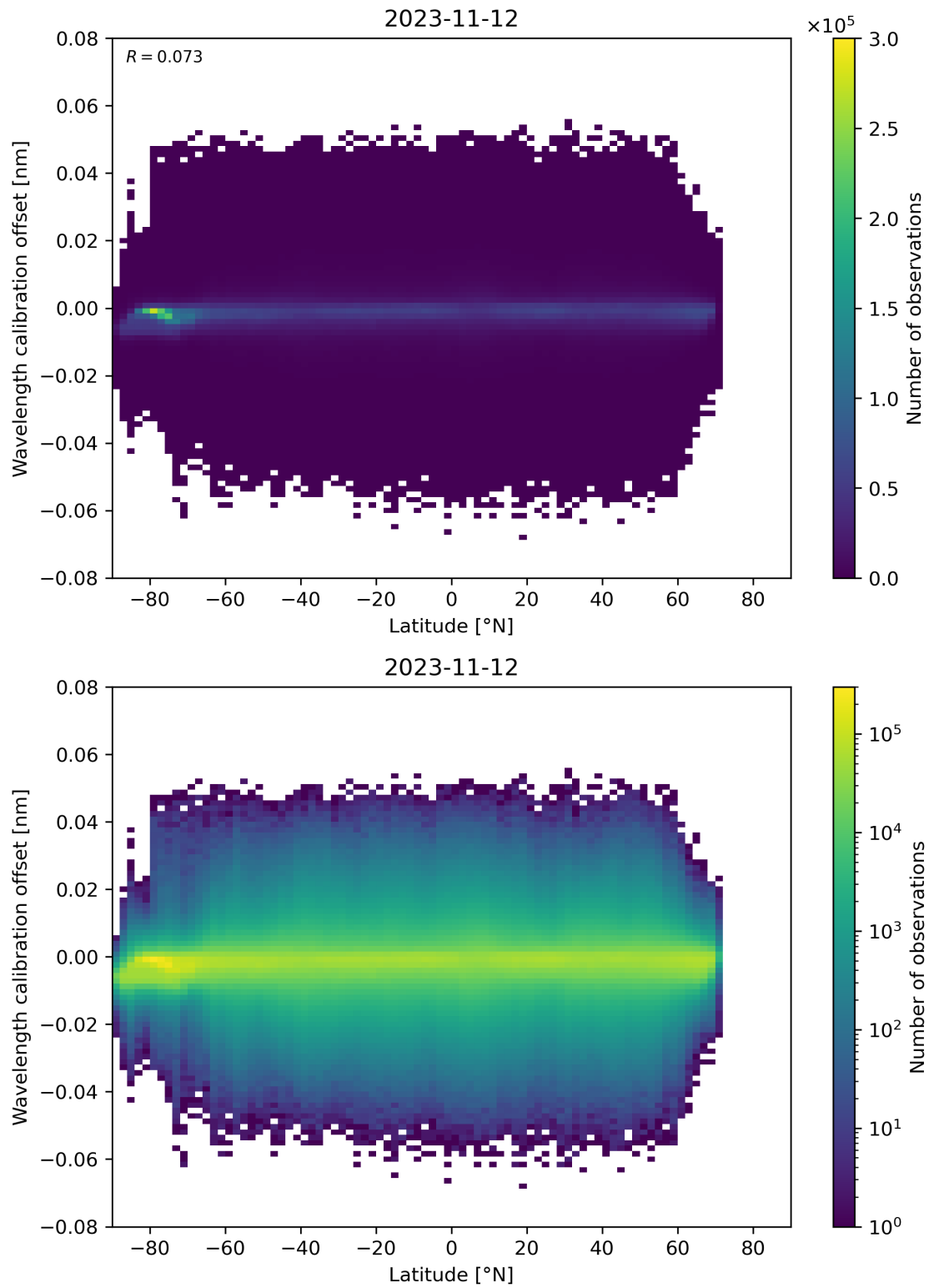
Figure 95: Scatter density plot of “Latitude” against “Wavelength calibration offset” for 2023-11-12 to 2023-11-13.
