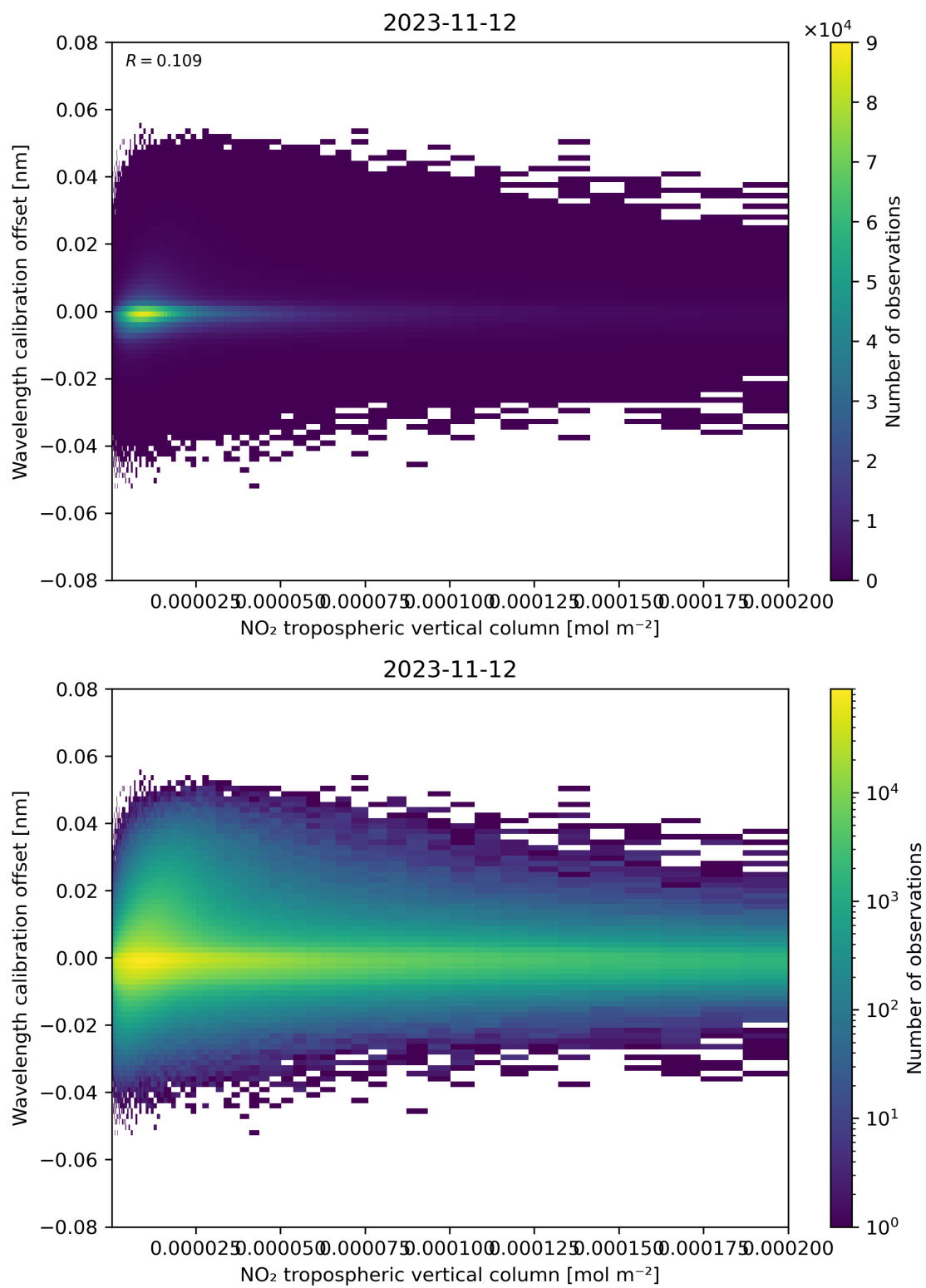
Figure 143: Scatter density plot of “NO 2 tropospheric vertical column” against “Wavelength calibration offset” for 2023-11-12 to 2023-11-13.
