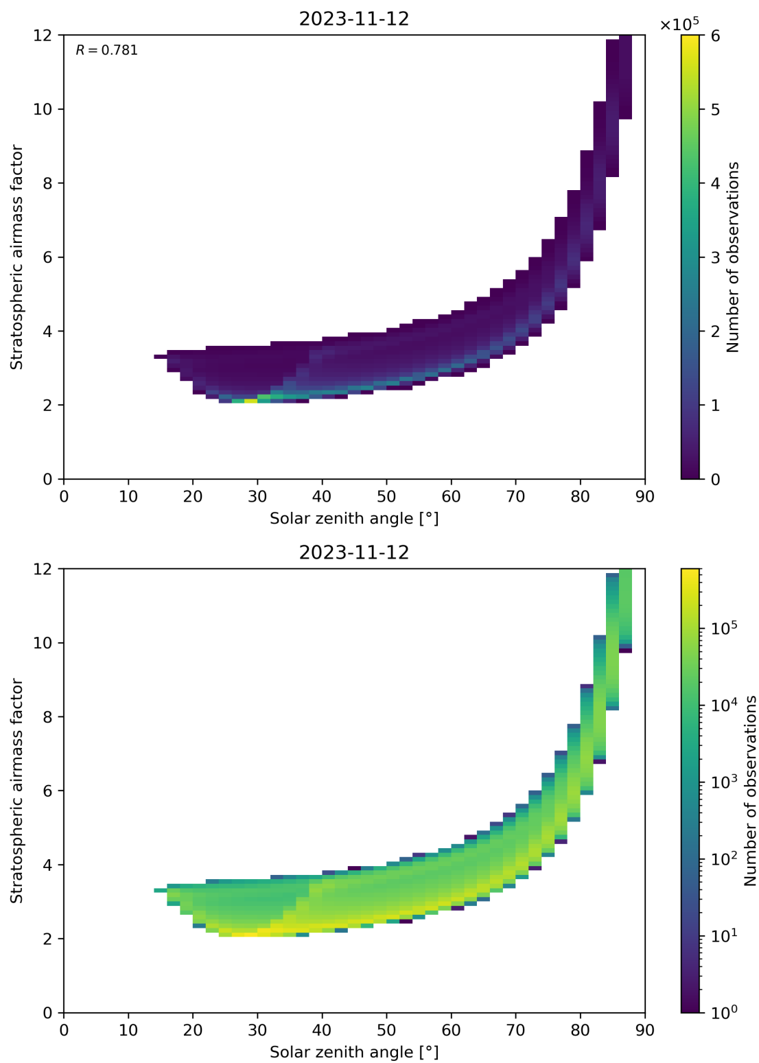
Figure 145: Scatter density plot of “Solar zenith angle” against “Stratospheric airmass factor” for 2023-11-12 to 2023-11-13.
