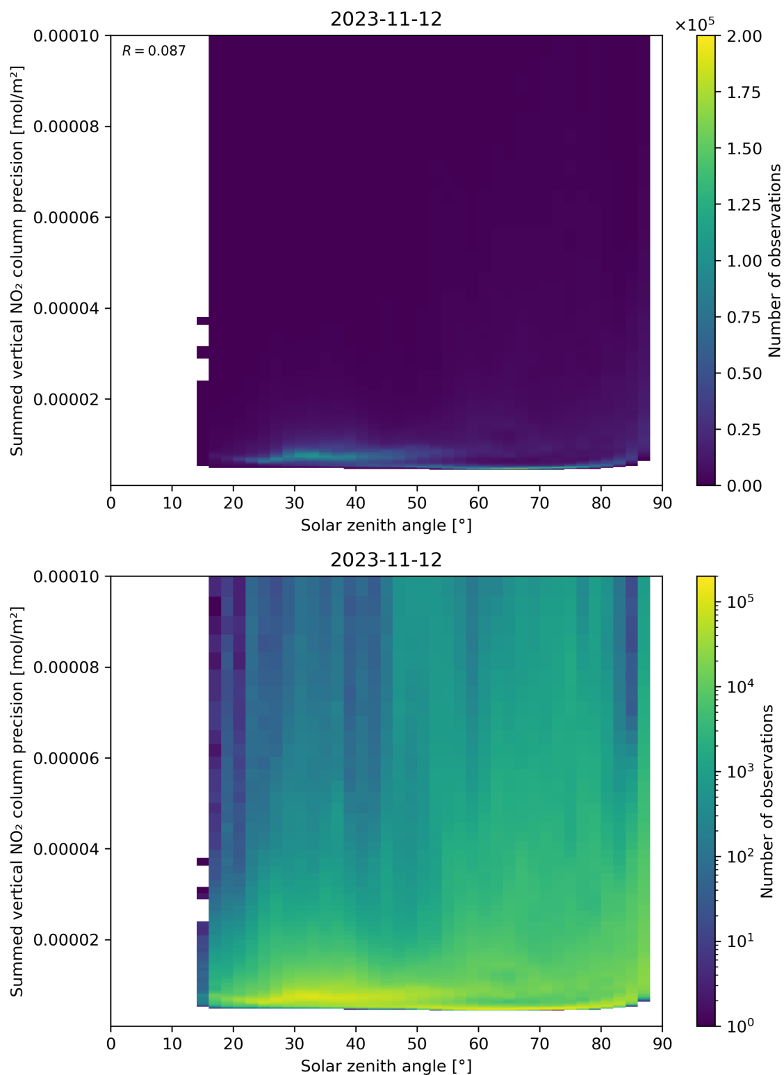
Figure 152: Scatter density plot of “Solar zenith angle” against “Summed vertical NO 2 column precision” for 2023-11-12 to 2023-11-13.
