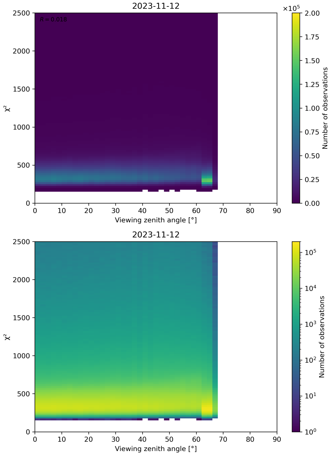
Figure 162: Scatter density plot of “Viewing zenith angle” against “ \chi^2 ” for 2023-11-12 to 2023-11-13.
