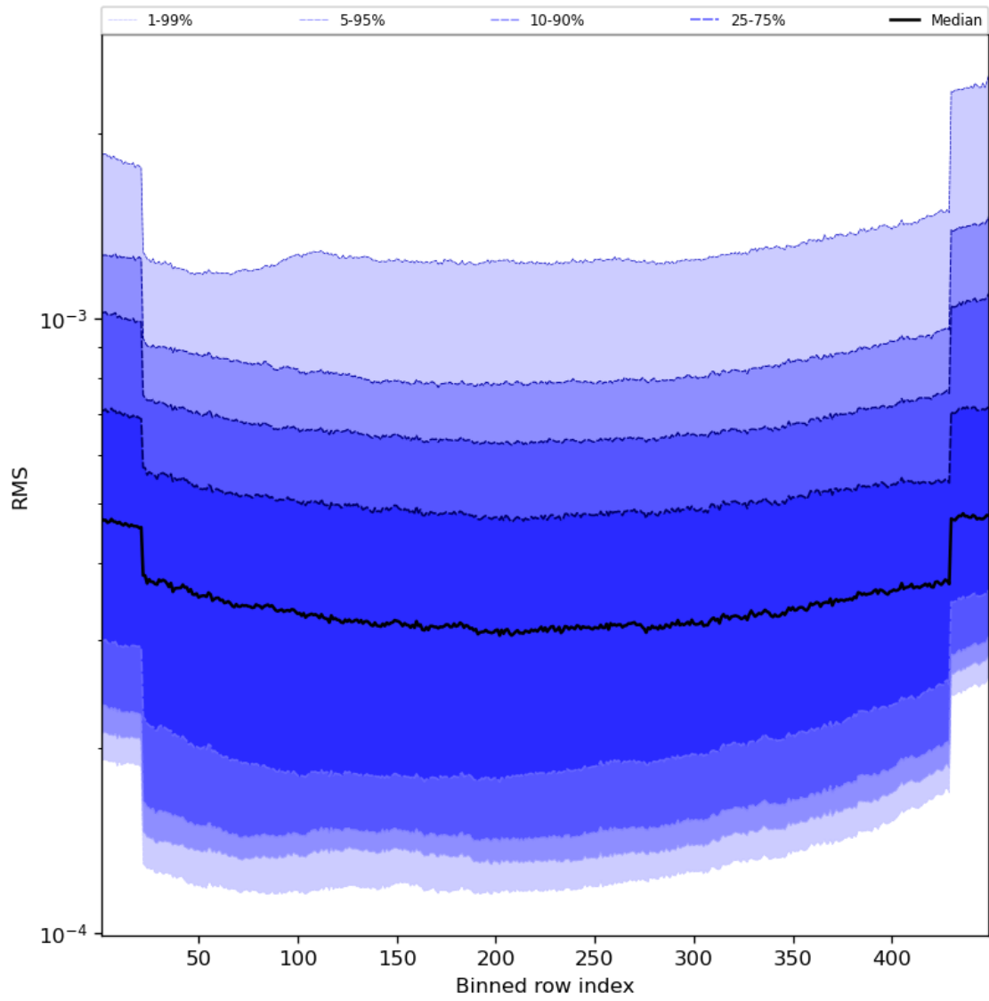
Figure 60: Along track statistics of “RMS” for 2023-11-12 to 2023-11-13
