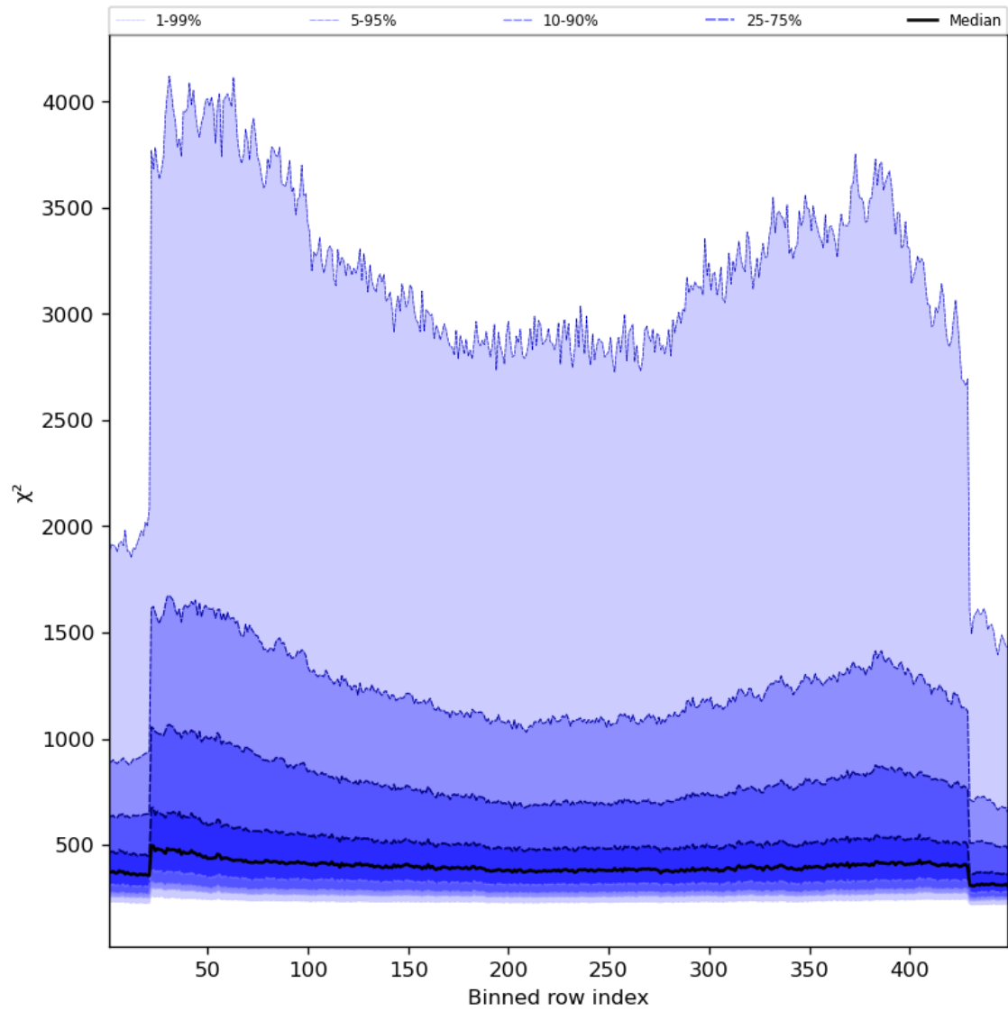
Figure 59: Along track statistics of “ \chi^2 ” for 2023-11-12 to 2023-11-13
