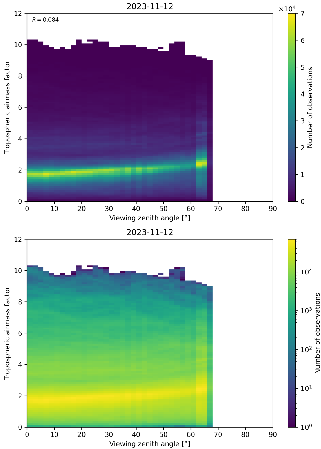
Figure 161: Scatter density plot of “Viewing zenith angle” against “Tropospheric airmass factor” for 2023-11-12 to 2023-11-13.
