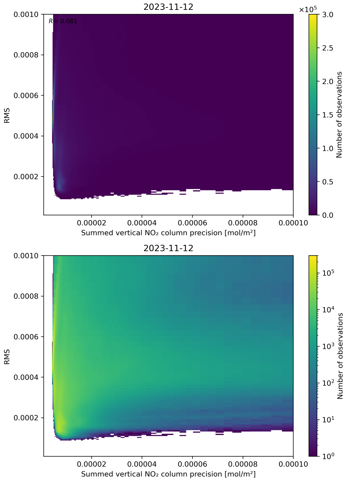
Figure 108: Scatter density plot of “Summed vertical NO 2 column precision” against “RMS” for 2023-11-12 to 2023-11-13.
