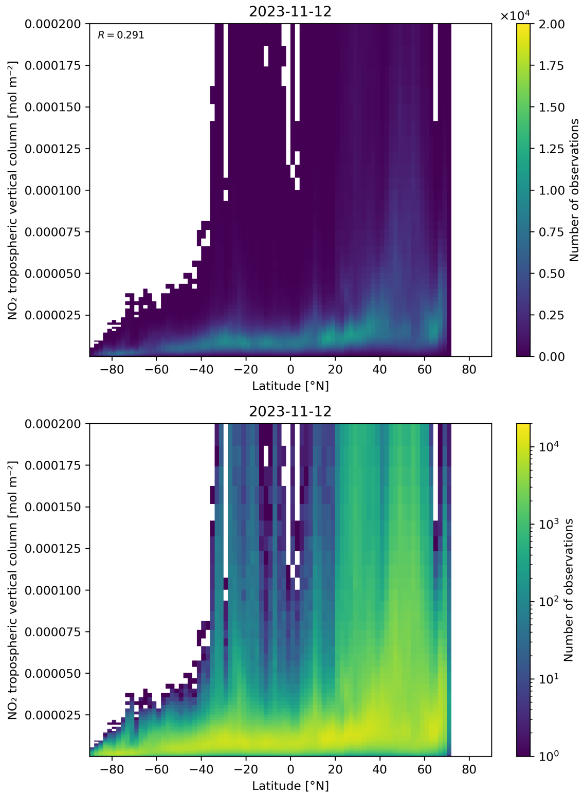
Figure 92: Scatter density plot of “Latitude” against “NO 2 tropospheric vertical column” for 2023-11-12 to 2023-11-13.
