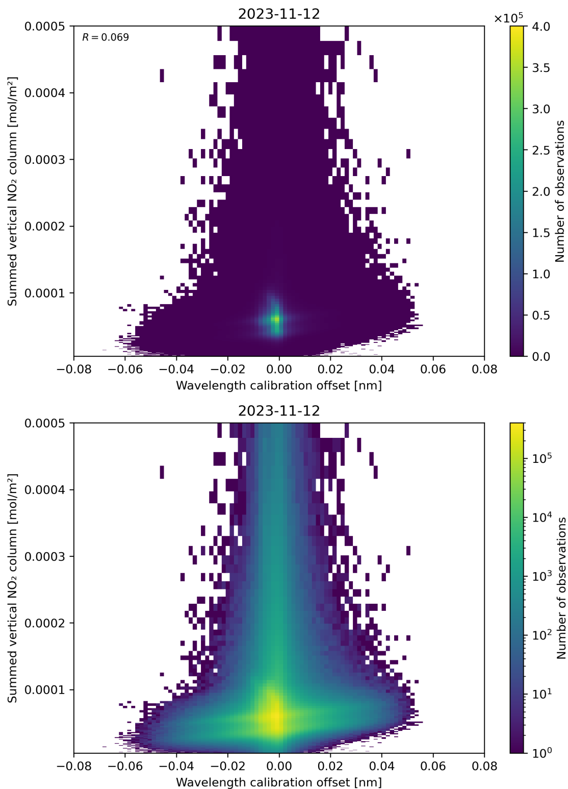
Figure 177: Scatter density plot of “Wavelength calibration offset” against “Summed vertical NO 2 column” for 2023-11-12 to 2023-11-13.
