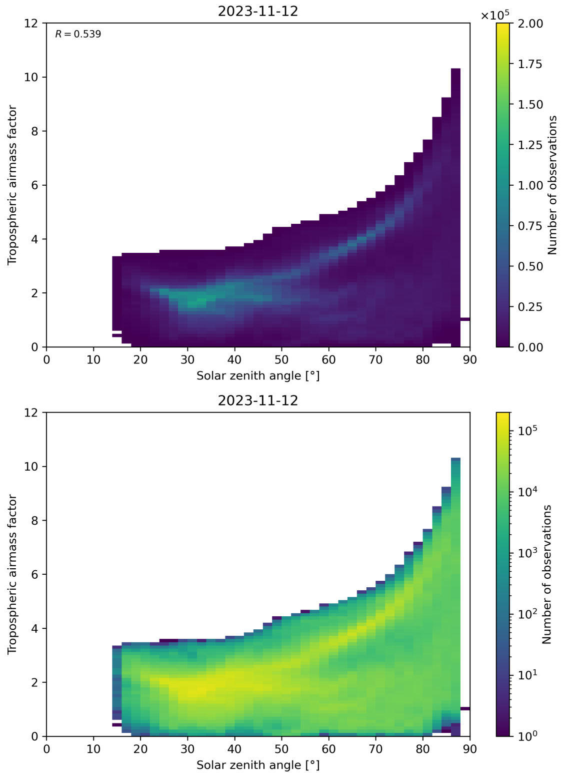
Figure 147: Scatter density plot of “Solar zenith angle” against “Tropospheric airmass factor” for 2023-11-12 to 2023-11-13.
