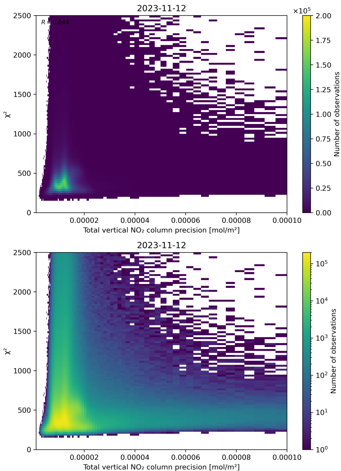
Figure 116: Scatter density plot of “Total vertical NO 2 column precision” against “ \chi^2 ” for 2023-11-12 to 2023-11-13.
