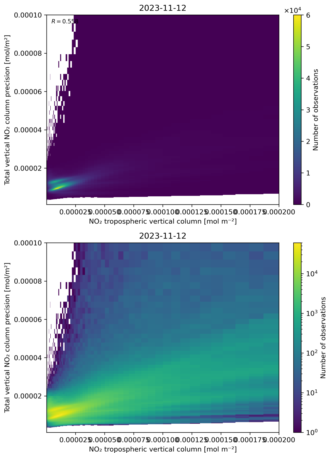
Figure 129: Scatter density plot of “NO 2 tropospheric vertical column” against “Total vertical NO 2 column precision” for 2023-11-12 to 2023-11-13.
