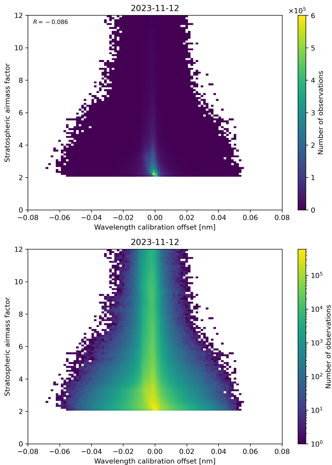
Figure 174: Scatter density plot of “Wavelength calibration offset” against “Stratospheric airmass factor” for 2023-11-12 to 2023-11-13.
