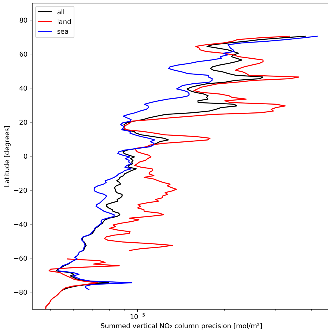
Figure 24: Zonal average of “Summed vertical NO 2 column precision” for 2023-11-12 to 2023-11-13.
