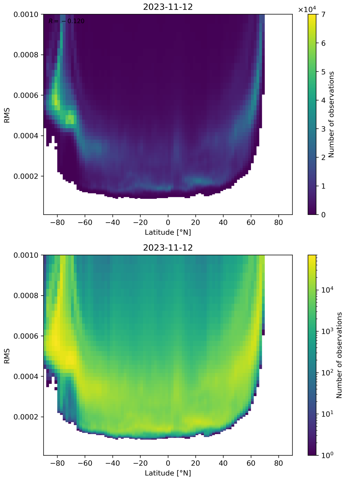
Figure 94: Scatter density plot of “Latitude” against “RMS” for 2023-11-12 to 2023-11-13.
