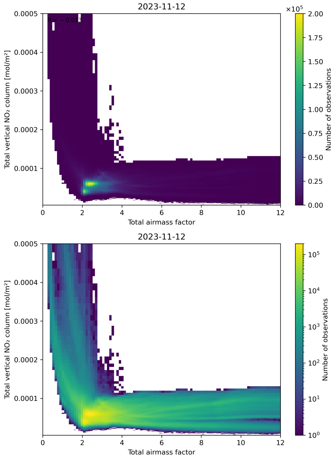
Figure 67: Scatter density plot of “Total airmass factor” against “Total vertical NO 2 column” for 2023-11-12 to 2023-11-13.
