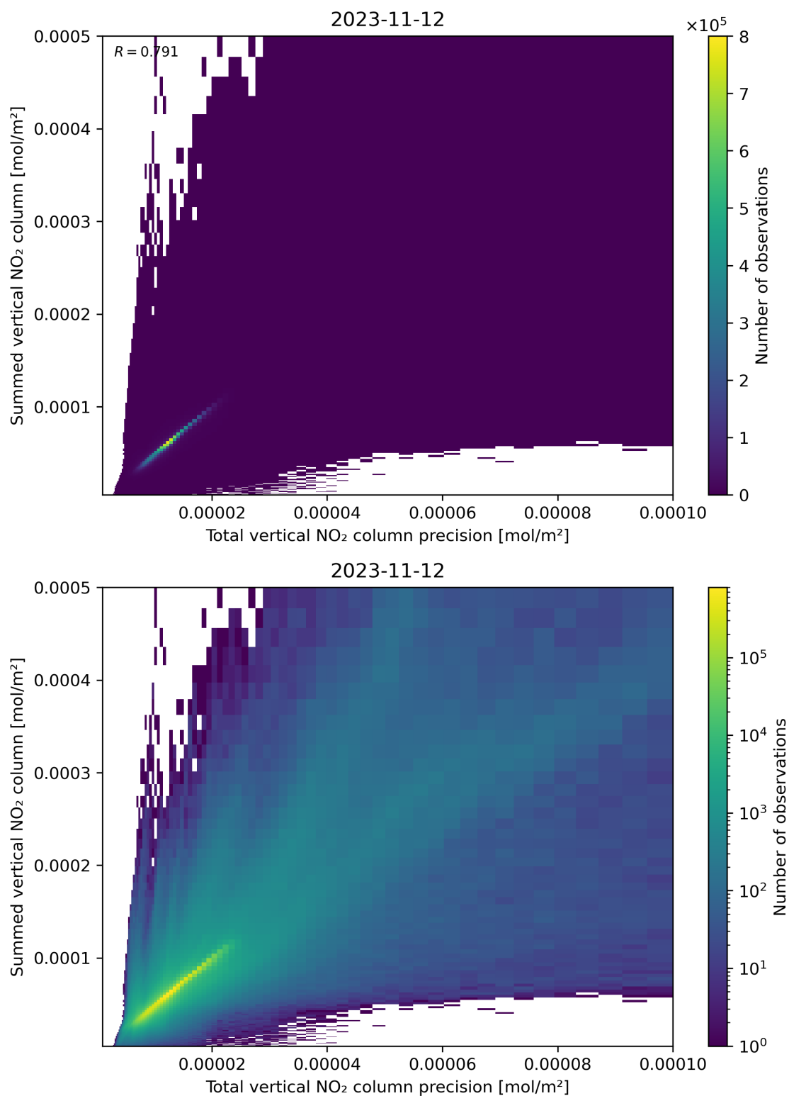
Figure 117: Scatter density plot of “Total vertical NO 2 column precision” against “Summed vertical NO 2 column” for 2023-11-12 to 2023-11-13.
