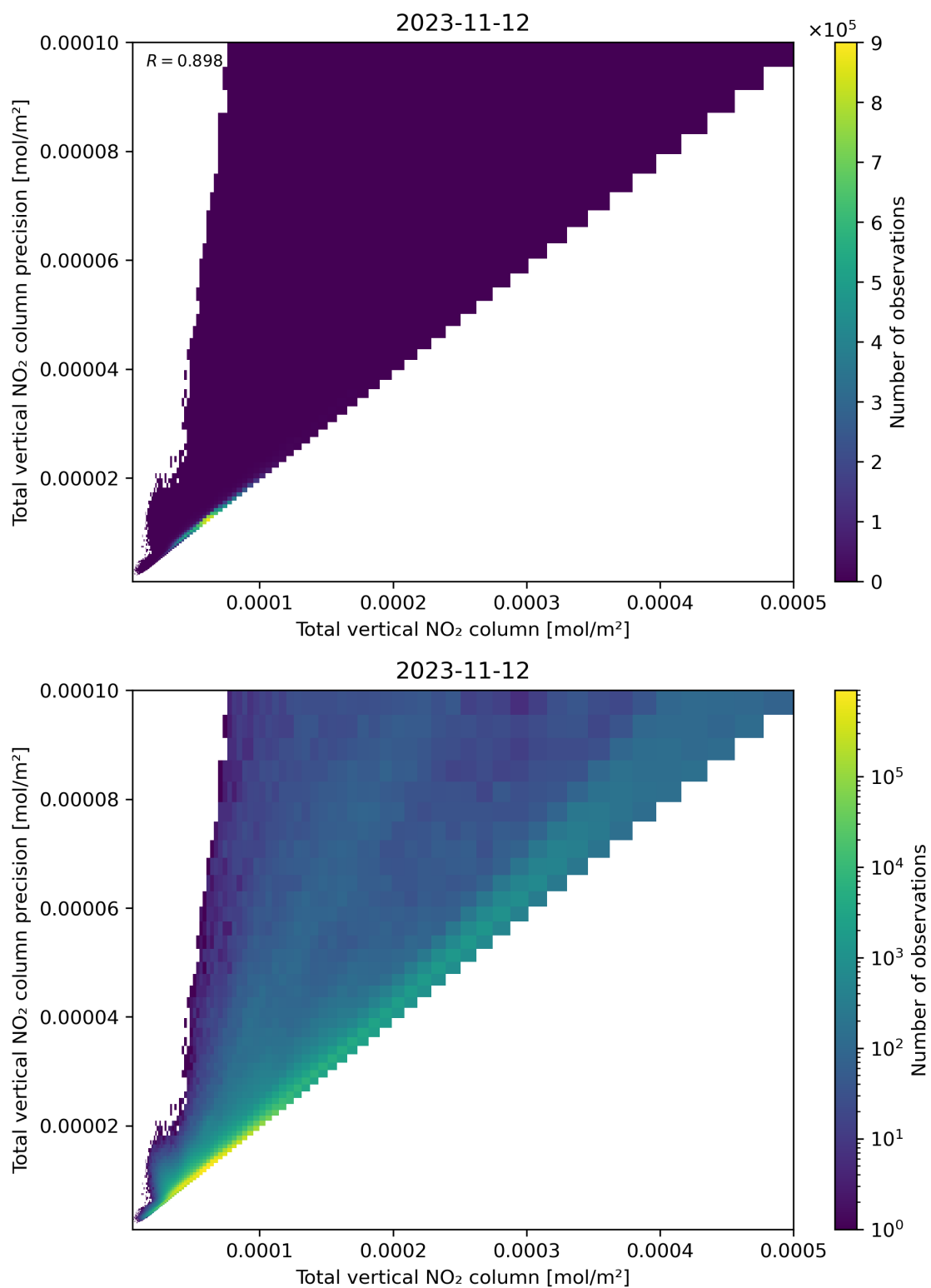
Figure 114: Scatter density plot of “Total vertical NO 2 column” against “Total vertical NO 2 column precision” for 2023-11-12 to 2023-11-13.
