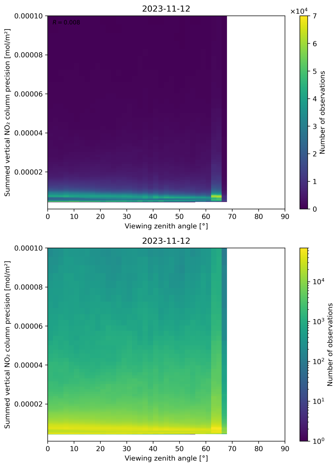
Figure 166: Scatter density plot of “Viewing zenith angle” against “Summed vertical NO 2 column precision” for 2023-11-12 to 2023-11-13.
