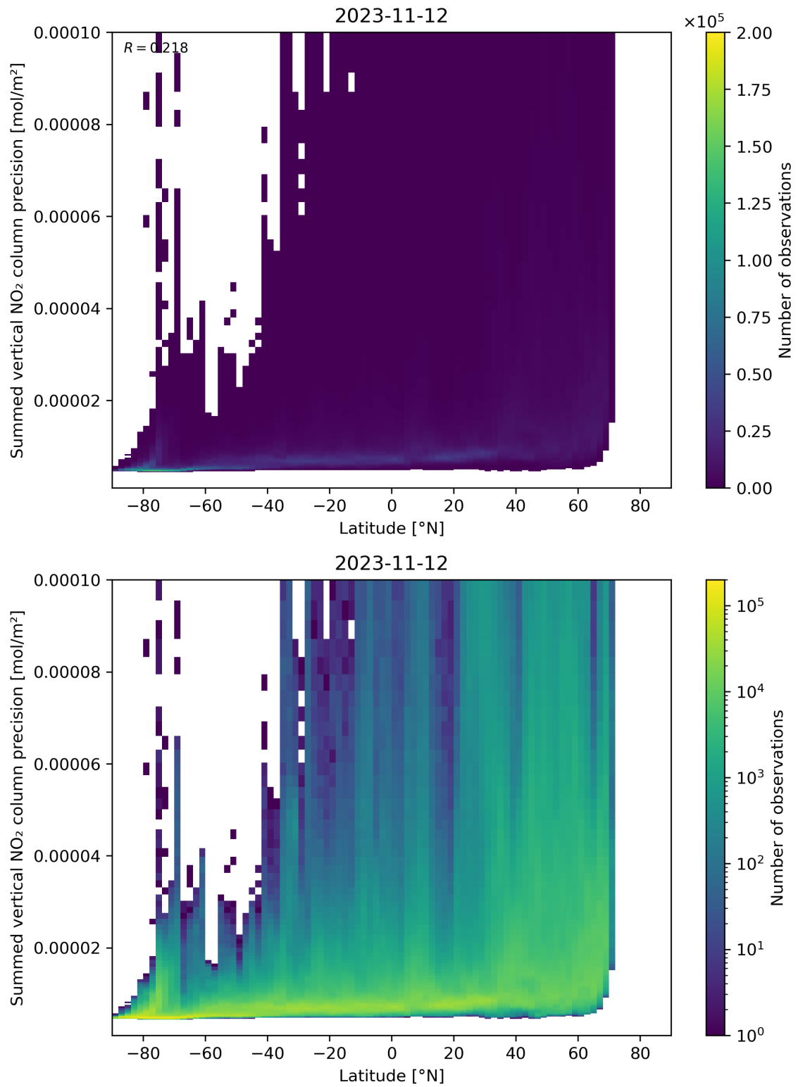
Figure 89: Scatter density plot of “Latitude” against “Summed vertical NO 2 column precision” for 2023-11-12 to 2023-11-13.
