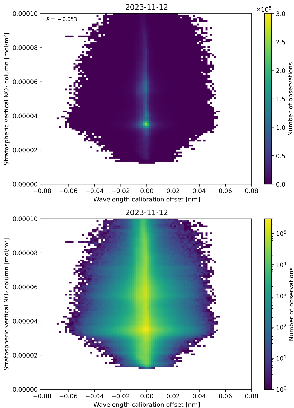
Figure 176: Scatter density plot of “Wavelength calibration offset” against “Stratospheric vertical NO 2 column” for 2023-11-12 to 2023-11-13.
