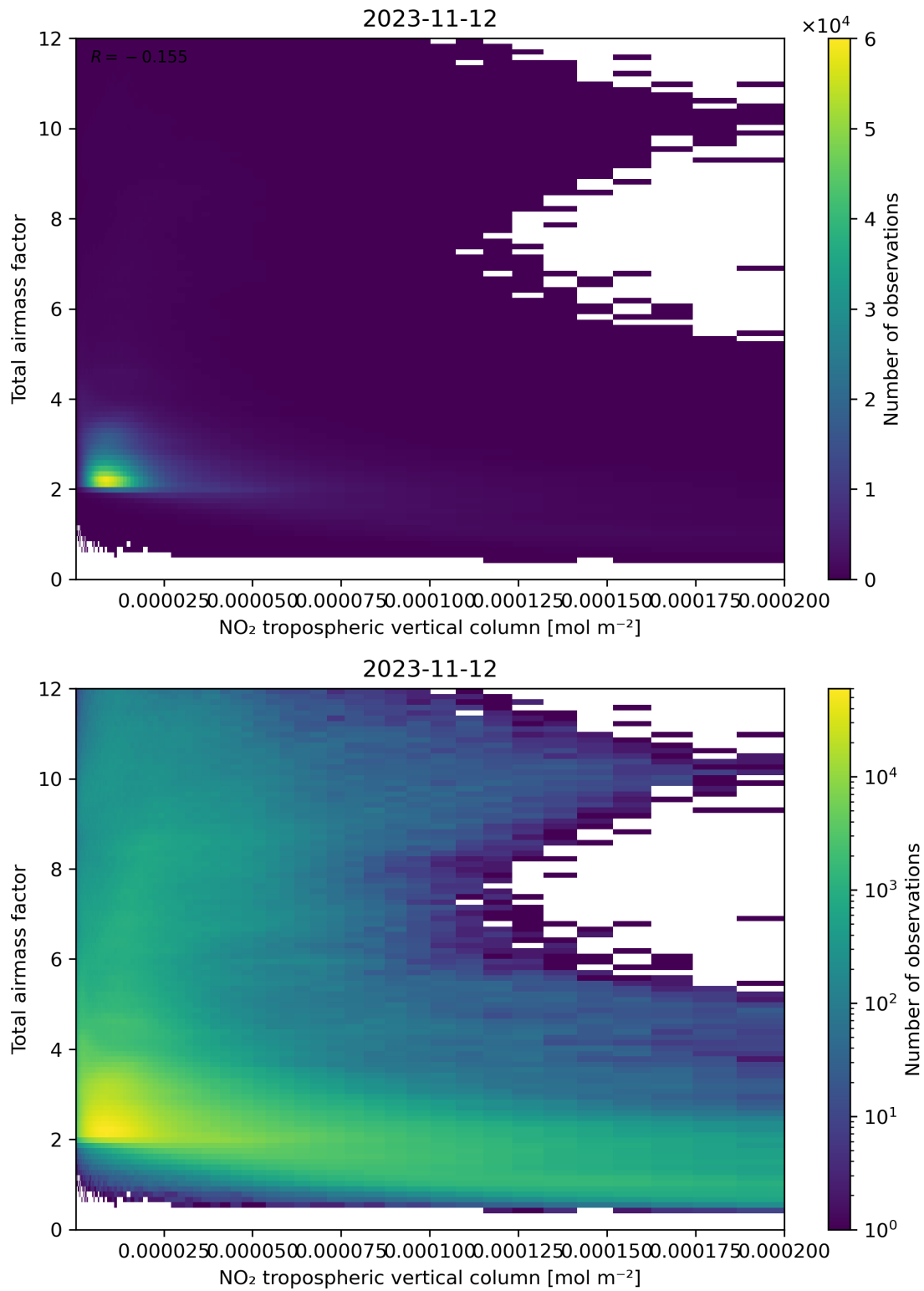
Figure 122: Scatter density plot of “NO 2 tropospheric vertical column” against “Total air mass factor” for 2023-11-12 to 2023-11-13.
