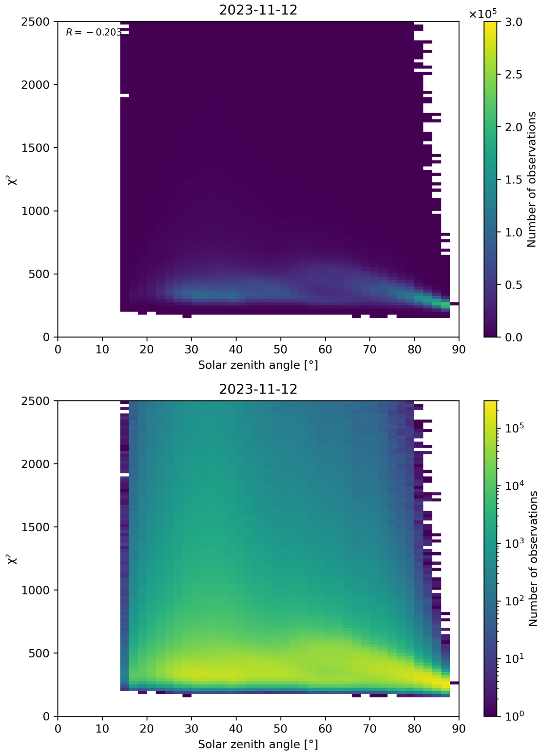
Figure 148: Scatter density plot of “Solar zenith angle” against “ \chi^2 ” for 2023-11-12 to 2023-11-13.
