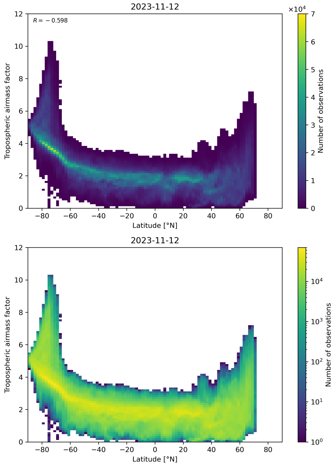
Figure 85: Scatter density plot of “Latitude” against “Tropospheric airmass factor” for 2023-11-12 to 2023-11-13.
