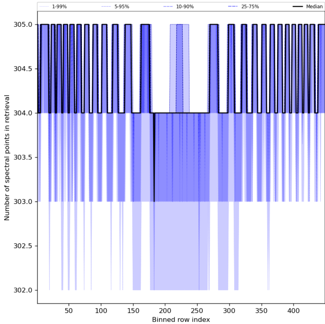
Figure 50: Along track statistics of “Number of spectral points in retrieval” for 2023-11-12 to 2023-11-13
