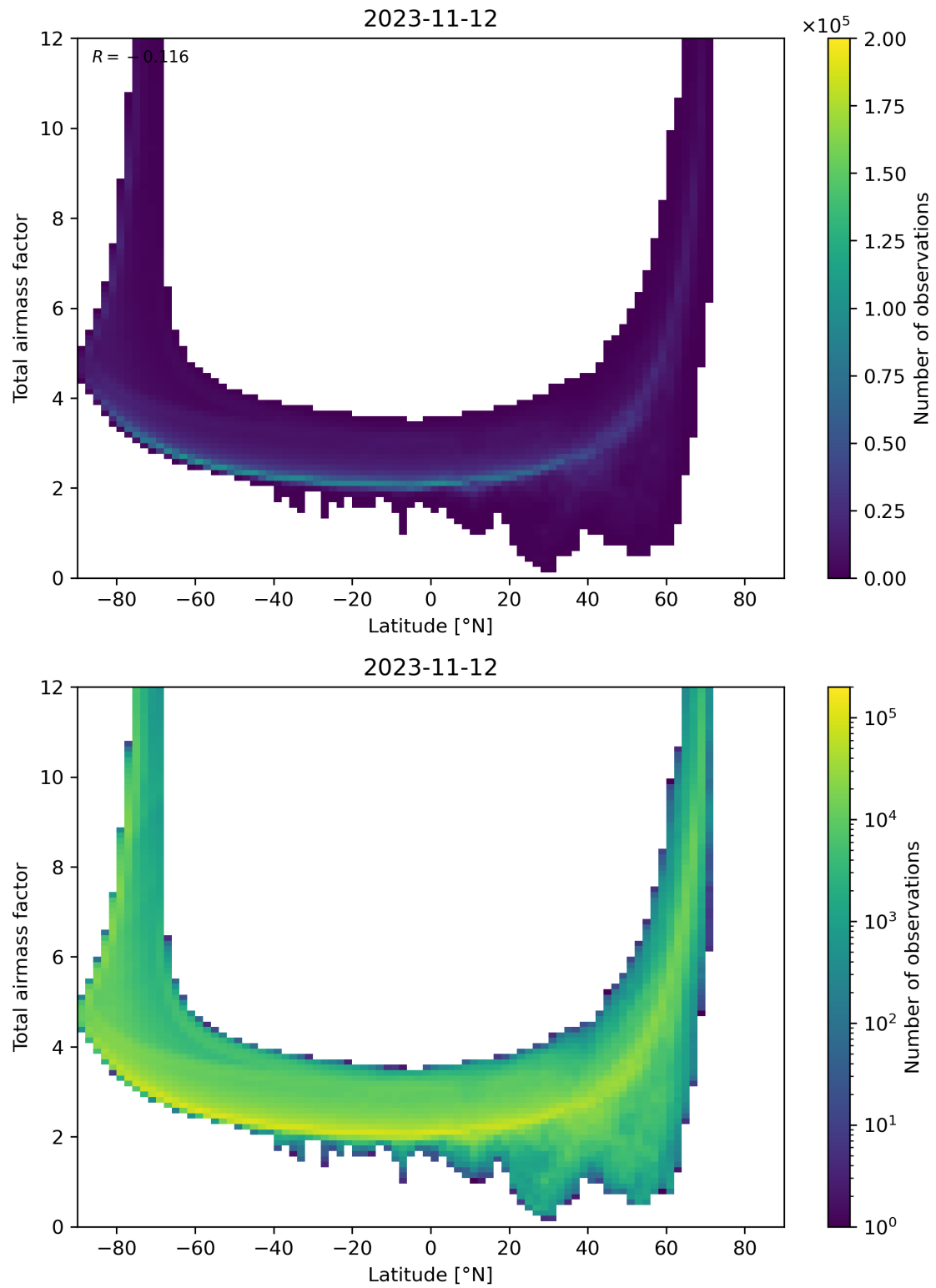
Figure 84: Scatter density plot of “Latitude” against “Total airmass factor” for 2023-11-12 to 2023-11-13.
