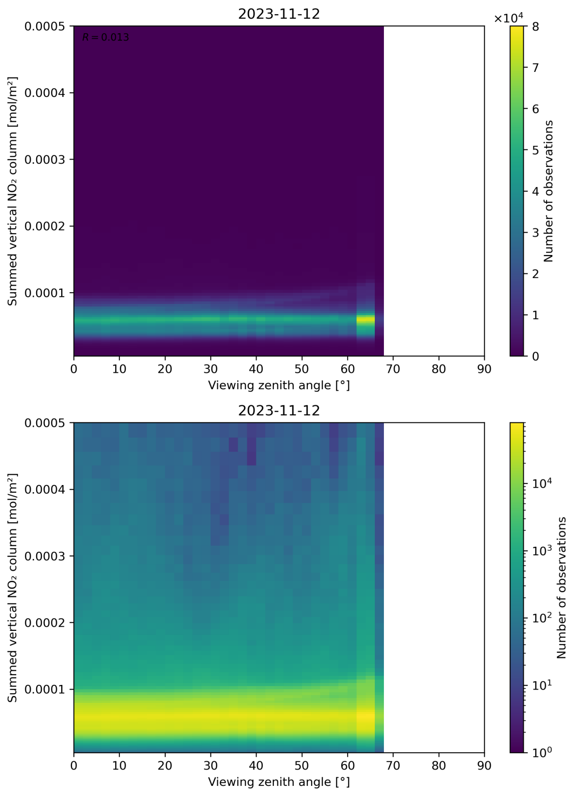
Figure 165: Scatter density plot of “Viewing zenith angle” against “Summed vertical NO 2 column” for 2023-11-12 to 2023-11-13.
