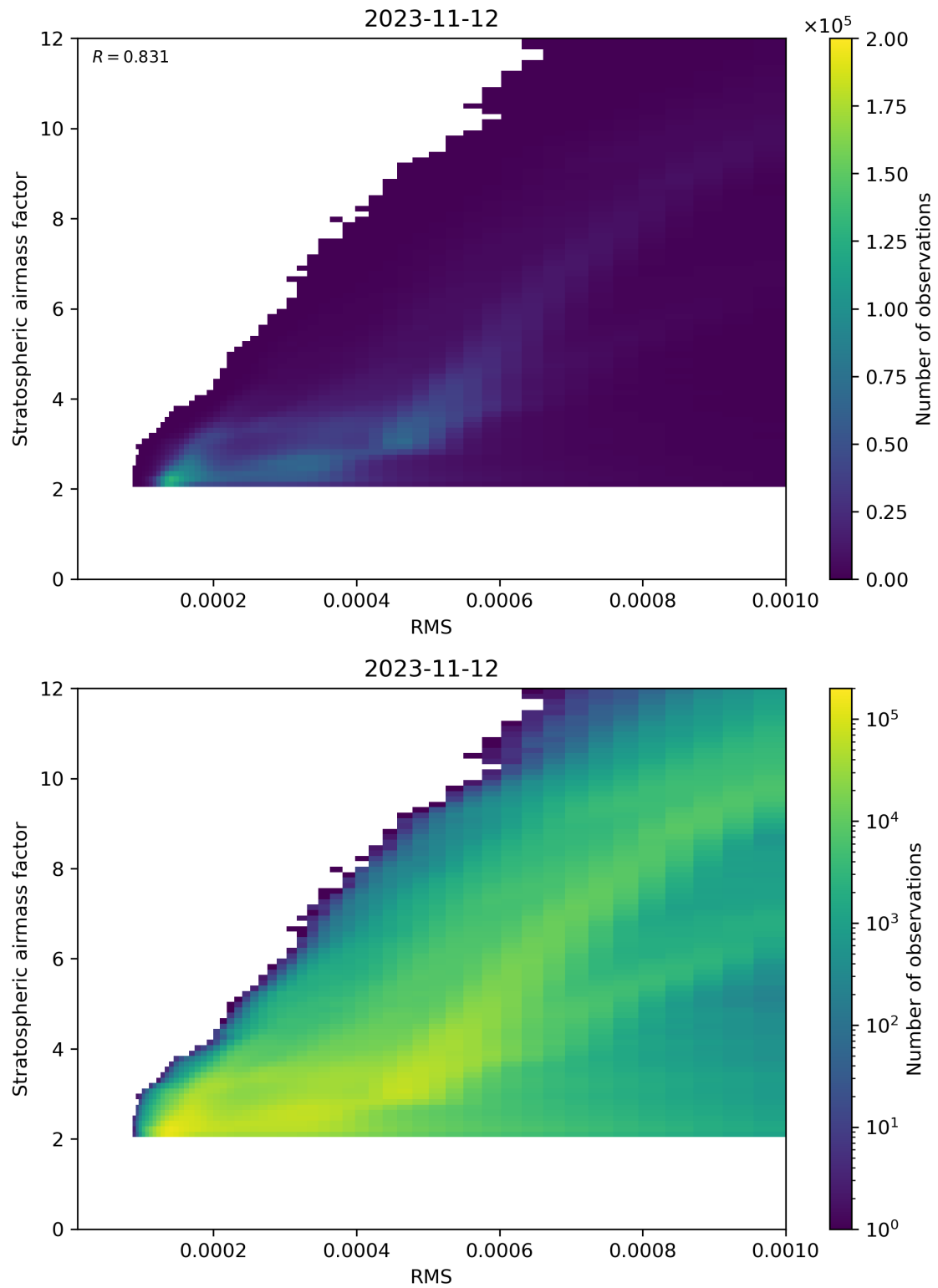
Figure 144: Scatter density plot of “RMS” against “Stratospheric airmass factor” for 2023-11-12 to 2023-11-13.
