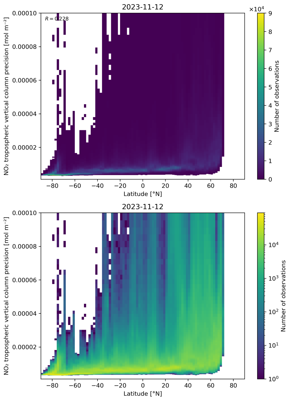
Figure 93: Scatter density plot of “Latitude” against “NO 2 tropospheric vertical column precision” for 2023-11-12 to 2023-11-13.
