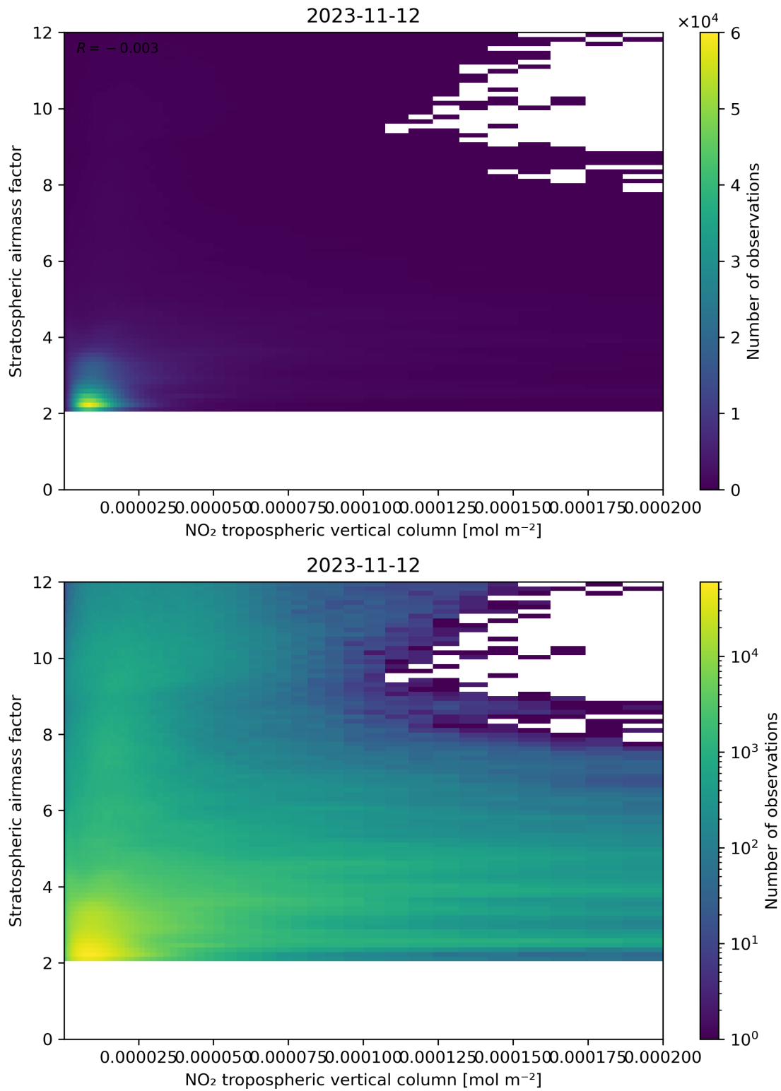
Figure 121: Scatter density plot of “NO 2 tropospheric vertical column” against “Stratospheric air mass factor” for 2023-11-12 to 2023-11-13.
