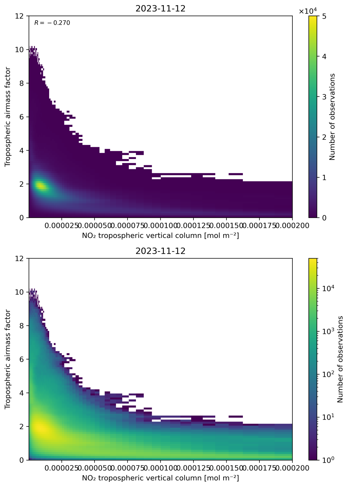
Figure 123: Scatter density plot of “NO 2 tropospheric vertical column” against “Tropospheric airmass factor” for 2023-11-12 to 2023-11-13.
