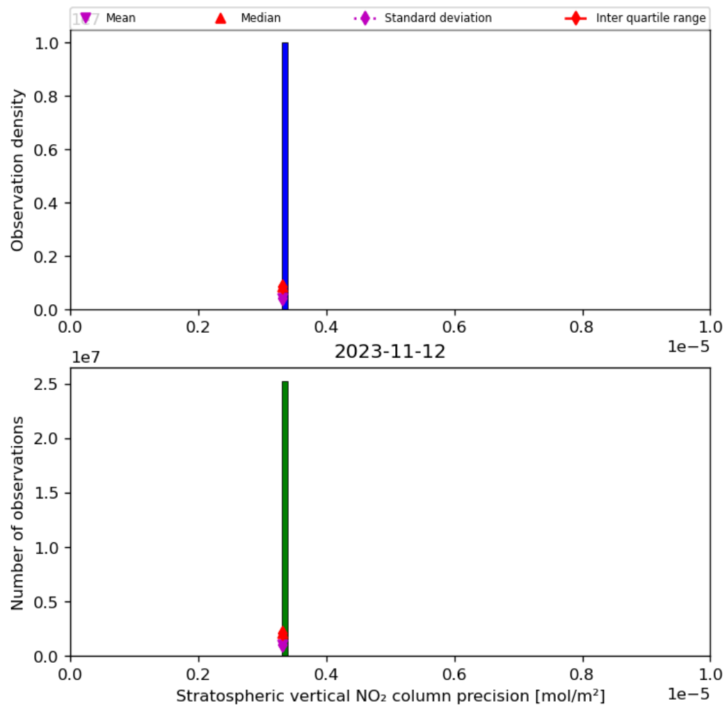
Figure 37: Histogram of “Stratospheric vertical NO 2 column precision” for 2023-11-12 to 2023-11-13
