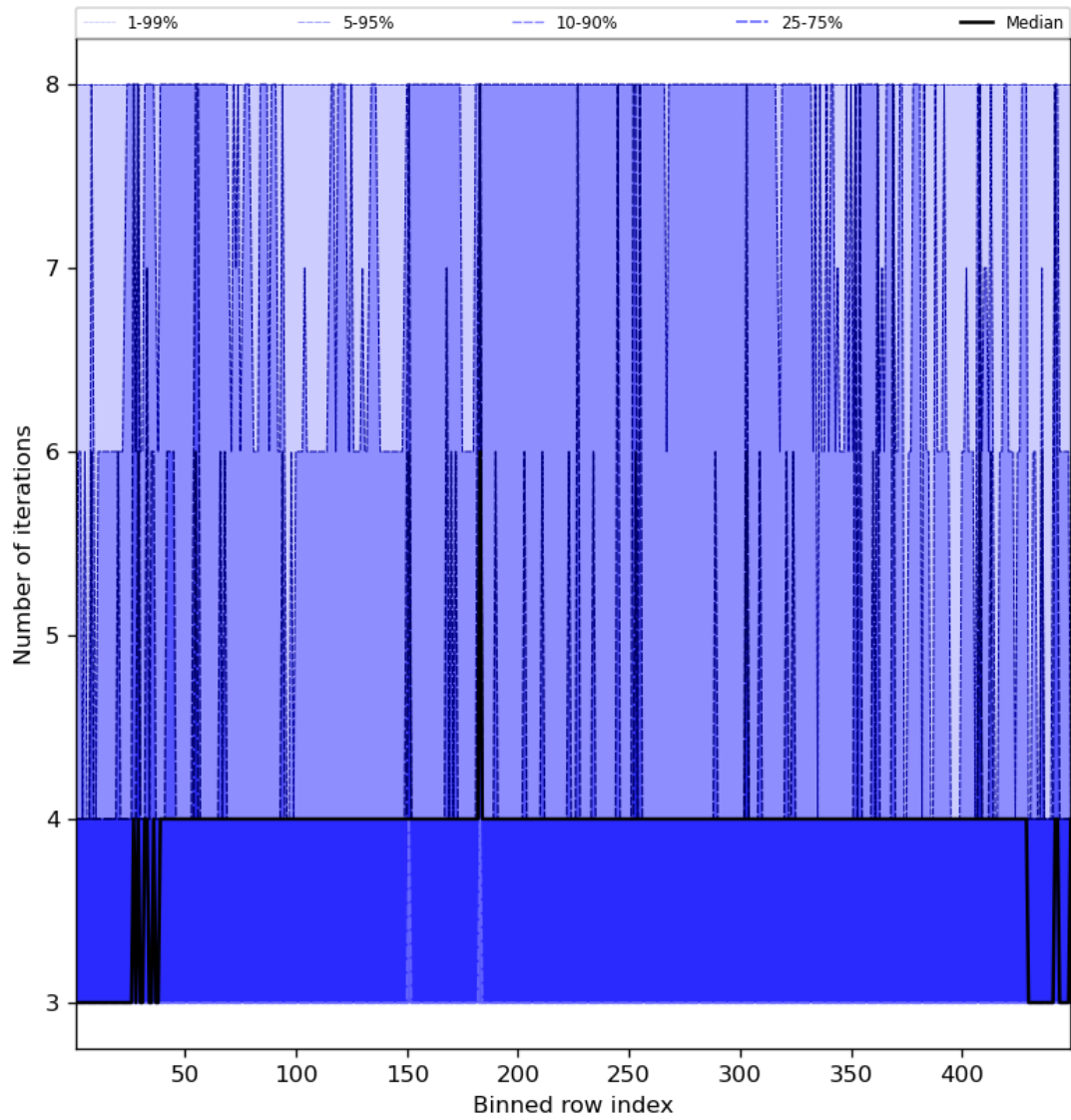
Figure 51: Along track statistics of “Number of iterations” for 2023-11-12 to 2023-11-13
