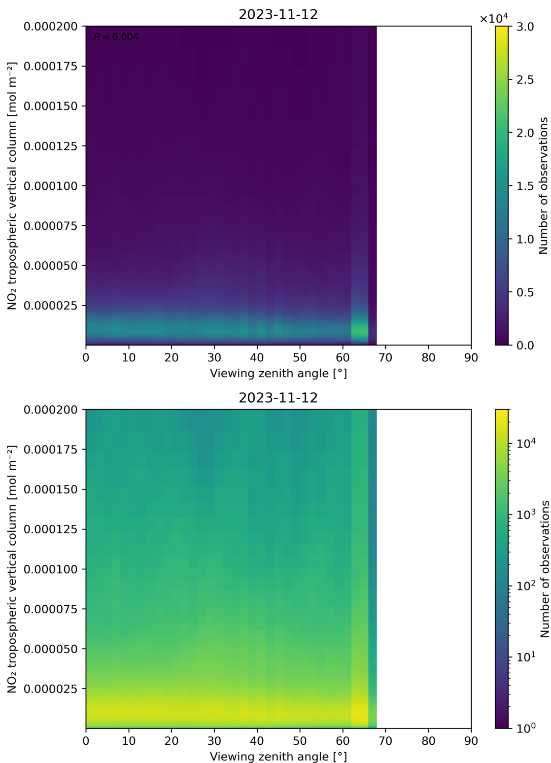
Figure 169: Scatter density plot of “Viewing zenith angle” against “NO 2 tropospheric vertical column” for 2023-11-12 to 2023-11-13.
