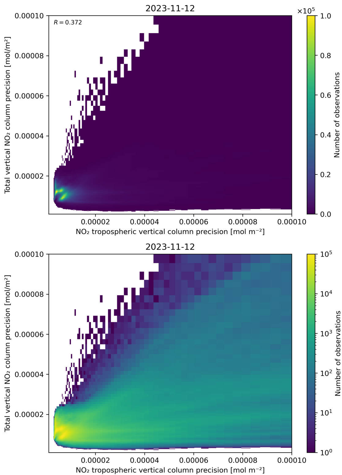
Figure 139: Scatter density plot of “NO 2 tropospheric vertical column precision” against “Total vertical NO 2 column precision” for 2023-11-12 to 2023-11-13.
