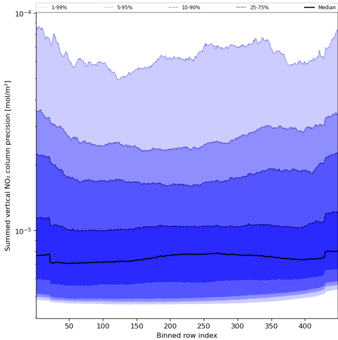
Figure 58: Along track statistics of “Summed vertical NO 2 column precision” for 2023-11-12 to 2023-11-13
