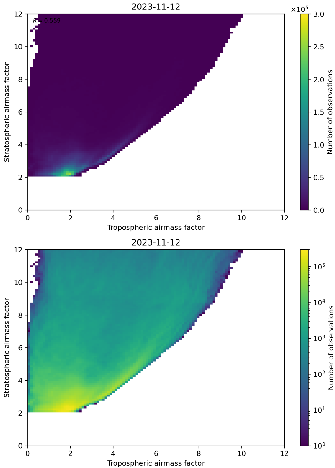
Figure 71: Scatter density plot of “Tropospheric airmass factor” against “Stratospheric airmass factor” for 2023-11-12 to 2023-11-13.
