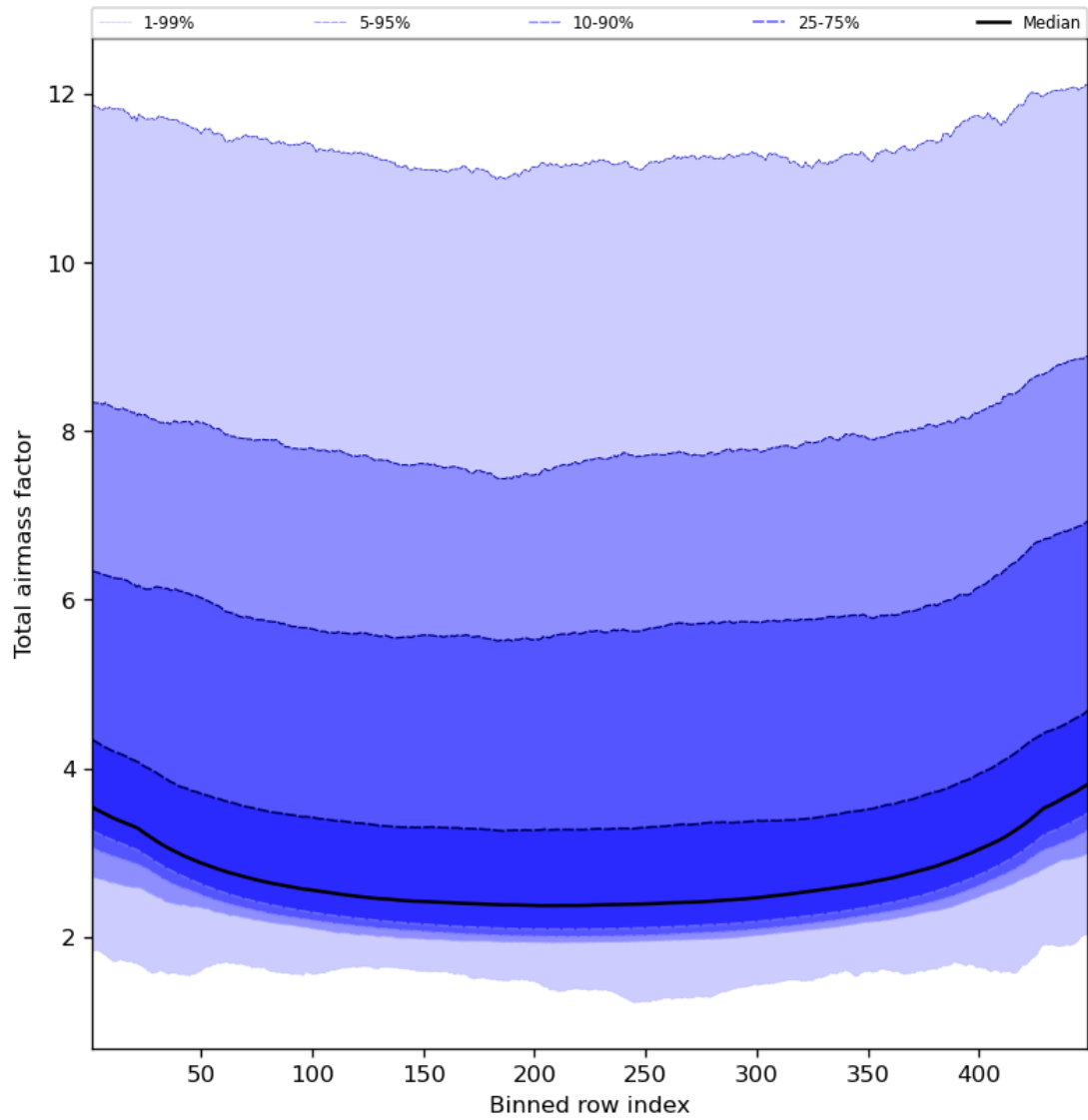
Figure 49: Along track statistics of “Total airmass factor” for 2023-11-12 to 2023-11-13
