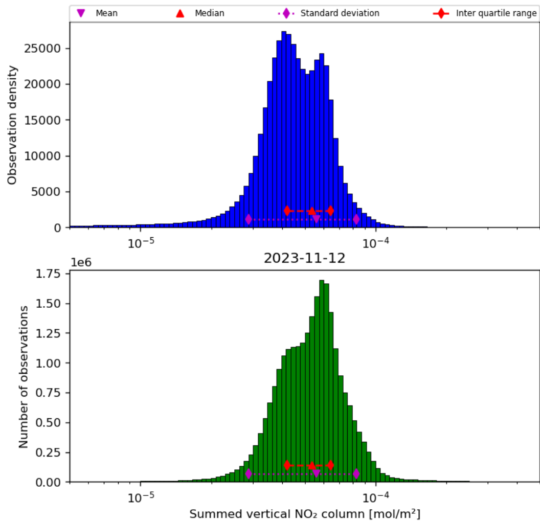
Figure 40: Histogram of “Summed vertical NO 2 column” for 2023-11-12 to 2023-11-13
