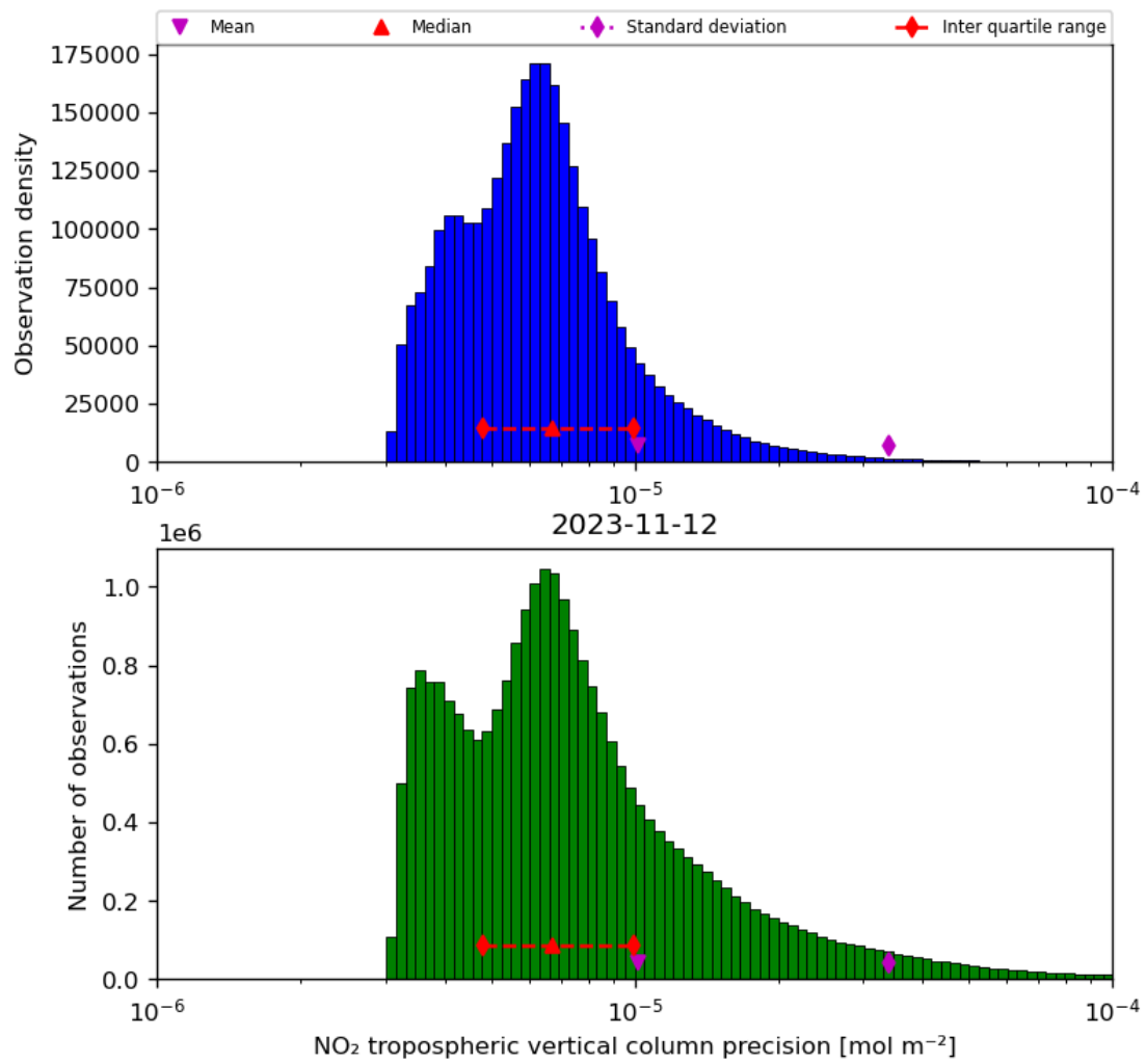
Figure 30: Histogram of “NO 2 tropospheric vertical column precision” for 2023-11-12 to 2023-11-13
