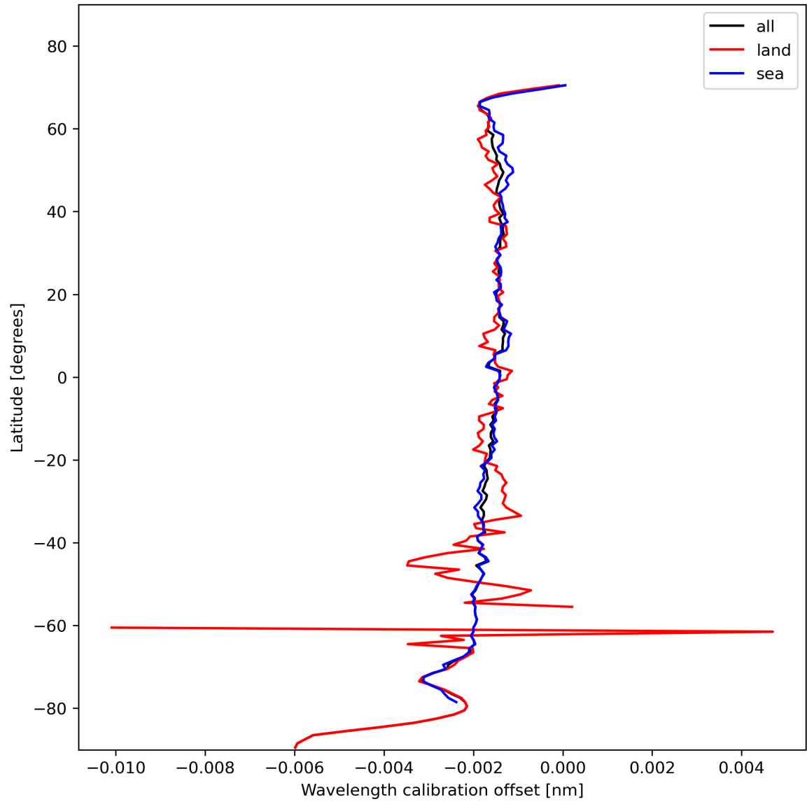
Figure 18: Zonal average of “Wavelength calibration offset” for 2023-11-12 to 2023-11-13.
