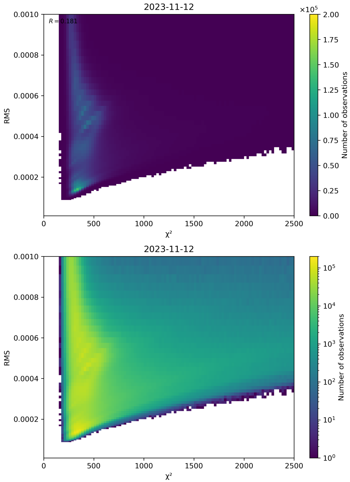
Figure 82: Scatter density plot of “ \chi^2 ” against “RMS” for 2023-11-12 to 2023-11-13.
