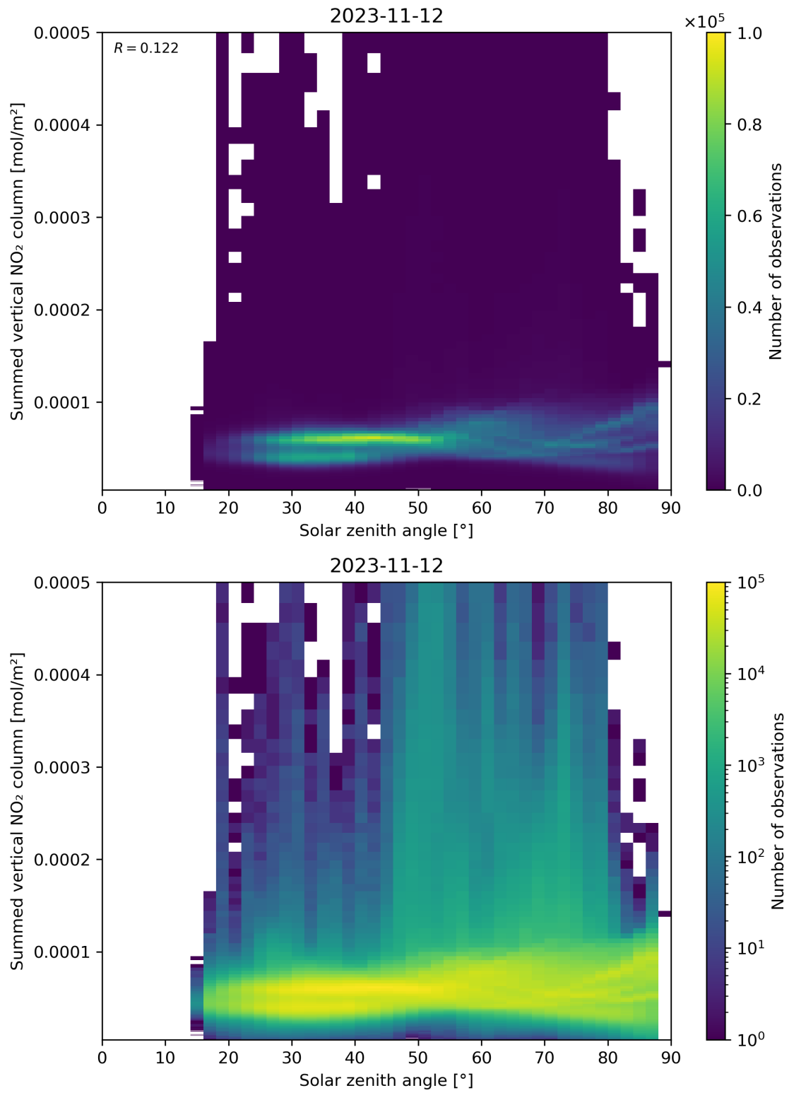
Figure 151: Scatter density plot of “Solar zenith angle” against “Summed vertical NO 2 column” for 2023-11-12 to 2023-11-13.
