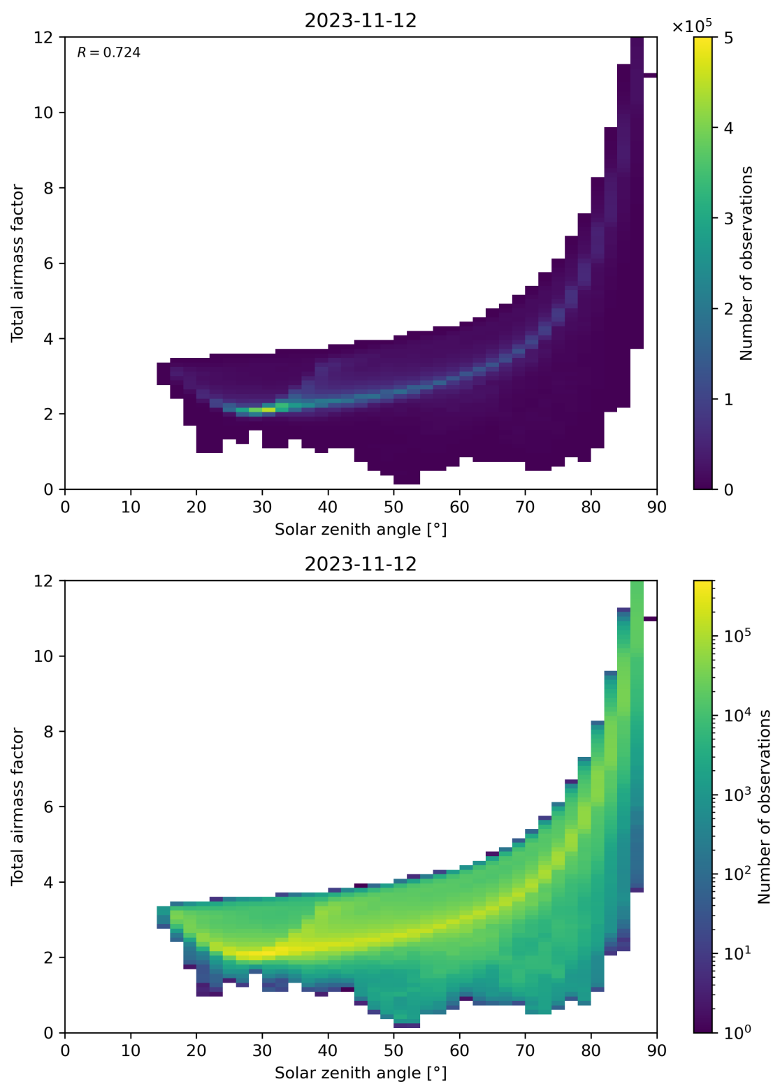
Figure 146: Scatter density plot of “Solar zenith angle” against “Total air mass factor” for 2023-11-12 to 2023-11-13.
