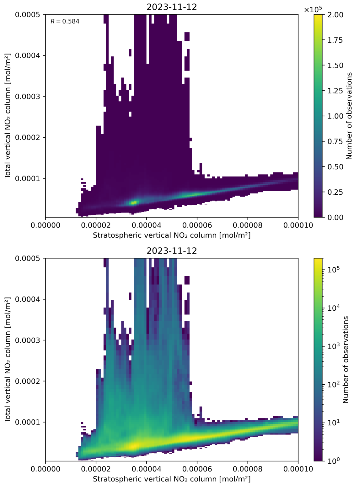
Figure 100: Scatter density plot of “Stratospheric vertical NO 2 column” against “Total vertical NO 2 column” for 2023-11-12 to 2023-11-13.
