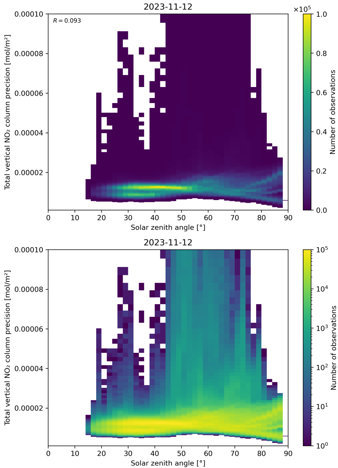
Figure 154: Scatter density plot of “Solar zenith angle” against “Total vertical NO 2 column precision” for 2023-11-12 to 2023-11-13.
