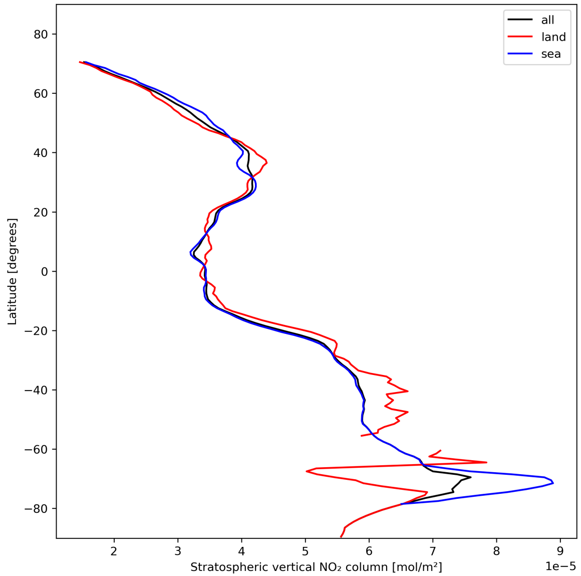
Figure 19: Zonal average of “Stratospheric vertical NO 2 column” for 2023-11-12 to 2023-11-13.
