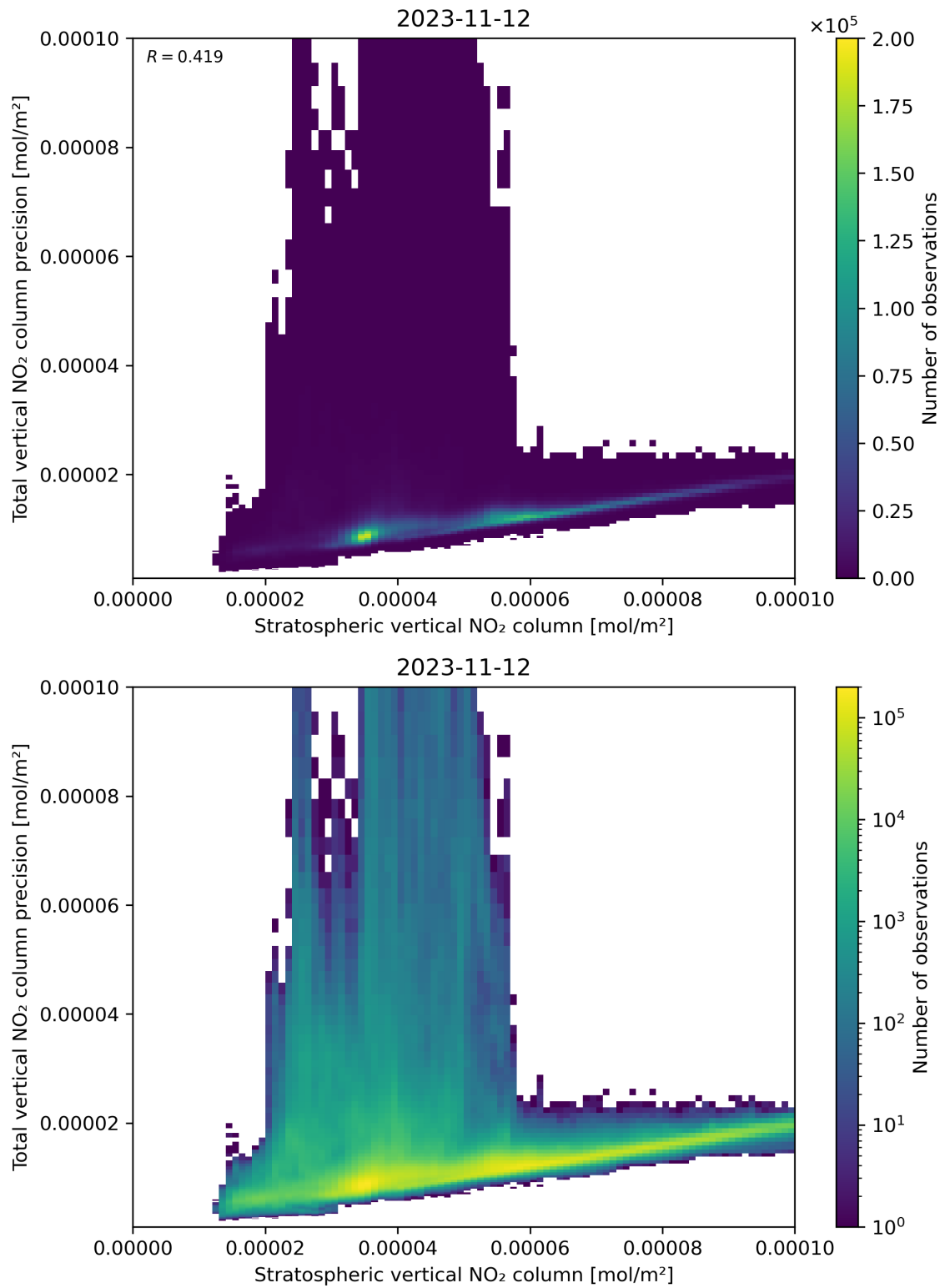
Figure 101: Scatter density plot of “Stratospheric vertical NO 2 column” against “Total vertical NO 2 column precision” for 2023-11-12 to 2023-11-13.
