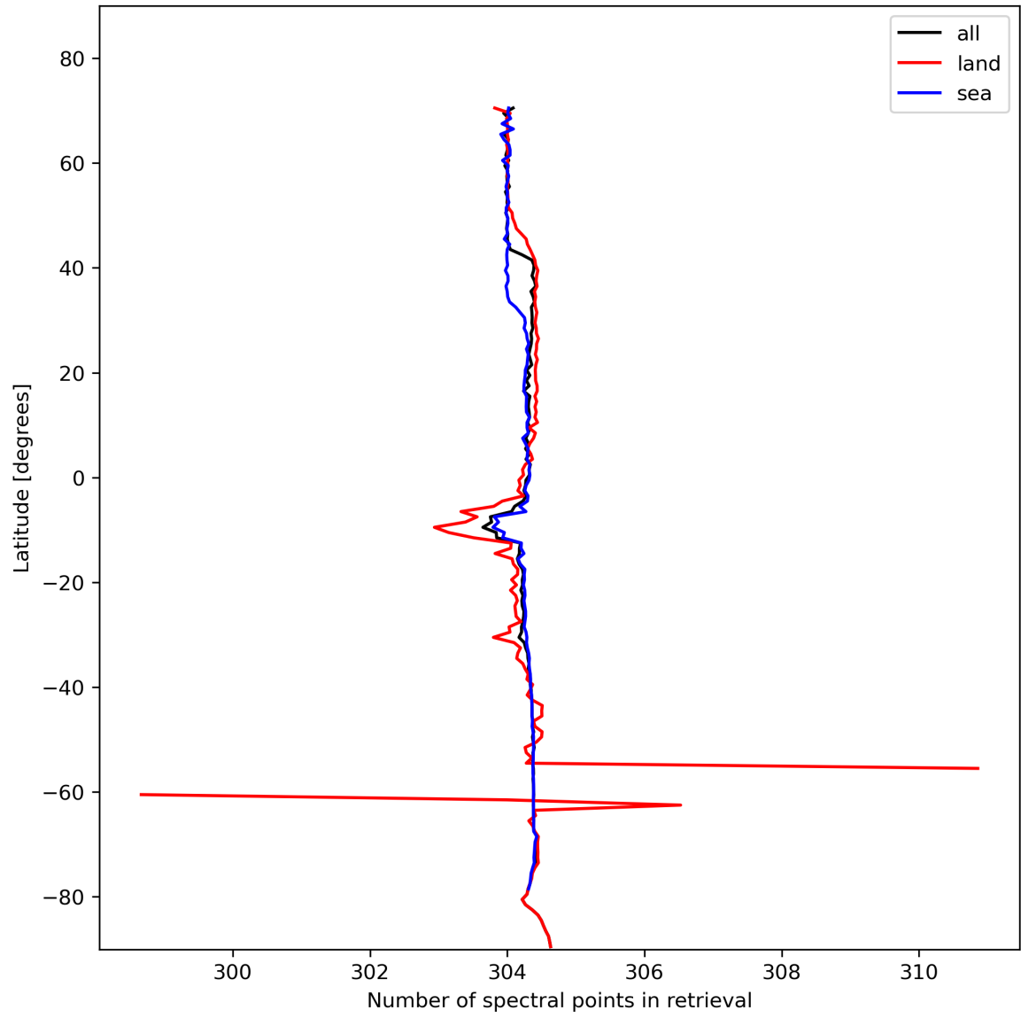
Figure 16: Zonal average of “Number of spectral points in retrieval” for 2023-11-12 to 2023-11-13.
