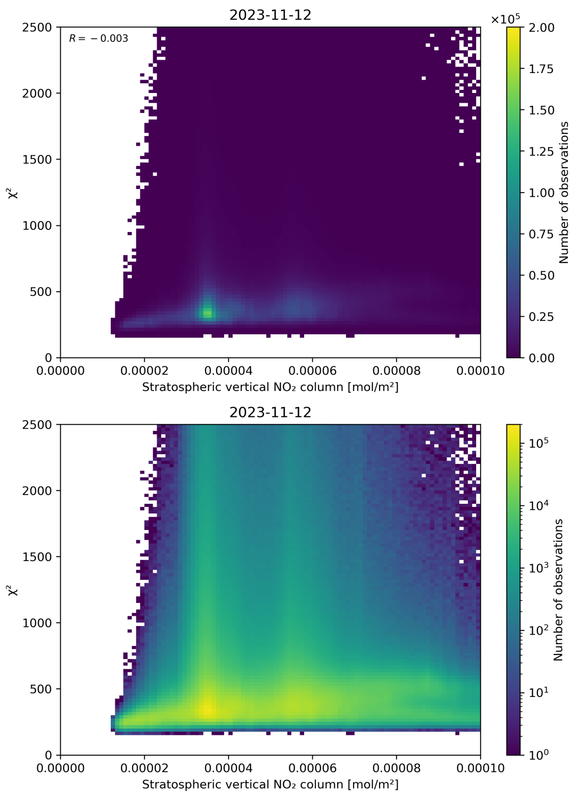
Figure 97: Scatter density plot of “Stratospheric vertical NO 2 column” against “ \chi^2 ” for 2023-11-12 to 2023-11-13.
