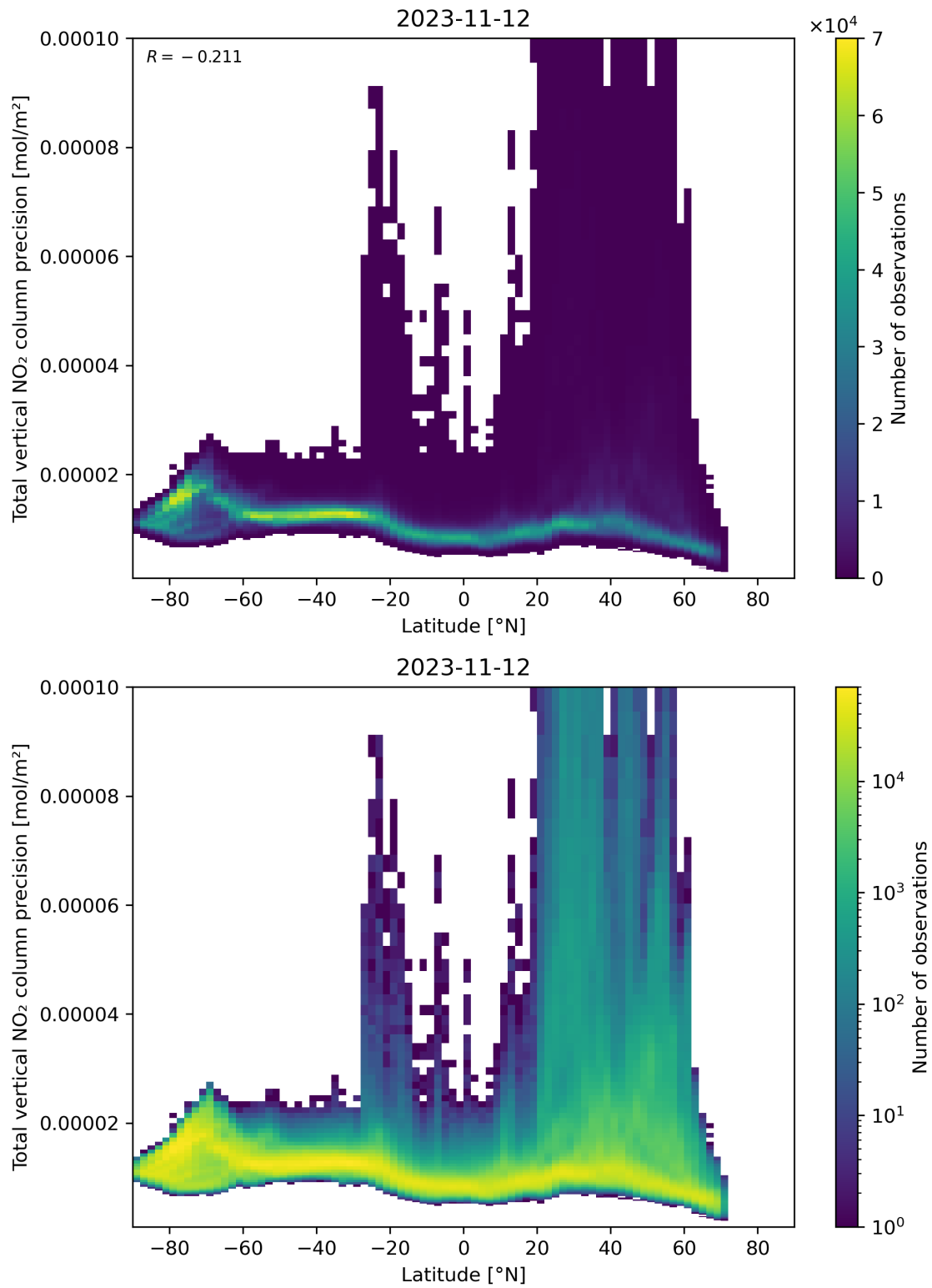
Figure 91: Scatter density plot of “Latitude” against “Total vertical NO 2 column precision” for 2023-11-12 to 2023-11-13.
