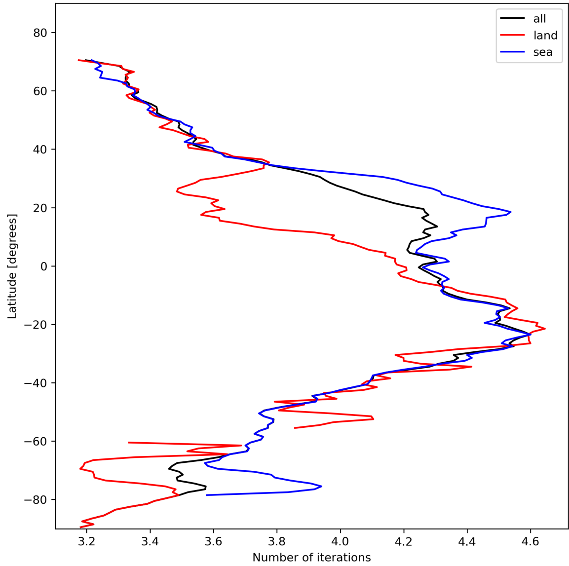
Figure 17: Zonal average of “Number of iterations” for 2023-11-12 to 2023-11-13.
