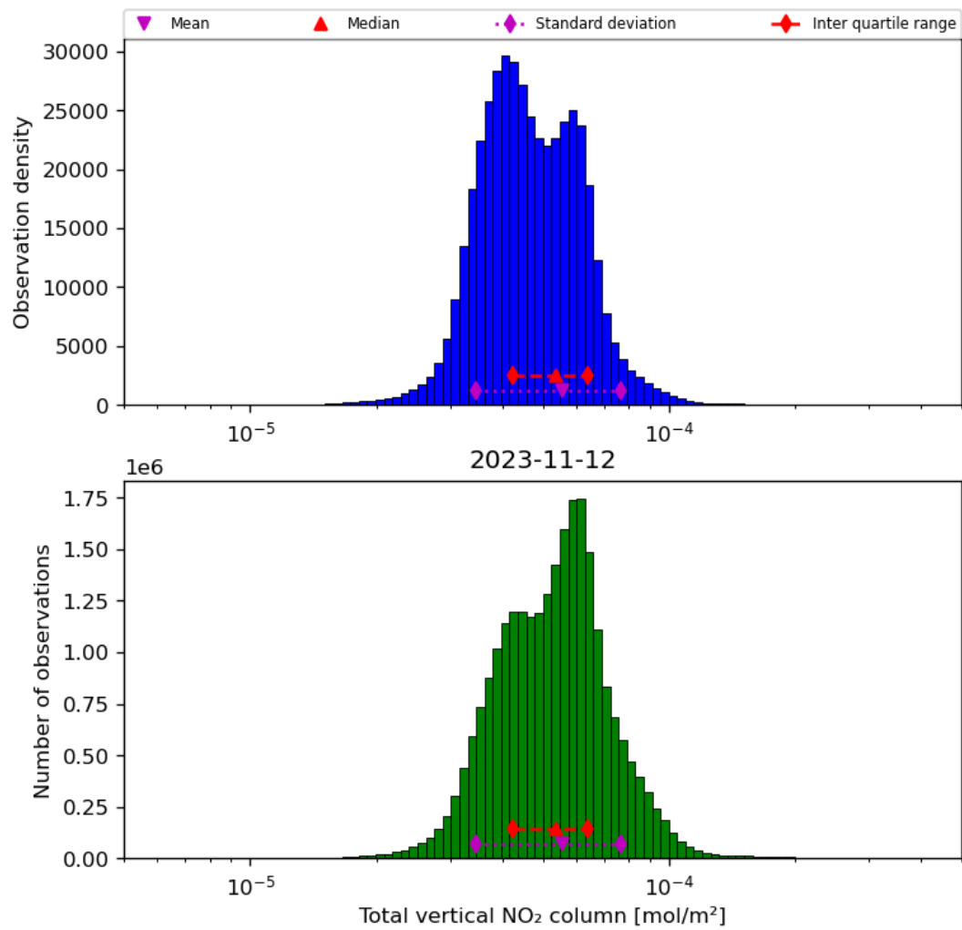
Figure 38: Histogram of “Total vertical NO 2 column” for 2023-11-12 to 2023-11-13
