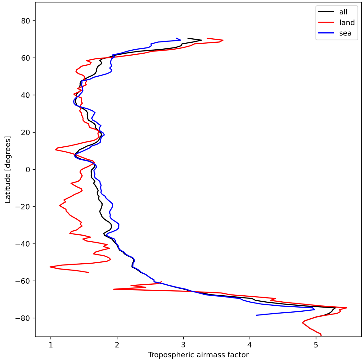
Figure 14: Zonal average of “Tropospheric airmass factor” for 2023-11-12 to 2023-11-13.
