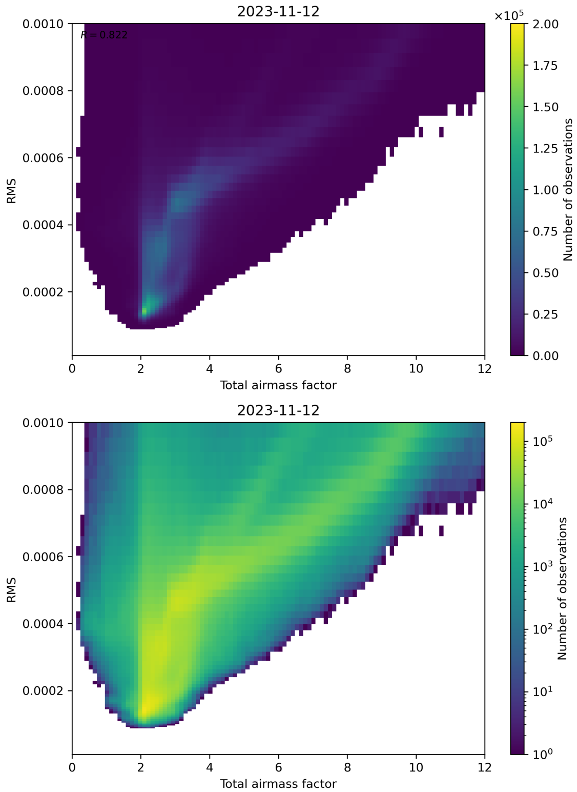
Figure 69: Scatter density plot of “Total airmass factor” against “RMS” for 2023-11-12 to 2023-11-13.
