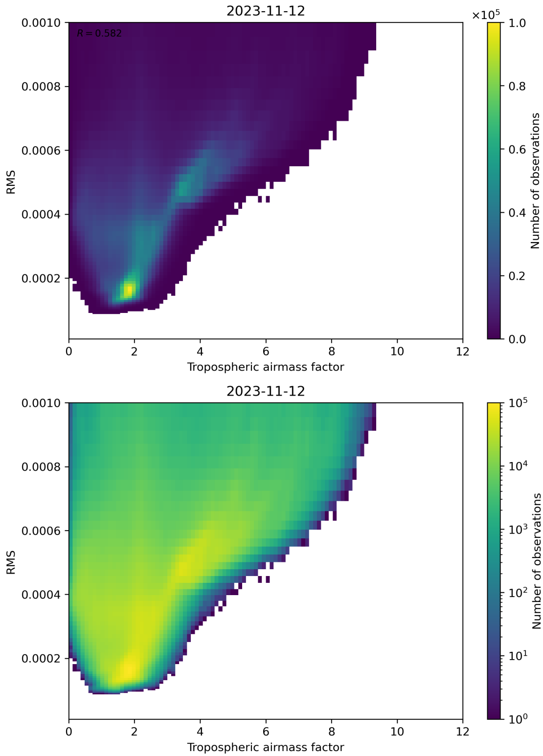
Figure 79: Scatter density plot of “Tropospheric airmass factor” against “RMS” for 2023-11-12 to 2023-11-13.
