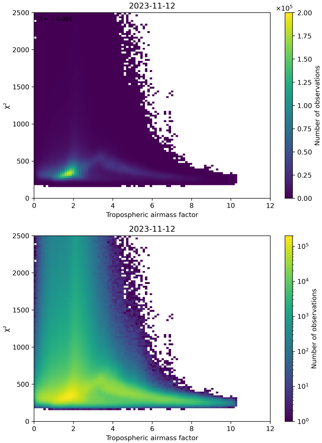
Figure 73: Scatter density plot of “Tropospheric airmass factor” against “ \chi^2 ” for 2023-11-12 to 2023-11-13.
