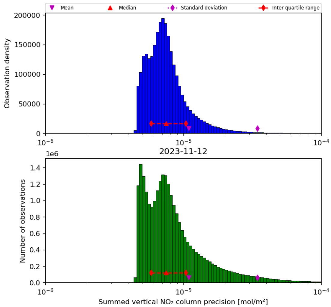
Figure 41: Histogram of “Summed vertical NO 2 column precision” for 2023-11-12 to 2023-11-13
