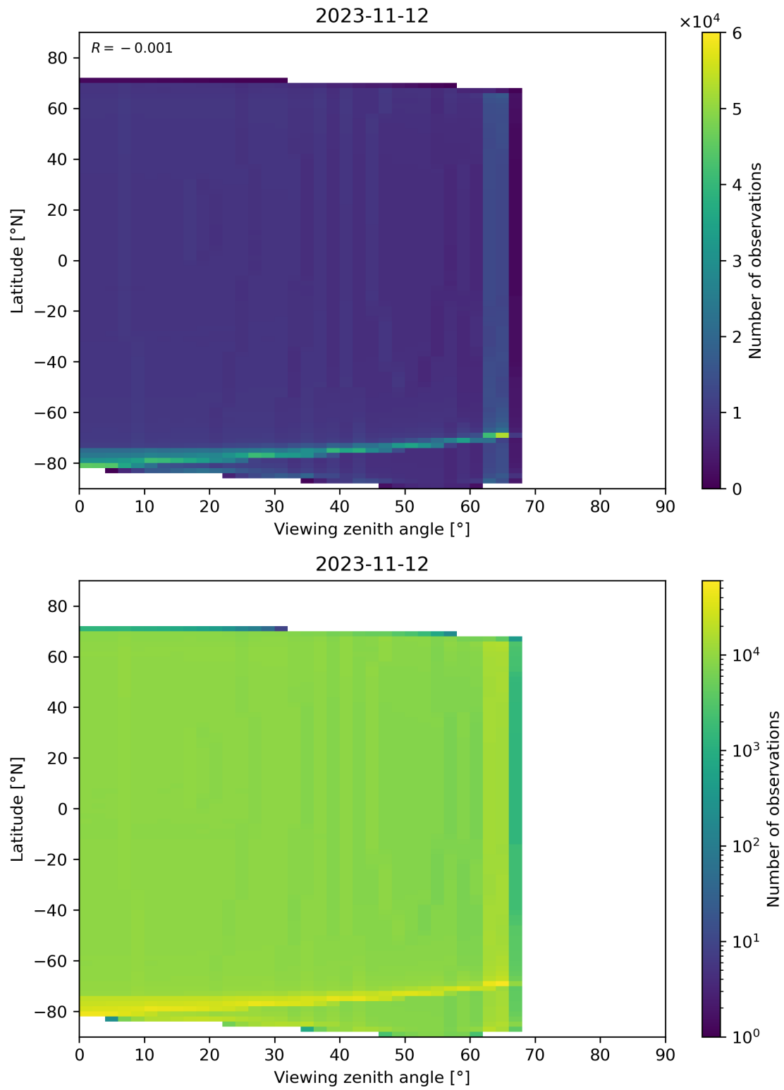
Figure 163: Scatter density plot of “Viewing zenith angle” against “Latitude” for 2023-11-12 to 2023-11-13.
