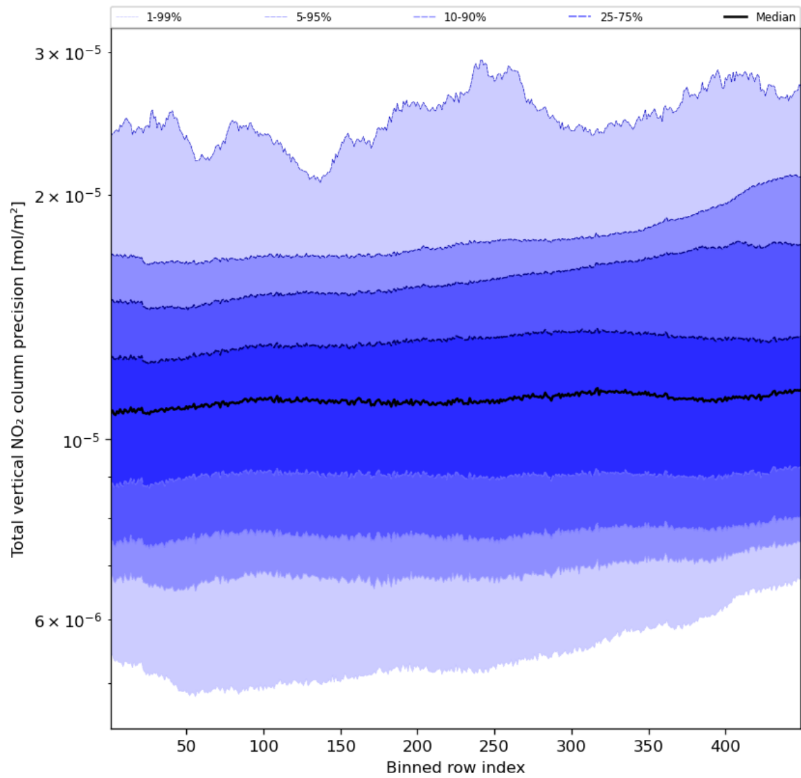
Figure 56: Along track statistics of “Total vertical NO 2 column precision” for 2023-11-12 to 2023-11-13
