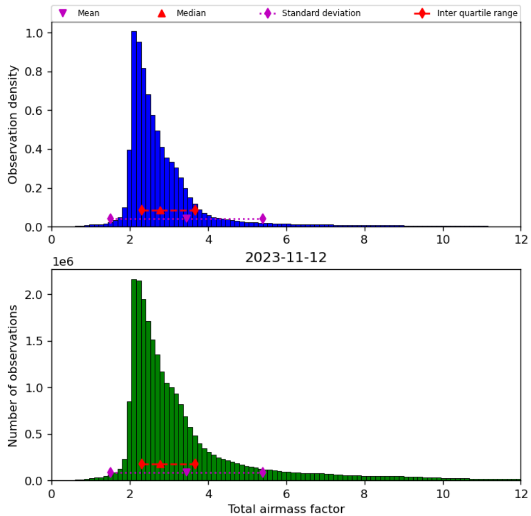
Figure 32: Histogram of “Total airmass factor” for 2023-11-12 to 2023-11-13
