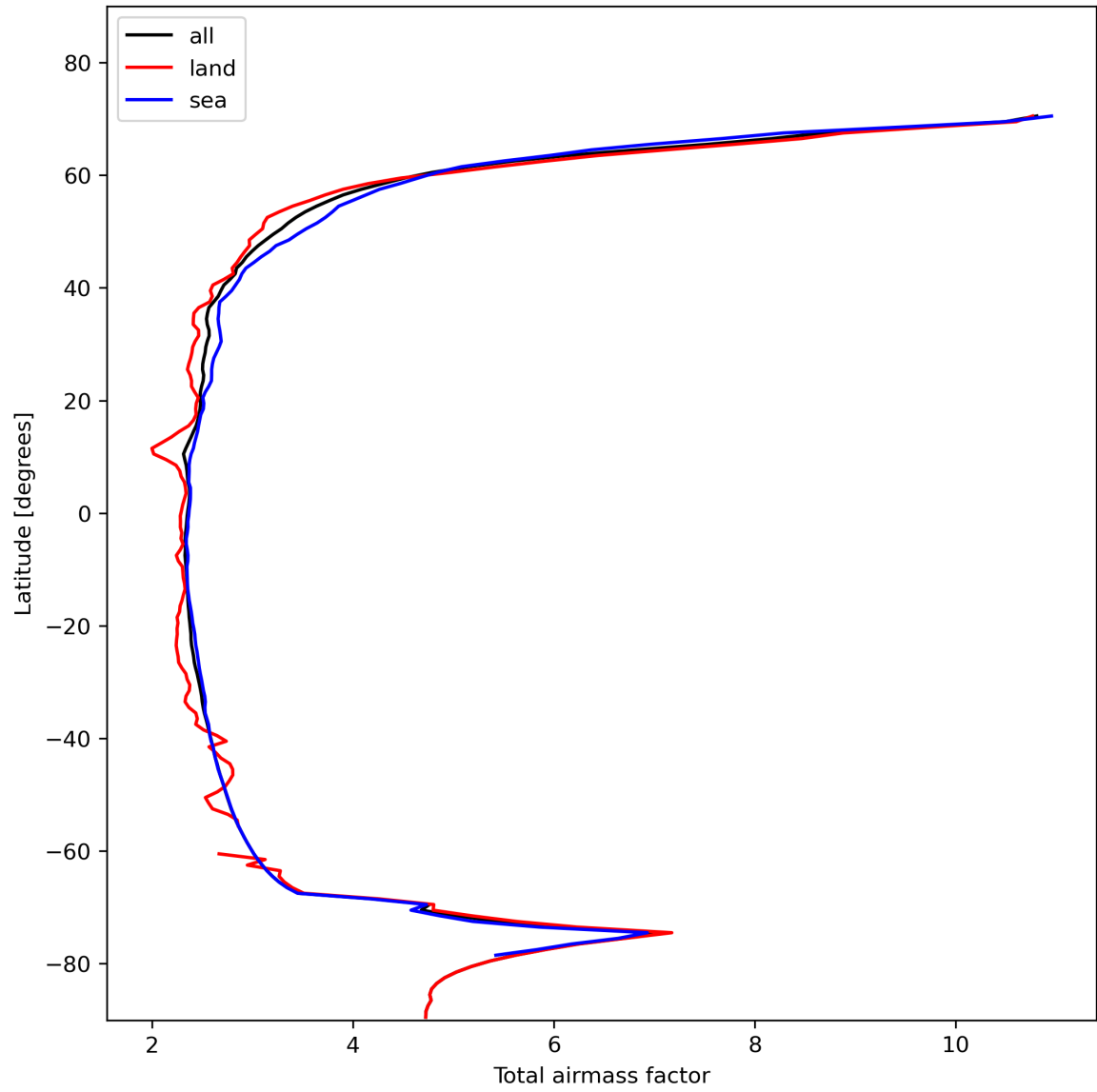
Figure 15: Zonal average of “Total airmass factor” for 2023-11-12 to 2023-11-13.
