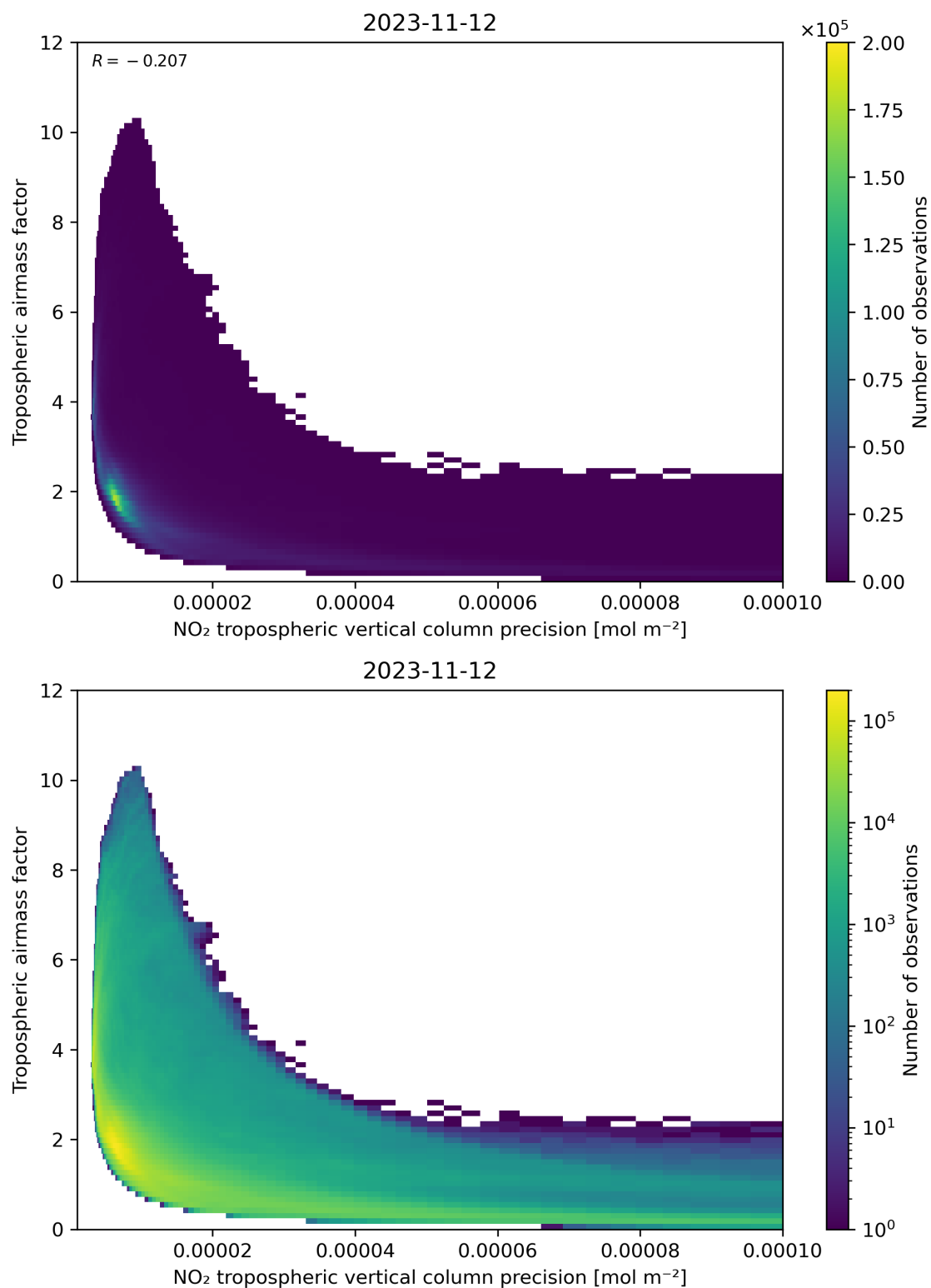
Figure 133: Scatter density plot of “NO 2 tropospheric vertical column precision” against “Tropospheric airmass factor” for 2023-11-12 to 2023-11-13.
