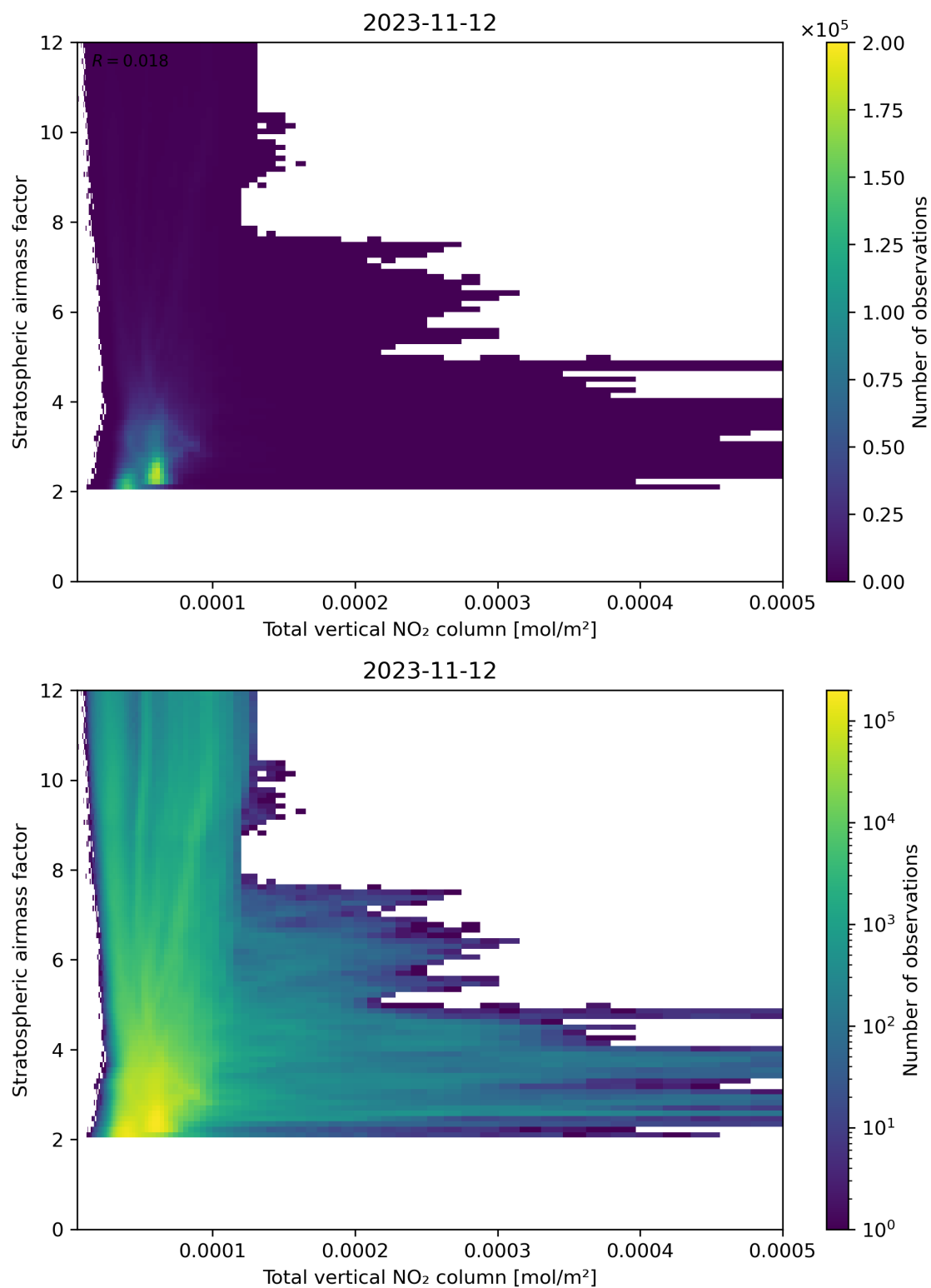
Figure 110: Scatter density plot of “Total vertical NO 2 column” against “Stratospheric airmass factor” for 2023-11-12 to 2023-11-13.
