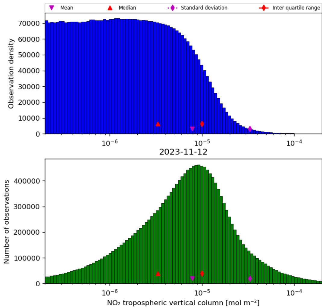
Figure 29: Histogram of “NO 2 tropospheric vertical column” for 2023-11-12 to 2023-11-13
