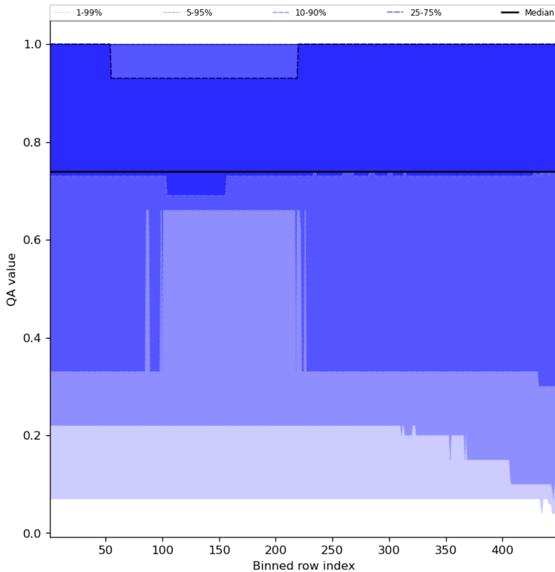
Figure 45: Along track statistics of “QA value” for 2023-11-12 to 2023-11-13
