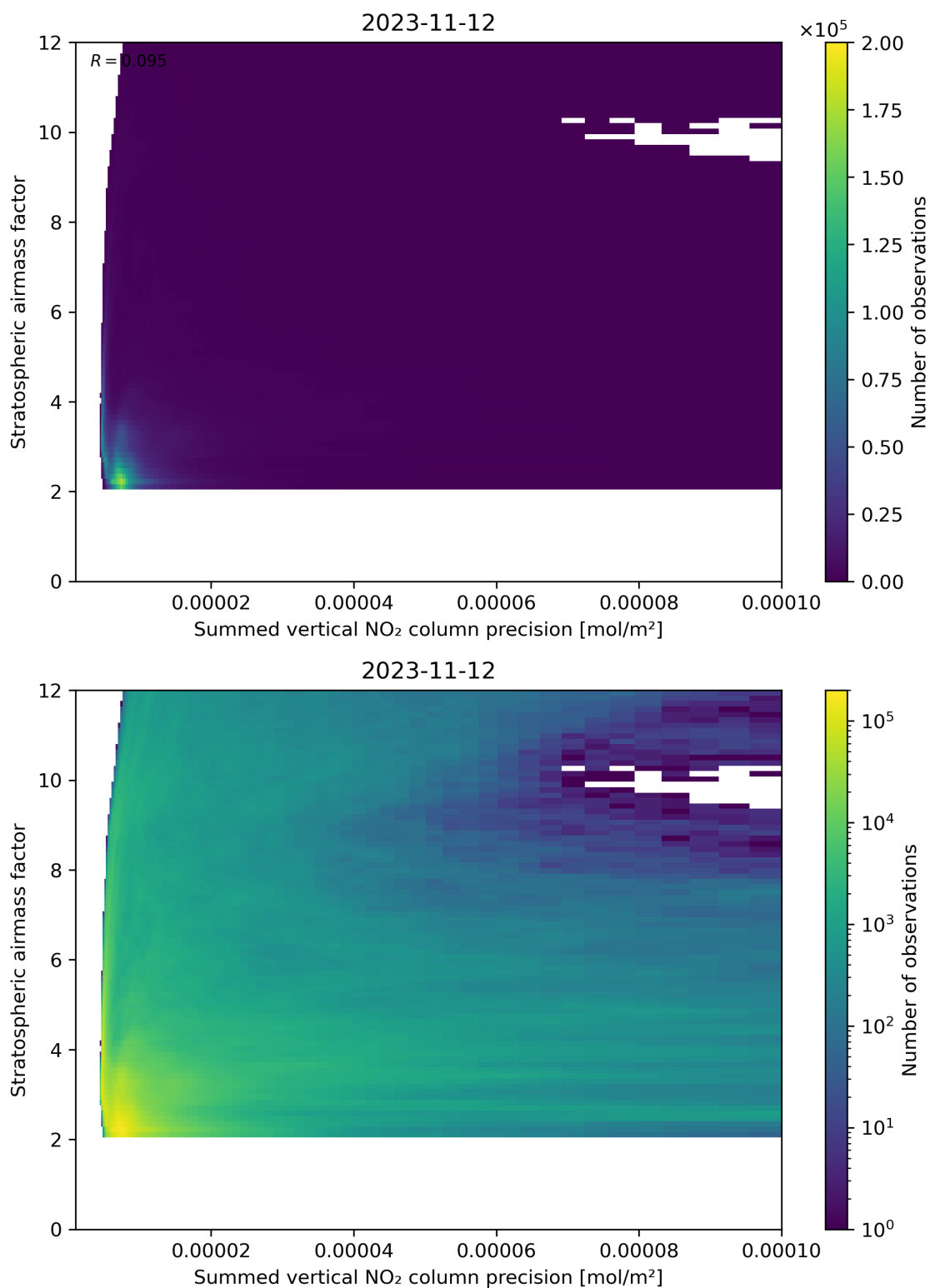
Figure 106: Scatter density plot of “Summed vertical NO 2 column precision” against “Stratospheric airmass factor” for 2023-11-12 to 2023-11-13.
