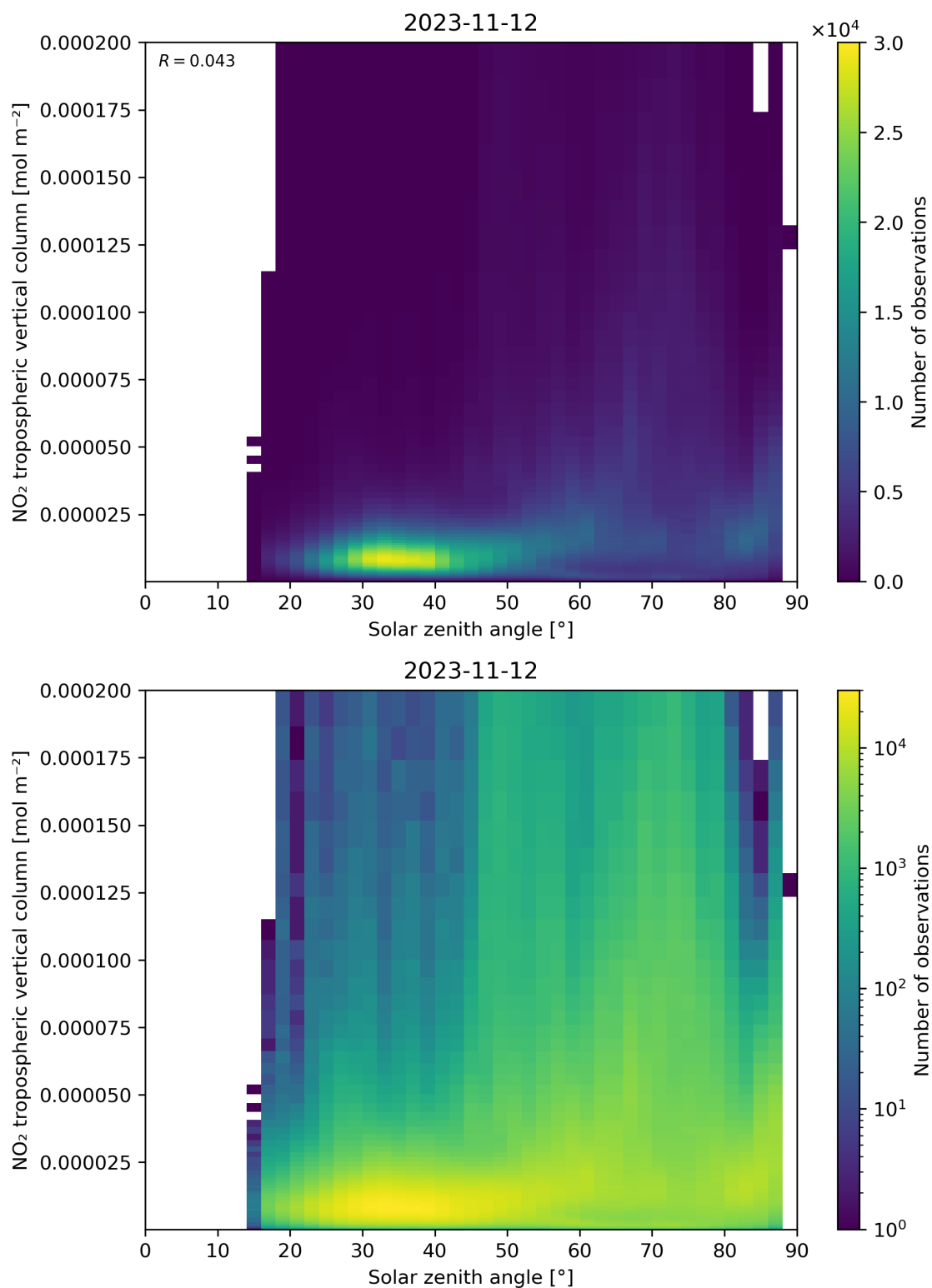
Figure 155: Scatter density plot of “Solar zenith angle” against “NO 2 tropospheric vertical column” for 2023-11-12 to 2023-11-13.
