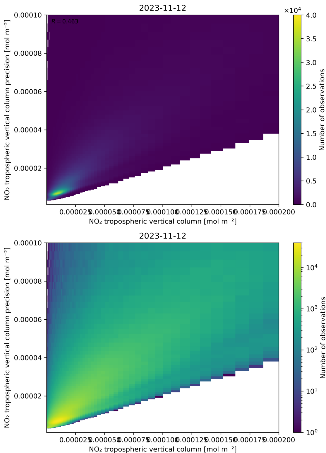
Figure 130: Scatter density plot of “NO 2 tropospheric vertical column” against “NO 2 tropospheric vertical column precision” for 2023-11-12 to 2023-11-13.
