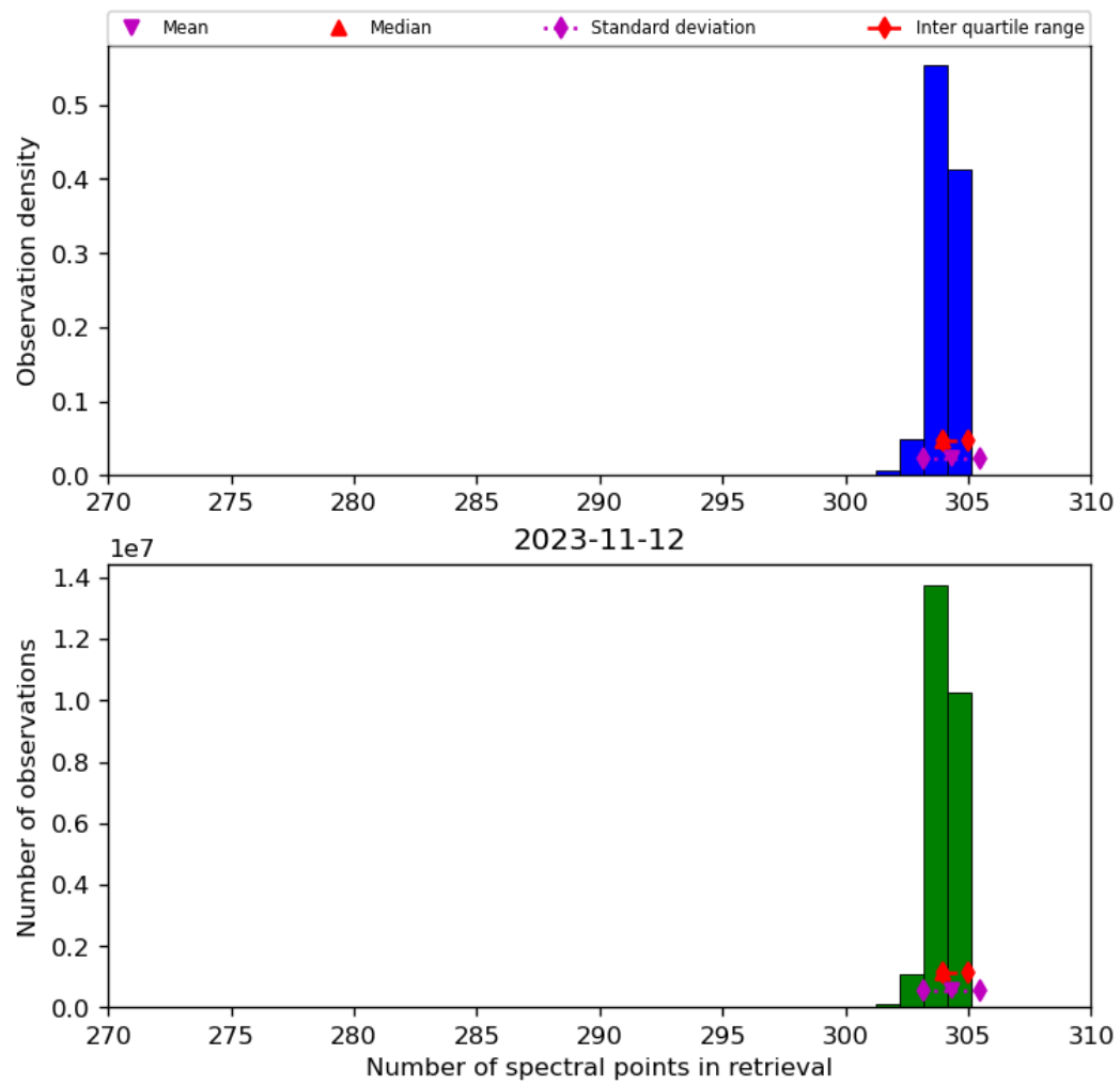
Figure 33: Histogram of “Number of spectral points in retrieval” for 2023-11-12 to 2023-11-13
