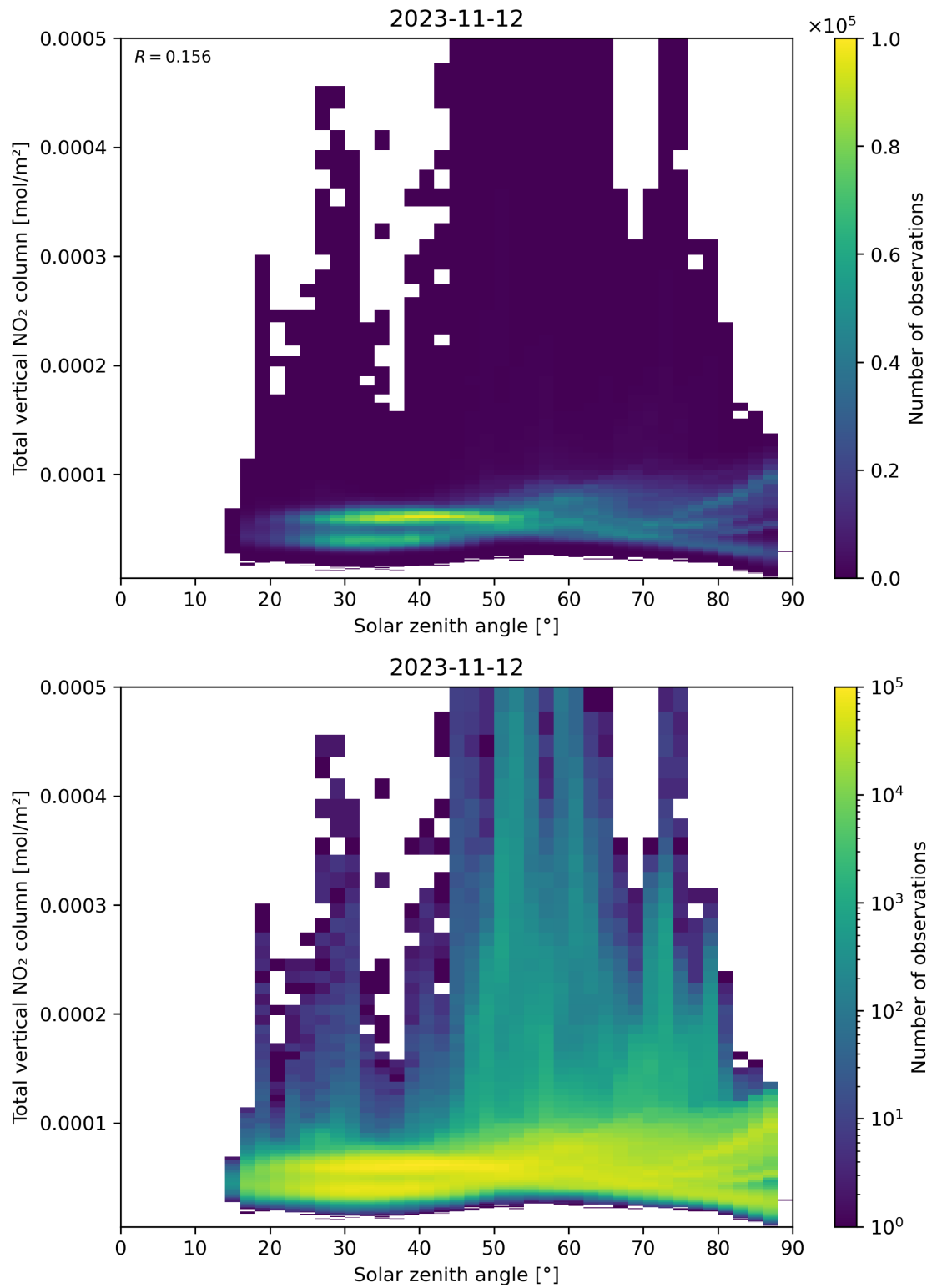
Figure 153: Scatter density plot of “Solar zenith angle” against “Total vertical NO 2 column” for 2023-11-12 to 2023-11-13.
