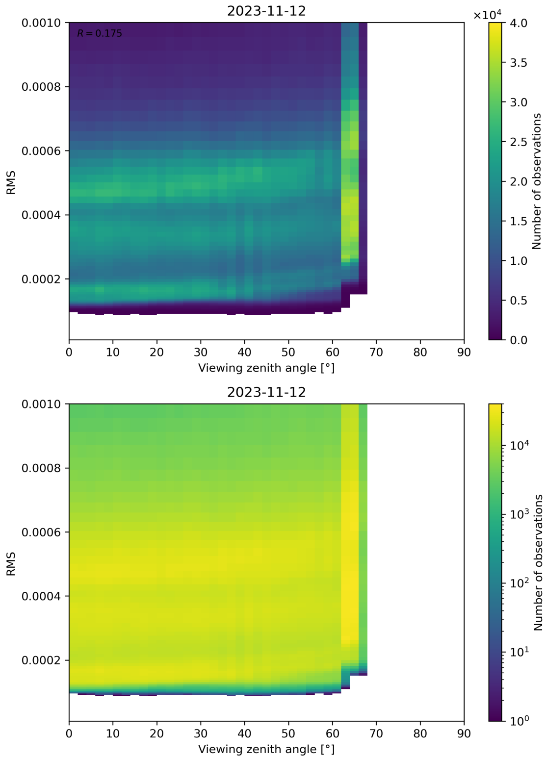
Figure 171: Scatter density plot of “Viewing zenith angle” against “RMS” for 2023-11-12 to 2023-11-13.
