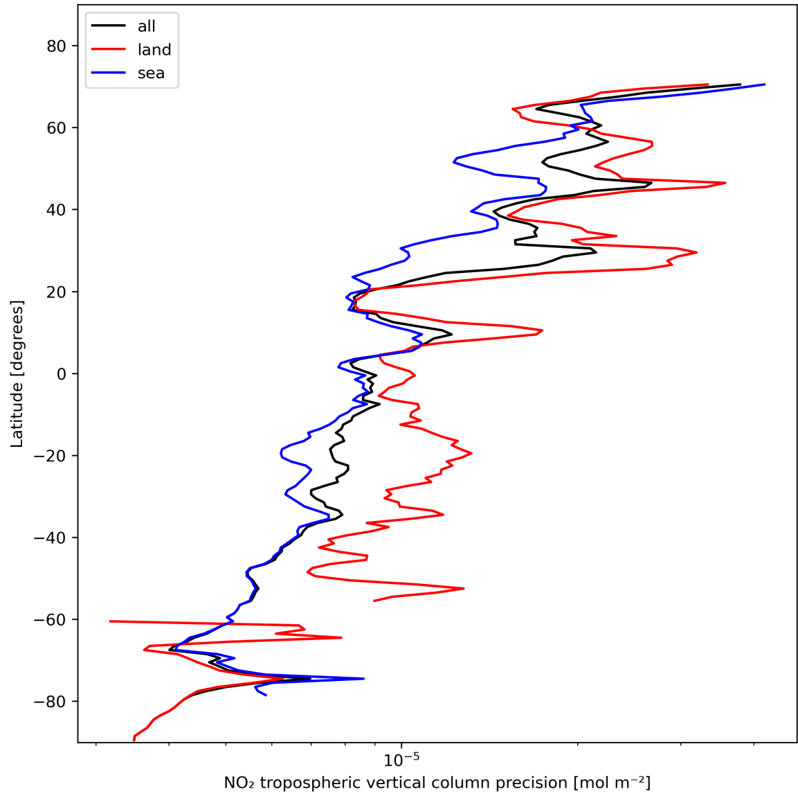
Figure 13: Zonal average of “NO 2 tropospheric vertical column precision” for 2023-11-12 to 2023-11-13.
