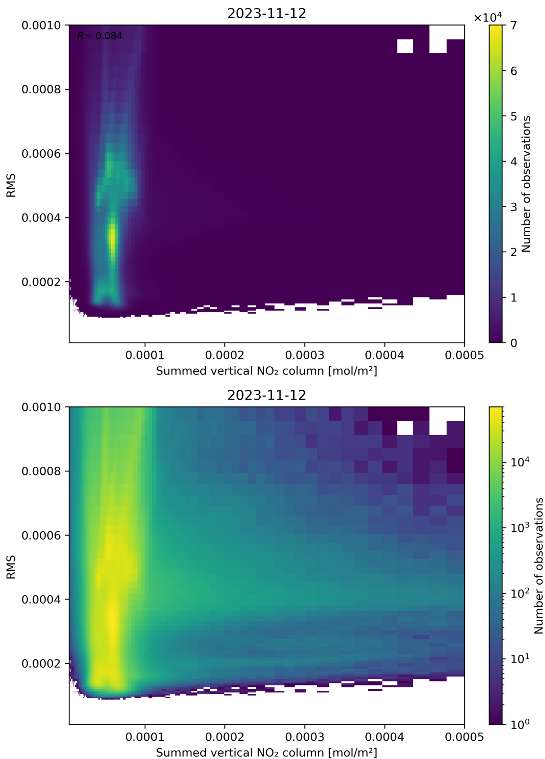
Figure 109: Scatter density plot of “Summed vertical NO 2 column” against “RMS” for 2023-11-12 to 2023-11-13.
