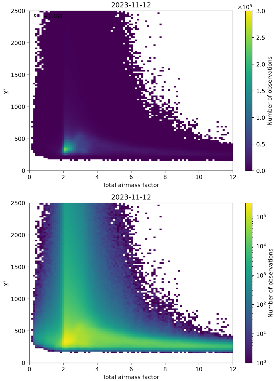
Figure 63: Scatter density plot of “Total airmass factor” against “ \chi^2 ” for 2023-11-12 to 2023-11-13.
