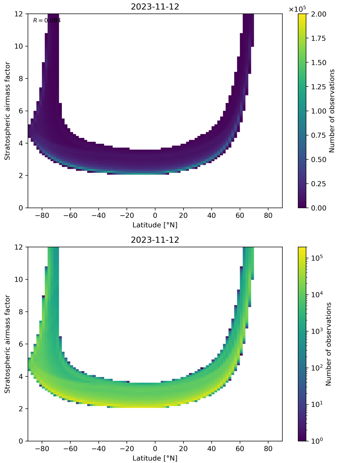
Figure 83: Scatter density plot of “Latitude” against “Stratospheric air mass factor” for 2023-11-12 to 2023-11-13.
