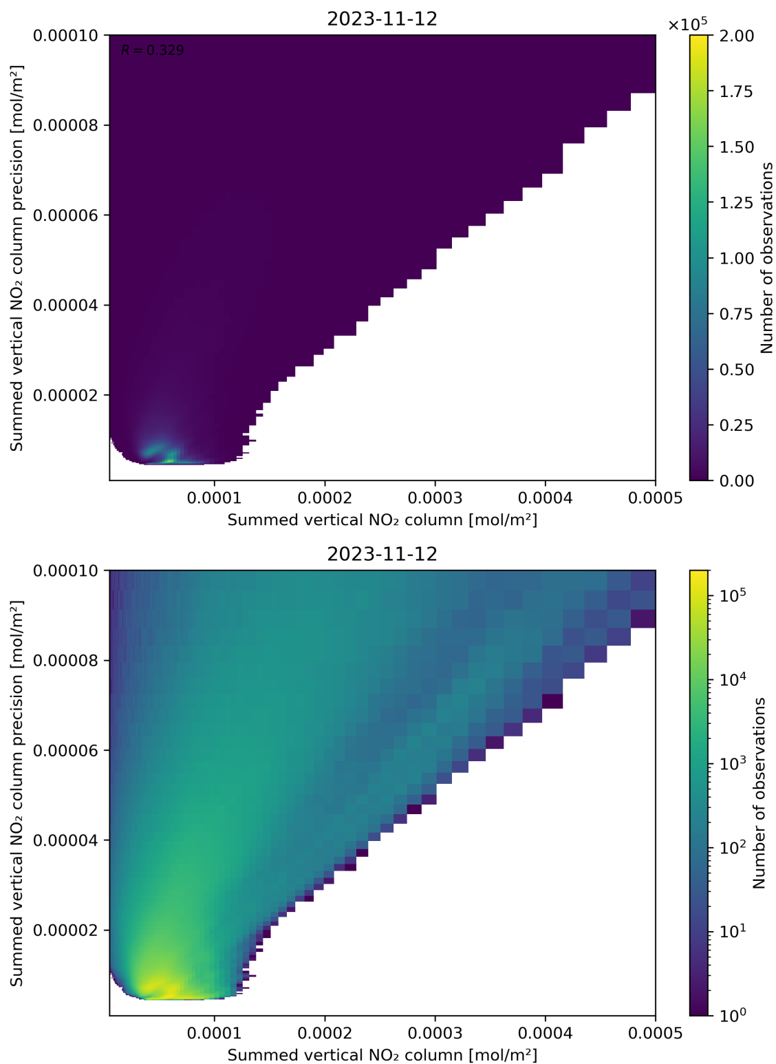
Figure 105: Scatter density plot of “Summed vertical NO 2 column” against “Summed vertical NO 2 column precision” for 2023-11-12 to 2023-11-13.
