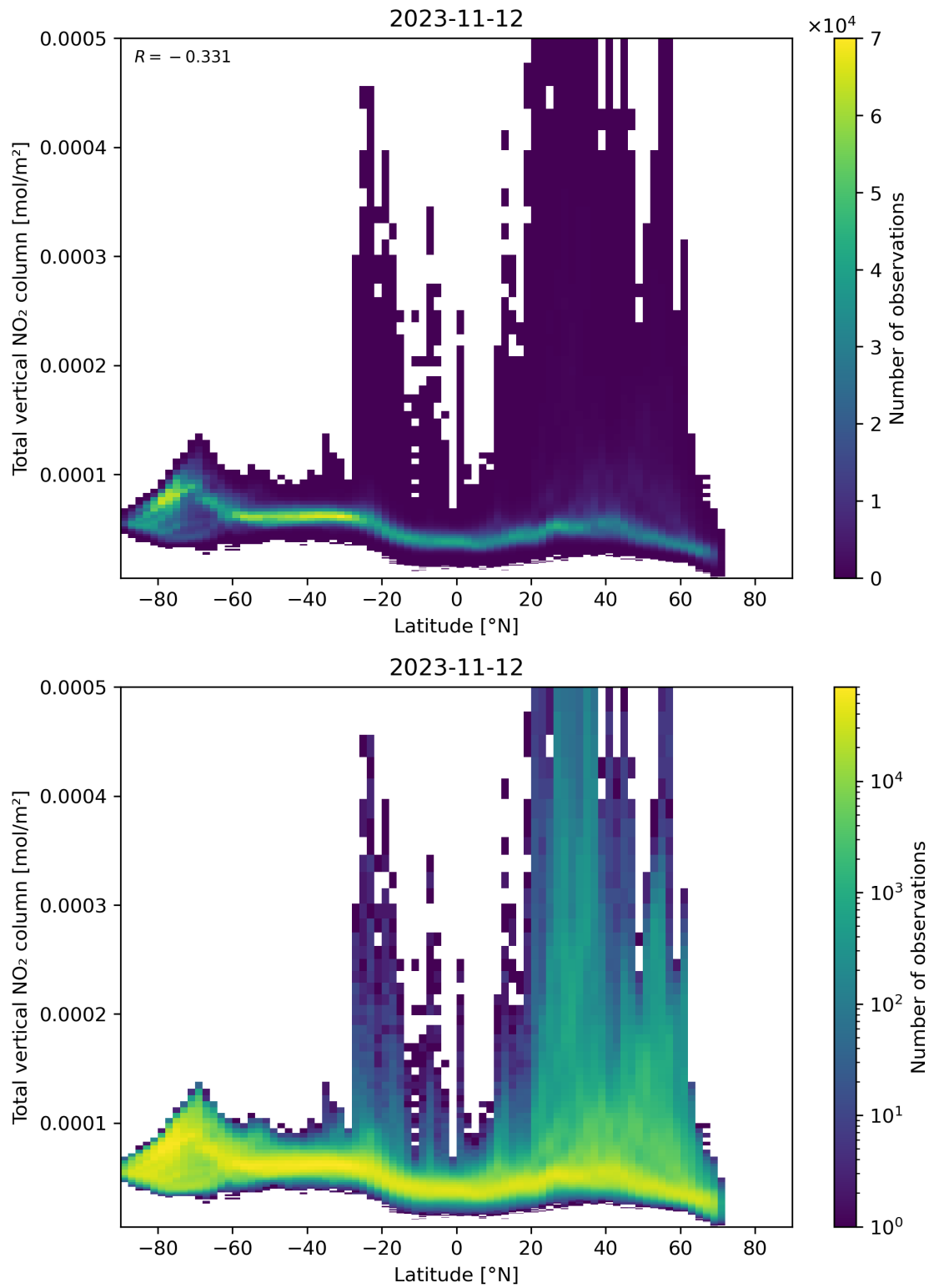
Figure 90: Scatter density plot of “Latitude” against “Total vertical NO 2 column” for 2023-11-12 to 2023-11-13.
