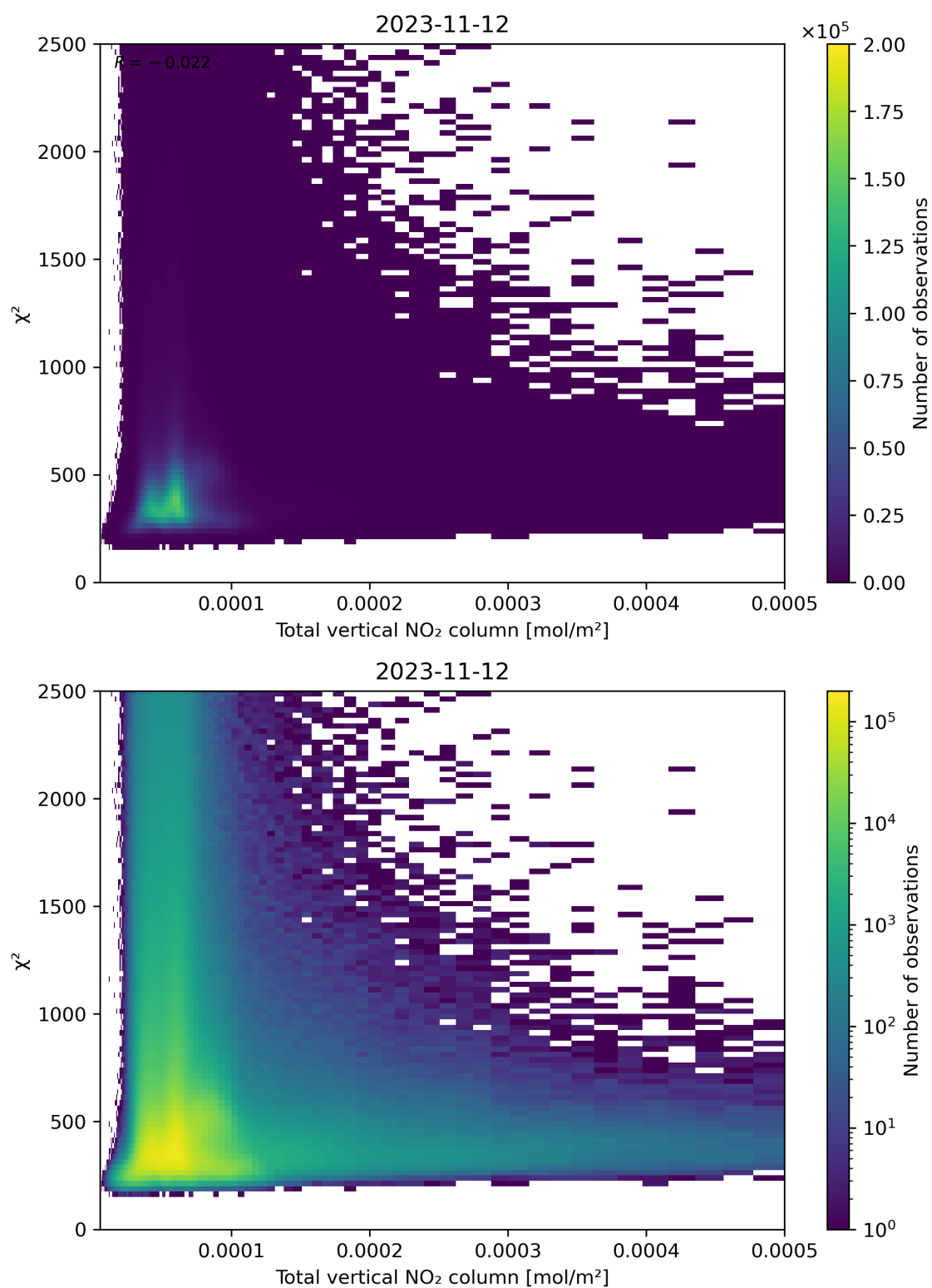
Figure 111: Scatter density plot of “Total vertical NO 2 column” against “ \chi^2 ” for 2023-11-12 to 2023-11-13.
