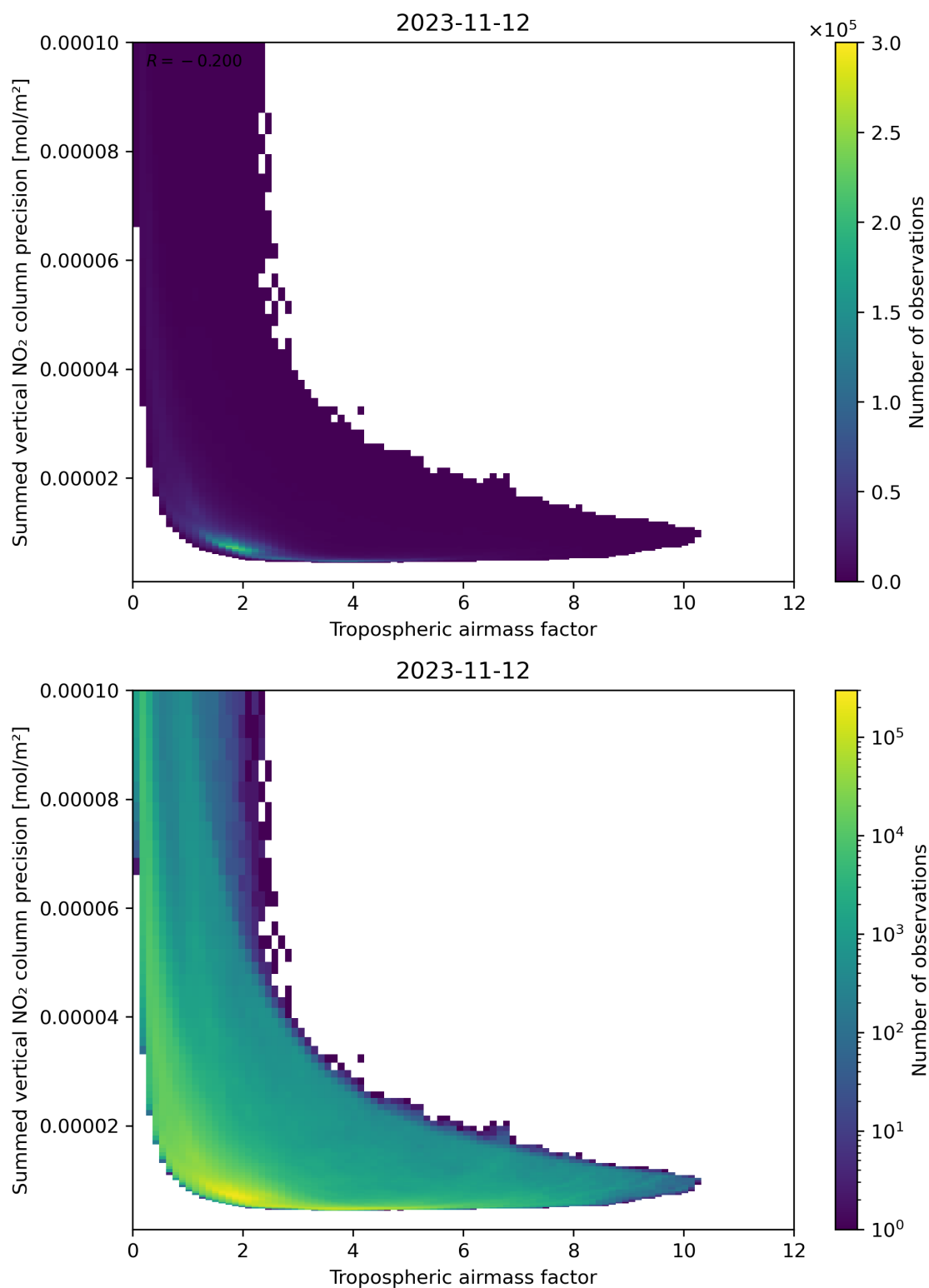
Figure 76: Scatter density plot of “Tropospheric air mass factor” against “Summed vertical NO 2 column precision” for 2023-11-12 to 2023-11-13.
