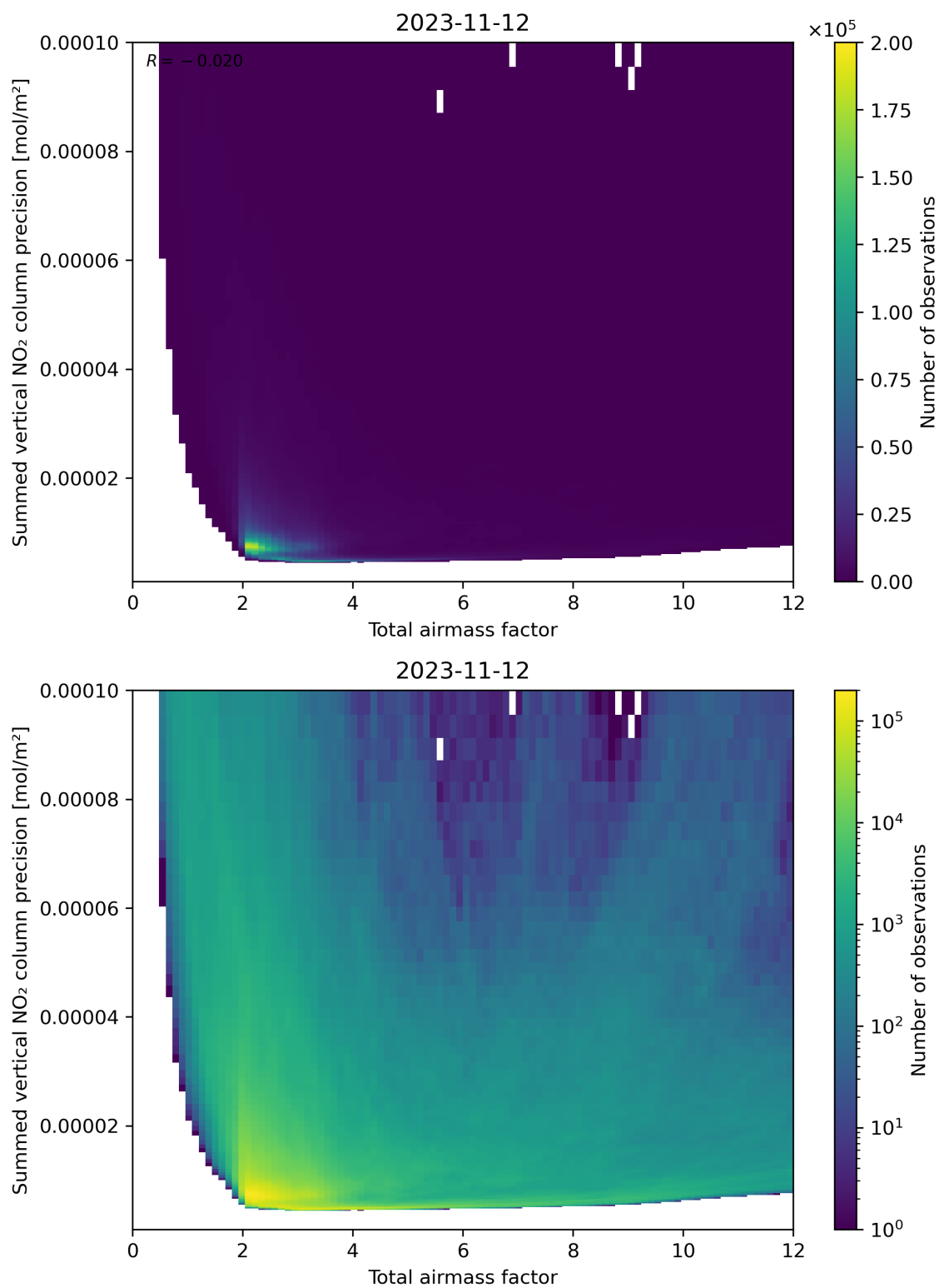
Figure 66: Scatter density plot of “Total airmass factor” against “Summed vertical NO 2 column precision” for 2023-11-12 to 2023-11-13.
