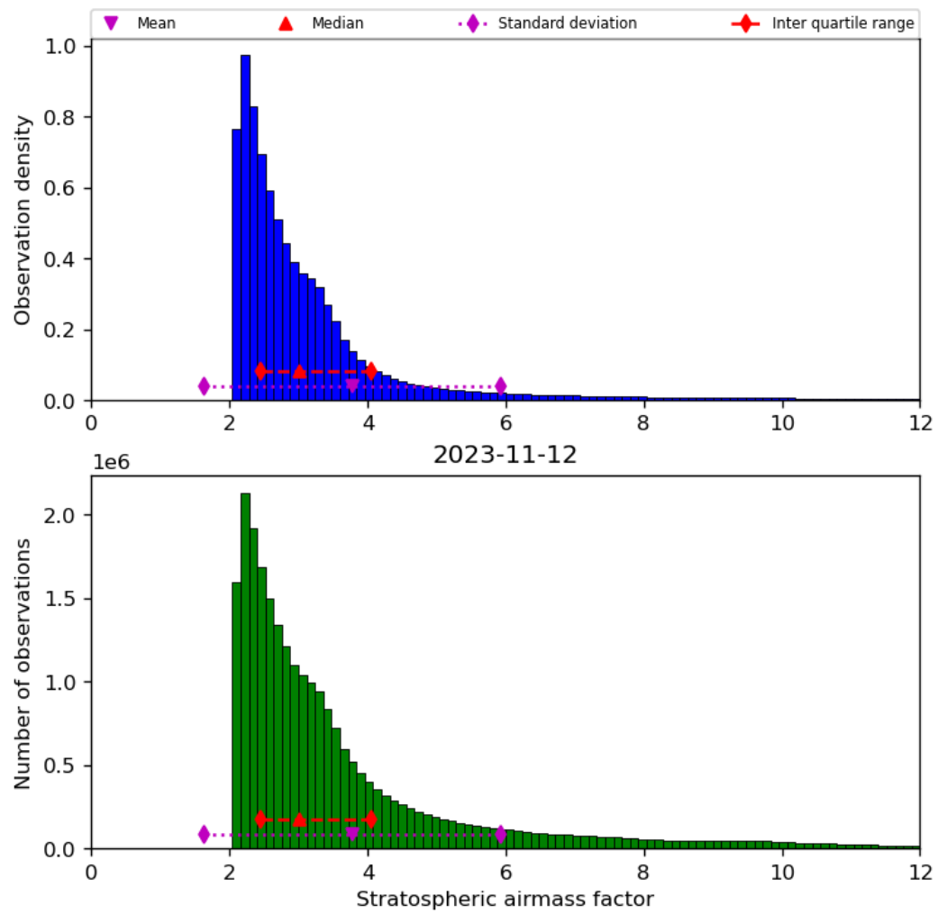
Figure 44: Histogram of “Stratospheric airmass factor” for 2023-11-12 to 2023-11-13
