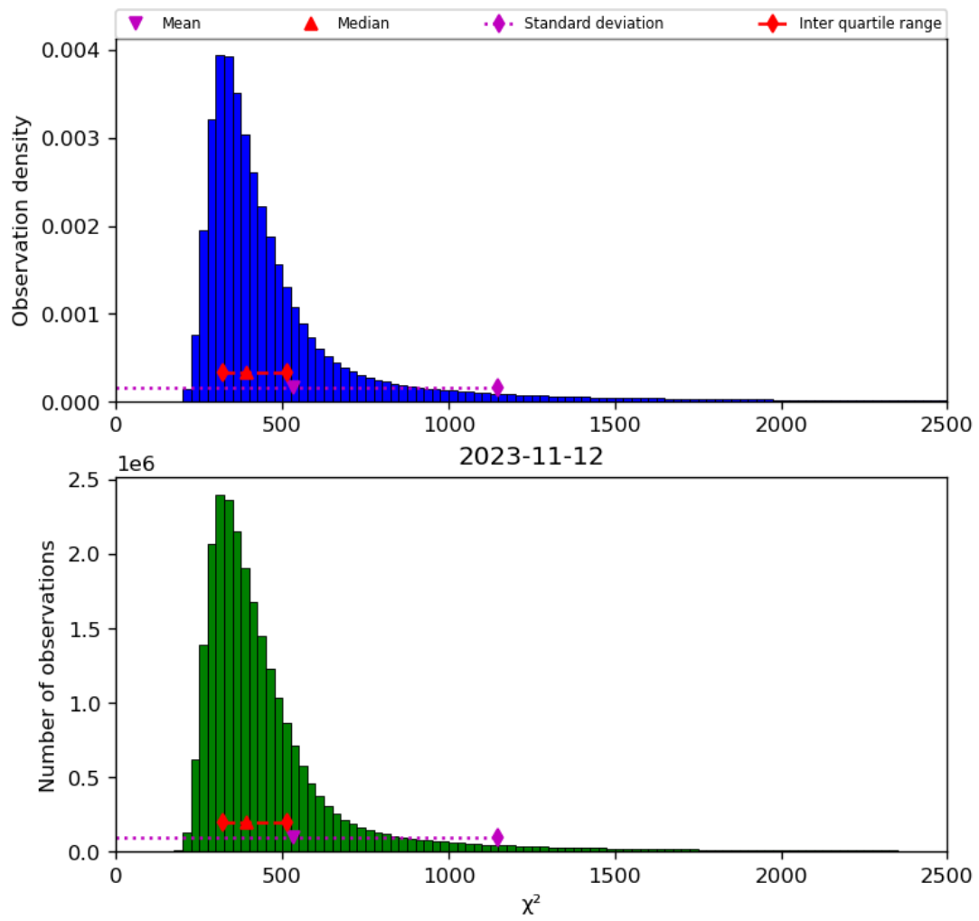
Figure 42: Histogram of “ \chi^2 ” for 2023-11-12 to 2023-11-13
