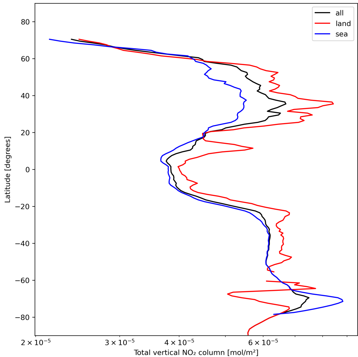
Figure 21: Zonal average of “Total vertical NO 2 column” for 2023-11-12 to 2023-11-13.
