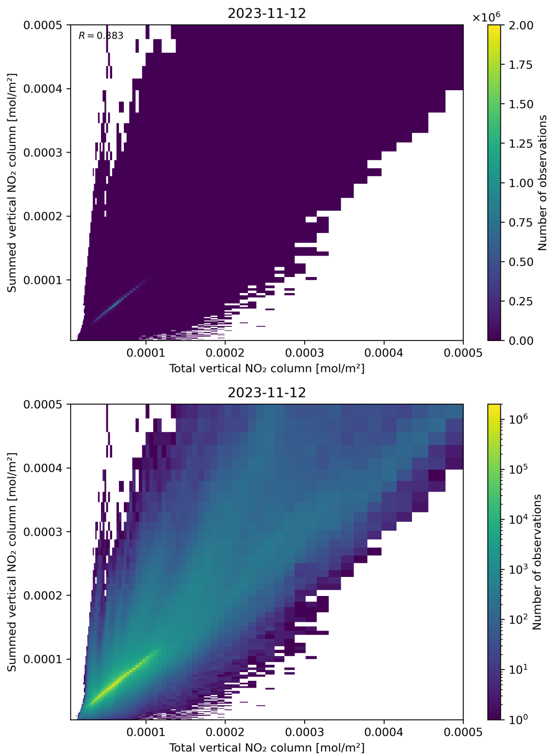
Figure 112: Scatter density plot of “Total vertical NO 2 column” against “Summed vertical NO 2 column” for 2023-11-12 to 2023-11-13.
