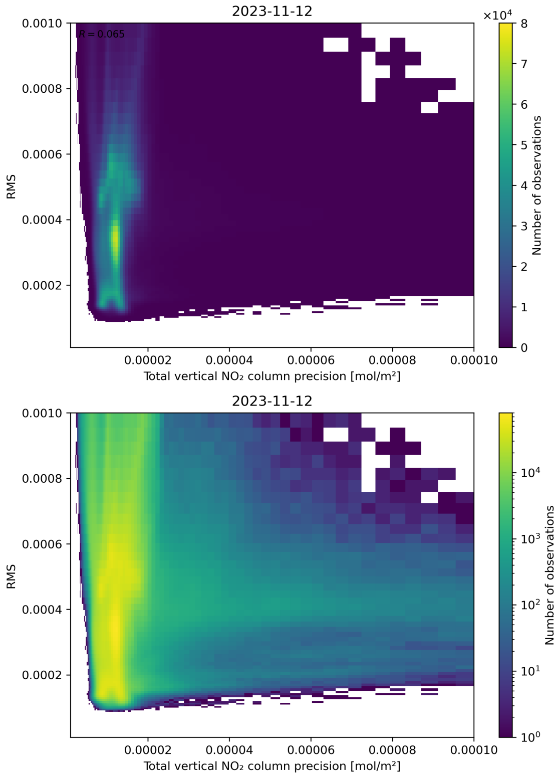
Figure 119: Scatter density plot of “Total vertical NO 2 column precision” against “RMS” for 2023-11-12 to 2023-11-13.
