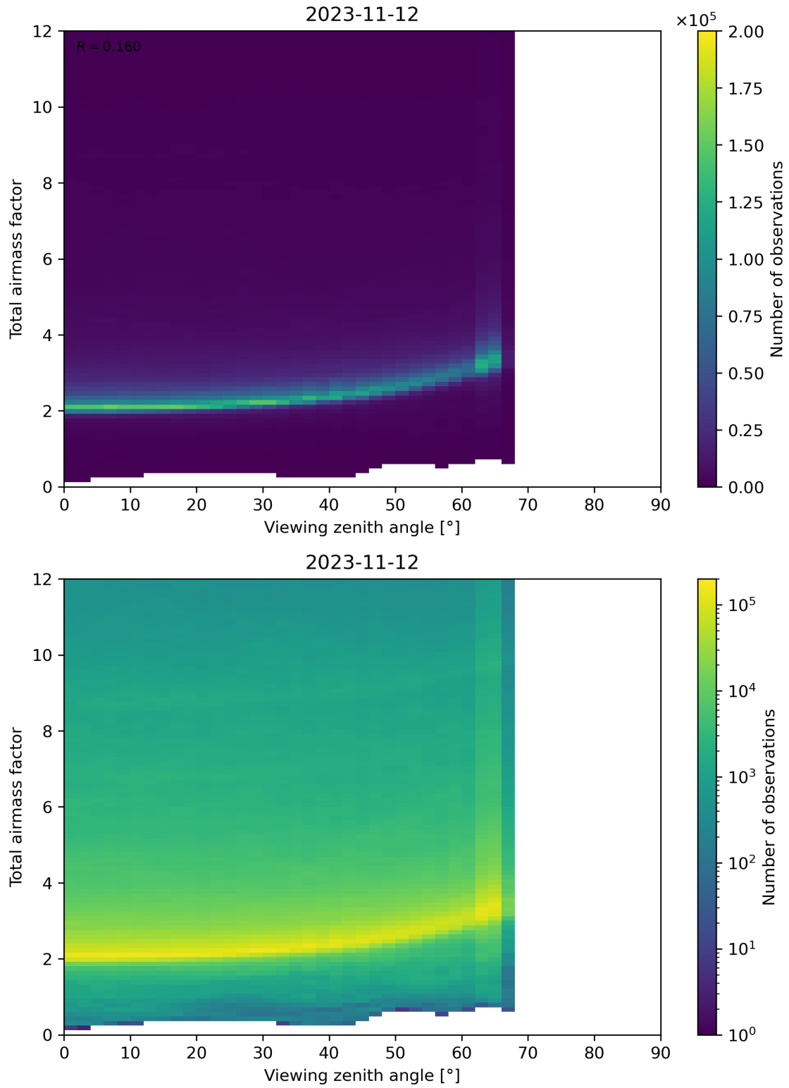
Figure 160: Scatter density plot of “Viewing zenith angle” against “Total airmass factor” for 2023-11-12 to 2023-11-13.
