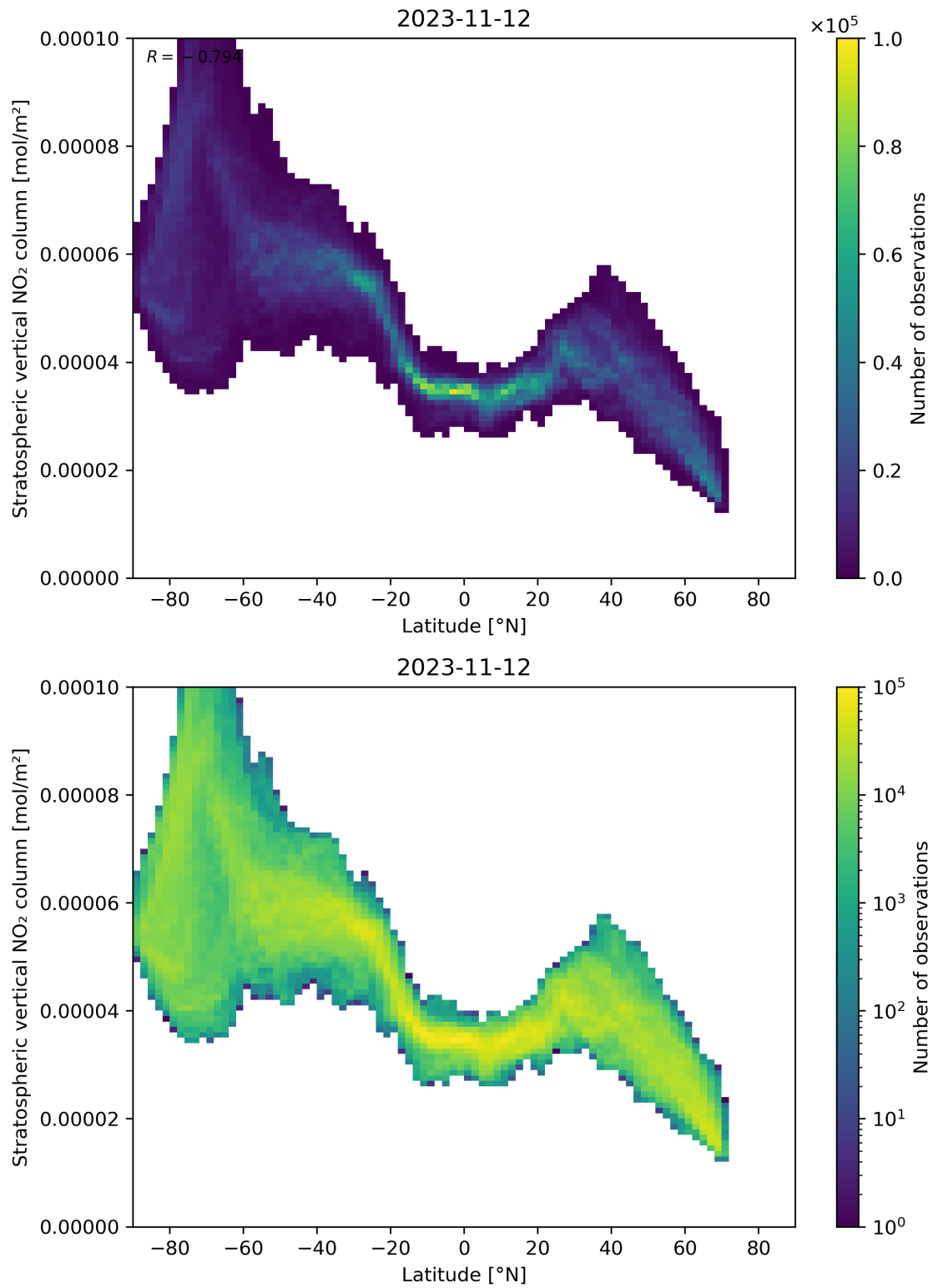
Figure 87: Scatter density plot of “Latitude” against “Stratospheric vertical NO 2 column” for 2023-11-12 to 2023-11-13.
