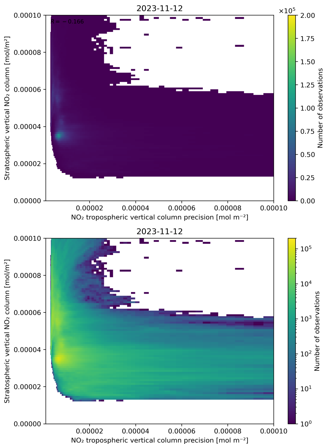
Figure 135: Scatter density plot of “NO 2 tropospheric vertical column precision” against “Stratospheric vertical NO 2 column” for 2023-11-12 to 2023-11-13.
