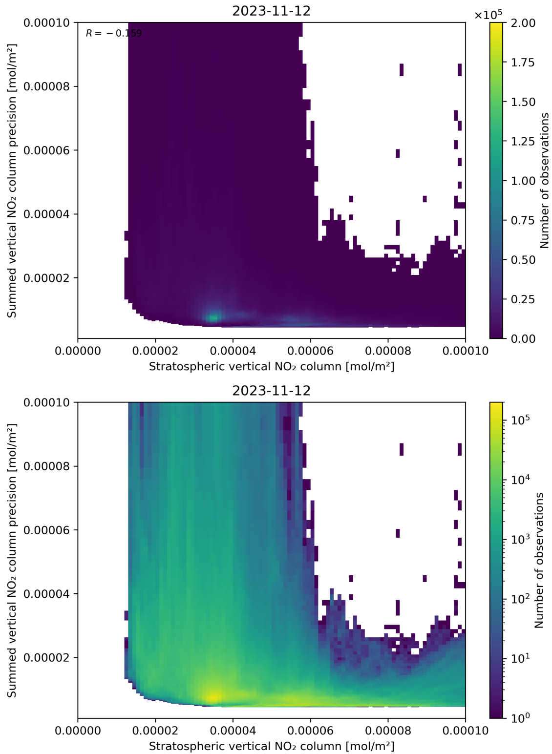
Figure 99: Scatter density plot of “Stratospheric vertical NO 2 column” against “Summed vertical NO 2 column precision” for 2023-11-12 to 2023-11-13.
