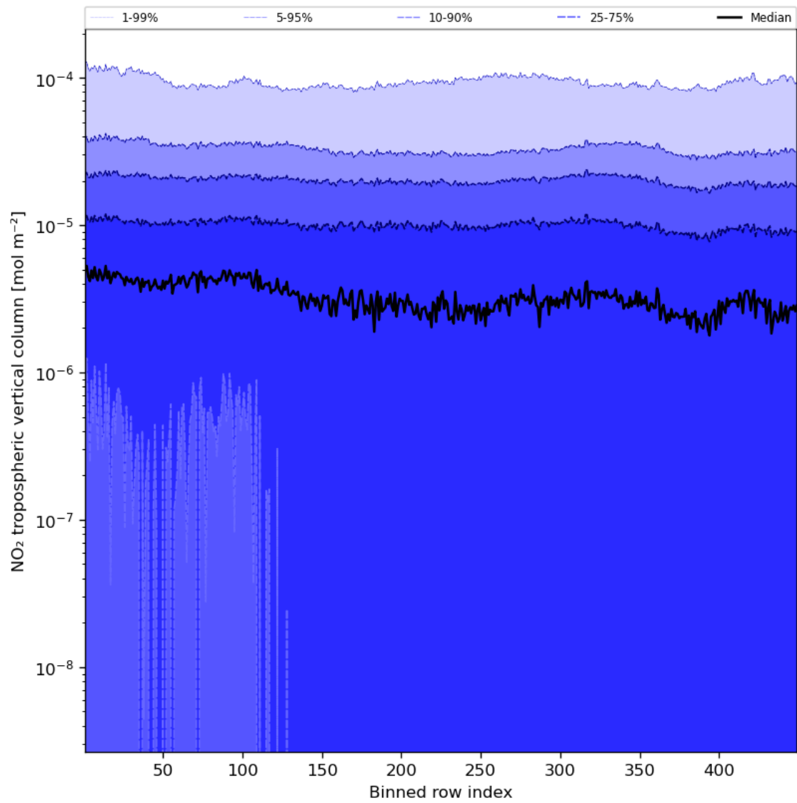
Figure 46: Along track statistics of “NO 2 tropospheric vertical column” for 2023-11-12 to 2023-11-13
