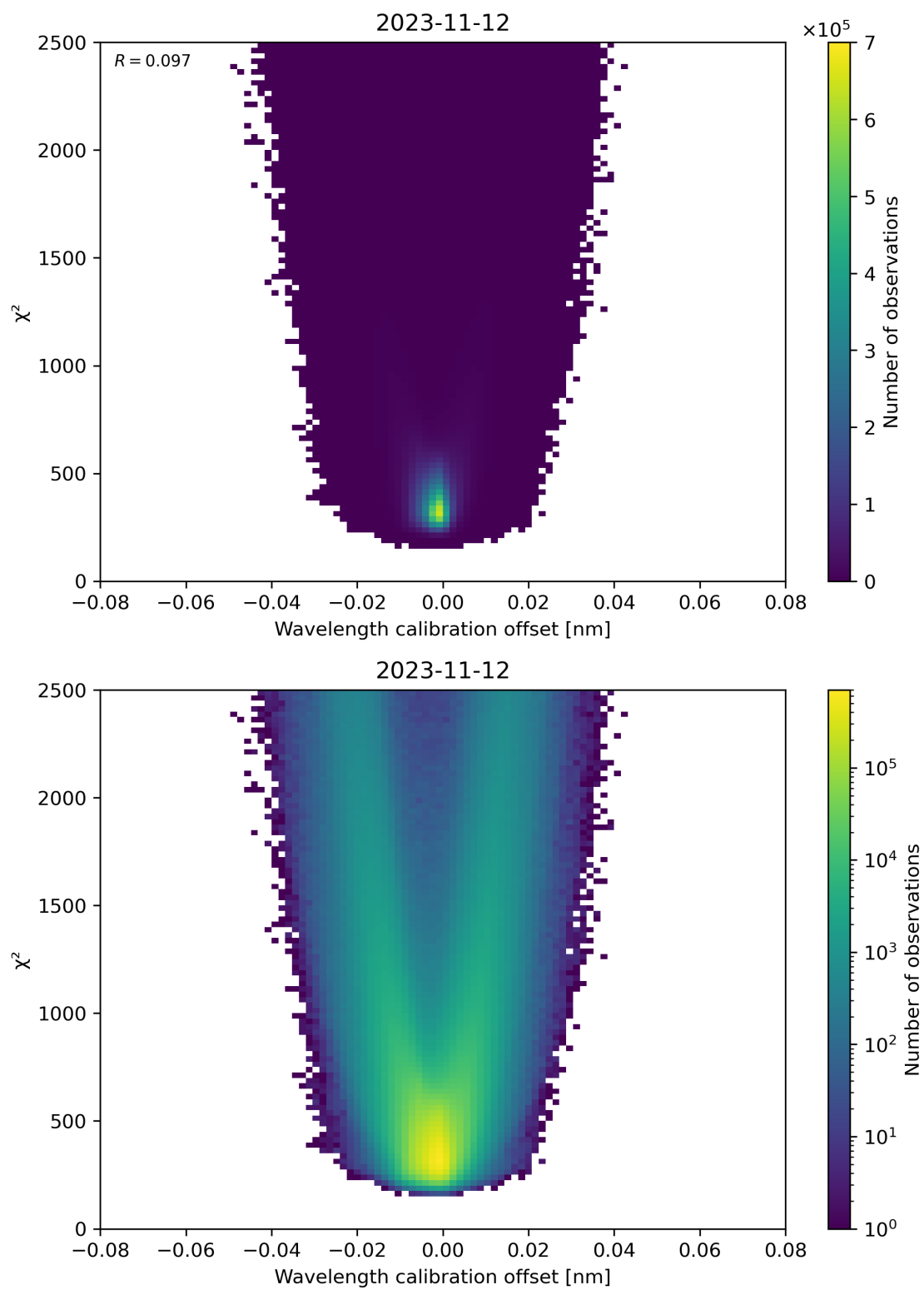
Figure 175: Scatter density plot of “Wavelength calibration offset” against “ \chi^2 ” for 2023-11-12 to 2023-11-13.
