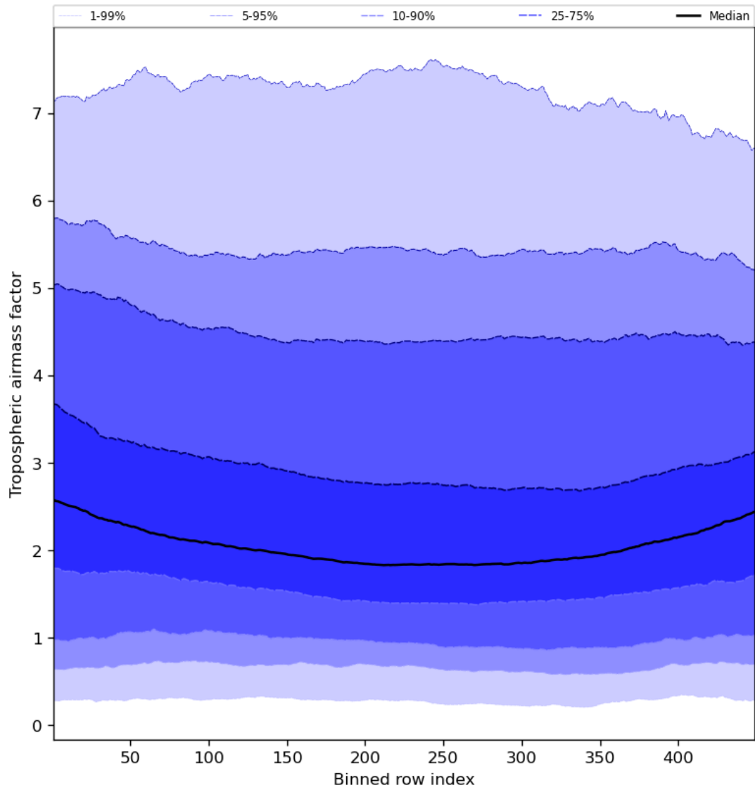
Figure 48: Along track statistics of “Tropospheric airmass factor” for 2023-11-12 to 2023-11-13
