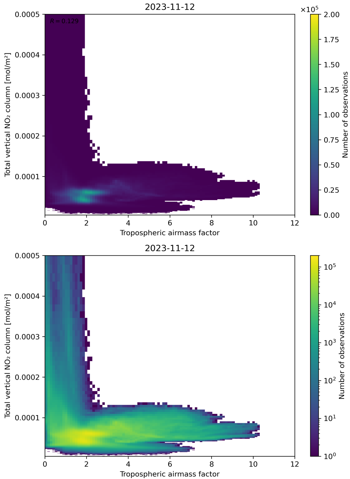
Figure 77: Scatter density plot of “Tropospheric airmass factor” against “Total vertical \text{NO}_2 column” for 2023-11-12 to 2023-11-13.
