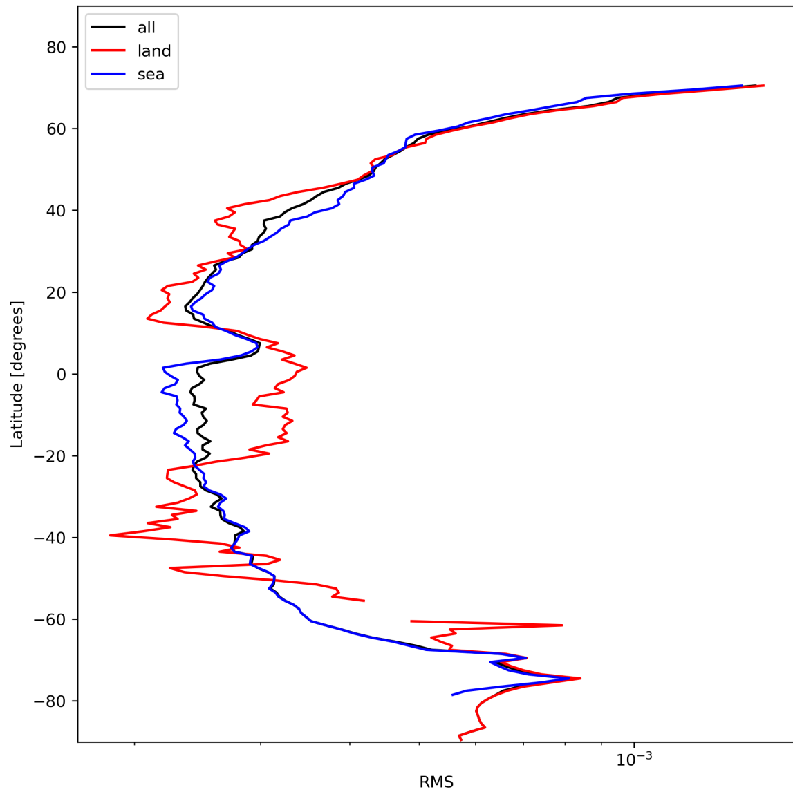
Figure 26: Zonal average of “RMS” for 2023-11-12 to 2023-11-13.
