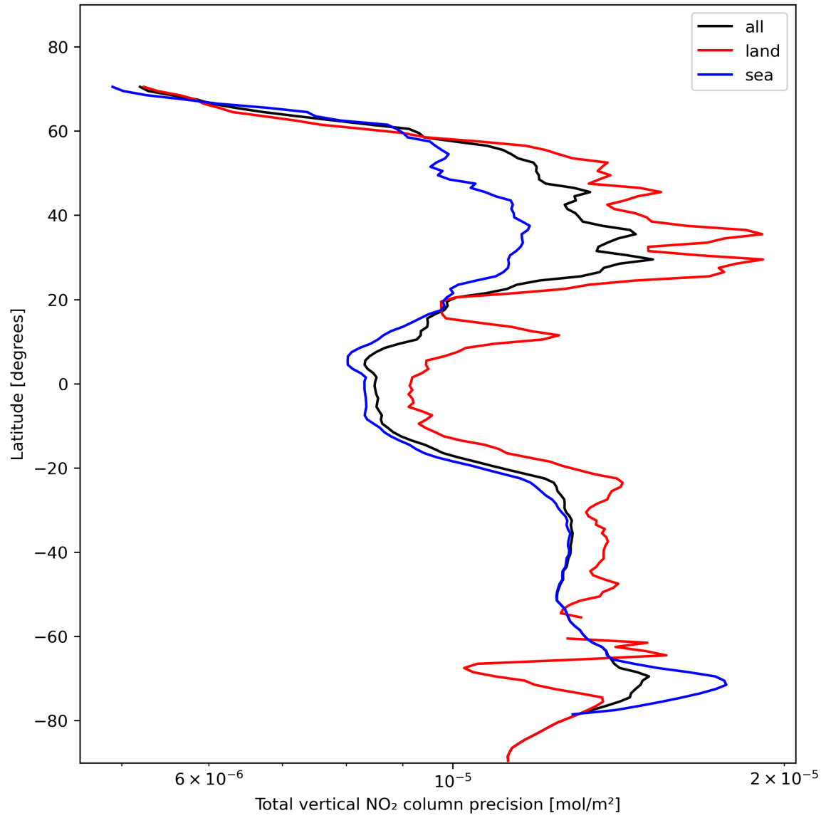
Figure 22: Zonal average of “Total vertical NO 2 column precision” for 2023-11-12 to 2023-11-13.
