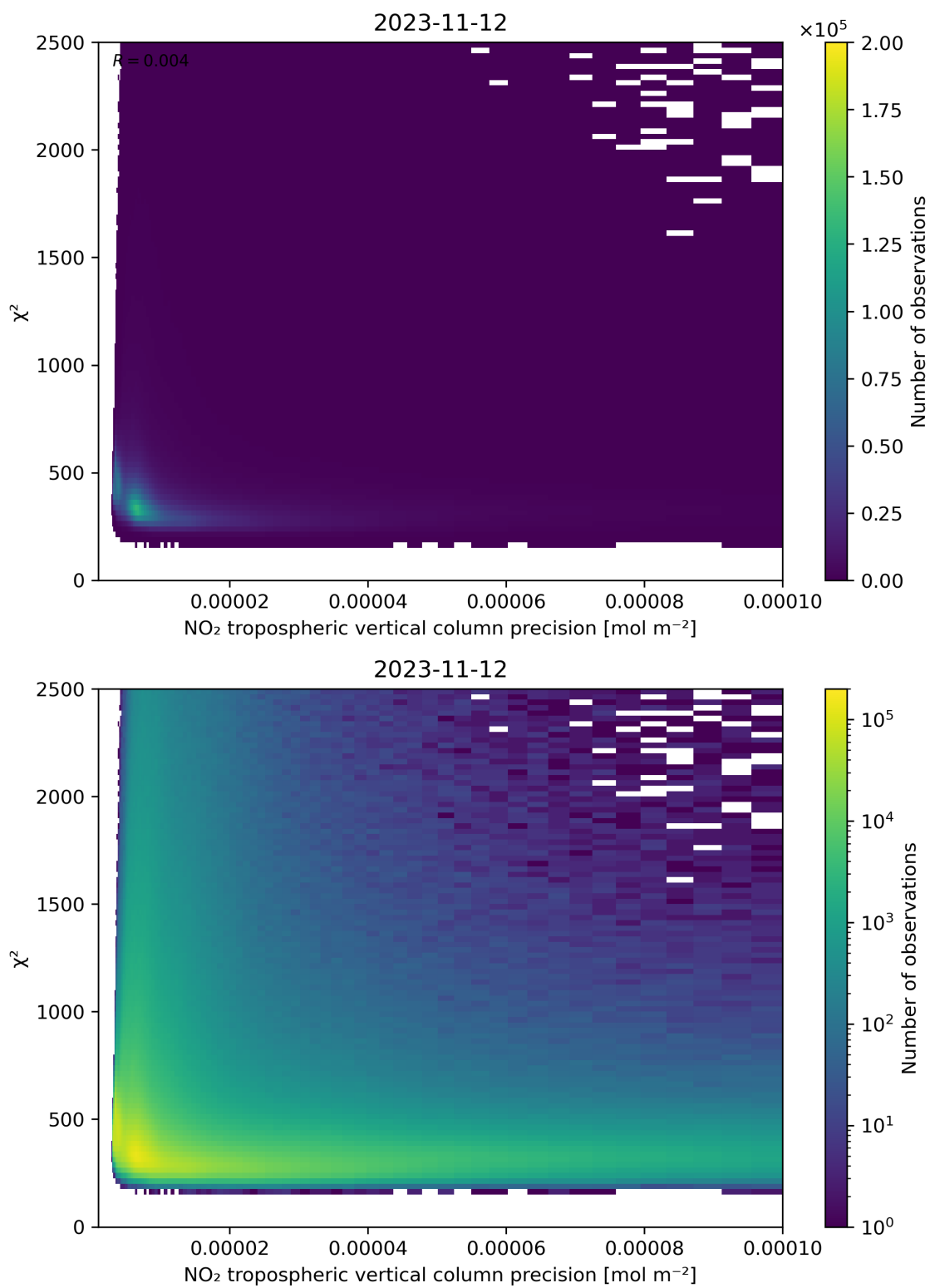
Figure 134: Scatter density plot of “NO 2 tropospheric vertical column precision” against “ \chi^2 ” for 2023-11-12 to 2023-11-13.
