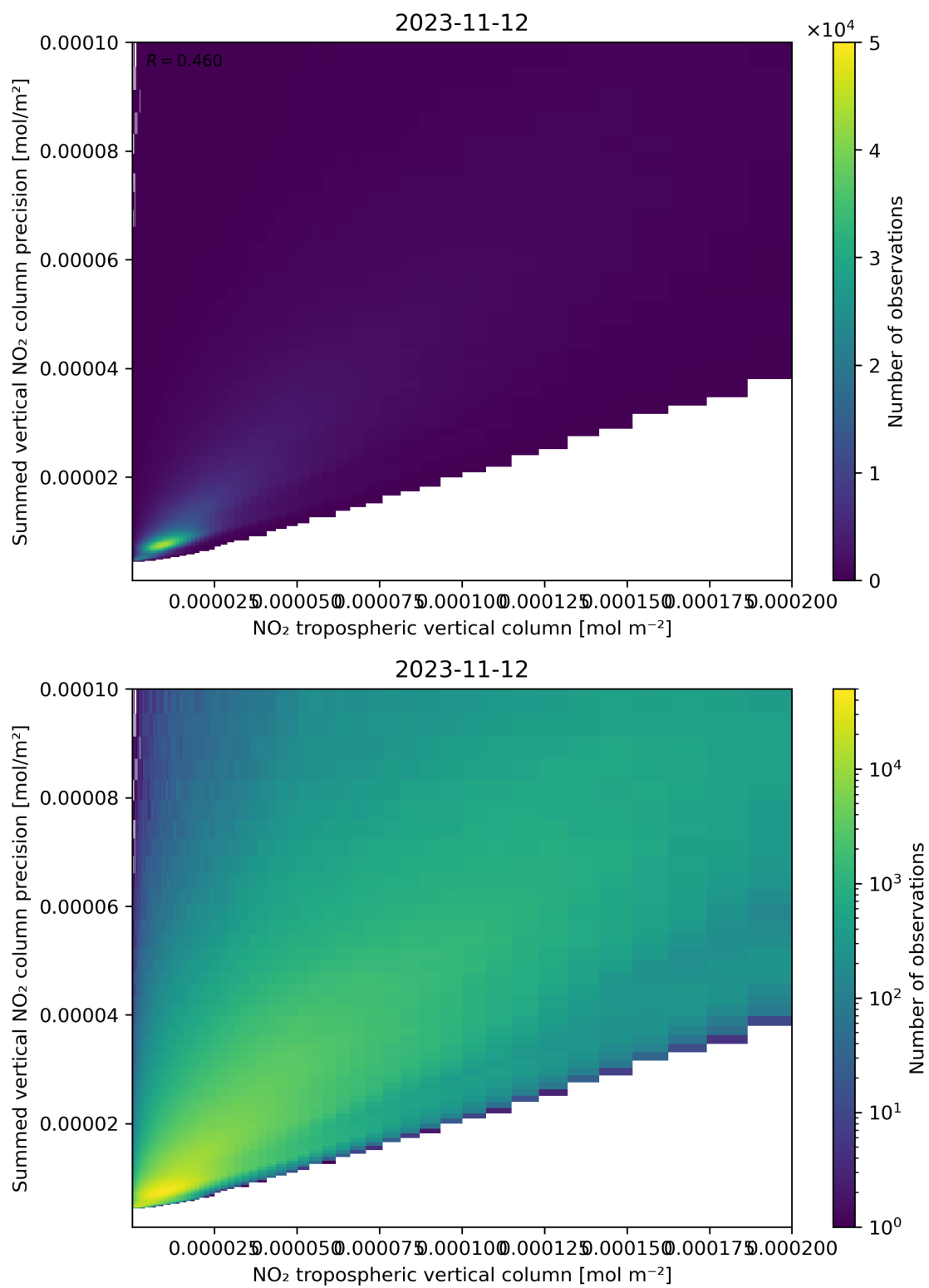
Figure 127: Scatter density plot of “NO 2 tropospheric vertical column” against “Summed vertical NO 2 column precision” for 2023-11-12 to 2023-11-13.
