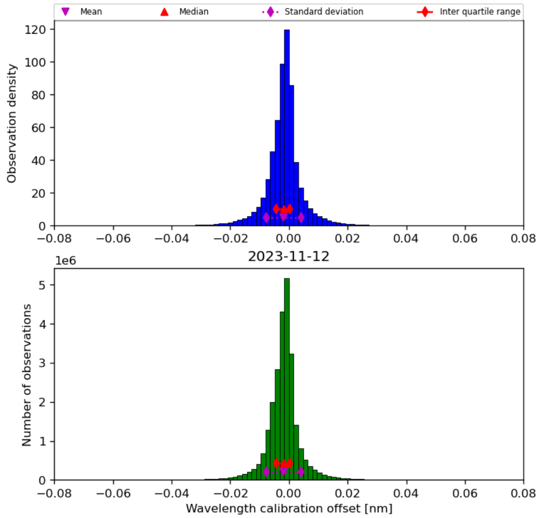
Figure 35: Histogram of “Wavelength calibration offset” for 2023-11-12 to 2023-11-13
