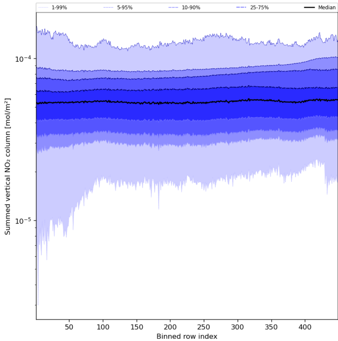
Figure 57: Along track statistics of “Summed vertical NO 2 column” for 2023-11-12 to 2023-11-13
