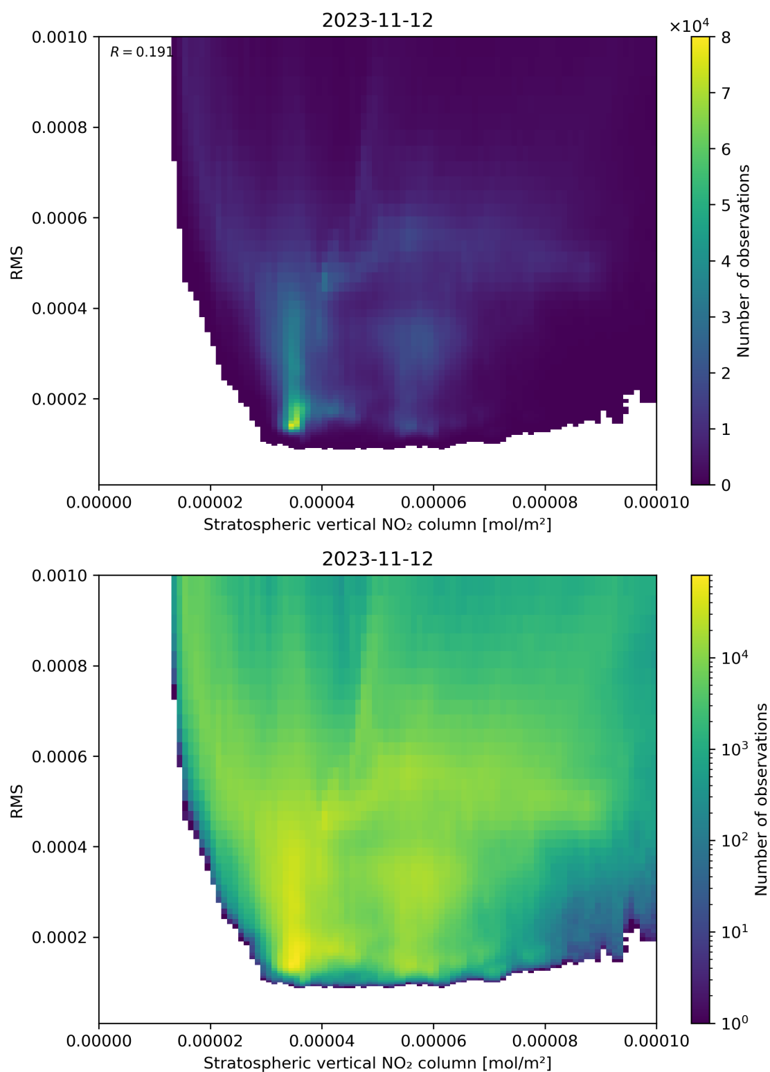
Figure 102: Scatter density plot of “Stratospheric vertical NO 2 column” against “RMS” for 2023-11-12 to 2023-11-13.
