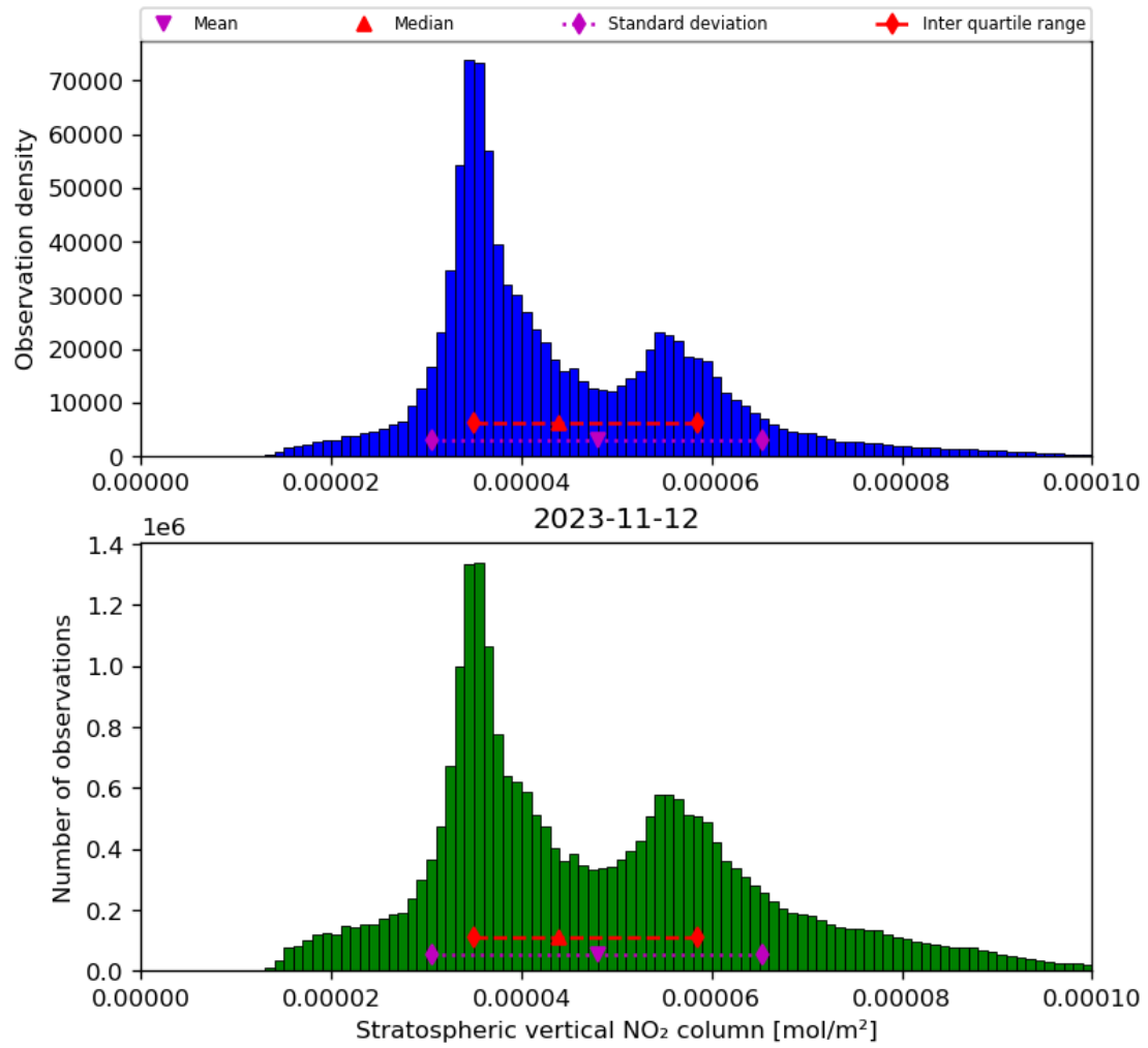
Figure 36: Histogram of “Stratospheric vertical NO 2 column” for 2023-11-12 to 2023-11-13
