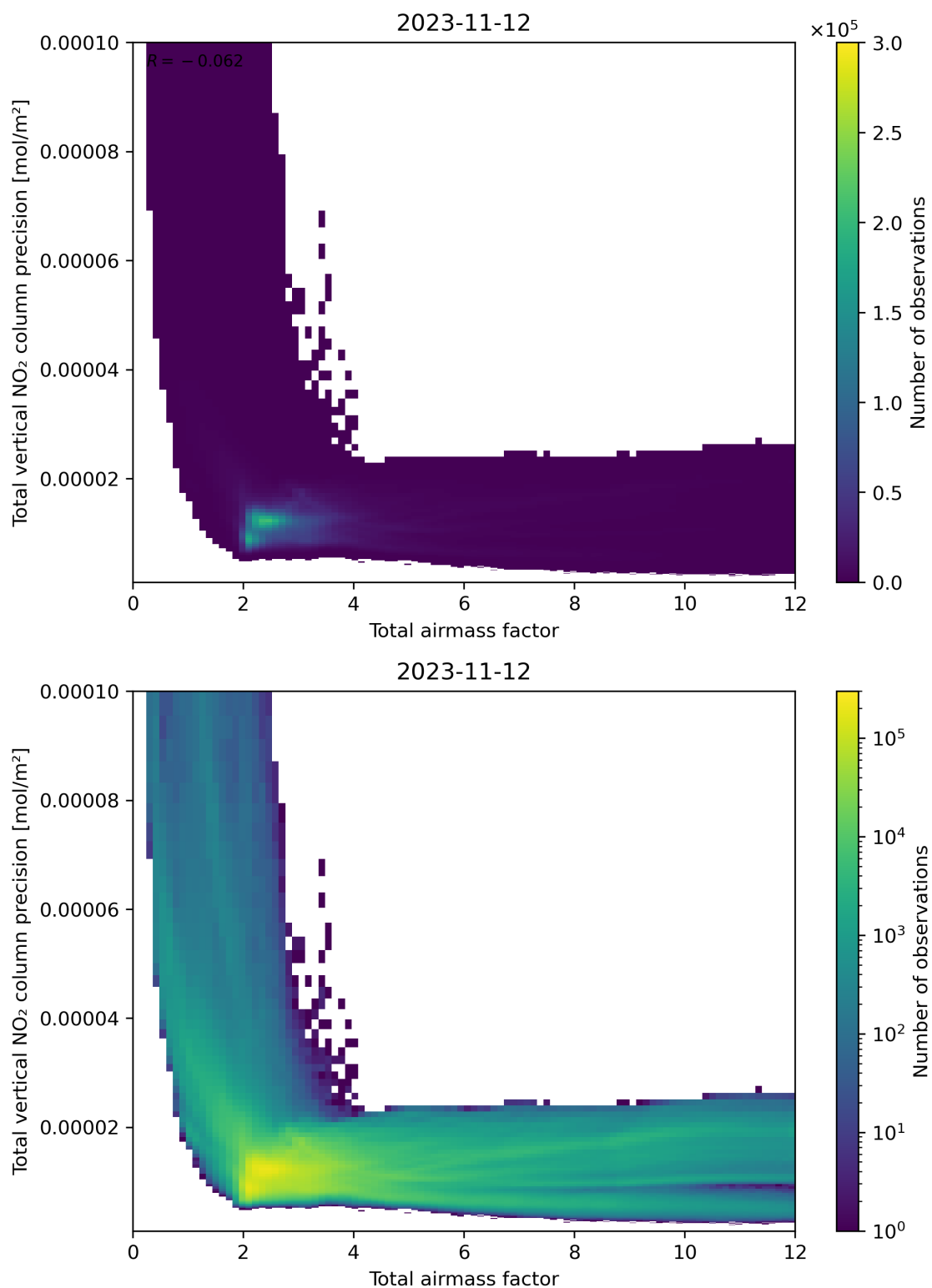
Figure 68: Scatter density plot of “Total airmass factor” against “Total vertical NO 2 column precision” for 2023-11-12 to 2023-11-13.
