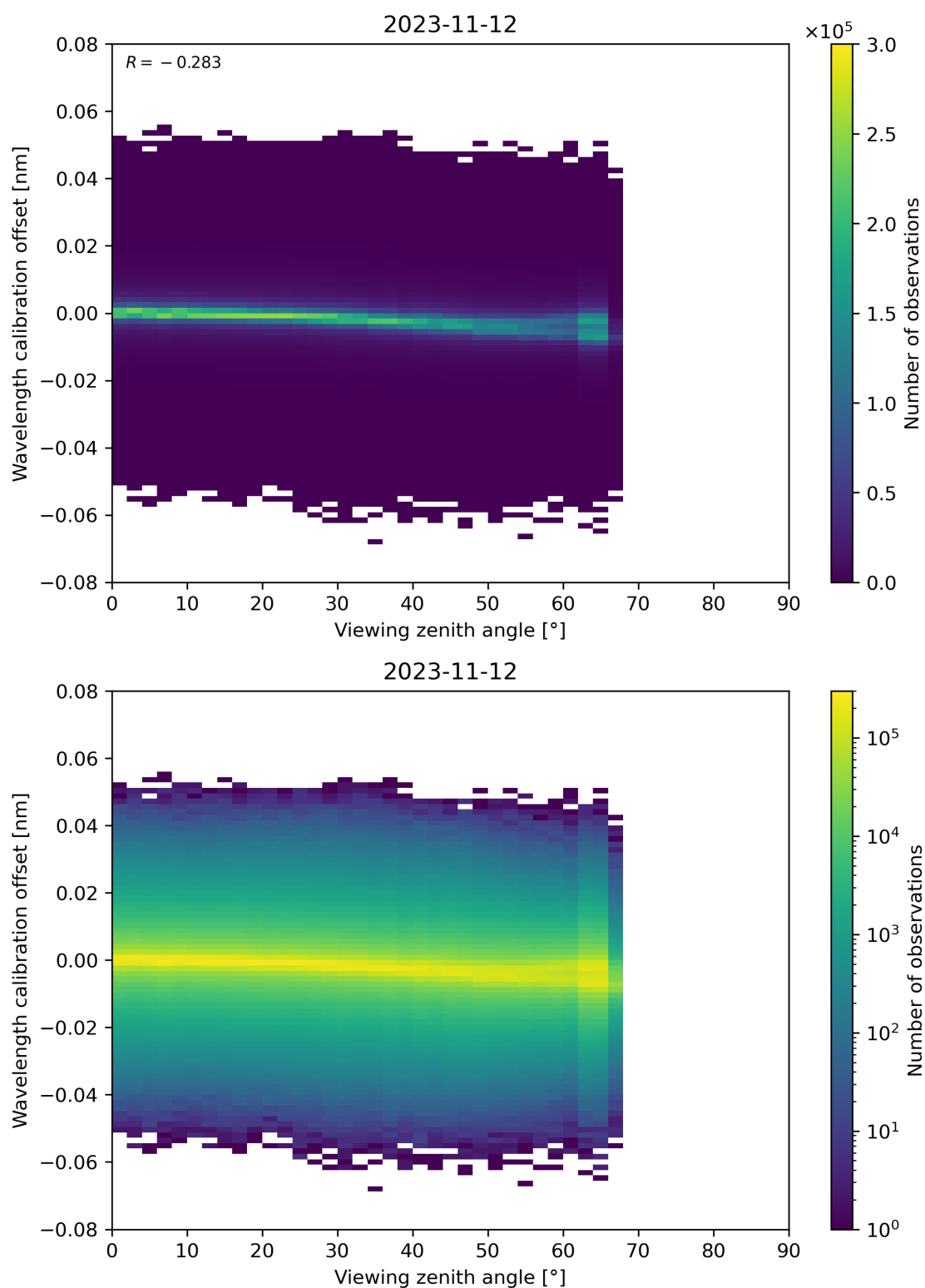
Figure 173: Scatter density plot of “Viewing zenith angle” against “Wavelength calibration offset” for 2023-11-12 to 2023-11-13.
