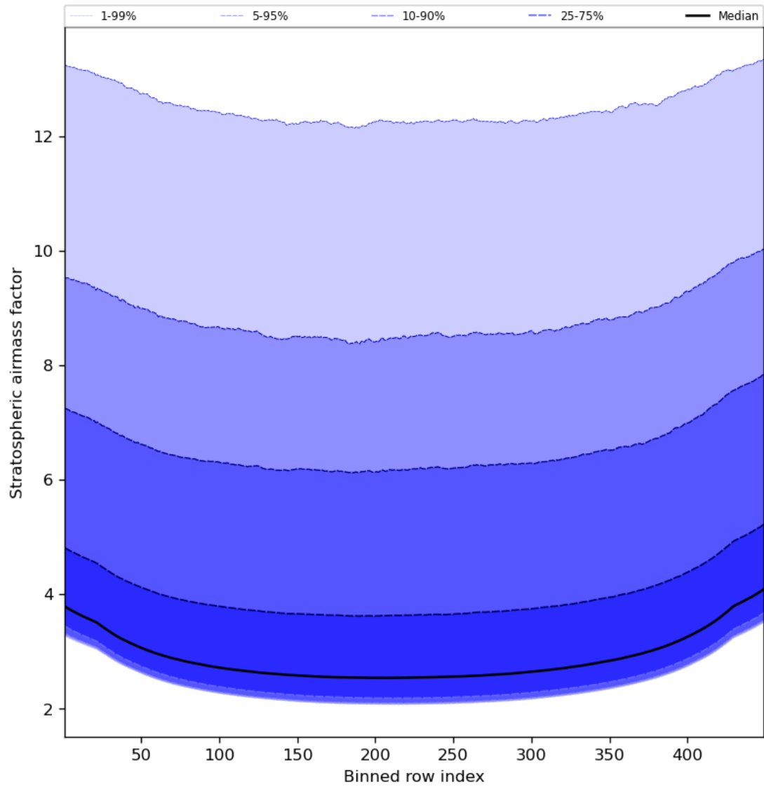
Figure 61: Along track statistics of “Stratospheric airmass factor” for 2023-11-12 to 2023-11-13
