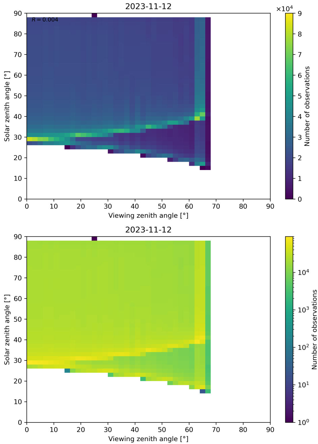
Figure 172: Scatter density plot of “Viewing zenith angle” against “Solar zenith angle” for 2023-11-12 to 2023-11-13.
