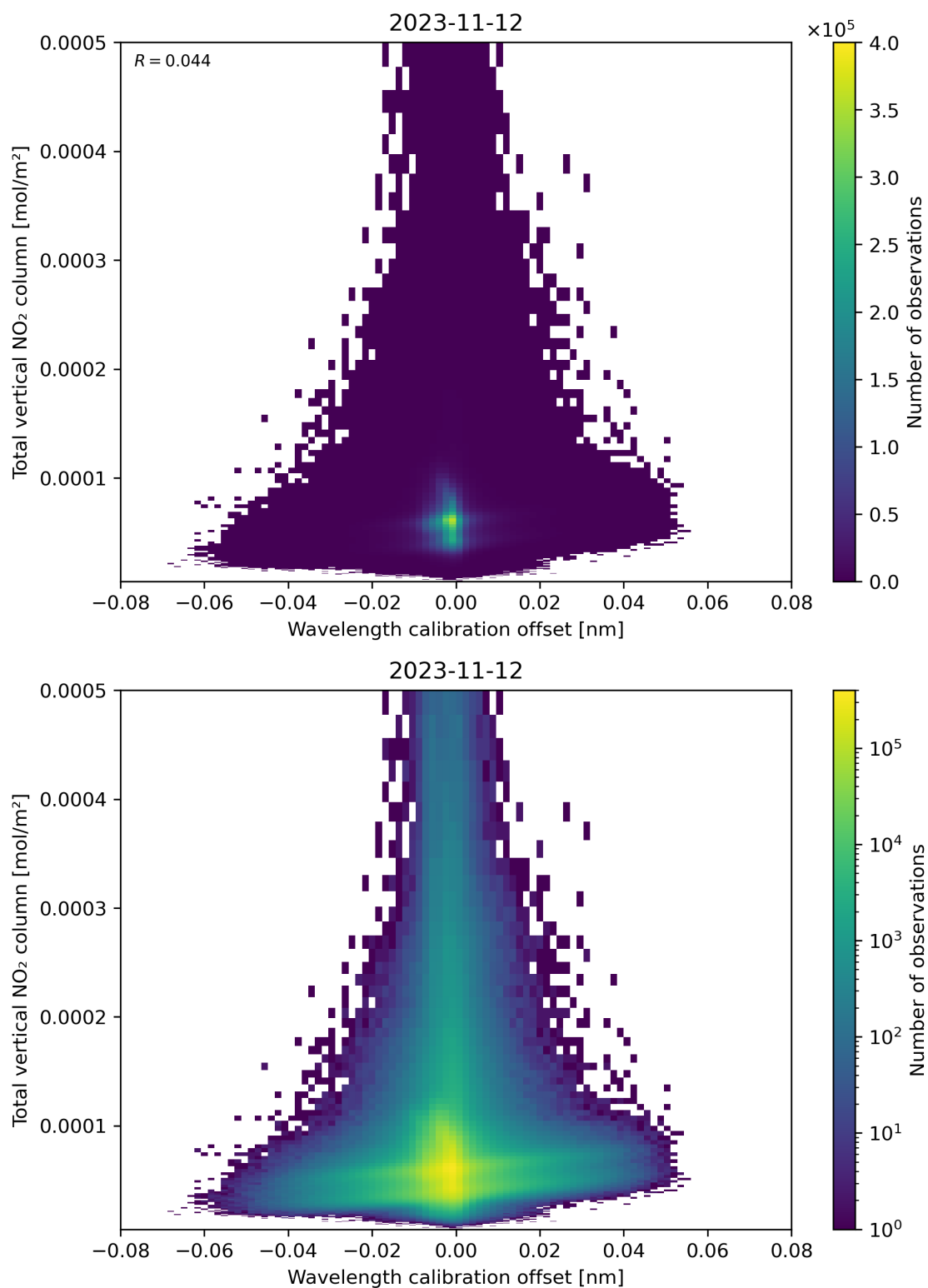
Figure 179: Scatter density plot of “Wavelength calibration offset” against “Total vertical NO 2 column” for 2023-11-12 to 2023-11-13.
