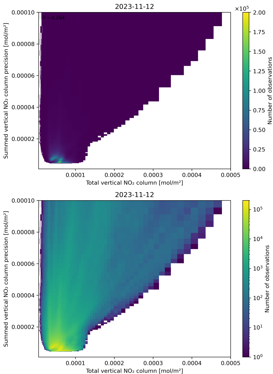
Figure 113: Scatter density plot of “Total vertical NO 2 column” against “Summed vertical NO 2 column precision” for 2023-11-12 to 2023-11-13.
