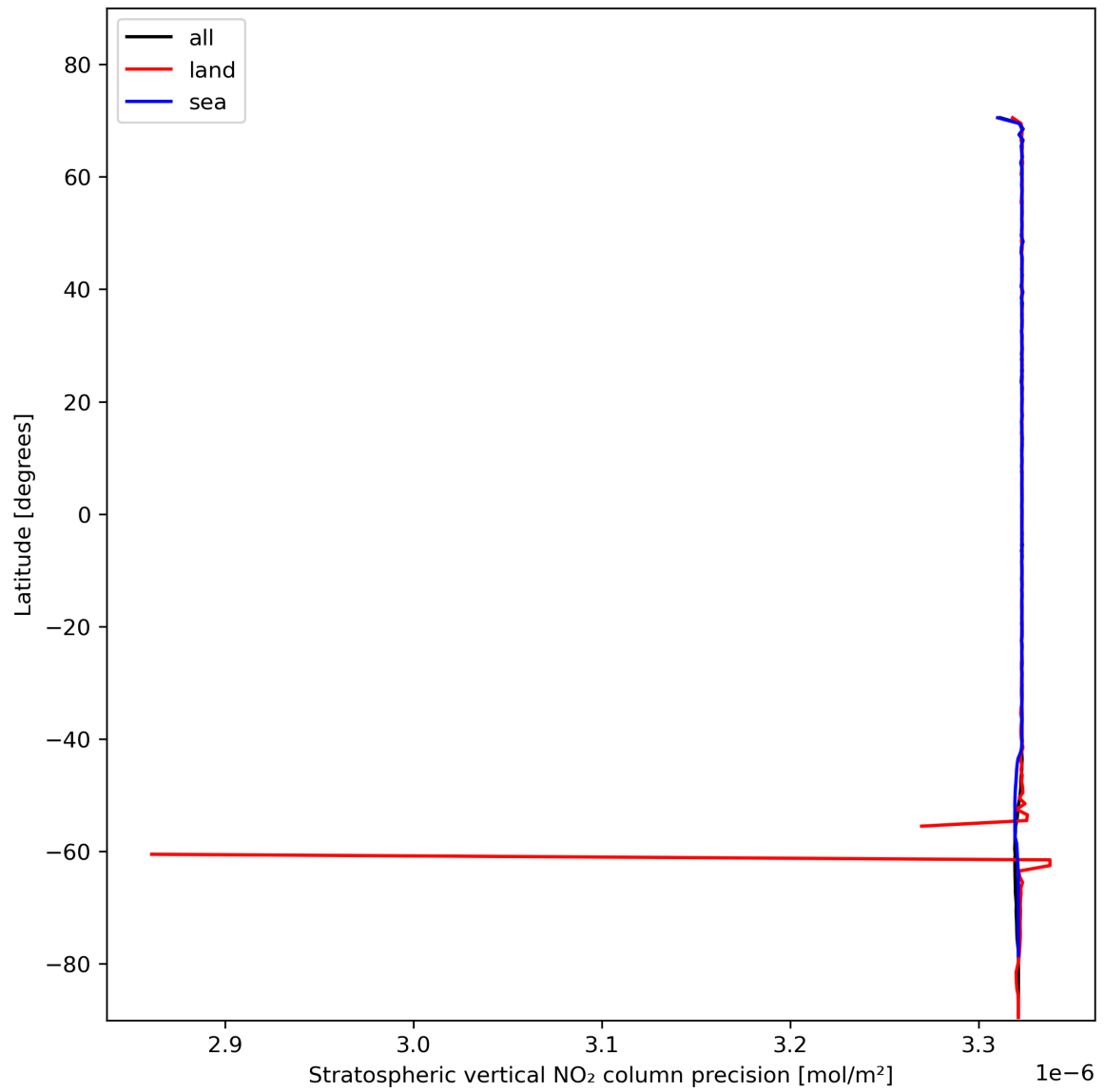
Figure 20: Zonal average of “Stratospheric vertical NO 2 column precision” for 2023-11-12 to 2023-11-13.
