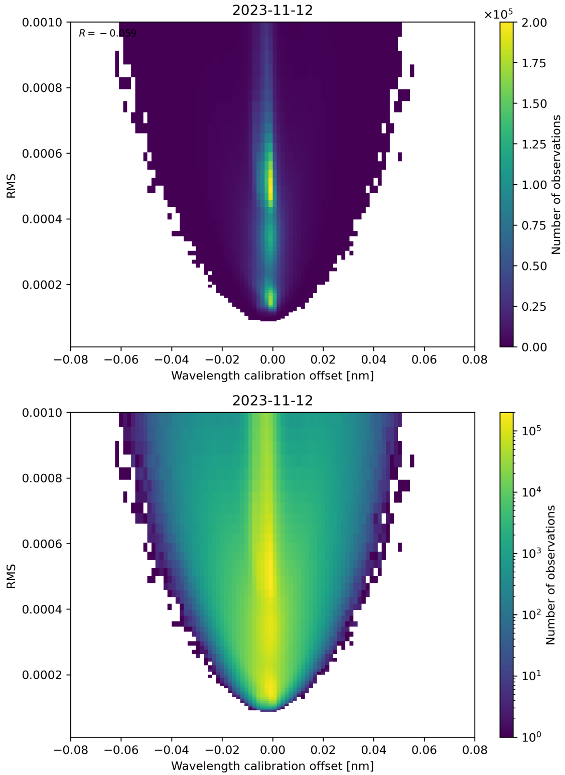
Figure 181: Scatter density plot of “Wavelength calibration offset” against “RMS” for 2023-11-12 to 2023-11-13.
