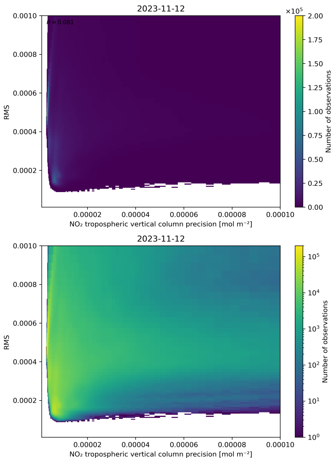
Figure 140: Scatter density plot of “NO 2 tropospheric vertical column precision” against “RMS” for 2023-11-12 to 2023-11-13.
