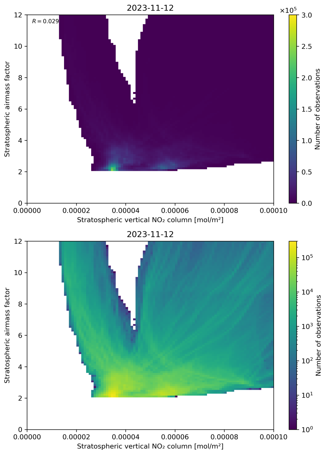
Figure 96: Scatter density plot of “Stratospheric vertical NO 2 column” against “Stratospheric airmass factor” for 2023-11-12 to 2023-11-13.
