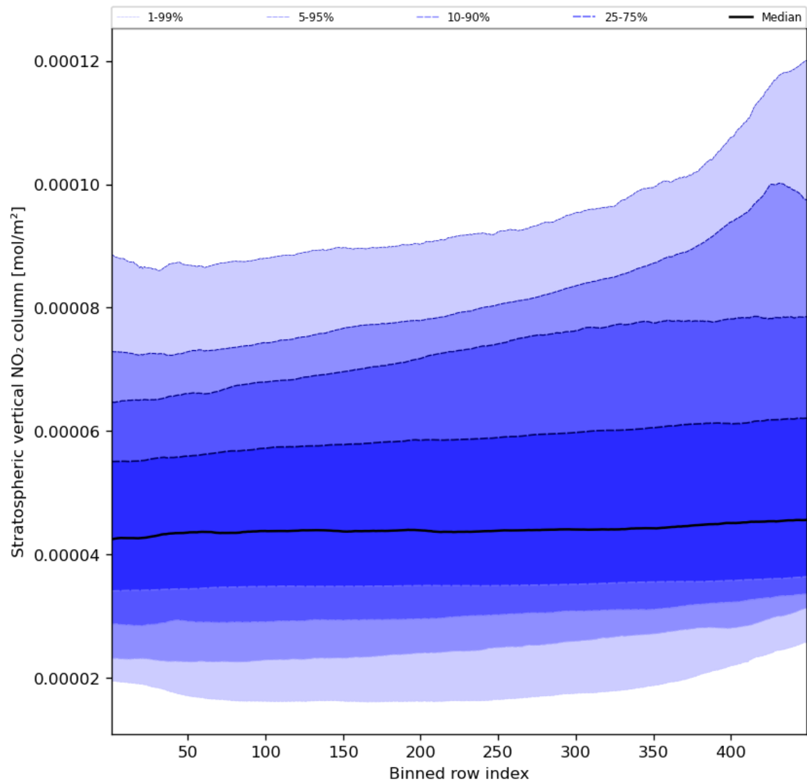
Figure 53: Along track statistics of “Stratospheric vertical NO 2 column” for 2023-11-12 to 2023-11-13
