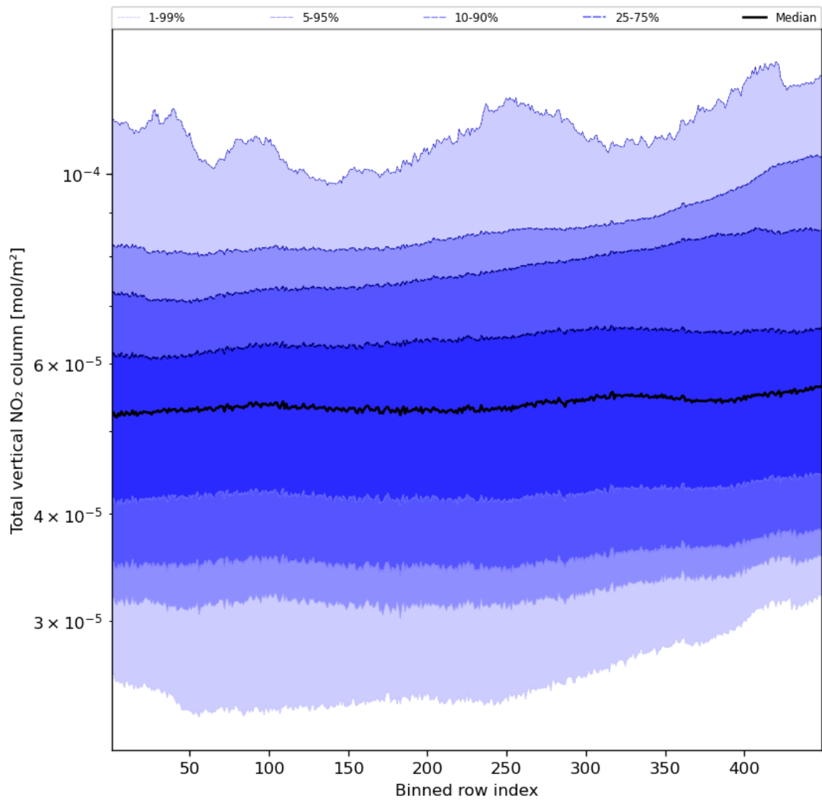
Figure 55: Along track statistics of “Total vertical NO 2 column” for 2023-11-12 to 2023-11-13
