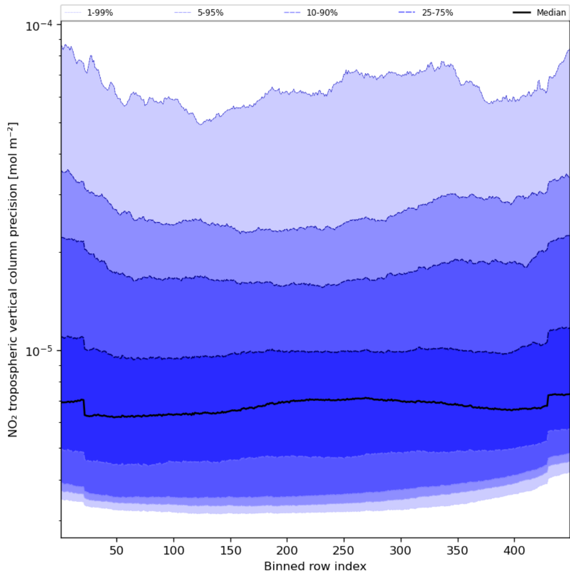
Figure 47: Along track statistics of “NO 2 tropospheric vertical column precision” for 2023-11-12 to 2023-11-13
