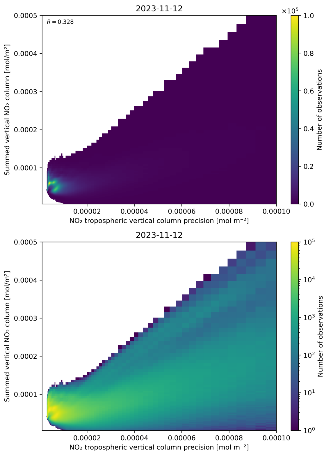
Figure 136: Scatter density plot of “NO 2 tropospheric vertical column precision” against “Summed vertical NO 2 column” for 2023-11-12 to 2023-11-13.
