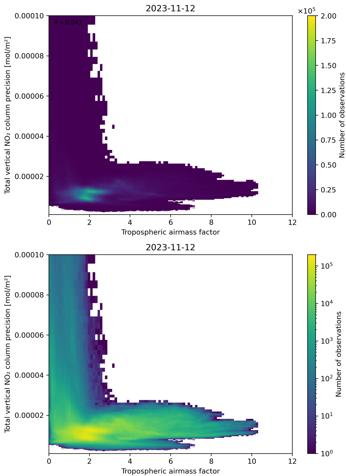
Figure 78: Scatter density plot of “Tropospheric air mass factor” against “Total vertical NO 2 column precision” for 2023-11-12 to 2023-11-13.
