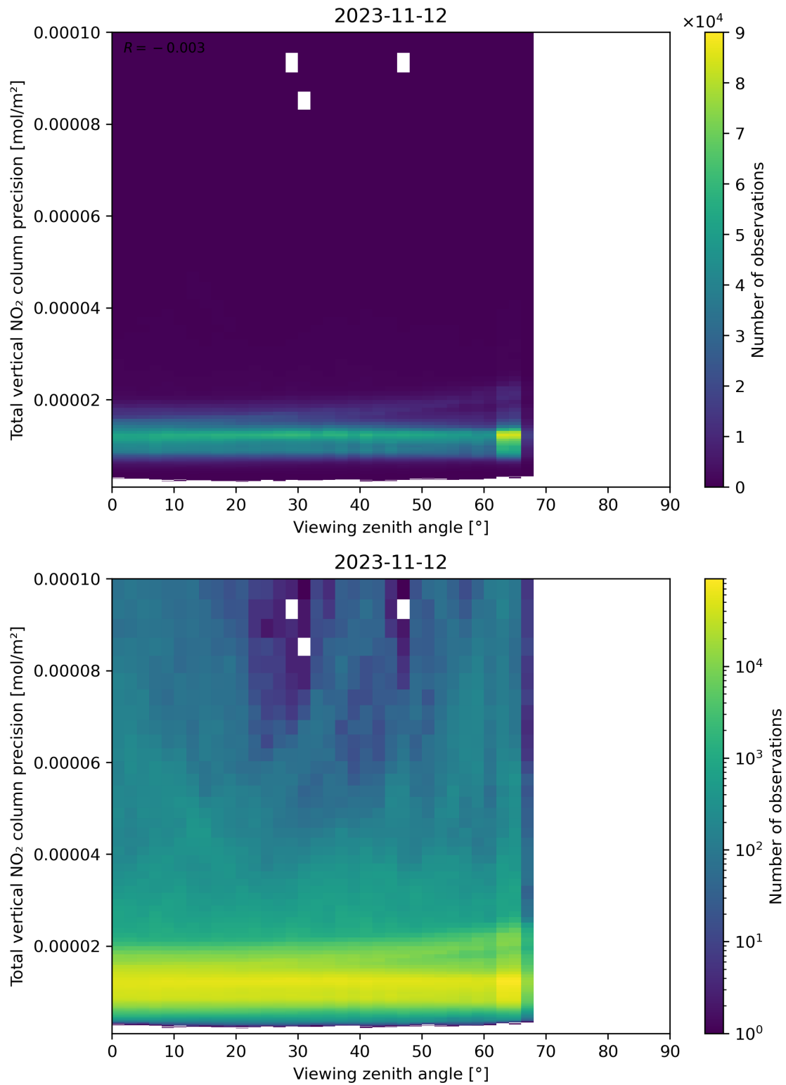
Figure 168: Scatter density plot of “Viewing zenith angle” against “Total vertical NO 2 column precision” for 2023-11-12 to 2023-11-13.
