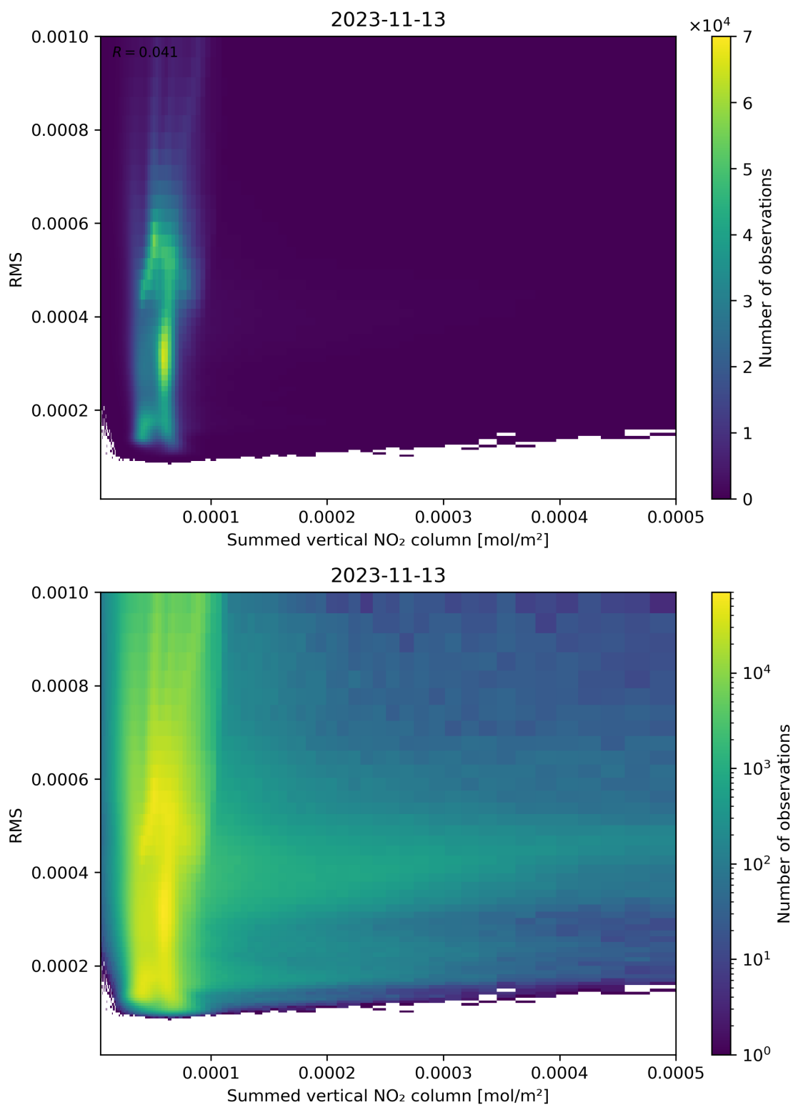
Figure 109: Scatter density plot of “Summed vertical NO 2 column” against “RMS” for 2023-11-13 to 2023-11-14.
