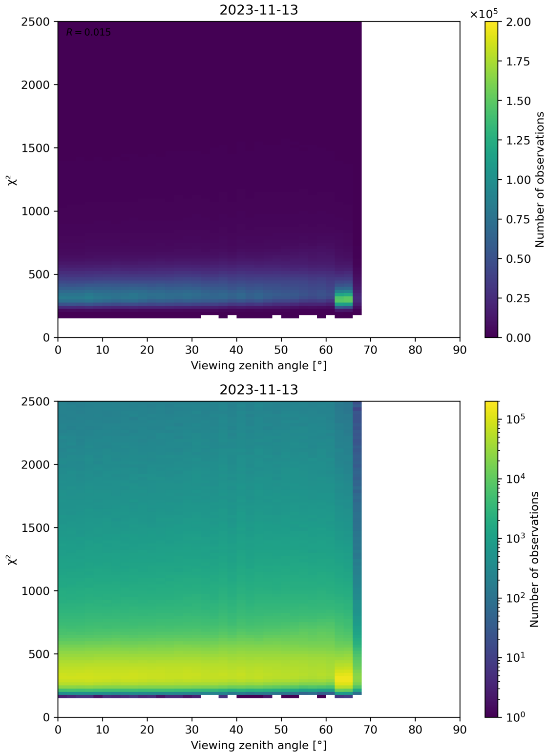
Figure 162: Scatter density plot of “Viewing zenith angle” against “ \chi^2 ” for 2023-11-13 to 2023-11-14.
