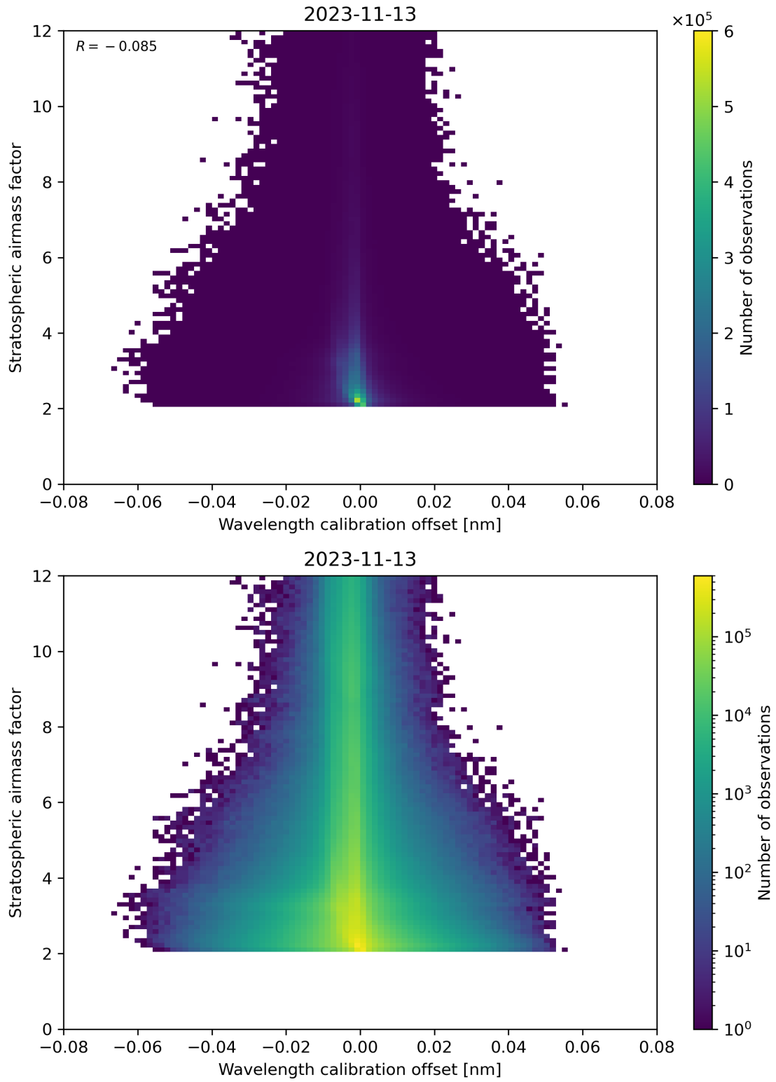
Figure 174: Scatter density plot of “Wavelength calibration offset” against “Stratospheric airmass factor” for 2023-11-13 to 2023-11-14.
