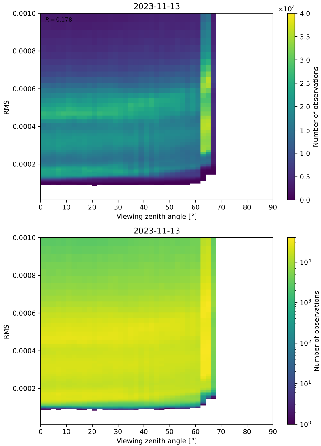
Figure 171: Scatter density plot of “Viewing zenith angle” against “RMS” for 2023-11-13 to 2023-11-14.
