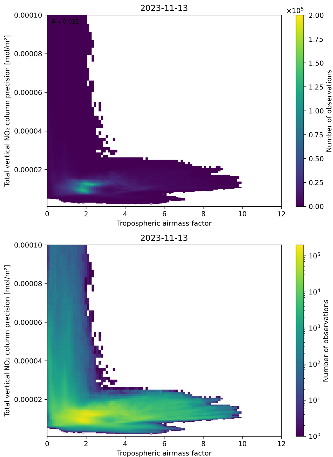
Figure 78: Scatter density plot of “Tropospheric air mass factor” against “Total vertical NO 2 column precision” for 2023-11-13 to 2023-11-14.
