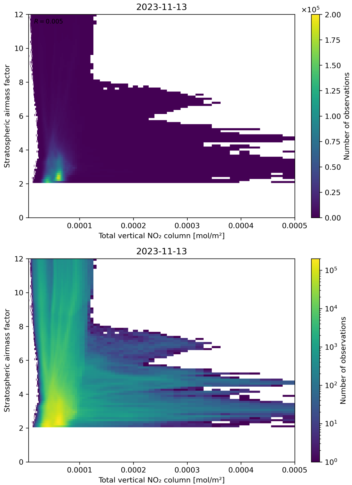
Figure 110: Scatter density plot of “Total vertical NO 2 column” against “Stratospheric air mass factor” for 2023-11-13 to 2023-11-14.
