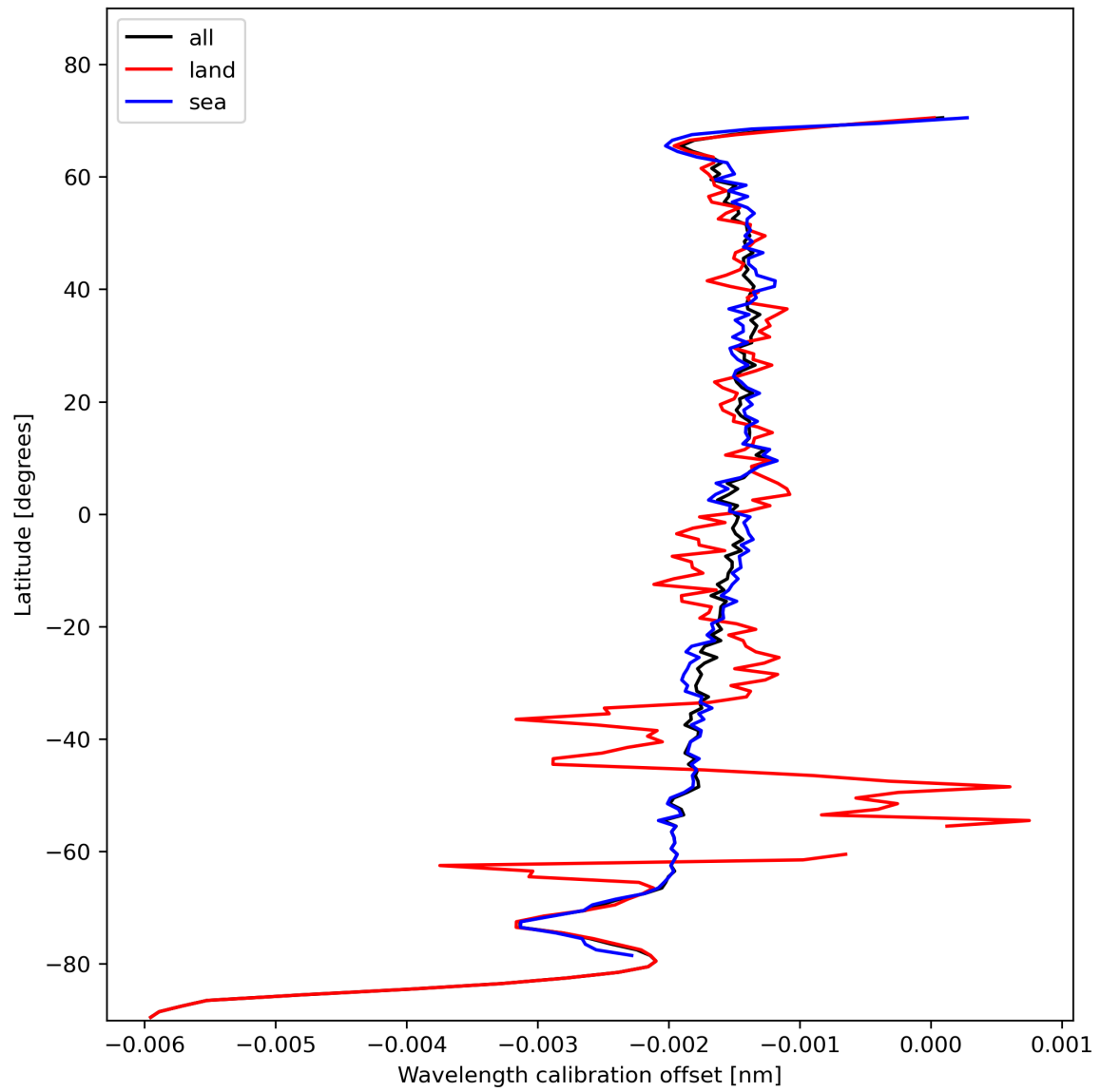
Figure 18: Zonal average of “Wavelength calibration offset” for 2023-11-13 to 2023-11-14.
