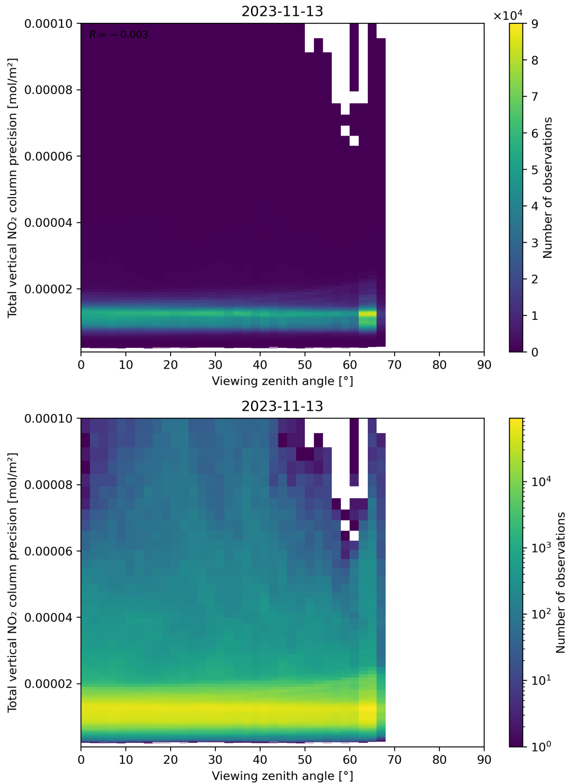
Figure 168: Scatter density plot of “Viewing zenith angle” against “Total vertical NO 2 column precision” for 2023-11-13 to 2023-11-14.
