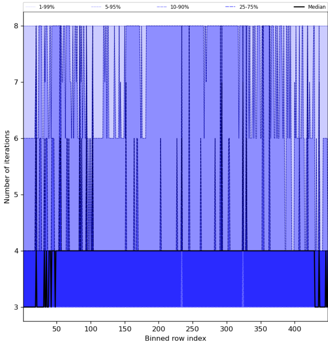
Figure 51: Along track statistics of “Number of iterations” for 2023-11-13 to 2023-11-14
