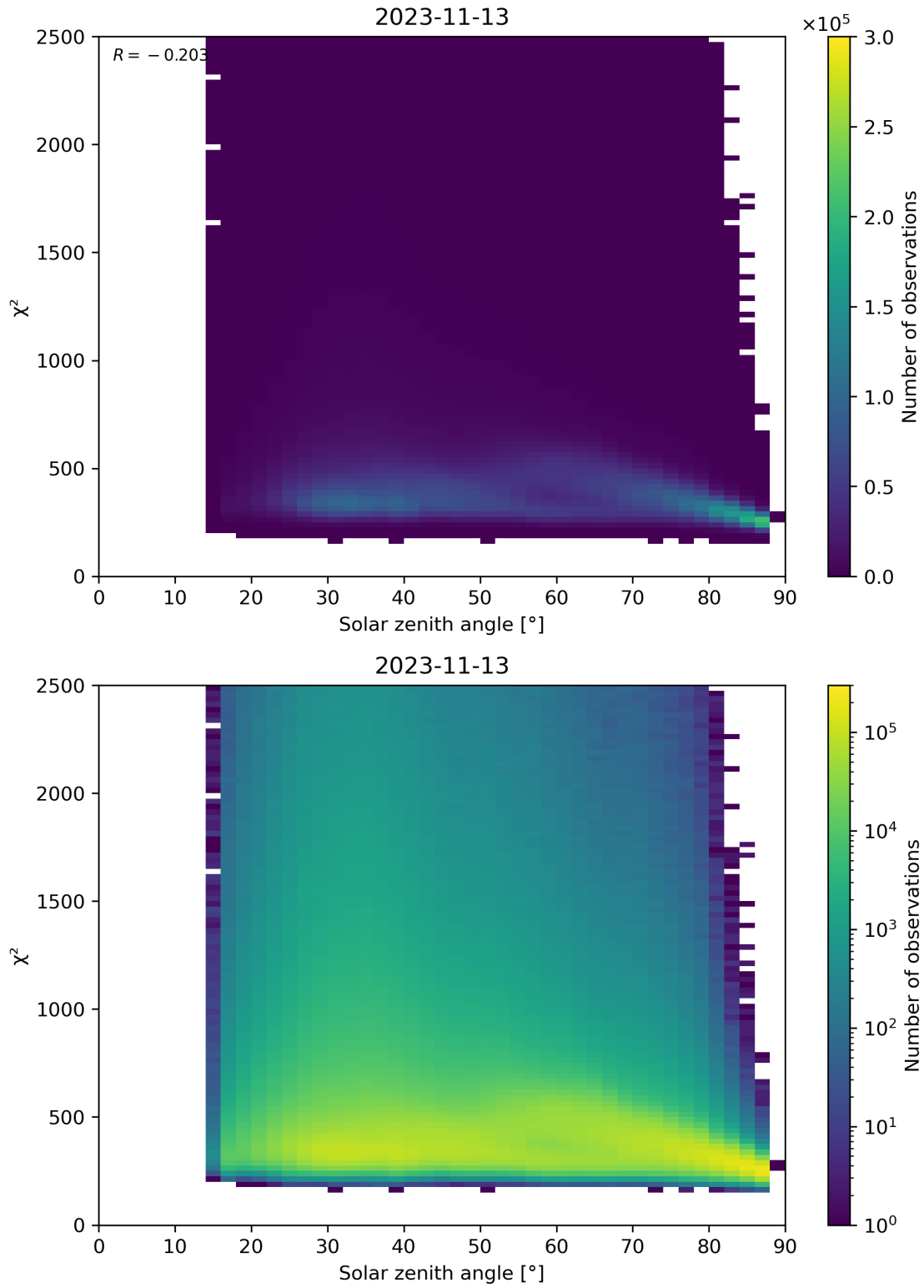
Figure 148: Scatter density plot of “Solar zenith angle” against “ \chi^2 ” for 2023-11-13 to 2023-11-14.
