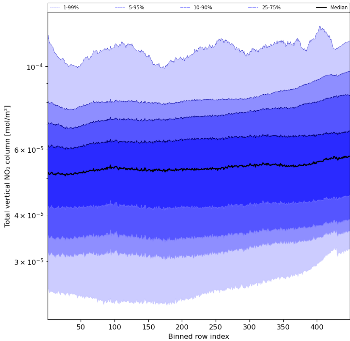
Figure 55: Along track statistics of “Total vertical NO 2 column” for 2023-11-13 to 2023-11-14
