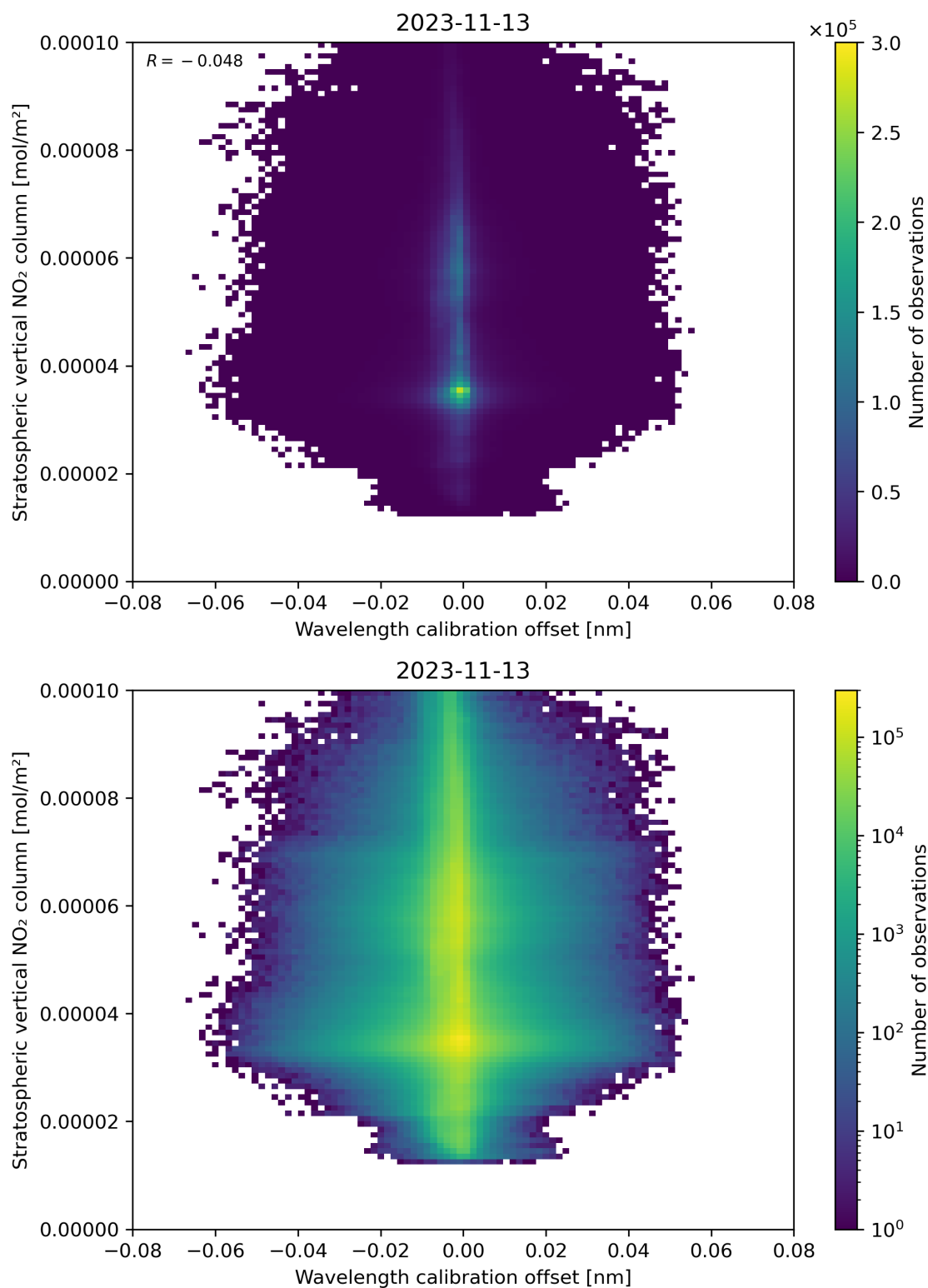
Figure 176: Scatter density plot of “Wavelength calibration offset” against “Stratospheric vertical NO 2 column” for 2023-11-13 to 2023-11-14.
