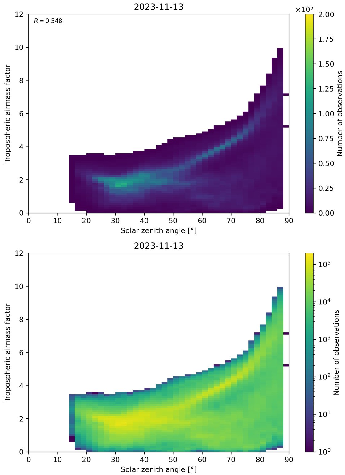
Figure 147: Scatter density plot of “Solar zenith angle” against “Tropospheric airmass factor” for 2023-11-13 to 2023-11-14.
