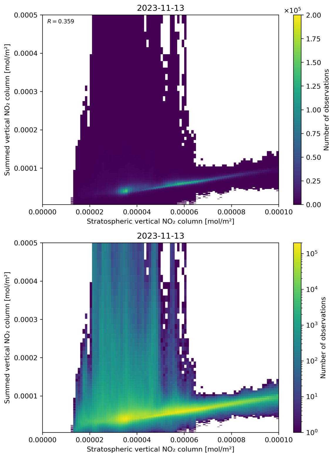
Figure 98: Scatter density plot of “Stratospheric vertical NO 2 column” against “Summed vertical NO 2 column” for 2023-11-13 to 2023-11-14.
