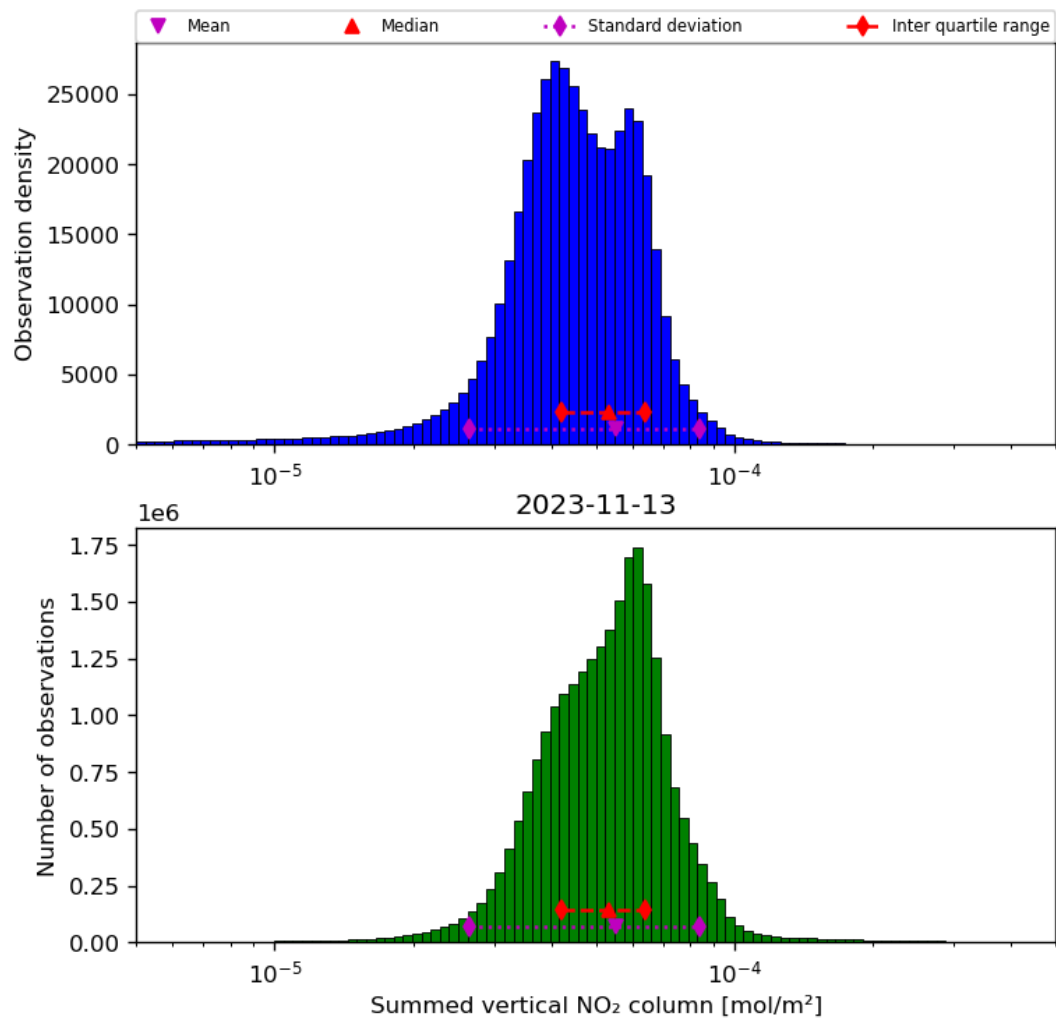
Figure 40: Histogram of “Summed vertical NO 2 column” for 2023-11-13 to 2023-11-14
