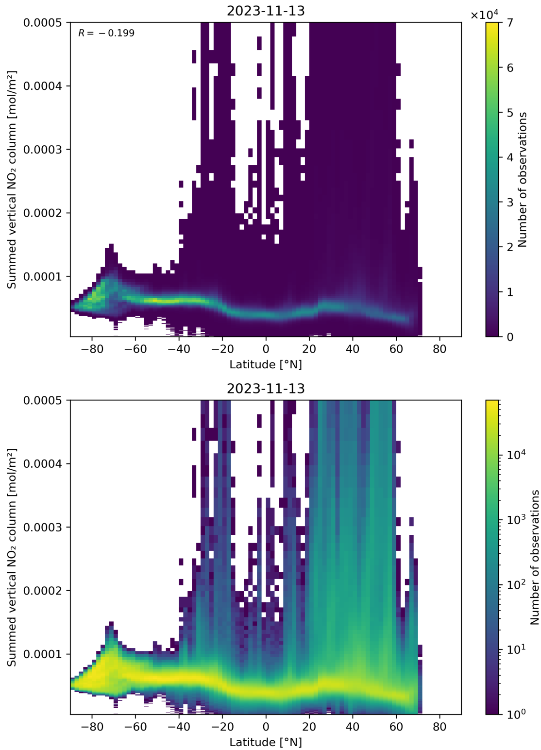
Figure 88: Scatter density plot of “Latitude” against “Summed vertical NO 2 column” for 2023-11-13 to 2023-11-14.
