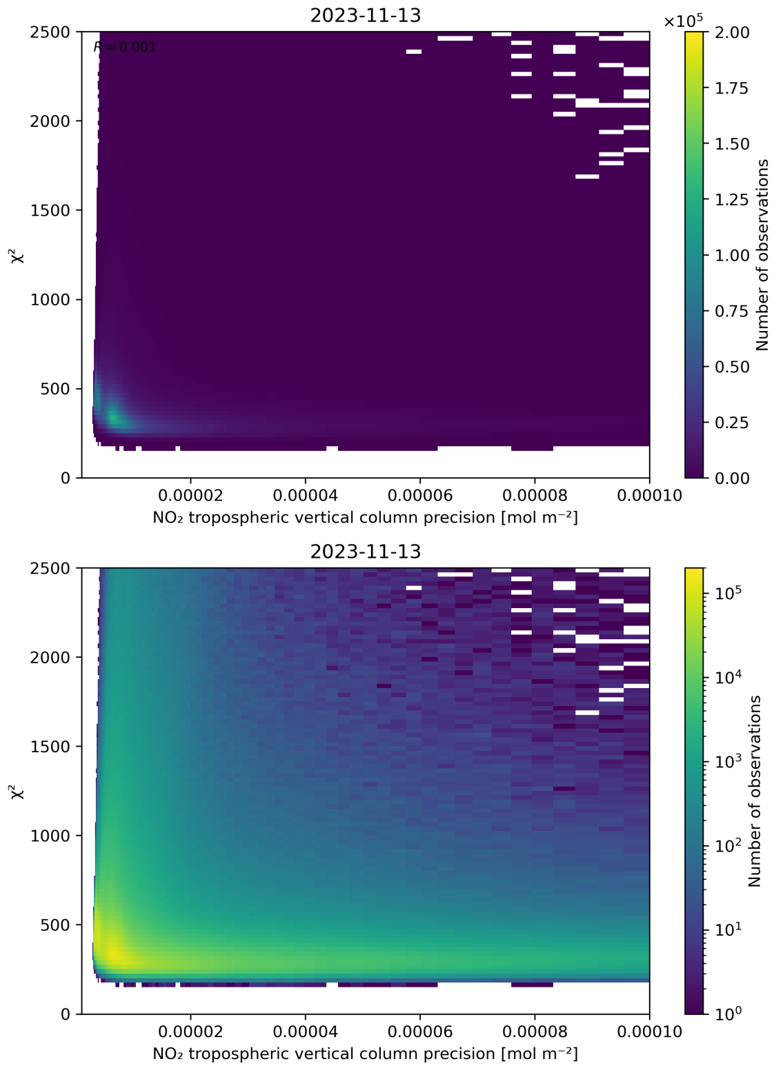
Figure 134: Scatter density plot of “NO 2 tropospheric vertical column precision” against “ \chi^2 ” for 2023-11-13 to 2023-11-14.
