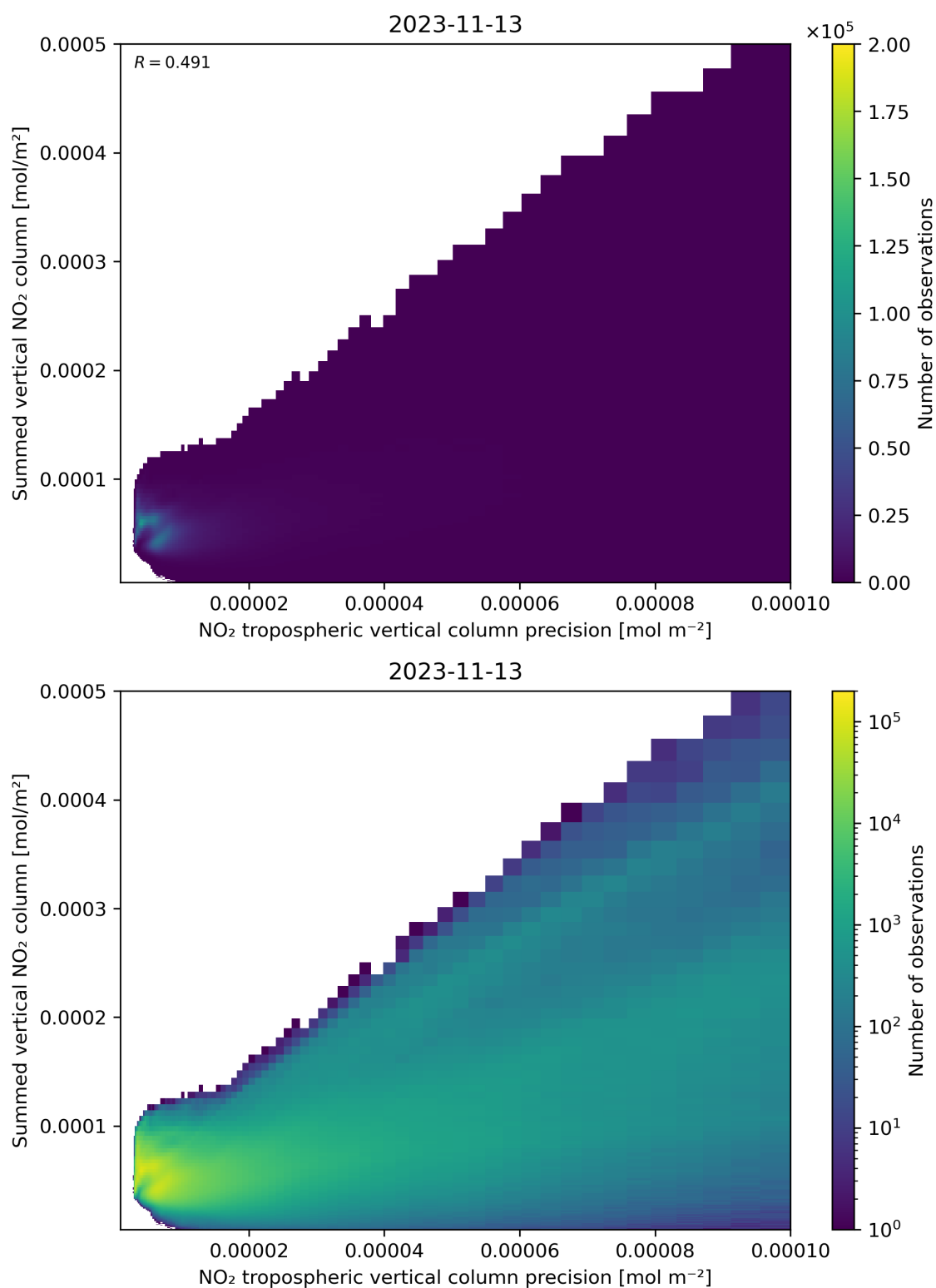
Figure 136: Scatter density plot of “NO 2 tropospheric vertical column precision” against “Summed vertical NO 2 column” for 2023-11-13 to 2023-11-14.
