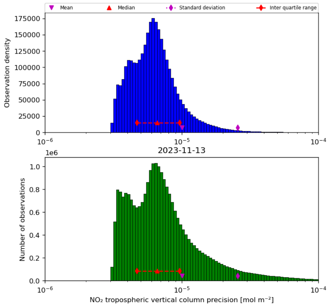
Figure 30: Histogram of “NO 2 tropospheric vertical column precision” for 2023-11-13 to 2023-11-14
