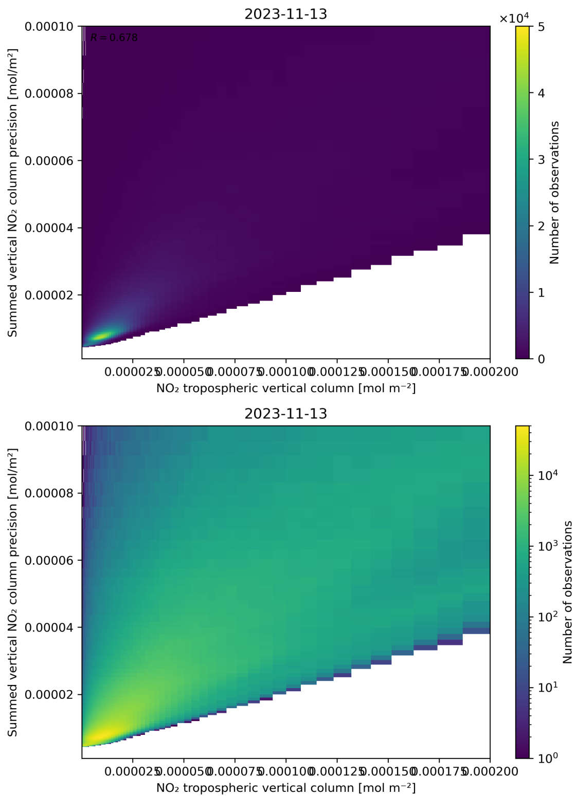
Figure 127: Scatter density plot of “NO 2 tropospheric vertical column” against “Summed vertical NO 2 column precision” for 2023-11-13 to 2023-11-14.
