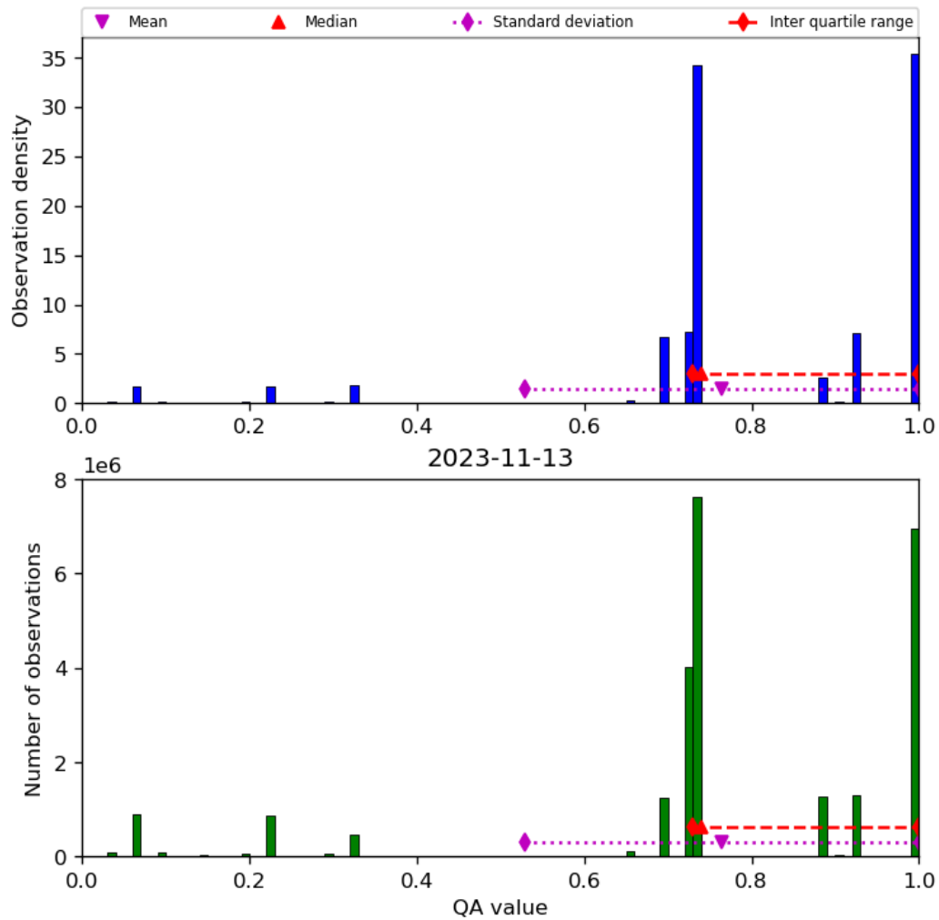
Figure 28: Histogram of “QA value” for 2023-11-13 to 2023-11-14
