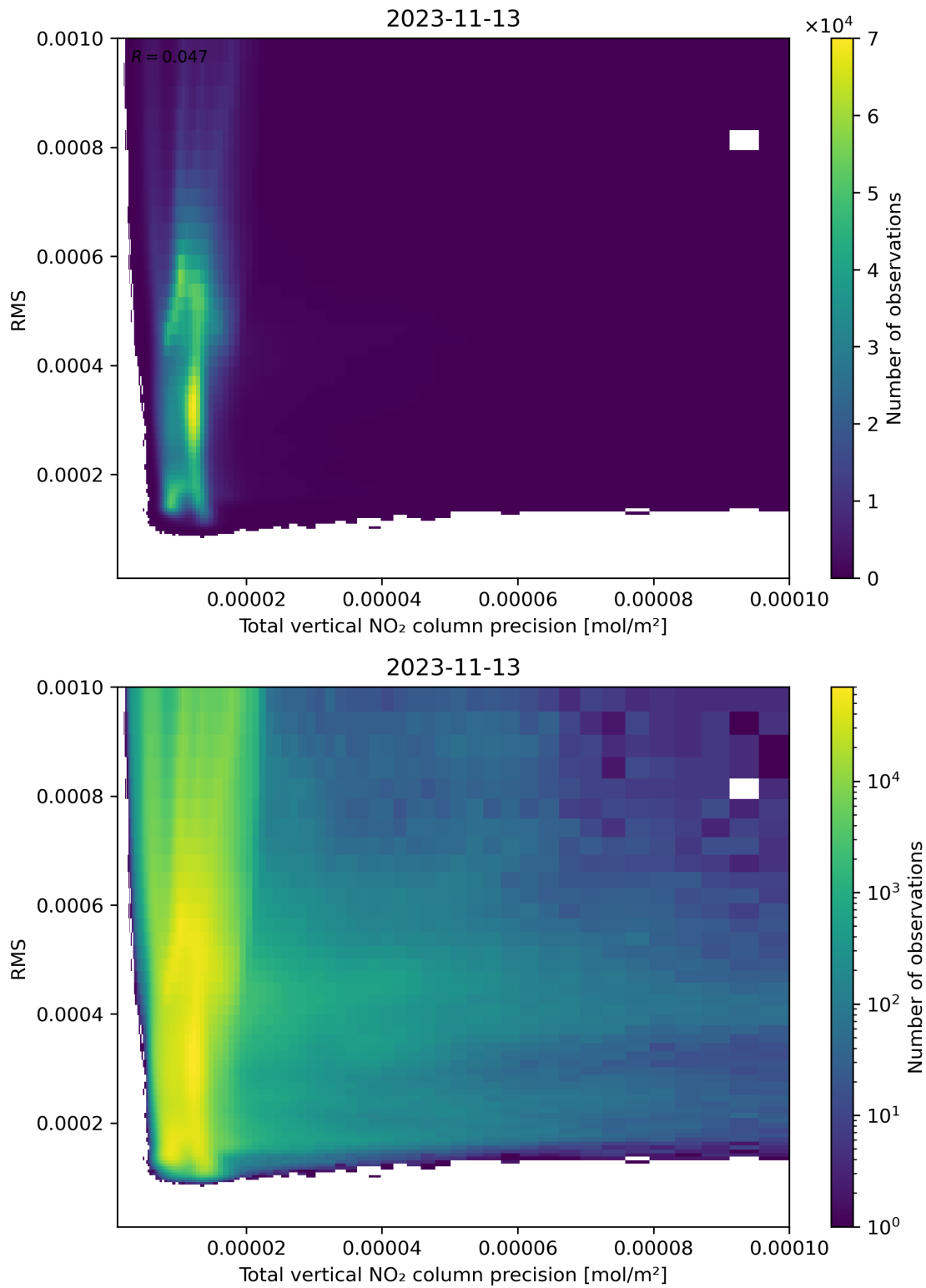
Figure 119: Scatter density plot of “Total vertical NO 2 column precision” against “RMS” for 2023-11-13 to 2023-11-14.
