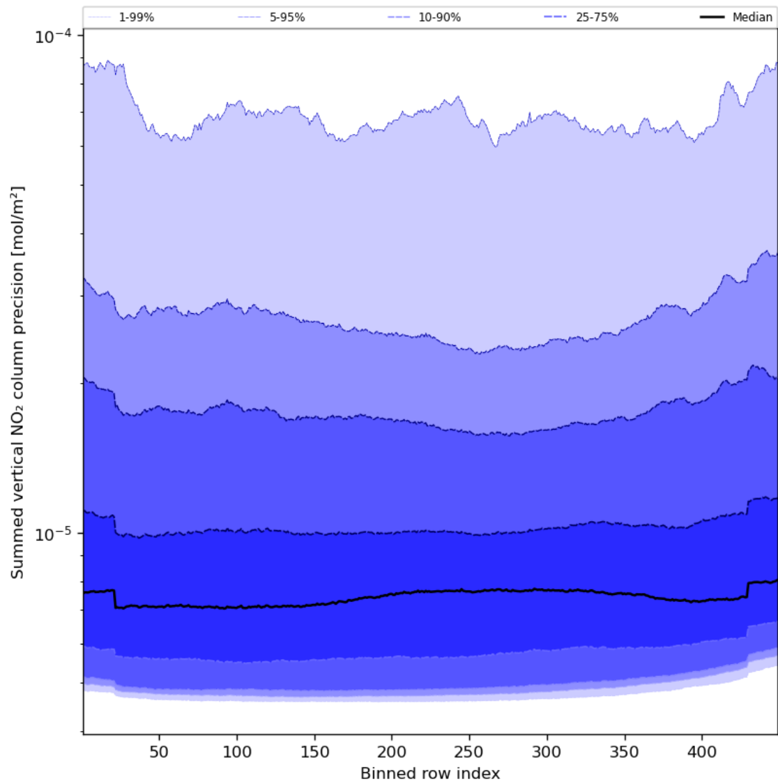
Figure 58: Along track statistics of “Summed vertical NO 2 column precision” for 2023-11-13 to 2023-11-14
