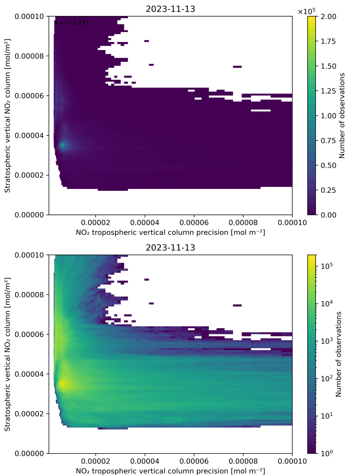
Figure 135: Scatter density plot of “NO 2 tropospheric vertical column precision” against “Stratospheric vertical NO 2 column” for 2023-11-13 to 2023-11-14.
