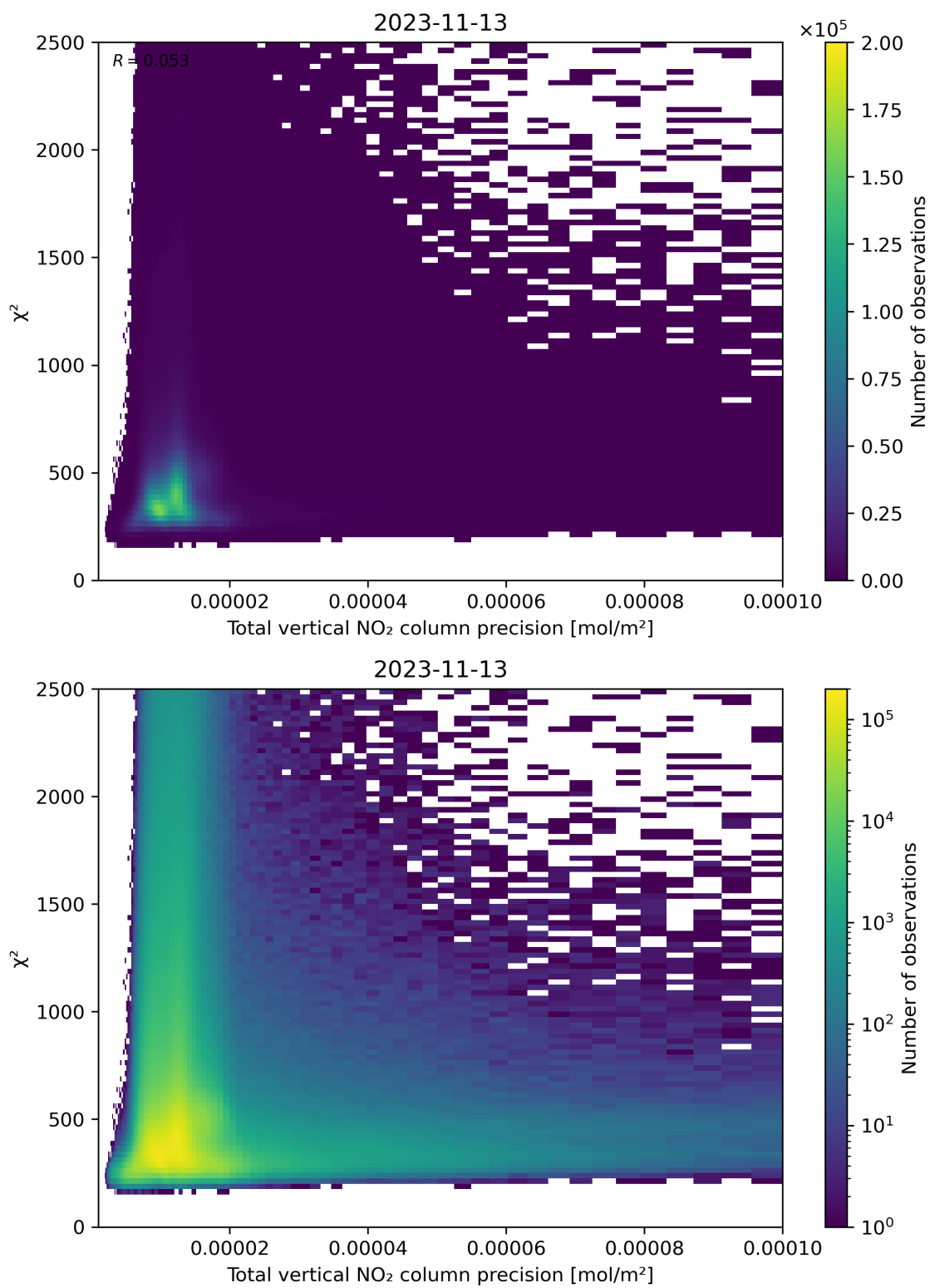
Figure 116: Scatter density plot of “Total vertical NO 2 column precision” against “ \chi^2 ” for 2023-11-13 to 2023-11-14.
