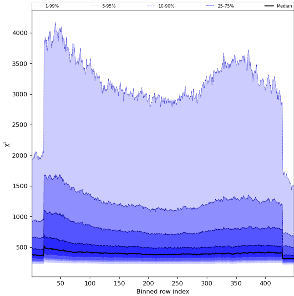
Figure 59: Along track statistics of “ \chi^2 ” for 2023-11-13 to 2023-11-14
