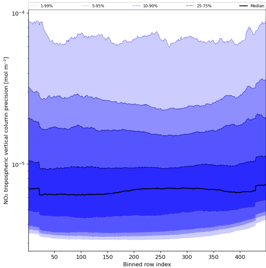
Figure 47: Along track statistics of “NO 2 tropospheric vertical column precision” for 2023-11-13 to 2023-11-14
