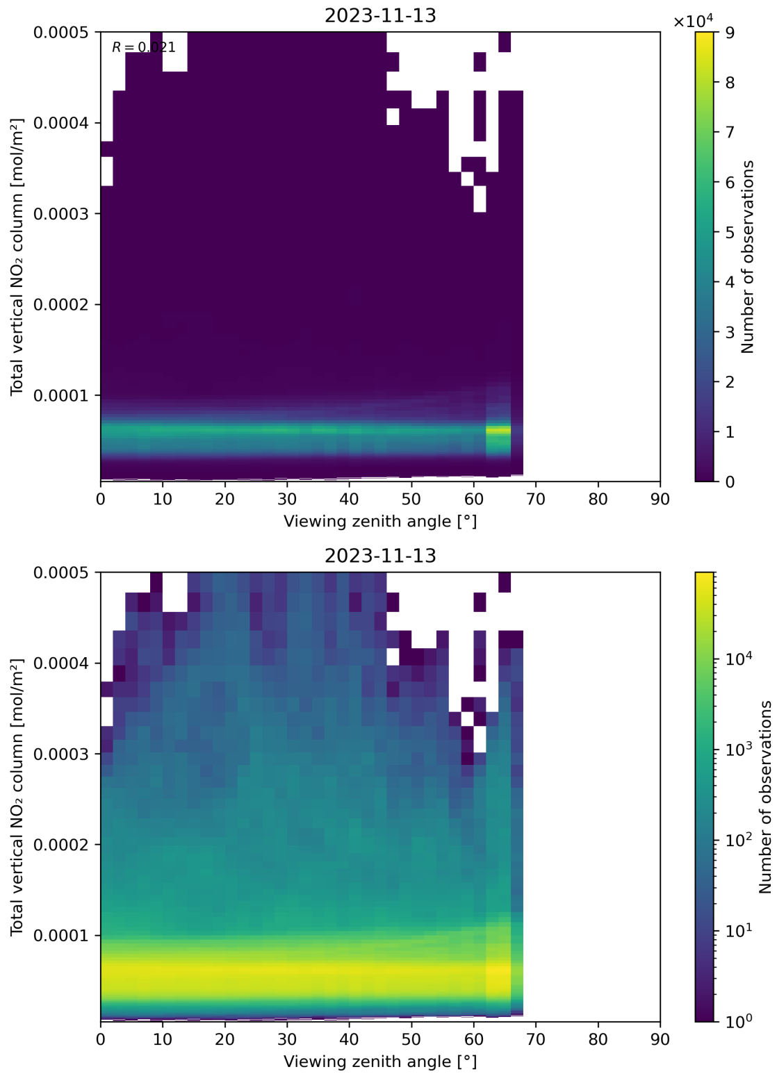
Figure 167: Scatter density plot of “Viewing zenith angle” against “Total vertical NO 2 column” for 2023-11-13 to 2023-11-14.
