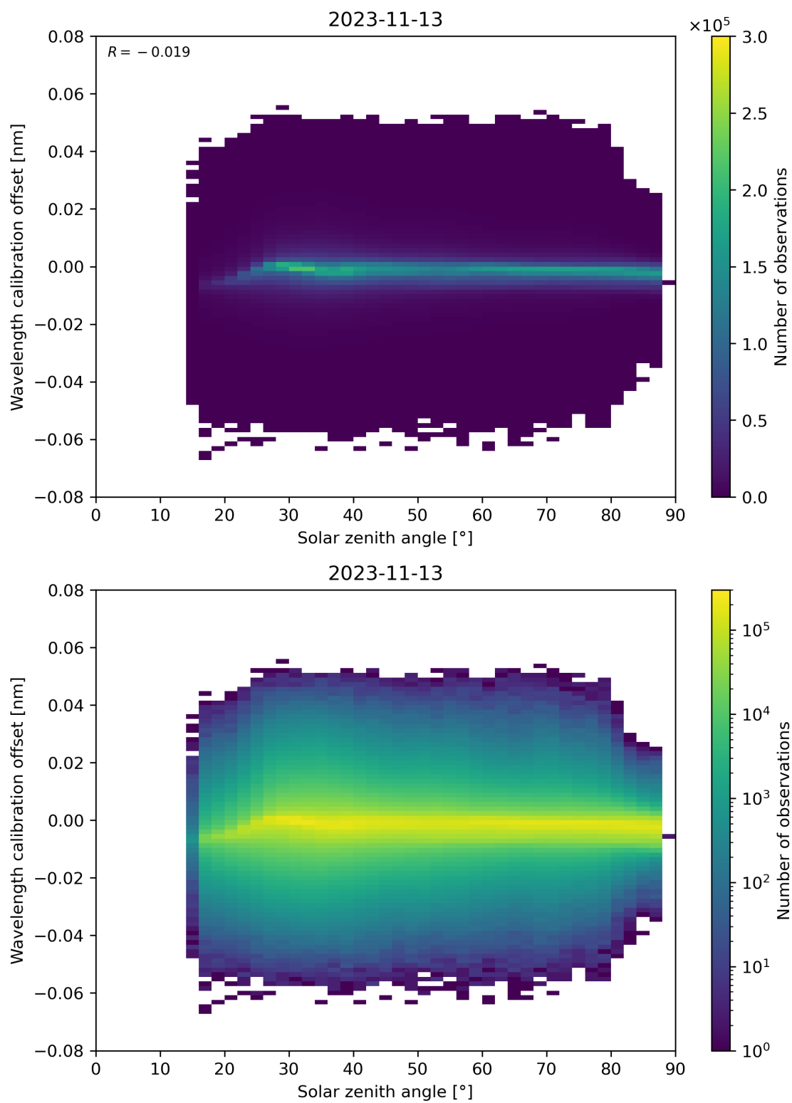
Figure 158: Scatter density plot of “Solar zenith angle” against “Wavelength calibration offset” for 2023-11-13 to 2023-11-14.
