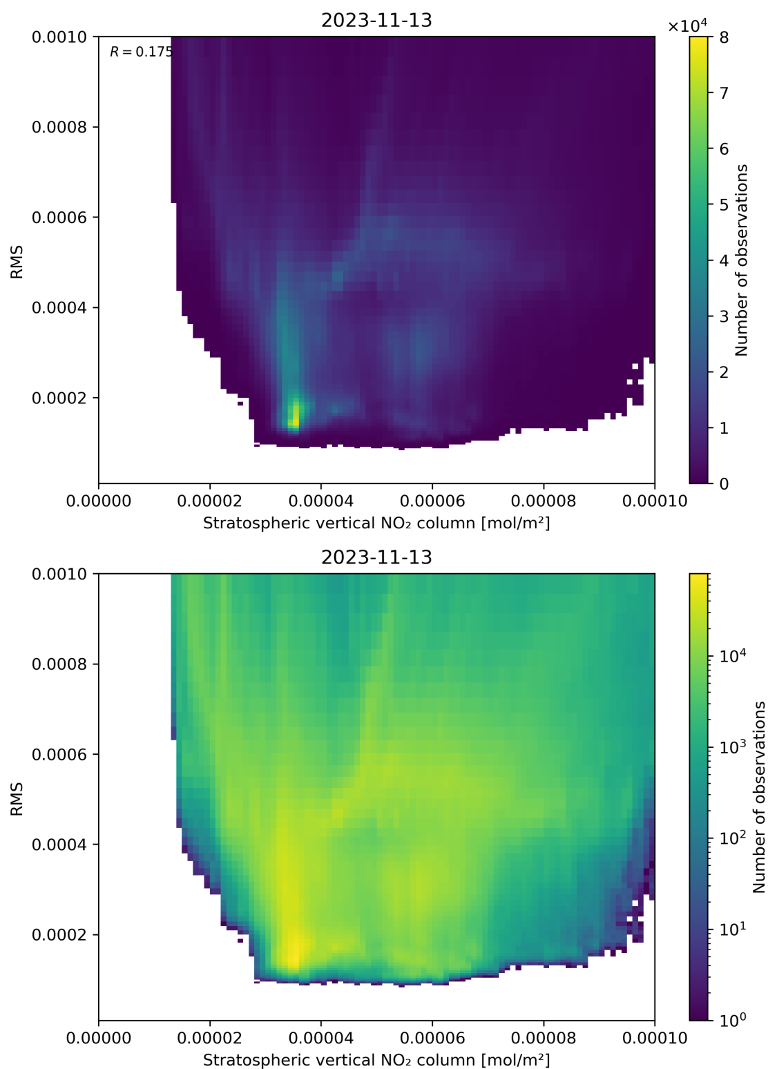
Figure 102: Scatter density plot of “Stratospheric vertical NO 2 column” against “RMS” for 2023-11-13 to 2023-11-14.
