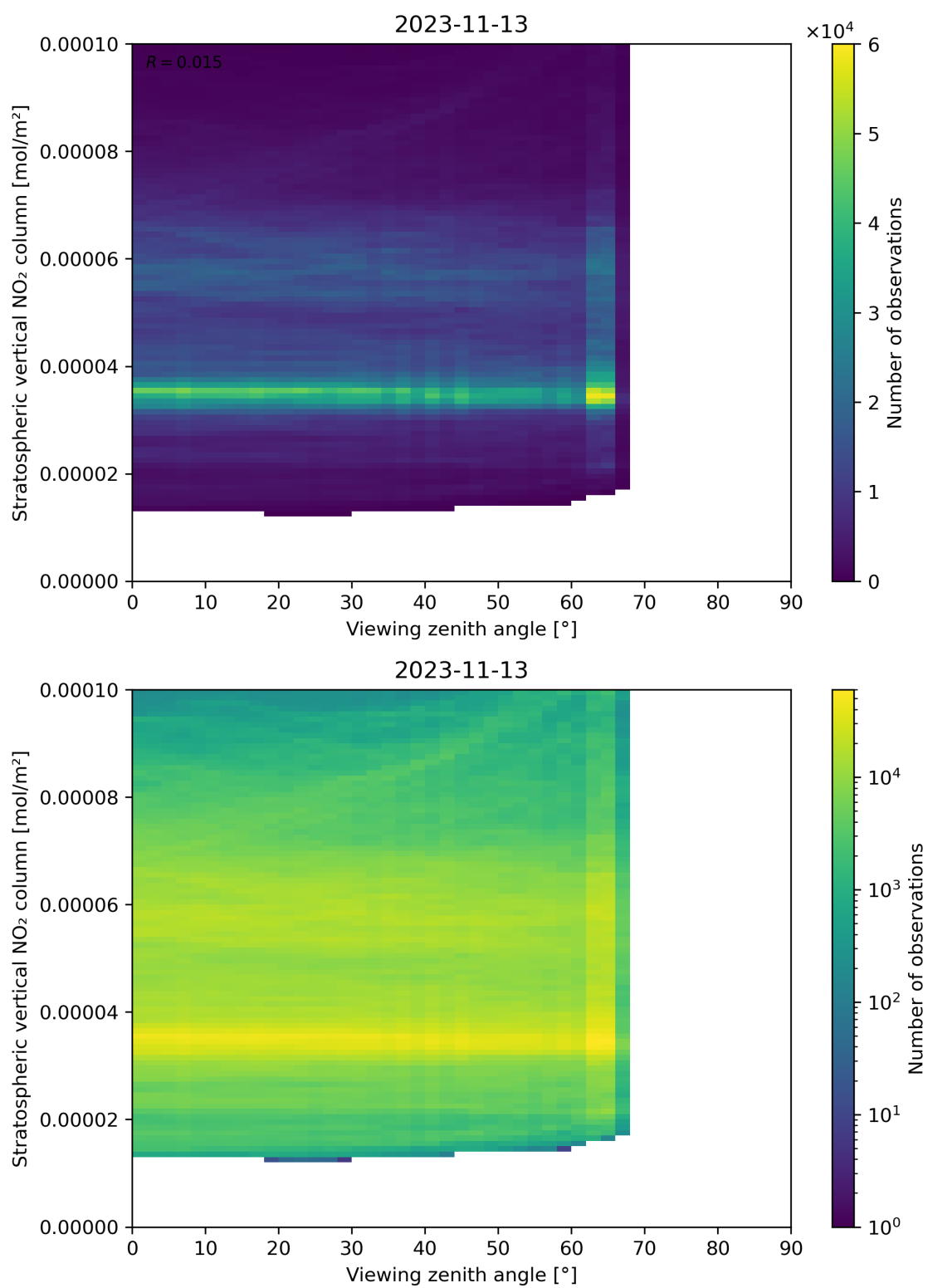
Figure 164: Scatter density plot of “Viewing zenith angle” against “Stratospheric vertical NO 2 column” for 2023-11-13 to 2023-11-14.
