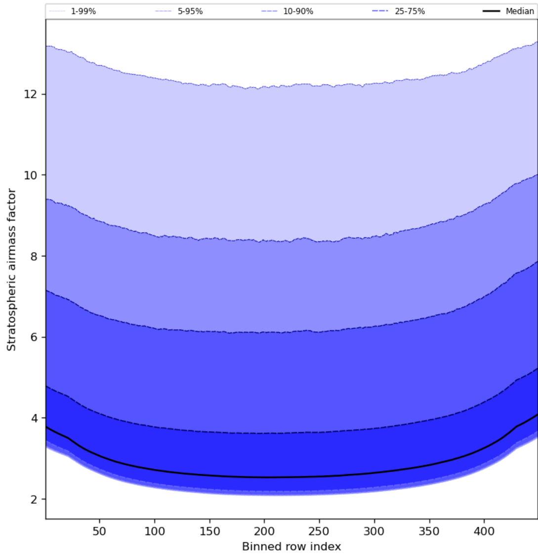
Figure 61: Along track statistics of “Stratospheric air mass factor” for 2023-11-13 to 2023-11-14
