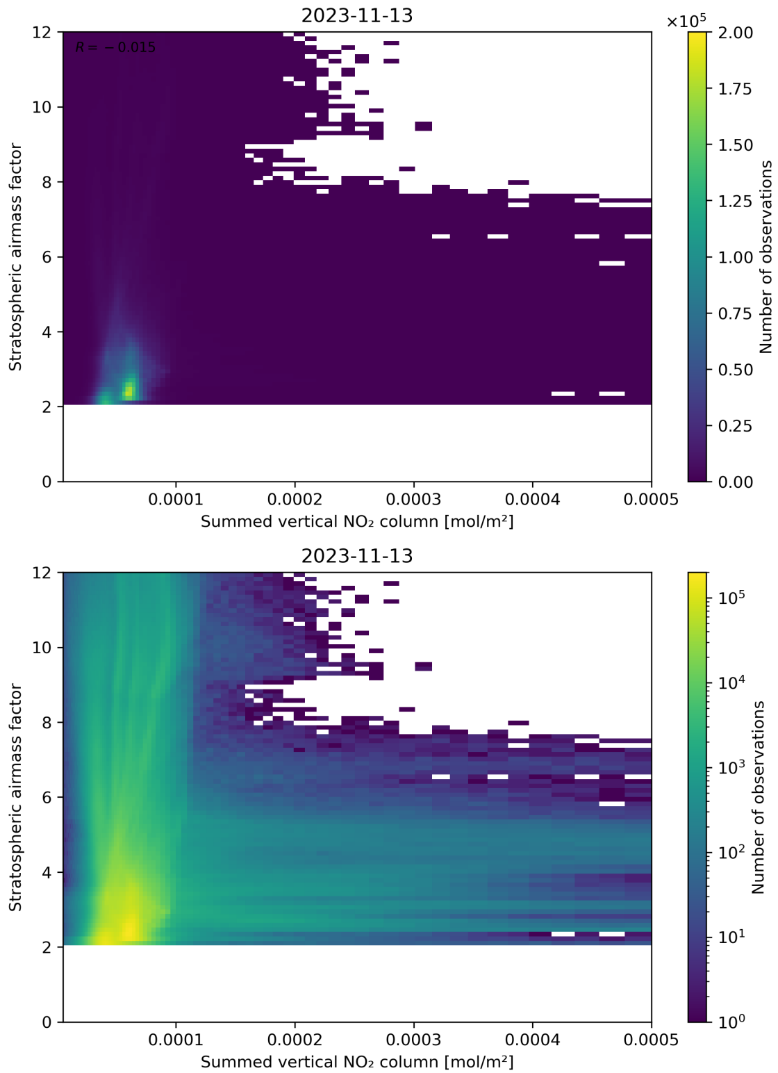
Figure 103: Scatter density plot of “Summed vertical NO 2 column” against “Stratospheric air mass factor” for 2023-11-13 to 2023-11-14.
