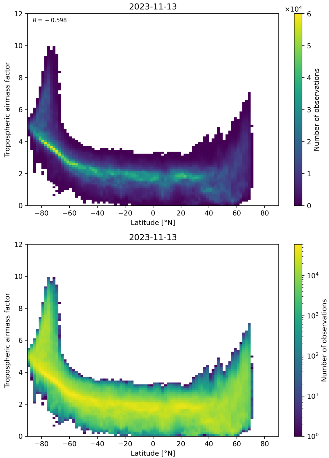
Figure 85: Scatter density plot of “Latitude” against “Tropospheric airmass factor” for 2023-11-13 to 2023-11-14.
