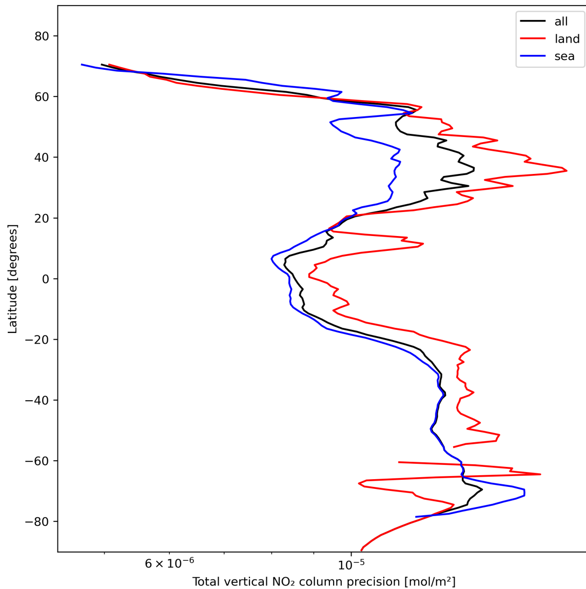
Figure 22: Zonal average of “Total vertical NO 2 column precision” for 2023-11-13 to 2023-11-14.
