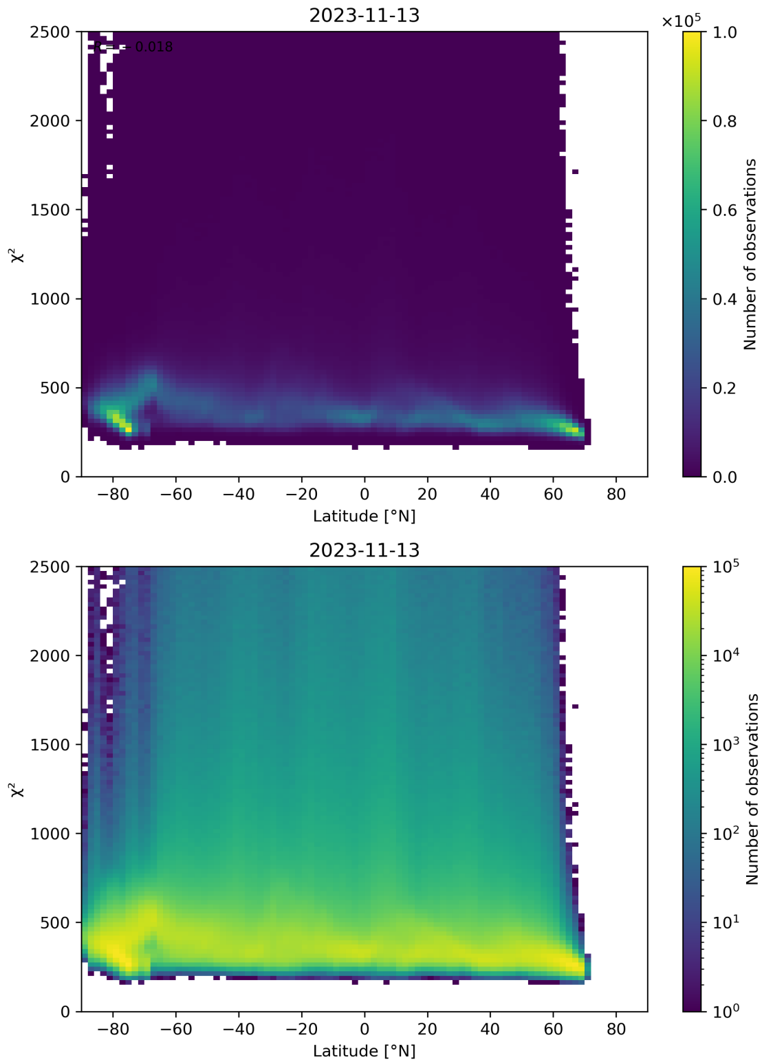
Figure 86: Scatter density plot of “Latitude” against “ \chi^2 ” for 2023-11-13 to 2023-11-14.
