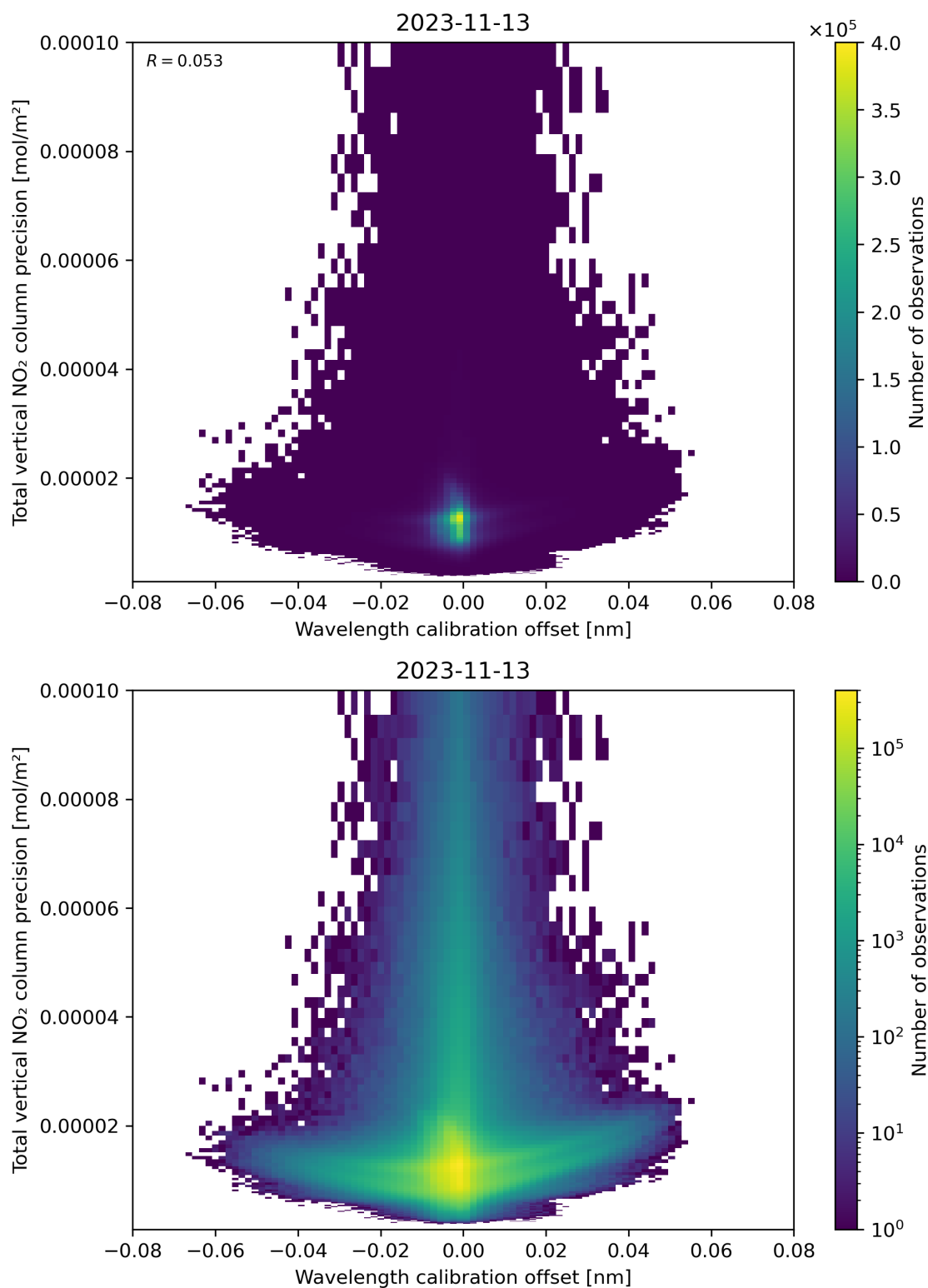
Figure 180: Scatter density plot of “Wavelength calibration offset” against “Total vertical NO 2 column precision” for 2023-11-13 to 2023-11-14.
