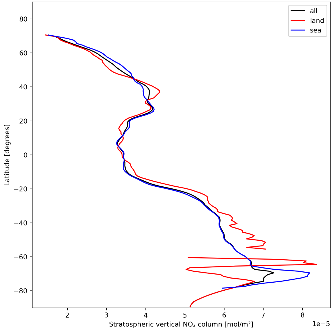
Figure 19: Zonal average of “Stratospheric vertical NO 2 column” for 2023-11-13 to 2023-11-14.
