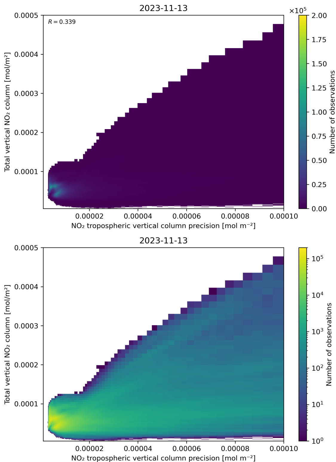
Figure 138: Scatter density plot of “NO 2 tropospheric vertical column precision” against “Total vertical NO 2 column” for 2023-11-13 to 2023-11-14.
