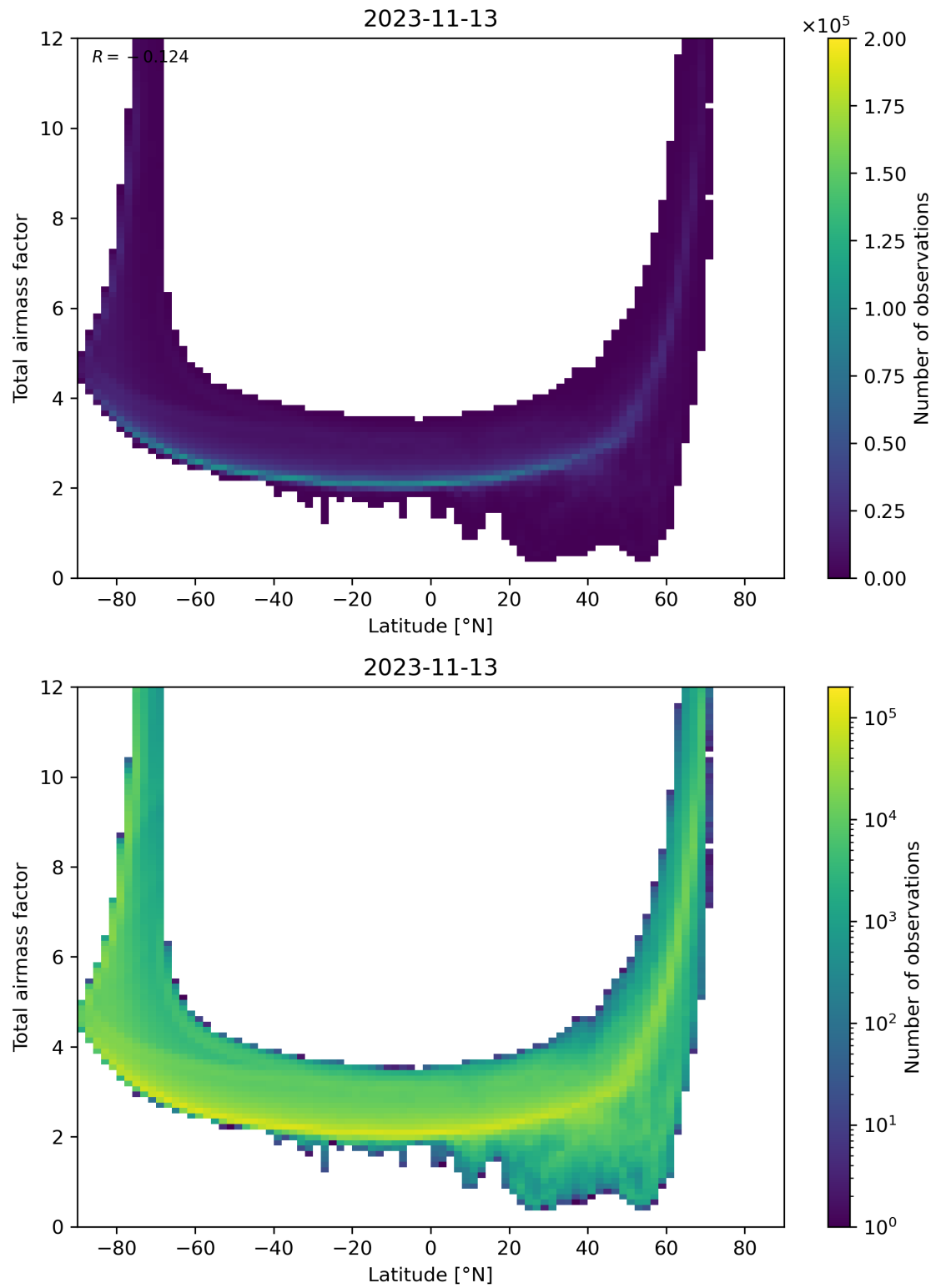
Figure 84: Scatter density plot of “Latitude” against “Total airmass factor” for 2023-11-13 to 2023-11-14.
