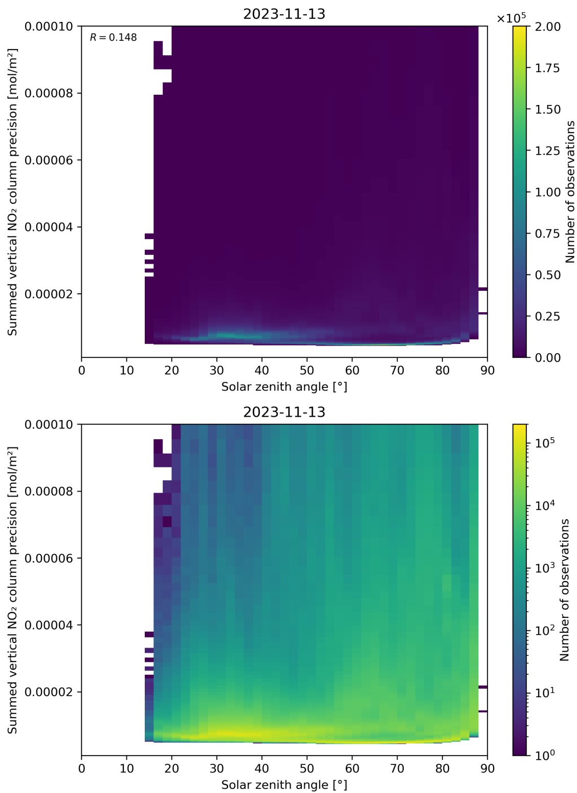
Figure 152: Scatter density plot of “Solar zenith angle” against “Summed vertical NO 2 column precision” for 2023-11-13 to 2023-11-14.
