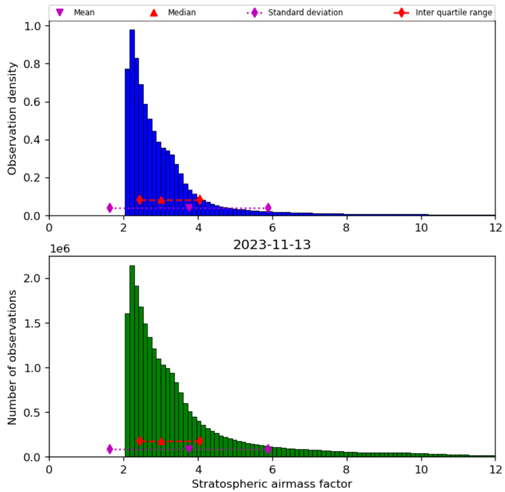
Figure 44: Histogram of “Stratospheric airmass factor” for 2023-11-13 to 2023-11-14
