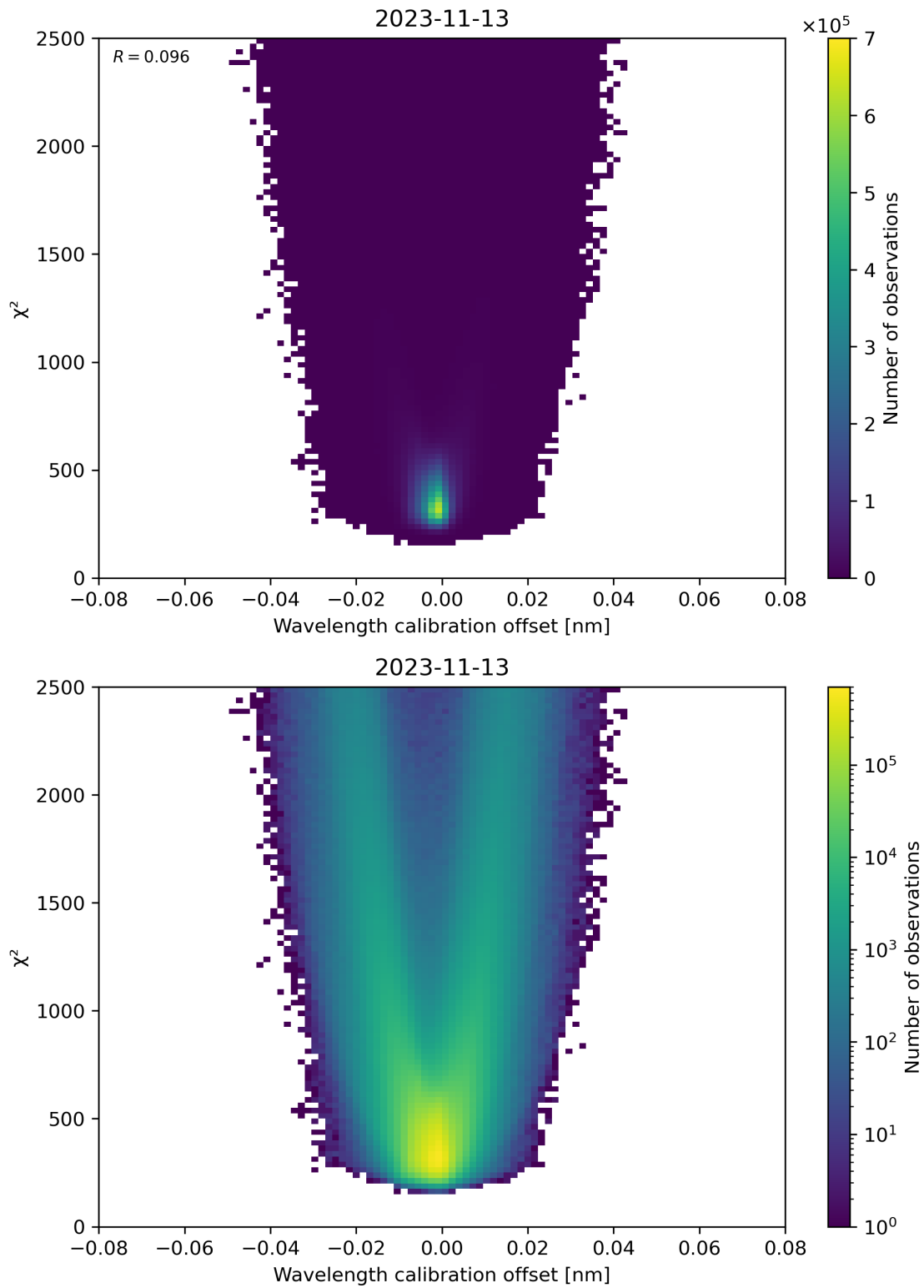
Figure 175: Scatter density plot of “Wavelength calibration offset” against “ \chi^2 ” for 2023-11-13 to 2023-11-14.
