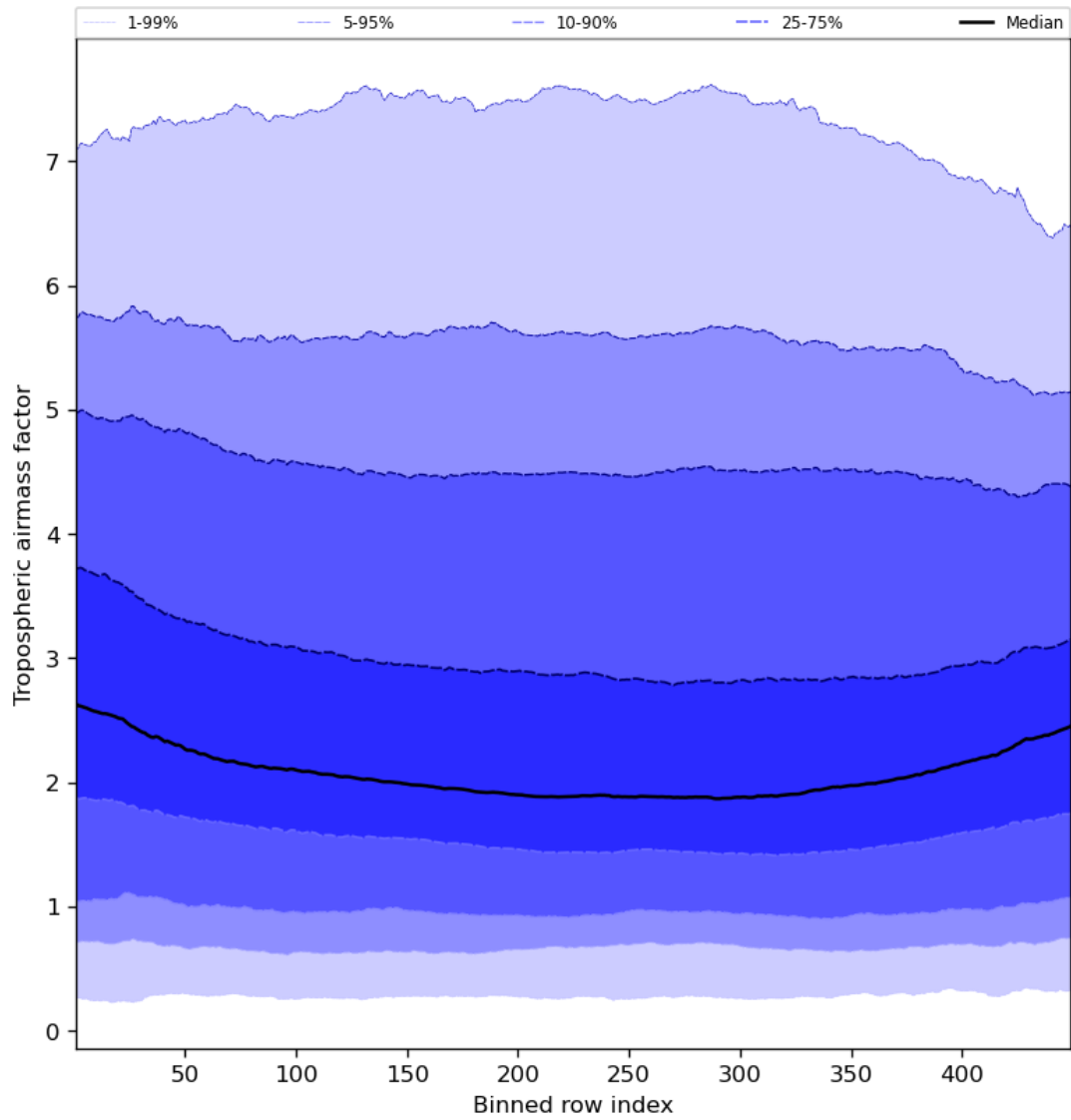
Figure 48: Along track statistics of “Tropospheric air mass factor” for 2023-11-13 to 2023-11-14
