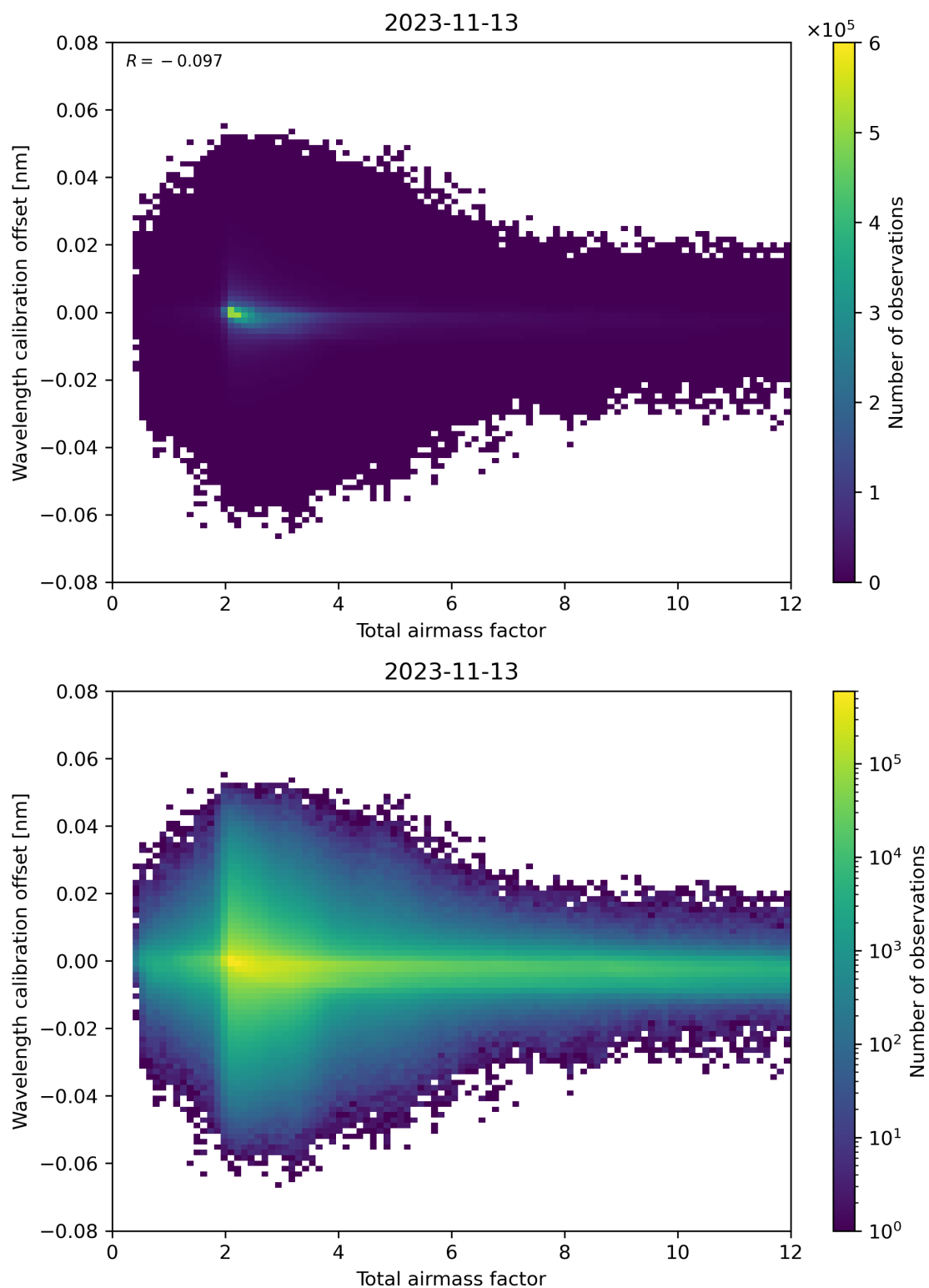
Figure 70: Scatter density plot of “Total airmass factor” against “Wavelength calibration offset” for 2023-11-13 to 2023-11-14.
