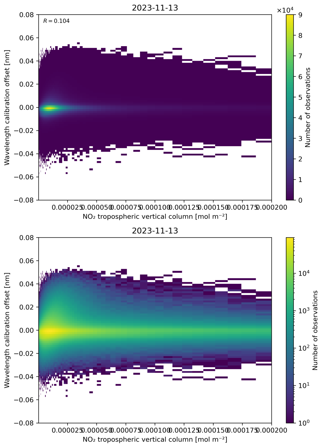
Figure 143: Scatter density plot of “NO 2 tropospheric vertical column” against “Wavelength calibration offset” for 2023-11-13 to 2023-11-14.
