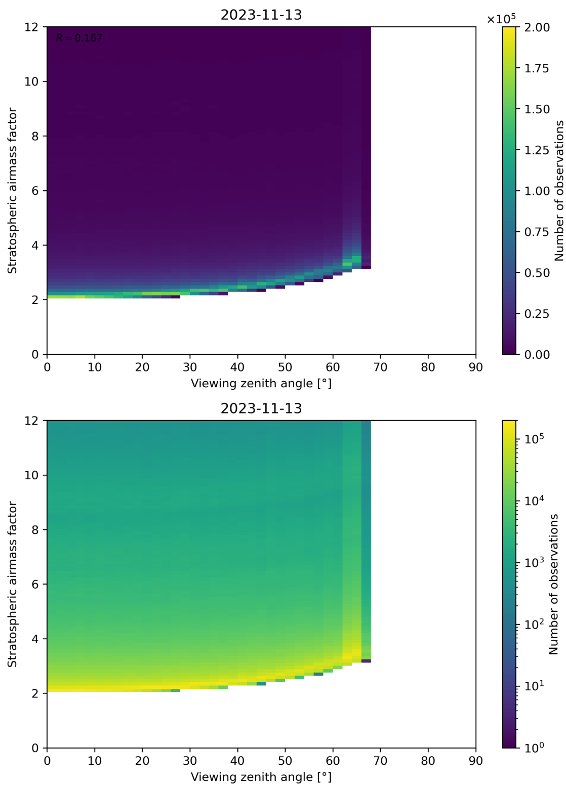
Figure 159: Scatter density plot of “Viewing zenith angle” against “Stratospheric airmass factor” for 2023-11-13 to 2023-11-14.
