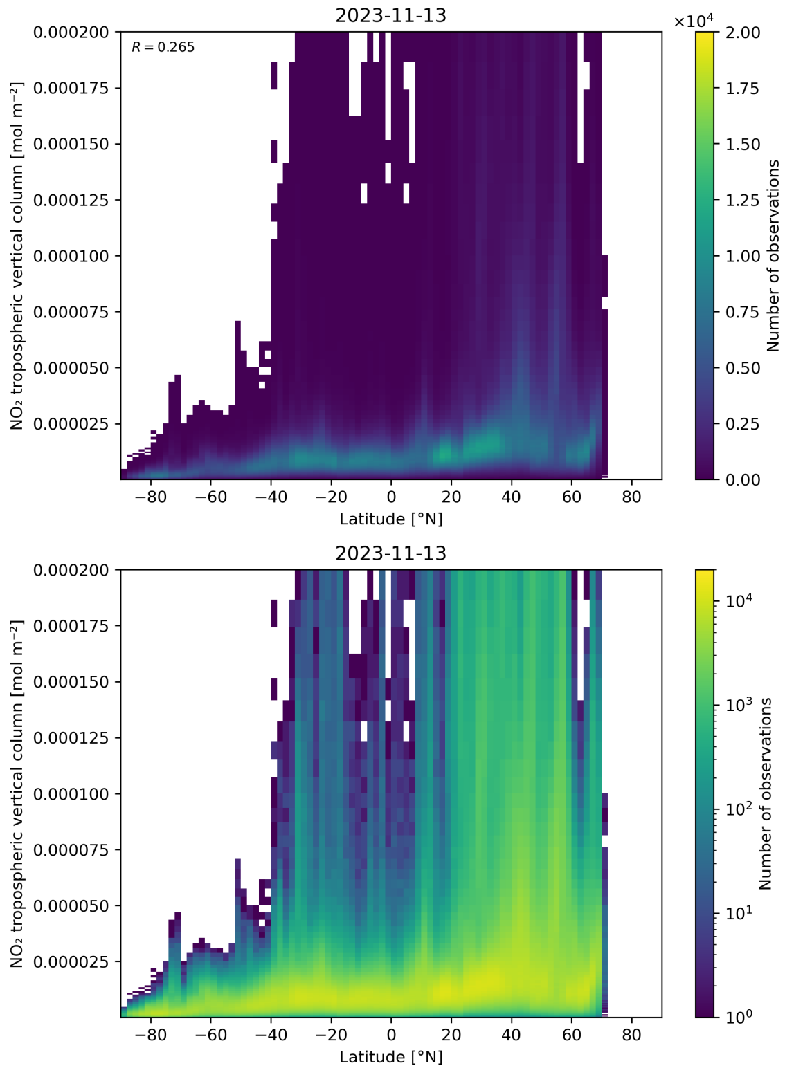
Figure 92: Scatter density plot of “Latitude” against “NO 2 tropospheric vertical column” for 2023-11-13 to 2023-11-14.
