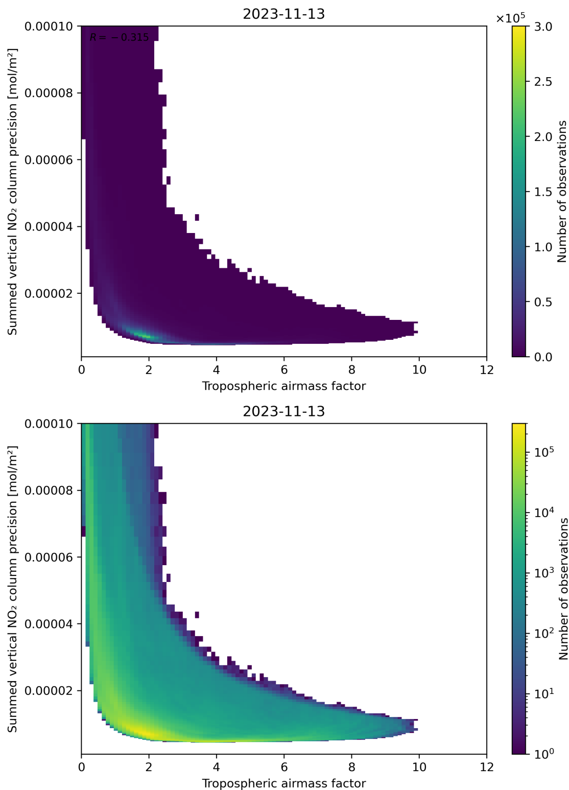
Figure 76: Scatter density plot of “Tropospheric air mass factor” against “Summed vertical NO 2 column precision” for 2023-11-13 to 2023-11-14.
