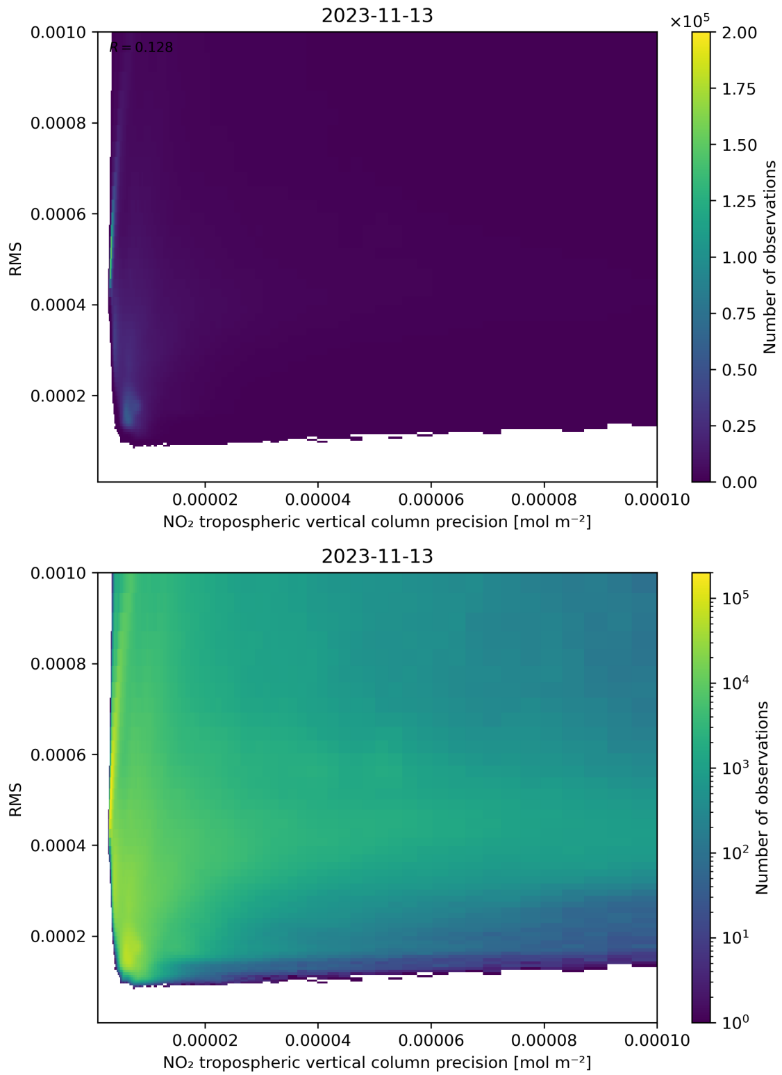
Figure 140: Scatter density plot of “NO 2 tropospheric vertical column precision” against “RMS” for 2023-11-13 to 2023-11-14.
