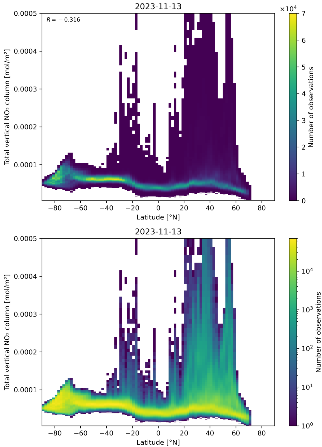
Figure 90: Scatter density plot of “Latitude” against “Total vertical NO 2 column” for 2023-11-13 to 2023-11-14.
