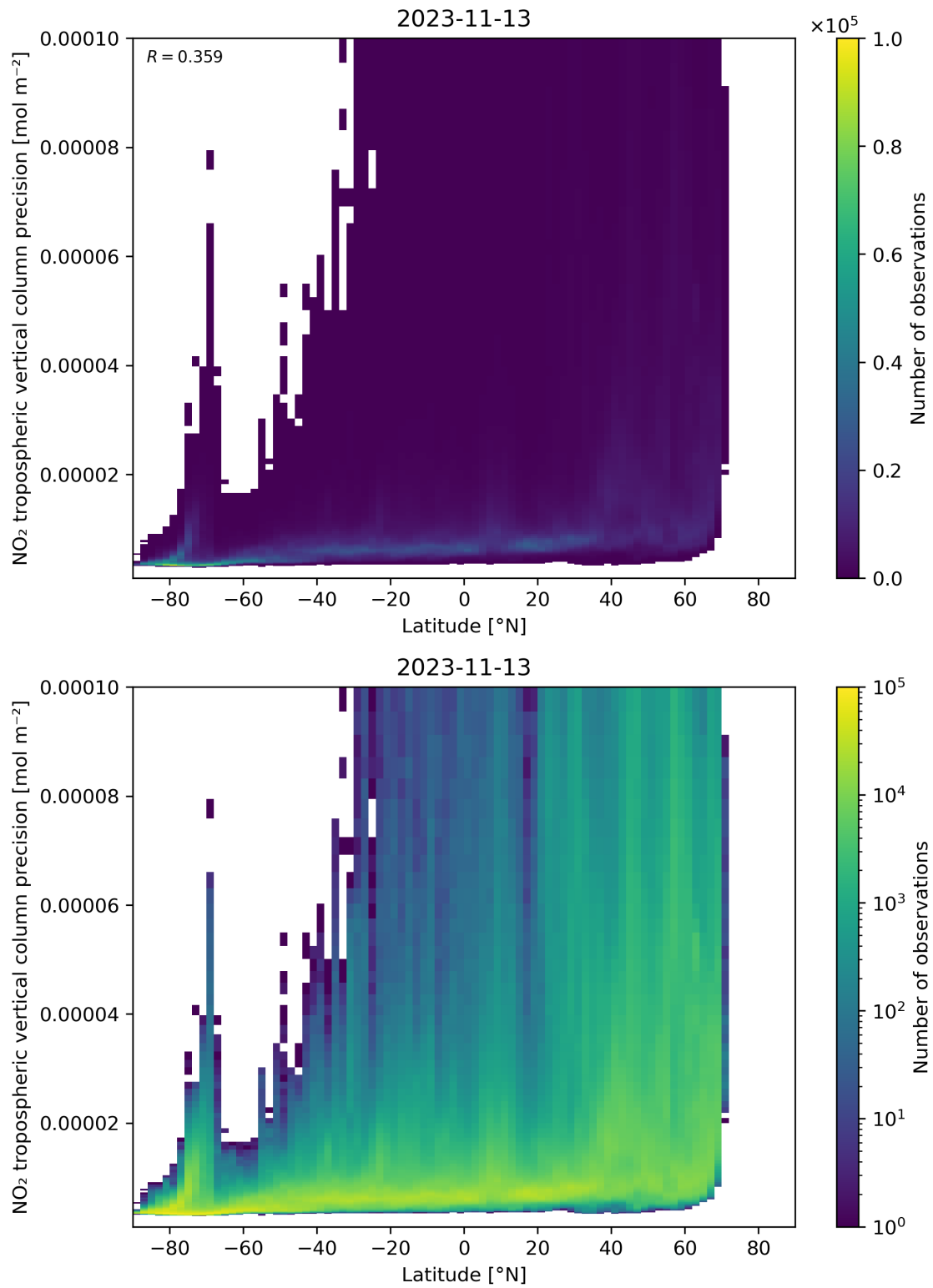
Figure 93: Scatter density plot of “Latitude” against “NO 2 tropospheric vertical column precision” for 2023-11-13 to 2023-11-14.
