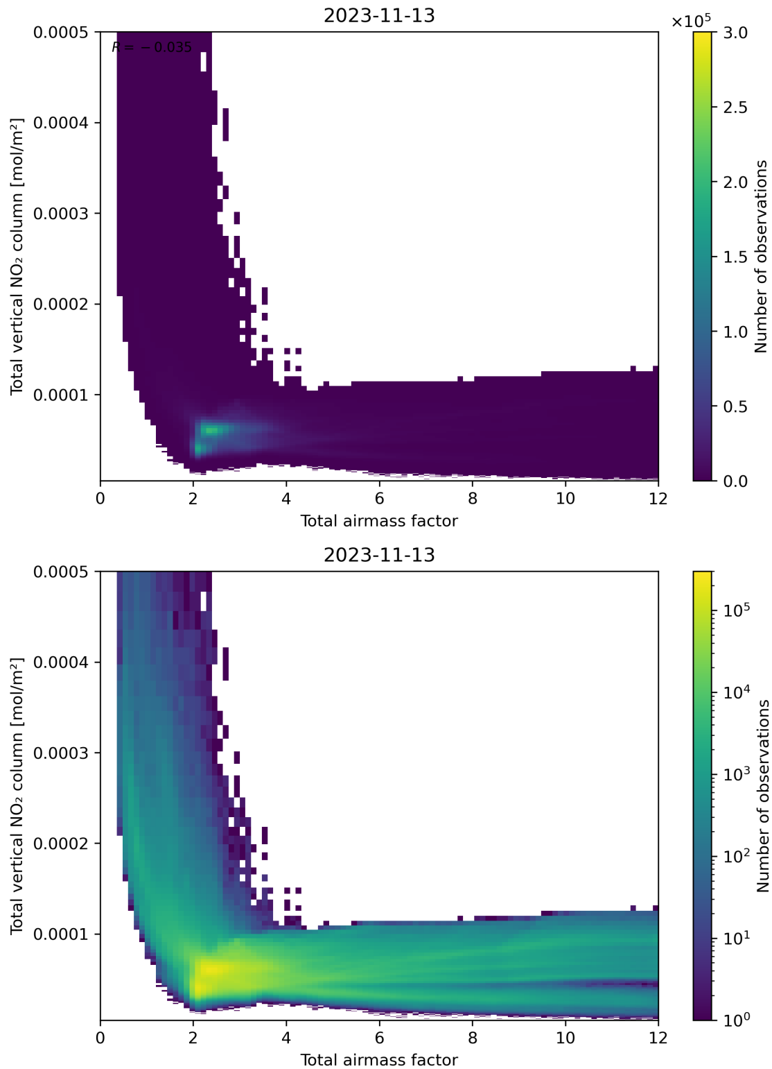
Figure 67: Scatter density plot of “Total airmass factor” against “Total vertical NO 2 column” for 2023-11-13 to 2023-11-14.
