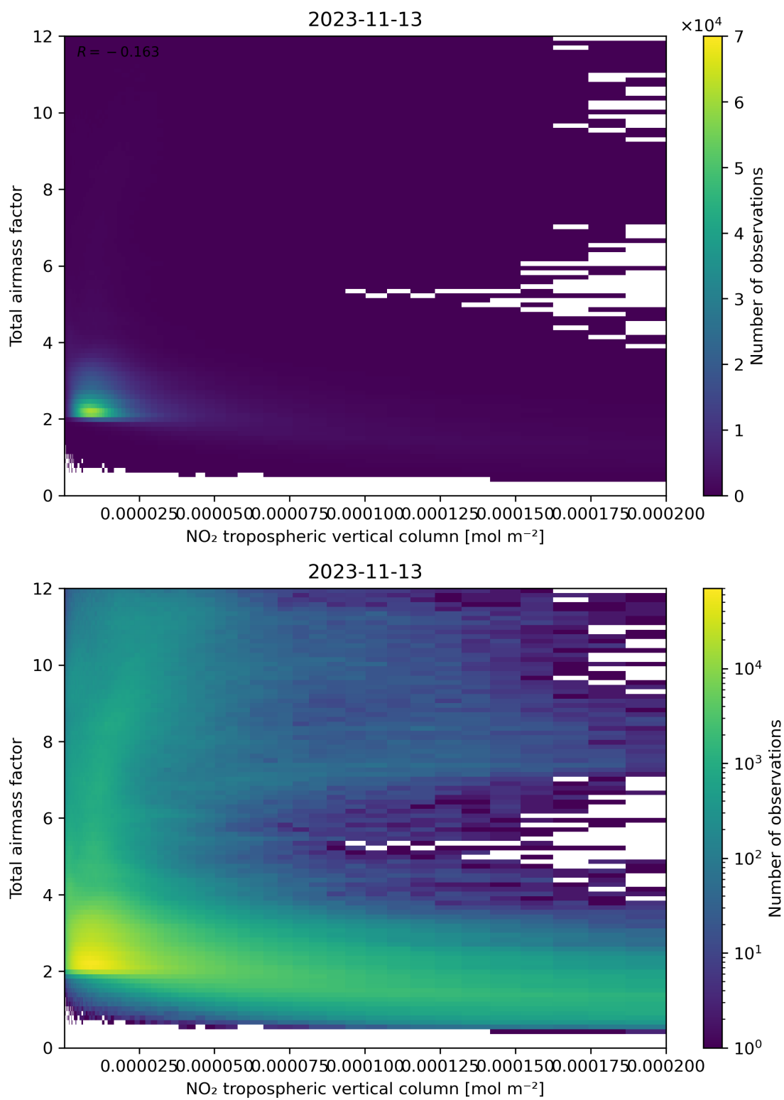
Figure 122: Scatter density plot of “NO 2 tropospheric vertical column” against “Total air mass factor” for 2023-11-13 to 2023-11-14.
