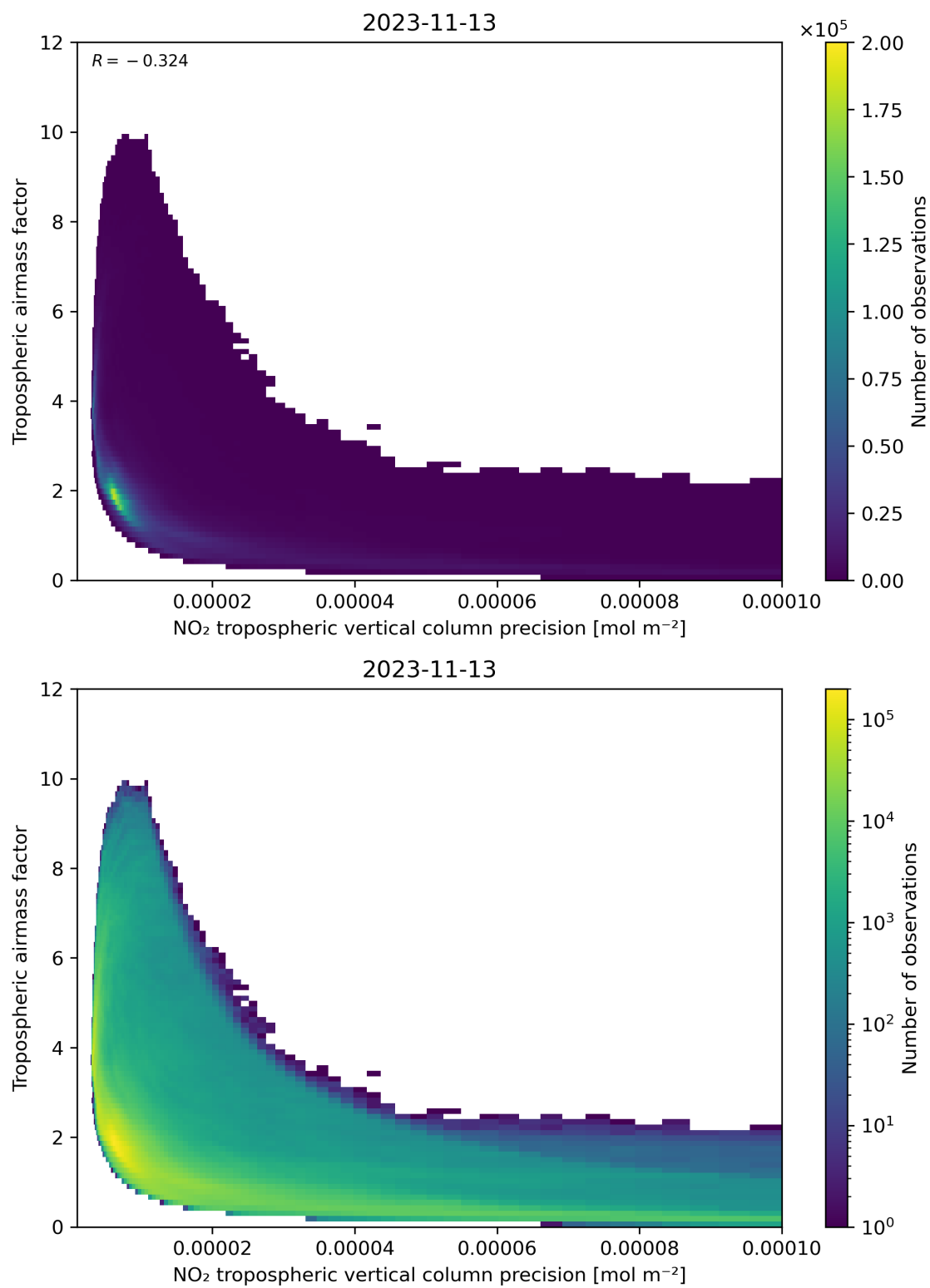
Figure 133: Scatter density plot of “NO 2 tropospheric vertical column precision” against “Tropospheric airmass factor” for 2023-11-13 to 2023-11-14.
