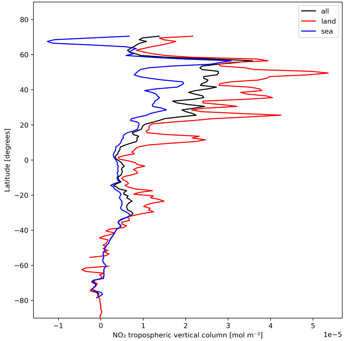
Figure 12: Zonal average of “NO 2 tropospheric vertical column” for 2023-11-13 to 2023-11-14.
