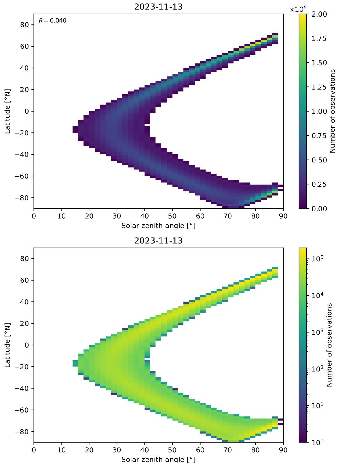
Figure 149: Scatter density plot of “Solar zenith angle” against “Latitude” for 2023-11-13 to 2023-11-14.
