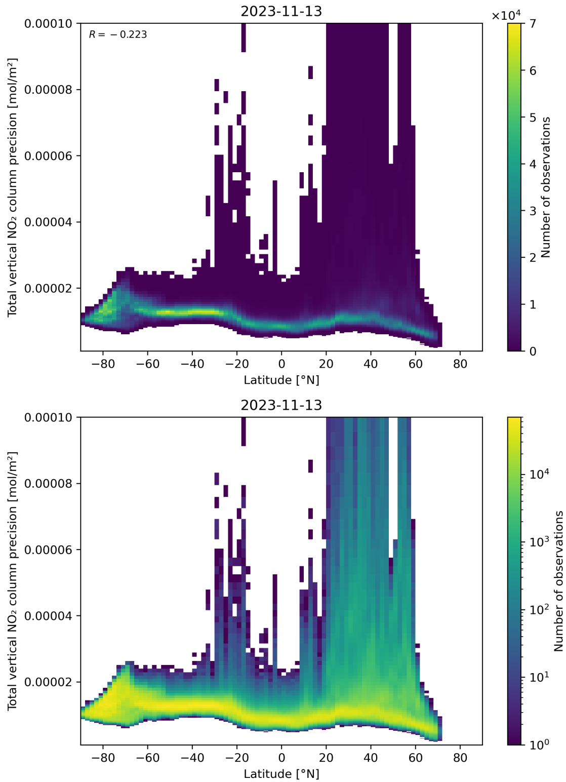
Figure 91: Scatter density plot of “Latitude” against “Total vertical NO 2 column precision” for 2023-11-13 to 2023-11-14.
