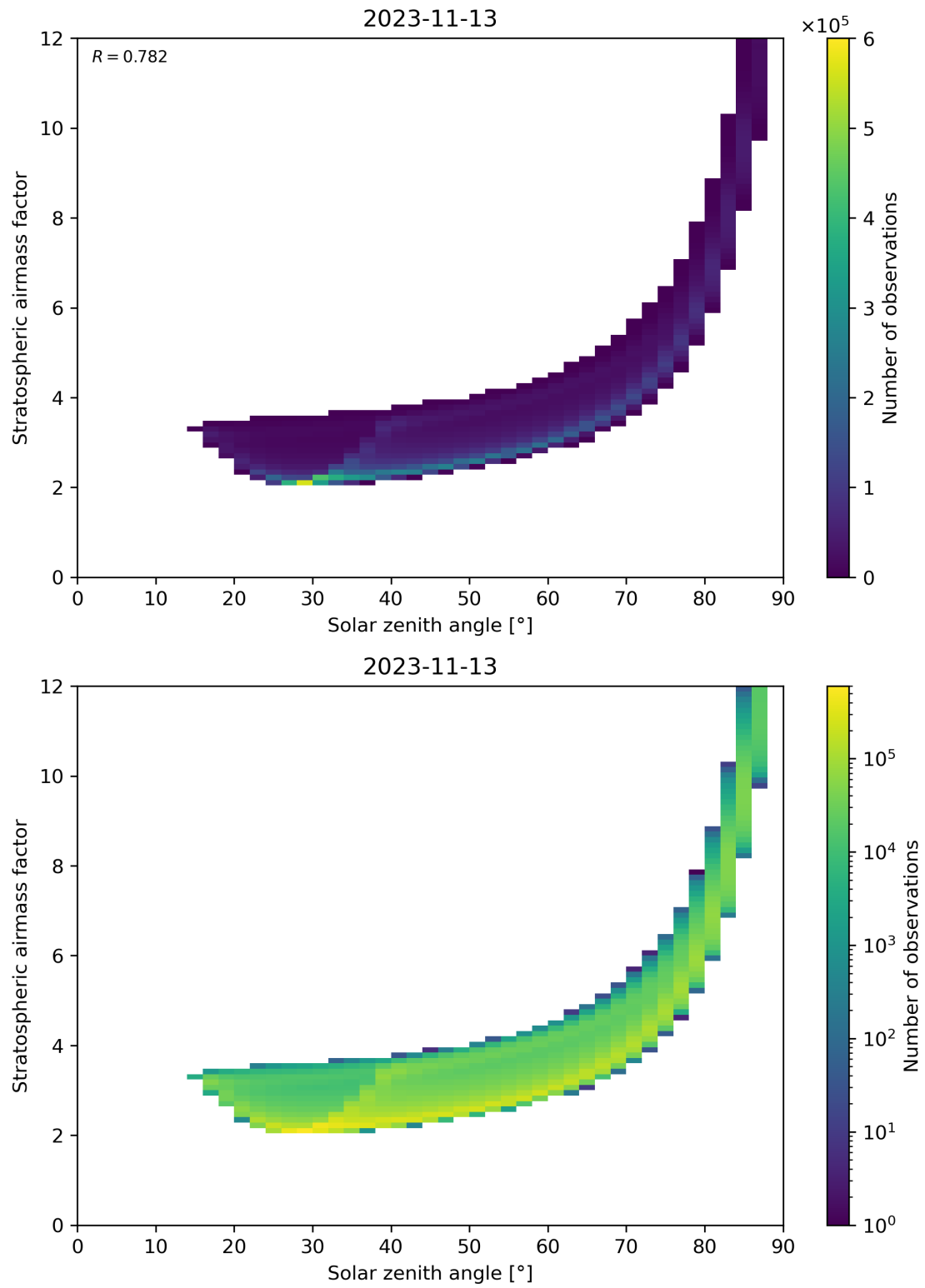
Figure 145: Scatter density plot of “Solar zenith angle” against “Stratospheric airmass factor” for 2023-11-13 to 2023-11-14.
