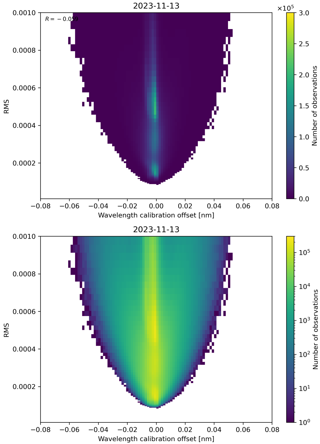
Figure 181: Scatter density plot of “Wavelength calibration offset” against “RMS” for 2023-11-13 to 2023-11-14.
