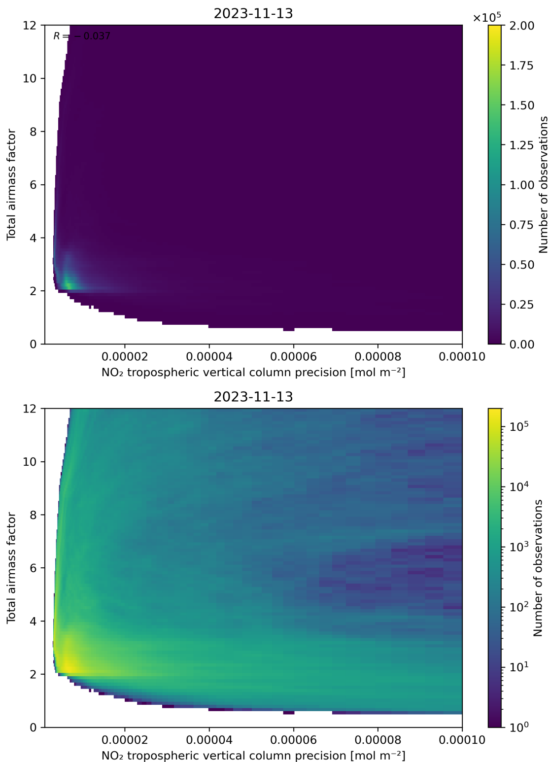
Figure 132: Scatter density plot of “NO 2 tropospheric vertical column precision” against “Total air mass factor” for 2023-11-13 to 2023-11-14.
