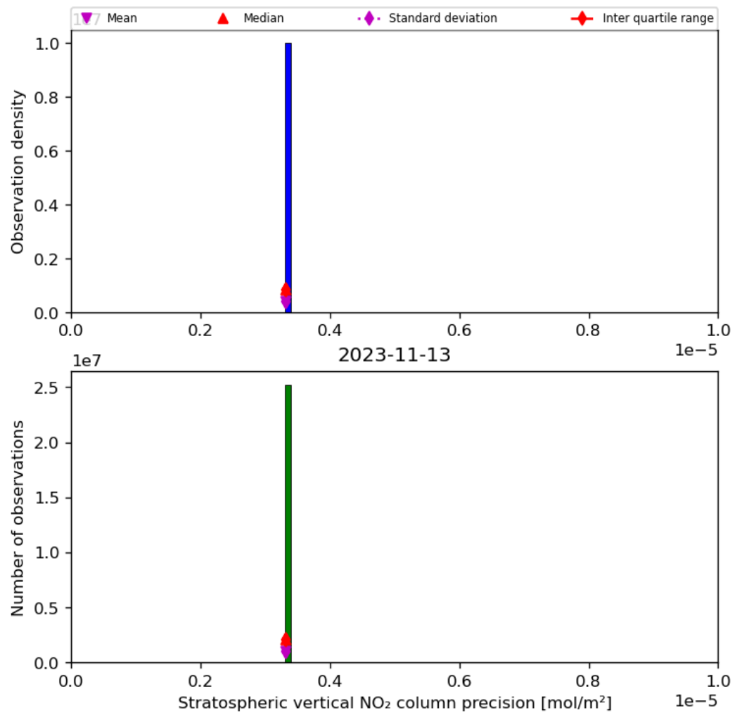
Figure 37: Histogram of “Stratospheric vertical NO 2 column precision” for 2023-11-13 to 2023-11-14
