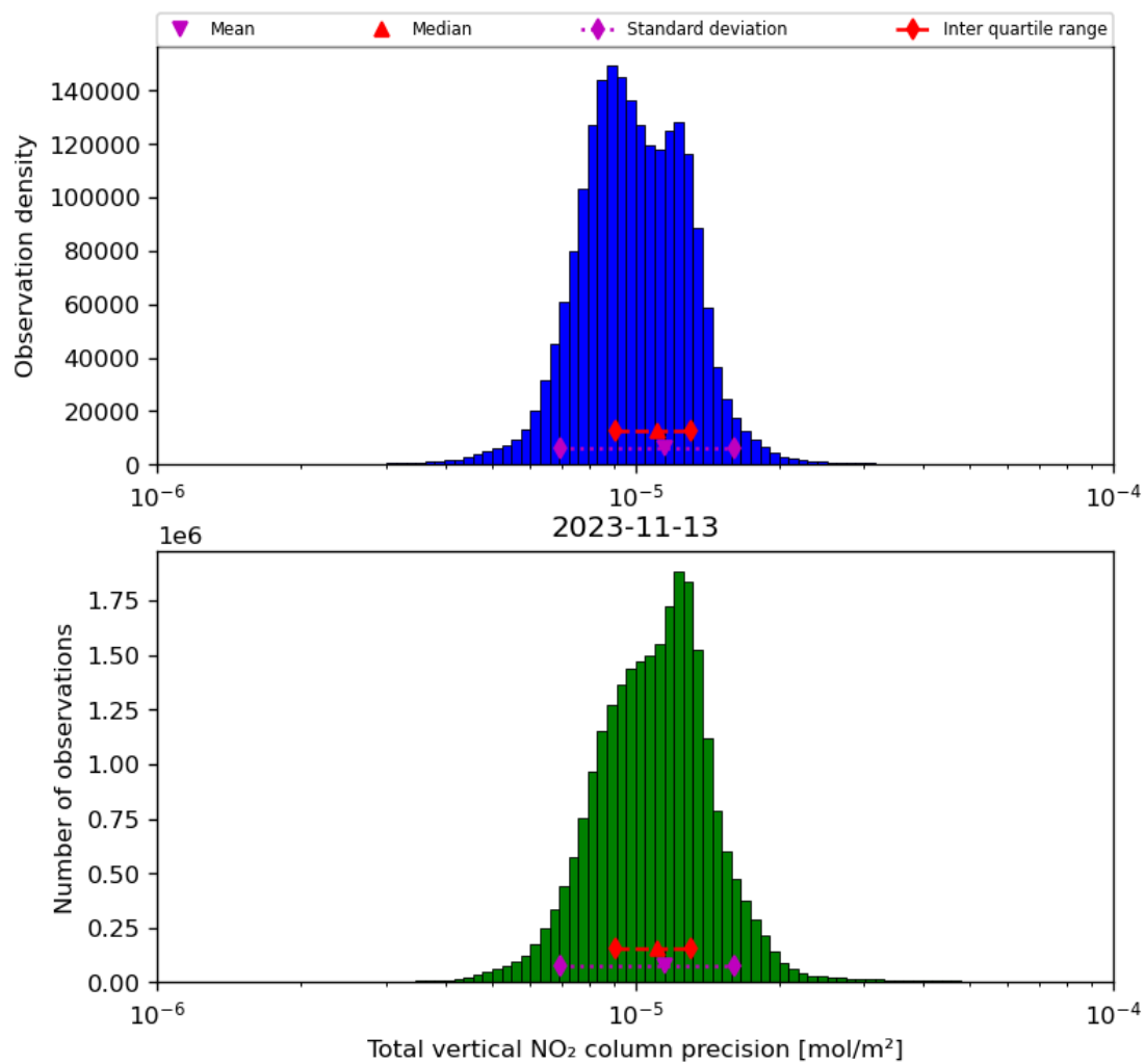
Figure 39: Histogram of “Total vertical NO 2 column precision” for 2023-11-13 to 2023-11-14
