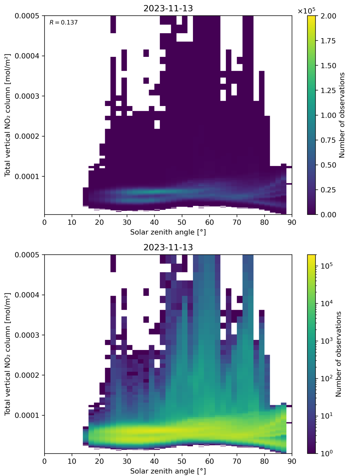
Figure 153: Scatter density plot of “Solar zenith angle” against “Total vertical NO 2 column” for 2023-11-13 to 2023-11-14.
