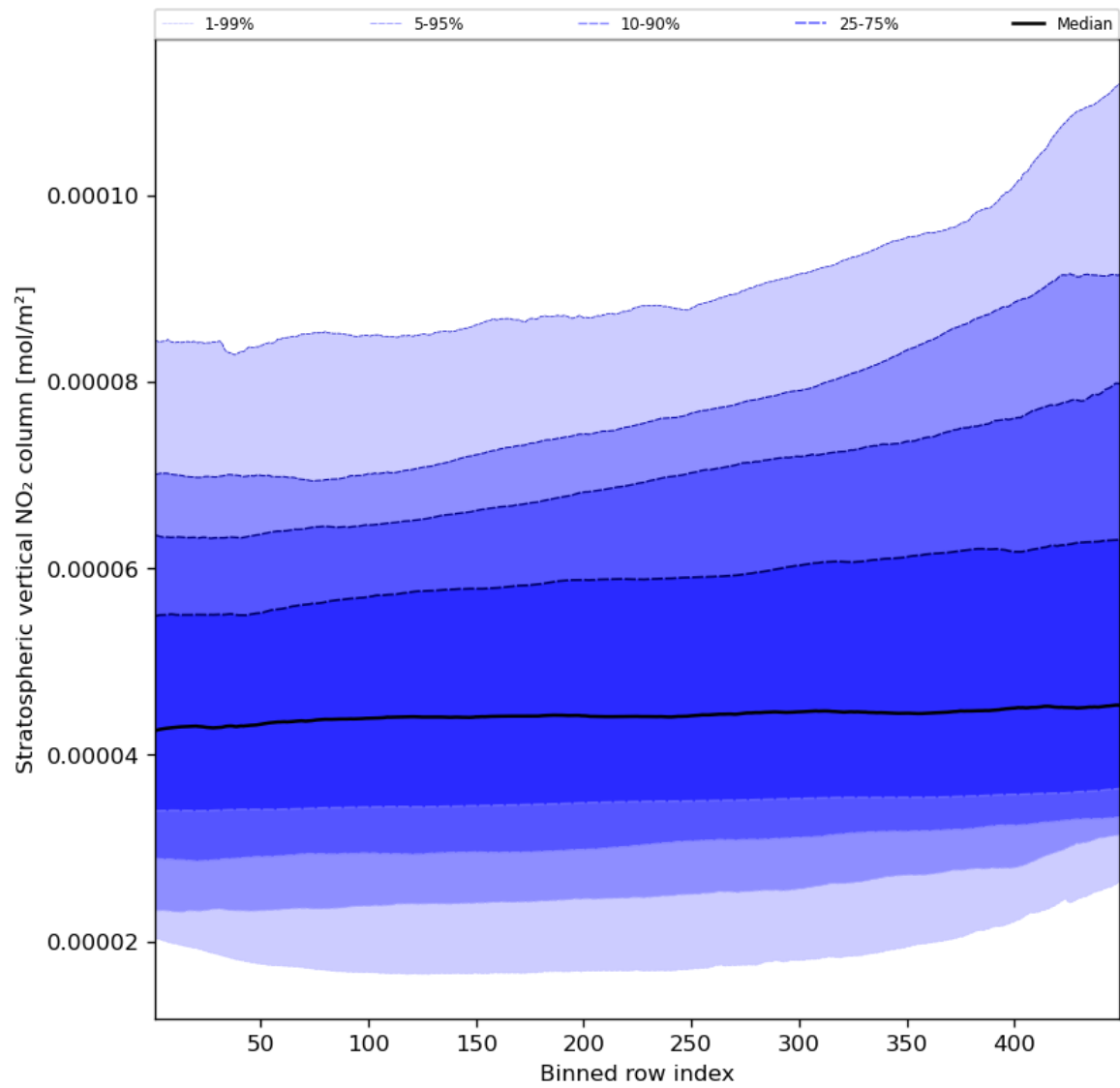
Figure 53: Along track statistics of “Stratospheric vertical NO 2 column” for 2023-11-13 to 2023-11-14
