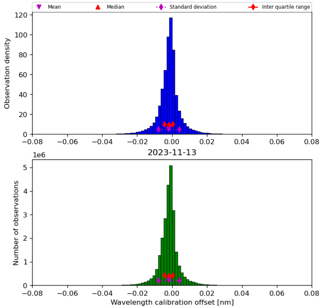
Figure 35: Histogram of “Wavelength calibration offset” for 2023-11-13 to 2023-11-14
