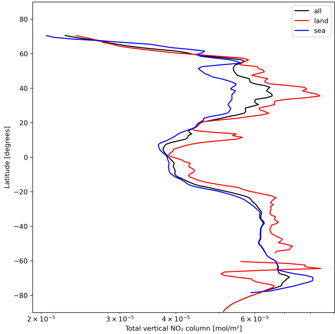
Figure 21: Zonal average of “Total vertical NO 2 column” for 2023-11-13 to 2023-11-14.
