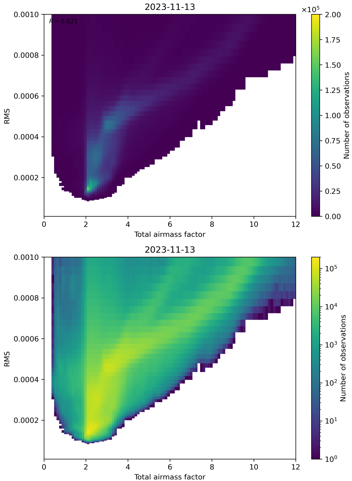
Figure 69: Scatter density plot of “Total airmass factor” against “RMS” for 2023-11-13 to 2023-11-14.
