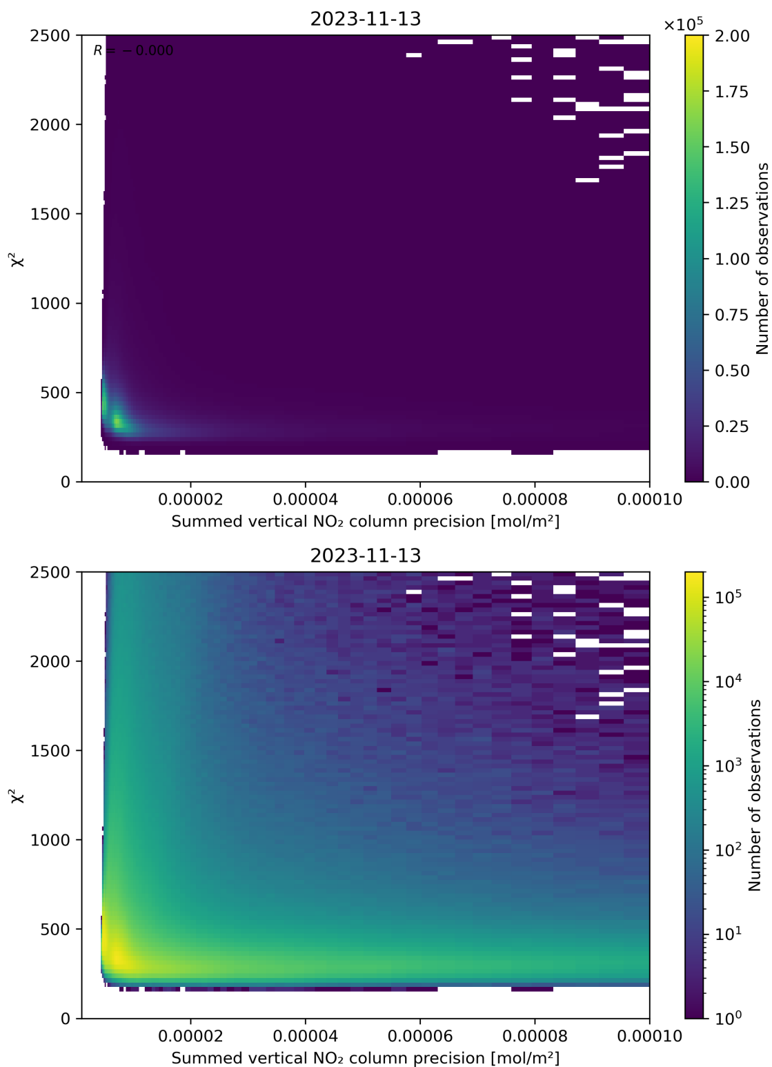
Figure 107: Scatter density plot of “Summed vertical NO 2 column precision” against “ \chi^2 ” for 2023-11-13 to 2023-11-14.
