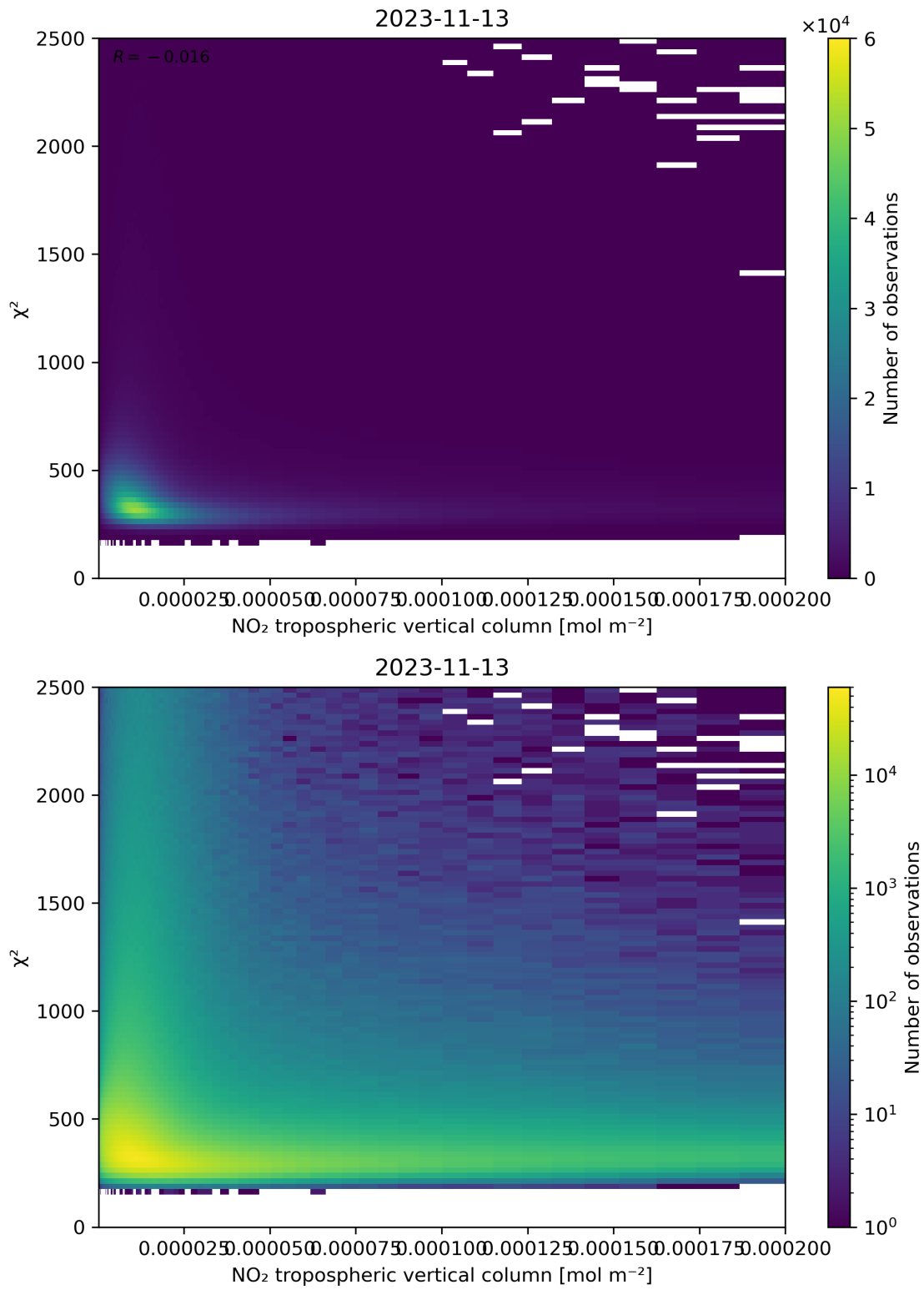
Figure 124: Scatter density plot of “NO 2 tropospheric vertical column” against “ \chi^2 ” for 2023-11-13 to 2023-11-14.
