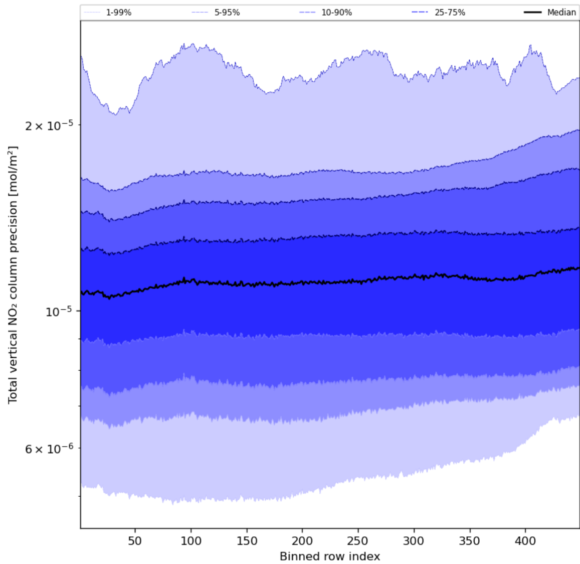
Figure 56: Along track statistics of "Total vertical NO 2 column precision" for 2023-11-13 to 2023-11-14
