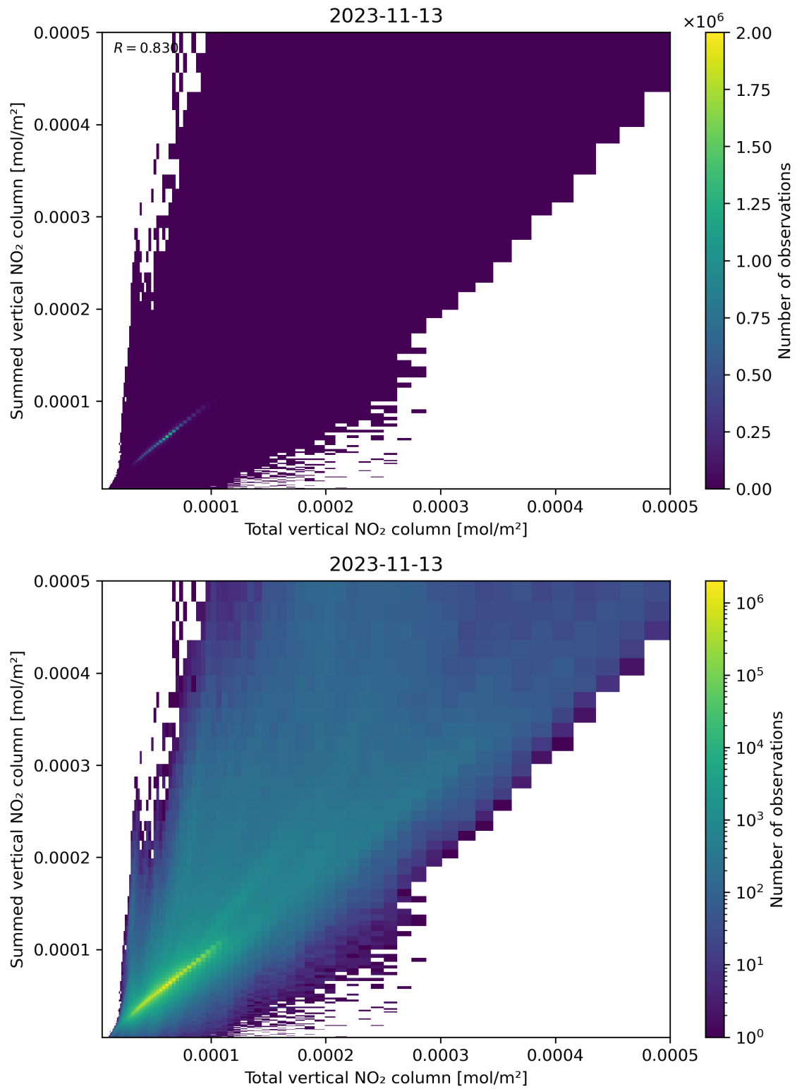
Figure 112: Scatter density plot of “Total vertical NO 2 column” against “Summed vertical NO 2 column” for 2023-11-13 to 2023-11-14.
