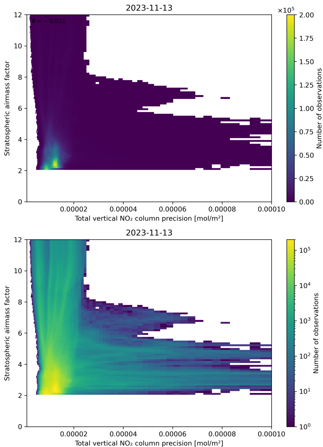
Figure 115: Scatter density plot of “Total vertical NO 2 column precision” against “Stratospheric airmass factor” for 2023-11-13 to 2023-11-14.
