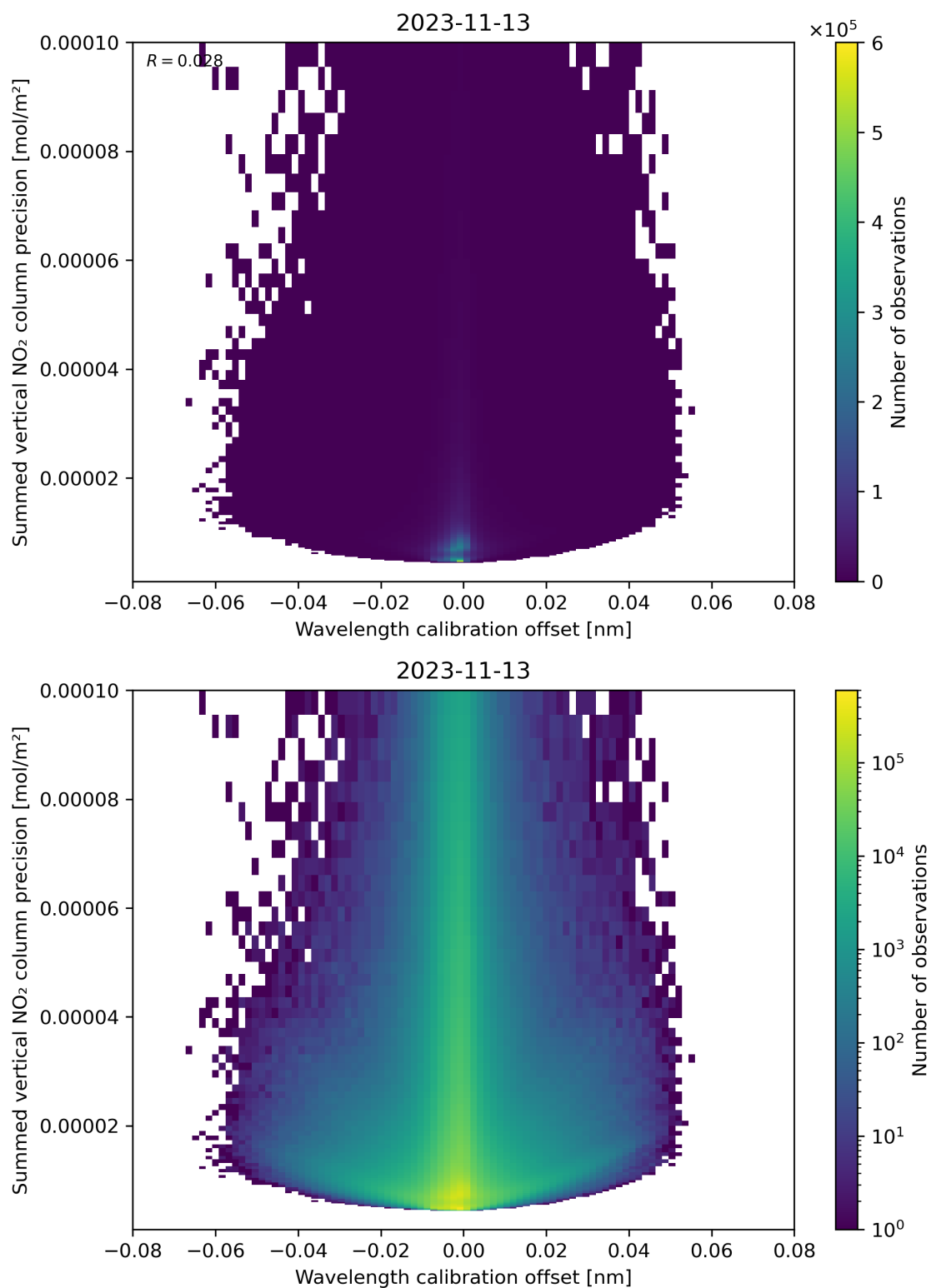
Figure 178: Scatter density plot of “Wavelength calibration offset” against “Summed vertical NO 2 column precision” for 2023-11-13 to 2023-11-14.
