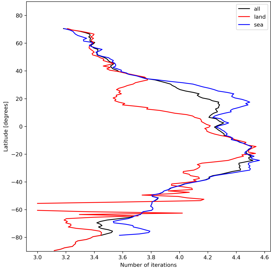
Figure 17: Zonal average of “Number of iterations” for 2023-11-13 to 2023-11-14.
