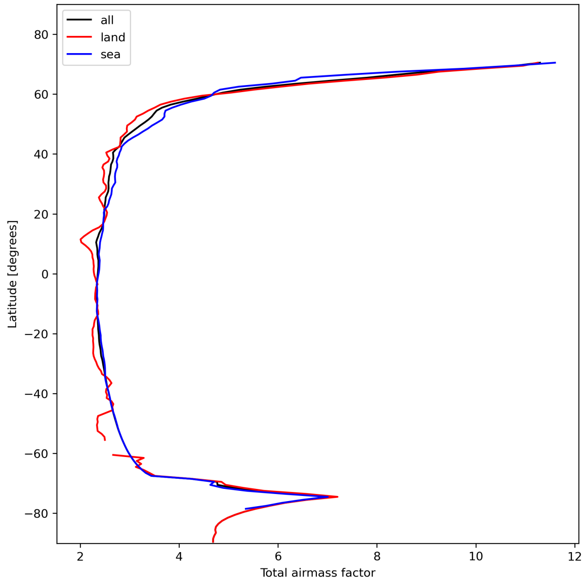
Figure 15: Zonal average of “Total airmass factor” for 2023-11-13 to 2023-11-14.
