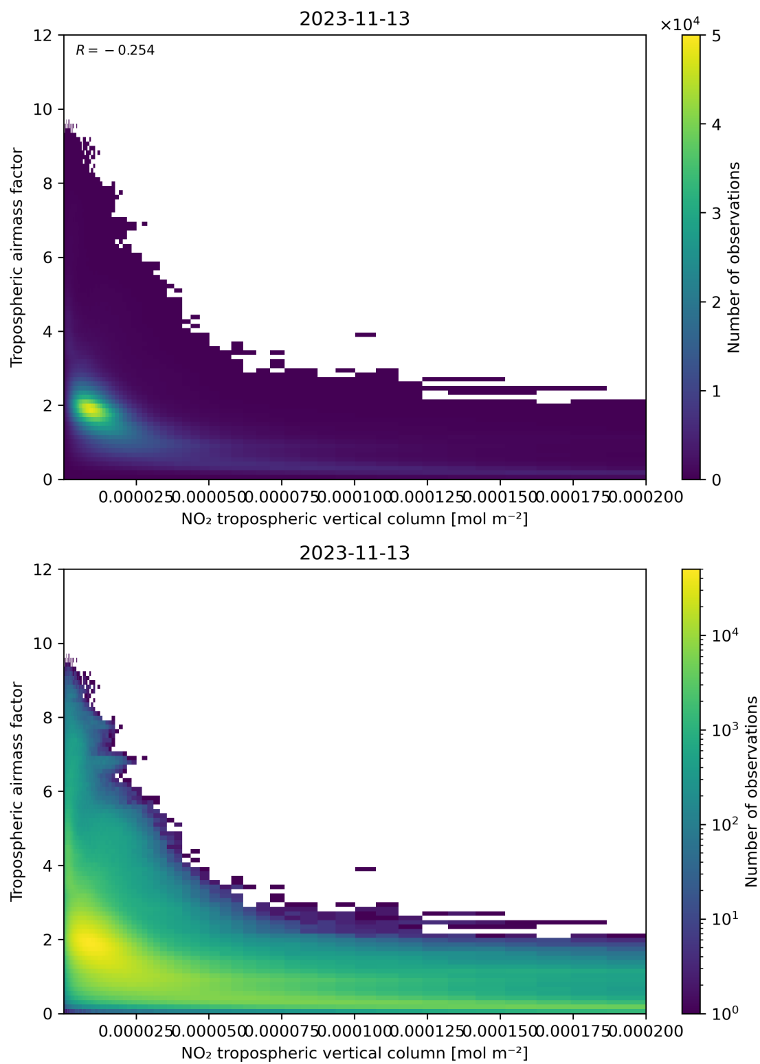
Figure 123: Scatter density plot of “NO 2 tropospheric vertical column” against “Tropospheric air mass factor” for 2023-11-13 to 2023-11-14.
