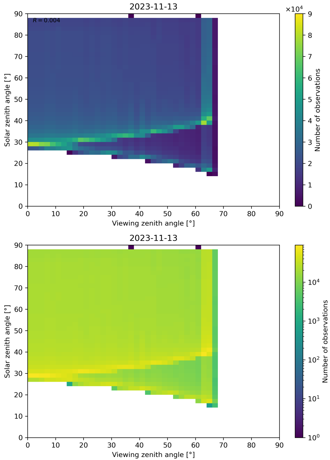
Figure 172: Scatter density plot of “Viewing zenith angle” against “Solar zenith angle” for 2023-11-13 to 2023-11-14.
