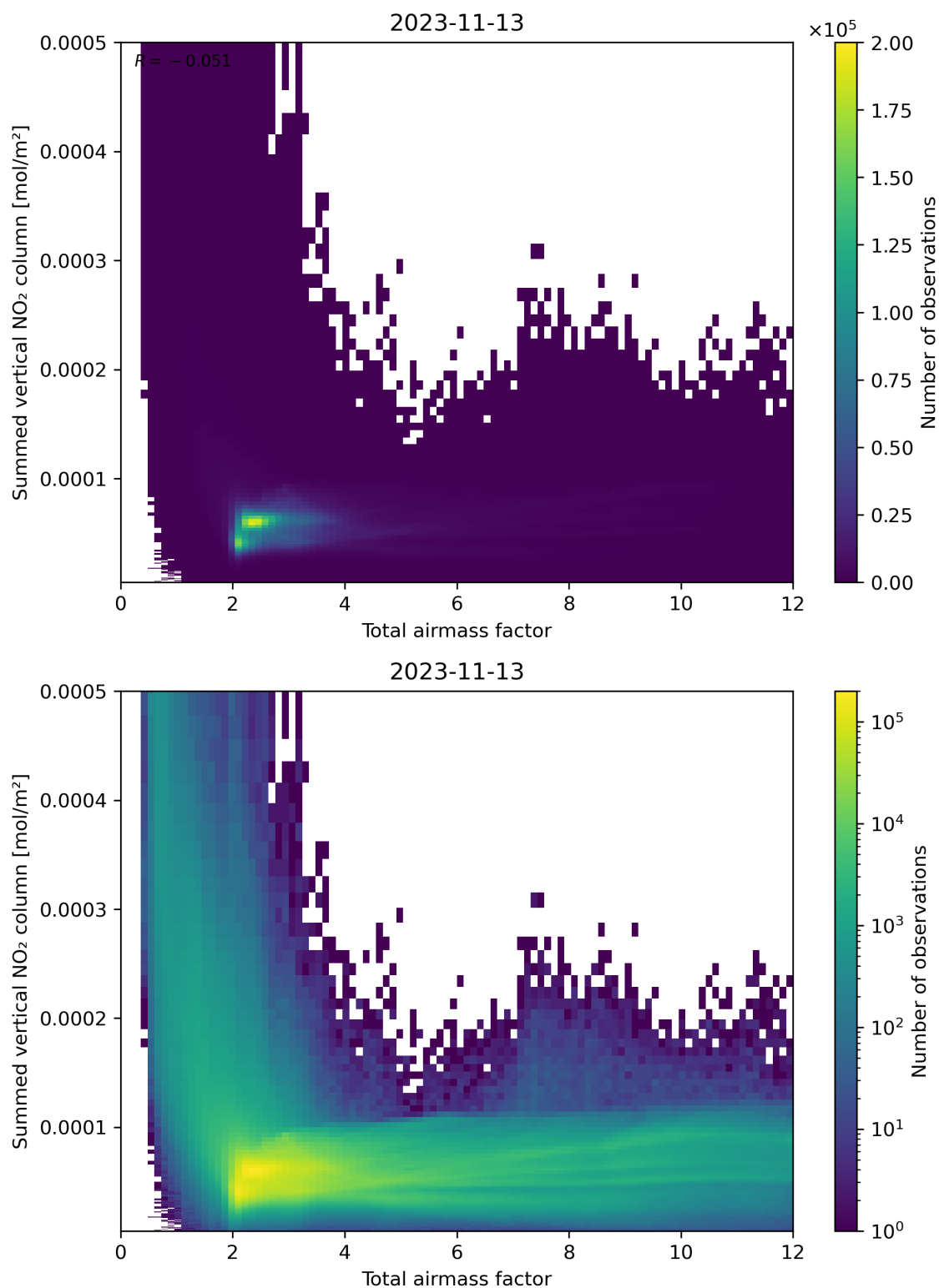
Figure 65: Scatter density plot of “Total airmass factor” against “Summed vertical NO 2 column” for 2023-11-13 to 2023-11-14.
