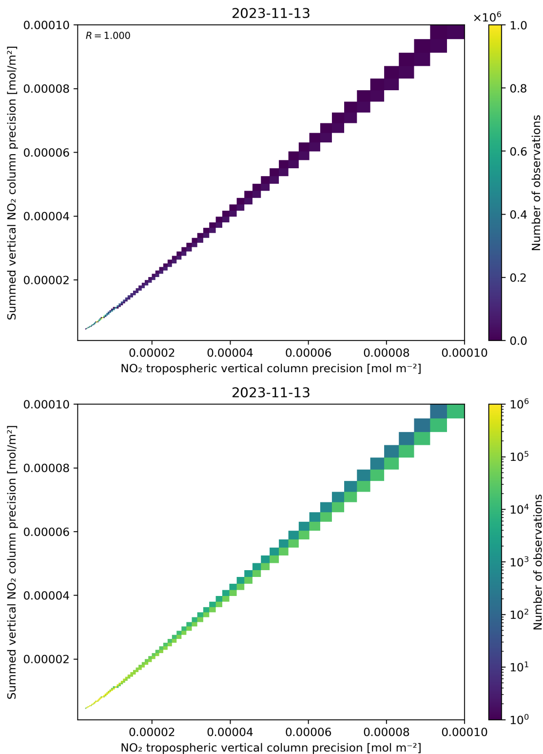
Figure 137: Scatter density plot of “NO 2 tropospheric vertical column precision” against “Summed vertical NO 2 column precision” for 2023-11-13 to 2023-11-14.
