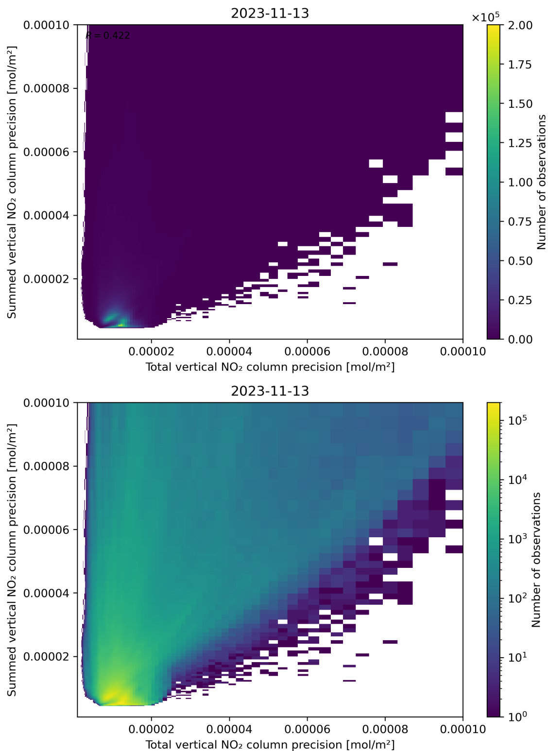
Figure 118: Scatter density plot of “Total vertical NO 2 column precision” against “Summed vertical NO 2 column precision” for 2023-11-13 to 2023-11-14.
