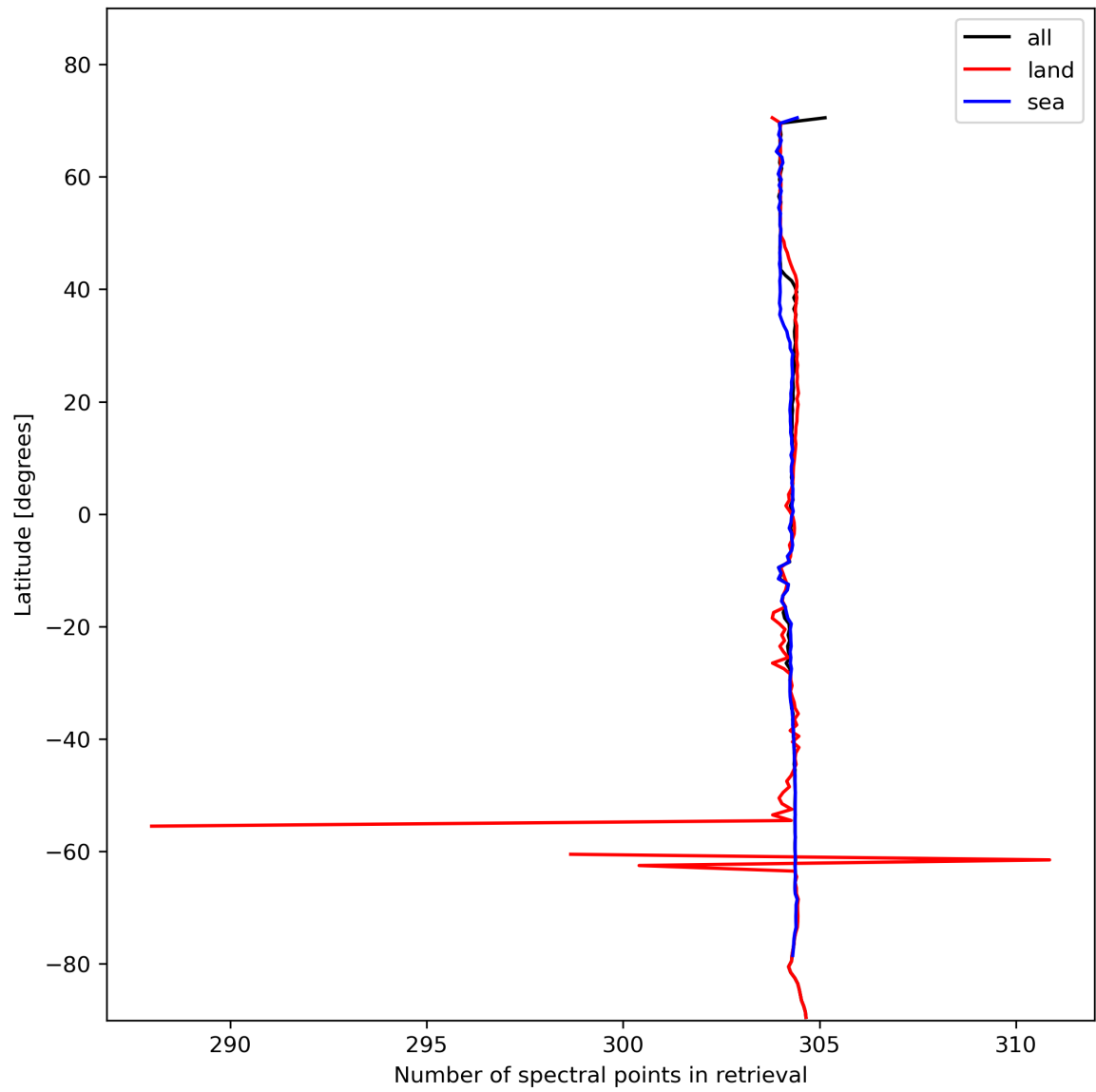
Figure 16: Zonal average of “Number of spectral points in retrieval” for 2023-11-13 to 2023-11-14.
