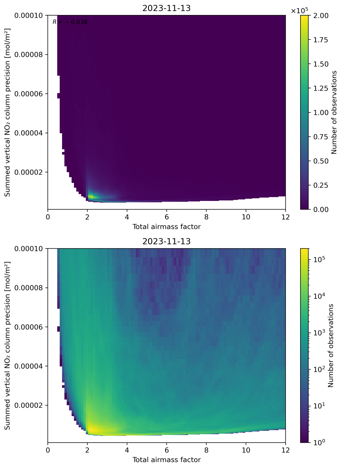
Figure 66: Scatter density plot of “Total airmass factor” against “Summed vertical NO 2 column precision” for 2023-11-13 to 2023-11-14.
