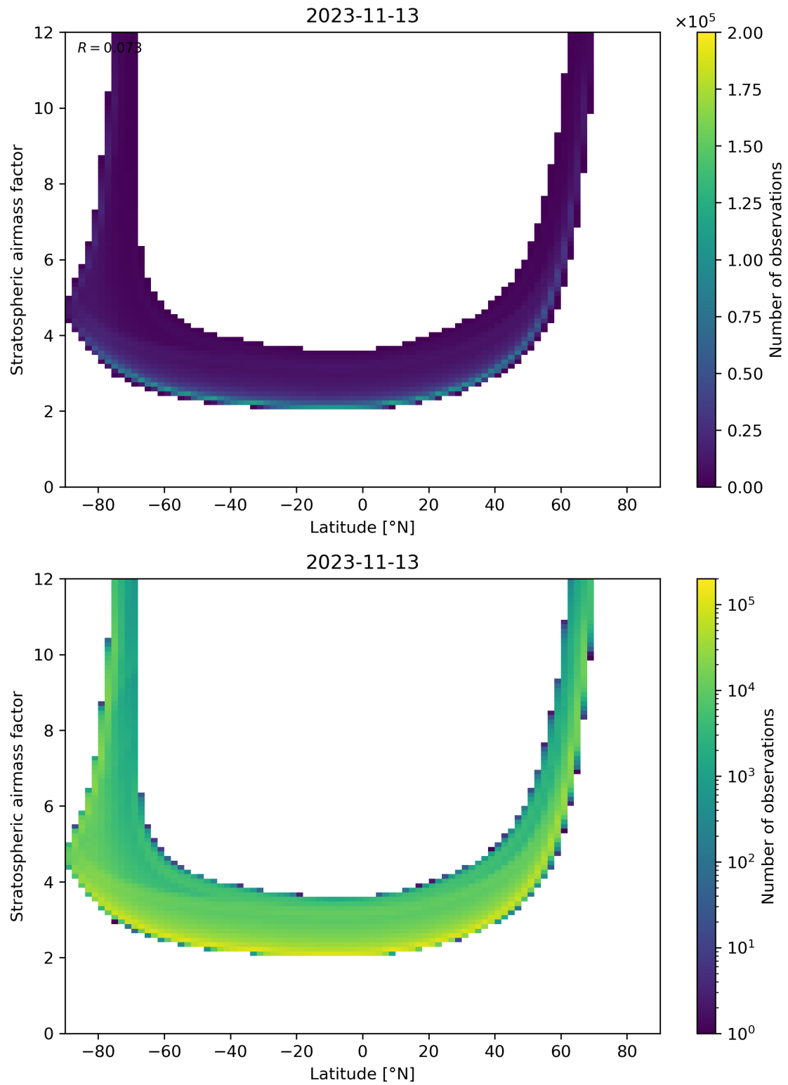
Figure 83: Scatter density plot of “Latitude” against “Stratospheric airmass factor” for 2023-11-13 to 2023-11-14.
