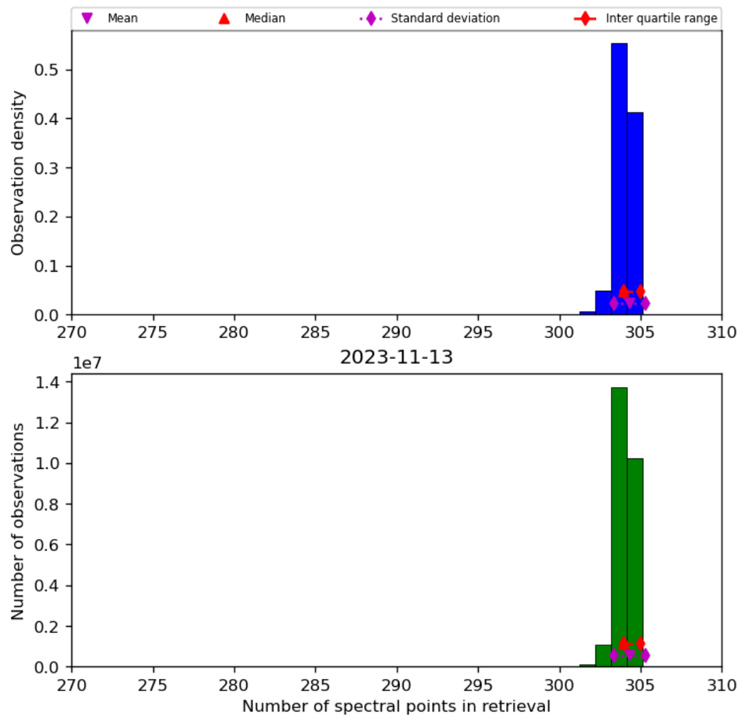
Figure 33: Histogram of “Number of spectral points in retrieval” for 2023-11-13 to 2023-11-14
