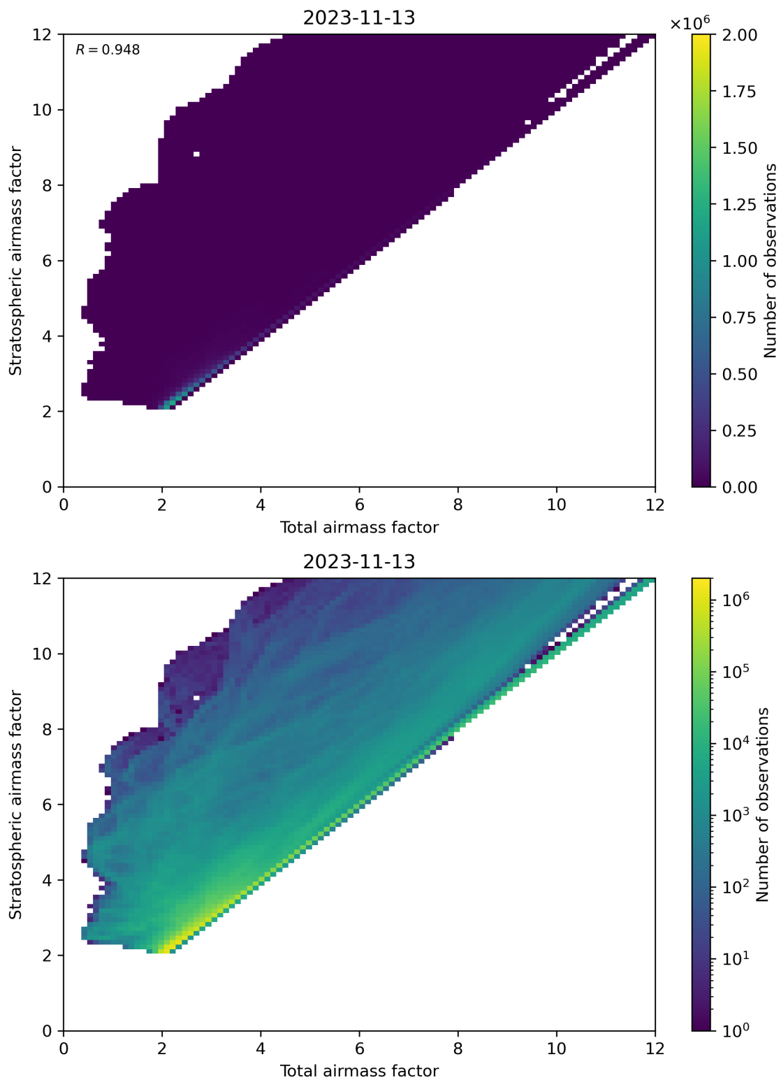
Figure 62: Scatter density plot of “Total airmass factor” against “Stratospheric airmass factor” for 2023-11-13 to 2023-11-14.
