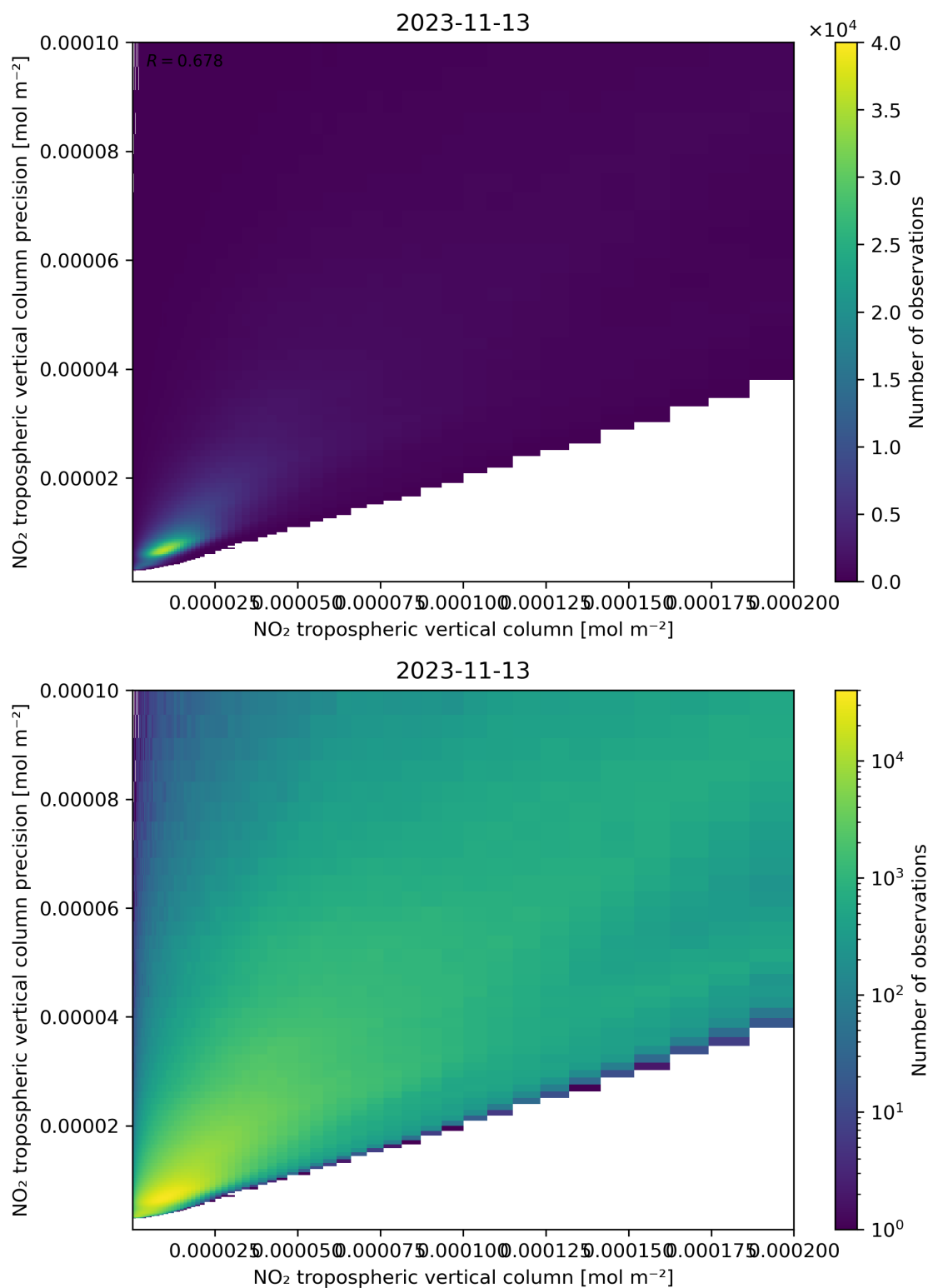
Figure 130: Scatter density plot of “NO 2 tropospheric vertical column” against “NO 2 tropospheric vertical column precision” for 2023-11-13 to 2023-11-14.
