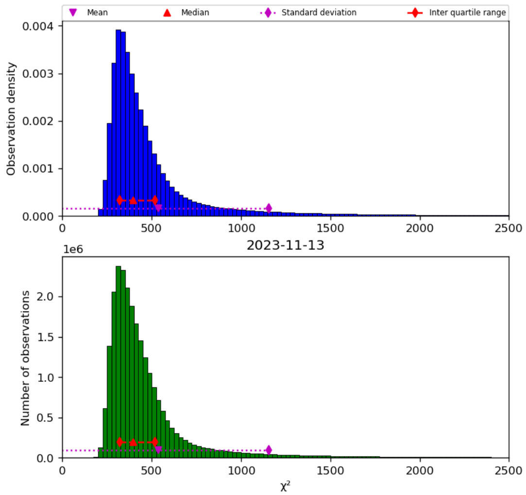
Figure 42: Histogram of “ \chi^2 ” for 2023-11-13 to 2023-11-14
