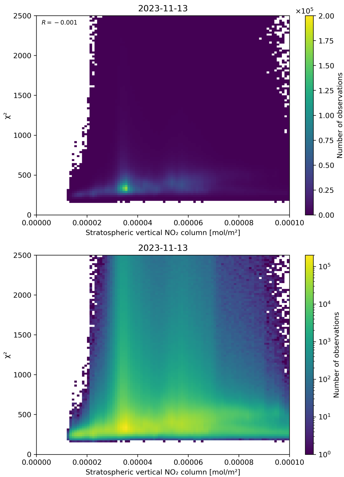
Figure 97: Scatter density plot of “Stratospheric vertical NO 2 column” against “ \chi^2 ” for 2023-11-13 to 2023-11-14.
