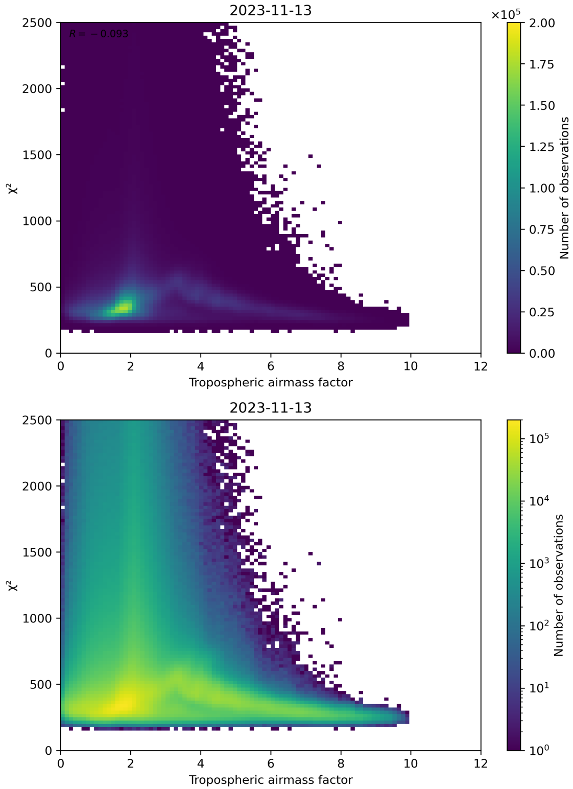
Figure 73: Scatter density plot of “Tropospheric airmass factor” against “ \chi^2 ” for 2023-11-13 to 2023-11-14.
