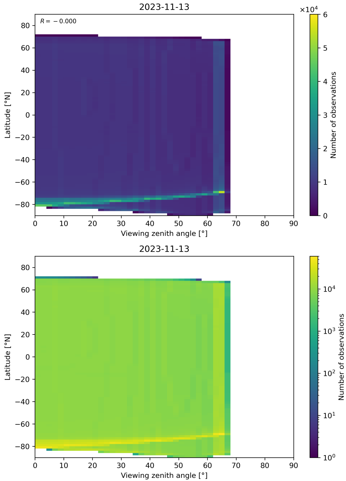
Figure 163: Scatter density plot of “Viewing zenith angle” against “Latitude” for 2023-11-13 to 2023-11-14.
