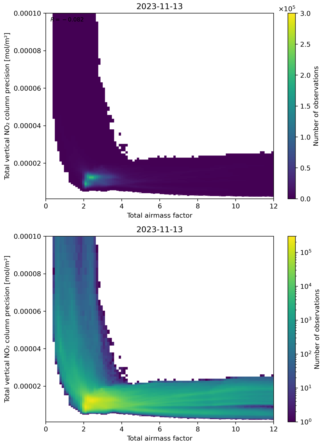
Figure 68: Scatter density plot of “Total airmass factor” against “Total vertical NO 2 column precision” for 2023-11-13 to 2023-11-14.
