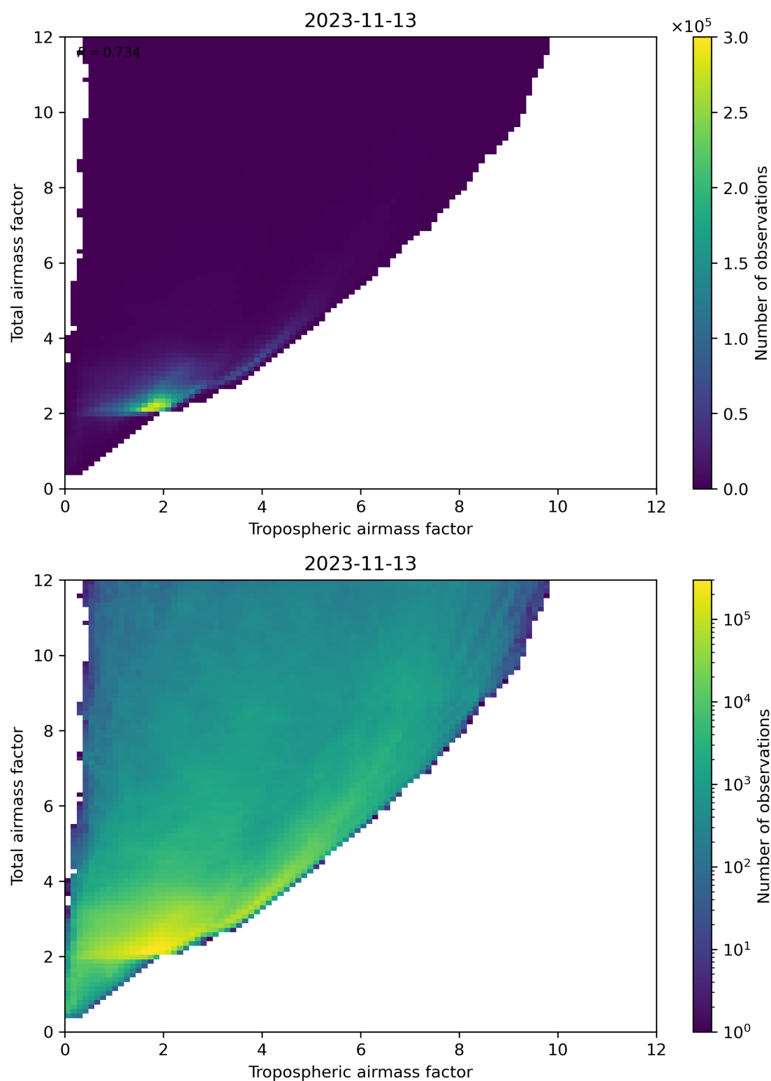
Figure 72: Scatter density plot of “Tropospheric airmass factor” against “Total airmass factor” for 2023-11-13 to 2023-11-14.
