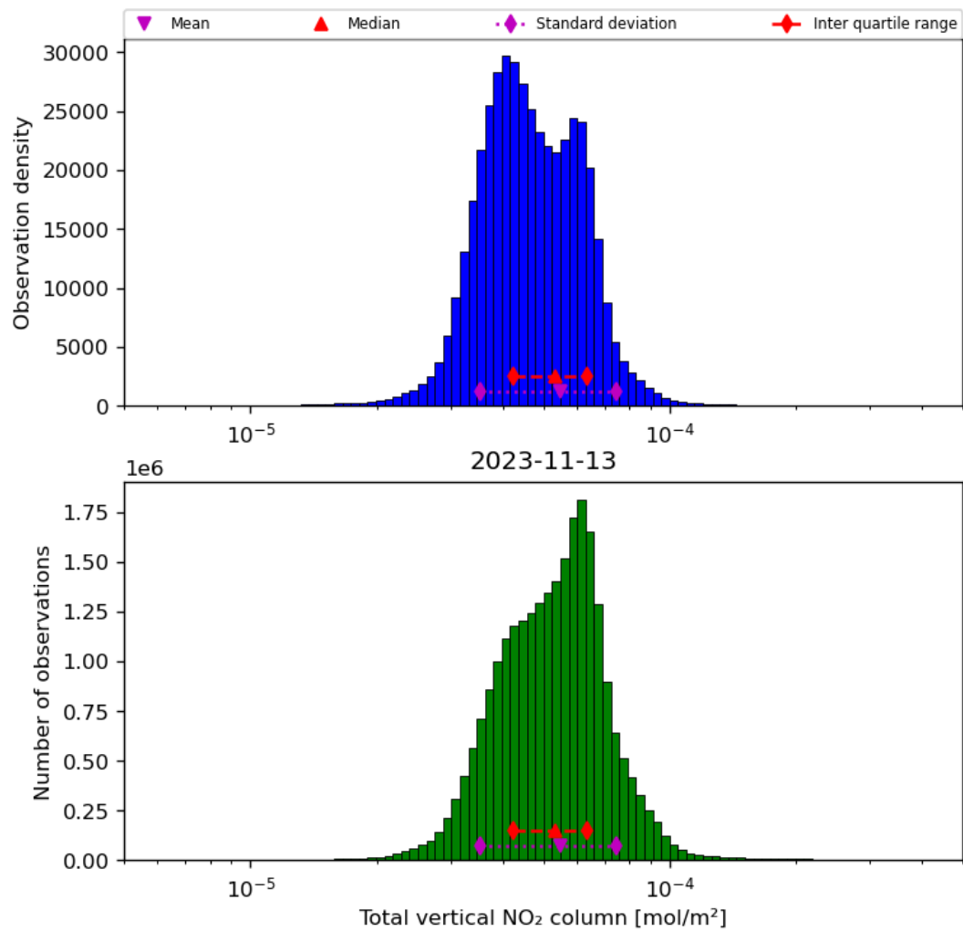
Figure 38: Histogram of “Total vertical NO 2 column” for 2023-11-13 to 2023-11-14
