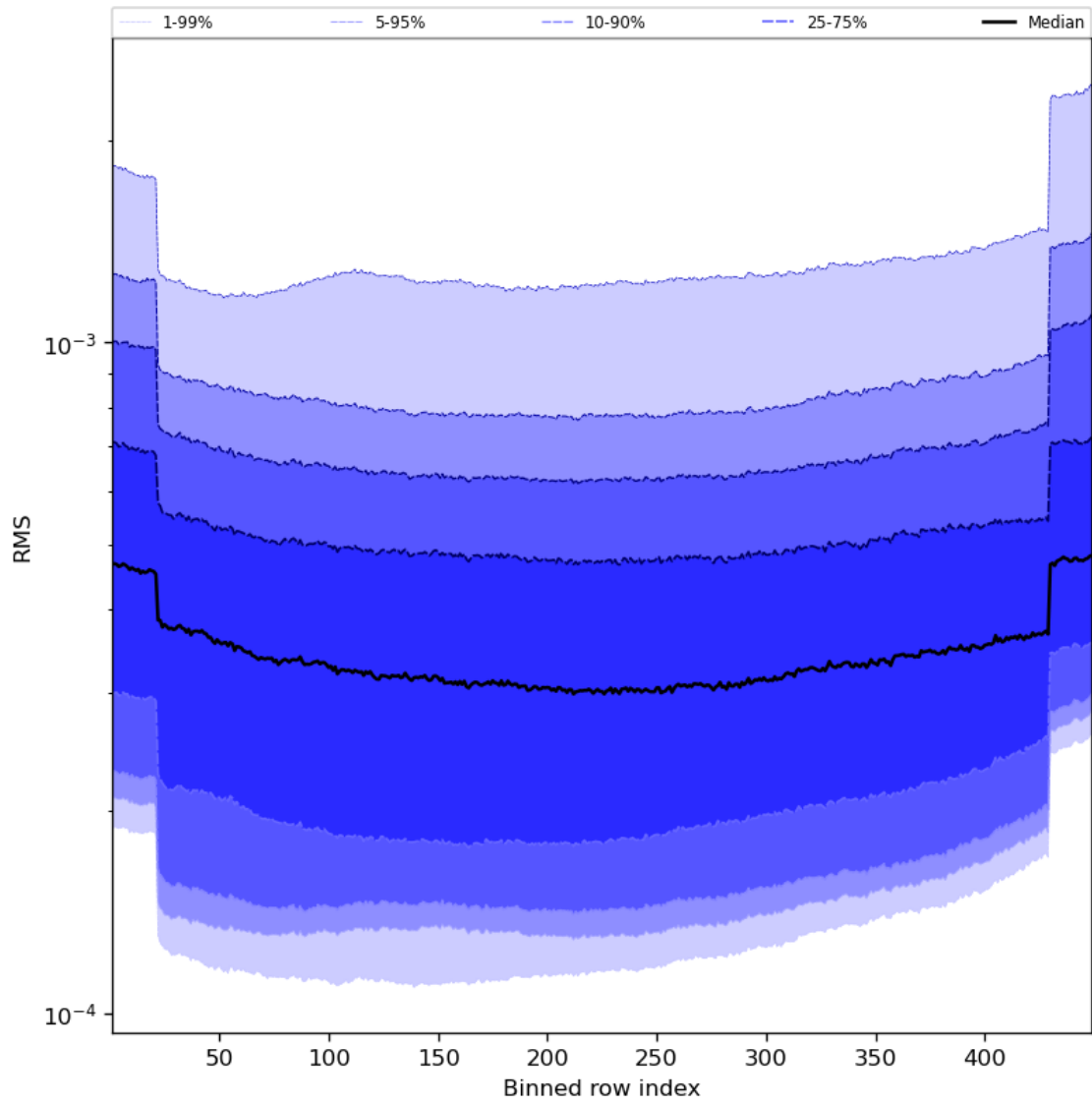
Figure 60: Along track statistics of “RMS” for 2023-11-13 to 2023-11-14
