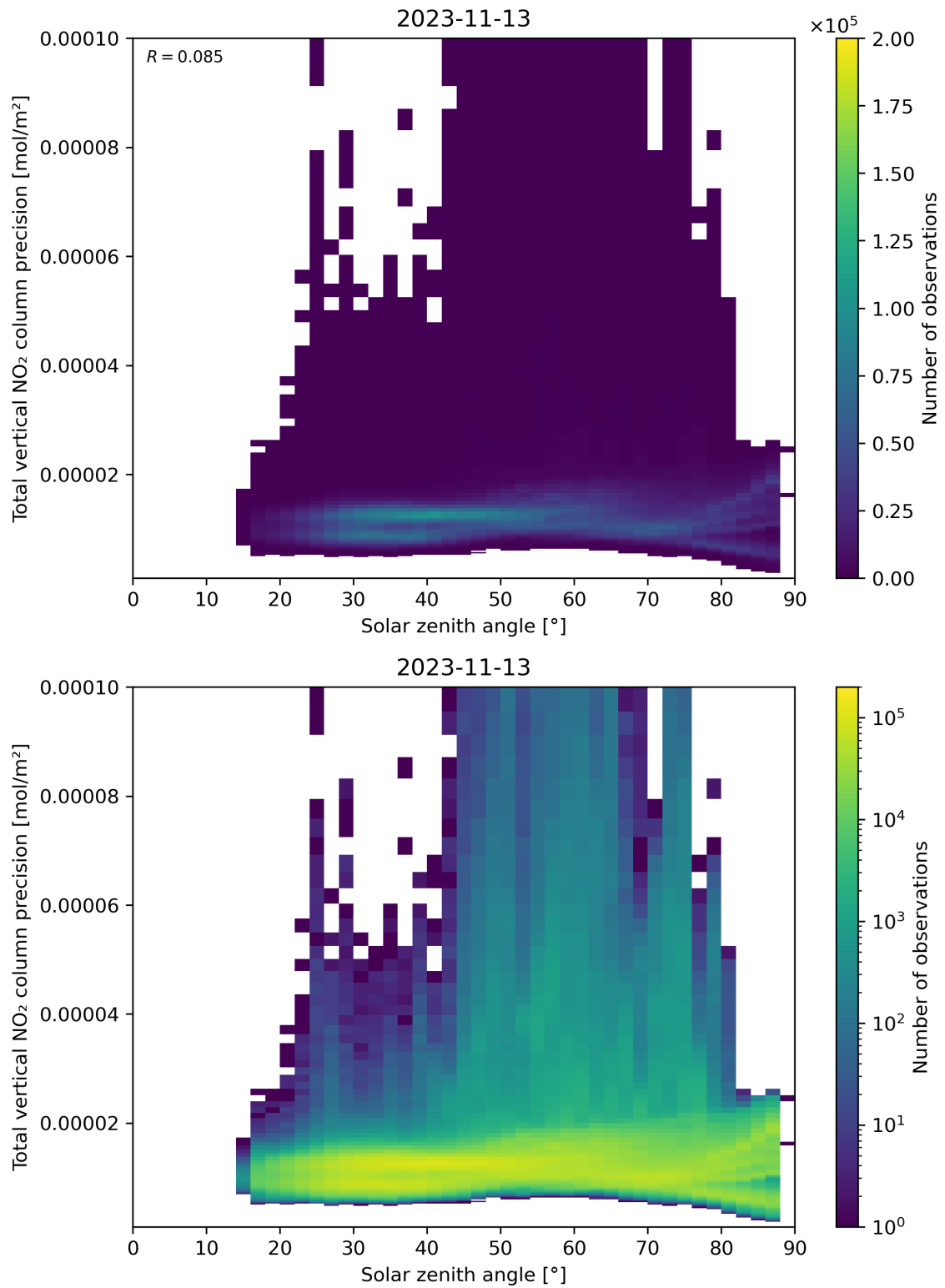
Figure 154: Scatter density plot of “Solar zenith angle” against “Total vertical NO 2 column precision” for 2023-11-13 to 2023-11-14.
