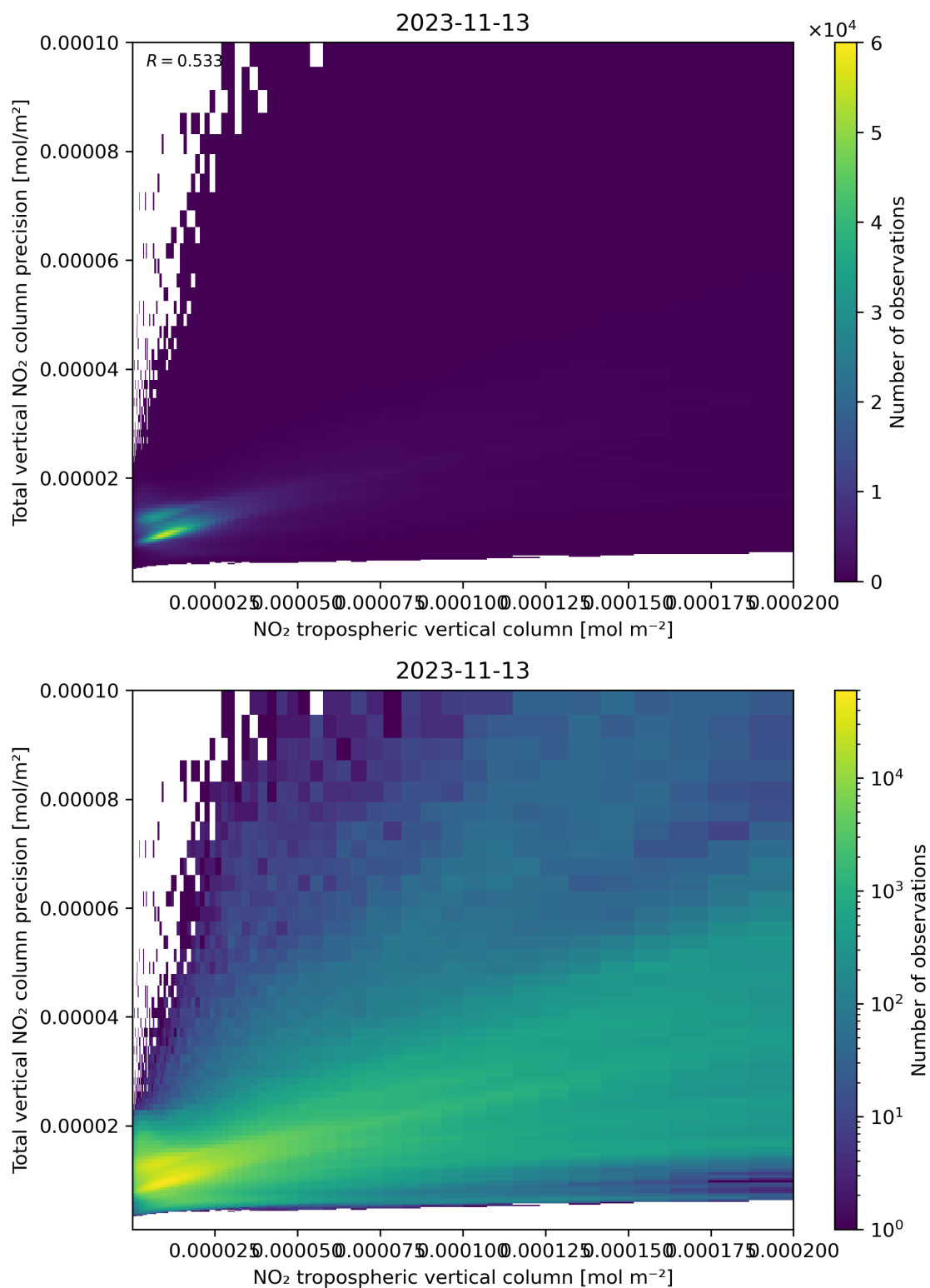
Figure 129: Scatter density plot of “NO 2 tropospheric vertical column” against “Total vertical NO 2 column precision” for 2023-11-13 to 2023-11-14.
