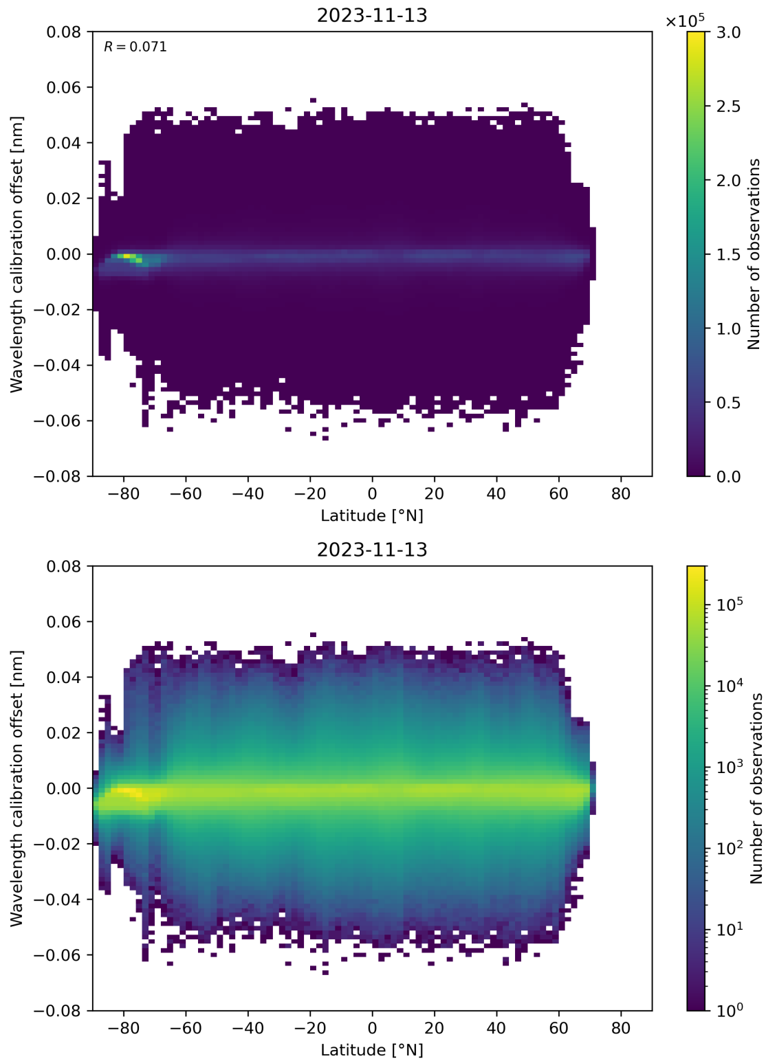
Figure 95: Scatter density plot of “Latitude” against “Wavelength calibration offset” for 2023-11-13 to 2023-11-14.
