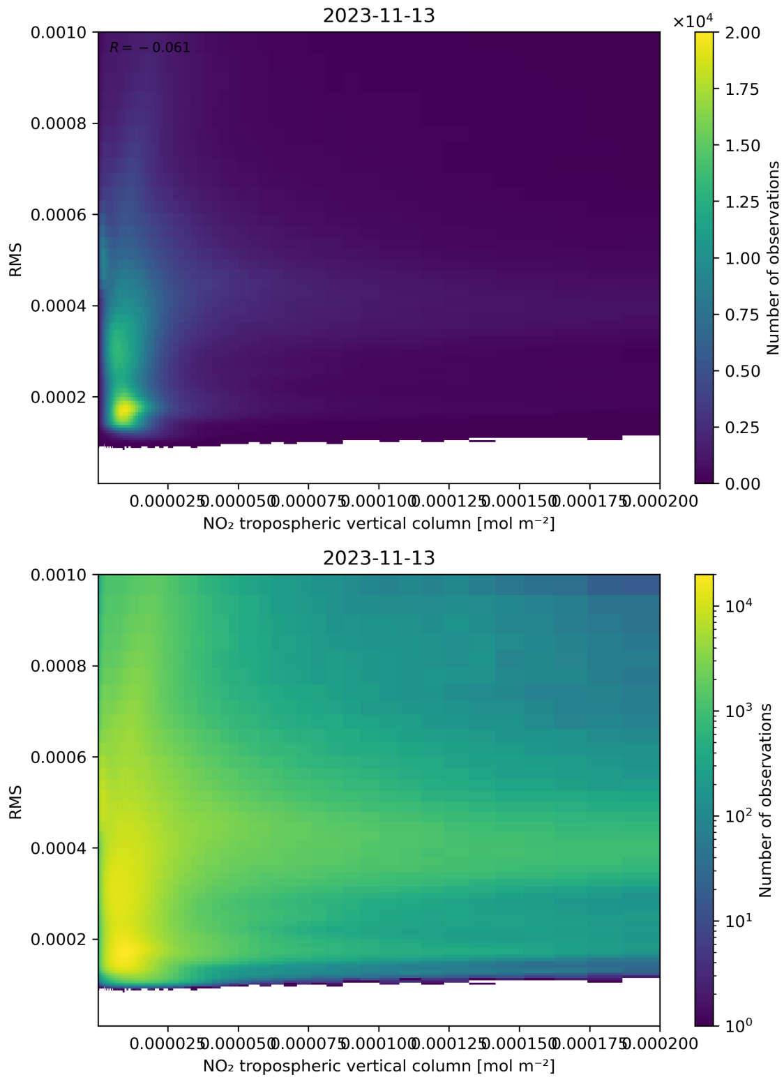
Figure 142: Scatter density plot of “NO 2 tropospheric vertical column” against “RMS” for 2023-11-13 to 2023-11-14.
