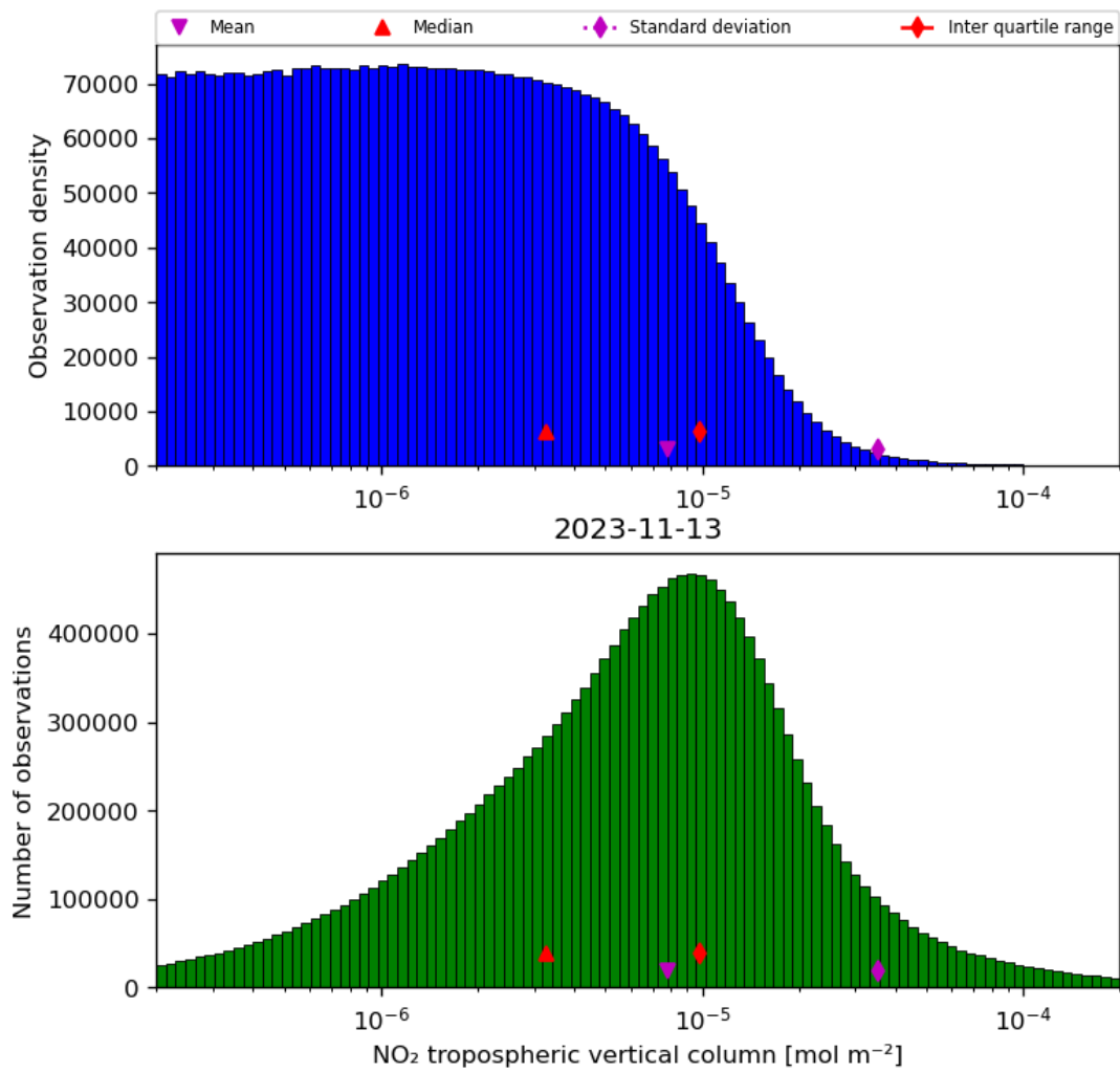
Figure 29: Histogram of “NO 2 tropospheric vertical column” for 2023-11-13 to 2023-11-14
