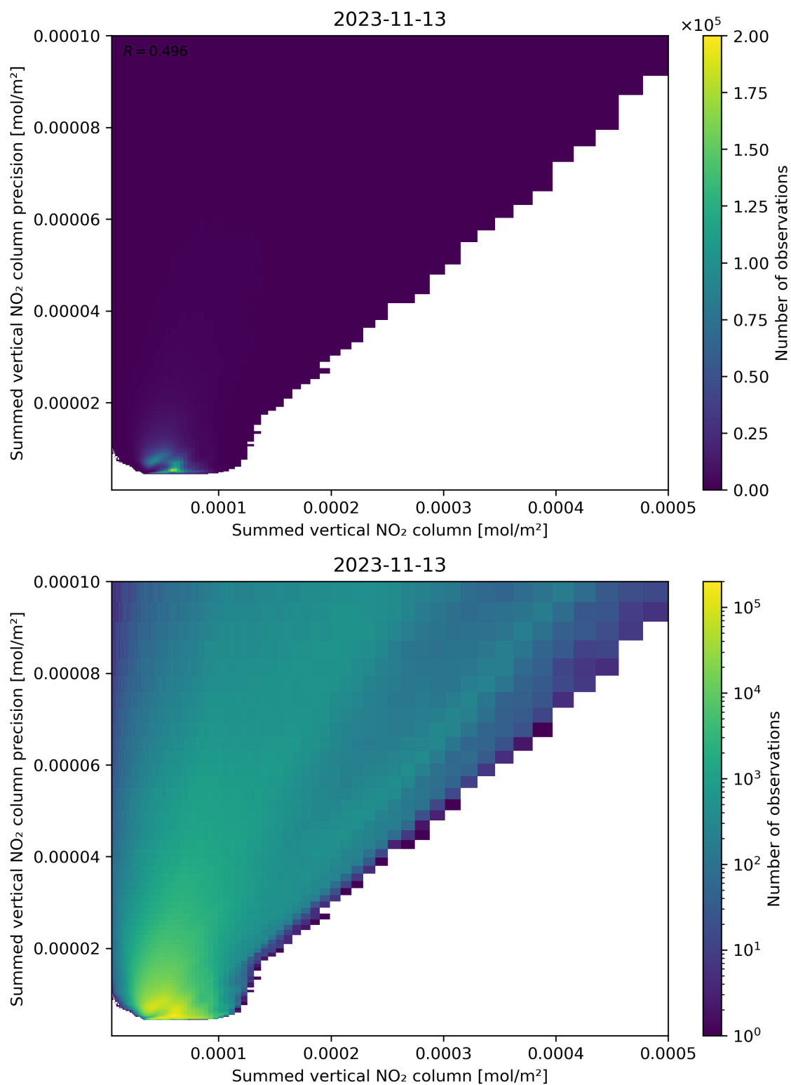
Figure 105: Scatter density plot of “Summed vertical NO 2 column” against “Summed vertical NO 2 column precision” for 2023-11-13 to 2023-11-14.
