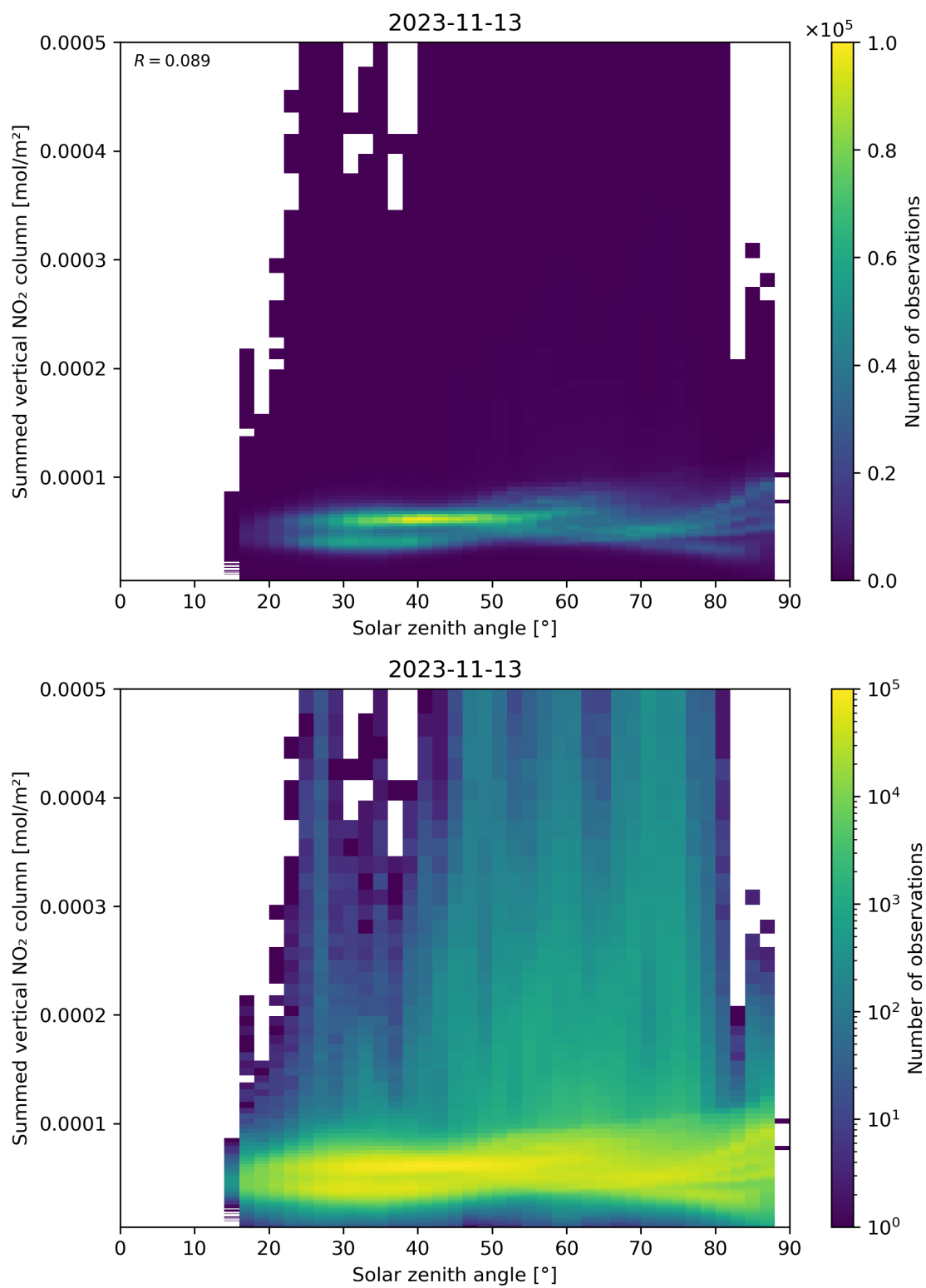
Figure 151: Scatter density plot of “Solar zenith angle” against “Summed vertical NO 2 column” for 2023-11-13 to 2023-11-14.
