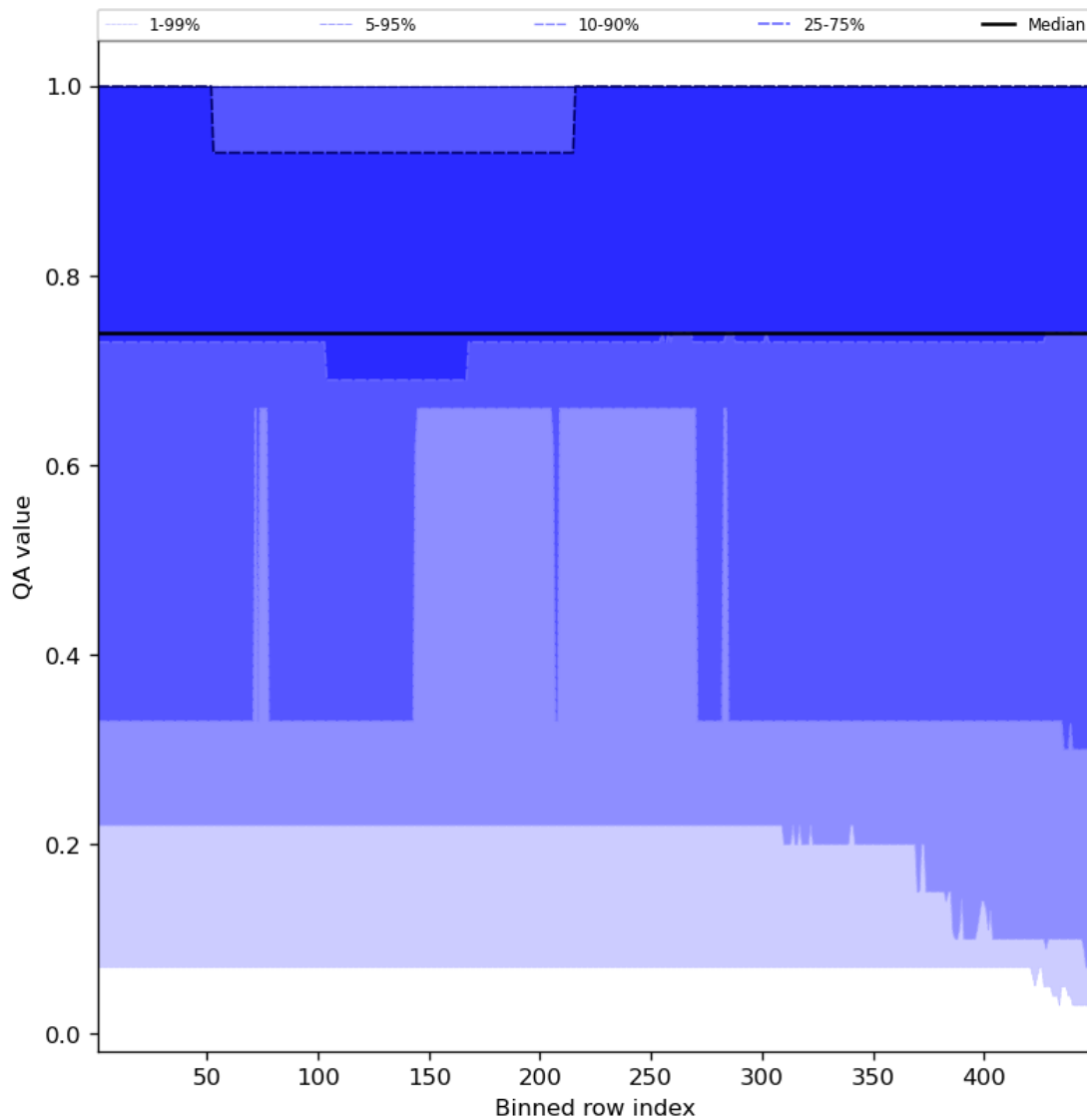
Figure 45: Along track statistics of “QA value” for 2023-11-13 to 2023-11-14
