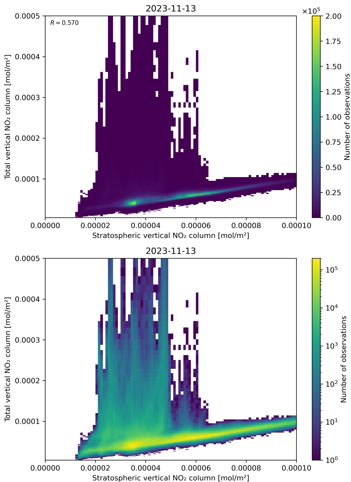
Figure 100: Scatter density plot of “Stratospheric vertical NO 2 column” against “Total vertical NO 2 column” for 2023-11-13 to 2023-11-14.
