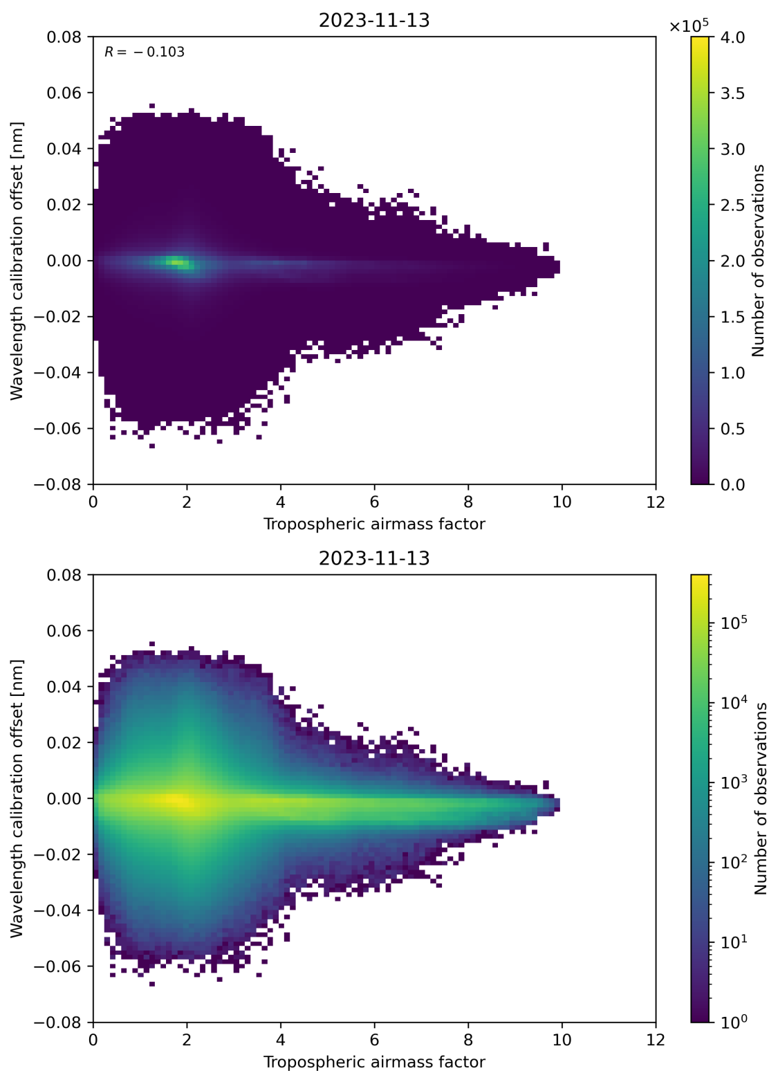
Figure 80: Scatter density plot of “Tropospheric airmass factor” against “Wavelength calibration offset” for 2023-11-13 to 2023-11-14.
