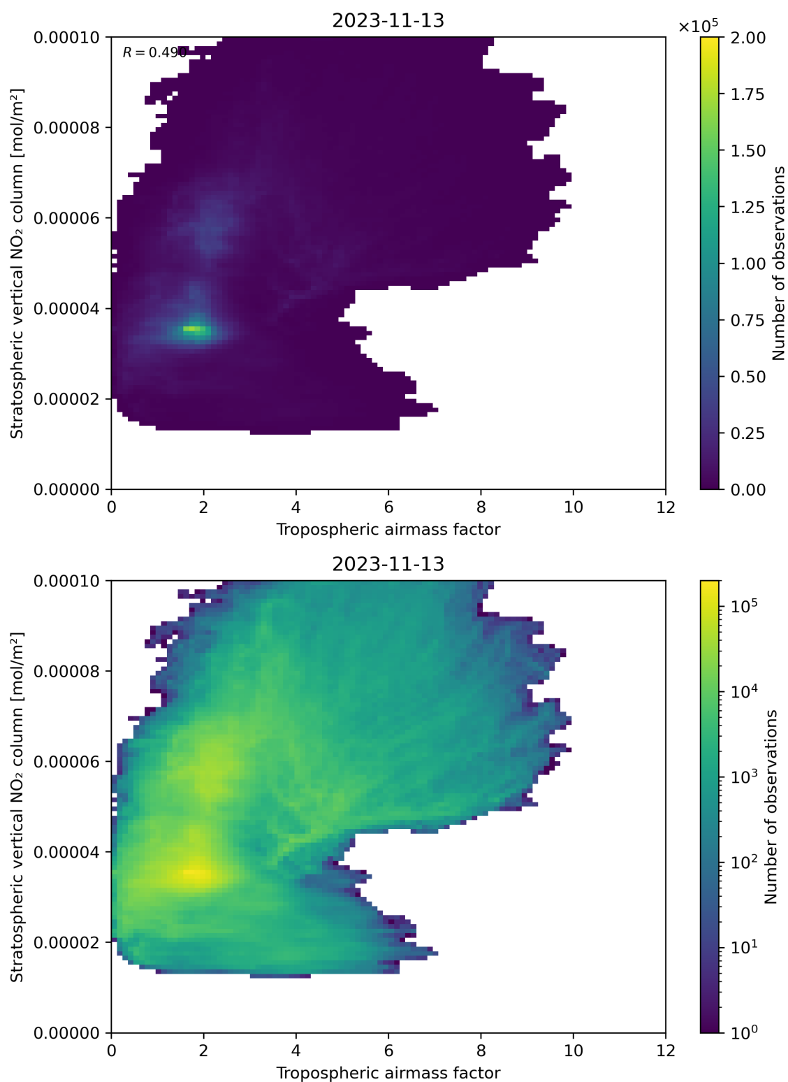
Figure 74: Scatter density plot of “Tropospheric air mass factor” against “Stratospheric vertical NO 2 column” for 2023-11-13 to 2023-11-14.
