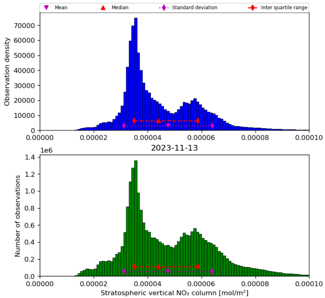
Figure 36: Histogram of “Stratospheric vertical NO 2 column” for 2023-11-13 to 2023-11-14
