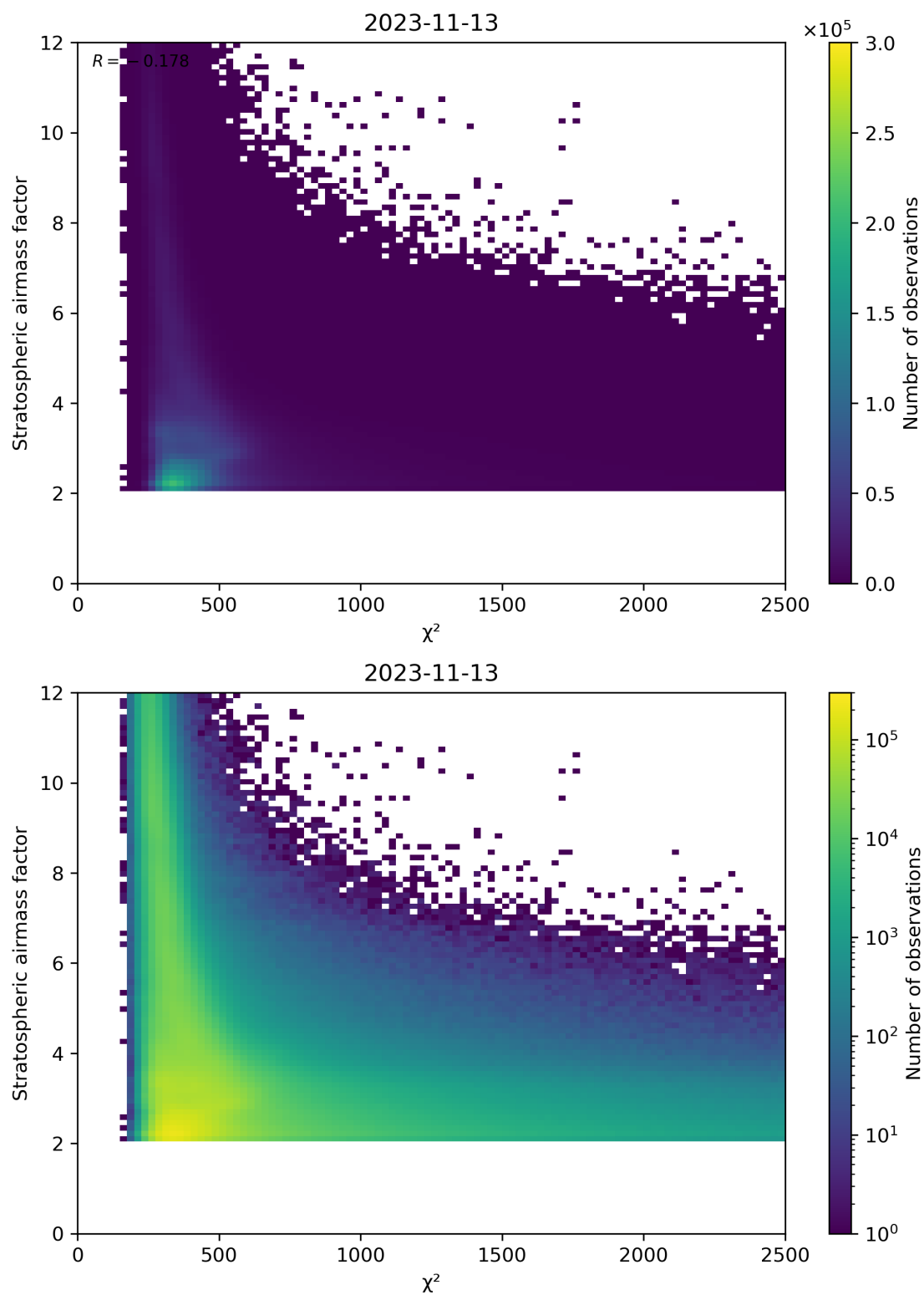
Figure 81: Scatter density plot of " \chi^2 " against "Stratospheric air mass factor" for 2023-11-13 to 2023-11-14.
