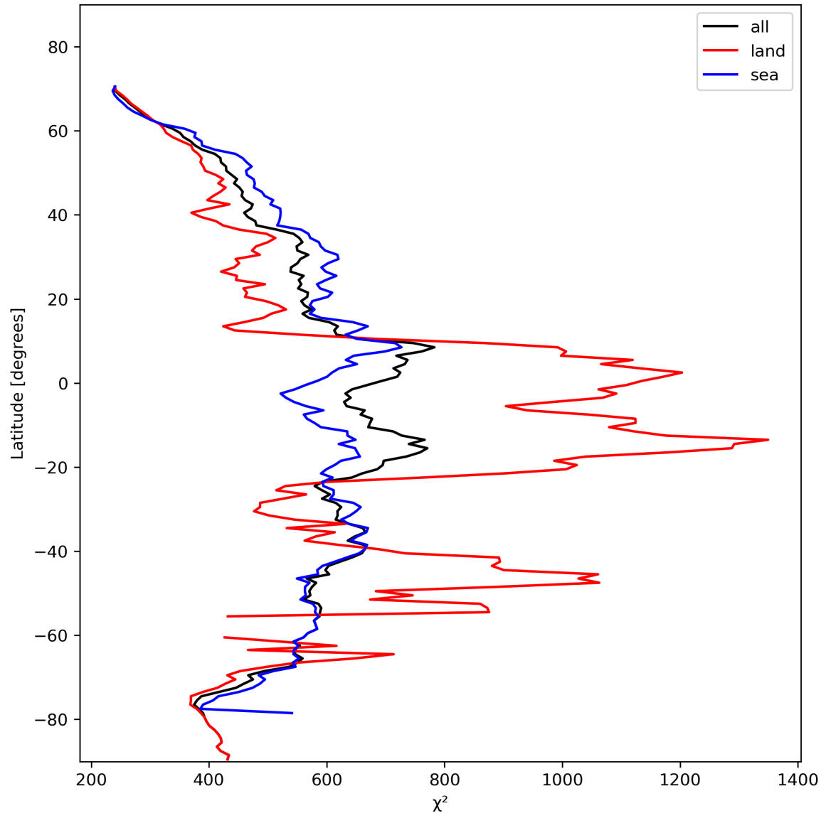
Figure 25: Zonal average of “ \chi^2 ” for 2023-11-13 to 2023-11-14.
