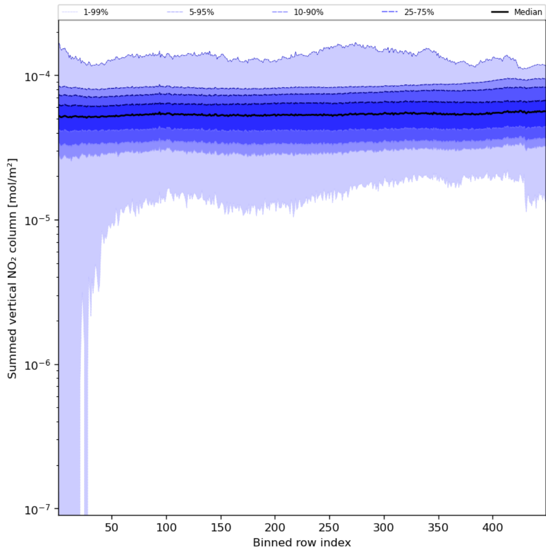
Figure 57: Along track statistics of “Summed vertical NO 2 column” for 2023-11-13 to 2023-11-14
