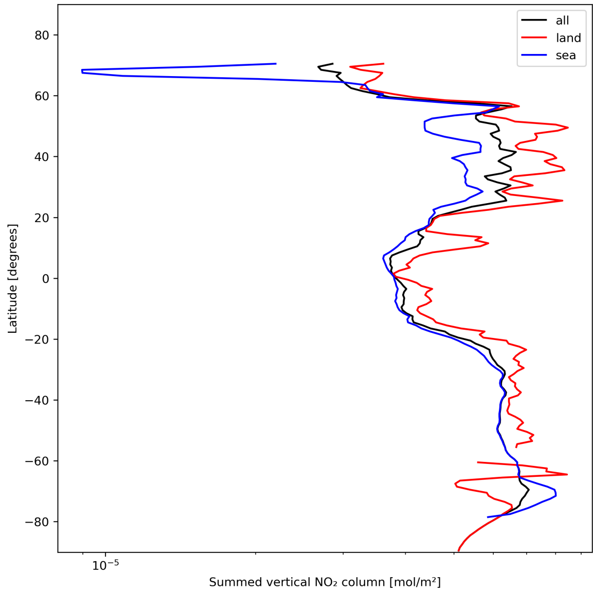
Figure 23: Zonal average of “Summed vertical NO 2 column” for 2023-11-13 to 2023-11-14.
