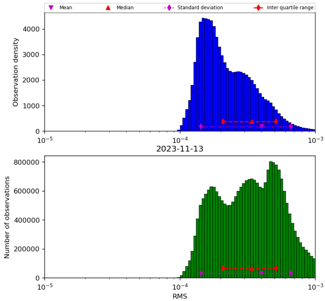
Figure 43: Histogram of “RMS” for 2023-11-13 to 2023-11-14
