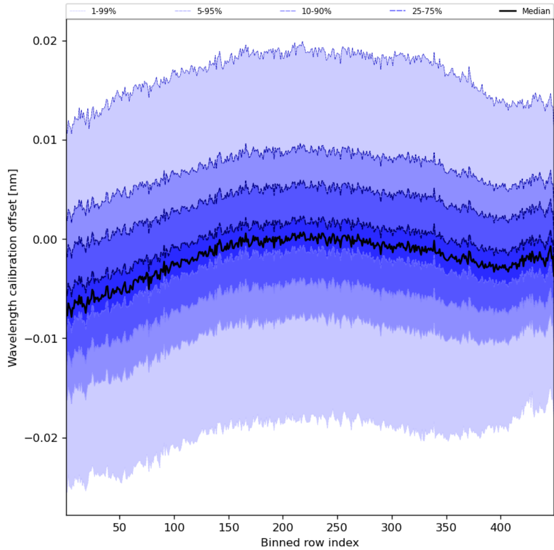
Figure 52: Along track statistics of “Wavelength calibration offset” for 2023-11-13 to 2023-11-14
