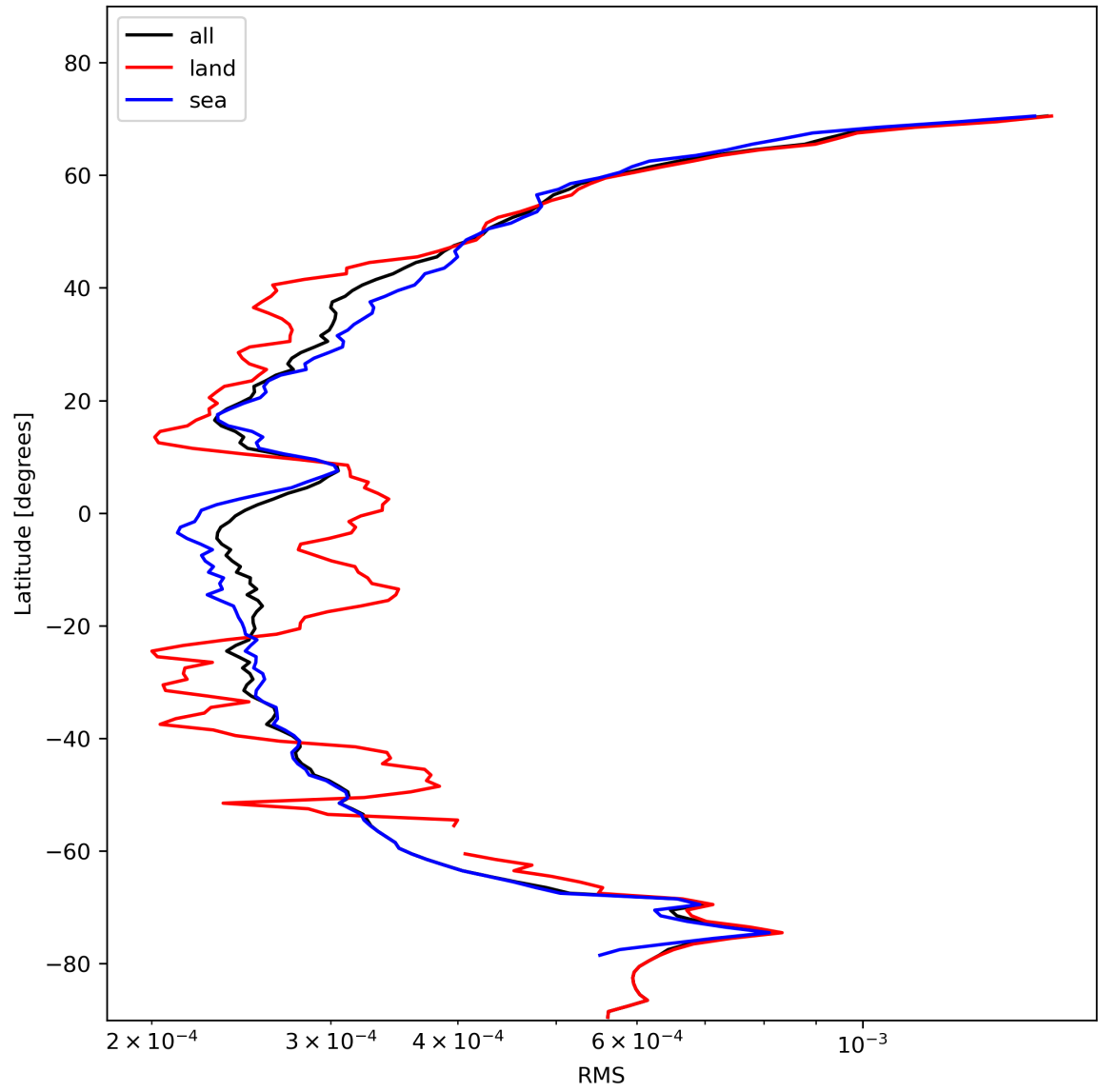
Figure 26: Zonal average of “RMS” for 2023-11-13 to 2023-11-14.
