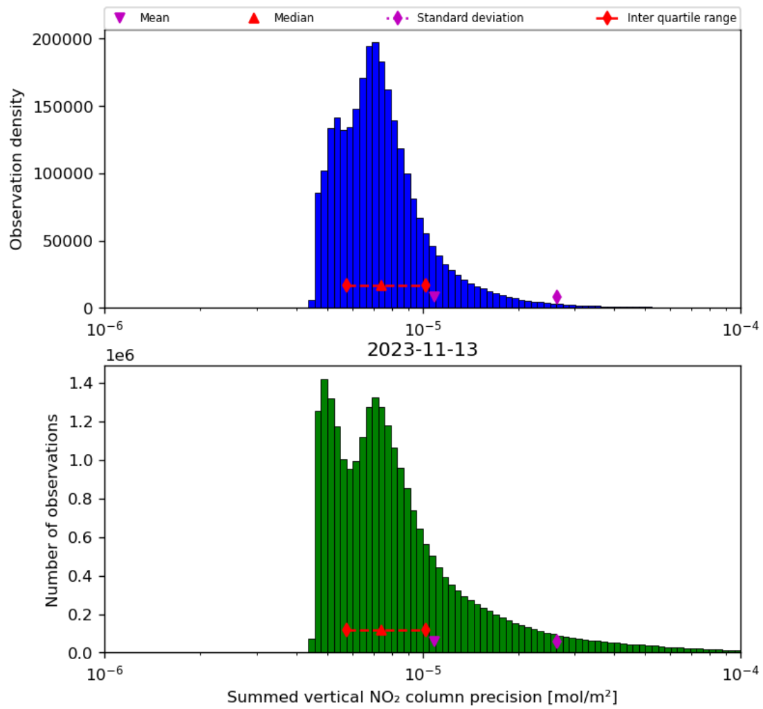
Figure 41: Histogram of “Summed vertical NO 2 column precision” for 2023-11-13 to 2023-11-14
