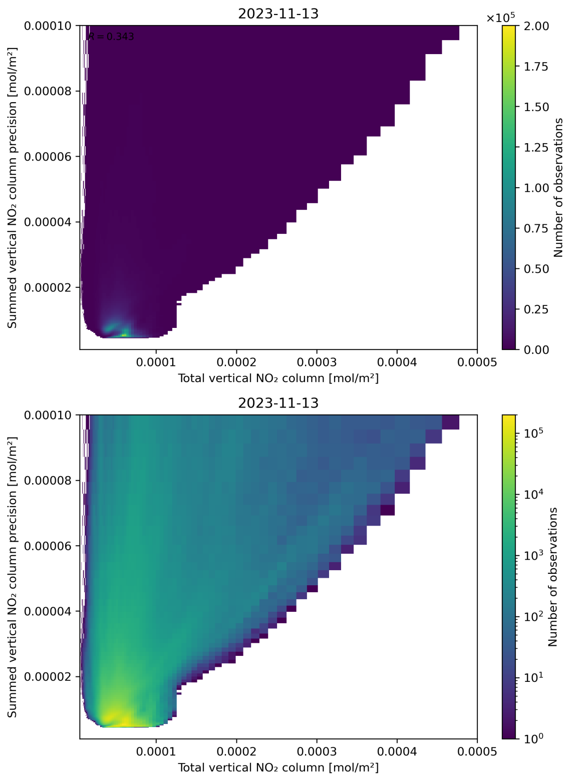
Figure 113: Scatter density plot of “Total vertical NO 2 column” against “Summed vertical NO 2 column precision” for 2023-11-13 to 2023-11-14.
