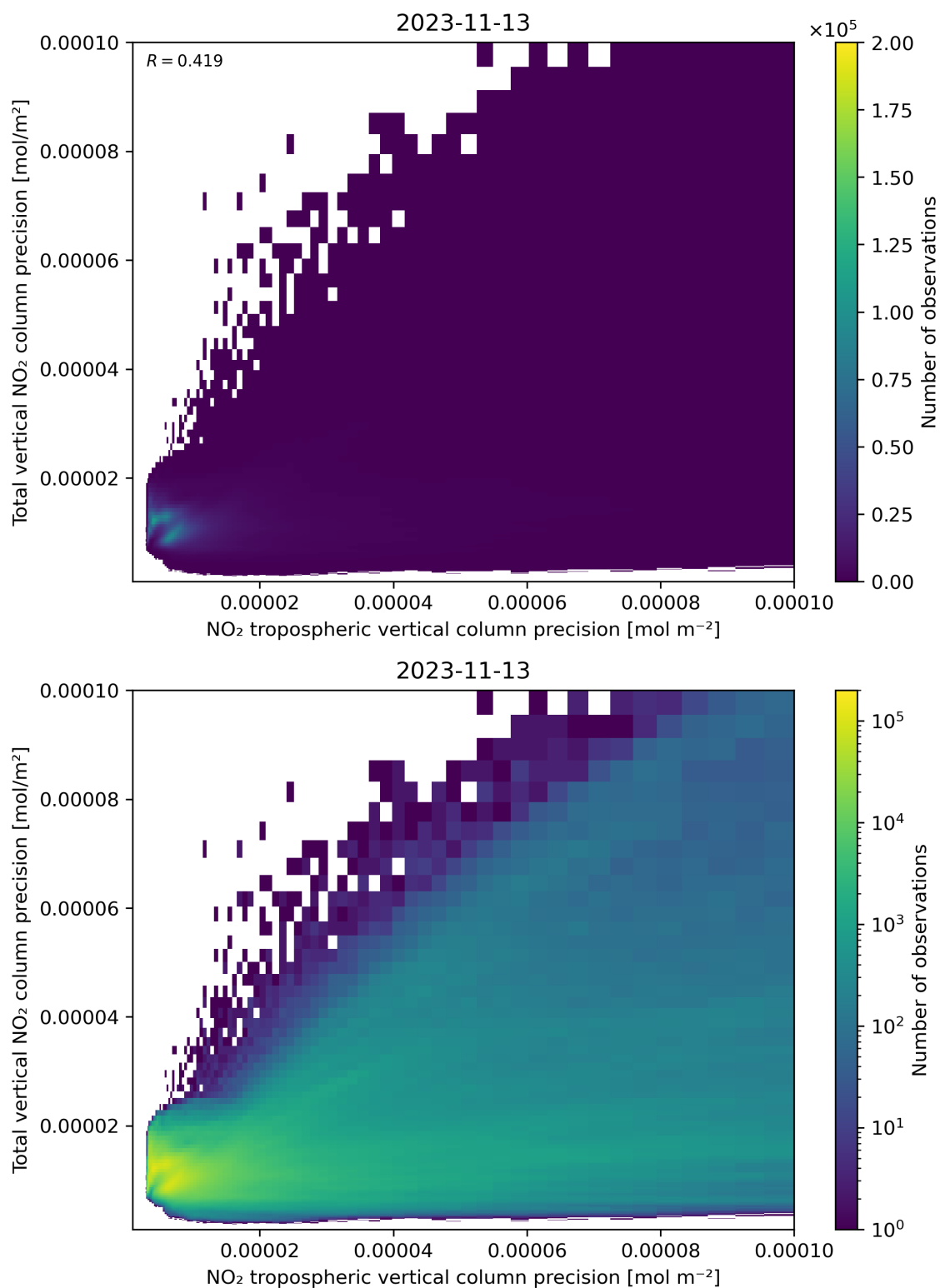
Figure 139: Scatter density plot of “NO 2 tropospheric vertical column precision” against “Total vertical NO 2 column precision” for 2023-11-13 to 2023-11-14.
