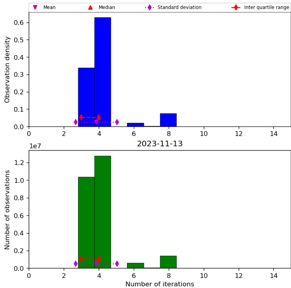
Figure 34: Histogram of “Number of iterations” for 2023-11-13 to 2023-11-14
