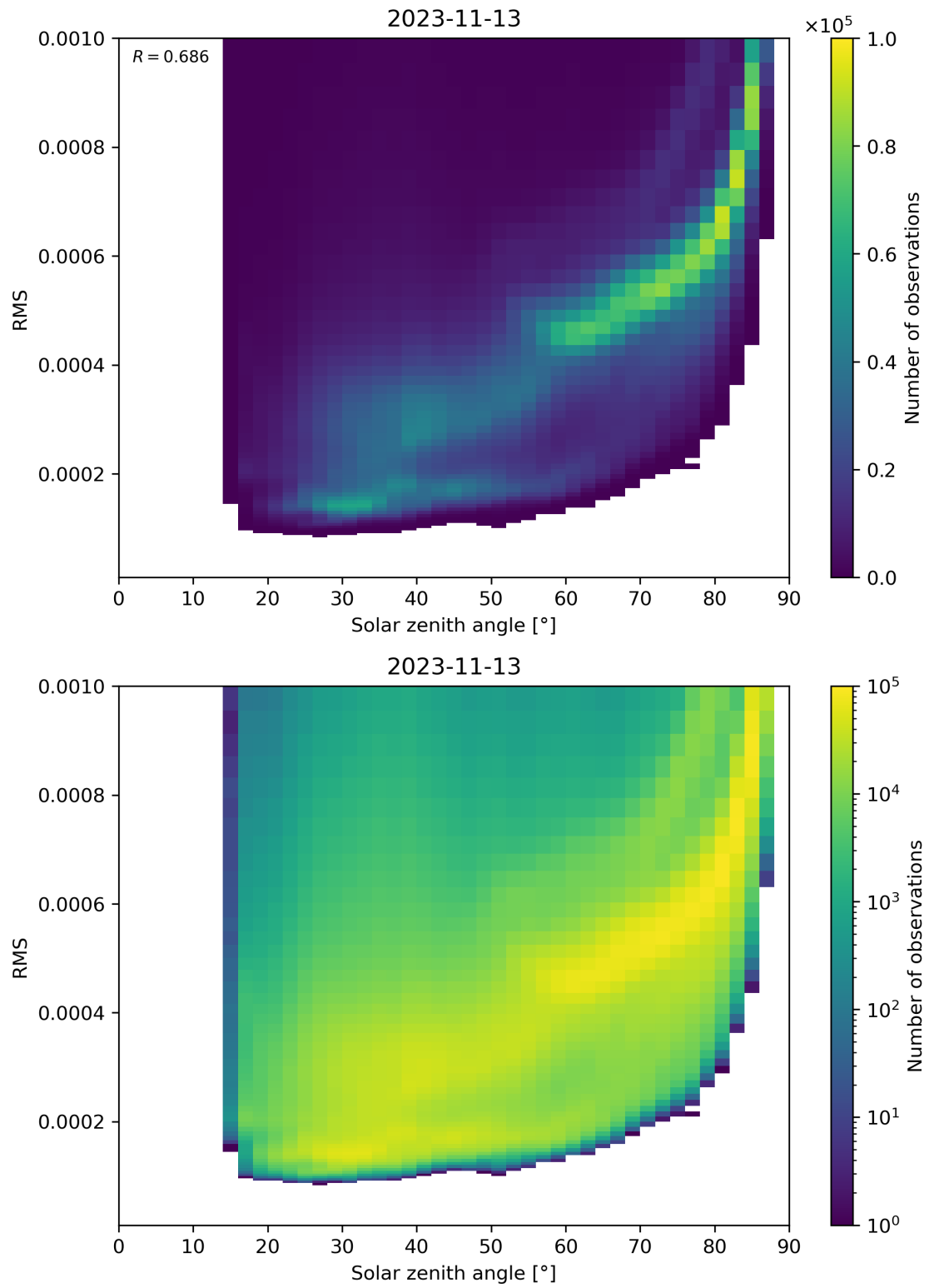
Figure 157: Scatter density plot of “Solar zenith angle” against “RMS” for 2023-11-13 to 2023-11-14.
