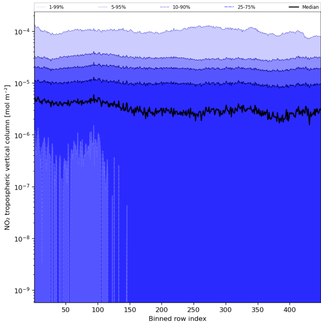
Figure 46: Along track statistics of “NO 2 tropospheric vertical column” for 2023-11-13 to 2023-11-14
