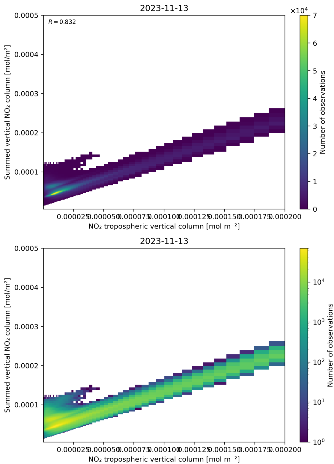
Figure 126: Scatter density plot of “NO 2 tropospheric vertical column” against “Summed vertical NO 2 column” for 2023-11-13 to 2023-11-14.
