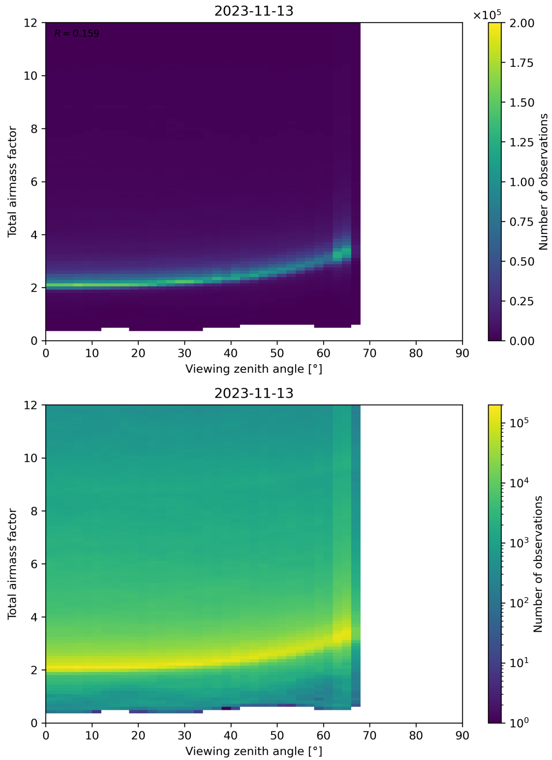
Figure 160: Scatter density plot of “Viewing zenith angle” against “Total airmass factor” for 2023-11-13 to 2023-11-14.
