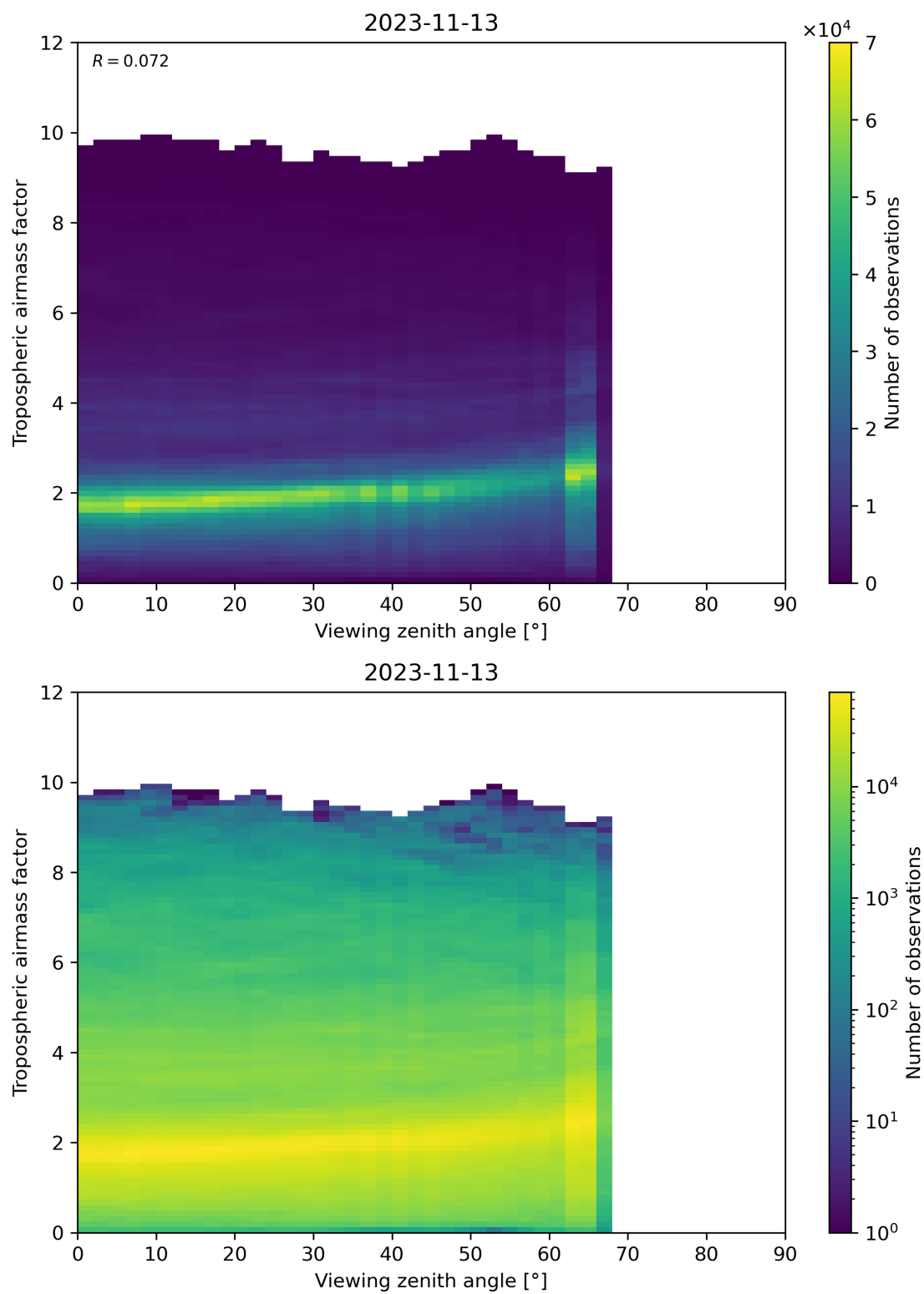
Figure 161: Scatter density plot of “Viewing zenith angle” against “Tropospheric airmass factor” for 2023-11-13 to 2023-11-14.
