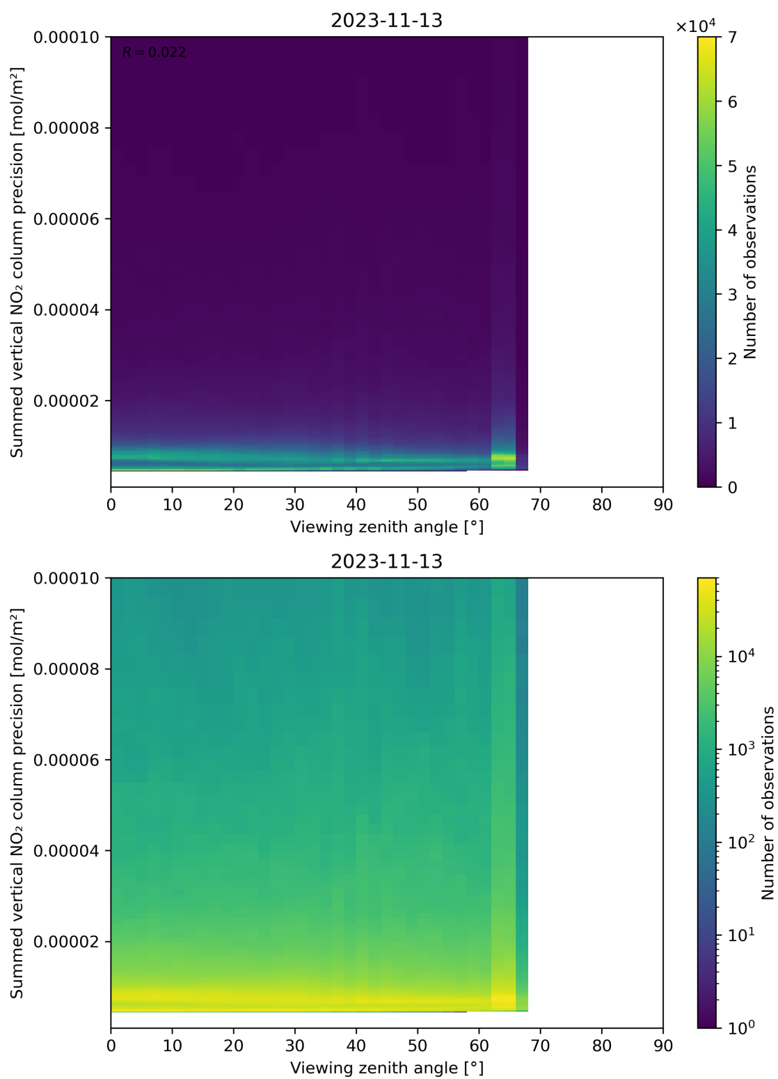
Figure 166: Scatter density plot of “Viewing zenith angle” against “Summed vertical NO 2 column precision” for 2023-11-13 to 2023-11-14.
