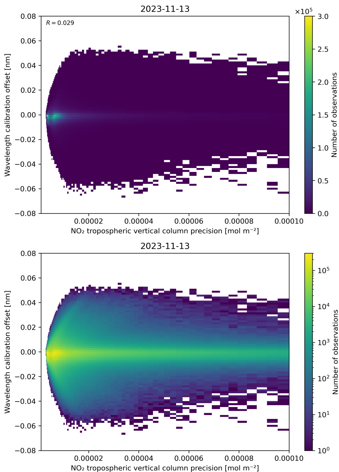
Figure 141: Scatter density plot of “NO 2 tropospheric vertical column precision” against “Wavelength calibration offset” for 2023-11-13 to 2023-11-14.
