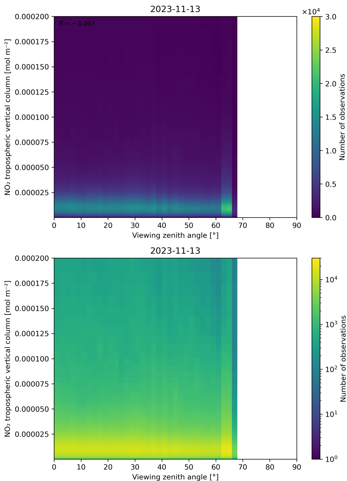
Figure 169: Scatter density plot of “Viewing zenith angle” against “NO 2 tropospheric vertical column” for 2023-11-13 to 2023-11-14.
