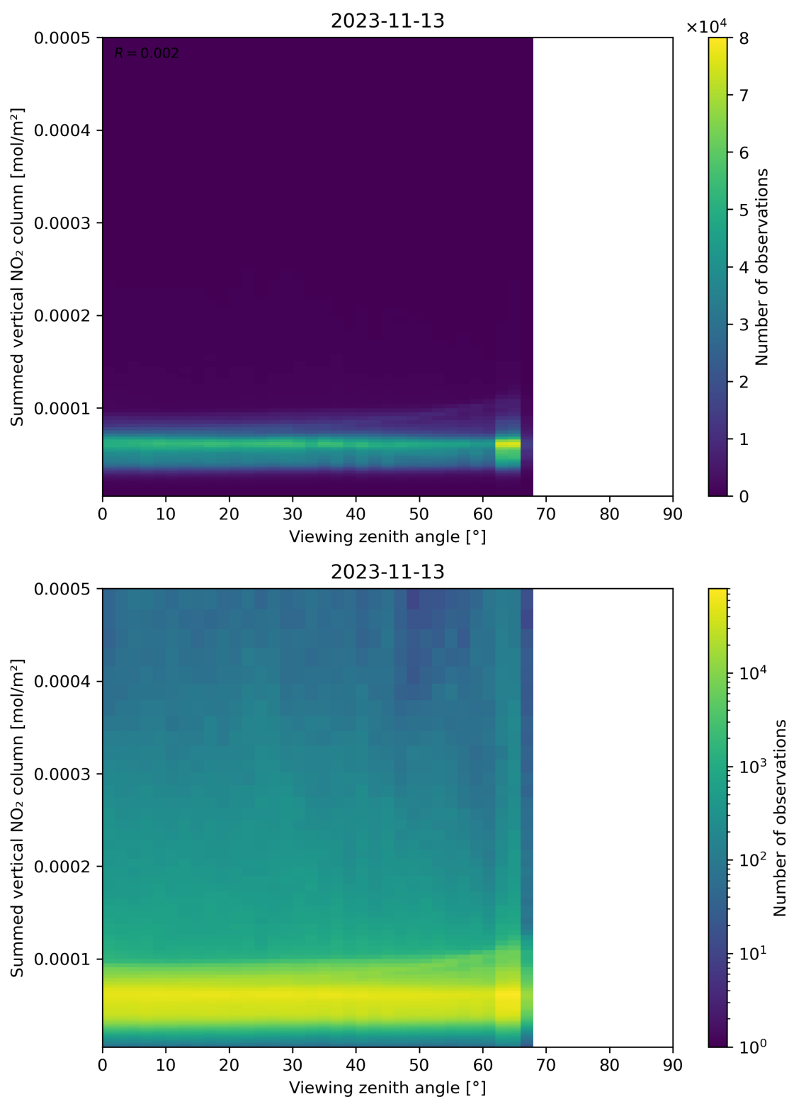
Figure 165: Scatter density plot of “Viewing zenith angle” against “Summed vertical NO 2 column” for 2023-11-13 to 2023-11-14.
