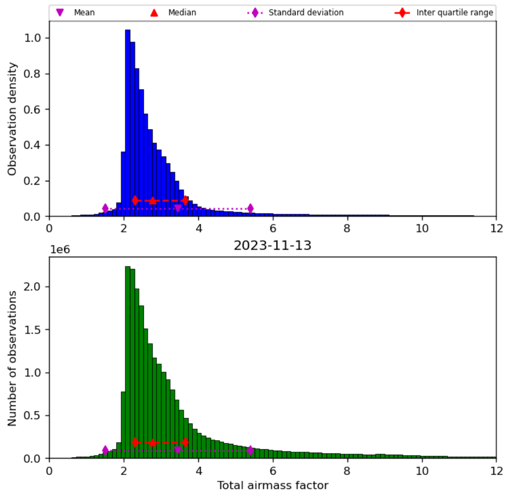
Figure 32: Histogram of “Total airmass factor” for 2023-11-13 to 2023-11-14
