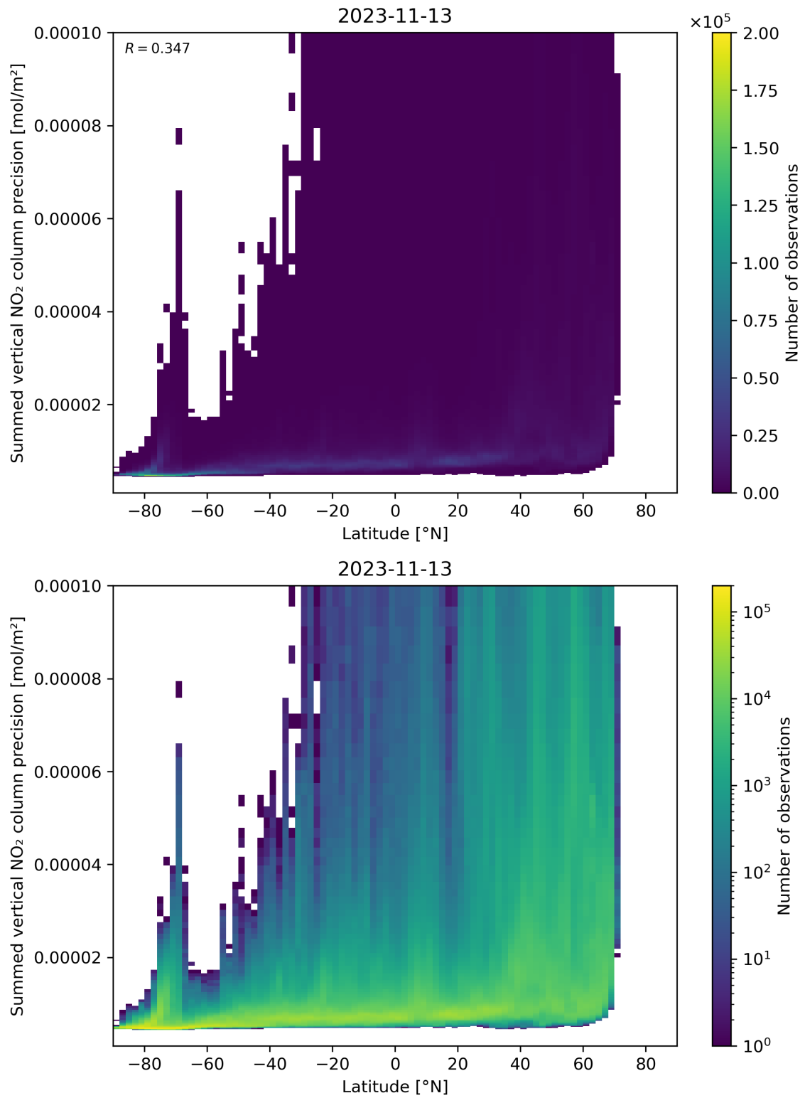
Figure 89: Scatter density plot of “Latitude” against “Summed vertical NO 2 column precision” for 2023-11-13 to 2023-11-14.
