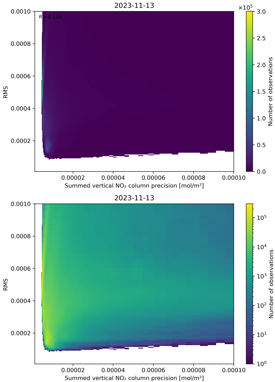
Figure 108: Scatter density plot of “Summed vertical NO 2 column precision” against “RMS” for 2023-11-13 to 2023-11-14.
