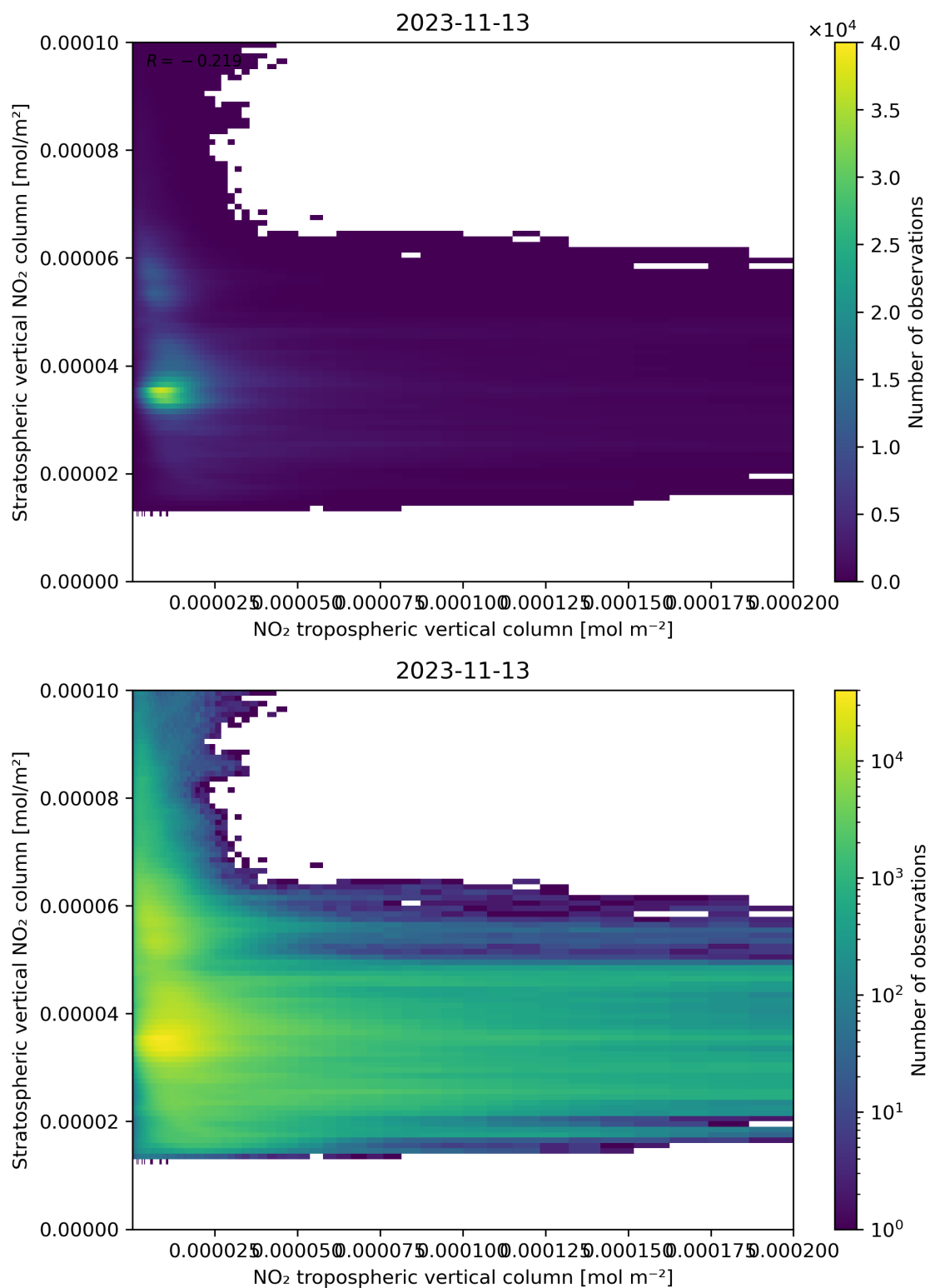
Figure 125: Scatter density plot of “NO 2 tropospheric vertical column” against “Stratospheric vertical NO 2 column” for 2023-11-13 to 2023-11-14.
