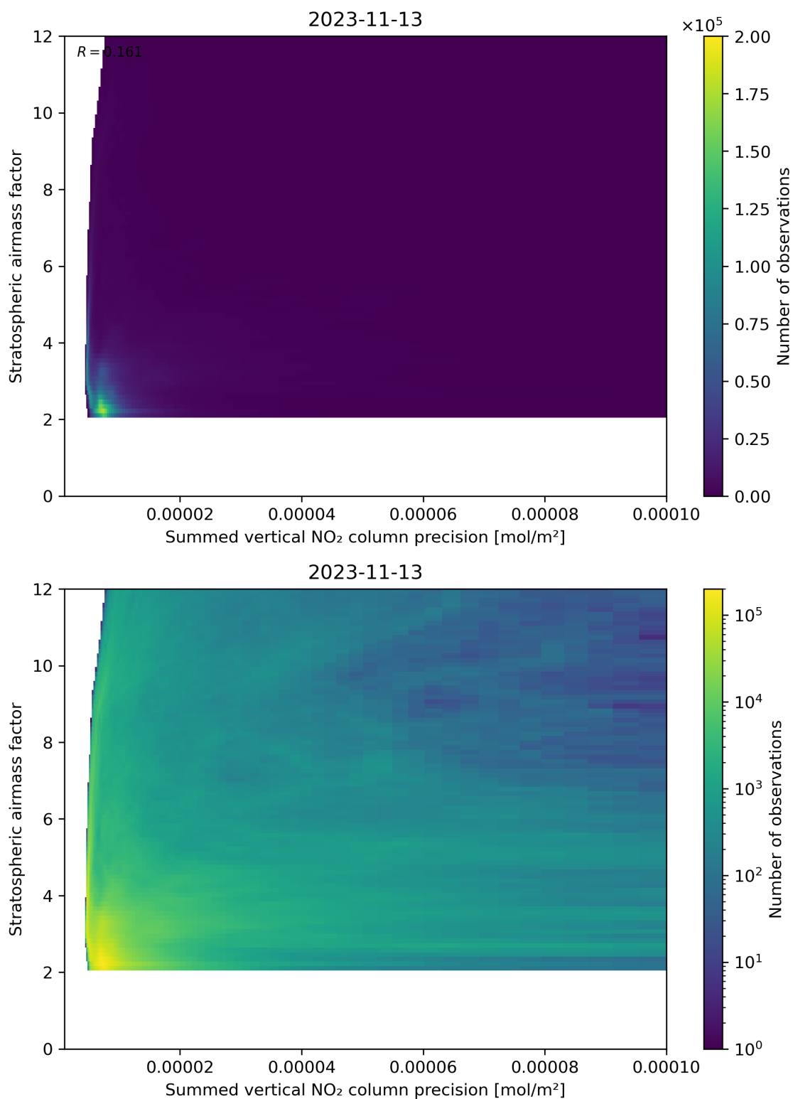
Figure 106: Scatter density plot of “Summed vertical NO 2 column precision” against “Stratospheric airmass factor” for 2023-11-13 to 2023-11-14.
