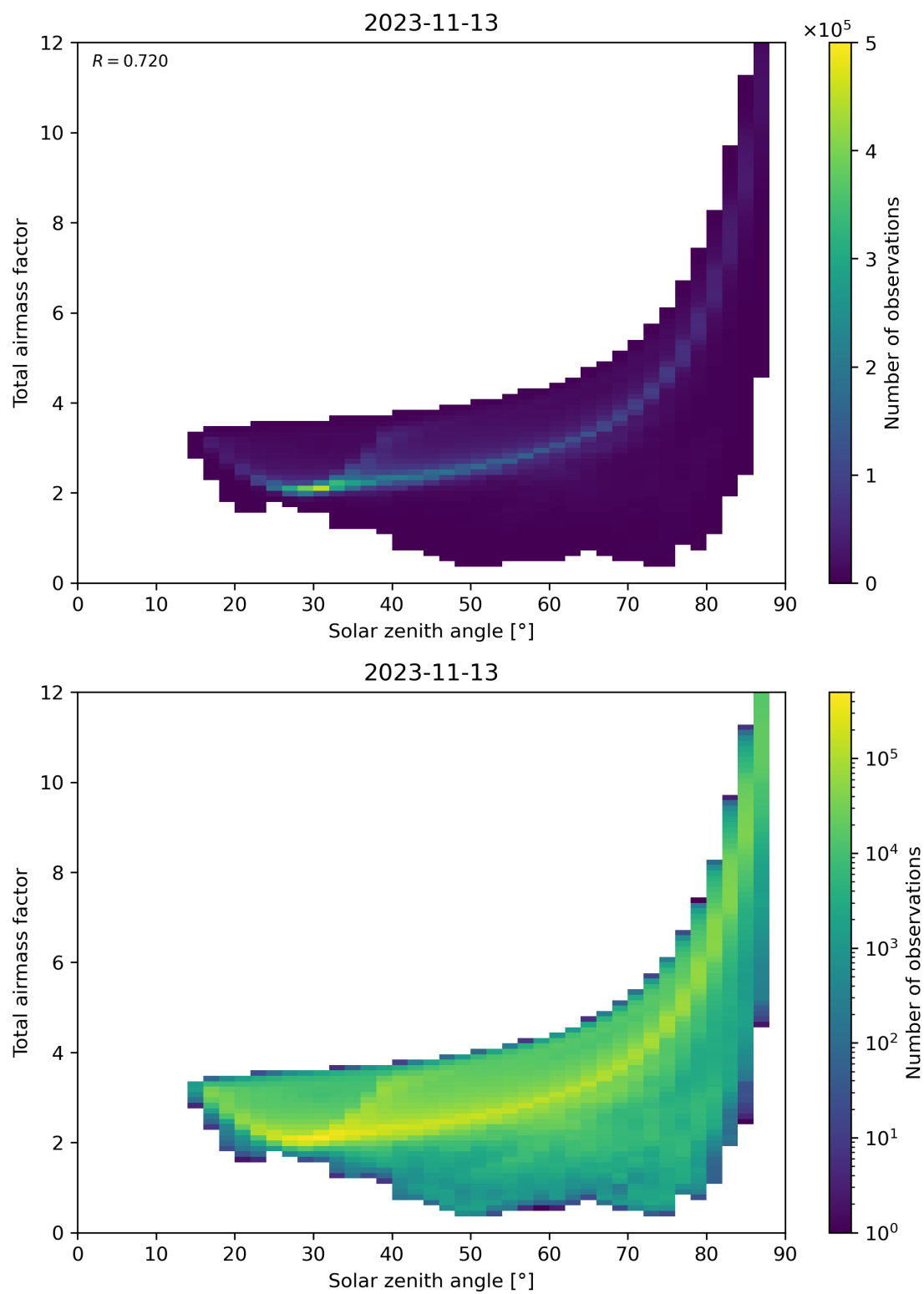
Figure 146: Scatter density plot of “Solar zenith angle” against “Total air mass factor” for 2023-11-13 to 2023-11-14.
