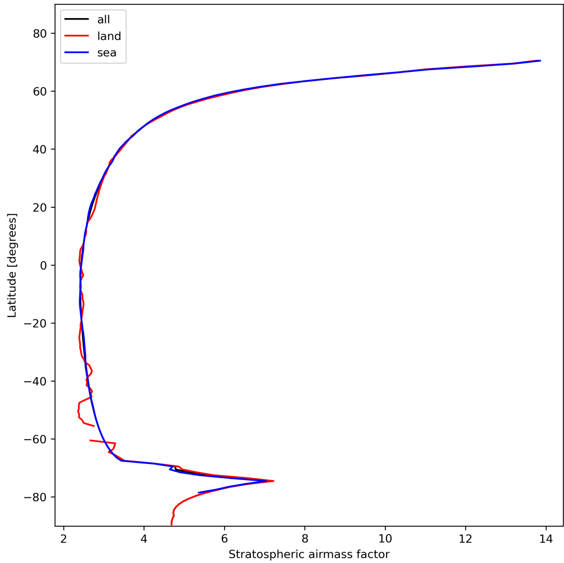
Figure 27: Zonal average of “Stratospheric airmass factor” for 2023-11-13 to 2023-11-14.
