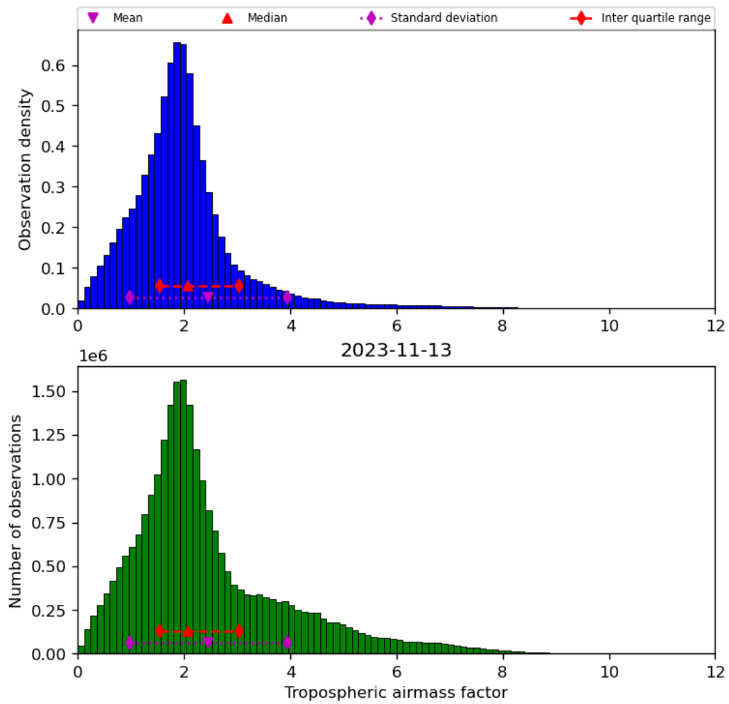
Figure 31: Histogram of “Tropospheric airmass factor” for 2023-11-13 to 2023-11-14
