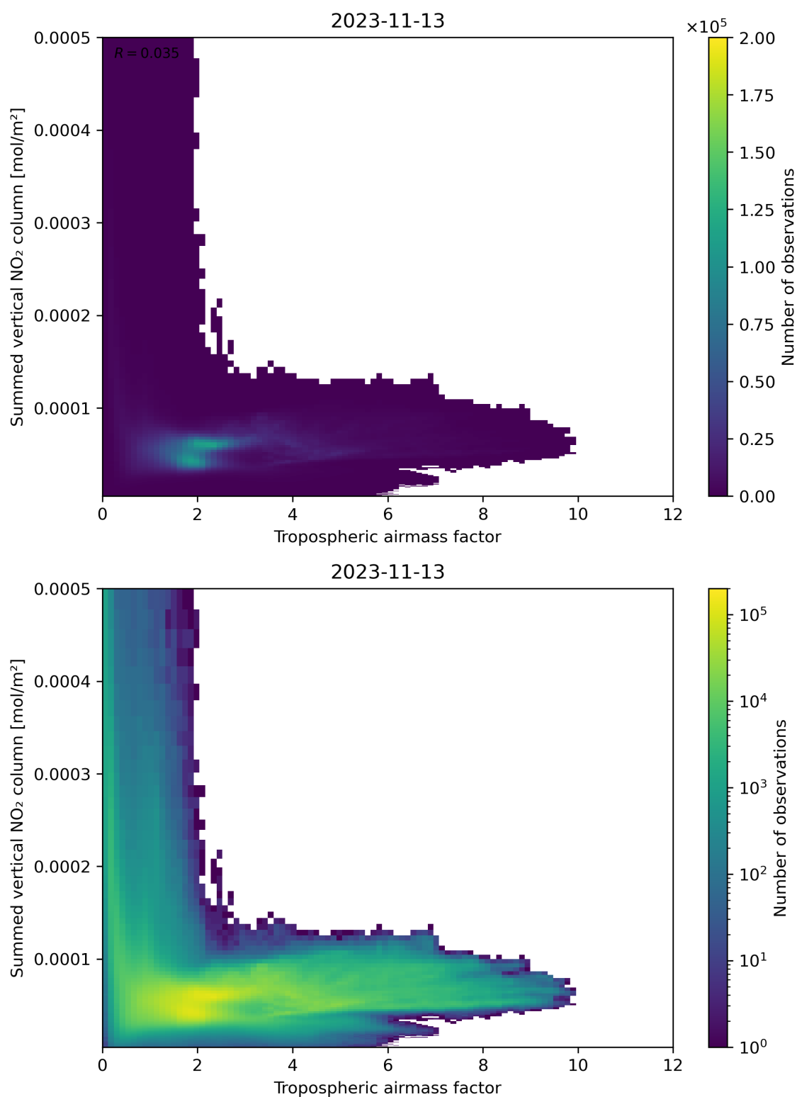
Figure 75: Scatter density plot of “Tropospheric airmass factor” against “Summed vertical NO 2 column” for 2023-11-13 to 2023-11-14.
