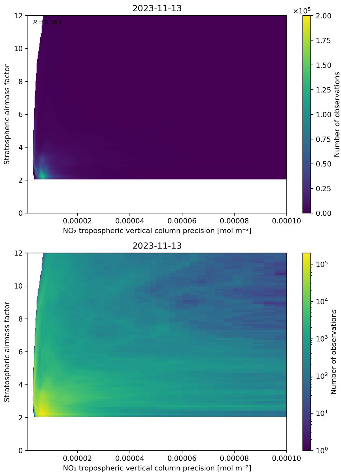
Figure 131: Scatter density plot of “NO 2 tropospheric vertical column precision” against “Stratospheric airmass factor” for 2023-11-13 to 2023-11-14.
