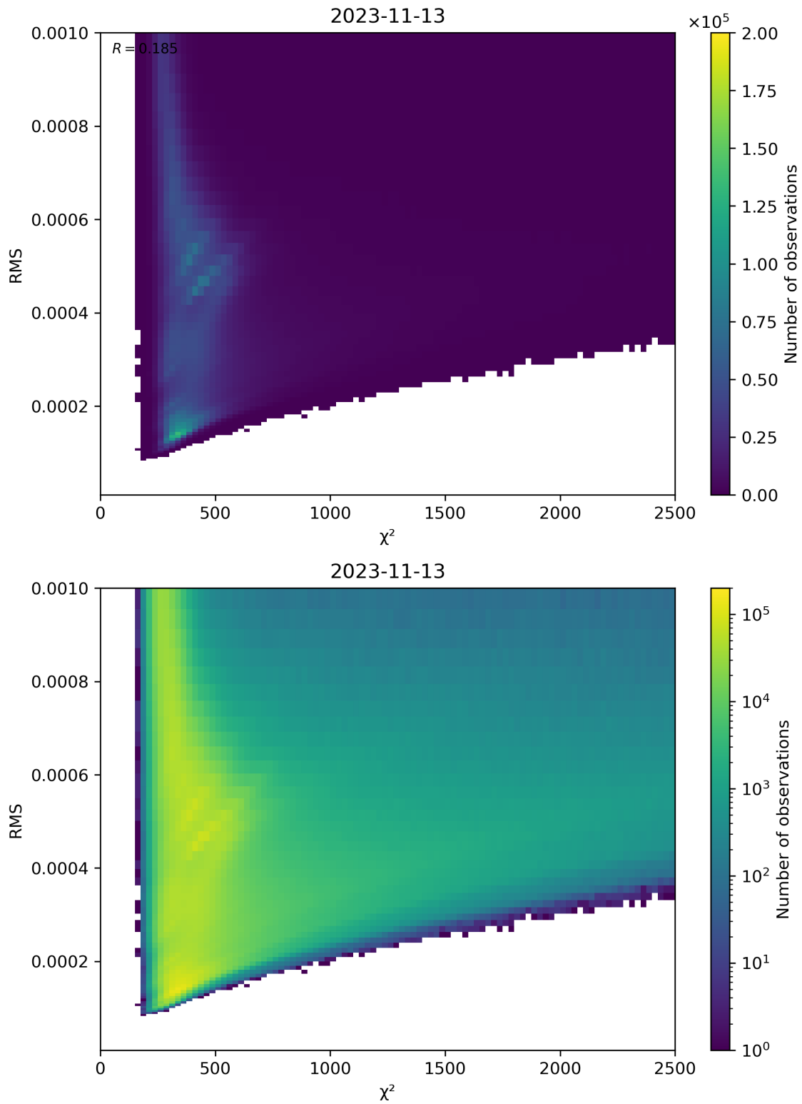
Figure 82: Scatter density plot of “ \chi^2 ” against “RMS” for 2023-11-13 to 2023-11-14.
