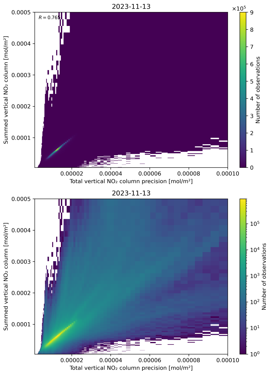
Figure 117: Scatter density plot of “Total vertical NO 2 column precision” against “Summed vertical NO 2 column” for 2023-11-13 to 2023-11-14.
