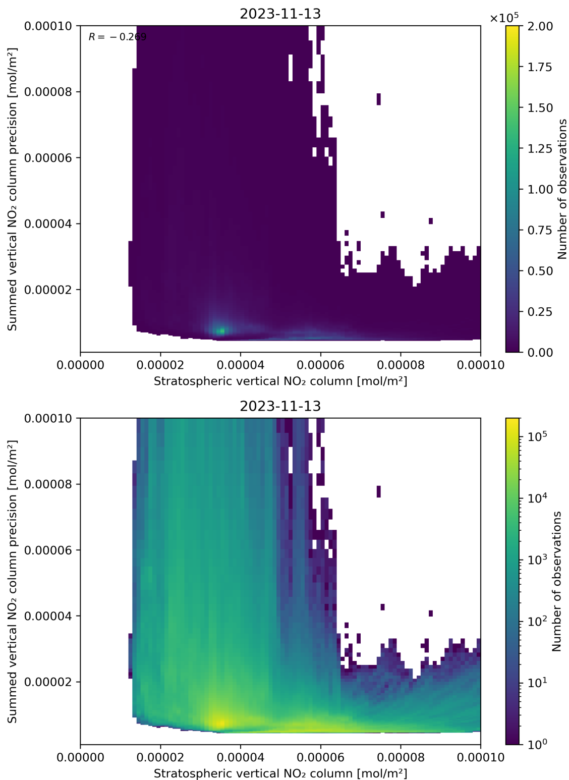
Figure 99: Scatter density plot of “Stratospheric vertical NO 2 column” against “Summed vertical NO 2 column precision” for 2023-11-13 to 2023-11-14.
