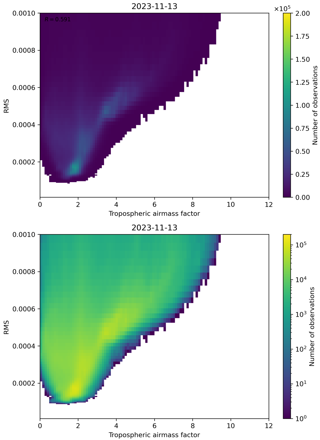
Figure 79: Scatter density plot of “Tropospheric airmass factor” against “RMS” for 2023-11-13 to 2023-11-14.
