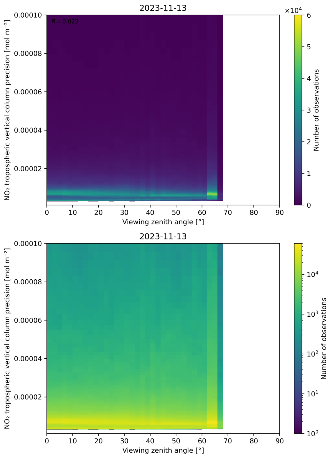
Figure 170: Scatter density plot of “Viewing zenith angle” against “NO 2 tropospheric vertical column precision” for 2023-11-13 to 2023-11-14.
