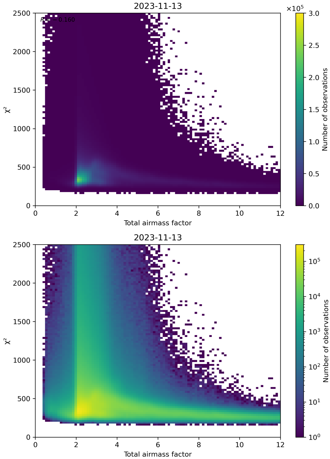
Figure 63: Scatter density plot of “Total airmass factor” against “ \chi^2 ” for 2023-11-13 to 2023-11-14.
