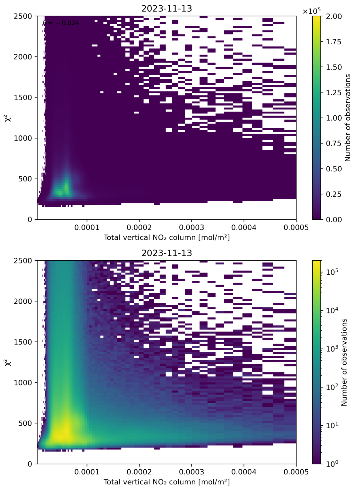
Figure 111: Scatter density plot of “Total vertical NO 2 column” against “ \chi^2 ” for 2023-11-13 to 2023-11-14.
