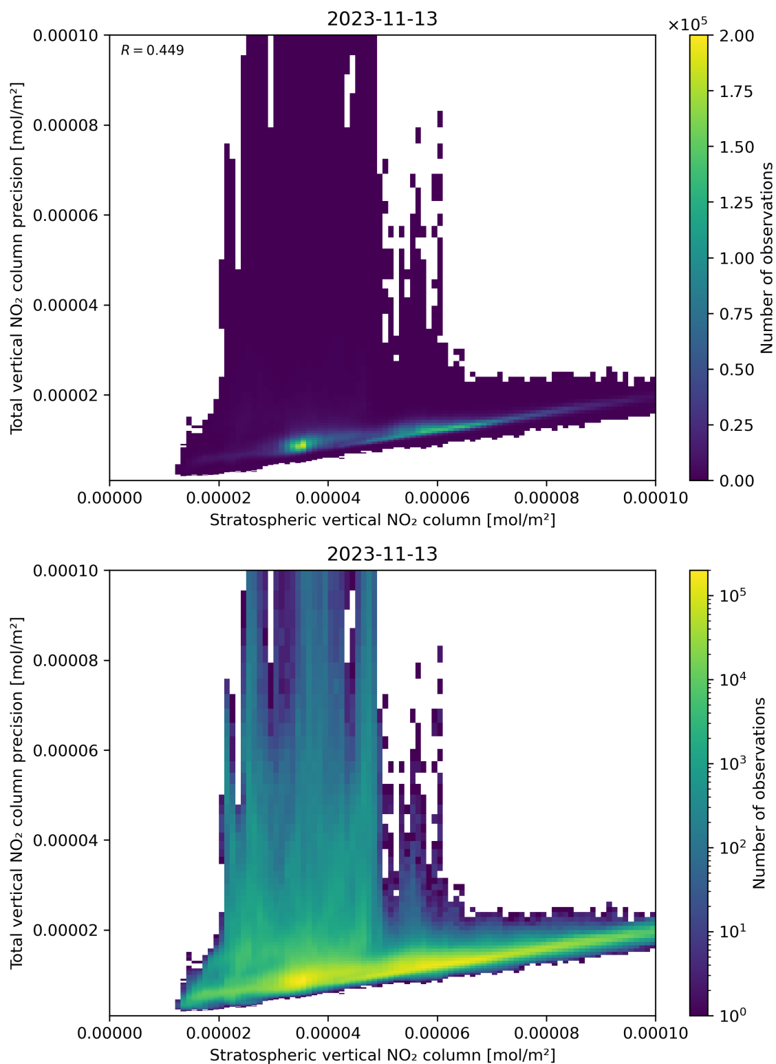
Figure 101: Scatter density plot of “Stratospheric vertical NO 2 column” against “Total vertical NO 2 column precision” for 2023-11-13 to 2023-11-14.
