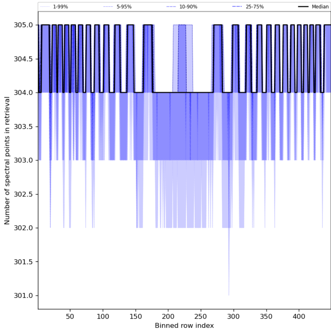
Figure 50: Along track statistics of “Number of spectral points in retrieval” for 2023-11-13 to 2023-11-14
