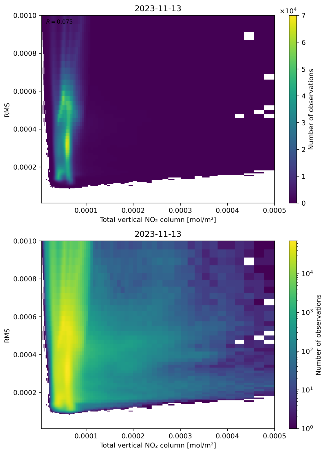
Figure 120: Scatter density plot of “Total vertical NO 2 column” against “RMS” for 2023-11-13 to 2023-11-14.
