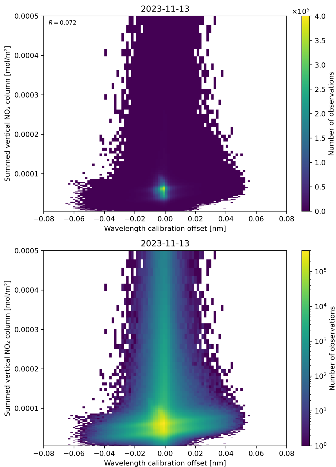
Figure 177: Scatter density plot of “Wavelength calibration offset” against “Summed vertical NO 2 column” for 2023-11-13 to 2023-11-14.
