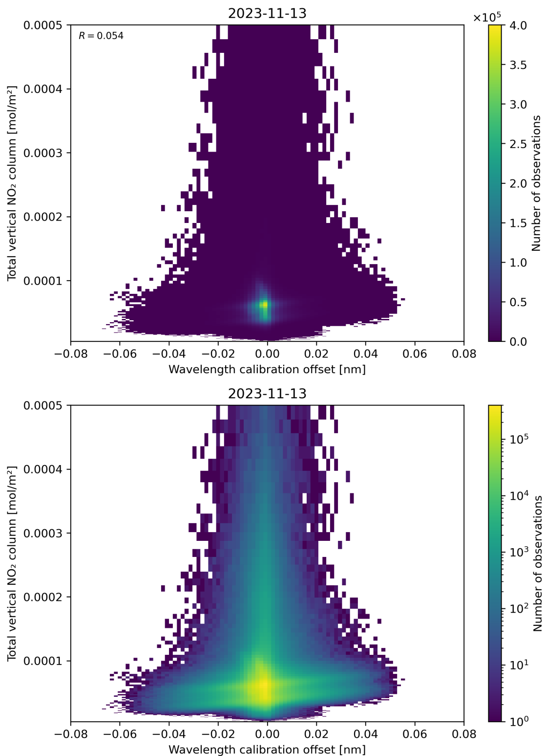
Figure 179: Scatter density plot of “Wavelength calibration offset” against “Total vertical NO 2 column” for 2023-11-13 to 2023-11-14.
