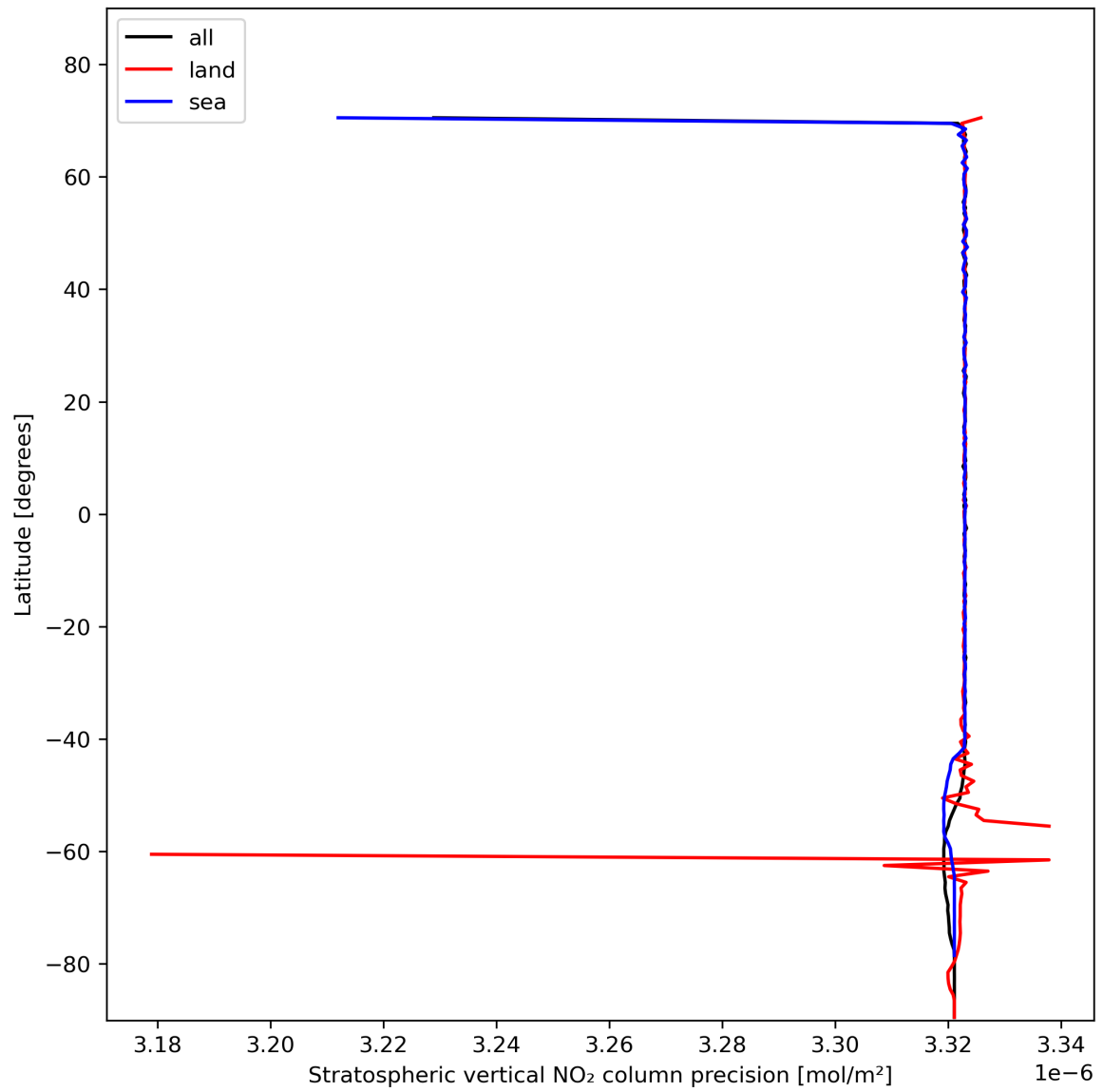
Figure 20: Zonal average of “Stratospheric vertical NO 2 column precision” for 2023-11-13 to 2023-11-14.
