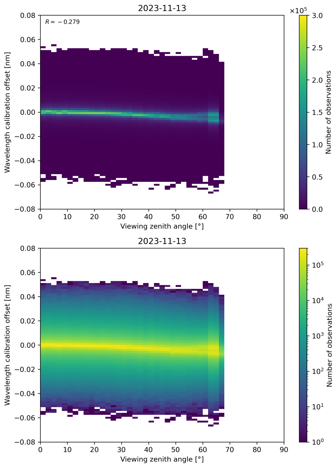
Figure 173: Scatter density plot of “Viewing zenith angle” against “Wavelength calibration offset” for 2023-11-13 to 2023-11-14.
