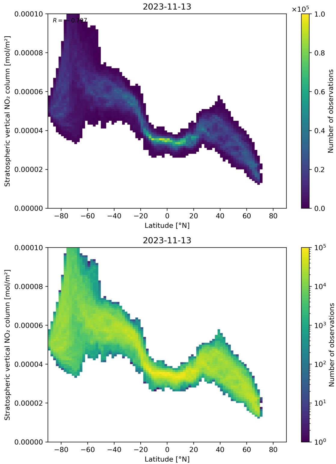
Figure 87: Scatter density plot of “Latitude” against “Stratospheric vertical NO 2 column” for 2023-11-13 to 2023-11-14.
