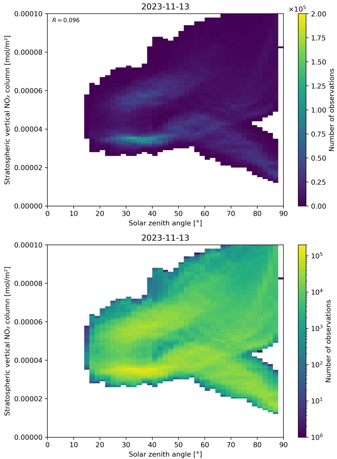
Figure 150: Scatter density plot of “Solar zenith angle” against “Stratospheric vertical NO 2 column” for 2023-11-13 to 2023-11-14.
