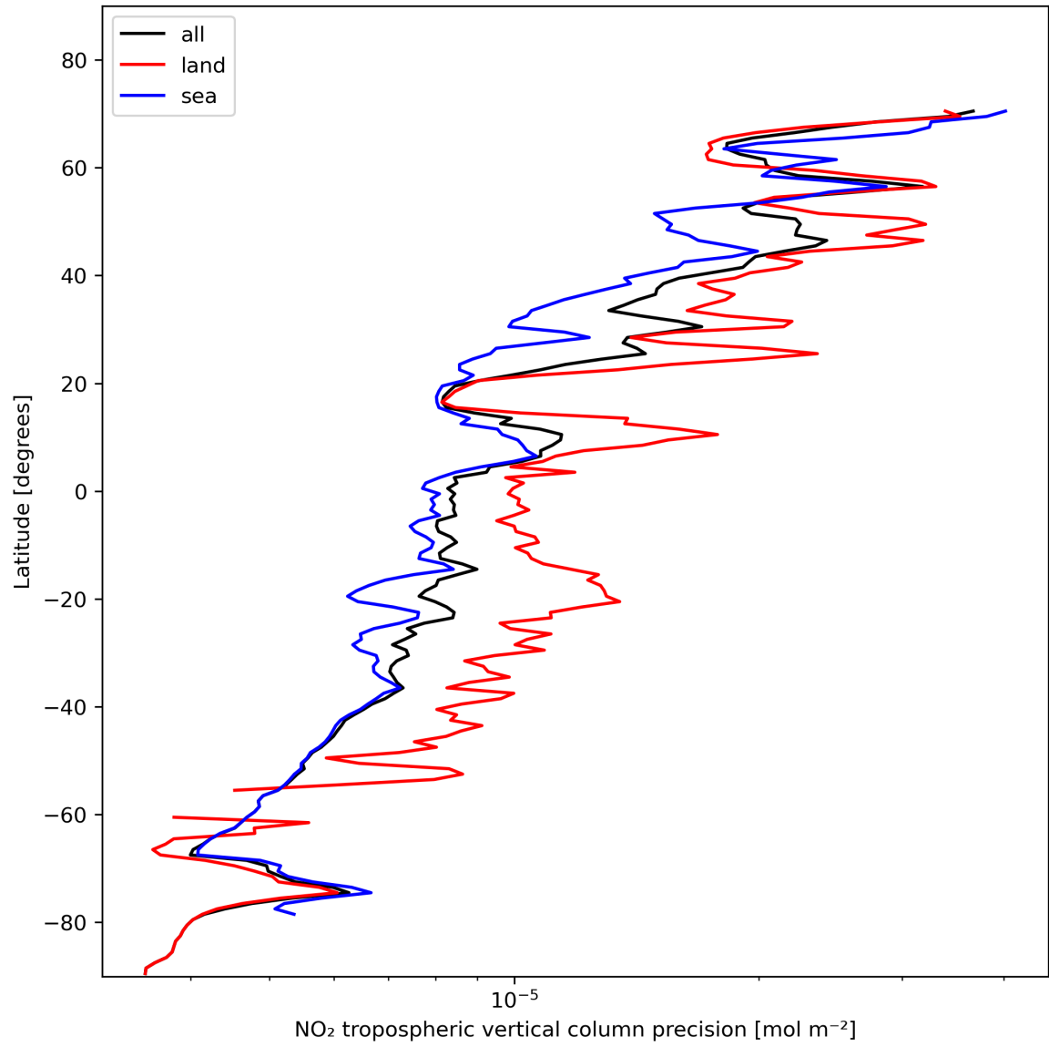
Figure 13: Zonal average of “NO 2 tropospheric vertical column precision” for 2023-11-13 to 2023-11-14.
