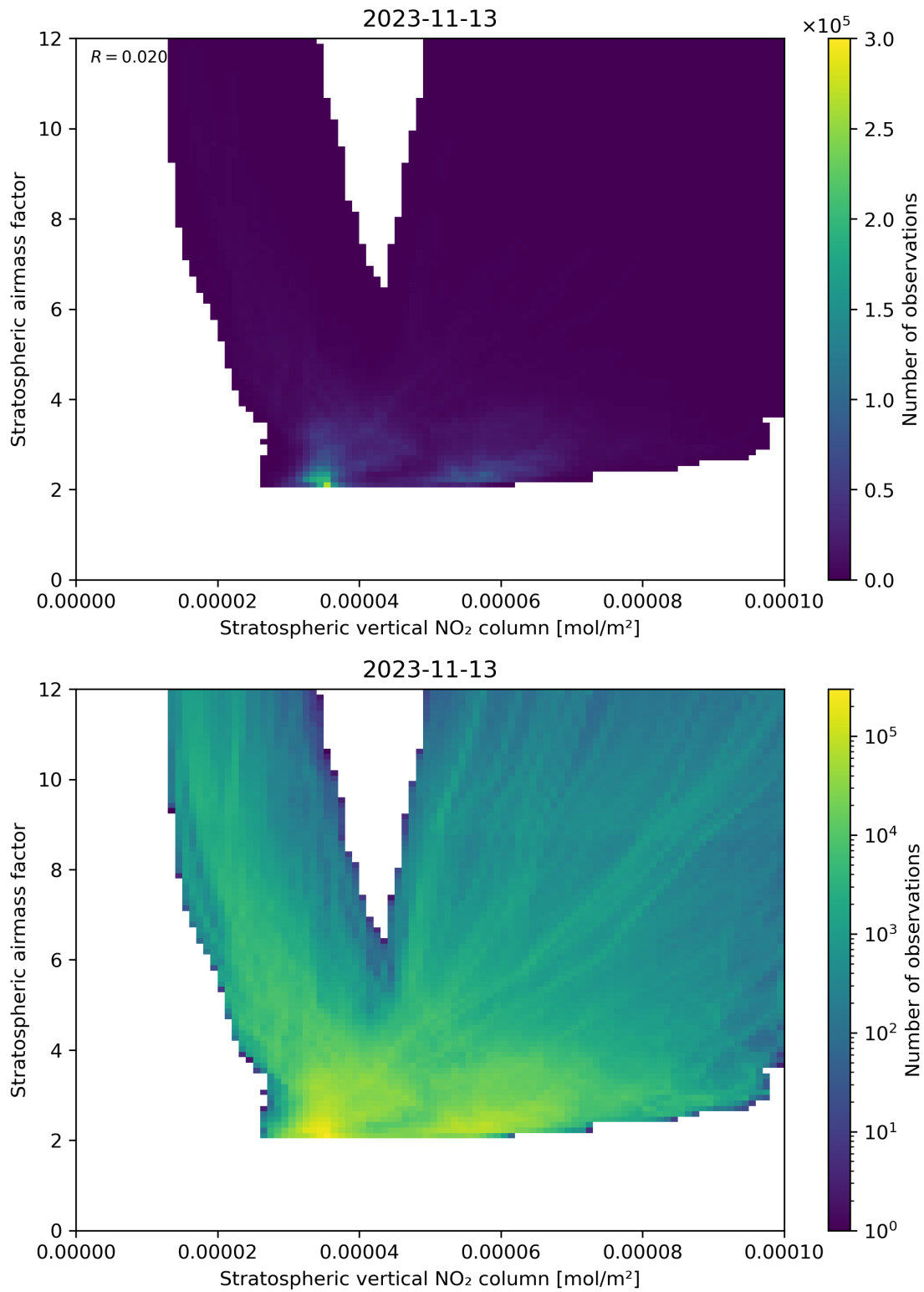
Figure 96: Scatter density plot of “Stratospheric vertical NO 2 column” against “Stratospheric airmass factor” for 2023-11-13 to 2023-11-14.
