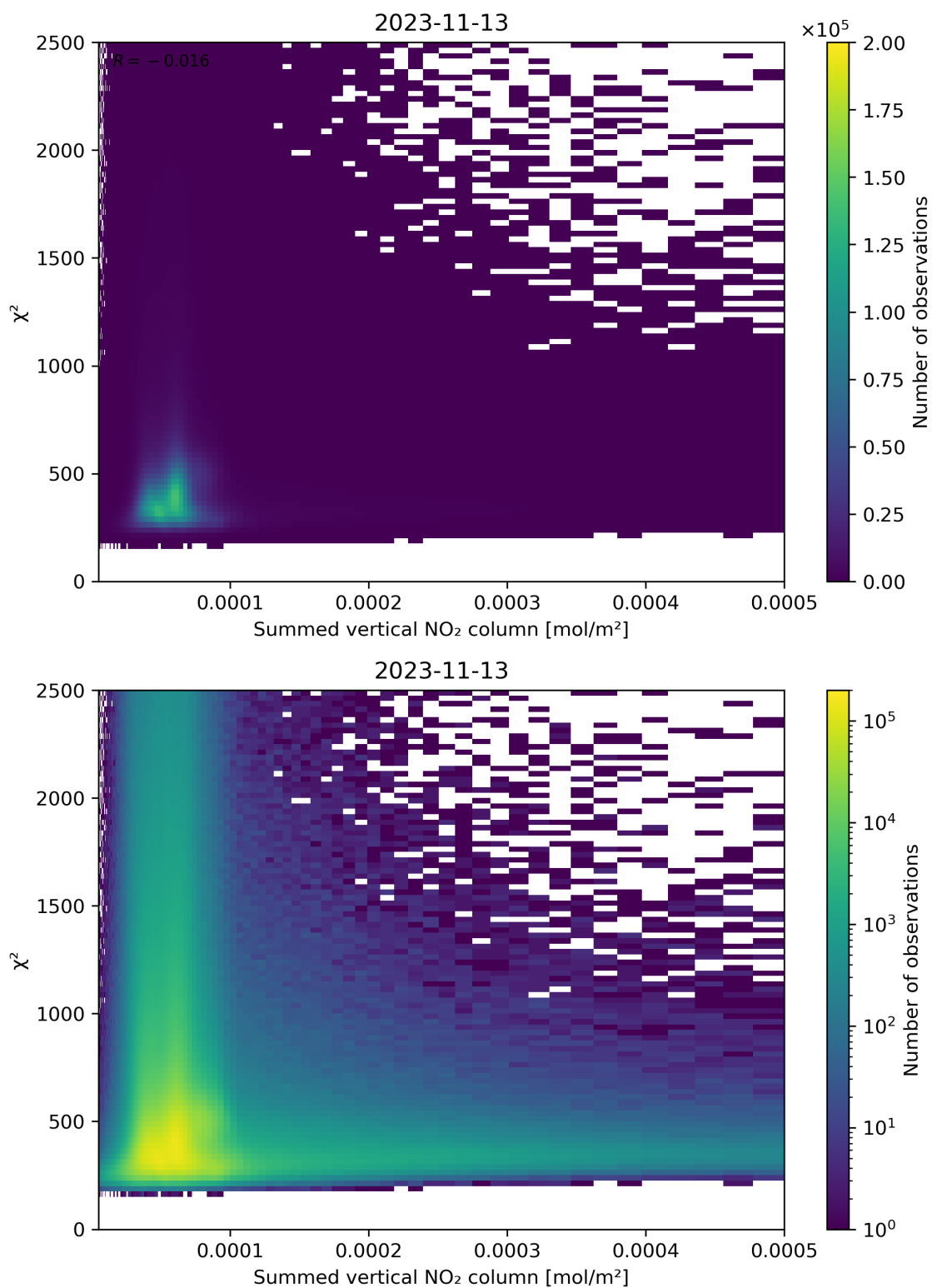
Figure 104: Scatter density plot of “Summed vertical NO 2 column” against “ \chi^2 ” for 2023-11-13 to 2023-11-14.
