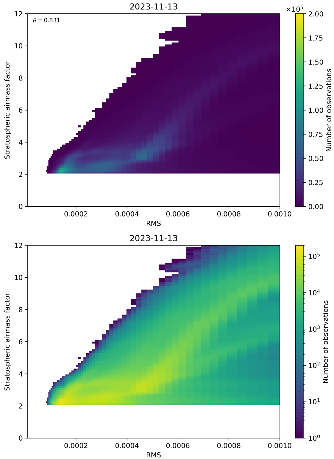
Figure 144: Scatter density plot of “RMS” against “Stratospheric airmass factor” for 2023-11-13 to 2023-11-14.
