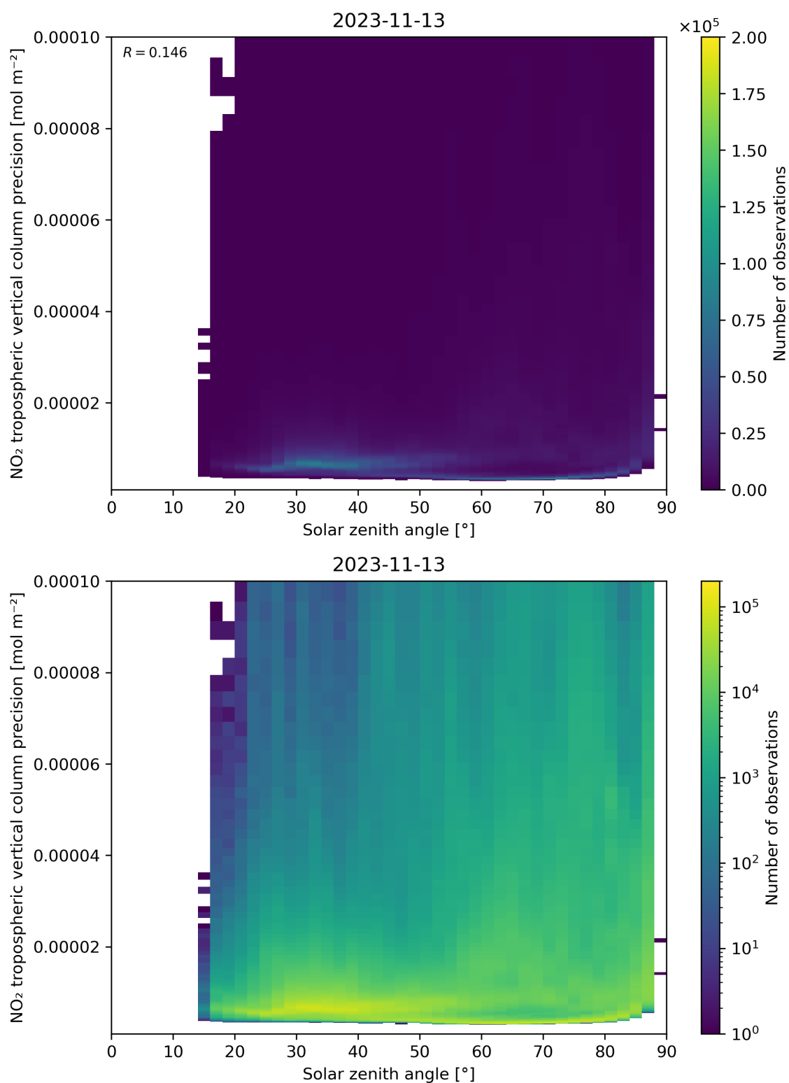
Figure 156: Scatter density plot of “Solar zenith angle” against “NO 2 tropospheric vertical column precision” for 2023-11-13 to 2023-11-14.
