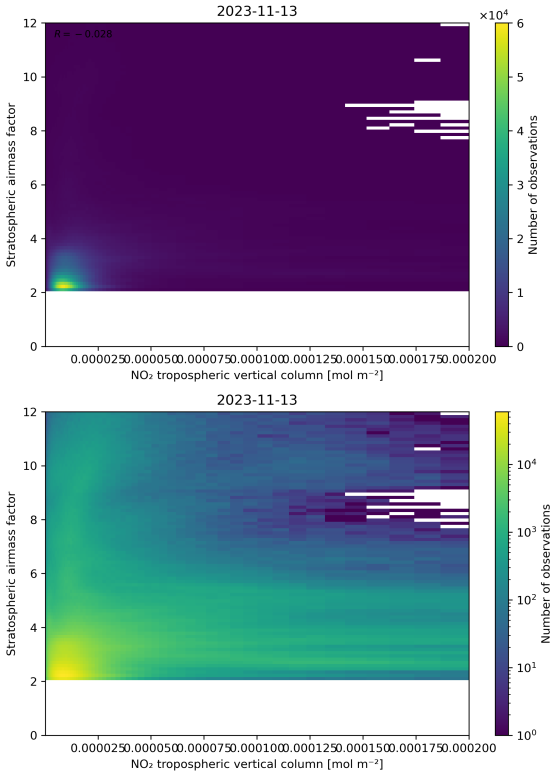
Figure 121: Scatter density plot of “NO 2 tropospheric vertical column” against “Stratospheric air mass factor” for 2023-11-13 to 2023-11-14.
