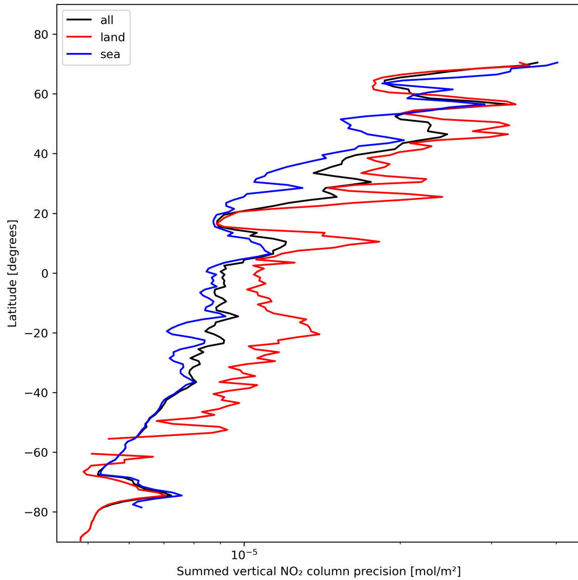
Figure 24: Zonal average of “Summed vertical NO 2 column precision” for 2023-11-13 to 2023-11-14.
