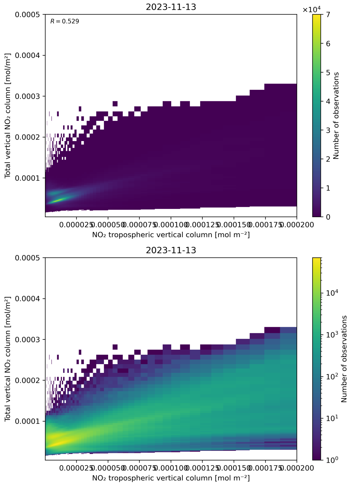
Figure 128: Scatter density plot of “NO 2 tropospheric vertical column” against “Total vertical NO 2 column” for 2023-11-13 to 2023-11-14.
