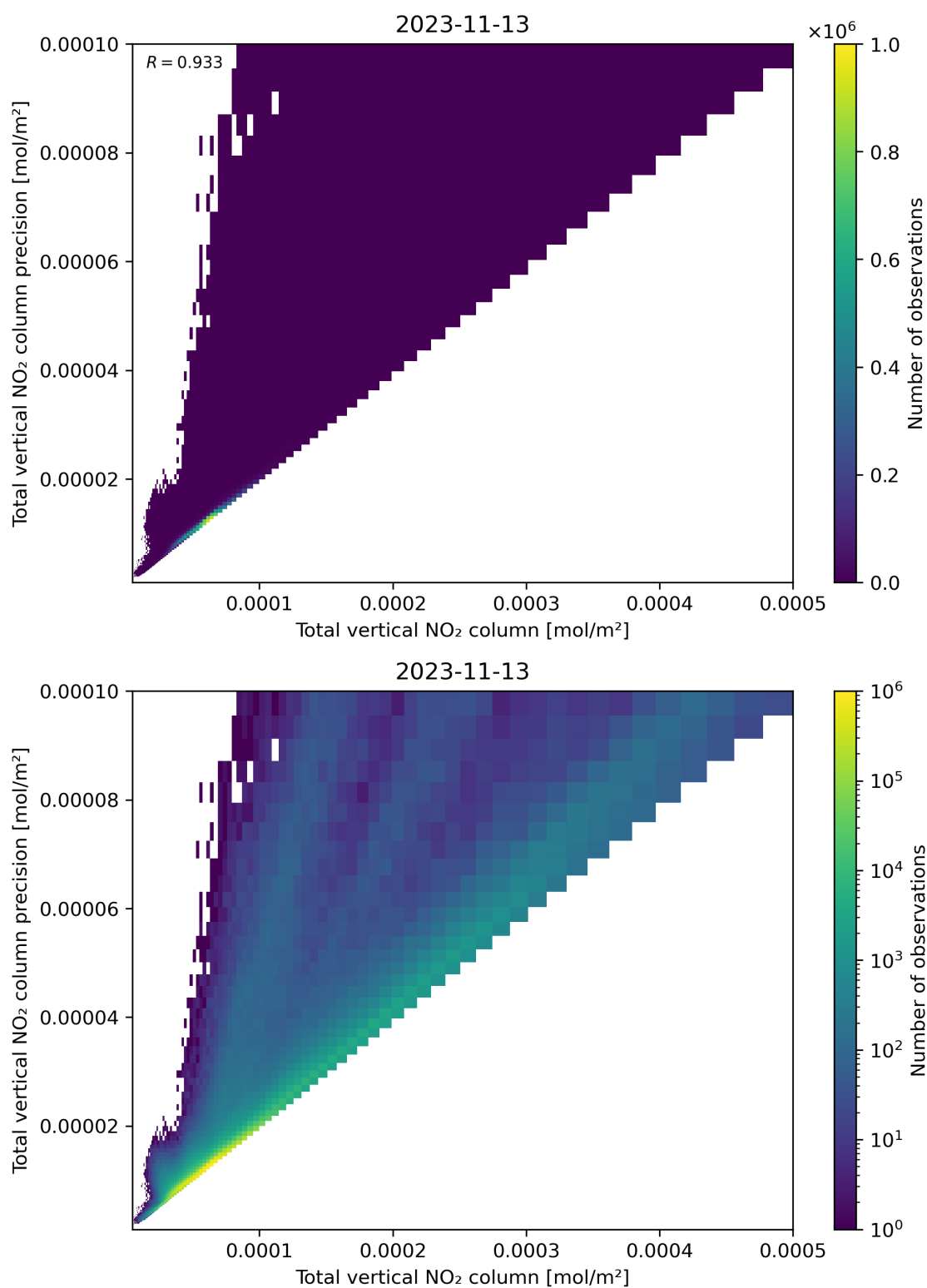
Figure 114: Scatter density plot of “Total vertical NO 2 column” against “Total vertical NO 2 column precision” for 2023-11-13 to 2023-11-14.
