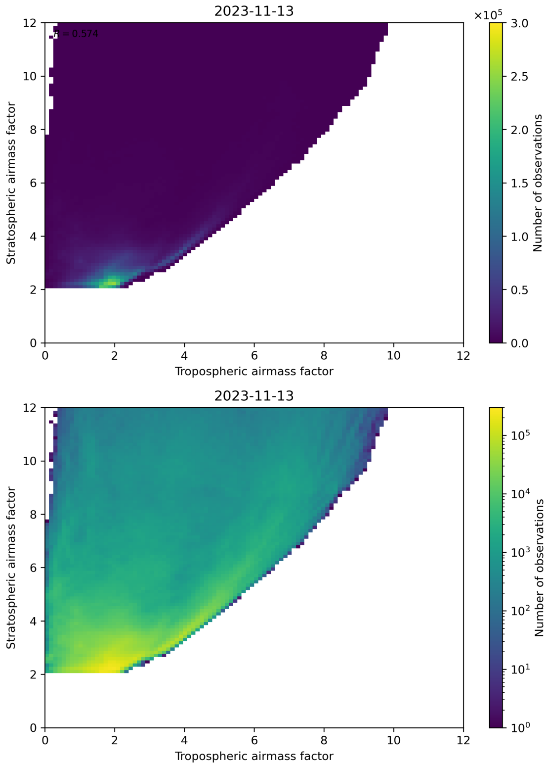
Figure 71: Scatter density plot of “Tropospheric airmass factor” against “Stratospheric airmass factor” for 2023-11-13 to 2023-11-14.
