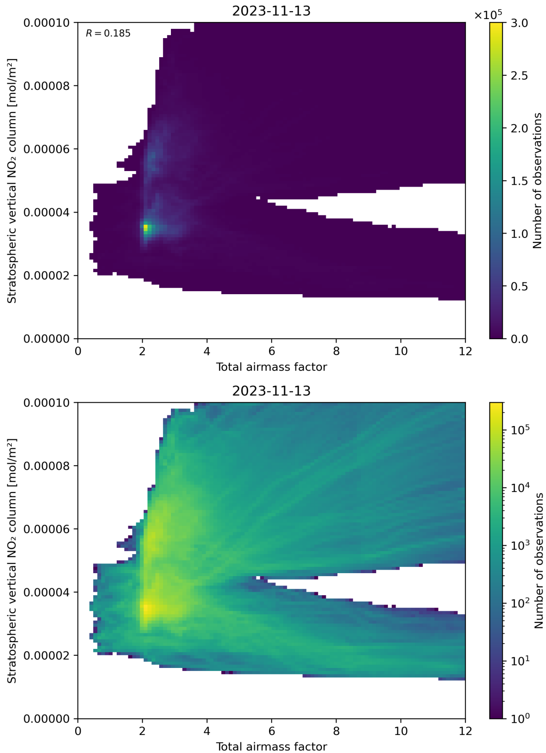
Figure 64: Scatter density plot of “Total airmass factor” against “Stratospheric vertical NO 2 column” for 2023-11-13 to 2023-11-14.
