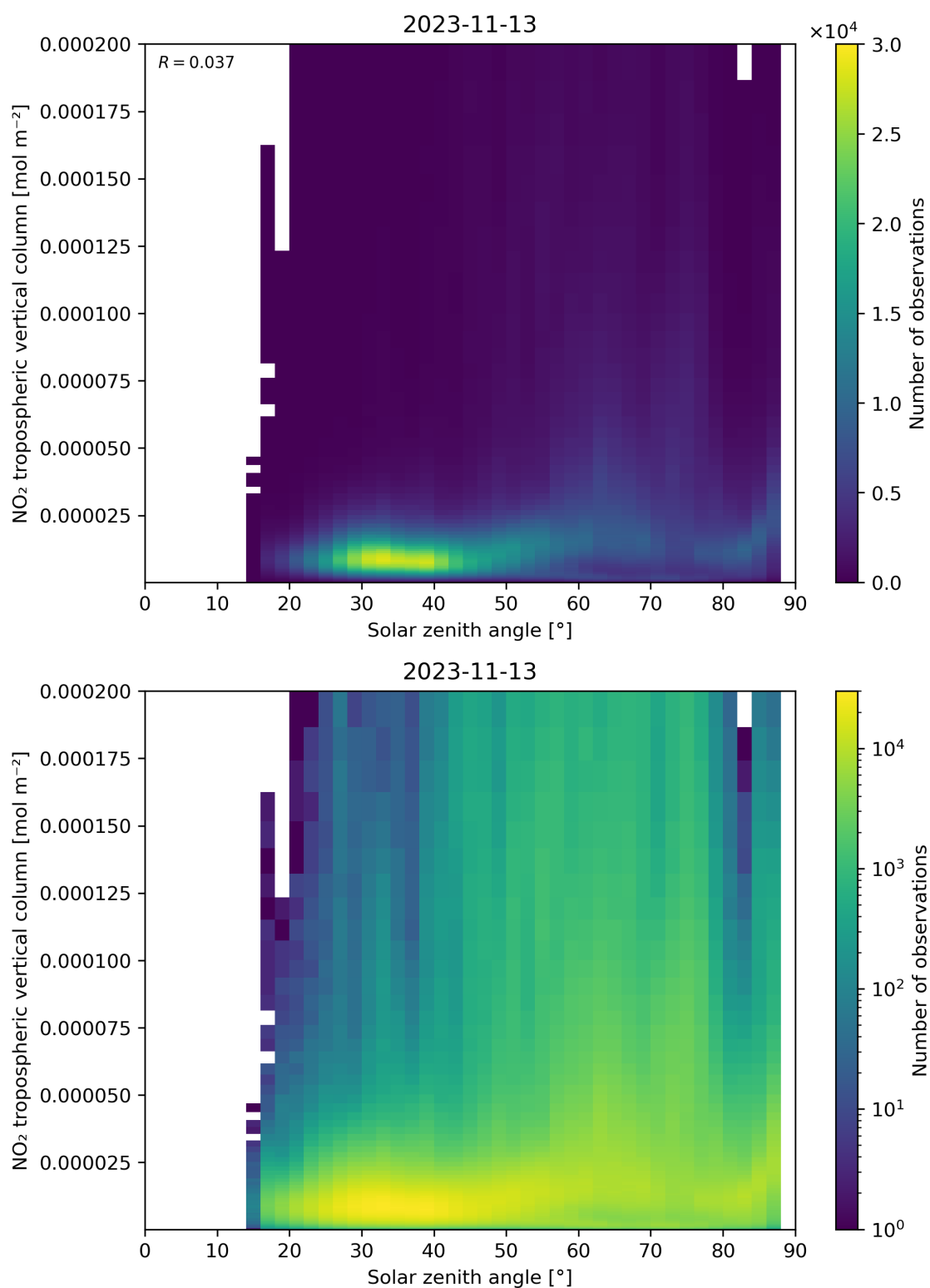
Figure 155: Scatter density plot of “Solar zenith angle” against “NO 2 tropospheric vertical column” for 2023-11-13 to 2023-11-14.
