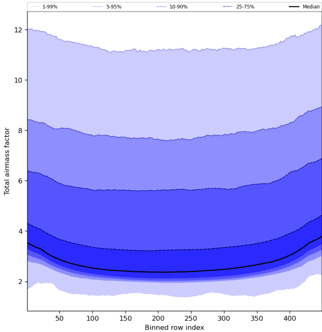
Figure 49: Along track statistics of “Total airmass factor” for 2023-11-13 to 2023-11-14
