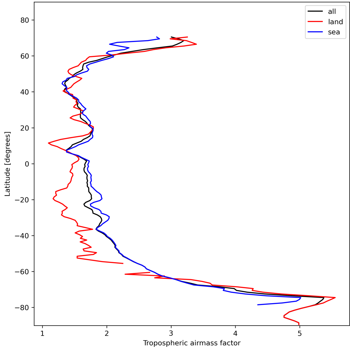
Figure 14: Zonal average of “Tropospheric airmass factor” for 2023-11-13 to 2023-11-14.
