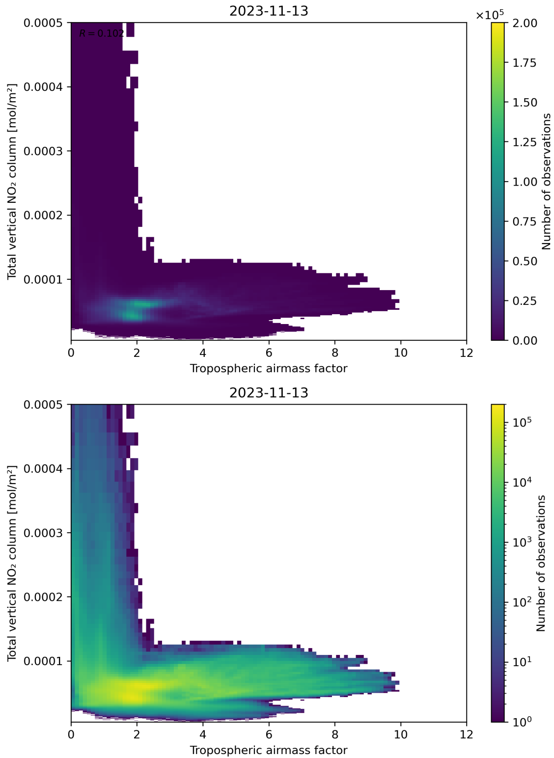
Figure 77: Scatter density plot of “Tropospheric airmass factor” against “Total vertical NO 2 column” for 2023-11-13 to 2023-11-14.
