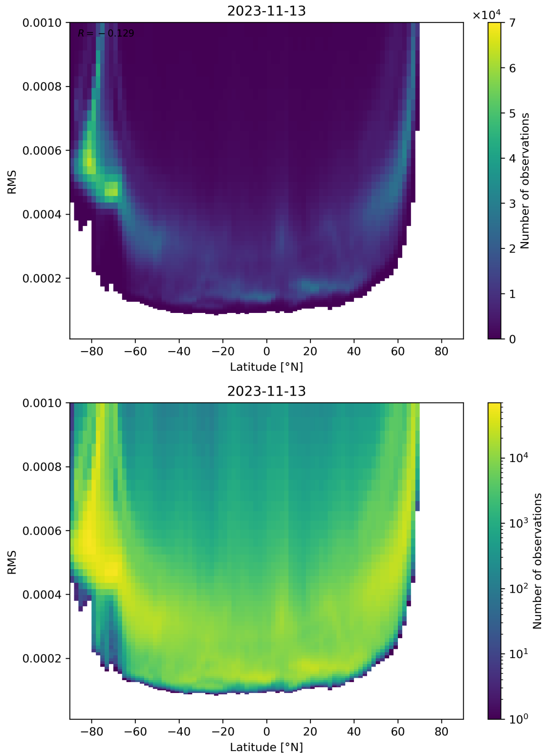
Figure 94: Scatter density plot of “Latitude” against “RMS” for 2023-11-13 to 2023-11-14.
