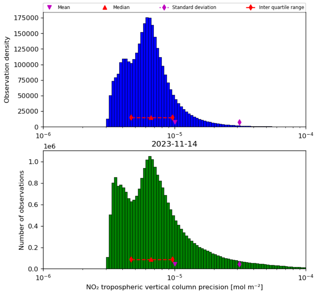
Figure 30: Histogram of “NO 2 tropospheric vertical column precision” for 2023-11-13 to 2023-11-15
