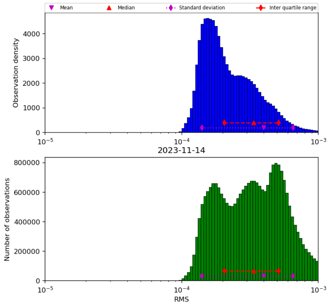
Figure 43: Histogram of “RMS” for 2023-11-13 to 2023-11-15
