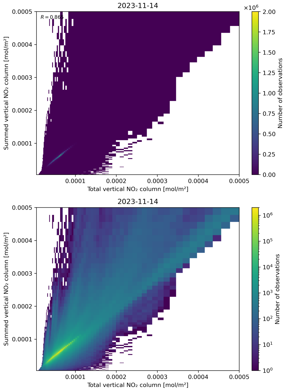
Figure 112: Scatter density plot of “Total vertical NO 2 column” against “Summed vertical NO 2 column” for 2023-11-13 to 2023-11-15.
