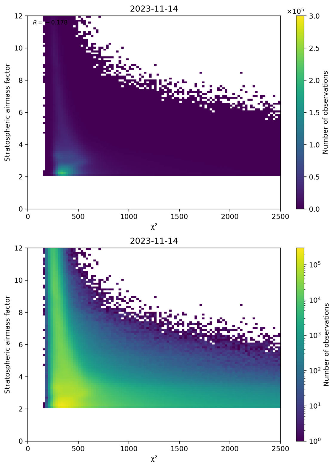
Figure 81: Scatter density plot of “ \chi^2 ” against “Stratospheric airmass factor” for 2023-11-13 to 2023-11-15.
