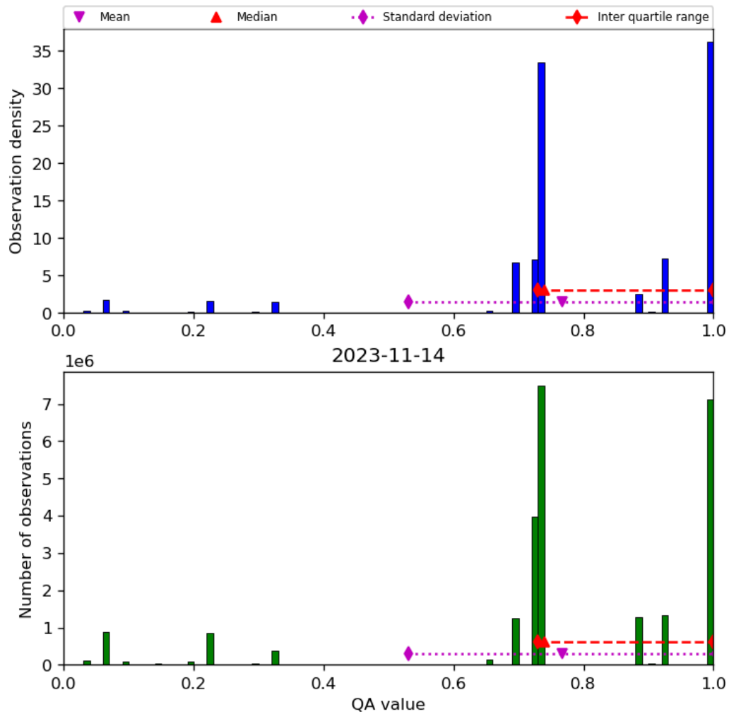
Figure 28: Histogram of “QA value” for 2023-11-13 to 2023-11-15
