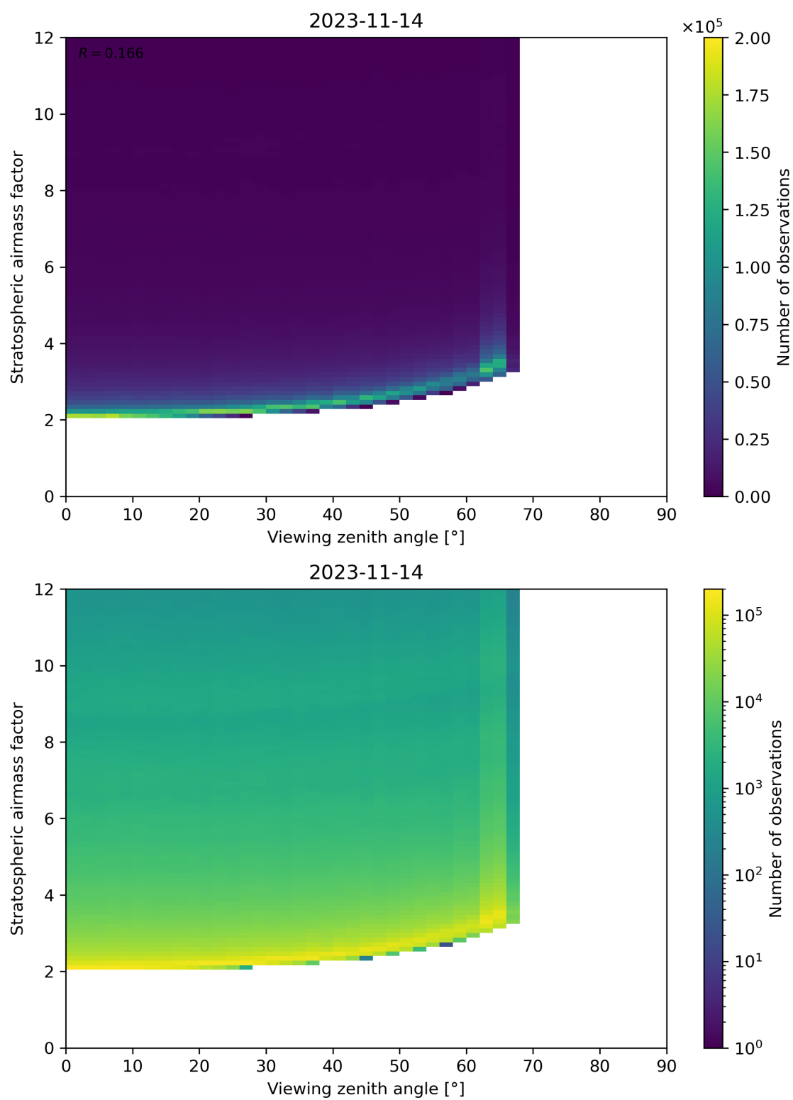
Figure 159: Scatter density plot of “Viewing zenith angle” against “Stratospheric airmass factor” for 2023-11-13 to 2023-11-15.
