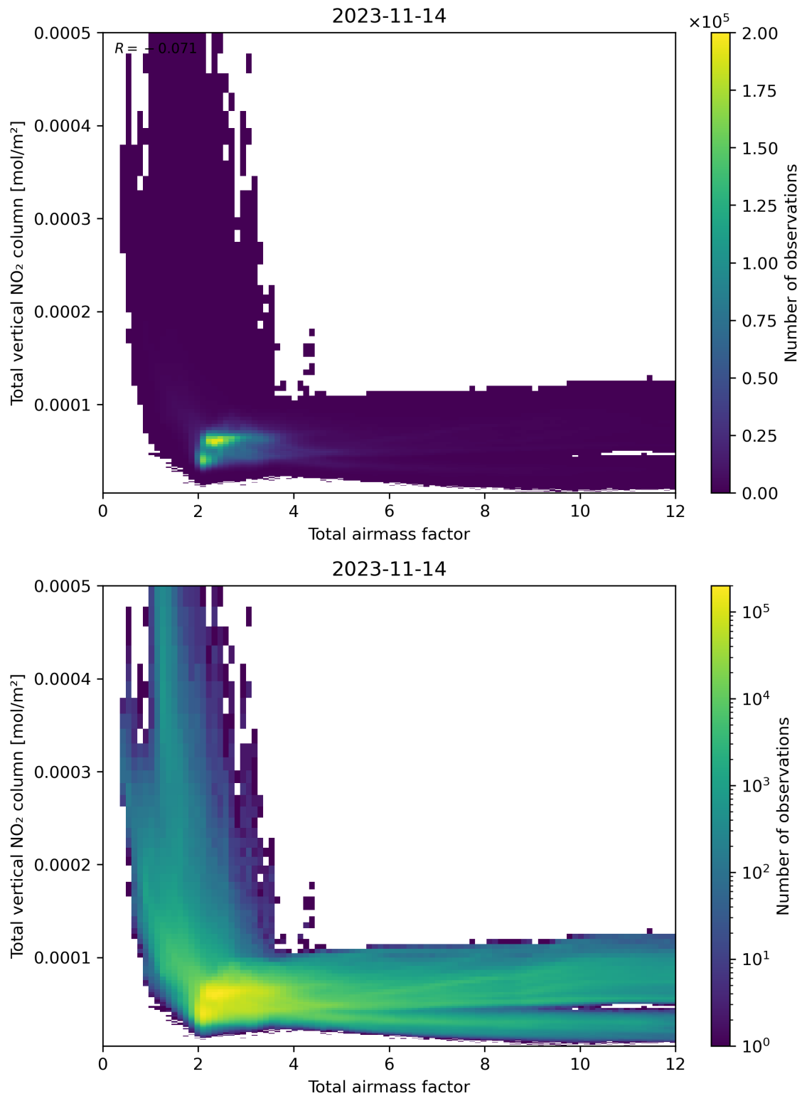
Figure 67: Scatter density plot of “Total airmass factor” against “Total vertical NO 2 column” for 2023-11-13 to 2023-11-15.
