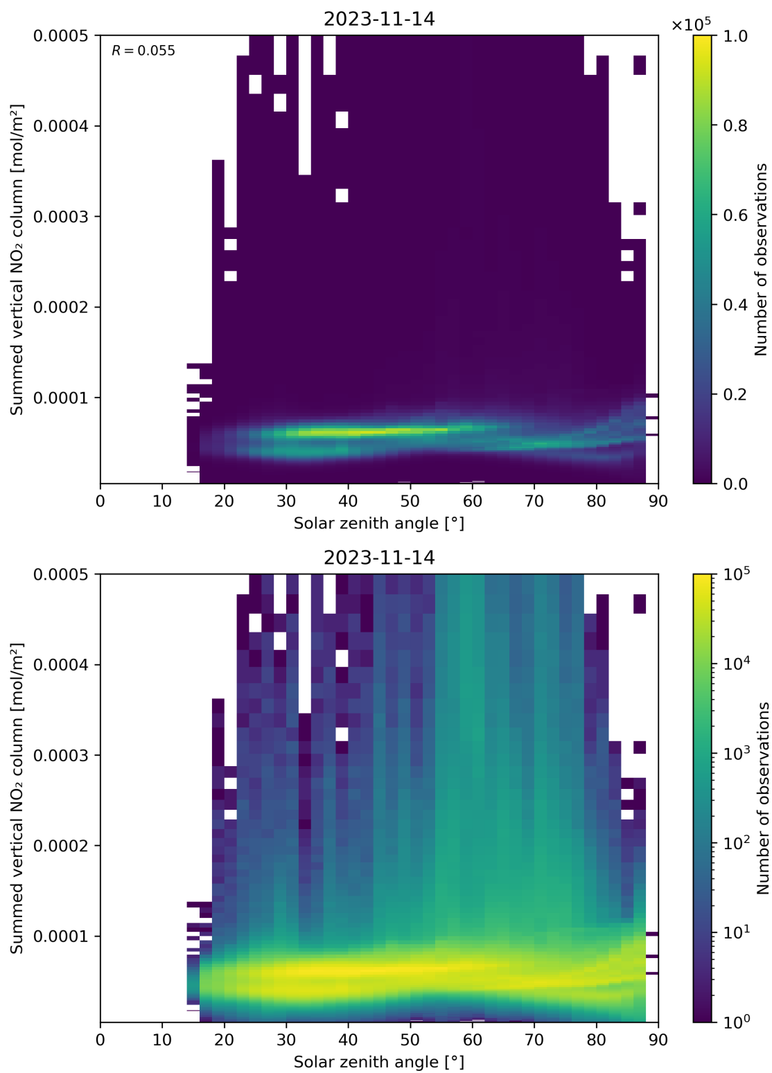
Figure 151: Scatter density plot of “Solar zenith angle” against “Summed vertical NO 2 column” for 2023-11-13 to 2023-11-15.
