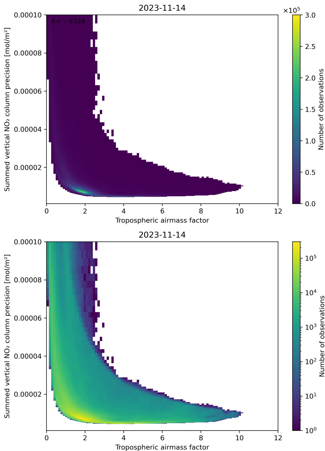
Figure 76: Scatter density plot of “Tropospheric air mass factor” against “Summed vertical NO 2 column precision” for 2023-11-13 to 2023-11-15.
