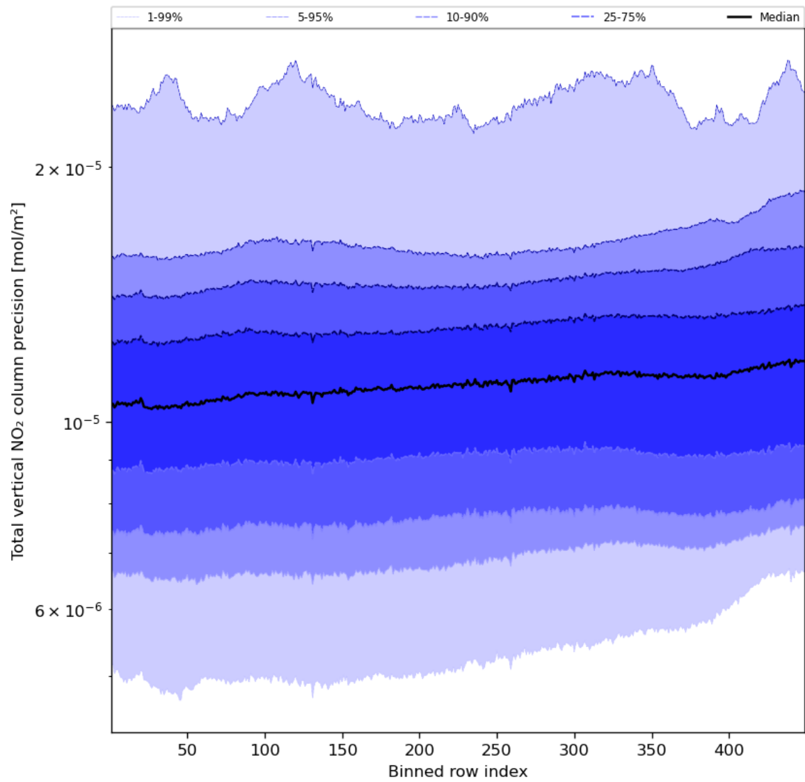
Figure 56: Along track statistics of “Total vertical NO 2 column precision” for 2023-11-13 to 2023-11-15
