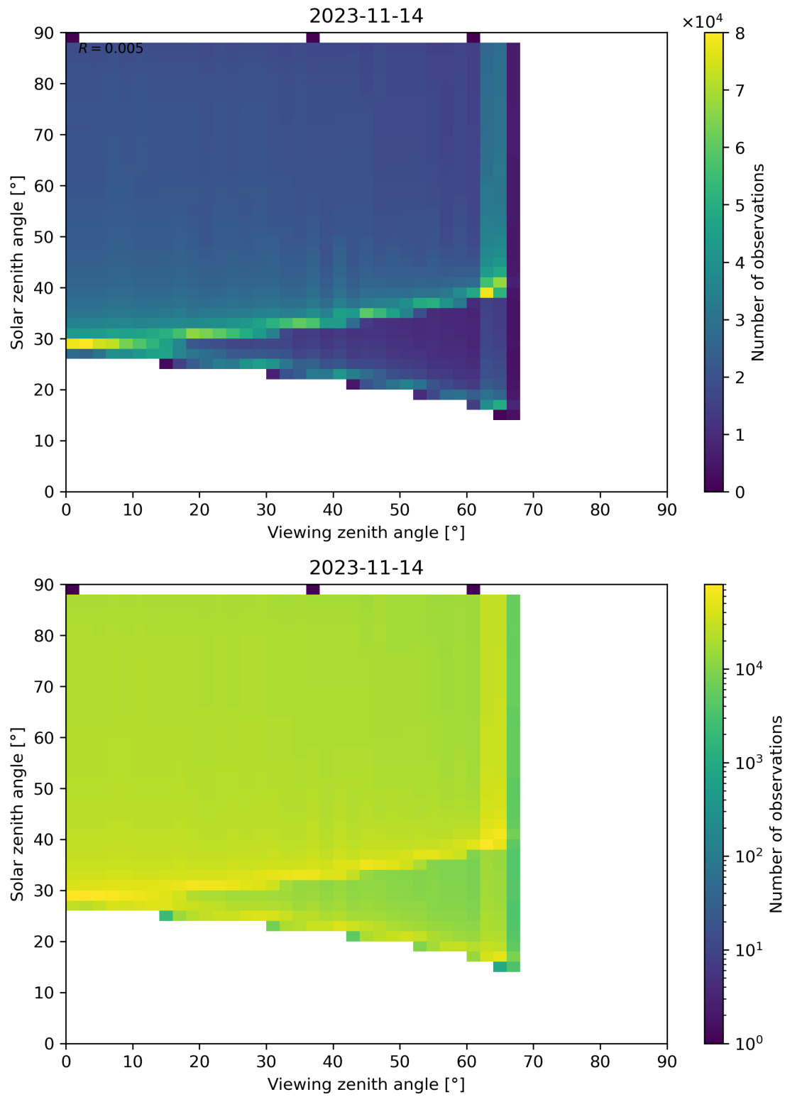
Figure 172: Scatter density plot of “Viewing zenith angle” against “Solar zenith angle” for 2023-11-13 to 2023-11-15.
