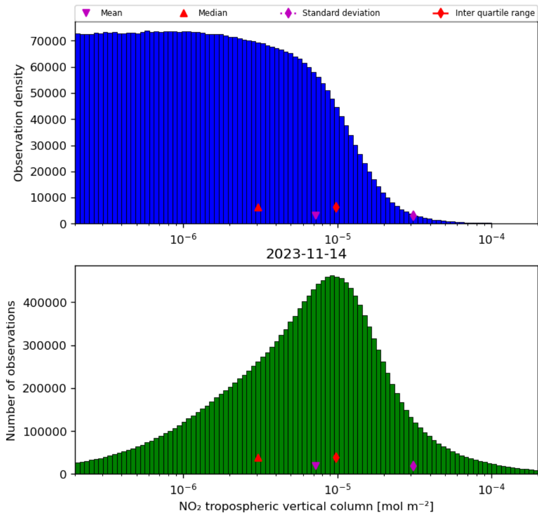
Figure 29: Histogram of “NO 2 tropospheric vertical column” for 2023-11-13 to 2023-11-15
