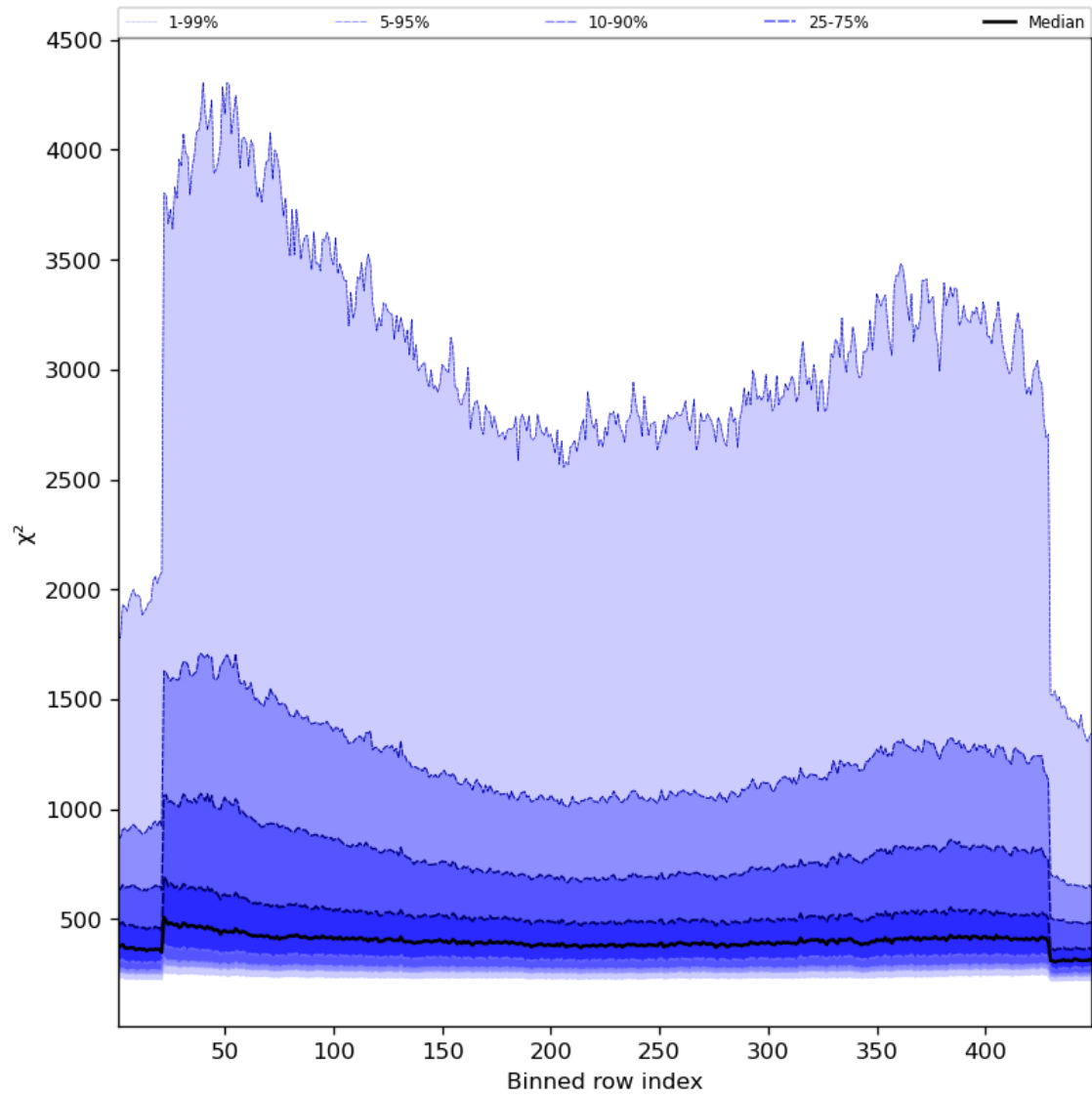
Figure 59: Along track statistics of “ \chi^2 ” for 2023-11-13 to 2023-11-15
