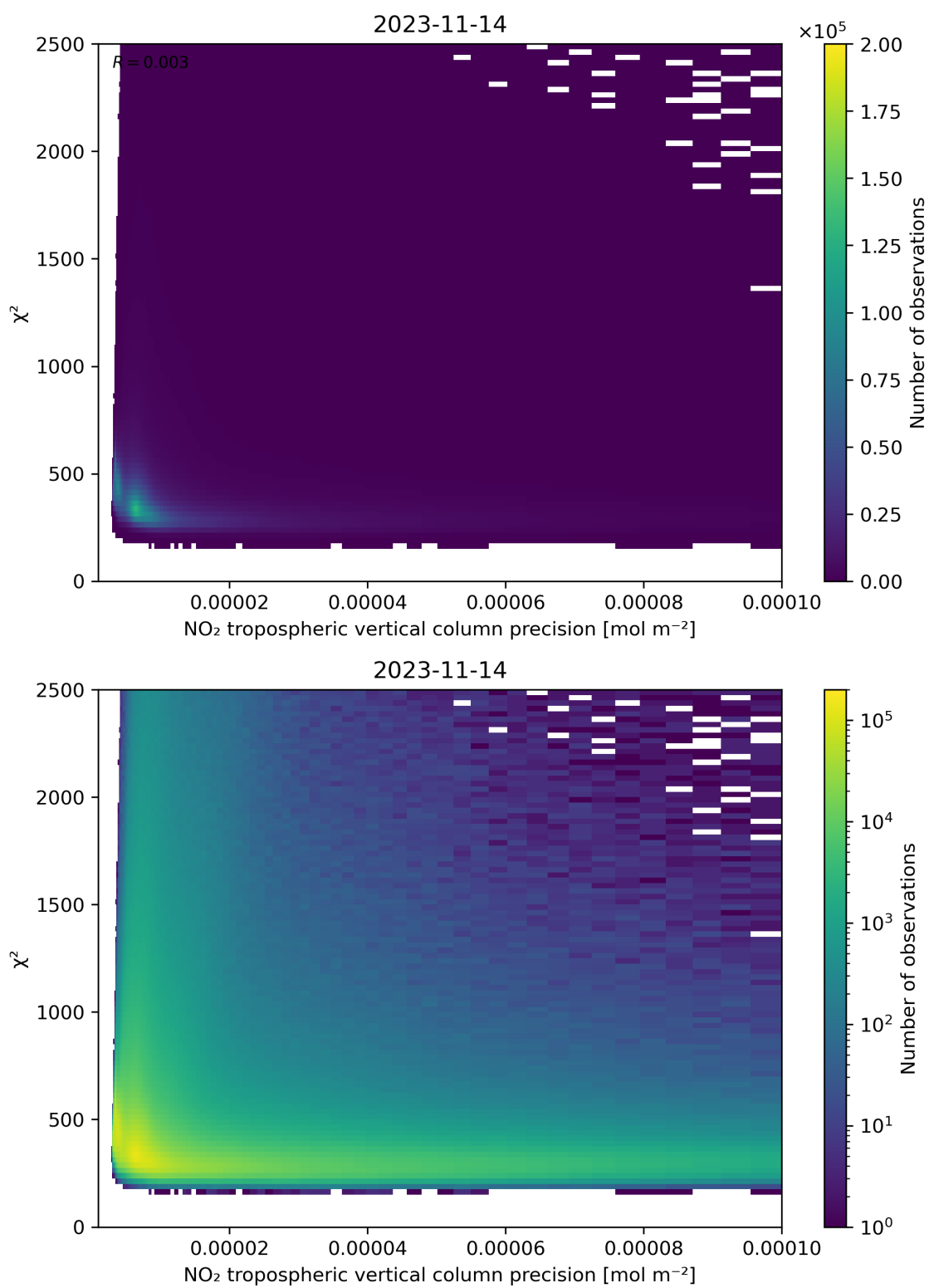
Figure 134: Scatter density plot of “NO 2 tropospheric vertical column precision” against “ \chi^2 ” for 2023-11-13 to 2023-11-15.
