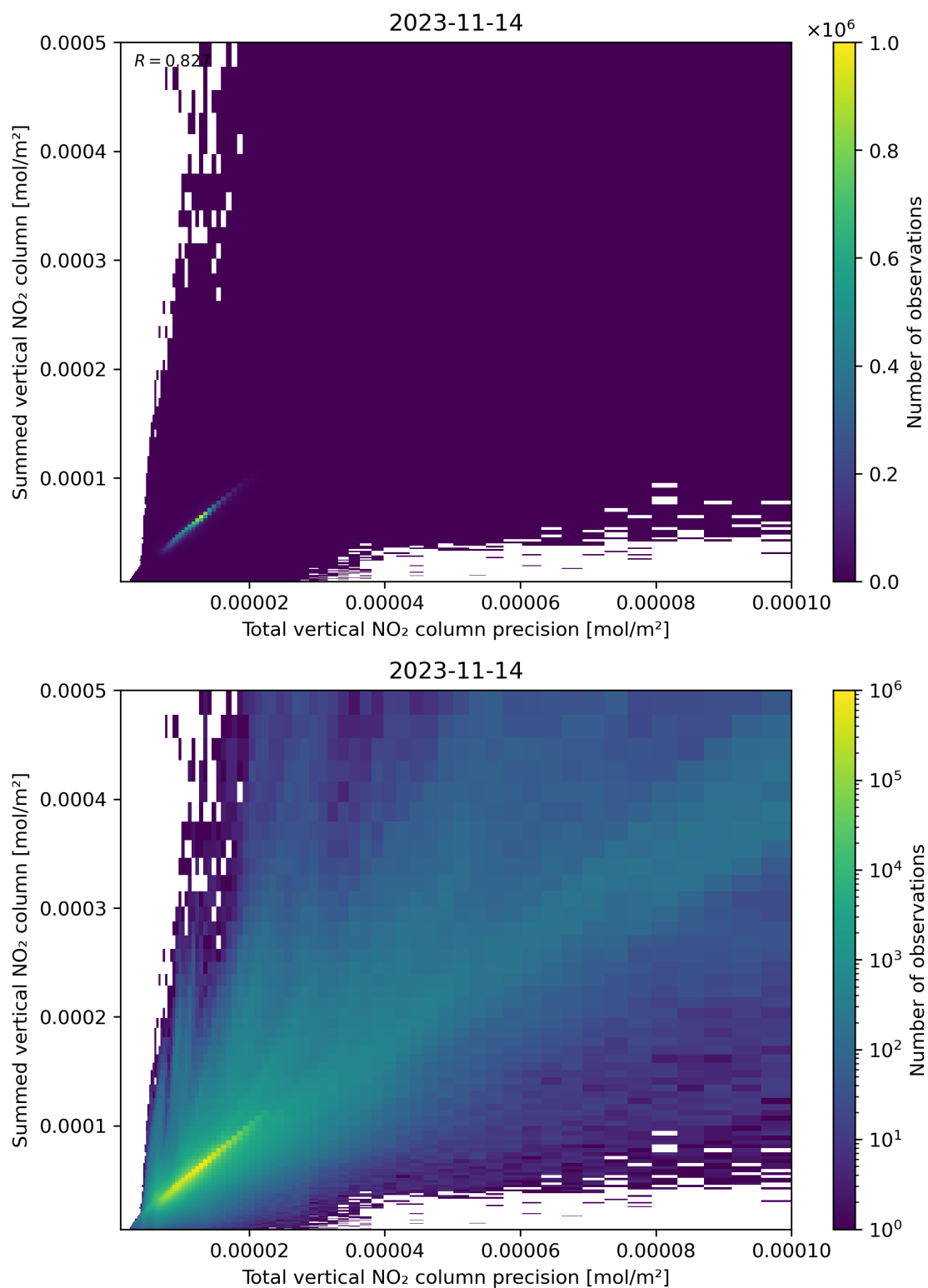
Figure 117: Scatter density plot of “Total vertical NO 2 column precision” against “Summed vertical NO 2 column” for 2023-11-13 to 2023-11-15.
