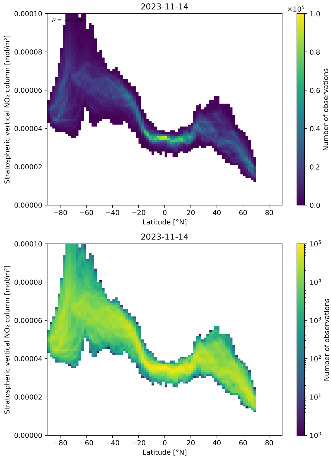
Figure 87: Scatter density plot of “Latitude” against “Stratospheric vertical NO 2 column” for 2023-11-13 to 2023-11-15.
