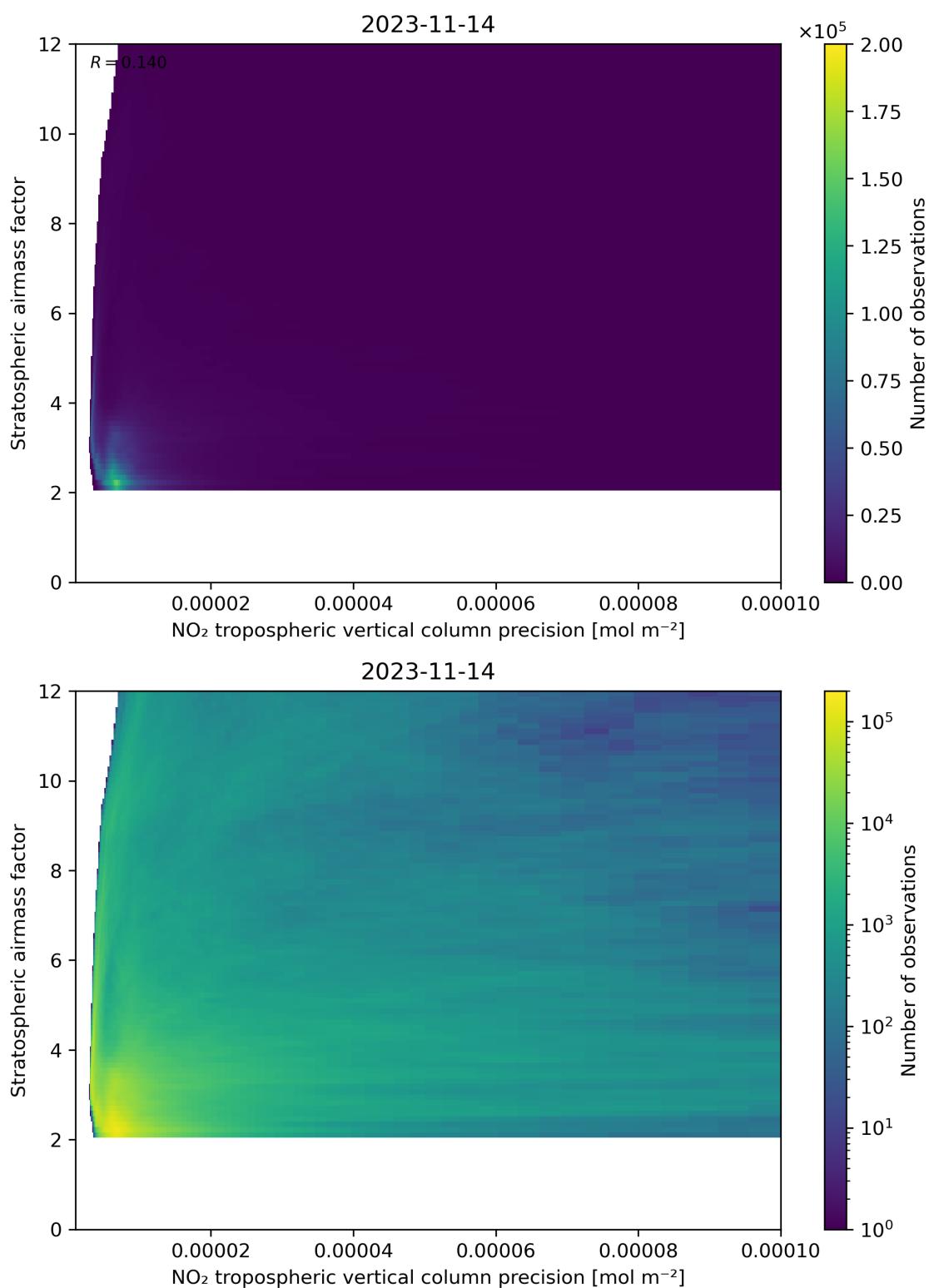
Figure 131: Scatter density plot of “NO 2 tropospheric vertical column precision” against “Stratospheric airmass factor” for 2023-11-13 to 2023-11-15.
