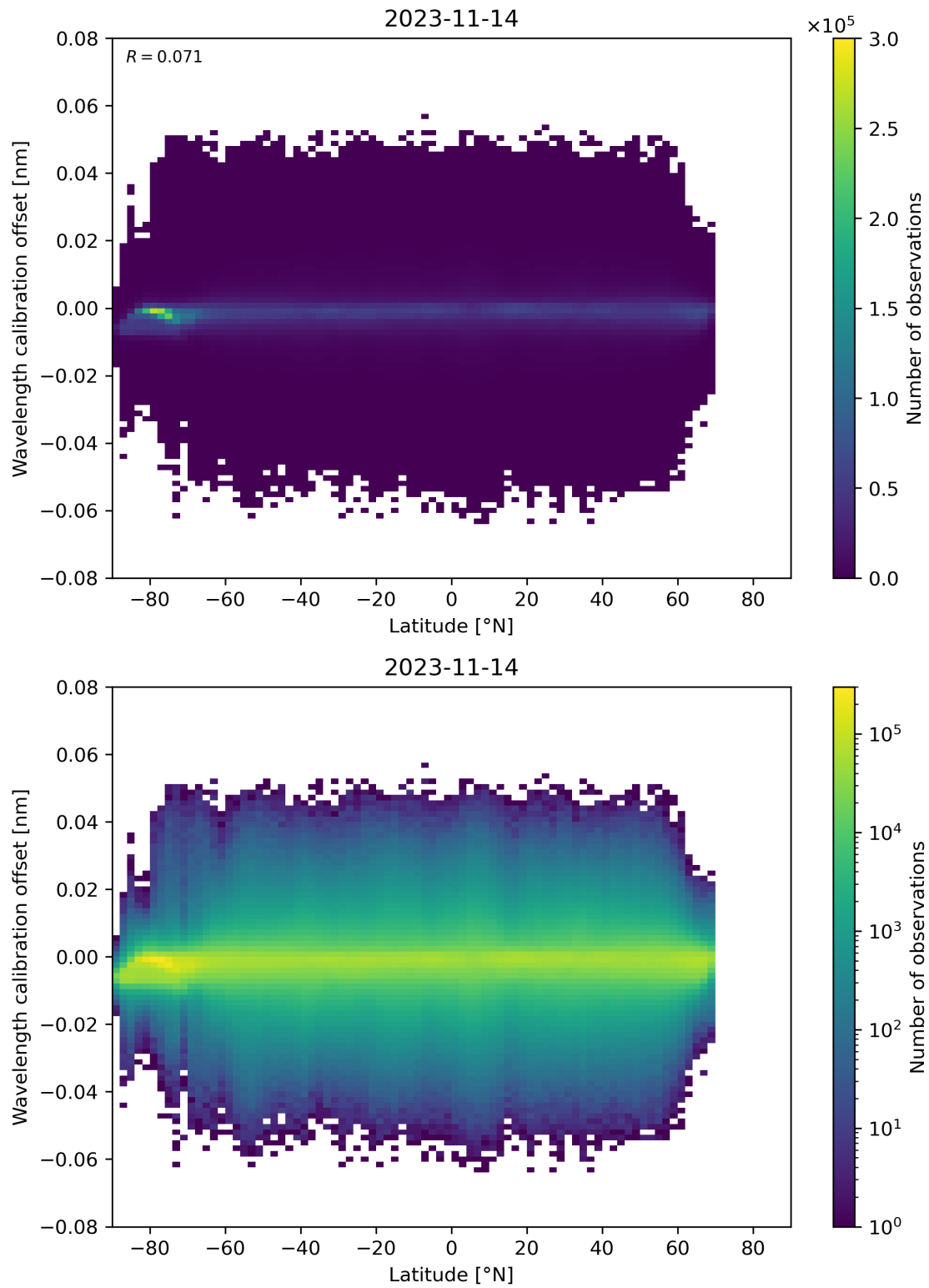
Figure 95: Scatter density plot of “Latitude” against “Wavelength calibration offset” for 2023-11-13 to 2023-11-15.
