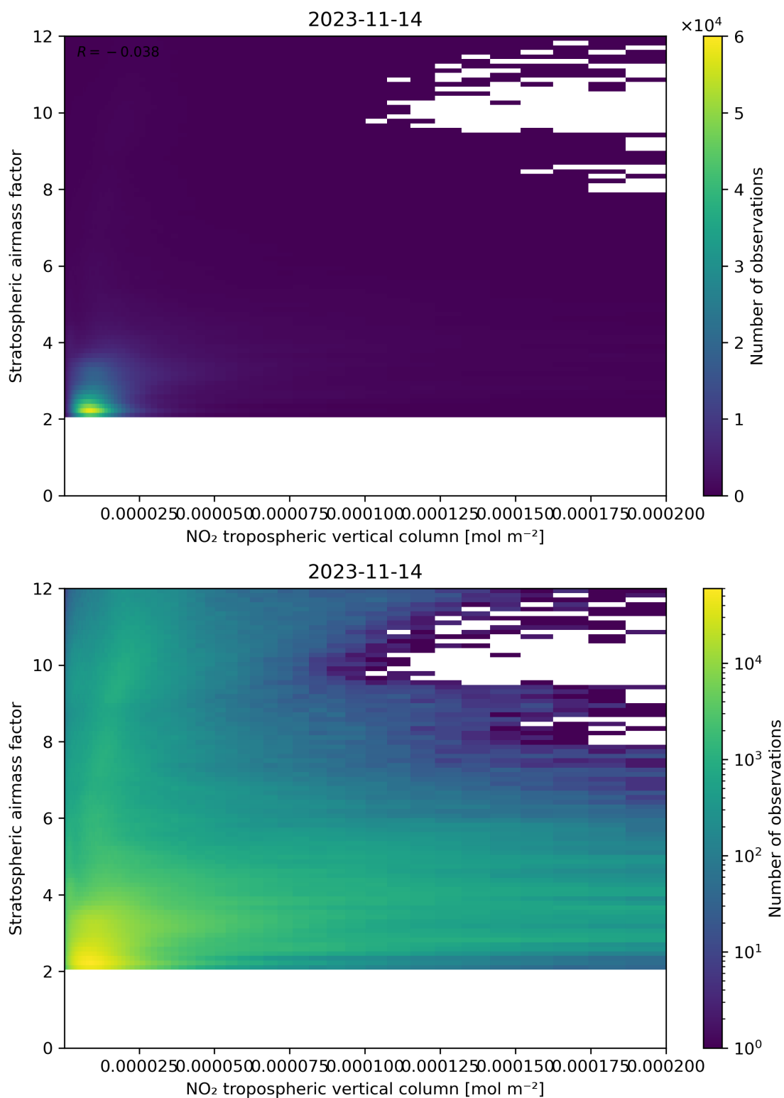
Figure 121: Scatter density plot of “NO 2 tropospheric vertical column” against “Stratospheric air mass factor” for 2023-11-13 to 2023-11-15.
