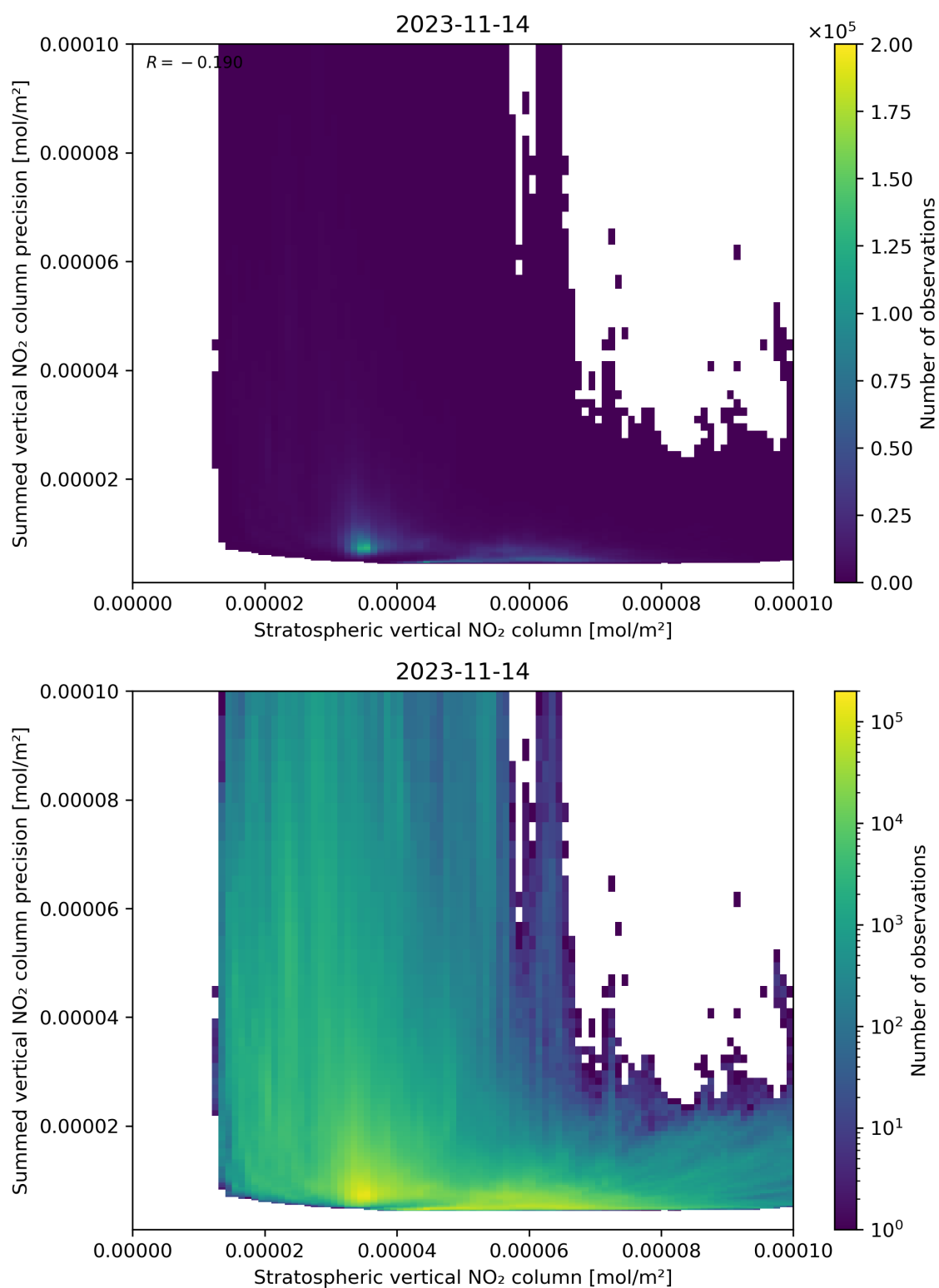
Figure 99: Scatter density plot of “Stratospheric vertical NO 2 column” against “Summed vertical NO 2 column precision” for 2023-11-13 to 2023-11-15.
