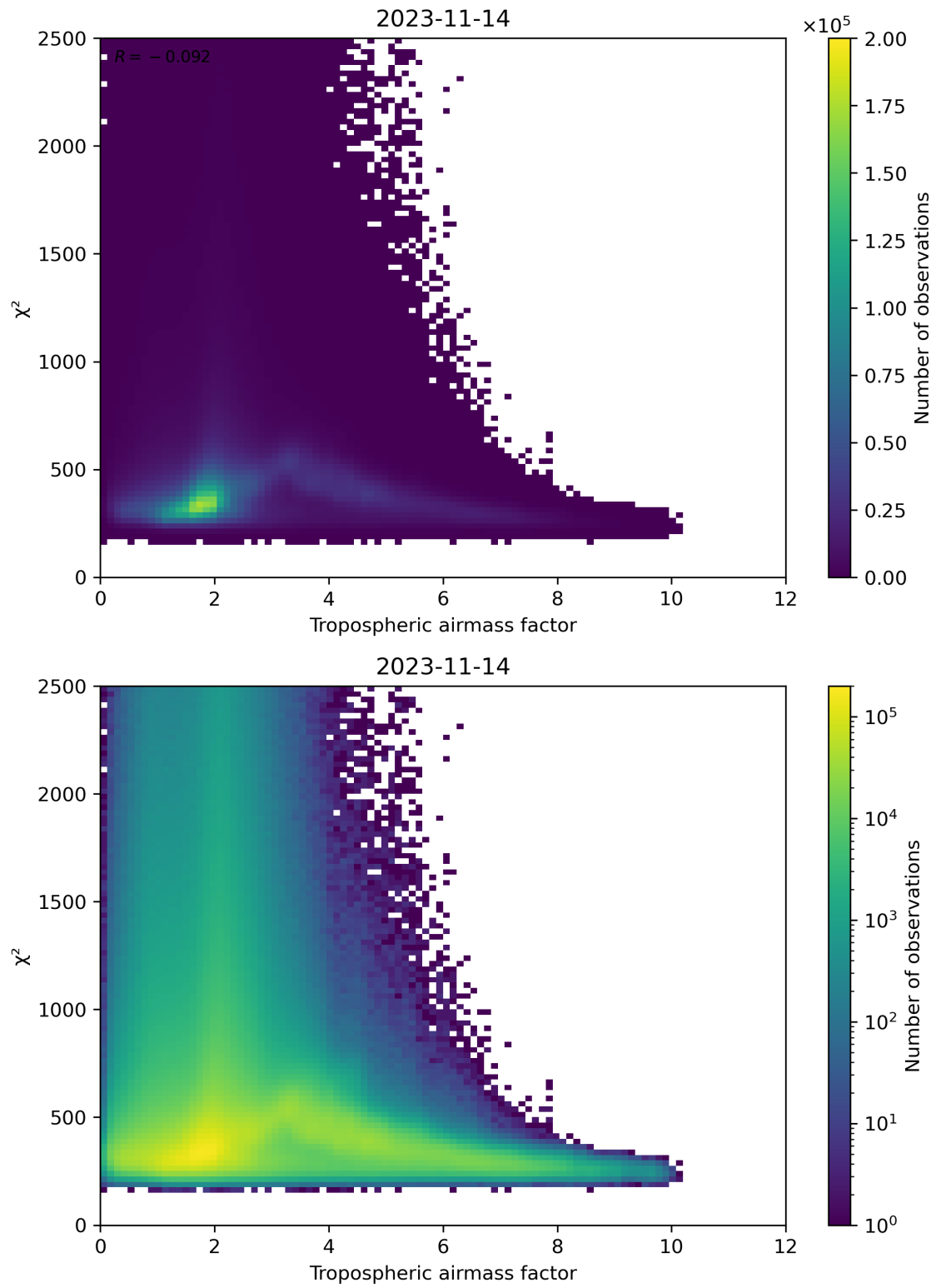
Figure 73: Scatter density plot of “Tropospheric airmass factor” against “ \chi^2 ” for 2023-11-13 to 2023-11-15.
