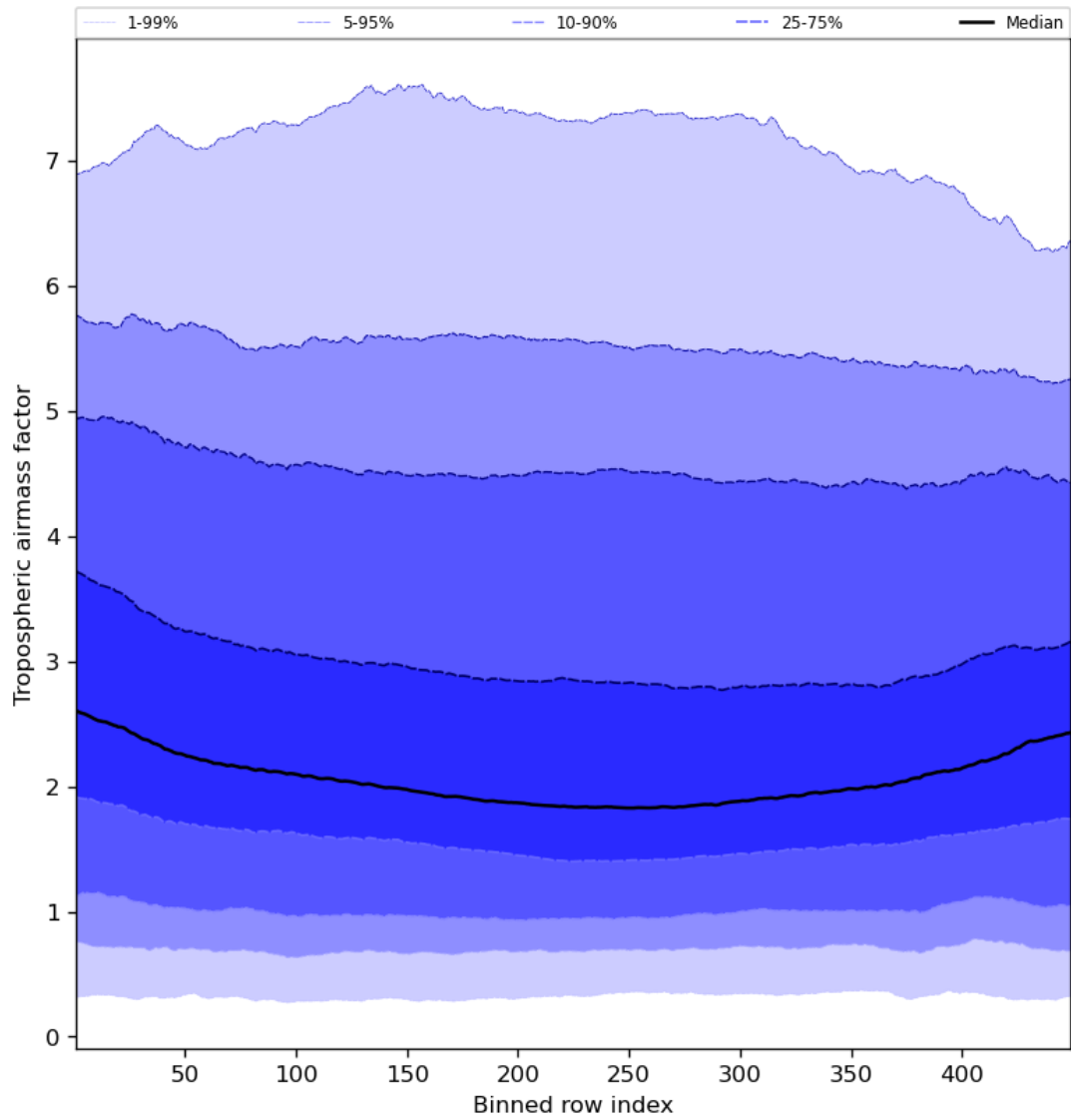
Figure 48: Along track statistics of “Tropospheric air mass factor” for 2023-11-13 to 2023-11-15
