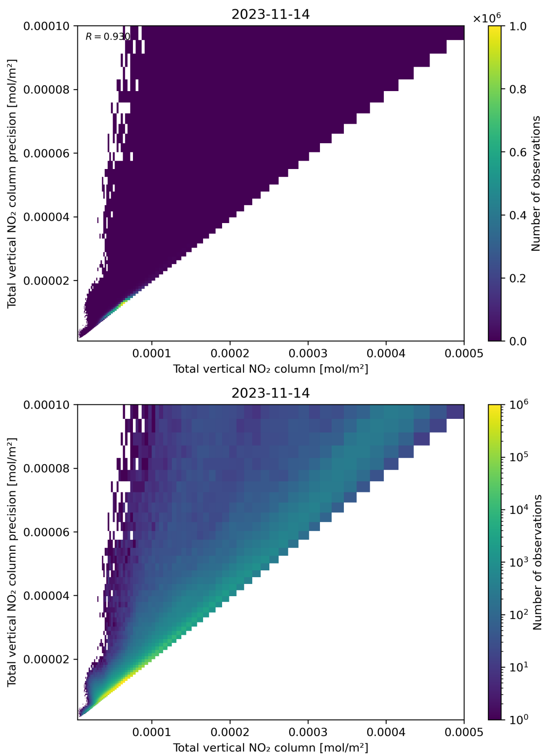
Figure 114: Scatter density plot of “Total vertical NO 2 column” against “Total vertical NO 2 column precision” for 2023-11-13 to 2023-11-15.
