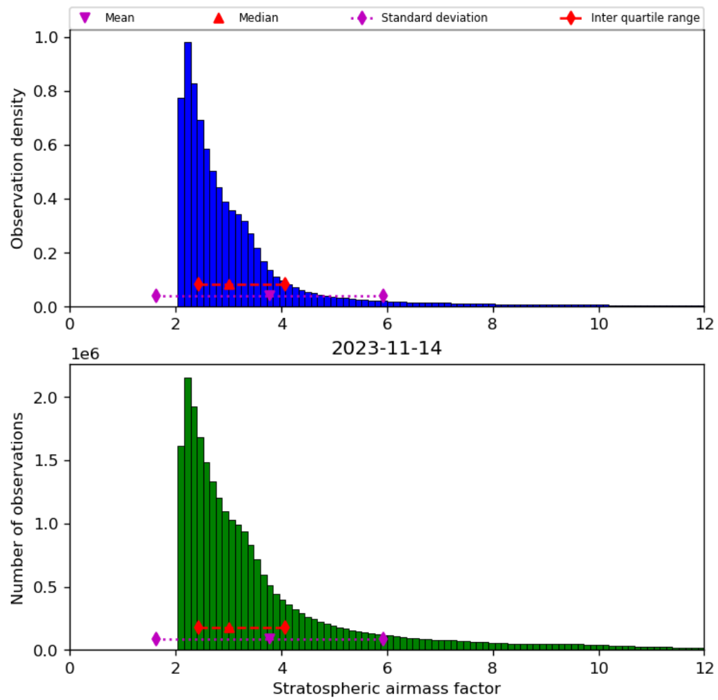
Figure 44: Histogram of “Stratospheric airmass factor” for 2023-11-13 to 2023-11-15
