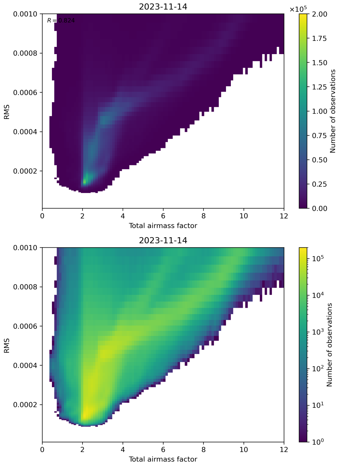
Figure 69: Scatter density plot of “Total airmass factor” against “RMS” for 2023-11-13 to 2023-11-15.
