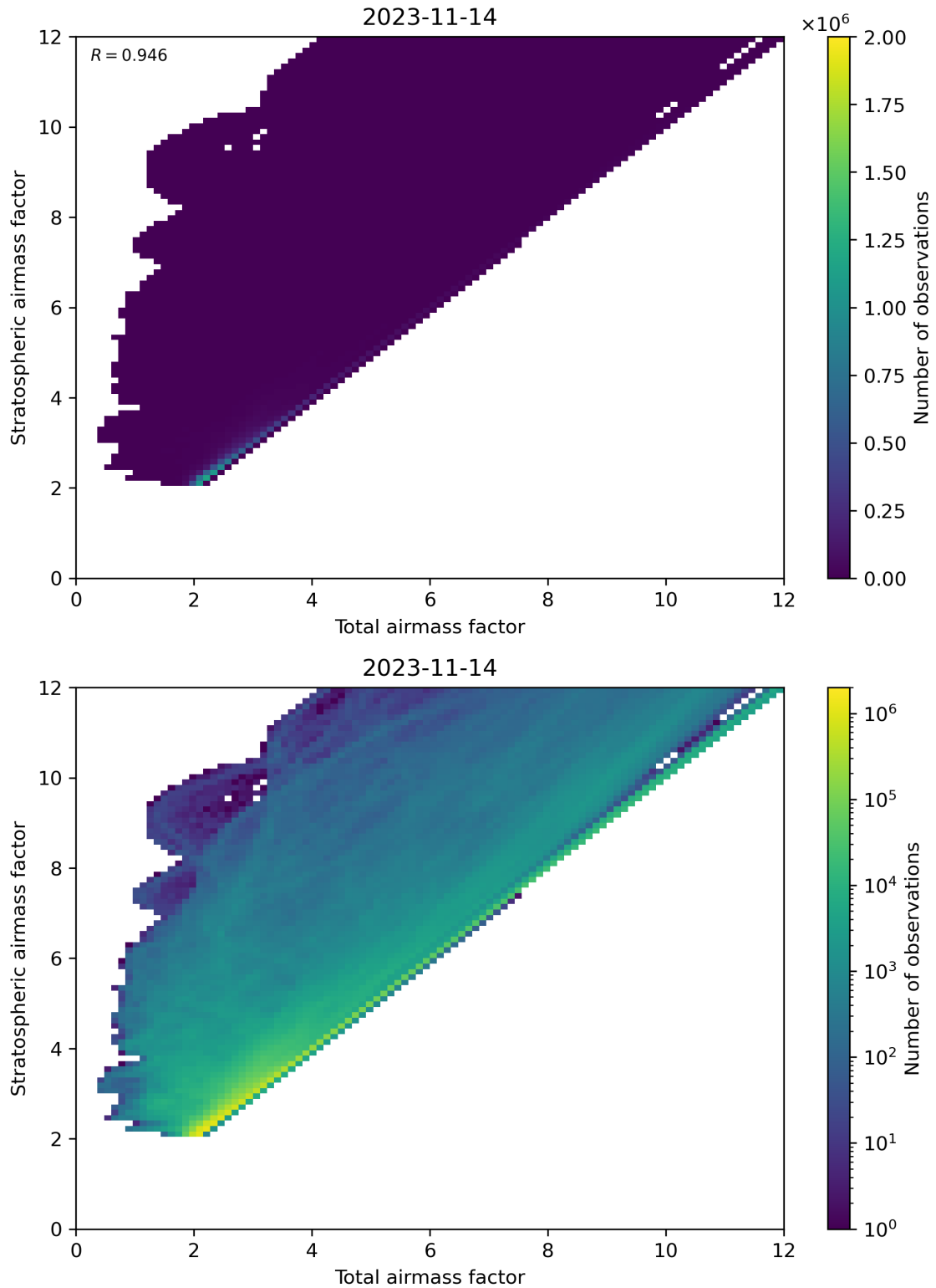
Figure 62: Scatter density plot of “Total airmass factor” against “Stratospheric airmass factor” for 2023-11-13 to 2023-11-15.
