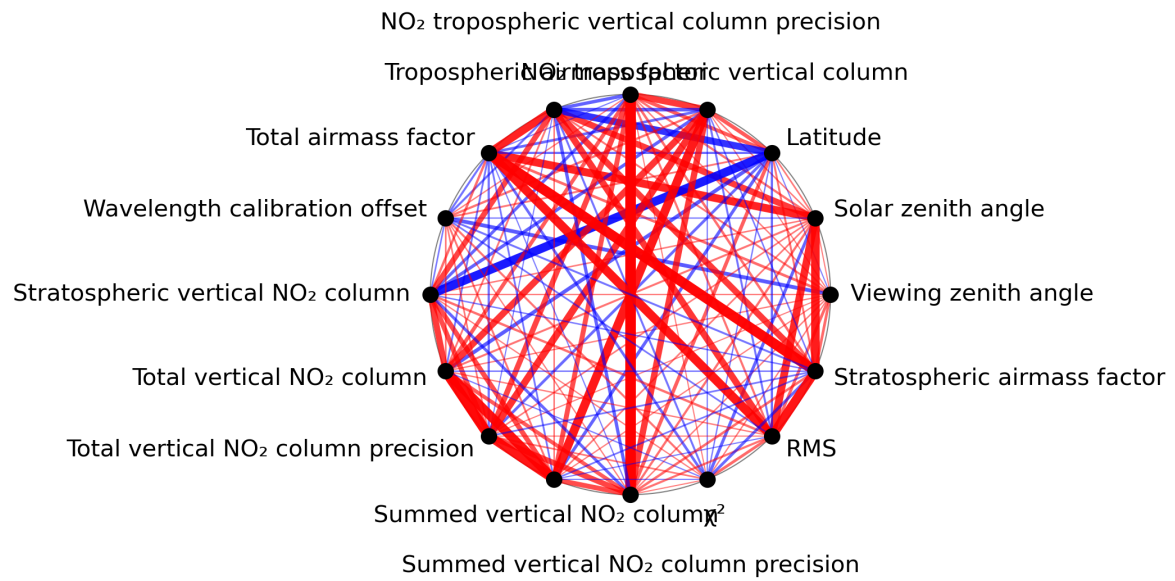
Figure 1: Map of correlation graph for 2023-11-13 to 2023-11-15.
