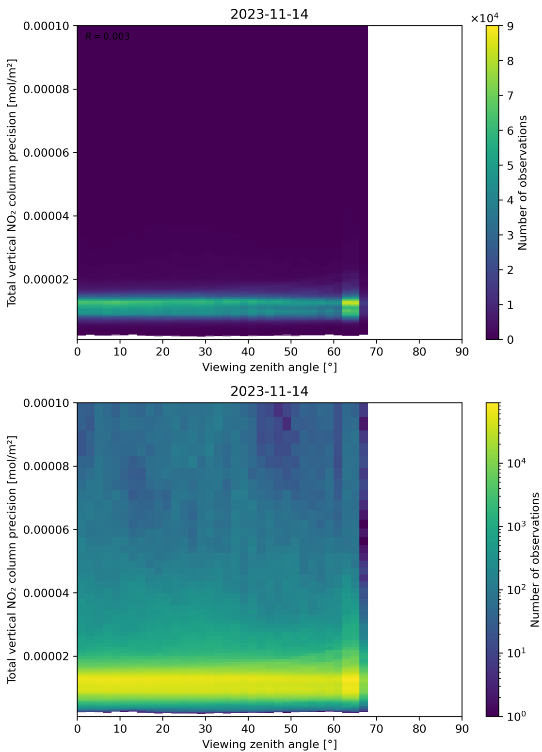
Figure 168: Scatter density plot of “Viewing zenith angle” against “Total vertical NO 2 column precision” for 2023-11-13 to 2023-11-15.
