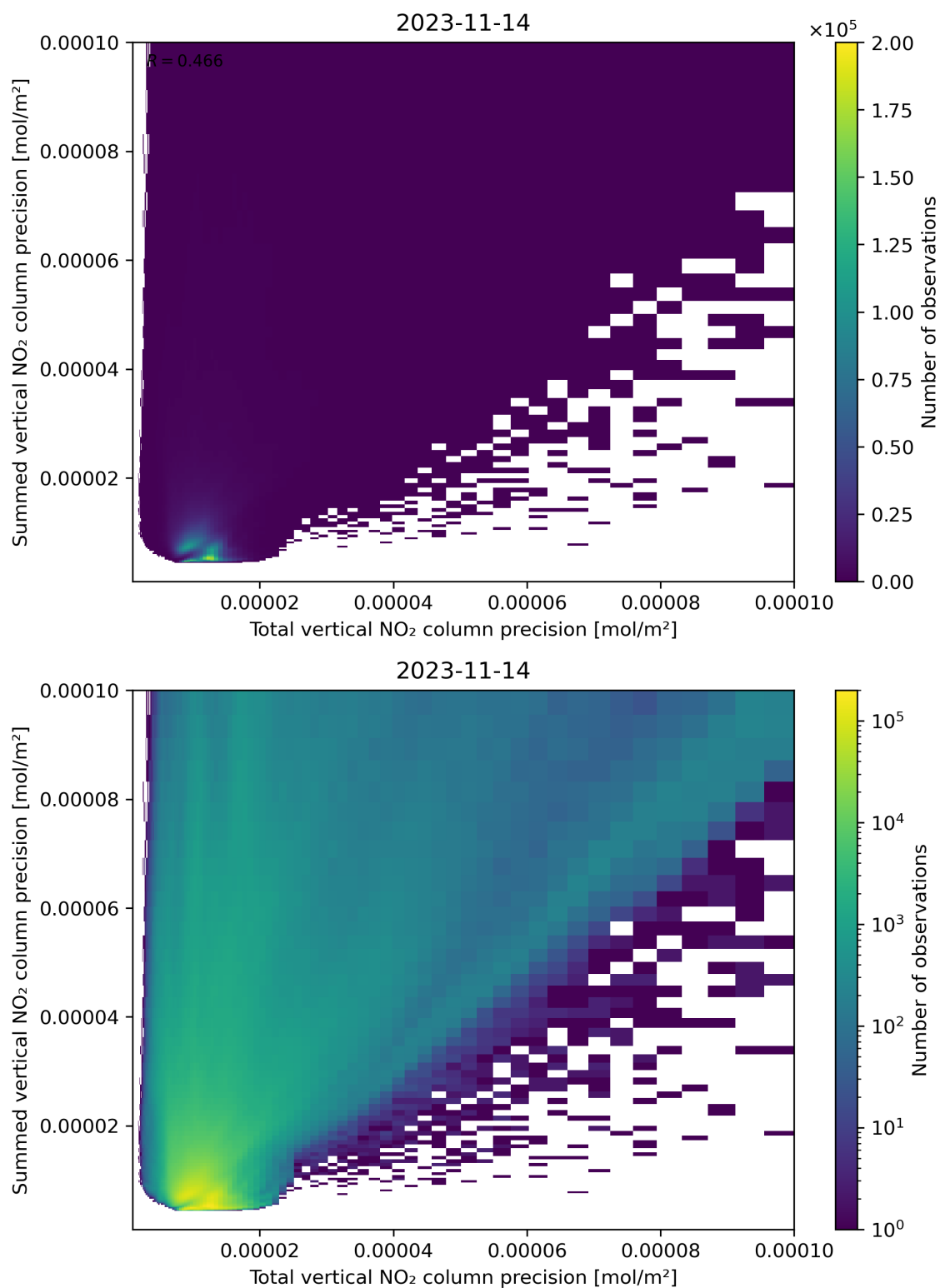
Figure 118: Scatter density plot of “Total vertical NO 2 column precision” against “Summed vertical NO 2 column precision” for 2023-11-13 to 2023-11-15.
