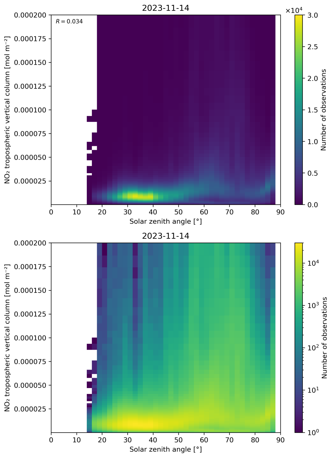
Figure 155: Scatter density plot of “Solar zenith angle” against “NO 2 tropospheric vertical column” for 2023-11-13 to 2023-11-15.
