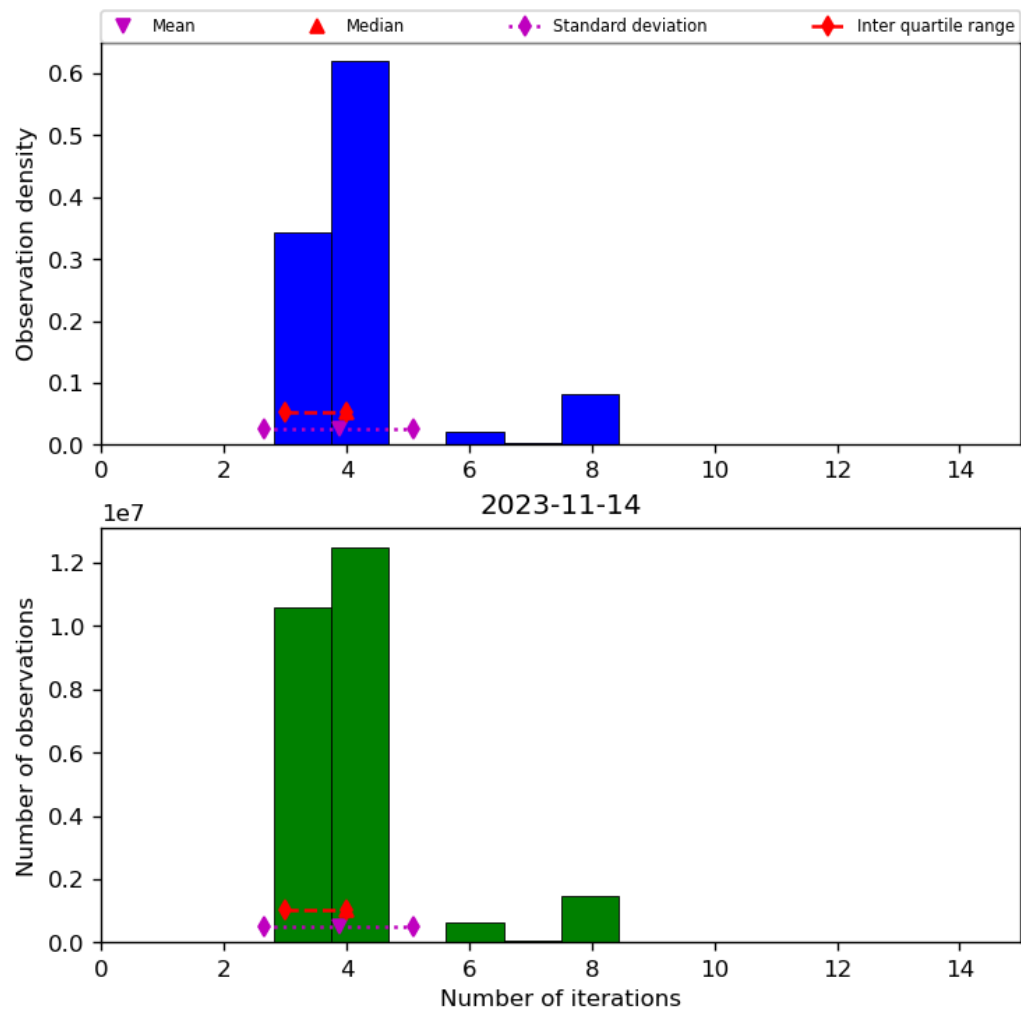
Figure 34: Histogram of “Number of iterations” for 2023-11-13 to 2023-11-15
