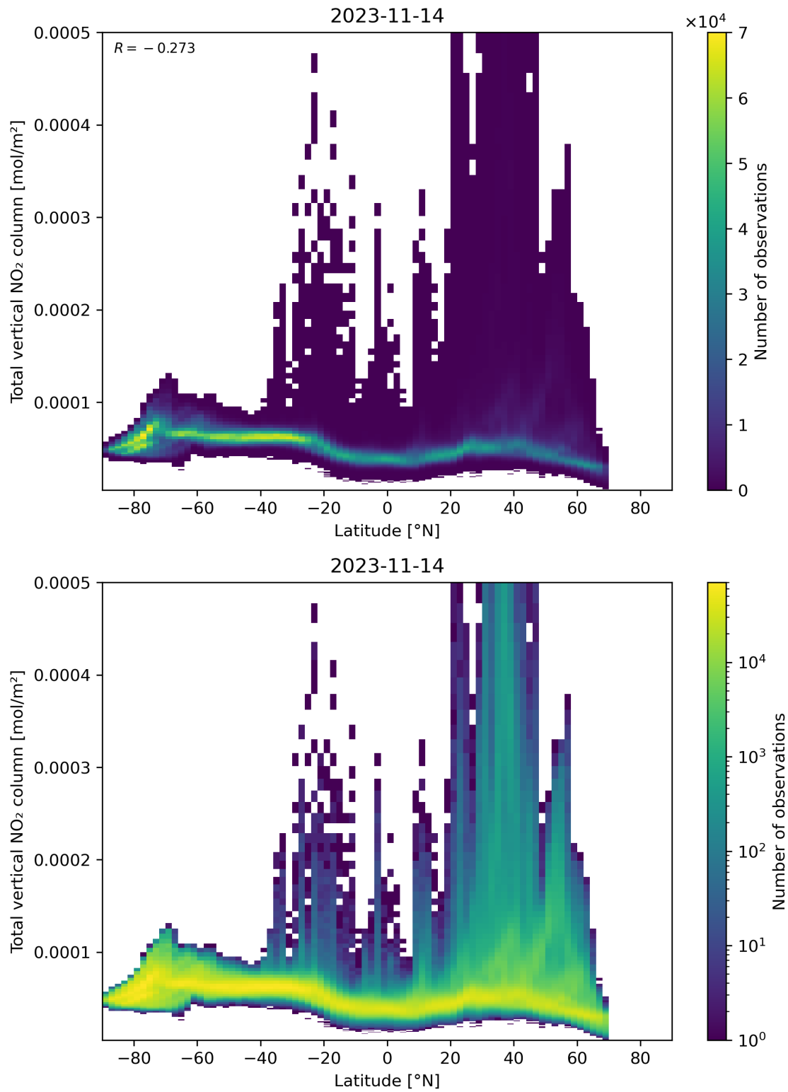
Figure 90: Scatter density plot of “Latitude” against “Total vertical NO 2 column” for 2023-11-13 to 2023-11-15.
