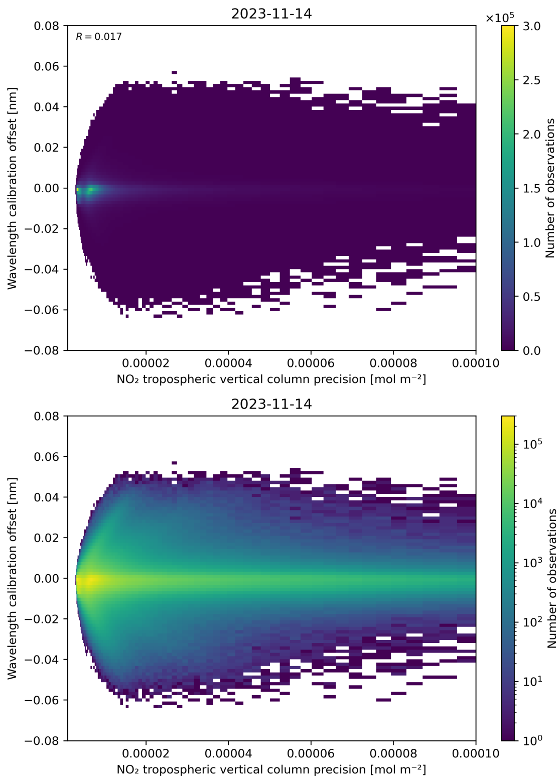
Figure 141: Scatter density plot of “NO 2 tropospheric vertical column precision” against “Wavelength calibration offset” for 2023-11-13 to 2023-11-15.
