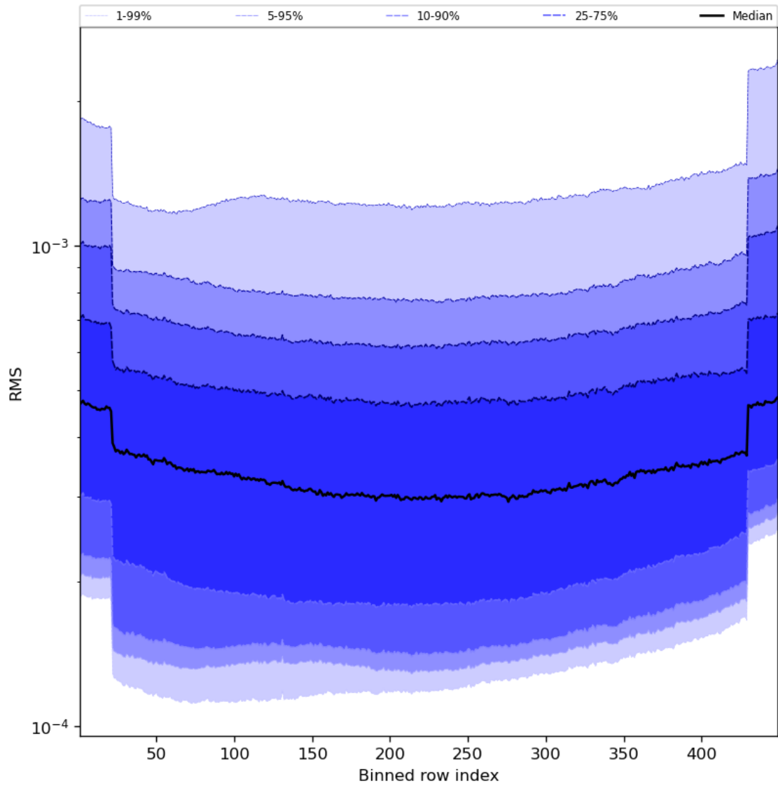
Figure 60: Along track statistics of “RMS” for 2023-11-13 to 2023-11-15
