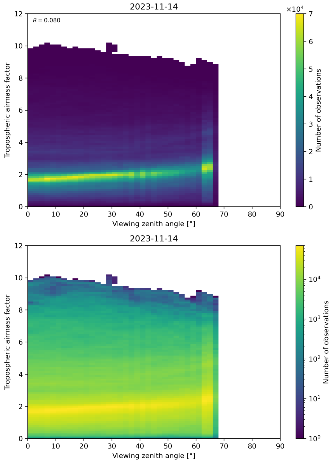
Figure 161: Scatter density plot of “Viewing zenith angle” against “Tropospheric airmass factor” for 2023-11-13 to 2023-11-15.
