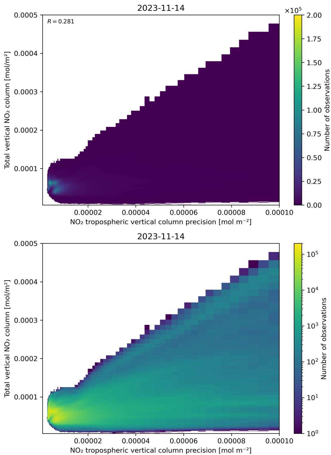
Figure 138: Scatter density plot of “NO 2 tropospheric vertical column precision” against “Total vertical NO 2 column” for 2023-11-13 to 2023-11-15.
