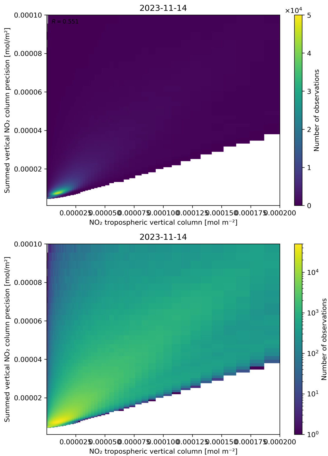
Figure 127: Scatter density plot of “NO 2 tropospheric vertical column” against “Summed vertical NO 2 column precision” for 2023-11-13 to 2023-11-15.
