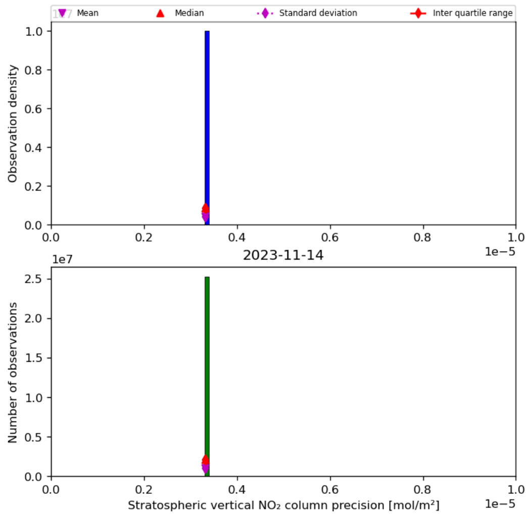
Figure 37: Histogram of “Stratospheric vertical NO 2 column precision” for 2023-11-13 to 2023-11-15
