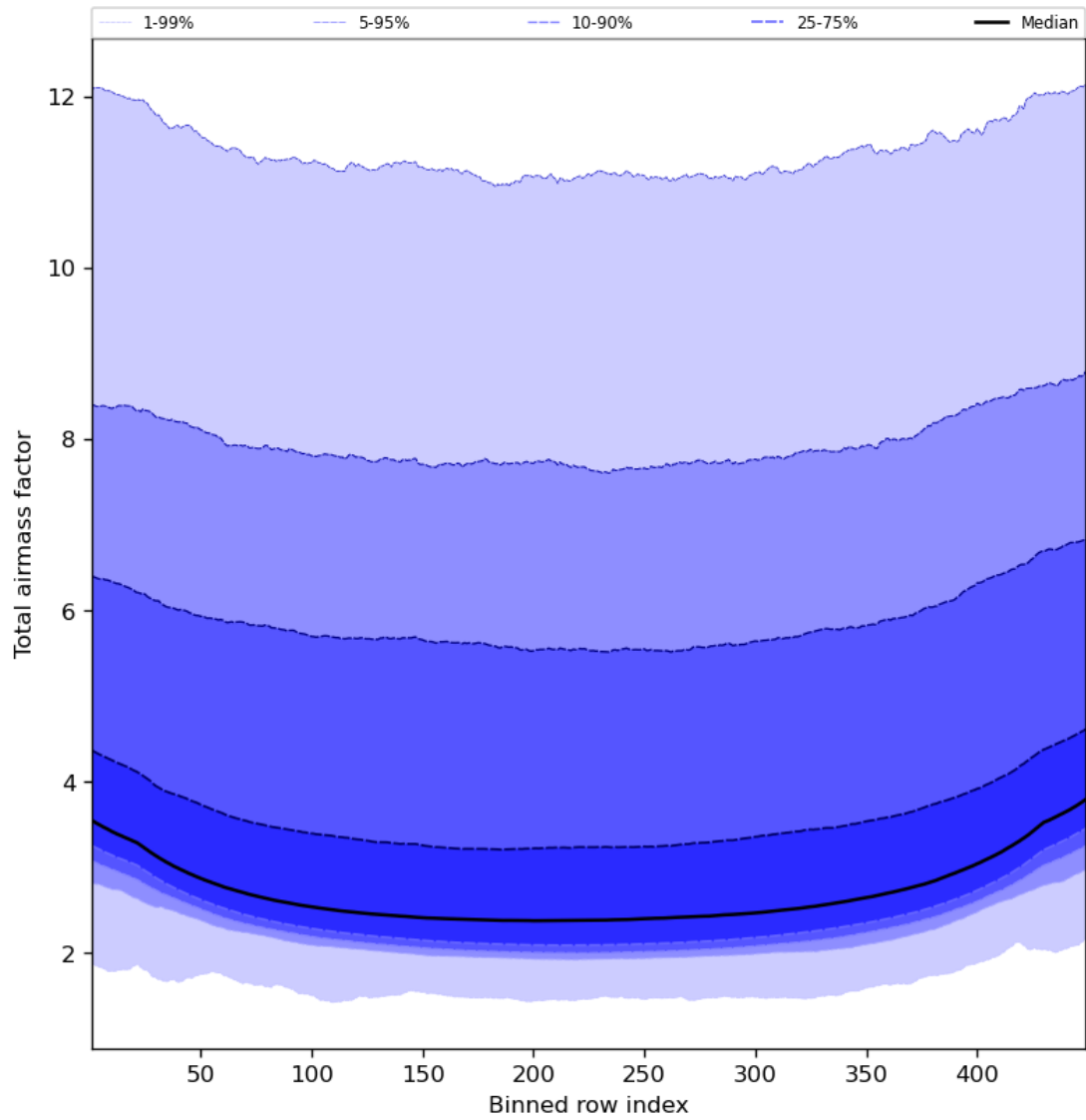
Figure 49: Along track statistics of “Total airmass factor” for 2023-11-13 to 2023-11-15
