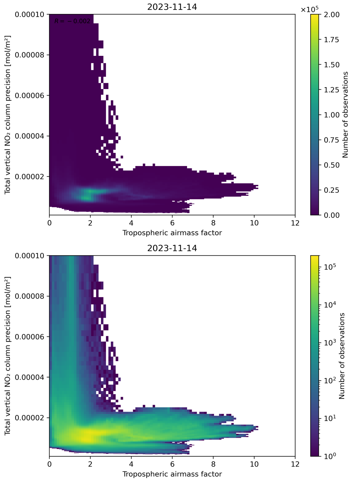
Figure 78: Scatter density plot of “Tropospheric air mass factor” against “Total vertical NO 2 column precision” for 2023-11-13 to 2023-11-15.
