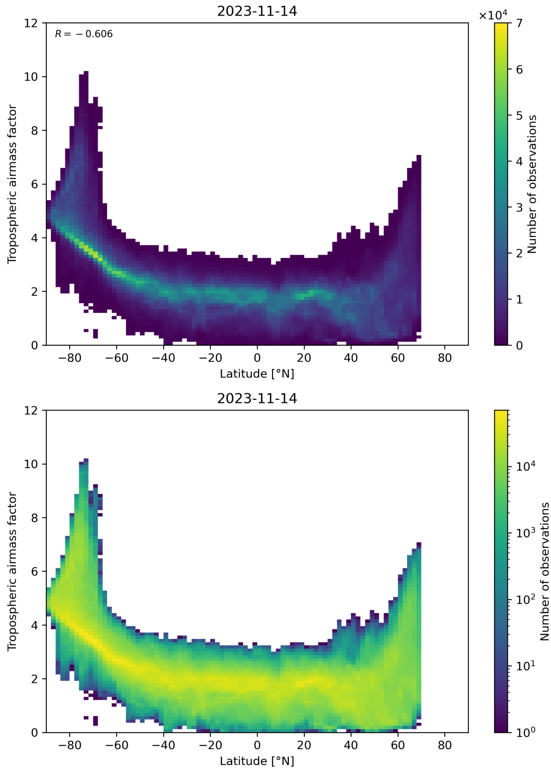
Figure 85: Scatter density plot of “Latitude” against “Tropospheric airmass factor” for 2023-11-13 to 2023-11-15.
