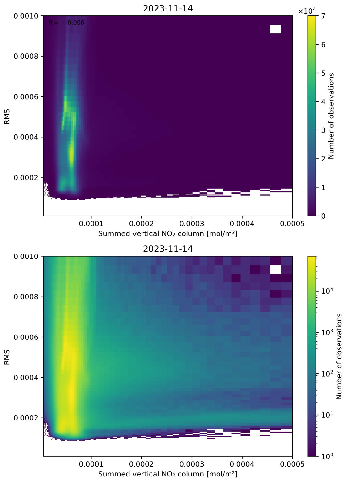
Figure 109: Scatter density plot of “Summed vertical NO 2 column” against “RMS” for 2023-11-13 to 2023-11-15.
