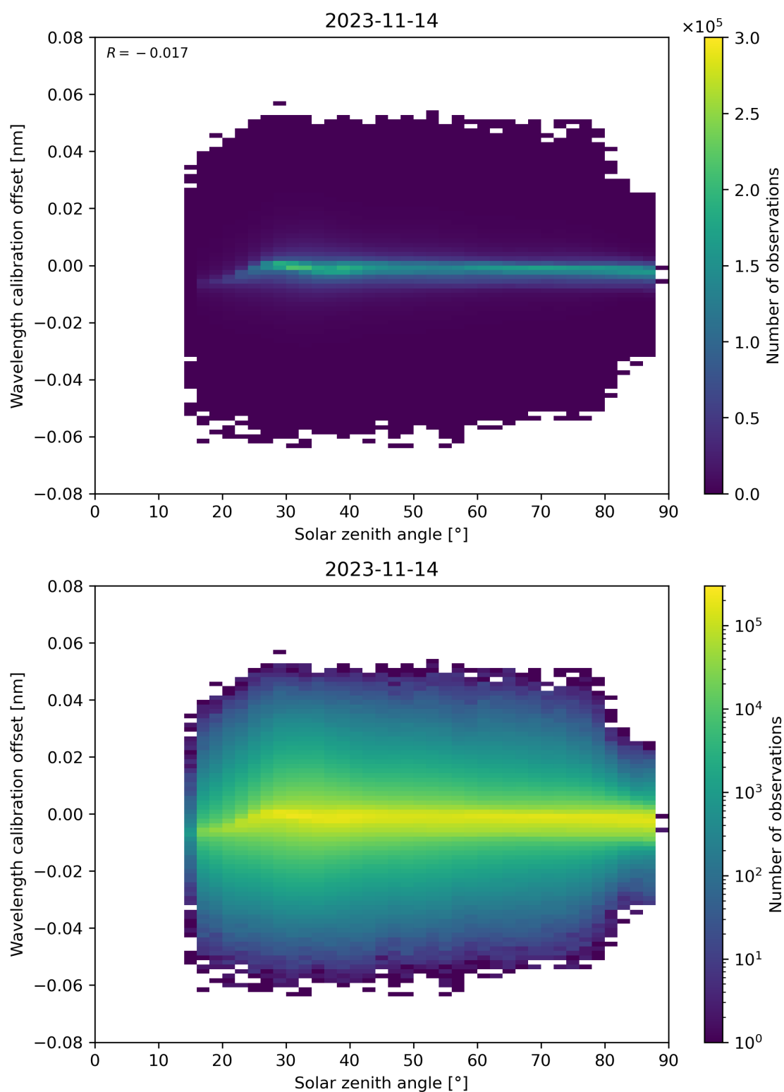
Figure 158: Scatter density plot of “Solar zenith angle” against “Wavelength calibration offset” for 2023-11-13 to 2023-11-15.
