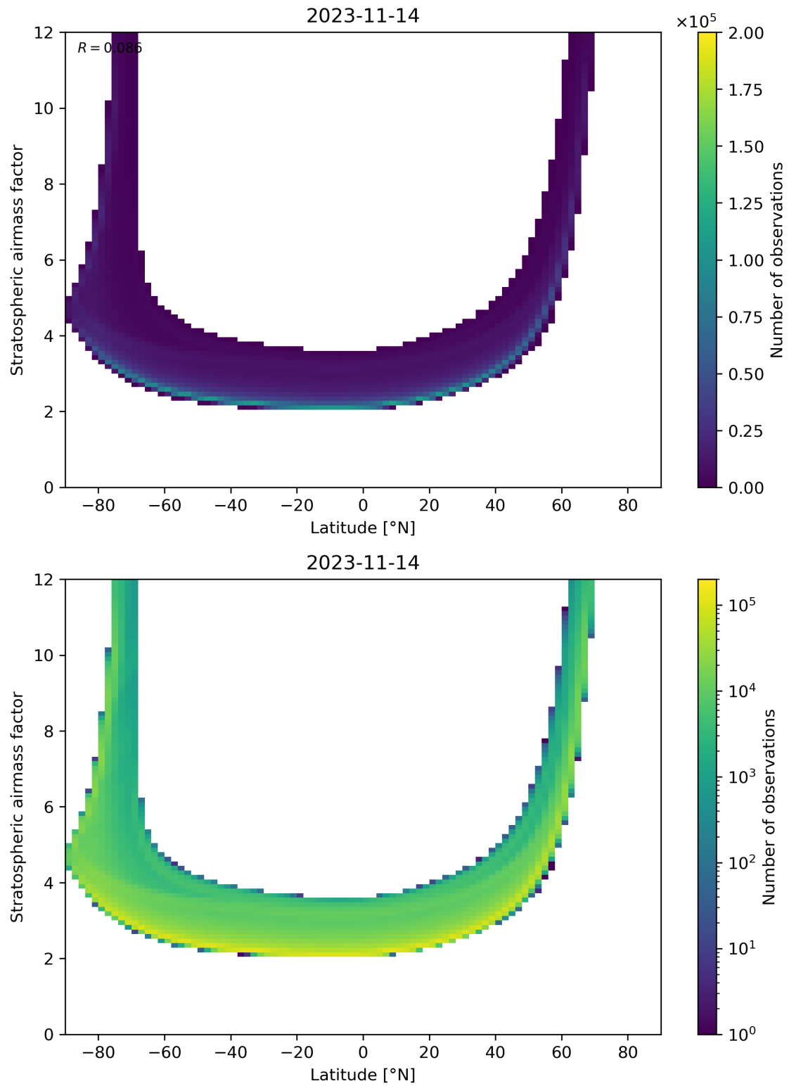
Figure 83: Scatter density plot of “Latitude” against “Stratospheric air mass factor” for 2023-11-13 to 2023-11-15.
