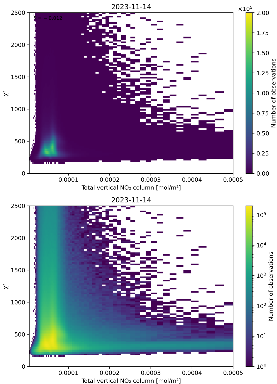
Figure 111: Scatter density plot of “Total vertical NO 2 column” against “ \chi^2 ” for 2023-11-13 to 2023-11-15.
