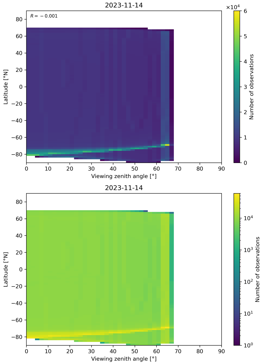
Figure 163: Scatter density plot of “Viewing zenith angle” against “Latitude” for 2023-11-13 to 2023-11-15.
