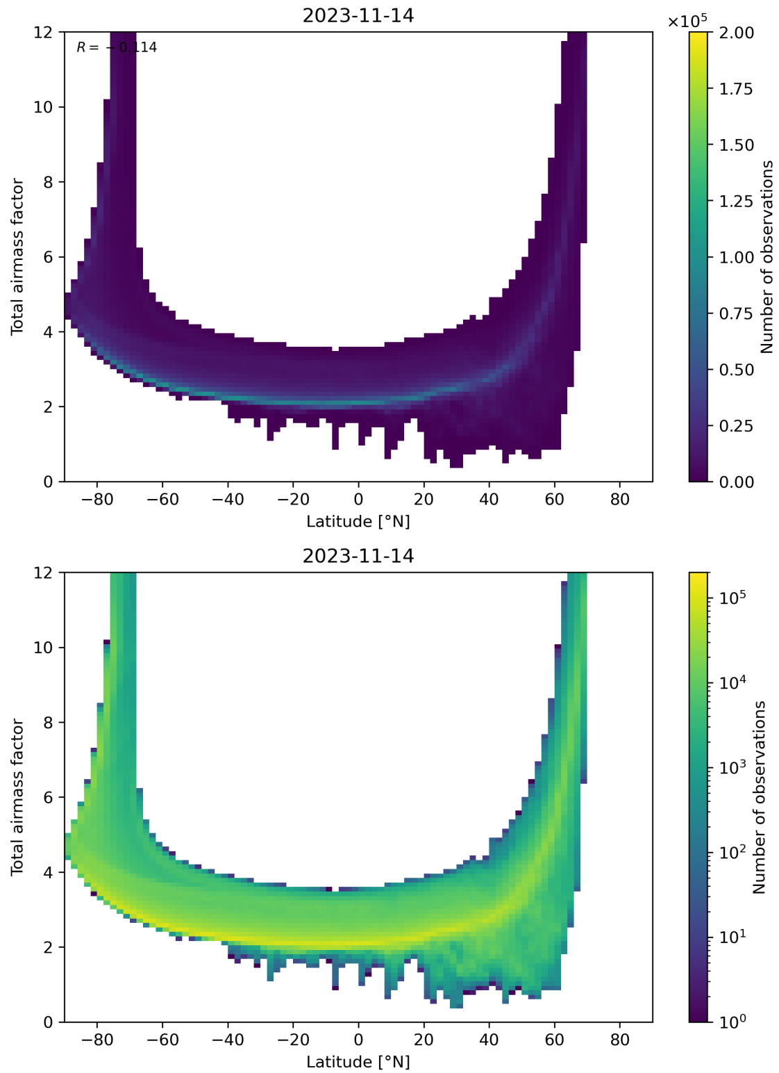
Figure 84: Scatter density plot of “Latitude” against “Total airmass factor” for 2023-11-13 to 2023-11-15.
