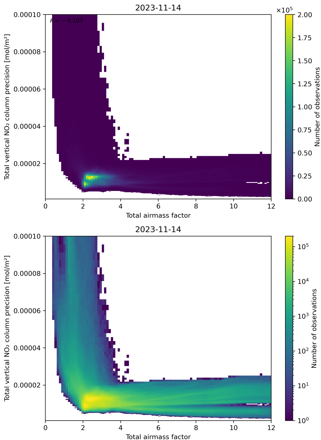
Figure 68: Scatter density plot of “Total airmass factor” against “Total vertical NO 2 column precision” for 2023-11-13 to 2023-11-15.
