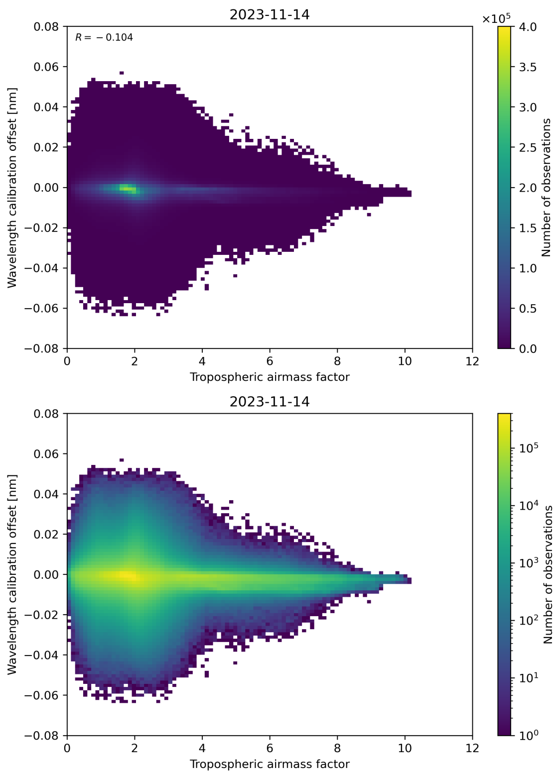
Figure 80: Scatter density plot of “Tropospheric airmass factor” against “Wavelength calibration offset” for 2023-11-13 to 2023-11-15.
