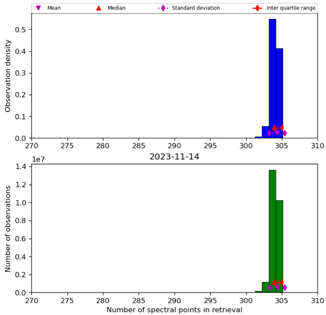
Figure 33: Histogram of “Number of spectral points in retrieval” for 2023-11-13 to 2023-11-15
