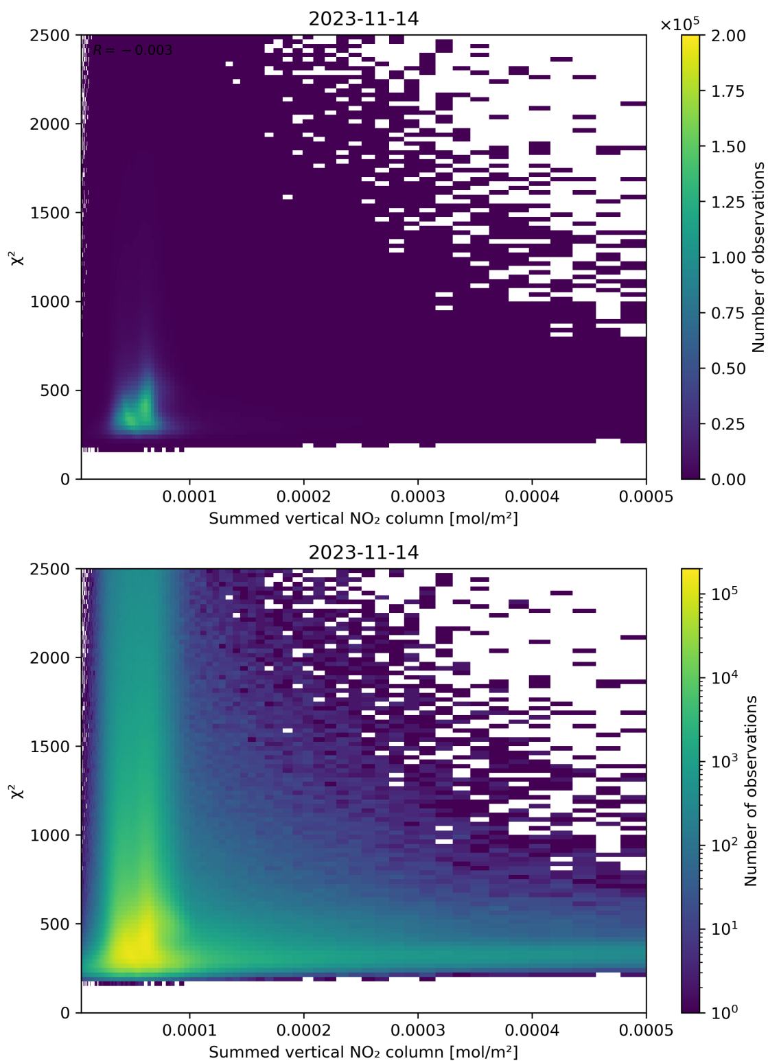
Figure 104: Scatter density plot of “Summed vertical NO 2 column” against “ \chi^2 ” for 2023-11-13 to 2023-11-15.
