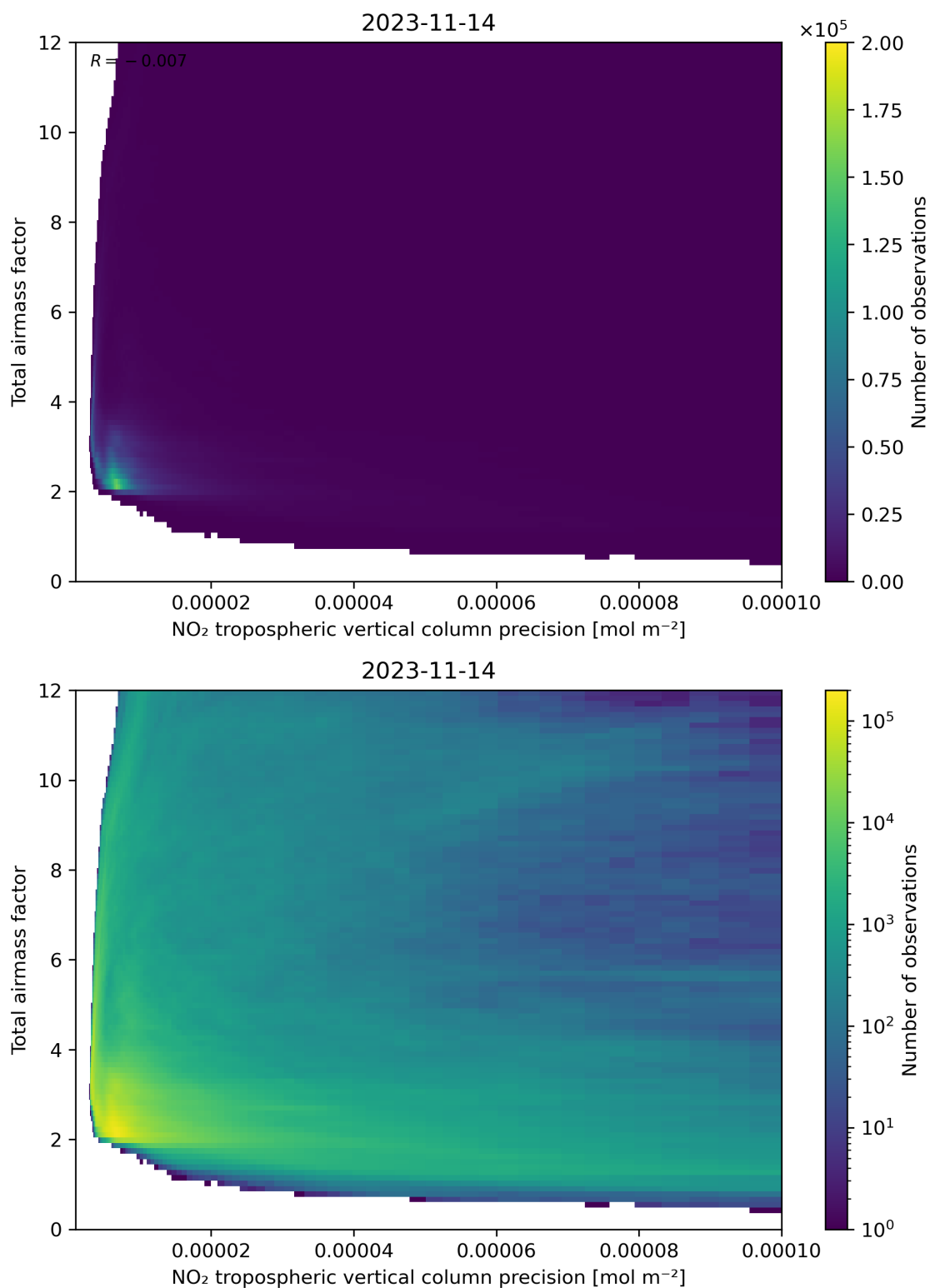
Figure 132: Scatter density plot of “NO 2 tropospheric vertical column precision” against “Total air mass factor” for 2023-11-13 to 2023-11-15.
