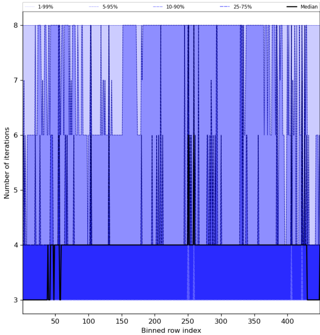
Figure 51: Along track statistics of “Number of iterations” for 2023-11-13 to 2023-11-15
