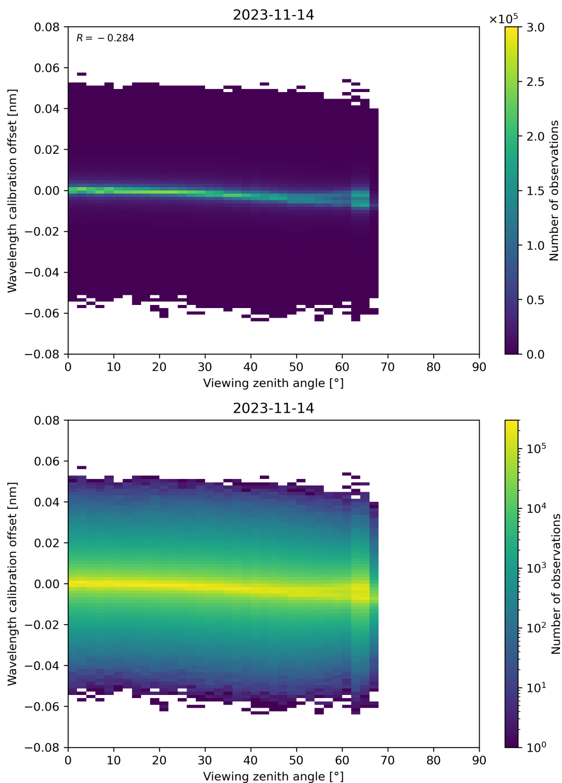
Figure 173: Scatter density plot of “Viewing zenith angle” against “Wavelength calibration offset” for 2023-11-13 to 2023-11-15.
