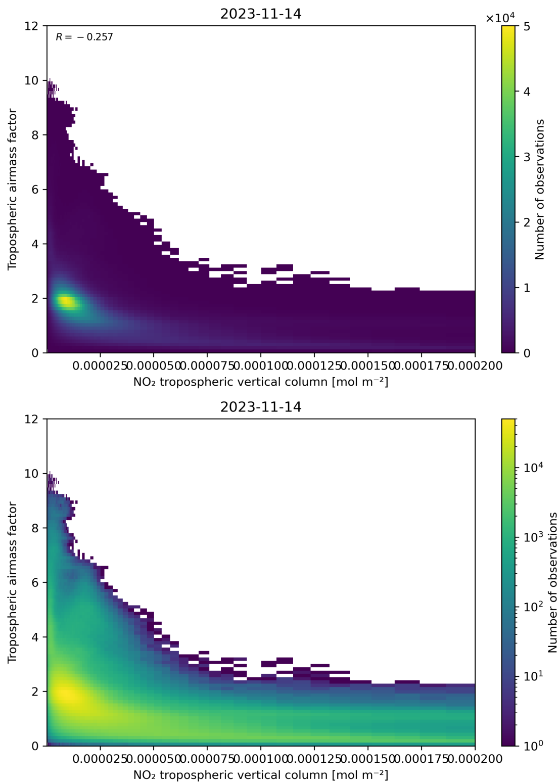
Figure 123: Scatter density plot of “NO 2 tropospheric vertical column” against “Tropospheric air mass factor” for 2023-11-13 to 2023-11-15.
