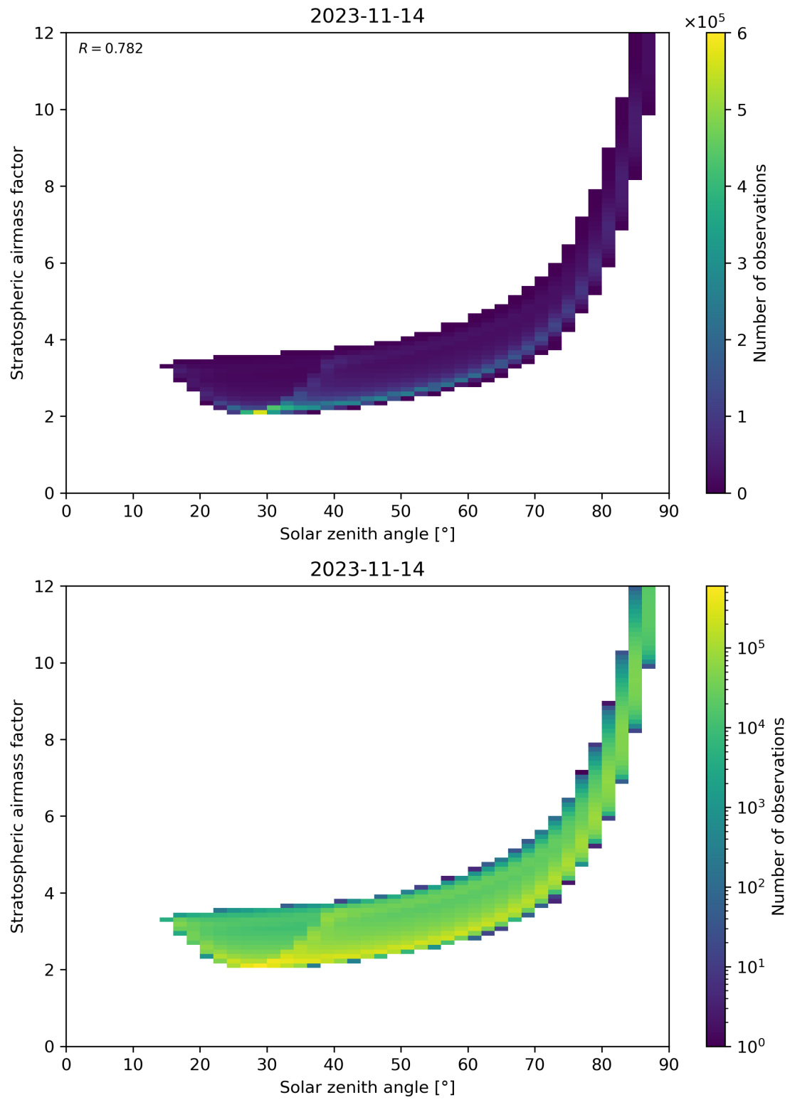
Figure 145: Scatter density plot of “Solar zenith angle” against “Stratospheric airmass factor” for 2023-11-13 to 2023-11-15.
