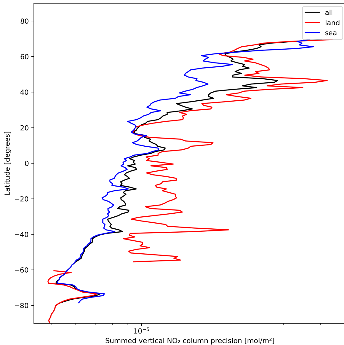
Figure 24: Zonal average of “Summed vertical NO 2 column precision” for 2023-11-13 to 2023-11-15.
