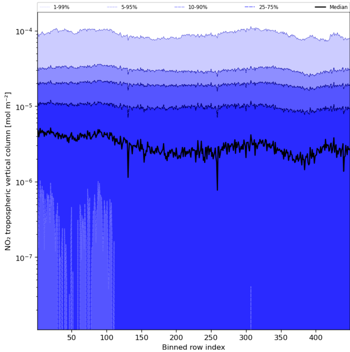
Figure 46: Along track statistics of “NO 2 tropospheric vertical column” for 2023-11-13 to 2023-11-15
