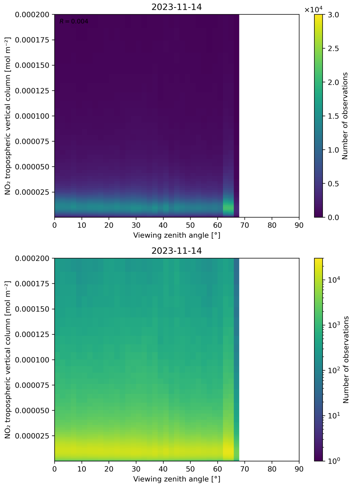
Figure 169: Scatter density plot of “Viewing zenith angle” against “NO 2 tropospheric vertical column” for 2023-11-13 to 2023-11-15.
