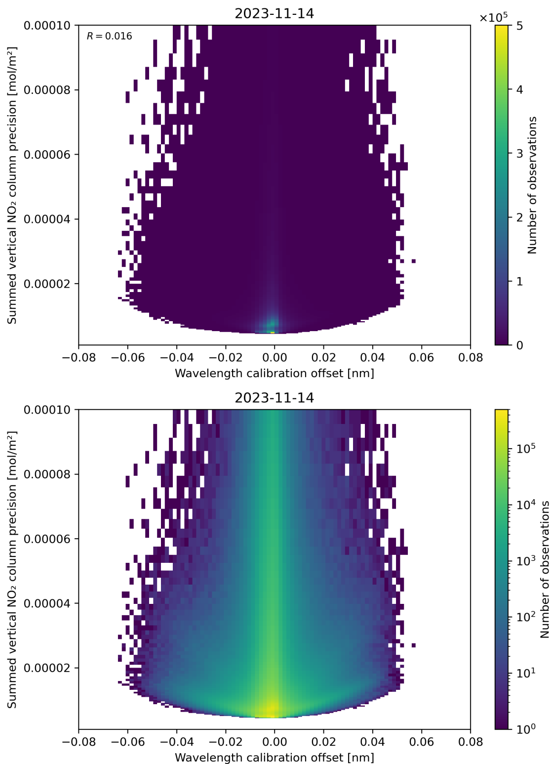
Figure 178: Scatter density plot of “Wavelength calibration offset” against “Summed vertical NO 2 column precision” for 2023-11-13 to 2023-11-15.
