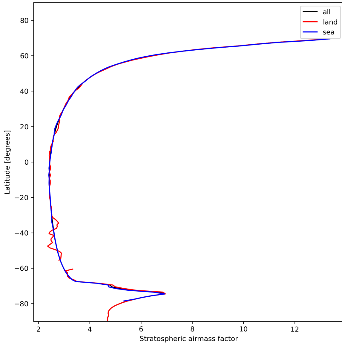
Figure 27: Zonal average of “Stratospheric airmass factor” for 2023-11-13 to 2023-11-15.
