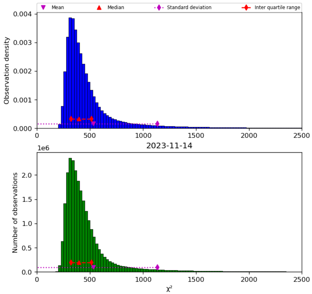
Figure 42: Histogram of “ \chi^2 ” for 2023-11-13 to 2023-11-15
