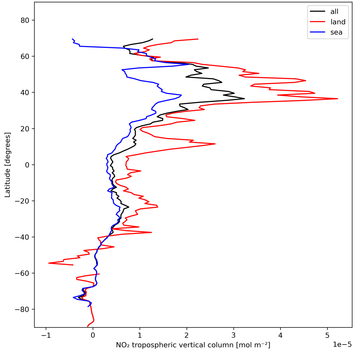
Figure 12: Zonal average of “NO 2 tropospheric vertical column” for 2023-11-13 to 2023-11-15.
