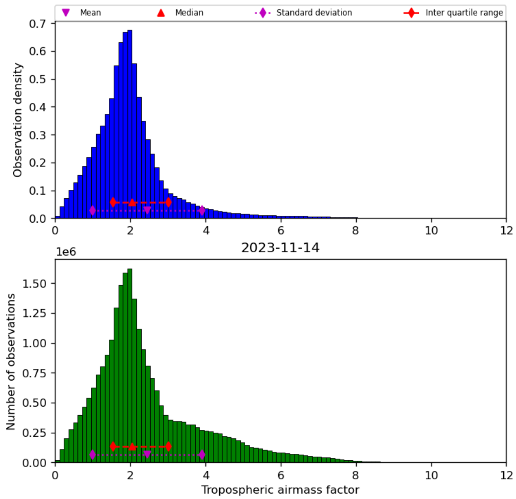
Figure 31: Histogram of “Tropospheric airmass factor” for 2023-11-13 to 2023-11-15
