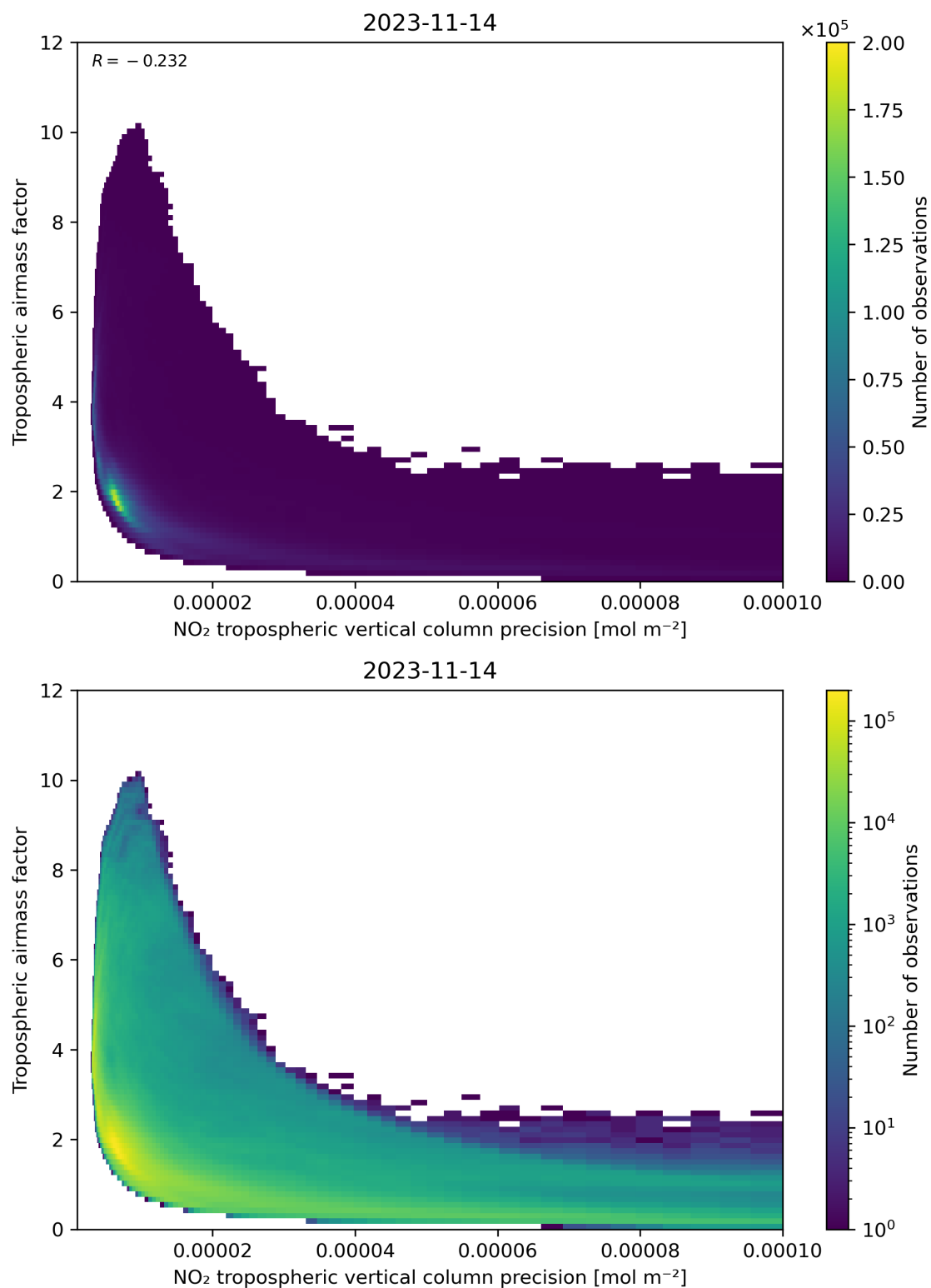
Figure 133: Scatter density plot of “NO 2 tropospheric vertical column precision” against “Tropospheric airmass factor” for 2023-11-13 to 2023-11-15.
