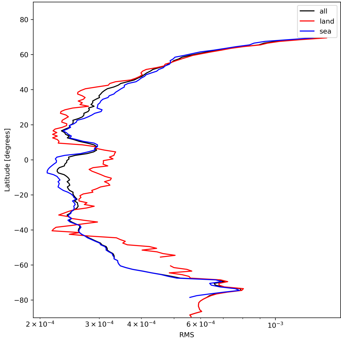
Figure 26: Zonal average of “RMS” for 2023-11-13 to 2023-11-15.
