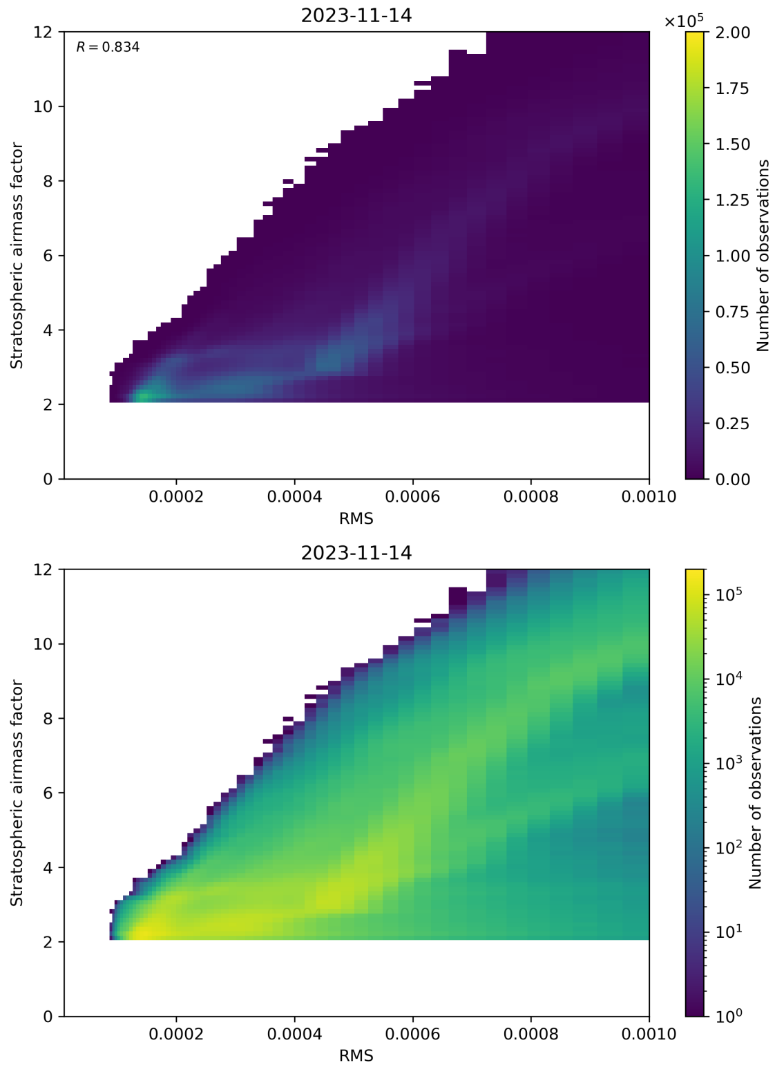
Figure 144: Scatter density plot of “RMS” against “Stratospheric airmass factor” for 2023-11-13 to 2023-11-15.
