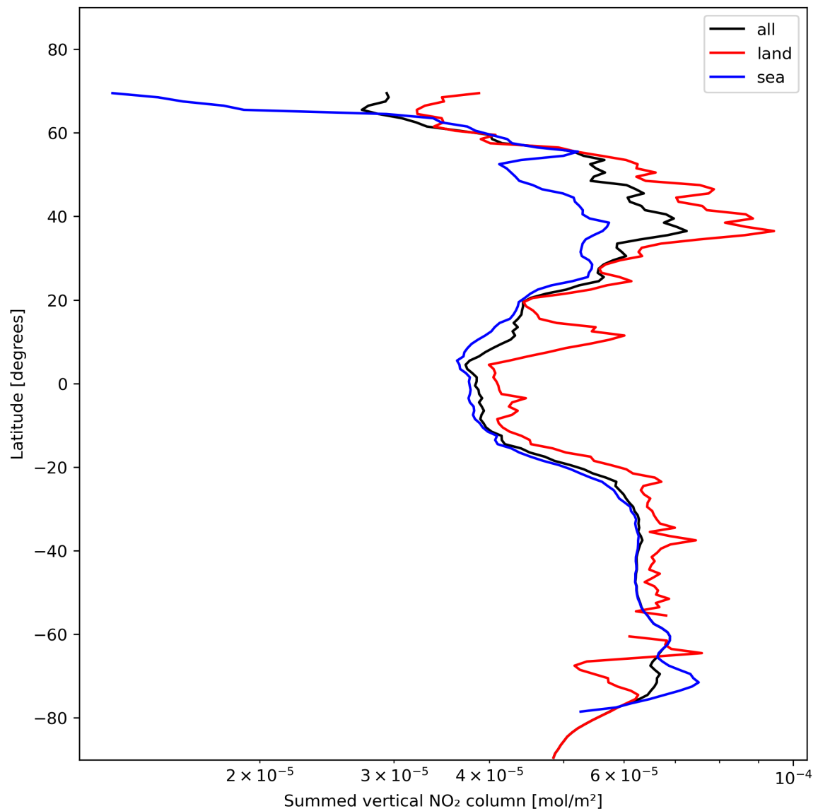
Figure 23: Zonal average of “Summed vertical NO 2 column” for 2023-11-13 to 2023-11-15.
