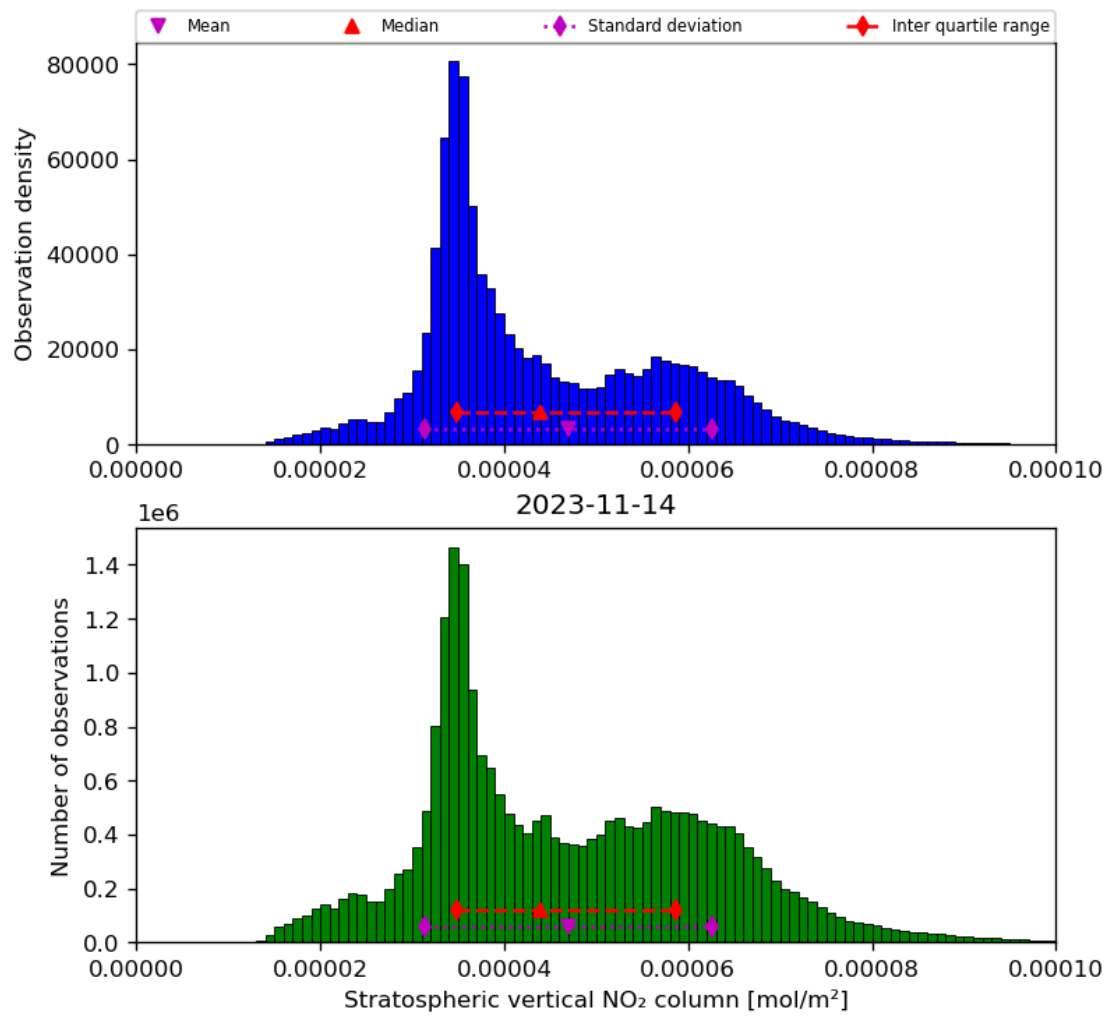
Figure 36: Histogram of “Stratospheric vertical NO 2 column” for 2023-11-13 to 2023-11-15
