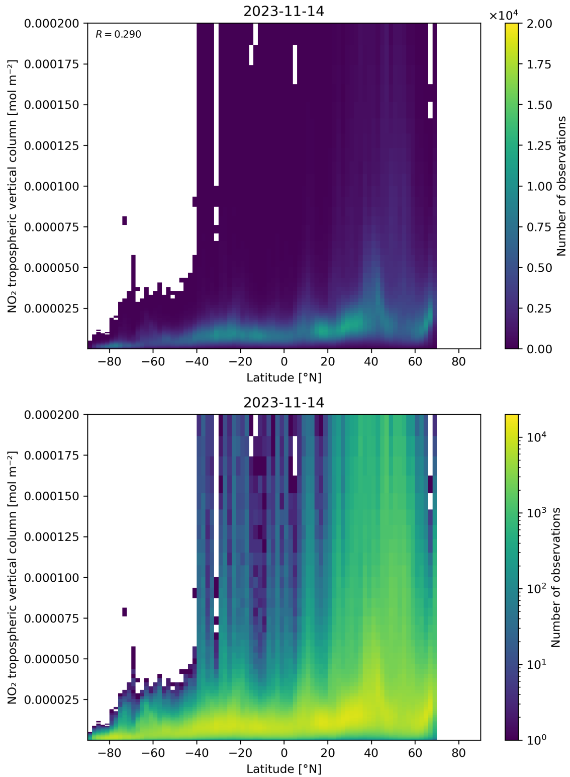
Figure 92: Scatter density plot of “Latitude” against “NO 2 tropospheric vertical column” for 2023-11-13 to 2023-11-15.
