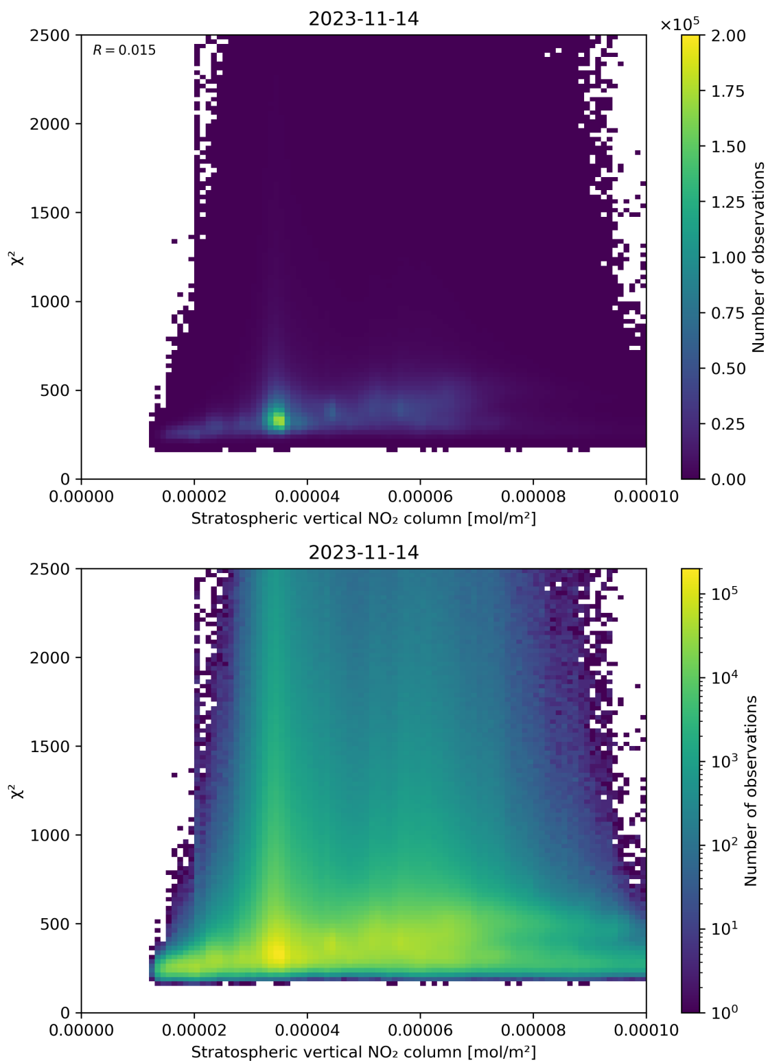
Figure 97: Scatter density plot of “Stratospheric vertical NO 2 column” against “ \chi^2 ” for 2023-11-13 to 2023-11-15.
