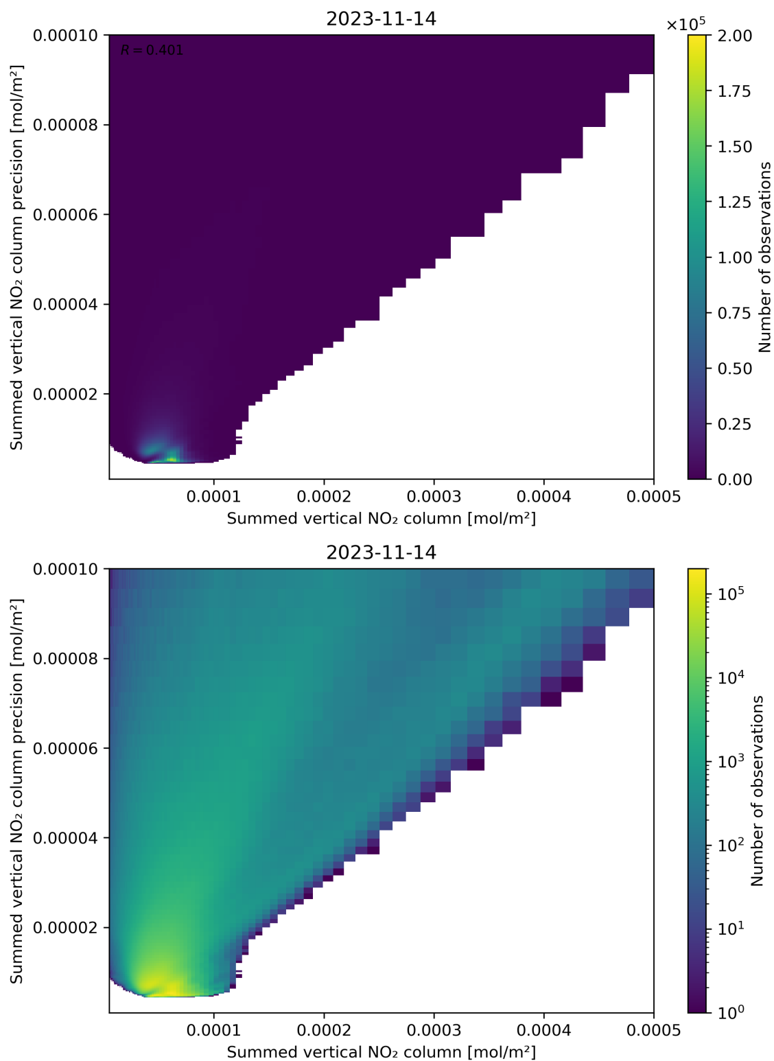
Figure 105: Scatter density plot of “Summed vertical NO 2 column” against “Summed vertical NO 2 column precision” for 2023-11-13 to 2023-11-15.
