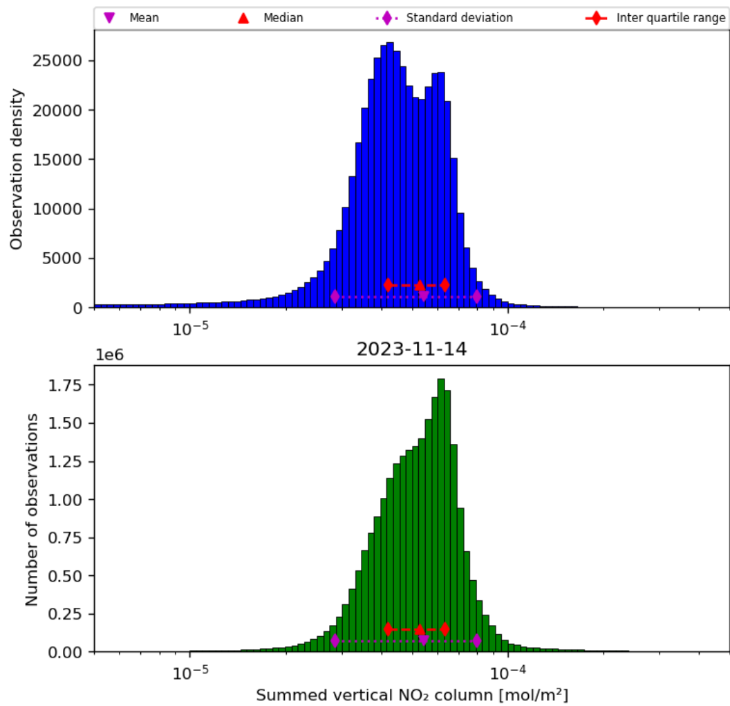
Figure 40: Histogram of “Summed vertical NO 2 column” for 2023-11-13 to 2023-11-15
