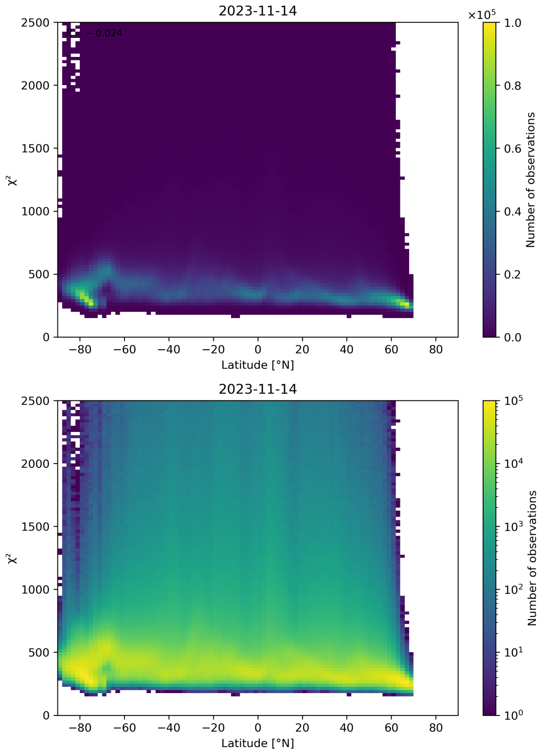
Figure 86: Scatter density plot of “Latitude” against “ \chi^2 ” for 2023-11-13 to 2023-11-15.
