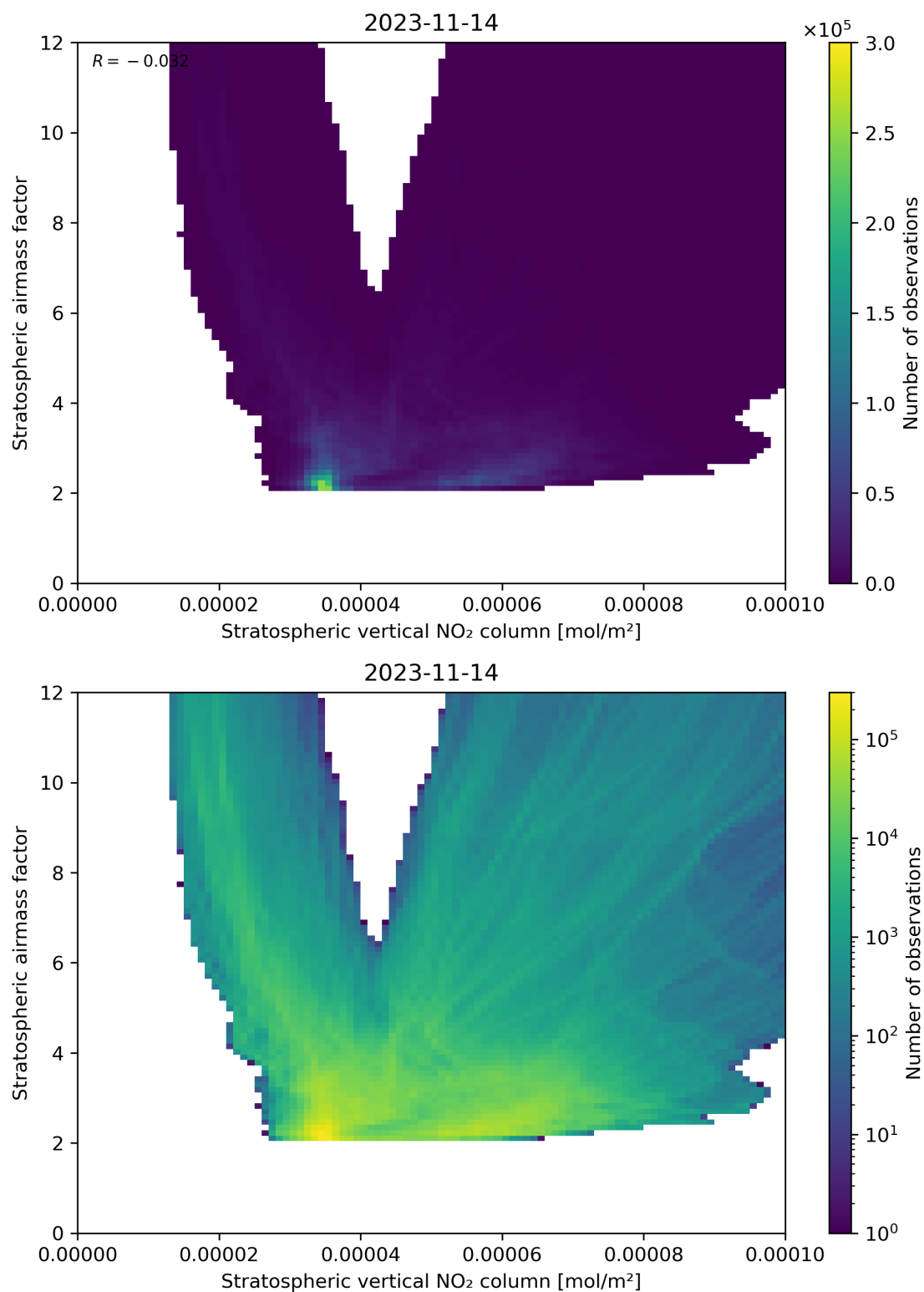
Figure 96: Scatter density plot of “Stratospheric vertical NO 2 column” against “Stratospheric airmass factor” for 2023-11-13 to 2023-11-15.
