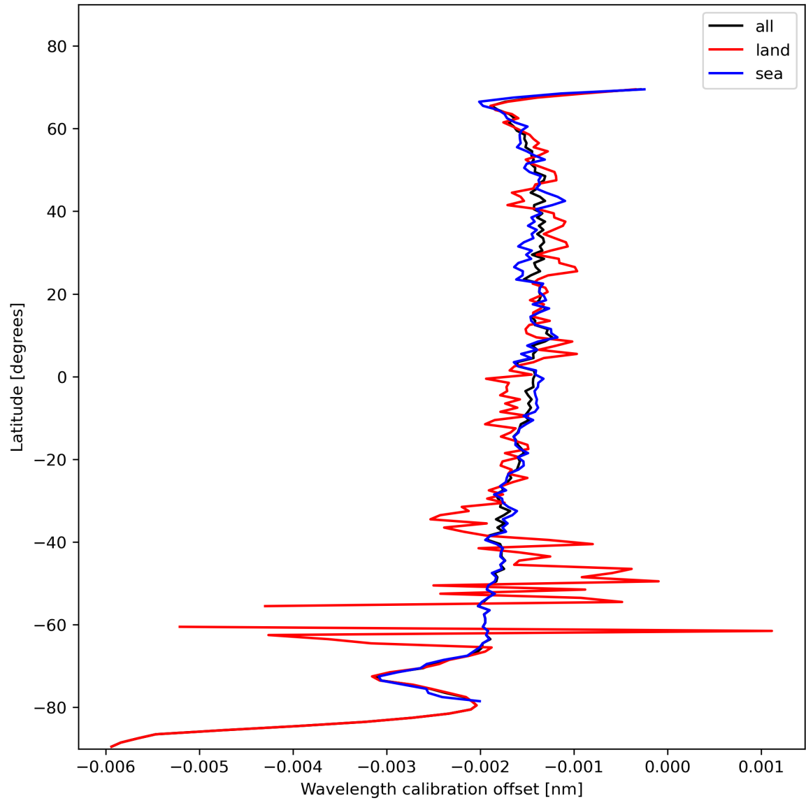
Figure 18: Zonal average of “Wavelength calibration offset” for 2023-11-13 to 2023-11-15.
