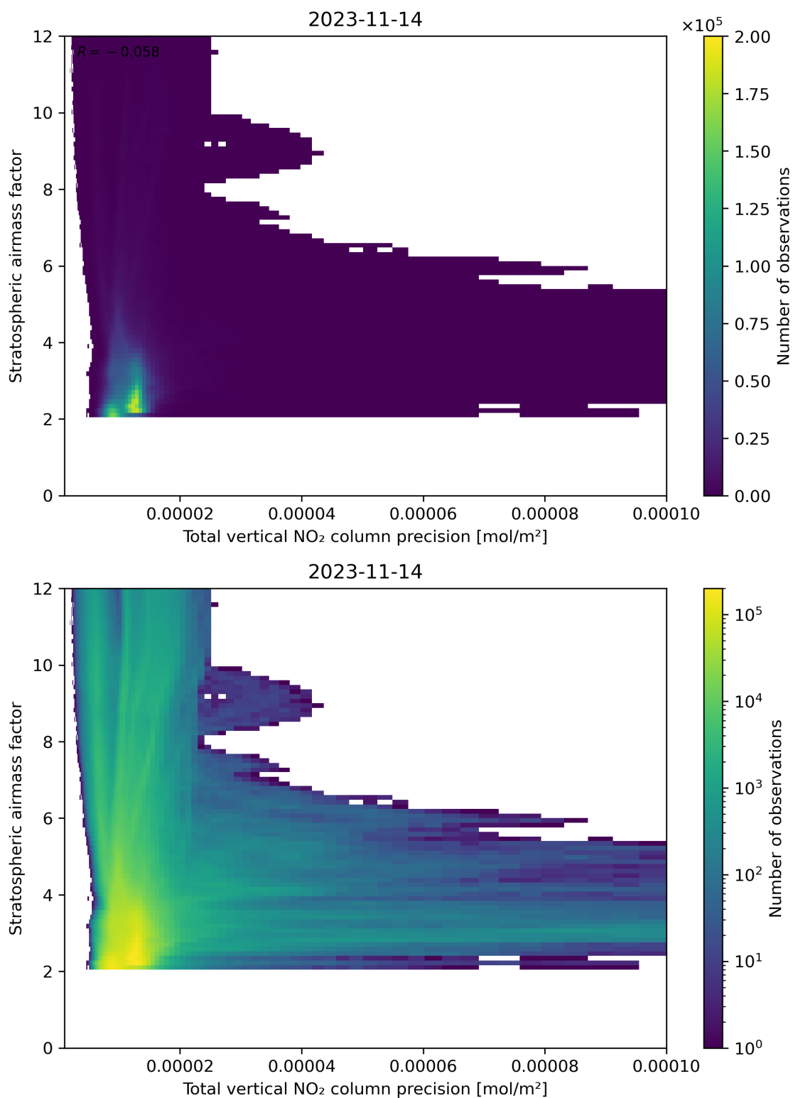
Figure 115: Scatter density plot of “Total vertical NO 2 column precision” against “Stratospheric air mass factor” for 2023-11-13 to 2023-11-15.
