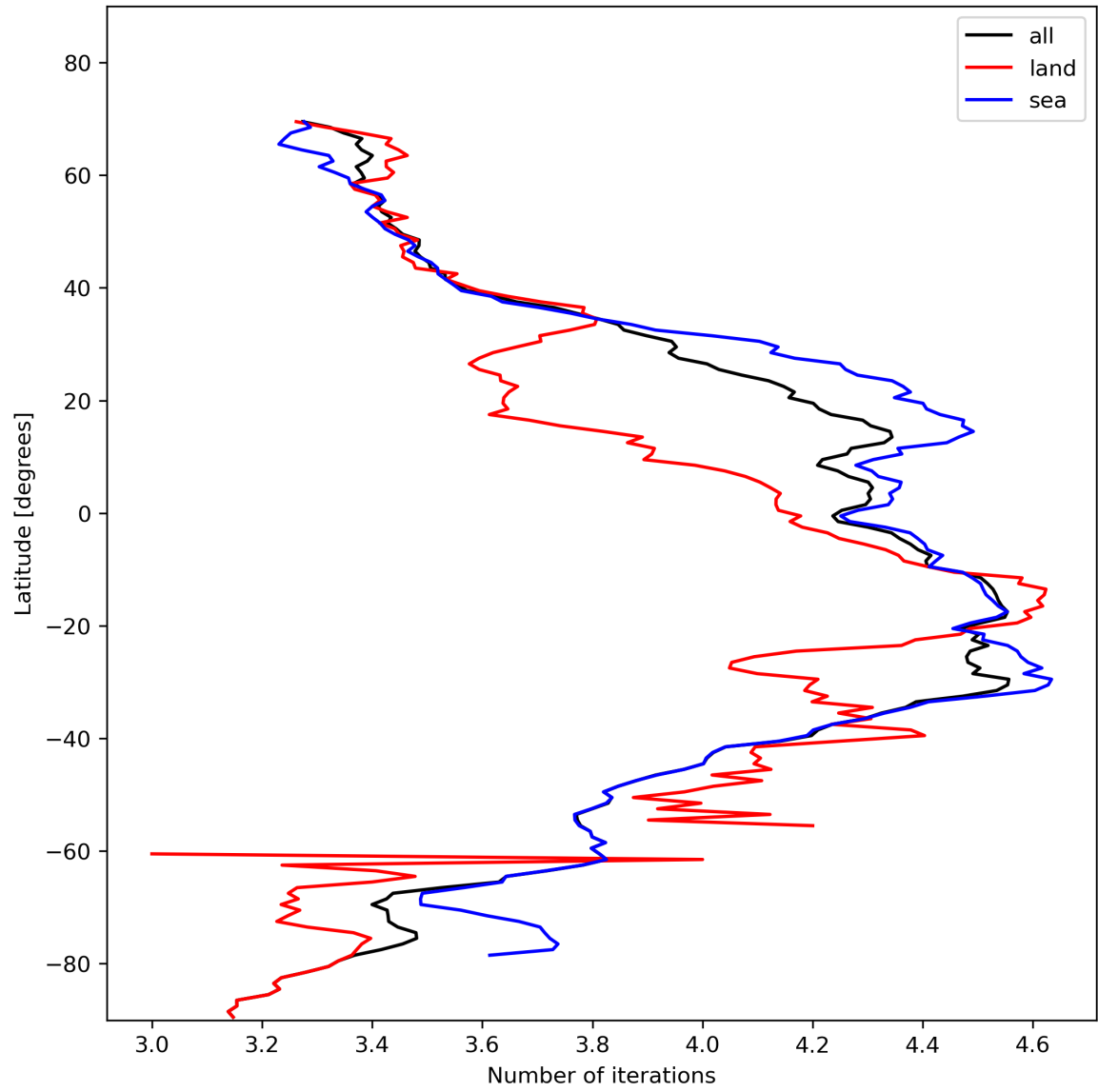
Figure 17: Zonal average of “Number of iterations” for 2023-11-13 to 2023-11-15.
