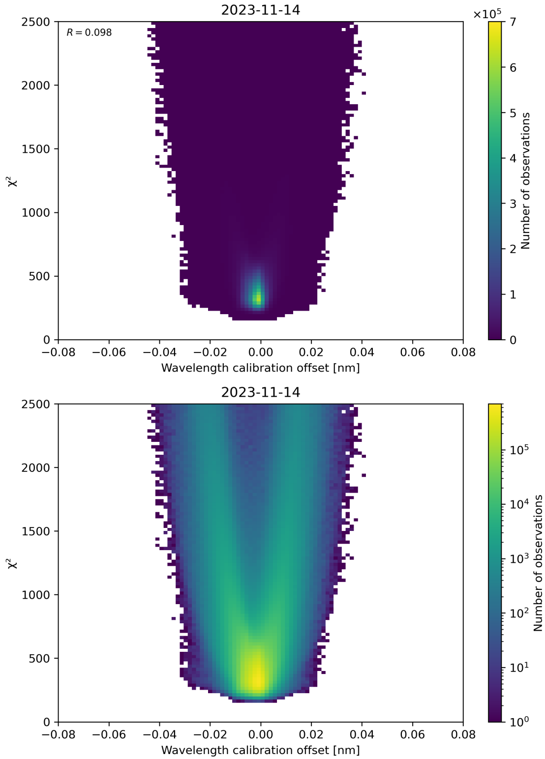
Figure 175: Scatter density plot of “Wavelength calibration offset” against “ \chi^2 ” for 2023-11-13 to 2023-11-15.
