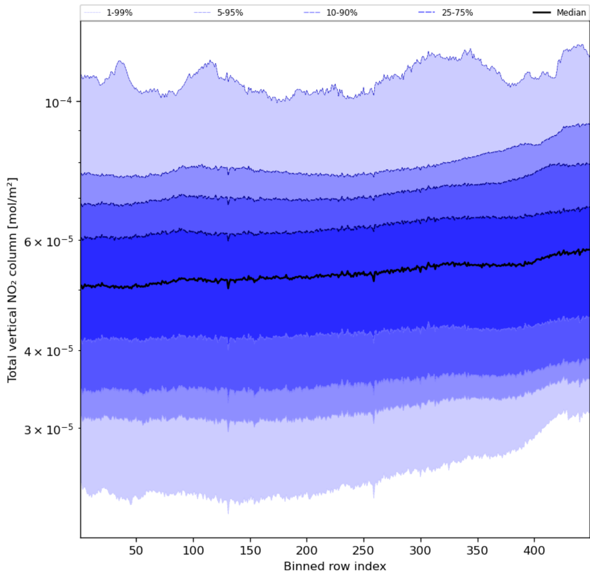
Figure 55: Along track statistics of “Total vertical NO 2 column” for 2023-11-13 to 2023-11-15
