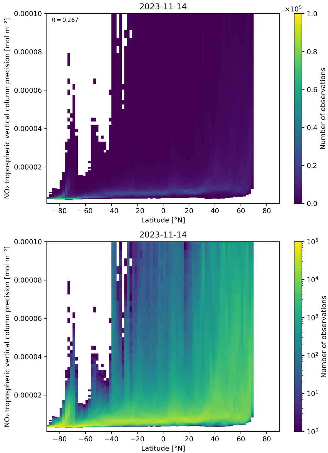
Figure 93: Scatter density plot of “Latitude” against “NO 2 tropospheric vertical column precision” for 2023-11-13 to 2023-11-15.
