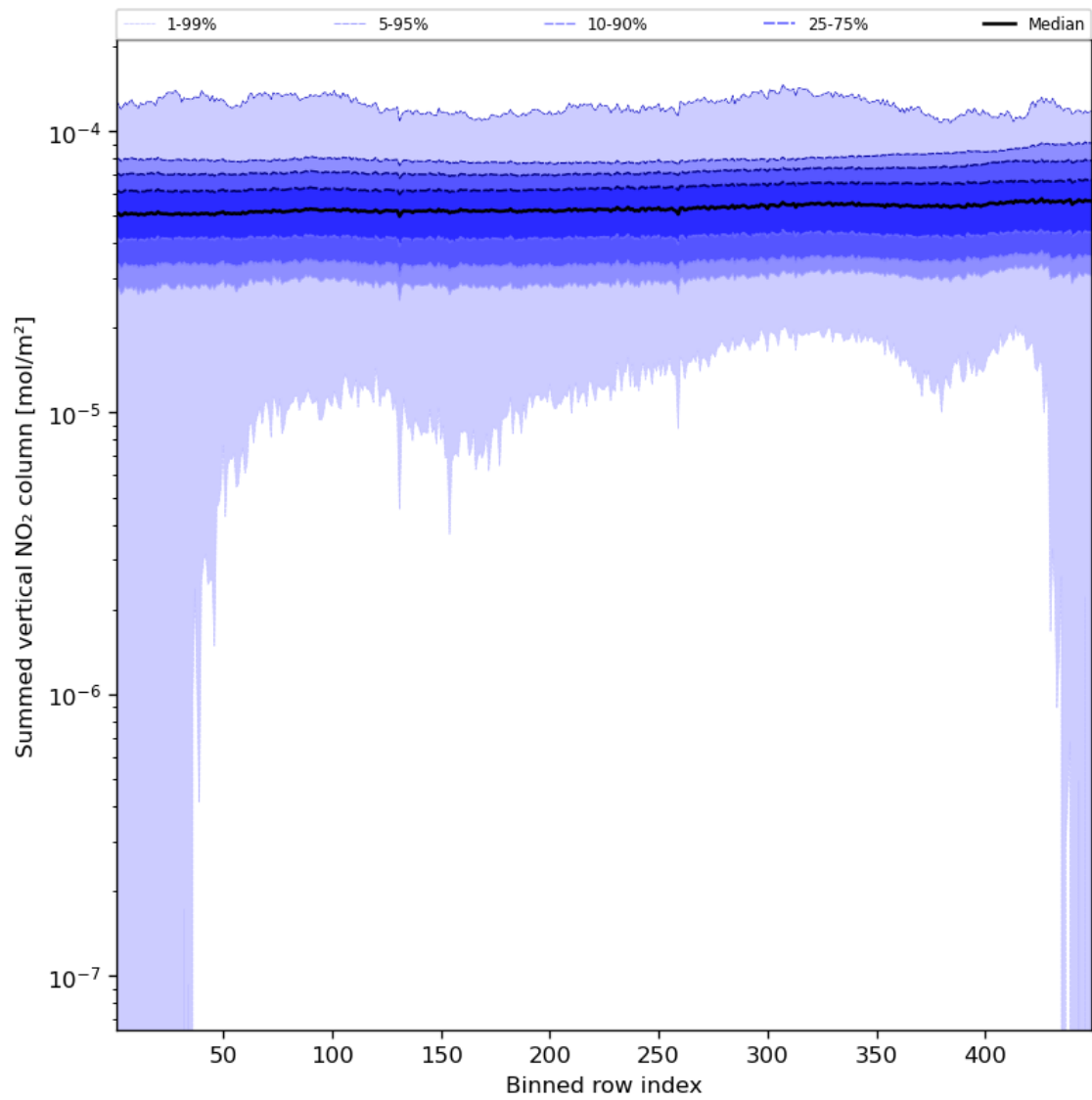
Figure 57: Along track statistics of “Summed vertical NO 2 column” for 2023-11-13 to 2023-11-15
