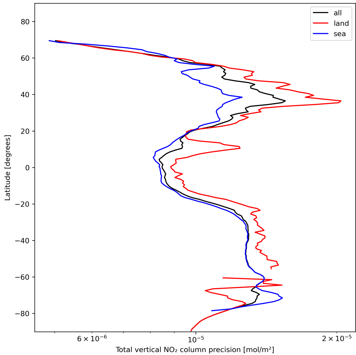
Figure 22: Zonal average of “Total vertical NO 2 column precision” for 2023-11-13 to 2023-11-15.
