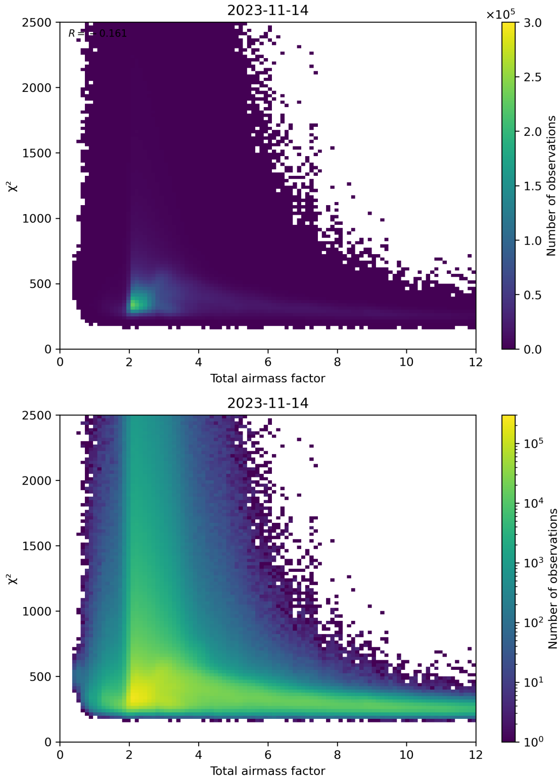
Figure 63: Scatter density plot of “Total airmass factor” against “ \chi^2 ” for 2023-11-13 to 2023-11-15.
