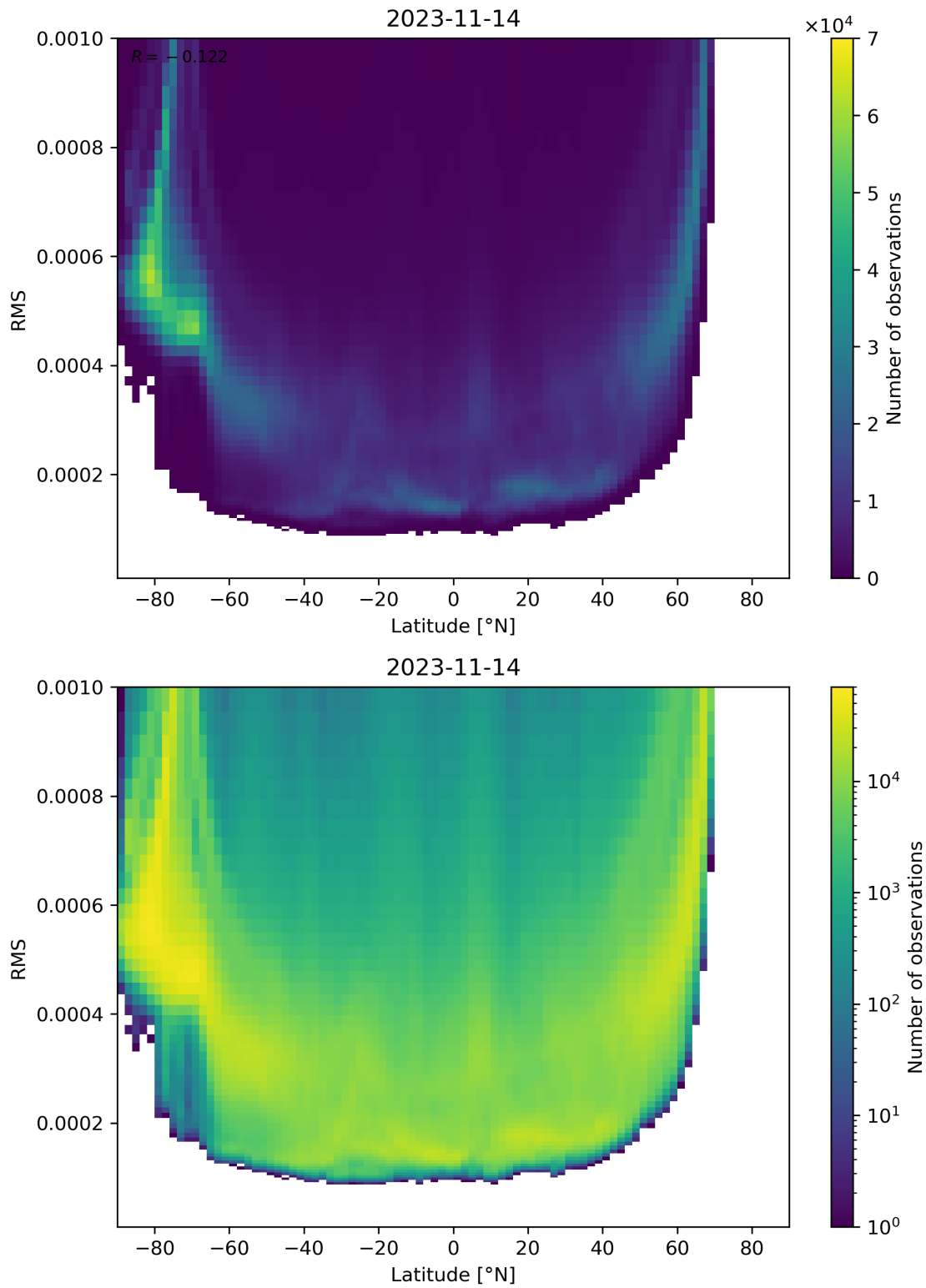
Figure 94: Scatter density plot of “Latitude” against “RMS” for 2023-11-13 to 2023-11-15.
