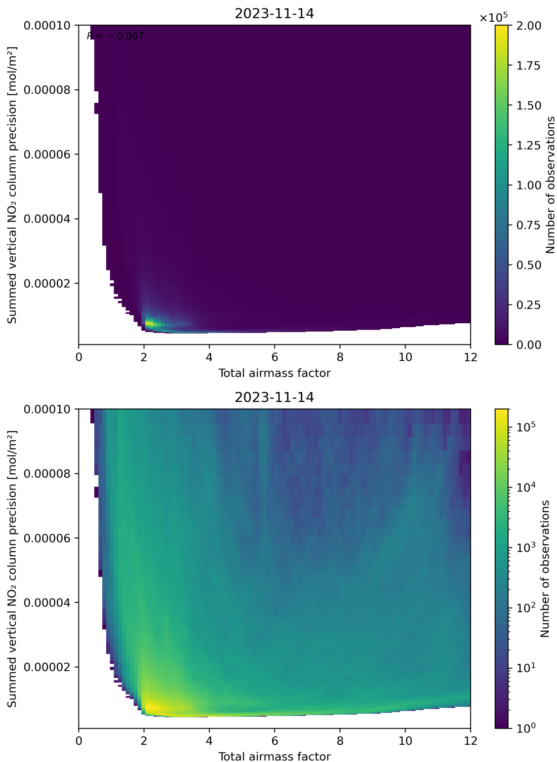
Figure 66: Scatter density plot of “Total airmass factor” against “Summed vertical NO 2 column precision” for 2023-11-13 to 2023-11-15.
