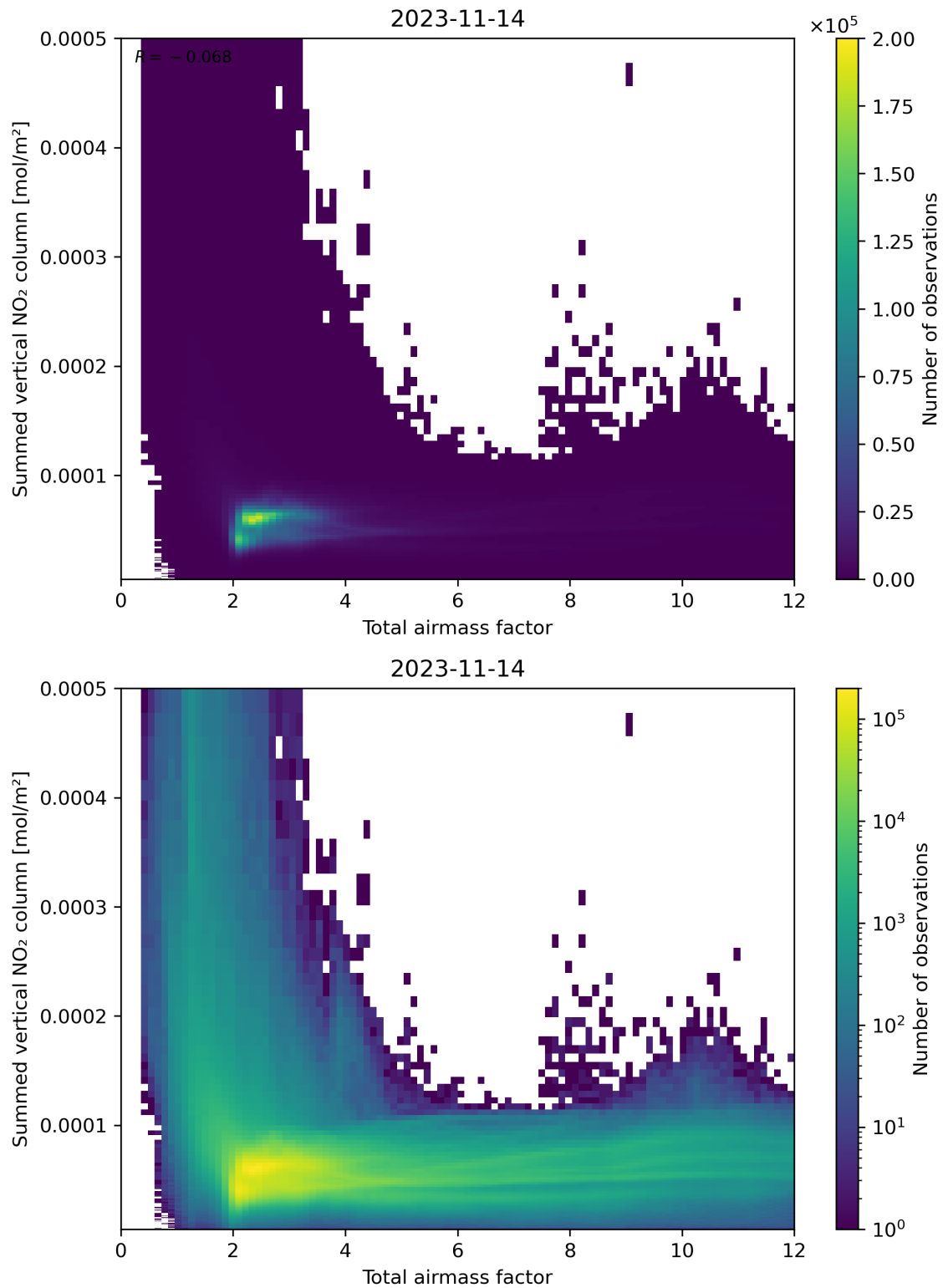
Figure 65: Scatter density plot of “Total airmass factor” against “Summed vertical NO 2 column” for 2023-11-13 to 2023-11-15.
