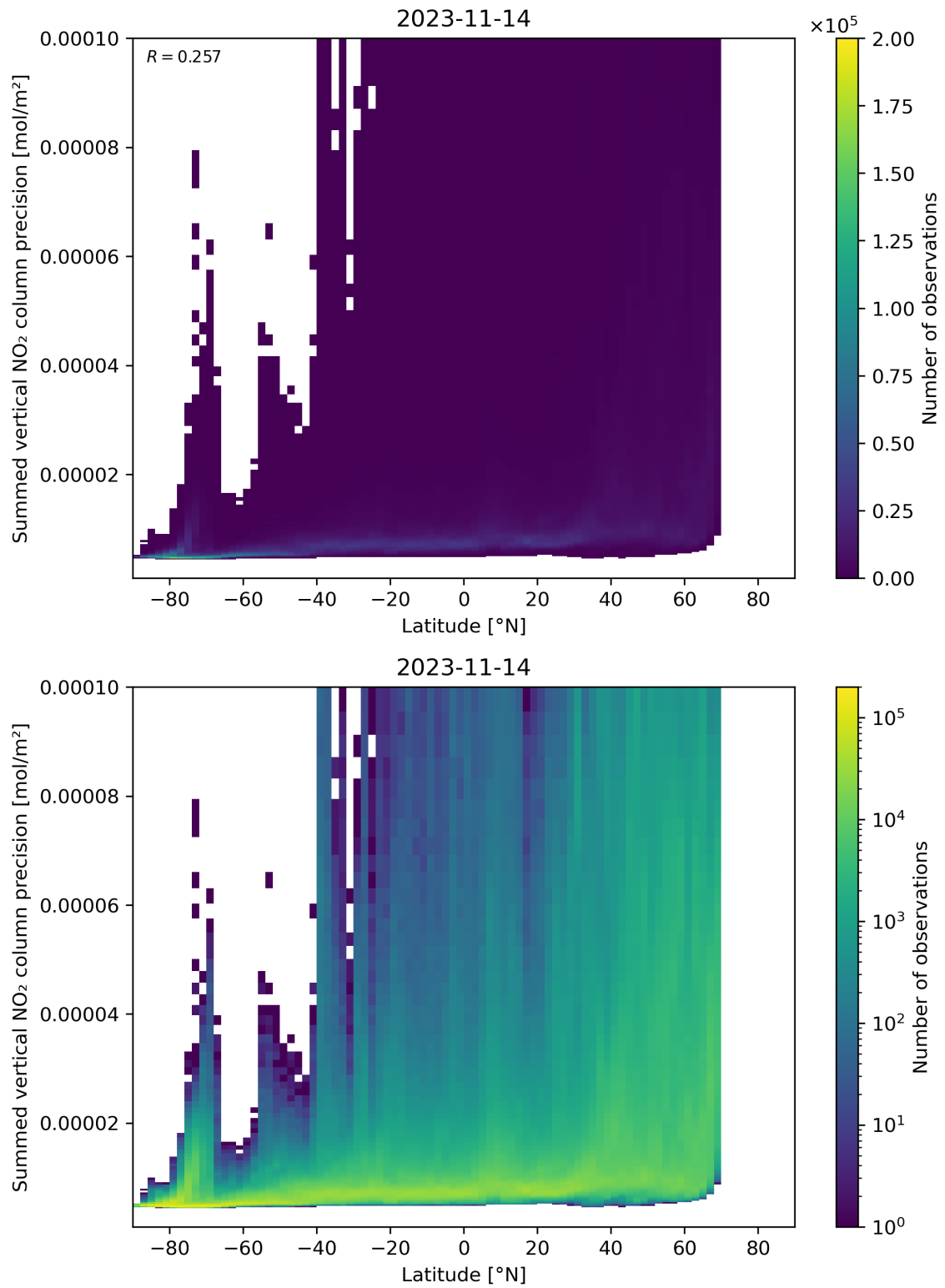
Figure 89: Scatter density plot of “Latitude” against “Summed vertical NO 2 column precision” for 2023-11-13 to 2023-11-15.
