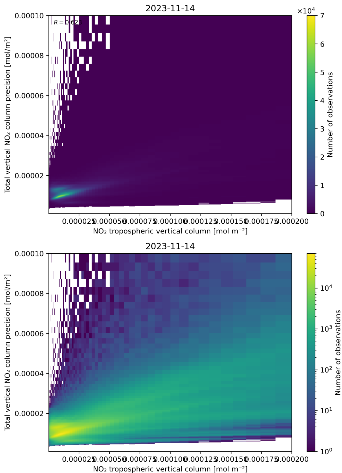
Figure 129: Scatter density plot of “NO 2 tropospheric vertical column” against “Total vertical NO 2 column precision” for 2023-11-13 to 2023-11-15.
