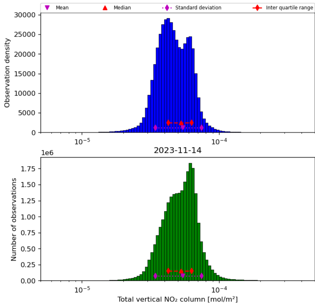
Figure 38: Histogram of “Total vertical NO 2 column” for 2023-11-13 to 2023-11-15
