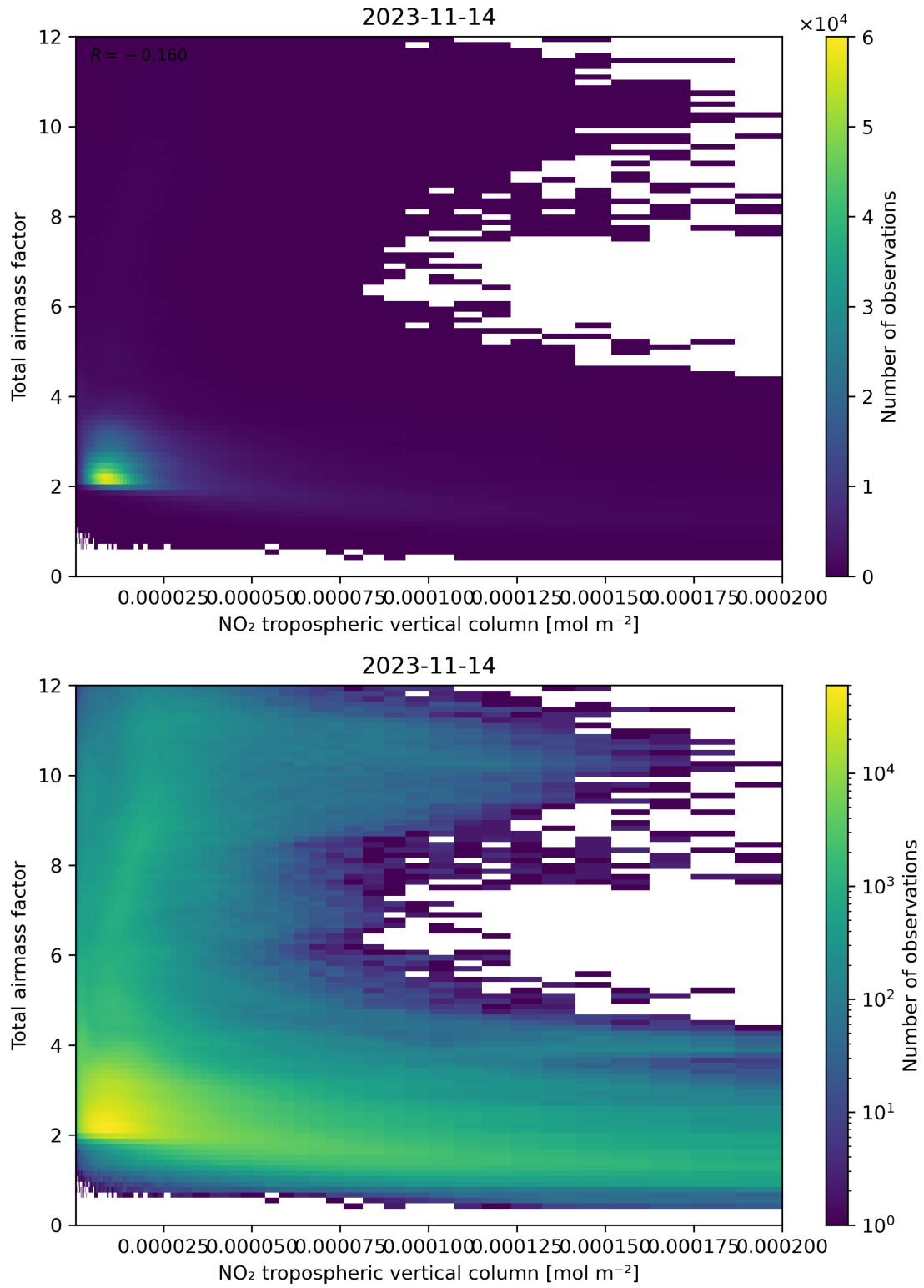
Figure 122: Scatter density plot of “NO 2 tropospheric vertical column” against “Total air mass factor” for 2023-11-13 to 2023-11-15.
