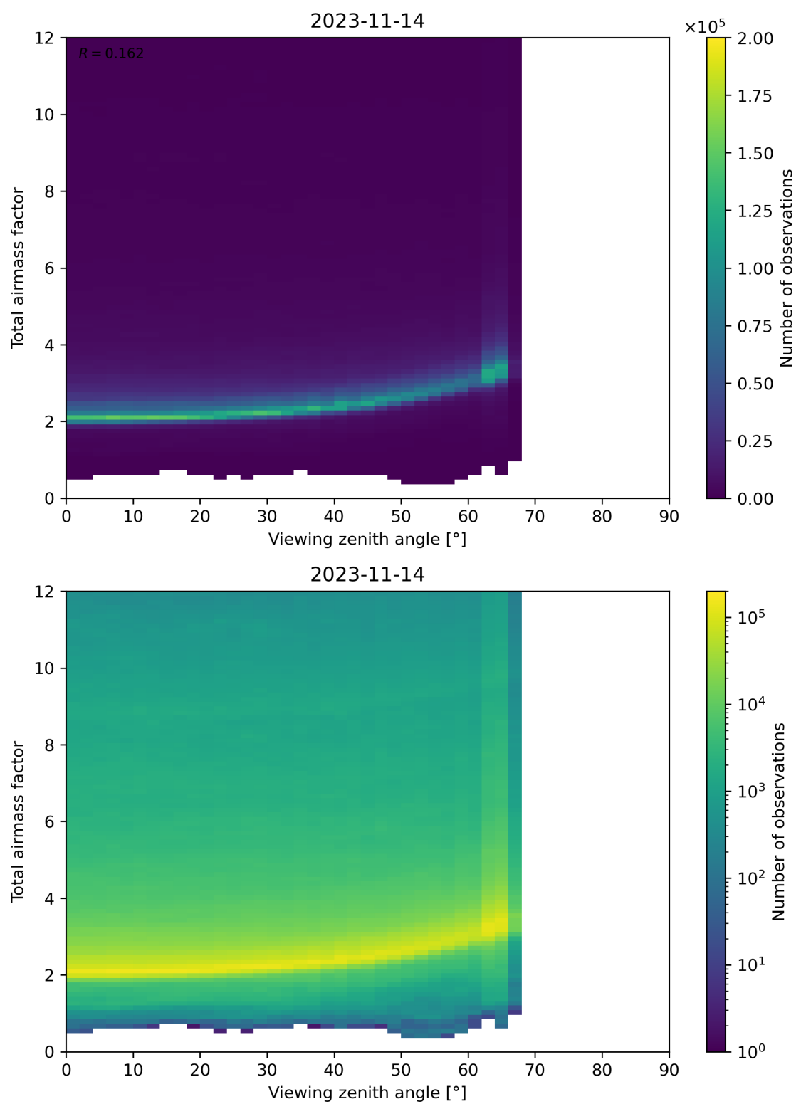
Figure 160: Scatter density plot of “Viewing zenith angle” against “Total airmass factor” for 2023-11-13 to 2023-11-15.
