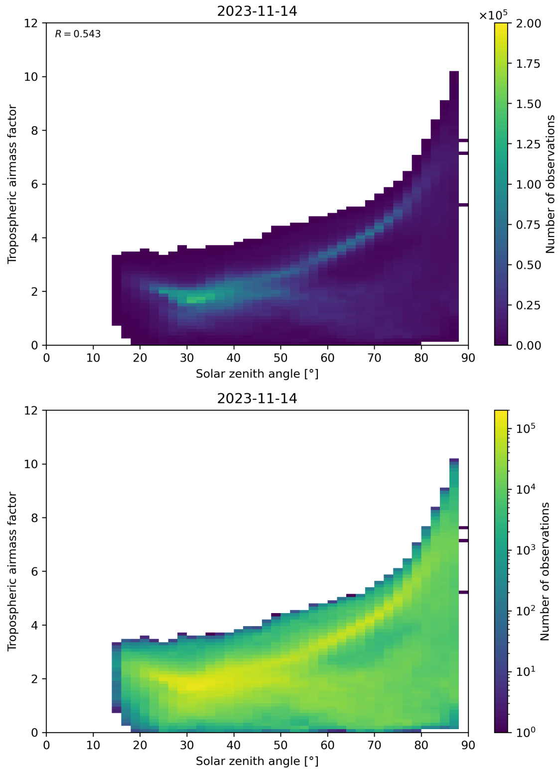
Figure 147: Scatter density plot of “Solar zenith angle” against “Tropospheric airmass factor” for 2023-11-13 to 2023-11-15.
