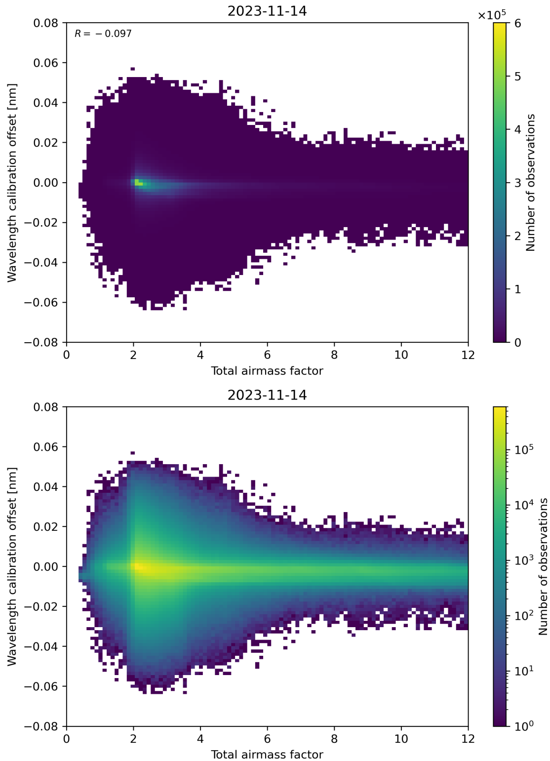
Figure 70: Scatter density plot of “Total airmass factor” against “Wavelength calibration offset” for 2023-11-13 to 2023-11-15.
