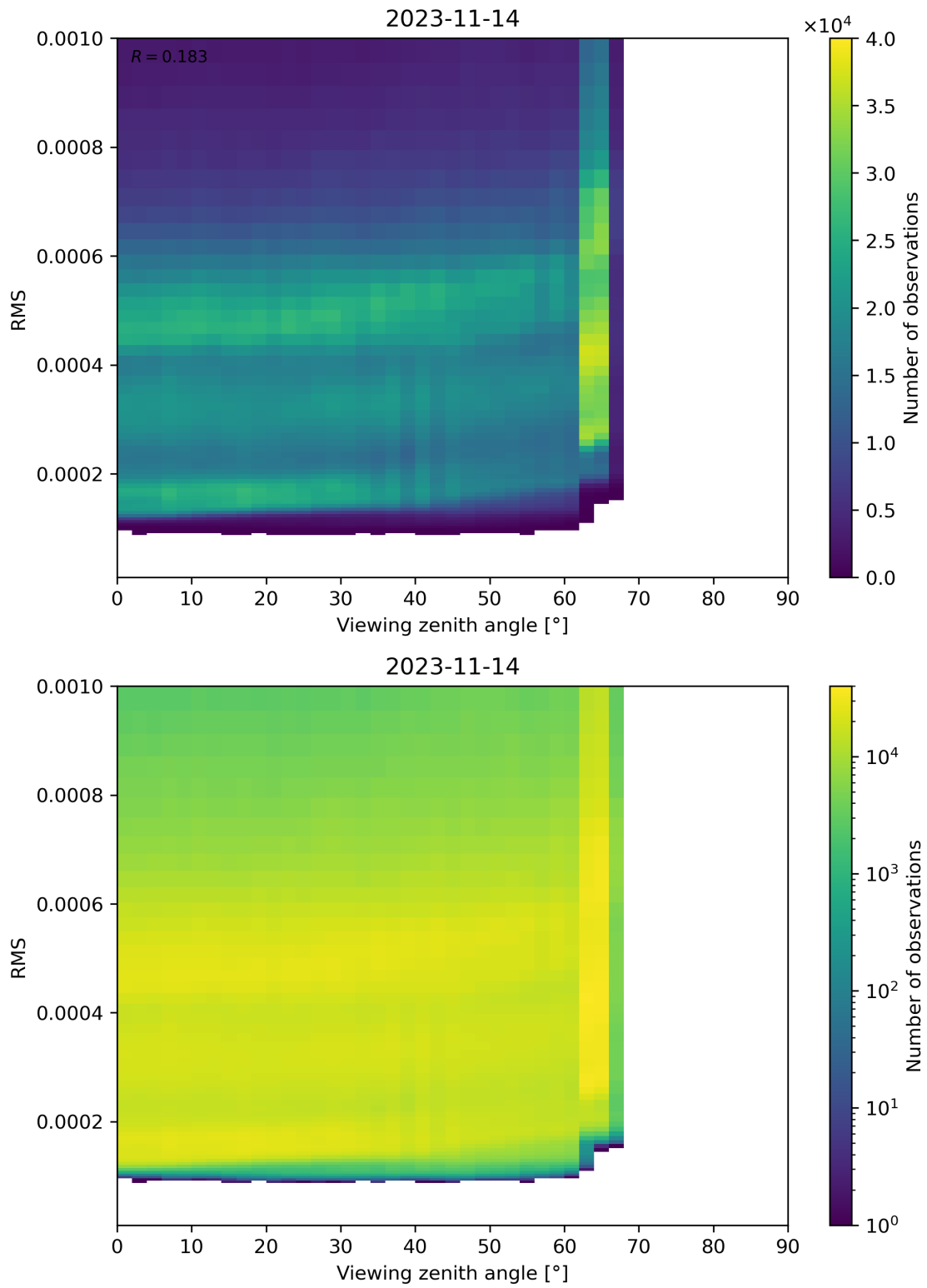
Figure 171: Scatter density plot of “Viewing zenith angle” against “RMS” for 2023-11-13 to 2023-11-15.
