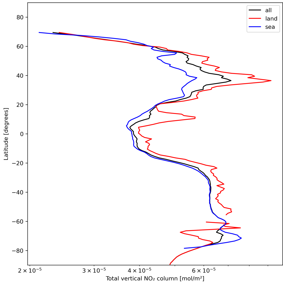
Figure 21: Zonal average of “Total vertical NO 2 column” for 2023-11-13 to 2023-11-15.
