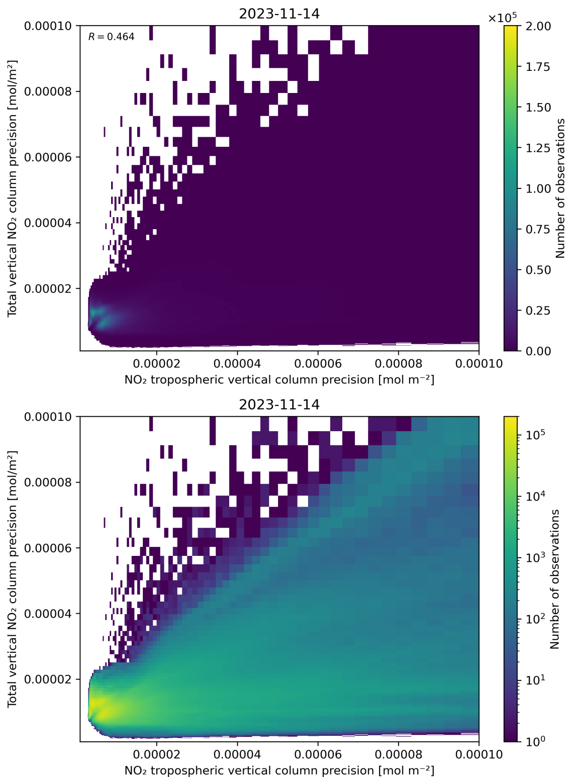
Figure 139: Scatter density plot of “NO 2 tropospheric vertical column precision” against “Total vertical NO 2 column precision” for 2023-11-13 to 2023-11-15.
