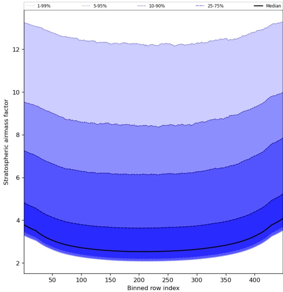
Figure 61: Along track statistics of “Stratospheric airmass factor” for 2023-11-13 to 2023-11-15
