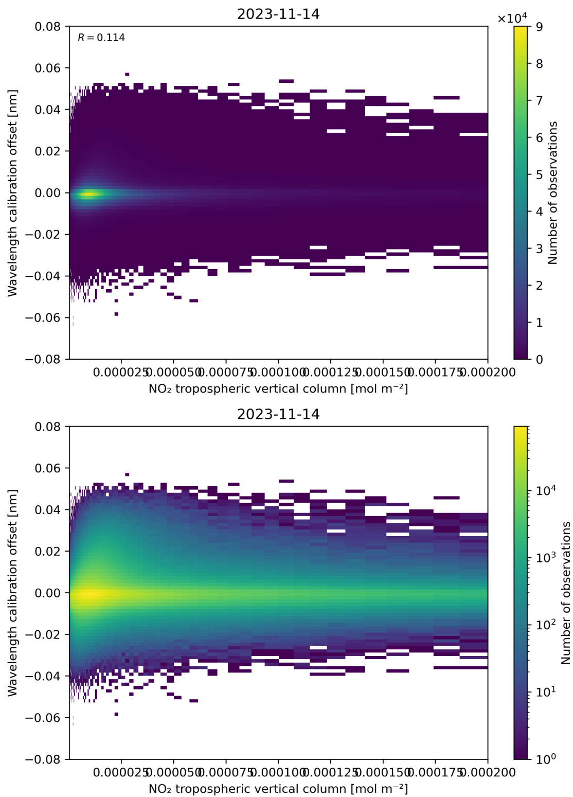
Figure 143: Scatter density plot of “NO 2 tropospheric vertical column” against “Wavelength calibration offset” for 2023-11-13 to 2023-11-15.
