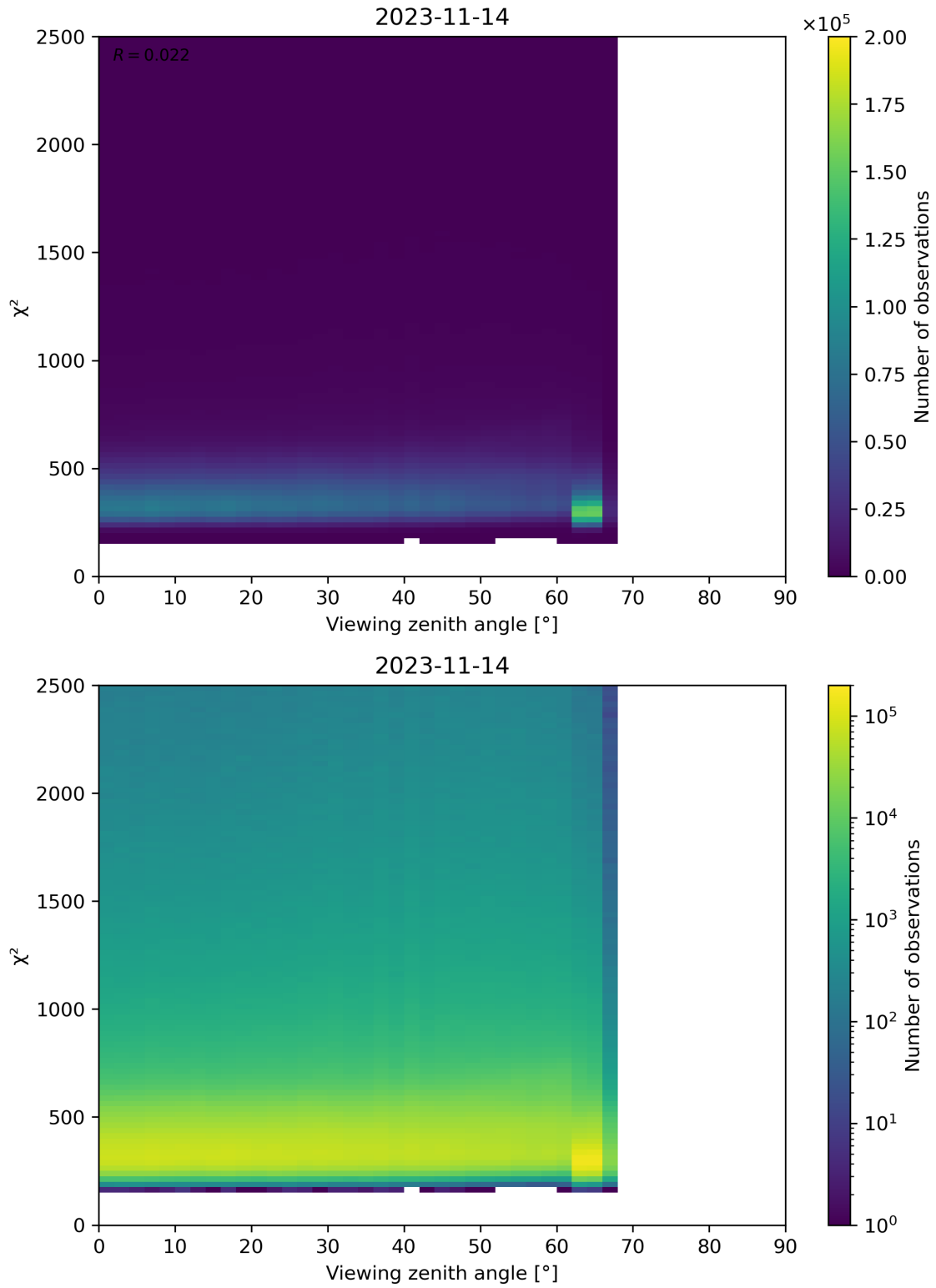
Figure 162: Scatter density plot of “Viewing zenith angle” against “ \chi^2 ” for 2023-11-13 to 2023-11-15.
