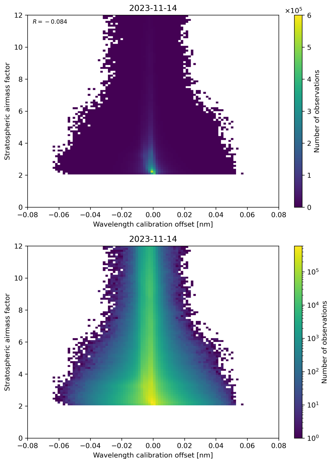
Figure 174: Scatter density plot of “Wavelength calibration offset” against “Stratospheric airmass factor” for 2023-11-13 to 2023-11-15.
