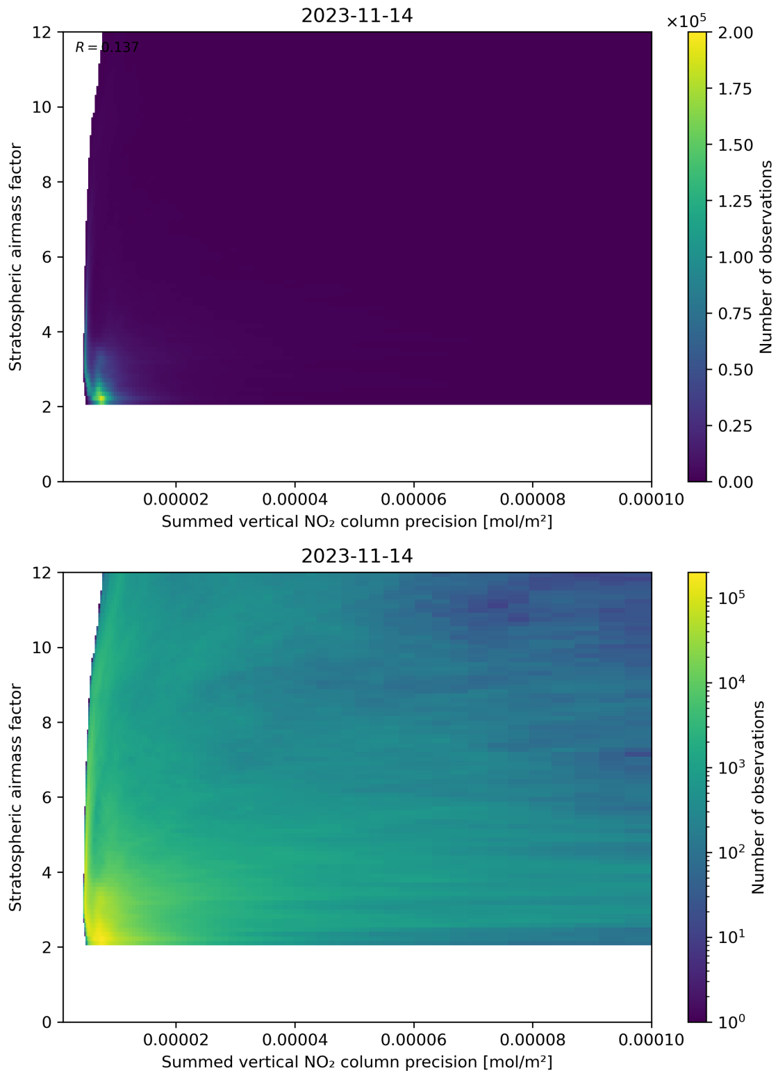
Figure 106: Scatter density plot of “Summed vertical NO 2 column precision” against “Stratospheric airmass factor” for 2023-11-13 to 2023-11-15.
