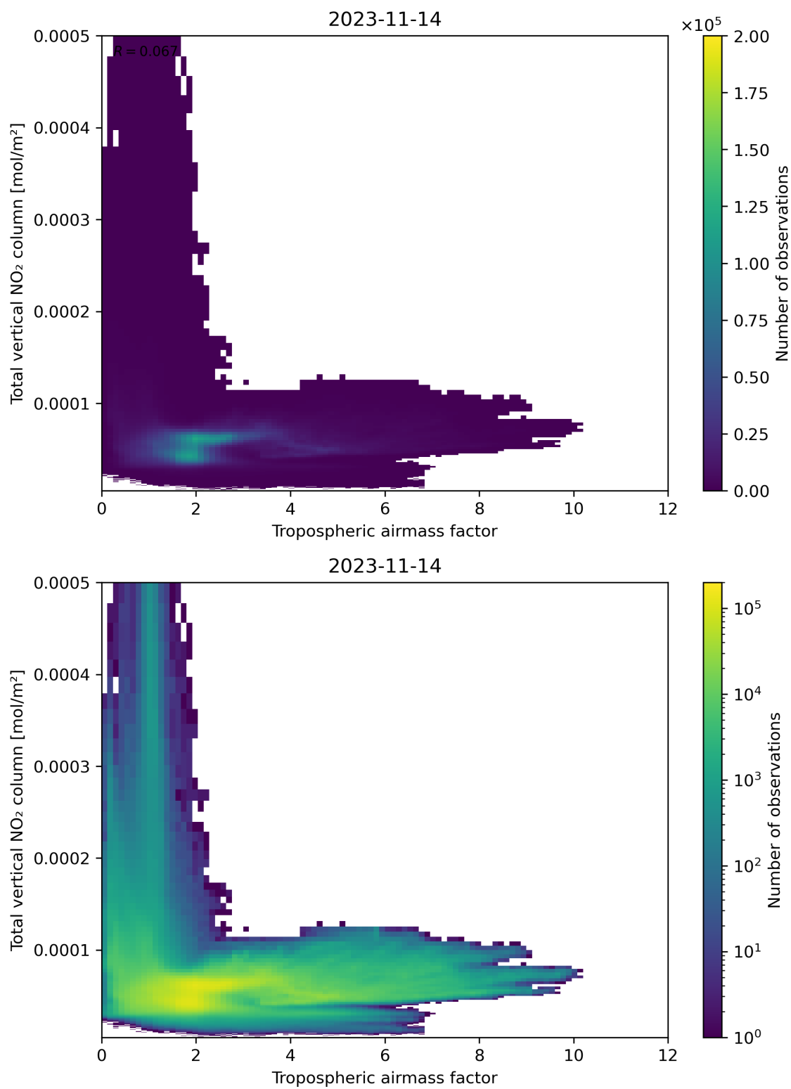
Figure 77: Scatter density plot of “Tropospheric airmass factor” against “Total vertical NO 2 column” for 2023-11-13 to 2023-11-15.
