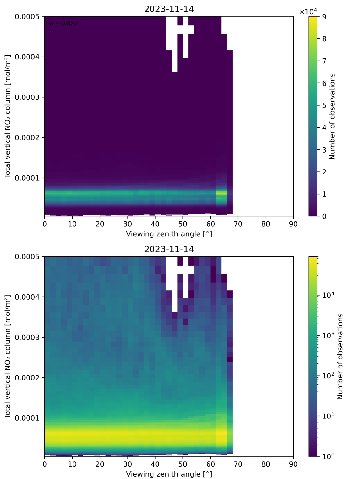
Figure 167: Scatter density plot of “Viewing zenith angle” against “Total vertical NO 2 column” for 2023-11-13 to 2023-11-15.
