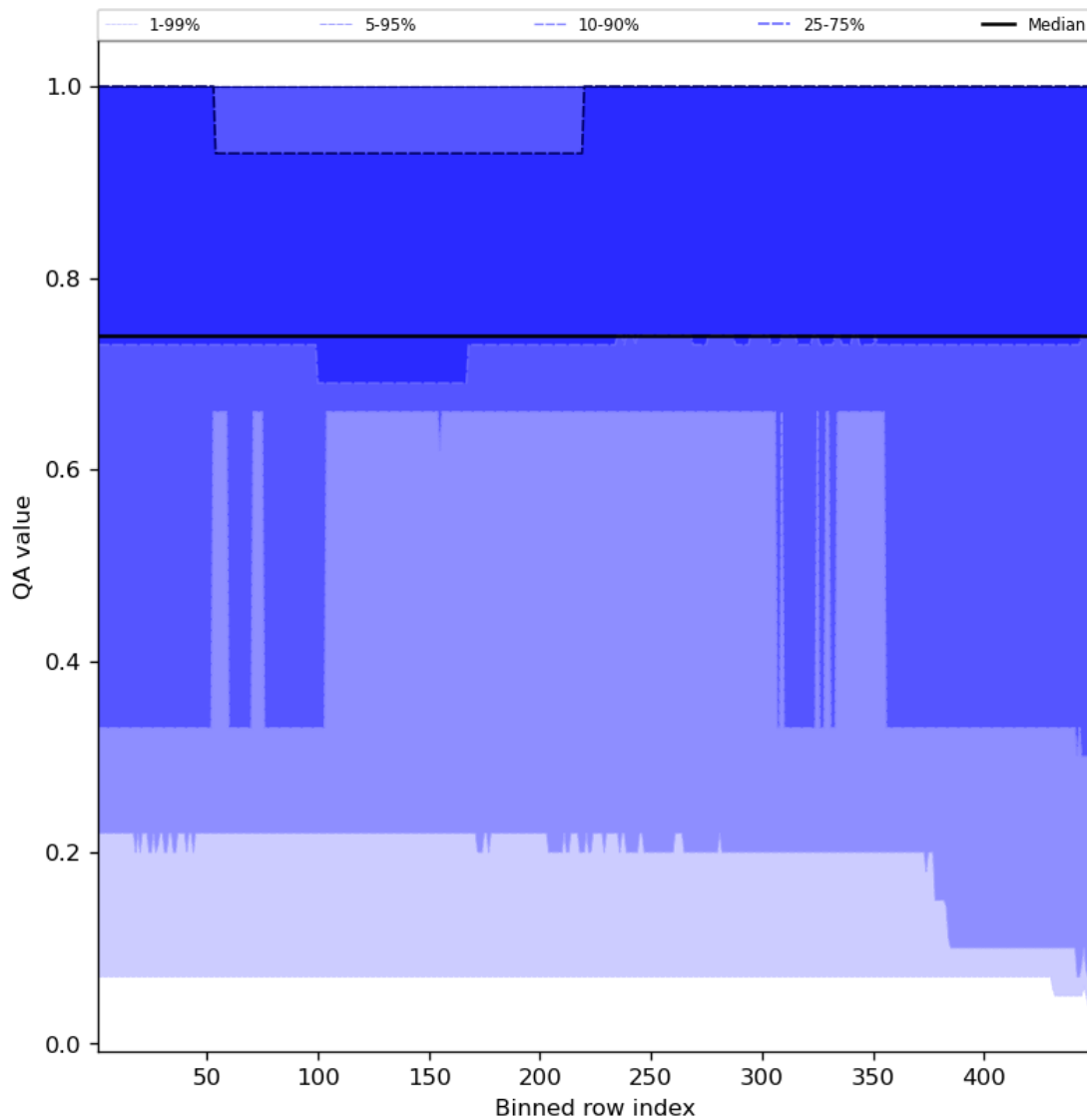
Figure 45: Along track statistics of “QA value” for 2023-11-13 to 2023-11-15
