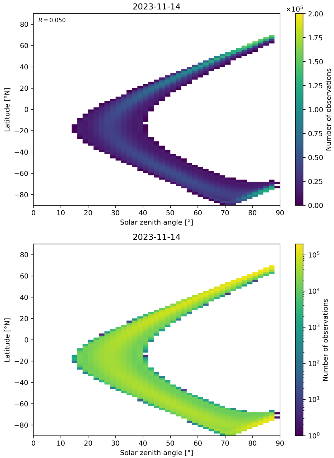
Figure 149: Scatter density plot of “Solar zenith angle” against “Latitude” for 2023-11-13 to 2023-11-15.
