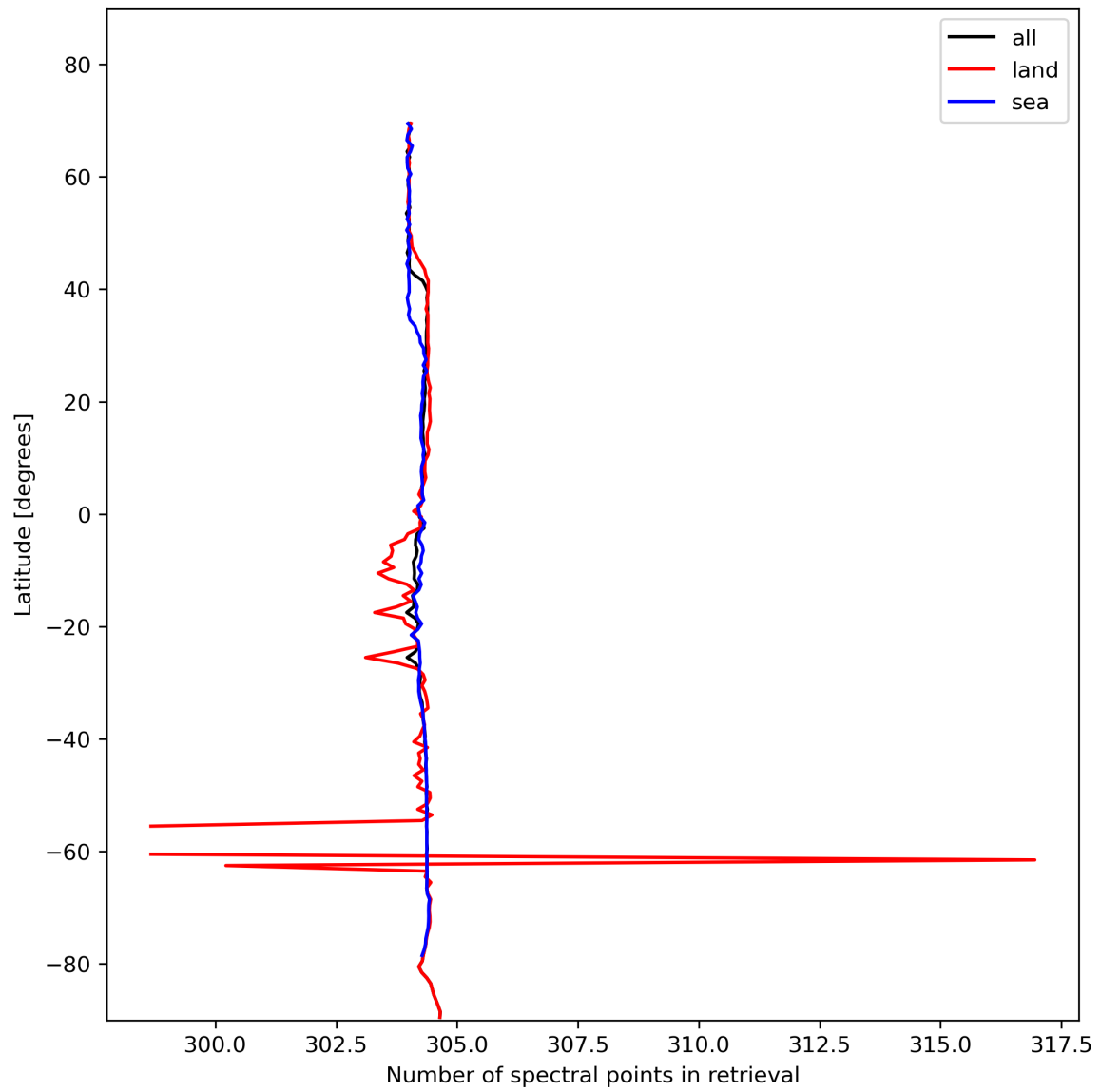
Figure 16: Zonal average of “Number of spectral points in retrieval” for 2023-11-13 to 2023-11-15.
