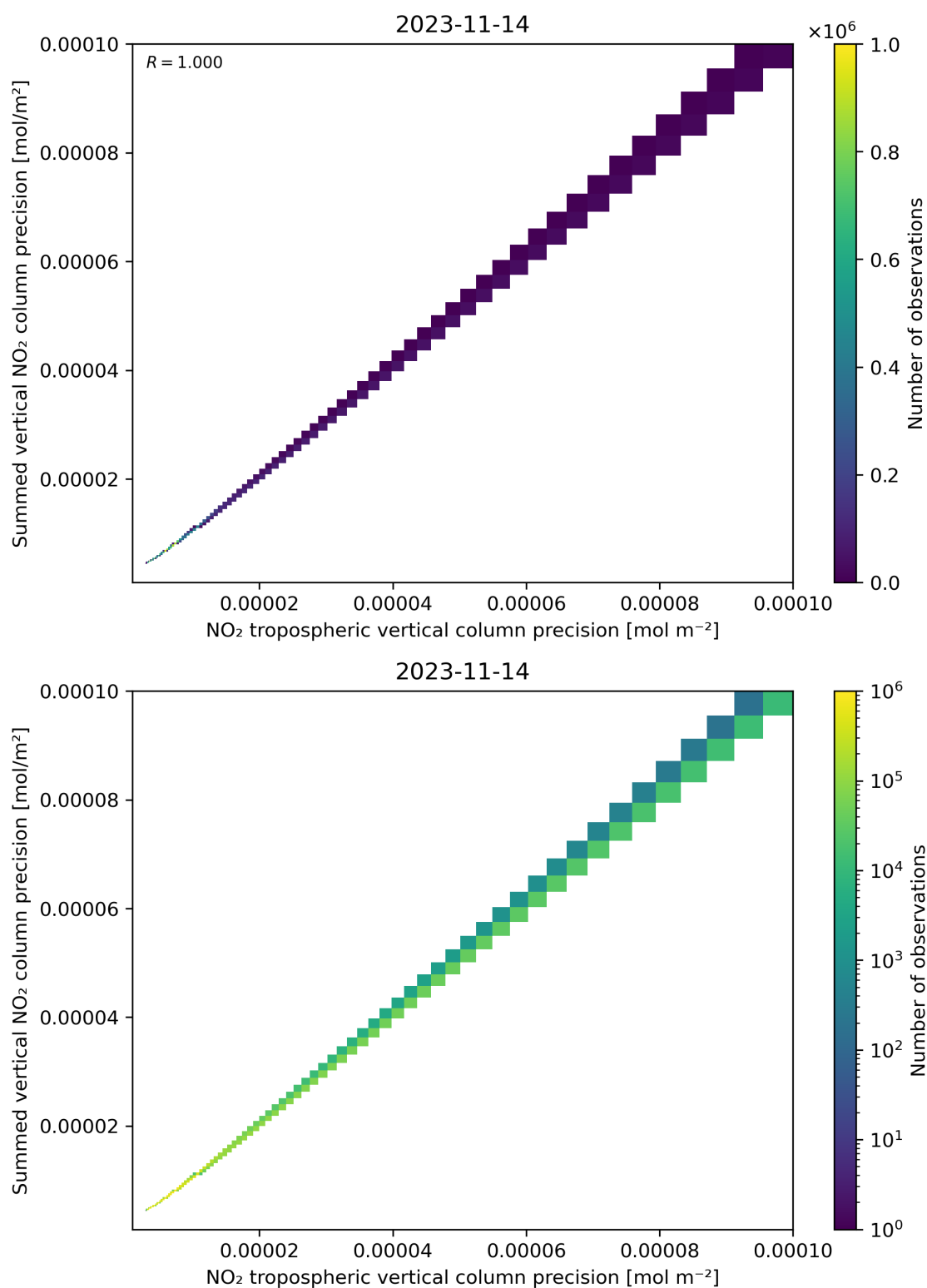
Figure 137: Scatter density plot of “NO 2 tropospheric vertical column precision” against “Summed vertical NO 2 column precision” for 2023-11-13 to 2023-11-15.
