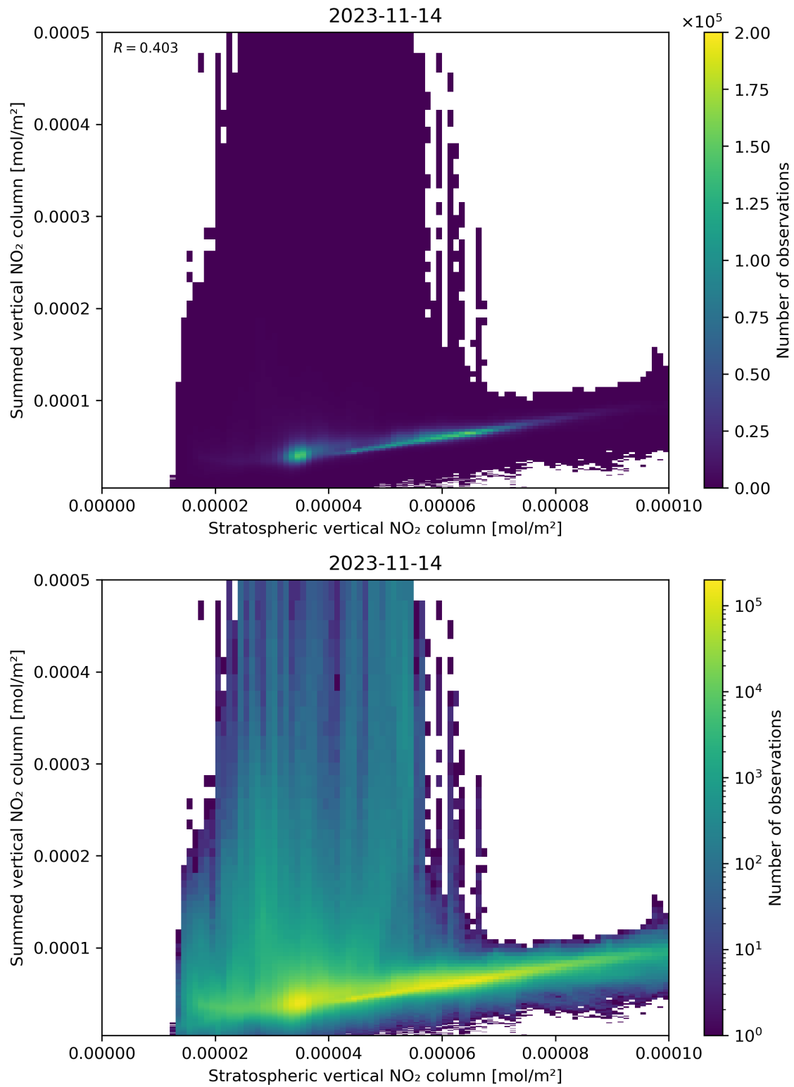
Figure 98: Scatter density plot of “Stratospheric vertical NO 2 column” against “Summed vertical NO 2 column” for 2023-11-13 to 2023-11-15.
