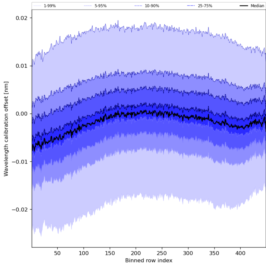
Figure 52: Along track statistics of “Wavelength calibration offset” for 2023-11-13 to 2023-11-15
