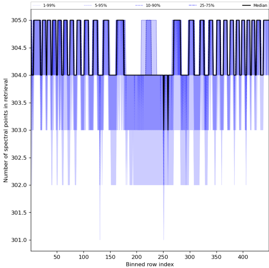
Figure 50: Along track statistics of “Number of spectral points in retrieval” for 2023-11-13 to 2023-11-15
