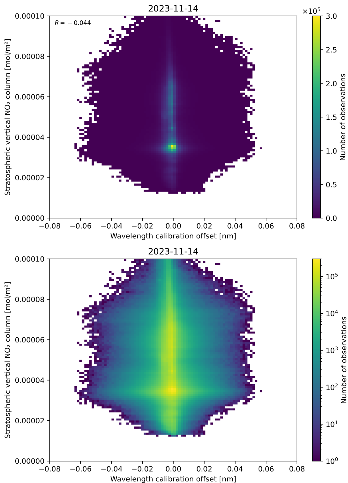
Figure 176: Scatter density plot of “Wavelength calibration offset” against “Stratospheric vertical NO 2 column” for 2023-11-13 to 2023-11-15.
