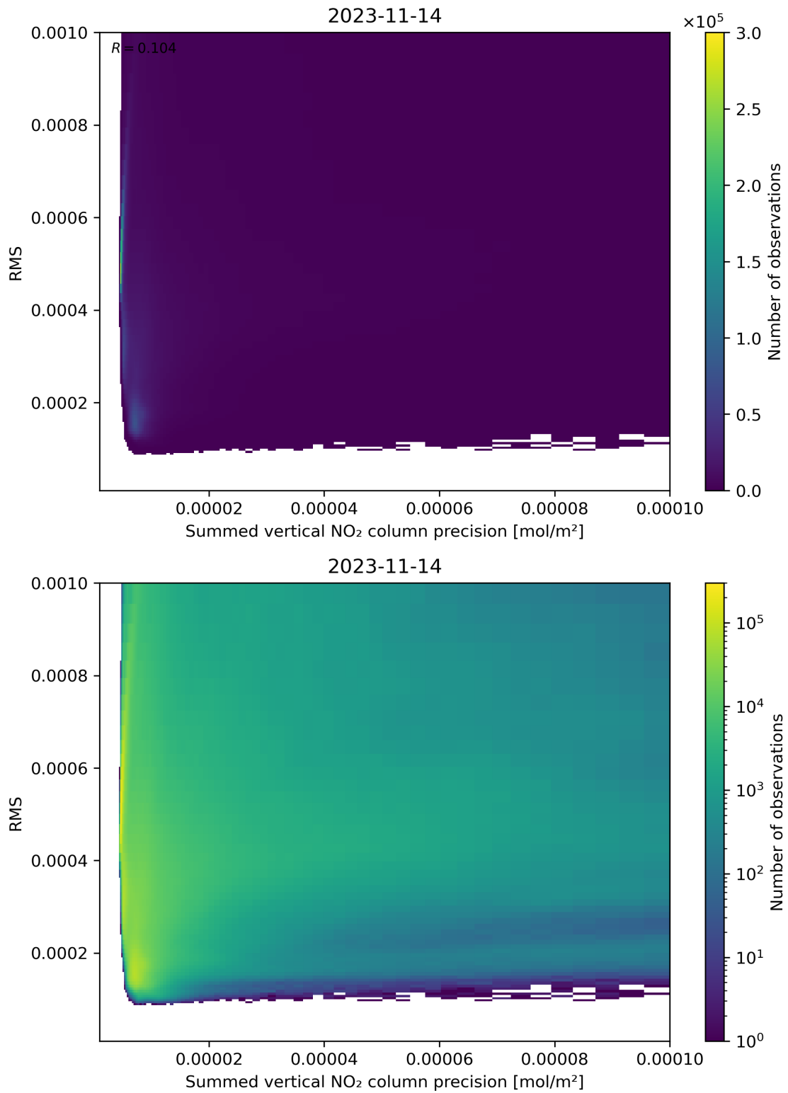
Figure 108: Scatter density plot of “Summed vertical NO 2 column precision” against “RMS” for 2023-11-13 to 2023-11-15.
