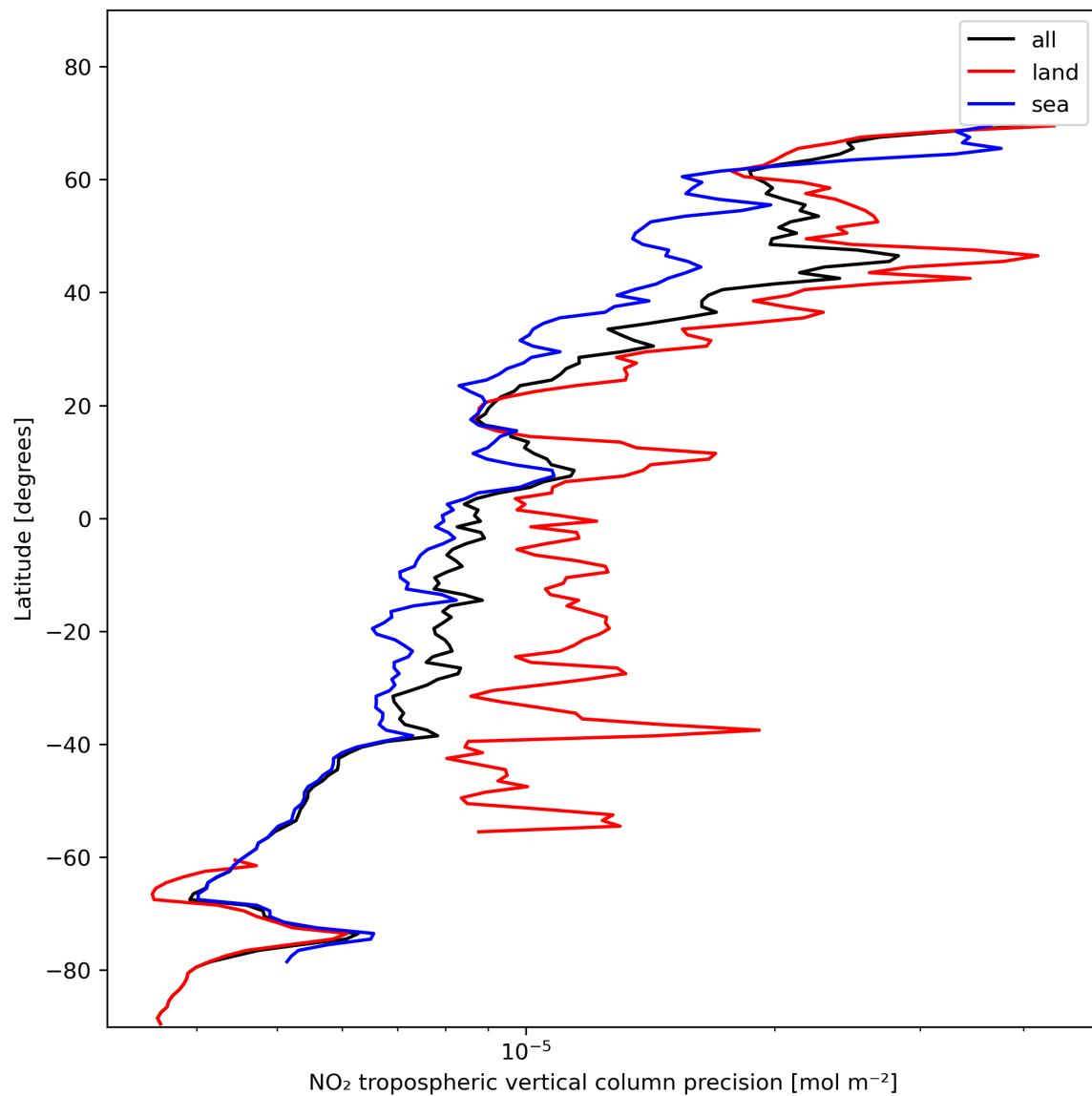
Figure 13: Zonal average of “NO 2 tropospheric vertical column precision” for 2023-11-13 to 2023-11-15.
