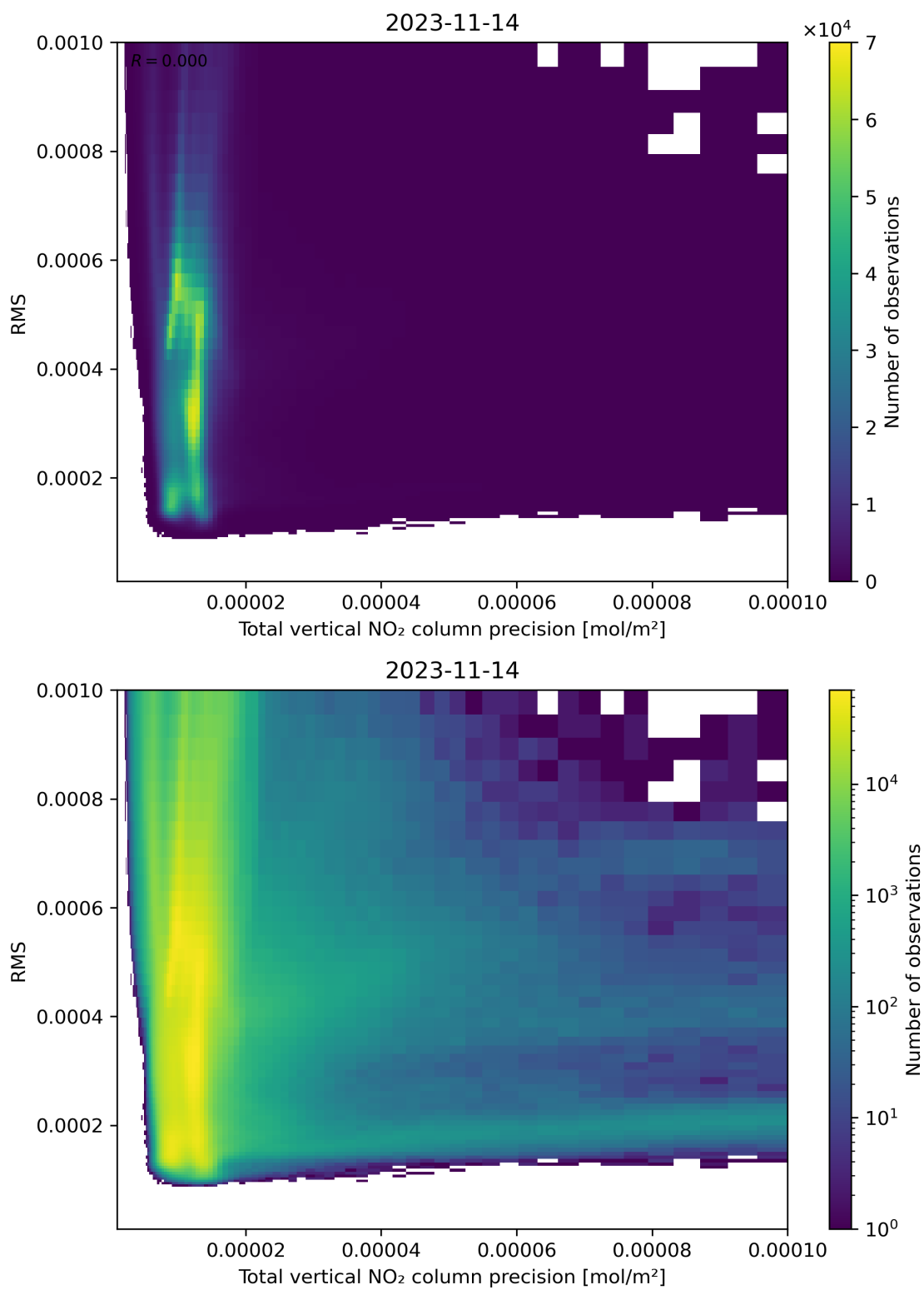
Figure 119: Scatter density plot of “Total vertical NO 2 column precision” against “RMS” for 2023-11-13 to 2023-11-15.
