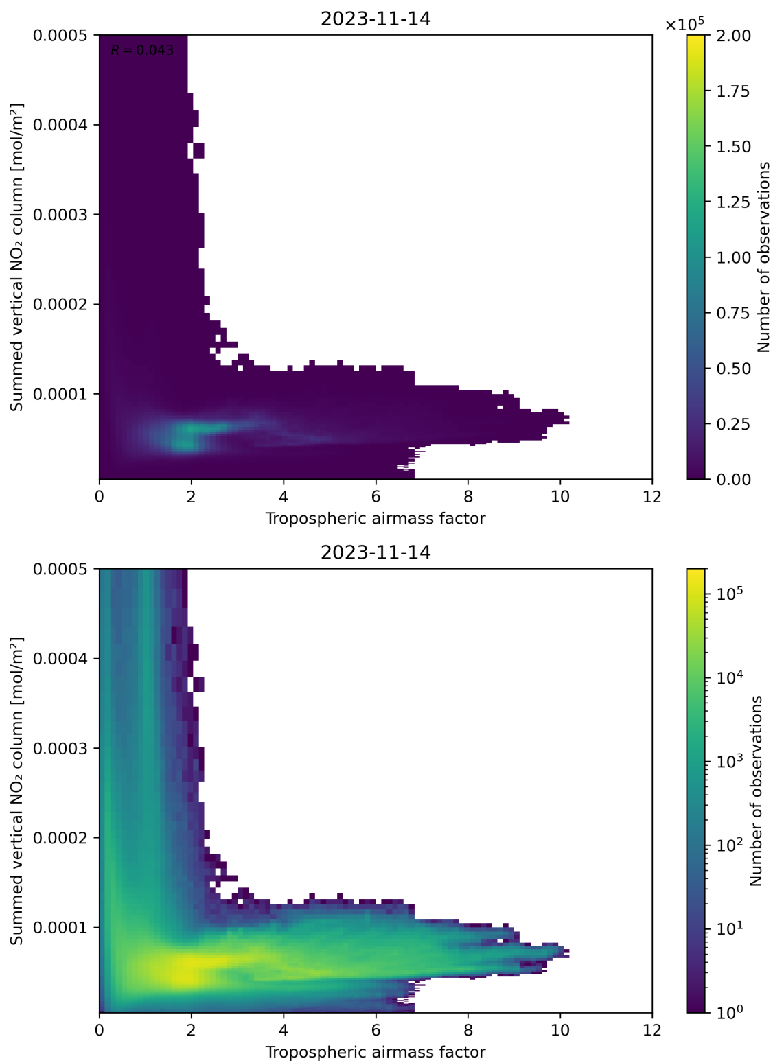
Figure 75: Scatter density plot of “Tropospheric airmass factor” against “Summed vertical NO 2 column” for 2023-11-13 to 2023-11-15.
