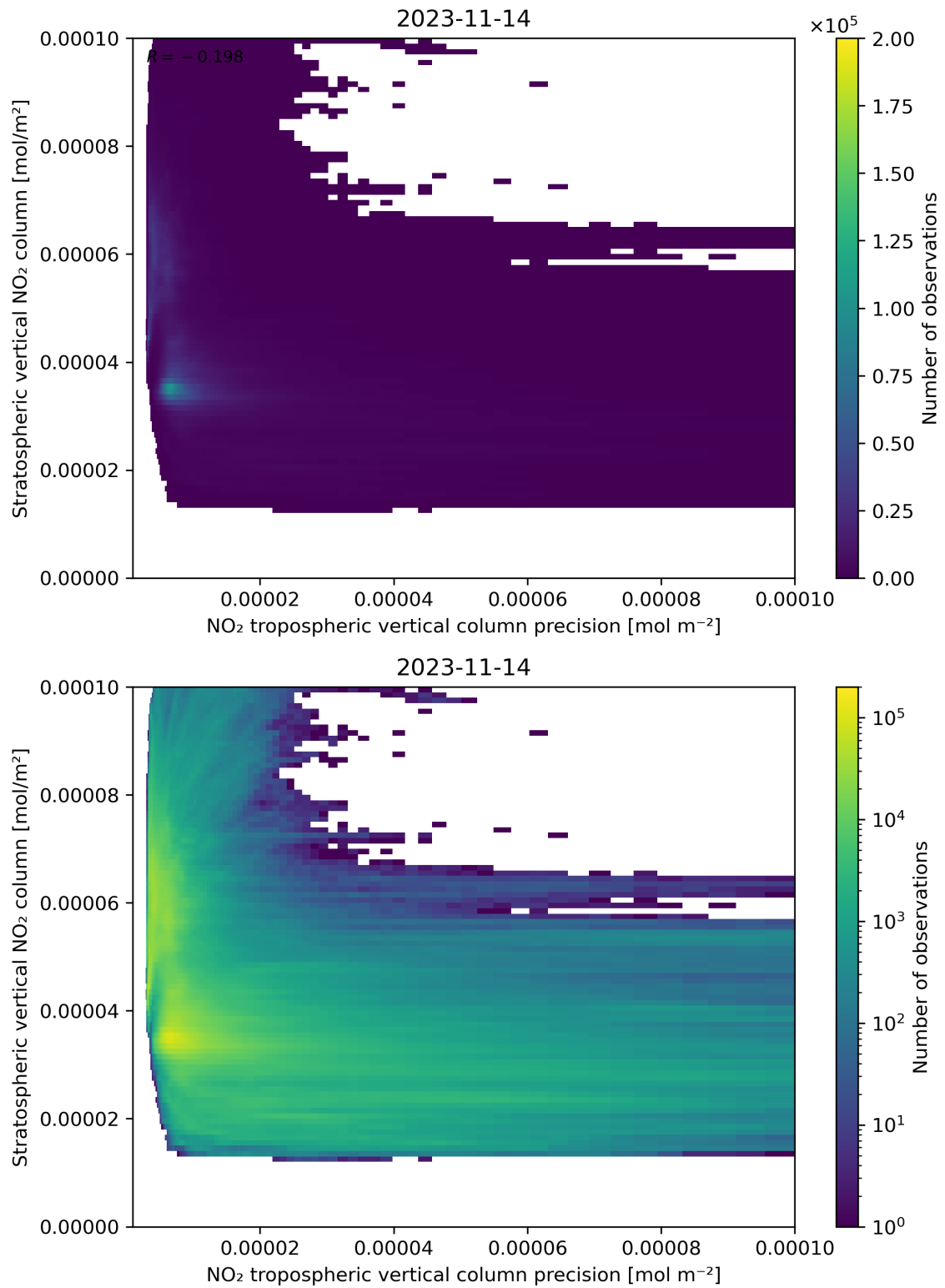
Figure 135: Scatter density plot of “NO 2 tropospheric vertical column precision” against “Stratospheric vertical NO 2 column” for 2023-11-13 to 2023-11-15.
