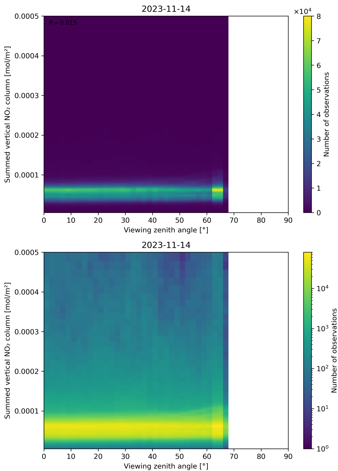
Figure 165: Scatter density plot of “Viewing zenith angle” against “Summed vertical NO 2 column” for 2023-11-13 to 2023-11-15.
