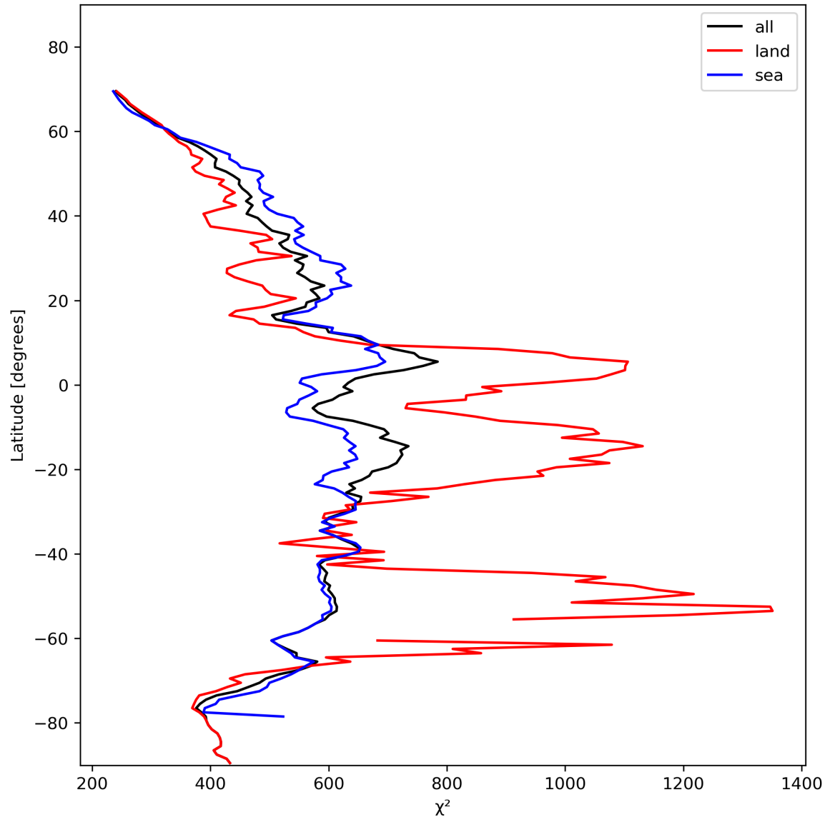
Figure 25: Zonal average of “ \chi^2 ” for 2023-11-13 to 2023-11-15.
