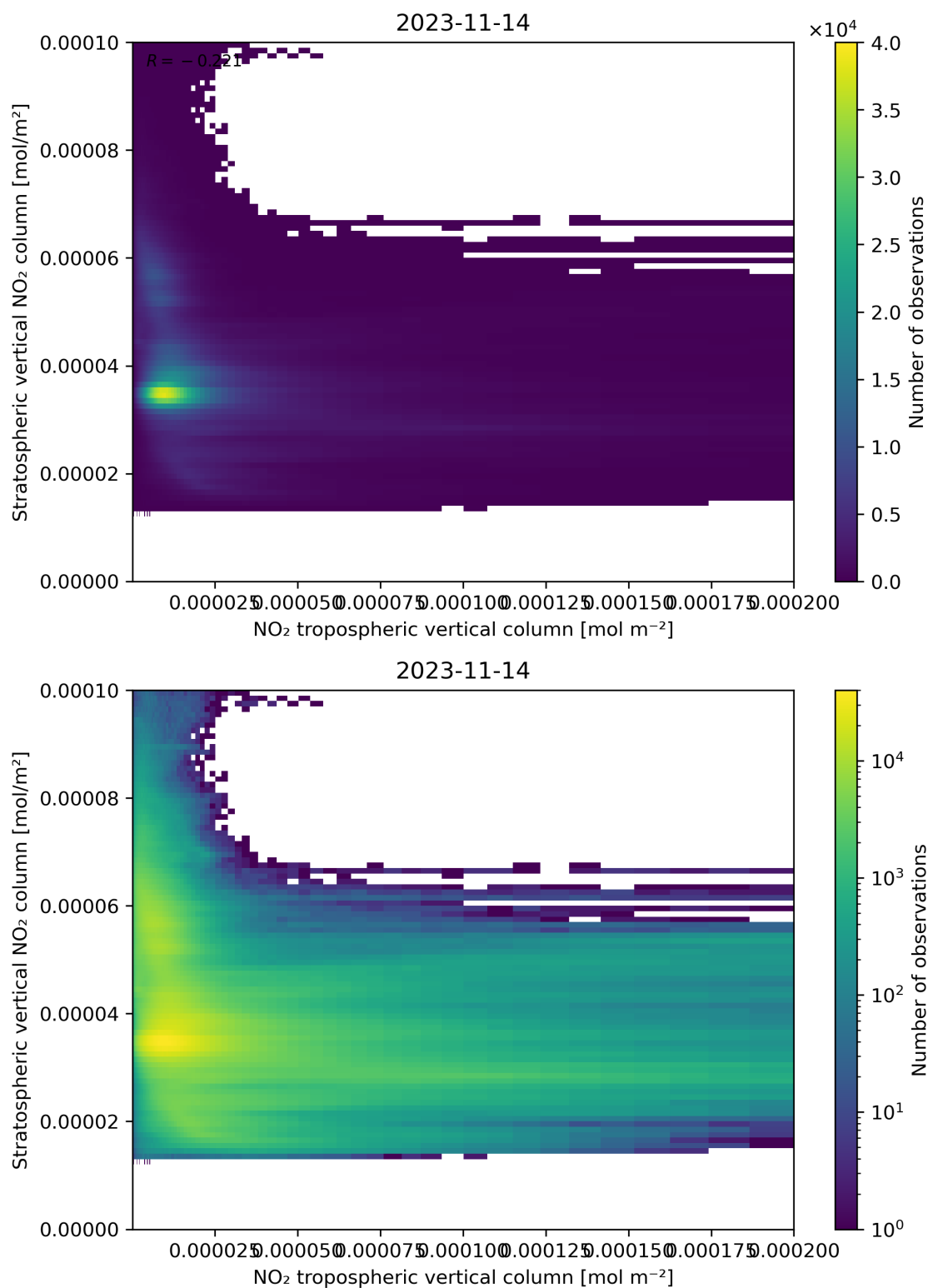
Figure 125: Scatter density plot of “NO 2 tropospheric vertical column” against “Stratospheric vertical NO 2 column” for 2023-11-13 to 2023-11-15.
