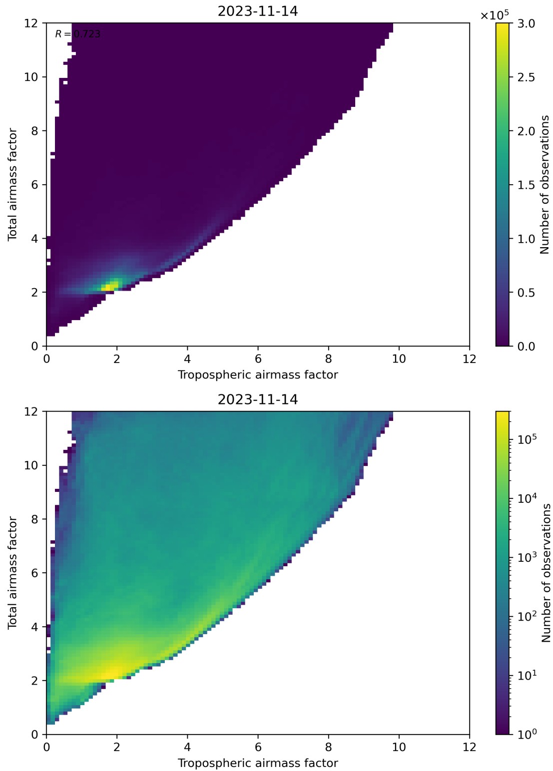
Figure 72: Scatter density plot of “Tropospheric airmass factor” against “Total airmass factor” for 2023-11-13 to 2023-11-15.
