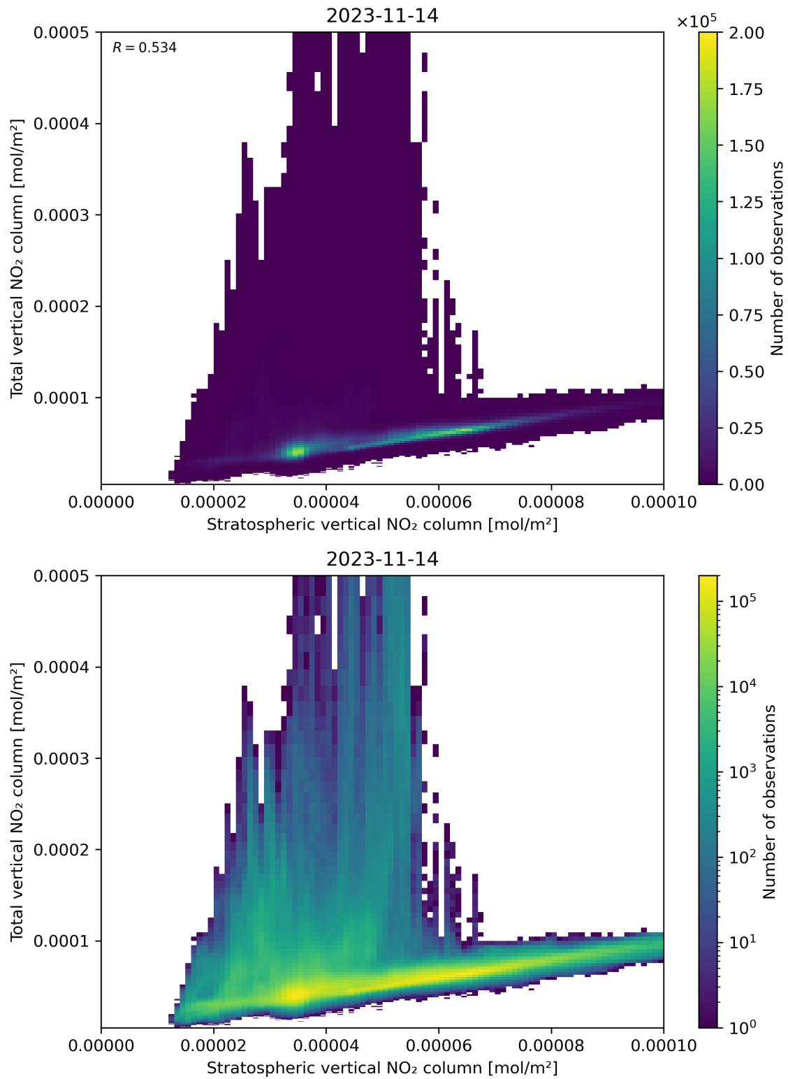
Figure 100: Scatter density plot of “Stratospheric vertical NO 2 column” against “Total vertical NO 2 column” for 2023-11-13 to 2023-11-15.
