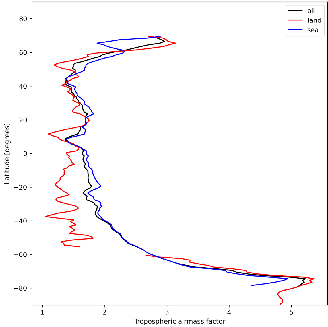
Figure 14: Zonal average of “Tropospheric airmass factor” for 2023-11-13 to 2023-11-15.
