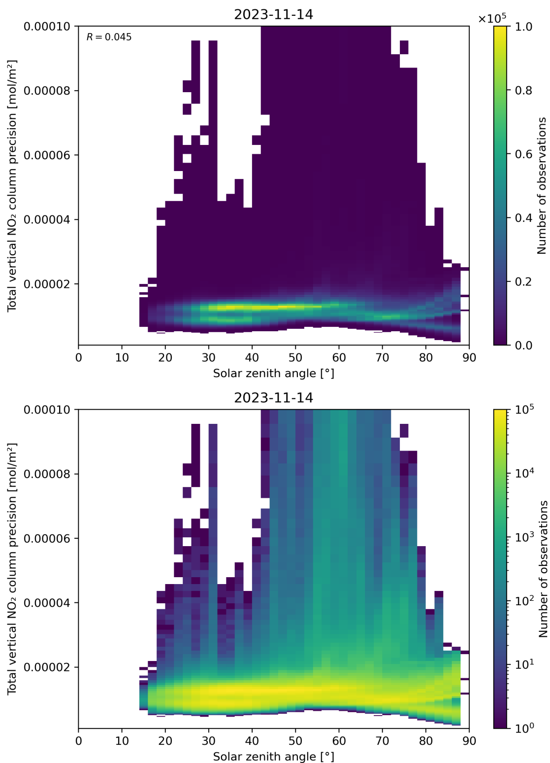
Figure 154: Scatter density plot of “Solar zenith angle” against “Total vertical NO 2 column precision” for 2023-11-13 to 2023-11-15.
