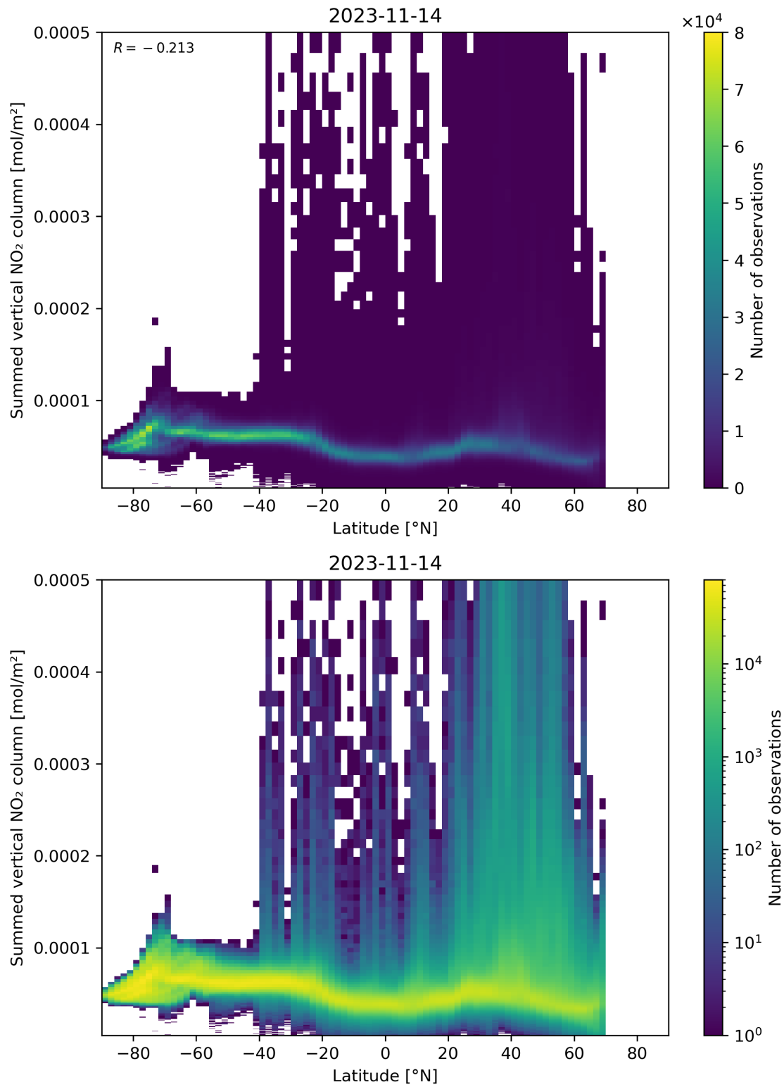
Figure 88: Scatter density plot of “Latitude” against “Summed vertical NO 2 column” for 2023-11-13 to 2023-11-15.
