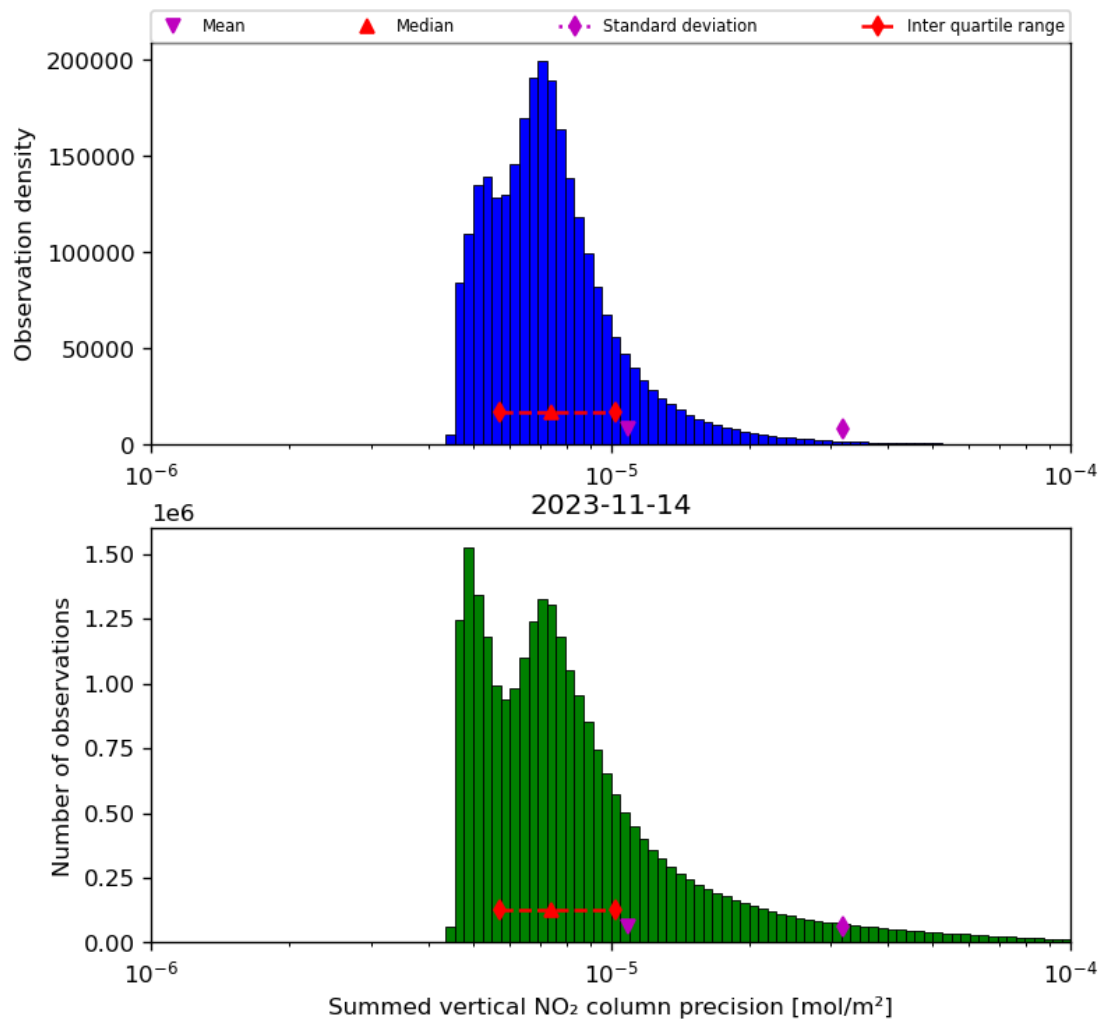
Figure 41: Histogram of "Summed vertical NO 2 column precision" for 2023-11-13 to 2023-11-15
