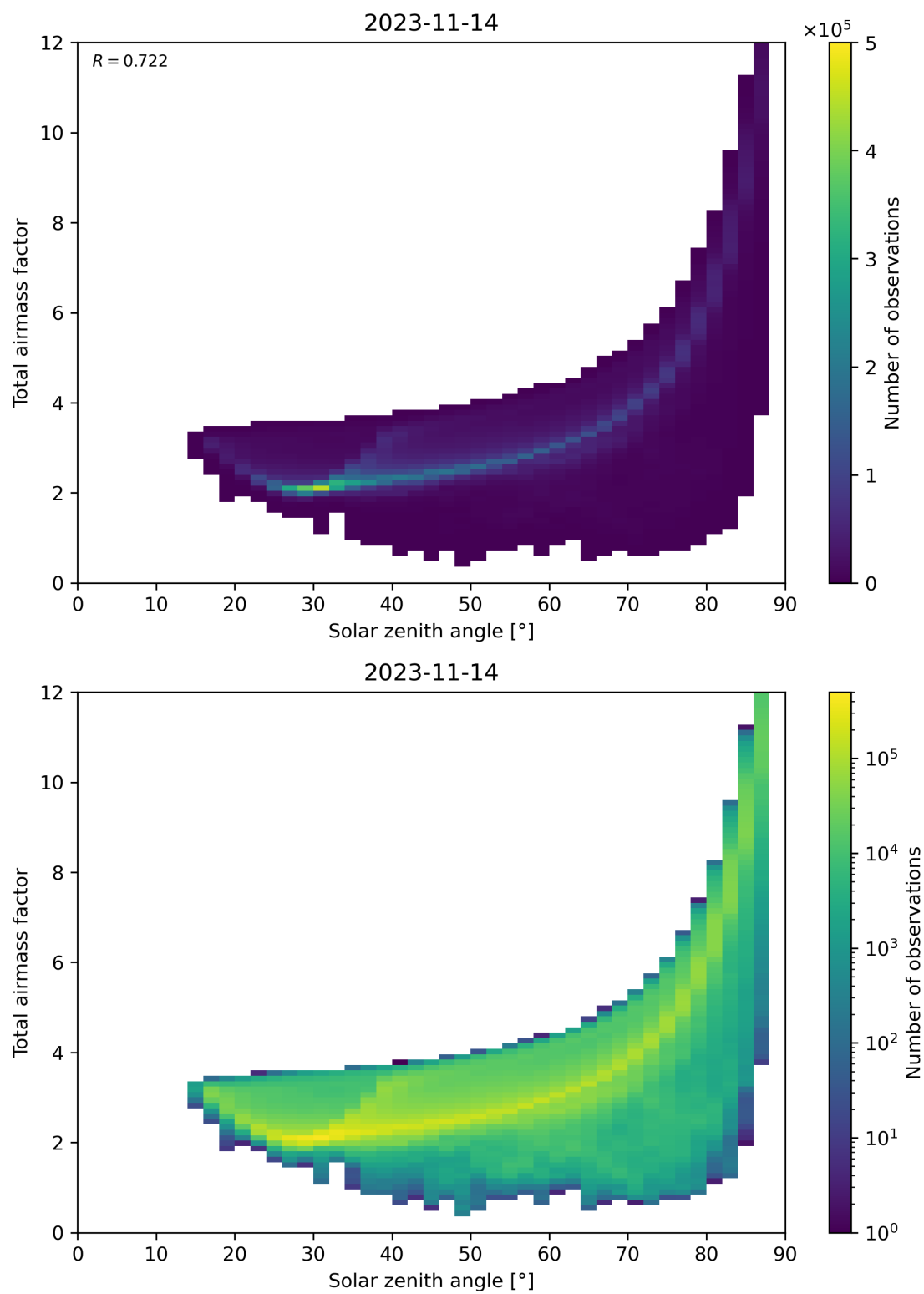
Figure 146: Scatter density plot of “Solar zenith angle” against “Total air mass factor” for 2023-11-13 to 2023-11-15.
