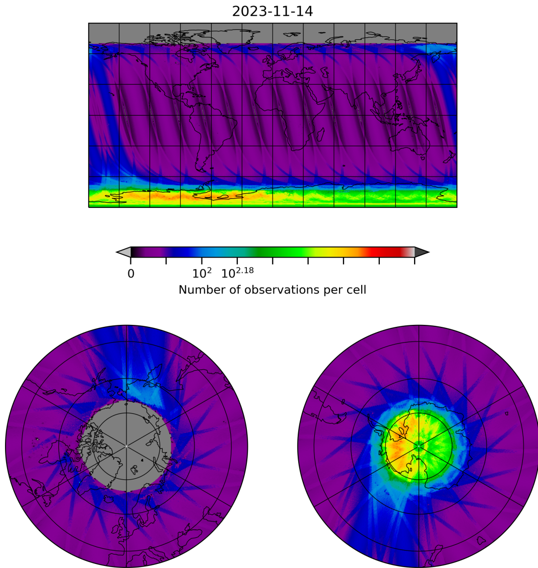
Figure 10: Map of the number of observations for 2023-11-13 to 2023-11-15
