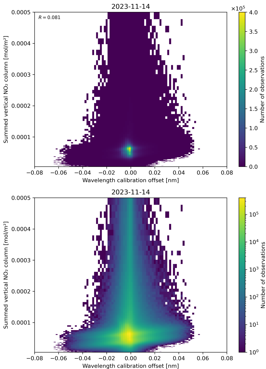
Figure 177: Scatter density plot of “Wavelength calibration offset” against “Summed vertical NO 2 column” for 2023-11-13 to 2023-11-15.
