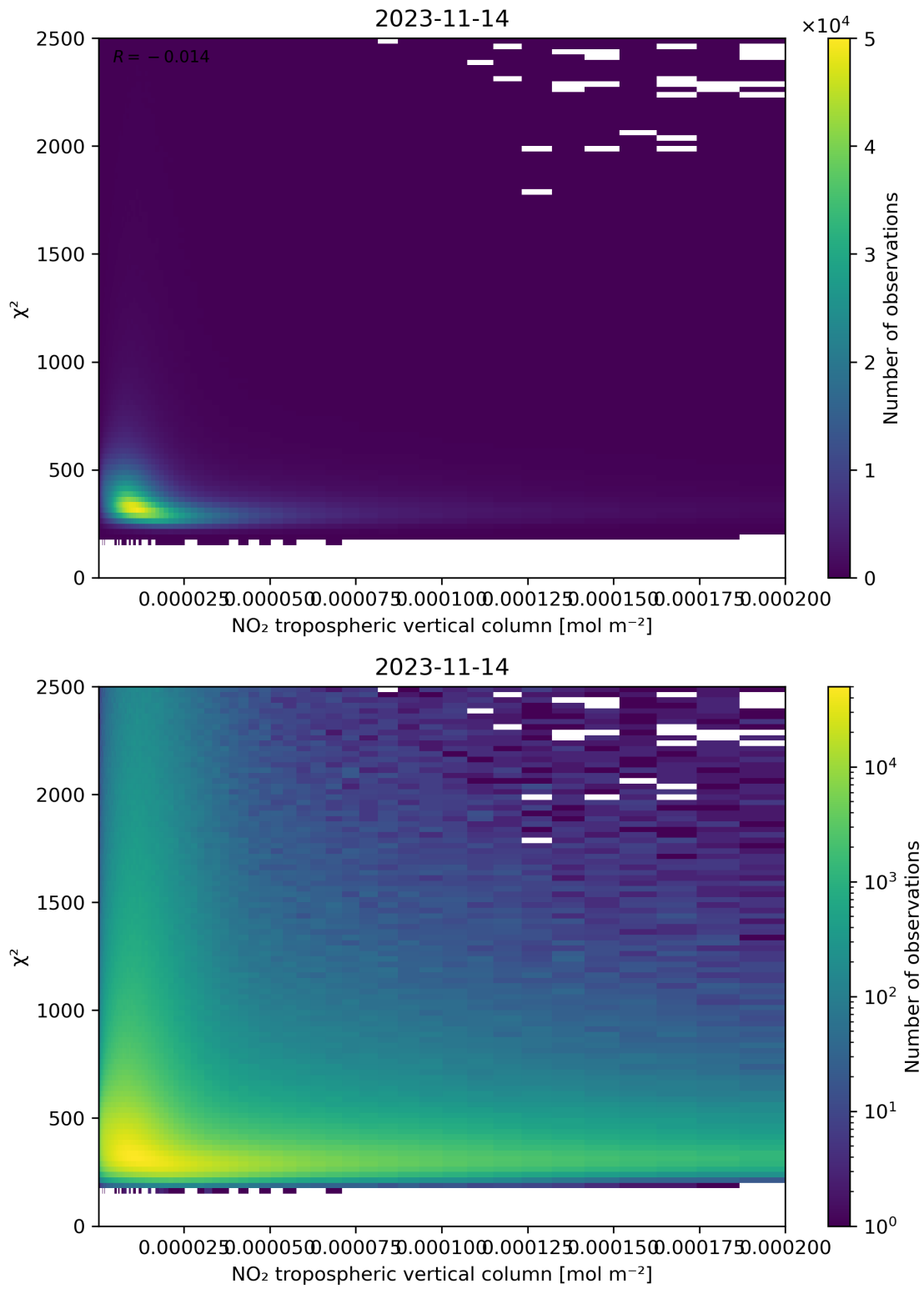
Figure 124: Scatter density plot of “NO 2 tropospheric vertical column” against “ \chi^2 ” for 2023-11-13 to 2023-11-15.
