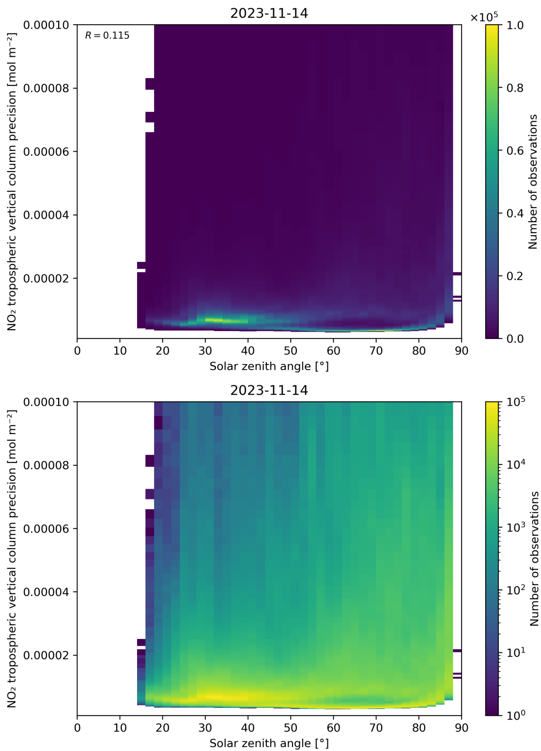
Figure 156: Scatter density plot of “Solar zenith angle” against “NO 2 tropospheric vertical column precision” for 2023-11-13 to 2023-11-15.
