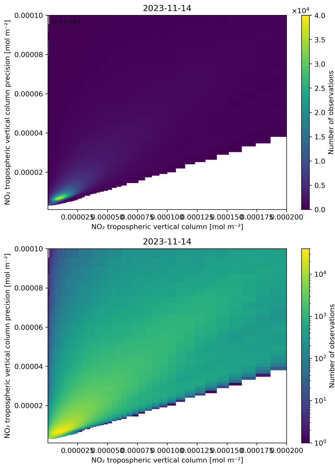
Figure 130: Scatter density plot of “NO 2 tropospheric vertical column” against “NO 2 tropospheric vertical column precision” for 2023-11-13 to 2023-11-15.
