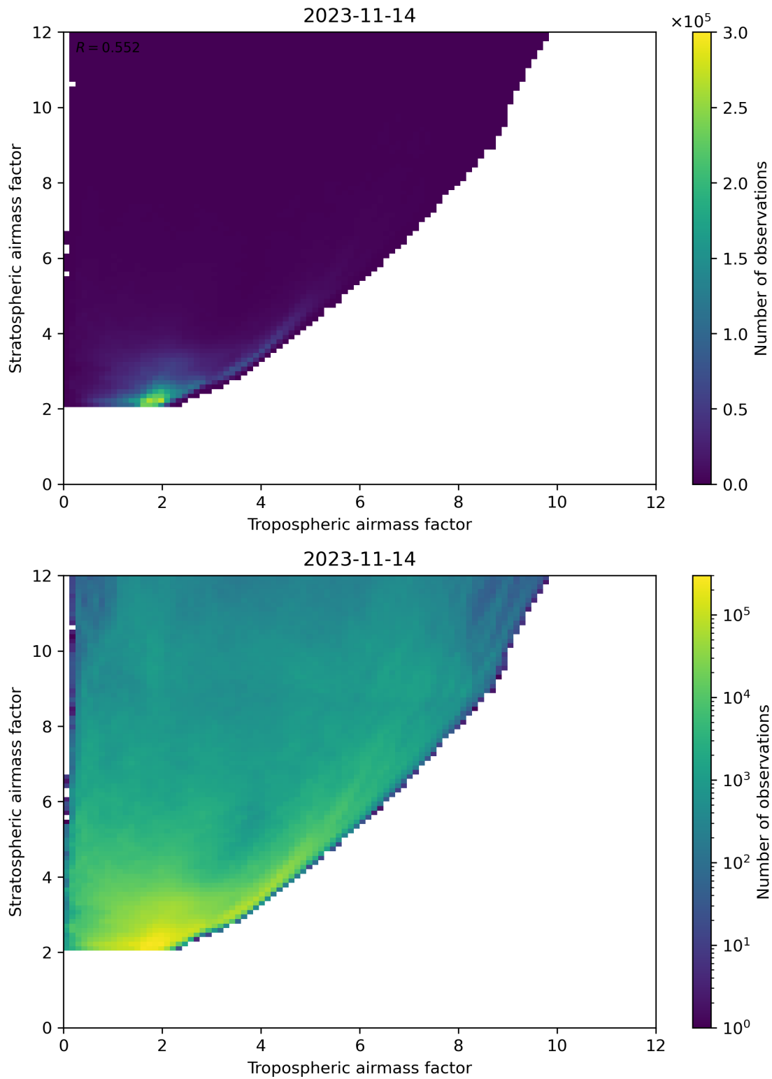
Figure 71: Scatter density plot of “Tropospheric airmass factor” against “Stratospheric airmass factor” for 2023-11-13 to 2023-11-15.
