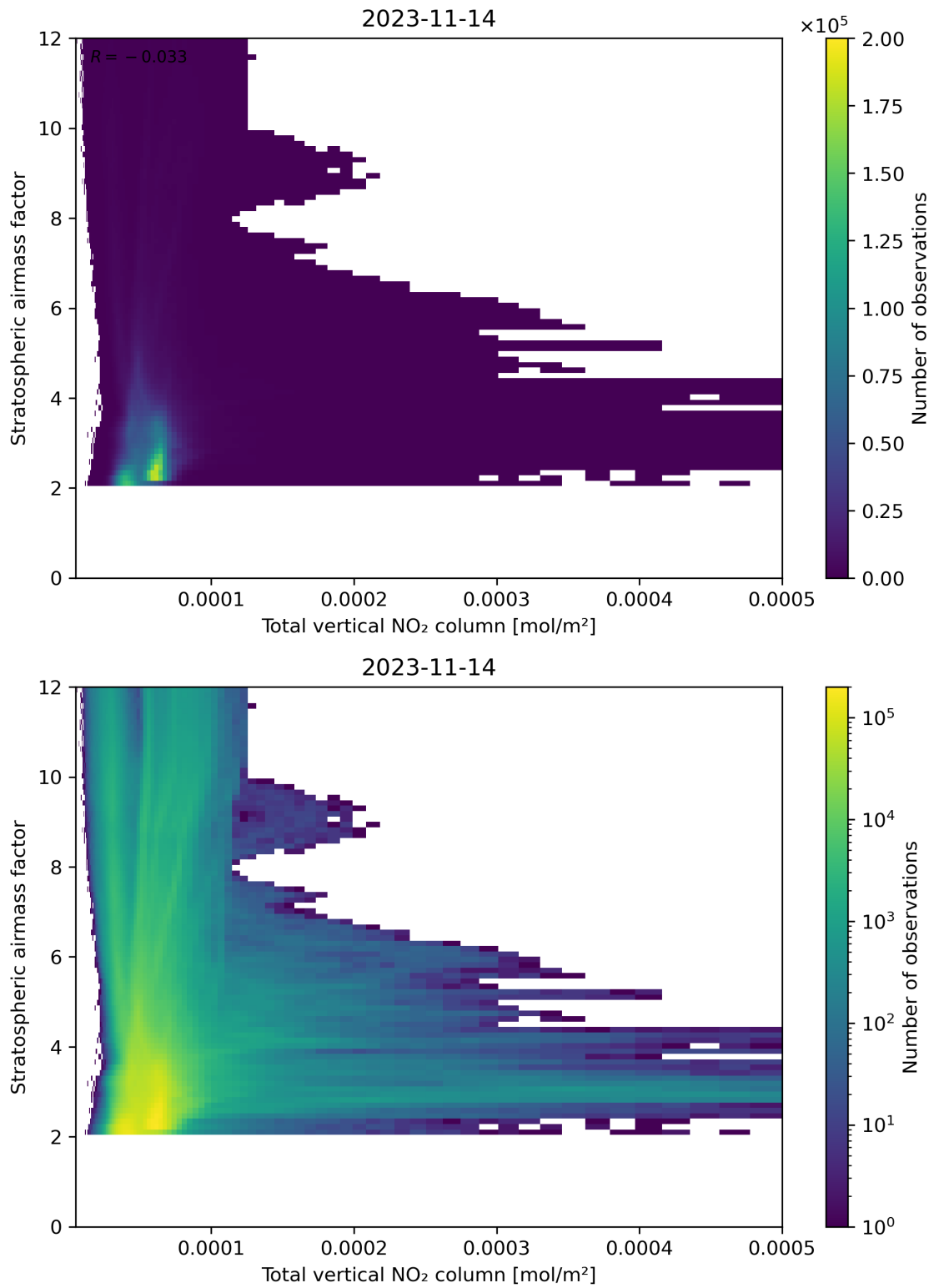
Figure 110: Scatter density plot of “Total vertical NO 2 column” against “Stratospheric airmass factor” for 2023-11-13 to 2023-11-15.
