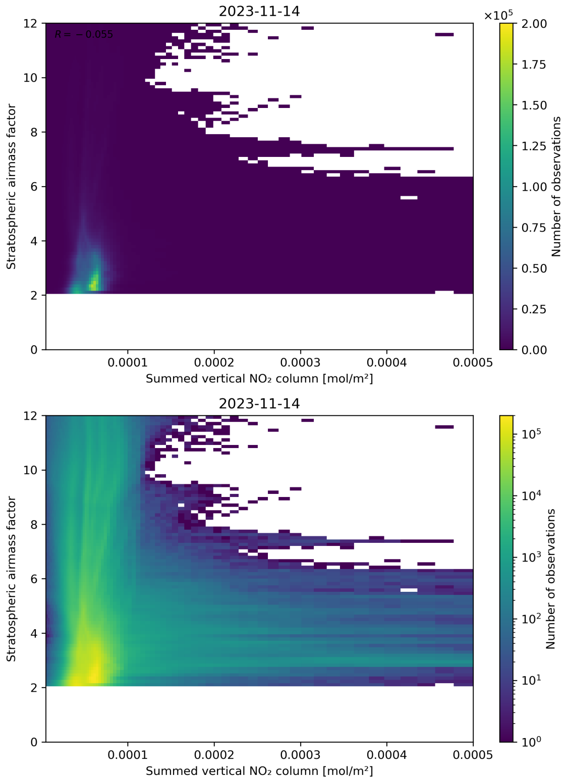
Figure 103: Scatter density plot of “Summed vertical NO 2 column” against “Stratospheric airmass factor” for 2023-11-13 to 2023-11-15.
