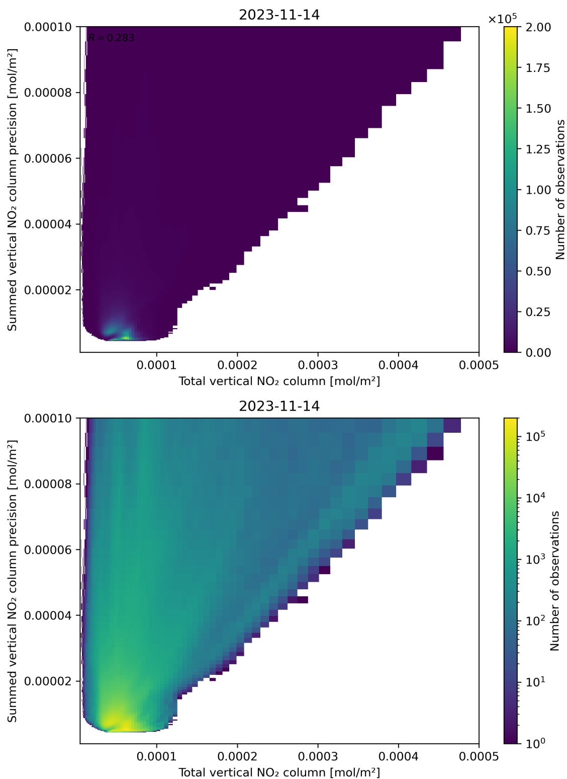
Figure 113: Scatter density plot of “Total vertical NO 2 column” against “Summed vertical NO 2 column precision” for 2023-11-13 to 2023-11-15.
