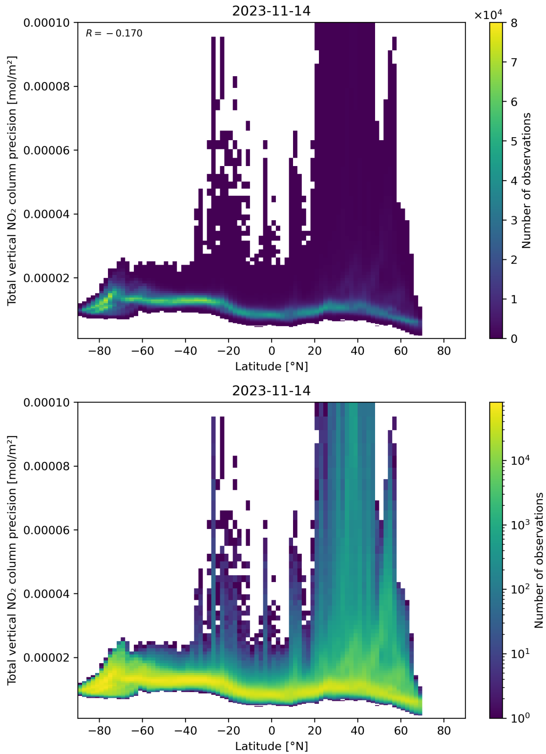
Figure 91: Scatter density plot of “Latitude” against “Total vertical NO 2 column precision” for 2023-11-13 to 2023-11-15.
