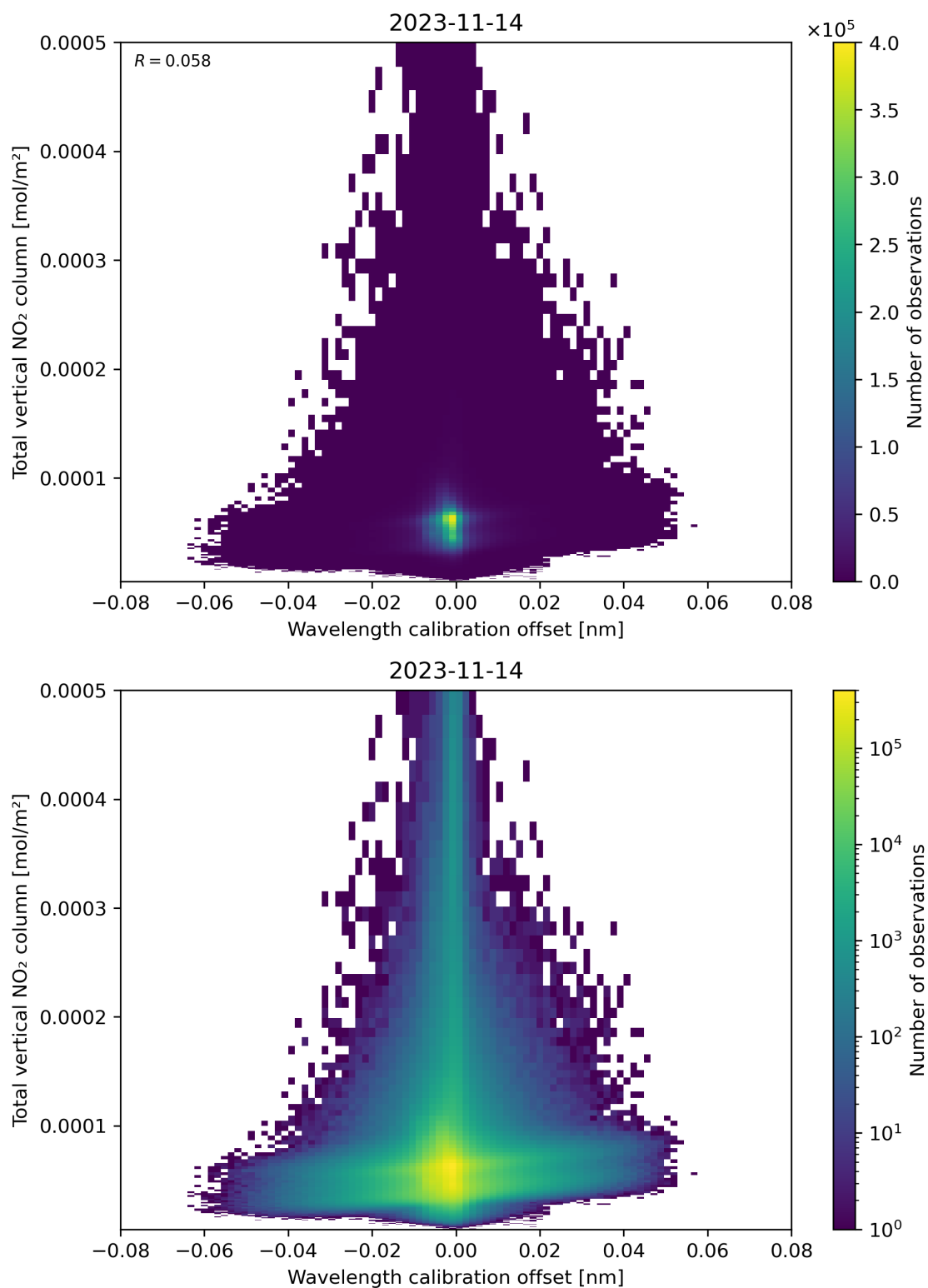
Figure 179: Scatter density plot of “Wavelength calibration offset” against “Total vertical NO 2 column” for 2023-11-13 to 2023-11-15.
