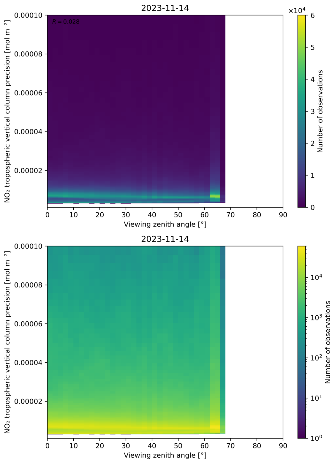
Figure 170: Scatter density plot of “Viewing zenith angle” against “NO 2 tropospheric vertical column precision” for 2023-11-13 to 2023-11-15.
