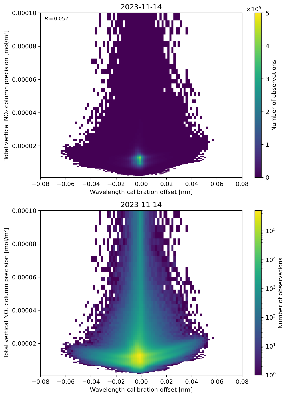
Figure 180: Scatter density plot of “Wavelength calibration offset” against “Total vertical NO 2 column precision” for 2023-11-13 to 2023-11-15.
