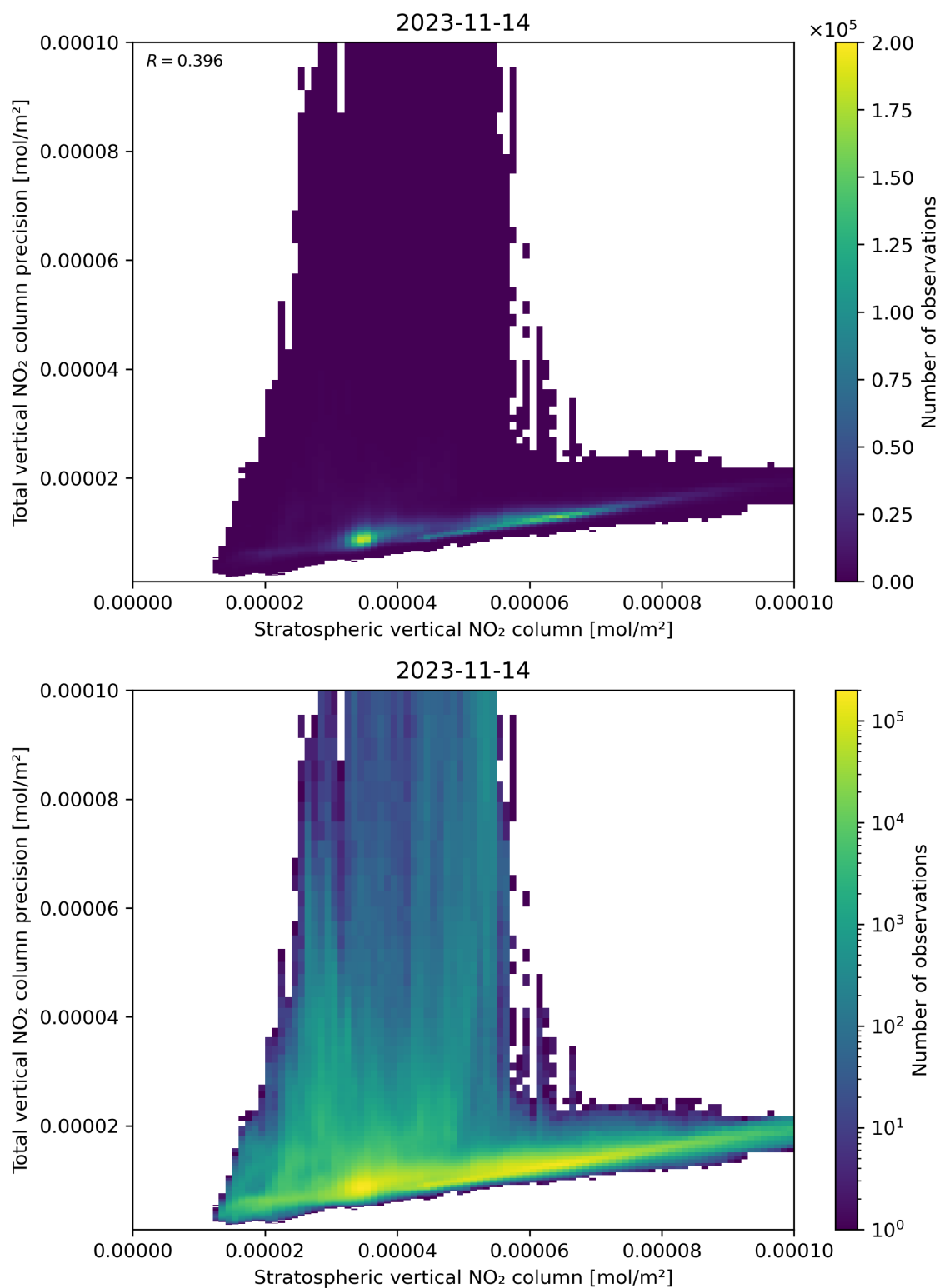
Figure 101: Scatter density plot of “Stratospheric vertical NO 2 column” against “Total vertical NO 2 column precision” for 2023-11-13 to 2023-11-15.
