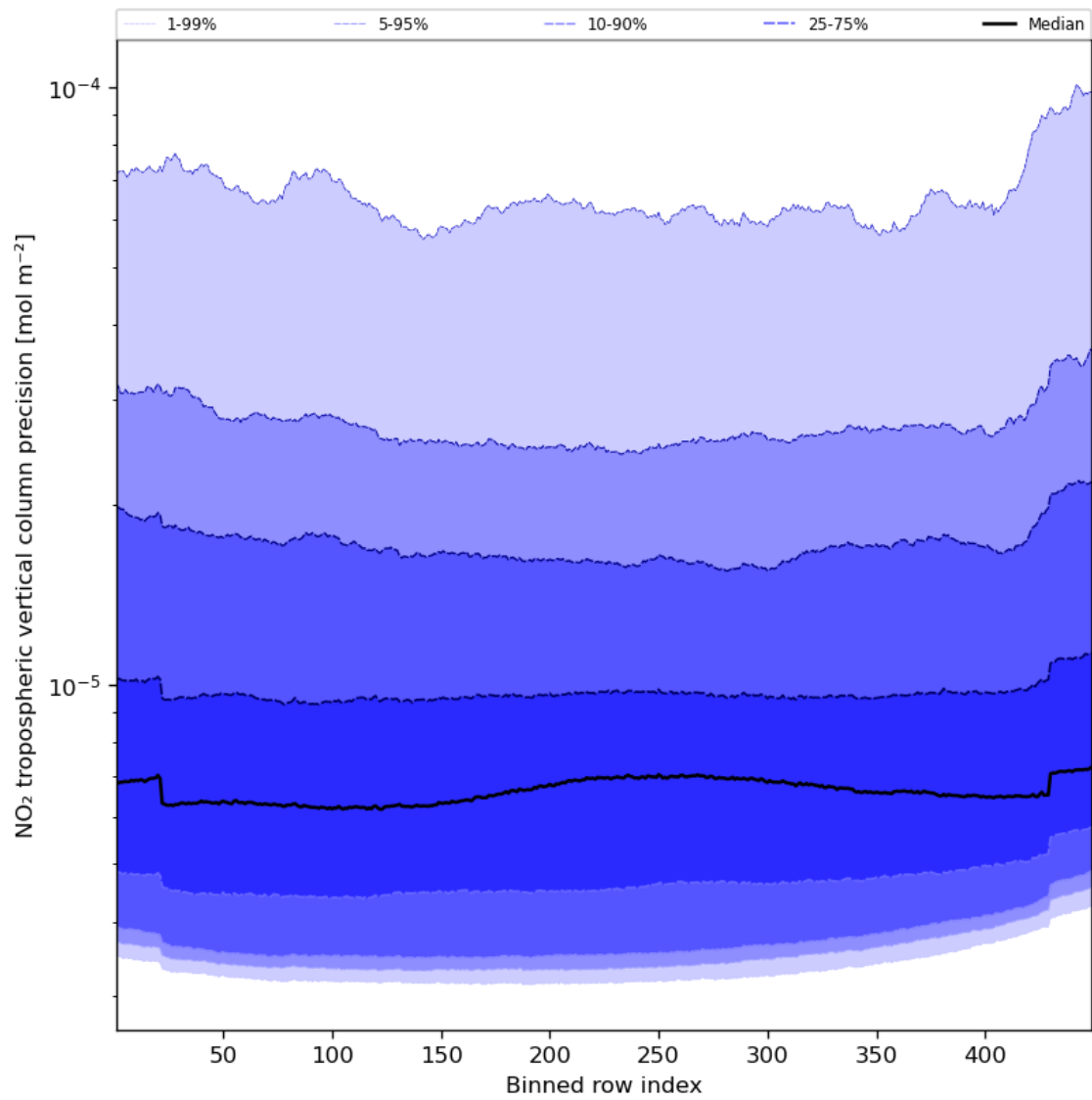
Figure 47: Along track statistics of “NO 2 tropospheric vertical column precision” for 2023-11-13 to 2023-11-15
