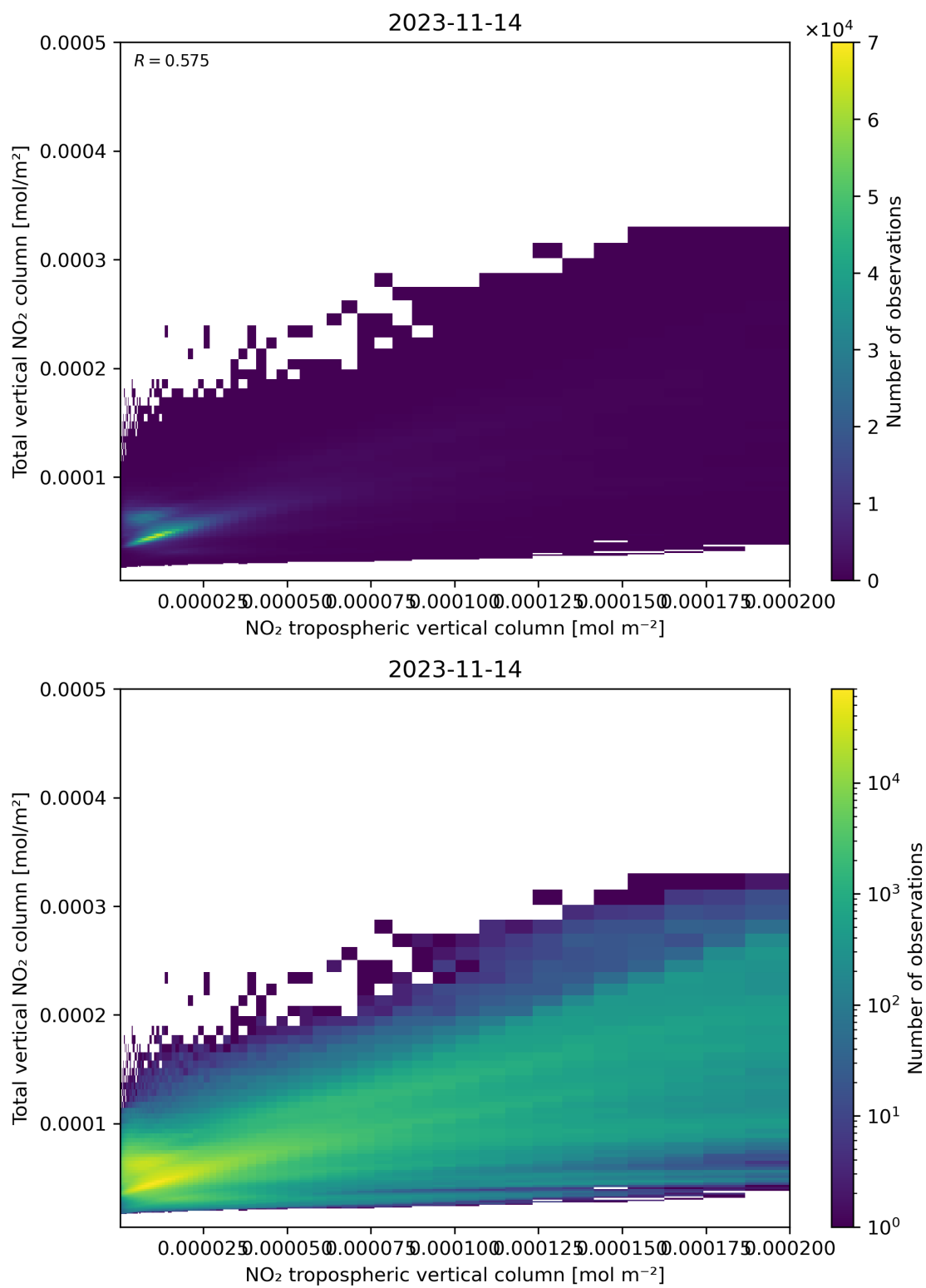
Figure 128: Scatter density plot of “NO 2 tropospheric vertical column” against “Total vertical NO 2 column” for 2023-11-13 to 2023-11-15.
