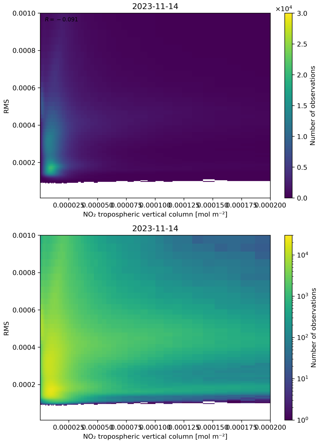
Figure 142: Scatter density plot of “NO 2 tropospheric vertical column” against “RMS” for 2023-11-13 to 2023-11-15.
