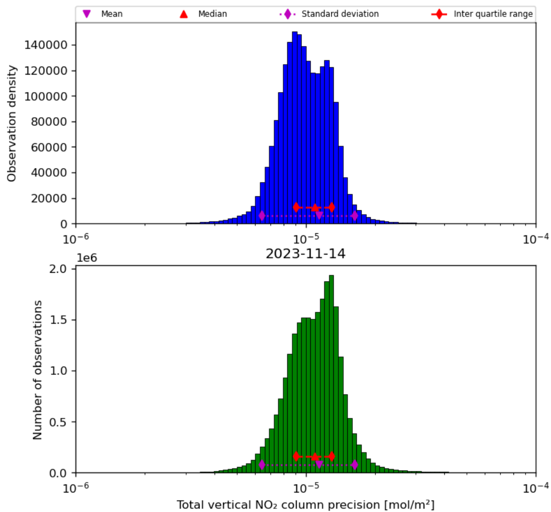
Figure 39: Histogram of “Total vertical NO 2 column precision” for 2023-11-13 to 2023-11-15
