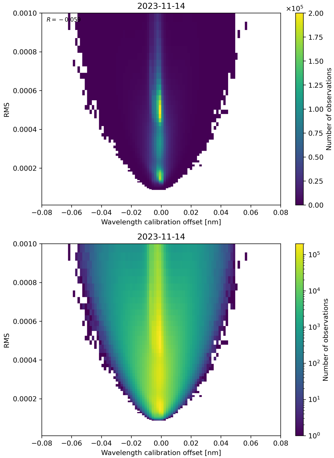
Figure 181: Scatter density plot of “Wavelength calibration offset” against “RMS” for 2023-11-13 to 2023-11-15.
