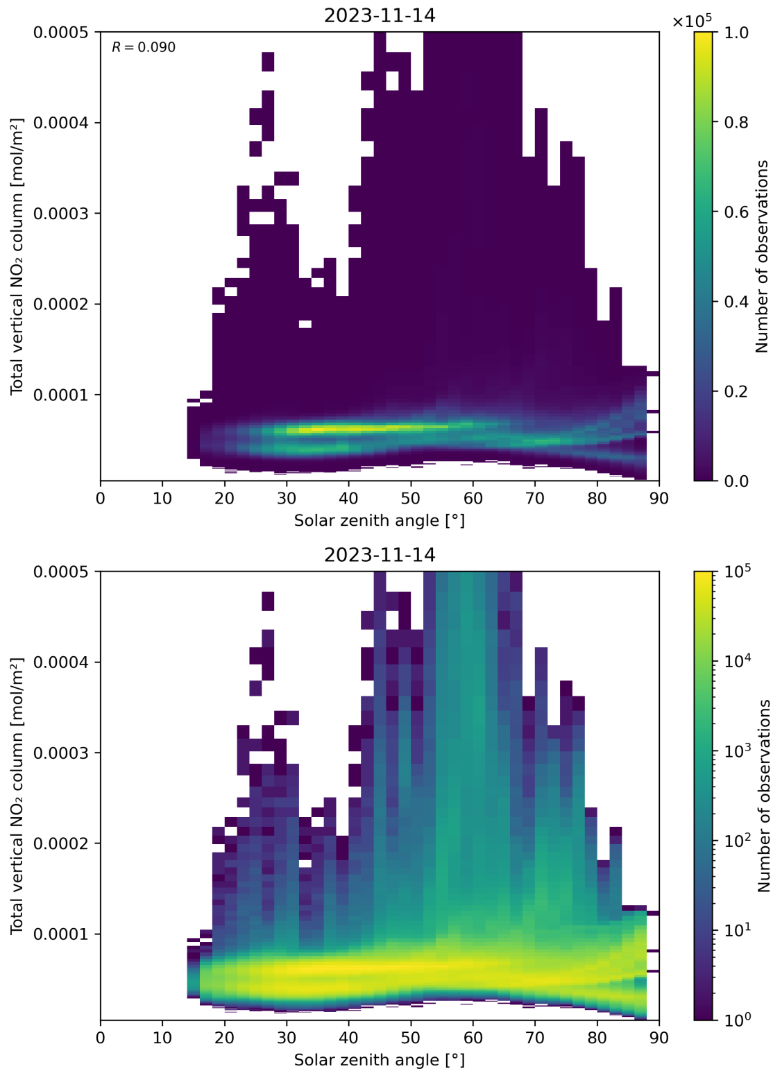
Figure 153: Scatter density plot of “Solar zenith angle” against “Total vertical NO 2 column” for 2023-11-13 to 2023-11-15.
