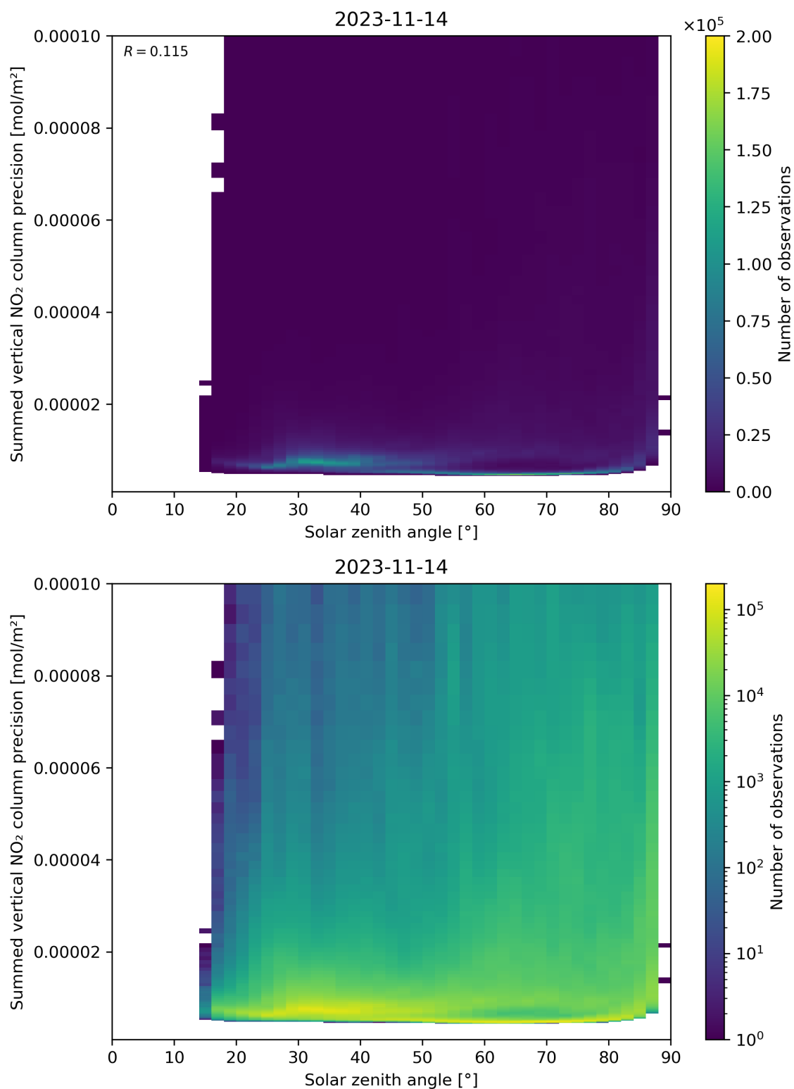
Figure 152: Scatter density plot of “Solar zenith angle” against “Summed vertical NO 2 column precision” for 2023-11-13 to 2023-11-15.
