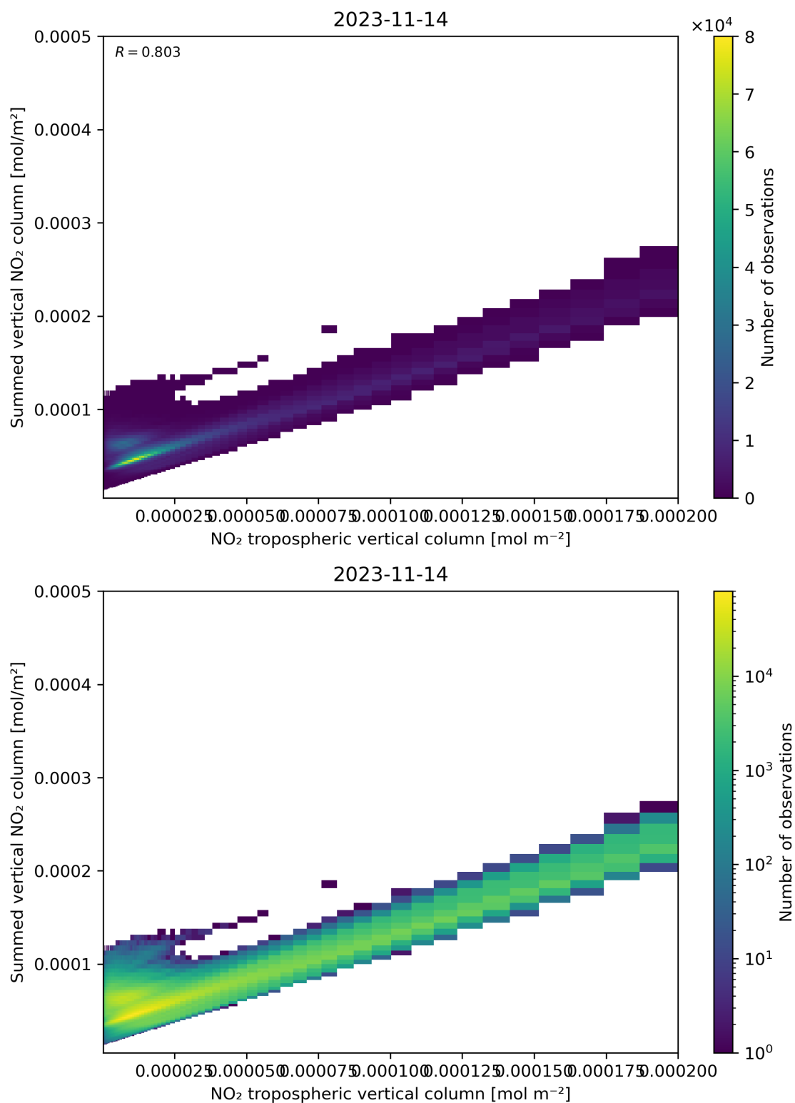
Figure 126: Scatter density plot of “NO 2 tropospheric vertical column” against “Summed vertical NO 2 column” for 2023-11-13 to 2023-11-15.
