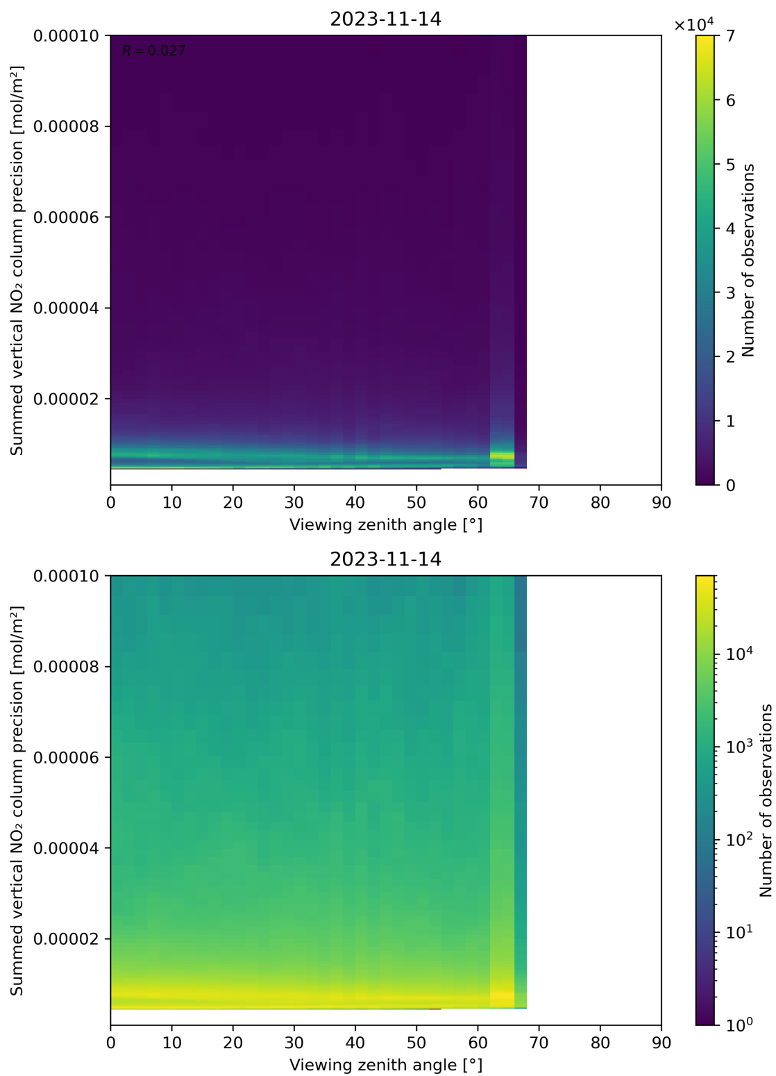
Figure 166: Scatter density plot of “Viewing zenith angle” against “Summed vertical NO 2 column precision” for 2023-11-13 to 2023-11-15.
