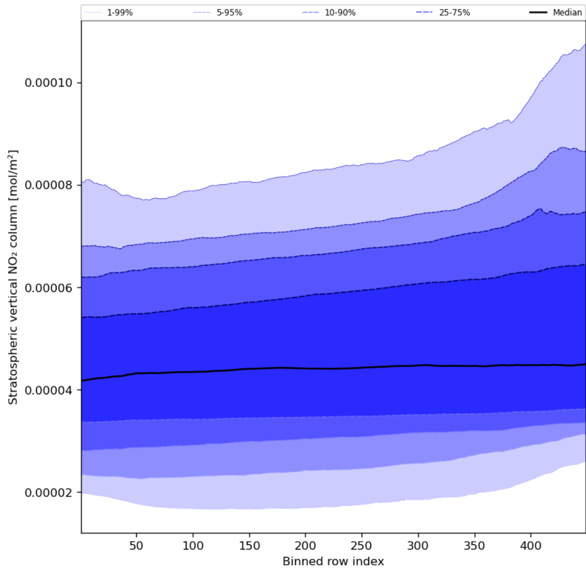
Figure 53: Along track statistics of “Stratospheric vertical NO 2 column” for 2023-11-13 to 2023-11-15
