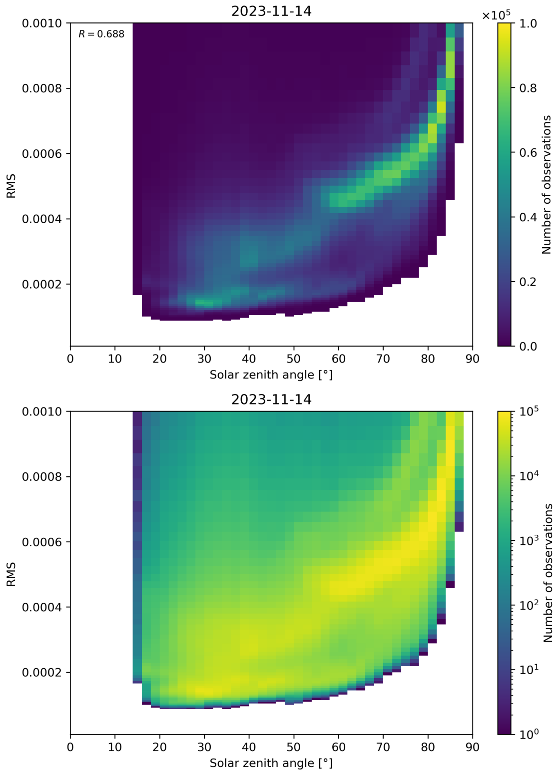
Figure 157: Scatter density plot of “Solar zenith angle” against “RMS” for 2023-11-13 to 2023-11-15.
