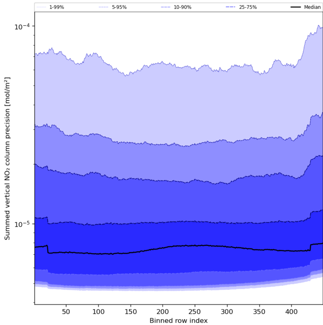
Figure 58: Along track statistics of “Summed vertical NO 2 column precision” for 2023-11-13 to 2023-11-15
