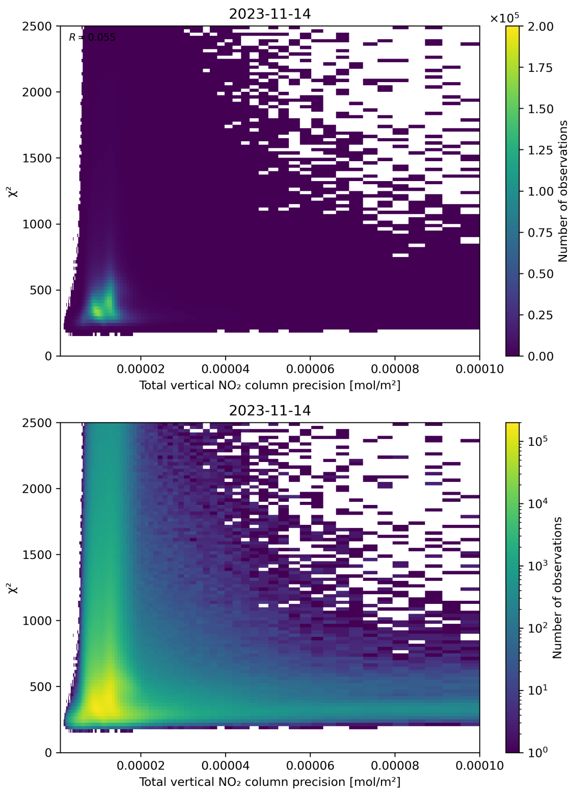
Figure 116: Scatter density plot of “Total vertical NO 2 column precision” against “ \chi^2 ” for 2023-11-13 to 2023-11-15.
