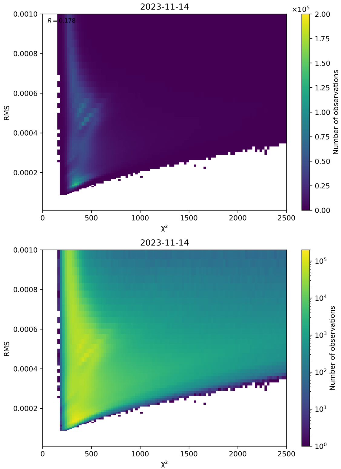
Figure 82: Scatter density plot of “ \chi^2 ” against “RMS” for 2023-11-13 to 2023-11-15.
