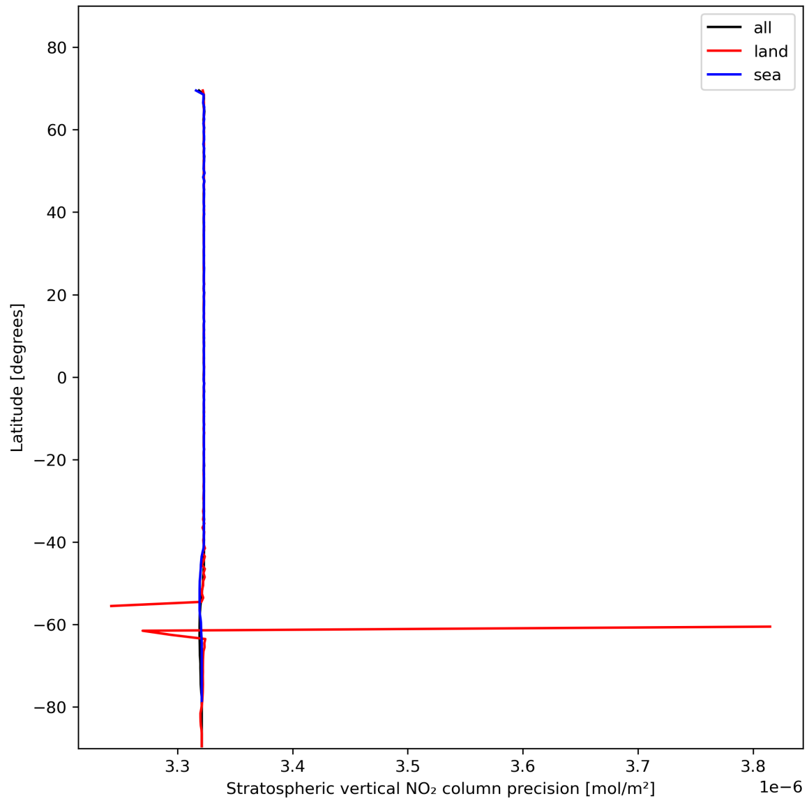
Figure 20: Zonal average of “Stratospheric vertical NO 2 column precision” for 2023-11-13 to 2023-11-15.
