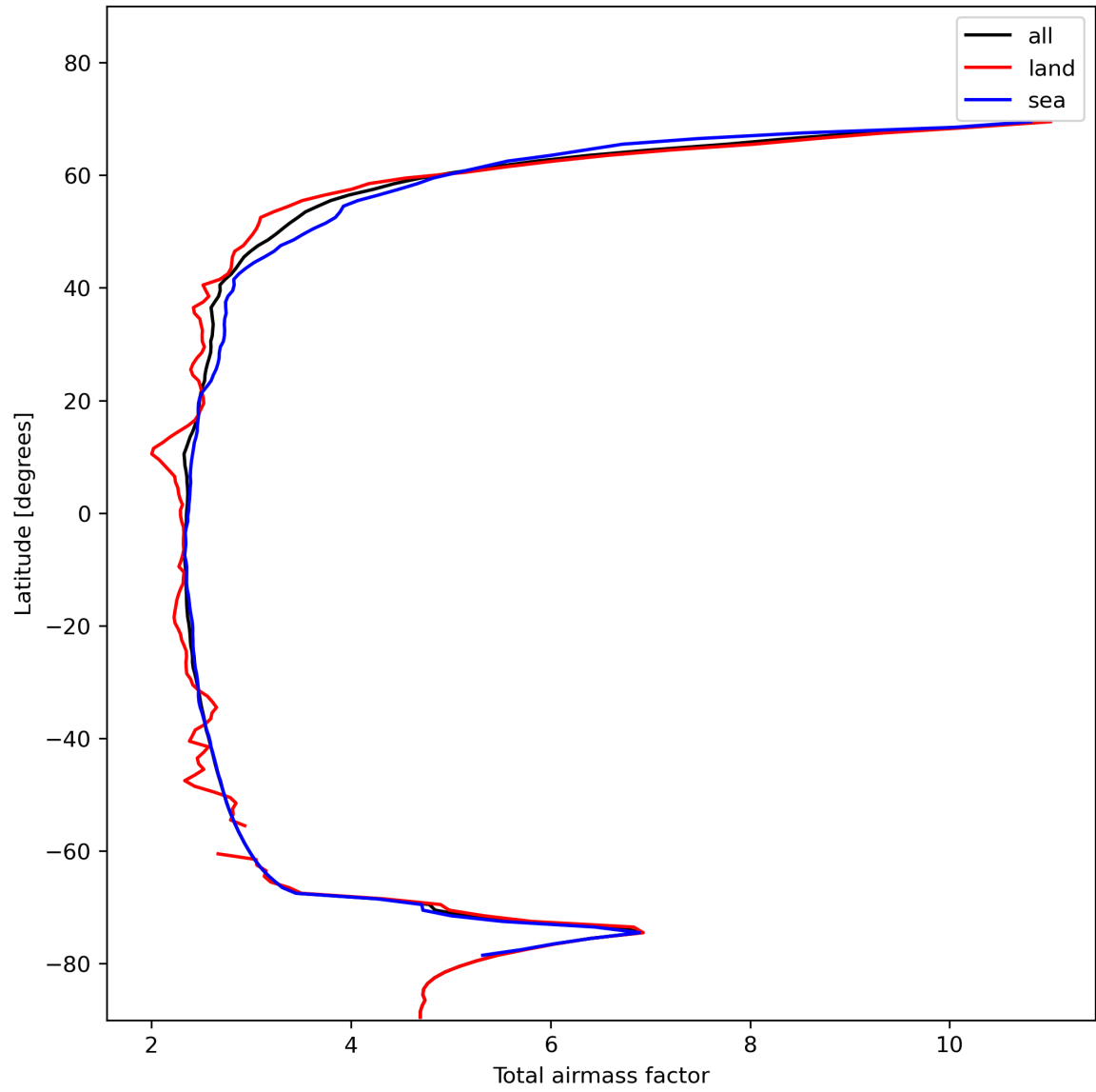
Figure 15: Zonal average of “Total airmass factor” for 2023-11-13 to 2023-11-15.
