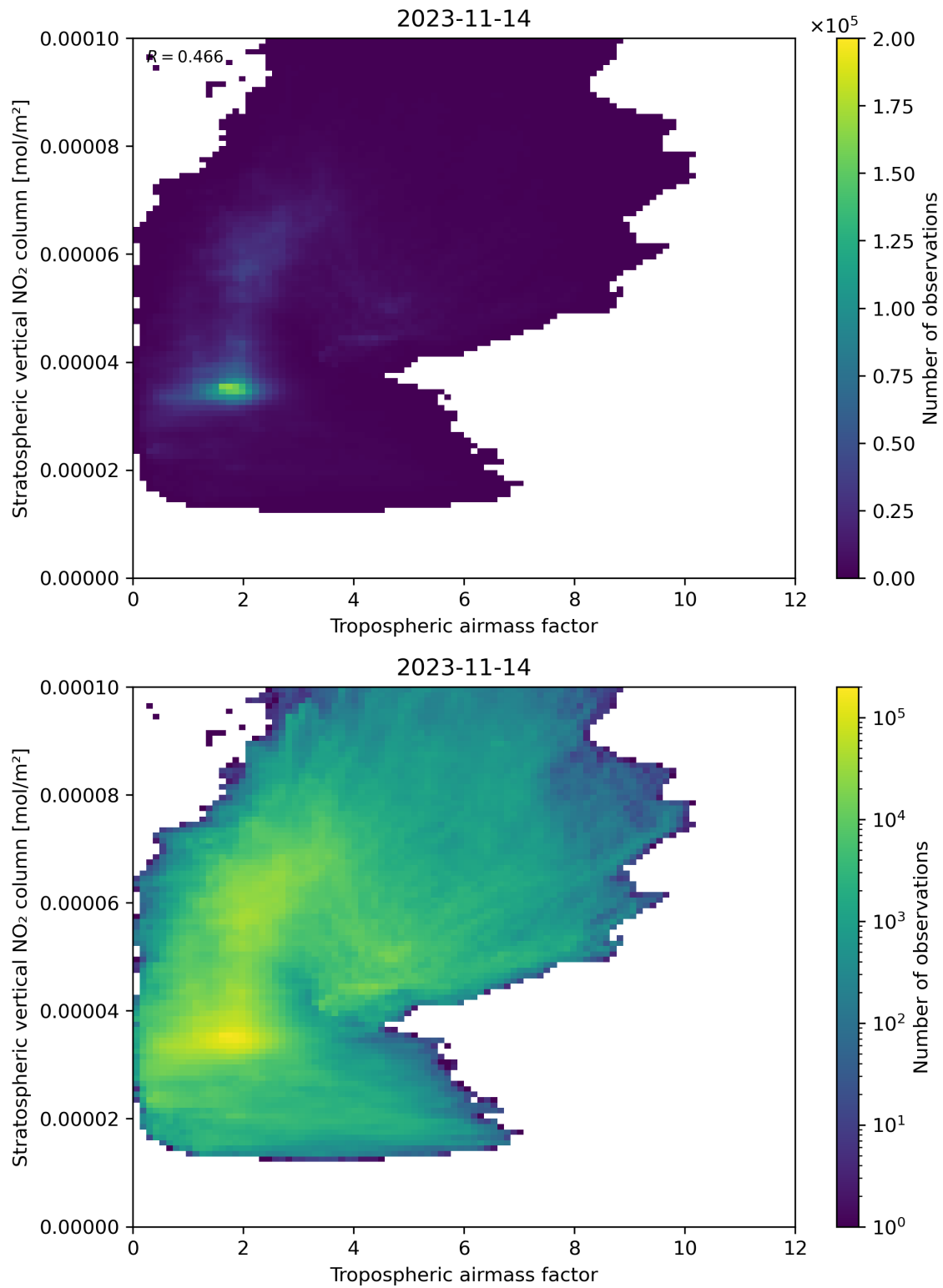
Figure 74: Scatter density plot of “Tropospheric air mass factor” against “Stratospheric vertical NO 2 column” for 2023-11-13 to 2023-11-15.
