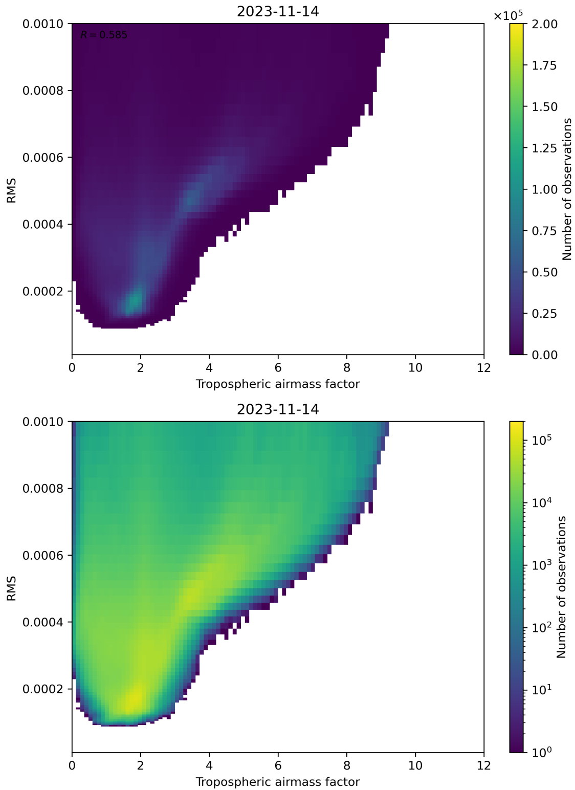
Figure 79: Scatter density plot of “Tropospheric airmass factor” against “RMS” for 2023-11-13 to 2023-11-15.
