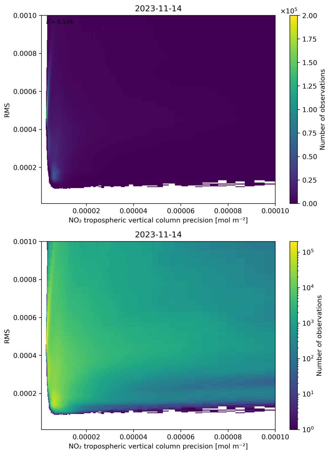
Figure 140: Scatter density plot of “NO 2 tropospheric vertical column precision” against “RMS” for 2023-11-13 to 2023-11-15.
