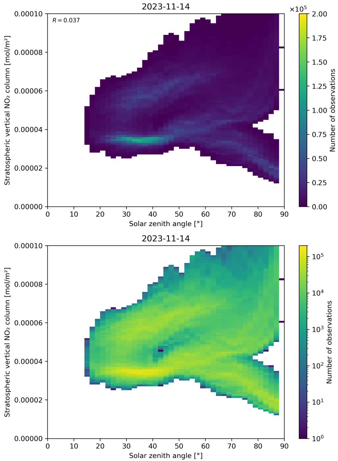
Figure 150: Scatter density plot of “Solar zenith angle” against “Stratospheric vertical NO 2 column” for 2023-11-13 to 2023-11-15.
