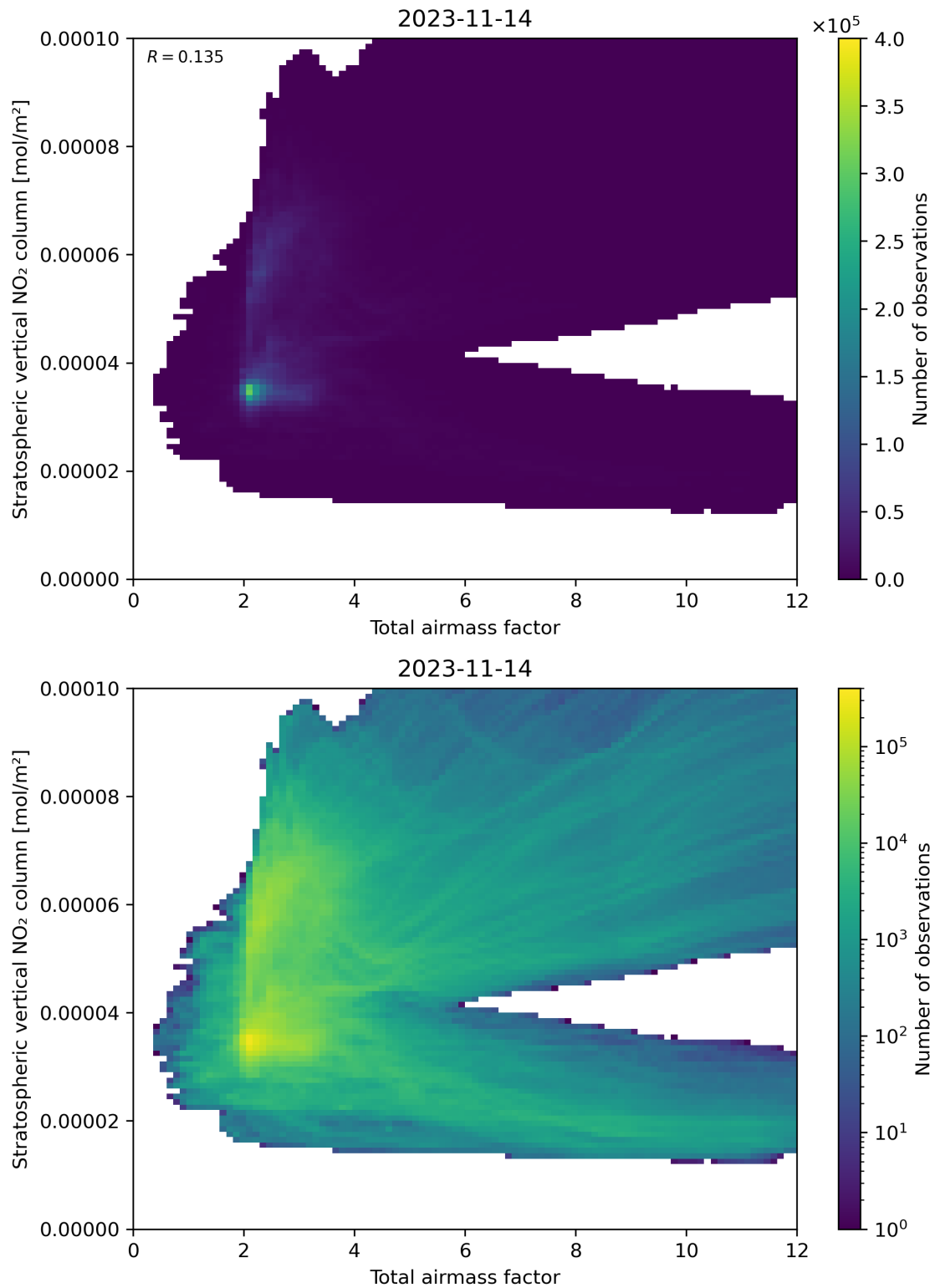
Figure 64: Scatter density plot of “Total airmass factor” against “Stratospheric vertical NO 2 column” for 2023-11-13 to 2023-11-15.
