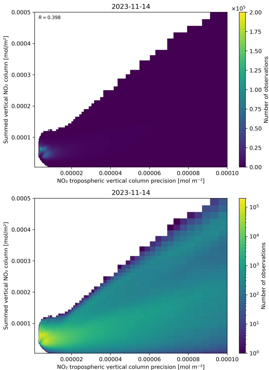
Figure 136: Scatter density plot of “NO 2 tropospheric vertical column precision” against “Summed vertical NO 2 column” for 2023-11-13 to 2023-11-15.
