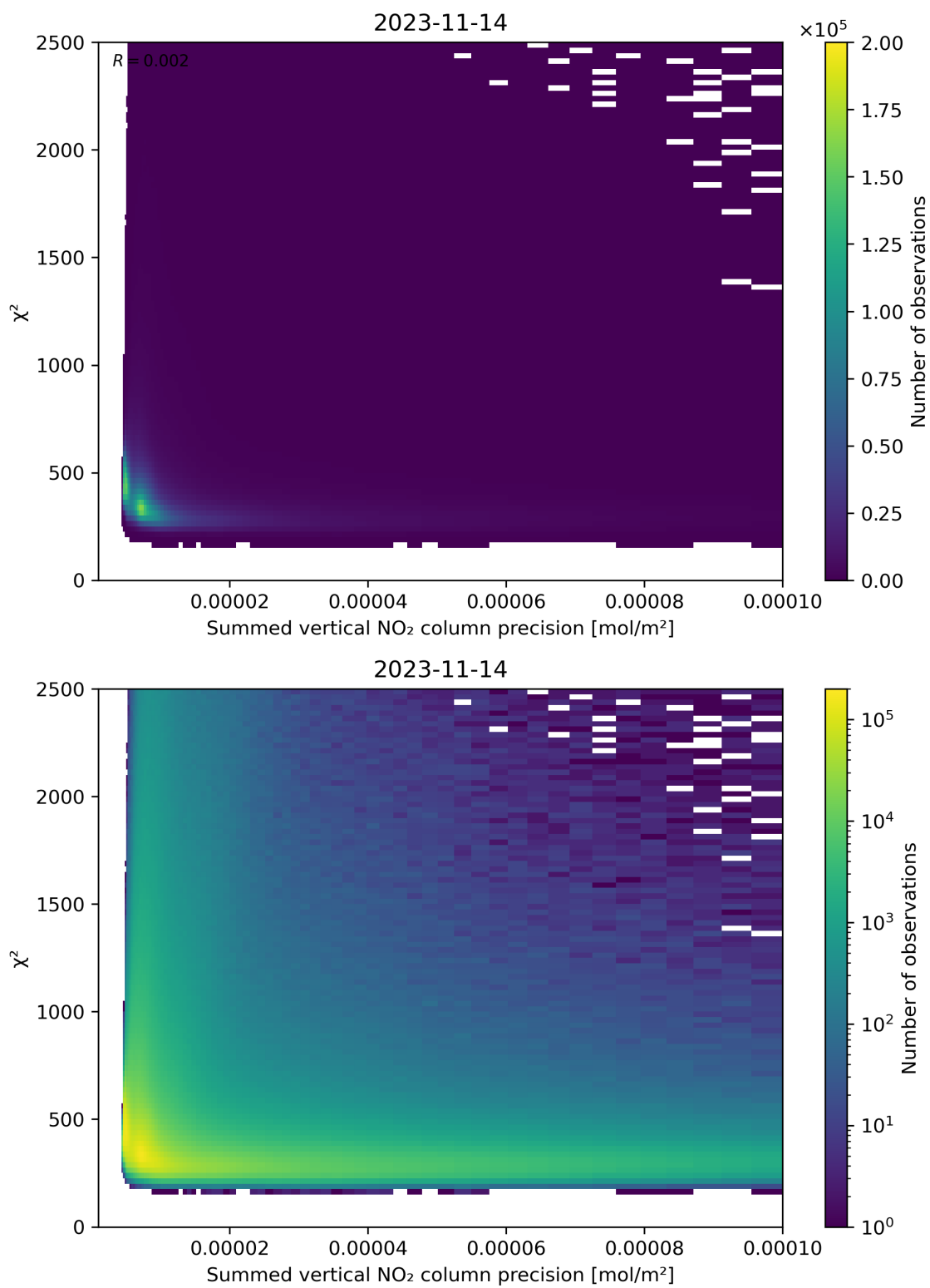
Figure 107: Scatter density plot of “Summed vertical NO 2 column precision” against “ \chi^2 ” for 2023-11-13 to 2023-11-15.
