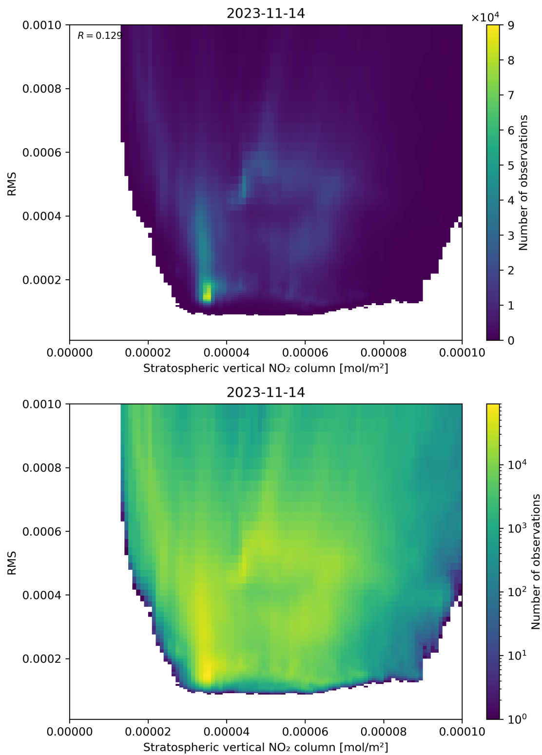
Figure 102: Scatter density plot of “Stratospheric vertical NO 2 column” against “RMS” for 2023-11-13 to 2023-11-15.
