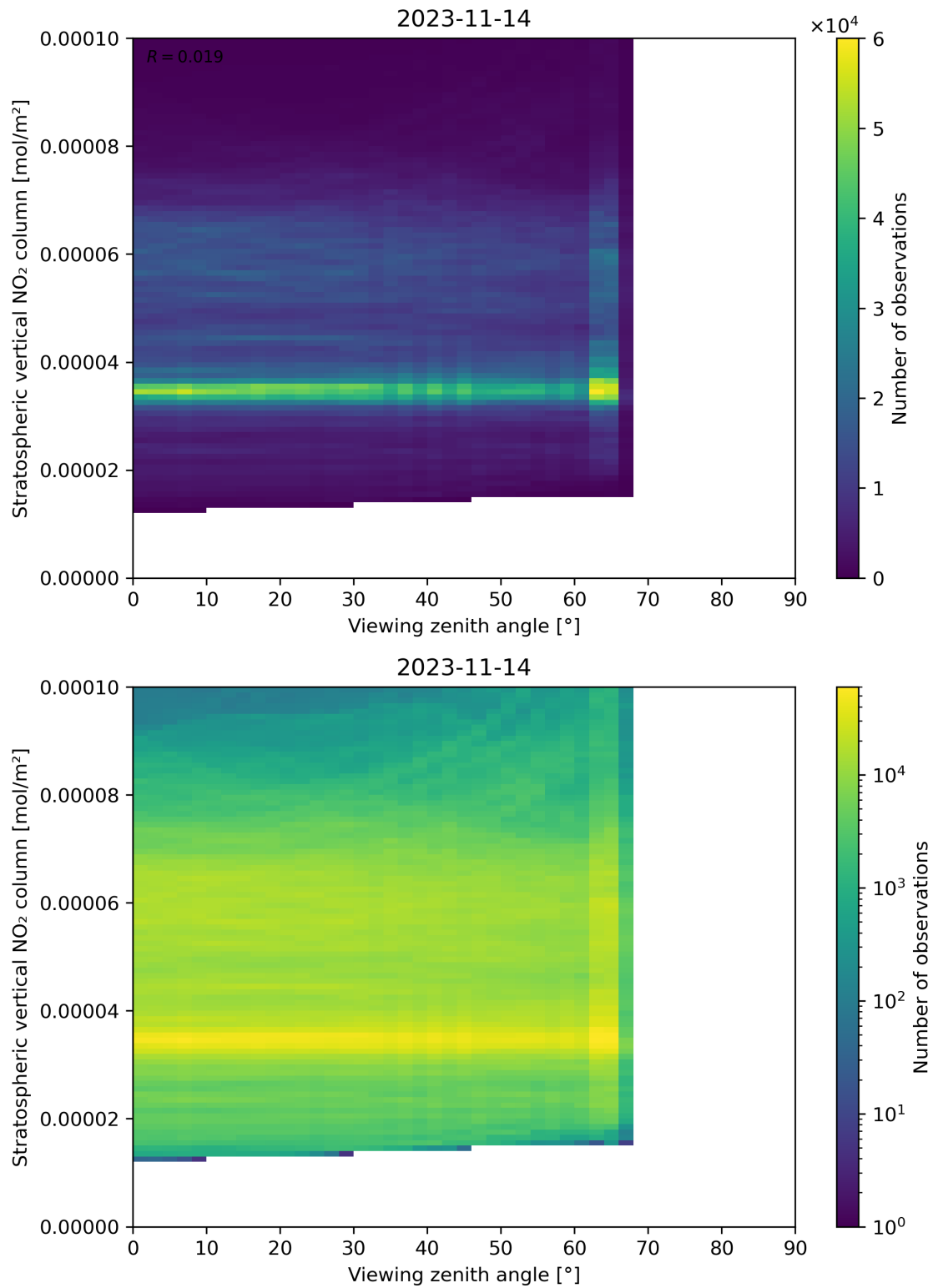
Figure 164: Scatter density plot of “Viewing zenith angle” against “Stratospheric vertical NO 2 column” for 2023-11-13 to 2023-11-15.
