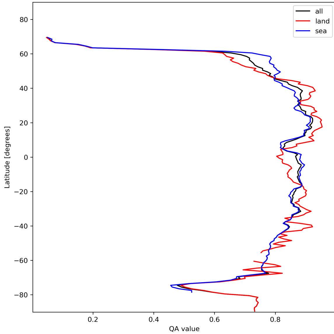
Figure 11: Zonal average of “QA value” for 2023-11-13 to 2023-11-15.
