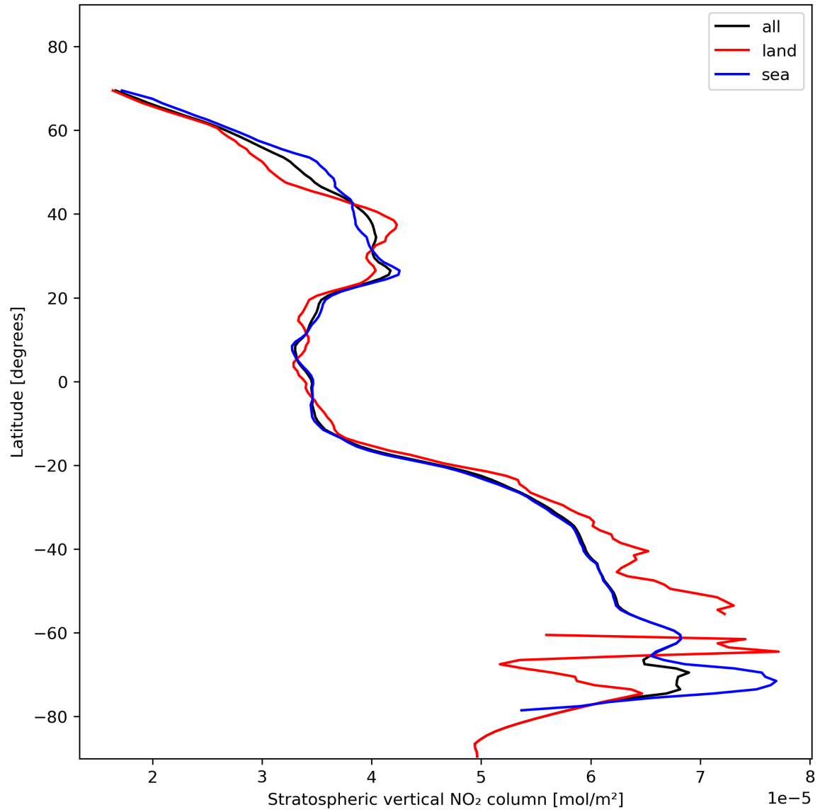
Figure 19: Zonal average of “Stratospheric vertical NO 2 column” for 2023-11-13 to 2023-11-15.
