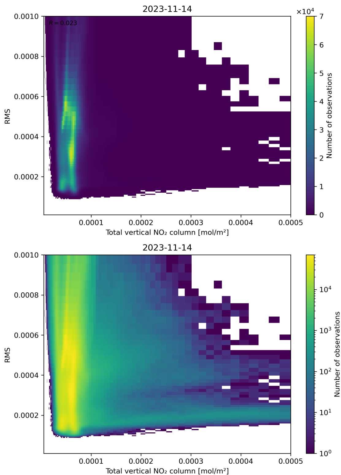
Figure 120: Scatter density plot of “Total vertical NO 2 column” against “RMS” for 2023-11-13 to 2023-11-15.
