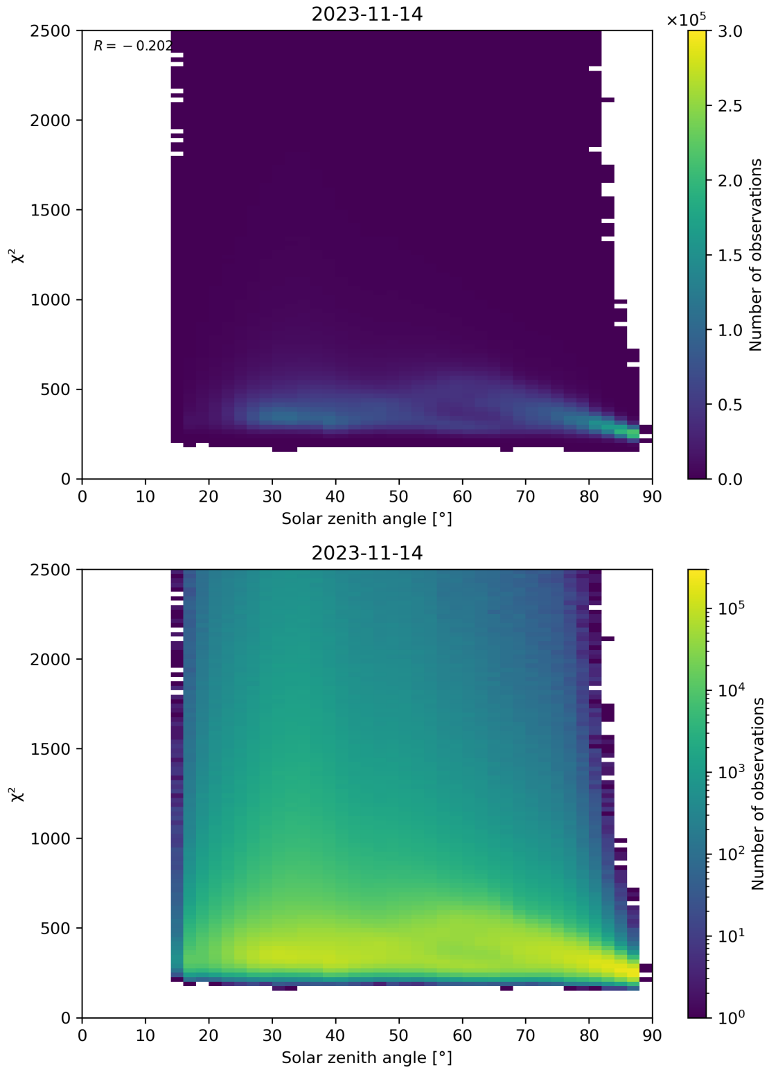
Figure 148: Scatter density plot of “Solar zenith angle” against “ \chi^2 ” for 2023-11-13 to 2023-11-15.
