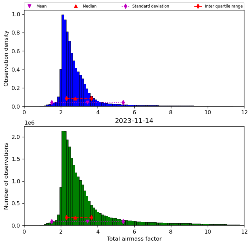
Figure 32: Histogram of “Total airmass factor” for 2023-11-13 to 2023-11-15
