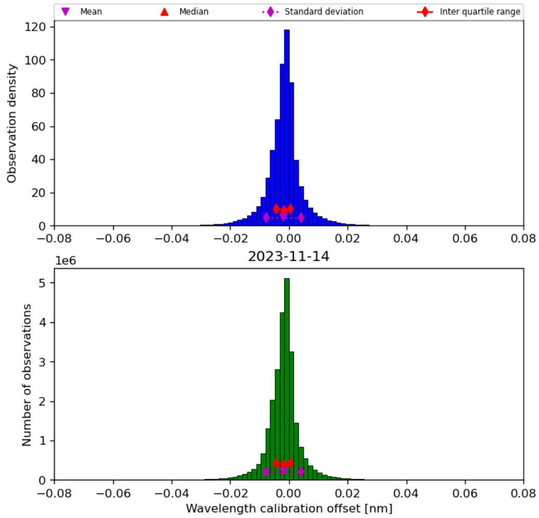
Figure 35: Histogram of “Wavelength calibration offset” for 2023-11-13 to 2023-11-15
