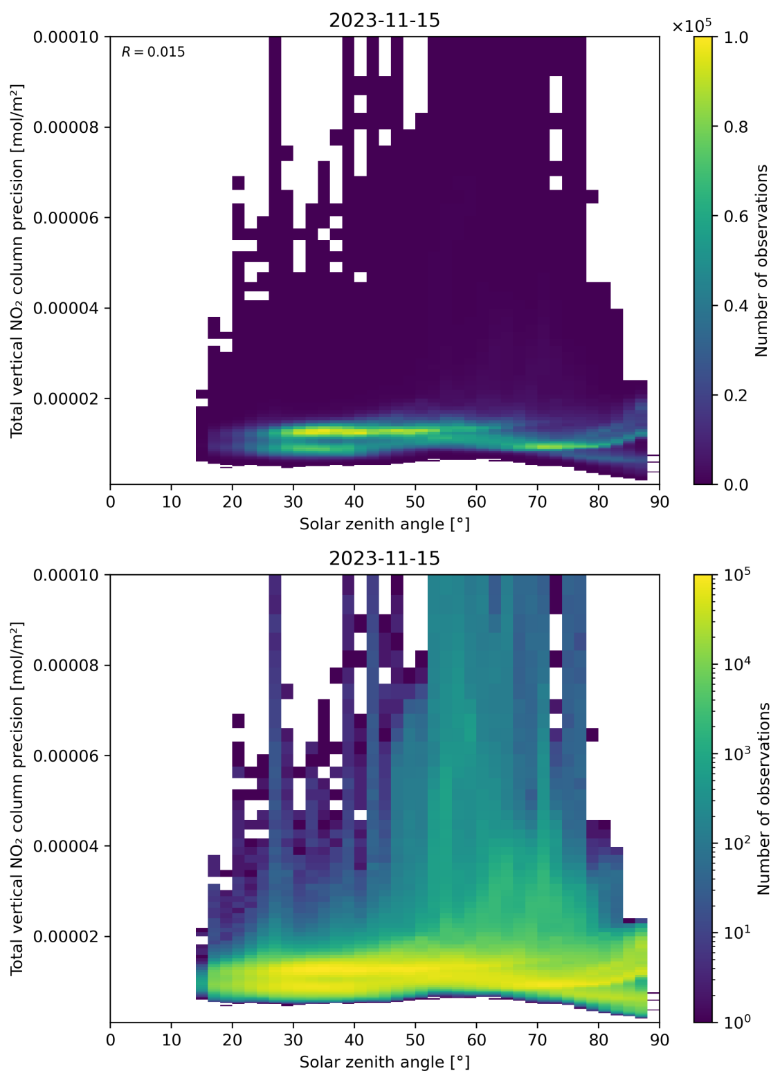
Figure 154: Scatter density plot of “Solar zenith angle” against “Total vertical NO 2 column precision” for 2023-11-14 to 2023-11-16.
