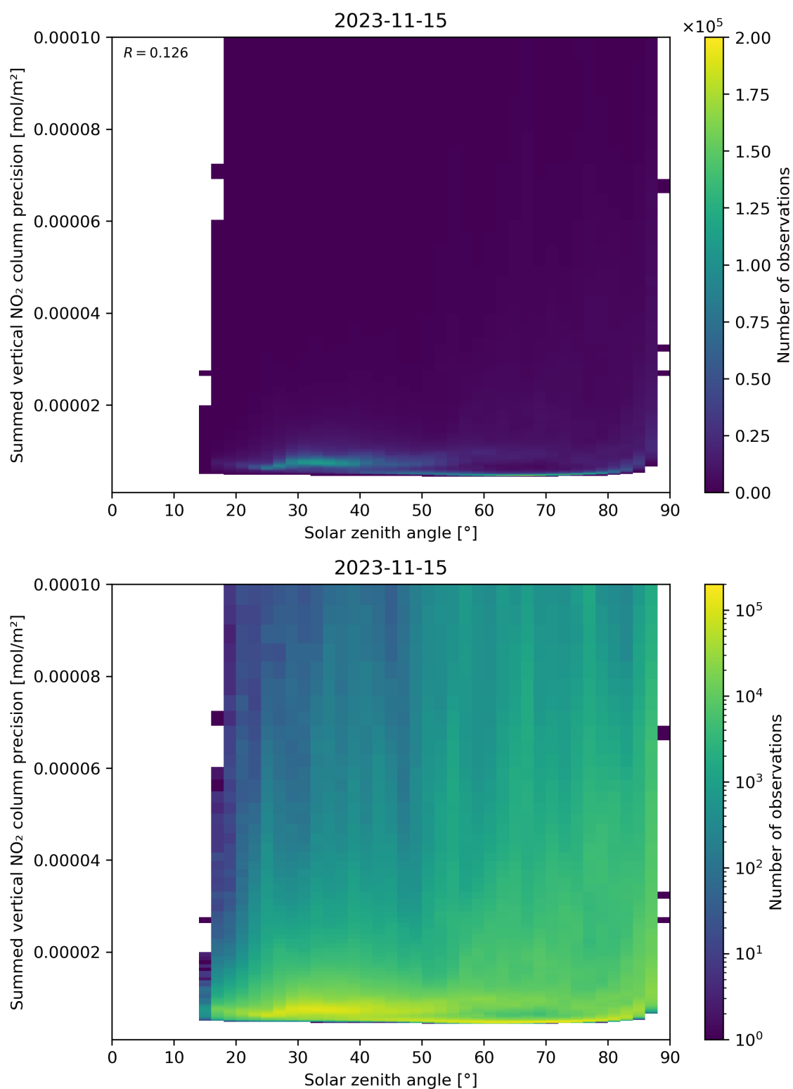
Figure 152: Scatter density plot of “Solar zenith angle” against “Summed vertical NO 2 column precision” for 2023-11-14 to 2023-11-16.
