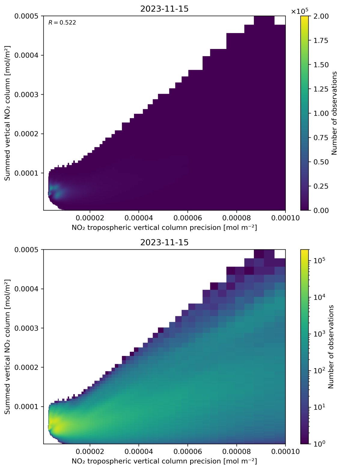
Figure 136: Scatter density plot of “NO 2 tropospheric vertical column precision” against “Summed vertical NO 2 column” for 2023-11-14 to 2023-11-16.
