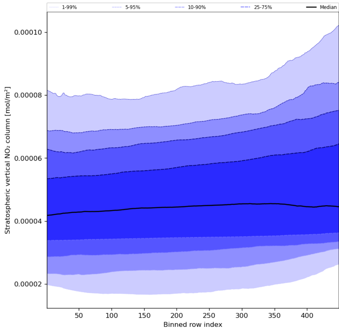
Figure 53: Along track statistics of “Stratospheric vertical NO 2 column” for 2023-11-14 to 2023-11-16
