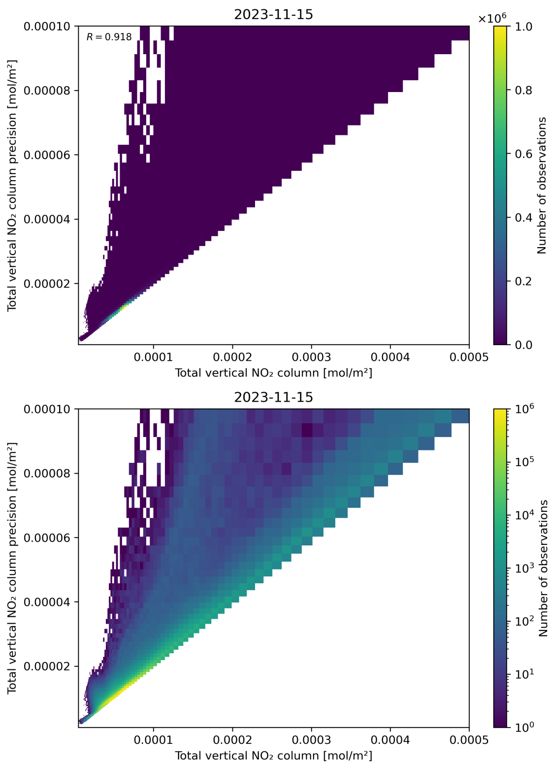
Figure 114: Scatter density plot of “Total vertical NO 2 column” against “Total vertical NO 2 column precision” for 2023-11-14 to 2023-11-16.
