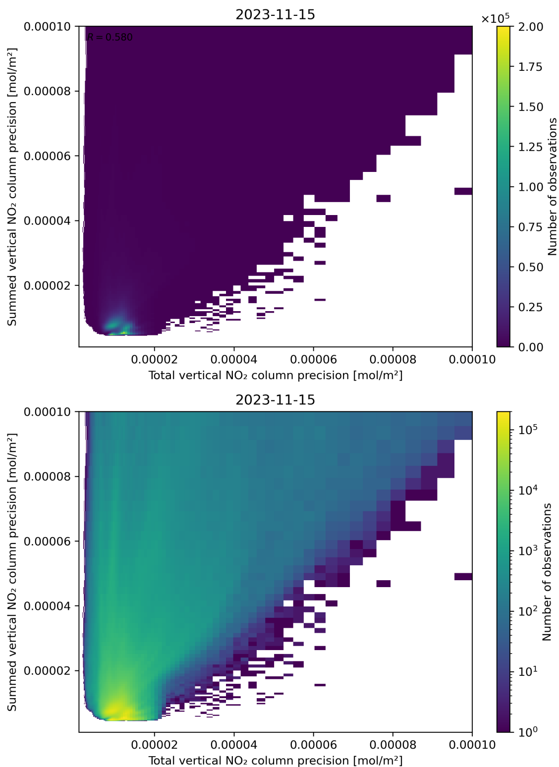
Figure 118: Scatter density plot of “Total vertical NO 2 column precision” against “Summed vertical NO 2 column precision” for 2023-11-14 to 2023-11-16.
