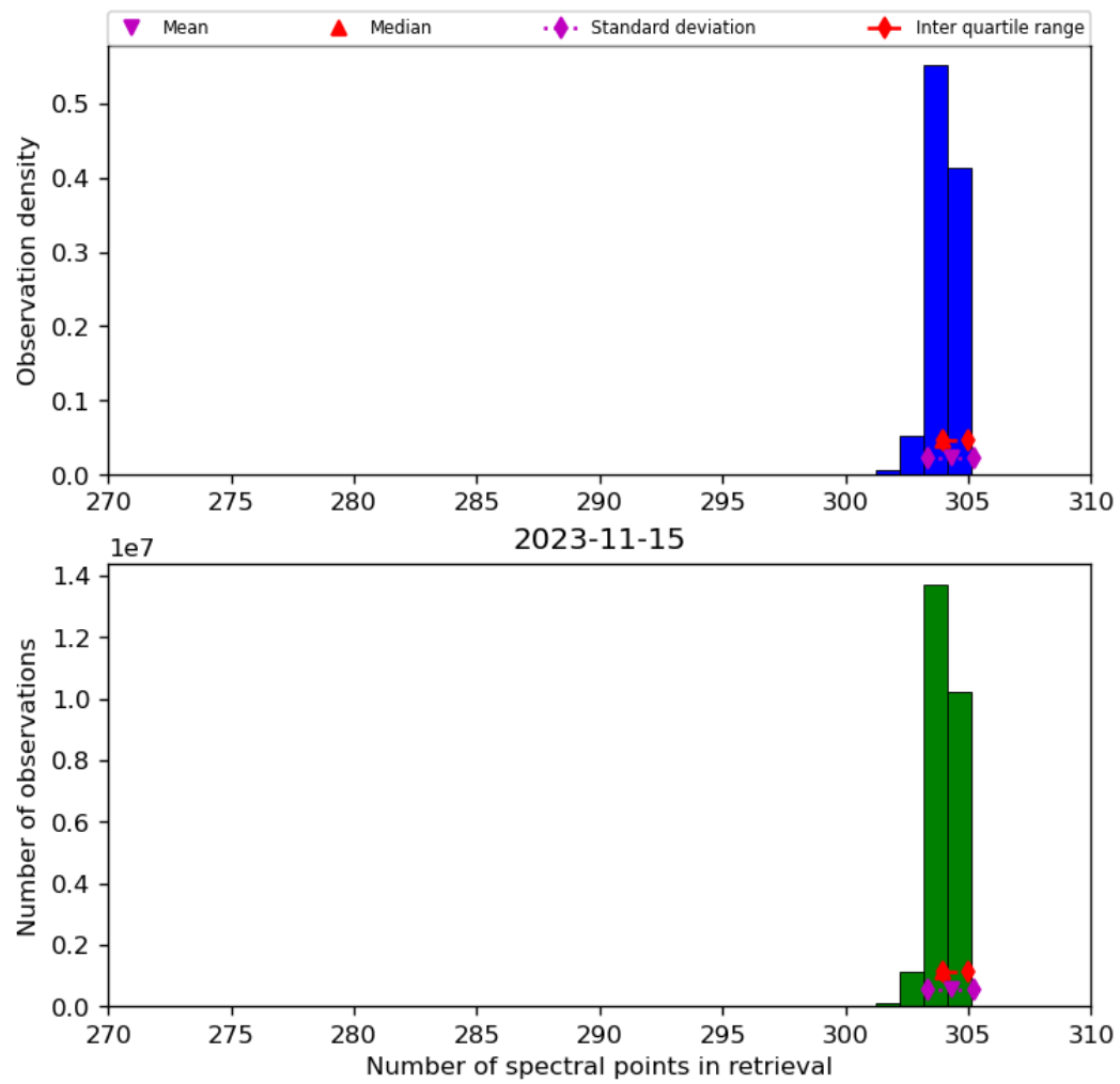
Figure 33: Histogram of “Number of spectral points in retrieval” for 2023-11-14 to 2023-11-16
