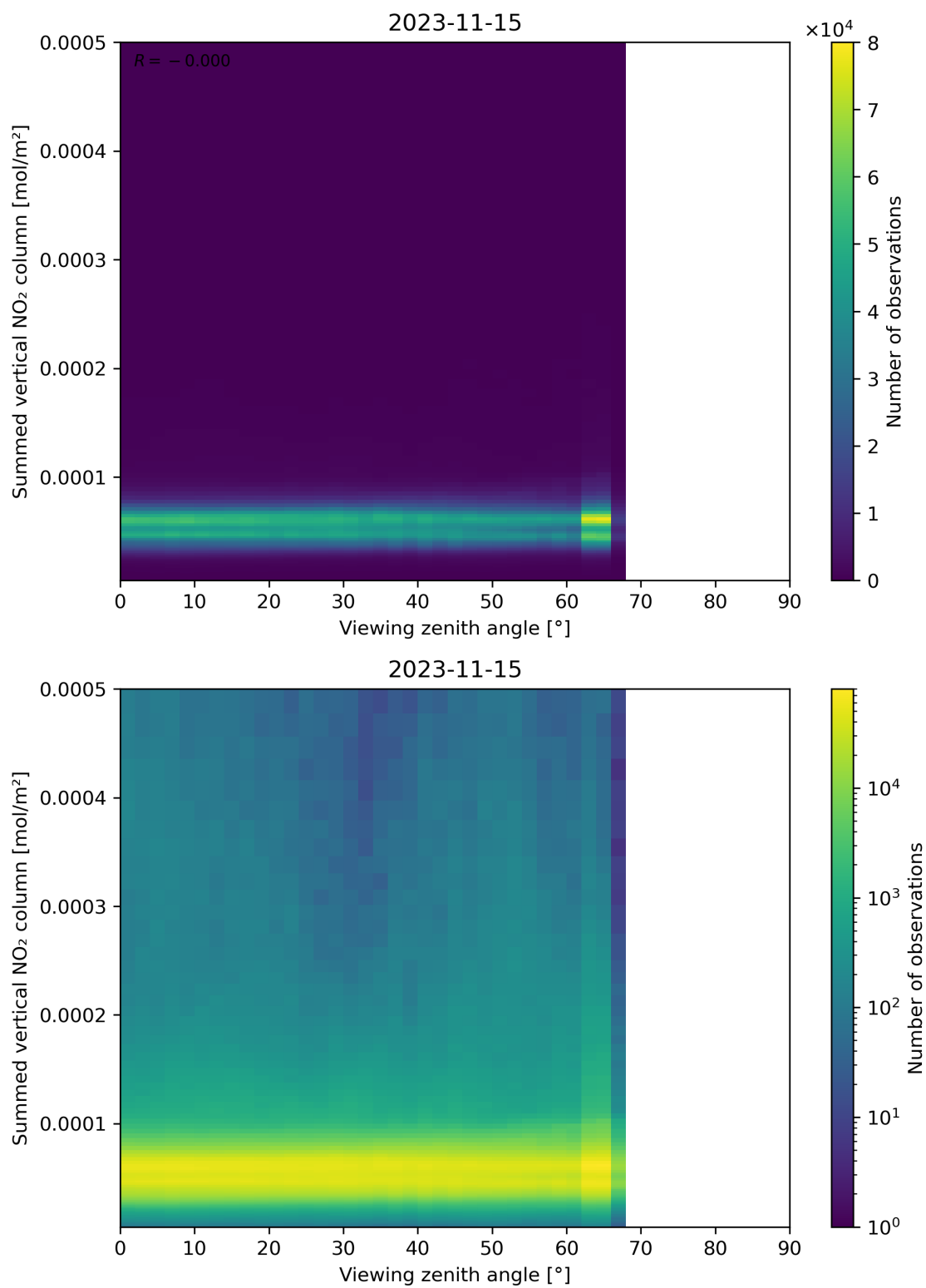
Figure 165: Scatter density plot of “Viewing zenith angle” against “Summed vertical NO 2 column” for 2023-11-14 to 2023-11-16.
