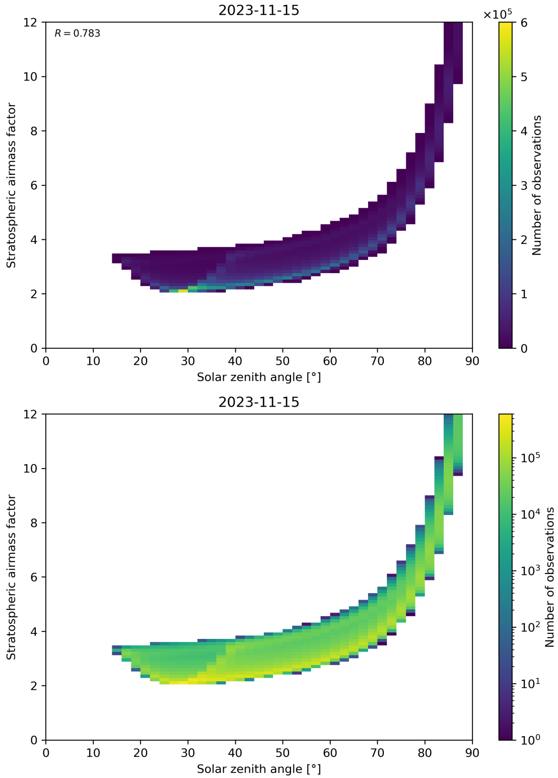
Figure 145: Scatter density plot of “Solar zenith angle” against “Stratospheric airmass factor” for 2023-11-14 to 2023-11-16.
