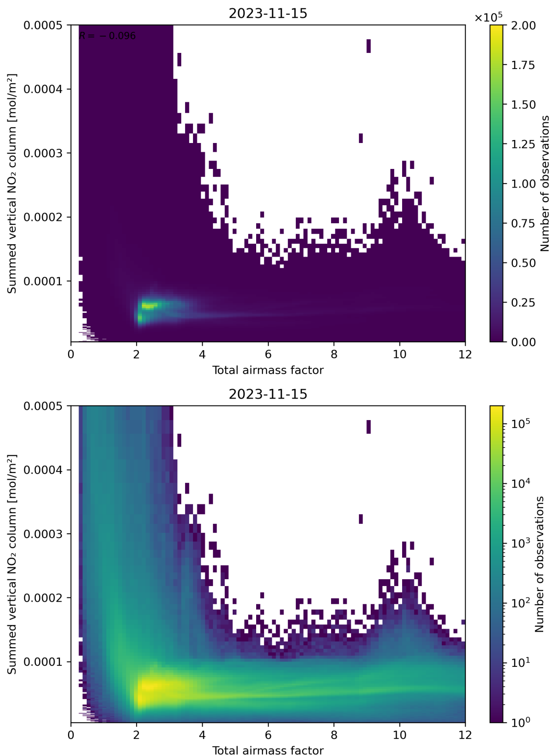
Figure 65: Scatter density plot of “Total airmass factor” against “Summed vertical NO 2 column” for 2023-11-14 to 2023-11-16.
