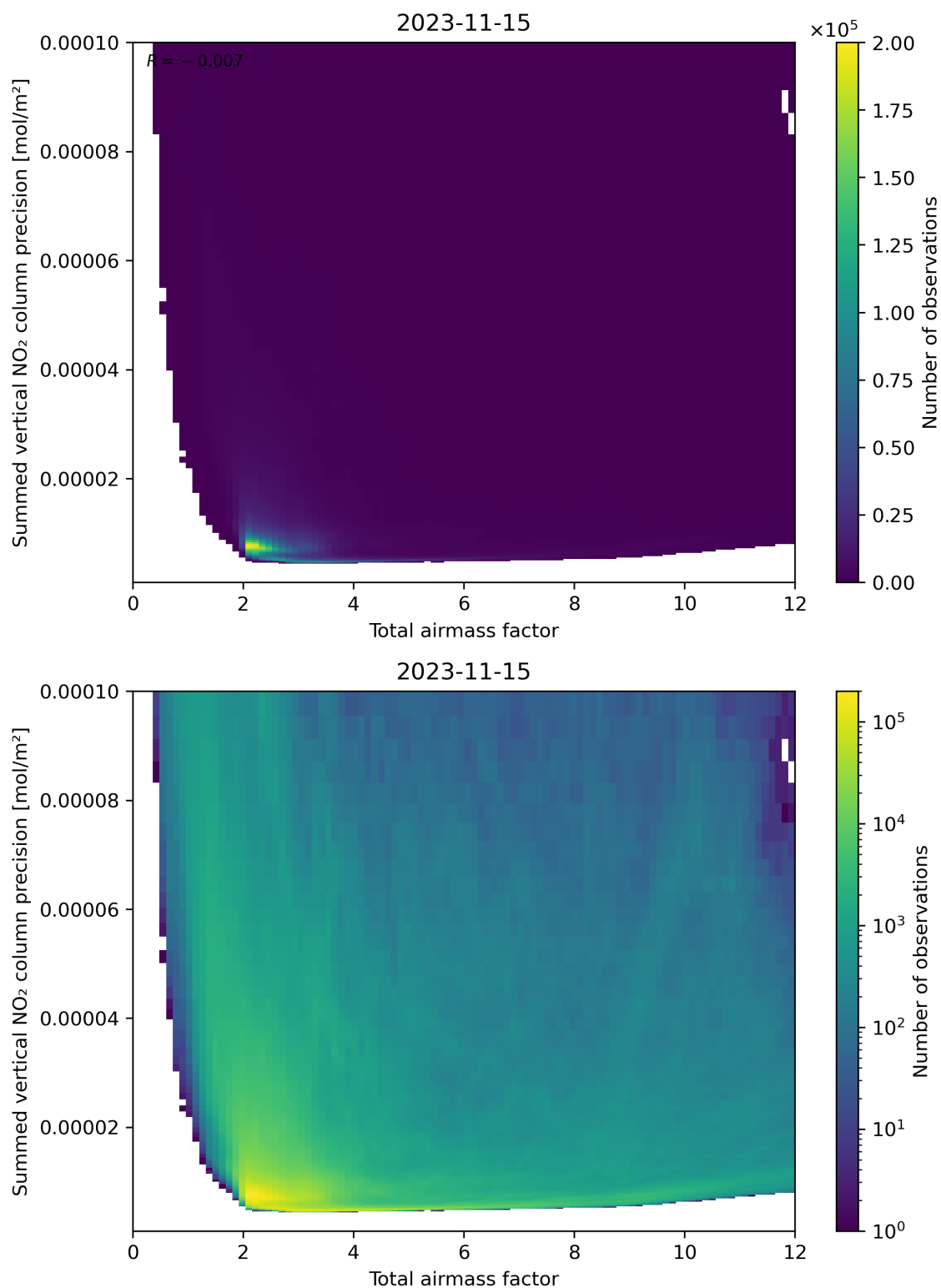
Figure 66: Scatter density plot of “Total airmass factor” against “Summed vertical NO 2 column precision” for 2023-11-14 to 2023-11-16.
