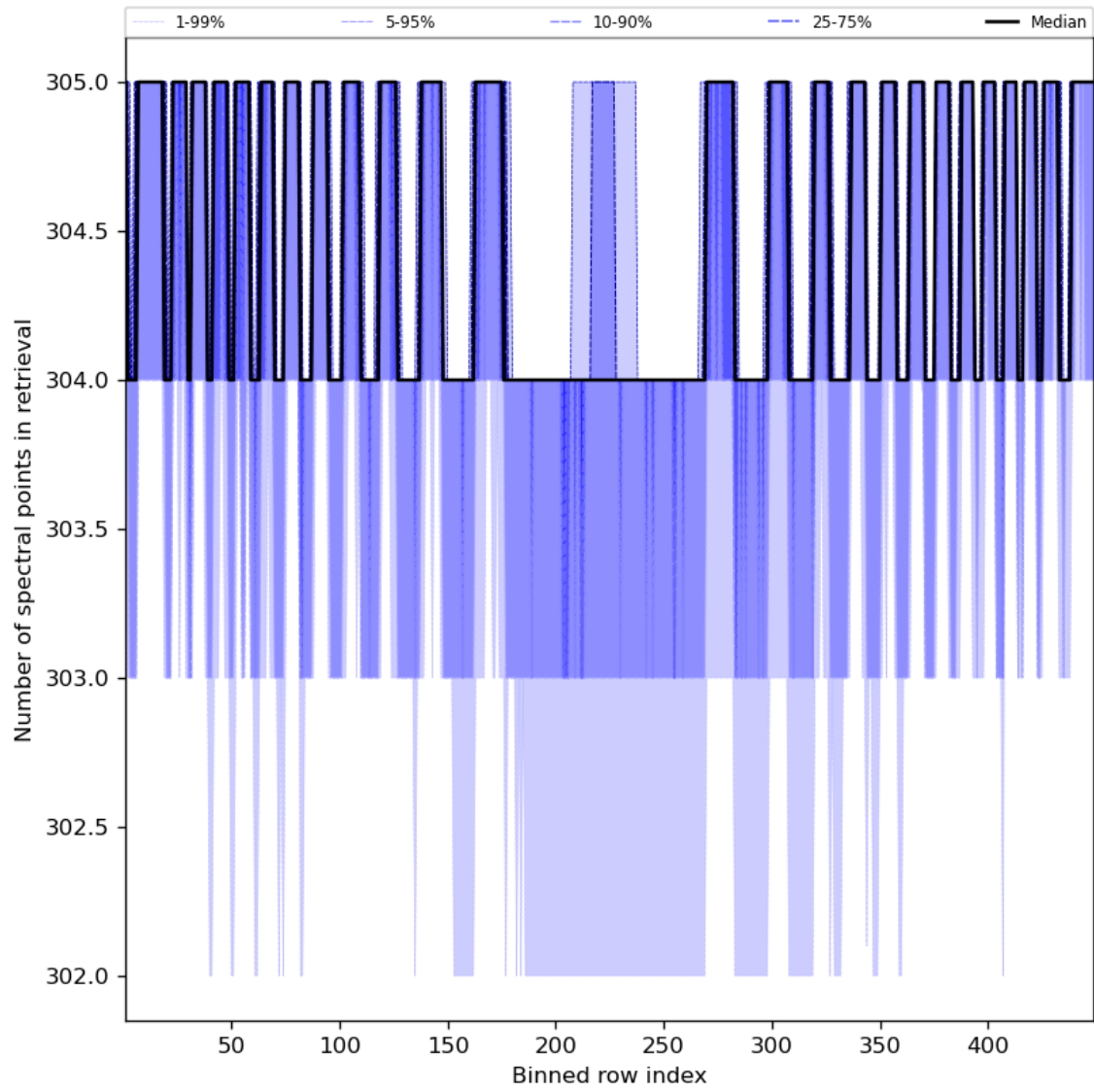
Figure 50: Along track statistics of “Number of spectral points in retrieval” for 2023-11-14 to 2023-11-16
