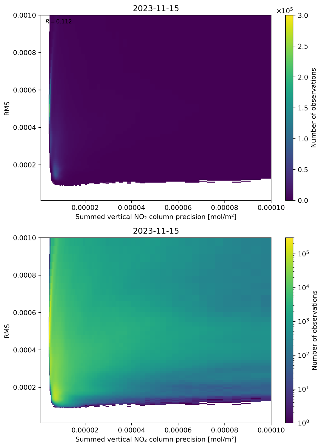
Figure 108: Scatter density plot of “Summed vertical NO 2 column precision” against “RMS” for 2023-11-14 to 2023-11-16.
