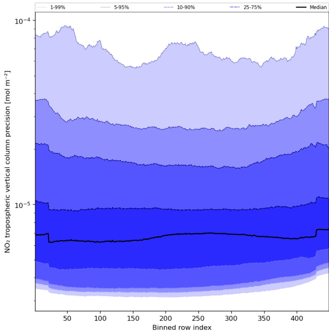
Figure 47: Along track statistics of “NO 2 tropospheric vertical column precision” for 2023-11-14 to 2023-11-16
