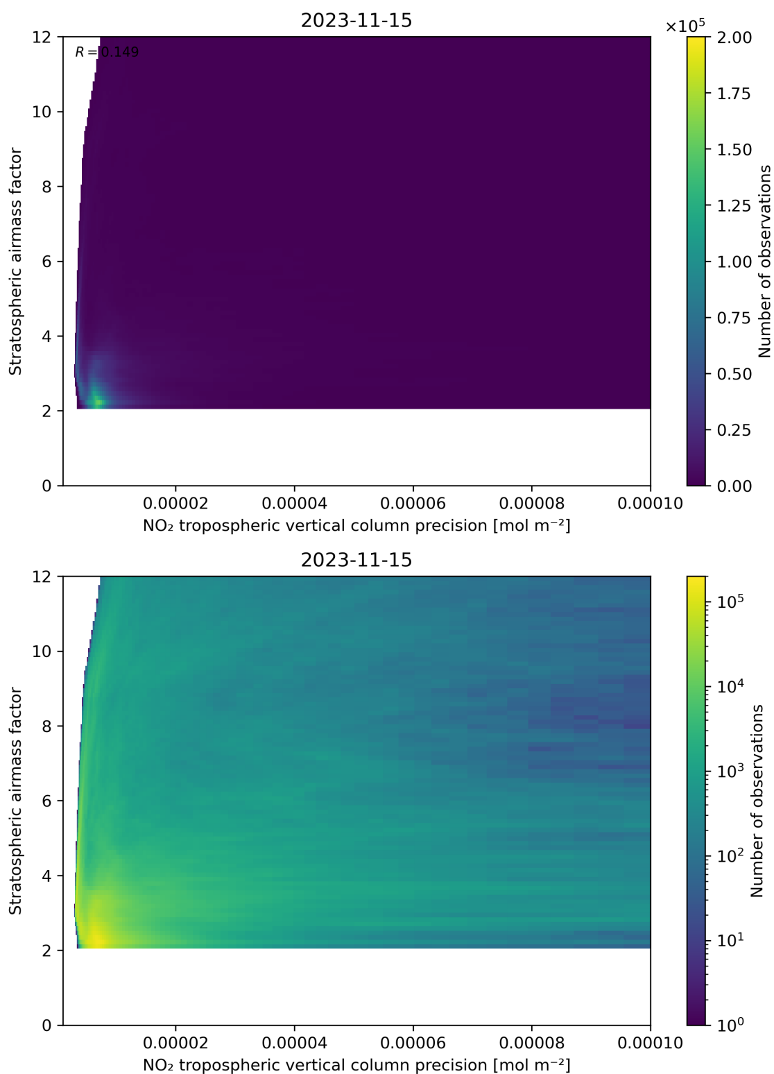
Figure 131: Scatter density plot of “NO 2 tropospheric vertical column precision” against “Stratospheric airmass factor” for 2023-11-14 to 2023-11-16.
