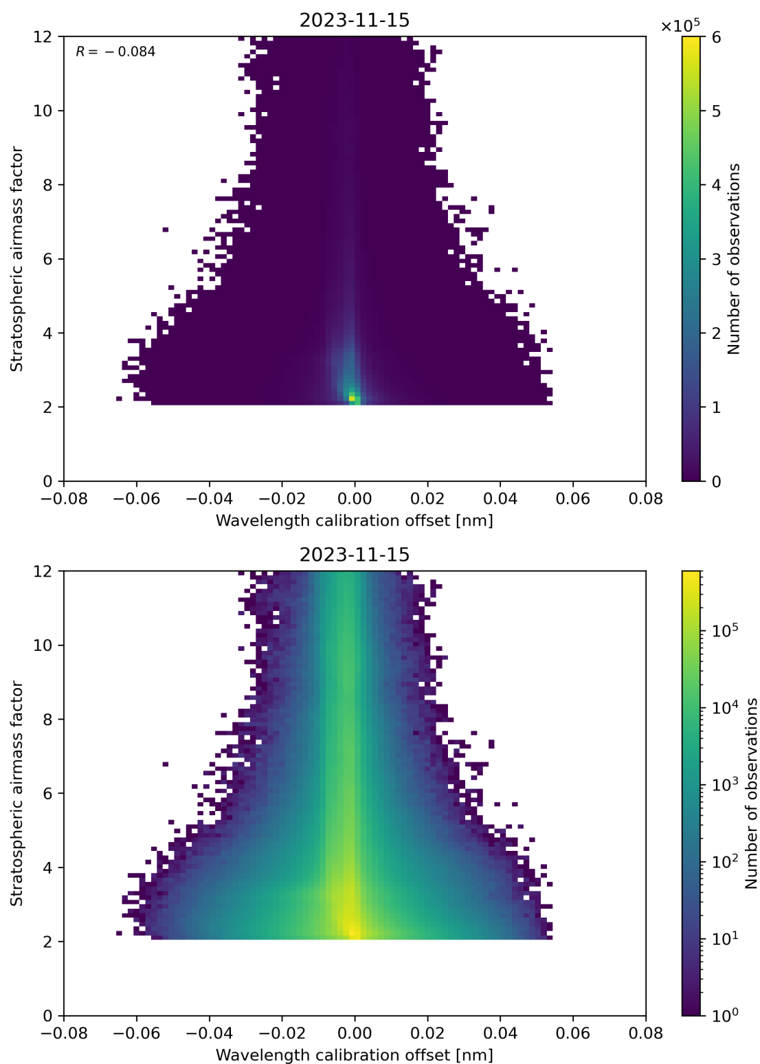
Figure 174: Scatter density plot of “Wavelength calibration offset” against “Stratospheric airmass factor” for 2023-11-14 to 2023-11-16.
