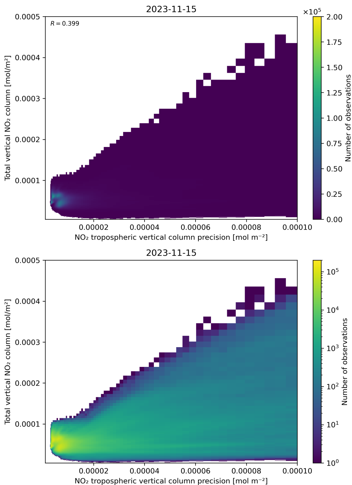
Figure 138: Scatter density plot of “NO 2 tropospheric vertical column precision” against “Total vertical NO 2 column” for 2023-11-14 to 2023-11-16.
