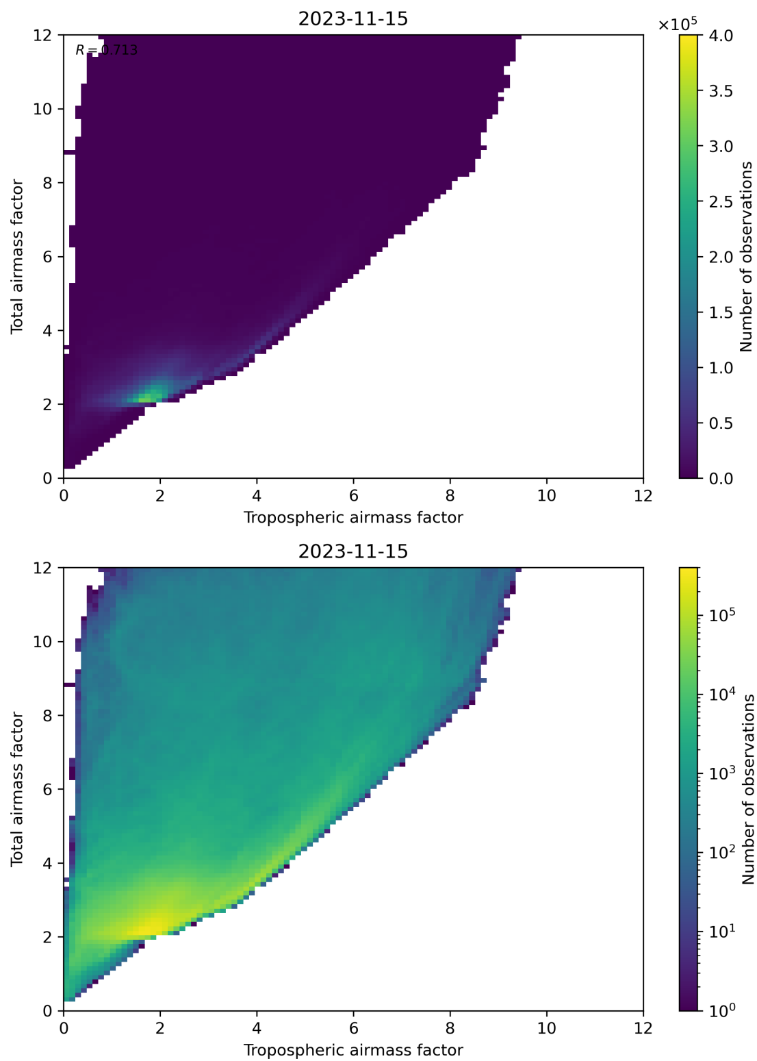
Figure 72: Scatter density plot of “Tropospheric airmass factor” against “Total airmass factor” for 2023-11-14 to 2023-11-16.
