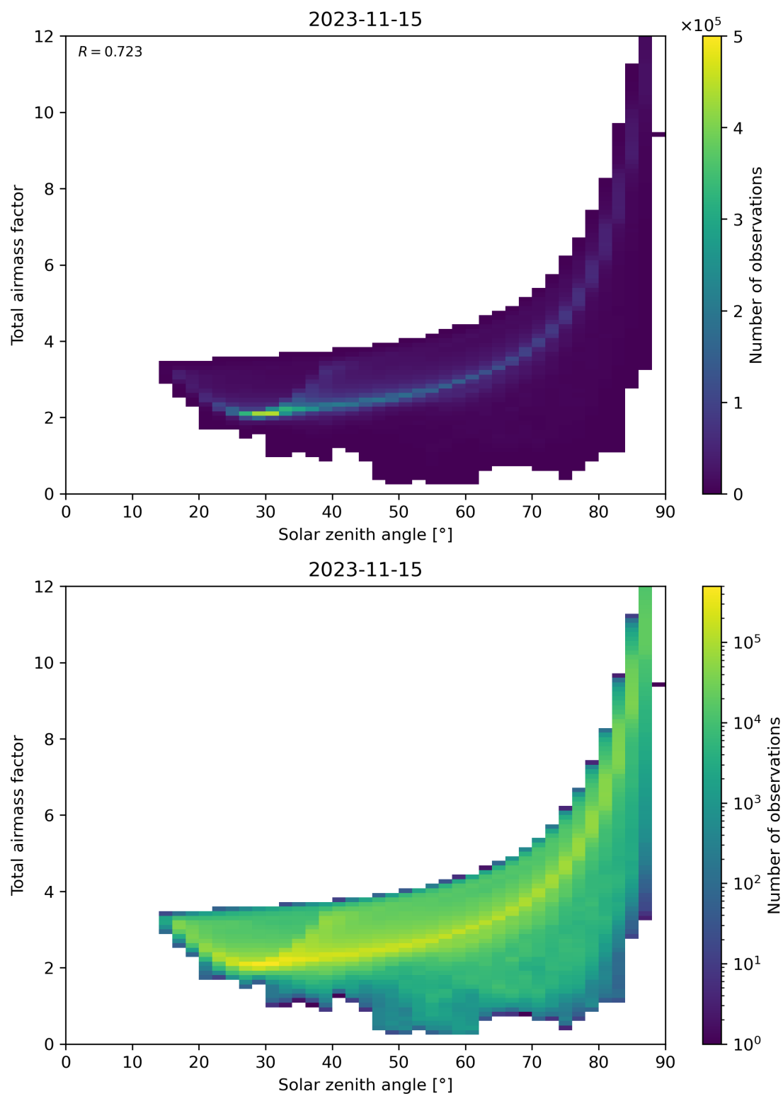
Figure 146: Scatter density plot of “Solar zenith angle” against “Total air mass factor” for 2023-11-14 to 2023-11-16.
