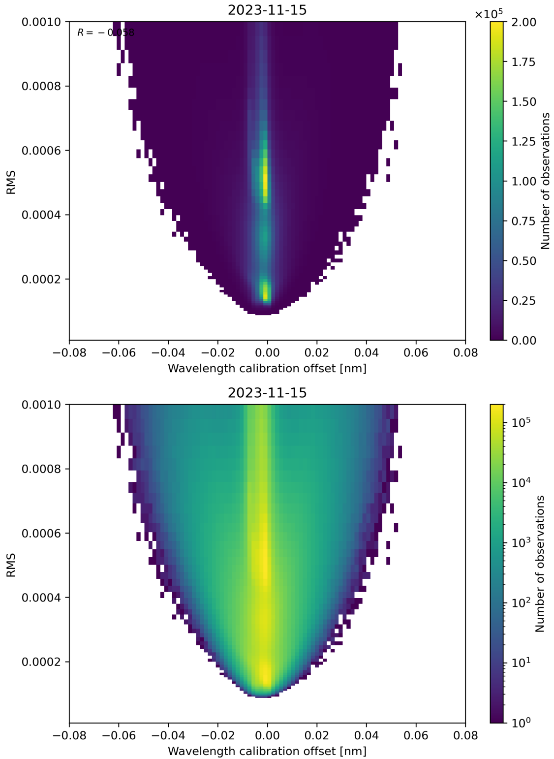
Figure 181: Scatter density plot of “Wavelength calibration offset” against “RMS” for 2023-11-14 to 2023-11-16.
