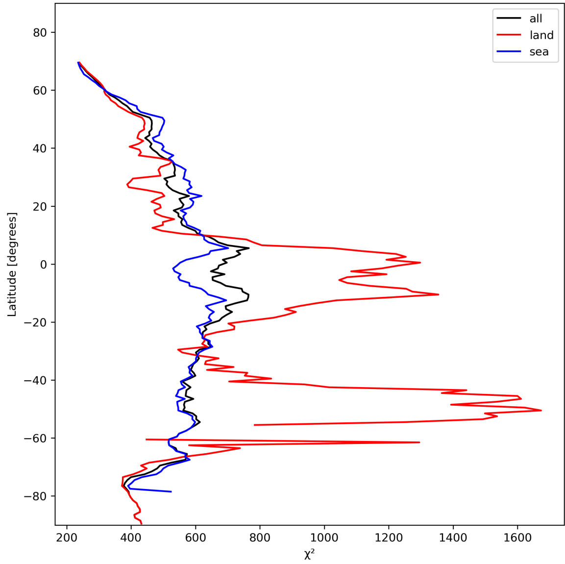
Figure 25: Zonal average of “ \chi^2 ” for 2023-11-14 to 2023-11-16.
