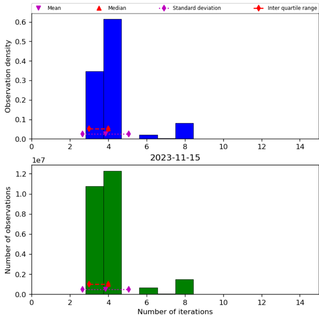
Figure 34: Histogram of “Number of iterations” for 2023-11-14 to 2023-11-16
