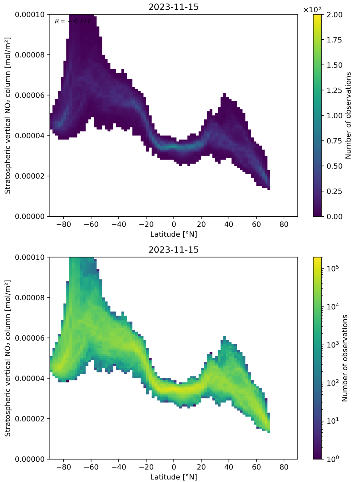
Figure 87: Scatter density plot of “Latitude” against “Stratospheric vertical NO 2 column” for 2023-11-14 to 2023-11-16.
