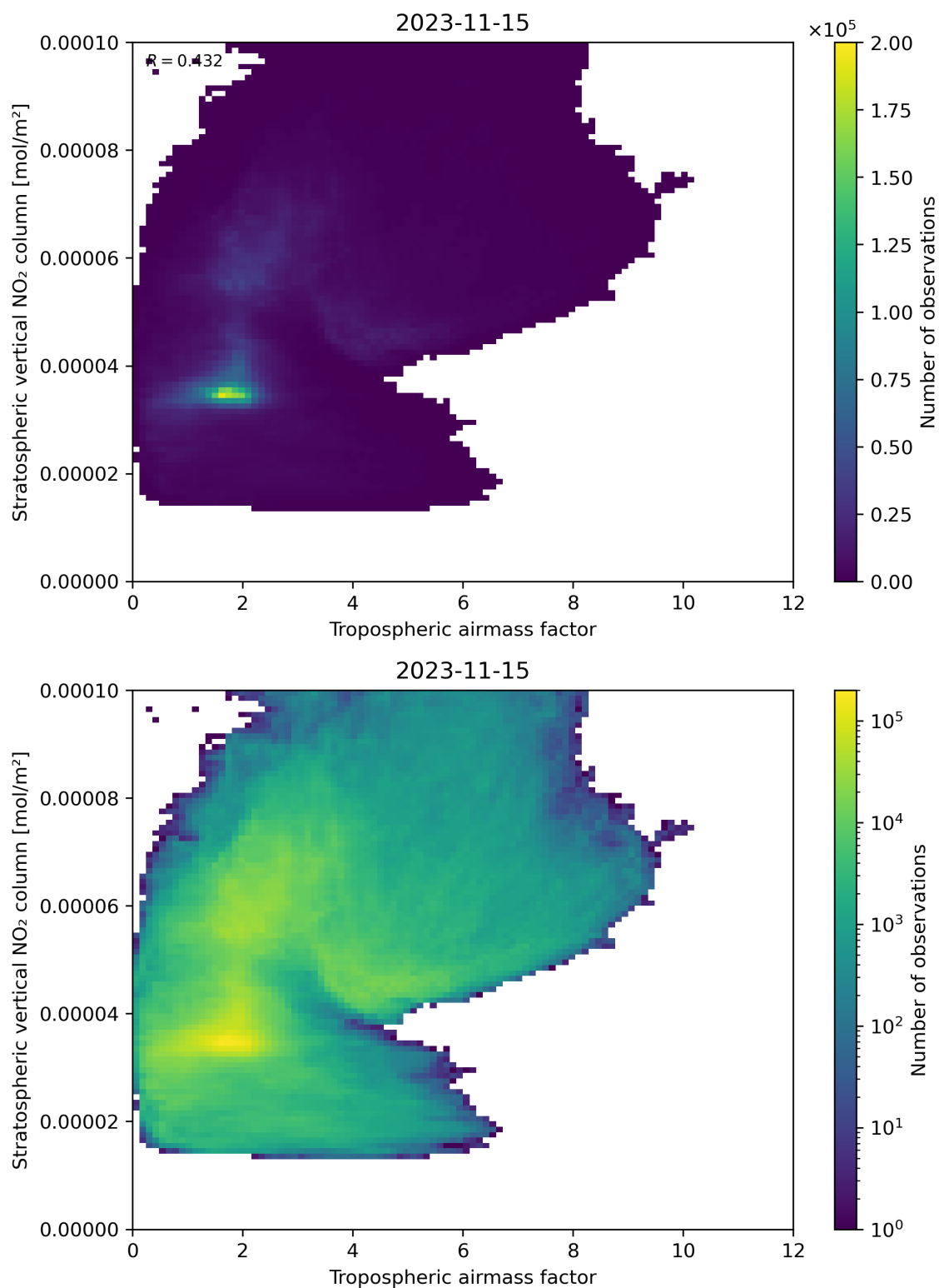
Figure 74: Scatter density plot of “Tropospheric air mass factor” against “Stratospheric vertical NO 2 column” for 2023-11-14 to 2023-11-16.
