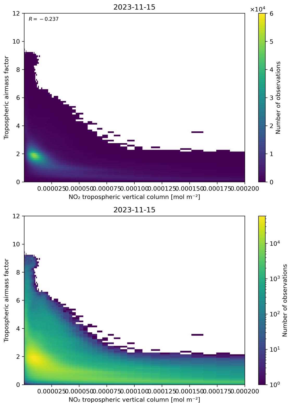
Figure 123: Scatter density plot of “NO 2 tropospheric vertical column” against “Tropospheric air mass factor” for 2023-11-14 to 2023-11-16.
