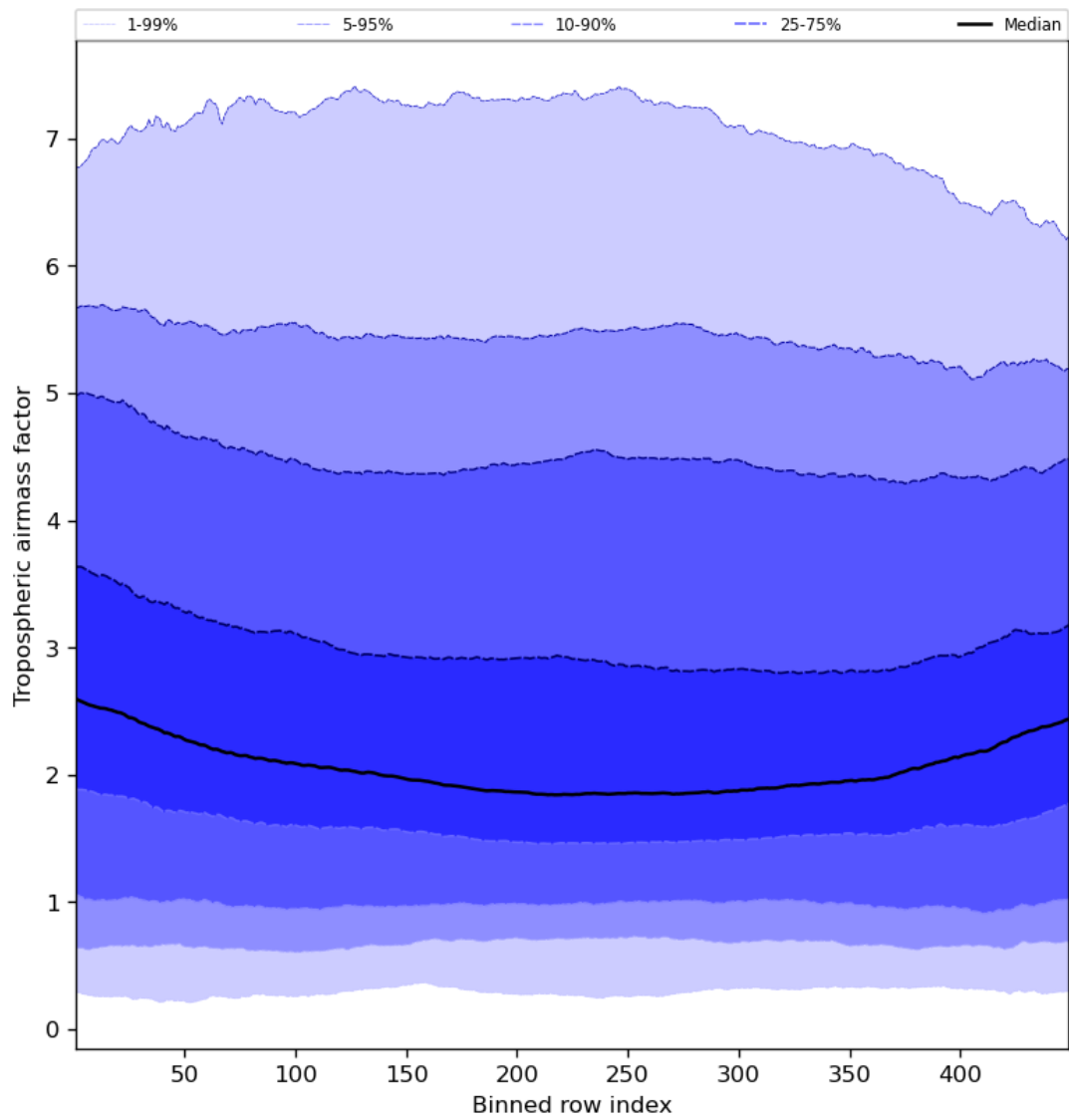
Figure 48: Along track statistics of “Tropospheric airmass factor” for 2023-11-14 to 2023-11-16
