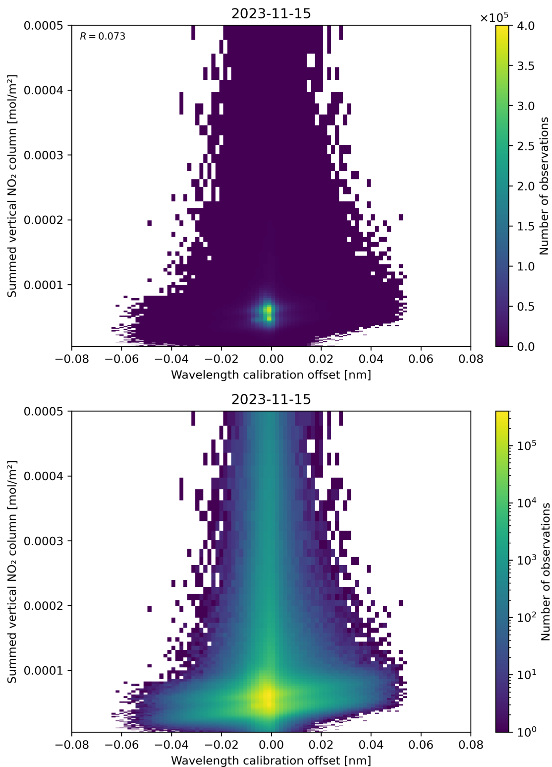
Figure 177: Scatter density plot of “Wavelength calibration offset” against “Summed vertical NO 2 column” for 2023-11-14 to 2023-11-16.
