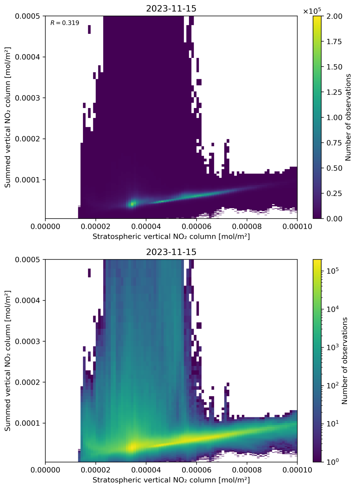
Figure 98: Scatter density plot of “Stratospheric vertical NO 2 column” against “Summed vertical NO 2 column” for 2023-11-14 to 2023-11-16.
