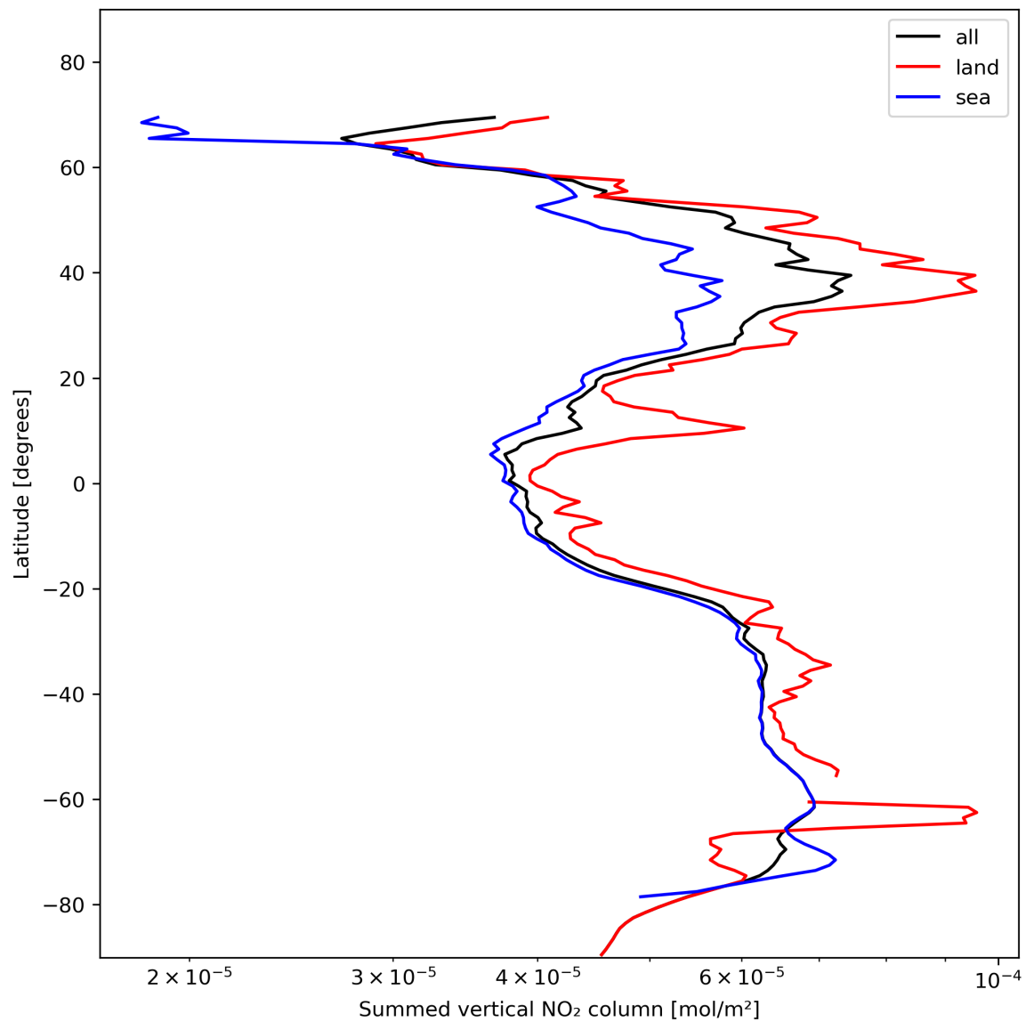
Figure 23: Zonal average of “Summed vertical NO 2 column” for 2023-11-14 to 2023-11-16.
