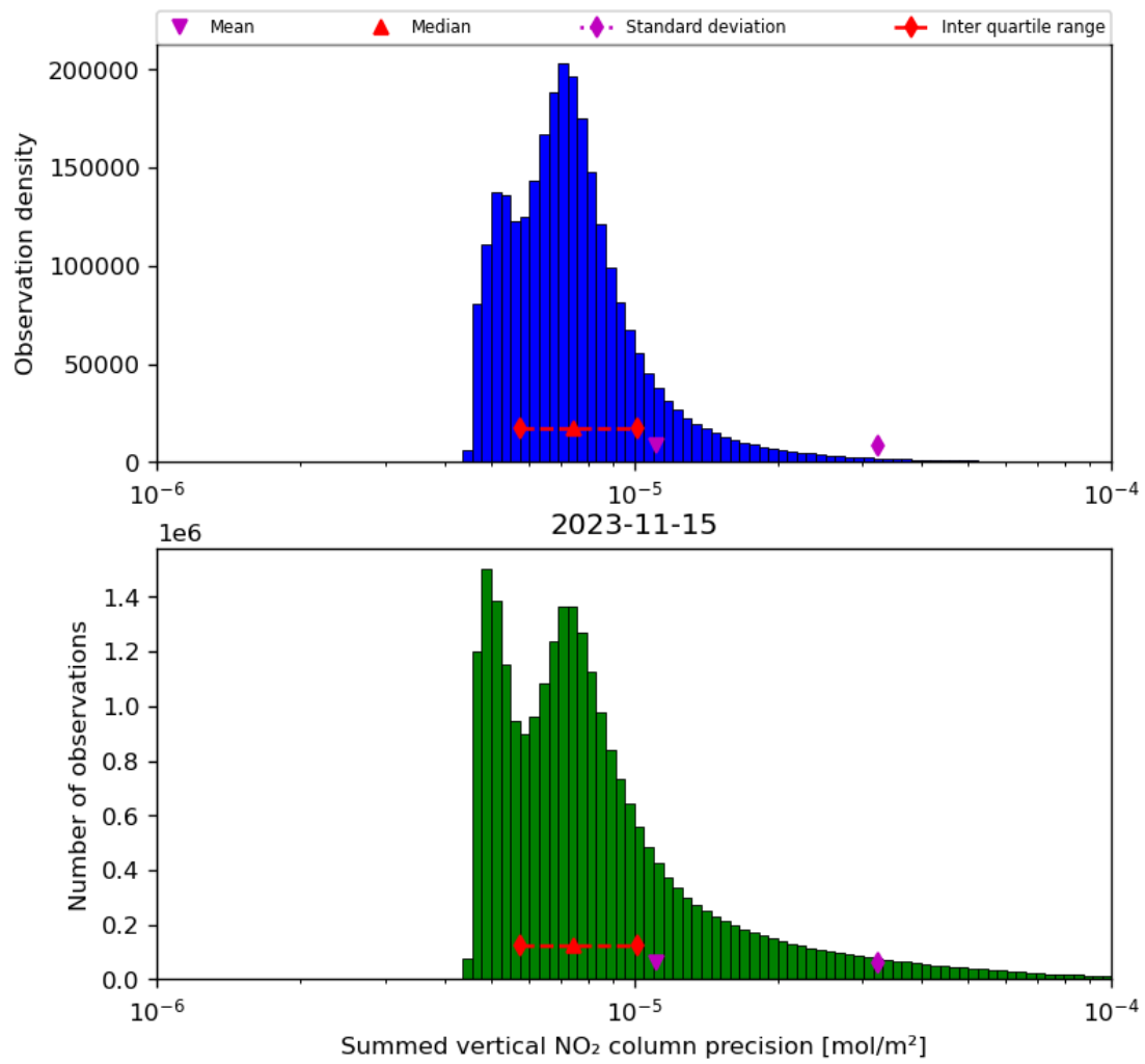
Figure 41: Histogram of "Summed vertical NO 2 column precision" for 2023-11-14 to 2023-11-16
