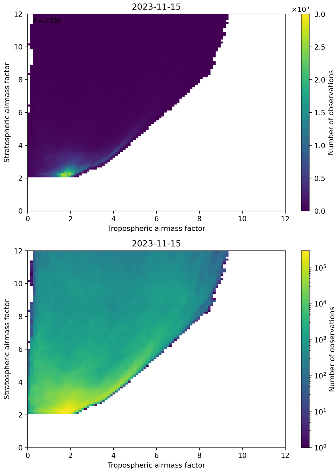
Figure 71: Scatter density plot of “Tropospheric airmass factor” against “Stratospheric airmass factor” for 2023-11-14 to 2023-11-16.
