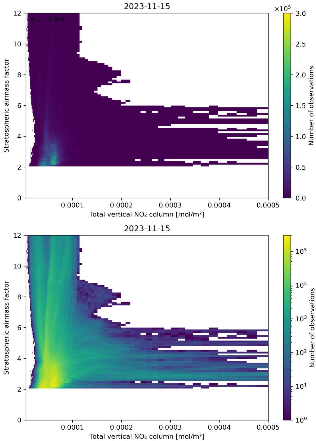
Figure 110: Scatter density plot of “Total vertical NO 2 column” against “Stratospheric airmass factor” for 2023-11-14 to 2023-11-16.
