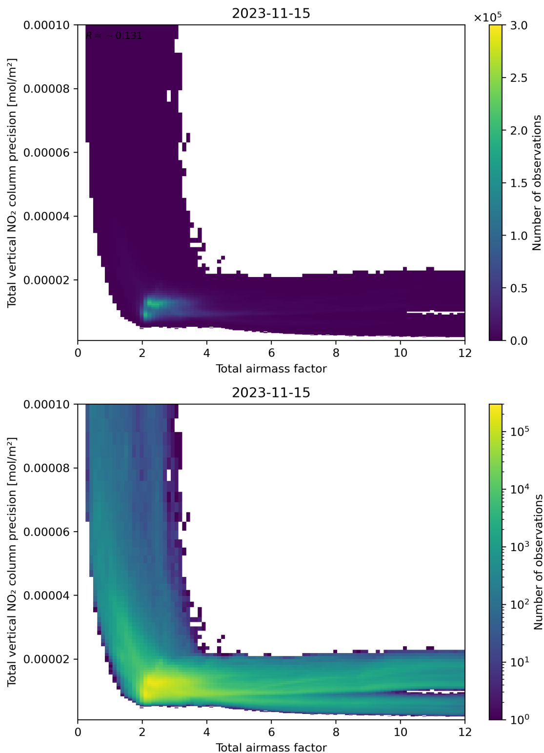
Figure 68: Scatter density plot of “Total airmass factor” against “Total vertical NO 2 column precision” for 2023-11-14 to 2023-11-16.
