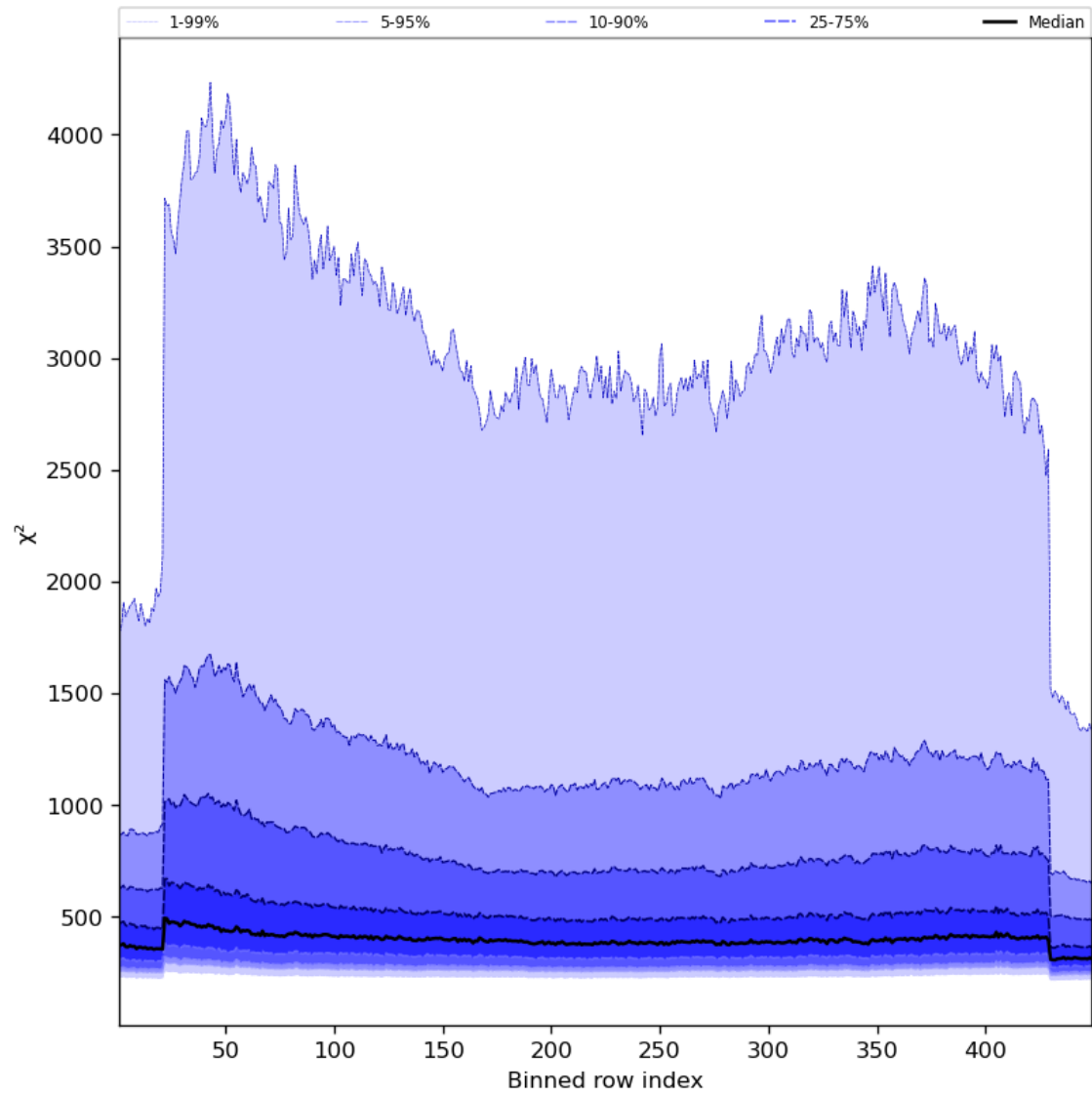
Figure 59: Along track statistics of “ \chi^2 ” for 2023-11-14 to 2023-11-16
