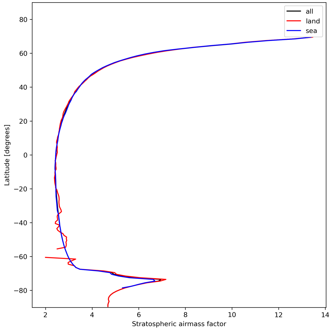
Figure 27: Zonal average of “Stratospheric airmass factor” for 2023-11-14 to 2023-11-16.
