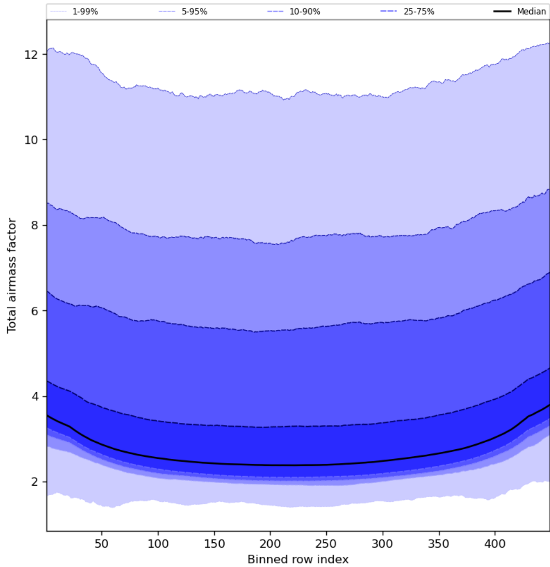
Figure 49: Along track statistics of “Total airmass factor” for 2023-11-14 to 2023-11-16
