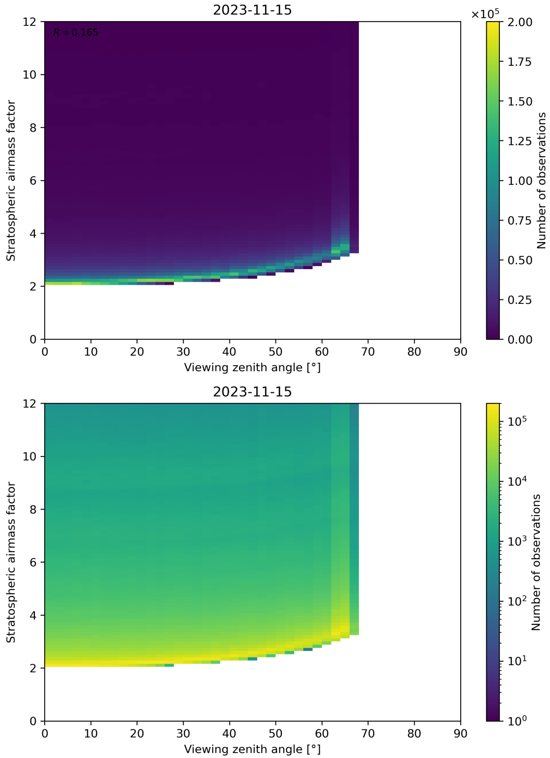
Figure 159: Scatter density plot of “Viewing zenith angle” against “Stratospheric airmass factor” for 2023-11-14 to 2023-11-16.
