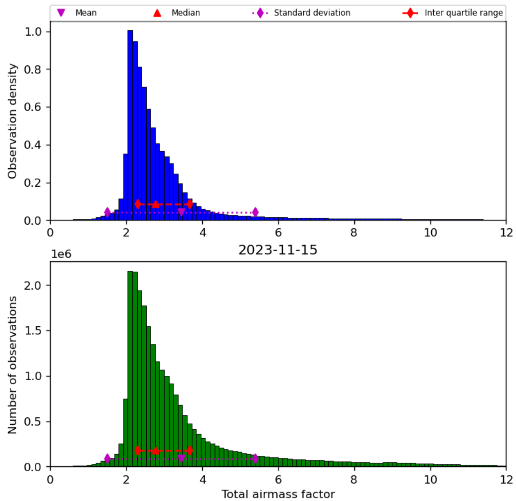
Figure 32: Histogram of “Total airmass factor” for 2023-11-14 to 2023-11-16
