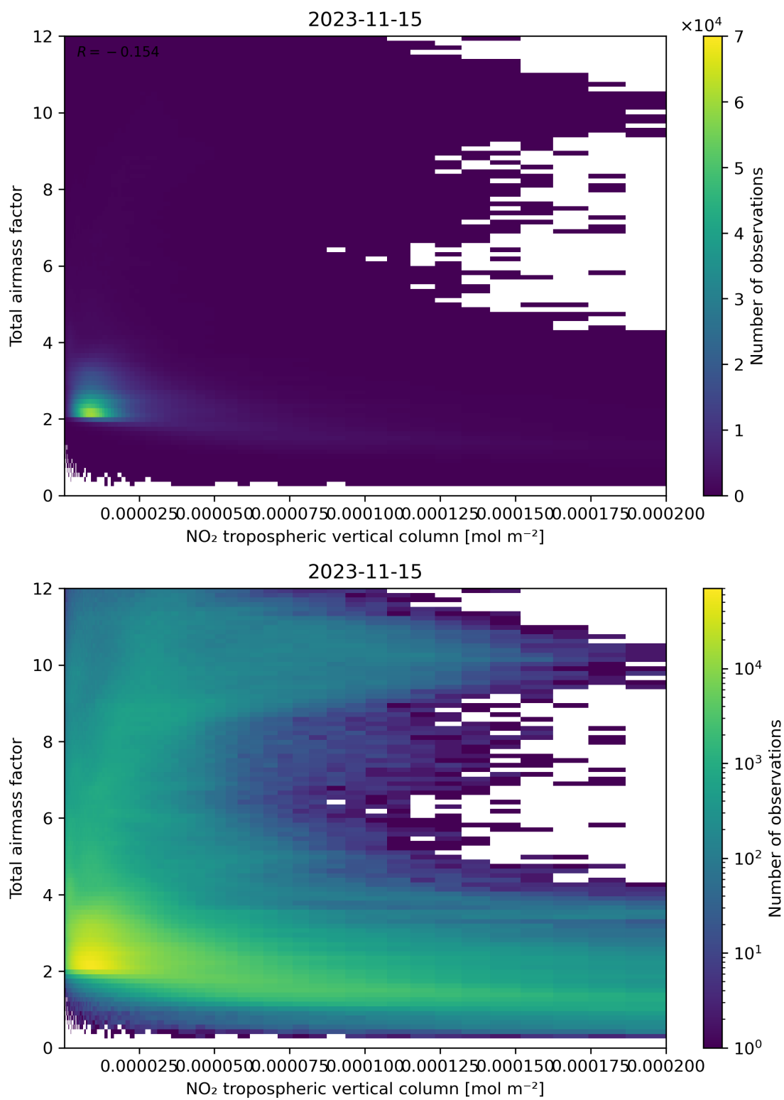
Figure 122: Scatter density plot of “NO 2 tropospheric vertical column” against “Total air mass factor” for 2023-11-14 to 2023-11-16.
