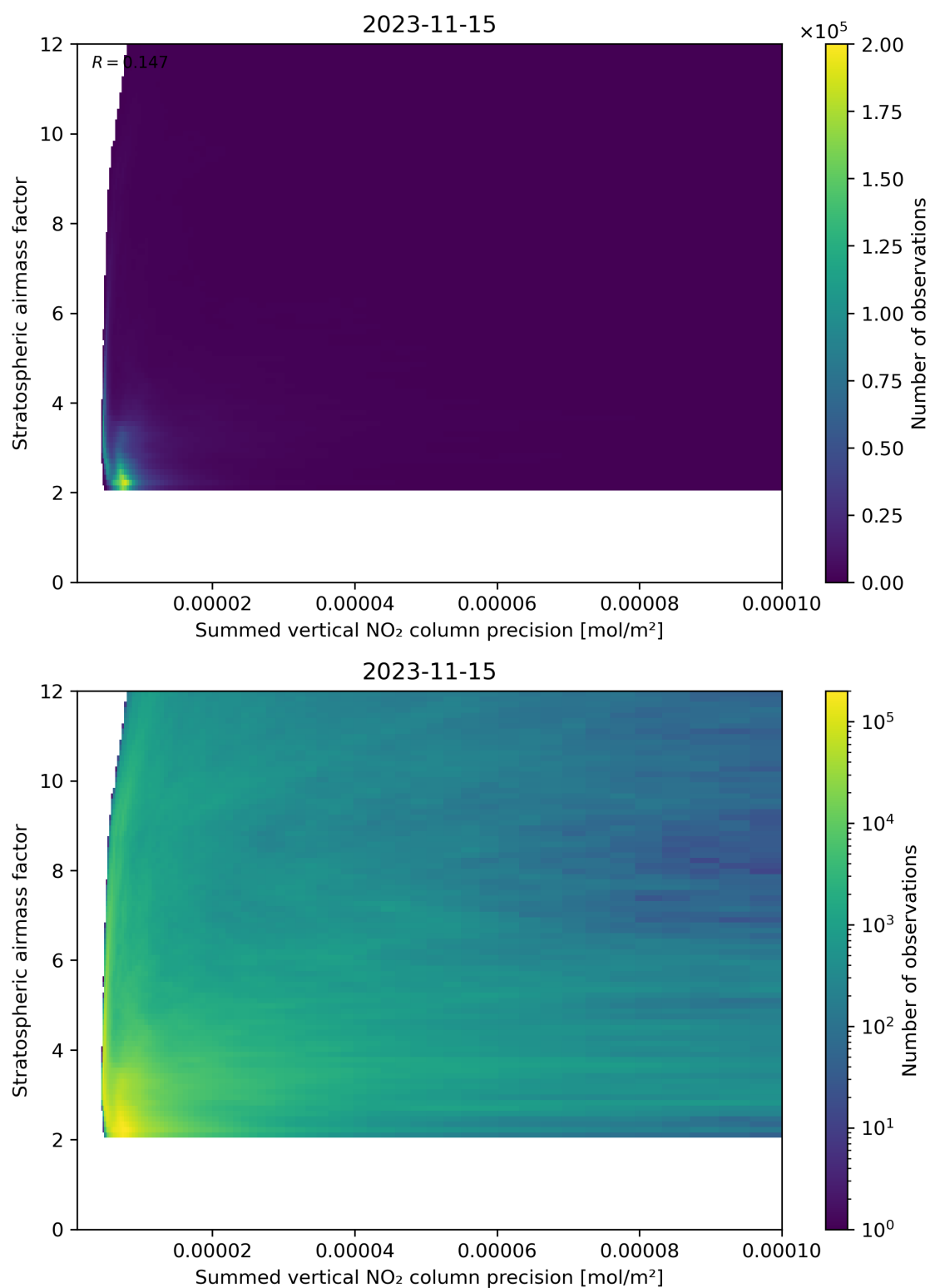
Figure 106: Scatter density plot of “Summed vertical NO 2 column precision” against “Stratospheric airmass factor” for 2023-11-14 to 2023-11-16.
