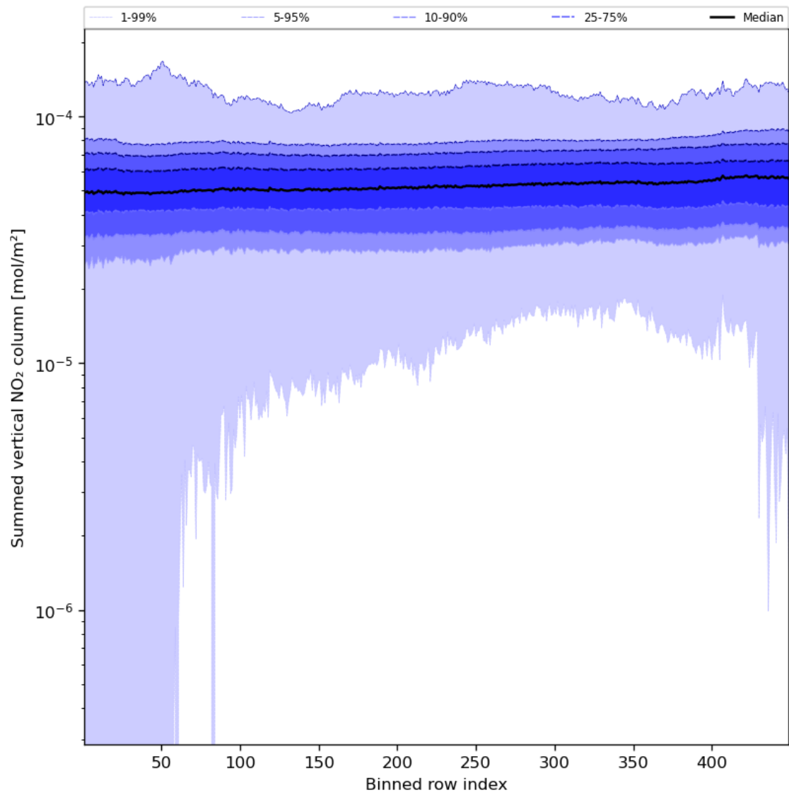
Figure 57: Along track statistics of “Summed vertical NO 2 column” for 2023-11-14 to 2023-11-16
