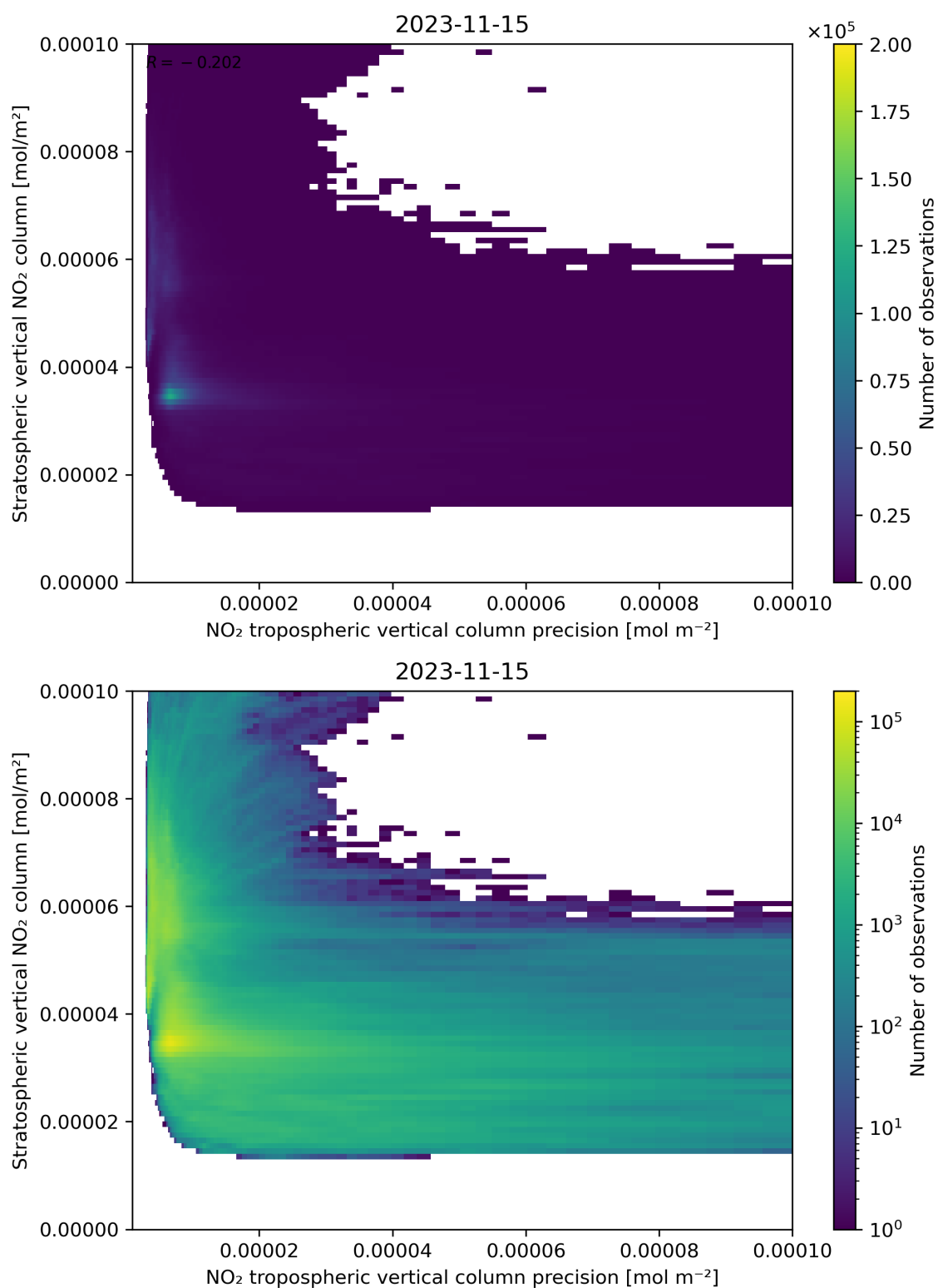
Figure 135: Scatter density plot of “NO 2 tropospheric vertical column precision” against “Stratospheric vertical NO 2 column” for 2023-11-14 to 2023-11-16.
