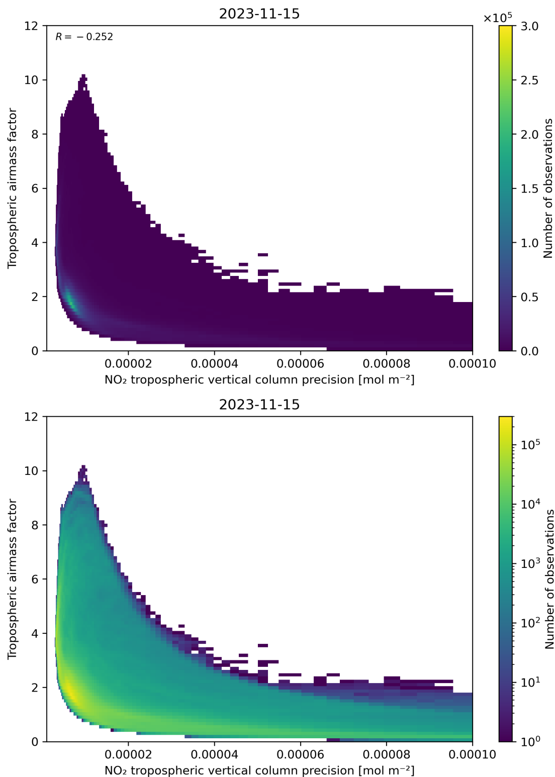
Figure 133: Scatter density plot of “NO 2 tropospheric vertical column precision” against “Tropospheric airmass factor” for 2023-11-14 to 2023-11-16.
