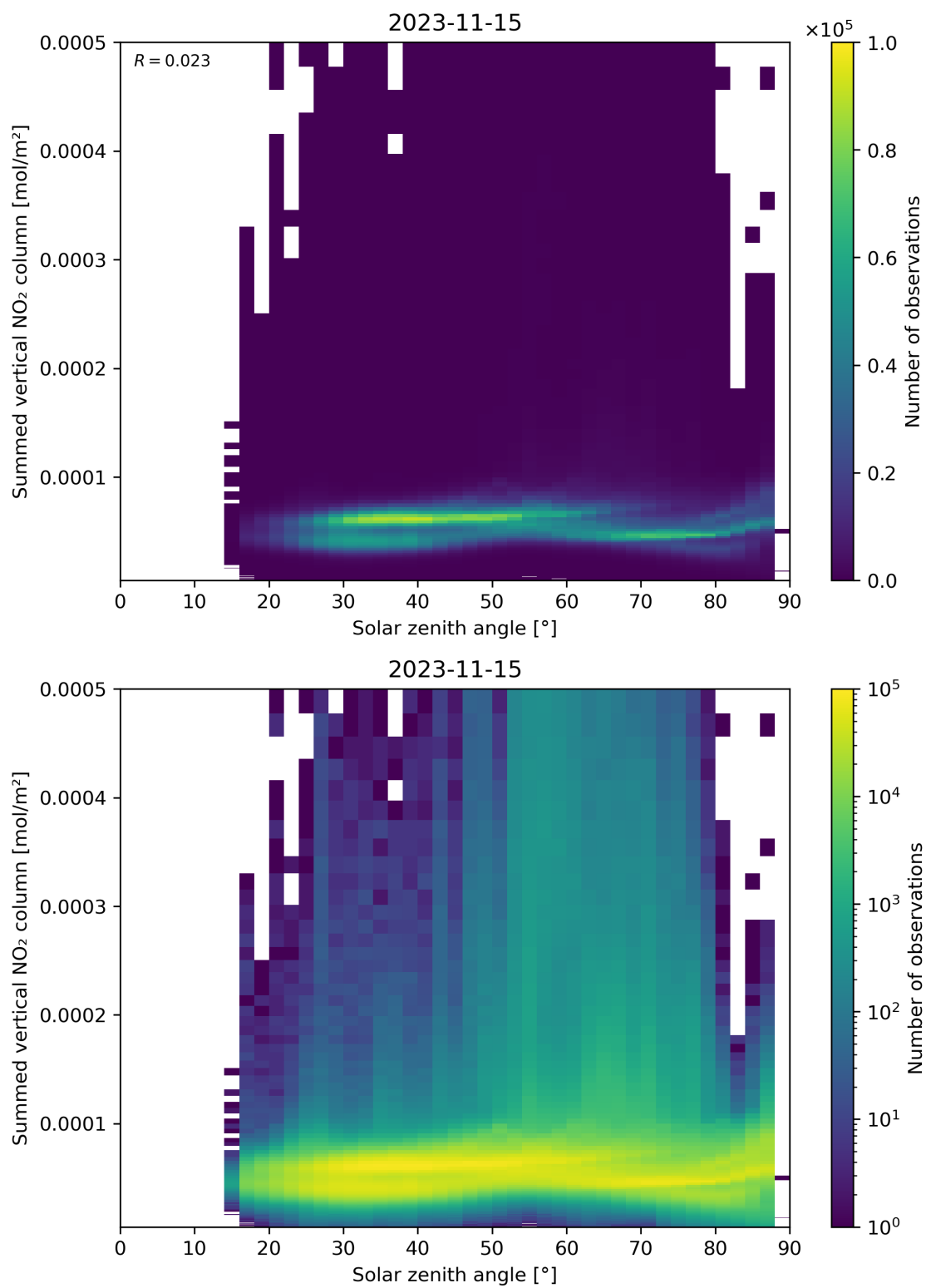
Figure 151: Scatter density plot of “Solar zenith angle” against “Summed vertical NO 2 column” for 2023-11-14 to 2023-11-16.
