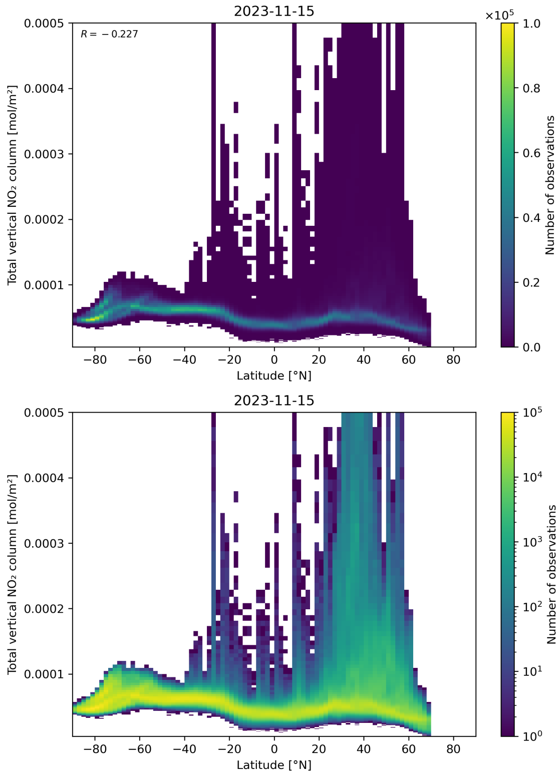
Figure 90: Scatter density plot of “Latitude” against “Total vertical NO 2 column” for 2023-11-14 to 2023-11-16.
