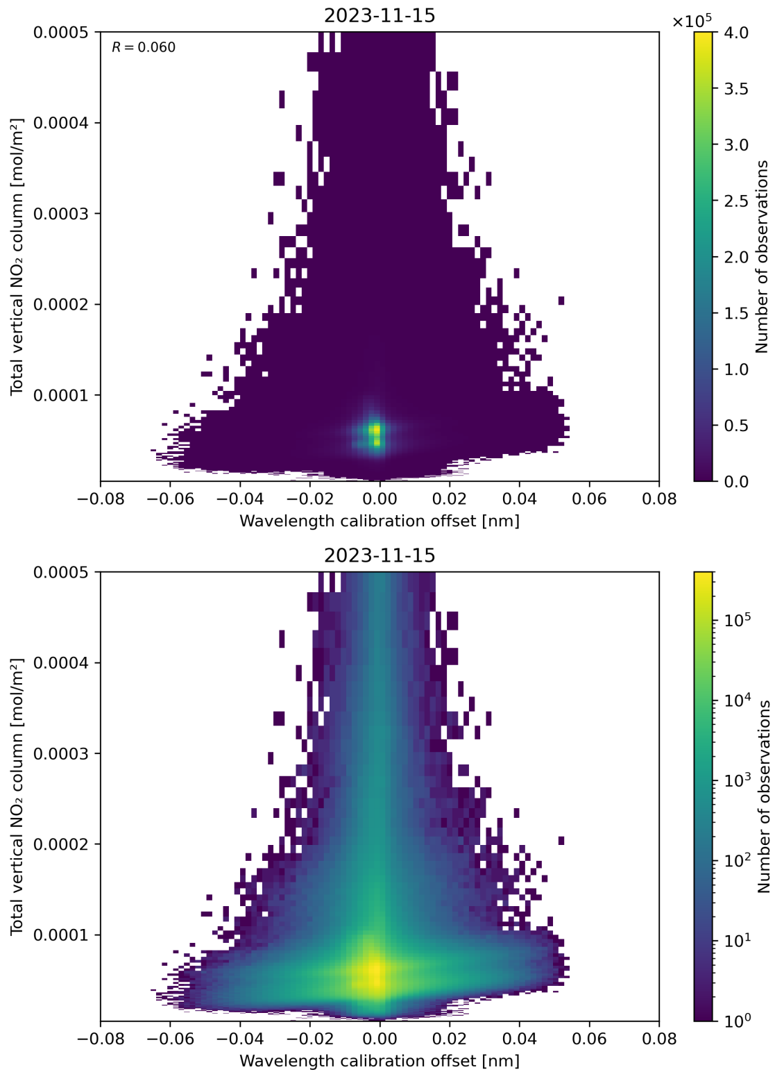
Figure 179: Scatter density plot of “Wavelength calibration offset” against “Total vertical NO 2 column” for 2023-11-14 to 2023-11-16.
