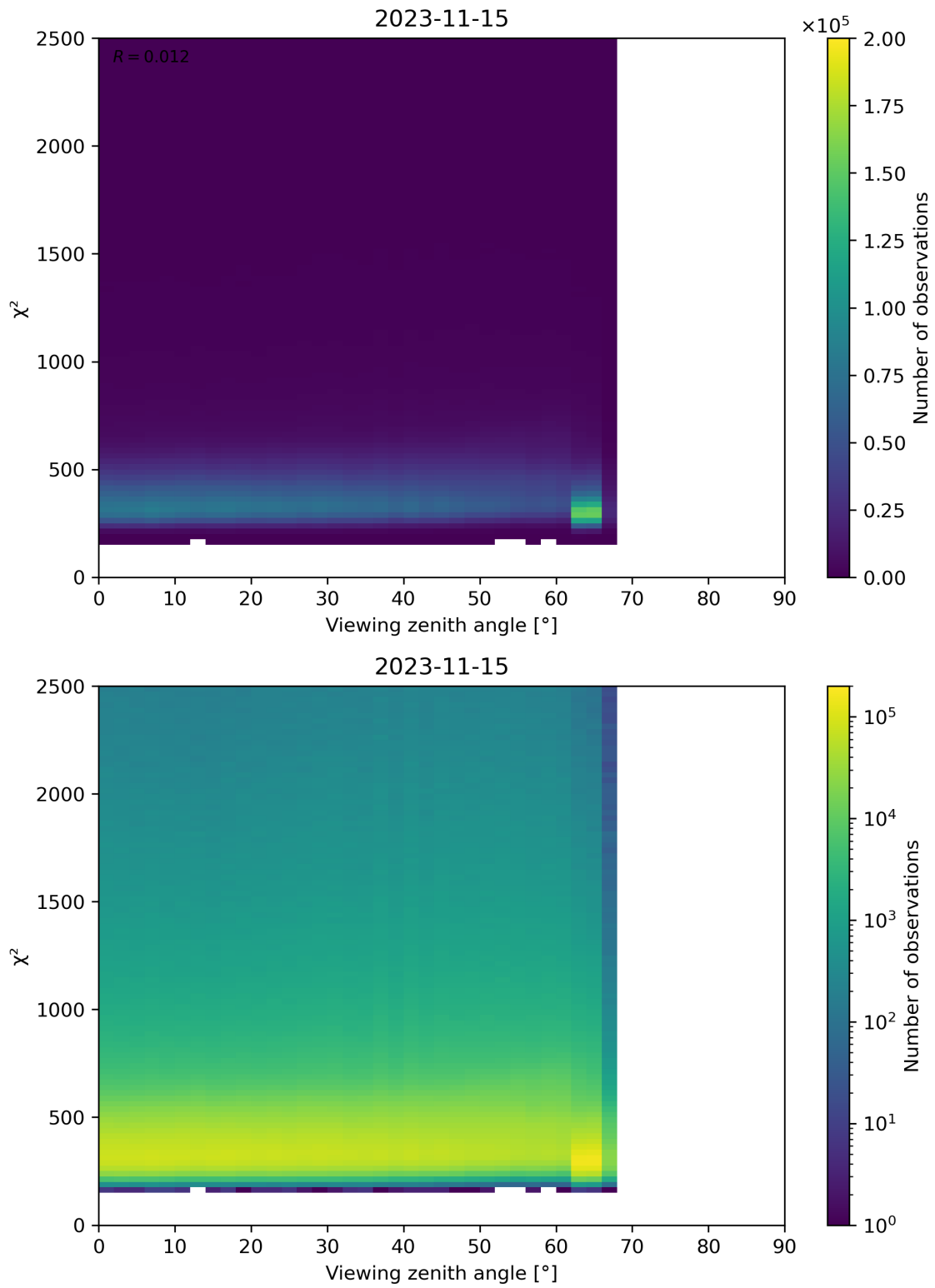
Figure 162: Scatter density plot of “Viewing zenith angle” against “ \chi^2 ” for 2023-11-14 to 2023-11-16.
