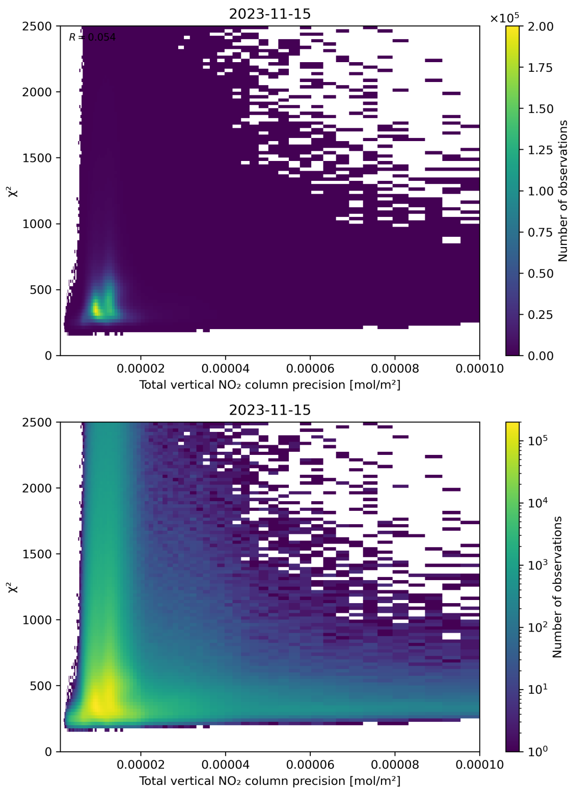
Figure 116: Scatter density plot of “Total vertical NO 2 column precision” against “ \chi^2 ” for 2023-11-14 to 2023-11-16.
