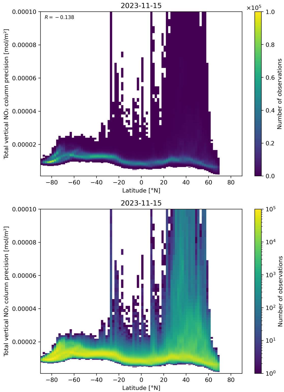
Figure 91: Scatter density plot of “Latitude” against “Total vertical NO 2 column precision” for 2023-11-14 to 2023-11-16.
