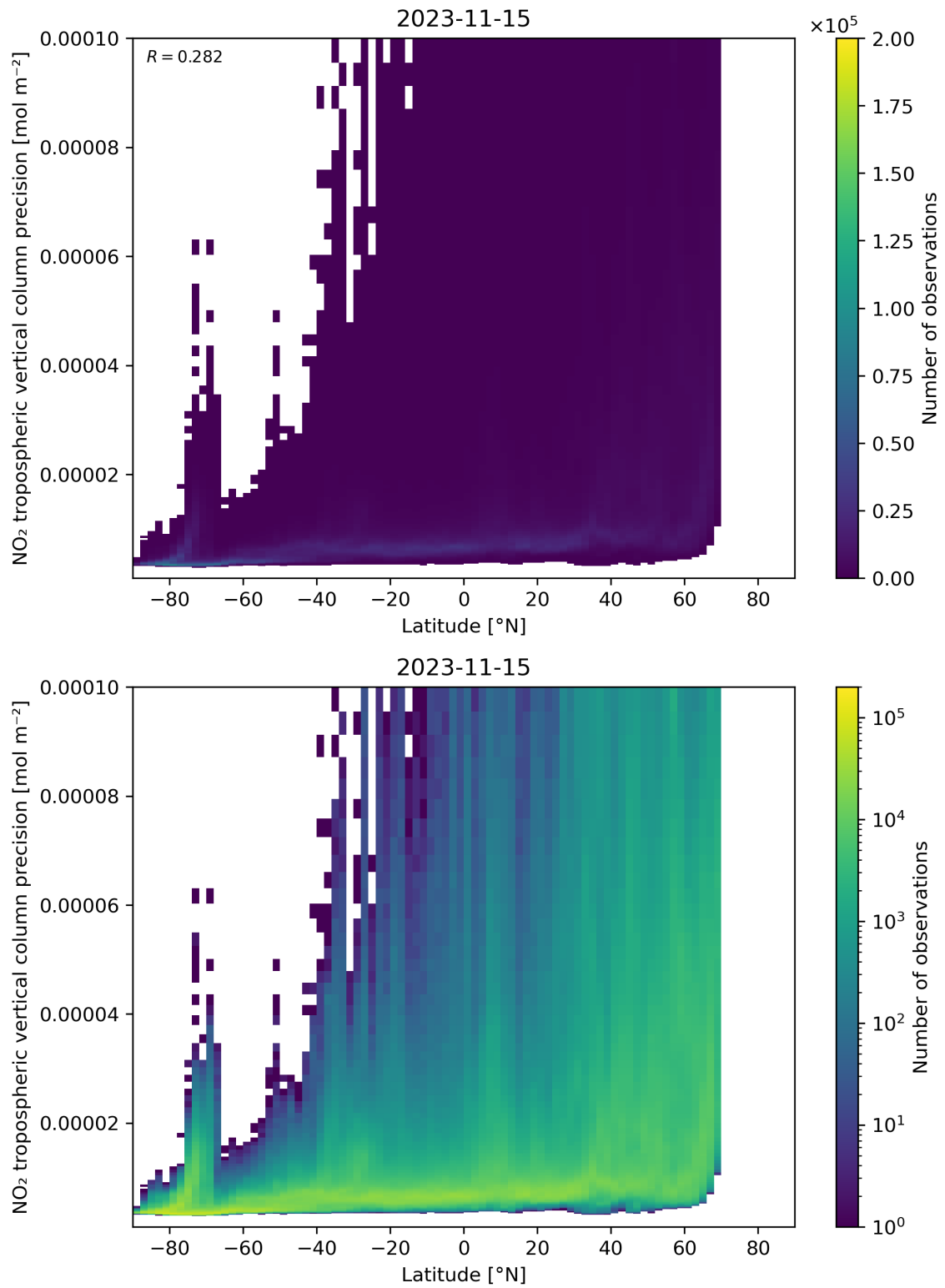
Figure 93: Scatter density plot of “Latitude” against “NO 2 tropospheric vertical column precision” for 2023-11-14 to 2023-11-16.
