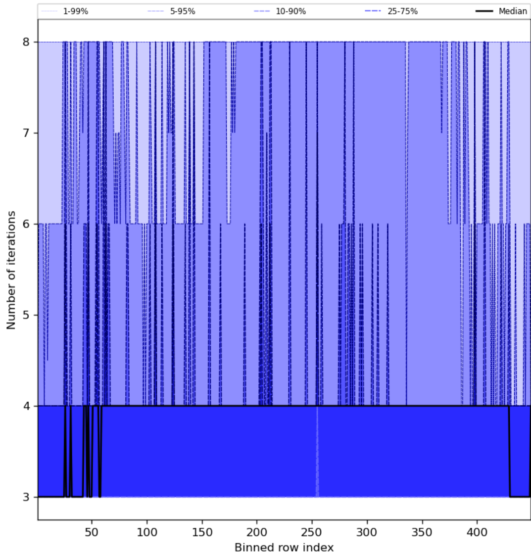
Figure 51: Along track statistics of "Number of iterations" for 2023-11-14 to 2023-11-16
