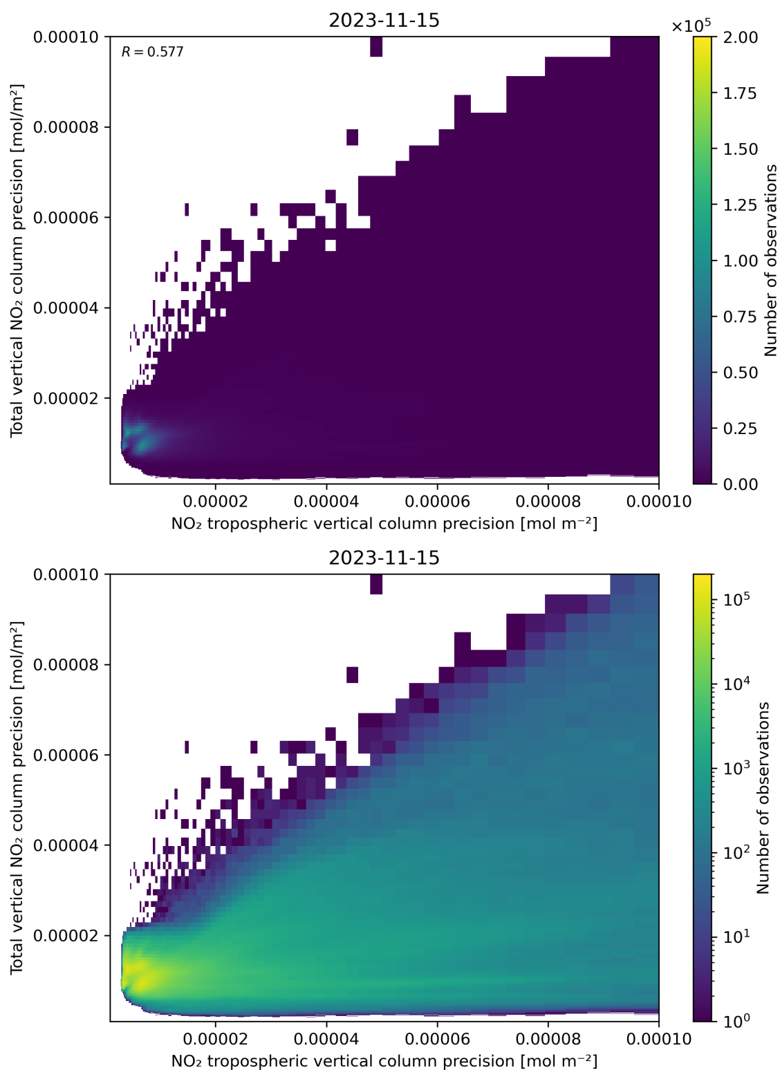
Figure 139: Scatter density plot of “NO 2 tropospheric vertical column precision” against “Total vertical NO 2 column precision” for 2023-11-14 to 2023-11-16.
