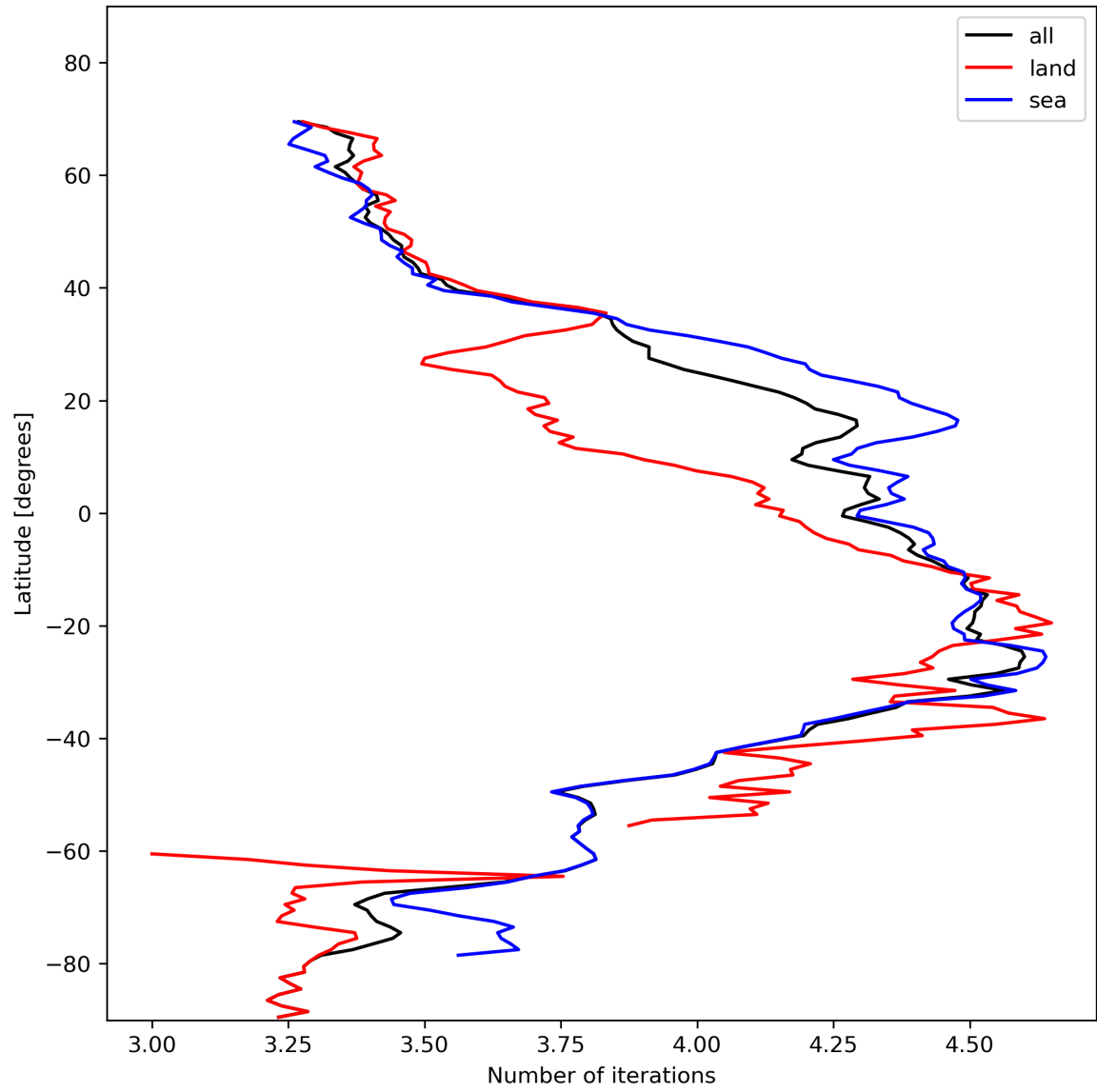
Figure 17: Zonal average of “Number of iterations” for 2023-11-14 to 2023-11-16.
