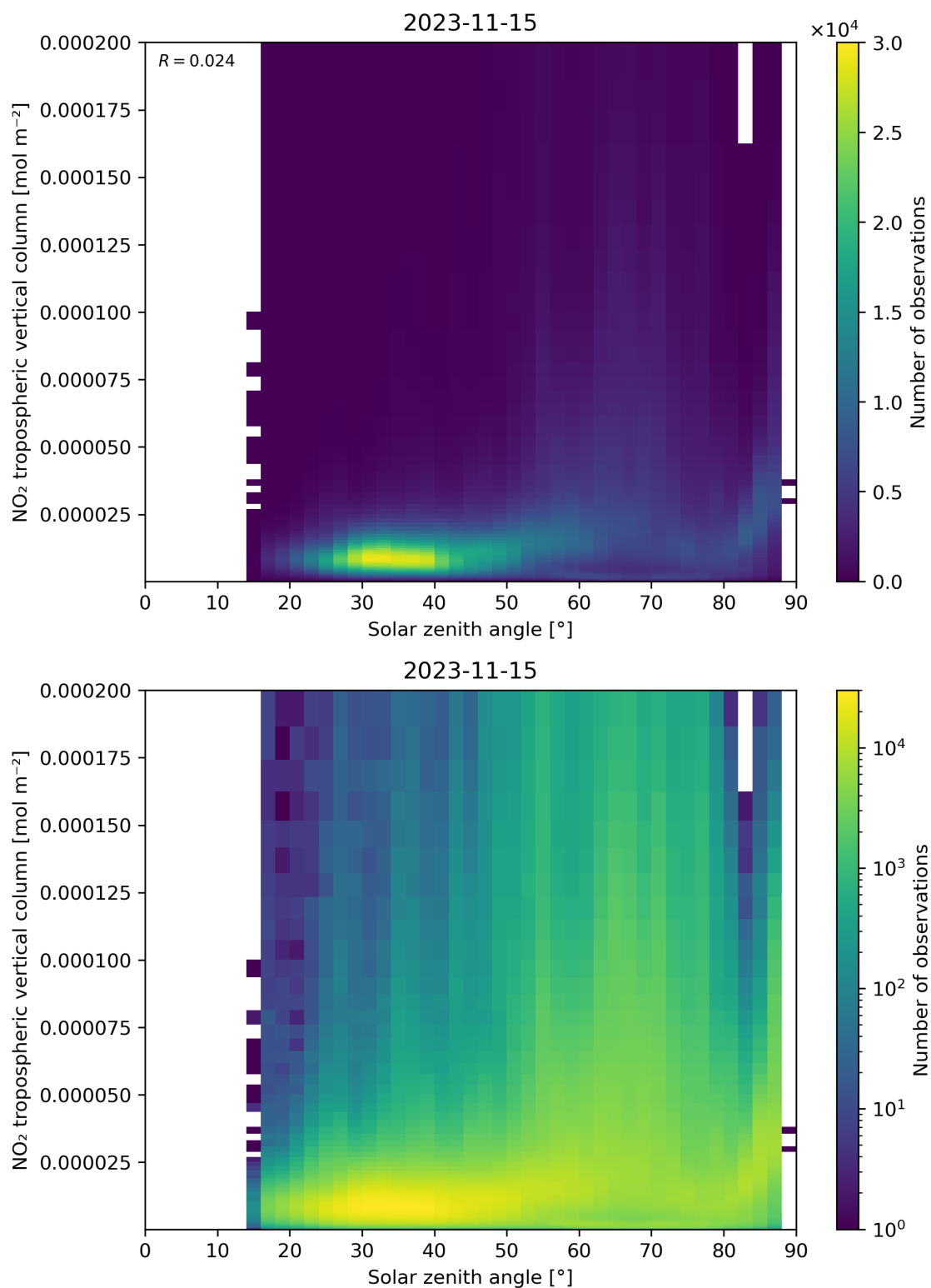
Figure 155: Scatter density plot of “Solar zenith angle” against “NO 2 tropospheric vertical column” for 2023-11-14 to 2023-11-16.
