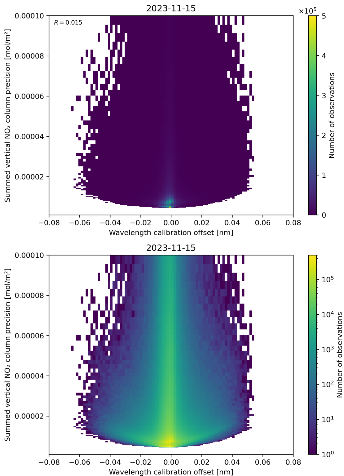
Figure 178: Scatter density plot of “Wavelength calibration offset” against “Summed vertical NO 2 column precision” for 2023-11-14 to 2023-11-16.
