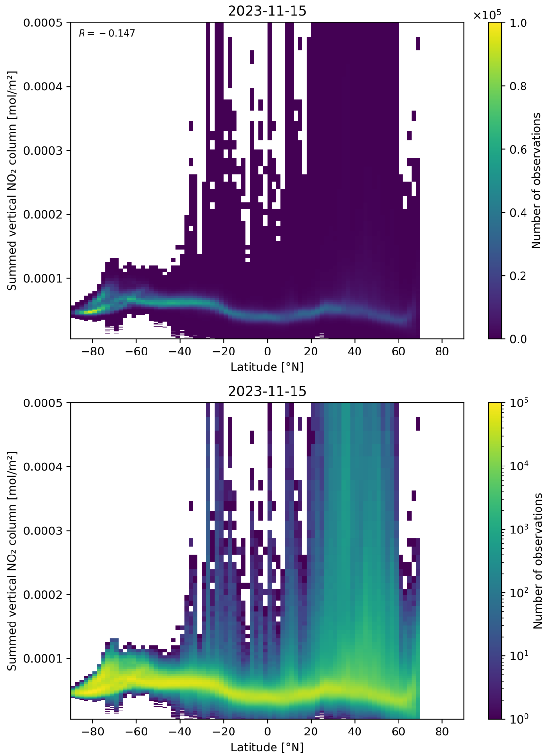
Figure 88: Scatter density plot of “Latitude” against “Summed vertical NO 2 column” for 2023-11-14 to 2023-11-16.
