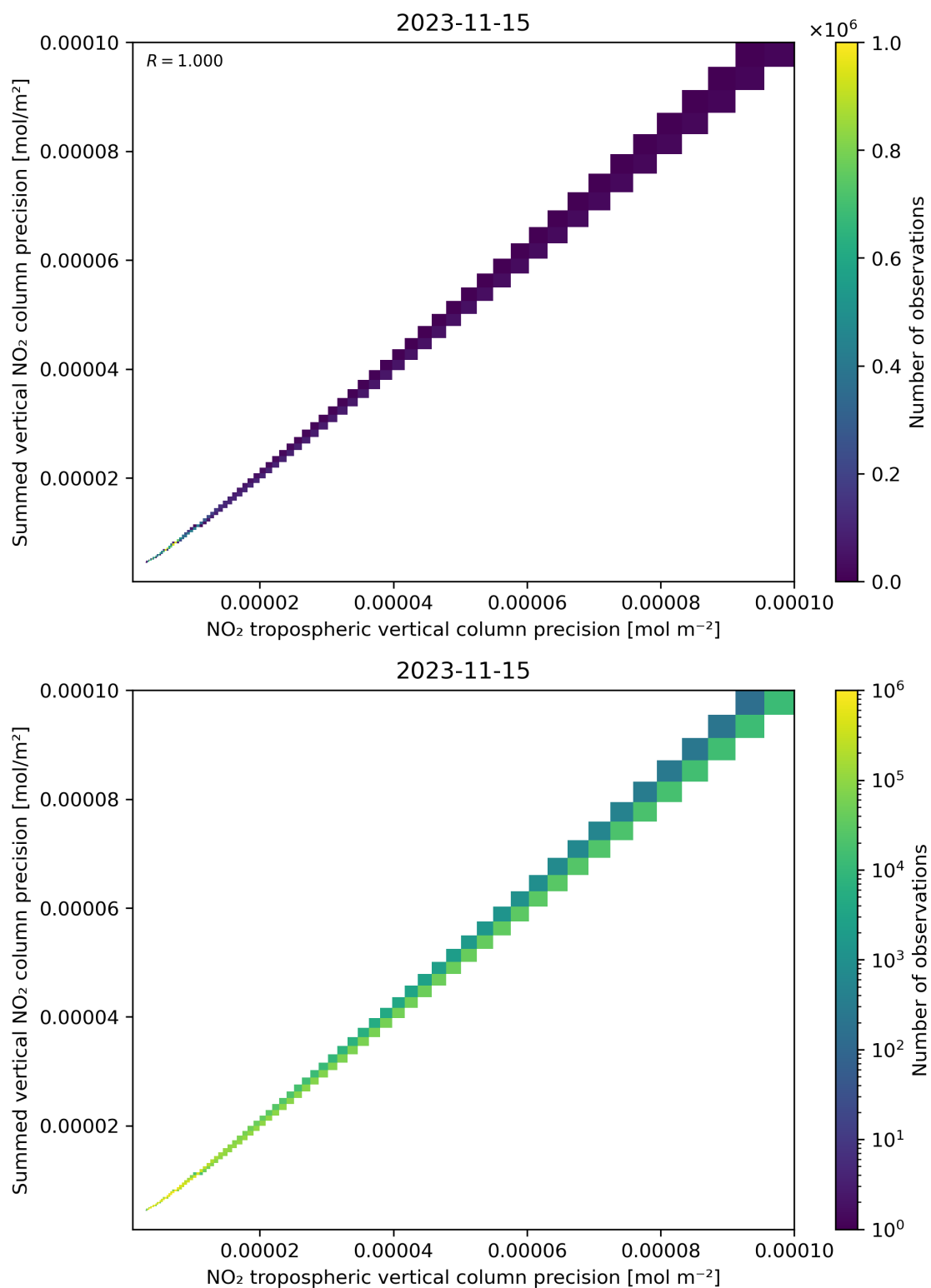
Figure 137: Scatter density plot of “NO 2 tropospheric vertical column precision” against “Summed vertical NO 2 column precision” for 2023-11-14 to 2023-11-16.
