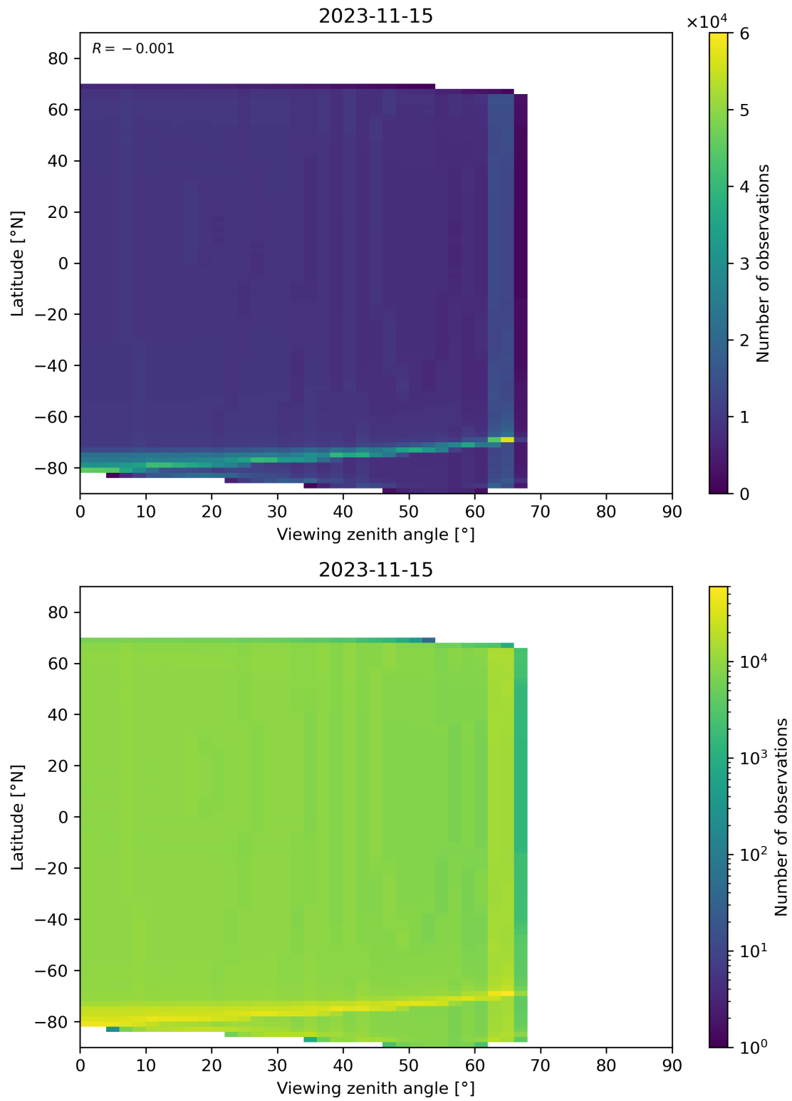
Figure 163: Scatter density plot of “Viewing zenith angle” against “Latitude” for 2023-11-14 to 2023-11-16.
