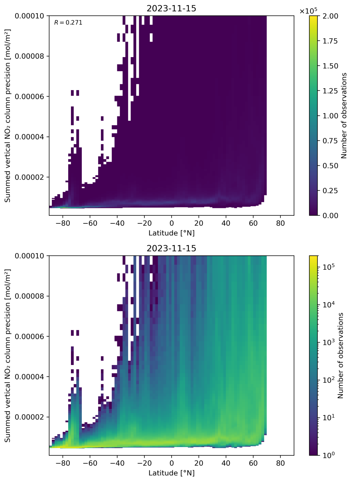
Figure 89: Scatter density plot of “Latitude” against “Summed vertical NO 2 column precision” for 2023-11-14 to 2023-11-16.
