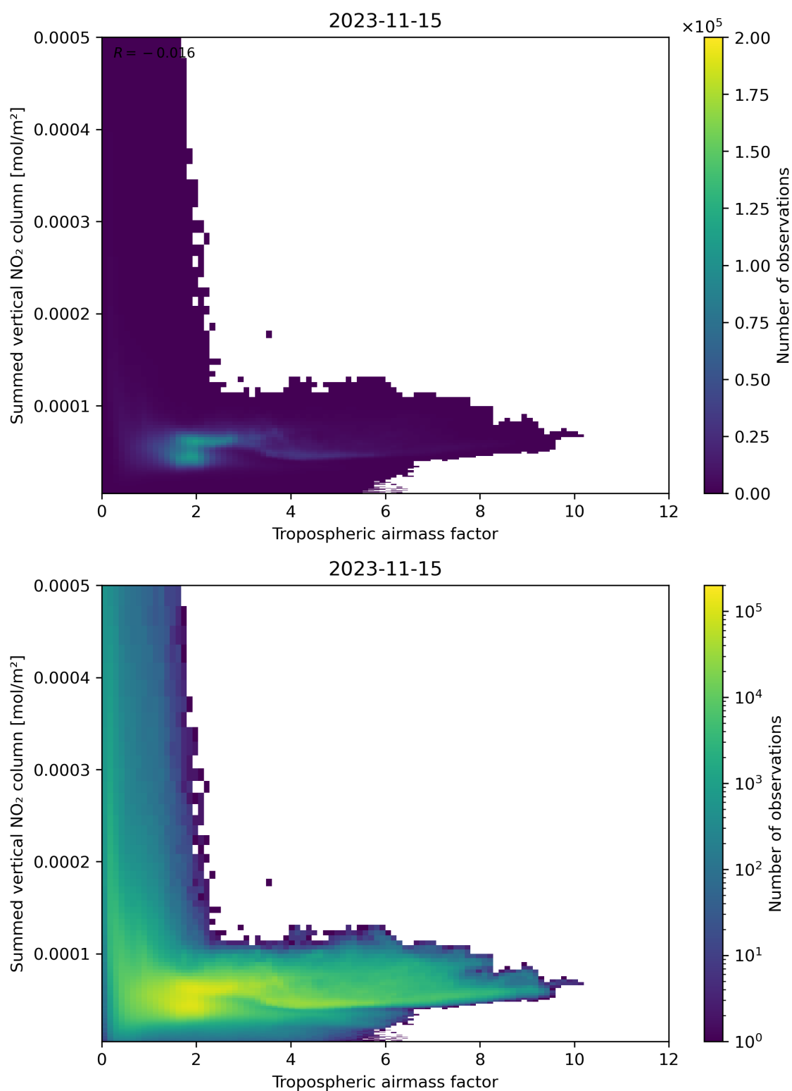
Figure 75: Scatter density plot of “Tropospheric air mass factor” against “Summed vertical NO 2 column” for 2023-11-14 to 2023-11-16.
