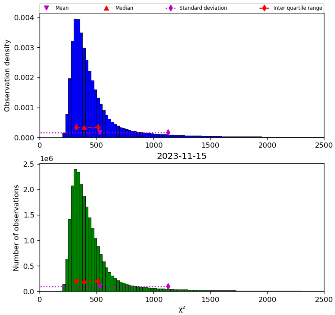
Figure 42: Histogram of “ \chi^2 ” for 2023-11-14 to 2023-11-16
