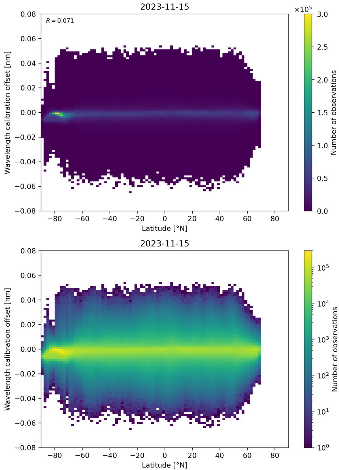
Figure 95: Scatter density plot of “Latitude” against “Wavelength calibration offset” for 2023-11-14 to 2023-11-16.
