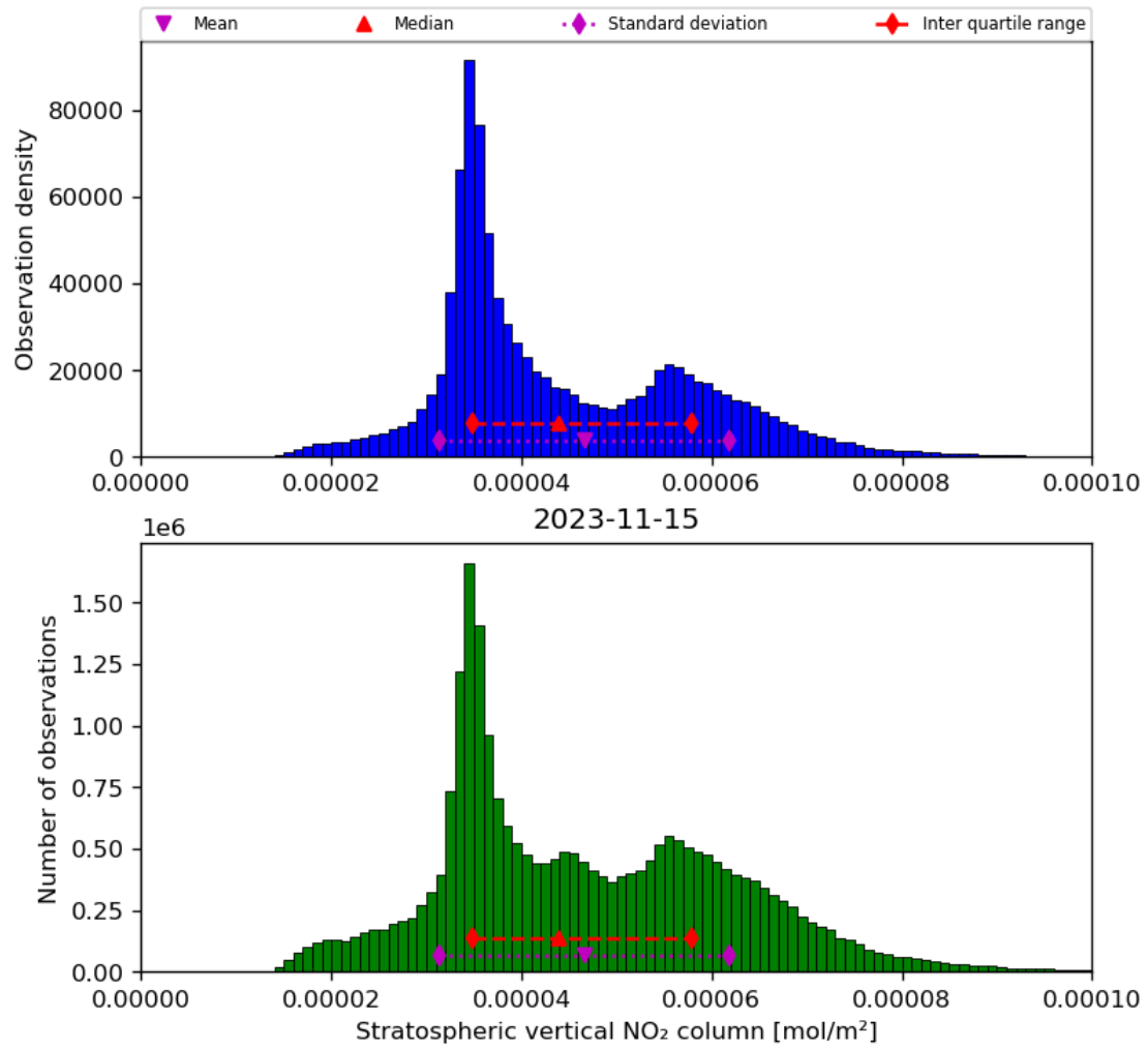
Figure 36: Histogram of “Stratospheric vertical NO 2 column” for 2023-11-14 to 2023-11-16
