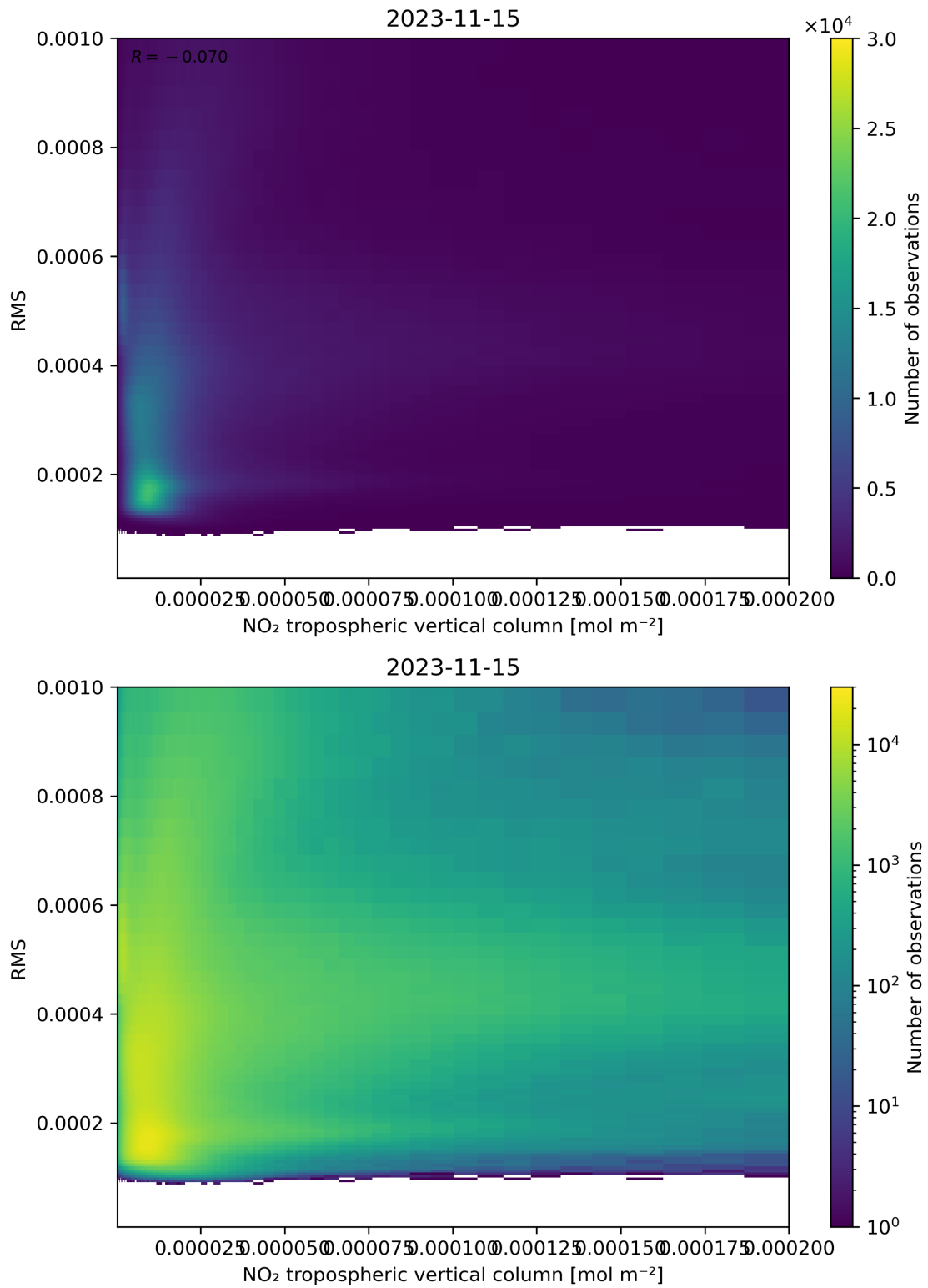
Figure 142: Scatter density plot of “NO 2 tropospheric vertical column” against “RMS” for 2023-11-14 to 2023-11-16.
