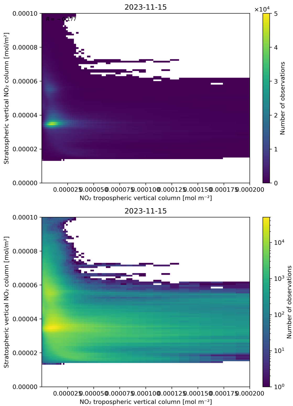
Figure 125: Scatter density plot of “NO 2 tropospheric vertical column” against “Stratospheric vertical NO 2 column” for 2023-11-14 to 2023-11-16.
