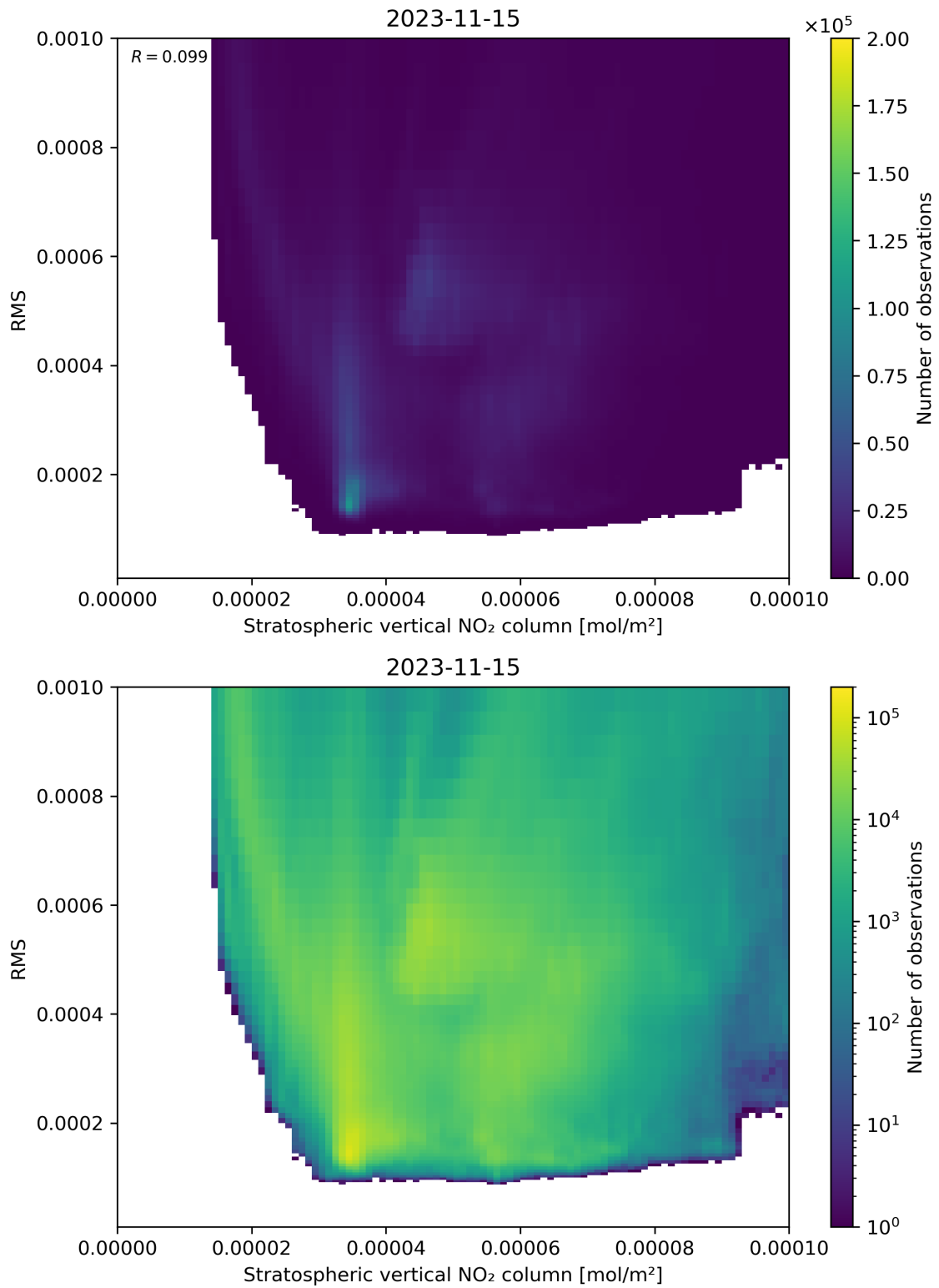
Figure 102: Scatter density plot of “Stratospheric vertical NO 2 column” against “RMS” for 2023-11-14 to 2023-11-16.
