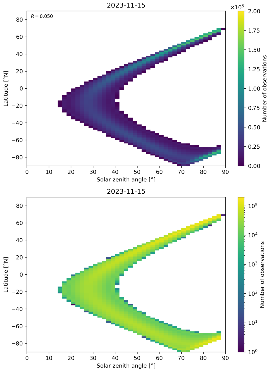
Figure 149: Scatter density plot of “Solar zenith angle” against “Latitude” for 2023-11-14 to 2023-11-16.
