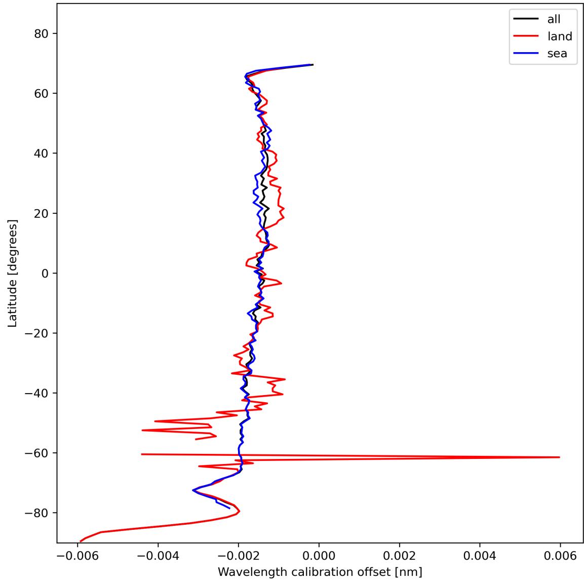
Figure 18: Zonal average of “Wavelength calibration offset” for 2023-11-14 to 2023-11-16.
