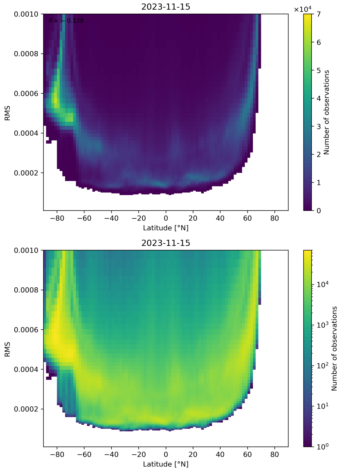
Figure 94: Scatter density plot of “Latitude” against “RMS” for 2023-11-14 to 2023-11-16.
