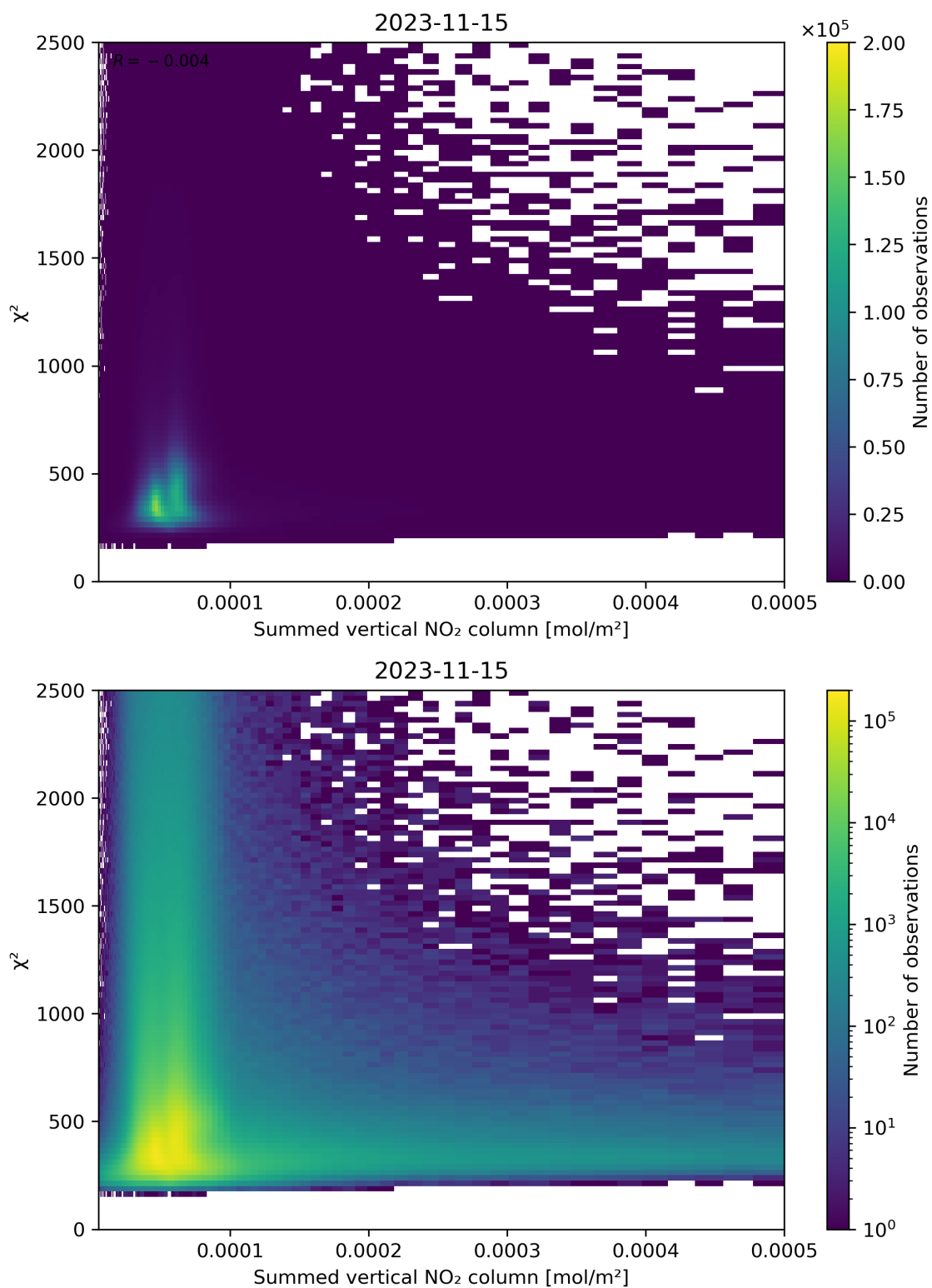
Figure 104: Scatter density plot of “Summed vertical NO 2 column” against “ \chi^2 ” for 2023-11-14 to 2023-11-16.
