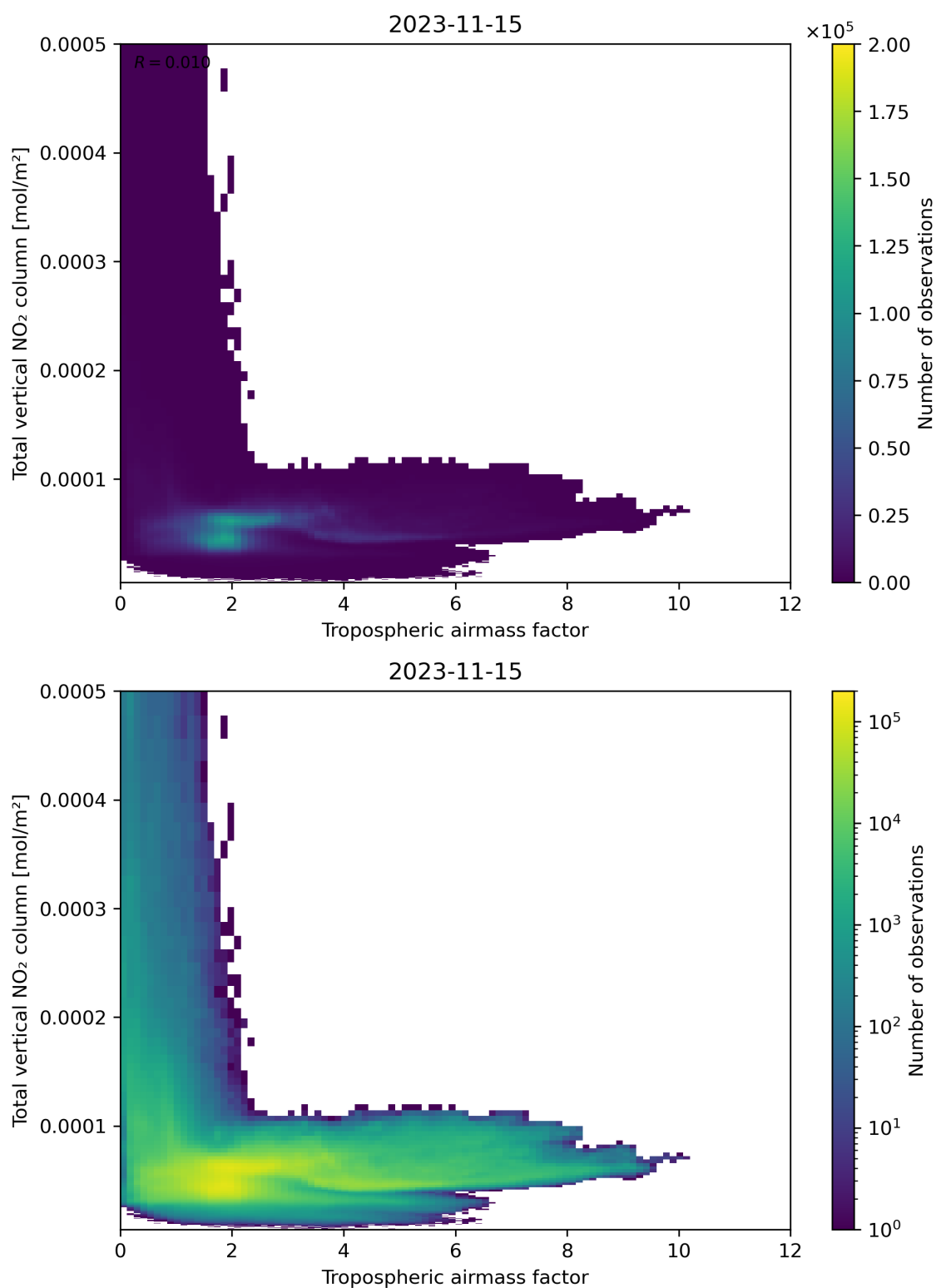
Figure 77: Scatter density plot of “Tropospheric airmass factor” against “Total vertical NO 2 column” for 2023-11-14 to 2023-11-16.
