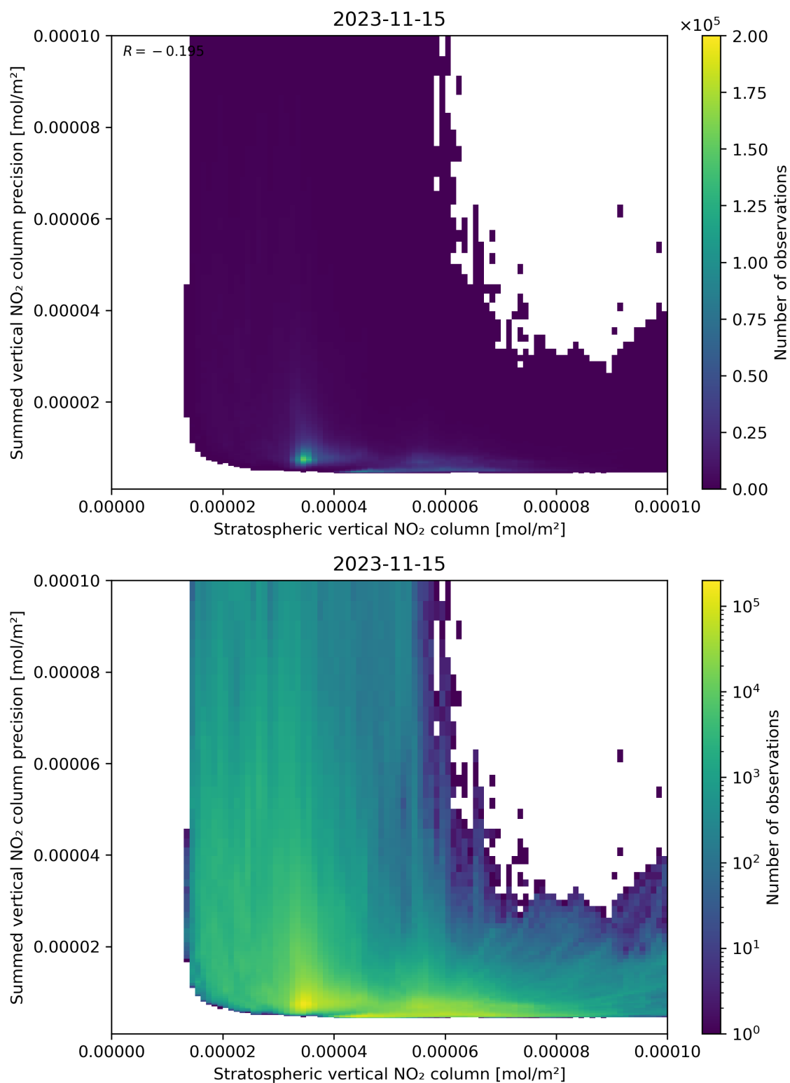
Figure 99: Scatter density plot of “Stratospheric vertical NO 2 column” against “Summed vertical NO 2 column precision” for 2023-11-14 to 2023-11-16.
