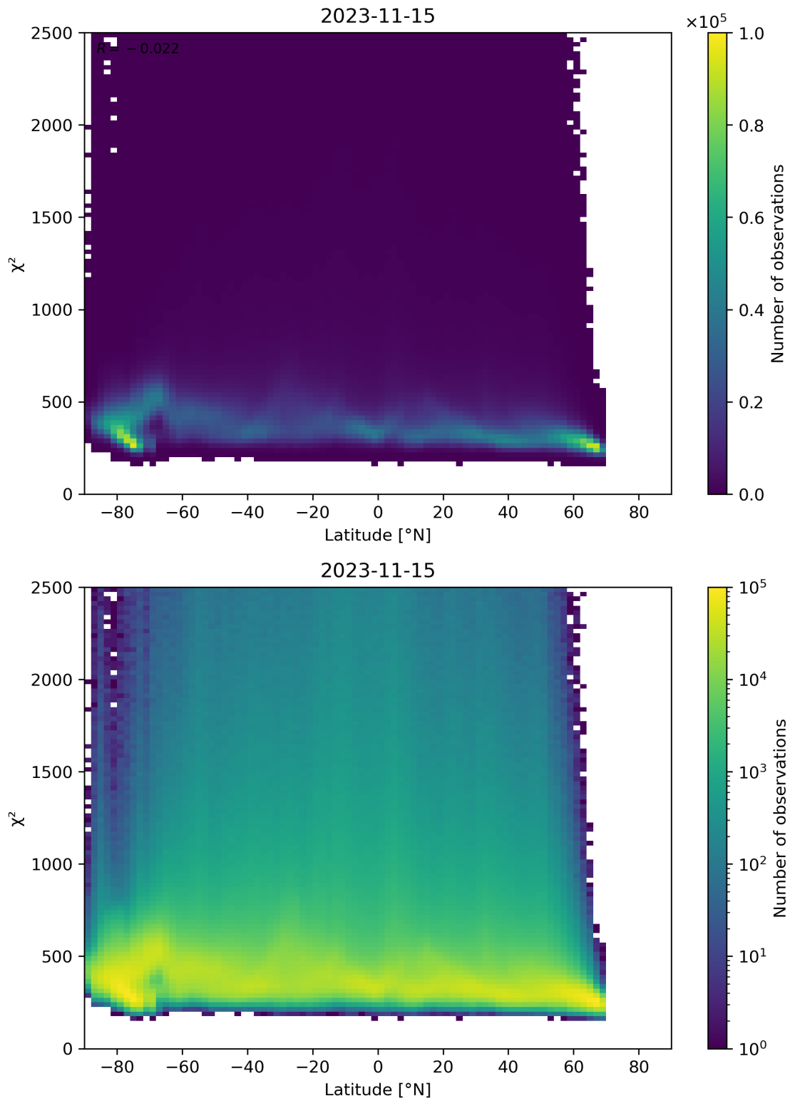
Figure 86: Scatter density plot of “Latitude” against “ \chi^2 ” for 2023-11-14 to 2023-11-16.
