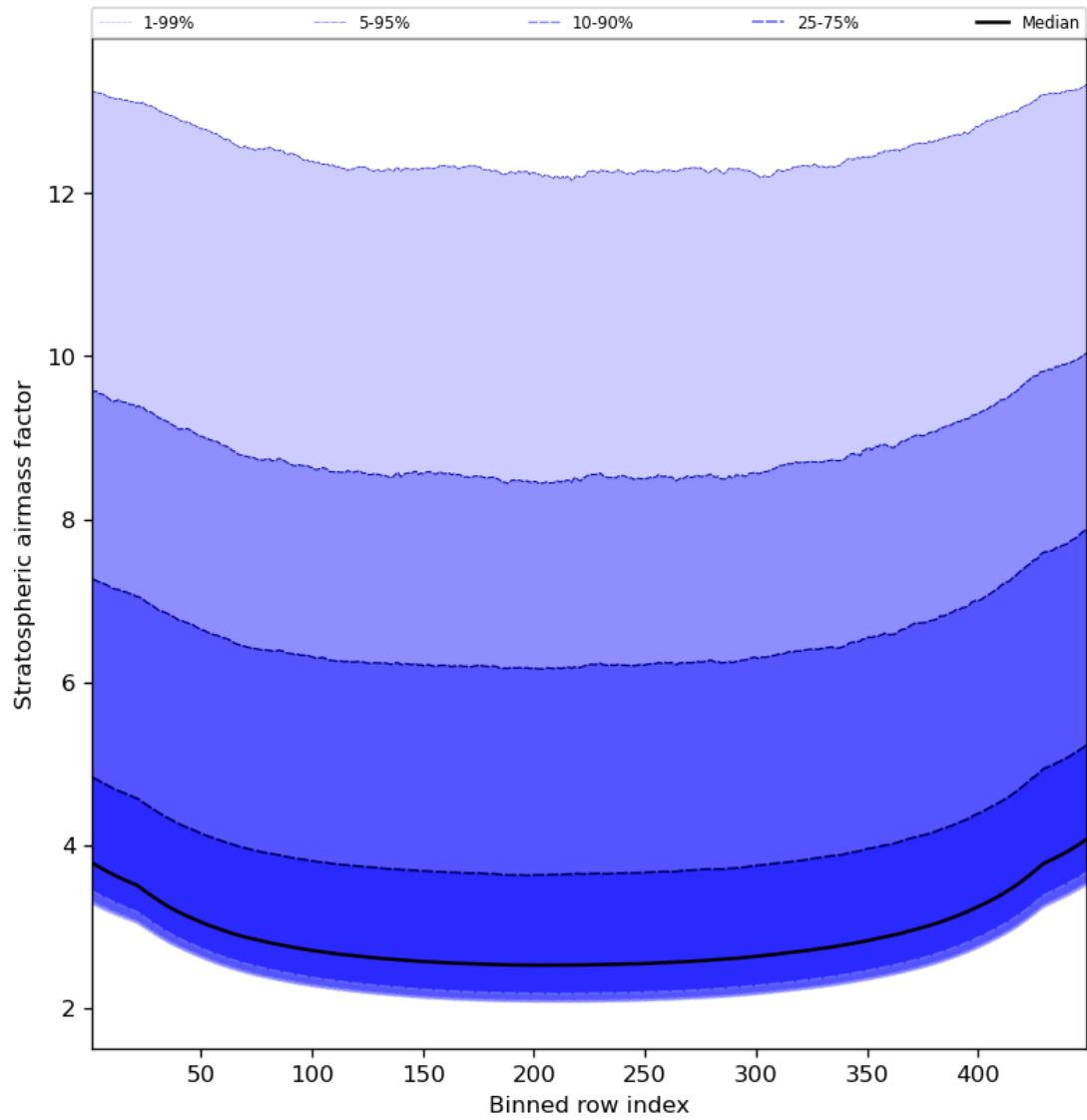
Figure 61: Along track statistics of “Stratospheric airmass factor” for 2023-11-14 to 2023-11-16
