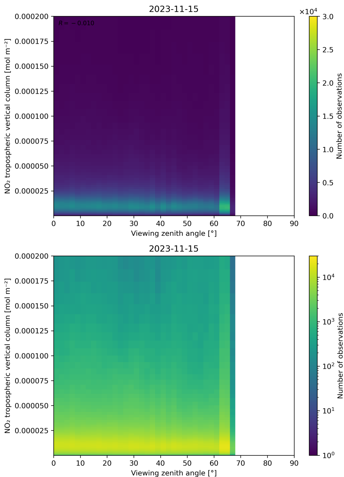
Figure 169: Scatter density plot of “Viewing zenith angle” against “NO 2 tropospheric vertical column” for 2023-11-14 to 2023-11-16.
