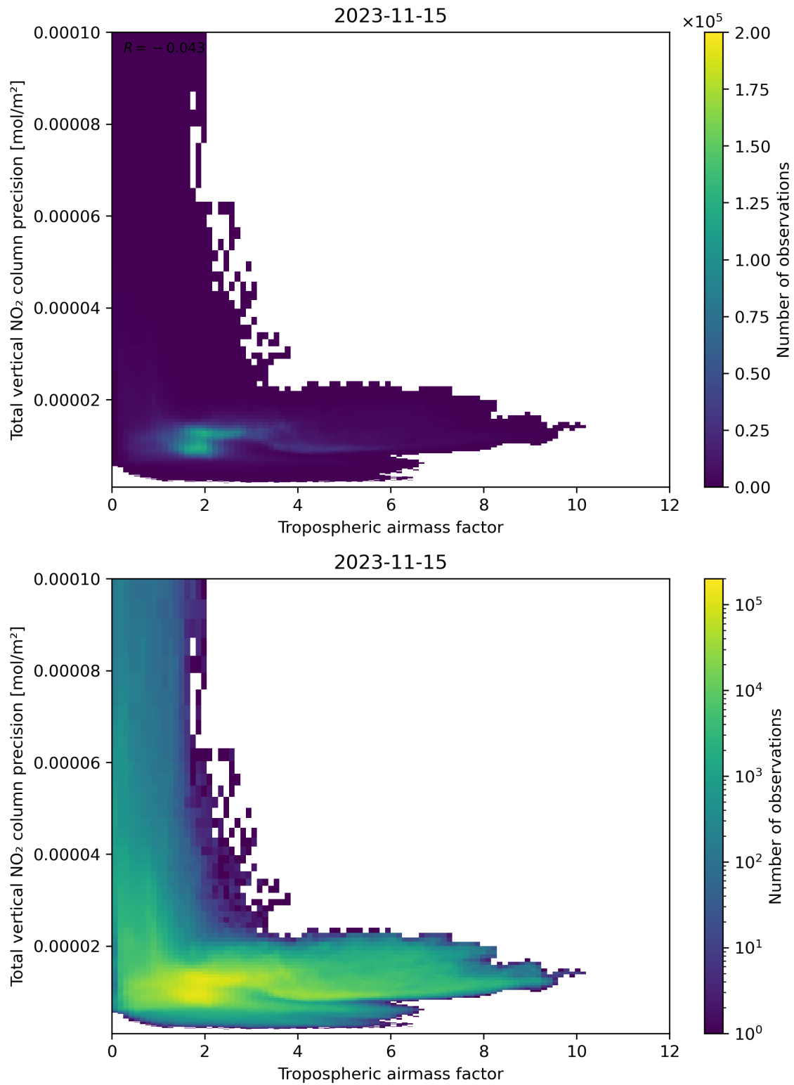
Figure 78: Scatter density plot of “Tropospheric air mass factor” against “Total vertical NO 2 column precision” for 2023-11-14 to 2023-11-16.
