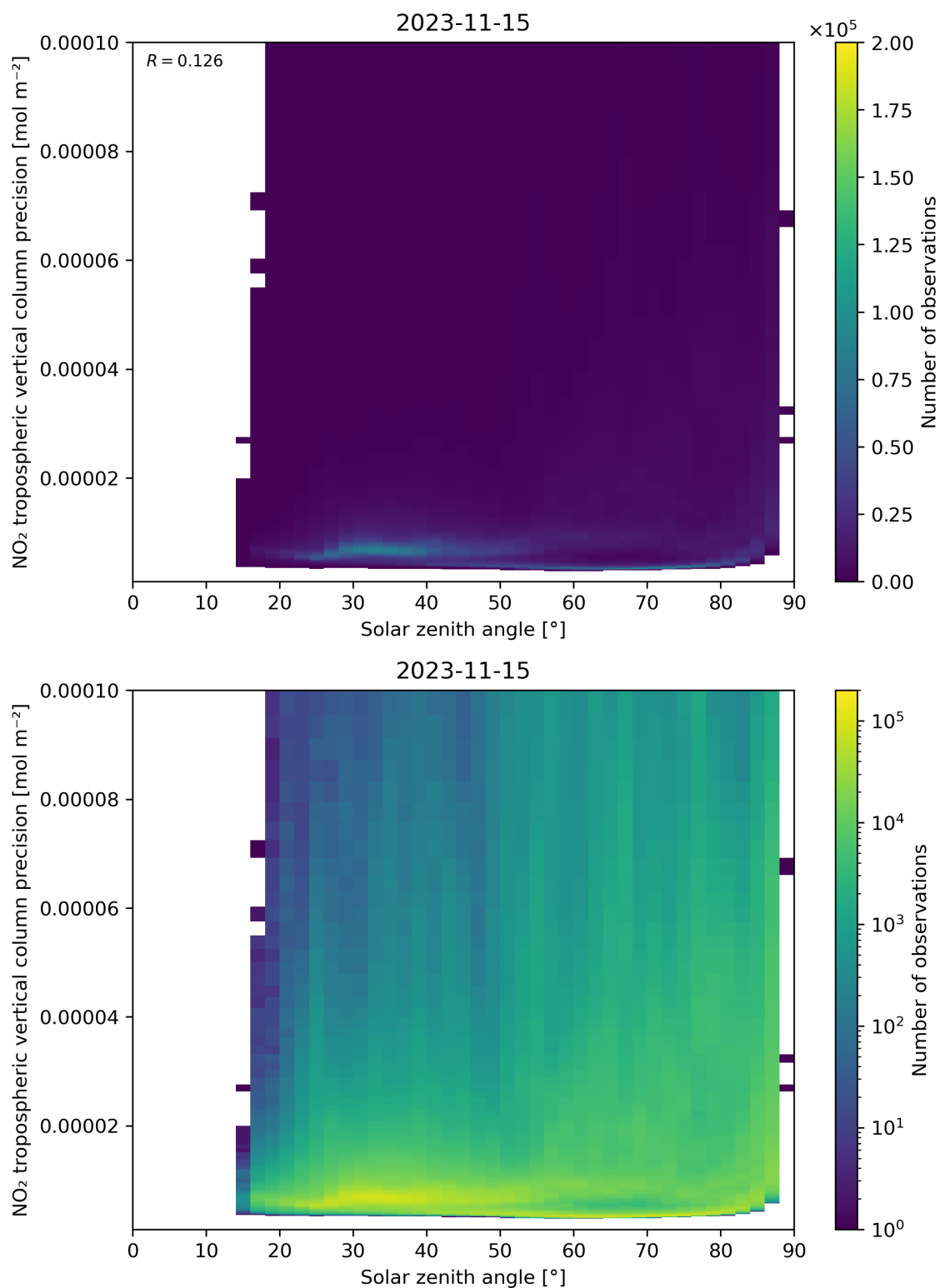
Figure 156: Scatter density plot of “Solar zenith angle” against “NO 2 tropospheric vertical column precision” for 2023-11-14 to 2023-11-16.
