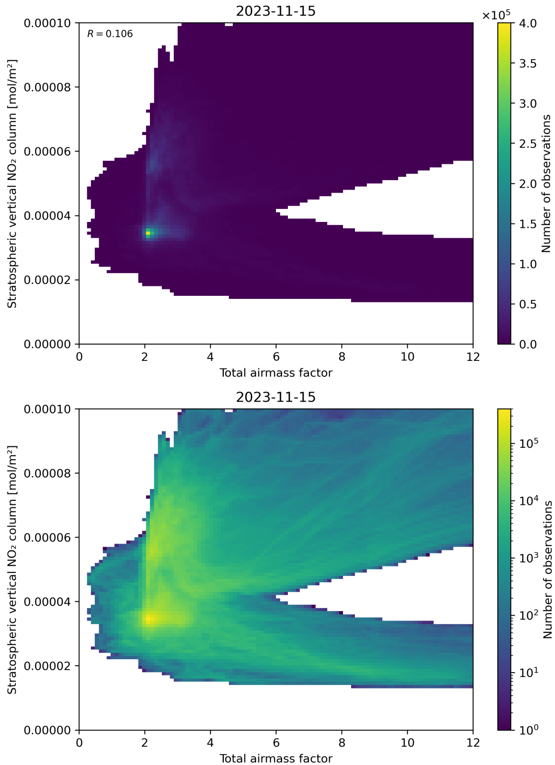
Figure 64: Scatter density plot of “Total airmass factor” against “Stratospheric vertical NO 2 column” for 2023-11-14 to 2023-11-16.
