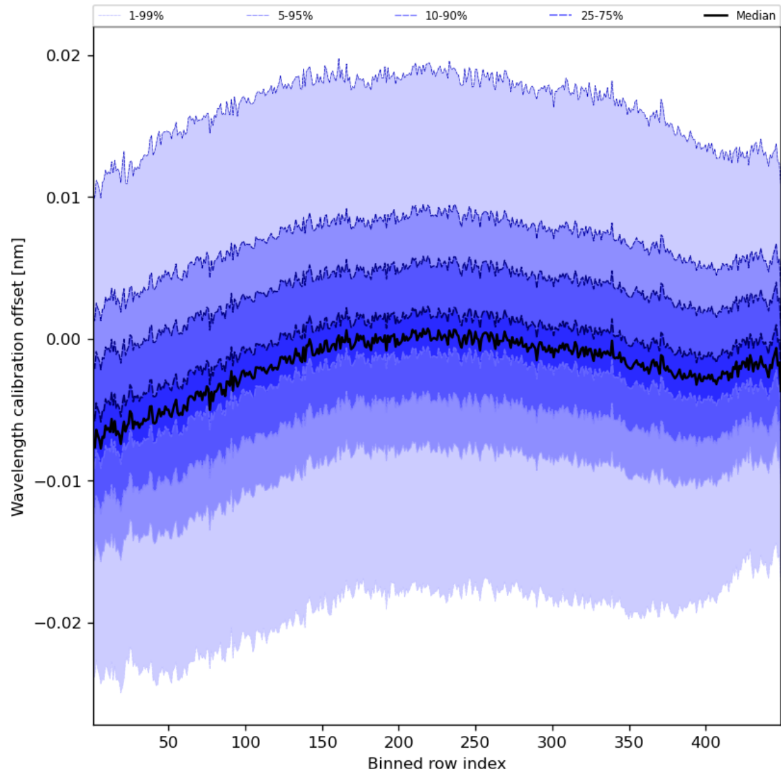
Figure 52: Along track statistics of “Wavelength calibration offset” for 2023-11-14 to 2023-11-16
