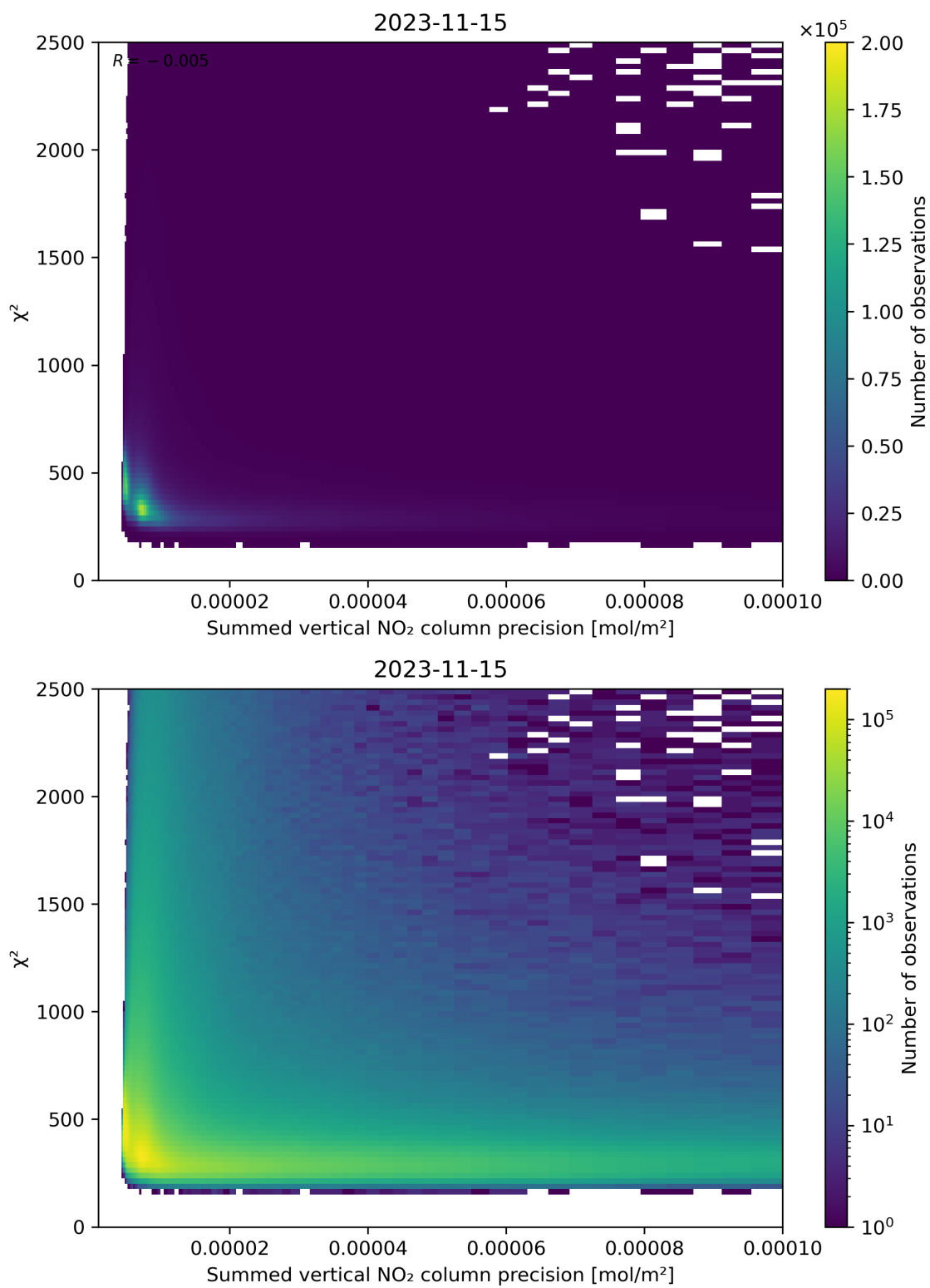
Figure 107: Scatter density plot of “Summed vertical NO 2 column precision” against “ \chi^2 ” for 2023-11-14 to 2023-11-16.
