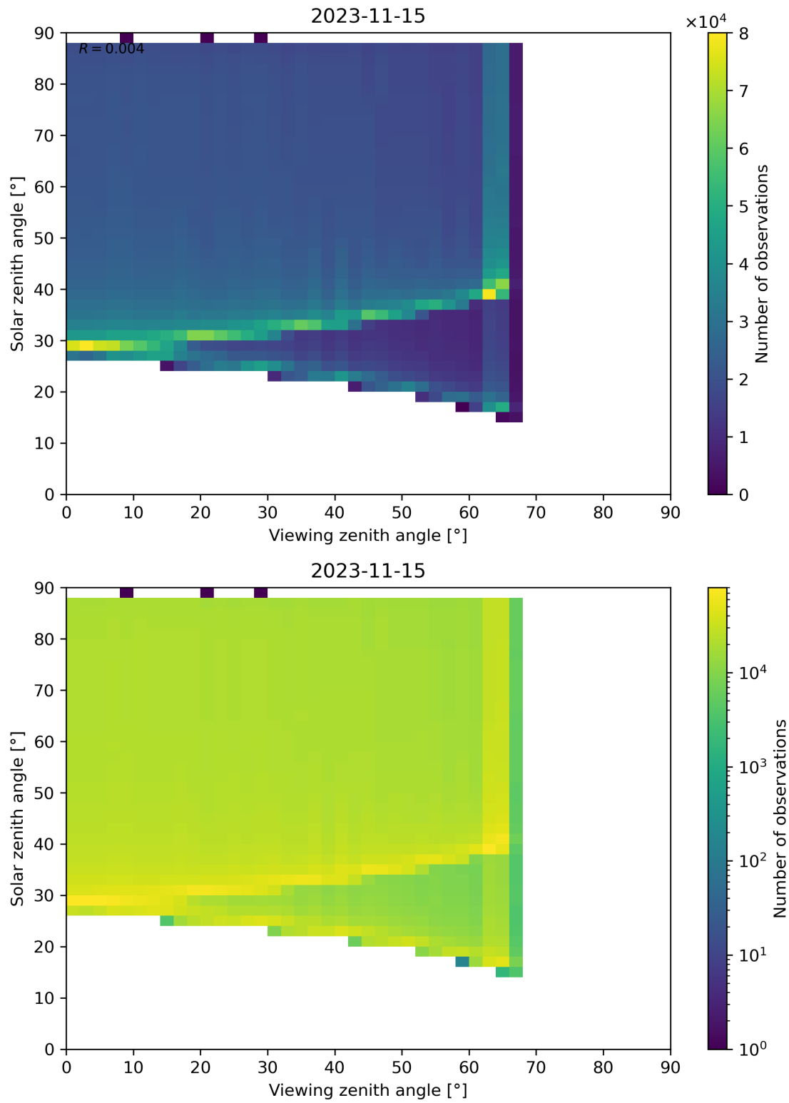
Figure 172: Scatter density plot of “Viewing zenith angle” against “Solar zenith angle” for 2023-11-14 to 2023-11-16.
