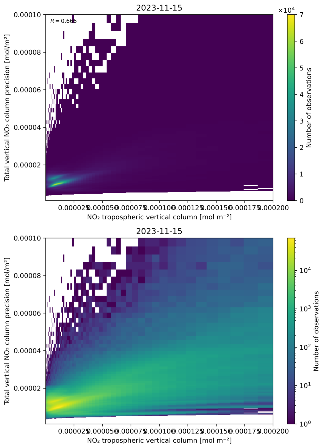
Figure 129: Scatter density plot of “NO 2 tropospheric vertical column” against “Total vertical NO 2 column precision” for 2023-11-14 to 2023-11-16.
