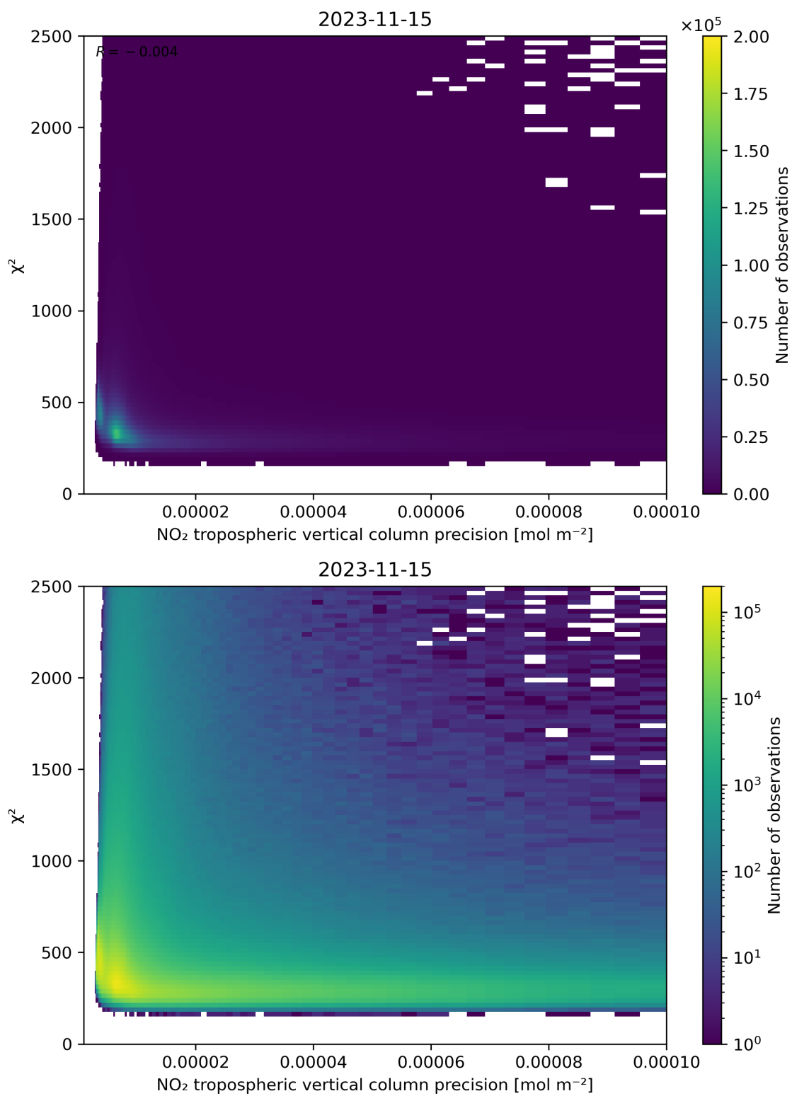
Figure 134: Scatter density plot of “NO 2 tropospheric vertical column precision” against “ \chi^2 ” for 2023-11-14 to 2023-11-16.
