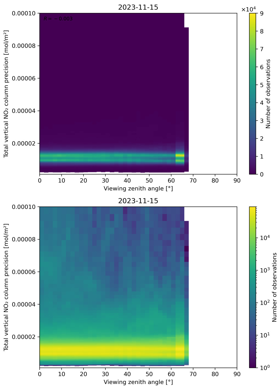
Figure 168: Scatter density plot of “Viewing zenith angle” against “Total vertical NO 2 column precision” for 2023-11-14 to 2023-11-16.
