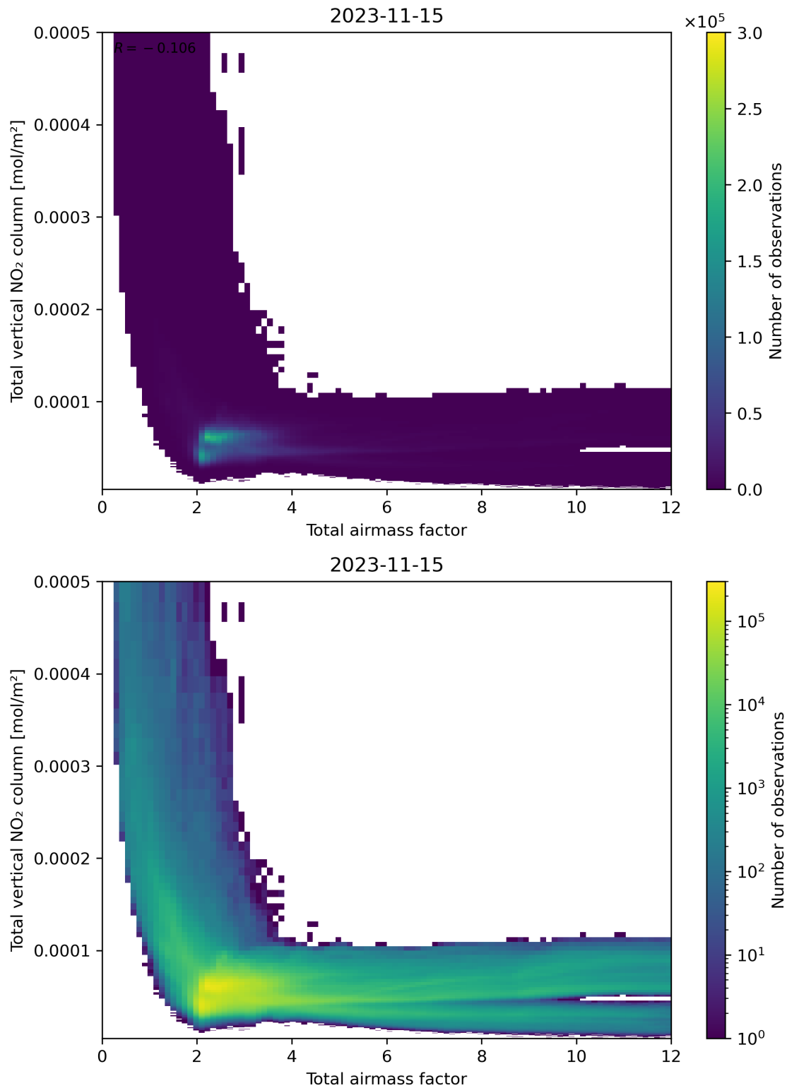
Figure 67: Scatter density plot of “Total airmass factor” against “Total vertical NO 2 column” for 2023-11-14 to 2023-11-16.
