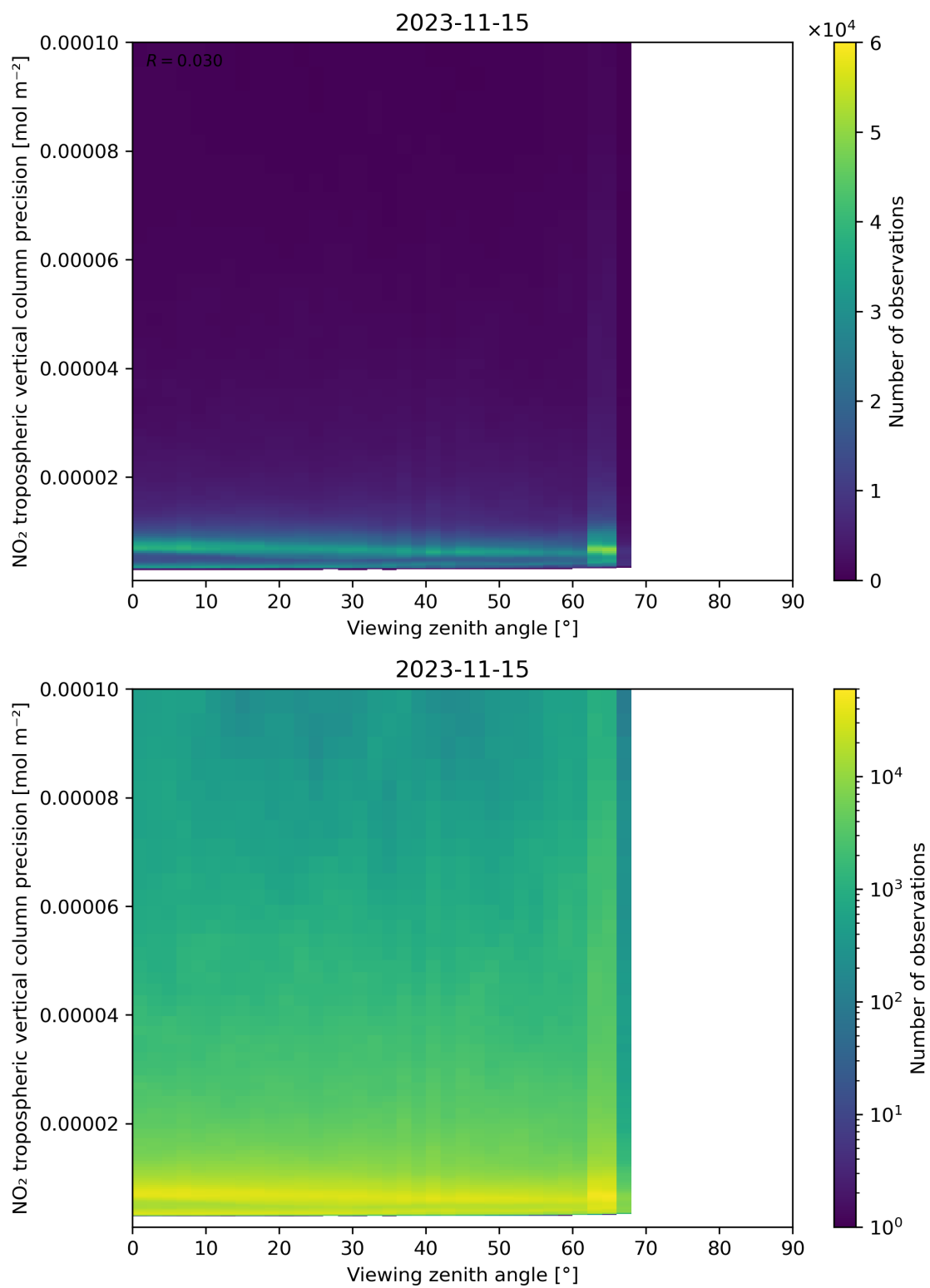
Figure 170: Scatter density plot of “Viewing zenith angle” against “NO 2 tropospheric vertical column precision” for 2023-11-14 to 2023-11-16.
