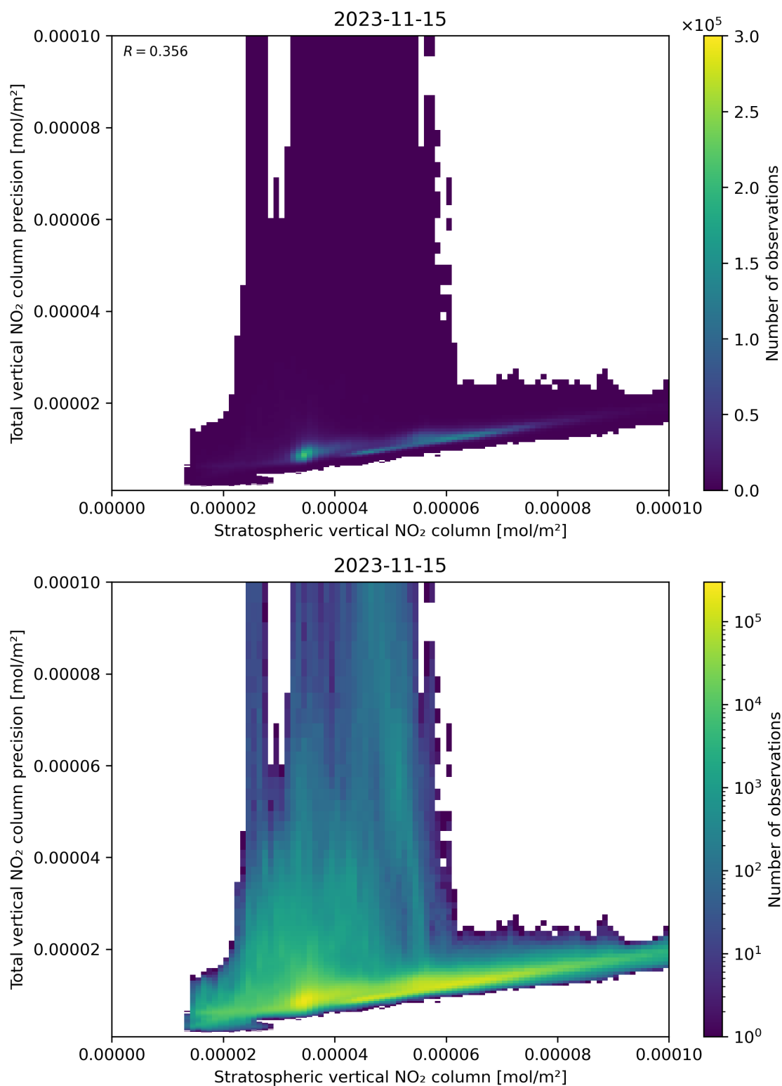
Figure 101: Scatter density plot of “Stratospheric vertical NO 2 column” against “Total vertical NO 2 column precision” for 2023-11-14 to 2023-11-16.
