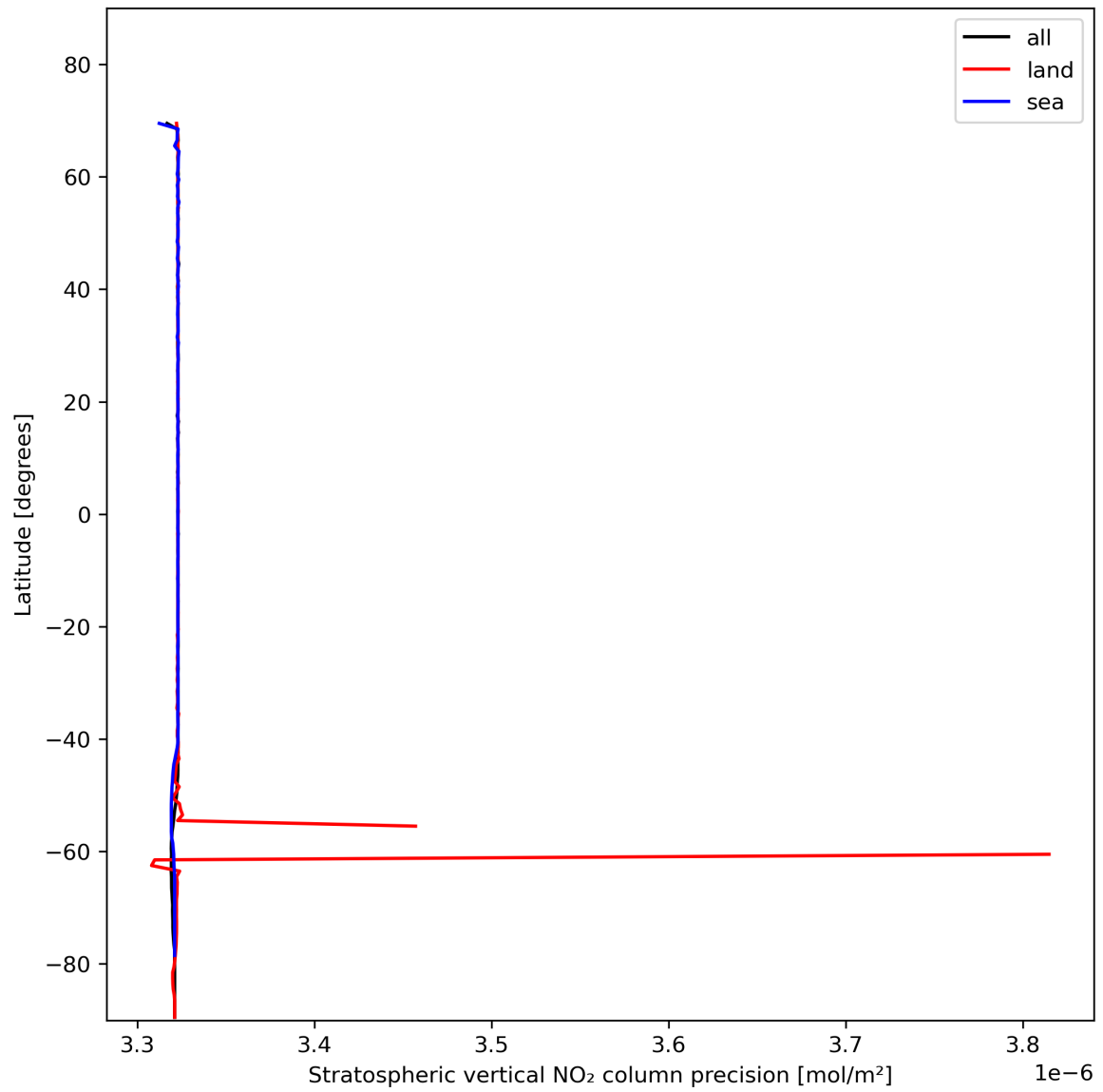
Figure 20: Zonal average of “Stratospheric vertical NO 2 column precision” for 2023-11-14 to 2023-11-16.
