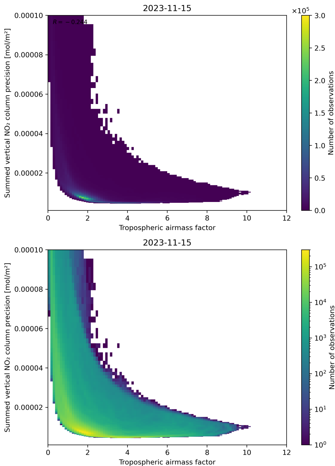
Figure 76: Scatter density plot of “Tropospheric air mass factor” against “Summed vertical NO 2 column precision” for 2023-11-14 to 2023-11-16.
