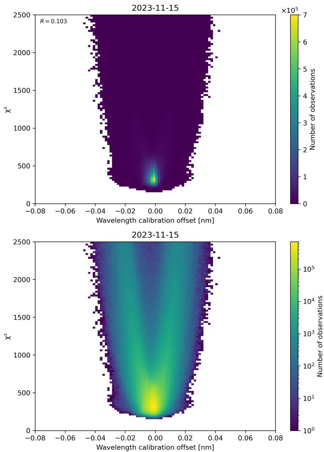
Figure 175: Scatter density plot of “Wavelength calibration offset” against “ \chi^2 ” for 2023-11-14 to 2023-11-16.
