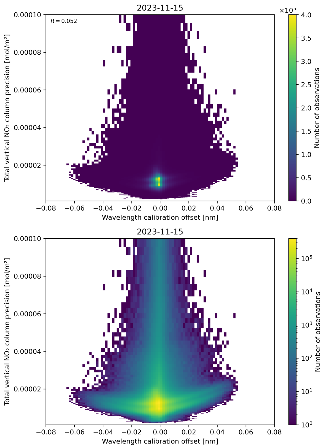
Figure 180: Scatter density plot of “Wavelength calibration offset” against “Total vertical NO 2 column precision” for 2023-11-14 to 2023-11-16.
