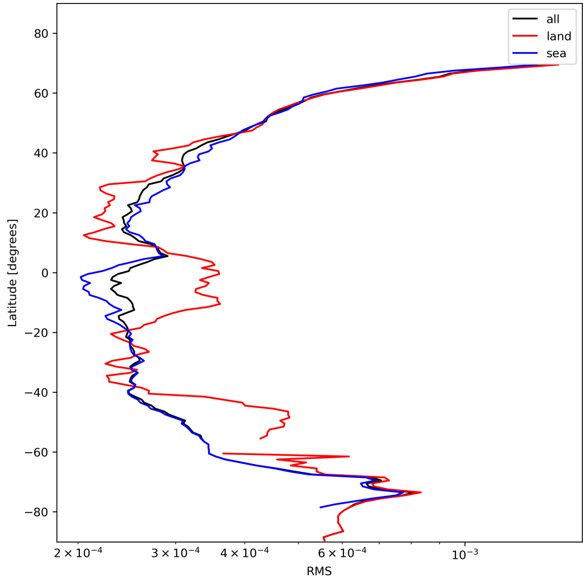
Figure 26: Zonal average of “RMS” for 2023-11-14 to 2023-11-16.
