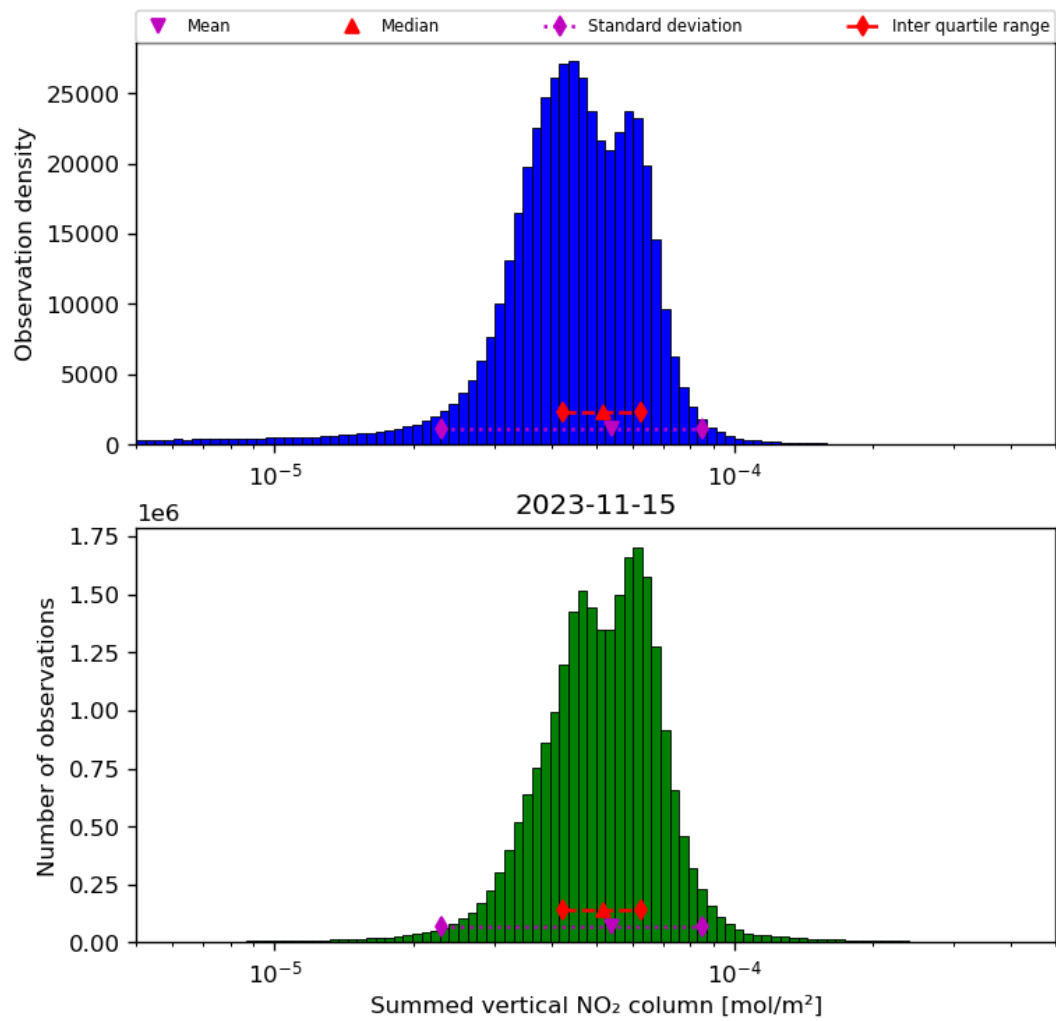
Figure 40: Histogram of “Summed vertical NO 2 column” for 2023-11-14 to 2023-11-16
