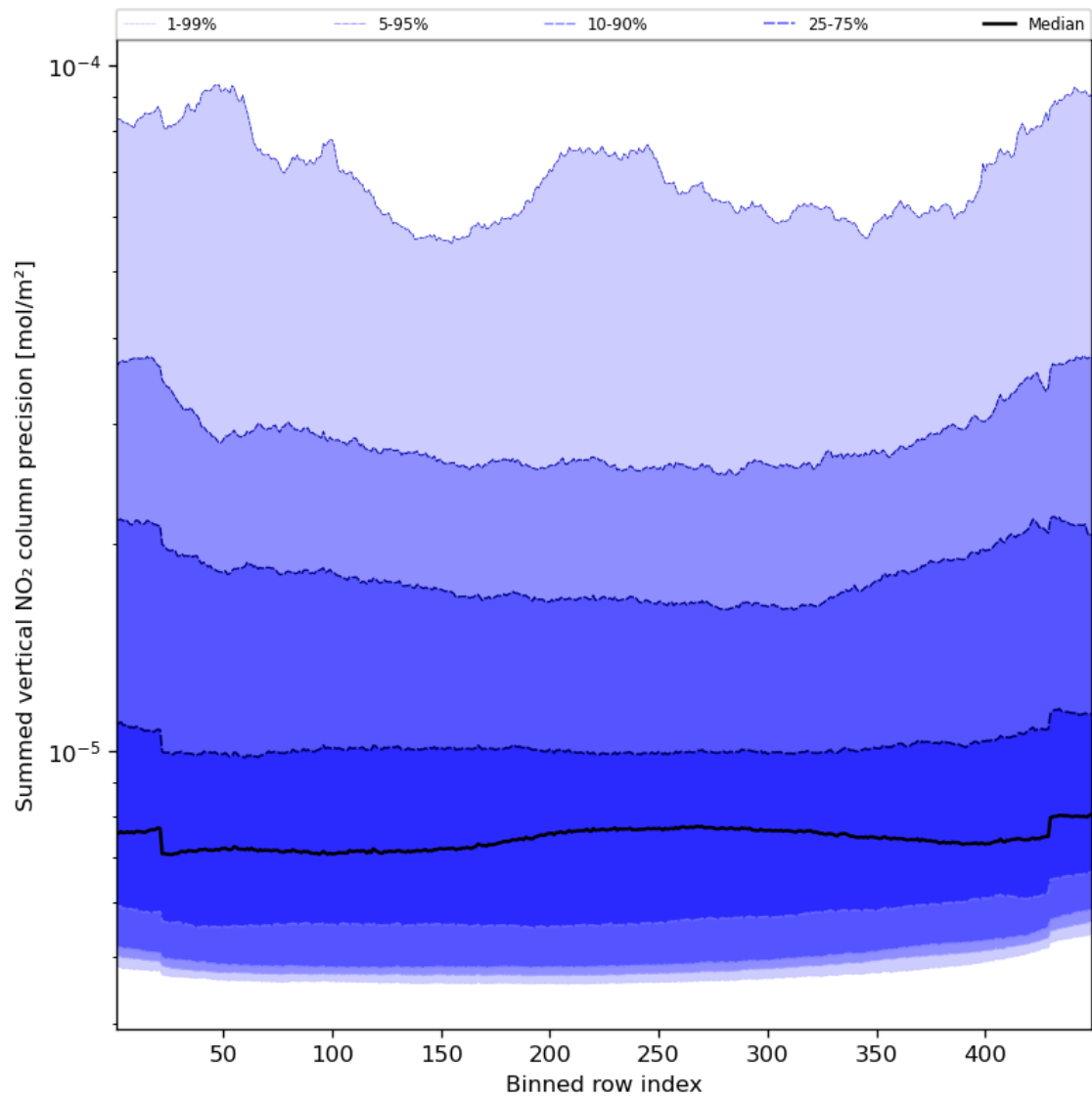
Figure 58: Along track statistics of “Summed vertical NO 2 column precision” for 2023-11-14 to 2023-11-16
