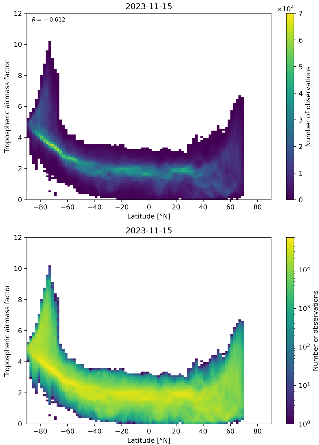
Figure 85: Scatter density plot of “Latitude” against “Tropospheric air mass factor” for 2023-11-14 to 2023-11-16.
