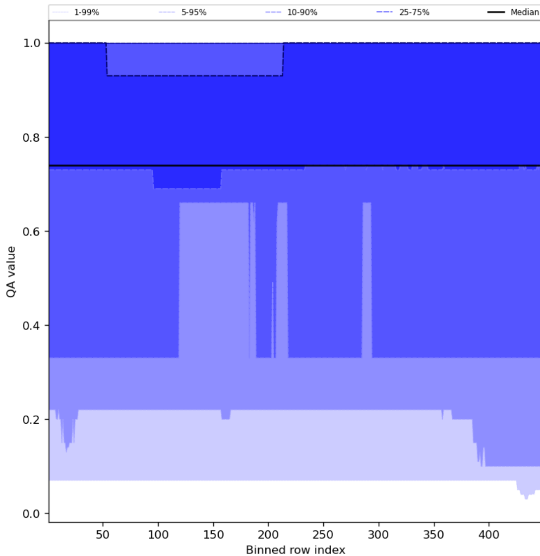
Figure 45: Along track statistics of “QA value” for 2023-11-14 to 2023-11-16
