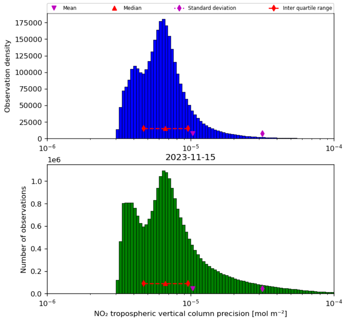
Figure 30: Histogram of “NO 2 tropospheric vertical column precision” for 2023-11-14 to 2023-11-16
