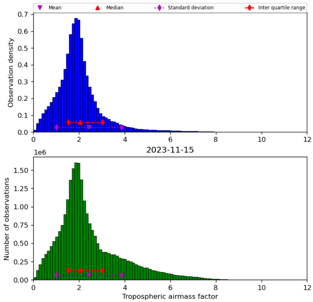
Figure 31: Histogram of “Tropospheric airmass factor” for 2023-11-14 to 2023-11-16
