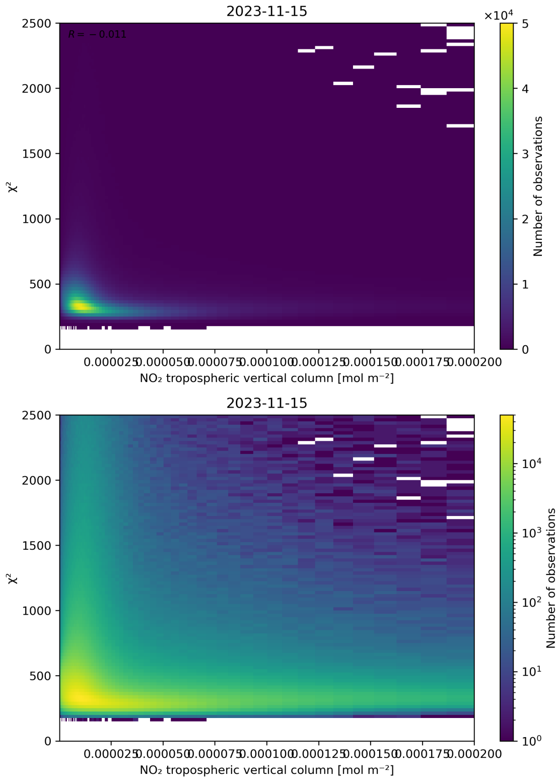
Figure 124: Scatter density plot of “NO 2 tropospheric vertical column” against “ \chi^2 ” for 2023-11-14 to 2023-11-16.
