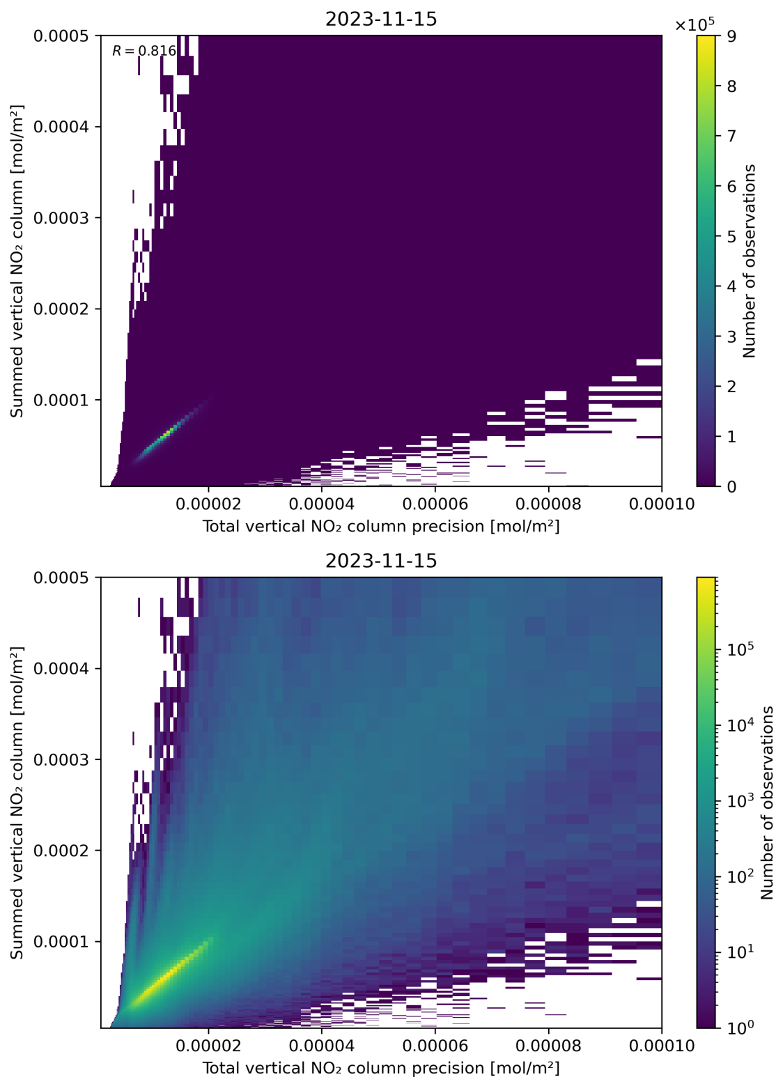
Figure 117: Scatter density plot of “Total vertical NO 2 column precision” against “Summed vertical NO 2 column” for 2023-11-14 to 2023-11-16.
