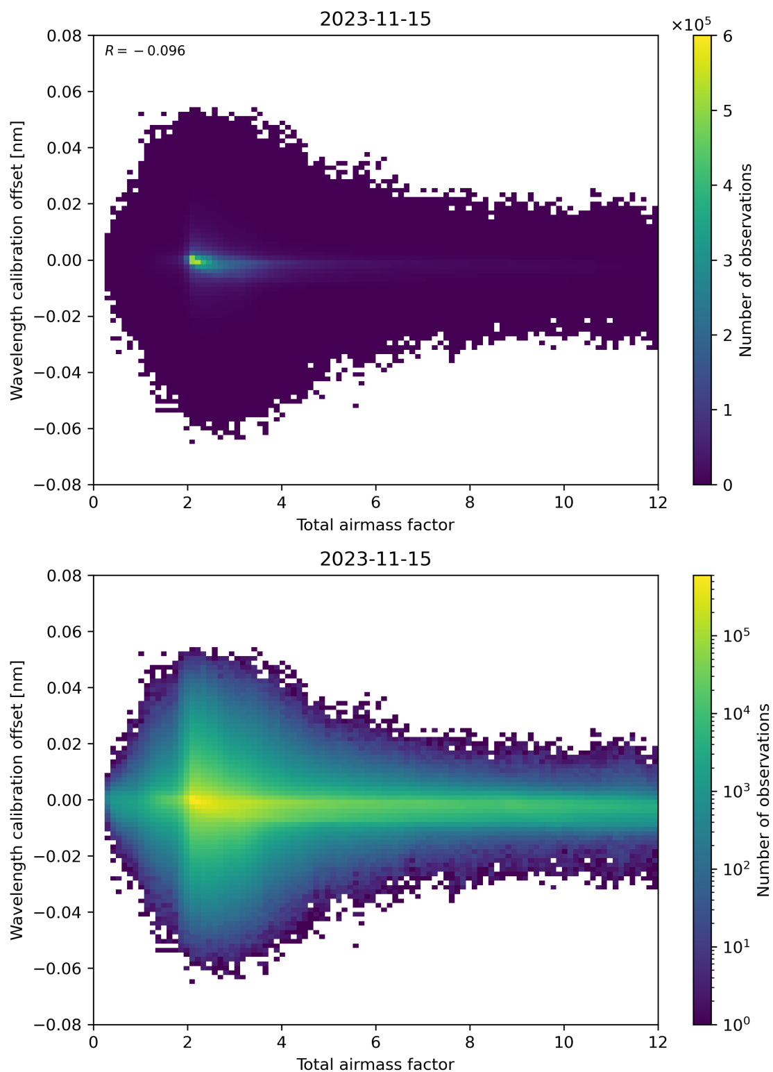
Figure 70: Scatter density plot of “Total airmass factor” against “Wavelength calibration offset” for 2023-11-14 to 2023-11-16.
