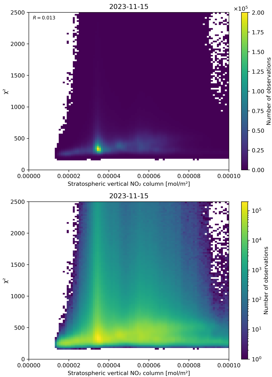
Figure 97: Scatter density plot of “Stratospheric vertical NO 2 column” against “ \chi^2 ” for 2023-11-14 to 2023-11-16.
