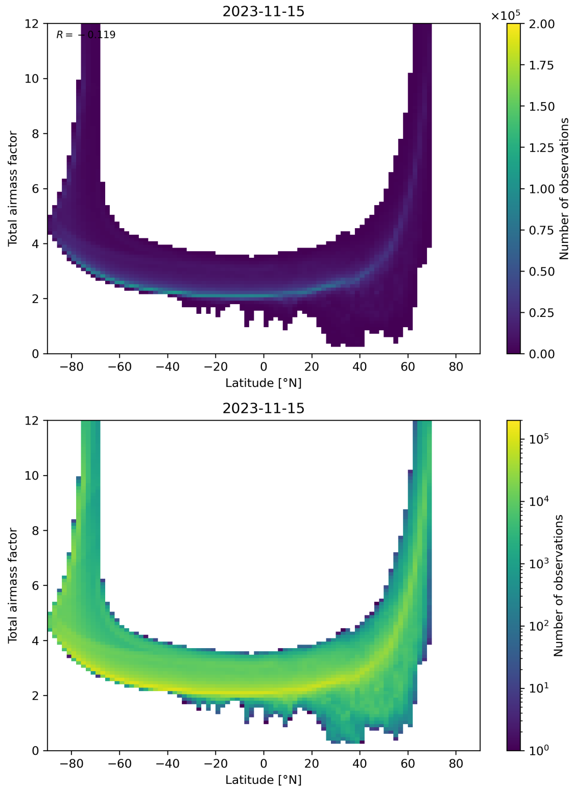
Figure 84: Scatter density plot of “Latitude” against “Total airmass factor” for 2023-11-14 to 2023-11-16.
