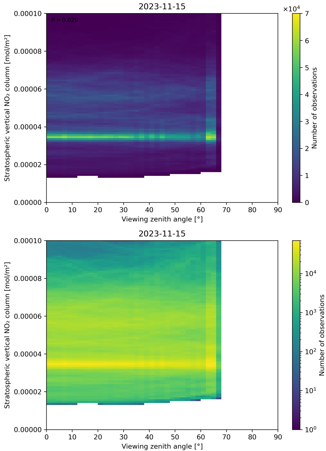
Figure 164: Scatter density plot of “Viewing zenith angle” against “Stratospheric vertical NO 2 column” for 2023-11-14 to 2023-11-16.
