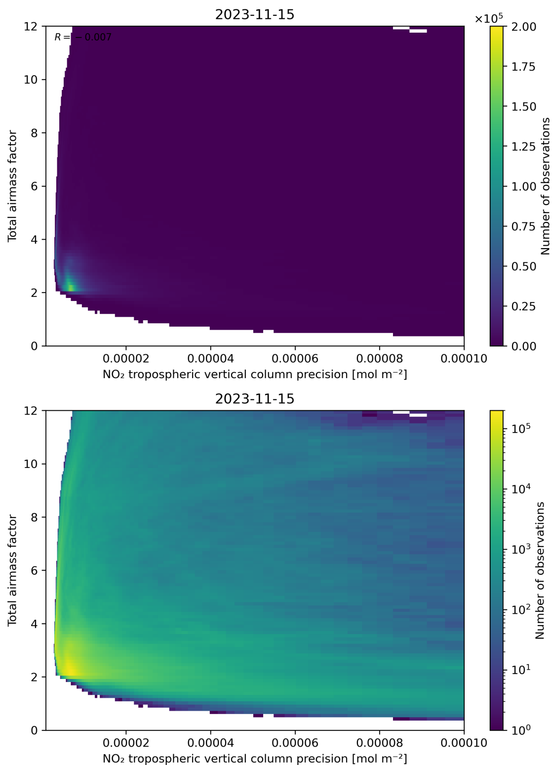
Figure 132: Scatter density plot of “NO 2 tropospheric vertical column precision” against “Total air mass factor” for 2023-11-14 to 2023-11-16.
