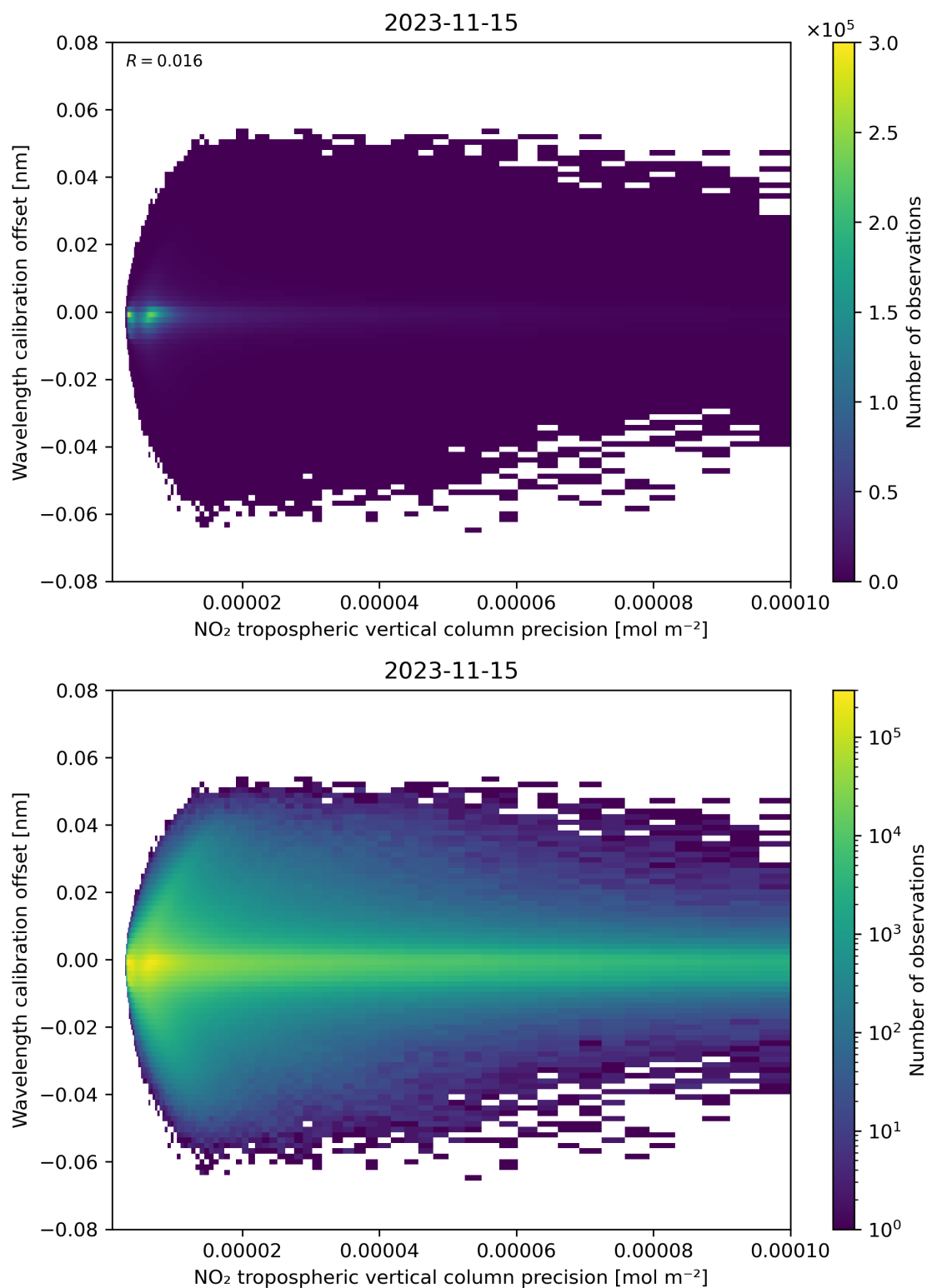
Figure 141: Scatter density plot of “NO 2 tropospheric vertical column precision” against “Wavelength calibration offset” for 2023-11-14 to 2023-11-16.
