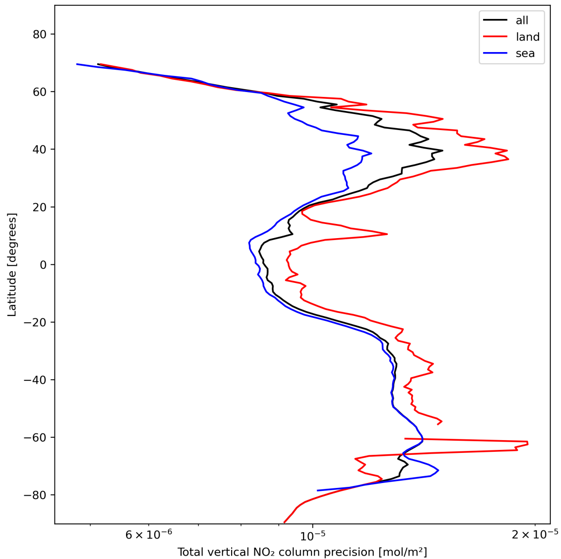
Figure 22: Zonal average of “Total vertical NO 2 column precision” for 2023-11-14 to 2023-11-16.
