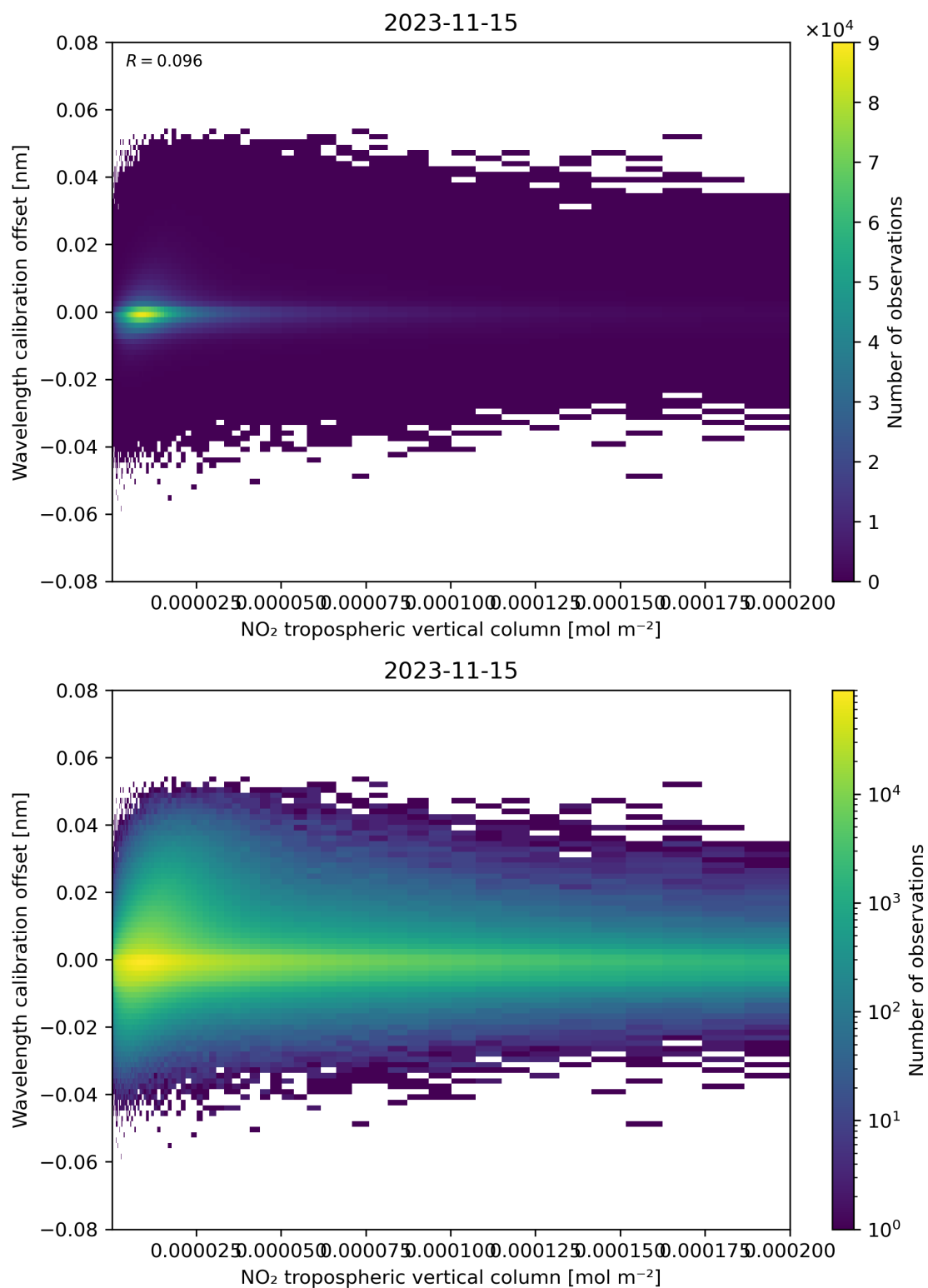
Figure 143: Scatter density plot of “NO 2 tropospheric vertical column” against “Wavelength calibration offset” for 2023-11-14 to 2023-11-16.
