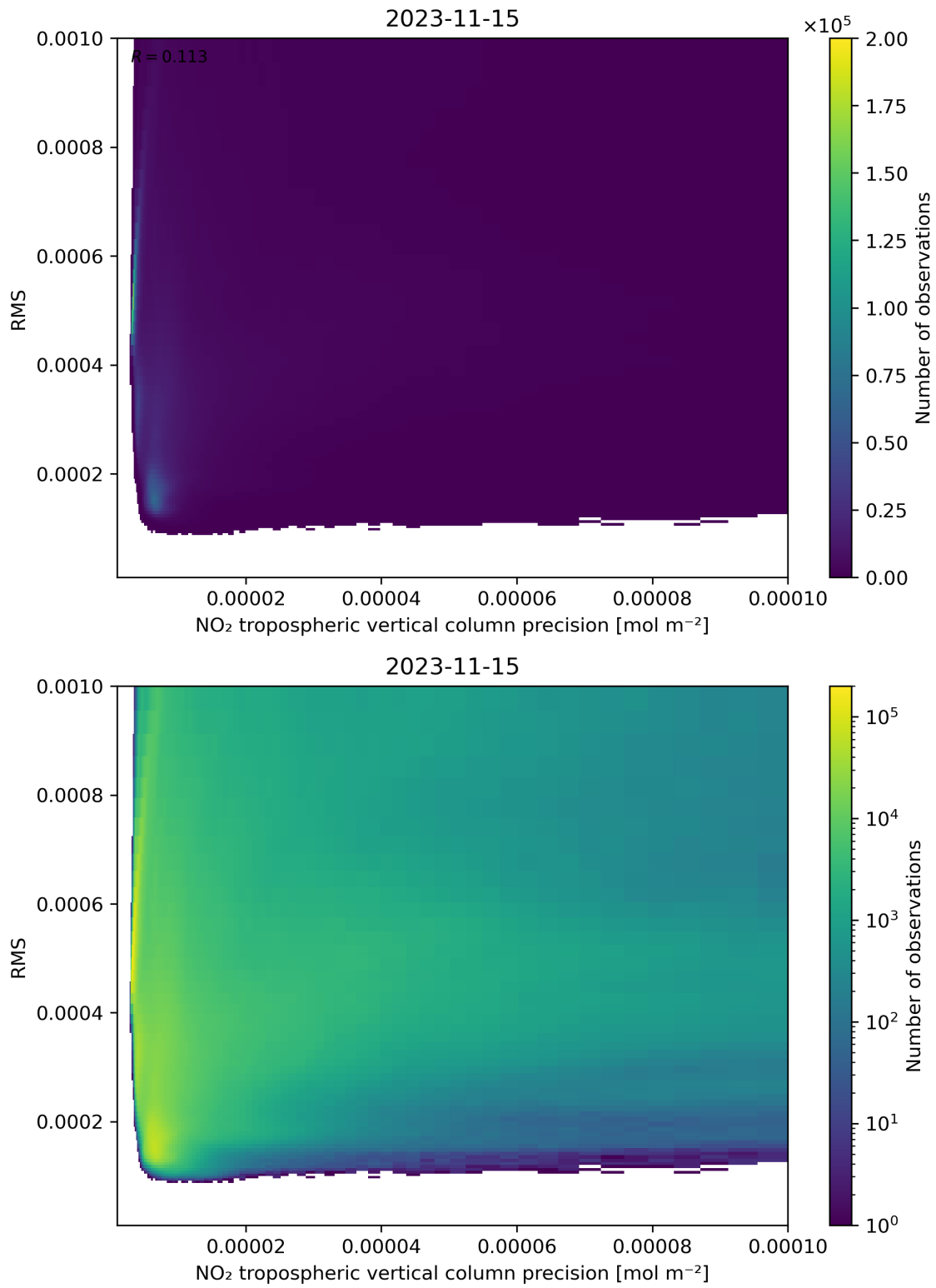
Figure 140: Scatter density plot of “NO 2 tropospheric vertical column precision” against “RMS” for 2023-11-14 to 2023-11-16.
