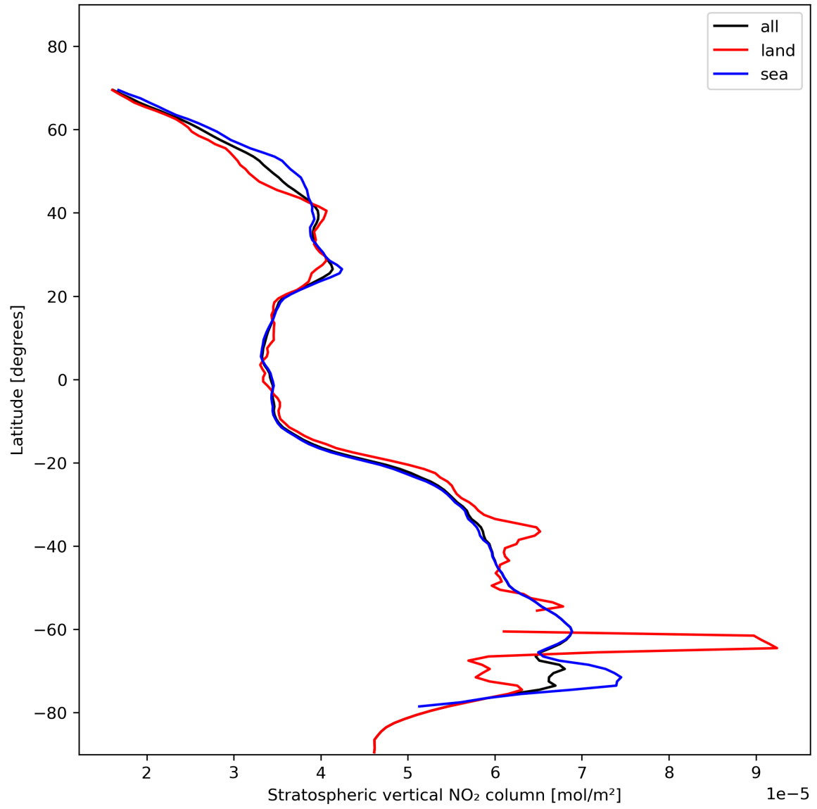
Figure 19: Zonal average of “Stratospheric vertical NO 2 column” for 2023-11-14 to 2023-11-16.
