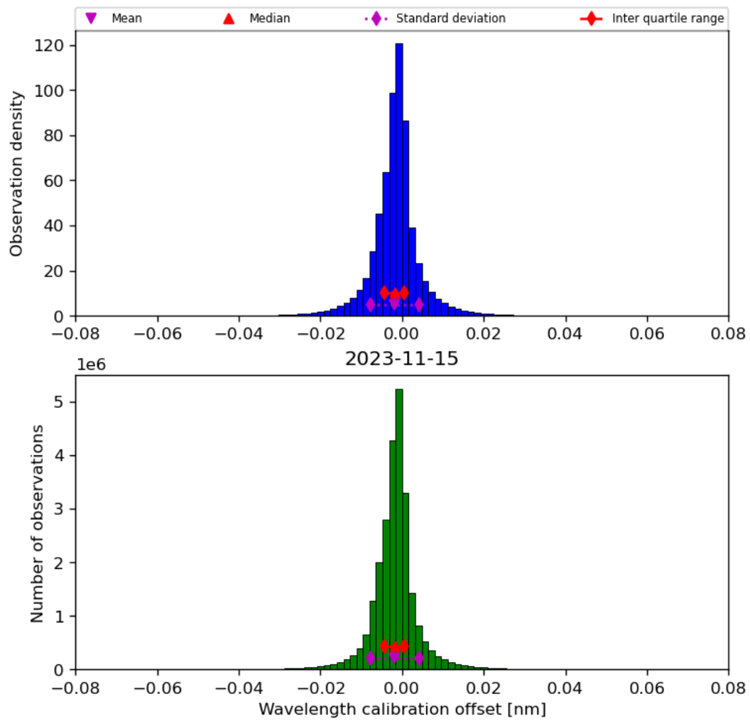
Figure 35: Histogram of “Wavelength calibration offset” for 2023-11-14 to 2023-11-16
