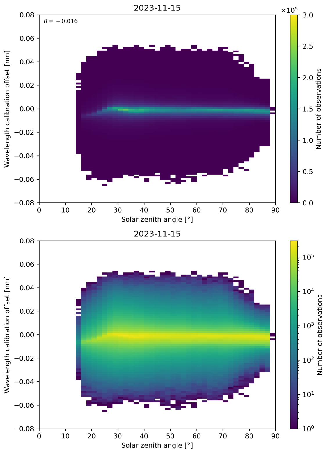
Figure 158: Scatter density plot of “Solar zenith angle” against “Wavelength calibration offset” for 2023-11-14 to 2023-11-16.
