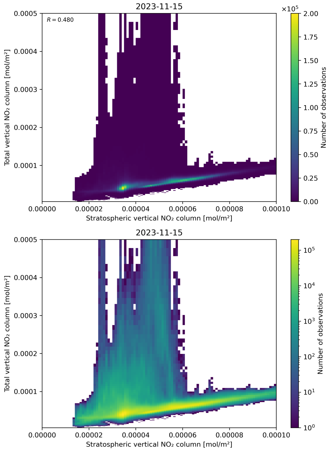
Figure 100: Scatter density plot of “Stratospheric vertical NO 2 column” against “Total vertical NO 2 column” for 2023-11-14 to 2023-11-16.
