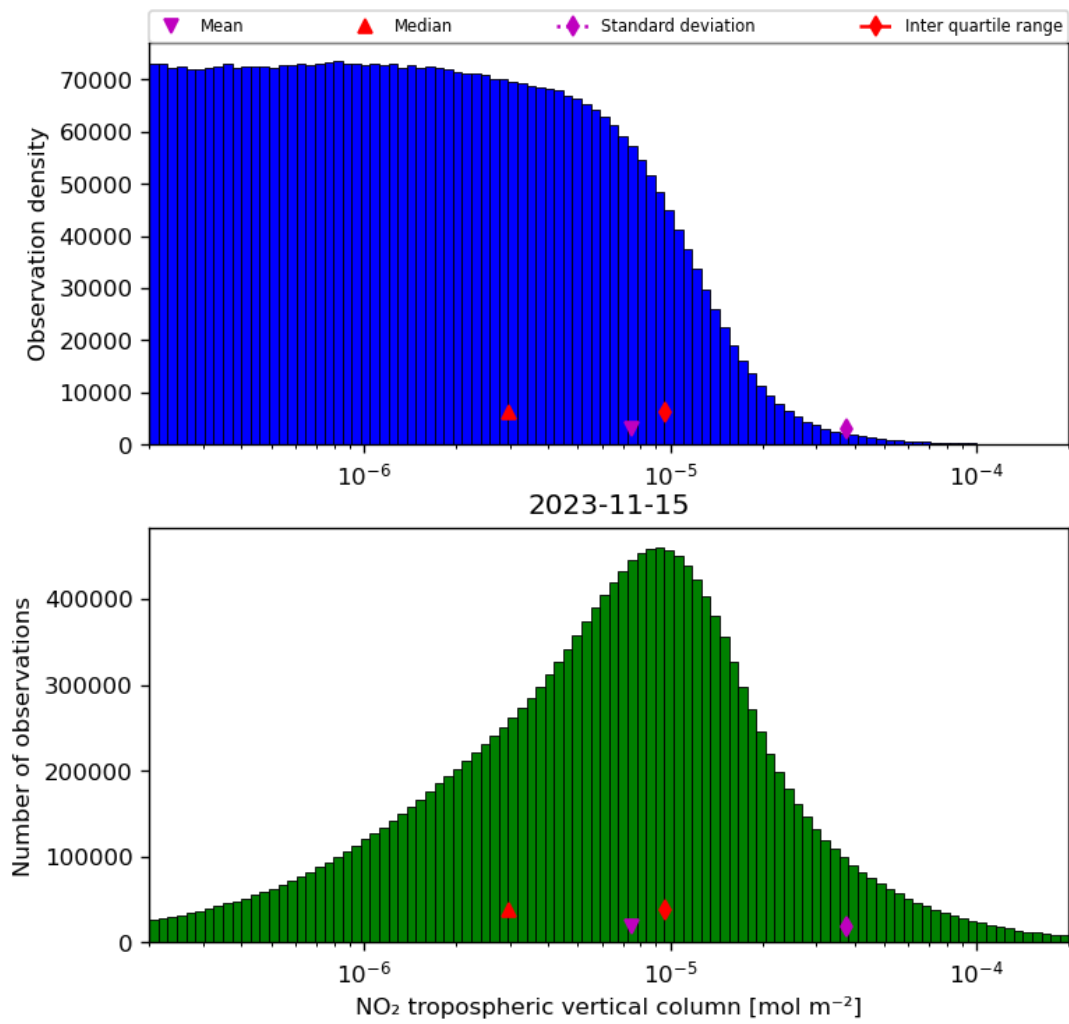
Figure 29: Histogram of “NO 2 tropospheric vertical column” for 2023-11-14 to 2023-11-16
