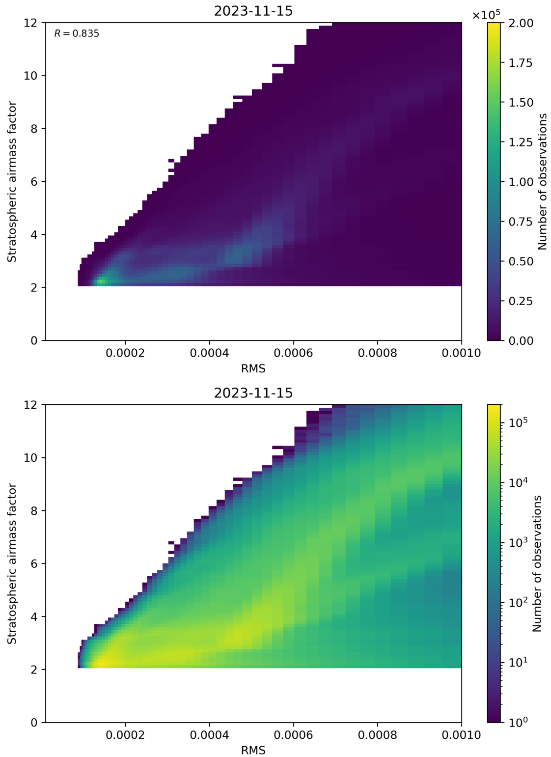
Figure 144: Scatter density plot of “RMS” against “Stratospheric airmass factor” for 2023-11-14 to 2023-11-16.
