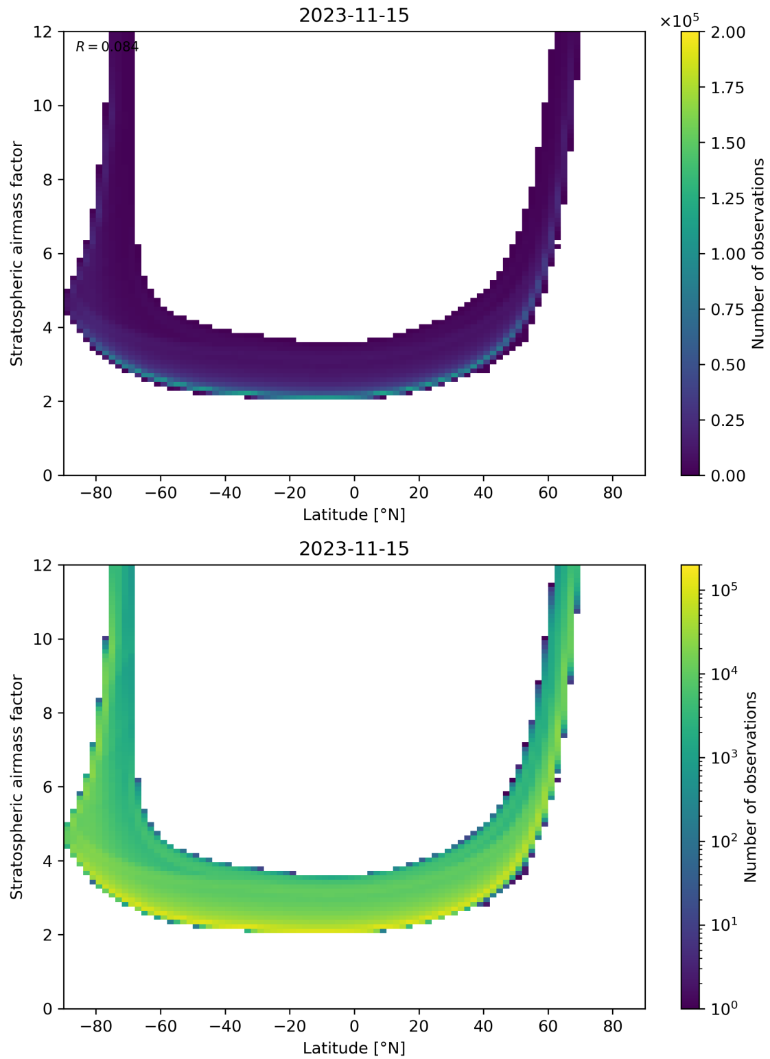
Figure 83: Scatter density plot of “Latitude” against “Stratospheric airmass factor” for 2023-11-14 to 2023-11-16.
