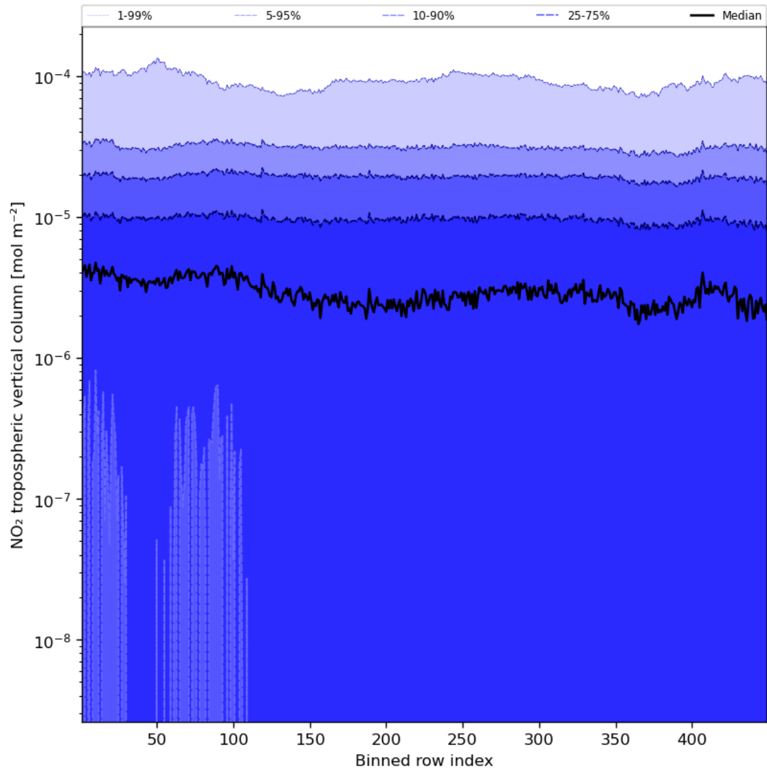
Figure 46: Along track statistics of “NO 2 tropospheric vertical column” for 2023-11-14 to 2023-11-16
