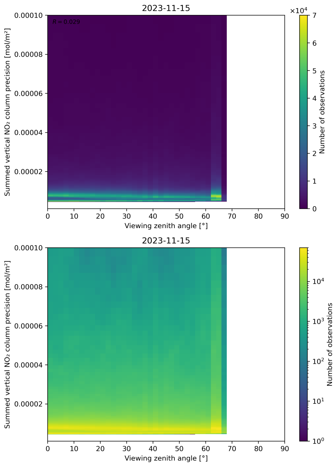
Figure 166: Scatter density plot of “Viewing zenith angle” against “Summed vertical NO 2 column precision” for 2023-11-14 to 2023-11-16.
