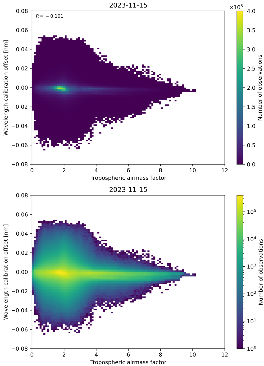
Figure 80: Scatter density plot of “Tropospheric airmass factor” against “Wavelength calibration offset” for 2023-11-14 to 2023-11-16.
