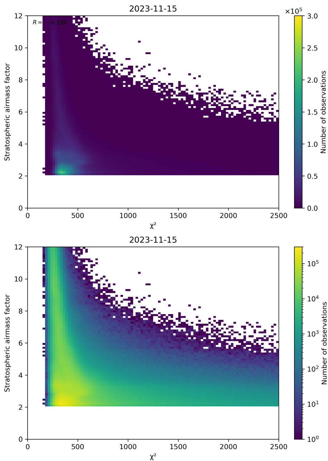
Figure 81: Scatter density plot of “ \chi^2 ” against “Stratospheric airmass factor” for 2023-11-14 to 2023-11-16.
