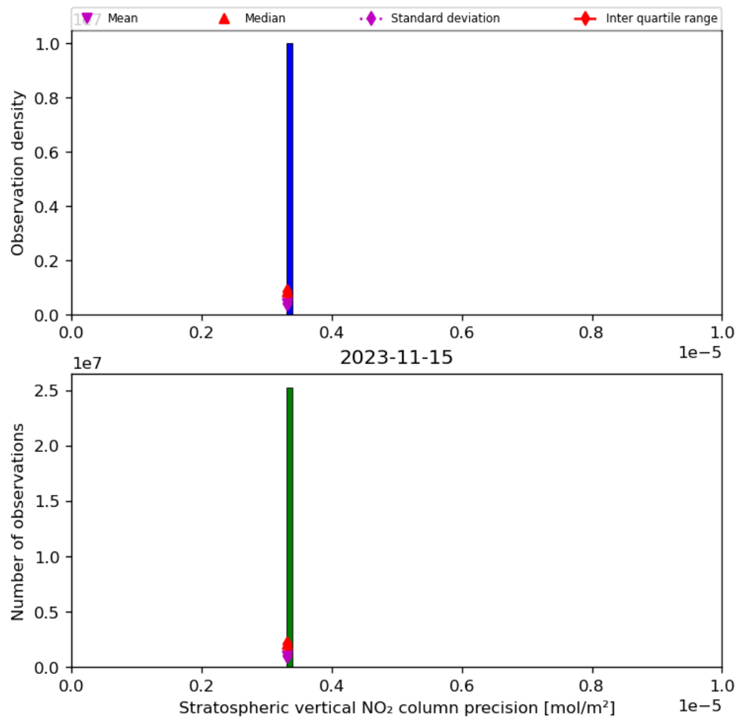
Figure 37: Histogram of “Stratospheric vertical NO 2 column precision” for 2023-11-14 to 2023-11-16
