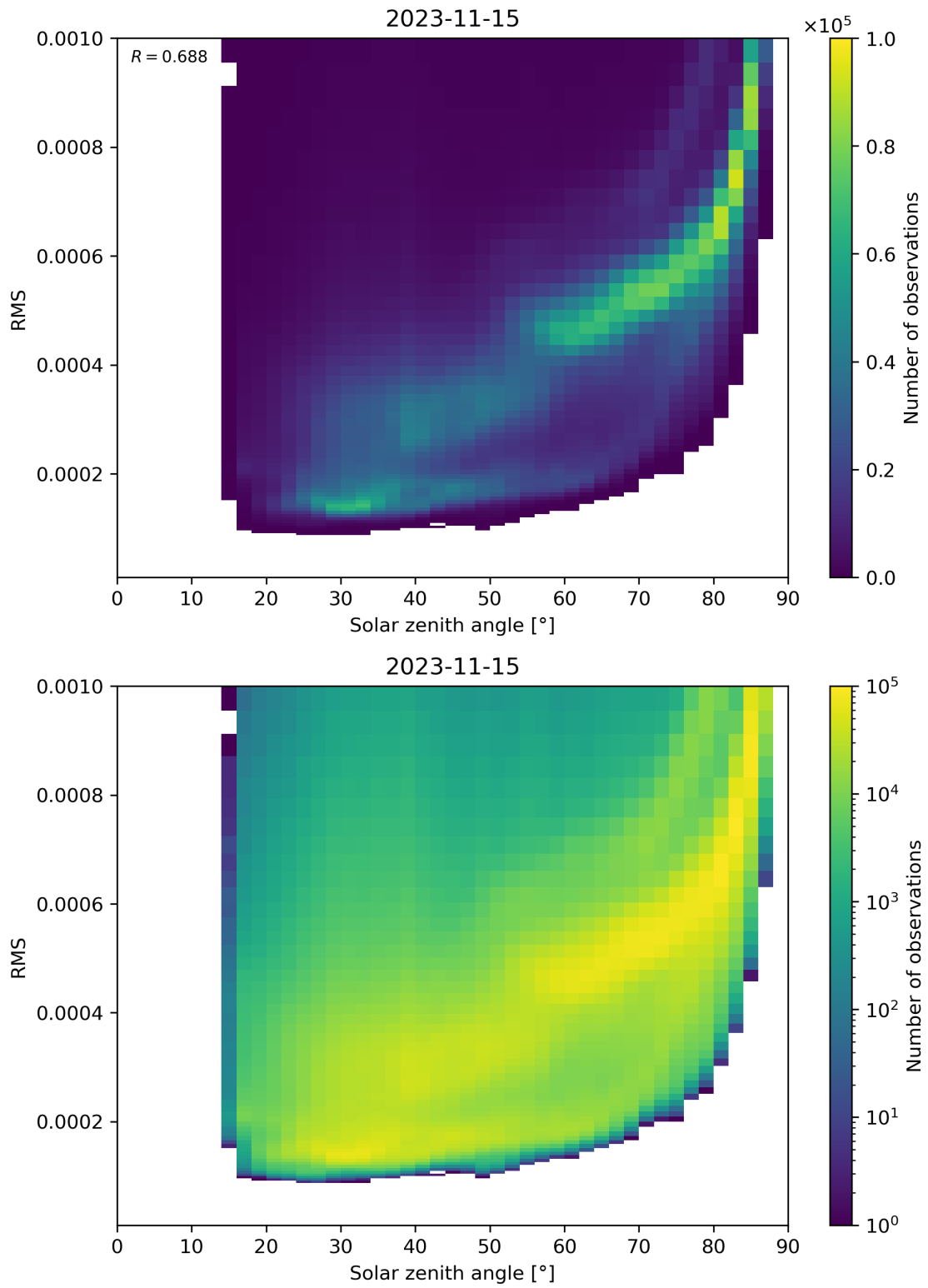
Figure 157: Scatter density plot of “Solar zenith angle” against “RMS” for 2023-11-14 to 2023-11-16.
