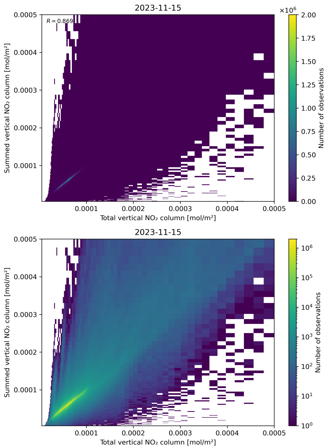
Figure 112: Scatter density plot of “Total vertical NO 2 column” against “Summed vertical NO 2 column” for 2023-11-14 to 2023-11-16.
