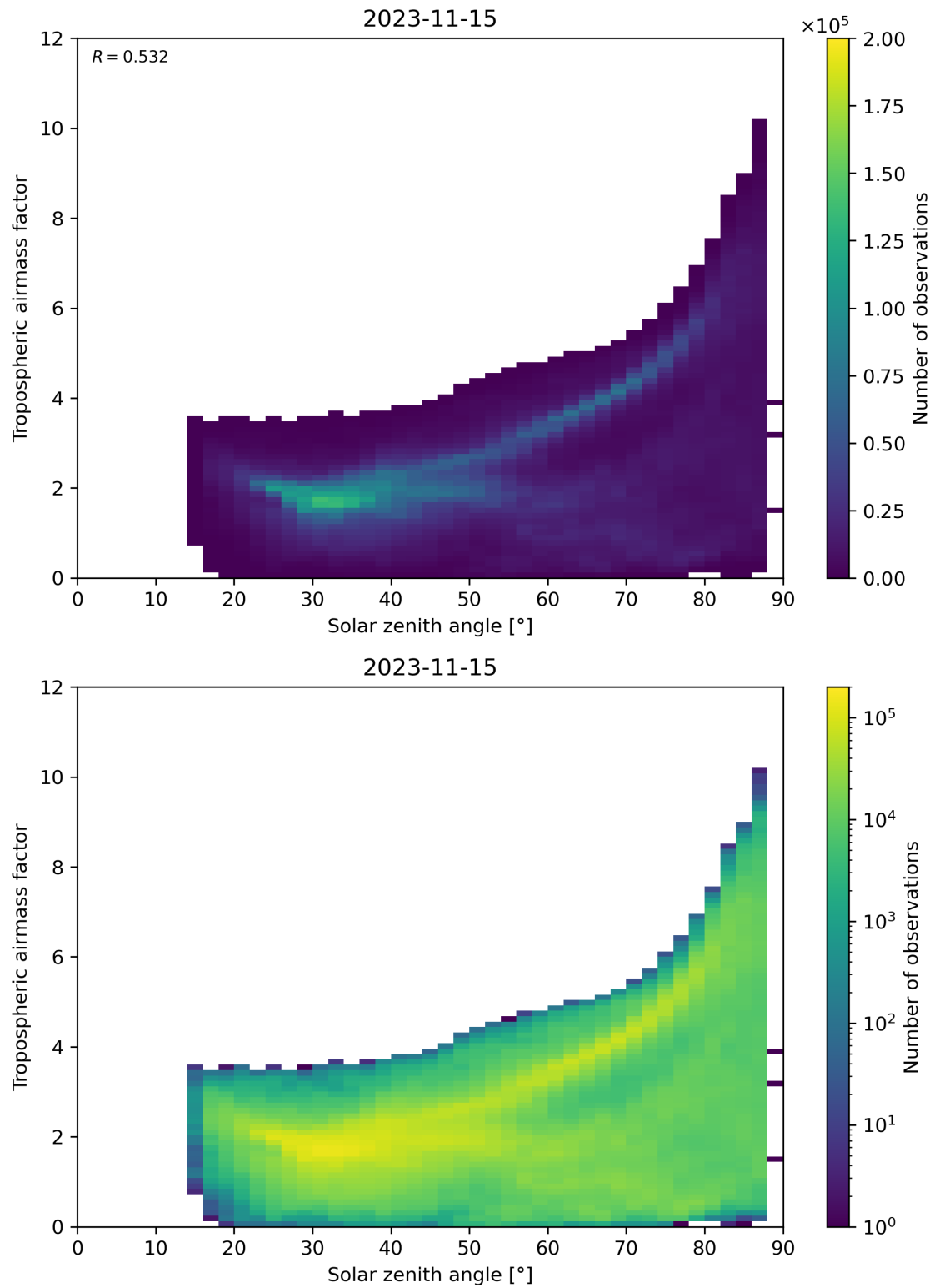
Figure 147: Scatter density plot of “Solar zenith angle” against “Tropospheric airmass factor” for 2023-11-14 to 2023-11-16.
