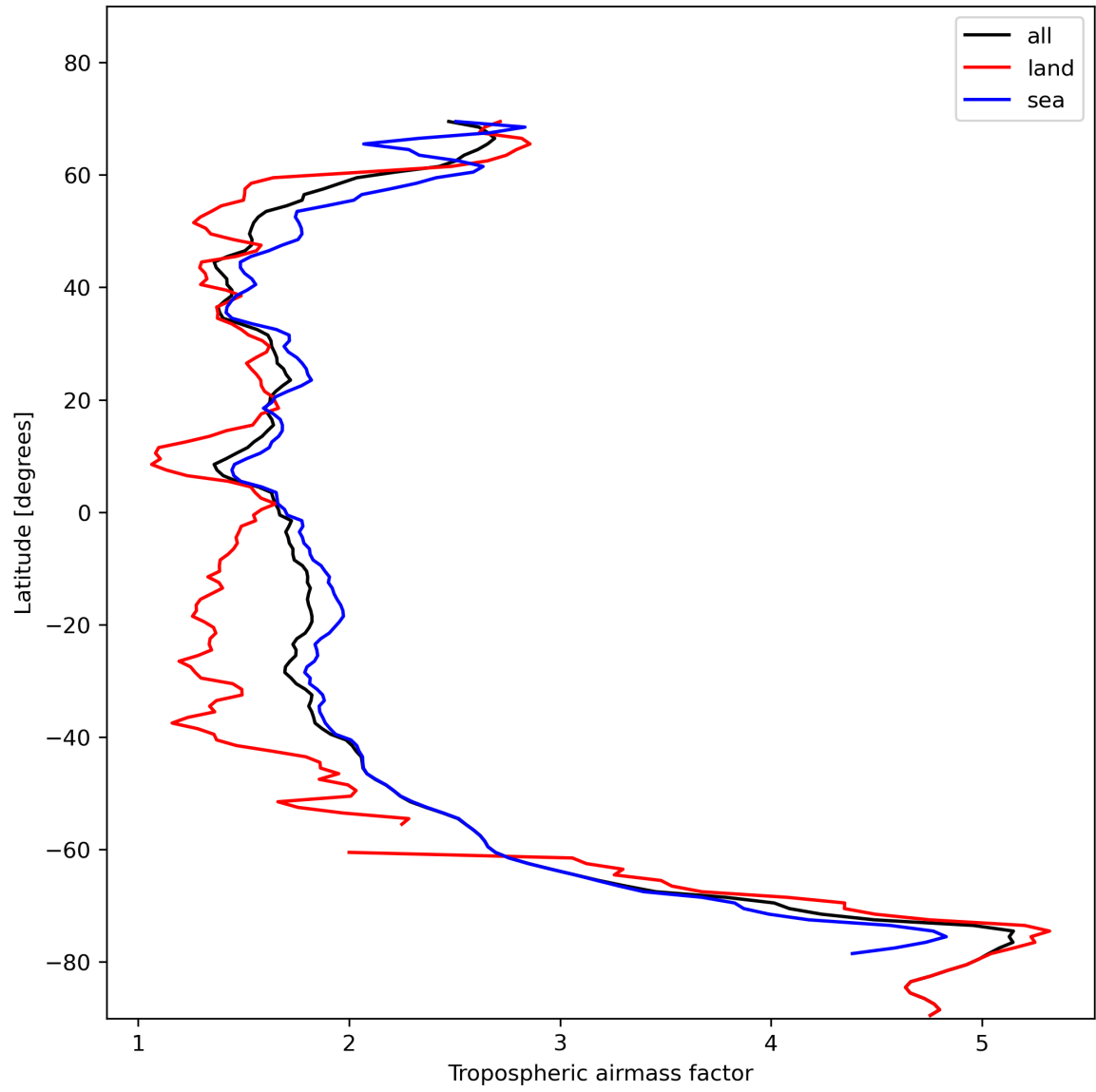
Figure 14: Zonal average of “Tropospheric airmass factor” for 2023-11-14 to 2023-11-16.
