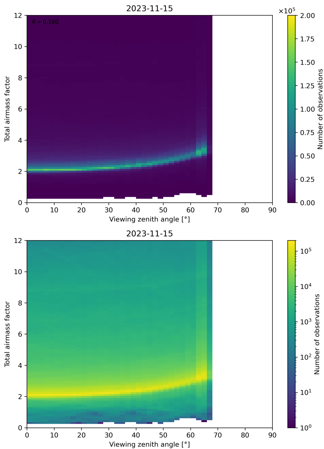
Figure 160: Scatter density plot of “Viewing zenith angle” against “Total airmass factor” for 2023-11-14 to 2023-11-16.
