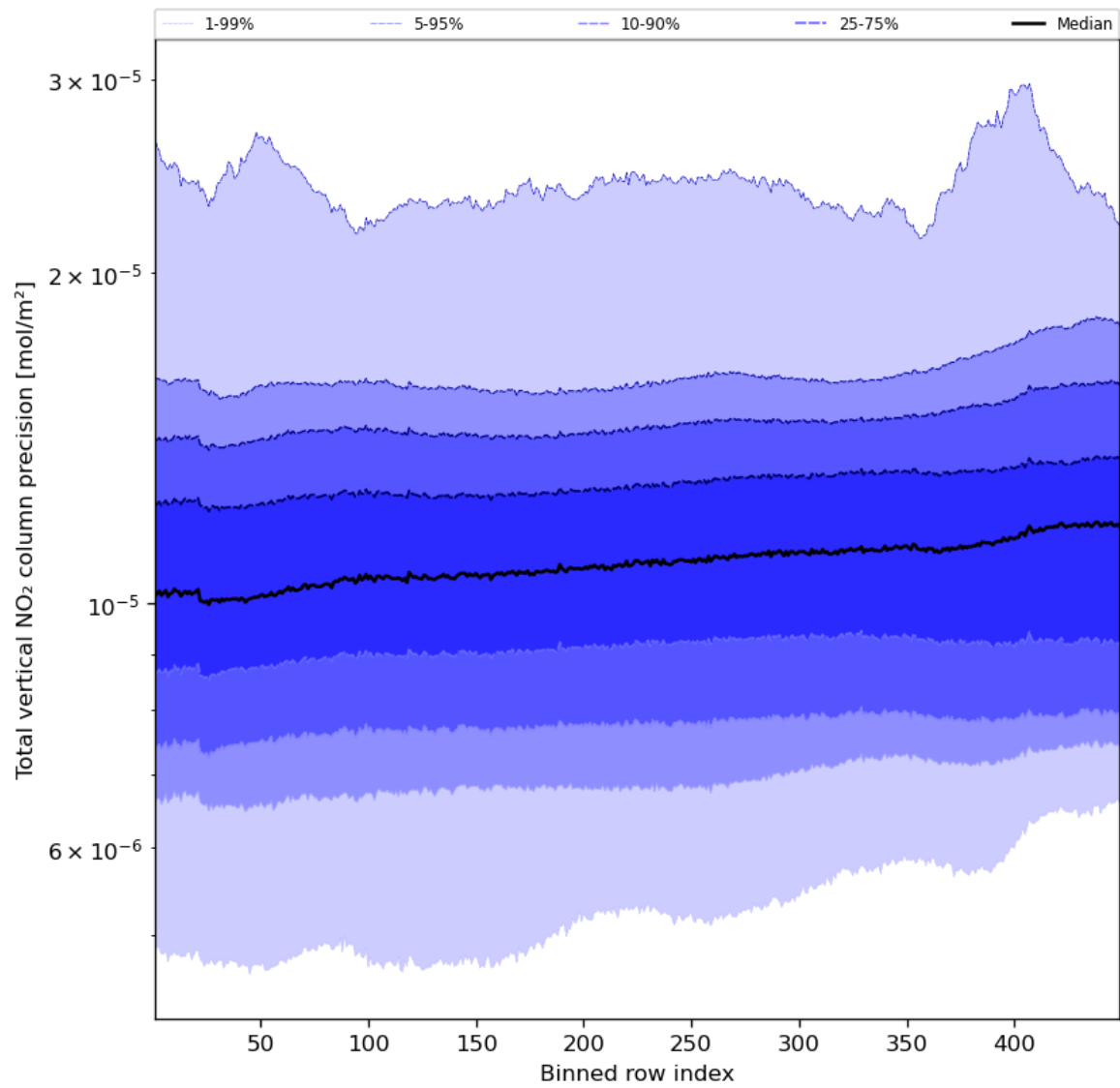
Figure 56: Along track statistics of “Total vertical NO 2 column precision” for 2023-11-14 to 2023-11-16
