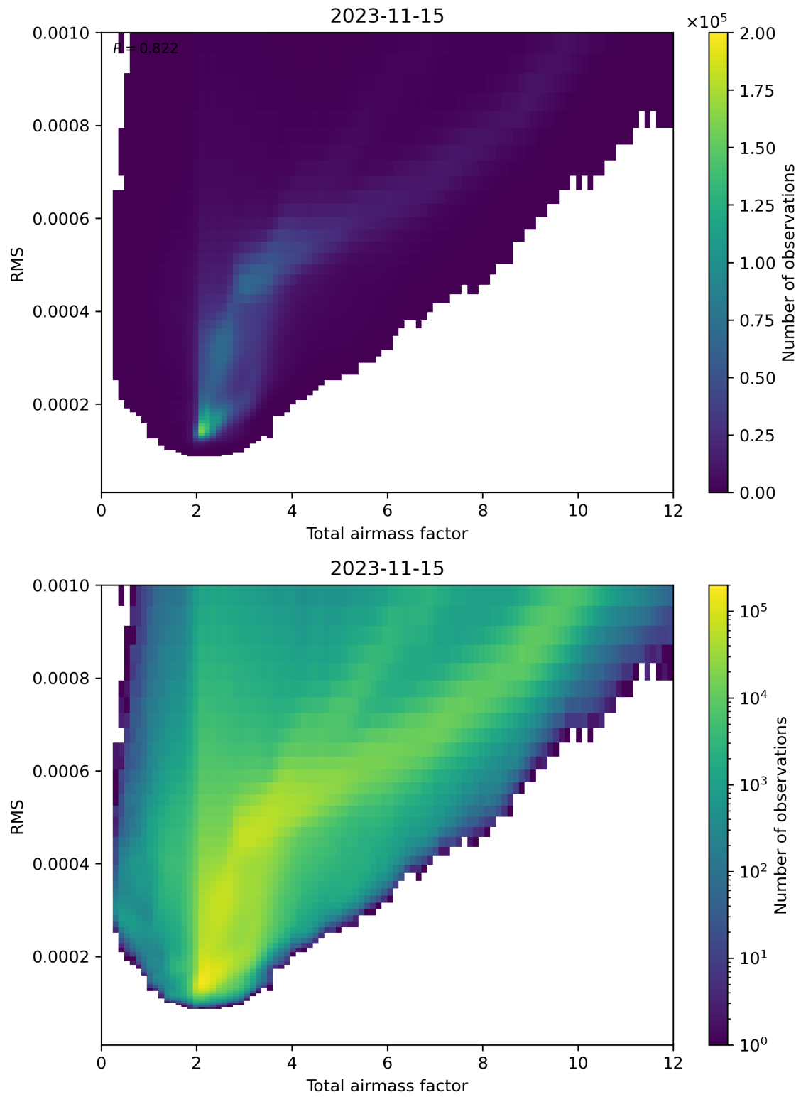
Figure 69: Scatter density plot of “Total airmass factor” against “RMS” for 2023-11-14 to 2023-11-16.
