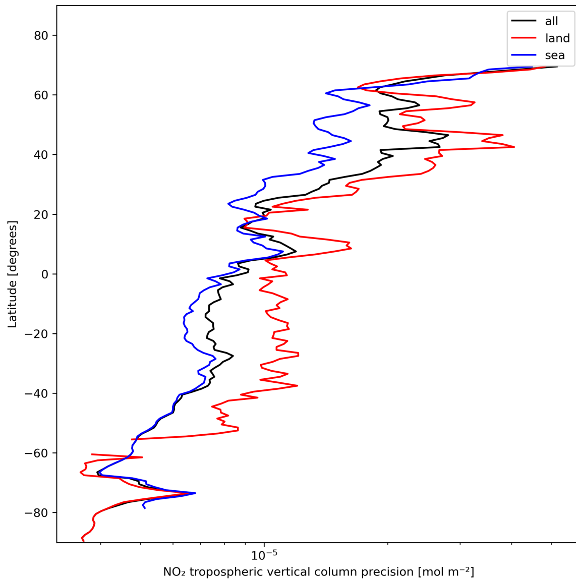
Figure 13: Zonal average of “NO 2 tropospheric vertical column precision” for 2023-11-14 to 2023-11-16.
