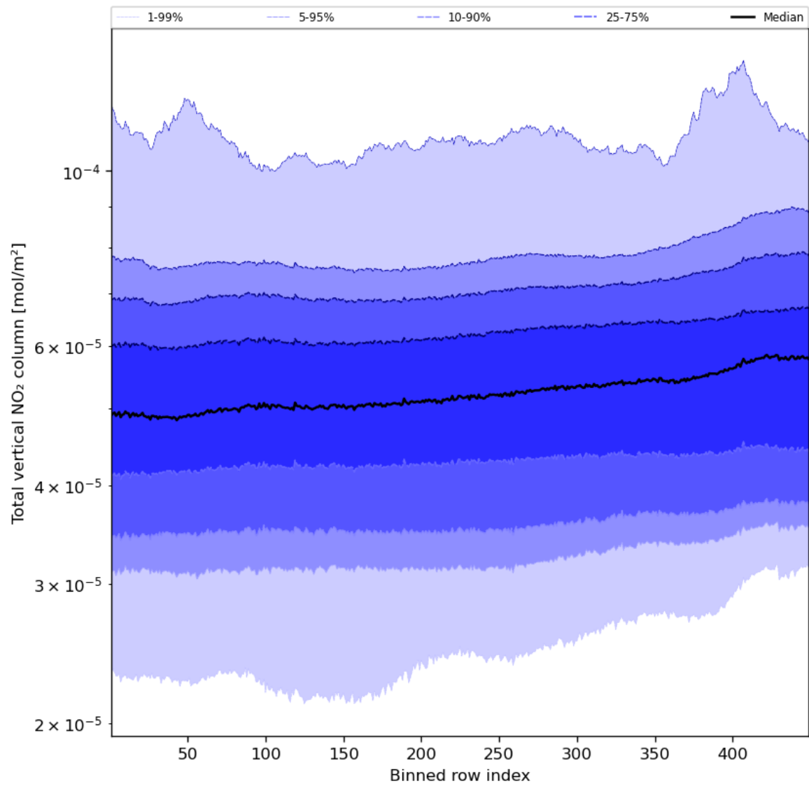
Figure 55: Along track statistics of “Total vertical NO 2 column” for 2023-11-14 to 2023-11-16
