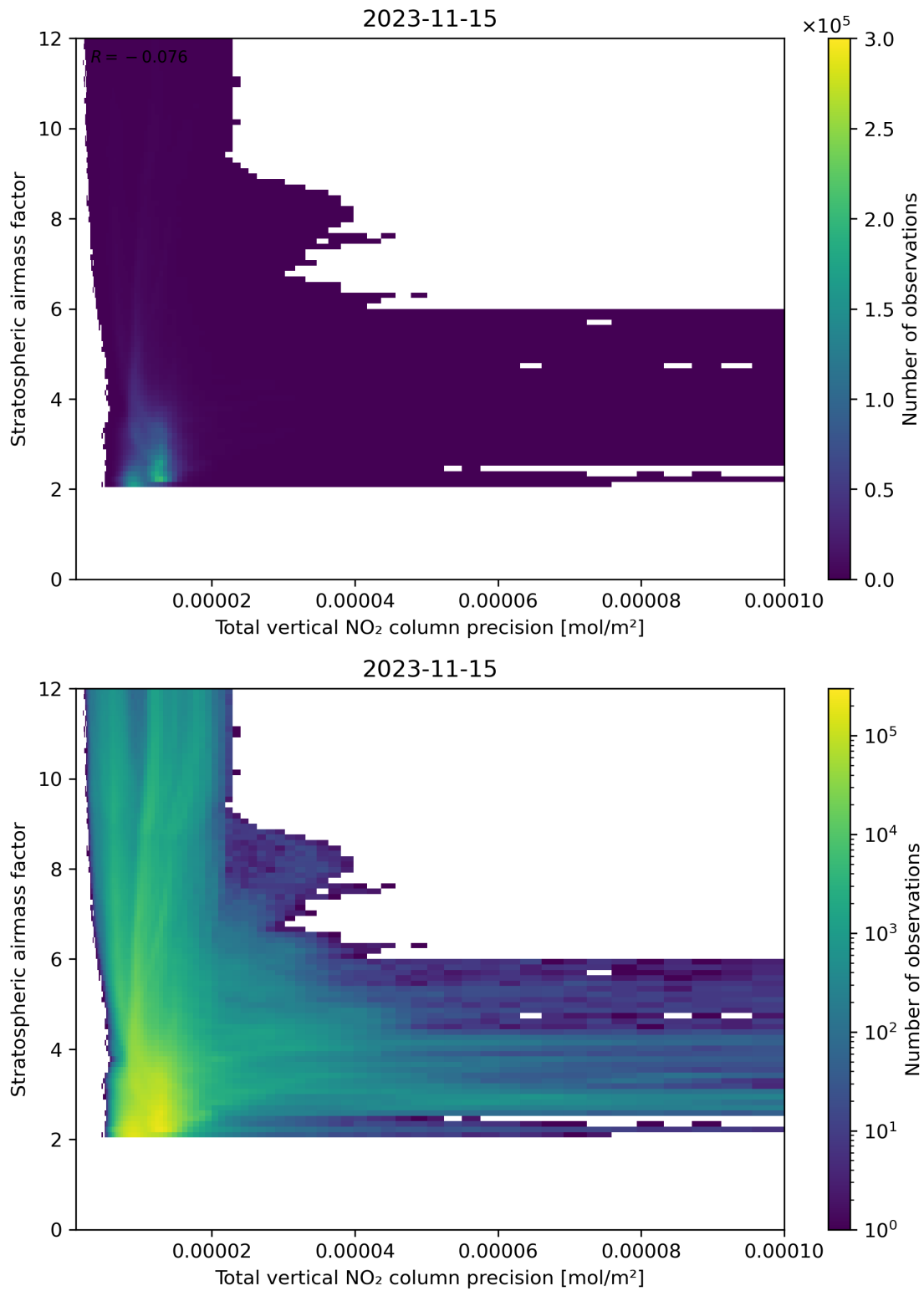
Figure 115: Scatter density plot of “Total vertical NO 2 column precision” against “Stratospheric air mass factor” for 2023-11-14 to 2023-11-16.
