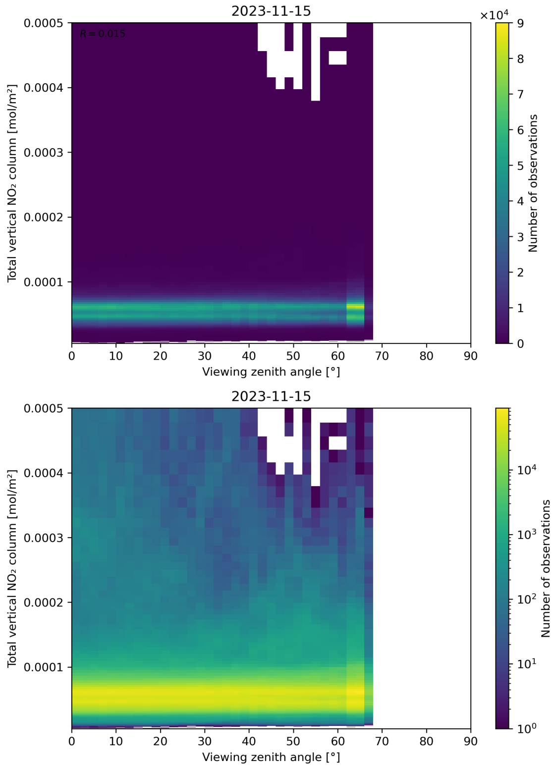
Figure 167: Scatter density plot of “Viewing zenith angle” against “Total vertical NO 2 column” for 2023-11-14 to 2023-11-16.
