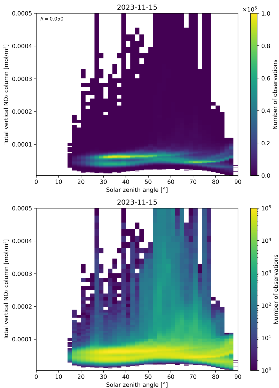
Figure 153: Scatter density plot of “Solar zenith angle” against “Total vertical NO 2 column” for 2023-11-14 to 2023-11-16.
