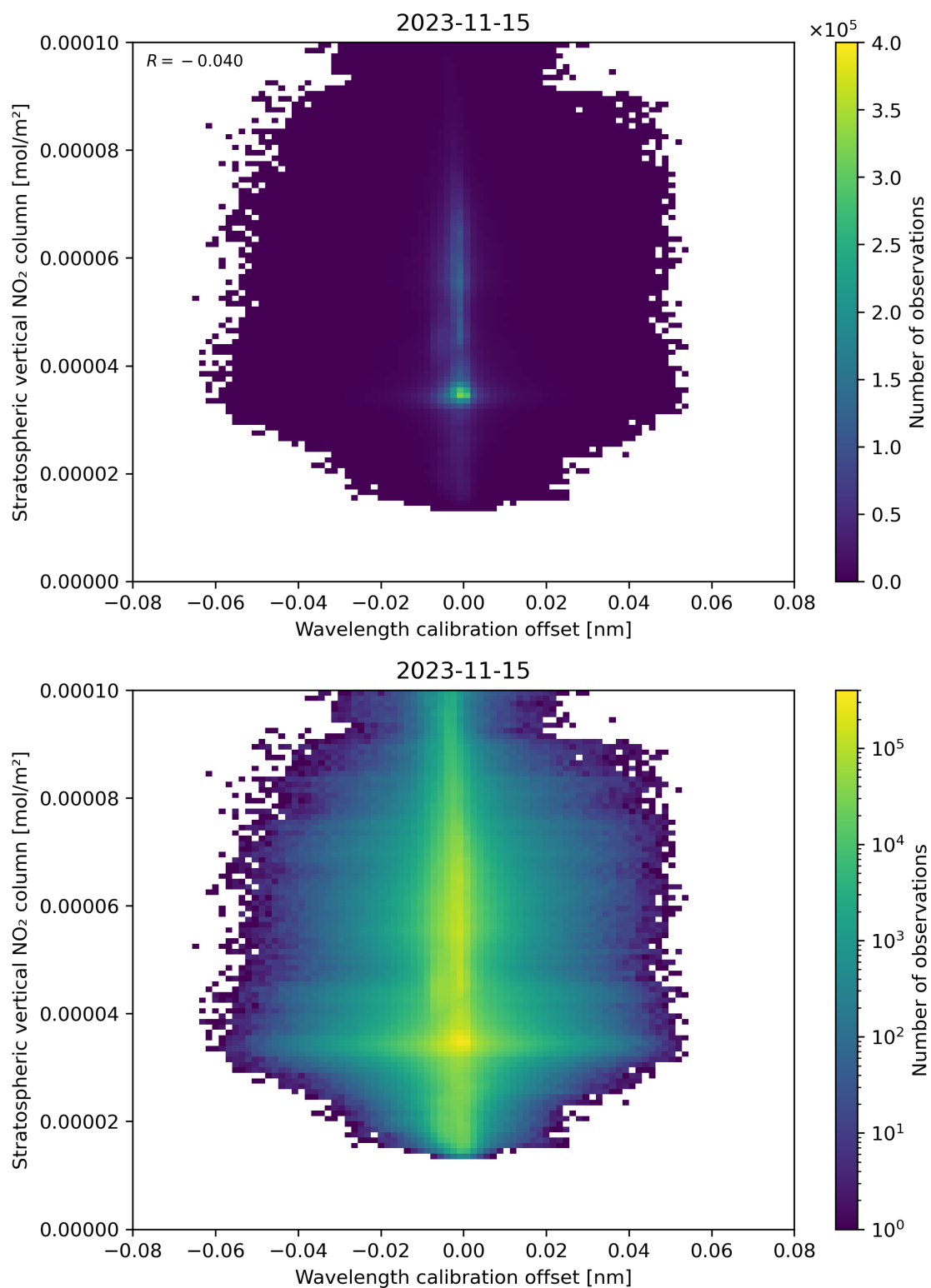
Figure 176: Scatter density plot of “Wavelength calibration offset” against “Stratospheric vertical NO 2 column” for 2023-11-14 to 2023-11-16.
