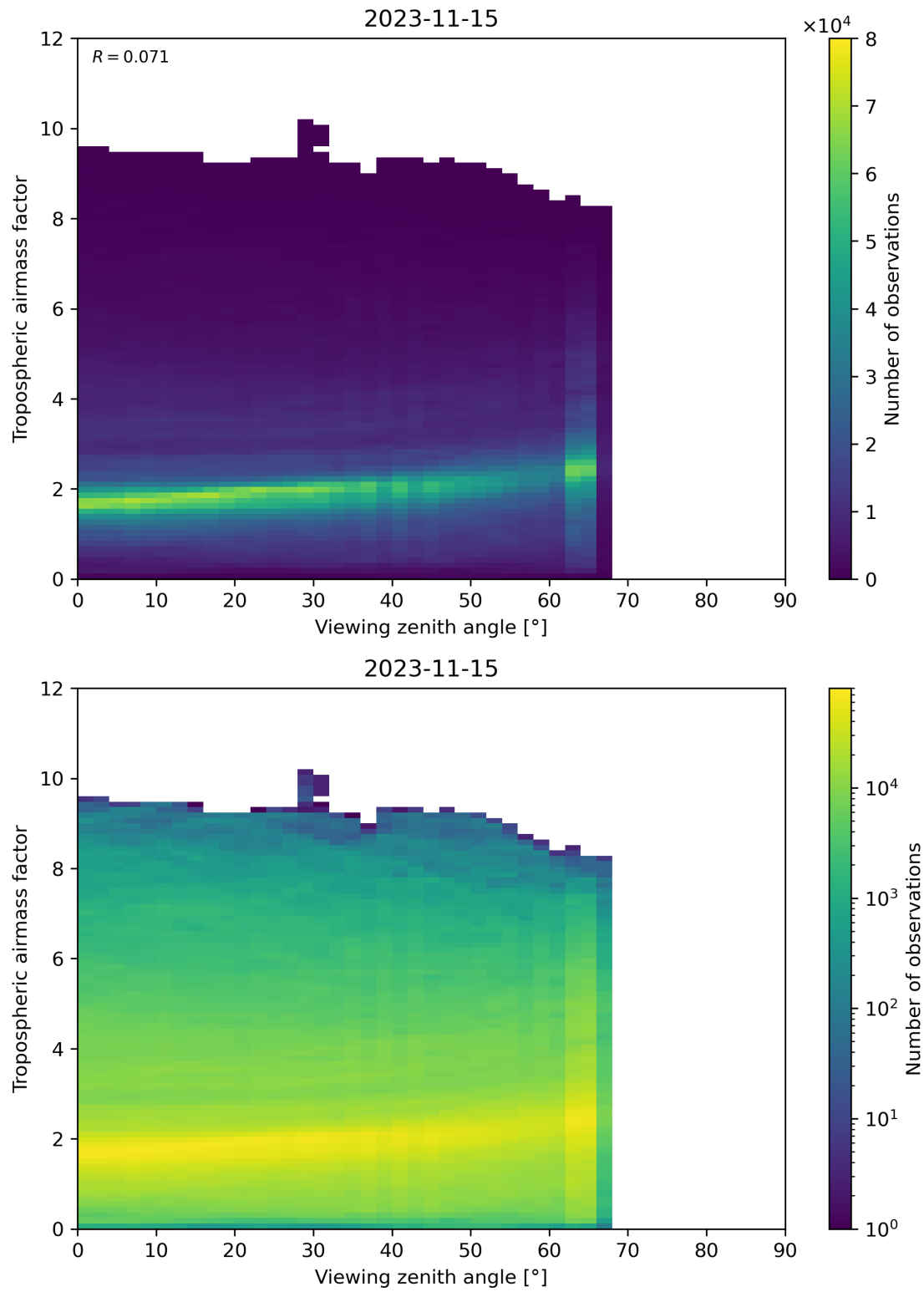
Figure 161: Scatter density plot of “Viewing zenith angle” against “Tropospheric airmass factor” for 2023-11-14 to 2023-11-16.
