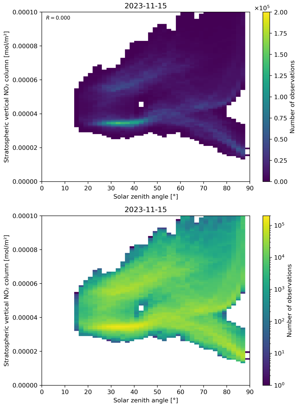
Figure 150: Scatter density plot of “Solar zenith angle” against “Stratospheric vertical NO 2 column” for 2023-11-14 to 2023-11-16.
