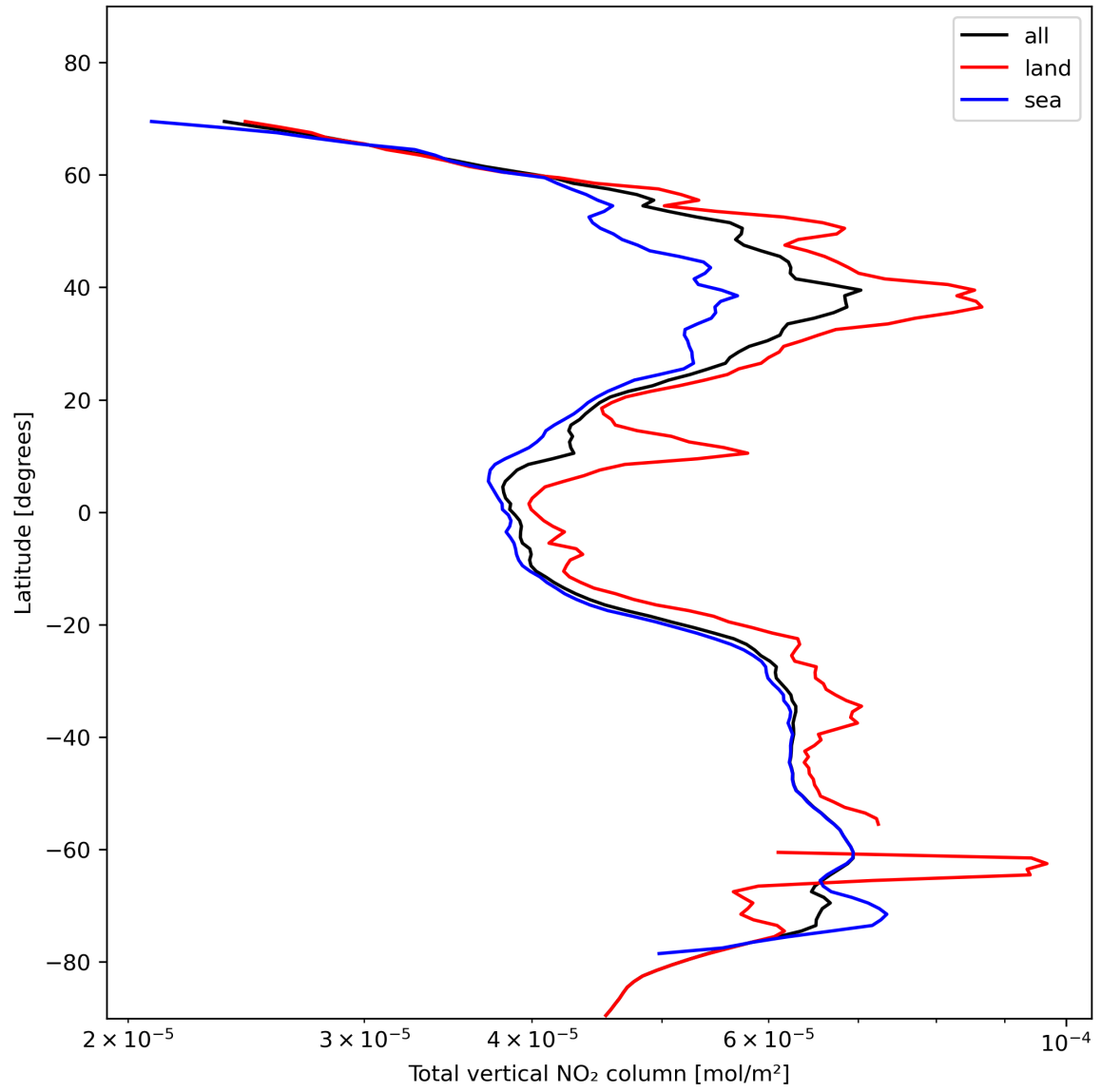
Figure 21: Zonal average of “Total vertical NO 2 column” for 2023-11-14 to 2023-11-16.
