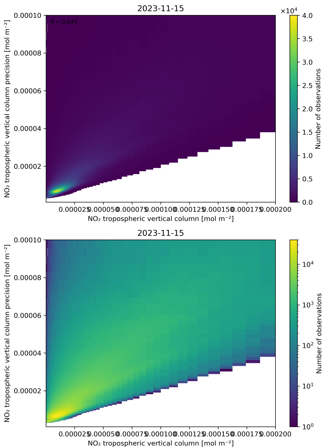
Figure 130: Scatter density plot of “NO 2 tropospheric vertical column” against “NO 2 tropospheric vertical column precision” for 2023-11-14 to 2023-11-16.
