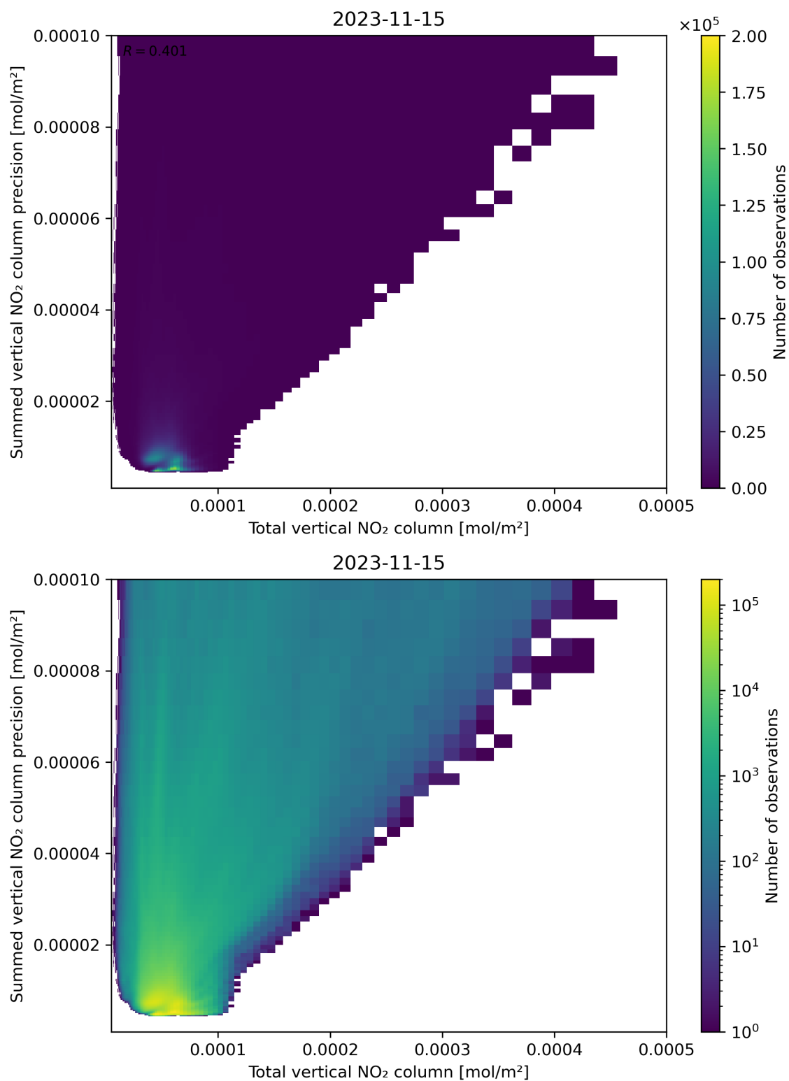
Figure 113: Scatter density plot of “Total vertical NO 2 column” against “Summed vertical NO 2 column precision” for 2023-11-14 to 2023-11-16.
