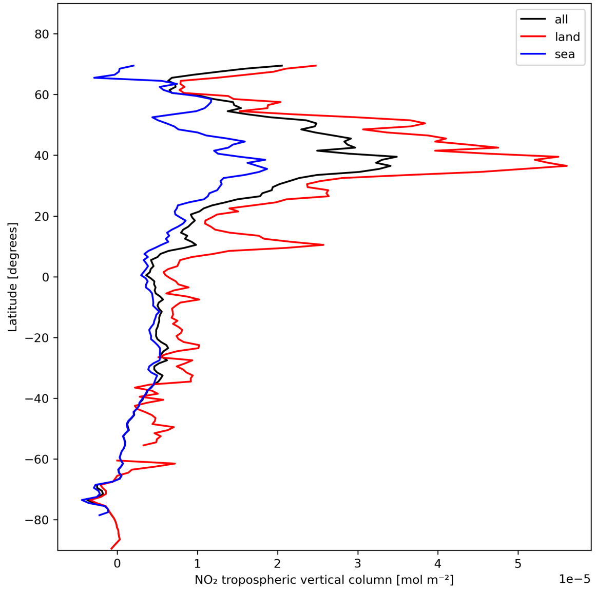
Figure 12: Zonal average of “NO 2 tropospheric vertical column” for 2023-11-14 to 2023-11-16.
