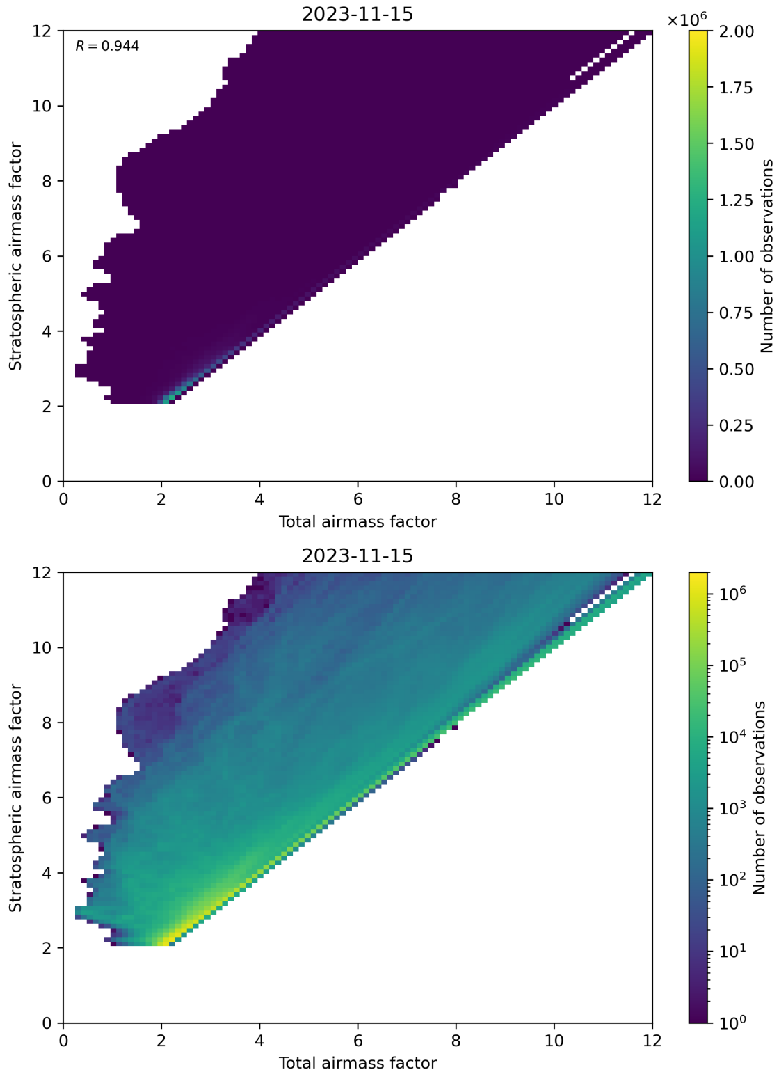
Figure 62: Scatter density plot of “Total airmass factor” against “Stratospheric airmass factor” for 2023-11-14 to 2023-11-16.
