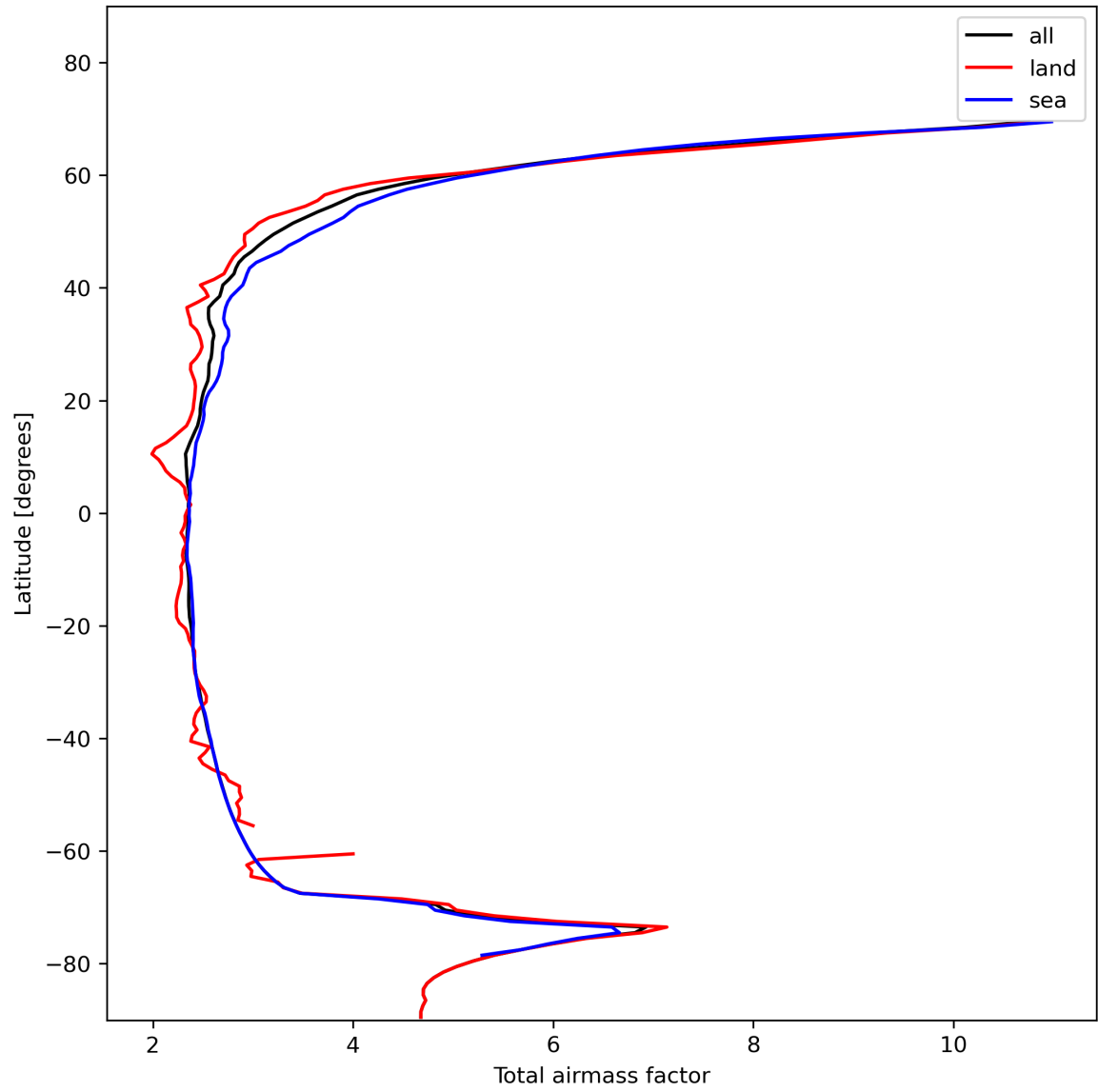
Figure 15: Zonal average of “Total airmass factor” for 2023-11-14 to 2023-11-16.
