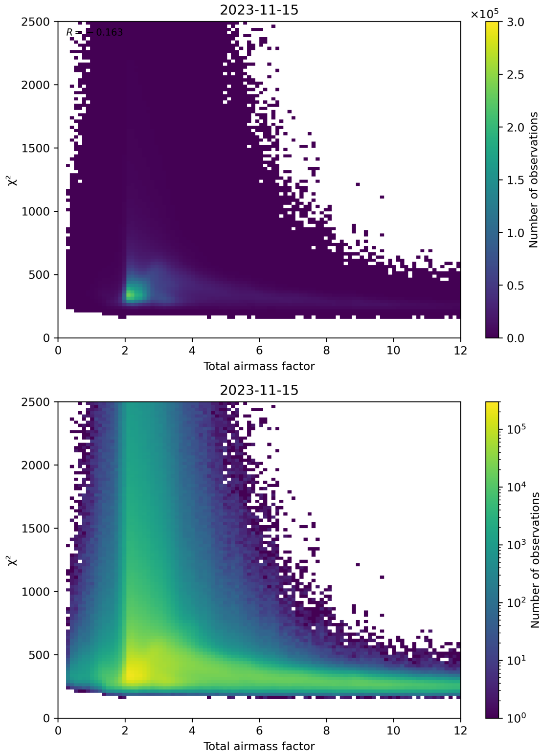
Figure 63: Scatter density plot of “Total airmass factor” against “ \chi^2 ” for 2023-11-14 to 2023-11-16.
