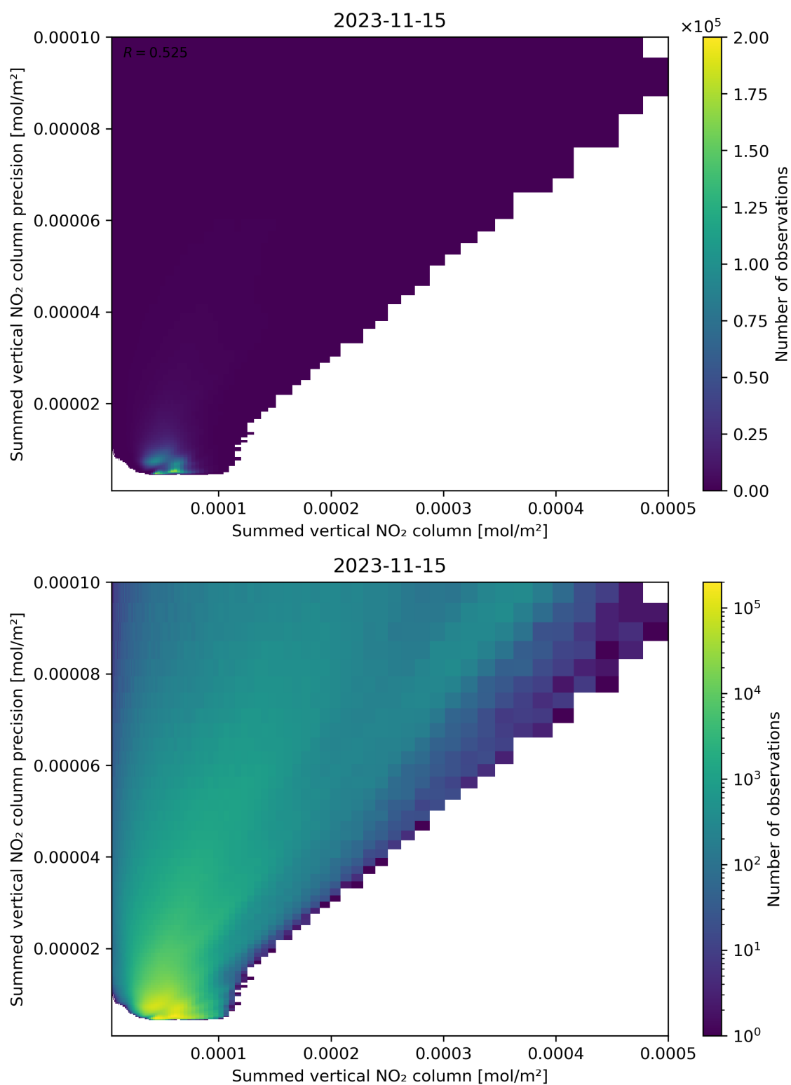
Figure 105: Scatter density plot of “Summed vertical NO 2 column” against “Summed vertical NO 2 column precision” for 2023-11-14 to 2023-11-16.
