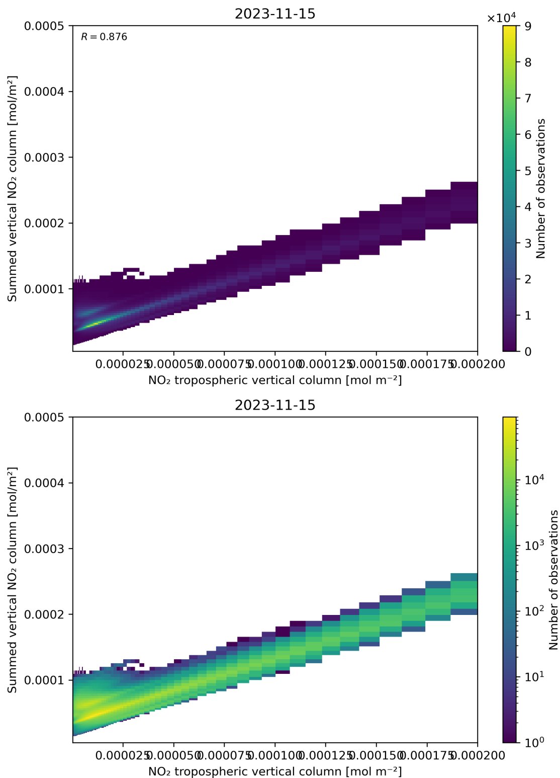
Figure 126: Scatter density plot of “NO 2 tropospheric vertical column” against “Summed vertical NO 2 column” for 2023-11-14 to 2023-11-16.
