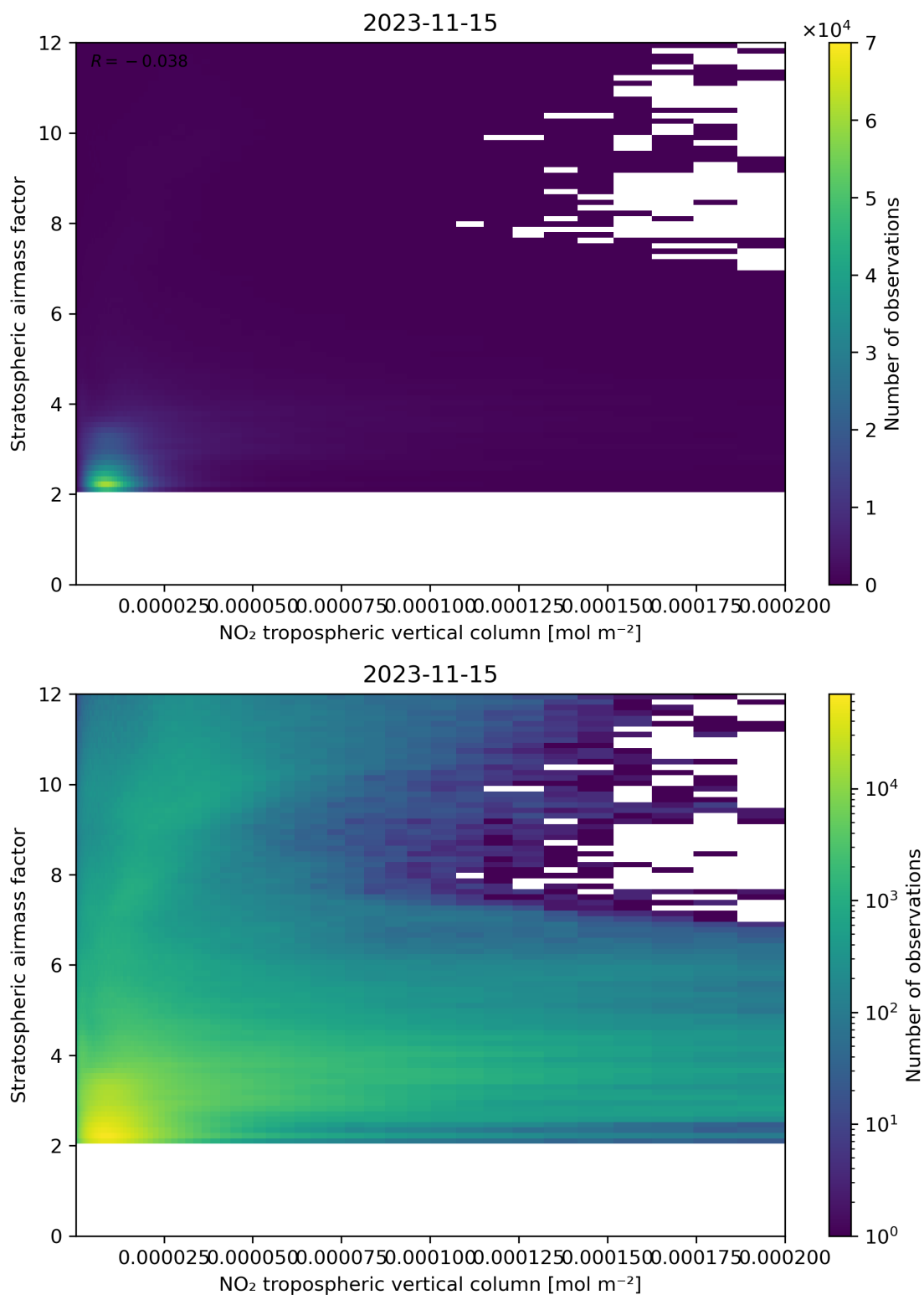
Figure 121: Scatter density plot of “NO 2 tropospheric vertical column” against “Stratospheric airmass factor” for 2023-11-14 to 2023-11-16.
