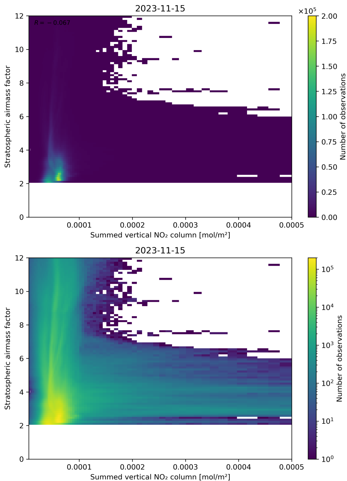
Figure 103: Scatter density plot of “Summed vertical NO 2 column” against “Stratospheric air mass factor” for 2023-11-14 to 2023-11-16.
