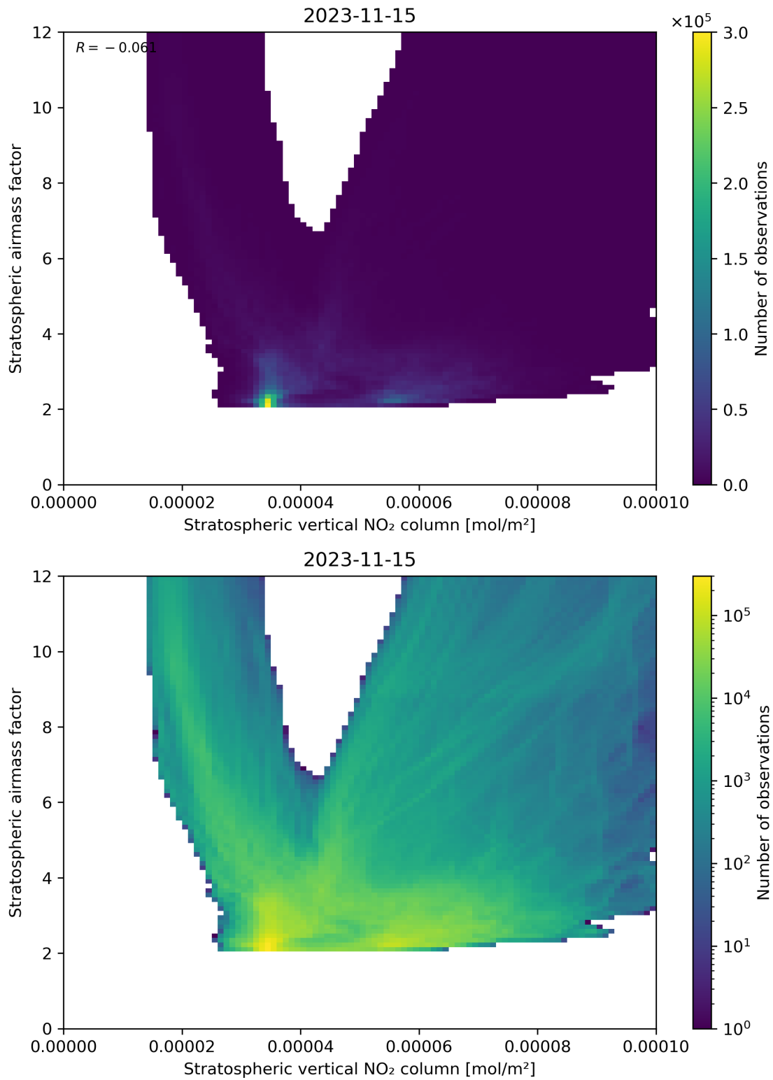
Figure 96: Scatter density plot of “Stratospheric vertical NO 2 column” against “Stratospheric airmass factor” for 2023-11-14 to 2023-11-16.
