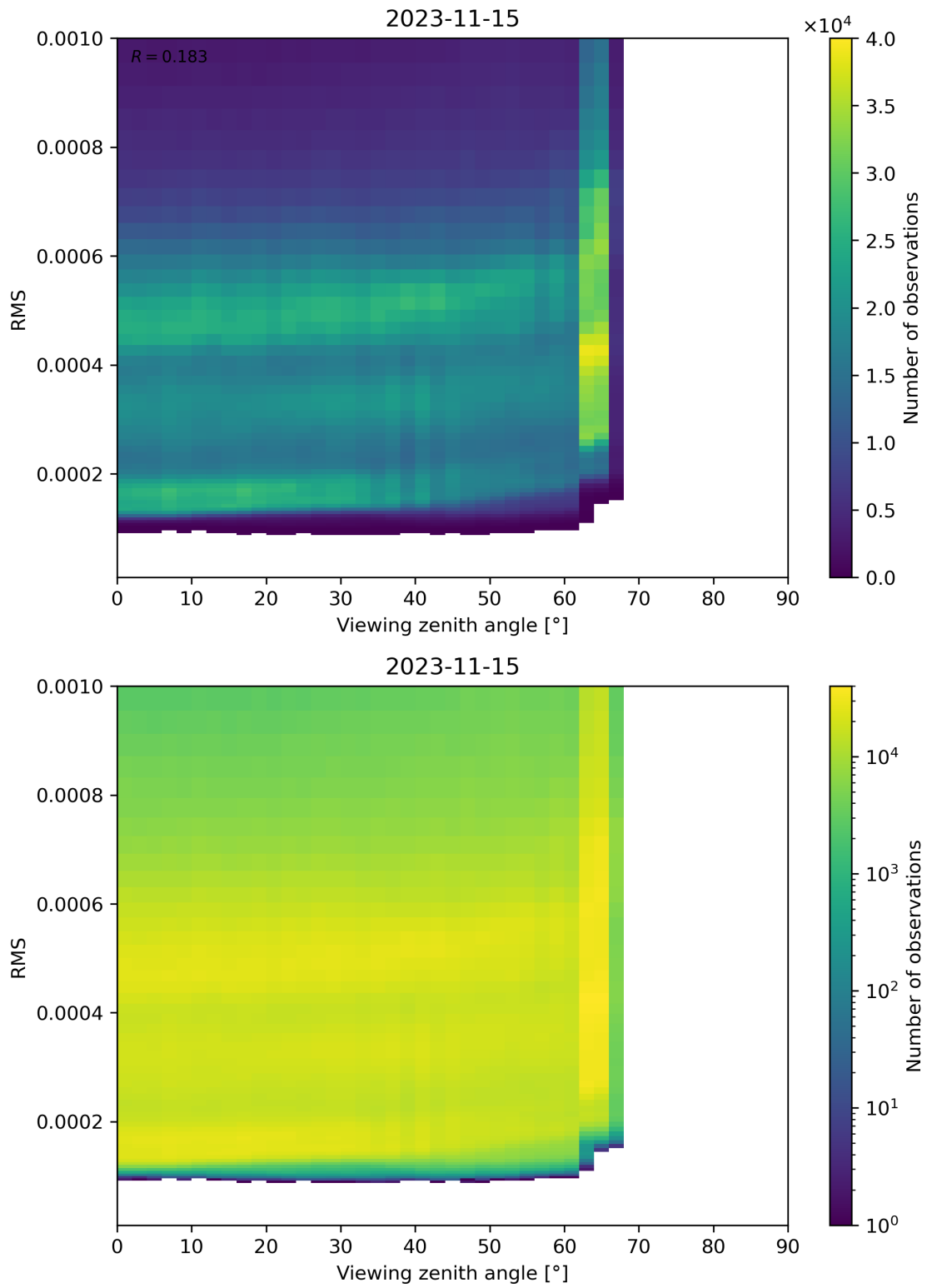
Figure 171: Scatter density plot of “Viewing zenith angle” against “RMS” for 2023-11-14 to 2023-11-16.
