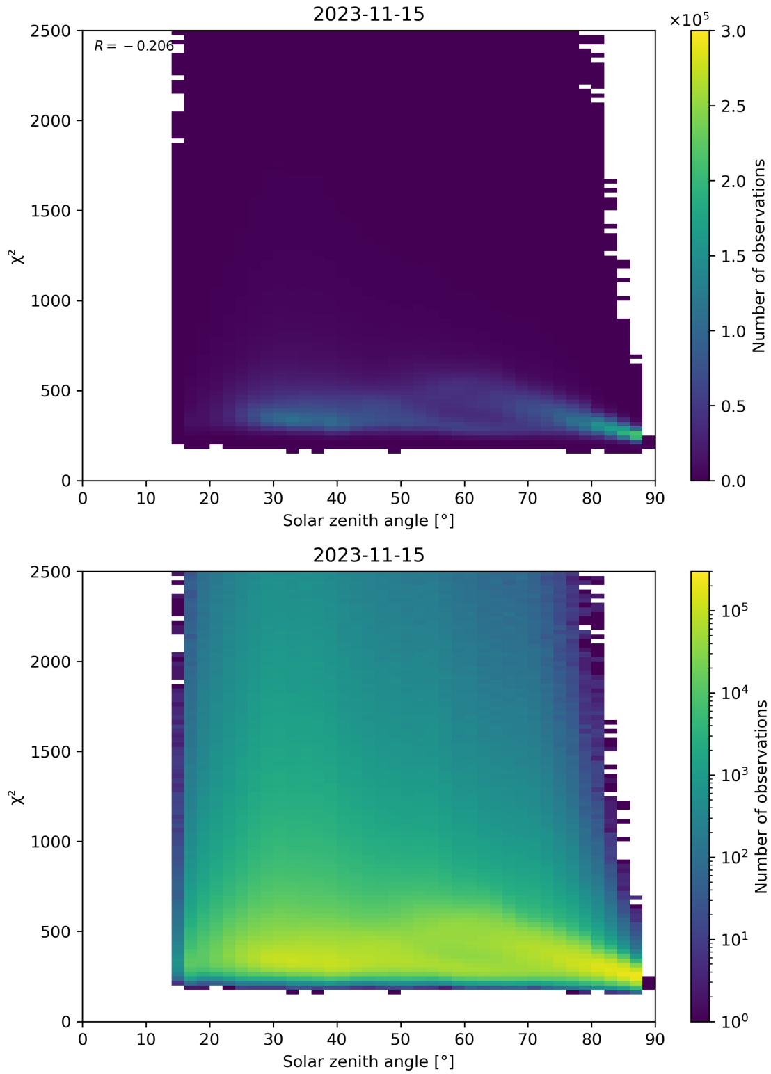
Figure 148: Scatter density plot of “Solar zenith angle” against “ \chi^2 ” for 2023-11-14 to 2023-11-16.
