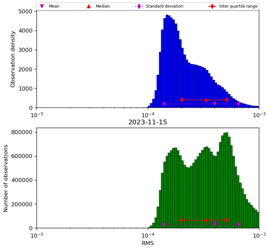
Figure 43: Histogram of “RMS” for 2023-11-14 to 2023-11-16
