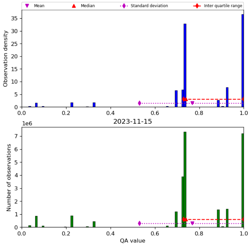
Figure 28: Histogram of “QA value” for 2023-11-14 to 2023-11-16
