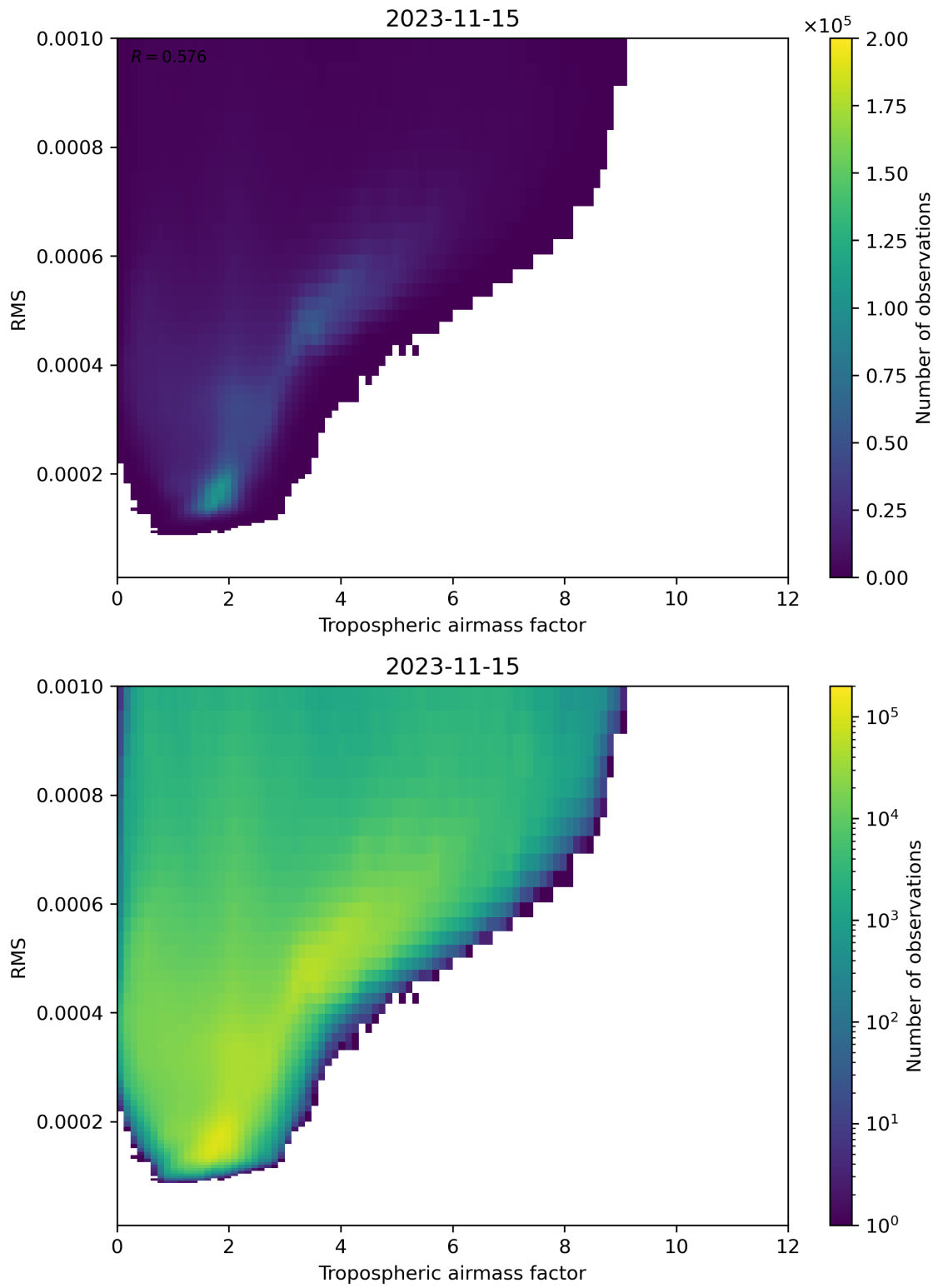
Figure 79: Scatter density plot of “Tropospheric airmass factor” against “RMS” for 2023-11-14 to 2023-11-16.
