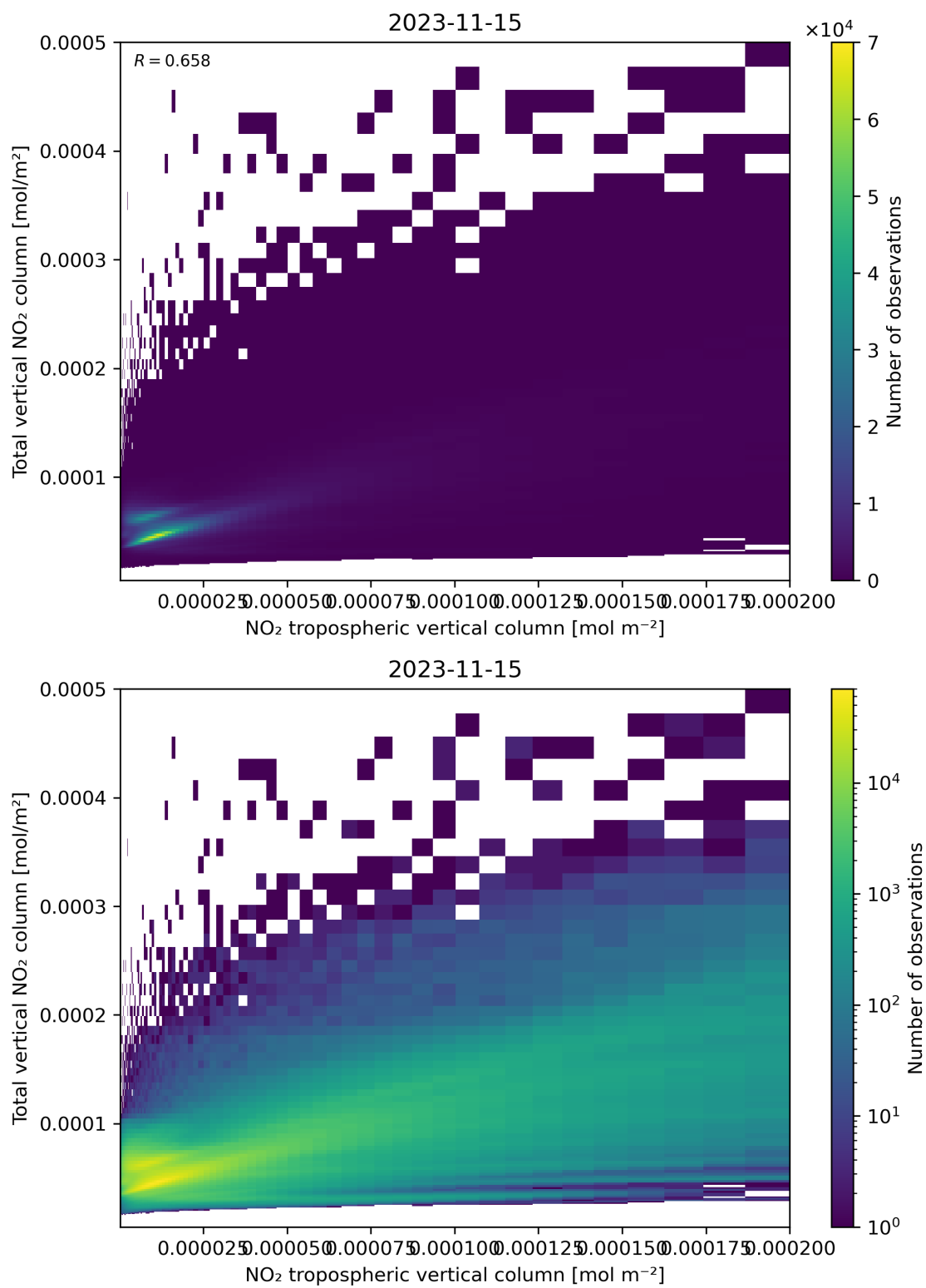
Figure 128: Scatter density plot of “NO 2 tropospheric vertical column” against “Total vertical NO 2 column” for 2023-11-14 to 2023-11-16.
