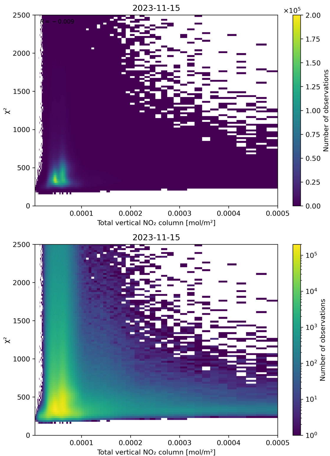
Figure 111: Scatter density plot of “Total vertical NO 2 column” against “ \chi^2 ” for 2023-11-14 to 2023-11-16.
