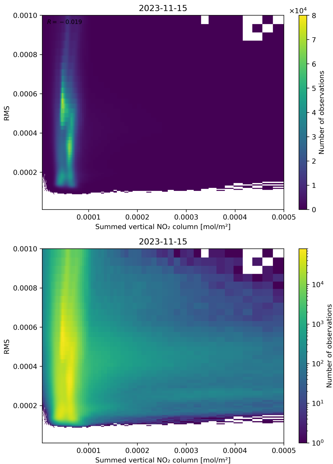
Figure 109: Scatter density plot of “Summed vertical NO 2 column” against “RMS” for 2023-11-14 to 2023-11-16.
