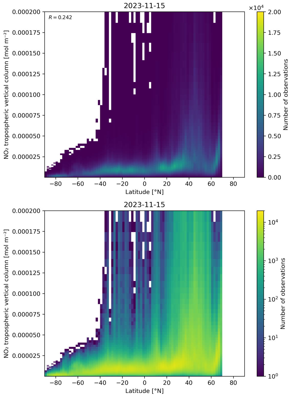
Figure 92: Scatter density plot of “Latitude” against “NO 2 tropospheric vertical column” for 2023-11-14 to 2023-11-16.
