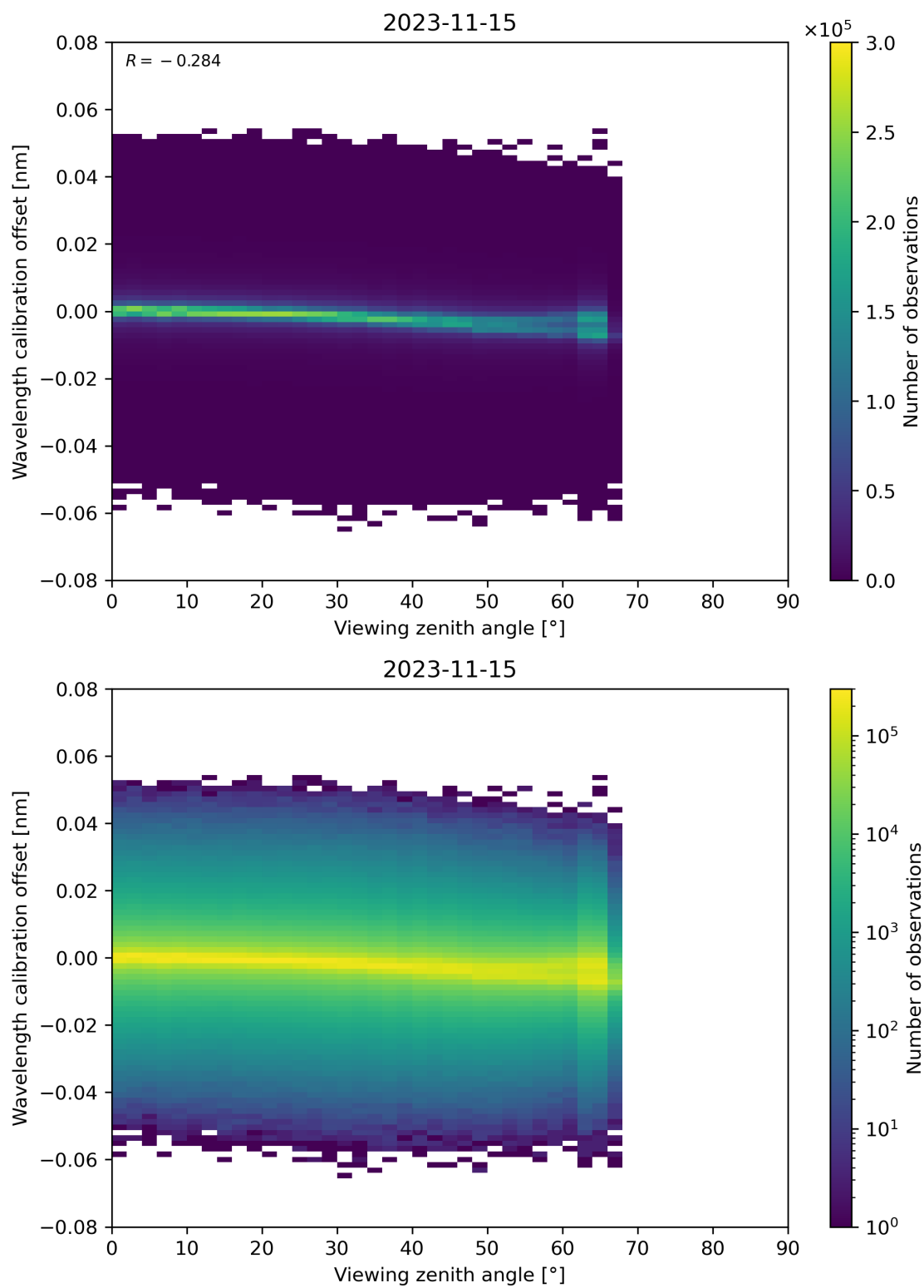
Figure 173: Scatter density plot of “Viewing zenith angle” against “Wavelength calibration offset” for 2023-11-14 to 2023-11-16.
