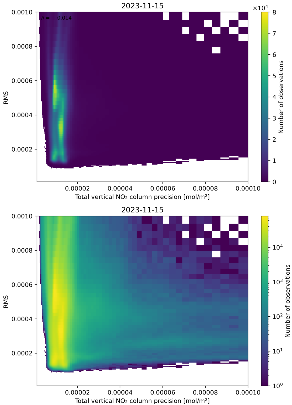
Figure 119: Scatter density plot of “Total vertical NO 2 column precision” against “RMS” for 2023-11-14 to 2023-11-16.
