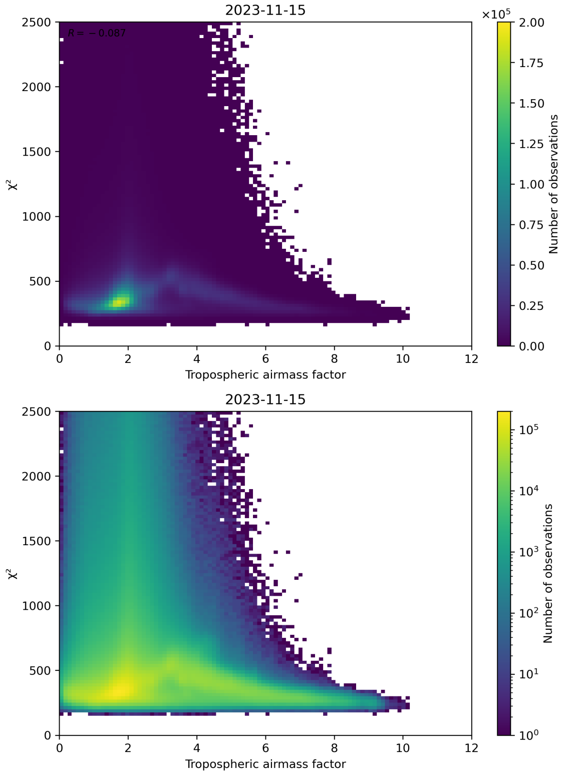
Figure 73: Scatter density plot of “Tropospheric airmass factor” against “ \chi^2 ” for 2023-11-14 to 2023-11-16.
