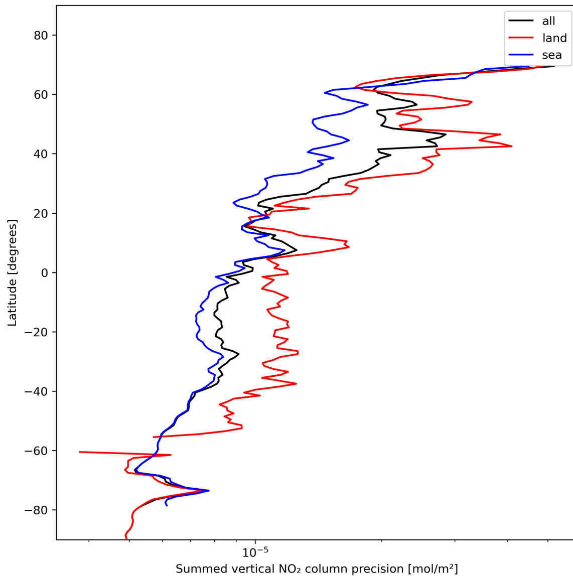
Figure 24: Zonal average of “Summed vertical NO 2 column precision” for 2023-11-14 to 2023-11-16.
