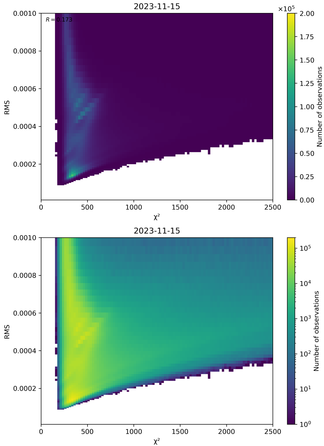
Figure 82: Scatter density plot of “ \chi^2 ” against “RMS” for 2023-11-14 to 2023-11-16.
