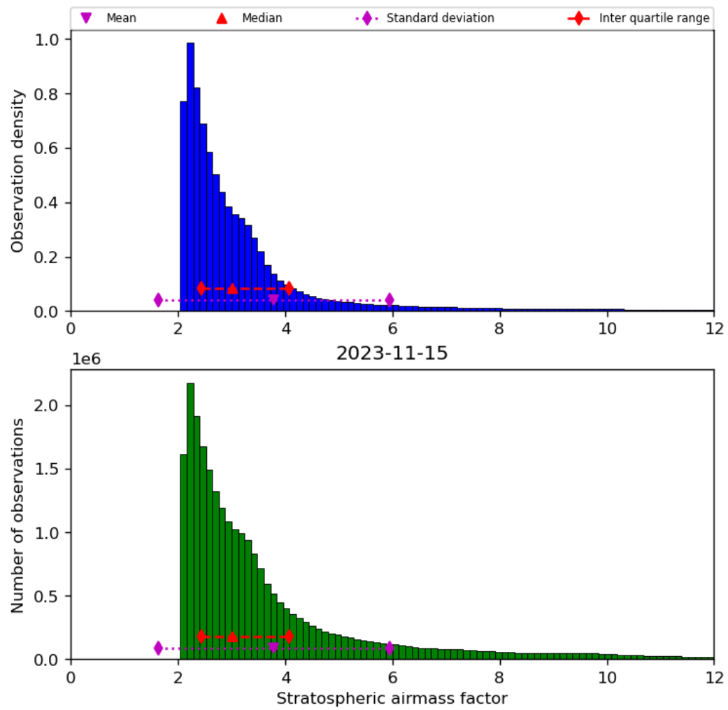
Figure 44: Histogram of “Stratospheric airmass factor” for 2023-11-14 to 2023-11-16
