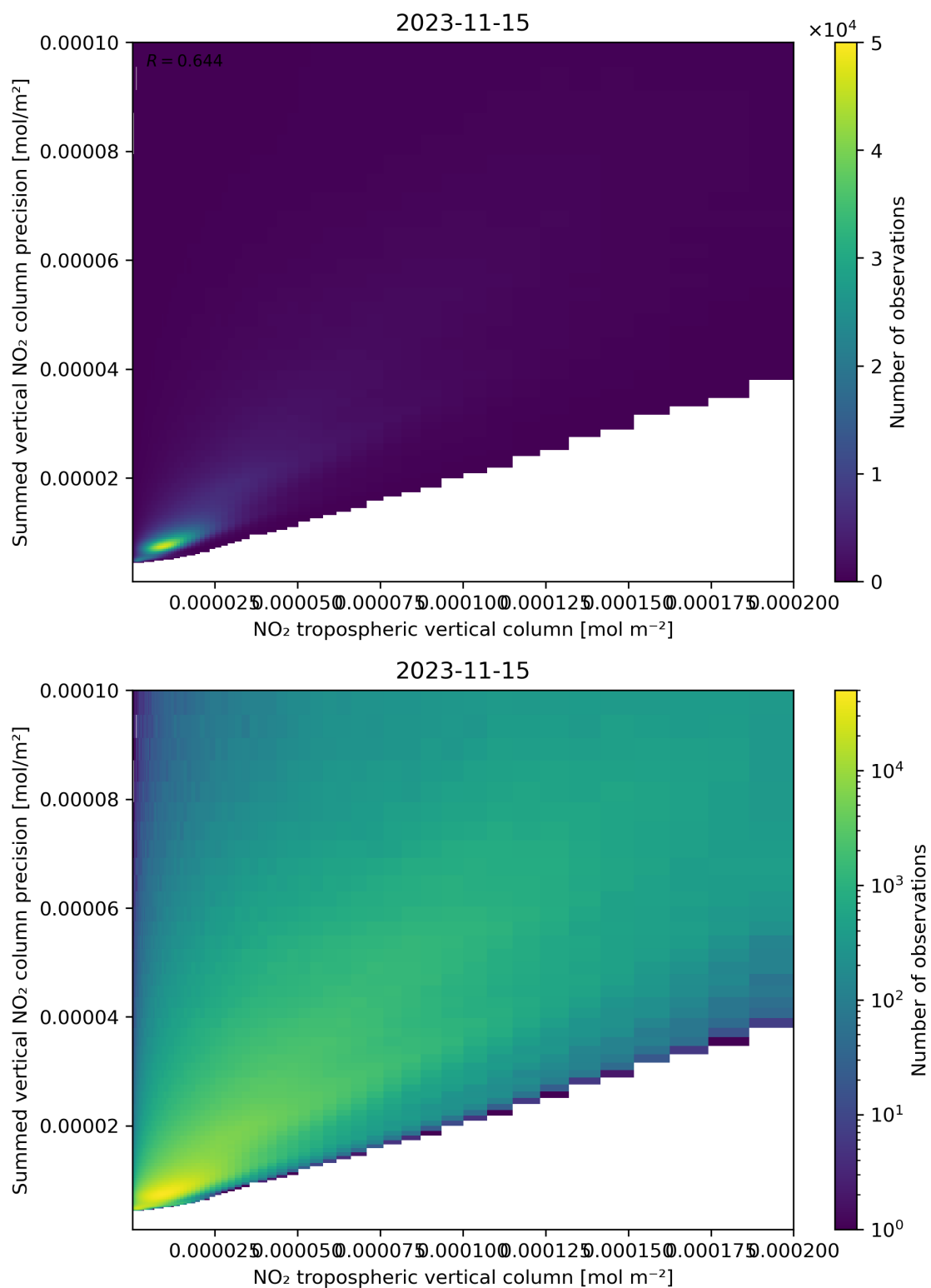
Figure 127: Scatter density plot of “NO 2 tropospheric vertical column” against “Summed vertical NO 2 column precision” for 2023-11-14 to 2023-11-16.
