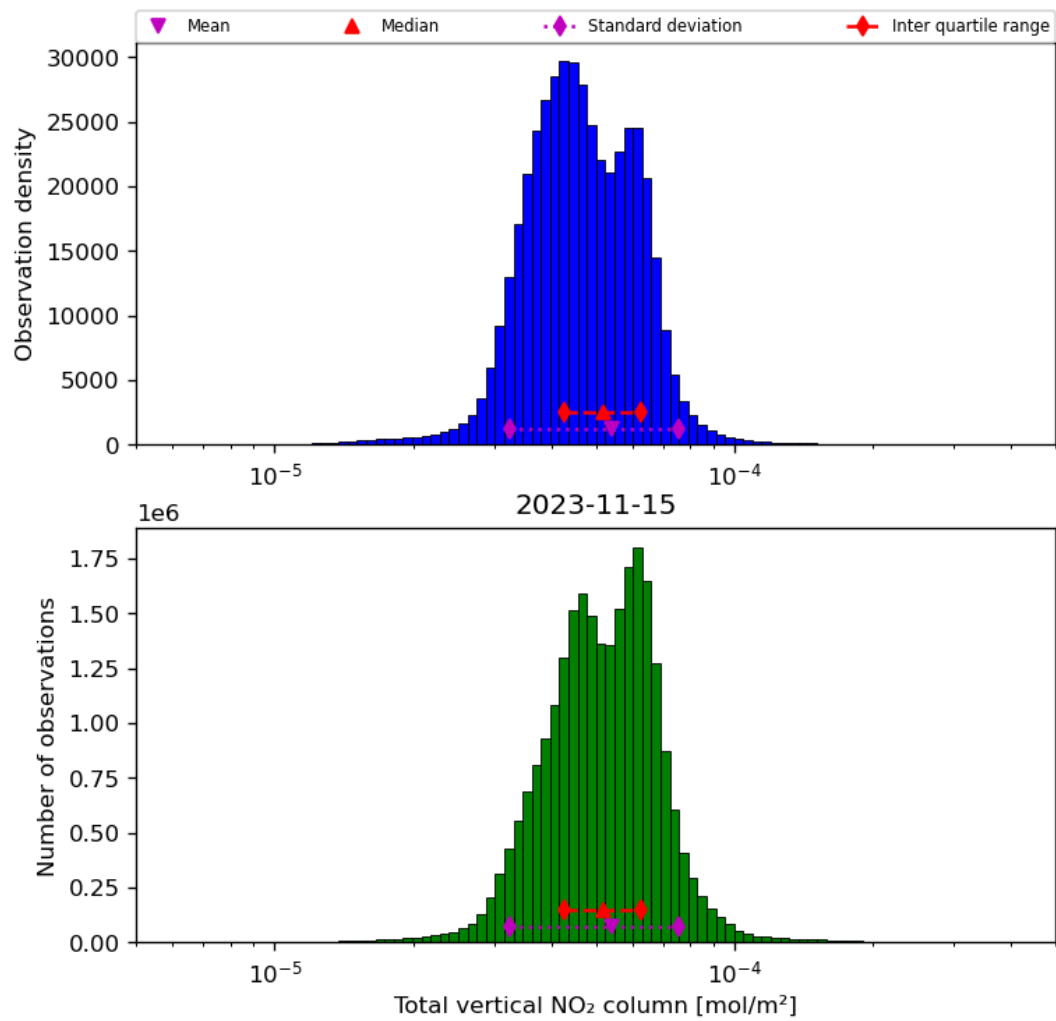
Figure 38: Histogram of “Total vertical NO 2 column” for 2023-11-14 to 2023-11-16
