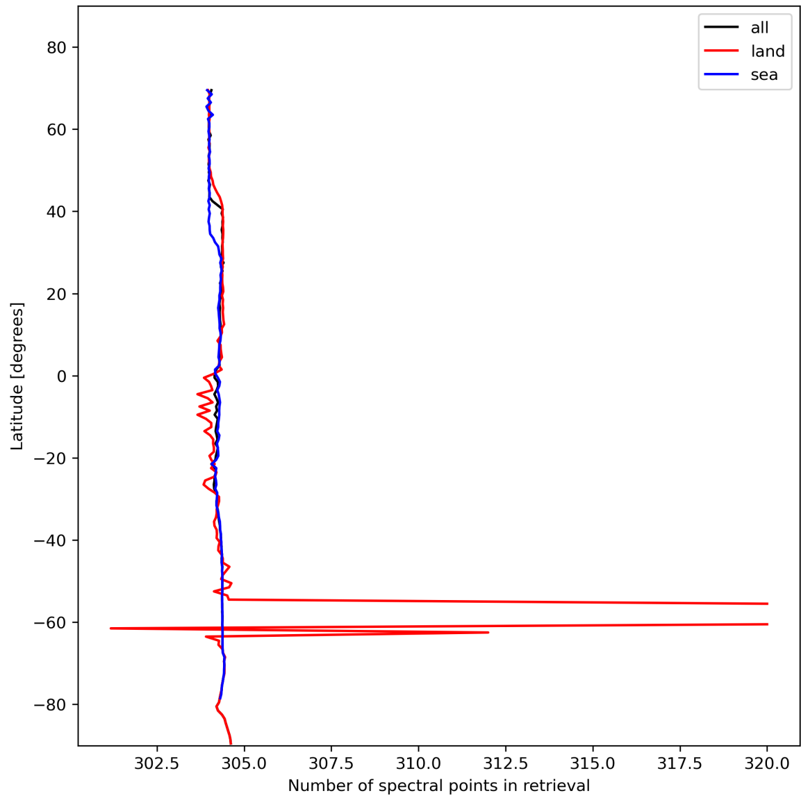
Figure 16: Zonal average of “Number of spectral points in retrieval” for 2023-11-14 to 2023-11-16.
