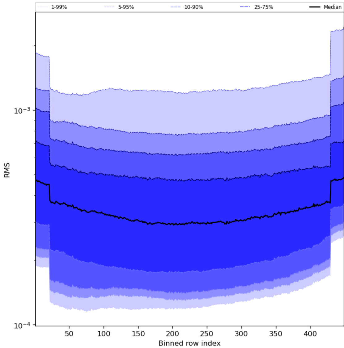
Figure 60: Along track statistics of “RMS” for 2023-11-14 to 2023-11-16
