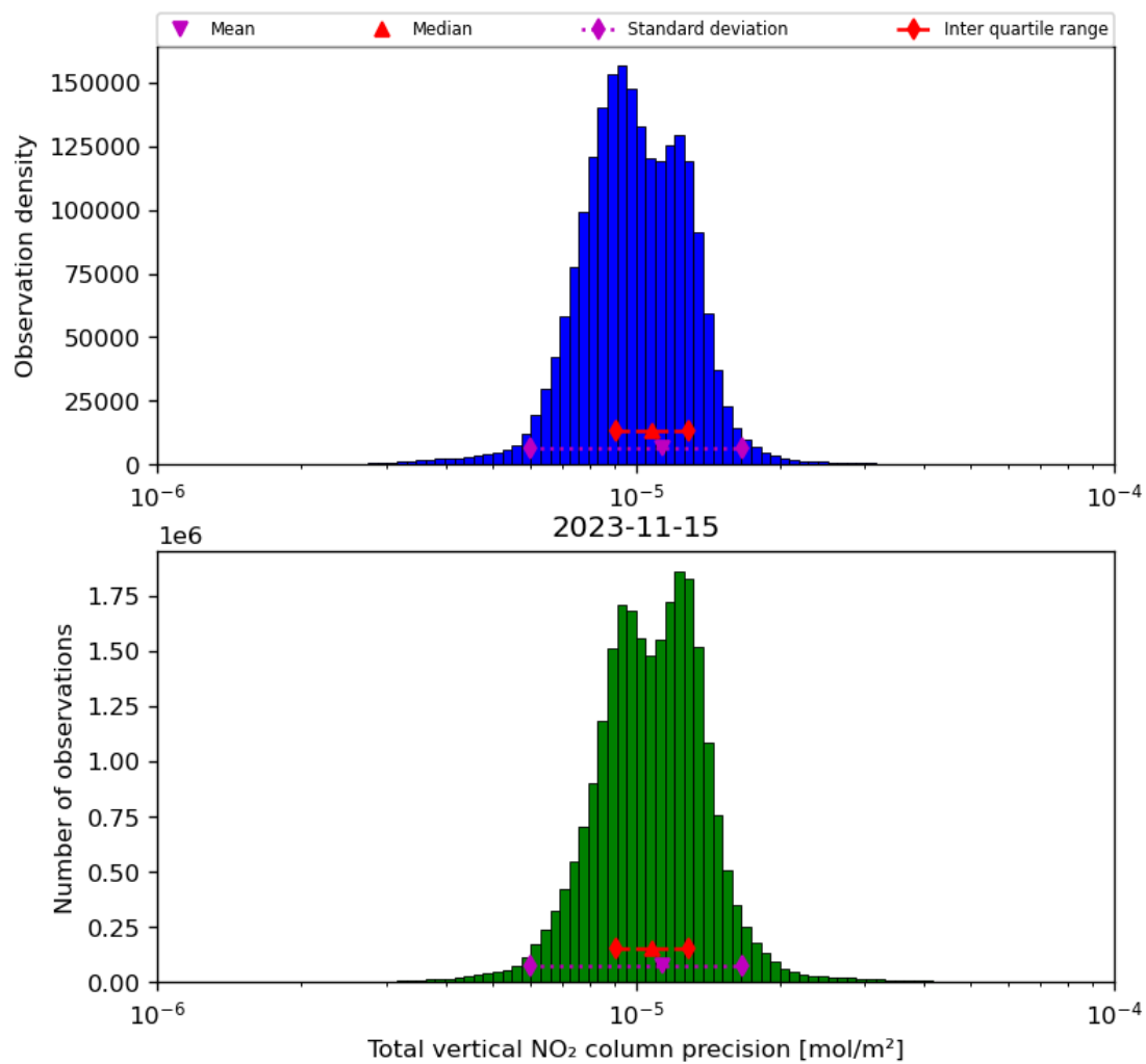
Figure 39: Histogram of “Total vertical NO 2 column precision” for 2023-11-14 to 2023-11-16
