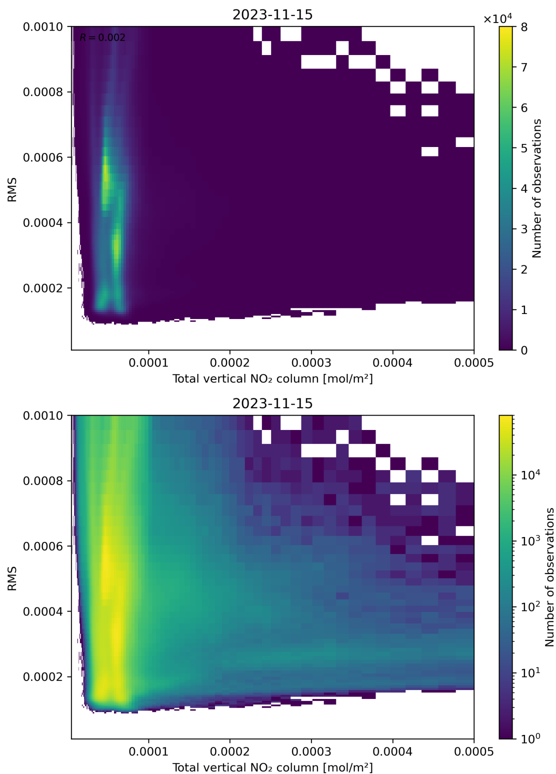
Figure 120: Scatter density plot of “Total vertical NO 2 column” against “RMS” for 2023-11-14 to 2023-11-16.
