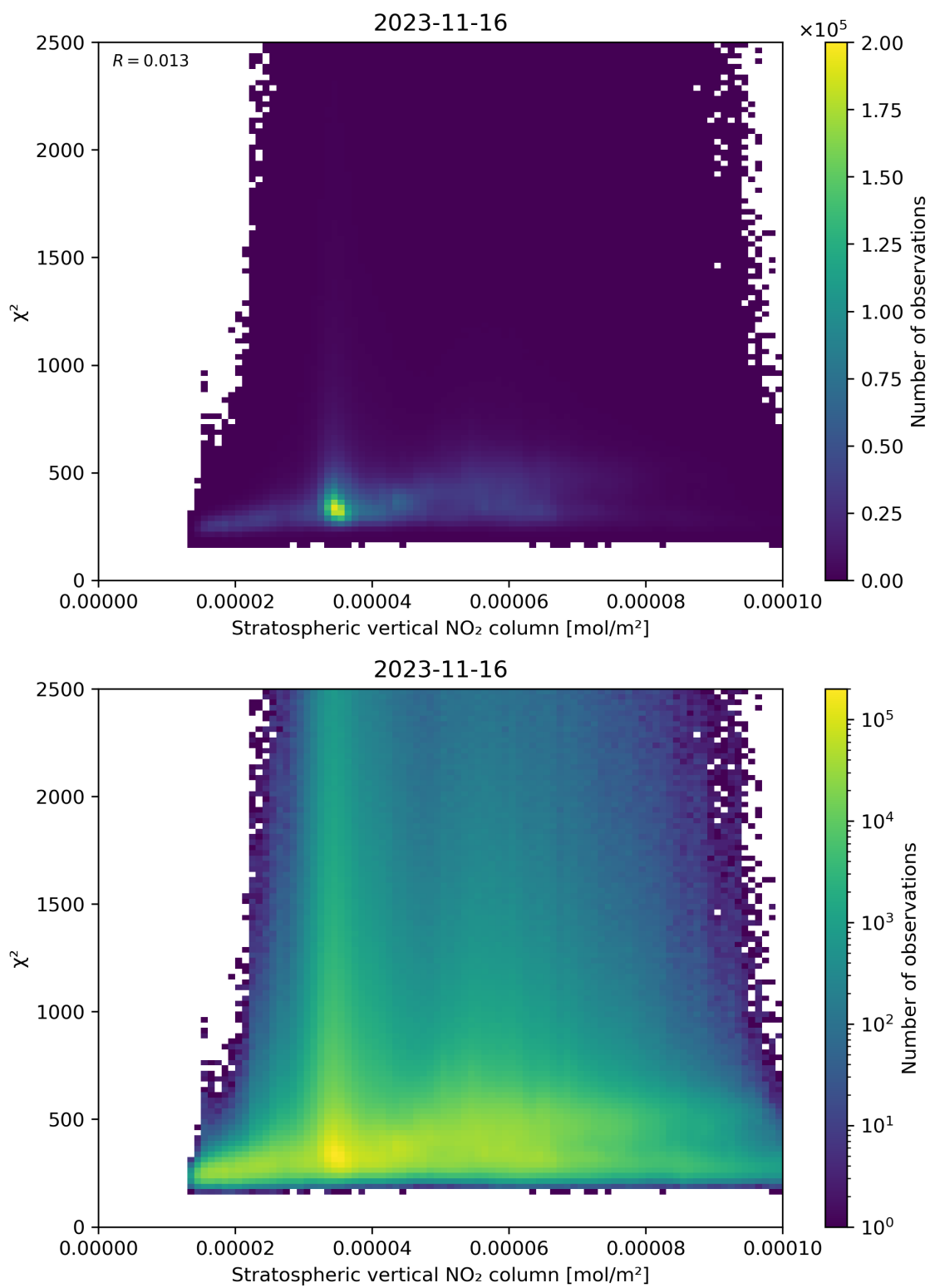
Figure 97: Scatter density plot of “Stratospheric vertical NO 2 column” against “ \chi^2 ” for 2023-11-15 to 2023-11-17.
