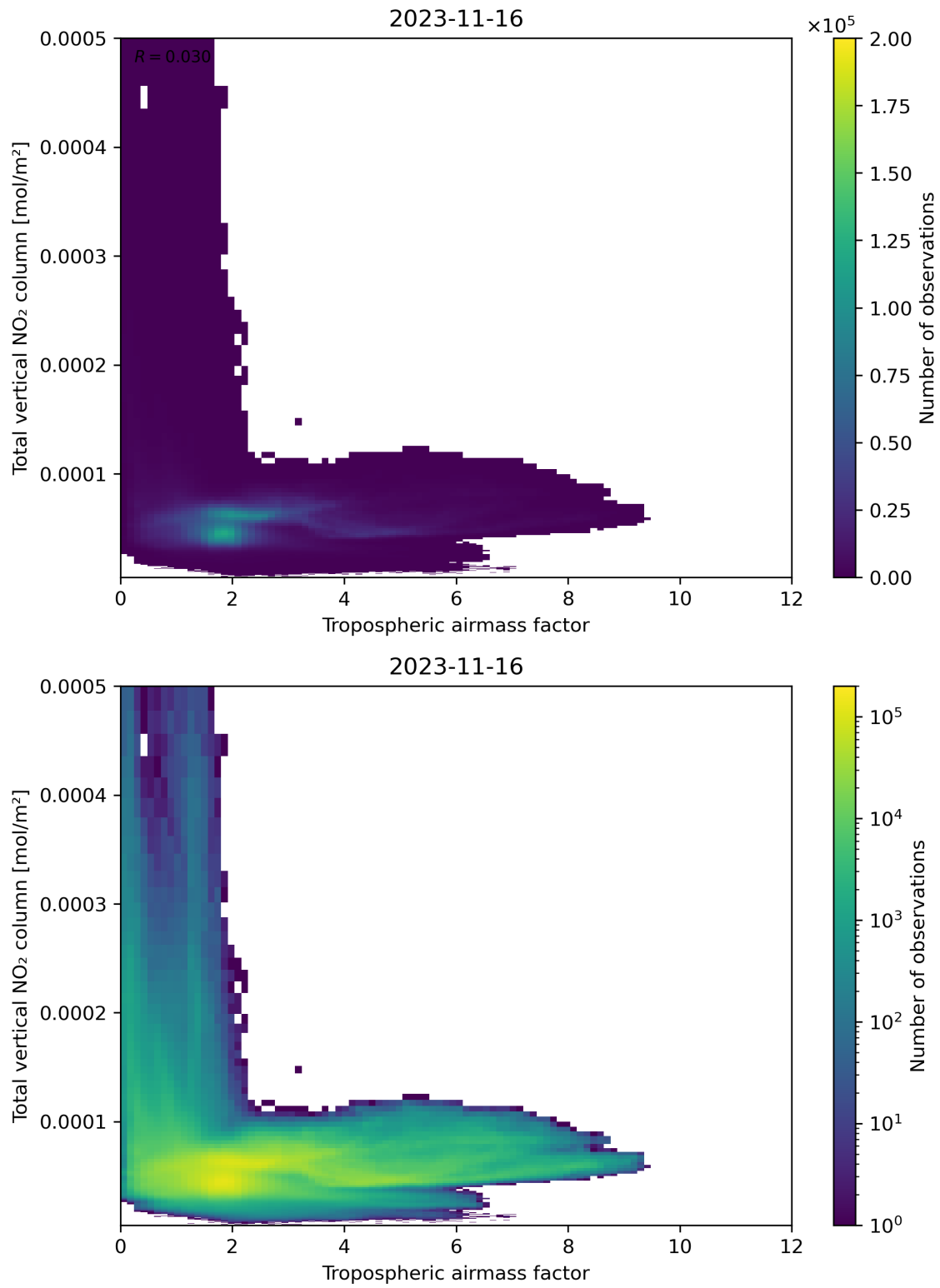
Figure 77: Scatter density plot of “Tropospheric airmass factor” against “Total vertical NO 2 column” for 2023-11-15 to 2023-11-17.
