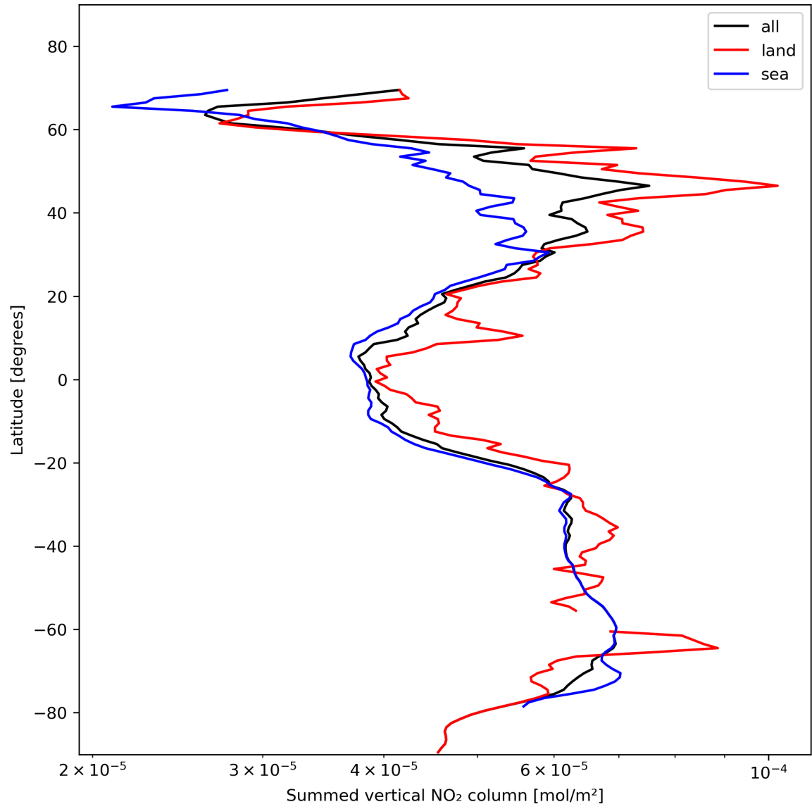
Figure 23: Zonal average of “Summed vertical NO 2 column” for 2023-11-15 to 2023-11-17.
