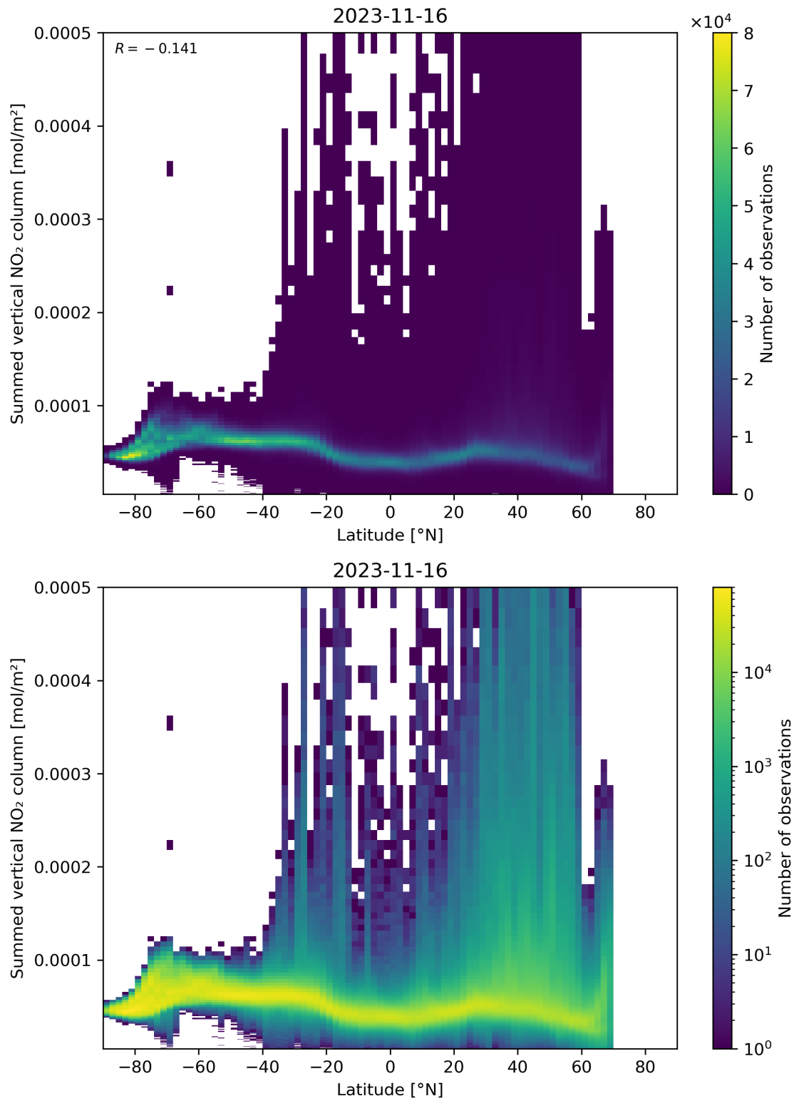
Figure 88: Scatter density plot of “Latitude” against “Summed vertical NO 2 column” for 2023-11-15 to 2023-11-17.
