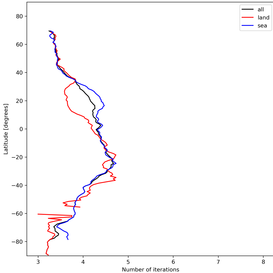
Figure 17: Zonal average of “Number of iterations” for 2023-11-15 to 2023-11-17.
