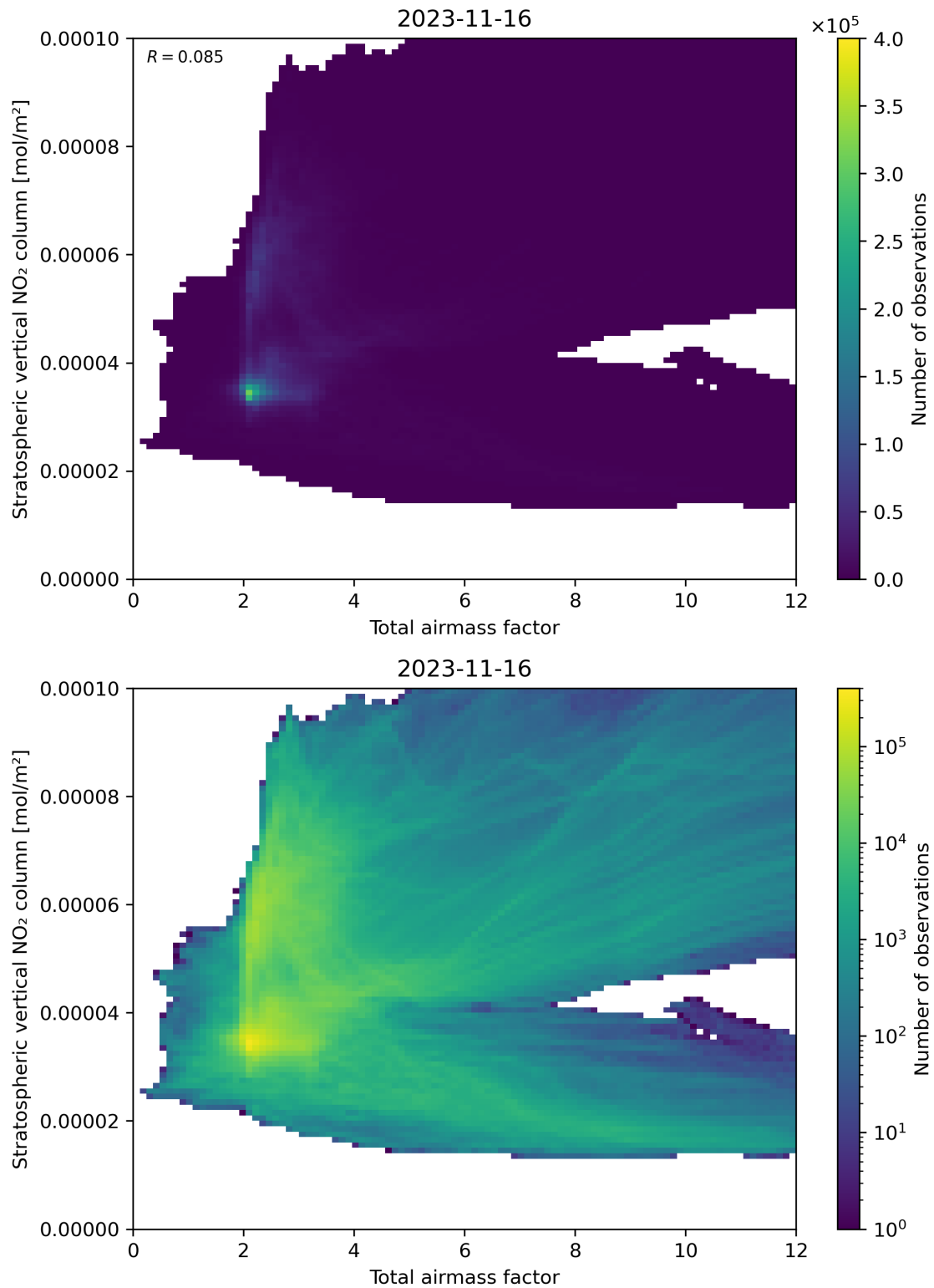
Figure 64: Scatter density plot of “Total airmass factor” against “Stratospheric vertical NO 2 column” for 2023-11-15 to 2023-11-17.
