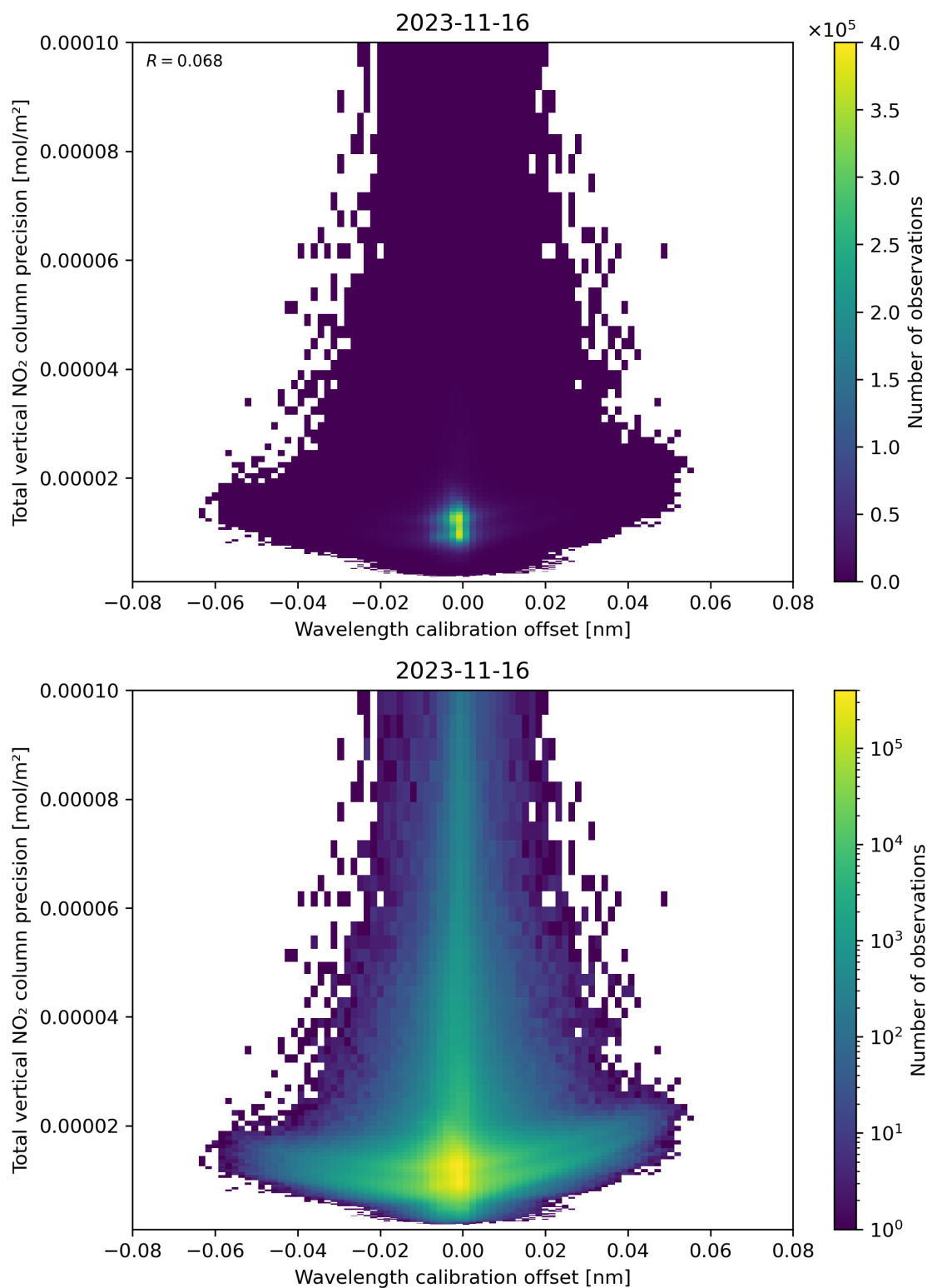
Figure 180: Scatter density plot of “Wavelength calibration offset” against “Total vertical NO 2 column precision” for 2023-11-15 to 2023-11-17.
