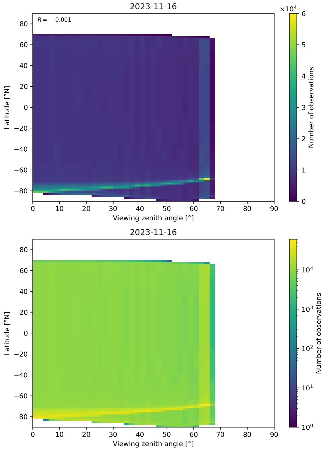
Figure 163: Scatter density plot of “Viewing zenith angle” against “Latitude” for 2023-11-15 to 2023-11-17.
