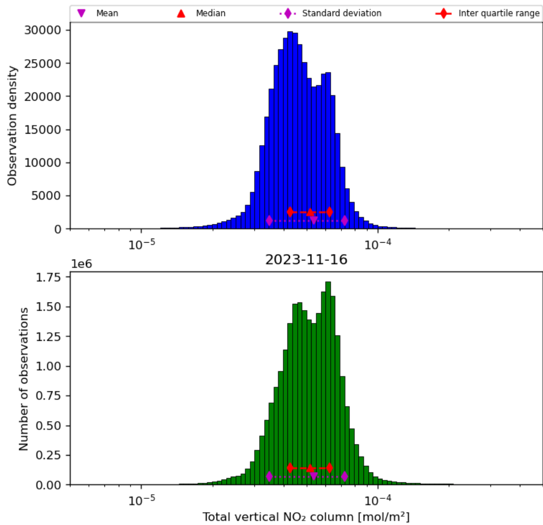
Figure 38: Histogram of “Total vertical NO 2 column” for 2023-11-15 to 2023-11-17
