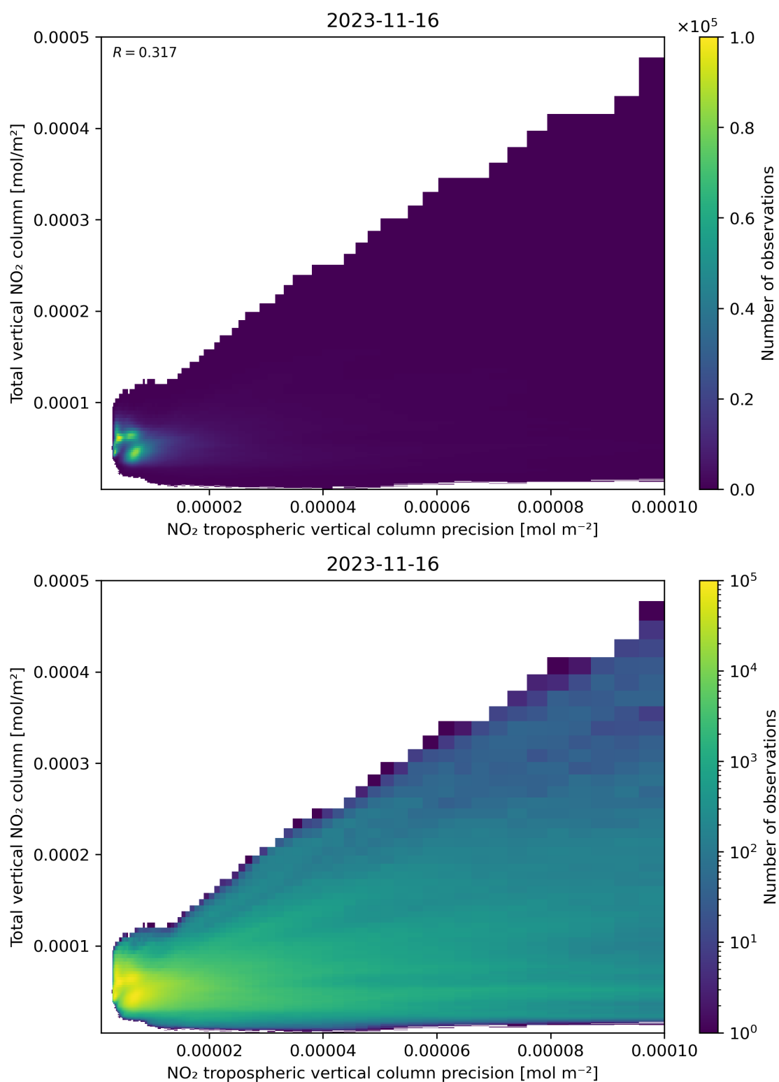
Figure 138: Scatter density plot of “NO 2 tropospheric vertical column precision” against “Total vertical NO 2 column” for 2023-11-15 to 2023-11-17.
