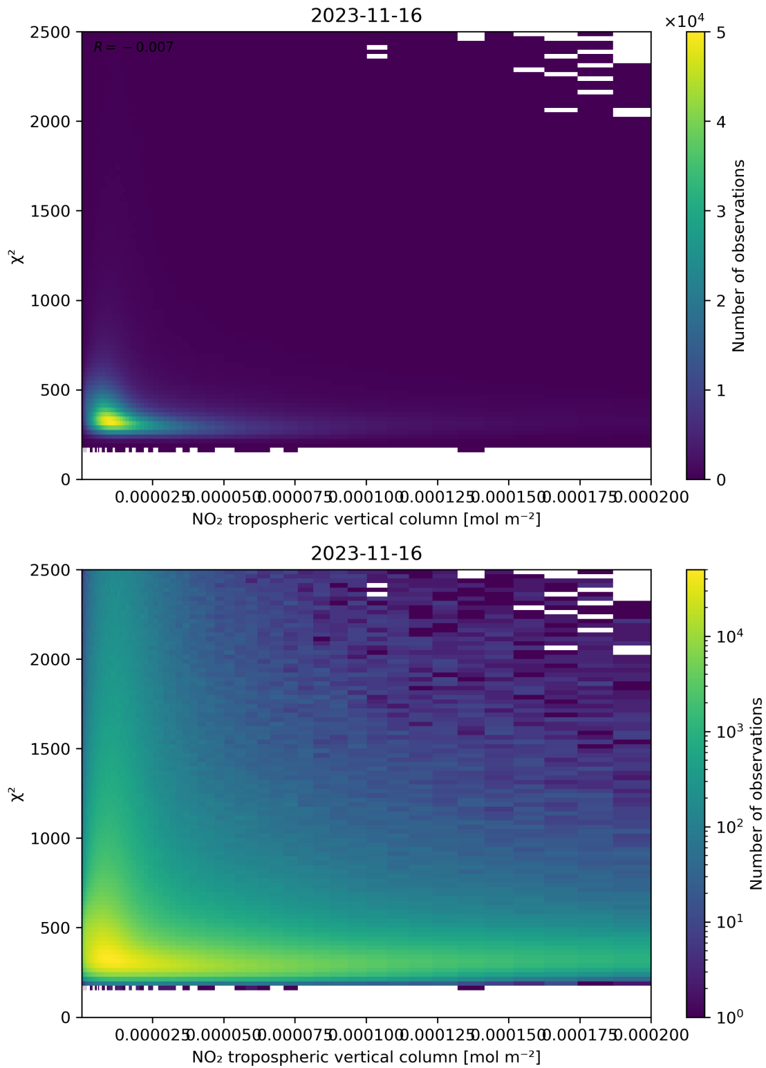
Figure 124: Scatter density plot of “NO 2 tropospheric vertical column” against “ \chi^2 ” for 2023-11-15 to 2023-11-17.
