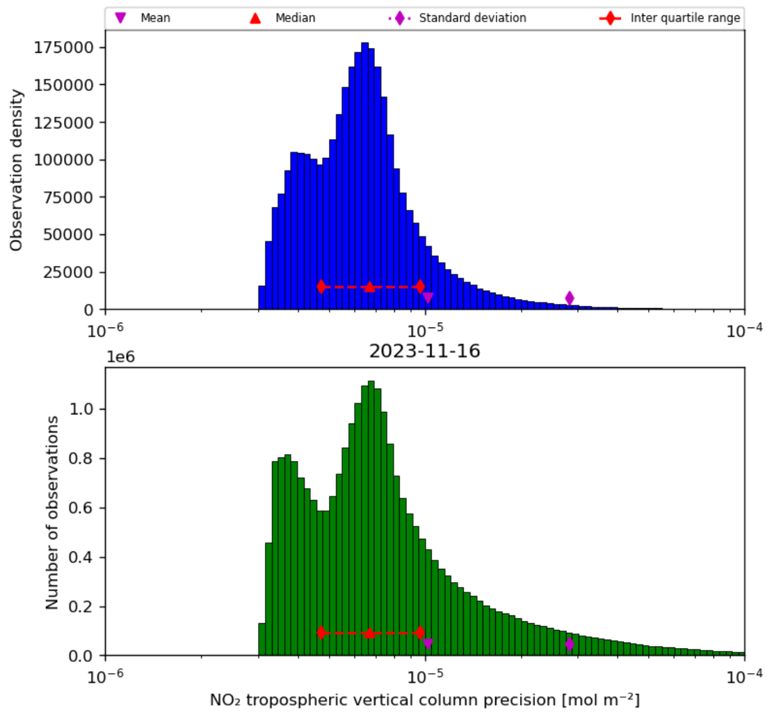
Figure 30: Histogram of “NO 2 tropospheric vertical column precision” for 2023-11-15 to 2023-11-17
