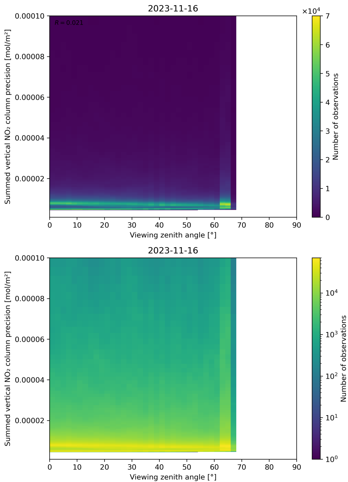
Figure 166: Scatter density plot of “Viewing zenith angle” against “Summed vertical NO 2 column precision” for 2023-11-15 to 2023-11-17.
