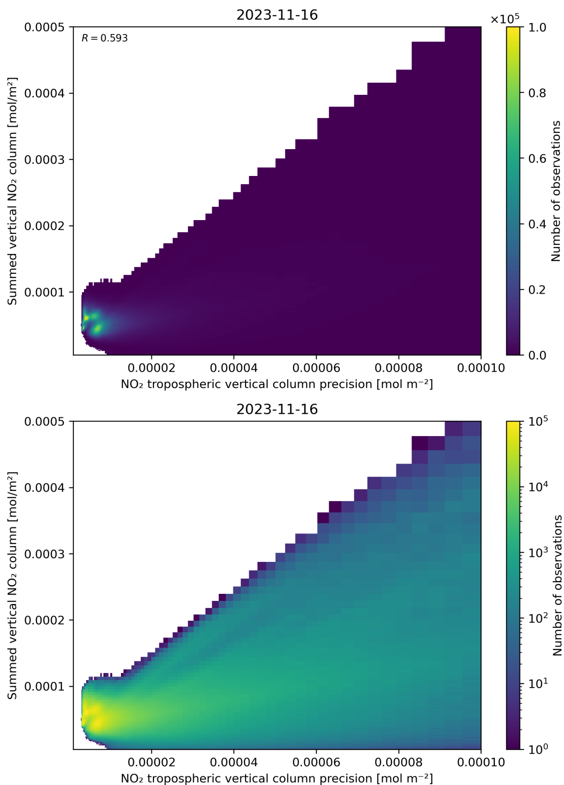
Figure 136: Scatter density plot of “NO 2 tropospheric vertical column precision” against “Summed vertical NO 2 column” for 2023-11-15 to 2023-11-17.
