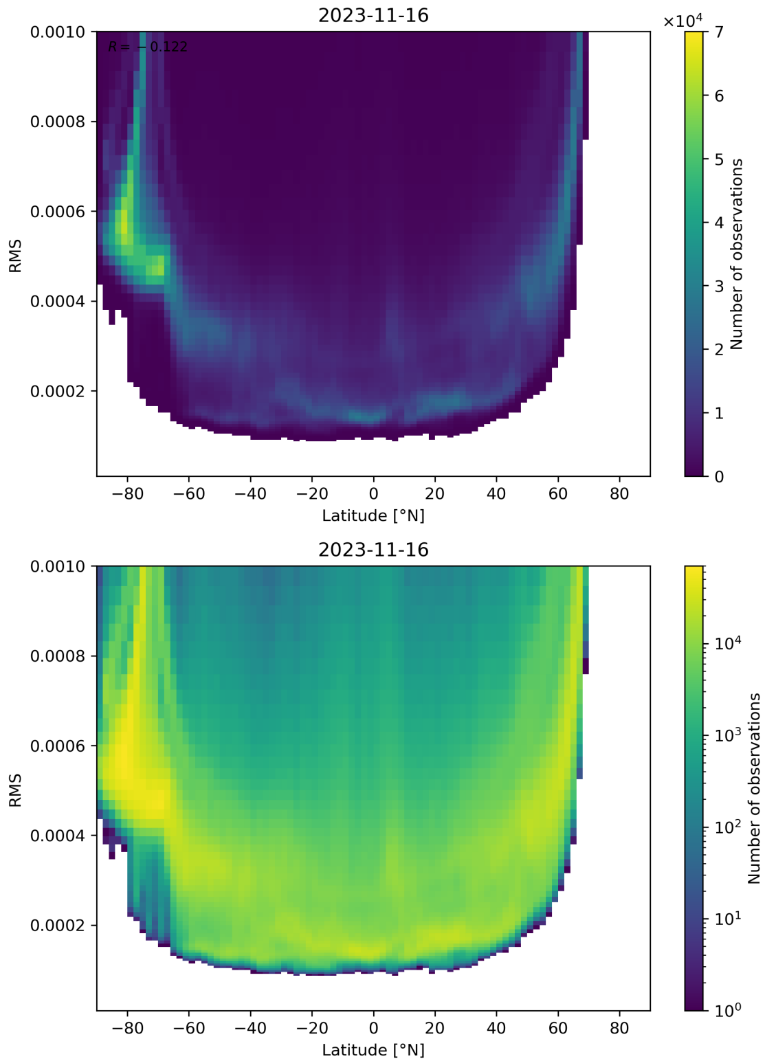
Figure 94: Scatter density plot of “Latitude” against “RMS” for 2023-11-15 to 2023-11-17.
