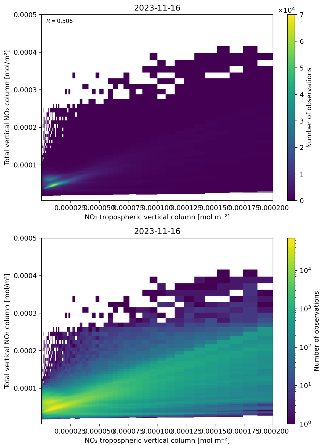
Figure 128: Scatter density plot of “NO 2 tropospheric vertical column” against “Total vertical NO 2 column” for 2023-11-15 to 2023-11-17.
