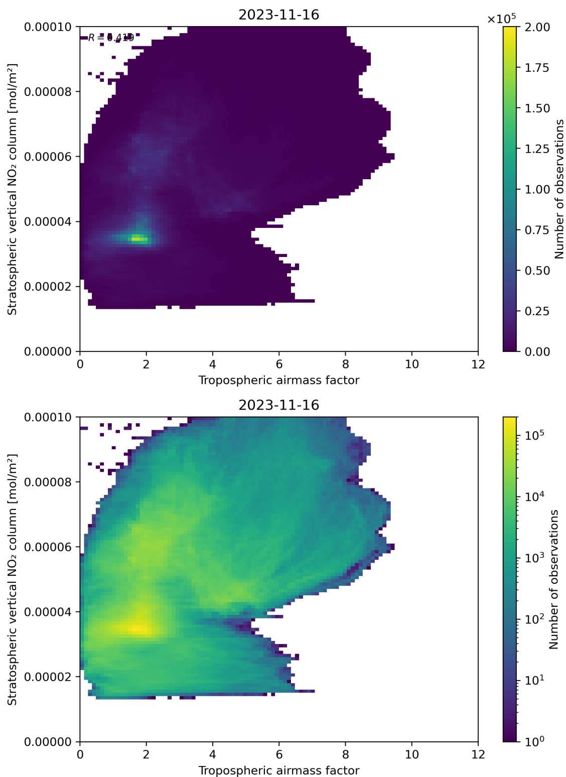
Figure 74: Scatter density plot of “Tropospheric air mass factor” against “Stratospheric vertical NO 2 column” for 2023-11-15 to 2023-11-17.
