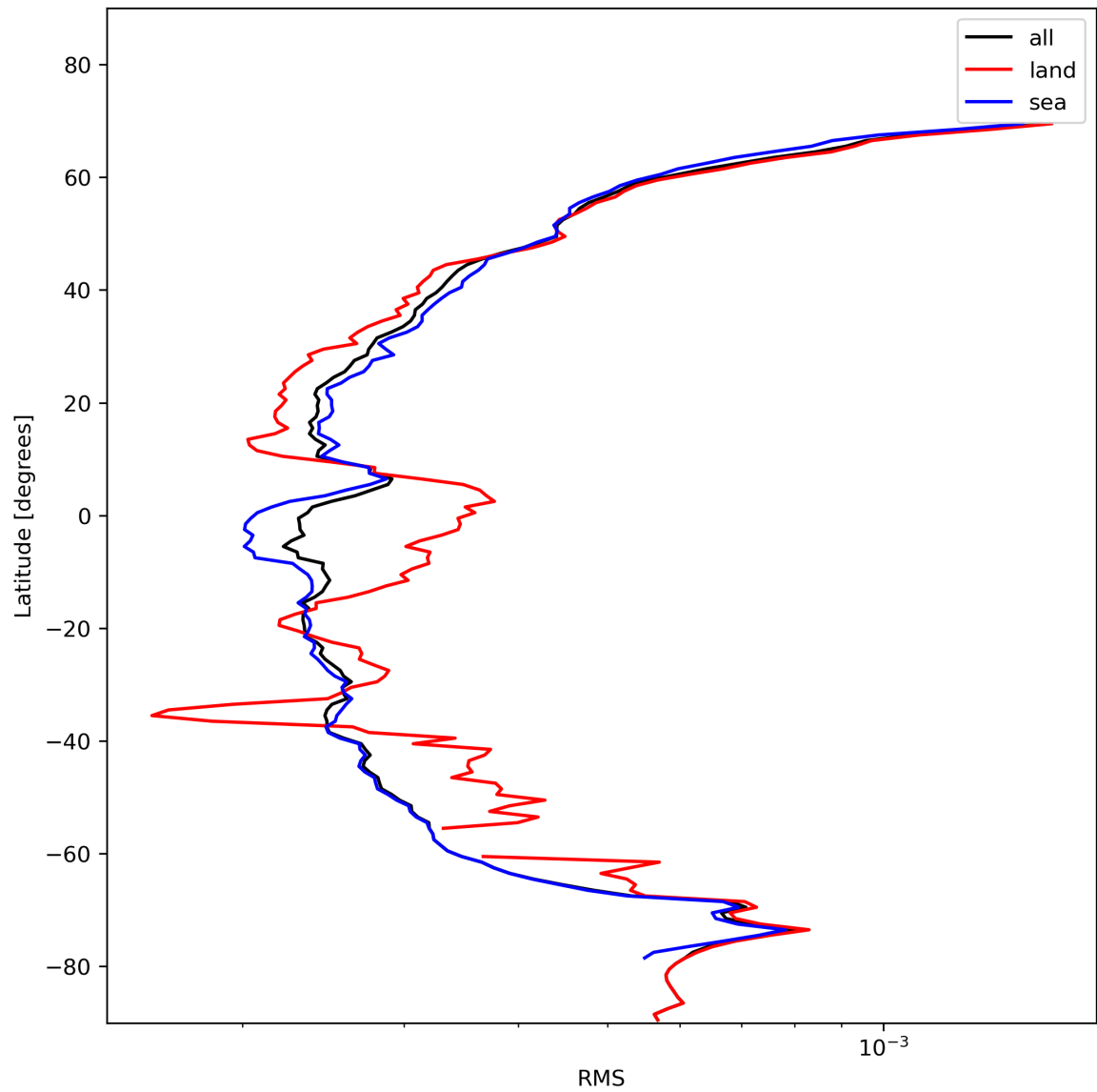
Figure 26: Zonal average of “RMS” for 2023-11-15 to 2023-11-17.
