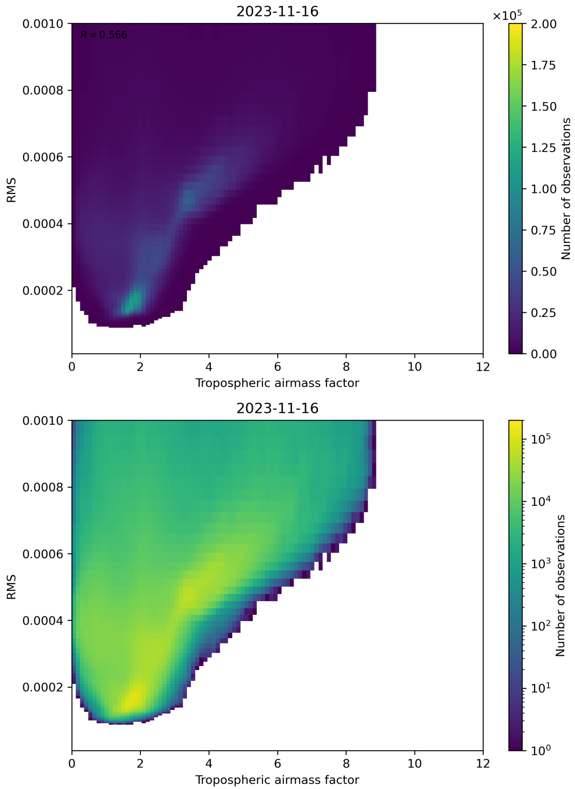
Figure 79: Scatter density plot of “Tropospheric airmass factor” against “RMS” for 2023-11-15 to 2023-11-17.
