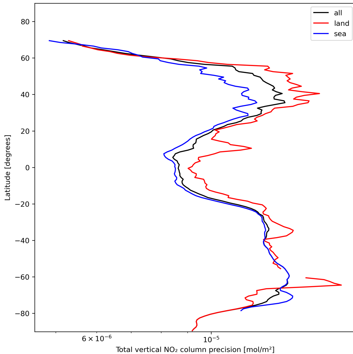
Figure 22: Zonal average of “Total vertical NO 2 column precision” for 2023-11-15 to 2023-11-17.
