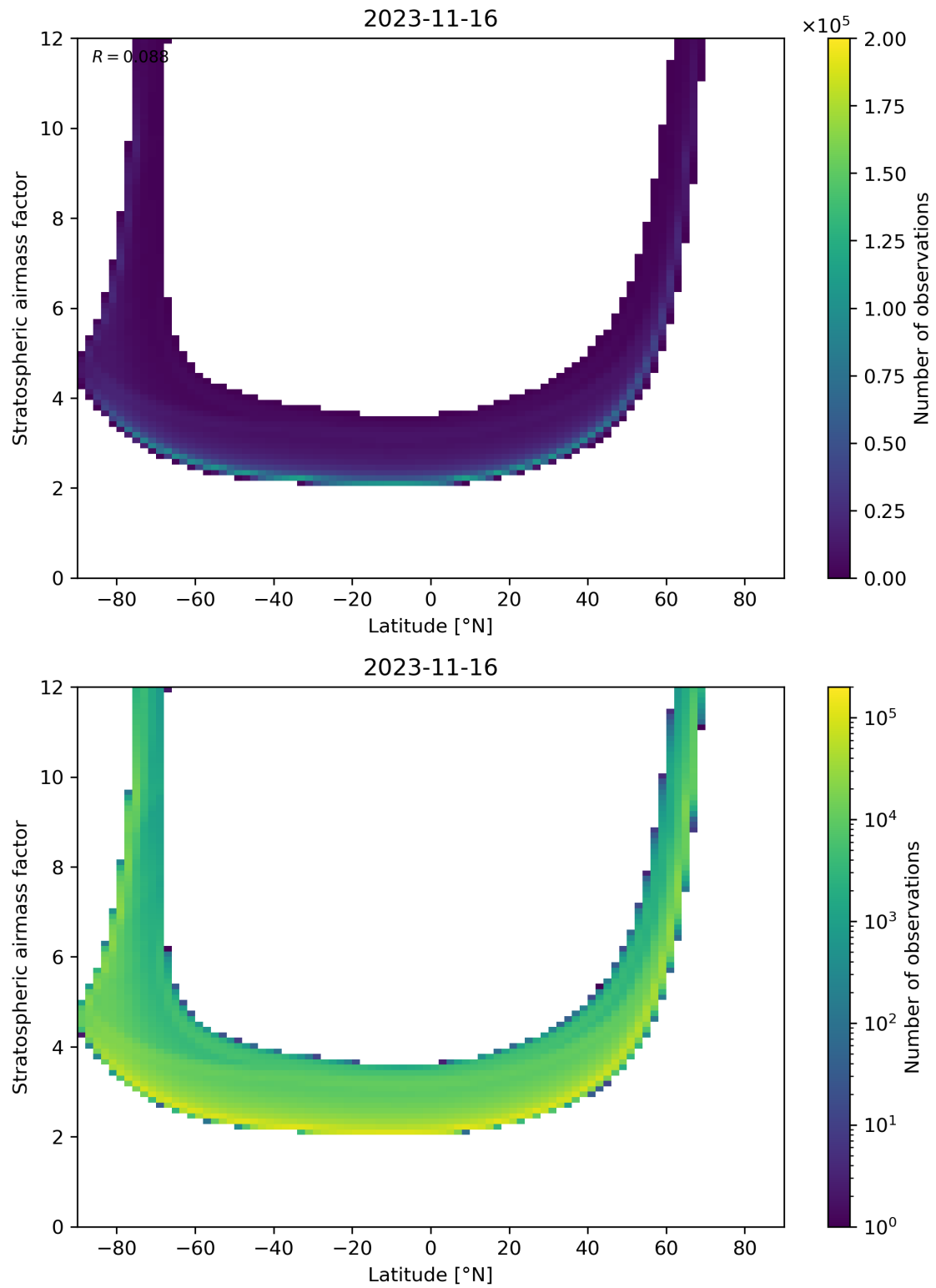
Figure 83: Scatter density plot of “Latitude” against “Stratospheric airmass factor” for 2023-11-15 to 2023-11-17.
