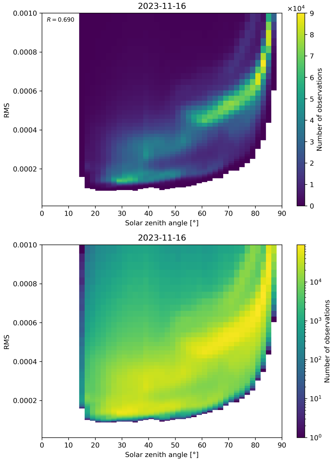
Figure 157: Scatter density plot of “Solar zenith angle” against “RMS” for 2023-11-15 to 2023-11-17.
