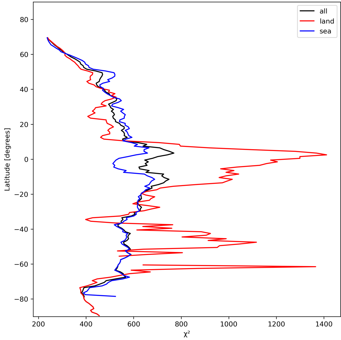
Figure 25: Zonal average of “ \chi^2 ” for 2023-11-15 to 2023-11-17.
