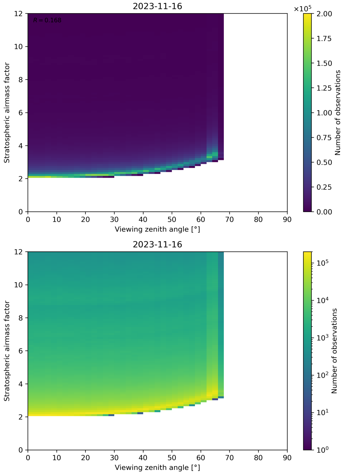
Figure 159: Scatter density plot of “Viewing zenith angle” against “Stratospheric airmass factor” for 2023-11-15 to 2023-11-17.
