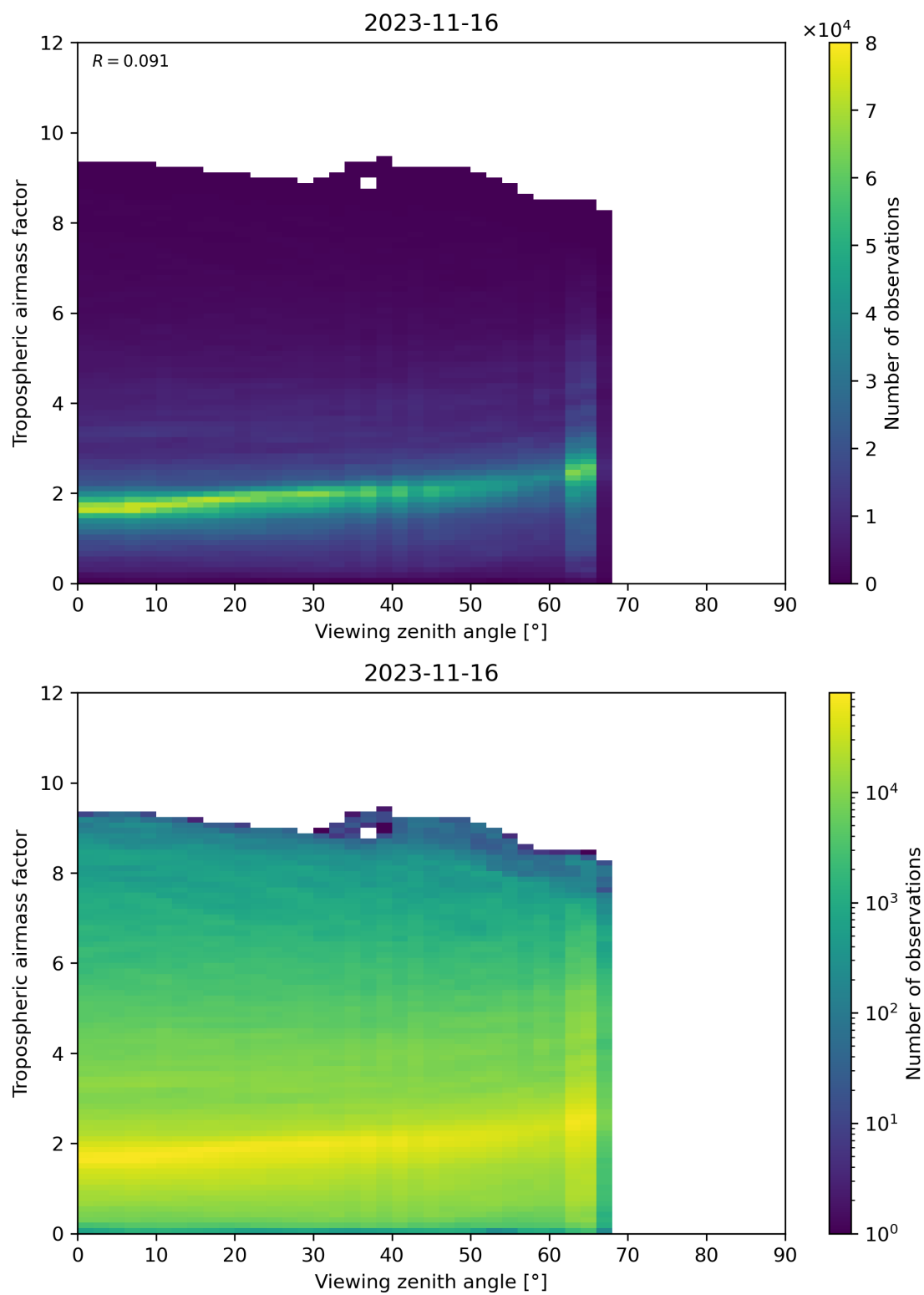
Figure 161: Scatter density plot of “Viewing zenith angle” against “Tropospheric airmass factor” for 2023-11-15 to 2023-11-17.
