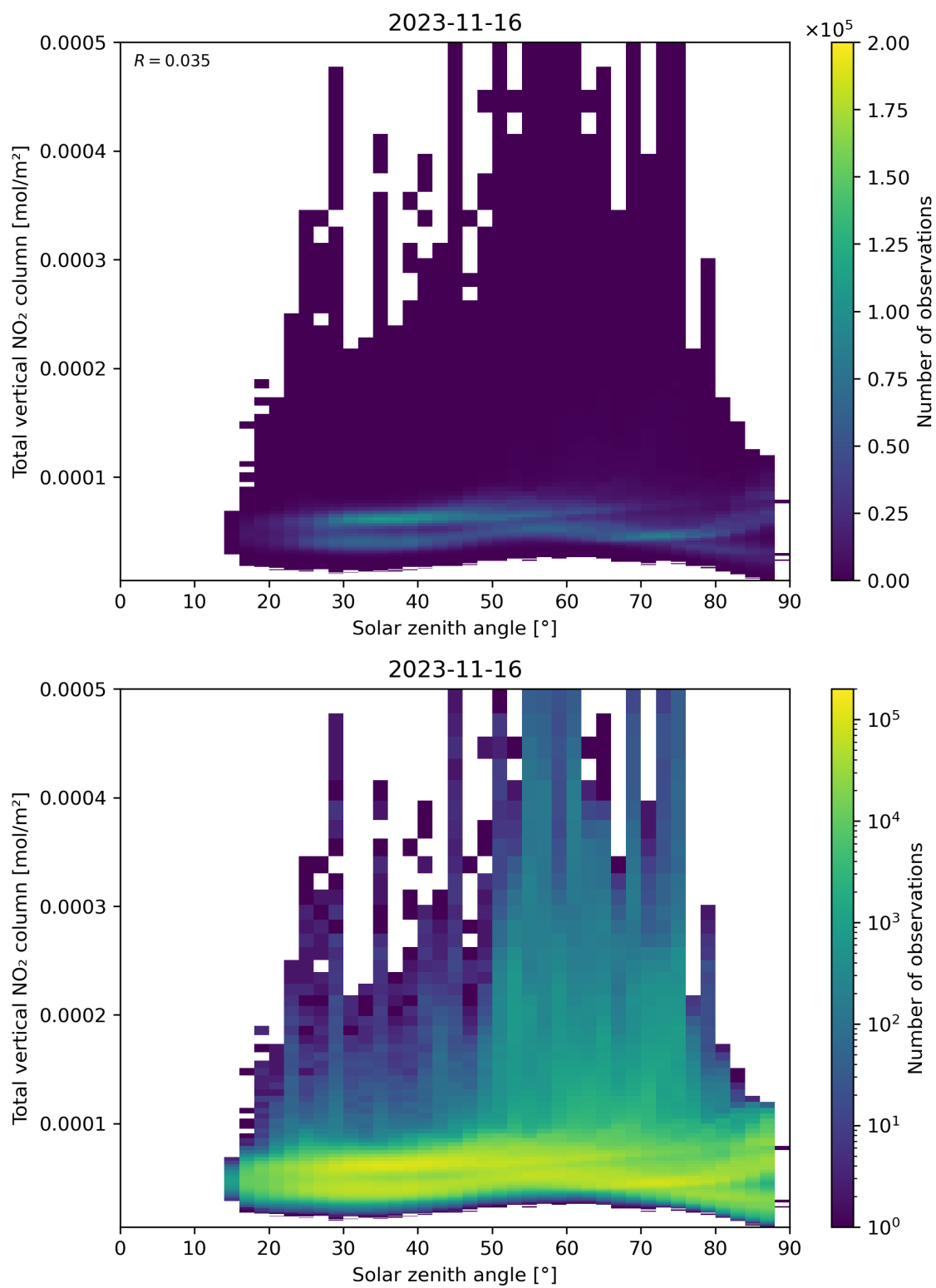
Figure 153: Scatter density plot of “Solar zenith angle” against “Total vertical NO 2 column” for 2023-11-15 to 2023-11-17.
