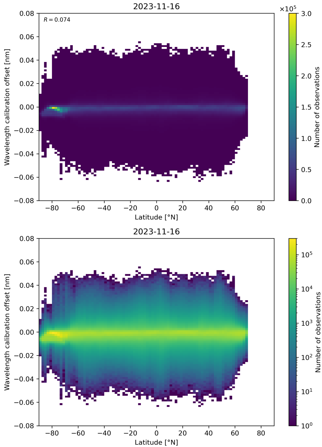
Figure 95: Scatter density plot of “Latitude” against “Wavelength calibration offset” for 2023-11-15 to 2023-11-17.
