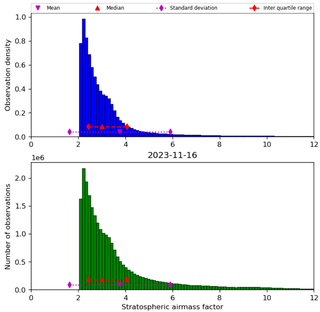
Figure 44: Histogram of “Stratospheric airmass factor” for 2023-11-15 to 2023-11-17
