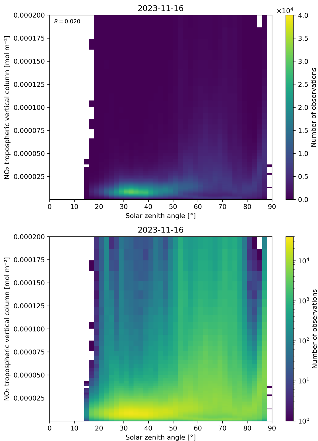
Figure 155: Scatter density plot of “Solar zenith angle” against “NO 2 tropospheric vertical column” for 2023-11-15 to 2023-11-17.
