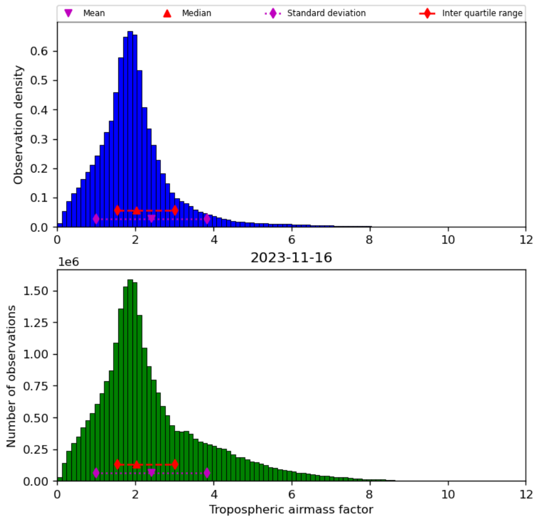
Figure 31: Histogram of “Tropospheric airmass factor” for 2023-11-15 to 2023-11-17
