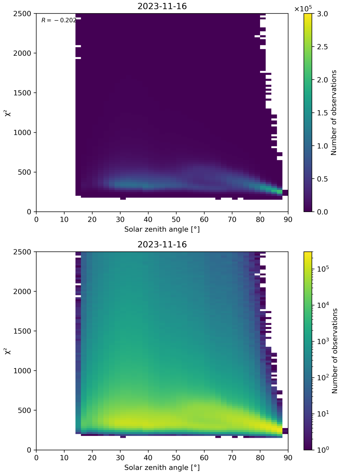
Figure 148: Scatter density plot of “Solar zenith angle” against “ \chi^2 ” for 2023-11-15 to 2023-11-17.
