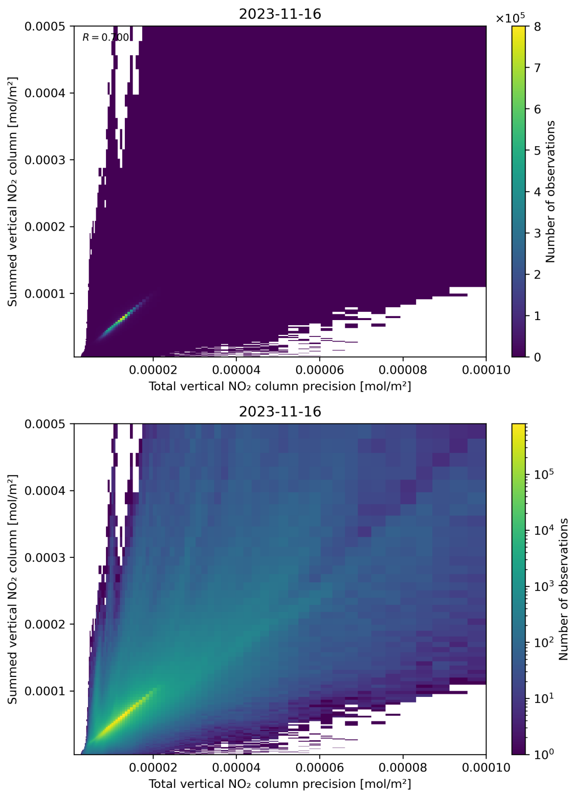
Figure 117: Scatter density plot of “Total vertical NO 2 column precision” against “Summed vertical NO 2 column” for 2023-11-15 to 2023-11-17.
