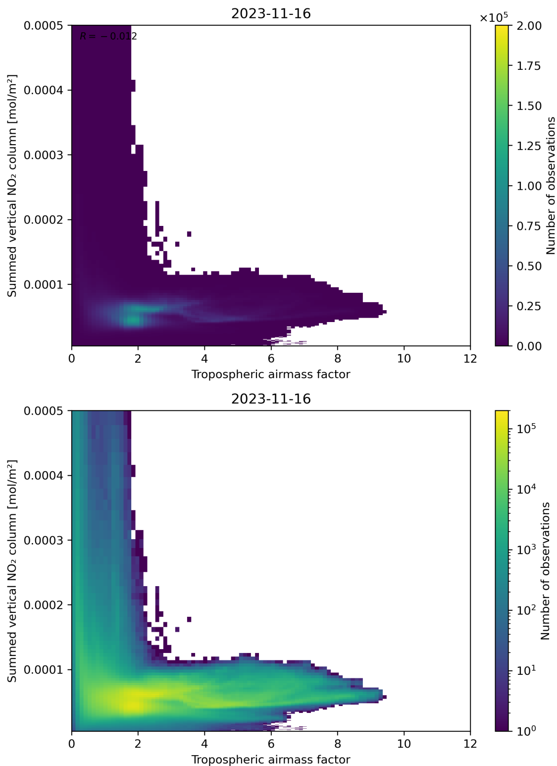
Figure 75: Scatter density plot of “Tropospheric airmass factor” against “Summed vertical NO 2 column” for 2023-11-15 to 2023-11-17.
