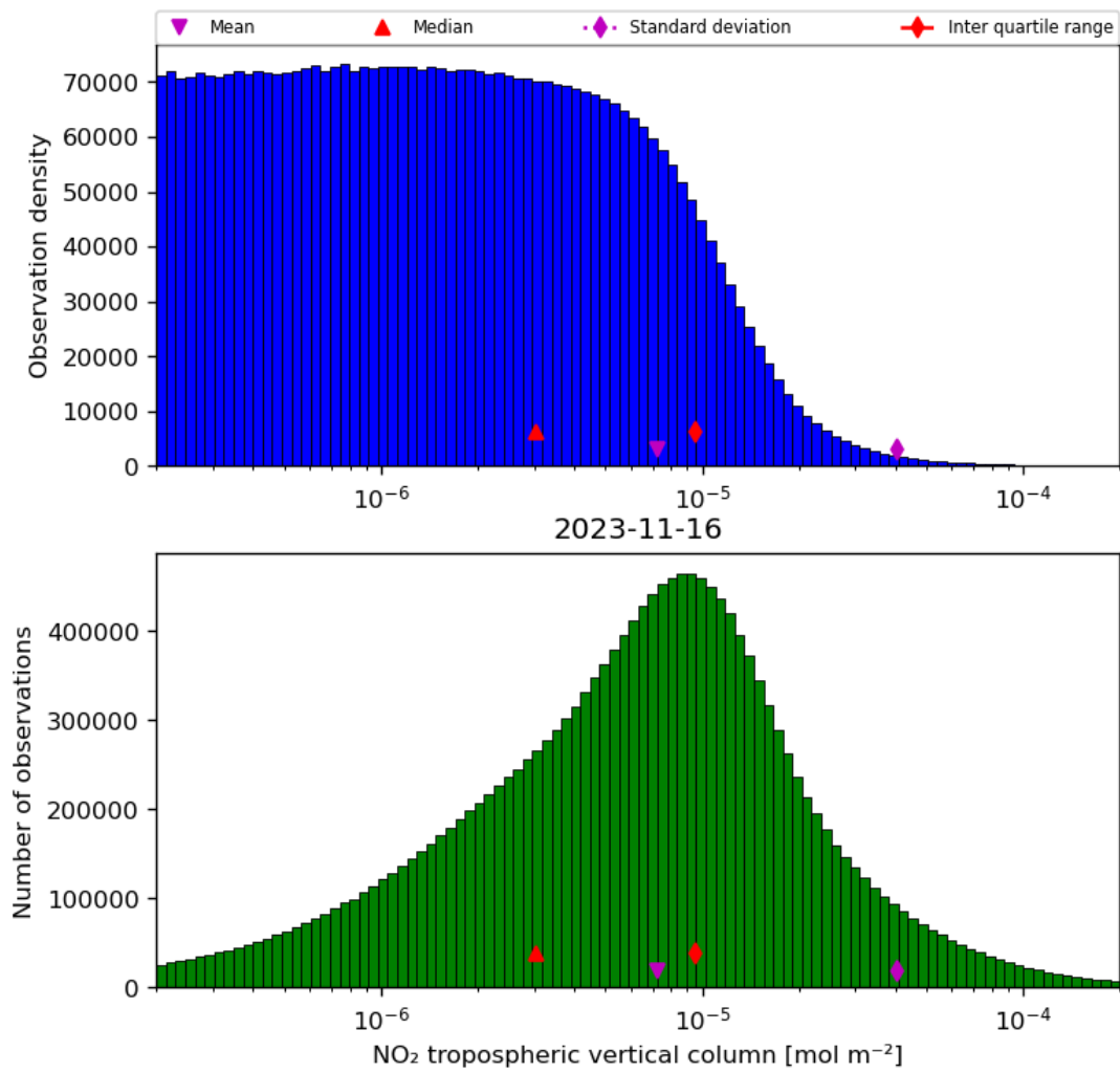
Figure 29: Histogram of “NO 2 tropospheric vertical column” for 2023-11-15 to 2023-11-17
