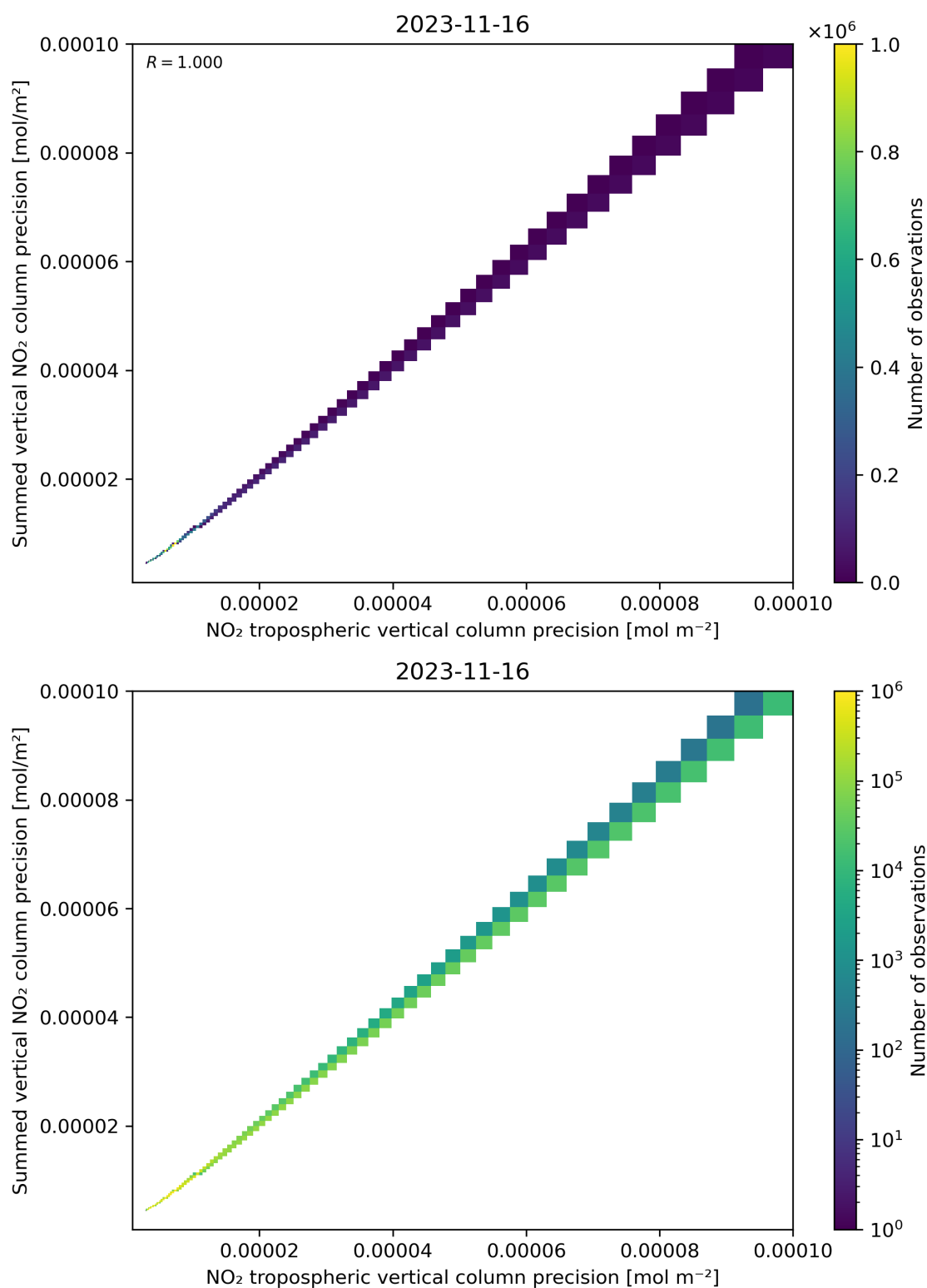
Figure 137: Scatter density plot of “NO 2 tropospheric vertical column precision” against “Summed vertical NO 2 column precision” for 2023-11-15 to 2023-11-17.
