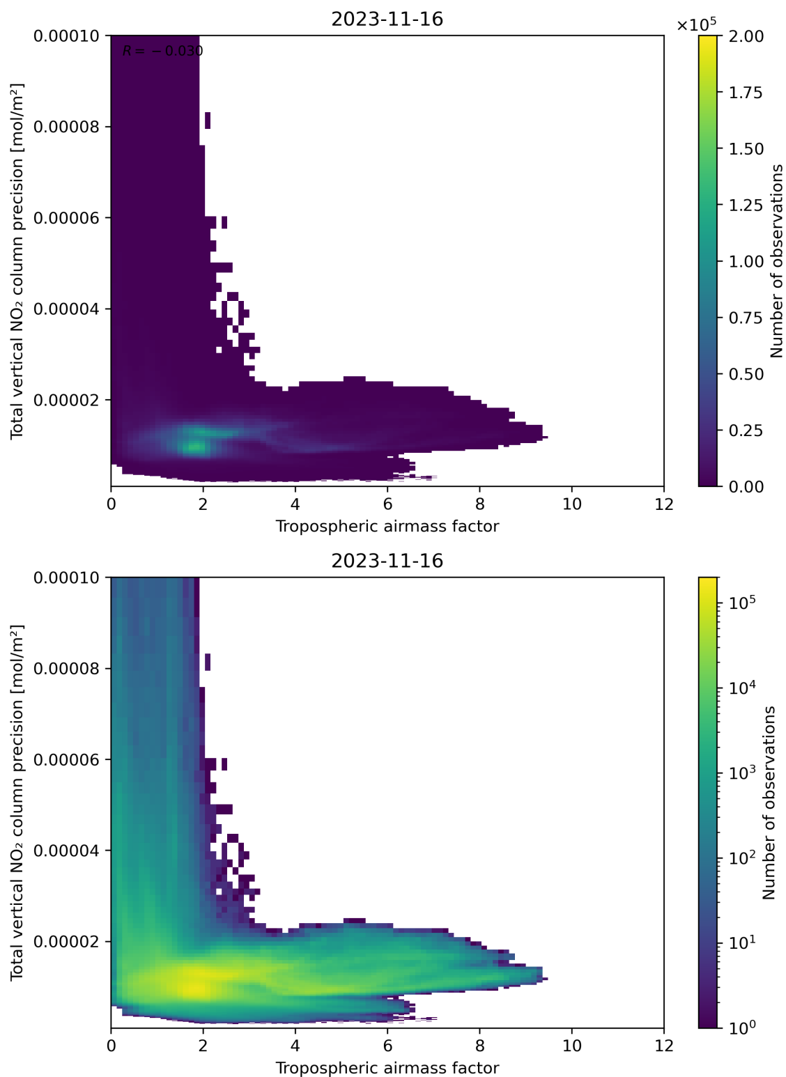
Figure 78: Scatter density plot of “Tropospheric air mass factor” against “Total vertical NO 2 column precision” for 2023-11-15 to 2023-11-17.
