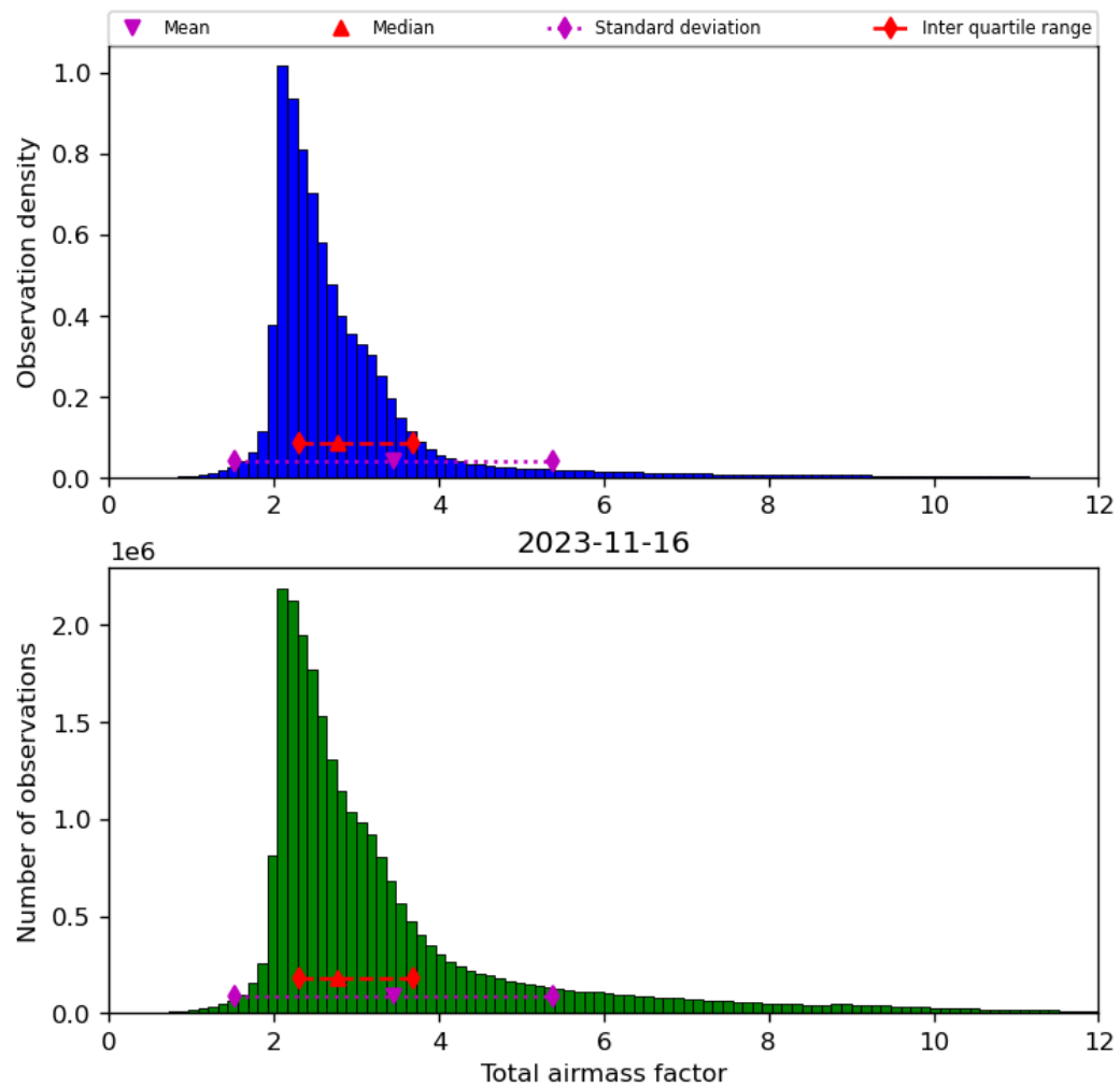
Figure 32: Histogram of “Total airmass factor” for 2023-11-15 to 2023-11-17
