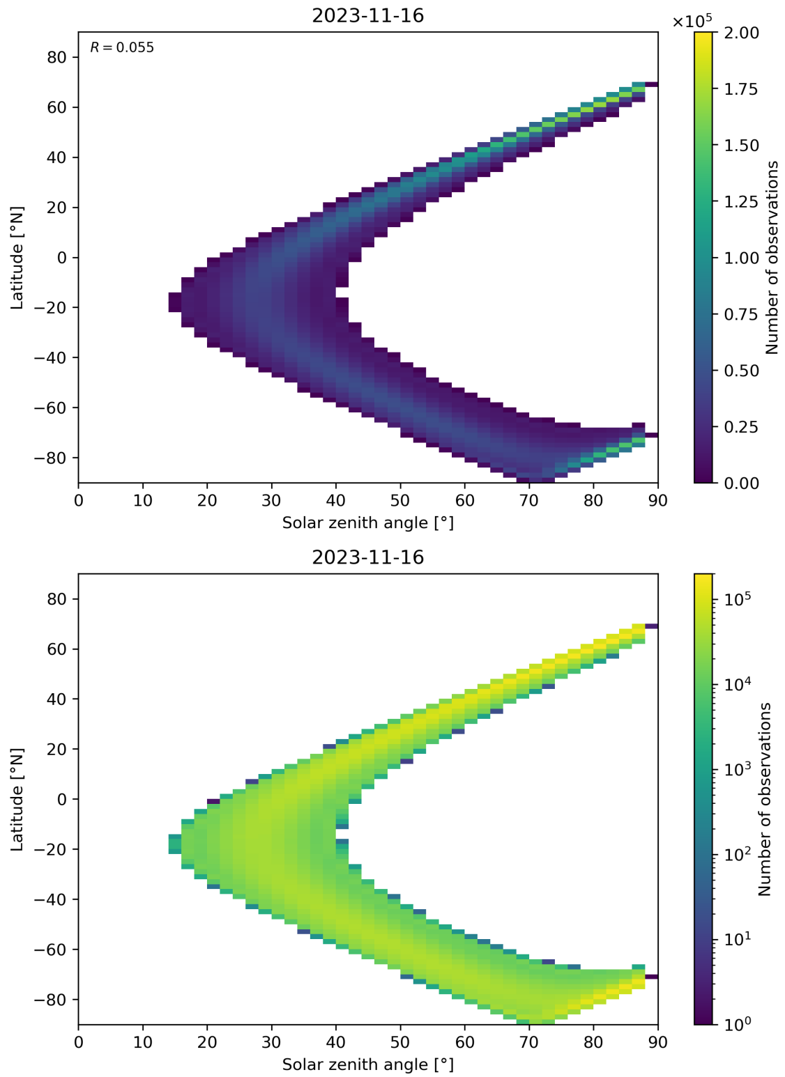
Figure 149: Scatter density plot of “Solar zenith angle” against “Latitude” for 2023-11-15 to 2023-11-17.
