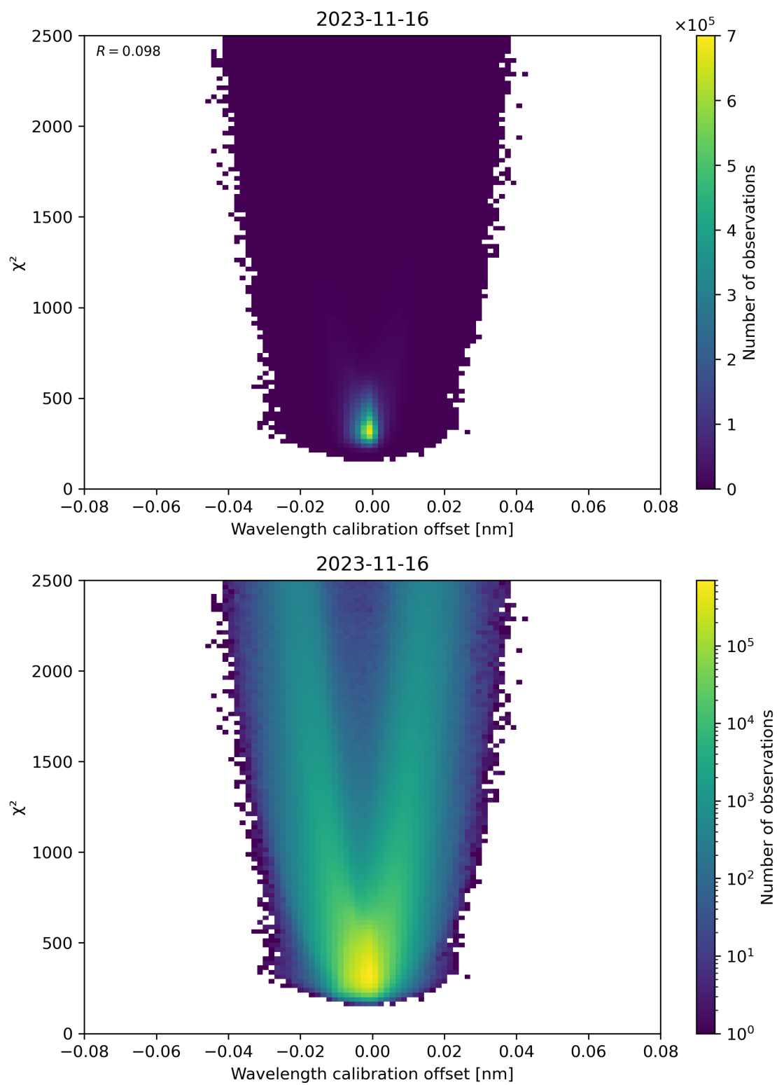
Figure 175: Scatter density plot of “Wavelength calibration offset” against “ \chi^2 ” for 2023-11-15 to 2023-11-17.
