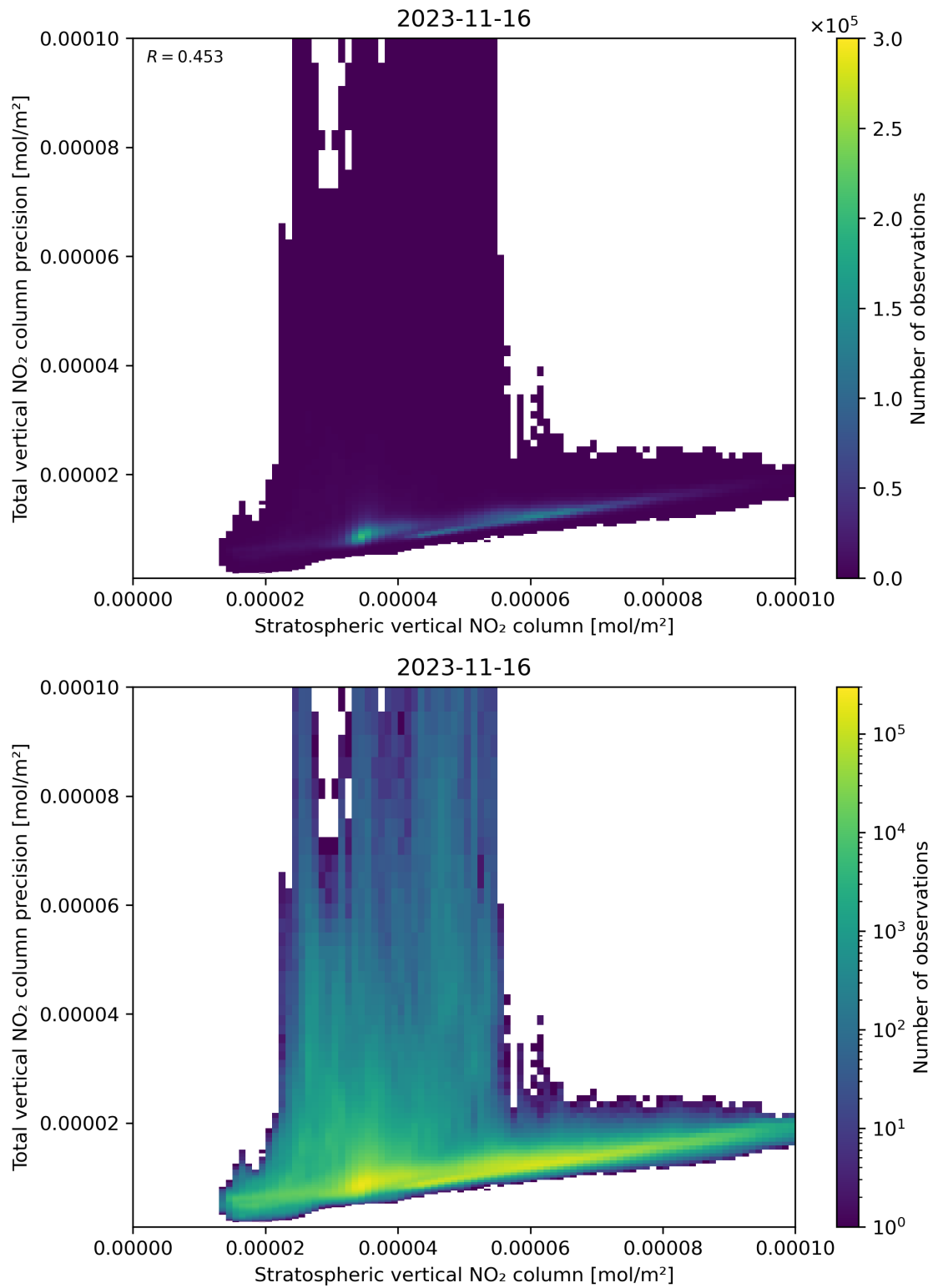
Figure 101: Scatter density plot of “Stratospheric vertical NO 2 column” against “Total vertical NO 2 column precision” for 2023-11-15 to 2023-11-17.
