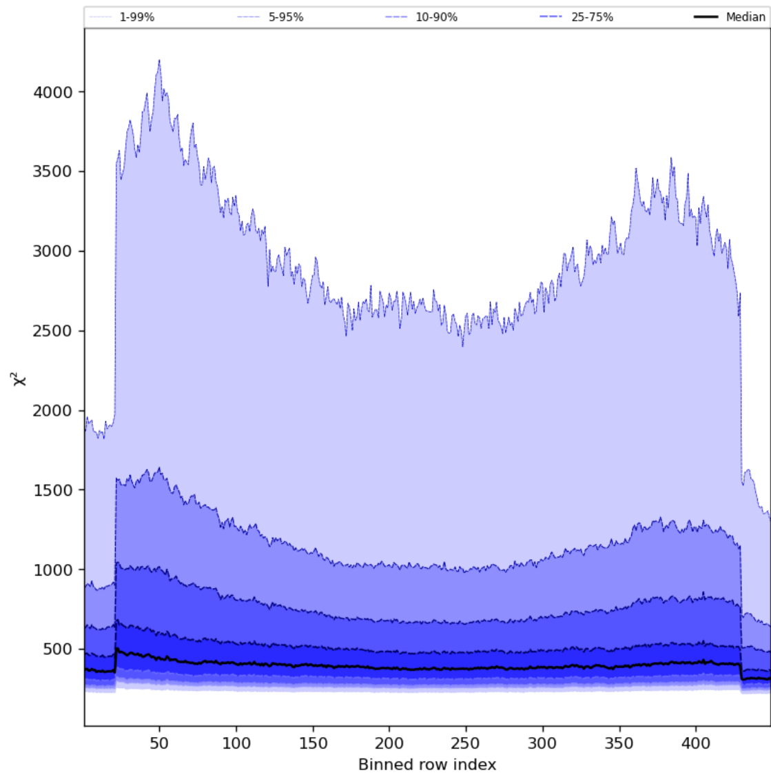
Figure 59: Along track statistics of “ \chi^2 ” for 2023-11-15 to 2023-11-17
