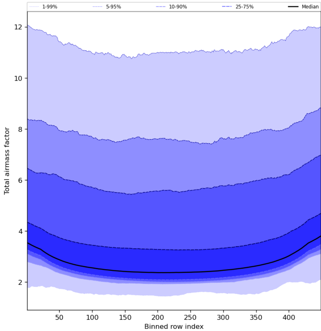
Figure 49: Along track statistics of “Total airmass factor” for 2023-11-15 to 2023-11-17
