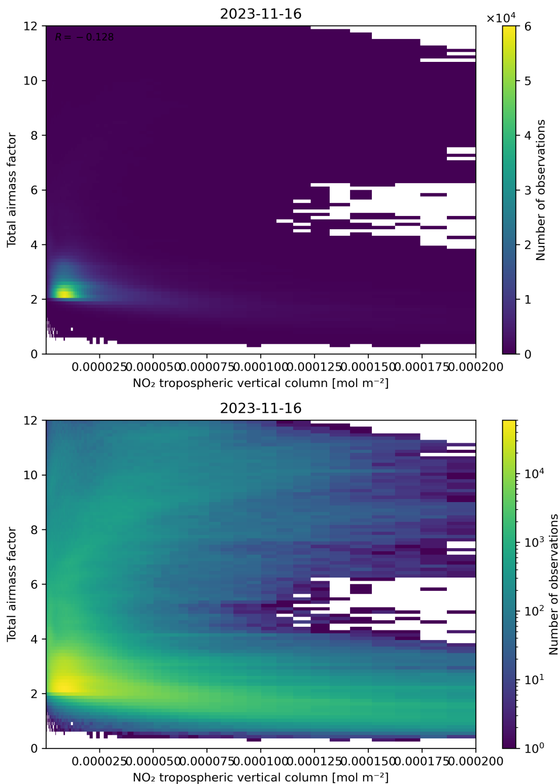
Figure 122: Scatter density plot of “NO 2 tropospheric vertical column” against “Total air mass factor” for 2023-11-15 to 2023-11-17.
