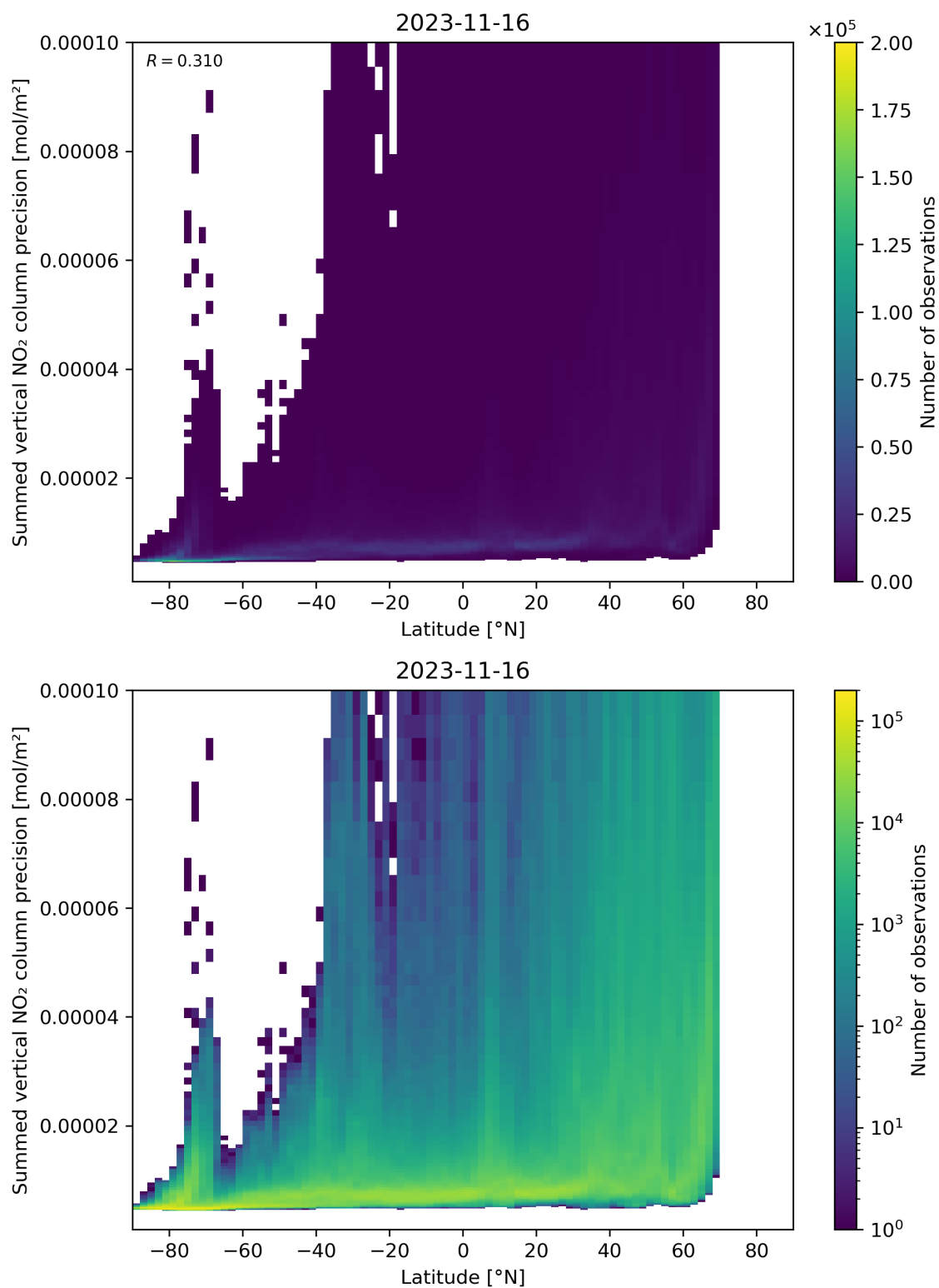
Figure 89: Scatter density plot of “Latitude” against “Summed vertical NO 2 column precision” for 2023-11-15 to 2023-11-17.
