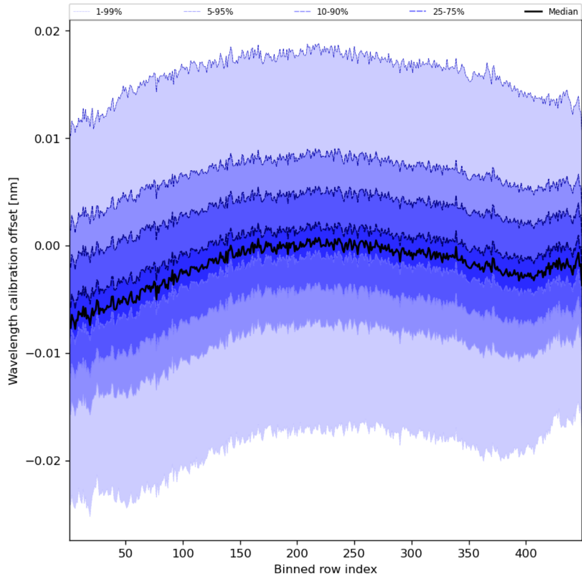
Figure 52: Along track statistics of “Wavelength calibration offset” for 2023-11-15 to 2023-11-17
