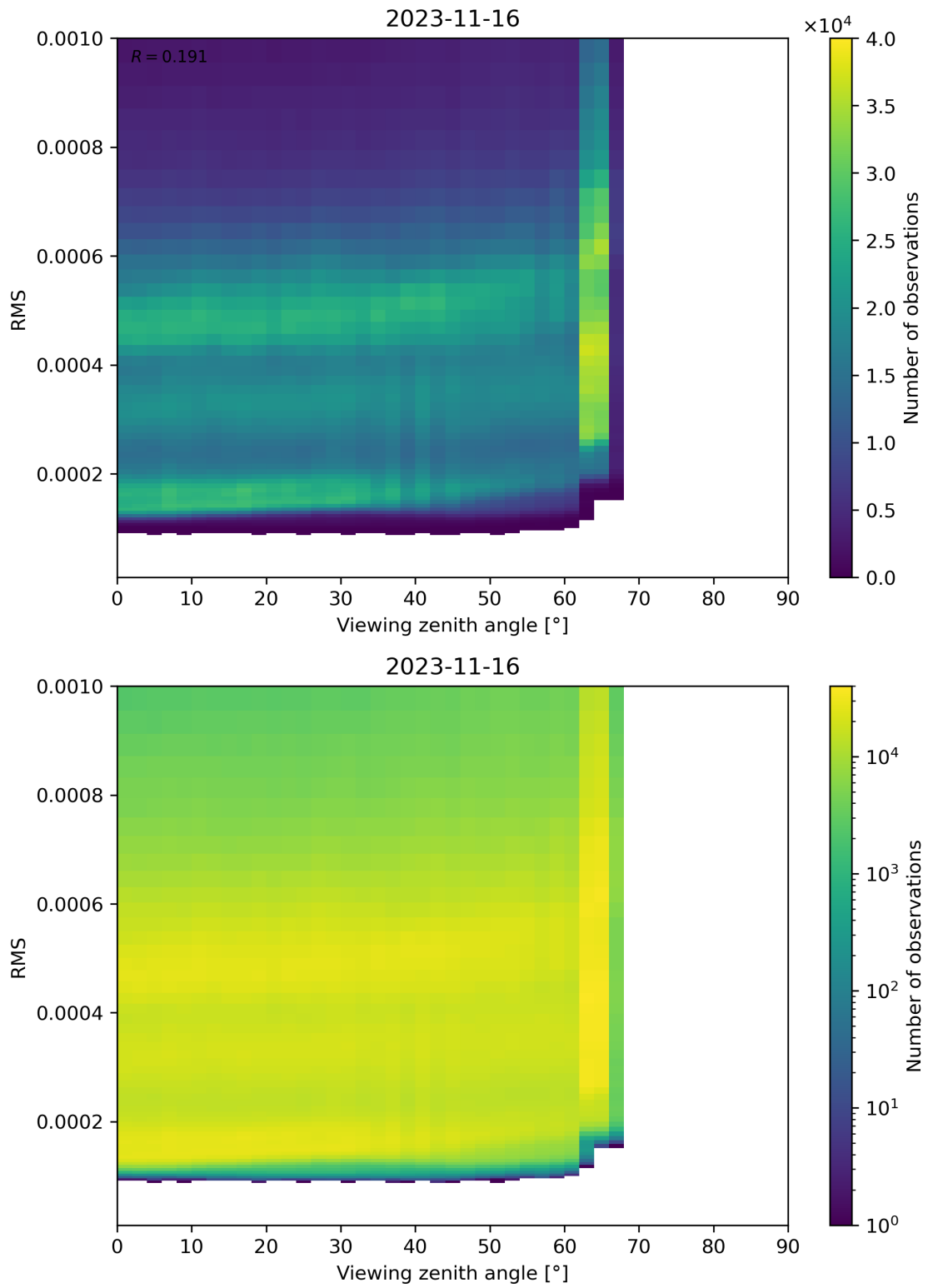
Figure 171: Scatter density plot of “Viewing zenith angle” against “RMS” for 2023-11-15 to 2023-11-17.
