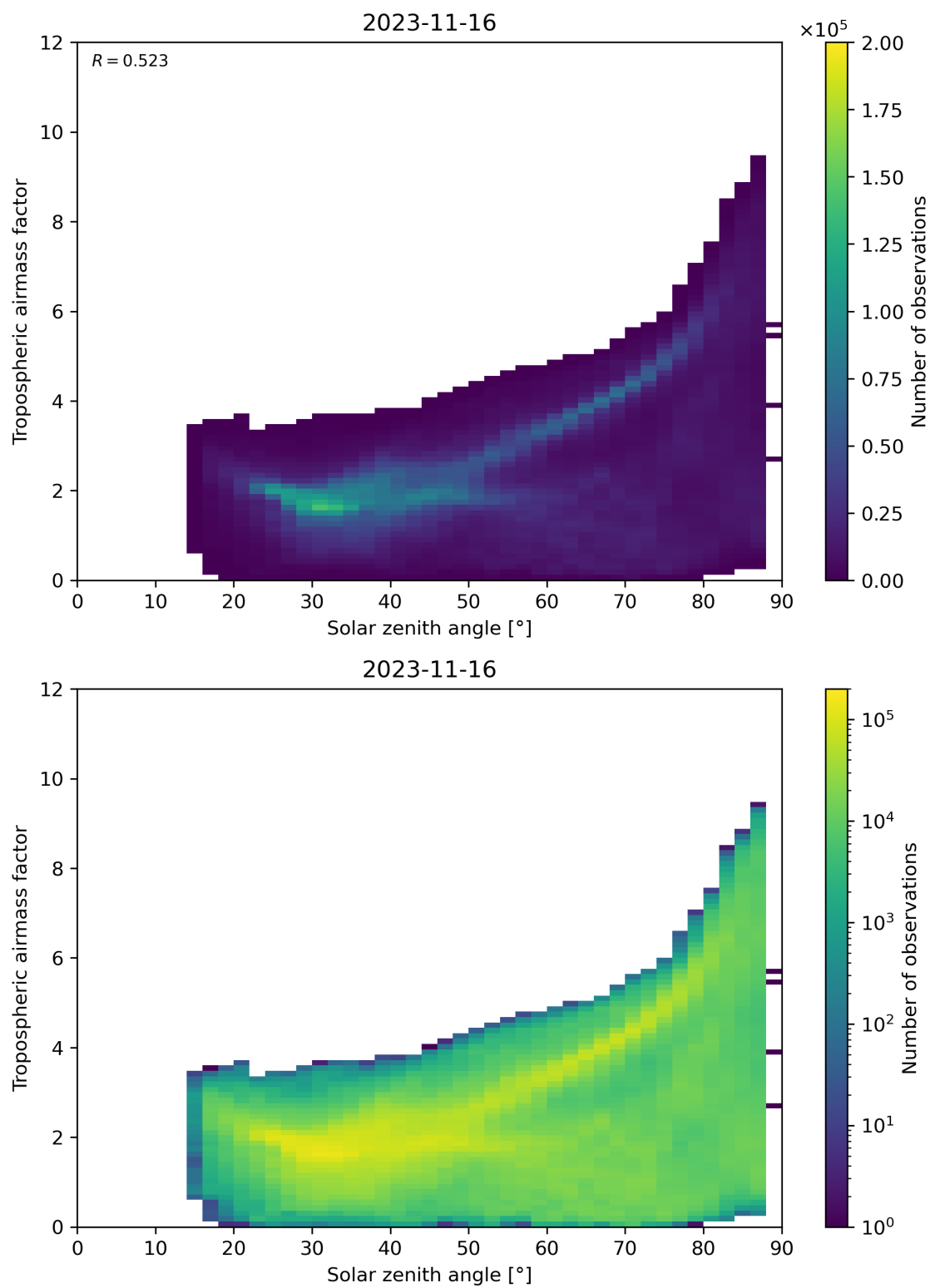
Figure 147: Scatter density plot of “Solar zenith angle” against “Tropospheric airmass factor” for 2023-11-15 to 2023-11-17.
