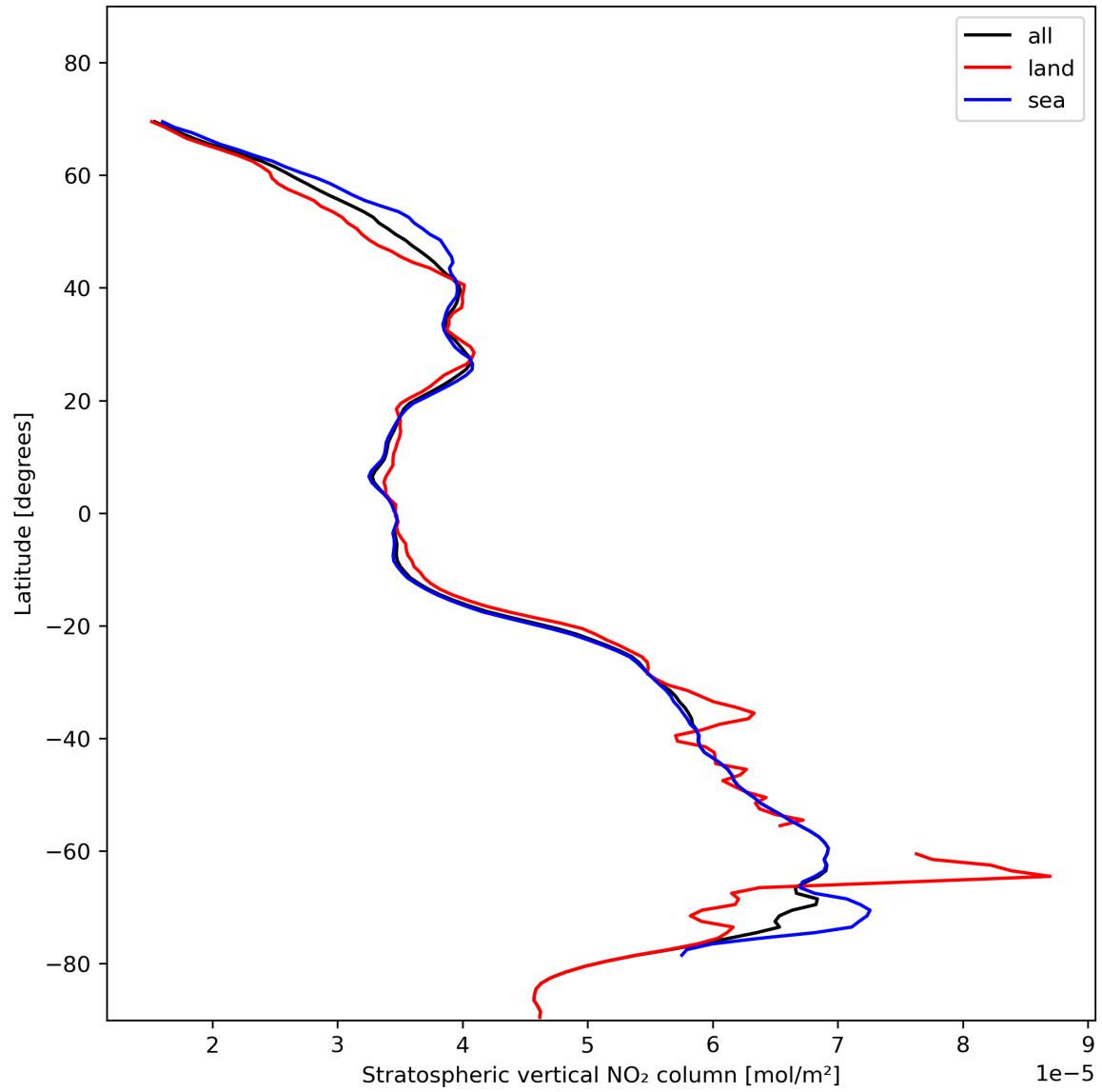
Figure 19: Zonal average of “Stratospheric vertical NO 2 column” for 2023-11-15 to 2023-11-17.
