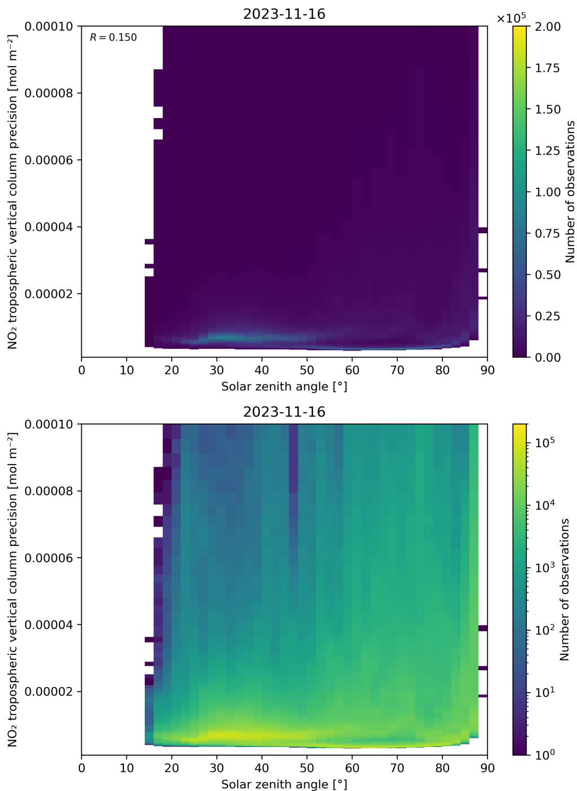
Figure 156: Scatter density plot of “Solar zenith angle” against “NO 2 tropospheric vertical column precision” for 2023-11-15 to 2023-11-17.
