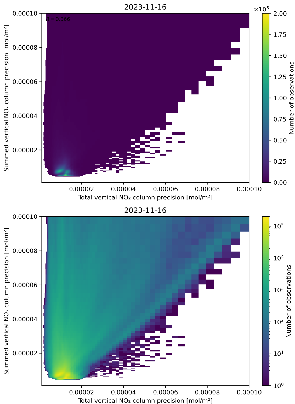
Figure 118: Scatter density plot of “Total vertical NO 2 column precision” against “Summed vertical NO 2 column precision” for 2023-11-15 to 2023-11-17.
