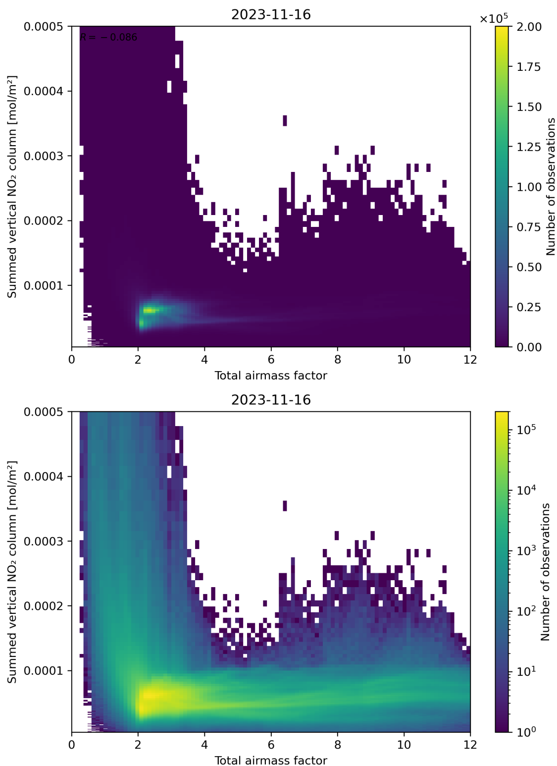
Figure 65: Scatter density plot of “Total airmass factor” against “Summed vertical NO 2 column” for 2023-11-15 to 2023-11-17.
