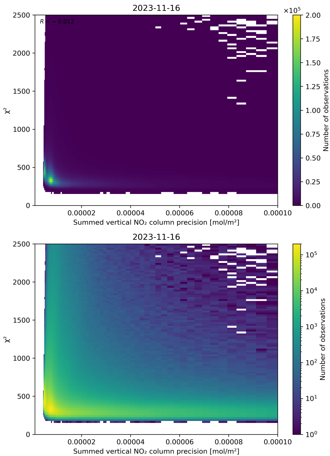
Figure 107: Scatter density plot of “Summed vertical NO 2 column precision” against “ \chi^2 ” for 2023-11-15 to 2023-11-17.
