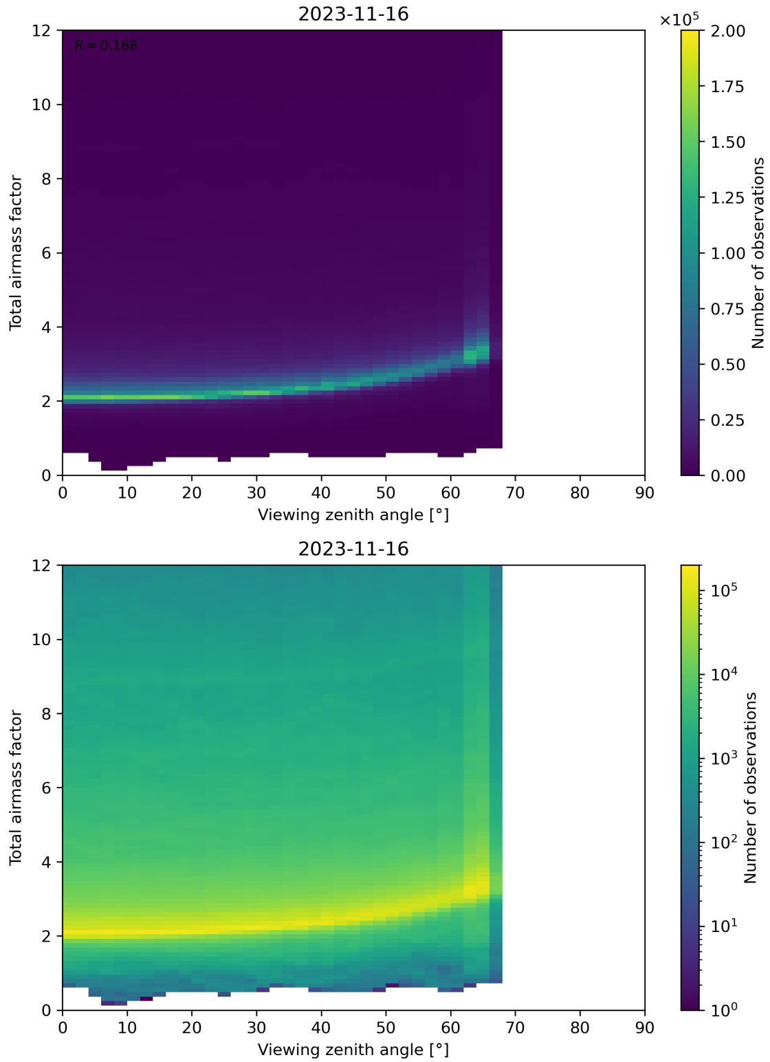
Figure 160: Scatter density plot of “Viewing zenith angle” against “Total airmass factor” for 2023-11-15 to 2023-11-17.
