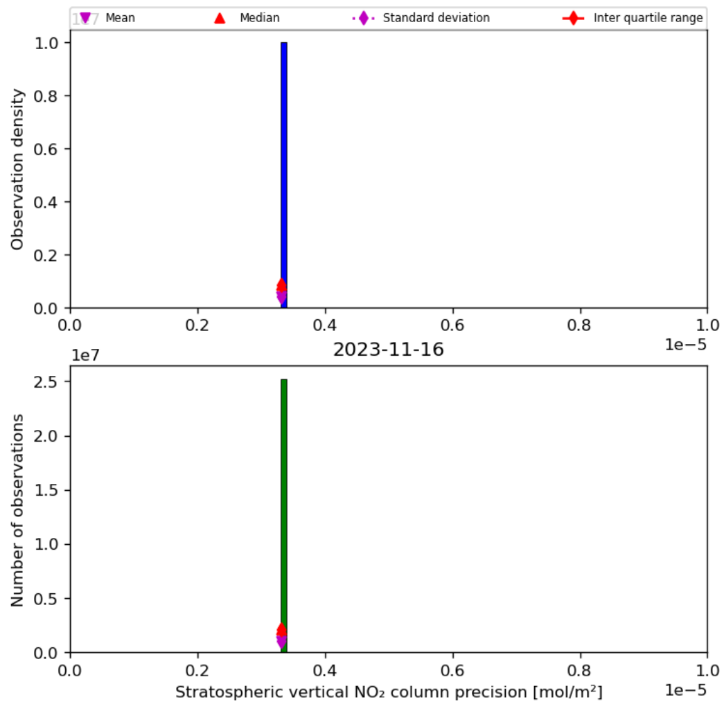
Figure 37: Histogram of “Stratospheric vertical NO 2 column precision” for 2023-11-15 to 2023-11-17
