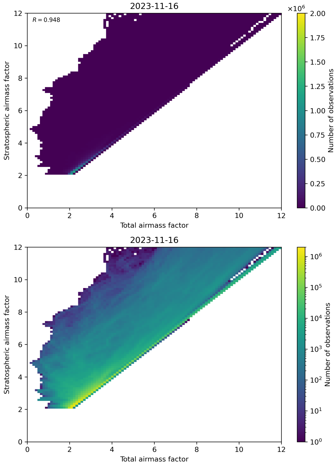
Figure 62: Scatter density plot of “Total airmass factor” against “Stratospheric airmass factor” for 2023-11-15 to 2023-11-17.
