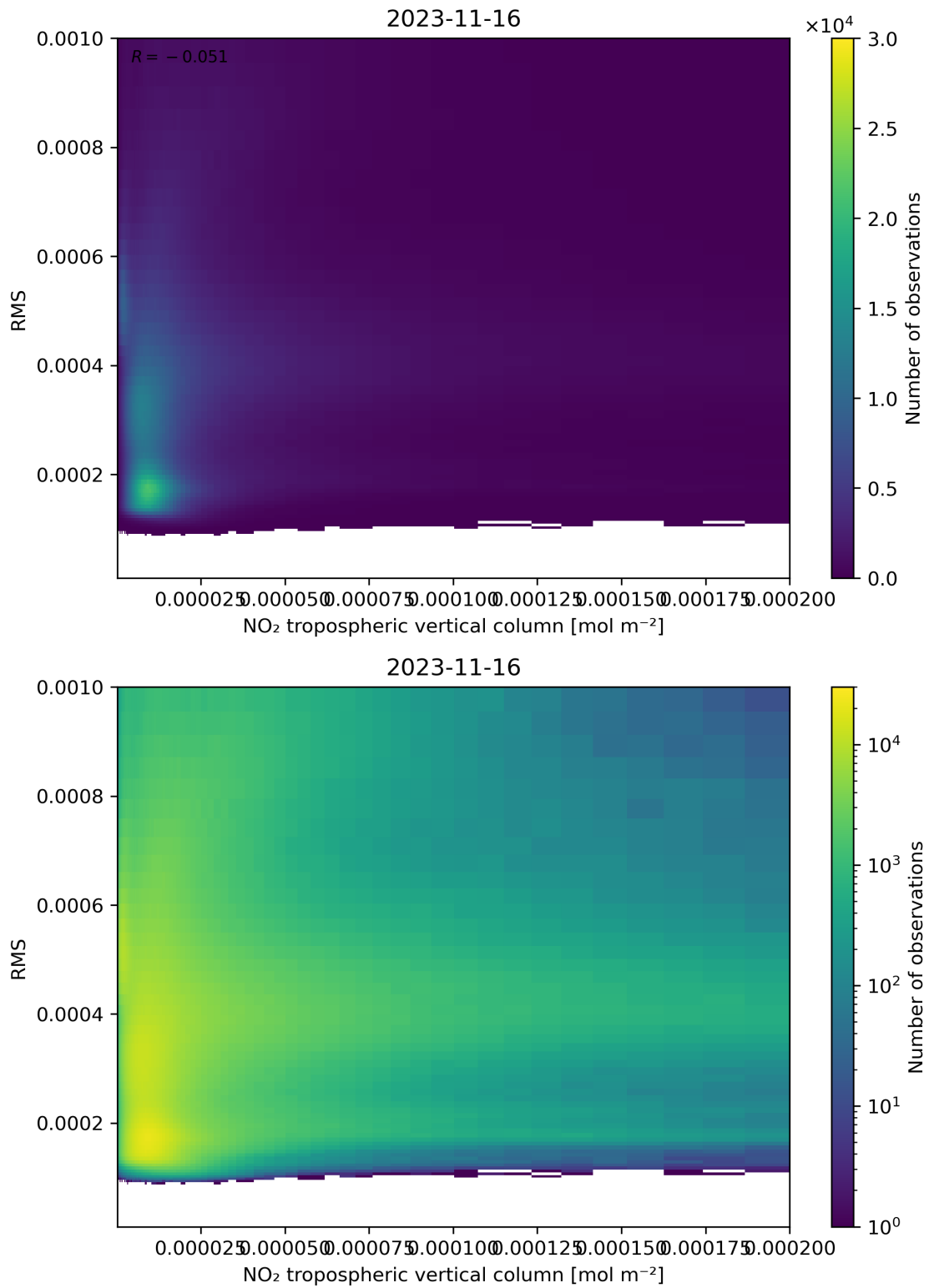
Figure 142: Scatter density plot of “NO 2 tropospheric vertical column” against “RMS” for 2023-11-15 to 2023-11-17.
