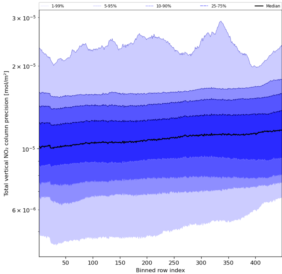
Figure 56: Along track statistics of “Total vertical NO 2 column precision” for 2023-11-15 to 2023-11-17
