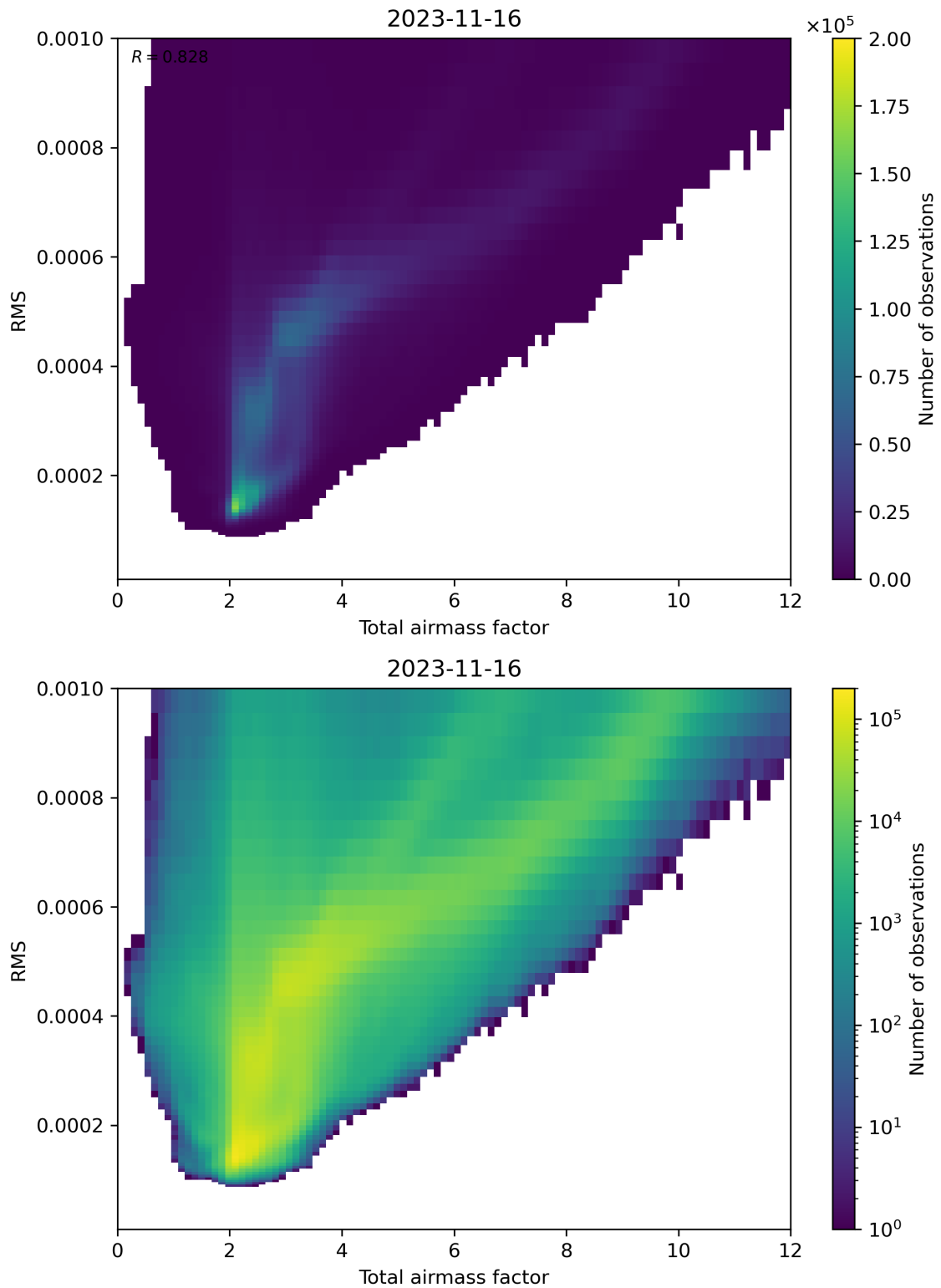
Figure 69: Scatter density plot of “Total airmass factor” against “RMS” for 2023-11-15 to 2023-11-17.
