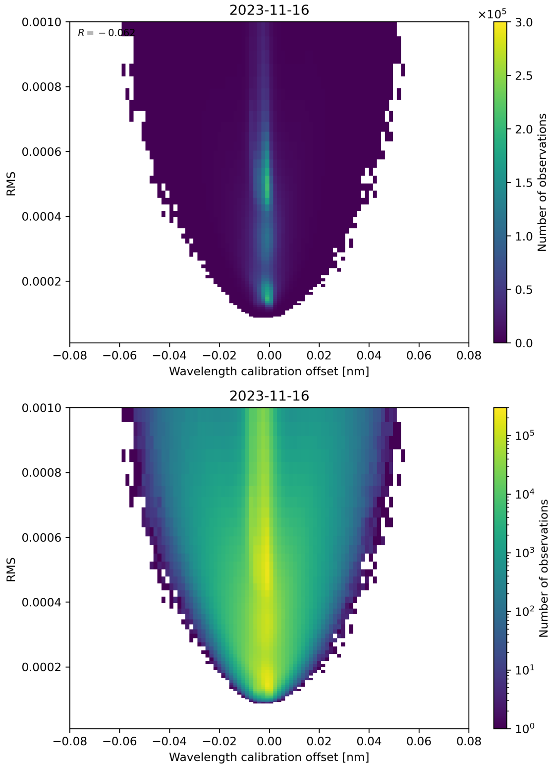
Figure 181: Scatter density plot of “Wavelength calibration offset” against “RMS” for 2023-11-15 to 2023-11-17.
