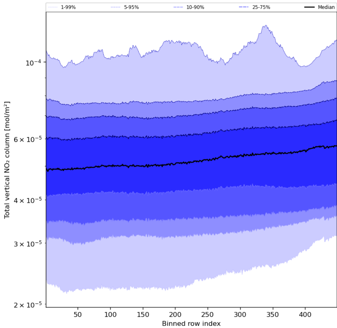
Figure 55: Along track statistics of “Total vertical NO 2 column” for 2023-11-15 to 2023-11-17
