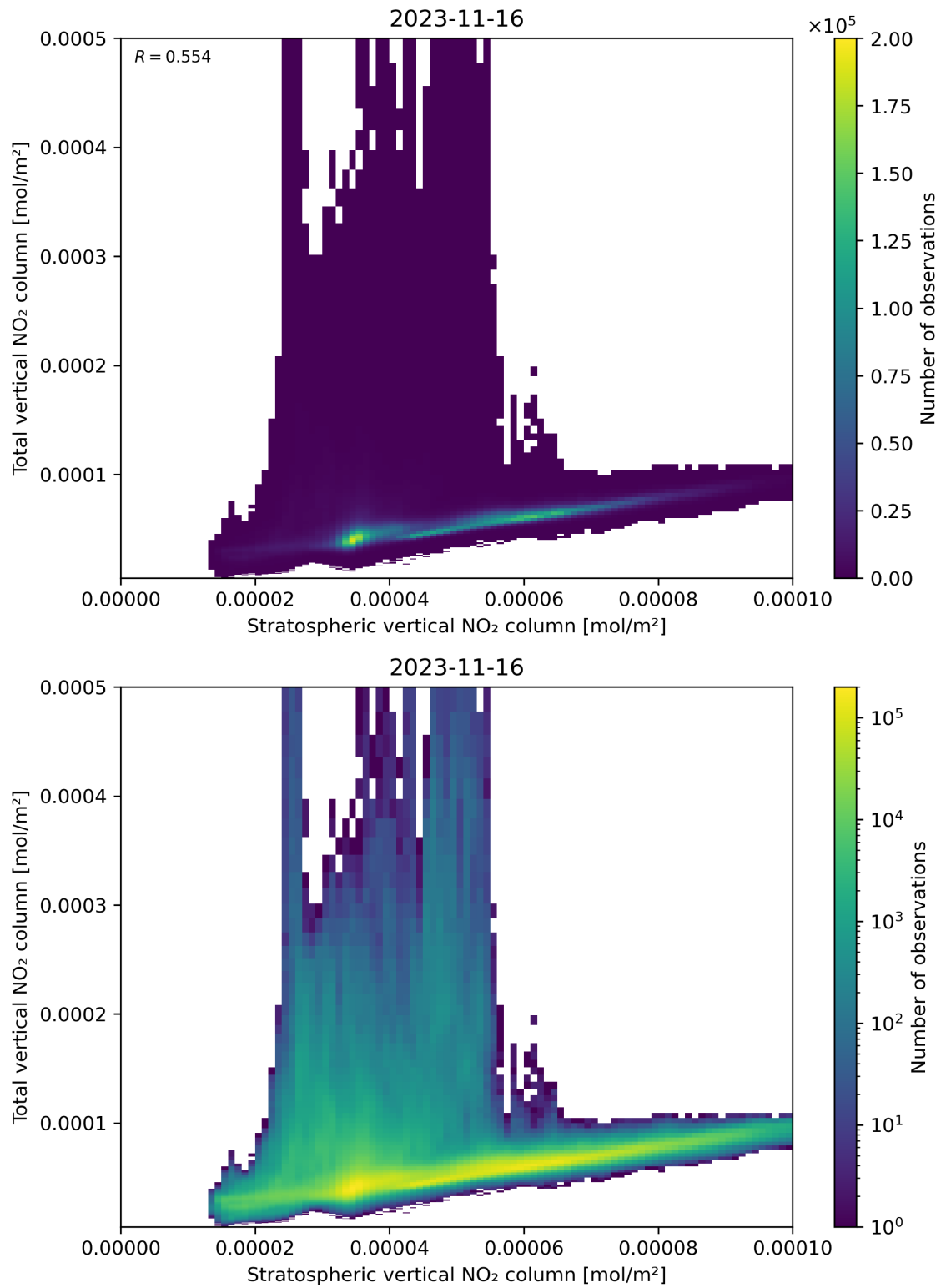
Figure 100: Scatter density plot of “Stratospheric vertical NO 2 column” against “Total vertical NO 2 column” for 2023-11-15 to 2023-11-17.
