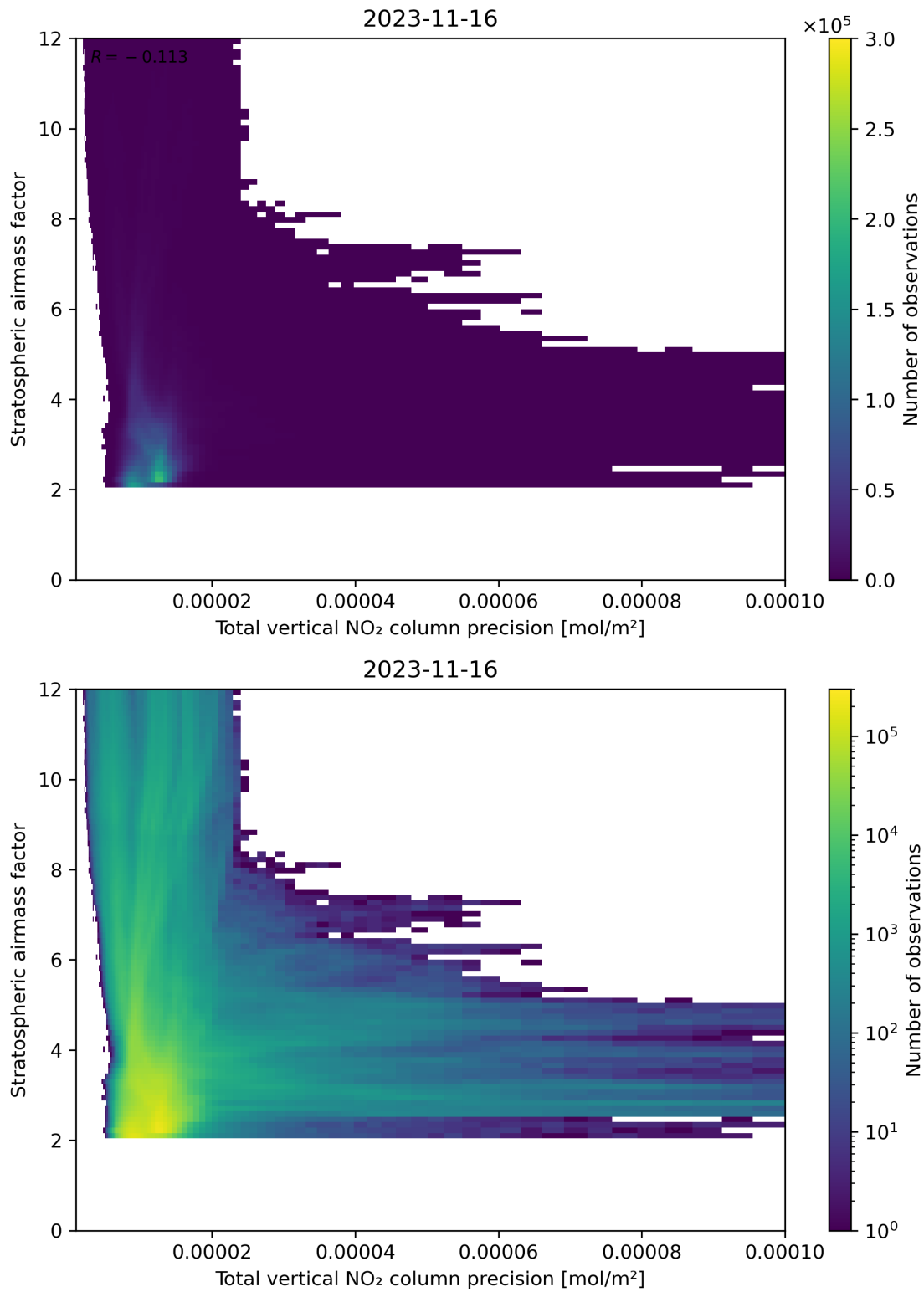
Figure 115: Scatter density plot of “Total vertical NO 2 column precision” against “Stratospheric air mass factor” for 2023-11-15 to 2023-11-17.
