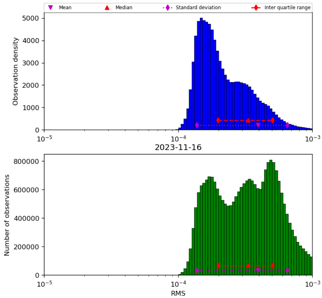
Figure 43: Histogram of “RMS” for 2023-11-15 to 2023-11-17
