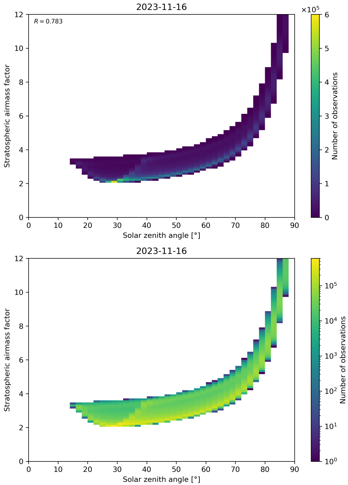
Figure 145: Scatter density plot of “Solar zenith angle” against “Stratospheric airmass factor” for 2023-11-15 to 2023-11-17.
