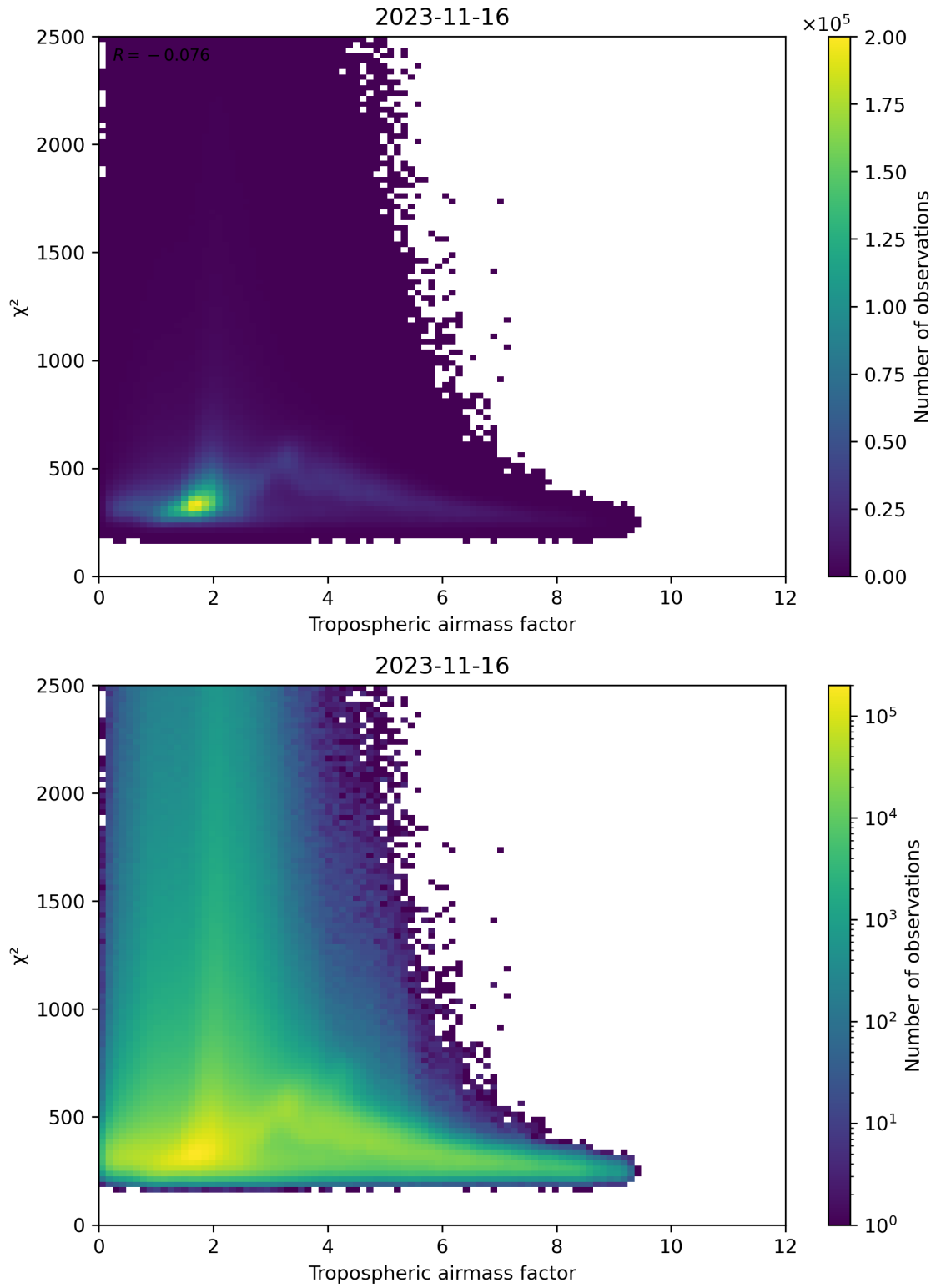
Figure 73: Scatter density plot of “Tropospheric airmass factor” against “ \chi^2 ” for 2023-11-15 to 2023-11-17.
