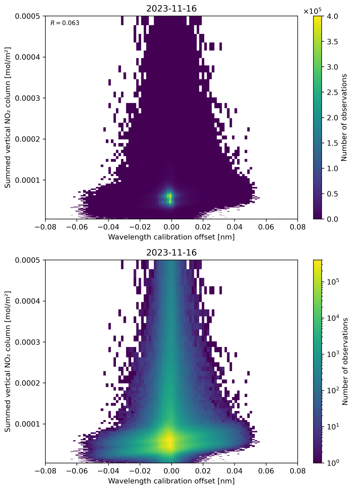
Figure 177: Scatter density plot of “Wavelength calibration offset” against “Summed vertical NO 2 column” for 2023-11-15 to 2023-11-17.
