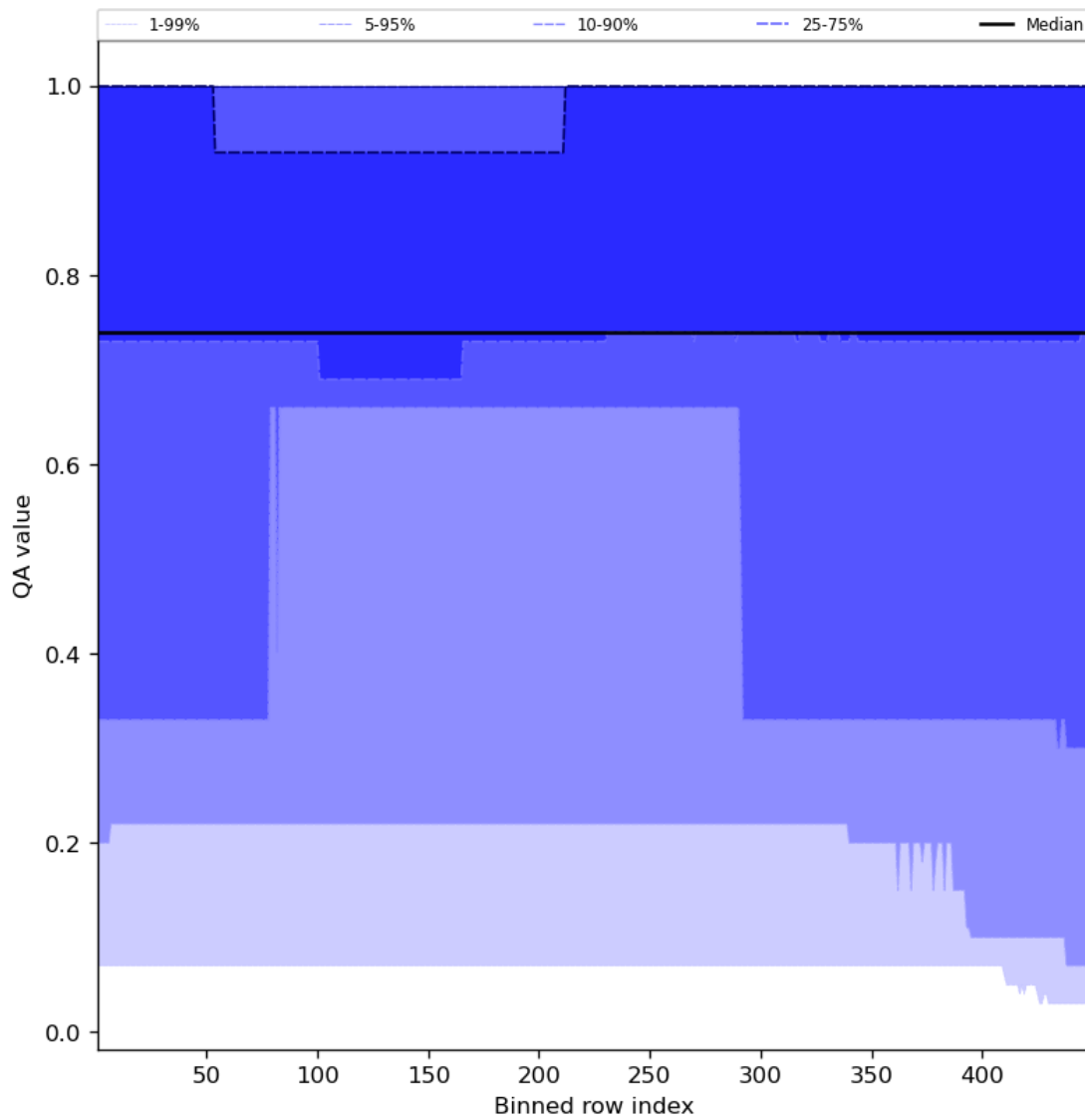
Figure 45: Along track statistics of “QA value” for 2023-11-15 to 2023-11-17
