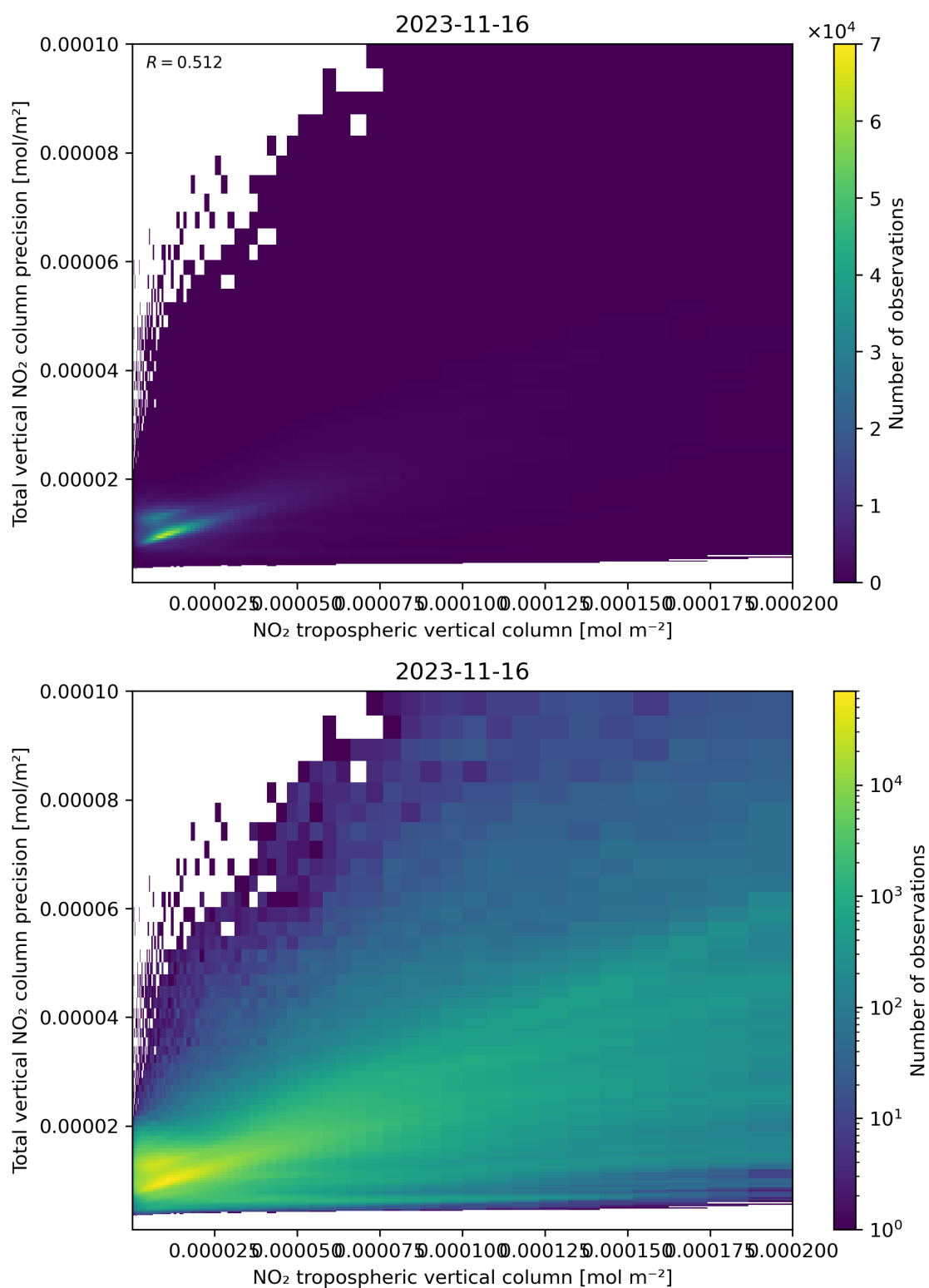
Figure 129: Scatter density plot of “NO 2 tropospheric vertical column” against “Total vertical NO 2 column precision” for 2023-11-15 to 2023-11-17.
