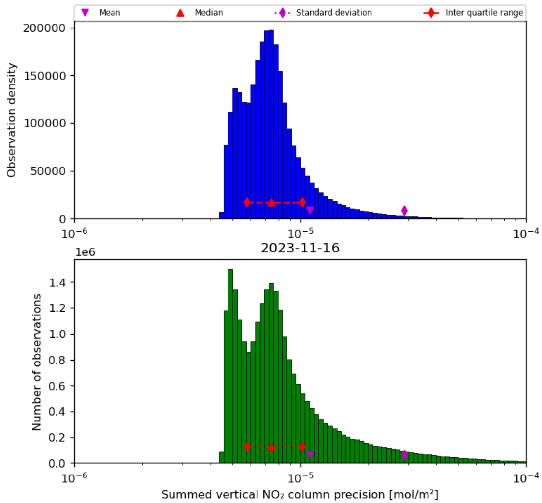
Figure 41: Histogram of “Summed vertical NO 2 column precision” for 2023-11-15 to 2023-11-17
