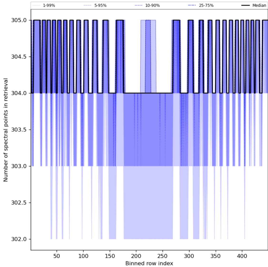
Figure 50: Along track statistics of “Number of spectral points in retrieval” for 2023-11-15 to 2023-11-17
