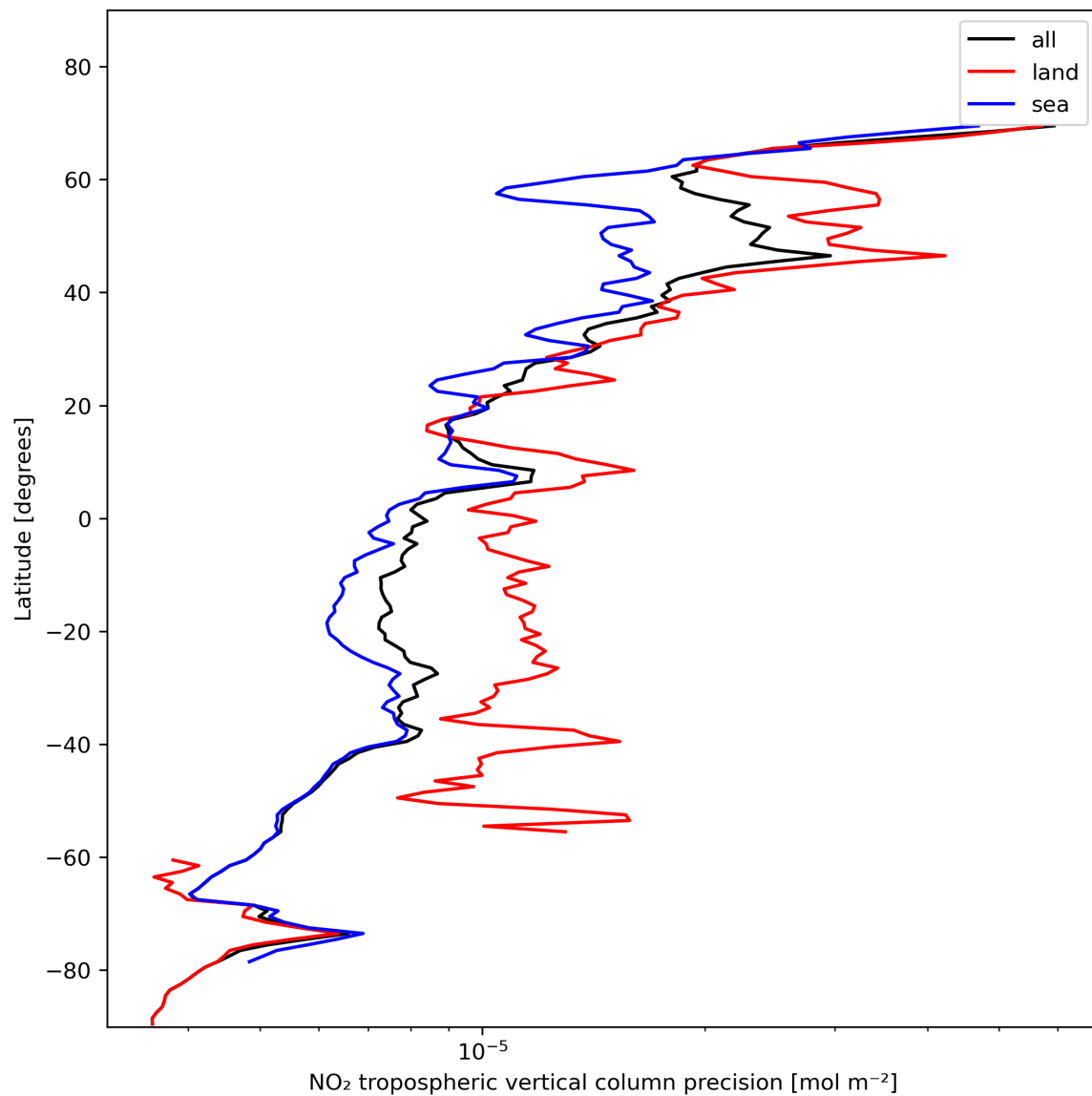
Figure 13: Zonal average of “NO 2 tropospheric vertical column precision” for 2023-11-15 to 2023-11-17.
