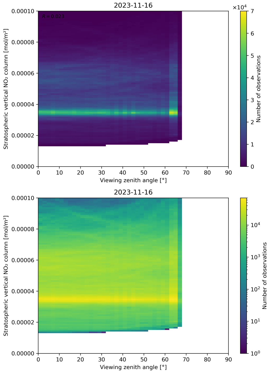
Figure 164: Scatter density plot of “Viewing zenith angle” against “Stratospheric vertical NO 2 column” for 2023-11-15 to 2023-11-17.
