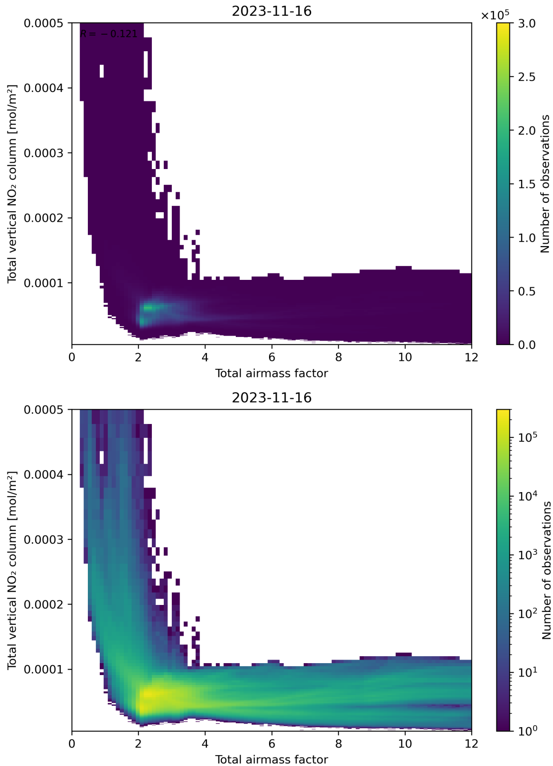
Figure 67: Scatter density plot of “Total airmass factor” against “Total vertical NO 2 column” for 2023-11-15 to 2023-11-17.
