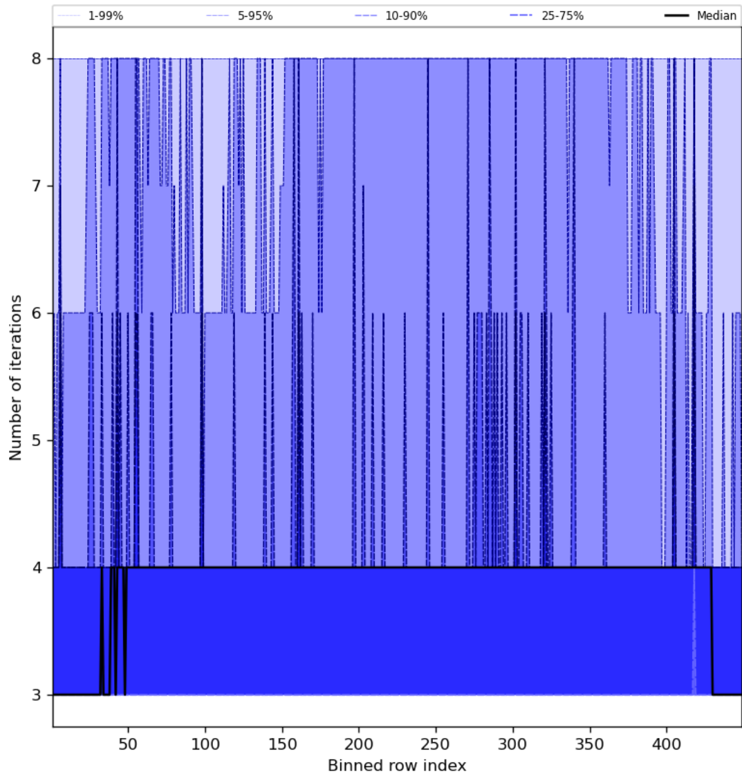
Figure 51: Along track statistics of “Number of iterations” for 2023-11-15 to 2023-11-17
