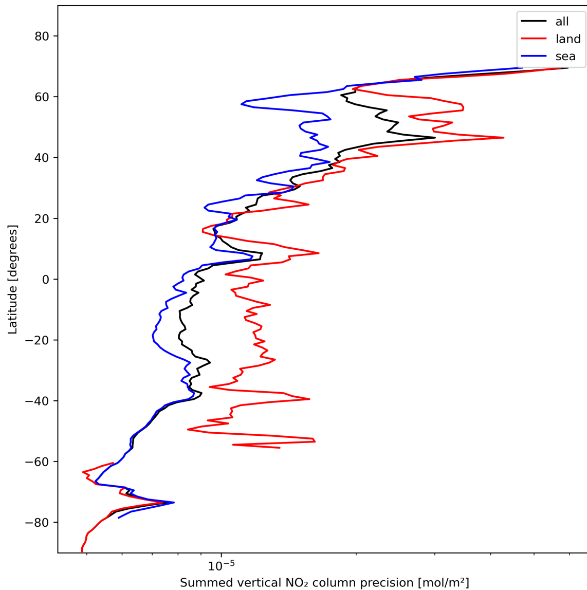
Figure 24: Zonal average of “Summed vertical NO 2 column precision” for 2023-11-15 to 2023-11-17.
