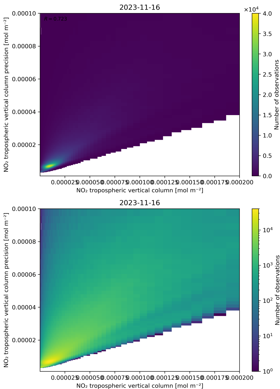
Figure 130: Scatter density plot of “NO 2 tropospheric vertical column” against “NO 2 tropospheric vertical column precision” for 2023-11-15 to 2023-11-17.
