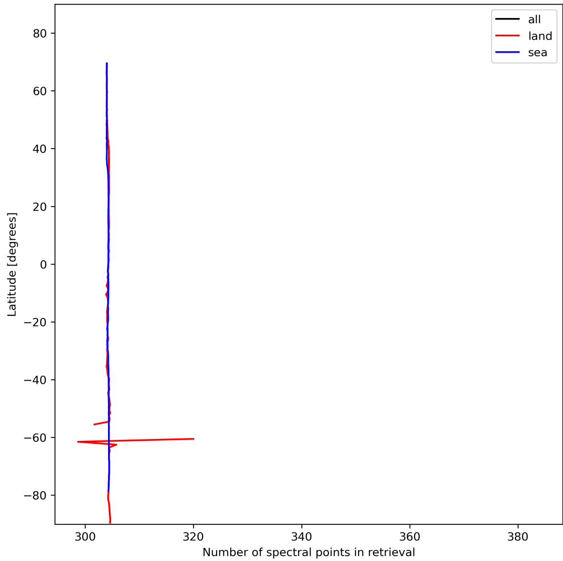
Figure 16: Zonal average of “Number of spectral points in retrieval” for 2023-11-15 to 2023-11-17.
