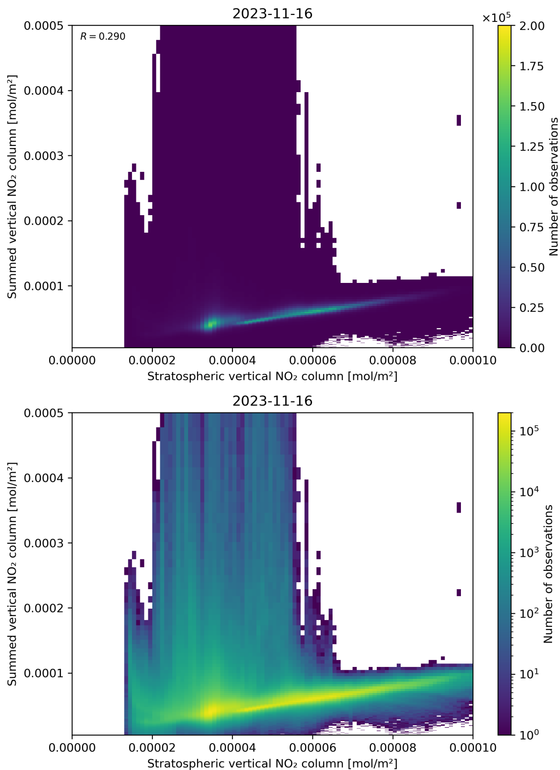
Figure 98: Scatter density plot of “Stratospheric vertical NO 2 column” against “Summed vertical NO 2 column” for 2023-11-15 to 2023-11-17.
