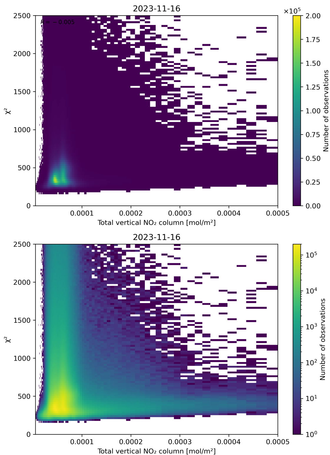
Figure 111: Scatter density plot of “Total vertical NO 2 column” against “ \chi^2 ” for 2023-11-15 to 2023-11-17.
