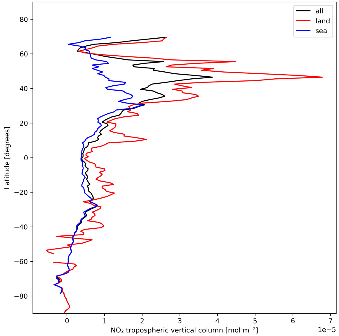
Figure 12: Zonal average of “NO 2 tropospheric vertical column” for 2023-11-15 to 2023-11-17.
