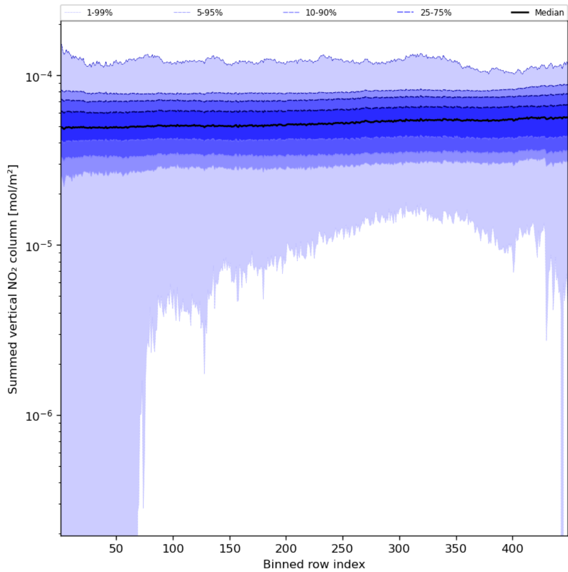
Figure 57: Along track statistics of “Summed vertical NO 2 column” for 2023-11-15 to 2023-11-17
