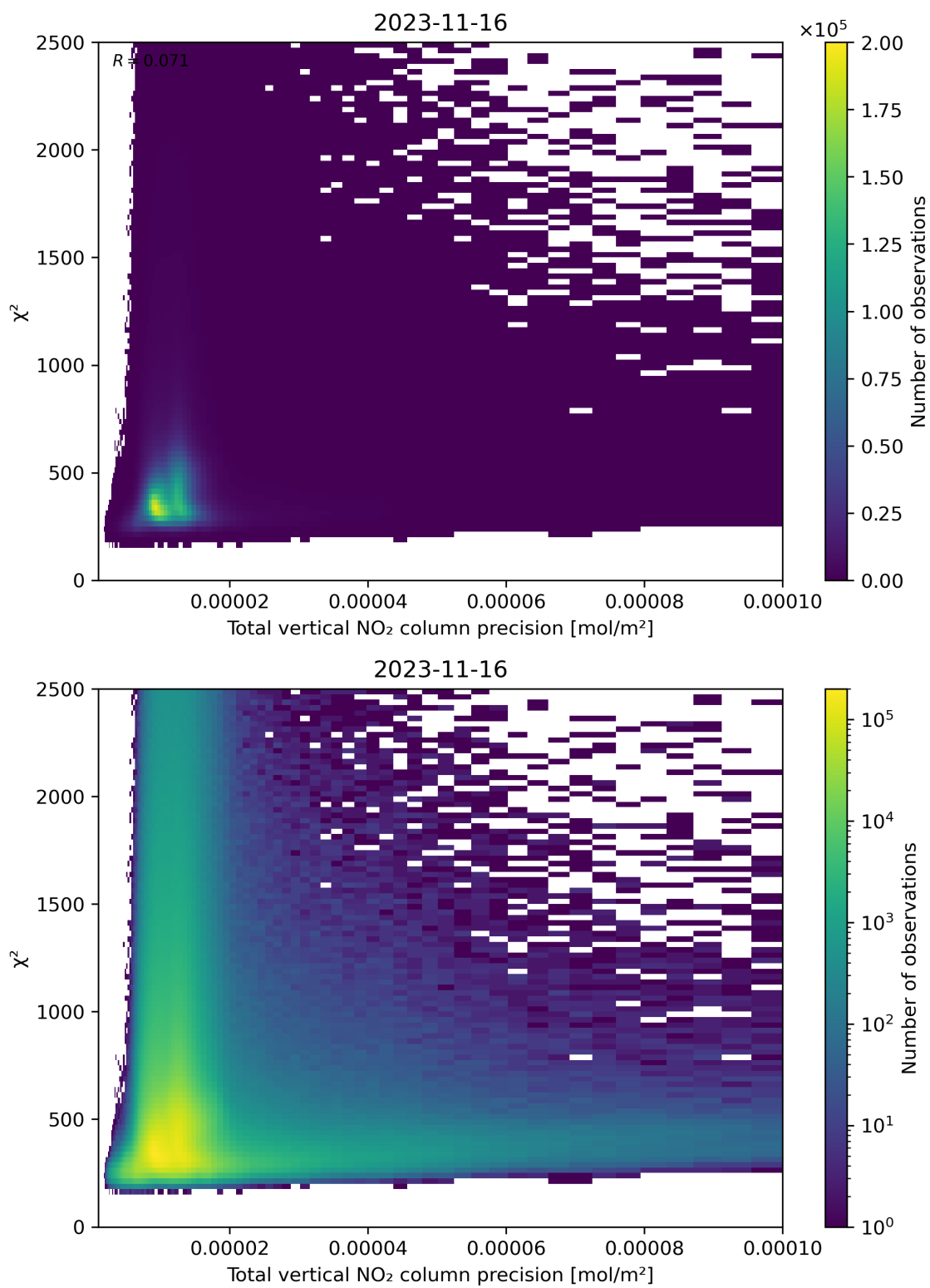
Figure 116: Scatter density plot of “Total vertical NO 2 column precision” against “ \chi^2 ” for 2023-11-15 to 2023-11-17.
