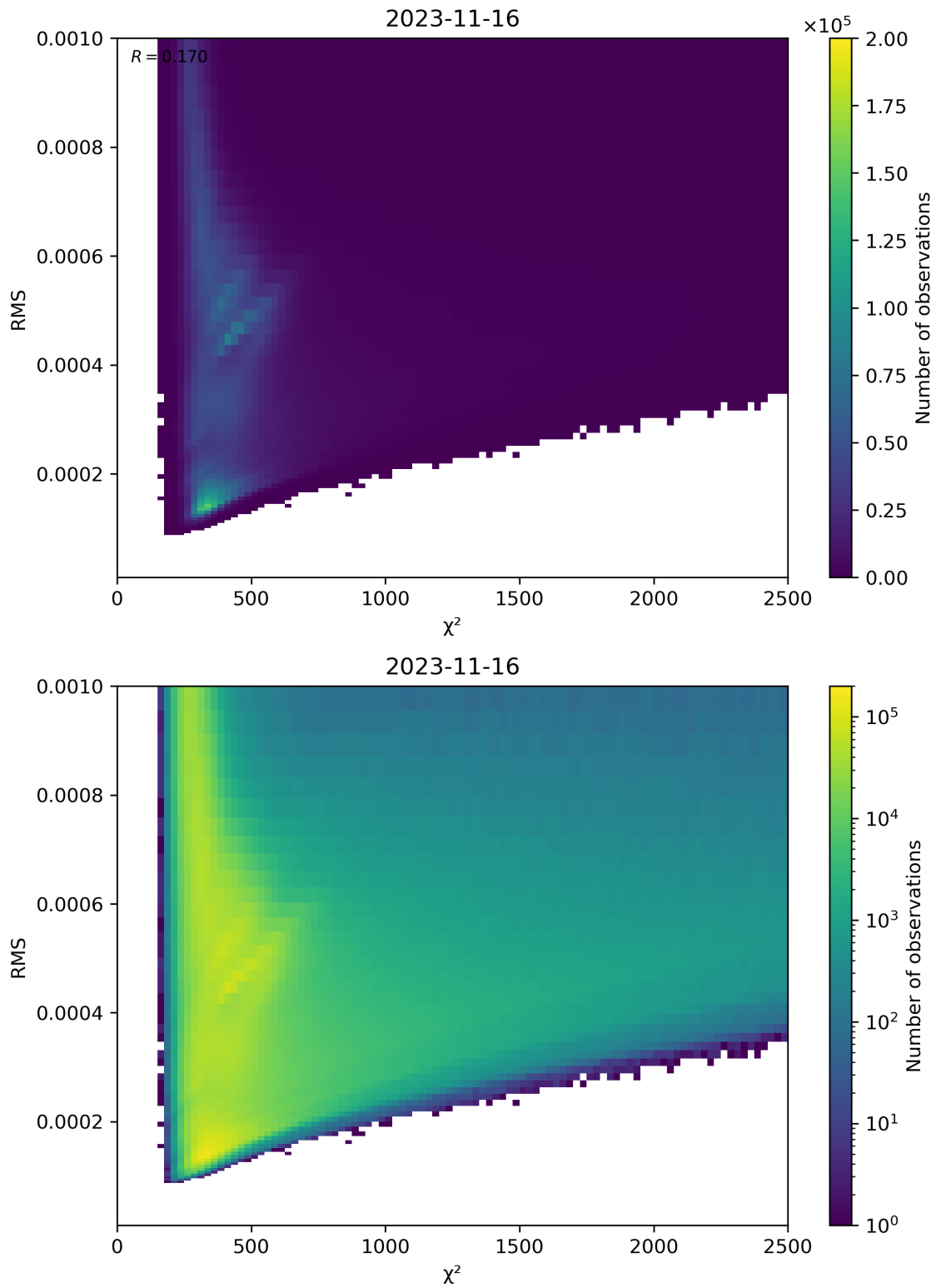
Figure 82: Scatter density plot of “ \chi^2 ” against “RMS” for 2023-11-15 to 2023-11-17.
