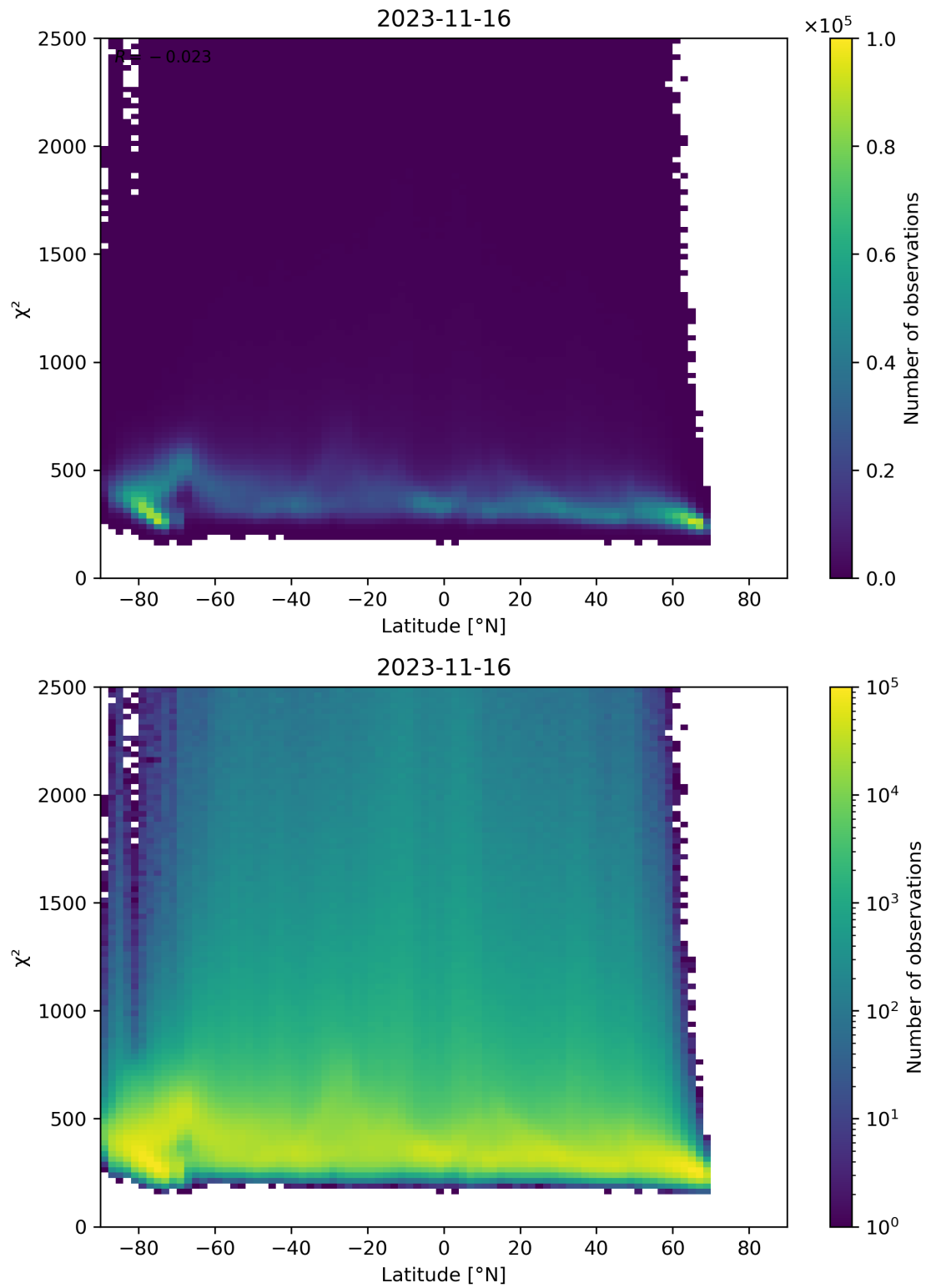
Figure 86: Scatter density plot of “Latitude” against “ \chi^2 ” for 2023-11-15 to 2023-11-17.
