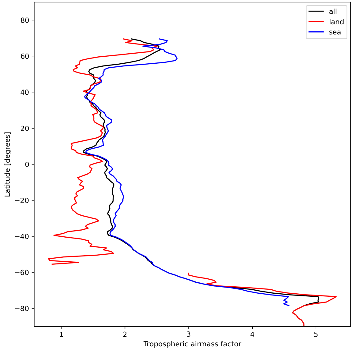
Figure 14: Zonal average of “Tropospheric airmass factor” for 2023-11-15 to 2023-11-17.
