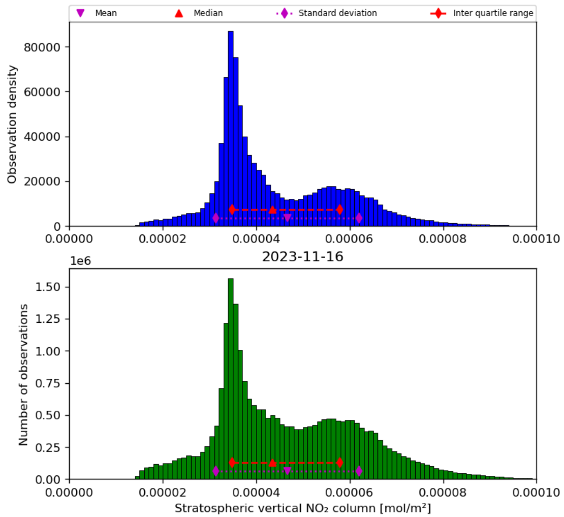
Figure 36: Histogram of “Stratospheric vertical NO 2 column” for 2023-11-15 to 2023-11-17
