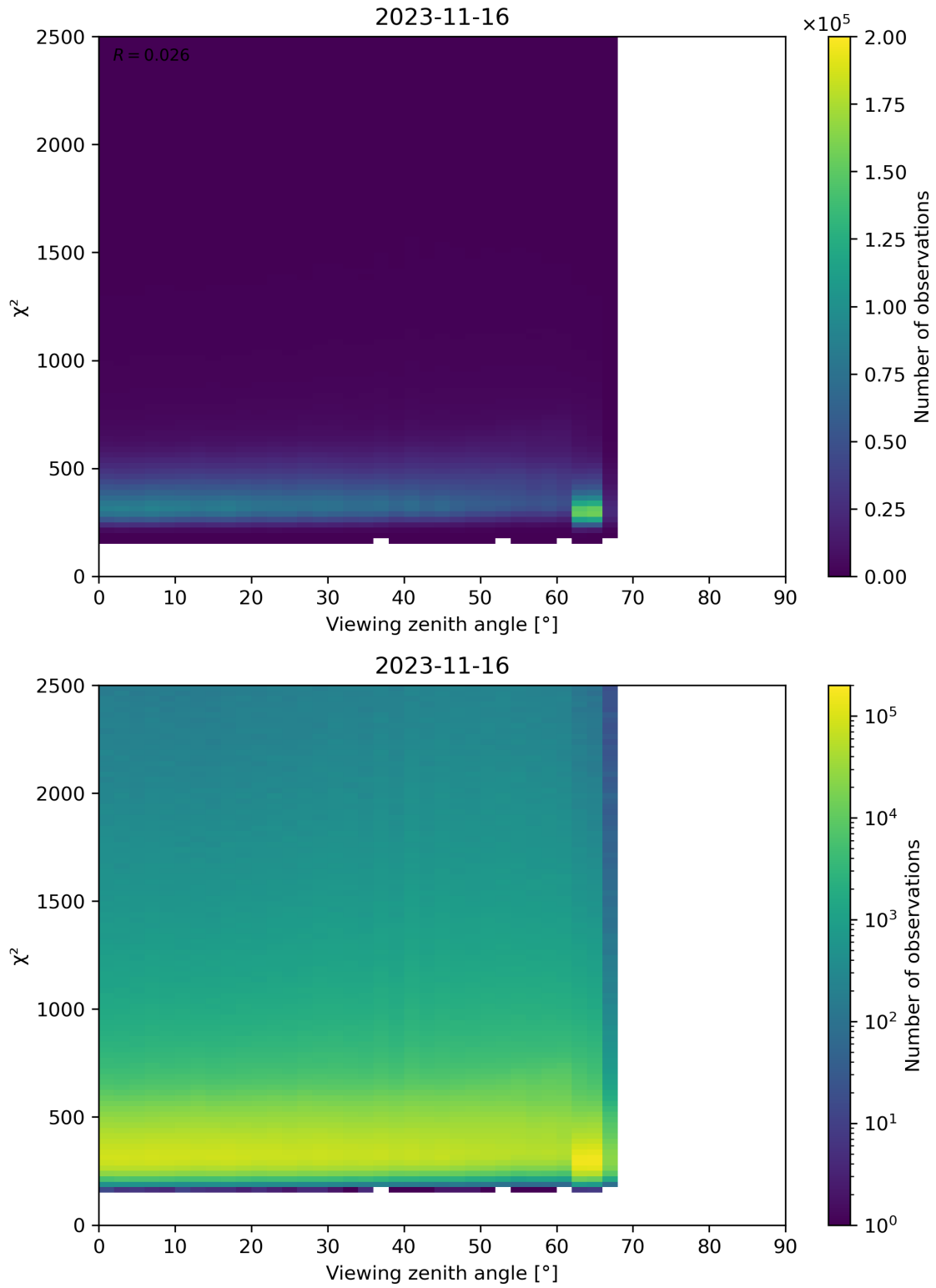
Figure 162: Scatter density plot of “Viewing zenith angle” against “ \chi^2 ” for 2023-11-15 to 2023-11-17.
