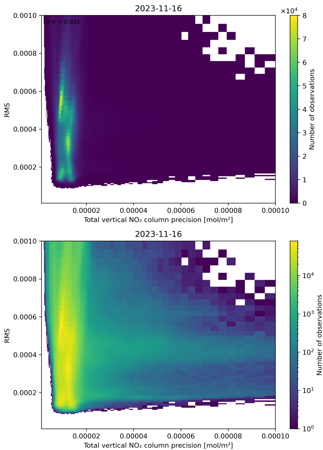
Figure 119: Scatter density plot of “Total vertical NO 2 column precision” against “RMS” for 2023-11-15 to 2023-11-17.
