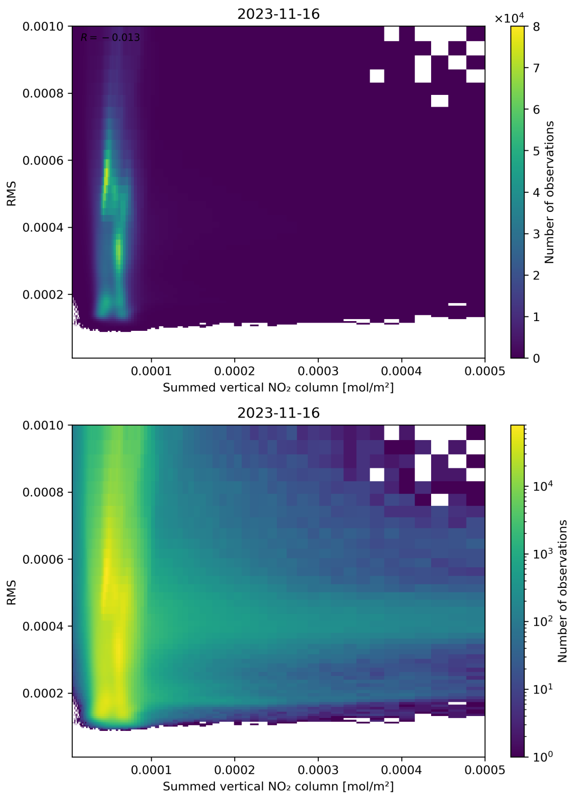
Figure 109: Scatter density plot of “Summed vertical NO 2 column” against “RMS” for 2023-11-15 to 2023-11-17.
