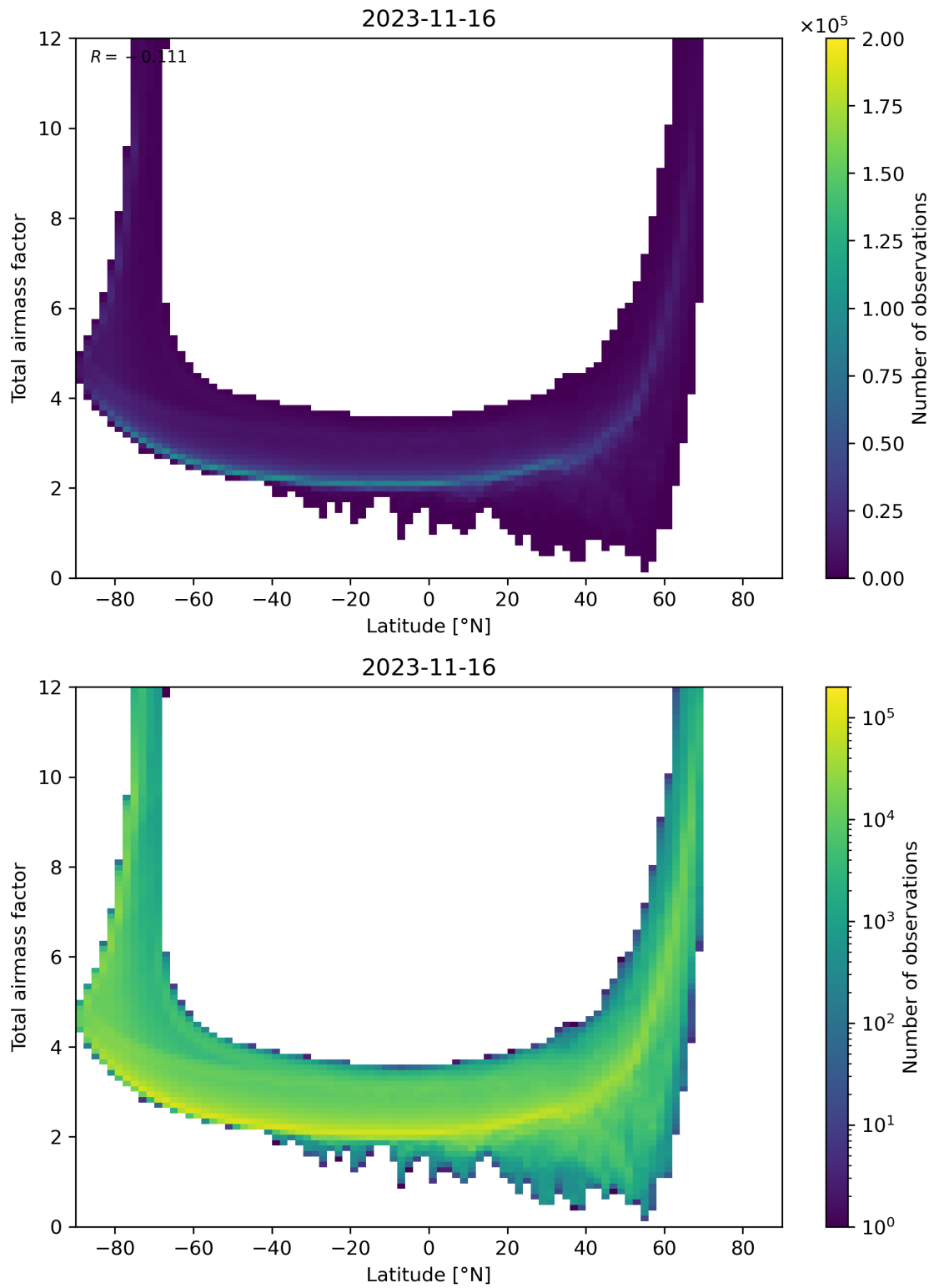
Figure 84: Scatter density plot of “Latitude” against “Total airmass factor” for 2023-11-15 to 2023-11-17.
