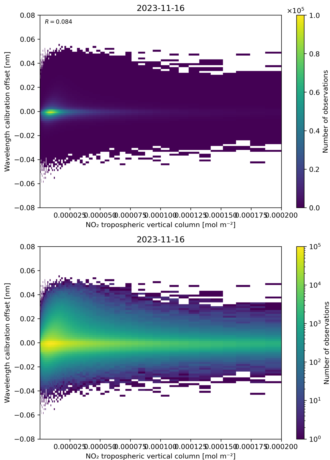
Figure 143: Scatter density plot of “NO 2 tropospheric vertical column” against “Wavelength calibration offset” for 2023-11-15 to 2023-11-17.
