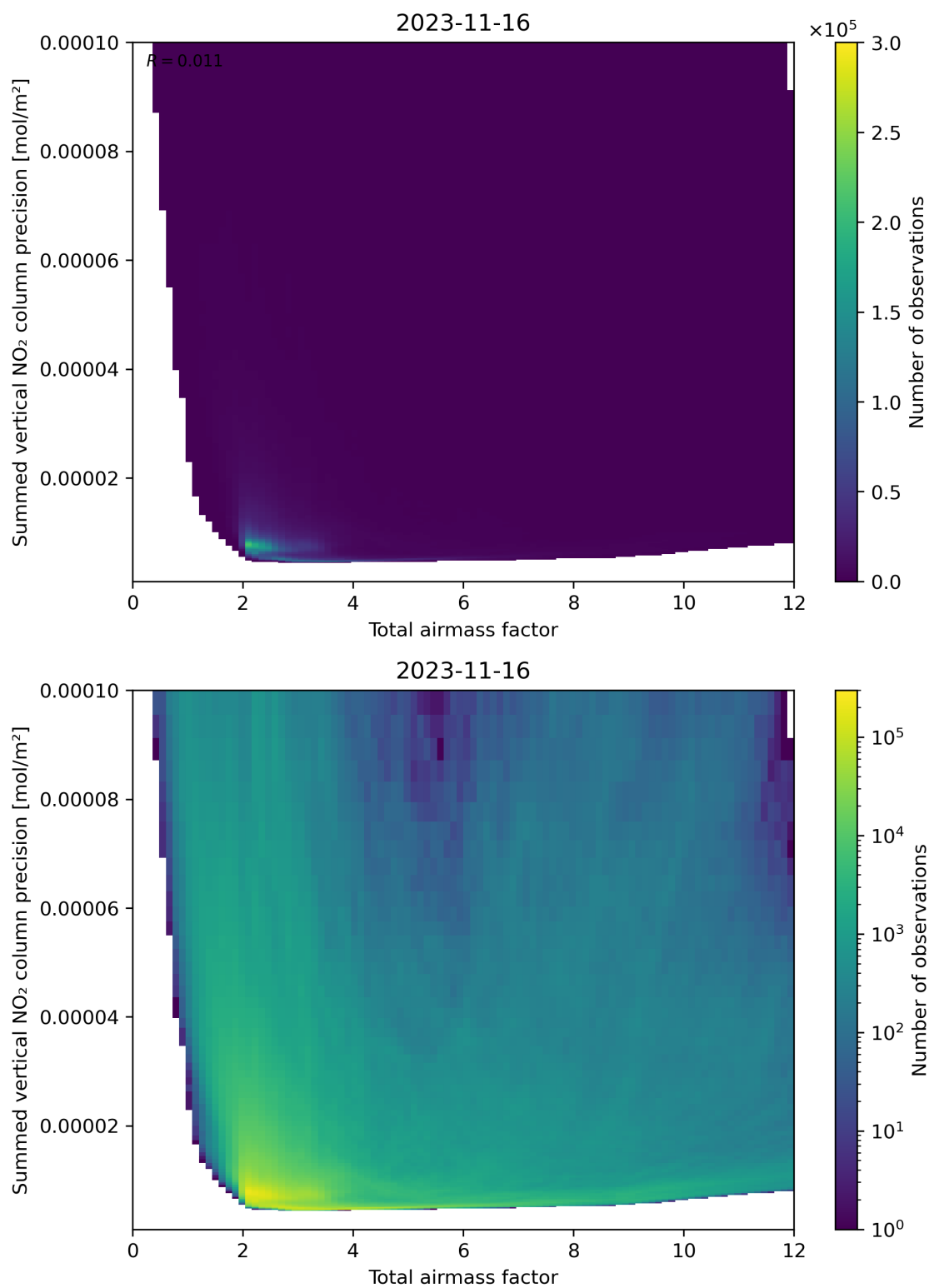
Figure 66: Scatter density plot of “Total airmass factor” against “Summed vertical NO 2 column precision” for 2023-11-15 to 2023-11-17.
