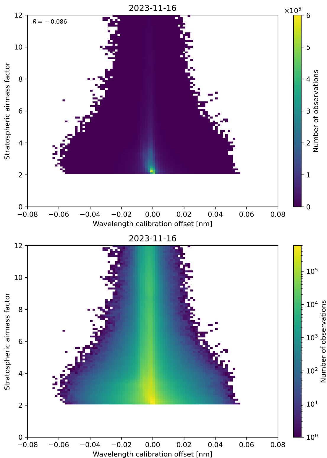
Figure 174: Scatter density plot of “Wavelength calibration offset” against “Stratospheric airmass factor” for 2023-11-15 to 2023-11-17.
