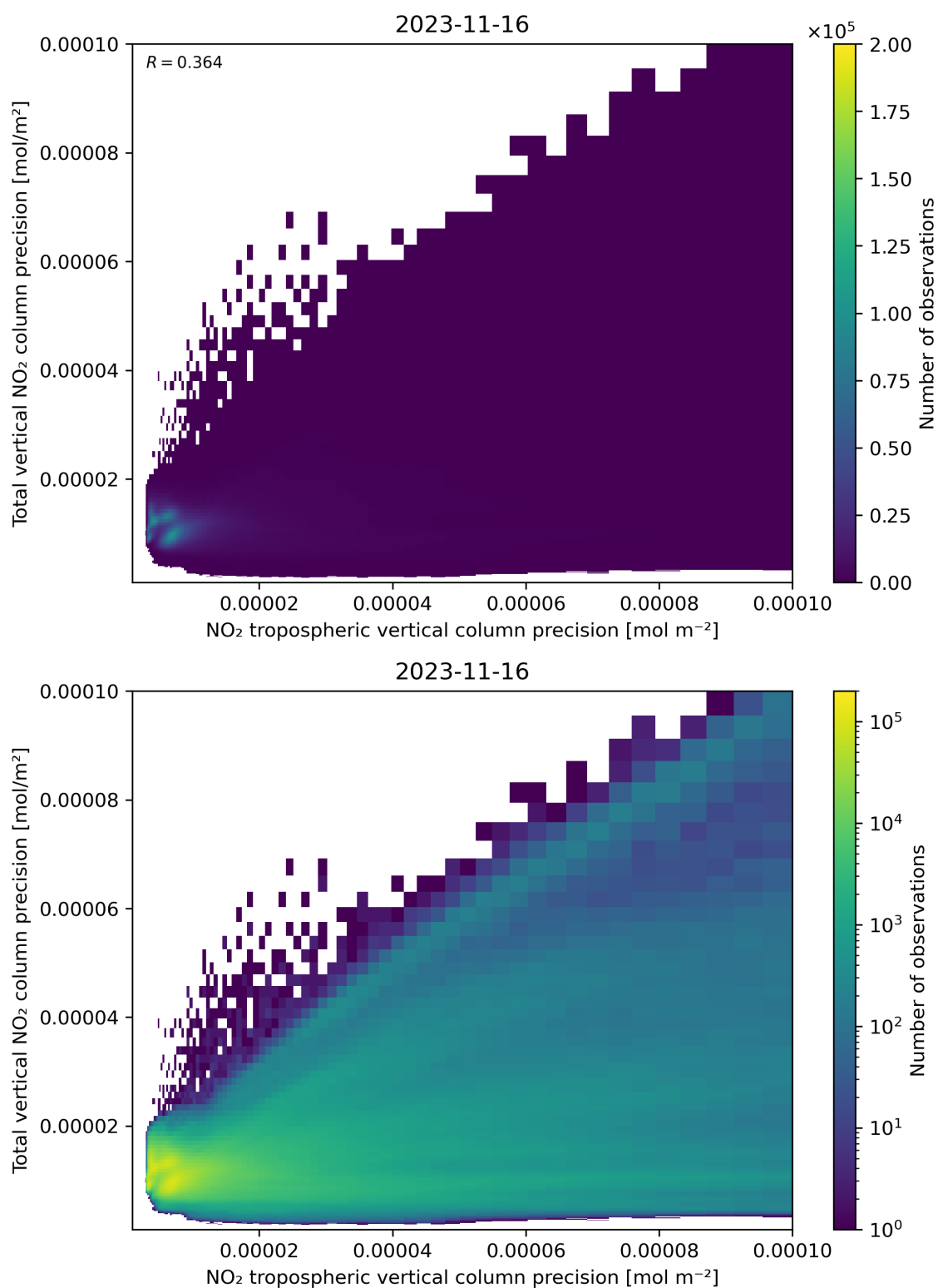
Figure 139: Scatter density plot of “NO 2 tropospheric vertical column precision” against “Total vertical NO 2 column precision” for 2023-11-15 to 2023-11-17.
