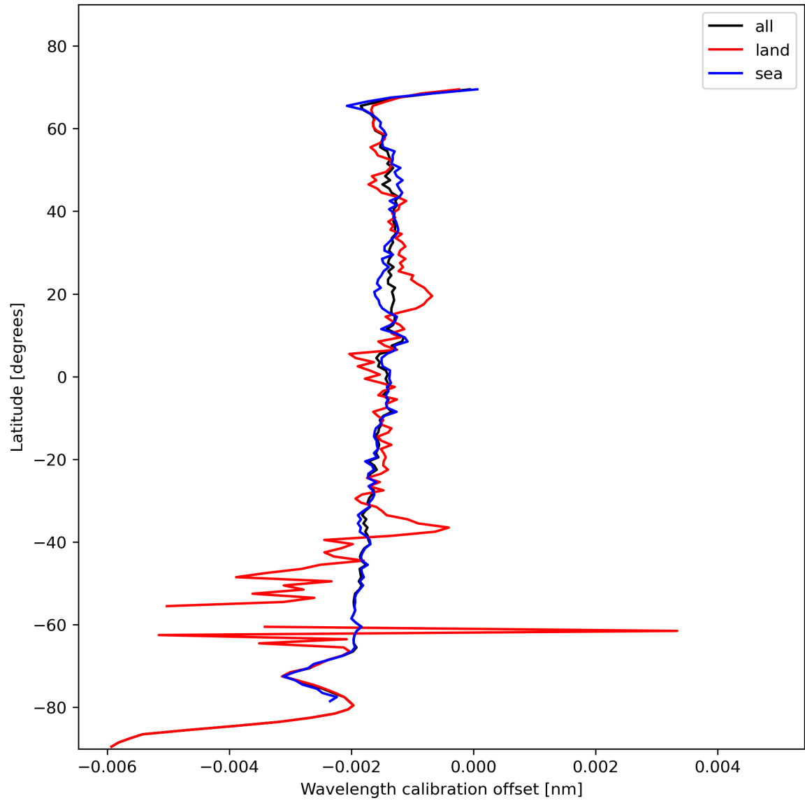
Figure 18: Zonal average of “Wavelength calibration offset” for 2023-11-15 to 2023-11-17.
