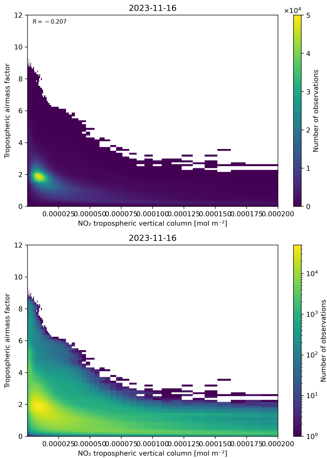
Figure 123: Scatter density plot of “NO 2 tropospheric vertical column” against “Tropospheric air mass factor” for 2023-11-15 to 2023-11-17.
