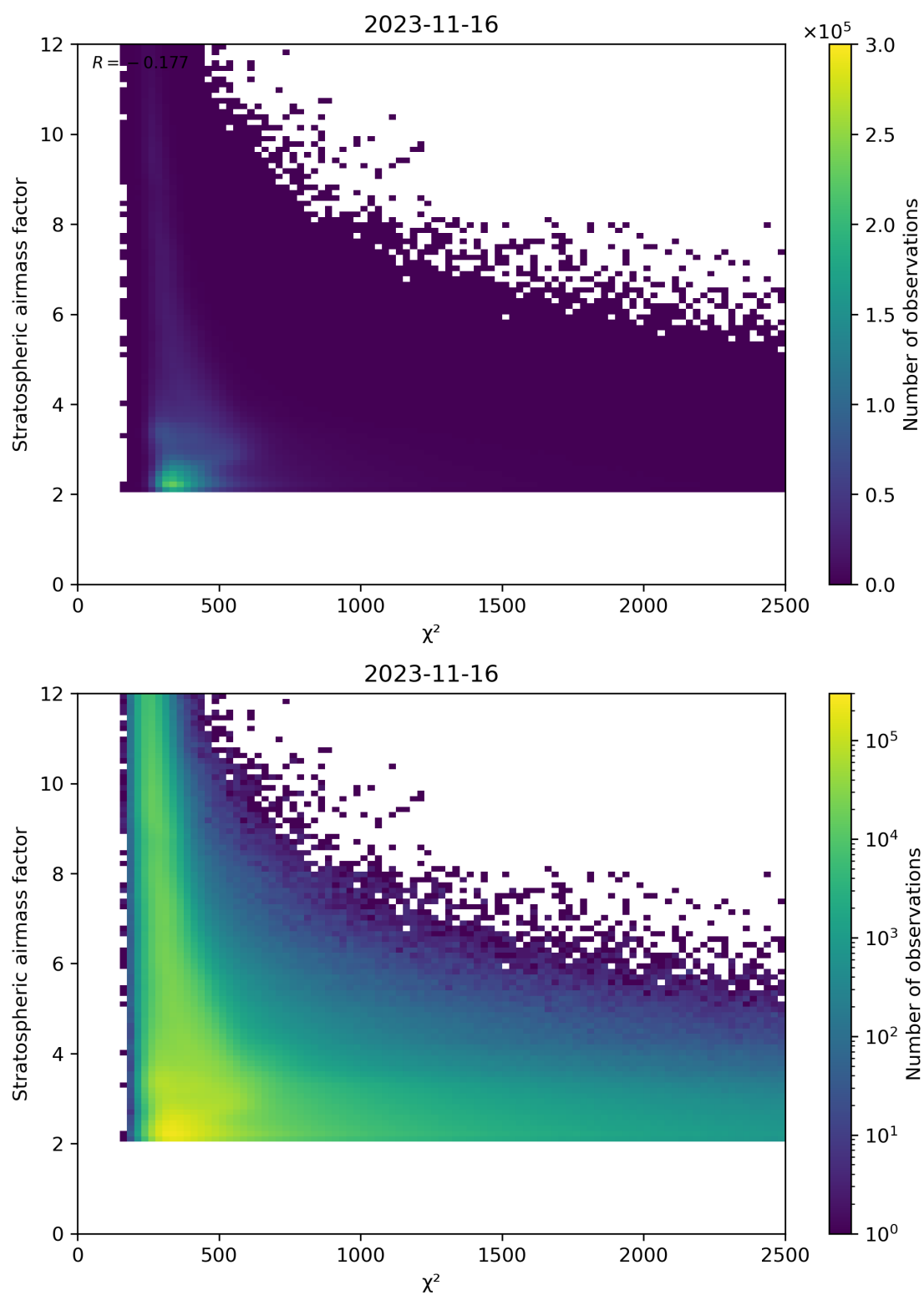
Figure 81: Scatter density plot of “ \chi^2 ” against “Stratospheric airmass factor” for 2023-11-15 to 2023-11-17.
