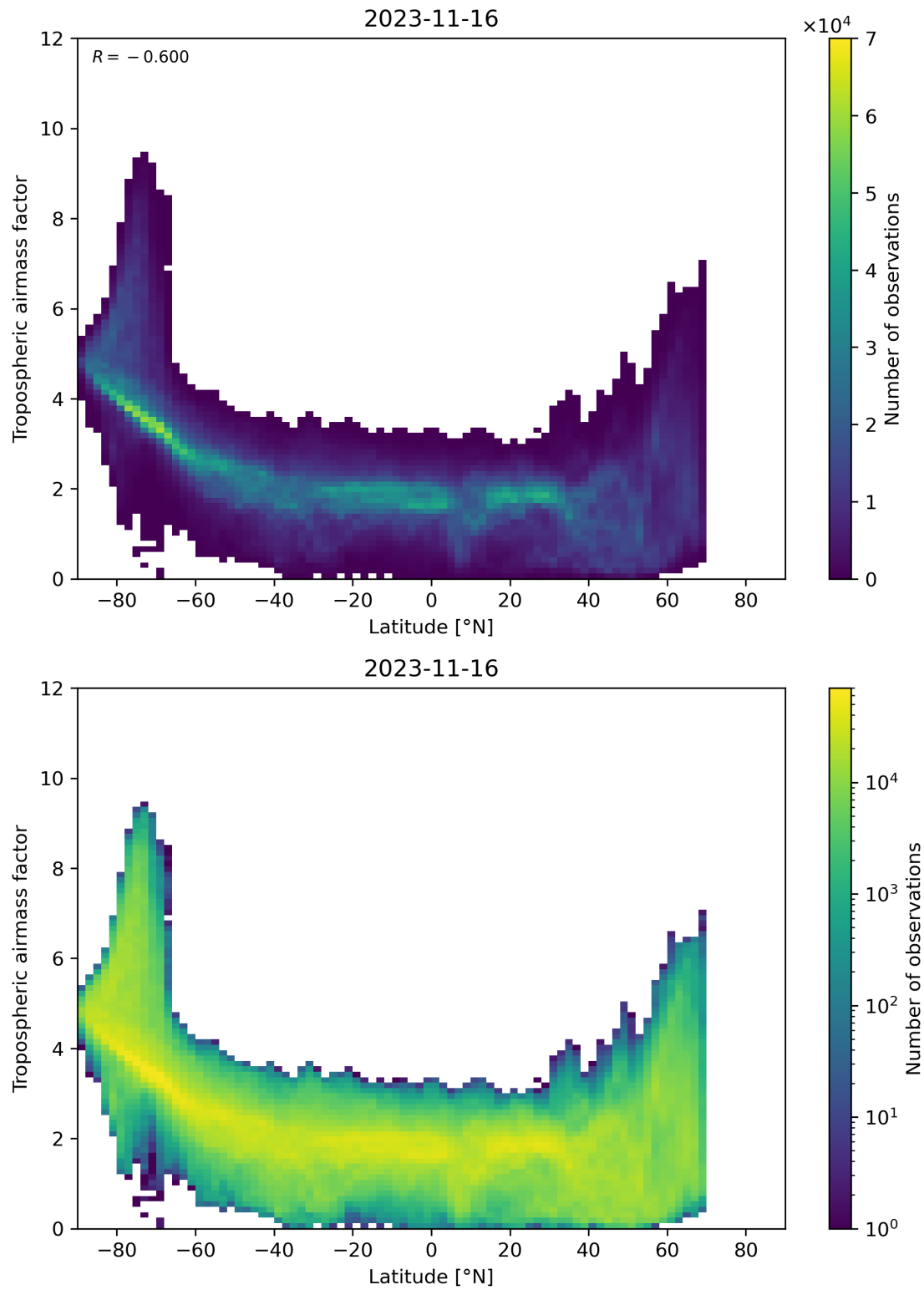
Figure 85: Scatter density plot of “Latitude” against “Tropospheric air mass factor” for 2023-11-15 to 2023-11-17.
