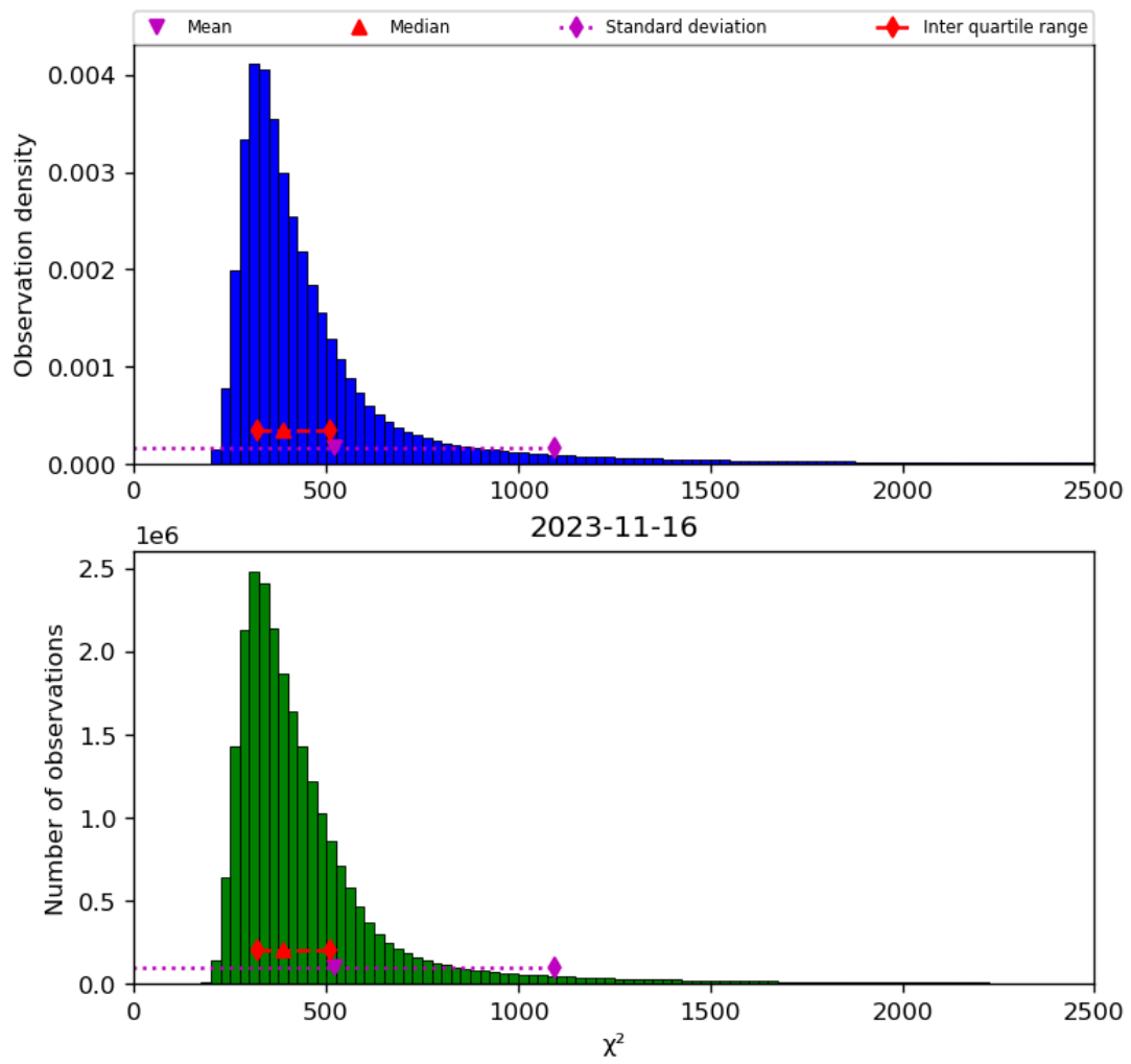
Figure 42: Histogram of “ \chi^2 ” for 2023-11-15 to 2023-11-17
