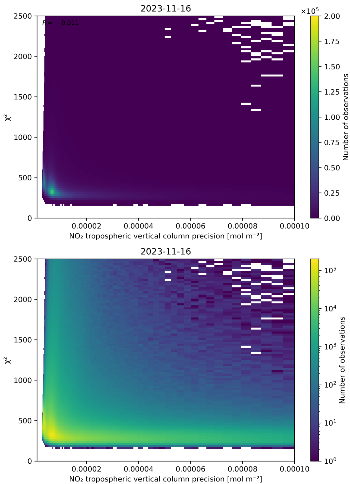
Figure 134: Scatter density plot of “NO 2 tropospheric vertical column precision” against “ \chi^2 ” for 2023-11-15 to 2023-11-17.
