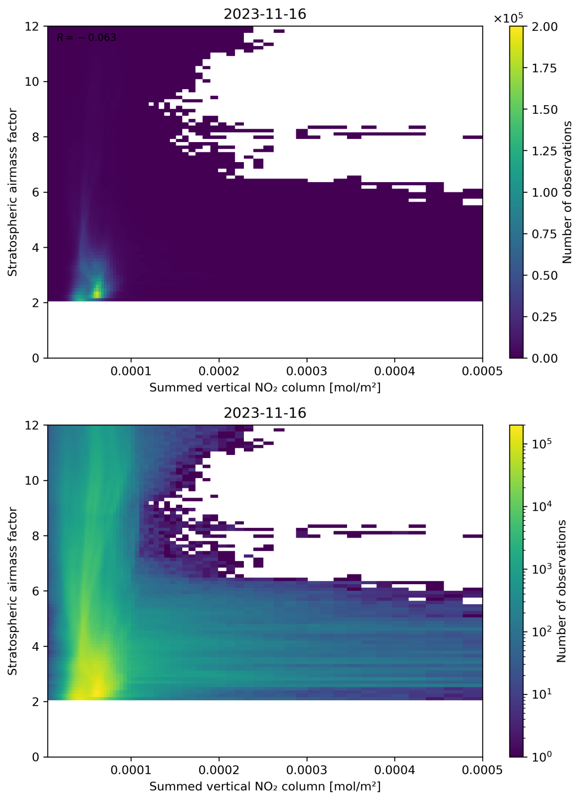
Figure 103: Scatter density plot of “Summed vertical NO 2 column” against “Stratospheric air mass factor” for 2023-11-15 to 2023-11-17.
