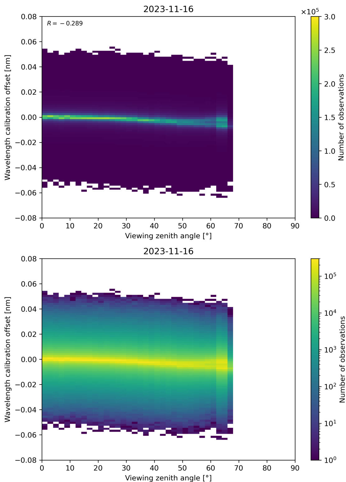
Figure 173: Scatter density plot of “Viewing zenith angle” against “Wavelength calibration offset” for 2023-11-15 to 2023-11-17.
