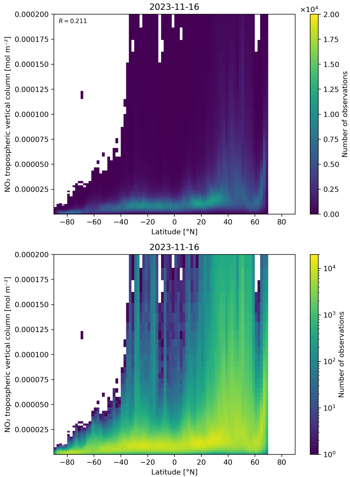
Figure 92: Scatter density plot of “Latitude” against “NO 2 tropospheric vertical column” for 2023-11-15 to 2023-11-17.
