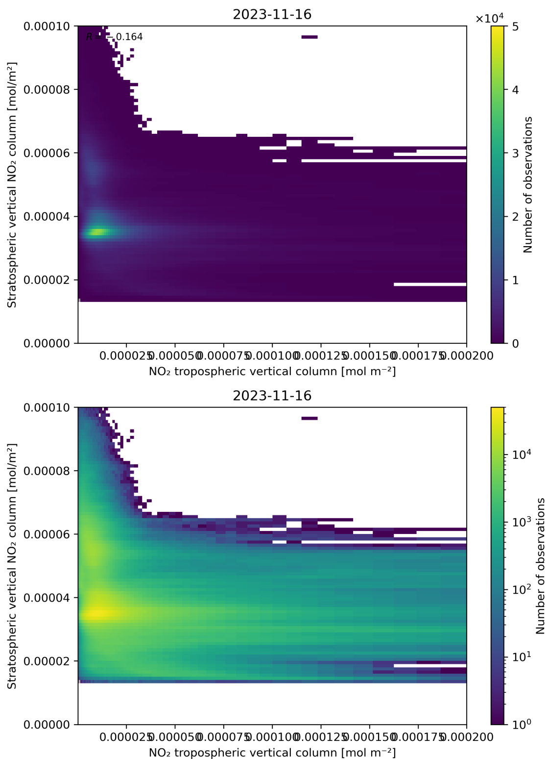
Figure 125: Scatter density plot of “NO 2 tropospheric vertical column” against “Stratospheric vertical NO 2 column” for 2023-11-15 to 2023-11-17.
