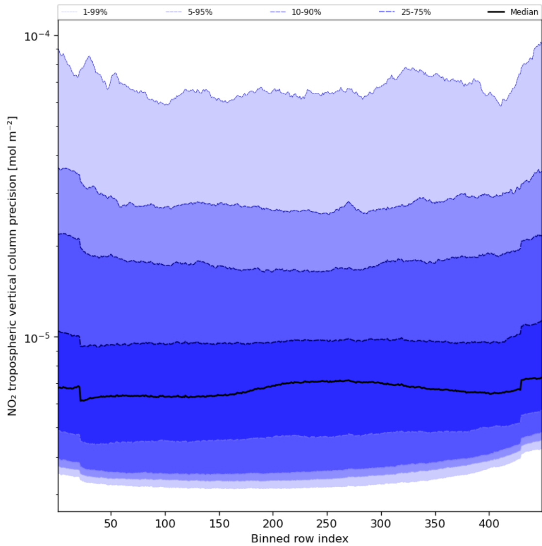
Figure 47: Along track statistics of “NO 2 tropospheric vertical column precision” for 2023-11-15 to 2023-11-17
