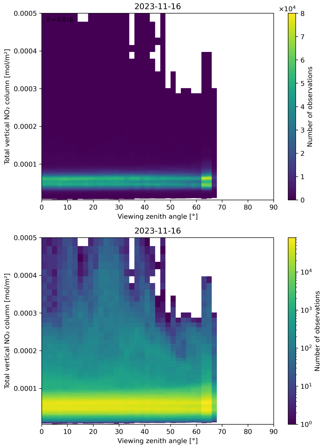
Figure 167: Scatter density plot of “Viewing zenith angle” against “Total vertical NO 2 column” for 2023-11-15 to 2023-11-17.
