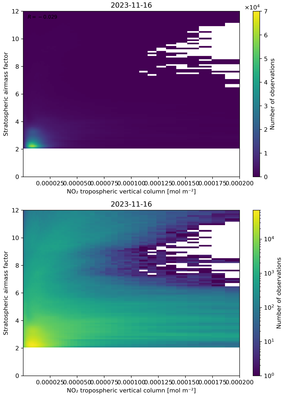
Figure 121: Scatter density plot of “NO 2 tropospheric vertical column” against “Stratospheric airmass factor” for 2023-11-15 to 2023-11-17.
