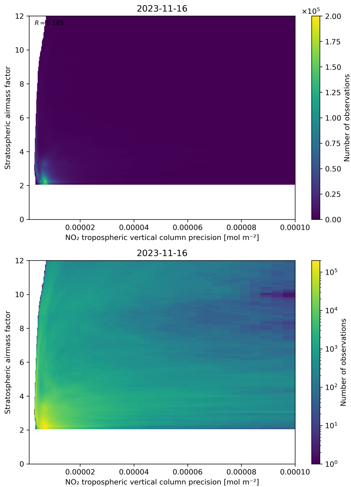
Figure 131: Scatter density plot of “NO 2 tropospheric vertical column precision” against “Stratospheric airmass factor” for 2023-11-15 to 2023-11-17.
