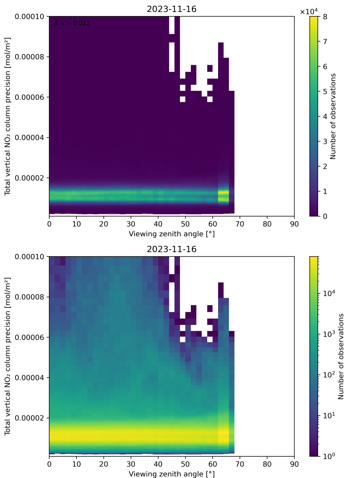
Figure 168: Scatter density plot of “Viewing zenith angle” against “Total vertical NO 2 column precision” for 2023-11-15 to 2023-11-17.
