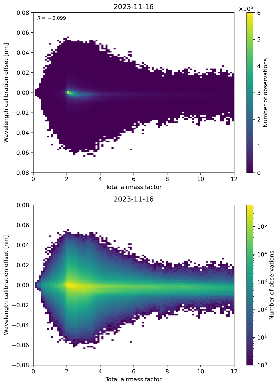
Figure 70: Scatter density plot of “Total airmass factor” against “Wavelength calibration offset” for 2023-11-15 to 2023-11-17.
