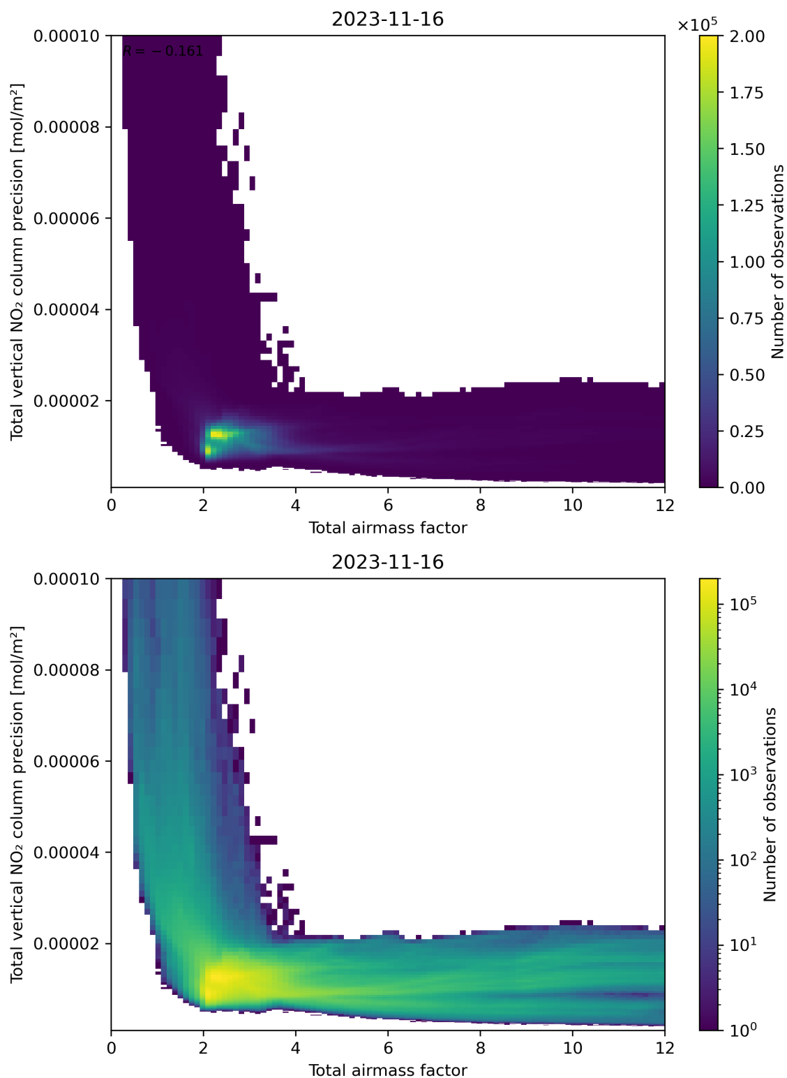
Figure 68: Scatter density plot of “Total airmass factor” against “Total vertical NO 2 column precision” for 2023-11-15 to 2023-11-17.
