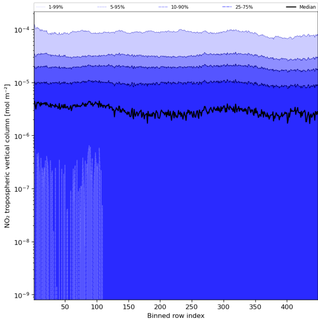
Figure 46: Along track statistics of “NO 2 tropospheric vertical column” for 2023-11-15 to 2023-11-17
