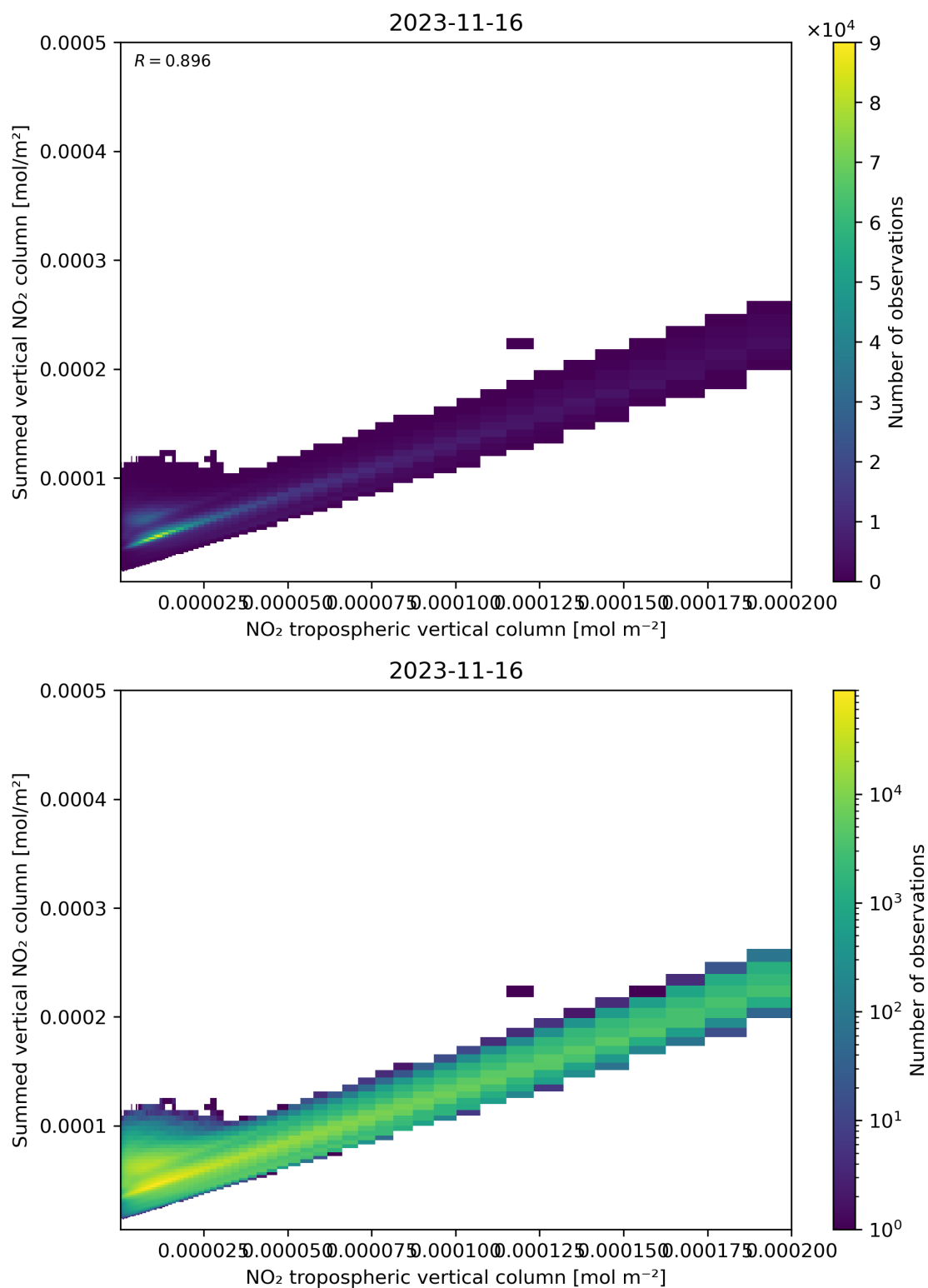
Figure 126: Scatter density plot of “NO 2 tropospheric vertical column” against “Summed vertical NO 2 column” for 2023-11-15 to 2023-11-17.
