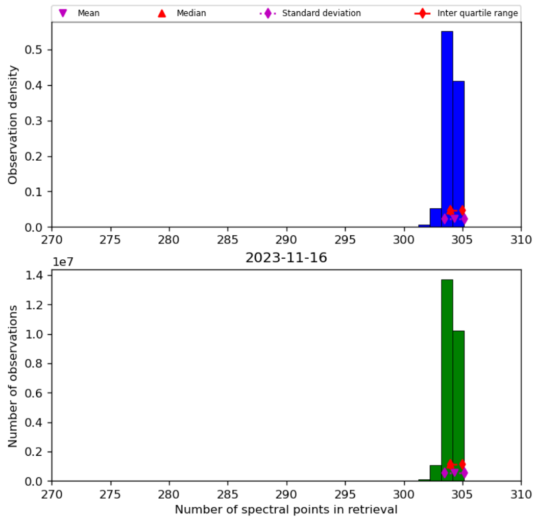
Figure 33: Histogram of “Number of spectral points in retrieval” for 2023-11-15 to 2023-11-17
