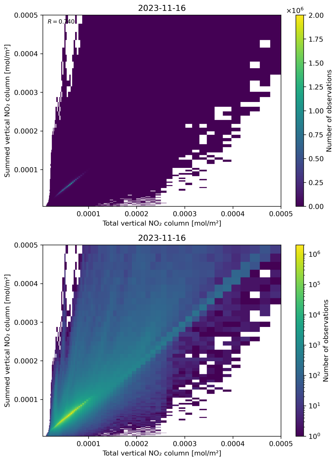
Figure 112: Scatter density plot of “Total vertical NO 2 column” against “Summed vertical NO 2 column” for 2023-11-15 to 2023-11-17.
