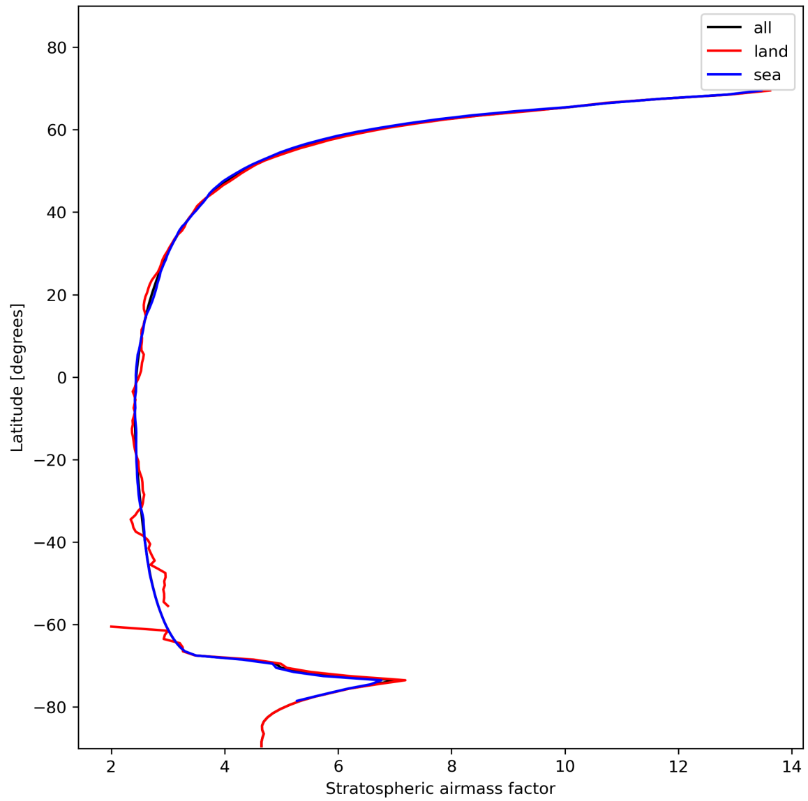
Figure 27: Zonal average of “Stratospheric air mass factor” for 2023-11-15 to 2023-11-17.
