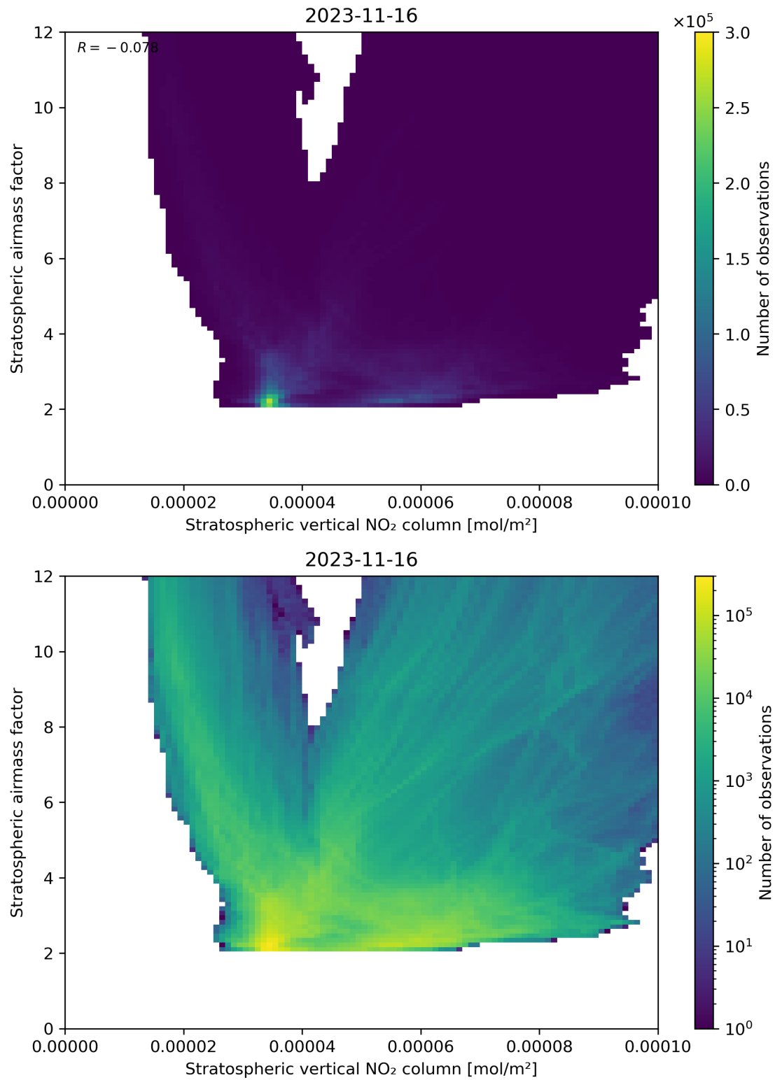
Figure 96: Scatter density plot of “Stratospheric vertical NO 2 column” against “Stratospheric airmass factor” for 2023-11-15 to 2023-11-17.
