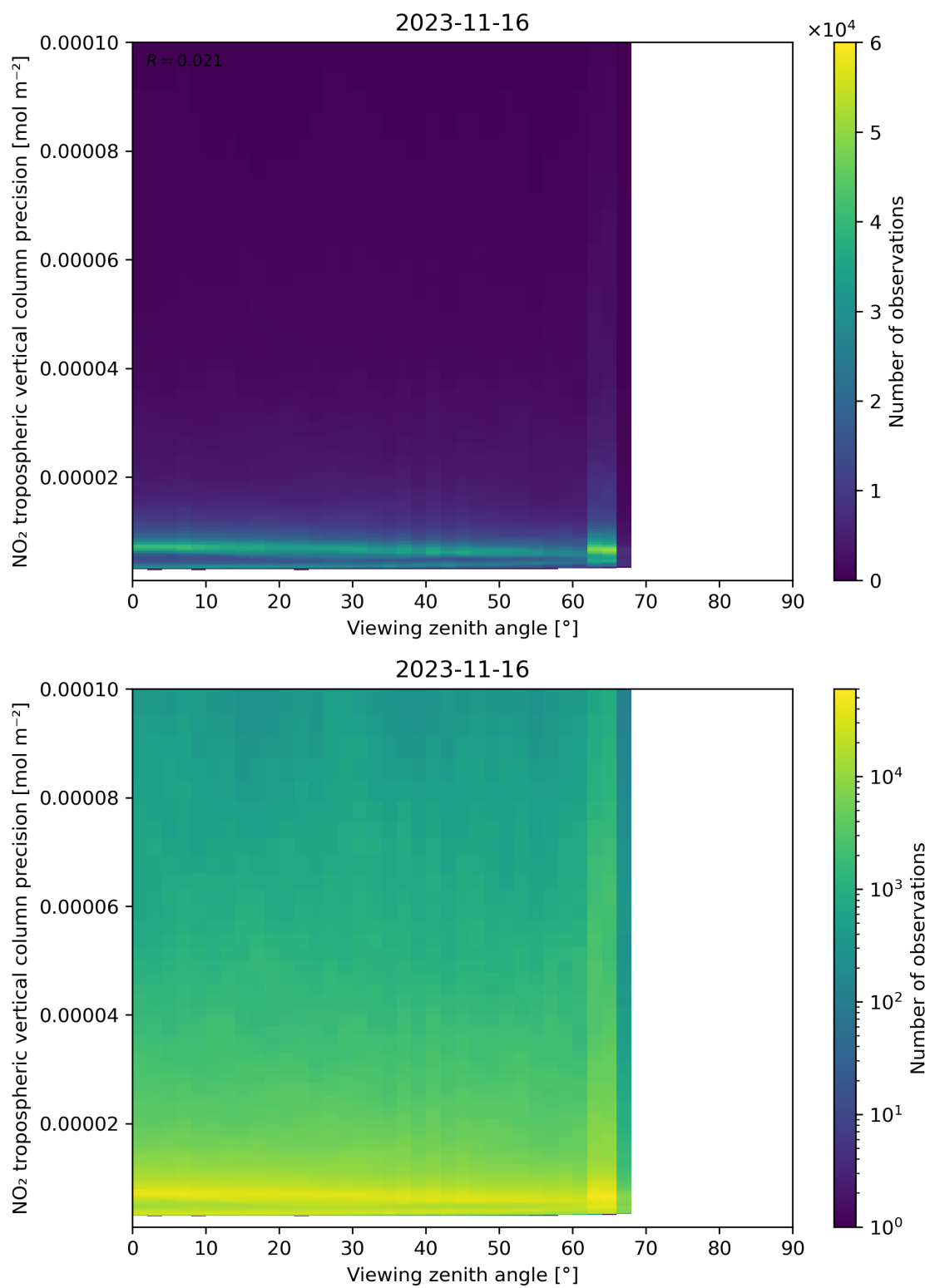
Figure 170: Scatter density plot of “Viewing zenith angle” against “NO 2 tropospheric vertical column precision” for 2023-11-15 to 2023-11-17.
