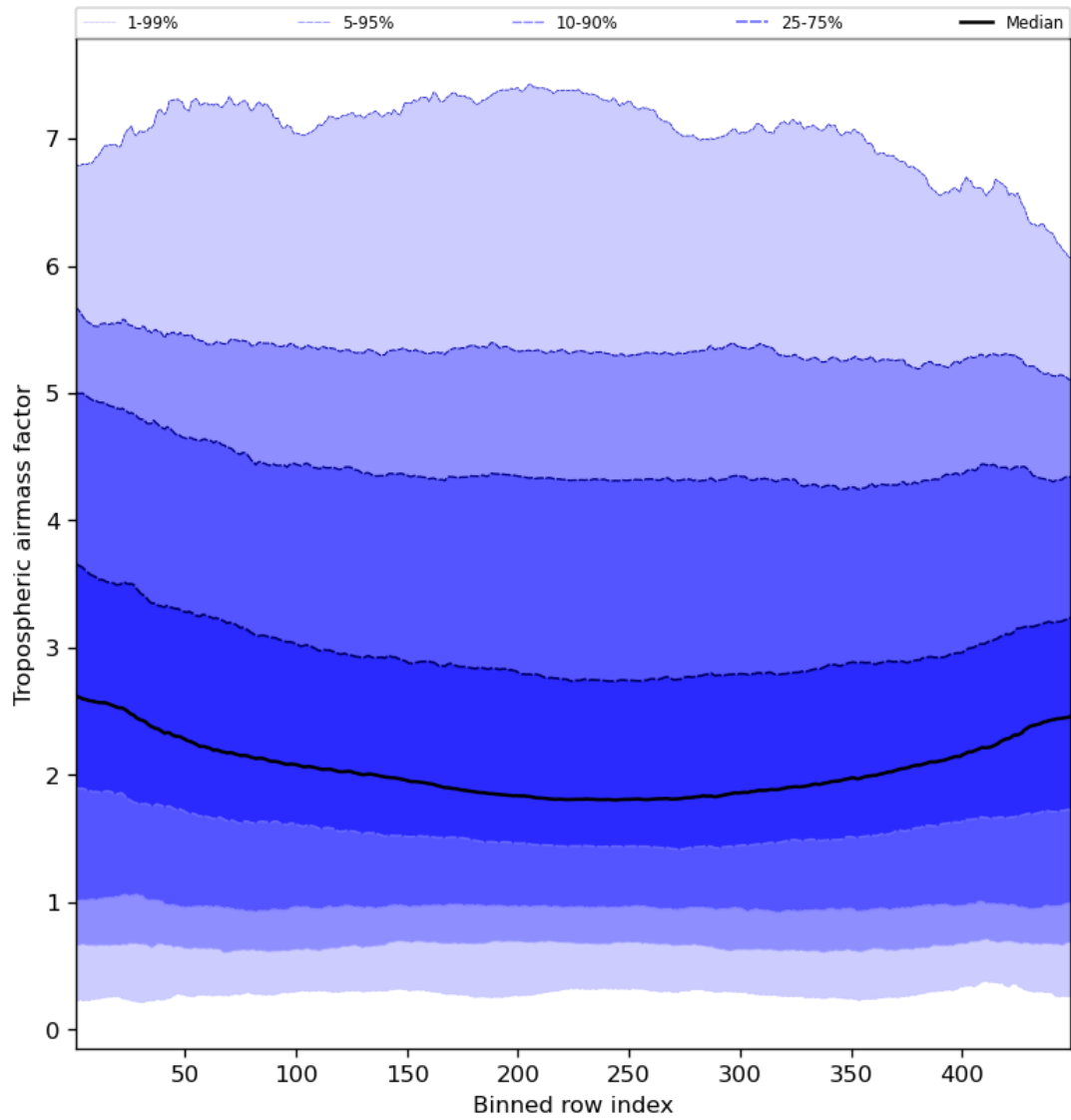
Figure 48: Along track statistics of “Tropospheric air mass factor” for 2023-11-15 to 2023-11-17
