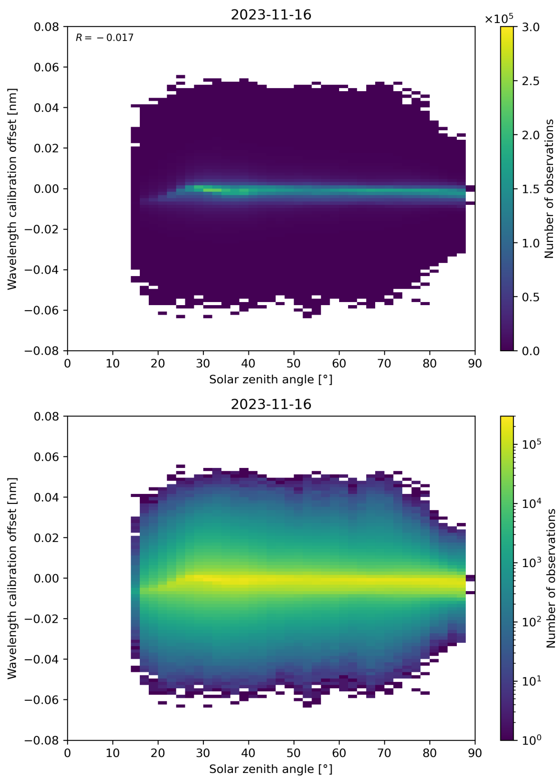
Figure 158: Scatter density plot of “Solar zenith angle” against “Wavelength calibration offset” for 2023-11-15 to 2023-11-17.
