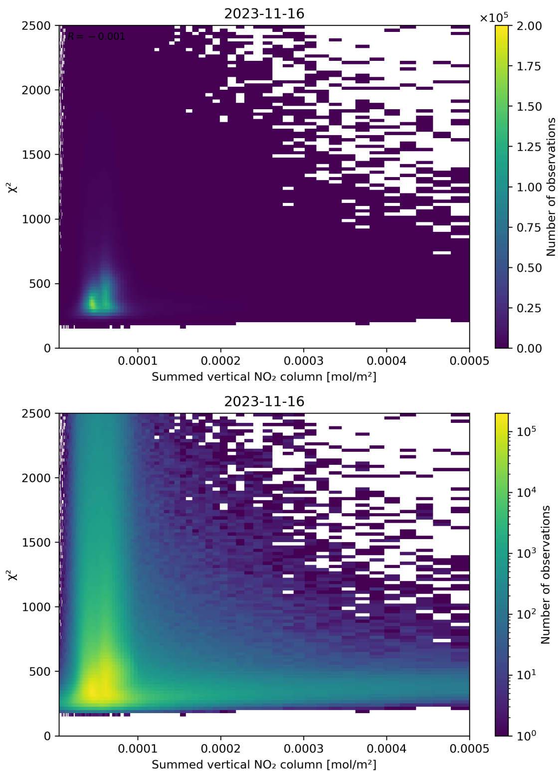
Figure 104: Scatter density plot of “Summed vertical NO 2 column” against “ \chi^2 ” for 2023-11-15 to 2023-11-17.
