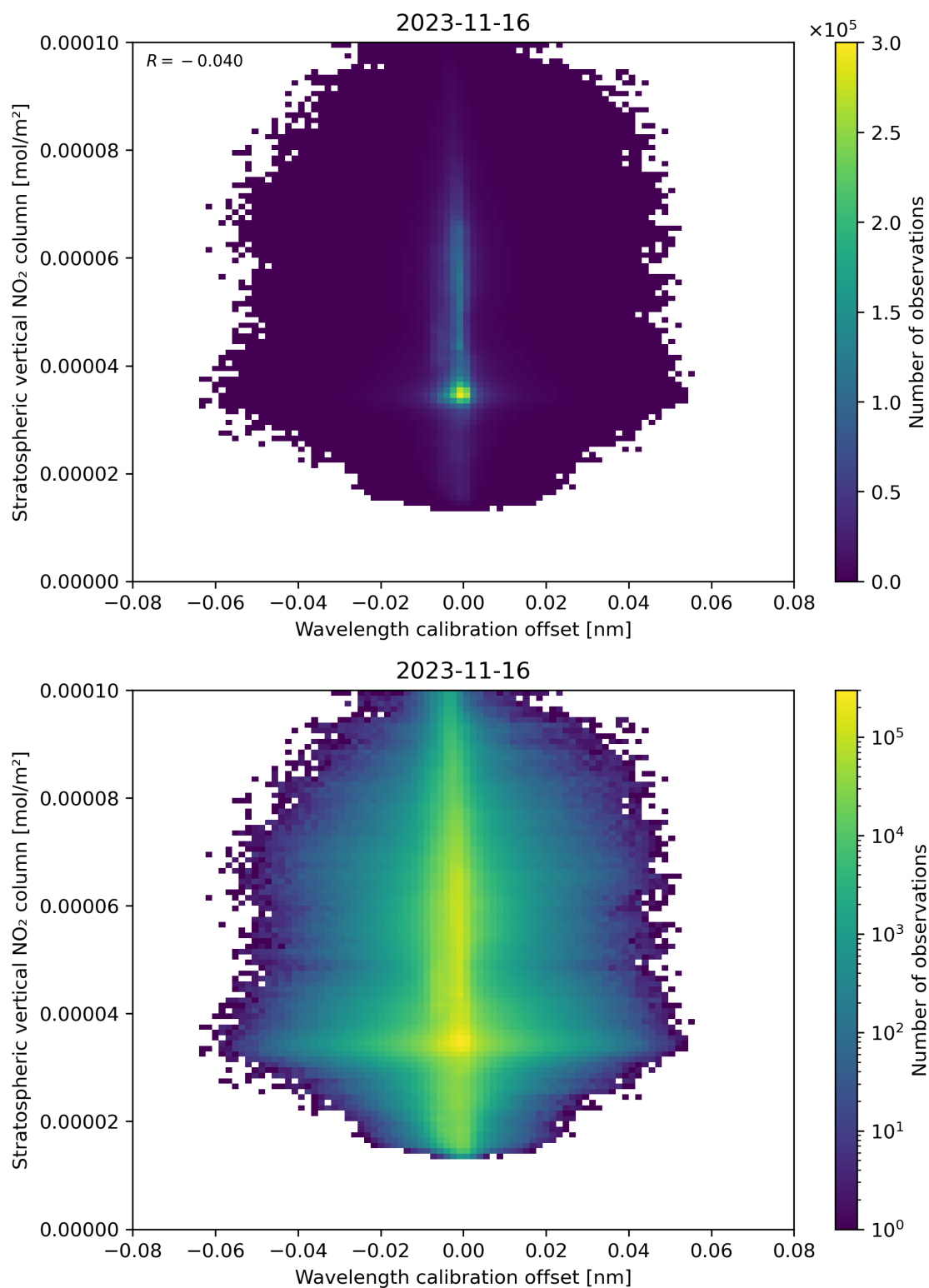
Figure 176: Scatter density plot of “Wavelength calibration offset” against “Stratospheric vertical NO 2 column” for 2023-11-15 to 2023-11-17.
