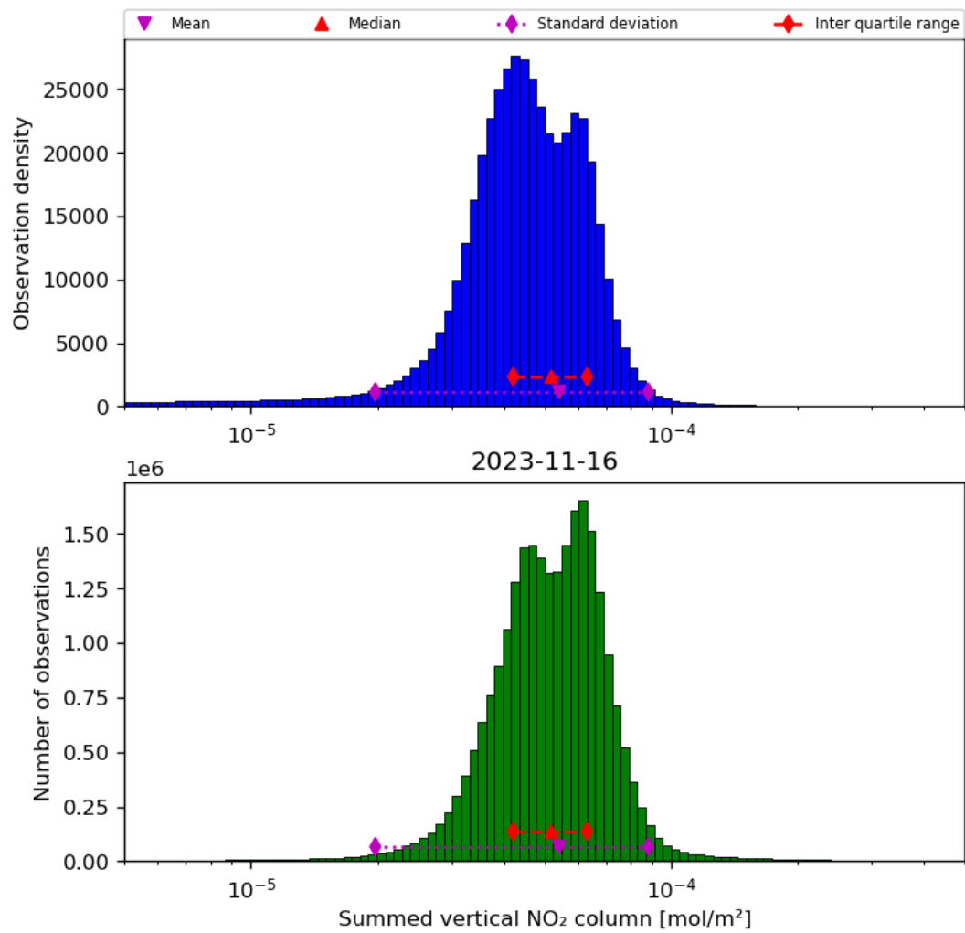
Figure 40: Histogram of “Summed vertical NO 2 column” for 2023-11-15 to 2023-11-17
