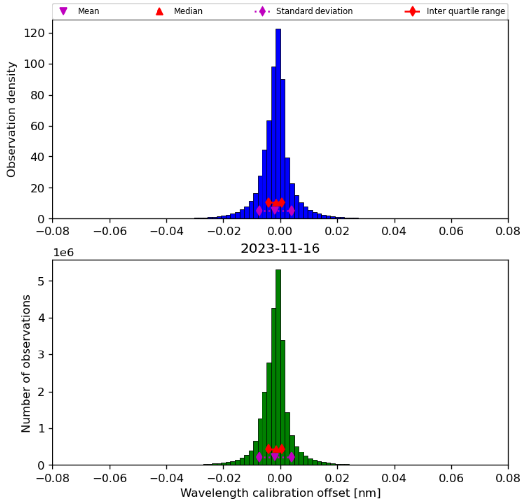
Figure 35: Histogram of “Wavelength calibration offset” for 2023-11-15 to 2023-11-17
