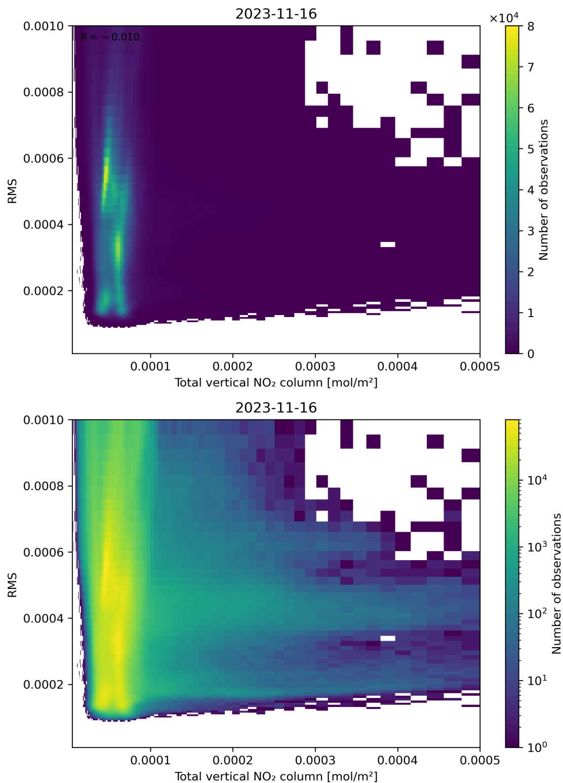
Figure 120: Scatter density plot of “Total vertical NO 2 column” against “RMS” for 2023-11-15 to 2023-11-17.
