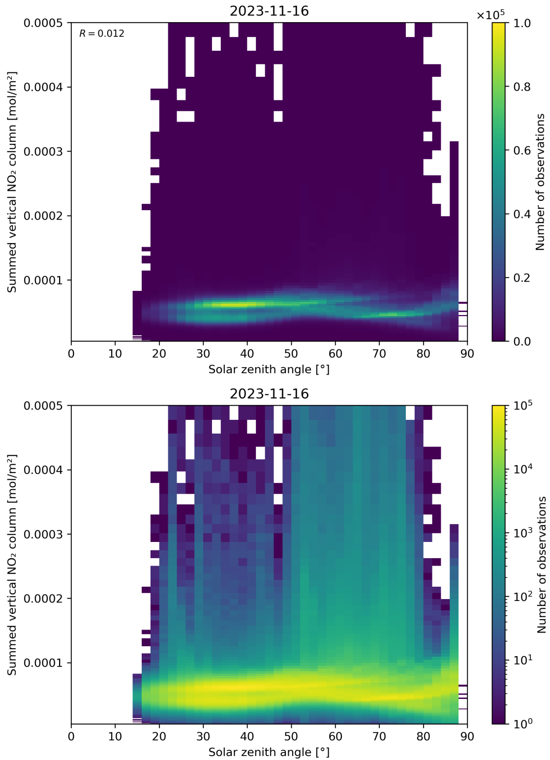
Figure 151: Scatter density plot of “Solar zenith angle” against “Summed vertical NO 2 column” for 2023-11-15 to 2023-11-17.
