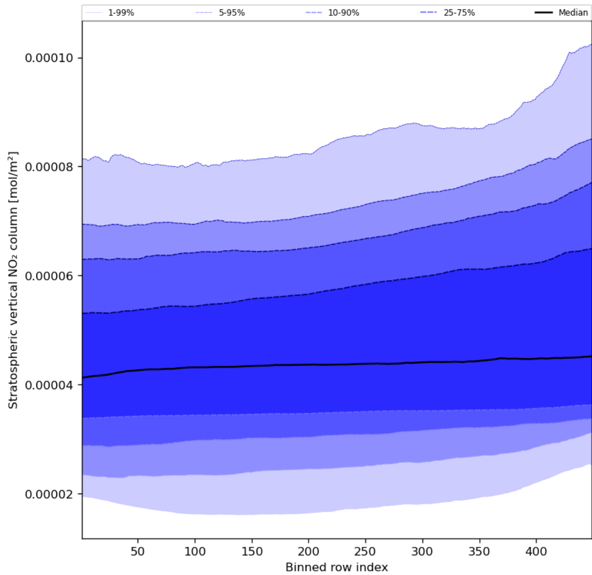
Figure 53: Along track statistics of “Stratospheric vertical NO 2 column” for 2023-11-15 to 2023-11-17
