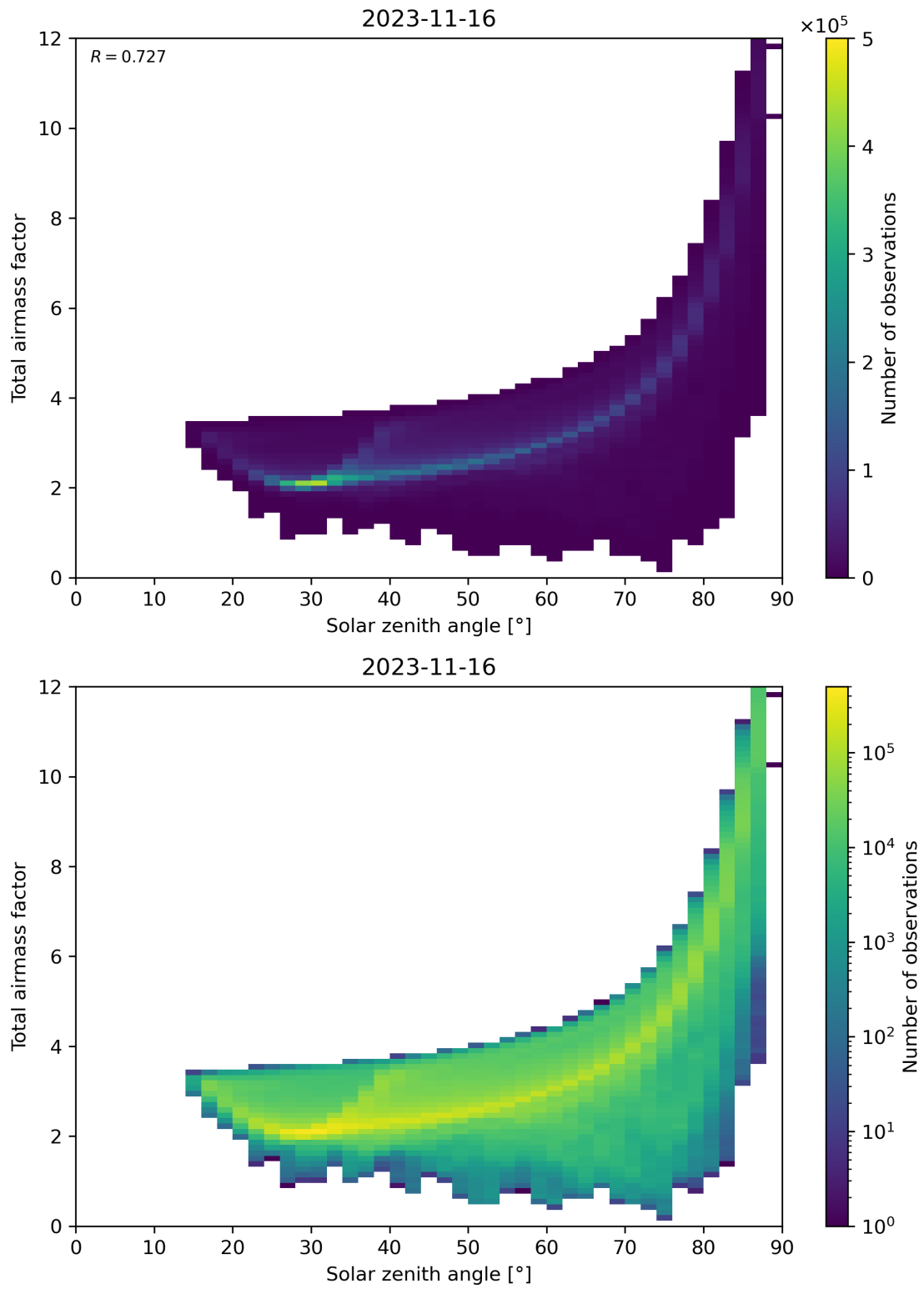
Figure 146: Scatter density plot of “Solar zenith angle” against “Total airmass factor” for 2023-11-15 to 2023-11-17.
