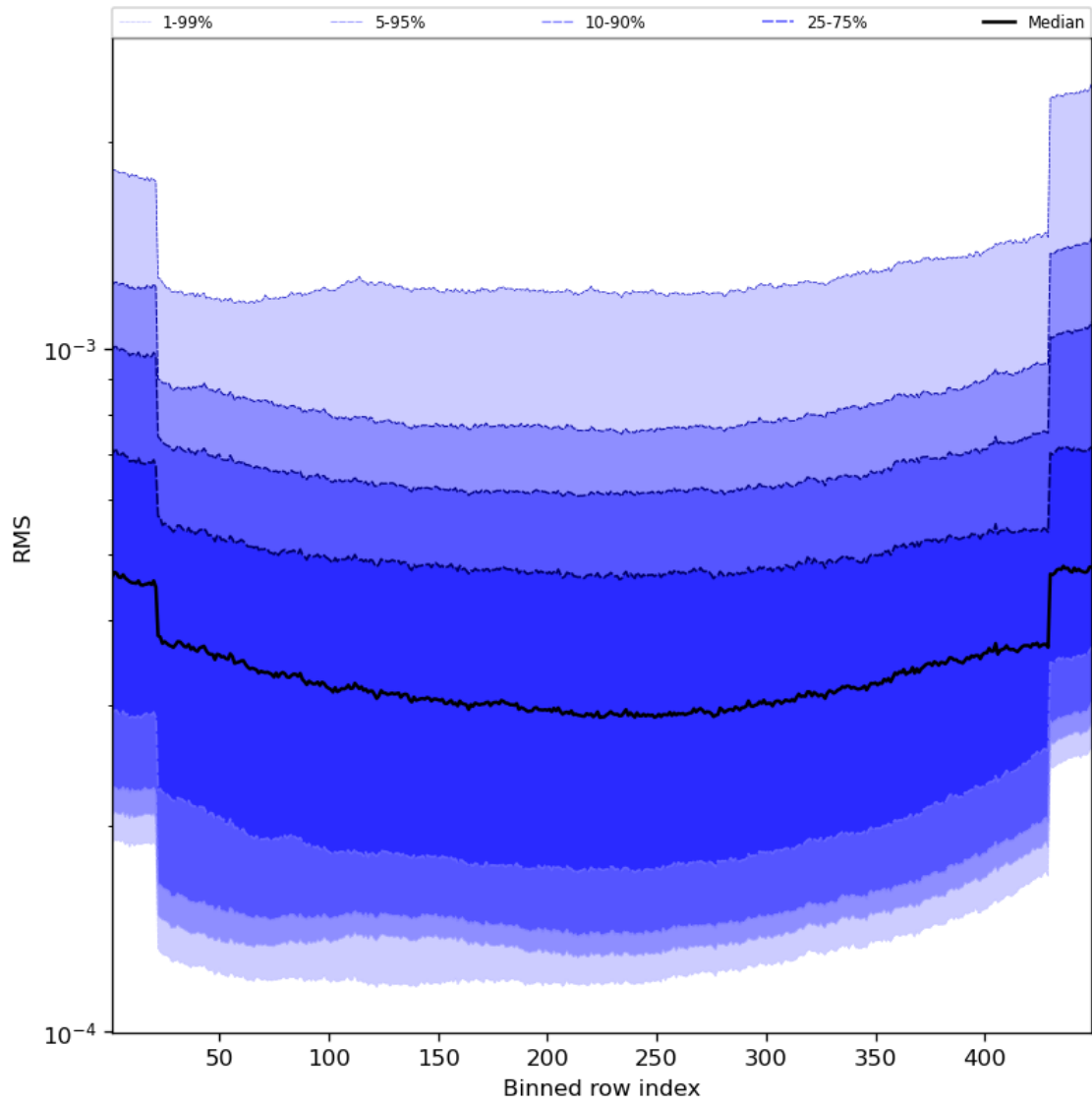
Figure 60: Along track statistics of “RMS” for 2023-11-15 to 2023-11-17
