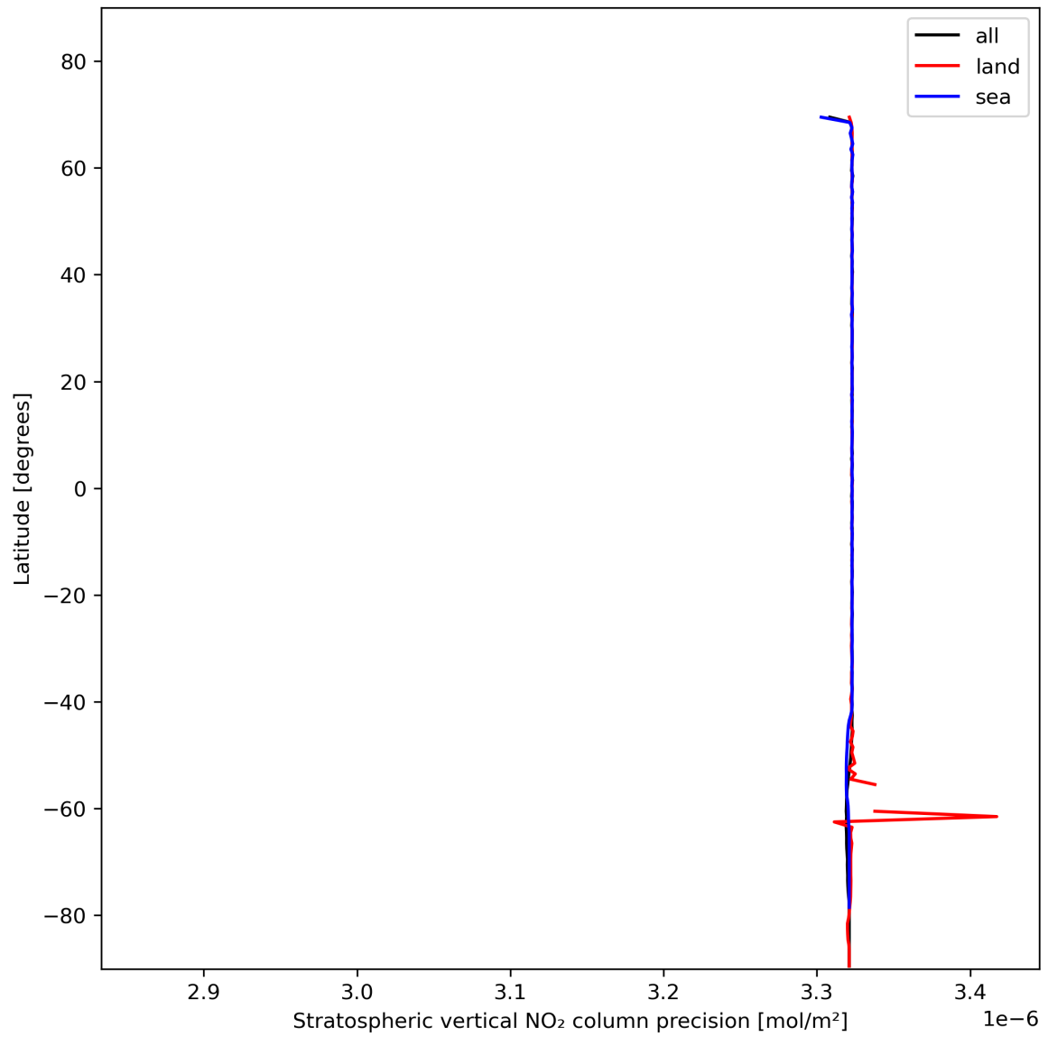
Figure 20: Zonal average of “Stratospheric vertical NO 2 column precision” for 2023-11-15 to 2023-11-17.
