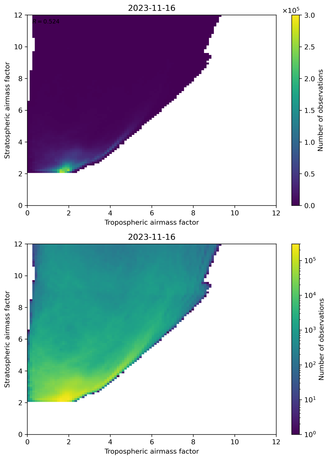
Figure 71: Scatter density plot of “Tropospheric airmass factor” against “Stratospheric airmass factor” for 2023-11-15 to 2023-11-17.
