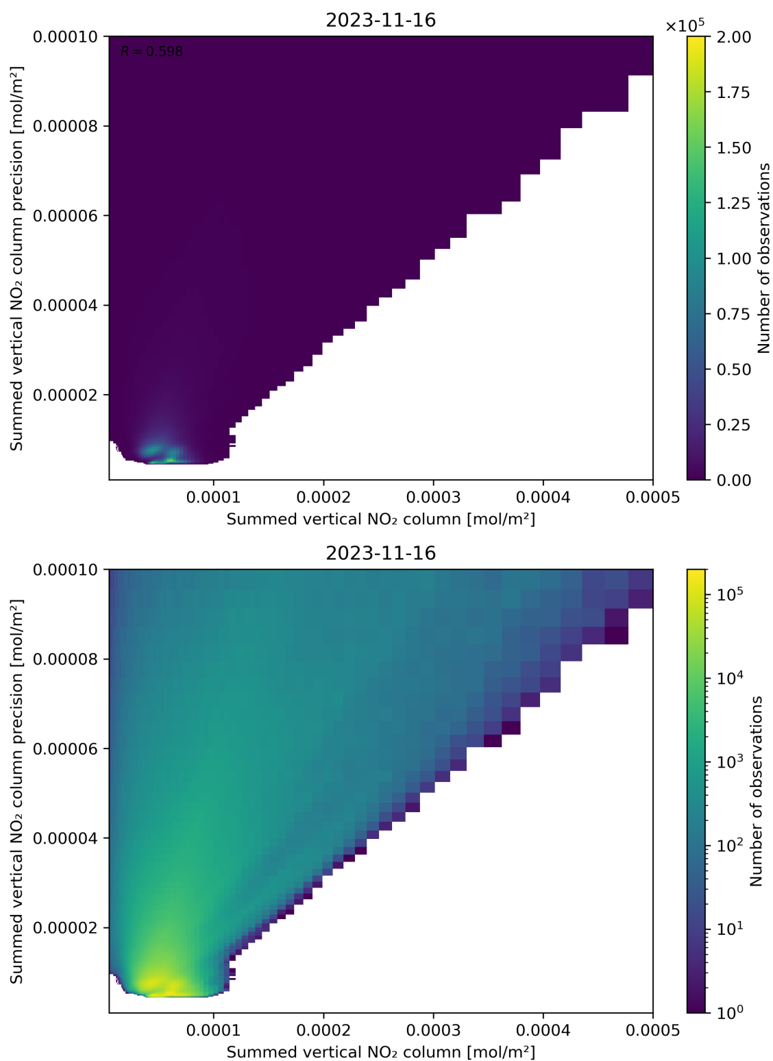
Figure 105: Scatter density plot of “Summed vertical NO 2 column” against “Summed vertical NO 2 column precision” for 2023-11-15 to 2023-11-17.
