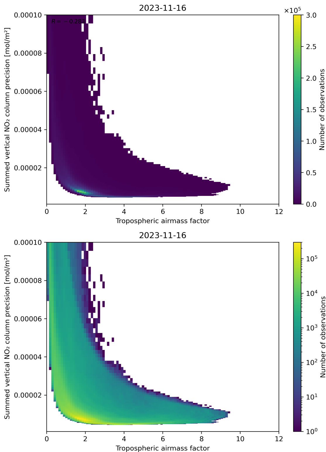
Figure 76: Scatter density plot of “Tropospheric air mass factor” against “Summed vertical NO 2 column precision” for 2023-11-15 to 2023-11-17.
