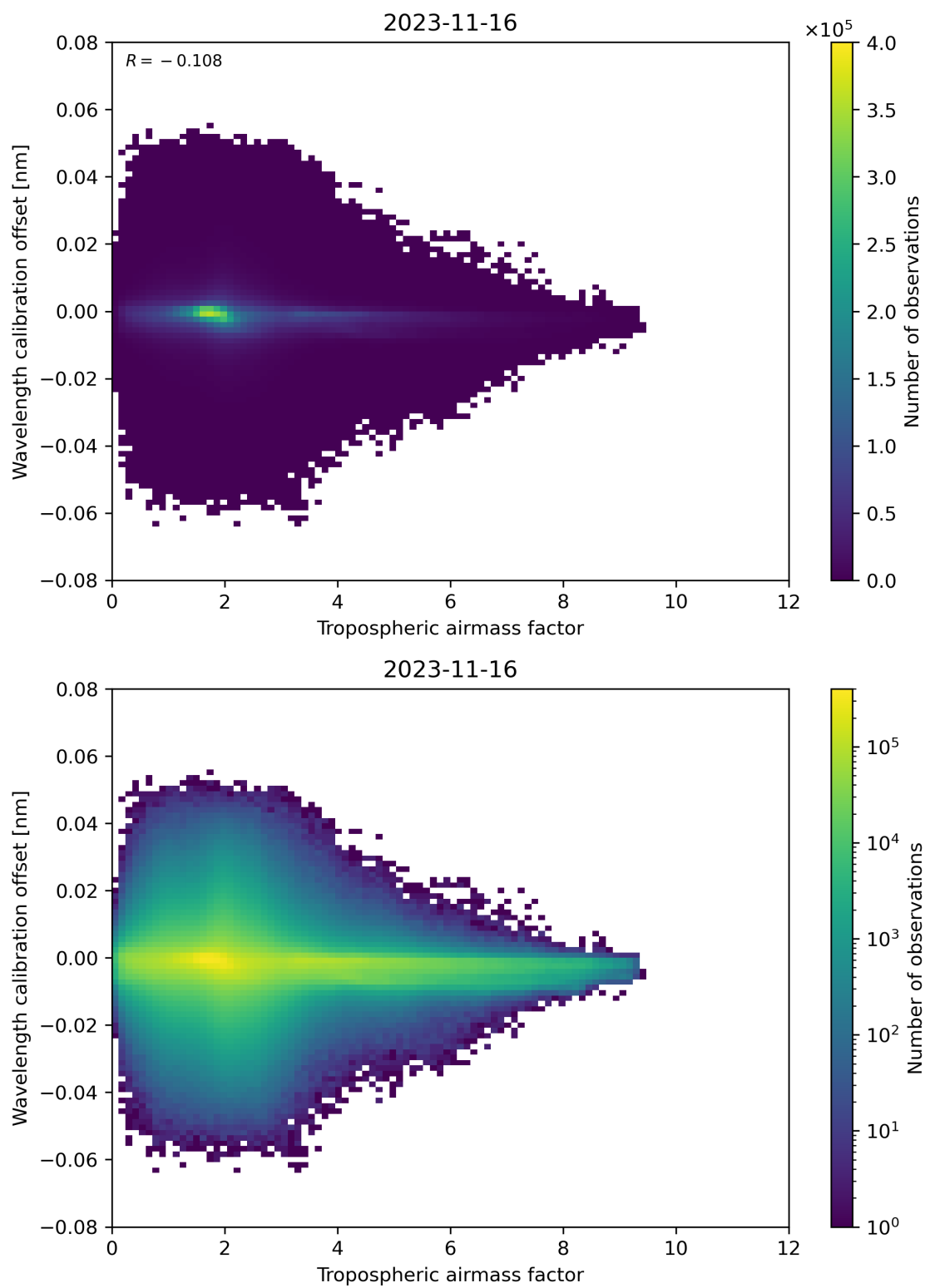
Figure 80: Scatter density plot of “Tropospheric airmass factor” against “Wavelength calibration offset” for 2023-11-15 to 2023-11-17.
