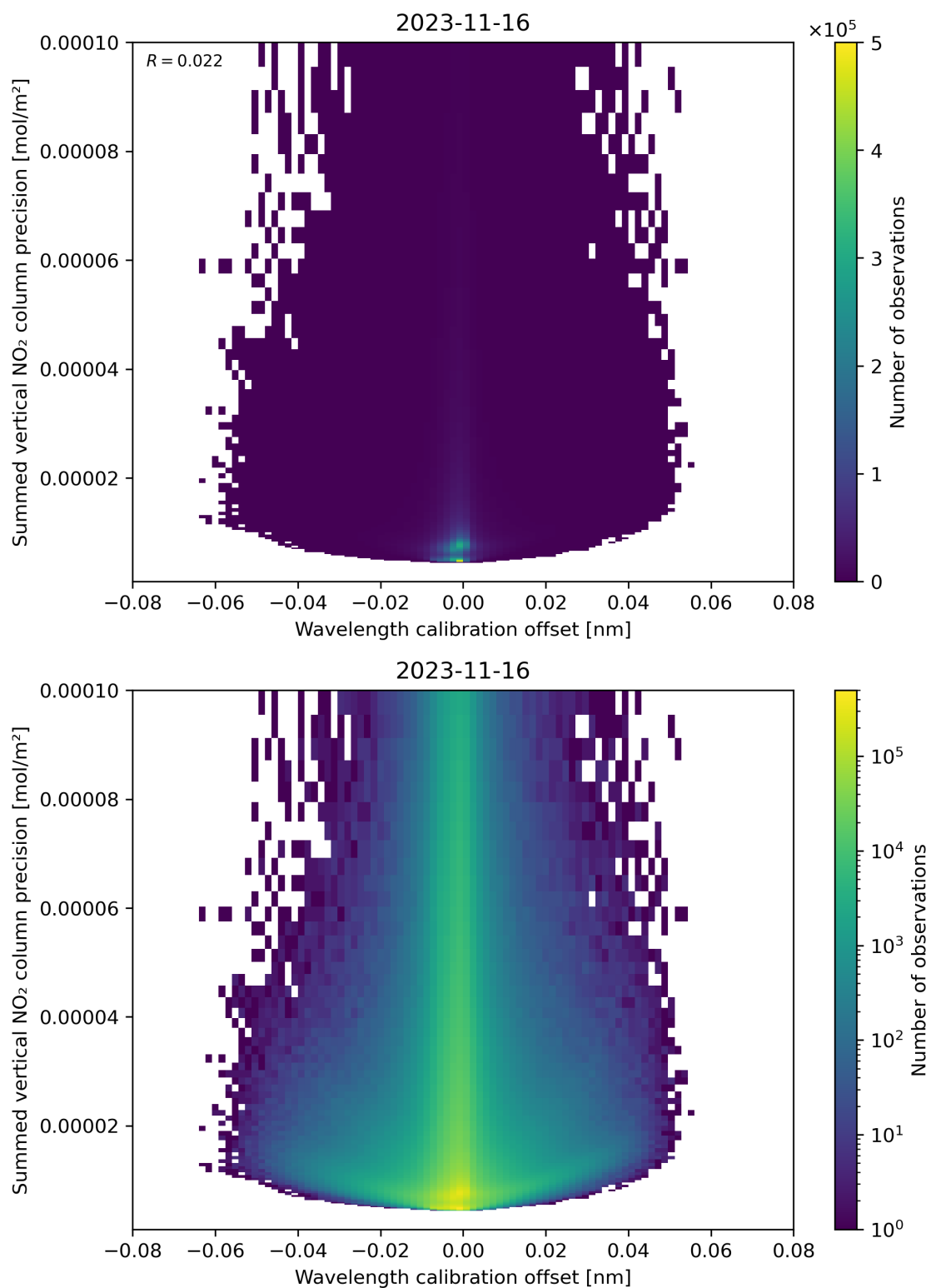
Figure 178: Scatter density plot of “Wavelength calibration offset” against “Summed vertical NO 2 column precision” for 2023-11-15 to 2023-11-17.
