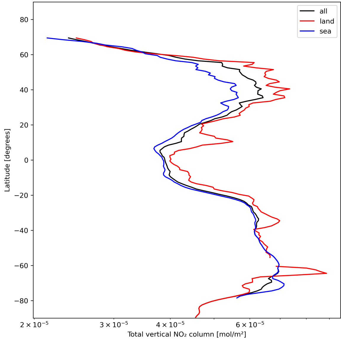
Figure 21: Zonal average of “Total vertical NO 2 column” for 2023-11-15 to 2023-11-17.
