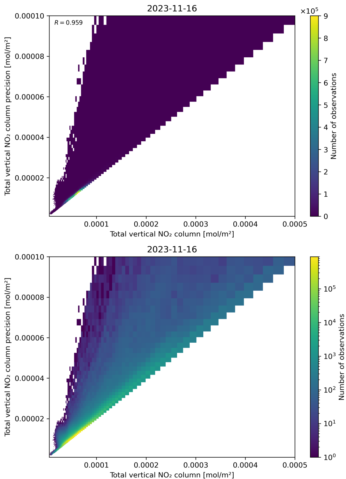
Figure 114: Scatter density plot of “Total vertical NO 2 column” against “Total vertical NO 2 column precision” for 2023-11-15 to 2023-11-17.
