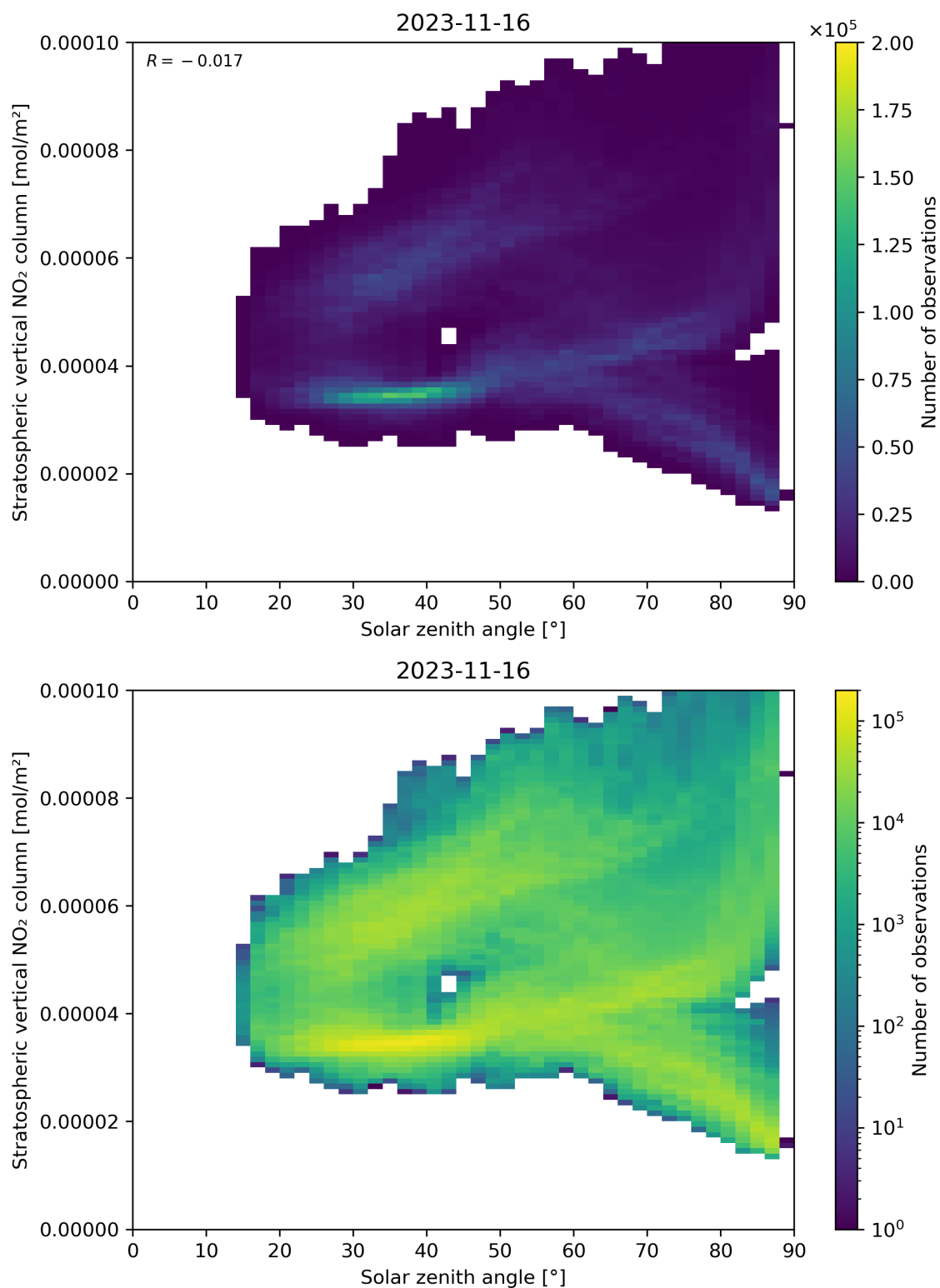
Figure 150: Scatter density plot of “Solar zenith angle” against “Stratospheric vertical NO 2 column” for 2023-11-15 to 2023-11-17.
