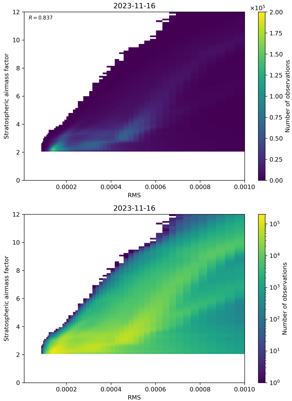
Figure 144: Scatter density plot of “RMS” against “Stratospheric airmass factor” for 2023-11-15 to 2023-11-17.
