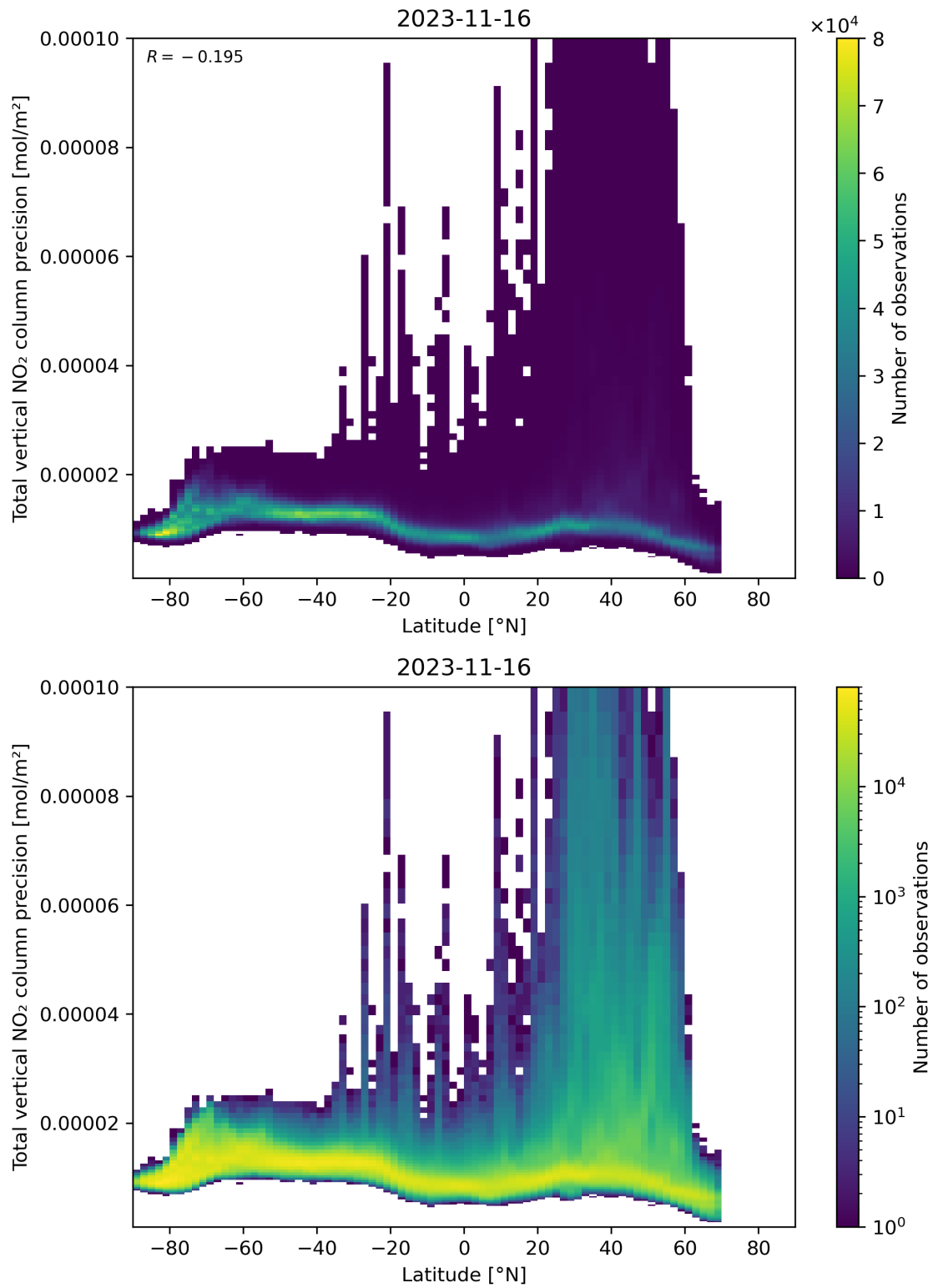
Figure 91: Scatter density plot of “Latitude” against “Total vertical NO 2 column precision” for 2023-11-15 to 2023-11-17.
