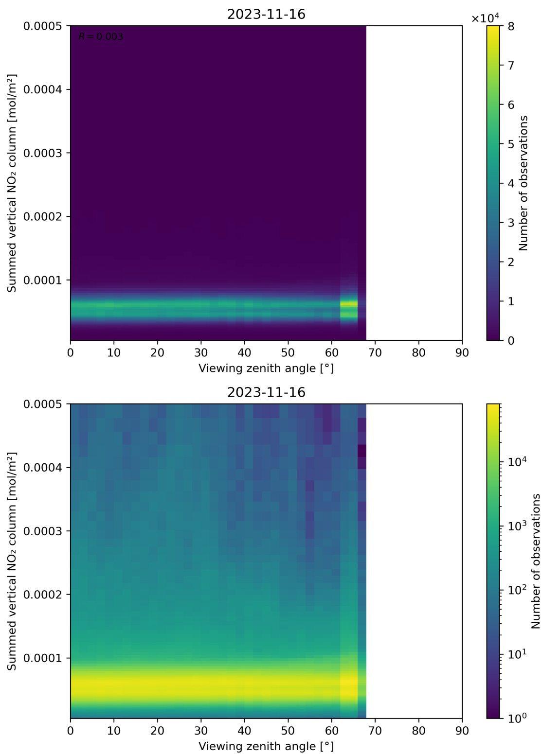
Figure 165: Scatter density plot of “Viewing zenith angle” against “Summed vertical NO 2 column” for 2023-11-15 to 2023-11-17.
