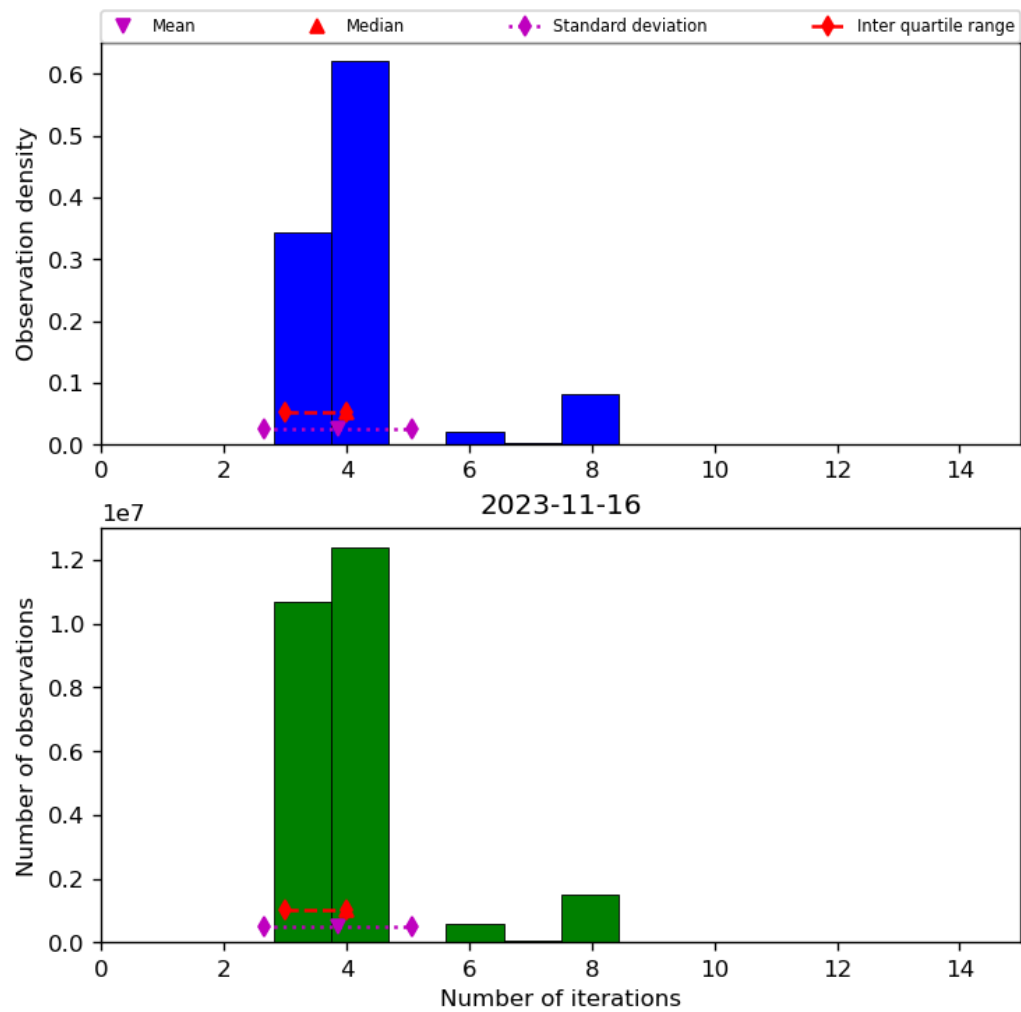
Figure 34: Histogram of “Number of iterations” for 2023-11-15 to 2023-11-17
