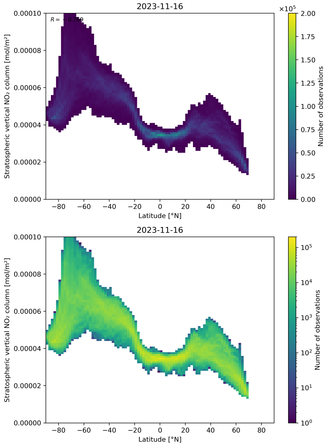
Figure 87: Scatter density plot of “Latitude” against “Stratospheric vertical NO 2 column” for 2023-11-15 to 2023-11-17.
