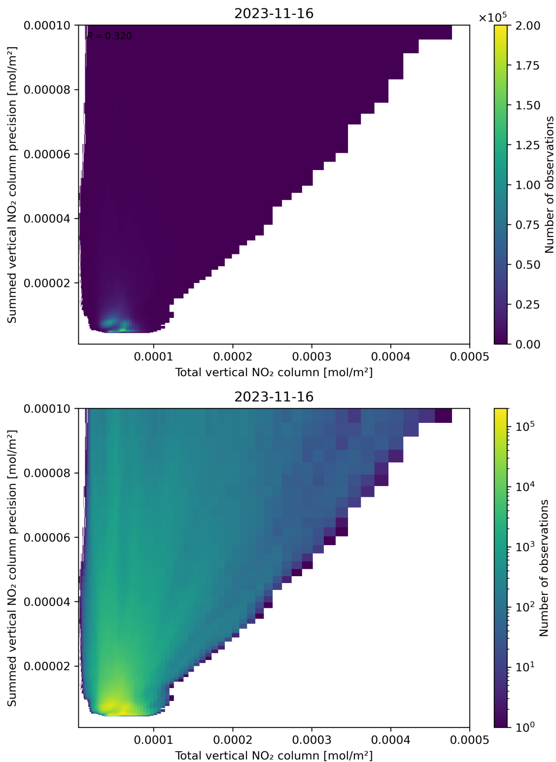
Figure 113: Scatter density plot of “Total vertical NO 2 column” against “Summed vertical NO 2 column precision” for 2023-11-15 to 2023-11-17.
