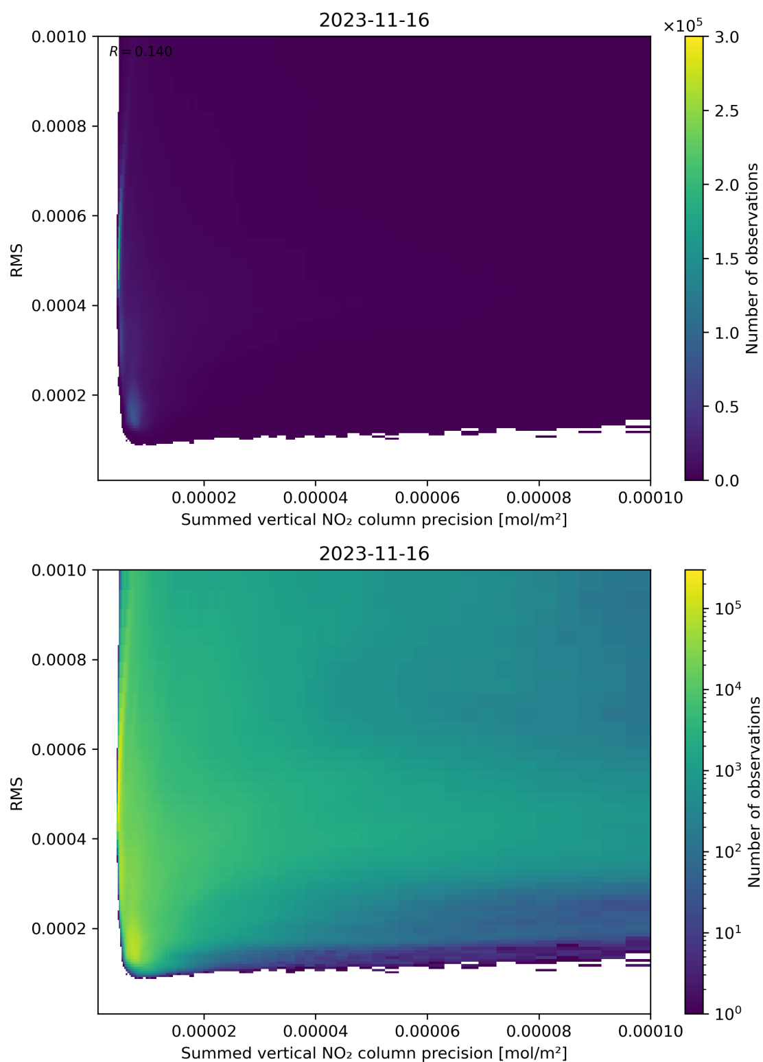
Figure 108: Scatter density plot of “Summed vertical NO 2 column precision” against “RMS” for 2023-11-15 to 2023-11-17.
