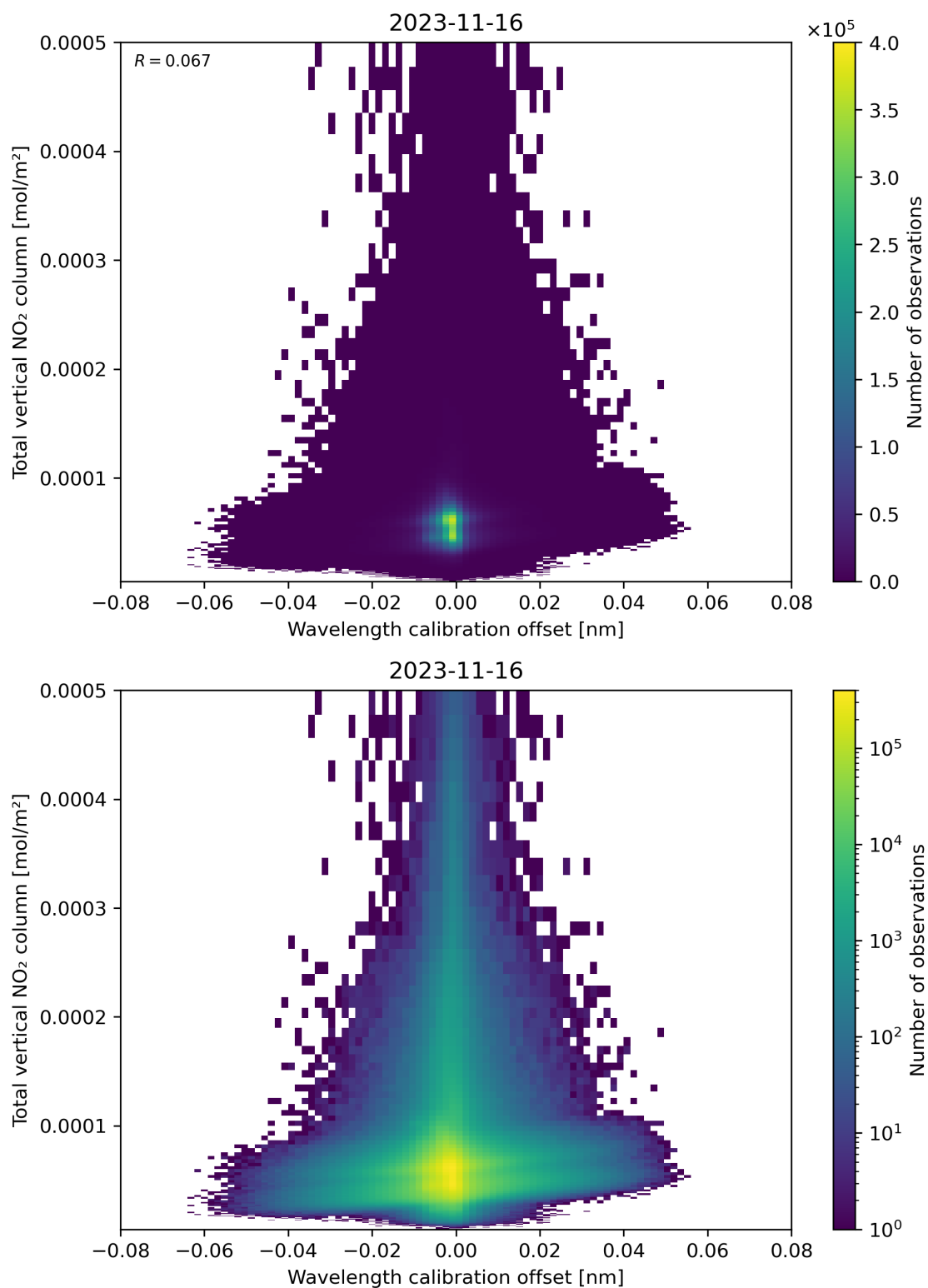
Figure 179: Scatter density plot of “Wavelength calibration offset” against “Total vertical NO 2 column” for 2023-11-15 to 2023-11-17.
