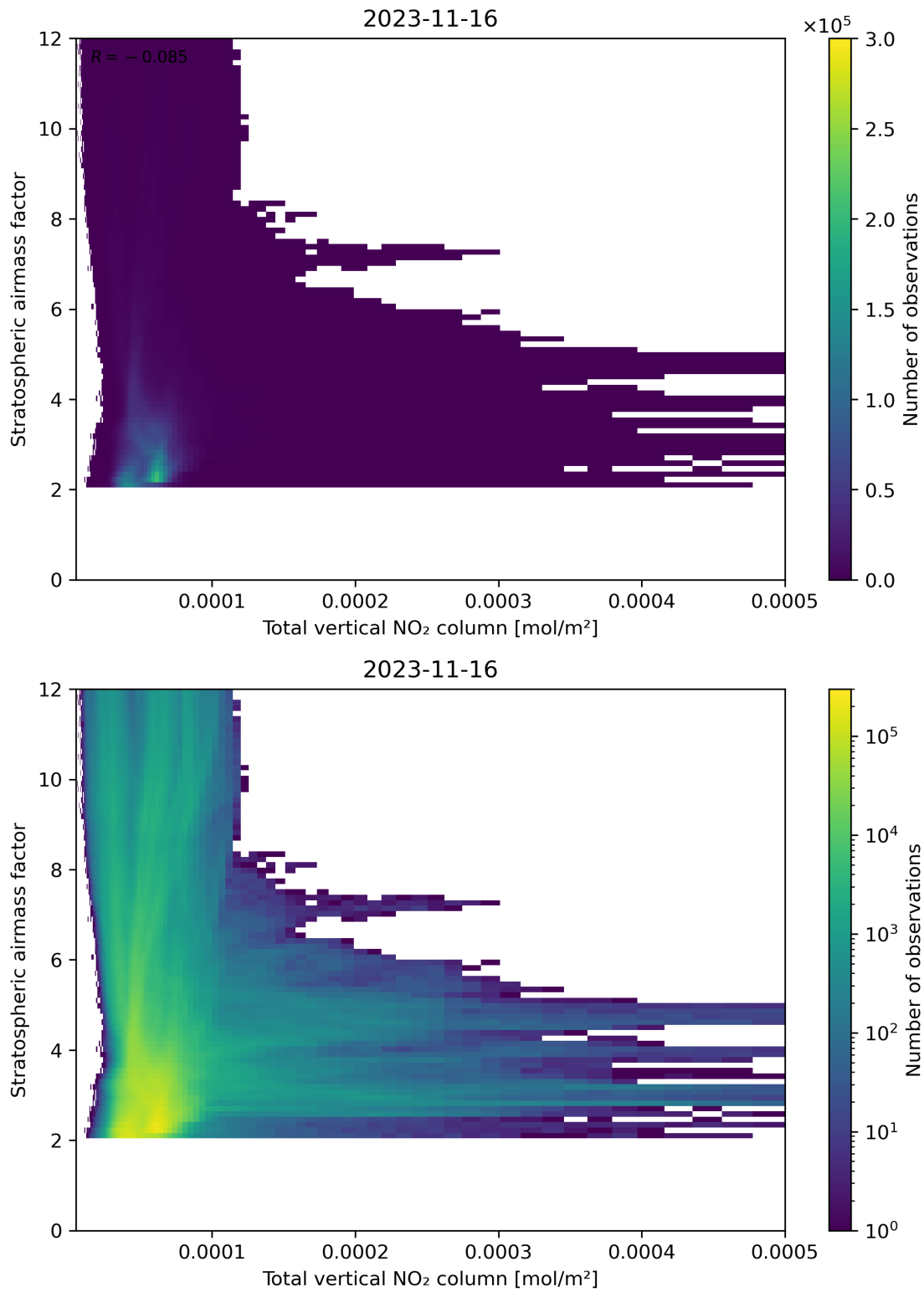
Figure 110: Scatter density plot of “Total vertical NO 2 column” against “Stratospheric airmass factor” for 2023-11-15 to 2023-11-17.
