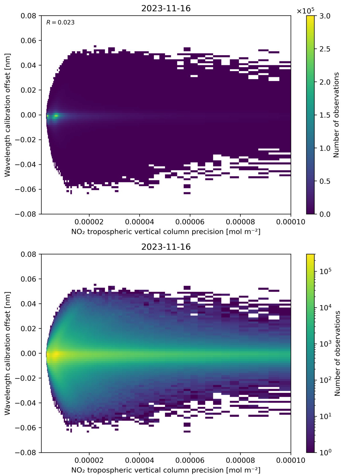
Figure 141: Scatter density plot of “NO 2 tropospheric vertical column precision” against “Wavelength calibration offset” for 2023-11-15 to 2023-11-17.
