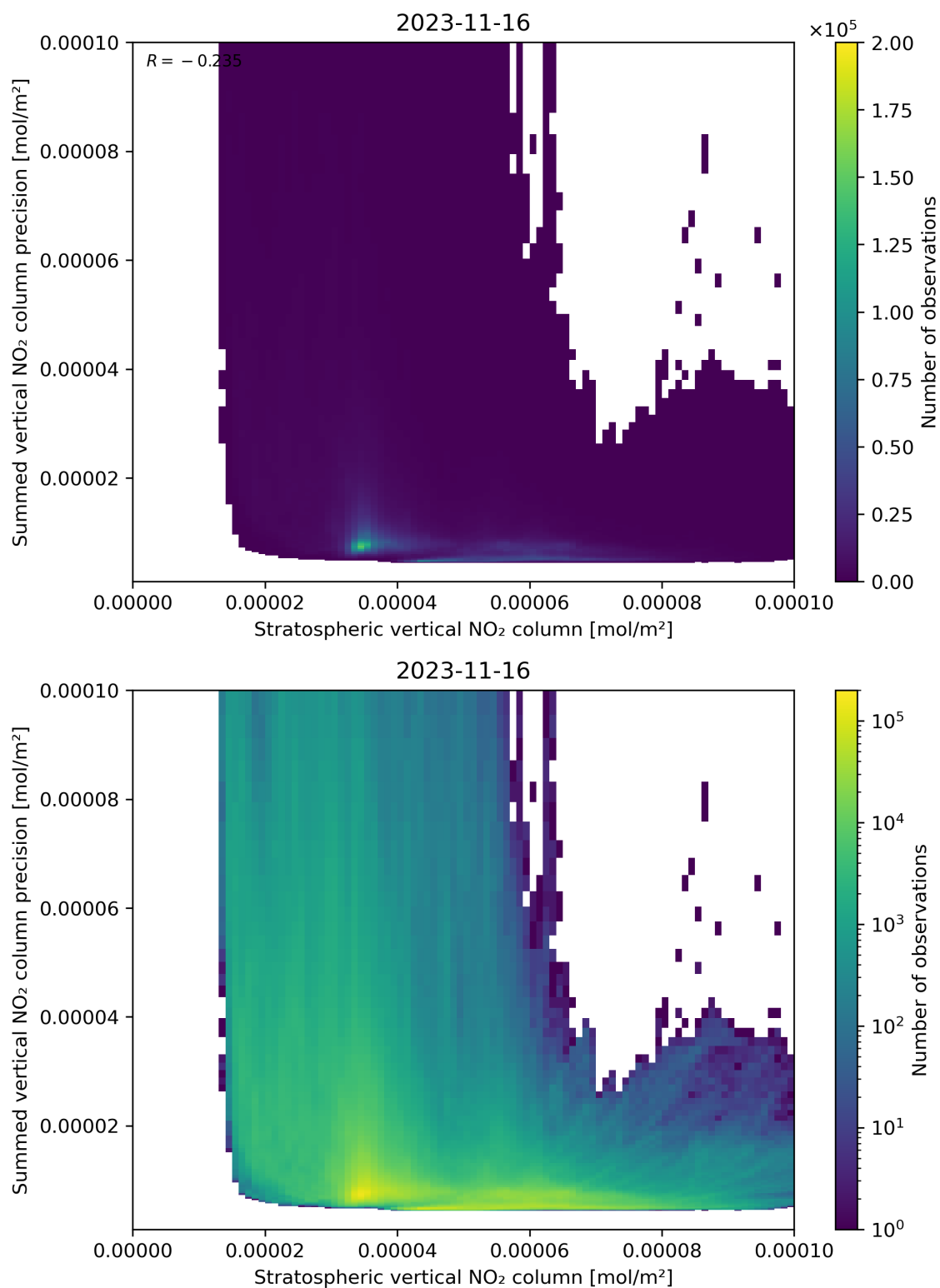
Figure 99: Scatter density plot of “Stratospheric vertical NO 2 column” against “Summed vertical NO 2 column precision” for 2023-11-15 to 2023-11-17.
