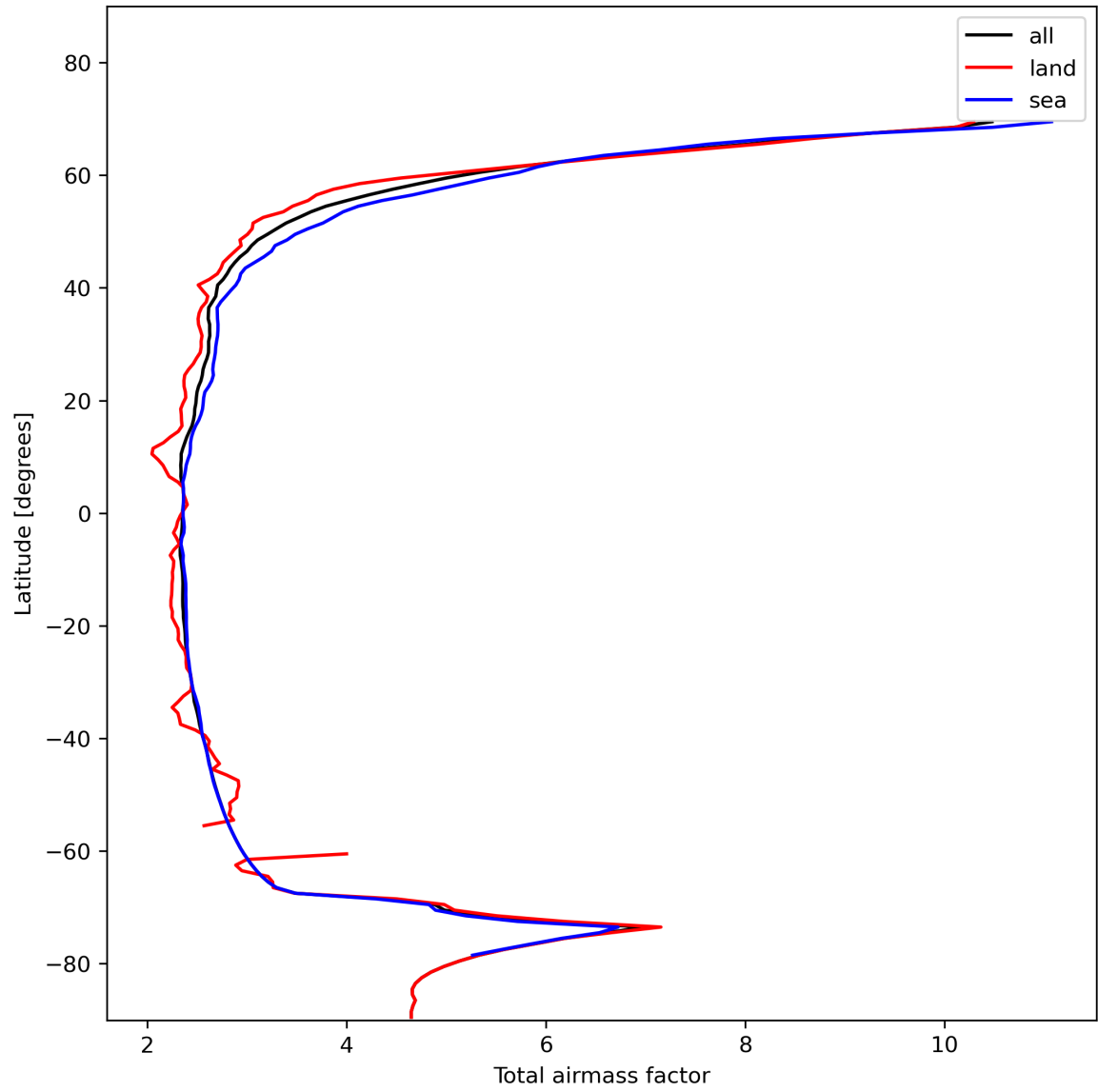
Figure 15: Zonal average of “Total airmass factor” for 2023-11-15 to 2023-11-17.
