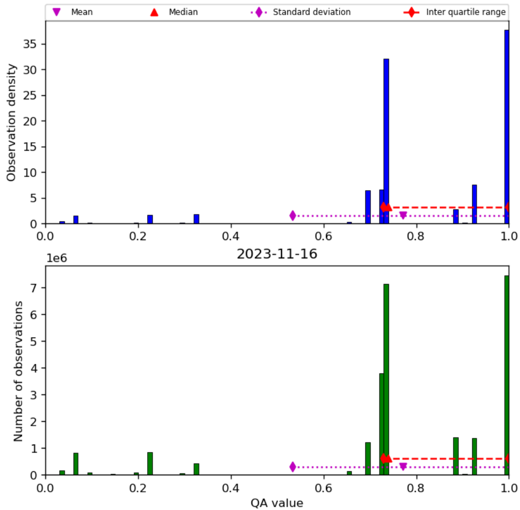
Figure 28: Histogram of “QA value” for 2023-11-15 to 2023-11-17
