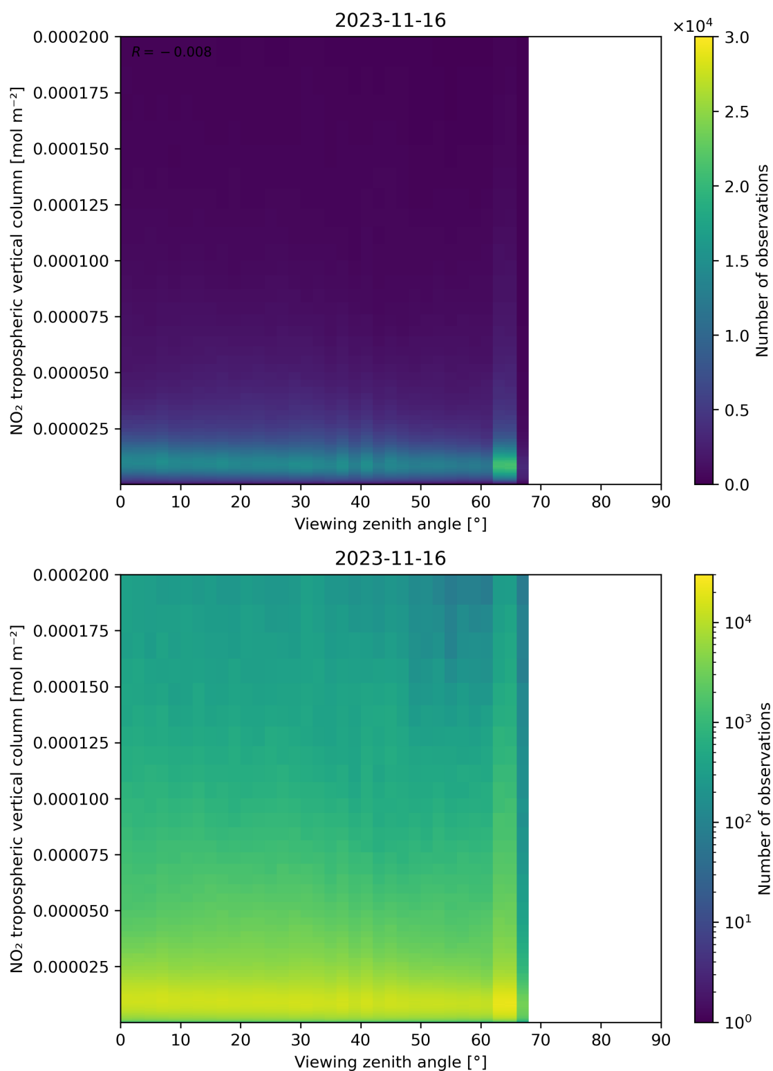
Figure 169: Scatter density plot of “Viewing zenith angle” against “NO 2 tropospheric vertical column” for 2023-11-15 to 2023-11-17.
