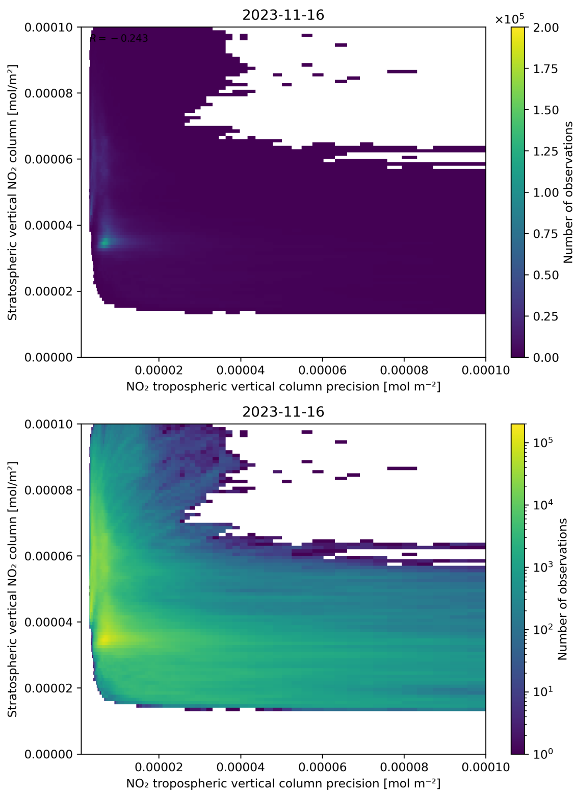
Figure 135: Scatter density plot of “NO 2 tropospheric vertical column precision” against “Stratospheric vertical NO 2 column” for 2023-11-15 to 2023-11-17.
