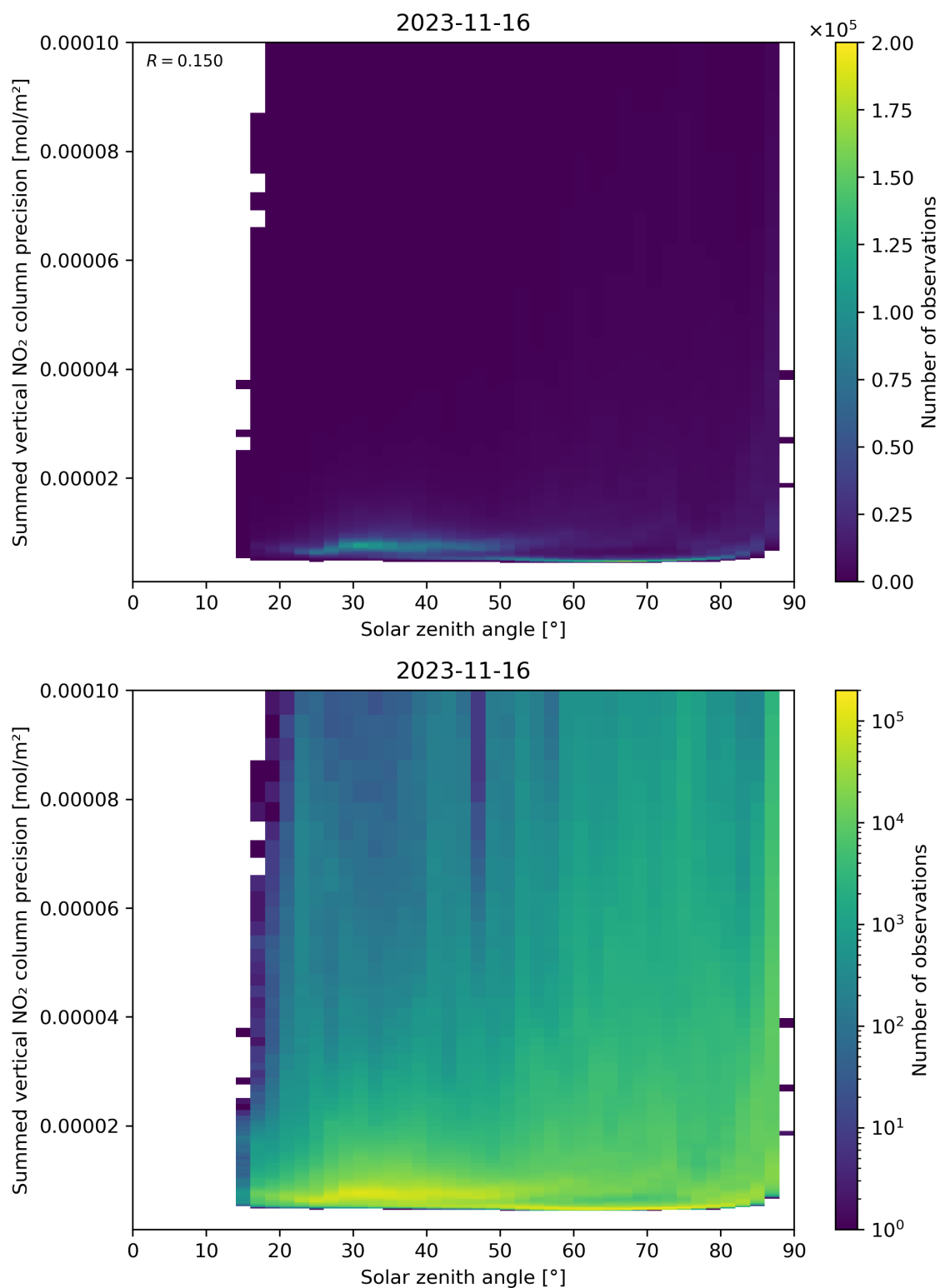
Figure 152: Scatter density plot of “Solar zenith angle” against “Summed vertical NO 2 column precision” for 2023-11-15 to 2023-11-17.
