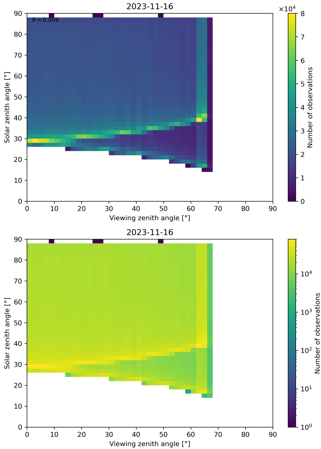
Figure 172: Scatter density plot of “Viewing zenith angle” against “Solar zenith angle” for 2023-11-15 to 2023-11-17.
