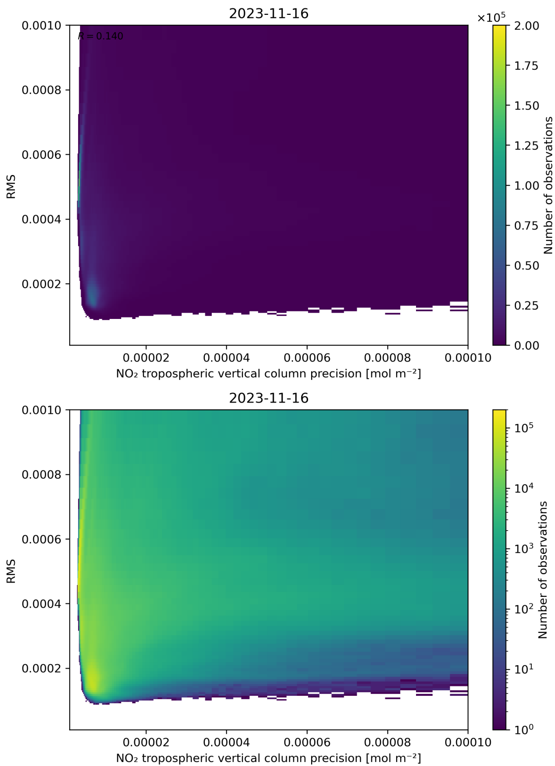
Figure 140: Scatter density plot of “NO 2 tropospheric vertical column precision” against “RMS” for 2023-11-15 to 2023-11-17.
