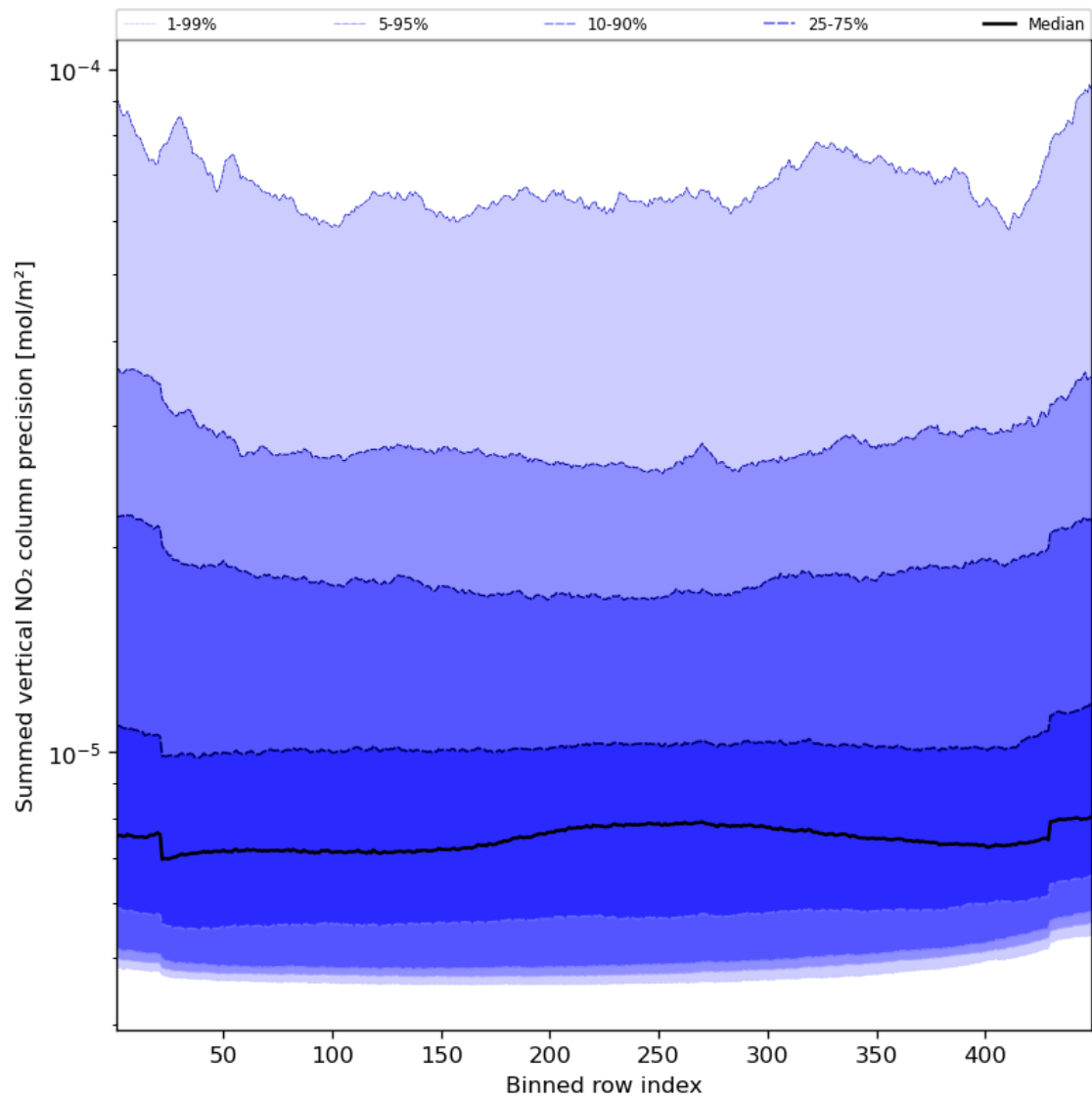
Figure 58: Along track statistics of “Summed vertical NO 2 column precision” for 2023-11-15 to 2023-11-17
