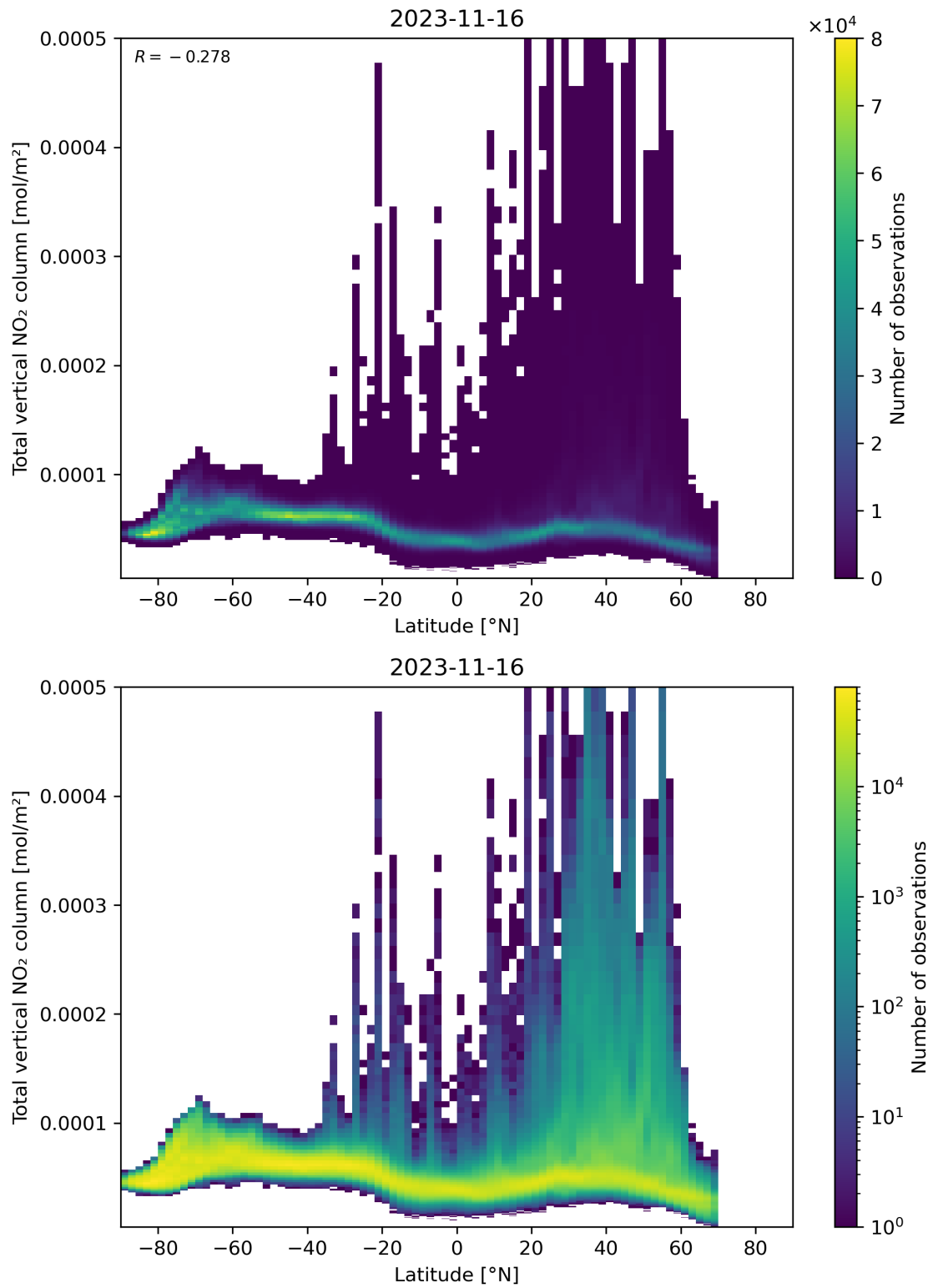
Figure 90: Scatter density plot of “Latitude” against “Total vertical NO 2 column” for 2023-11-15 to 2023-11-17.
