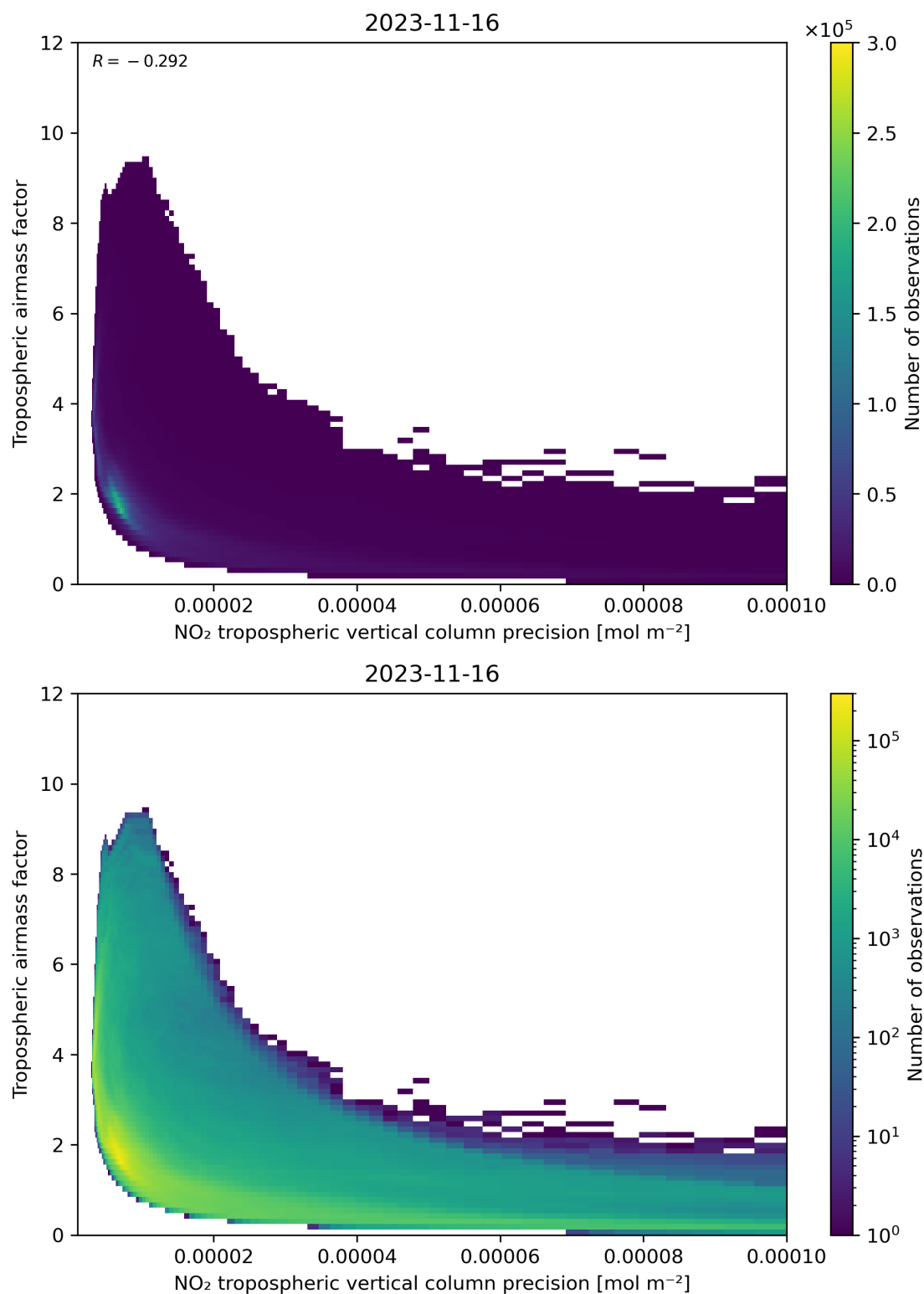
Figure 133: Scatter density plot of “NO 2 tropospheric vertical column precision” against “Tropospheric airmass factor” for 2023-11-15 to 2023-11-17.
