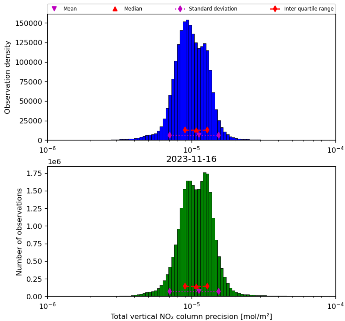
Figure 39: Histogram of "Total vertical NO 2 column precision" for 2023-11-15 to 2023-11-17
