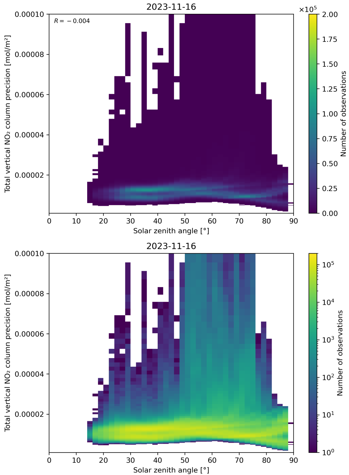
Figure 154: Scatter density plot of “Solar zenith angle” against “Total vertical NO 2 column precision” for 2023-11-15 to 2023-11-17.
