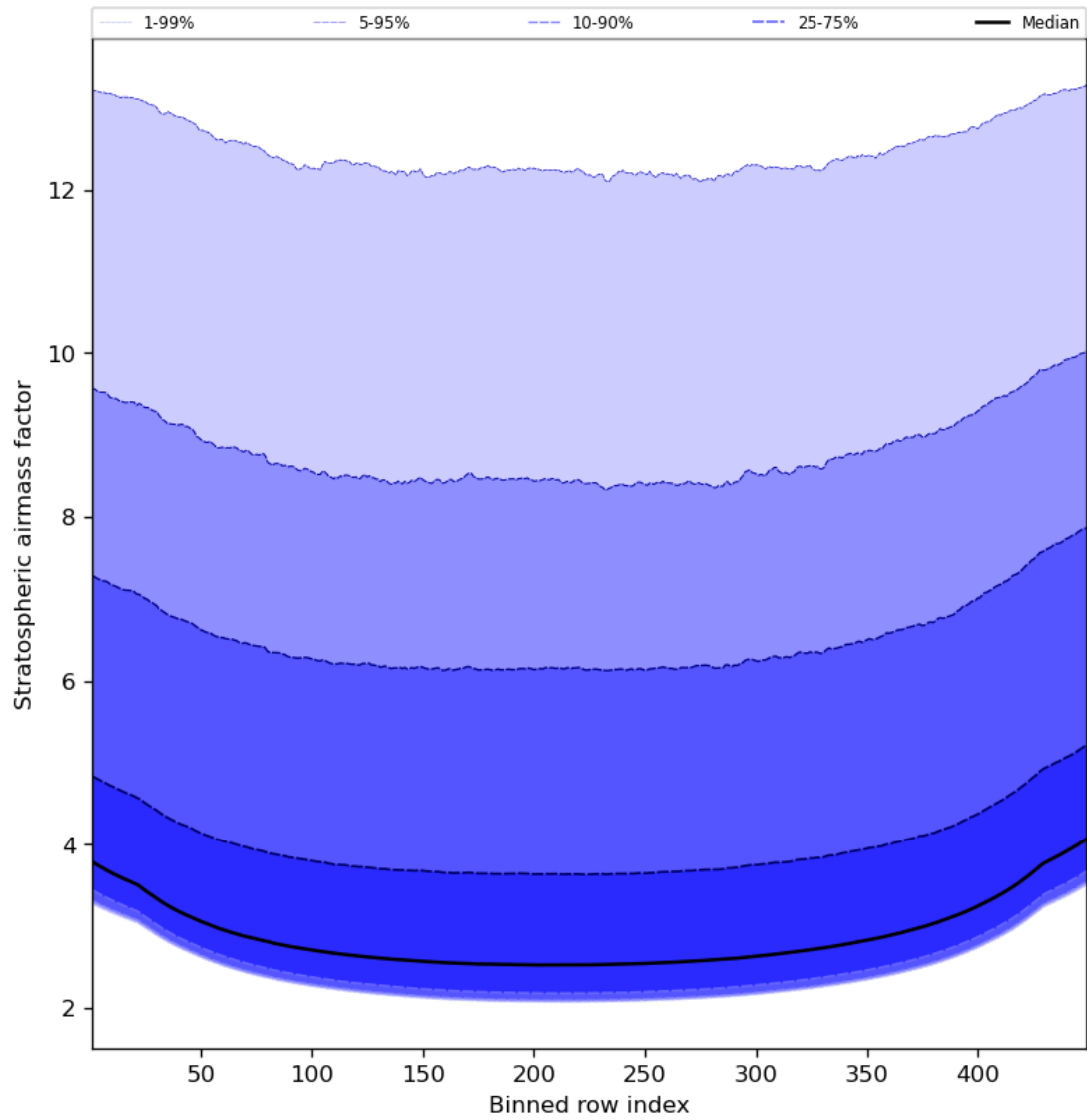
Figure 61: Along track statistics of “Stratospheric airmass factor” for 2023-11-15 to 2023-11-17
