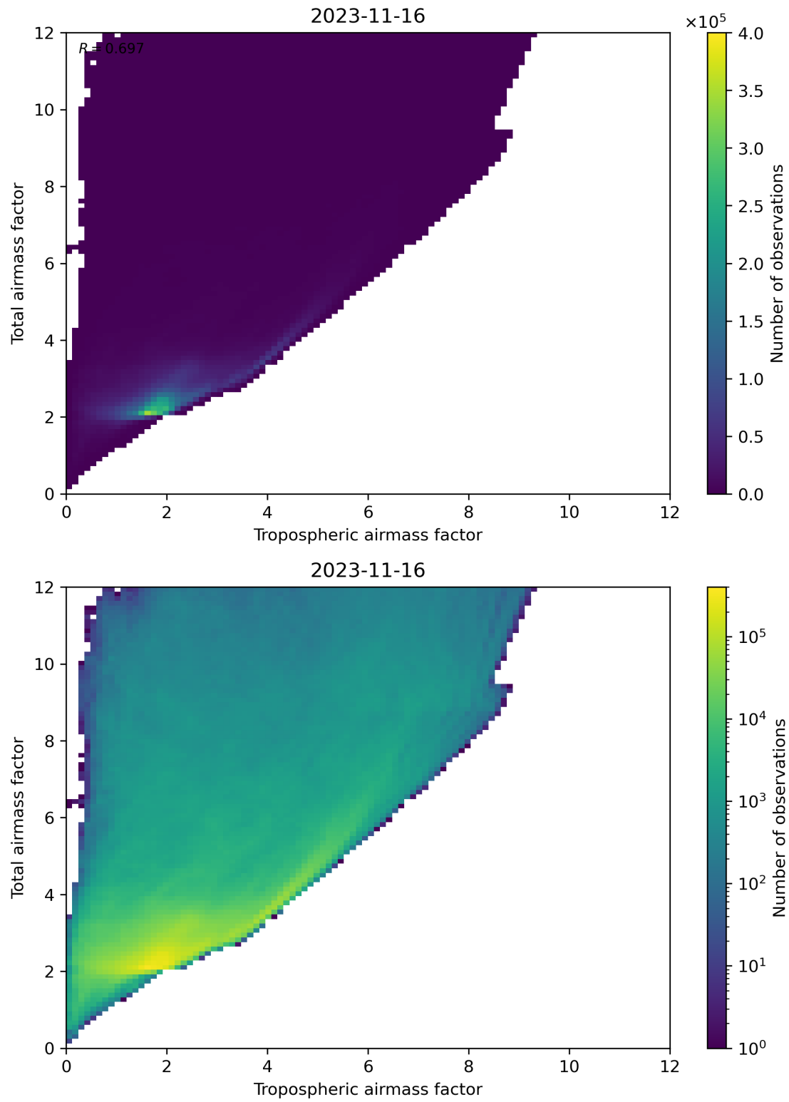
Figure 72: Scatter density plot of “Tropospheric airmass factor” against “Total airmass factor” for 2023-11-15 to 2023-11-17.
