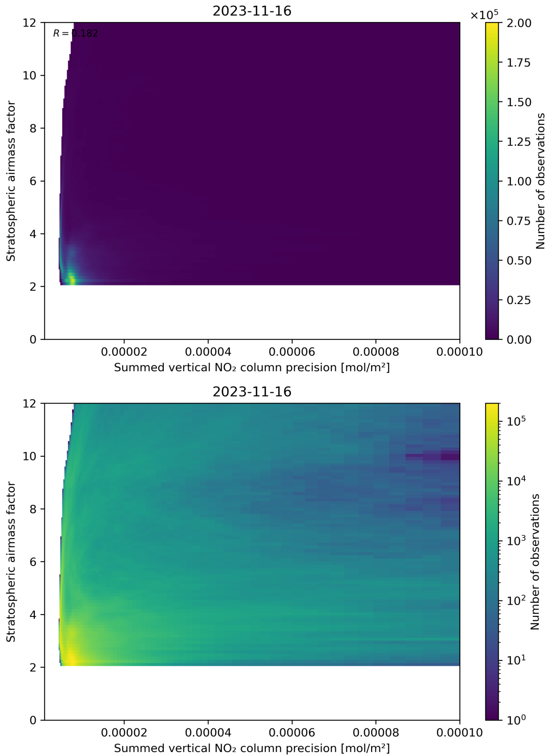
Figure 106: Scatter density plot of “Summed vertical NO 2 column precision” against “Stratospheric airmass factor” for 2023-11-15 to 2023-11-17.
