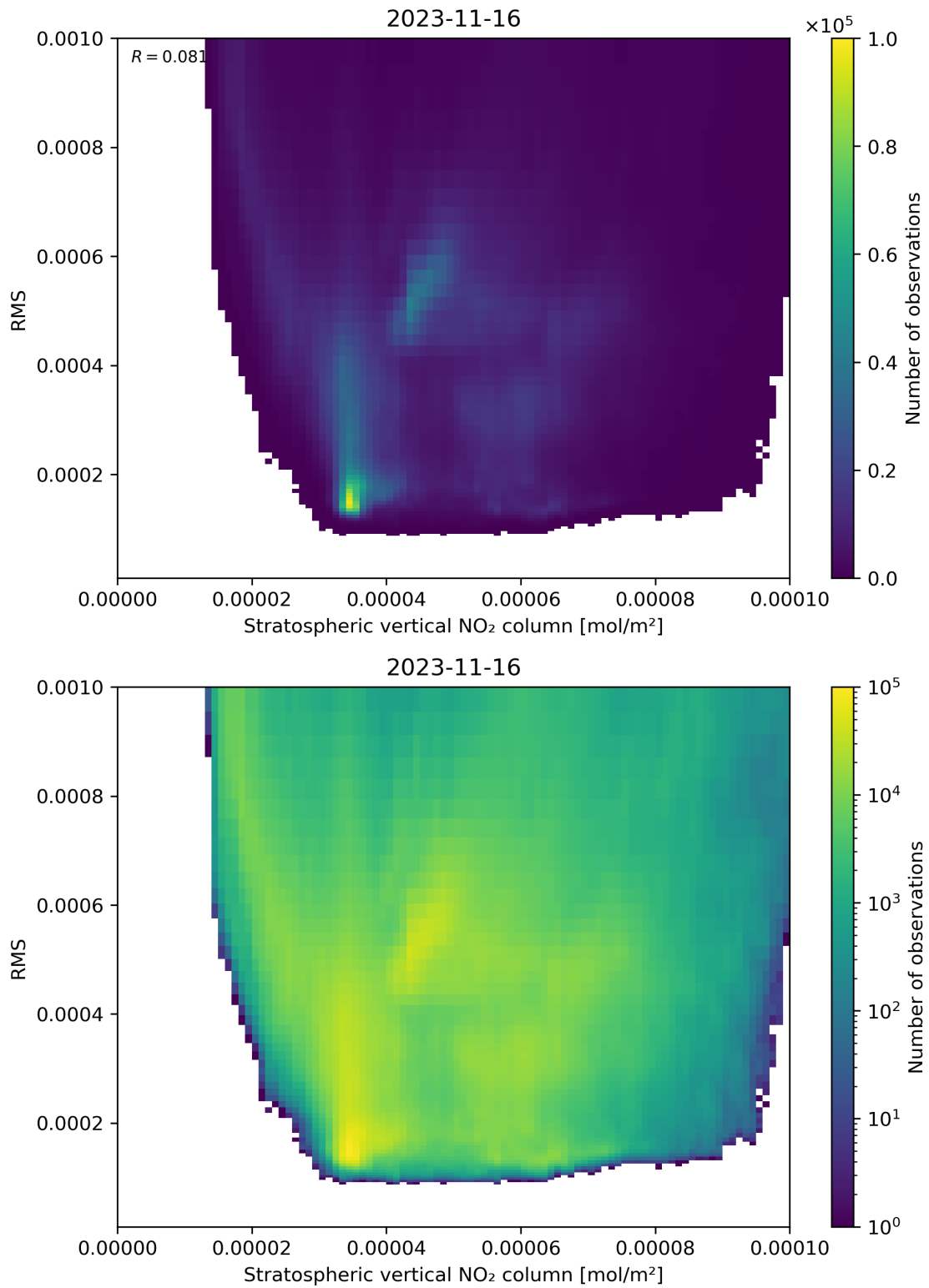
Figure 102: Scatter density plot of “Stratospheric vertical NO 2 column” against “RMS” for 2023-11-15 to 2023-11-17.
