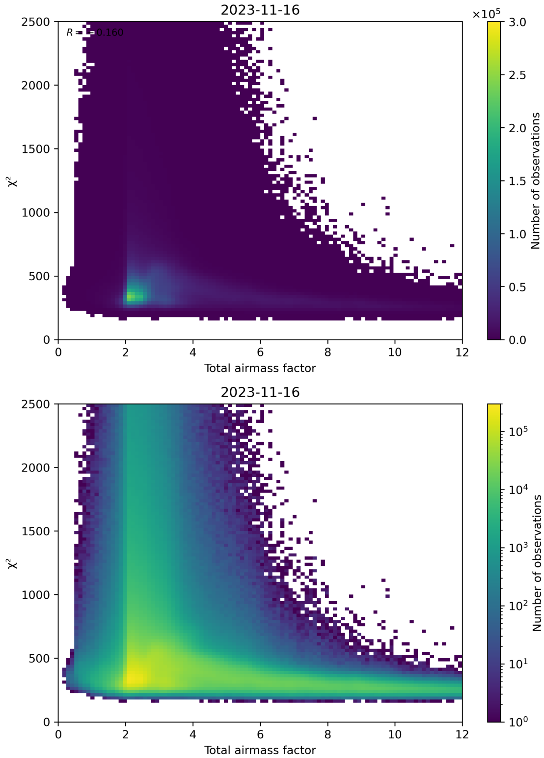
Figure 63: Scatter density plot of “Total airmass factor” against “ \chi^2 ” for 2023-11-15 to 2023-11-17.
