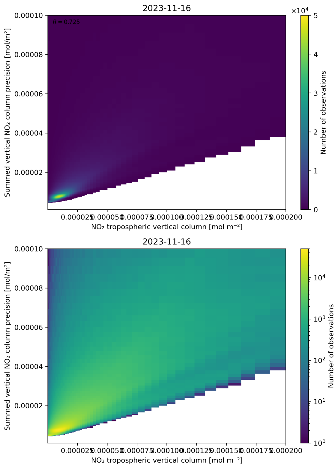
Figure 127: Scatter density plot of “NO 2 tropospheric vertical column” against “Summed vertical NO 2 column precision” for 2023-11-15 to 2023-11-17.
