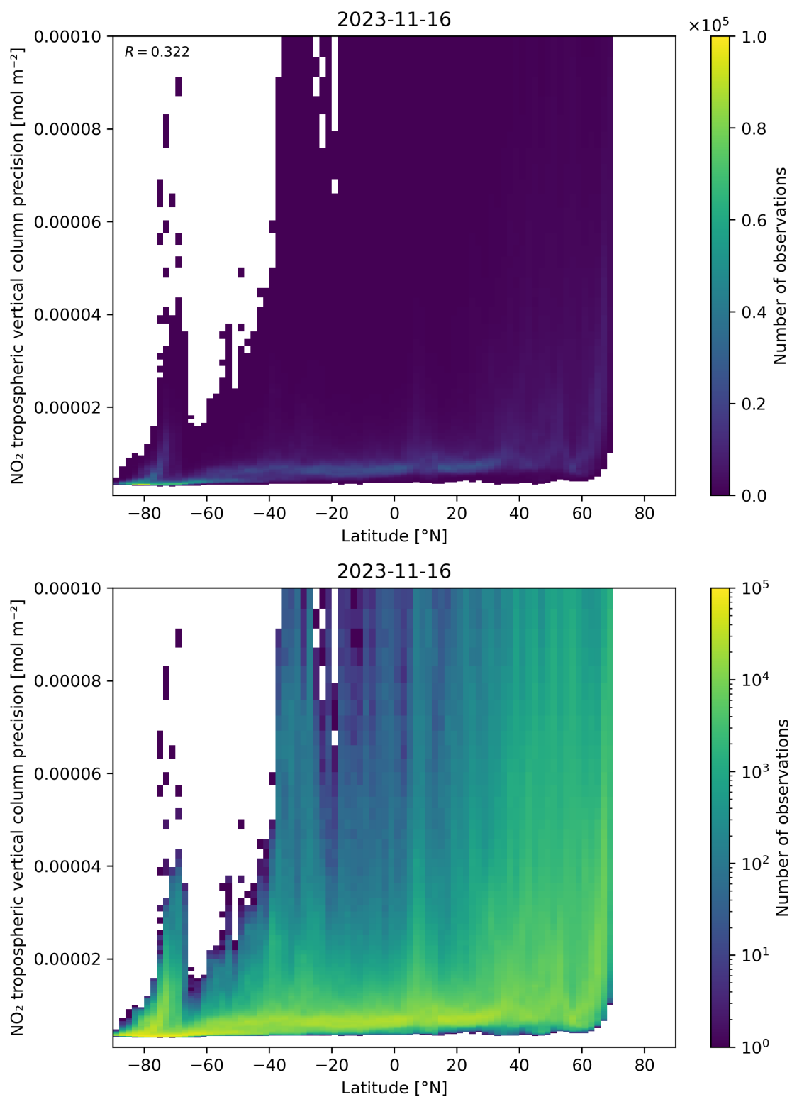
Figure 93: Scatter density plot of “Latitude” against “NO 2 tropospheric vertical column precision” for 2023-11-15 to 2023-11-17.
