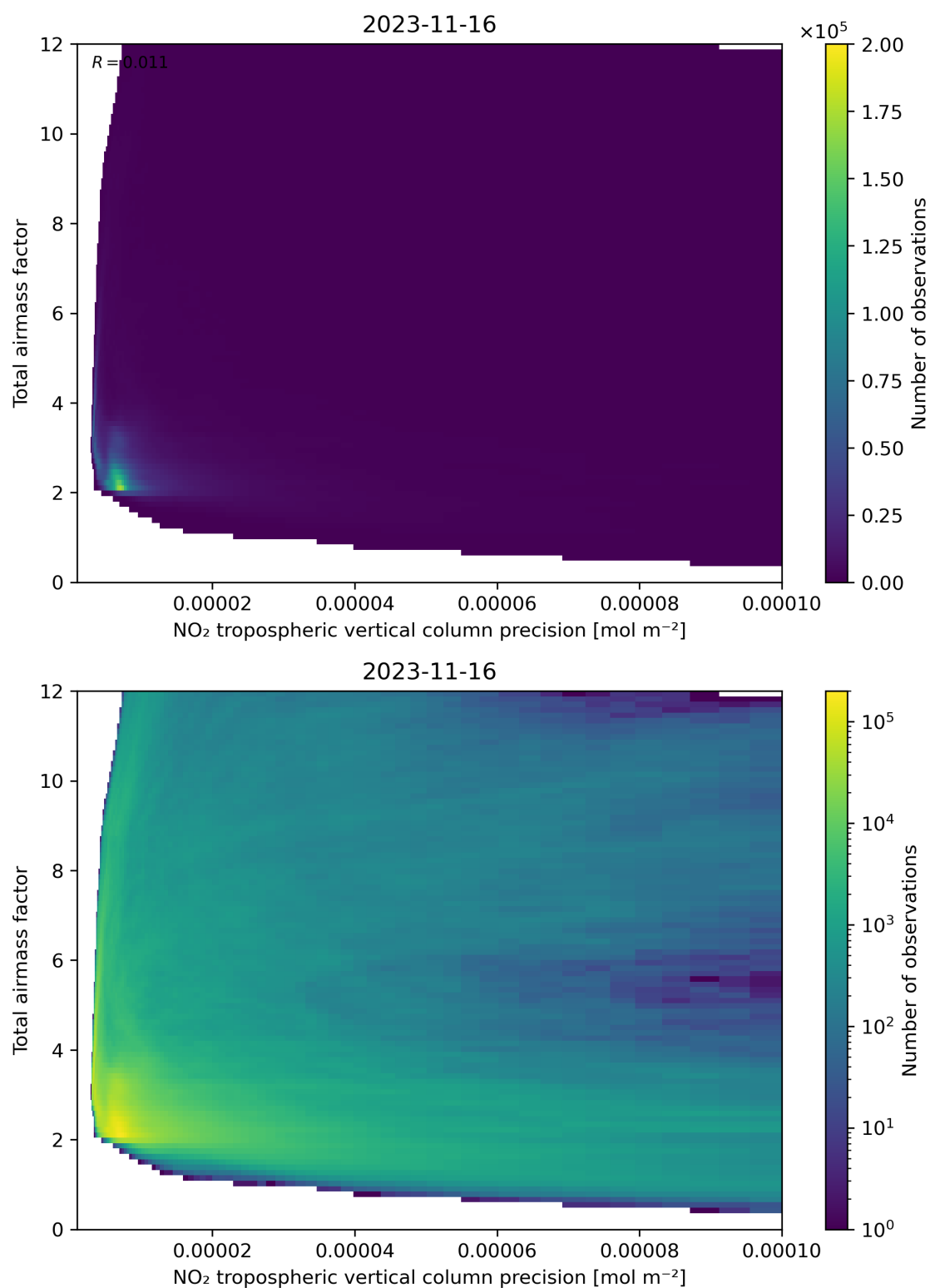
Figure 132: Scatter density plot of “NO 2 tropospheric vertical column precision” against “Total air mass factor” for 2023-11-15 to 2023-11-17.
