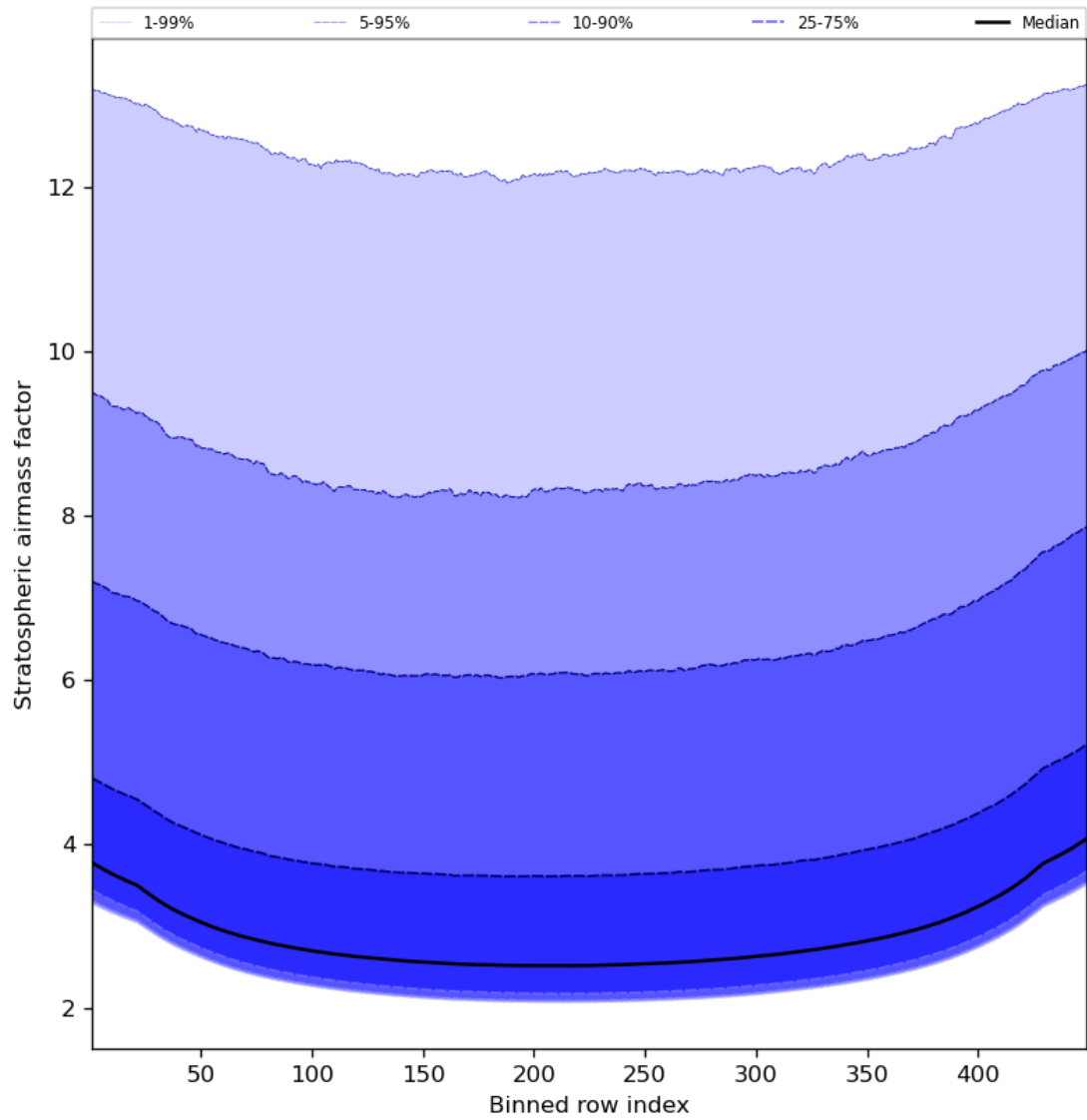
Figure 61: Along track statistics of “Stratospheric airmass factor” for 2023-11-16 to 2023-11-18
