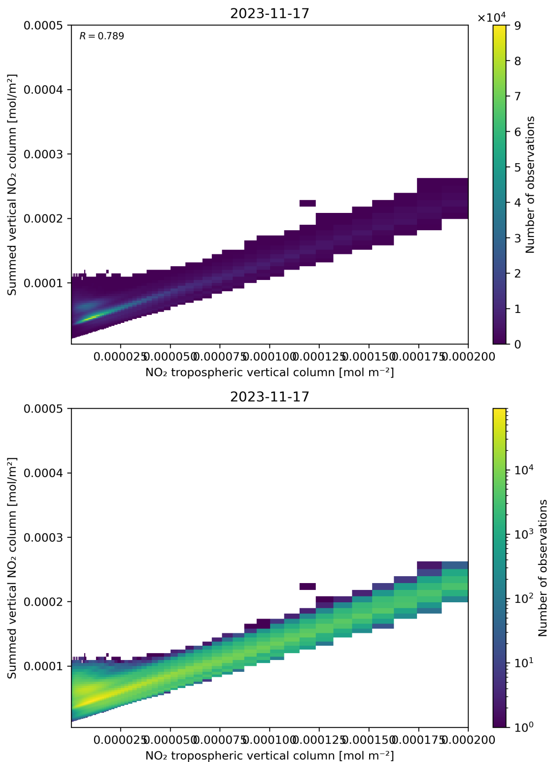
Figure 126: Scatter density plot of “NO 2 tropospheric vertical column” against “Summed vertical NO 2 column” for 2023-11-16 to 2023-11-18.
