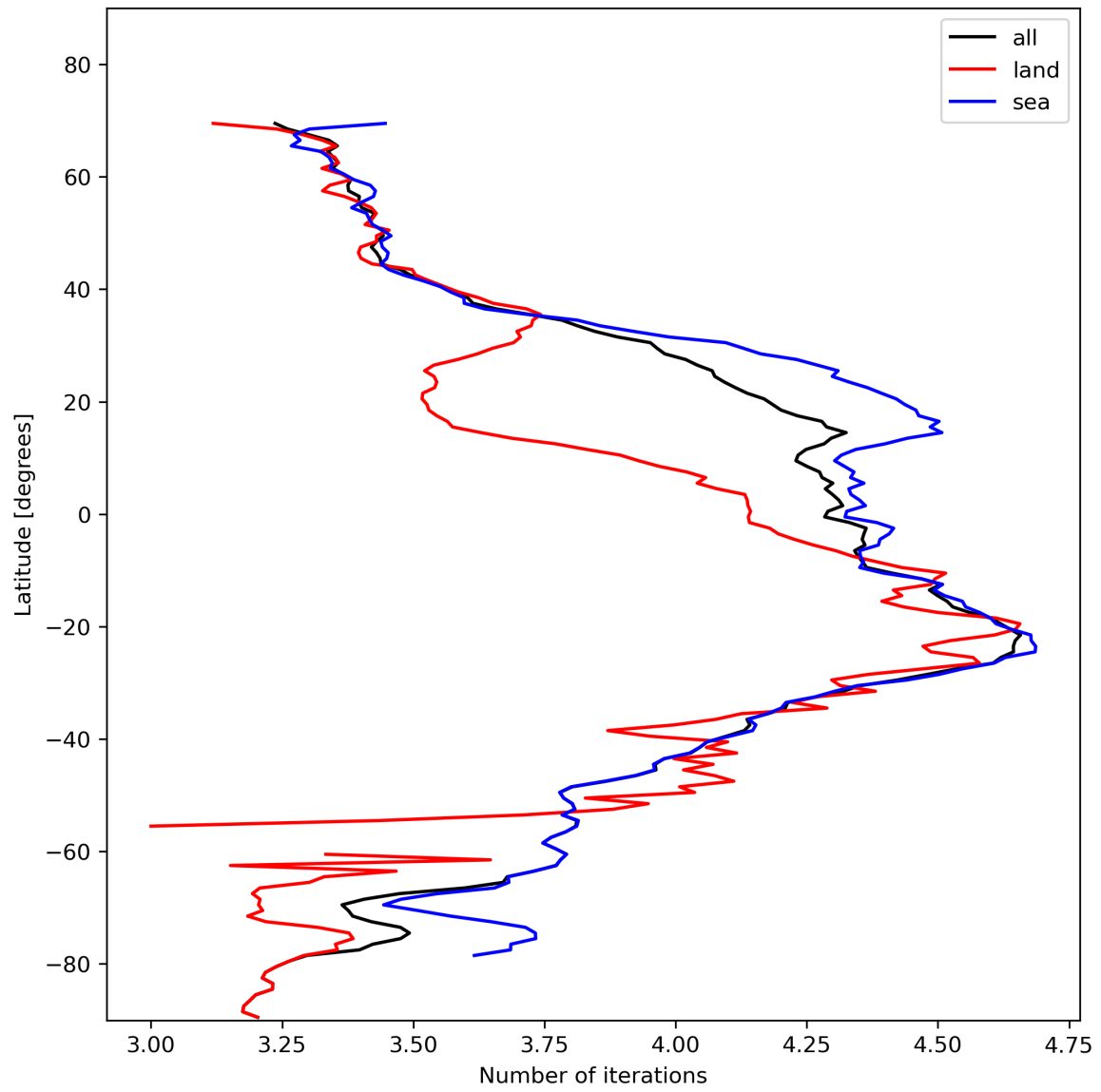
Figure 17: Zonal average of “Number of iterations” for 2023-11-16 to 2023-11-18.
