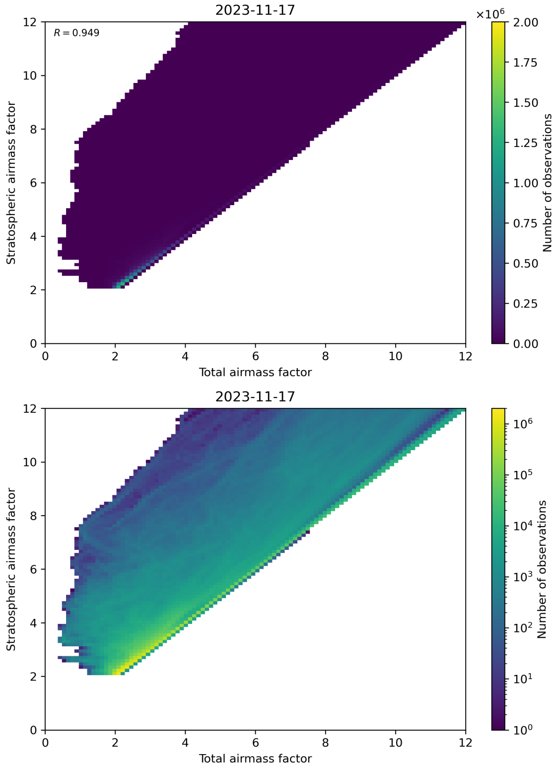
Figure 62: Scatter density plot of “Total airmass factor” against “Stratospheric airmass factor” for 2023-11-16 to 2023-11-18.
