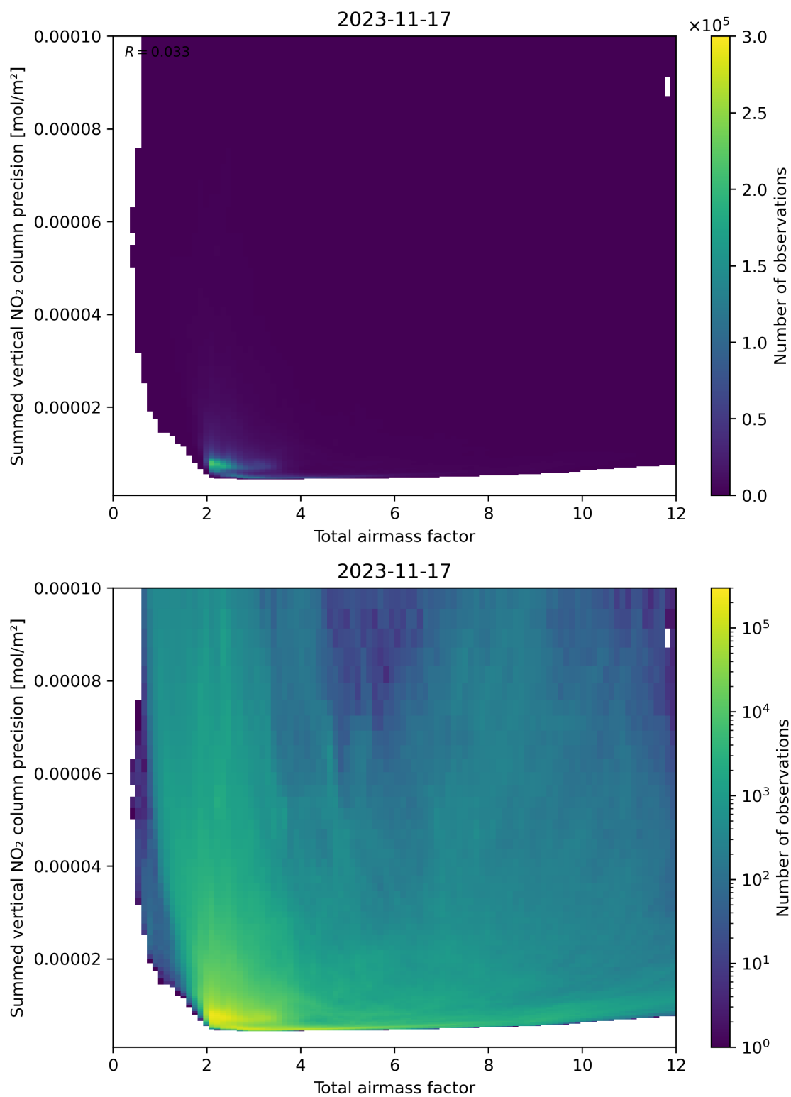
Figure 66: Scatter density plot of “Total airmass factor” against “Summed vertical NO 2 column precision” for 2023-11-16 to 2023-11-18.
