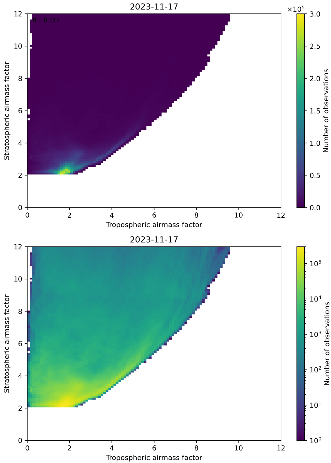
Figure 71: Scatter density plot of “Tropospheric airmass factor” against “Stratospheric airmass factor” for 2023-11-16 to 2023-11-18.
