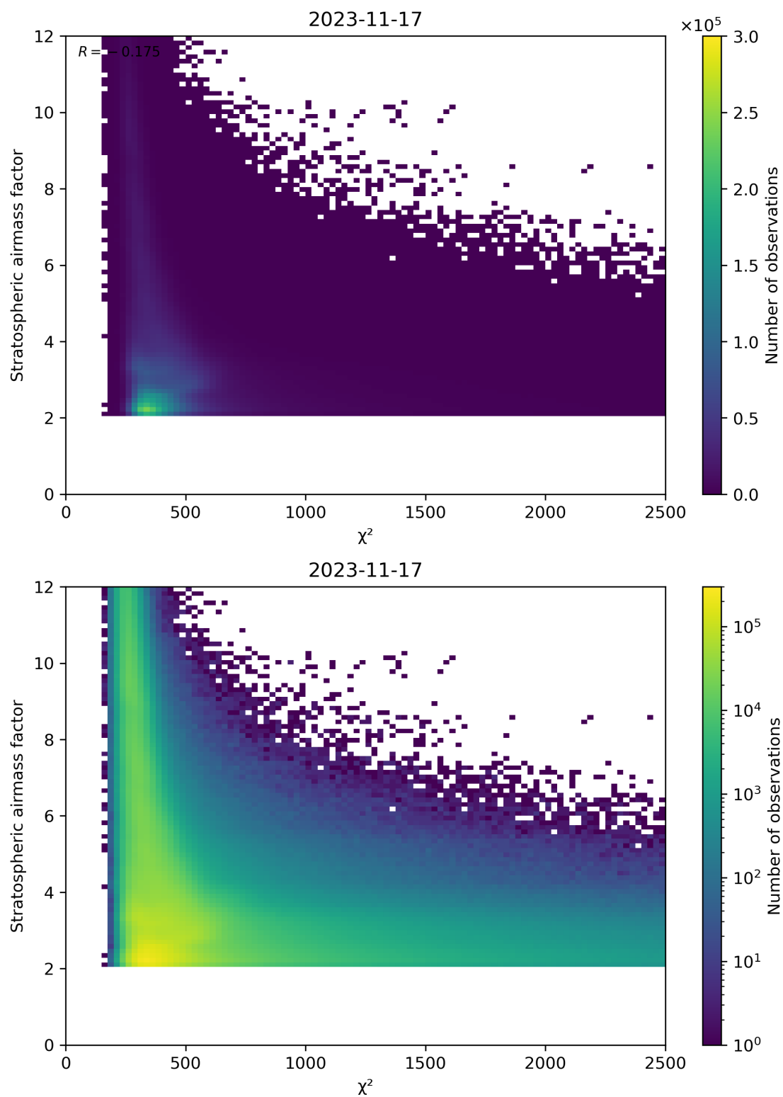
Figure 81: Scatter density plot of “ \chi^2 ” against “Stratospheric airmass factor” for 2023-11-16 to 2023-11-18.
