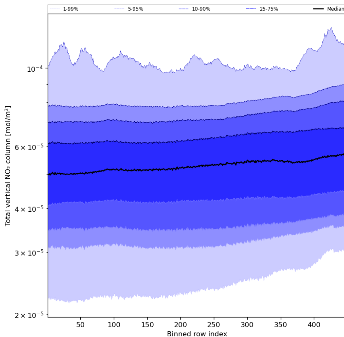
Figure 55: Along track statistics of "Total vertical NO 2 column" for 2023-11-16 to 2023-11-18
