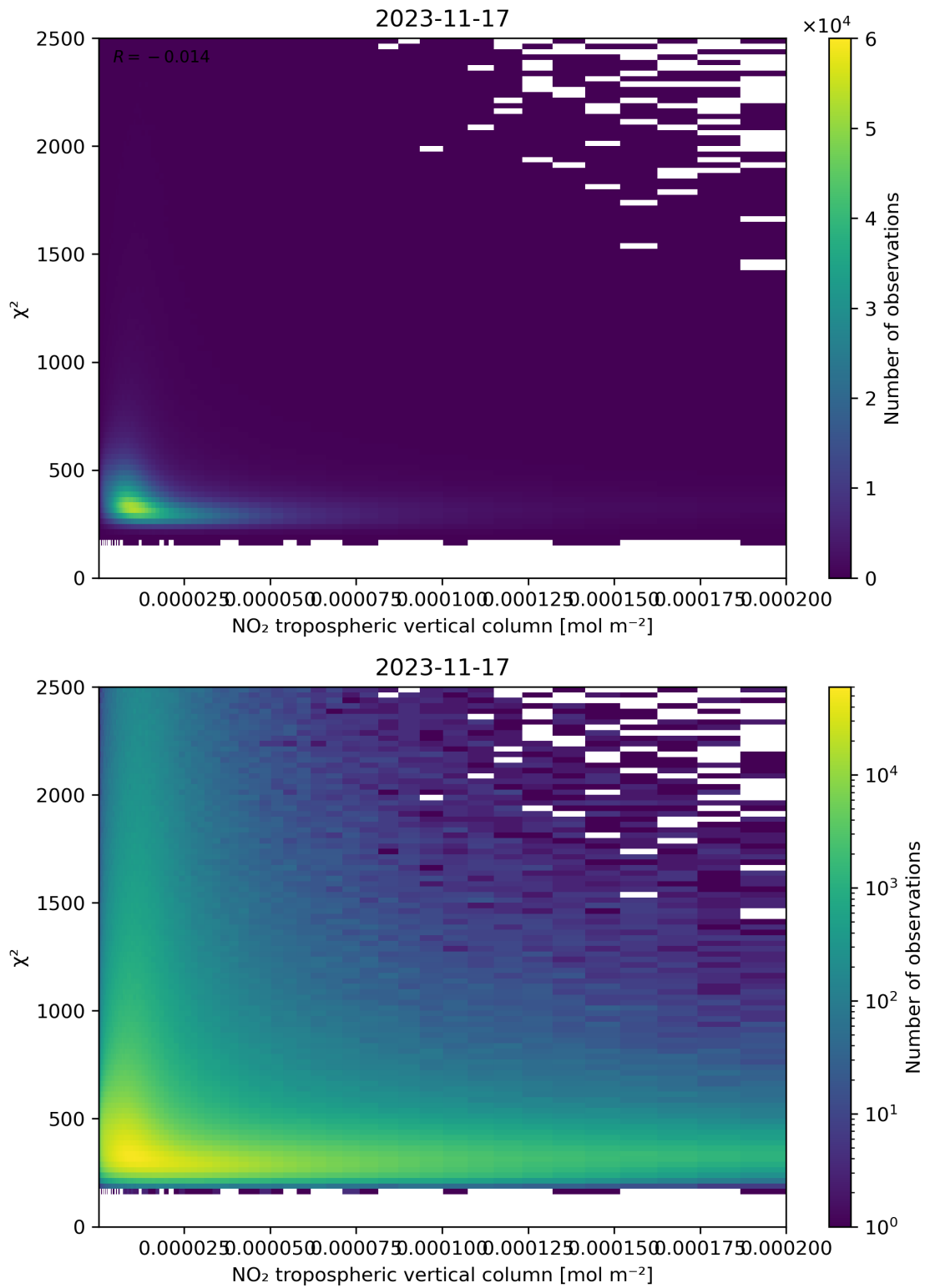
Figure 124: Scatter density plot of “NO 2 tropospheric vertical column” against “ \chi^2 ” for 2023-11-16 to 2023-11-18.
