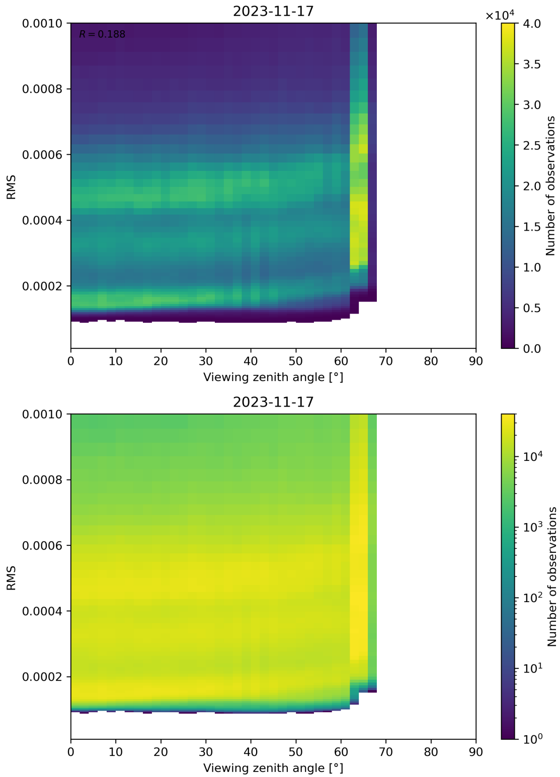
Figure 171: Scatter density plot of “Viewing zenith angle” against “RMS” for 2023-11-16 to 2023-11-18.
