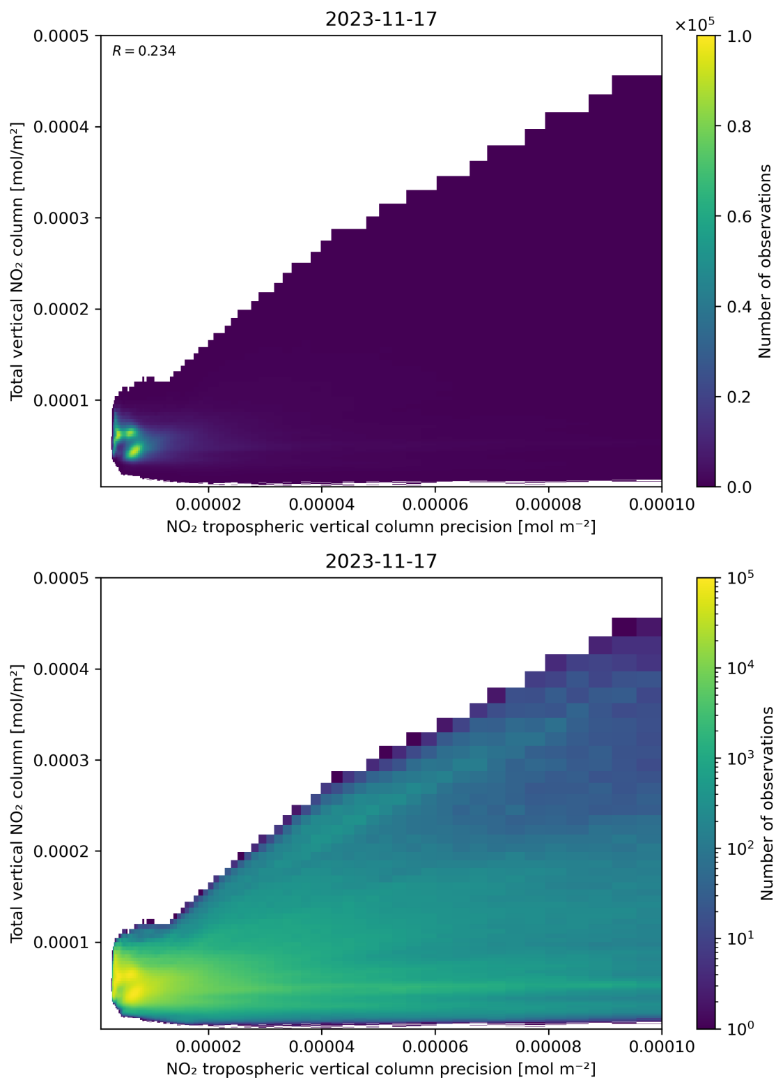
Figure 138: Scatter density plot of “NO 2 tropospheric vertical column precision” against “Total vertical NO 2 column” for 2023-11-16 to 2023-11-18.
