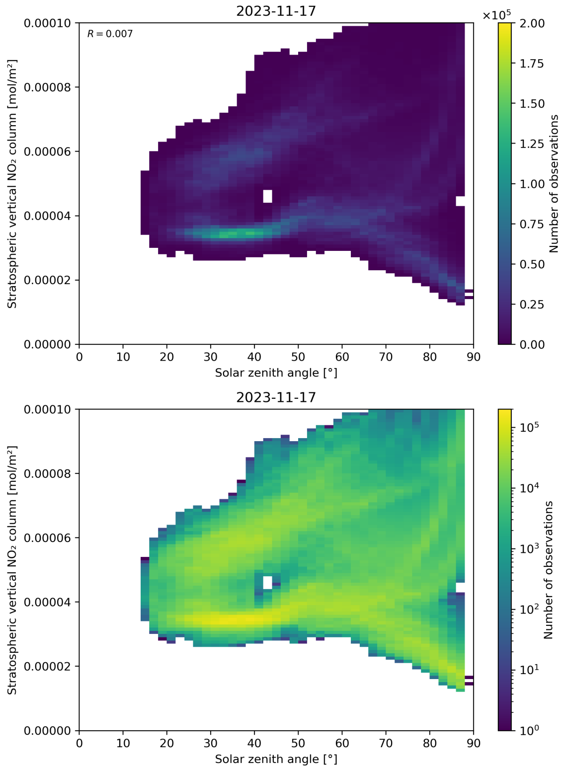
Figure 150: Scatter density plot of “Solar zenith angle” against “Stratospheric vertical NO 2 column” for 2023-11-16 to 2023-11-18.
