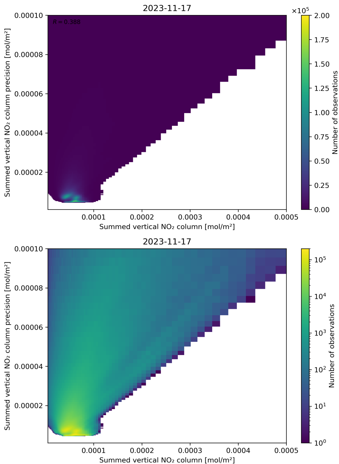
Figure 105: Scatter density plot of “Summed vertical NO 2 column” against “Summed vertical NO 2 column precision” for 2023-11-16 to 2023-11-18.
