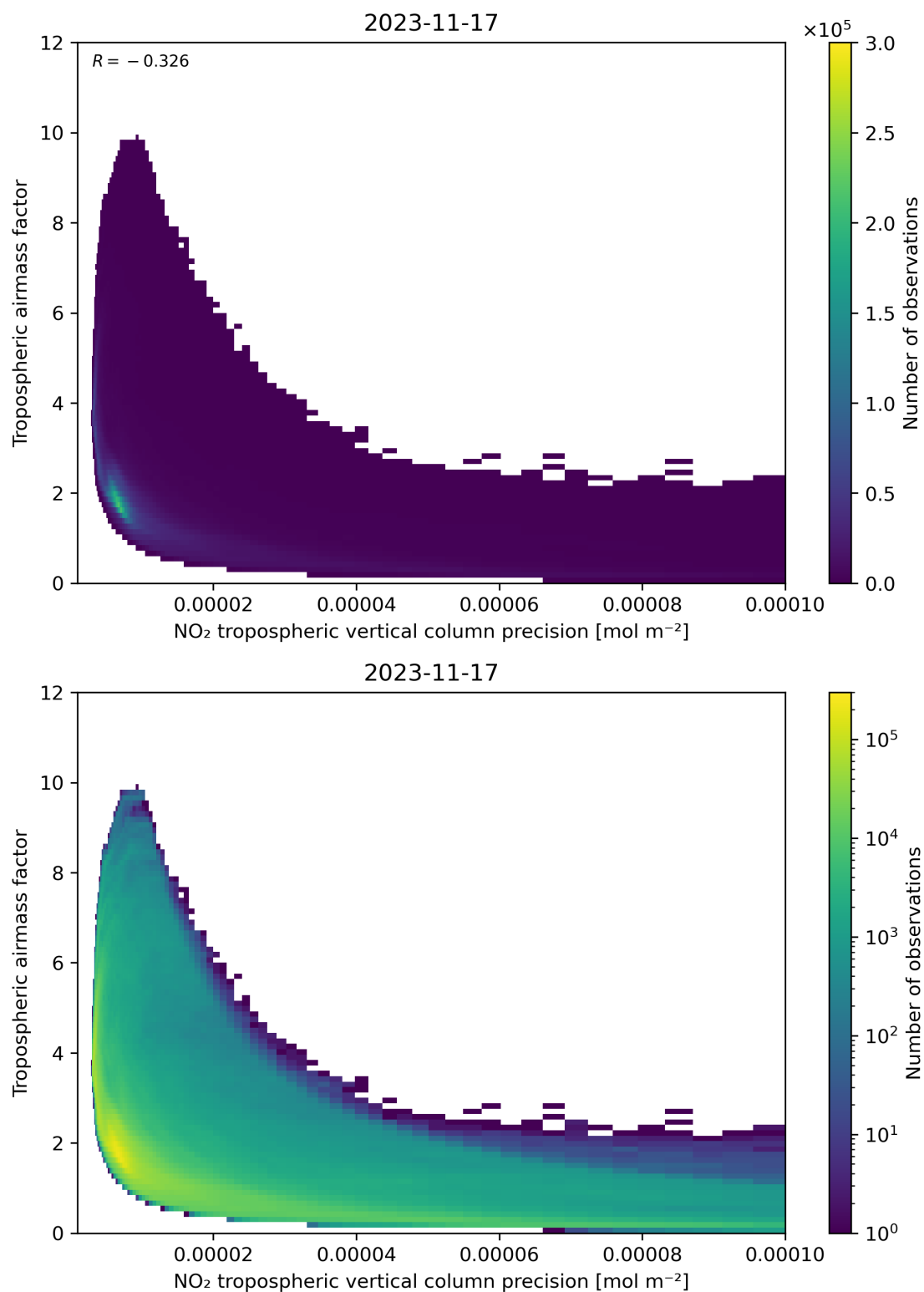
Figure 133: Scatter density plot of “NO 2 tropospheric vertical column precision” against “Tropospheric airmass factor” for 2023-11-16 to 2023-11-18.
