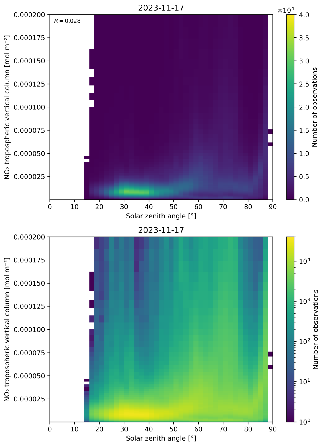
Figure 155: Scatter density plot of “Solar zenith angle” against “NO 2 tropospheric vertical column” for 2023-11-16 to 2023-11-18.
