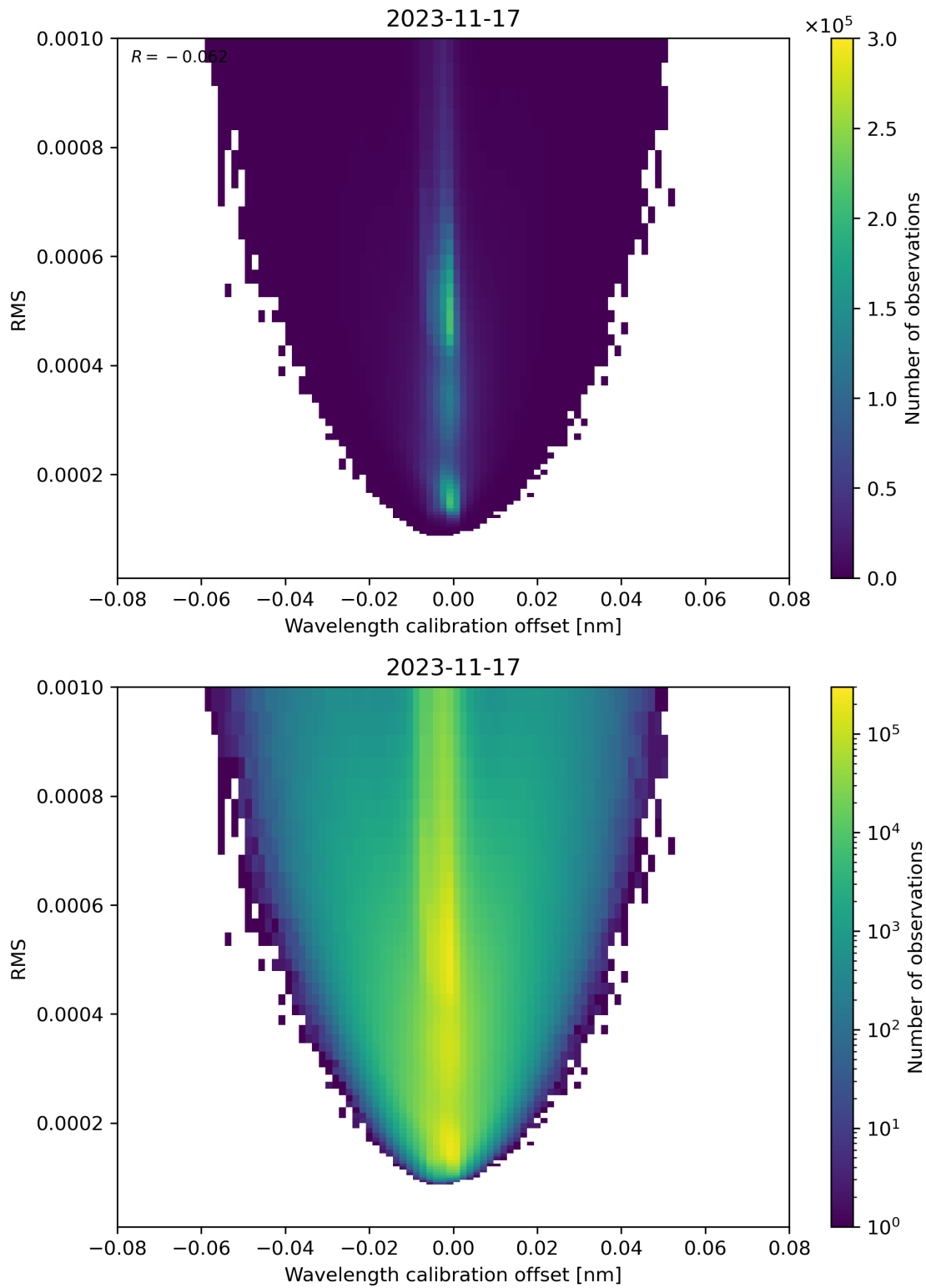
Figure 181: Scatter density plot of “Wavelength calibration offset” against “RMS” for 2023-11-16 to 2023-11-18.
