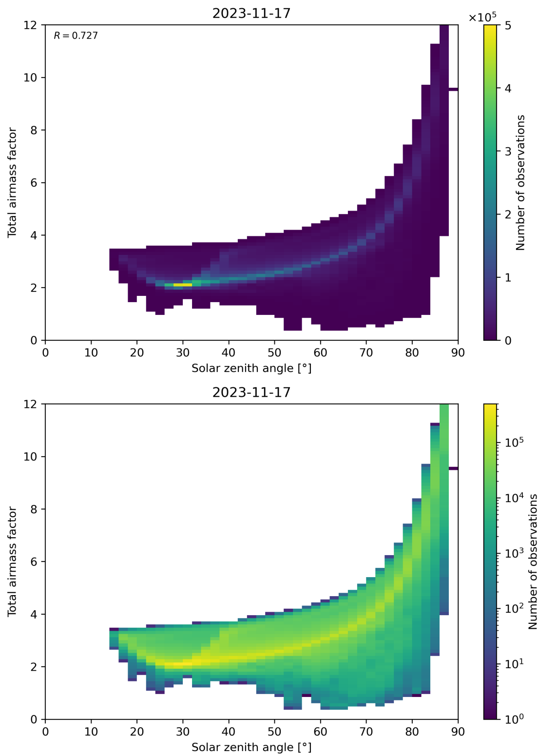
Figure 146: Scatter density plot of “Solar zenith angle” against “Total airmass factor” for 2023-11-16 to 2023-11-18.
