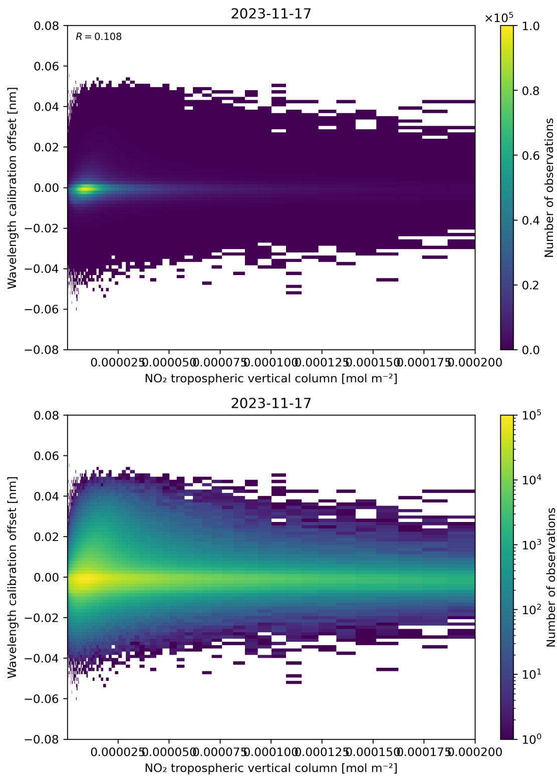
Figure 143: Scatter density plot of “NO 2 tropospheric vertical column” against “Wavelength calibration offset” for 2023-11-16 to 2023-11-18.
