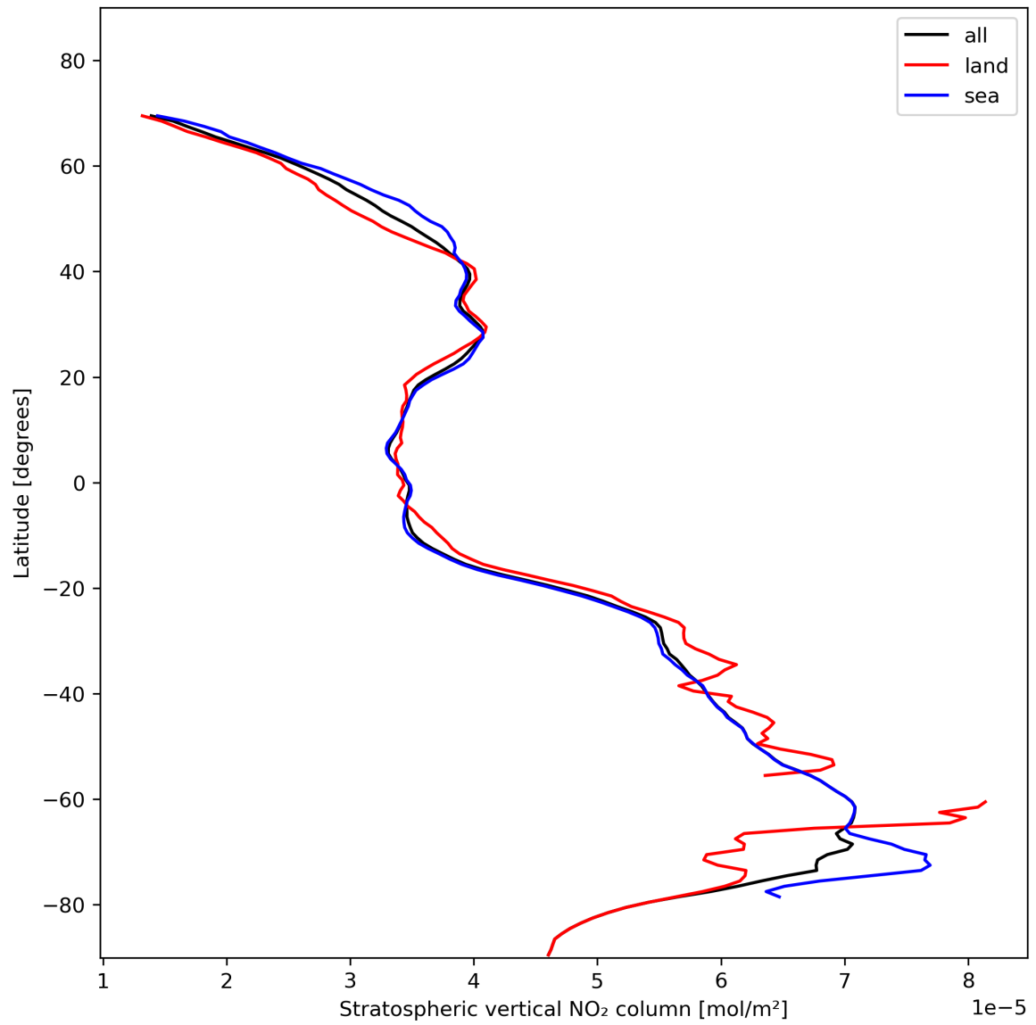
Figure 19: Zonal average of “Stratospheric vertical NO 2 column” for 2023-11-16 to 2023-11-18.
