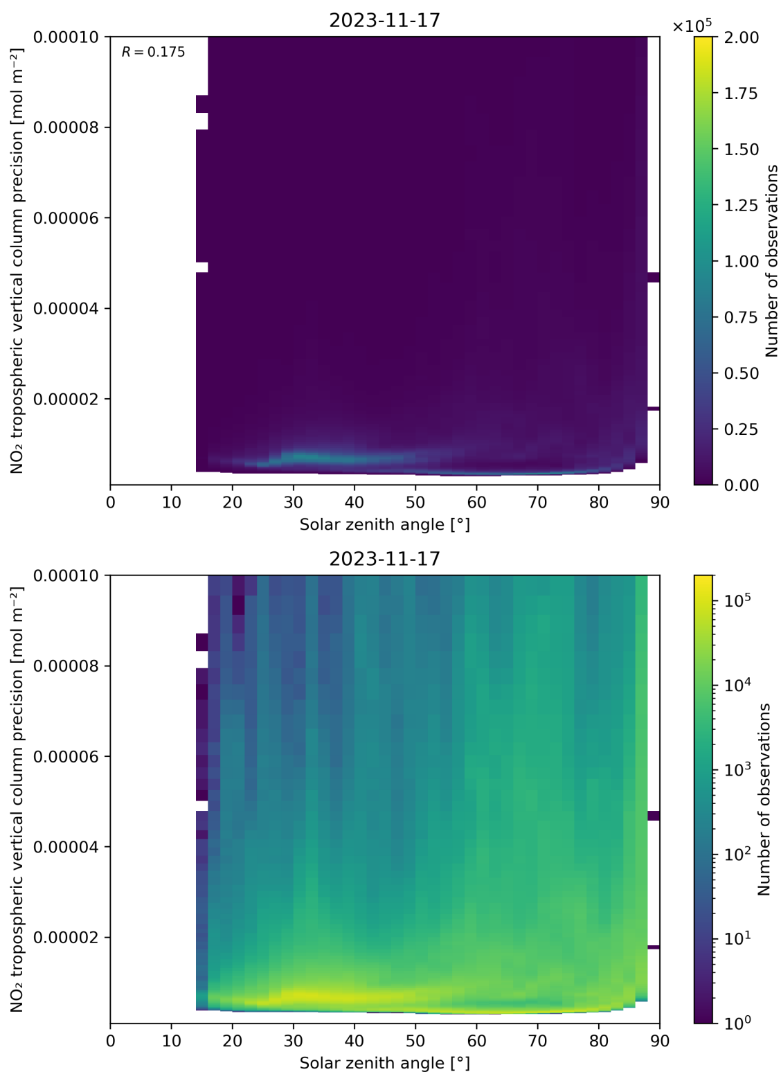
Figure 156: Scatter density plot of “Solar zenith angle” against “NO 2 tropospheric vertical column precision” for 2023-11-16 to 2023-11-18.
