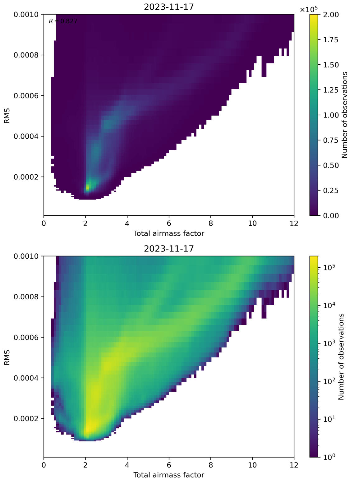
Figure 69: Scatter density plot of “Total airmass factor” against “RMS” for 2023-11-16 to 2023-11-18.
