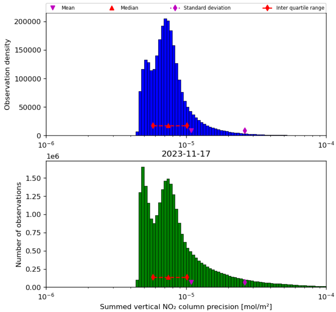
Figure 41: Histogram of "Summed vertical NO 2 column precision" for 2023-11-16 to 2023-11-18
