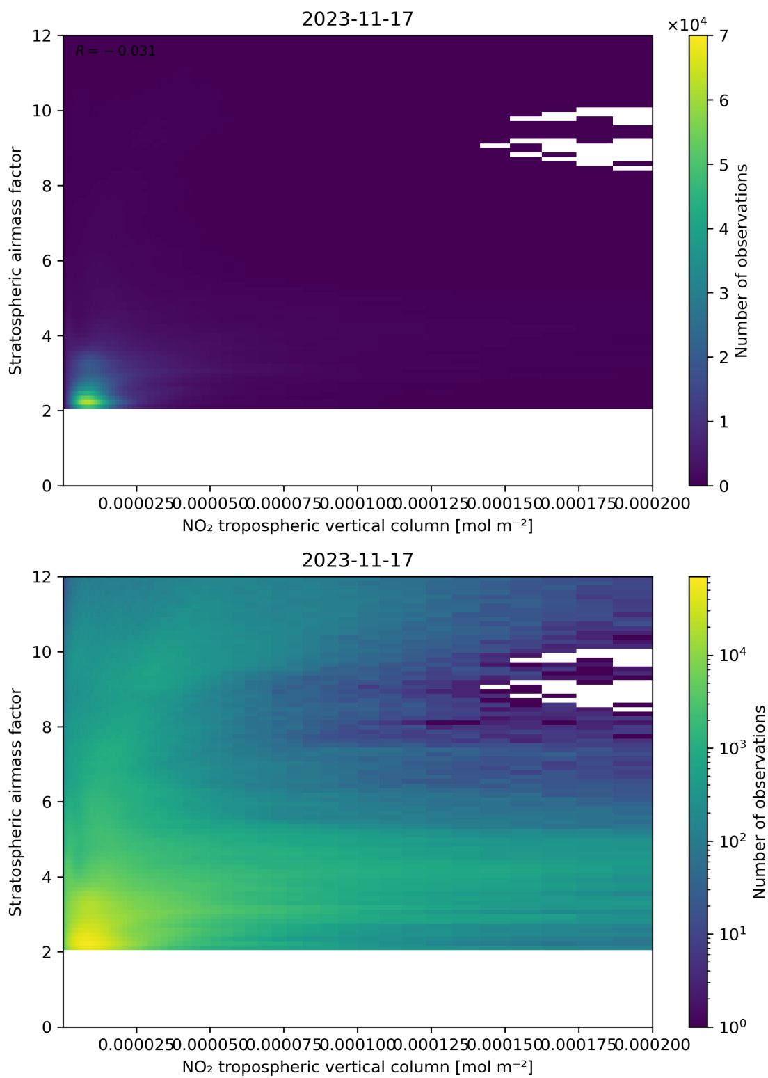
Figure 121: Scatter density plot of “NO 2 tropospheric vertical column” against “Stratospheric airmass factor” for 2023-11-16 to 2023-11-18.
