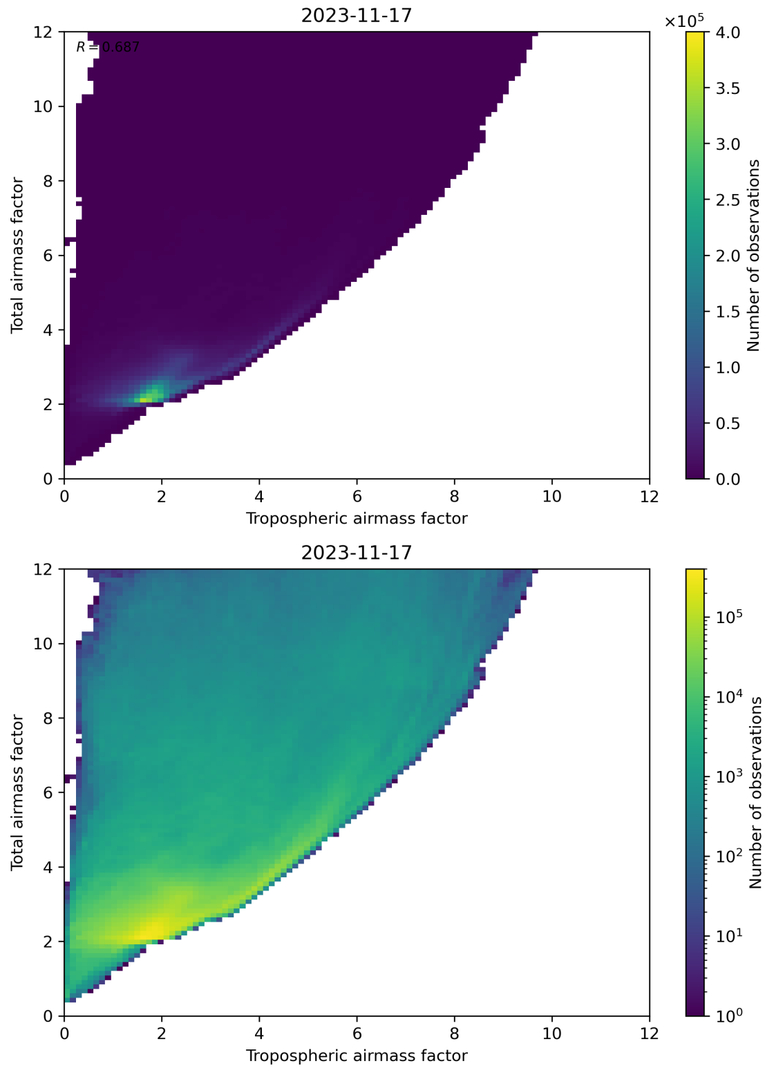
Figure 72: Scatter density plot of “Tropospheric airmass factor” against “Total airmass factor” for 2023-11-16 to 2023-11-18.
