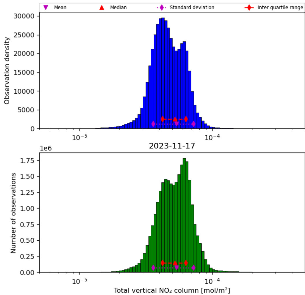
Figure 38: Histogram of “Total vertical NO 2 column” for 2023-11-16 to 2023-11-18
