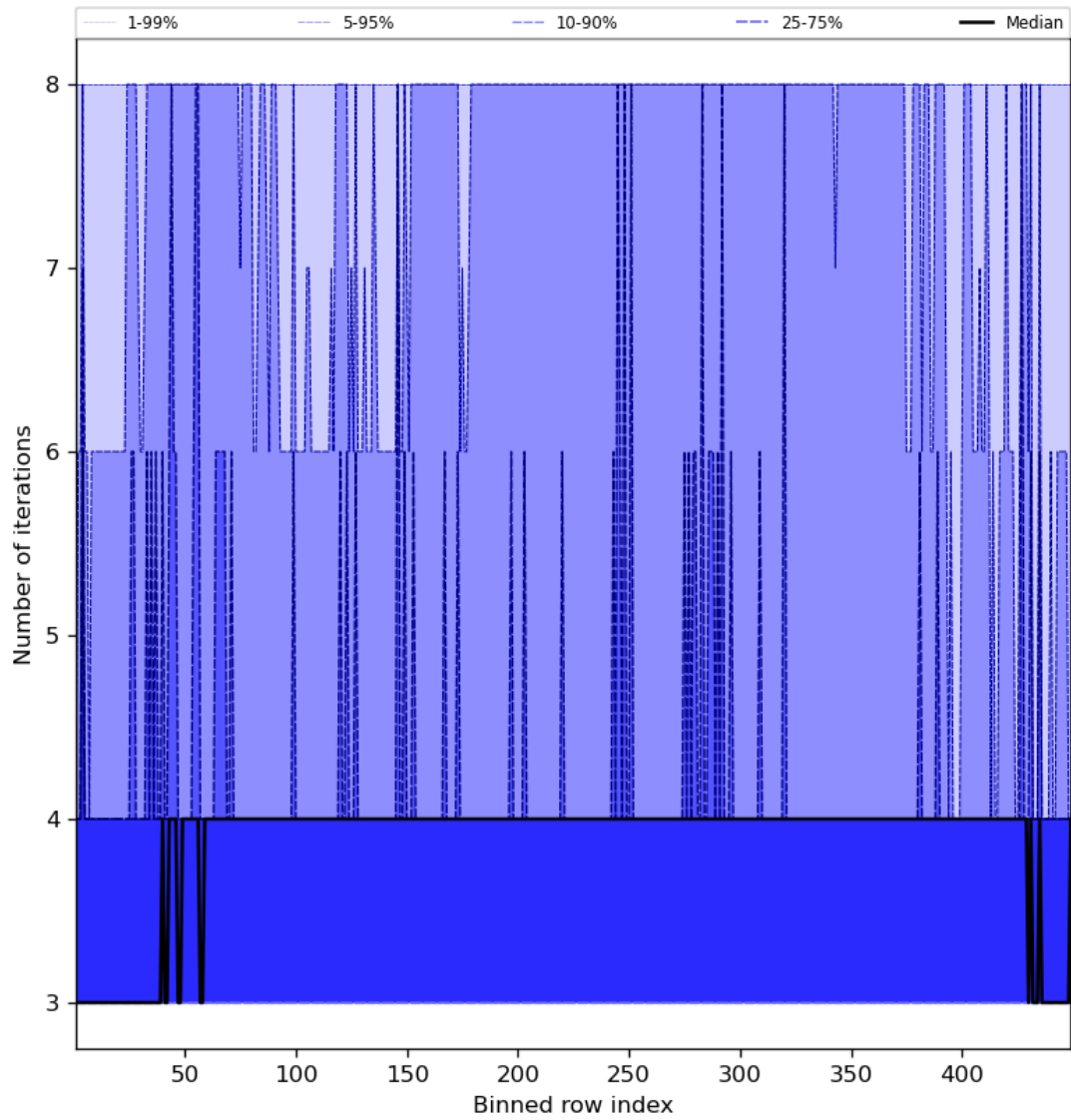
Figure 51: Along track statistics of “Number of iterations” for 2023-11-16 to 2023-11-18
