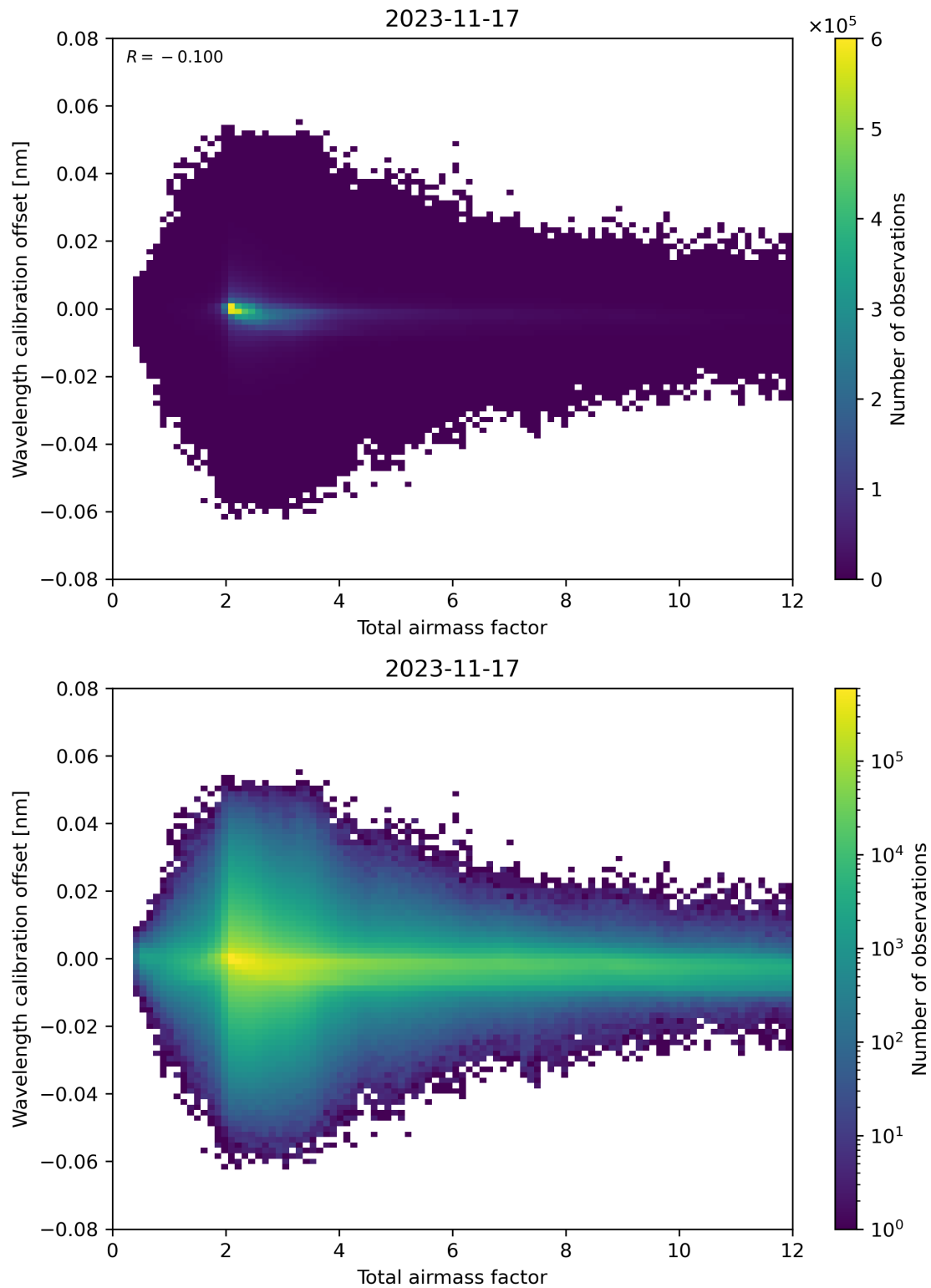
Figure 70: Scatter density plot of “Total airmass factor” against “Wavelength calibration offset” for 2023-11-16 to 2023-11-18.
