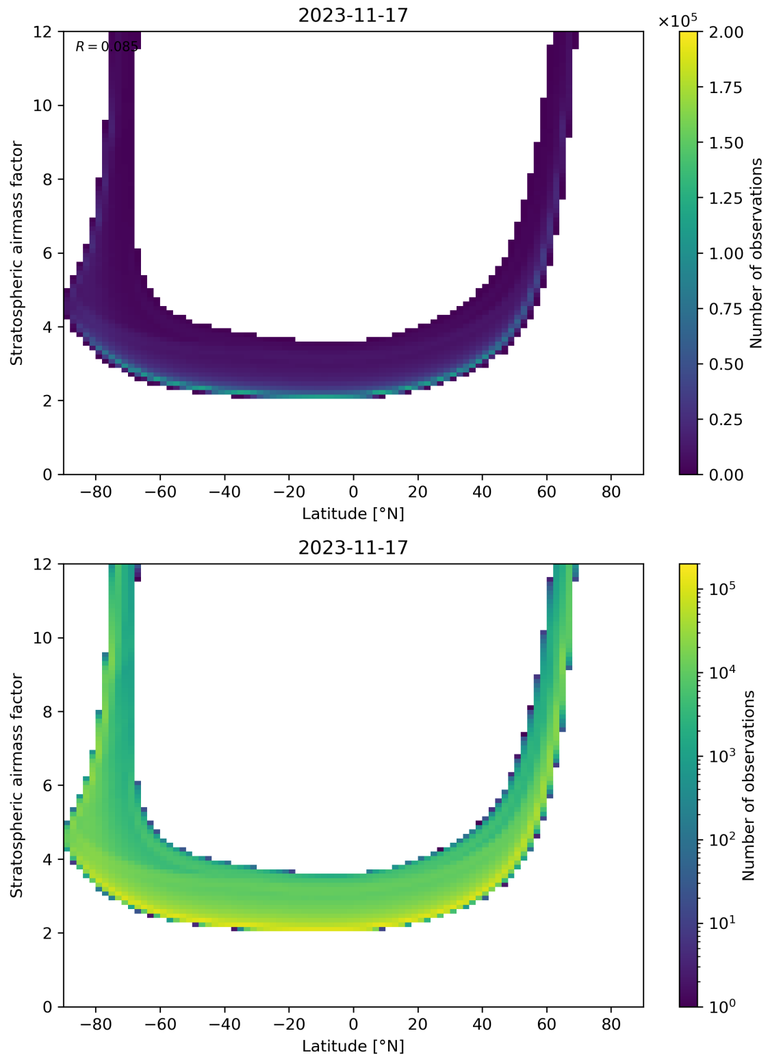
Figure 83: Scatter density plot of “Latitude” against “Stratospheric airmass factor” for 2023-11-16 to 2023-11-18.
