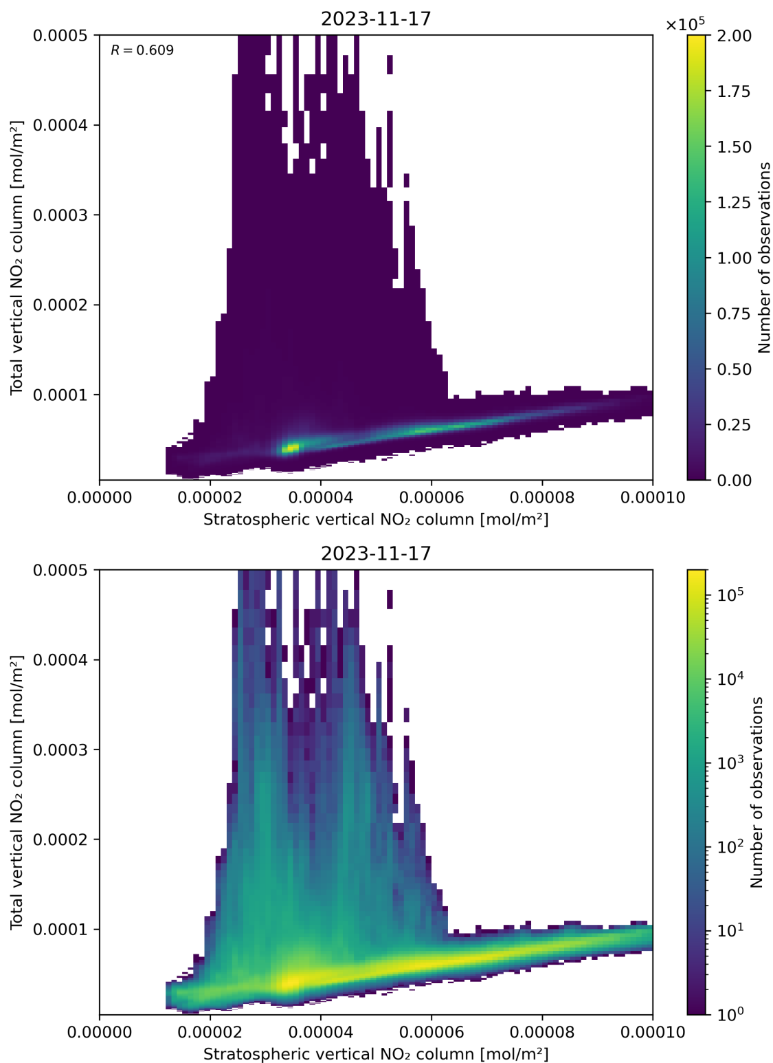
Figure 100: Scatter density plot of “Stratospheric vertical NO 2 column” against “Total vertical NO 2 column” for 2023-11-16 to 2023-11-18.
