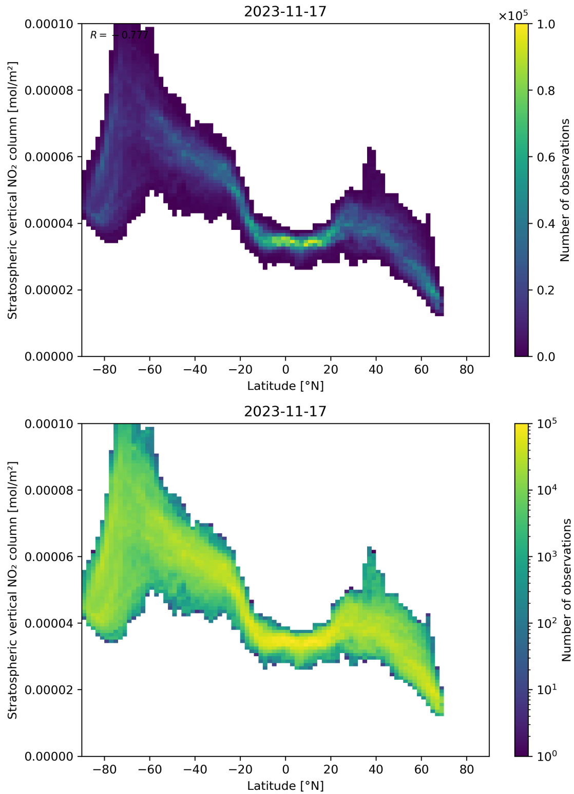
Figure 87: Scatter density plot of “Latitude” against “Stratospheric vertical NO 2 column” for 2023-11-16 to 2023-11-18.
