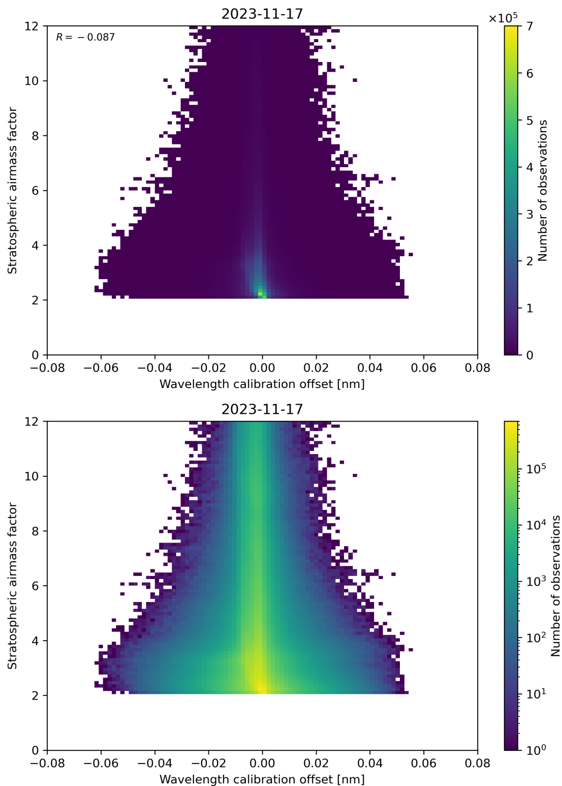
Figure 174: Scatter density plot of “Wavelength calibration offset” against “Stratospheric air mass factor” for 2023-11-16 to 2023-11-18.
