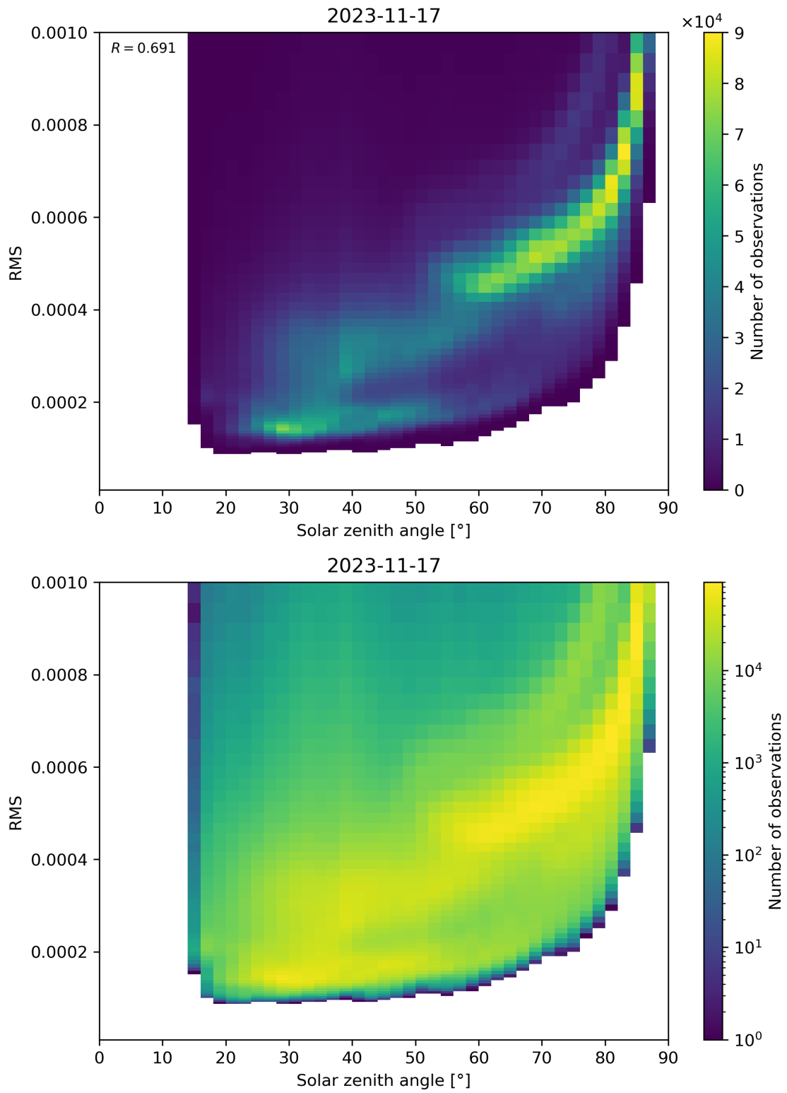
Figure 157: Scatter density plot of “Solar zenith angle” against “RMS” for 2023-11-16 to 2023-11-18.
