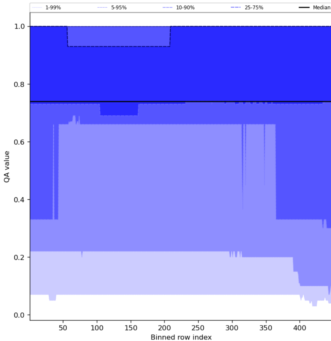
Figure 45: Along track statistics of “QA value” for 2023-11-16 to 2023-11-18
