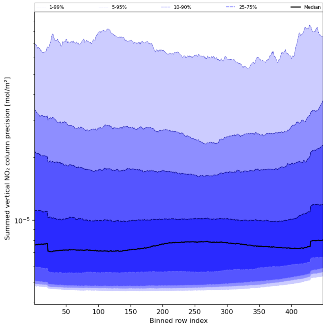
Figure 58: Along track statistics of “Summed vertical NO 2 column precision” for 2023-11-16 to 2023-11-18
