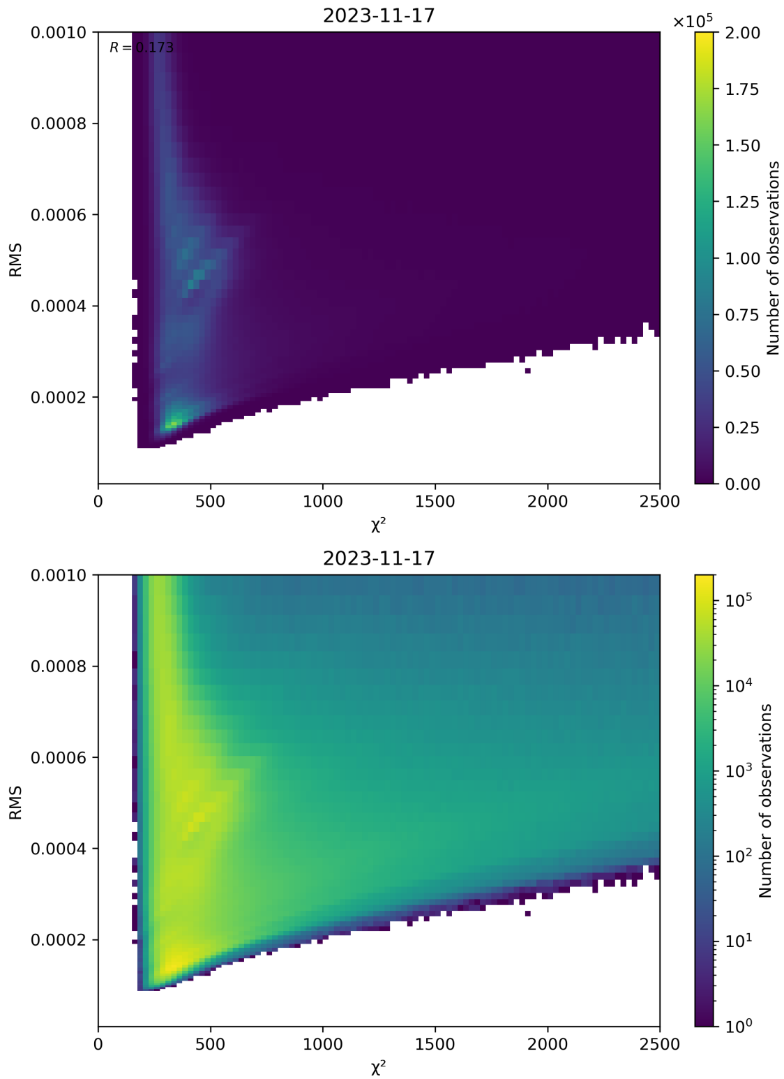
Figure 82: Scatter density plot of “ \chi^2 ” against “RMS” for 2023-11-16 to 2023-11-18.
