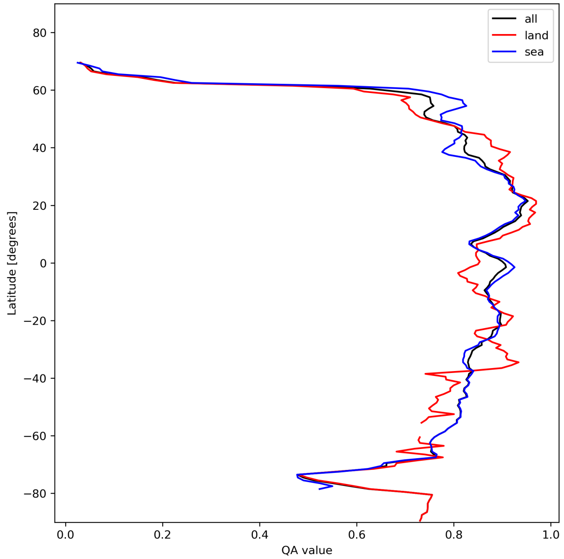
Figure 11: Zonal average of “QA value” for 2023-11-16 to 2023-11-18.
