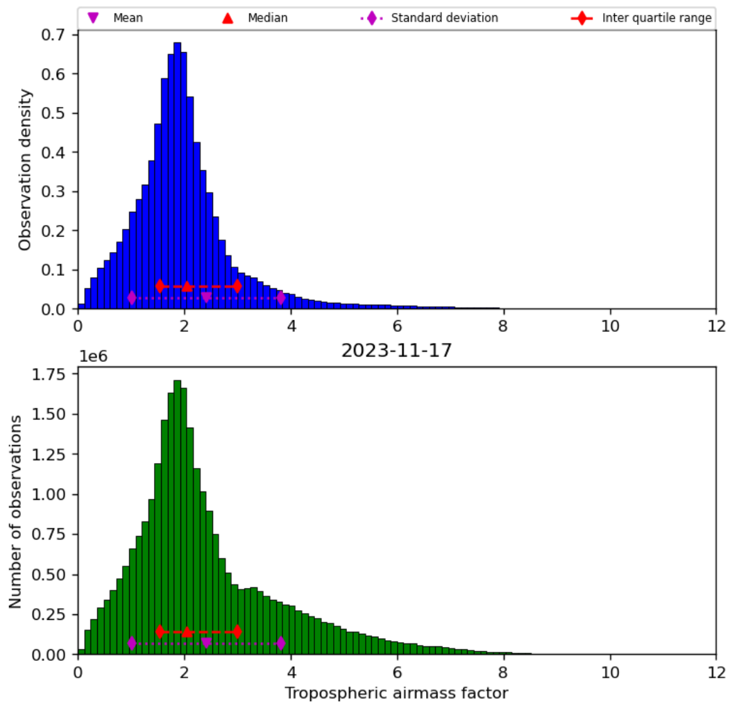
Figure 31: Histogram of “Tropospheric airmass factor” for 2023-11-16 to 2023-11-18
