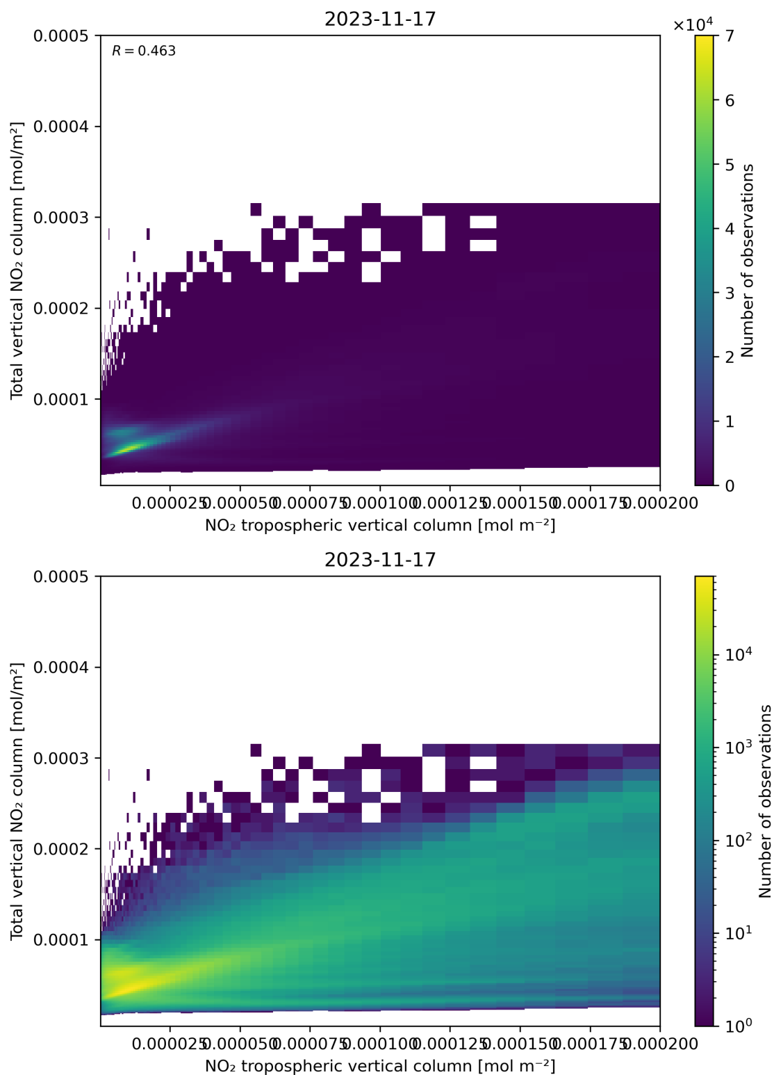
Figure 128: Scatter density plot of “NO 2 tropospheric vertical column” against “Total vertical NO 2 column” for 2023-11-16 to 2023-11-18.
