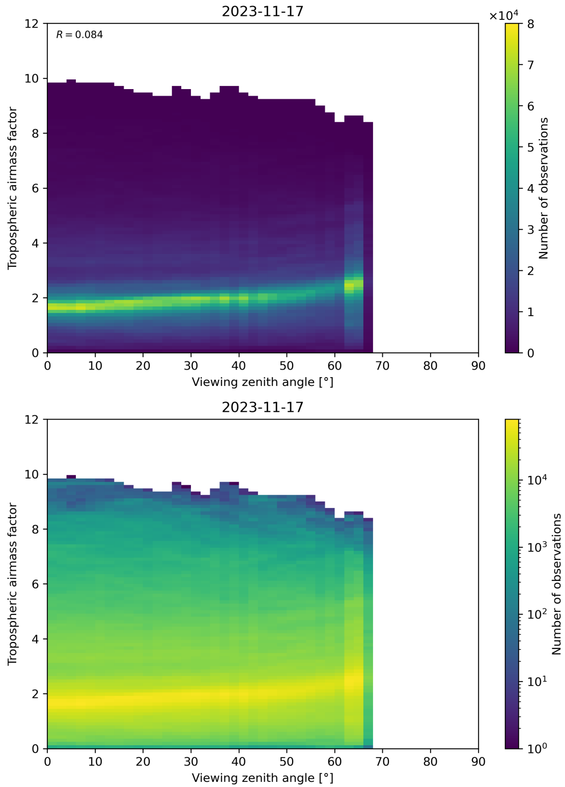
Figure 161: Scatter density plot of “Viewing zenith angle” against “Tropospheric airmass factor” for 2023-11-16 to 2023-11-18.
