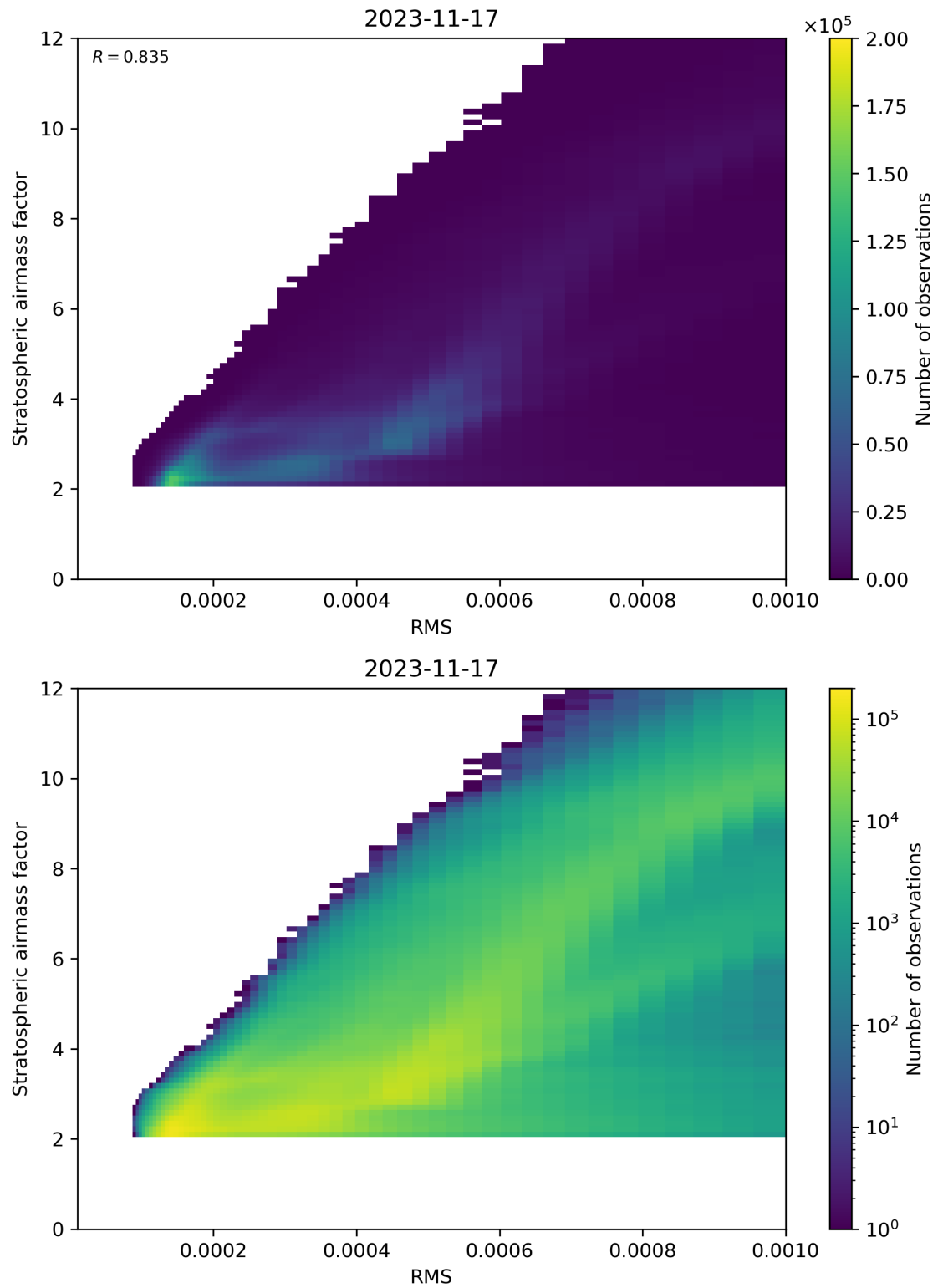
Figure 144: Scatter density plot of “RMS” against “Stratospheric airmass factor” for 2023-11-16 to 2023-11-18.
