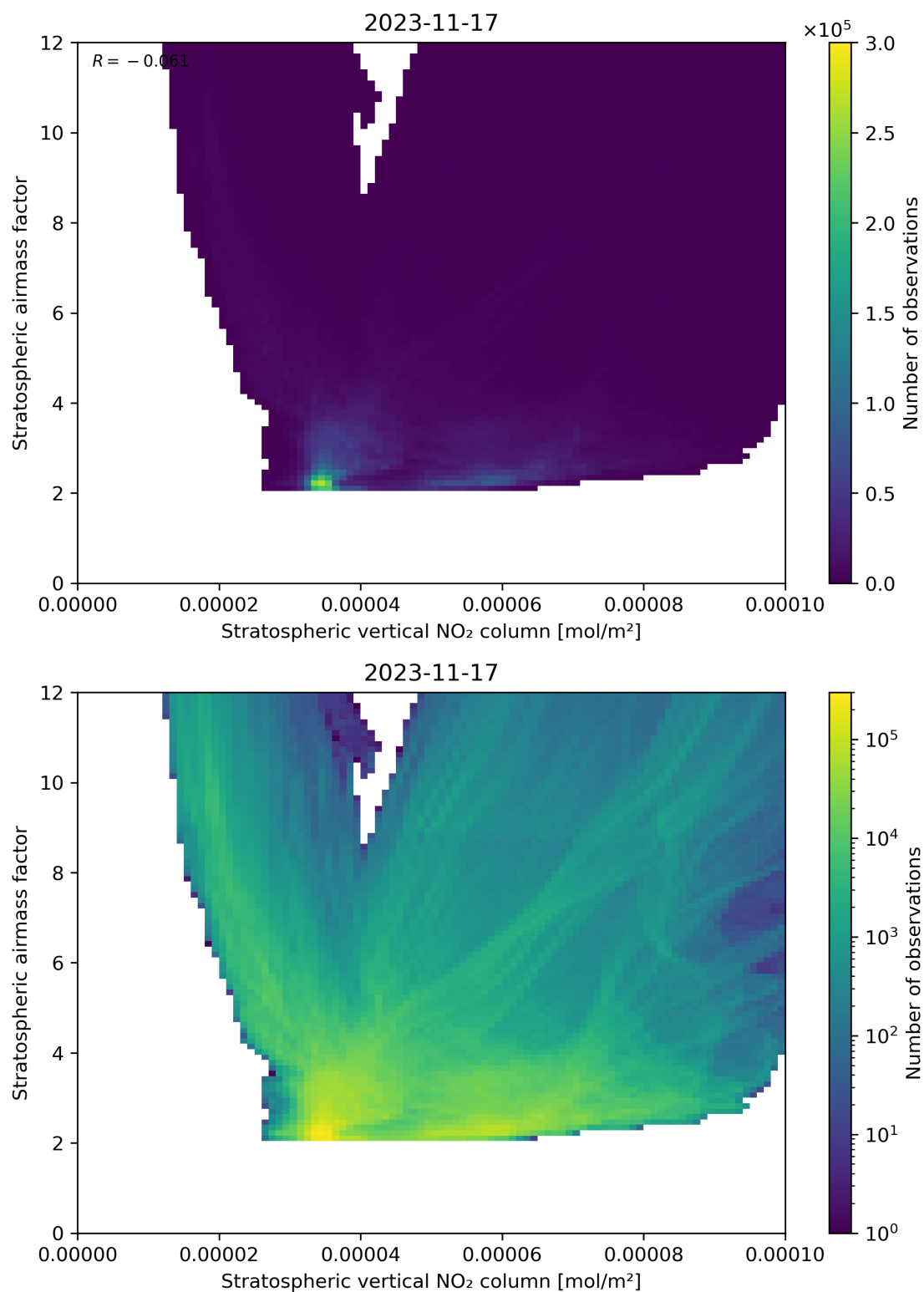
Figure 96: Scatter density plot of “Stratospheric vertical NO 2 column” against “Stratospheric airmass factor” for 2023-11-16 to 2023-11-18.
