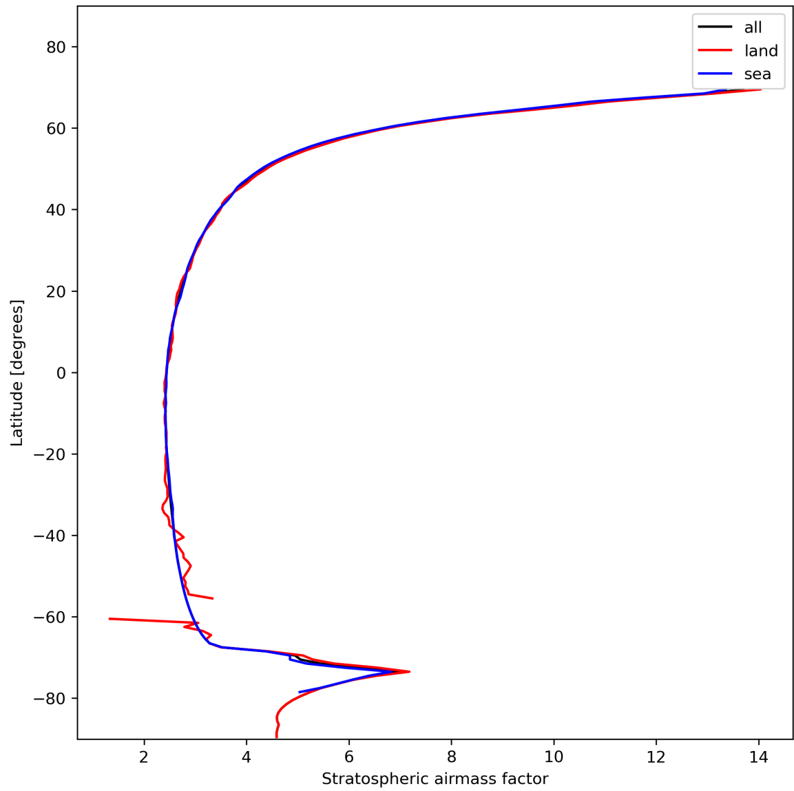
Figure 27: Zonal average of “Stratospheric air mass factor” for 2023-11-16 to 2023-11-18.
