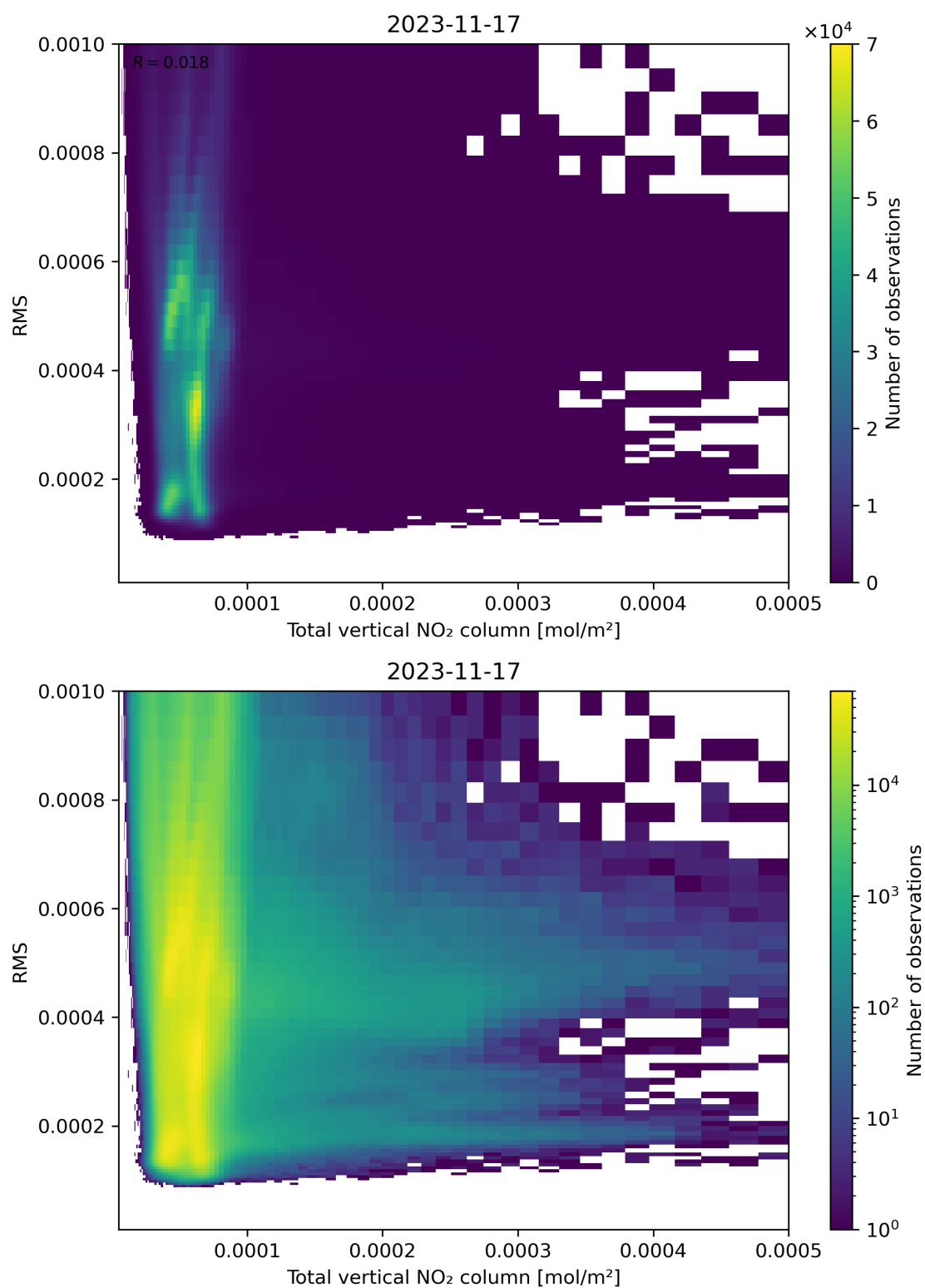
Figure 120: Scatter density plot of “Total vertical NO 2 column” against “RMS” for 2023-11-16 to 2023-11-18.
