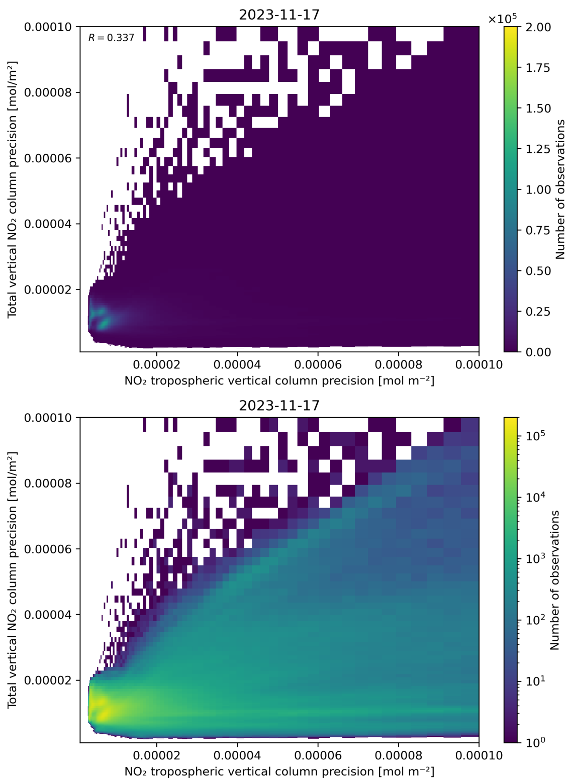
Figure 139: Scatter density plot of “NO 2 tropospheric vertical column precision” against “Total vertical NO 2 column precision” for 2023-11-16 to 2023-11-18.
