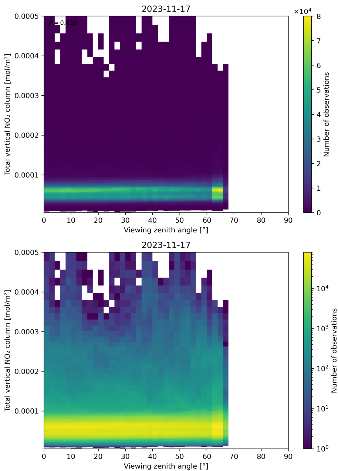
Figure 167: Scatter density plot of “Viewing zenith angle” against “Total vertical NO 2 column” for 2023-11-16 to 2023-11-18.
