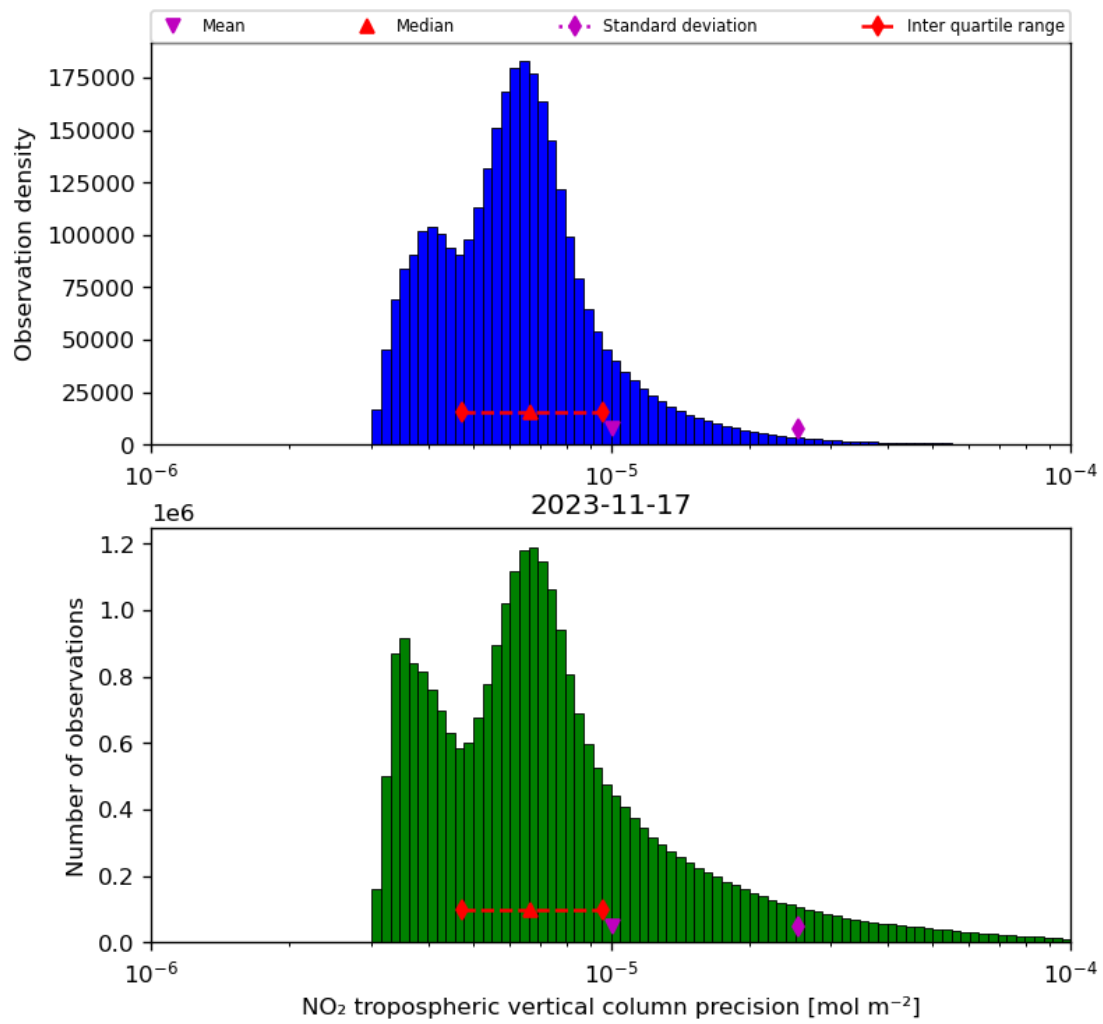
Figure 30: Histogram of “NO 2 tropospheric vertical column precision” for 2023-11-16 to 2023-11-18
