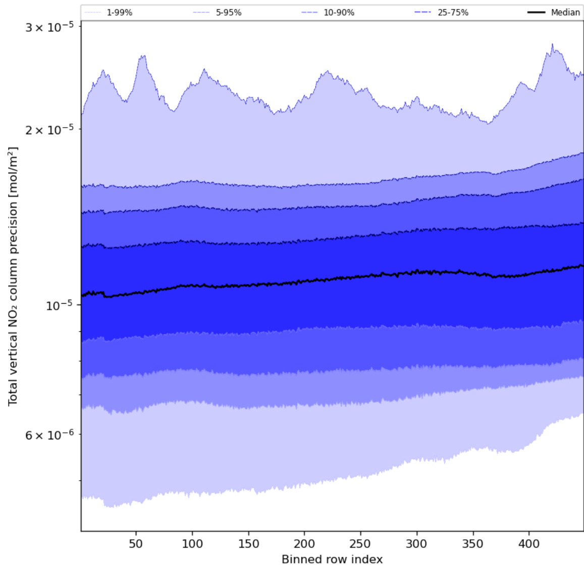
Figure 56: Along track statistics of “Total vertical NO 2 column precision” for 2023-11-16 to 2023-11-18
