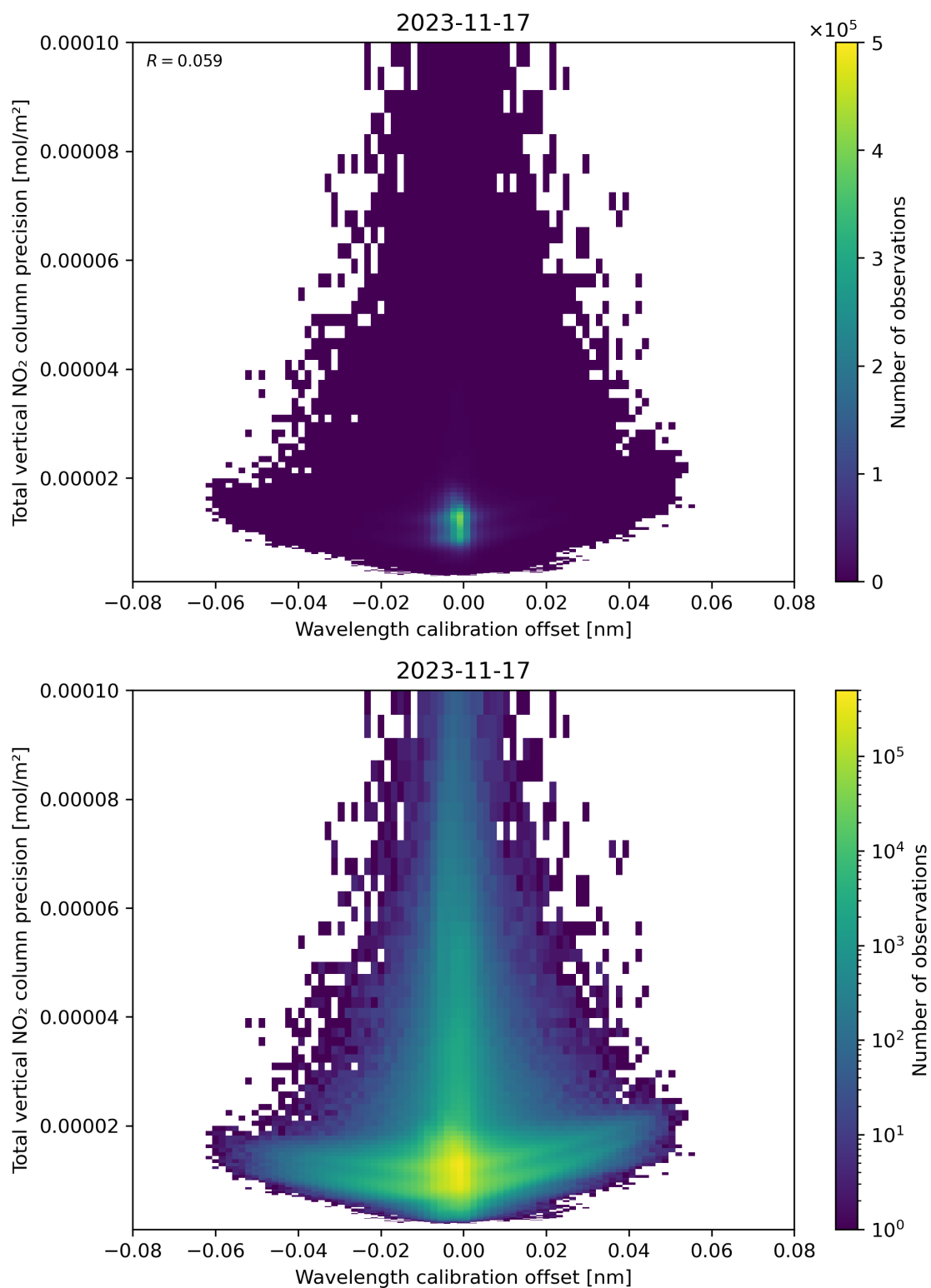
Figure 180: Scatter density plot of “Wavelength calibration offset” against “Total vertical NO 2 column precision” for 2023-11-16 to 2023-11-18.
