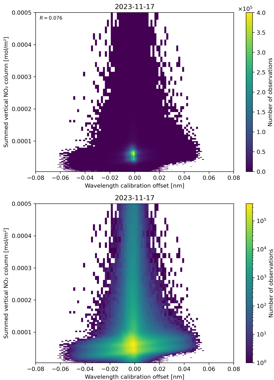
Figure 177: Scatter density plot of “Wavelength calibration offset” against “Summed vertical NO 2 column” for 2023-11-16 to 2023-11-18.
