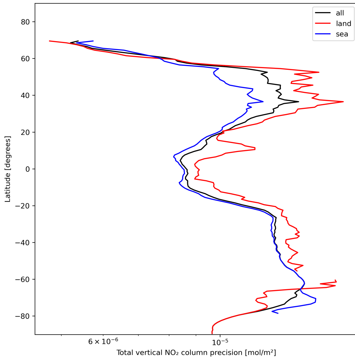
Figure 22: Zonal average of “Total vertical NO 2 column precision” for 2023-11-16 to 2023-11-18.
