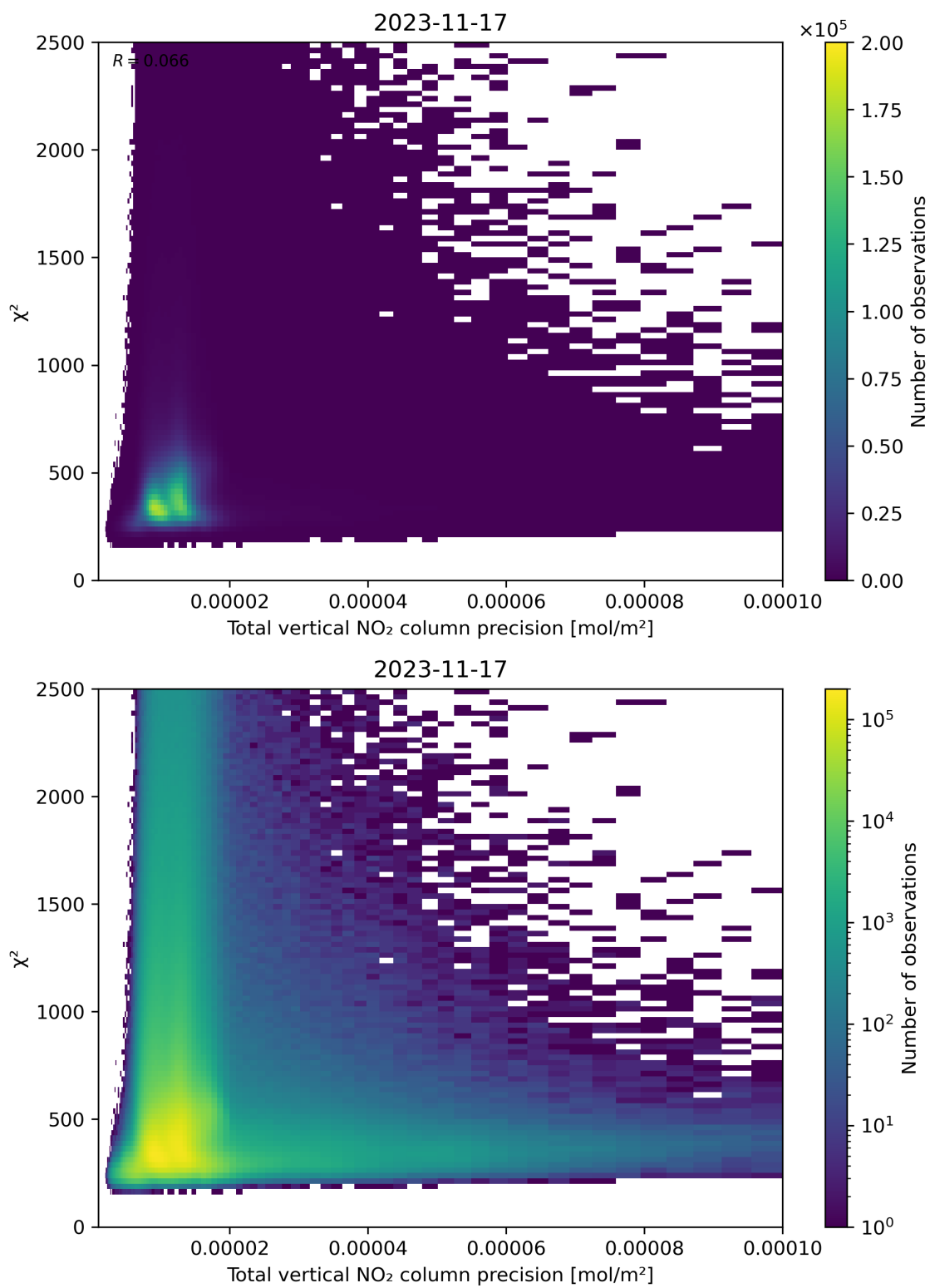
Figure 116: Scatter density plot of “Total vertical NO 2 column precision” against “ \chi^2 ” for 2023-11-16 to 2023-11-18.
