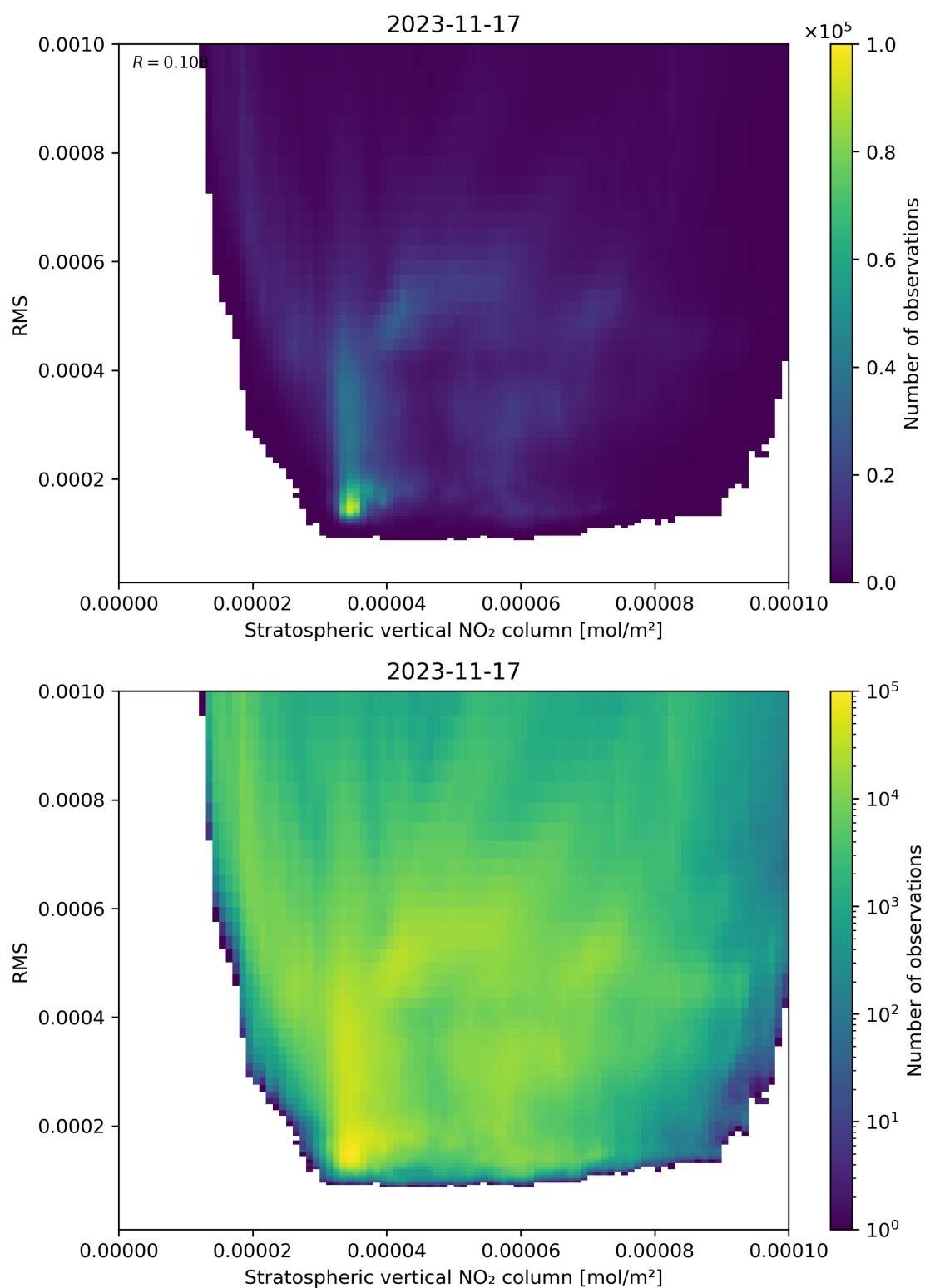
Figure 102: Scatter density plot of “Stratospheric vertical NO 2 column” against “RMS” for 2023-11-16 to 2023-11-18.
