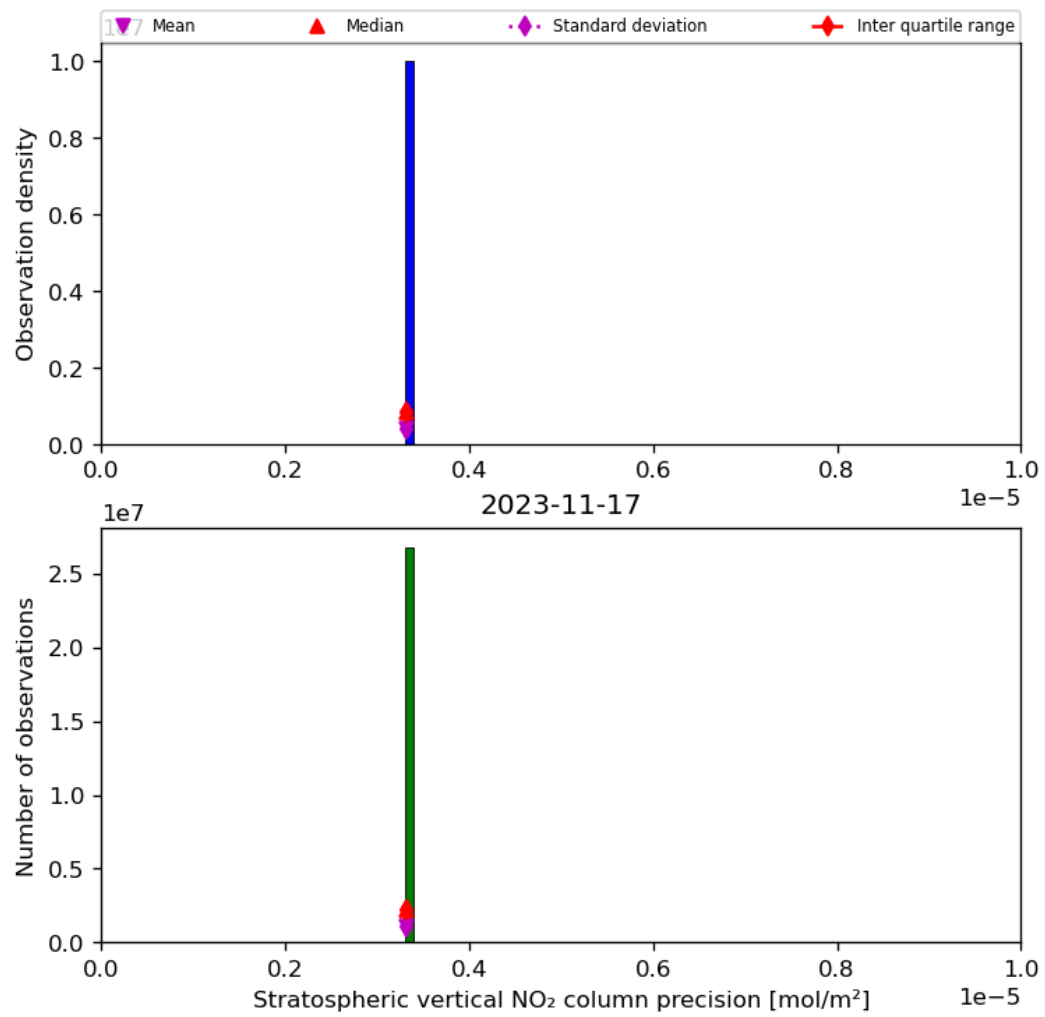
Figure 37: Histogram of “Stratospheric vertical NO 2 column precision” for 2023-11-16 to 2023-11-18
