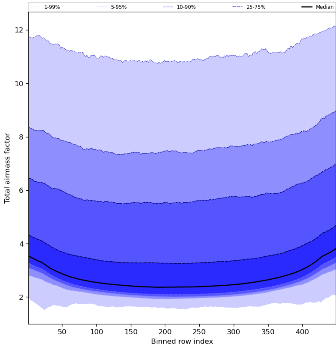
Figure 49: Along track statistics of “Total airmass factor” for 2023-11-16 to 2023-11-18
