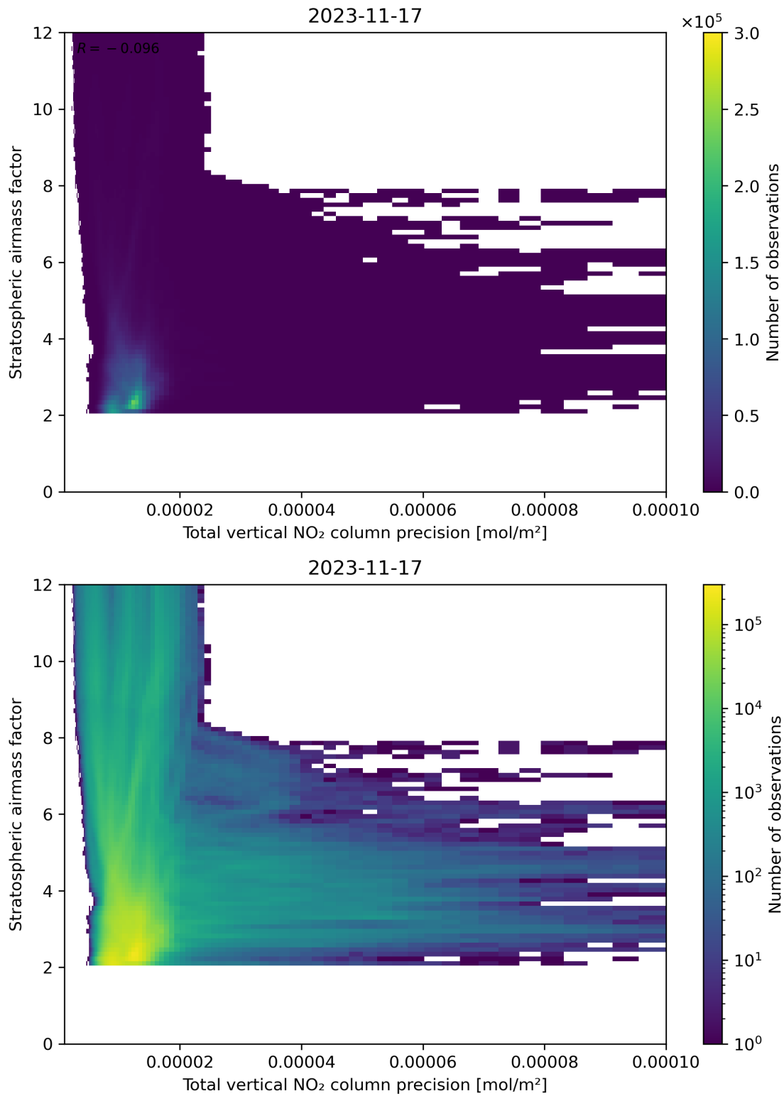
Figure 115: Scatter density plot of “Total vertical NO 2 column precision” against “Stratospheric air mass factor” for 2023-11-16 to 2023-11-18.
