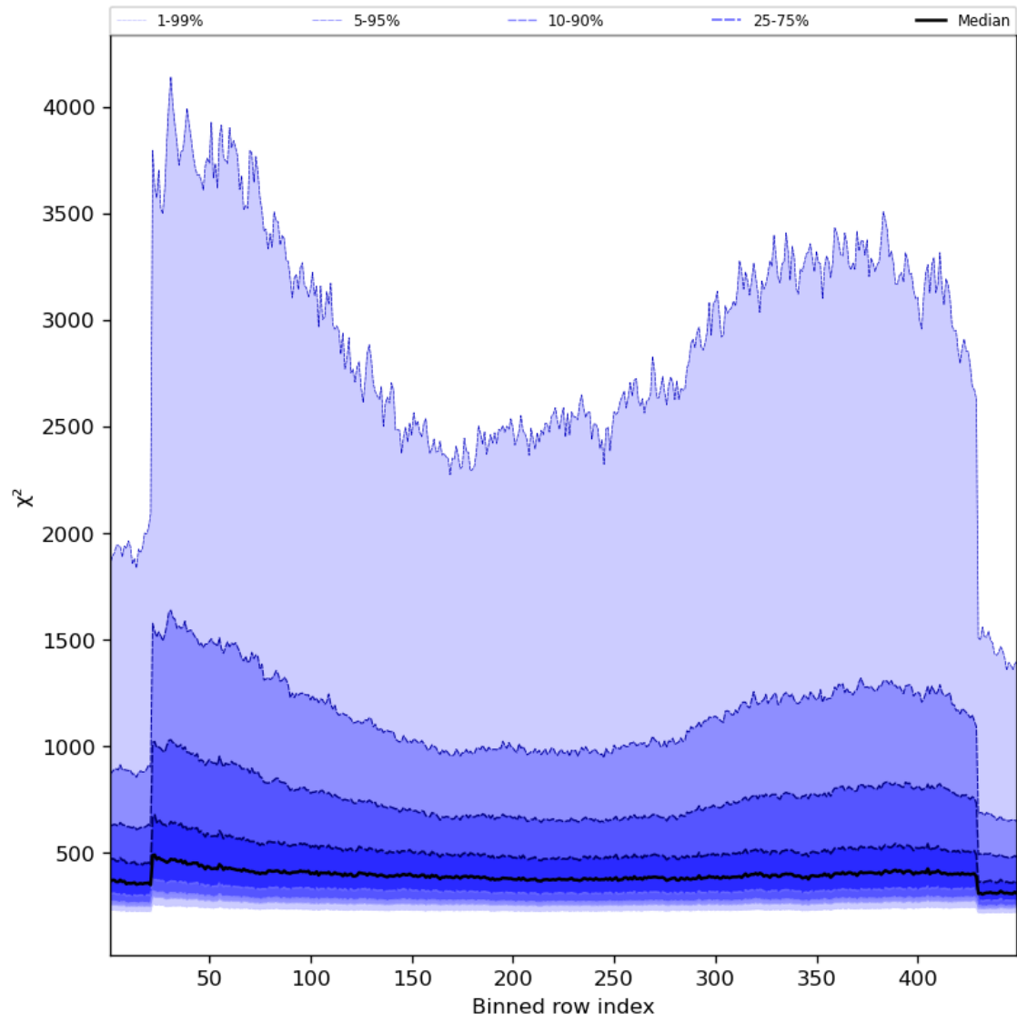
Figure 59: Along track statistics of “ \chi^2 ” for 2023-11-16 to 2023-11-18
