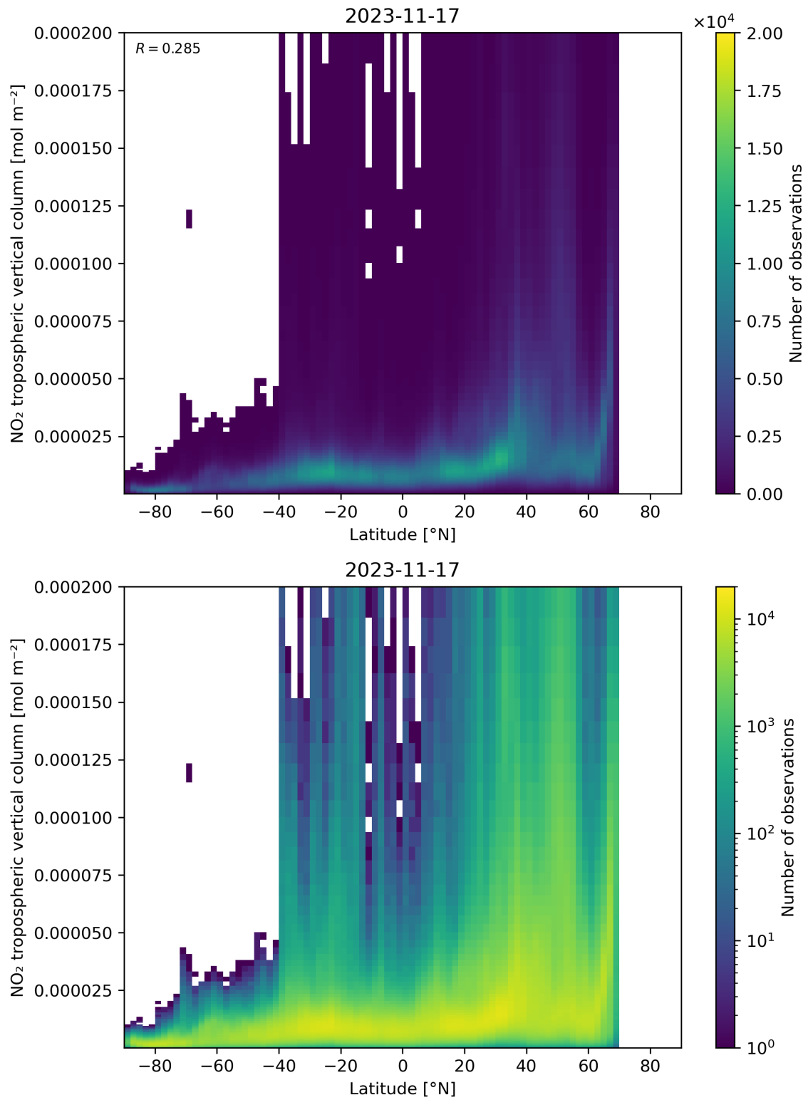
Figure 92: Scatter density plot of “Latitude” against “NO 2 tropospheric vertical column” for 2023-11-16 to 2023-11-18.
