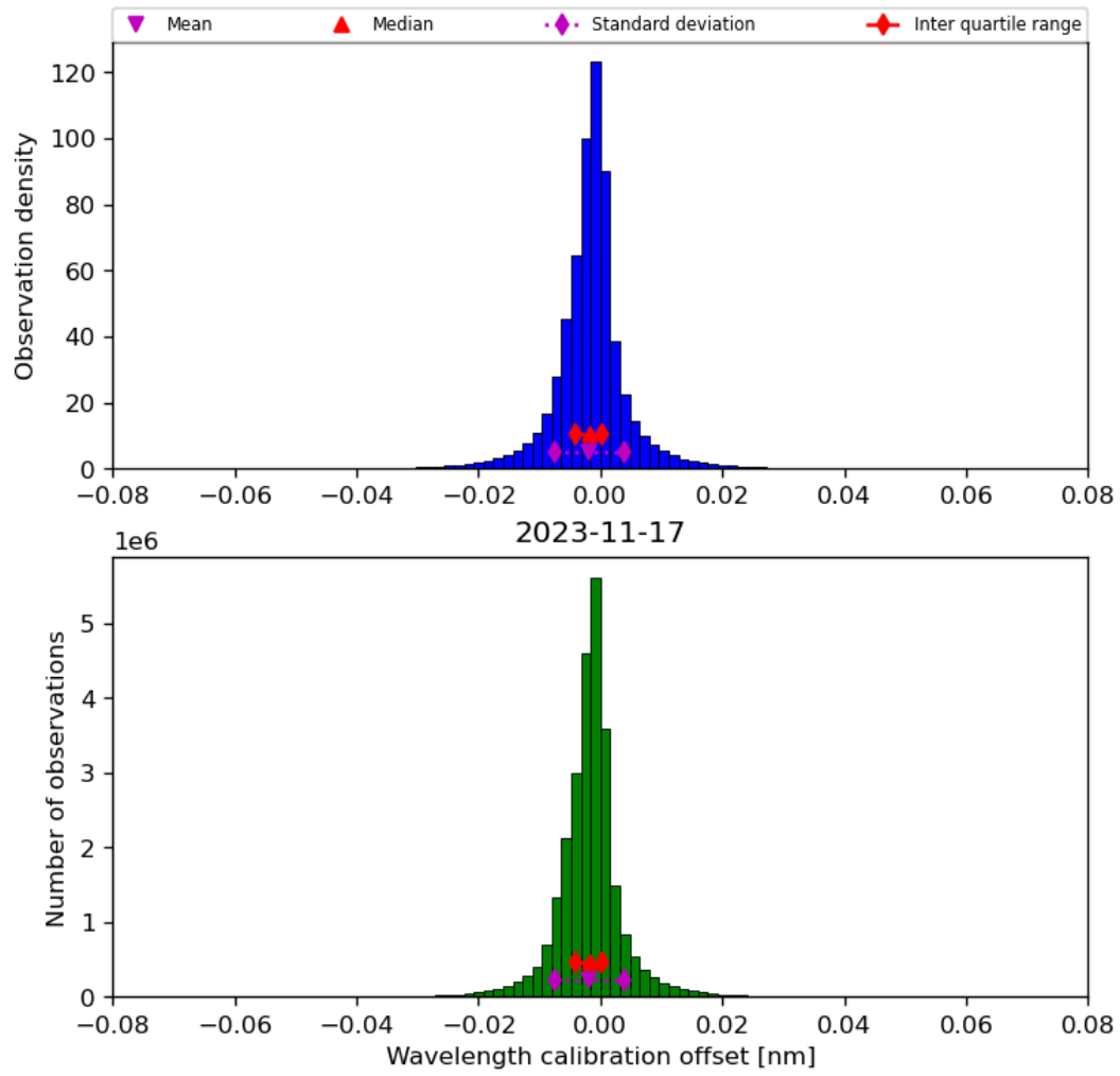
Figure 35: Histogram of “Wavelength calibration offset” for 2023-11-16 to 2023-11-18
