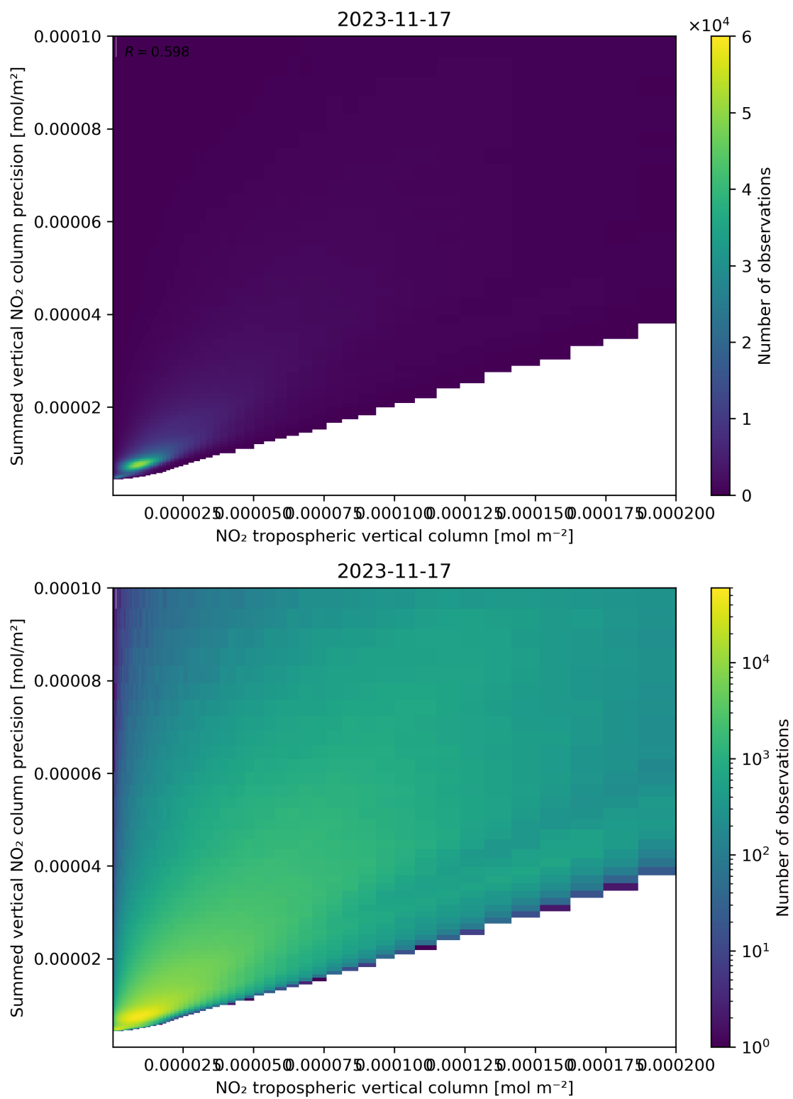
Figure 127: Scatter density plot of “NO 2 tropospheric vertical column” against “Summed vertical NO 2 column precision” for 2023-11-16 to 2023-11-18.
