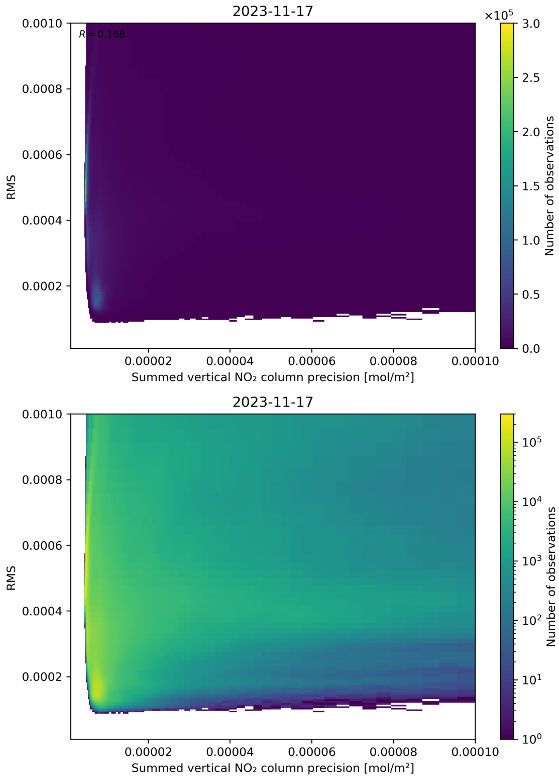
Figure 108: Scatter density plot of “Summed vertical NO 2 column precision” against “RMS” for 2023-11-16 to 2023-11-18.
