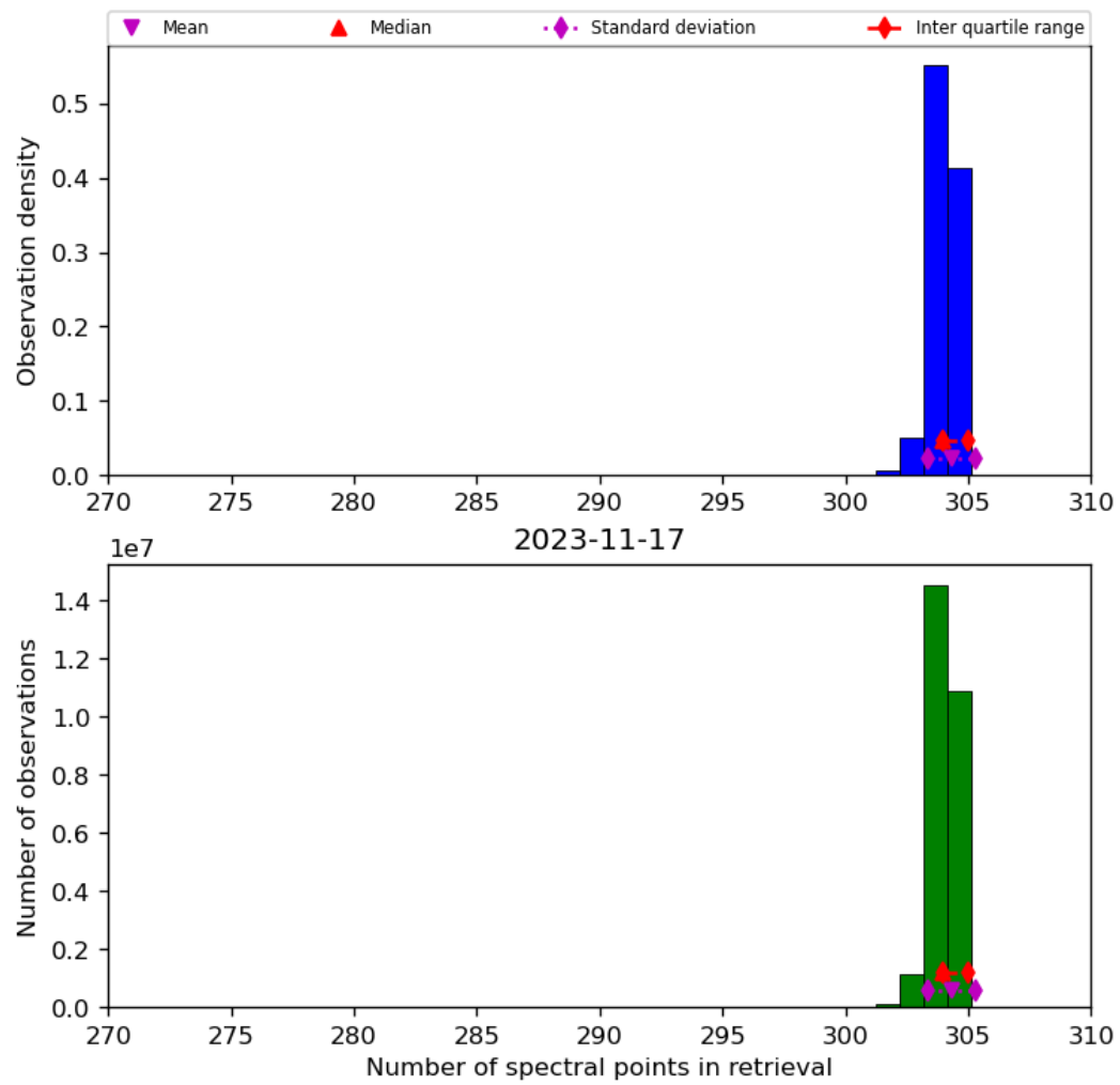
Figure 33: Histogram of “Number of spectral points in retrieval” for 2023-11-16 to 2023-11-18
