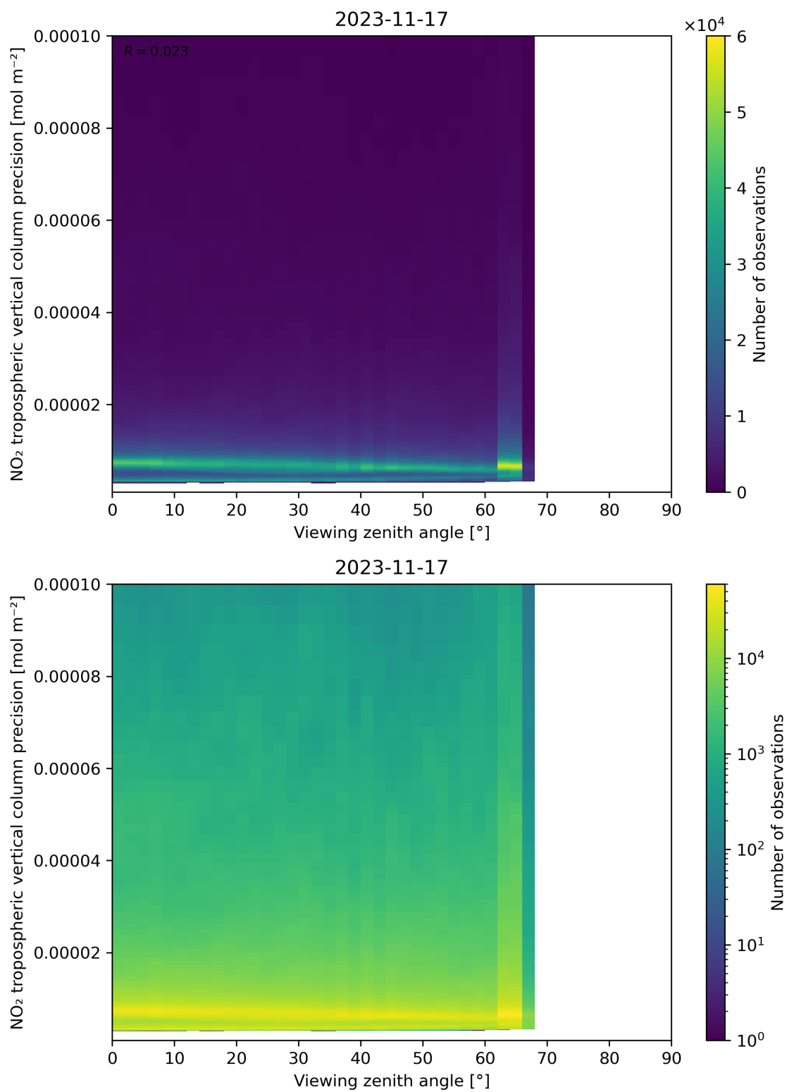
Figure 170: Scatter density plot of “Viewing zenith angle” against “NO 2 tropospheric vertical column precision” for 2023-11-16 to 2023-11-18.
