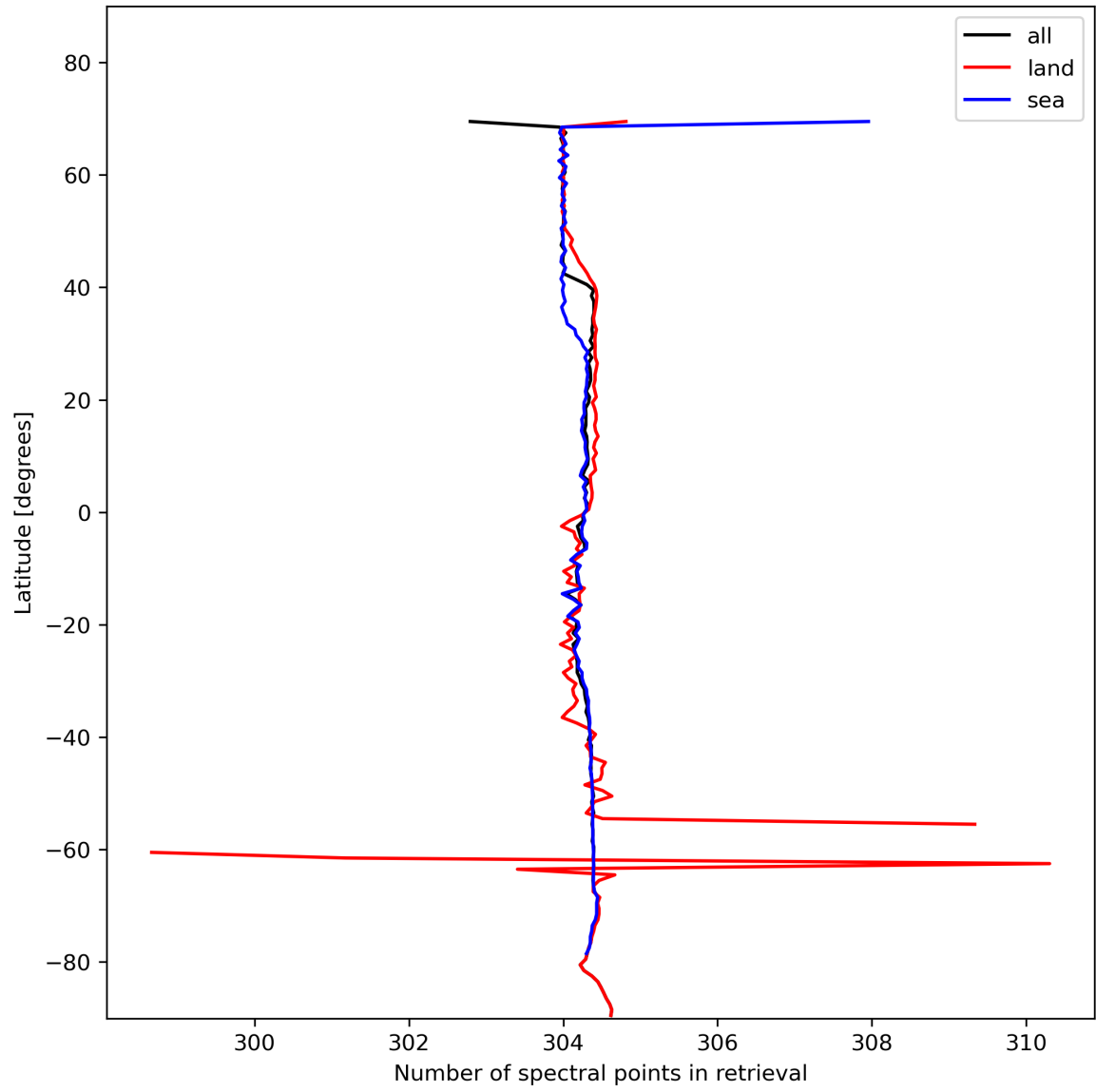
Figure 16: Zonal average of “Number of spectral points in retrieval” for 2023-11-16 to 2023-11-18.
