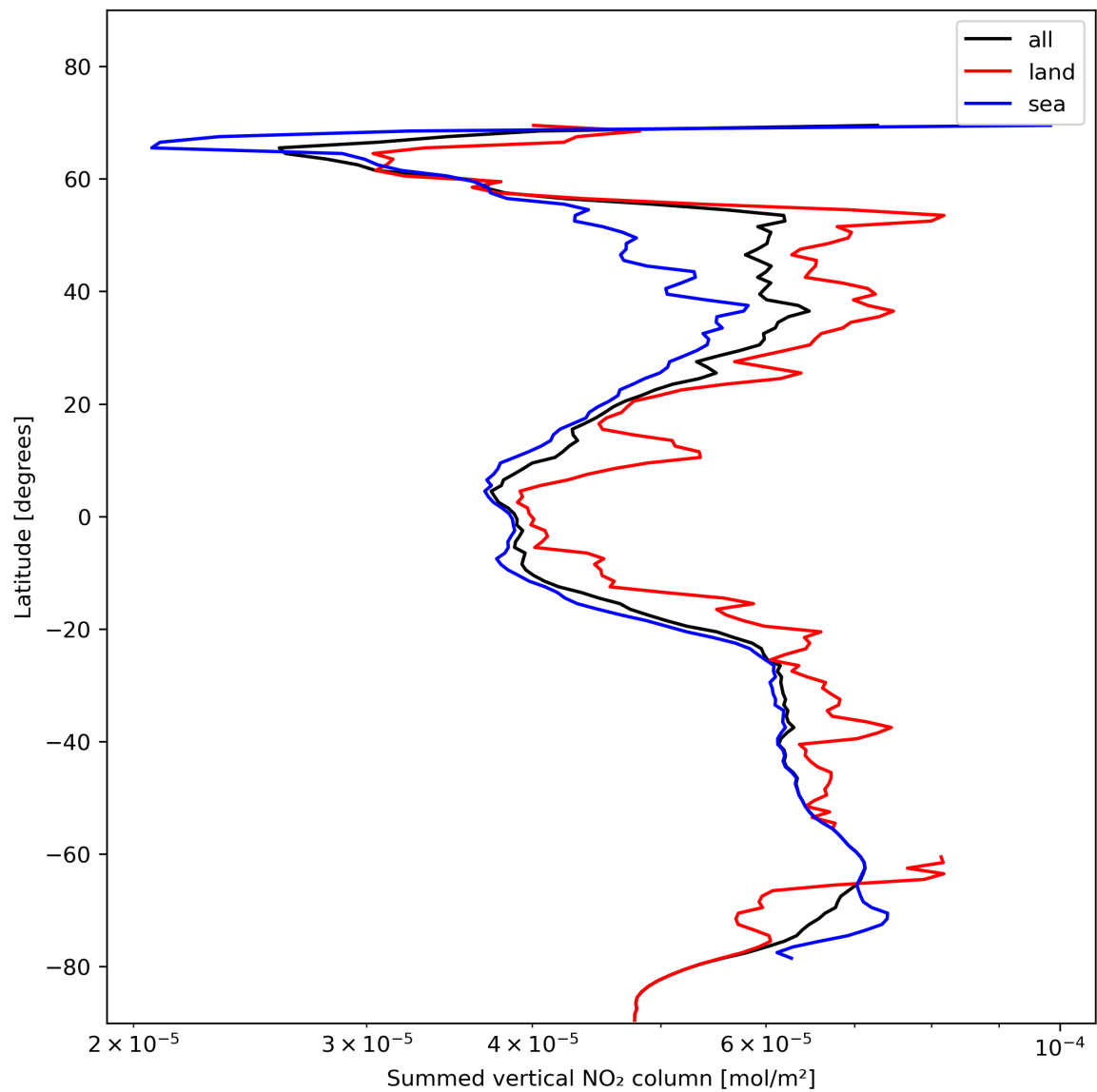
Figure 23: Zonal average of “Summed vertical NO 2 column” for 2023-11-16 to 2023-11-18.
