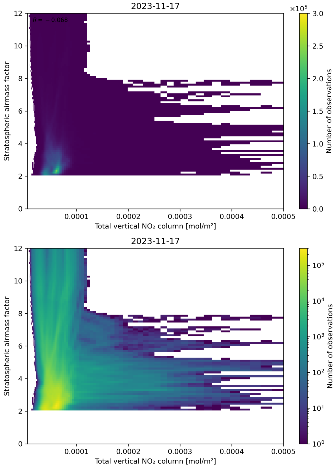
Figure 110: Scatter density plot of “Total vertical NO 2 column” against “Stratospheric airmass factor” for 2023-11-16 to 2023-11-18.
