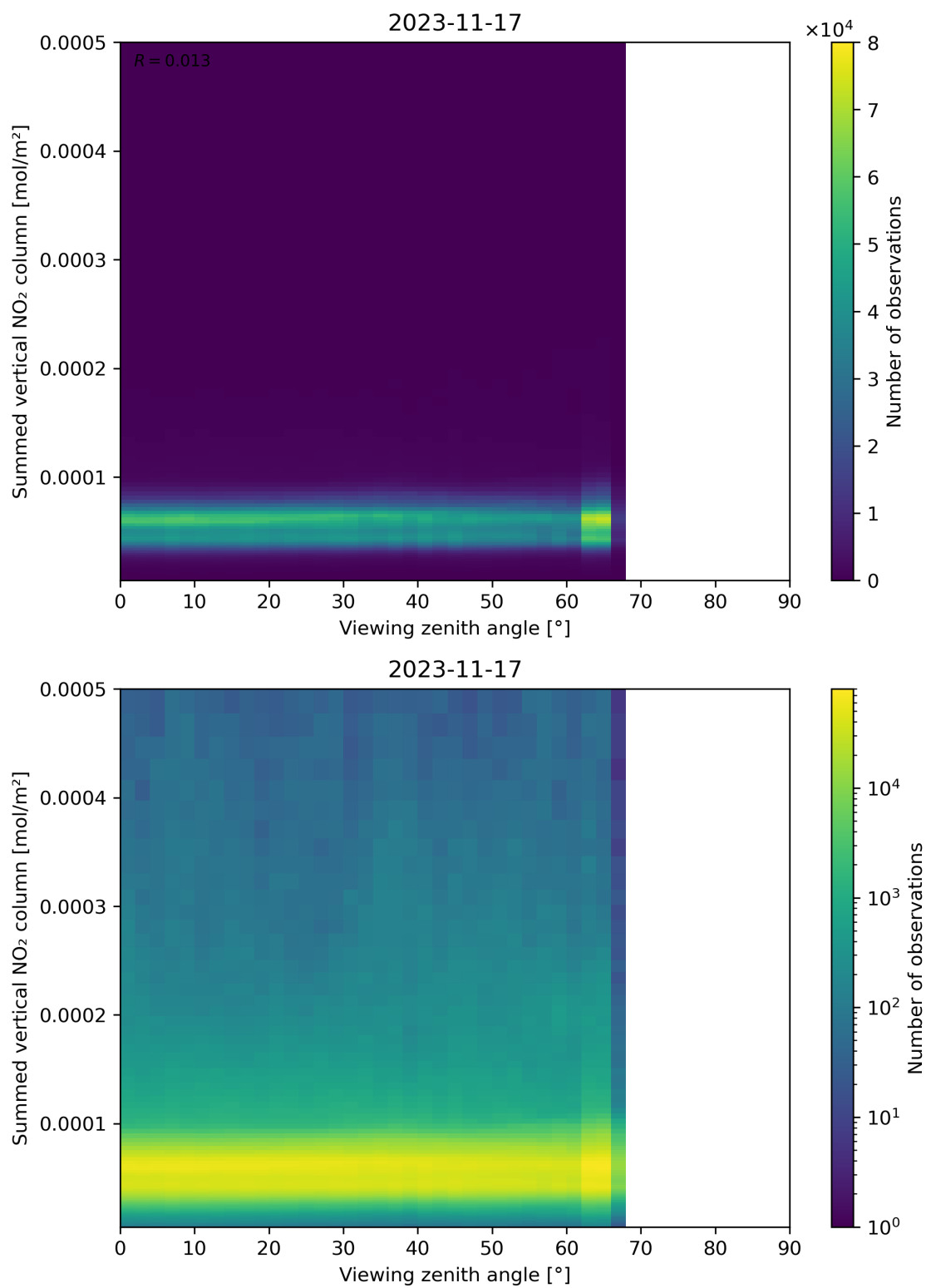
Figure 165: Scatter density plot of “Viewing zenith angle” against “Summed vertical NO 2 column” for 2023-11-16 to 2023-11-18.
