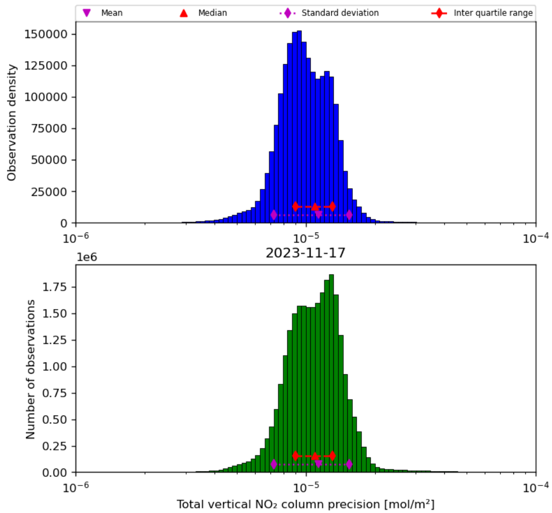
Figure 39: Histogram of “Total vertical NO 2 column precision” for 2023-11-16 to 2023-11-18
