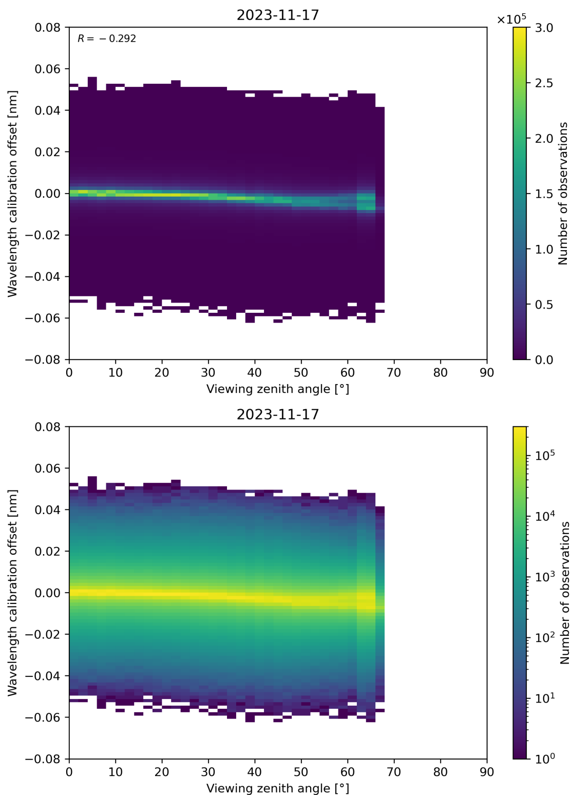
Figure 173: Scatter density plot of “Viewing zenith angle” against “Wavelength calibration offset” for 2023-11-16 to 2023-11-18.
