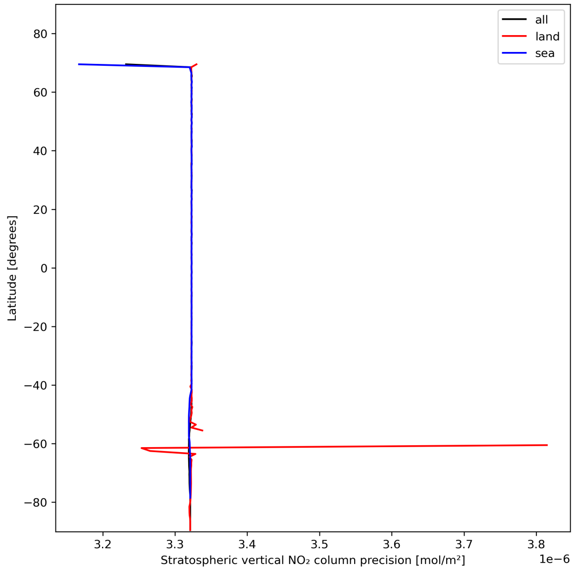
Figure 20: Zonal average of “Stratospheric vertical NO 2 column precision” for 2023-11-16 to 2023-11-18.
