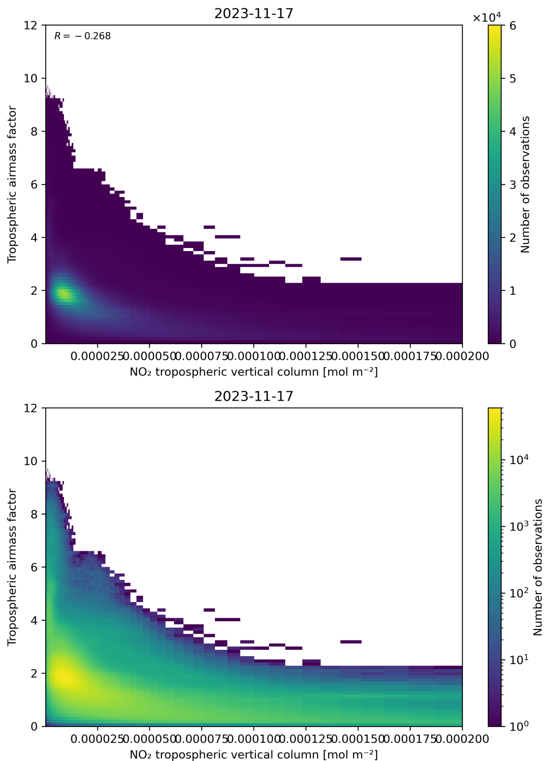
Figure 123: Scatter density plot of “NO 2 tropospheric vertical column” against “Tropospheric air mass factor” for 2023-11-16 to 2023-11-18.
