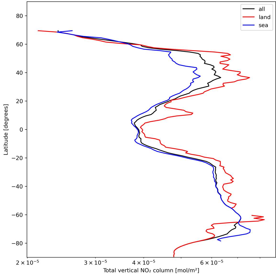
Figure 21: Zonal average of “Total vertical NO 2 column” for 2023-11-16 to 2023-11-18.
