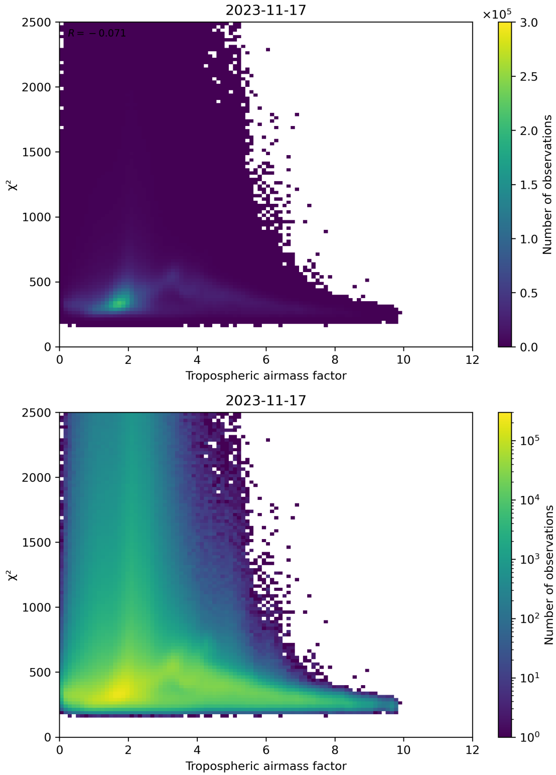
Figure 73: Scatter density plot of “Tropospheric airmass factor” against “ \chi^2 ” for 2023-11-16 to 2023-11-18.
