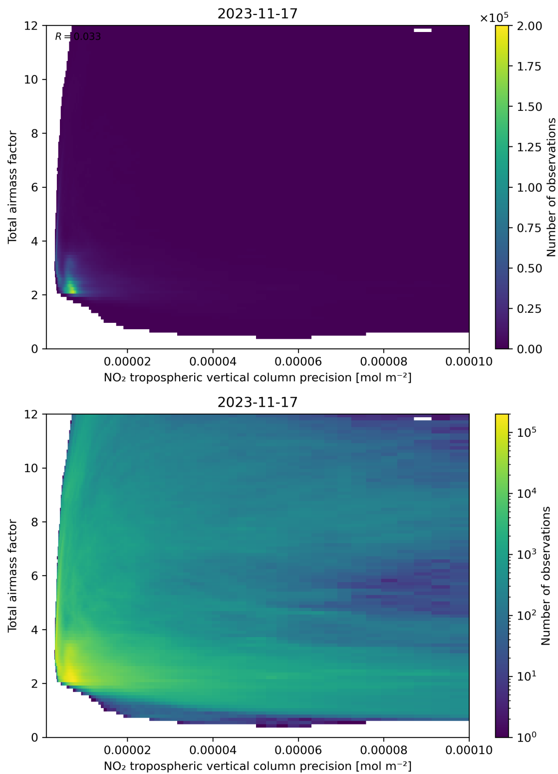
Figure 132: Scatter density plot of “NO 2 tropospheric vertical column precision” against “Total air mass factor” for 2023-11-16 to 2023-11-18.
