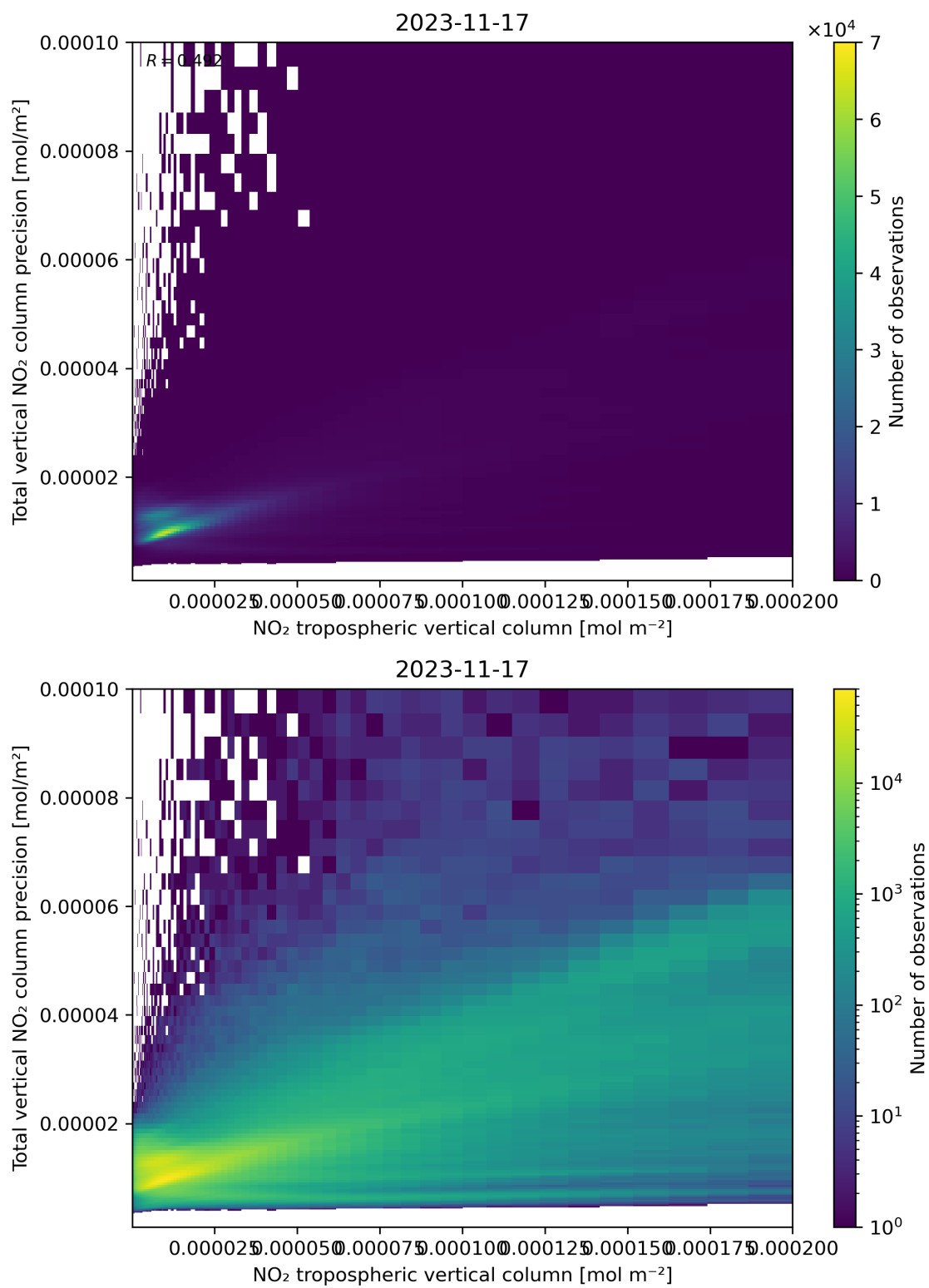
Figure 129: Scatter density plot of “NO 2 tropospheric vertical column” against “Total vertical NO 2 column precision” for 2023-11-16 to 2023-11-18.
