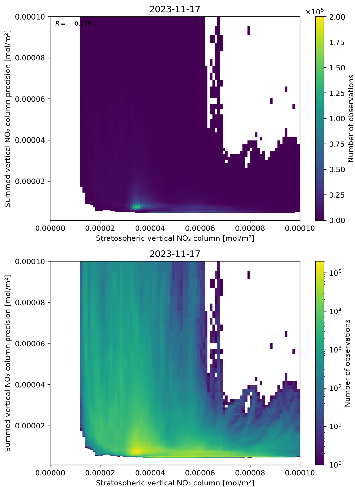
Figure 99: Scatter density plot of “Stratospheric vertical NO 2 column” against “Summed vertical NO 2 column precision” for 2023-11-16 to 2023-11-18.
