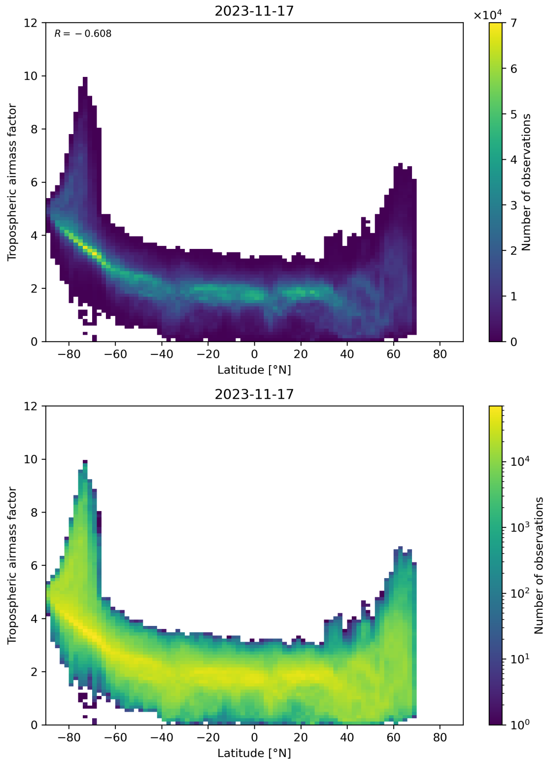
Figure 85: Scatter density plot of “Latitude” against “Tropospheric airmass factor” for 2023-11-16 to 2023-11-18.
