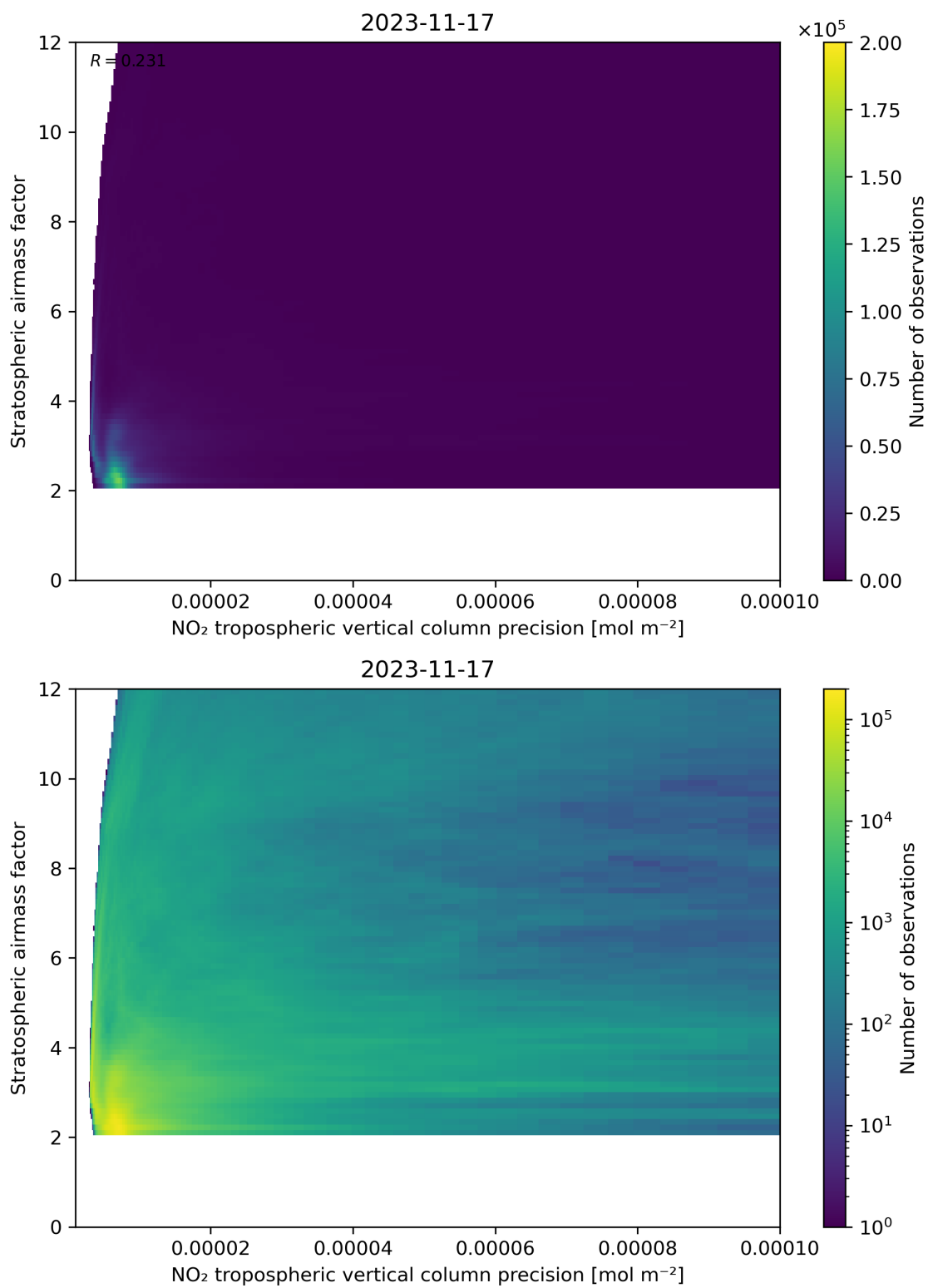
Figure 131: Scatter density plot of “NO 2 tropospheric vertical column precision” against “Stratospheric airmass factor” for 2023-11-16 to 2023-11-18.
