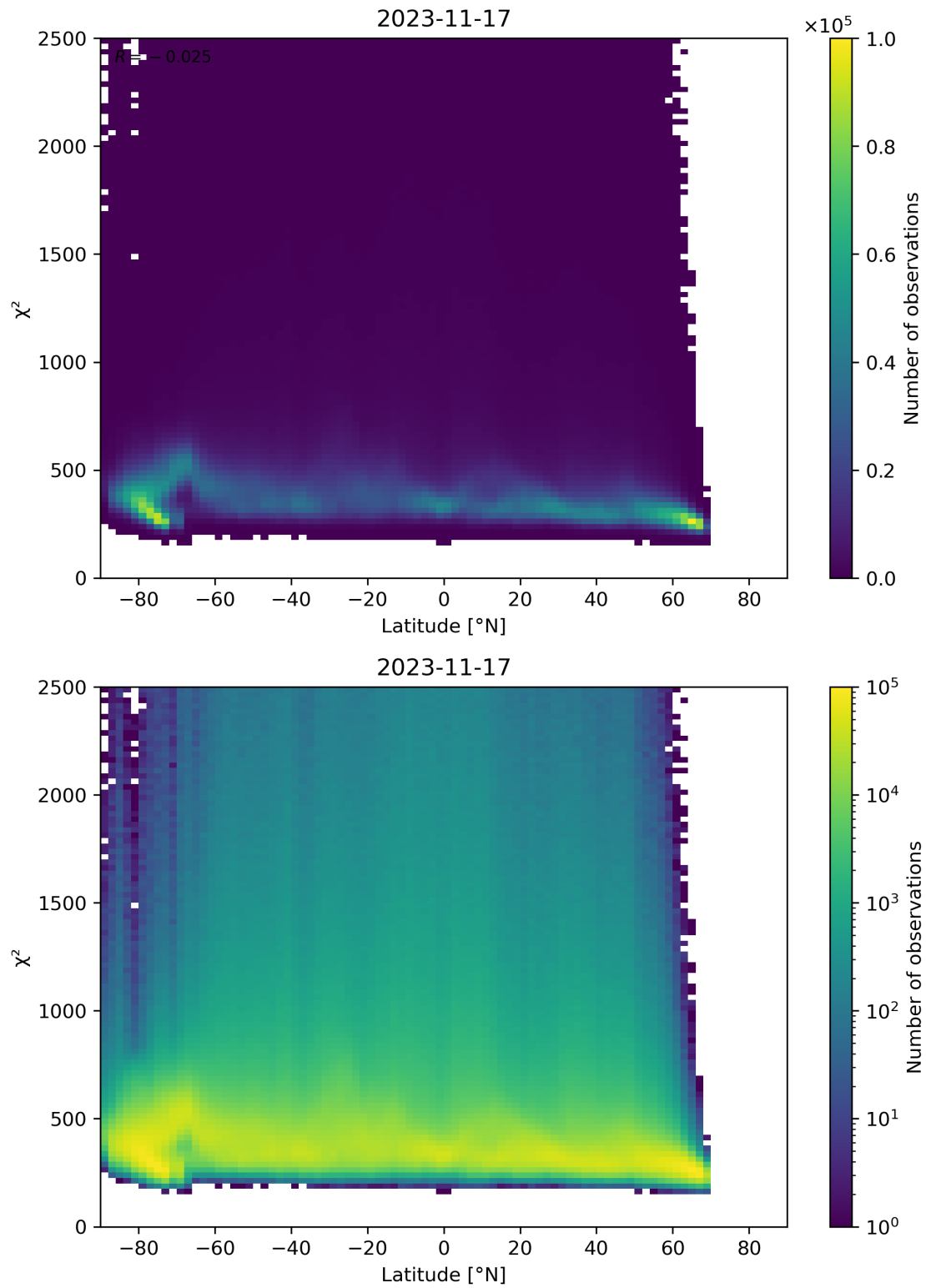
Figure 86: Scatter density plot of “Latitude” against “ \chi^2 ” for 2023-11-16 to 2023-11-18.
