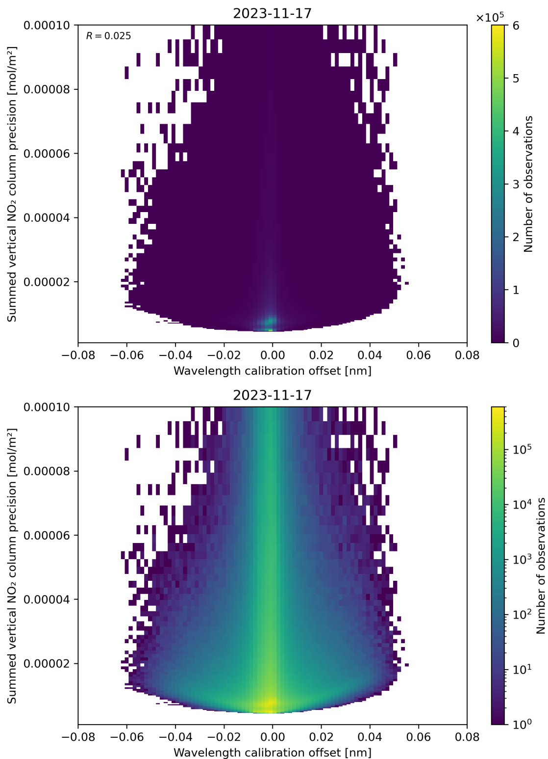
Figure 178: Scatter density plot of “Wavelength calibration offset” against “Summed vertical NO 2 column precision” for 2023-11-16 to 2023-11-18.
