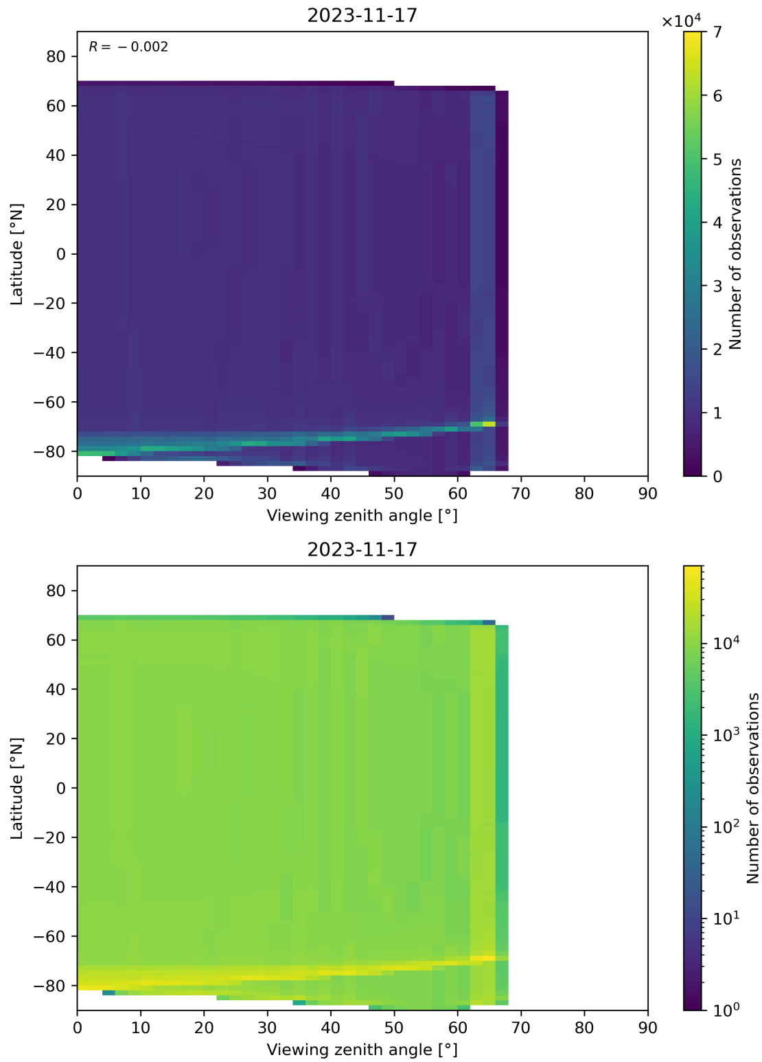
Figure 163: Scatter density plot of “Viewing zenith angle” against “Latitude” for 2023-11-16 to 2023-11-18.
