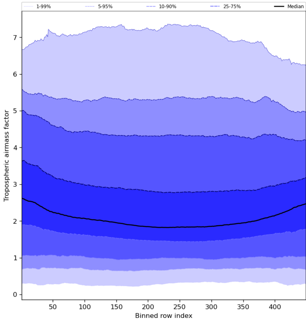
Figure 48: Along track statistics of “Tropospheric air mass factor” for 2023-11-16 to 2023-11-18
