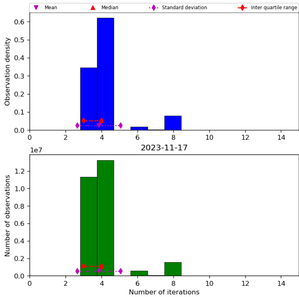
Figure 34: Histogram of “Number of iterations” for 2023-11-16 to 2023-11-18
