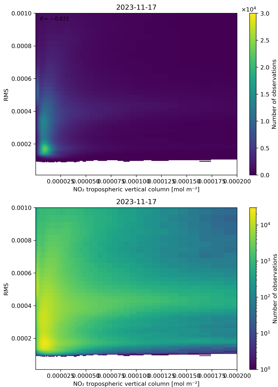
Figure 142: Scatter density plot of “NO 2 tropospheric vertical column” against “RMS” for 2023-11-16 to 2023-11-18.
