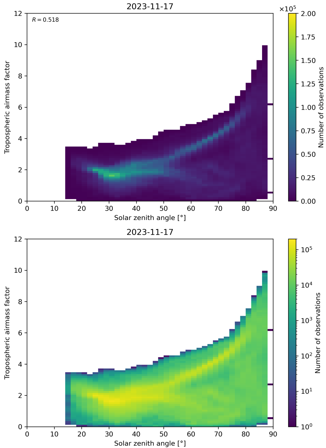
Figure 147: Scatter density plot of “Solar zenith angle” against “Tropospheric airmass factor” for 2023-11-16 to 2023-11-18.
