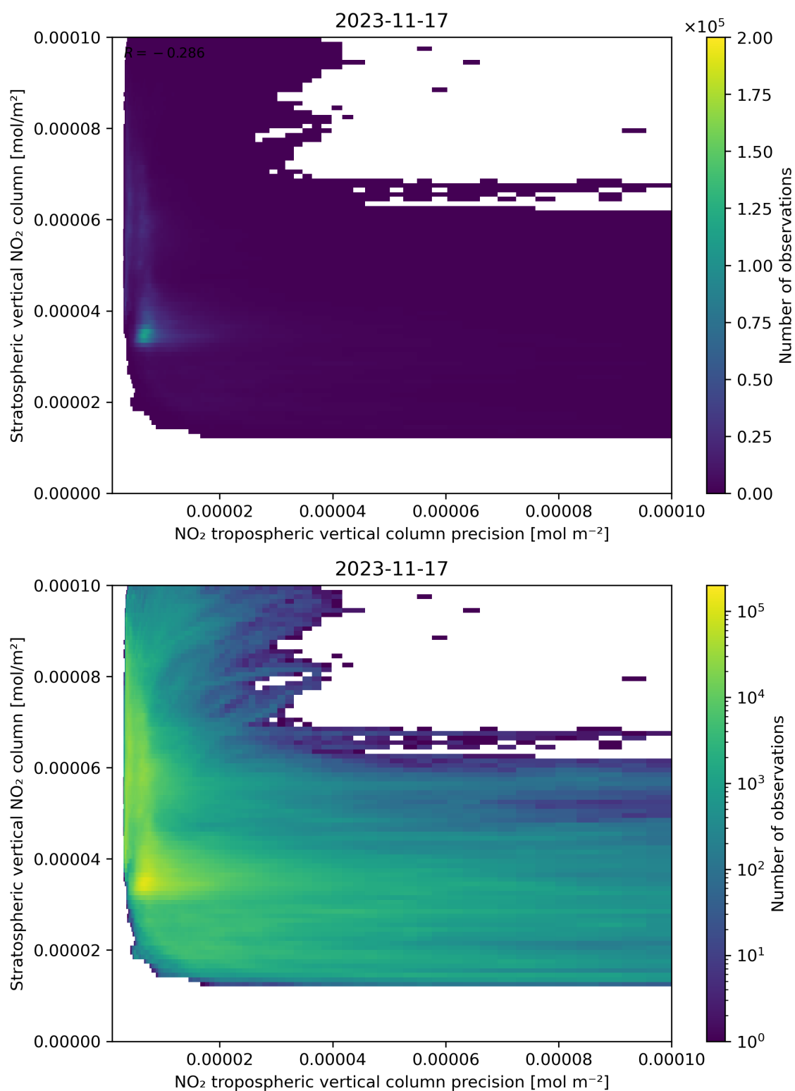
Figure 135: Scatter density plot of “NO 2 tropospheric vertical column precision” against “Stratospheric vertical NO 2 column” for 2023-11-16 to 2023-11-18.
