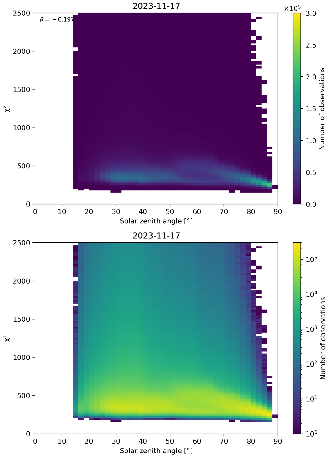
Figure 148: Scatter density plot of “Solar zenith angle” against “ \chi^2 ” for 2023-11-16 to 2023-11-18.
