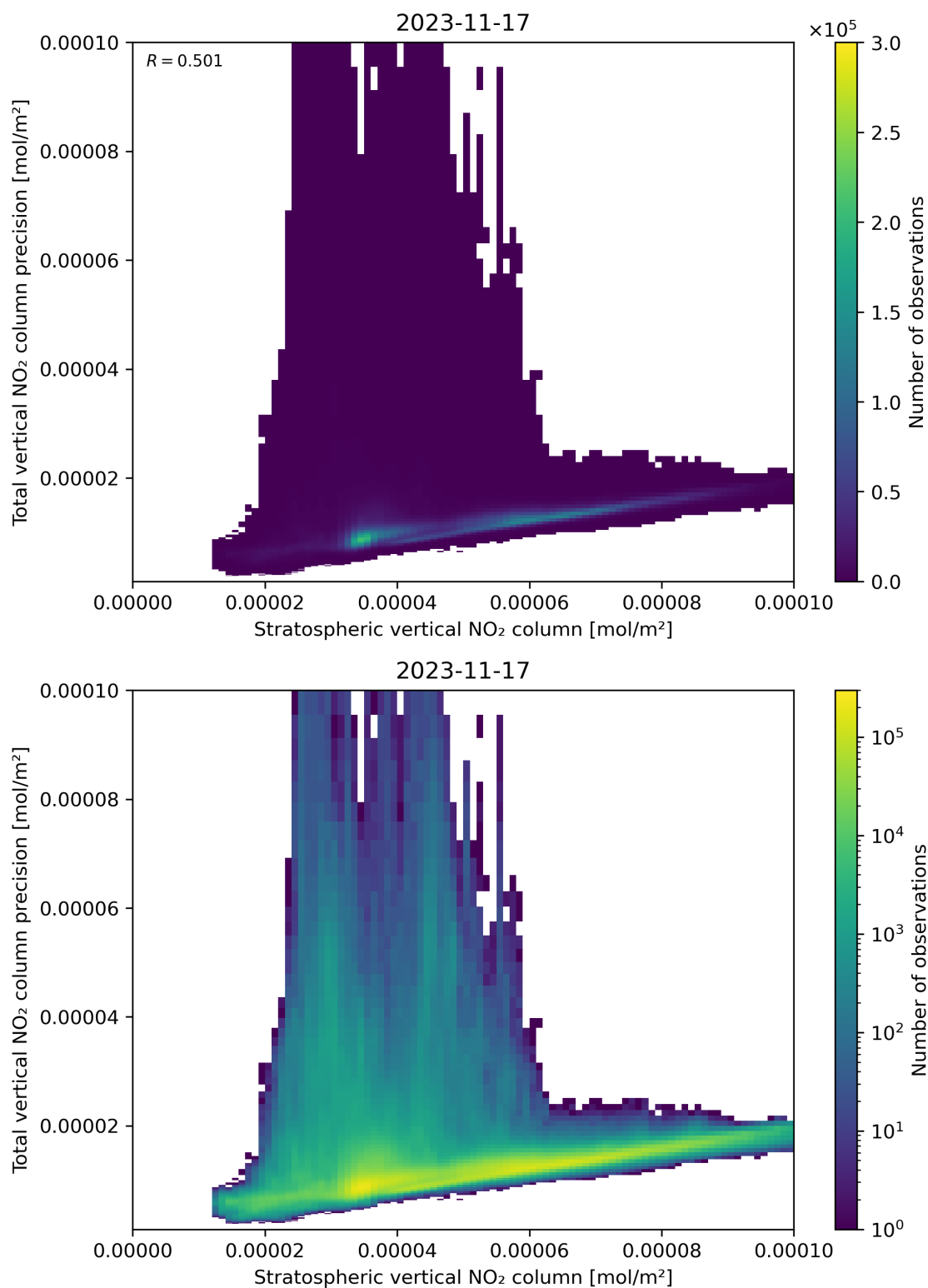
Figure 101: Scatter density plot of “Stratospheric vertical NO 2 column” against “Total vertical NO 2 column precision” for 2023-11-16 to 2023-11-18.
