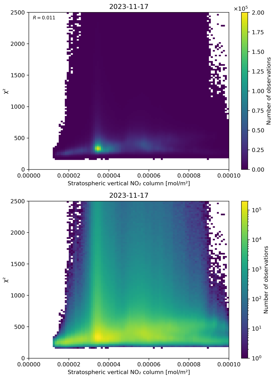
Figure 97: Scatter density plot of “Stratospheric vertical NO 2 column” against “ \chi^2 ” for 2023-11-16 to 2023-11-18.
