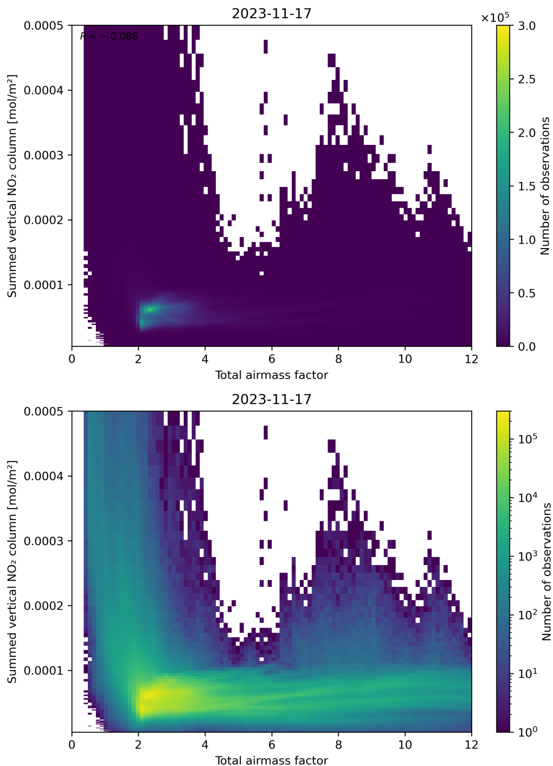
Figure 65: Scatter density plot of “Total airmass factor” against “Summed vertical NO 2 column” for 2023-11-16 to 2023-11-18.
