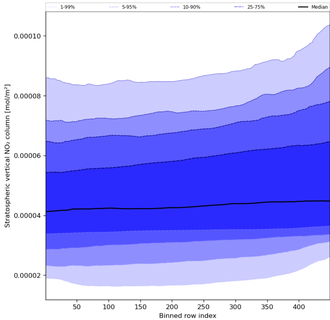
Figure 53: Along track statistics of “Stratospheric vertical NO 2 column” for 2023-11-16 to 2023-11-18
