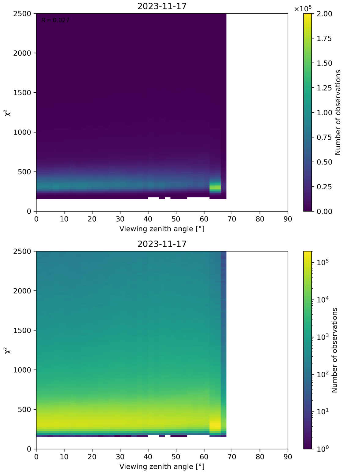
Figure 162: Scatter density plot of “Viewing zenith angle” against “ \chi^2 ” for 2023-11-16 to 2023-11-18.
