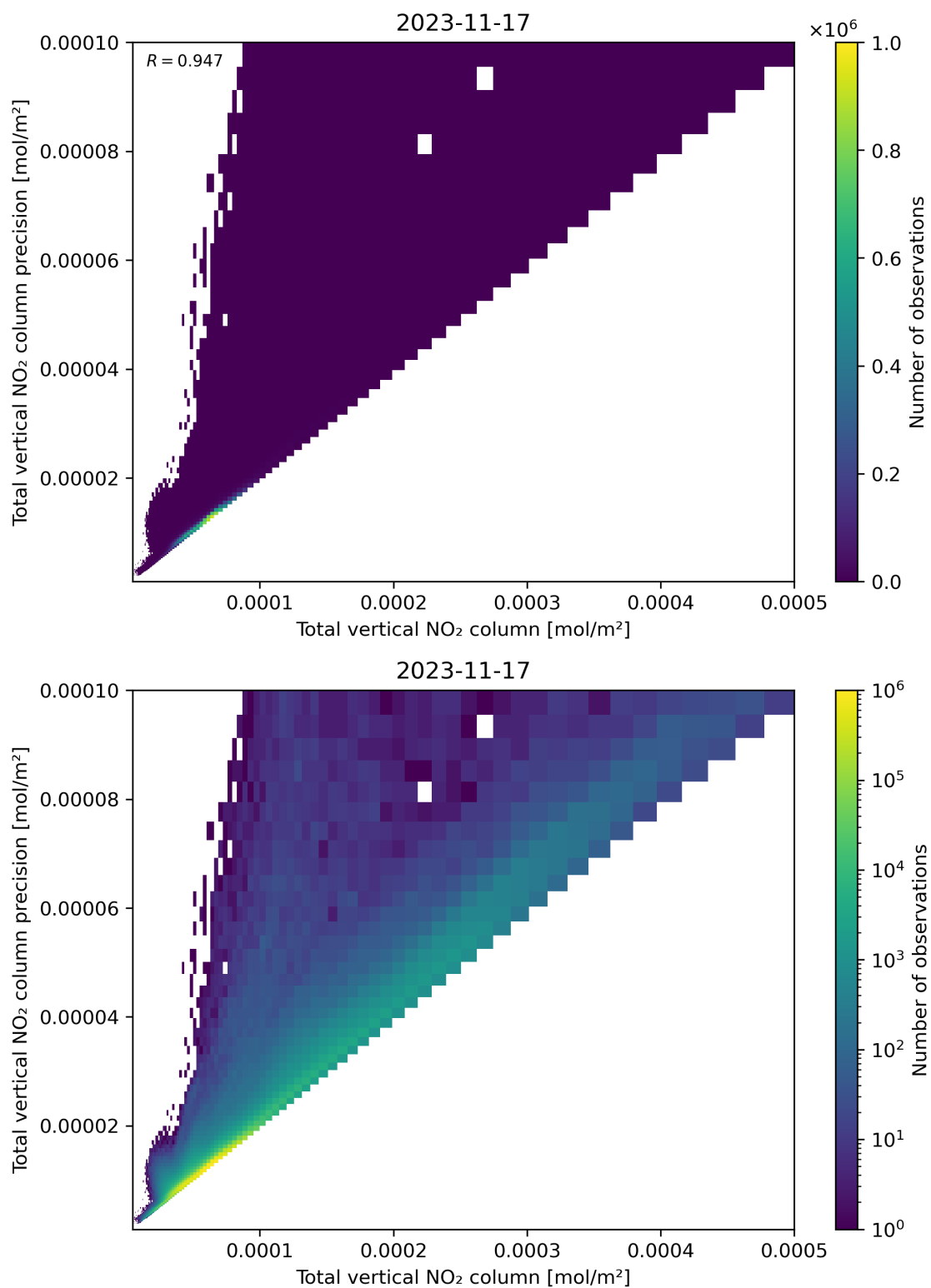
Figure 114: Scatter density plot of “Total vertical NO 2 column” against “Total vertical NO 2 column precision” for 2023-11-16 to 2023-11-18.
