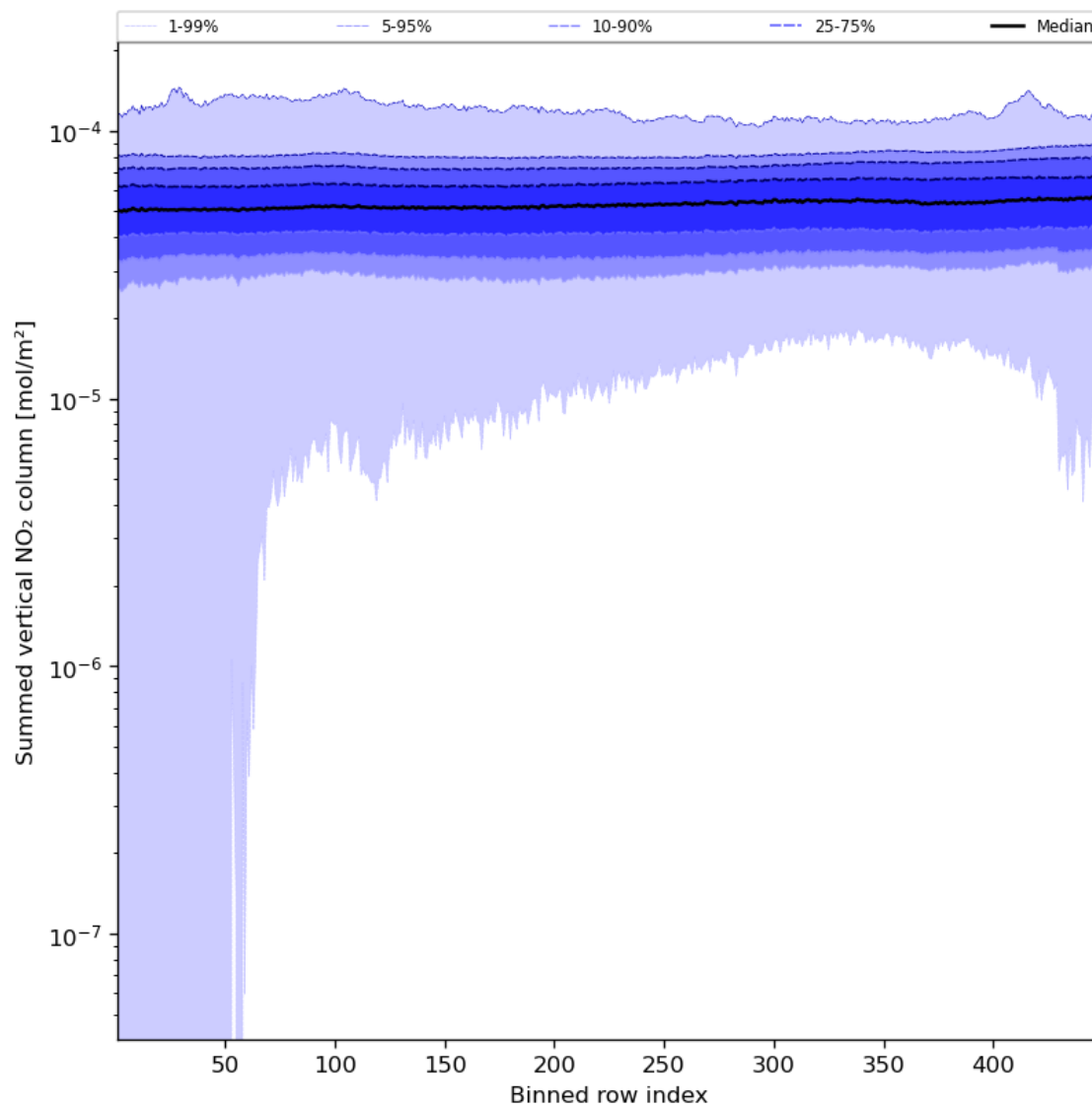
Figure 57: Along track statistics of “Summed vertical NO 2 column” for 2023-11-16 to 2023-11-18
