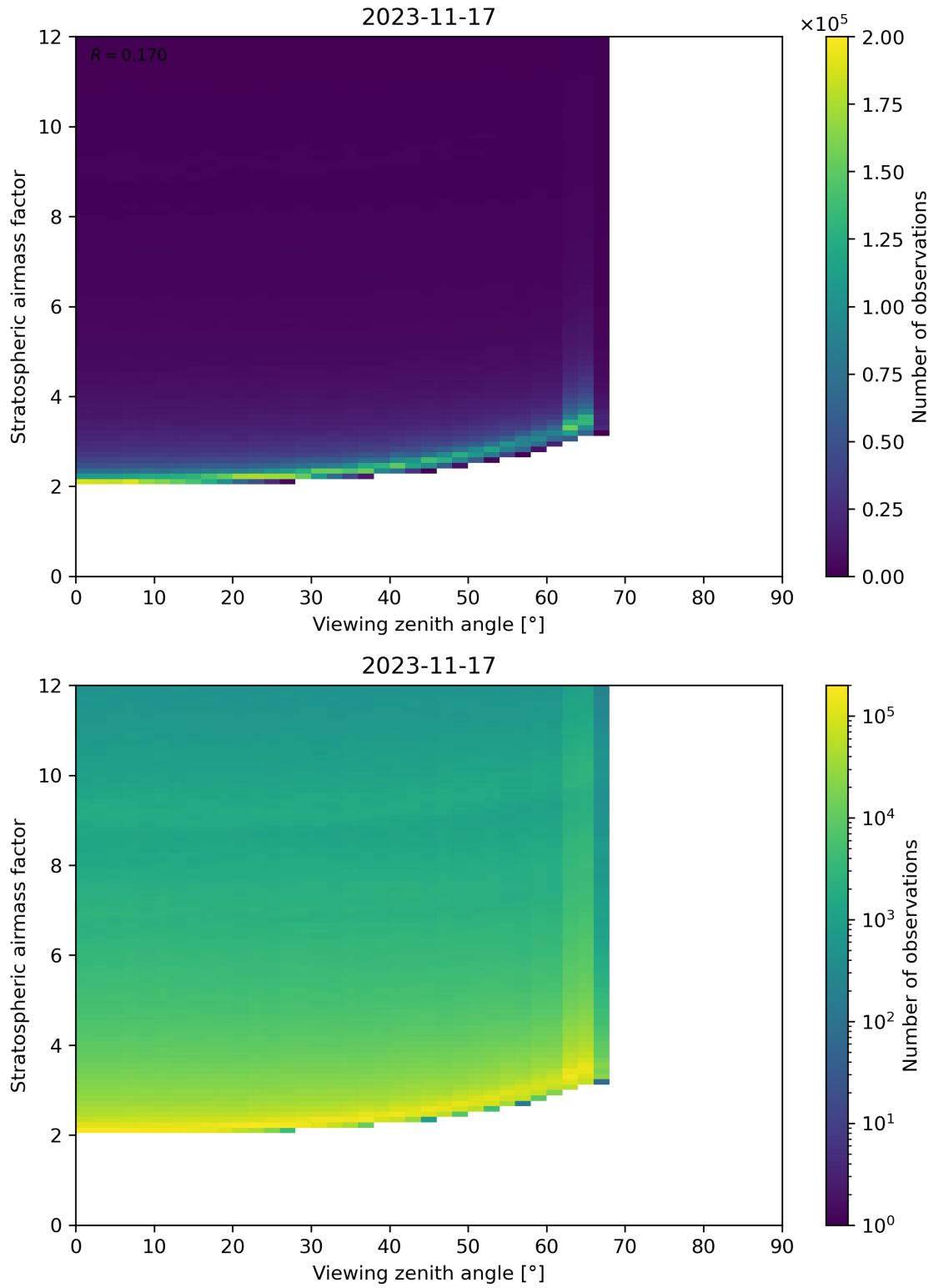
Figure 159: Scatter density plot of “Viewing zenith angle” against “Stratospheric airmass factor” for 2023-11-16 to 2023-11-18.
