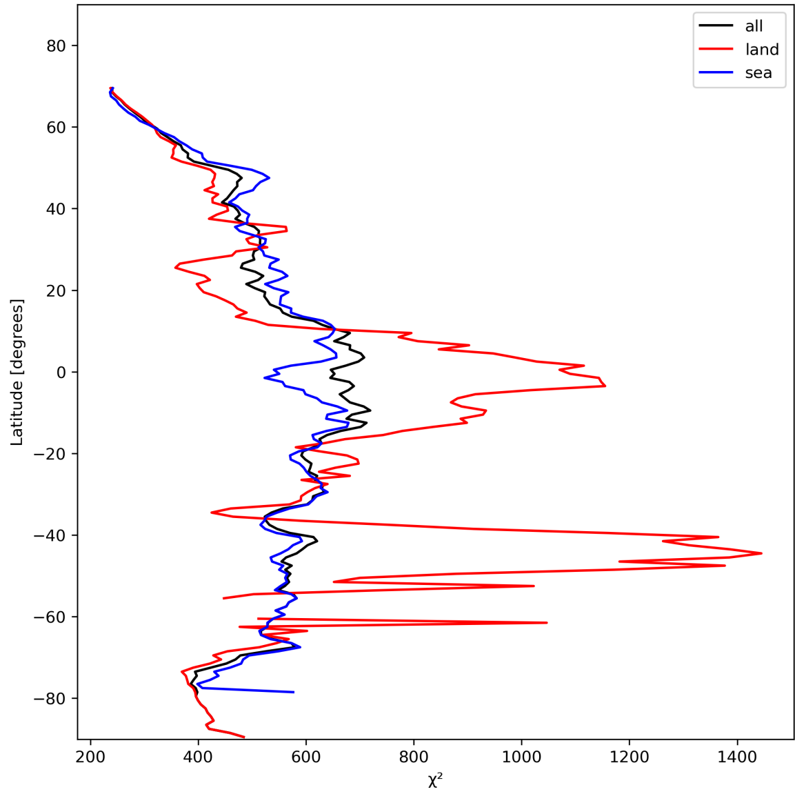
Figure 25: Zonal average of “ \chi^2 ” for 2023-11-16 to 2023-11-18.
