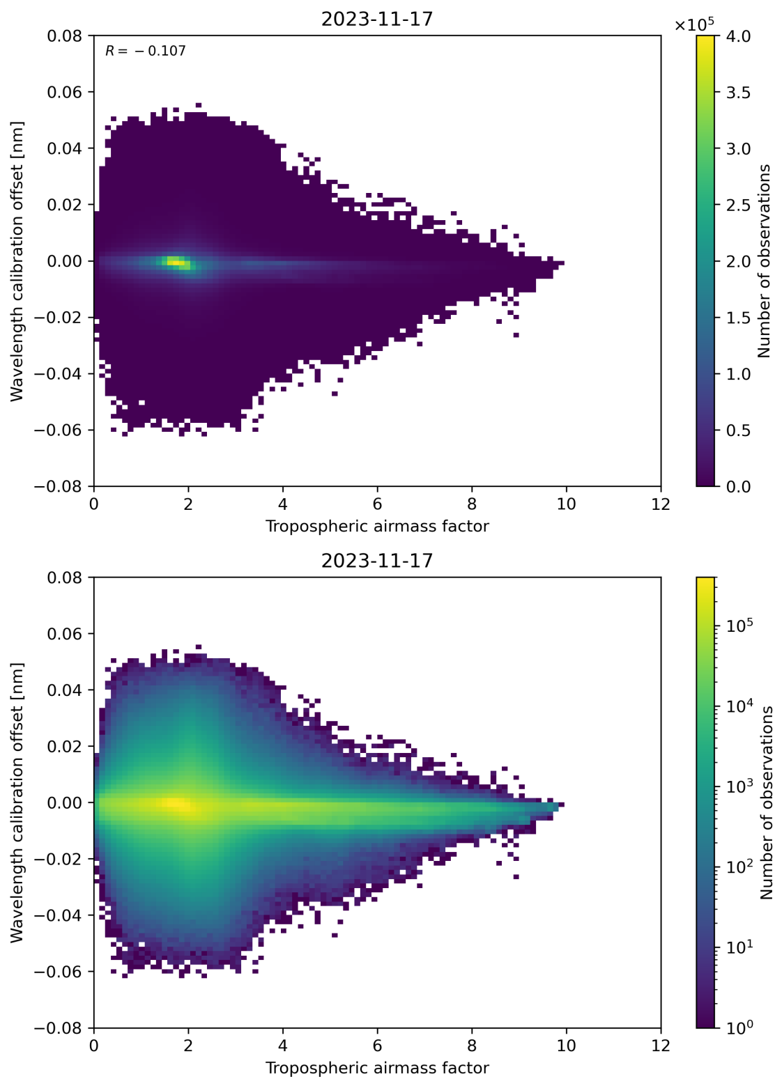
Figure 80: Scatter density plot of “Tropospheric airmass factor” against “Wavelength calibration offset” for 2023-11-16 to 2023-11-18.
