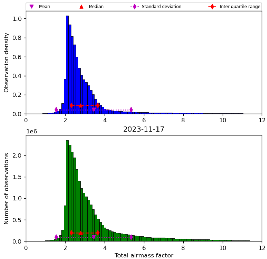
Figure 32: Histogram of “Total airmass factor” for 2023-11-16 to 2023-11-18
