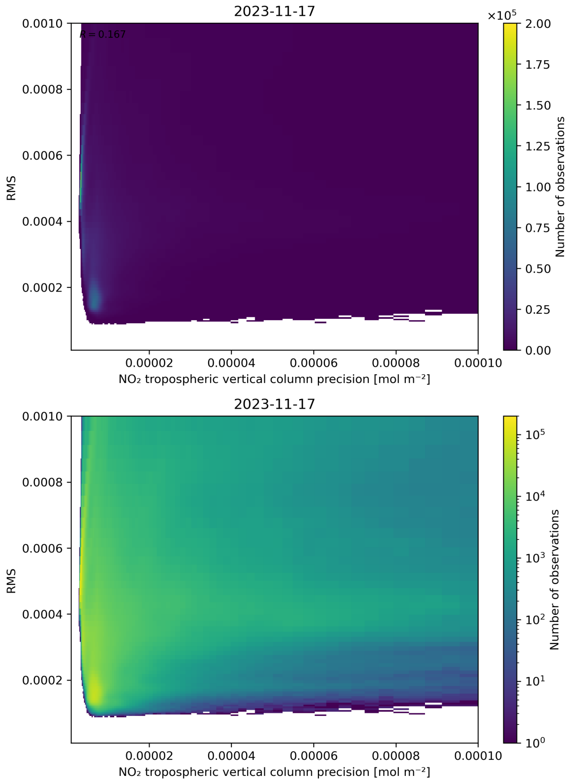
Figure 140: Scatter density plot of “NO 2 tropospheric vertical column precision” against “RMS” for 2023-11-16 to 2023-11-18.
