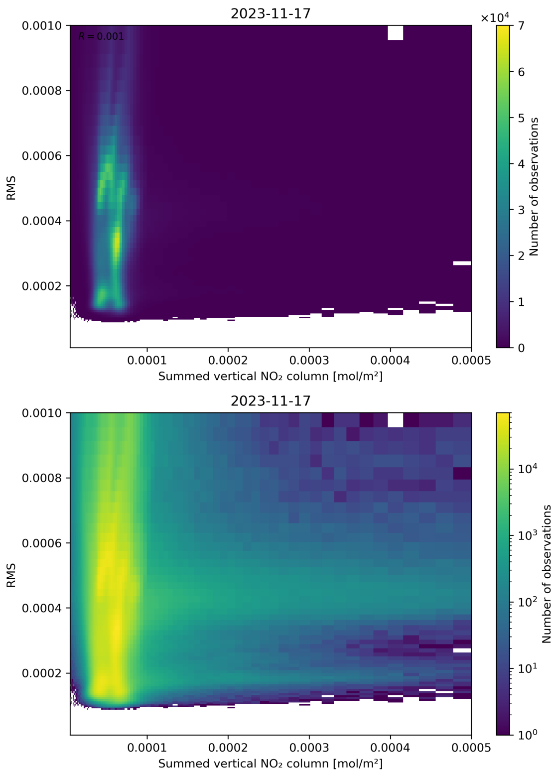
Figure 109: Scatter density plot of “Summed vertical NO 2 column” against “RMS” for 2023-11-16 to 2023-11-18.
