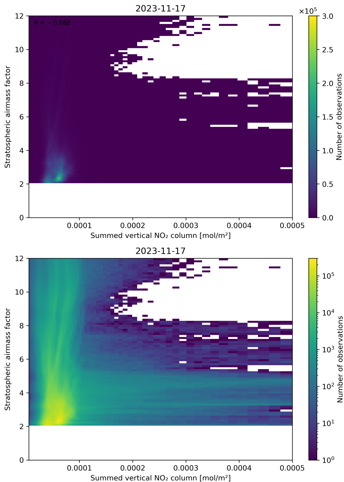
Figure 103: Scatter density plot of “Summed vertical NO 2 column” against “Stratospheric airmass factor” for 2023-11-16 to 2023-11-18.
