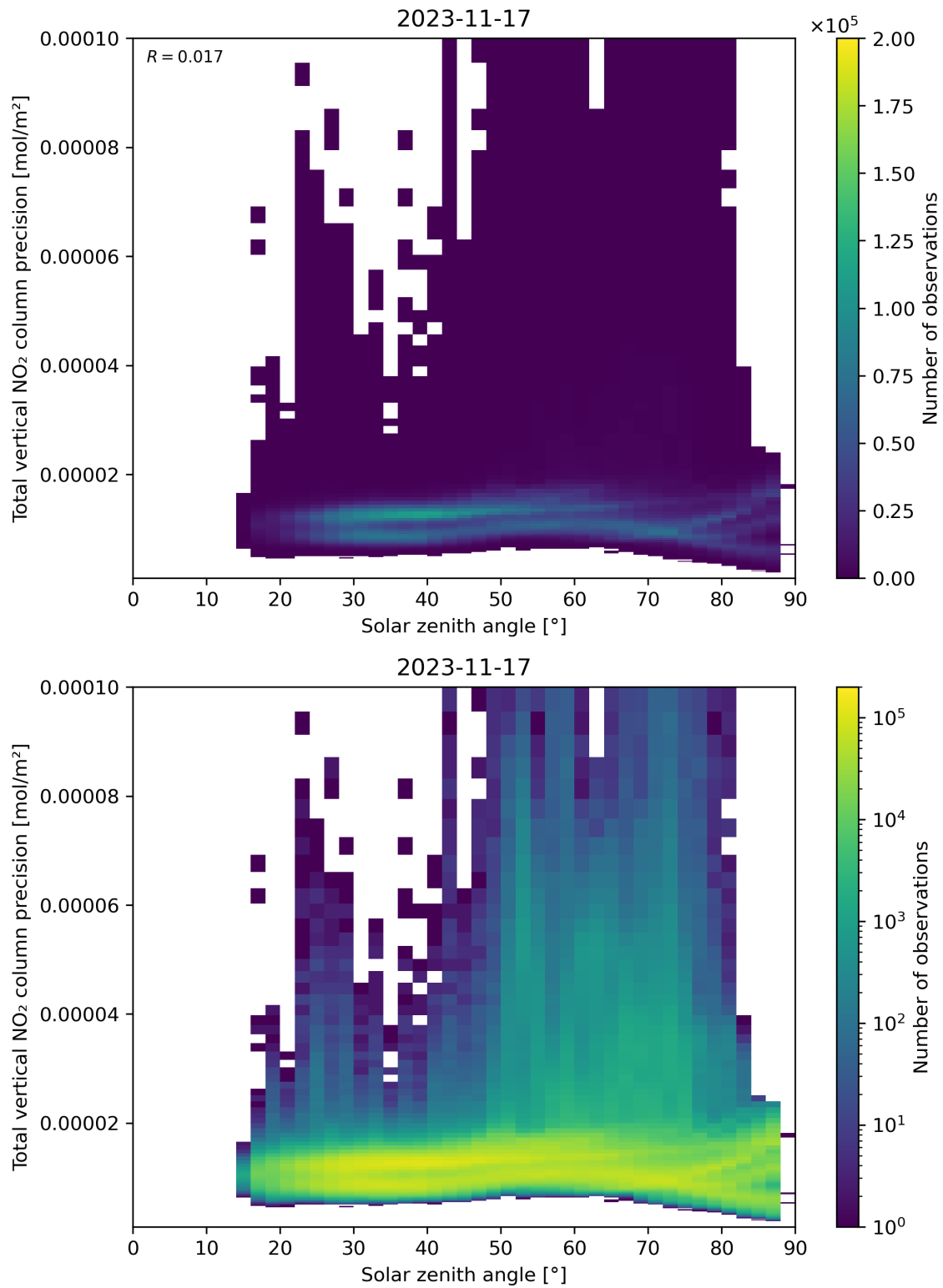
Figure 154: Scatter density plot of “Solar zenith angle” against “Total vertical NO 2 column precision” for 2023-11-16 to 2023-11-18.
