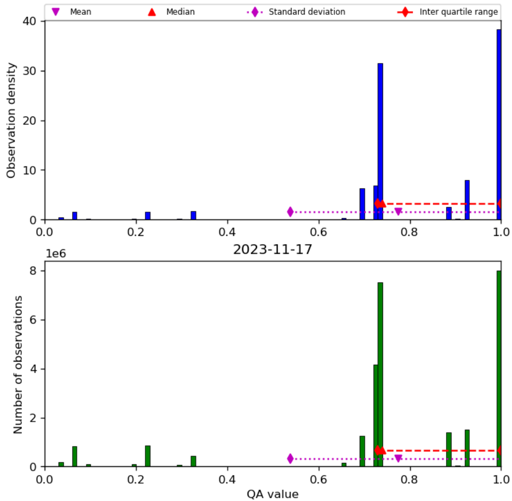
Figure 28: Histogram of “QA value” for 2023-11-16 to 2023-11-18
