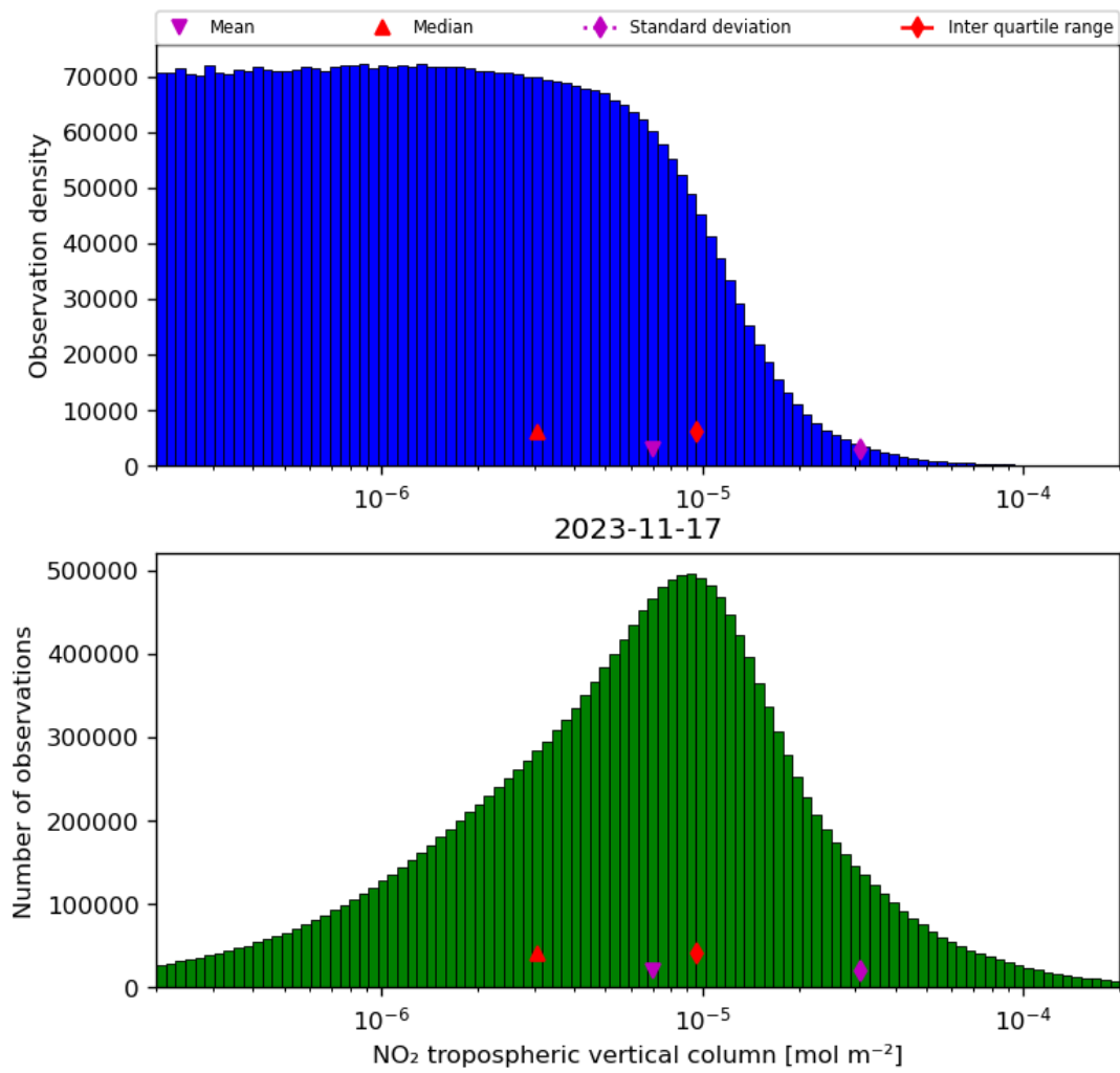
Figure 29: Histogram of “NO 2 tropospheric vertical column” for 2023-11-16 to 2023-11-18
