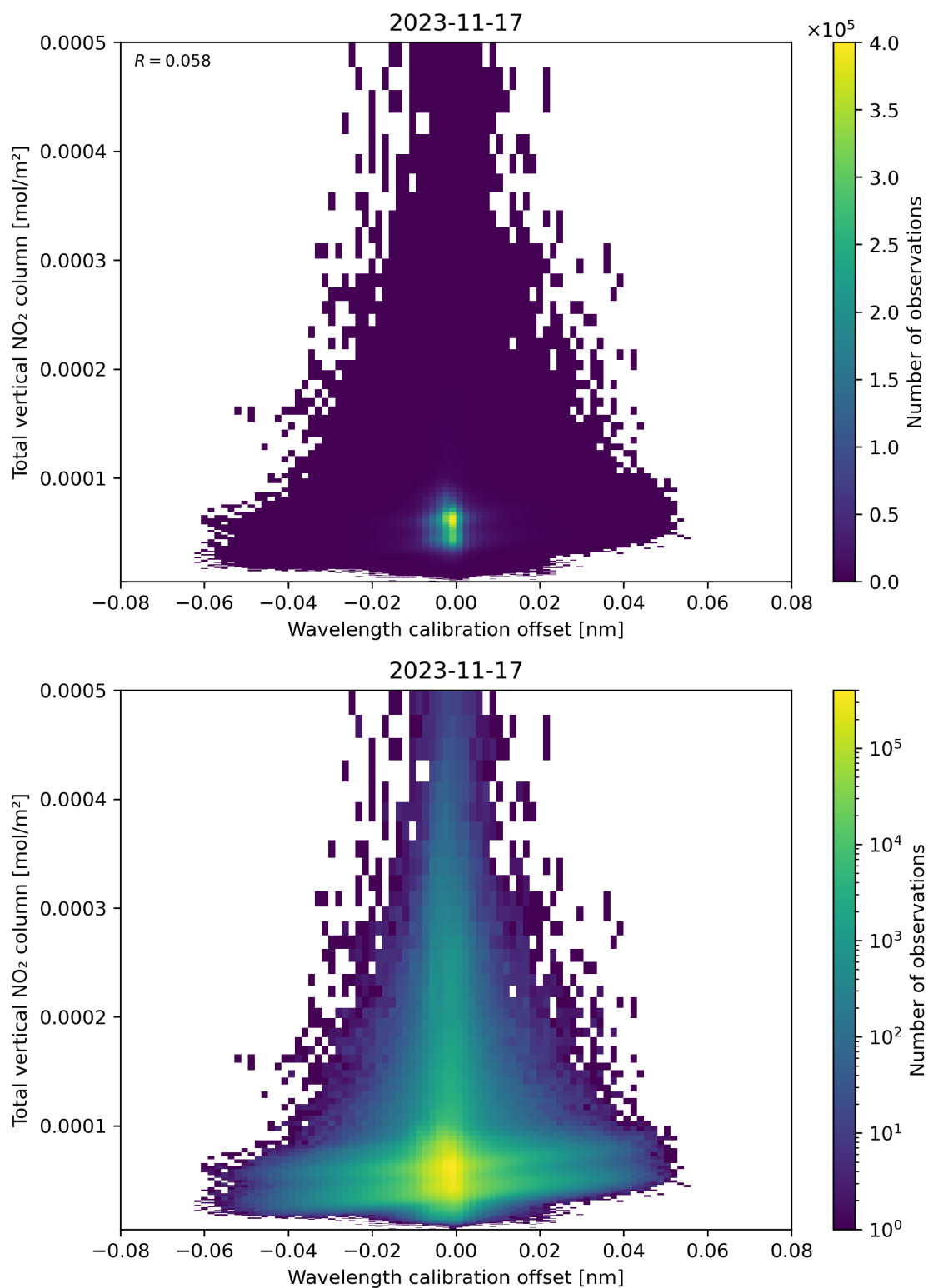
Figure 179: Scatter density plot of “Wavelength calibration offset” against “Total vertical NO 2 column” for 2023-11-16 to 2023-11-18.
