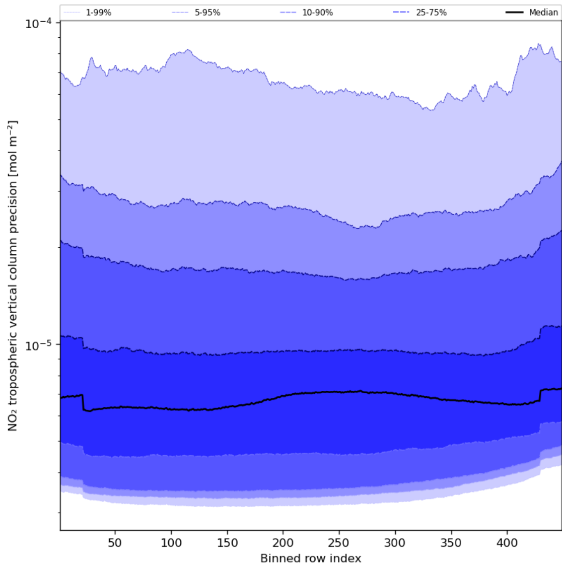
Figure 47: Along track statistics of “NO 2 tropospheric vertical column precision” for 2023-11-16 to 2023-11-18
