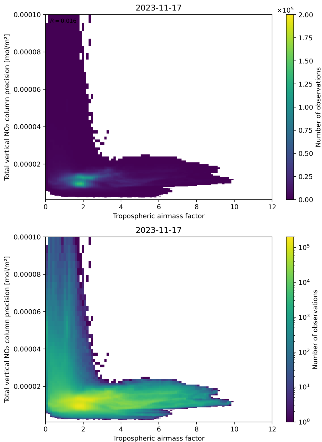
Figure 78: Scatter density plot of “Tropospheric air mass factor” against “Total vertical NO 2 column precision” for 2023-11-16 to 2023-11-18.
