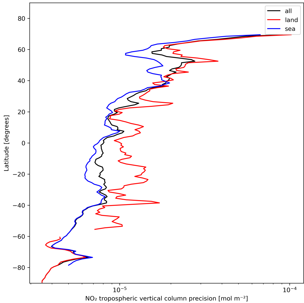
Figure 13: Zonal average of “NO 2 tropospheric vertical column precision” for 2023-11-16 to 2023-11-18.
