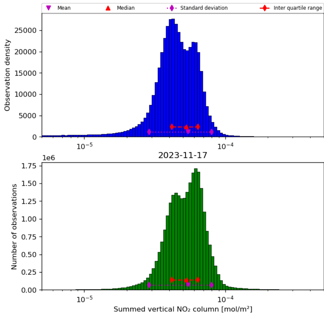
Figure 40: Histogram of "Summed vertical NO 2 column" for 2023-11-16 to 2023-11-18
