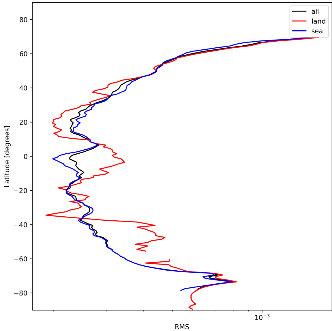
Figure 26: Zonal average of “RMS” for 2023-11-16 to 2023-11-18.
