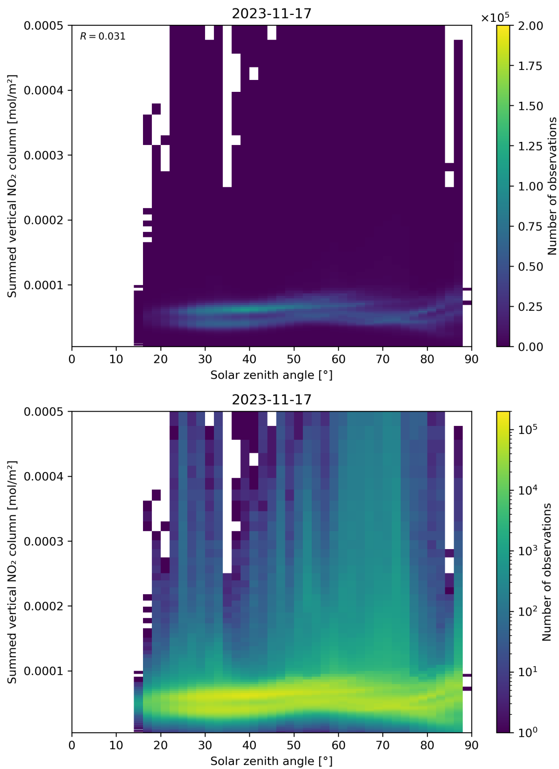
Figure 151: Scatter density plot of “Solar zenith angle” against “Summed vertical NO 2 column” for 2023-11-16 to 2023-11-18.
