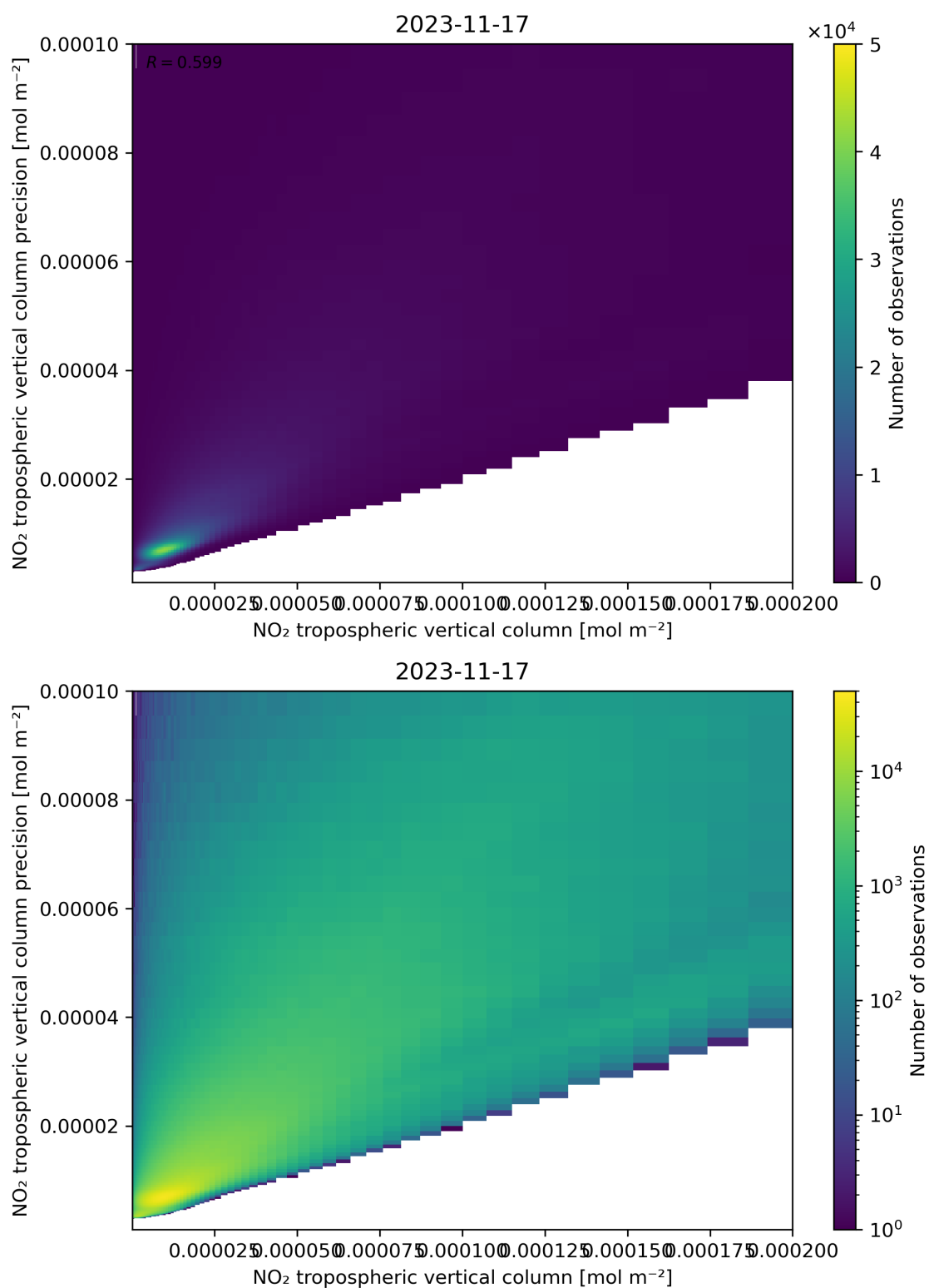
Figure 130: Scatter density plot of “NO 2 tropospheric vertical column” against “NO 2 tropospheric vertical column precision” for 2023-11-16 to 2023-11-18.
