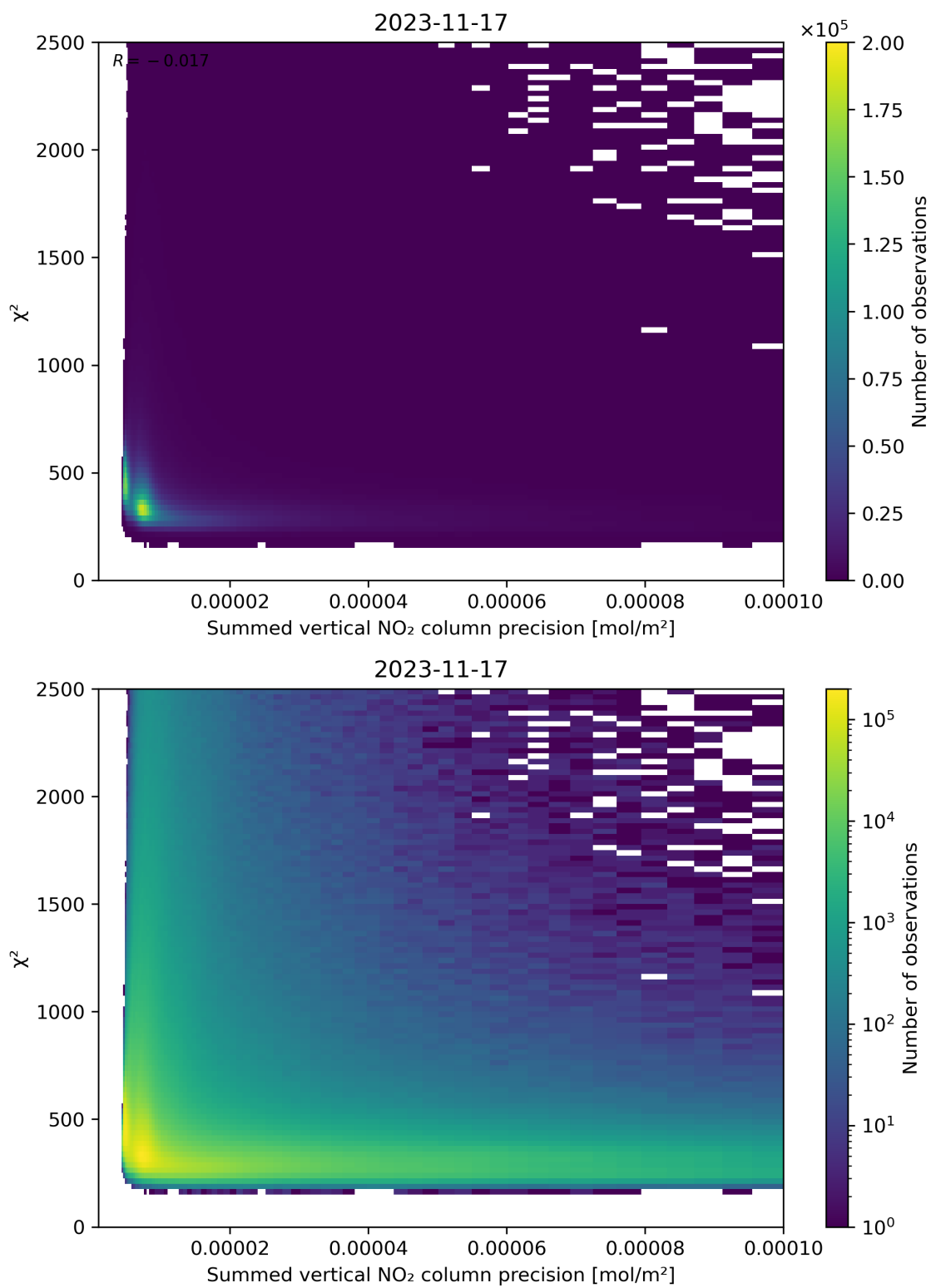
Figure 107: Scatter density plot of “Summed vertical NO 2 column precision” against “ \chi^2 ” for 2023-11-16 to 2023-11-18.
