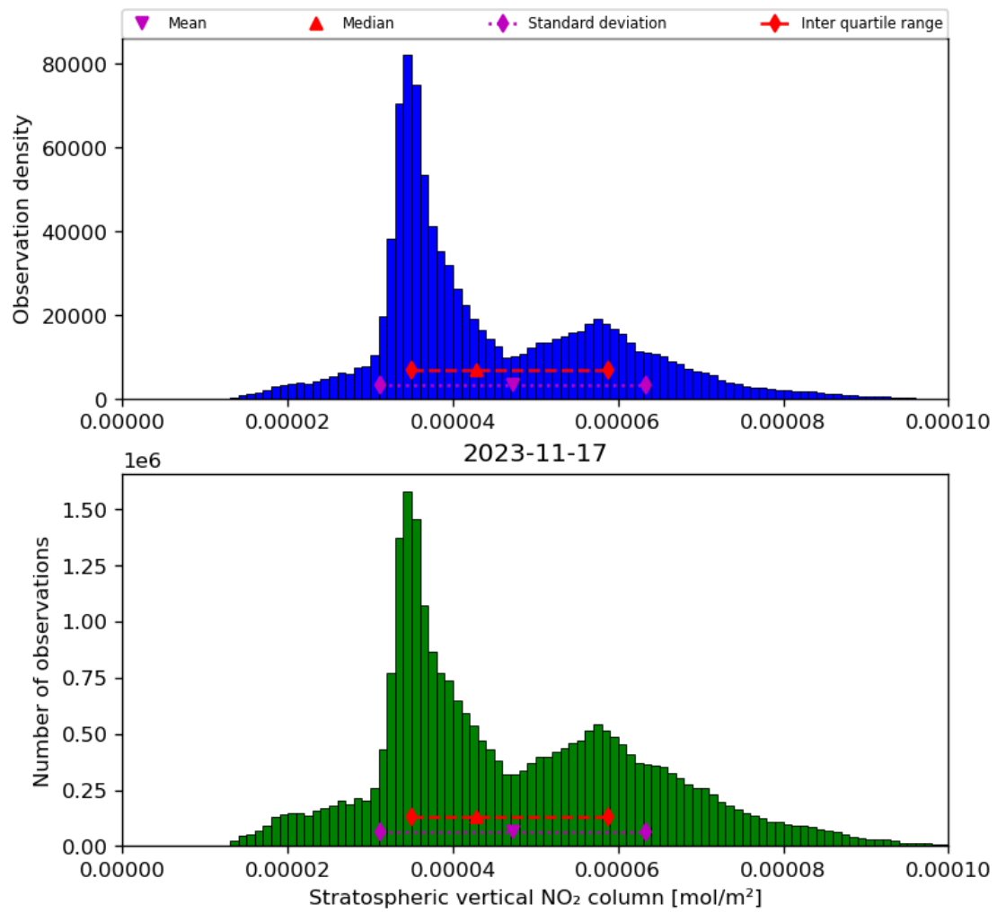
Figure 36: Histogram of “Stratospheric vertical NO 2 column” for 2023-11-16 to 2023-11-18
