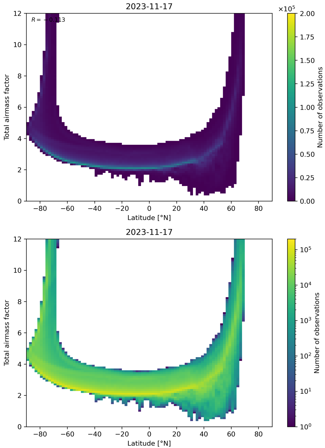
Figure 84: Scatter density plot of “Latitude” against “Total airmass factor” for 2023-11-16 to 2023-11-18.
