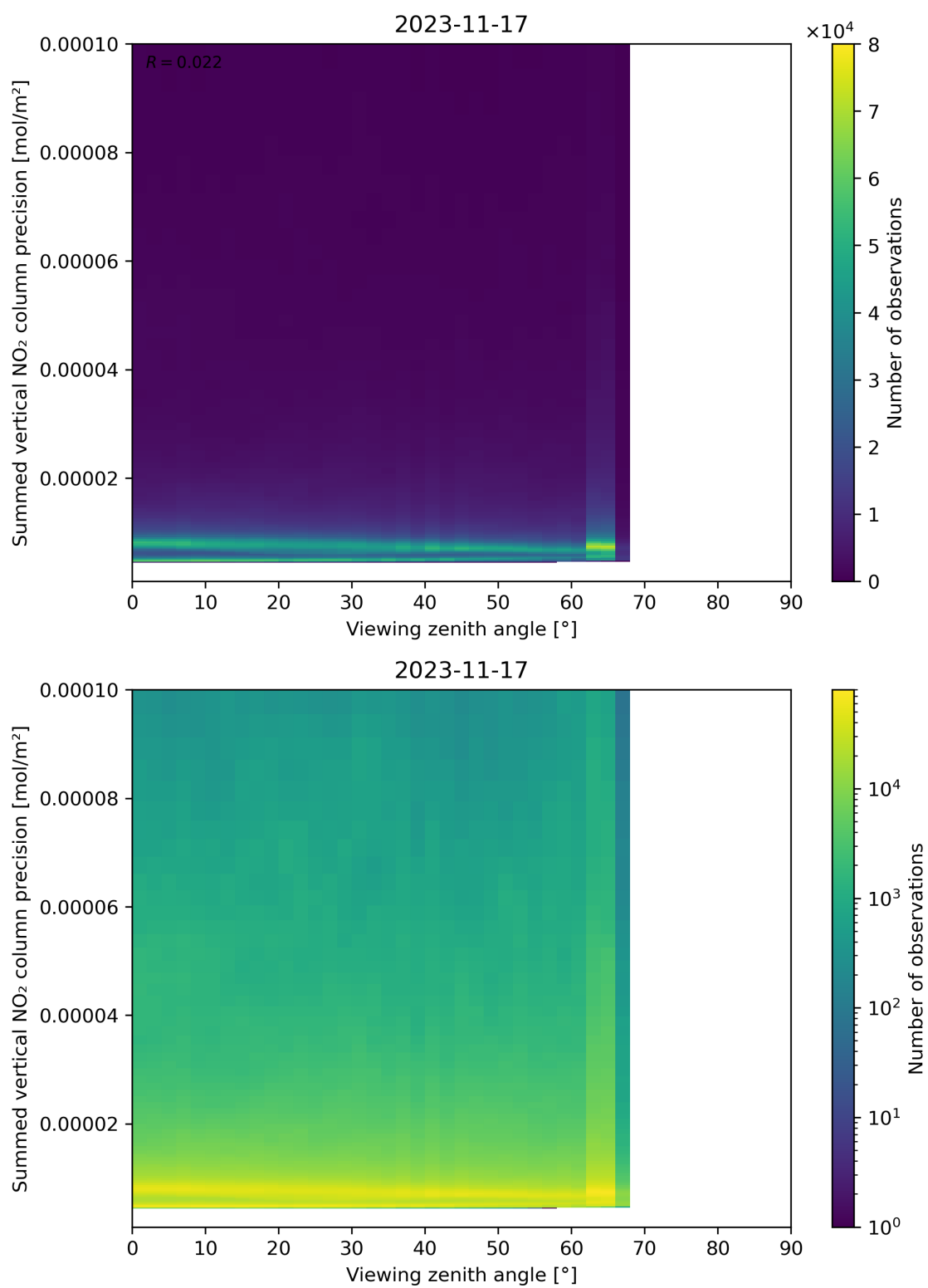
Figure 166: Scatter density plot of “Viewing zenith angle” against “Summed vertical NO 2 column precision” for 2023-11-16 to 2023-11-18.
