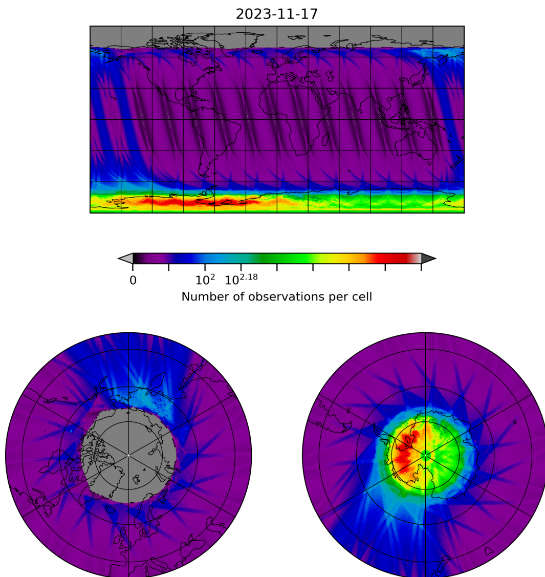
Figure 10: Map of the number of observations for 2023-11-16 to 2023-11-18
