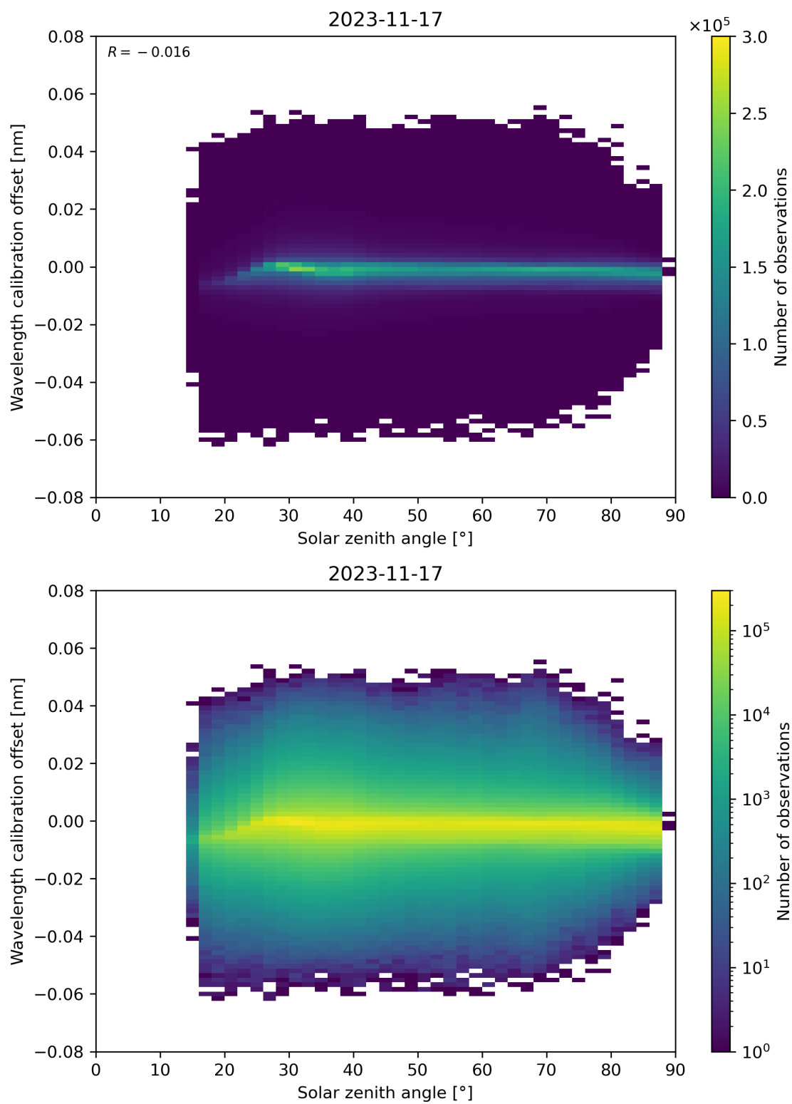
Figure 158: Scatter density plot of “Solar zenith angle” against “Wavelength calibration offset” for 2023-11-16 to 2023-11-18.
