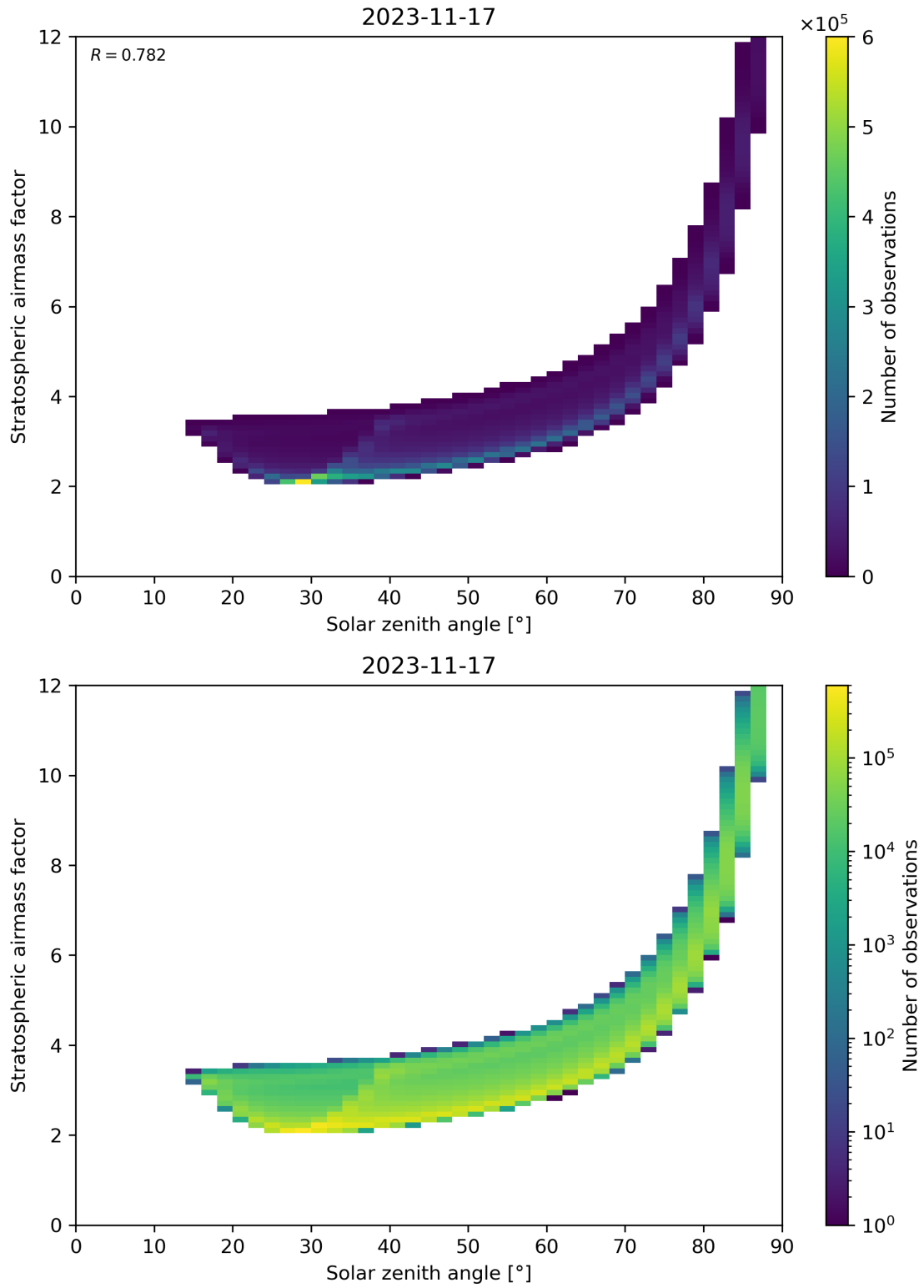
Figure 145: Scatter density plot of “Solar zenith angle” against “Stratospheric airmass factor” for 2023-11-16 to 2023-11-18.
