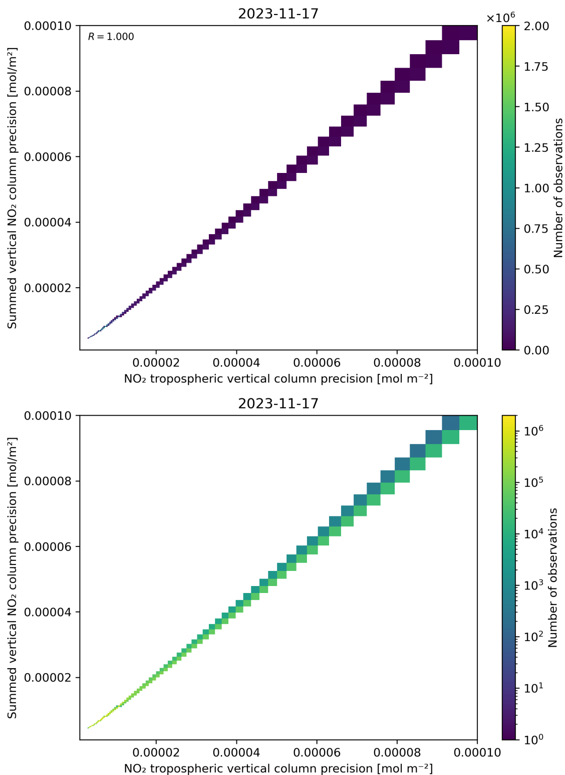
Figure 137: Scatter density plot of “NO 2 tropospheric vertical column precision” against “Summed vertical NO 2 column precision” for 2023-11-16 to 2023-11-18.
