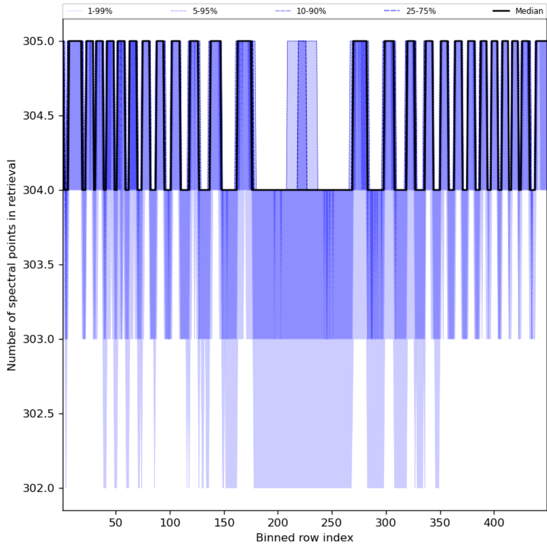
Figure 50: Along track statistics of “Number of spectral points in retrieval” for 2023-11-16 to 2023-11-18
