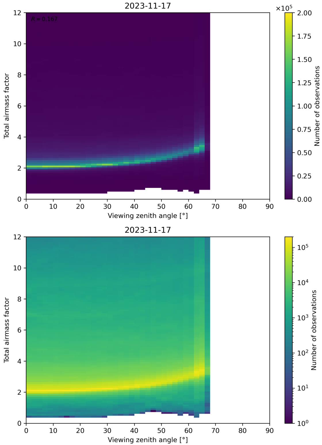
Figure 160: Scatter density plot of “Viewing zenith angle” against “Total airmass factor” for 2023-11-16 to 2023-11-18.
