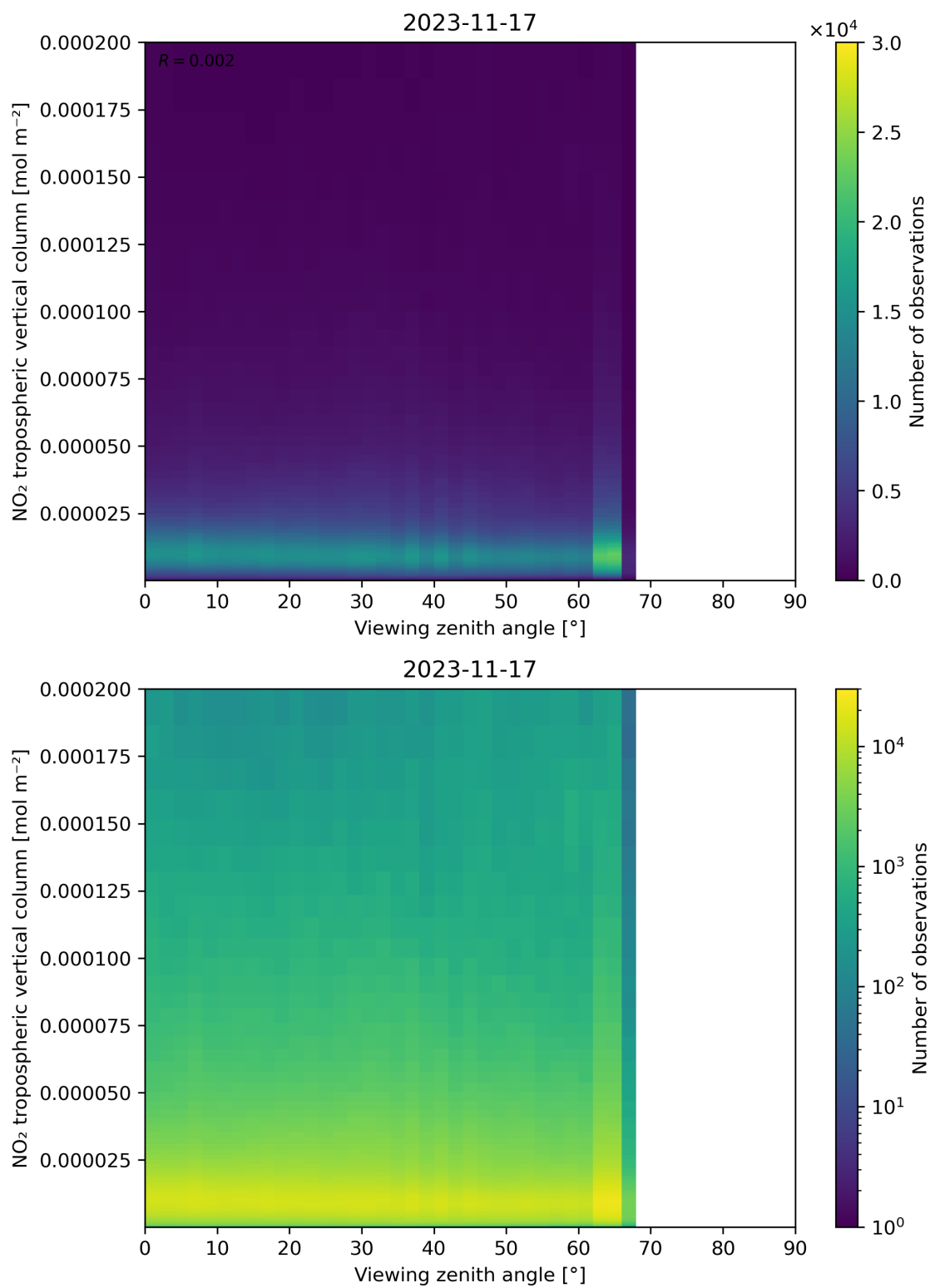
Figure 169: Scatter density plot of “Viewing zenith angle” against “NO 2 tropospheric vertical column” for 2023-11-16 to 2023-11-18.
