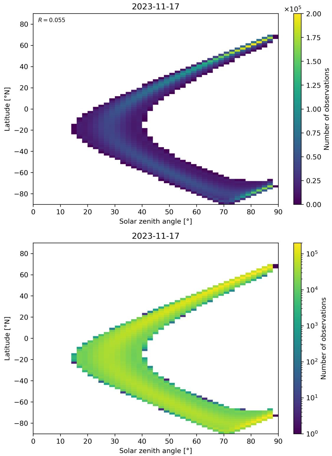
Figure 149: Scatter density plot of “Solar zenith angle” against “Latitude” for 2023-11-16 to 2023-11-18.
