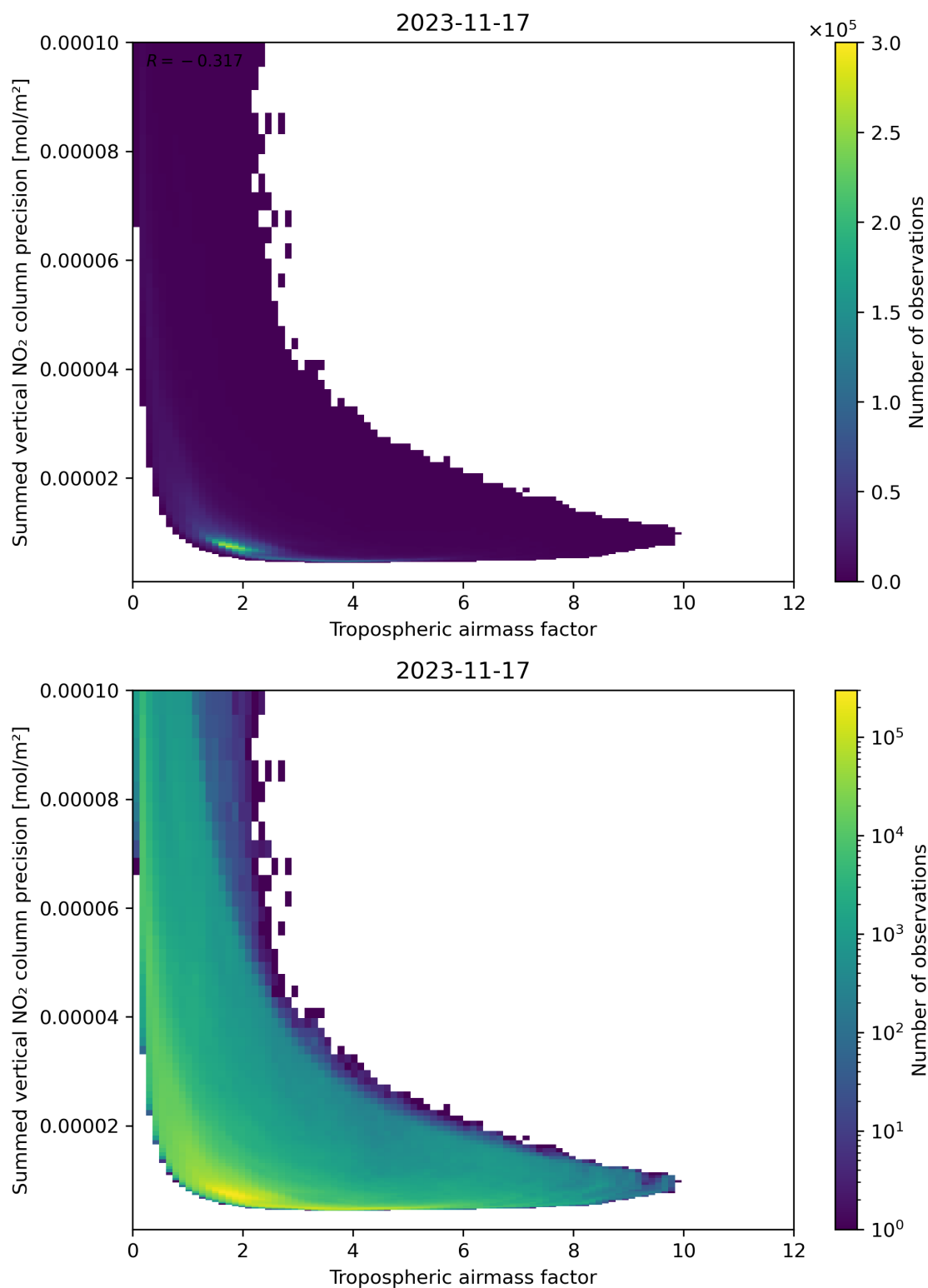
Figure 76: Scatter density plot of “Tropospheric air mass factor” against “Summed vertical NO 2 column precision” for 2023-11-16 to 2023-11-18.
