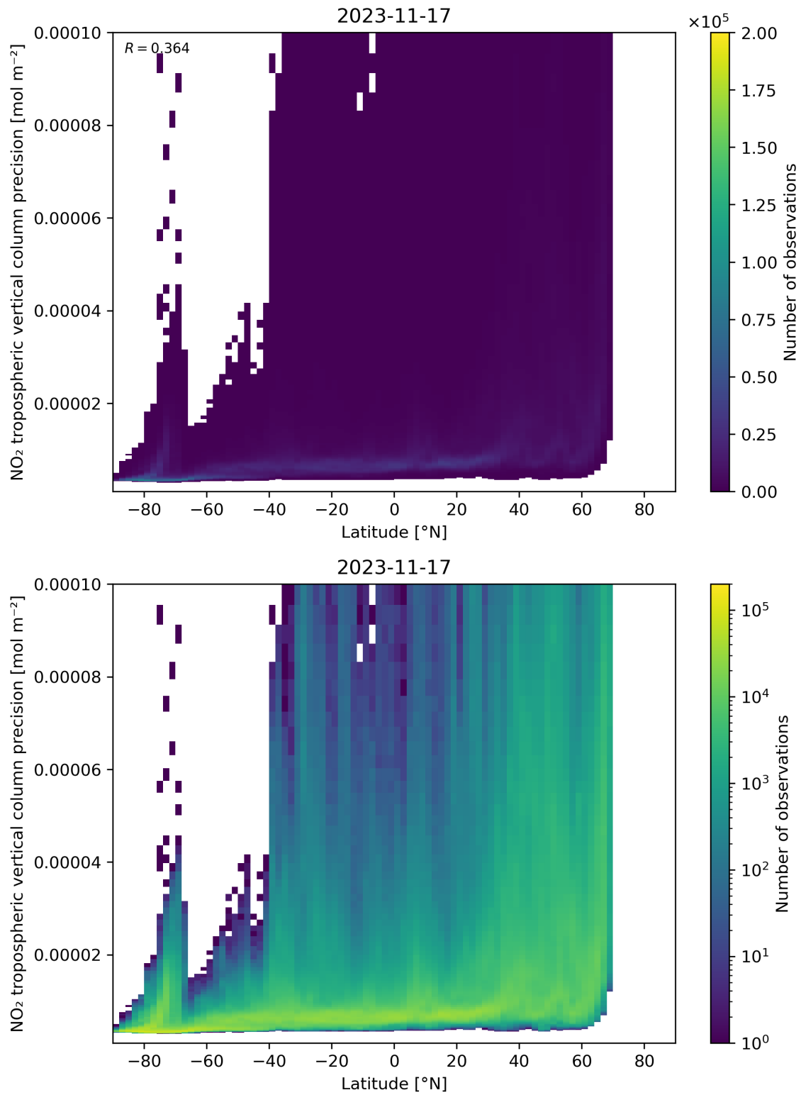
Figure 93: Scatter density plot of “Latitude” against “NO 2 tropospheric vertical column precision” for 2023-11-16 to 2023-11-18.
