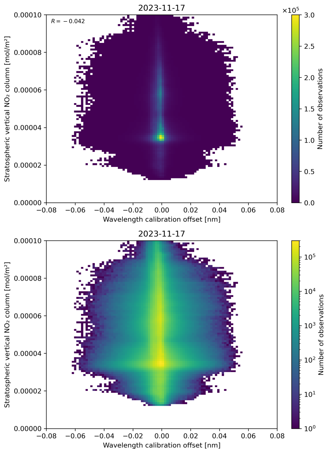
Figure 176: Scatter density plot of “Wavelength calibration offset” against “Stratospheric vertical NO 2 column” for 2023-11-16 to 2023-11-18.
