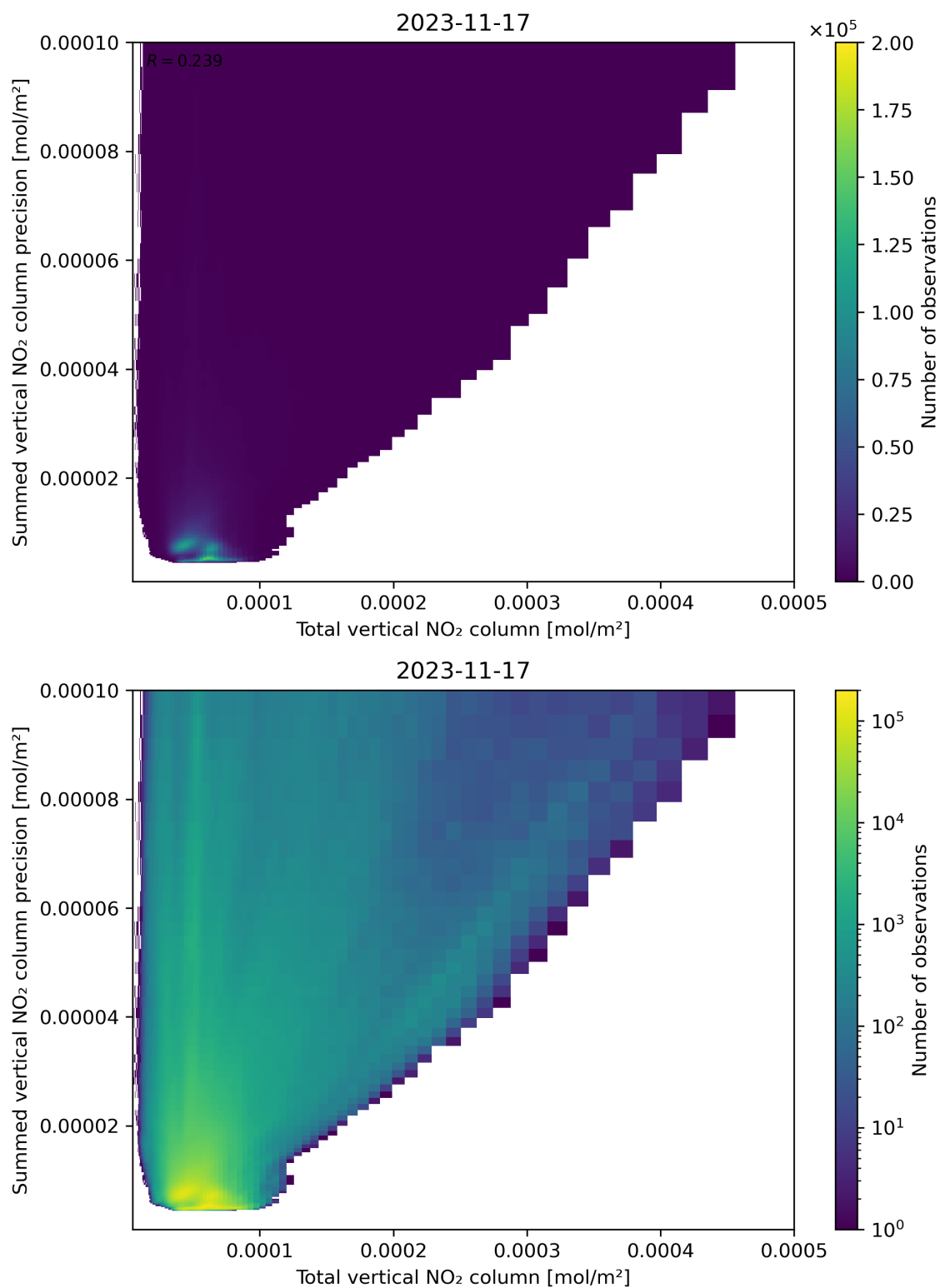
Figure 113: Scatter density plot of “Total vertical NO 2 column” against “Summed vertical NO 2 column precision” for 2023-11-16 to 2023-11-18.
