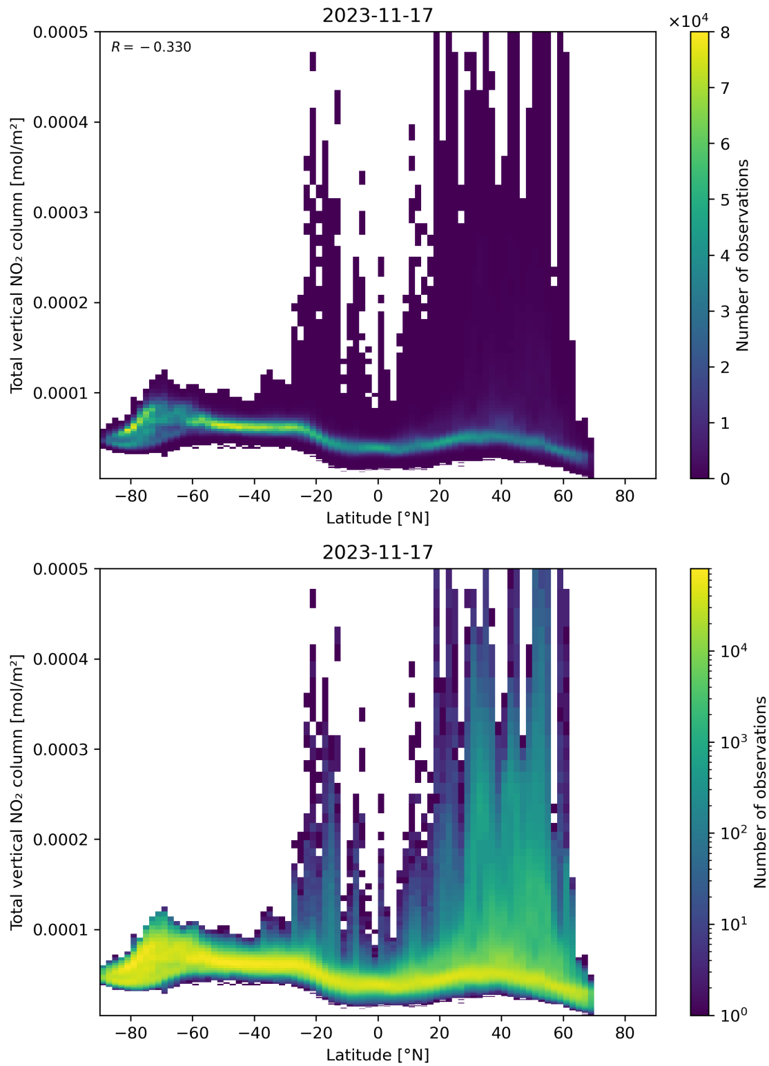
Figure 90: Scatter density plot of “Latitude” against “Total vertical NO 2 column” for 2023-11-16 to 2023-11-18.
