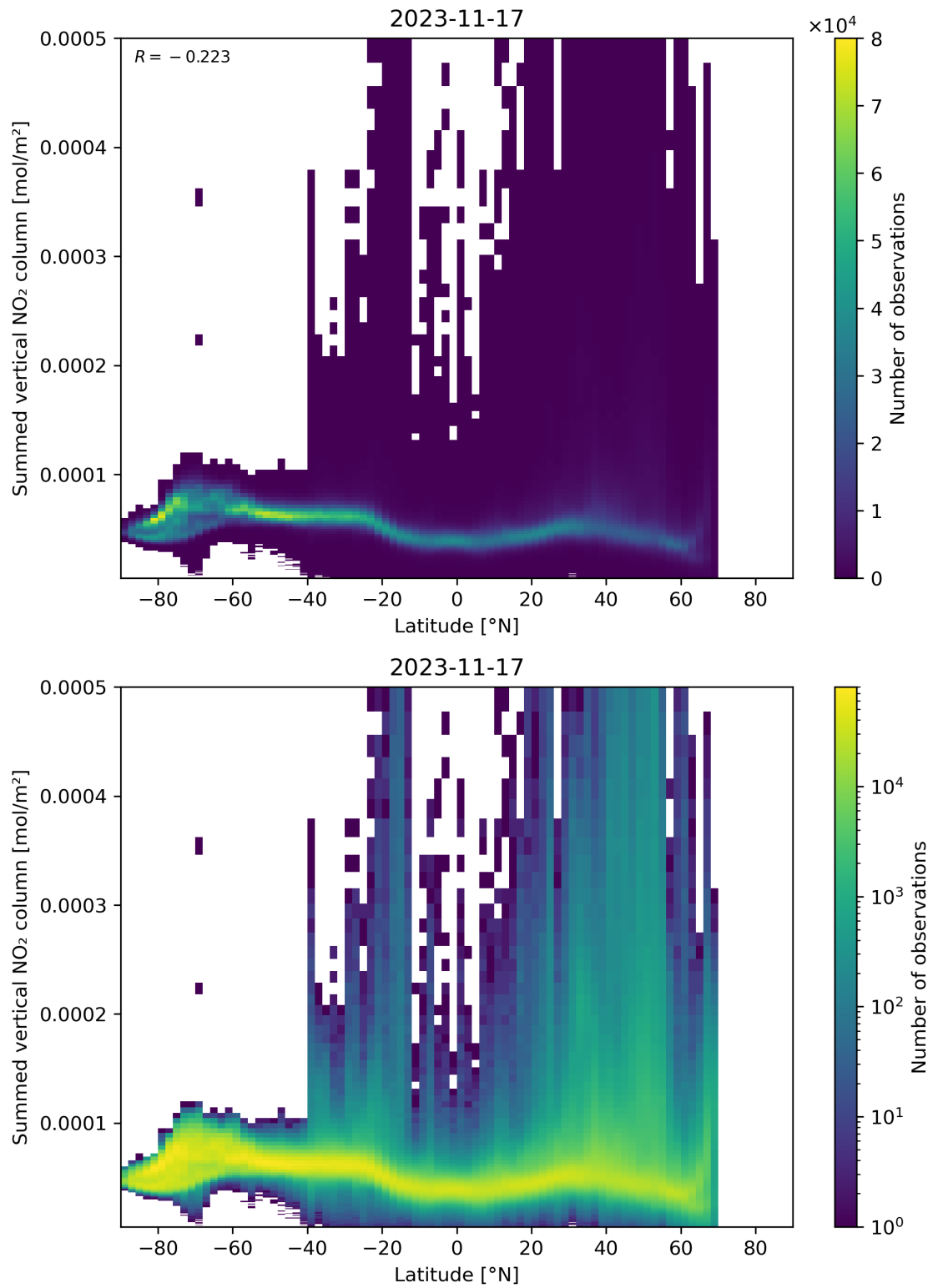
Figure 88: Scatter density plot of “Latitude” against “Summed vertical NO 2 column” for 2023-11-16 to 2023-11-18.
