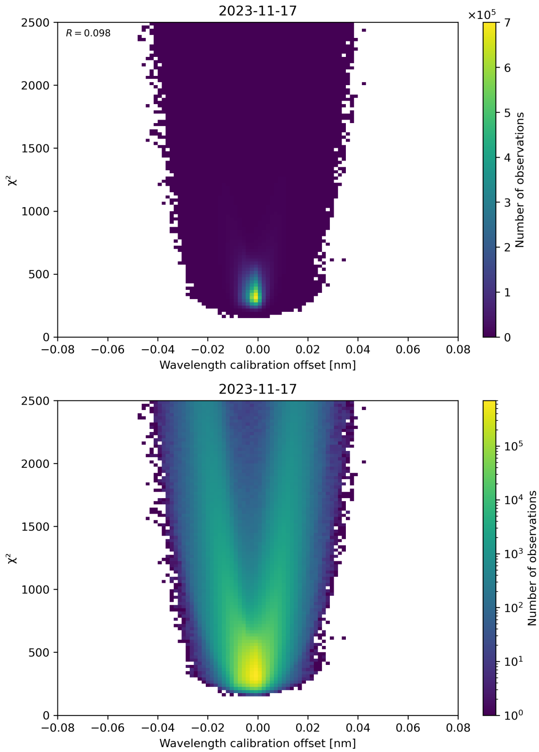
Figure 175: Scatter density plot of “Wavelength calibration offset” against “ \chi^2 ” for 2023-11-16 to 2023-11-18.
