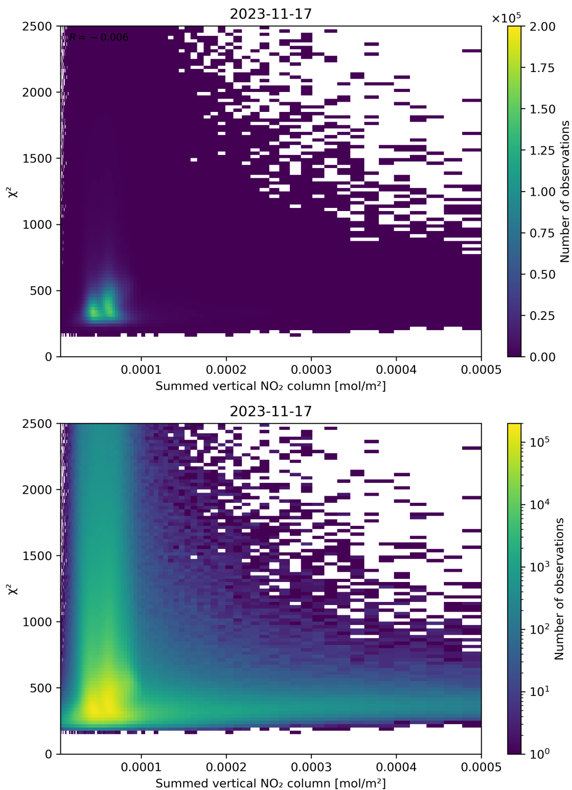
Figure 104: Scatter density plot of “Summed vertical NO 2 column” against “ \chi^2 ” for 2023-11-16 to 2023-11-18.
