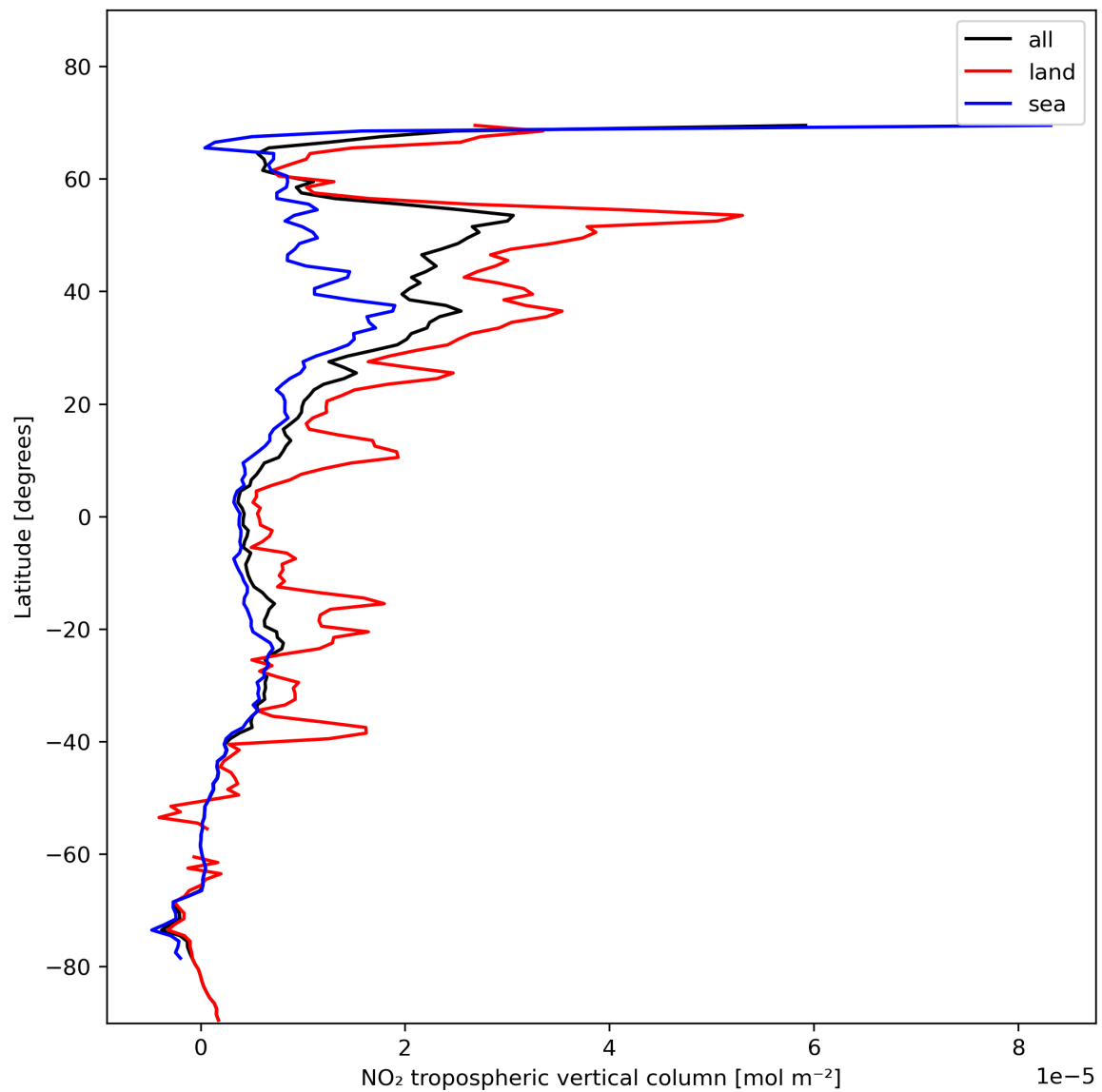
Figure 12: Zonal average of “NO 2 tropospheric vertical column” for 2023-11-16 to 2023-11-18.
