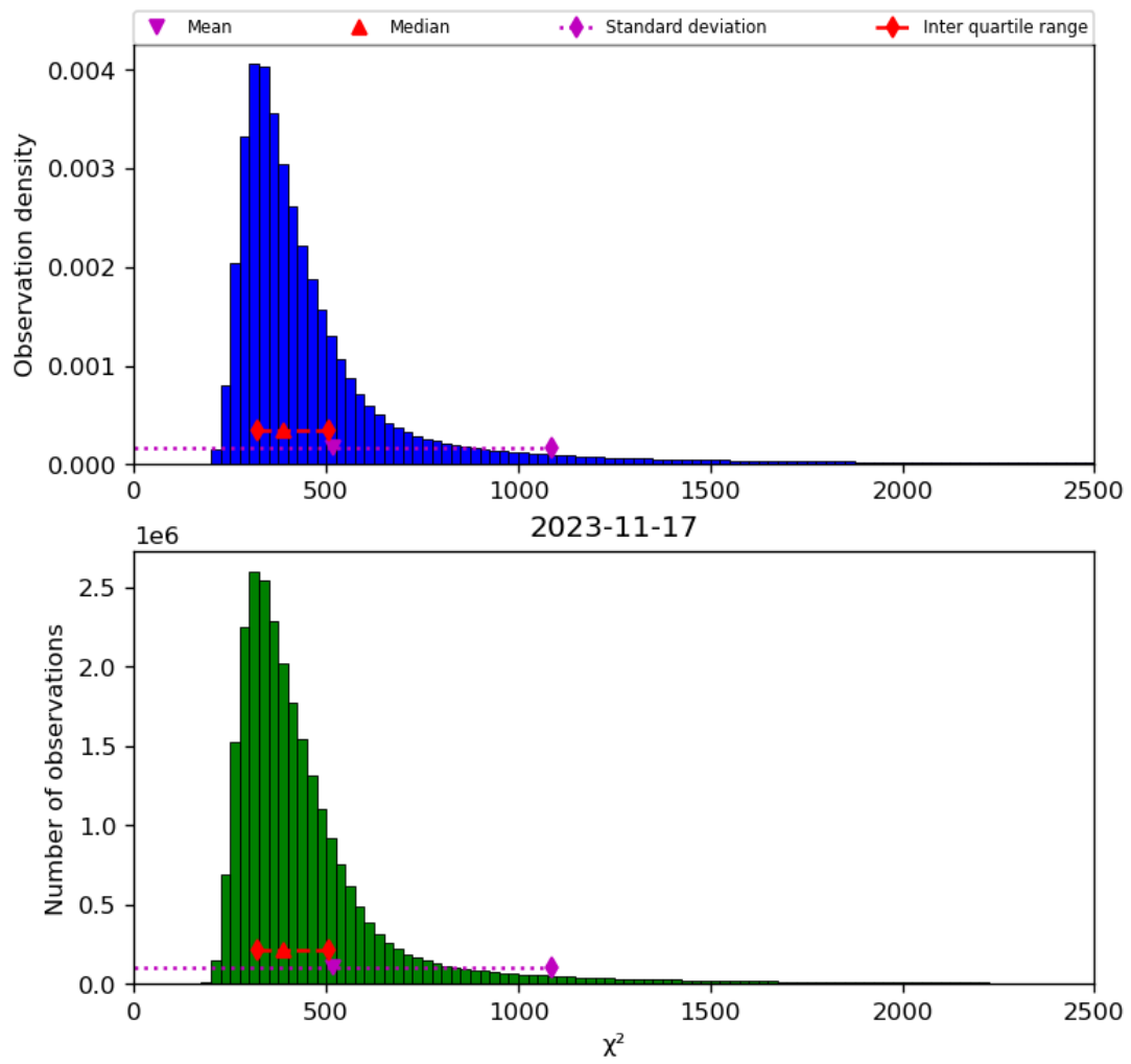
Figure 42: Histogram of “ \chi^2 ” for 2023-11-16 to 2023-11-18
