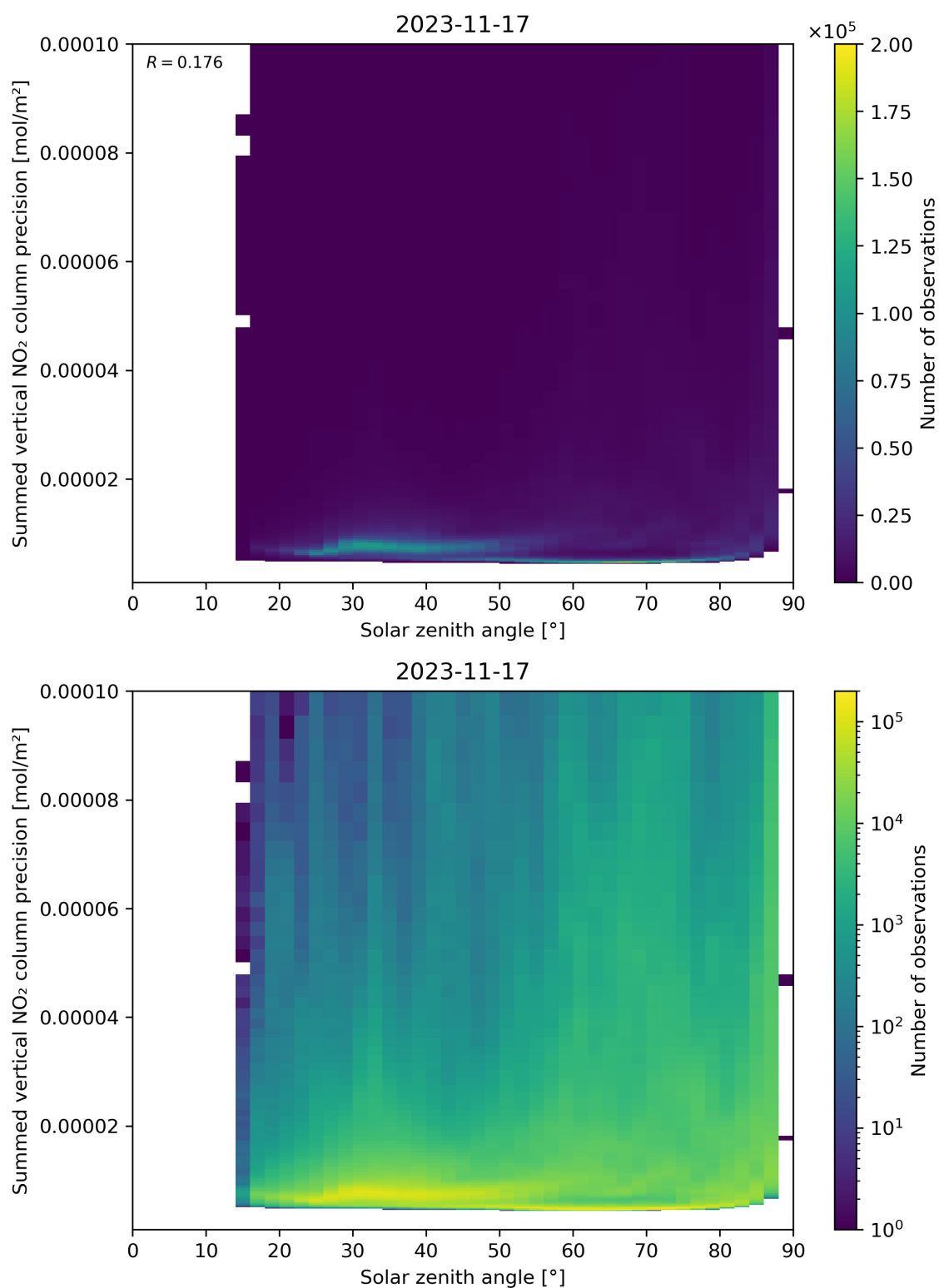
Figure 152: Scatter density plot of “Solar zenith angle” against “Summed vertical NO 2 column precision” for 2023-11-16 to 2023-11-18.
