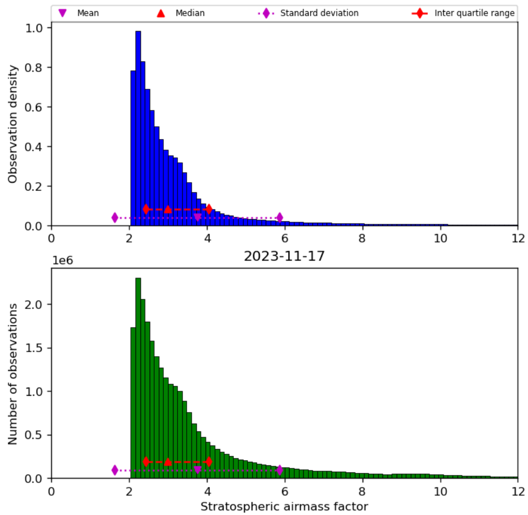
Figure 44: Histogram of “Stratospheric airmass factor” for 2023-11-16 to 2023-11-18
