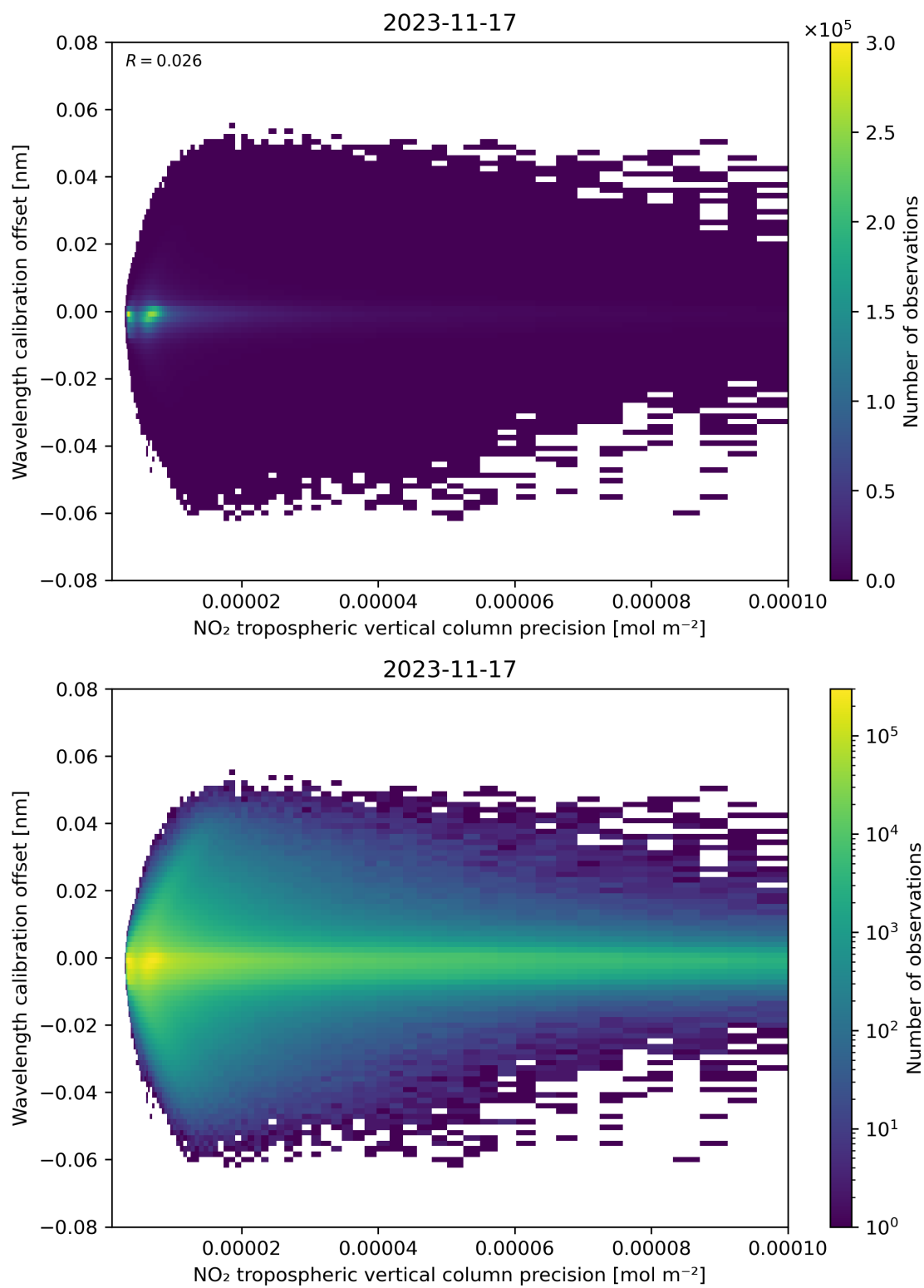
Figure 141: Scatter density plot of “NO 2 tropospheric vertical column precision” against “Wavelength calibration offset” for 2023-11-16 to 2023-11-18.
