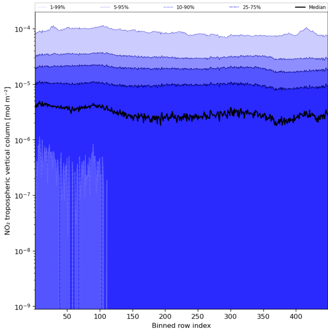
Figure 46: Along track statistics of “NO 2 tropospheric vertical column” for 2023-11-16 to 2023-11-18
