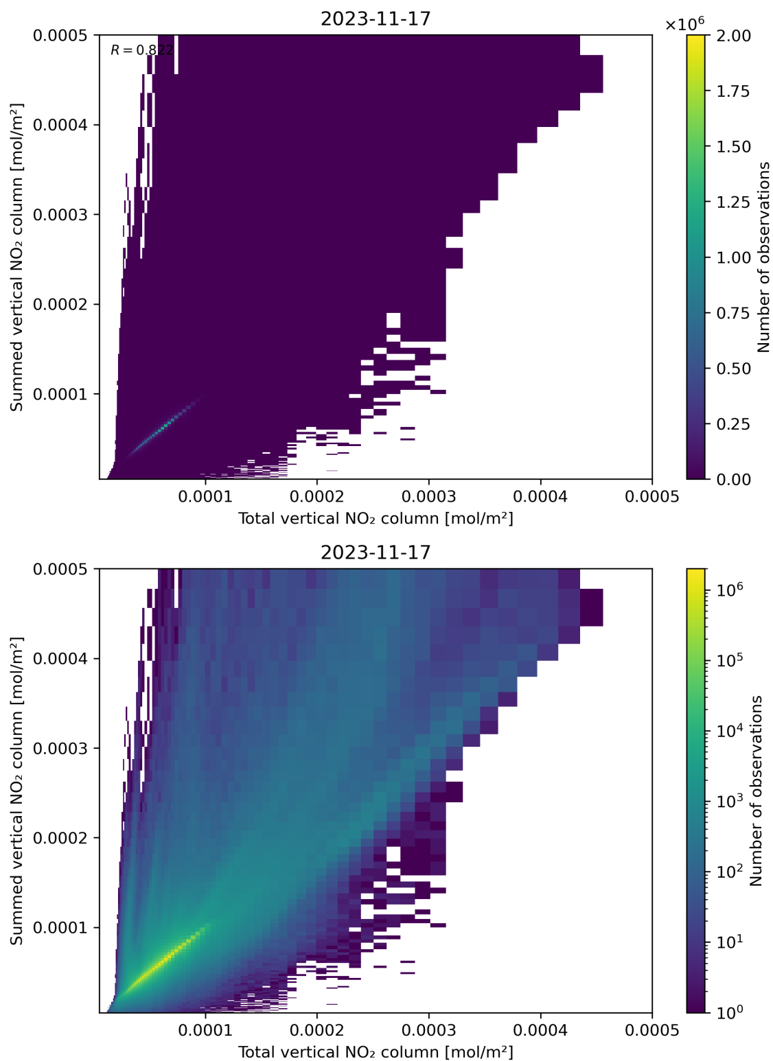
Figure 112: Scatter density plot of “Total vertical NO 2 column” against “Summed vertical NO 2 column” for 2023-11-16 to 2023-11-18.
