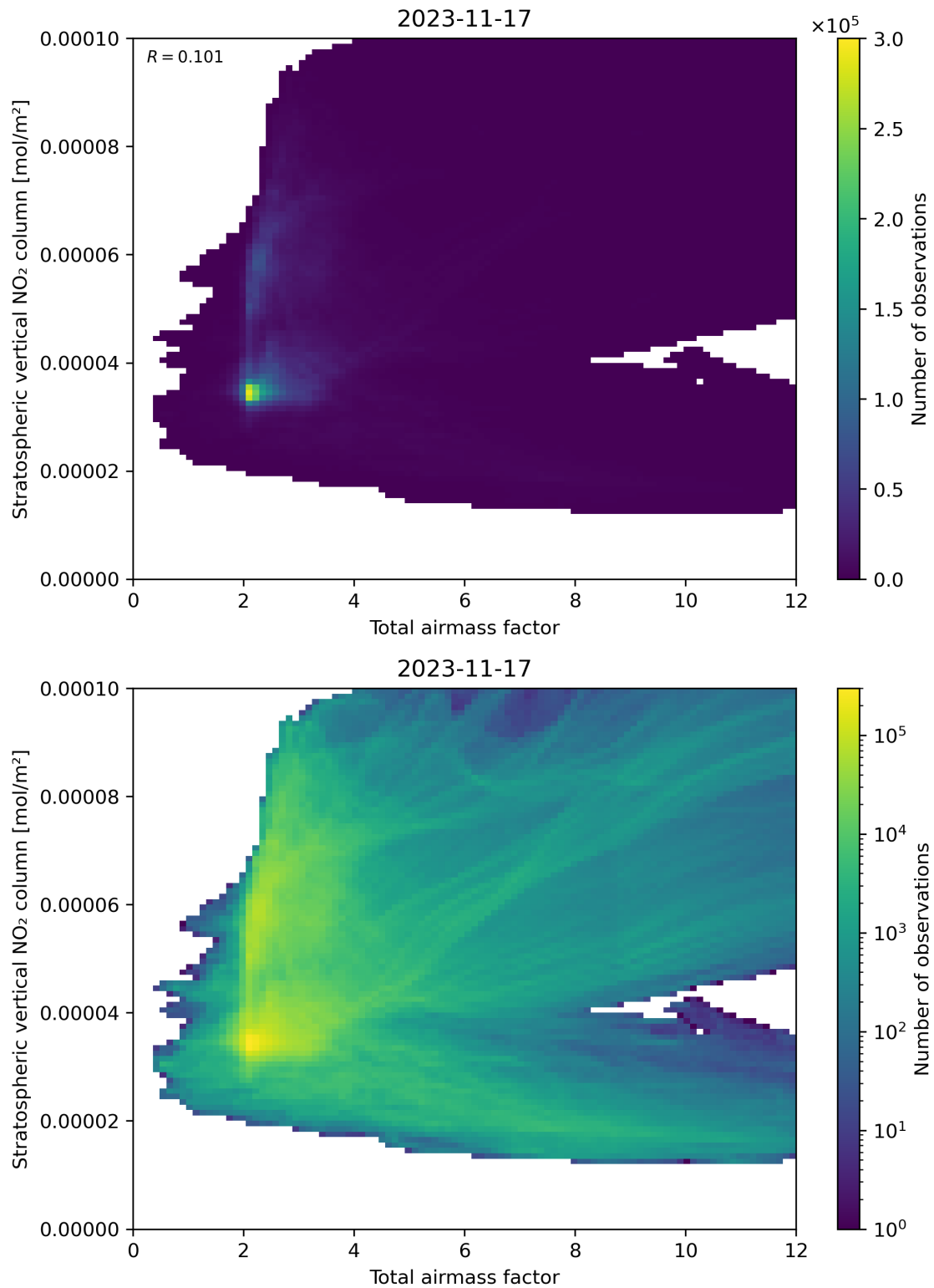
Figure 64: Scatter density plot of “Total airmass factor” against “Stratospheric vertical NO 2 column” for 2023-11-16 to 2023-11-18.
