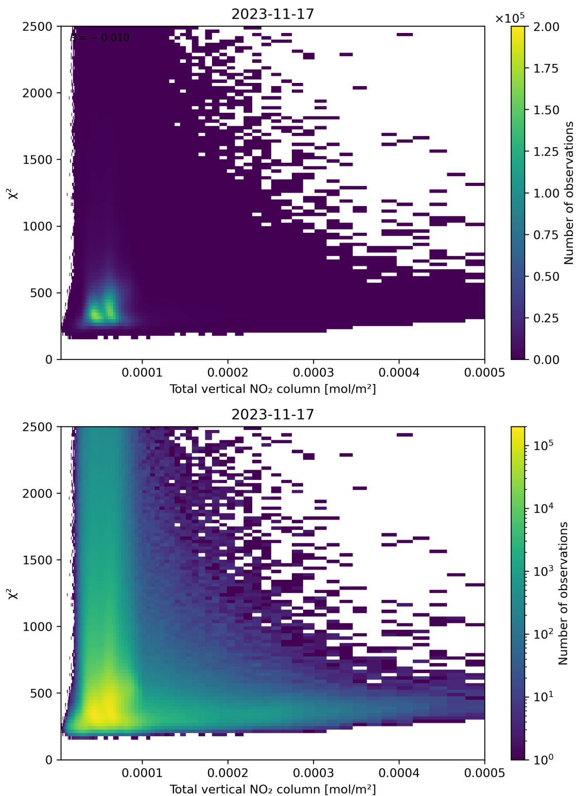
Figure 111: Scatter density plot of “Total vertical NO 2 column” against “ \chi^2 ” for 2023-11-16 to 2023-11-18.
