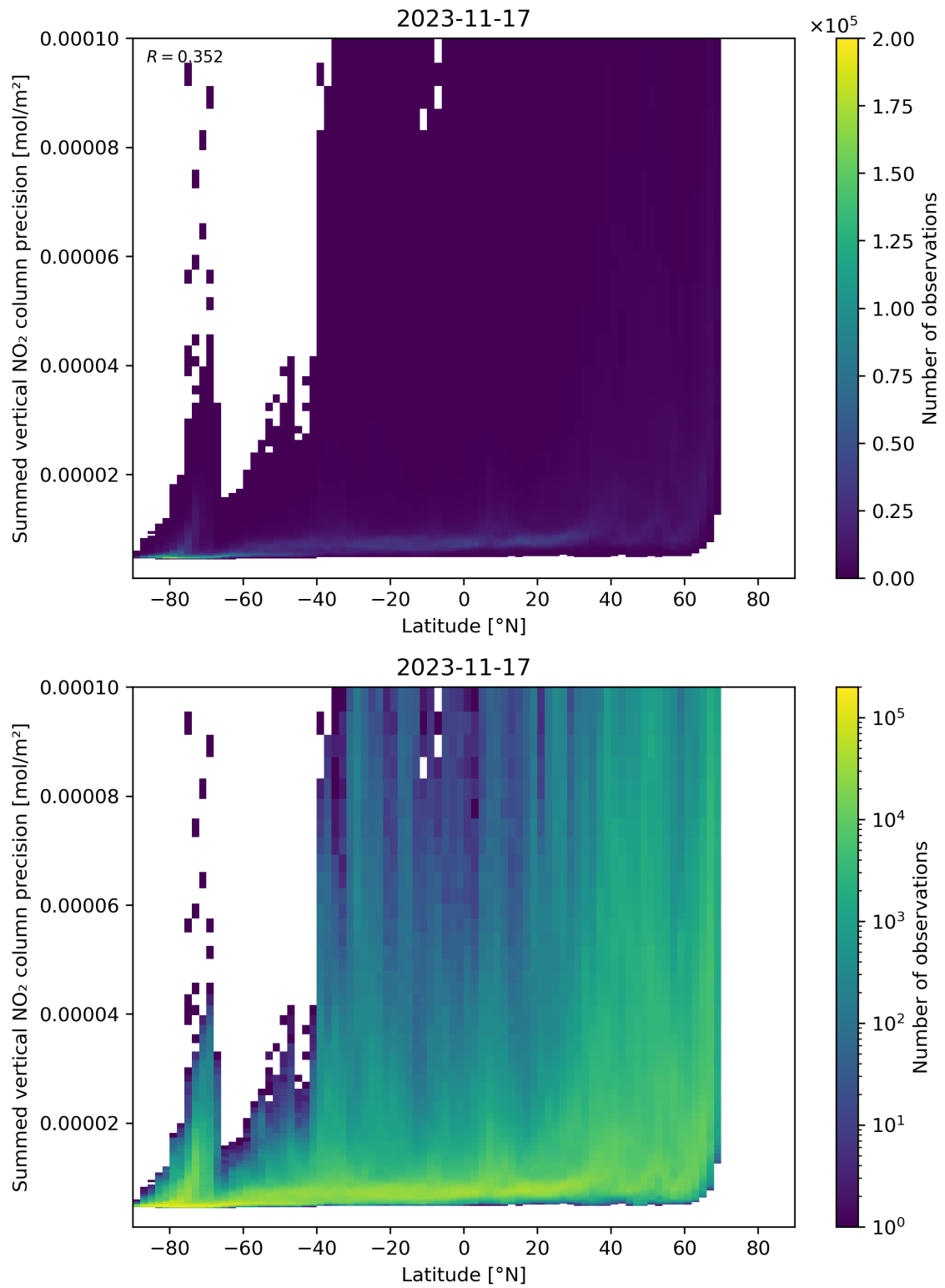
Figure 89: Scatter density plot of “Latitude” against “Summed vertical NO 2 column precision” for 2023-11-16 to 2023-11-18.
