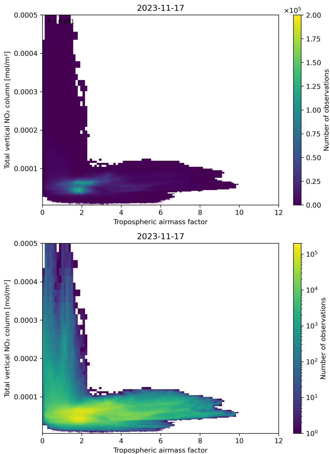
Figure 77: Scatter density plot of “Tropospheric airmass factor” against “Total vertical NO 2 column” for 2023-11-16 to 2023-11-18.
