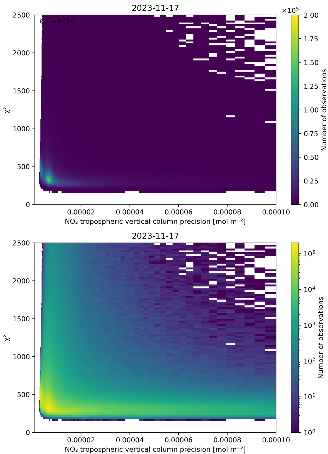
Figure 134: Scatter density plot of “NO 2 tropospheric vertical column precision” against “ \chi^2 ” for 2023-11-16 to 2023-11-18.
