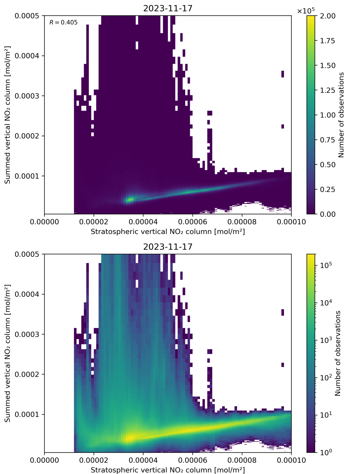
Figure 98: Scatter density plot of “Stratospheric vertical NO 2 column” against “Summed vertical NO 2 column” for 2023-11-16 to 2023-11-18.
