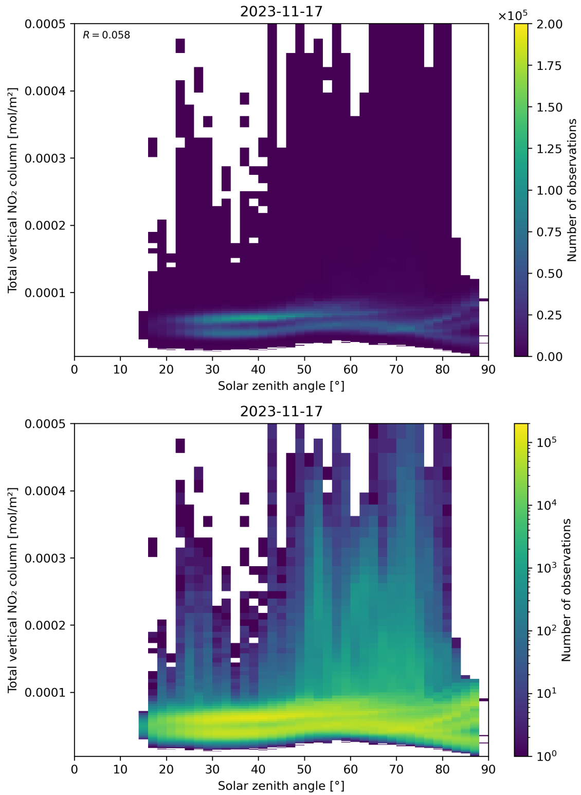
Figure 153: Scatter density plot of “Solar zenith angle” against “Total vertical NO 2 column” for 2023-11-16 to 2023-11-18.
