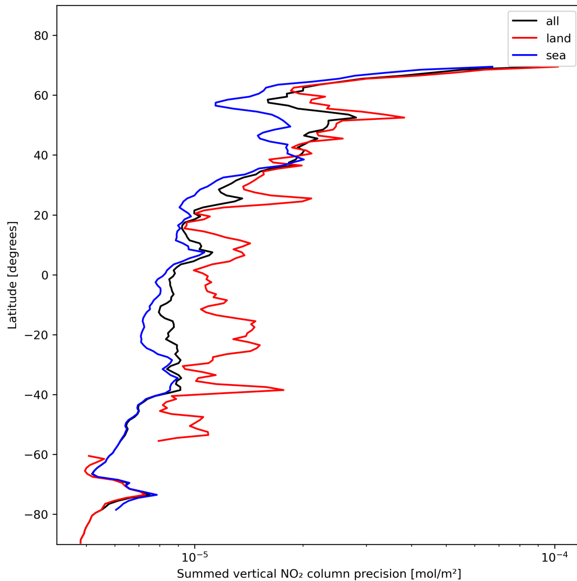
Figure 24: Zonal average of “Summed vertical NO 2 column precision” for 2023-11-16 to 2023-11-18.
