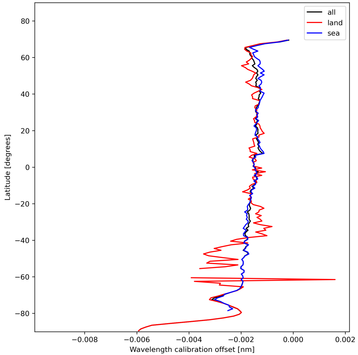
Figure 18: Zonal average of “Wavelength calibration offset” for 2023-11-16 to 2023-11-18.
