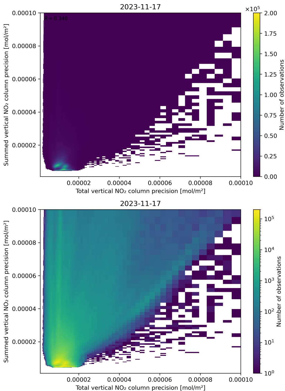
Figure 118: Scatter density plot of “Total vertical NO 2 column precision” against “Summed vertical NO 2 column precision” for 2023-11-16 to 2023-11-18.
