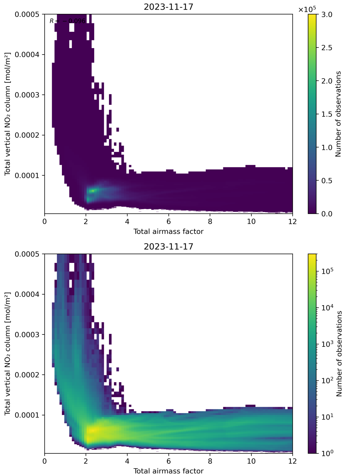
Figure 67: Scatter density plot of “Total air mass factor” against “Total vertical NO 2 column” for 2023-11-16 to 2023-11-18.
