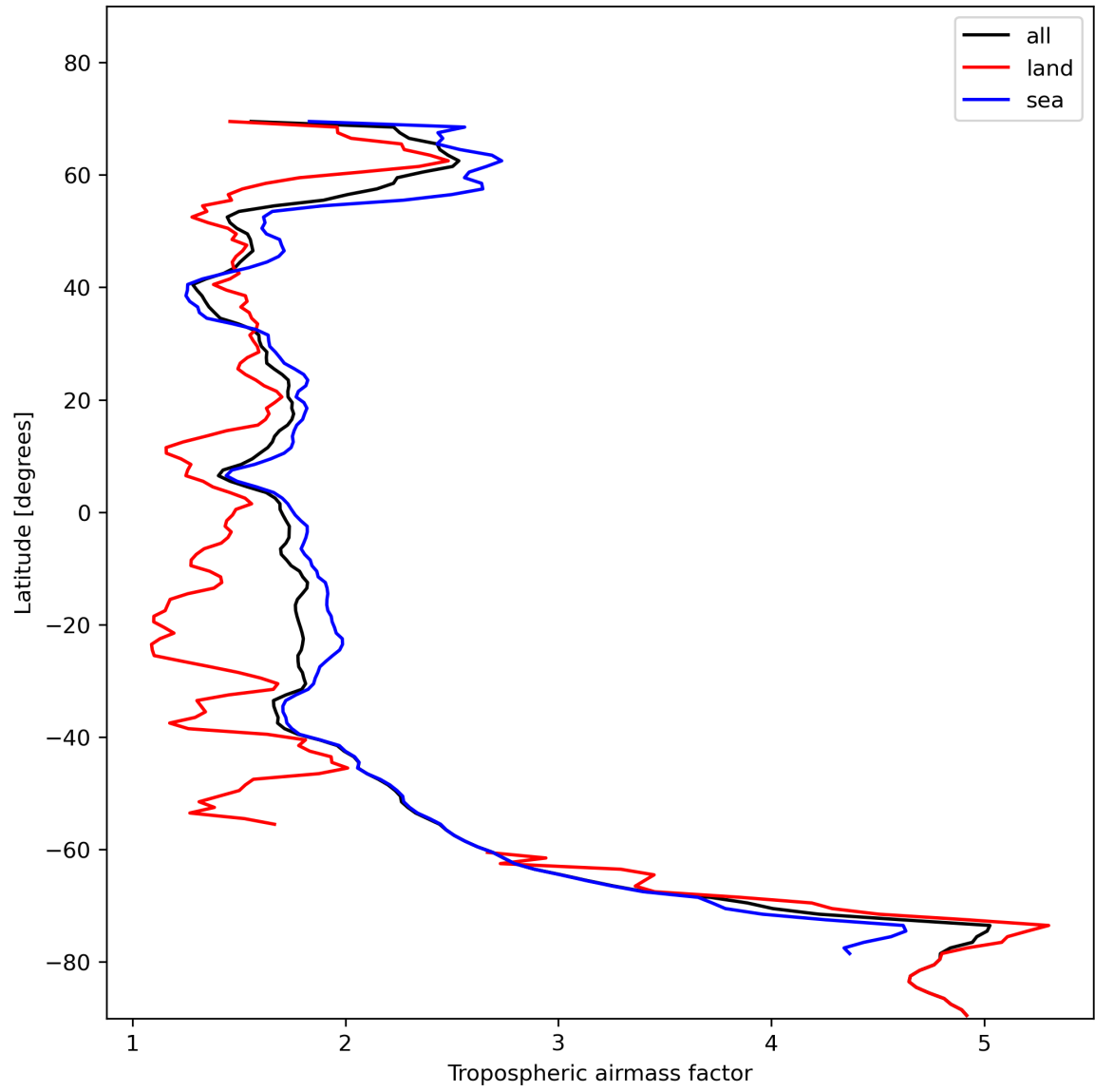
Figure 14: Zonal average of “Tropospheric airmass factor” for 2023-11-16 to 2023-11-18.
