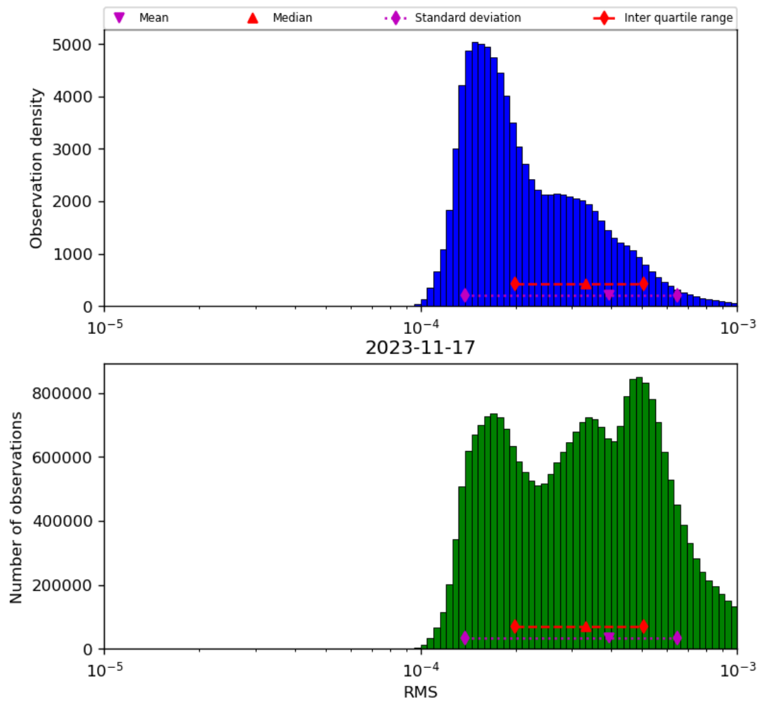
Figure 43: Histogram of “RMS” for 2023-11-16 to 2023-11-18
