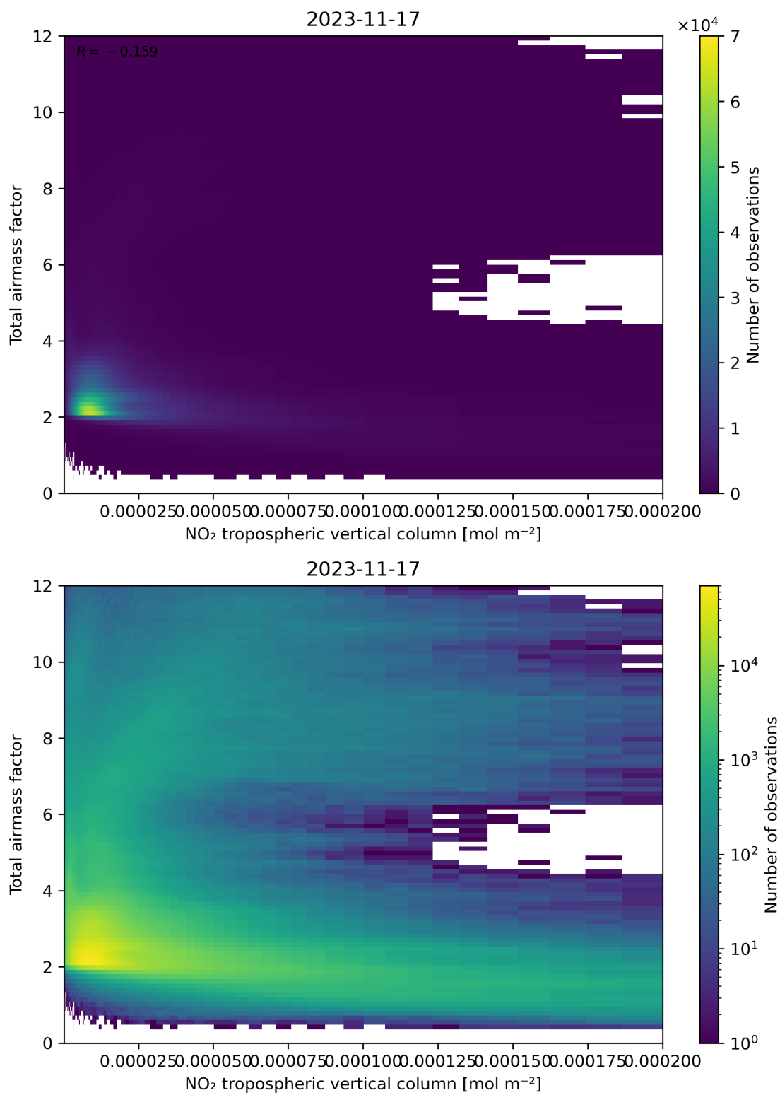
Figure 122: Scatter density plot of “NO 2 tropospheric vertical column” against “Total air mass factor” for 2023-11-16 to 2023-11-18.
