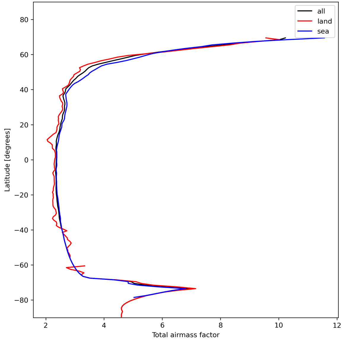
Figure 15: Zonal average of “Total airmass factor” for 2023-11-16 to 2023-11-18.
