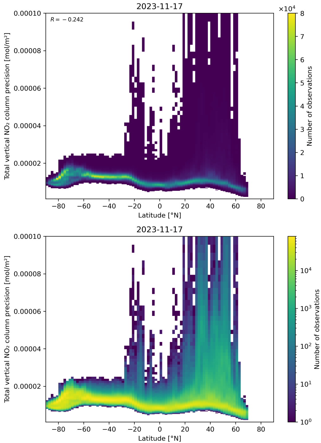
Figure 91: Scatter density plot of “Latitude” against “Total vertical NO 2 column precision” for 2023-11-16 to 2023-11-18.
