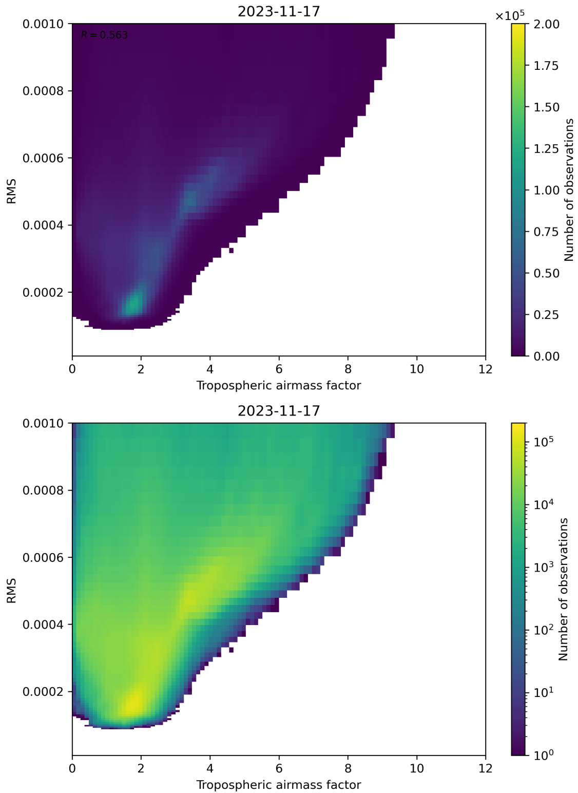
Figure 79: Scatter density plot of “Tropospheric airmass factor” against “RMS” for 2023-11-16 to 2023-11-18.
