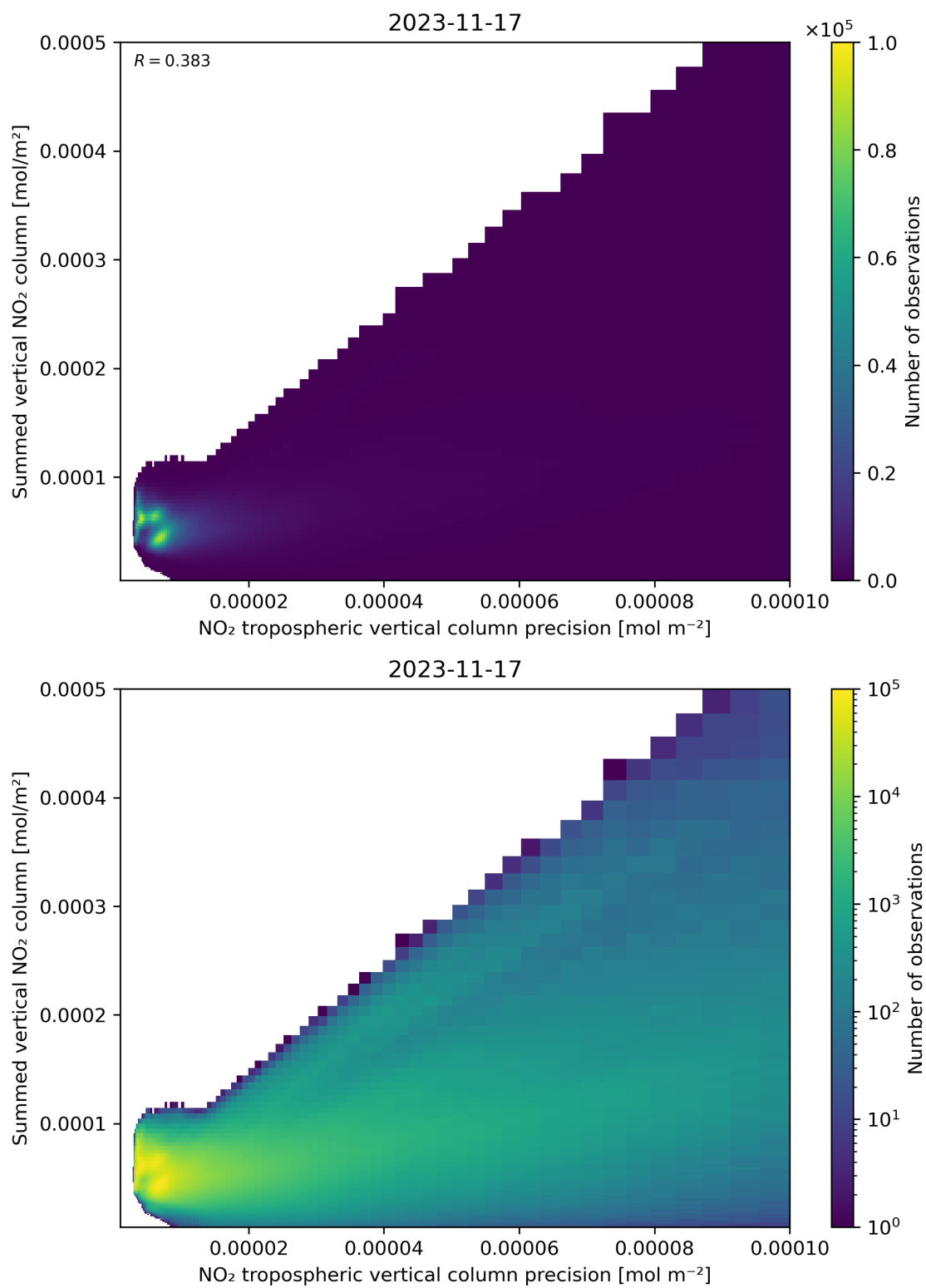
Figure 136: Scatter density plot of “NO 2 tropospheric vertical column precision” against “Summed vertical NO 2 column” for 2023-11-16 to 2023-11-18.
