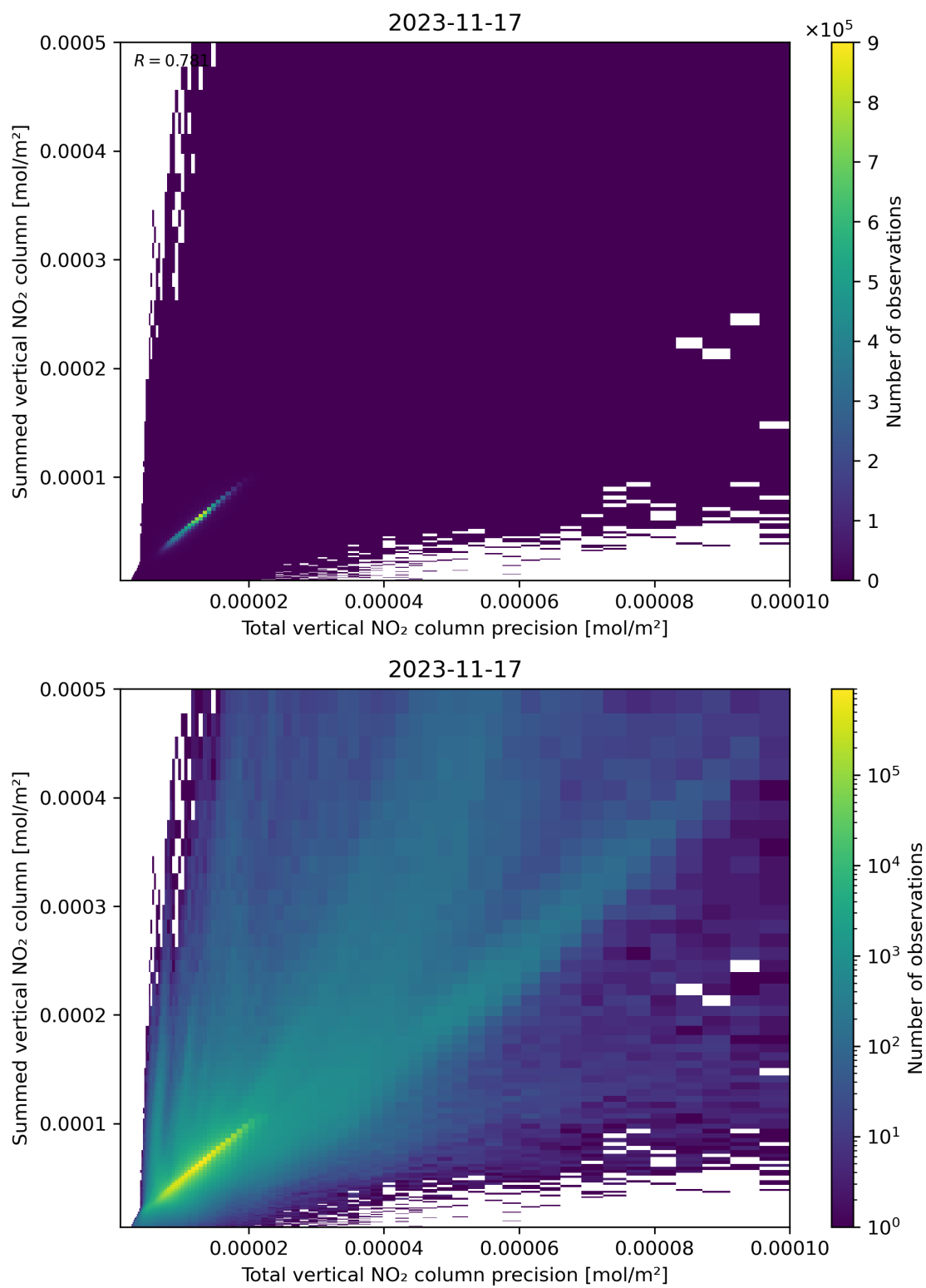
Figure 117: Scatter density plot of “Total vertical NO 2 column precision” against “Summed vertical NO 2 column” for 2023-11-16 to 2023-11-18.
