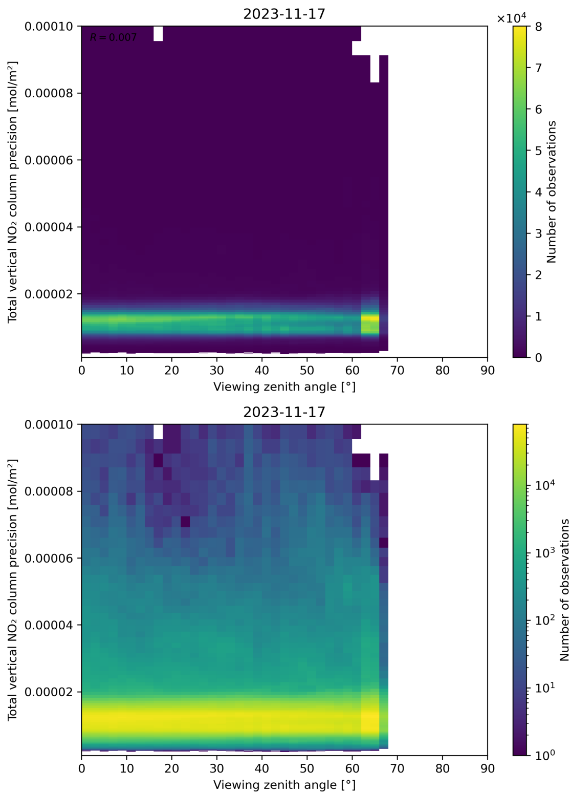
Figure 168: Scatter density plot of “Viewing zenith angle” against “Total vertical NO 2 column precision” for 2023-11-16 to 2023-11-18.
