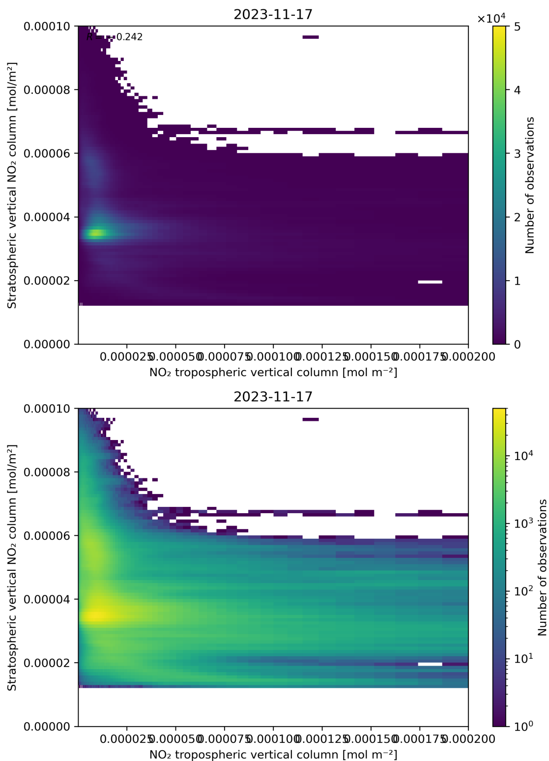
Figure 125: Scatter density plot of “NO 2 tropospheric vertical column” against “Stratospheric vertical NO 2 column” for 2023-11-16 to 2023-11-18.
