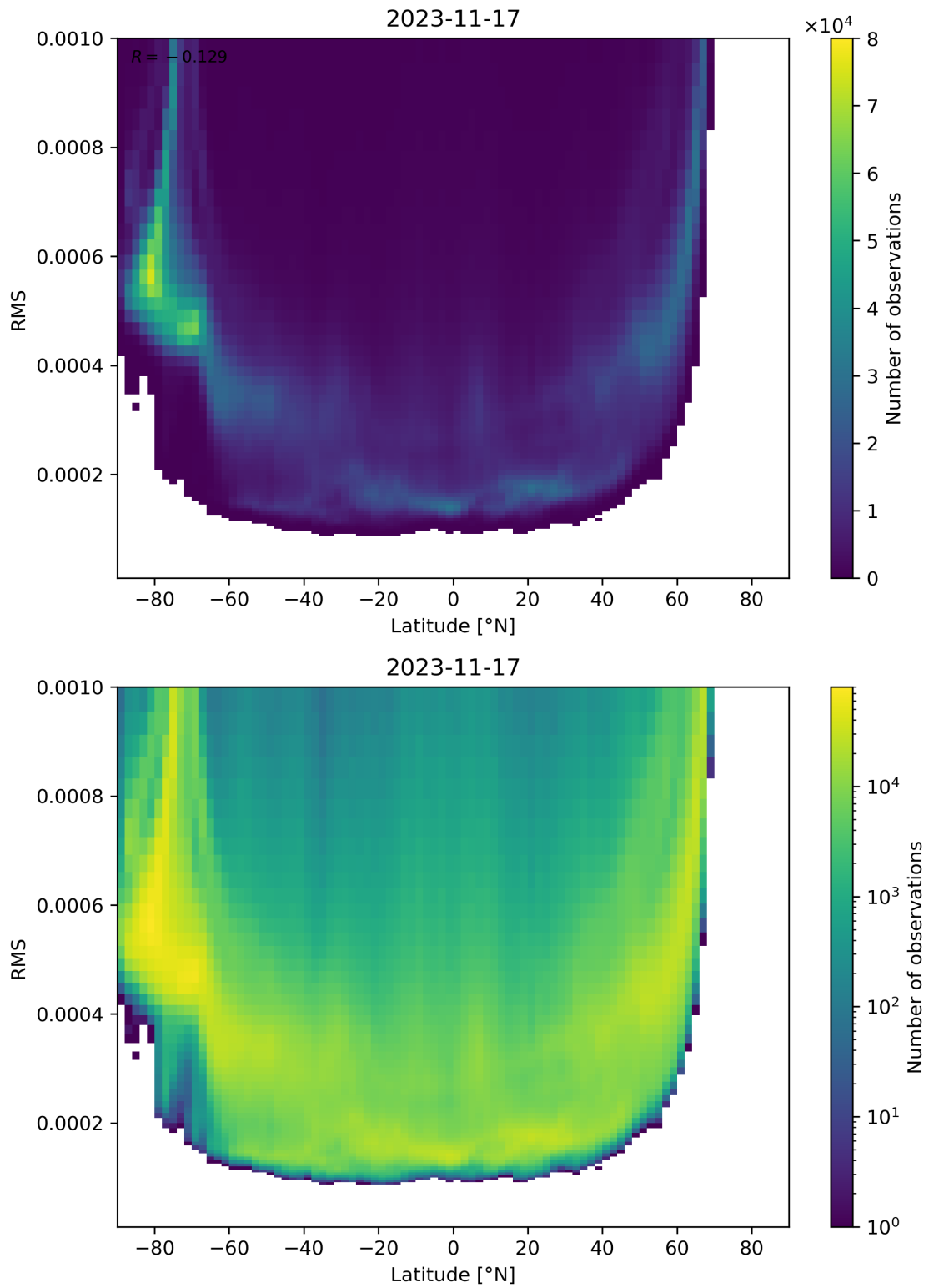
Figure 94: Scatter density plot of “Latitude” against “RMS” for 2023-11-16 to 2023-11-18.
