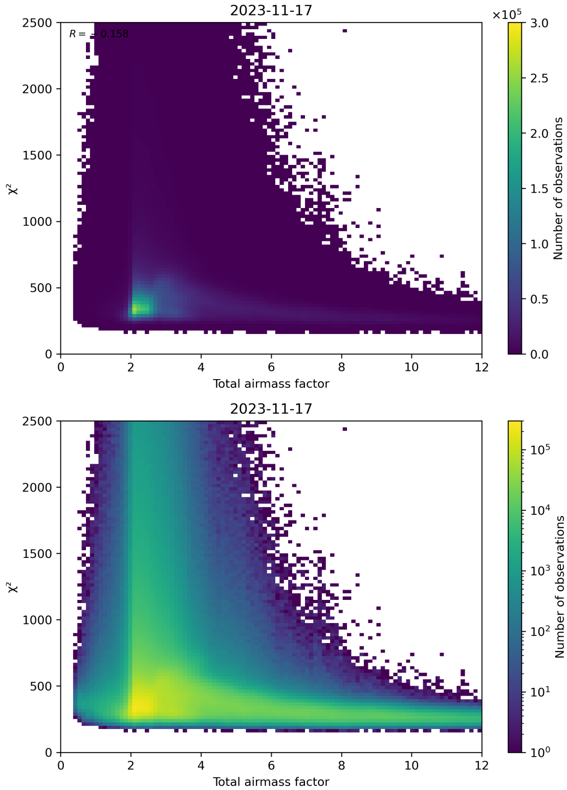
Figure 63: Scatter density plot of “Total airmass factor” against “ \chi^2 ” for 2023-11-16 to 2023-11-18.
