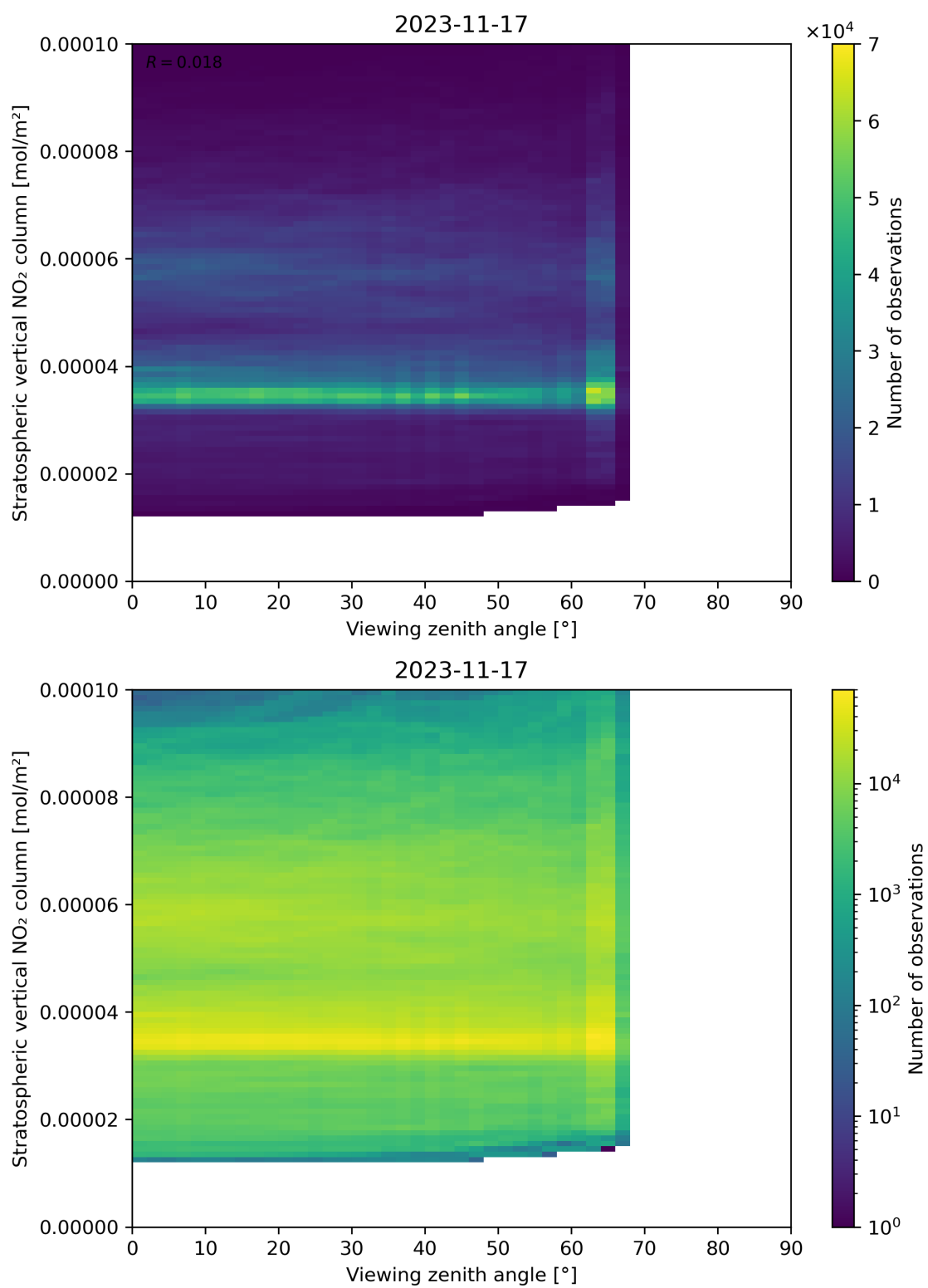
Figure 164: Scatter density plot of “Viewing zenith angle” against “Stratospheric vertical NO 2 column” for 2023-11-16 to 2023-11-18.
