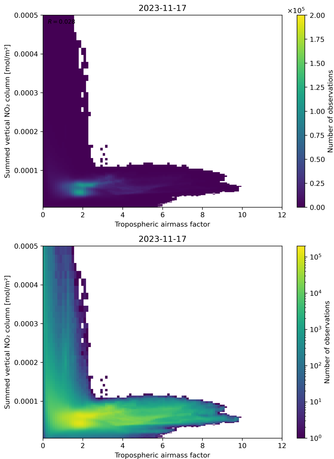
Figure 75: Scatter density plot of “Tropospheric air mass factor” against “Summed vertical NO 2 column” for 2023-11-16 to 2023-11-18.
