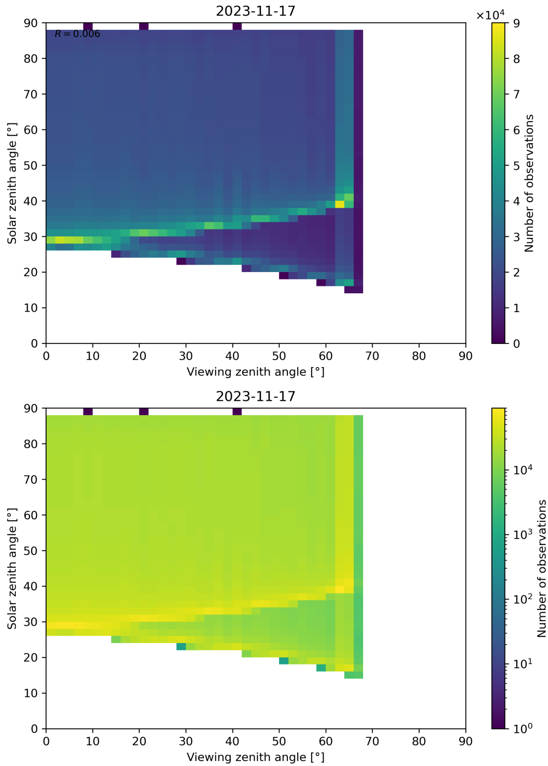
Figure 172: Scatter density plot of “Viewing zenith angle” against “Solar zenith angle” for 2023-11-16 to 2023-11-18.
