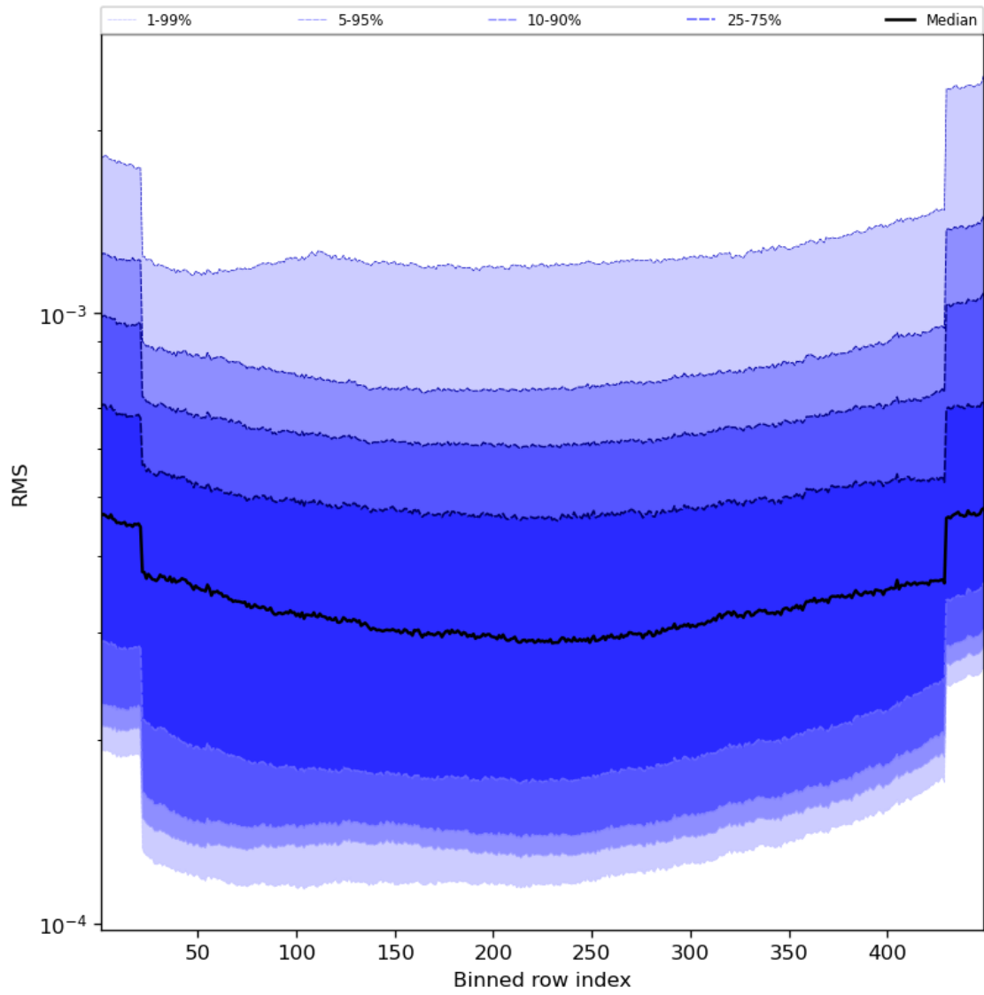
Figure 60: Along track statistics of “RMS” for 2023-11-16 to 2023-11-18
