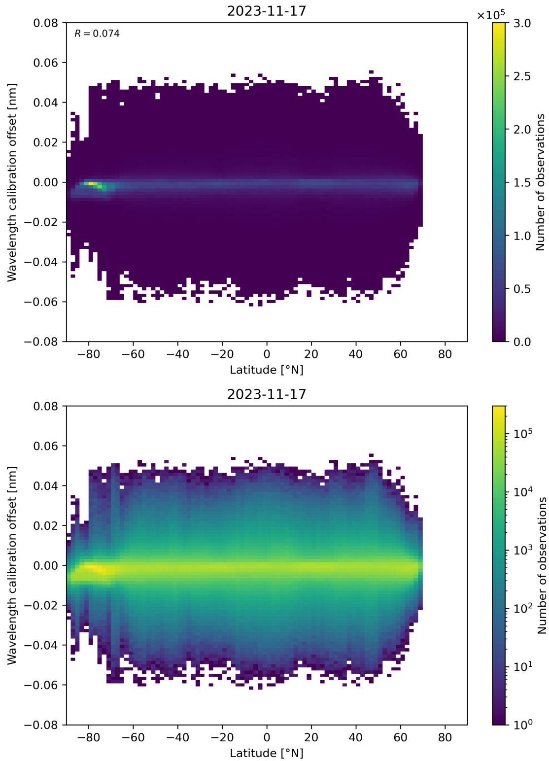
Figure 95: Scatter density plot of “Latitude” against “Wavelength calibration offset” for 2023-11-16 to 2023-11-18.
