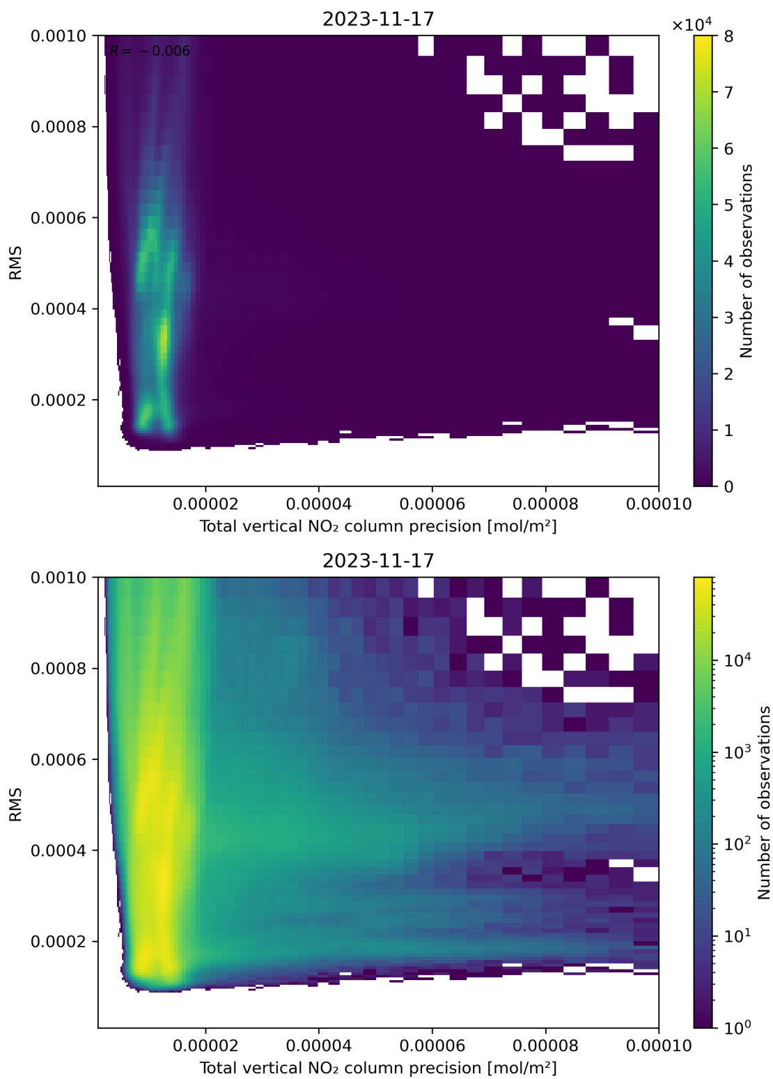
Figure 119: Scatter density plot of “Total vertical NO 2 column precision” against “RMS” for 2023-11-16 to 2023-11-18.
