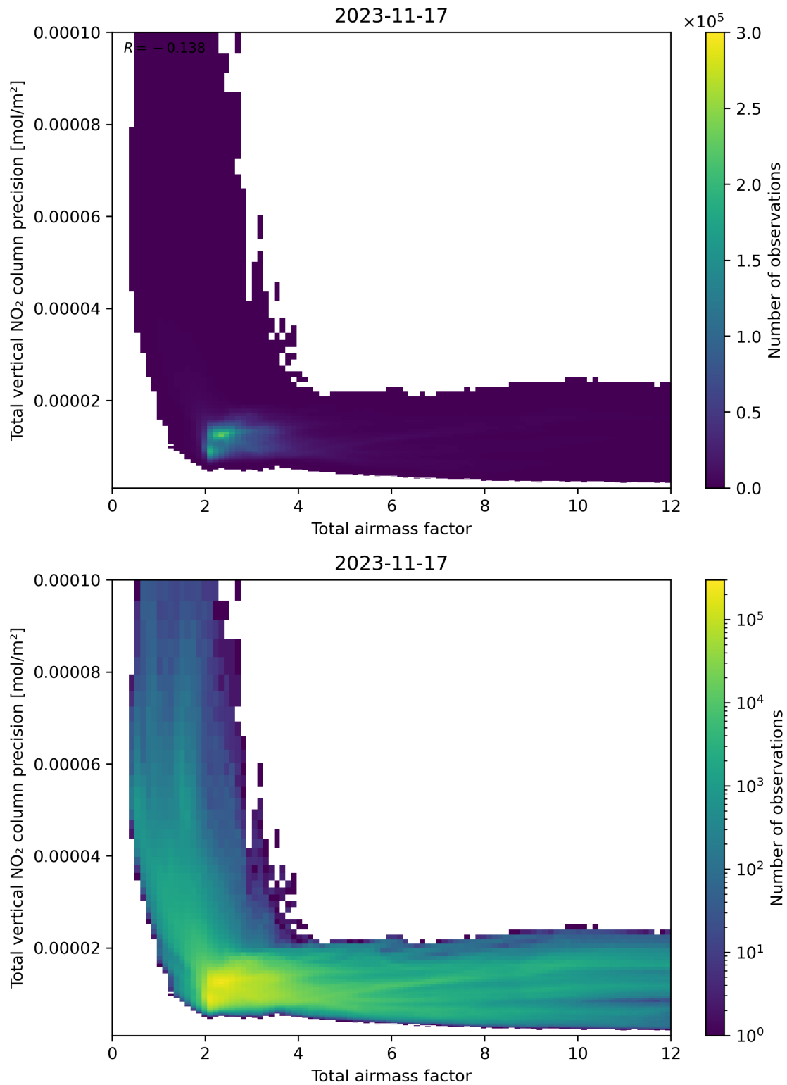
Figure 68: Scatter density plot of “Total airmass factor” against “Total vertical NO 2 column precision” for 2023-11-16 to 2023-11-18.
