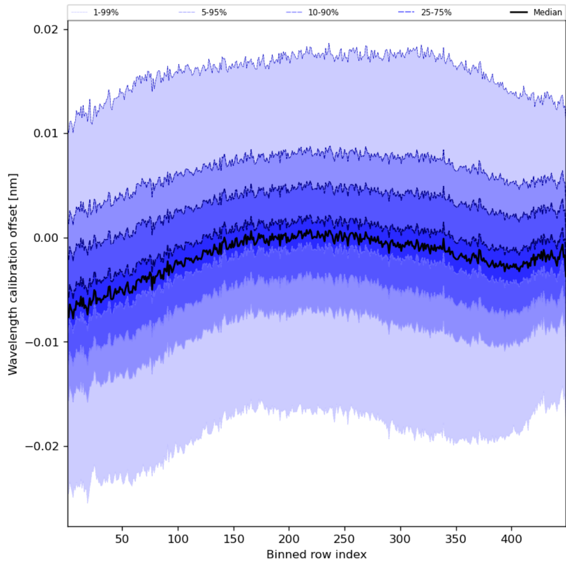
Figure 52: Along track statistics of “Wavelength calibration offset” for 2023-11-16 to 2023-11-18
