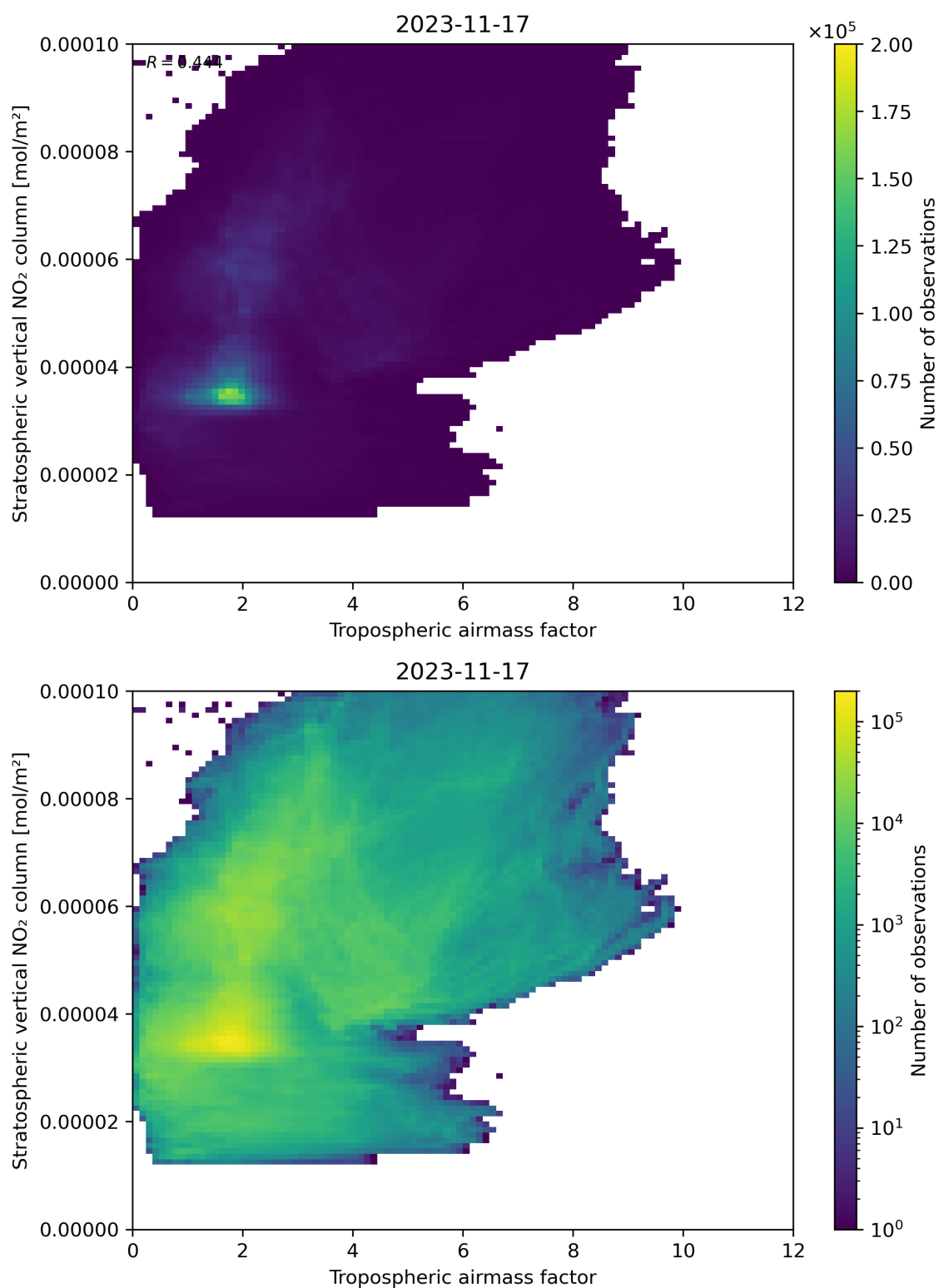
Figure 74: Scatter density plot of “Tropospheric air mass factor” against “Stratospheric vertical NO 2 column” for 2023-11-16 to 2023-11-18.
