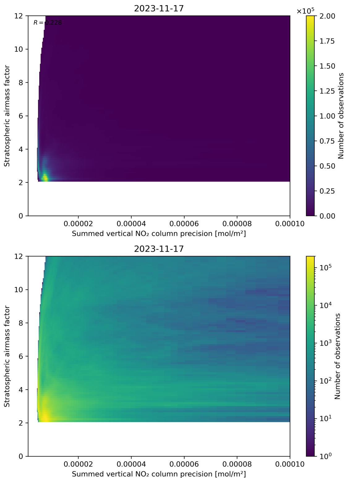
Figure 106: Scatter density plot of “Summed vertical NO 2 column precision” against “Stratospheric airmass factor” for 2023-11-16 to 2023-11-18.
