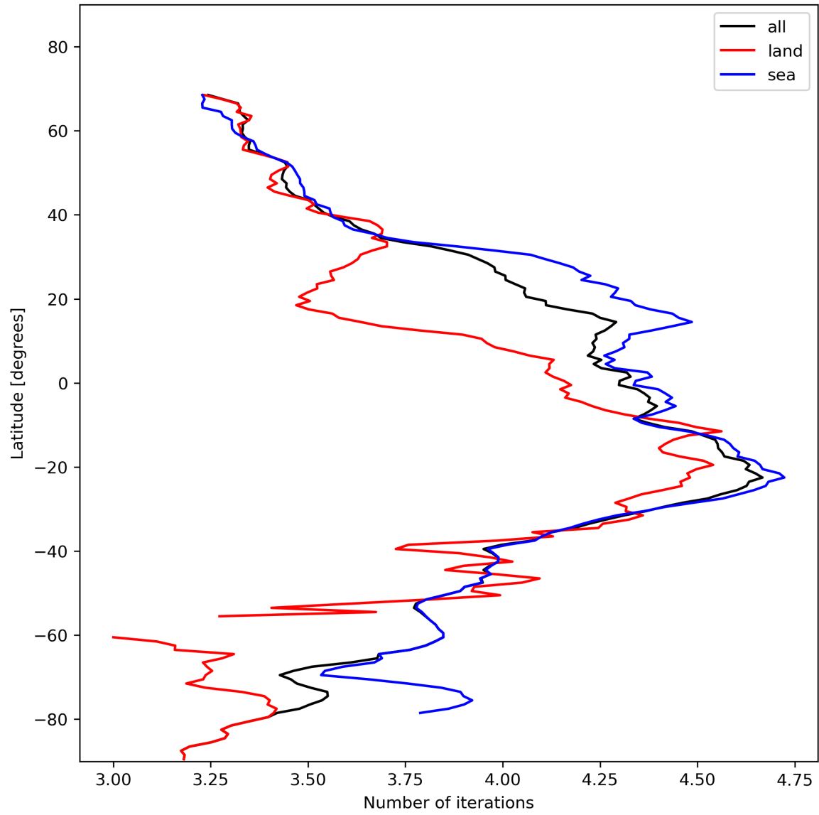
Figure 17: Zonal average of “Number of iterations” for 2023-11-18 to 2023-11-19.
