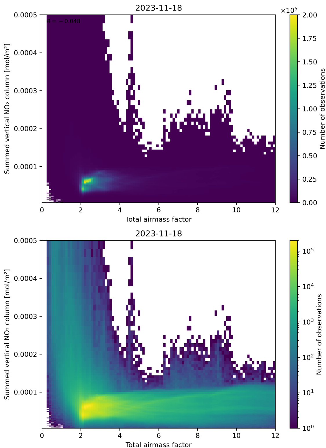
Figure 65: Scatter density plot of “Total airmass factor” against “Summed vertical NO 2 column” for 2023-11-18 to 2023-11-19.
