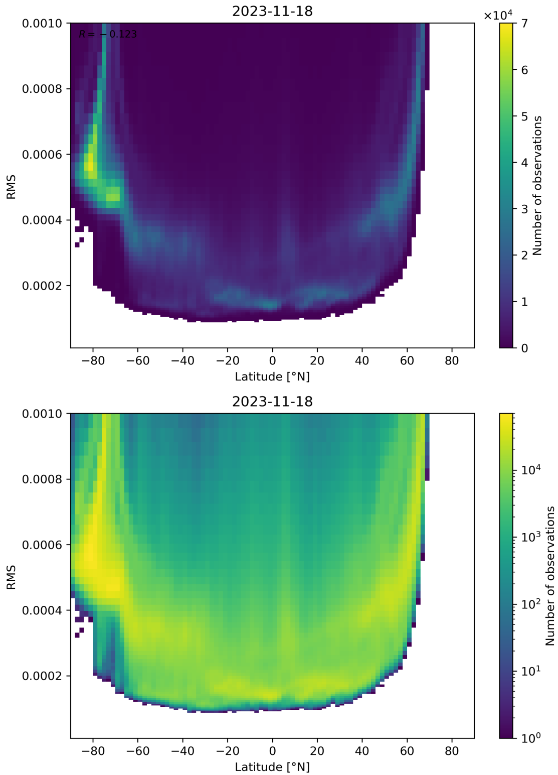
Figure 94: Scatter density plot of “Latitude” against “RMS” for 2023-11-18 to 2023-11-19.
