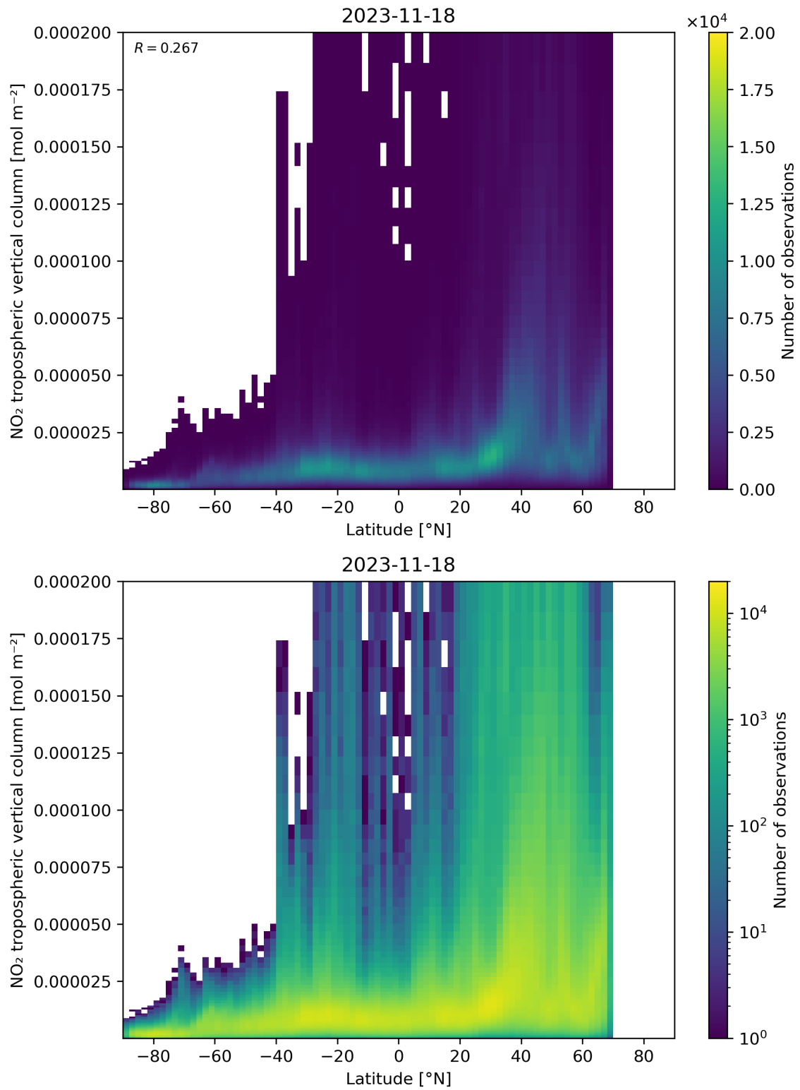
Figure 92: Scatter density plot of “Latitude” against “NO 2 tropospheric vertical column” for 2023-11-18 to 2023-11-19.
