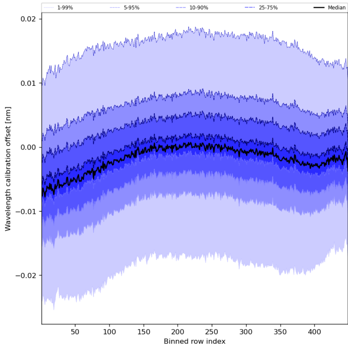
Figure 52: Along track statistics of “Wavelength calibration offset” for 2023-11-18 to 2023-11-19
