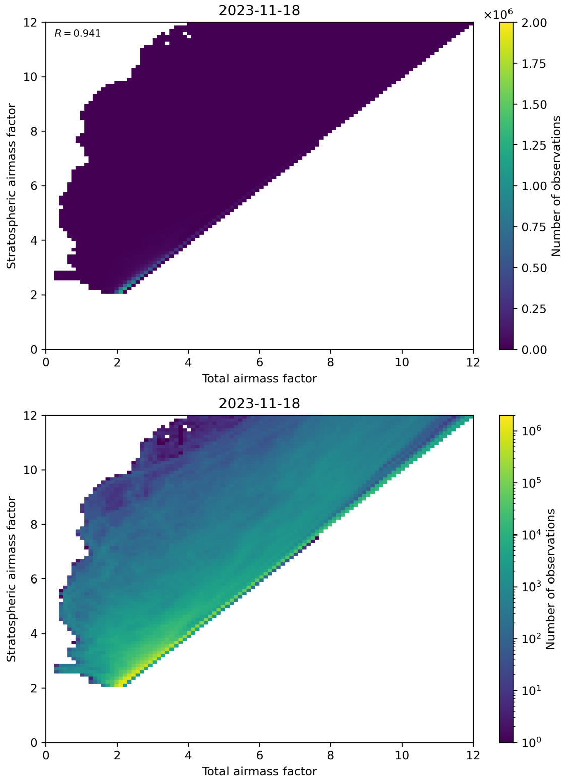
Figure 62: Scatter density plot of “Total airmass factor” against “Stratospheric airmass factor” for 2023-11-18 to 2023-11-19.
