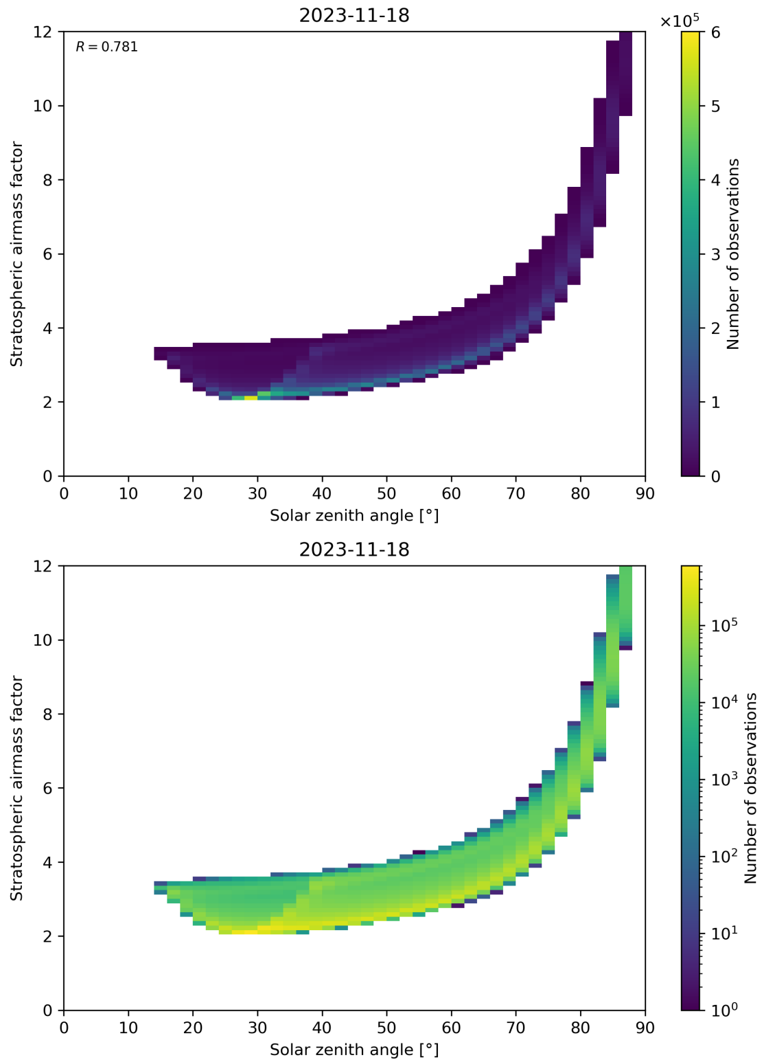
Figure 145: Scatter density plot of “Solar zenith angle” against “Stratospheric airmass factor” for 2023-11-18 to 2023-11-19.
