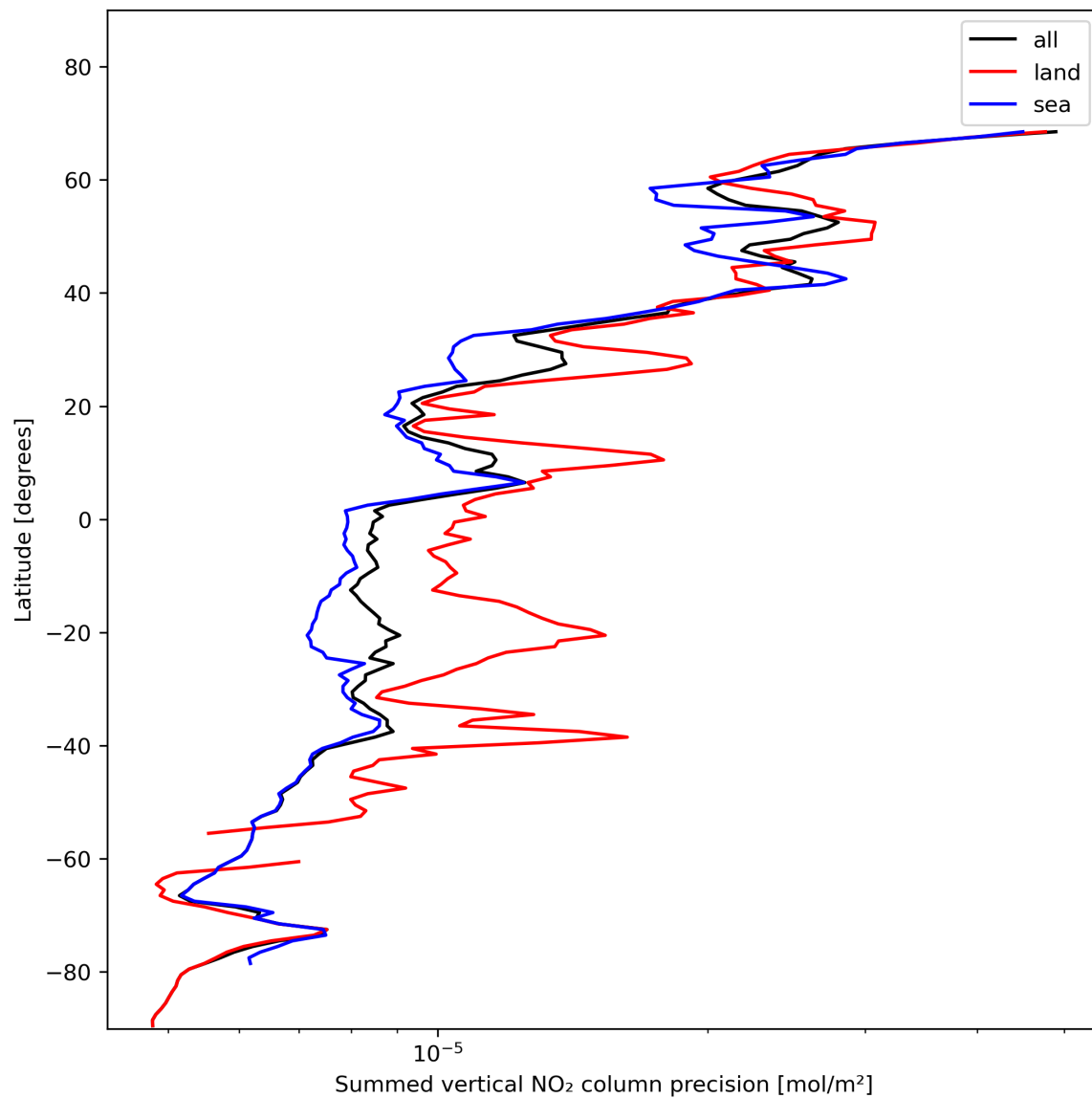
Figure 24: Zonal average of “Summed vertical NO 2 column precision” for 2023-11-18 to 2023-11-19.
