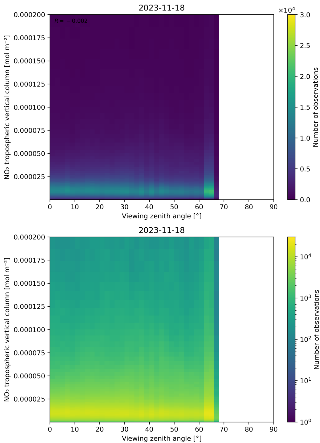
Figure 169: Scatter density plot of “Viewing zenith angle” against “NO 2 tropospheric vertical column” for 2023-11-18 to 2023-11-19.
