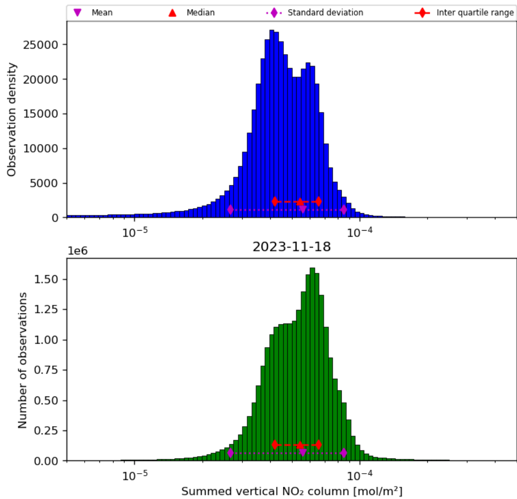
Figure 40: Histogram of “Summed vertical NO 2 column” for 2023-11-18 to 2023-11-19
