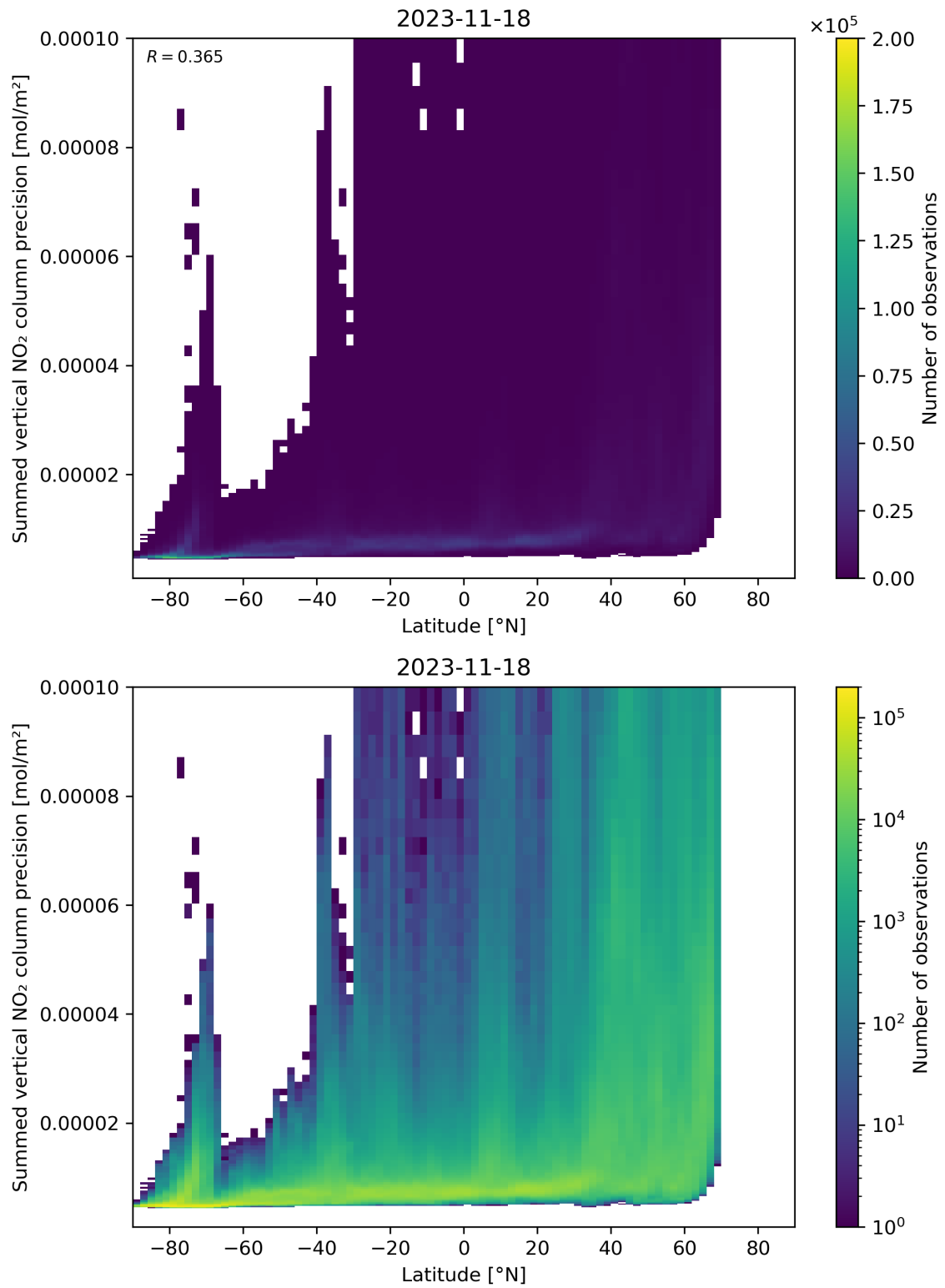
Figure 89: Scatter density plot of “Latitude” against “Summed vertical NO 2 column precision” for 2023-11-18 to 2023-11-19.
