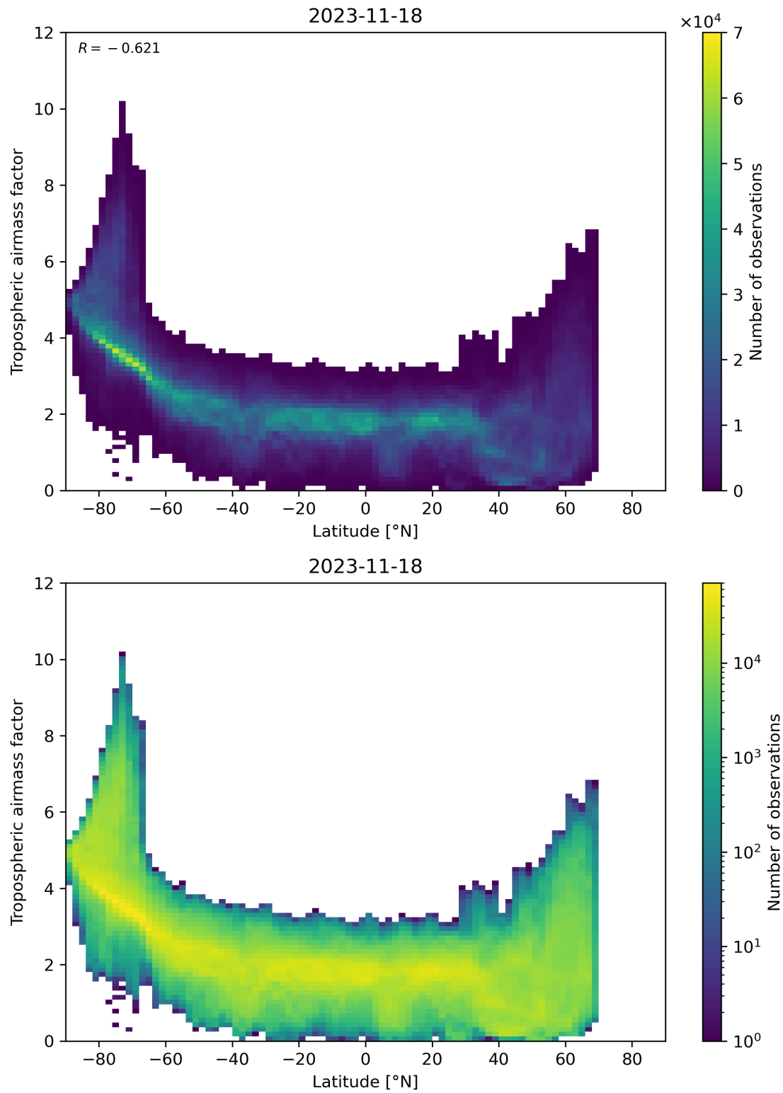
Figure 85: Scatter density plot of “Latitude” against “Tropospheric airmass factor” for 2023-11-18 to 2023-11-19.
