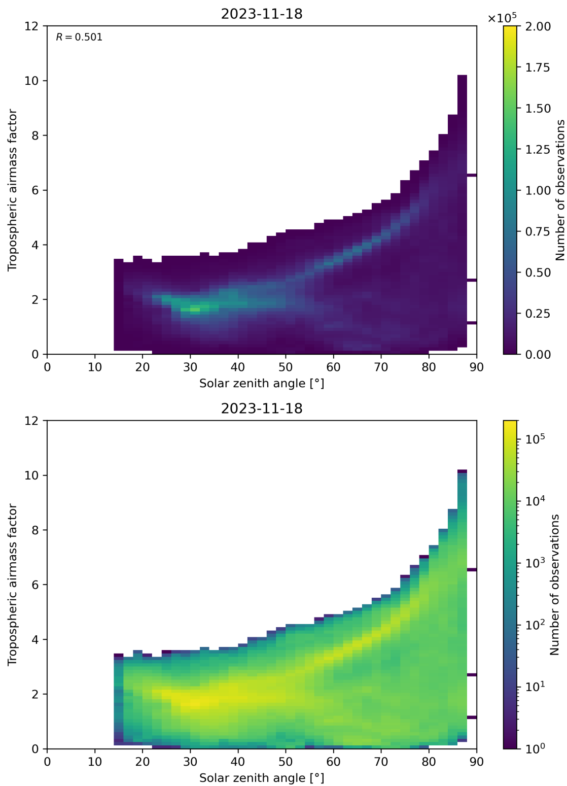
Figure 147: Scatter density plot of “Solar zenith angle” against “Tropospheric airmass factor” for 2023-11-18 to 2023-11-19.
