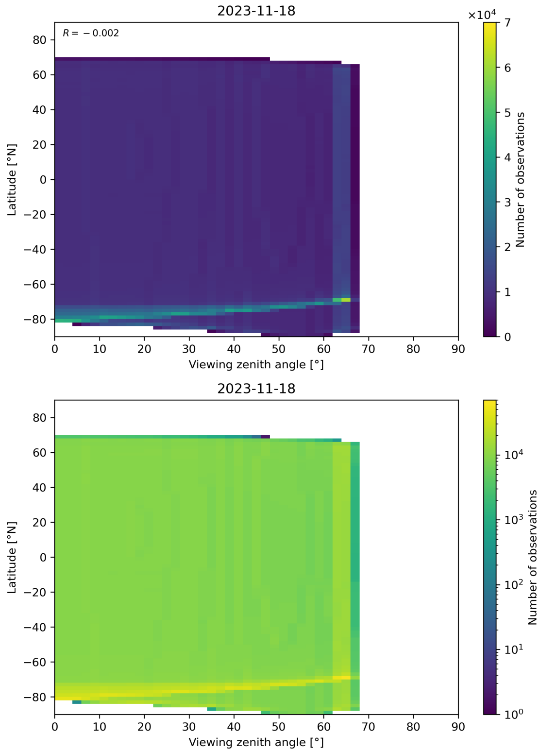
Figure 163: Scatter density plot of “Viewing zenith angle” against “Latitude” for 2023-11-18 to 2023-11-19.
