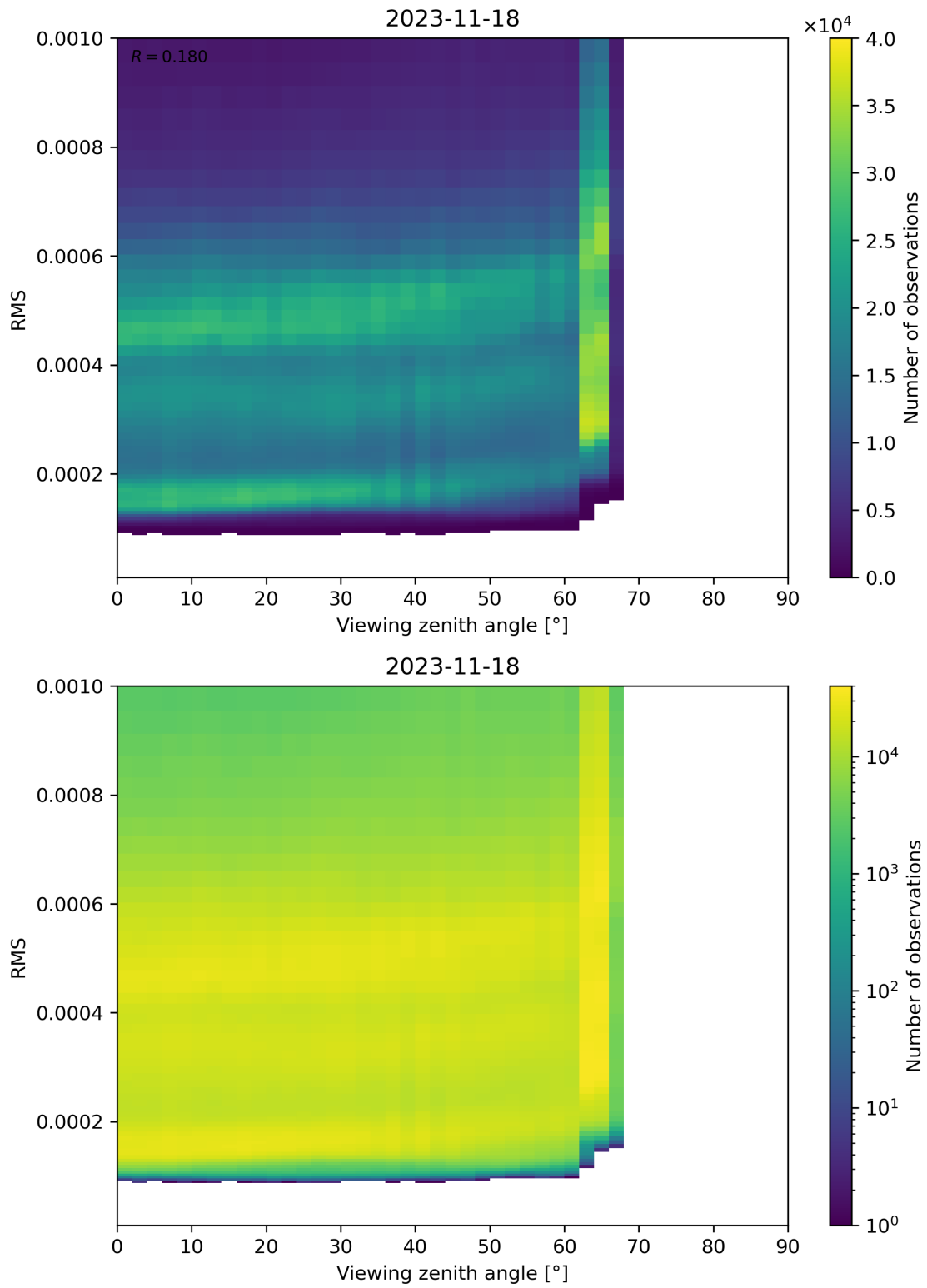
Figure 171: Scatter density plot of “Viewing zenith angle” against “RMS” for 2023-11-18 to 2023-11-19.
