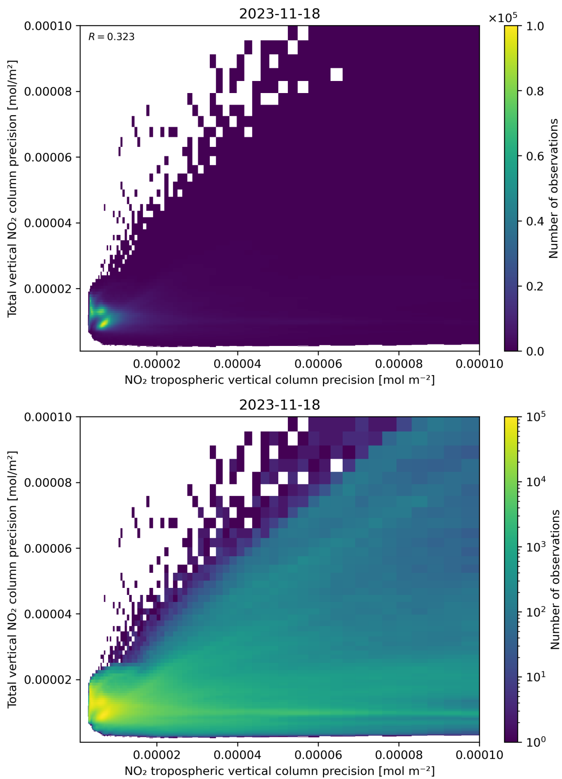
Figure 139: Scatter density plot of “NO 2 tropospheric vertical column precision” against “Total vertical NO 2 column precision” for 2023-11-18 to 2023-11-19.
