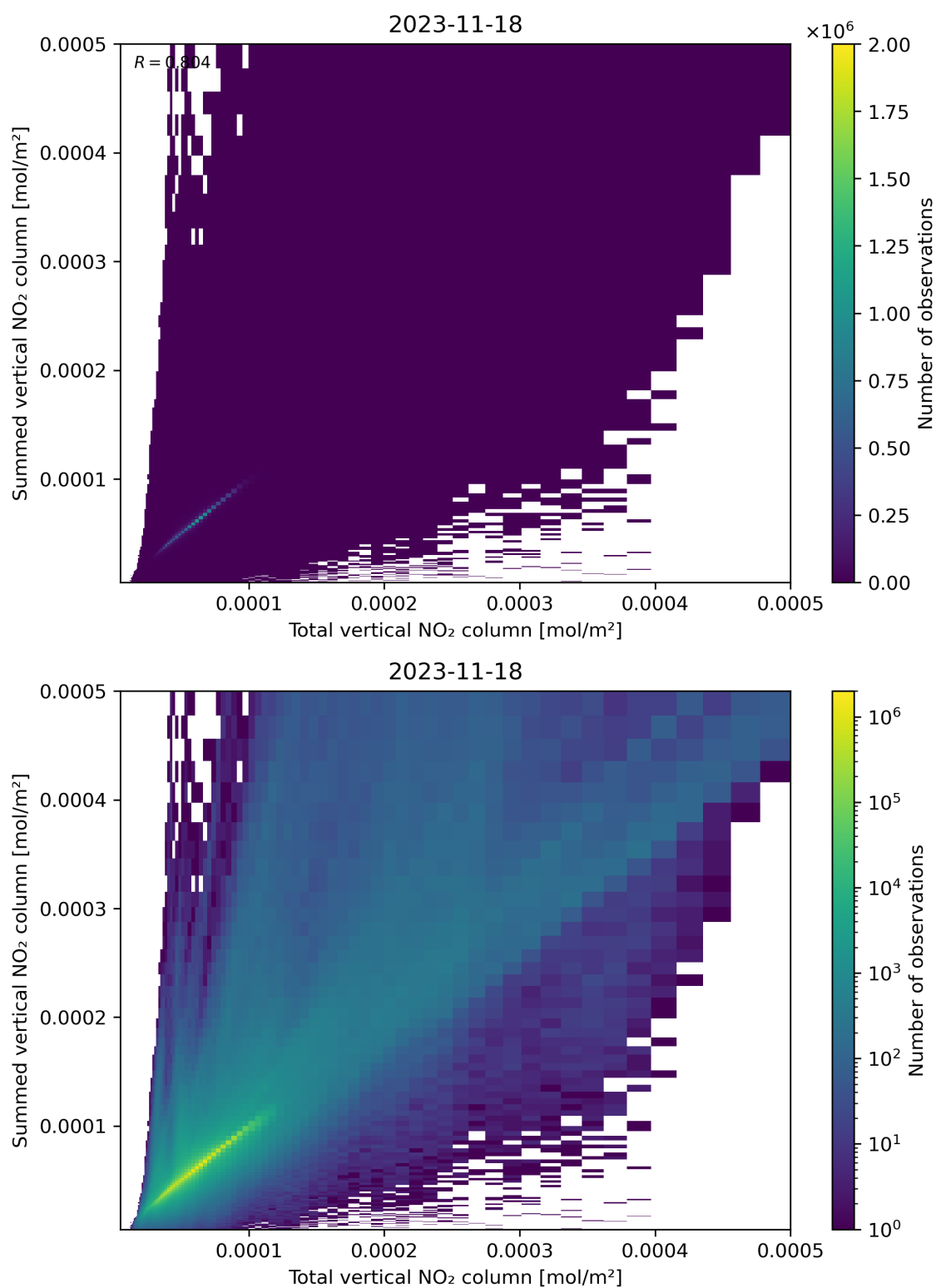
Figure 112: Scatter density plot of “Total vertical NO 2 column” against “Summed vertical NO 2 column” for 2023-11-18 to 2023-11-19.
