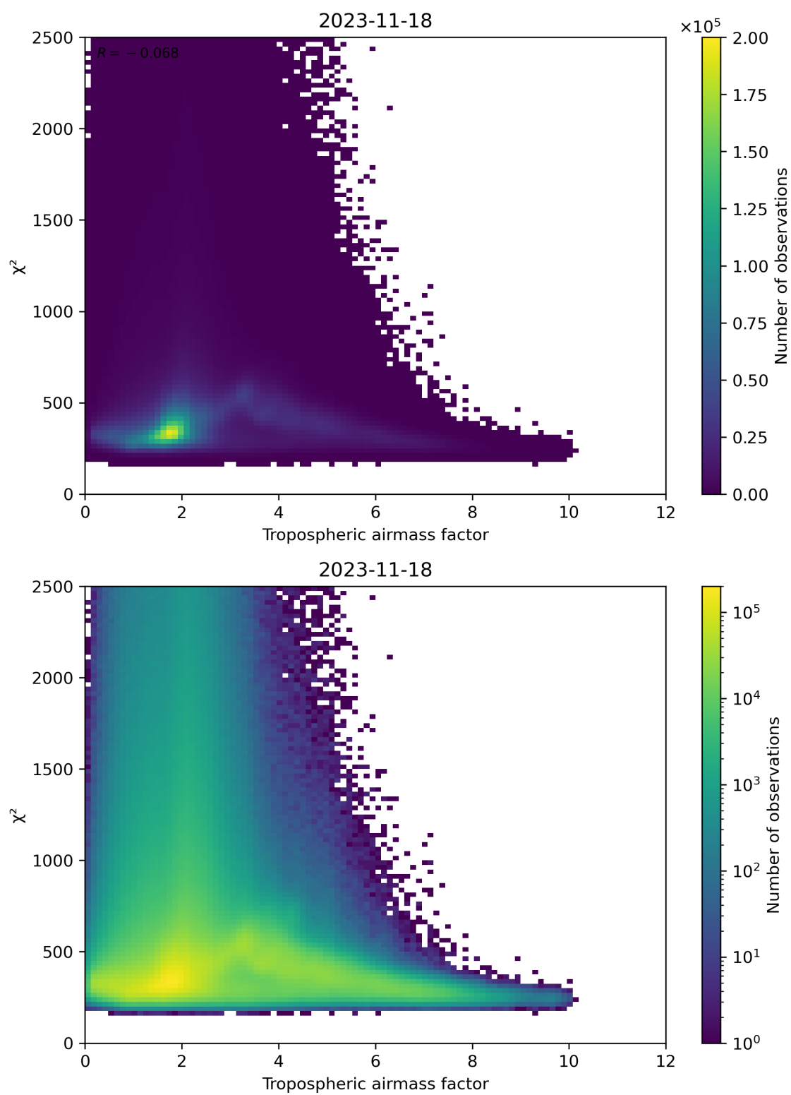
Figure 73: Scatter density plot of “Tropospheric airmass factor” against “ \chi^2 ” for 2023-11-18 to 2023-11-19.
