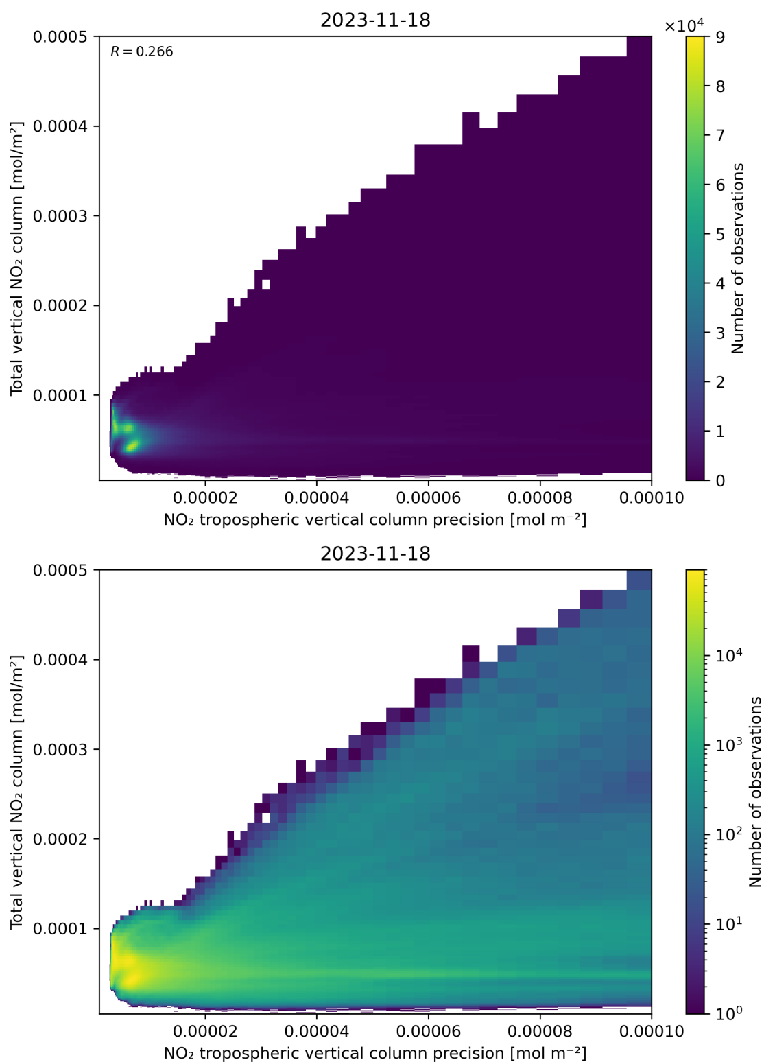
Figure 138: Scatter density plot of “NO 2 tropospheric vertical column precision” against “Total vertical NO 2 column” for 2023-11-18 to 2023-11-19.
