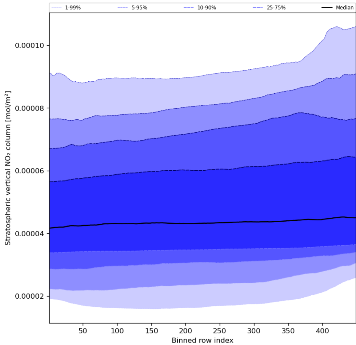
Figure 53: Along track statistics of “Stratospheric vertical NO 2 column” for 2023-11-18 to 2023-11-19
