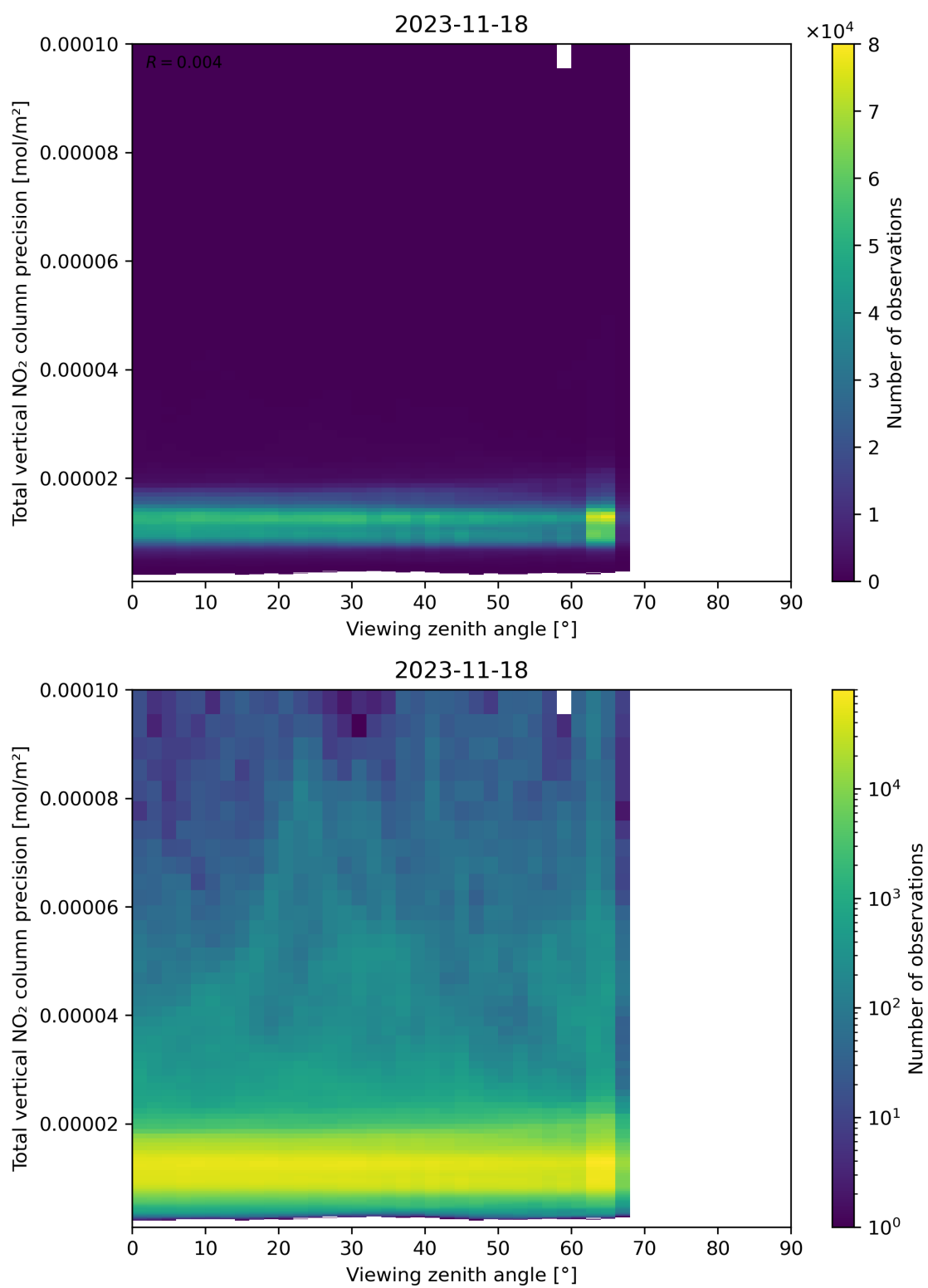
Figure 168: Scatter density plot of “Viewing zenith angle” against “Total vertical NO 2 column precision” for 2023-11-18 to 2023-11-19.
