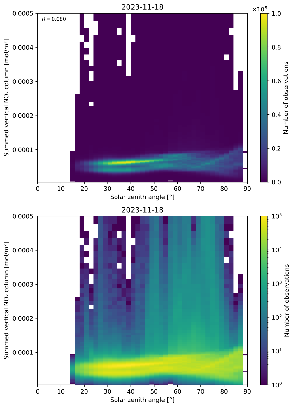
Figure 151: Scatter density plot of “Solar zenith angle” against “Summed vertical NO 2 column” for 2023-11-18 to 2023-11-19.
