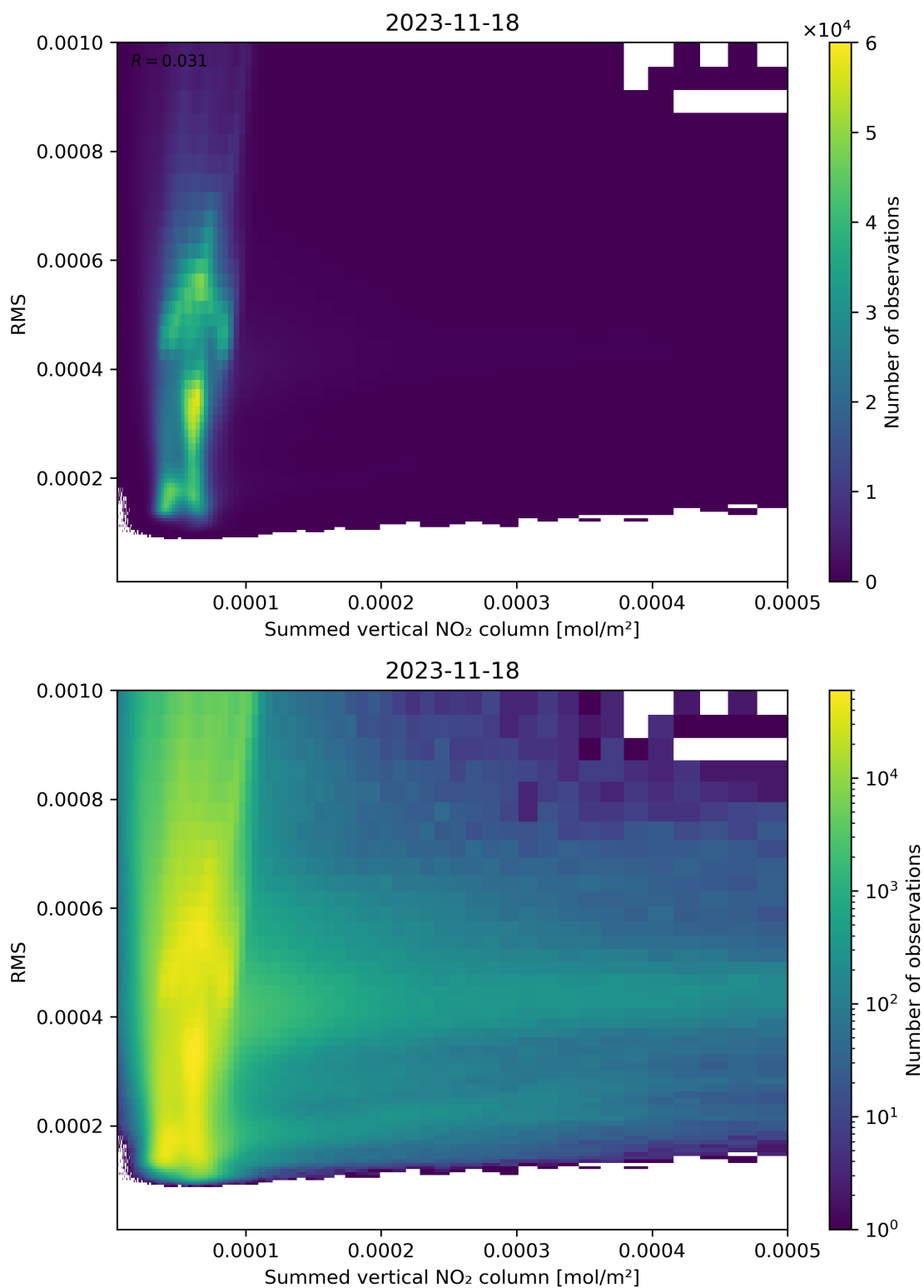
Figure 109: Scatter density plot of “Summed vertical NO 2 column” against “RMS” for 2023-11-18 to 2023-11-19.
