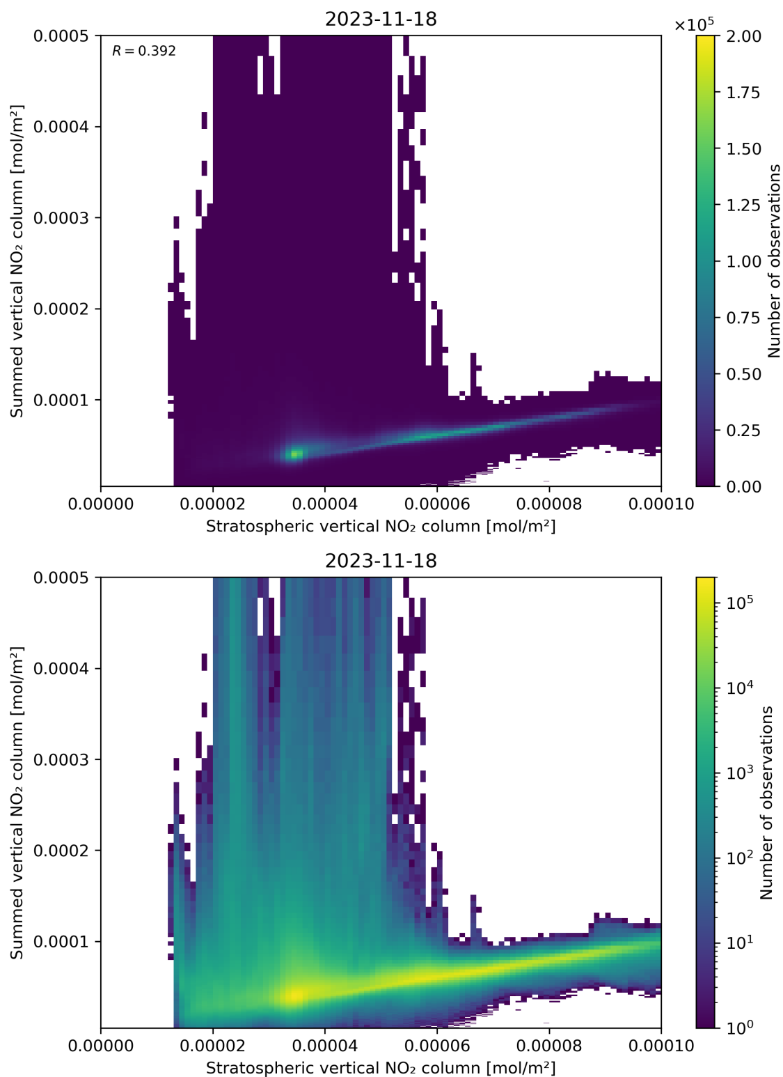
Figure 98: Scatter density plot of “Stratospheric vertical NO 2 column” against “Summed vertical NO 2 column” for 2023-11-18 to 2023-11-19.
