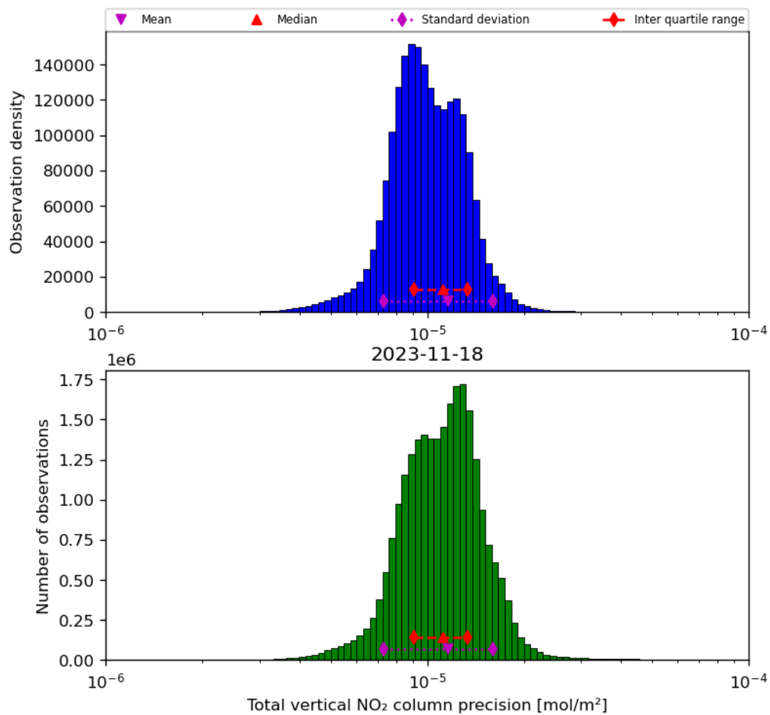
Figure 39: Histogram of “Total vertical NO 2 column precision” for 2023-11-18 to 2023-11-19
