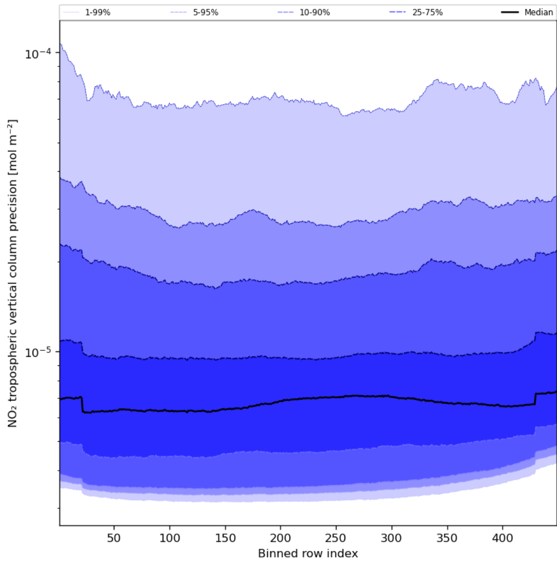
Figure 47: Along track statistics of “NO 2 tropospheric vertical column precision” for 2023-11-18 to 2023-11-19
