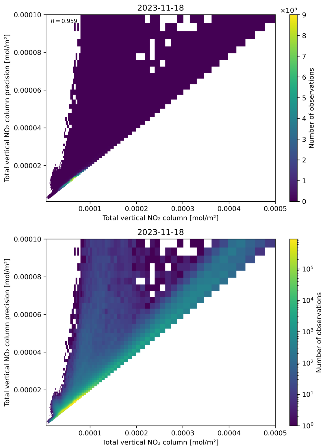
Figure 114: Scatter density plot of “Total vertical NO 2 column” against “Total vertical NO 2 column precision” for 2023-11-18 to 2023-11-19.
