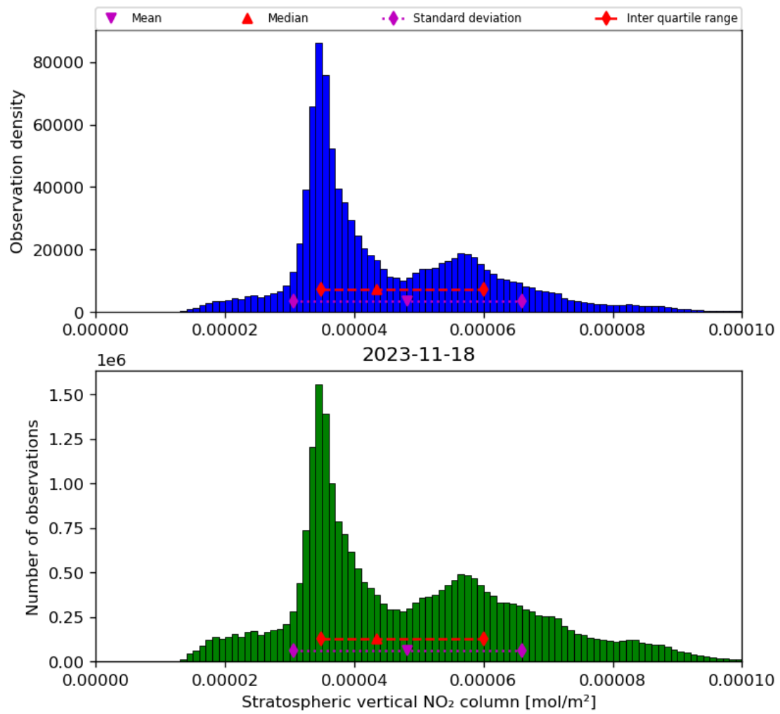
Figure 36: Histogram of “Stratospheric vertical NO 2 column” for 2023-11-18 to 2023-11-19
