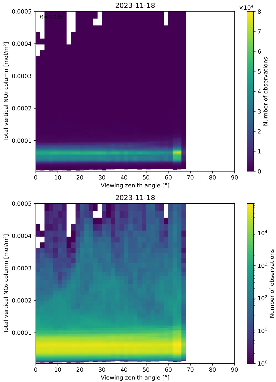
Figure 167: Scatter density plot of “Viewing zenith angle” against “Total vertical NO 2 column” for 2023-11-18 to 2023-11-19.
