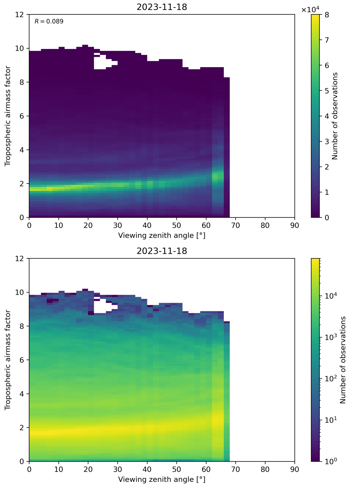
Figure 161: Scatter density plot of “Viewing zenith angle” against “Tropospheric airmass factor” for 2023-11-18 to 2023-11-19.
