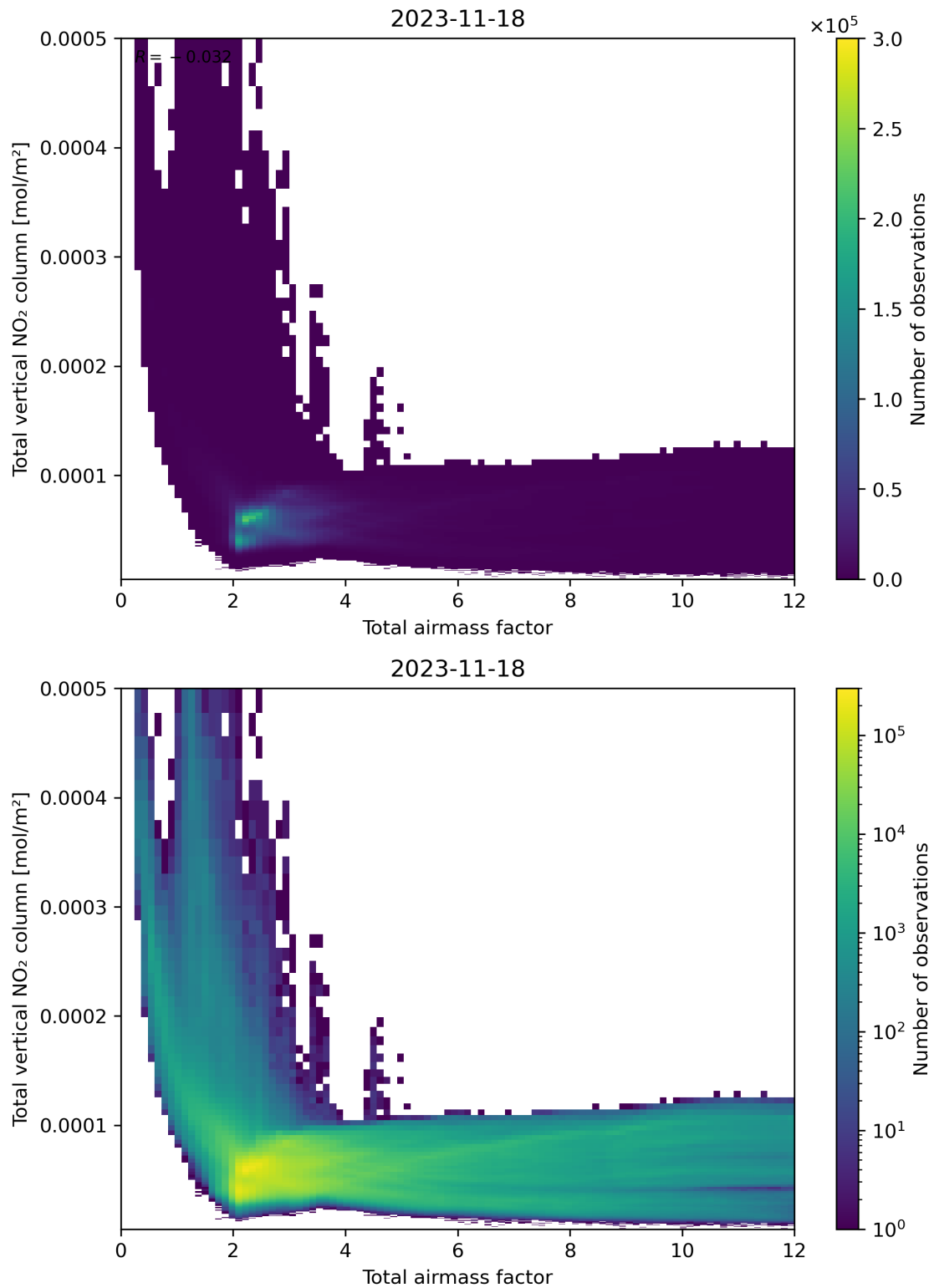
Figure 67: Scatter density plot of “Total airmass factor” against “Total vertical NO 2 column” for 2023-11-18 to 2023-11-19.
