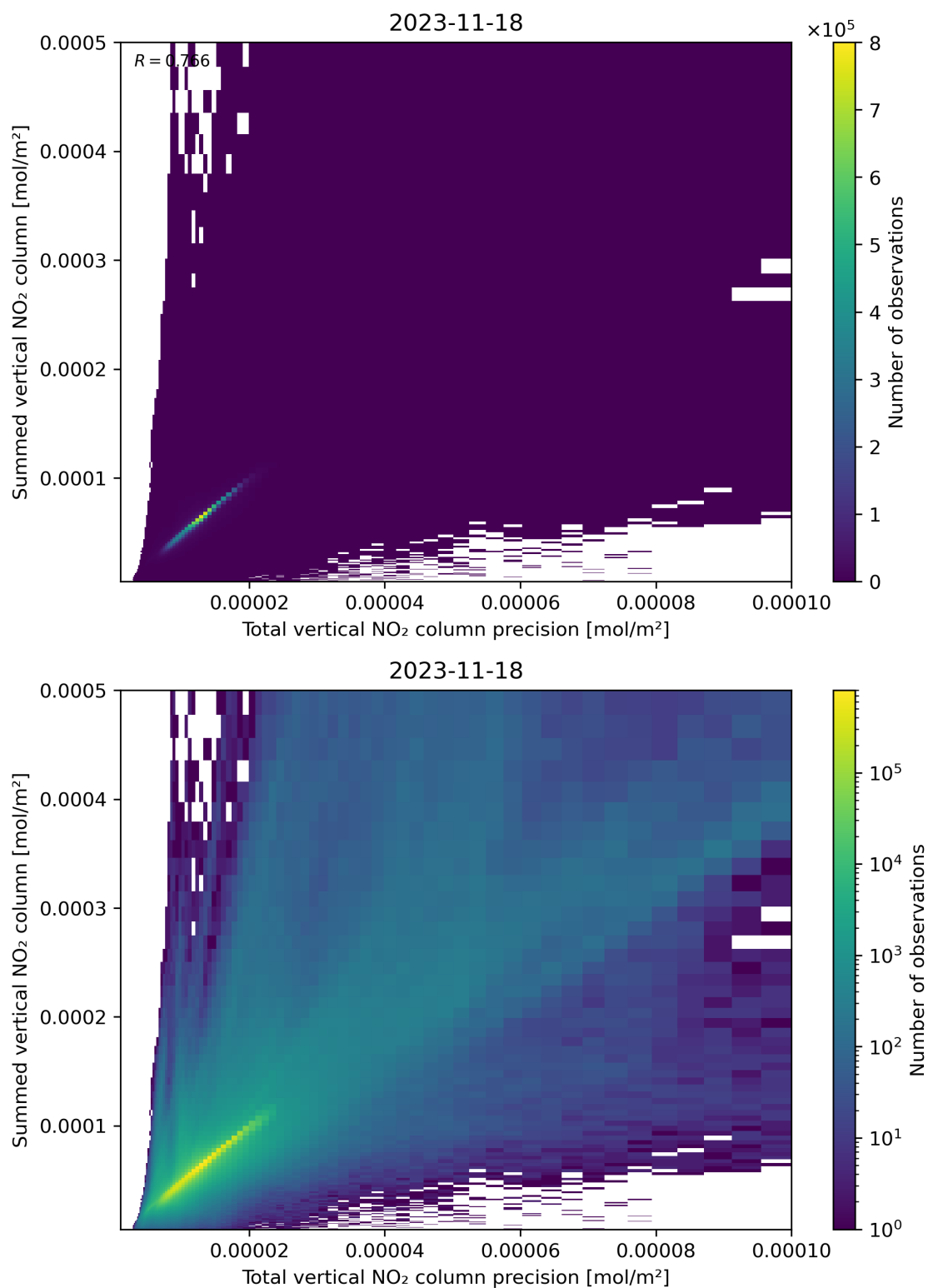
Figure 117: Scatter density plot of “Total vertical NO 2 column precision” against “Summed vertical NO 2 column” for 2023-11-18 to 2023-11-19.
