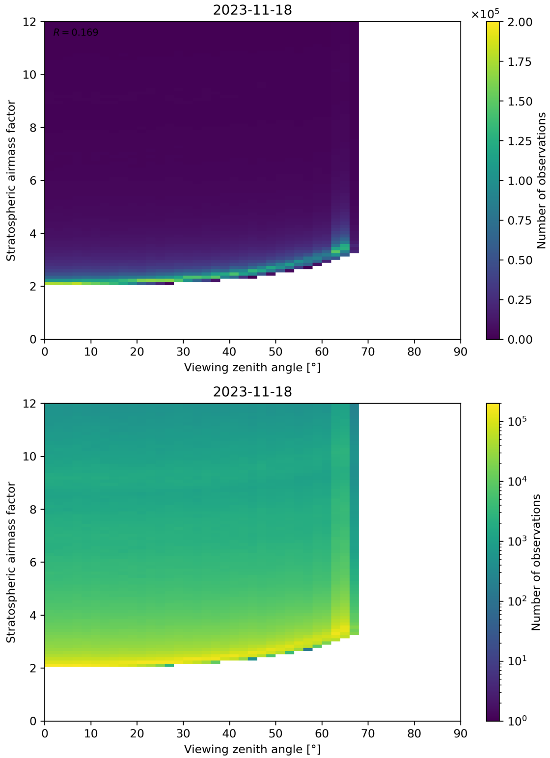
Figure 159: Scatter density plot of “Viewing zenith angle” against “Stratospheric airmass factor” for 2023-11-18 to 2023-11-19.
