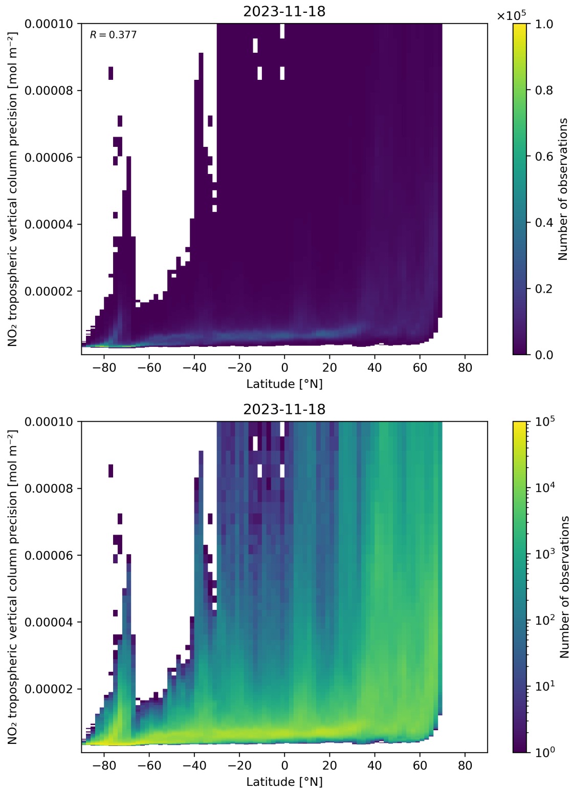
Figure 93: Scatter density plot of “Latitude” against “NO 2 tropospheric vertical column precision” for 2023-11-18 to 2023-11-19.
