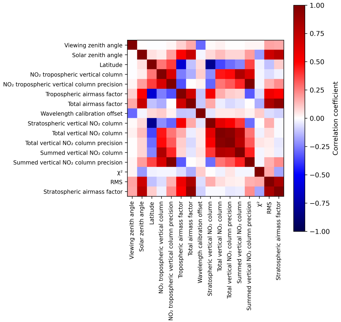
Figure 2: Map of correlation matrix for 2023-11-18 to 2023-11-19.
