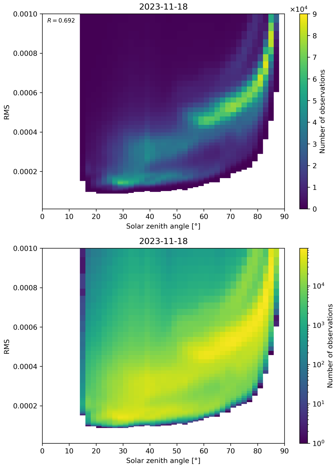
Figure 157: Scatter density plot of “Solar zenith angle” against “RMS” for 2023-11-18 to 2023-11-19.
