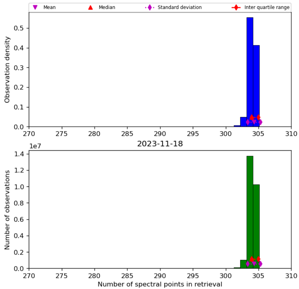
Figure 33: Histogram of “Number of spectral points in retrieval” for 2023-11-18 to 2023-11-19
