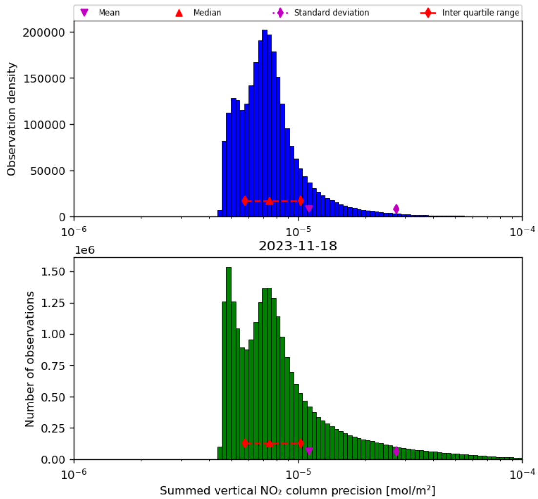
Figure 41: Histogram of “Summed vertical NO 2 column precision” for 2023-11-18 to 2023-11-19
