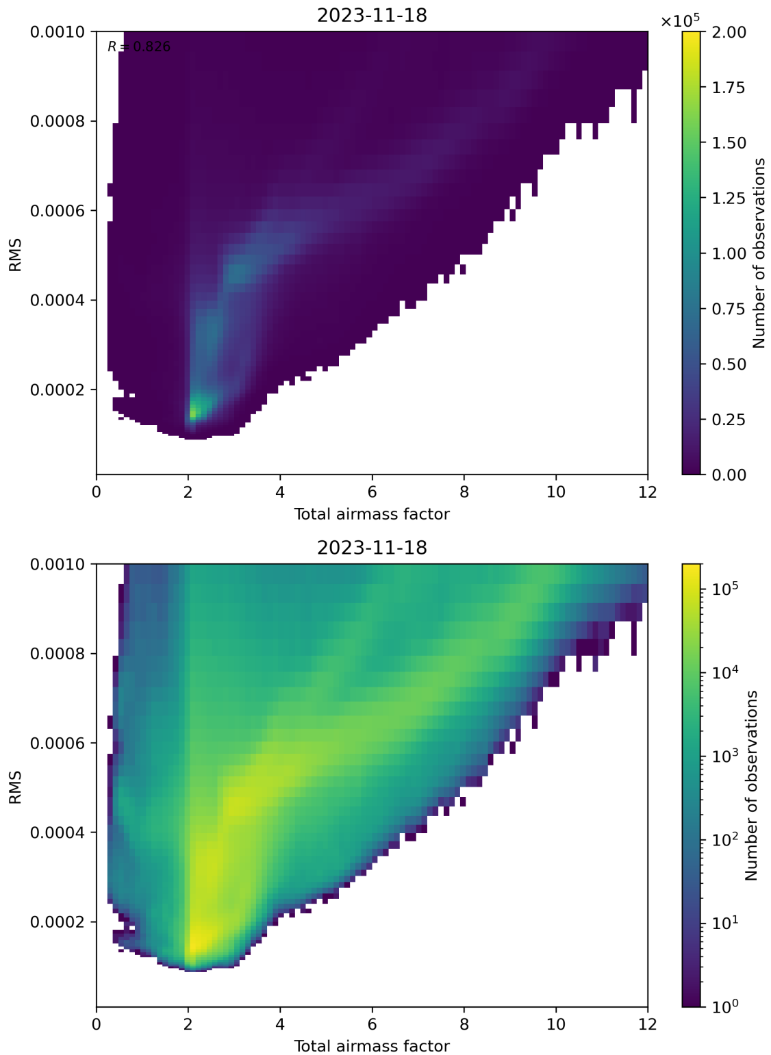
Figure 69: Scatter density plot of “Total airmass factor” against “RMS” for 2023-11-18 to 2023-11-19.
