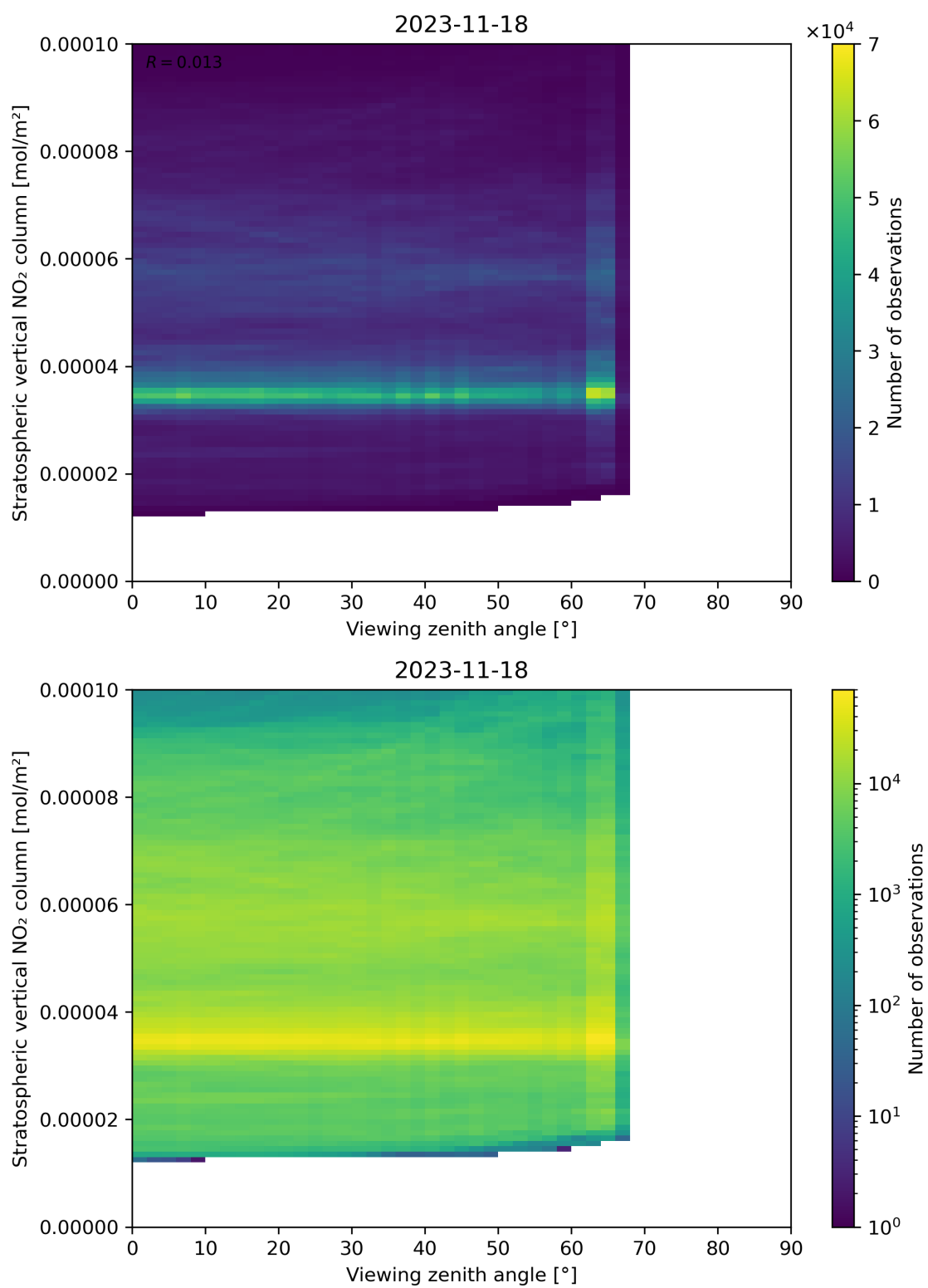
Figure 164: Scatter density plot of “Viewing zenith angle” against “Stratospheric vertical NO 2 column” for 2023-11-18 to 2023-11-19.
