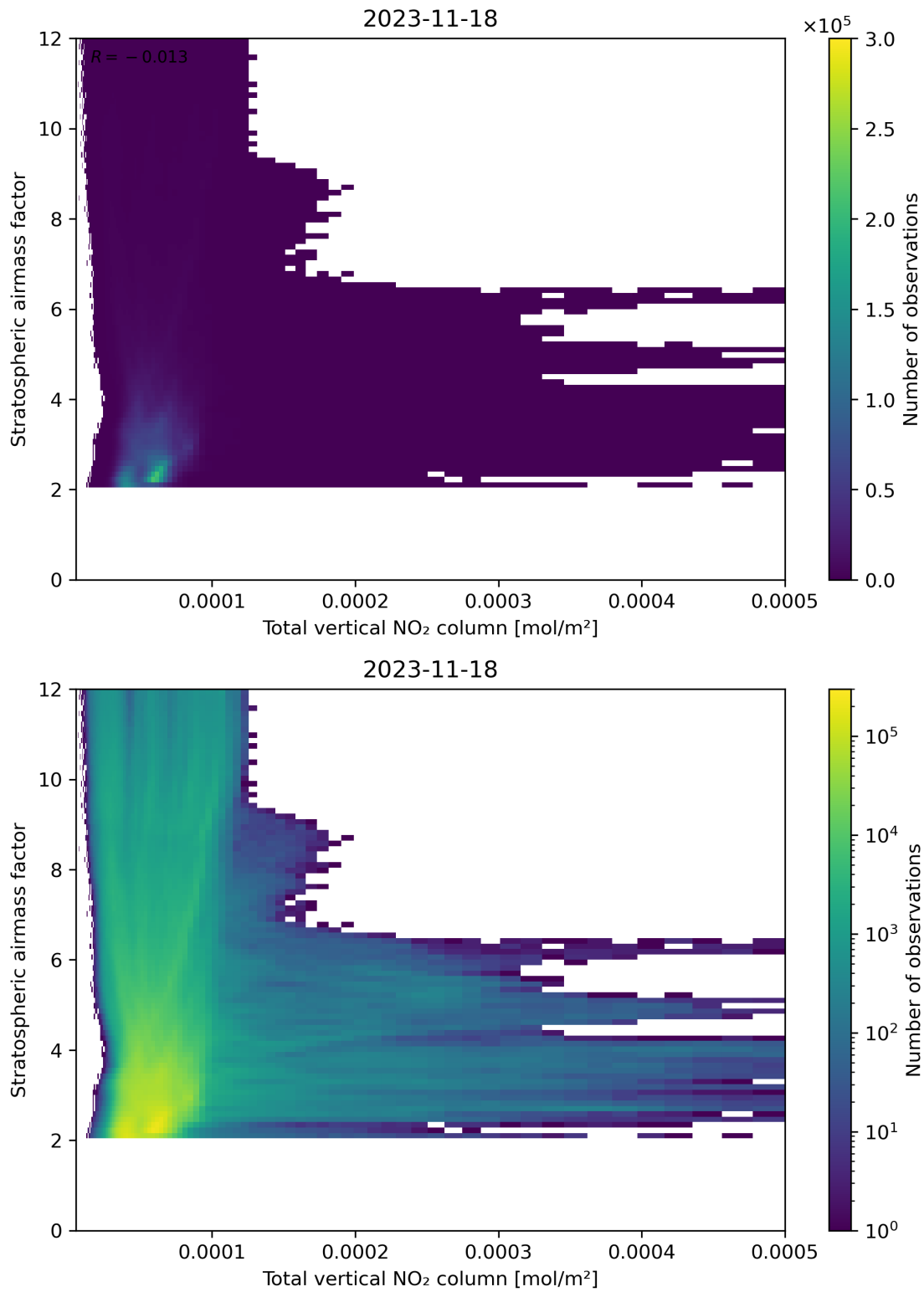
Figure 110: Scatter density plot of “Total vertical NO 2 column” against “Stratospheric airmass factor” for 2023-11-18 to 2023-11-19.
