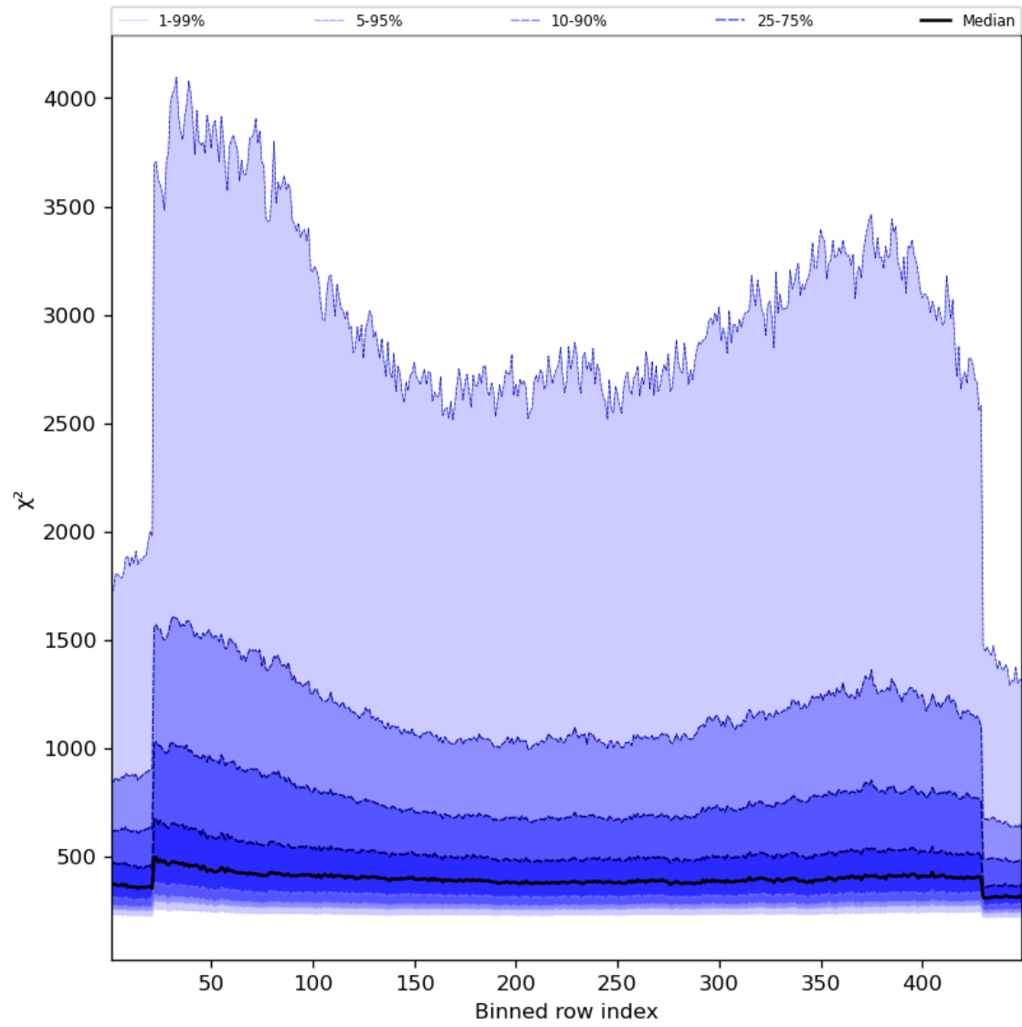
Figure 59: Along track statistics of “ \chi^2 ” for 2023-11-18 to 2023-11-19
