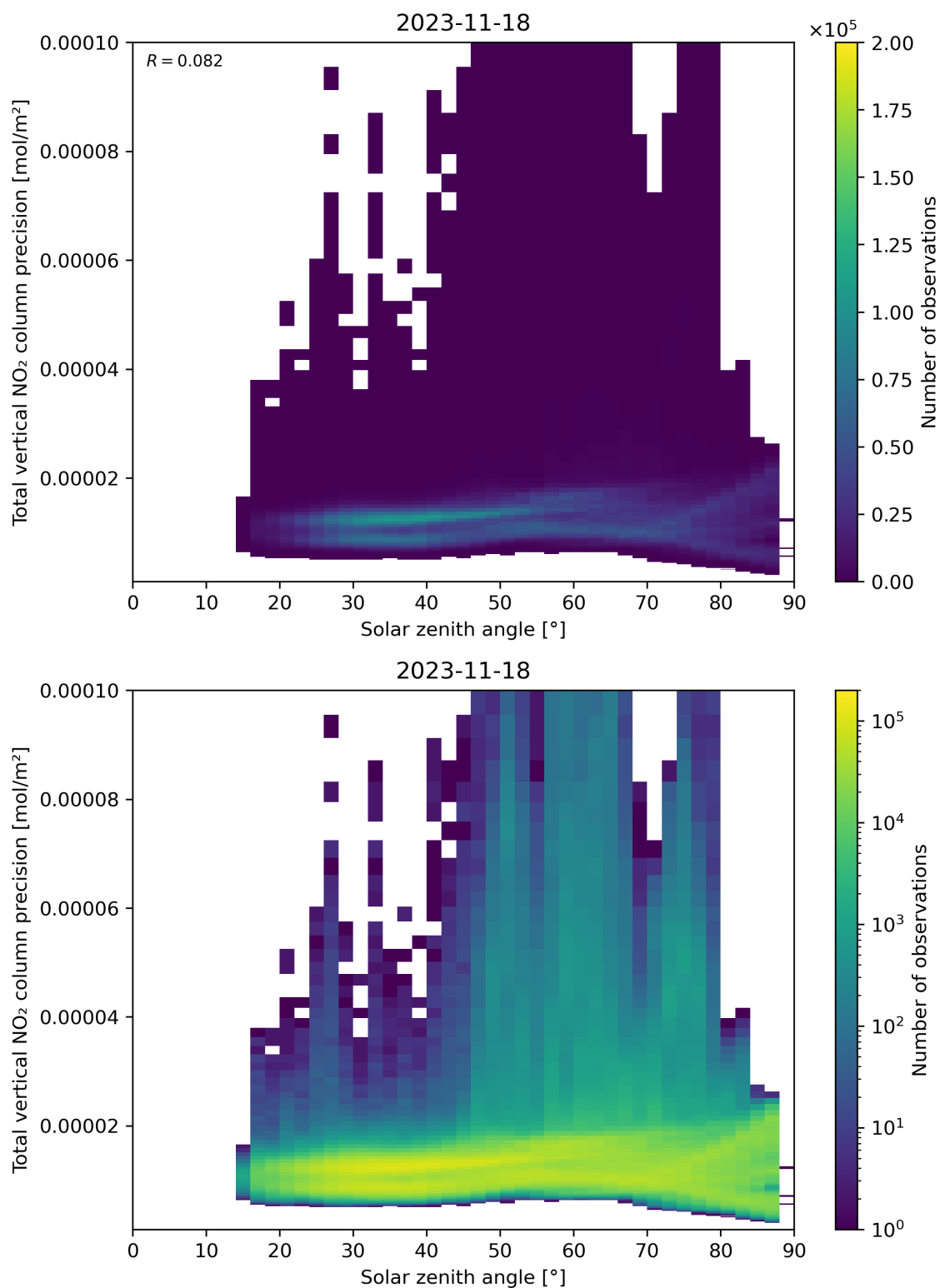
Figure 154: Scatter density plot of “Solar zenith angle” against “Total vertical NO 2 column precision” for 2023-11-18 to 2023-11-19.
