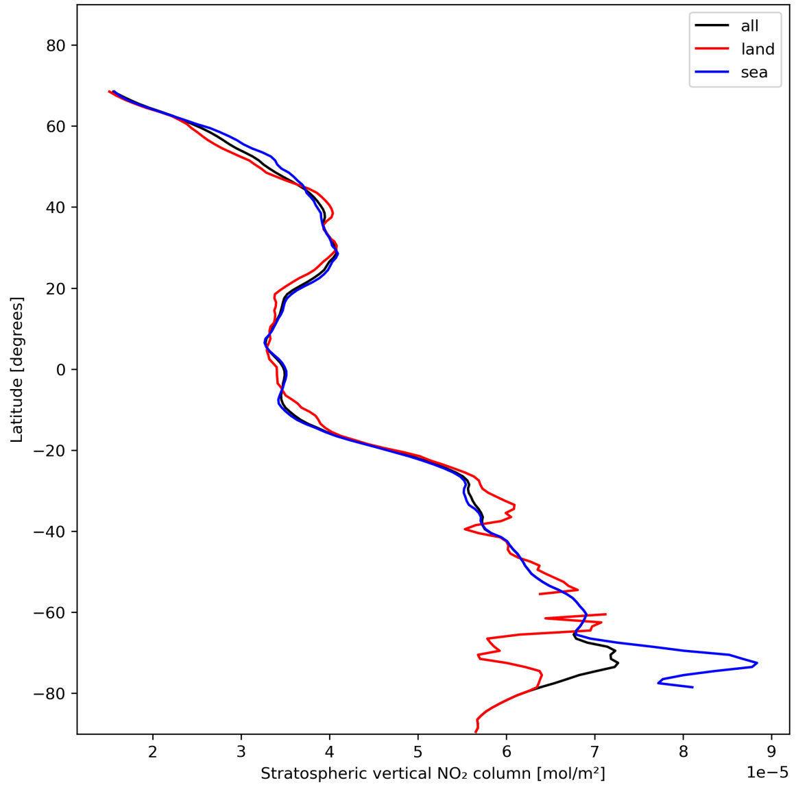
Figure 19: Zonal average of “Stratospheric vertical NO 2 column” for 2023-11-18 to 2023-11-19.
