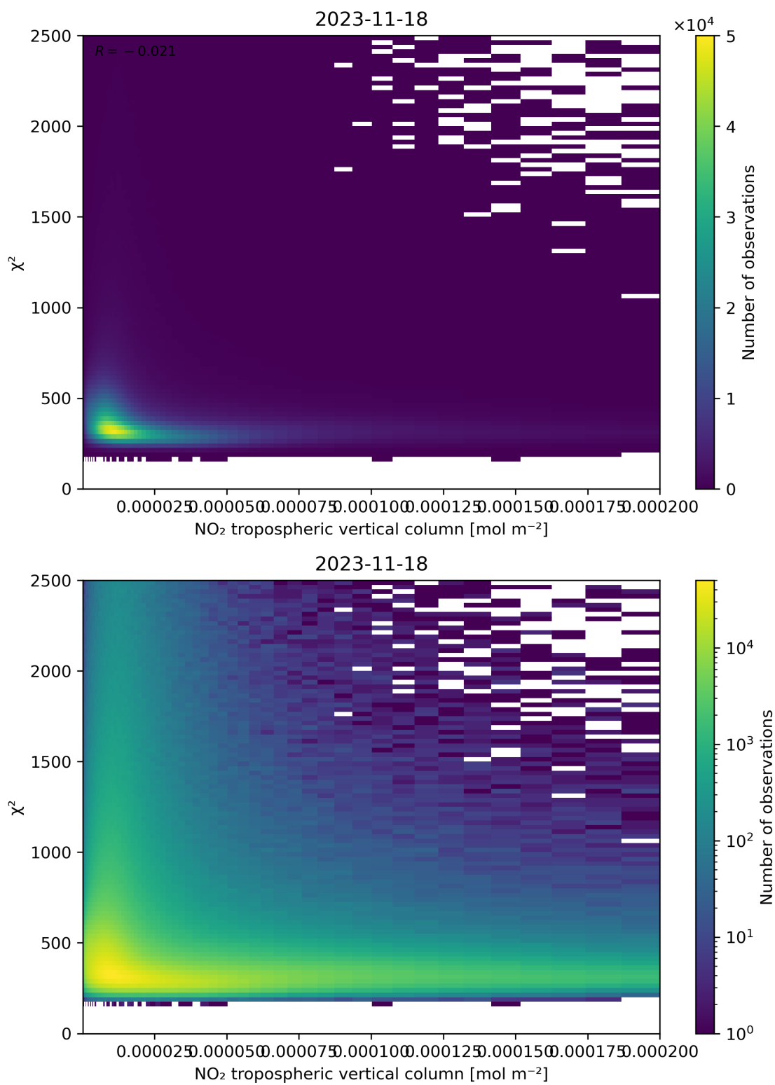
Figure 124: Scatter density plot of “NO 2 tropospheric vertical column” against “ \chi^2 ” for 2023-11-18 to 2023-11-19.
