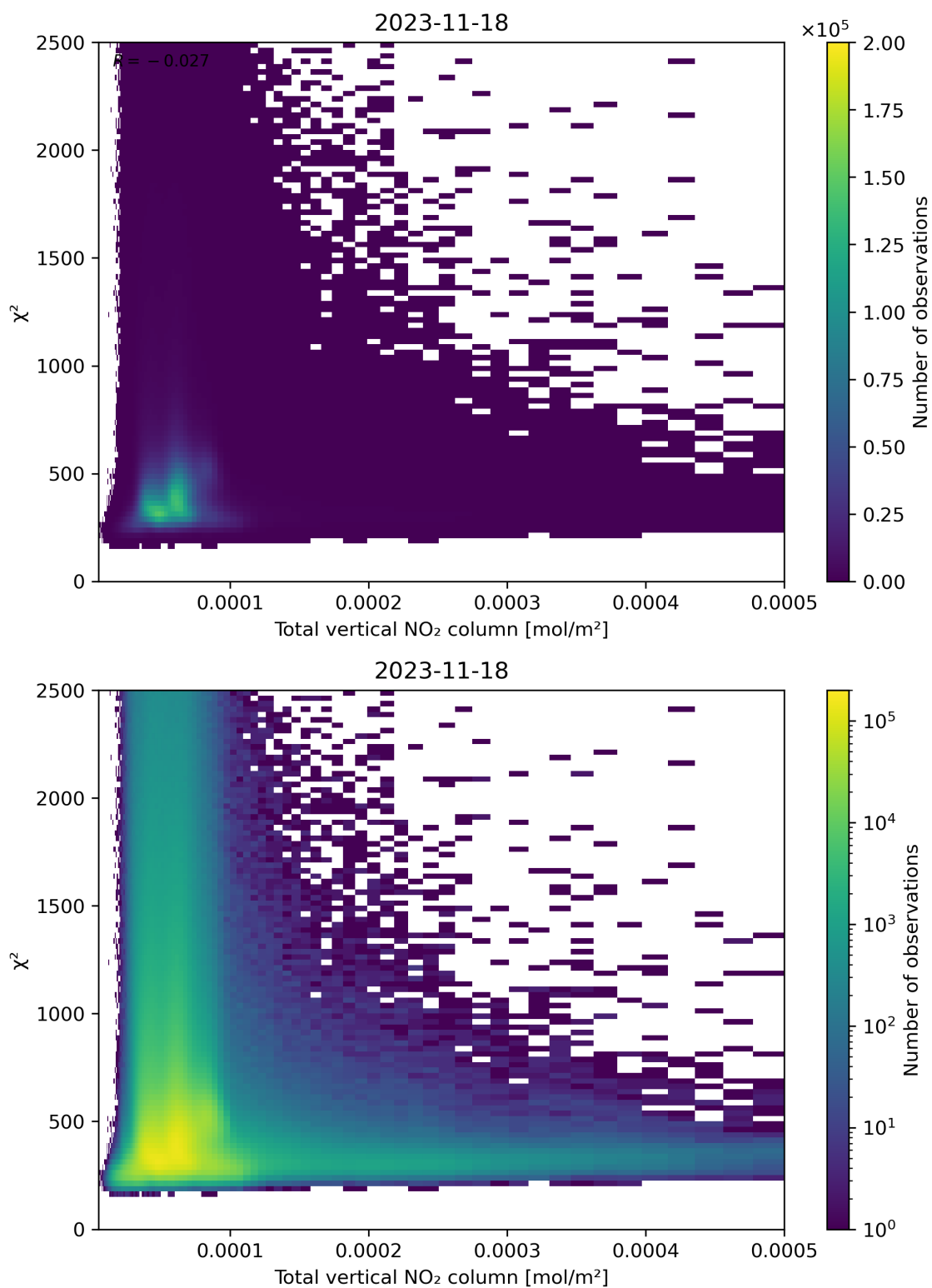
Figure 111: Scatter density plot of “Total vertical NO 2 column” against “ \chi^2 ” for 2023-11-18 to 2023-11-19.
