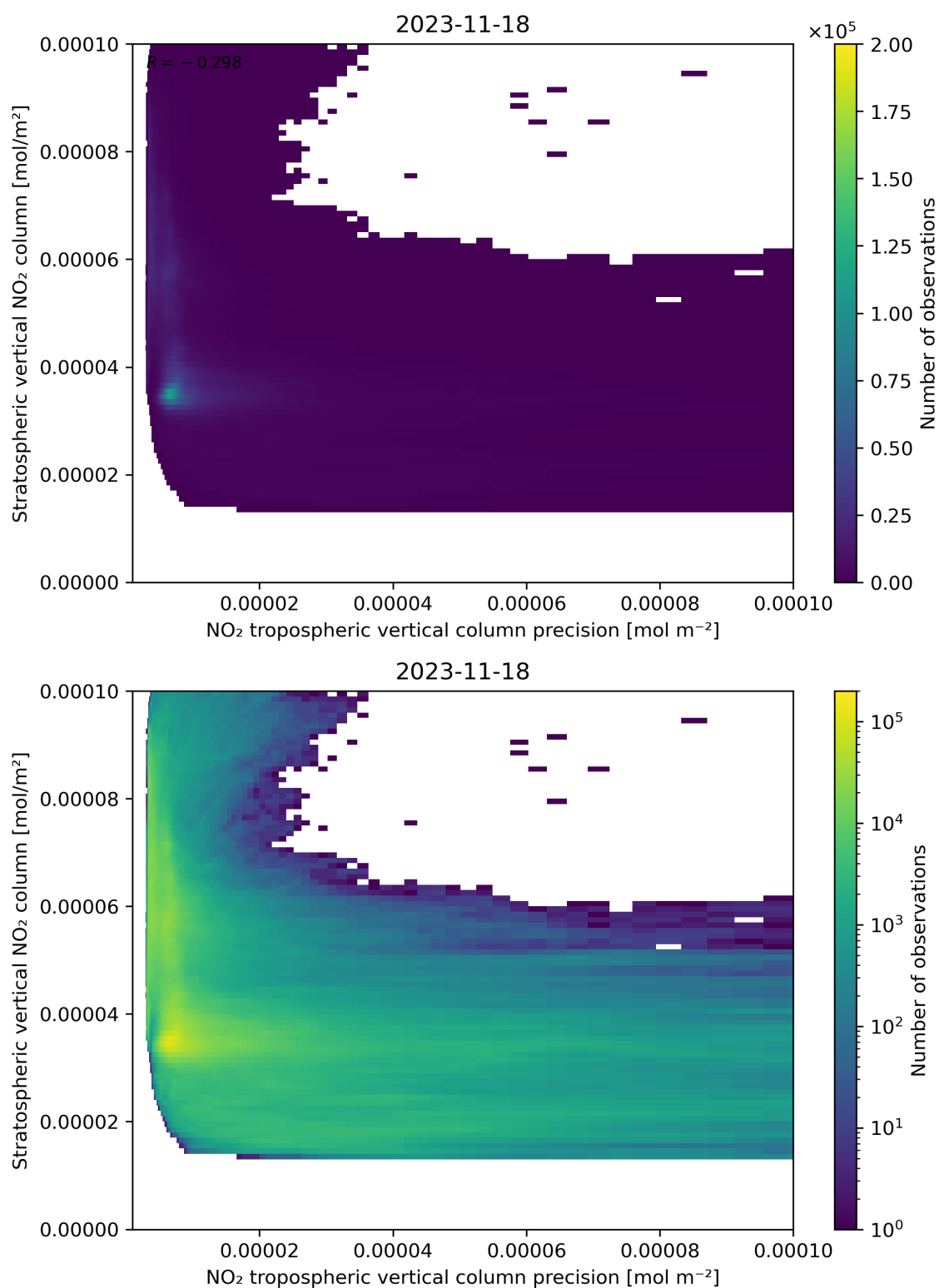
Figure 135: Scatter density plot of “NO 2 tropospheric vertical column precision” against “Stratospheric vertical NO 2 column” for 2023-11-18 to 2023-11-19.
