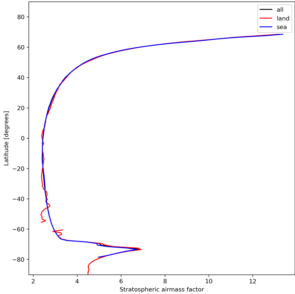
Figure 27: Zonal average of “Stratospheric airmass factor” for 2023-11-18 to 2023-11-19.
