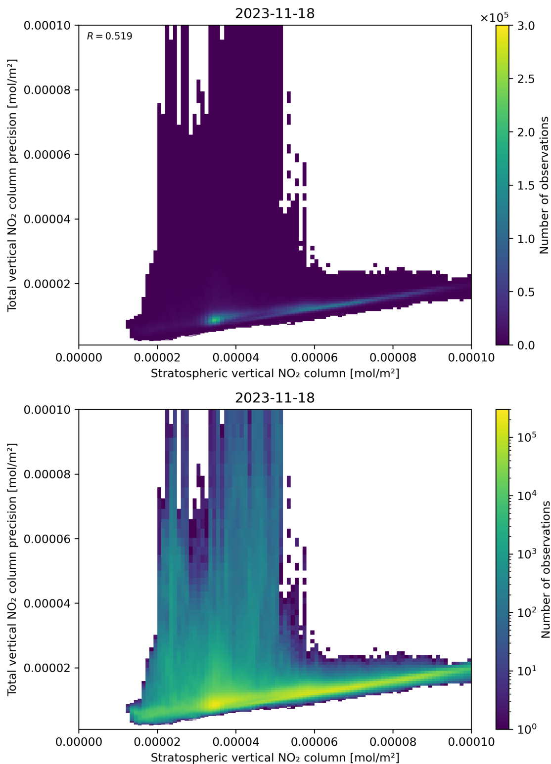
Figure 101: Scatter density plot of “Stratospheric vertical NO 2 column” against “Total vertical NO 2 column precision” for 2023-11-18 to 2023-11-19.
