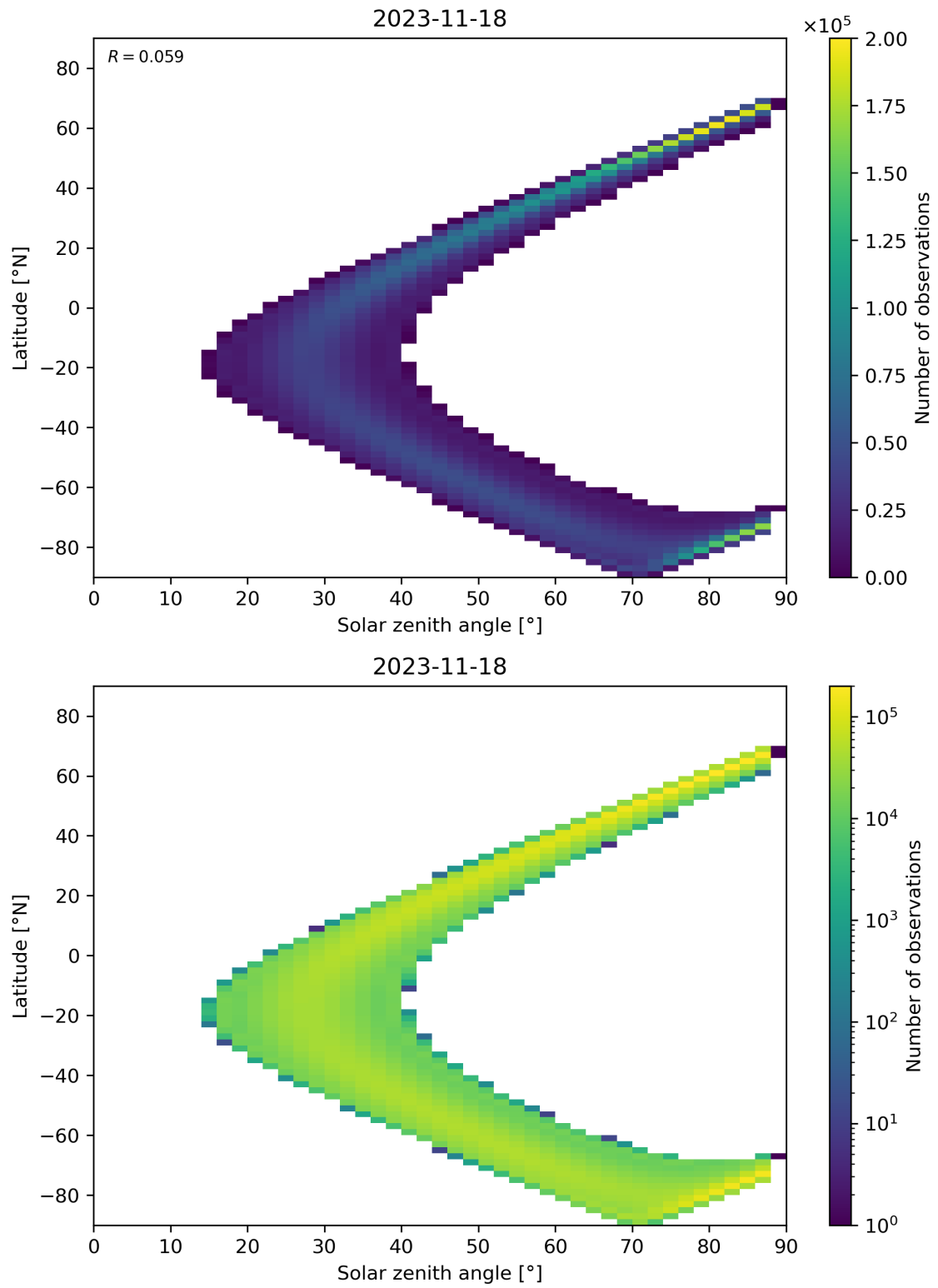
Figure 149: Scatter density plot of “Solar zenith angle” against “Latitude” for 2023-11-18 to 2023-11-19.
