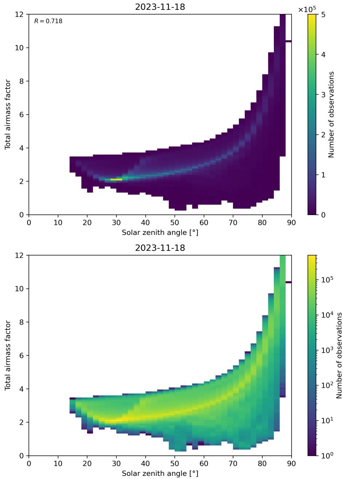
Figure 146: Scatter density plot of “Solar zenith angle” against “Total airmass factor” for 2023-11-18 to 2023-11-19.
