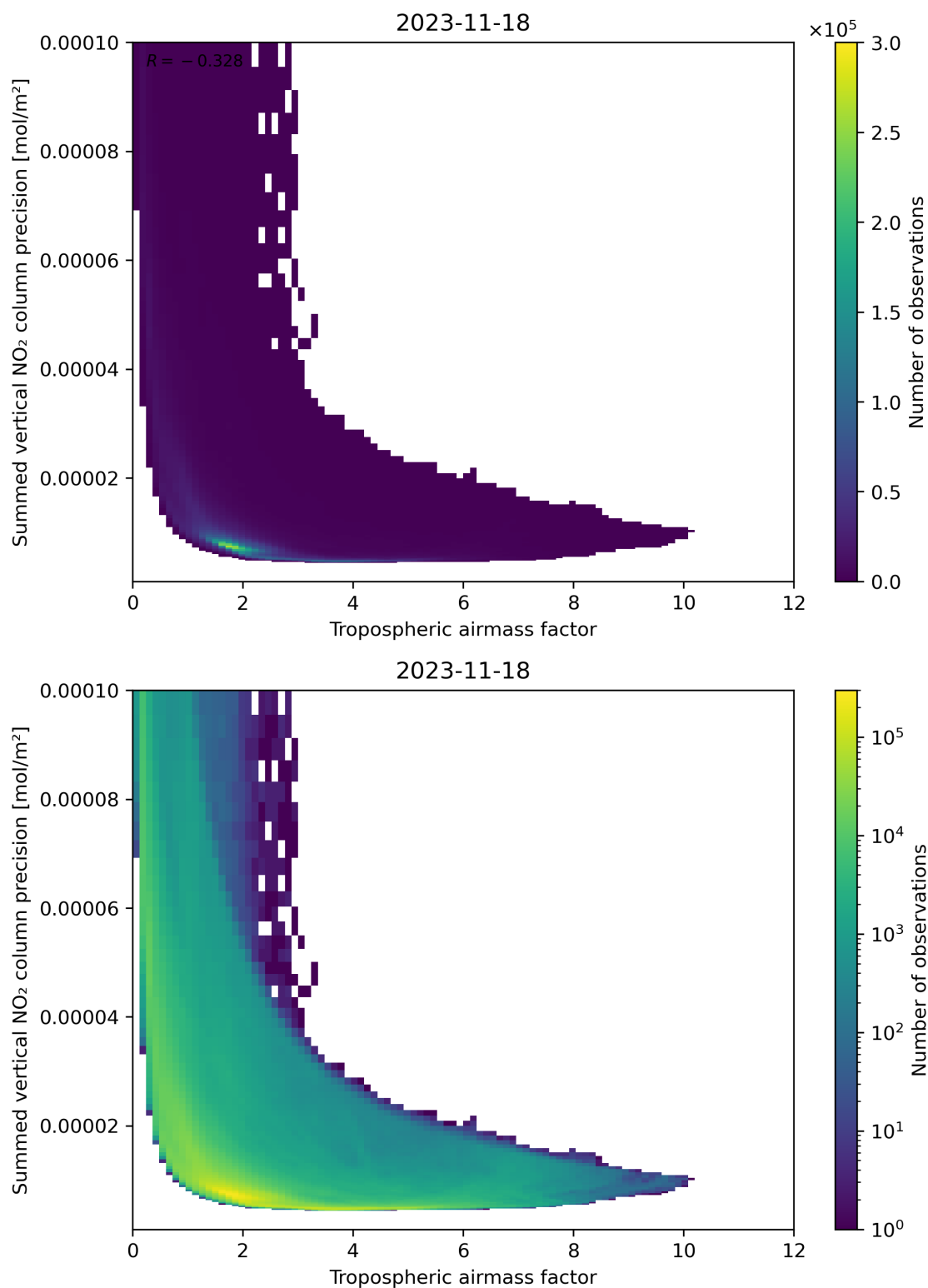
Figure 76: Scatter density plot of “Tropospheric airmass factor” against “Summed vertical NO 2 column precision” for 2023-11-18 to 2023-11-19.
