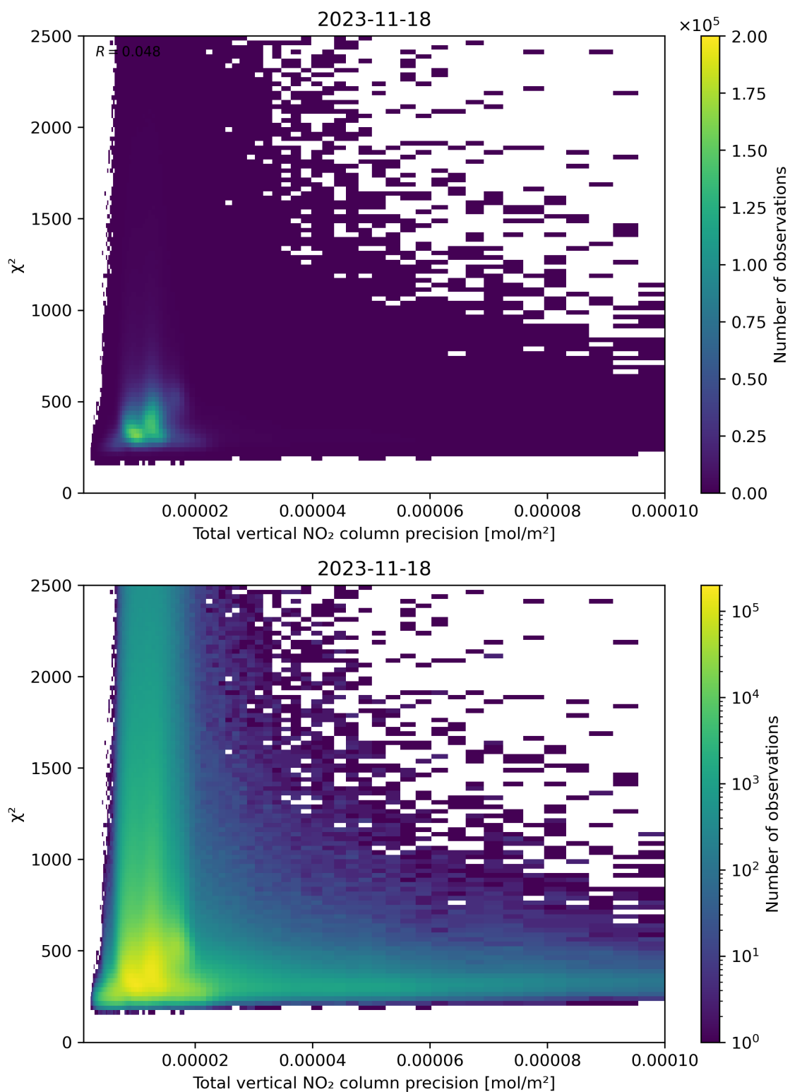
Figure 116: Scatter density plot of “Total vertical NO 2 column precision” against “ \chi^2 ” for 2023-11-18 to 2023-11-19.
