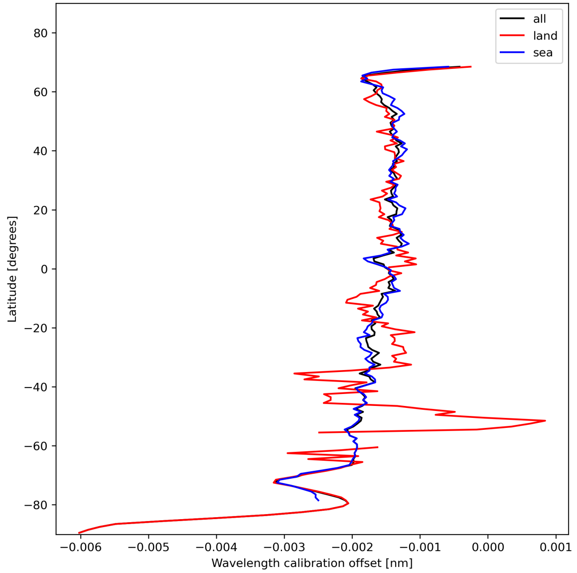
Figure 18: Zonal average of “Wavelength calibration offset” for 2023-11-18 to 2023-11-19.
