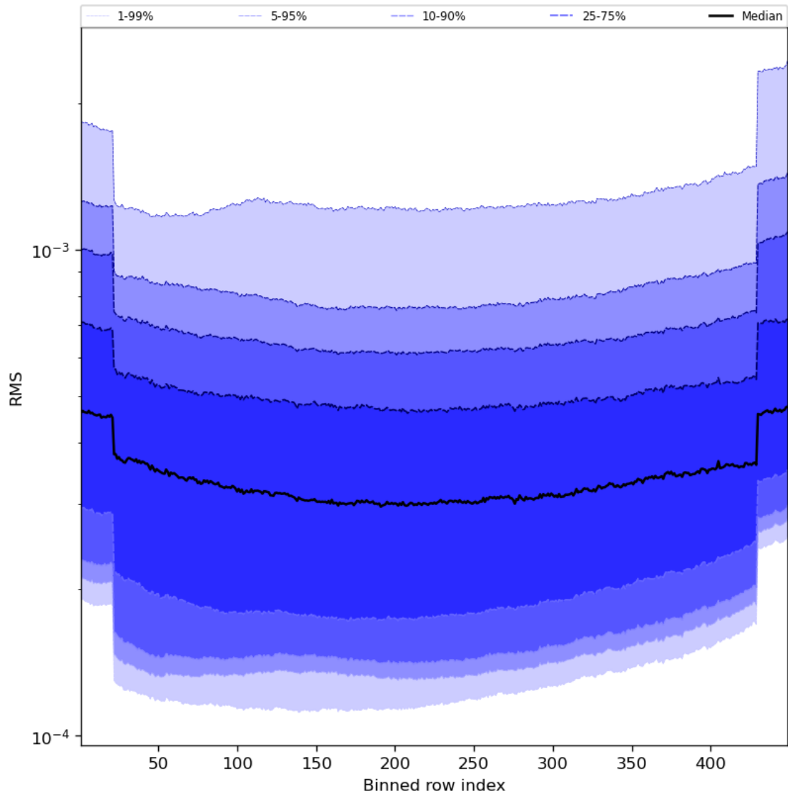
Figure 60: Along track statistics of “RMS” for 2023-11-18 to 2023-11-19
