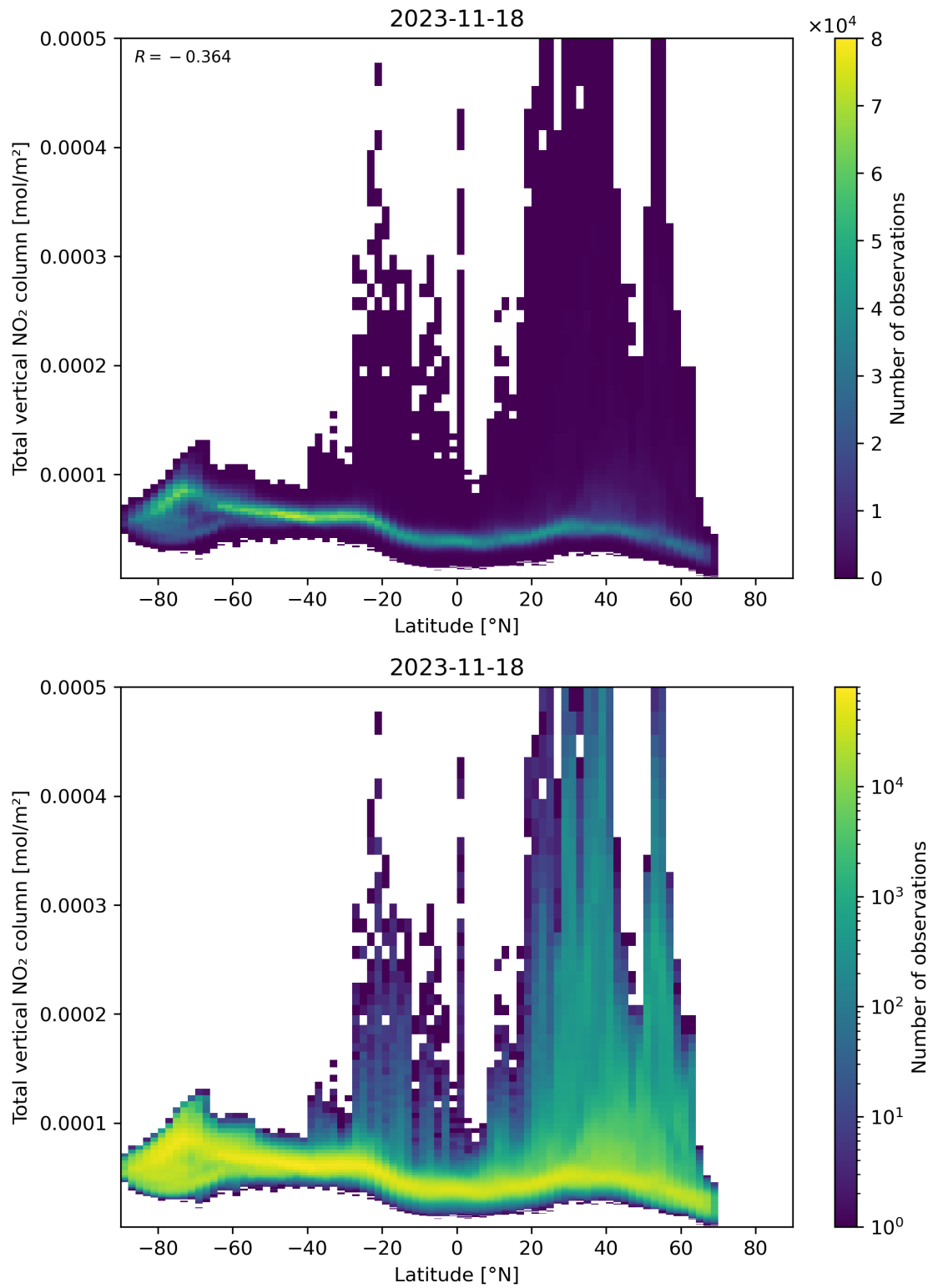
Figure 90: Scatter density plot of “Latitude” against “Total vertical NO 2 column” for 2023-11-18 to 2023-11-19.
