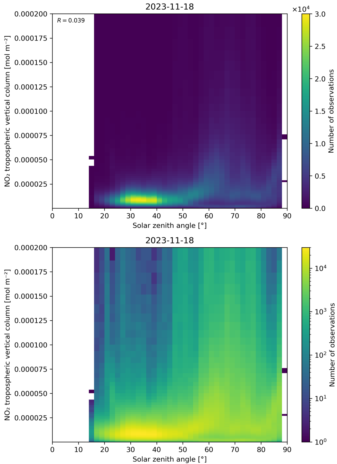
Figure 155: Scatter density plot of “Solar zenith angle” against “NO 2 tropospheric vertical column” for 2023-11-18 to 2023-11-19.
