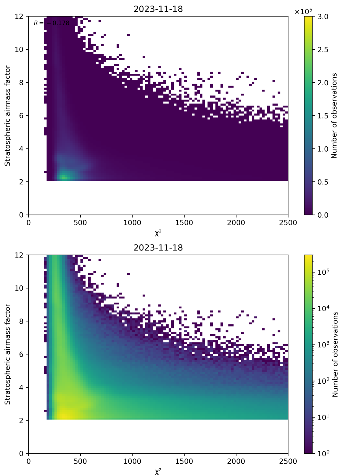
Figure 81: Scatter density plot of " \chi^2 " against "Stratospheric airmass factor" for 2023-11-18 to 2023-11-19.
