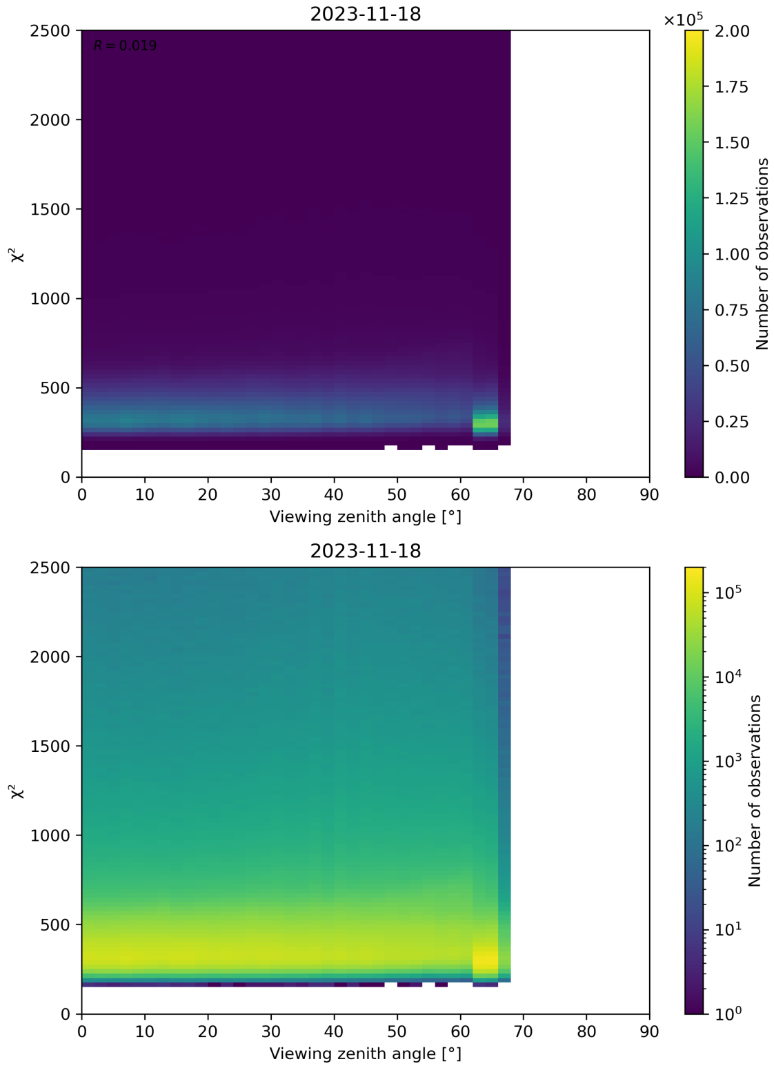
Figure 162: Scatter density plot of “Viewing zenith angle” against “ \chi^2 ” for 2023-11-18 to 2023-11-19.
