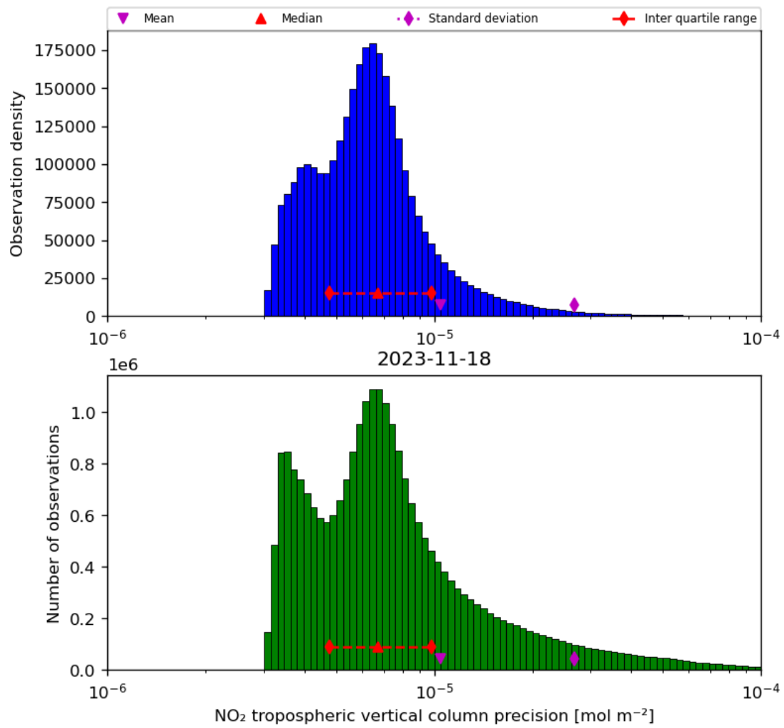
Figure 30: Histogram of “NO 2 tropospheric vertical column precision” for 2023-11-18 to 2023-11-19
