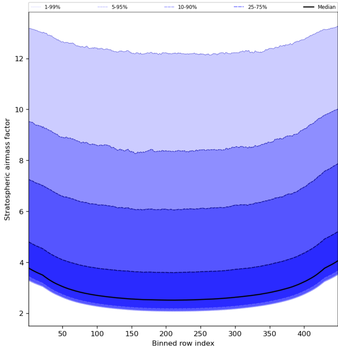
Figure 61: Along track statistics of “Stratospheric airmass factor” for 2023-11-18 to 2023-11-19
