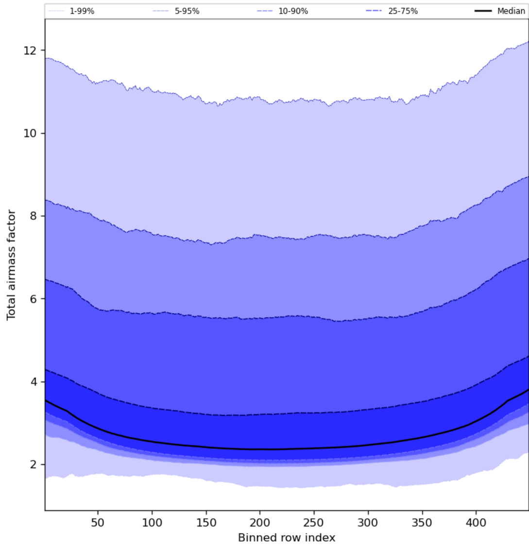
Figure 49: Along track statistics of “Total airmass factor” for 2023-11-18 to 2023-11-19
