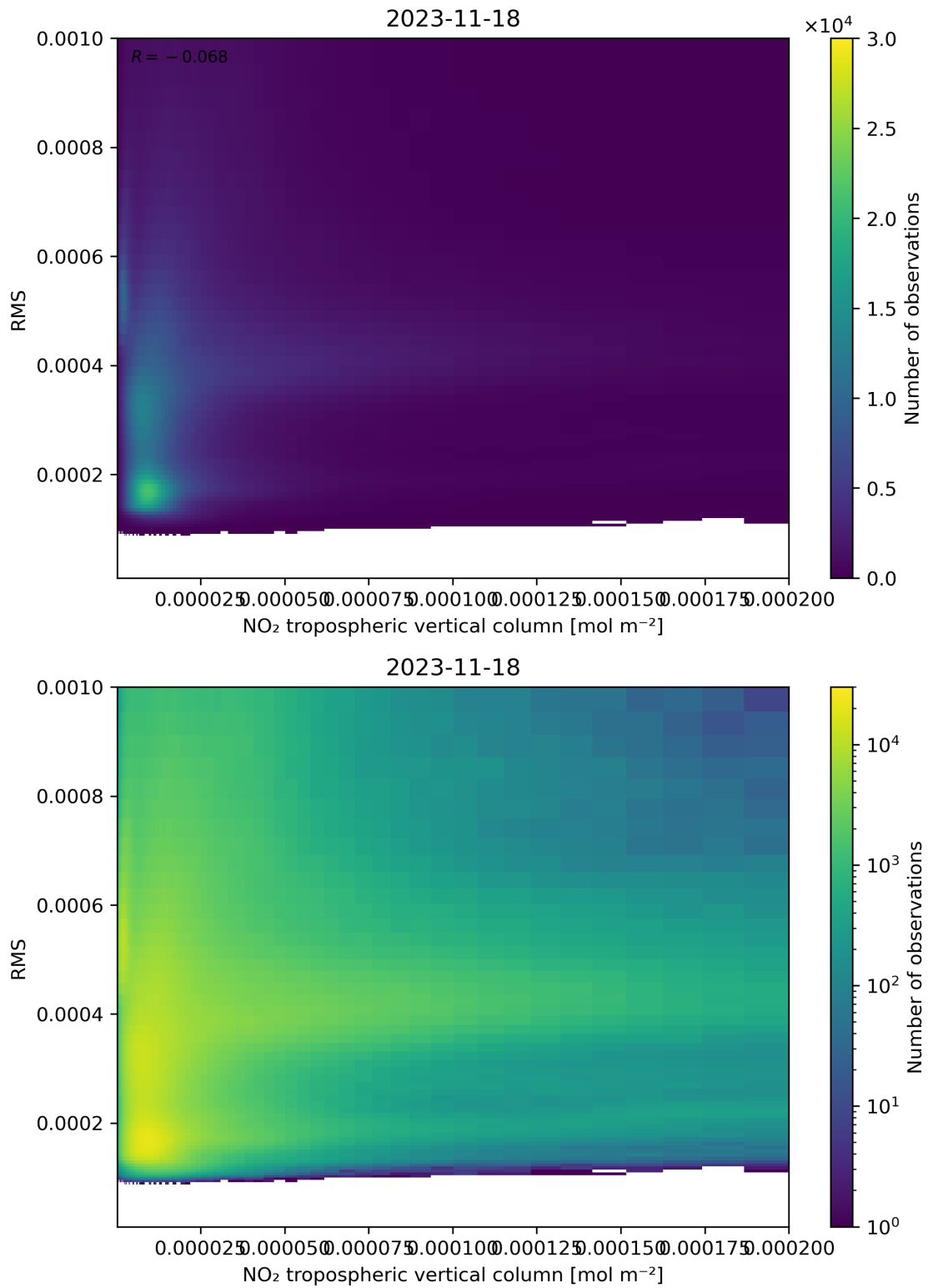
Figure 142: Scatter density plot of “NO 2 tropospheric vertical column” against “RMS” for 2023-11-18 to 2023-11-19.
