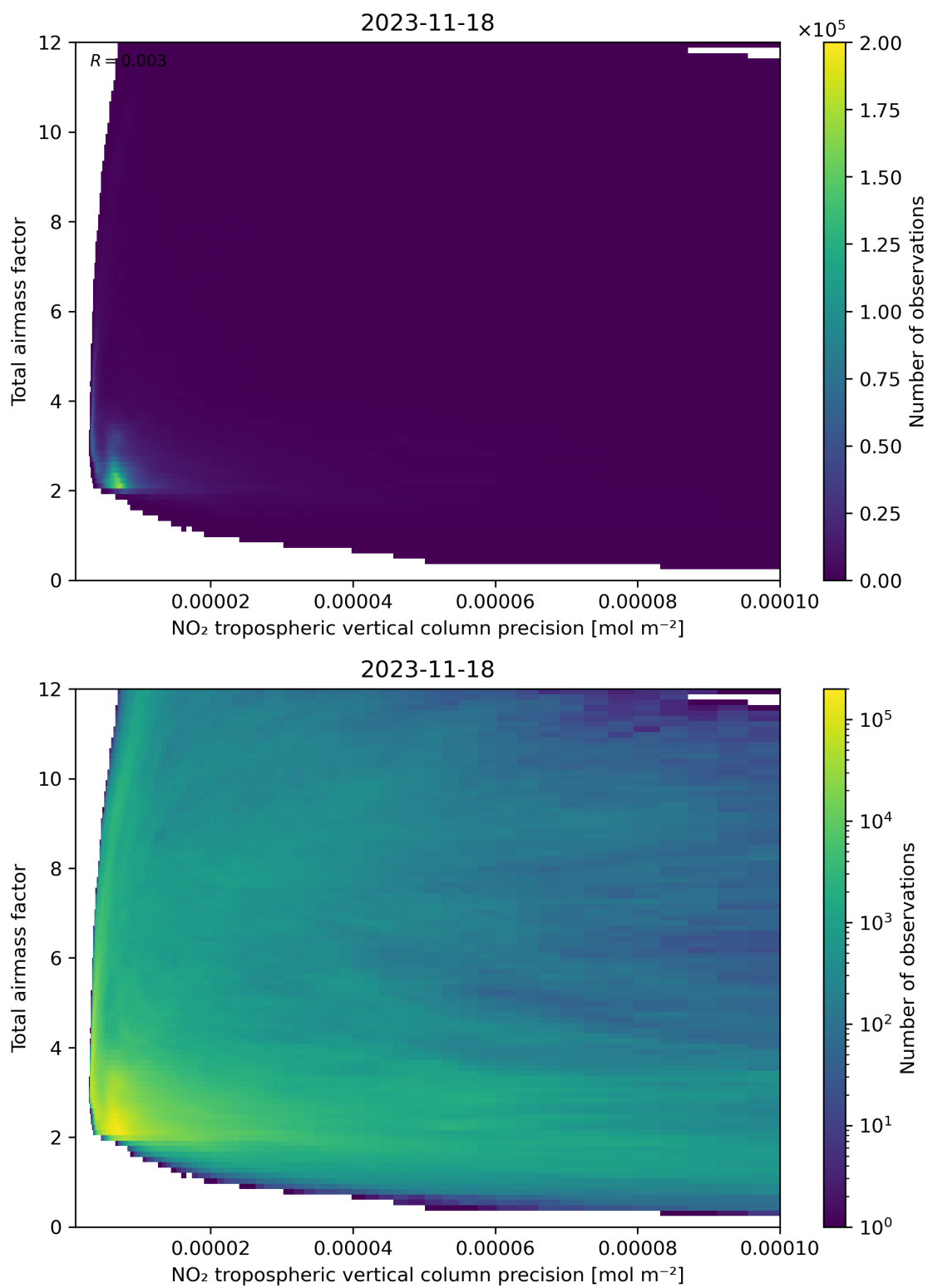
Figure 132: Scatter density plot of “NO 2 tropospheric vertical column precision” against “Total air mass factor” for 2023-11-18 to 2023-11-19.
