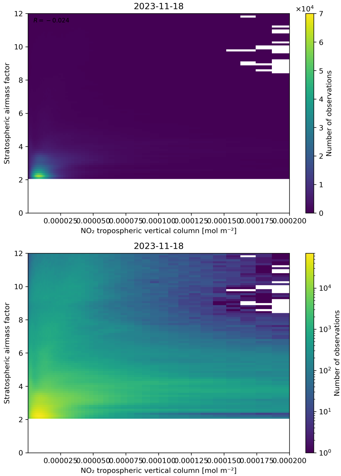
Figure 121: Scatter density plot of “NO 2 tropospheric vertical column” against “Stratospheric airmass factor” for 2023-11-18 to 2023-11-19.
