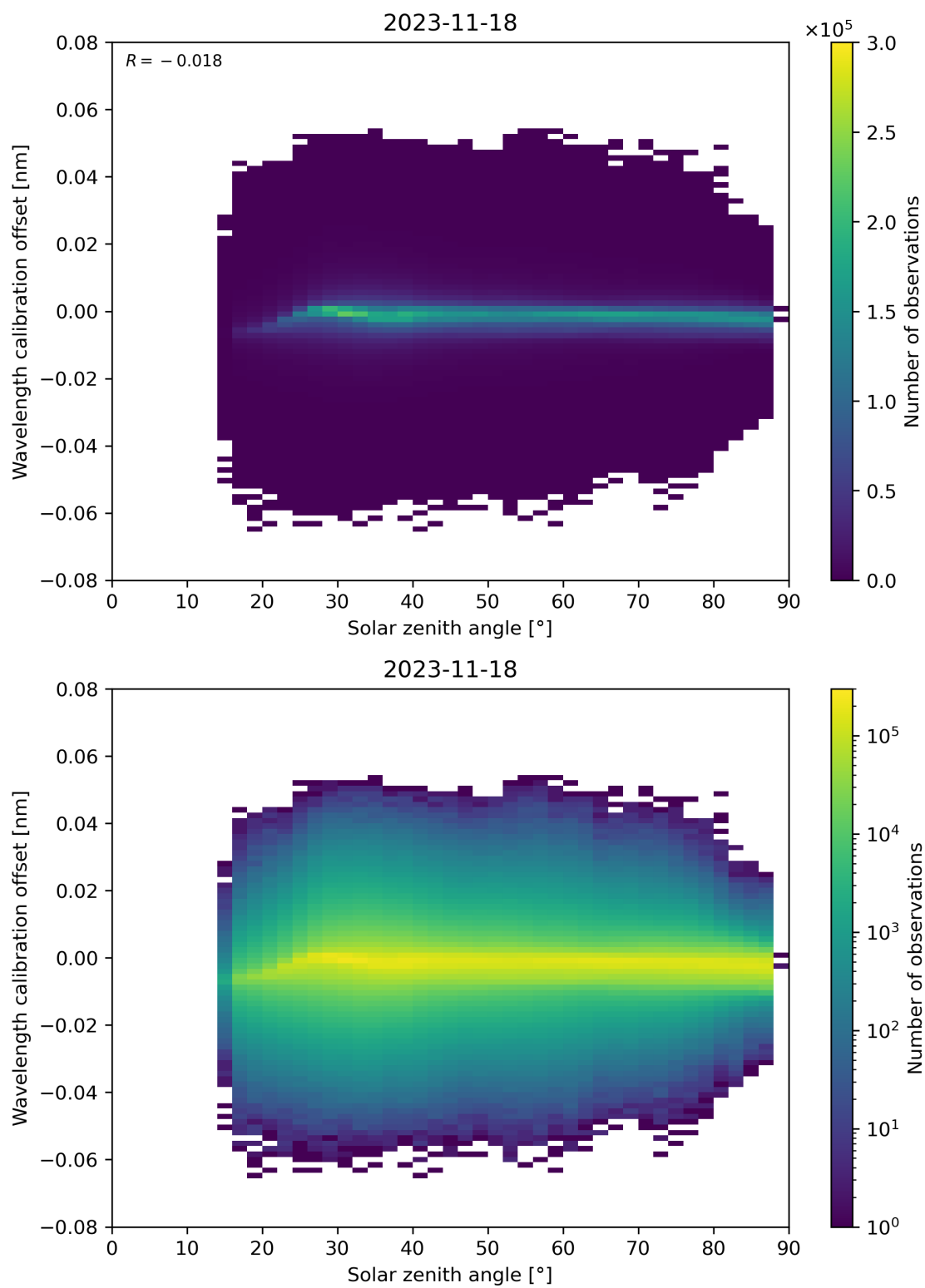
Figure 158: Scatter density plot of “Solar zenith angle” against “Wavelength calibration offset” for 2023-11-18 to 2023-11-19.
