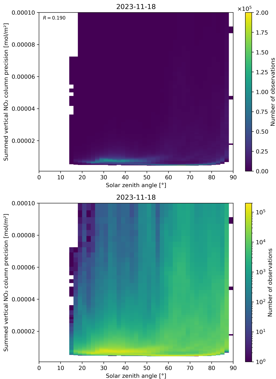
Figure 152: Scatter density plot of “Solar zenith angle” against “Summed vertical NO 2 column precision” for 2023-11-18 to 2023-11-19.
