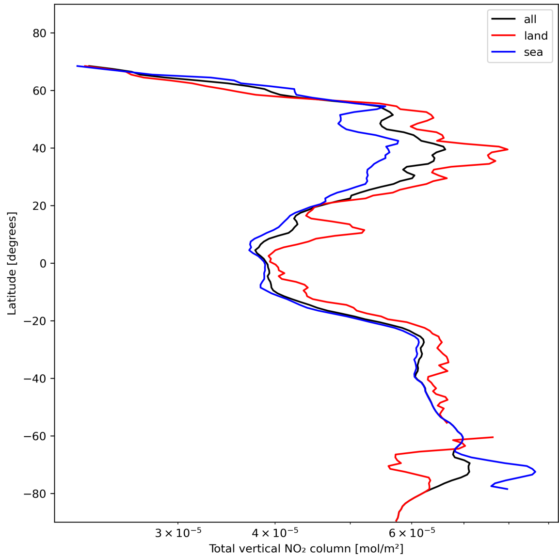
Figure 21: Zonal average of “Total vertical NO 2 column” for 2023-11-18 to 2023-11-19.
