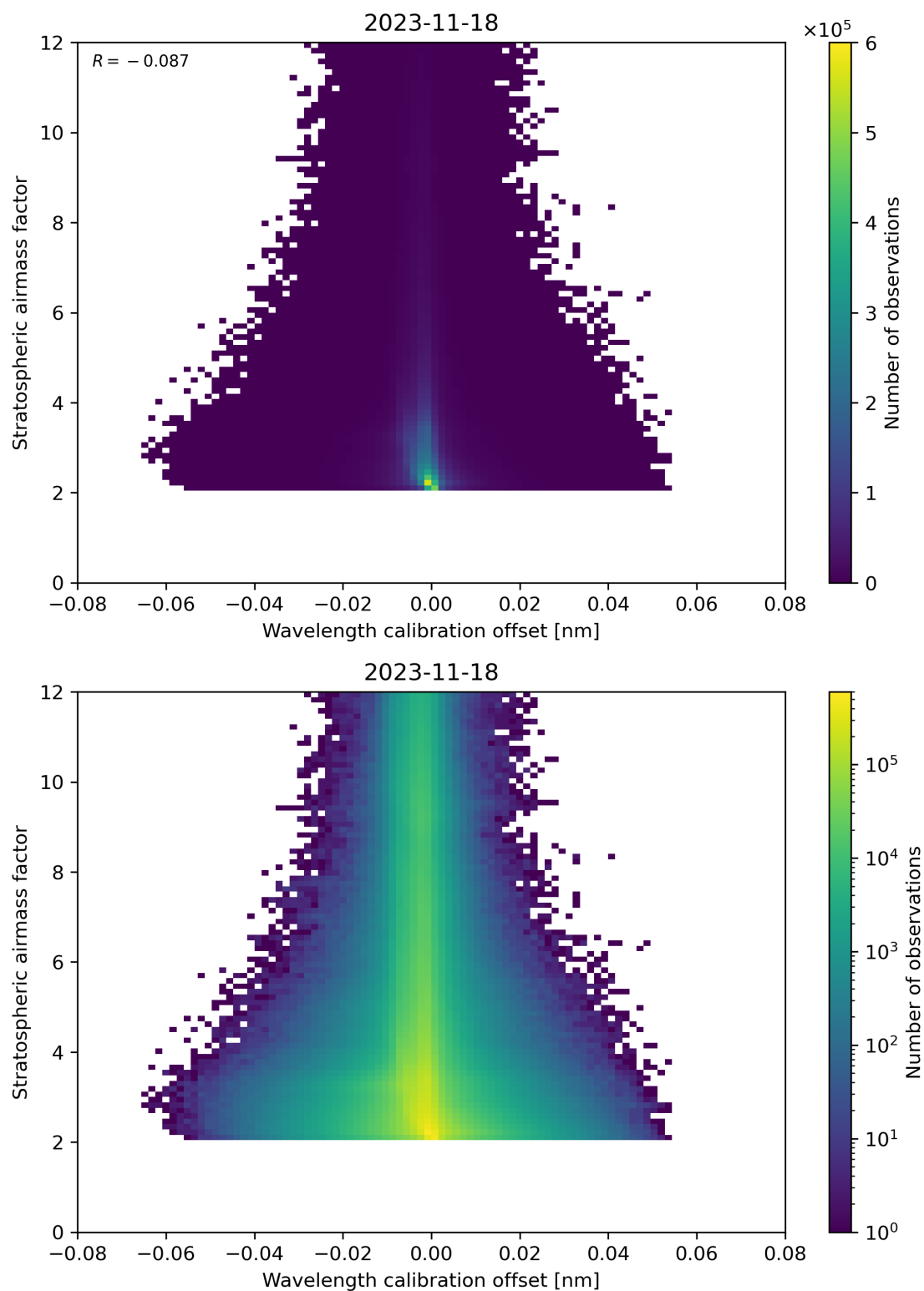
Figure 174: Scatter density plot of “Wavelength calibration offset” against “Stratospheric airmass factor” for 2023-11-18 to 2023-11-19.
