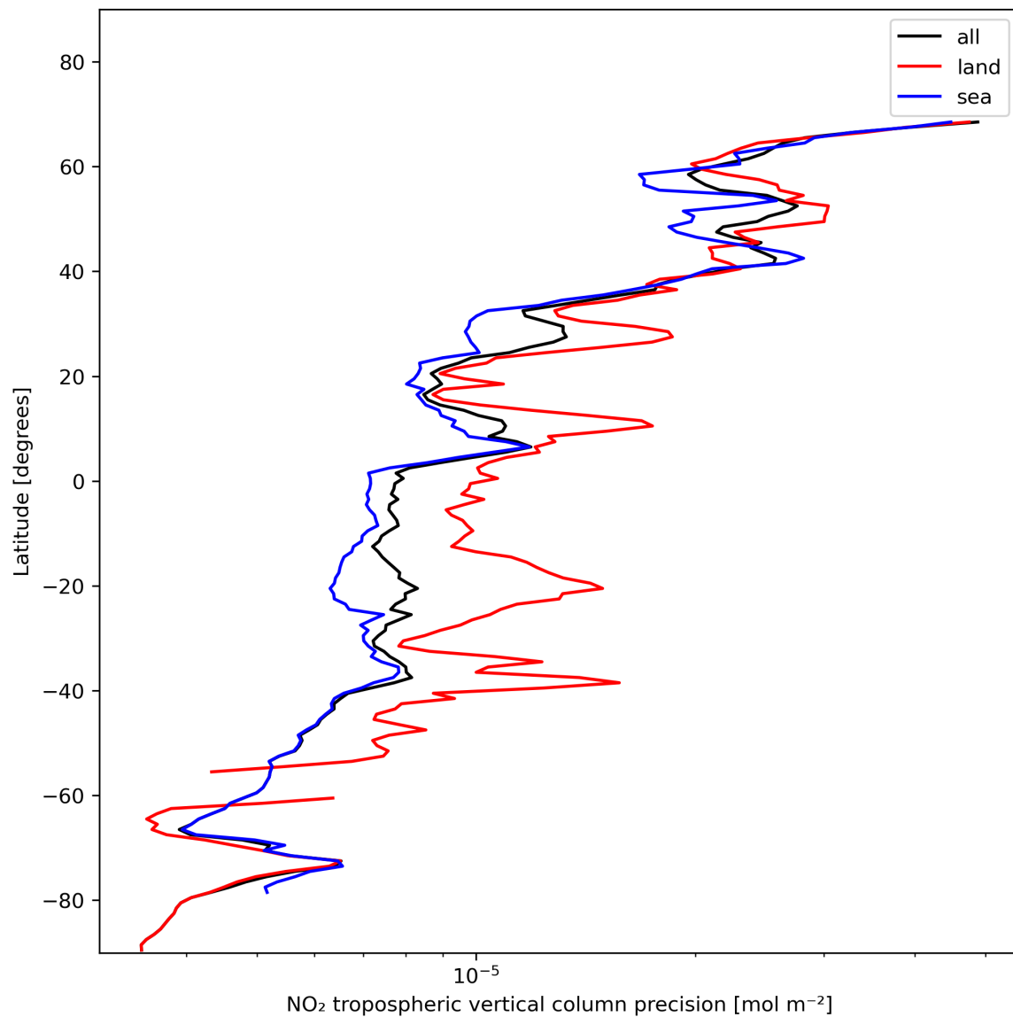
Figure 13: Zonal average of “NO 2 tropospheric vertical column precision” for 2023-11-18 to 2023-11-19.
