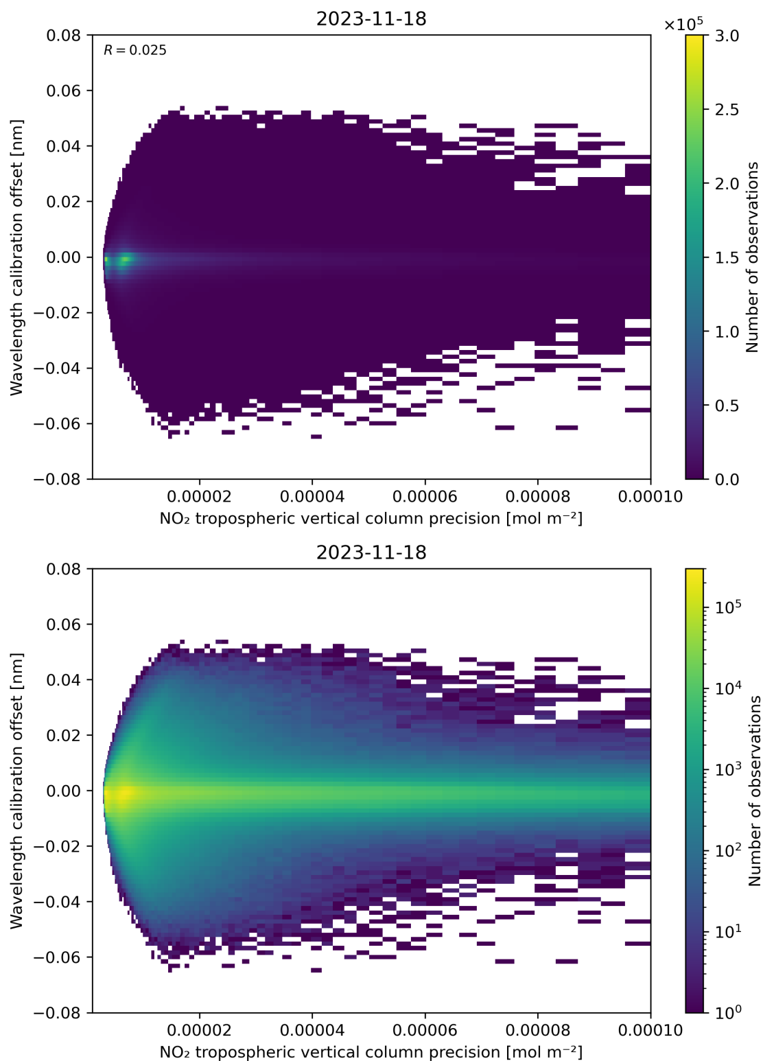
Figure 141: Scatter density plot of “NO 2 tropospheric vertical column precision” against “Wavelength calibration offset” for 2023-11-18 to 2023-11-19.
