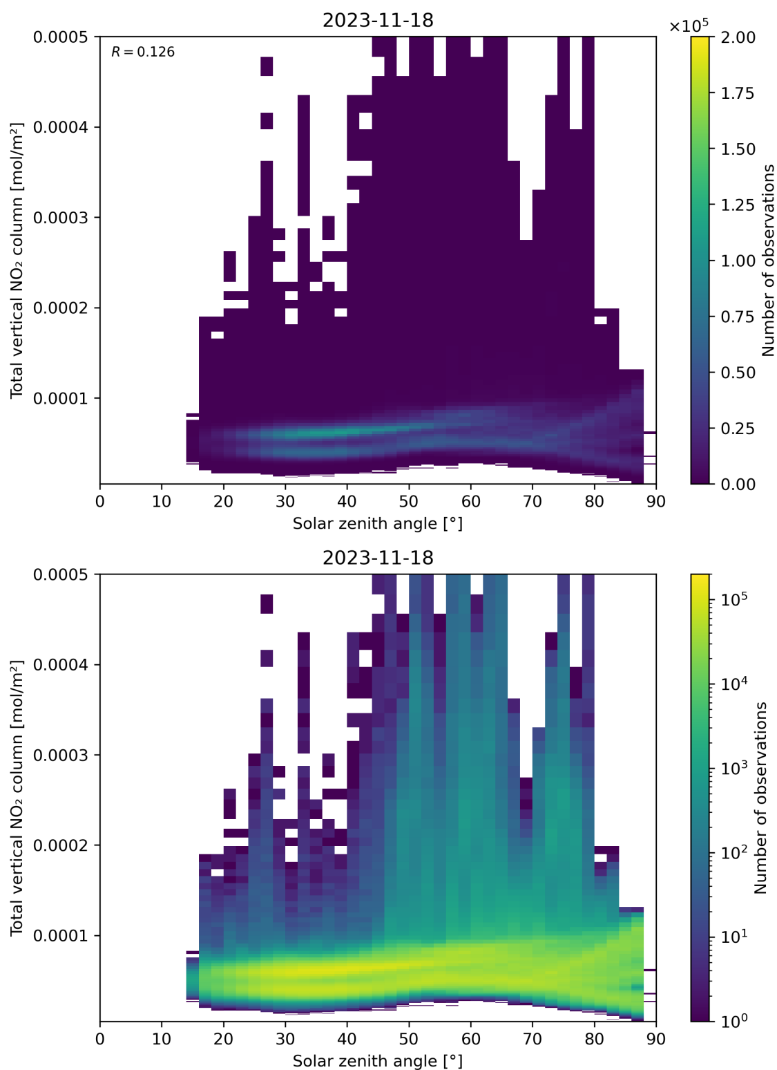
Figure 153: Scatter density plot of “Solar zenith angle” against “Total vertical NO 2 column” for 2023-11-18 to 2023-11-19.
