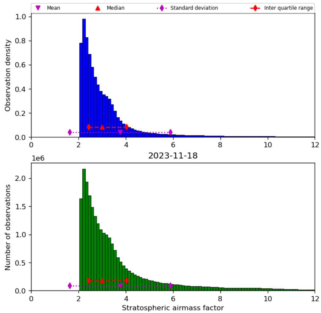
Figure 44: Histogram of “Stratospheric airmass factor” for 2023-11-18 to 2023-11-19
