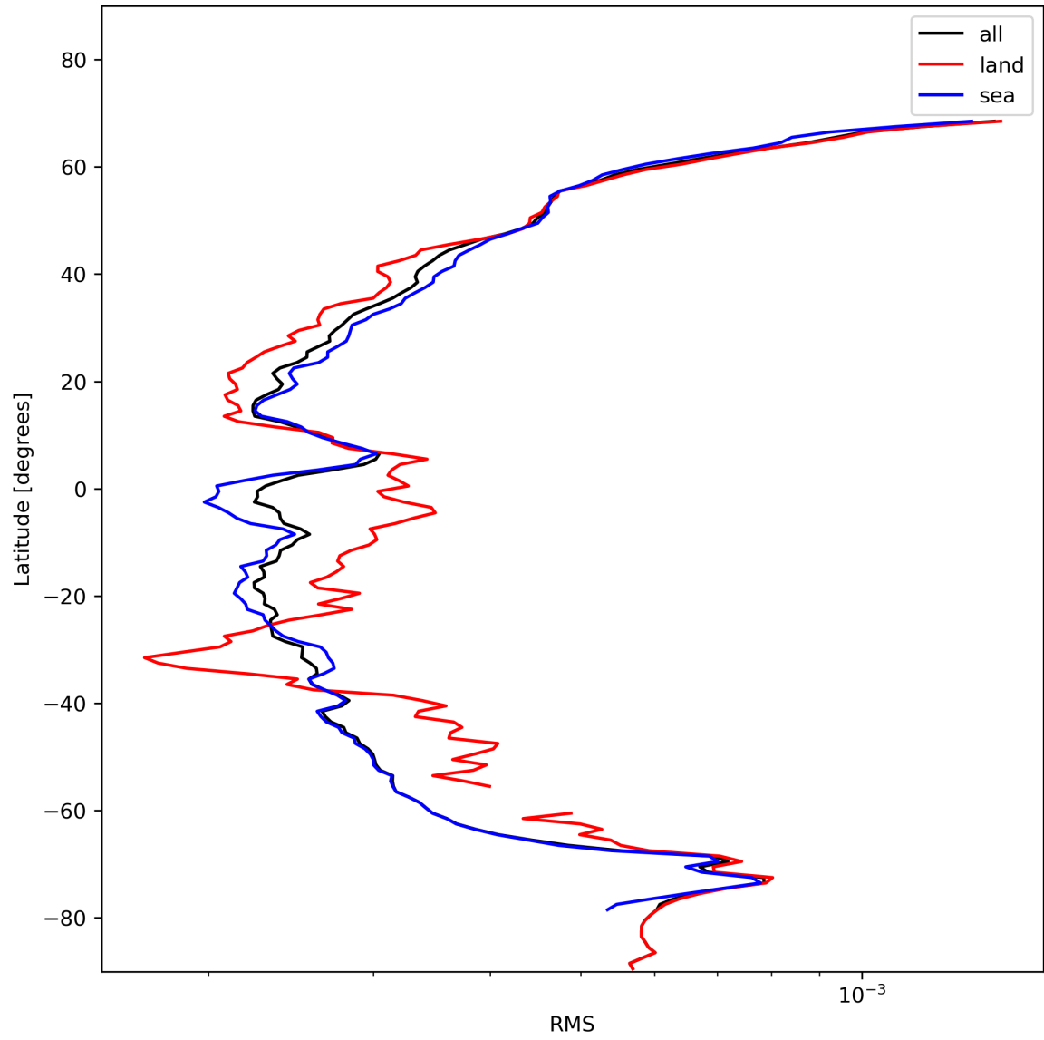
Figure 26: Zonal average of “RMS” for 2023-11-18 to 2023-11-19.
