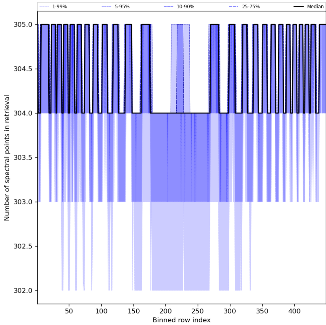
Figure 50: Along track statistics of “Number of spectral points in retrieval” for 2023-11-18 to 2023-11-19
