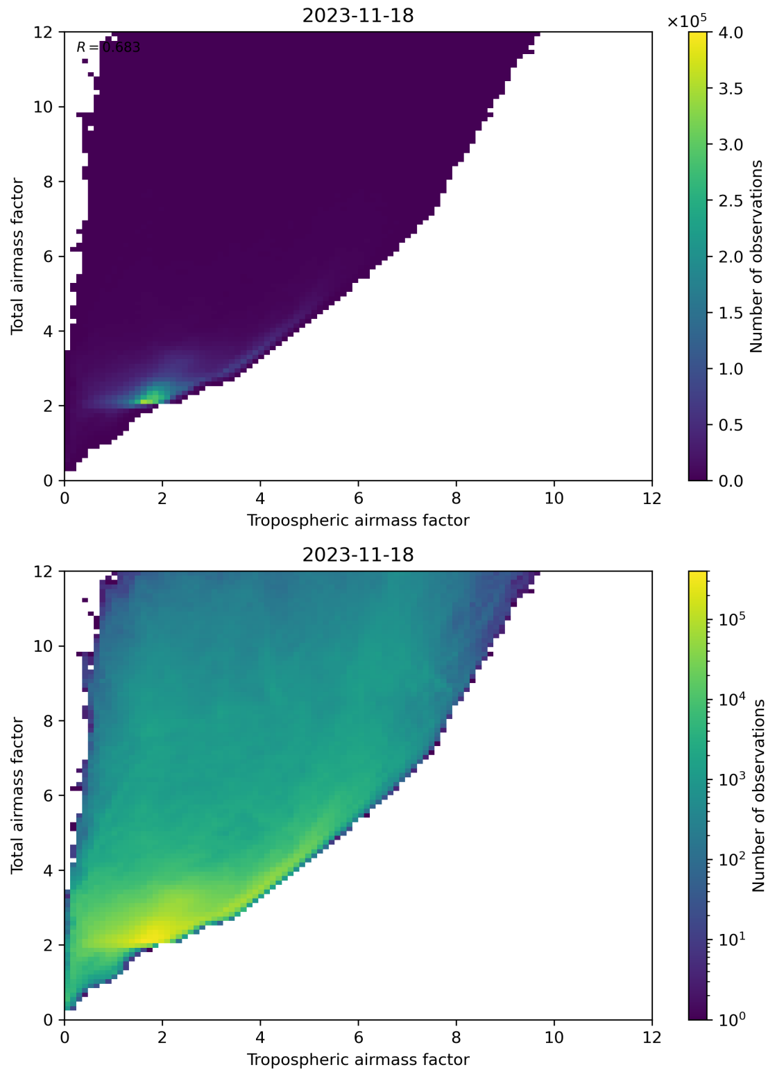
Figure 72: Scatter density plot of “Tropospheric airmass factor” against “Total airmass factor” for 2023-11-18 to 2023-11-19.
