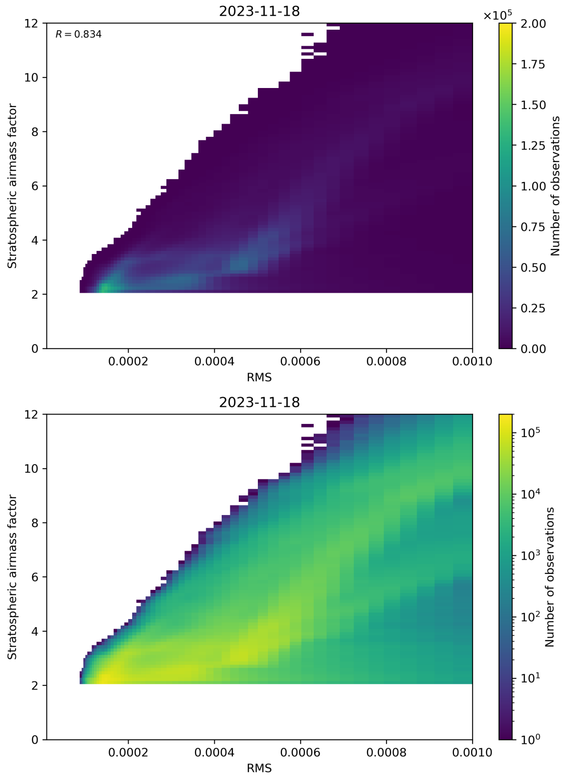
Figure 144: Scatter density plot of “RMS” against “Stratospheric airmass factor” for 2023-11-18 to 2023-11-19.
