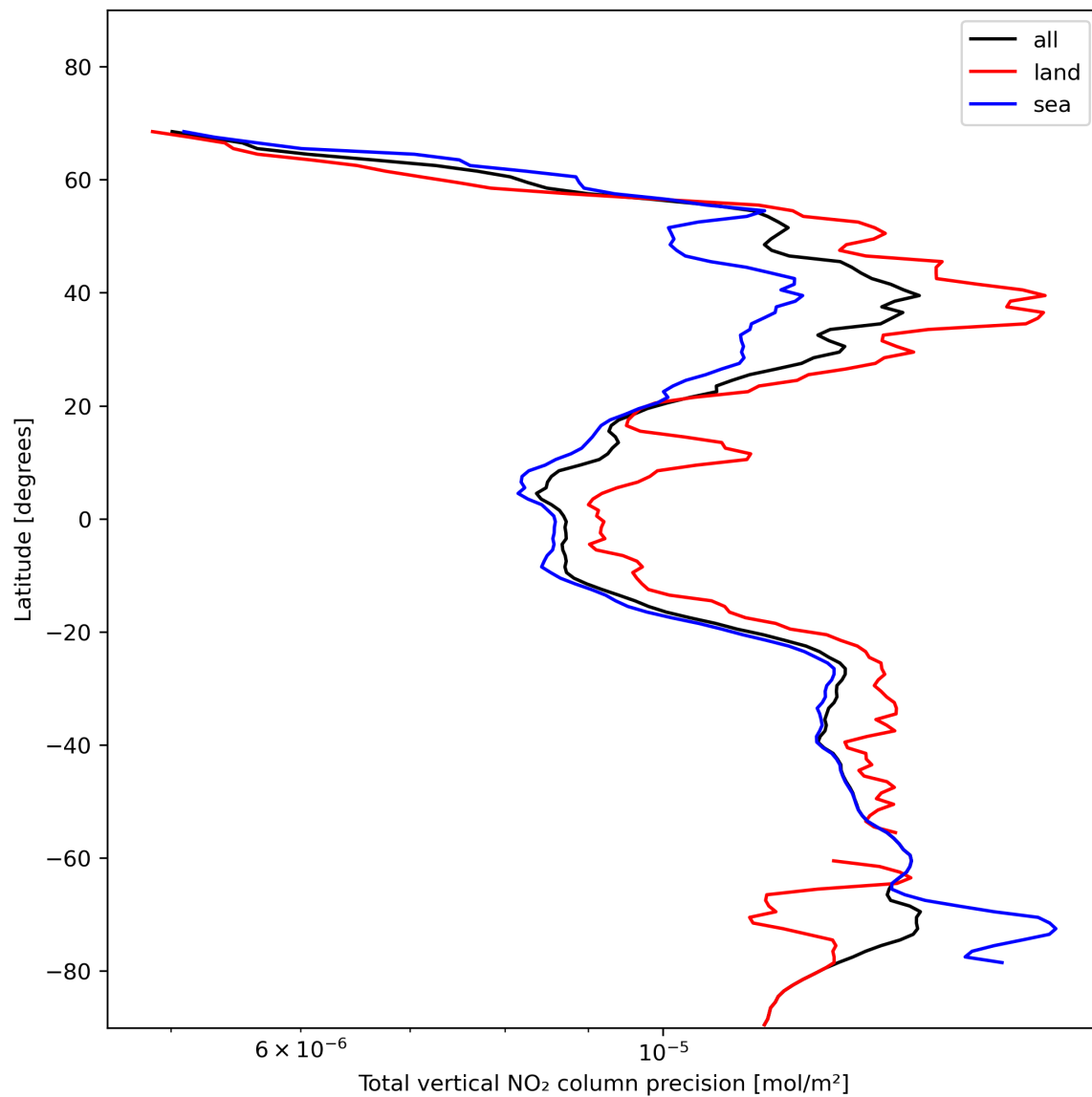
Figure 22: Zonal average of “Total vertical NO 2 column precision” for 2023-11-18 to 2023-11-19.
