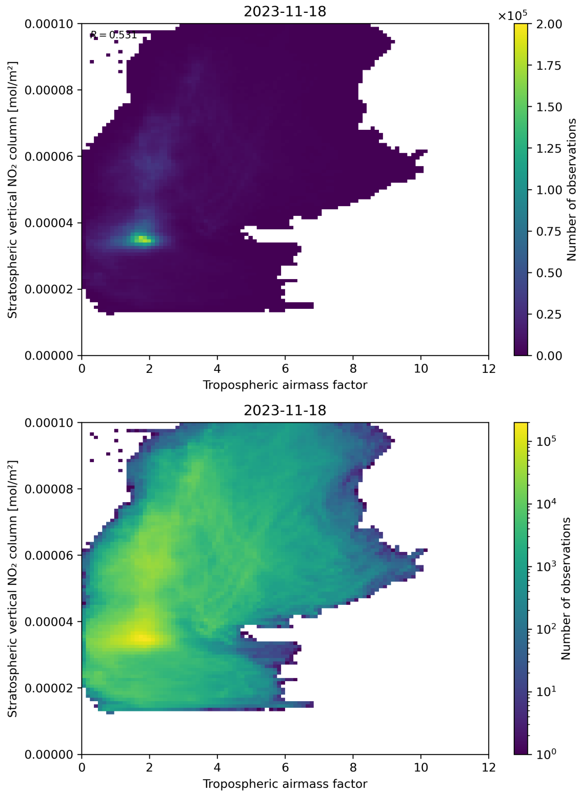
Figure 74: Scatter density plot of “Tropospheric air mass factor” against “Stratospheric vertical NO 2 column” for 2023-11-18 to 2023-11-19.
