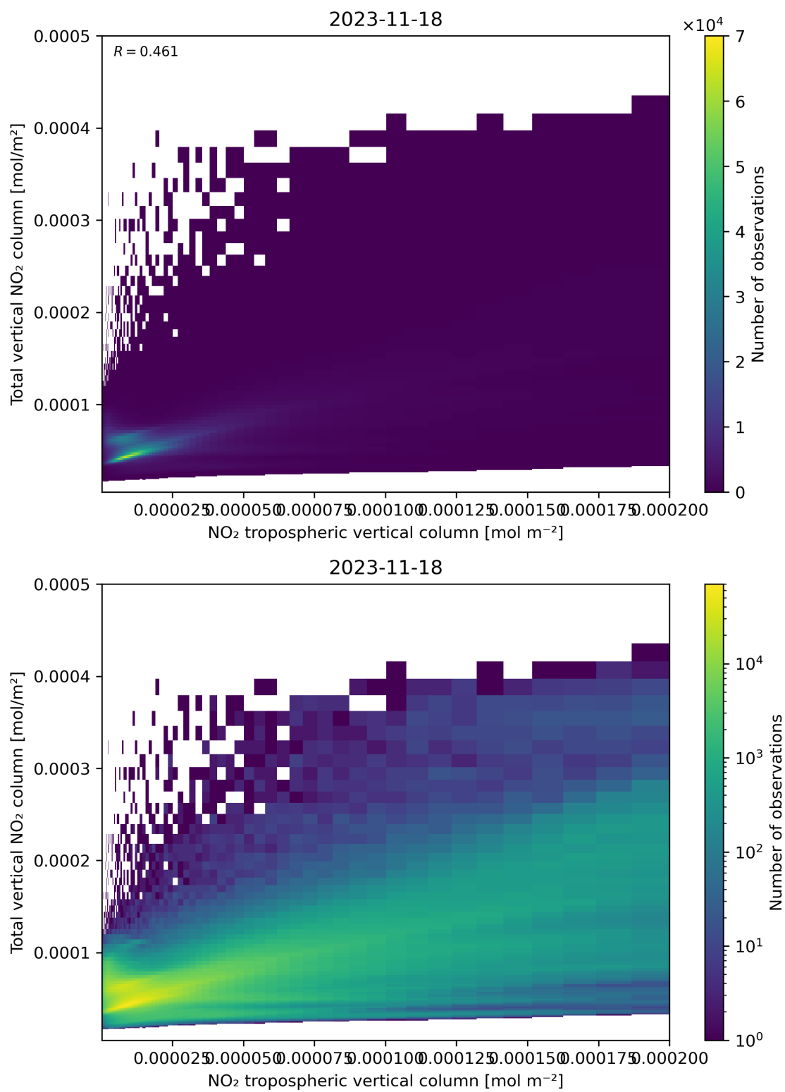
Figure 128: Scatter density plot of “NO 2 tropospheric vertical column” against “Total vertical NO 2 column” for 2023-11-18 to 2023-11-19.
