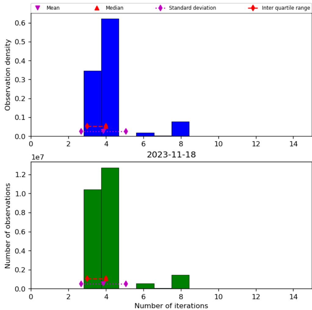
Figure 34: Histogram of “Number of iterations” for 2023-11-18 to 2023-11-19
