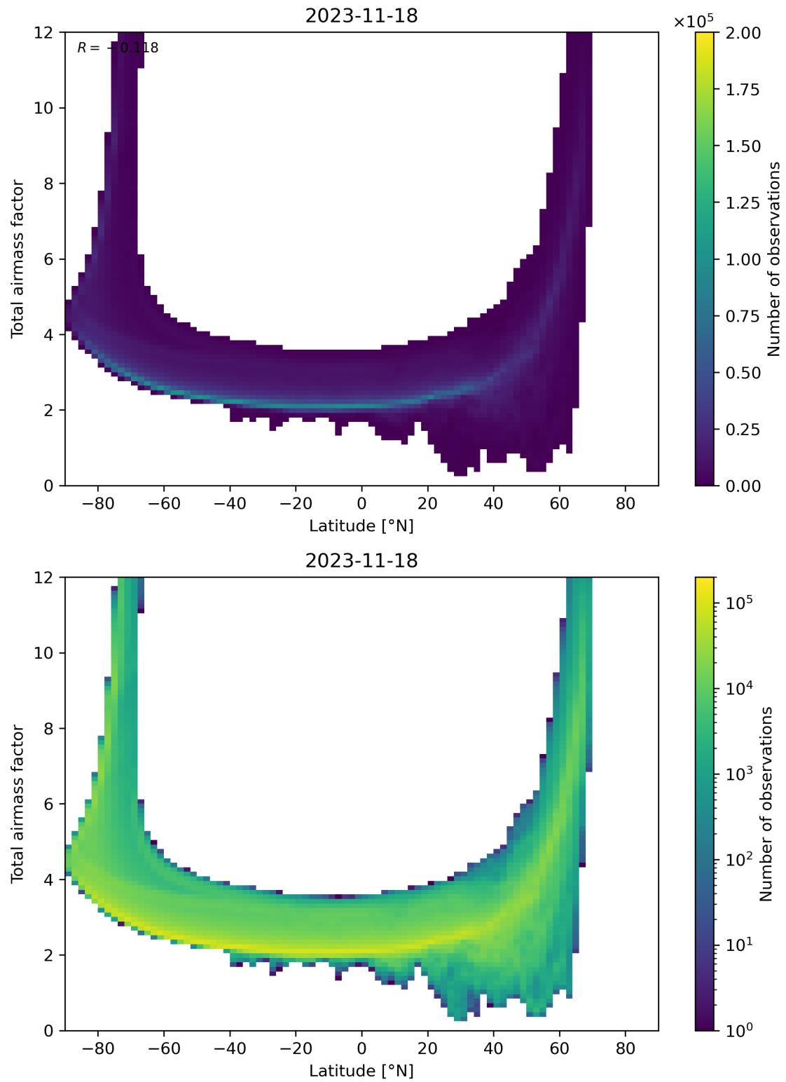
Figure 84: Scatter density plot of “Latitude” against “Total airmass factor” for 2023-11-18 to 2023-11-19.
