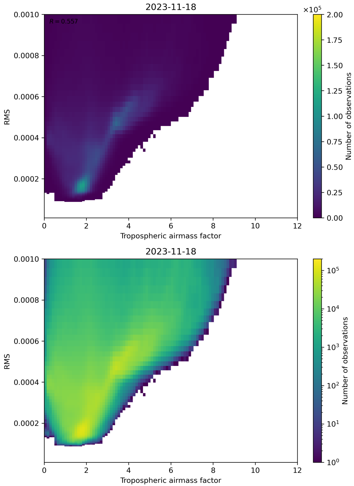
Figure 79: Scatter density plot of “Tropospheric airmass factor” against “RMS” for 2023-11-18 to 2023-11-19.
