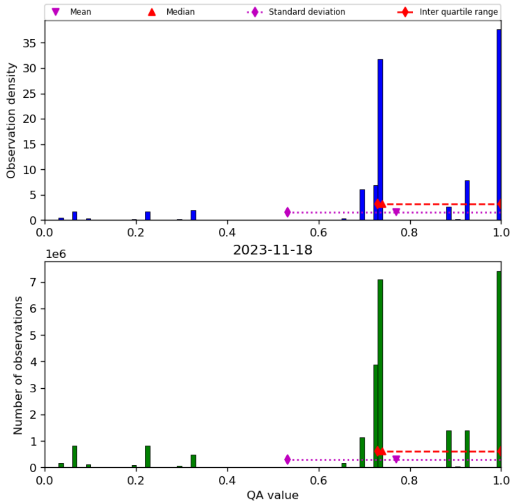
Figure 28: Histogram of “QA value” for 2023-11-18 to 2023-11-19
