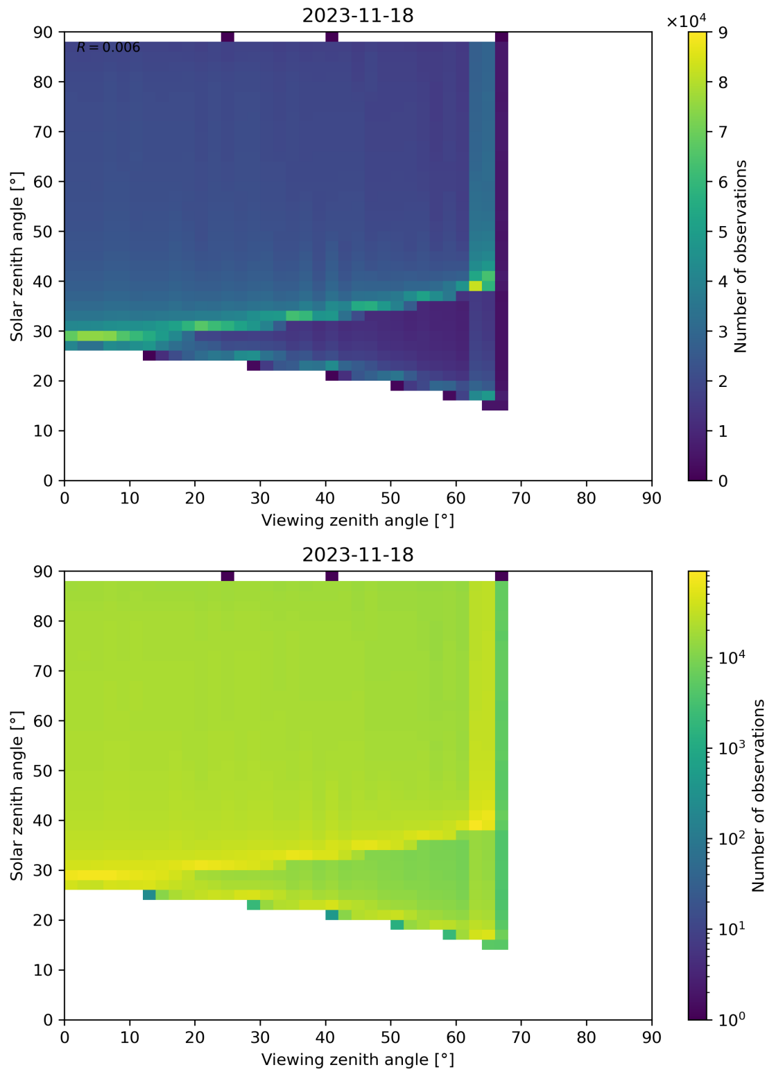
Figure 172: Scatter density plot of “Viewing zenith angle” against “Solar zenith angle” for 2023-11-18 to 2023-11-19.
