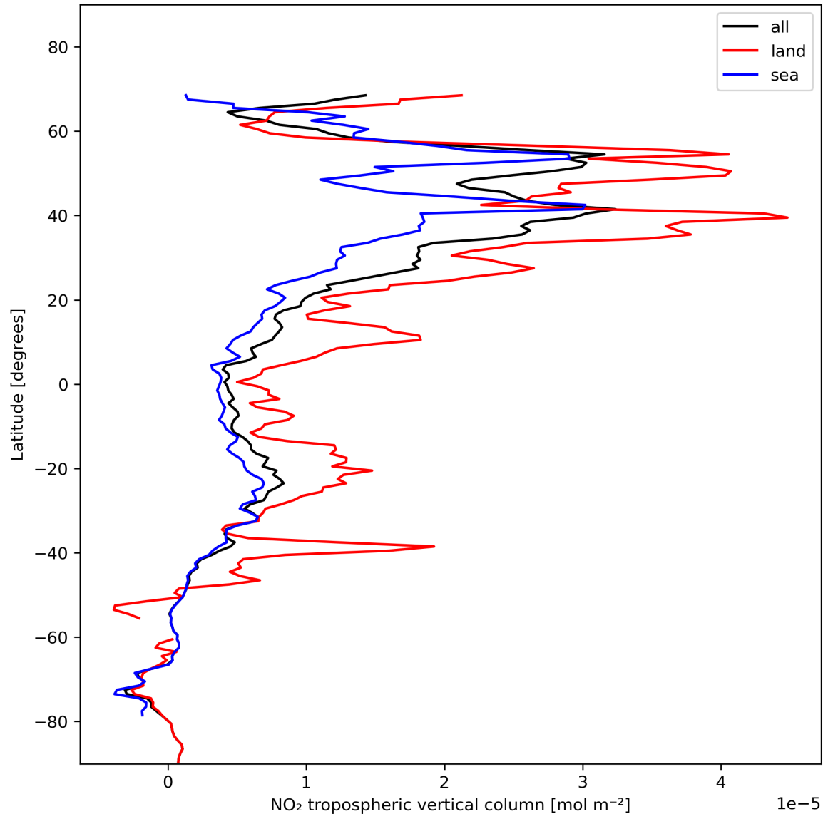
Figure 12: Zonal average of “NO 2 tropospheric vertical column” for 2023-11-18 to 2023-11-19.
