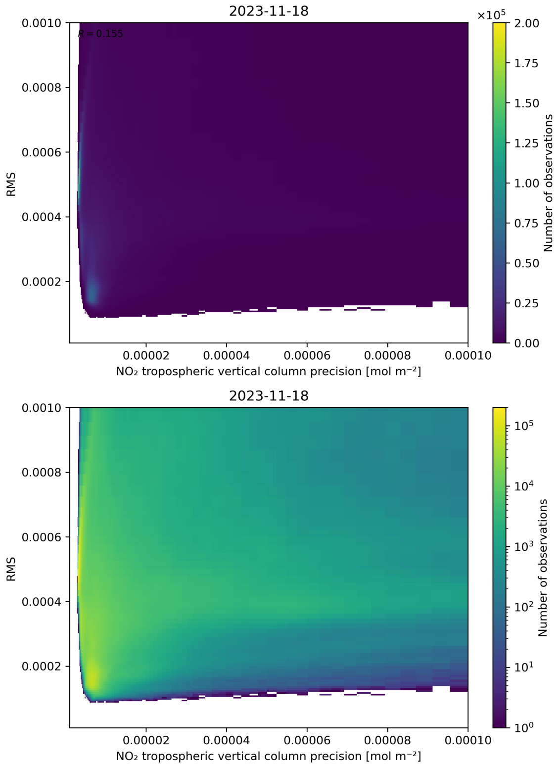
Figure 140: Scatter density plot of “NO 2 tropospheric vertical column precision” against “RMS” for 2023-11-18 to 2023-11-19.
