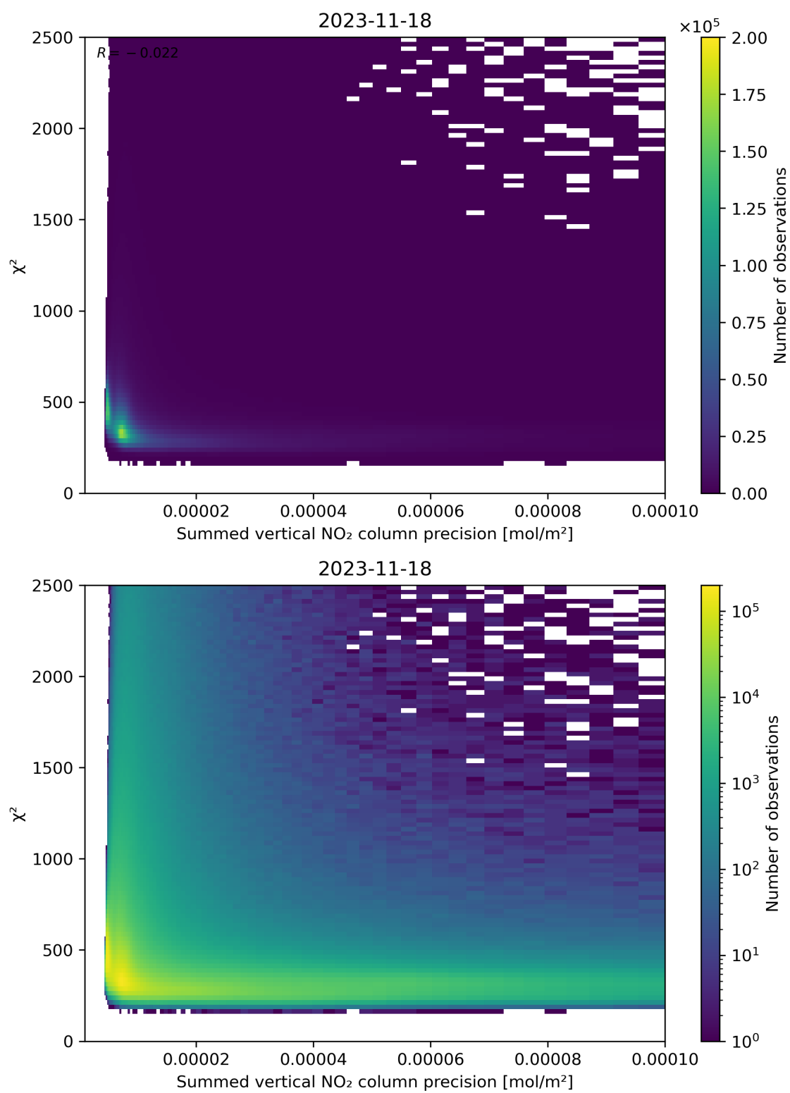
Figure 107: Scatter density plot of “Summed vertical NO 2 column precision” against “ \chi^2 ” for 2023-11-18 to 2023-11-19.
