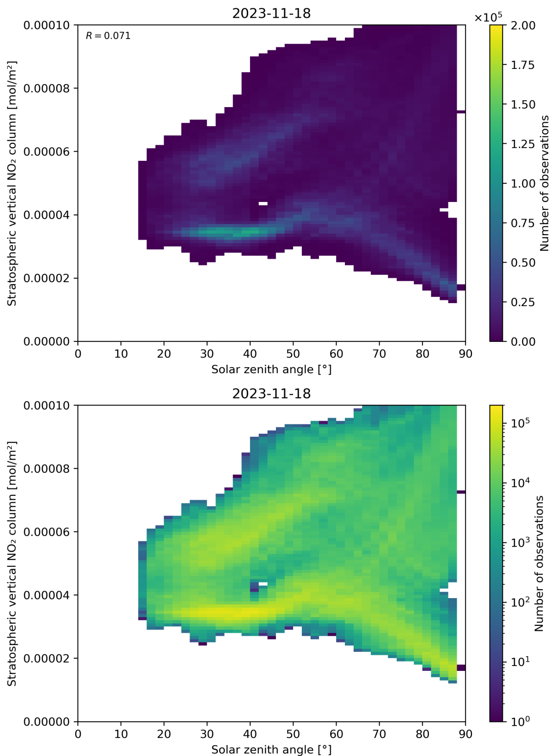
Figure 150: Scatter density plot of “Solar zenith angle” against “Stratospheric vertical NO 2 column” for 2023-11-18 to 2023-11-19.
