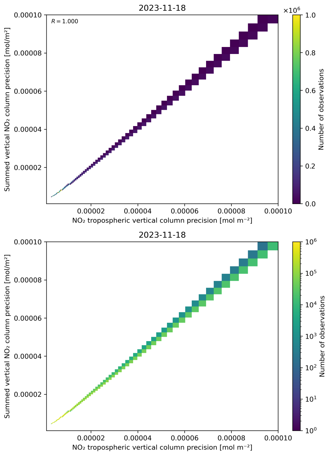
Figure 137: Scatter density plot of “NO 2 tropospheric vertical column precision” against “Summed vertical NO 2 column precision” for 2023-11-18 to 2023-11-19.
