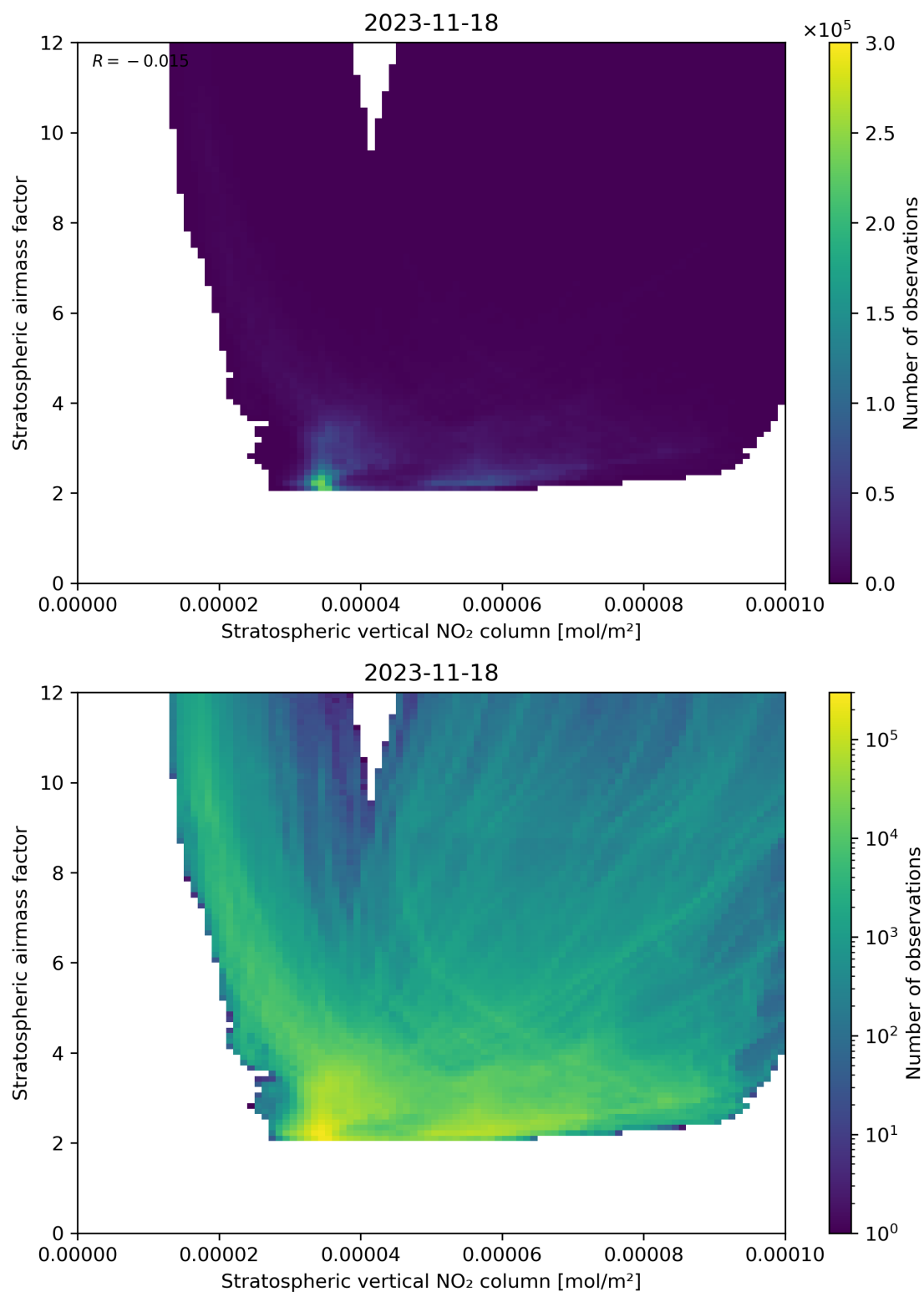
Figure 96: Scatter density plot of “Stratospheric vertical NO 2 column” against “Stratospheric airmass factor” for 2023-11-18 to 2023-11-19.
