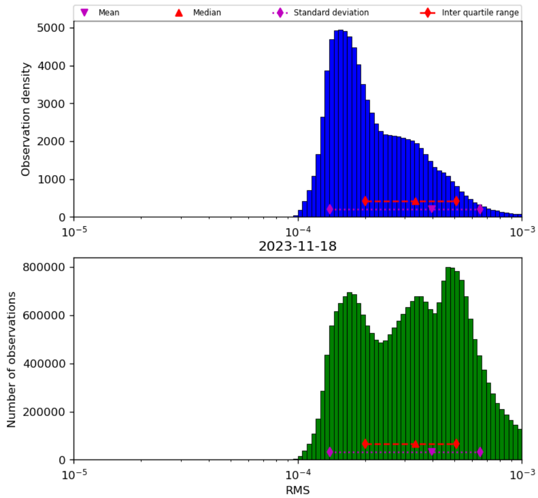
Figure 43: Histogram of “RMS” for 2023-11-18 to 2023-11-19
