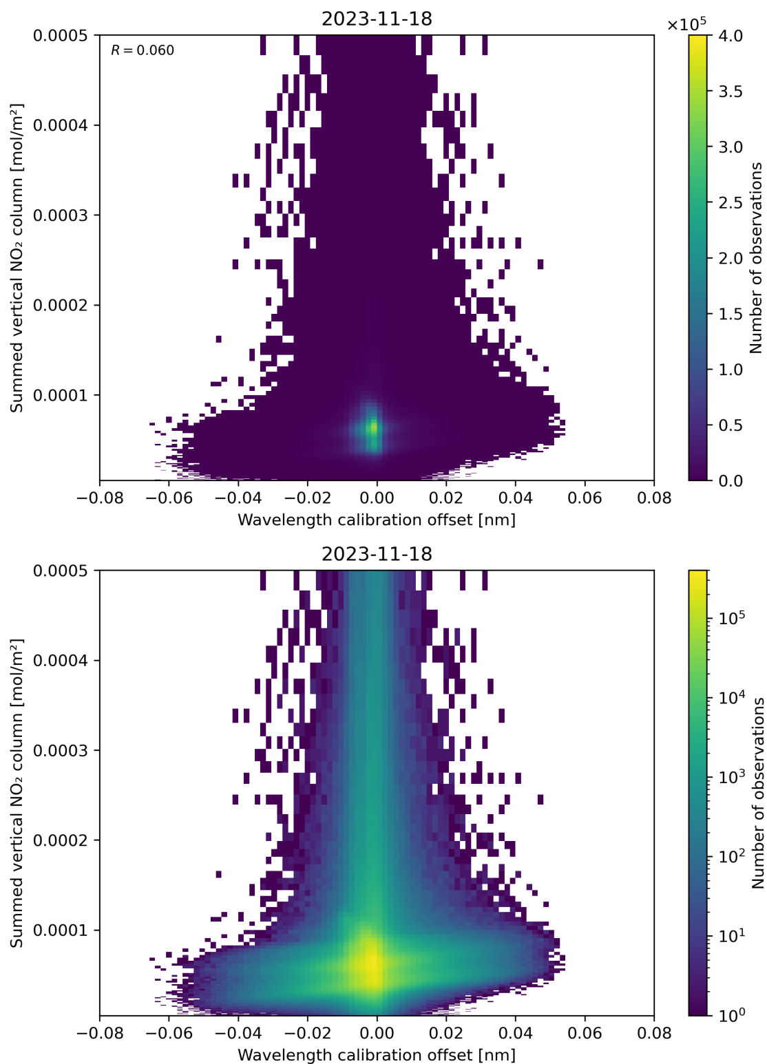
Figure 177: Scatter density plot of “Wavelength calibration offset” against “Summed vertical NO 2 column” for 2023-11-18 to 2023-11-19.
