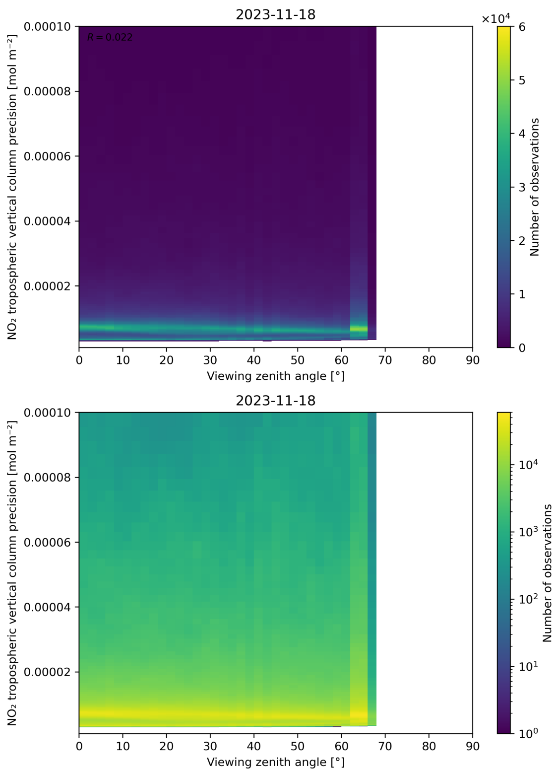
Figure 170: Scatter density plot of “Viewing zenith angle” against “NO 2 tropospheric vertical column precision” for 2023-11-18 to 2023-11-19.
