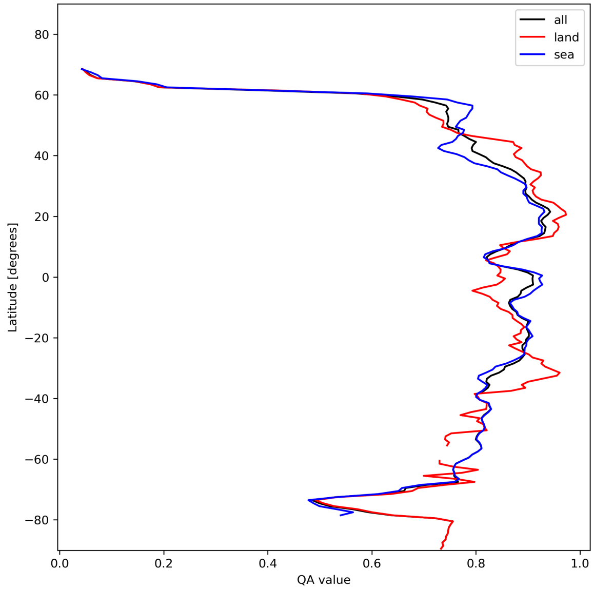
Figure 11: Zonal average of “QA value” for 2023-11-18 to 2023-11-19.
