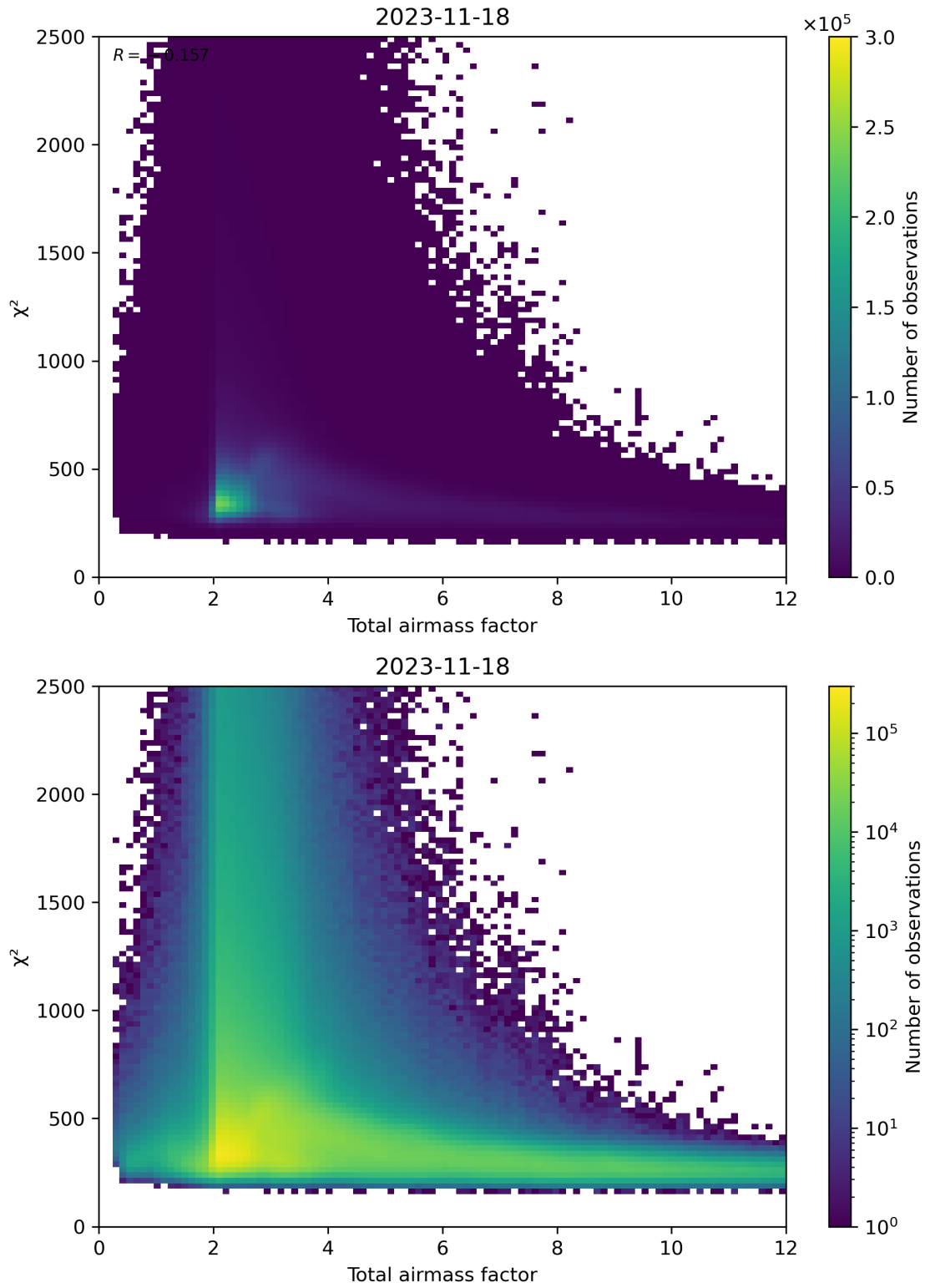
Figure 63: Scatter density plot of “Total airmass factor” against “ \chi^2 ” for 2023-11-18 to 2023-11-19.
