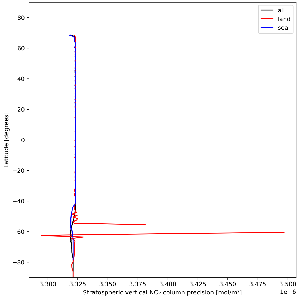
Figure 20: Zonal average of “Stratospheric vertical NO 2 column precision” for 2023-11-18 to 2023-11-19.
