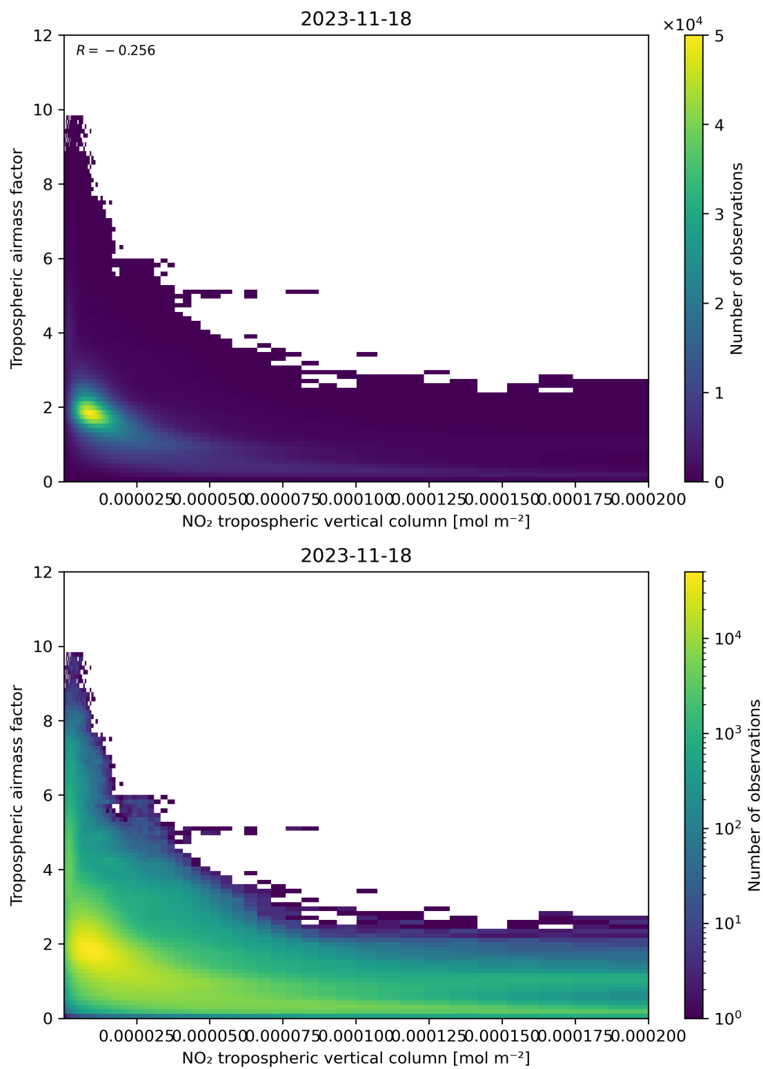
Figure 123: Scatter density plot of “NO 2 tropospheric vertical column” against “Tropospheric air mass factor” for 2023-11-18 to 2023-11-19.
