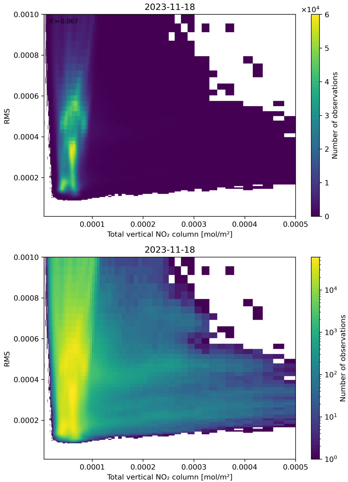
Figure 120: Scatter density plot of “Total vertical NO 2 column” against “RMS” for 2023-11-18 to 2023-11-19.
