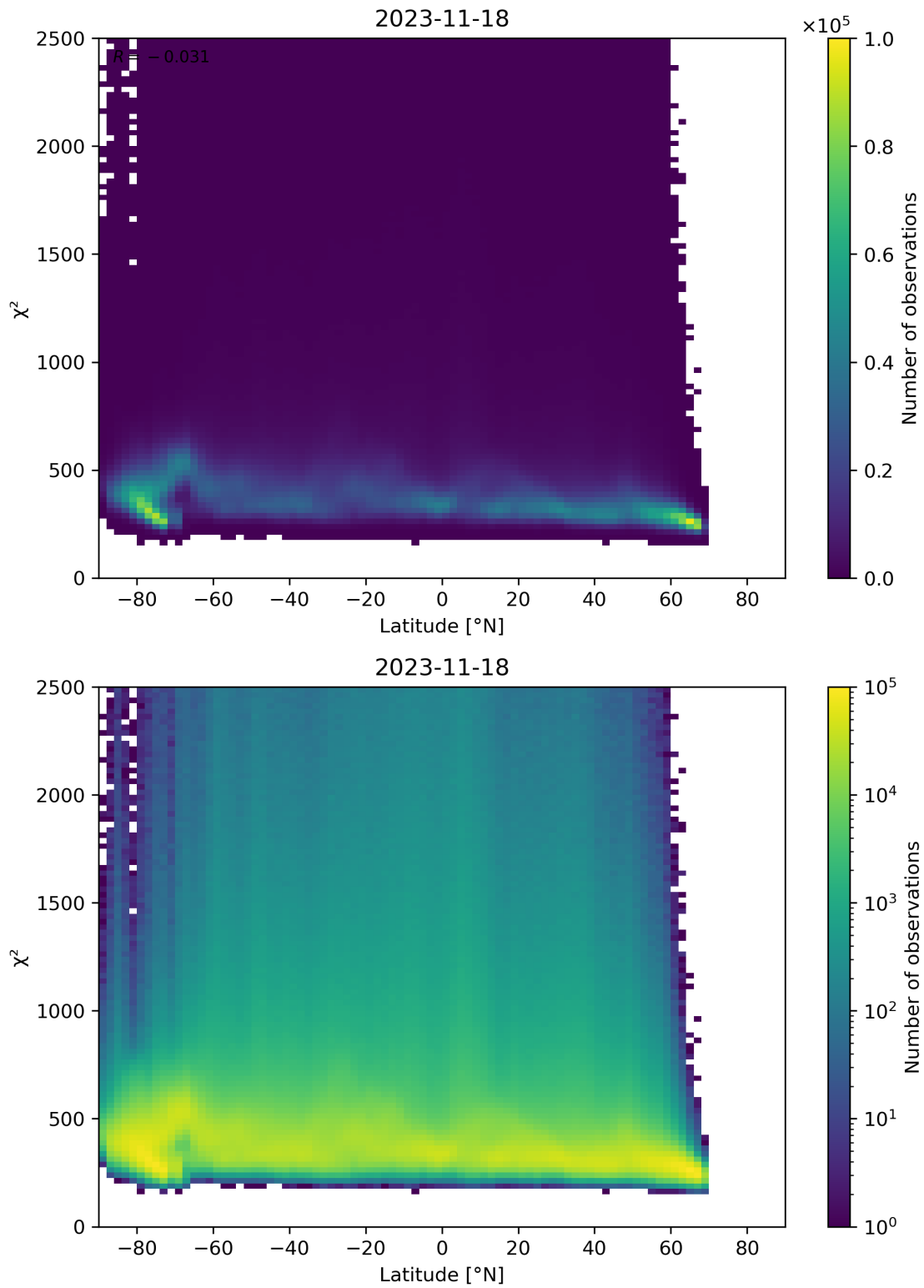
Figure 86: Scatter density plot of “Latitude” against “ \chi^2 ” for 2023-11-18 to 2023-11-19.
