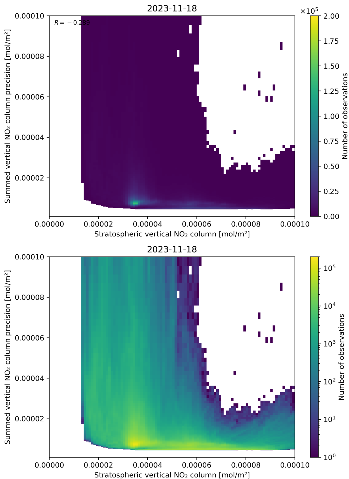
Figure 99: Scatter density plot of “Stratospheric vertical NO 2 column” against “Summed vertical NO 2 column precision” for 2023-11-18 to 2023-11-19.
