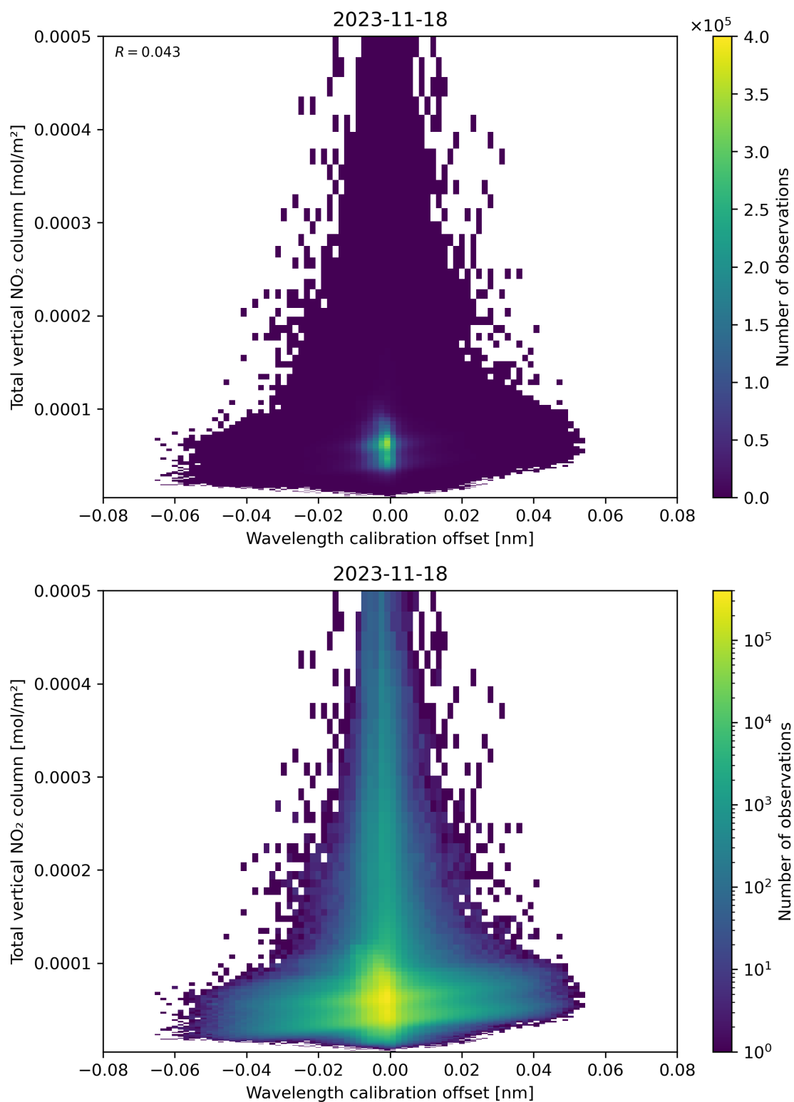
Figure 179: Scatter density plot of “Wavelength calibration offset” against “Total vertical NO 2 column” for 2023-11-18 to 2023-11-19.
