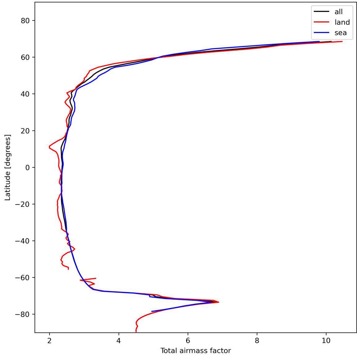
Figure 15: Zonal average of “Total airmass factor” for 2023-11-18 to 2023-11-19.
