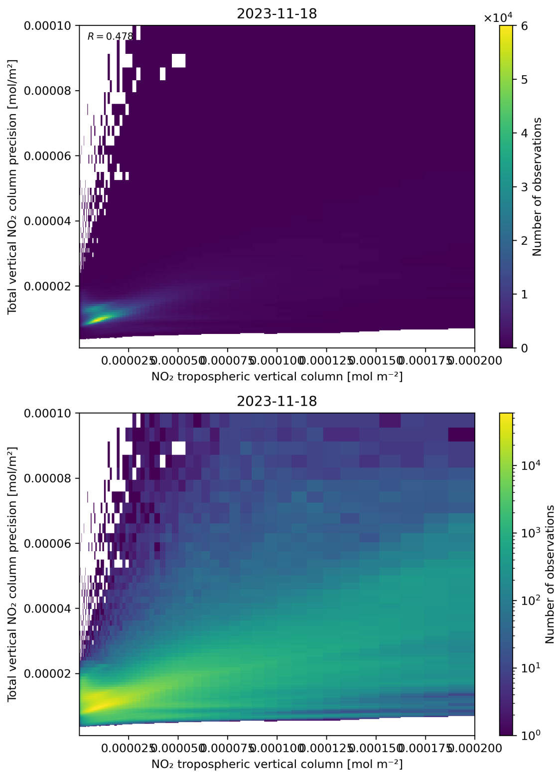
Figure 129: Scatter density plot of “NO 2 tropospheric vertical column” against “Total vertical NO 2 column precision” for 2023-11-18 to 2023-11-19.
