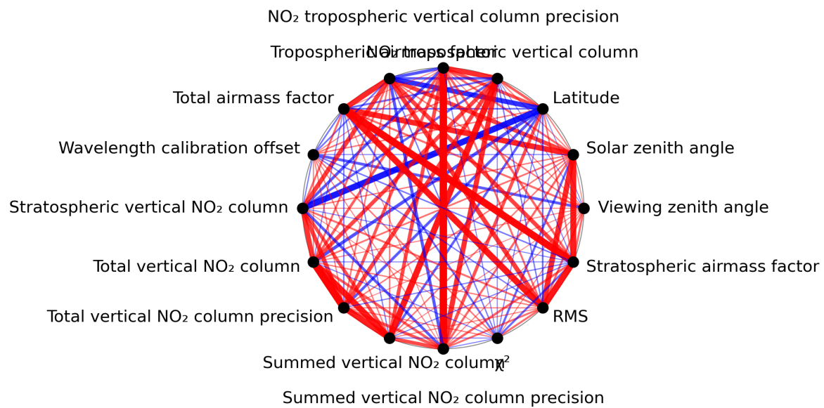
Figure 1: Map of correlation graph for 2023-11-18 to 2023-11-19.
