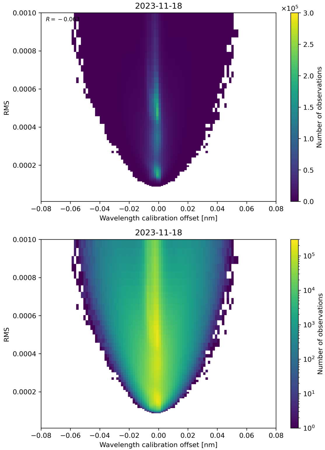
Figure 181: Scatter density plot of “Wavelength calibration offset” against “RMS” for 2023-11-18 to 2023-11-19.
