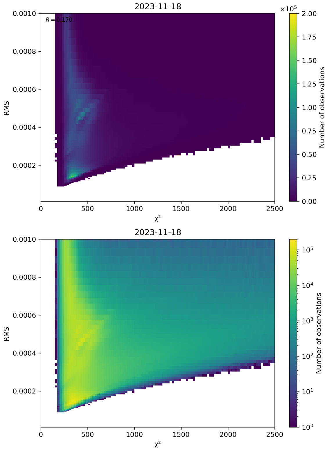
Figure 82: Scatter density plot of “ \chi^2 ” against “RMS” for 2023-11-18 to 2023-11-19.
