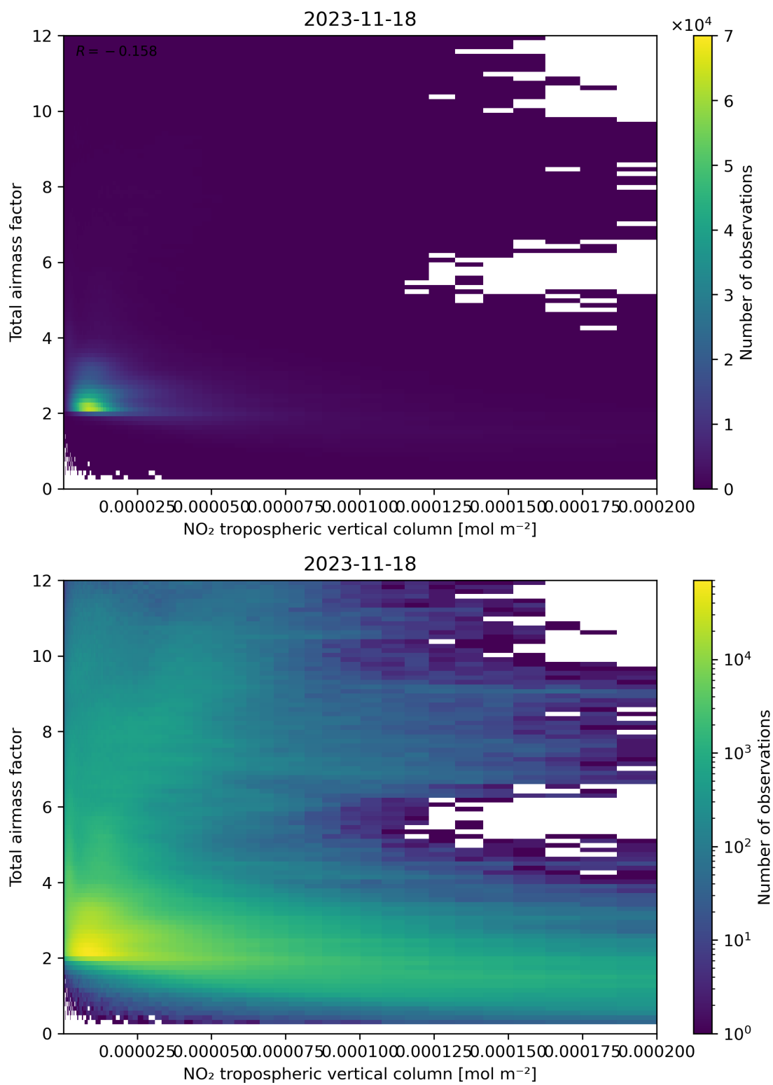
Figure 122: Scatter density plot of “NO 2 tropospheric vertical column” against “Total air mass factor” for 2023-11-18 to 2023-11-19.
