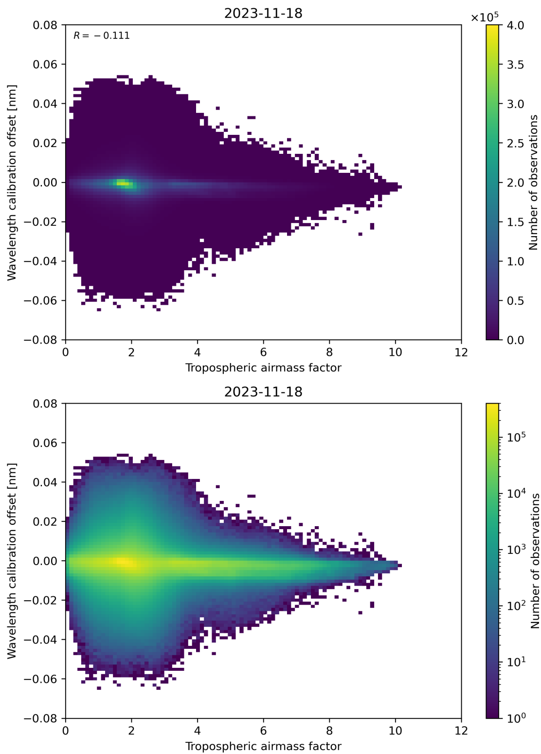
Figure 80: Scatter density plot of “Tropospheric airmass factor” against “Wavelength calibration offset” for 2023-11-18 to 2023-11-19.
