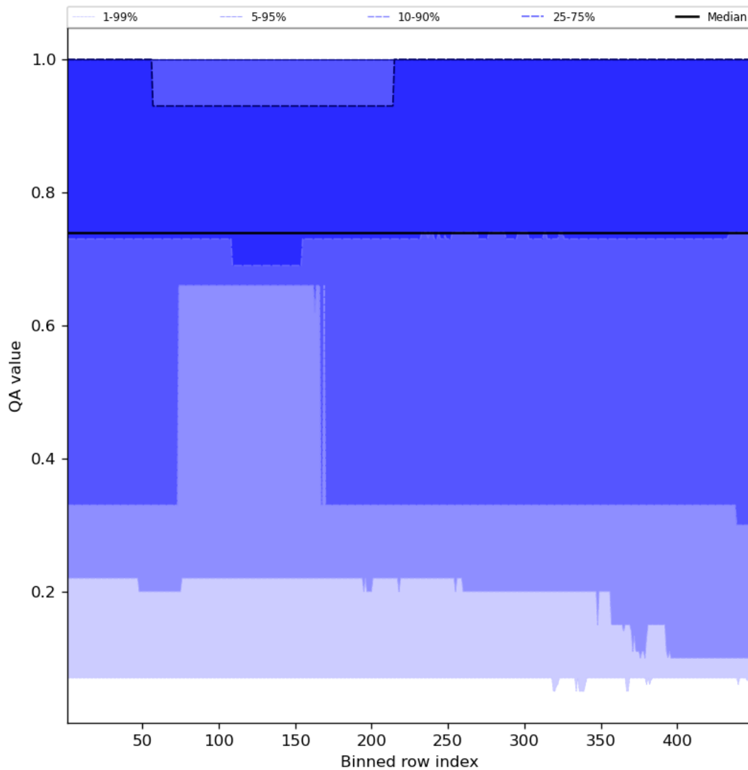
Figure 45: Along track statistics of “QA value” for 2023-11-18 to 2023-11-19
