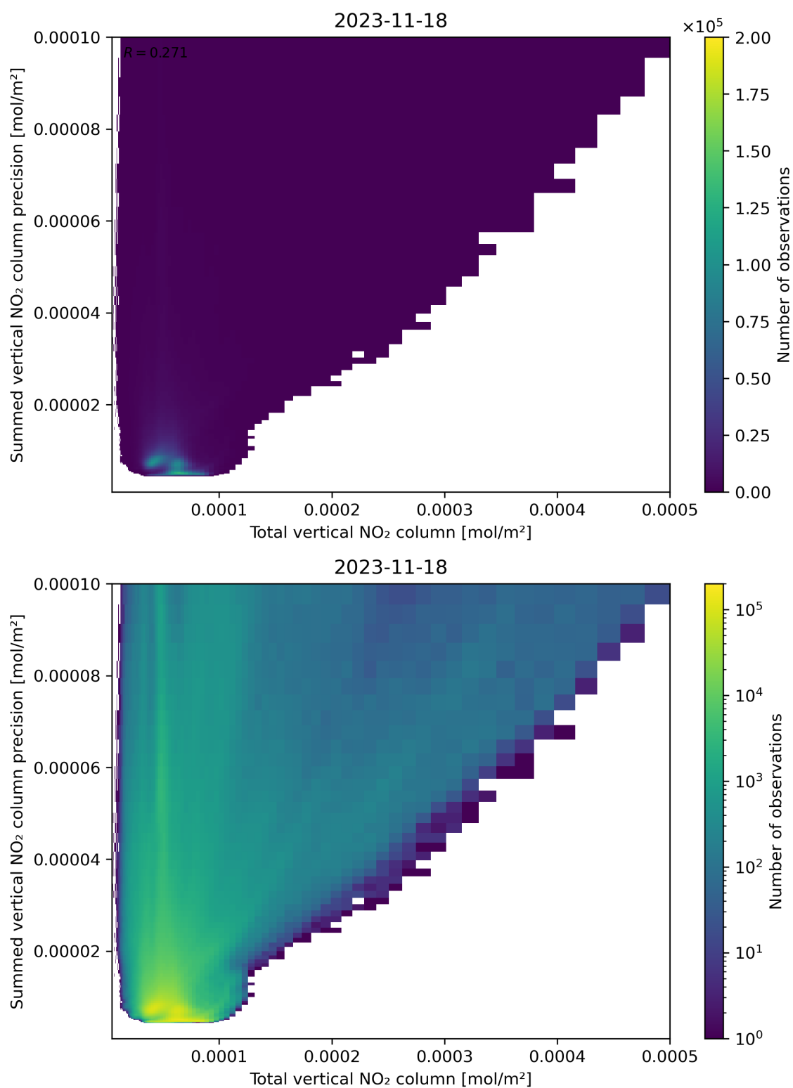
Figure 113: Scatter density plot of “Total vertical NO 2 column” against “Summed vertical NO 2 column precision” for 2023-11-18 to 2023-11-19.
