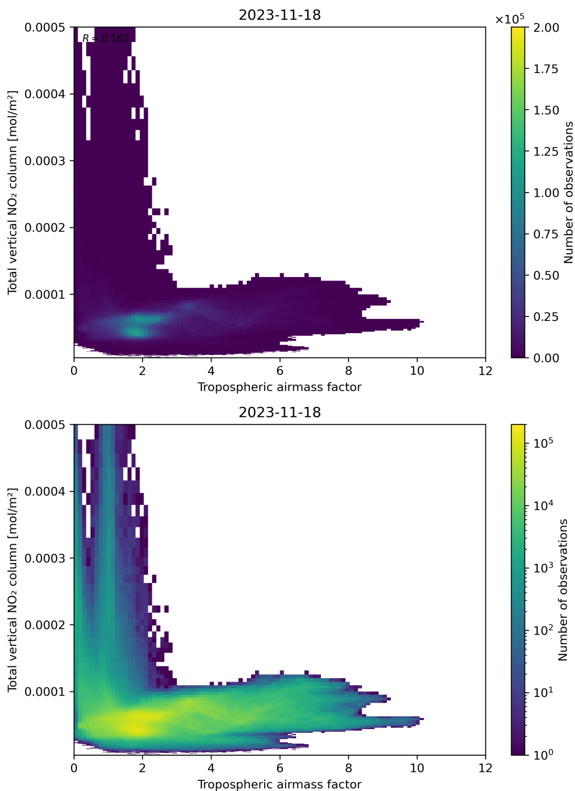
Figure 77: Scatter density plot of “Tropospheric airmass factor” against “Total vertical NO 2 column” for 2023-11-18 to 2023-11-19.
