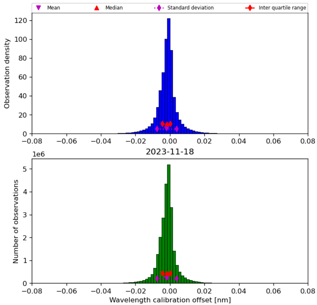
Figure 35: Histogram of “Wavelength calibration offset” for 2023-11-18 to 2023-11-19
