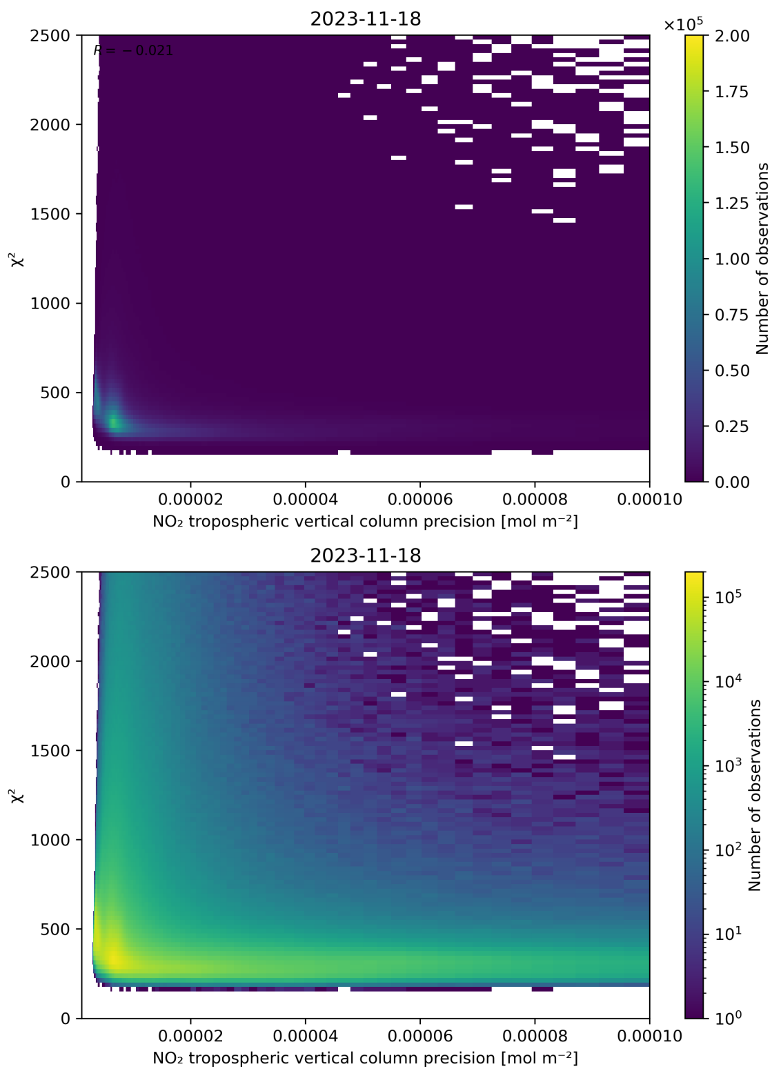
Figure 134: Scatter density plot of “NO 2 tropospheric vertical column precision” against “ \chi^2 ” for 2023-11-18 to 2023-11-19.
