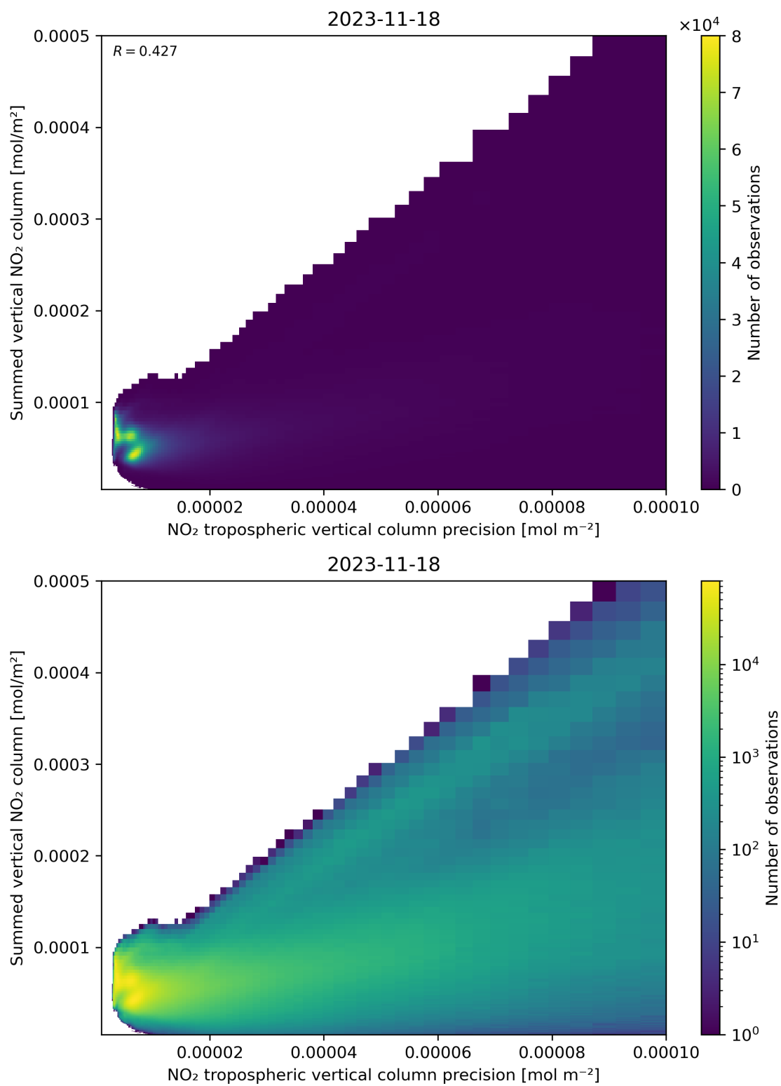
Figure 136: Scatter density plot of “NO 2 tropospheric vertical column precision” against “Summed vertical NO 2 column” for 2023-11-18 to 2023-11-19.
