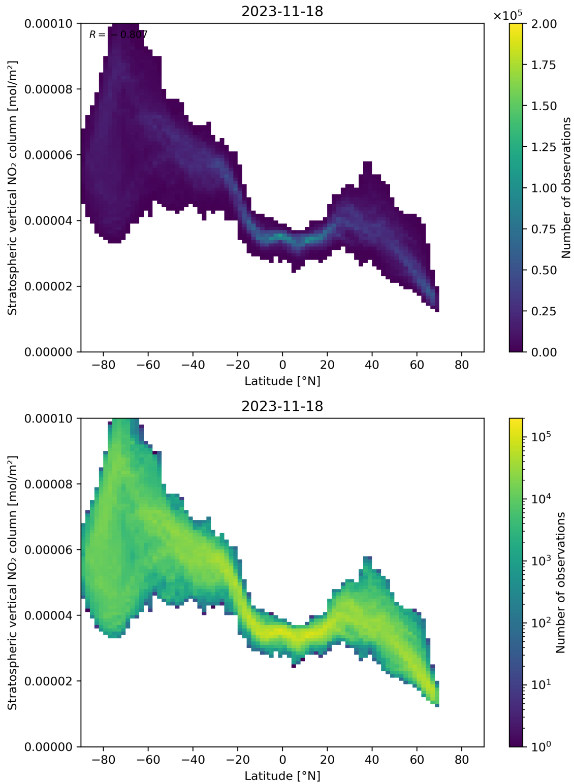
Figure 87: Scatter density plot of “Latitude” against “Stratospheric vertical NO 2 column” for 2023-11-18 to 2023-11-19.
