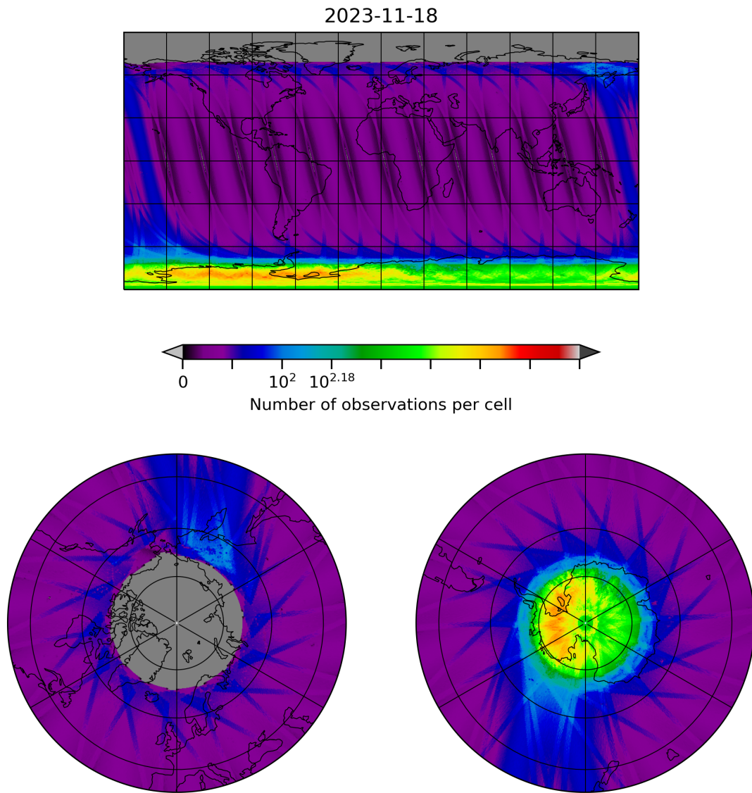
Figure 10: Map of the number of observations for 2023-11-18 to 2023-11-19
