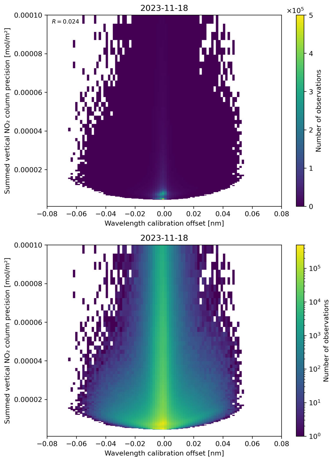
Figure 178: Scatter density plot of “Wavelength calibration offset” against “Summed vertical NO 2 column precision” for 2023-11-18 to 2023-11-19.
