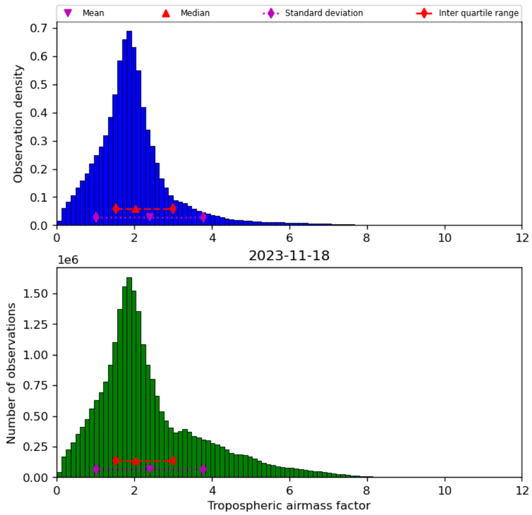
Figure 31: Histogram of “Tropospheric airmass factor” for 2023-11-18 to 2023-11-19
