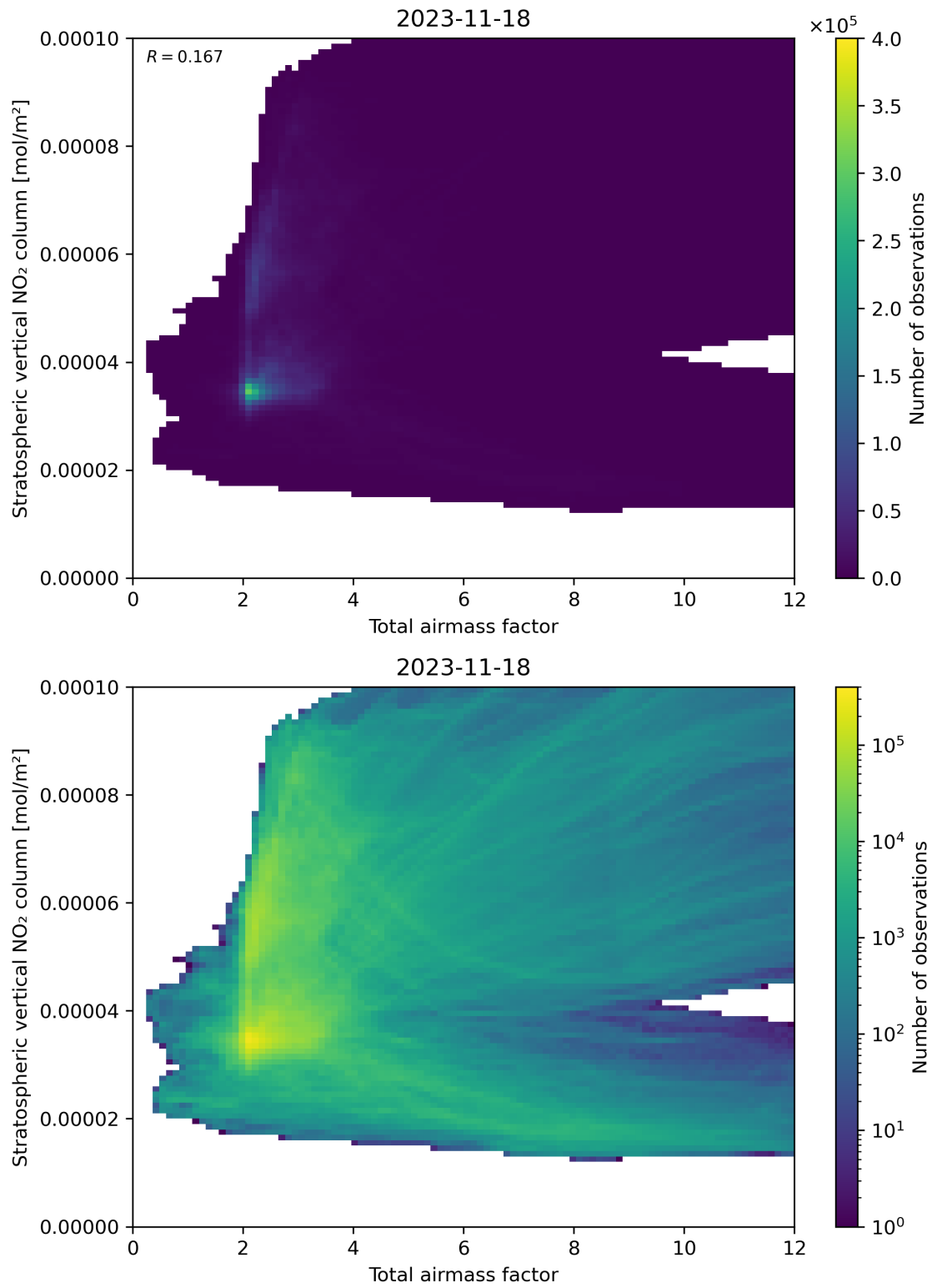
Figure 64: Scatter density plot of “Total airmass factor” against “Stratospheric vertical NO 2 column” for 2023-11-18 to 2023-11-19.
