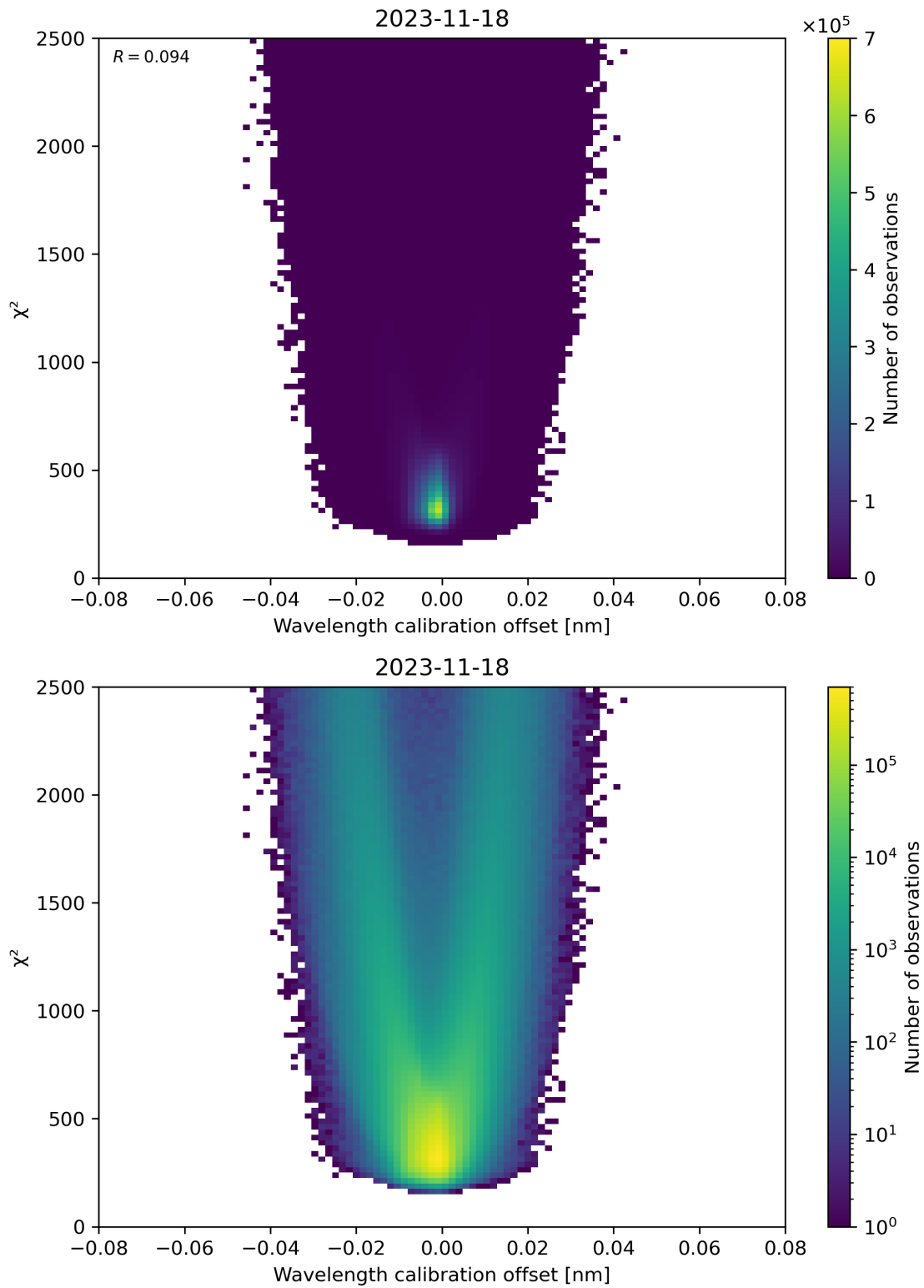
Figure 175: Scatter density plot of “Wavelength calibration offset” against “ \chi^2 ” for 2023-11-18 to 2023-11-19.
