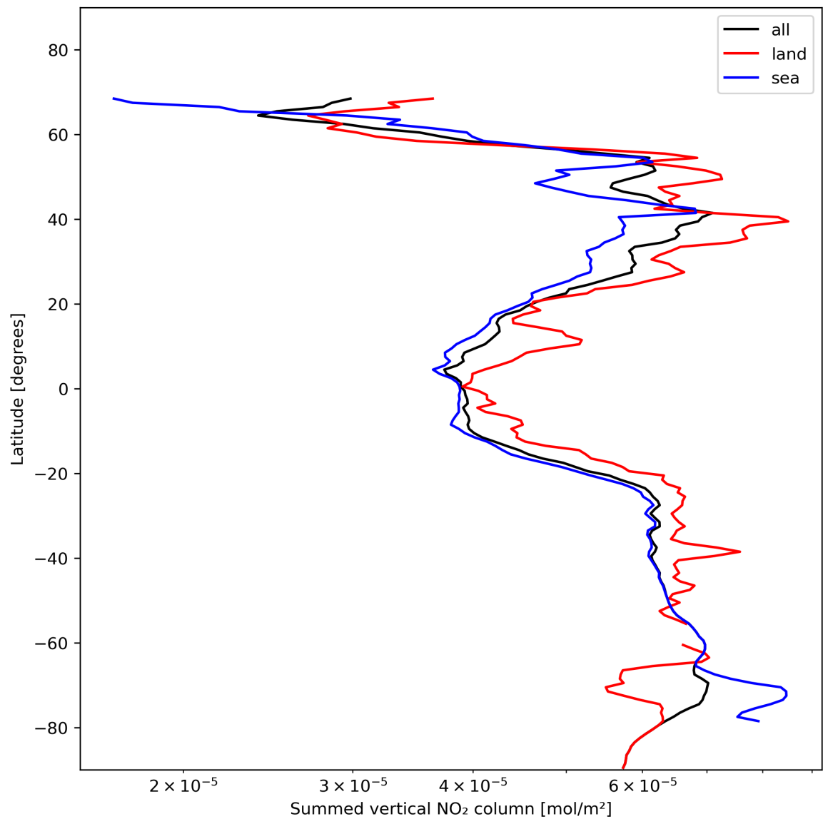
Figure 23: Zonal average of “Summed vertical NO 2 column” for 2023-11-18 to 2023-11-19.
