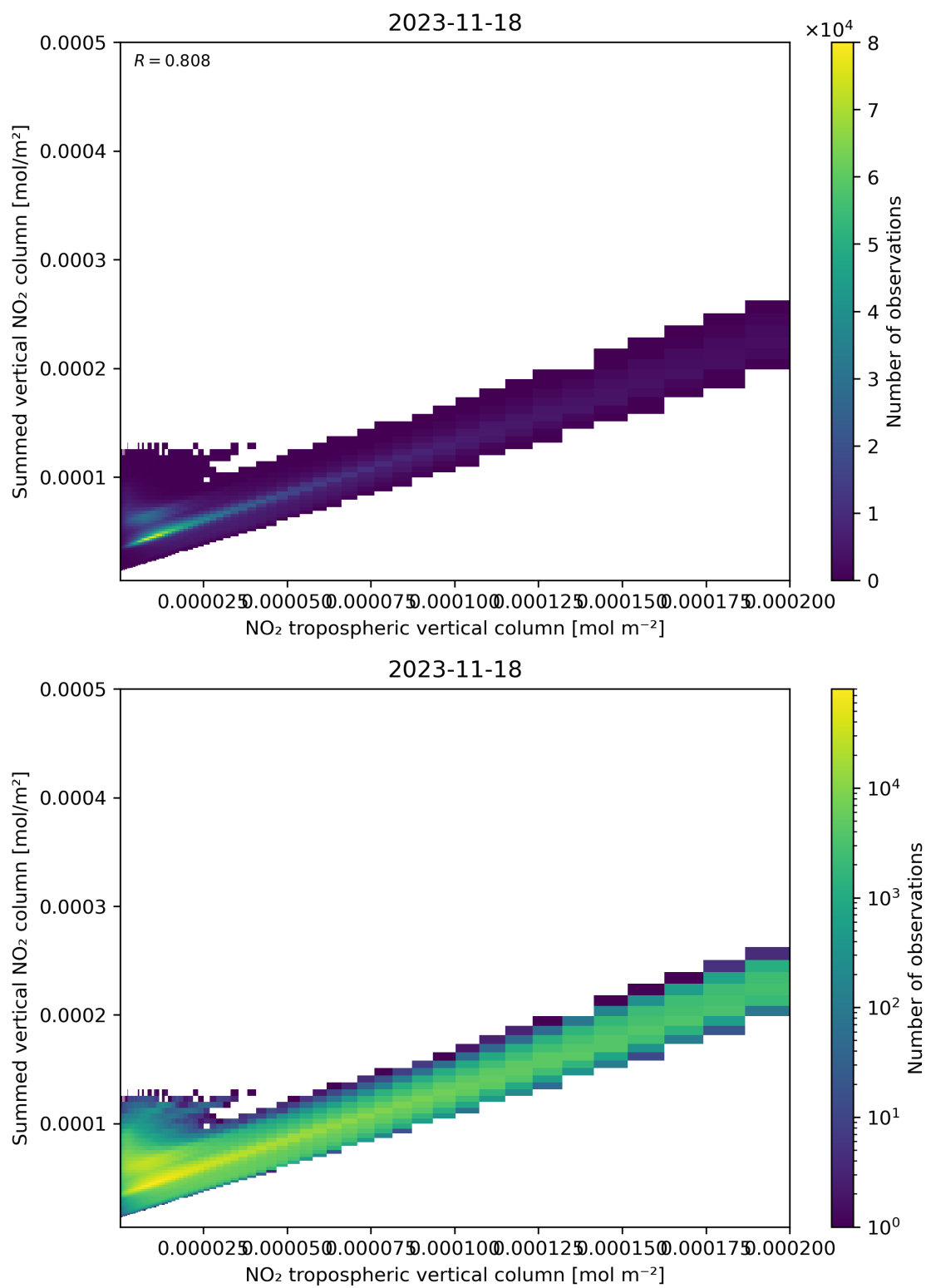
Figure 126: Scatter density plot of “NO 2 tropospheric vertical column” against “Summed vertical NO 2 column” for 2023-11-18 to 2023-11-19.
