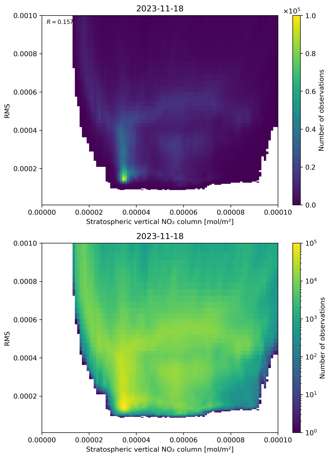
Figure 102: Scatter density plot of “Stratospheric vertical NO 2 column” against “RMS” for 2023-11-18 to 2023-11-19.
