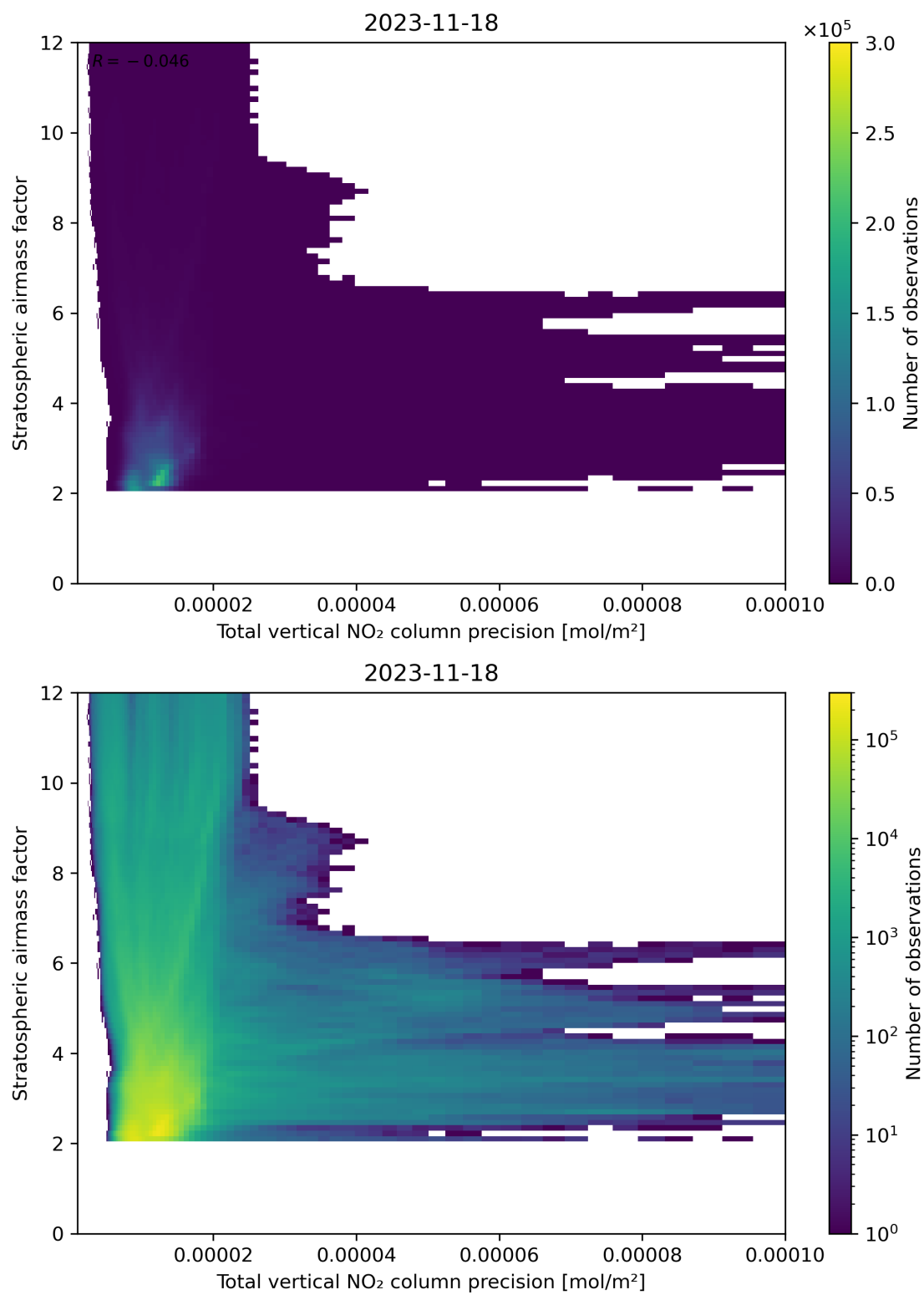
Figure 115: Scatter density plot of “Total vertical NO 2 column precision” against “Stratospheric air mass factor” for 2023-11-18 to 2023-11-19.
