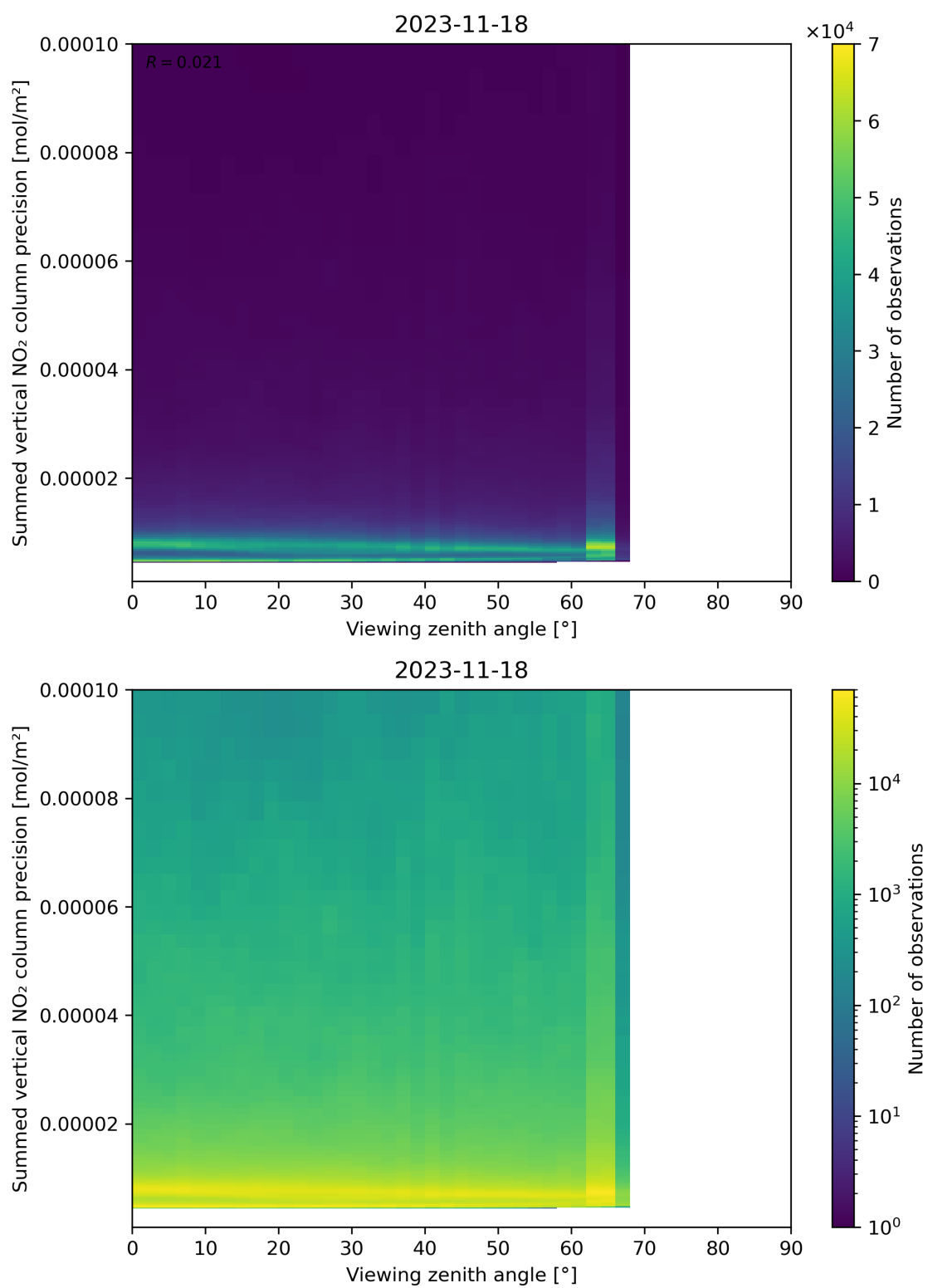
Figure 166: Scatter density plot of “Viewing zenith angle” against “Summed vertical NO 2 column precision” for 2023-11-18 to 2023-11-19.
