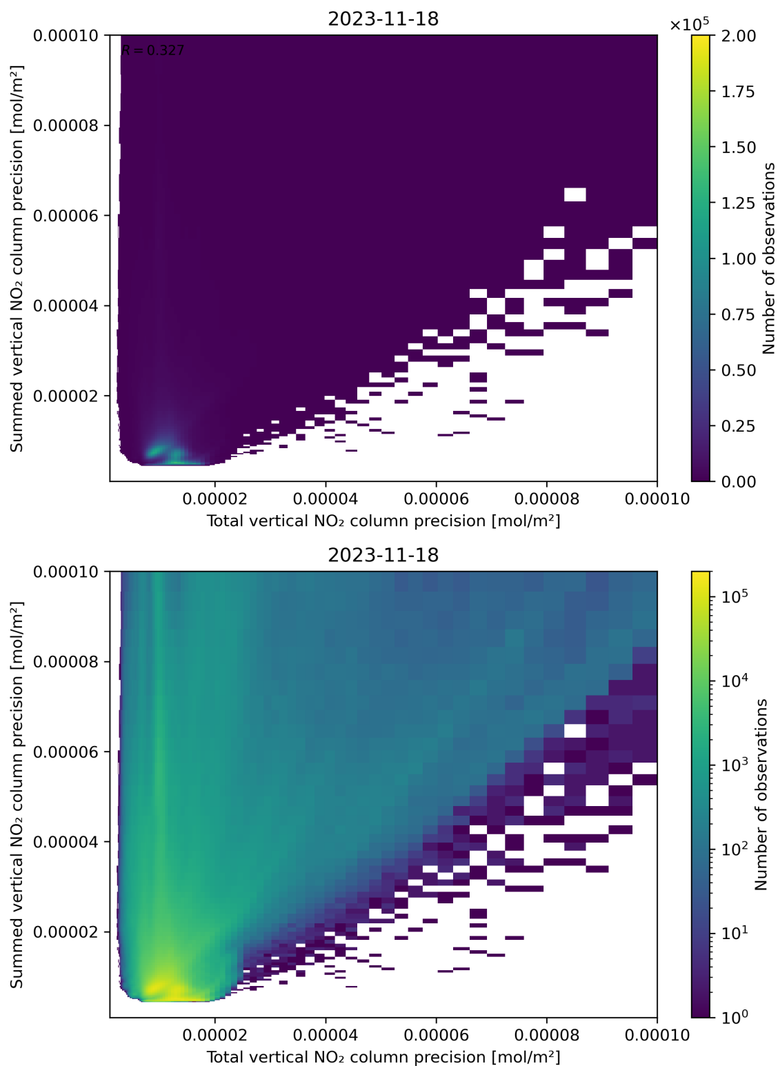
Figure 118: Scatter density plot of “Total vertical NO 2 column precision” against “Summed vertical NO 2 column precision” for 2023-11-18 to 2023-11-19.
