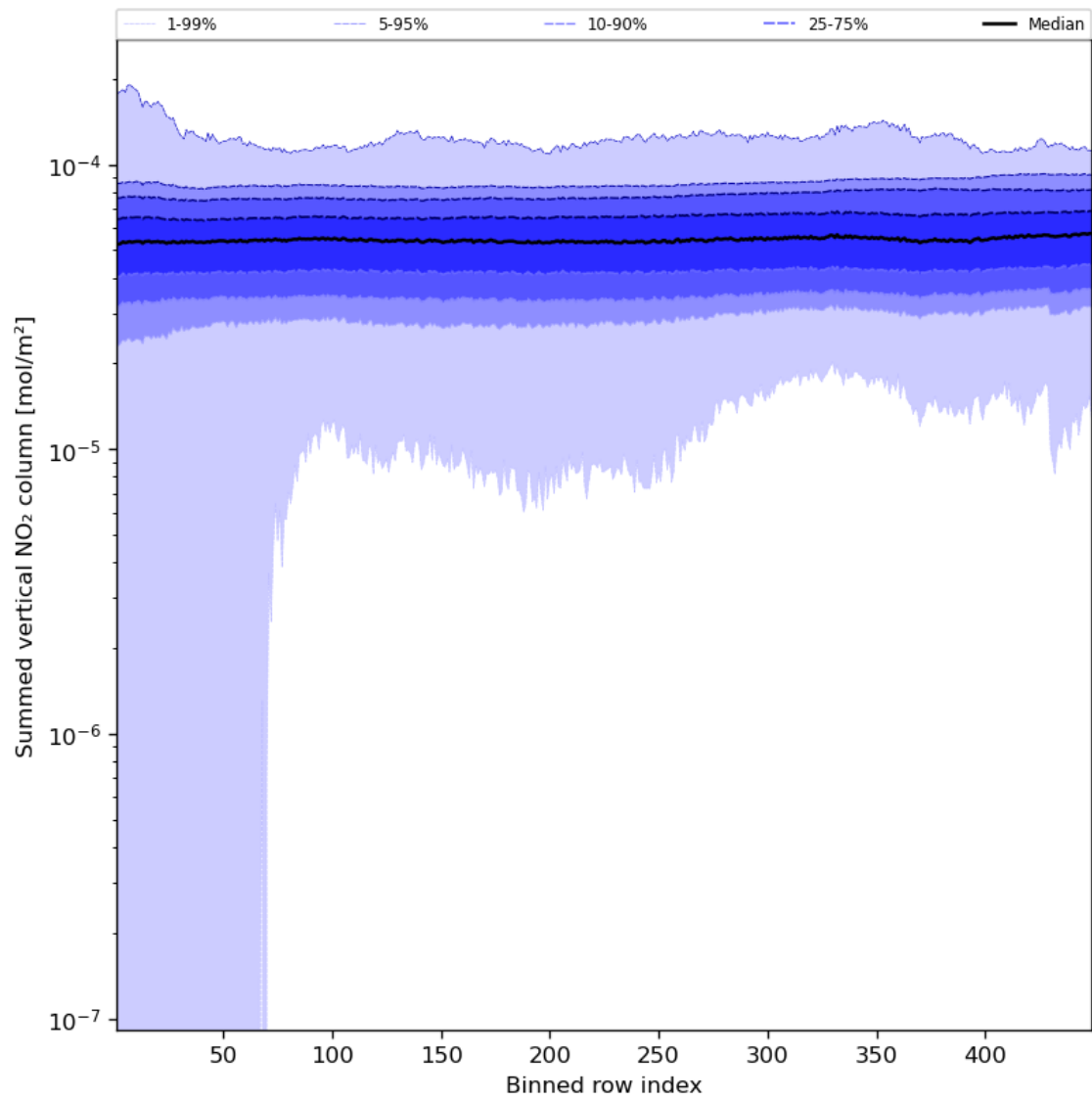
Figure 57: Along track statistics of “Summed vertical NO 2 column” for 2023-11-18 to 2023-11-19
