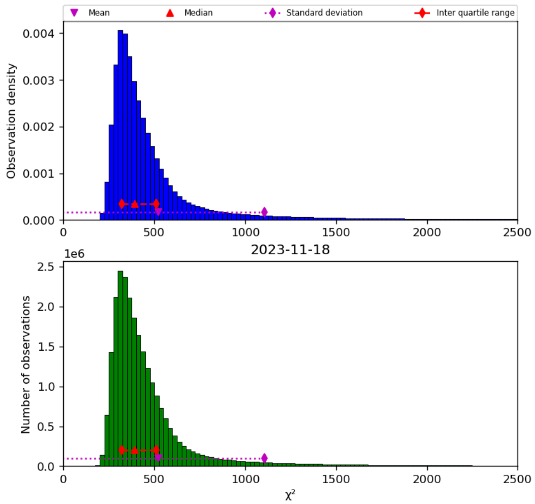
Figure 42: Histogram of “ \chi^2 ” for 2023-11-18 to 2023-11-19
