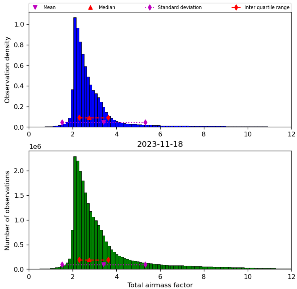
Figure 32: Histogram of “Total airmass factor” for 2023-11-18 to 2023-11-19
