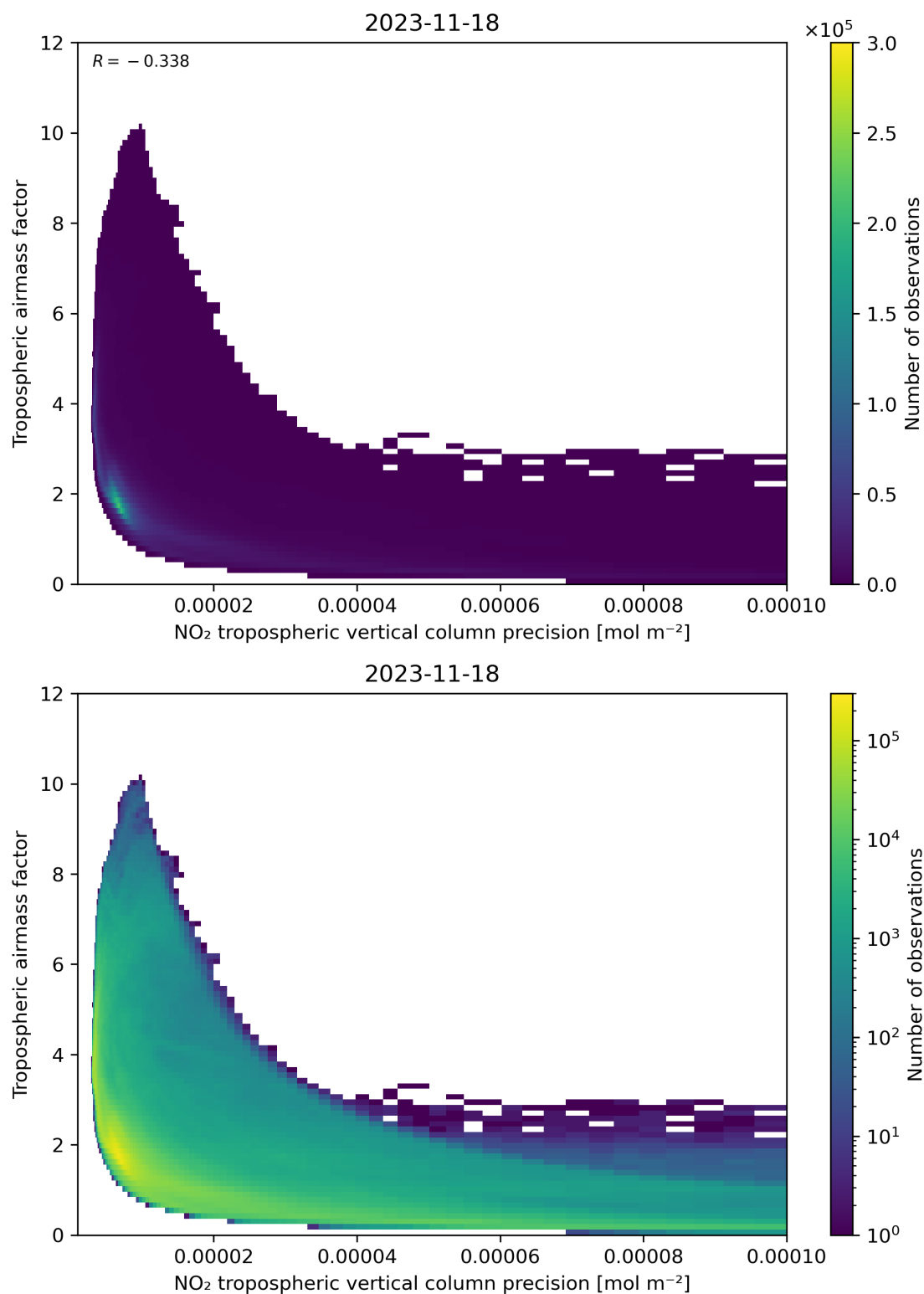
Figure 133: Scatter density plot of “NO 2 tropospheric vertical column precision” against “Tropospheric airmass factor” for 2023-11-18 to 2023-11-19.
