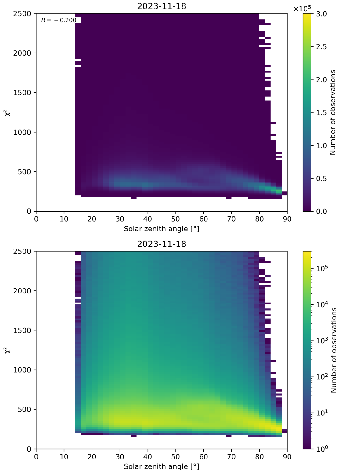
Figure 148: Scatter density plot of “Solar zenith angle” against “ \chi^2 ” for 2023-11-18 to 2023-11-19.
