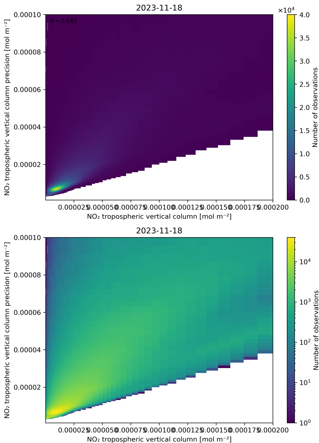
Figure 130: Scatter density plot of “NO 2 tropospheric vertical column” against “NO 2 tropospheric vertical column precision” for 2023-11-18 to 2023-11-19.
