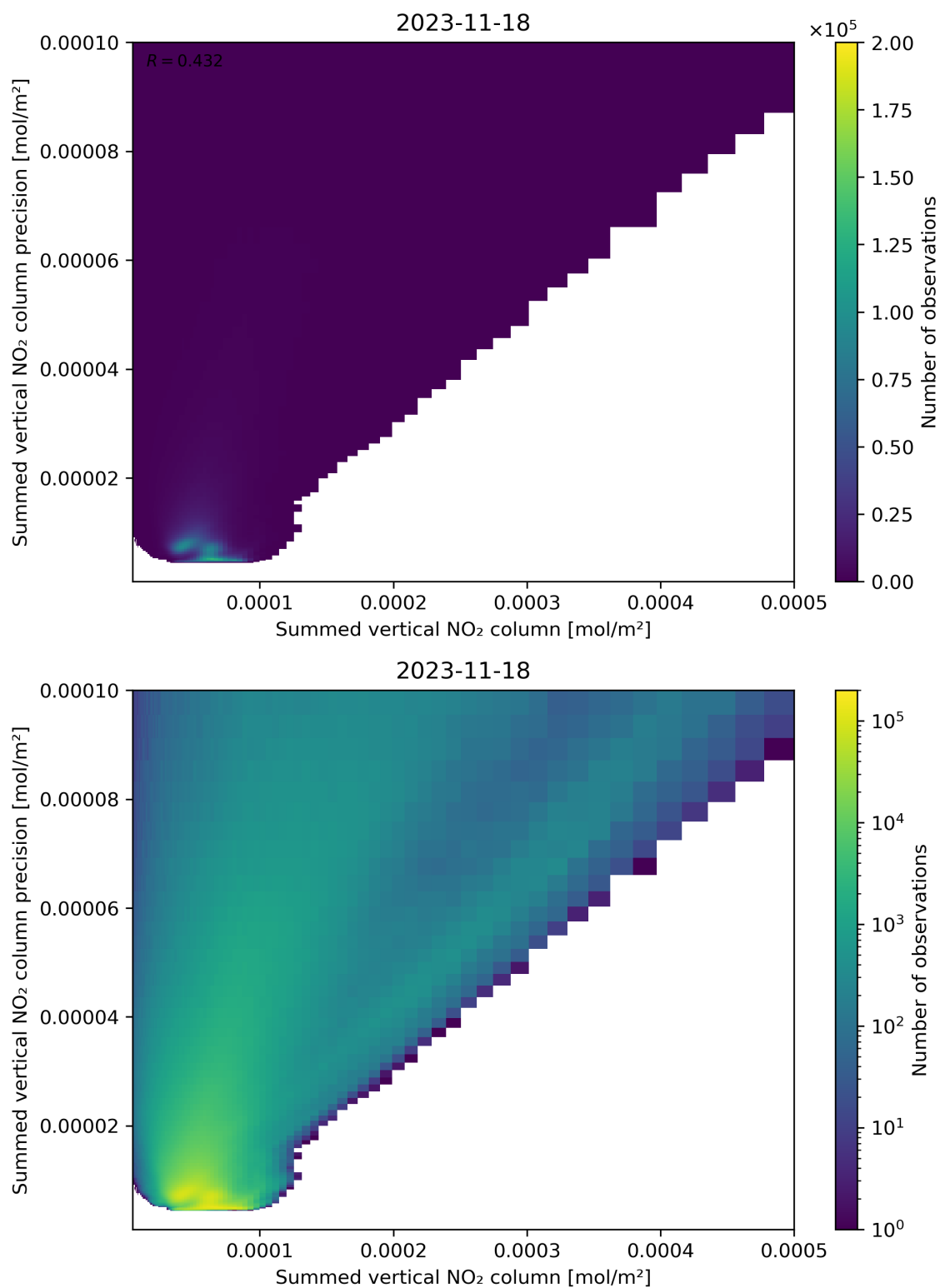
Figure 105: Scatter density plot of “Summed vertical NO 2 column” against “Summed vertical NO 2 column precision” for 2023-11-18 to 2023-11-19.
