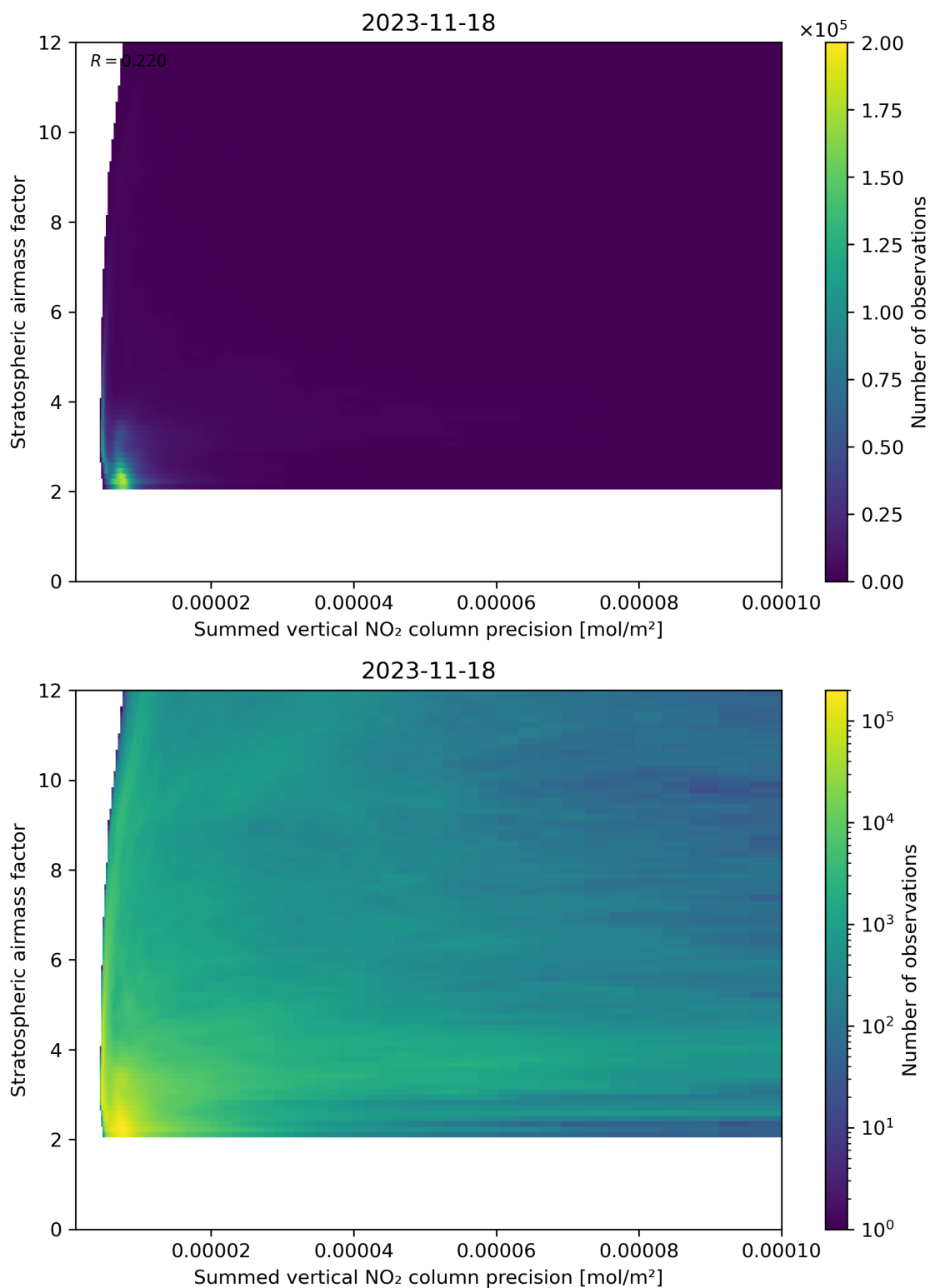
Figure 106: Scatter density plot of “Summed vertical NO 2 column precision” against “Stratospheric airmass factor” for 2023-11-18 to 2023-11-19.
