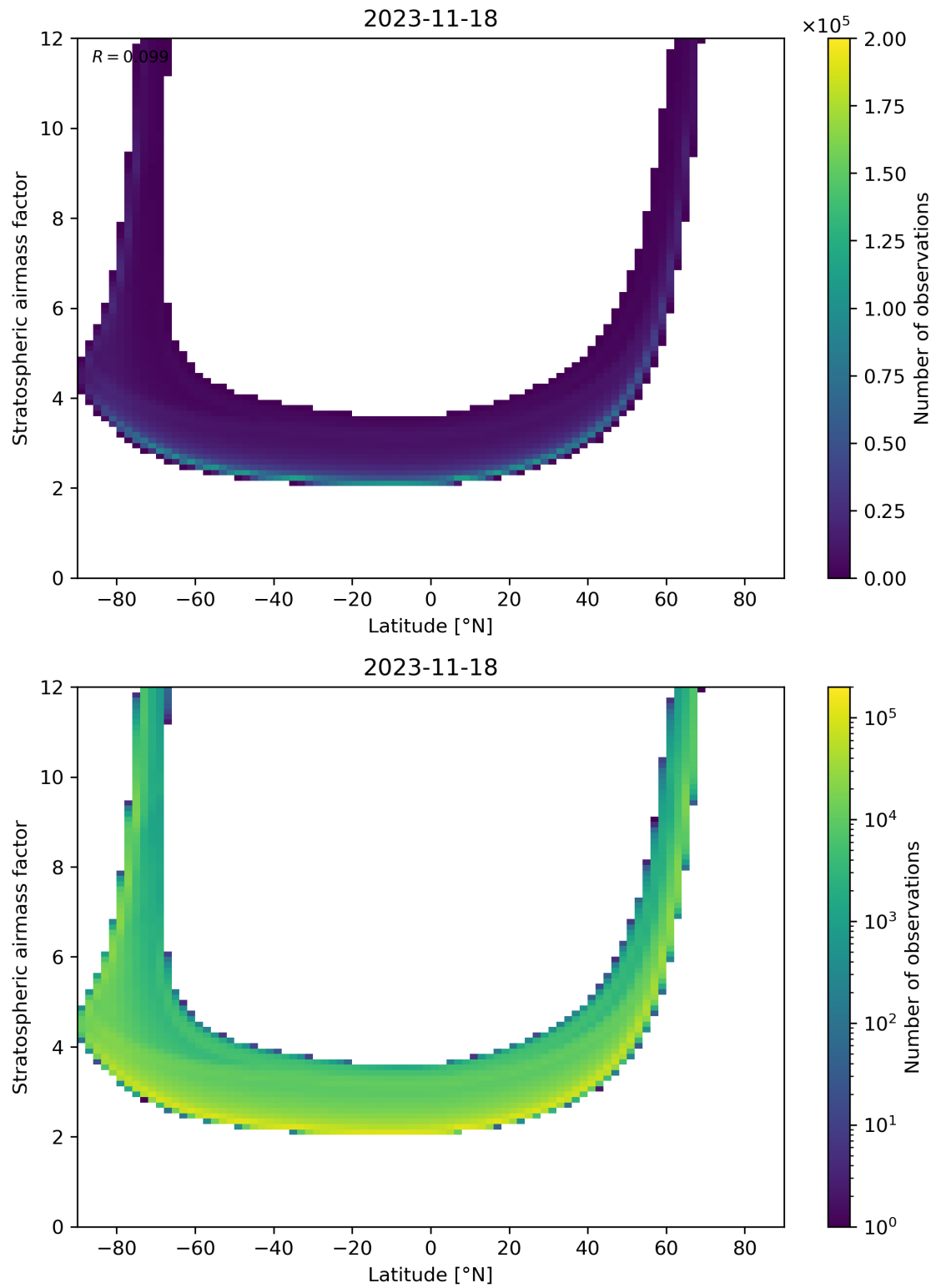
Figure 83: Scatter density plot of “Latitude” against “Stratospheric air mass factor” for 2023-11-18 to 2023-11-19.
