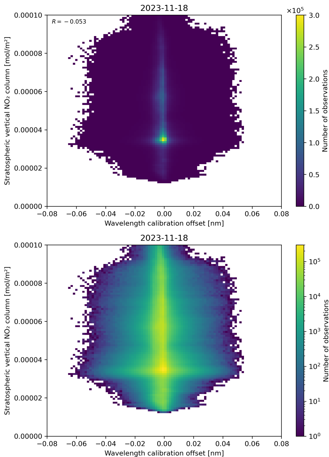
Figure 176: Scatter density plot of “Wavelength calibration offset” against “Stratospheric vertical NO 2 column” for 2023-11-18 to 2023-11-19.
