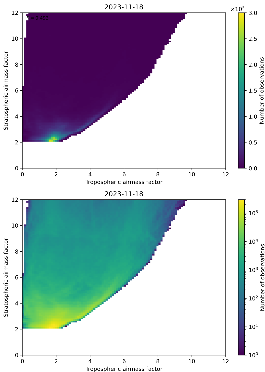
Figure 71: Scatter density plot of “Tropospheric airmass factor” against “Stratospheric airmass factor” for 2023-11-18 to 2023-11-19.
