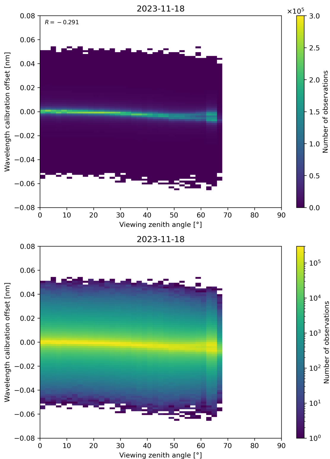
Figure 173: Scatter density plot of “Viewing zenith angle” against “Wavelength calibration offset” for 2023-11-18 to 2023-11-19.
