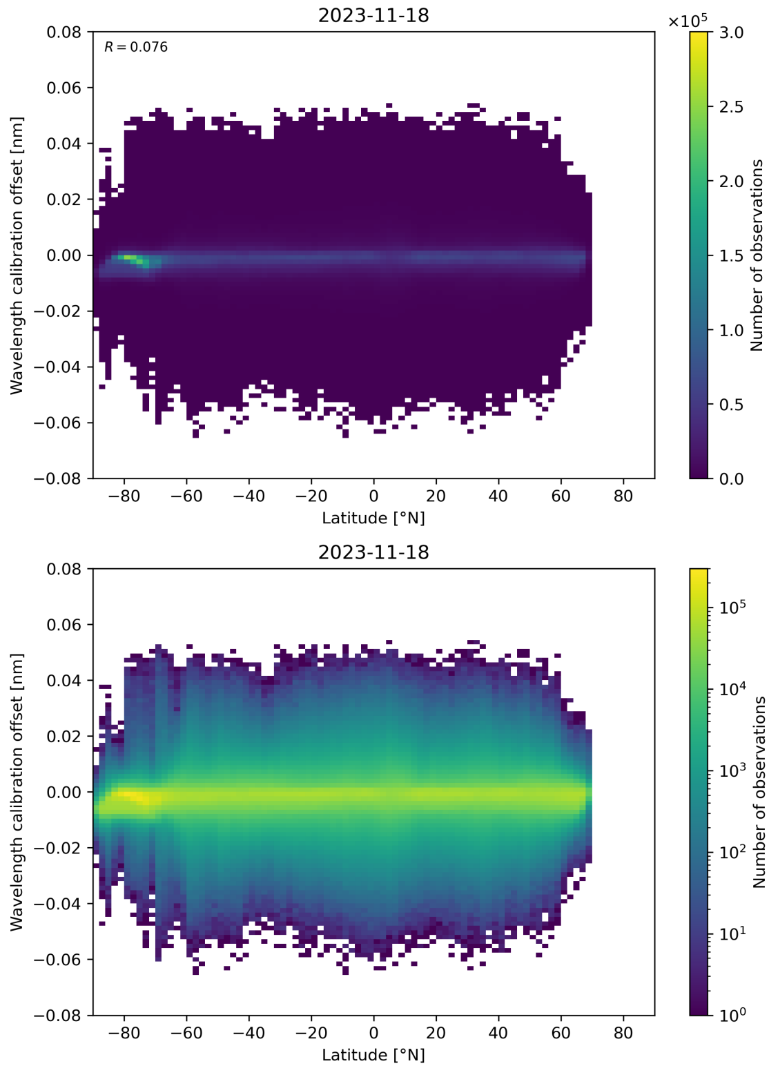
Figure 95: Scatter density plot of “Latitude” against “Wavelength calibration offset” for 2023-11-18 to 2023-11-19.
