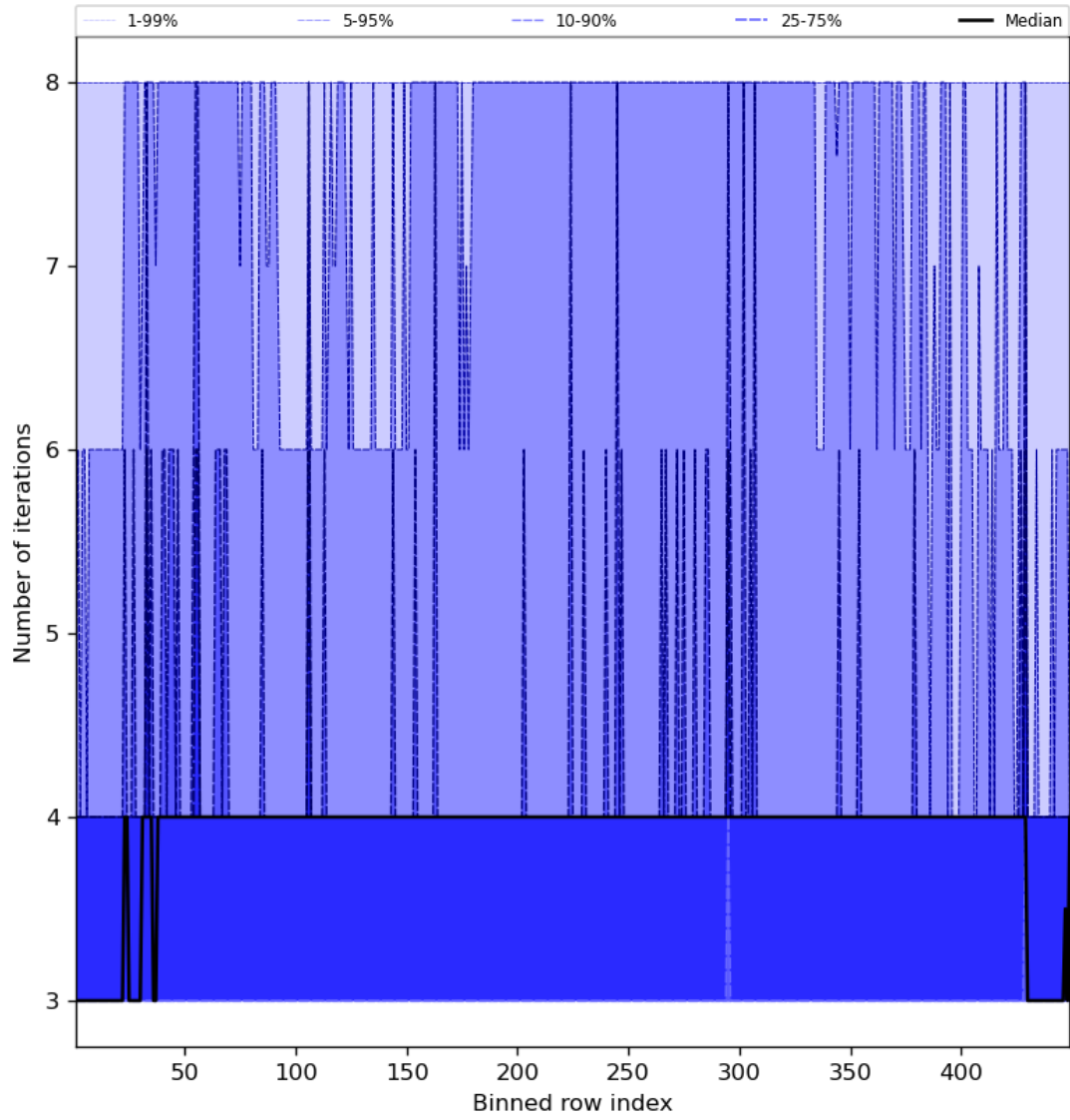
Figure 51: Along track statistics of “Number of iterations” for 2023-11-18 to 2023-11-19
