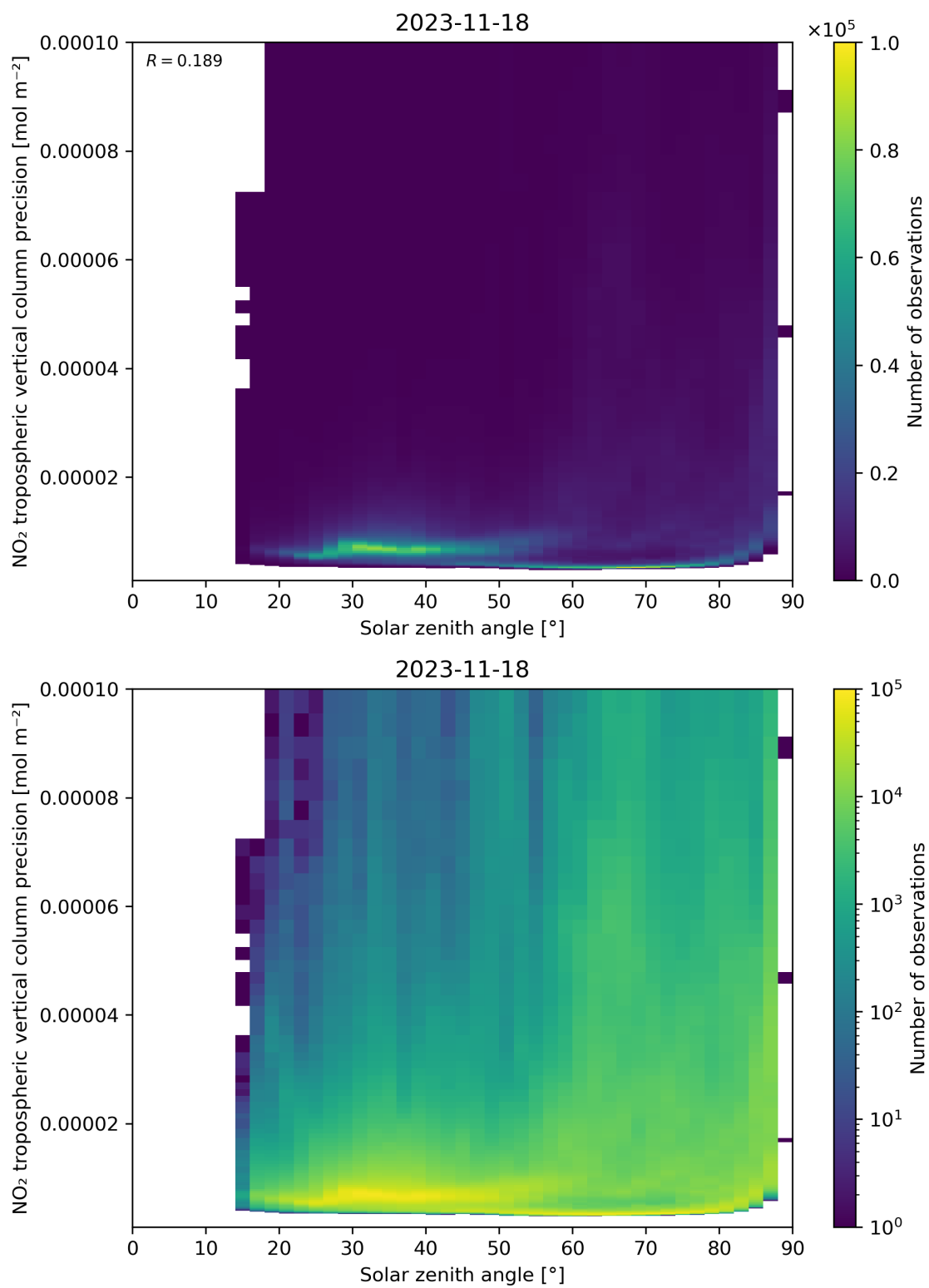
Figure 156: Scatter density plot of “Solar zenith angle” against “NO 2 tropospheric vertical column precision” for 2023-11-18 to 2023-11-19.
