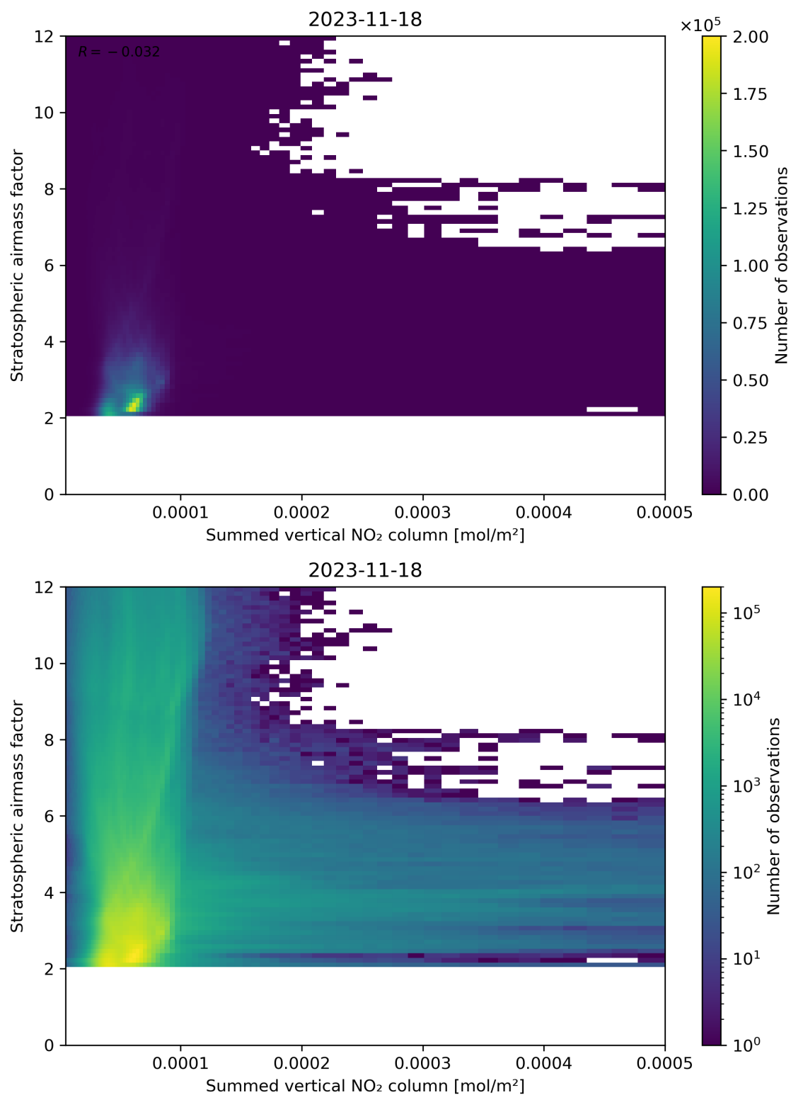
Figure 103: Scatter density plot of “Summed vertical NO 2 column” against “Stratospheric air mass factor” for 2023-11-18 to 2023-11-19.
