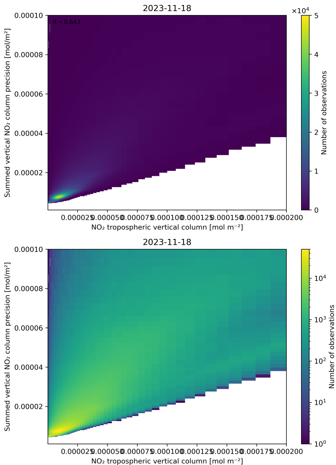
Figure 127: Scatter density plot of “NO 2 tropospheric vertical column” against “Summed vertical NO 2 column precision” for 2023-11-18 to 2023-11-19.
