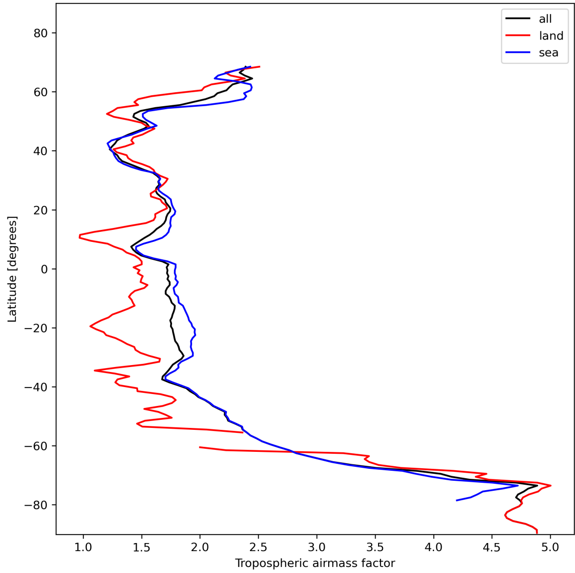
Figure 14: Zonal average of “Tropospheric airmass factor” for 2023-11-18 to 2023-11-19.
