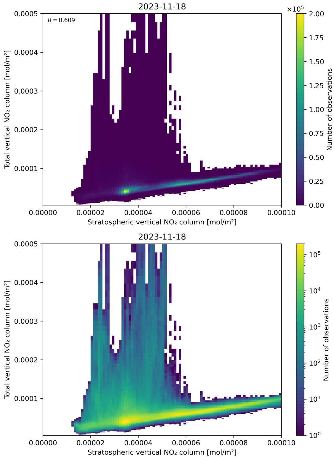
Figure 100: Scatter density plot of “Stratospheric vertical NO 2 column” against “Total vertical NO 2 column” for 2023-11-18 to 2023-11-19.
