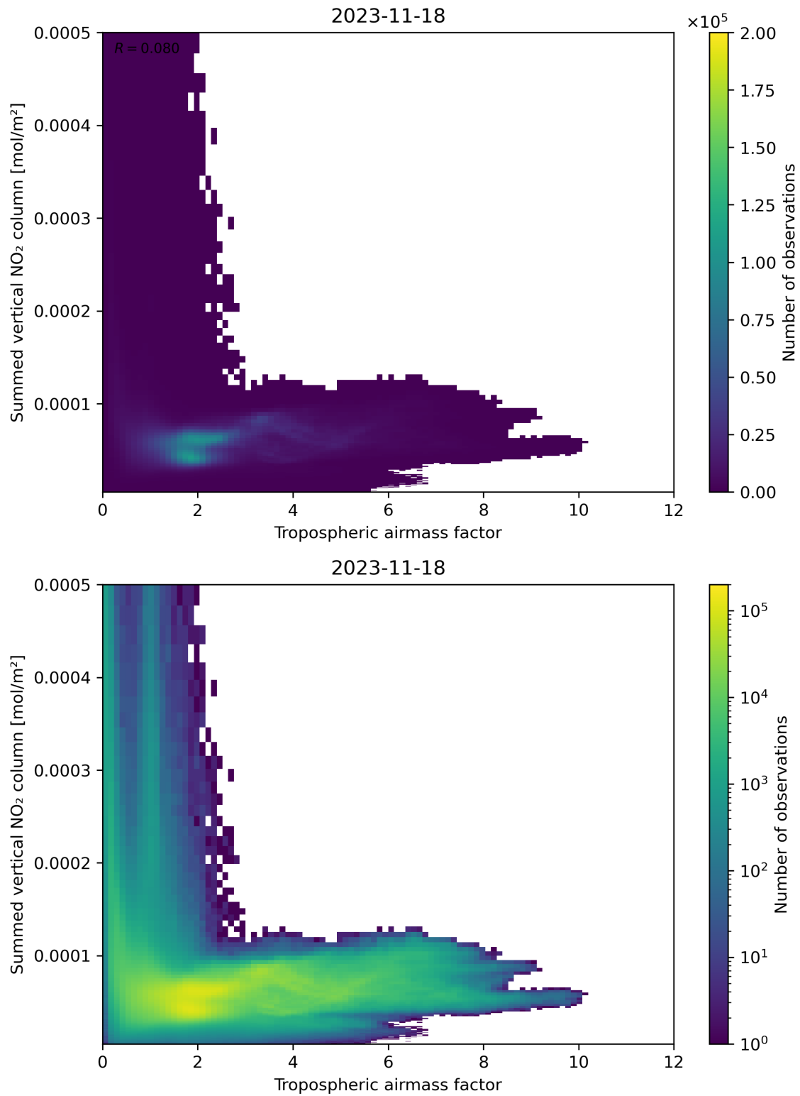
Figure 75: Scatter density plot of “Tropospheric airmass factor” against “Summed vertical NO 2 column” for 2023-11-18 to 2023-11-19.
