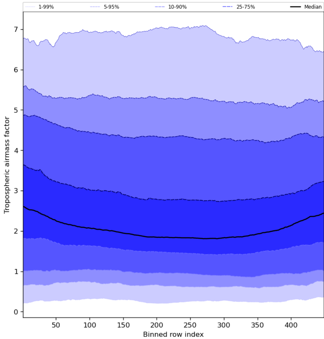
Figure 48: Along track statistics of “Tropospheric airmass factor” for 2023-11-18 to 2023-11-19
