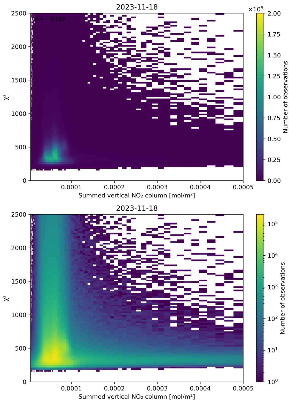
Figure 104: Scatter density plot of “Summed vertical NO 2 column” against “ \chi^2 ” for 2023-11-18 to 2023-11-19.
