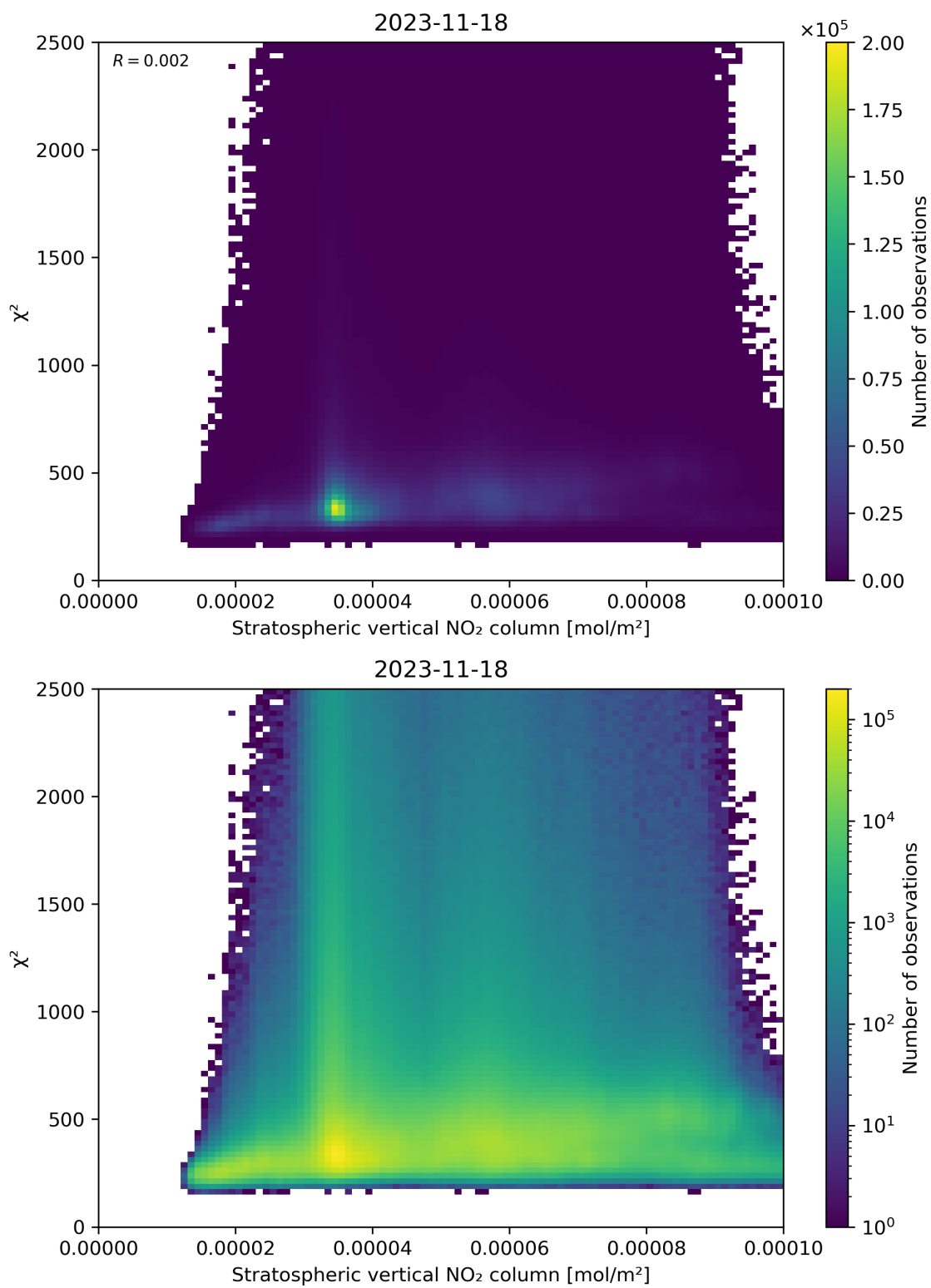
Figure 97: Scatter density plot of “Stratospheric vertical NO 2 column” against “ \chi^2 ” for 2023-11-18 to 2023-11-19.
