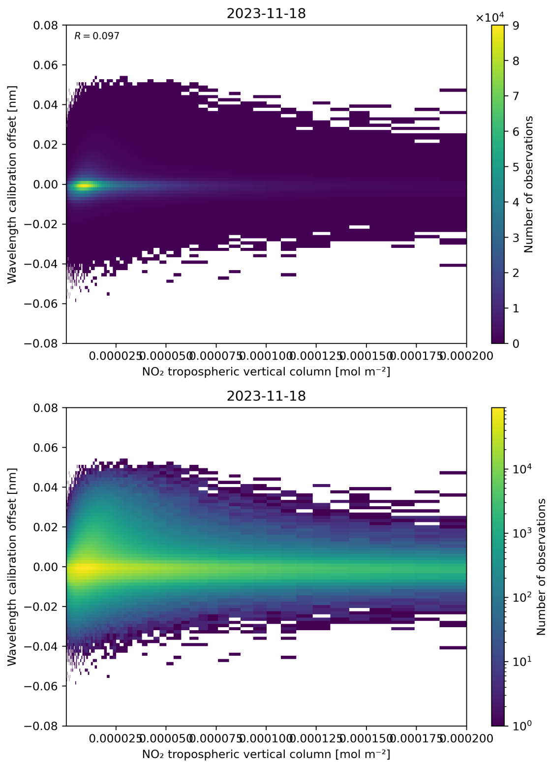
Figure 143: Scatter density plot of “NO 2 tropospheric vertical column” against “Wavelength calibration offset” for 2023-11-18 to 2023-11-19.
