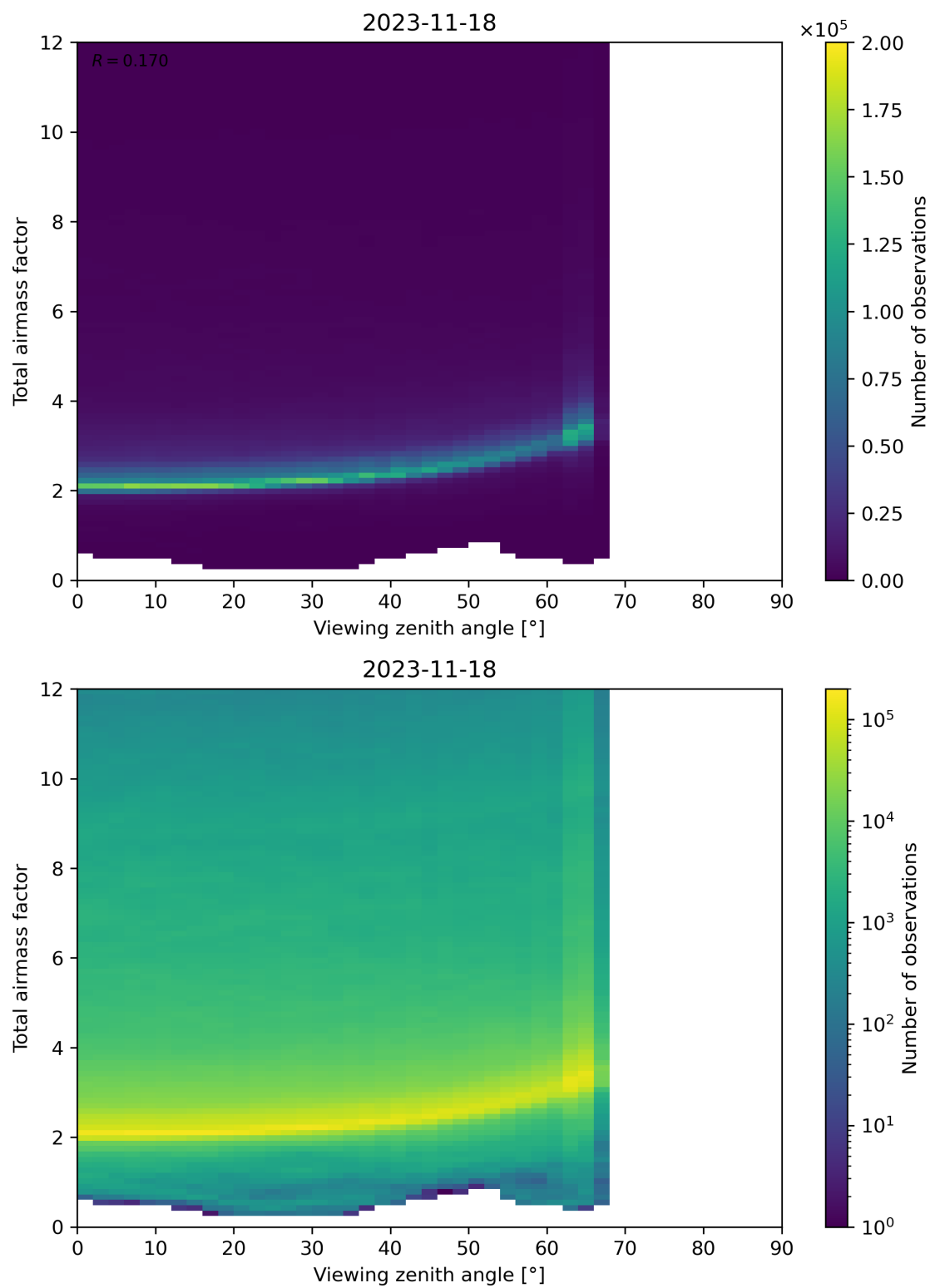
Figure 160: Scatter density plot of “Viewing zenith angle” against “Total airmass factor” for 2023-11-18 to 2023-11-19.
