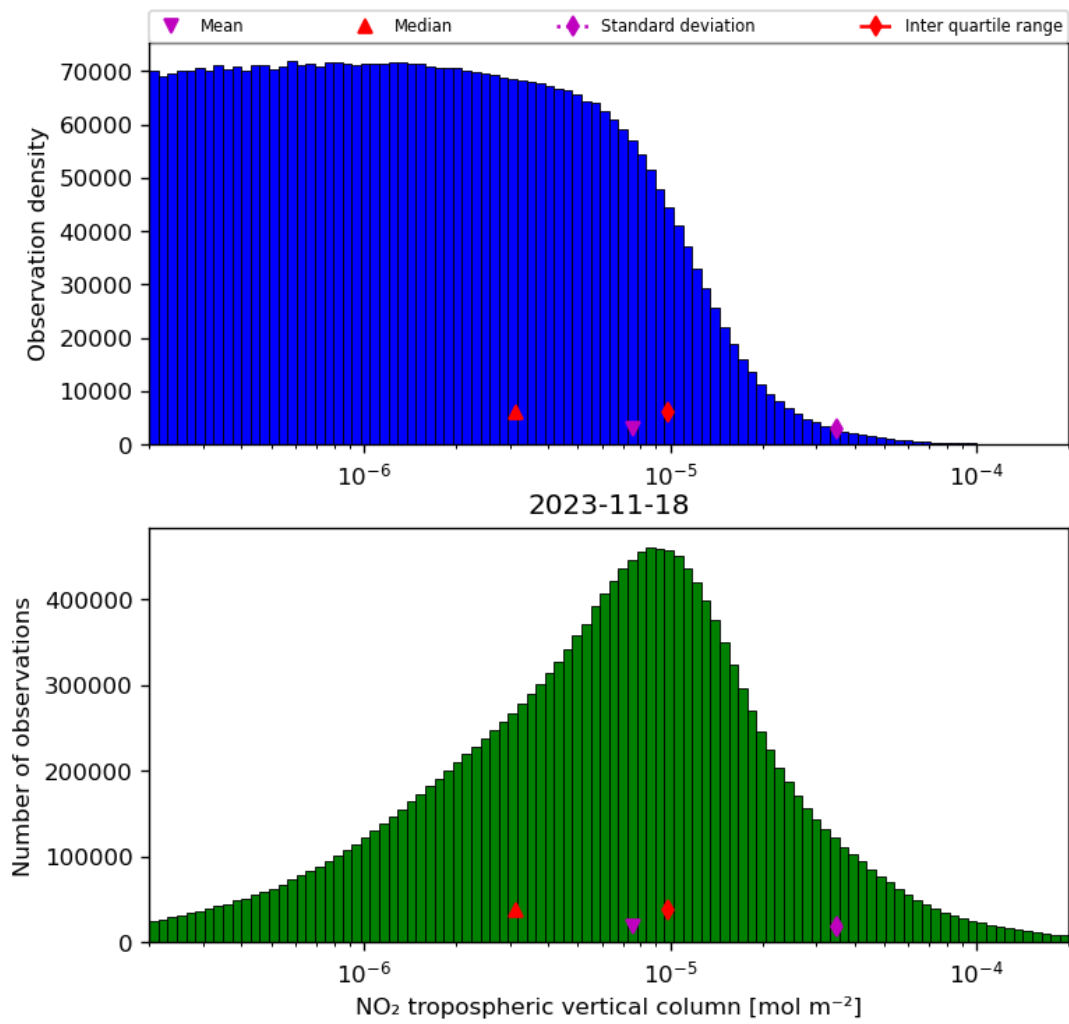
Figure 29: Histogram of “NO 2 tropospheric vertical column” for 2023-11-18 to 2023-11-19
