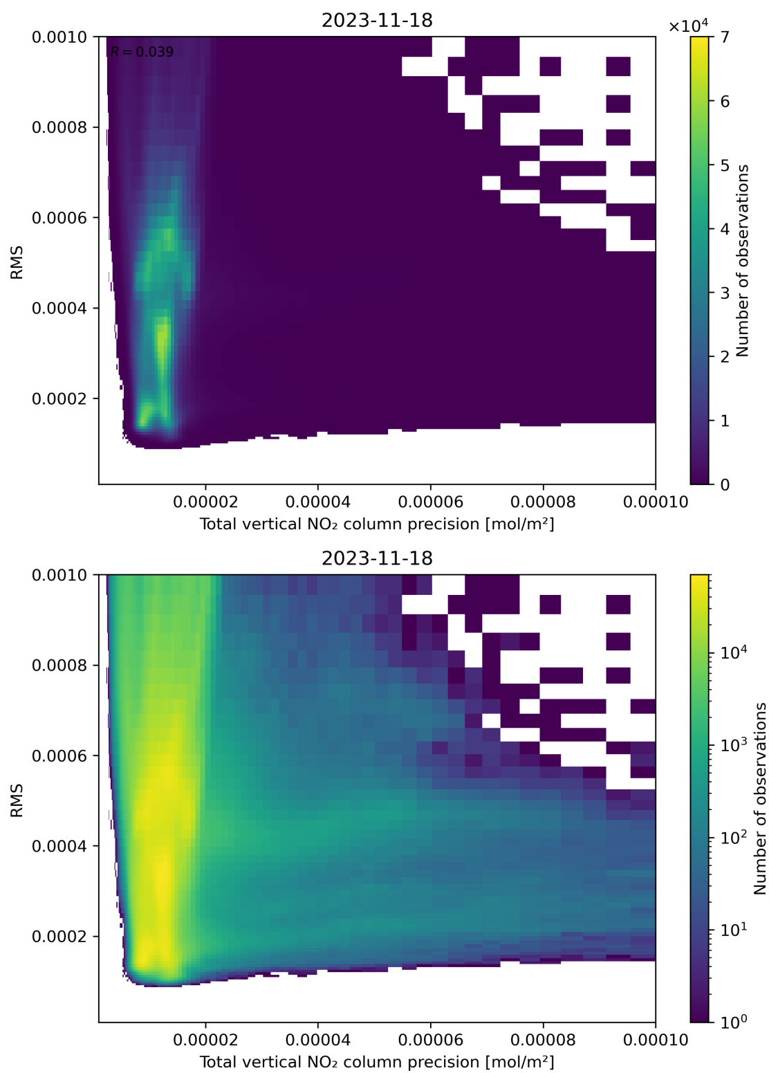
Figure 119: Scatter density plot of “Total vertical NO 2 column precision” against “RMS” for 2023-11-18 to 2023-11-19.
