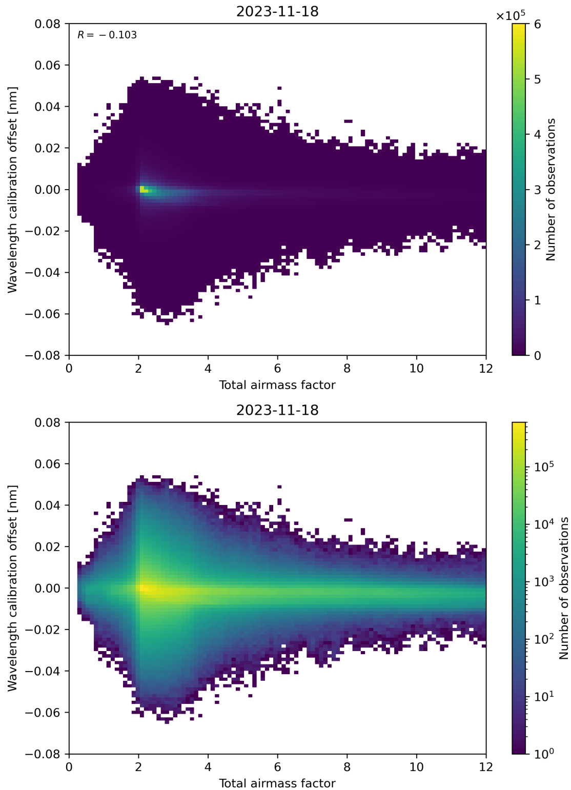
Figure 70: Scatter density plot of “Total airmass factor” against “Wavelength calibration offset” for 2023-11-18 to 2023-11-19.
