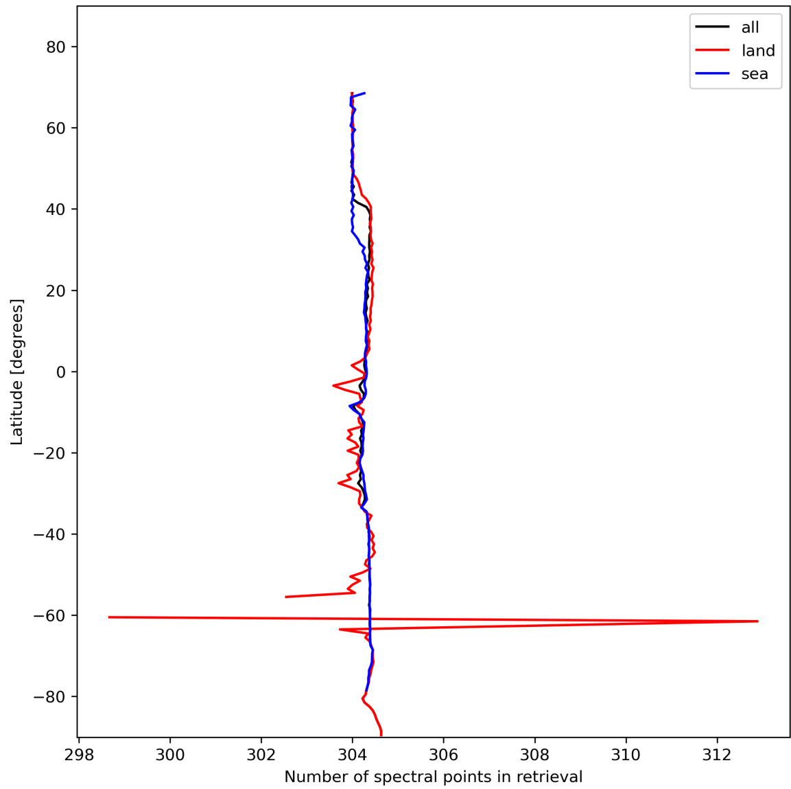
Figure 16: Zonal average of “Number of spectral points in retrieval” for 2023-11-18 to 2023-11-19.
