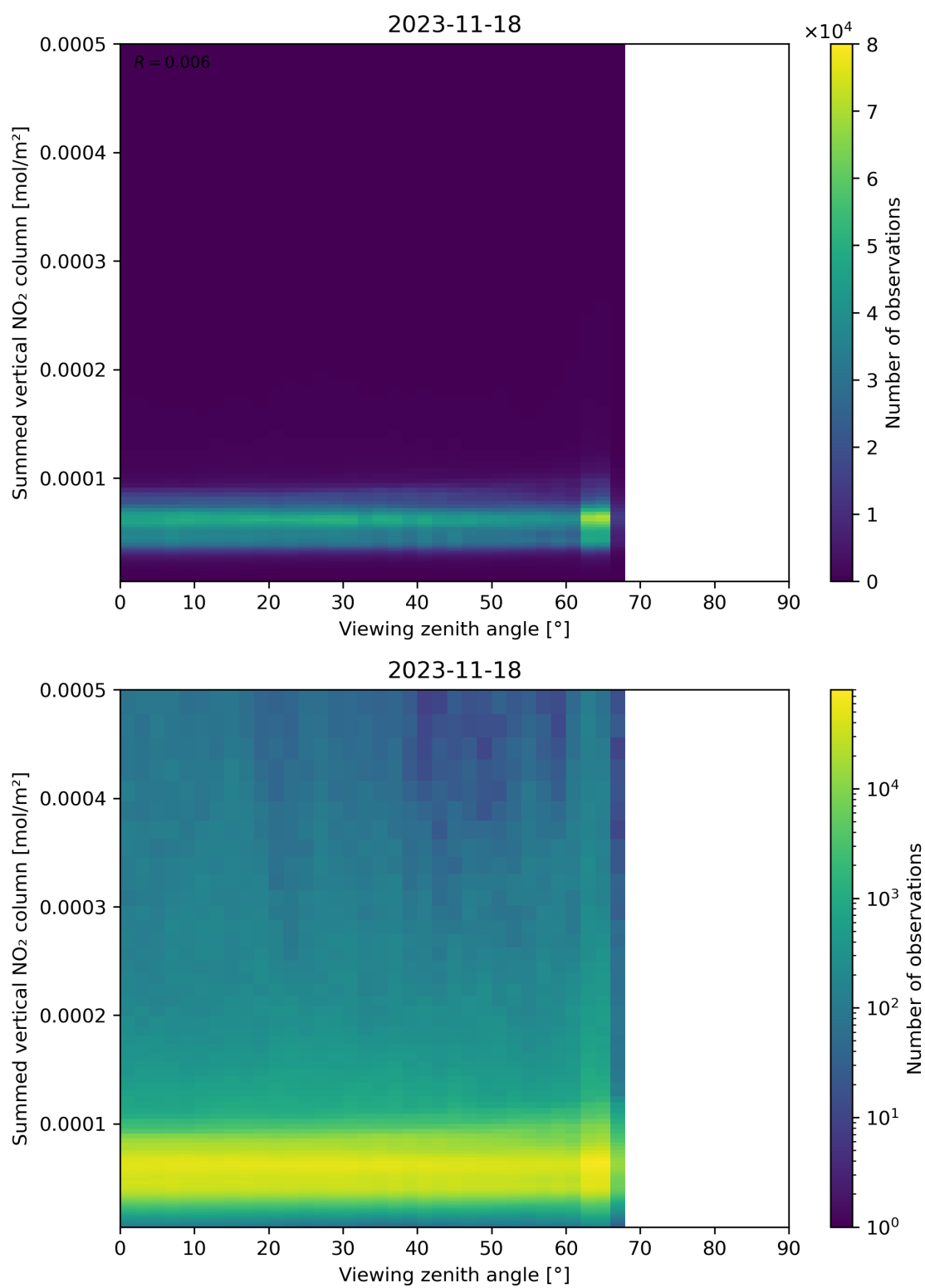
Figure 165: Scatter density plot of “Viewing zenith angle” against “Summed vertical NO 2 column” for 2023-11-18 to 2023-11-19.
