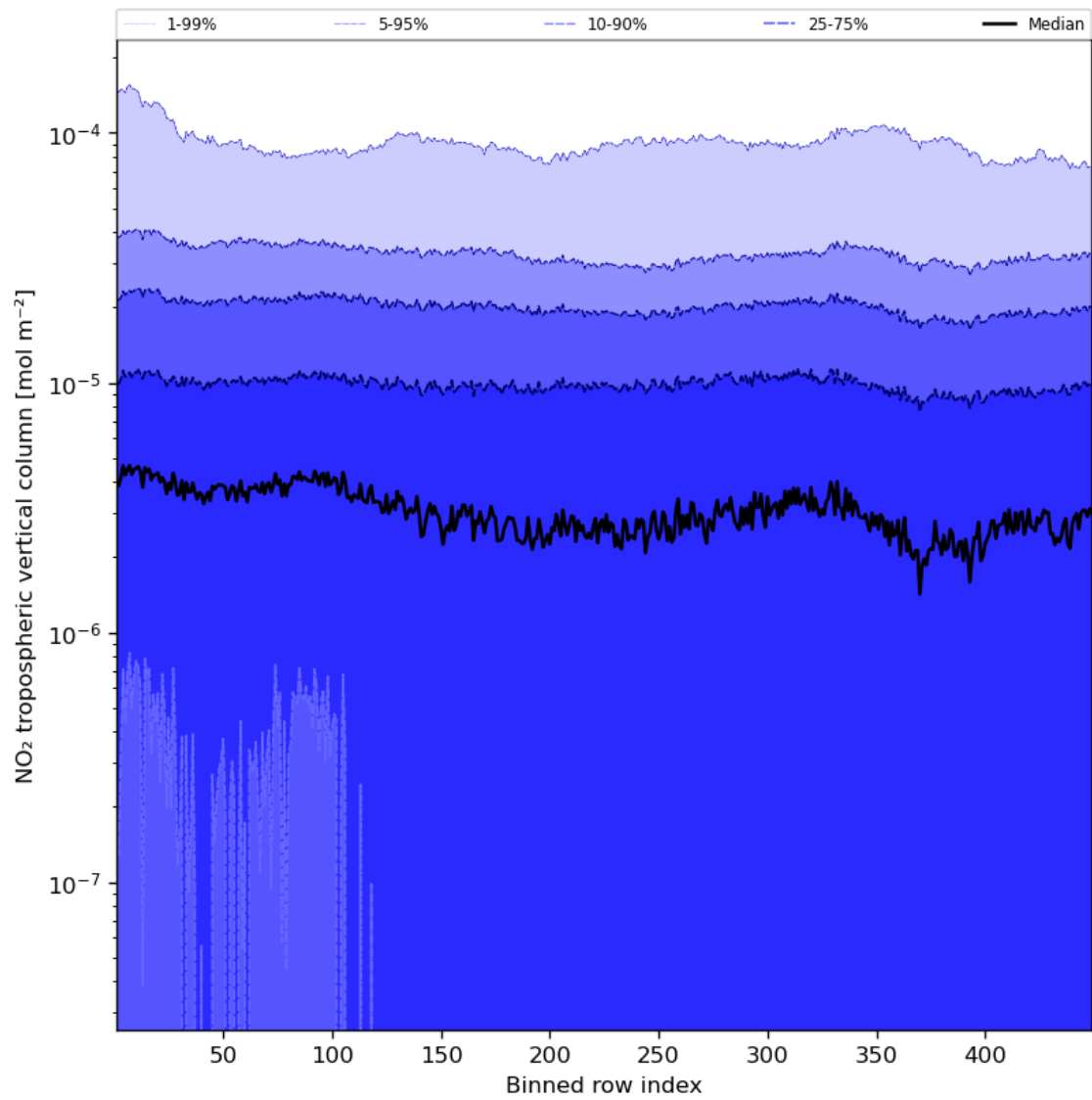
Figure 46: Along track statistics of “NO 2 tropospheric vertical column” for 2023-11-18 to 2023-11-19
