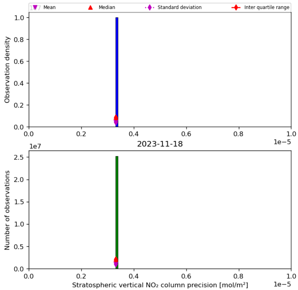
Figure 37: Histogram of “Stratospheric vertical NO 2 column precision” for 2023-11-18 to 2023-11-19
