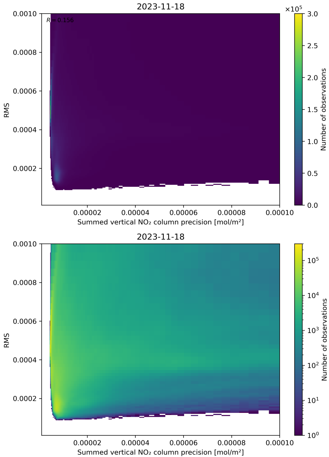
Figure 108: Scatter density plot of “Summed vertical NO 2 column precision” against “RMS” for 2023-11-18 to 2023-11-19.
