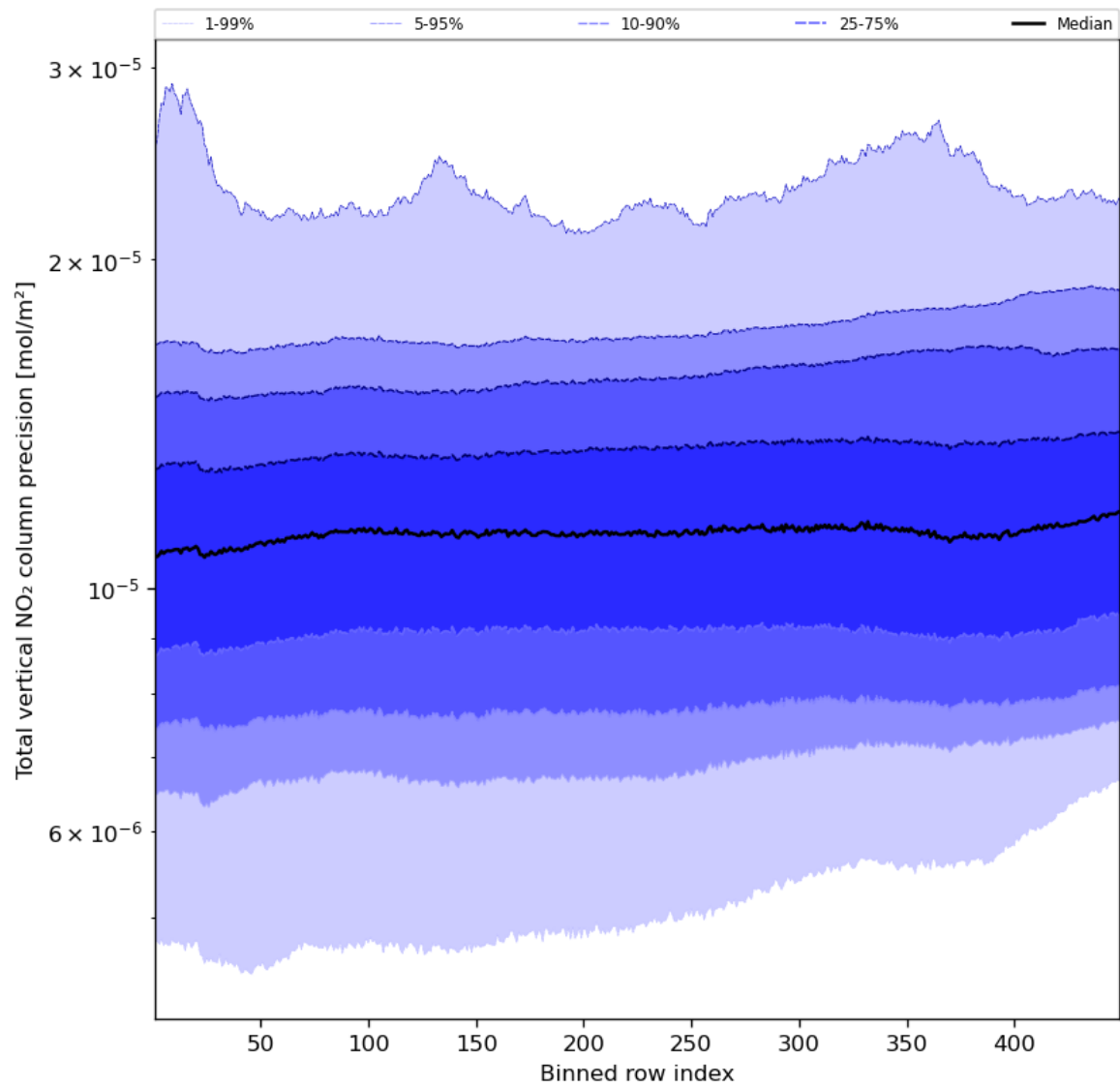
Figure 56: Along track statistics of "Total vertical NO 2 column precision" for 2023-11-18 to 2023-11-19
