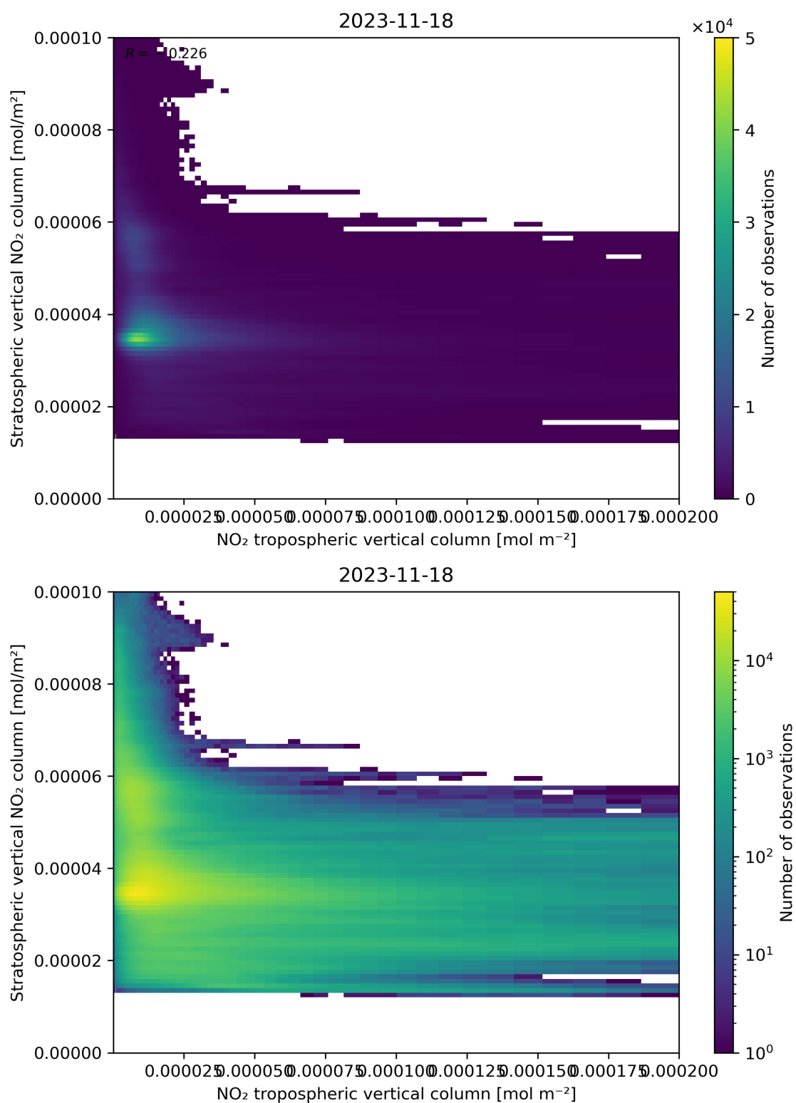
Figure 125: Scatter density plot of “NO 2 tropospheric vertical column” against “Stratospheric vertical NO 2 column” for 2023-11-18 to 2023-11-19.
