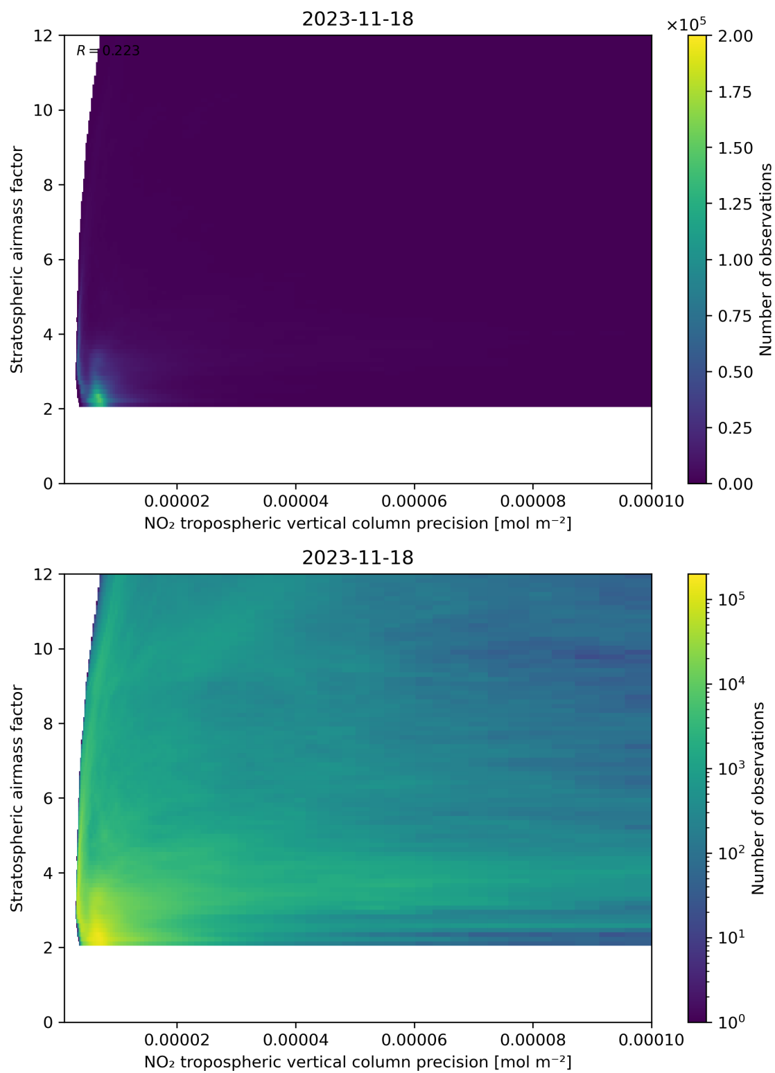
Figure 131: Scatter density plot of “NO 2 tropospheric vertical column precision” against “Stratospheric airmass factor” for 2023-11-18 to 2023-11-19.
