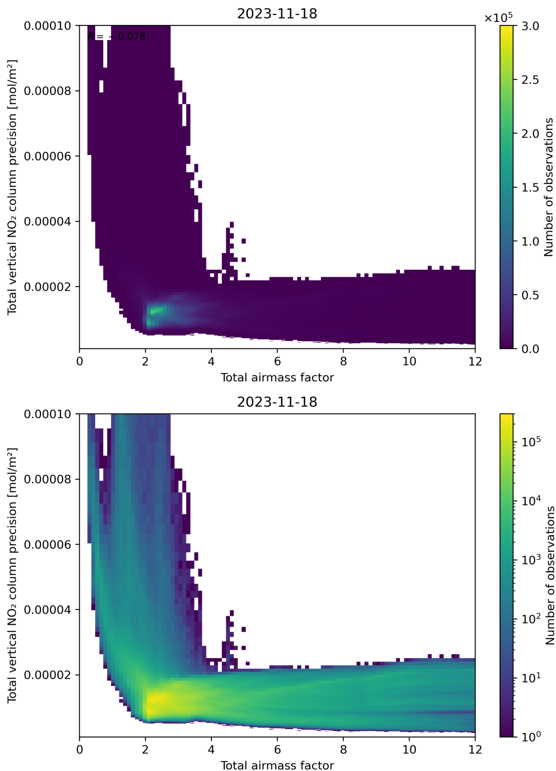
Figure 68: Scatter density plot of “Total airmass factor” against “Total vertical NO 2 column precision” for 2023-11-18 to 2023-11-19.
