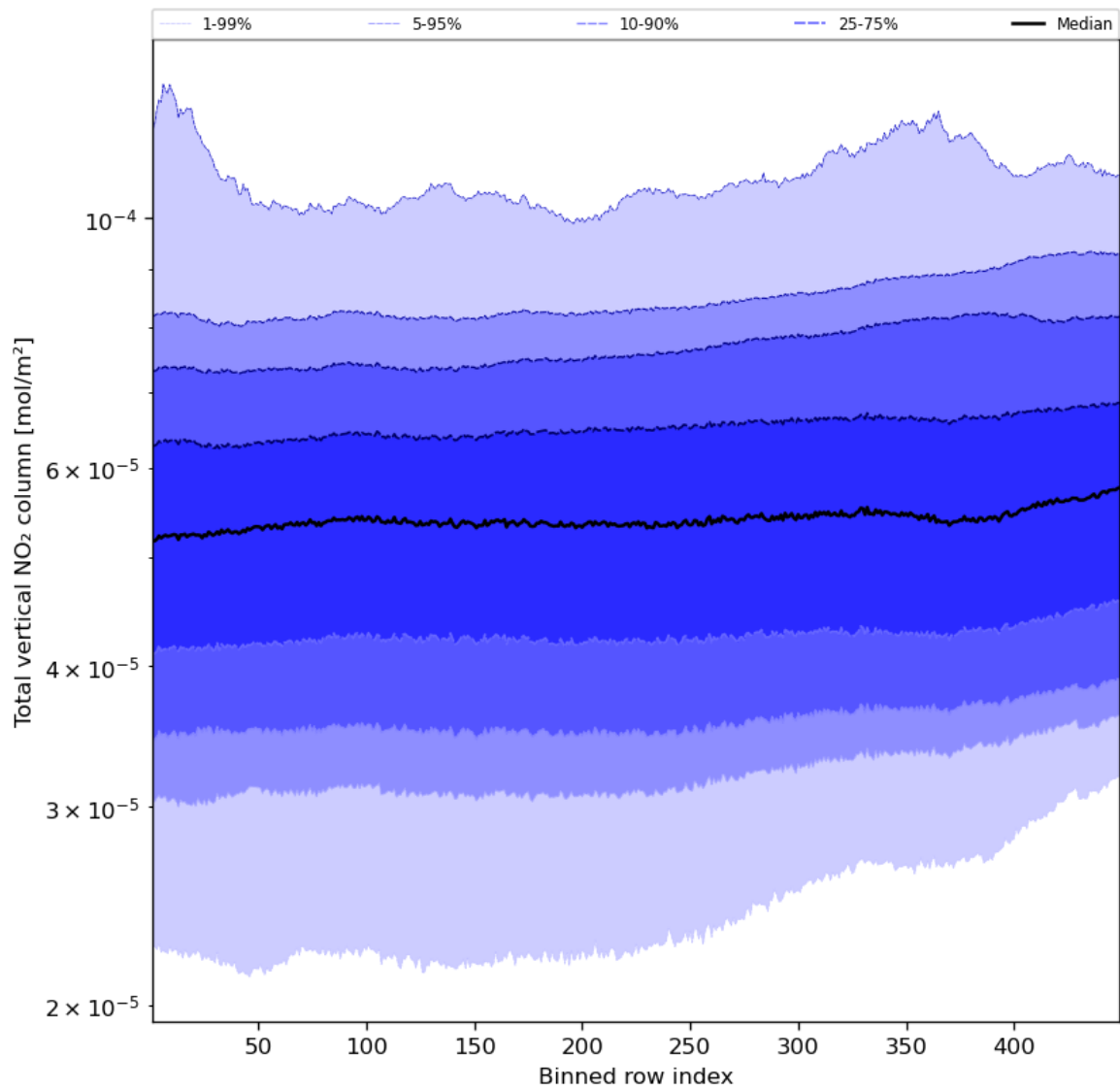
Figure 55: Along track statistics of “Total vertical NO 2 column” for 2023-11-18 to 2023-11-19
