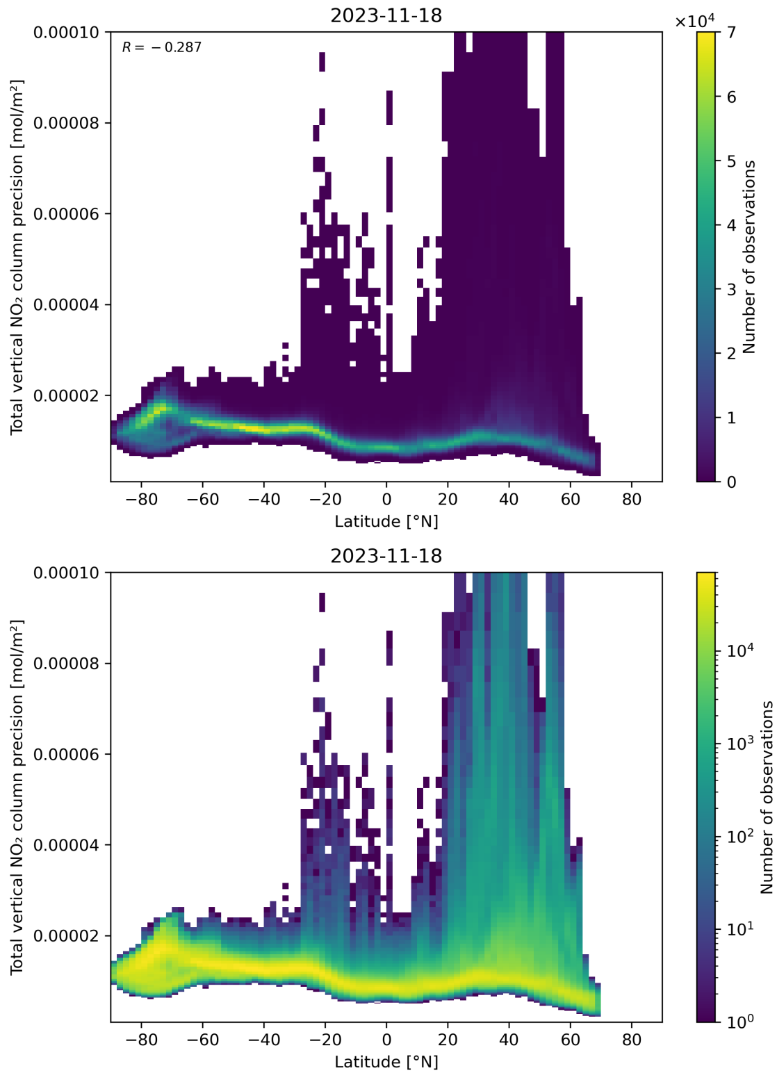
Figure 91: Scatter density plot of “Latitude” against “Total vertical NO 2 column precision” for 2023-11-18 to 2023-11-19.
