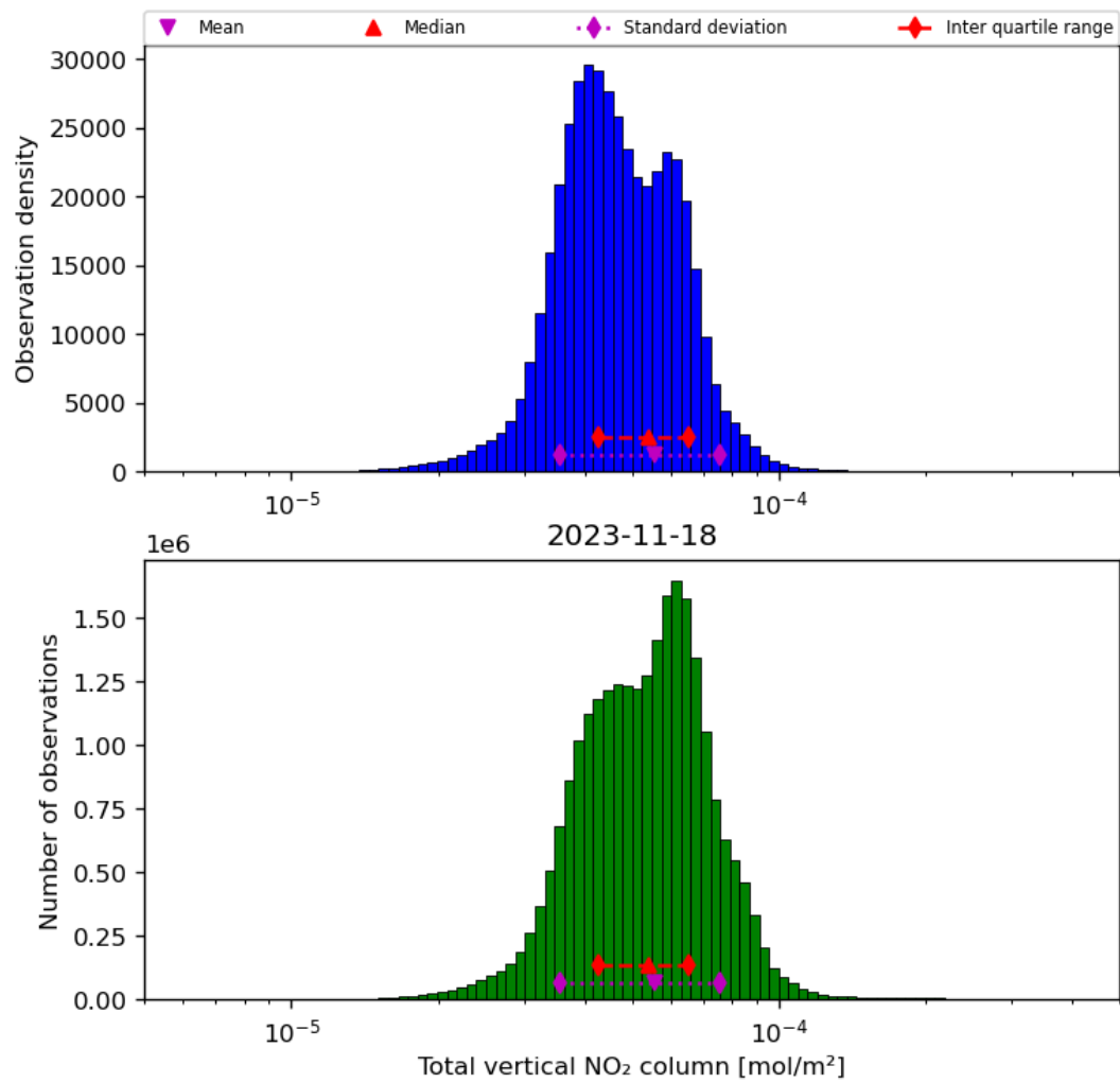
Figure 38: Histogram of “Total vertical NO 2 column” for 2023-11-18 to 2023-11-19
