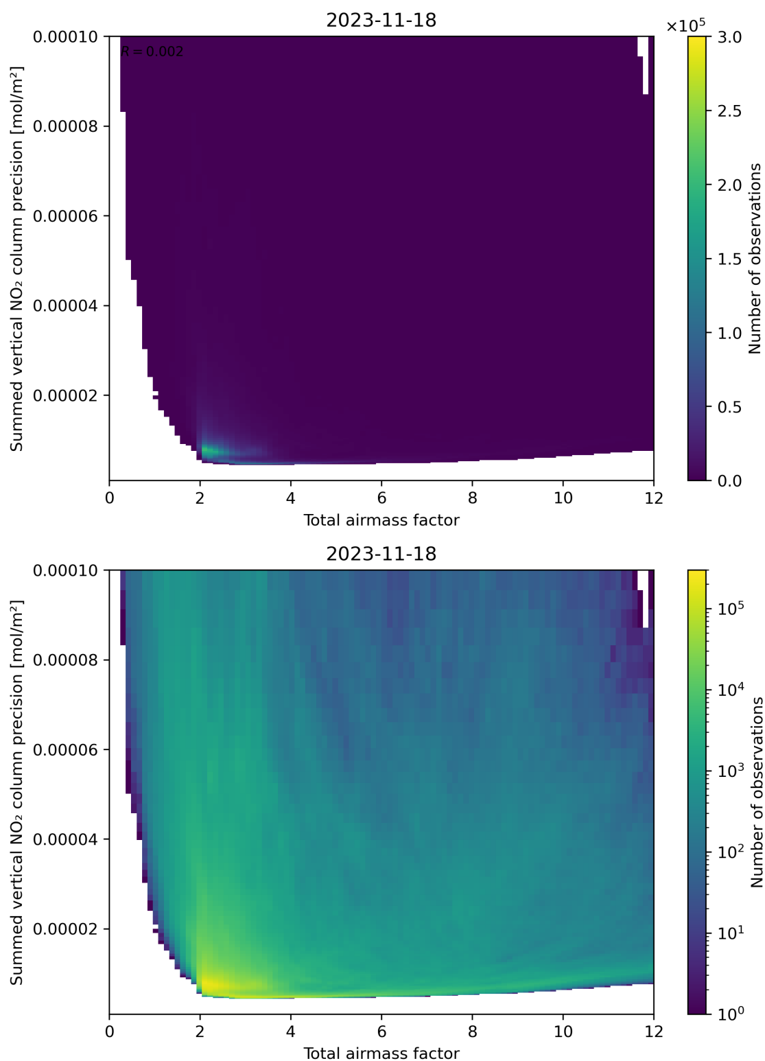
Figure 66: Scatter density plot of “Total airmass factor” against “Summed vertical NO 2 column precision” for 2023-11-18 to 2023-11-19.
