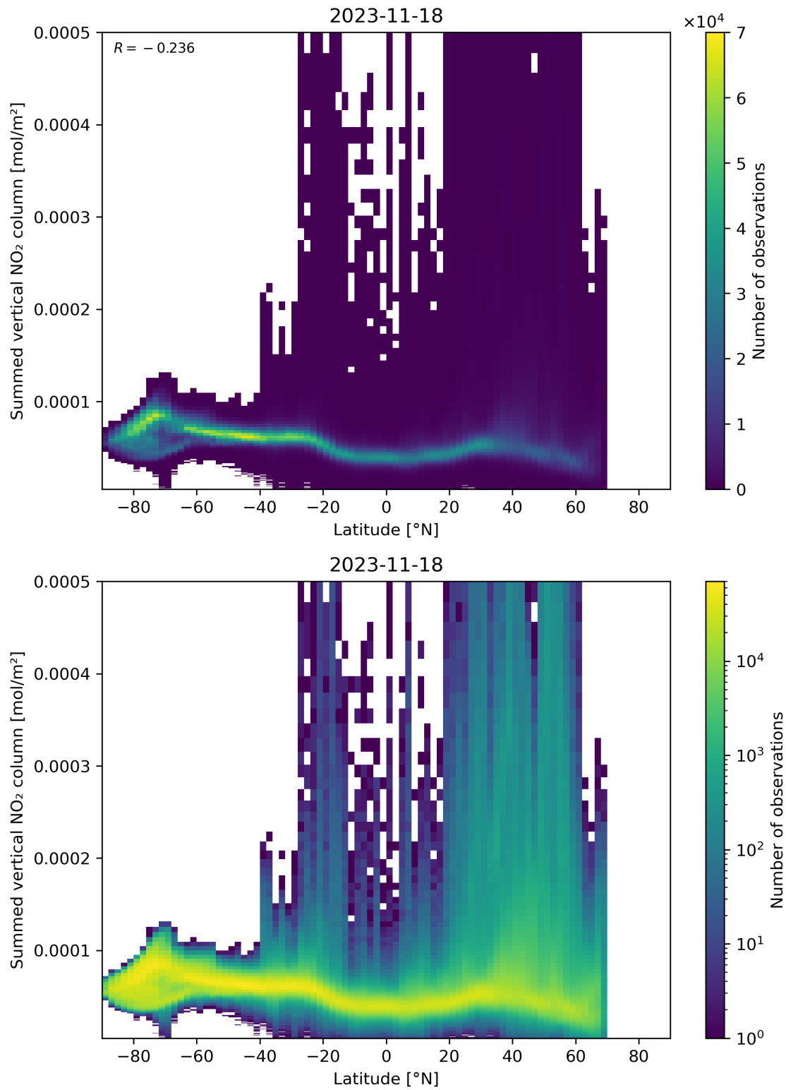
Figure 88: Scatter density plot of “Latitude” against “Summed vertical NO 2 column” for 2023-11-18 to 2023-11-19.
