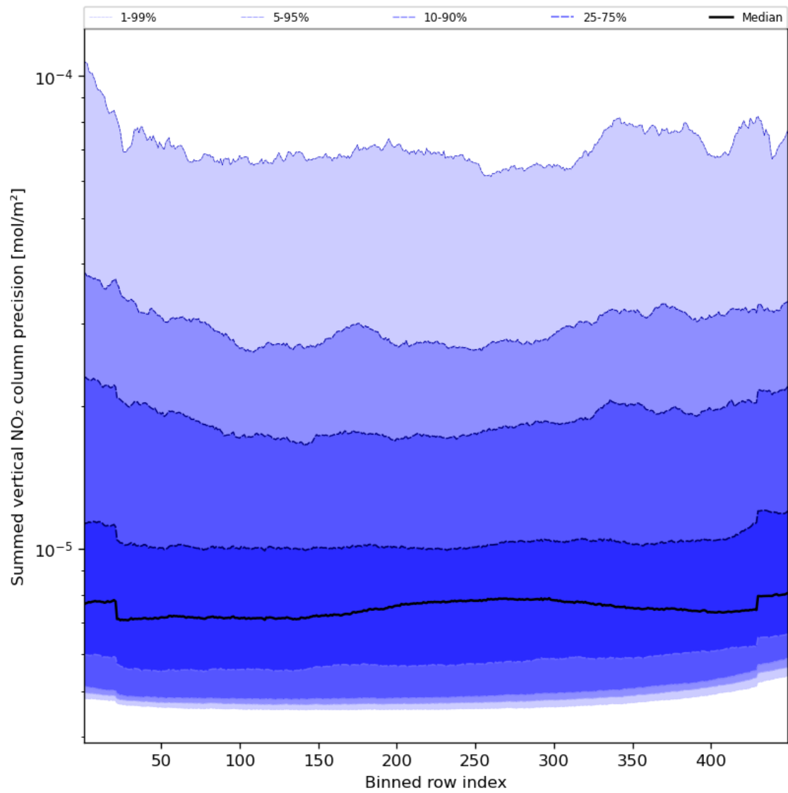
Figure 58: Along track statistics of “Summed vertical NO 2 column precision” for 2023-11-18 to 2023-11-19
