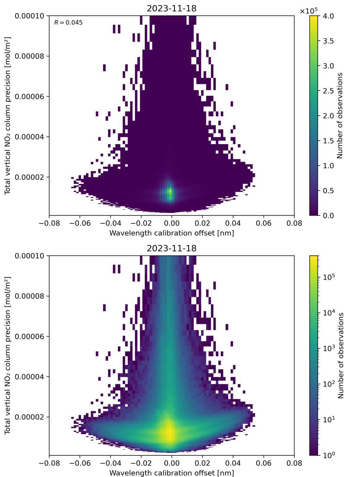
Figure 180: Scatter density plot of “Wavelength calibration offset” against “Total vertical NO 2 column precision” for 2023-11-18 to 2023-11-19.
