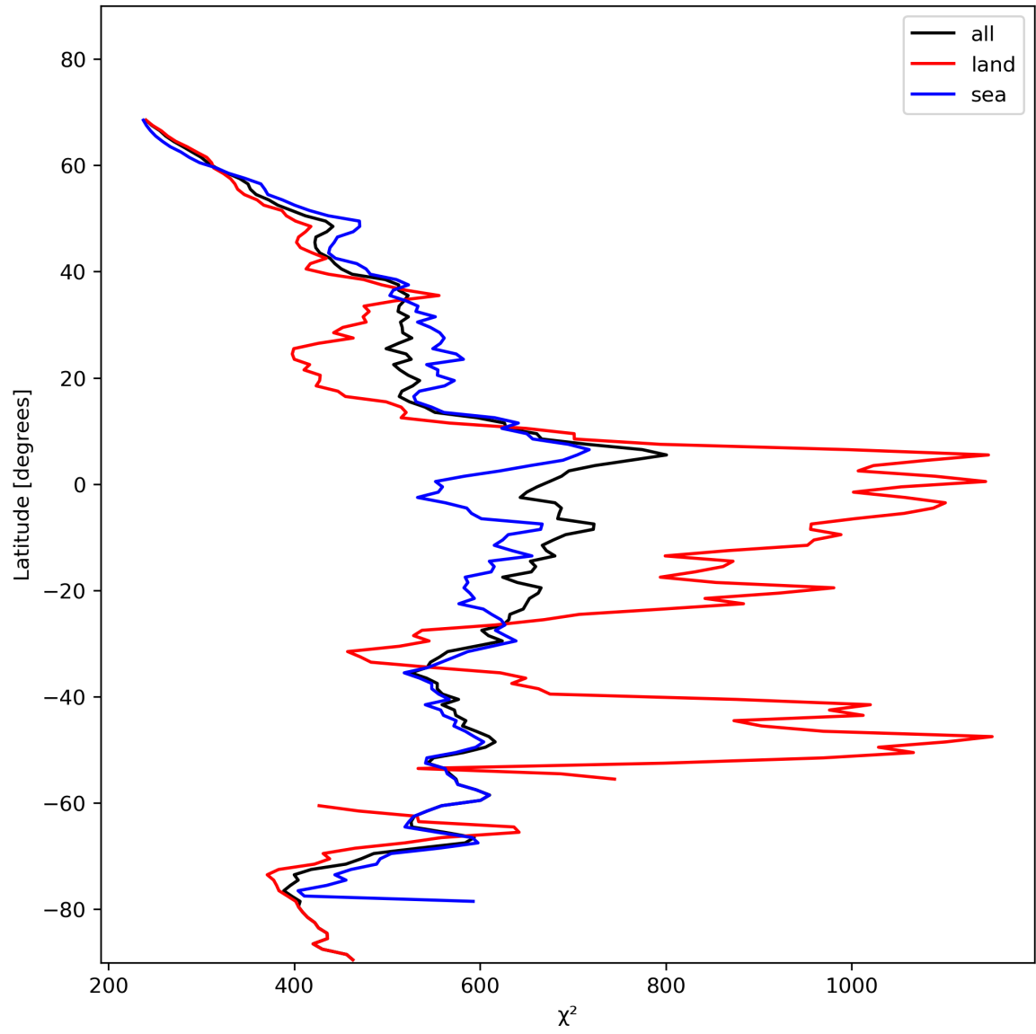
Figure 25: Zonal average of “ \chi^2 ” for 2023-11-18 to 2023-11-19.
