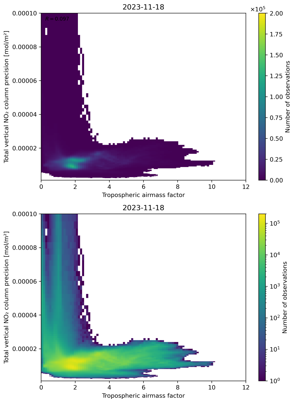
Figure 78: Scatter density plot of “Tropospheric air mass factor” against “Total vertical NO 2 column precision” for 2023-11-18 to 2023-11-19.
