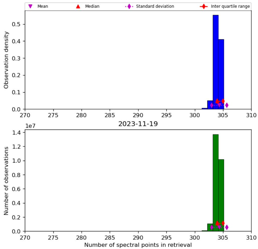
Figure 33: Histogram of “Number of spectral points in retrieval” for 2023-11-18 to 2023-11-20
