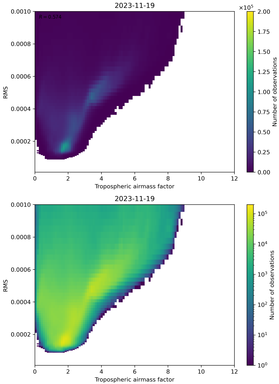
Figure 79: Scatter density plot of “Tropospheric airmass factor” against “RMS” for 2023-11-18 to 2023-11-20.
