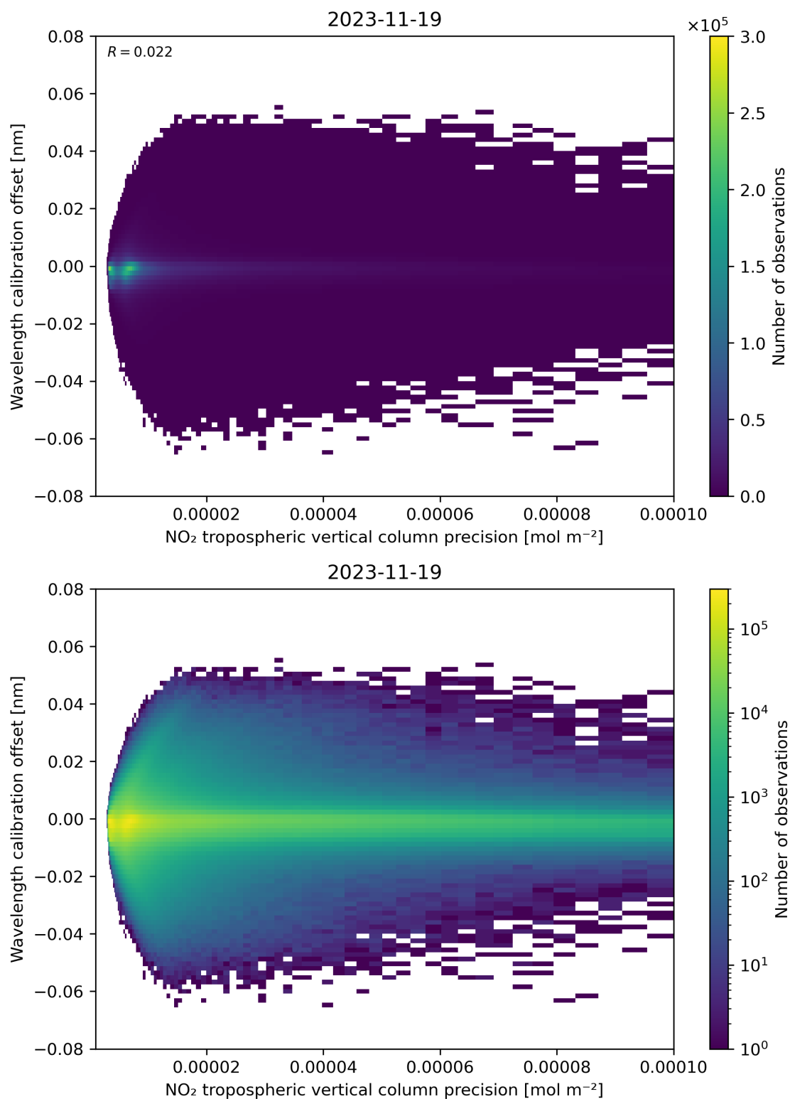
Figure 141: Scatter density plot of “NO 2 tropospheric vertical column precision” against “Wavelength calibration offset” for 2023-11-18 to 2023-11-20.
