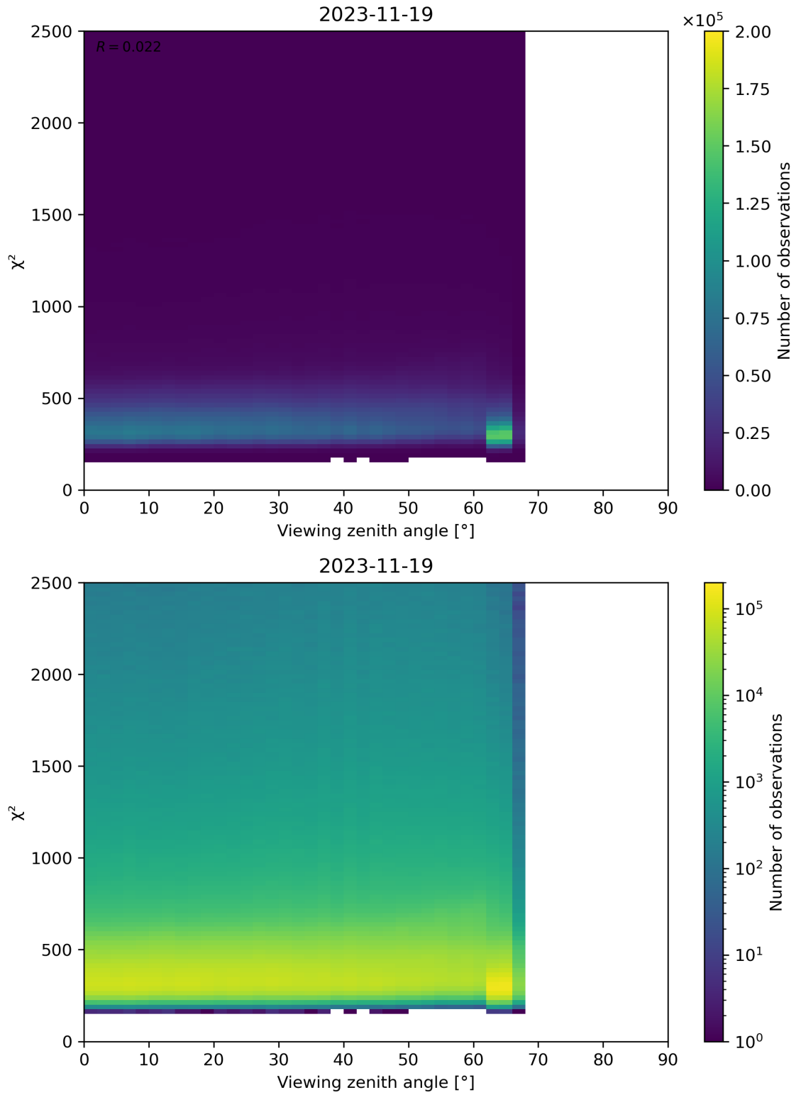
Figure 162: Scatter density plot of “Viewing zenith angle” against “ \chi^2 ” for 2023-11-18 to 2023-11-20.
