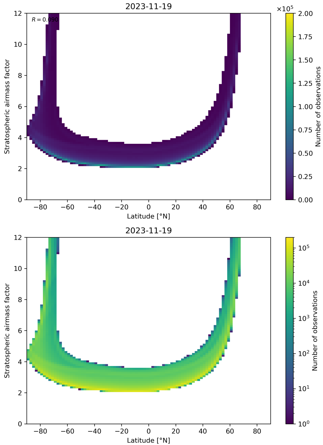
Figure 83: Scatter density plot of “Latitude” against “Stratospheric airmass factor” for 2023-11-18 to 2023-11-20.
