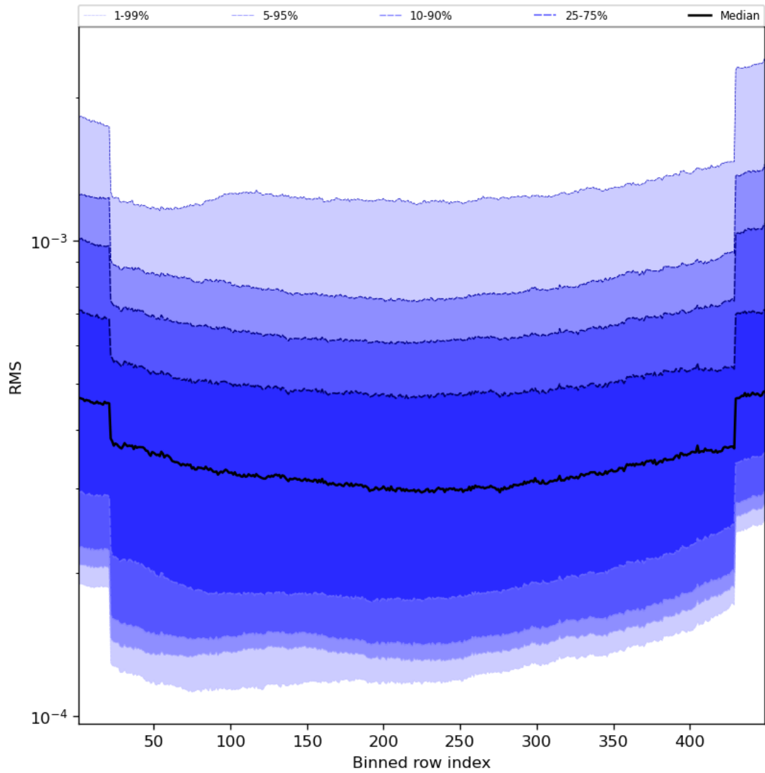
Figure 60: Along track statistics of “RMS” for 2023-11-18 to 2023-11-20
