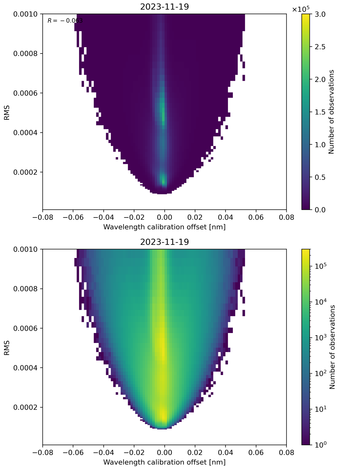
Figure 181: Scatter density plot of “Wavelength calibration offset” against “RMS” for 2023-11-18 to 2023-11-20.
