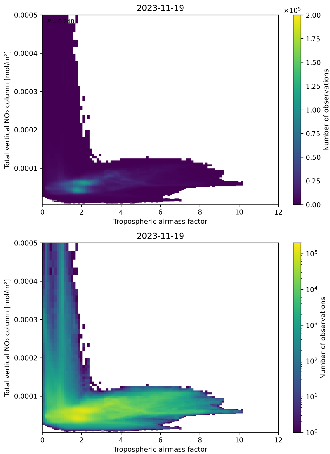
Figure 77: Scatter density plot of “Tropospheric airmass factor” against “Total vertical NO 2 column” for 2023-11-18 to 2023-11-20.
