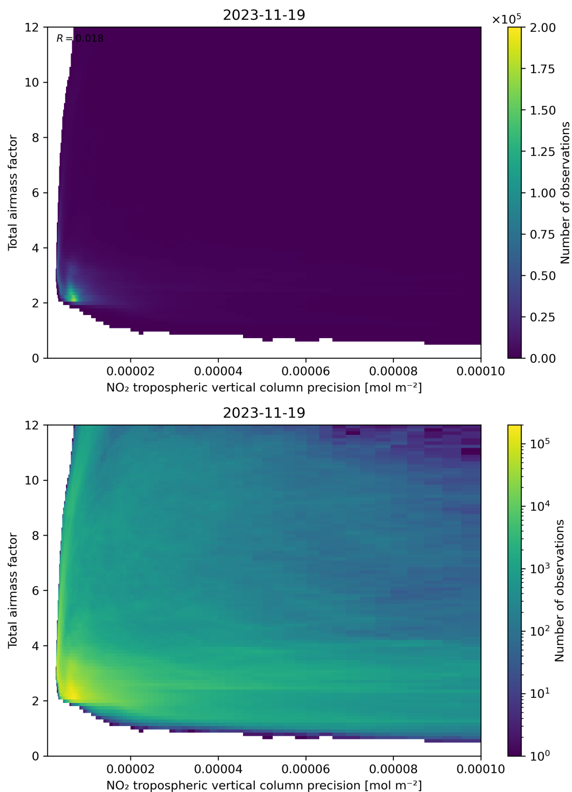
Figure 132: Scatter density plot of “NO 2 tropospheric vertical column precision” against “Total air mass factor” for 2023-11-18 to 2023-11-20.
