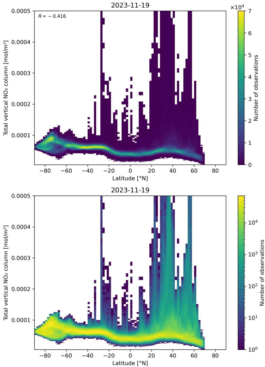
Figure 90: Scatter density plot of “Latitude” against “Total vertical NO 2 column” for 2023-11-18 to 2023-11-20.
