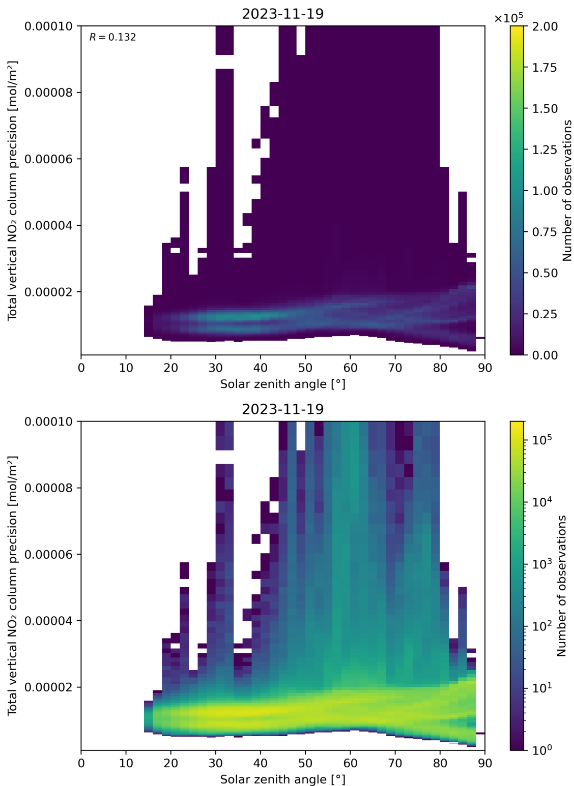
Figure 154: Scatter density plot of “Solar zenith angle” against “Total vertical NO 2 column precision” for 2023-11-18 to 2023-11-20.
