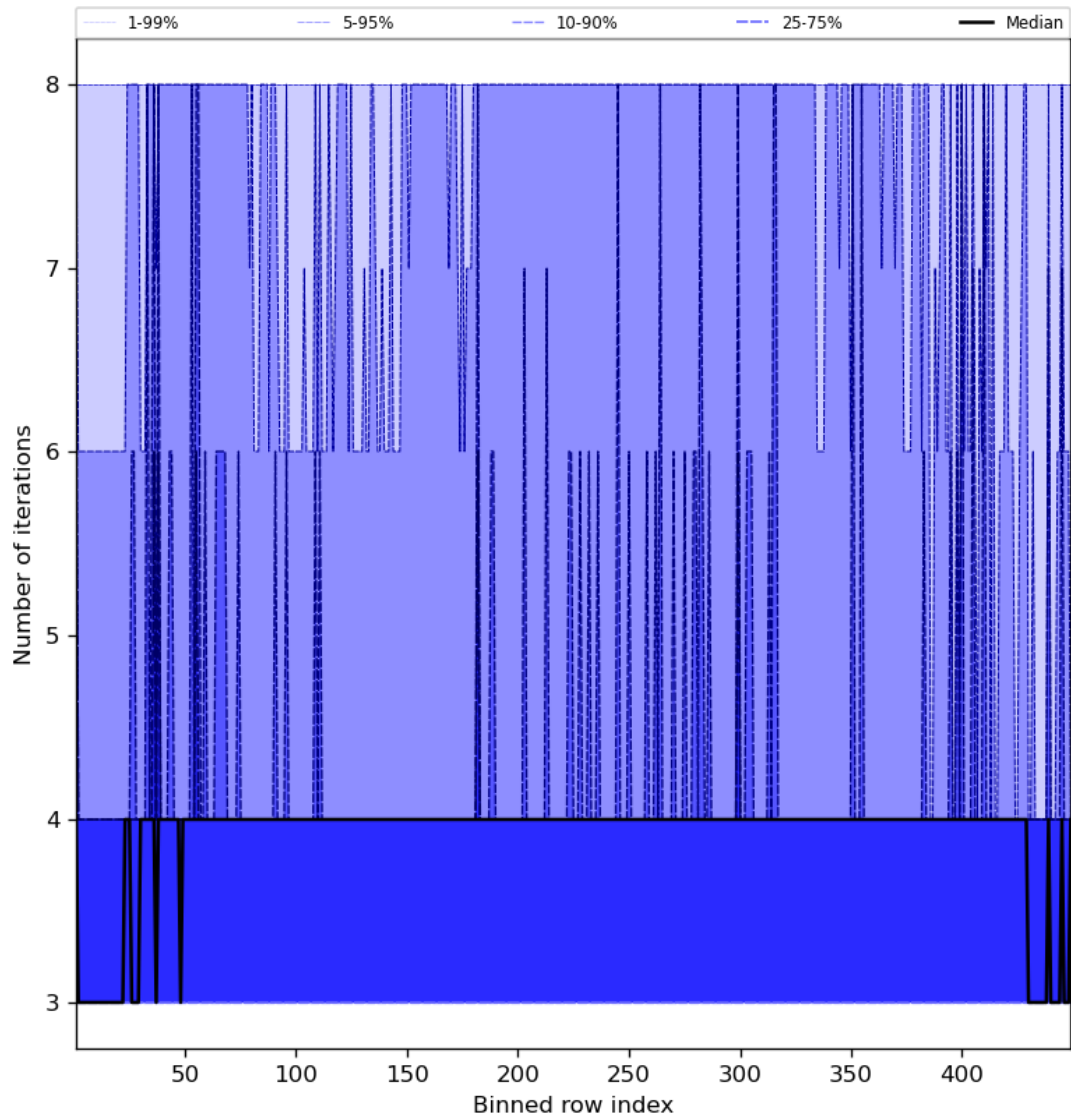
Figure 51: Along track statistics of “Number of iterations” for 2023-11-18 to 2023-11-20
