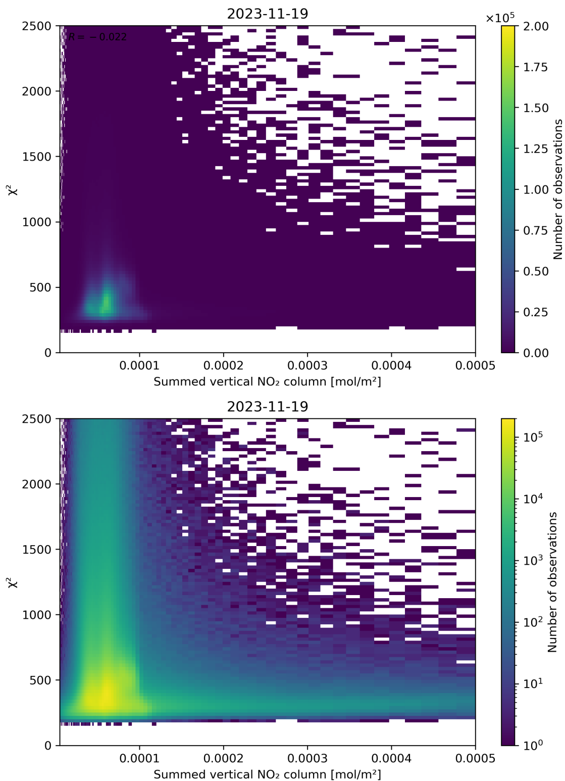
Figure 104: Scatter density plot of “Summed vertical NO 2 column” against “ \chi^2 ” for 2023-11-18 to 2023-11-20.
