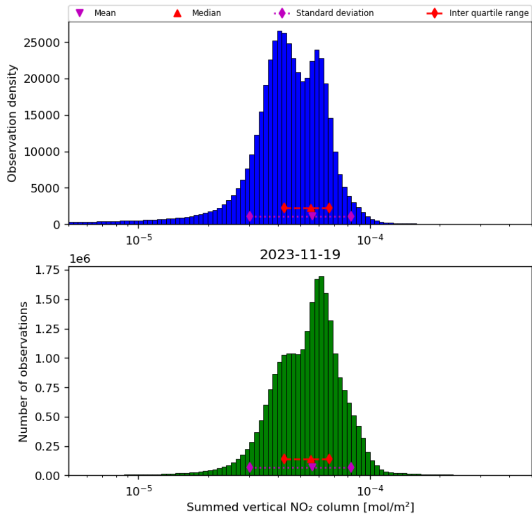
Figure 40: Histogram of “Summed vertical NO 2 column” for 2023-11-18 to 2023-11-20
