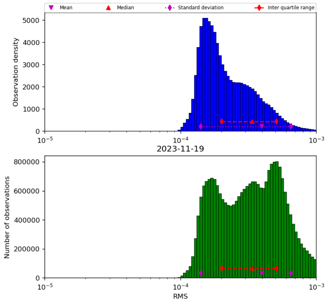
Figure 43: Histogram of “RMS” for 2023-11-18 to 2023-11-20
