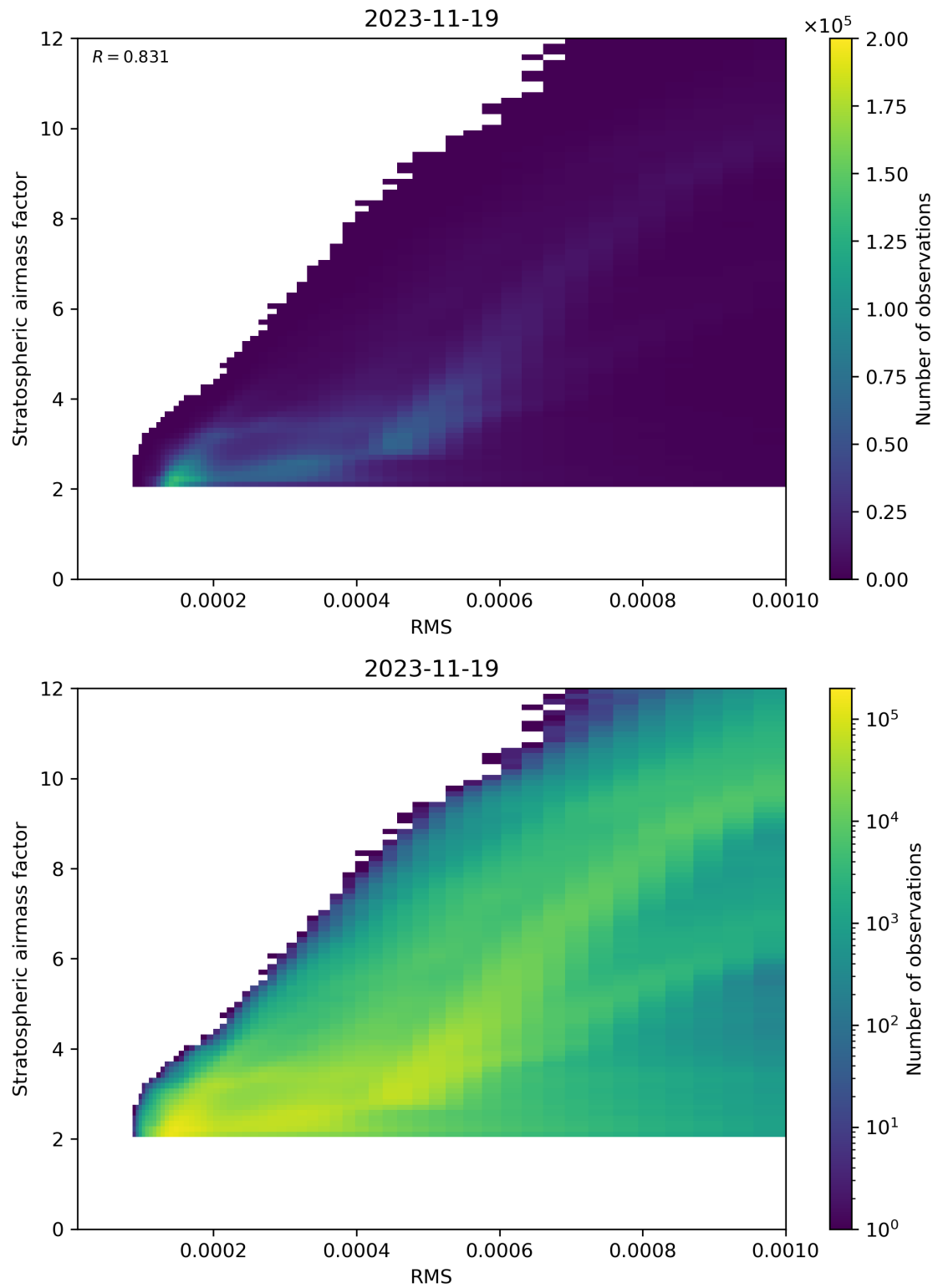
Figure 144: Scatter density plot of “RMS” against “Stratospheric airmass factor” for 2023-11-18 to 2023-11-20.
