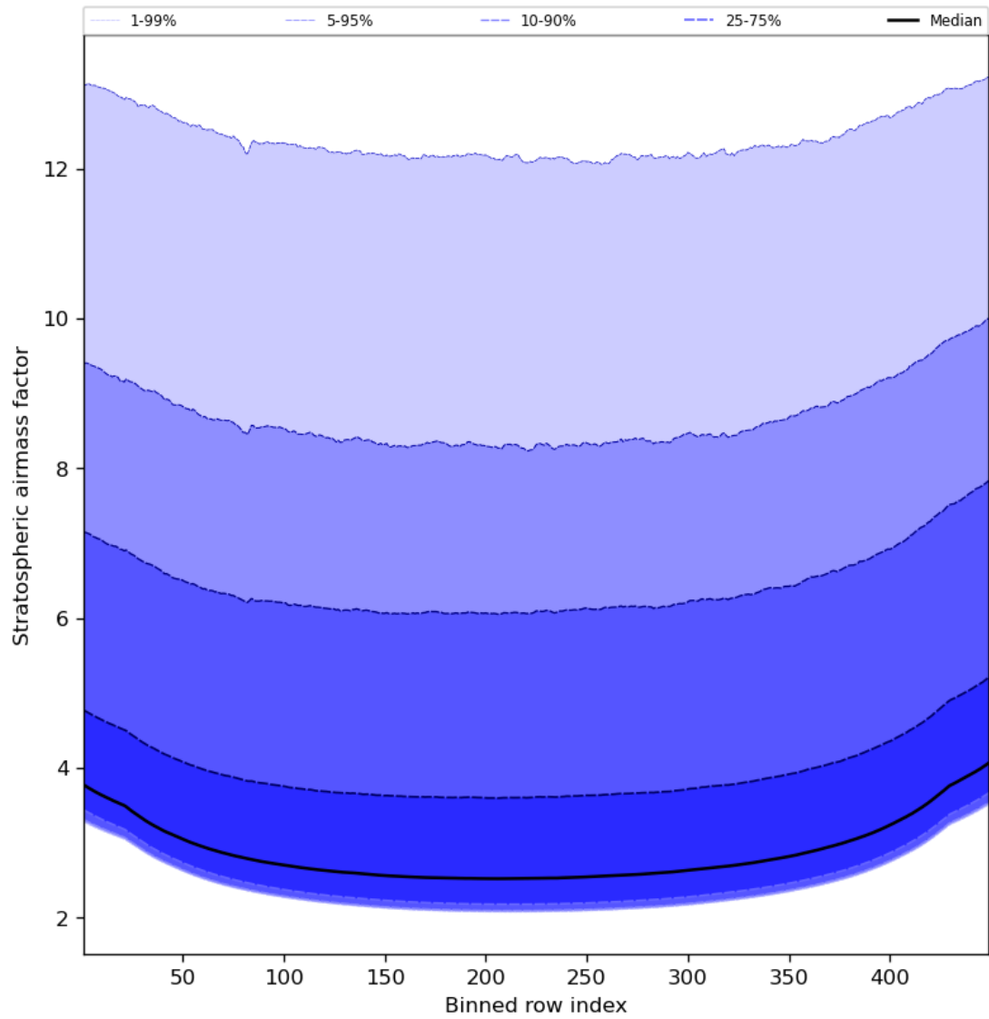
Figure 61: Along track statistics of “Stratospheric air mass factor” for 2023-11-18 to 2023-11-20
