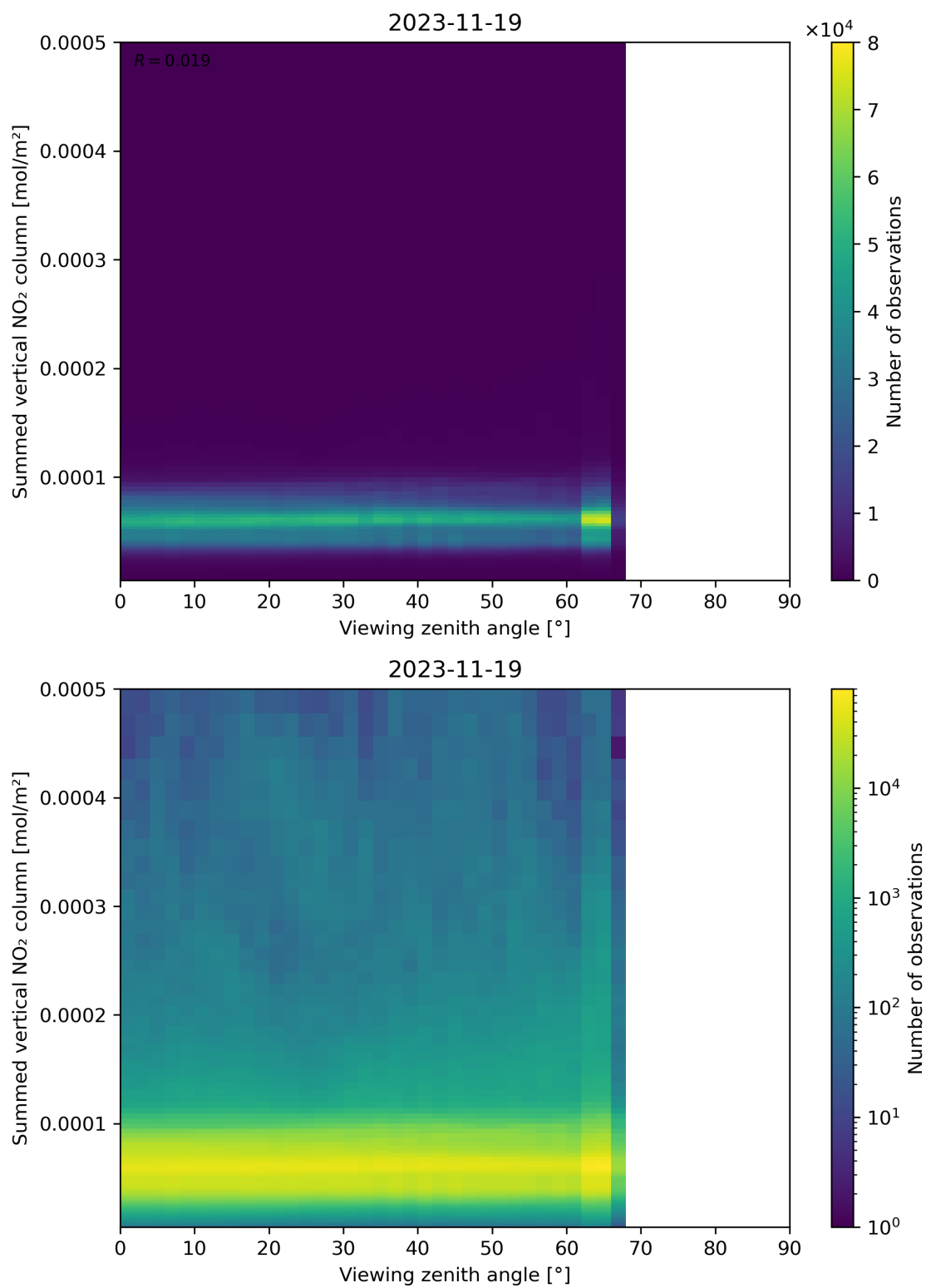
Figure 165: Scatter density plot of “Viewing zenith angle” against “Summed vertical NO 2 column” for 2023-11-18 to 2023-11-20.
