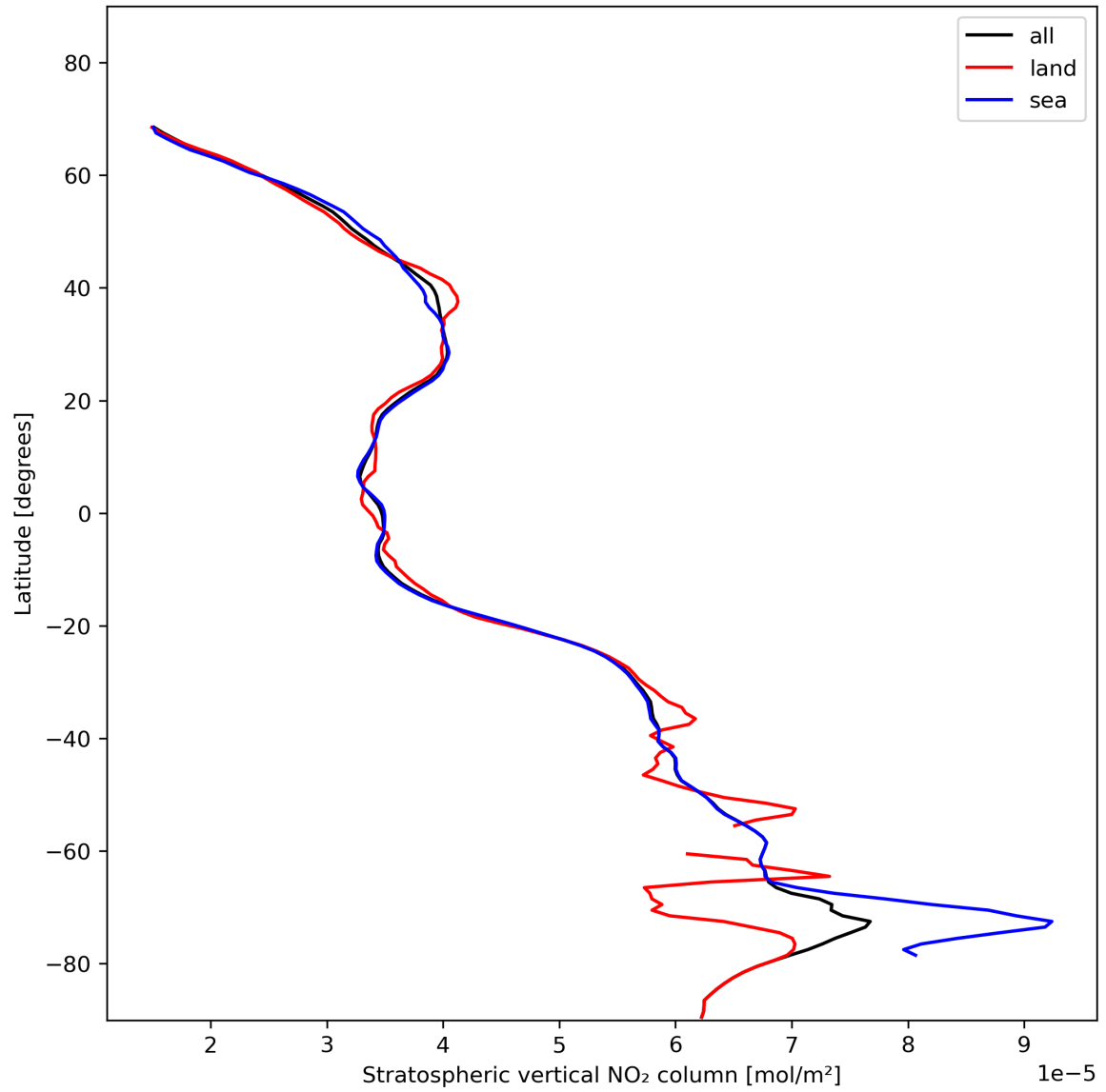
Figure 19: Zonal average of “Stratospheric vertical NO 2 column” for 2023-11-18 to 2023-11-20.
