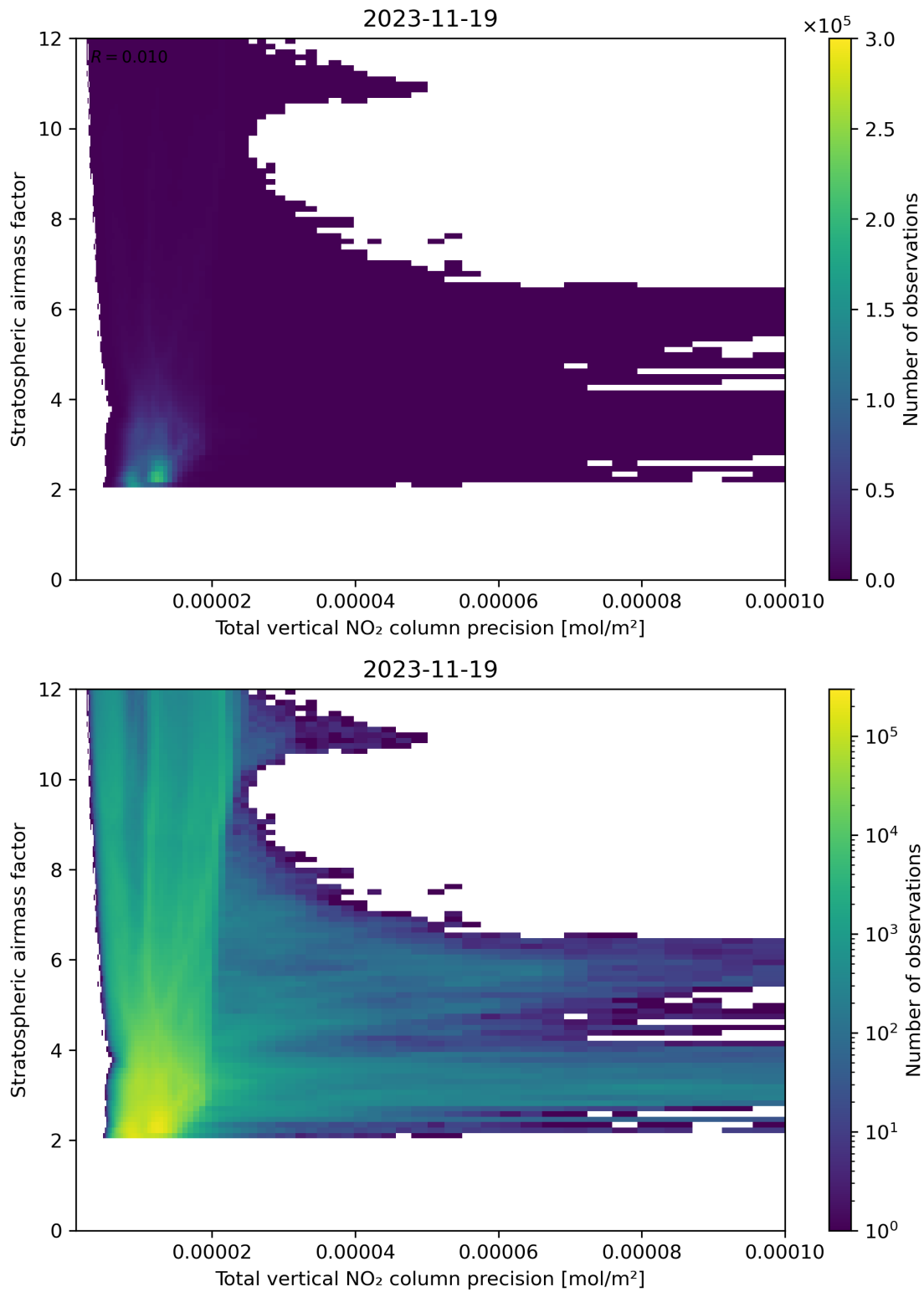
Figure 115: Scatter density plot of “Total vertical NO 2 column precision” against “Stratospheric air mass factor” for 2023-11-18 to 2023-11-20.
