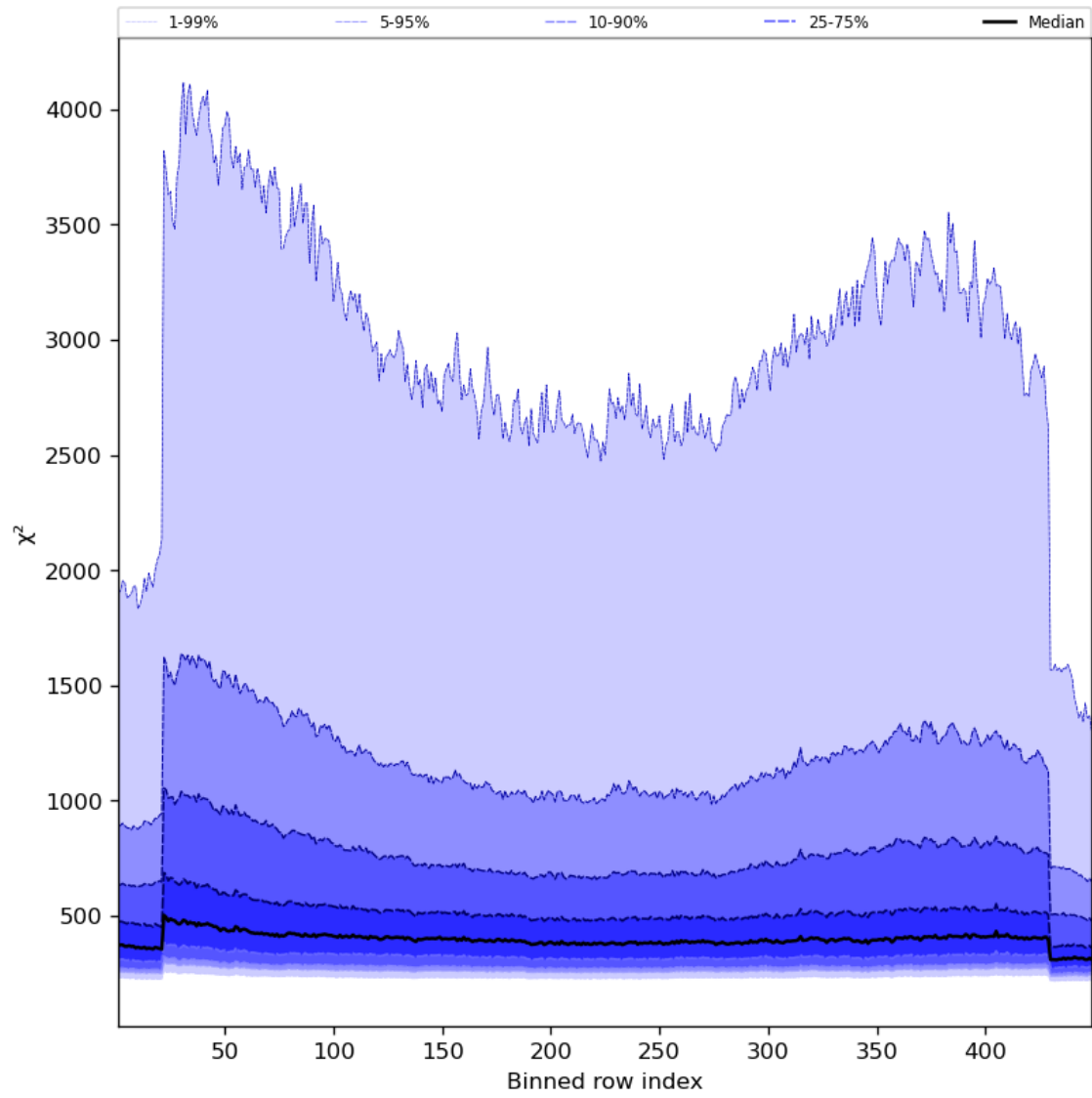
Figure 59: Along track statistics of “ \chi^2 ” for 2023-11-18 to 2023-11-20
