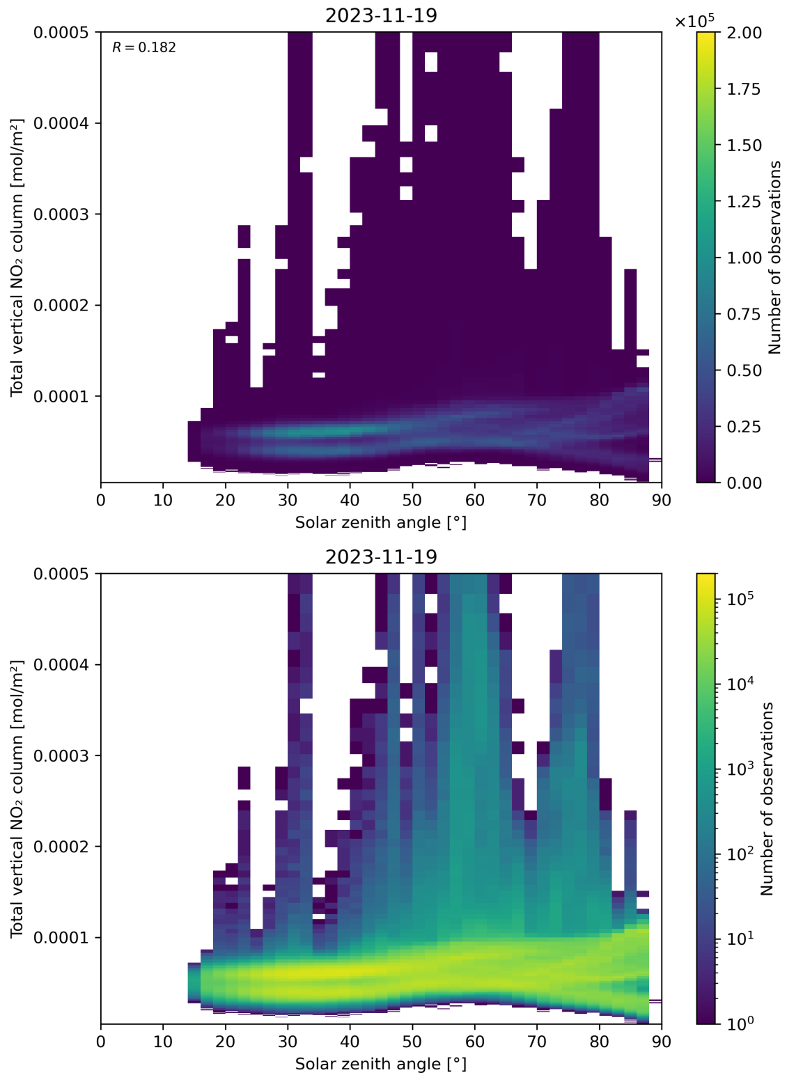
Figure 153: Scatter density plot of “Solar zenith angle” against “Total vertical NO 2 column” for 2023-11-18 to 2023-11-20.
