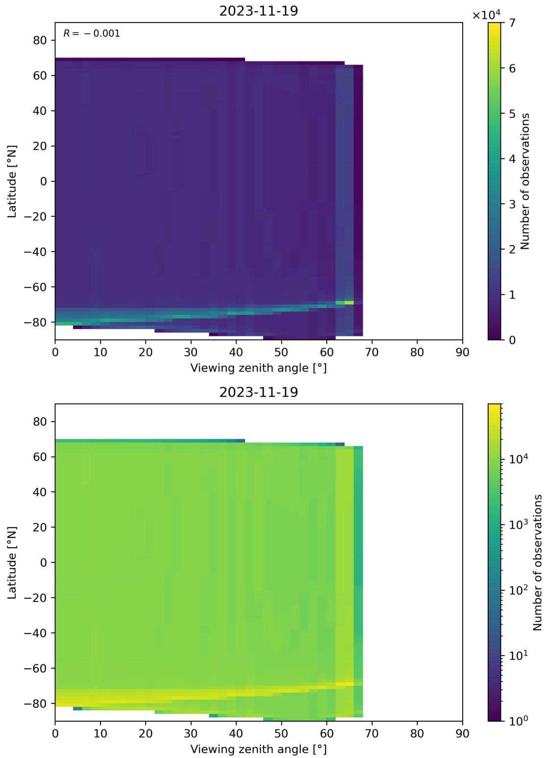
Figure 163: Scatter density plot of “Viewing zenith angle” against “Latitude” for 2023-11-18 to 2023-11-20.
