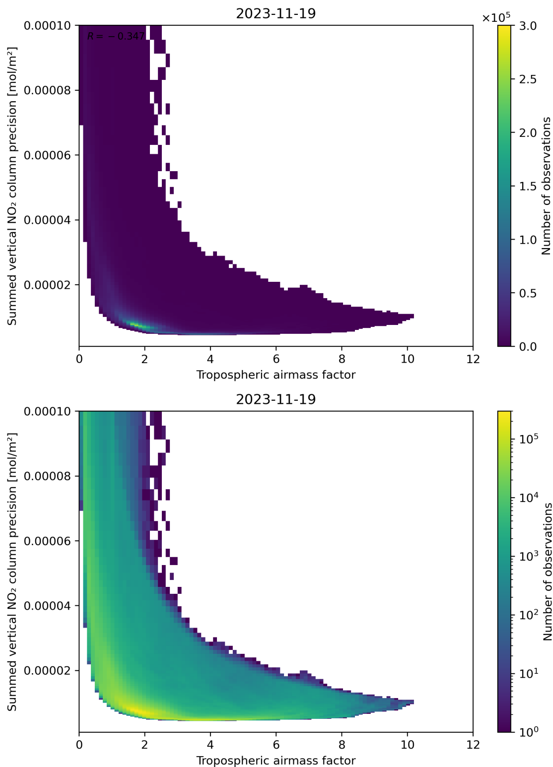
Figure 76: Scatter density plot of “Tropospheric air mass factor” against “Summed vertical NO 2 column precision” for 2023-11-18 to 2023-11-20.
