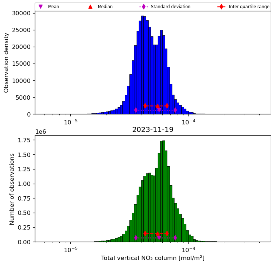
Figure 38: Histogram of “Total vertical NO 2 column” for 2023-11-18 to 2023-11-20
