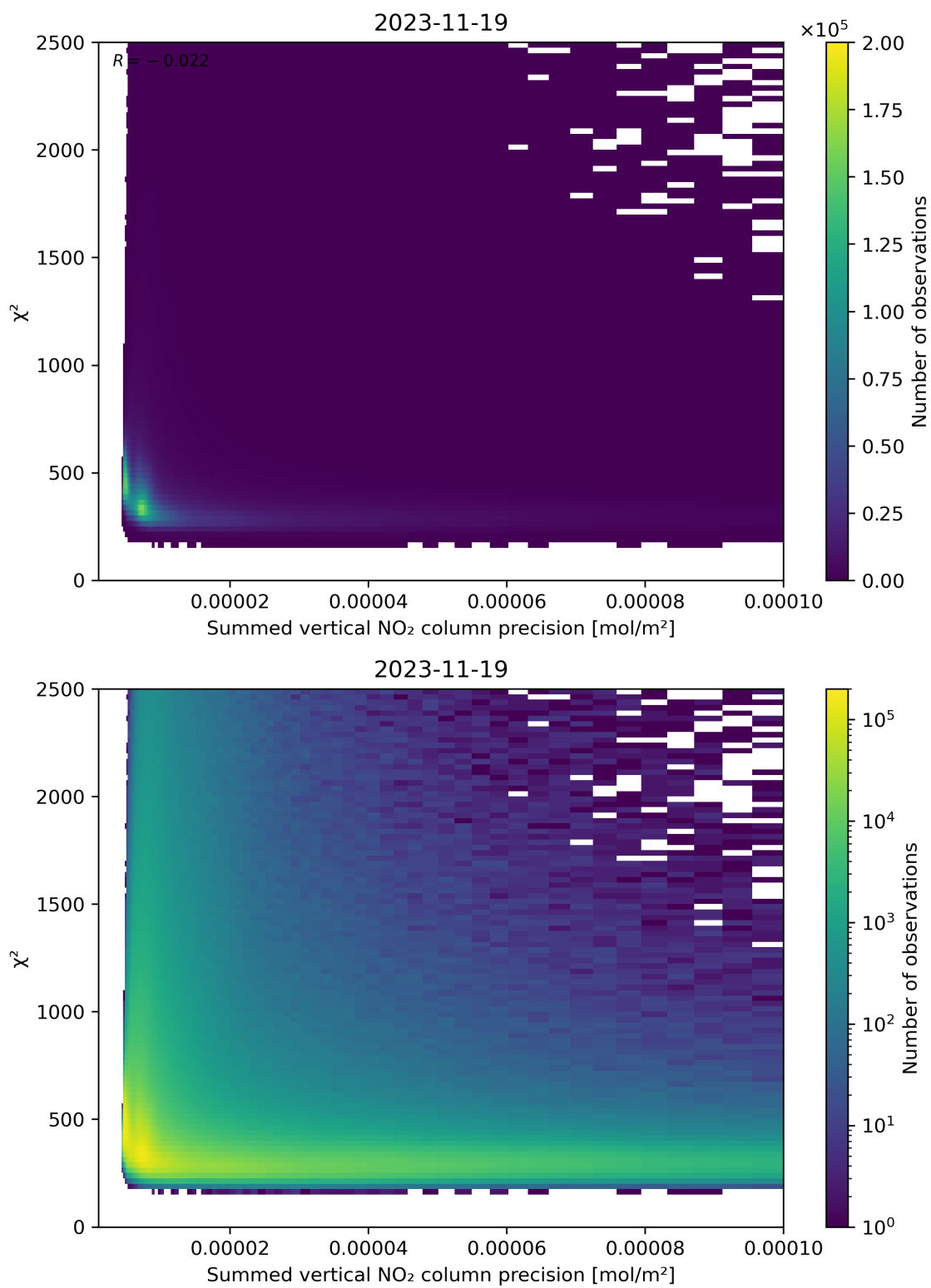
Figure 107: Scatter density plot of “Summed vertical NO 2 column precision” against “ \chi^2 ” for 2023-11-18 to 2023-11-20.
