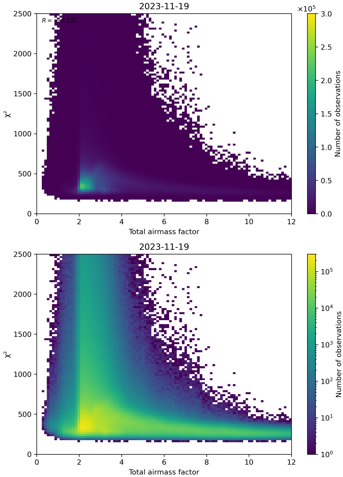
Figure 63: Scatter density plot of “Total airmass factor” against “ \chi^2 ” for 2023-11-18 to 2023-11-20.
