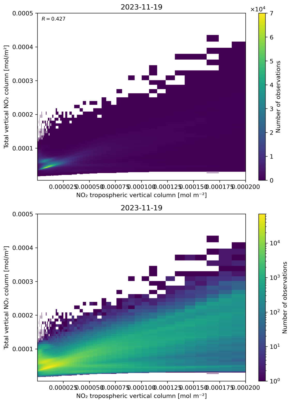
Figure 128: Scatter density plot of “NO 2 tropospheric vertical column” against “Total vertical NO 2 column” for 2023-11-18 to 2023-11-20.
