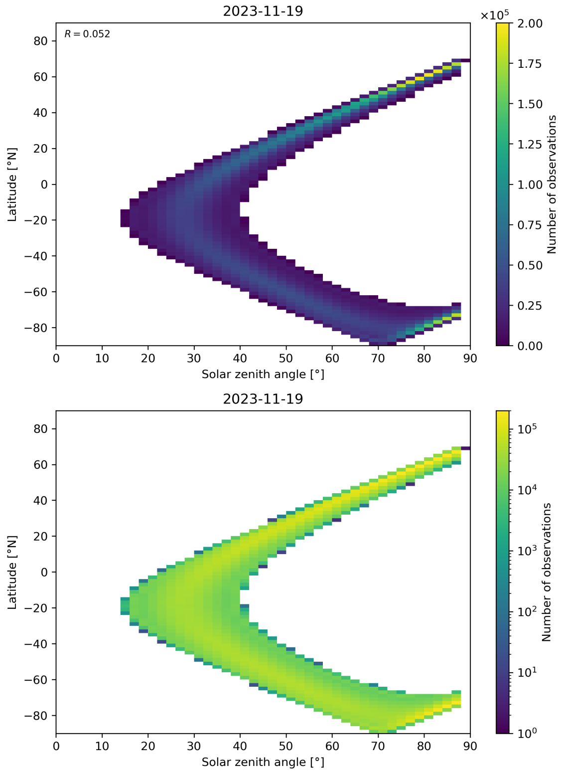
Figure 149: Scatter density plot of “Solar zenith angle” against “Latitude” for 2023-11-18 to 2023-11-20.
