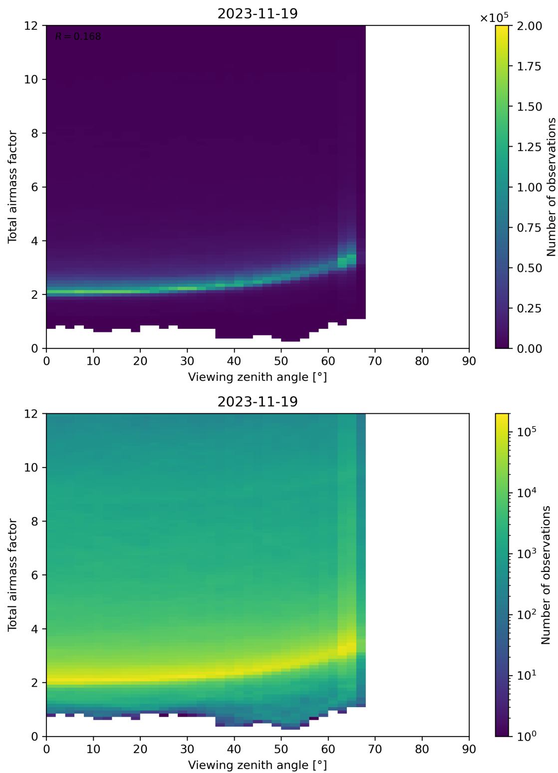
Figure 160: Scatter density plot of “Viewing zenith angle” against “Total airmass factor” for 2023-11-18 to 2023-11-20.
