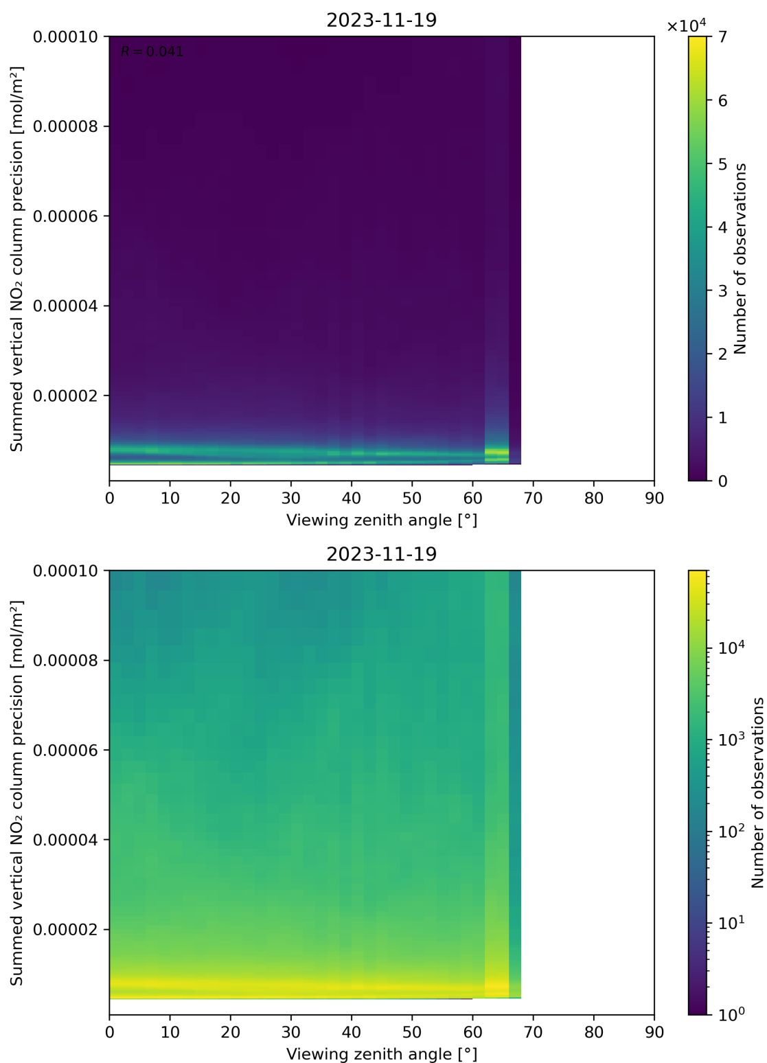
Figure 166: Scatter density plot of “Viewing zenith angle” against “Summed vertical NO 2 column precision” for 2023-11-18 to 2023-11-20.
