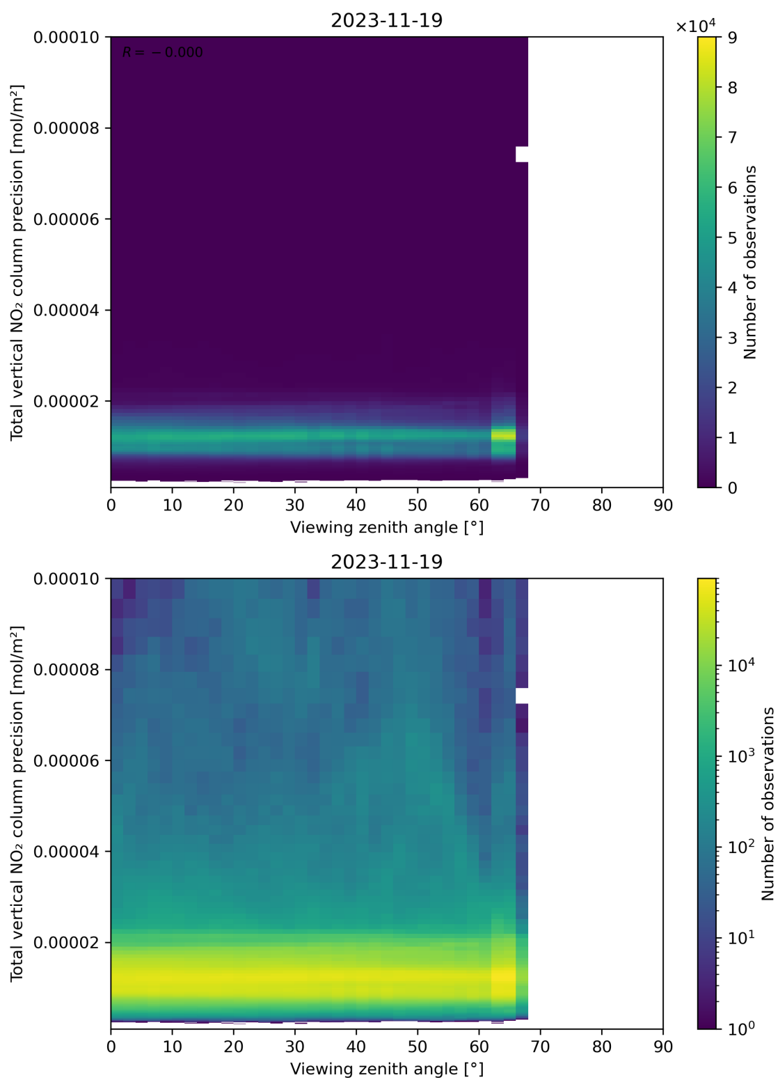
Figure 168: Scatter density plot of “Viewing zenith angle” against “Total vertical NO 2 column precision” for 2023-11-18 to 2023-11-20.
