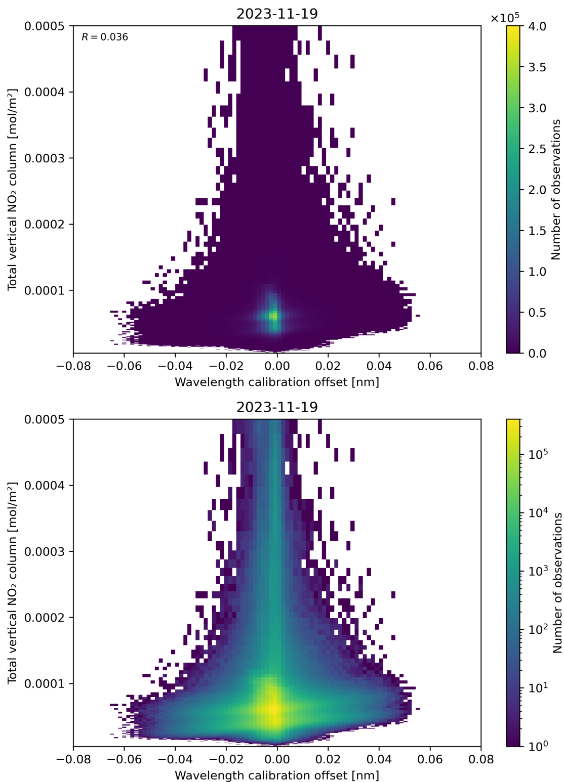
Figure 179: Scatter density plot of “Wavelength calibration offset” against “Total vertical NO 2 column” for 2023-11-18 to 2023-11-20.
