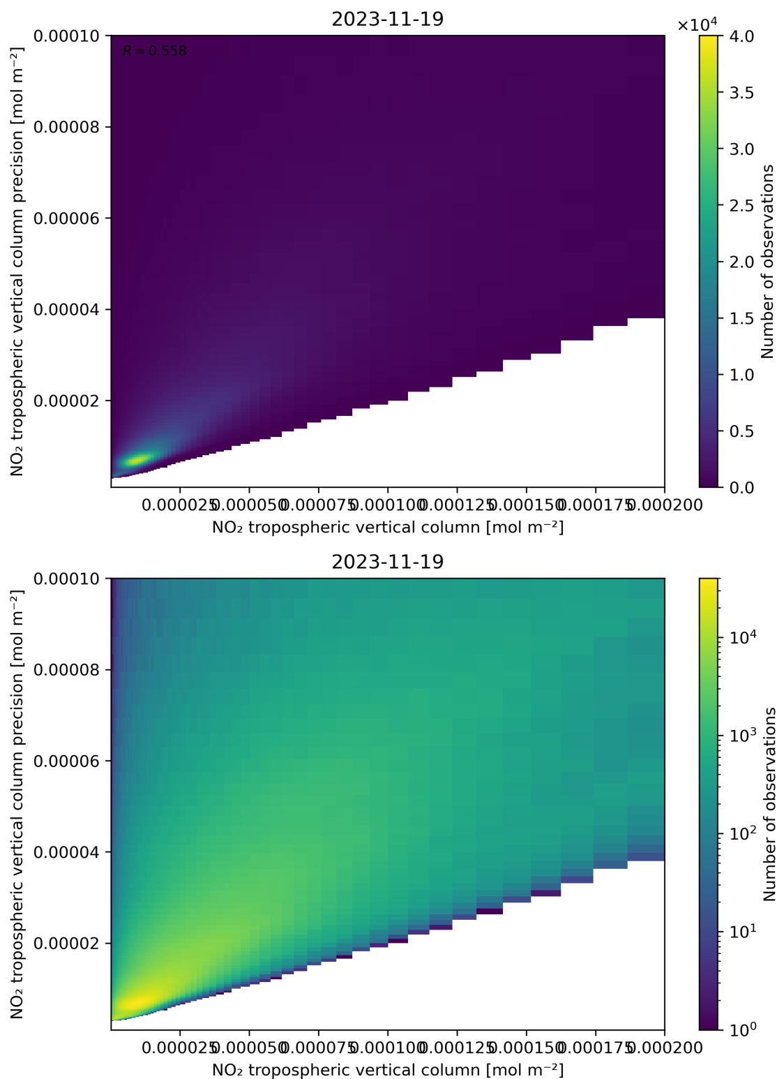
Figure 130: Scatter density plot of “NO 2 tropospheric vertical column” against “NO 2 tropospheric vertical column precision” for 2023-11-18 to 2023-11-20.
