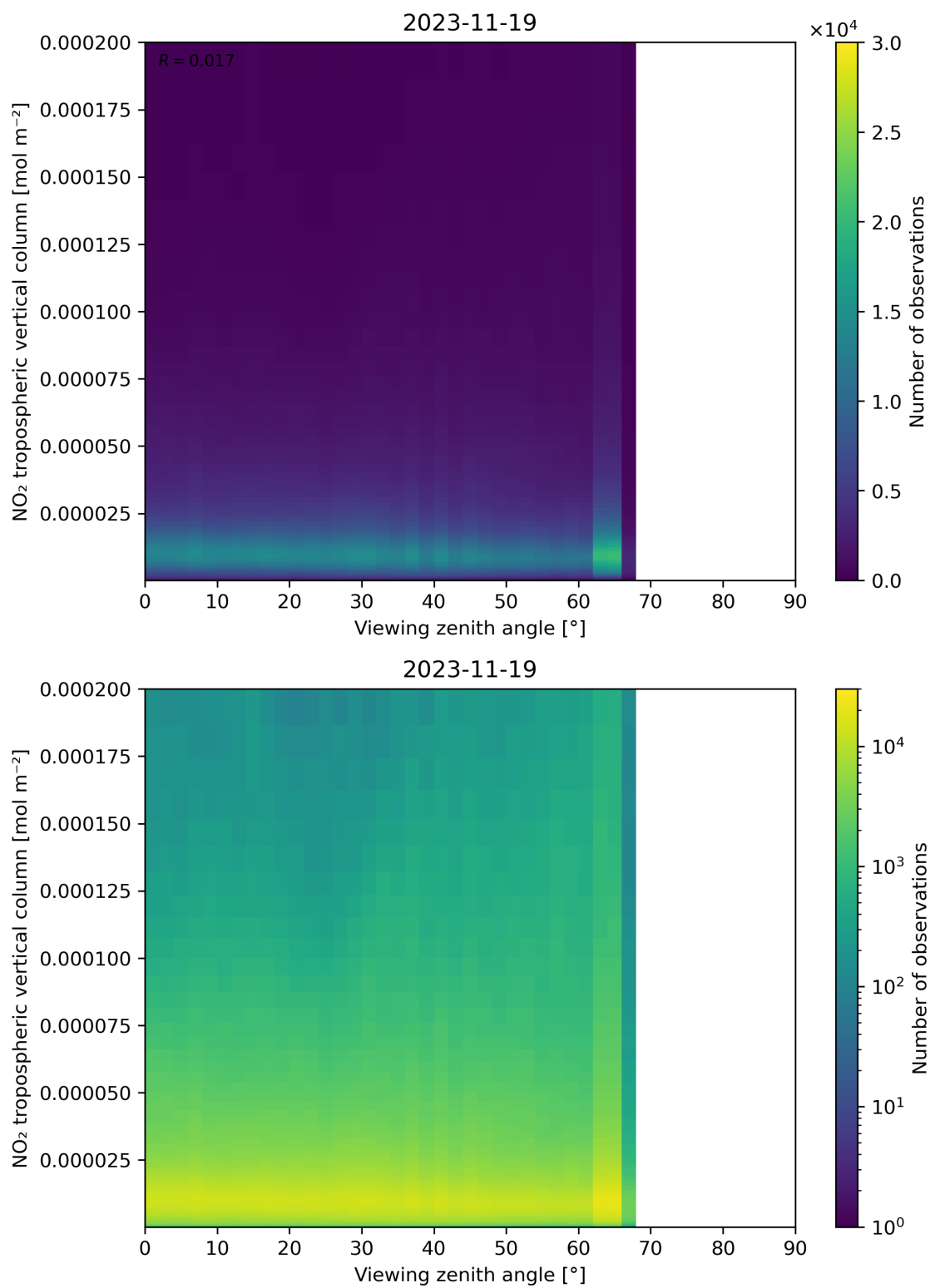
Figure 169: Scatter density plot of “Viewing zenith angle” against “NO 2 tropospheric vertical column” for 2023-11-18 to 2023-11-20.
