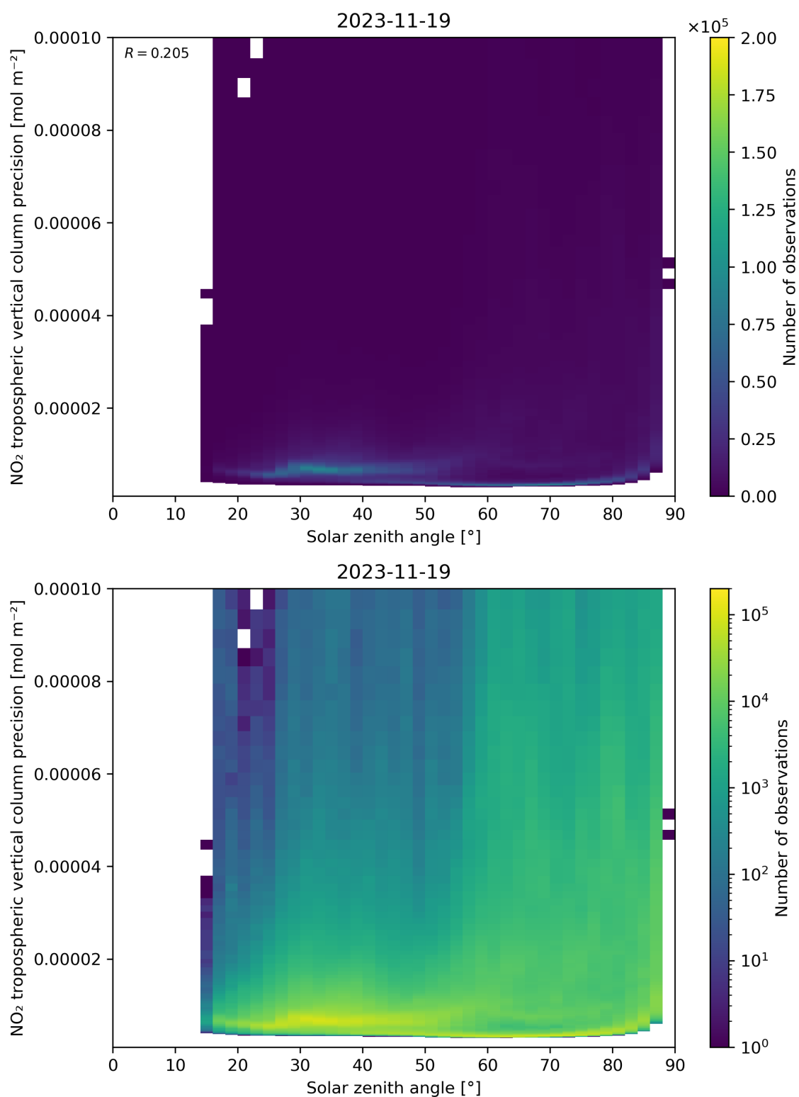
Figure 156: Scatter density plot of “Solar zenith angle” against “NO 2 tropospheric vertical column precision” for 2023-11-18 to 2023-11-20.
