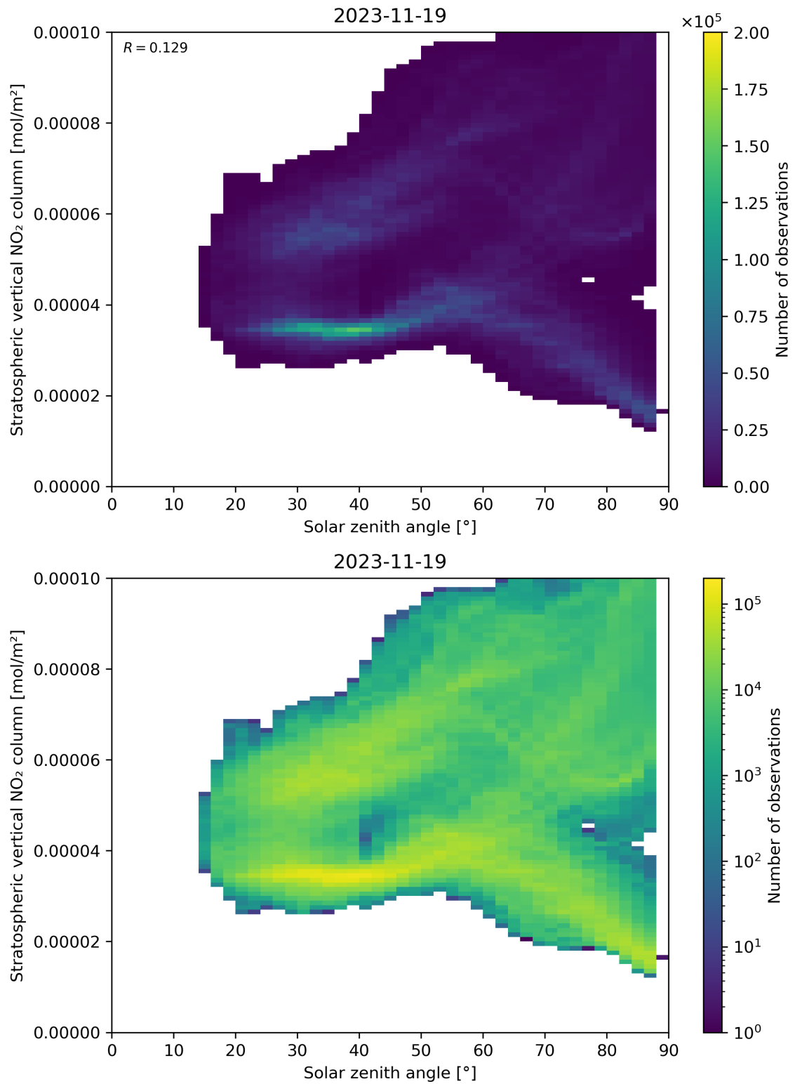
Figure 150: Scatter density plot of “Solar zenith angle” against “Stratospheric vertical NO 2 column” for 2023-11-18 to 2023-11-20.
