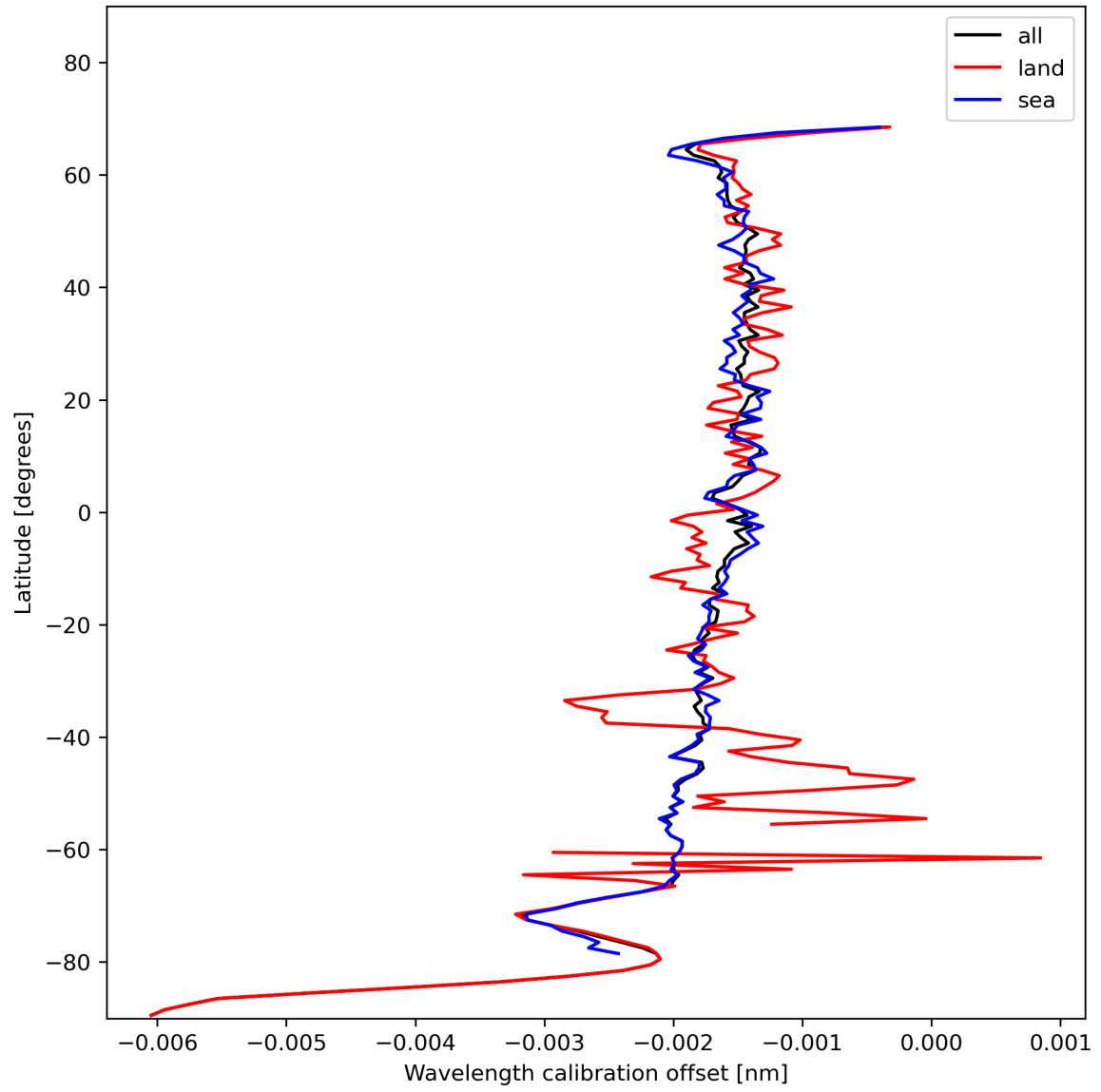
Figure 18: Zonal average of “Wavelength calibration offset” for 2023-11-18 to 2023-11-20.
