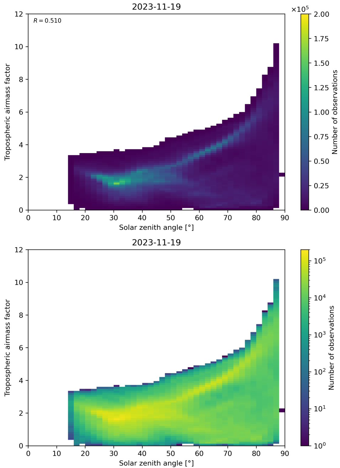
Figure 147: Scatter density plot of “Solar zenith angle” against “Tropospheric airmass factor” for 2023-11-18 to 2023-11-20.
