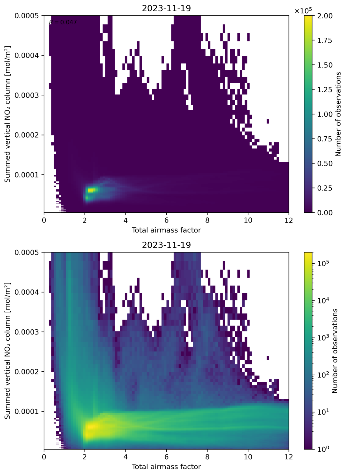
Figure 65: Scatter density plot of “Total airmass factor” against “Summed vertical NO 2 column” for 2023-11-18 to 2023-11-20.
