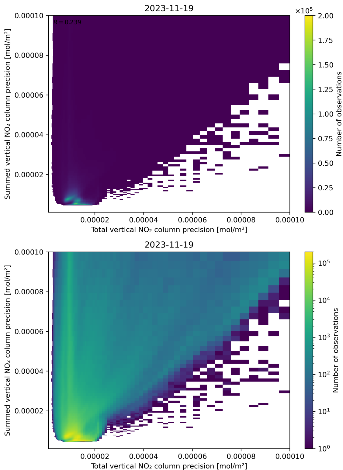
Figure 118: Scatter density plot of “Total vertical NO 2 column precision” against “Summed vertical NO 2 column precision” for 2023-11-18 to 2023-11-20.
