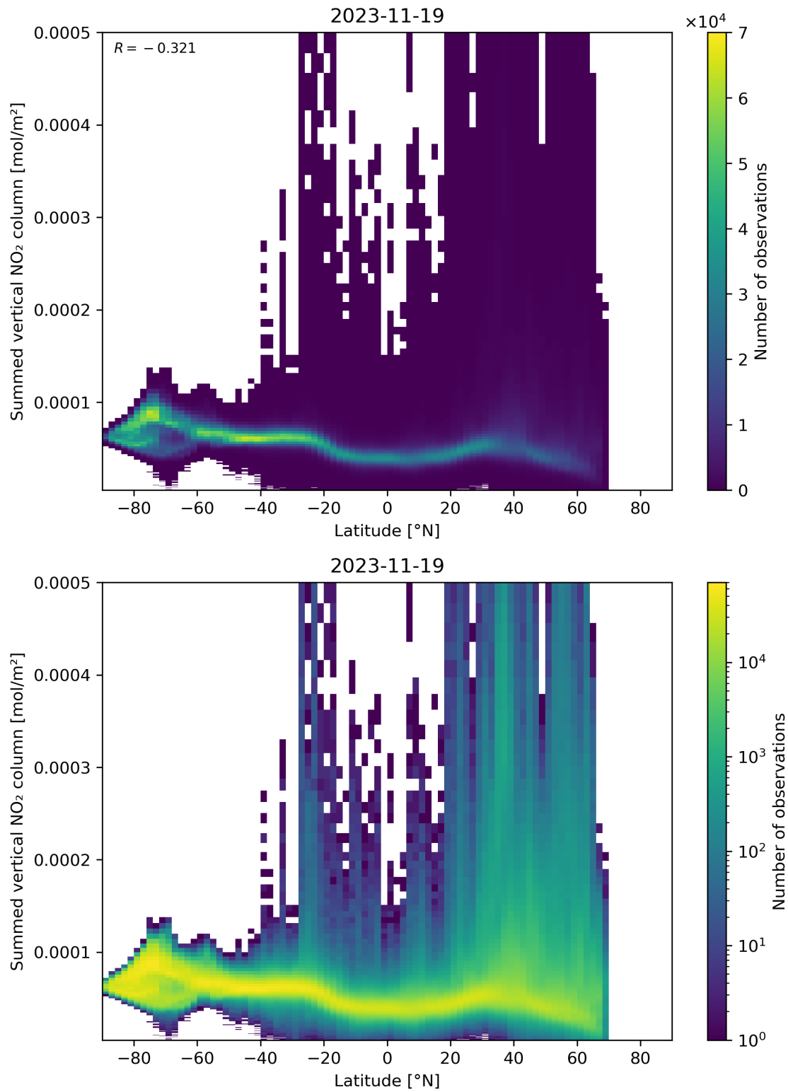
Figure 88: Scatter density plot of “Latitude” against “Summed vertical NO 2 column” for 2023-11-18 to 2023-11-20.
