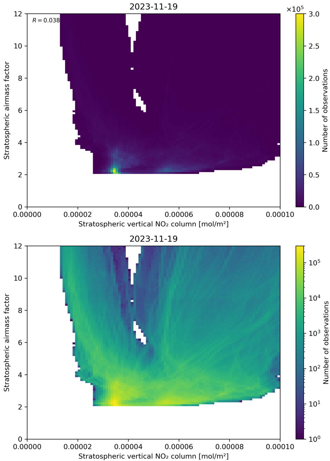
Figure 96: Scatter density plot of “Stratospheric vertical NO 2 column” against “Stratospheric airmass factor” for 2023-11-18 to 2023-11-20.
