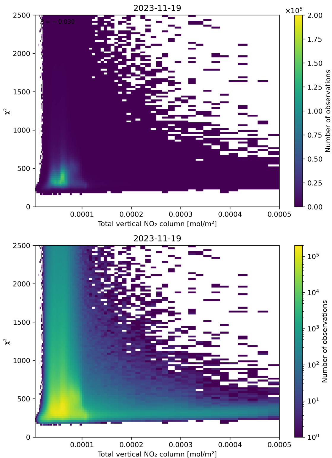
Figure 111: Scatter density plot of “Total vertical NO 2 column” against “ \chi^2 ” for 2023-11-18 to 2023-11-20.
