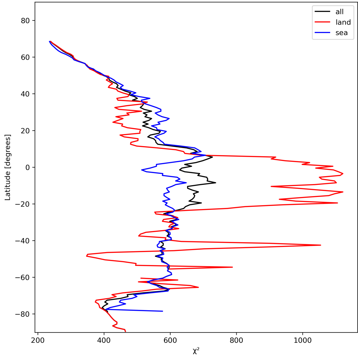
Figure 25: Zonal average of “ \chi^2 ” for 2023-11-18 to 2023-11-20.
