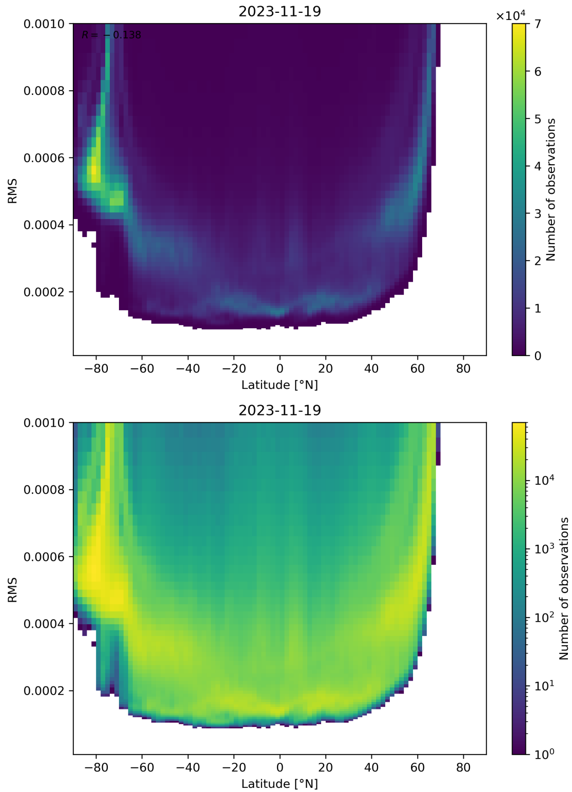
Figure 94: Scatter density plot of “Latitude” against “RMS” for 2023-11-18 to 2023-11-20.
