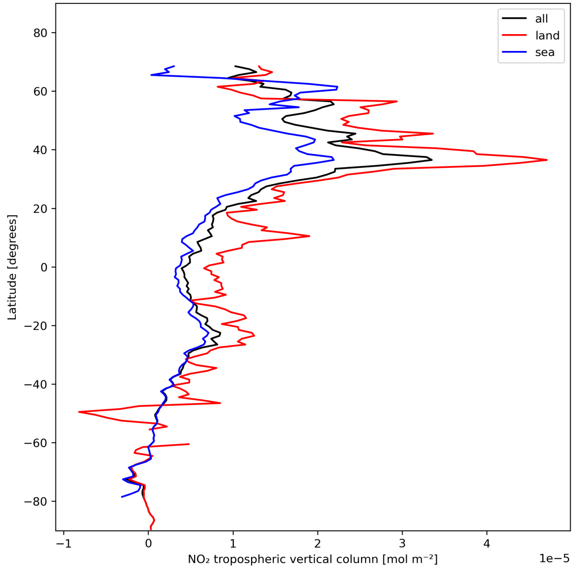
Figure 12: Zonal average of “NO 2 tropospheric vertical column” for 2023-11-18 to 2023-11-20.
