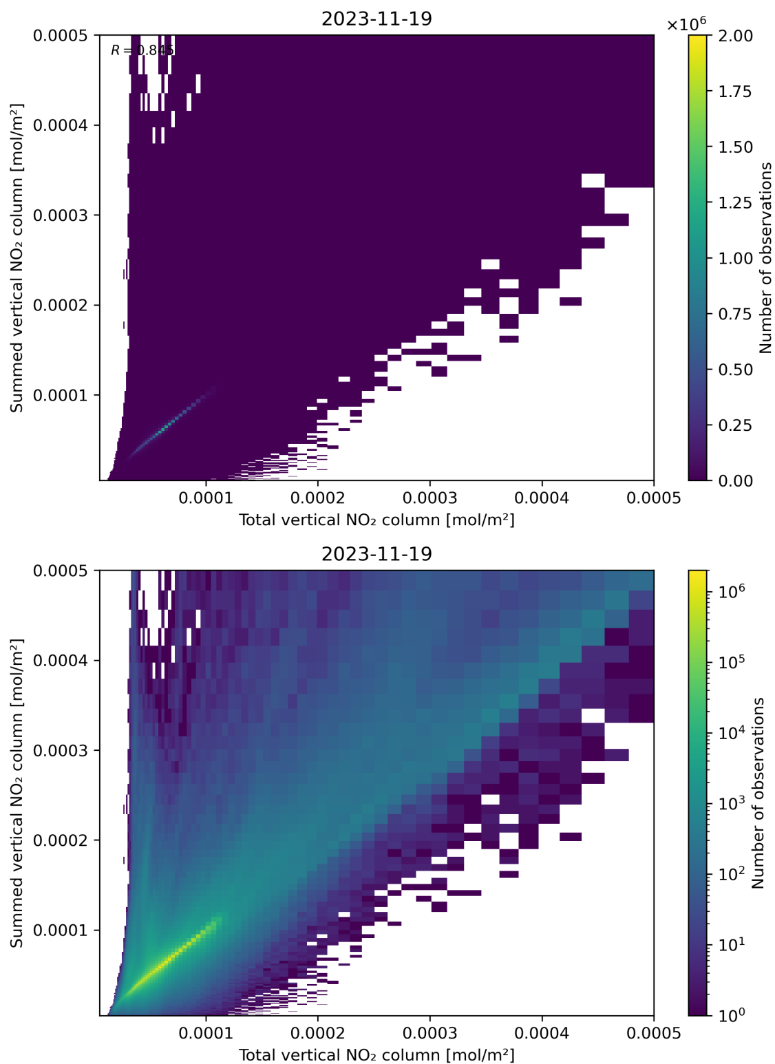
Figure 112: Scatter density plot of “Total vertical NO 2 column” against “Summed vertical NO 2 column” for 2023-11-18 to 2023-11-20.
