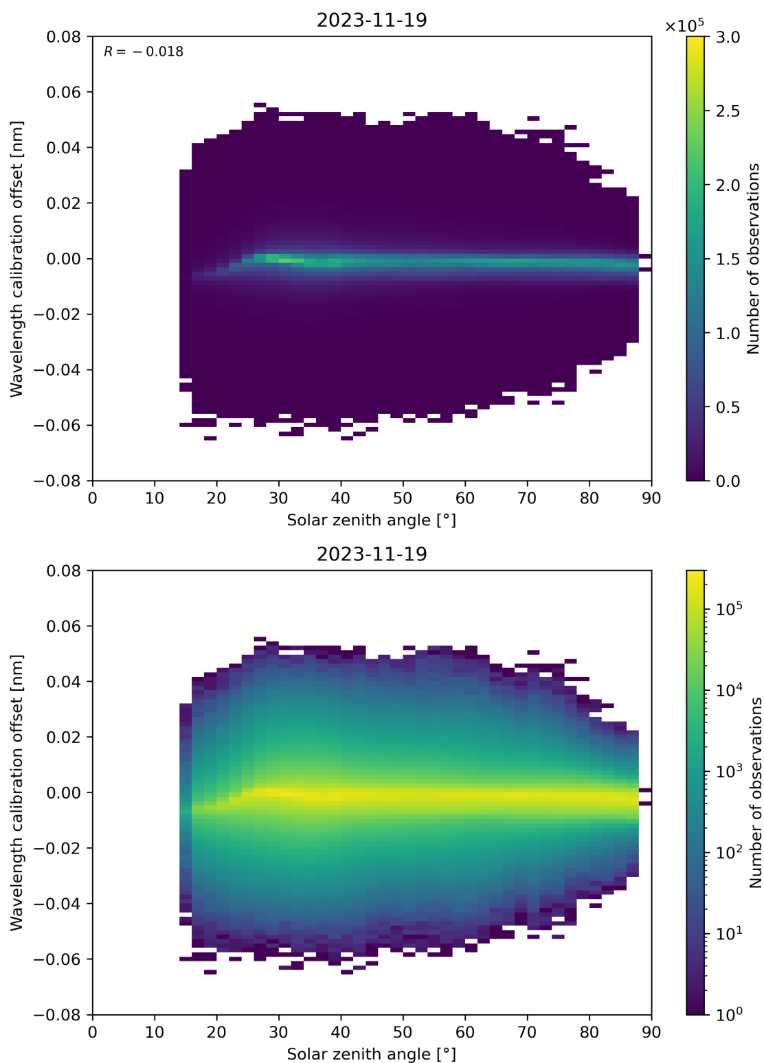
Figure 158: Scatter density plot of “Solar zenith angle” against “Wavelength calibration offset” for 2023-11-18 to 2023-11-20.
