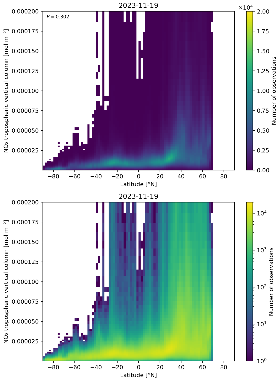
Figure 92: Scatter density plot of “Latitude” against “NO 2 tropospheric vertical column” for 2023-11-18 to 2023-11-20.
