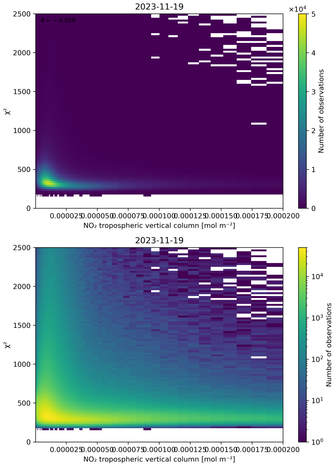
Figure 124: Scatter density plot of “NO 2 tropospheric vertical column” against “ \chi^2 ” for 2023-11-18 to 2023-11-20.
