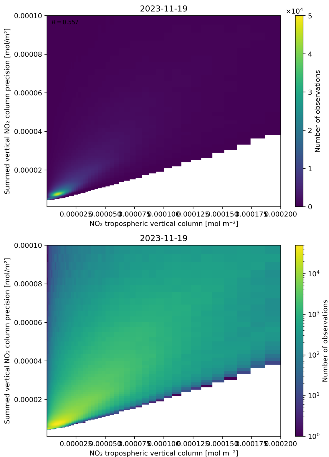
Figure 127: Scatter density plot of “NO 2 tropospheric vertical column” against “Summed vertical NO 2 column precision” for 2023-11-18 to 2023-11-20.
