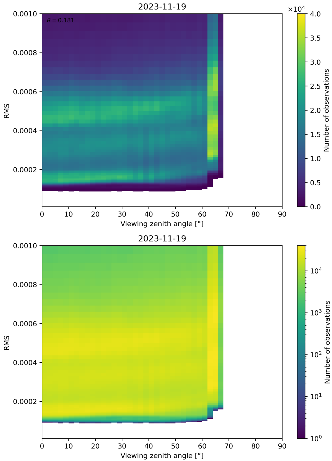
Figure 171: Scatter density plot of “Viewing zenith angle” against “RMS” for 2023-11-18 to 2023-11-20.
