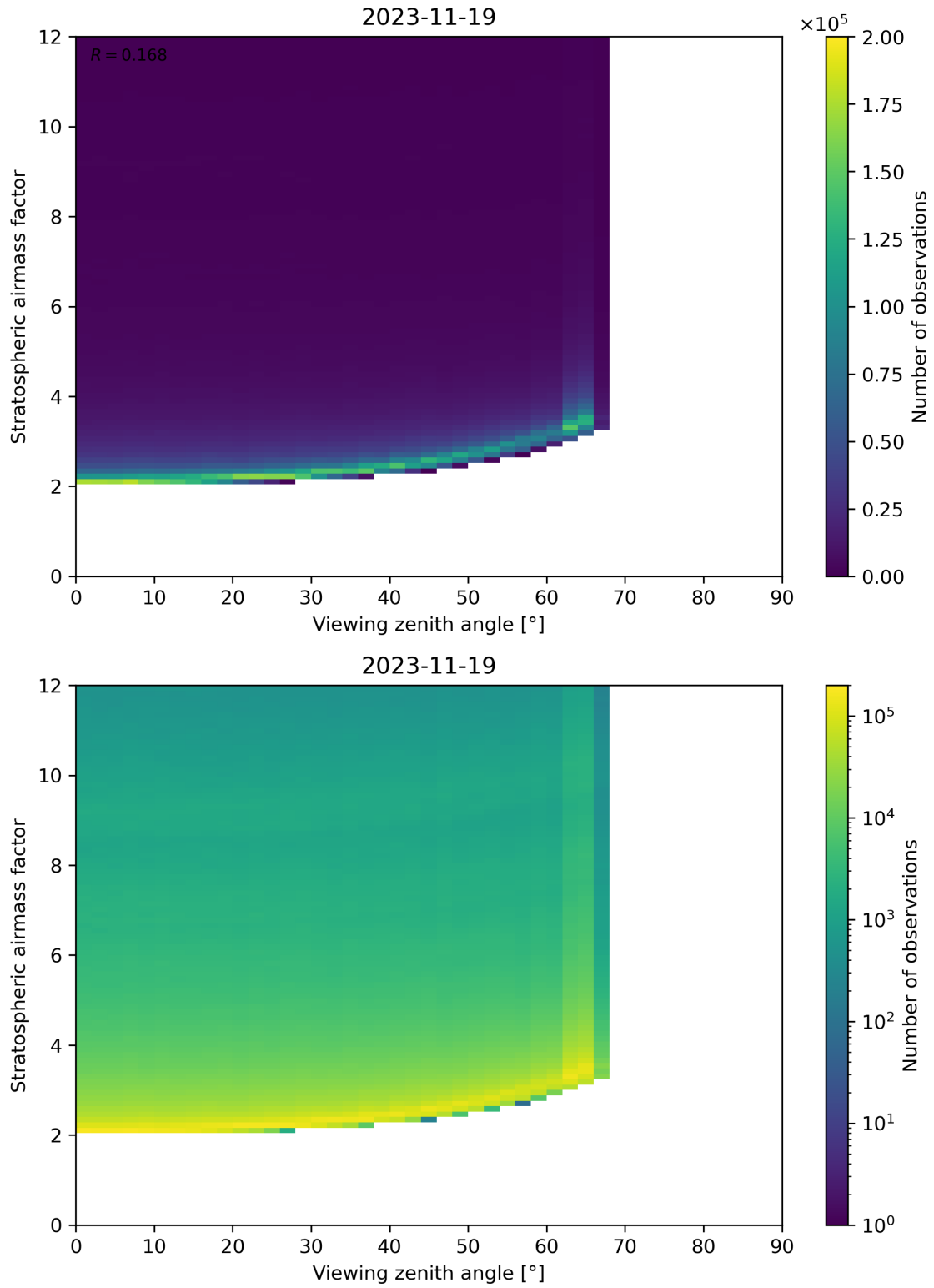
Figure 159: Scatter density plot of “Viewing zenith angle” against “Stratospheric airmass factor” for 2023-11-18 to 2023-11-20.
