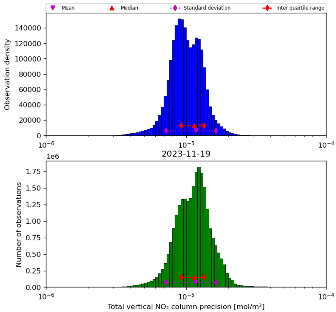
Figure 39: Histogram of “Total vertical NO 2 column precision” for 2023-11-18 to 2023-11-20
