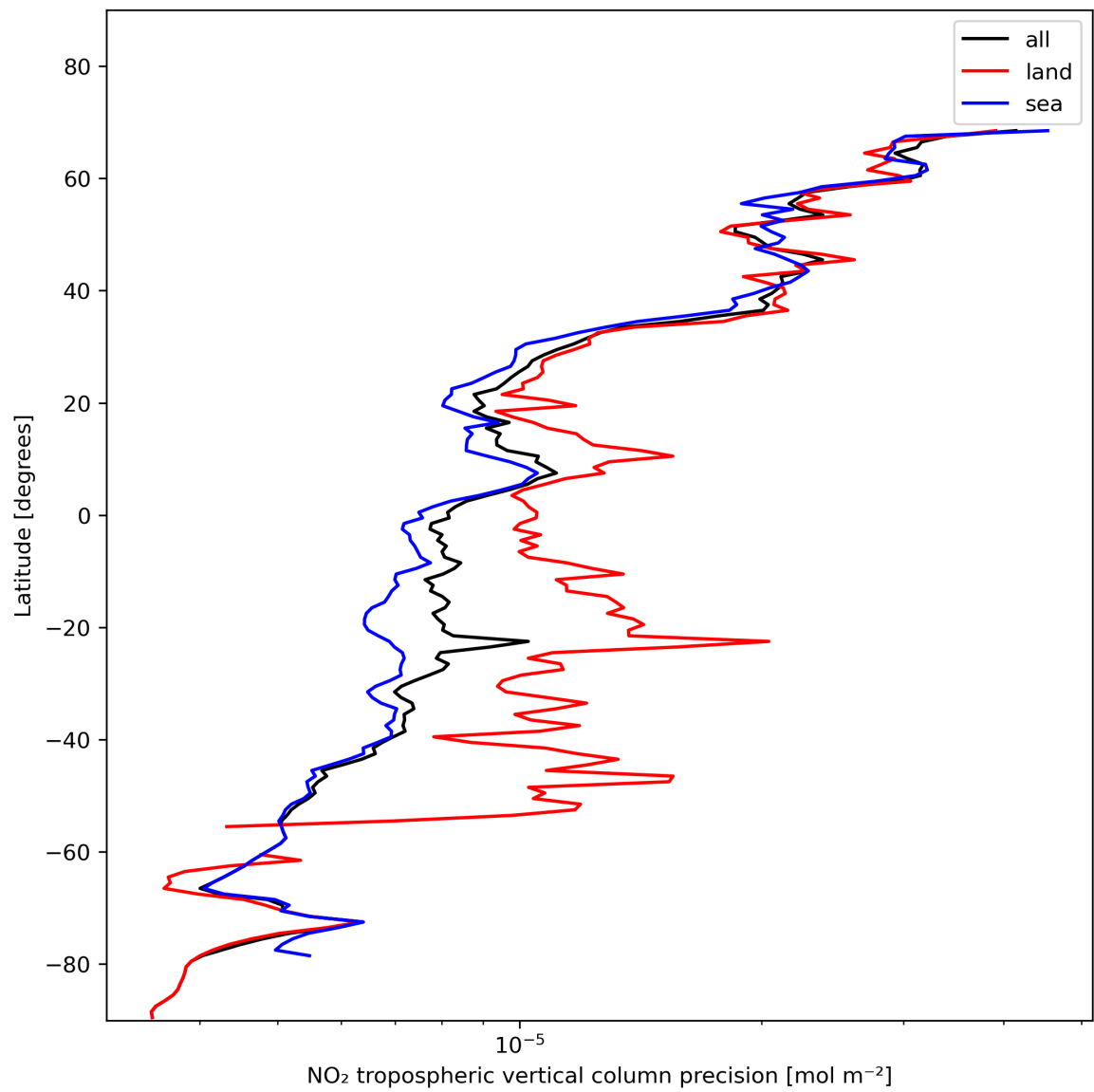
Figure 13: Zonal average of “NO 2 tropospheric vertical column precision” for 2023-11-18 to 2023-11-20.
