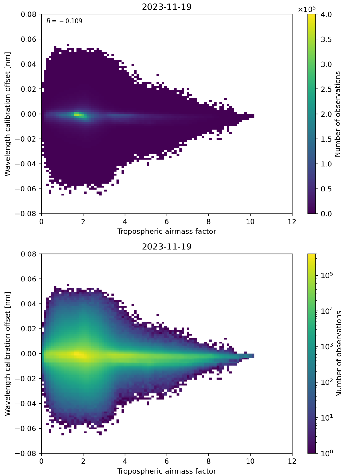
Figure 80: Scatter density plot of “Tropospheric airmass factor” against “Wavelength calibration offset” for 2023-11-18 to 2023-11-20.
