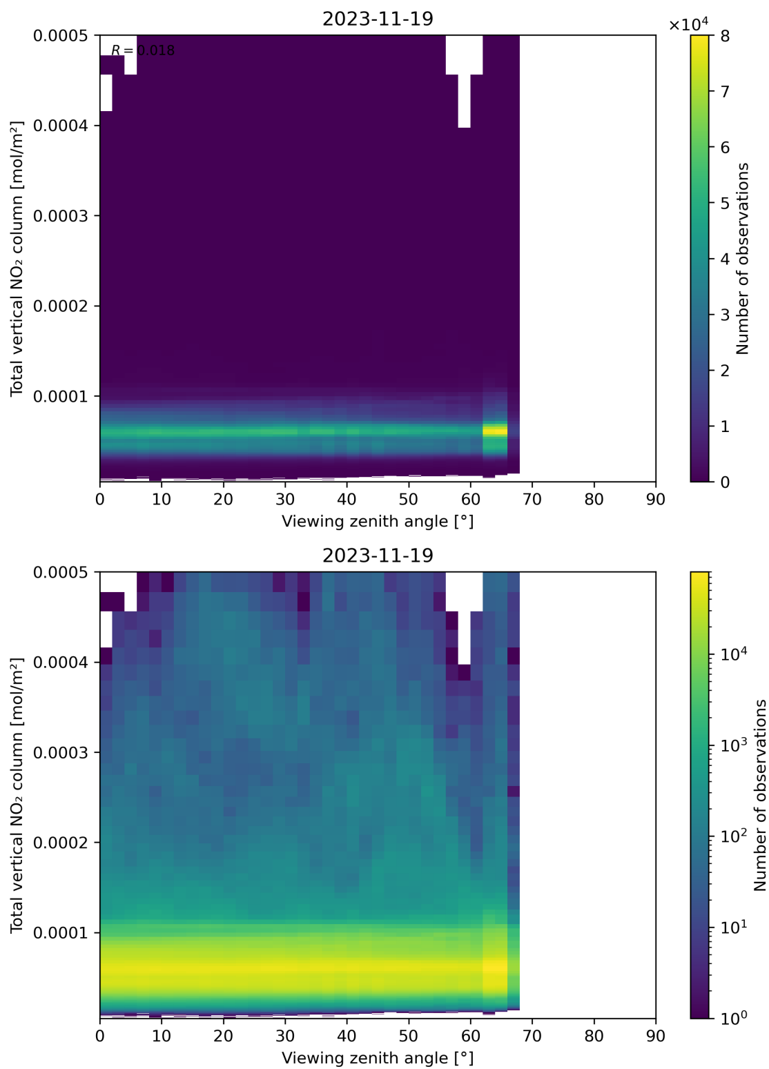
Figure 167: Scatter density plot of “Viewing zenith angle” against “Total vertical NO 2 column” for 2023-11-18 to 2023-11-20.
