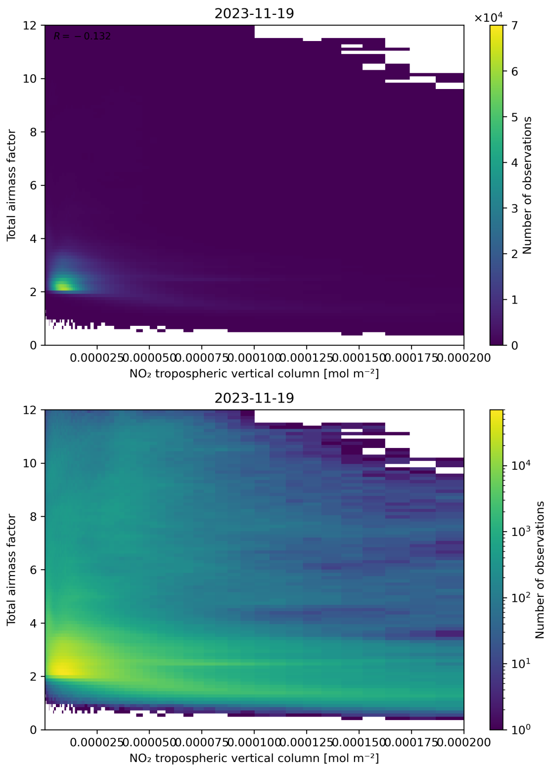
Figure 122: Scatter density plot of “NO 2 tropospheric vertical column” against “Total air mass factor” for 2023-11-18 to 2023-11-20.
