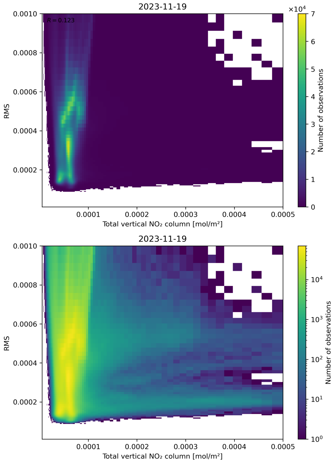
Figure 120: Scatter density plot of “Total vertical NO 2 column” against “RMS” for 2023-11-18 to 2023-11-20.
