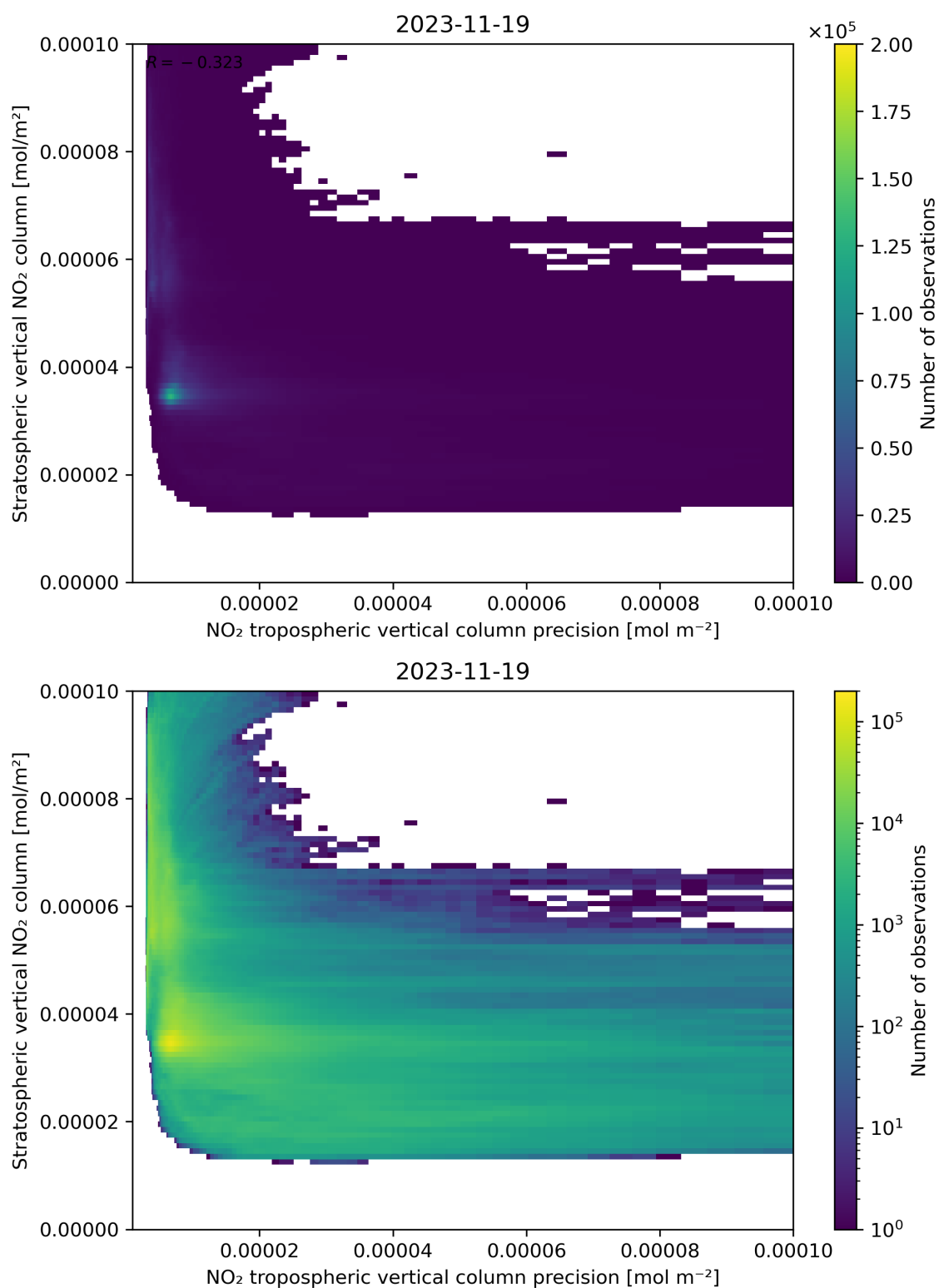
Figure 135: Scatter density plot of “NO 2 tropospheric vertical column precision” against “Stratospheric vertical NO 2 column” for 2023-11-18 to 2023-11-20.
