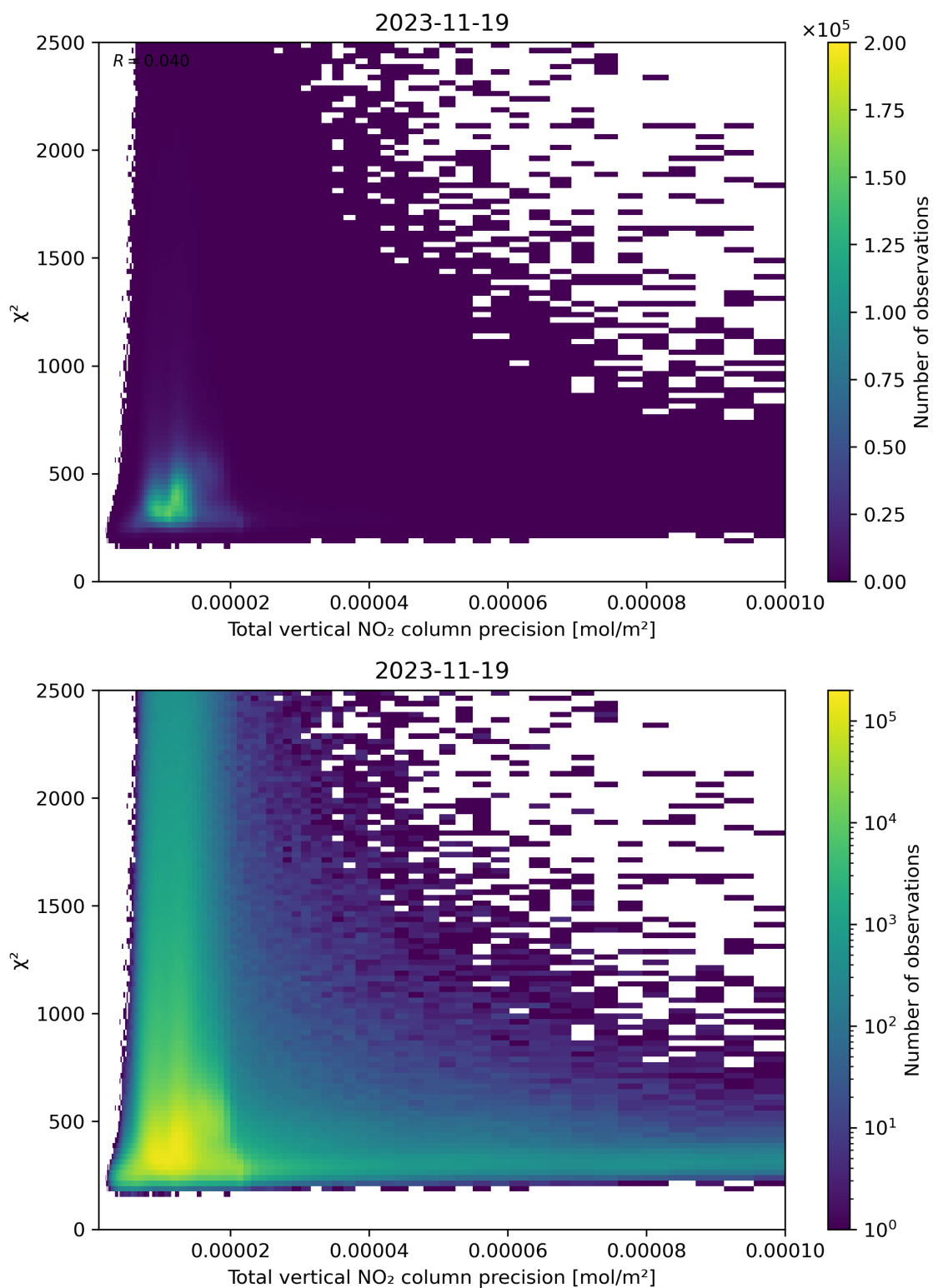
Figure 116: Scatter density plot of “Total vertical NO 2 column precision” against “ \chi^2 ” for 2023-11-18 to 2023-11-20.
