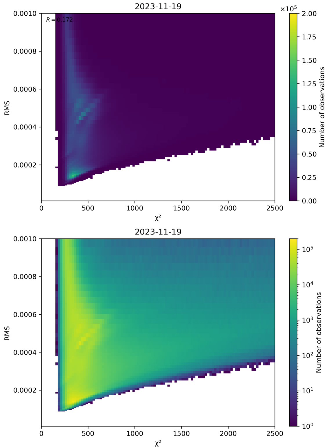
Figure 82: Scatter density plot of “ \chi^2 ” against “RMS” for 2023-11-18 to 2023-11-20.
