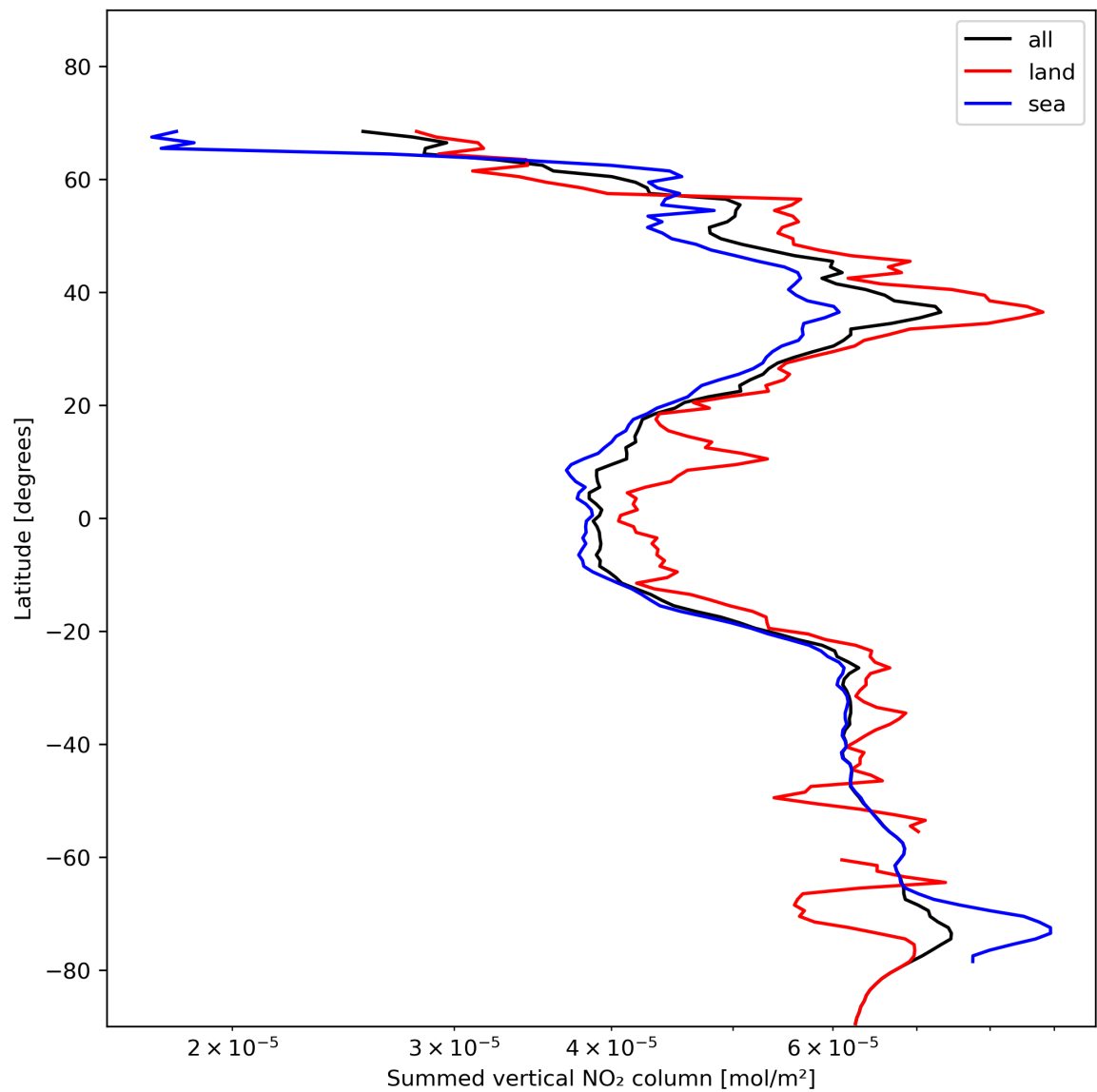
Figure 23: Zonal average of “Summed vertical NO 2 column” for 2023-11-18 to 2023-11-20.
