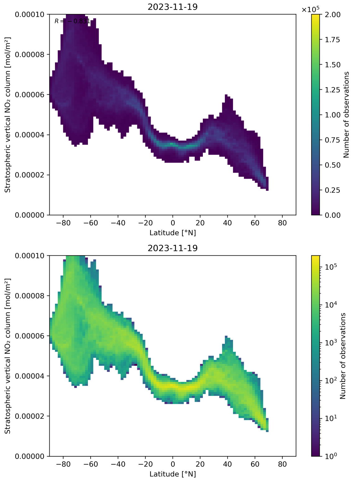
Figure 87: Scatter density plot of “Latitude” against “Stratospheric vertical NO 2 column” for 2023-11-18 to 2023-11-20.
