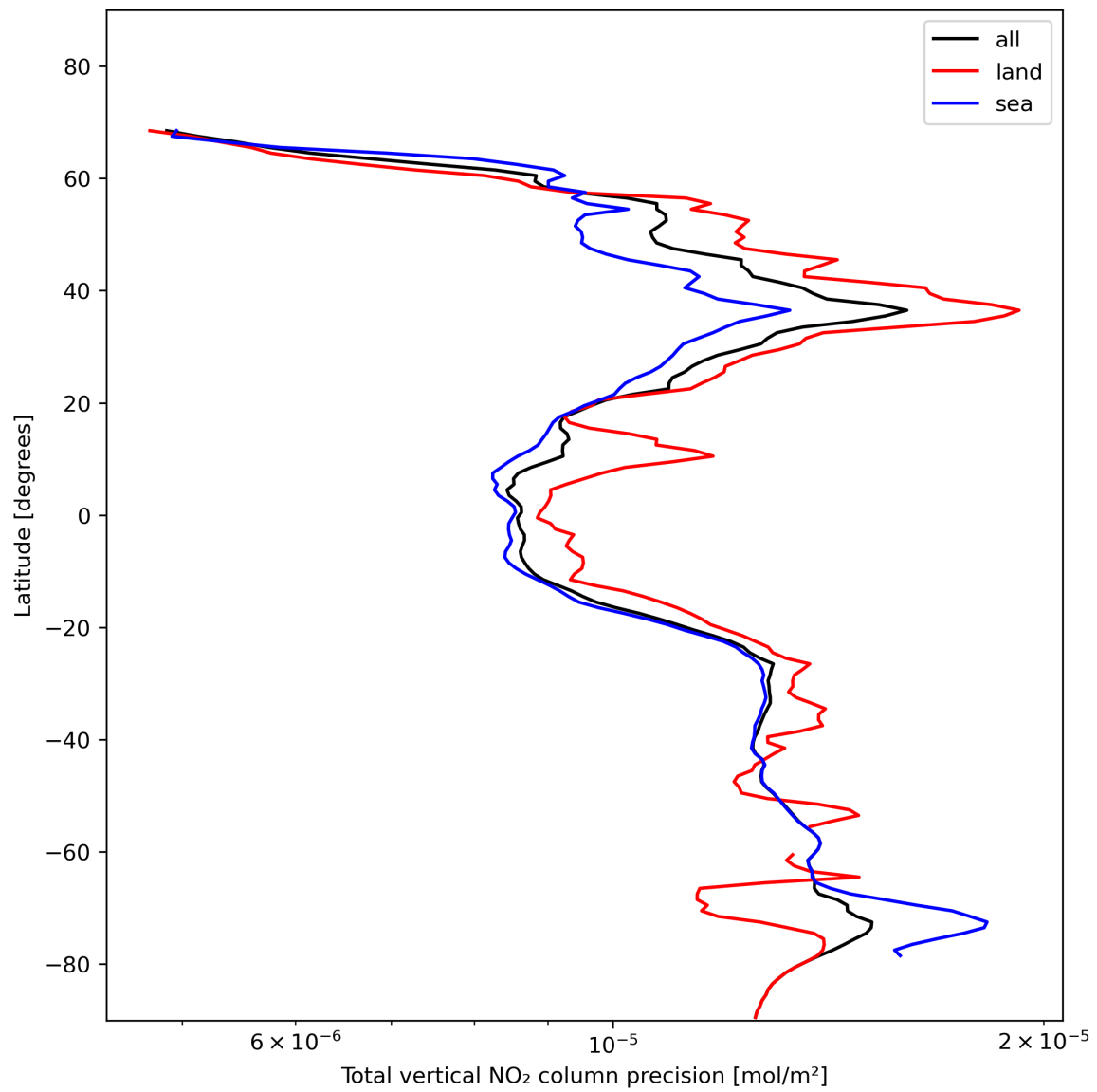
Figure 22: Zonal average of “Total vertical NO 2 column precision” for 2023-11-18 to 2023-11-20.
