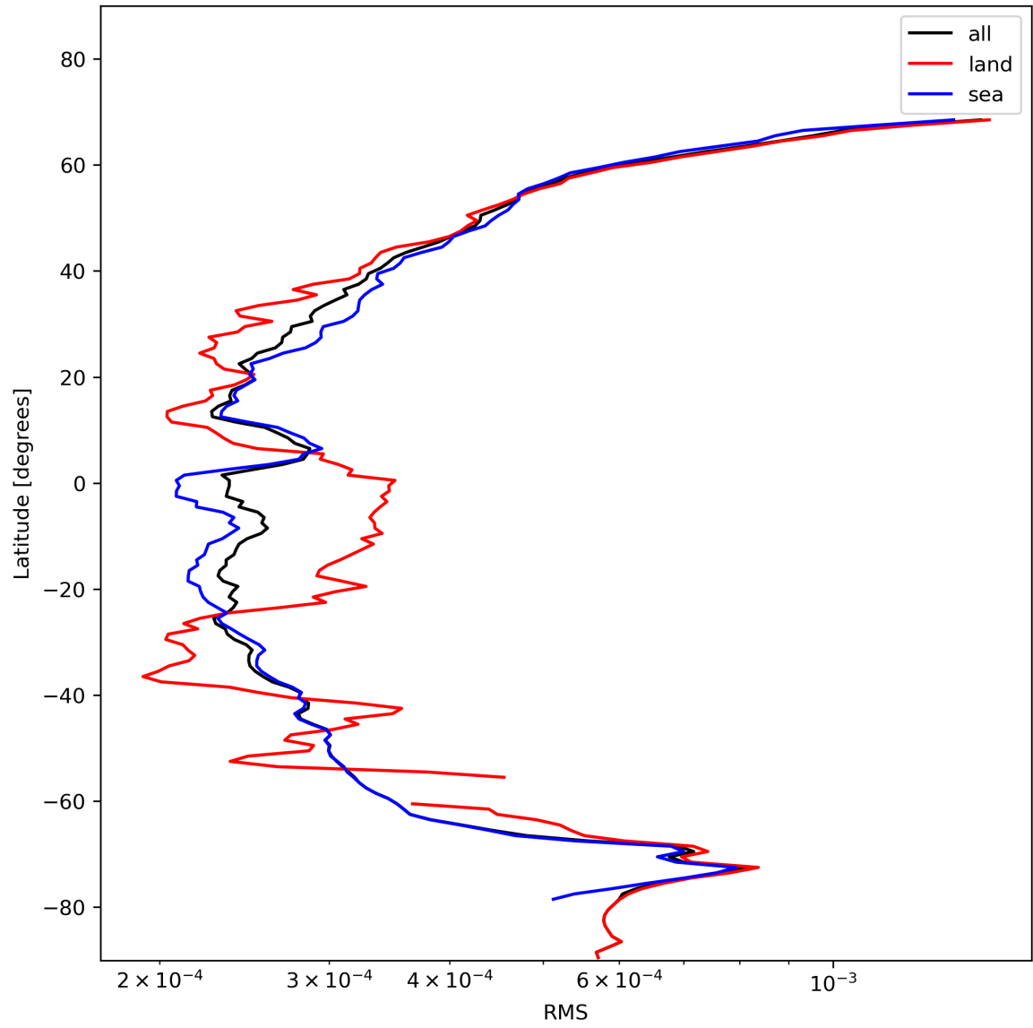
Figure 26: Zonal average of “RMS” for 2023-11-18 to 2023-11-20.
