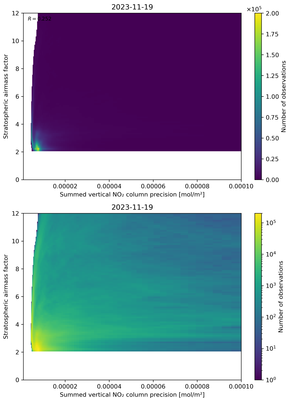
Figure 106: Scatter density plot of “Summed vertical NO 2 column precision” against “Stratospheric airmass factor” for 2023-11-18 to 2023-11-20.
