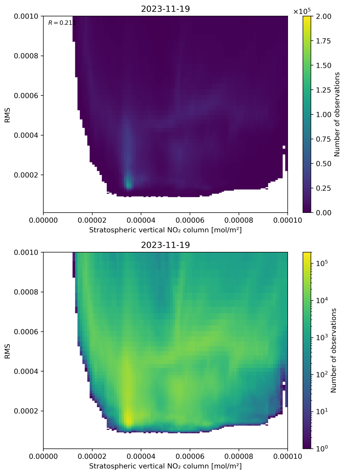
Figure 102: Scatter density plot of “Stratospheric vertical NO 2 column” against “RMS” for 2023-11-18 to 2023-11-20.
