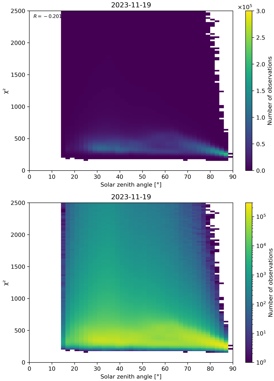
Figure 148: Scatter density plot of “Solar zenith angle” against “ \chi^2 ” for 2023-11-18 to 2023-11-20.
