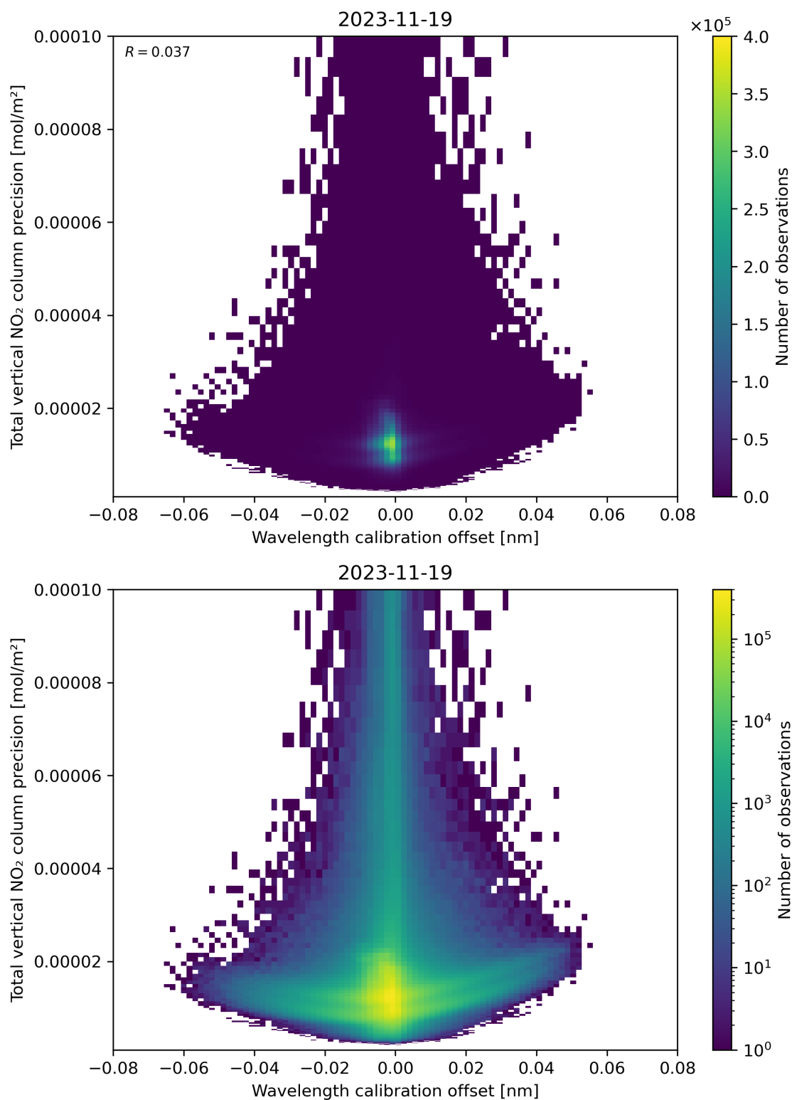
Figure 180: Scatter density plot of “Wavelength calibration offset” against “Total vertical NO 2 column precision” for 2023-11-18 to 2023-11-20.
