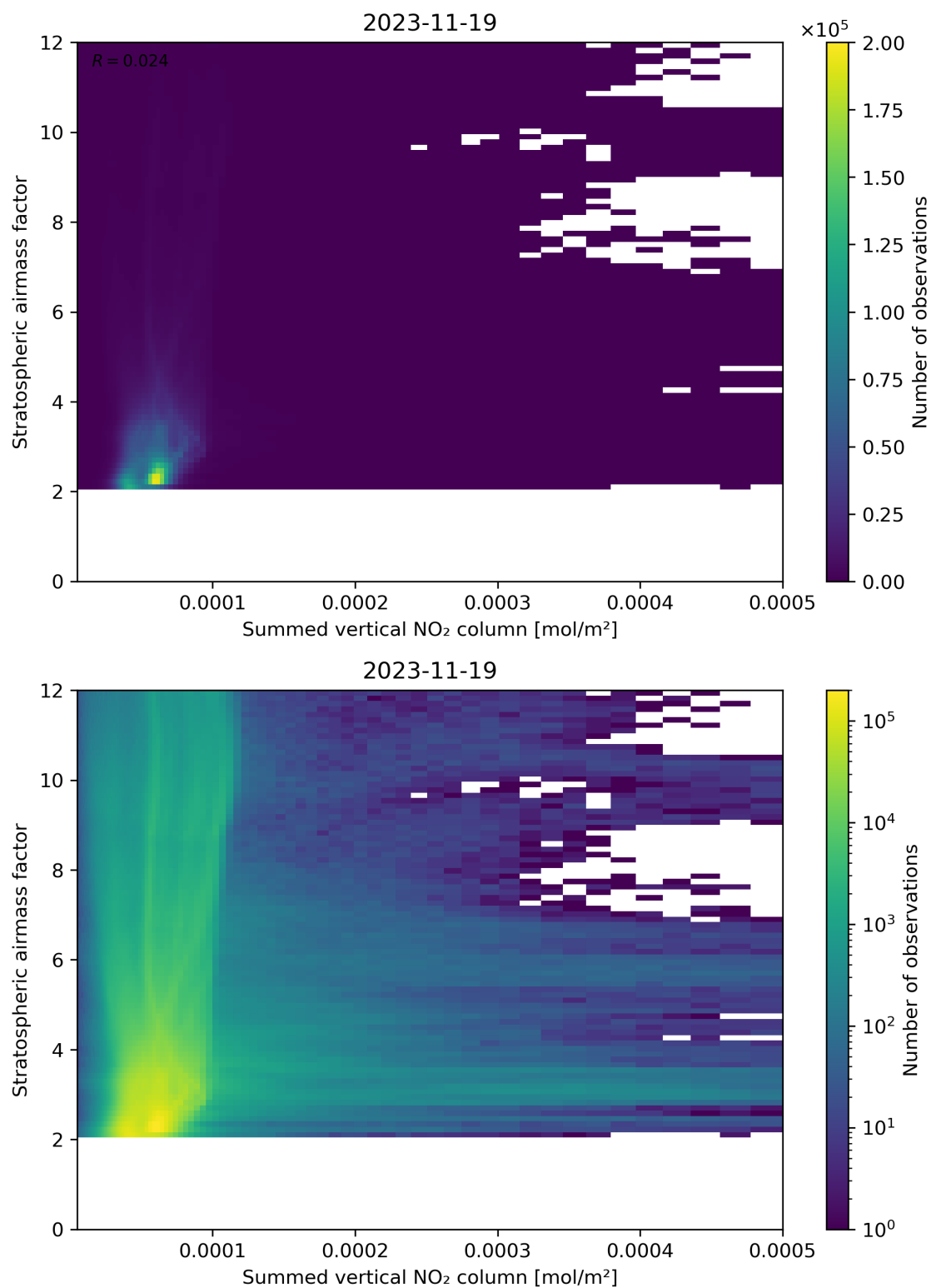
Figure 103: Scatter density plot of “Summed vertical NO 2 column” against “Stratospheric air mass factor” for 2023-11-18 to 2023-11-20.
