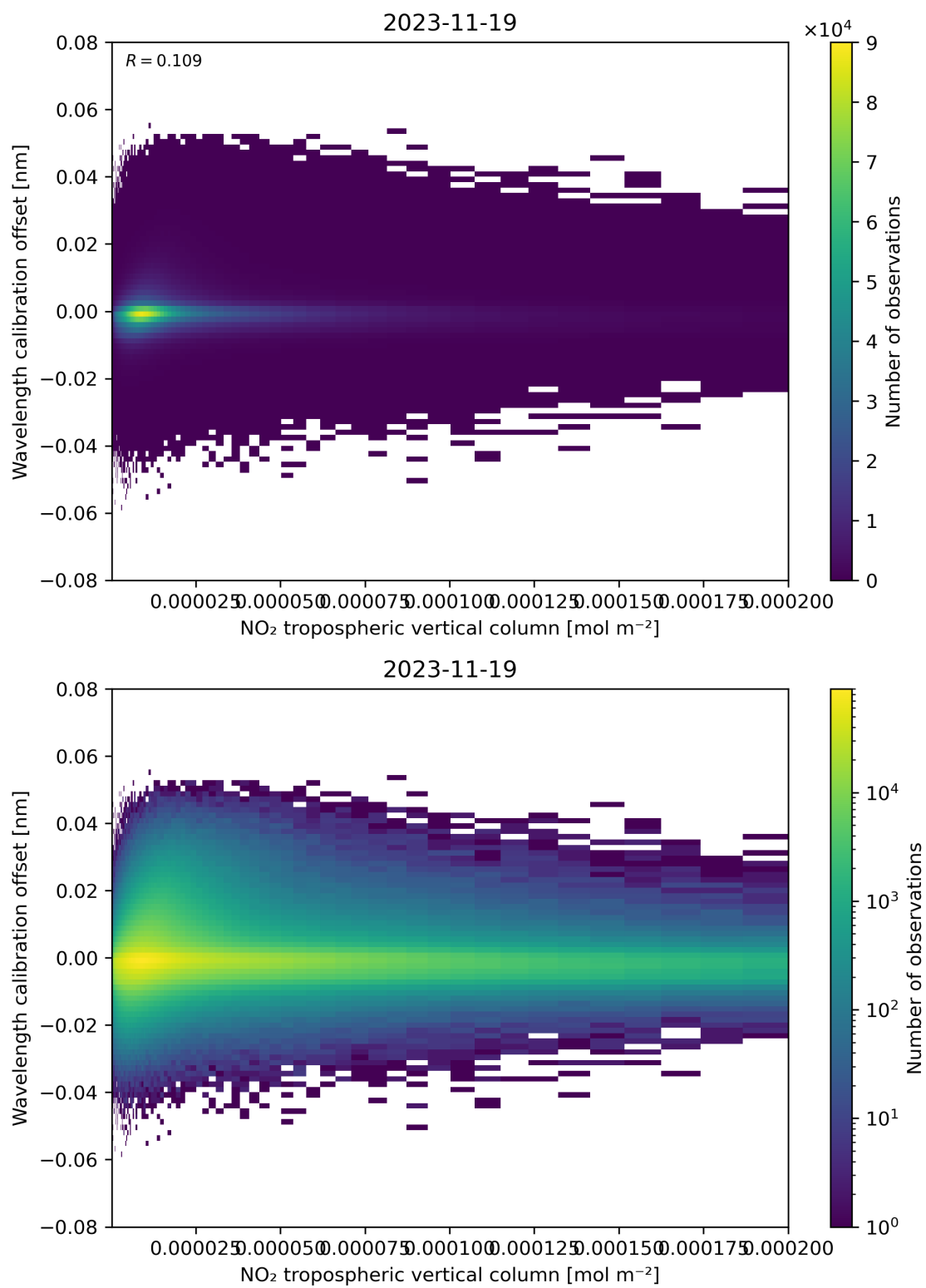
Figure 143: Scatter density plot of “NO 2 tropospheric vertical column” against “Wavelength calibration offset” for 2023-11-18 to 2023-11-20.
