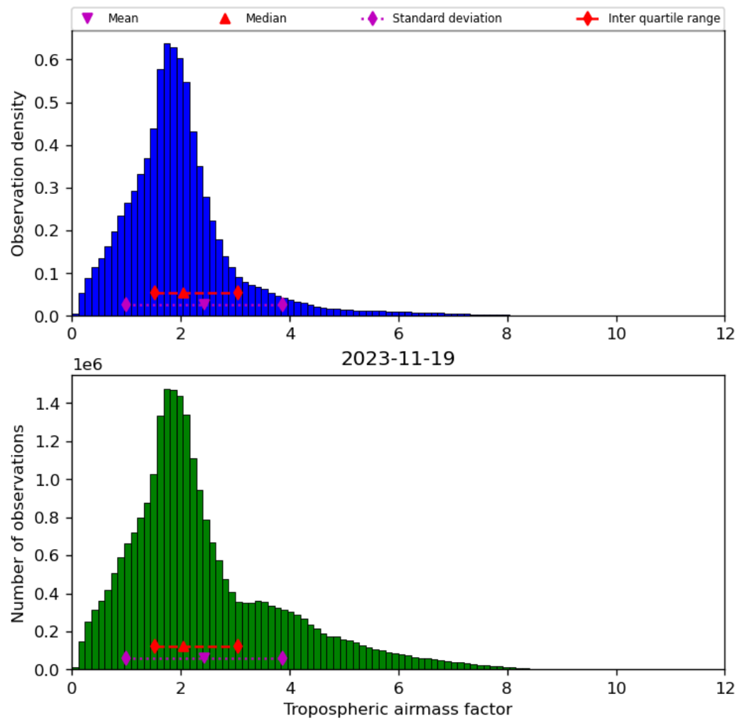
Figure 31: Histogram of “Tropospheric airmass factor” for 2023-11-18 to 2023-11-20
