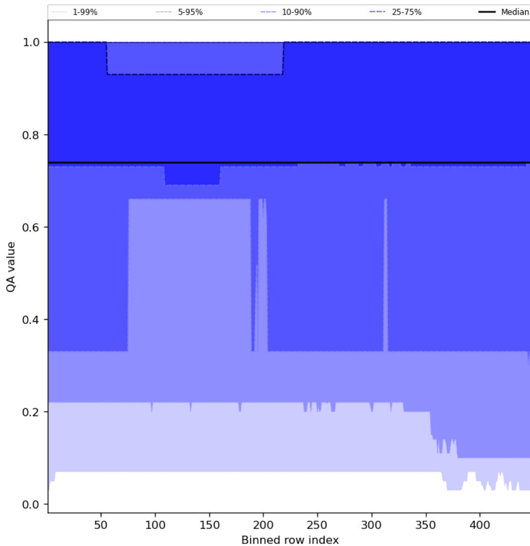
Figure 45: Along track statistics of “QA value” for 2023-11-18 to 2023-11-20
