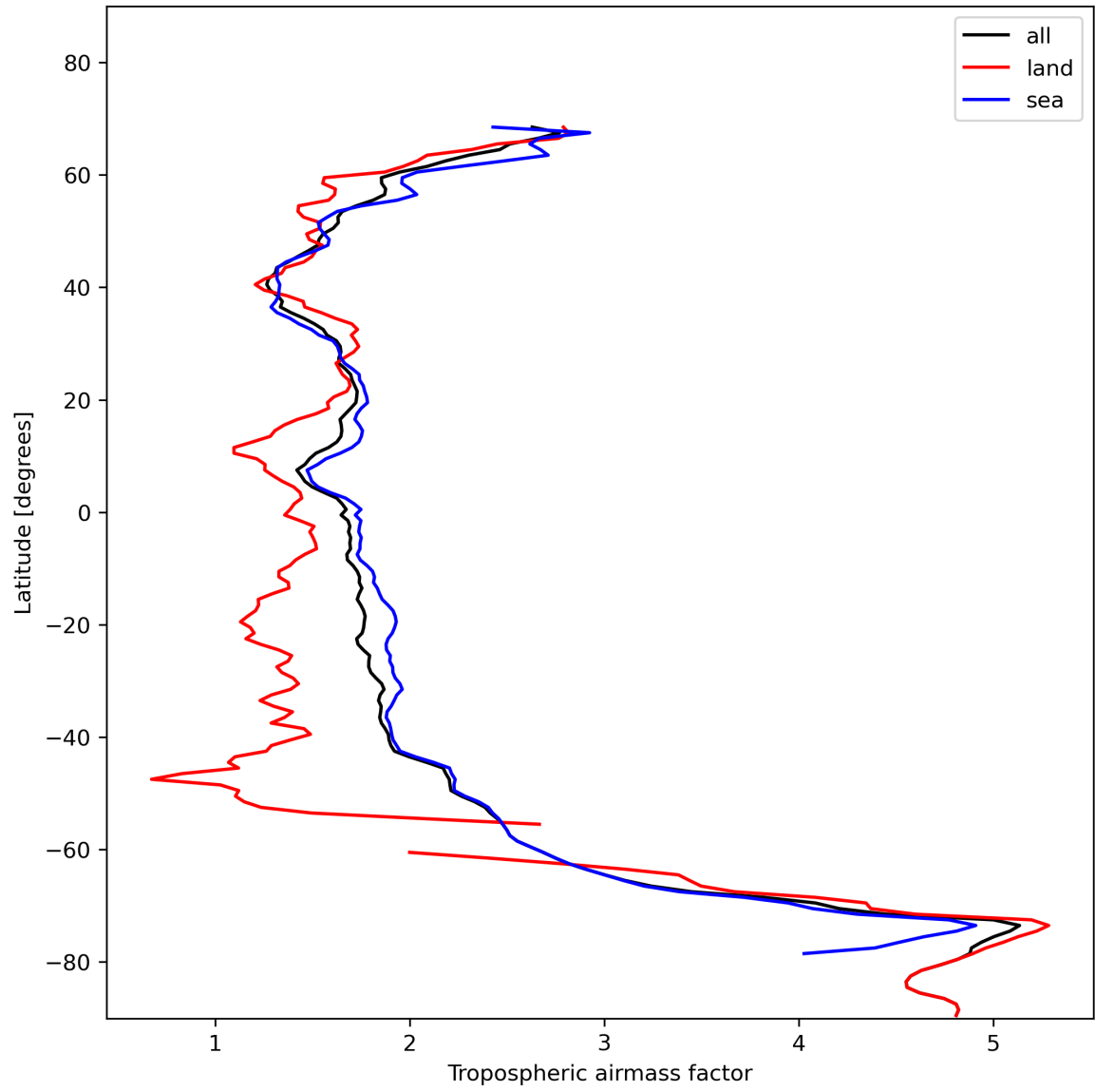
Figure 14: Zonal average of “Tropospheric airmass factor” for 2023-11-18 to 2023-11-20.
