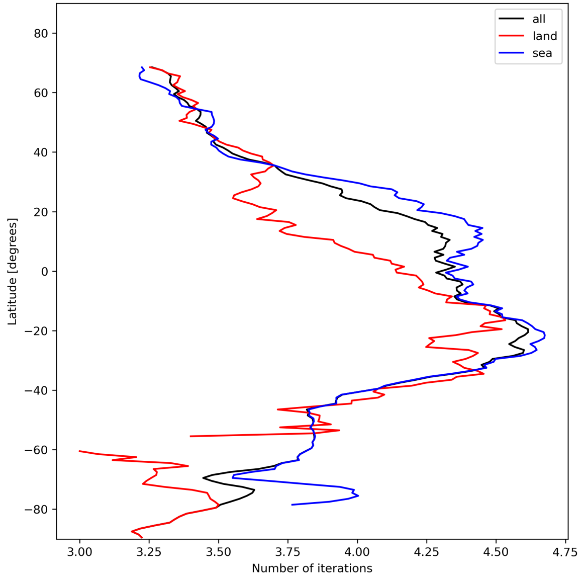
Figure 17: Zonal average of “Number of iterations” for 2023-11-18 to 2023-11-20.
