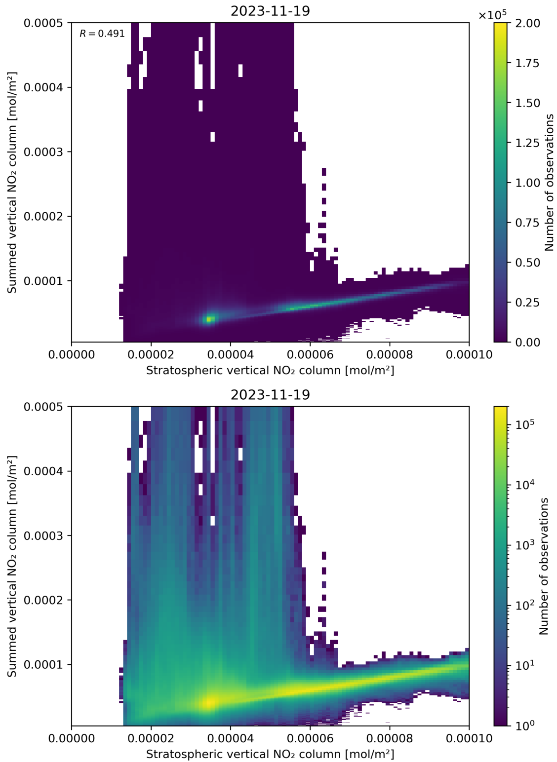
Figure 98: Scatter density plot of “Stratospheric vertical NO 2 column” against “Summed vertical NO 2 column” for 2023-11-18 to 2023-11-20.
