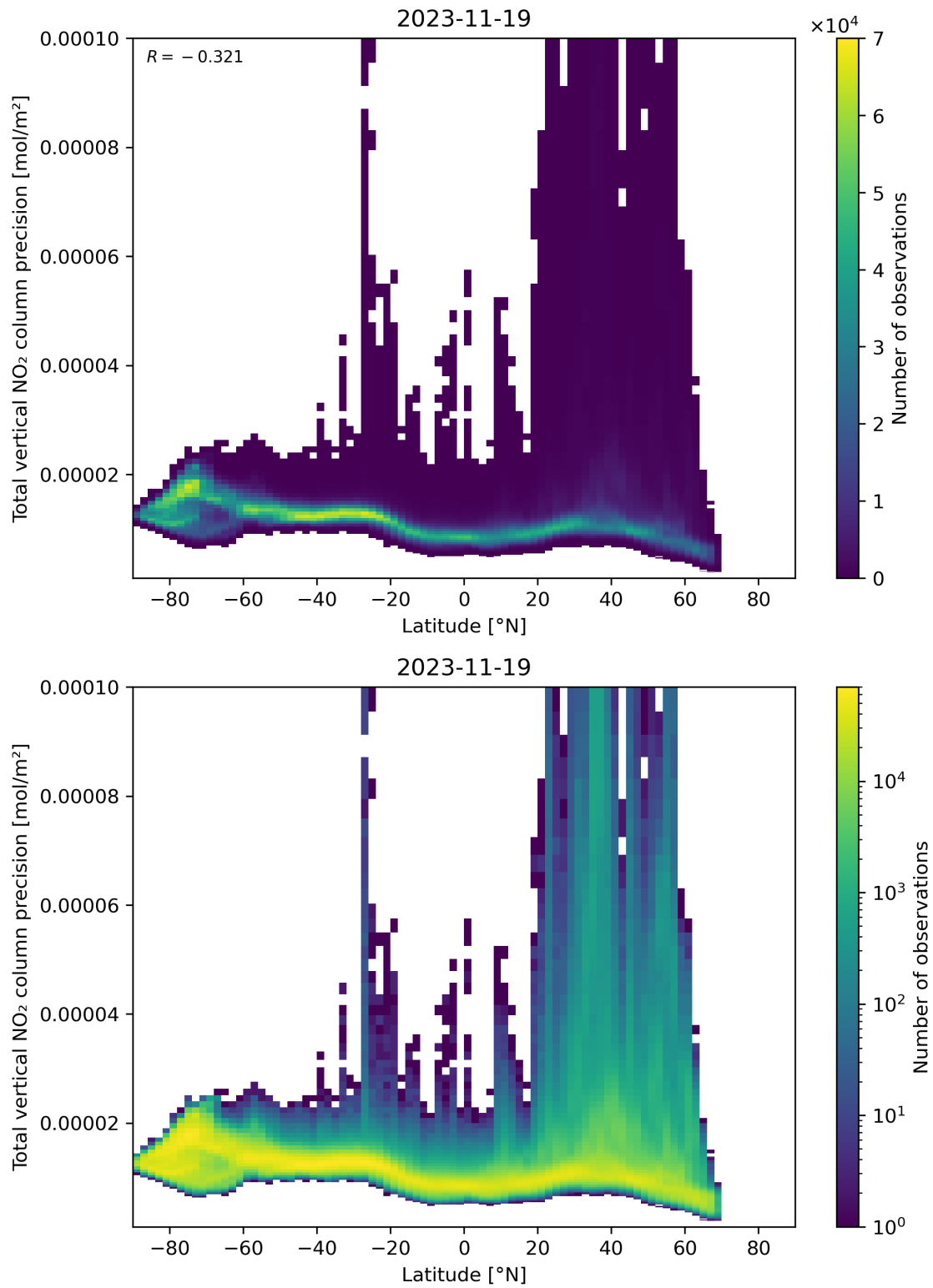
Figure 91: Scatter density plot of “Latitude” against “Total vertical NO 2 column precision” for 2023-11-18 to 2023-11-20.
