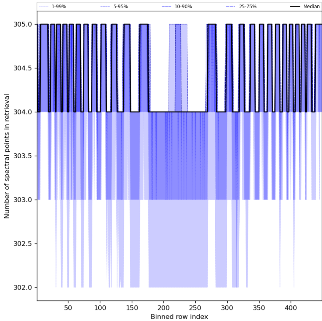
Figure 50: Along track statistics of “Number of spectral points in retrieval” for 2023-11-18 to 2023-11-20
