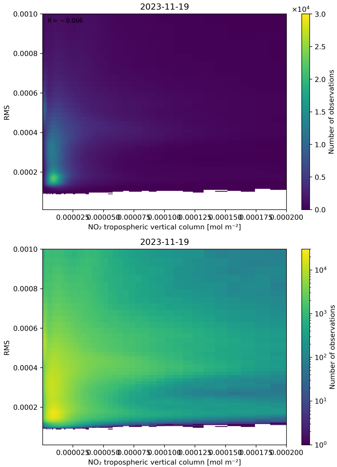
Figure 142: Scatter density plot of “NO 2 tropospheric vertical column” against “RMS” for 2023-11-18 to 2023-11-20.
