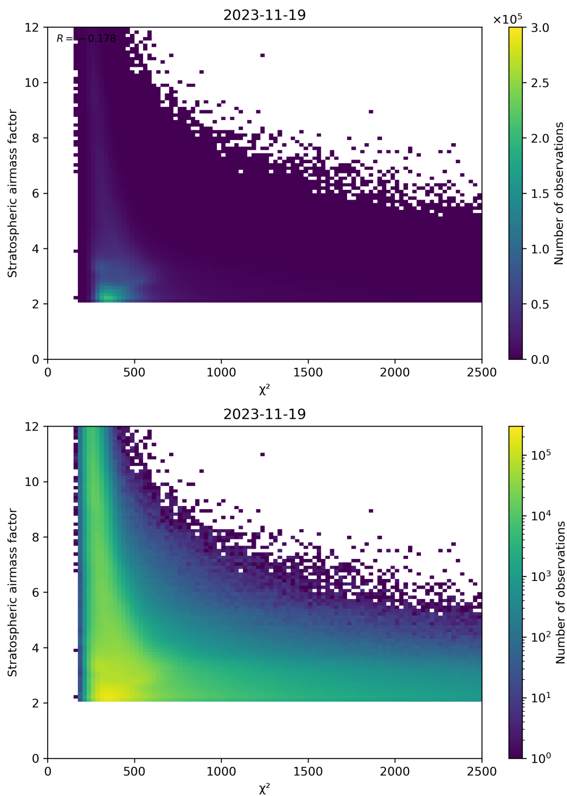
Figure 81: Scatter density plot of “ \chi^2 ” against “Stratospheric airmass factor” for 2023-11-18 to 2023-11-20.
