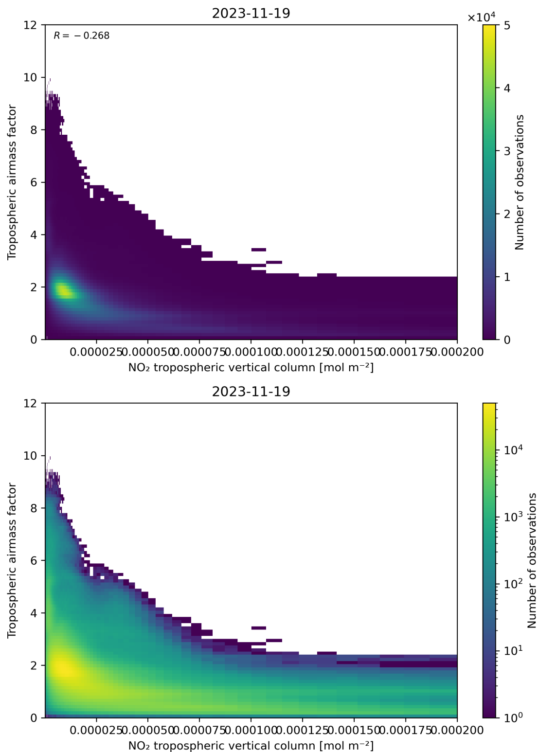
Figure 123: Scatter density plot of “NO 2 tropospheric vertical column” against “Tropospheric air mass factor” for 2023-11-18 to 2023-11-20.
