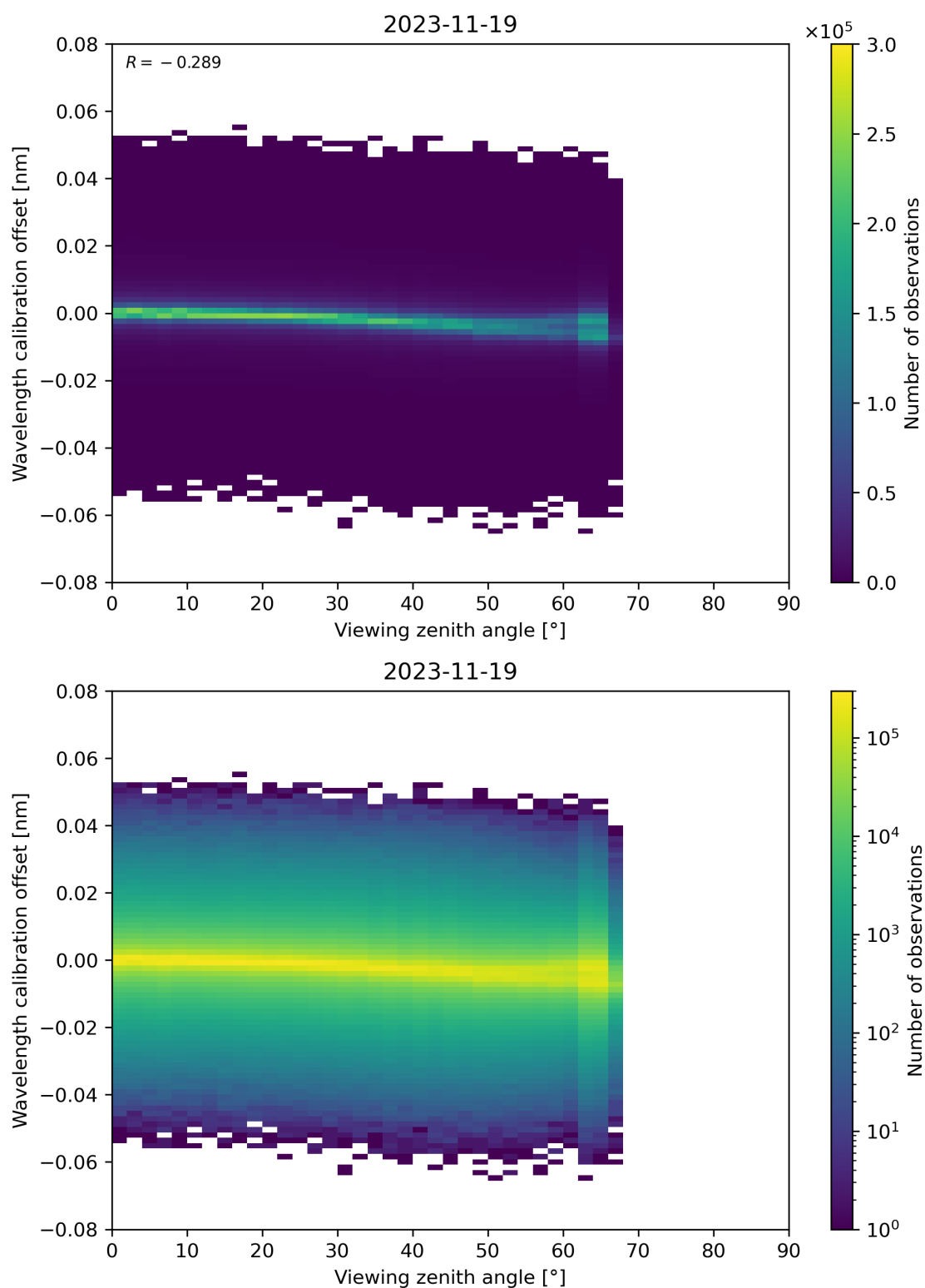
Figure 173: Scatter density plot of “Viewing zenith angle” against “Wavelength calibration offset” for 2023-11-18 to 2023-11-20.
