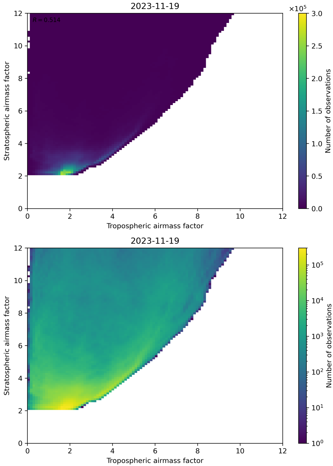
Figure 71: Scatter density plot of “Tropospheric airmass factor” against “Stratospheric airmass factor” for 2023-11-18 to 2023-11-20.
