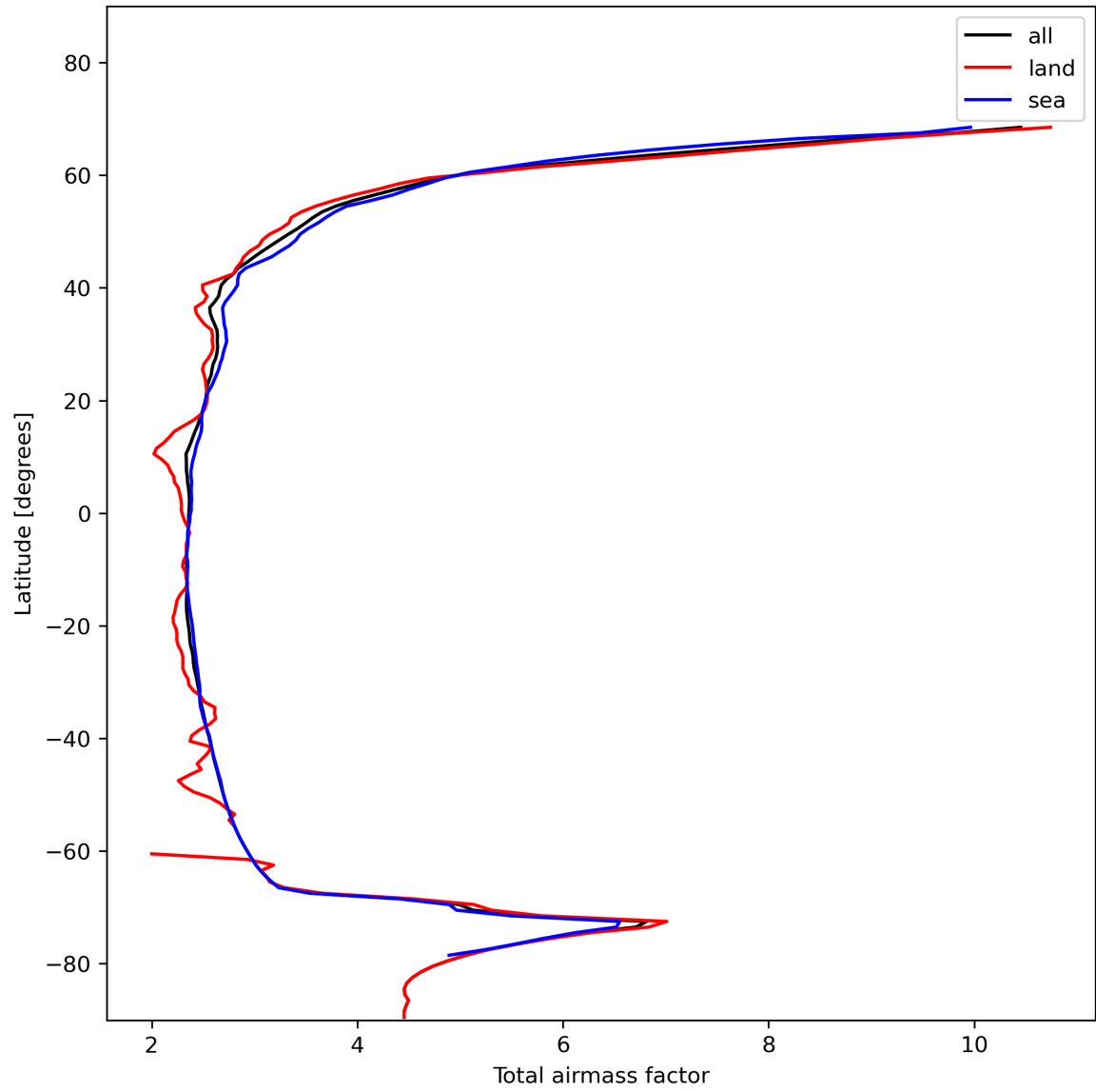
Figure 15: Zonal average of “Total airmass factor” for 2023-11-18 to 2023-11-20.
