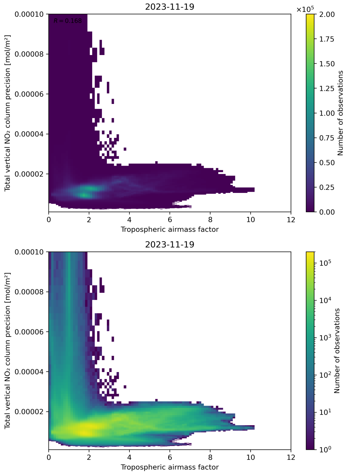
Figure 78: Scatter density plot of “Tropospheric airmass factor” against “Total vertical NO 2 column precision” for 2023-11-18 to 2023-11-20.
