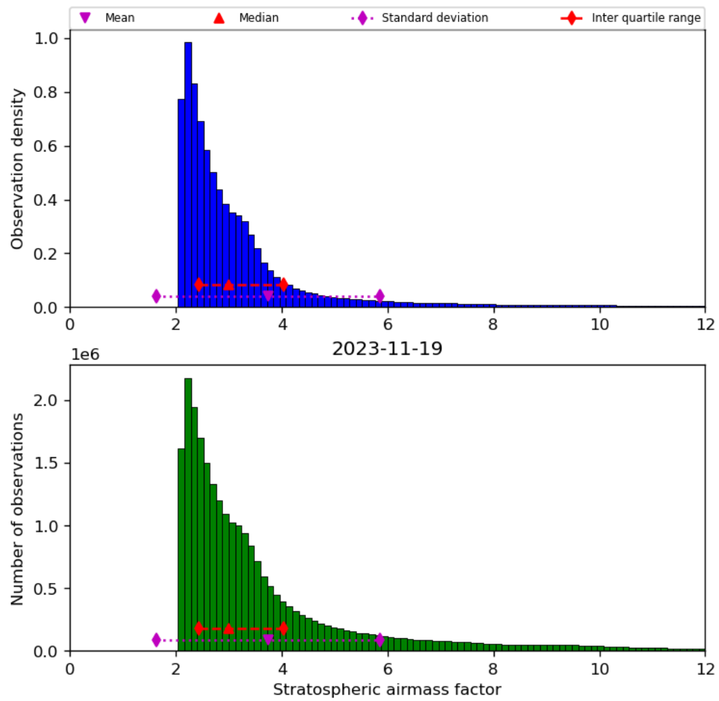
Figure 44: Histogram of “Stratospheric airmass factor” for 2023-11-18 to 2023-11-20
