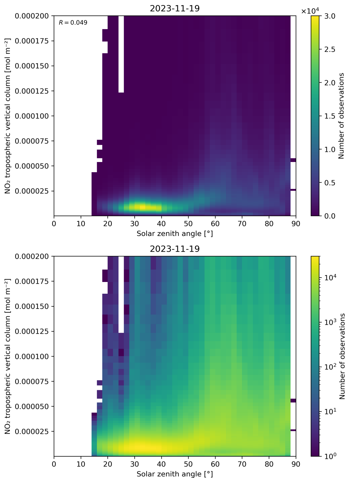
Figure 155: Scatter density plot of “Solar zenith angle” against “NO 2 tropospheric vertical column” for 2023-11-18 to 2023-11-20.
