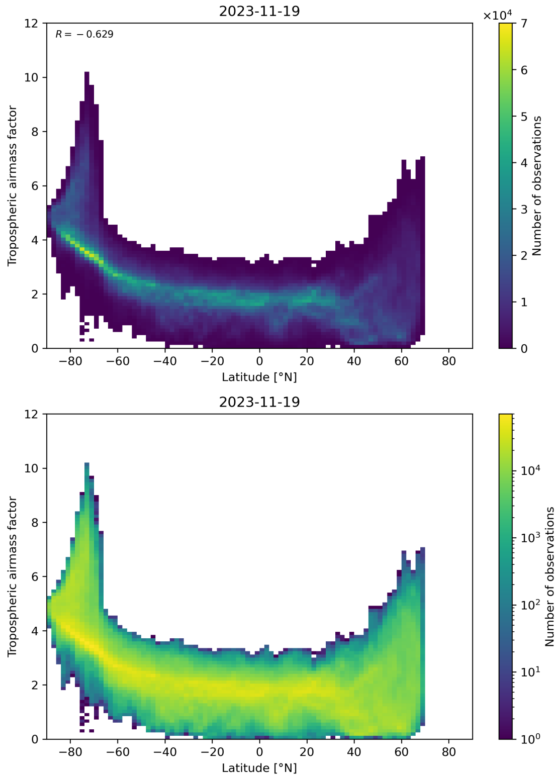
Figure 85: Scatter density plot of “Latitude” against “Tropospheric airmass factor” for 2023-11-18 to 2023-11-20.
