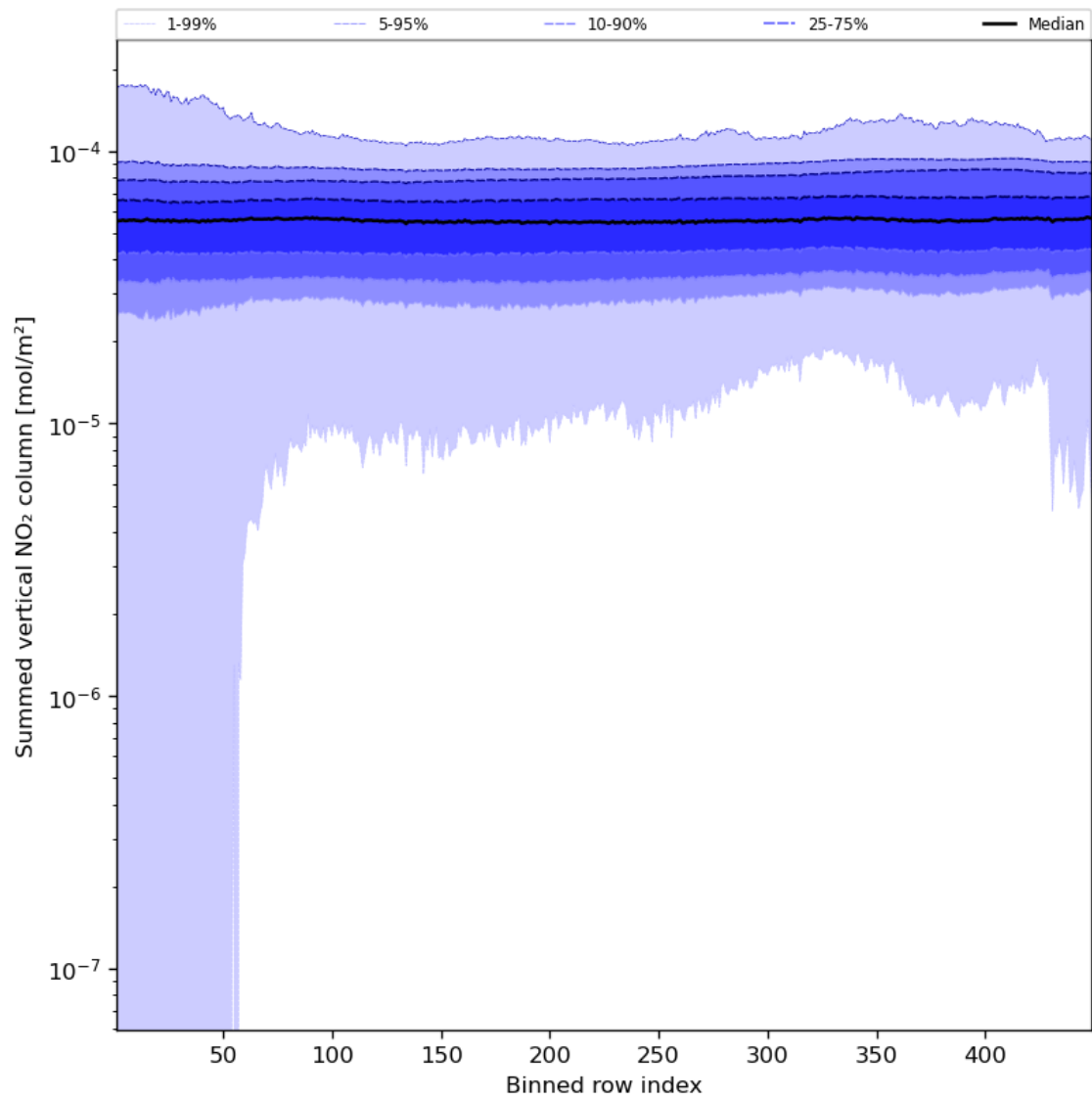
Figure 57: Along track statistics of “Summed vertical NO 2 column” for 2023-11-18 to 2023-11-20
