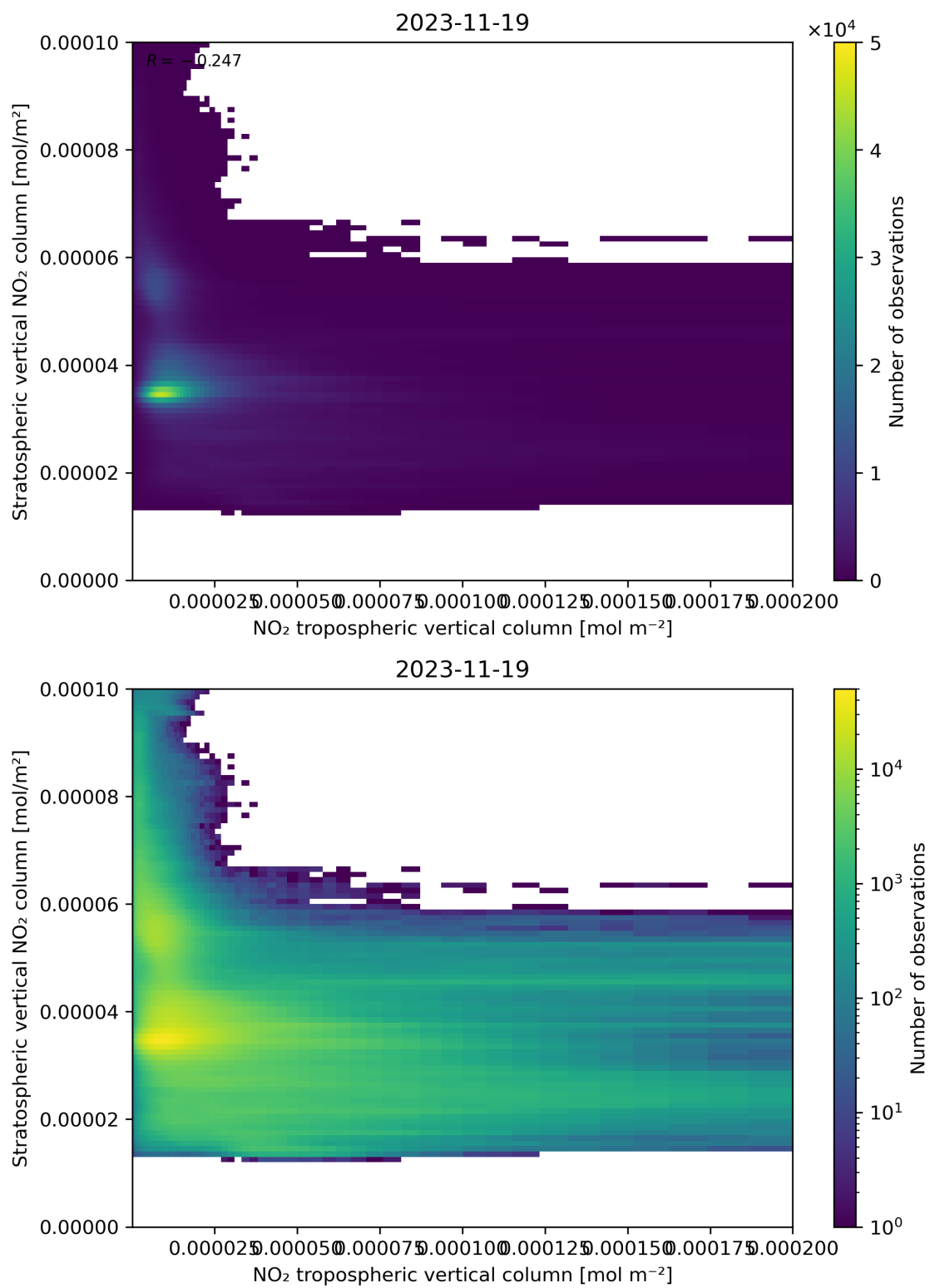
Figure 125: Scatter density plot of “NO 2 tropospheric vertical column” against “Stratospheric vertical NO 2 column” for 2023-11-18 to 2023-11-20.
