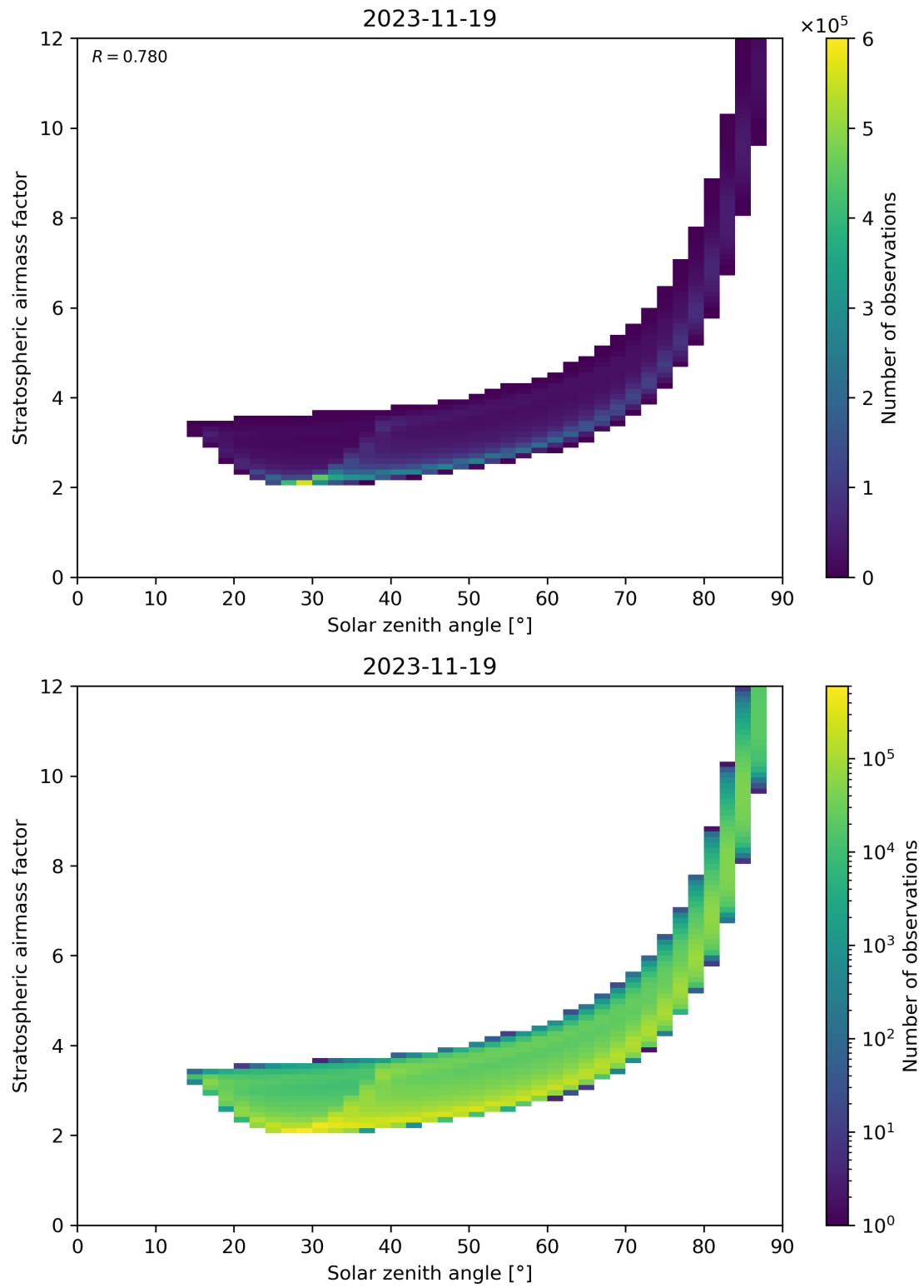
Figure 145: Scatter density plot of “Solar zenith angle” against “Stratospheric airmass factor” for 2023-11-18 to 2023-11-20.
