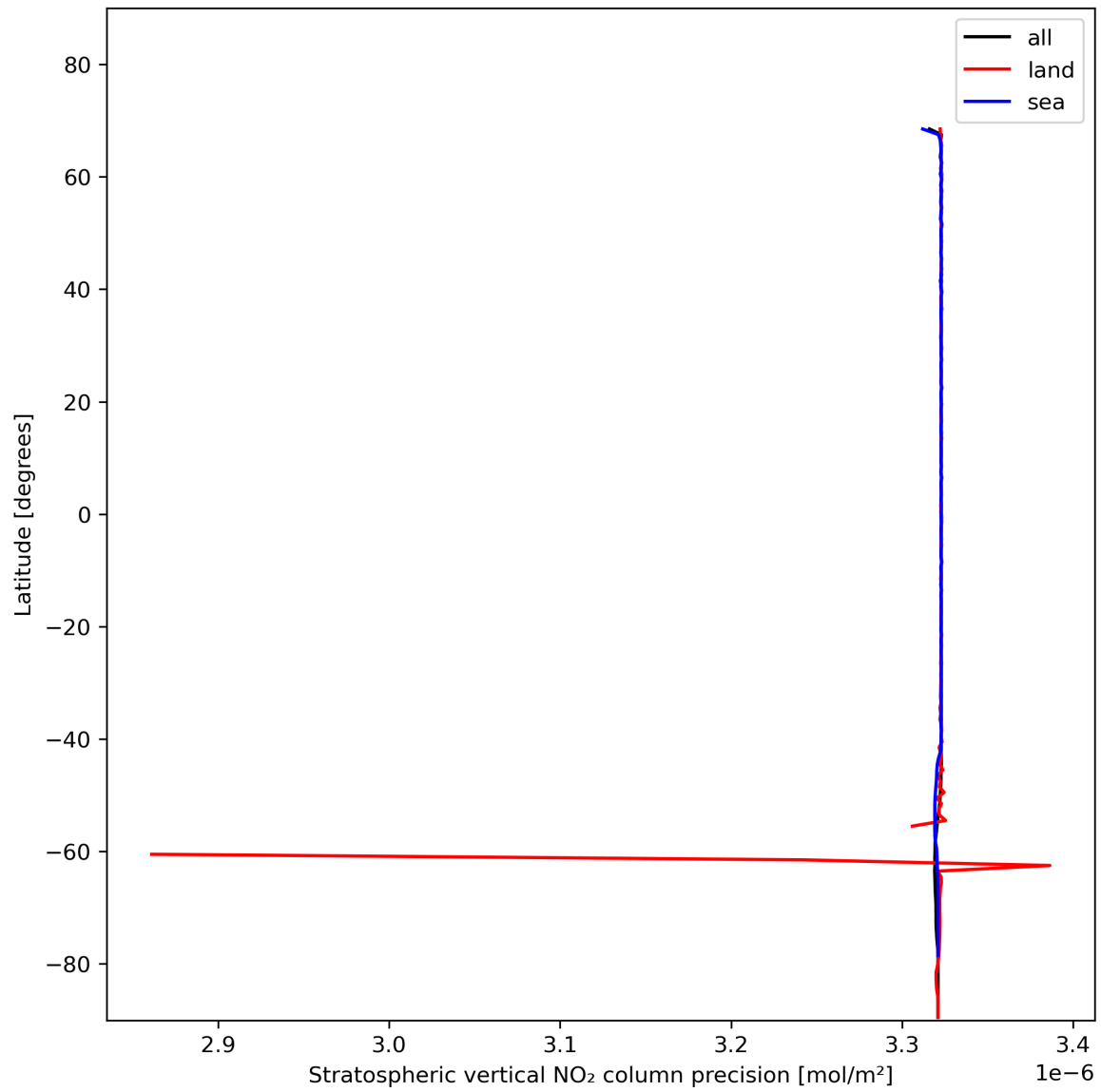
Figure 20: Zonal average of “Stratospheric vertical NO 2 column precision” for 2023-11-18 to 2023-11-20.
