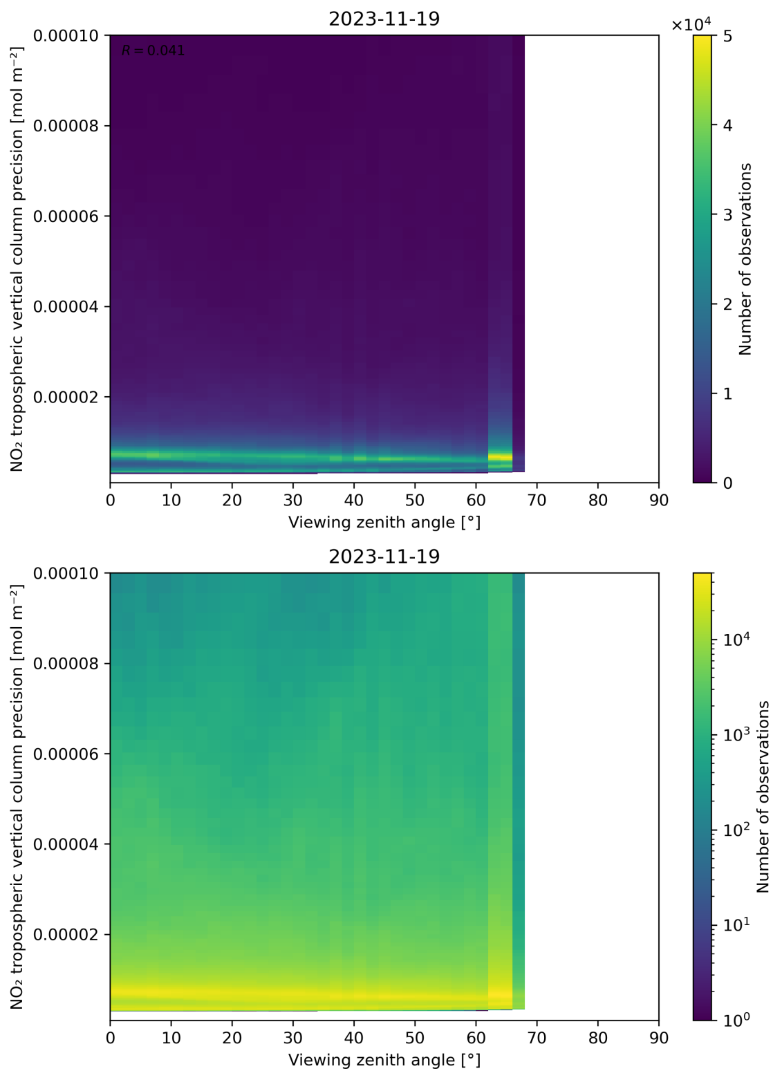
Figure 170: Scatter density plot of “Viewing zenith angle” against “NO 2 tropospheric vertical column precision” for 2023-11-18 to 2023-11-20.
