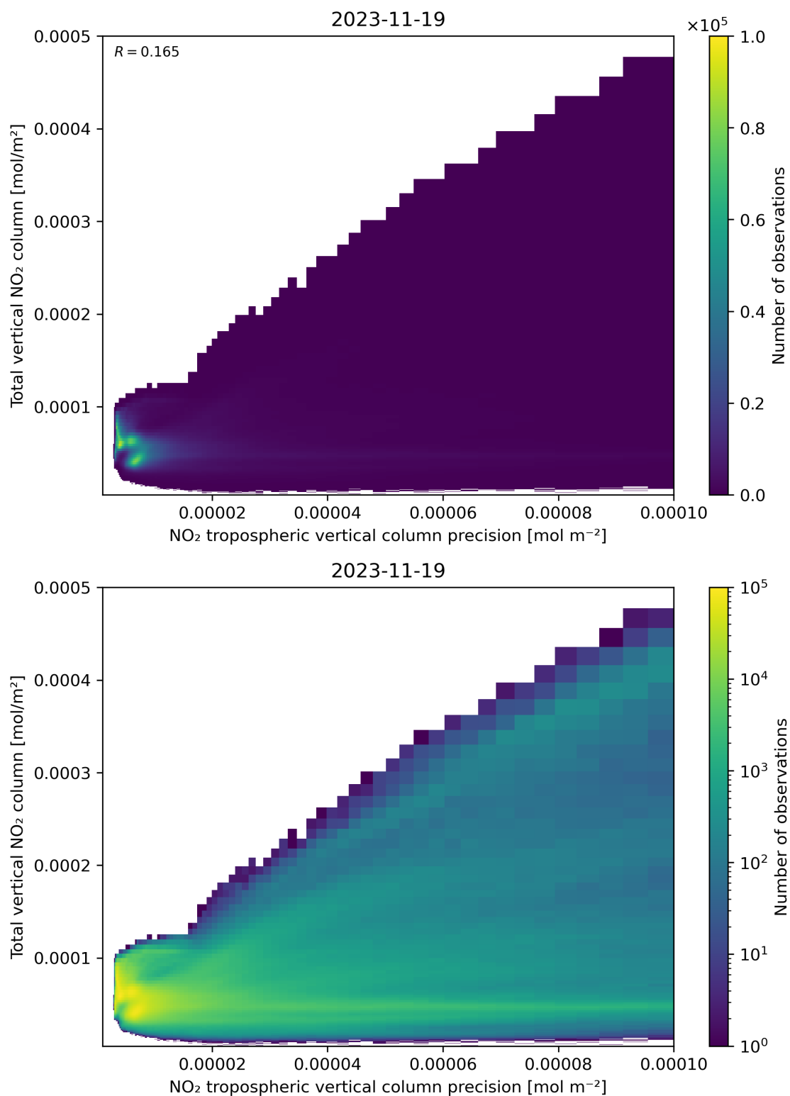
Figure 138: Scatter density plot of “NO 2 tropospheric vertical column precision” against “Total vertical NO 2 column” for 2023-11-18 to 2023-11-20.
