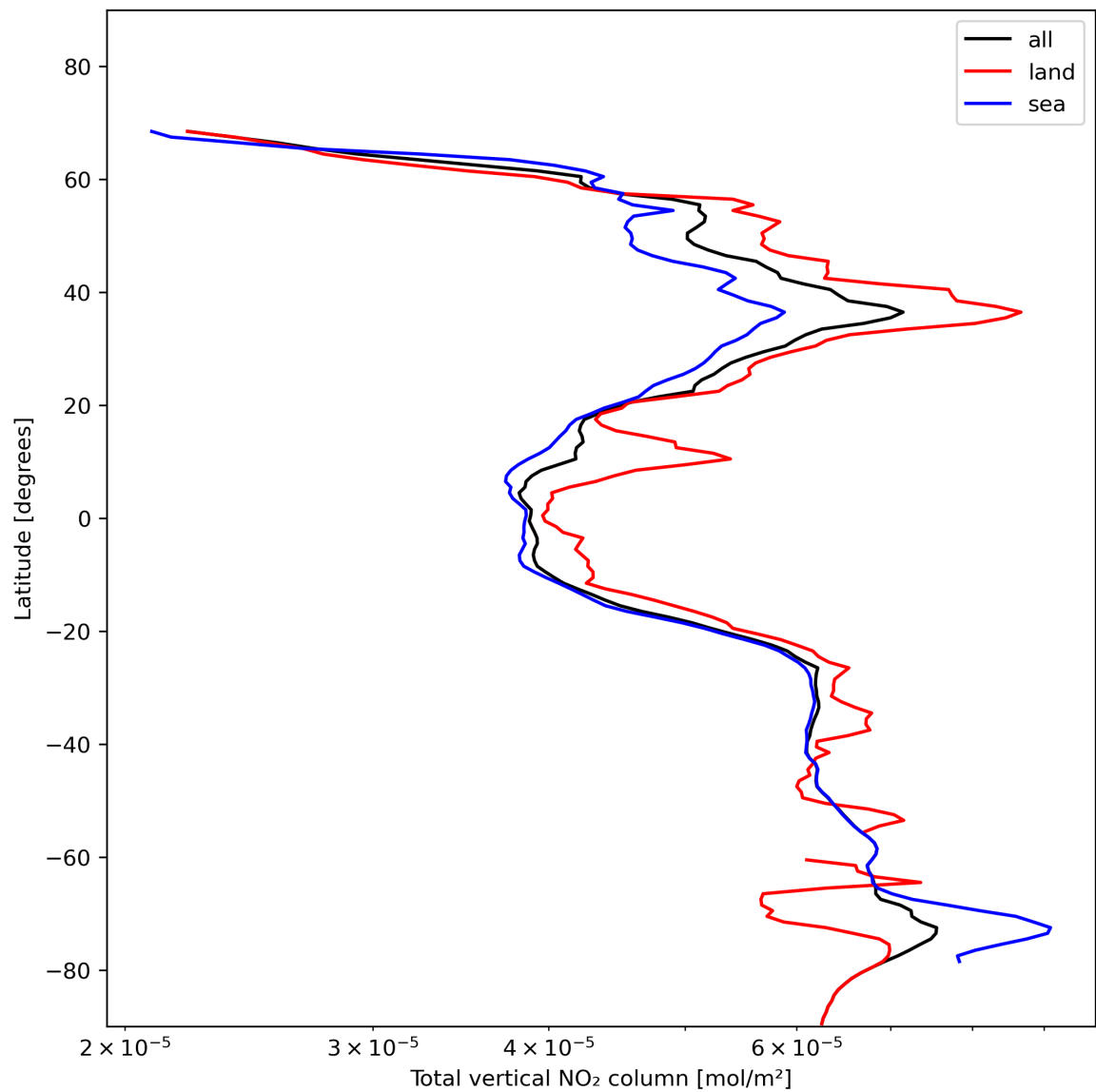
Figure 21: Zonal average of “Total vertical NO 2 column” for 2023-11-18 to 2023-11-20.
