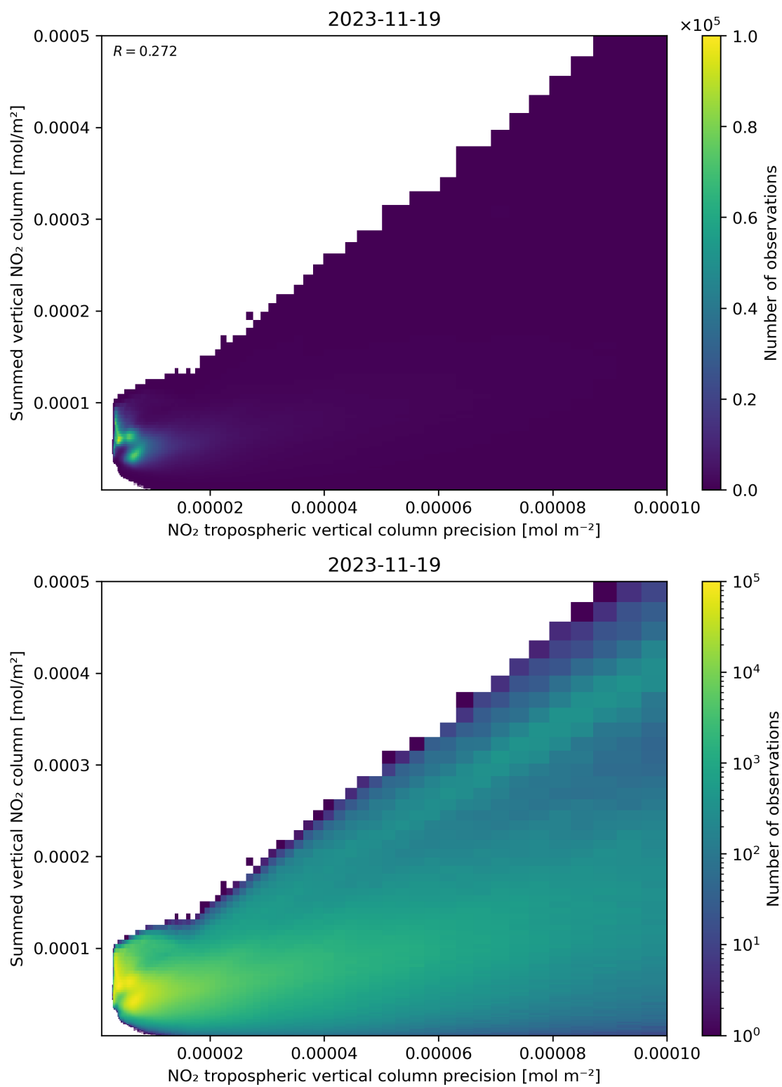
Figure 136: Scatter density plot of “NO 2 tropospheric vertical column precision” against “Summed vertical NO 2 column” for 2023-11-18 to 2023-11-20.
