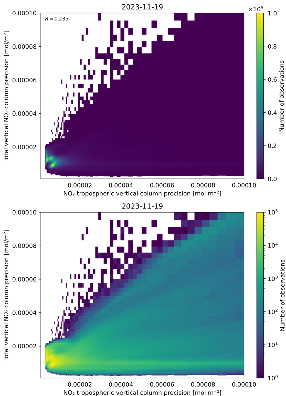
Figure 139: Scatter density plot of “NO 2 tropospheric vertical column precision” against “Total vertical NO 2 column precision” for 2023-11-18 to 2023-11-20.
