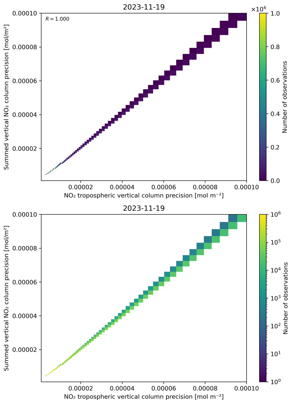
Figure 137: Scatter density plot of “NO 2 tropospheric vertical column precision” against “Summed vertical NO 2 column precision” for 2023-11-18 to 2023-11-20.
