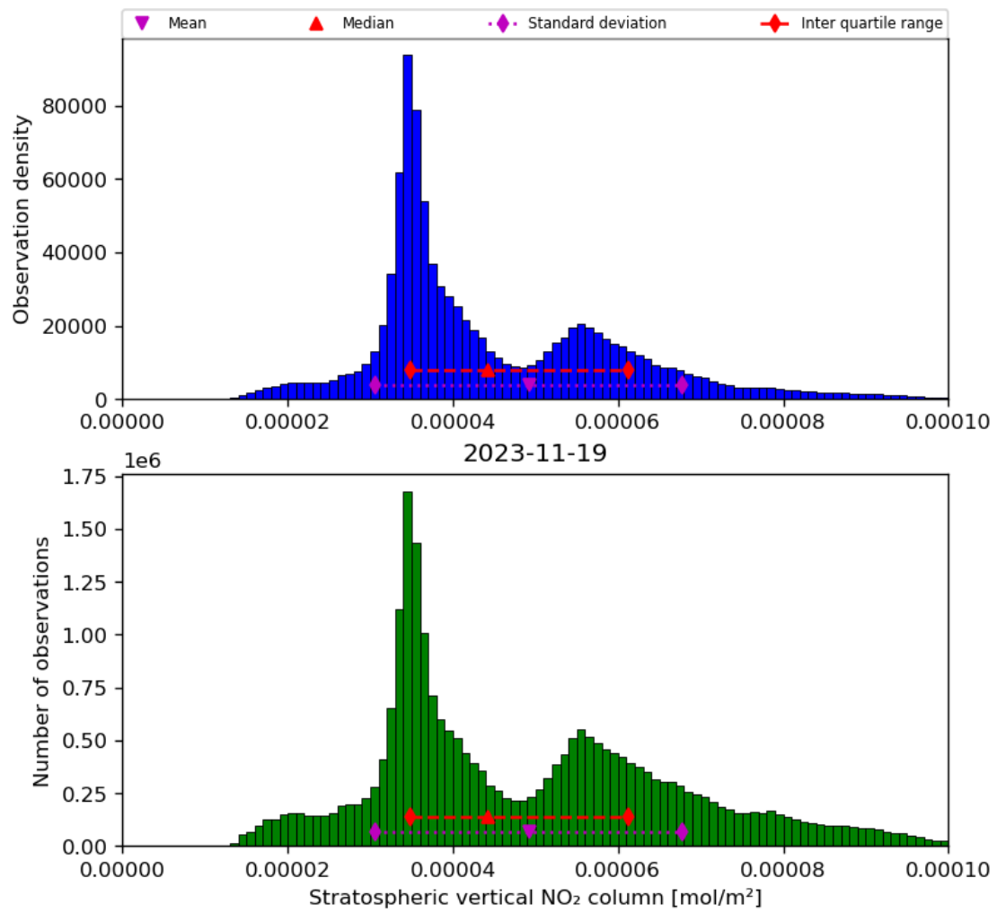
Figure 36: Histogram of “Stratospheric vertical NO 2 column” for 2023-11-18 to 2023-11-20
