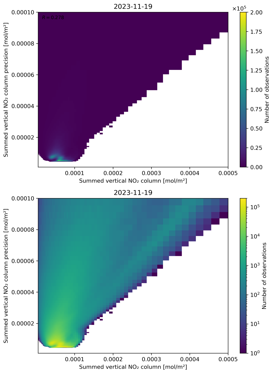
Figure 105: Scatter density plot of “Summed vertical NO 2 column” against “Summed vertical NO 2 column precision” for 2023-11-18 to 2023-11-20.
