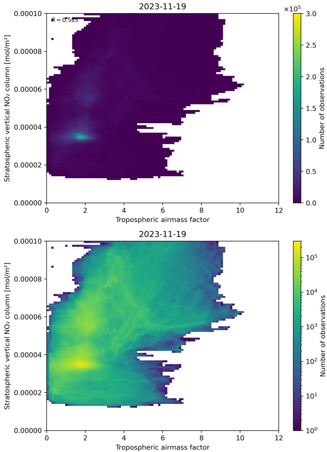
Figure 74: Scatter density plot of “Tropospheric air mass factor” against “Stratospheric vertical NO 2 column” for 2023-11-18 to 2023-11-20.
