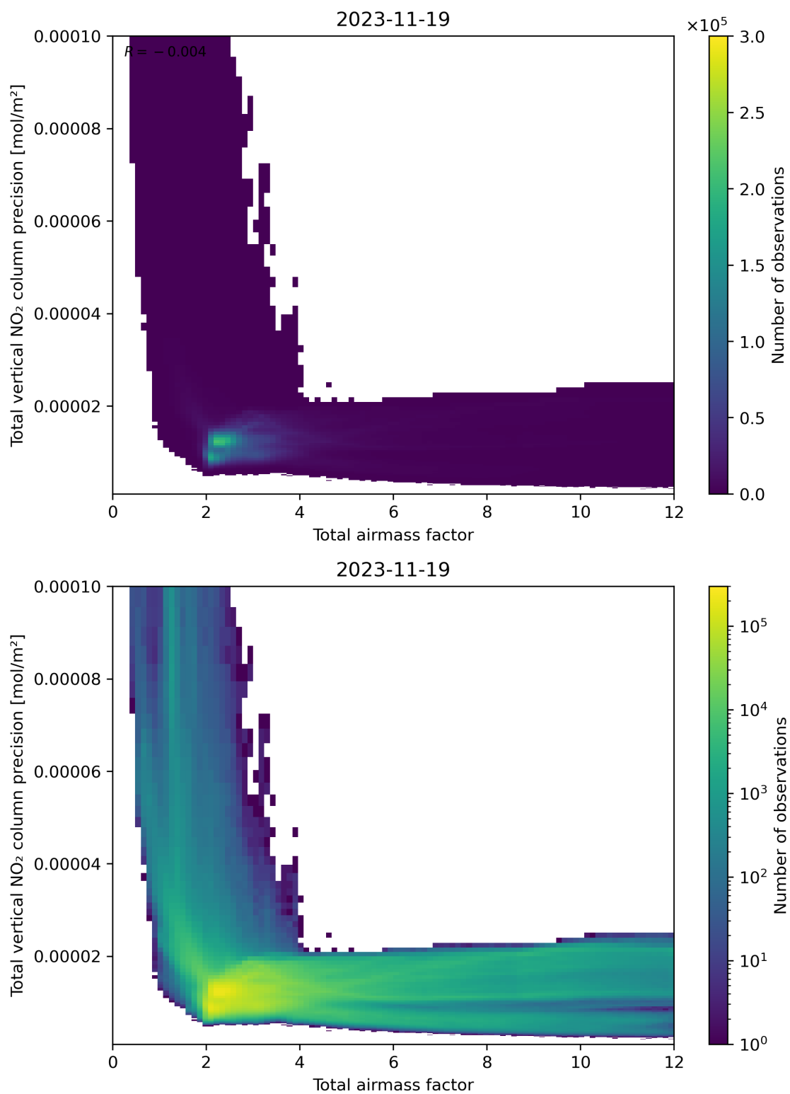
Figure 68: Scatter density plot of “Total airmass factor” against “Total vertical NO 2 column precision” for 2023-11-18 to 2023-11-20.
