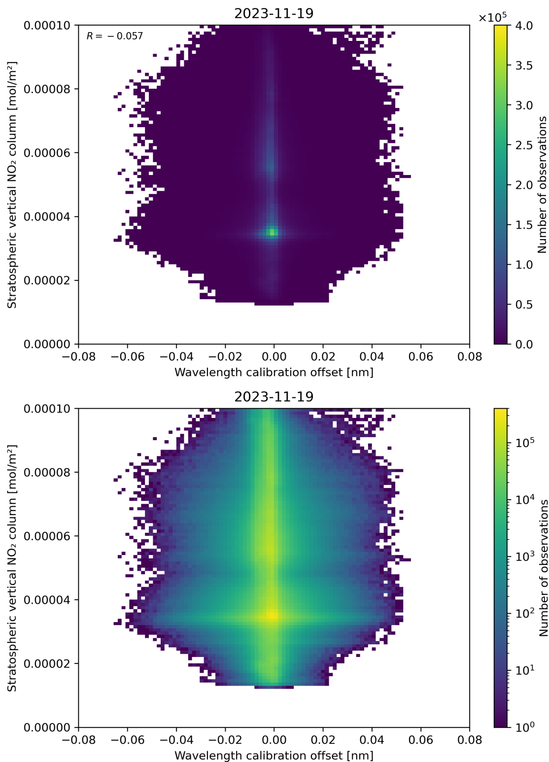
Figure 176: Scatter density plot of “Wavelength calibration offset” against “Stratospheric vertical NO 2 column” for 2023-11-18 to 2023-11-20.
