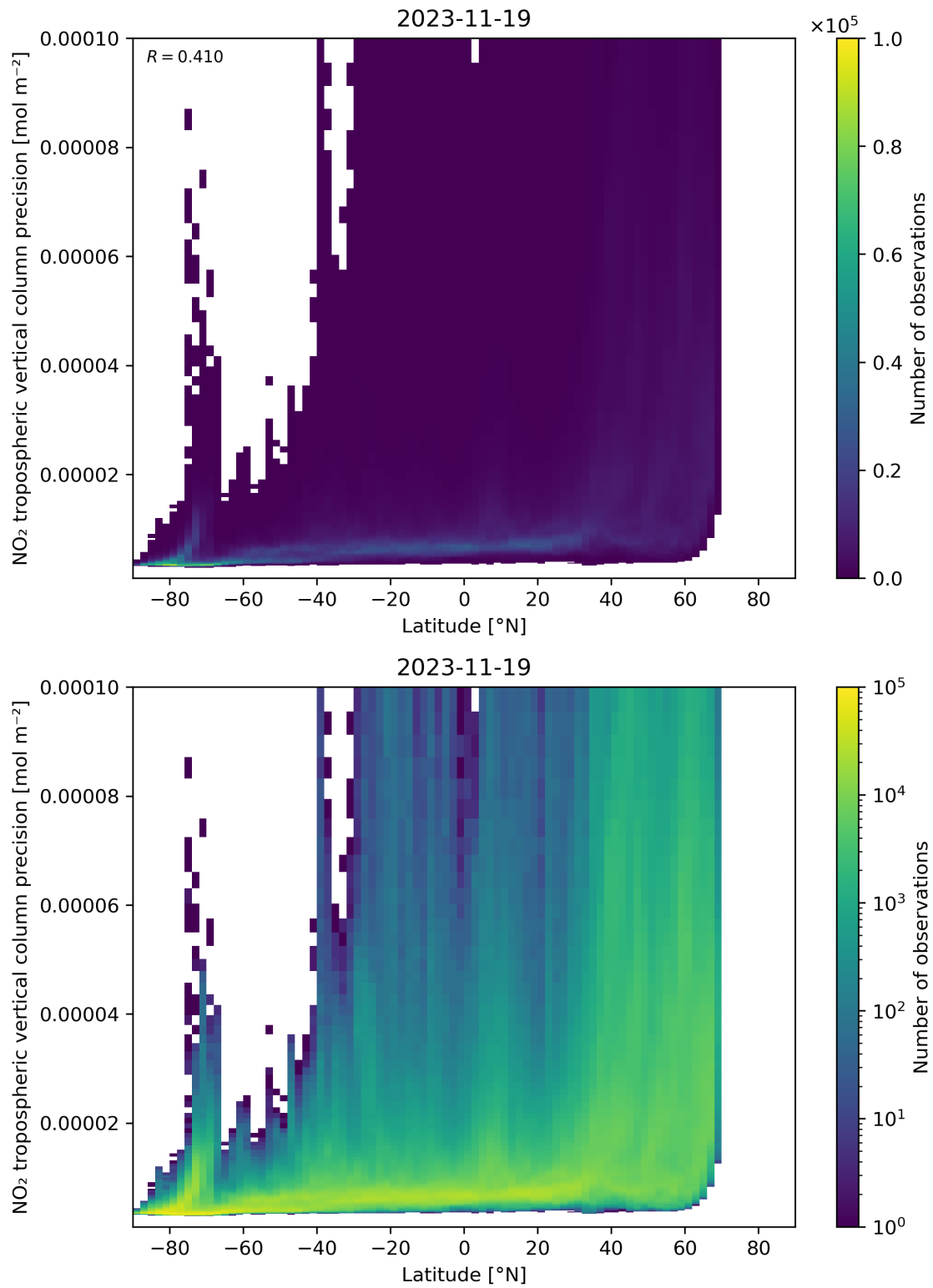
Figure 93: Scatter density plot of “Latitude” against “NO 2 tropospheric vertical column precision” for 2023-11-18 to 2023-11-20.
