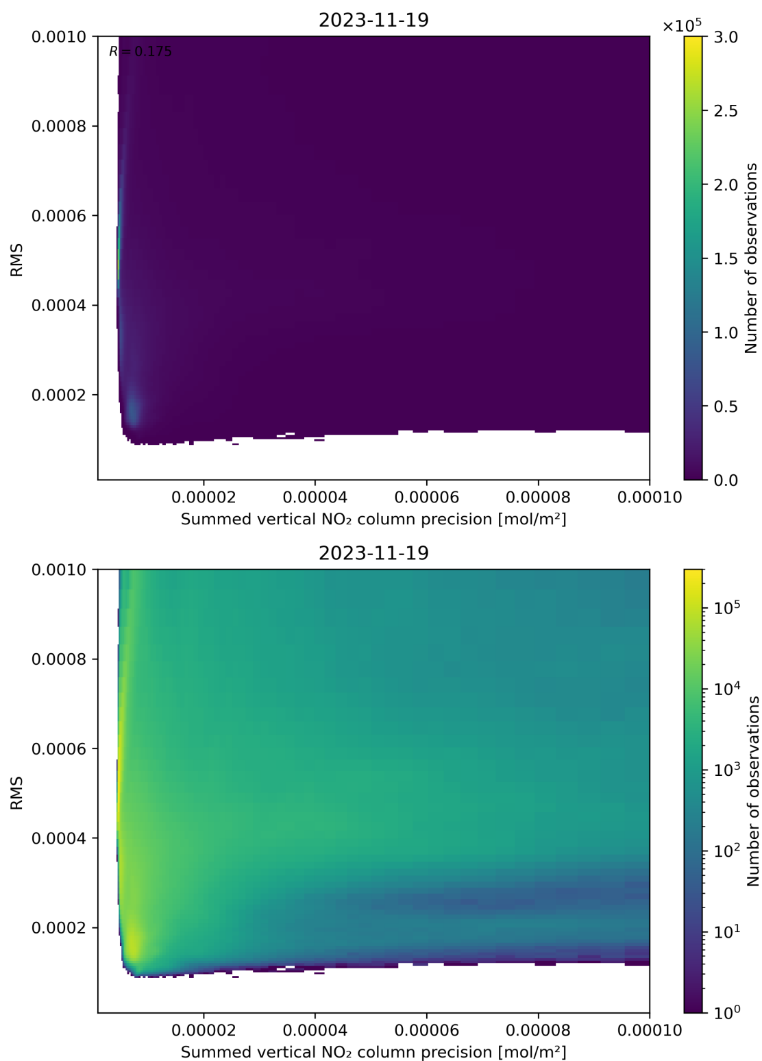
Figure 108: Scatter density plot of “Summed vertical NO 2 column precision” against “RMS” for 2023-11-18 to 2023-11-20.
