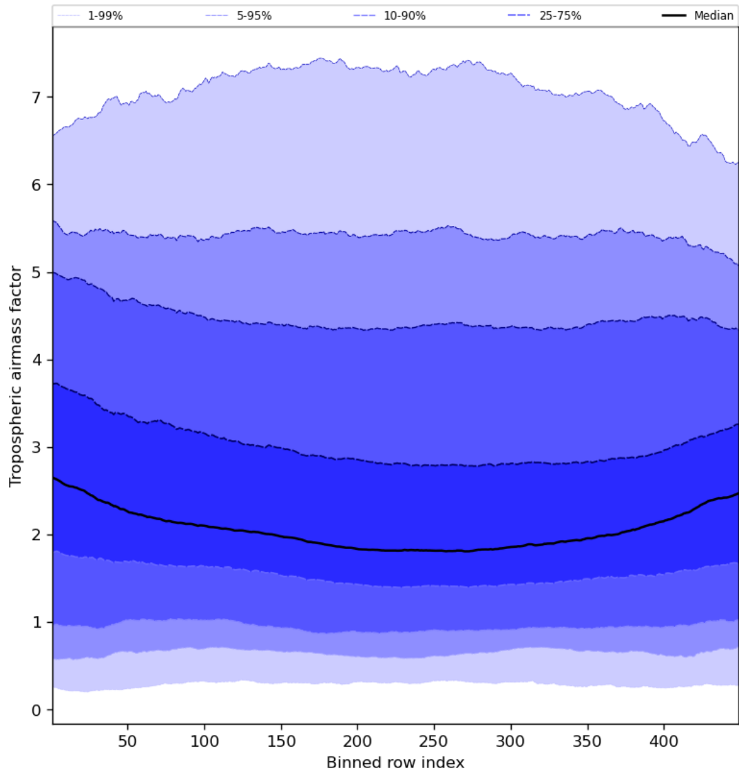
Figure 48: Along track statistics of “Tropospheric air mass factor” for 2023-11-18 to 2023-11-20
