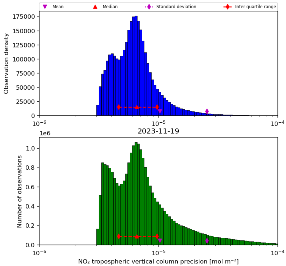
Figure 30: Histogram of “NO 2 tropospheric vertical column precision” for 2023-11-18 to 2023-11-20
