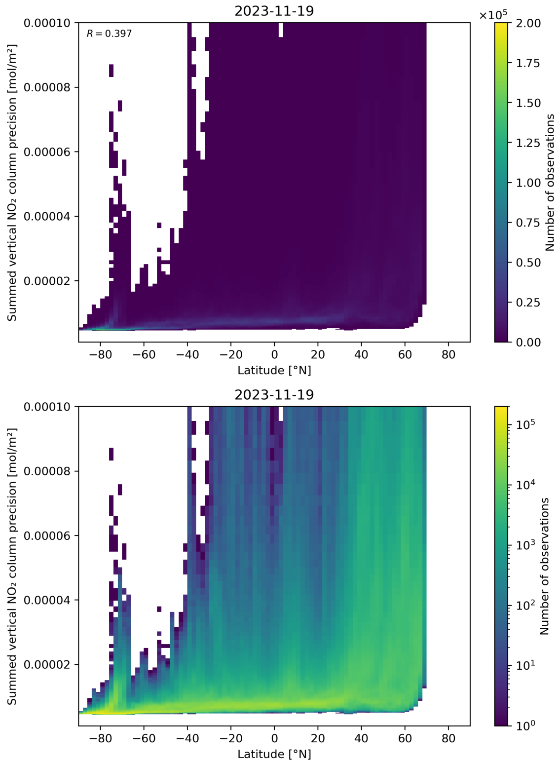
Figure 89: Scatter density plot of “Latitude” against “Summed vertical NO 2 column precision” for 2023-11-18 to 2023-11-20.
