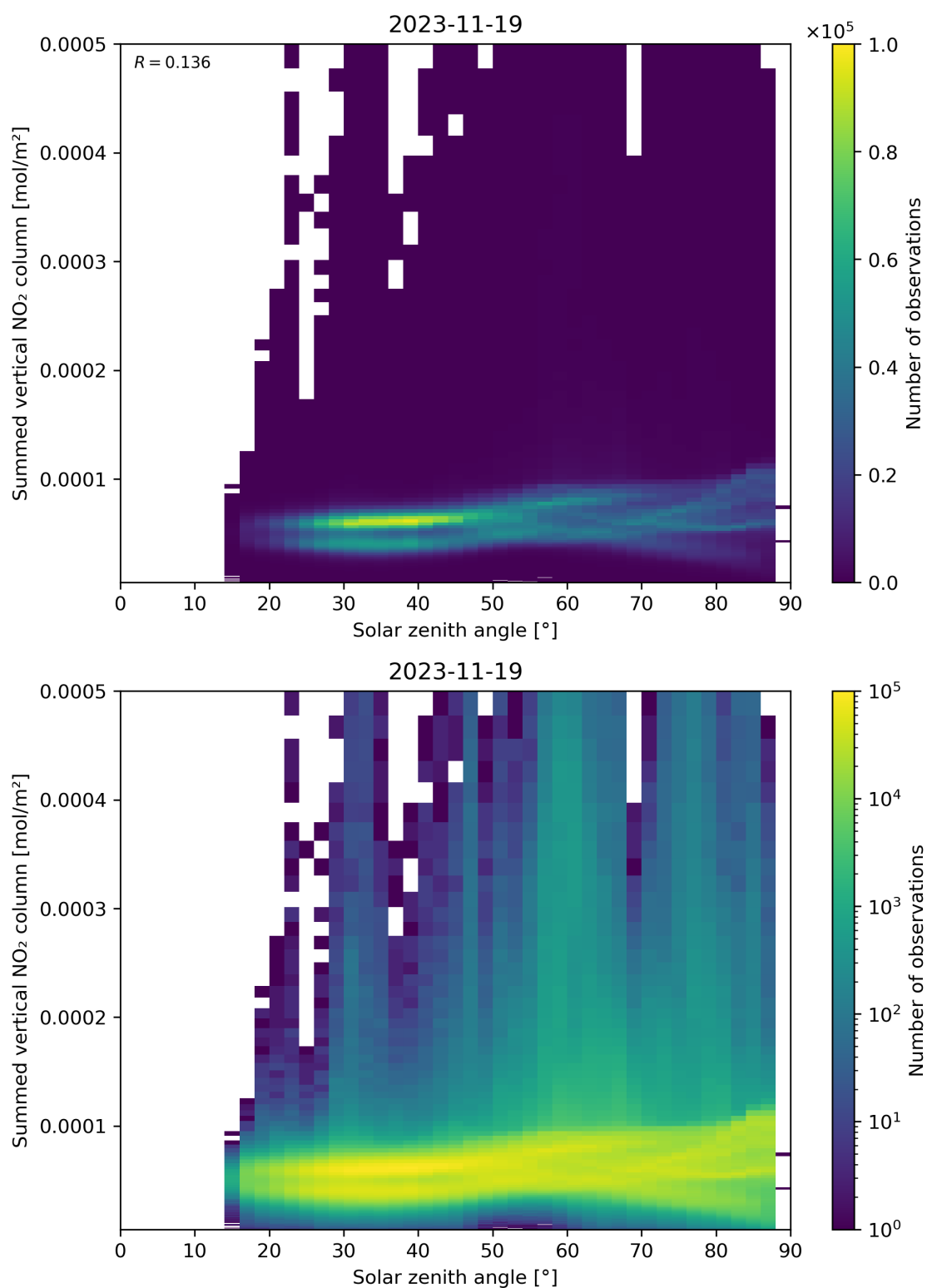
Figure 151: Scatter density plot of “Solar zenith angle” against “Summed vertical NO 2 column” for 2023-11-18 to 2023-11-20.
