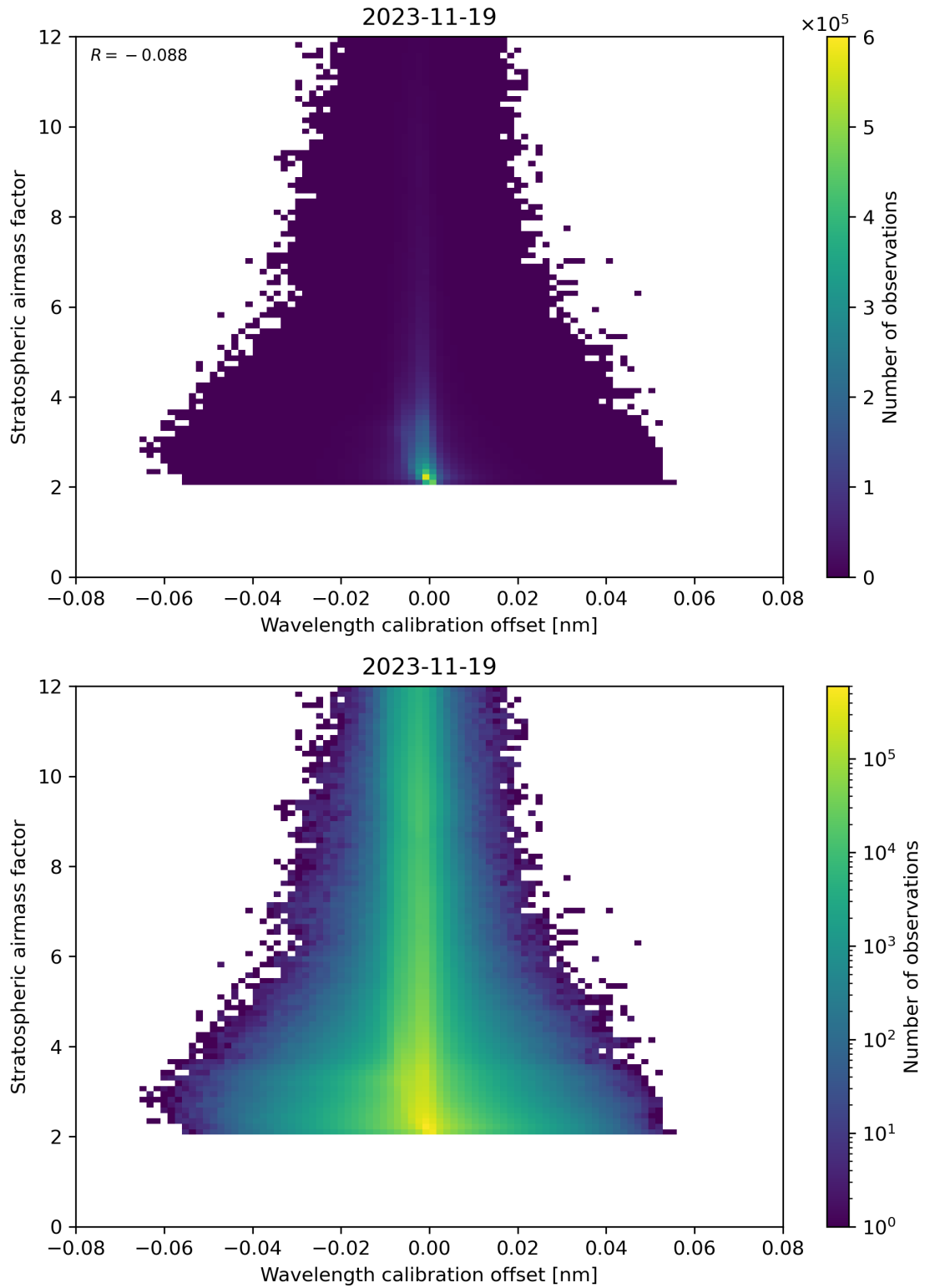
Figure 174: Scatter density plot of “Wavelength calibration offset” against “Stratospheric airmass factor” for 2023-11-18 to 2023-11-20.
