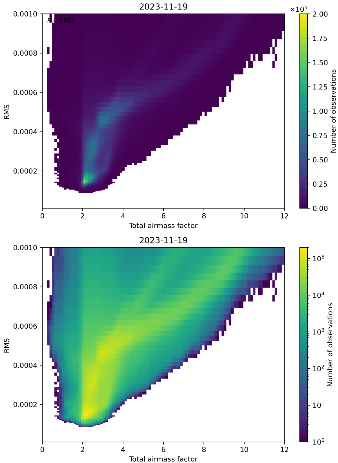
Figure 69: Scatter density plot of “Total airmass factor” against “RMS” for 2023-11-18 to 2023-11-20.
