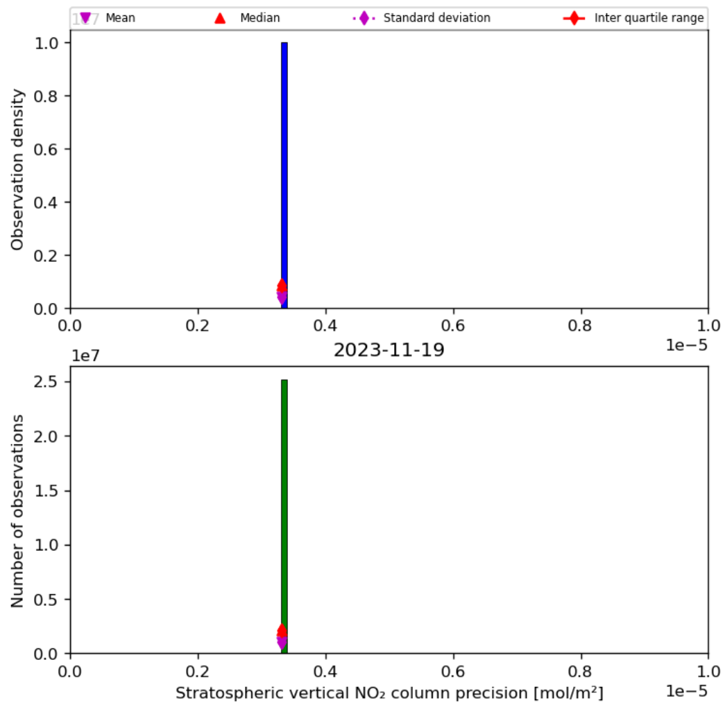
Figure 37: Histogram of “Stratospheric vertical NO 2 column precision” for 2023-11-18 to 2023-11-20
