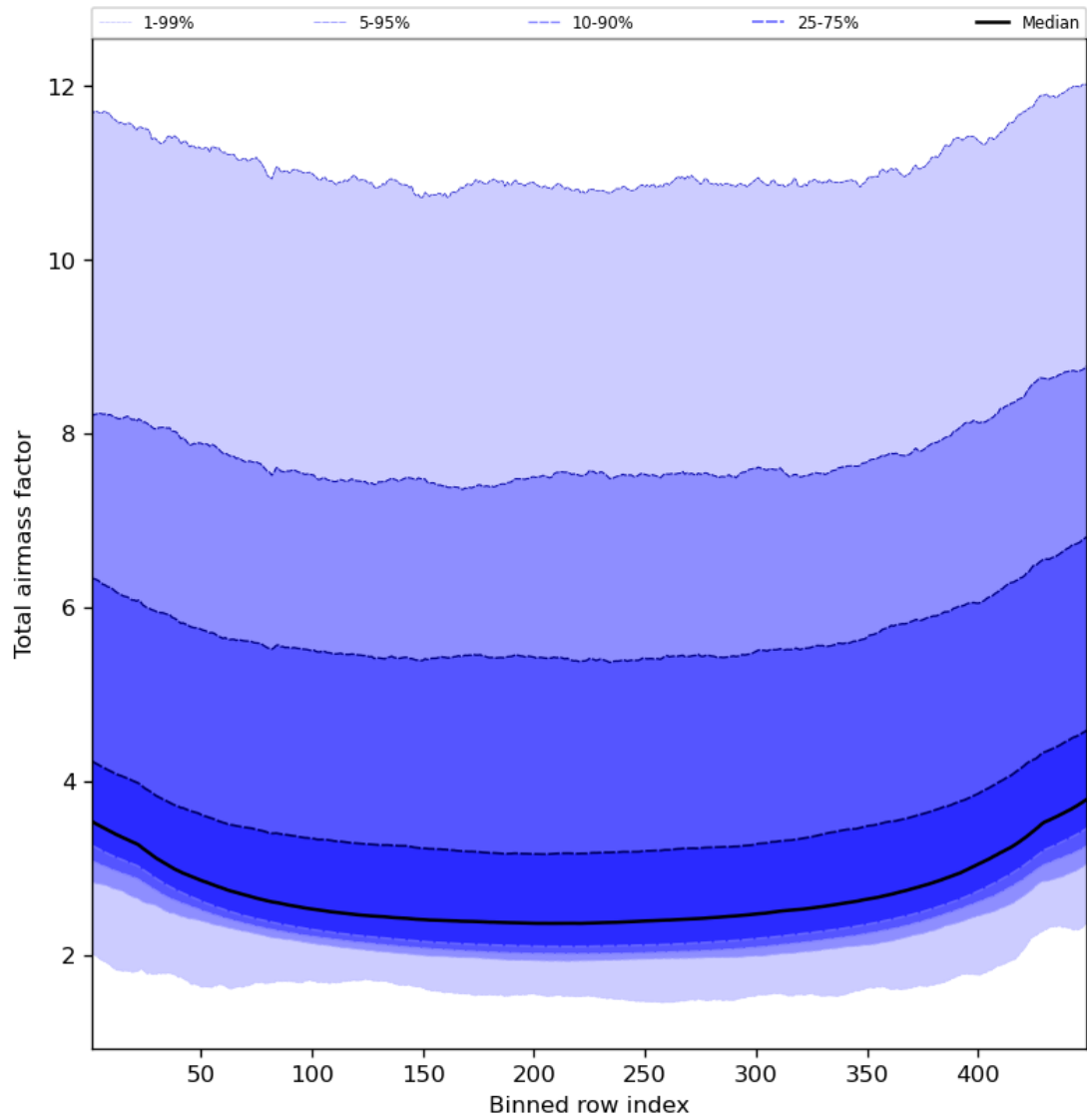
Figure 49: Along track statistics of “Total airmass factor” for 2023-11-18 to 2023-11-20
