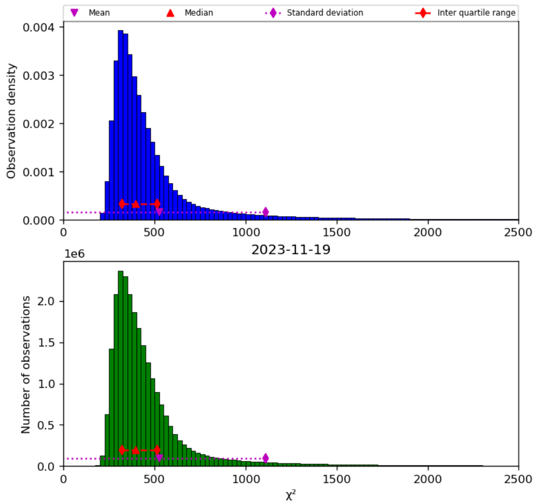
Figure 42: Histogram of “ \chi^2 ” for 2023-11-18 to 2023-11-20
