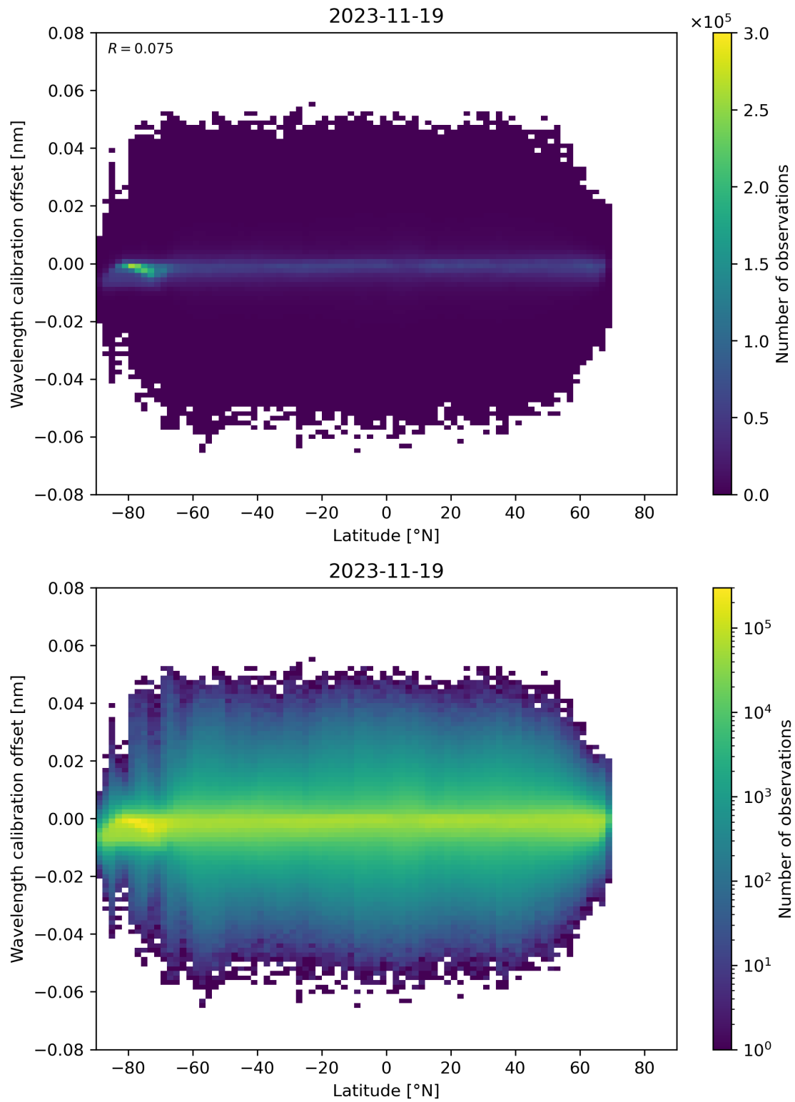
Figure 95: Scatter density plot of “Latitude” against “Wavelength calibration offset” for 2023-11-18 to 2023-11-20.
