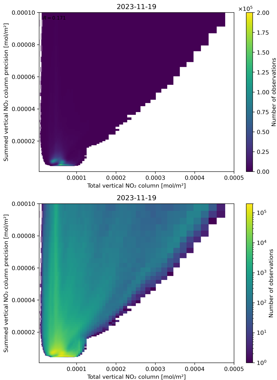
Figure 113: Scatter density plot of “Total vertical NO 2 column” against “Summed vertical NO 2 column precision” for 2023-11-18 to 2023-11-20.
