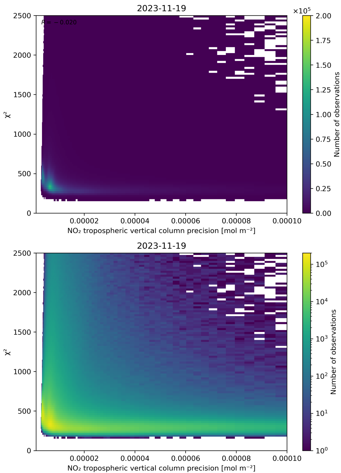
Figure 134: Scatter density plot of “NO 2 tropospheric vertical column precision” against “ \chi^2 ” for 2023-11-18 to 2023-11-20.
