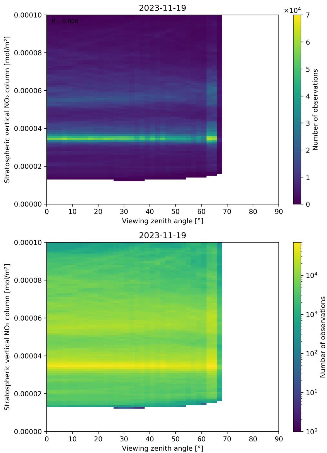
Figure 164: Scatter density plot of “Viewing zenith angle” against “Stratospheric vertical NO 2 column” for 2023-11-18 to 2023-11-20.
