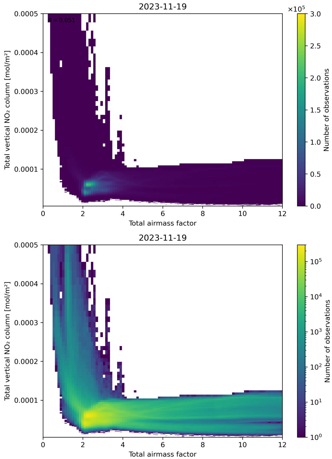
Figure 67: Scatter density plot of “Total airmass factor” against “Total vertical NO 2 column” for 2023-11-18 to 2023-11-20.
