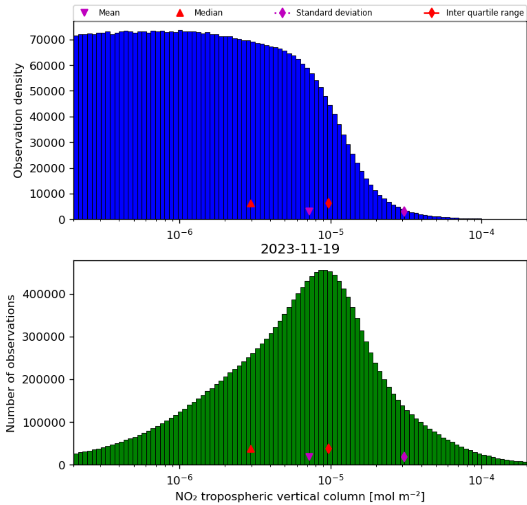
Figure 29: Histogram of “NO 2 tropospheric vertical column” for 2023-11-18 to 2023-11-20
