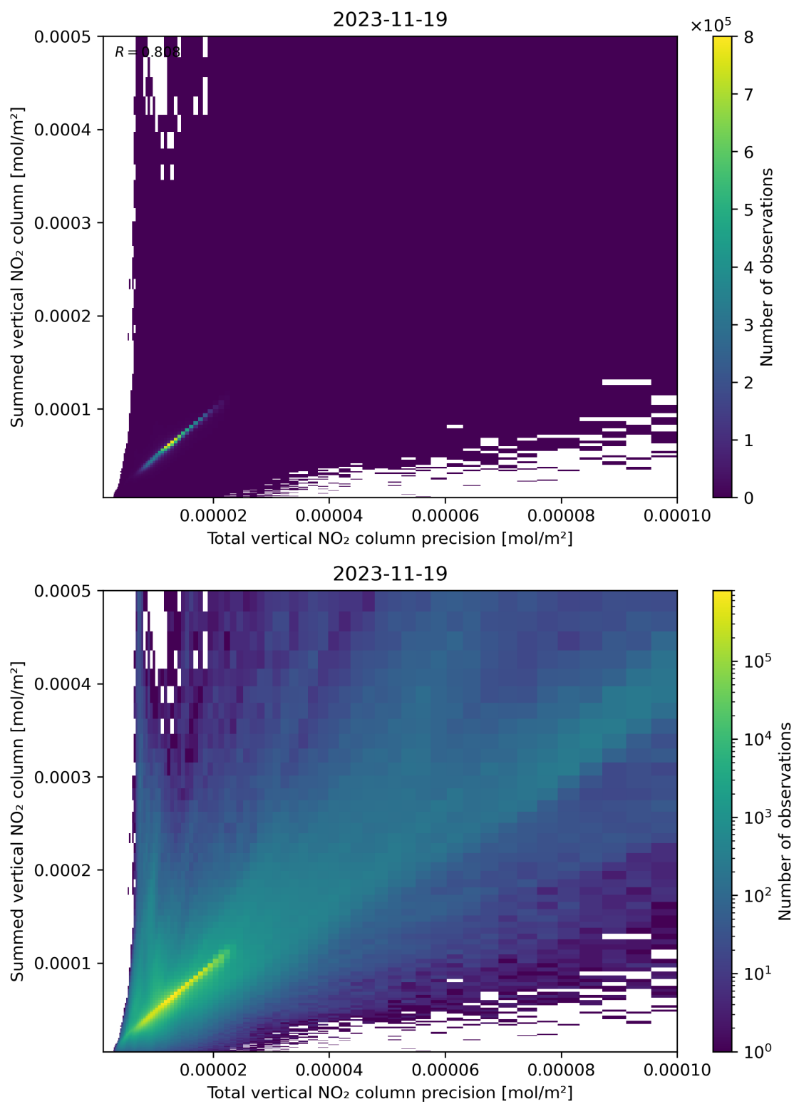
Figure 117: Scatter density plot of “Total vertical NO 2 column precision” against “Summed vertical NO 2 column” for 2023-11-18 to 2023-11-20.
