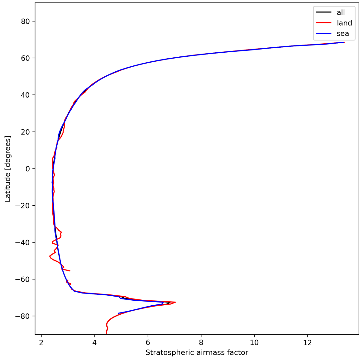
Figure 27: Zonal average of “Stratospheric airmass factor” for 2023-11-18 to 2023-11-20.
