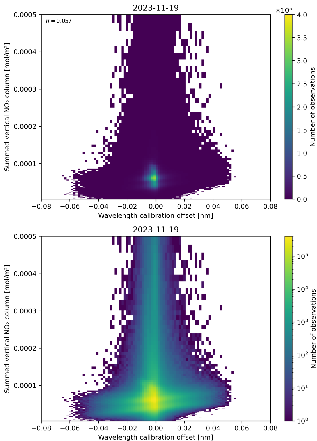
Figure 177: Scatter density plot of “Wavelength calibration offset” against “Summed vertical NO 2 column” for 2023-11-18 to 2023-11-20.
