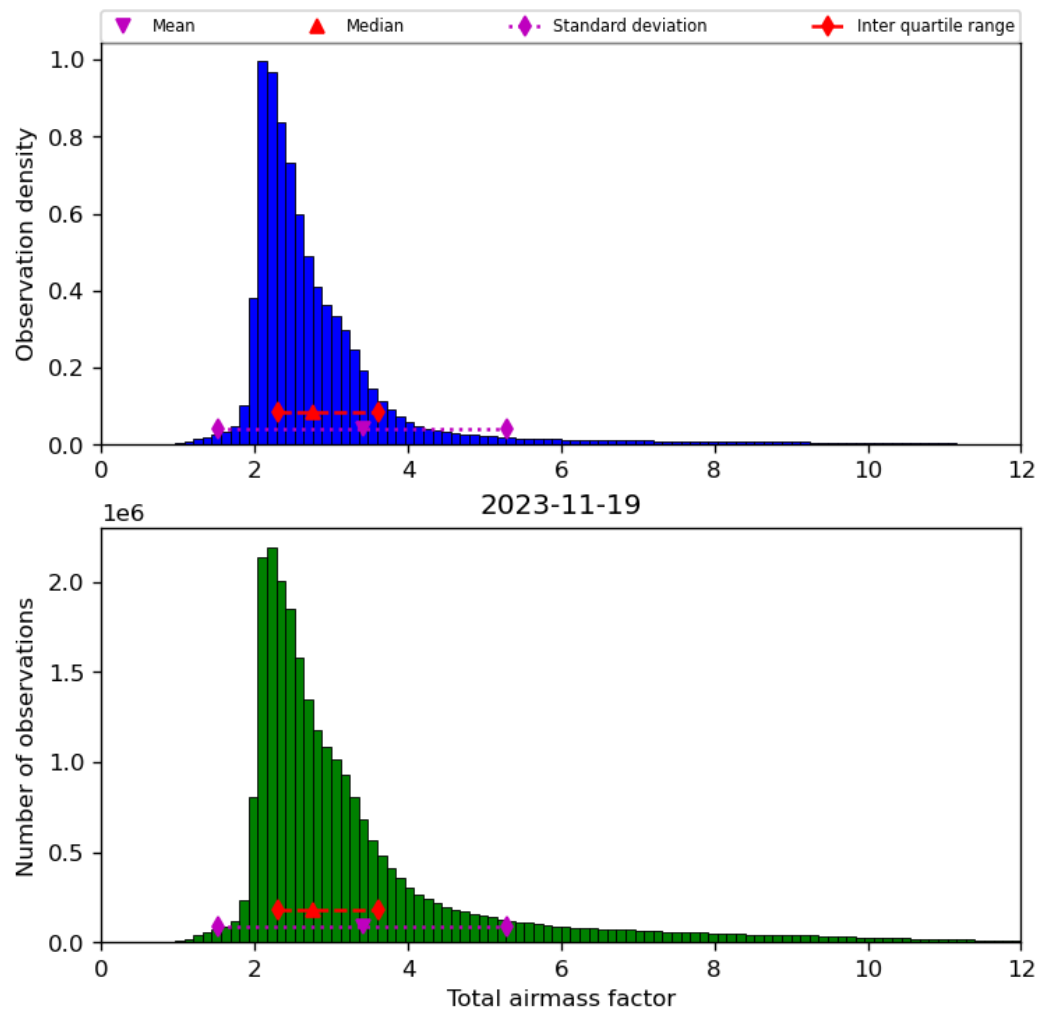
Figure 32: Histogram of “Total airmass factor” for 2023-11-18 to 2023-11-20
