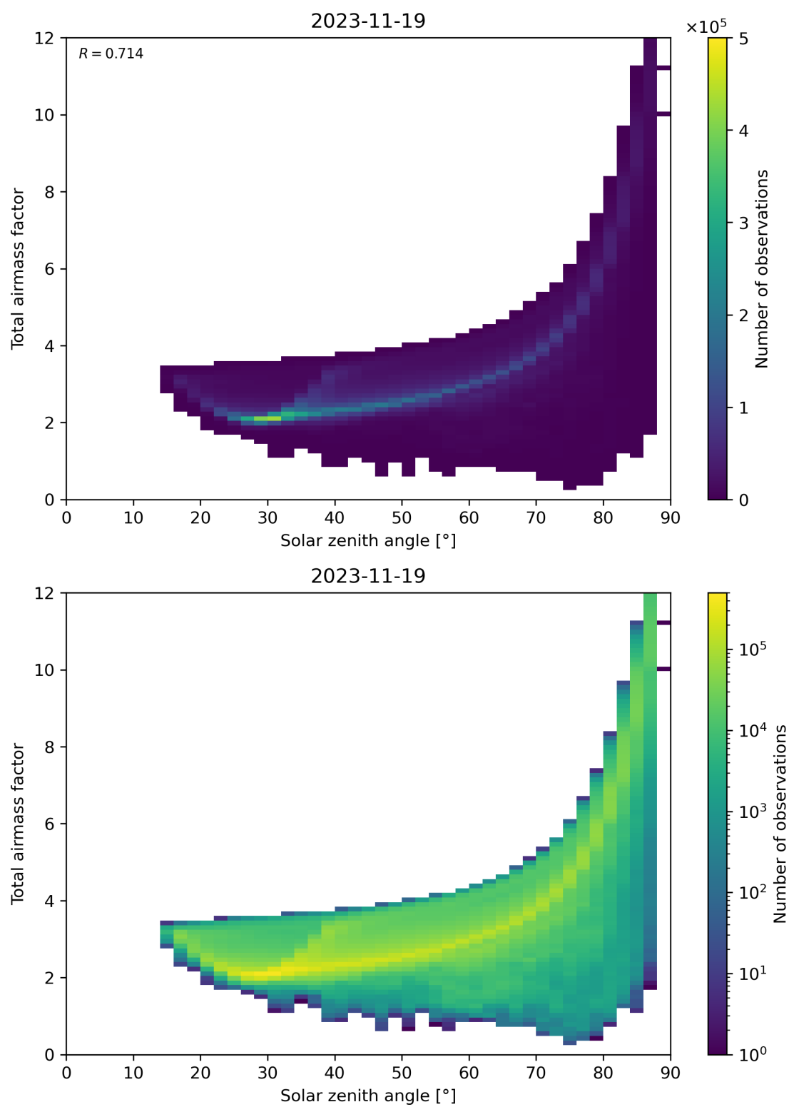
Figure 146: Scatter density plot of “Solar zenith angle” against “Total air mass factor” for 2023-11-18 to 2023-11-20.
