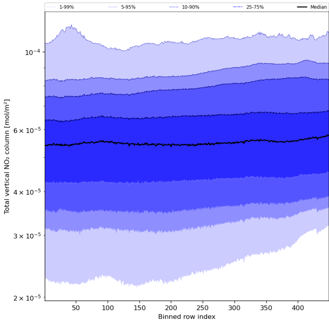
Figure 55: Along track statistics of “Total vertical NO 2 column” for 2023-11-18 to 2023-11-20
