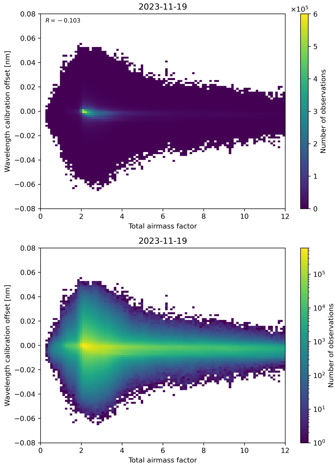
Figure 70: Scatter density plot of “Total airmass factor” against “Wavelength calibration offset” for 2023-11-18 to 2023-11-20.
