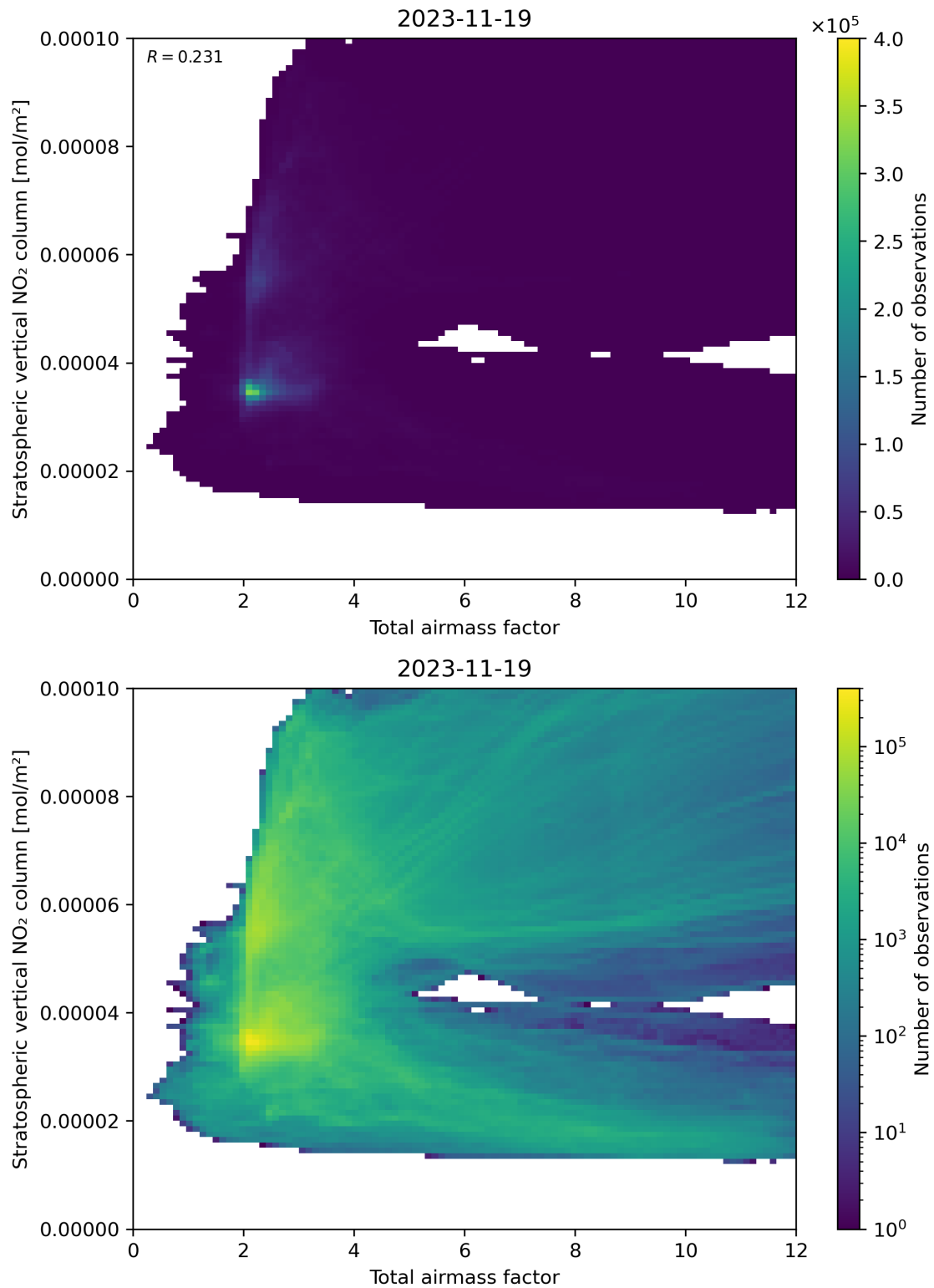
Figure 64: Scatter density plot of “Total airmass factor” against “Stratospheric vertical NO 2 column” for 2023-11-18 to 2023-11-20.
