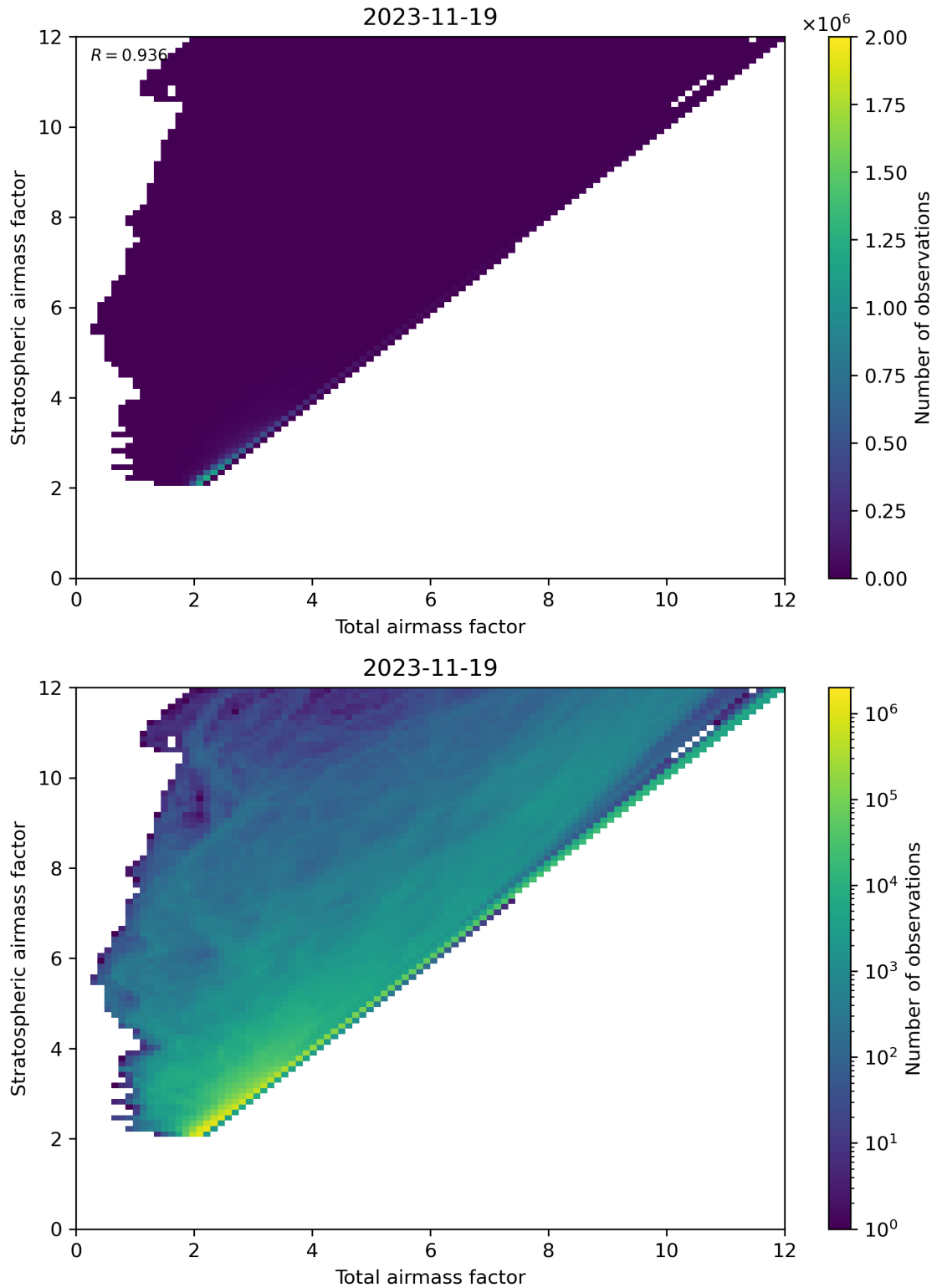
Figure 62: Scatter density plot of “Total airmass factor” against “Stratospheric airmass factor” for 2023-11-18 to 2023-11-20.
