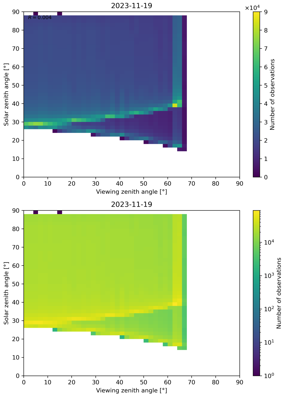
Figure 172: Scatter density plot of “Viewing zenith angle” against “Solar zenith angle” for 2023-11-18 to 2023-11-20.
