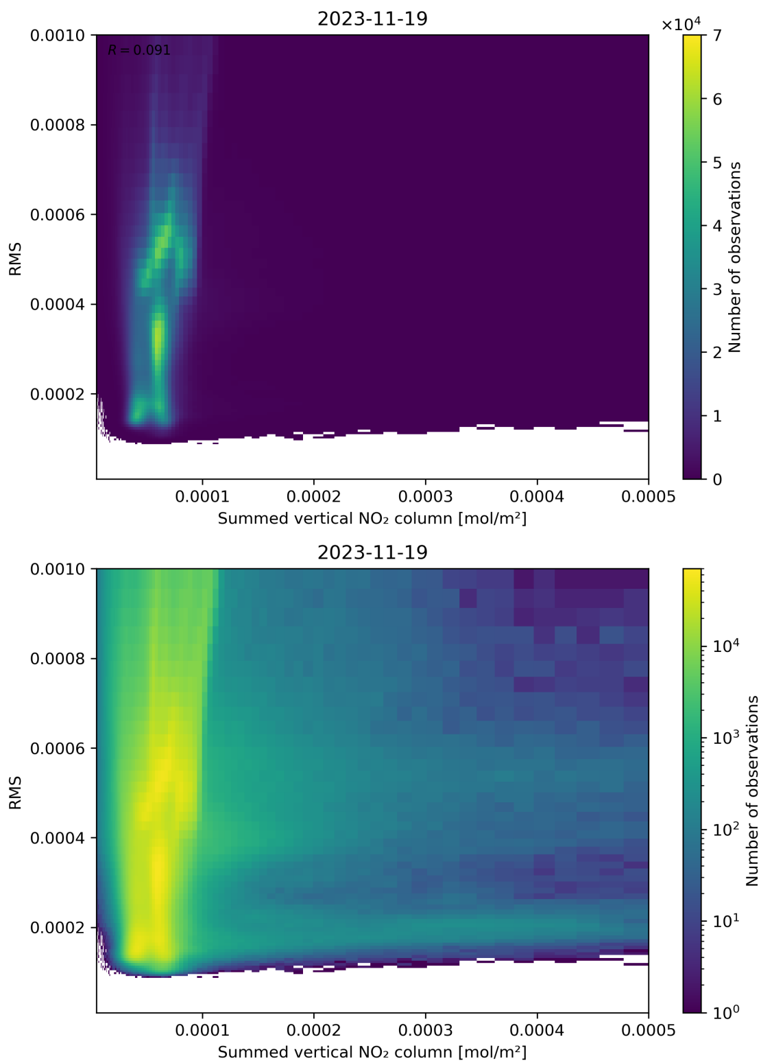
Figure 109: Scatter density plot of “Summed vertical NO 2 column” against “RMS” for 2023-11-18 to 2023-11-20.
