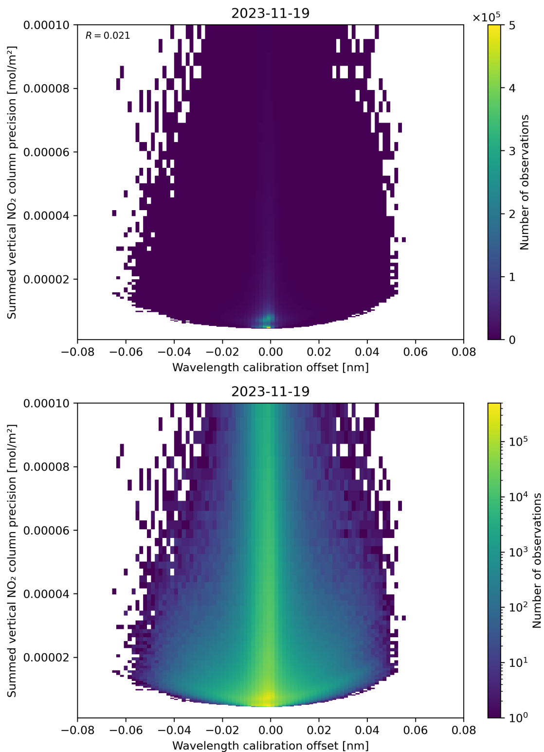
Figure 178: Scatter density plot of “Wavelength calibration offset” against “Summed vertical NO 2 column precision” for 2023-11-18 to 2023-11-20.
