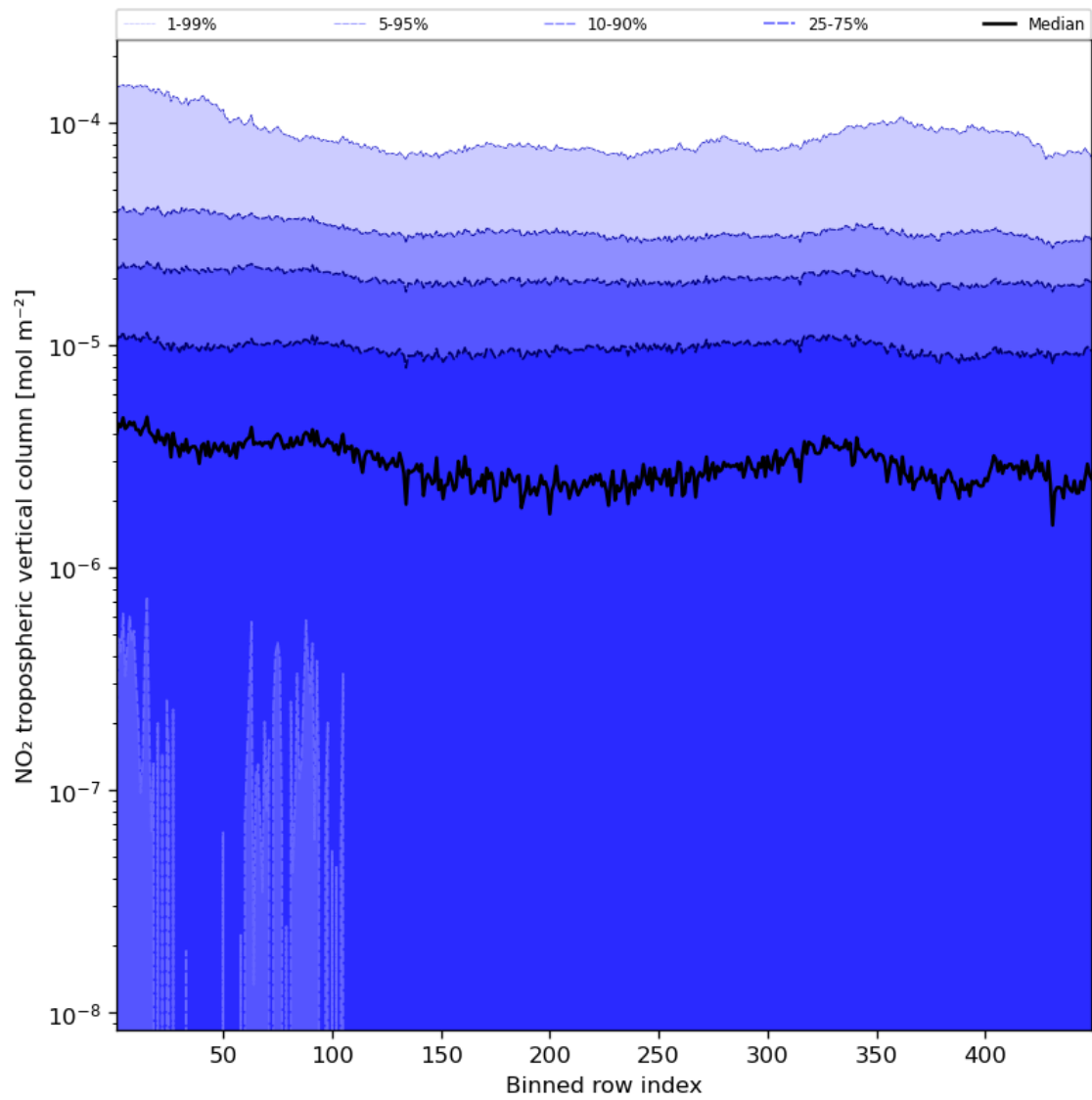
Figure 46: Along track statistics of “NO 2 tropospheric vertical column” for 2023-11-18 to 2023-11-20
