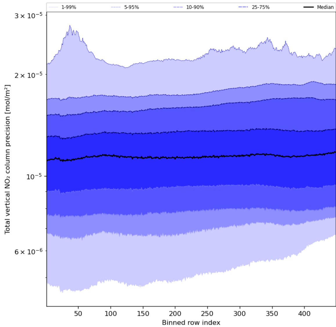
Figure 56: Along track statistics of “Total vertical NO 2 column precision” for 2023-11-18 to 2023-11-20
