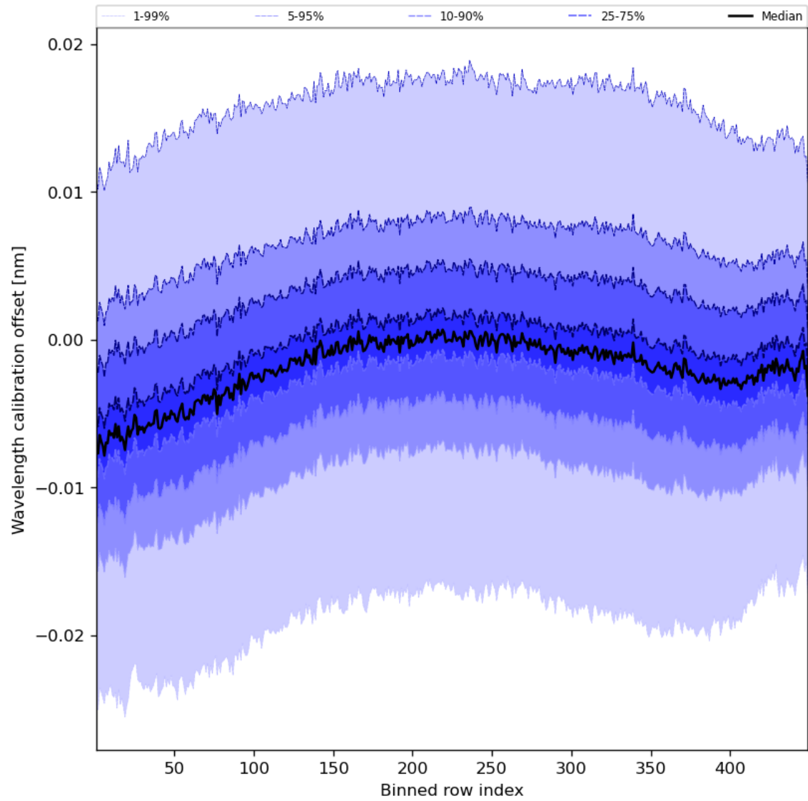
Figure 52: Along track statistics of “Wavelength calibration offset” for 2023-11-18 to 2023-11-20
