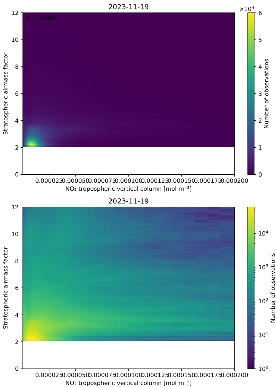
Figure 121: Scatter density plot of “NO 2 tropospheric vertical column” against “Stratospheric airmass factor” for 2023-11-18 to 2023-11-20.
