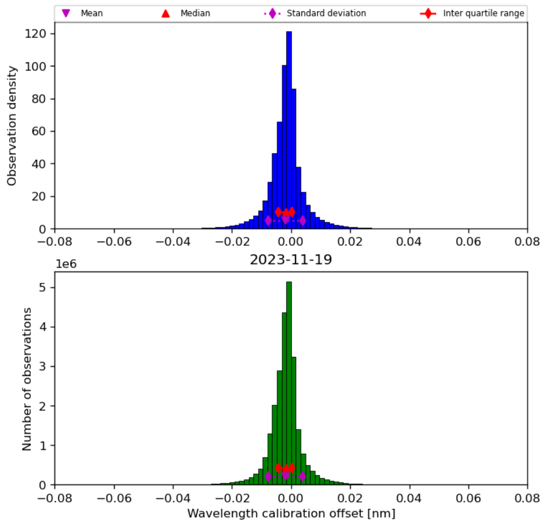
Figure 35: Histogram of “Wavelength calibration offset” for 2023-11-18 to 2023-11-20
