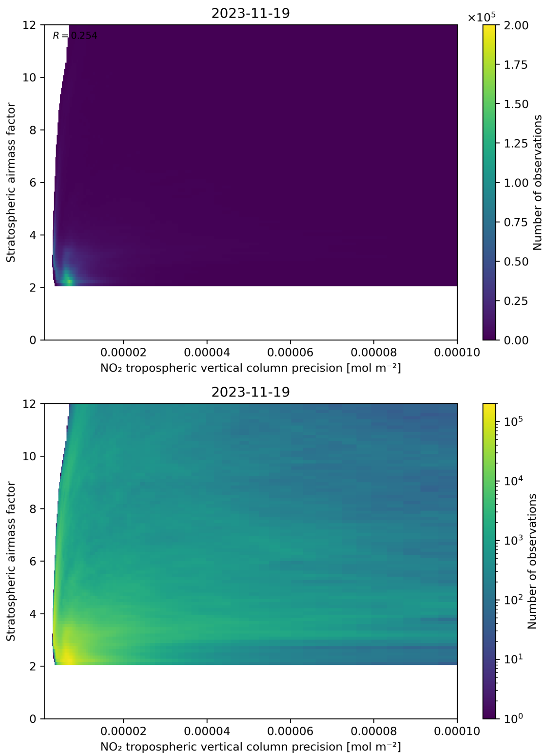
Figure 131: Scatter density plot of “NO 2 tropospheric vertical column precision” against “Stratospheric airmass factor” for 2023-11-18 to 2023-11-20.
