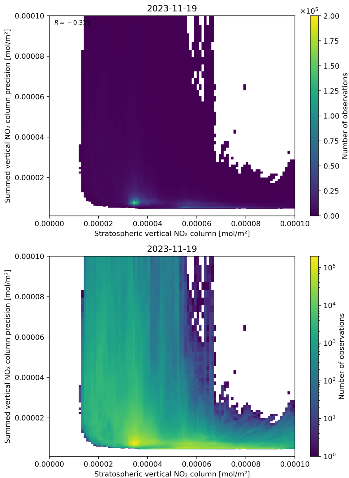
Figure 99: Scatter density plot of “Stratospheric vertical NO 2 column” against “Summed vertical NO 2 column precision” for 2023-11-18 to 2023-11-20.
