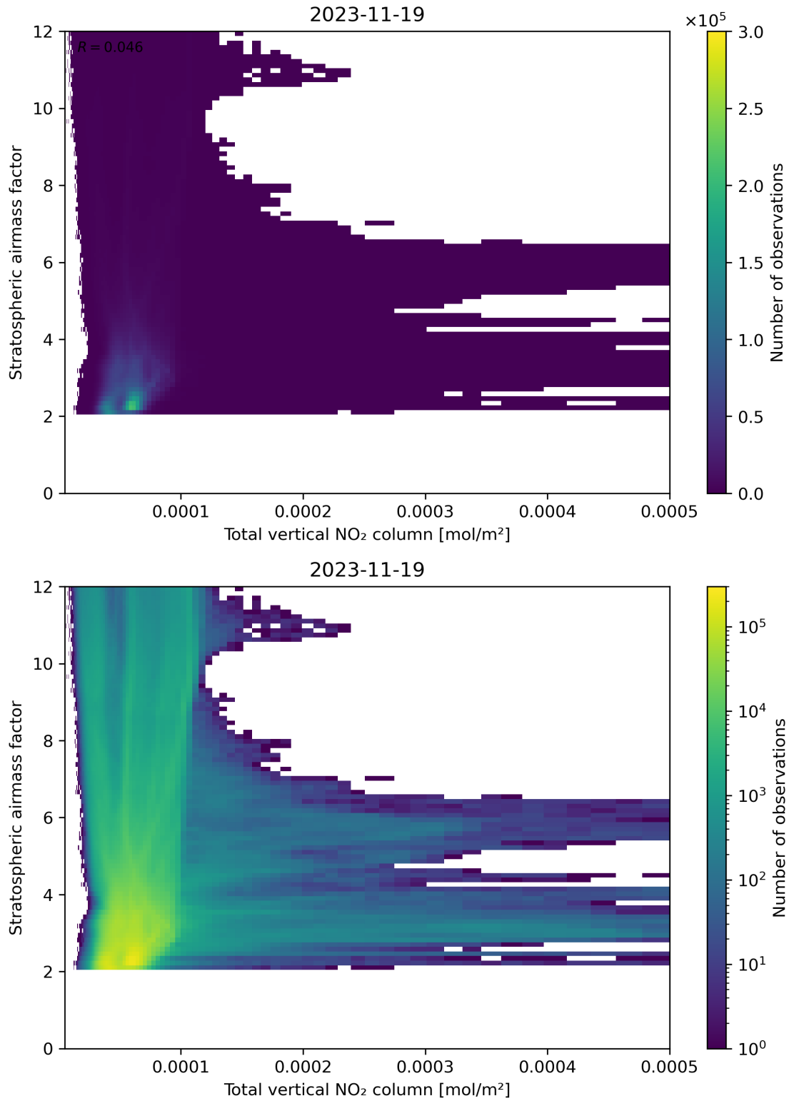
Figure 110: Scatter density plot of “Total vertical NO 2 column” against “Stratospheric air mass factor” for 2023-11-18 to 2023-11-20.
