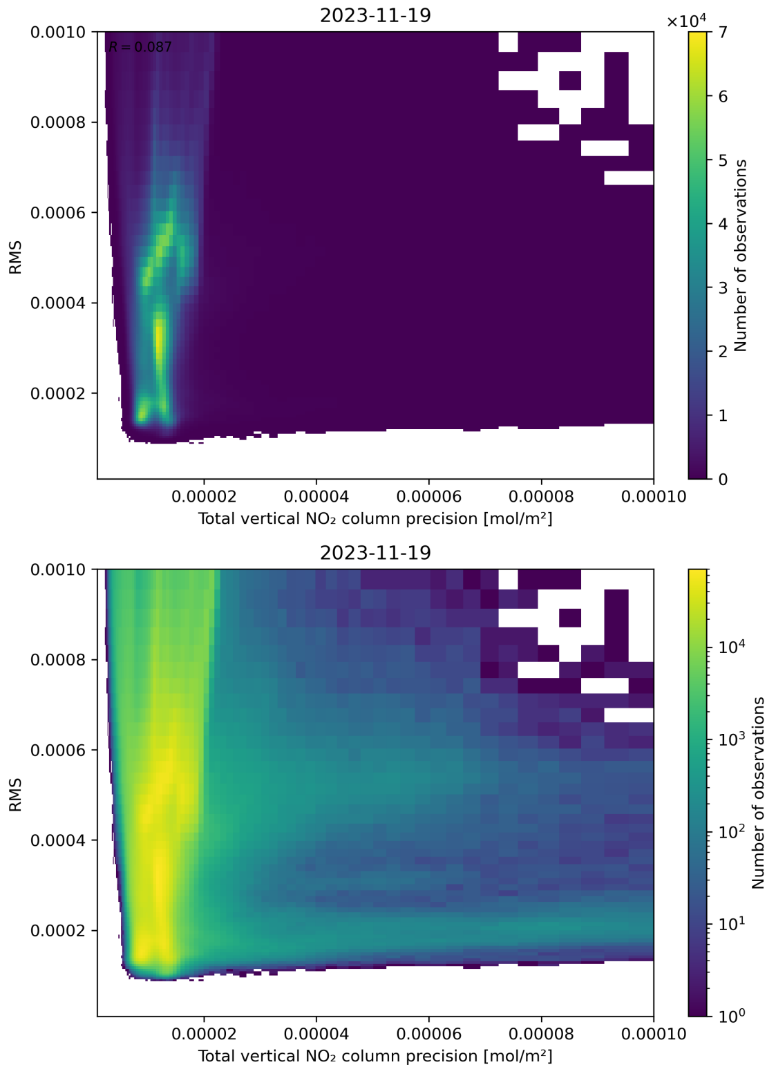
Figure 119: Scatter density plot of “Total vertical NO 2 column precision” against “RMS” for 2023-11-18 to 2023-11-20.
