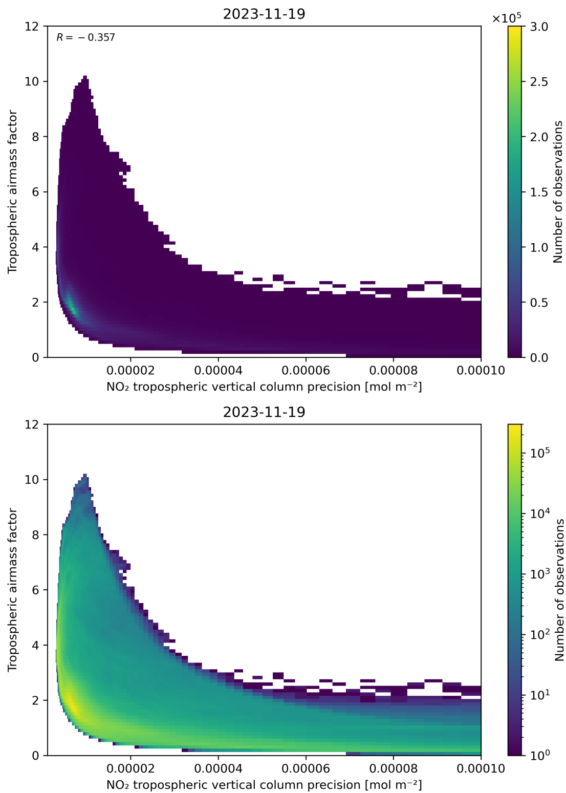
Figure 133: Scatter density plot of “NO 2 tropospheric vertical column precision” against “Tropospheric airmass factor” for 2023-11-18 to 2023-11-20.
