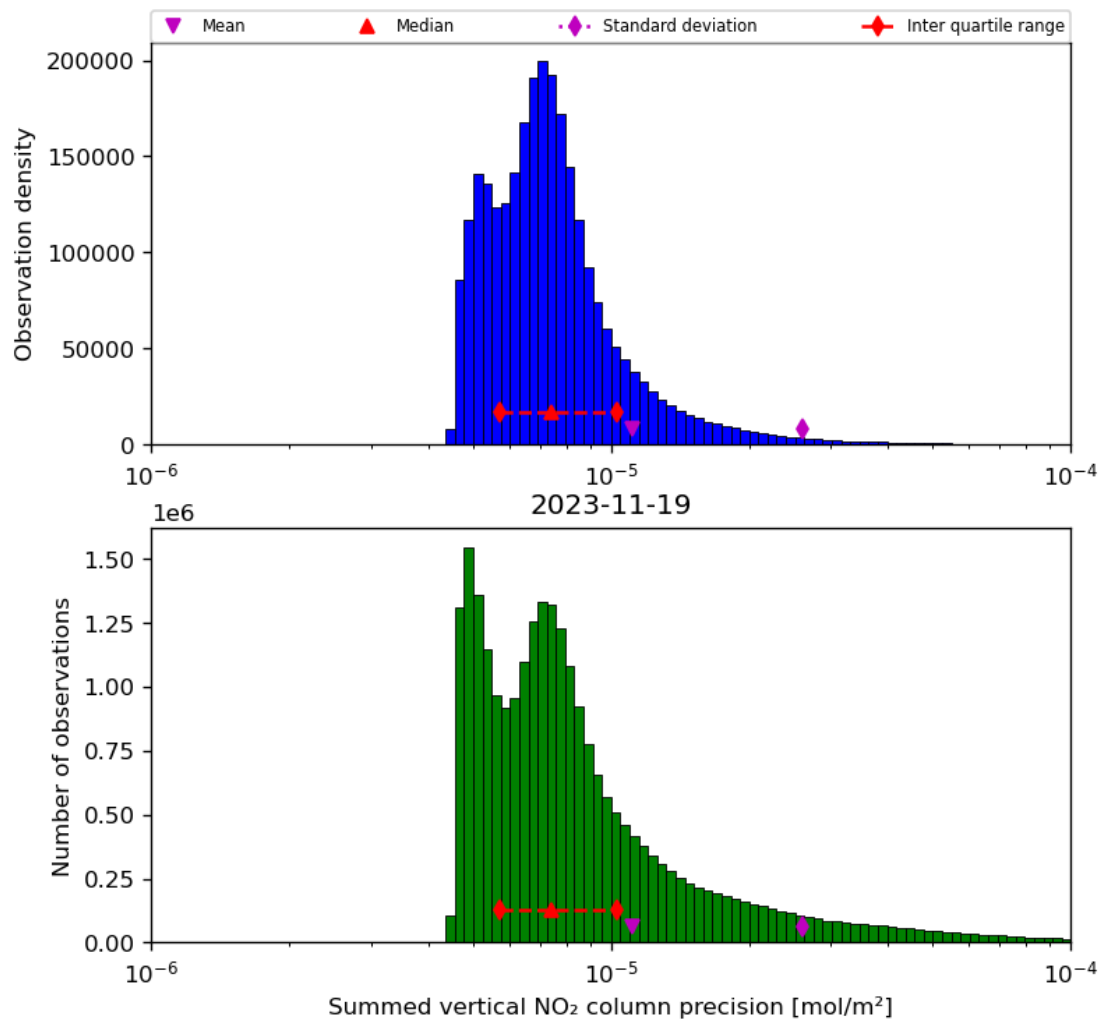
Figure 41: Histogram of “Summed vertical NO 2 column precision” for 2023-11-18 to 2023-11-20
