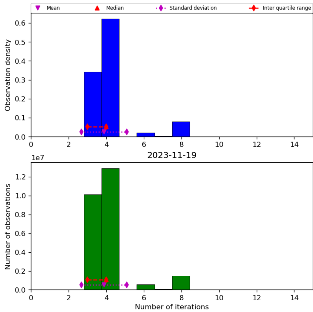
Figure 34: Histogram of “Number of iterations” for 2023-11-18 to 2023-11-20
