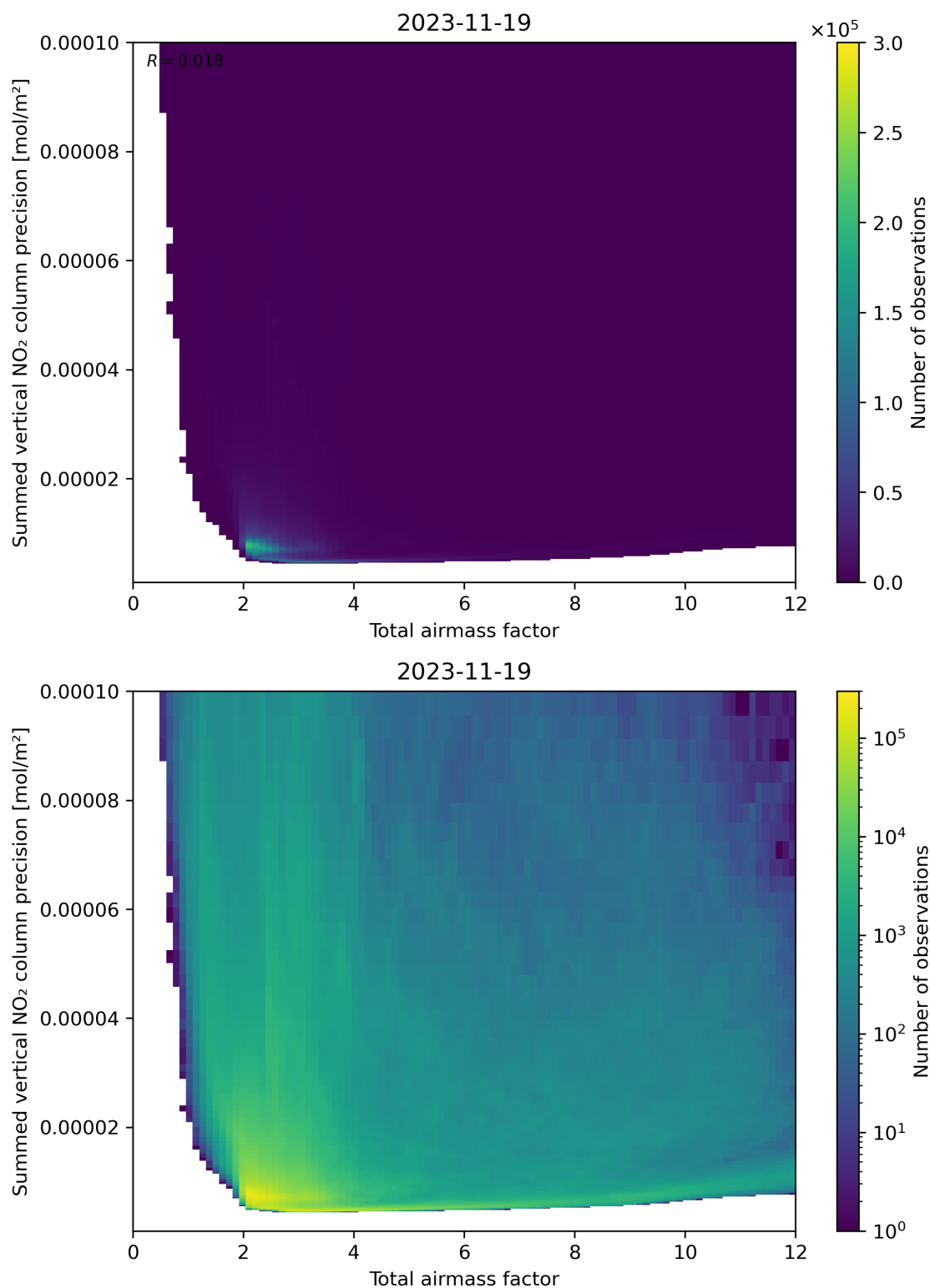
Figure 66: Scatter density plot of “Total airmass factor” against “Summed vertical NO 2 column precision” for 2023-11-18 to 2023-11-20.
