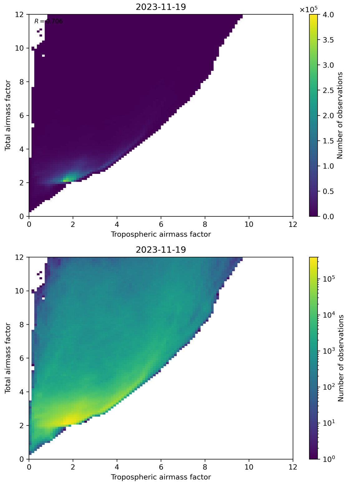
Figure 72: Scatter density plot of “Tropospheric airmass factor” against “Total airmass factor” for 2023-11-18 to 2023-11-20.
