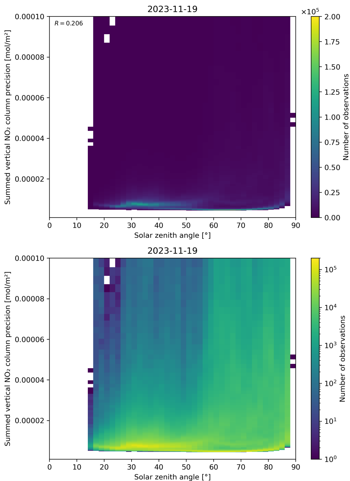
Figure 152: Scatter density plot of “Solar zenith angle” against “Summed vertical NO 2 column precision” for 2023-11-18 to 2023-11-20.
