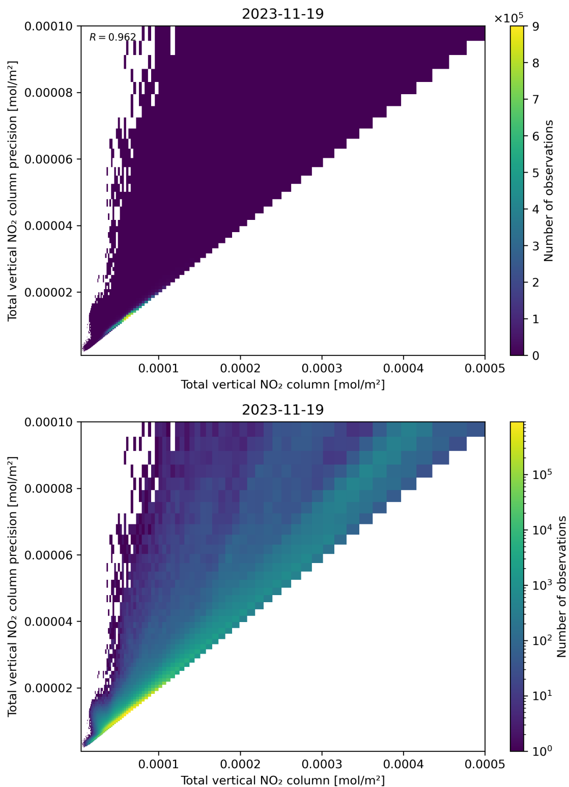
Figure 114: Scatter density plot of “Total vertical NO 2 column” against “Total vertical NO 2 column precision” for 2023-11-18 to 2023-11-20.
