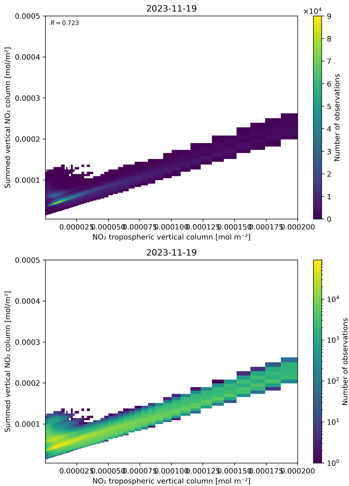
Figure 126: Scatter density plot of “NO 2 tropospheric vertical column” against “Summed vertical NO 2 column” for 2023-11-18 to 2023-11-20.
