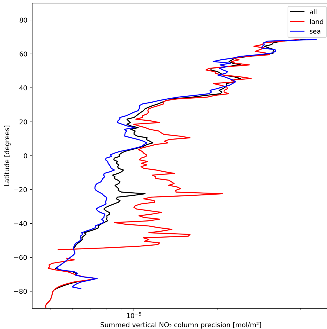
Figure 24: Zonal average of “Summed vertical NO 2 column precision” for 2023-11-18 to 2023-11-20.
