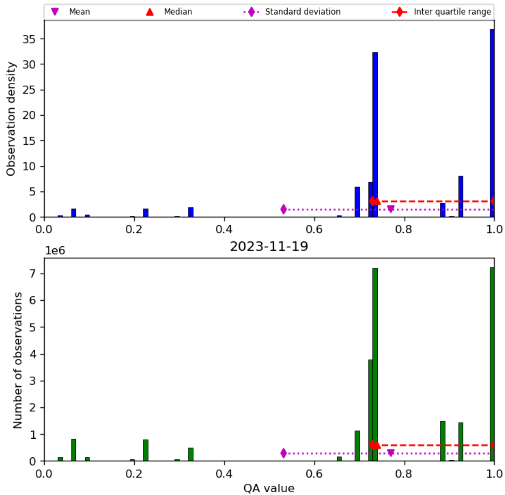
Figure 28: Histogram of “QA value” for 2023-11-18 to 2023-11-20
