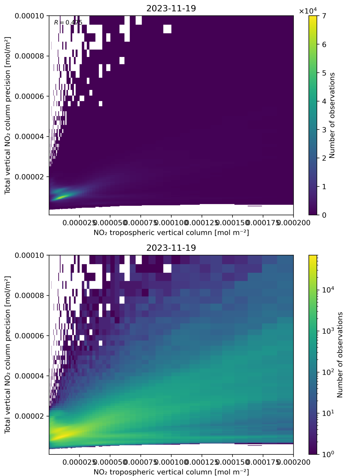
Figure 129: Scatter density plot of “NO 2 tropospheric vertical column” against “Total vertical NO 2 column precision” for 2023-11-18 to 2023-11-20.
