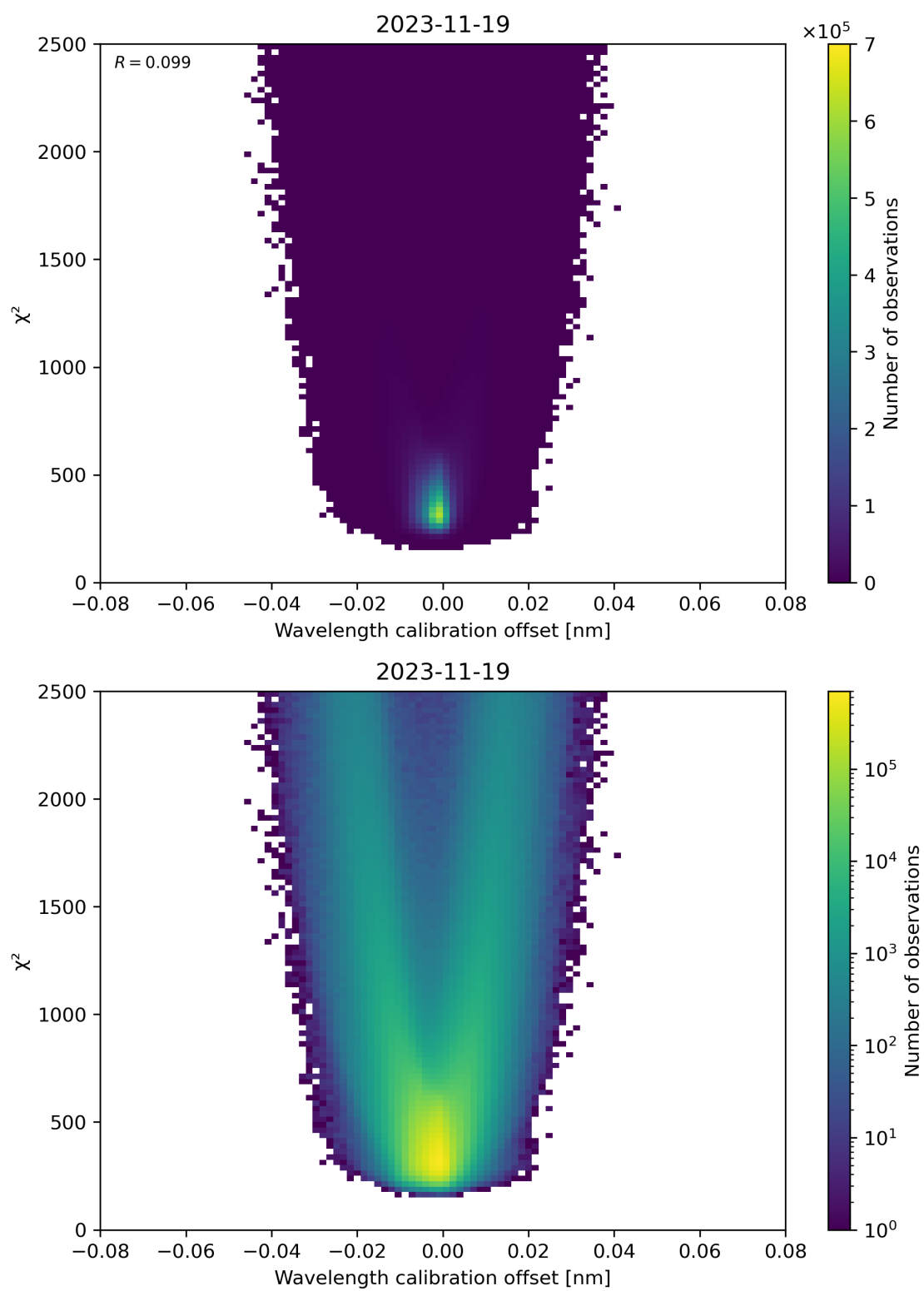
Figure 175: Scatter density plot of “Wavelength calibration offset” against “ \chi^2 ” for 2023-11-18 to 2023-11-20.
