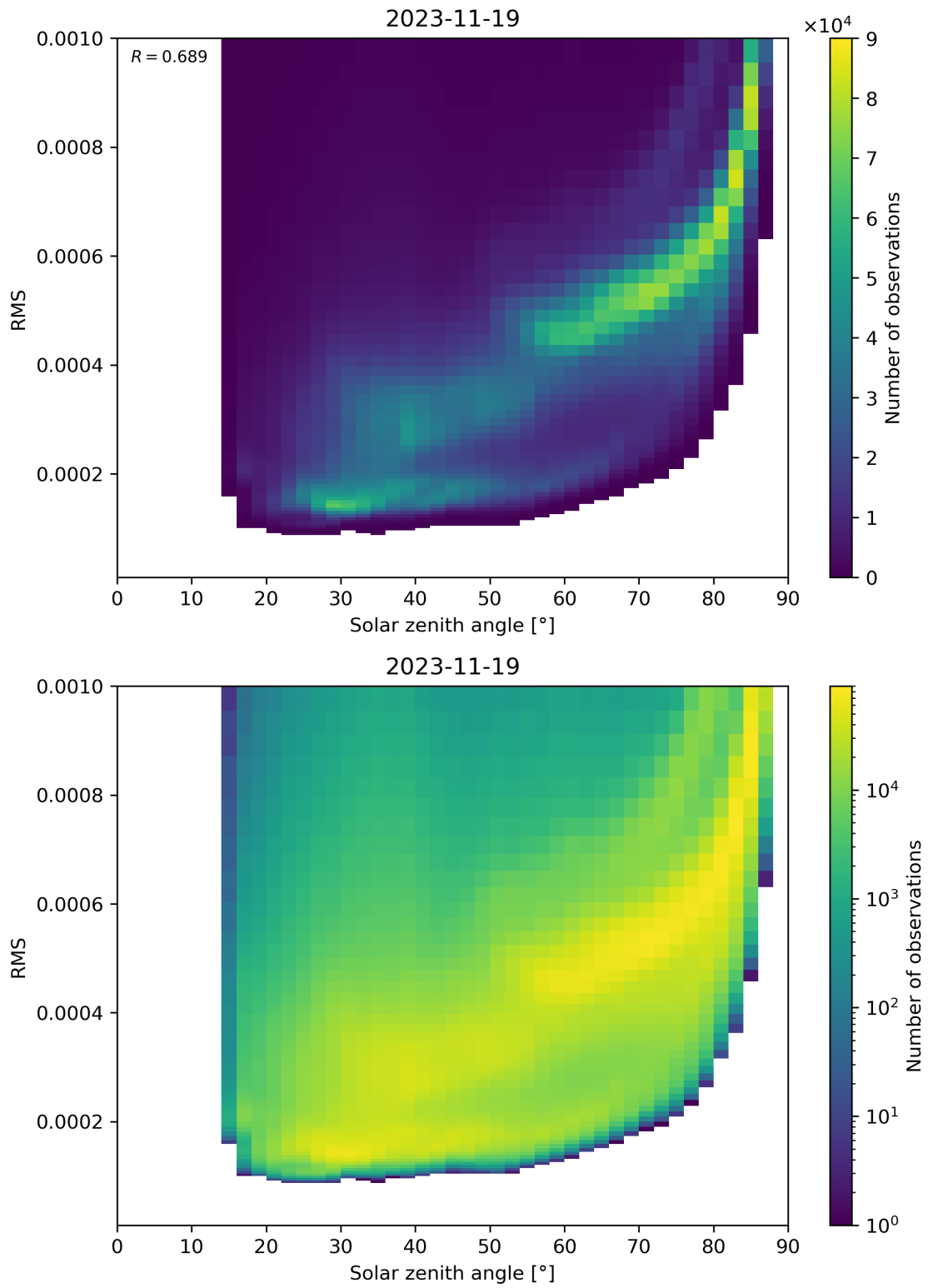
Figure 157: Scatter density plot of “Solar zenith angle” against “RMS” for 2023-11-18 to 2023-11-20.
