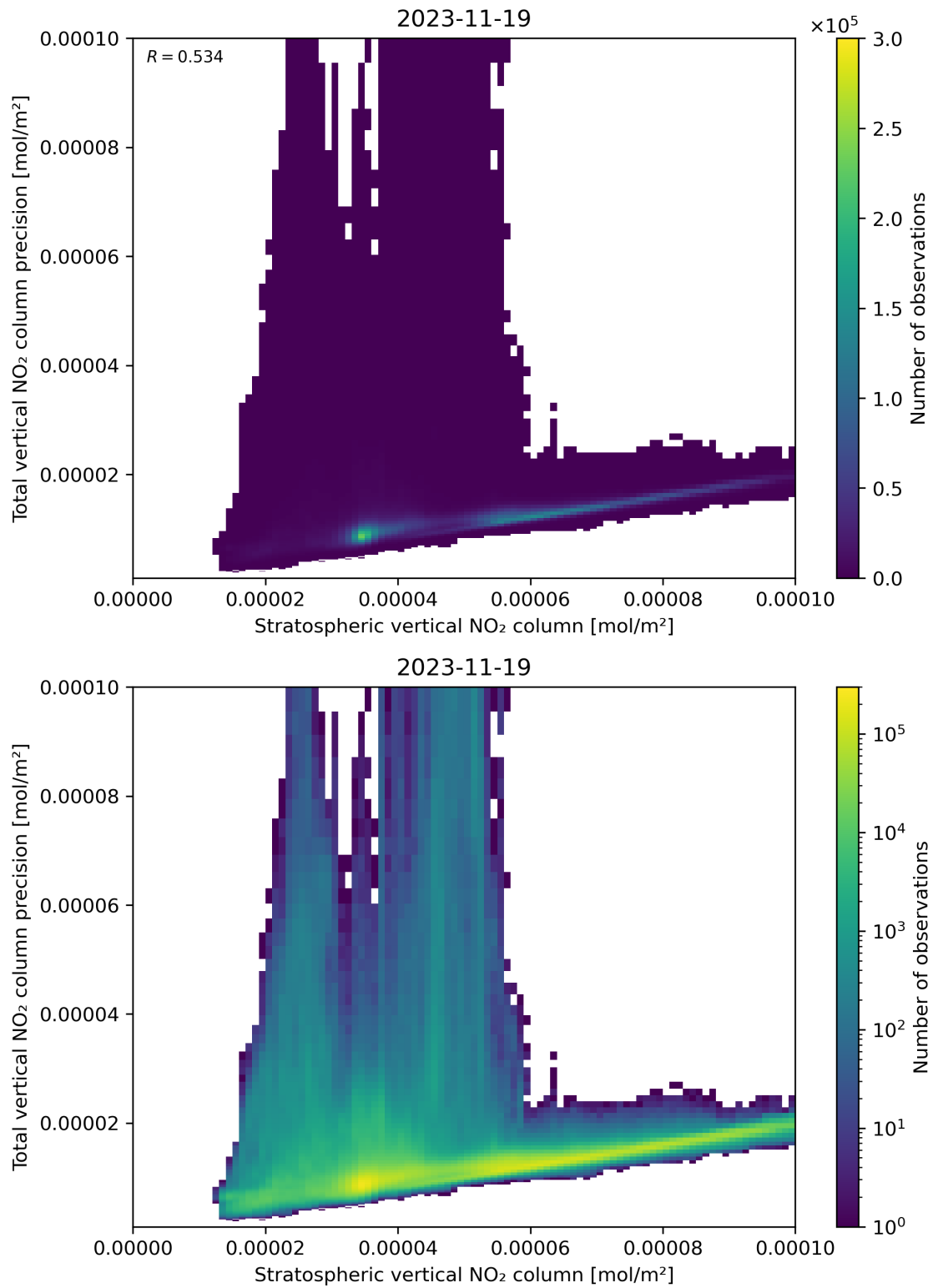
Figure 101: Scatter density plot of “Stratospheric vertical NO 2 column” against “Total vertical NO 2 column precision” for 2023-11-18 to 2023-11-20.
