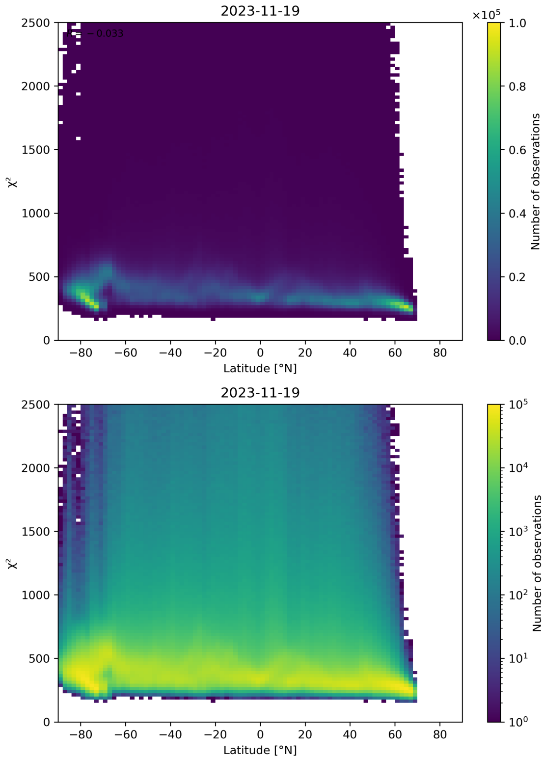
Figure 86: Scatter density plot of “Latitude” against “ \chi^2 ” for 2023-11-18 to 2023-11-20.
