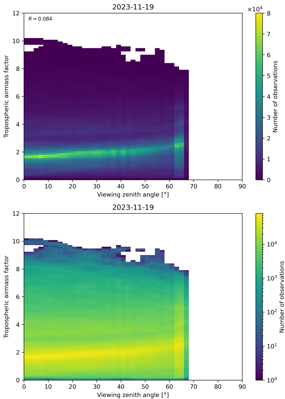
Figure 161: Scatter density plot of “Viewing zenith angle” against “Tropospheric airmass factor” for 2023-11-18 to 2023-11-20.
