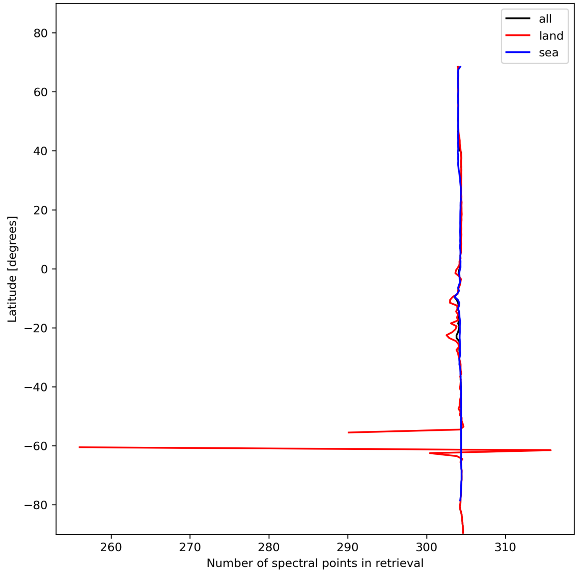
Figure 16: Zonal average of “Number of spectral points in retrieval” for 2023-11-18 to 2023-11-20.
