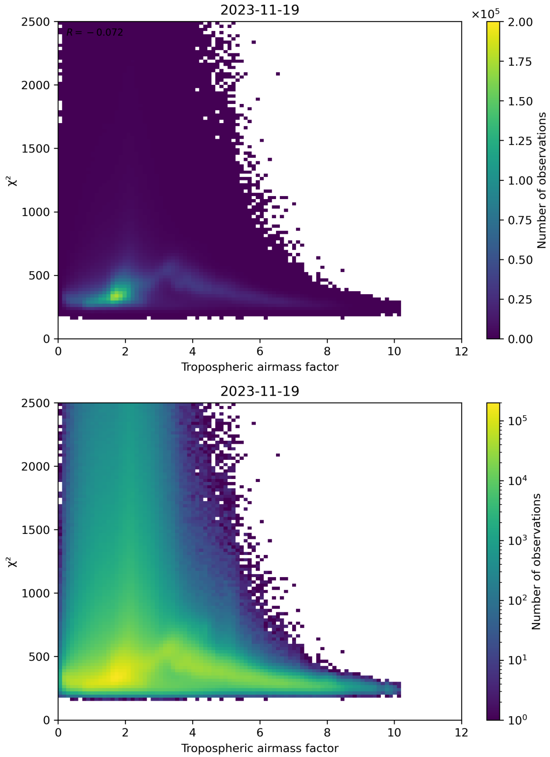
Figure 73: Scatter density plot of “Tropospheric airmass factor” against “ \chi^2 ” for 2023-11-18 to 2023-11-20.
