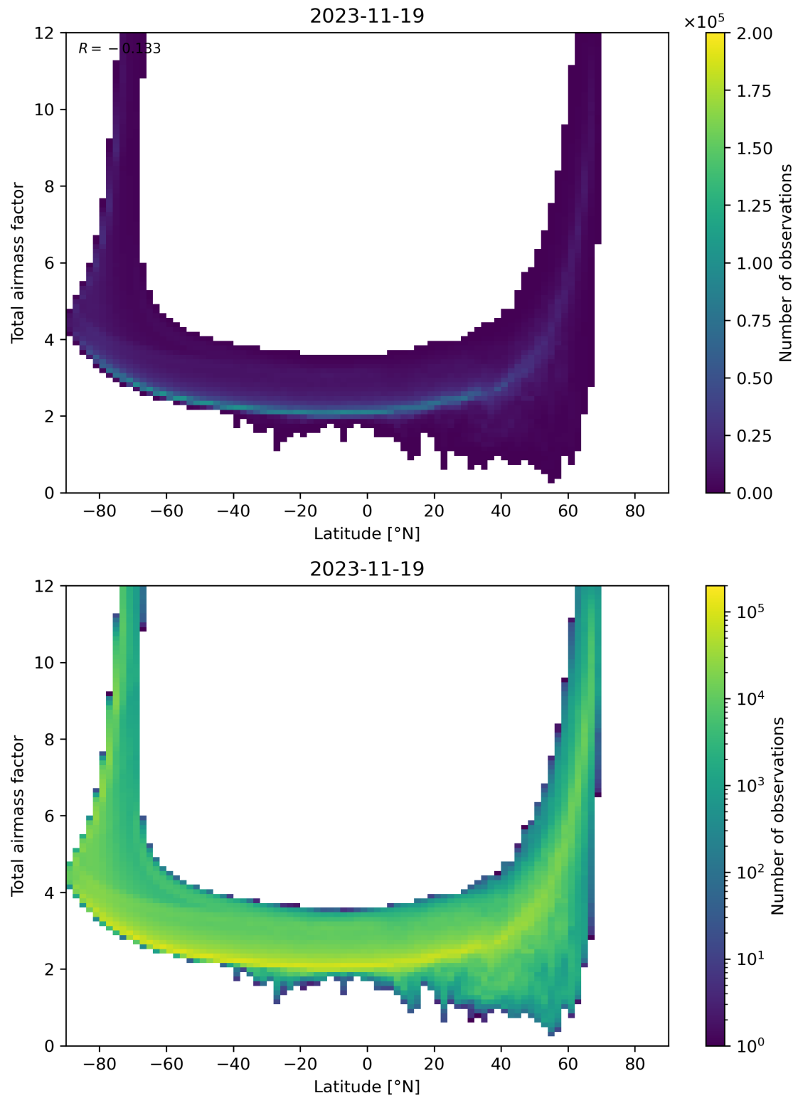
Figure 84: Scatter density plot of “Latitude” against “Total airmass factor” for 2023-11-18 to 2023-11-20.
