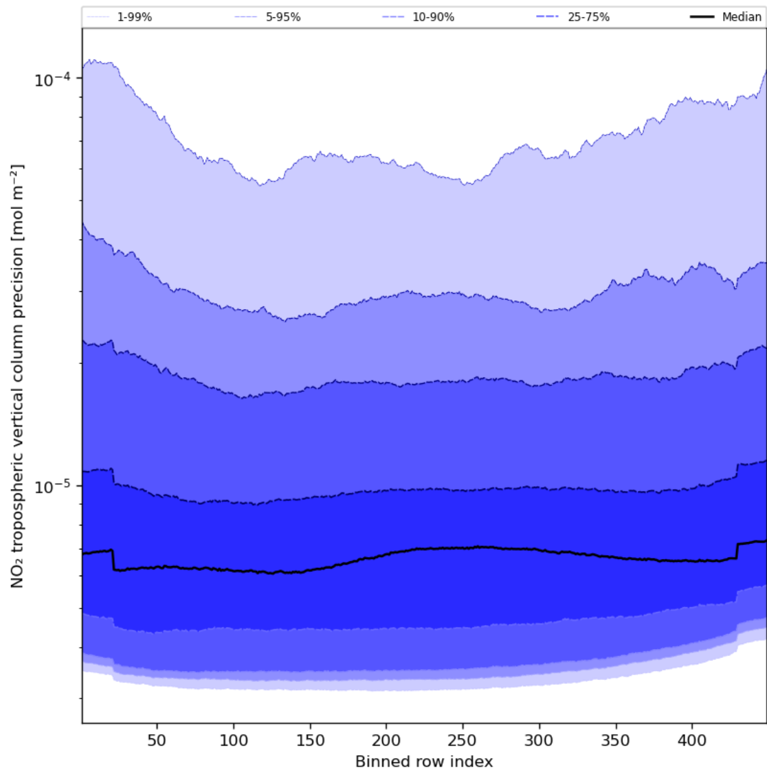
Figure 47: Along track statistics of “NO 2 tropospheric vertical column precision” for 2023-11-18 to 2023-11-20
