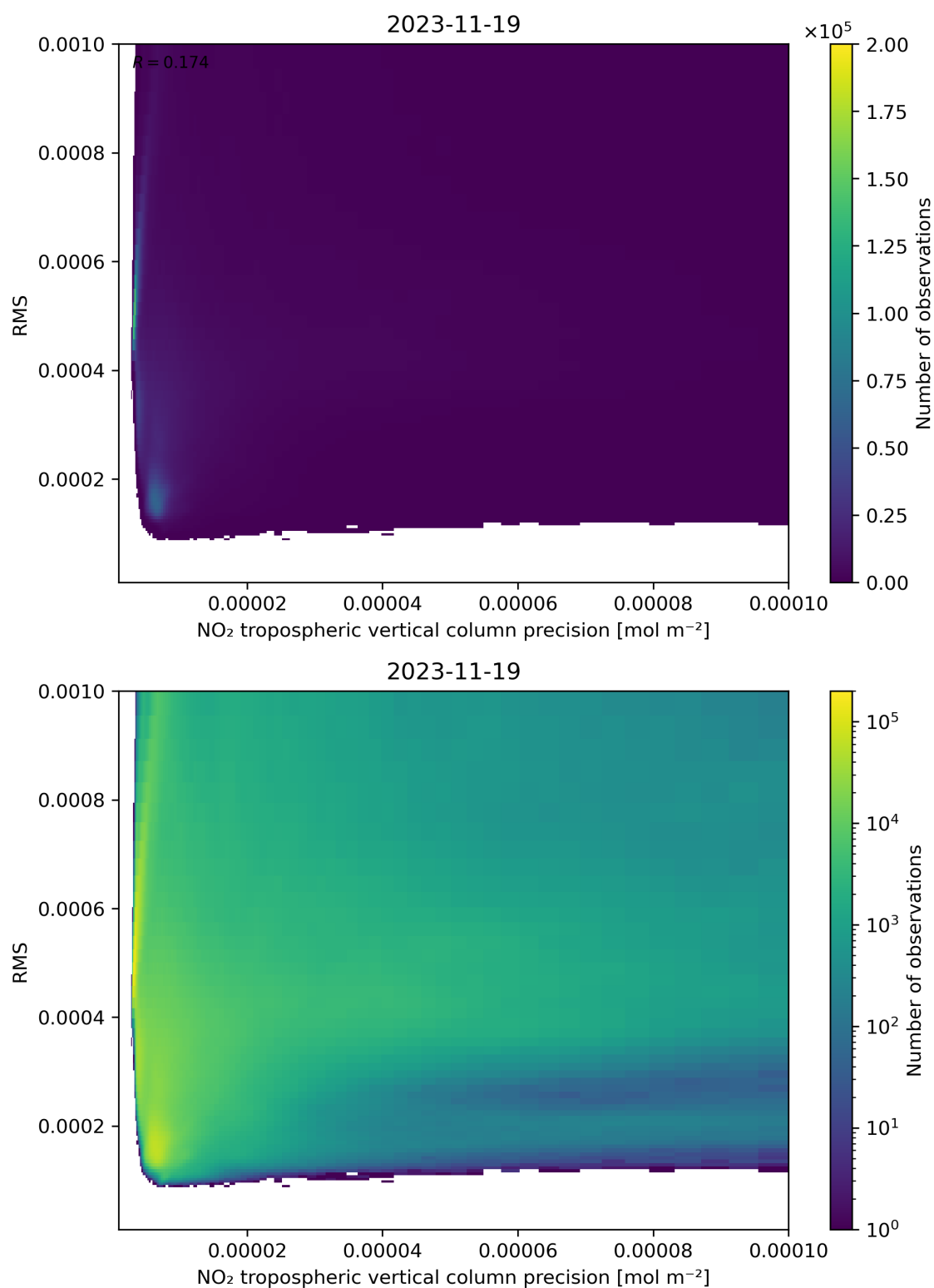
Figure 140: Scatter density plot of “NO 2 tropospheric vertical column precision” against “RMS” for 2023-11-18 to 2023-11-20.
