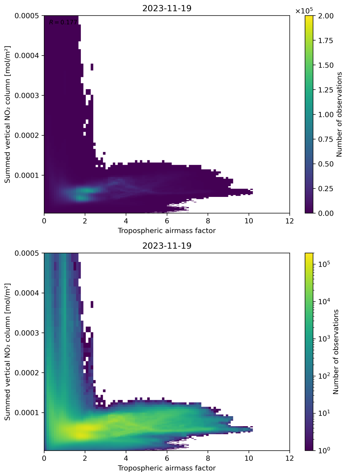
Figure 75: Scatter density plot of “Tropospheric airmass factor” against “Summed vertical NO 2 column” for 2023-11-18 to 2023-11-20.
