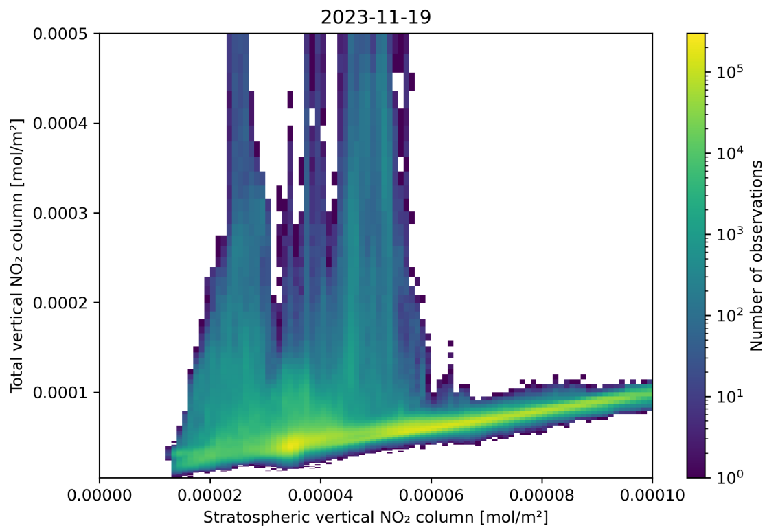
Figure 100: Scatter density plot of “Stratospheric vertical NO 2 column” against “Total vertical NO 2 column” for 2023-11-18 to 2023-11-20.
