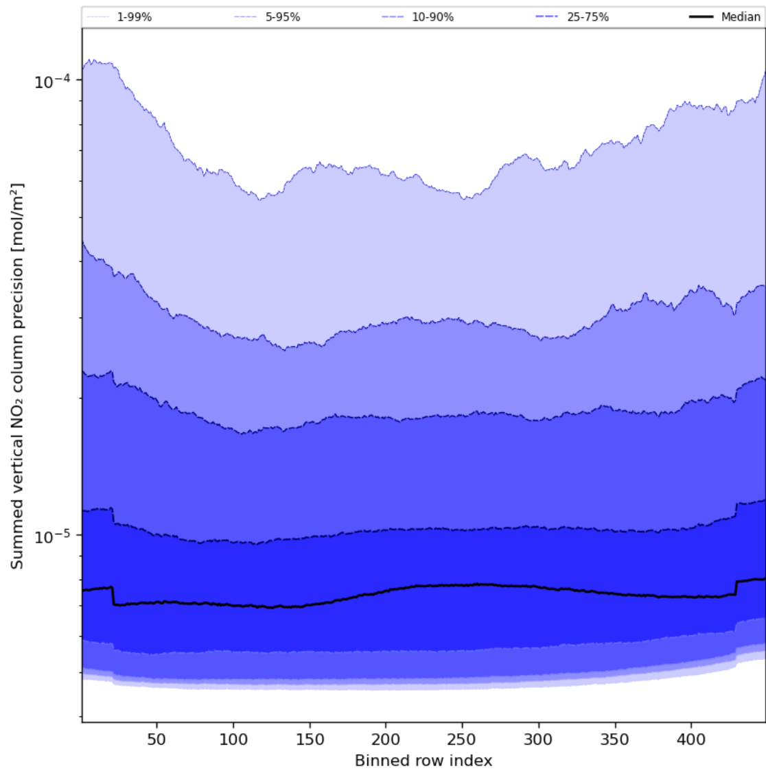
Figure 58: Along track statistics of “Summed vertical NO 2 column precision” for 2023-11-18 to 2023-11-20
