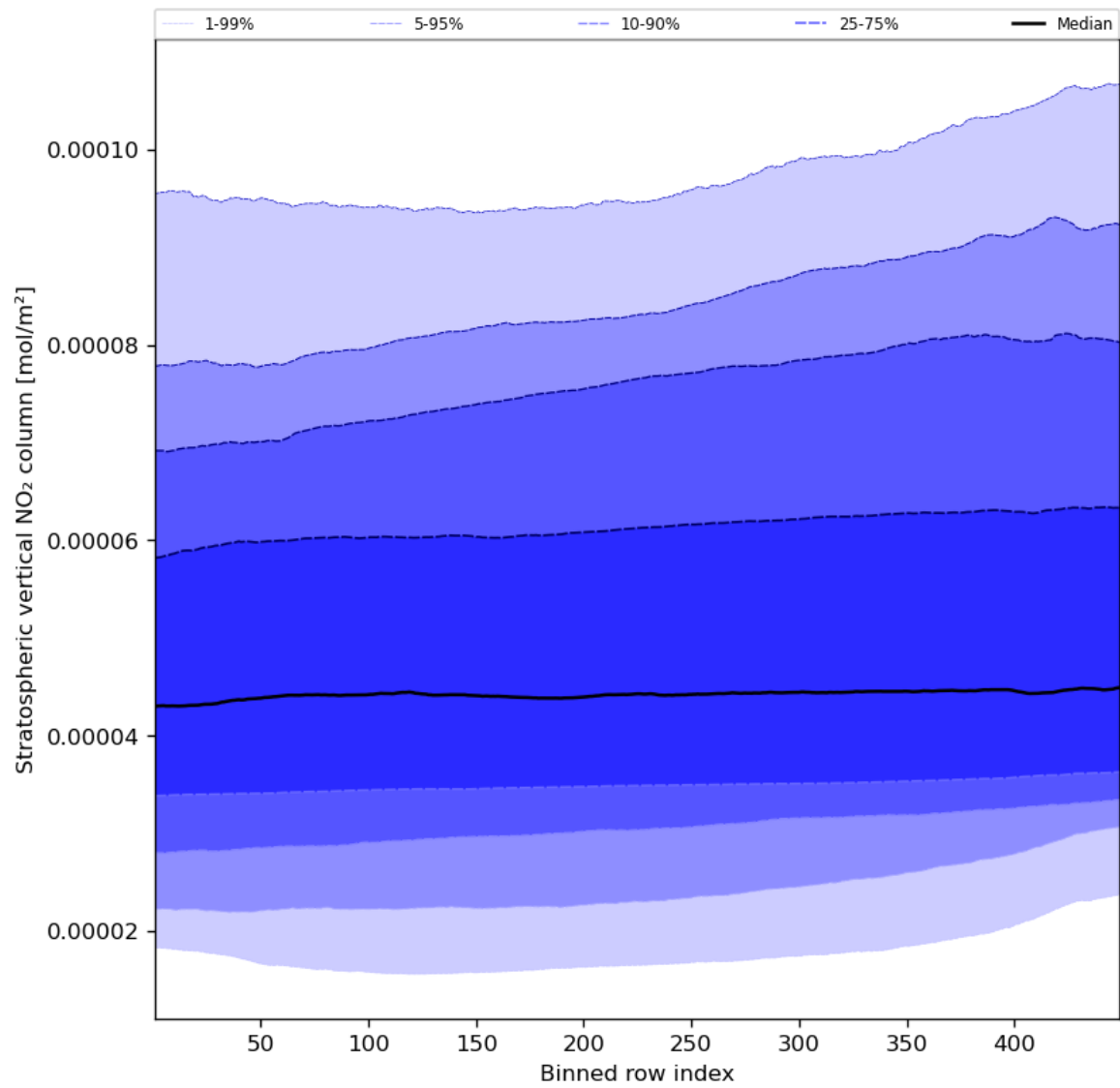
Figure 53: Along track statistics of “Stratospheric vertical NO 2 column” for 2023-11-18 to 2023-11-20
