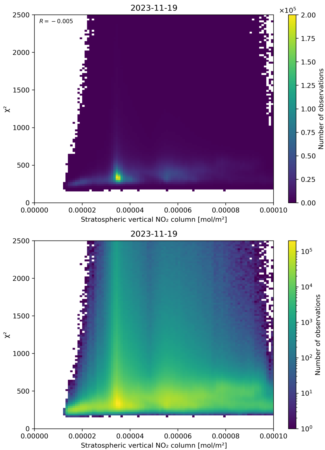
Figure 97: Scatter density plot of “Stratospheric vertical NO 2 column” against “ \chi^2 ” for 2023-11-18 to 2023-11-20.
