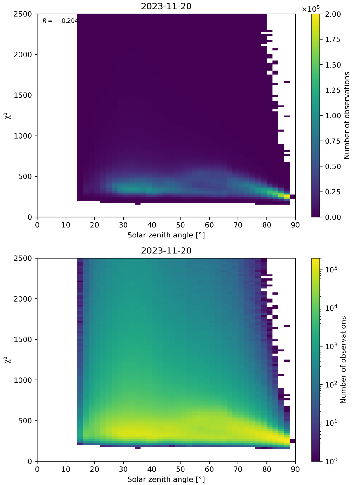
Figure 148: Scatter density plot of “Solar zenith angle” against “ \chi^2 ” for 2023-11-19 to 2023-11-21.
