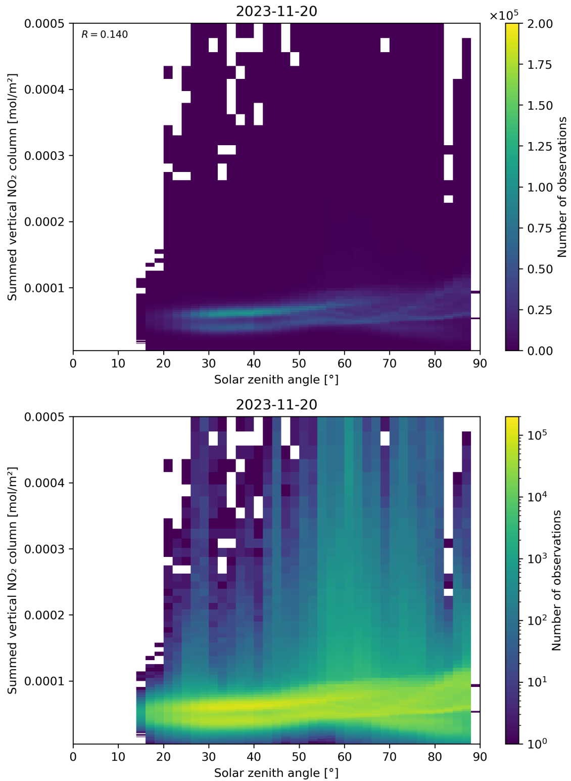
Figure 151: Scatter density plot of “Solar zenith angle” against “Summed vertical NO 2 column” for 2023-11-19 to 2023-11-21.
