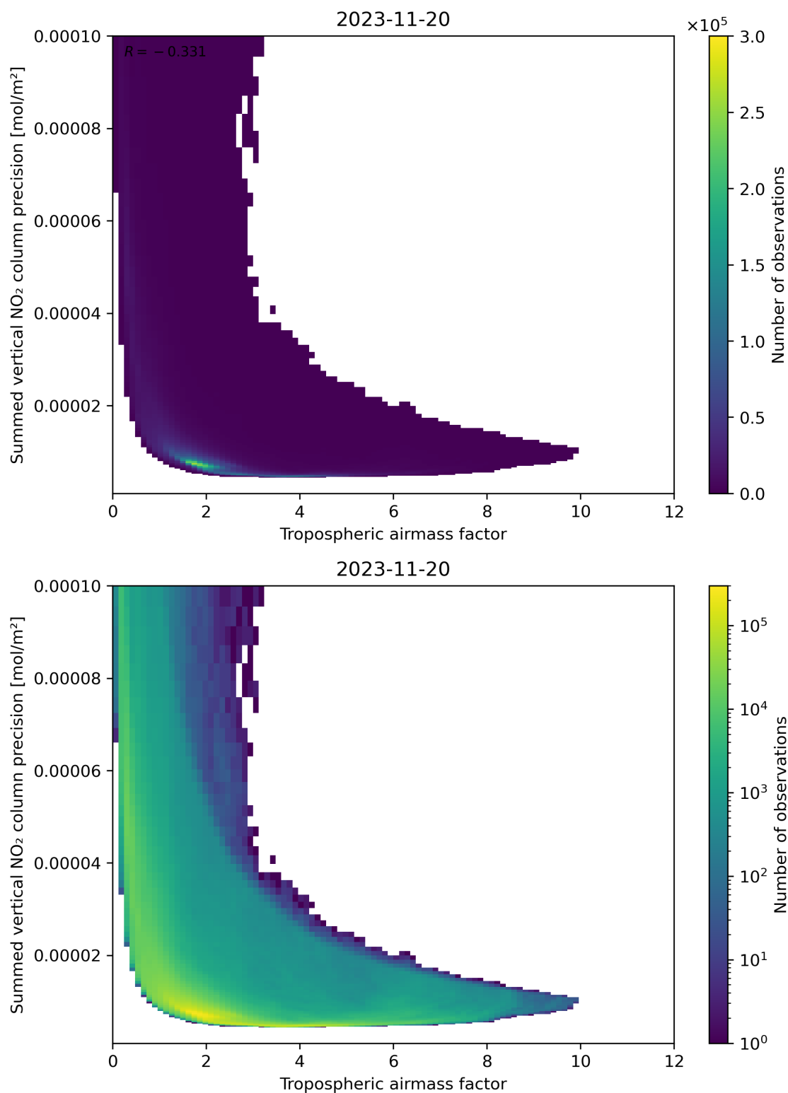
Figure 76: Scatter density plot of “Tropospheric air mass factor” against “Summed vertical NO 2 column precision” for 2023-11-19 to 2023-11-21.
