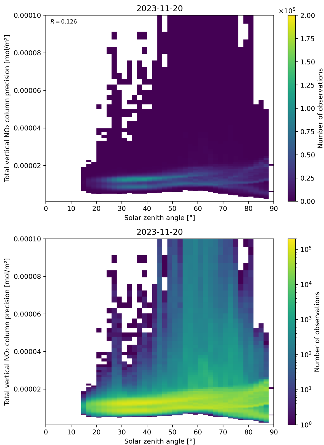
Figure 154: Scatter density plot of “Solar zenith angle” against “Total vertical NO 2 column precision” for 2023-11-19 to 2023-11-21.
