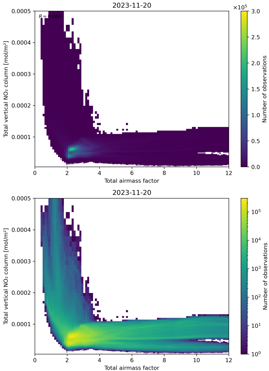
Figure 67: Scatter density plot of “Total airmass factor” against “Total vertical NO 2 column” for 2023-11-19 to 2023-11-21.
