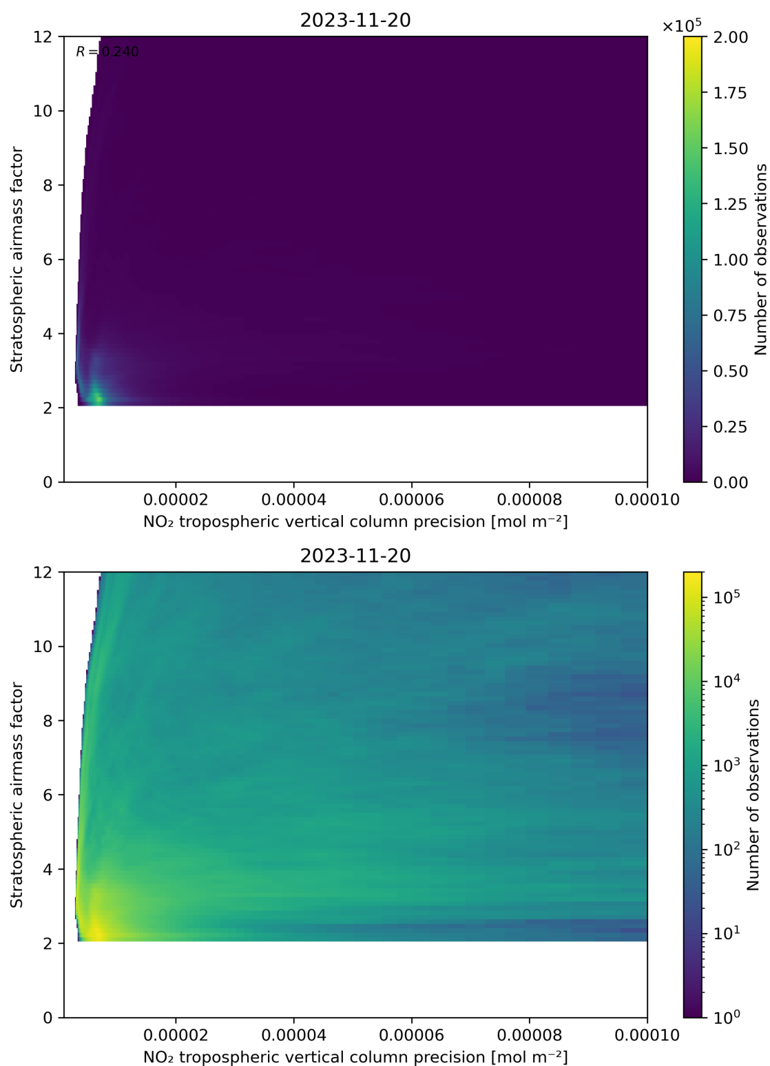
Figure 131: Scatter density plot of “NO 2 tropospheric vertical column precision” against “Stratospheric airmass factor” for 2023-11-19 to 2023-11-21.
