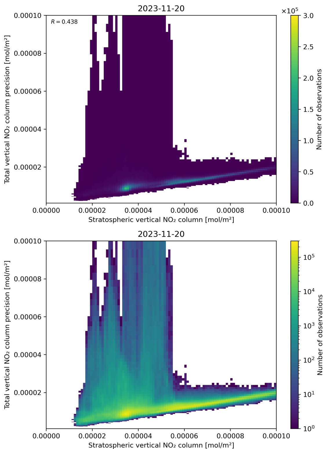
Figure 101: Scatter density plot of “Stratospheric vertical NO 2 column” against “Total vertical NO 2 column precision” for 2023-11-19 to 2023-11-21.
