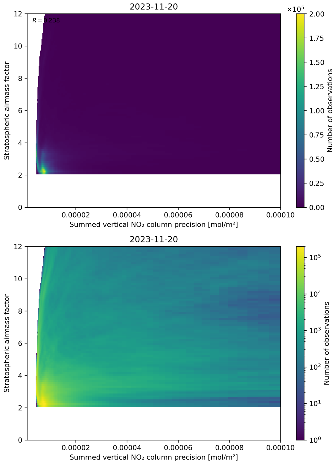
Figure 106: Scatter density plot of “Summed vertical NO 2 column precision” against “Stratospheric airmass factor” for 2023-11-19 to 2023-11-21.
