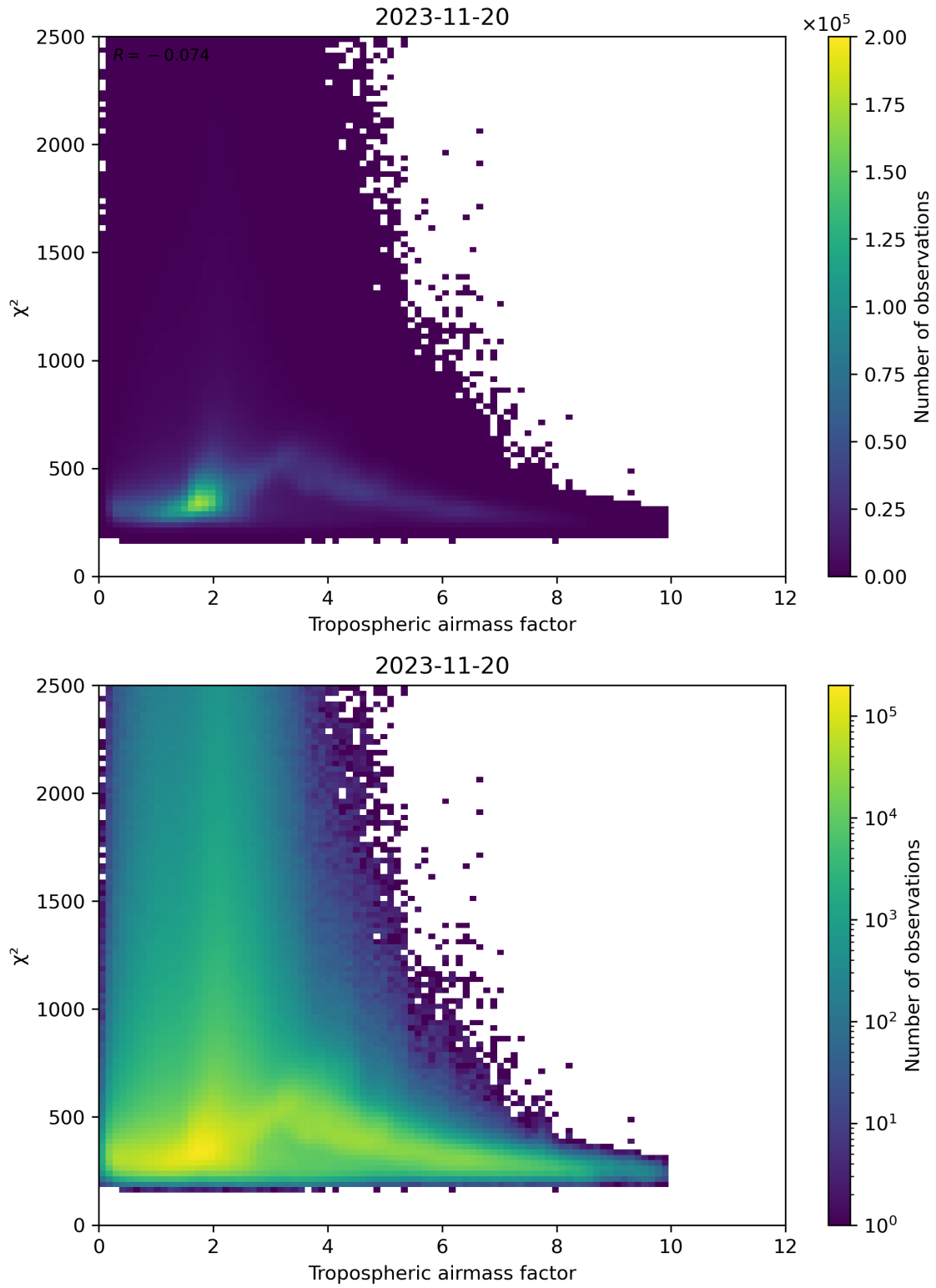
Figure 73: Scatter density plot of “Tropospheric airmass factor” against “ \chi^2 ” for 2023-11-19 to 2023-11-21.
