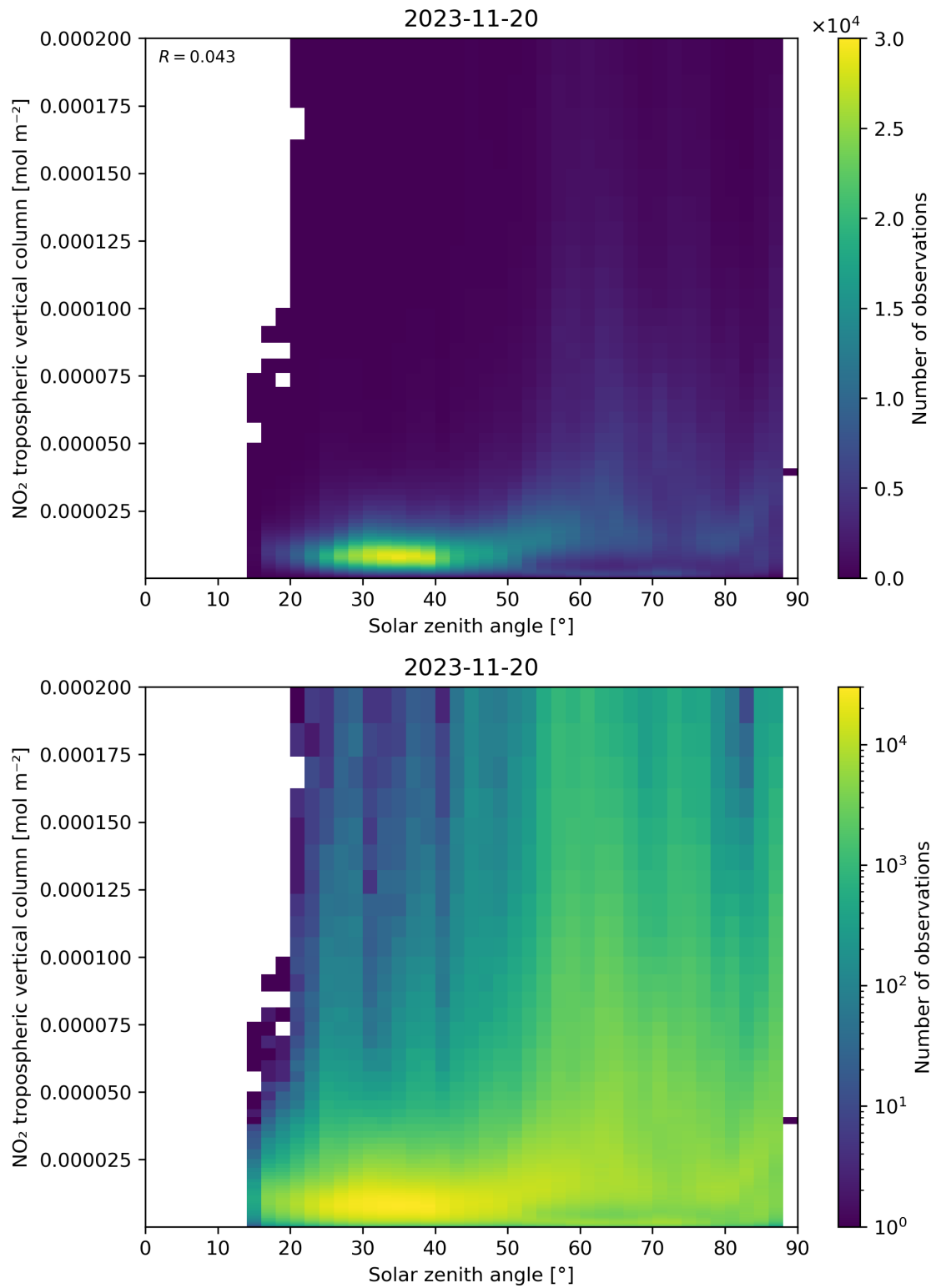
Figure 155: Scatter density plot of “Solar zenith angle” against “NO 2 tropospheric vertical column” for 2023-11-19 to 2023-11-21.
