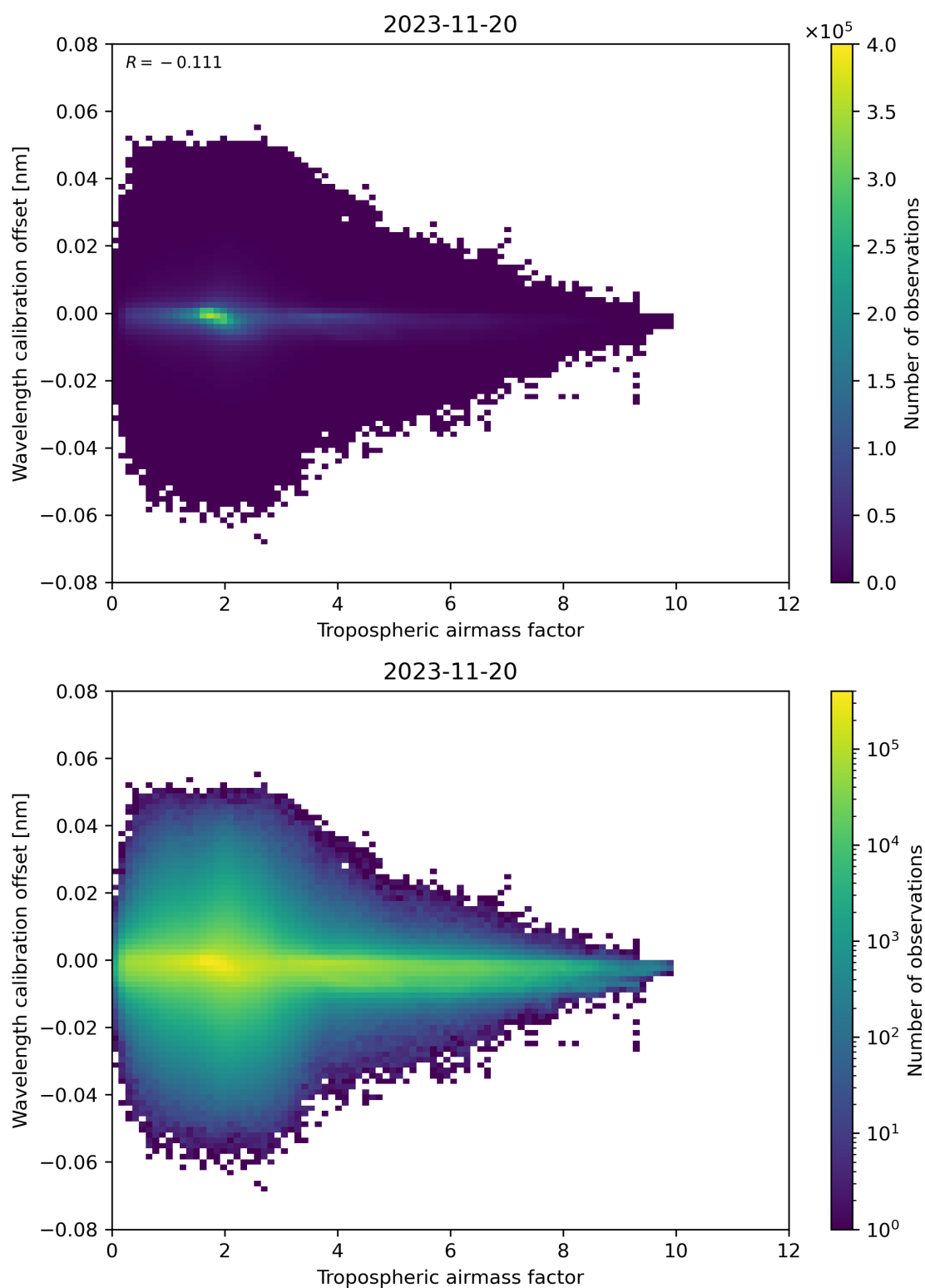
Figure 80: Scatter density plot of “Tropospheric airmass factor” against “Wavelength calibration offset” for 2023-11-19 to 2023-11-21.
