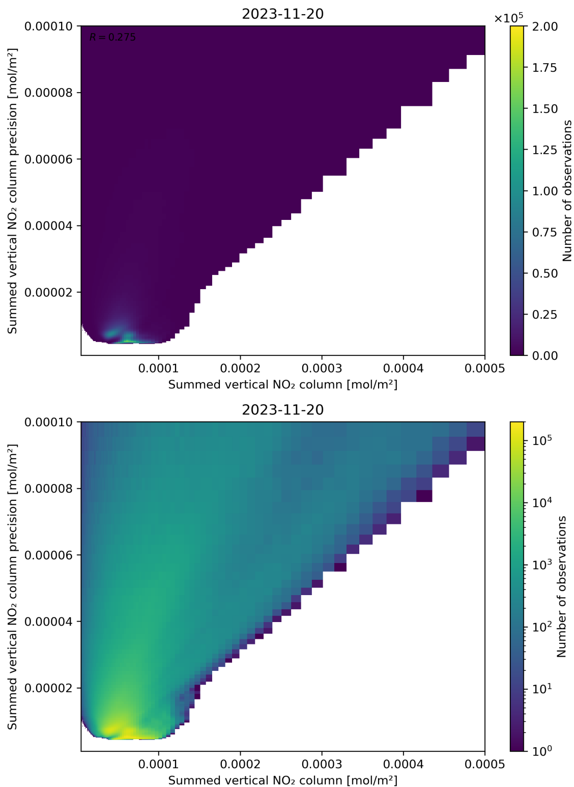
Figure 105: Scatter density plot of “Summed vertical NO 2 column” against “Summed vertical NO 2 column precision” for 2023-11-19 to 2023-11-21.
