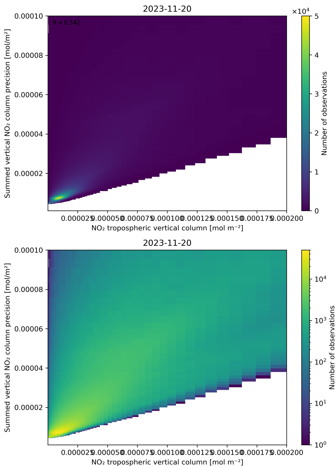
Figure 127: Scatter density plot of “NO 2 tropospheric vertical column” against “Summed vertical NO 2 column precision” for 2023-11-19 to 2023-11-21.
