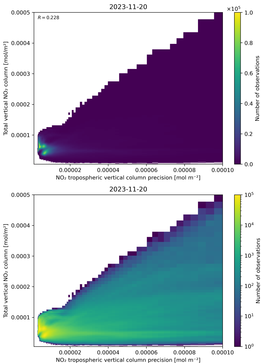
Figure 138: Scatter density plot of “NO 2 tropospheric vertical column precision” against “Total vertical NO 2 column” for 2023-11-19 to 2023-11-21.
