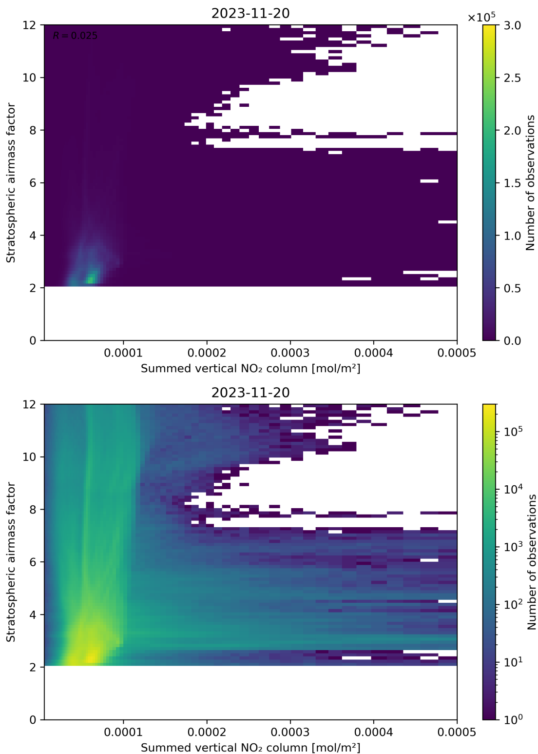
Figure 103: Scatter density plot of “Summed vertical NO 2 column” against “Stratospheric airmass factor” for 2023-11-19 to 2023-11-21.
