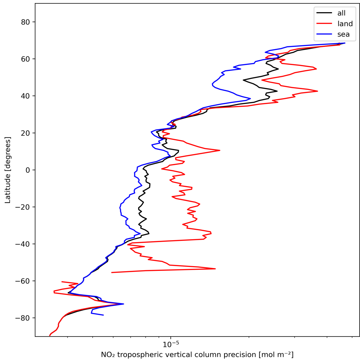
Figure 13: Zonal average of “NO 2 tropospheric vertical column precision” for 2023-11-19 to 2023-11-21.
