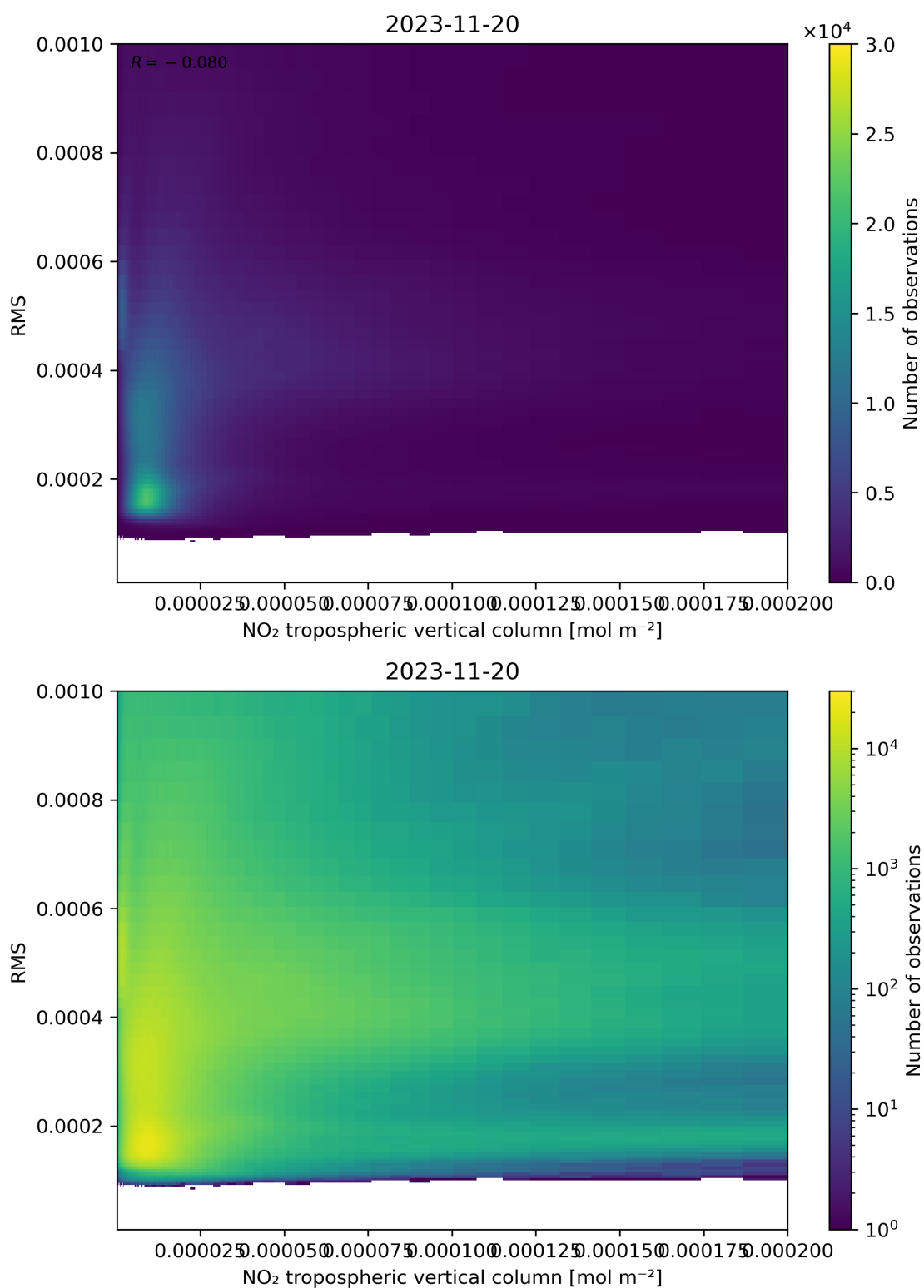
Figure 142: Scatter density plot of “NO 2 tropospheric vertical column” against “RMS” for 2023-11-19 to 2023-11-21.
