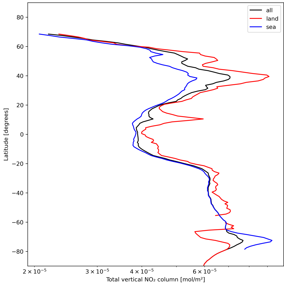
Figure 21: Zonal average of “Total vertical NO 2 column” for 2023-11-19 to 2023-11-21.
