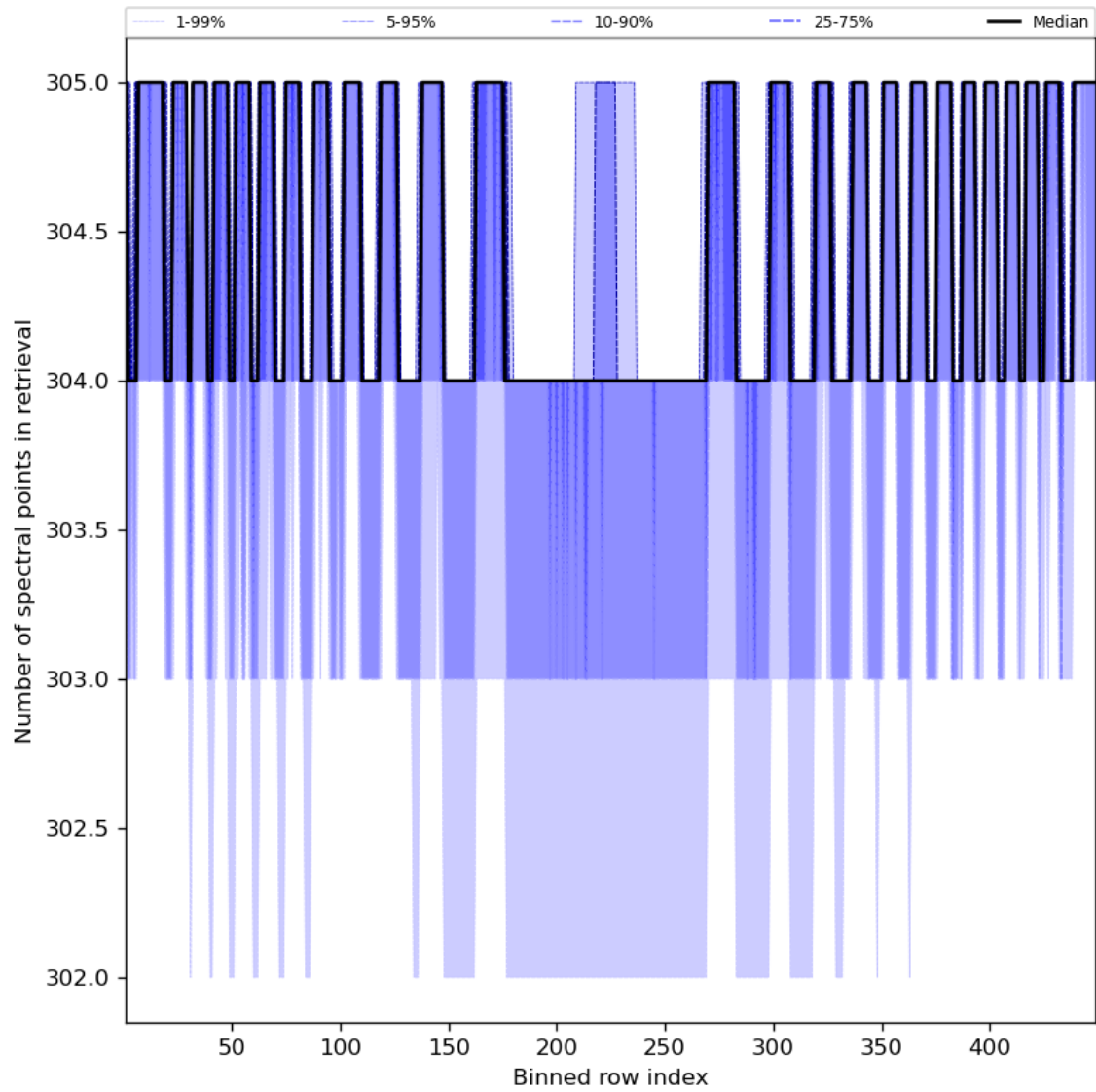
Figure 50: Along track statistics of “Number of spectral points in retrieval” for 2023-11-19 to 2023-11-21
