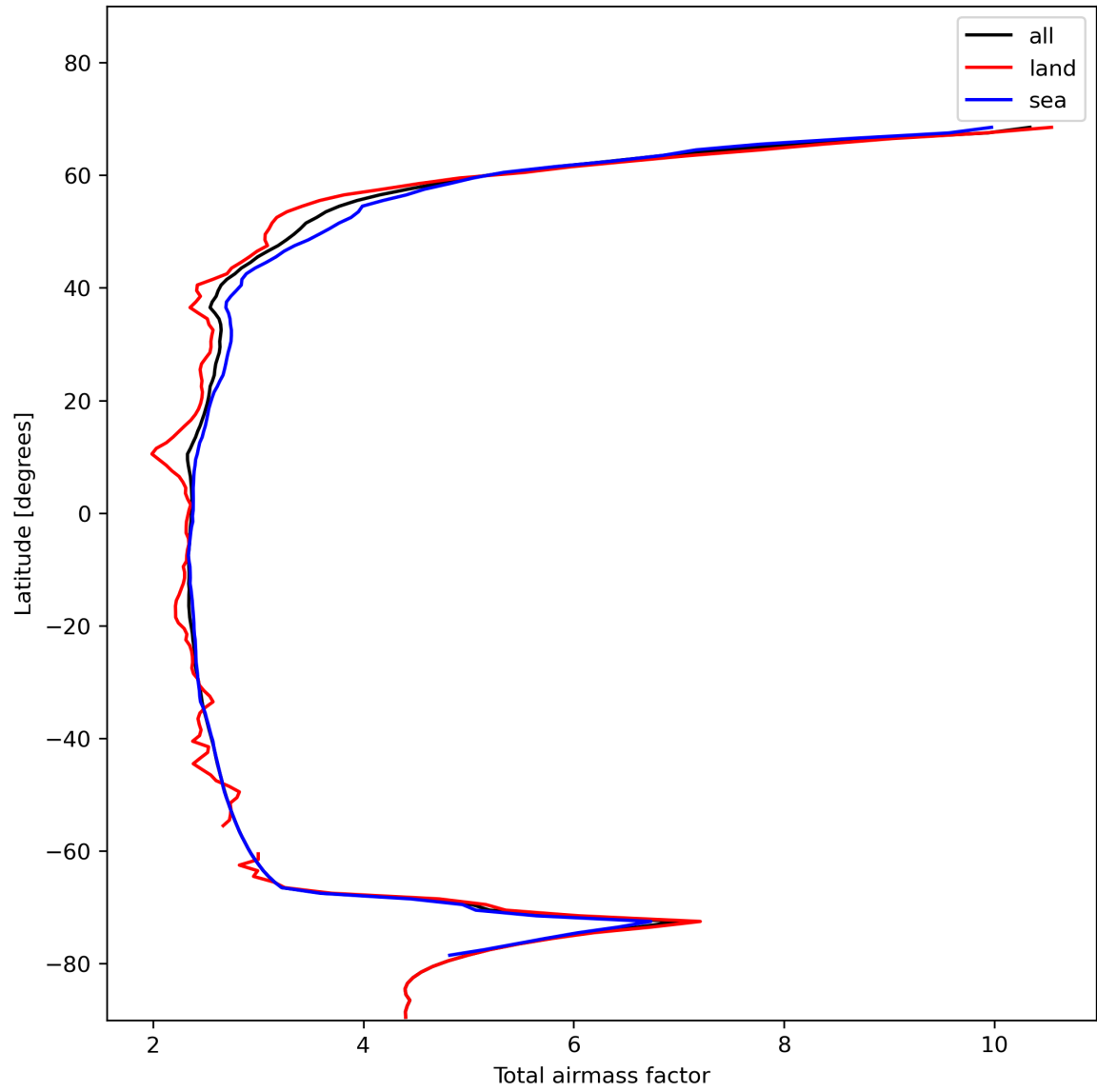
Figure 15: Zonal average of “Total airmass factor” for 2023-11-19 to 2023-11-21.
