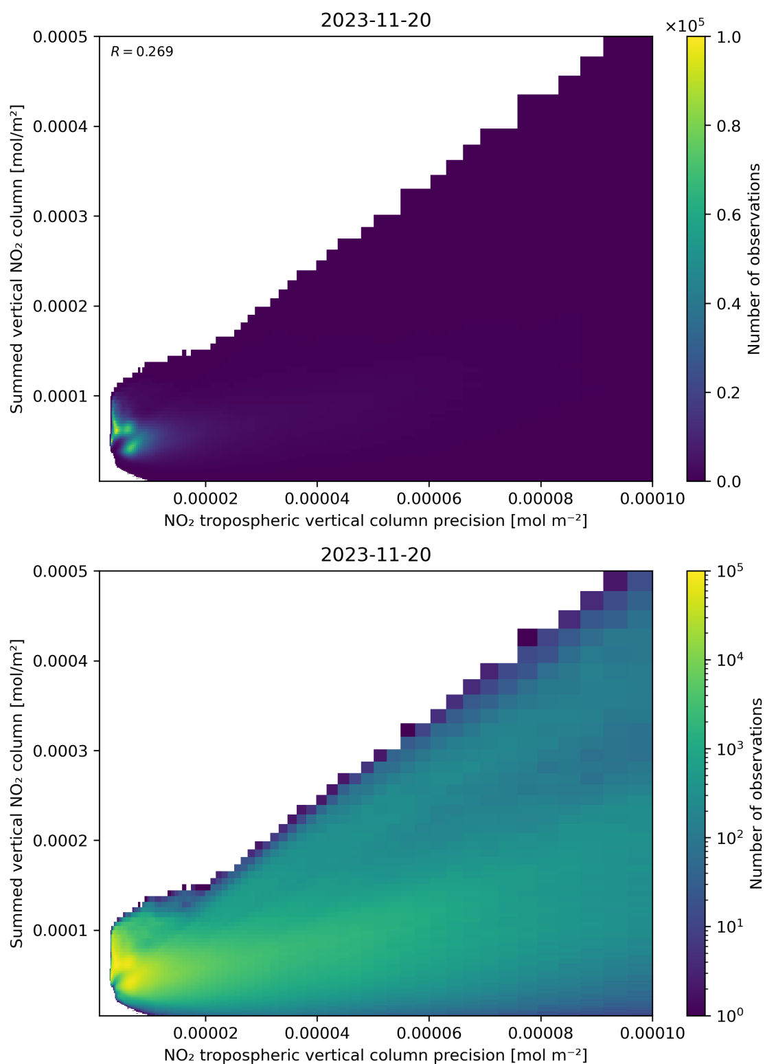
Figure 136: Scatter density plot of “NO 2 tropospheric vertical column precision” against “Summed vertical NO 2 column” for 2023-11-19 to 2023-11-21.
