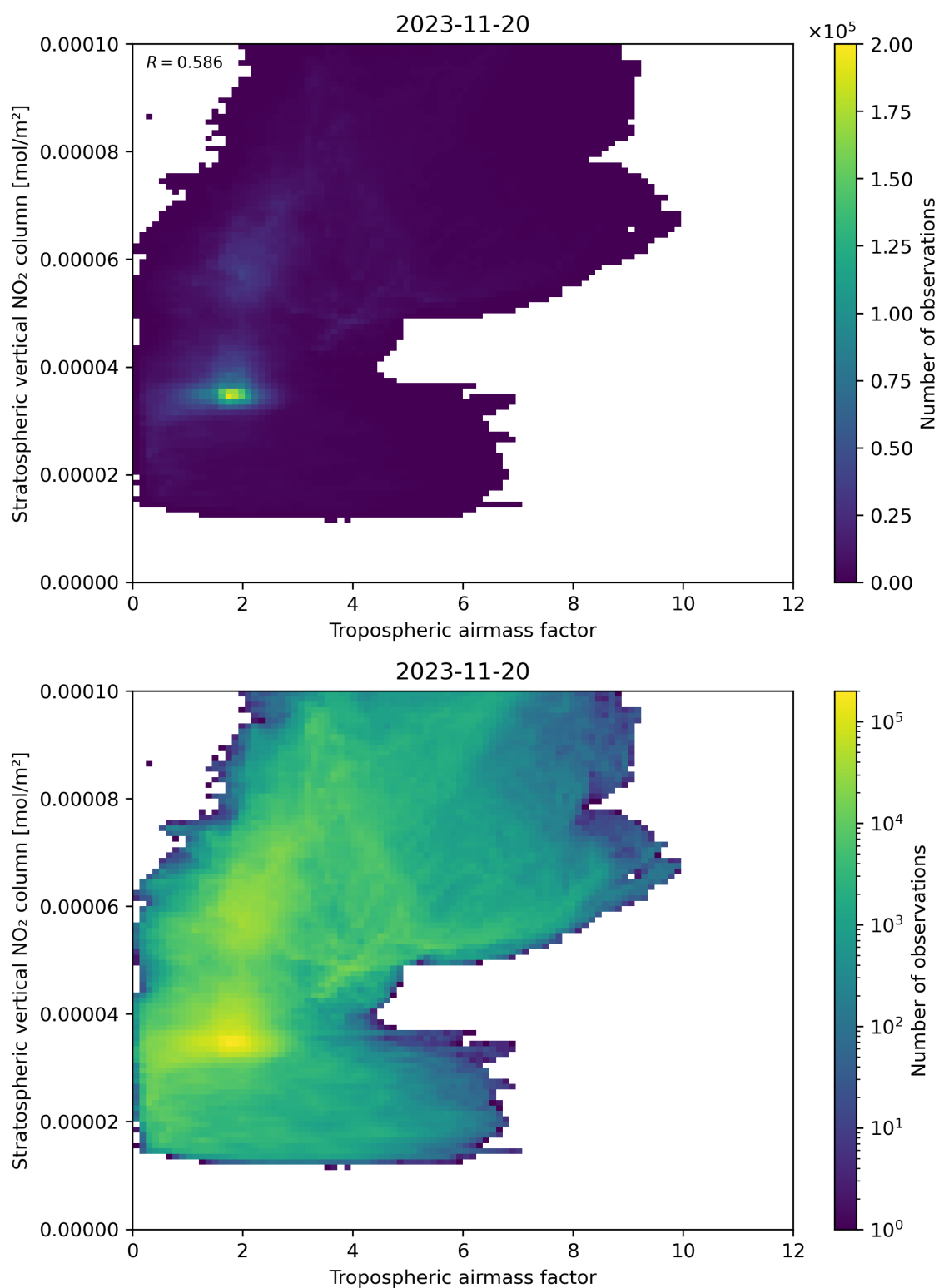
Figure 74: Scatter density plot of “Tropospheric airmass factor” against “Stratospheric vertical NO 2 column” for 2023-11-19 to 2023-11-21.
