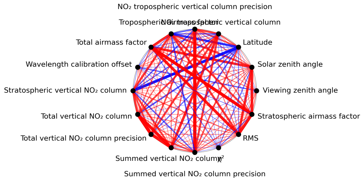
Figure 1: Map of correlation graph for 2023-11-19 to 2023-11-21.
