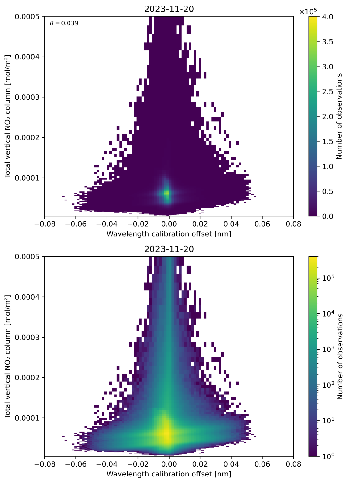
Figure 179: Scatter density plot of “Wavelength calibration offset” against “Total vertical NO 2 column” for 2023-11-19 to 2023-11-21.
