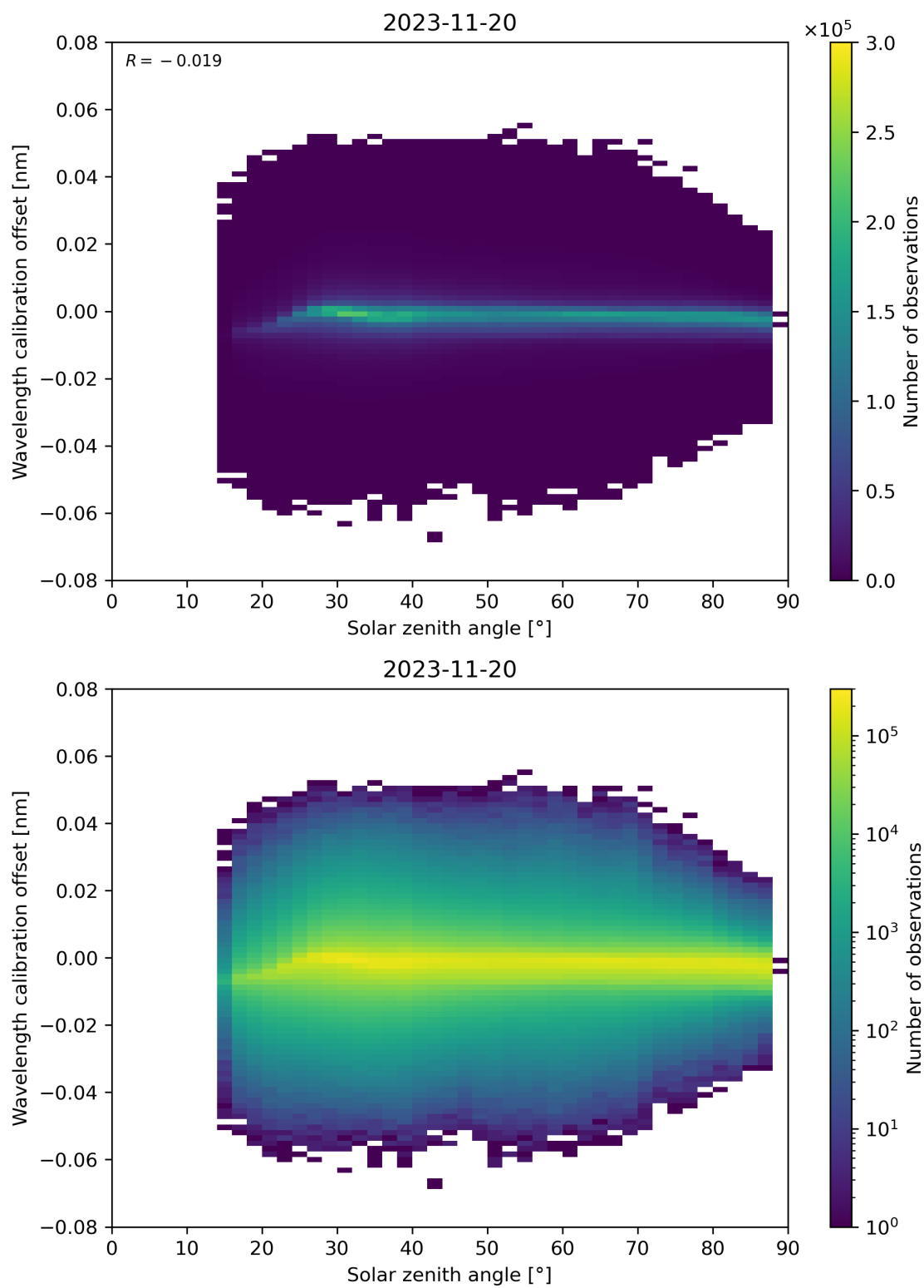
Figure 158: Scatter density plot of “Solar zenith angle” against “Wavelength calibration offset” for 2023-11-19 to 2023-11-21.
