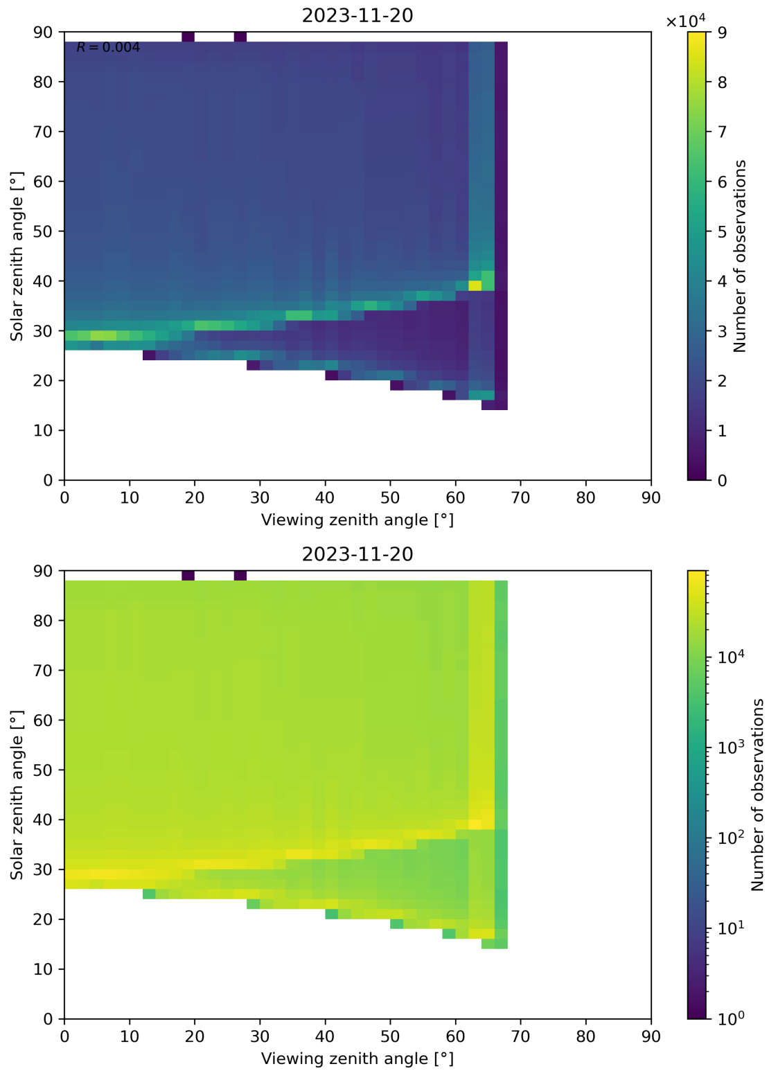
Figure 172: Scatter density plot of “Viewing zenith angle” against “Solar zenith angle” for 2023-11-19 to 2023-11-21.
