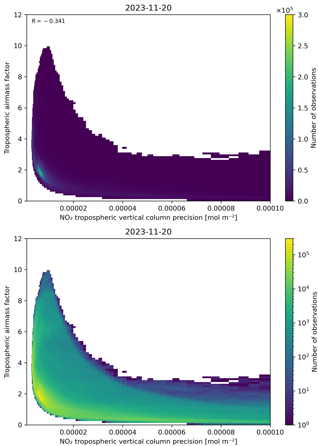
Figure 133: Scatter density plot of “NO 2 tropospheric vertical column precision” against “Tropospheric airmass factor” for 2023-11-19 to 2023-11-21.
