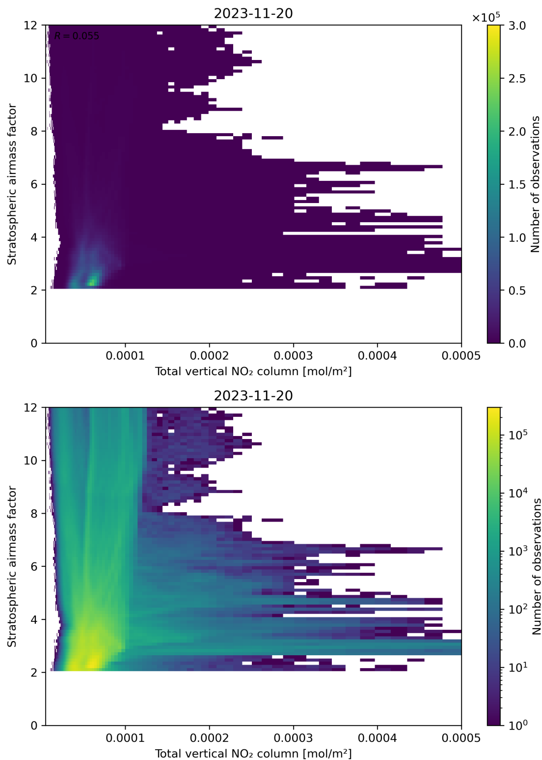
Figure 110: Scatter density plot of “Total vertical NO 2 column” against “Stratospheric airmass factor” for 2023-11-19 to 2023-11-21.
