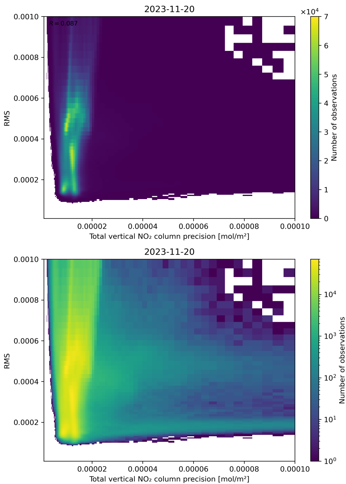
Figure 119: Scatter density plot of “Total vertical NO 2 column precision” against “RMS” for 2023-11-19 to 2023-11-21.
