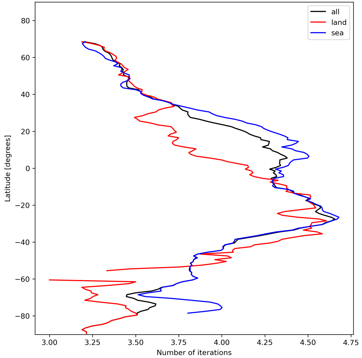
Figure 17: Zonal average of “Number of iterations” for 2023-11-19 to 2023-11-21.
