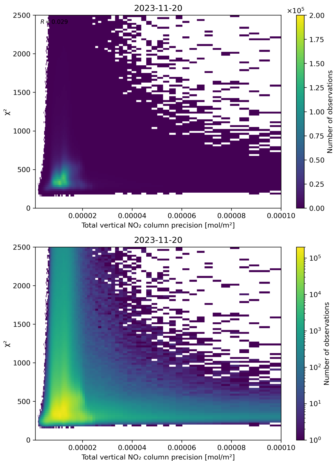
Figure 116: Scatter density plot of “Total vertical NO 2 column precision” against “ \chi^2 ” for 2023-11-19 to 2023-11-21.
