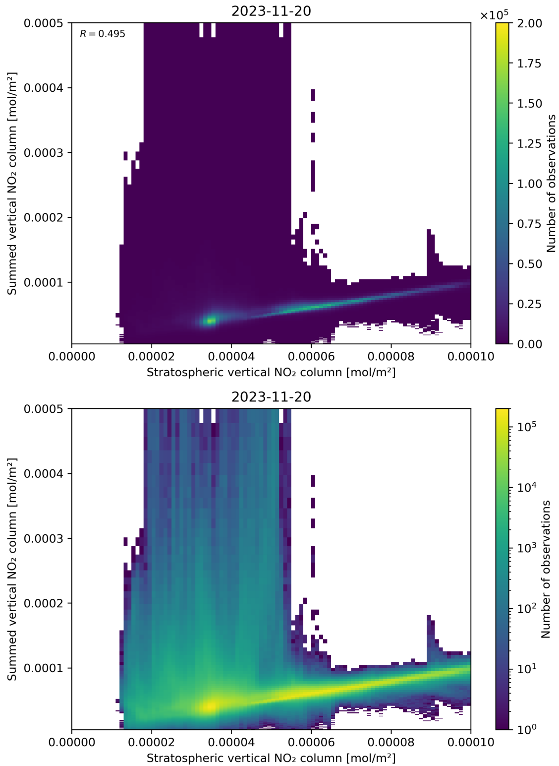
Figure 98: Scatter density plot of “Stratospheric vertical NO 2 column” against “Summed vertical NO 2 column” for 2023-11-19 to 2023-11-21.
