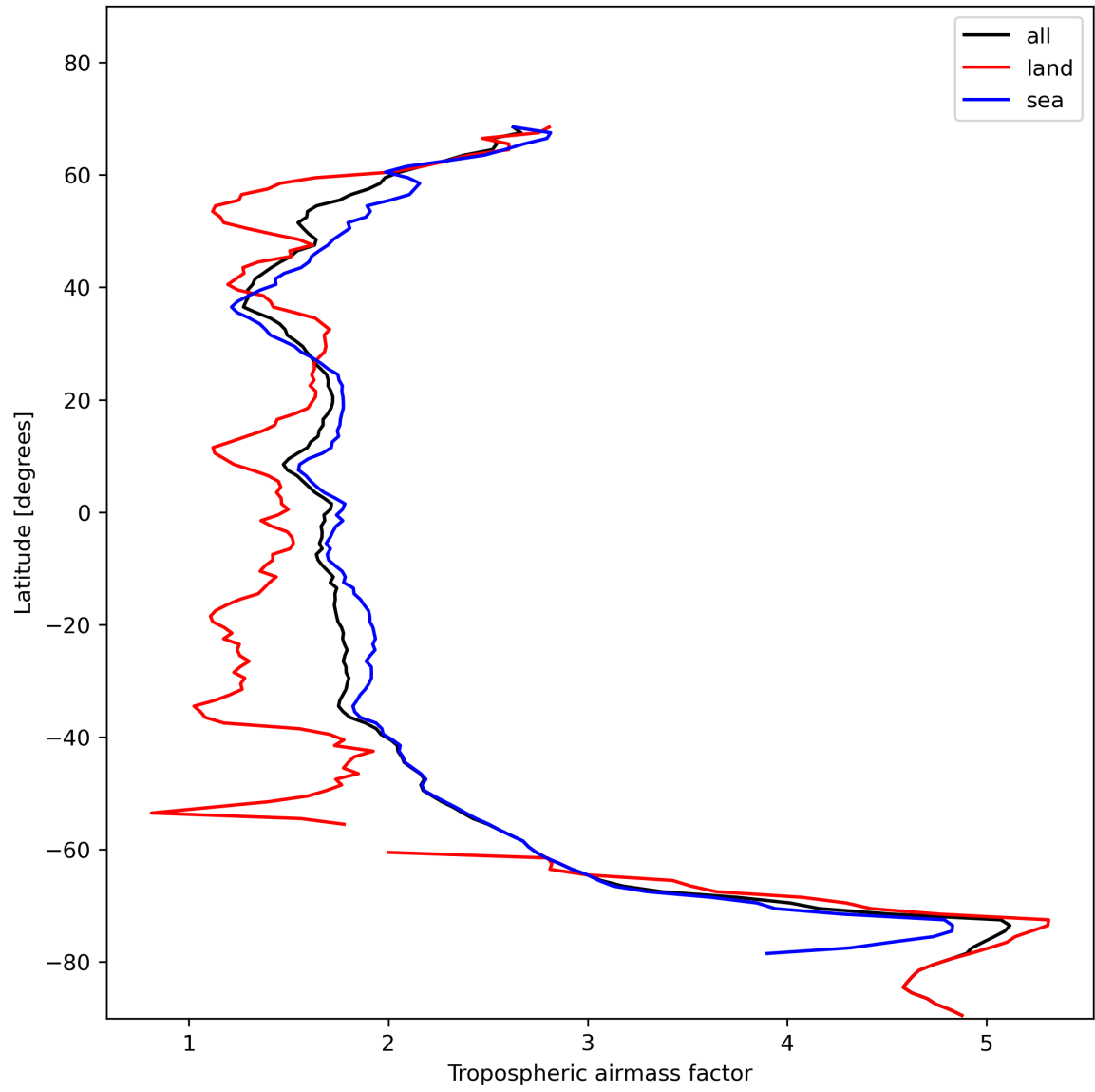
Figure 14: Zonal average of “Tropospheric airmass factor” for 2023-11-19 to 2023-11-21.
