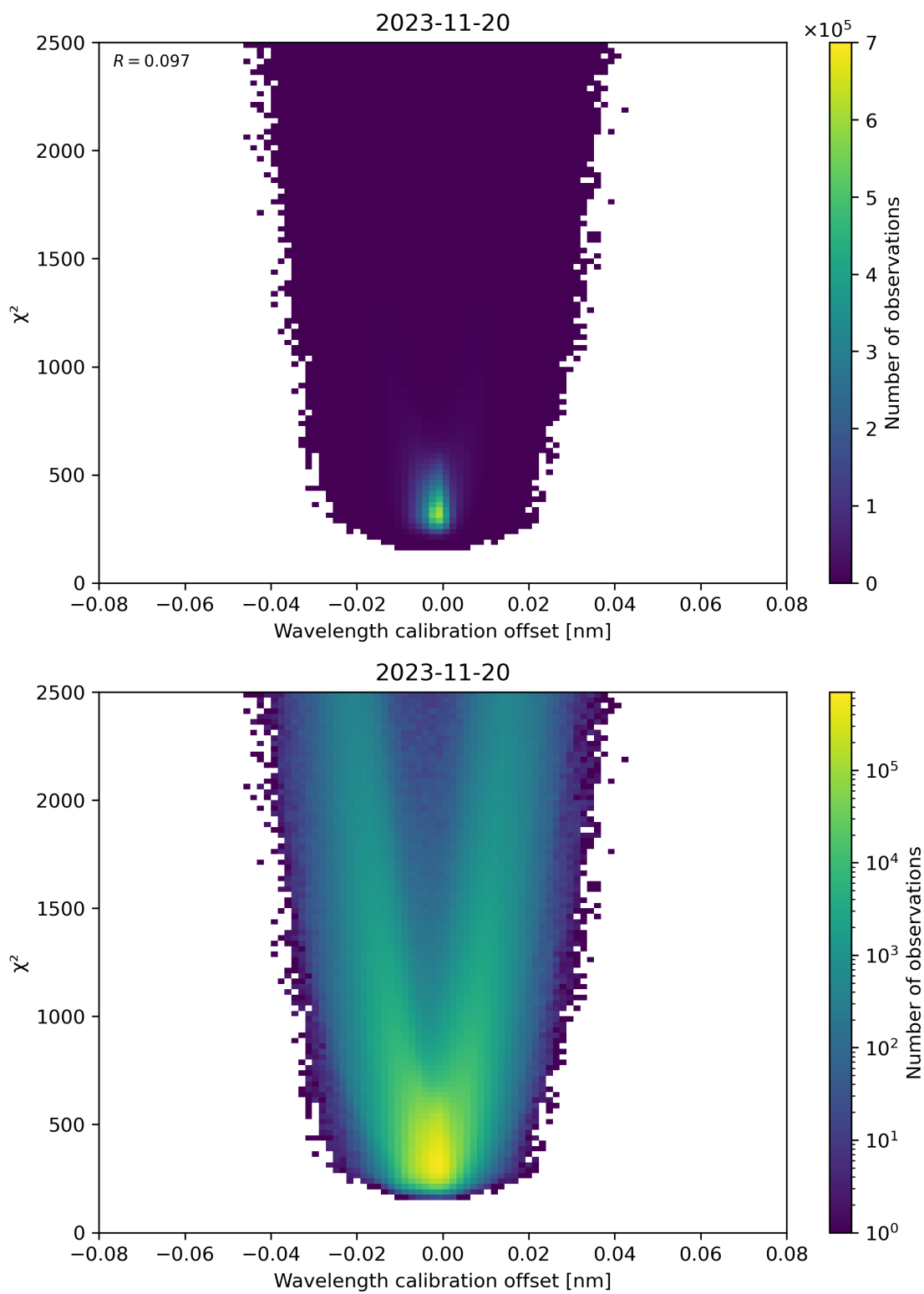
Figure 175: Scatter density plot of “Wavelength calibration offset” against “ \chi^2 ” for 2023-11-19 to 2023-11-21.
