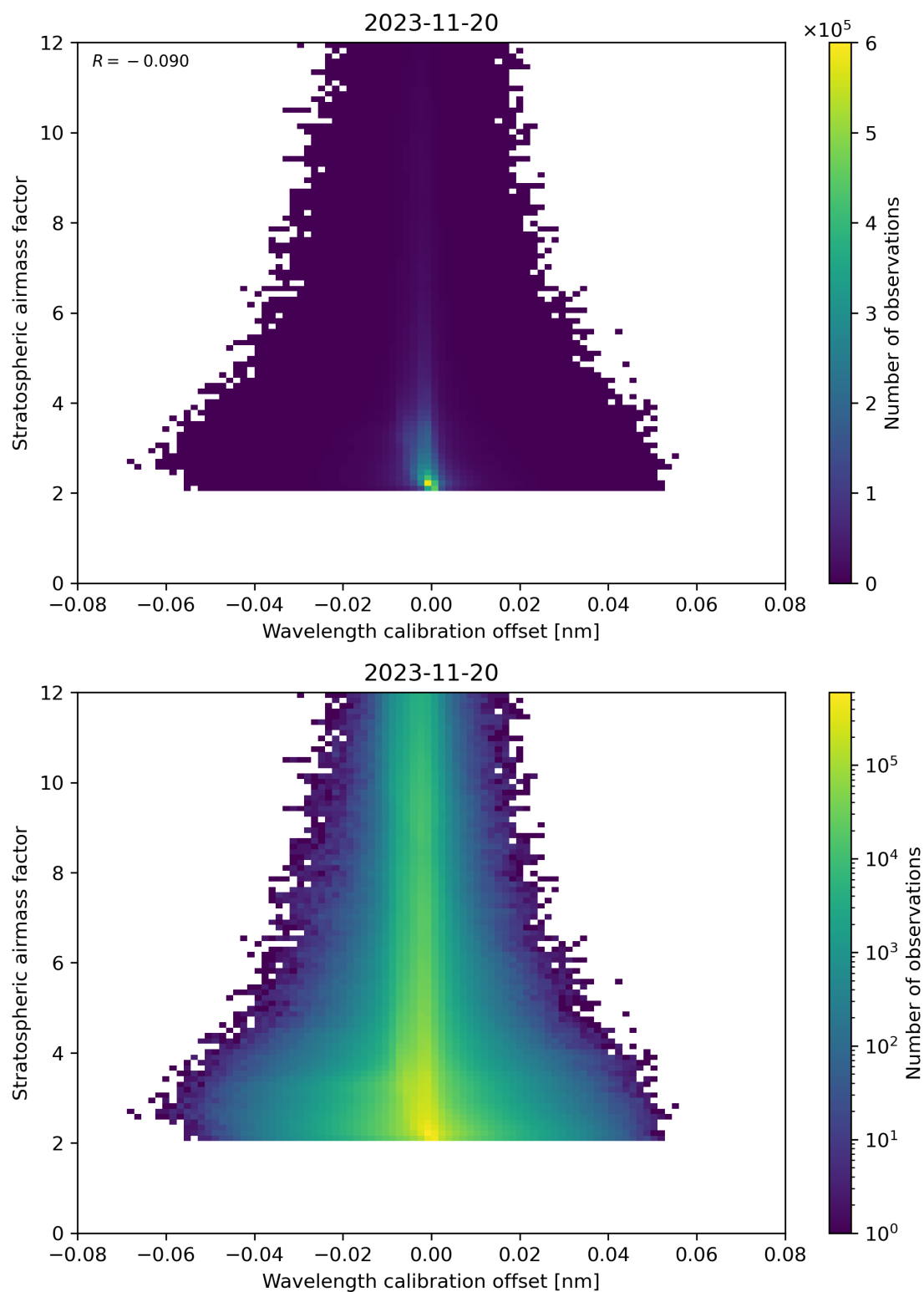
Figure 174: Scatter density plot of “Wavelength calibration offset” against “Stratospheric airmass factor” for 2023-11-19 to 2023-11-21.
