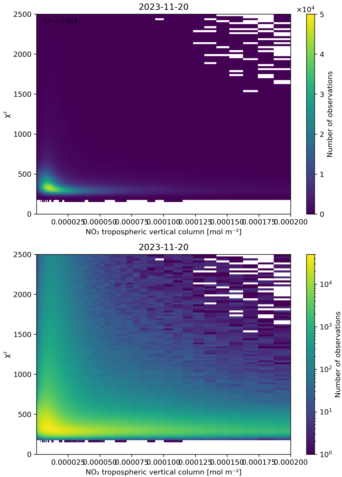
Figure 124: Scatter density plot of “NO 2 tropospheric vertical column” against “ \chi^2 ” for 2023-11-19 to 2023-11-21.
