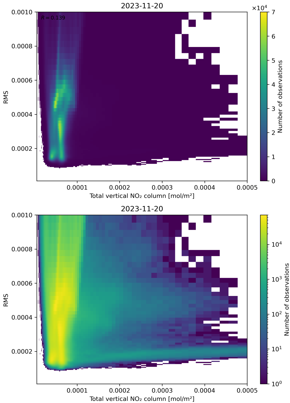
Figure 120: Scatter density plot of “Total vertical NO 2 column” against “RMS” for 2023-11-19 to 2023-11-21.
