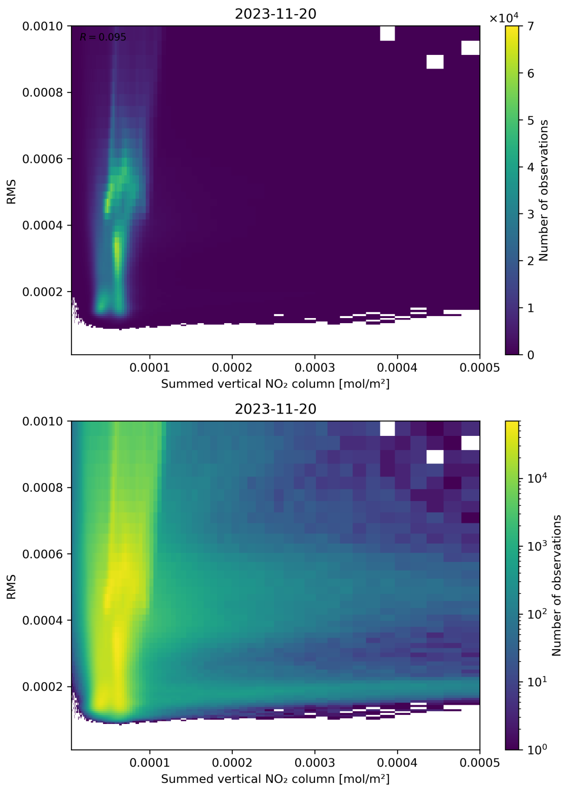
Figure 109: Scatter density plot of “Summed vertical NO 2 column” against “RMS” for 2023-11-19 to 2023-11-21.
