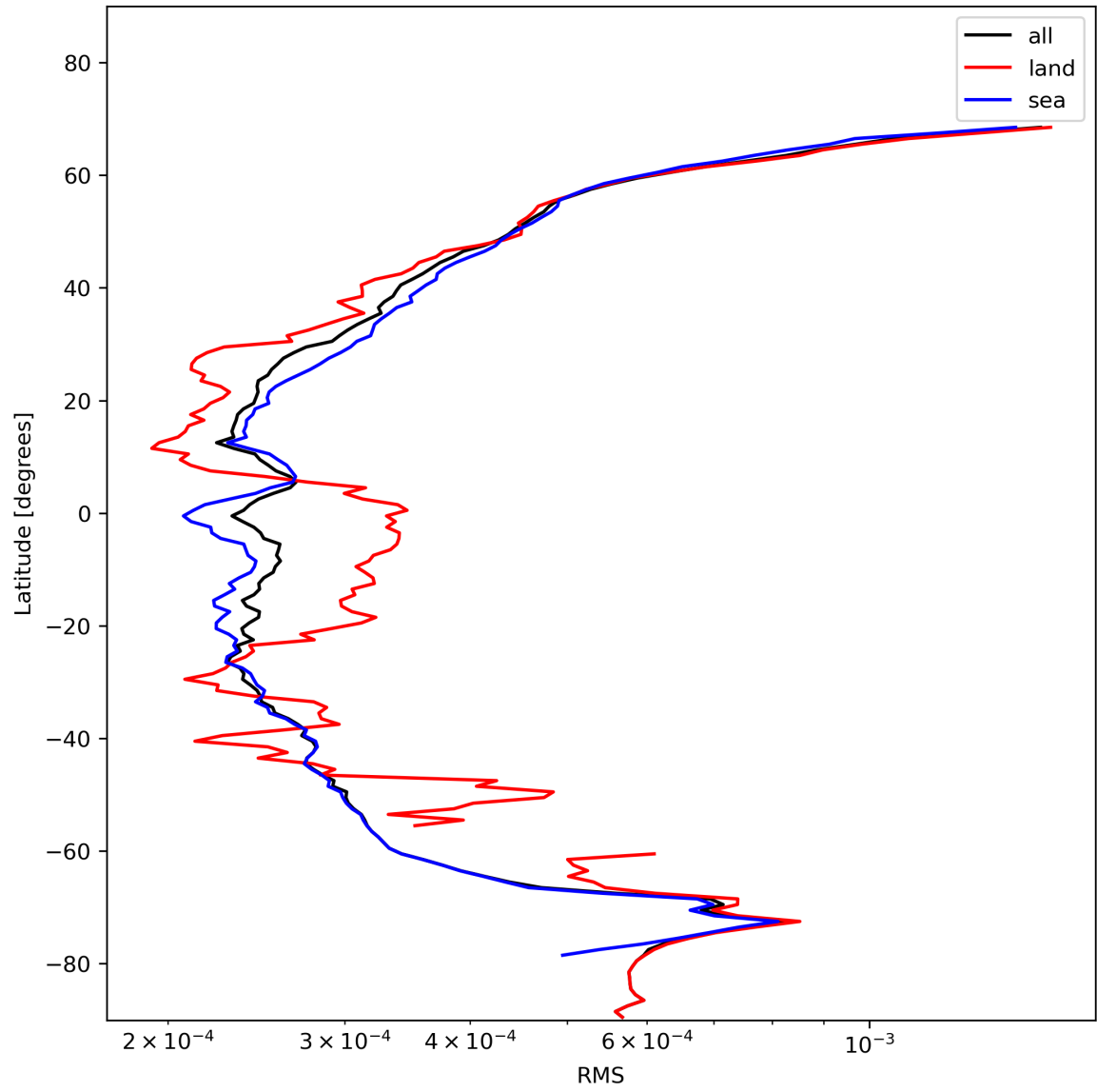
Figure 26: Zonal average of “RMS” for 2023-11-19 to 2023-11-21.
