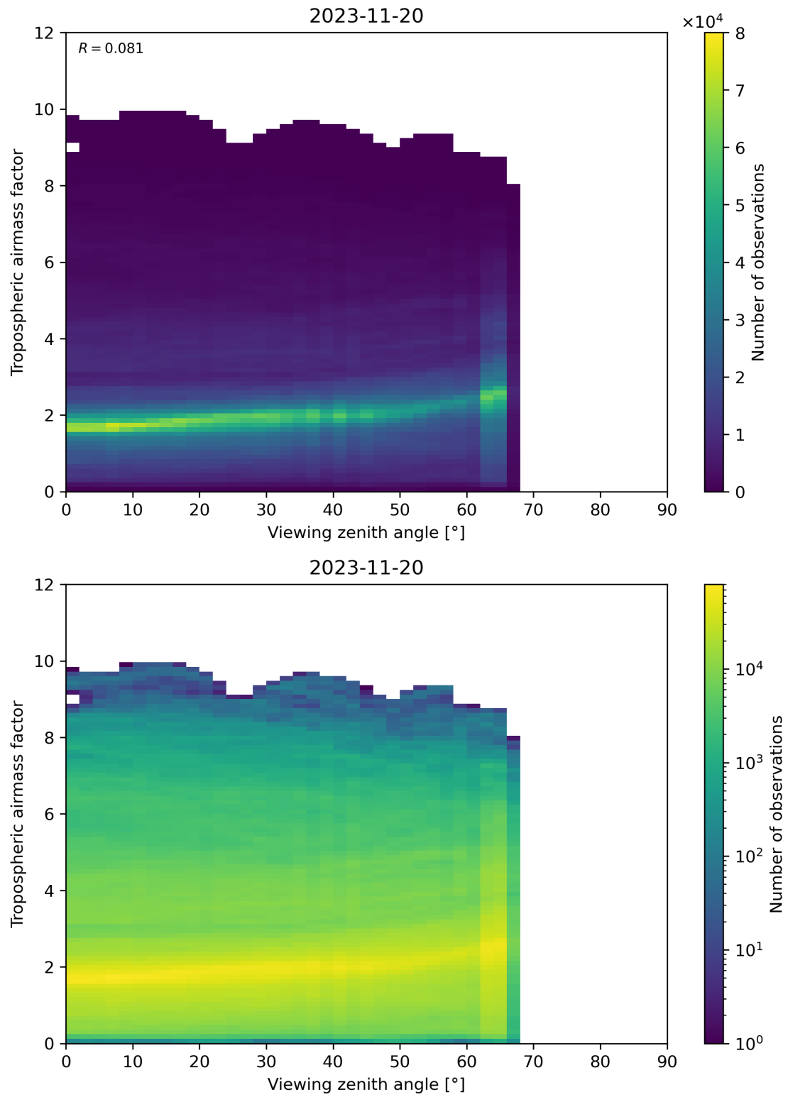
Figure 161: Scatter density plot of “Viewing zenith angle” against “Tropospheric airmass factor” for 2023-11-19 to 2023-11-21.
