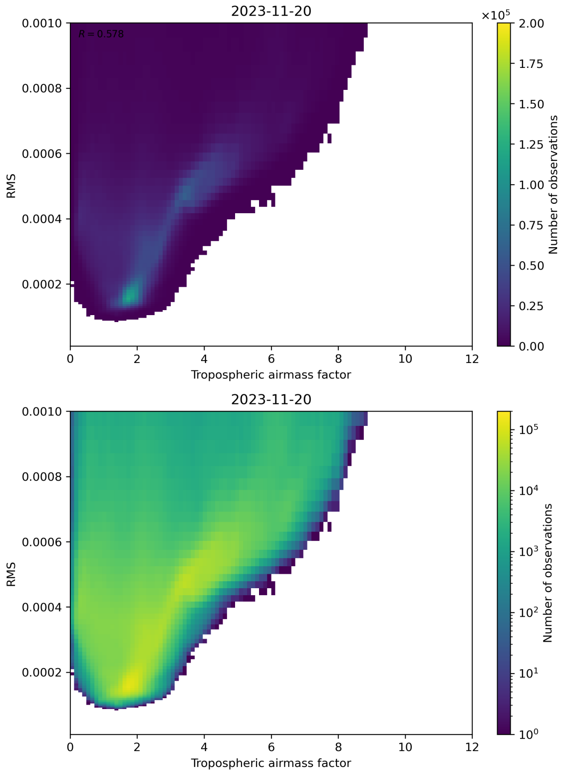
Figure 79: Scatter density plot of “Tropospheric airmass factor” against “RMS” for 2023-11-19 to 2023-11-21.
