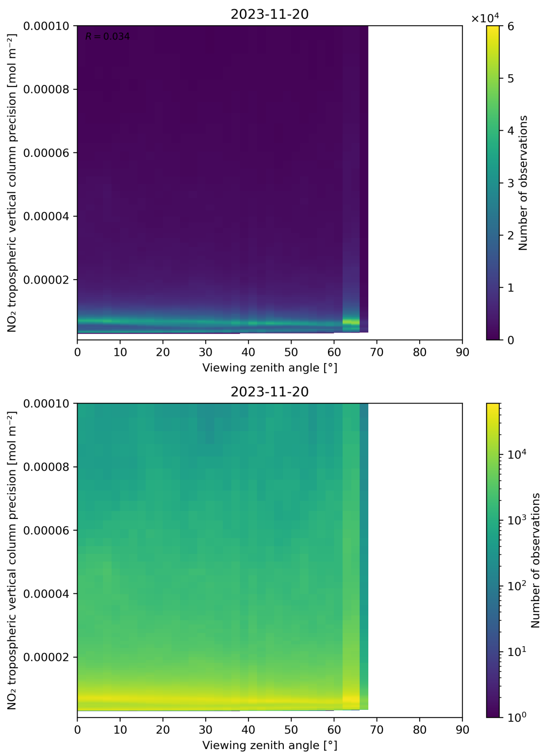
Figure 170: Scatter density plot of “Viewing zenith angle” against “NO 2 tropospheric vertical column precision” for 2023-11-19 to 2023-11-21.
