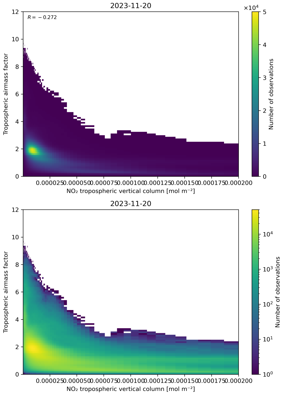
Figure 123: Scatter density plot of “NO 2 tropospheric vertical column” against “Tropospheric air mass factor” for 2023-11-19 to 2023-11-21.
