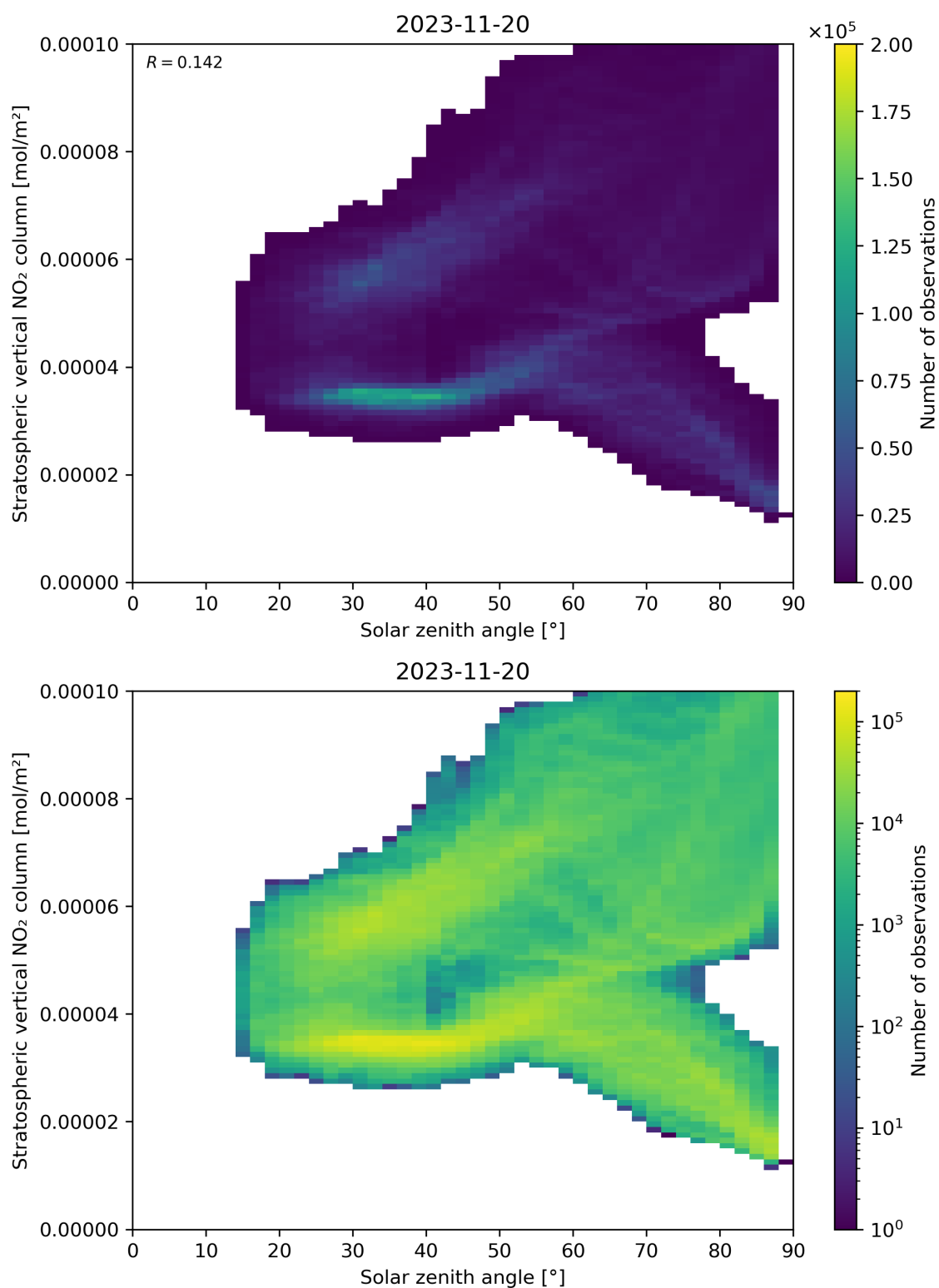
Figure 150: Scatter density plot of “Solar zenith angle” against “Stratospheric vertical NO 2 column” for 2023-11-19 to 2023-11-21.
