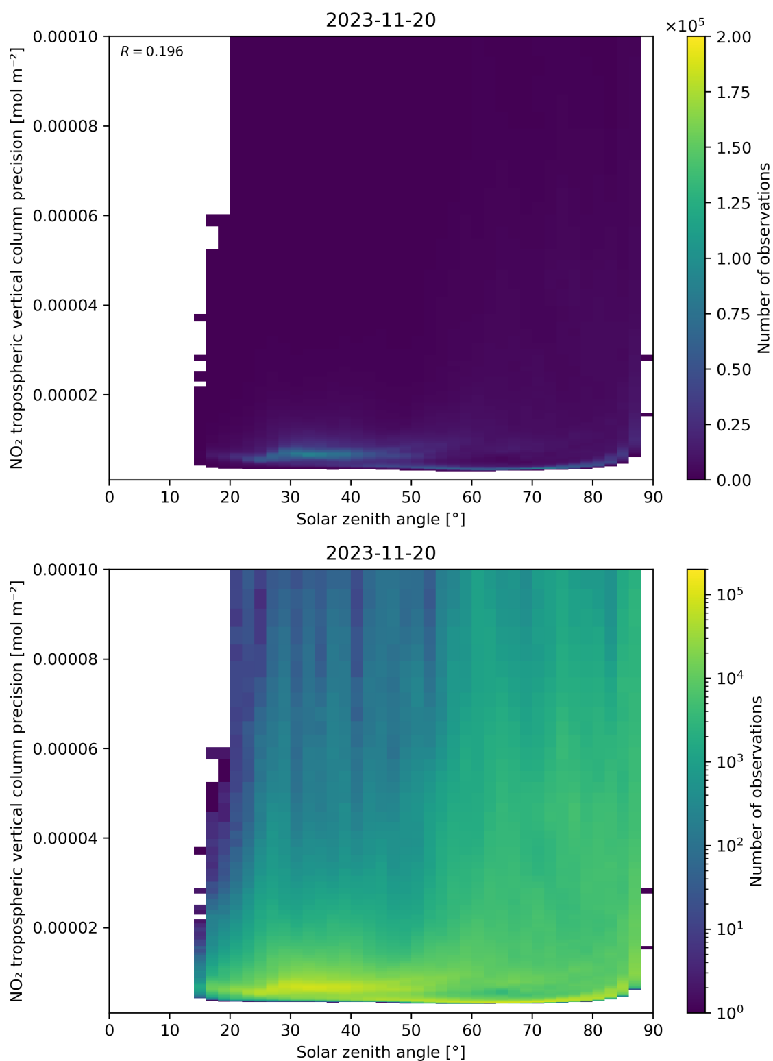
Figure 156: Scatter density plot of “Solar zenith angle” against “NO 2 tropospheric vertical column precision” for 2023-11-19 to 2023-11-21.
