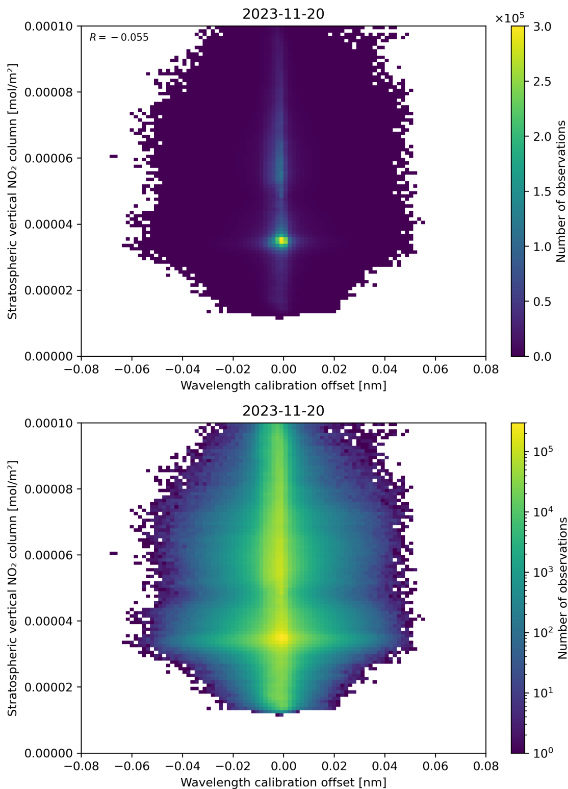
Figure 176: Scatter density plot of “Wavelength calibration offset” against “Stratospheric vertical NO 2 column” for 2023-11-19 to 2023-11-21.
