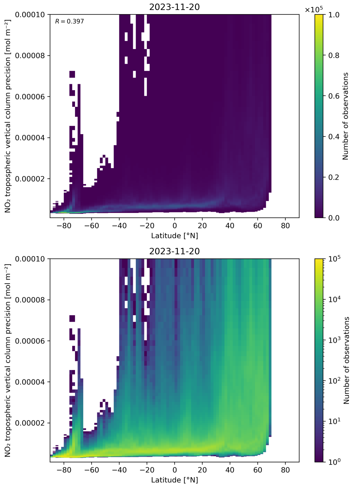
Figure 93: Scatter density plot of “Latitude” against “NO 2 tropospheric vertical column precision” for 2023-11-19 to 2023-11-21.
