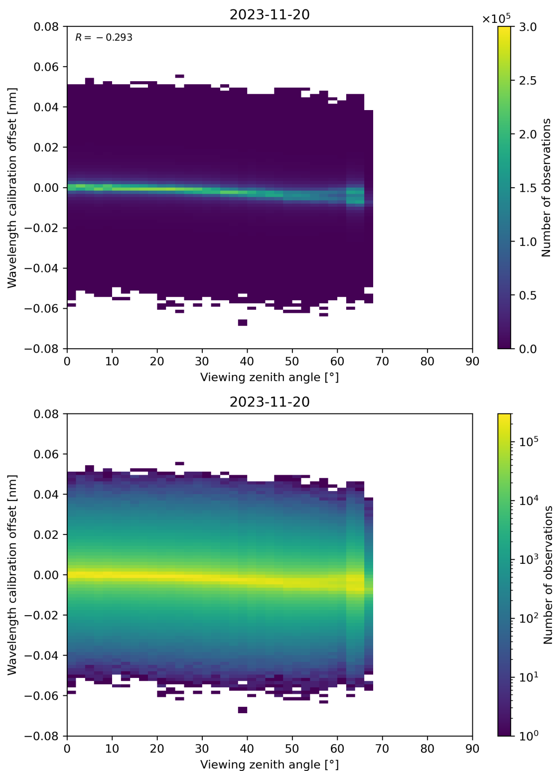
Figure 173: Scatter density plot of “Viewing zenith angle” against “Wavelength calibration offset” for 2023-11-19 to 2023-11-21.
