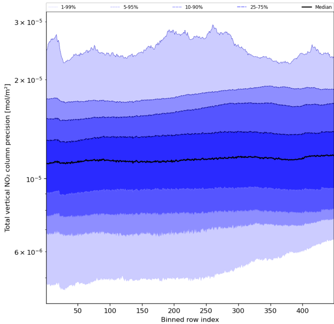
Figure 56: Along track statistics of “Total vertical NO 2 column precision” for 2023-11-19 to 2023-11-21
