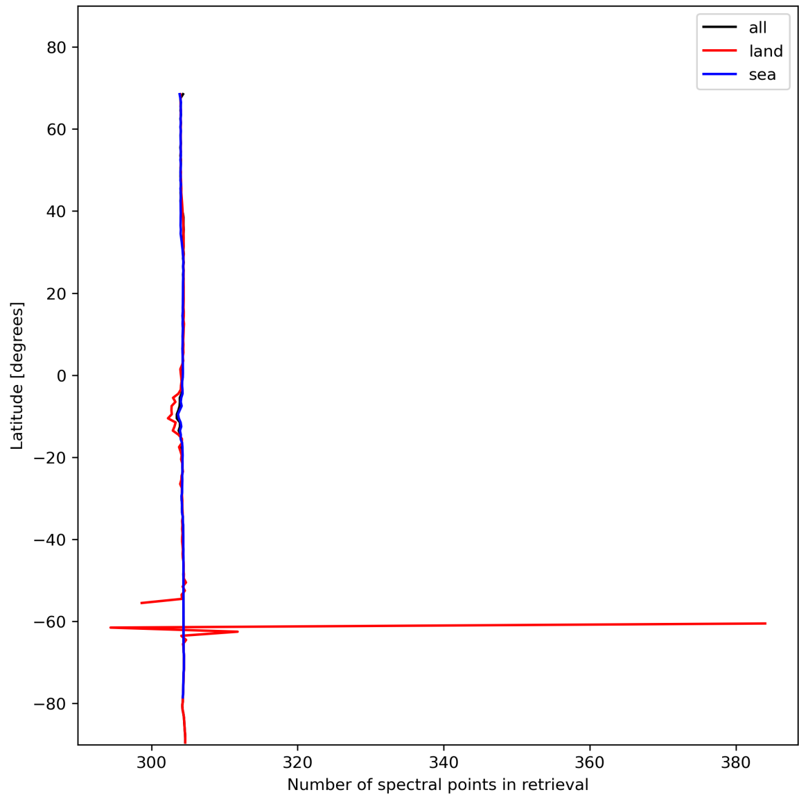
Figure 16: Zonal average of “Number of spectral points in retrieval” for 2023-11-19 to 2023-11-21.
