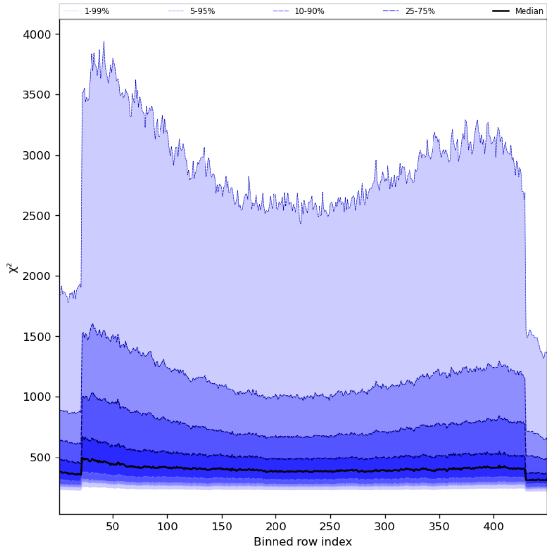
Figure 59: Along track statistics of “ \chi^2 ” for 2023-11-19 to 2023-11-21
