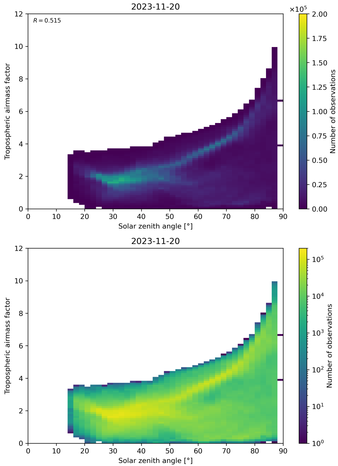
Figure 147: Scatter density plot of “Solar zenith angle” against “Tropospheric airmass factor” for 2023-11-19 to 2023-11-21.
