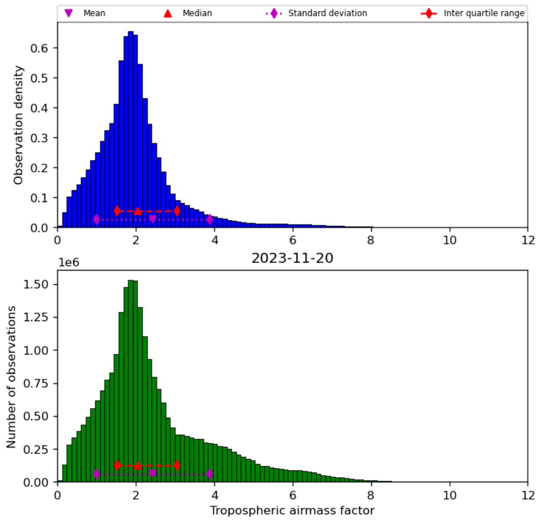
Figure 31: Histogram of “Tropospheric airmass factor” for 2023-11-19 to 2023-11-21
