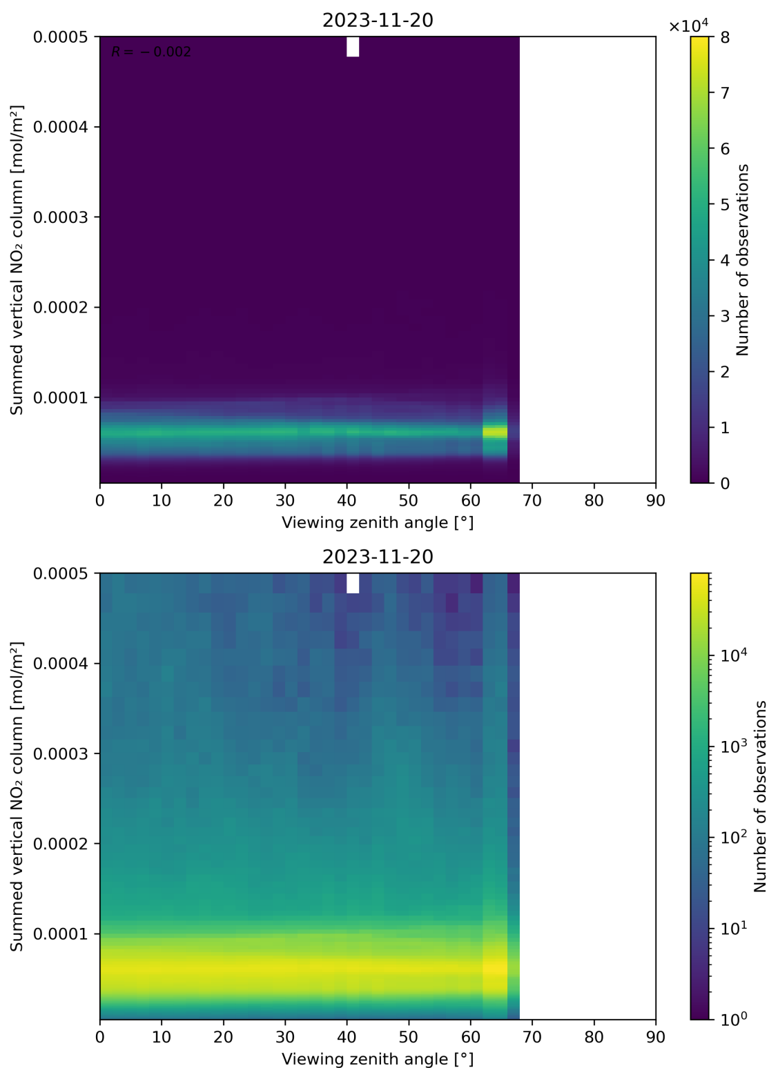
Figure 165: Scatter density plot of “Viewing zenith angle” against “Summed vertical NO 2 column” for 2023-11-19 to 2023-11-21.
