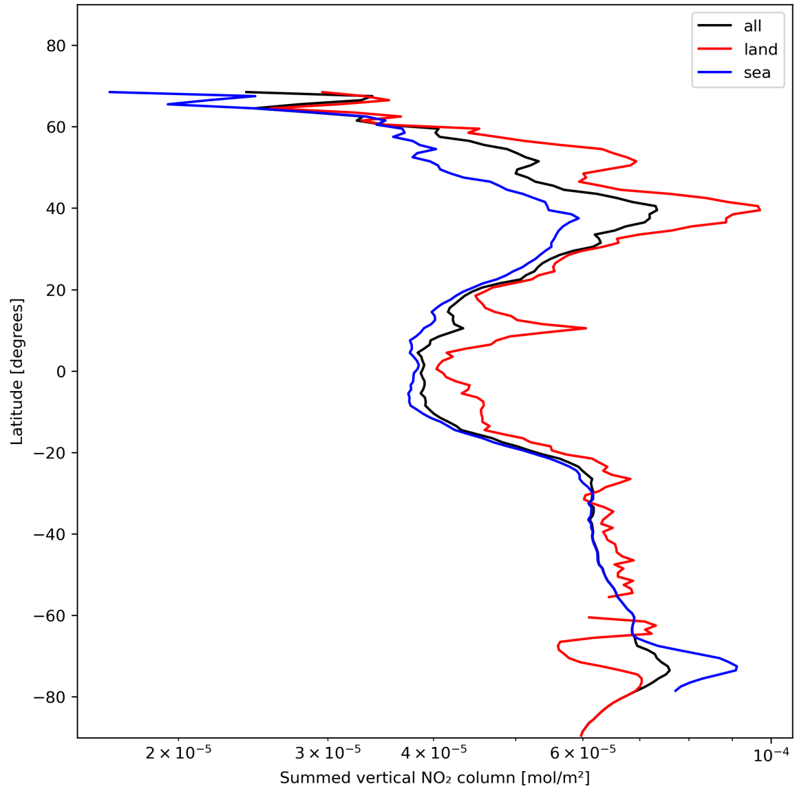
Figure 23: Zonal average of “Summed vertical NO 2 column” for 2023-11-19 to 2023-11-21.
