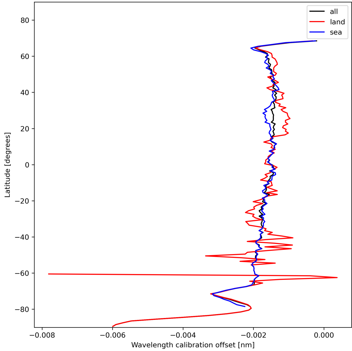
Figure 18: Zonal average of “Wavelength calibration offset” for 2023-11-19 to 2023-11-21.
