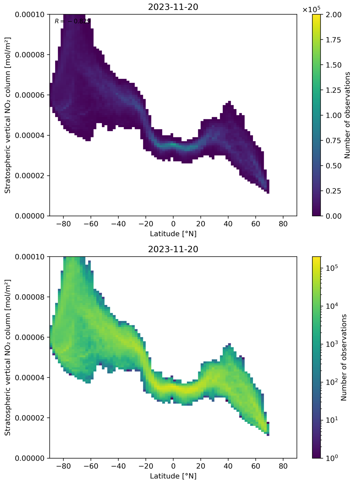
Figure 87: Scatter density plot of “Latitude” against “Stratospheric vertical NO 2 column” for 2023-11-19 to 2023-11-21.
