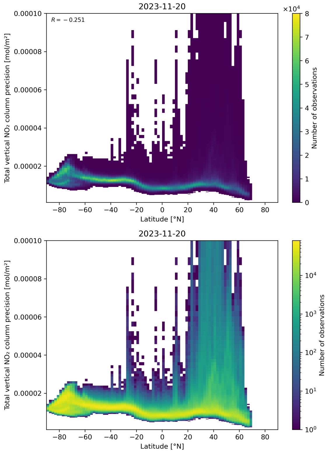
Figure 91: Scatter density plot of “Latitude” against “Total vertical NO 2 column precision” for 2023-11-19 to 2023-11-21.
