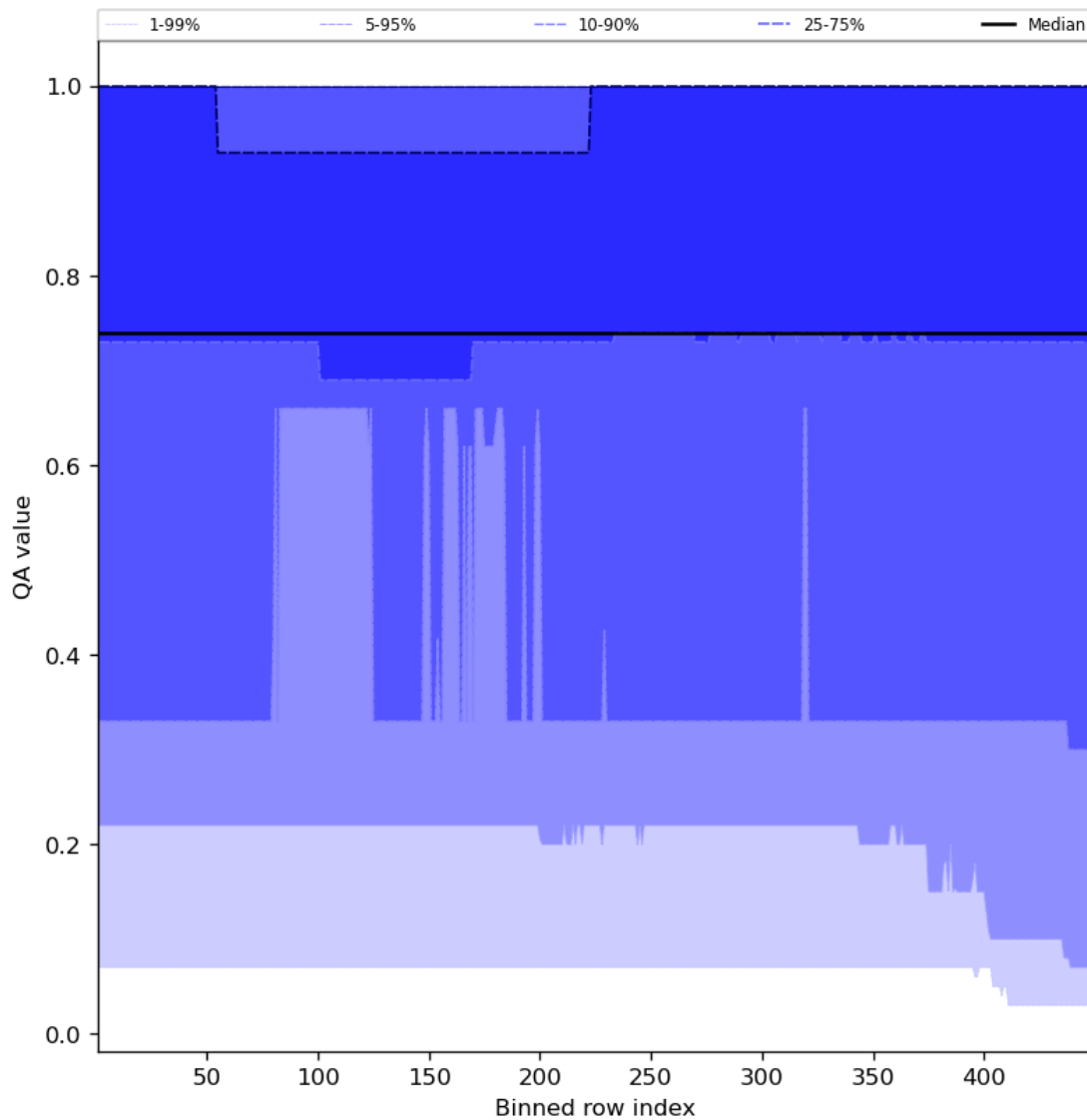
Figure 45: Along track statistics of “QA value” for 2023-11-19 to 2023-11-21
