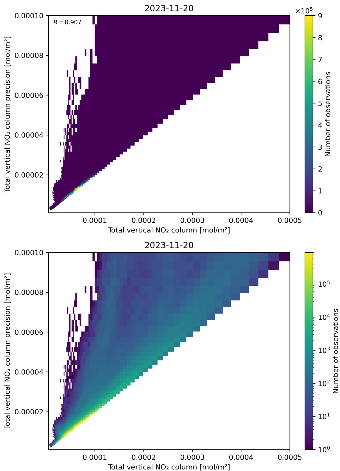
Figure 114: Scatter density plot of “Total vertical NO 2 column” against “Total vertical NO 2 column precision” for 2023-11-19 to 2023-11-21.
