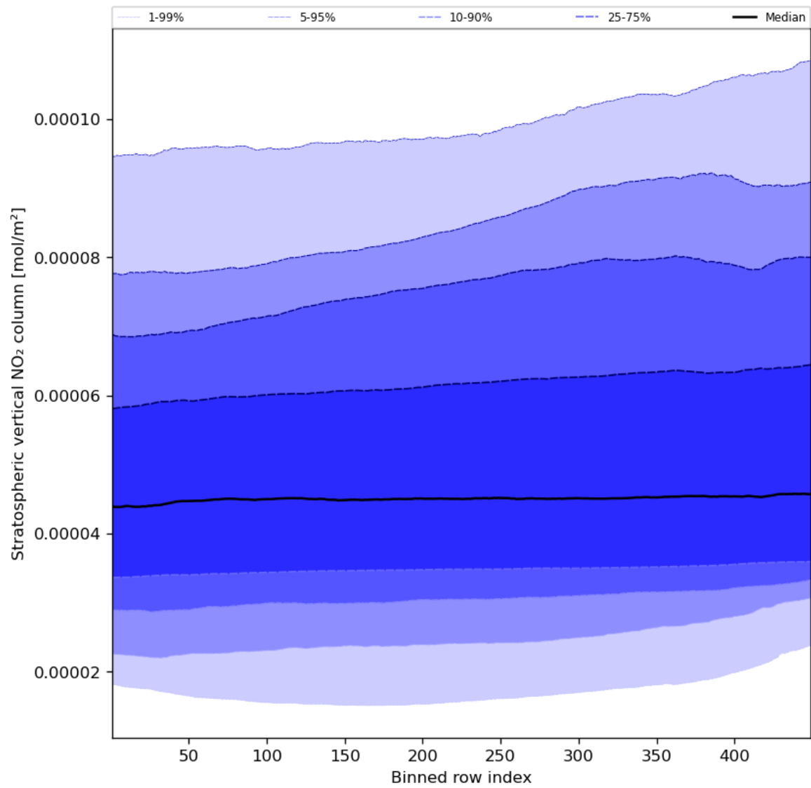
Figure 53: Along track statistics of “Stratospheric vertical NO 2 column” for 2023-11-19 to 2023-11-21
