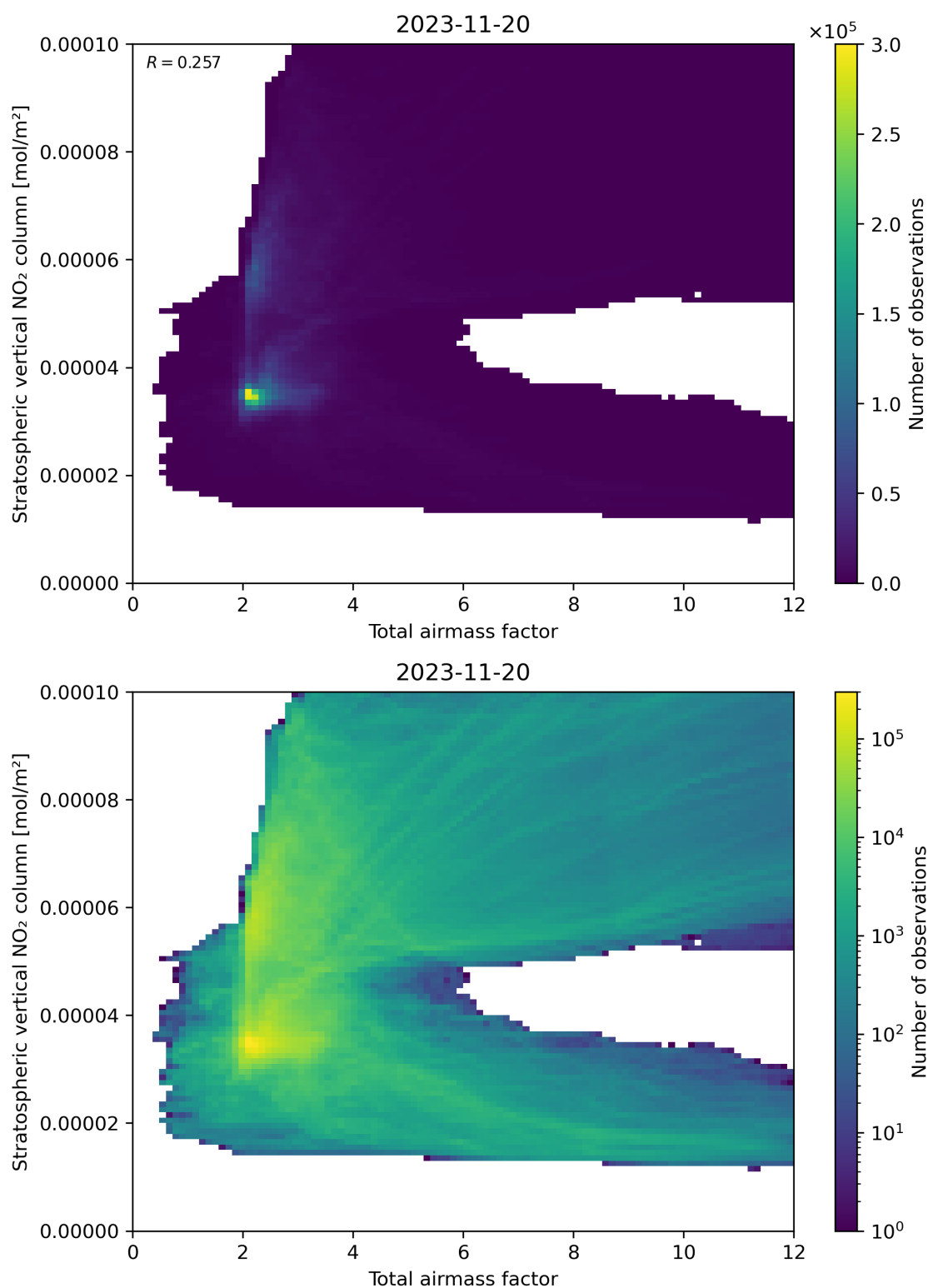
Figure 64: Scatter density plot of “Total airmass factor” against “Stratospheric vertical \text{NO}_2 column” for 2023-11-19 to 2023-11-21.
