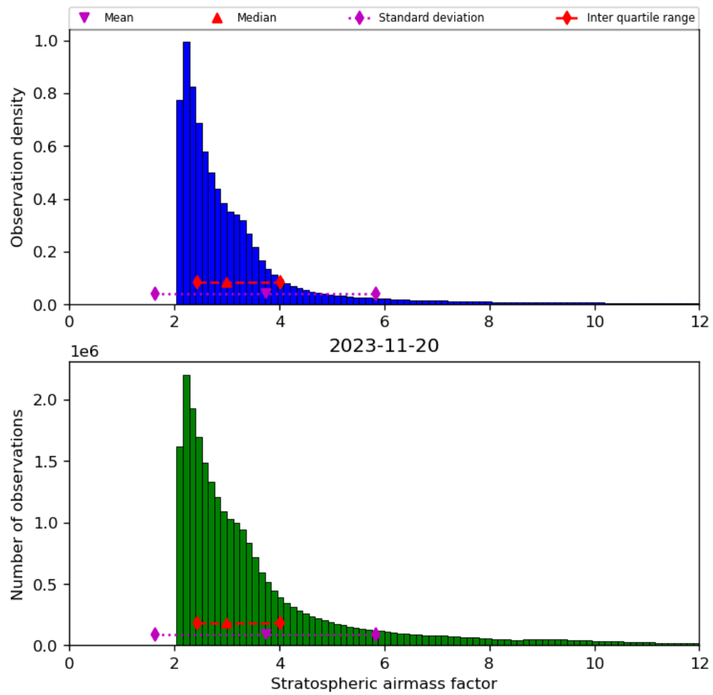
Figure 44: Histogram of “Stratospheric airmass factor” for 2023-11-19 to 2023-11-21
