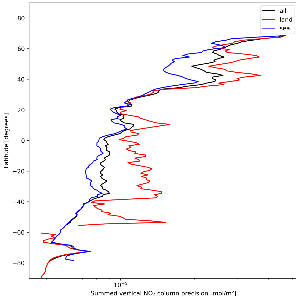
Figure 24: Zonal average of “Summed vertical NO 2 column precision” for 2023-11-19 to 2023-11-21.
