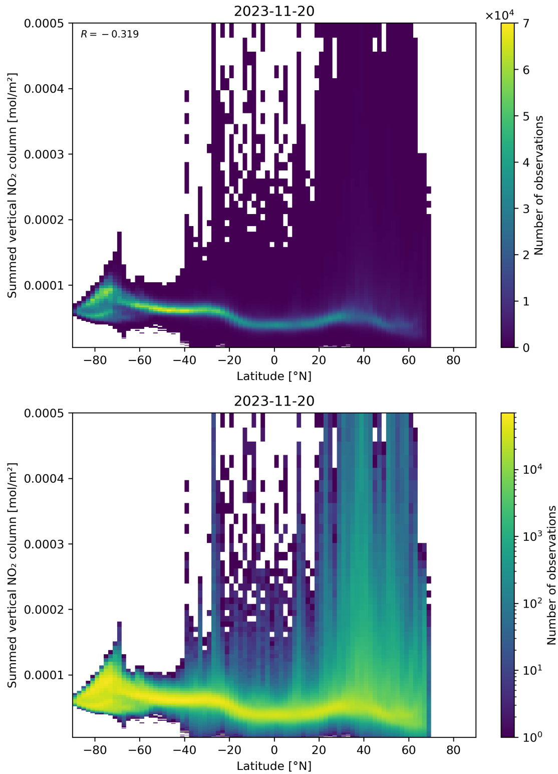
Figure 88: Scatter density plot of “Latitude” against “Summed vertical NO 2 column” for 2023-11-19 to 2023-11-21.
