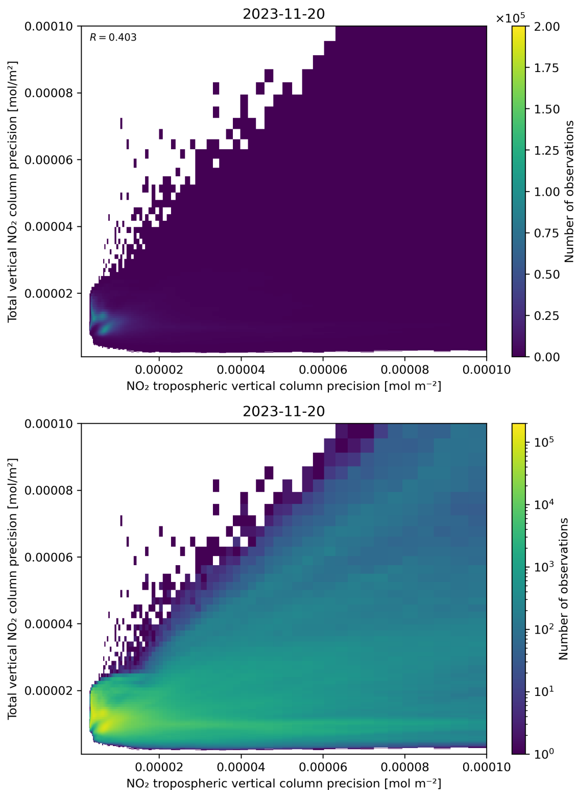
Figure 139: Scatter density plot of “NO 2 tropospheric vertical column precision” against “Total vertical NO 2 column precision” for 2023-11-19 to 2023-11-21.
