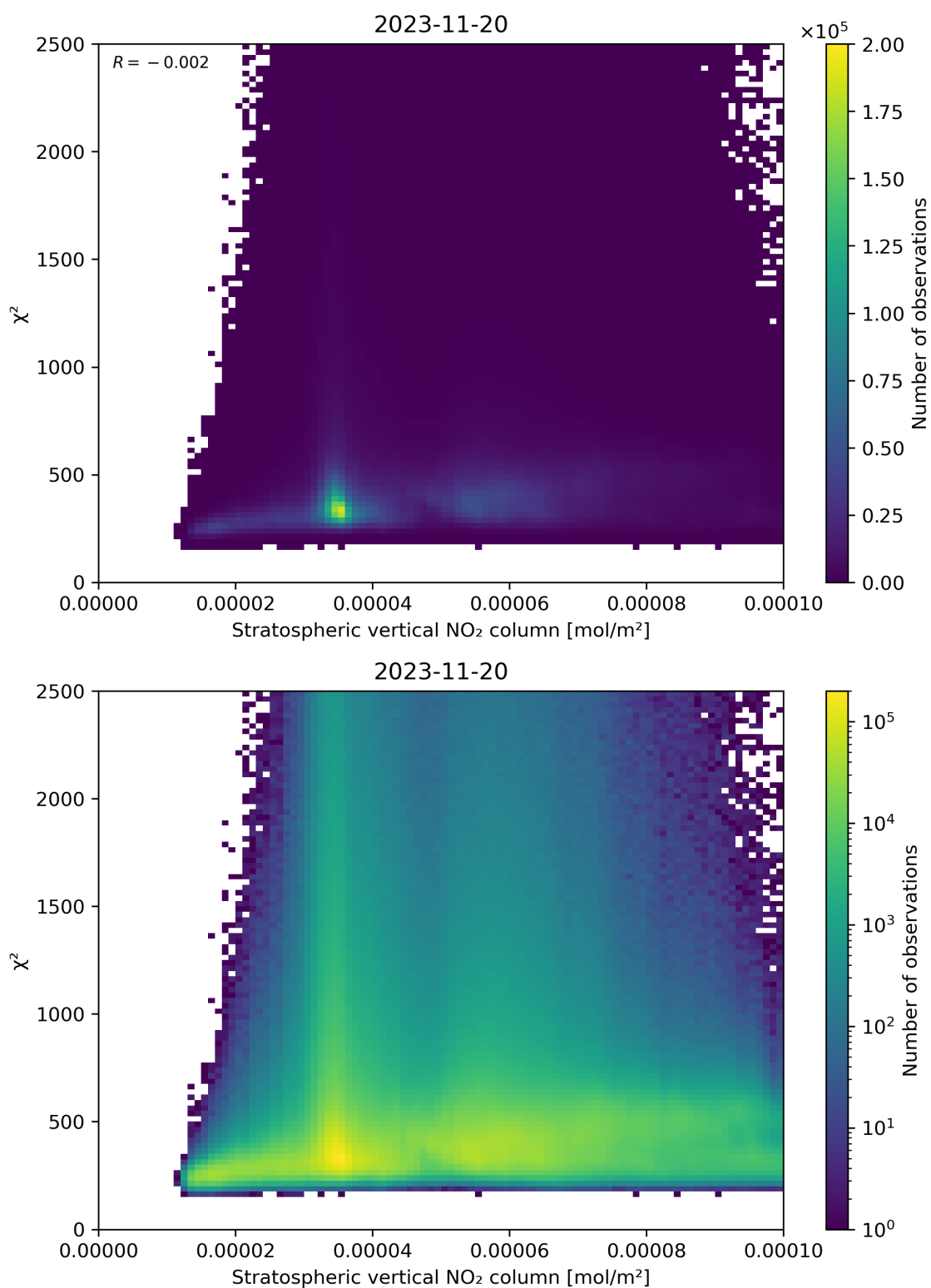
Figure 97: Scatter density plot of “Stratospheric vertical NO 2 column” against “ \chi^2 ” for 2023-11-19 to 2023-11-21.
