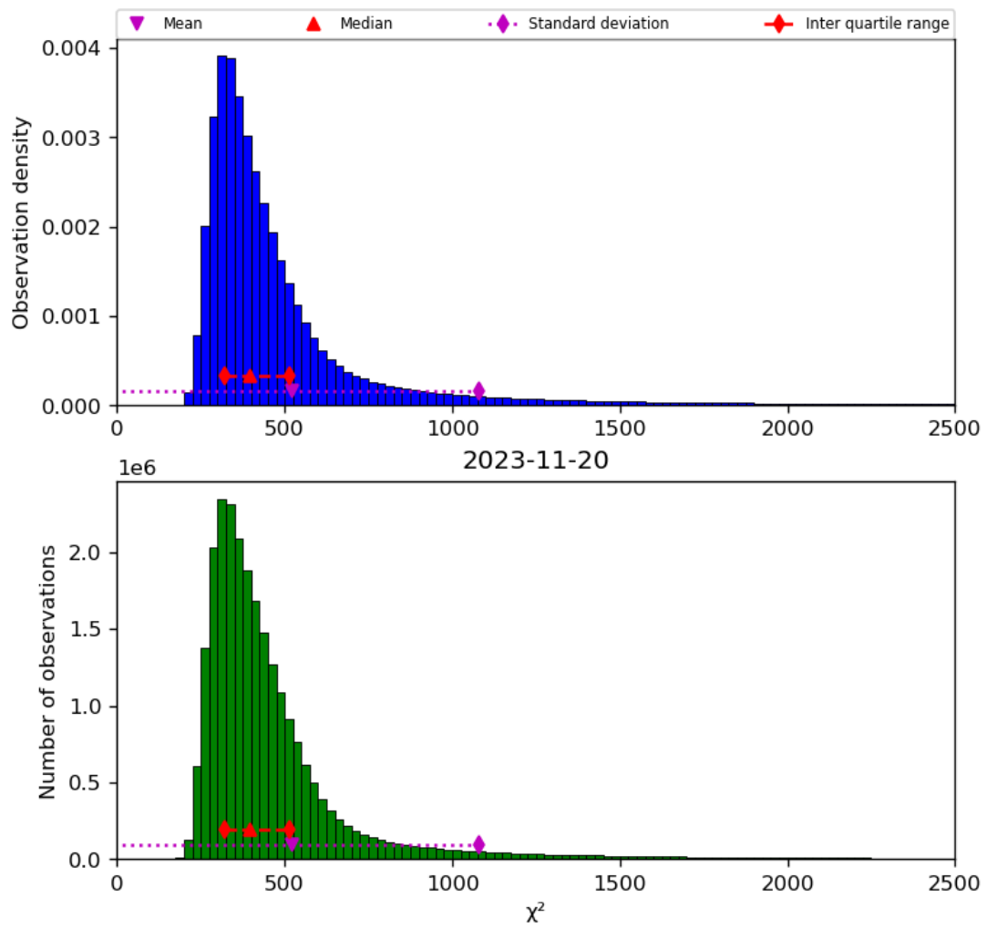
Figure 42: Histogram of “ \chi^2 ” for 2023-11-19 to 2023-11-21
