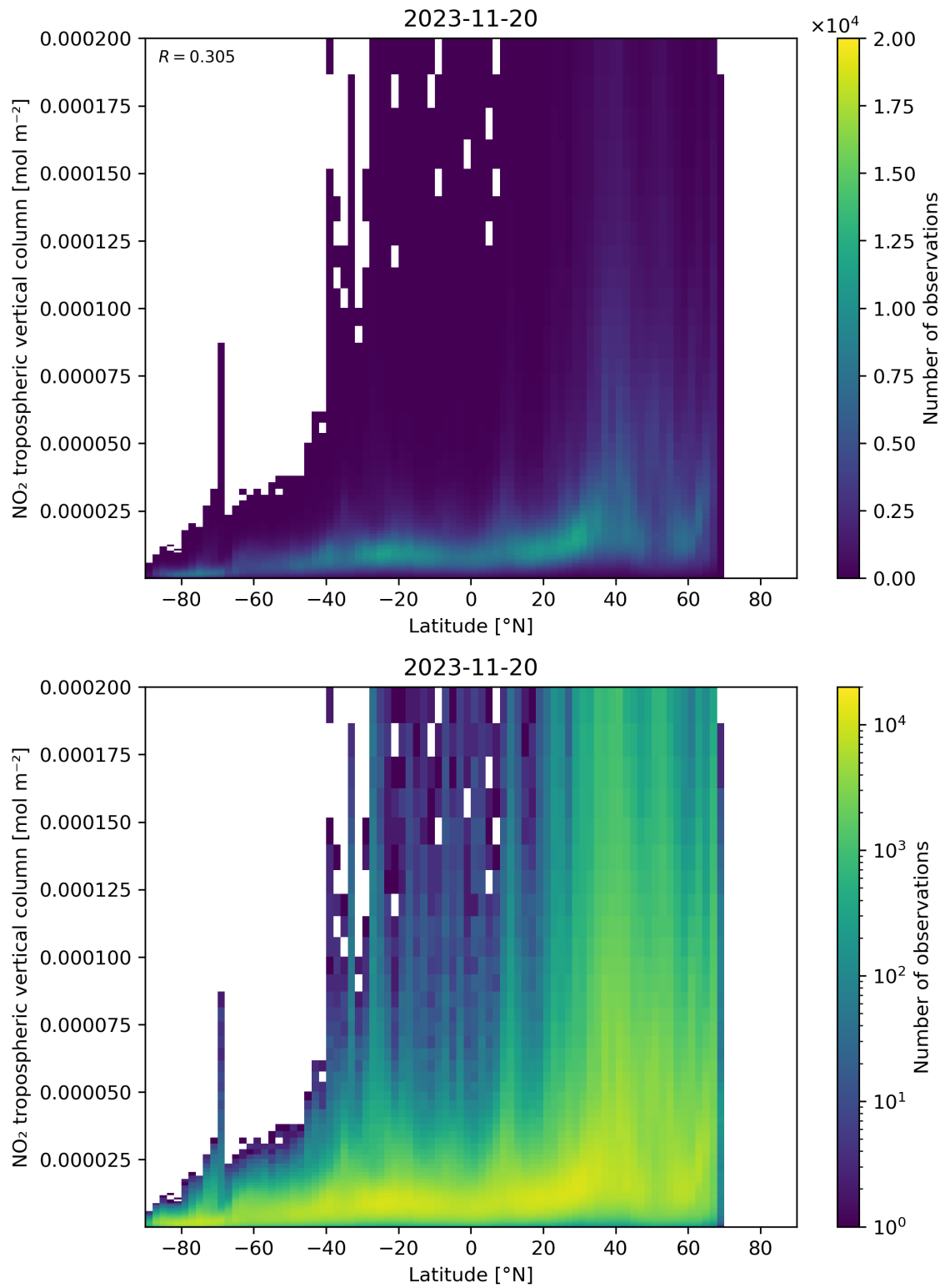
Figure 92: Scatter density plot of “Latitude” against “NO 2 tropospheric vertical column” for 2023-11-19 to 2023-11-21.
