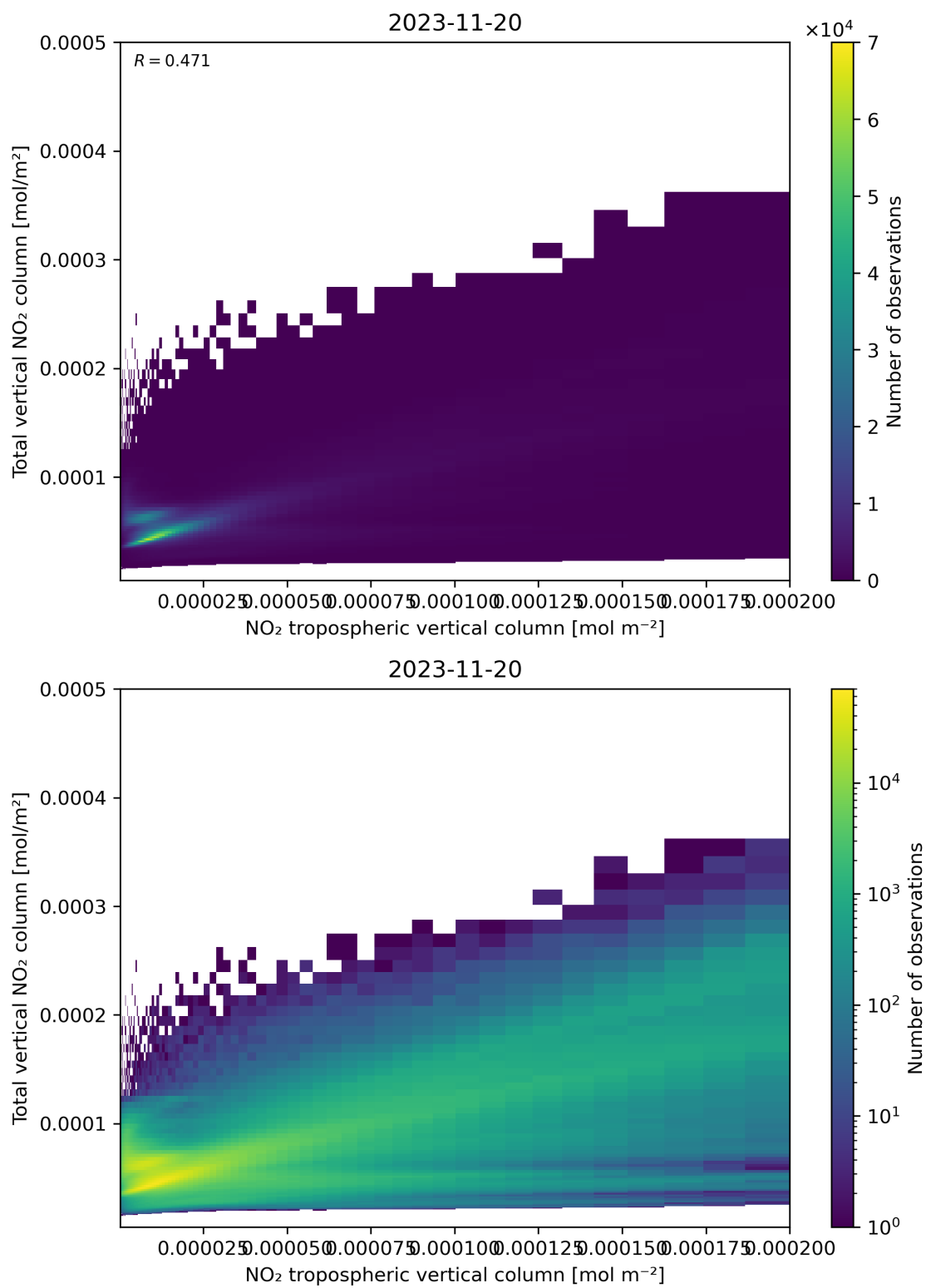
Figure 128: Scatter density plot of “NO 2 tropospheric vertical column” against “Total vertical NO 2 column” for 2023-11-19 to 2023-11-21.
