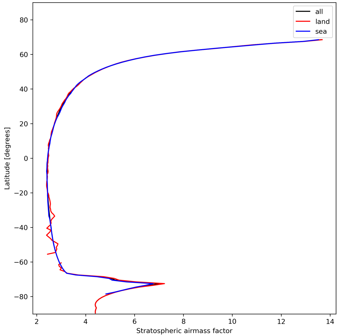
Figure 27: Zonal average of “Stratospheric airmass factor” for 2023-11-19 to 2023-11-21.
