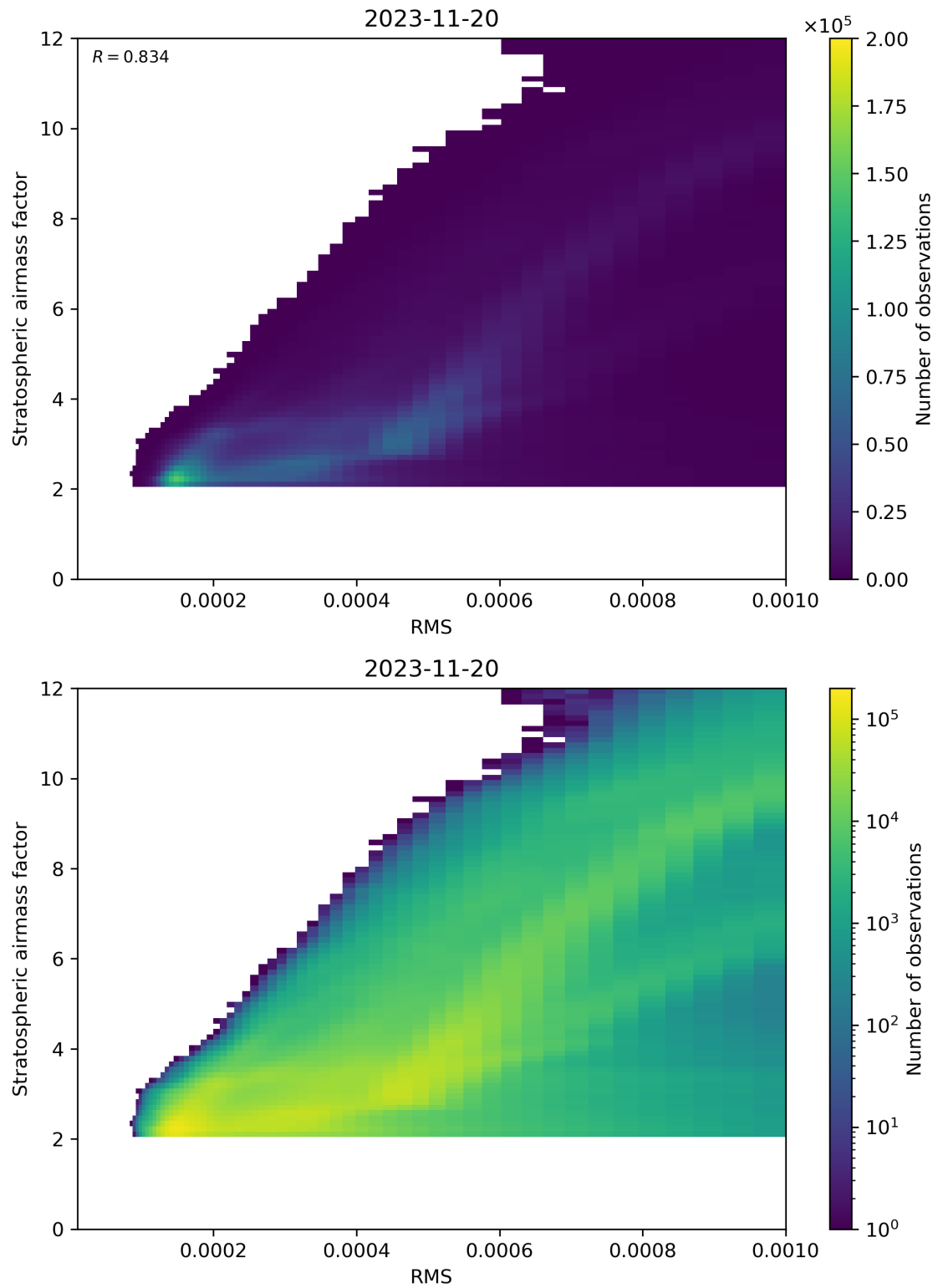
Figure 144: Scatter density plot of “RMS” against “Stratospheric airmass factor” for 2023-11-19 to 2023-11-21.
