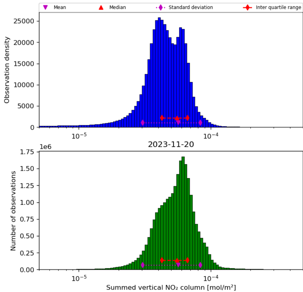
Figure 40: Histogram of “Summed vertical NO 2 column” for 2023-11-19 to 2023-11-21
