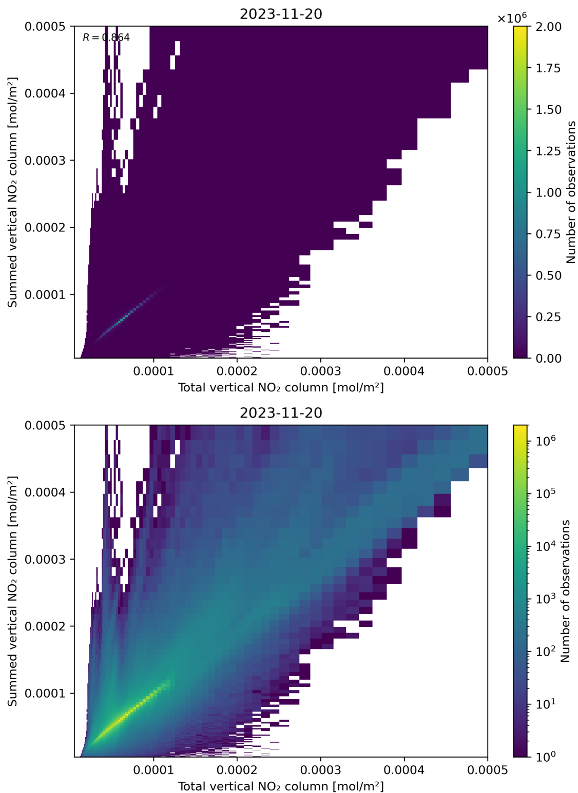
Figure 112: Scatter density plot of “Total vertical NO 2 column” against “Summed vertical NO 2 column” for 2023-11-19 to 2023-11-21.
