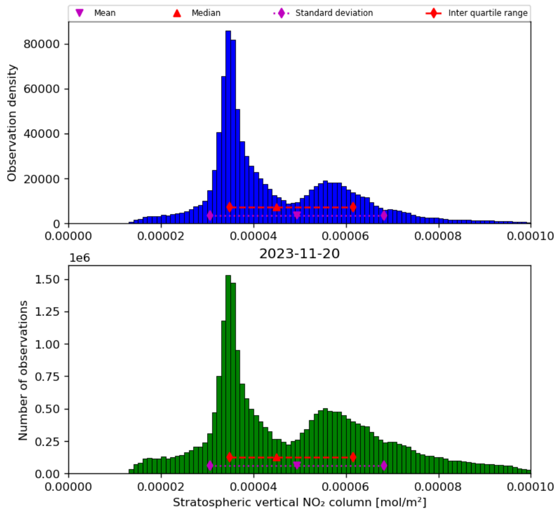
Figure 36: Histogram of “Stratospheric vertical NO 2 column” for 2023-11-19 to 2023-11-21
