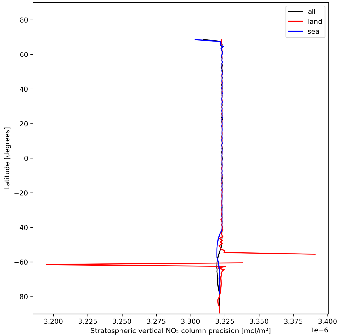
Figure 20: Zonal average of “Stratospheric vertical NO 2 column precision” for 2023-11-19 to 2023-11-21.
