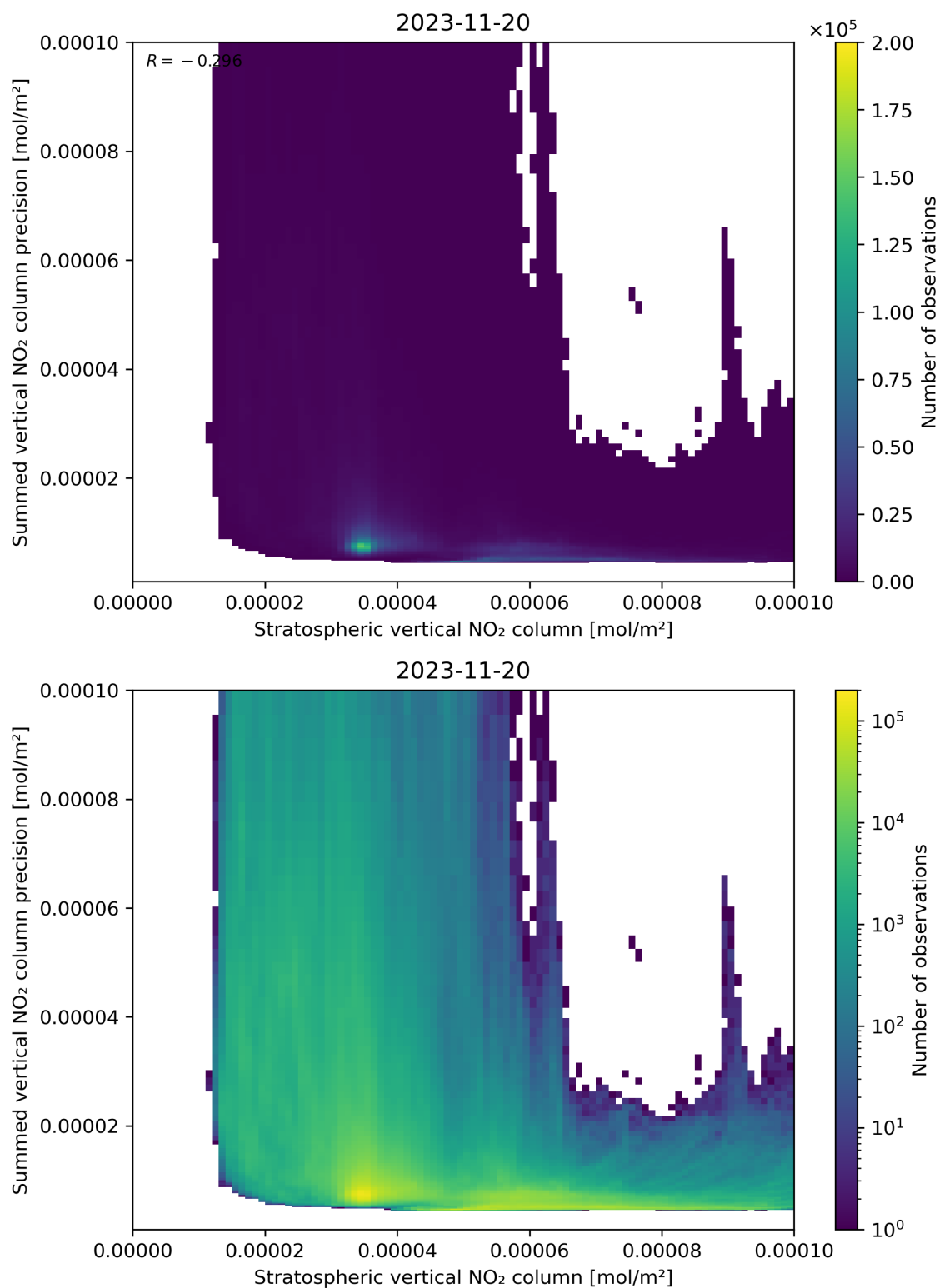
Figure 99: Scatter density plot of “Stratospheric vertical NO 2 column” against “Summed vertical NO 2 column precision” for 2023-11-19 to 2023-11-21.
