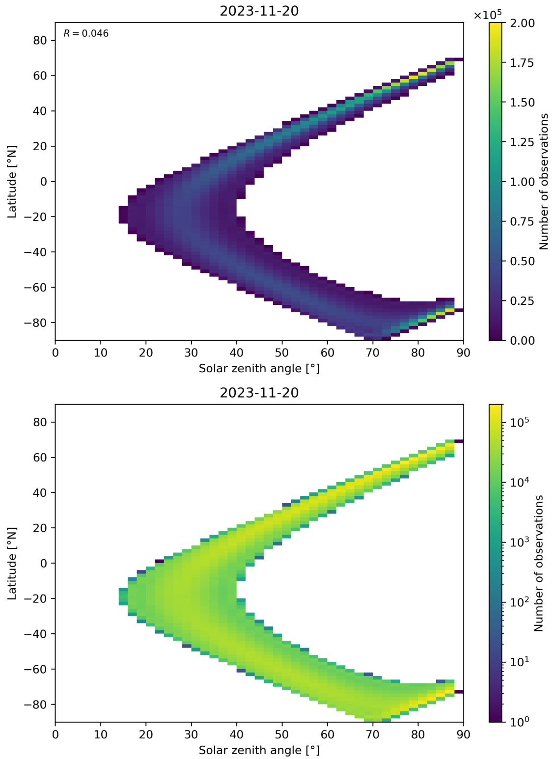
Figure 149: Scatter density plot of “Solar zenith angle” against “Latitude” for 2023-11-19 to 2023-11-21.
