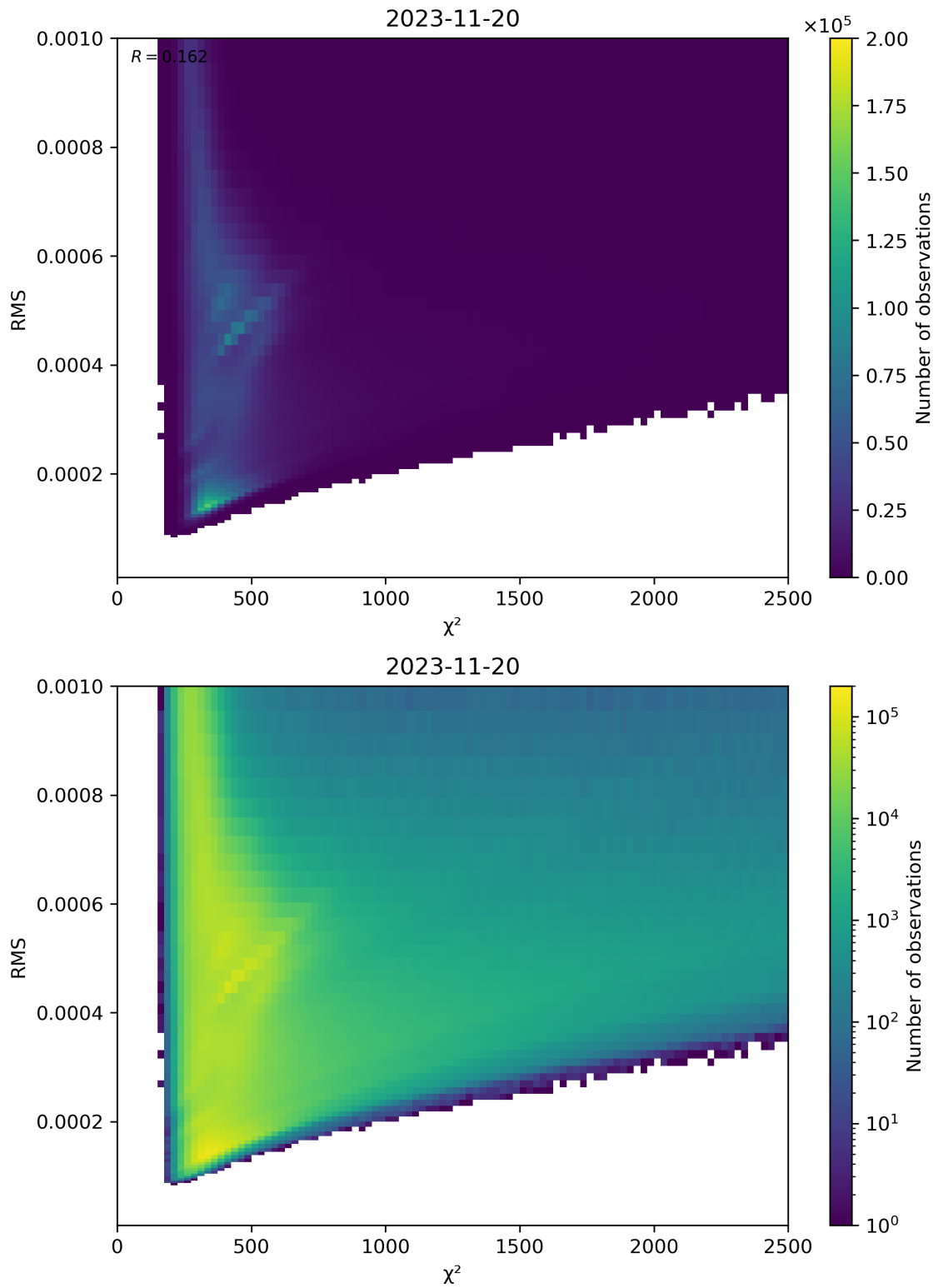
Figure 82: Scatter density plot of “ \chi^2 ” against “RMS” for 2023-11-19 to 2023-11-21.
