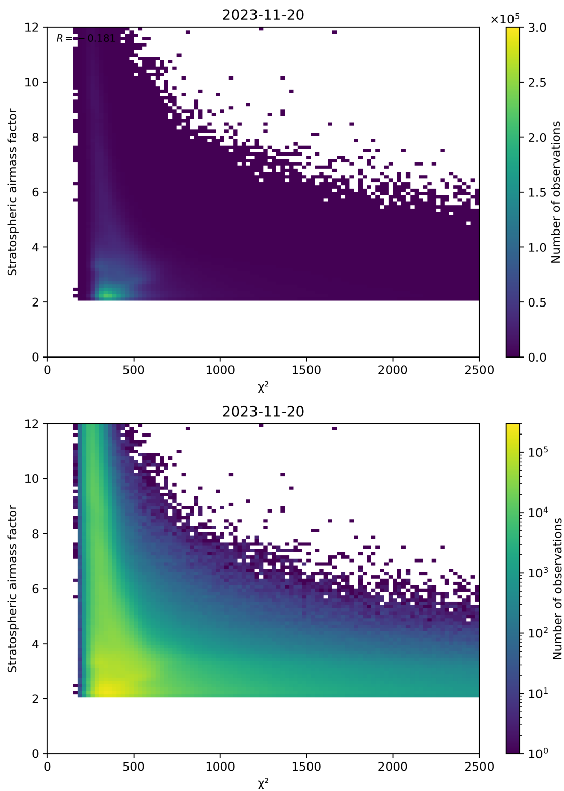
Figure 81: Scatter density plot of “ \chi^2 ” against “Stratospheric airmass factor” for 2023-11-19 to 2023-11-21.
