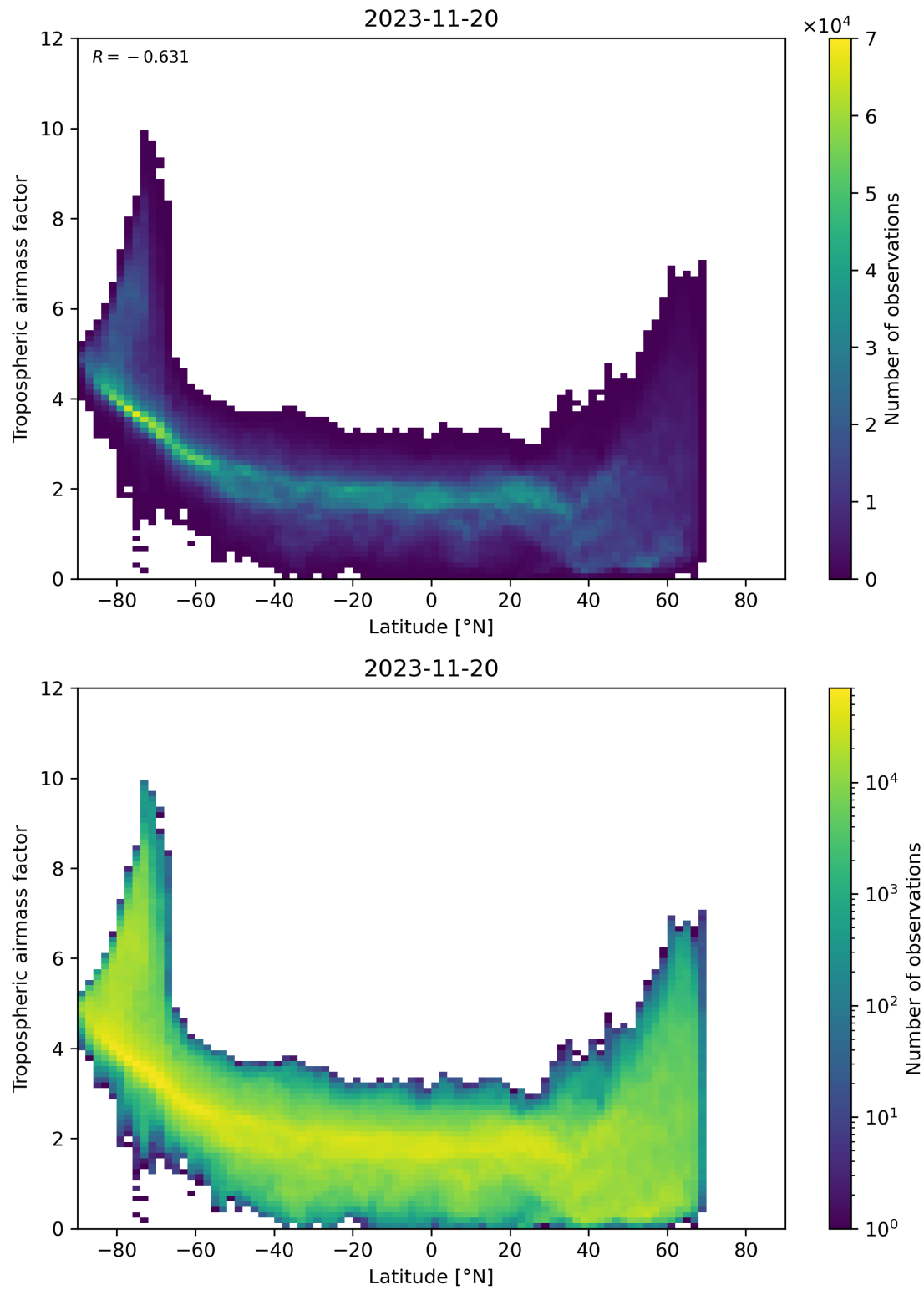
Figure 85: Scatter density plot of “Latitude” against “Tropospheric airmass factor” for 2023-11-19 to 2023-11-21.
