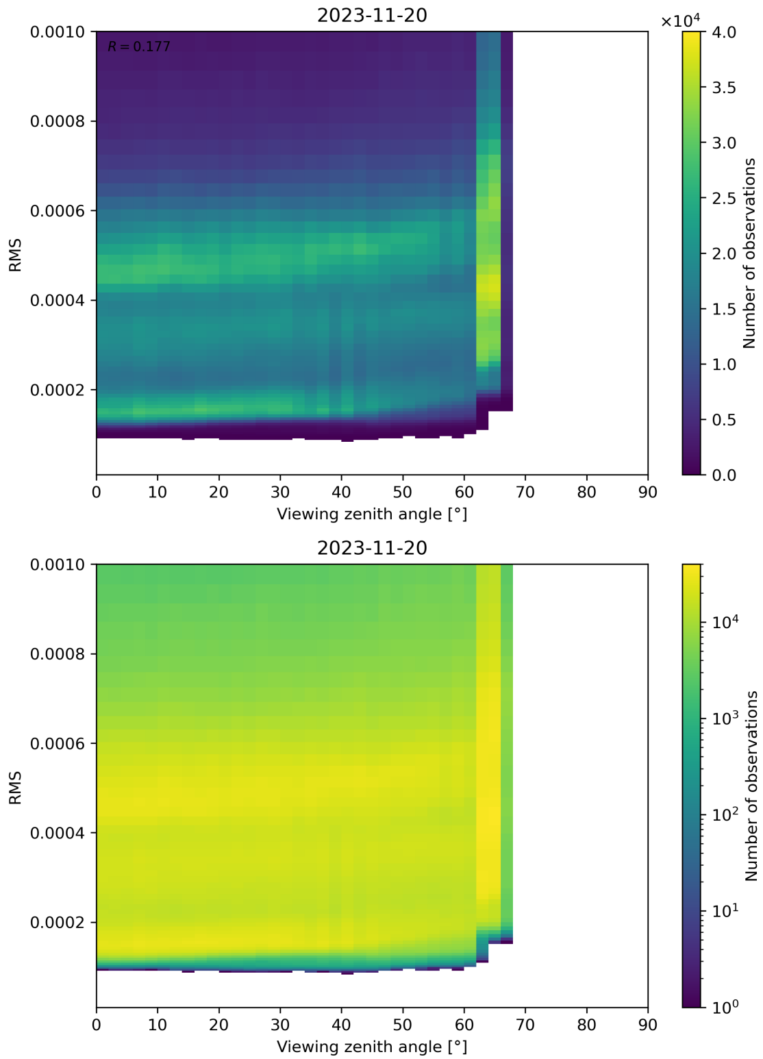
Figure 171: Scatter density plot of “Viewing zenith angle” against “RMS” for 2023-11-19 to 2023-11-21.
