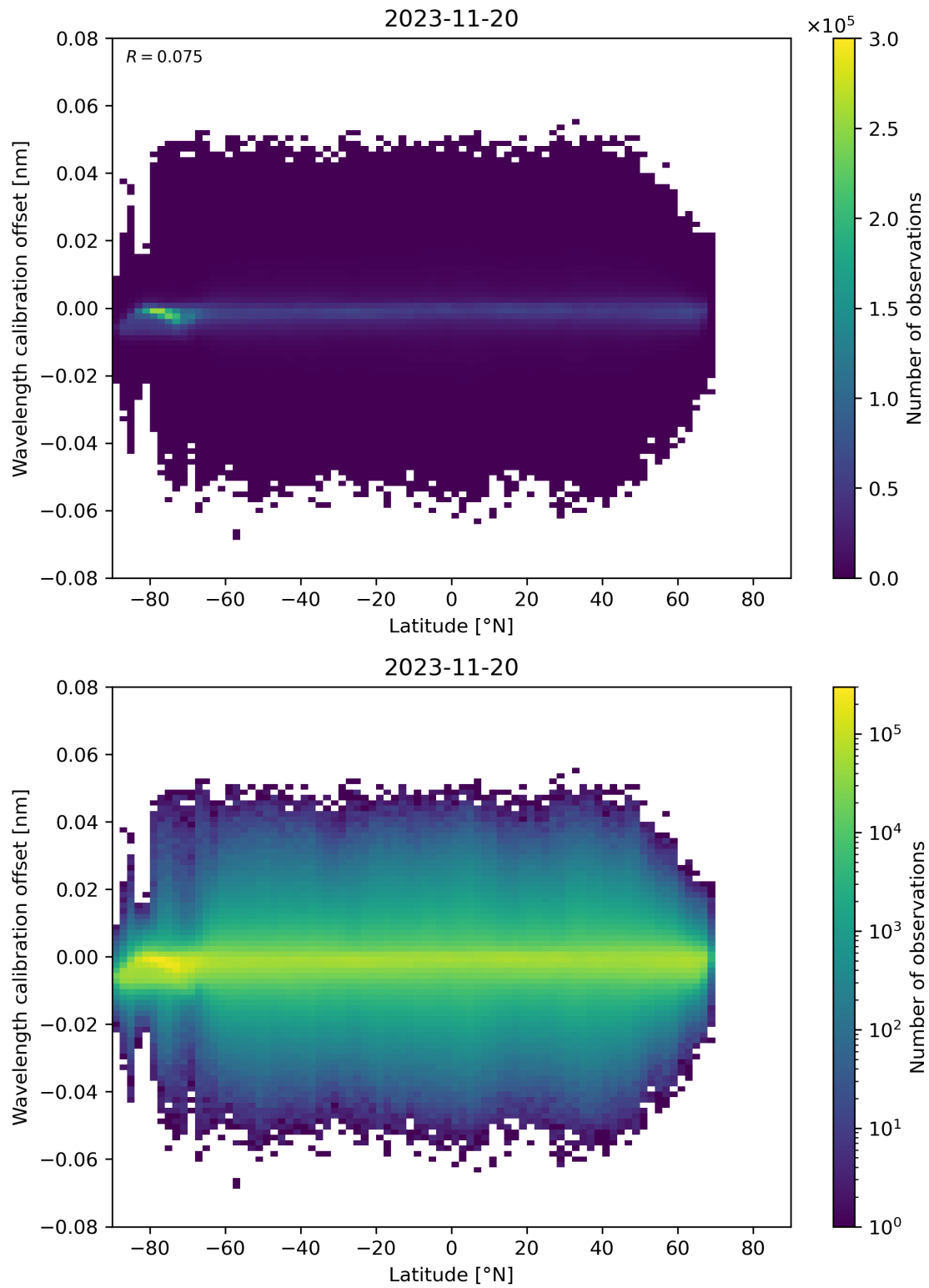
Figure 95: Scatter density plot of “Latitude” against “Wavelength calibration offset” for 2023-11-19 to 2023-11-21.
