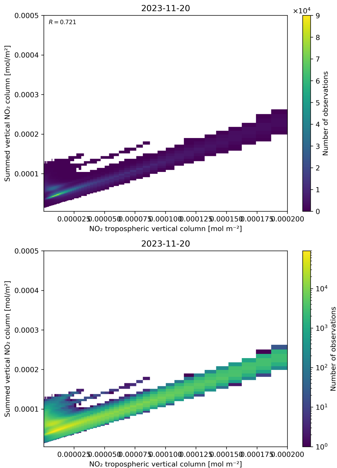
Figure 126: Scatter density plot of “NO 2 tropospheric vertical column” against “Summed vertical NO 2 column” for 2023-11-19 to 2023-11-21.
