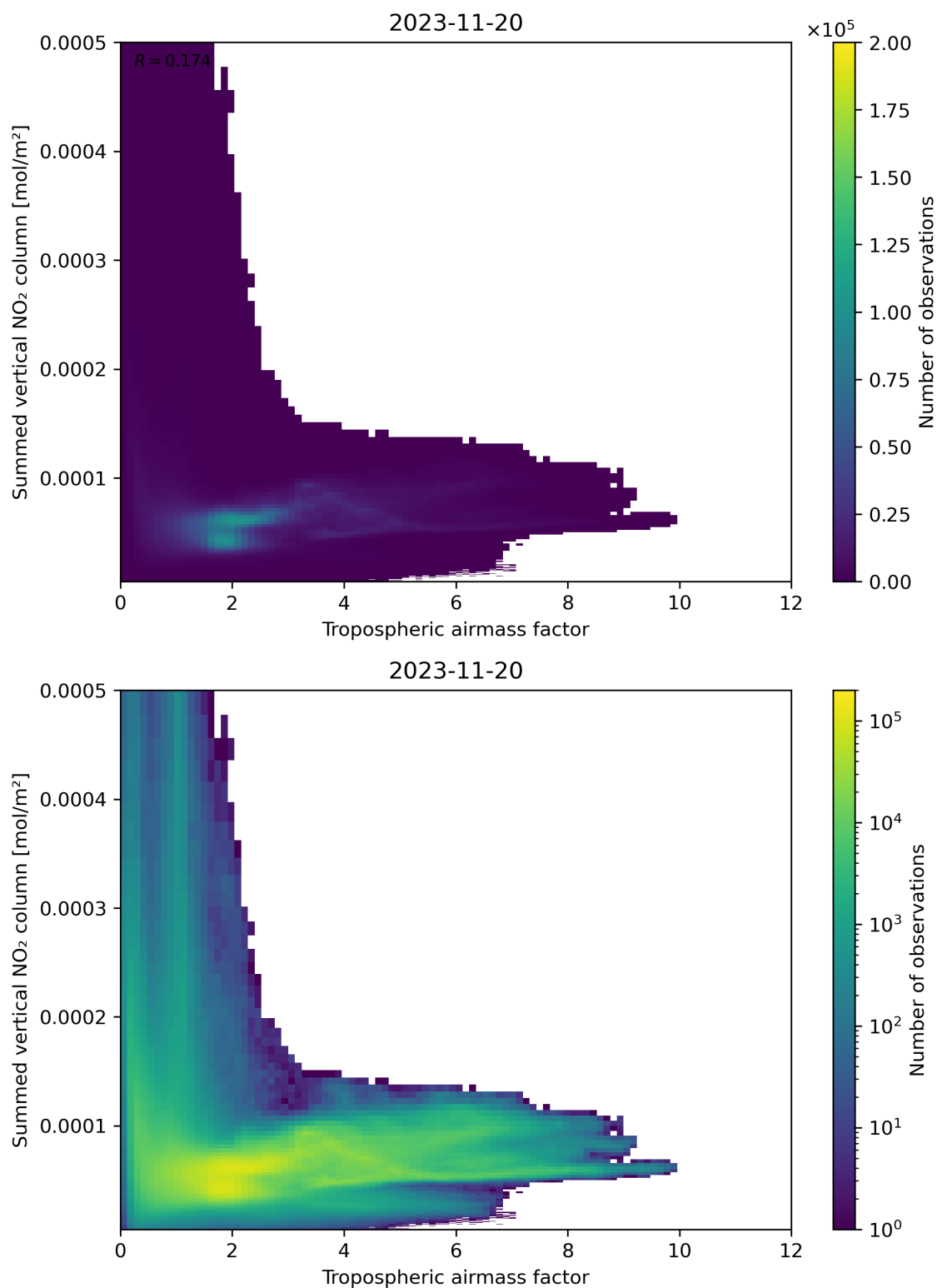
Figure 75: Scatter density plot of “Tropospheric airmass factor” against “Summed vertical NO 2 column” for 2023-11-19 to 2023-11-21.
