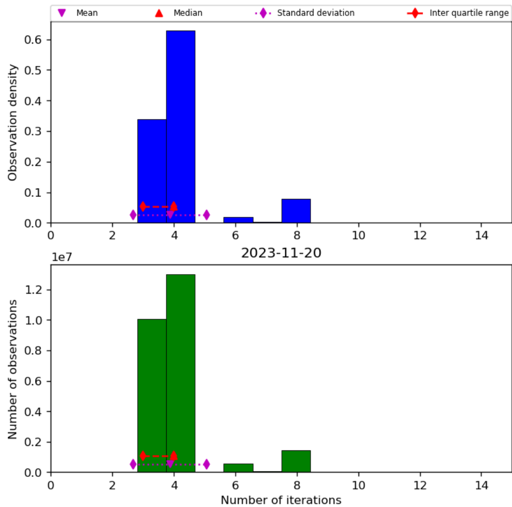
Figure 34: Histogram of “Number of iterations” for 2023-11-19 to 2023-11-21
