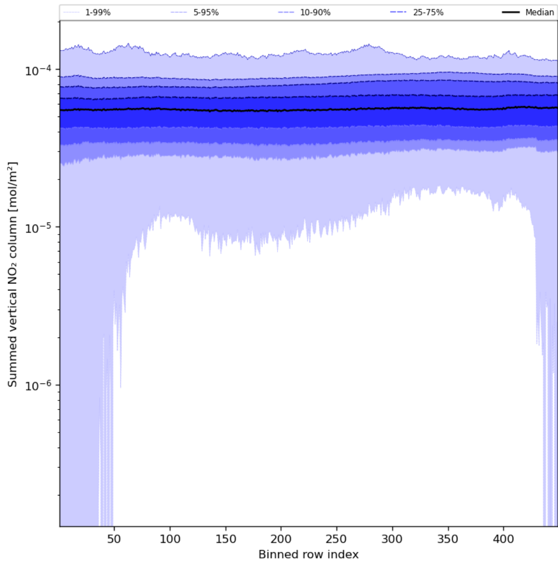
Figure 57: Along track statistics of “Summed vertical NO 2 column” for 2023-11-19 to 2023-11-21
