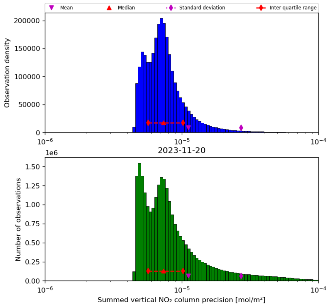
Figure 41: Histogram of "Summed vertical NO 2 column precision" for 2023-11-19 to 2023-11-21
