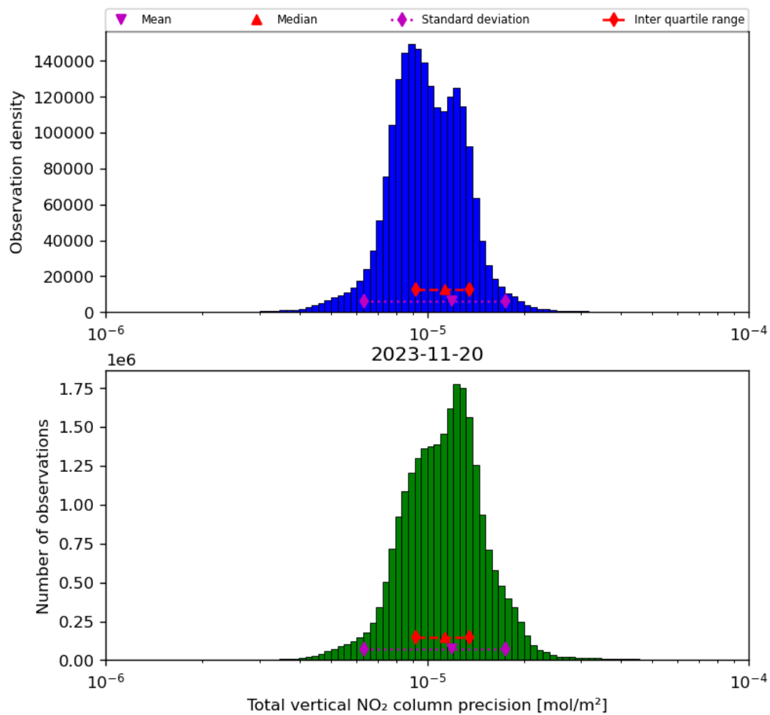
Figure 39: Histogram of “Total vertical NO 2 column precision” for 2023-11-19 to 2023-11-21
