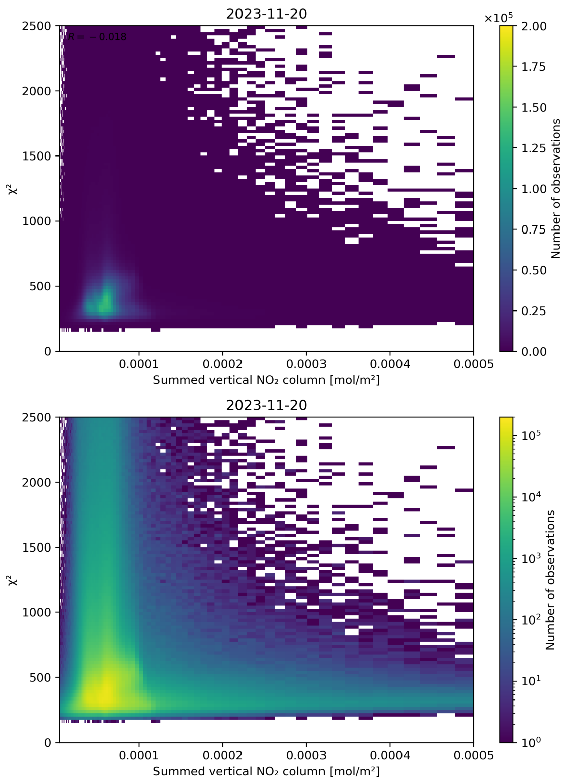
Figure 104: Scatter density plot of “Summed vertical NO 2 column” against “ \chi^2 ” for 2023-11-19 to 2023-11-21.
