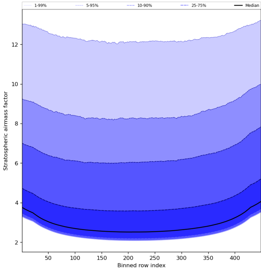
Figure 61: Along track statistics of “Stratospheric airmass factor” for 2023-11-19 to 2023-11-21
