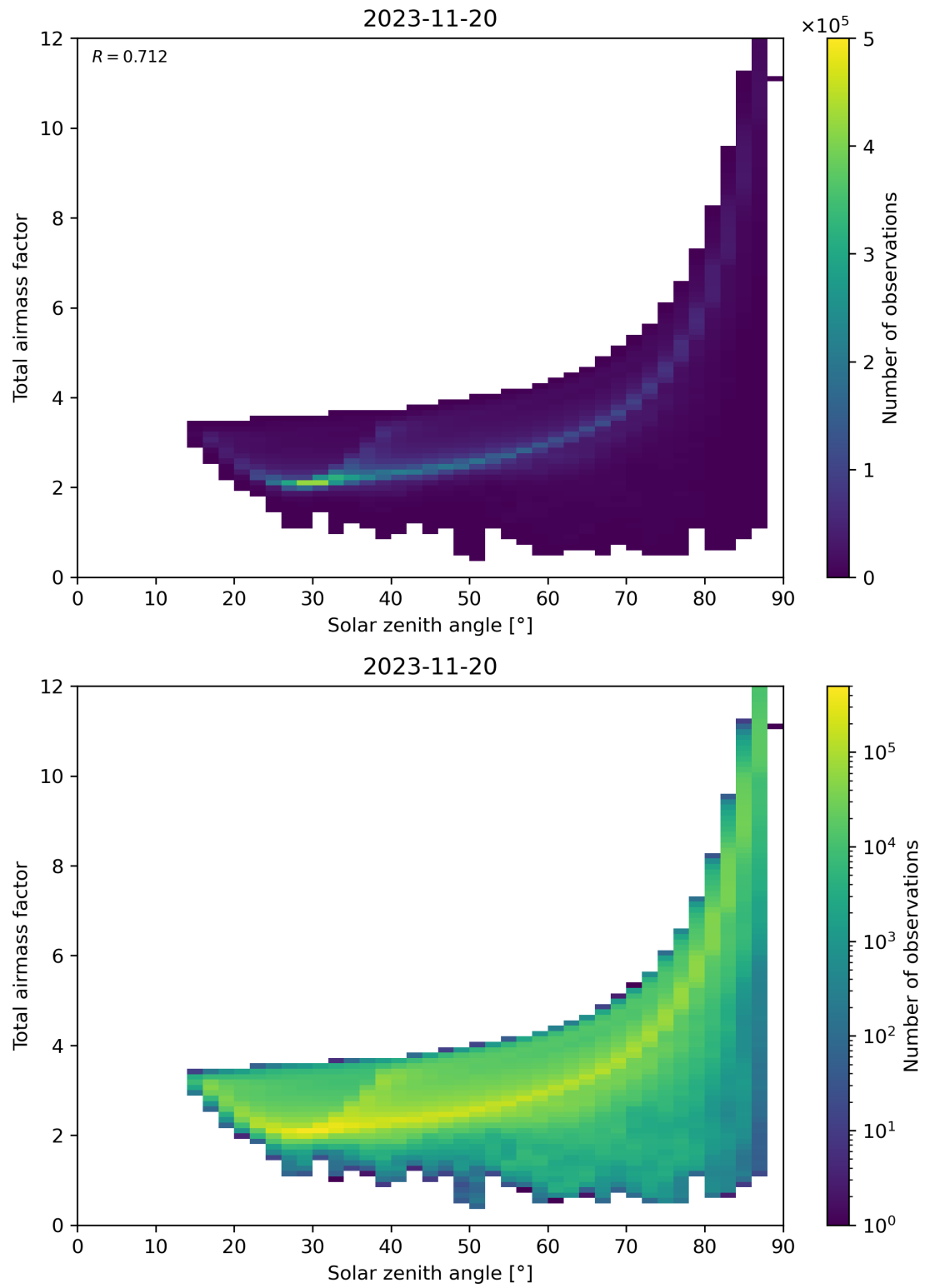
Figure 146: Scatter density plot of “Solar zenith angle” against “Total air mass factor” for 2023-11-19 to 2023-11-21.
