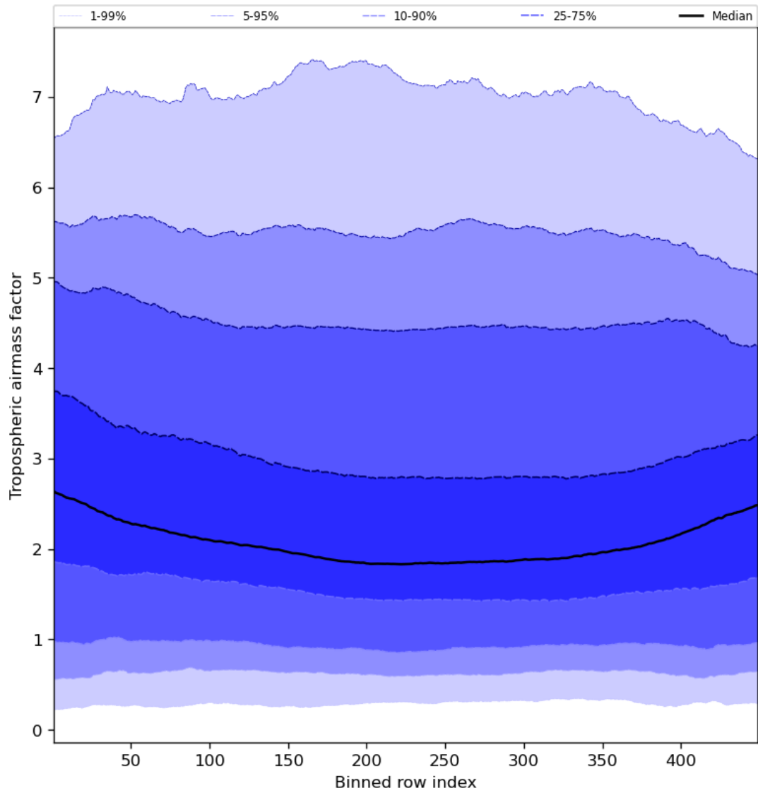
Figure 48: Along track statistics of “Tropospheric air mass factor” for 2023-11-19 to 2023-11-21
