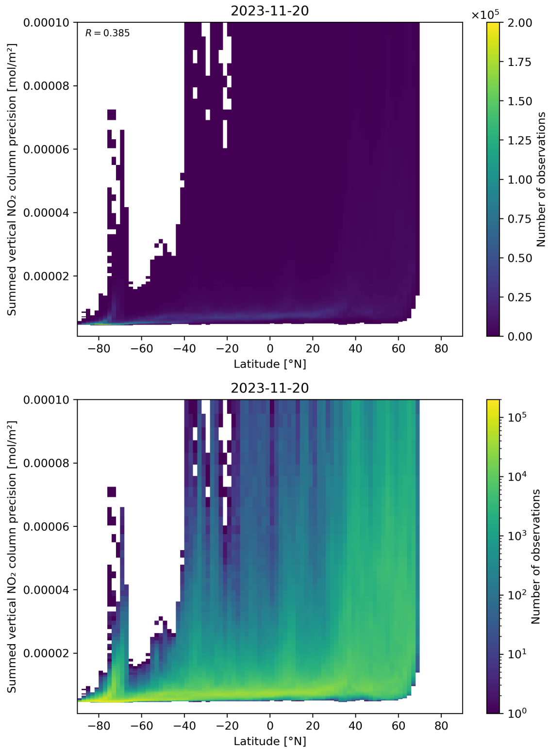
Figure 89: Scatter density plot of “Latitude” against “Summed vertical NO 2 column precision” for 2023-11-19 to 2023-11-21.
