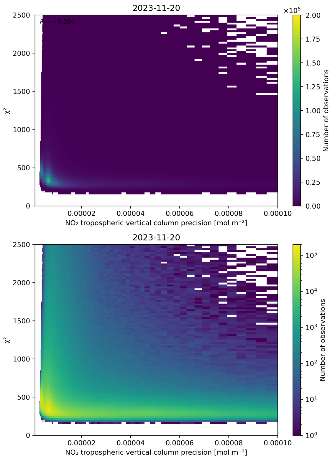
Figure 134: Scatter density plot of “NO 2 tropospheric vertical column precision” against “ \chi^2 ” for 2023-11-19 to 2023-11-21.
