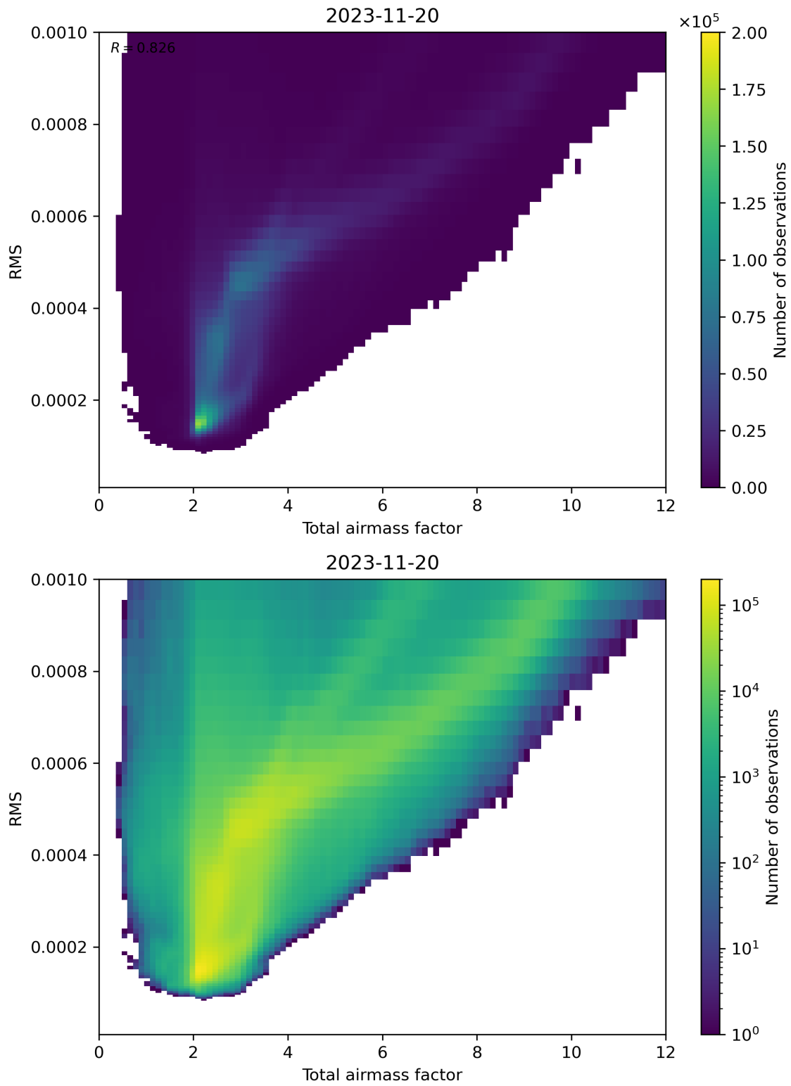
Figure 69: Scatter density plot of “Total airmass factor” against “RMS” for 2023-11-19 to 2023-11-21.
