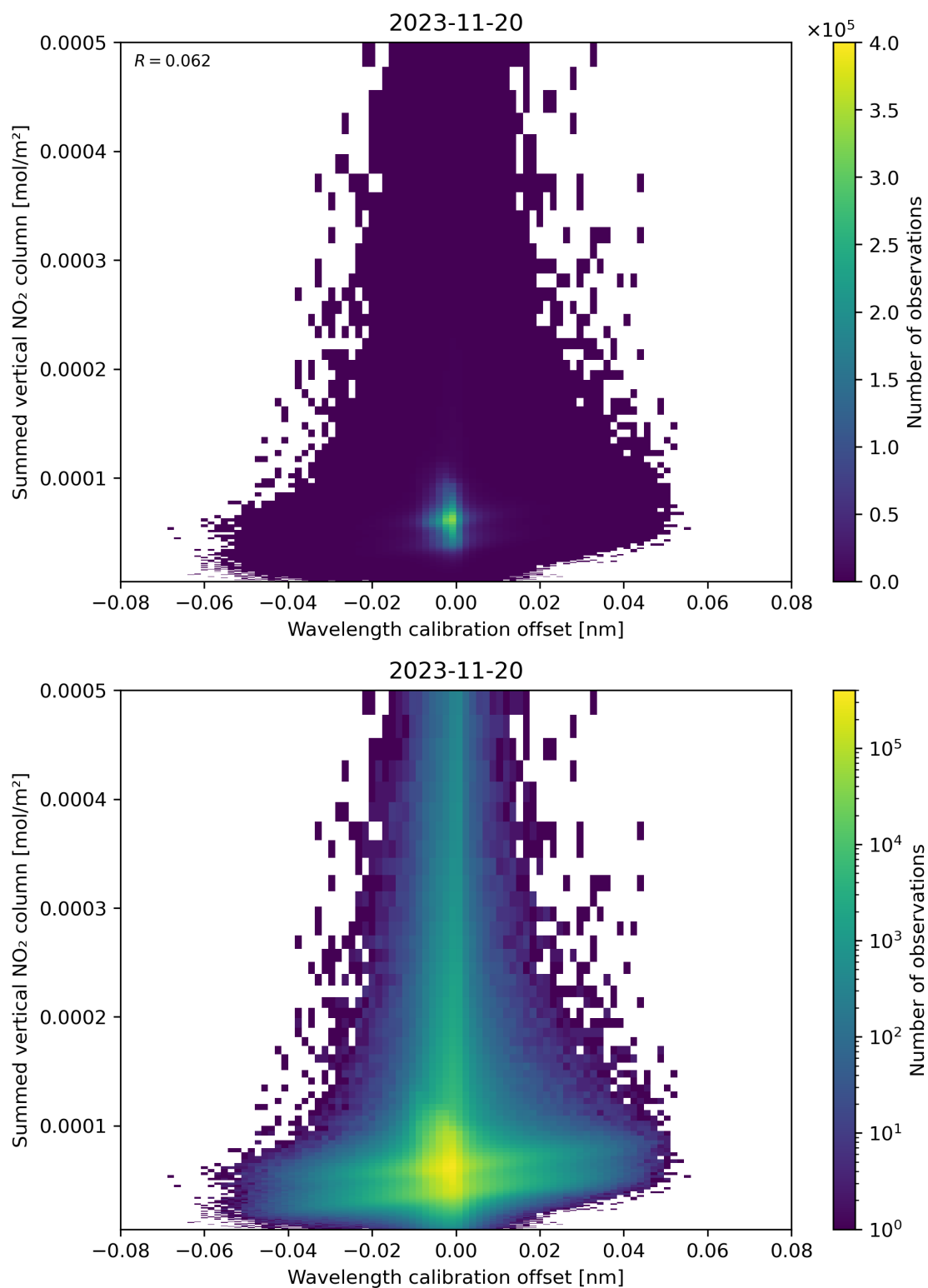
Figure 177: Scatter density plot of “Wavelength calibration offset” against “Summed vertical NO 2 column” for 2023-11-19 to 2023-11-21.
