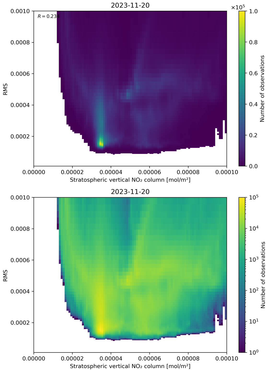
Figure 102: Scatter density plot of “Stratospheric vertical NO 2 column” against “RMS” for 2023-11-19 to 2023-11-21.
