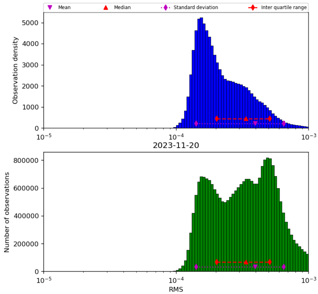
Figure 43: Histogram of “RMS” for 2023-11-19 to 2023-11-21
