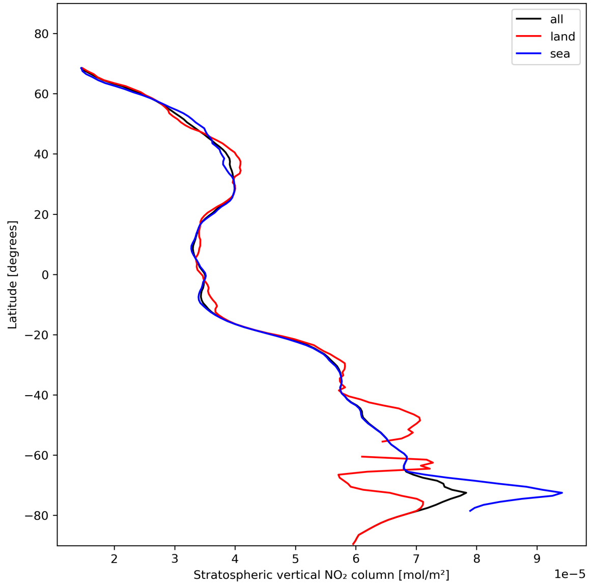
Figure 19: Zonal average of “Stratospheric vertical NO 2 column” for 2023-11-19 to 2023-11-21.
