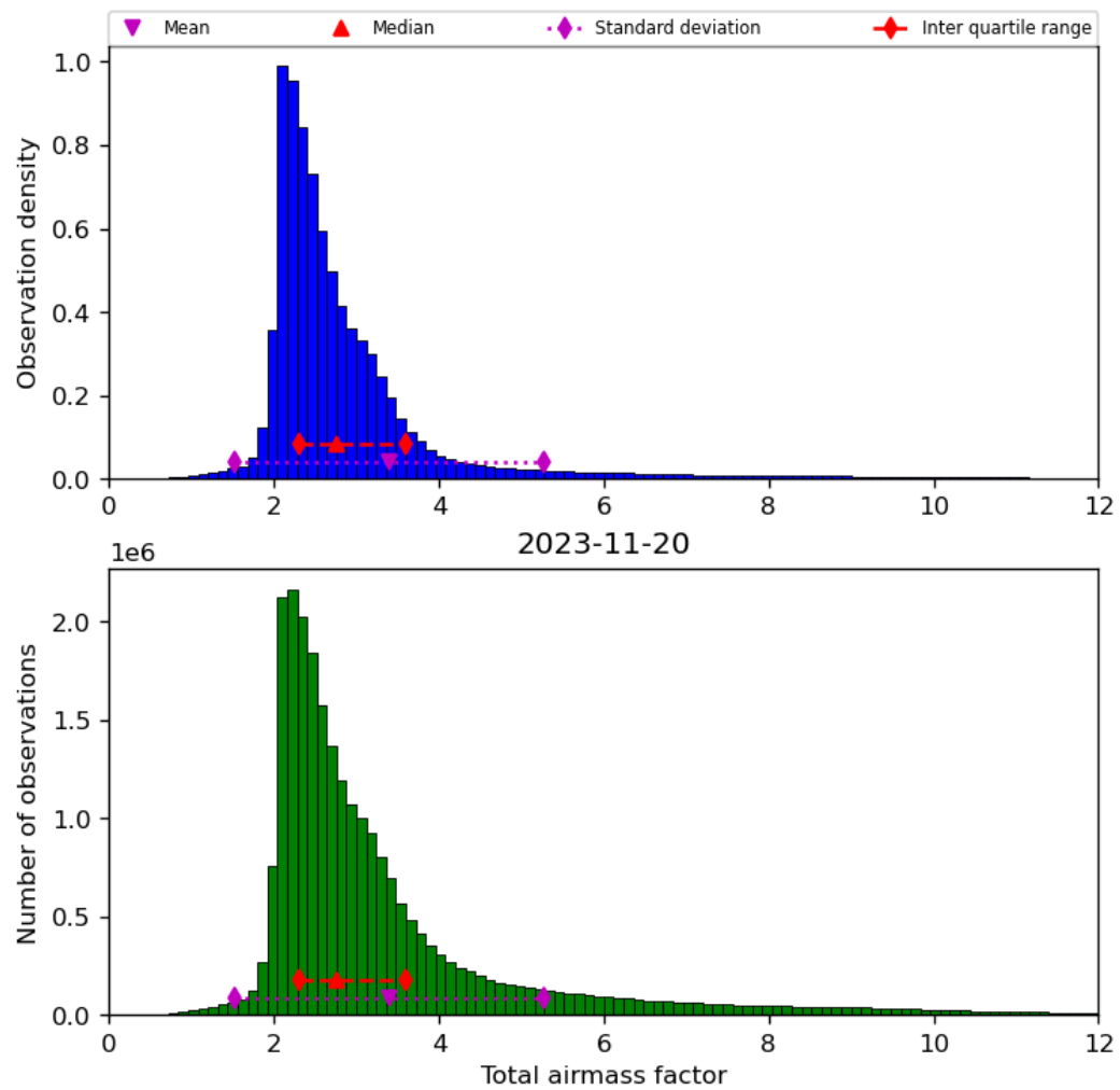
Figure 32: Histogram of “Total airmass factor” for 2023-11-19 to 2023-11-21
