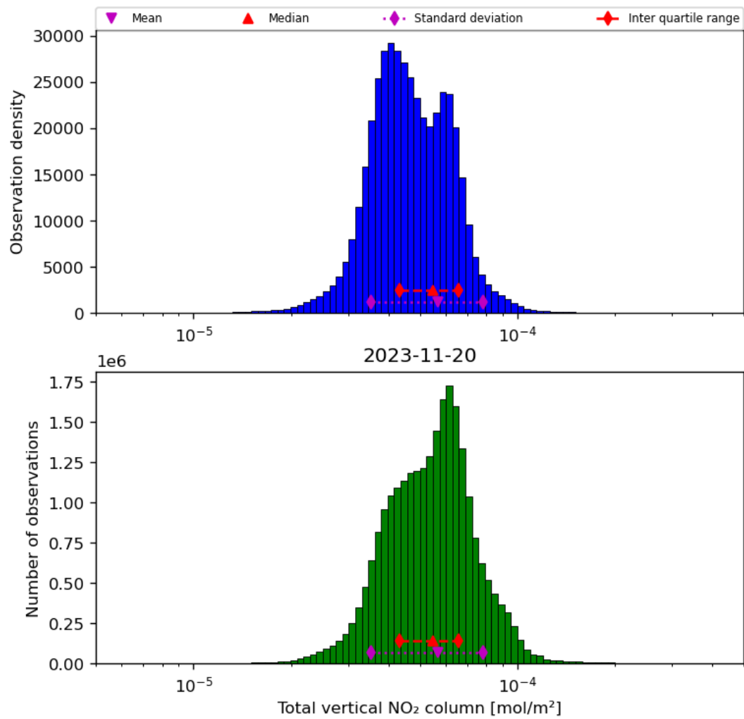
Figure 38: Histogram of “Total vertical NO 2 column” for 2023-11-19 to 2023-11-21
