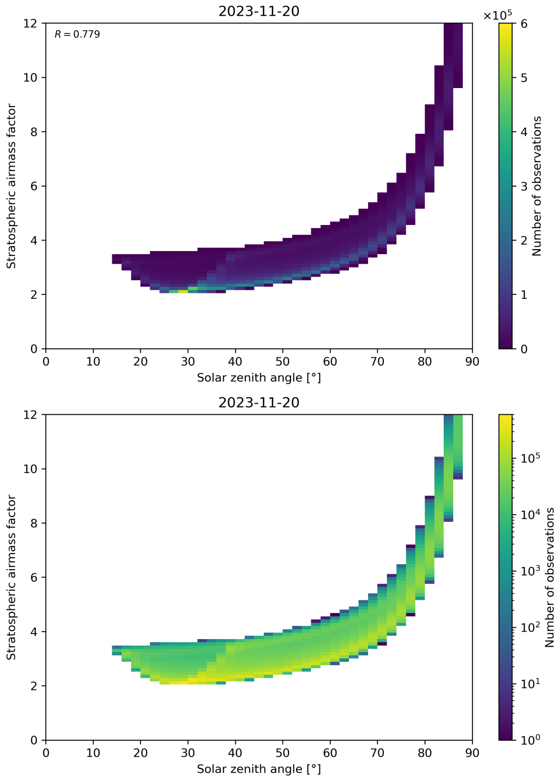
Figure 145: Scatter density plot of “Solar zenith angle” against “Stratospheric airmass factor” for 2023-11-19 to 2023-11-21.
