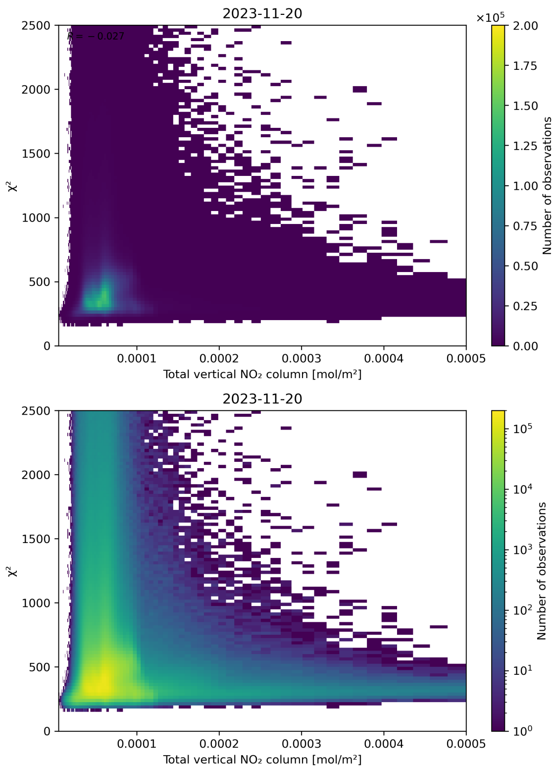
Figure 111: Scatter density plot of “Total vertical NO 2 column” against “ \chi^2 ” for 2023-11-19 to 2023-11-21.
