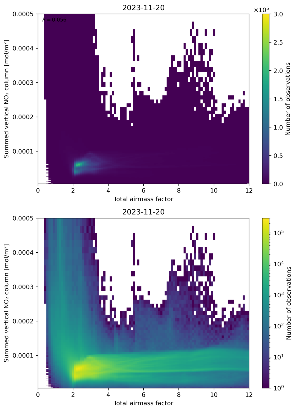
Figure 65: Scatter density plot of “Total airmass factor” against “Summed vertical NO 2 column” for 2023-11-19 to 2023-11-21.
