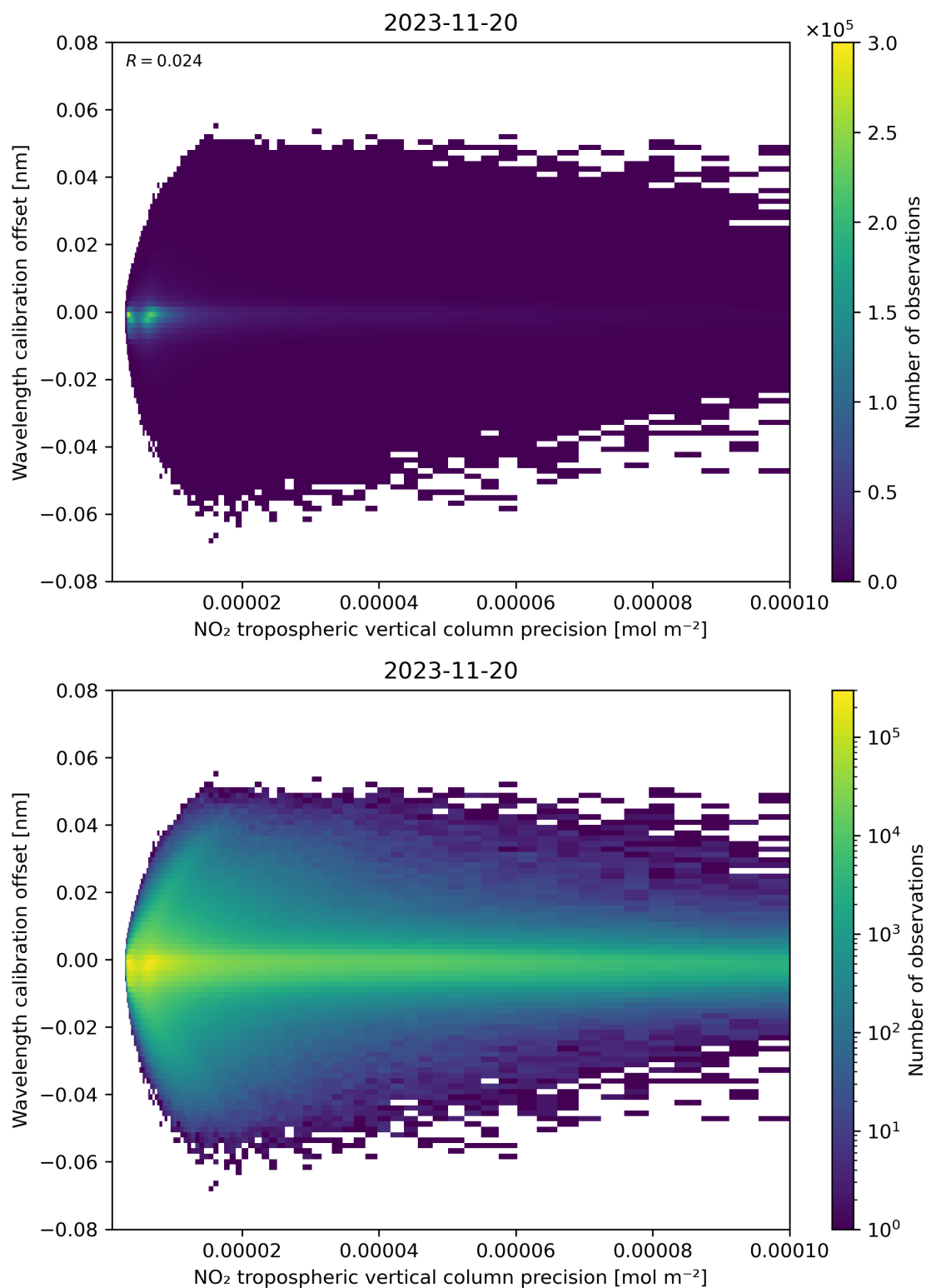
Figure 141: Scatter density plot of “NO 2 tropospheric vertical column precision” against “Wavelength calibration offset” for 2023-11-19 to 2023-11-21.
