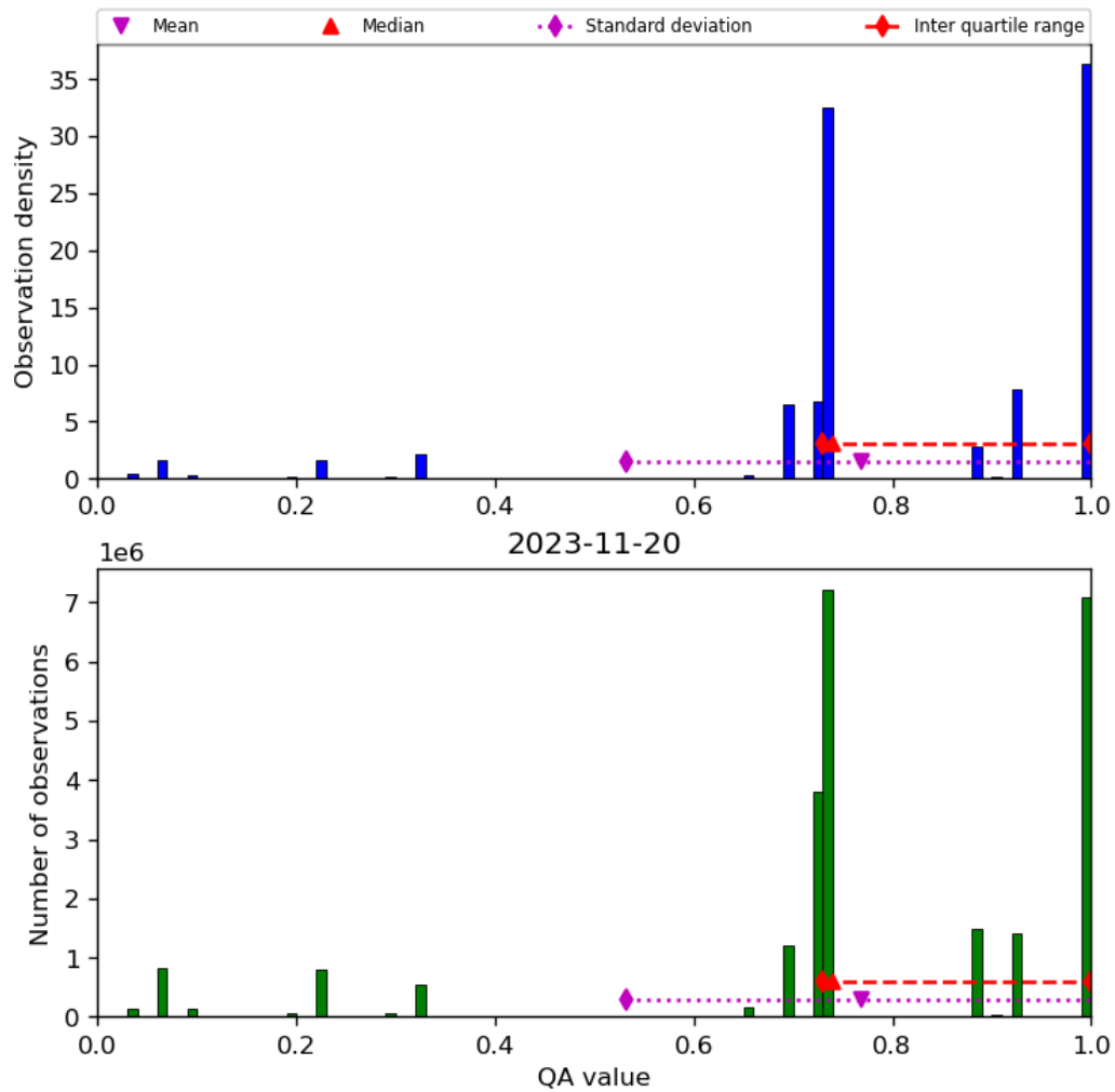
Figure 28: Histogram of “QA value” for 2023-11-19 to 2023-11-21
