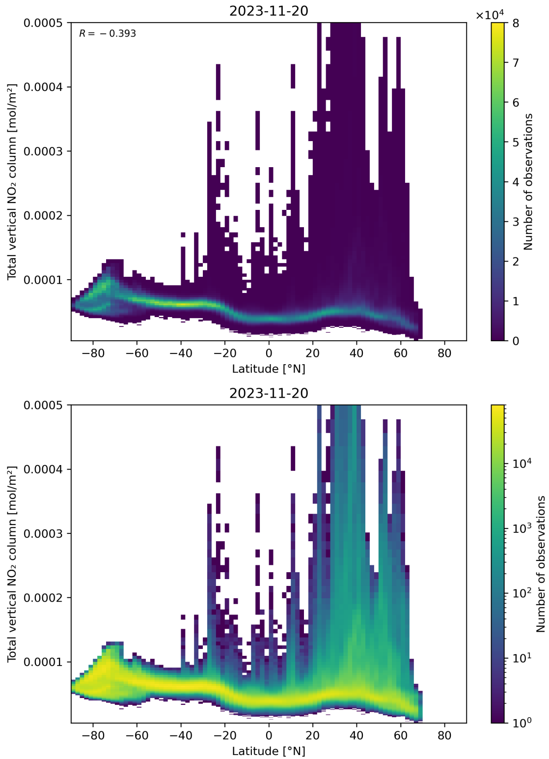
Figure 90: Scatter density plot of “Latitude” against “Total vertical NO 2 column” for 2023-11-19 to 2023-11-21.
