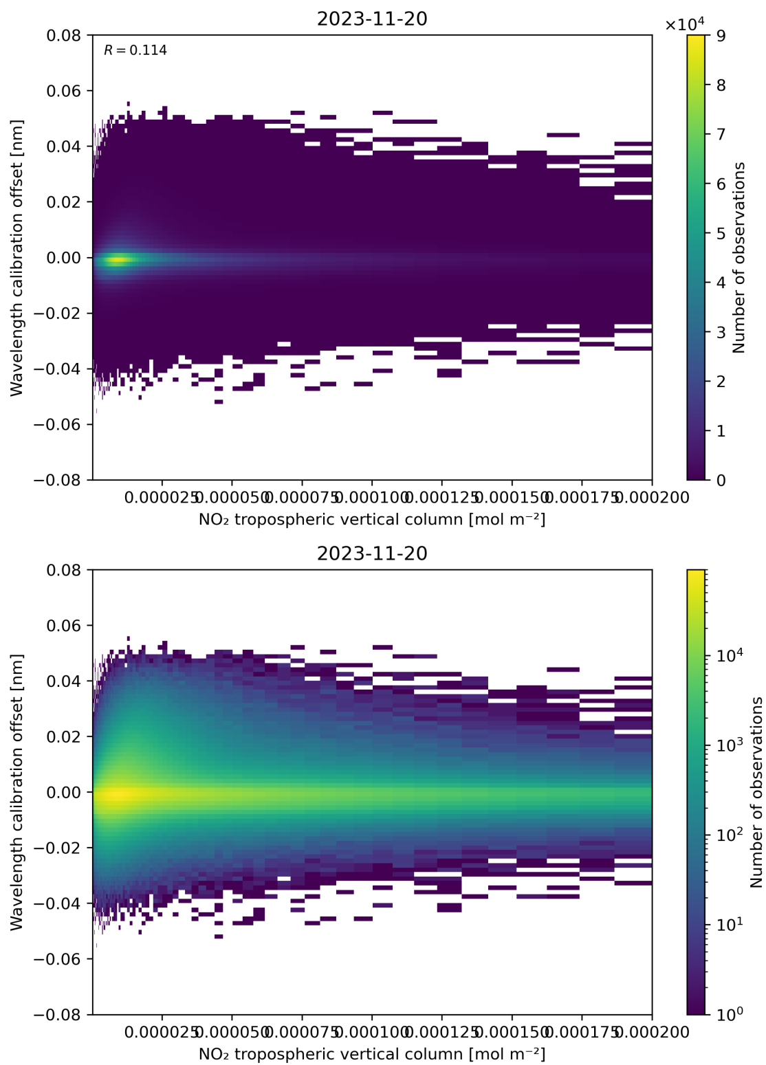
Figure 143: Scatter density plot of “NO 2 tropospheric vertical column” against “Wavelength calibration offset” for 2023-11-19 to 2023-11-21.
