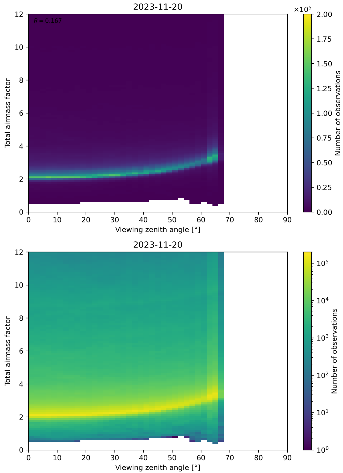
Figure 160: Scatter density plot of “Viewing zenith angle” against “Total airmass factor” for 2023-11-19 to 2023-11-21.
