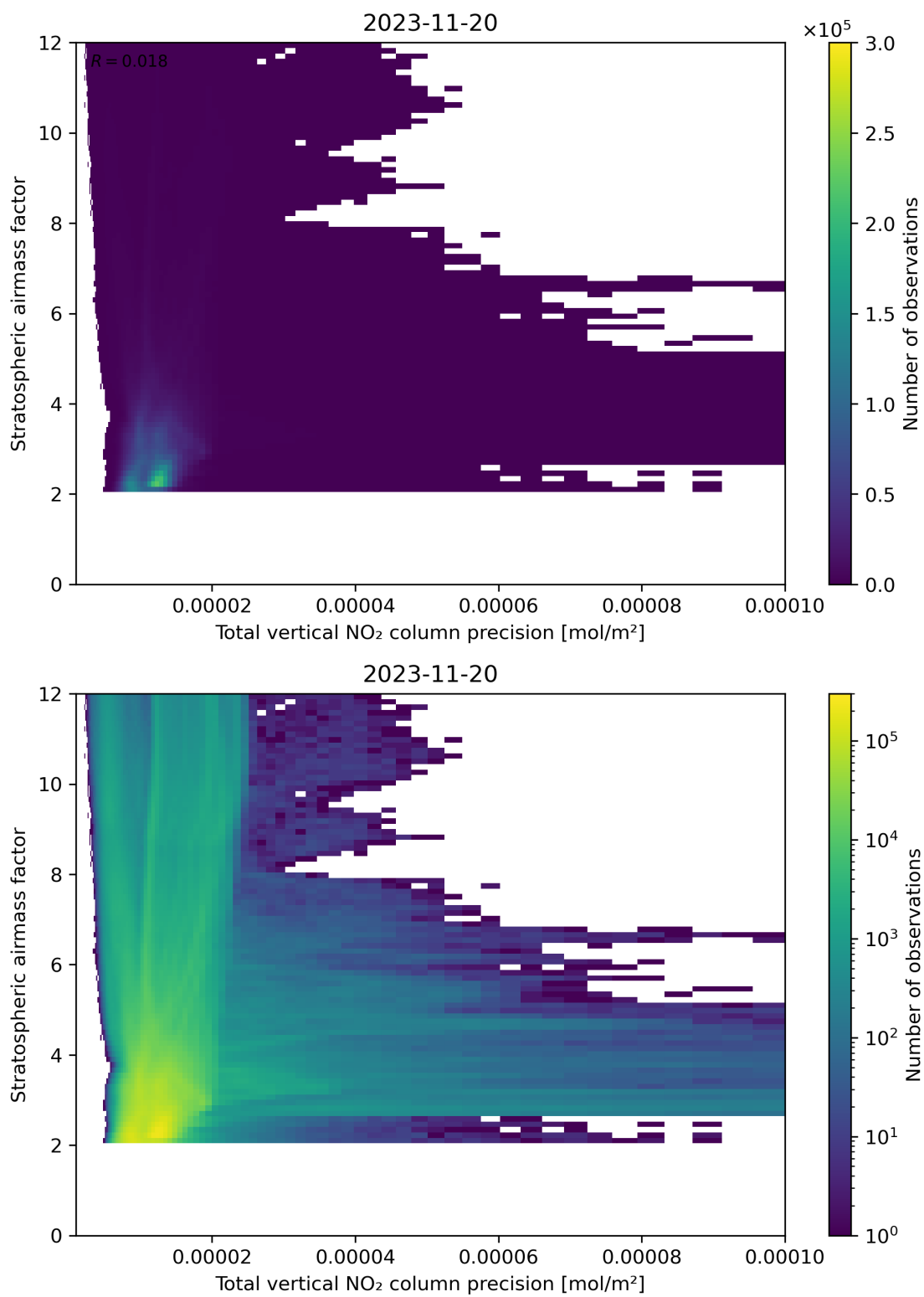
Figure 115: Scatter density plot of “Total vertical NO 2 column precision” against “Stratospheric air mass factor” for 2023-11-19 to 2023-11-21.
