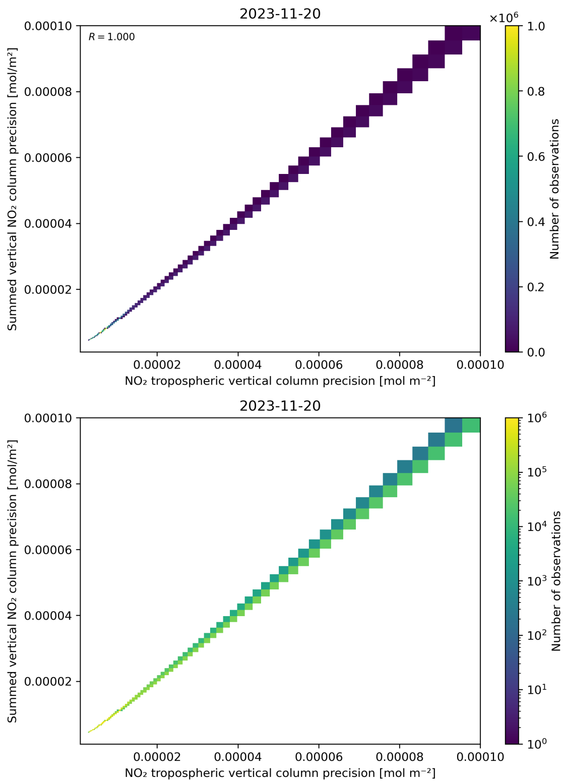
Figure 137: Scatter density plot of “NO 2 tropospheric vertical column precision” against “Summed vertical NO 2 column precision” for 2023-11-19 to 2023-11-21.
