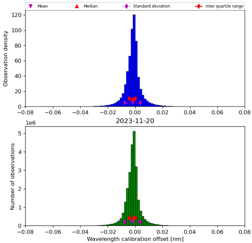
Figure 35: Histogram of “Wavelength calibration offset” for 2023-11-19 to 2023-11-21
