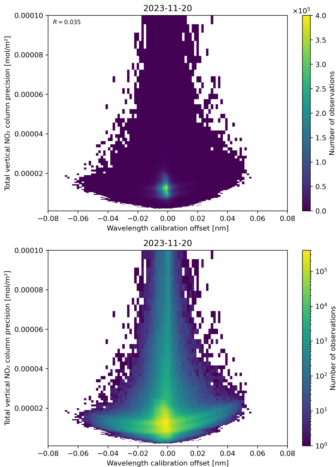
Figure 180: Scatter density plot of “Wavelength calibration offset” against “Total vertical NO 2 column precision” for 2023-11-19 to 2023-11-21.
