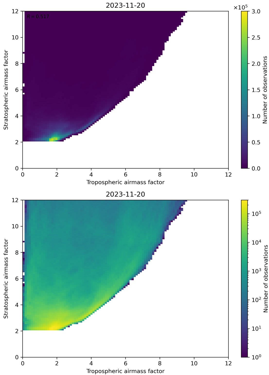
Figure 71: Scatter density plot of “Tropospheric airmass factor” against “Stratospheric airmass factor” for 2023-11-19 to 2023-11-21.
