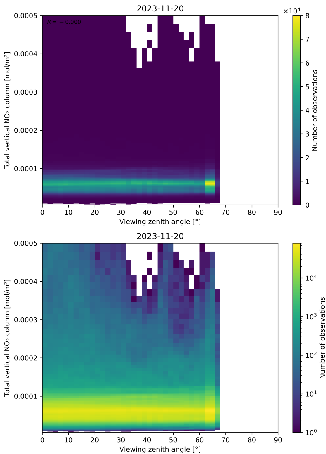
Figure 167: Scatter density plot of “Viewing zenith angle” against “Total vertical NO 2 column” for 2023-11-19 to 2023-11-21.
