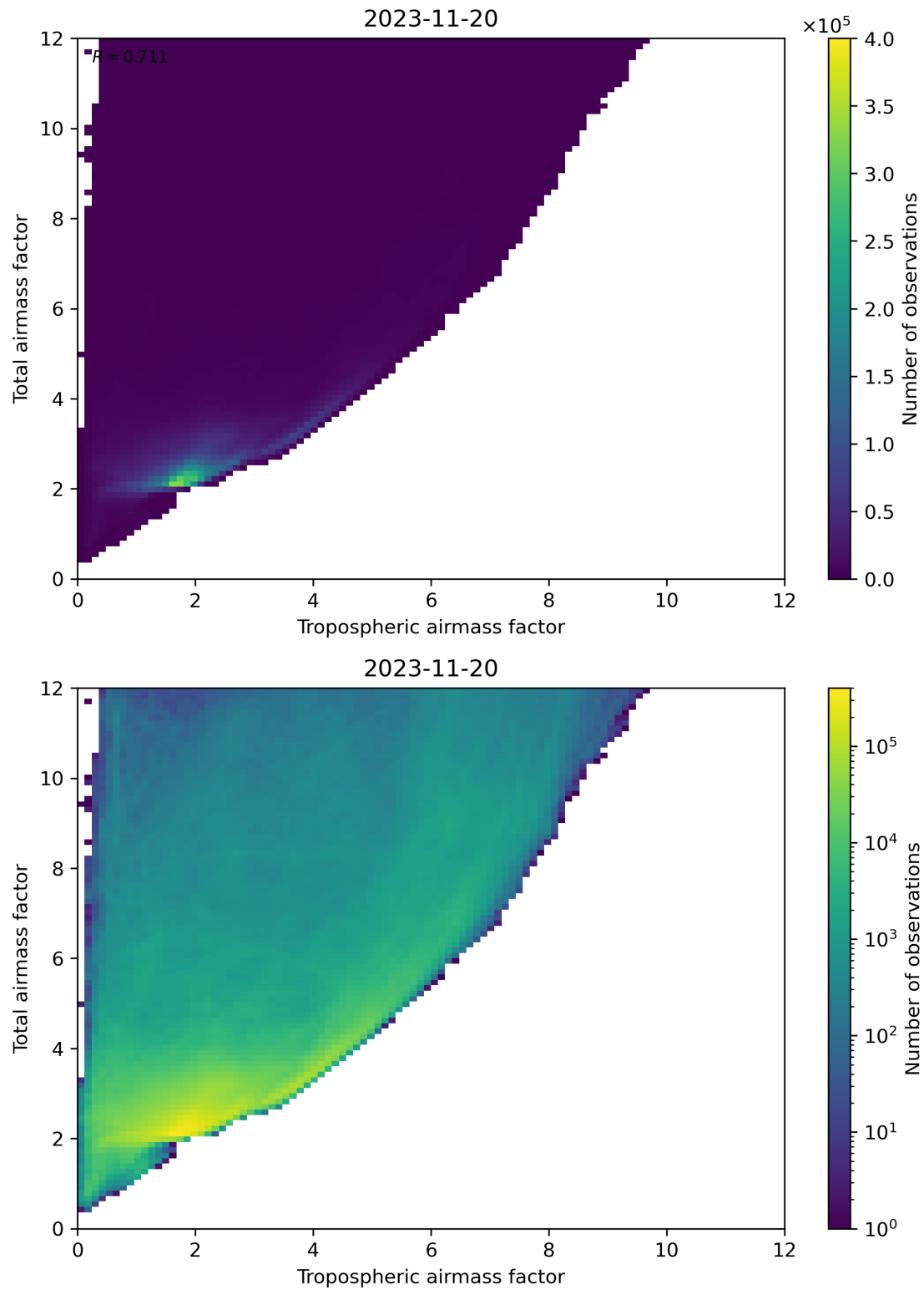
Figure 72: Scatter density plot of “Tropospheric airmass factor” against “Total airmass factor” for 2023-11-19 to 2023-11-21.
