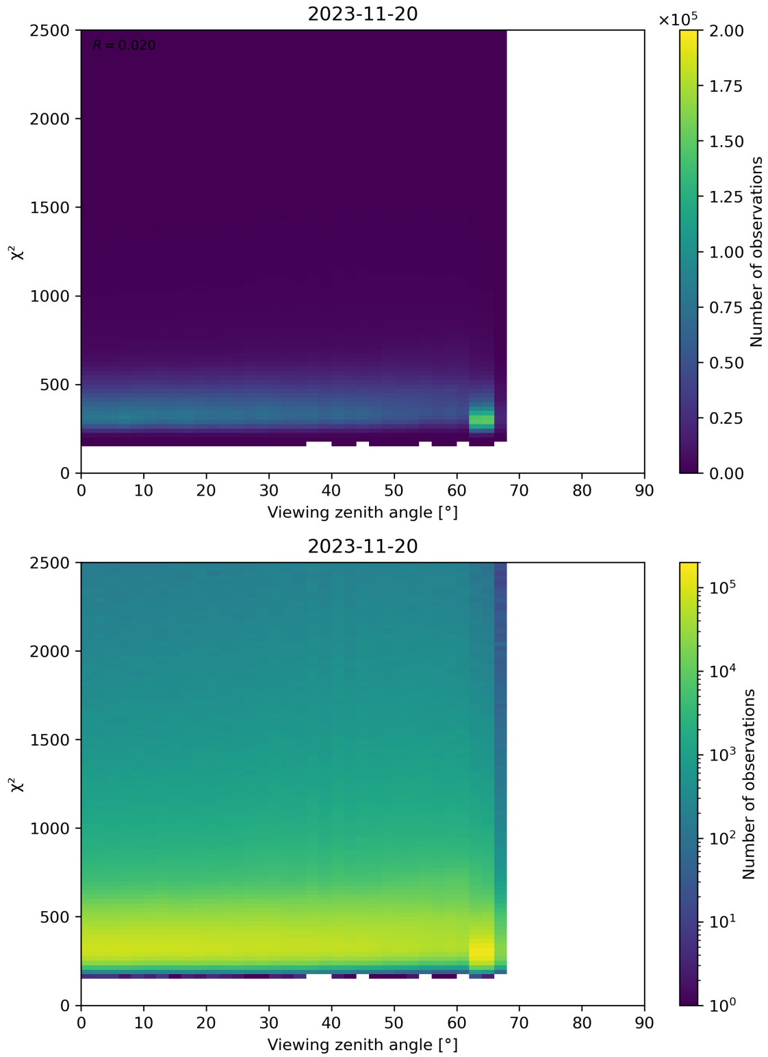
Figure 162: Scatter density plot of “Viewing zenith angle” against “ \chi^2 ” for 2023-11-19 to 2023-11-21.
