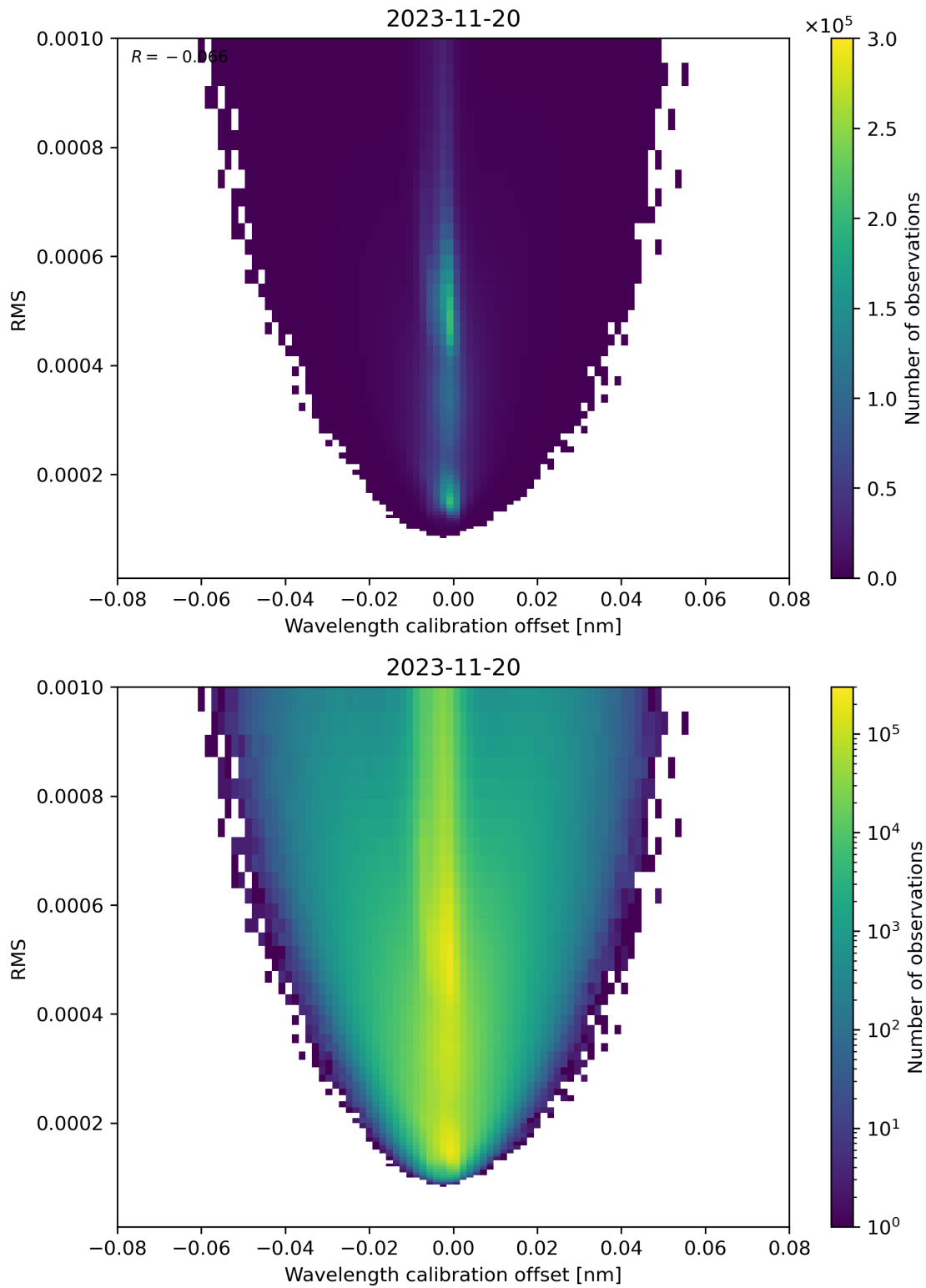
Figure 181: Scatter density plot of “Wavelength calibration offset” against “RMS” for 2023-11-19 to 2023-11-21.
