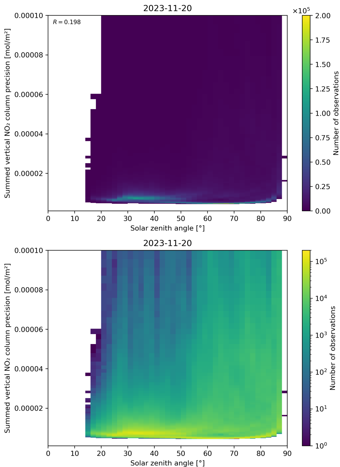
Figure 152: Scatter density plot of “Solar zenith angle” against “Summed vertical NO 2 column precision” for 2023-11-19 to 2023-11-21.
