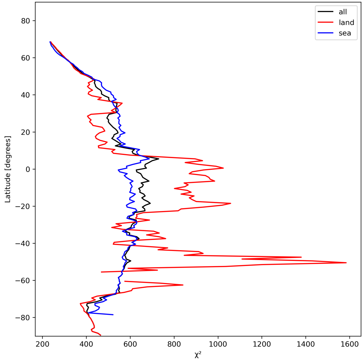
Figure 25: Zonal average of “ \chi^2 ” for 2023-11-19 to 2023-11-21.
