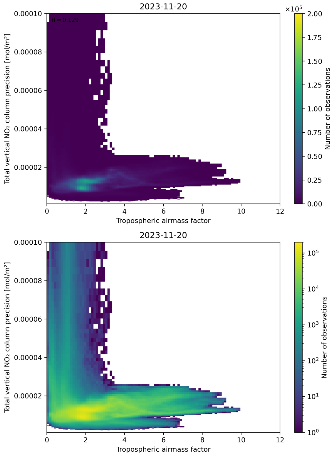
Figure 78: Scatter density plot of “Tropospheric air mass factor” against “Total vertical NO 2 column precision” for 2023-11-19 to 2023-11-21.
