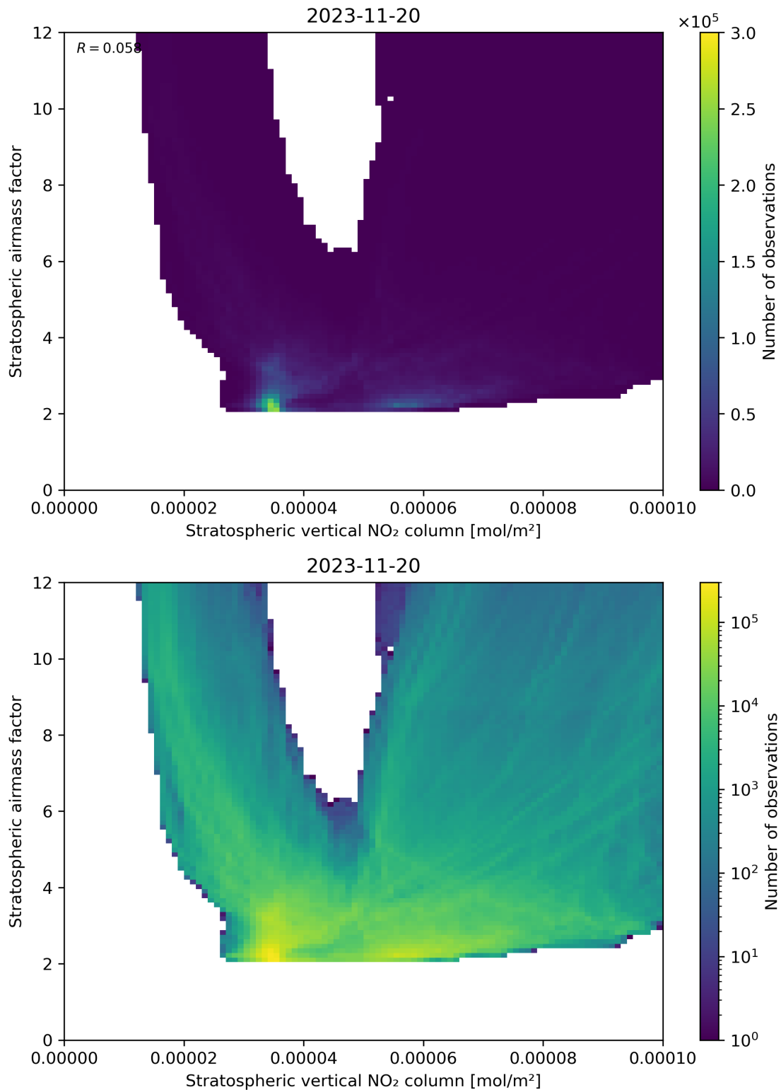
Figure 96: Scatter density plot of “Stratospheric vertical NO 2 column” against “Stratospheric airmass factor” for 2023-11-19 to 2023-11-21.
