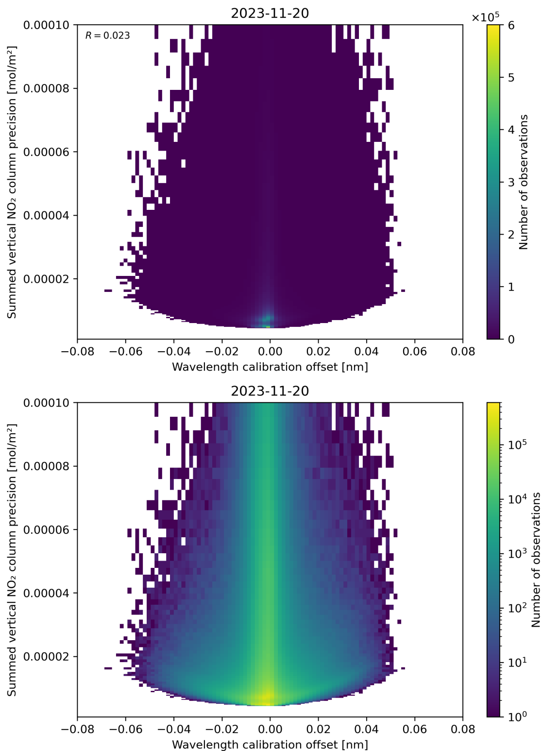
Figure 178: Scatter density plot of “Wavelength calibration offset” against “Summed vertical NO 2 column precision” for 2023-11-19 to 2023-11-21.
