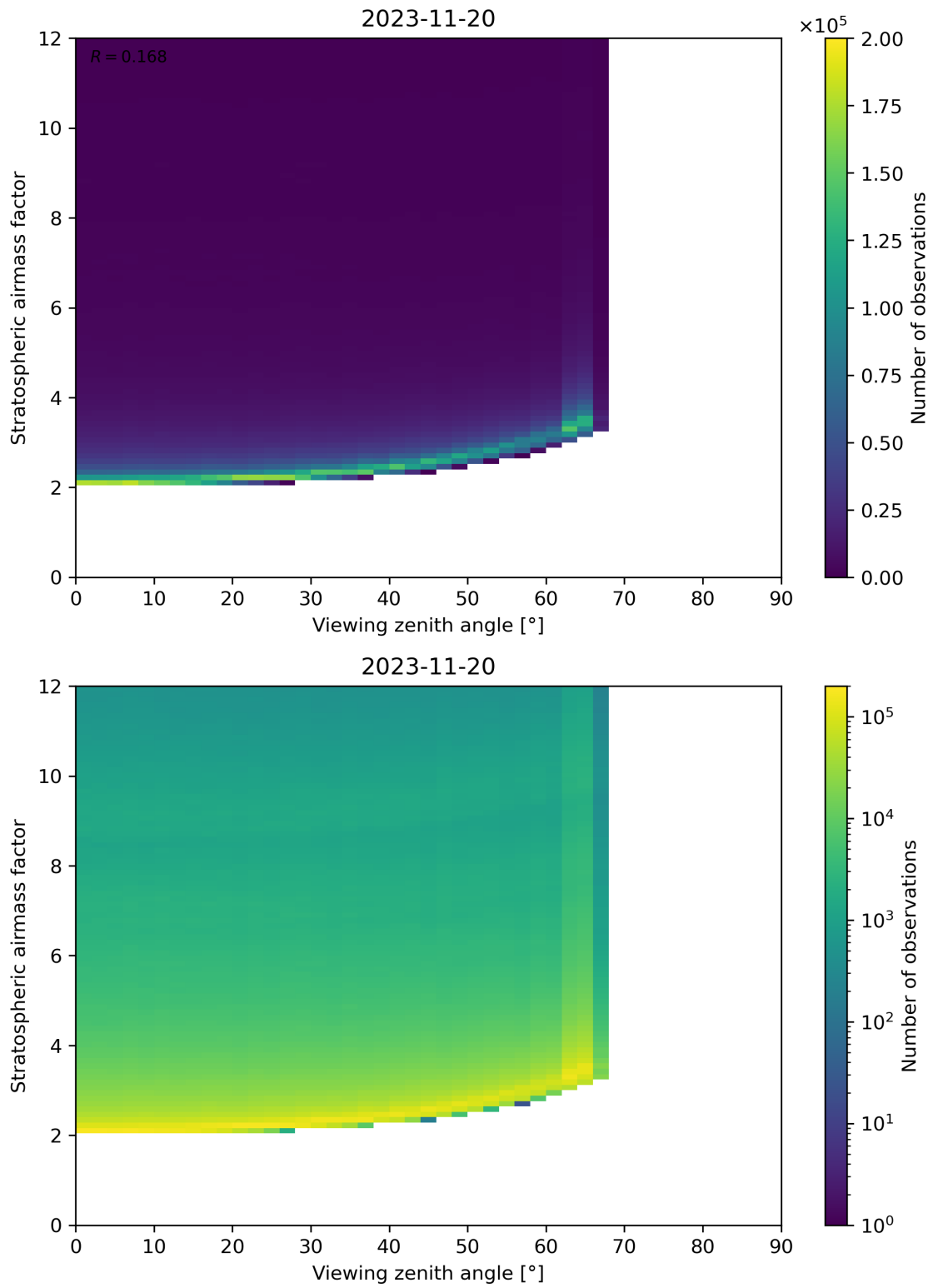
Figure 159: Scatter density plot of “Viewing zenith angle” against “Stratospheric airmass factor” for 2023-11-19 to 2023-11-21.
