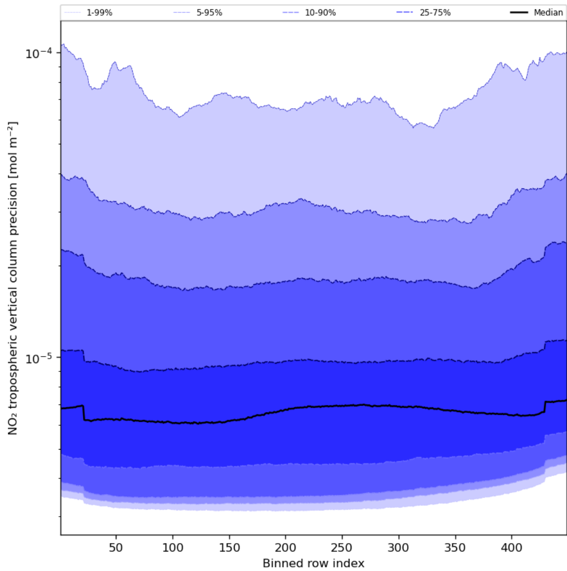
Figure 47: Along track statistics of “NO 2 tropospheric vertical column precision” for 2023-11-19 to 2023-11-21
