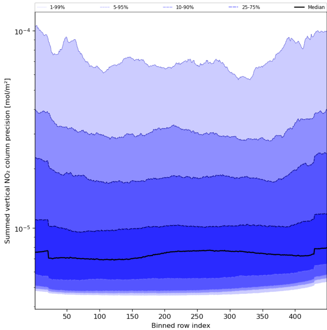
Figure 58: Along track statistics of “Summed vertical NO 2 column precision” for 2023-11-19 to 2023-11-21
