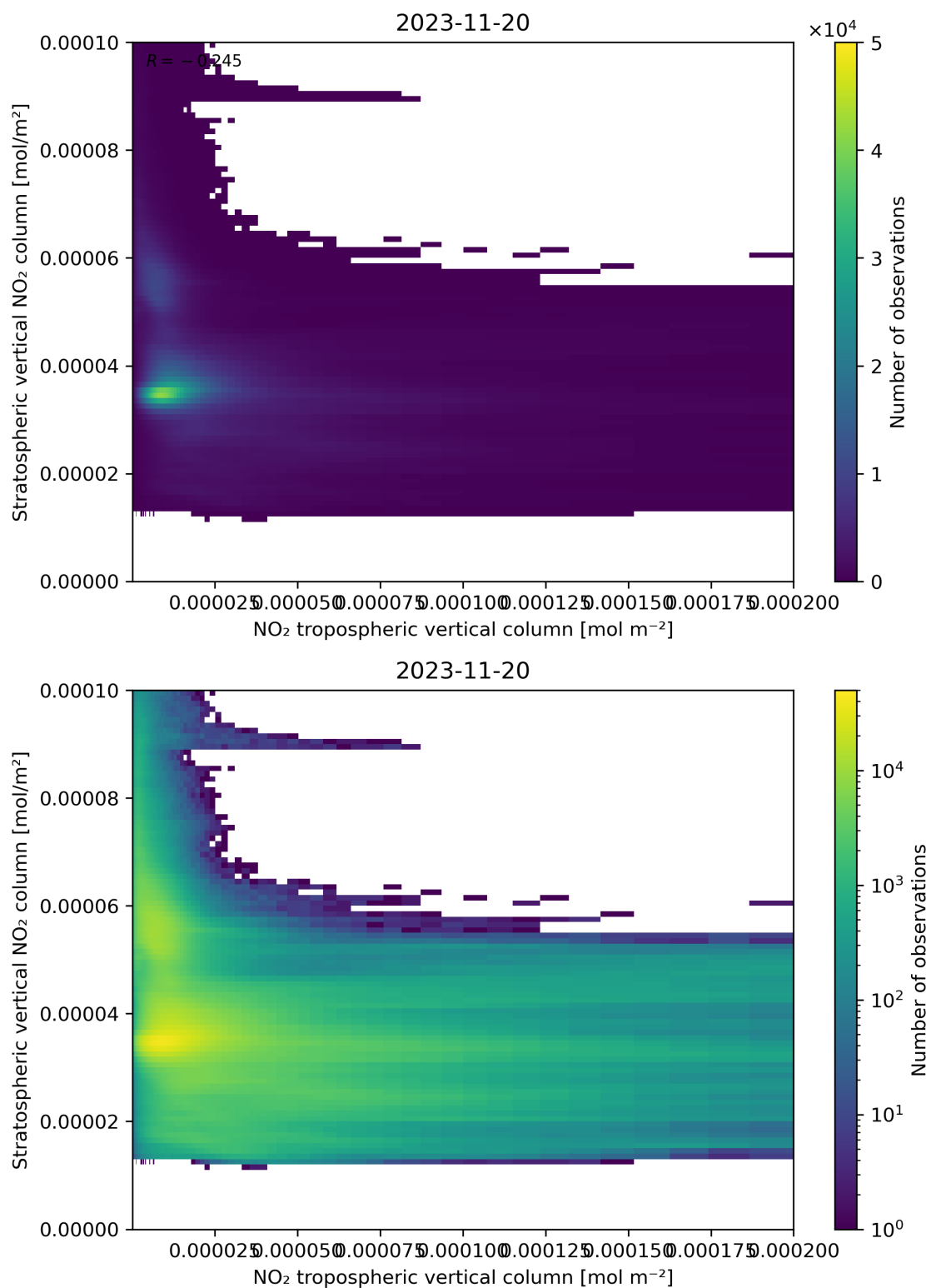
Figure 125: Scatter density plot of “NO 2 tropospheric vertical column” against “Stratospheric vertical NO 2 column” for 2023-11-19 to 2023-11-21.
