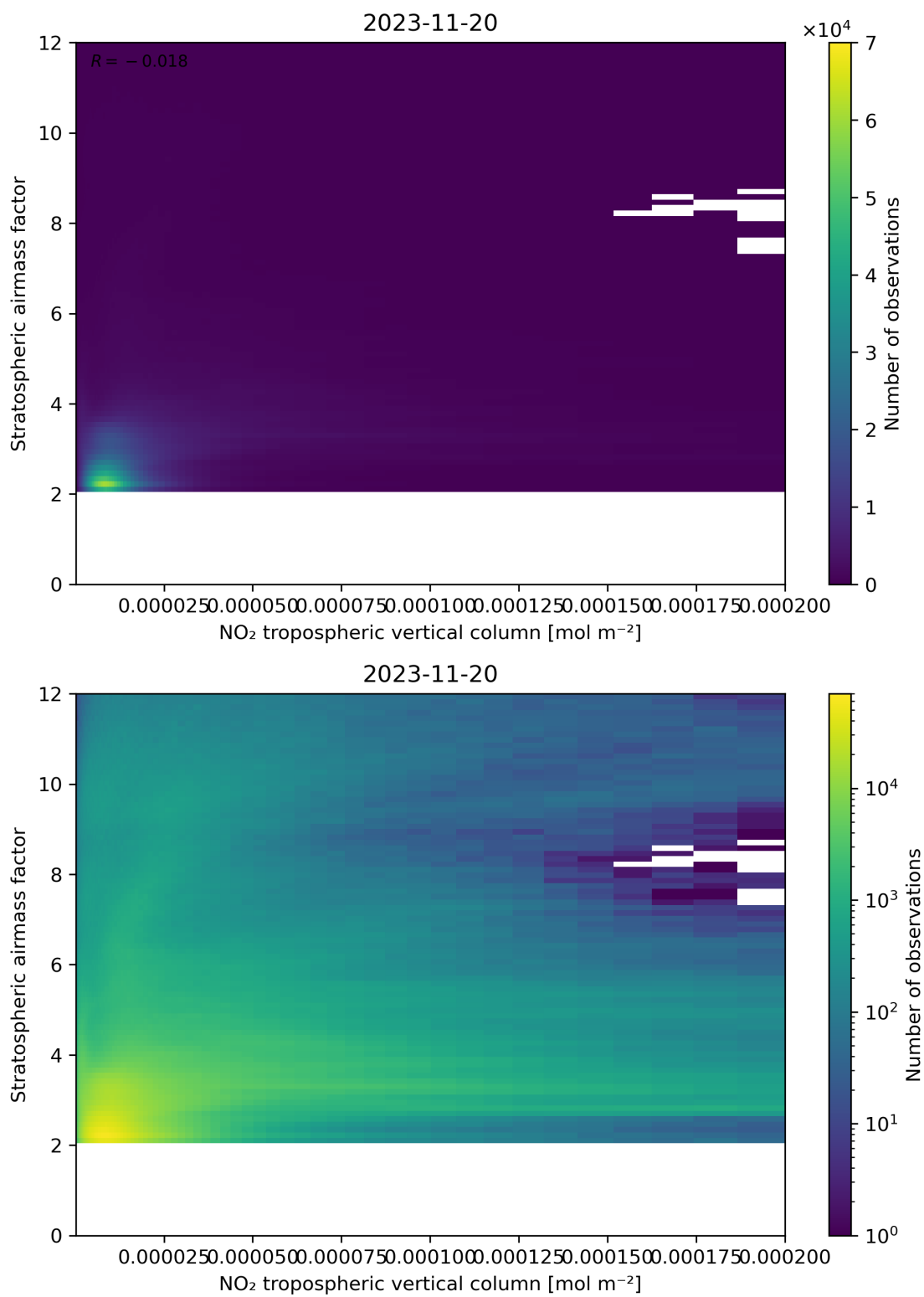
Figure 121: Scatter density plot of “NO 2 tropospheric vertical column” against “Stratospheric air mass factor” for 2023-11-19 to 2023-11-21.
