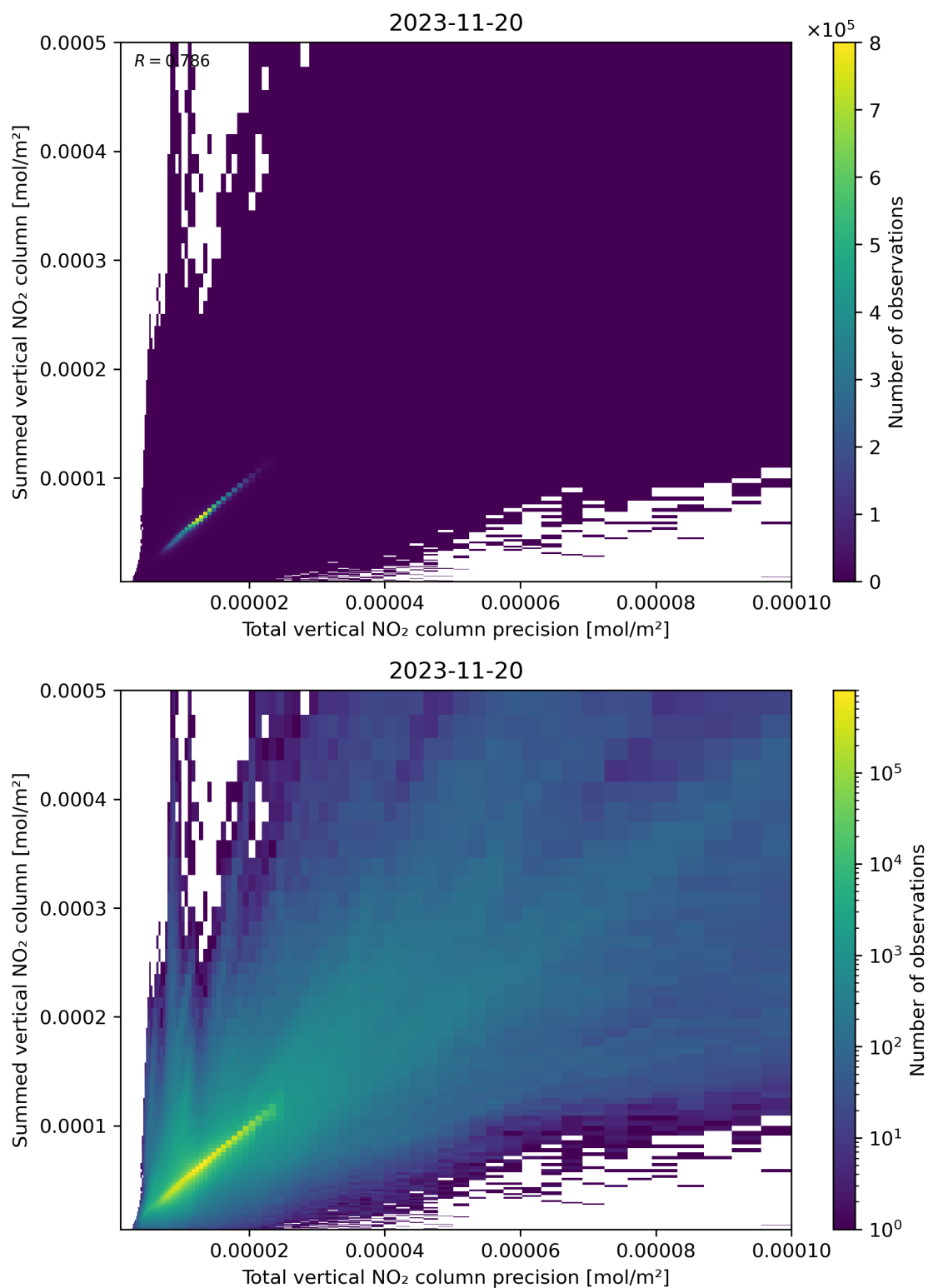
Figure 117: Scatter density plot of “Total vertical NO 2 column precision” against “Summed vertical NO 2 column” for 2023-11-19 to 2023-11-21.
