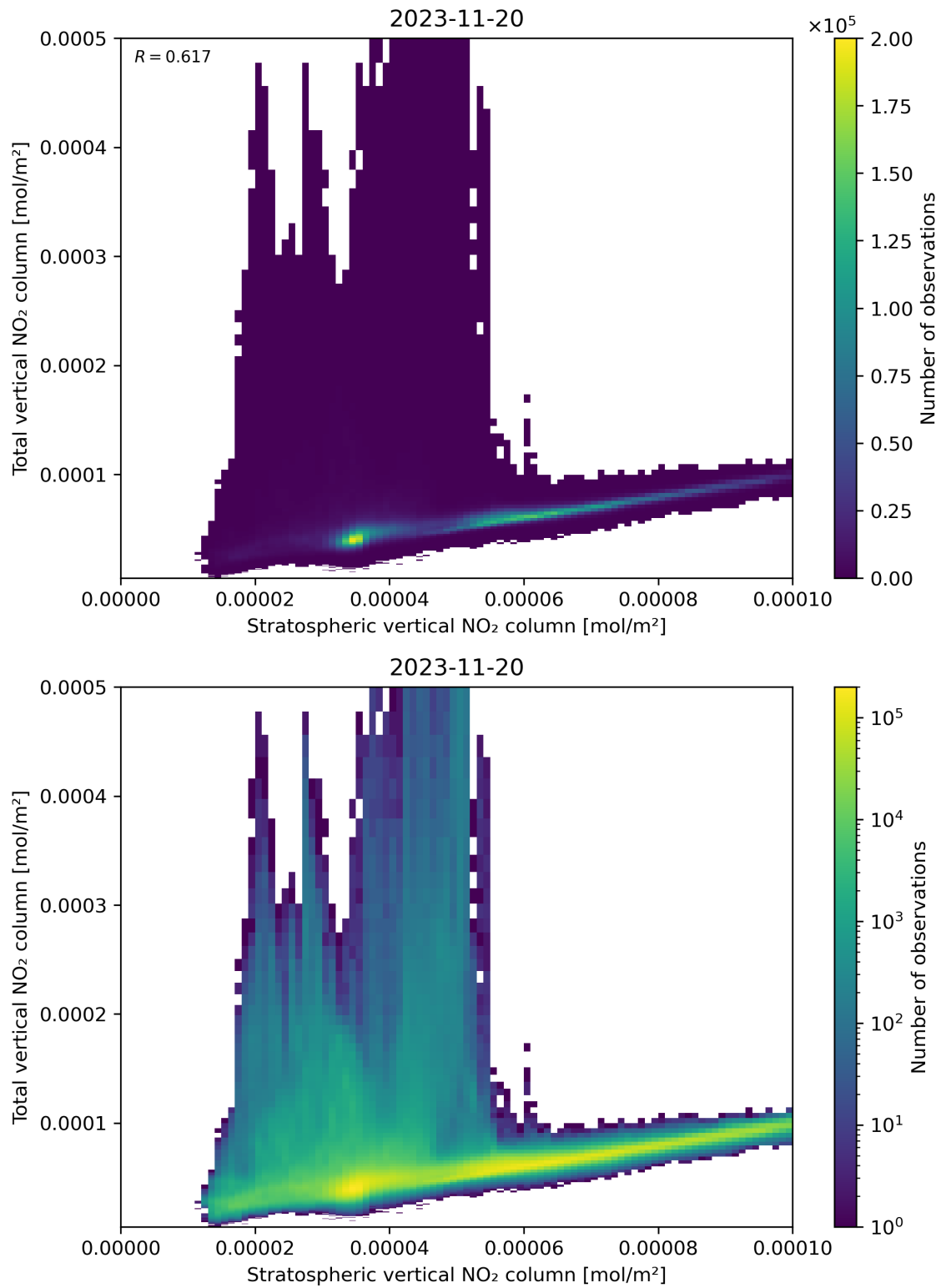
Figure 100: Scatter density plot of “Stratospheric vertical NO 2 column” against “Total vertical NO 2 column” for 2023-11-19 to 2023-11-21.
