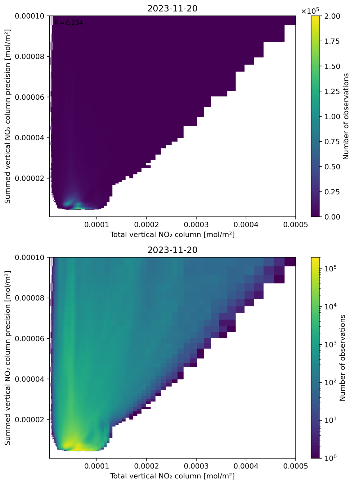
Figure 113: Scatter density plot of “Total vertical NO 2 column” against “Summed vertical NO 2 column precision” for 2023-11-19 to 2023-11-21.
