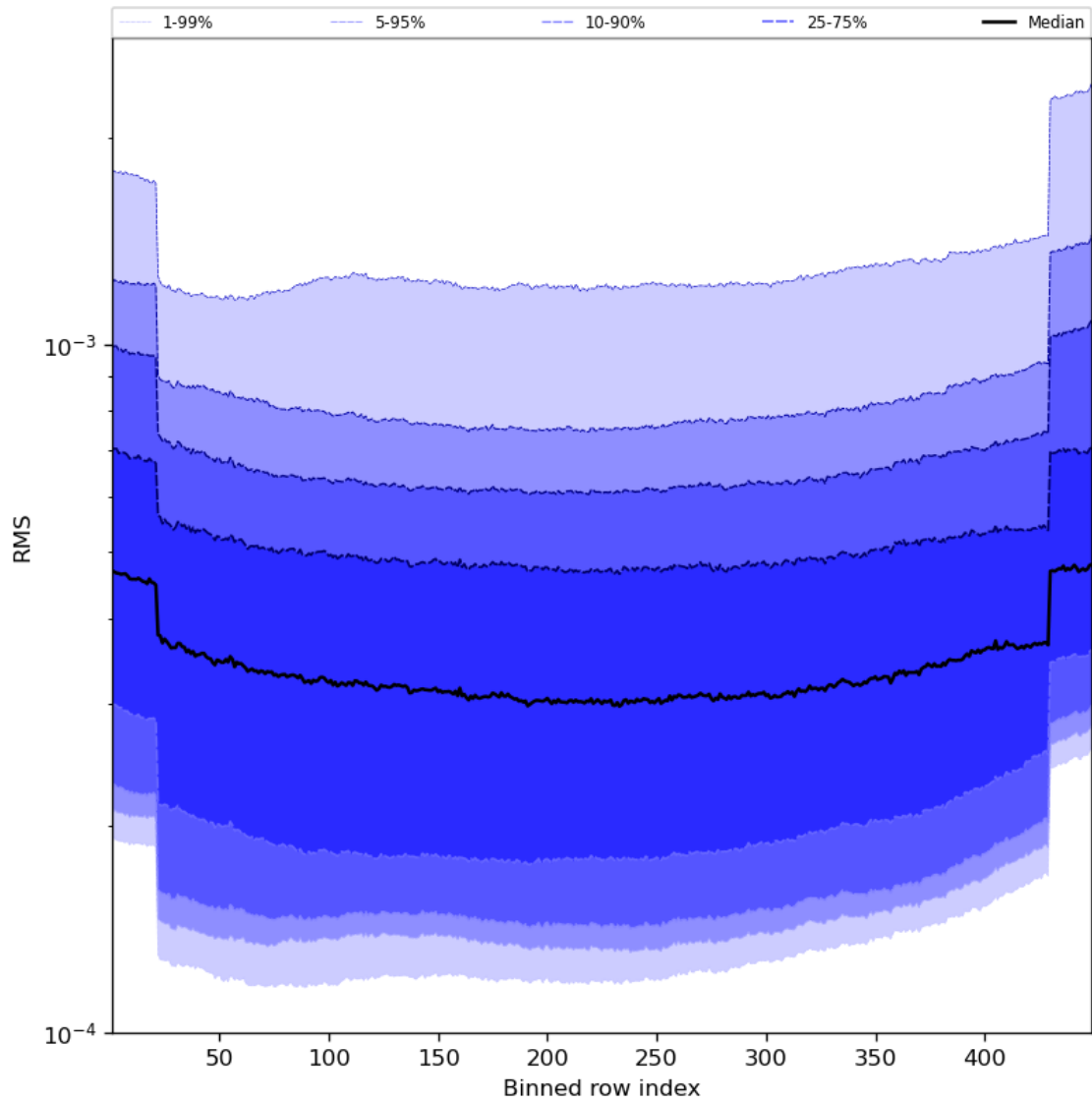
Figure 60: Along track statistics of “RMS” for 2023-11-19 to 2023-11-21
