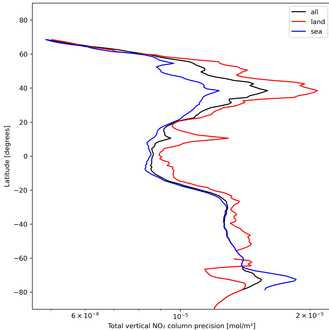
Figure 22: Zonal average of "Total vertical NO 2 column precision" for 2023-11-19 to 2023-11-21.
