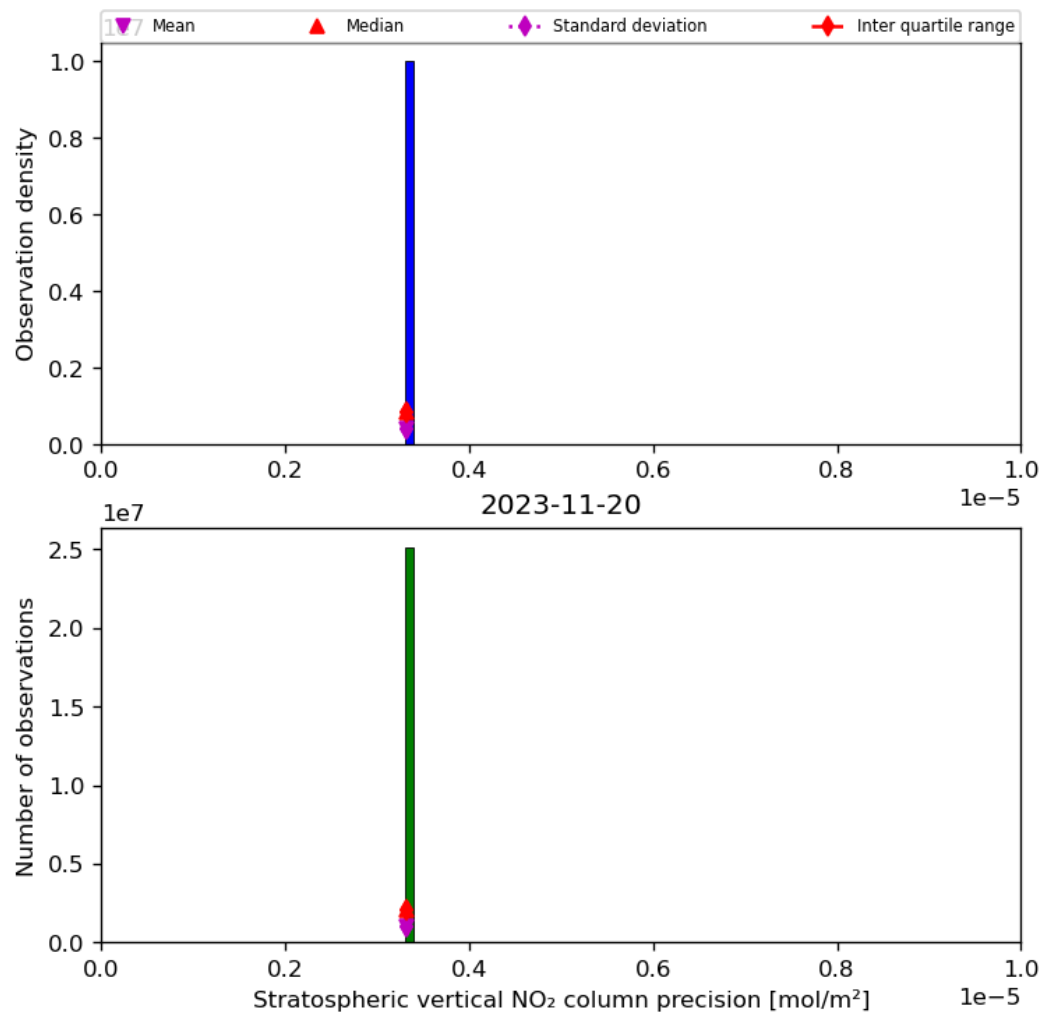
Figure 37: Histogram of “Stratospheric vertical NO 2 column precision” for 2023-11-19 to 2023-11-21
