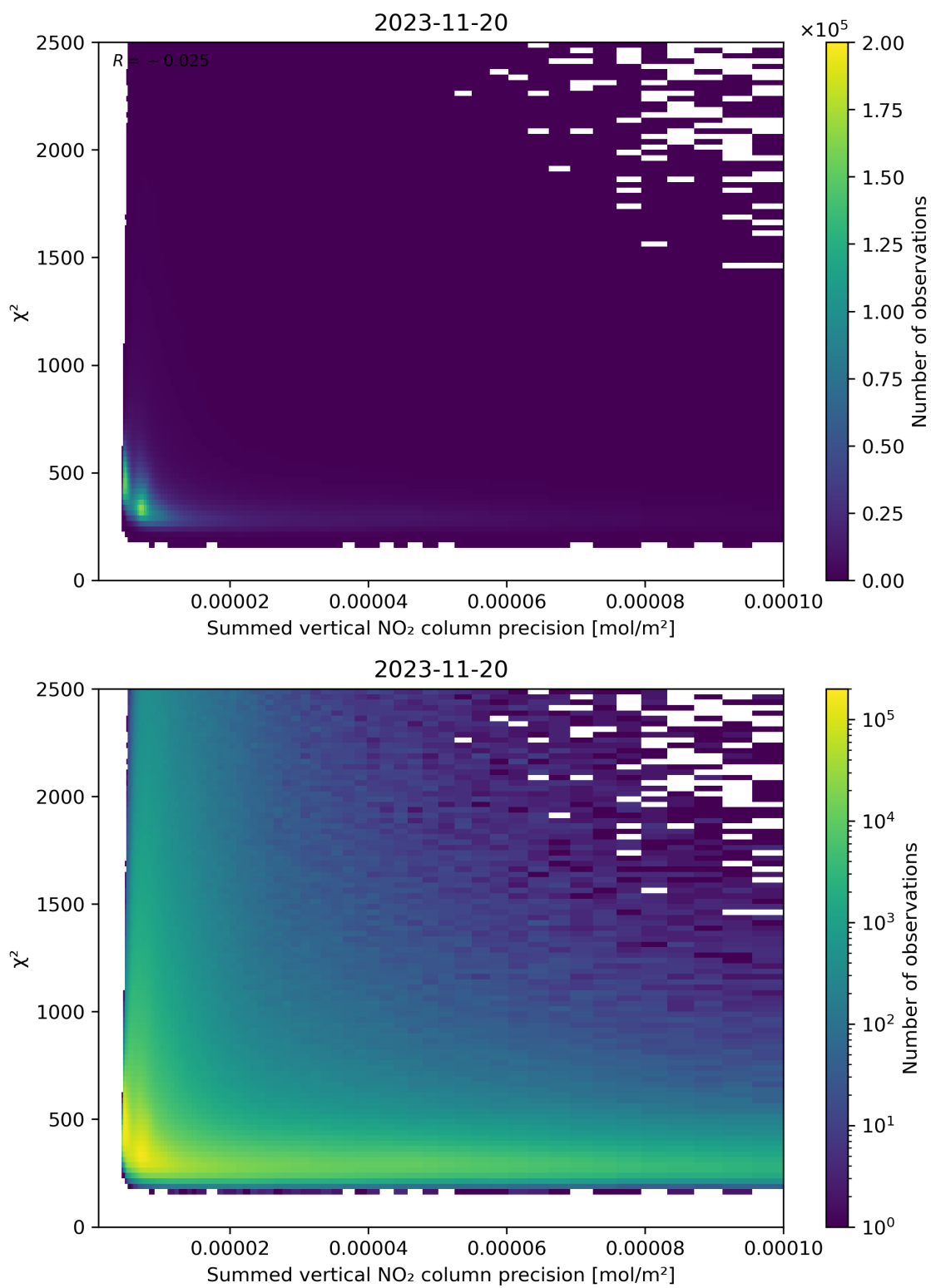
Figure 107: Scatter density plot of “Summed vertical NO 2 column precision” against “ \chi^2 ” for 2023-11-19 to 2023-11-21.
