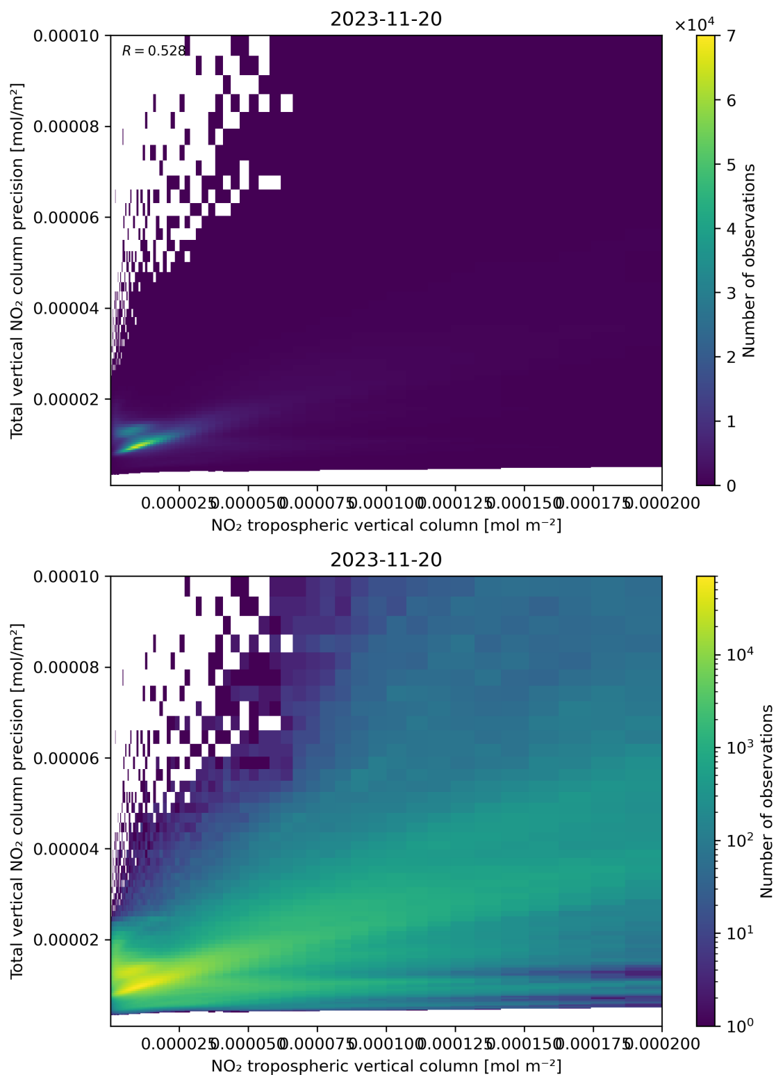
Figure 129: Scatter density plot of “NO 2 tropospheric vertical column” against “Total vertical NO 2 column precision” for 2023-11-19 to 2023-11-21.
