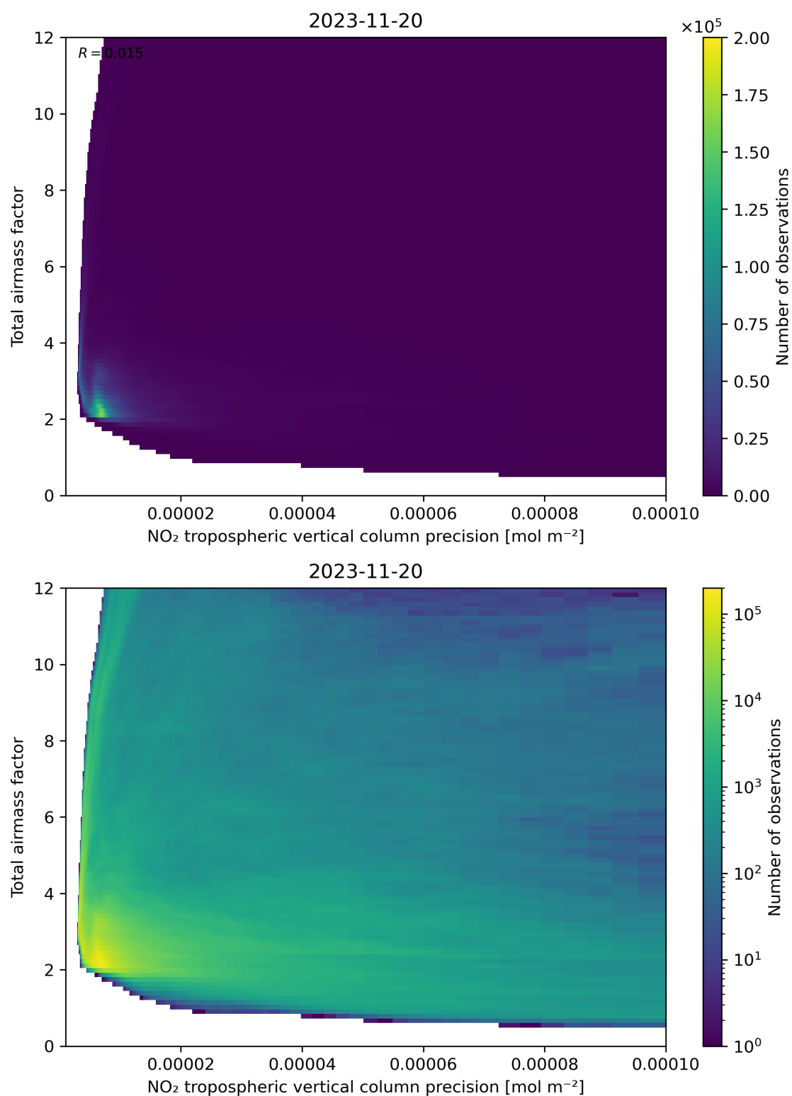
Figure 132: Scatter density plot of “NO 2 tropospheric vertical column precision” against “Total air mass factor” for 2023-11-19 to 2023-11-21.
