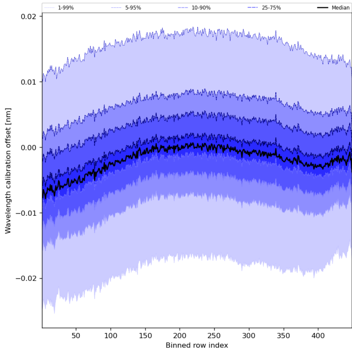
Figure 52: Along track statistics of “Wavelength calibration offset” for 2023-11-19 to 2023-11-21
