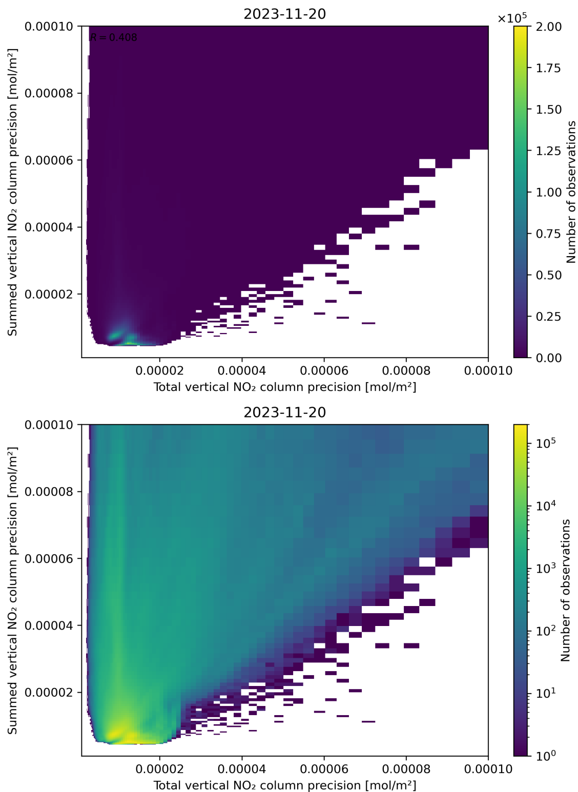
Figure 118: Scatter density plot of “Total vertical NO 2 column precision” against “Summed vertical NO 2 column precision” for 2023-11-19 to 2023-11-21.
