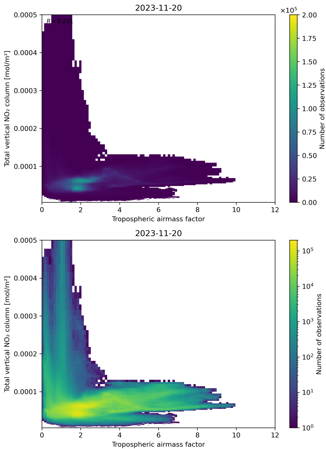
Figure 77: Scatter density plot of “Tropospheric airmass factor” against “Total vertical NO 2 column” for 2023-11-19 to 2023-11-21.
