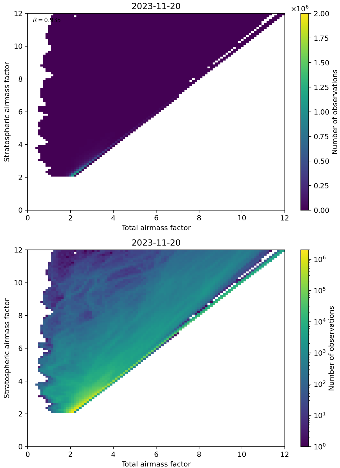
Figure 62: Scatter density plot of “Total airmass factor” against “Stratospheric airmass factor” for 2023-11-19 to 2023-11-21.
