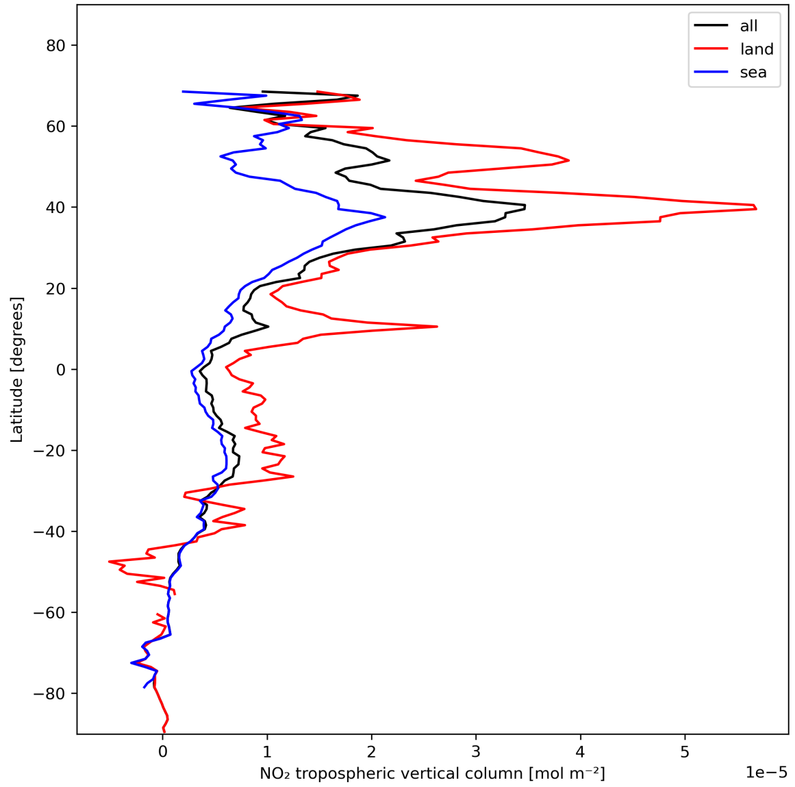
Figure 12: Zonal average of “NO 2 tropospheric vertical column” for 2023-11-19 to 2023-11-21.
