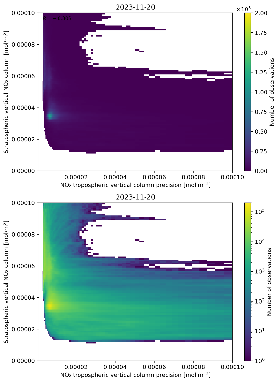
Figure 135: Scatter density plot of “NO 2 tropospheric vertical column precision” against “Stratospheric vertical NO 2 column” for 2023-11-19 to 2023-11-21.
