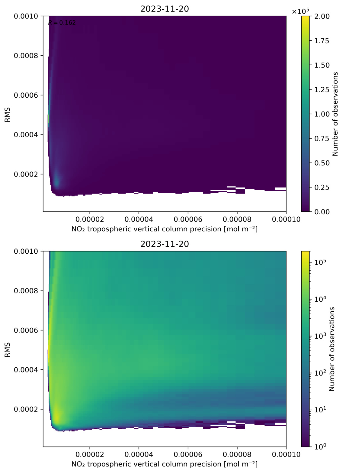
Figure 140: Scatter density plot of “NO 2 tropospheric vertical column precision” against “RMS” for 2023-11-19 to 2023-11-21.
