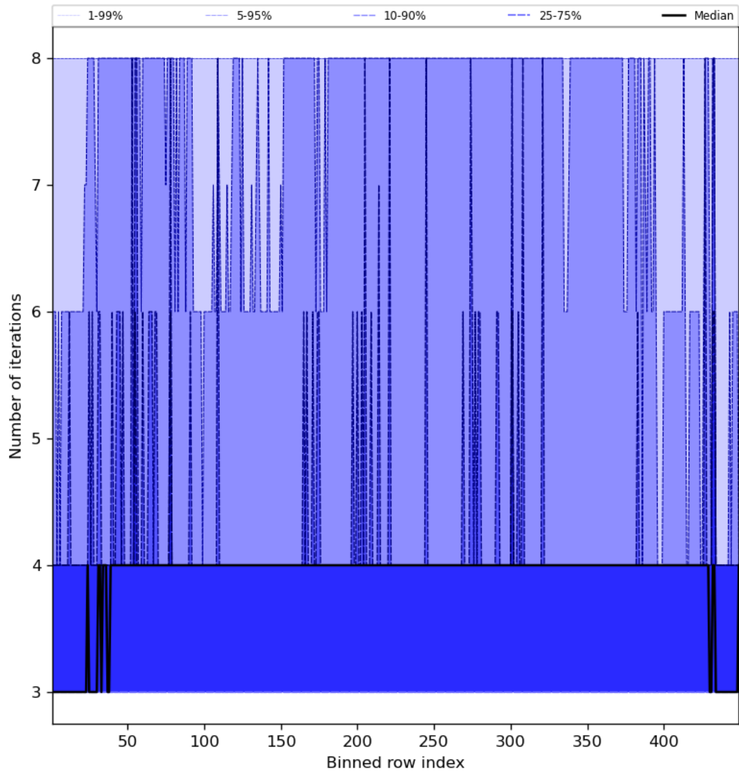
Figure 51: Along track statistics of “Number of iterations” for 2023-11-19 to 2023-11-21
