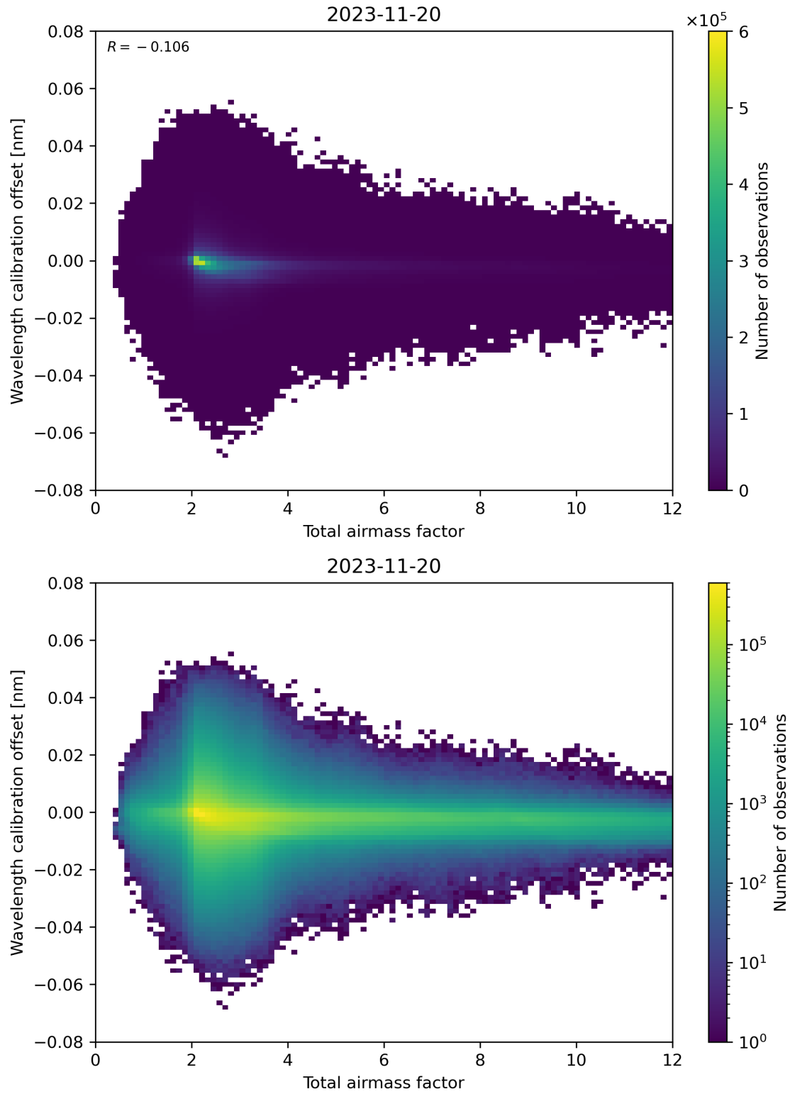
Figure 70: Scatter density plot of “Total airmass factor” against “Wavelength calibration offset” for 2023-11-19 to 2023-11-21.
