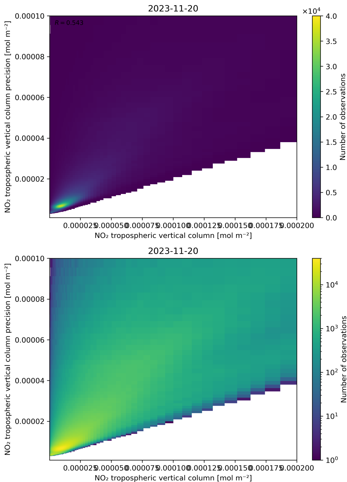
Figure 130: Scatter density plot of “NO 2 tropospheric vertical column” against “NO 2 tropospheric vertical column precision” for 2023-11-19 to 2023-11-21.
