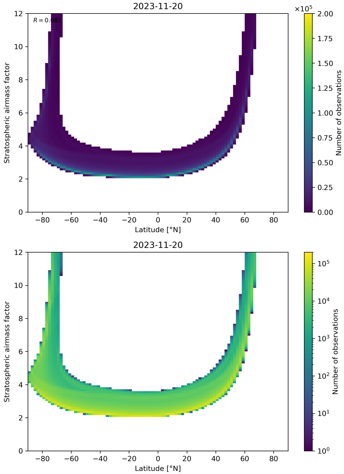
Figure 83: Scatter density plot of “Latitude” against “Stratospheric air mass factor” for 2023-11-19 to 2023-11-21.
