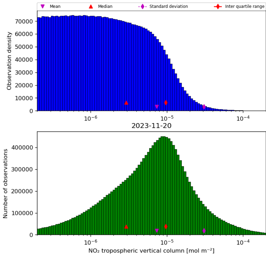
Figure 29: Histogram of “NO 2 tropospheric vertical column” for 2023-11-19 to 2023-11-21
