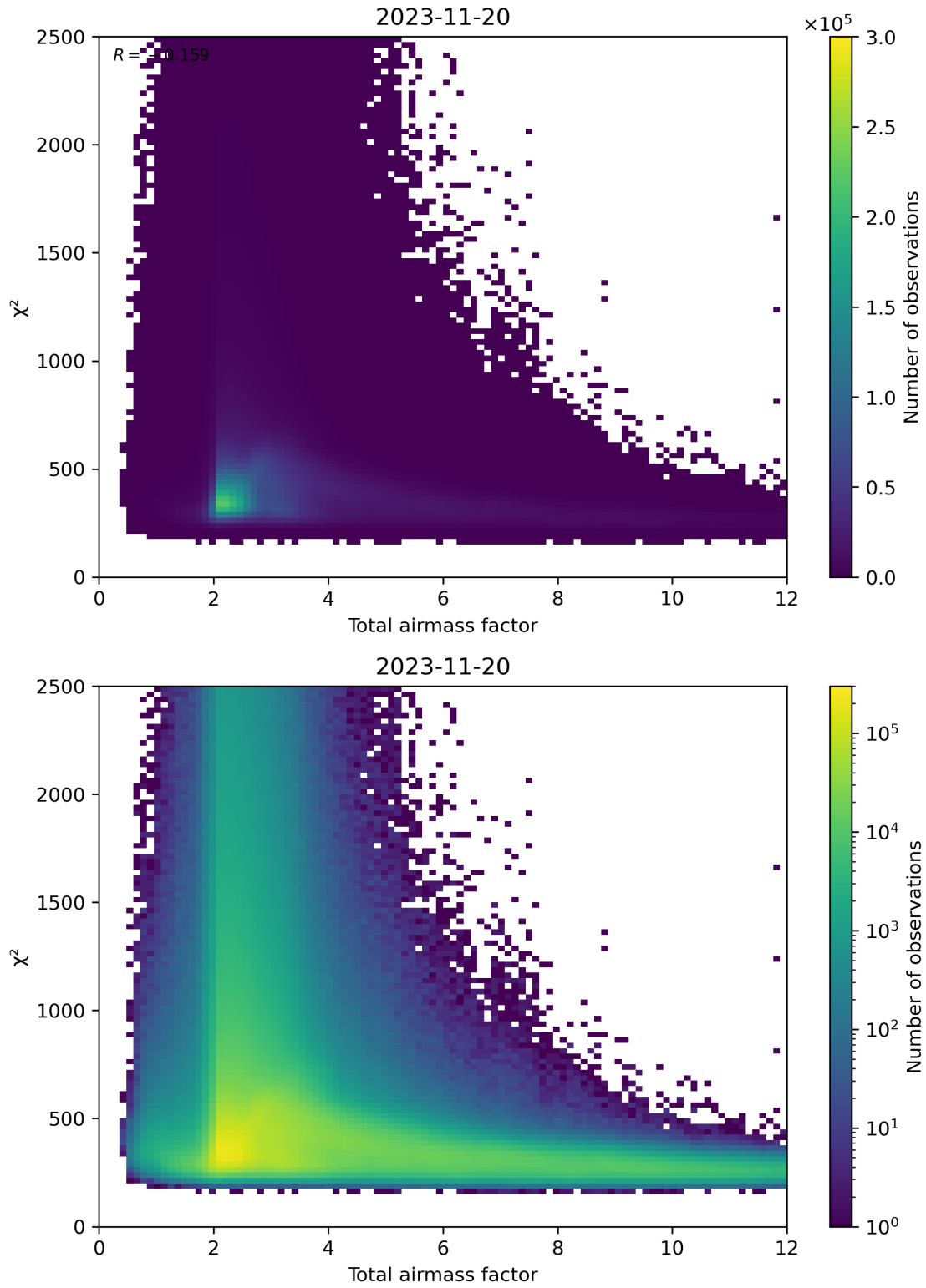
Figure 63: Scatter density plot of “Total airmass factor” against “ \chi^2 ” for 2023-11-19 to 2023-11-21.
