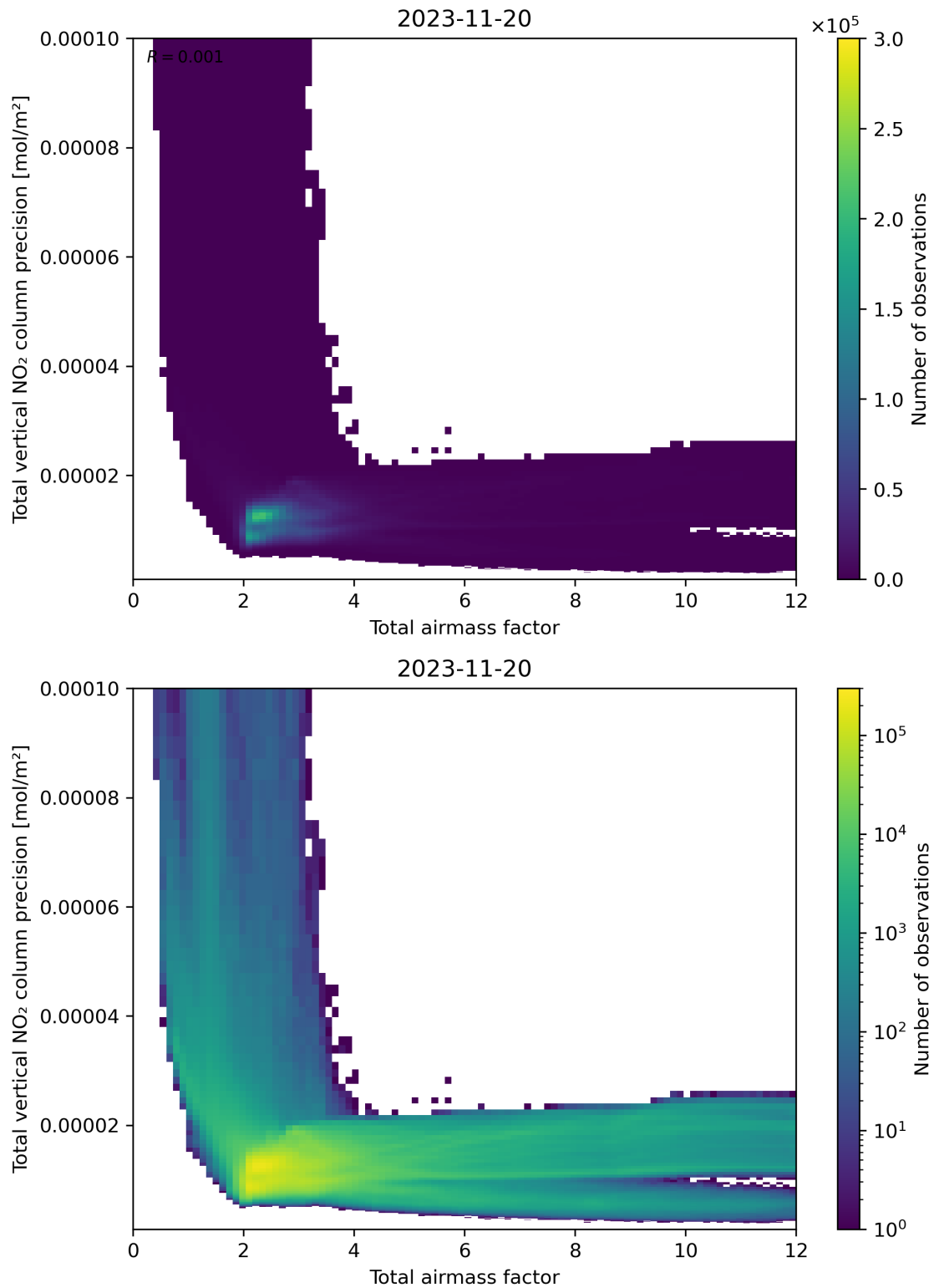
Figure 68: Scatter density plot of “Total airmass factor” against “Total vertical NO 2 column precision” for 2023-11-19 to 2023-11-21.
