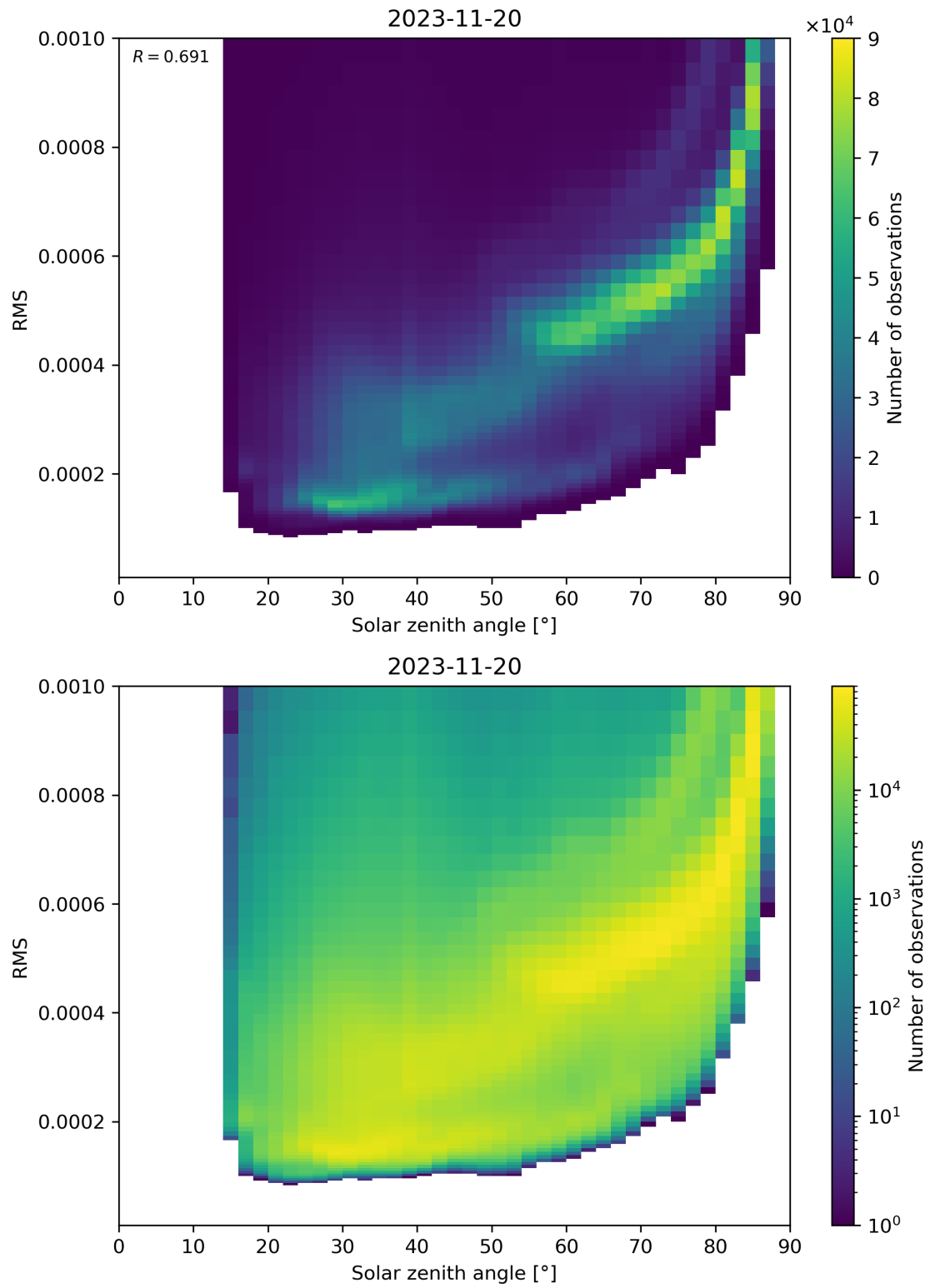
Figure 157: Scatter density plot of “Solar zenith angle” against “RMS” for 2023-11-19 to 2023-11-21.
