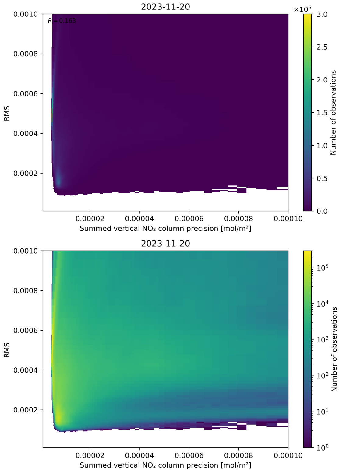
Figure 108: Scatter density plot of “Summed vertical NO 2 column precision” against “RMS” for 2023-11-19 to 2023-11-21.
