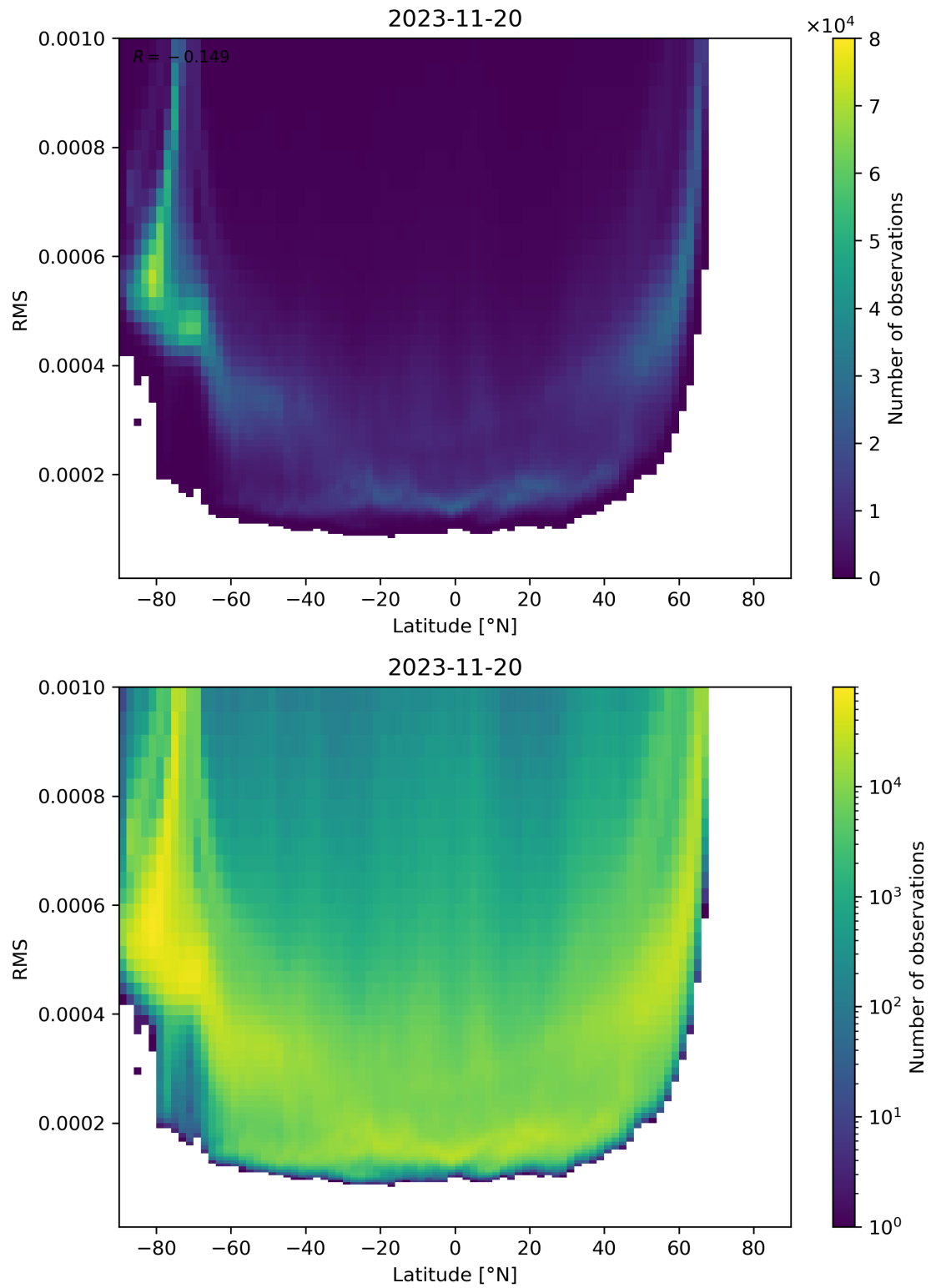
Figure 94: Scatter density plot of “Latitude” against “RMS” for 2023-11-19 to 2023-11-21.
