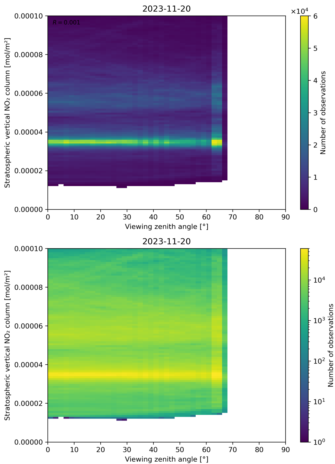
Figure 164: Scatter density plot of “Viewing zenith angle” against “Stratospheric vertical NO 2 column” for 2023-11-19 to 2023-11-21.
