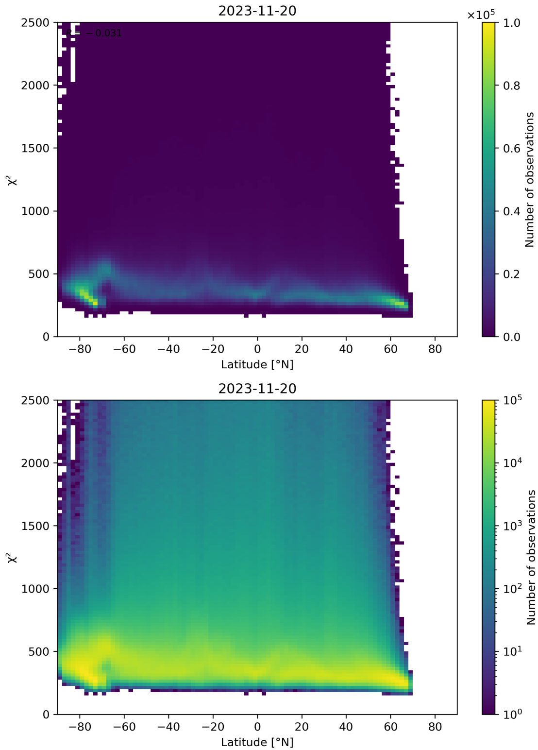
Figure 86: Scatter density plot of “Latitude” against “ \chi^2 ” for 2023-11-19 to 2023-11-21.
