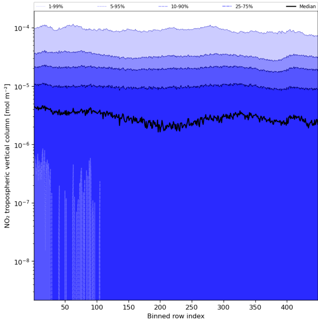
Figure 46: Along track statistics of “NO 2 tropospheric vertical column” for 2023-11-19 to 2023-11-21
