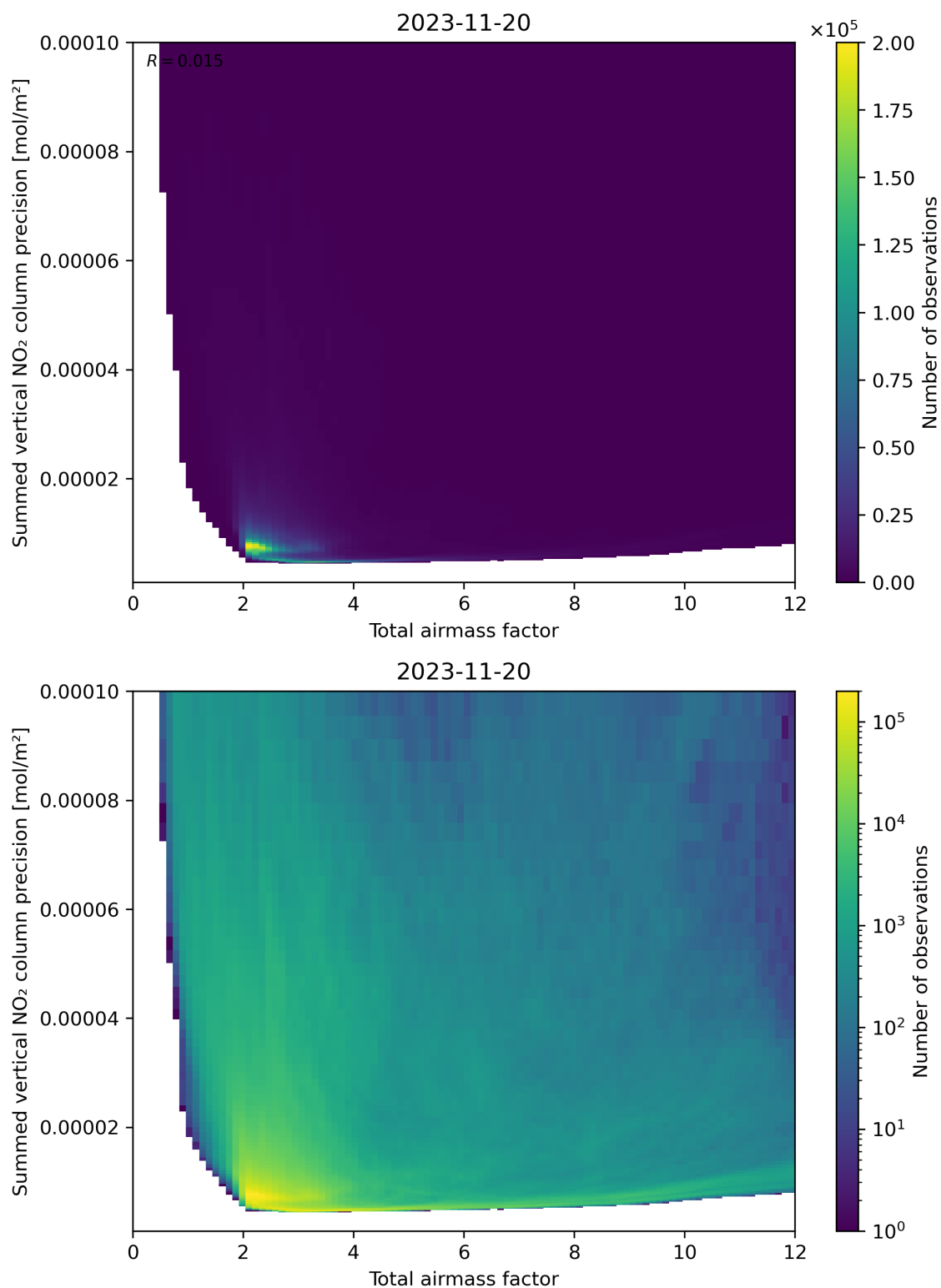
Figure 66: Scatter density plot of “Total airmass factor” against “Summed vertical NO 2 column precision” for 2023-11-19 to 2023-11-21.
