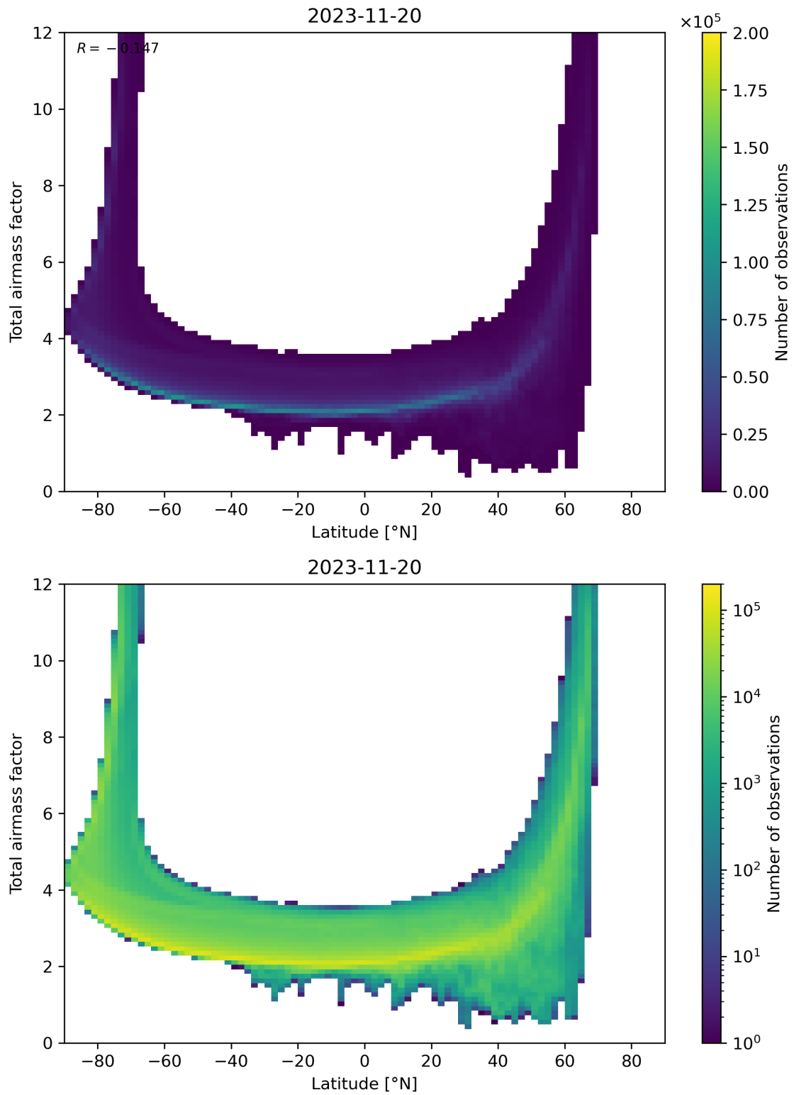
Figure 84: Scatter density plot of “Latitude” against “Total airmass factor” for 2023-11-19 to 2023-11-21.
