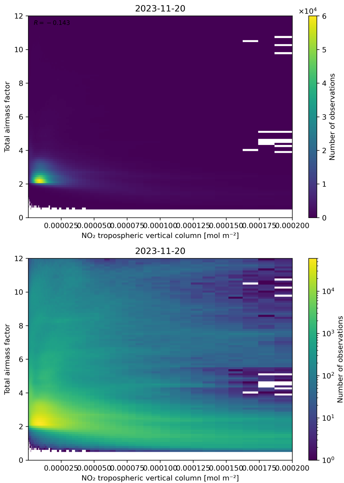
Figure 122: Scatter density plot of “NO 2 tropospheric vertical column” against “Total air mass factor” for 2023-11-19 to 2023-11-21.
