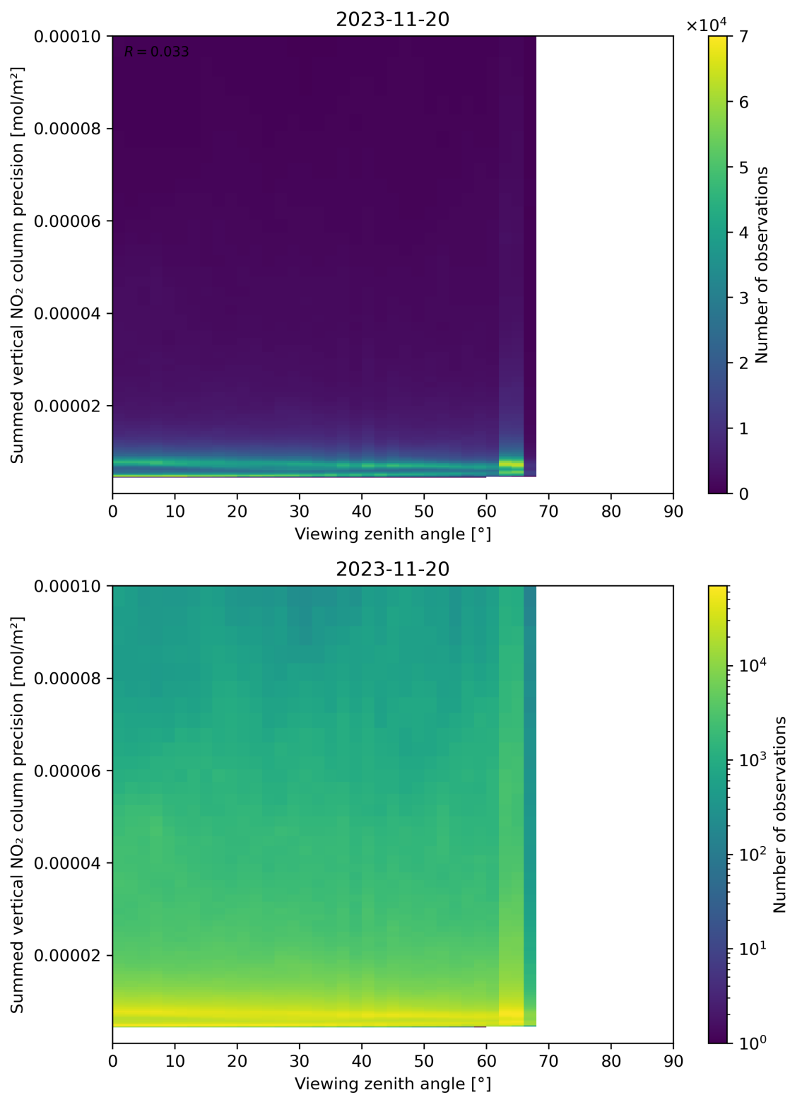
Figure 166: Scatter density plot of “Viewing zenith angle” against “Summed vertical NO 2 column precision” for 2023-11-19 to 2023-11-21.
