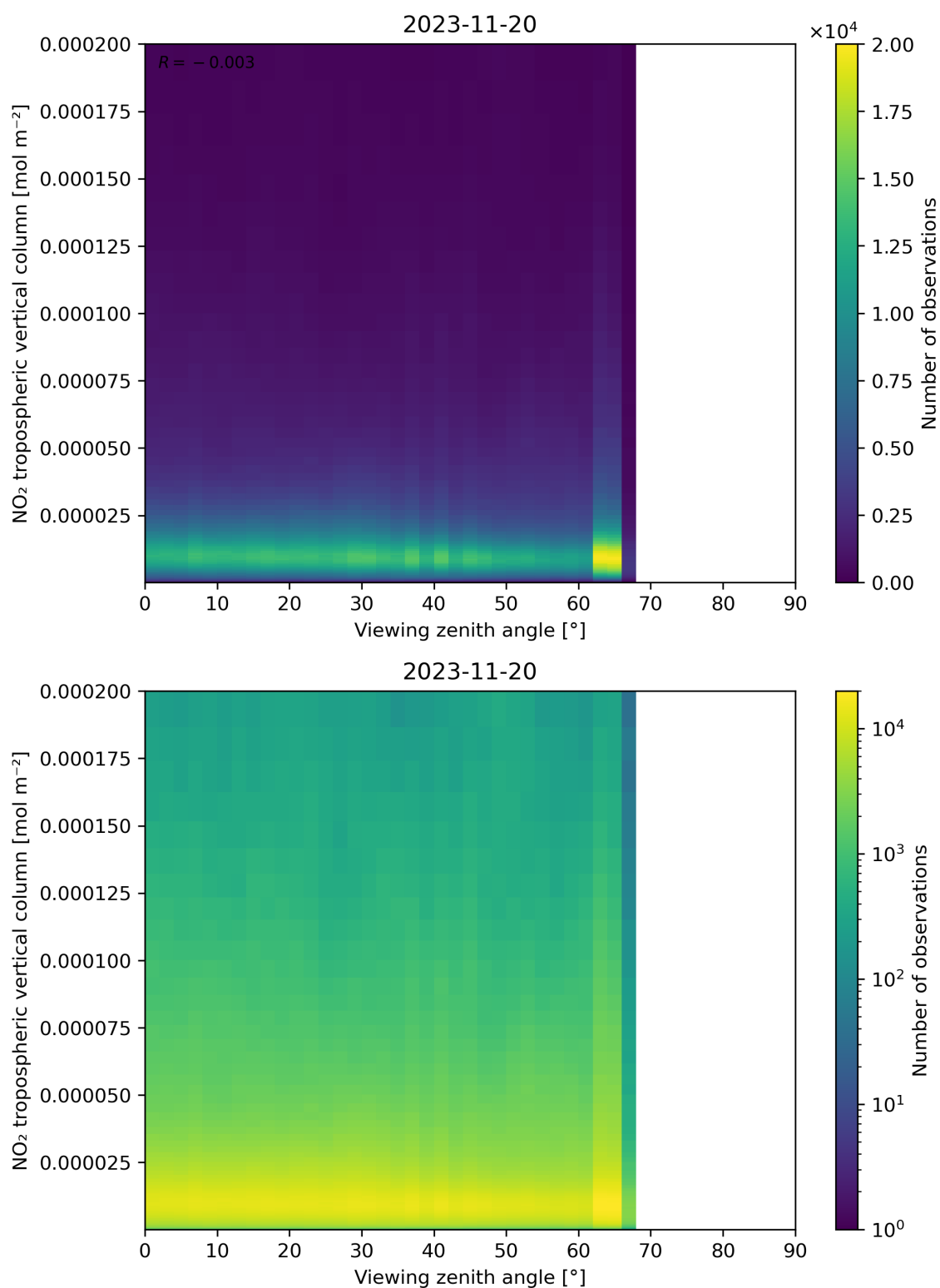
Figure 169: Scatter density plot of “Viewing zenith angle” against “NO 2 tropospheric vertical column” for 2023-11-19 to 2023-11-21.
