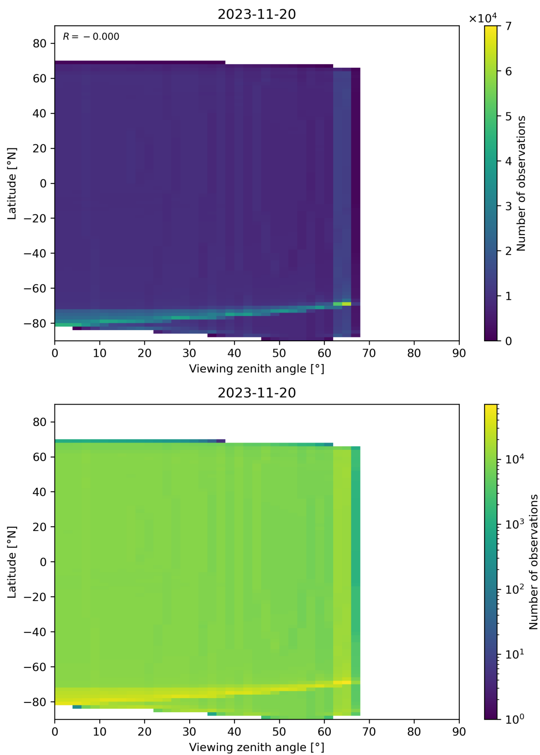
Figure 163: Scatter density plot of “Viewing zenith angle” against “Latitude” for 2023-11-19 to 2023-11-21.
