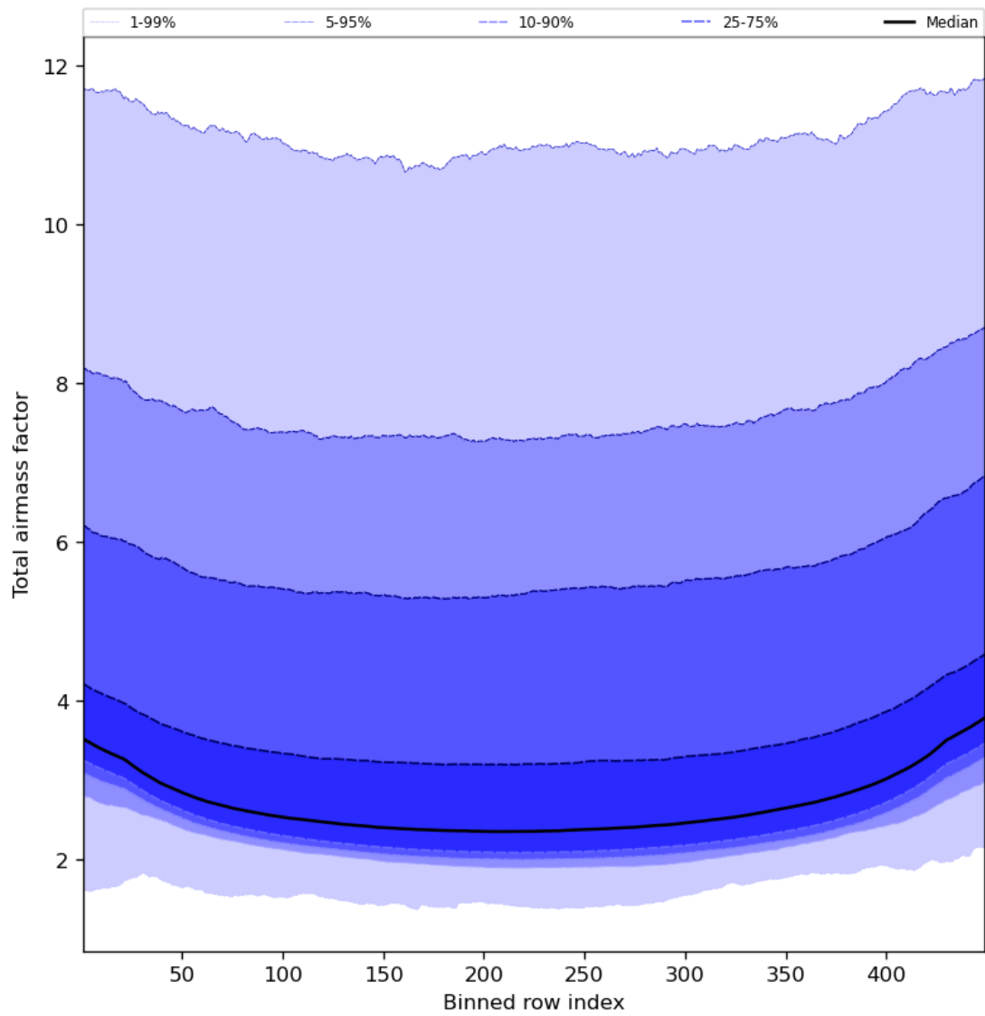
Figure 49: Along track statistics of “Total airmass factor” for 2023-11-19 to 2023-11-21
