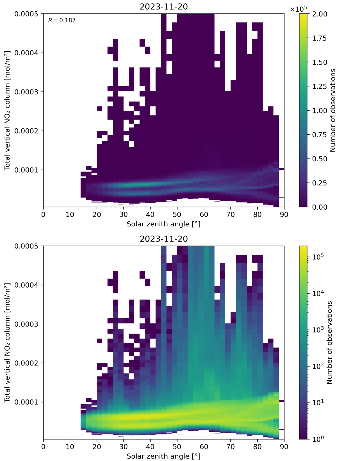
Figure 153: Scatter density plot of “Solar zenith angle” against “Total vertical NO 2 column” for 2023-11-19 to 2023-11-21.
