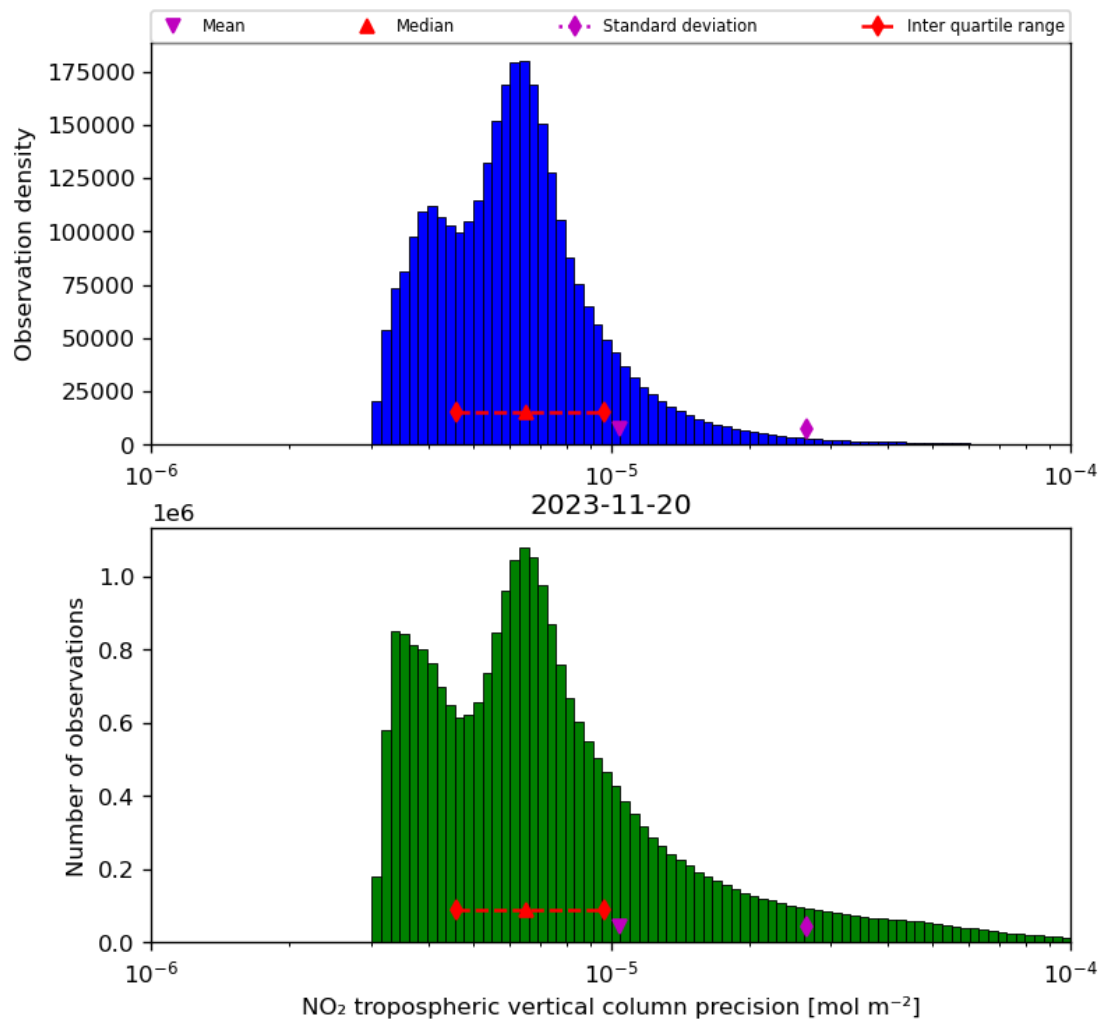
Figure 30: Histogram of “NO 2 tropospheric vertical column precision” for 2023-11-19 to 2023-11-21
