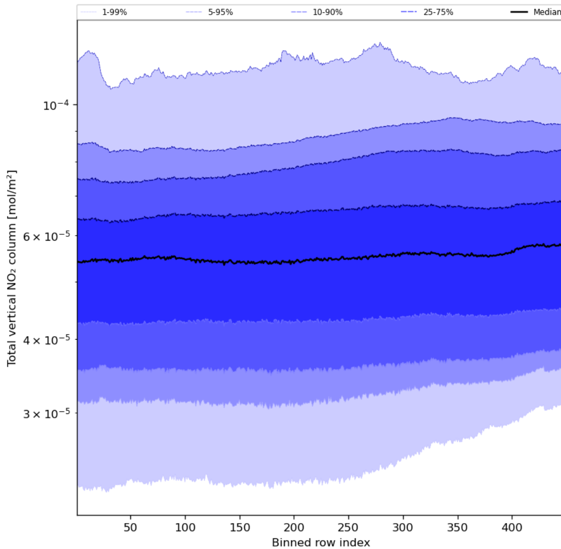
Figure 55: Along track statistics of “Total vertical NO 2 column” for 2023-11-19 to 2023-11-21
