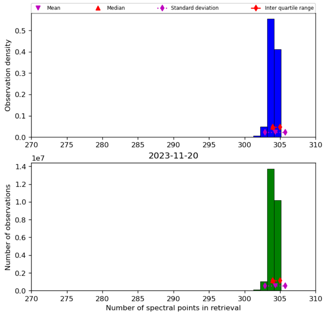
Figure 33: Histogram of “Number of spectral points in retrieval” for 2023-11-19 to 2023-11-21
