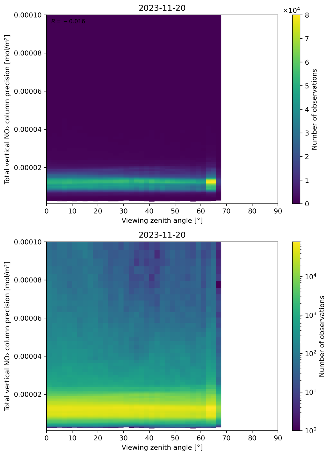
Figure 168: Scatter density plot of “Viewing zenith angle” against “Total vertical NO 2 column precision” for 2023-11-19 to 2023-11-21.
