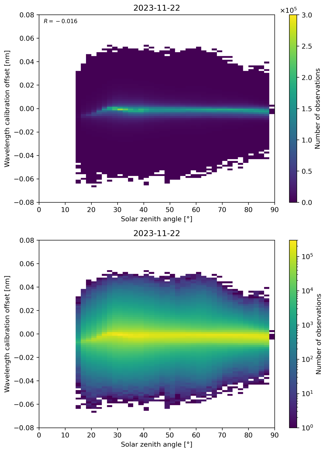
Figure 158: Scatter density plot of “Solar zenith angle” against “Wavelength calibration offset” for 2023-11-21 to 2023-11-23.
