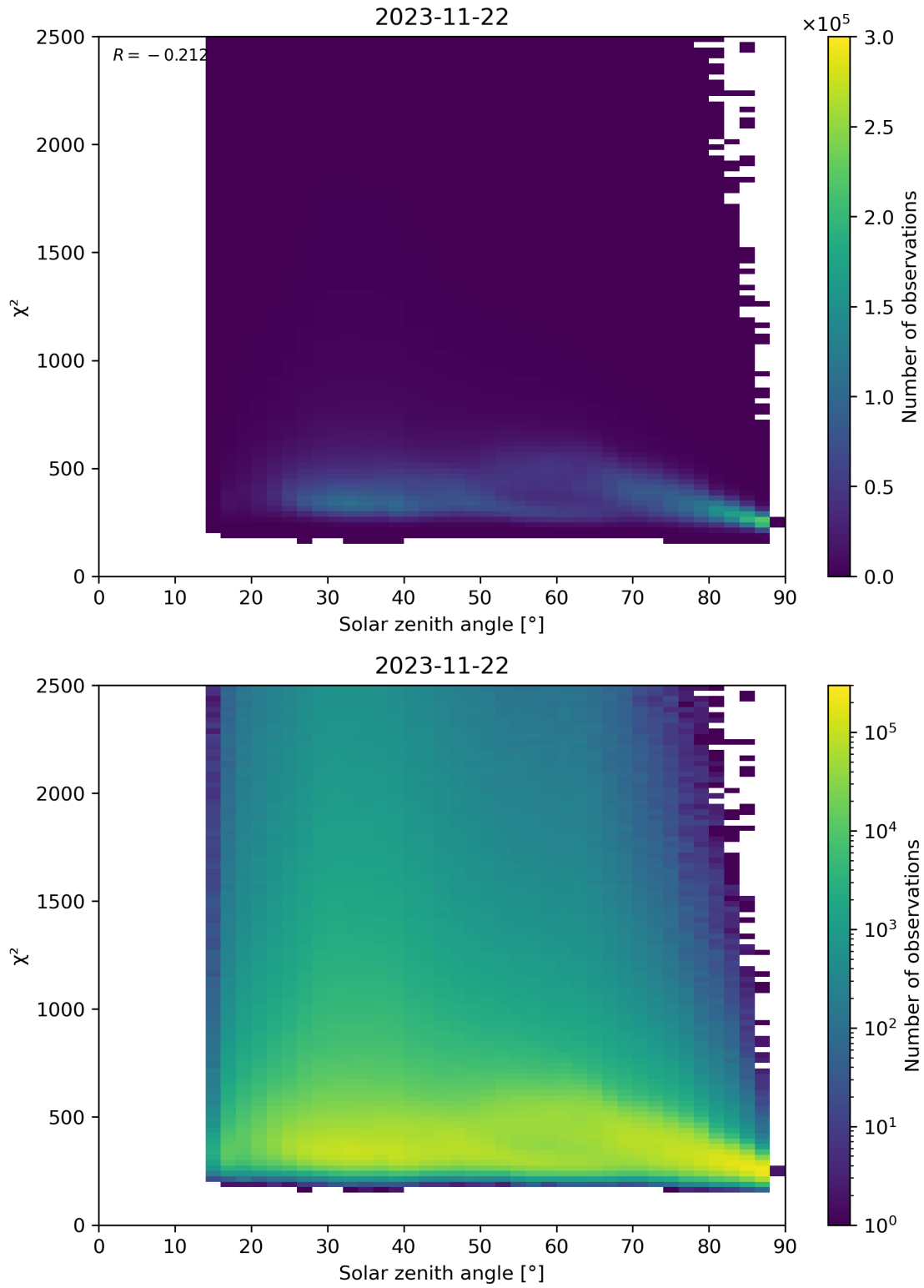
Figure 148: Scatter density plot of “Solar zenith angle” against “ \chi^2 ” for 2023-11-21 to 2023-11-23.
