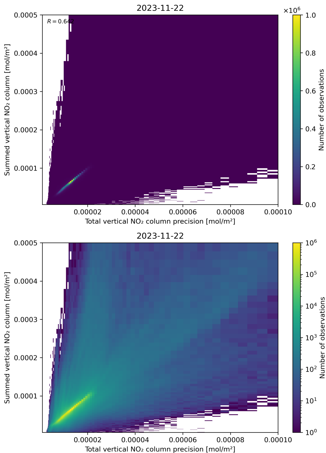
Figure 117: Scatter density plot of “Total vertical NO 2 column precision” against “Summed vertical NO 2 column” for 2023-11-21 to 2023-11-23.
