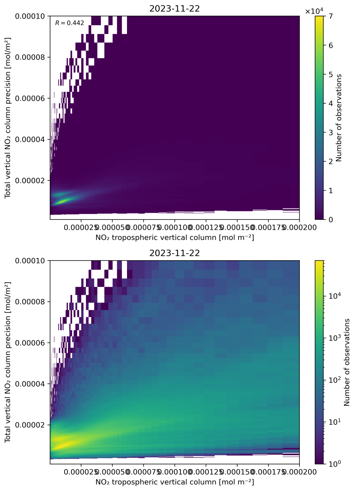
Figure 129: Scatter density plot of “NO 2 tropospheric vertical column” against “Total vertical NO 2 column precision” for 2023-11-21 to 2023-11-23.
