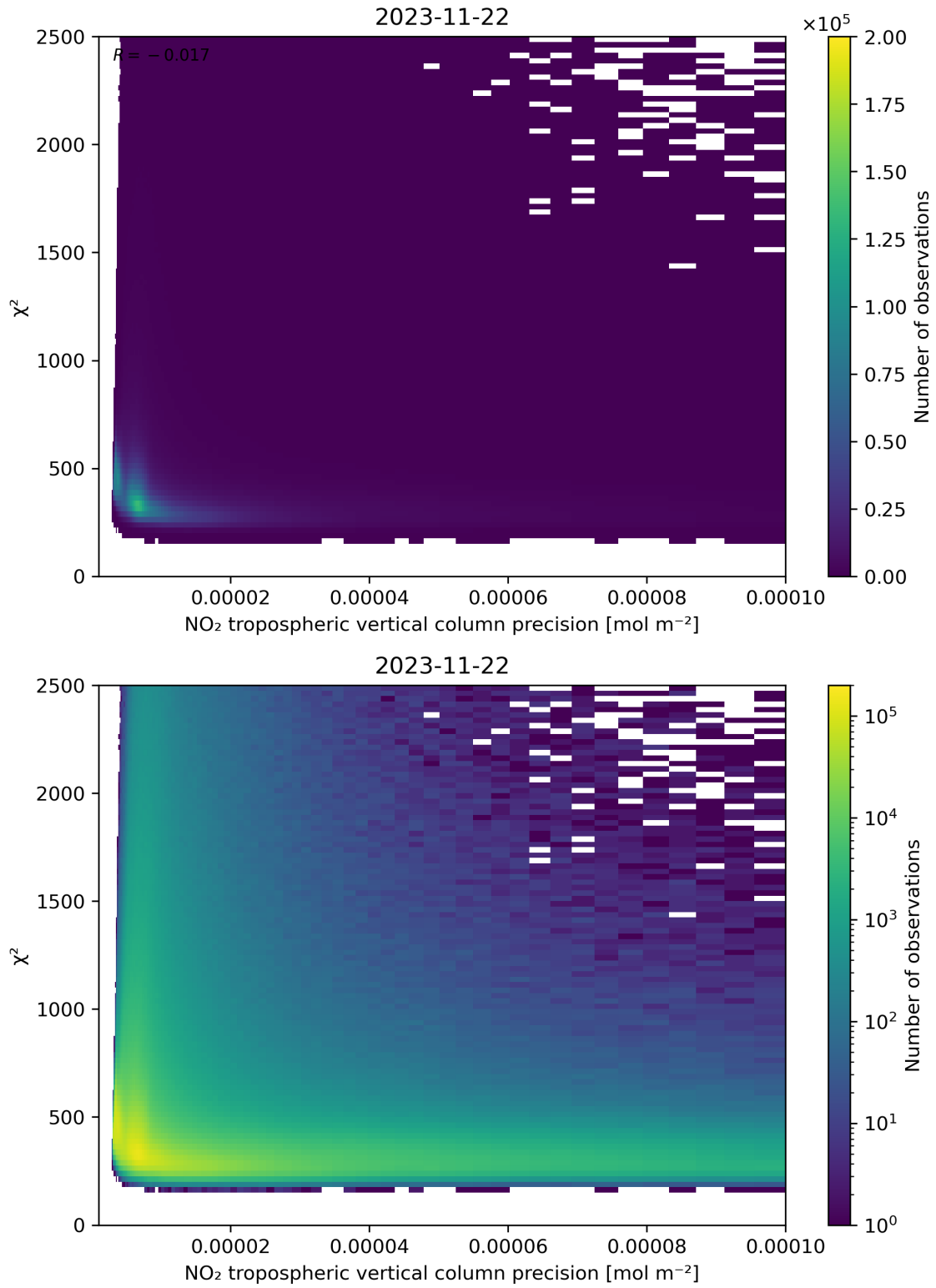
Figure 134: Scatter density plot of “NO 2 tropospheric vertical column precision” against “ \chi^2 ” for 2023-11-21 to 2023-11-23.
