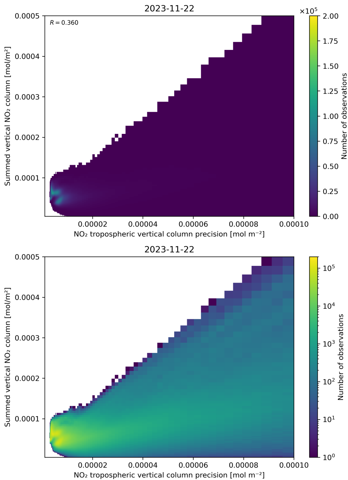
Figure 136: Scatter density plot of “NO 2 tropospheric vertical column precision” against “Summed vertical NO 2 column” for 2023-11-21 to 2023-11-23.
