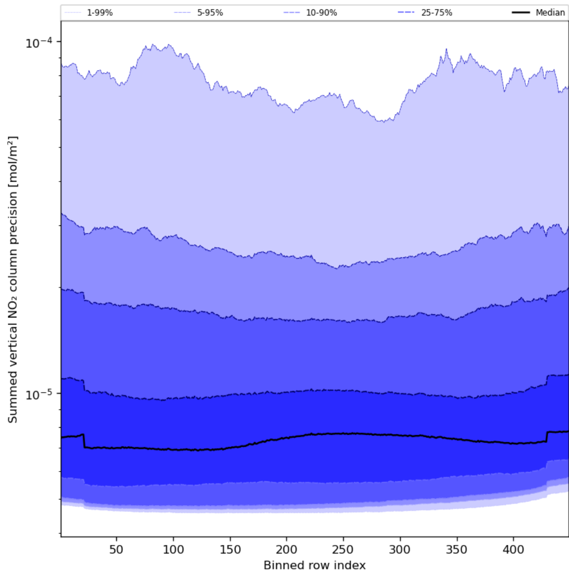
Figure 58: Along track statistics of “Summed vertical NO 2 column precision” for 2023-11-21 to 2023-11-23
