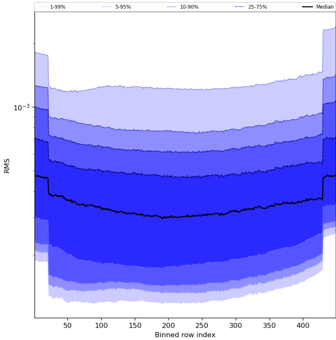
Figure 60: Along track statistics of “RMS” for 2023-11-21 to 2023-11-23
