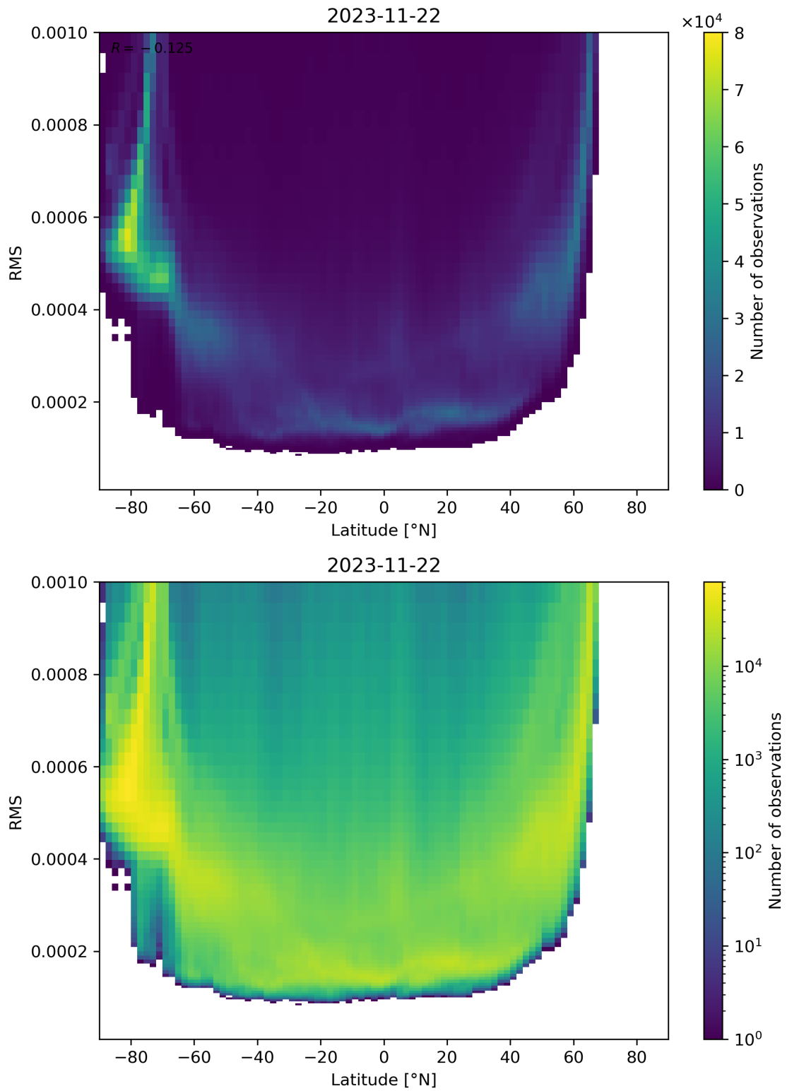
Figure 94: Scatter density plot of “Latitude” against “RMS” for 2023-11-21 to 2023-11-23.
