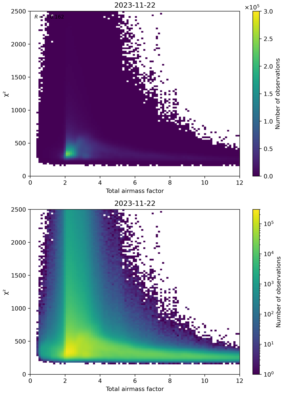
Figure 63: Scatter density plot of “Total airmass factor” against “ \chi^2 ” for 2023-11-21 to 2023-11-23.
