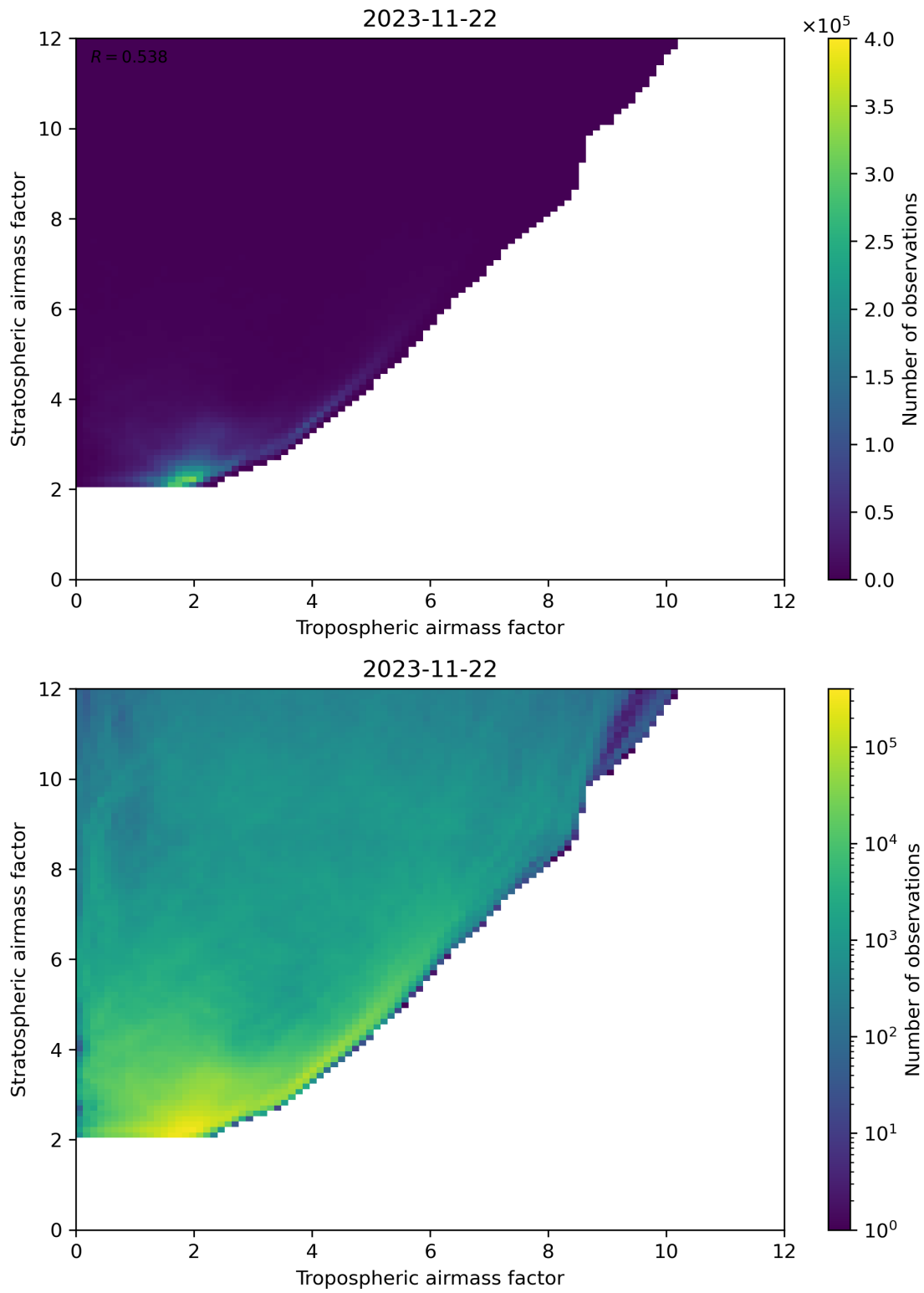
Figure 71: Scatter density plot of “Tropospheric airmass factor” against “Stratospheric airmass factor” for 2023-11-21 to 2023-11-23.
