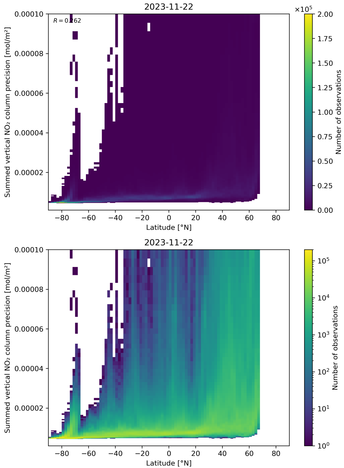
Figure 89: Scatter density plot of “Latitude” against “Summed vertical NO 2 column precision” for 2023-11-21 to 2023-11-23.
