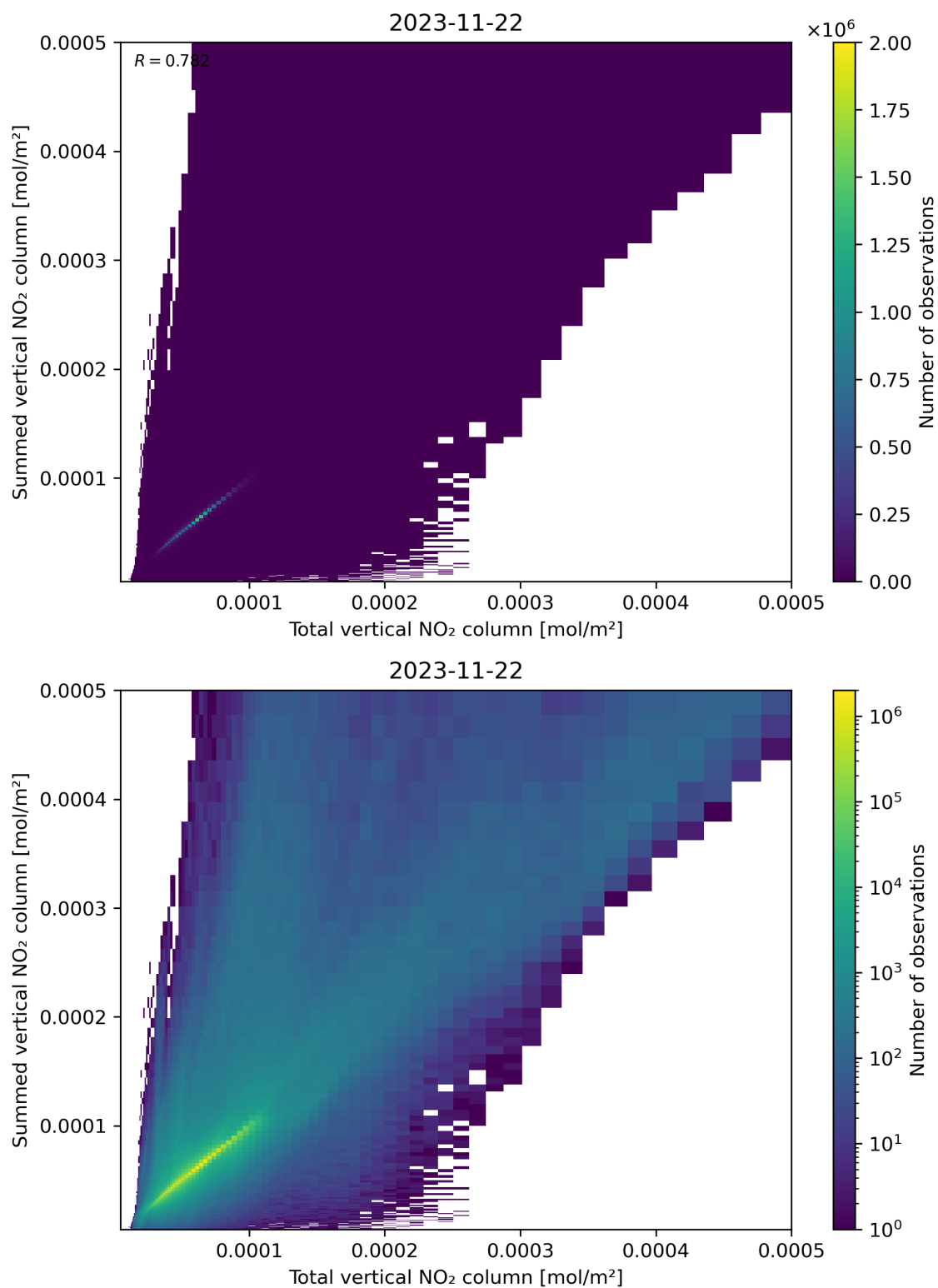
Figure 112: Scatter density plot of “Total vertical NO 2 column” against “Summed vertical NO 2 column” for 2023-11-21 to 2023-11-23.
