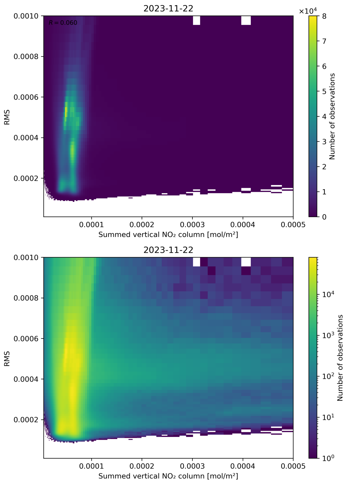
Figure 109: Scatter density plot of “Summed vertical NO 2 column” against “RMS” for 2023-11-21 to 2023-11-23.
