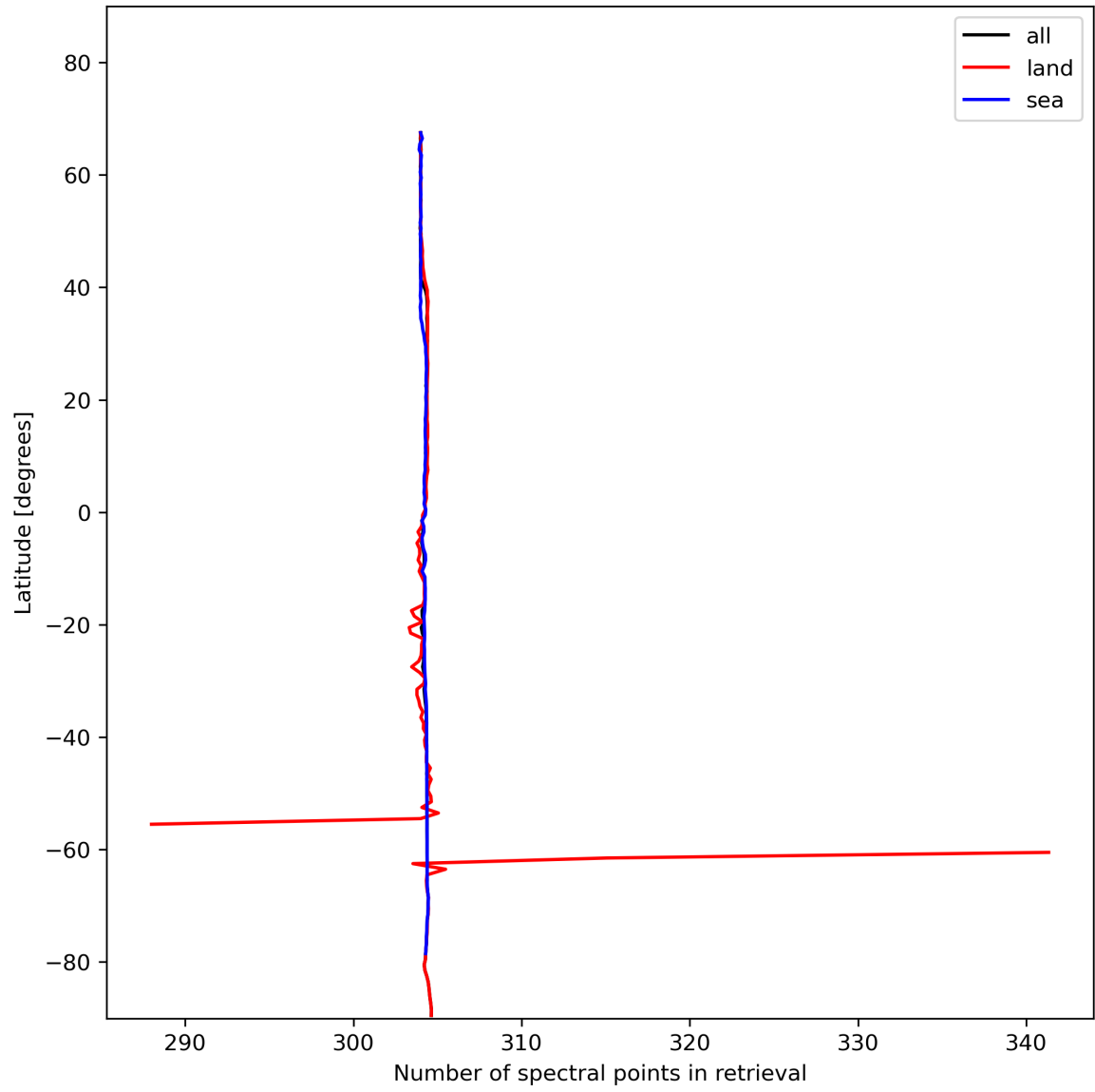
Figure 16: Zonal average of “Number of spectral points in retrieval” for 2023-11-21 to 2023-11-23.
