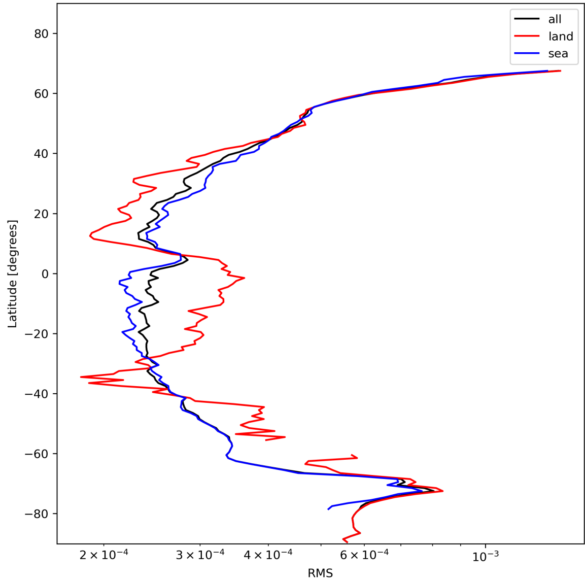
Figure 26: Zonal average of “RMS” for 2023-11-21 to 2023-11-23.
