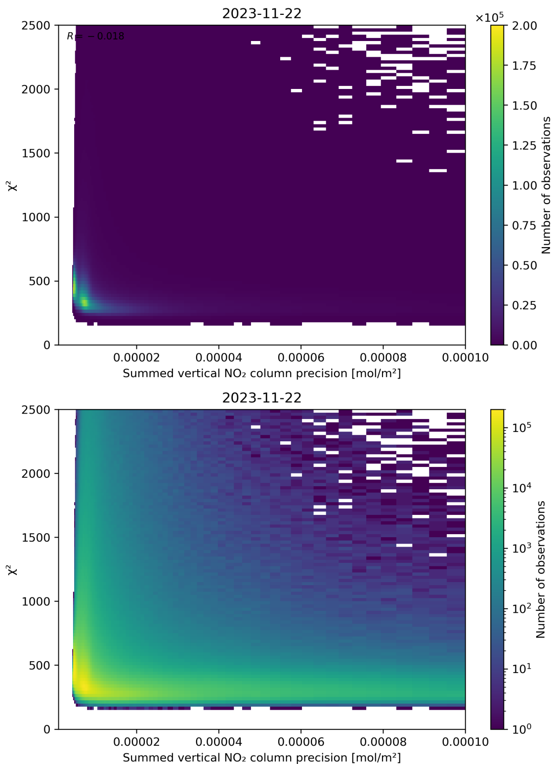
Figure 107: Scatter density plot of “Summed vertical NO 2 column precision” against “ \chi^2 ” for 2023-11-21 to 2023-11-23.
