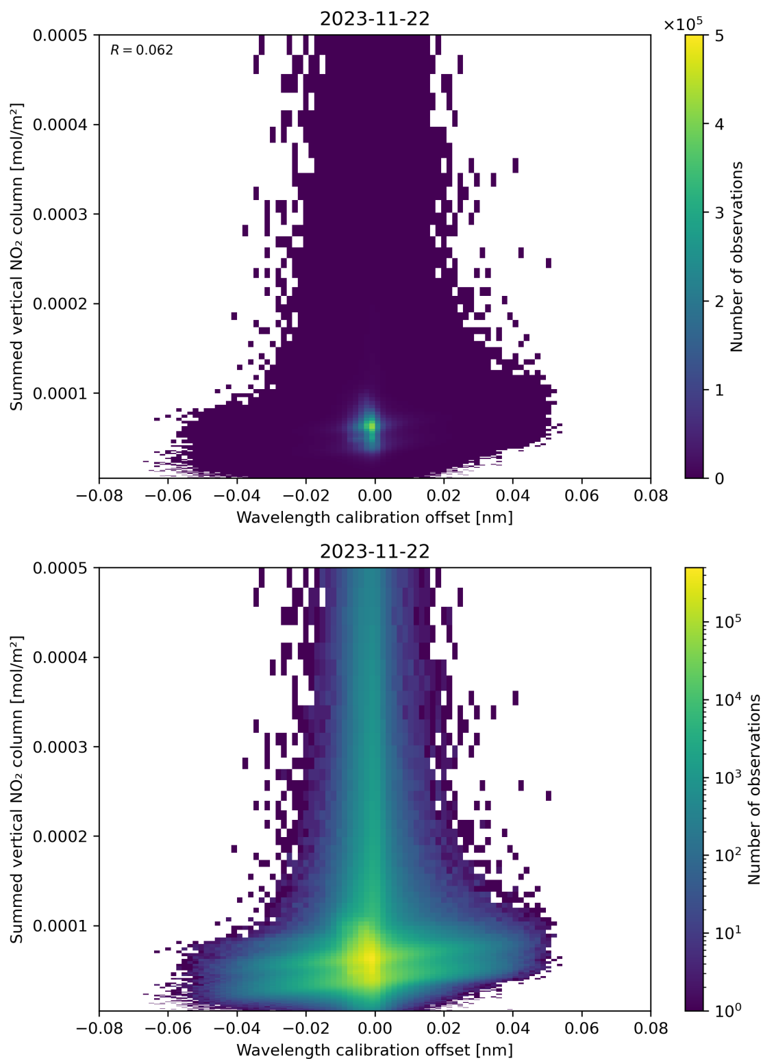
Figure 177: Scatter density plot of “Wavelength calibration offset” against “Summed vertical NO 2 column” for 2023-11-21 to 2023-11-23.
