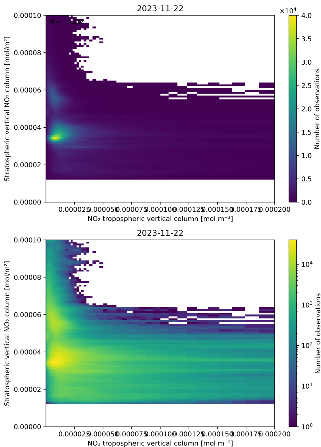
Figure 125: Scatter density plot of “NO 2 tropospheric vertical column” against “Stratospheric vertical NO 2 column” for 2023-11-21 to 2023-11-23.
