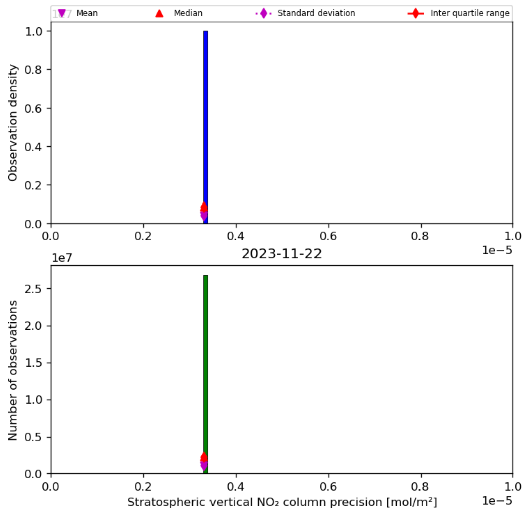
Figure 37: Histogram of “Stratospheric vertical NO 2 column precision” for 2023-11-21 to 2023-11-23
