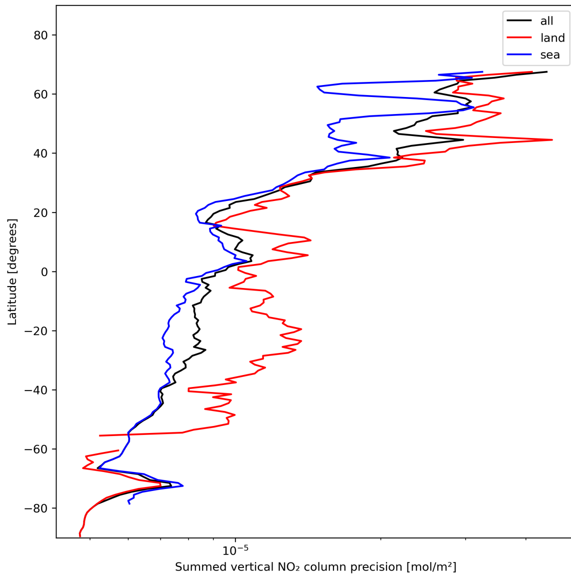
Figure 24: Zonal average of “Summed vertical NO 2 column precision” for 2023-11-21 to 2023-11-23.
