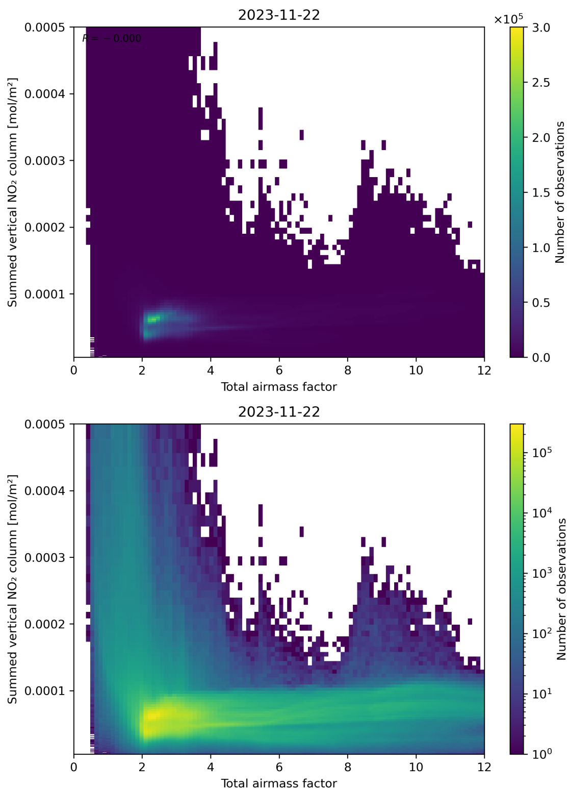
Figure 65: Scatter density plot of “Total airmass factor” against “Summed vertical NO 2 column” for 2023-11-21 to 2023-11-23.
