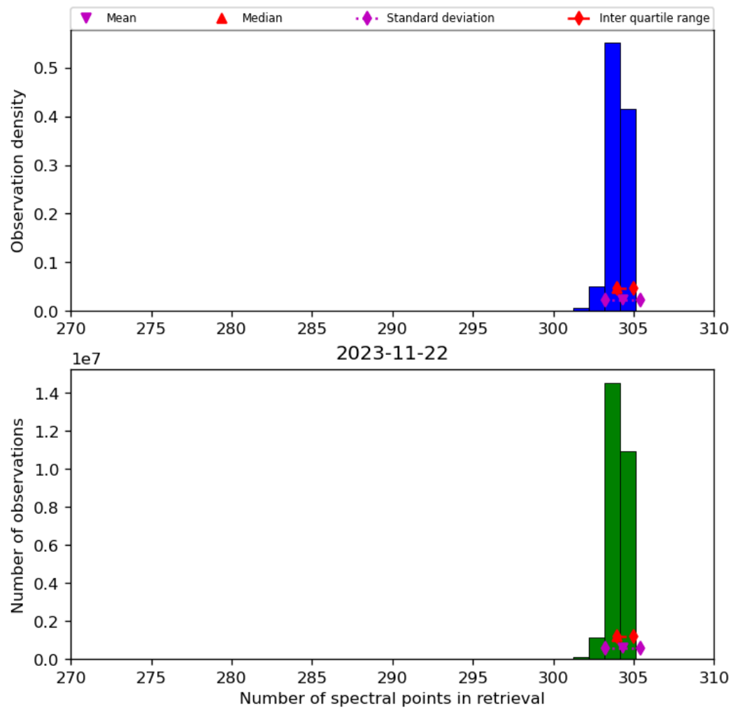
Figure 33: Histogram of “Number of spectral points in retrieval” for 2023-11-21 to 2023-11-23
