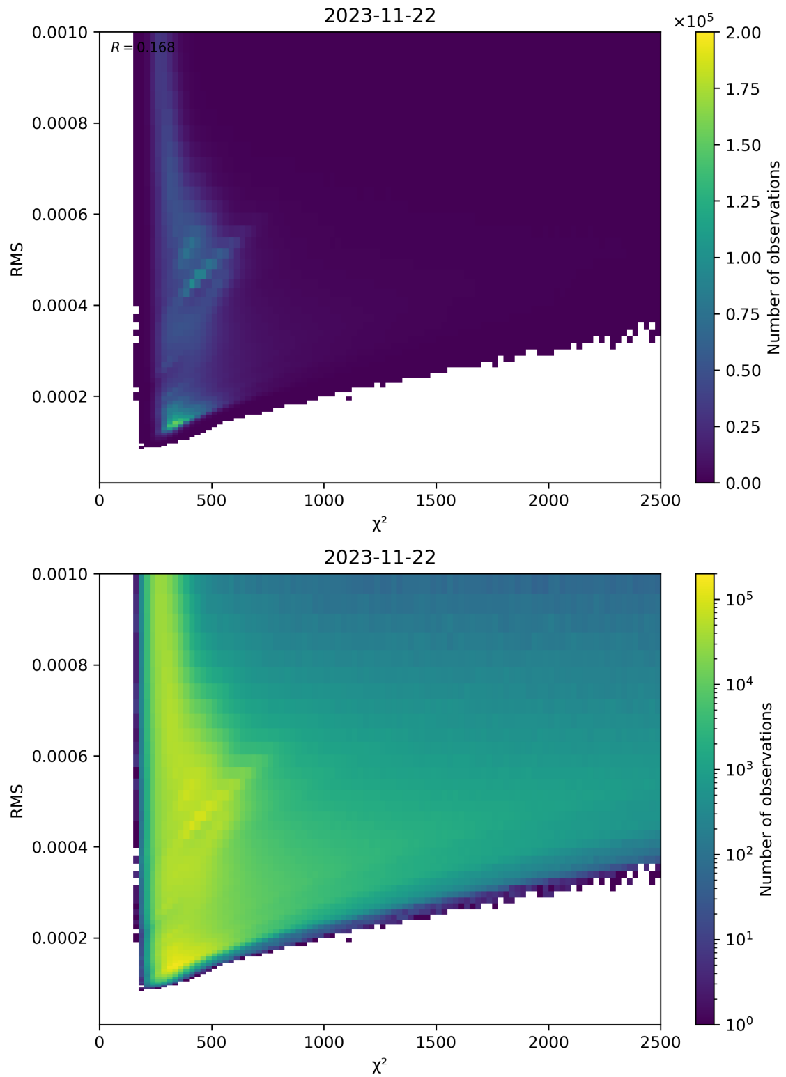
Figure 82: Scatter density plot of “ \chi^2 ” against “RMS” for 2023-11-21 to 2023-11-23.
