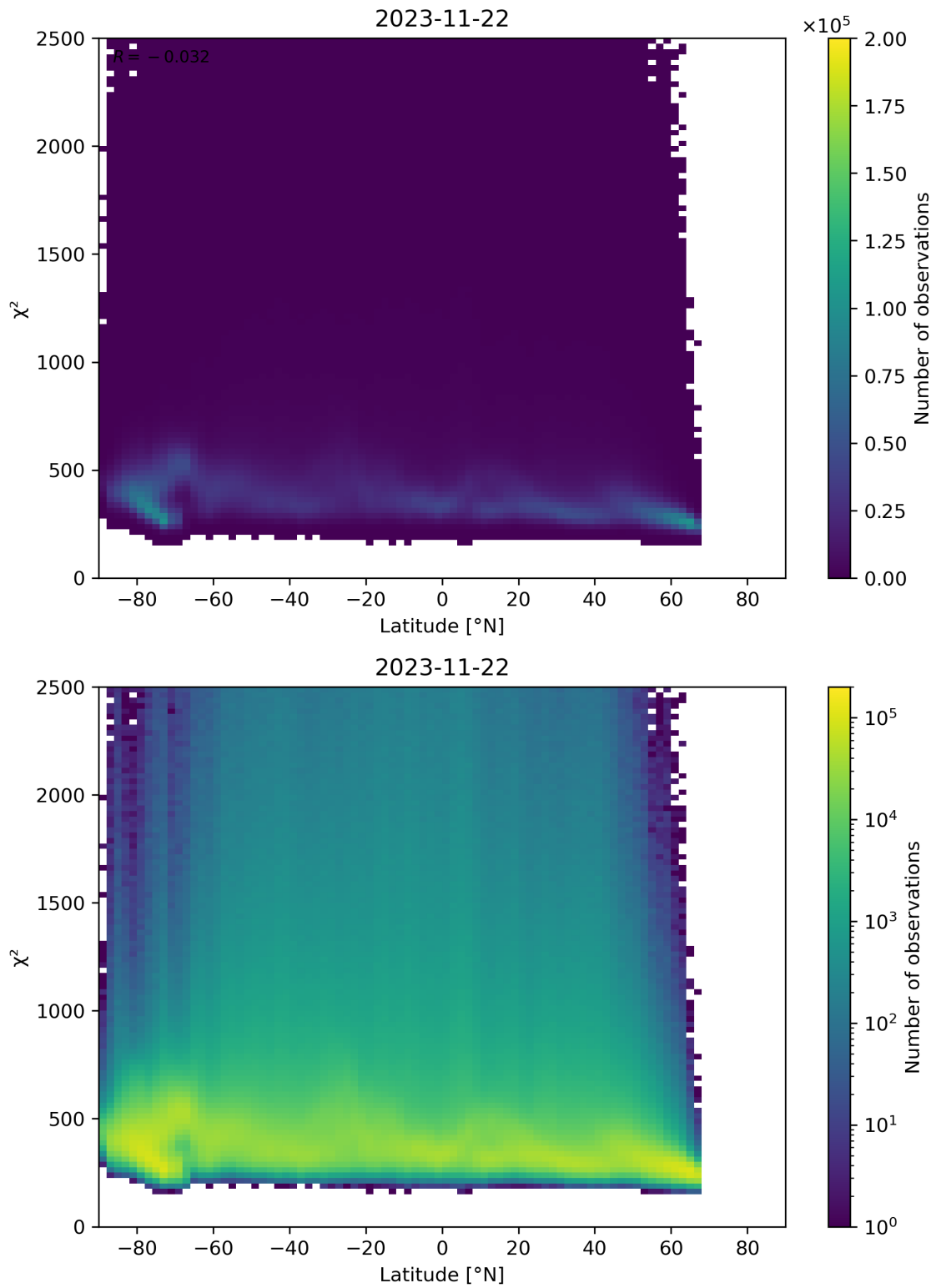
Figure 86: Scatter density plot of “Latitude” against “ \chi^2 ” for 2023-11-21 to 2023-11-23.
