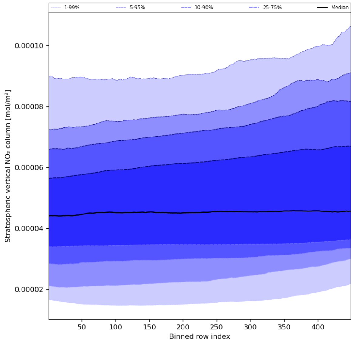
Figure 53: Along track statistics of “Stratospheric vertical NO 2 column” for 2023-11-21 to 2023-11-23
