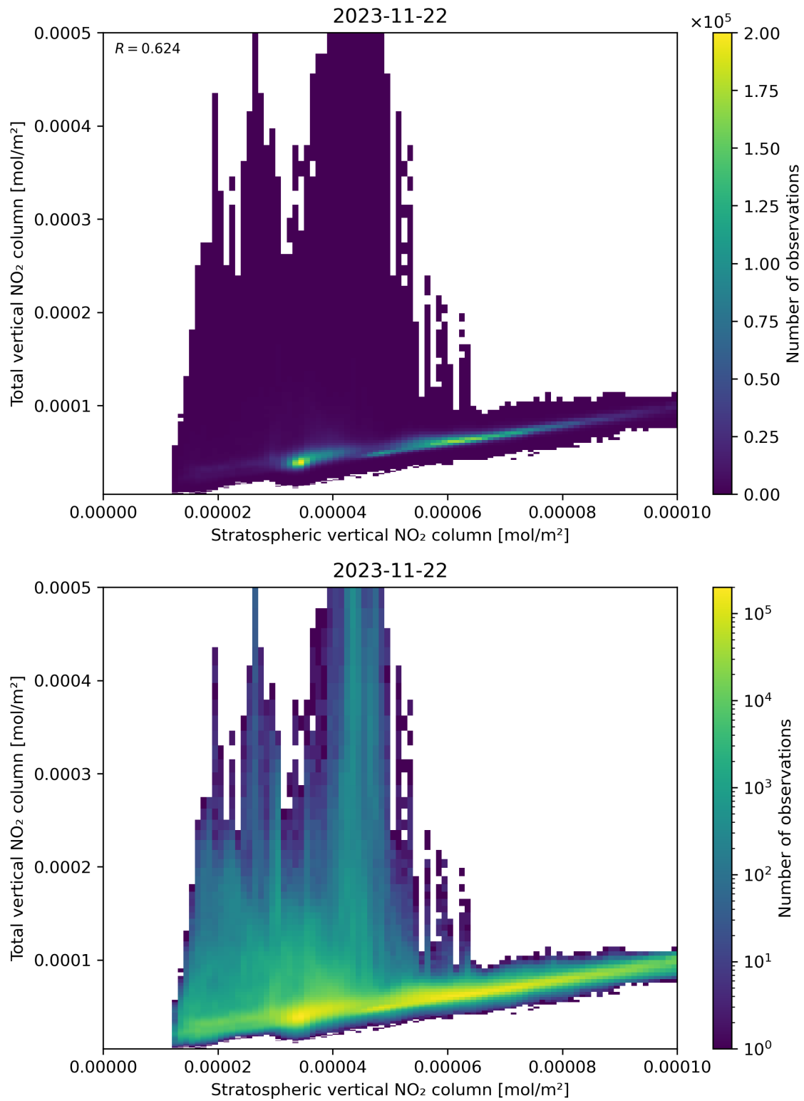
Figure 100: Scatter density plot of “Stratospheric vertical NO 2 column” against “Total vertical NO 2 column” for 2023-11-21 to 2023-11-23.
