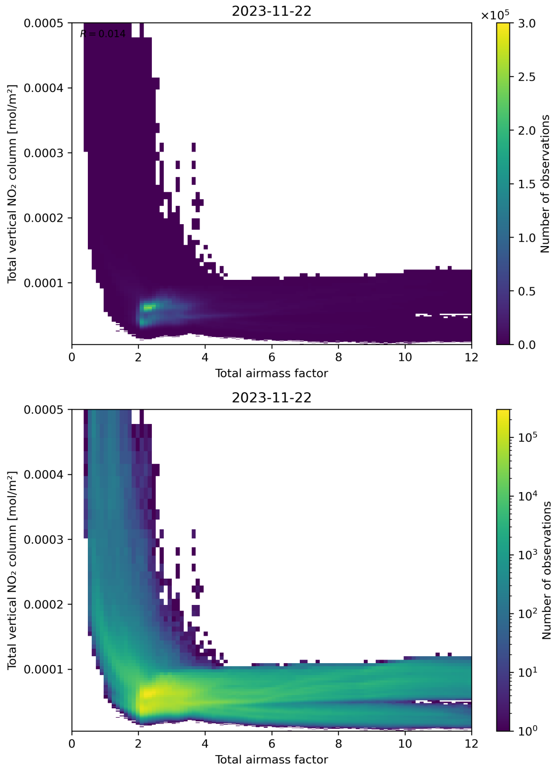
Figure 67: Scatter density plot of “Total airmass factor” against “Total vertical NO 2 column” for 2023-11-21 to 2023-11-23.
