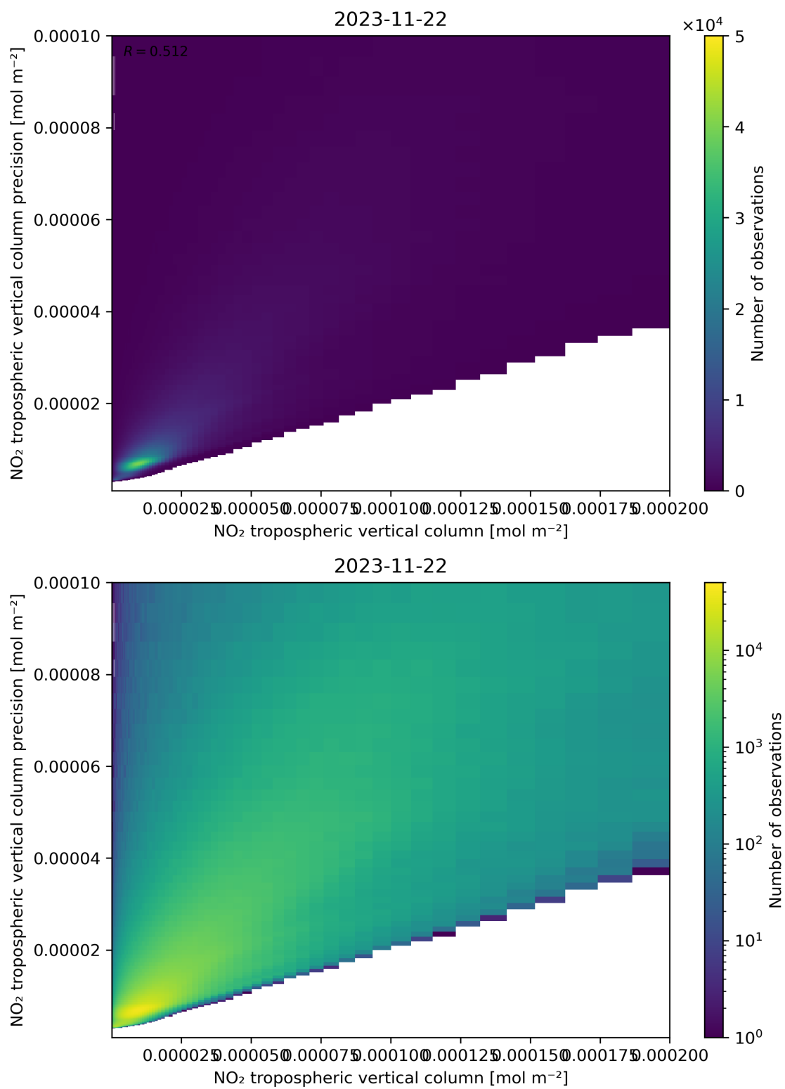
Figure 130: Scatter density plot of “NO 2 tropospheric vertical column” against “NO 2 tropospheric vertical column precision” for 2023-11-21 to 2023-11-23.
