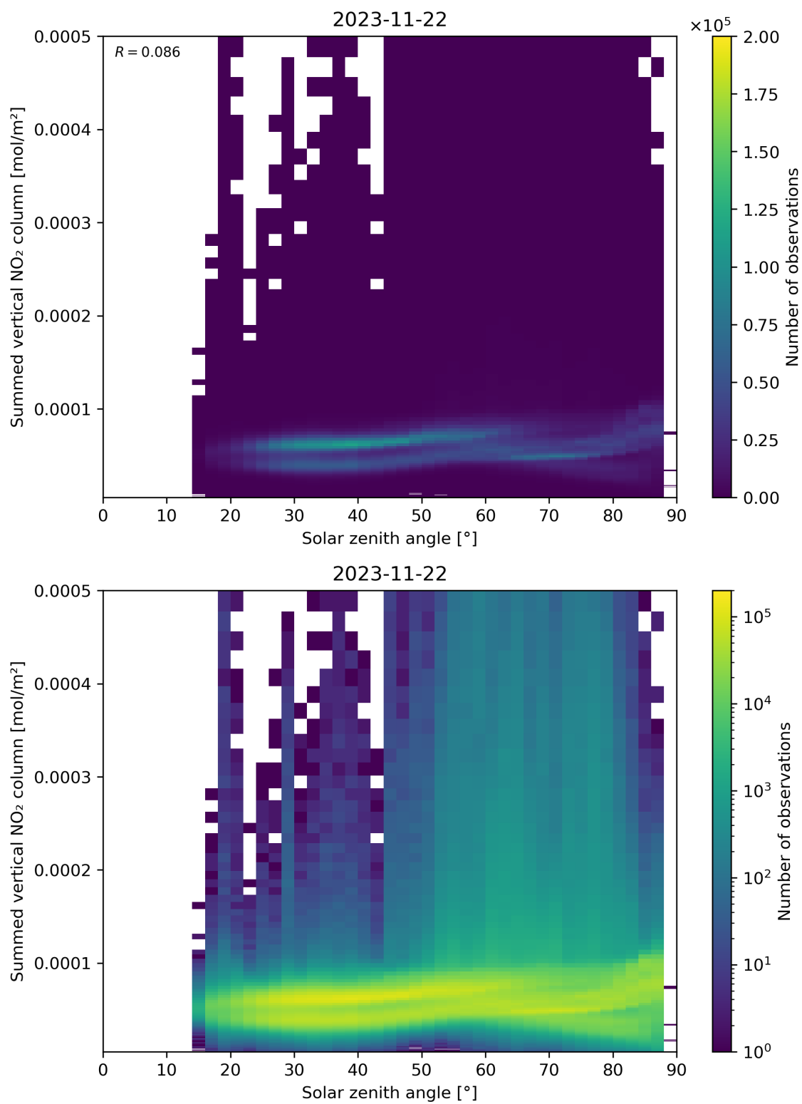
Figure 151: Scatter density plot of “Solar zenith angle” against “Summed vertical NO 2 column” for 2023-11-21 to 2023-11-23.
