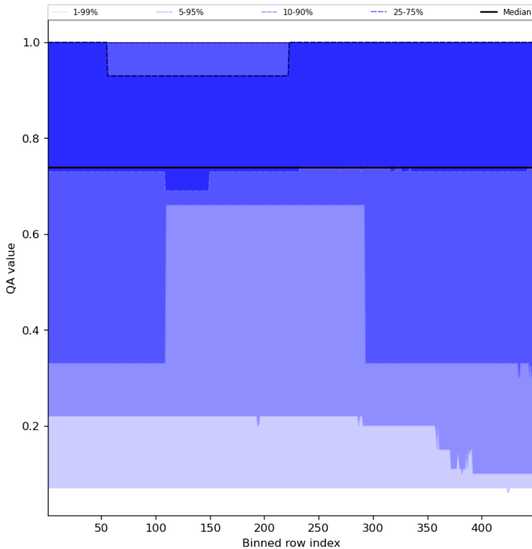
Figure 45: Along track statistics of “QA value” for 2023-11-21 to 2023-11-23
