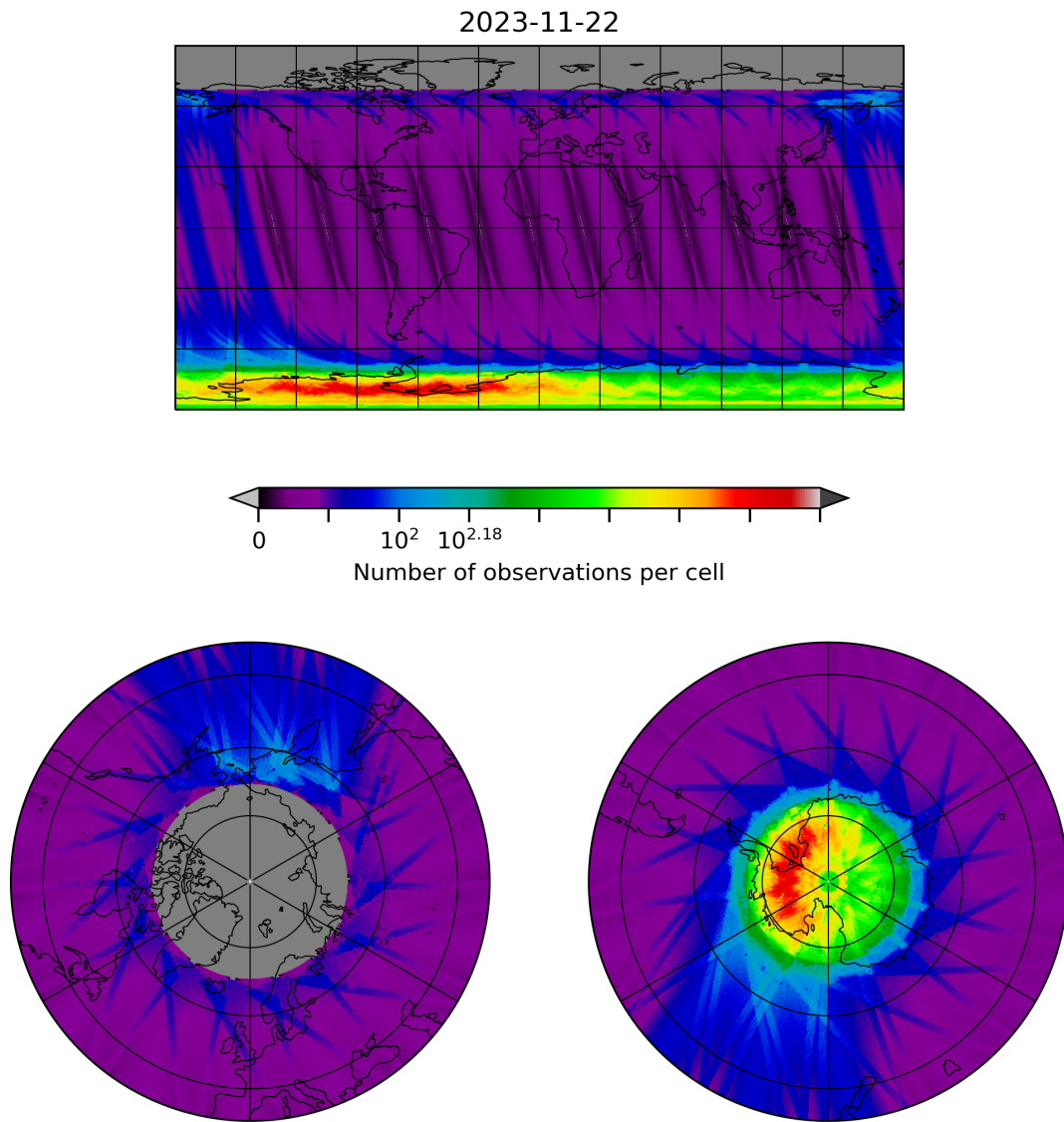
Figure 10: Map of the number of observations for 2023-11-21 to 2023-11-23
