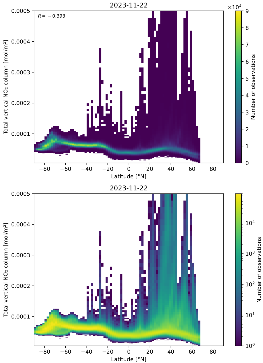
Figure 90: Scatter density plot of “Latitude” against “Total vertical NO 2 column” for 2023-11-21 to 2023-11-23.
