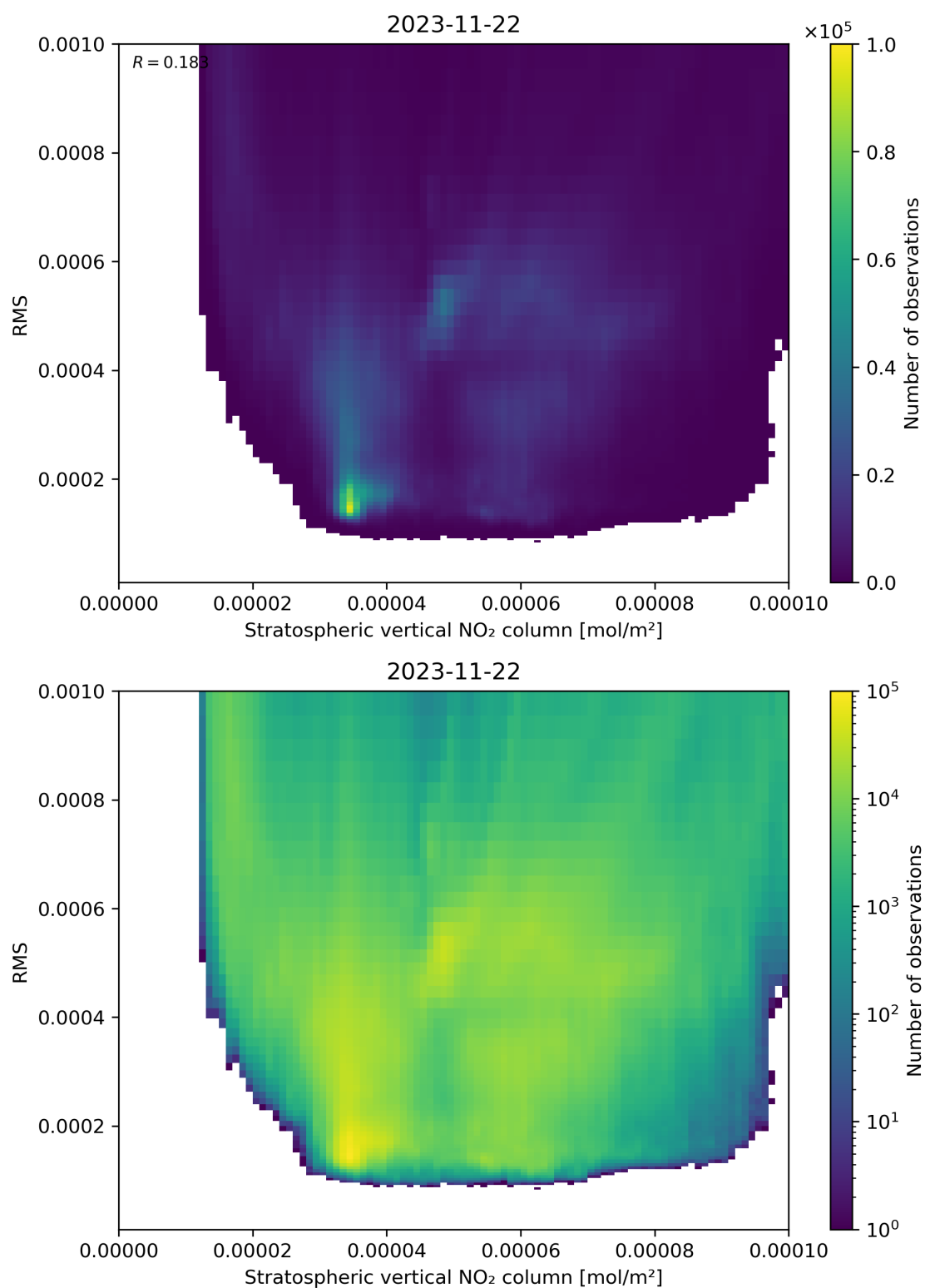
Figure 102: Scatter density plot of “Stratospheric vertical NO 2 column” against “RMS” for 2023-11-21 to 2023-11-23.
