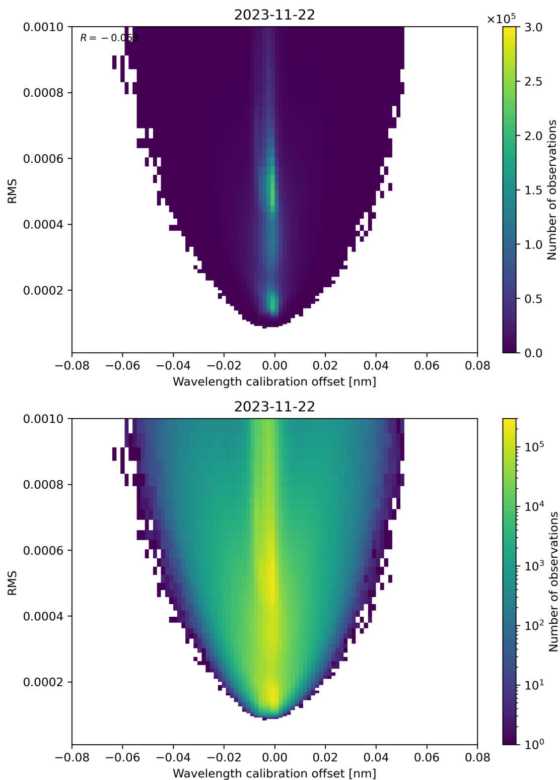
Figure 181: Scatter density plot of “Wavelength calibration offset” against “RMS” for 2023-11-21 to 2023-11-23.
