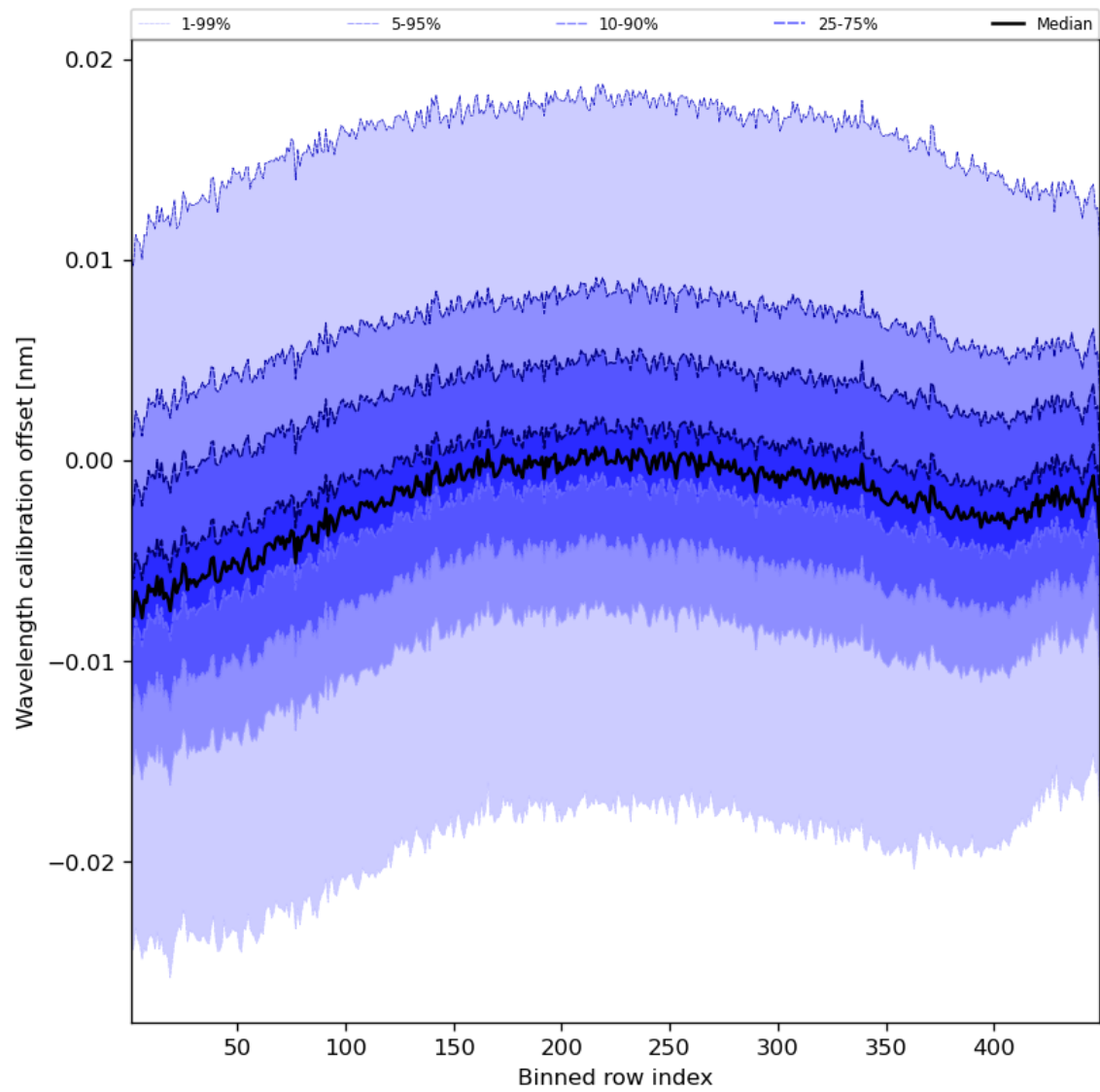
Figure 52: Along track statistics of “Wavelength calibration offset” for 2023-11-21 to 2023-11-23
