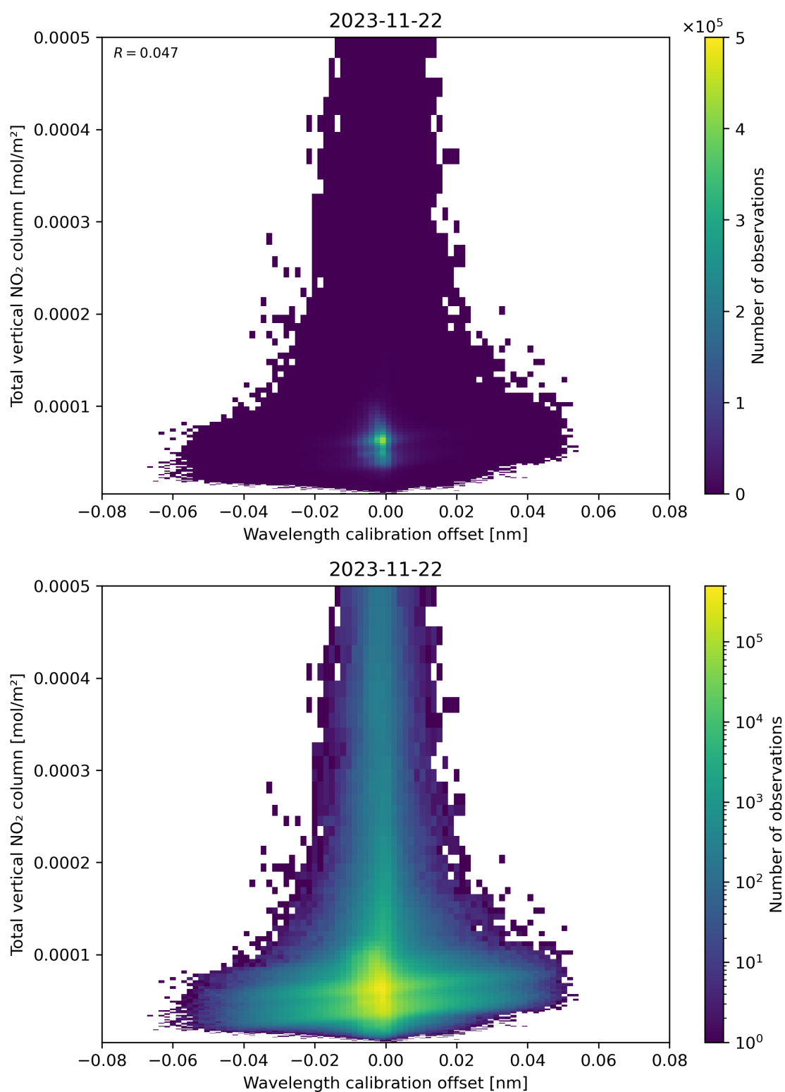
Figure 179: Scatter density plot of “Wavelength calibration offset” against “Total vertical NO 2 column” for 2023-11-21 to 2023-11-23.
