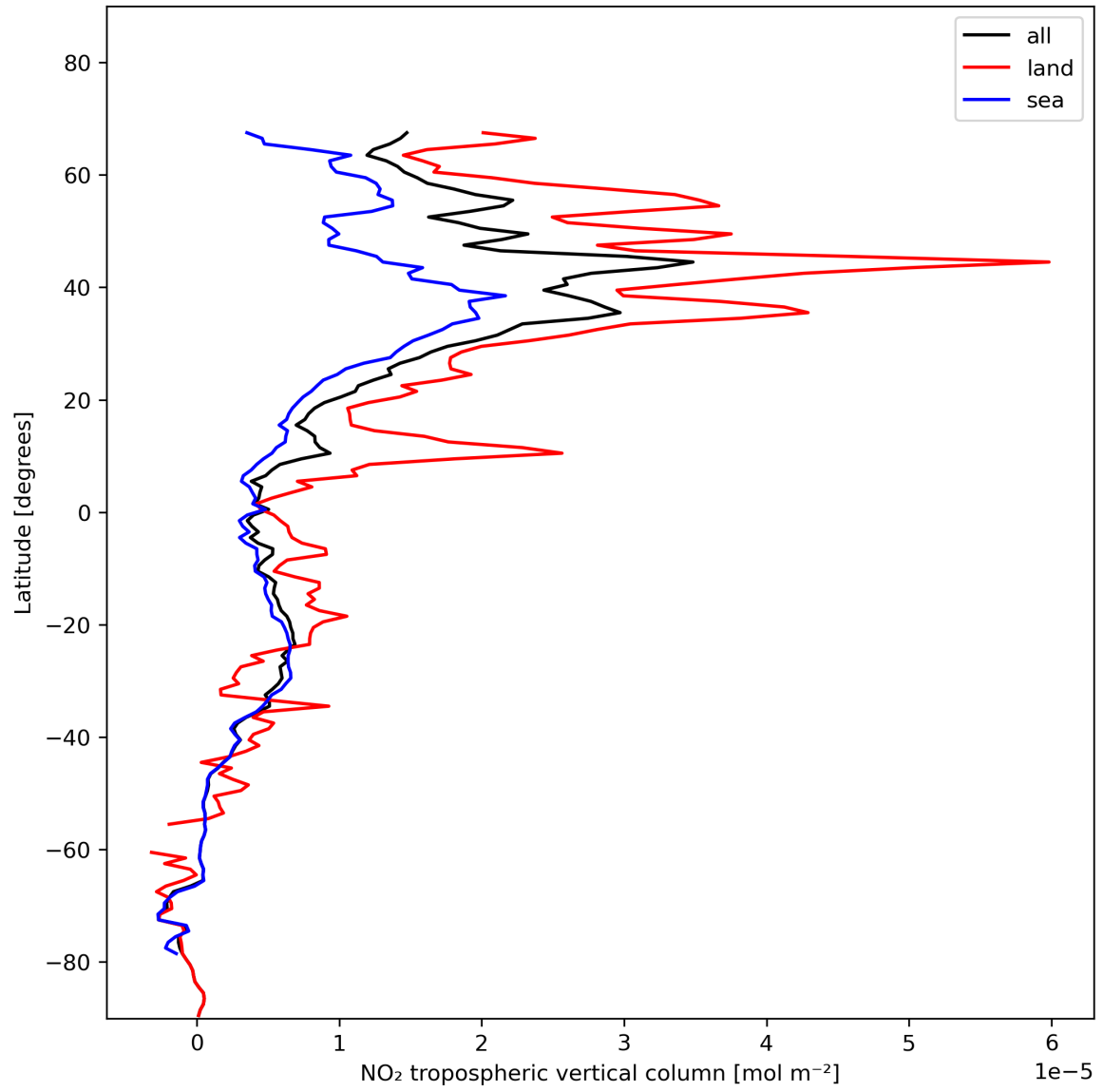
Figure 12: Zonal average of “NO 2 tropospheric vertical column” for 2023-11-21 to 2023-11-23.
