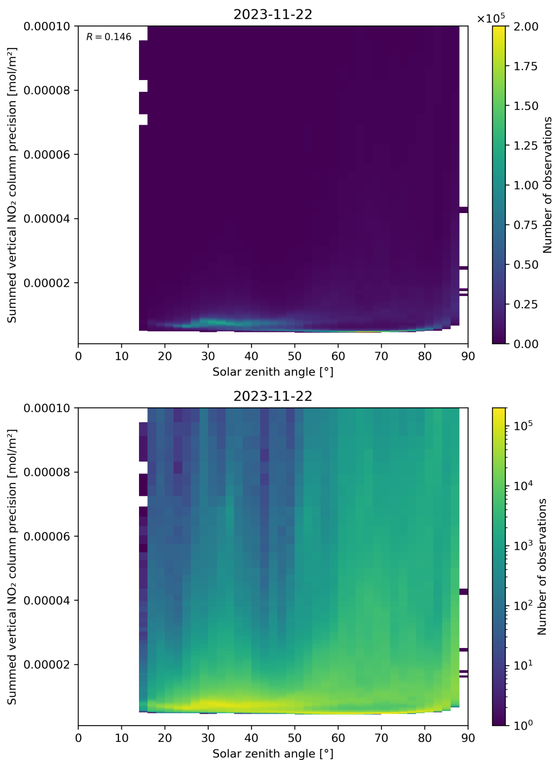
Figure 152: Scatter density plot of “Solar zenith angle” against “Summed vertical NO 2 column precision” for 2023-11-21 to 2023-11-23.
