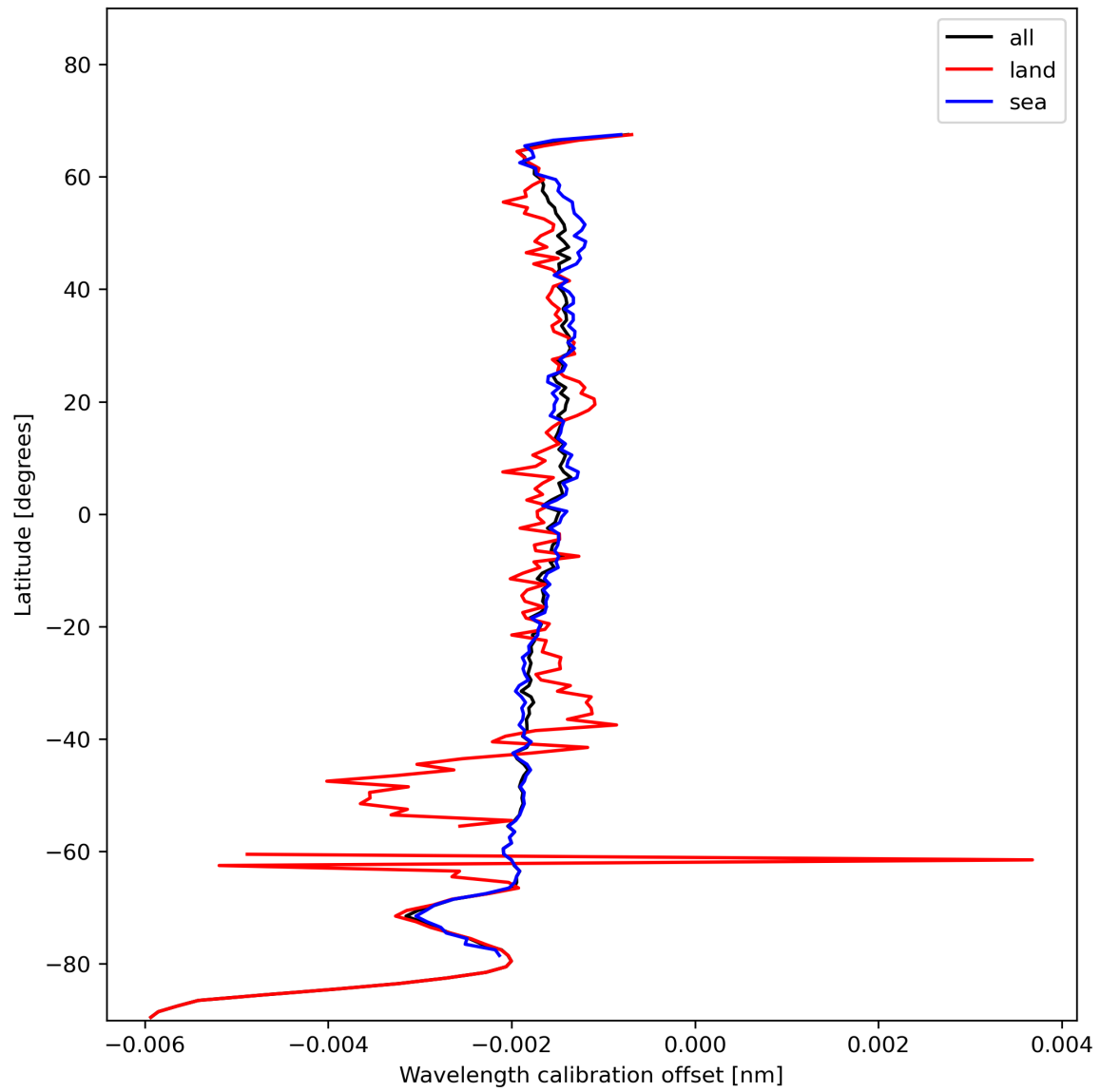
Figure 18: Zonal average of “Wavelength calibration offset” for 2023-11-21 to 2023-11-23.
