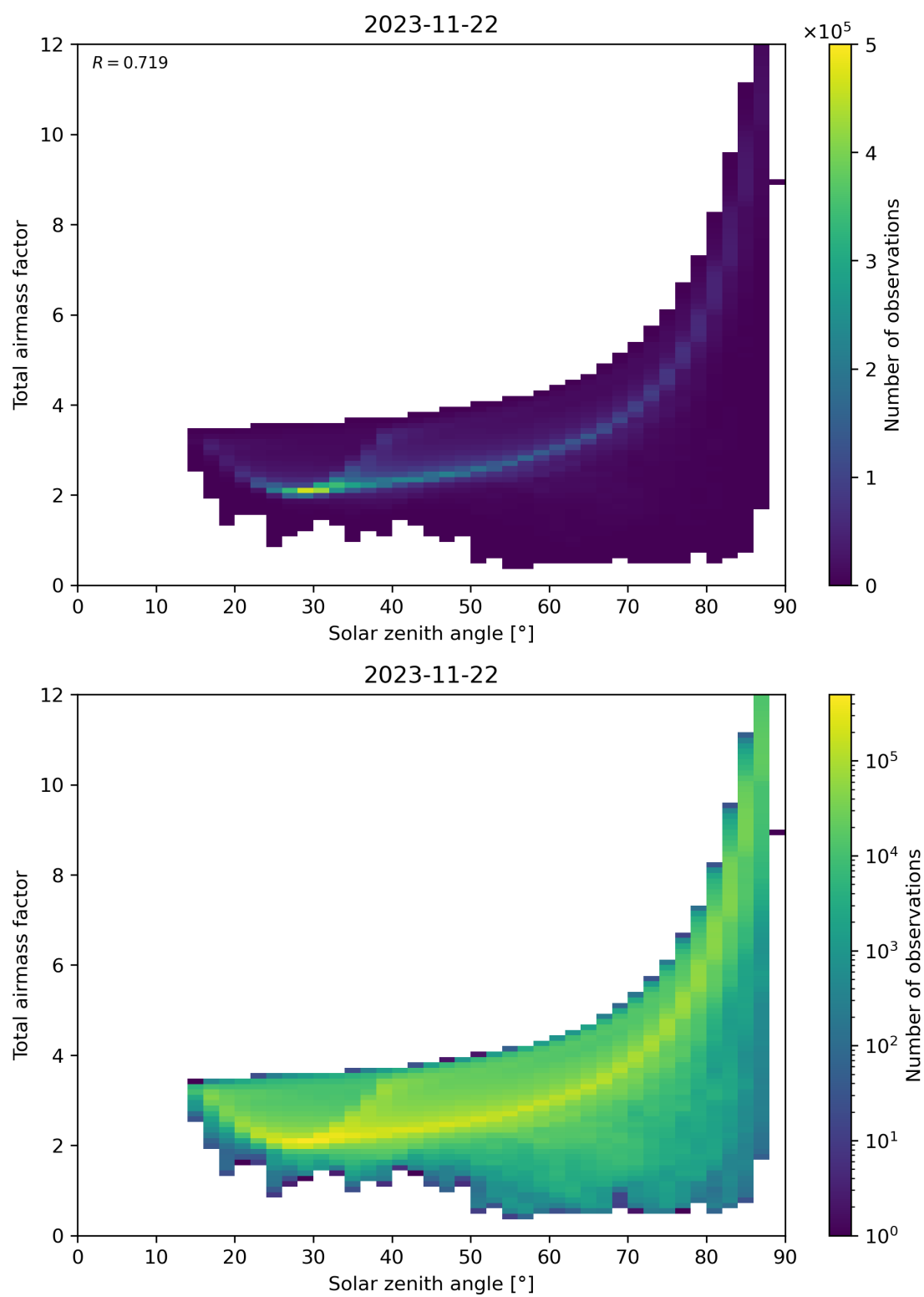
Figure 146: Scatter density plot of “Solar zenith angle” against “Total airmass factor” for 2023-11-21 to 2023-11-23.
