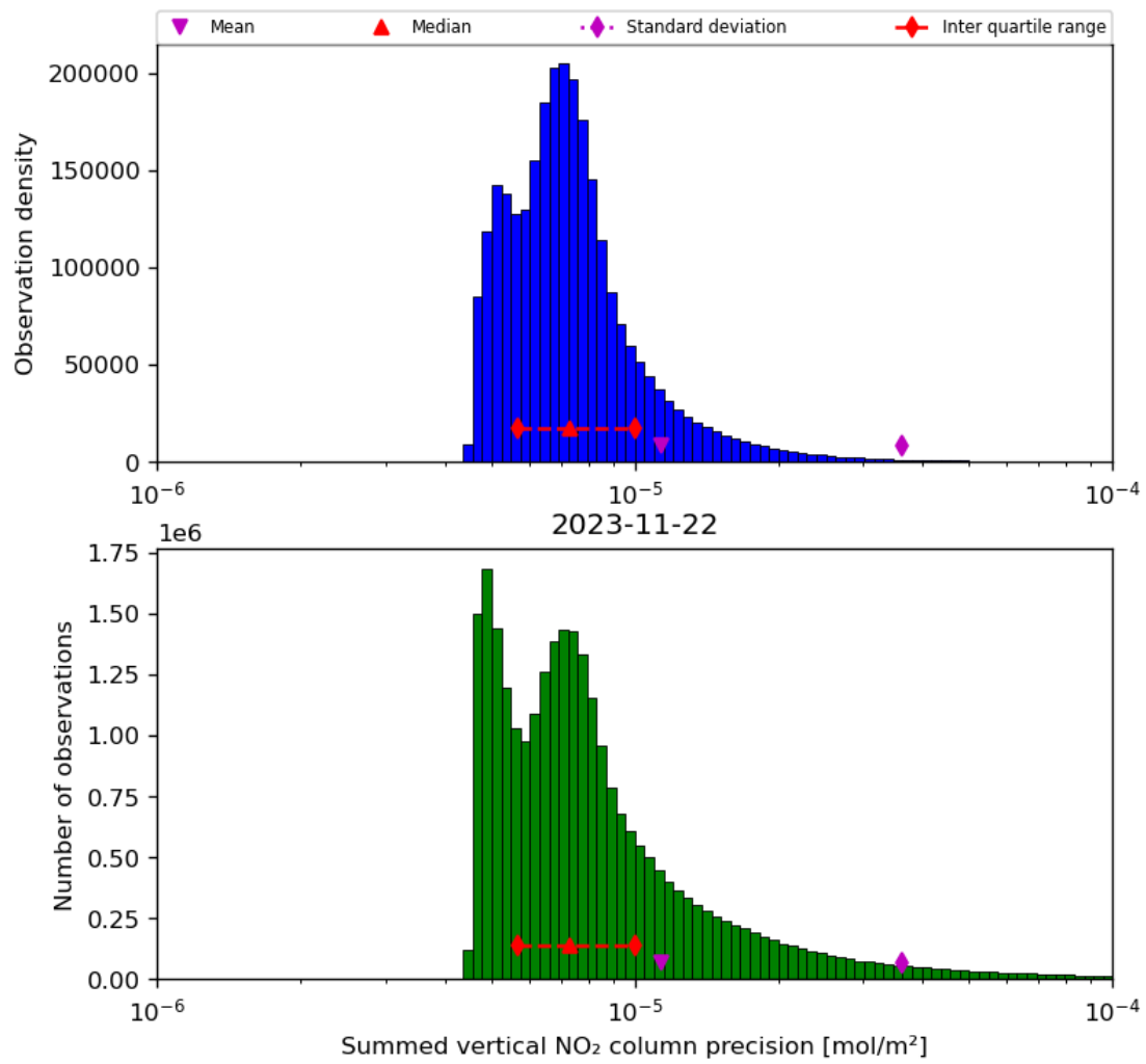
Figure 41: Histogram of “Summed vertical NO 2 column precision” for 2023-11-21 to 2023-11-23
