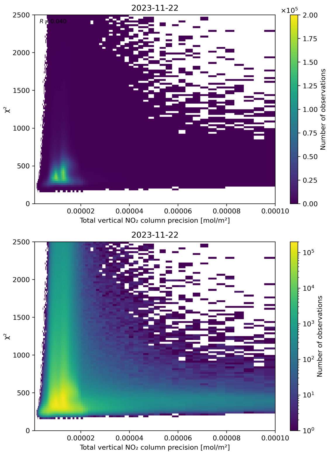
Figure 116: Scatter density plot of “Total vertical NO 2 column precision” against “ \chi^2 ” for 2023-11-21 to 2023-11-23.
