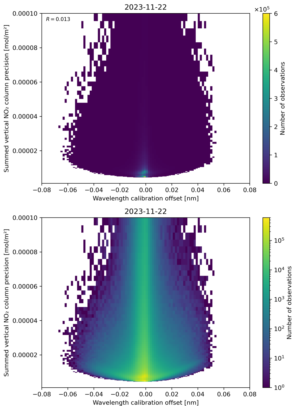
Figure 178: Scatter density plot of “Wavelength calibration offset” against “Summed vertical NO 2 column precision” for 2023-11-21 to 2023-11-23.
