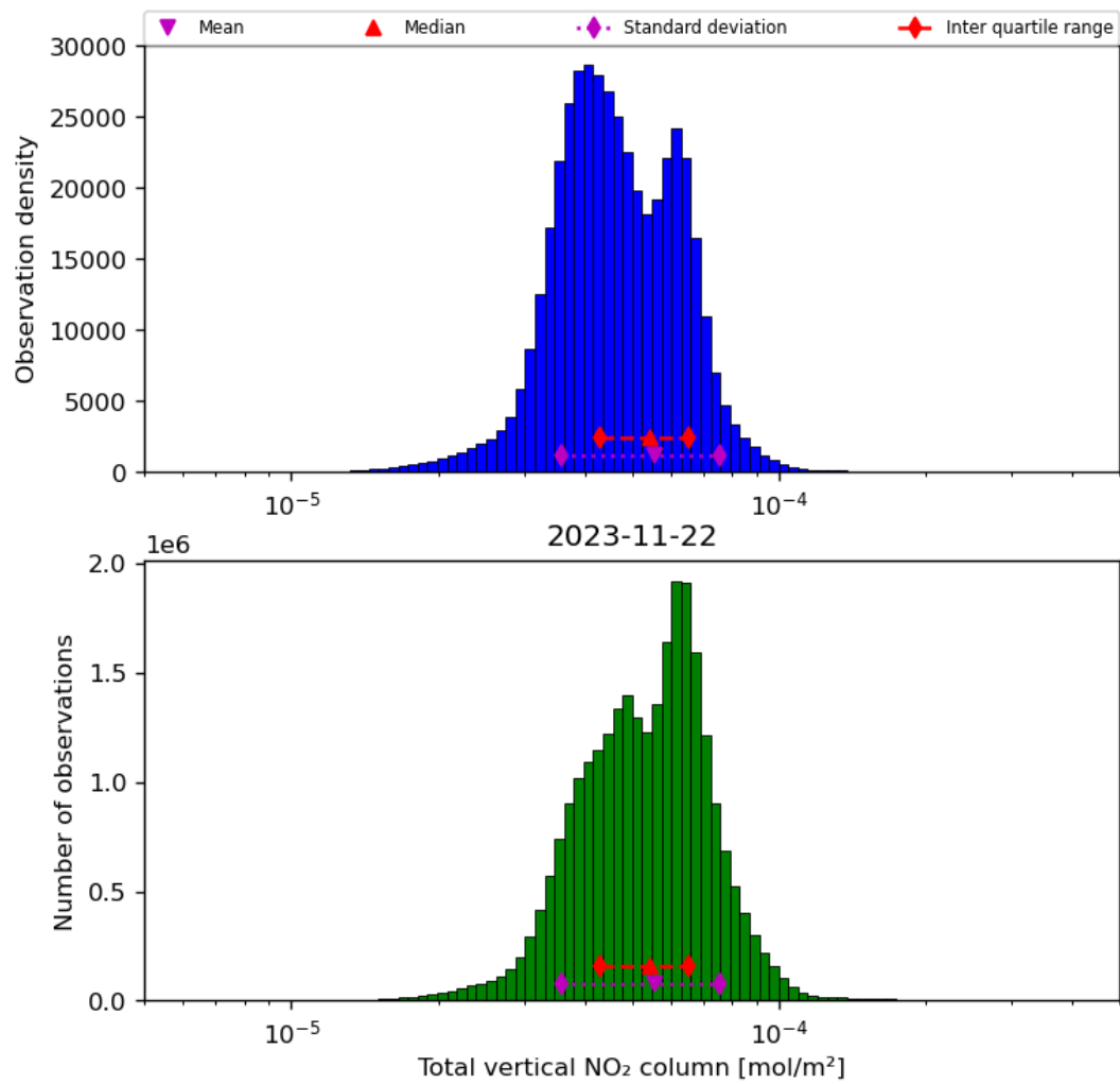
Figure 38: Histogram of “Total vertical NO 2 column” for 2023-11-21 to 2023-11-23
