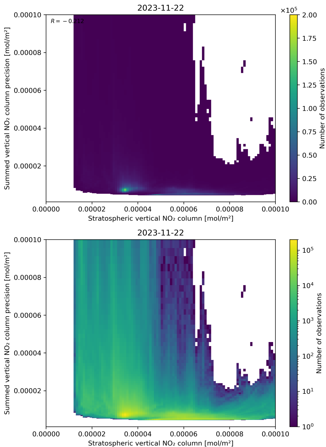
Figure 99: Scatter density plot of “Stratospheric vertical NO 2 column” against “Summed vertical NO 2 column precision” for 2023-11-21 to 2023-11-23.
