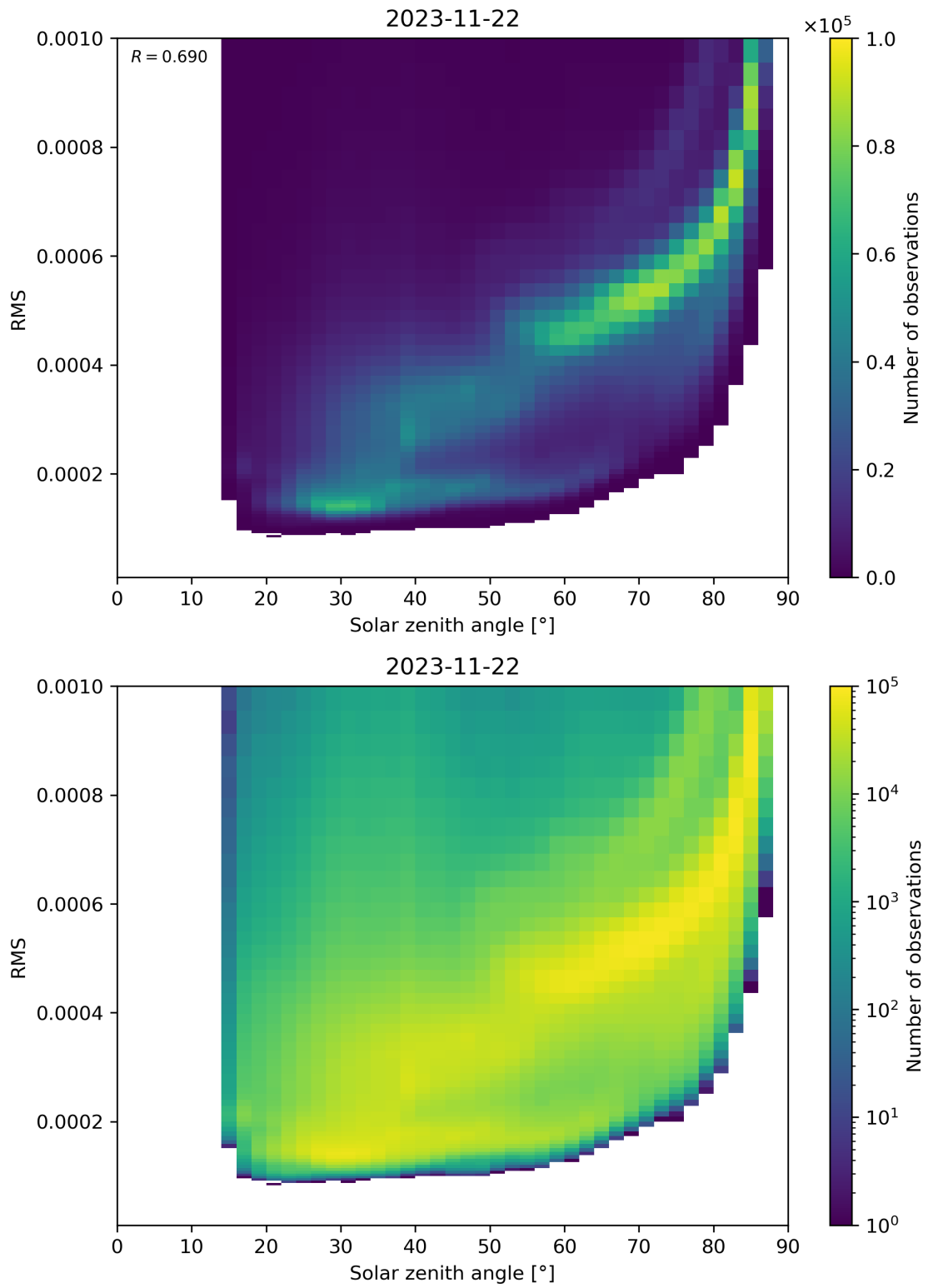
Figure 157: Scatter density plot of “Solar zenith angle” against “RMS” for 2023-11-21 to 2023-11-23.
