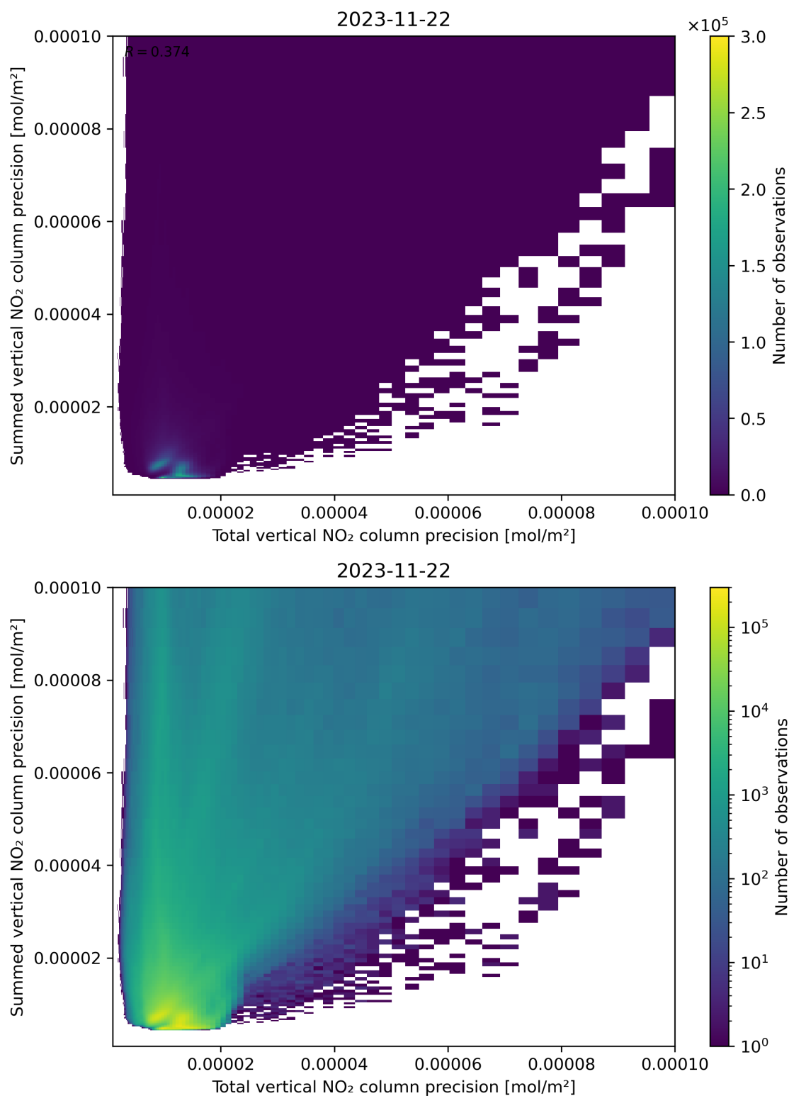
Figure 118: Scatter density plot of “Total vertical NO 2 column precision” against “Summed vertical NO 2 column precision” for 2023-11-21 to 2023-11-23.
