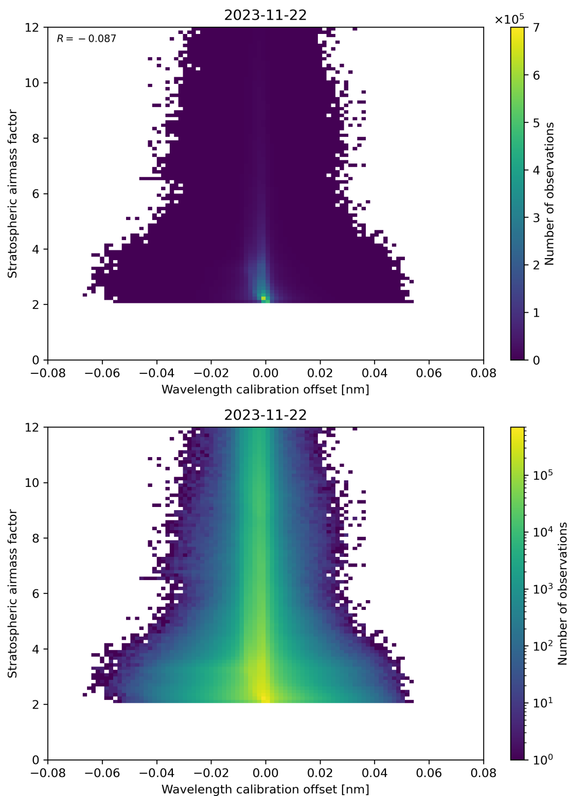
Figure 174: Scatter density plot of “Wavelength calibration offset” against “Stratospheric airmass factor” for 2023-11-21 to 2023-11-23.
