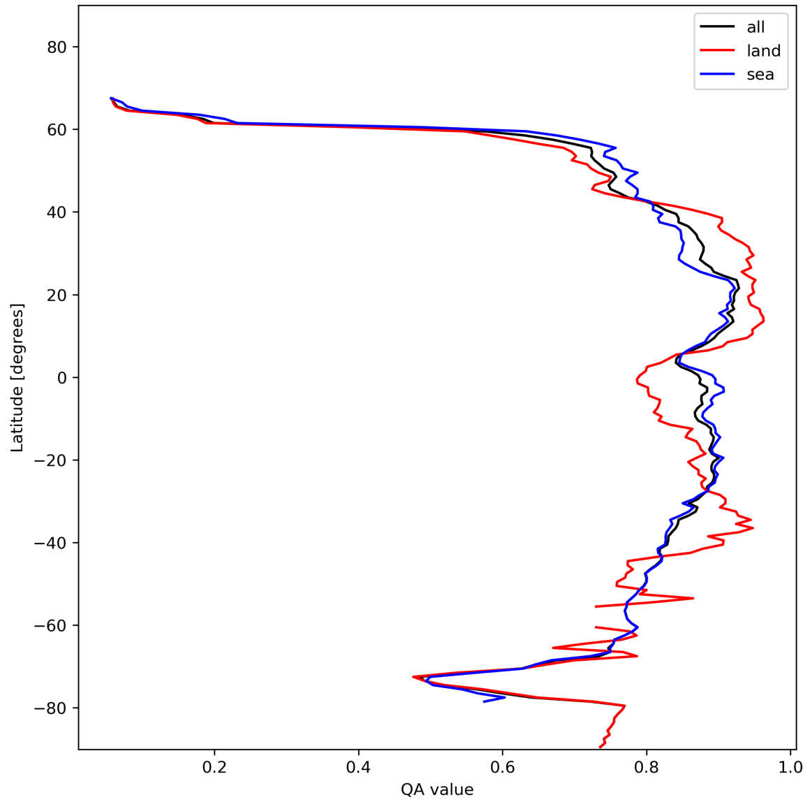
Figure 11: Zonal average of “QA value” for 2023-11-21 to 2023-11-23.
