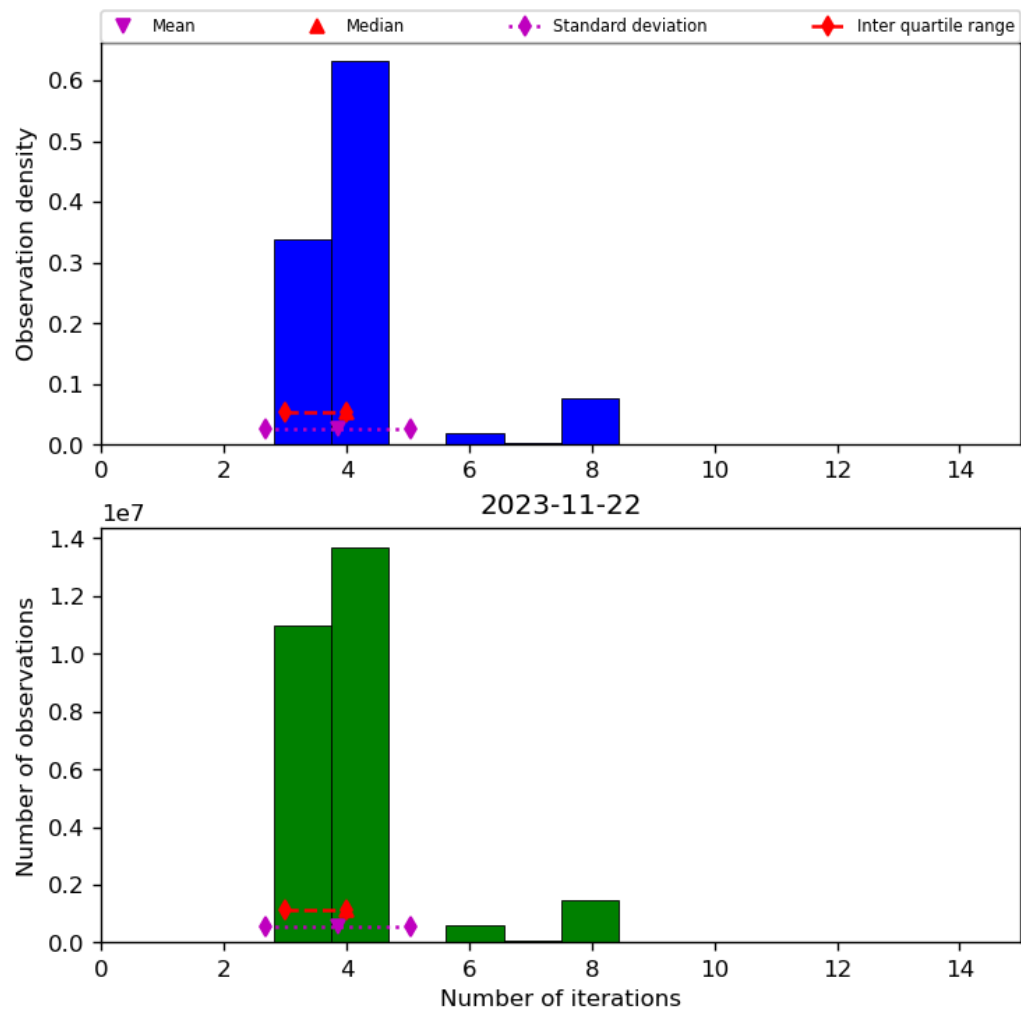
Figure 34: Histogram of “Number of iterations” for 2023-11-21 to 2023-11-23
