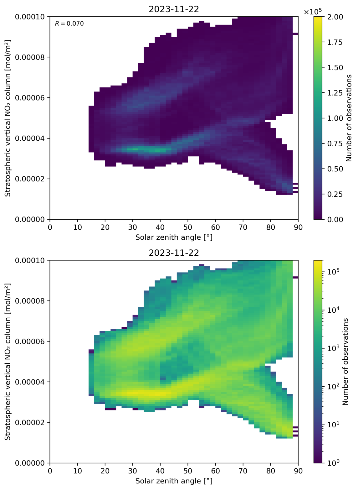
Figure 150: Scatter density plot of “Solar zenith angle” against “Stratospheric vertical NO 2 column” for 2023-11-21 to 2023-11-23.
