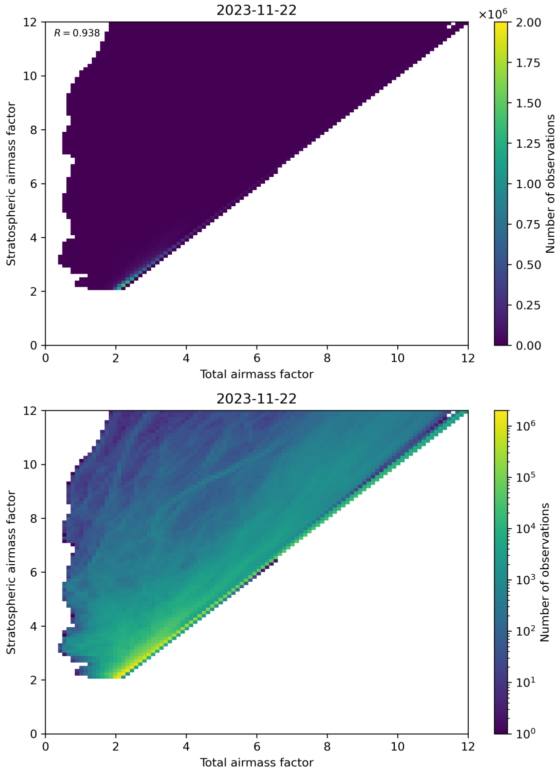
Figure 62: Scatter density plot of “Total airmass factor” against “Stratospheric airmass factor” for 2023-11-21 to 2023-11-23.
