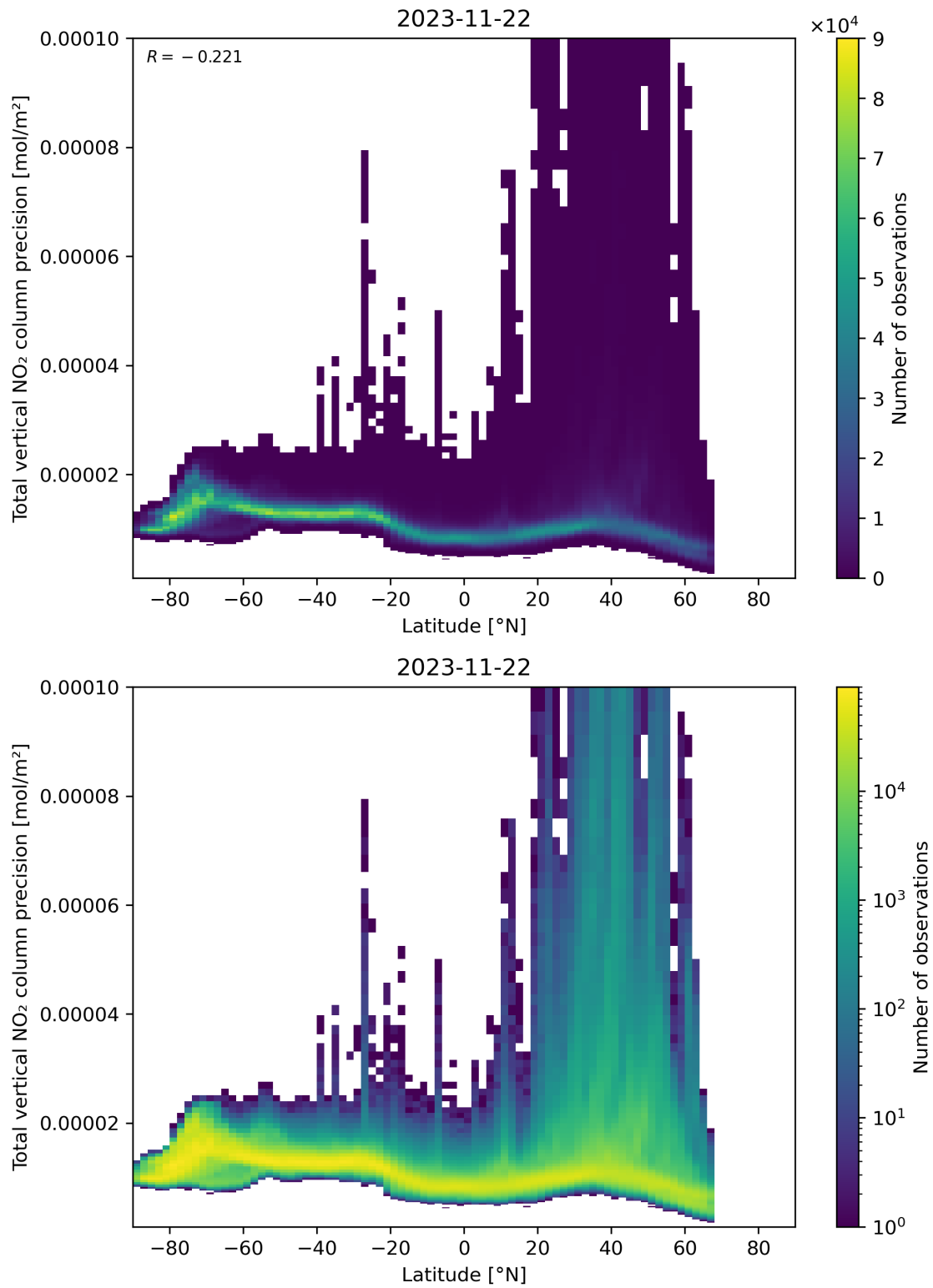
Figure 91: Scatter density plot of “Latitude” against “Total vertical NO 2 column precision” for 2023-11-21 to 2023-11-23.
