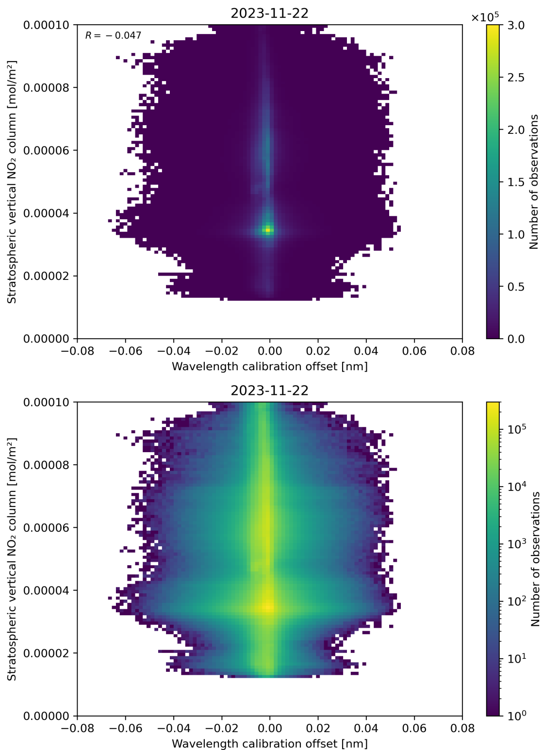
Figure 176: Scatter density plot of “Wavelength calibration offset” against “Stratospheric vertical NO 2 column” for 2023-11-21 to 2023-11-23.
