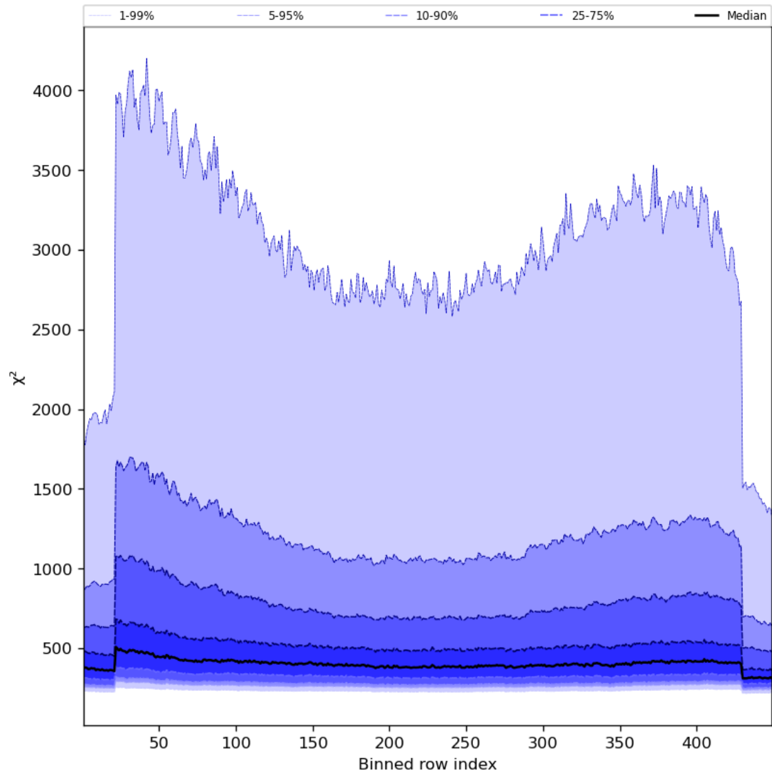
Figure 59: Along track statistics of “ \chi^2 ” for 2023-11-21 to 2023-11-23
