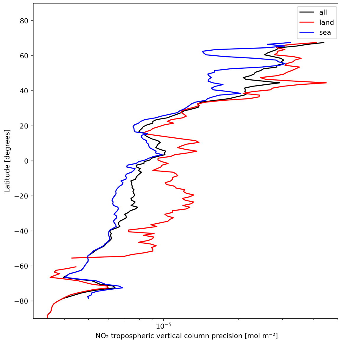
Figure 13: Zonal average of “NO 2 tropospheric vertical column precision” for 2023-11-21 to 2023-11-23.
