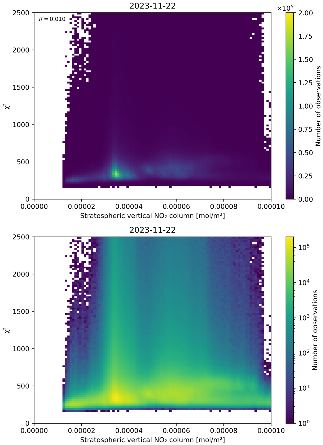
Figure 97: Scatter density plot of “Stratospheric vertical NO 2 column” against “ \chi^2 ” for 2023-11-21 to 2023-11-23.
