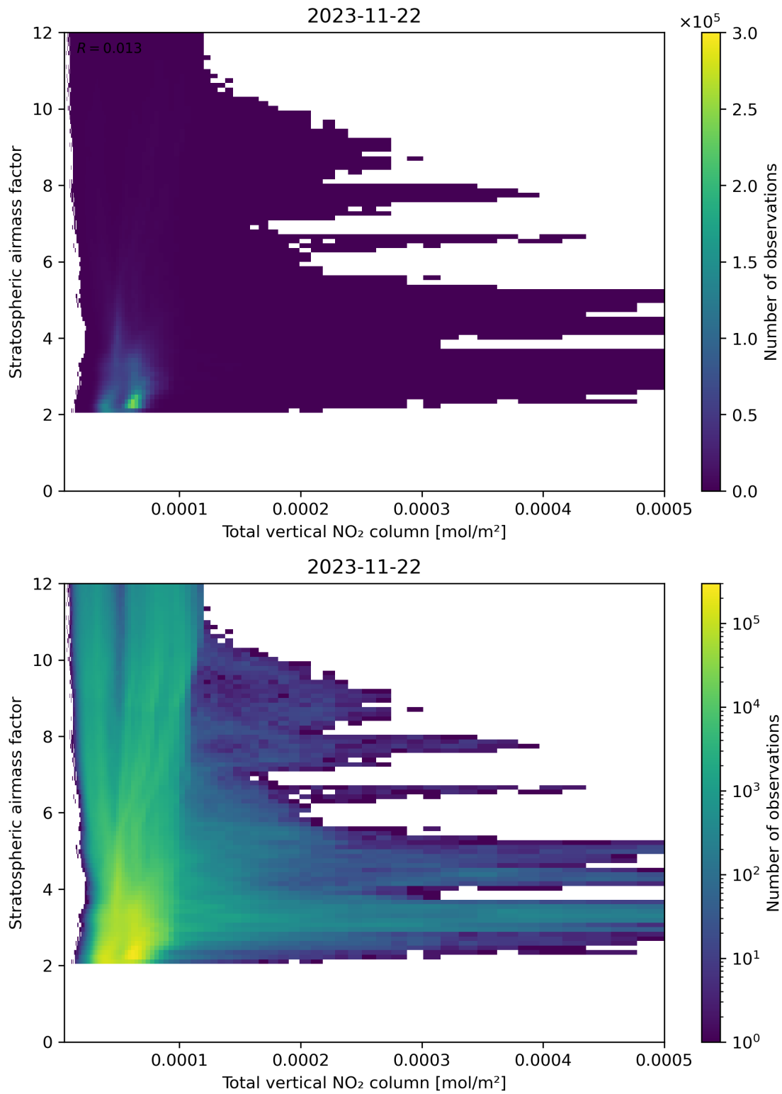
Figure 110: Scatter density plot of “Total vertical NO 2 column” against “Stratospheric airmass factor” for 2023-11-21 to 2023-11-23.
