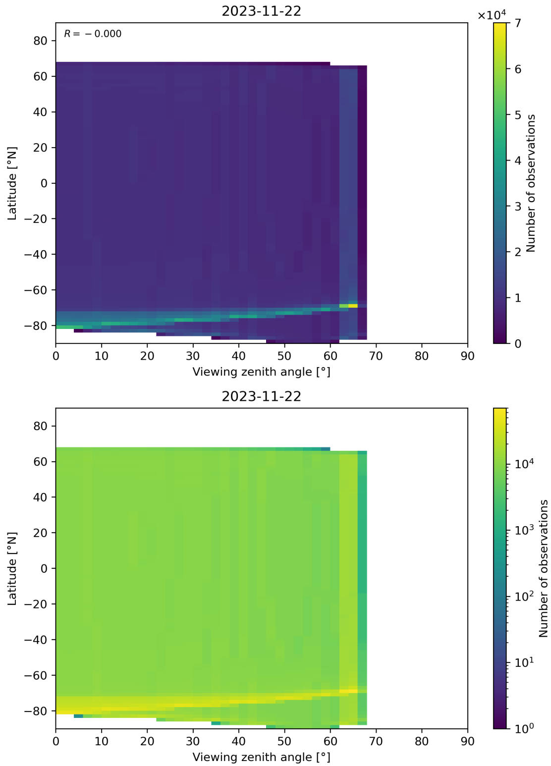
Figure 163: Scatter density plot of “Viewing zenith angle” against “Latitude” for 2023-11-21 to 2023-11-23.
