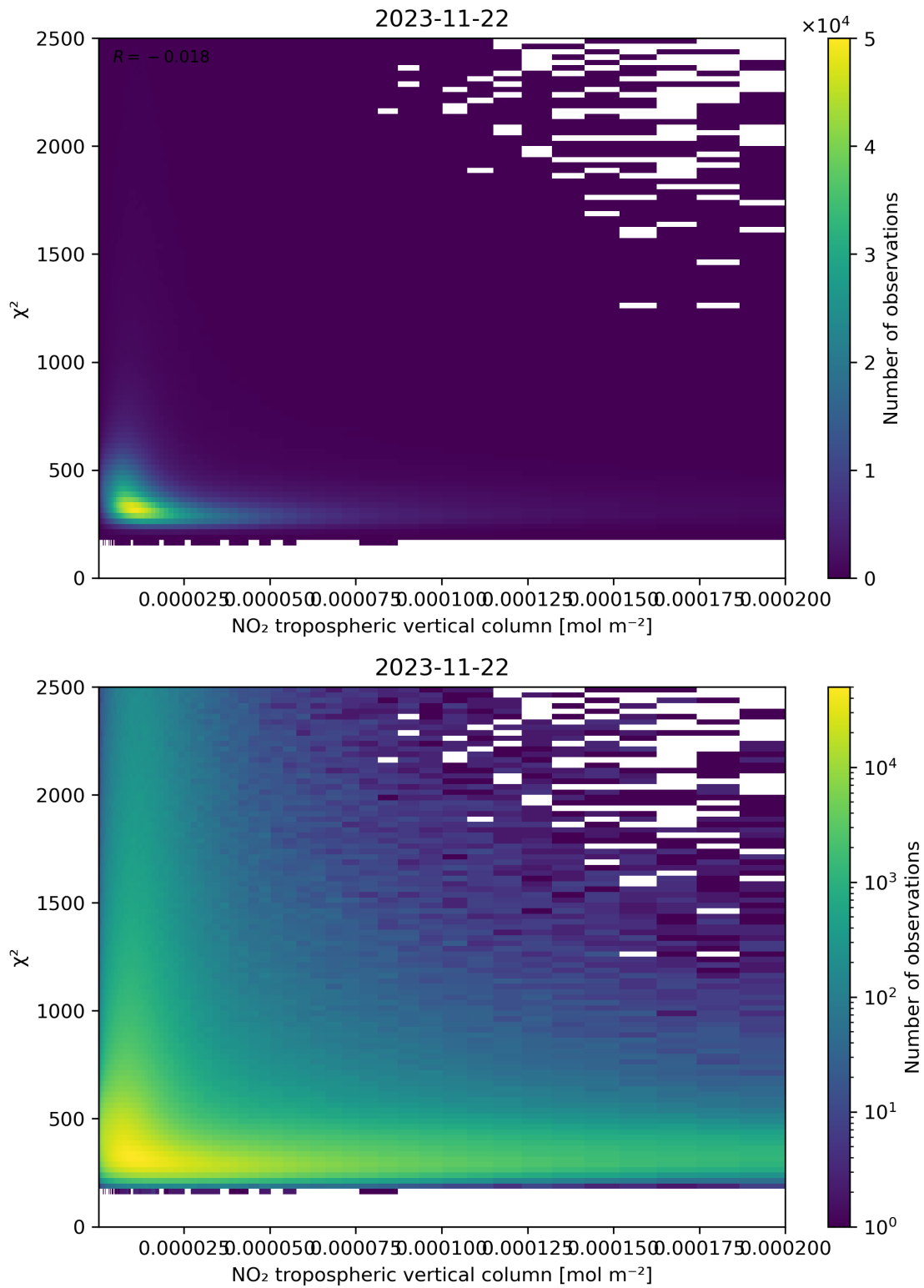
Figure 124: Scatter density plot of “NO 2 tropospheric vertical column” against “ \chi^2 ” for 2023-11-21 to 2023-11-23.
