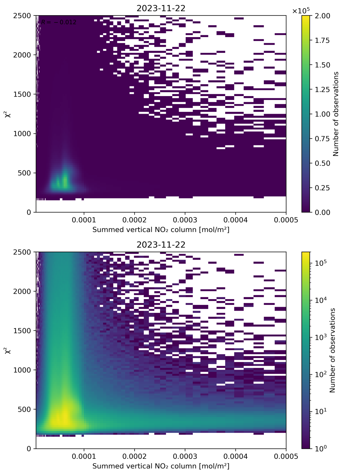
Figure 104: Scatter density plot of “Summed vertical NO 2 column” against “ \chi^2 ” for 2023-11-21 to 2023-11-23.
