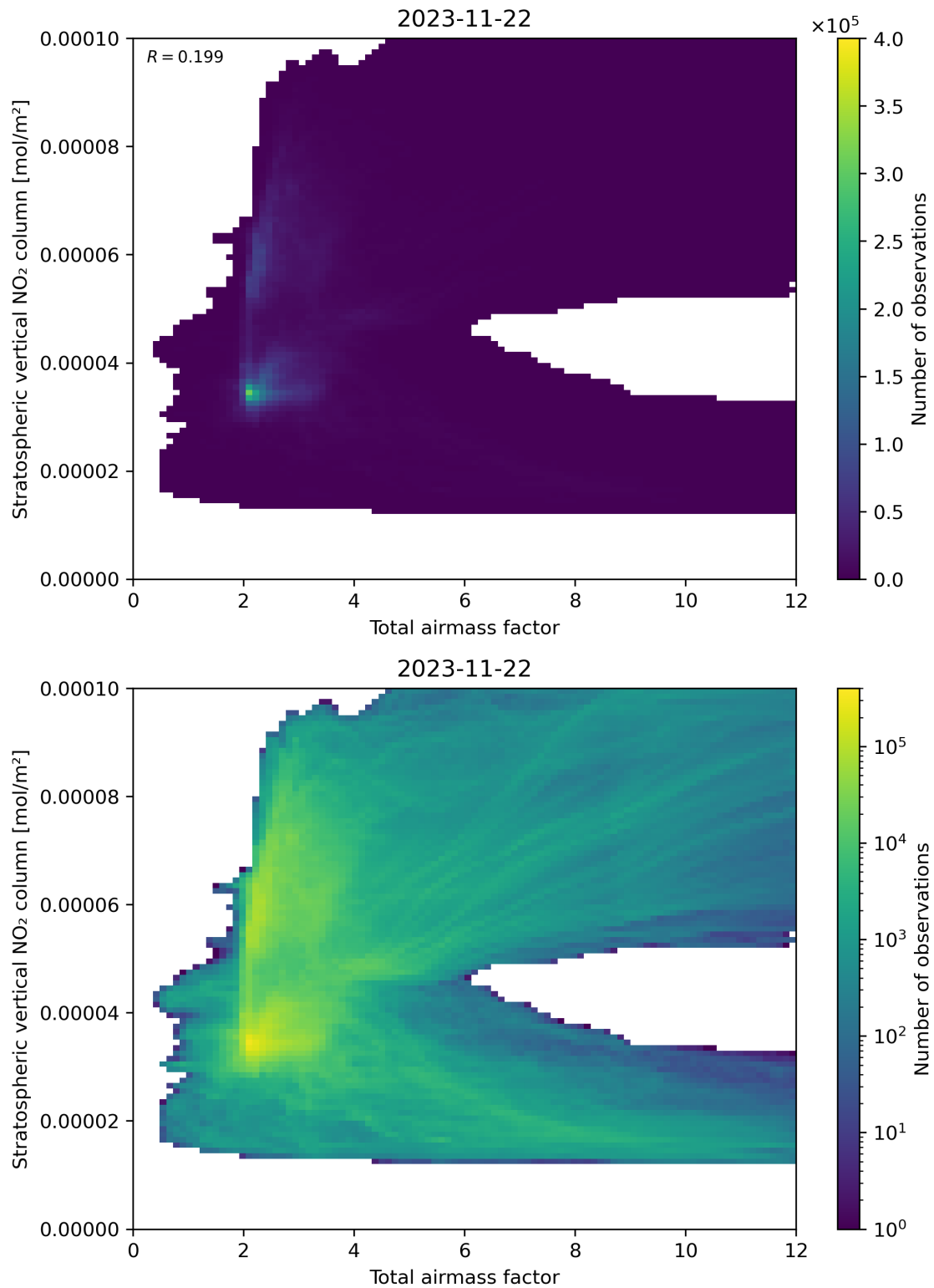
Figure 64: Scatter density plot of “Total airmass factor” against “Stratospheric vertical NO 2 column” for 2023-11-21 to 2023-11-23.
