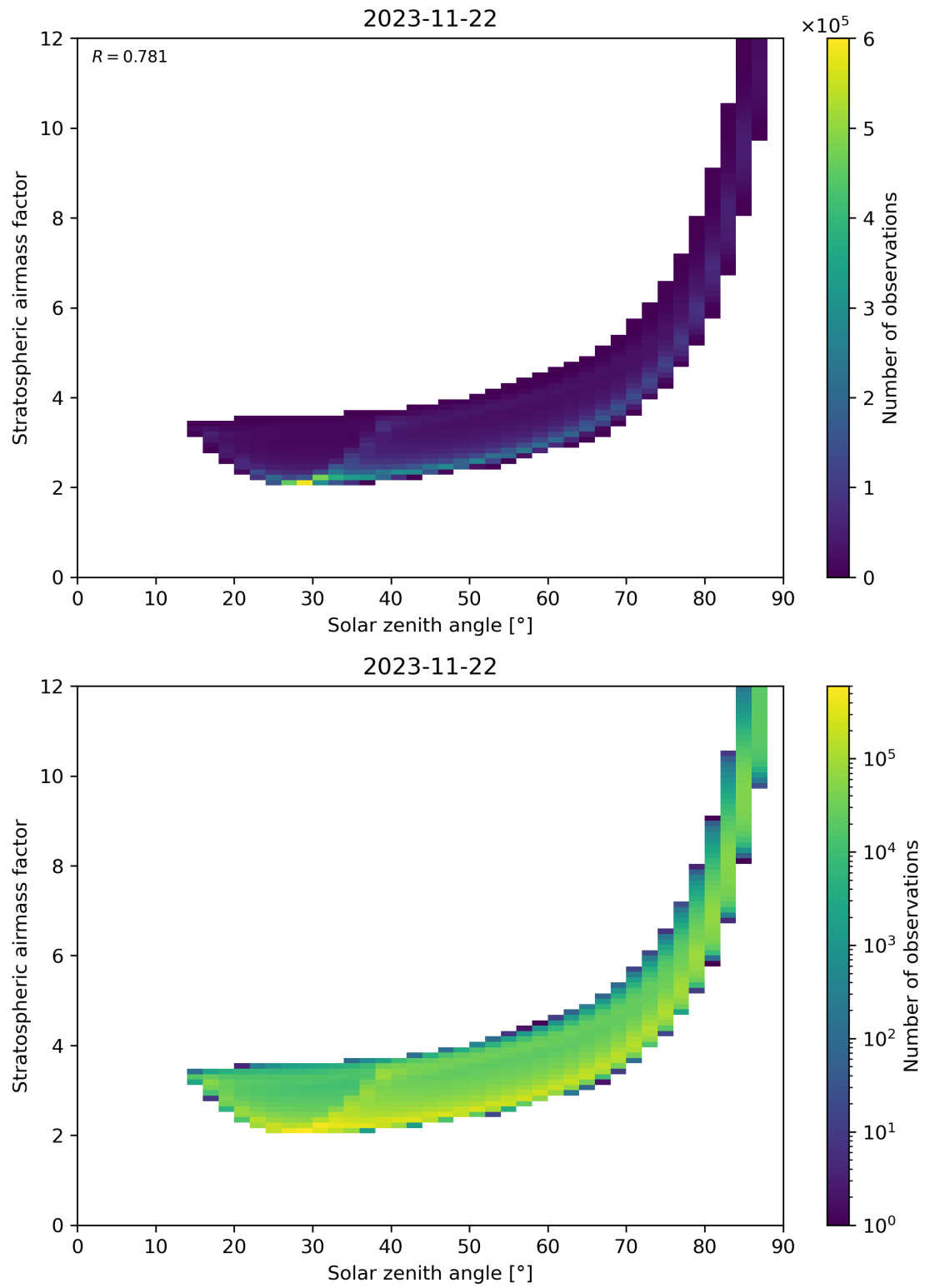
Figure 145: Scatter density plot of “Solar zenith angle” against “Stratospheric airmass factor” for 2023-11-21 to 2023-11-23.
