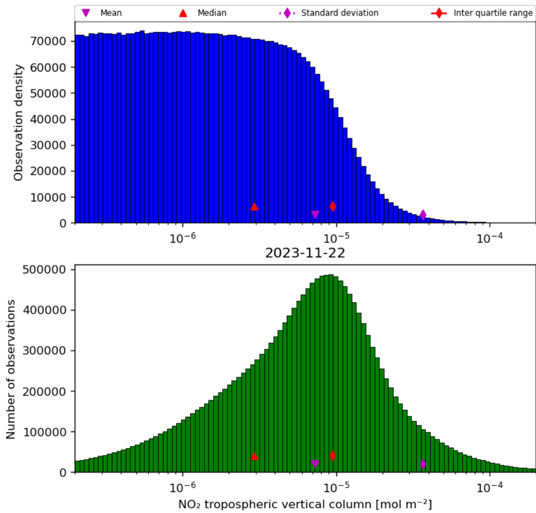
Figure 29: Histogram of “NO 2 tropospheric vertical column” for 2023-11-21 to 2023-11-23
