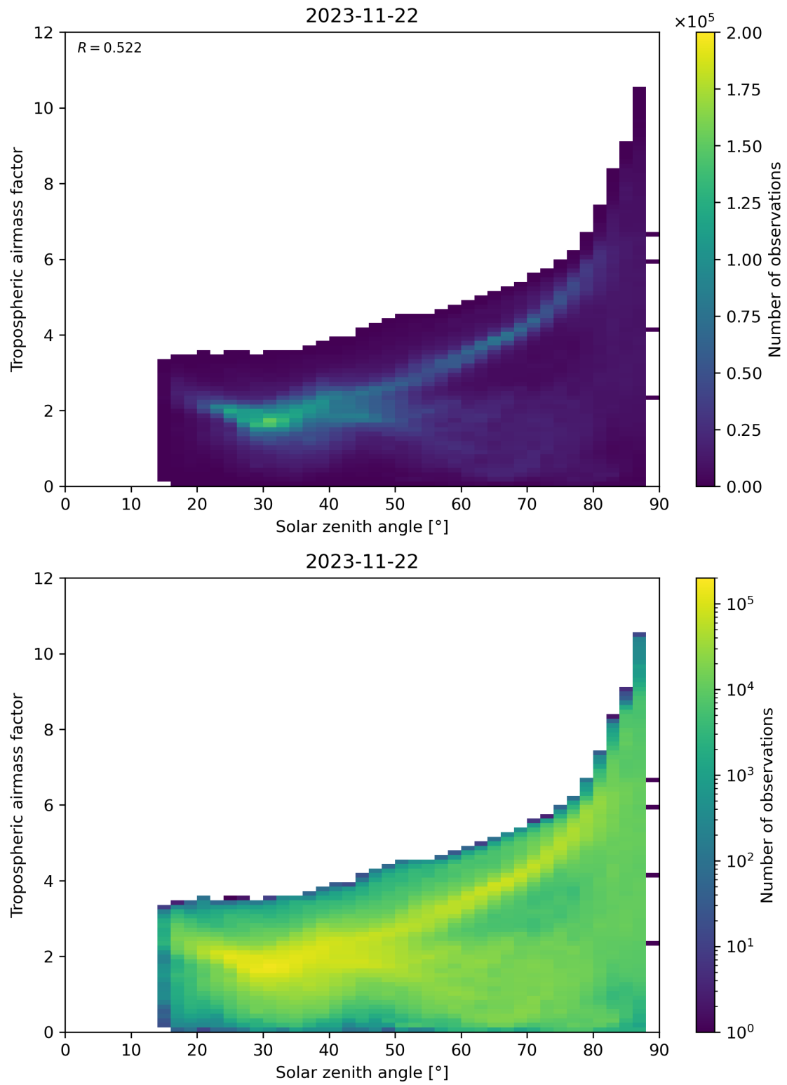
Figure 147: Scatter density plot of “Solar zenith angle” against “Tropospheric airmass factor” for 2023-11-21 to 2023-11-23.
