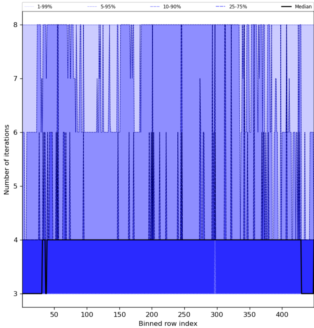
Figure 51: Along track statistics of “Number of iterations” for 2023-11-21 to 2023-11-23
