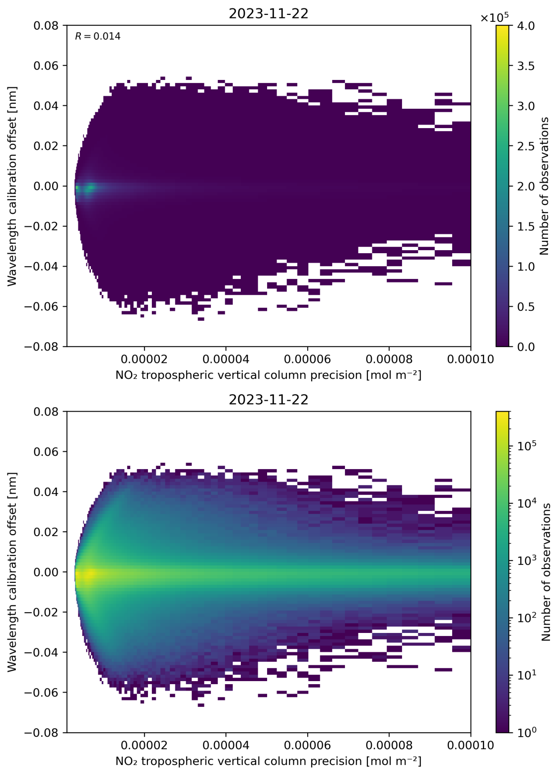
Figure 141: Scatter density plot of “NO 2 tropospheric vertical column precision” against “Wavelength calibration offset” for 2023-11-21 to 2023-11-23.
