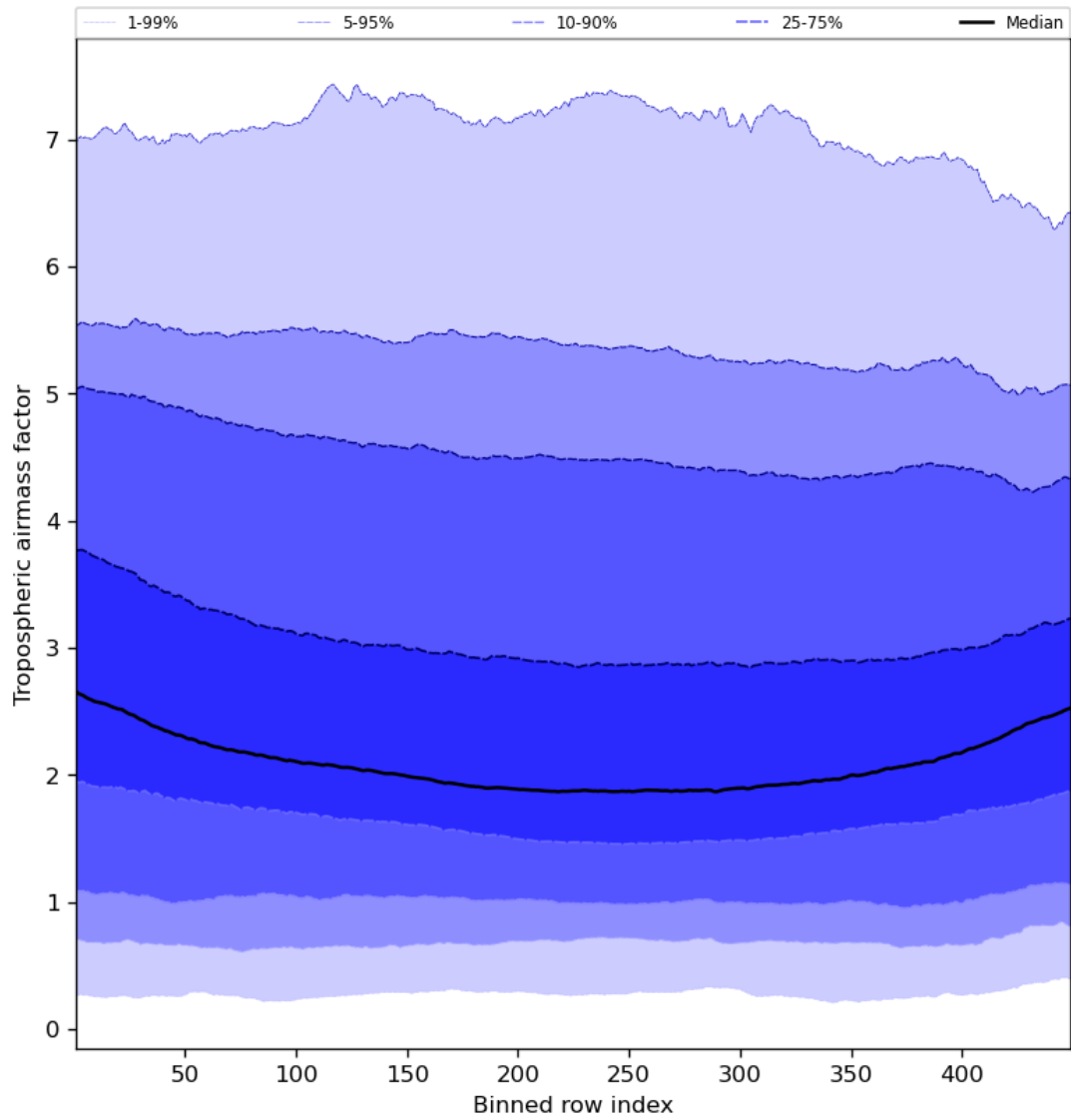
Figure 48: Along track statistics of “Tropospheric airmass factor” for 2023-11-21 to 2023-11-23
