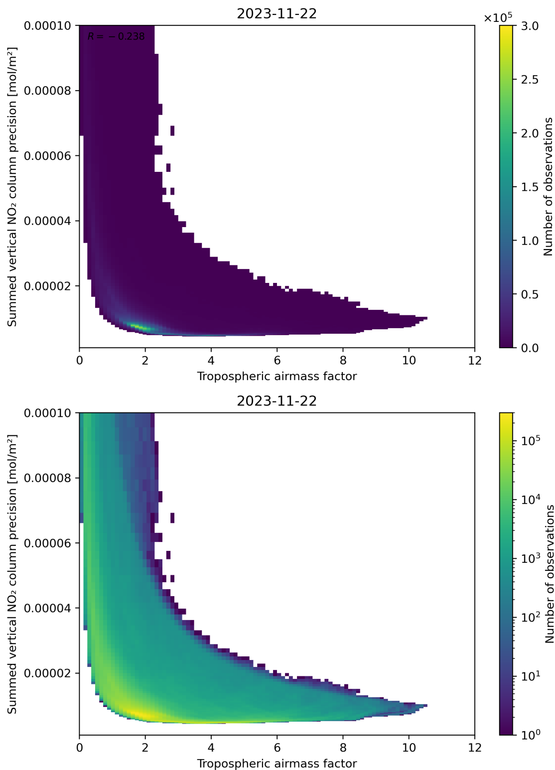
Figure 76: Scatter density plot of “Tropospheric air mass factor” against “Summed vertical NO 2 column precision” for 2023-11-21 to 2023-11-23.
