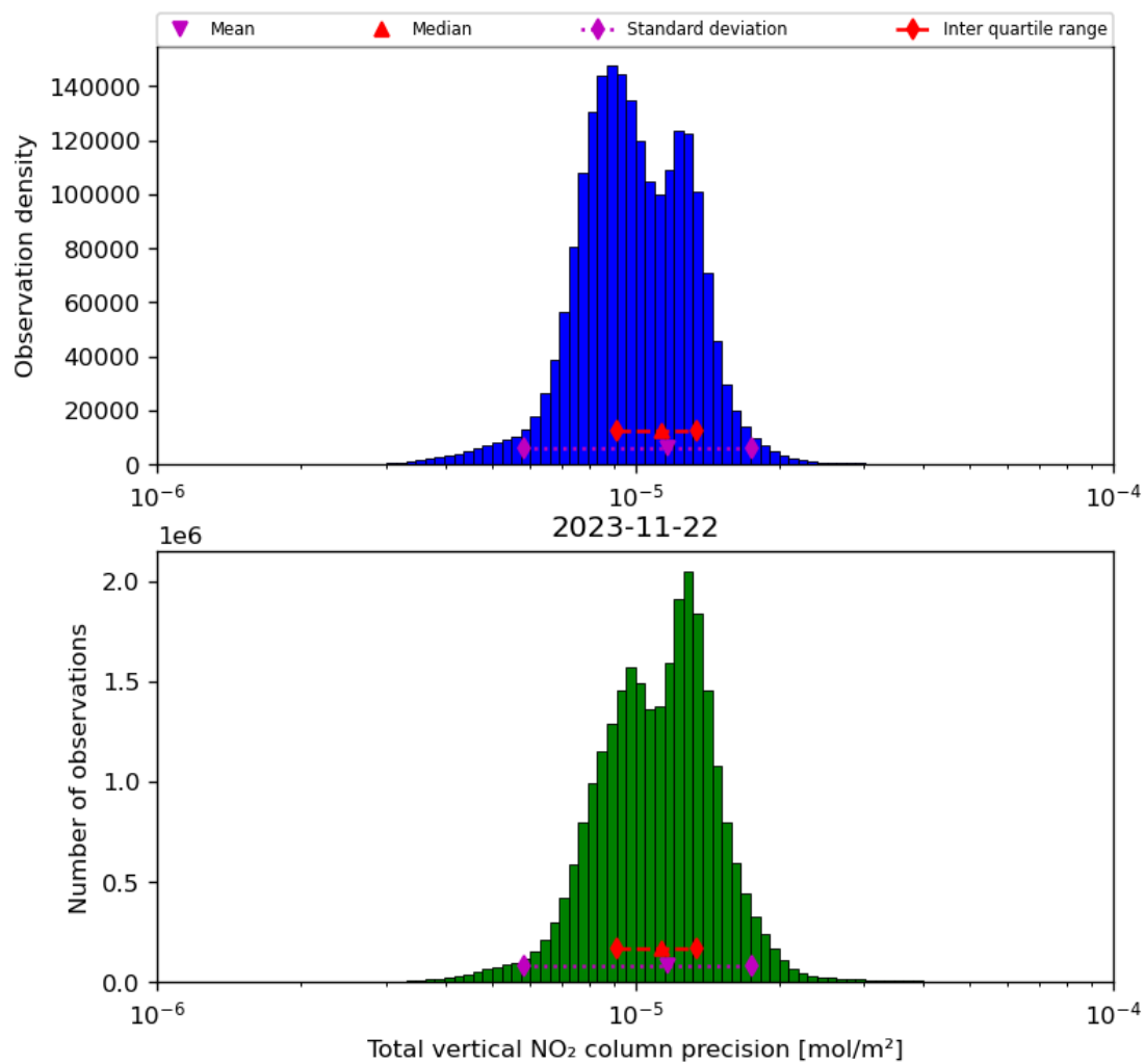
Figure 39: Histogram of “Total vertical NO 2 column precision” for 2023-11-21 to 2023-11-23
