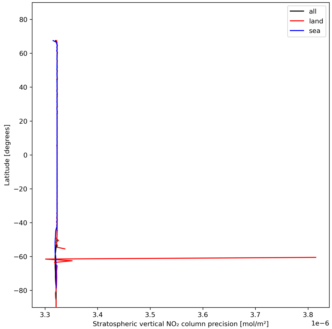
Figure 20: Zonal average of “Stratospheric vertical NO 2 column precision” for 2023-11-21 to 2023-11-23.
