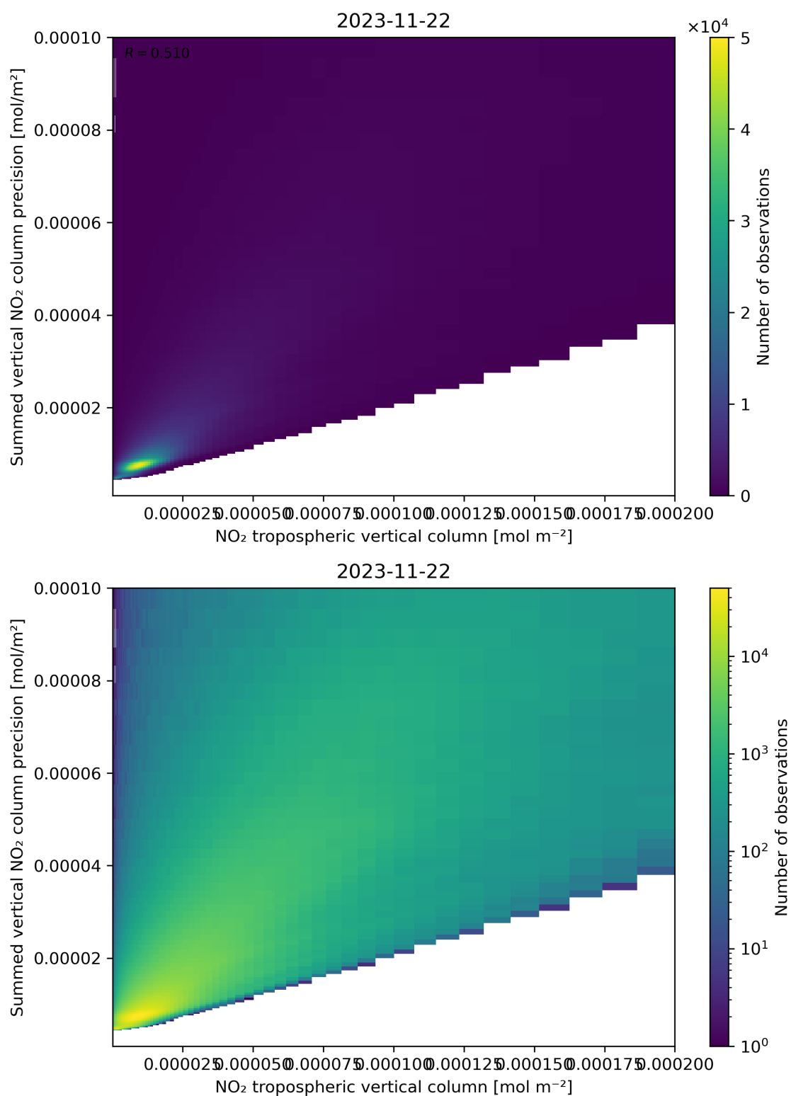
Figure 127: Scatter density plot of “NO 2 tropospheric vertical column” against “Summed vertical NO 2 column precision” for 2023-11-21 to 2023-11-23.
