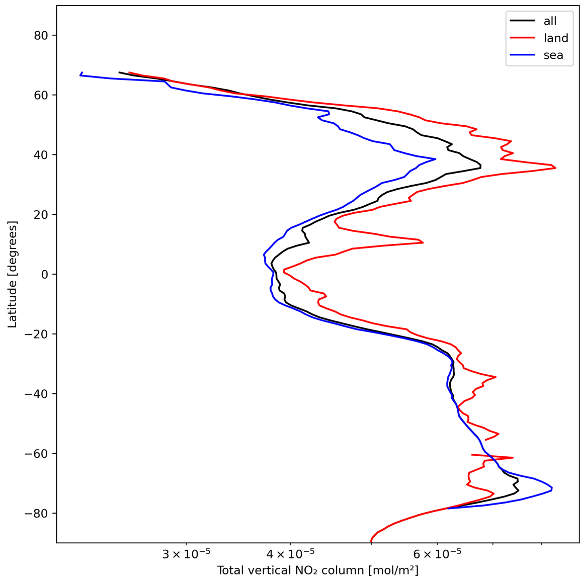
Figure 21: Zonal average of “Total vertical NO 2 column” for 2023-11-21 to 2023-11-23.
