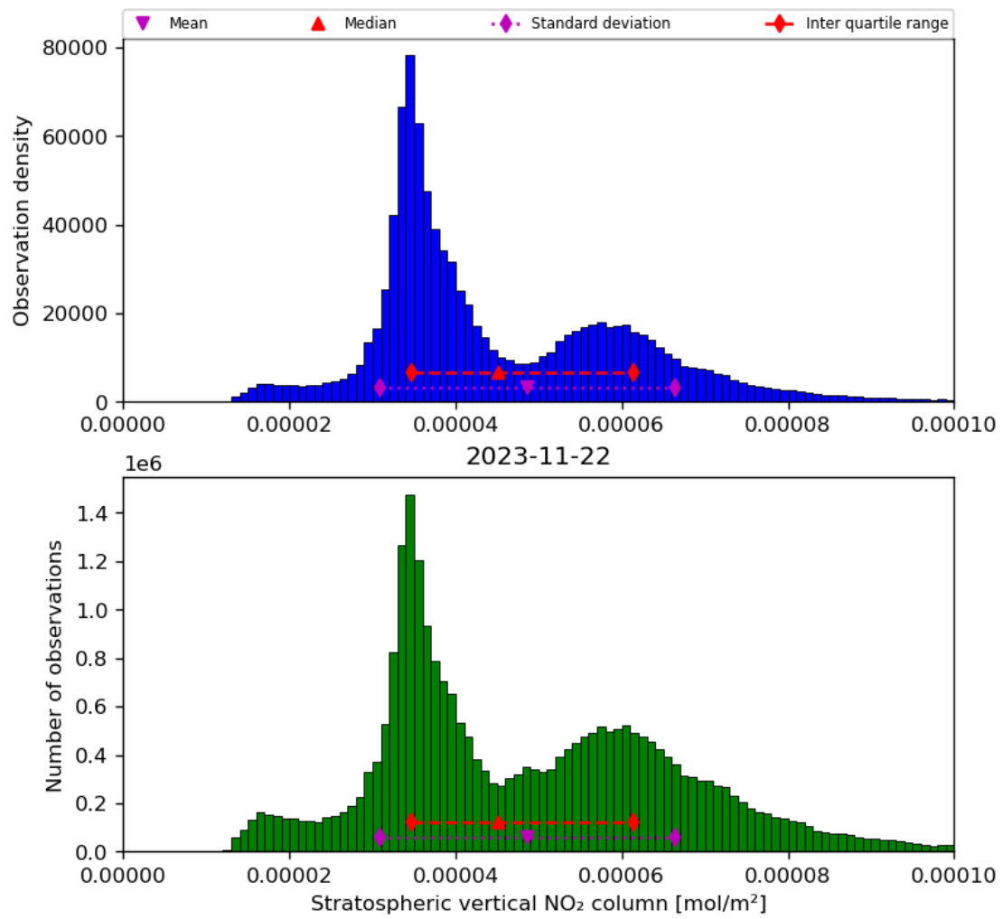
Figure 36: Histogram of “Stratospheric vertical NO 2 column” for 2023-11-21 to 2023-11-23
