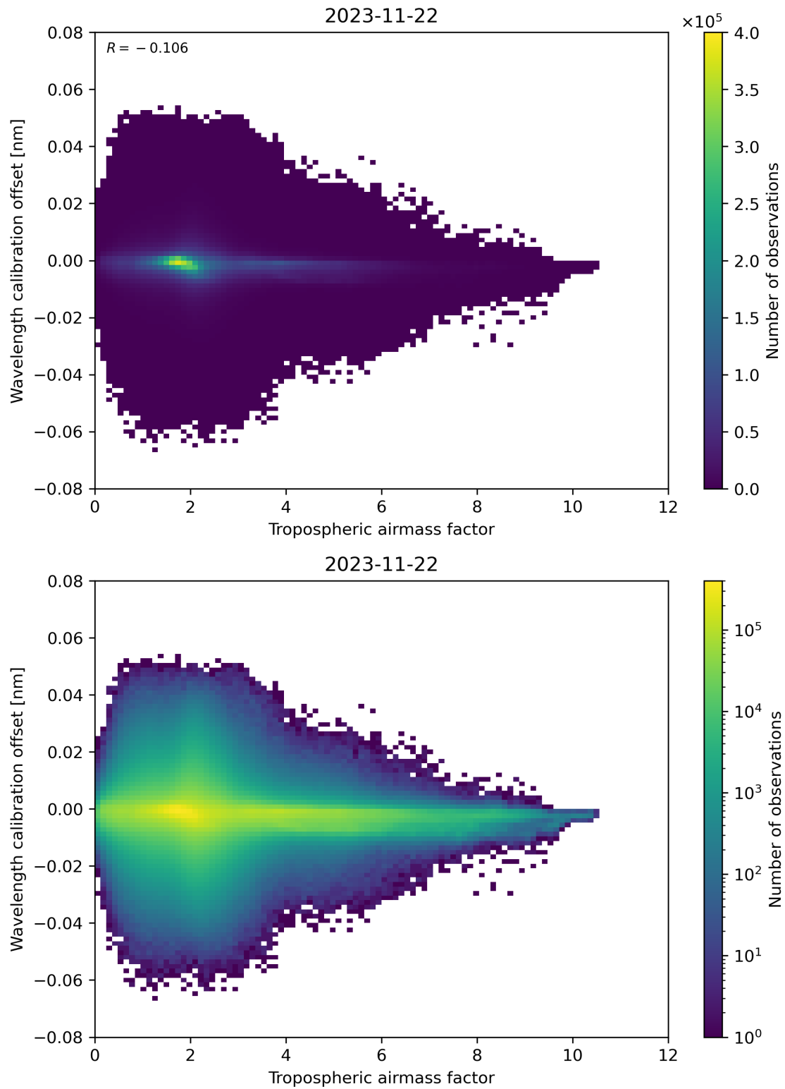
Figure 80: Scatter density plot of “Tropospheric airmass factor” against “Wavelength calibration offset” for 2023-11-21 to 2023-11-23.
