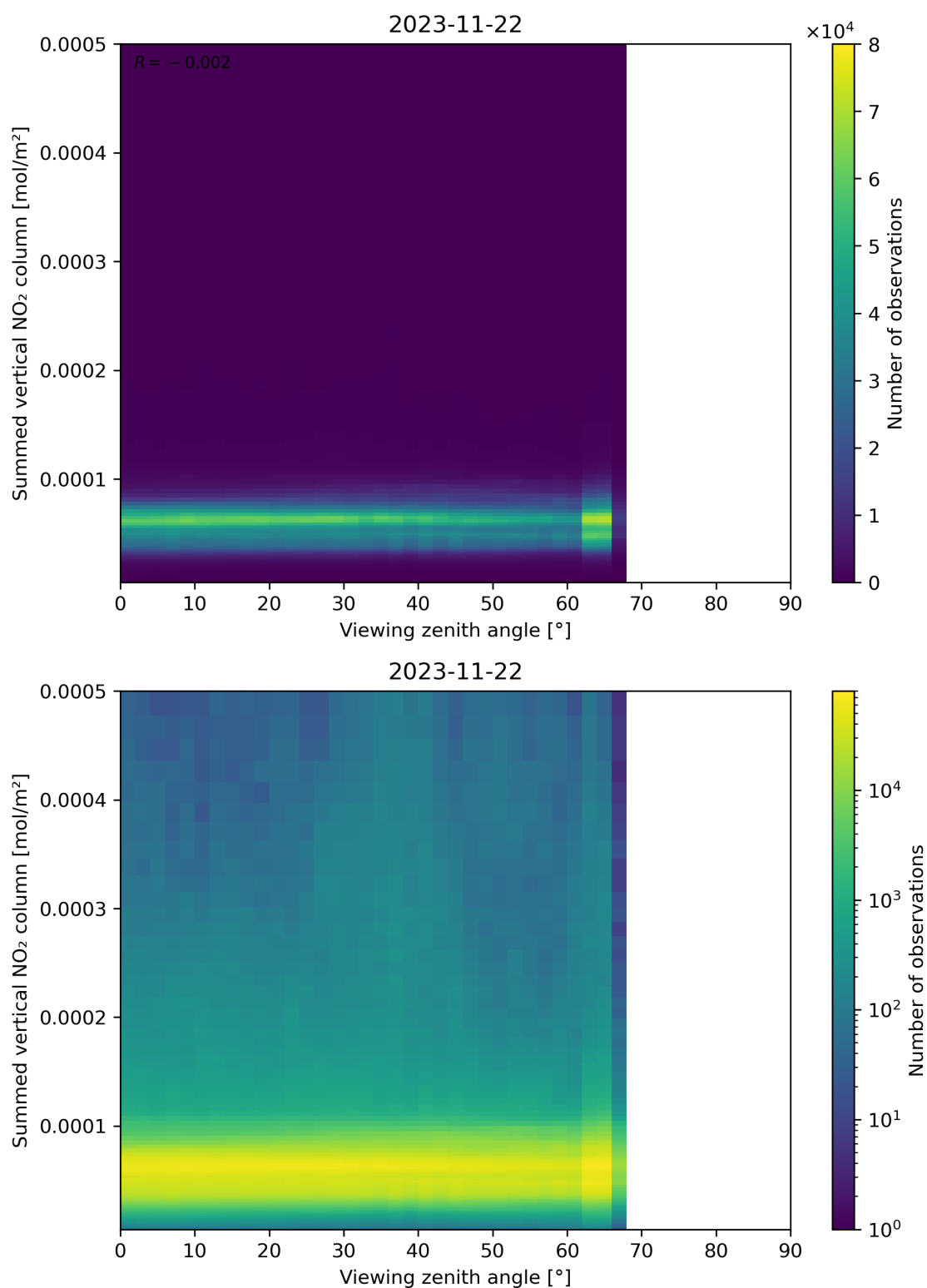
Figure 165: Scatter density plot of “Viewing zenith angle” against “Summed vertical NO 2 column” for 2023-11-21 to 2023-11-23.
