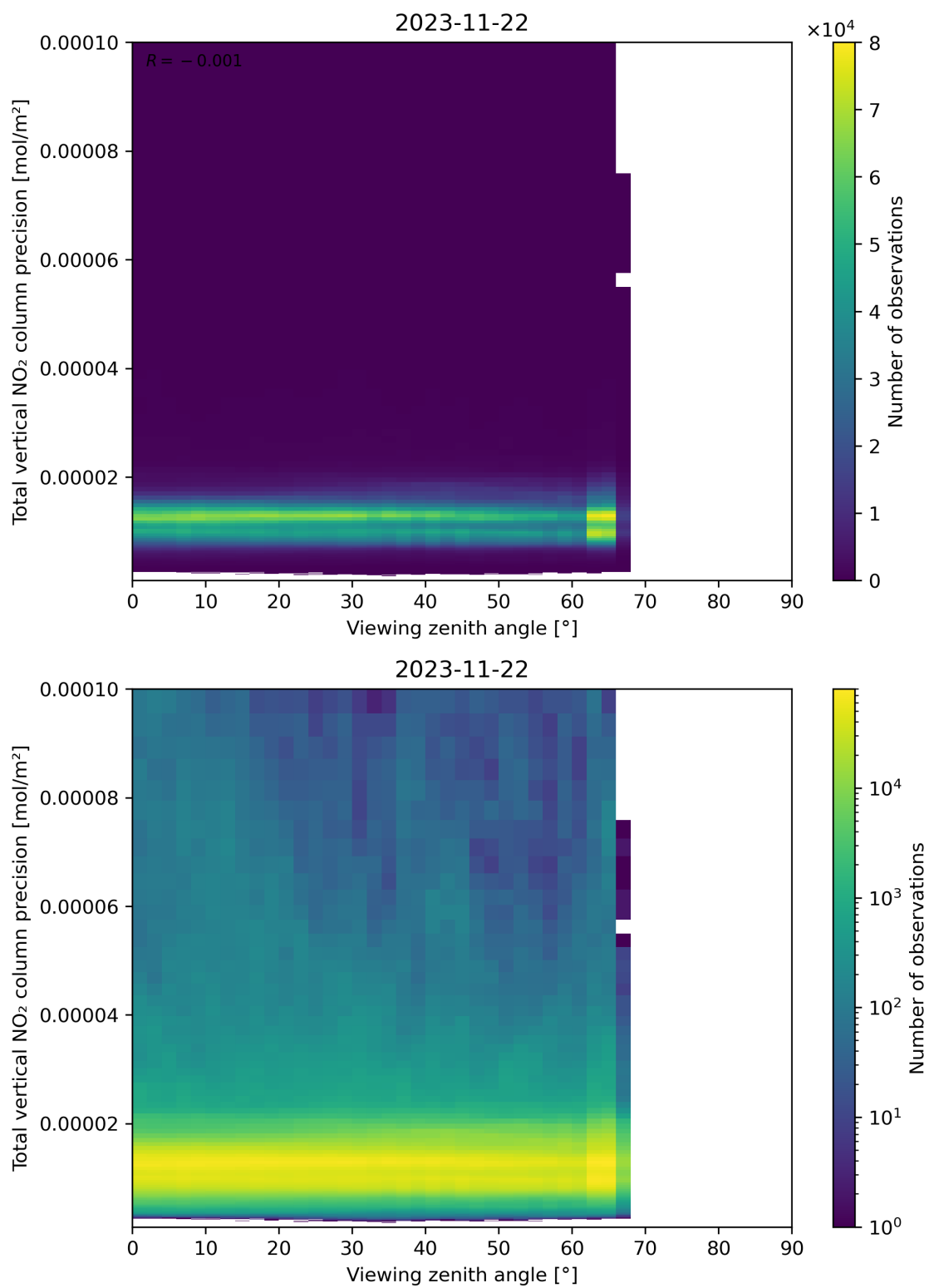
Figure 168: Scatter density plot of “Viewing zenith angle” against “Total vertical NO 2 column precision” for 2023-11-21 to 2023-11-23.
