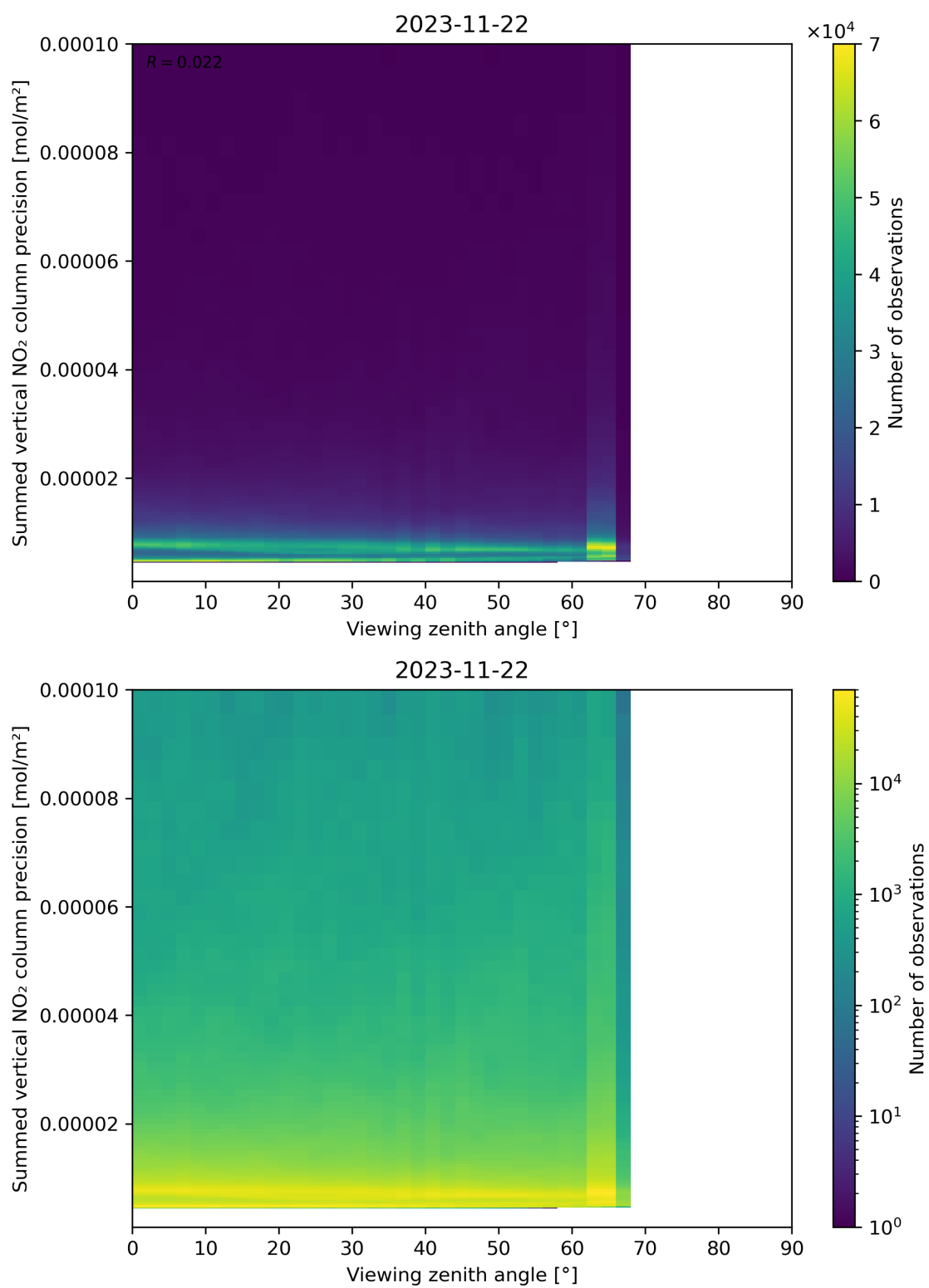
Figure 166: Scatter density plot of “Viewing zenith angle” against “Summed vertical NO 2 column precision” for 2023-11-21 to 2023-11-23.
