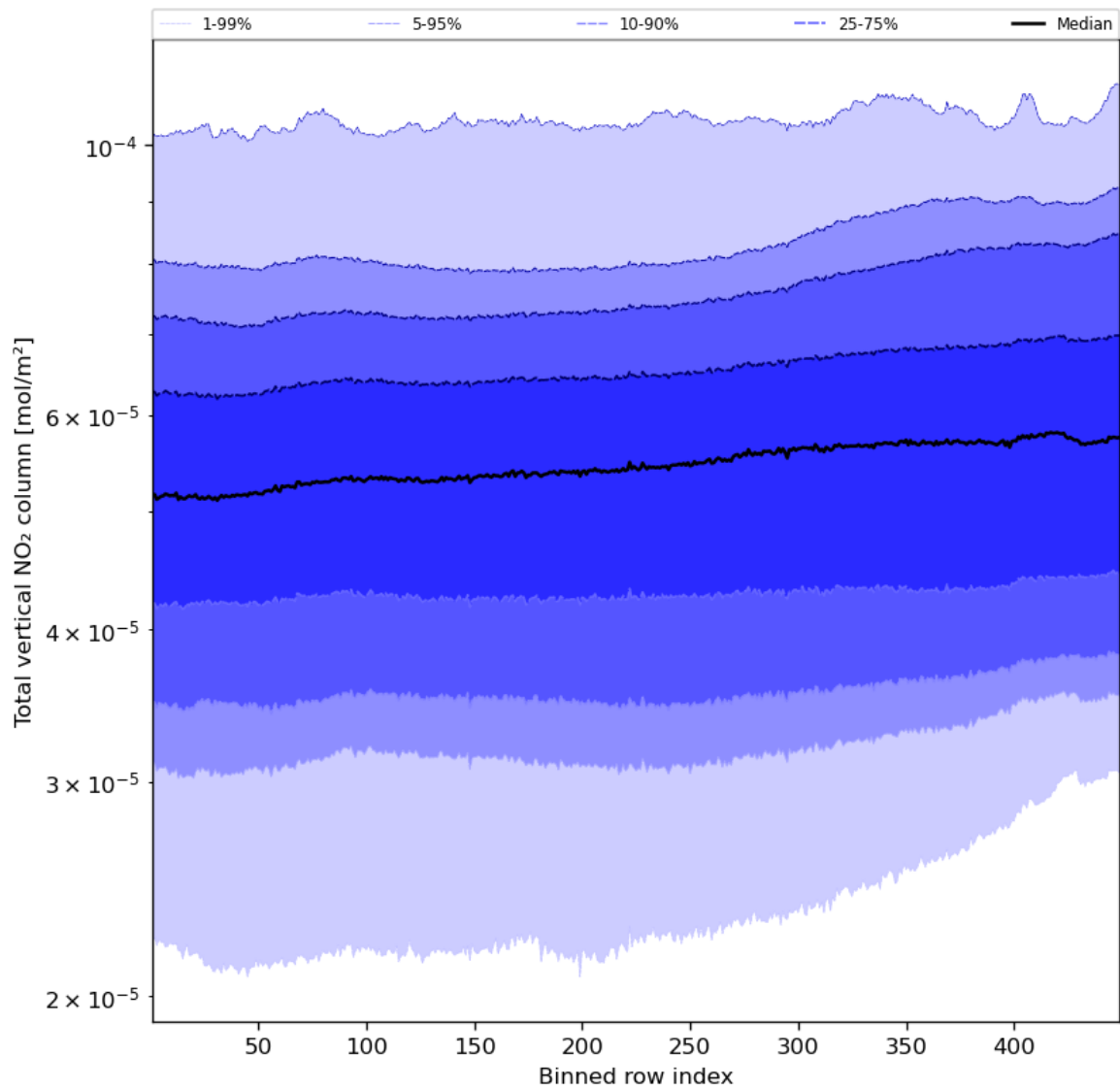
Figure 55: Along track statistics of “Total vertical NO 2 column” for 2023-11-21 to 2023-11-23
