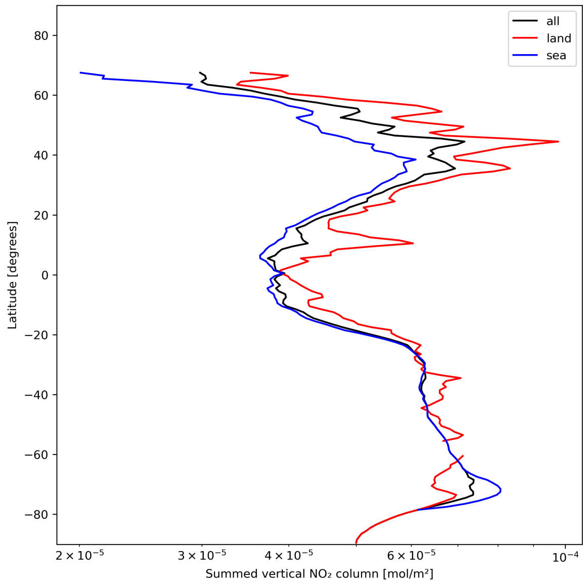
Figure 23: Zonal average of “Summed vertical NO 2 column” for 2023-11-21 to 2023-11-23.
