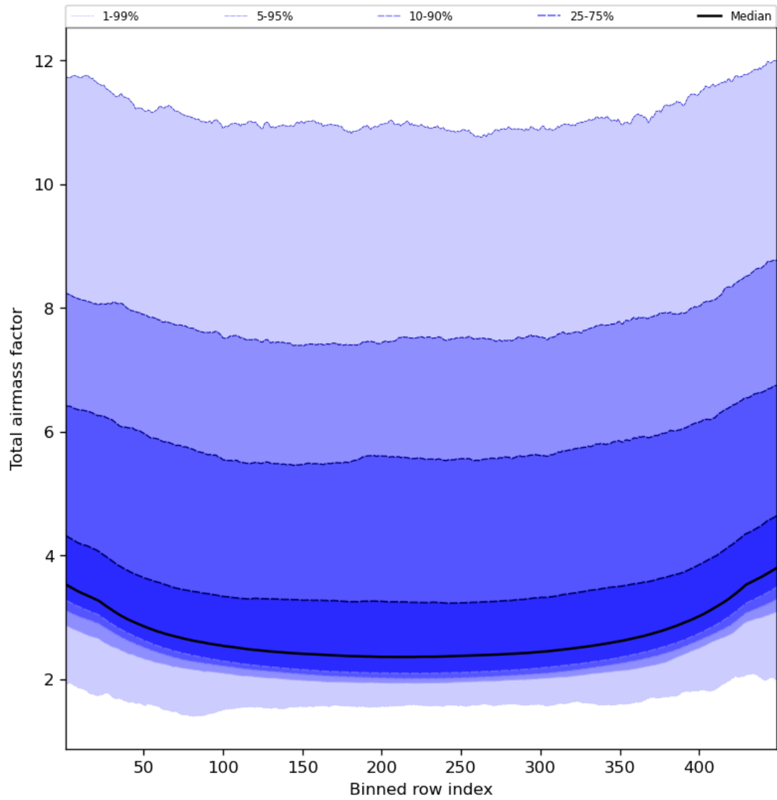
Figure 49: Along track statistics of “Total airmass factor” for 2023-11-21 to 2023-11-23
