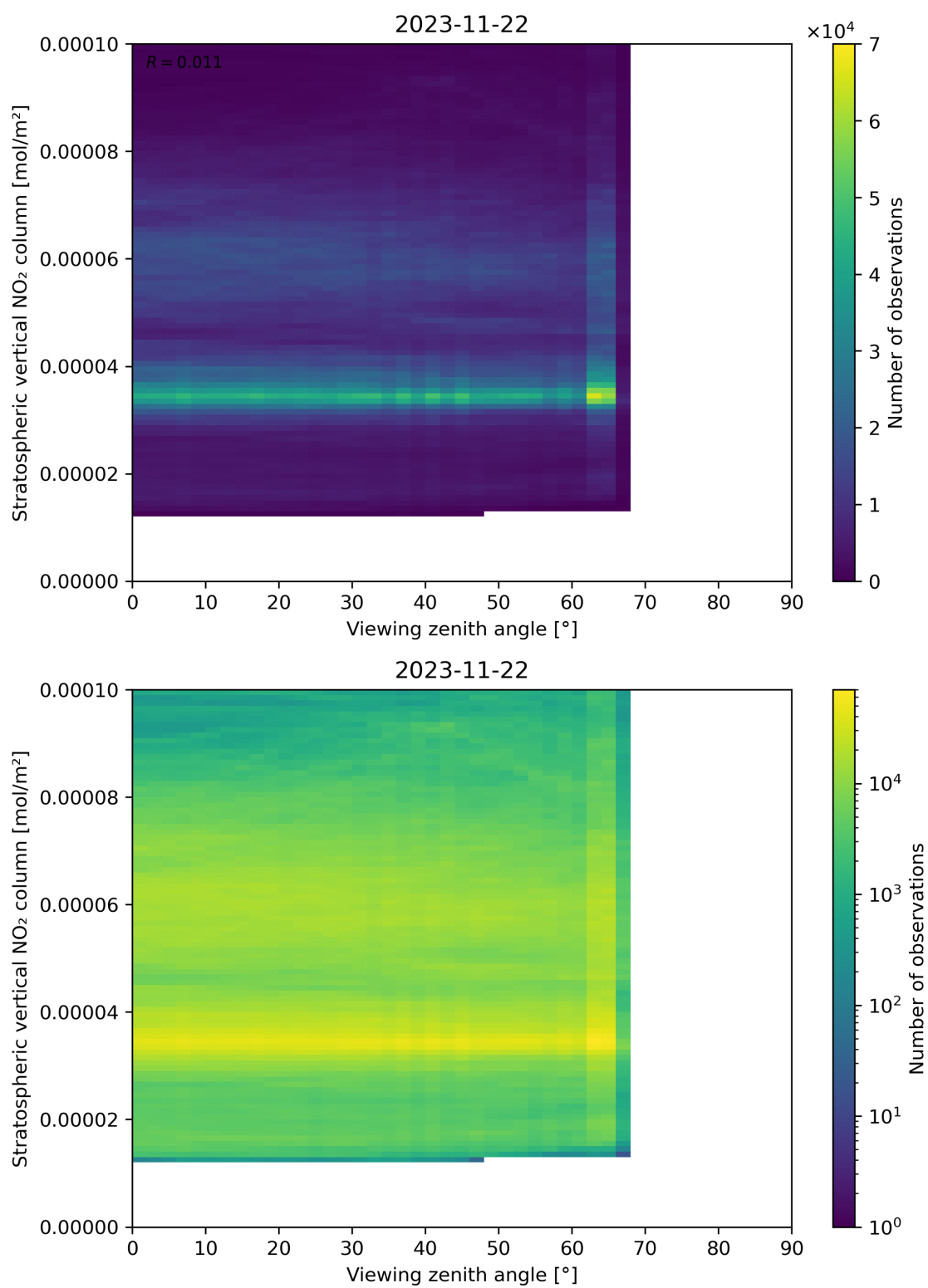
Figure 164: Scatter density plot of “Viewing zenith angle” against “Stratospheric vertical NO 2 column” for 2023-11-21 to 2023-11-23.
