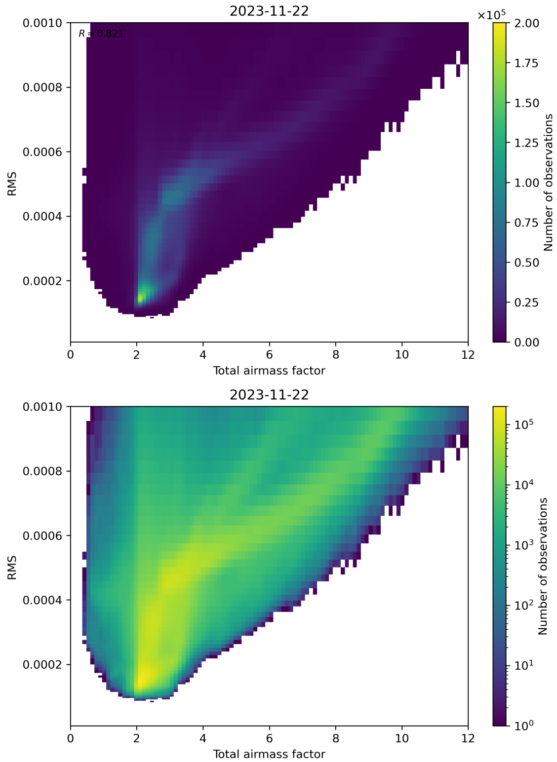
Figure 69: Scatter density plot of “Total airmass factor” against “RMS” for 2023-11-21 to 2023-11-23.
