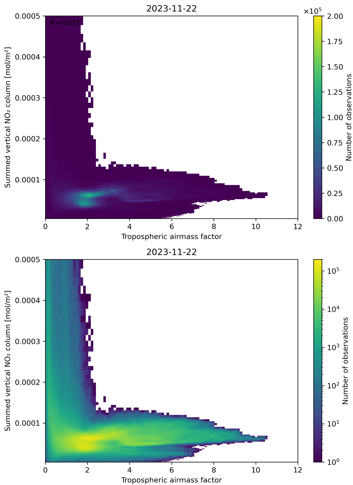
Figure 75: Scatter density plot of “Tropospheric airmass factor” against “Summed vertical NO 2 column” for 2023-11-21 to 2023-11-23.
