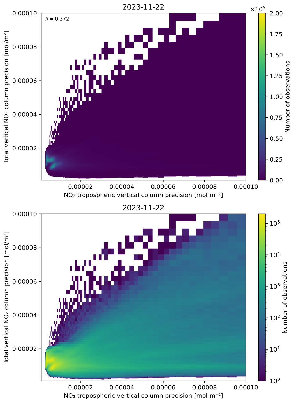
Figure 139: Scatter density plot of “NO 2 tropospheric vertical column precision” against “Total vertical NO 2 column precision” for 2023-11-21 to 2023-11-23.
