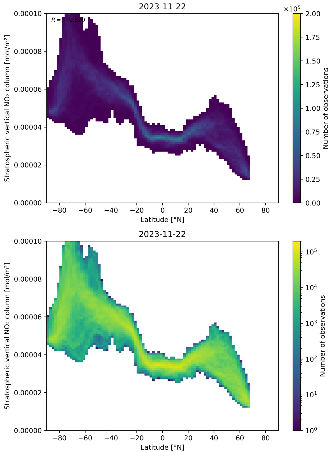
Figure 87: Scatter density plot of “Latitude” against “Stratospheric vertical NO 2 column” for 2023-11-21 to 2023-11-23.
