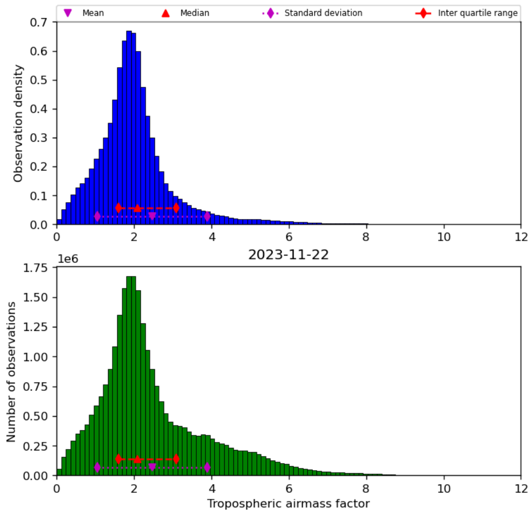
Figure 31: Histogram of “Tropospheric airmass factor” for 2023-11-21 to 2023-11-23
