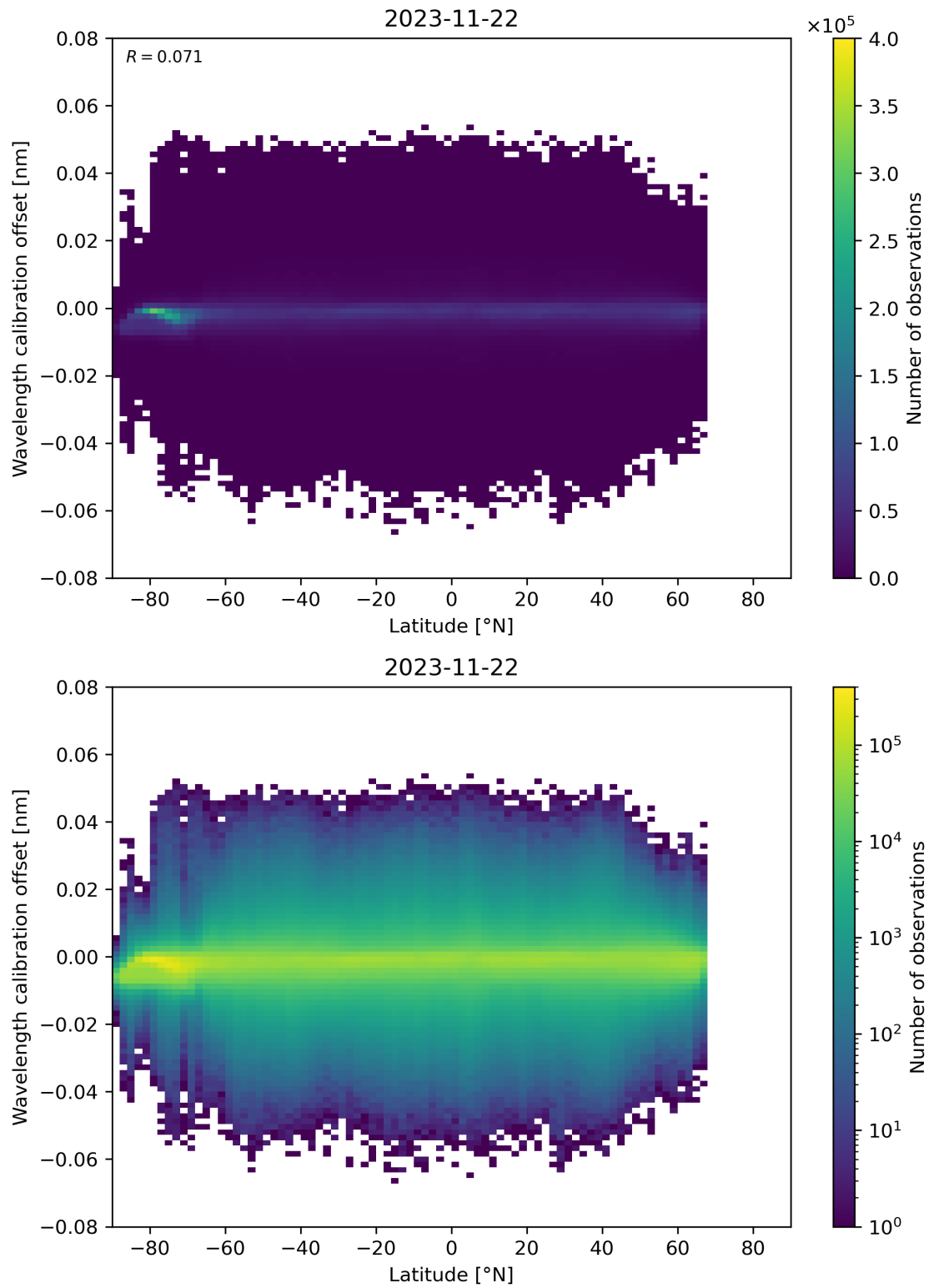
Figure 95: Scatter density plot of “Latitude” against “Wavelength calibration offset” for 2023-11-21 to 2023-11-23.
