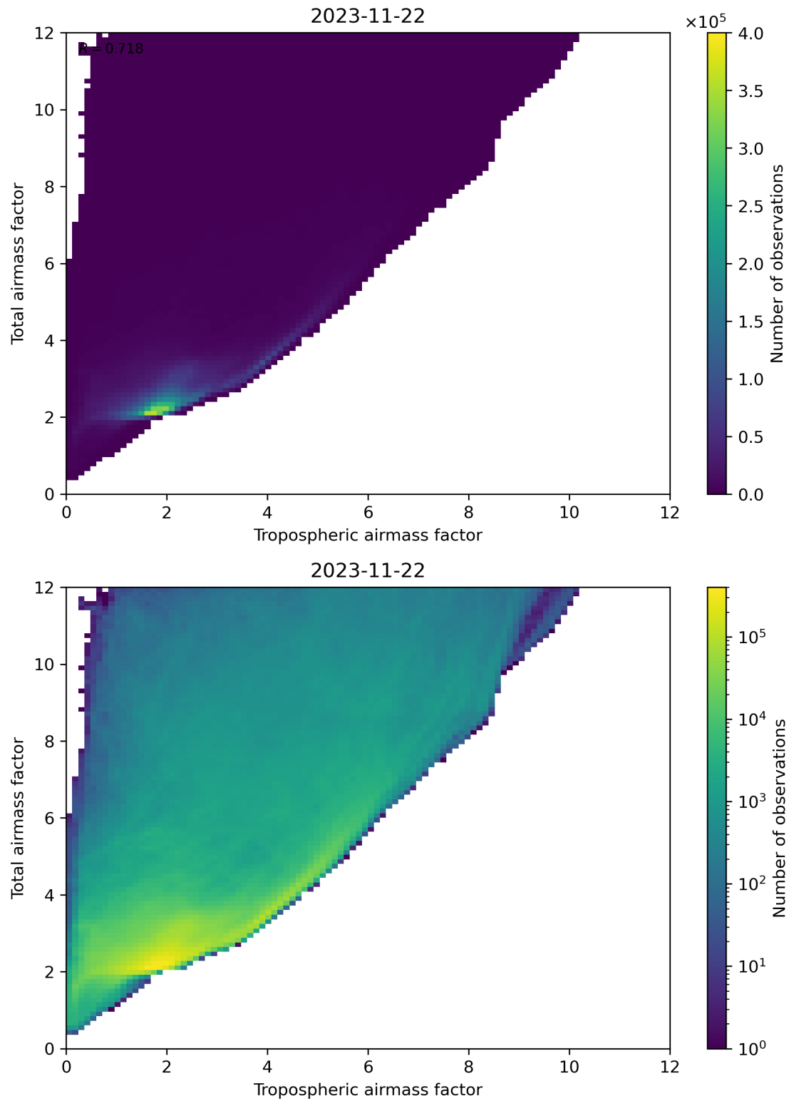
Figure 72: Scatter density plot of “Tropospheric airmass factor” against “Total airmass factor” for 2023-11-21 to 2023-11-23.
