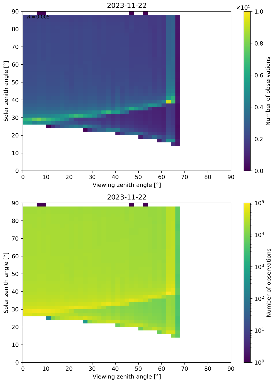
Figure 172: Scatter density plot of “Viewing zenith angle” against “Solar zenith angle” for 2023-11-21 to 2023-11-23.
