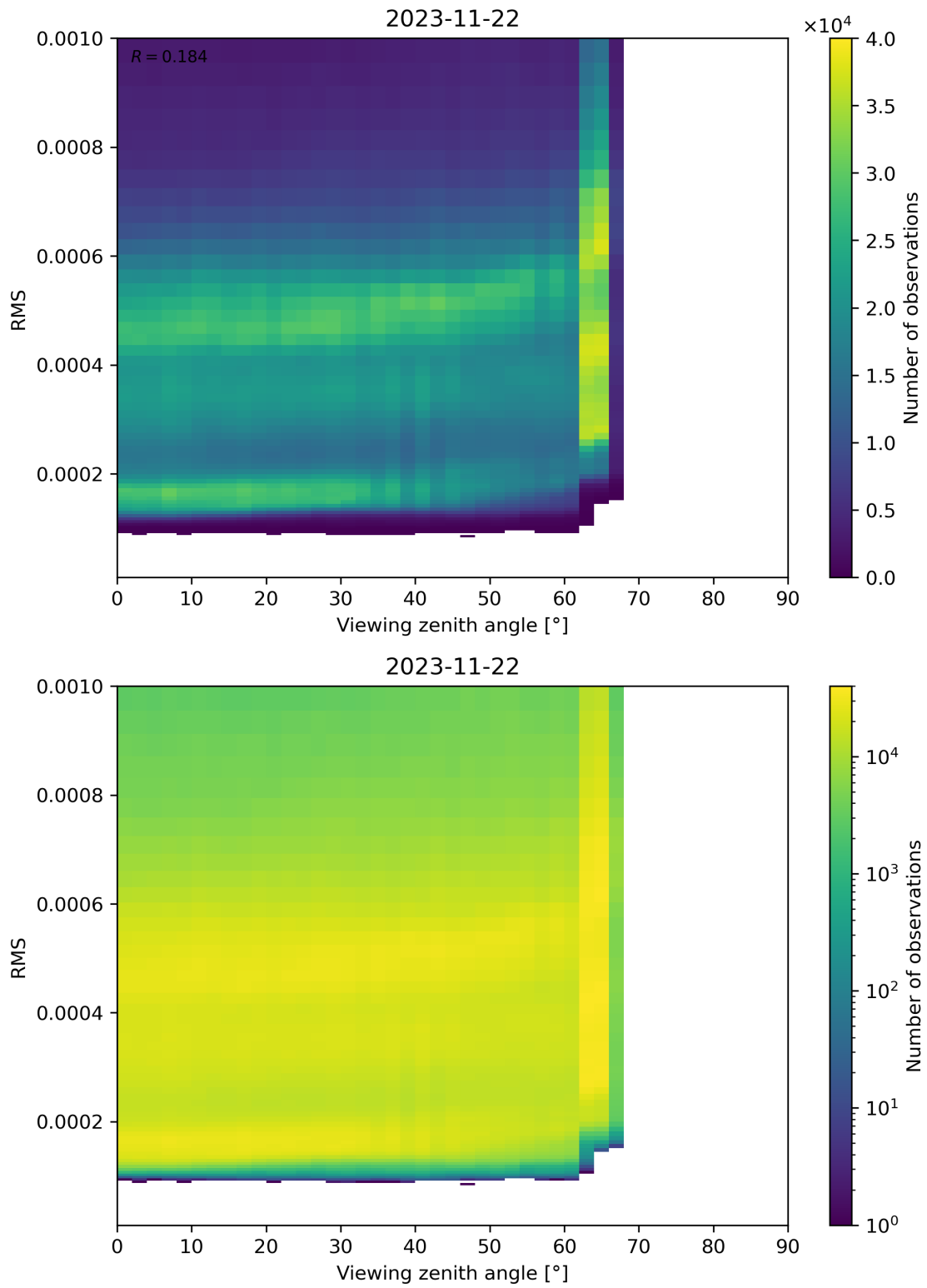
Figure 171: Scatter density plot of “Viewing zenith angle” against “RMS” for 2023-11-21 to 2023-11-23.
