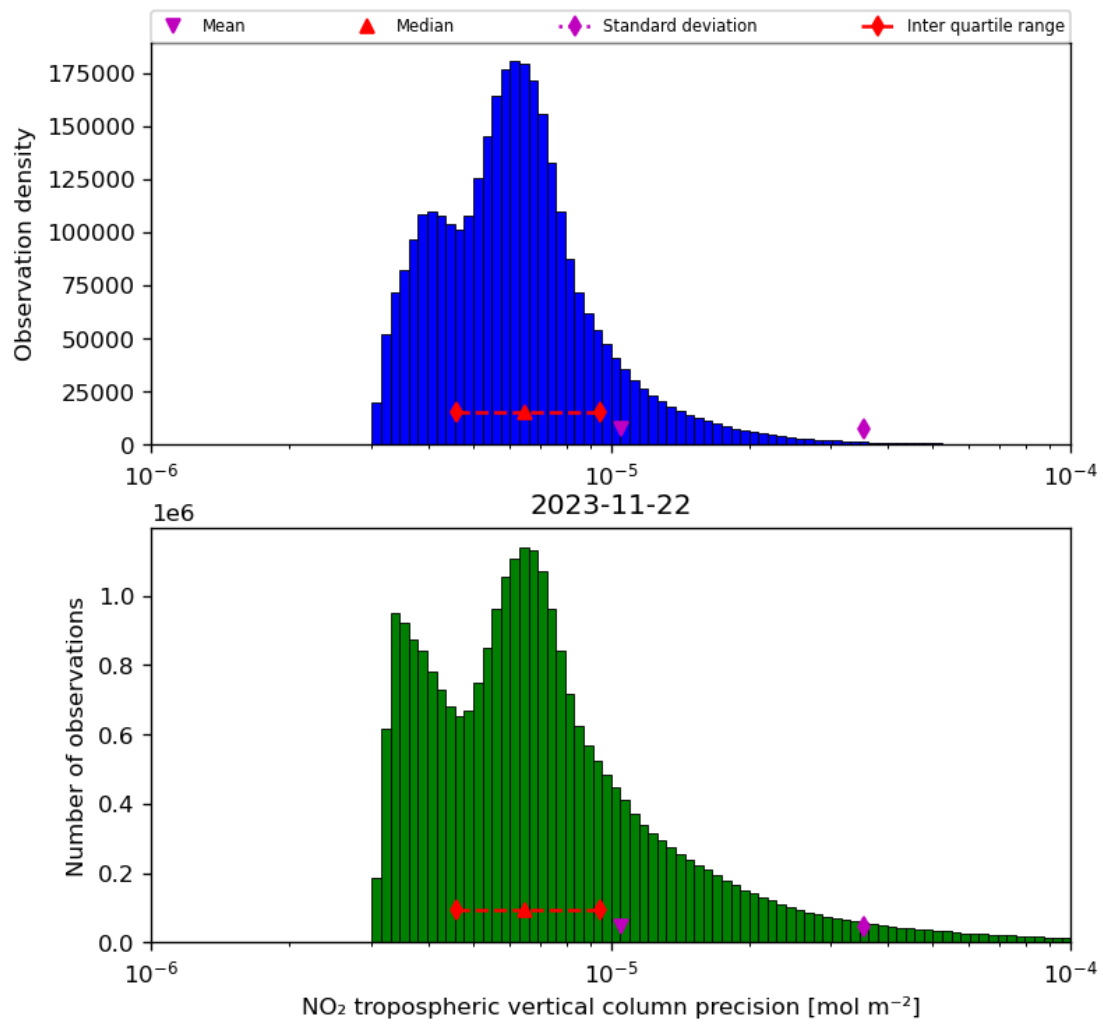
Figure 30: Histogram of “NO 2 tropospheric vertical column precision” for 2023-11-21 to 2023-11-23
