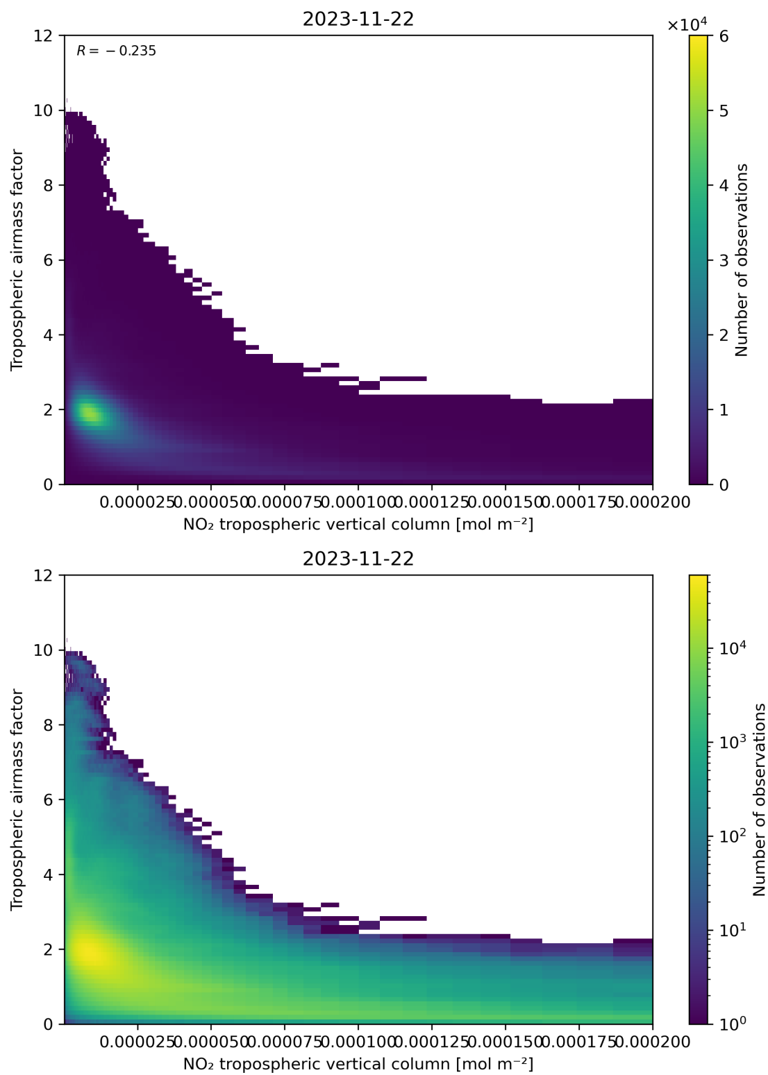
Figure 123: Scatter density plot of “NO 2 tropospheric vertical column” against “Tropospheric airmass factor” for 2023-11-21 to 2023-11-23.
