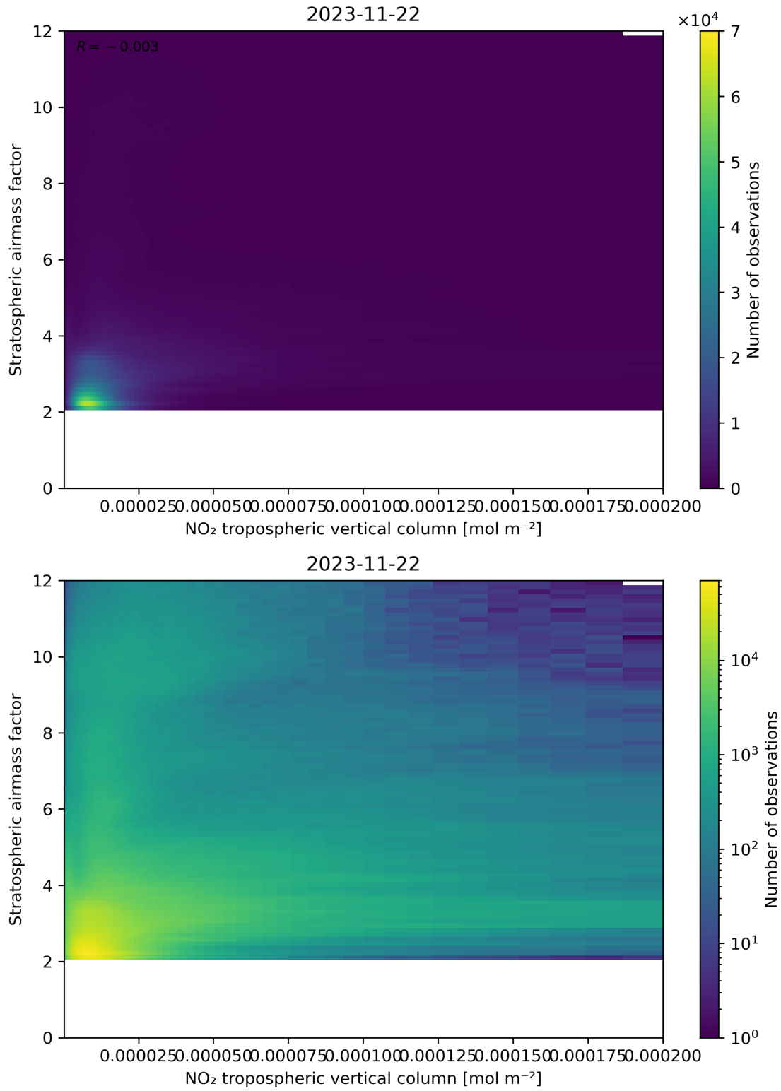
Figure 121: Scatter density plot of “NO 2 tropospheric vertical column” against “Stratospheric airmass factor” for 2023-11-21 to 2023-11-23.
