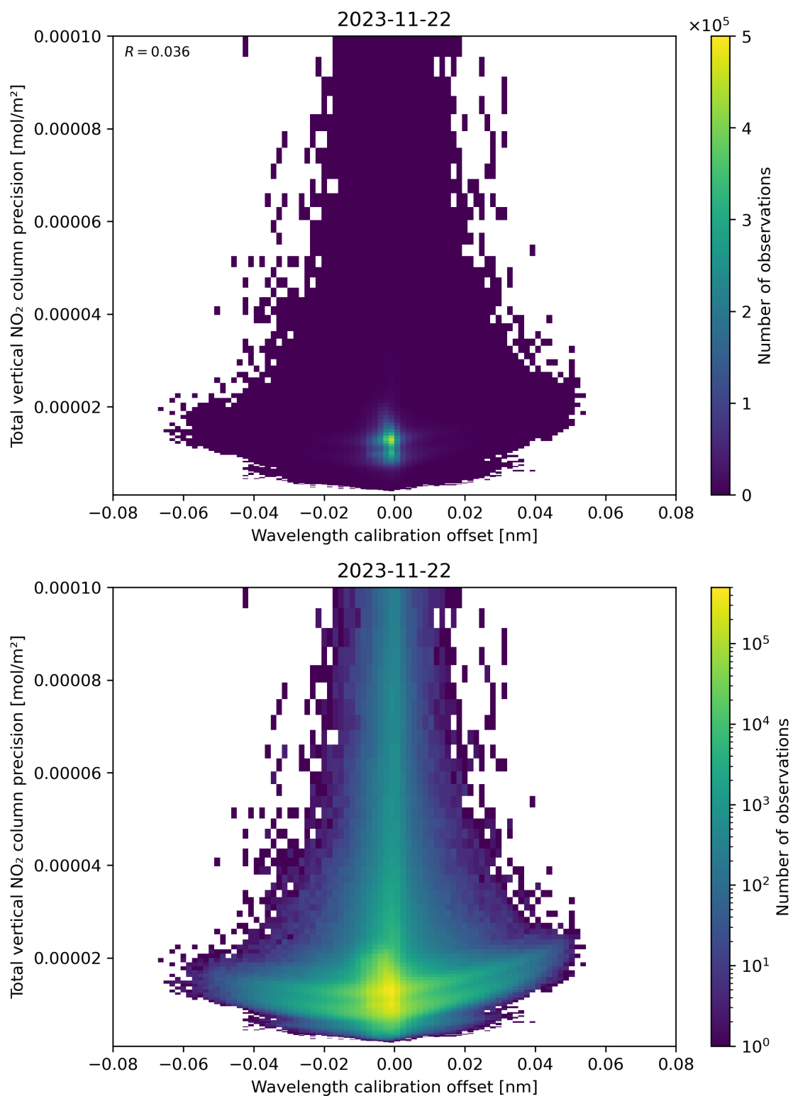
Figure 180: Scatter density plot of “Wavelength calibration offset” against “Total vertical NO 2 column precision” for 2023-11-21 to 2023-11-23.
