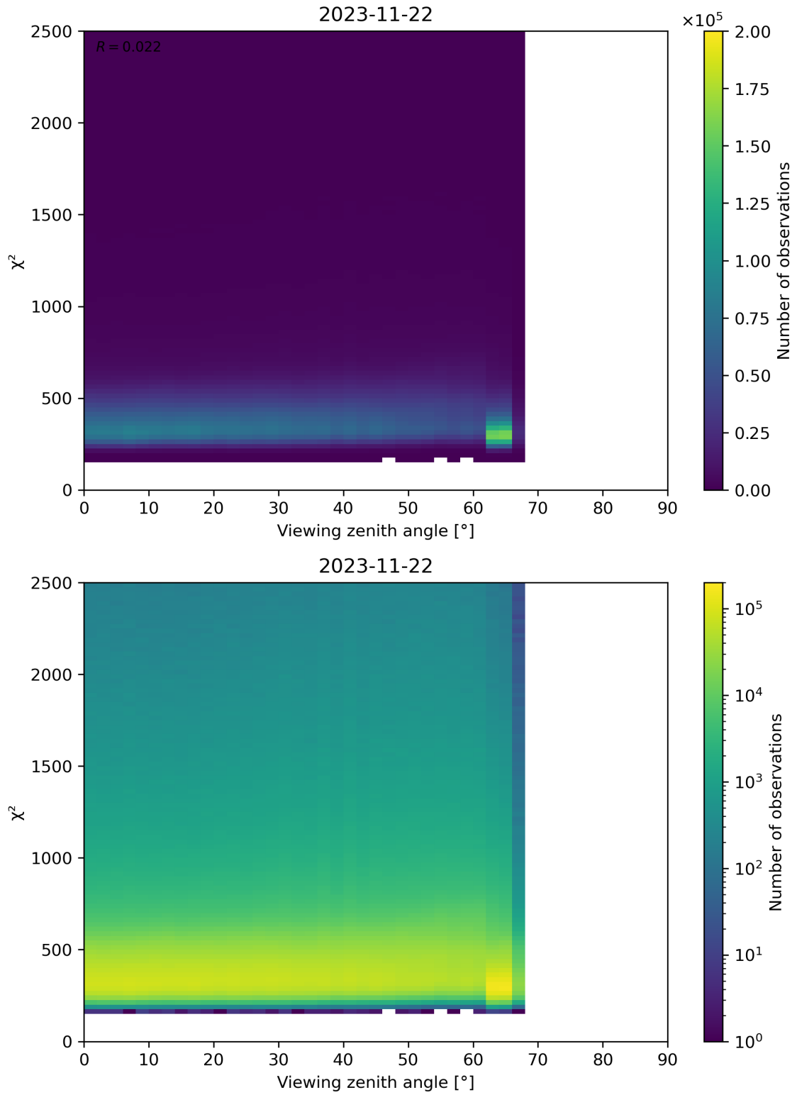
Figure 162: Scatter density plot of “Viewing zenith angle” against “ \chi^2 ” for 2023-11-21 to 2023-11-23.
