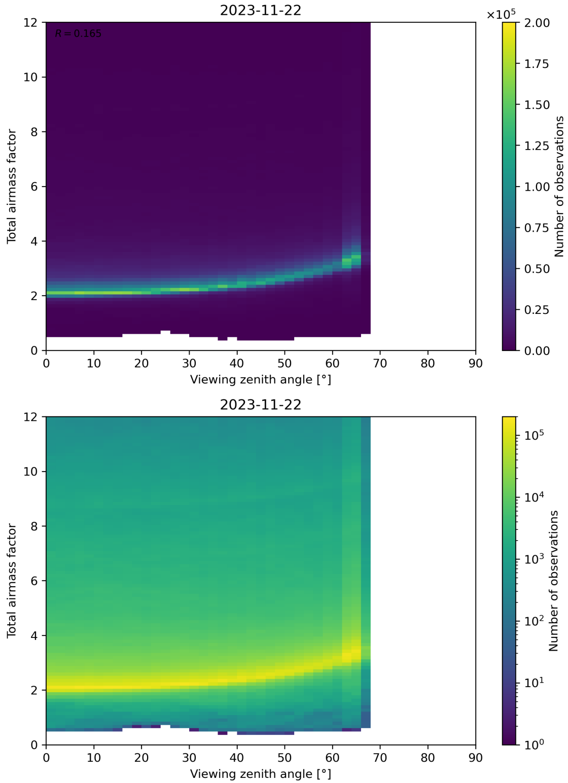
Figure 160: Scatter density plot of “Viewing zenith angle” against “Total airmass factor” for 2023-11-21 to 2023-11-23.
