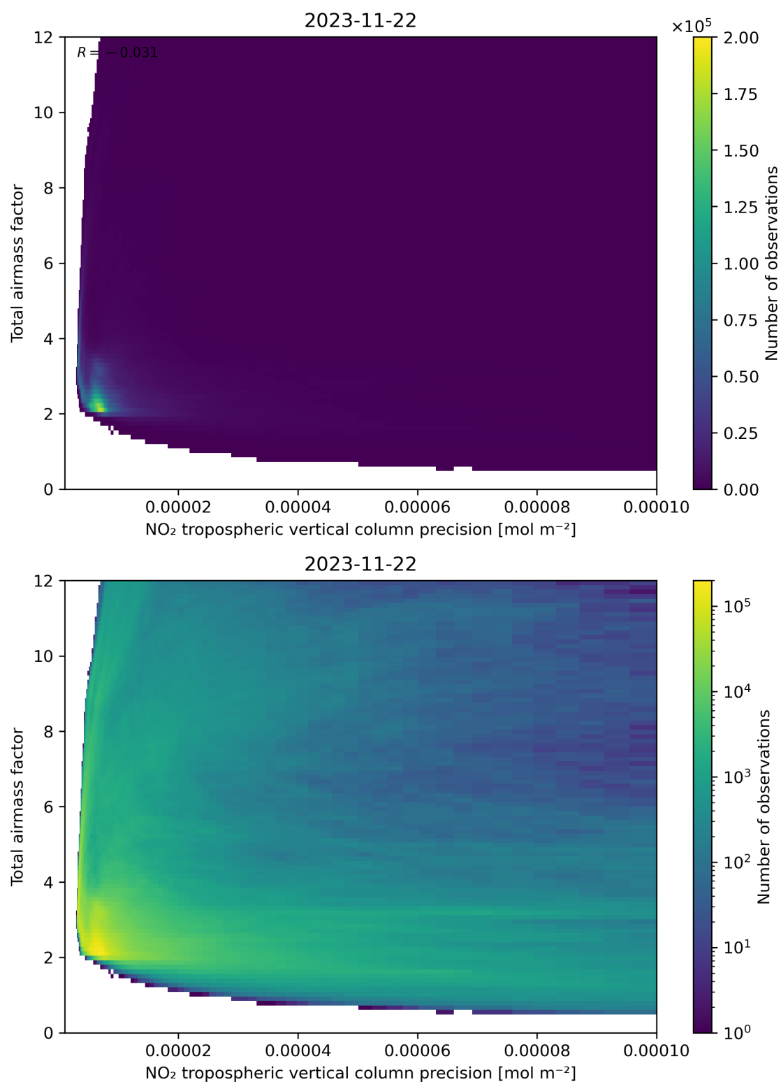
Figure 132: Scatter density plot of “NO 2 tropospheric vertical column precision” against “Total air mass factor” for 2023-11-21 to 2023-11-23.
