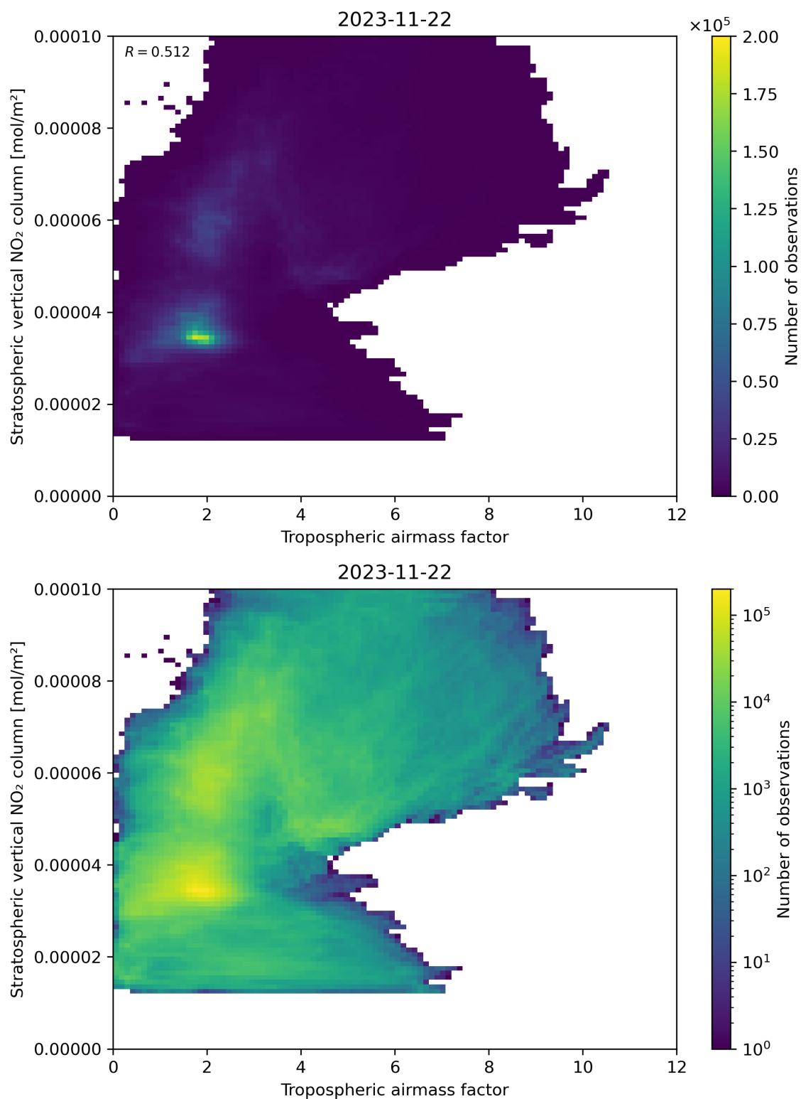
Figure 74: Scatter density plot of “Tropospheric airmass factor” against “Stratospheric vertical NO 2 column” for 2023-11-21 to 2023-11-23.
