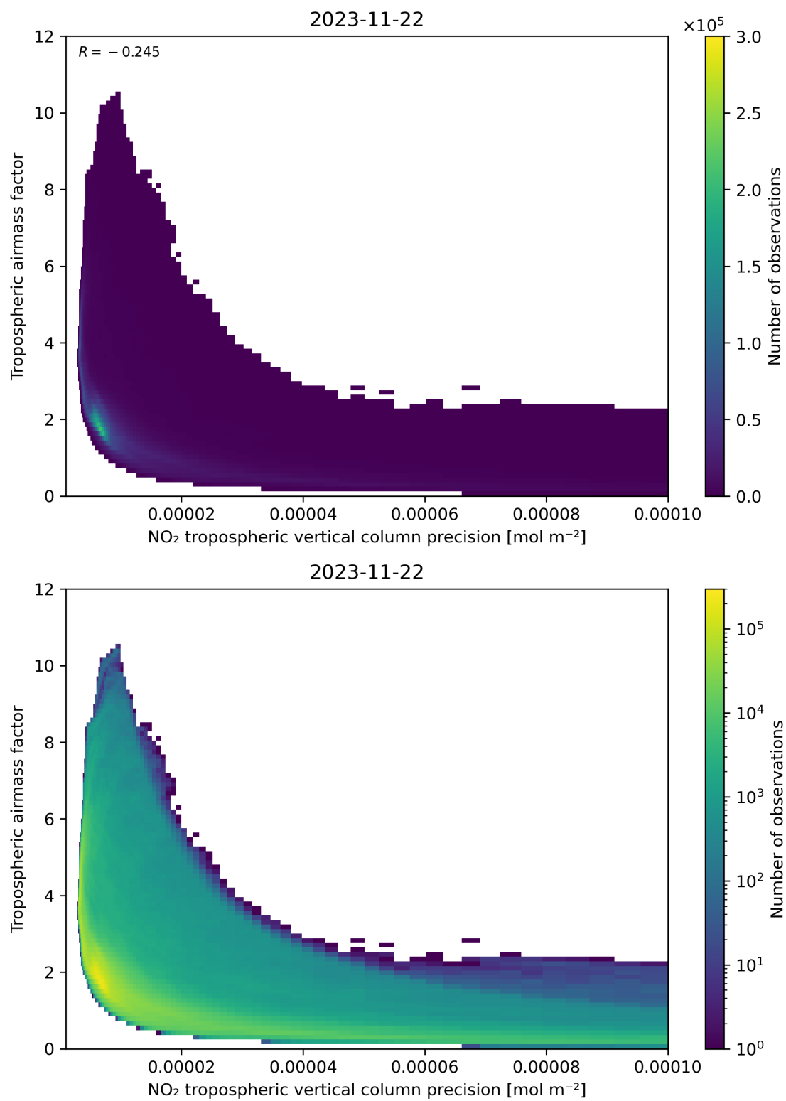
Figure 133: Scatter density plot of “NO 2 tropospheric vertical column precision” against “Tropospheric airmass factor” for 2023-11-21 to 2023-11-23.
