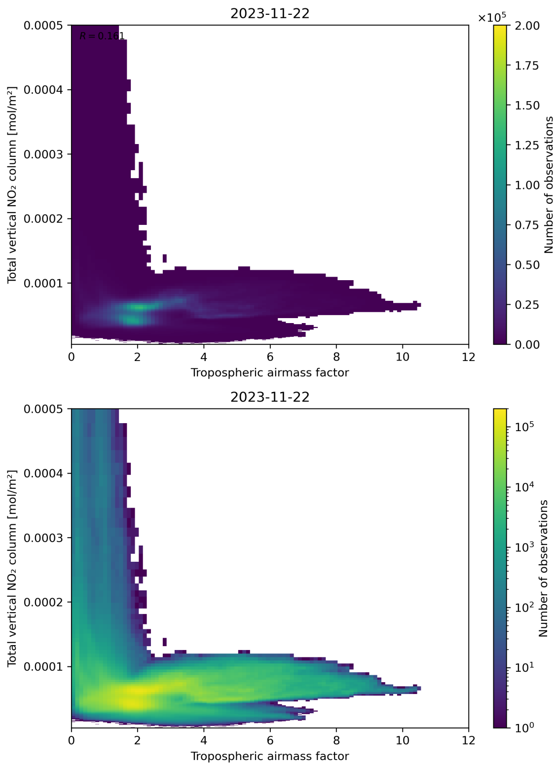
Figure 77: Scatter density plot of “Tropospheric airmass factor” against “Total vertical NO 2 column” for 2023-11-21 to 2023-11-23.
