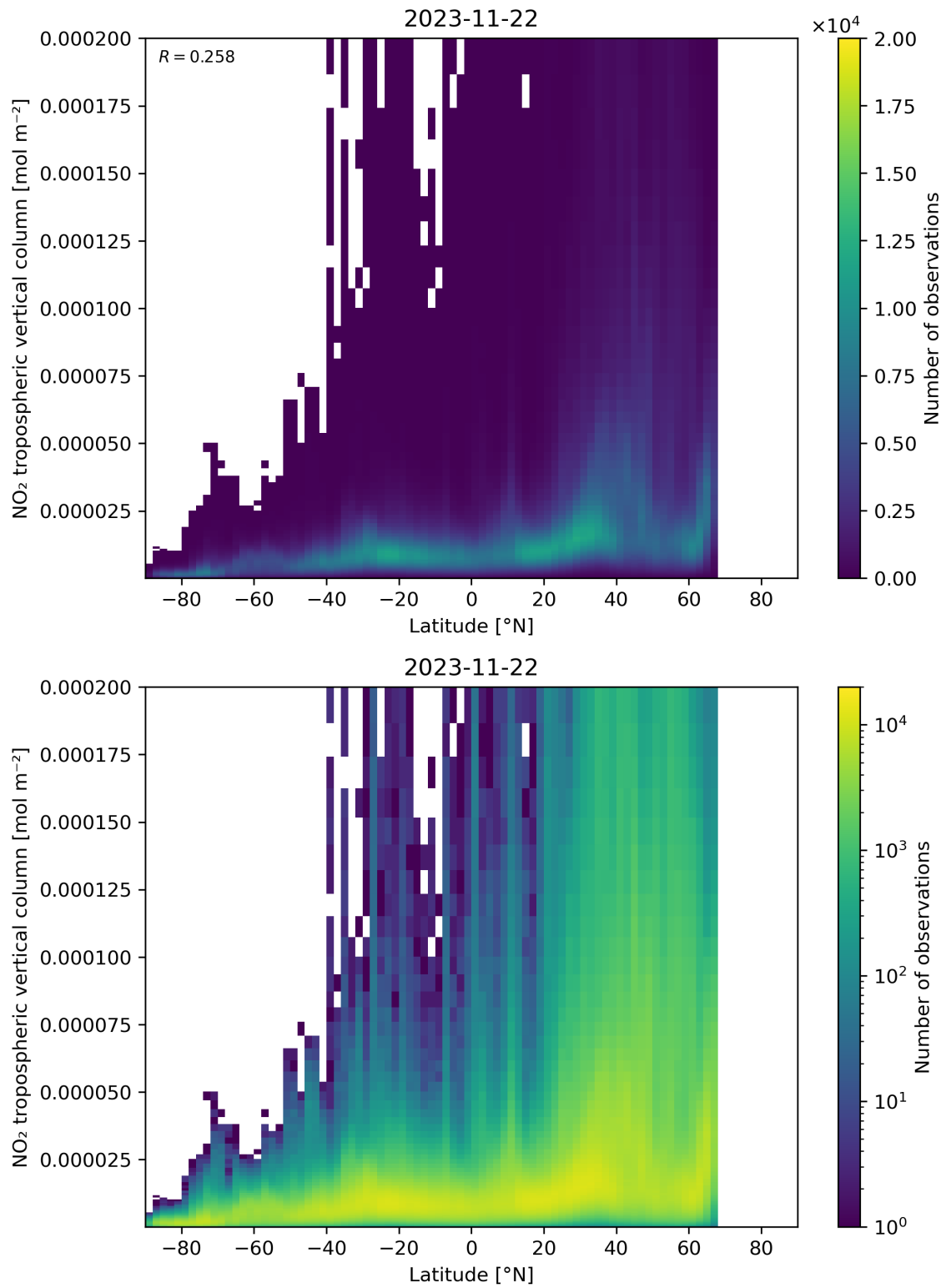
Figure 92: Scatter density plot of “Latitude” against “NO 2 tropospheric vertical column” for 2023-11-21 to 2023-11-23.
