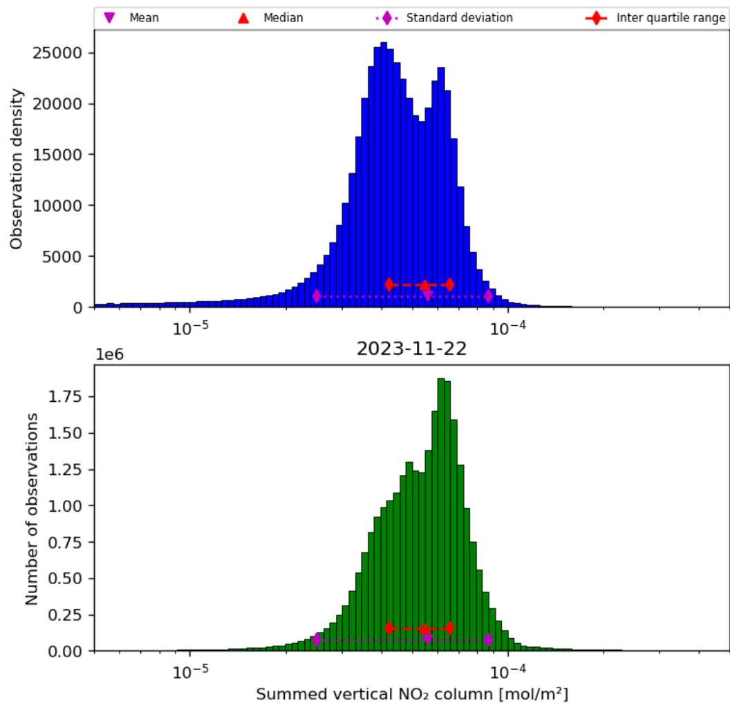
Figure 40: Histogram of “Summed vertical NO 2 column” for 2023-11-21 to 2023-11-23
