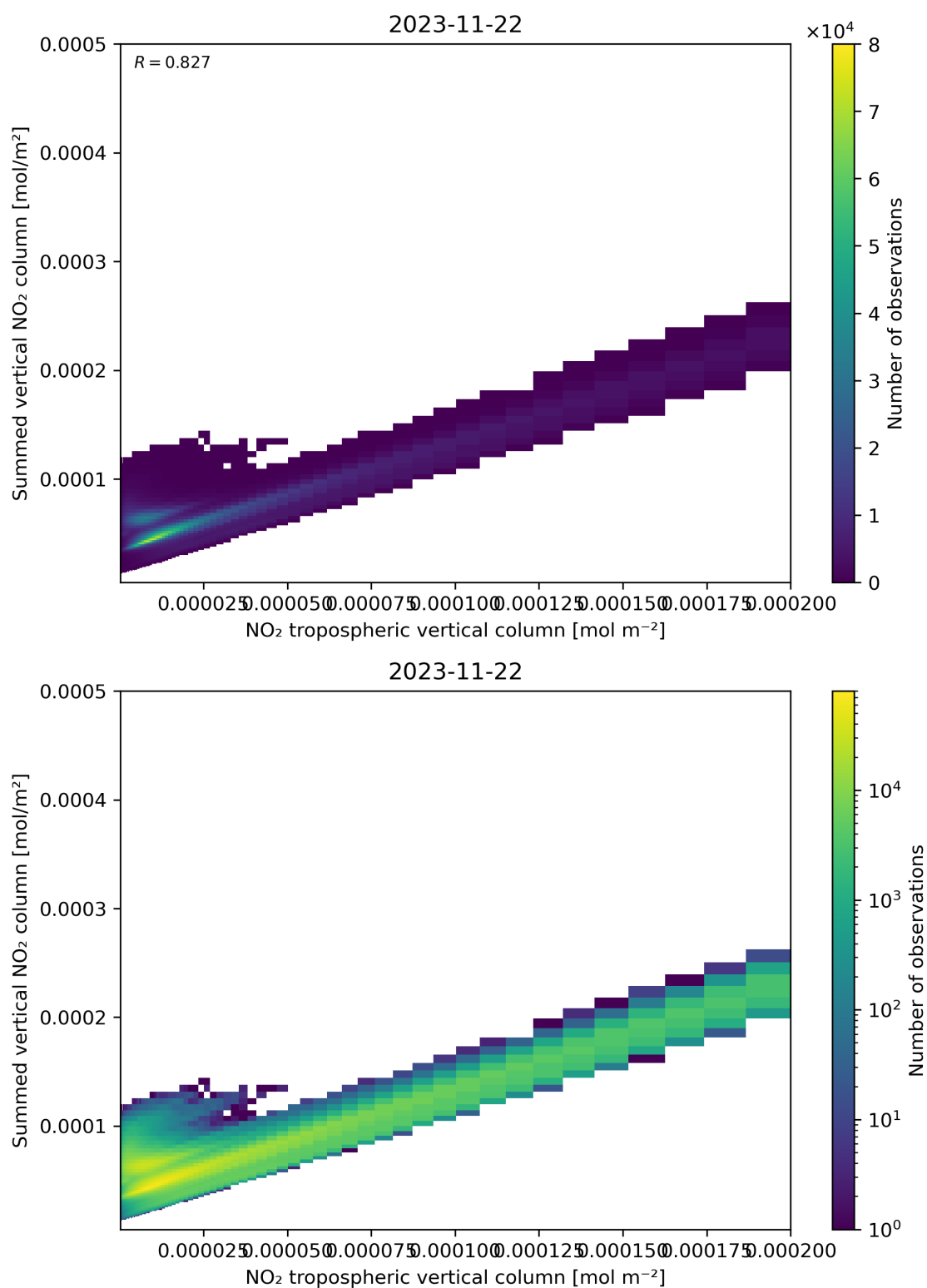
Figure 126: Scatter density plot of “NO 2 tropospheric vertical column” against “Summed vertical NO 2 column” for 2023-11-21 to 2023-11-23.
