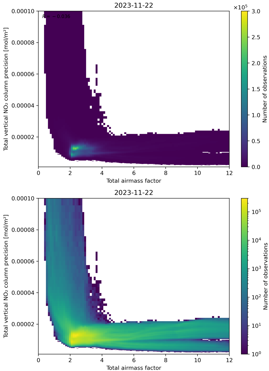
Figure 68: Scatter density plot of “Total airmass factor” against “Total vertical NO 2 column precision” for 2023-11-21 to 2023-11-23.
