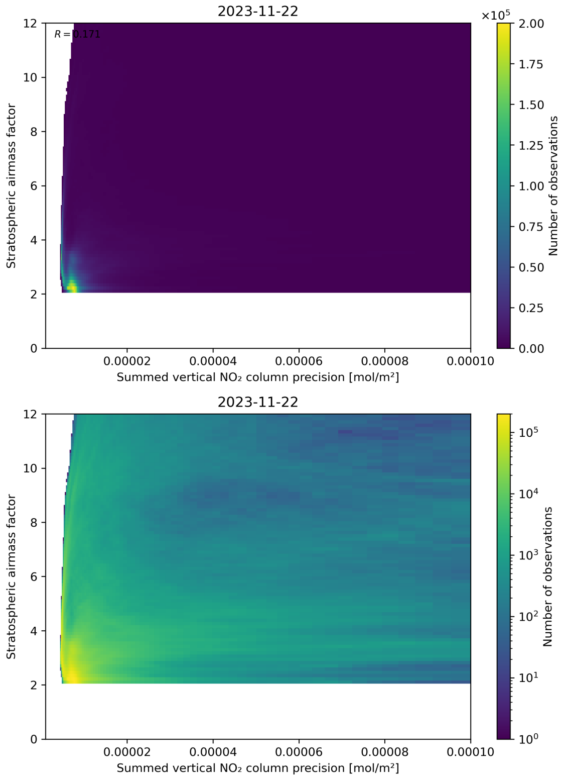
Figure 106: Scatter density plot of “Summed vertical NO 2 column precision” against “Stratospheric airmass factor” for 2023-11-21 to 2023-11-23.
