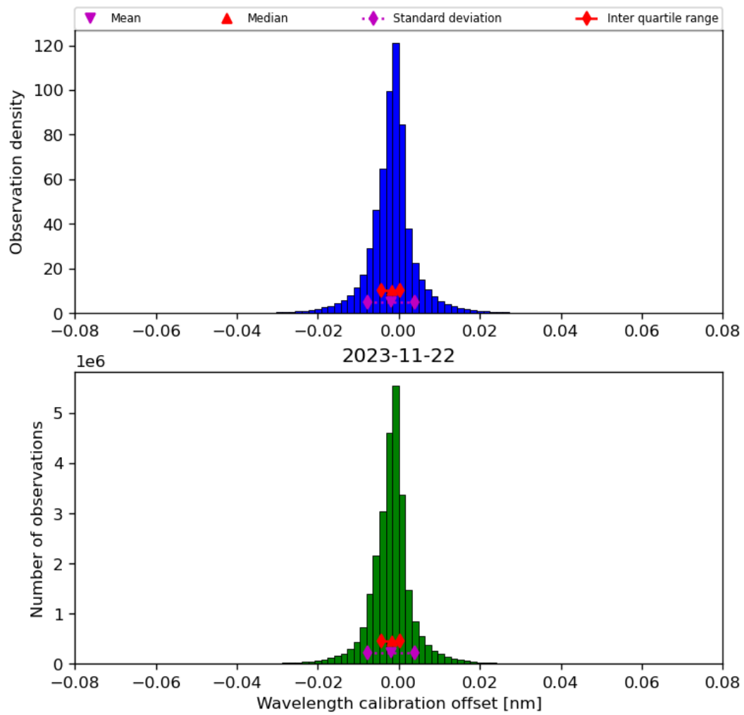
Figure 35: Histogram of “Wavelength calibration offset” for 2023-11-21 to 2023-11-23
