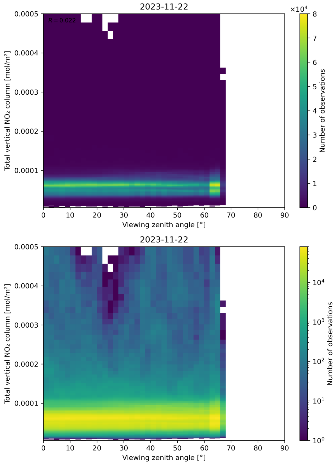
Figure 167: Scatter density plot of “Viewing zenith angle” against “Total vertical NO 2 column” for 2023-11-21 to 2023-11-23.
