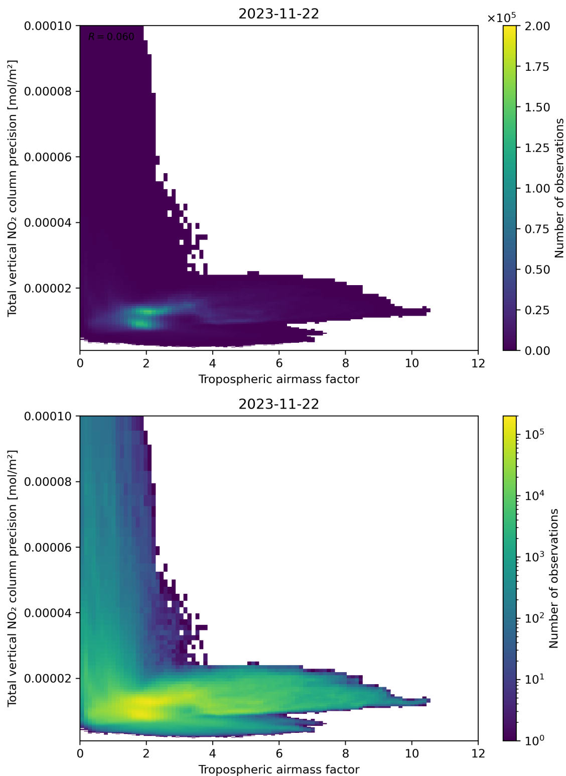
Figure 78: Scatter density plot of “Tropospheric airmass factor” against “Total vertical NO 2 column precision” for 2023-11-21 to 2023-11-23.
