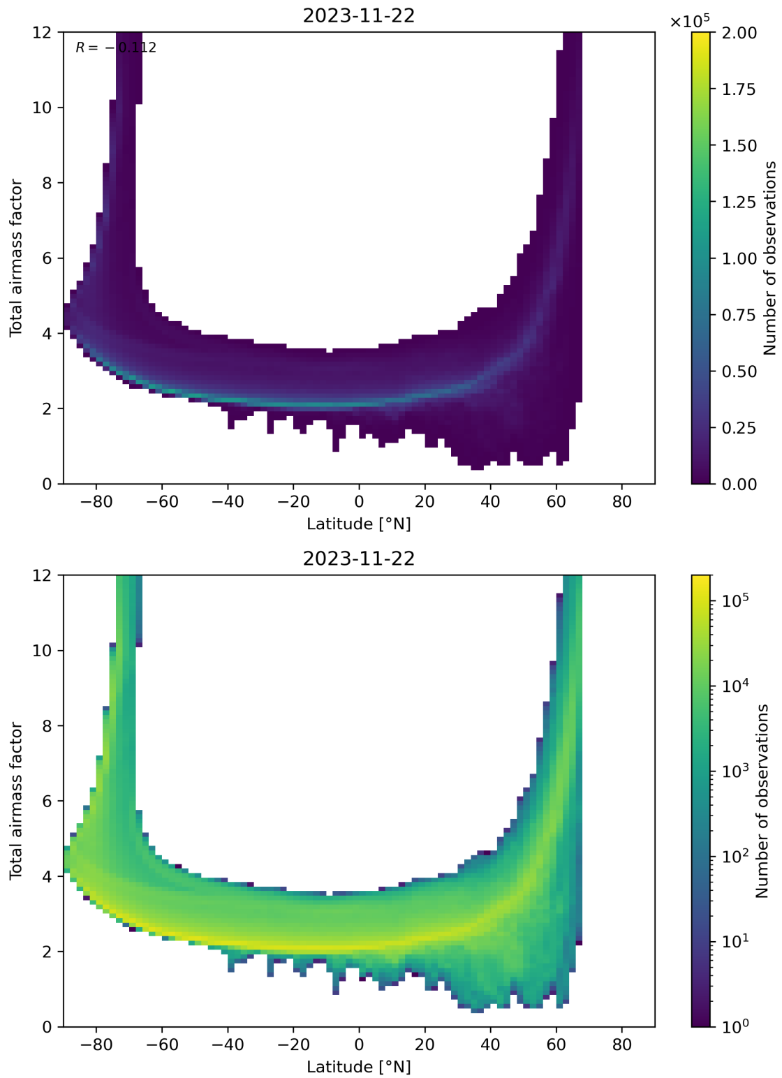
Figure 84: Scatter density plot of “Latitude” against “Total airmass factor” for 2023-11-21 to 2023-11-23.
