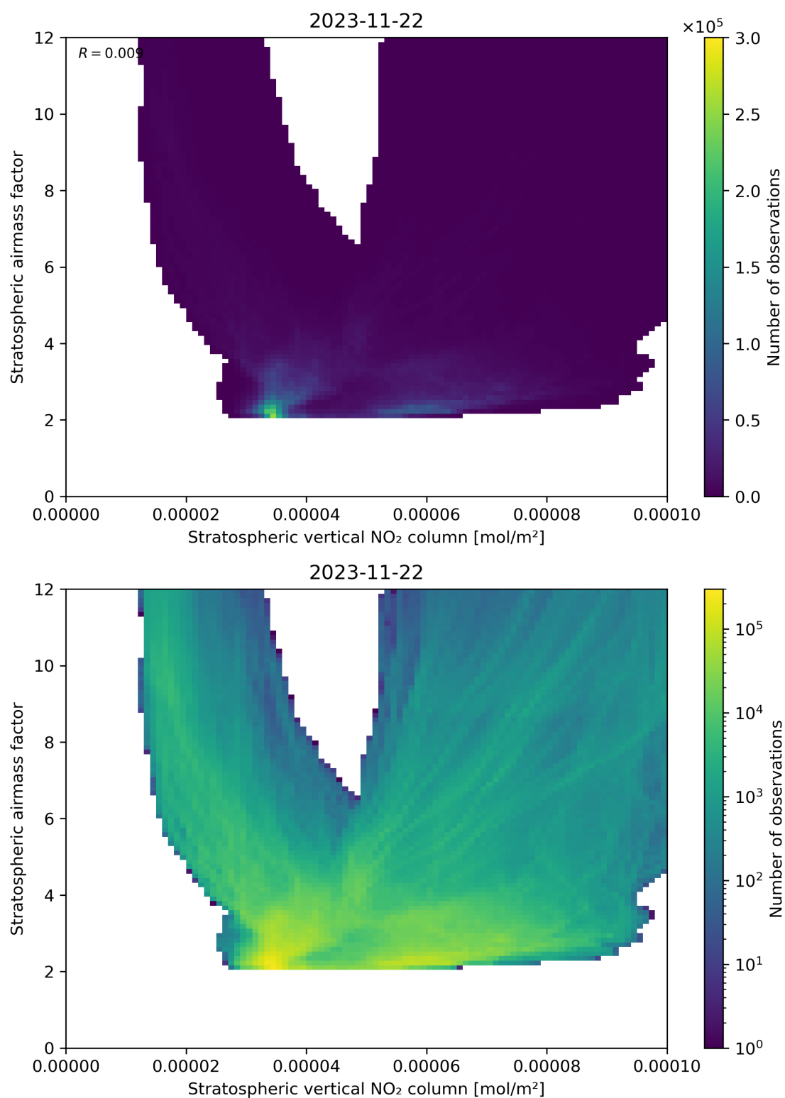
Figure 96: Scatter density plot of “Stratospheric vertical NO 2 column” against “Stratospheric airmass factor” for 2023-11-21 to 2023-11-23.
