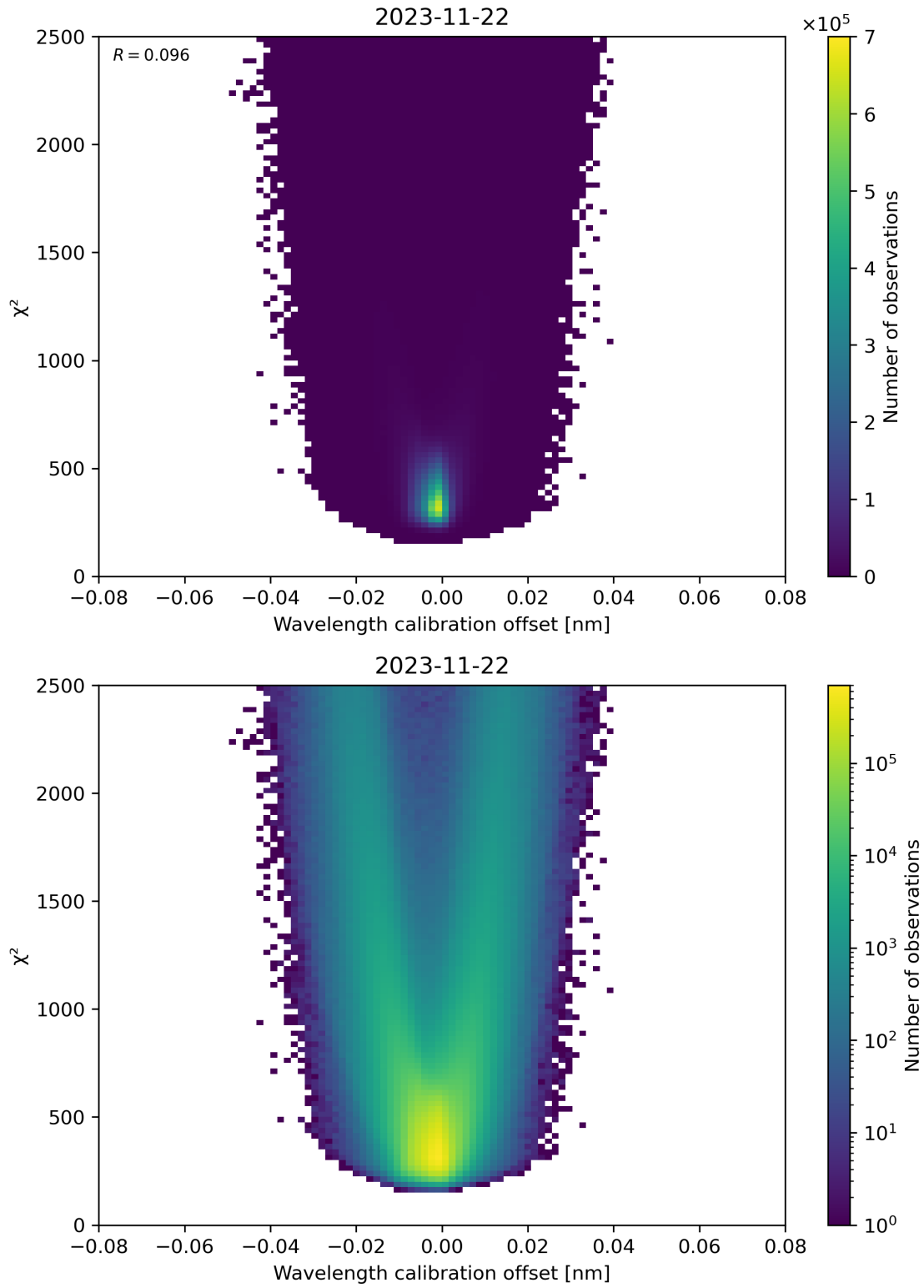
Figure 175: Scatter density plot of “Wavelength calibration offset” against “ \chi^2 ” for 2023-11-21 to 2023-11-23.
