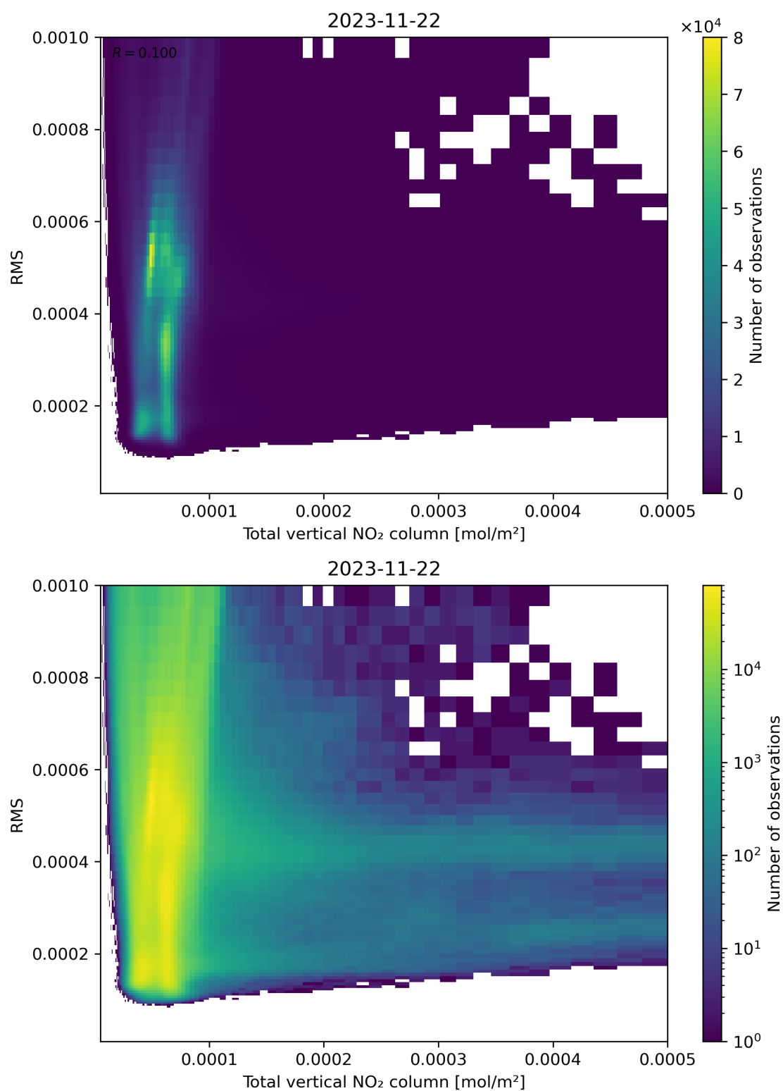
Figure 120: Scatter density plot of “Total vertical NO 2 column” against “RMS” for 2023-11-21 to 2023-11-23.
