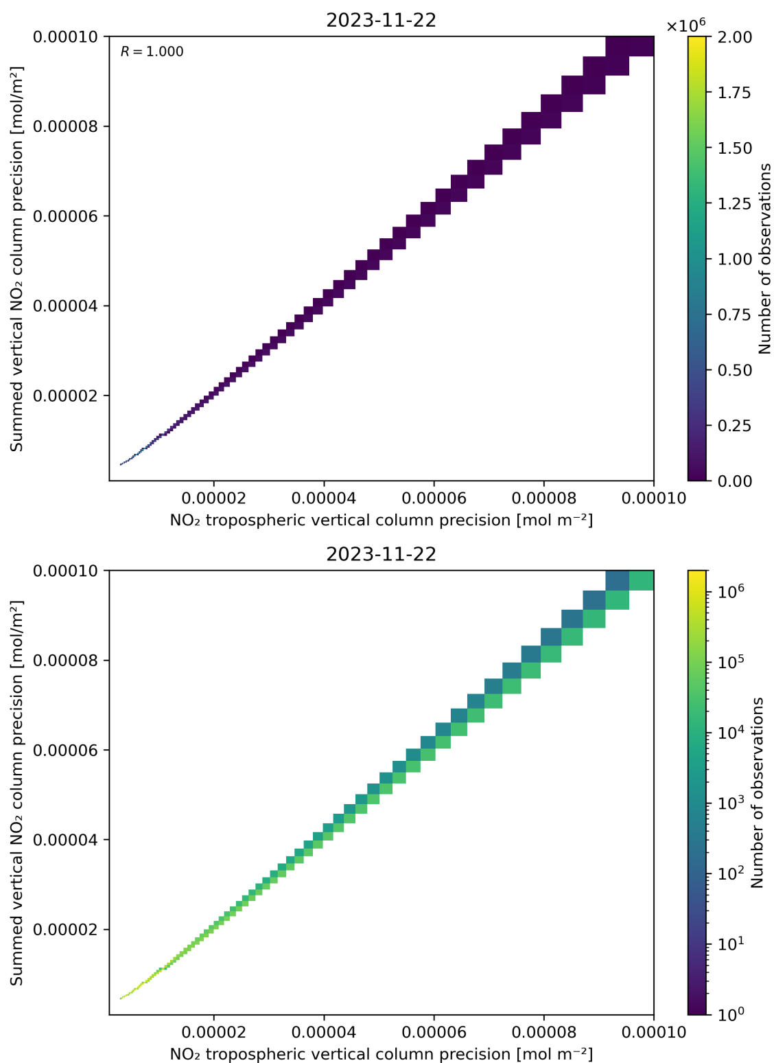
Figure 137: Scatter density plot of “NO 2 tropospheric vertical column precision” against “Summed vertical NO 2 column precision” for 2023-11-21 to 2023-11-23.
