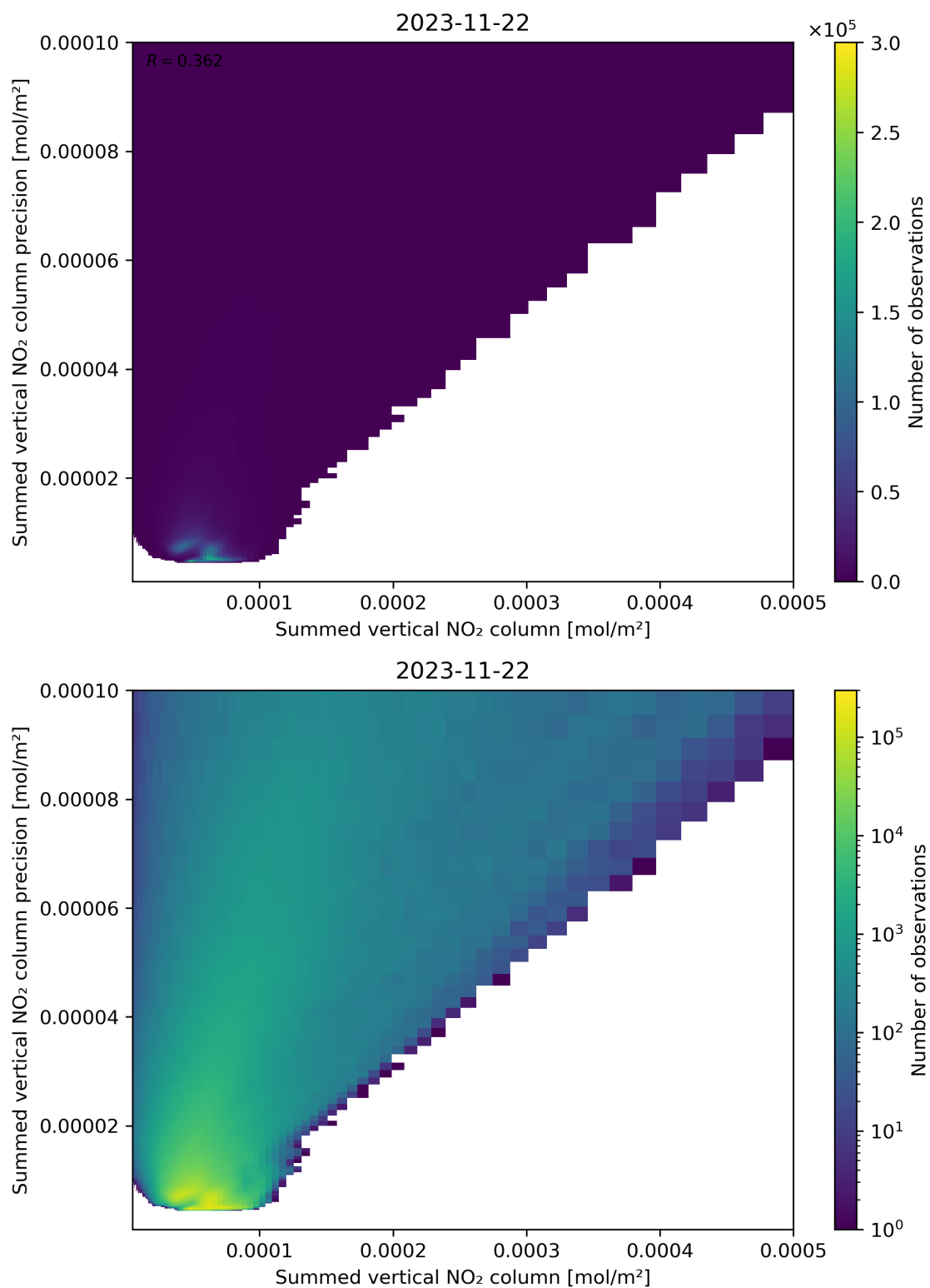
Figure 105: Scatter density plot of “Summed vertical NO 2 column” against “Summed vertical NO 2 column precision” for 2023-11-21 to 2023-11-23.
