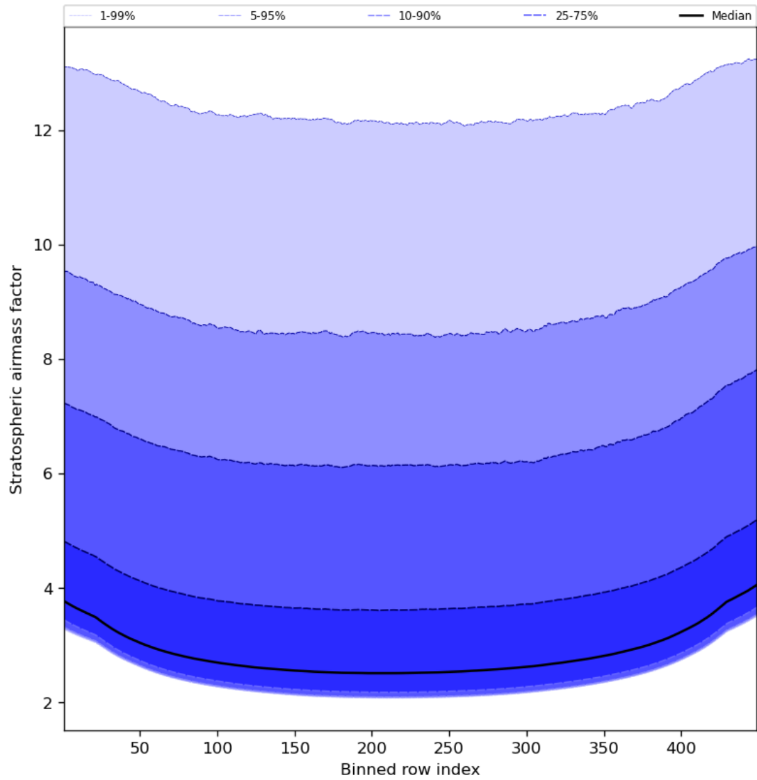
Figure 61: Along track statistics of “Stratospheric airmass factor” for 2023-11-21 to 2023-11-23
