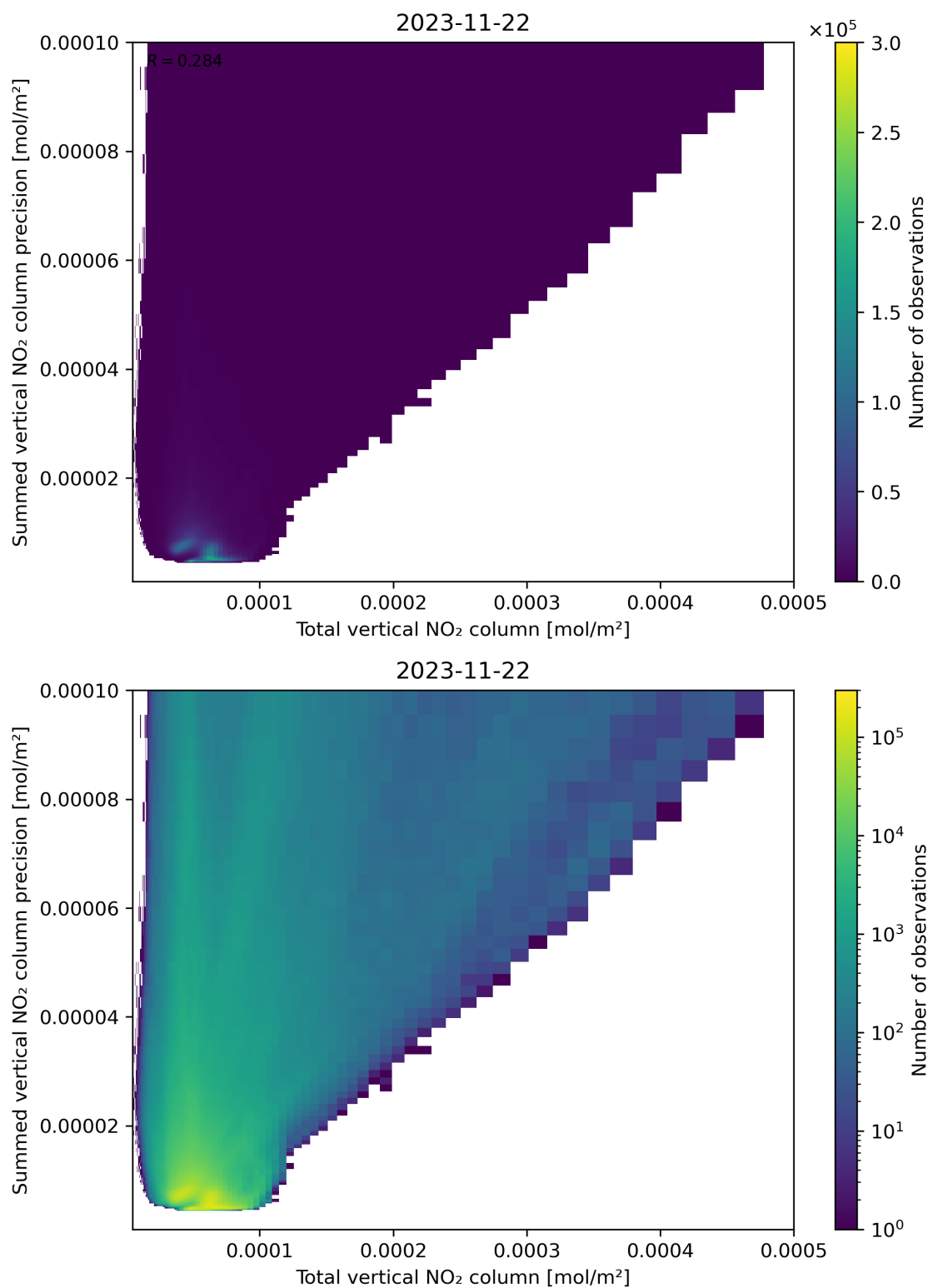
Figure 113: Scatter density plot of “Total vertical NO 2 column” against “Summed vertical NO 2 column precision” for 2023-11-21 to 2023-11-23.
