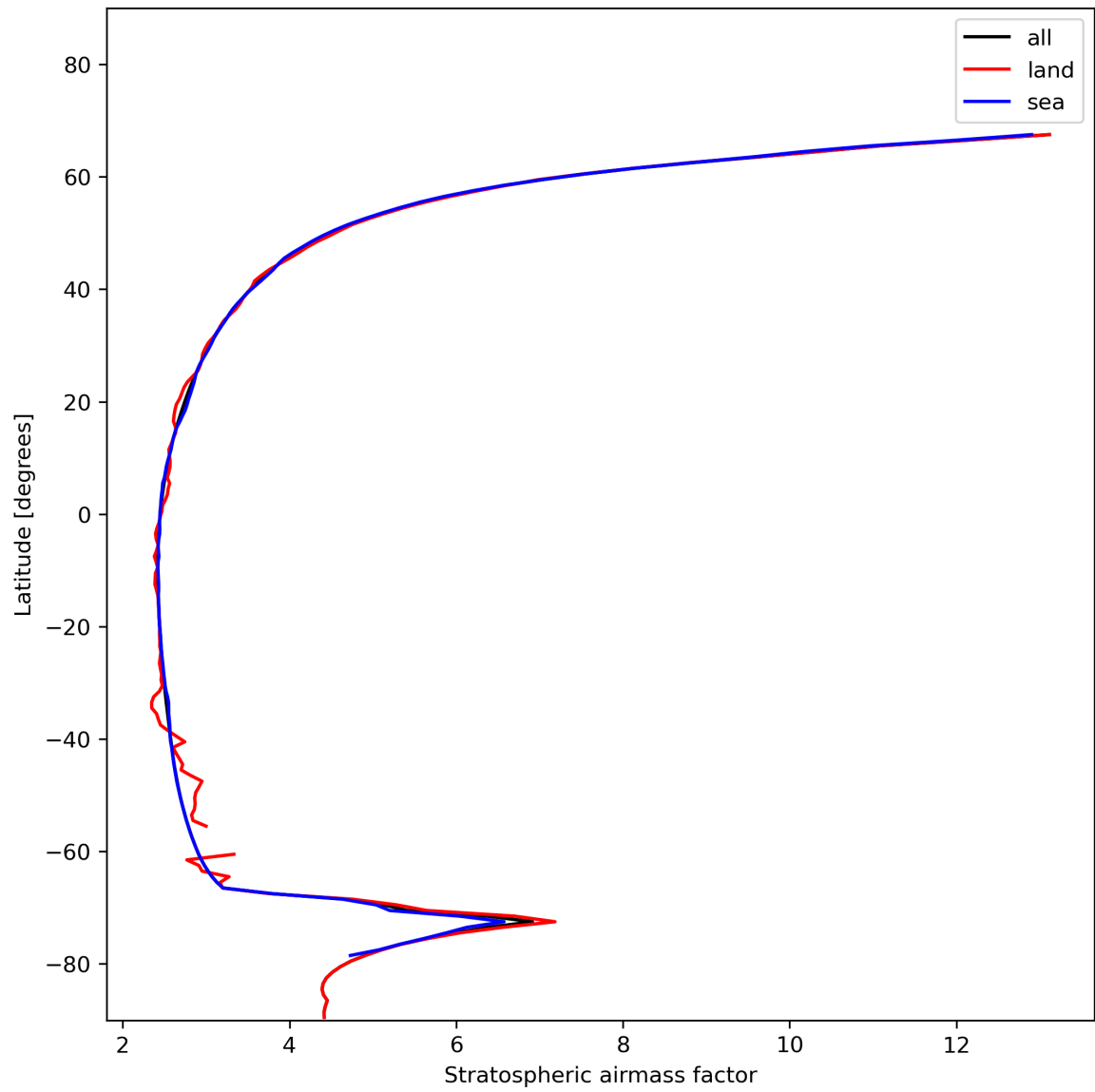
Figure 27: Zonal average of “Stratospheric airmass factor” for 2023-11-21 to 2023-11-23.
