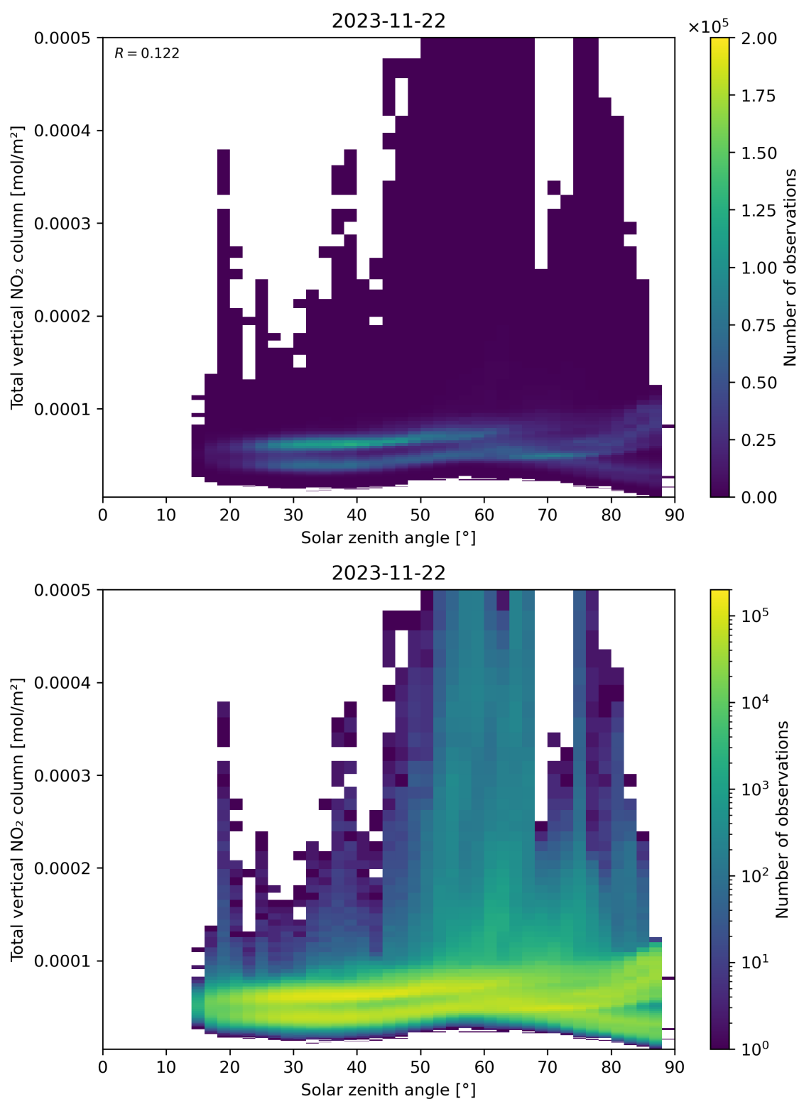
Figure 153: Scatter density plot of “Solar zenith angle” against “Total vertical NO 2 column” for 2023-11-21 to 2023-11-23.
