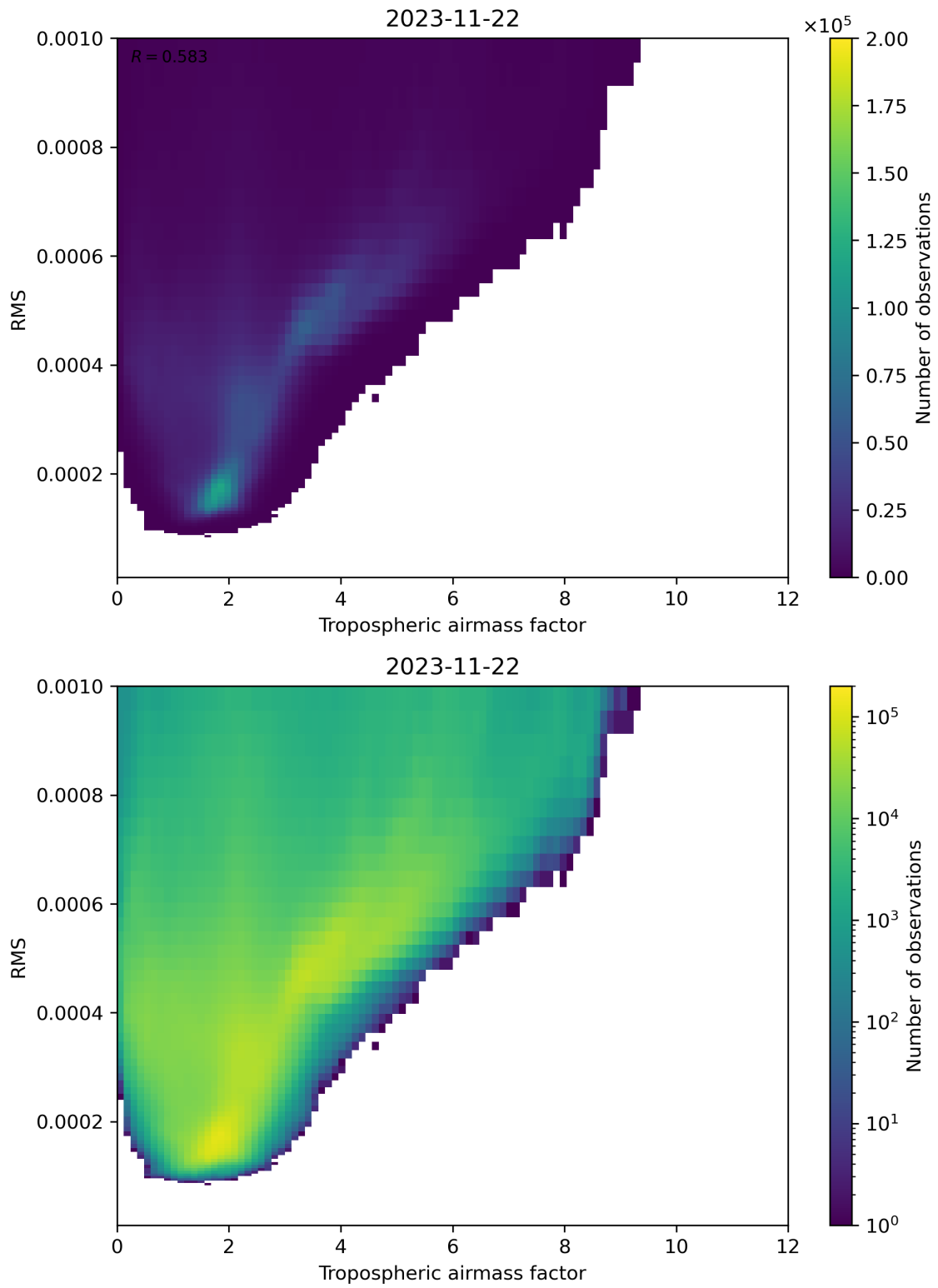
Figure 79: Scatter density plot of “Tropospheric airmass factor” against “RMS” for 2023-11-21 to 2023-11-23.
