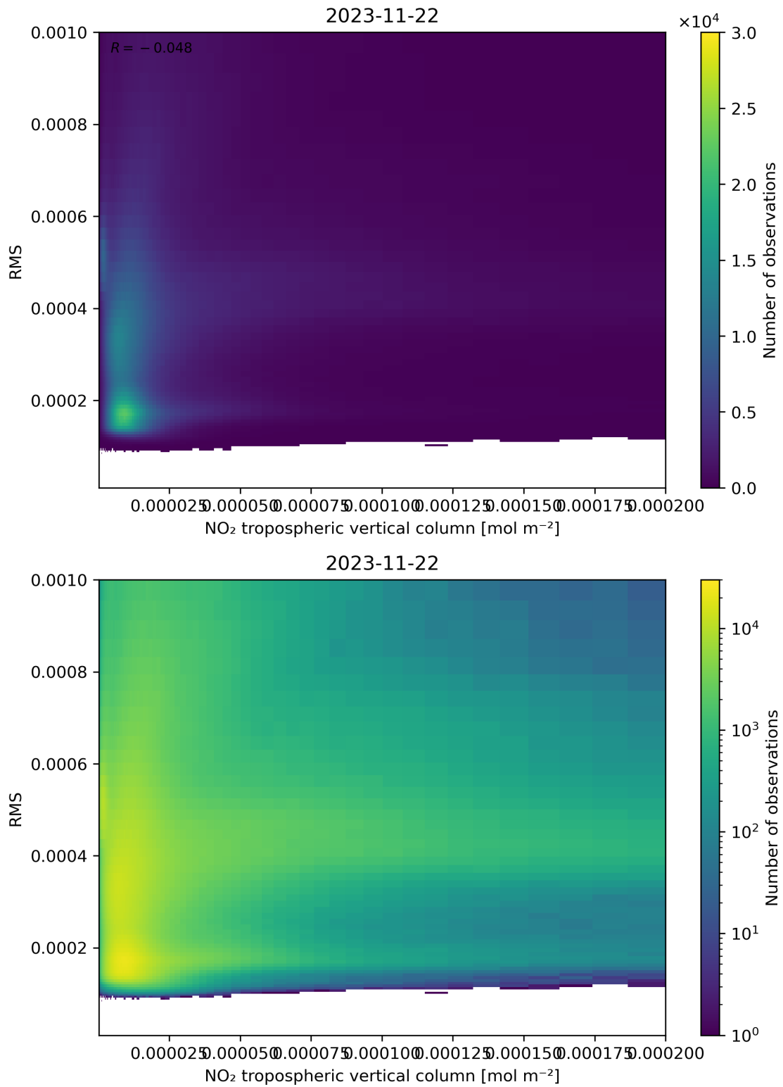
Figure 142: Scatter density plot of “NO 2 tropospheric vertical column” against “RMS” for 2023-11-21 to 2023-11-23.
