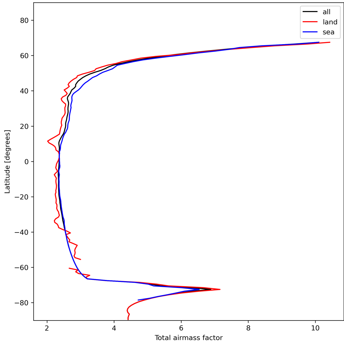
Figure 15: Zonal average of “Total airmass factor” for 2023-11-21 to 2023-11-23.
