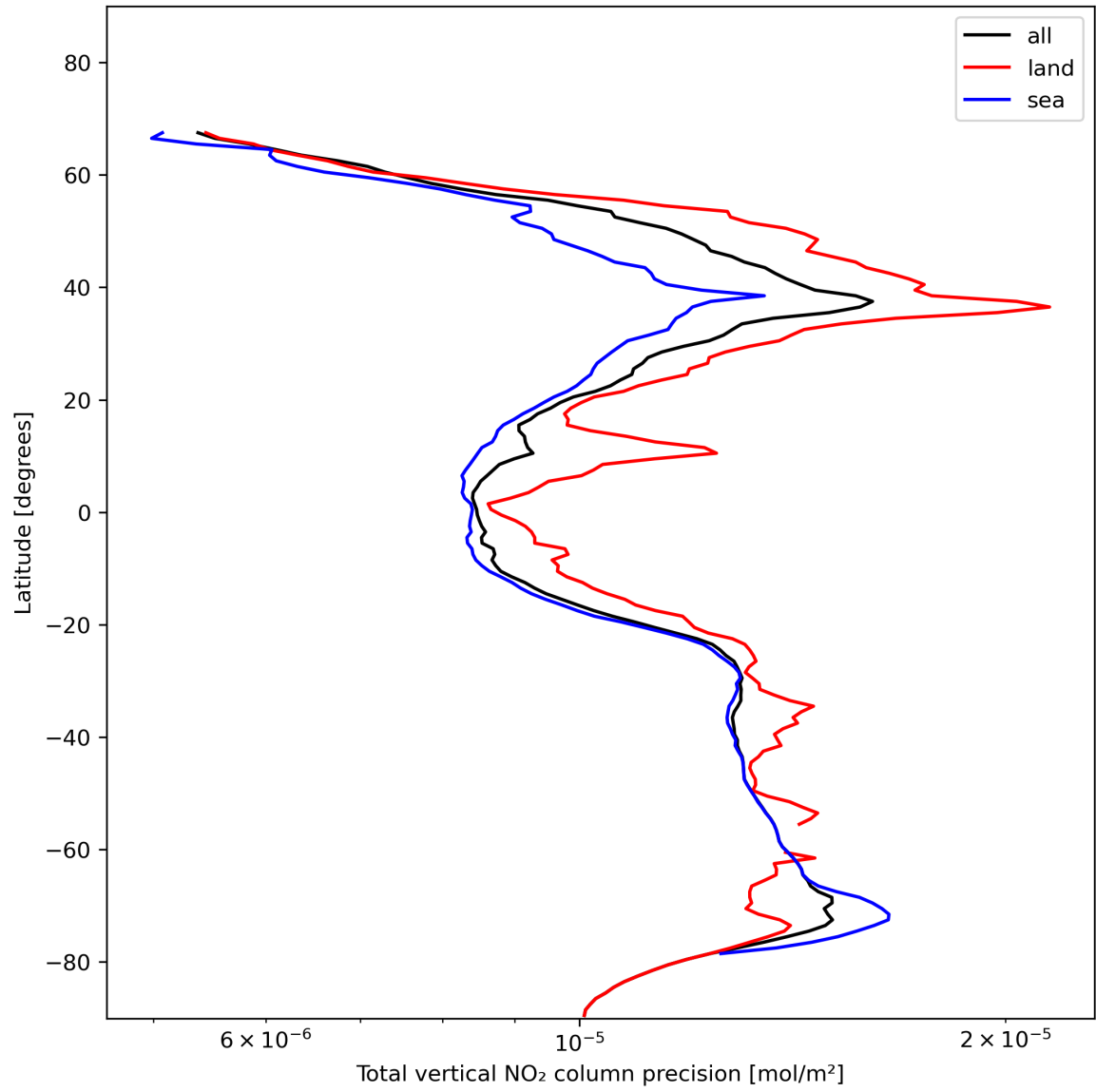
Figure 22: Zonal average of “Total vertical NO 2 column precision” for 2023-11-21 to 2023-11-23.
