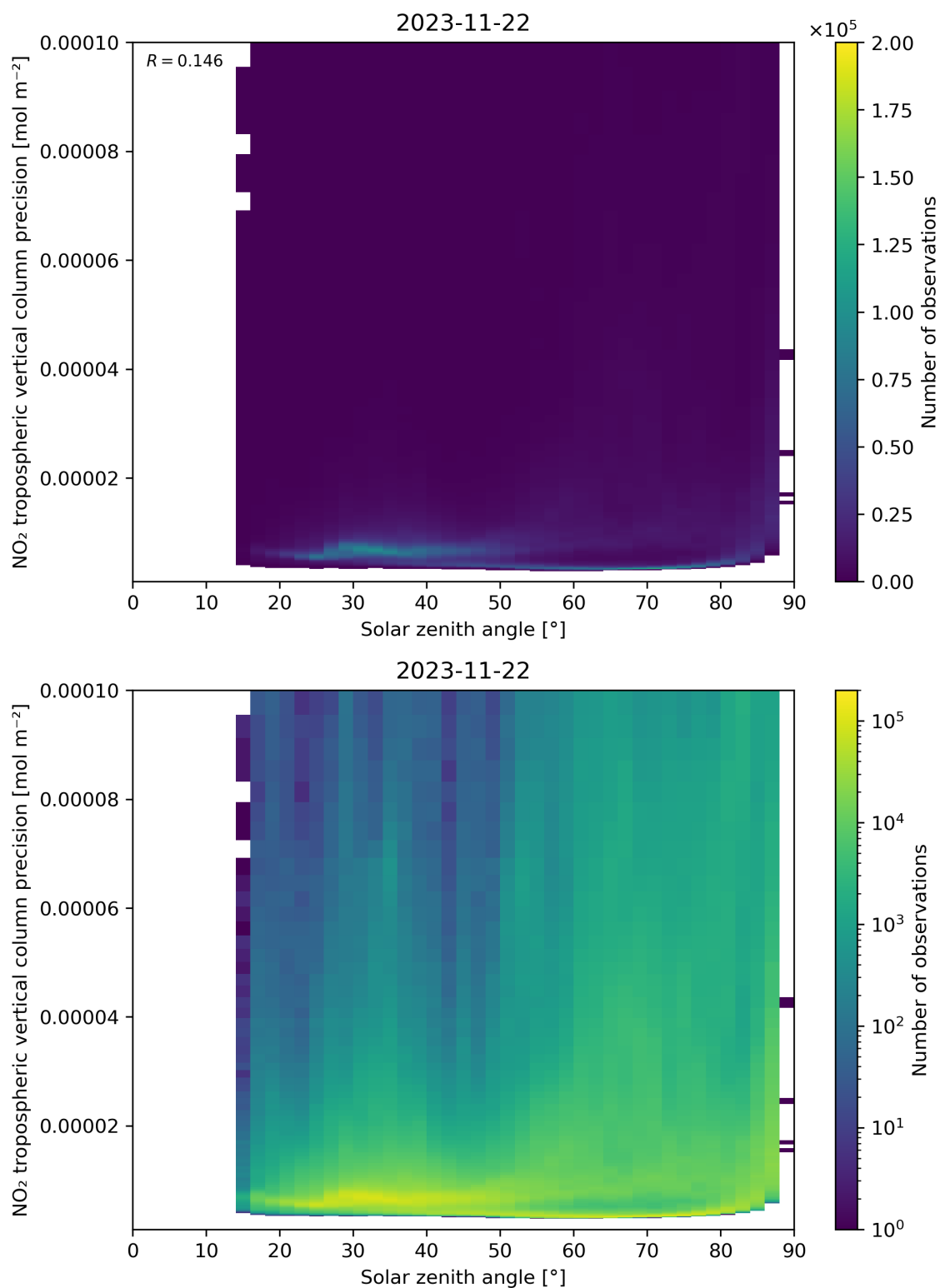
Figure 156: Scatter density plot of “Solar zenith angle” against “NO 2 tropospheric vertical column precision” for 2023-11-21 to 2023-11-23.
