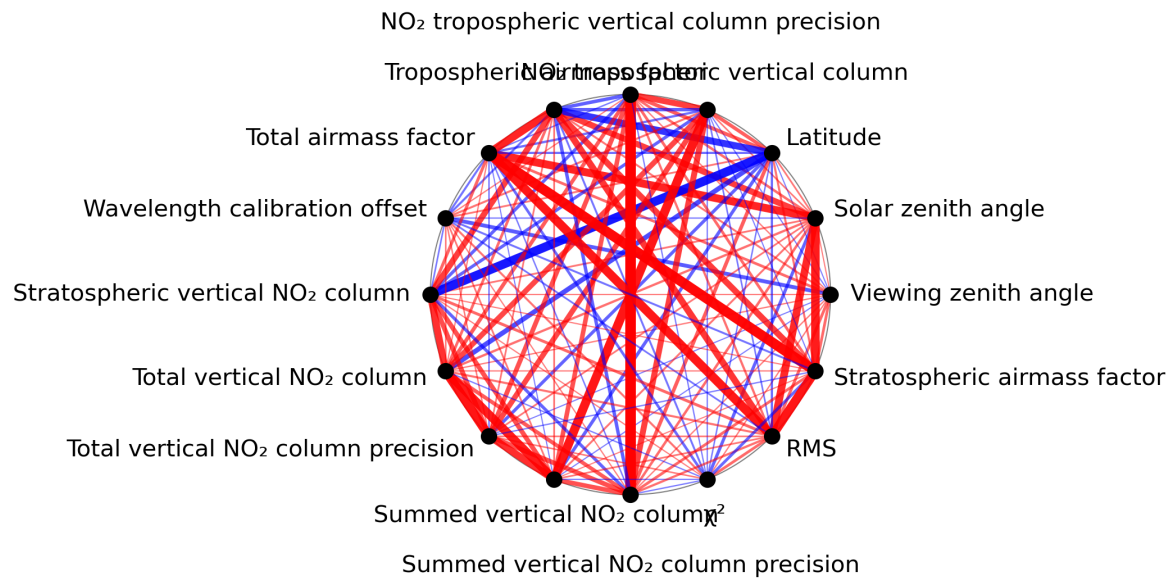
Figure 1: Map of correlation graph for 2023-11-21 to 2023-11-23.
