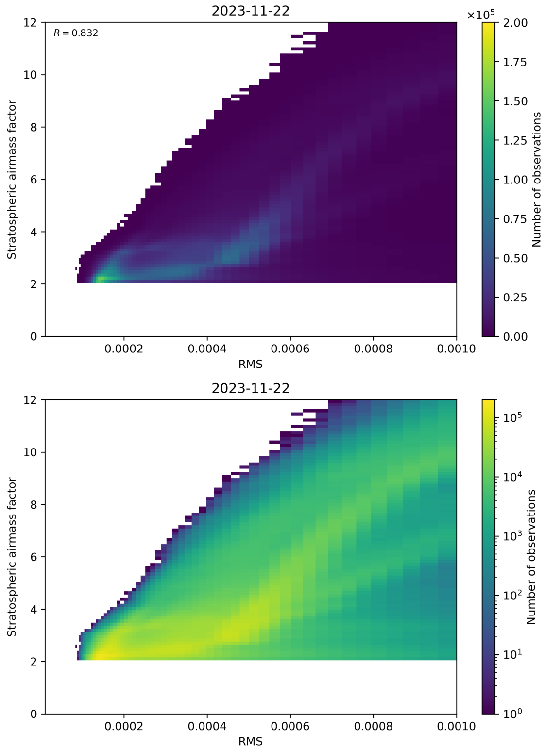
Figure 144: Scatter density plot of “RMS” against “Stratospheric airmass factor” for 2023-11-21 to 2023-11-23.
