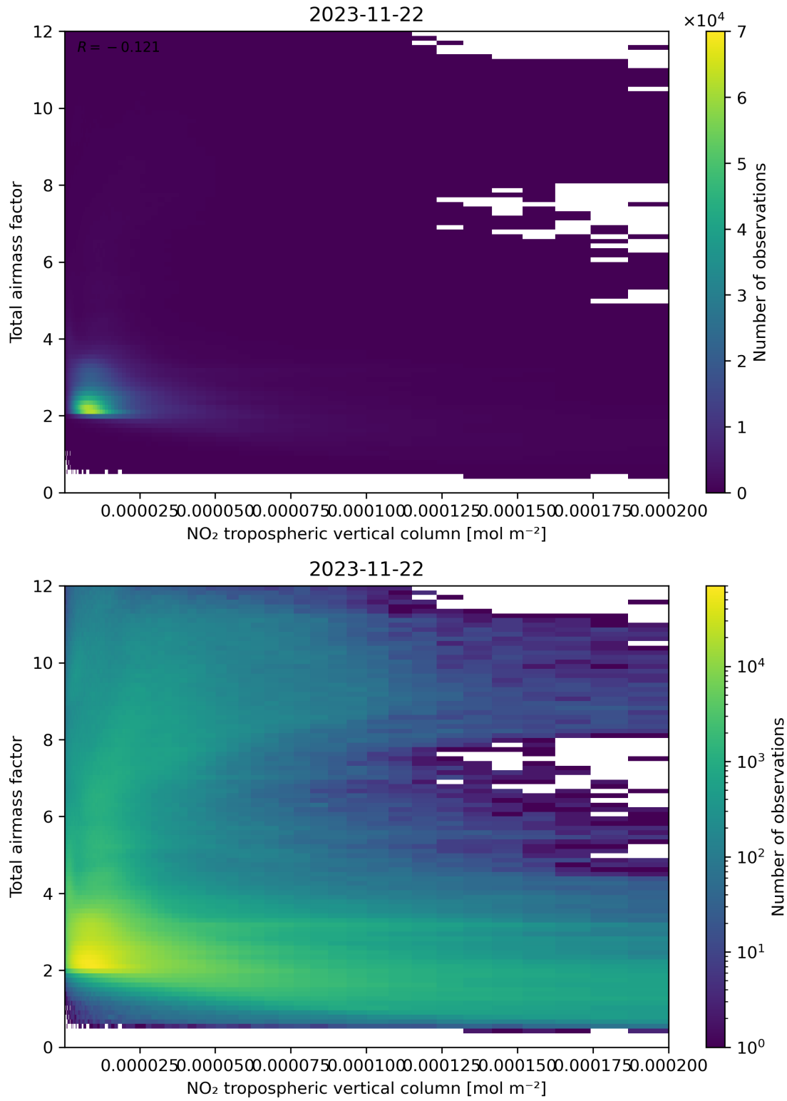
Figure 122: Scatter density plot of “NO 2 tropospheric vertical column” against “Total air mass factor” for 2023-11-21 to 2023-11-23.
