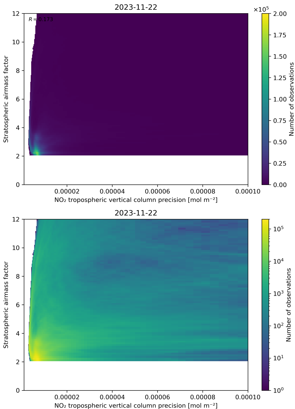
Figure 131: Scatter density plot of “NO 2 tropospheric vertical column precision” against “Stratospheric airmass factor” for 2023-11-21 to 2023-11-23.
