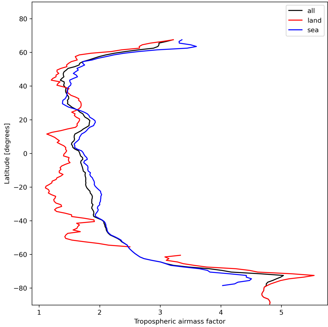
Figure 14: Zonal average of “Tropospheric airmass factor” for 2023-11-21 to 2023-11-23.
