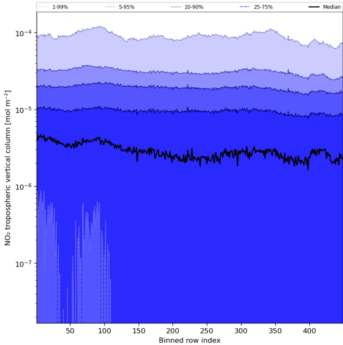
Figure 46: Along track statistics of “NO 2 tropospheric vertical column” for 2023-11-21 to 2023-11-23
