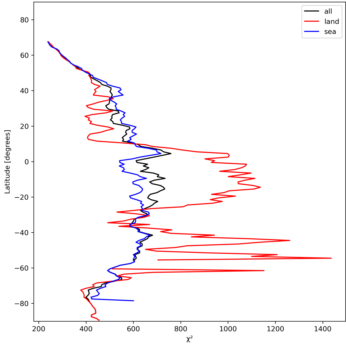
Figure 25: Zonal average of “ \chi^2 ” for 2023-11-21 to 2023-11-23.
