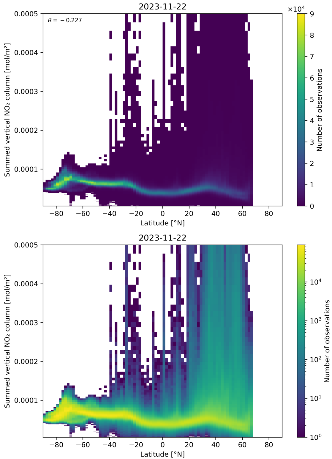
Figure 88: Scatter density plot of “Latitude” against “Summed vertical NO 2 column” for 2023-11-21 to 2023-11-23.
