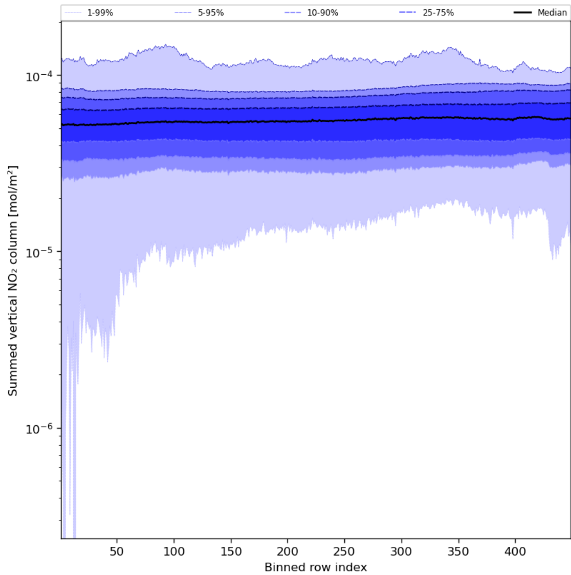
Figure 57: Along track statistics of “Summed vertical NO 2 column” for 2023-11-21 to 2023-11-23
