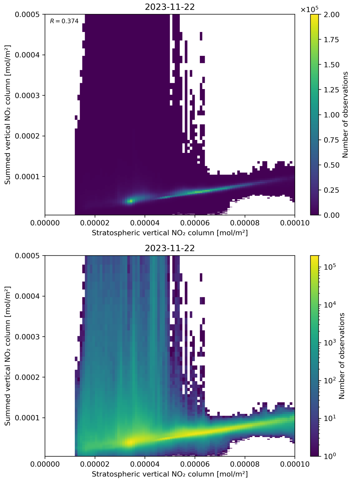
Figure 98: Scatter density plot of “Stratospheric vertical NO 2 column” against “Summed vertical NO 2 column” for 2023-11-21 to 2023-11-23.
