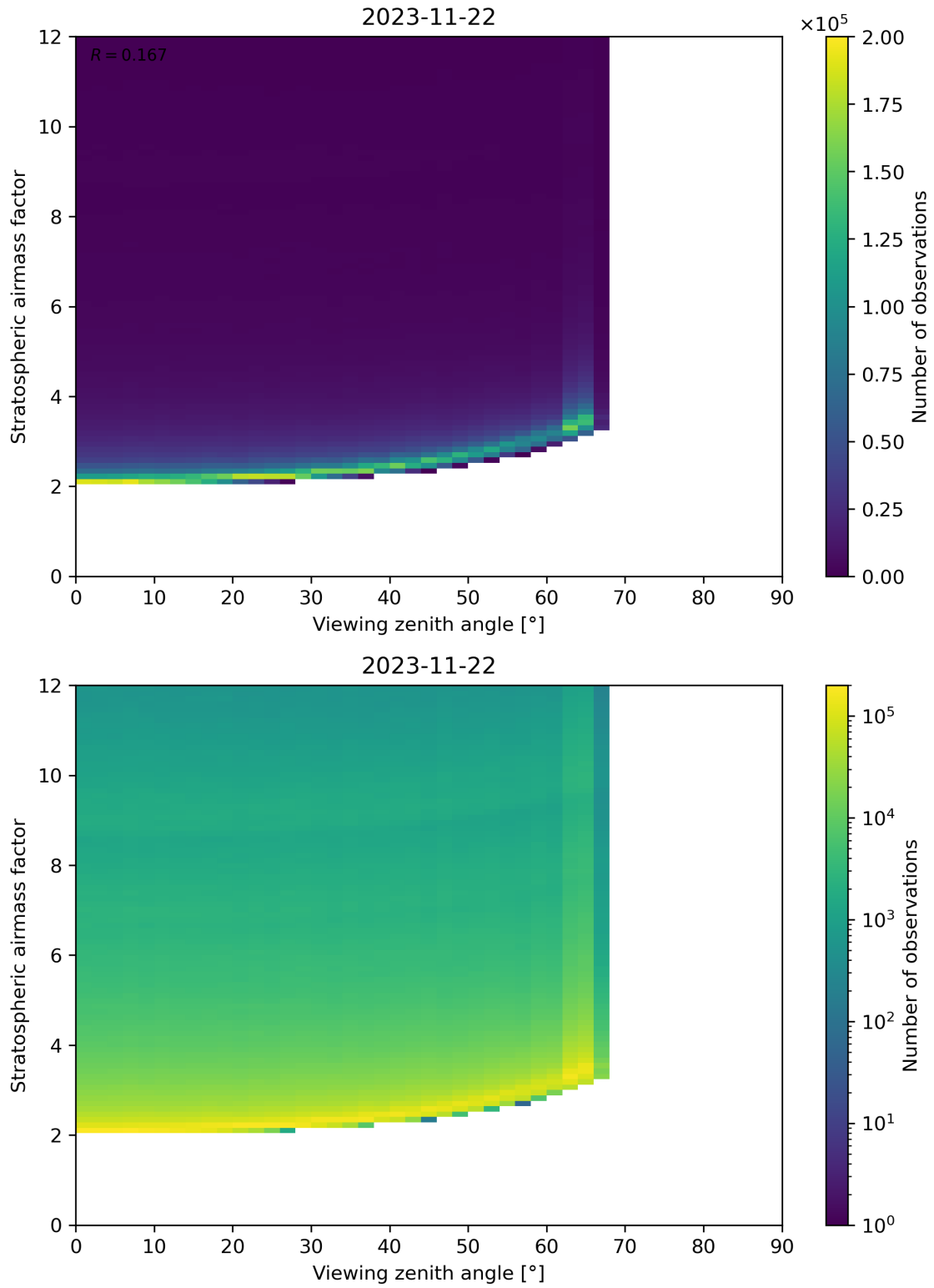
Figure 159: Scatter density plot of “Viewing zenith angle” against “Stratospheric airmass factor” for 2023-11-21 to 2023-11-23.
