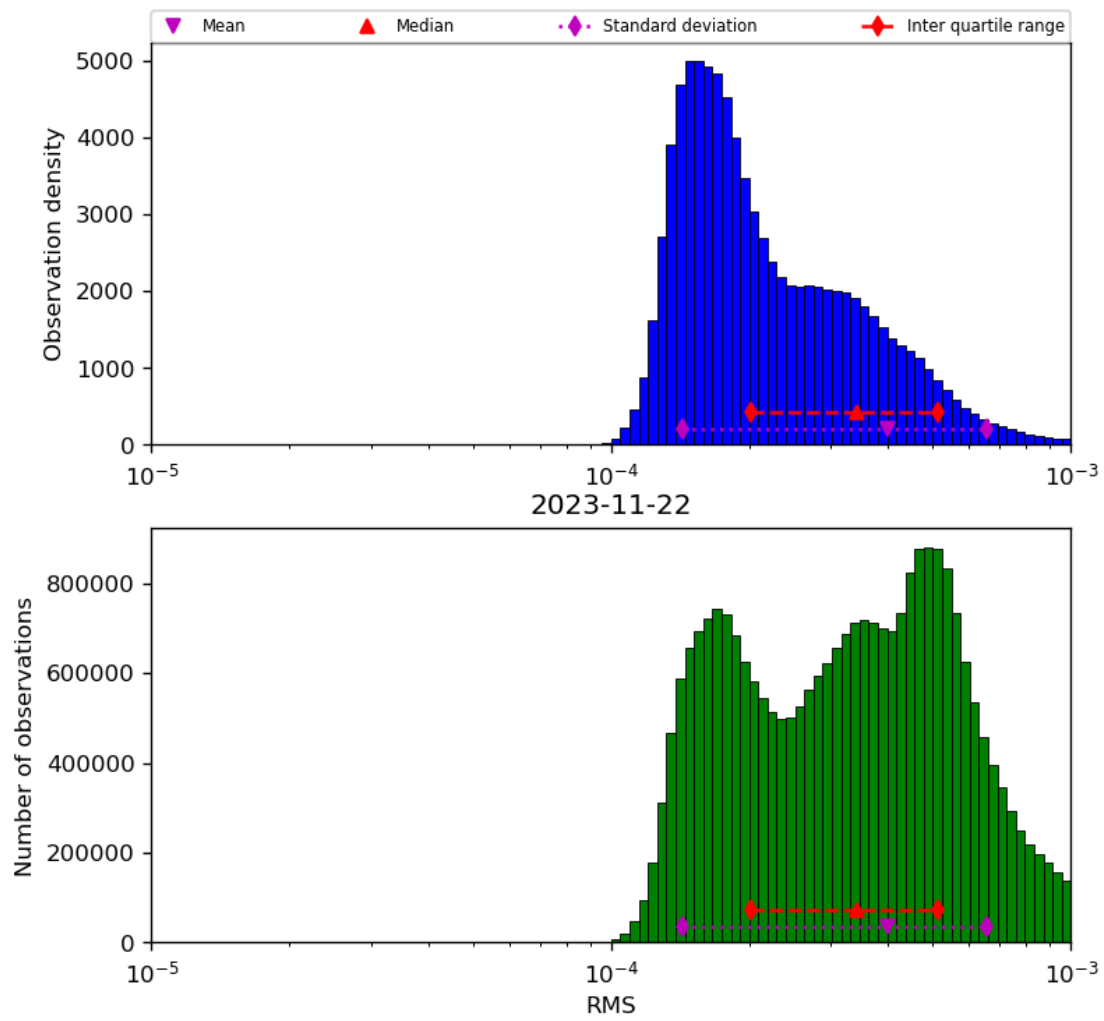
Figure 43: Histogram of “RMS” for 2023-11-21 to 2023-11-23
