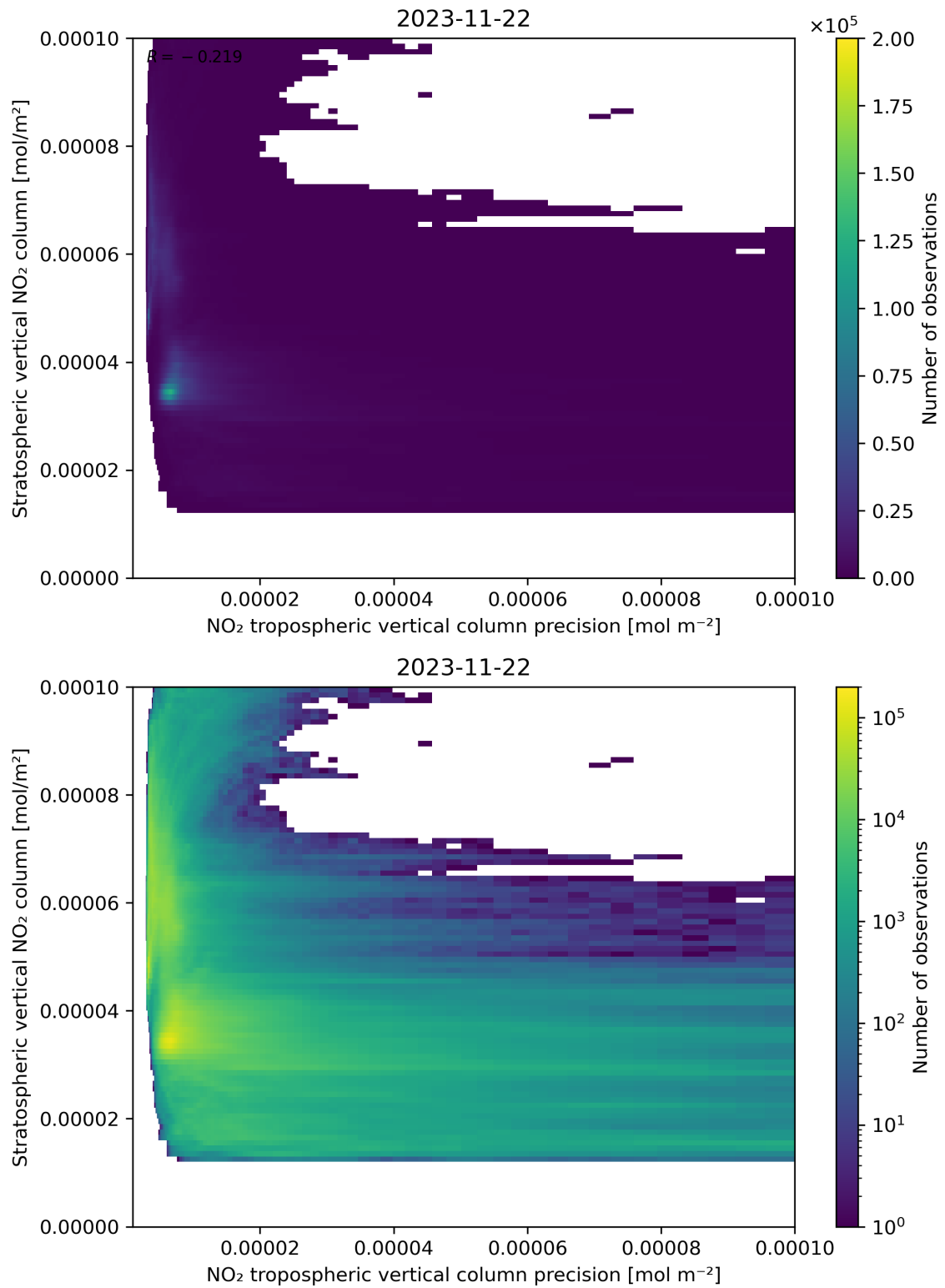
Figure 135: Scatter density plot of “NO 2 tropospheric vertical column precision” against “Stratospheric vertical NO 2 column” for 2023-11-21 to 2023-11-23.
