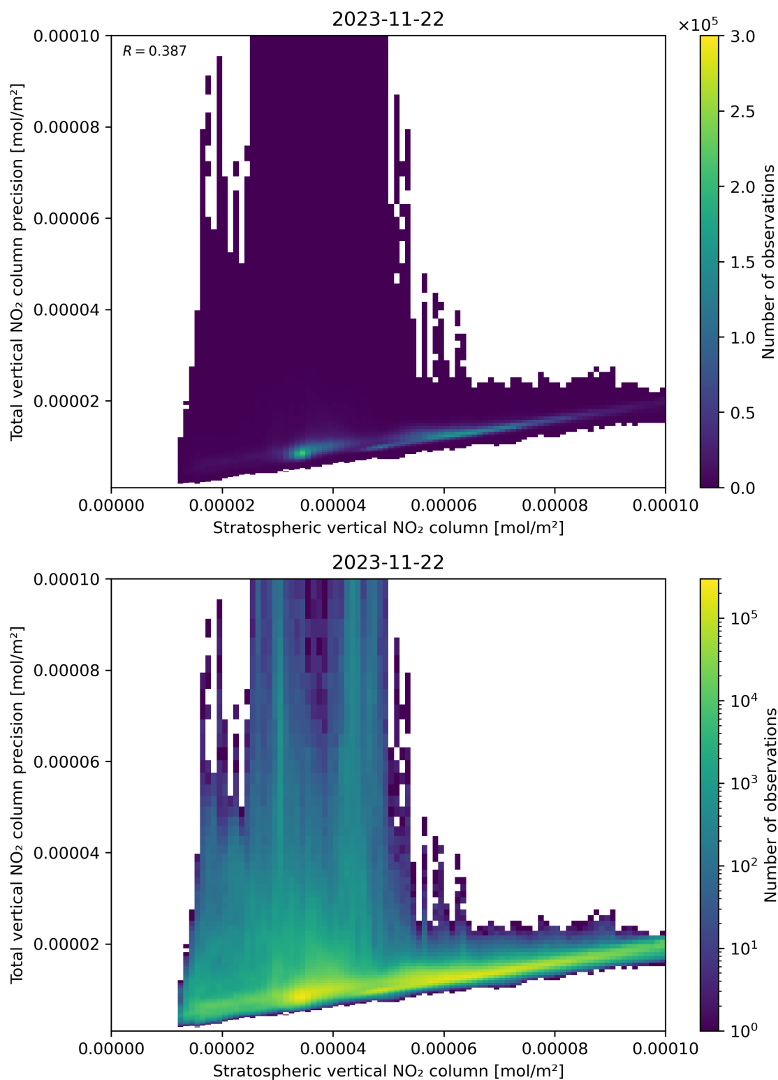
Figure 101: Scatter density plot of “Stratospheric vertical NO 2 column” against “Total vertical NO 2 column precision” for 2023-11-21 to 2023-11-23.
