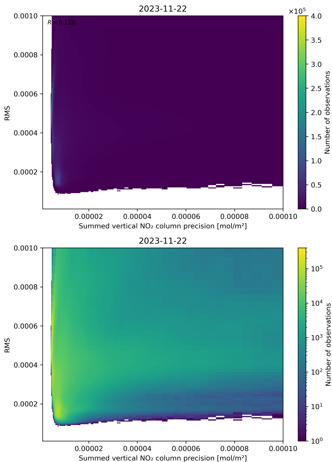
Figure 108: Scatter density plot of “Summed vertical NO 2 column precision” against “RMS” for 2023-11-21 to 2023-11-23.
