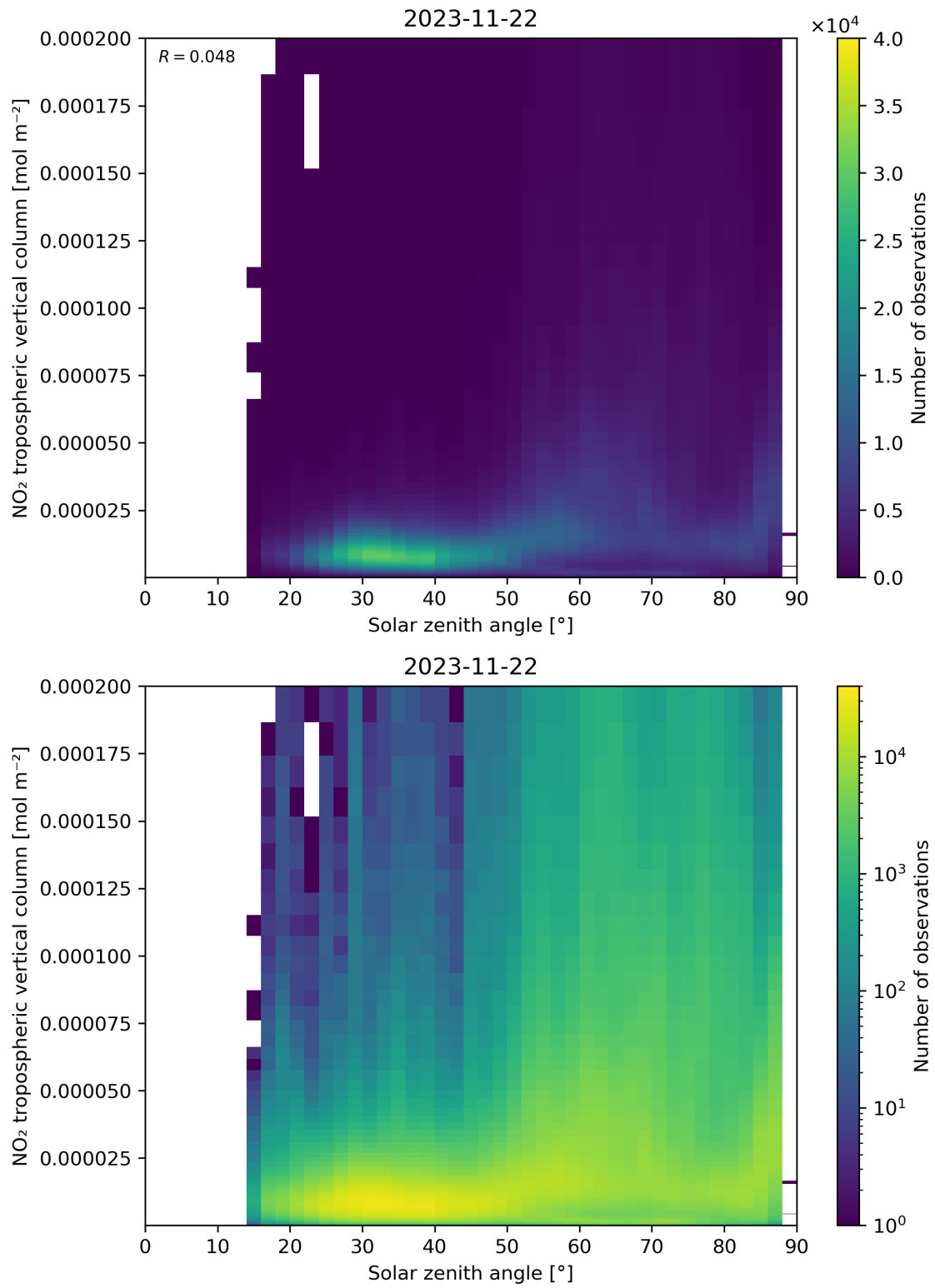
Figure 155: Scatter density plot of “Solar zenith angle” against “NO 2 tropospheric vertical column” for 2023-11-21 to 2023-11-23.
