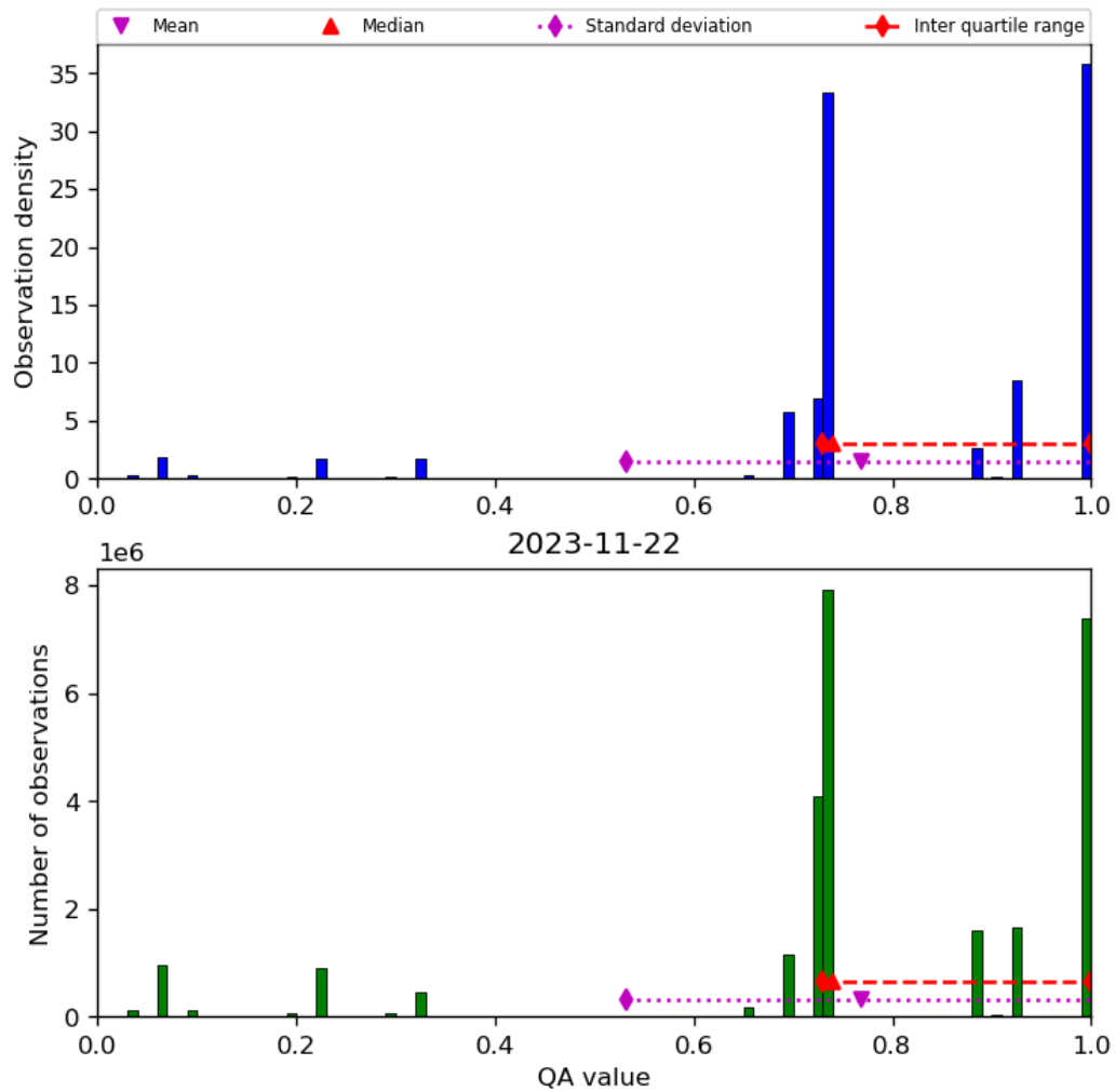
Figure 28: Histogram of “QA value” for 2023-11-21 to 2023-11-23
