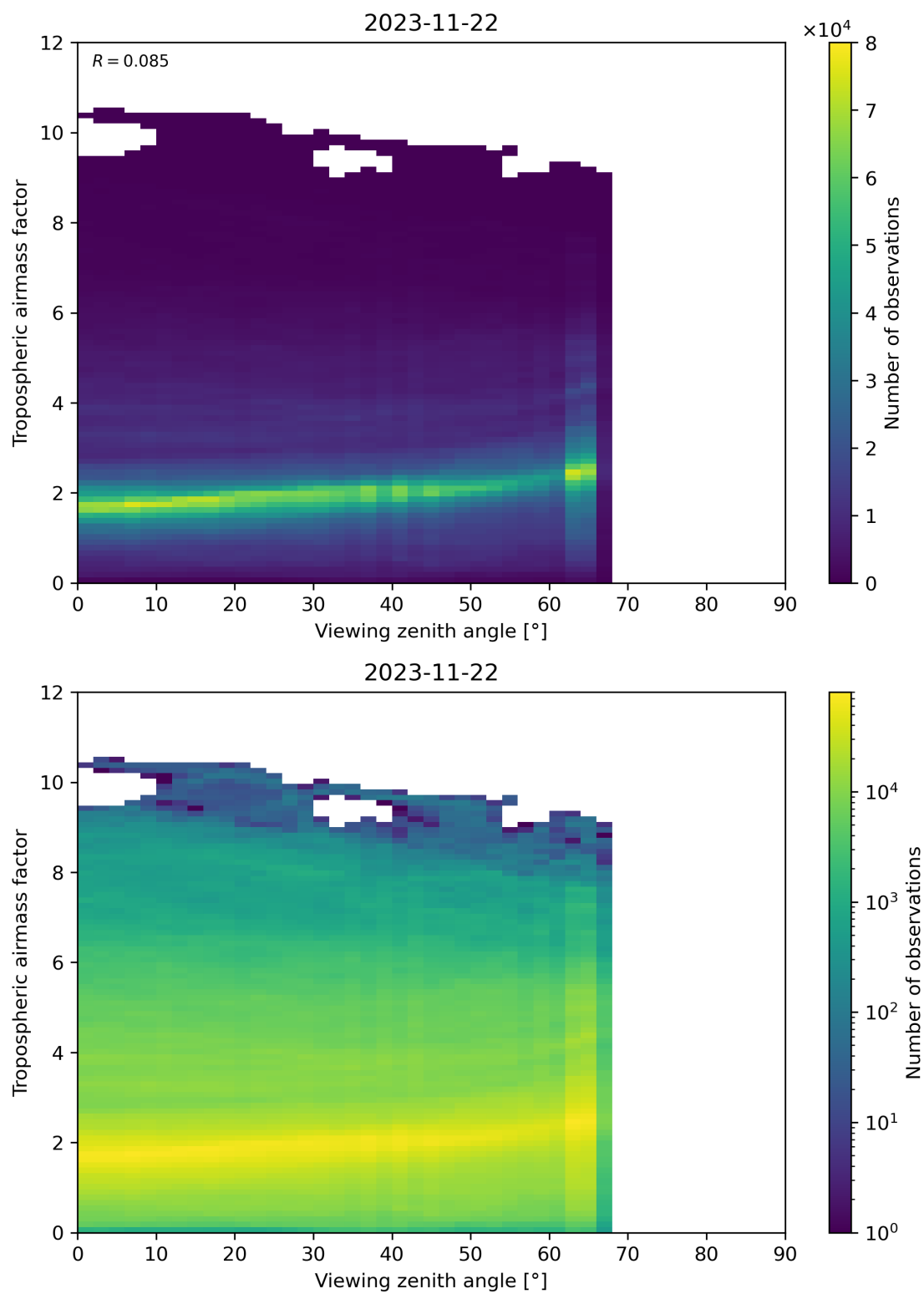
Figure 161: Scatter density plot of “Viewing zenith angle” against “Tropospheric airmass factor” for 2023-11-21 to 2023-11-23.
