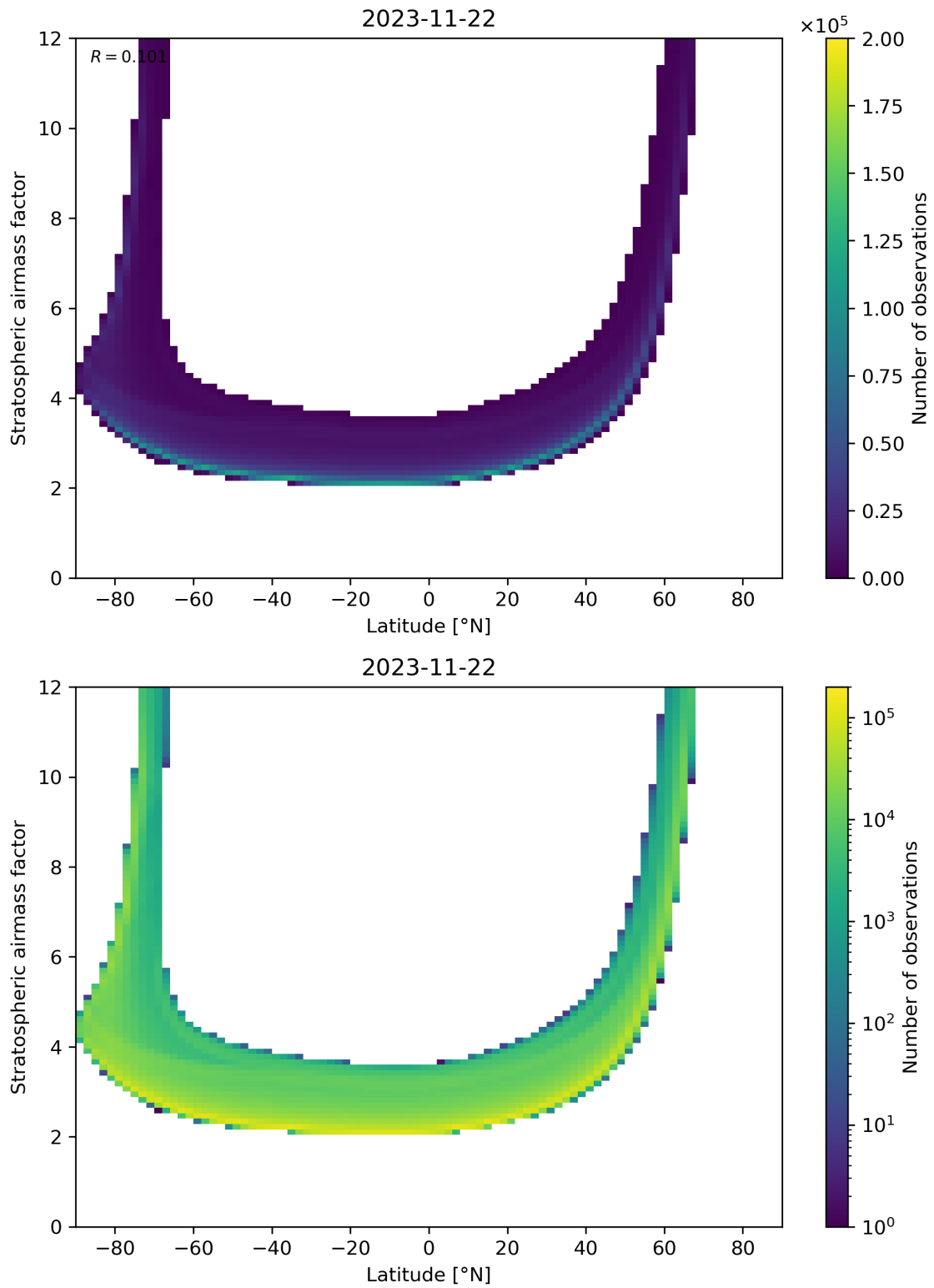
Figure 83: Scatter density plot of “Latitude” against “Stratospheric airmass factor” for 2023-11-21 to 2023-11-23.
