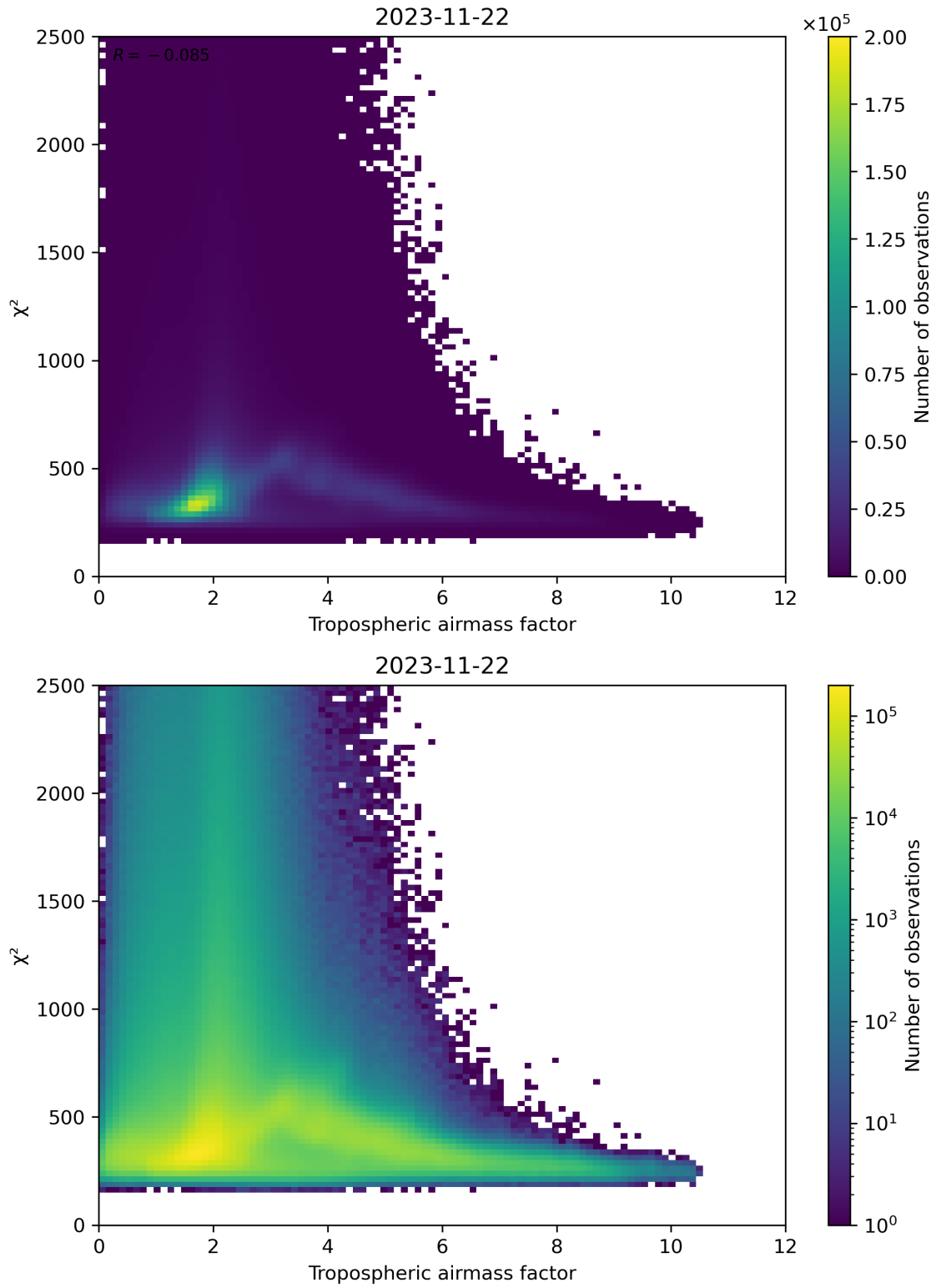
Figure 73: Scatter density plot of “Tropospheric airmass factor” against “ \chi^2 ” for 2023-11-21 to 2023-11-23.
