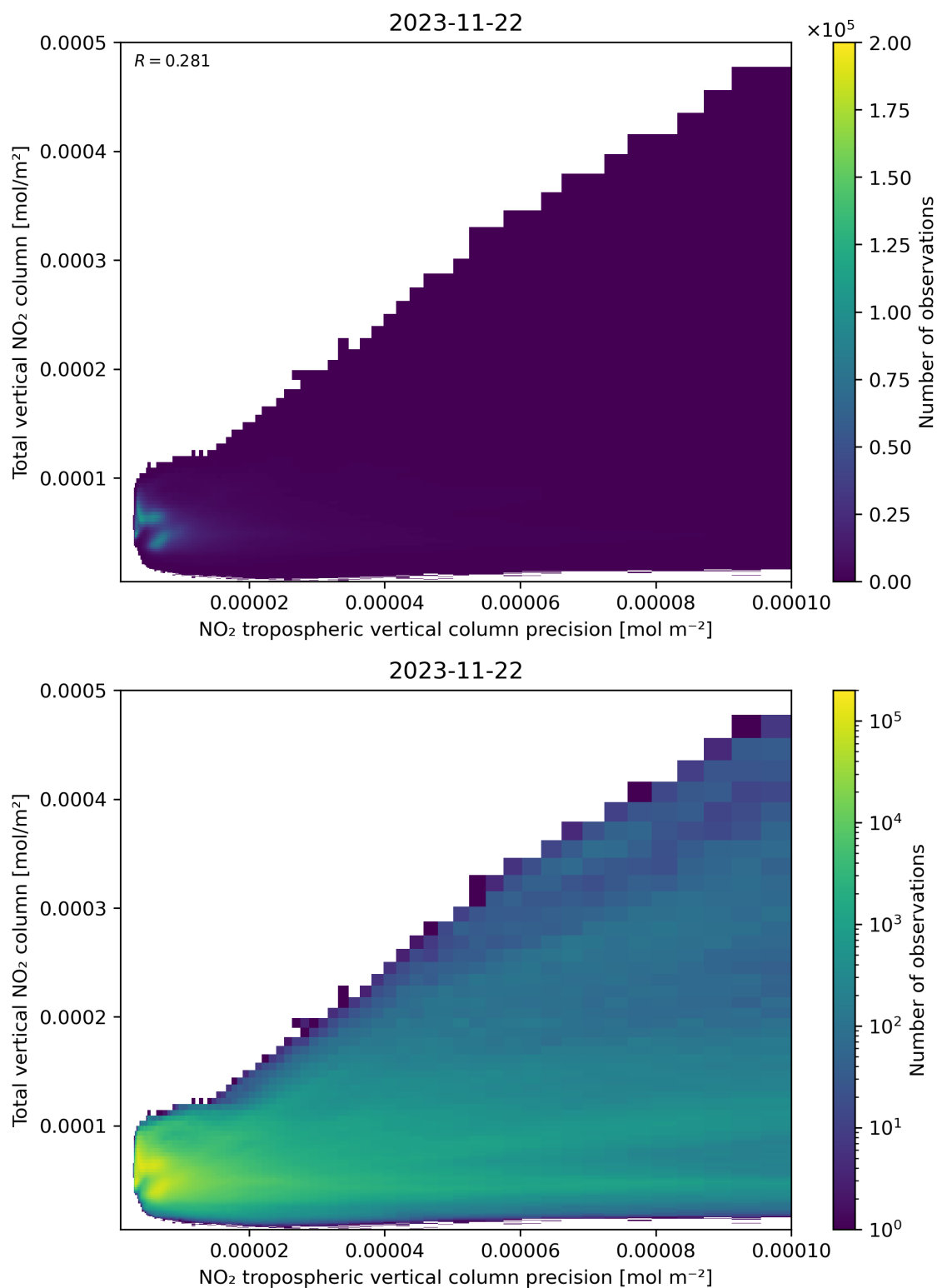
Figure 138: Scatter density plot of “NO 2 tropospheric vertical column precision” against “Total vertical NO 2 column” for 2023-11-21 to 2023-11-23.
