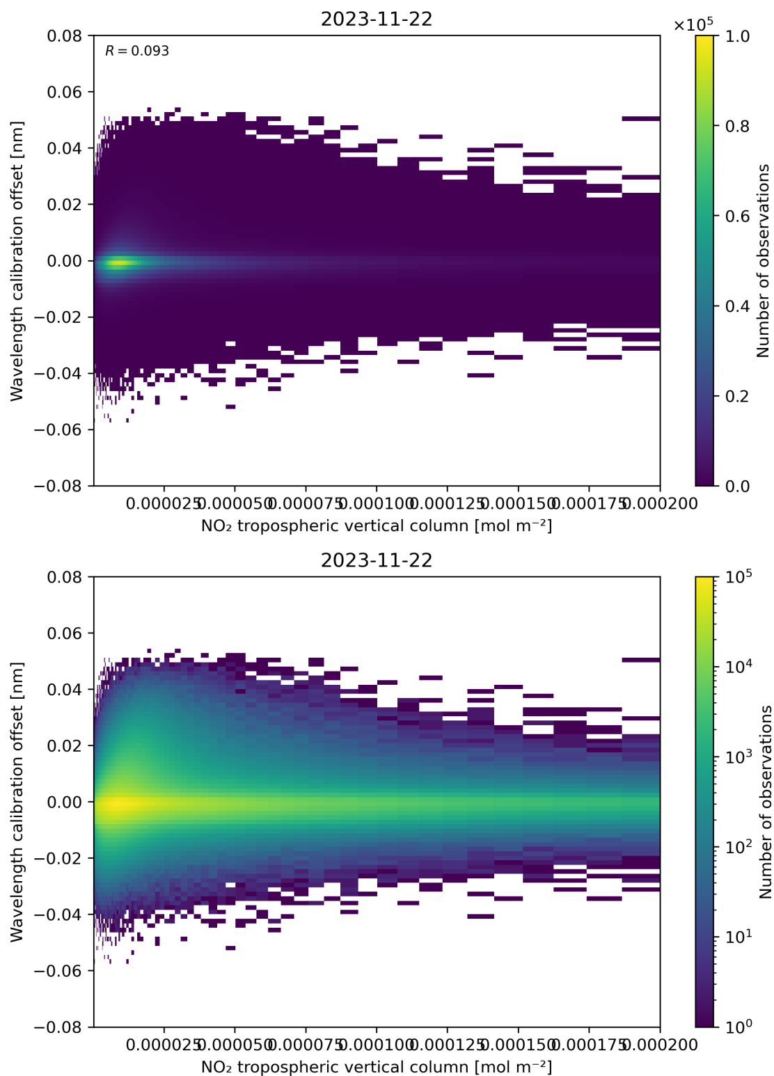
Figure 143: Scatter density plot of “NO 2 tropospheric vertical column” against “Wavelength calibration offset” for 2023-11-21 to 2023-11-23.
