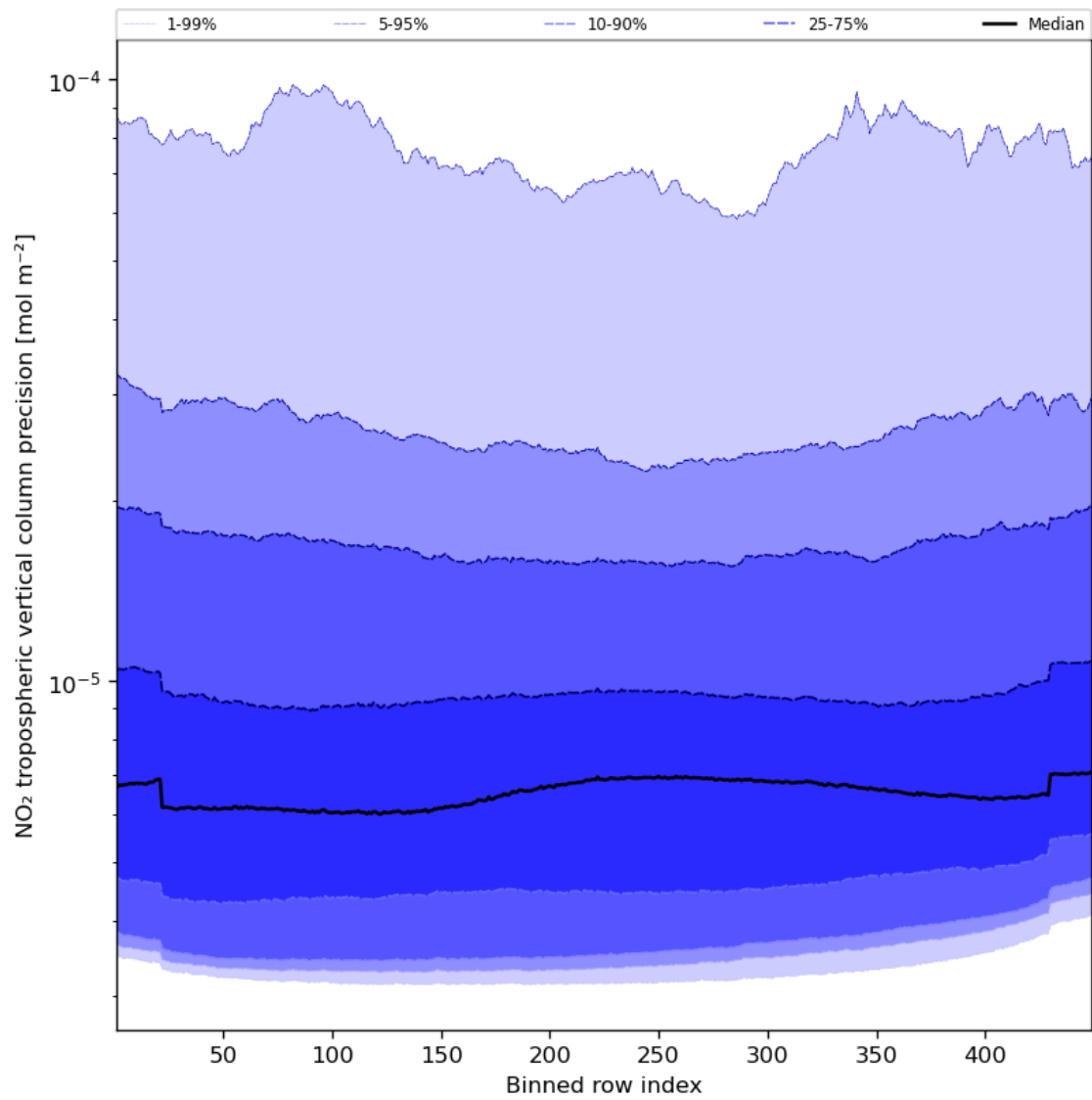
Figure 47: Along track statistics of “NO 2 tropospheric vertical column precision” for 2023-11-21 to 2023-11-23
