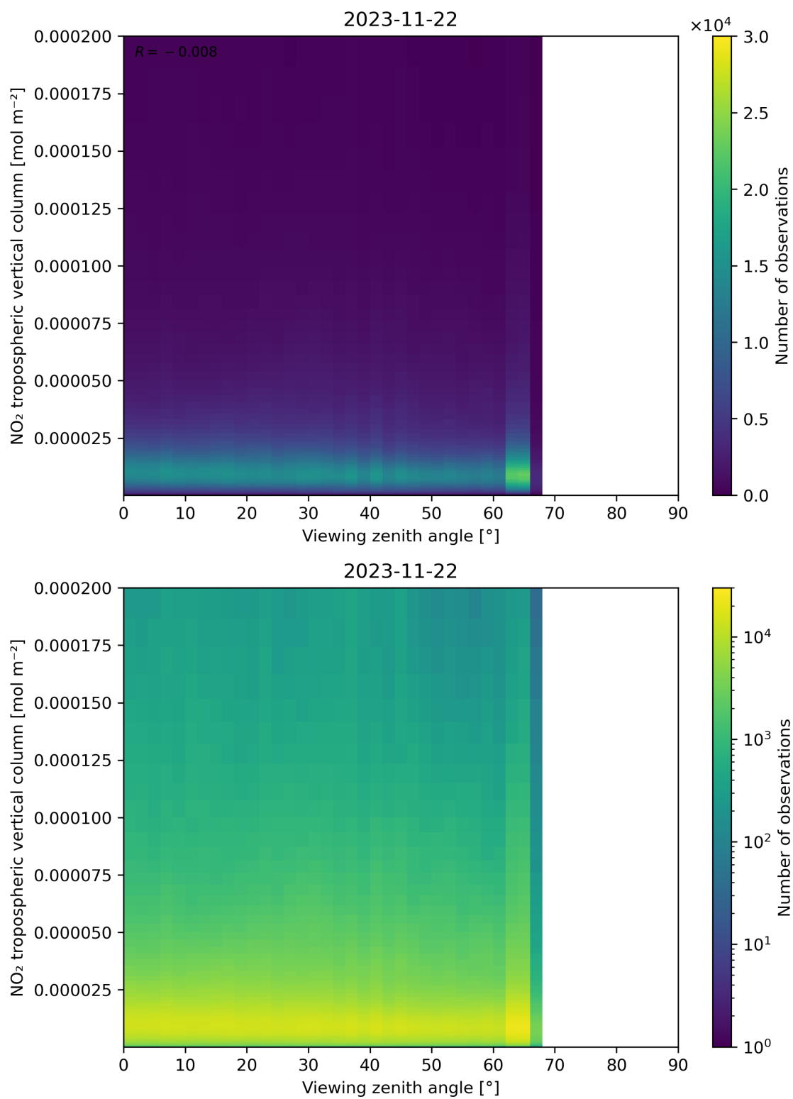
Figure 169: Scatter density plot of “Viewing zenith angle” against “NO 2 tropospheric vertical column” for 2023-11-21 to 2023-11-23.
