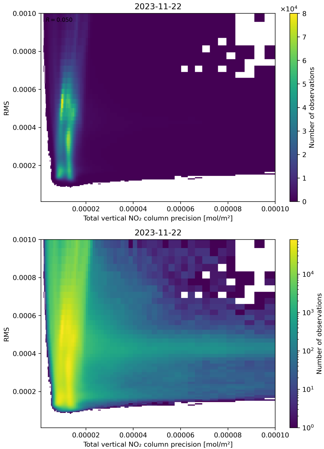
Figure 119: Scatter density plot of “Total vertical NO 2 column precision” against “RMS” for 2023-11-21 to 2023-11-23.
