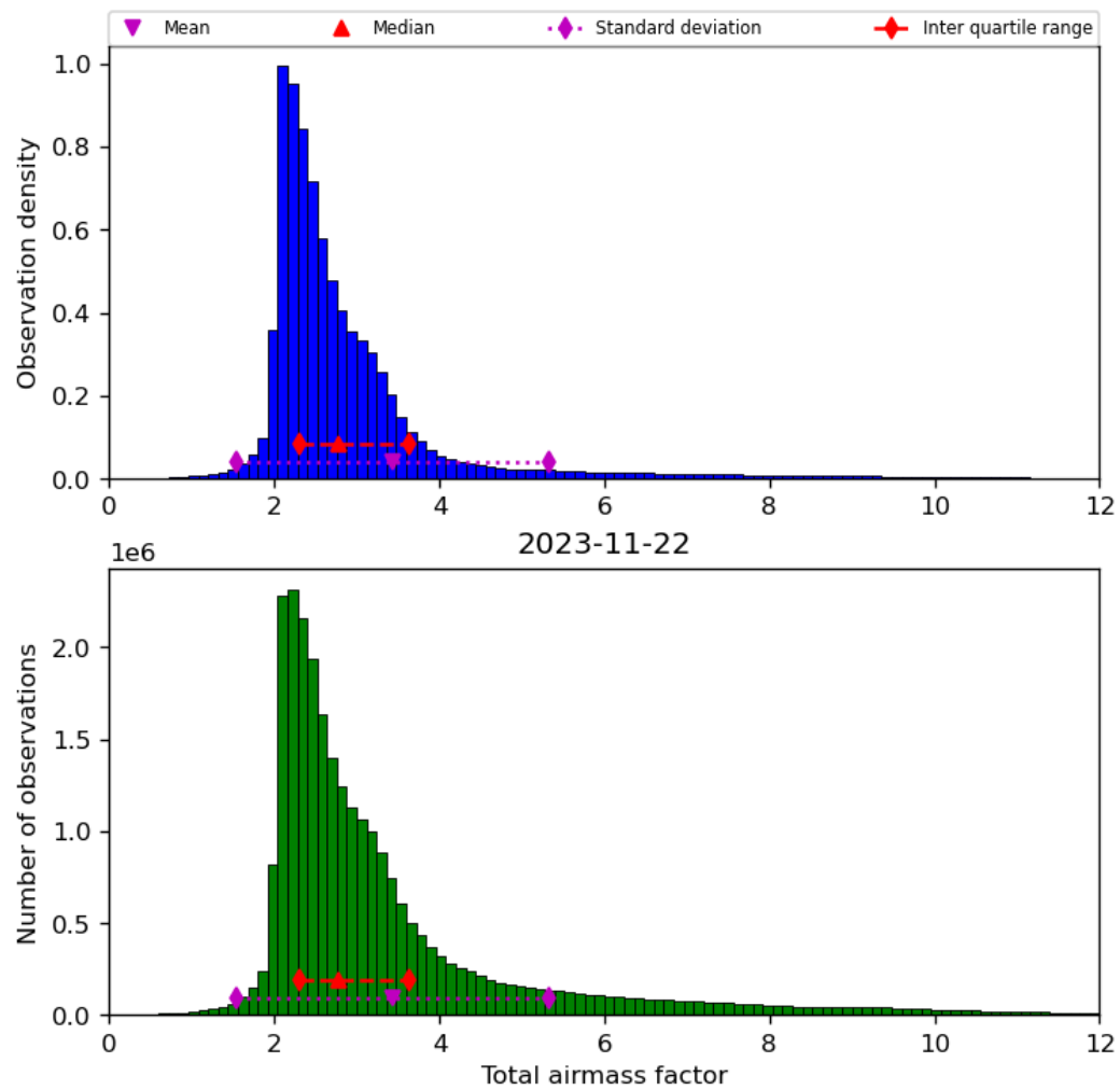
Figure 32: Histogram of “Total airmass factor” for 2023-11-21 to 2023-11-23
