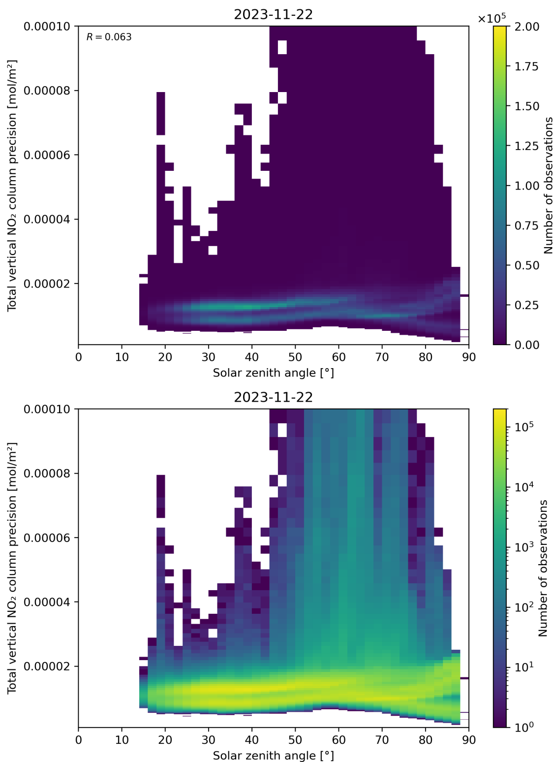
Figure 154: Scatter density plot of “Solar zenith angle” against “Total vertical NO 2 column precision” for 2023-11-21 to 2023-11-23.
