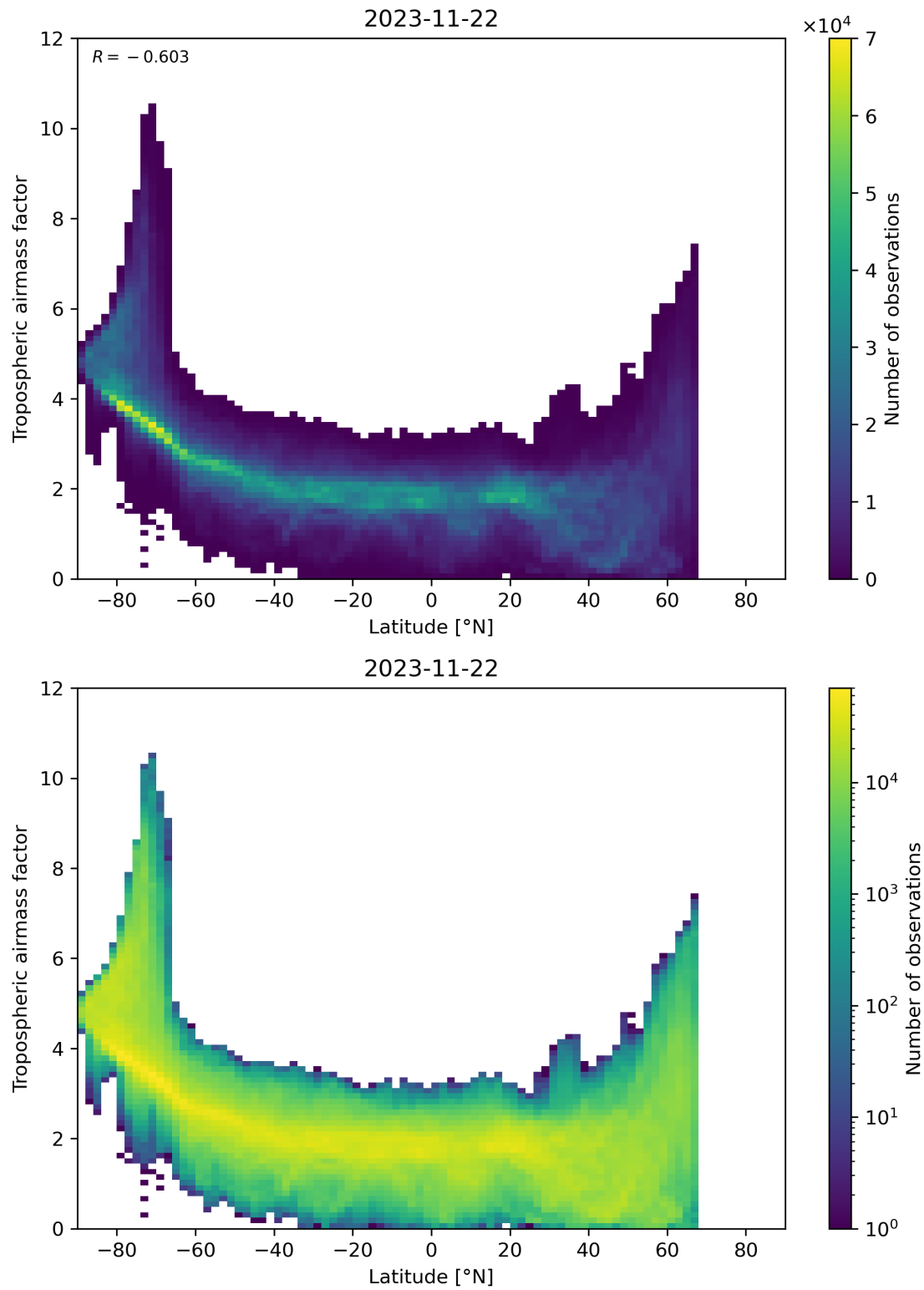
Figure 85: Scatter density plot of “Latitude” against “Tropospheric airmass factor” for 2023-11-21 to 2023-11-23.
