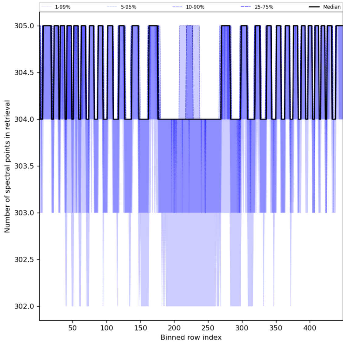
Figure 50: Along track statistics of “Number of spectral points in retrieval” for 2023-11-21 to 2023-11-23
