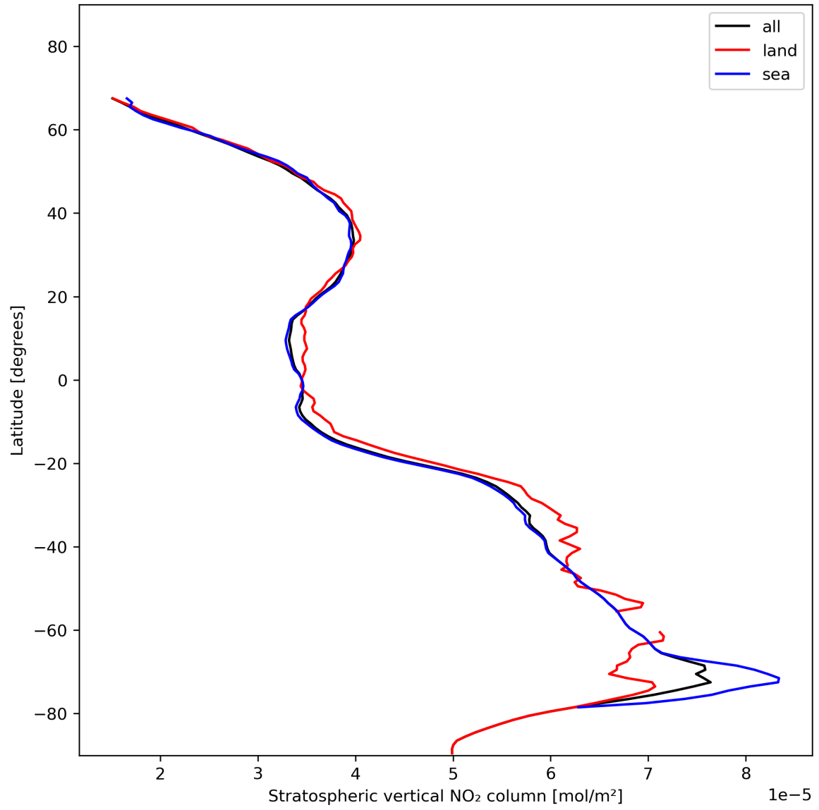
Figure 19: Zonal average of “Stratospheric vertical NO 2 column” for 2023-11-21 to 2023-11-23.
