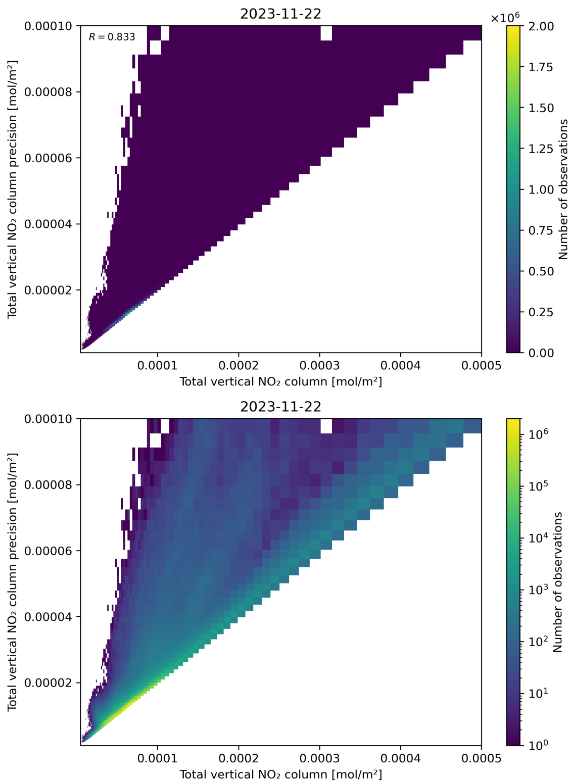
Figure 114: Scatter density plot of “Total vertical NO 2 column” against “Total vertical NO 2 column precision” for 2023-11-21 to 2023-11-23.
