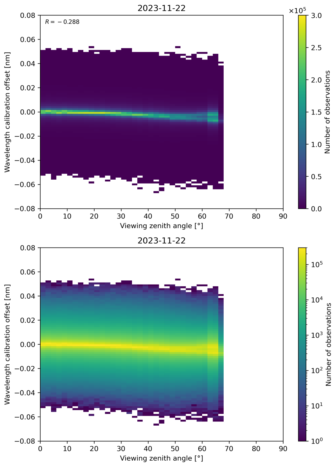
Figure 173: Scatter density plot of “Viewing zenith angle” against “Wavelength calibration offset” for 2023-11-21 to 2023-11-23.
