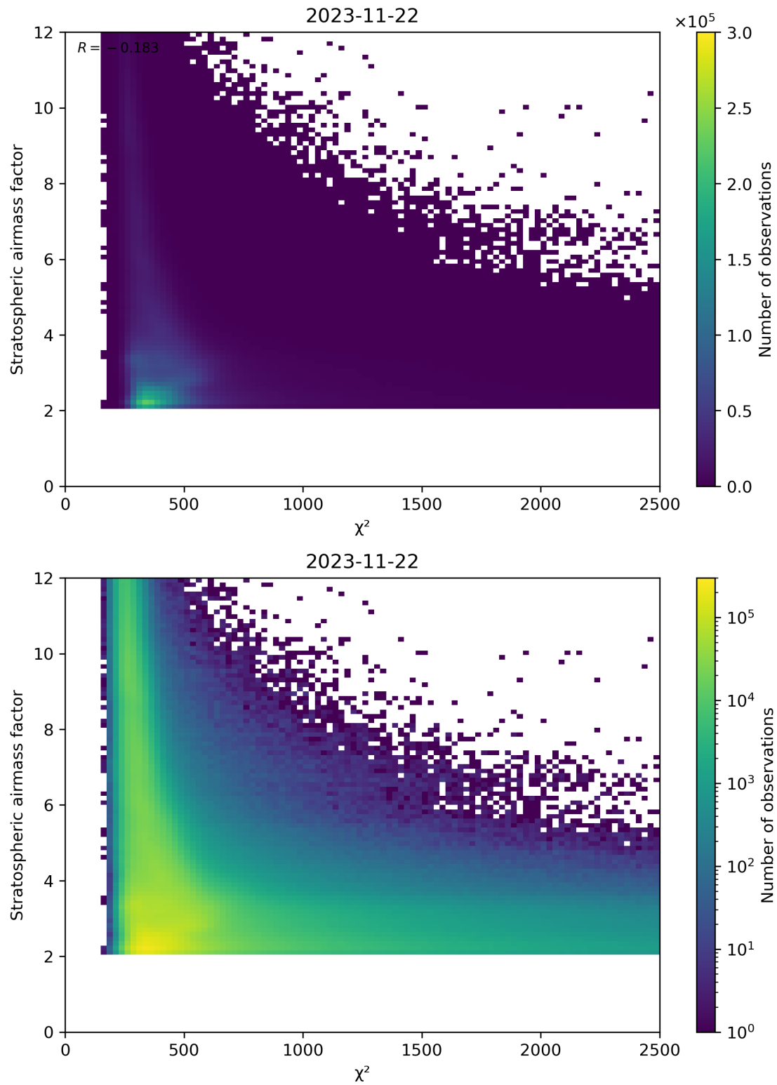
Figure 81: Scatter density plot of “ \chi^2 ” against “Stratospheric airmass factor” for 2023-11-21 to 2023-11-23.
