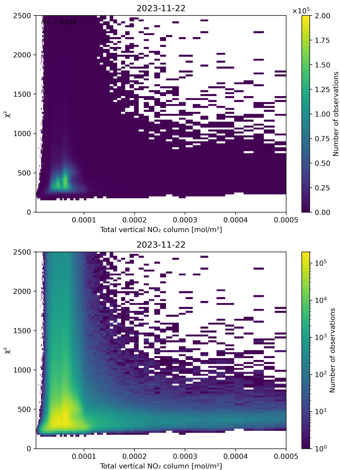
Figure 111: Scatter density plot of “Total vertical NO 2 column” against “ \chi^2 ” for 2023-11-21 to 2023-11-23.
