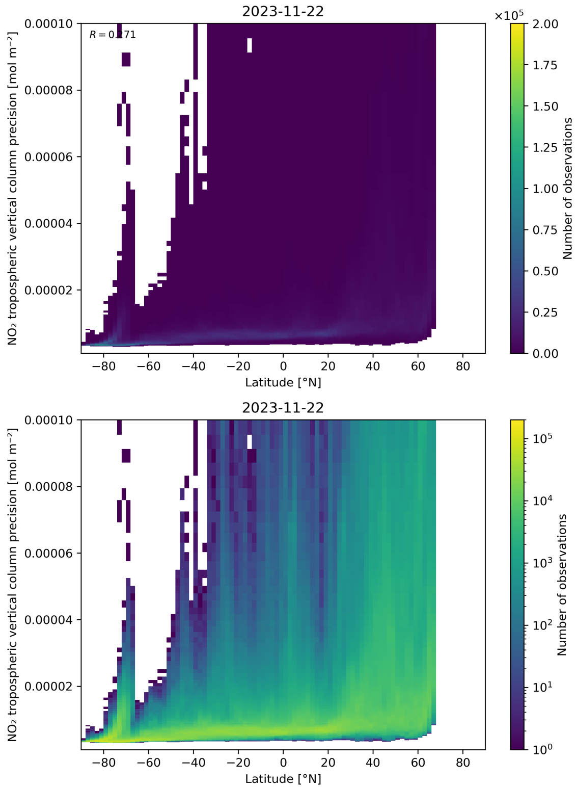
Figure 93: Scatter density plot of “Latitude” against “NO 2 tropospheric vertical column precision” for 2023-11-21 to 2023-11-23.
