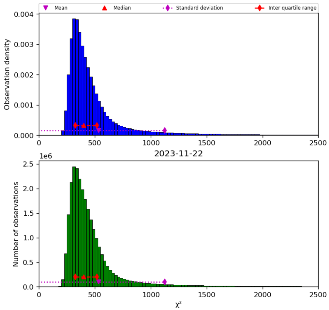
Figure 42: Histogram of “ \chi^2 ” for 2023-11-21 to 2023-11-23
