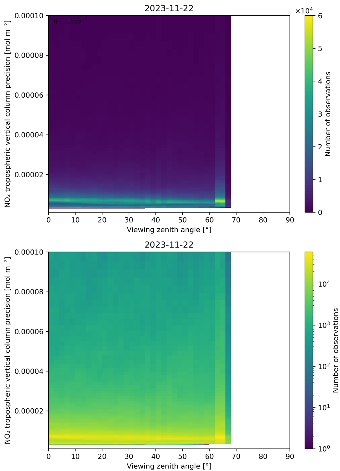
Figure 170: Scatter density plot of “Viewing zenith angle” against “NO 2 tropospheric vertical column precision” for 2023-11-21 to 2023-11-23.
