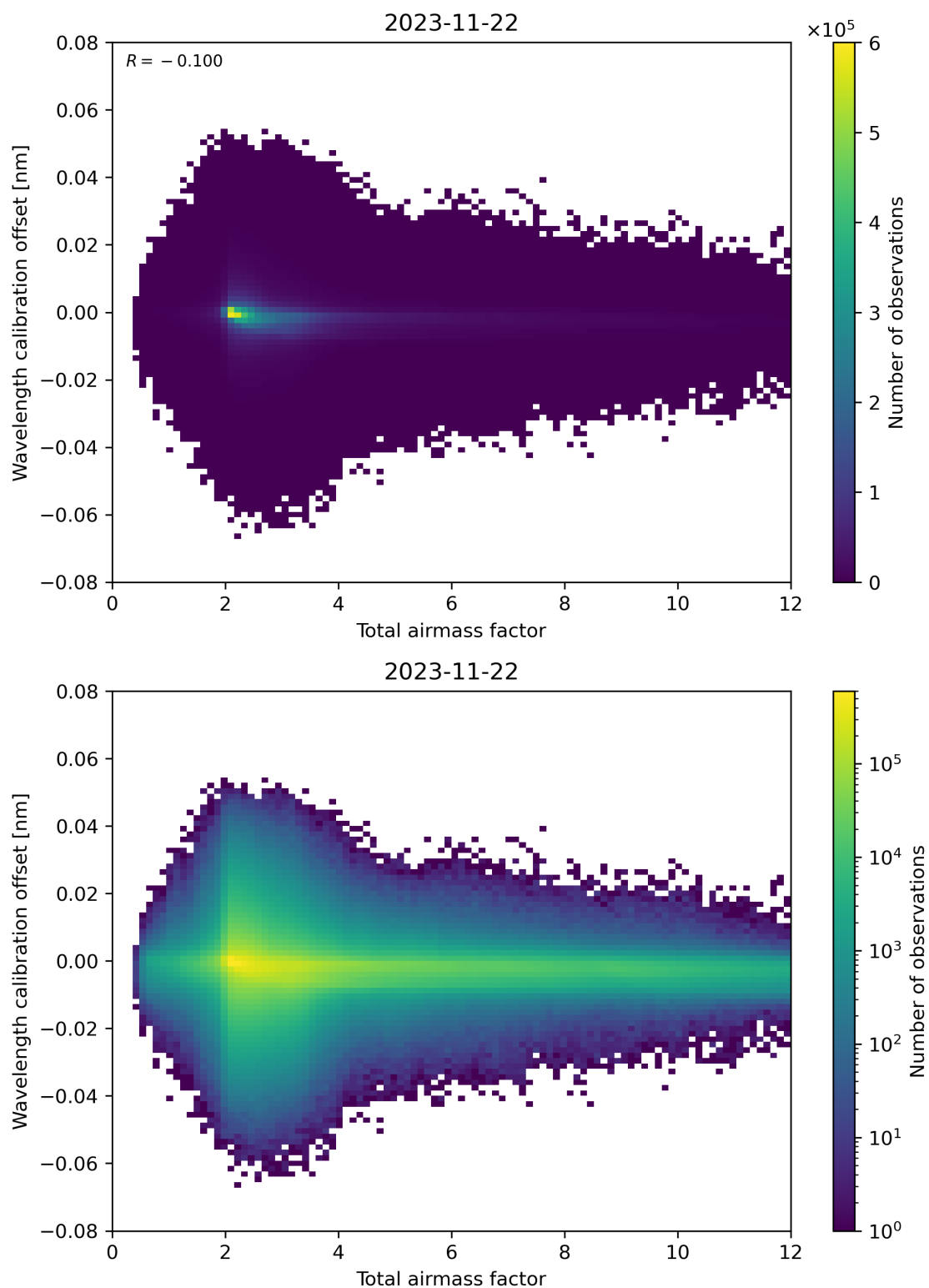
Figure 70: Scatter density plot of “Total airmass factor” against “Wavelength calibration offset” for 2023-11-21 to 2023-11-23.
