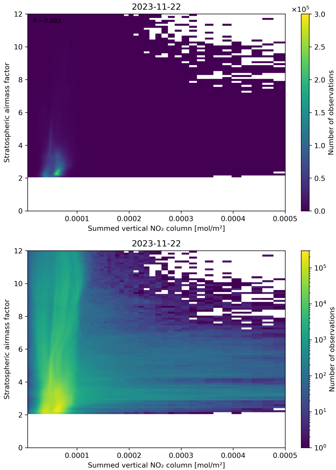
Figure 103: Scatter density plot of “Summed vertical NO 2 column” against “Stratospheric airmass factor” for 2023-11-21 to 2023-11-23.
