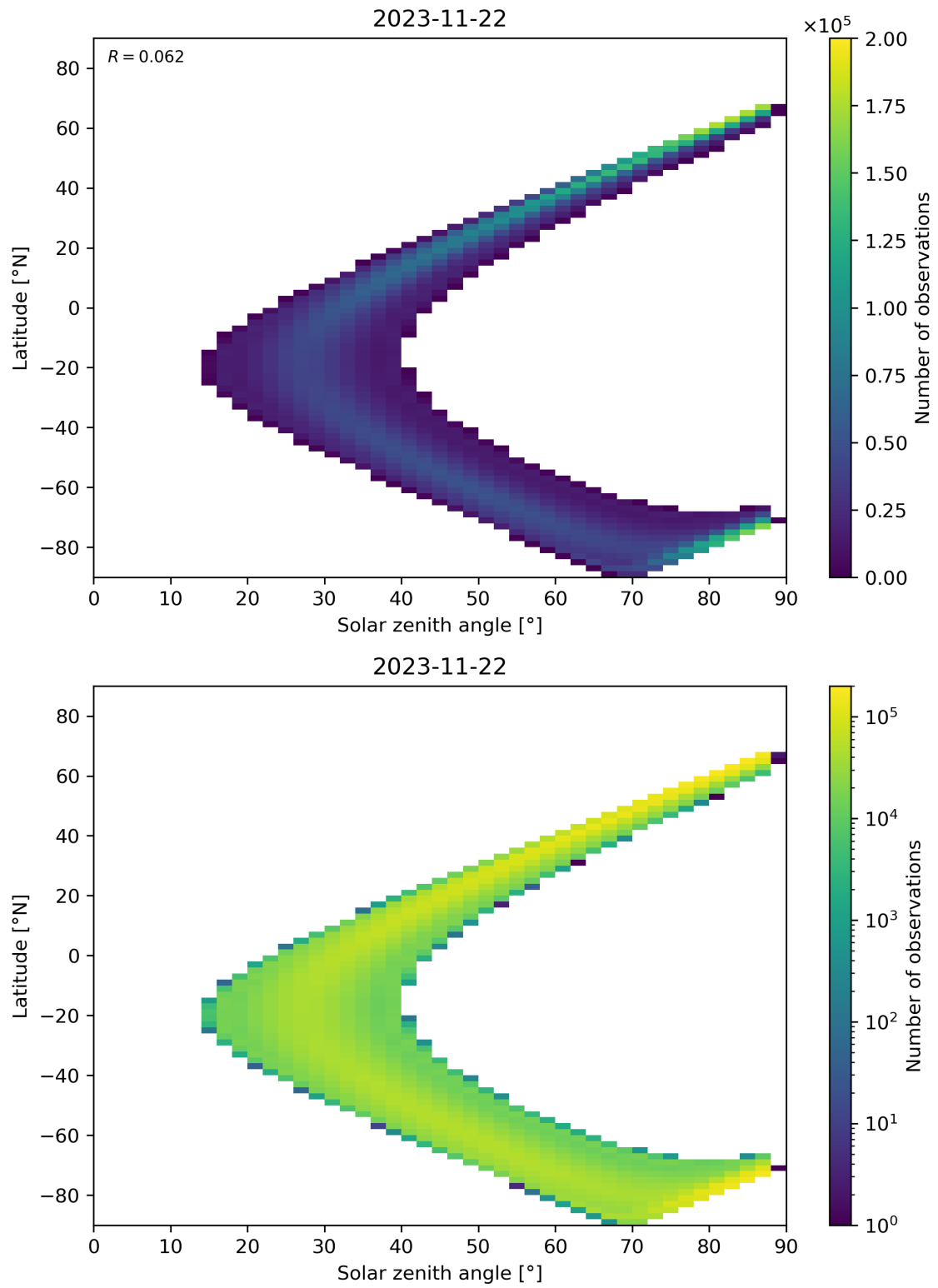
Figure 149: Scatter density plot of “Solar zenith angle” against “Latitude” for 2023-11-21 to 2023-11-23.
