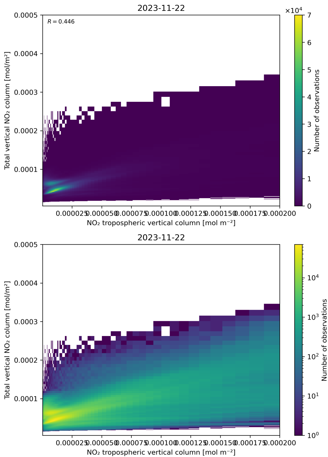
Figure 128: Scatter density plot of “NO 2 tropospheric vertical column” against “Total vertical NO 2 column” for 2023-11-21 to 2023-11-23.
