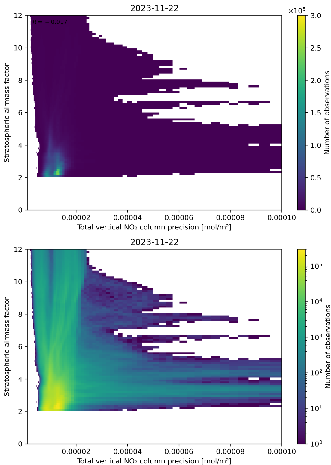
Figure 115: Scatter density plot of “Total vertical NO 2 column precision” against “Stratospheric air mass factor” for 2023-11-21 to 2023-11-23.
