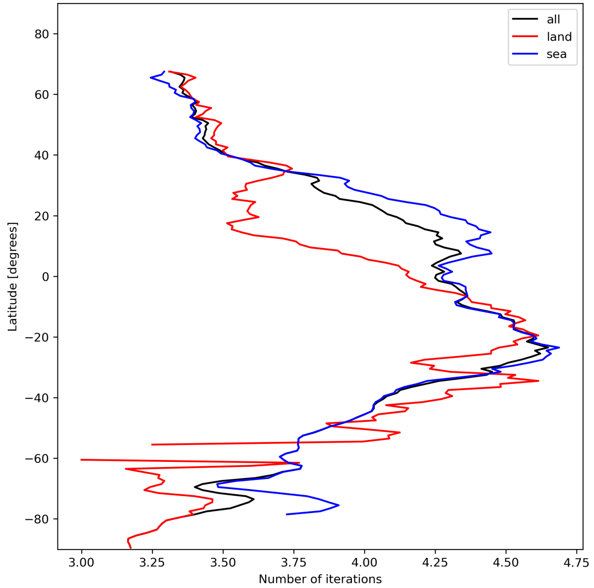
Figure 17: Zonal average of “Number of iterations” for 2023-11-21 to 2023-11-23.
