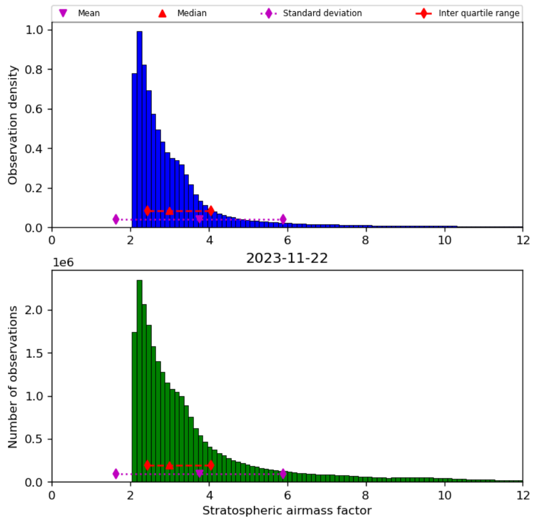
Figure 44: Histogram of “Stratospheric airmass factor” for 2023-11-21 to 2023-11-23
