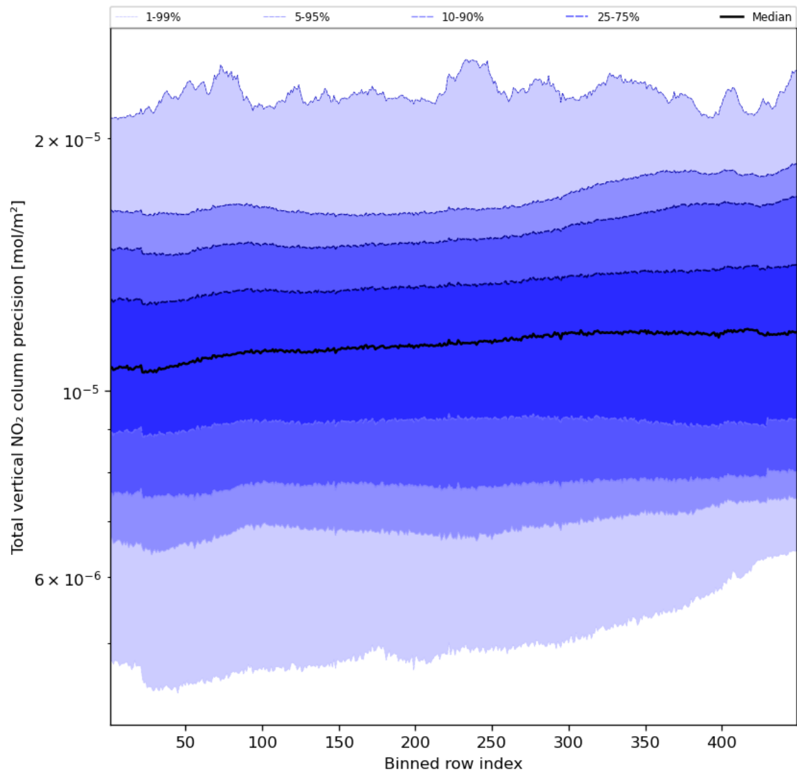
Figure 56: Along track statistics of "Total vertical NO 2 column precision" for 2023-11-21 to 2023-11-23
