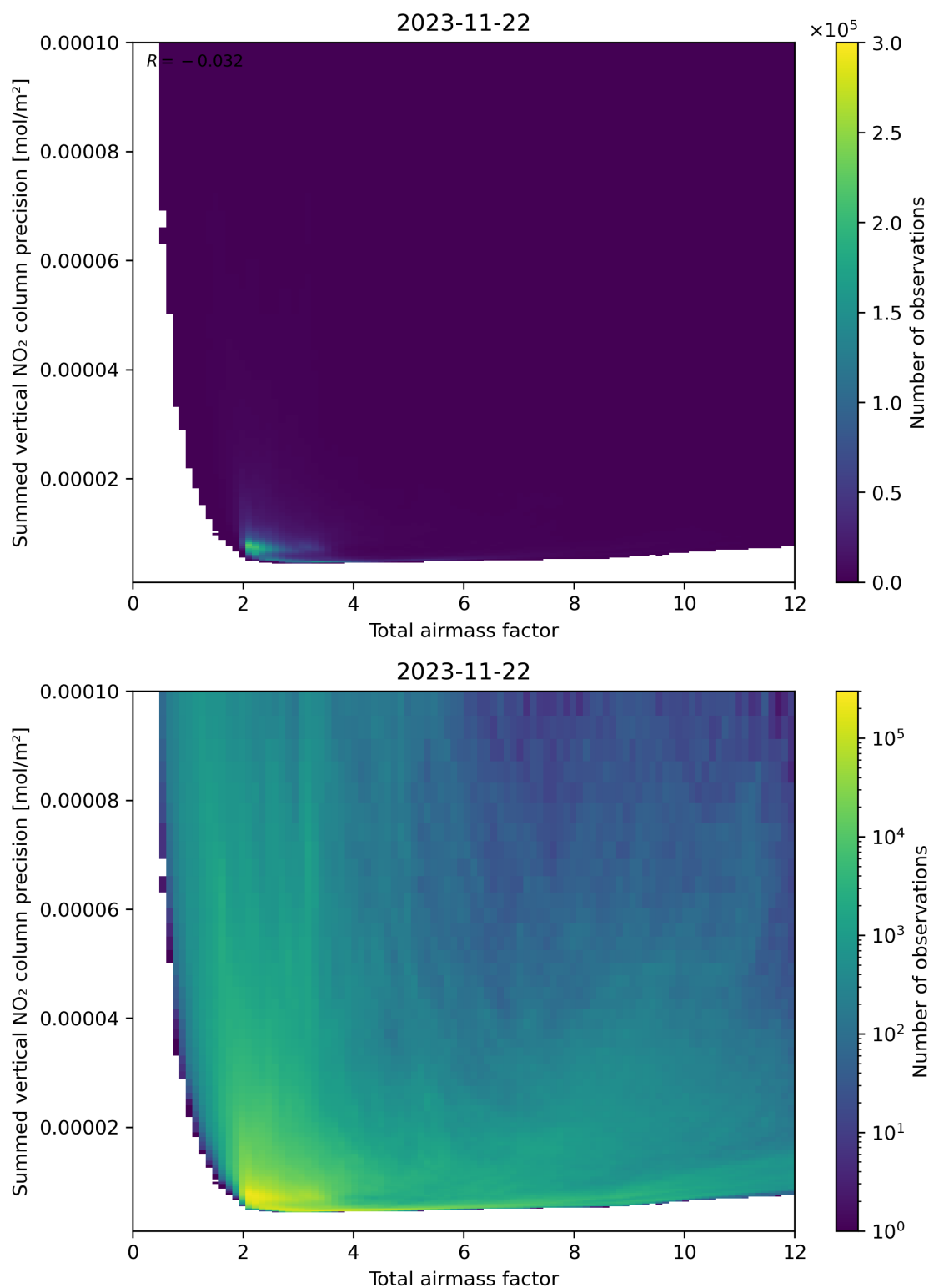
Figure 66: Scatter density plot of “Total airmass factor” against “Summed vertical NO 2 column precision” for 2023-11-21 to 2023-11-23.
