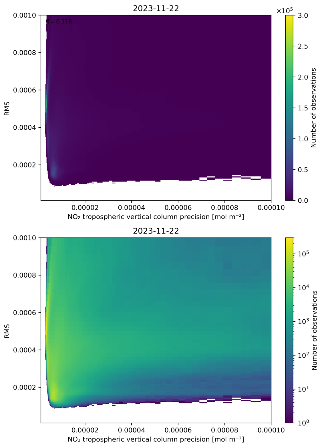
Figure 140: Scatter density plot of “NO 2 tropospheric vertical column precision” against “RMS” for 2023-11-21 to 2023-11-23.
