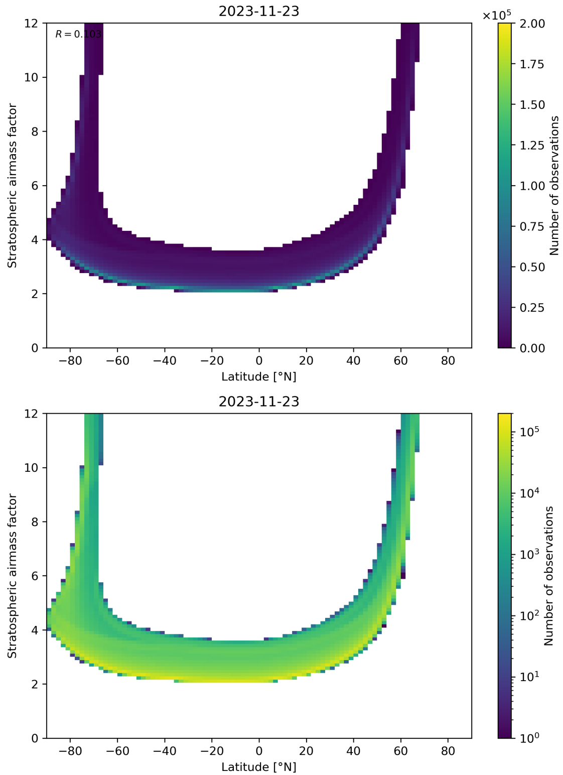
Figure 83: Scatter density plot of “Latitude” against “Stratospheric air mass factor” for 2023-11-23 to 2023-11-24.
