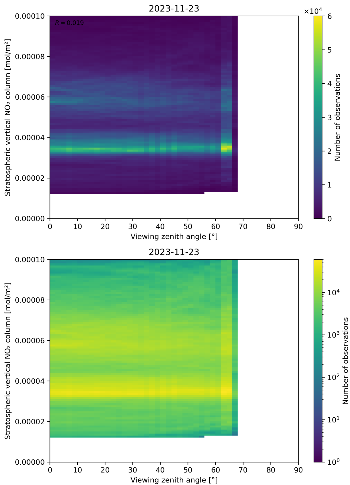
Figure 164: Scatter density plot of “Viewing zenith angle” against “Stratospheric vertical NO 2 column” for 2023-11-23 to 2023-11-24.
