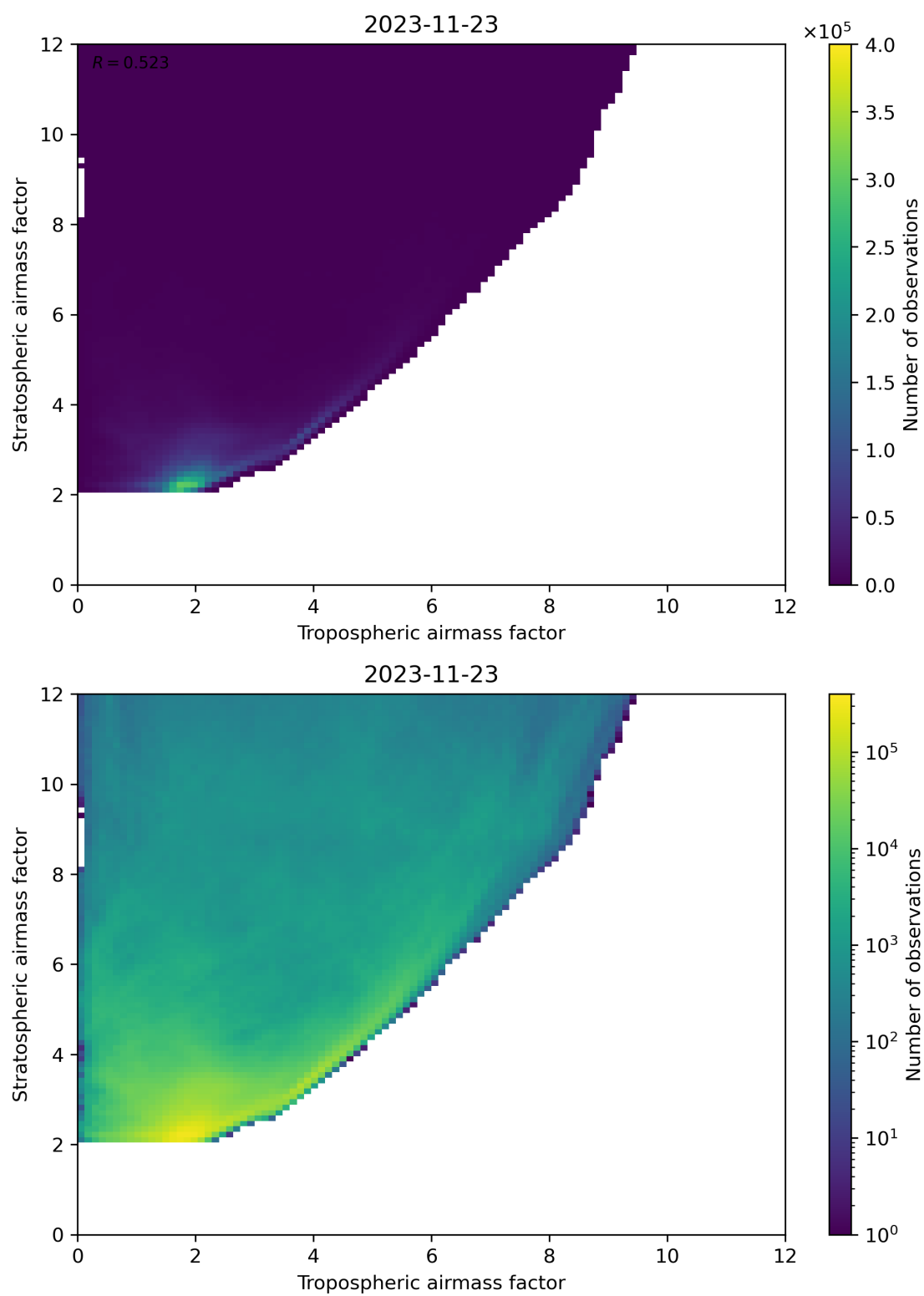
Figure 71: Scatter density plot of “Tropospheric airmass factor” against “Stratospheric airmass factor” for 2023-11-23 to 2023-11-24.
