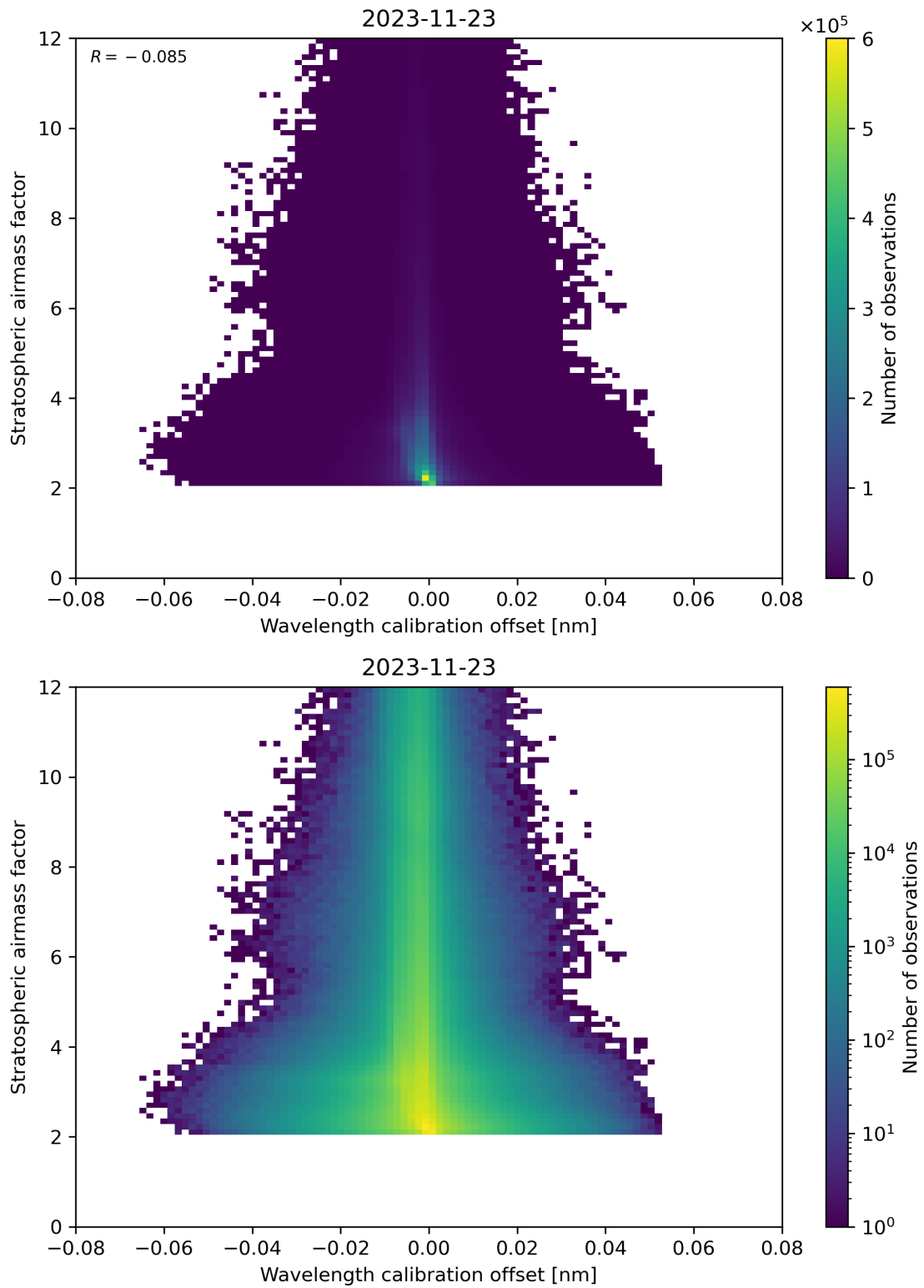
Figure 174: Scatter density plot of “Wavelength calibration offset” against “Stratospheric airmass factor” for 2023-11-23 to 2023-11-24.
