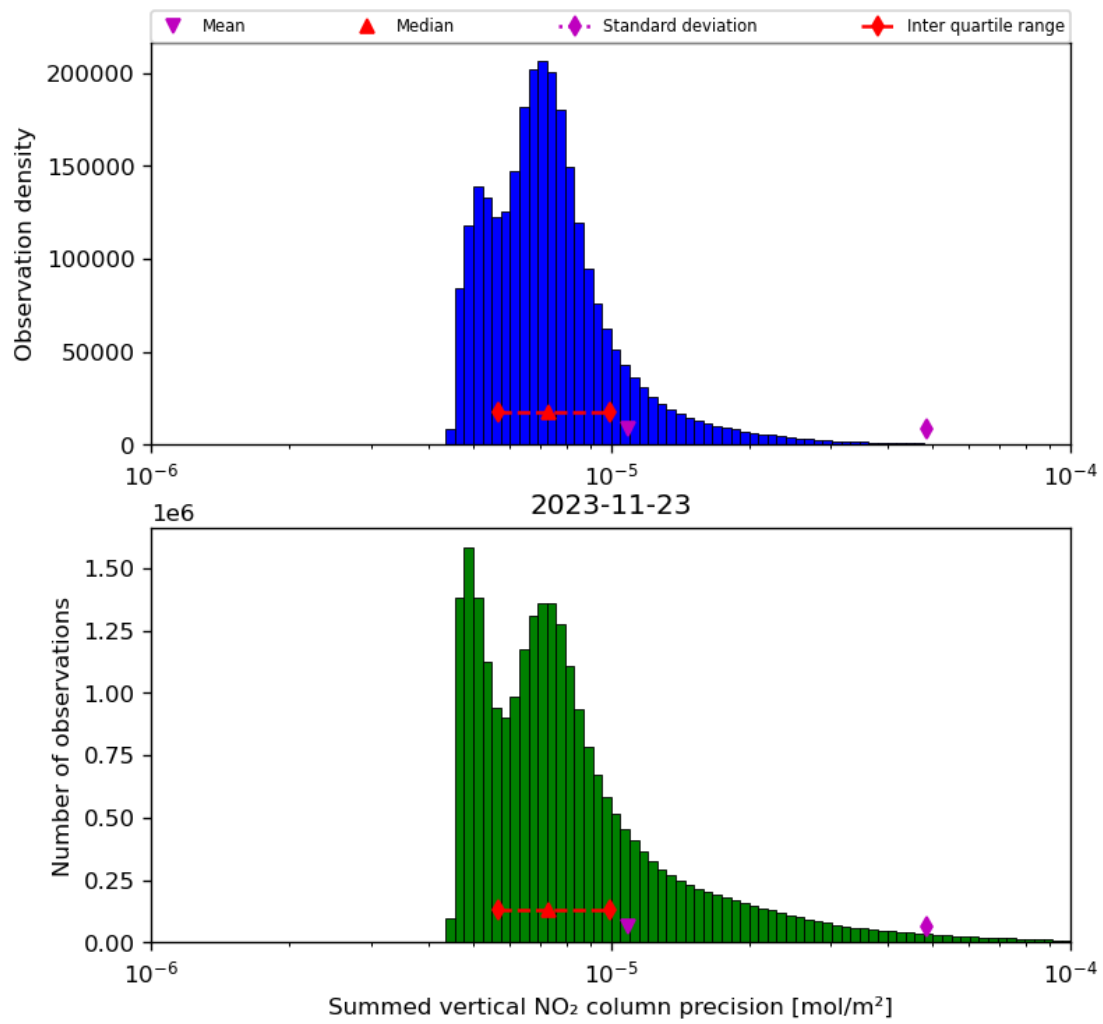
Figure 41: Histogram of “Summed vertical NO 2 column precision” for 2023-11-23 to 2023-11-24
