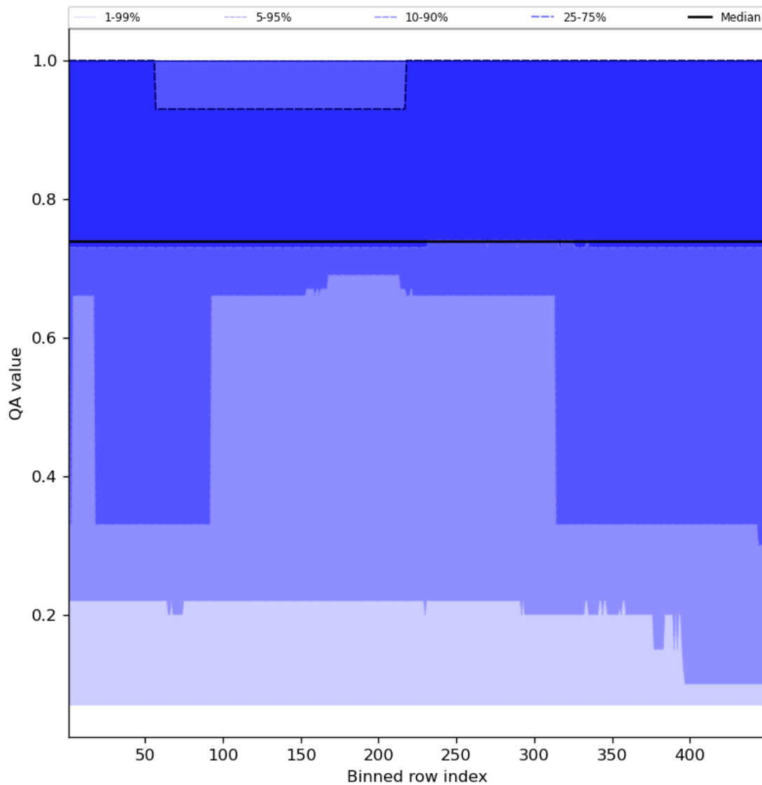
Figure 45: Along track statistics of “QA value” for 2023-11-23 to 2023-11-24
