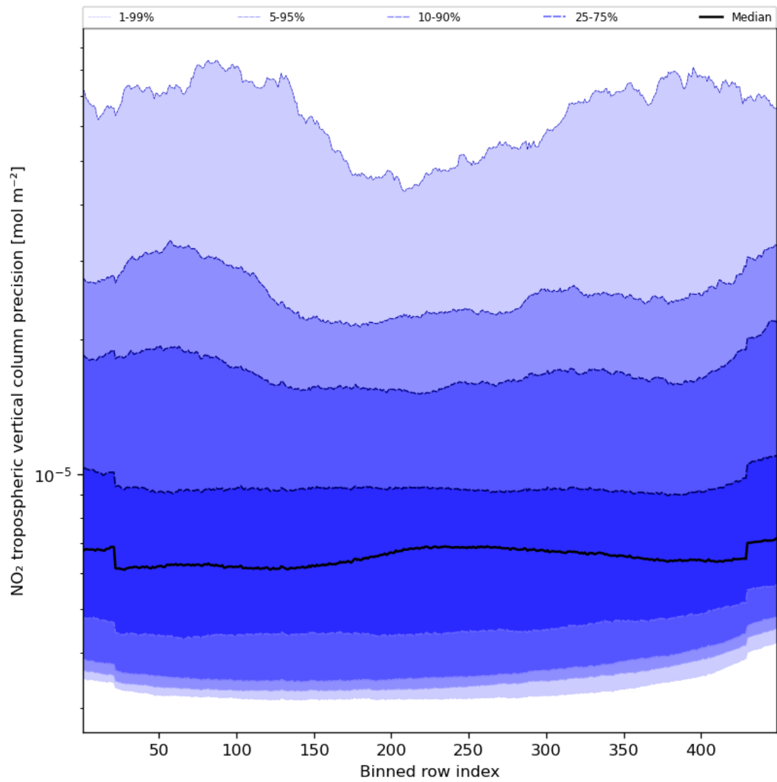
Figure 47: Along track statistics of “NO 2 tropospheric vertical column precision” for 2023-11-23 to 2023-11-24
