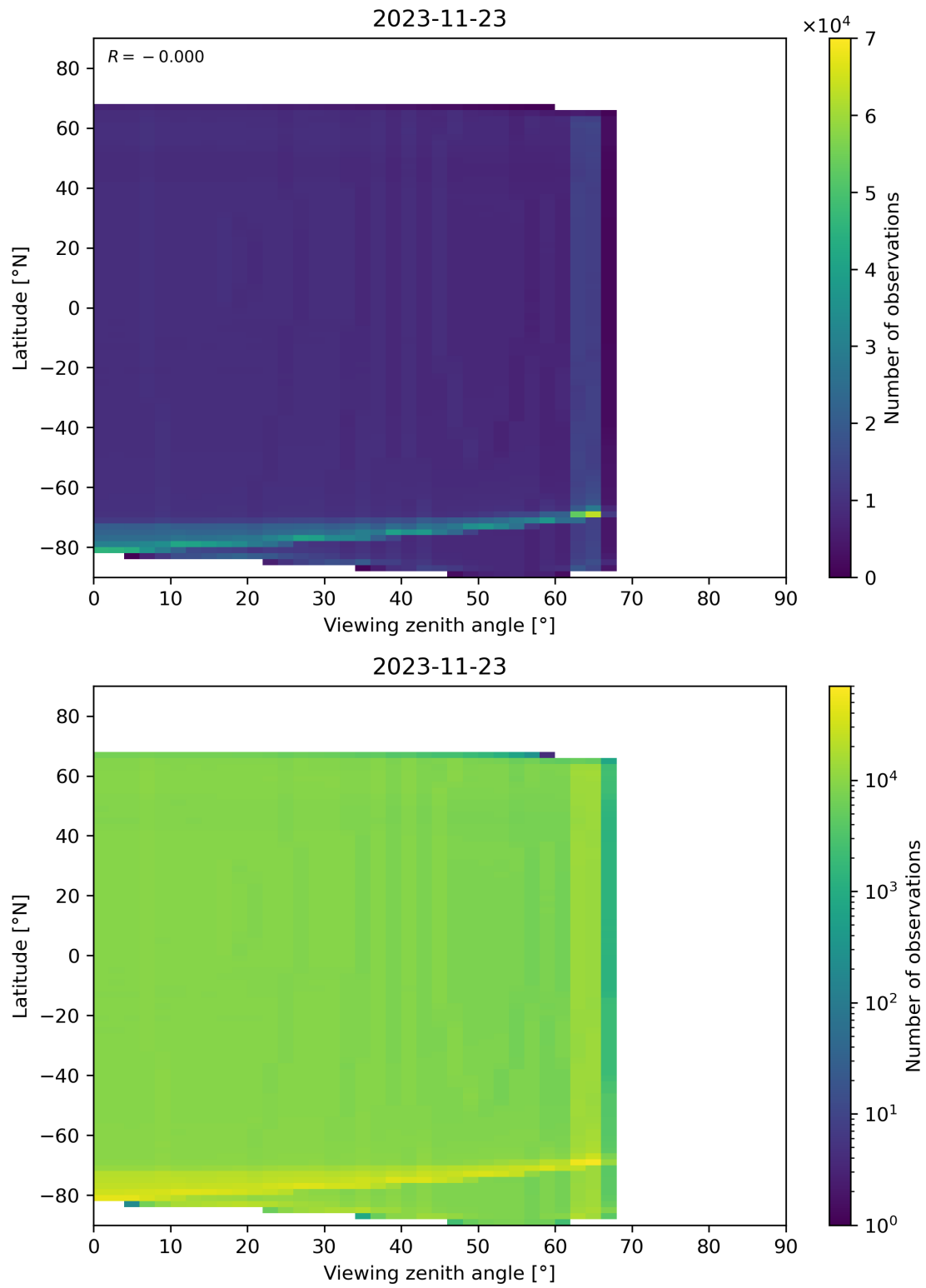
Figure 163: Scatter density plot of “Viewing zenith angle” against “Latitude” for 2023-11-23 to 2023-11-24.
