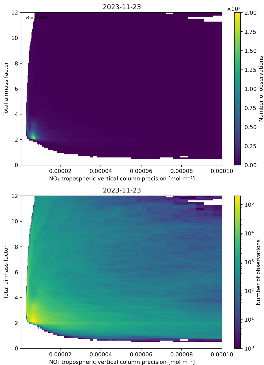
Figure 132: Scatter density plot of “NO 2 tropospheric vertical column precision” against “Total air mass factor” for 2023-11-23 to 2023-11-24.
