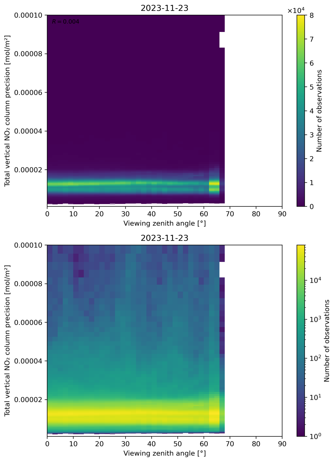
Figure 168: Scatter density plot of “Viewing zenith angle” against “Total vertical NO 2 column precision” for 2023-11-23 to 2023-11-24.
