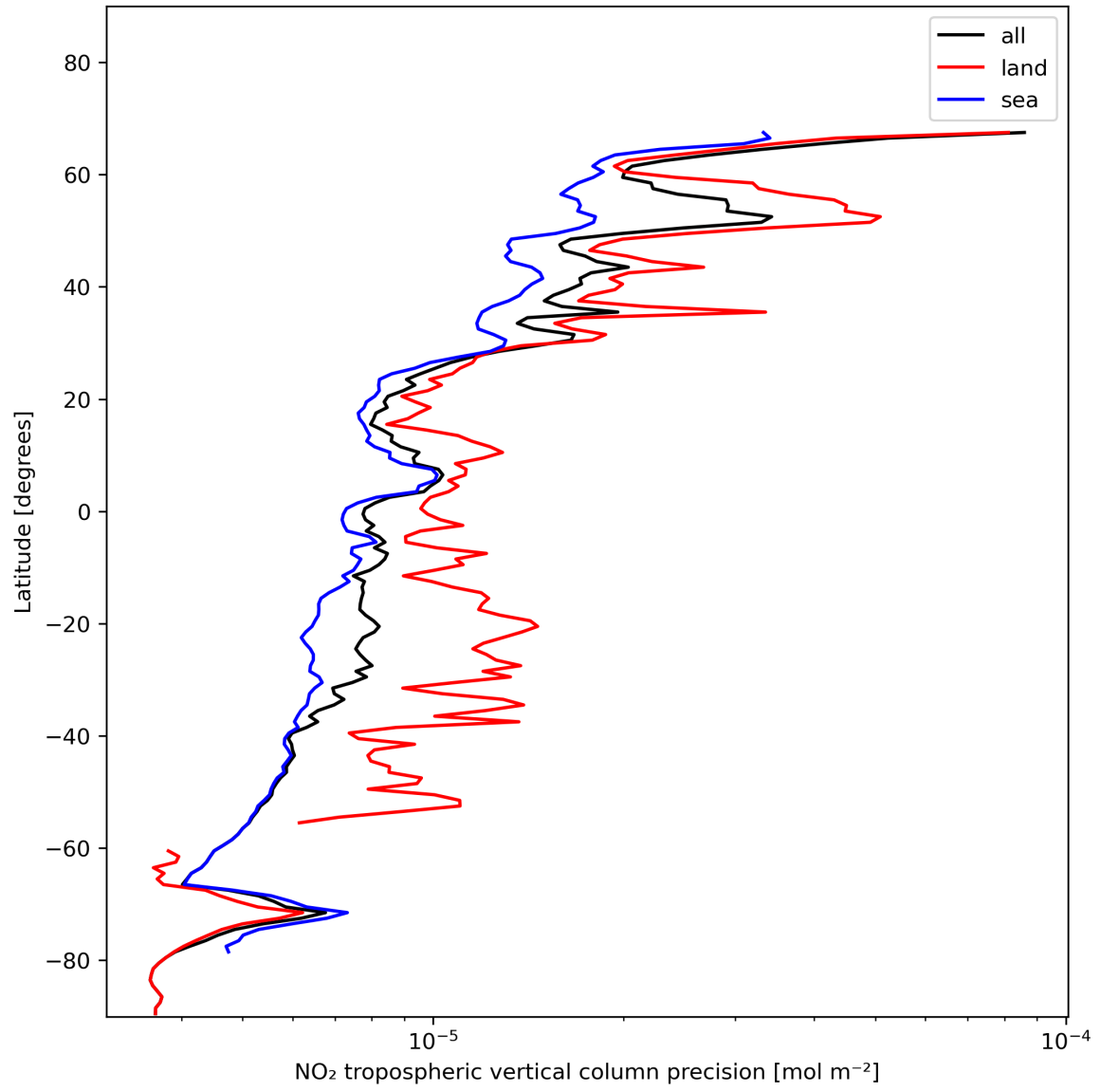
Figure 13: Zonal average of “NO 2 tropospheric vertical column precision” for 2023-11-23 to 2023-11-24.
