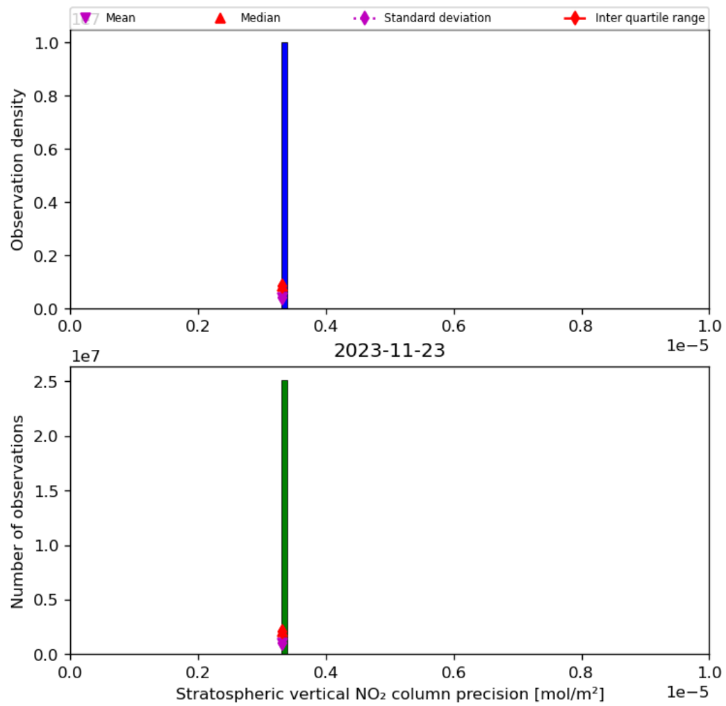
Figure 37: Histogram of “Stratospheric vertical NO 2 column precision” for 2023-11-23 to 2023-11-24
