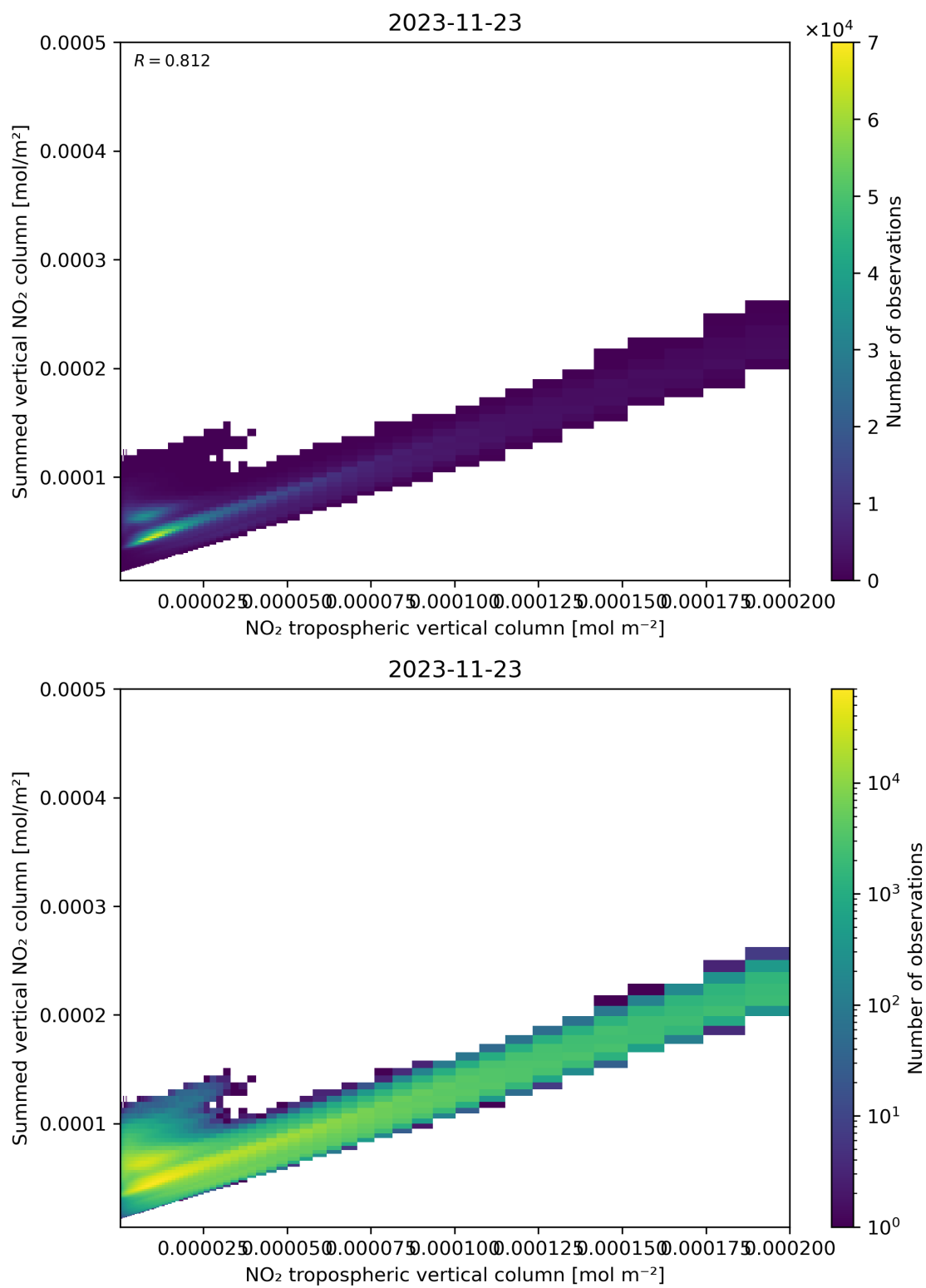
Figure 126: Scatter density plot of “NO 2 tropospheric vertical column” against “Summed vertical NO 2 column” for 2023-11-23 to 2023-11-24.
