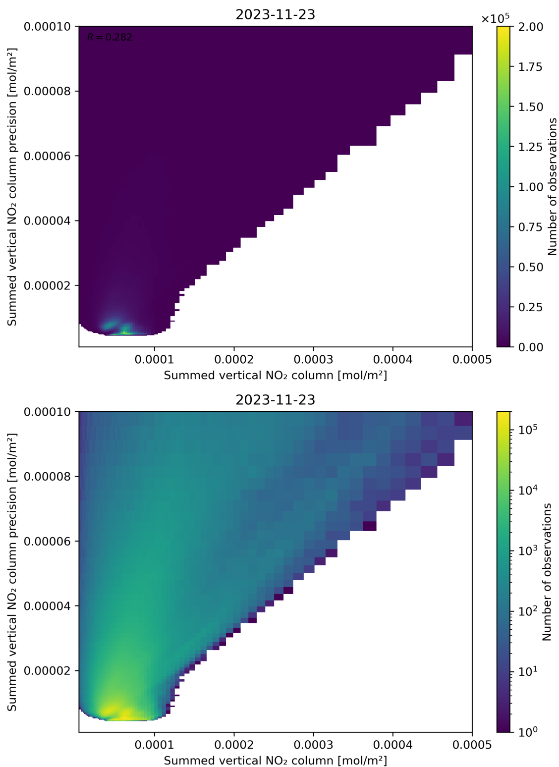
Figure 105: Scatter density plot of “Summed vertical NO 2 column” against “Summed vertical NO 2 column precision” for 2023-11-23 to 2023-11-24.
