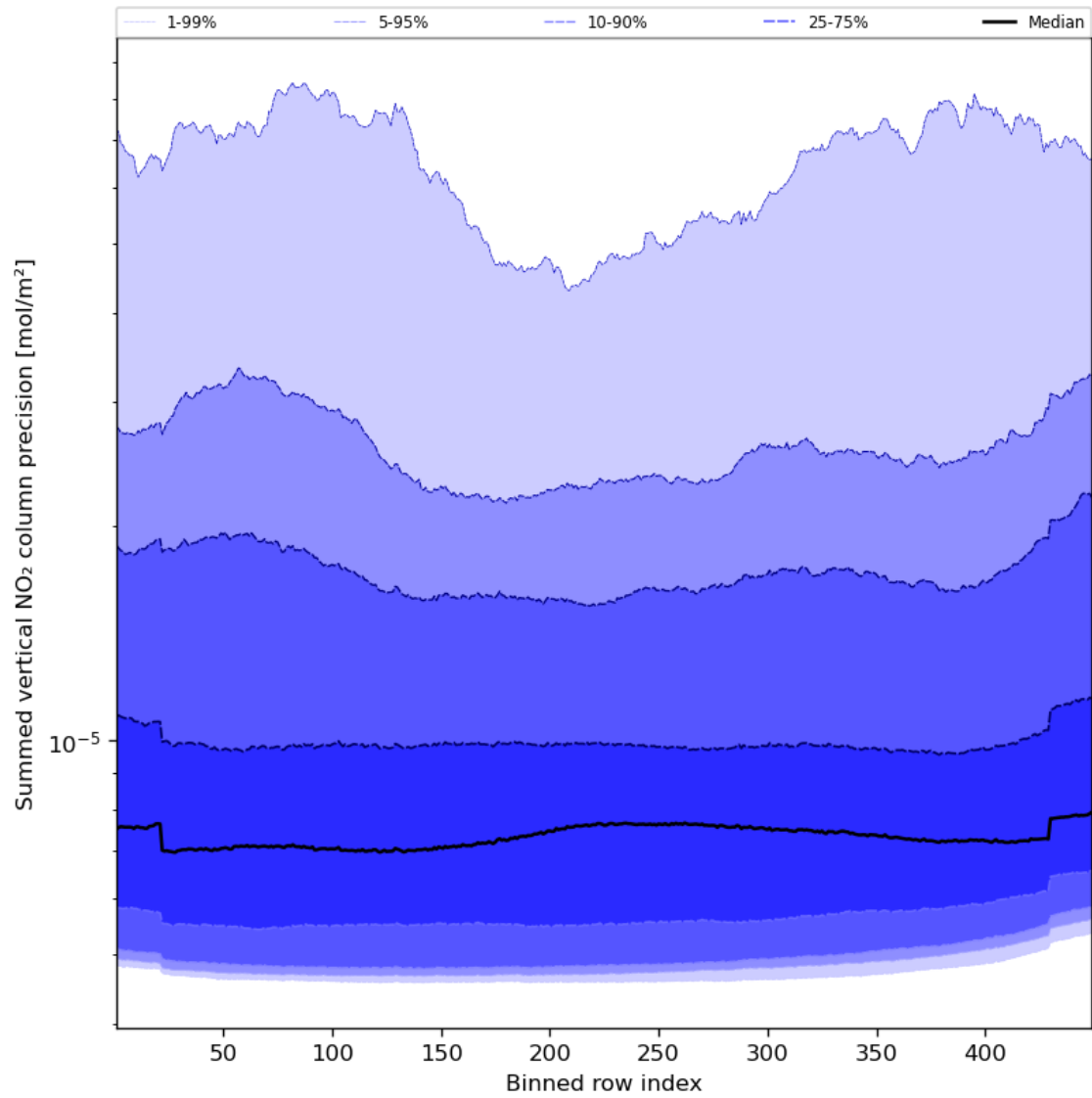
Figure 58: Along track statistics of “Summed vertical NO 2 column precision” for 2023-11-23 to 2023-11-24
