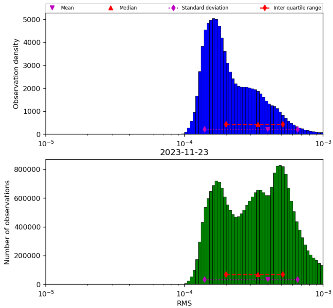
Figure 43: Histogram of “RMS” for 2023-11-23 to 2023-11-24
