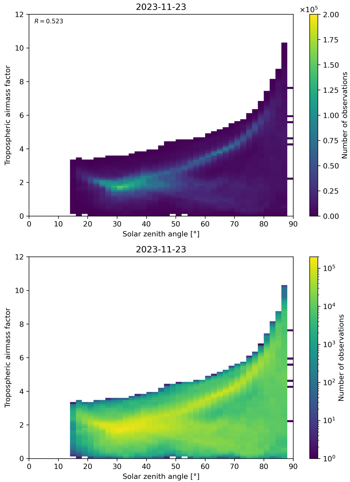
Figure 147: Scatter density plot of “Solar zenith angle” against “Tropospheric airmass factor” for 2023-11-23 to 2023-11-24.
