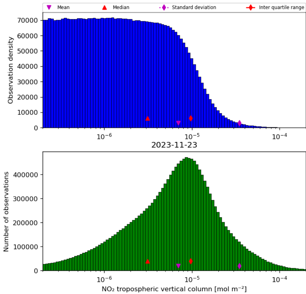
Figure 29: Histogram of “NO 2 tropospheric vertical column” for 2023-11-23 to 2023-11-24
