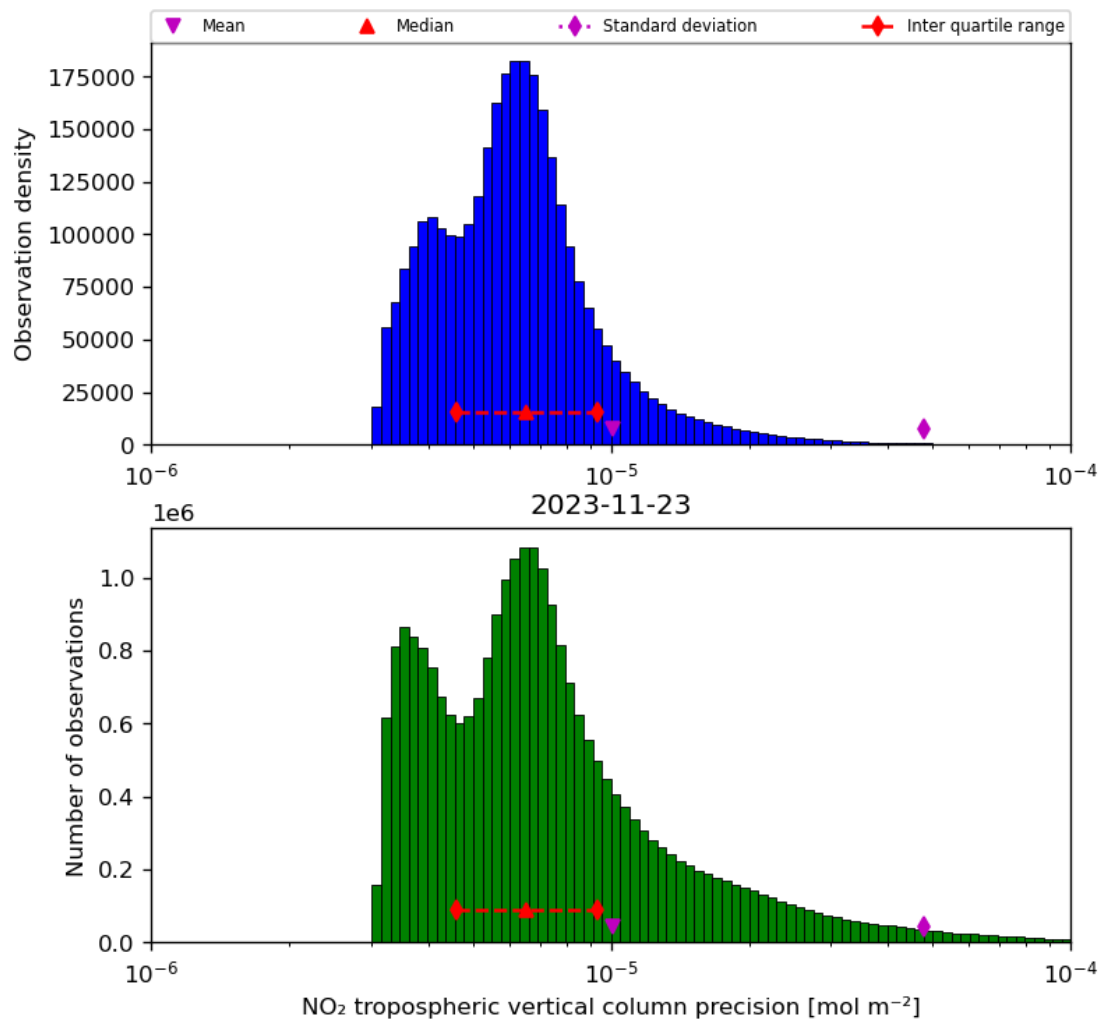
Figure 30: Histogram of “NO 2 tropospheric vertical column precision” for 2023-11-23 to 2023-11-24
