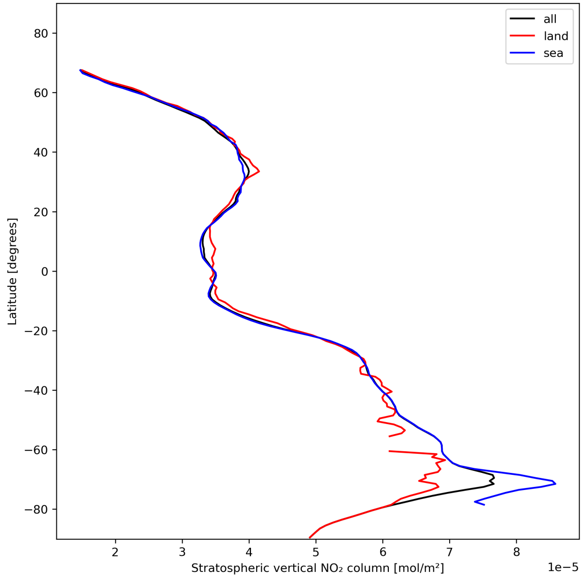
Figure 19: Zonal average of “Stratospheric vertical NO 2 column” for 2023-11-23 to 2023-11-24.
