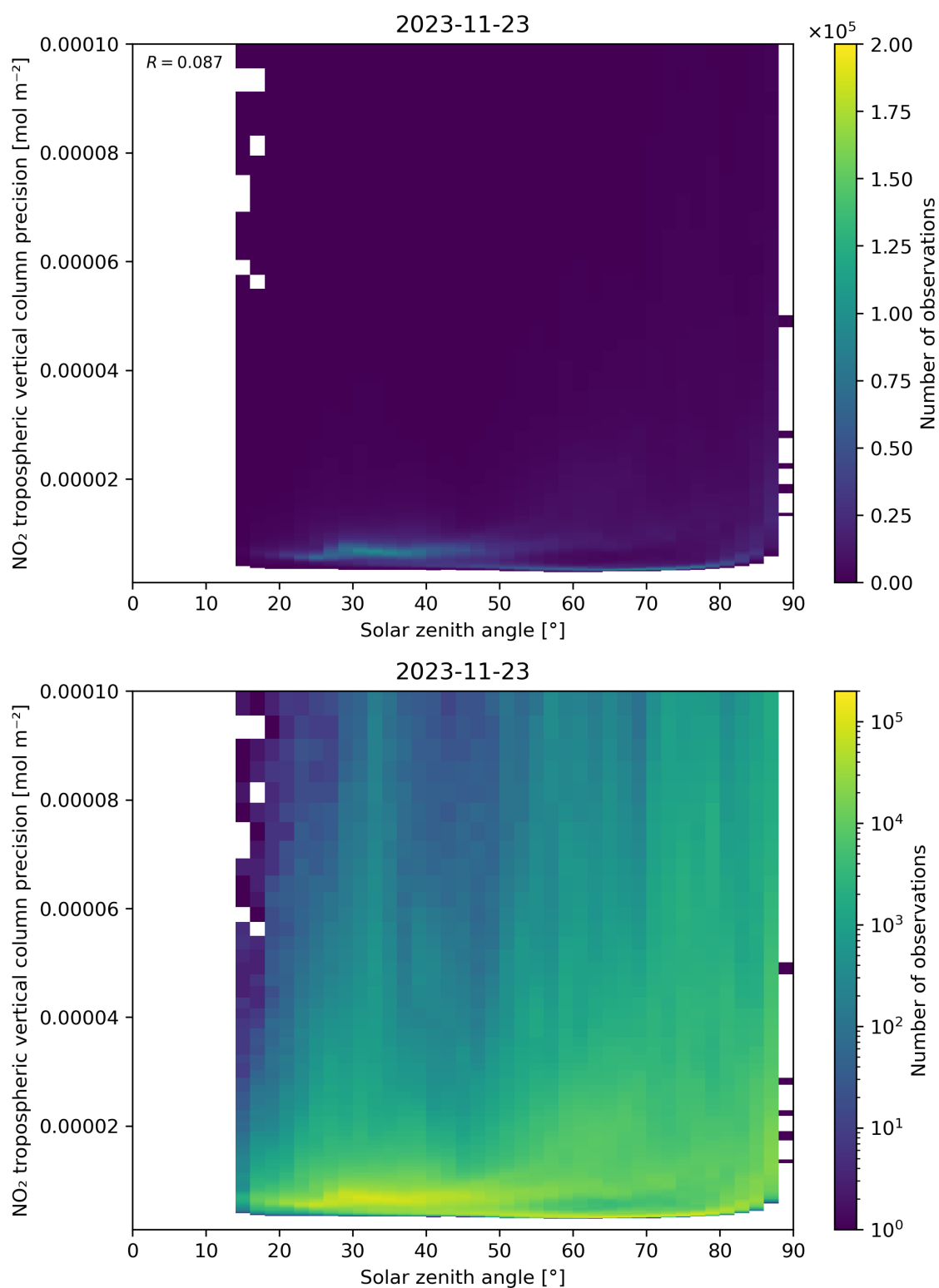
Figure 156: Scatter density plot of “Solar zenith angle” against “NO 2 tropospheric vertical column precision” for 2023-11-23 to 2023-11-24.
