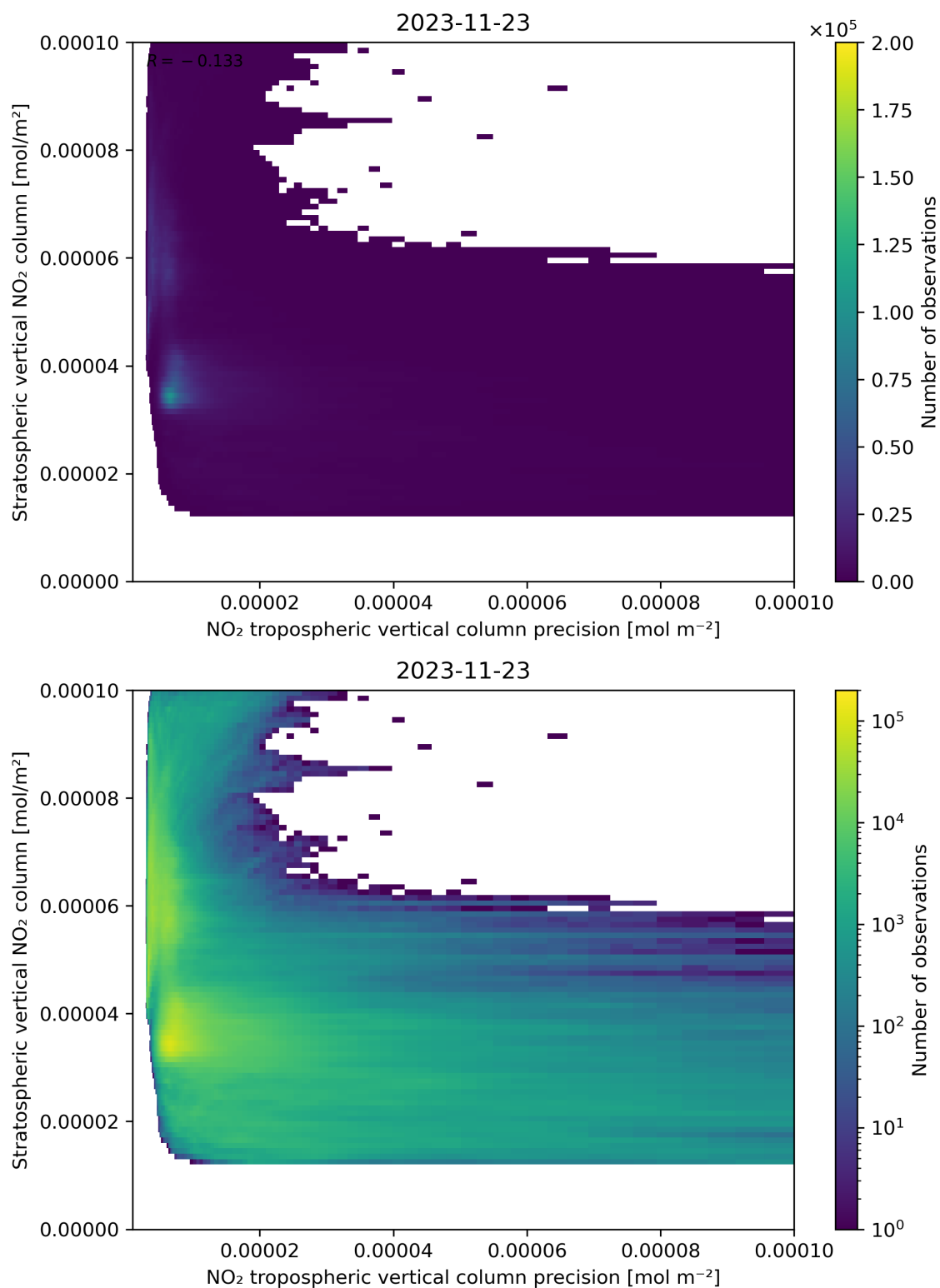
Figure 135: Scatter density plot of “NO 2 tropospheric vertical column precision” against “Stratospheric vertical NO 2 column” for 2023-11-23 to 2023-11-24.
