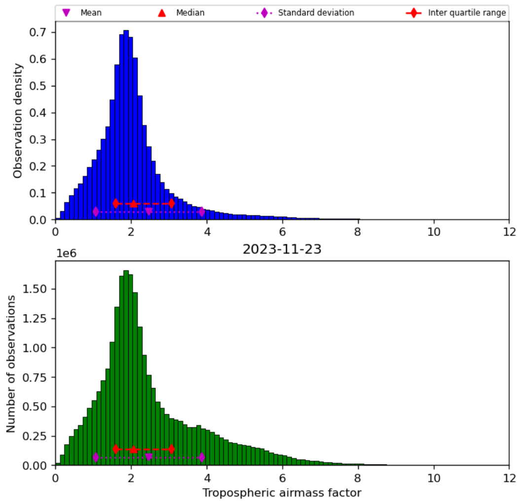
Figure 31: Histogram of “Tropospheric airmass factor” for 2023-11-23 to 2023-11-24
