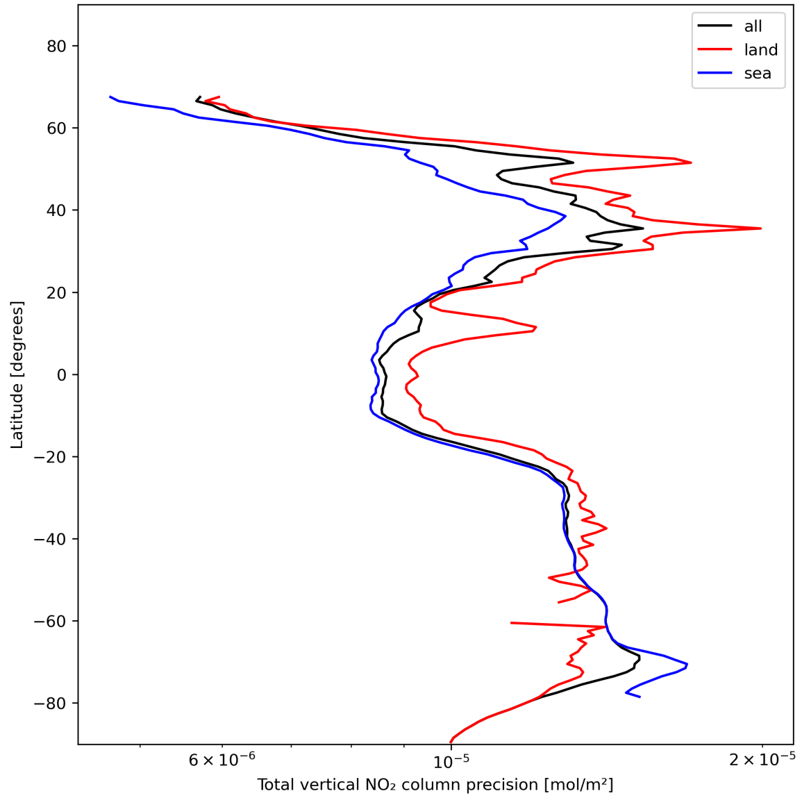
Figure 22: Zonal average of “Total vertical NO 2 column precision” for 2023-11-23 to 2023-11-24.
