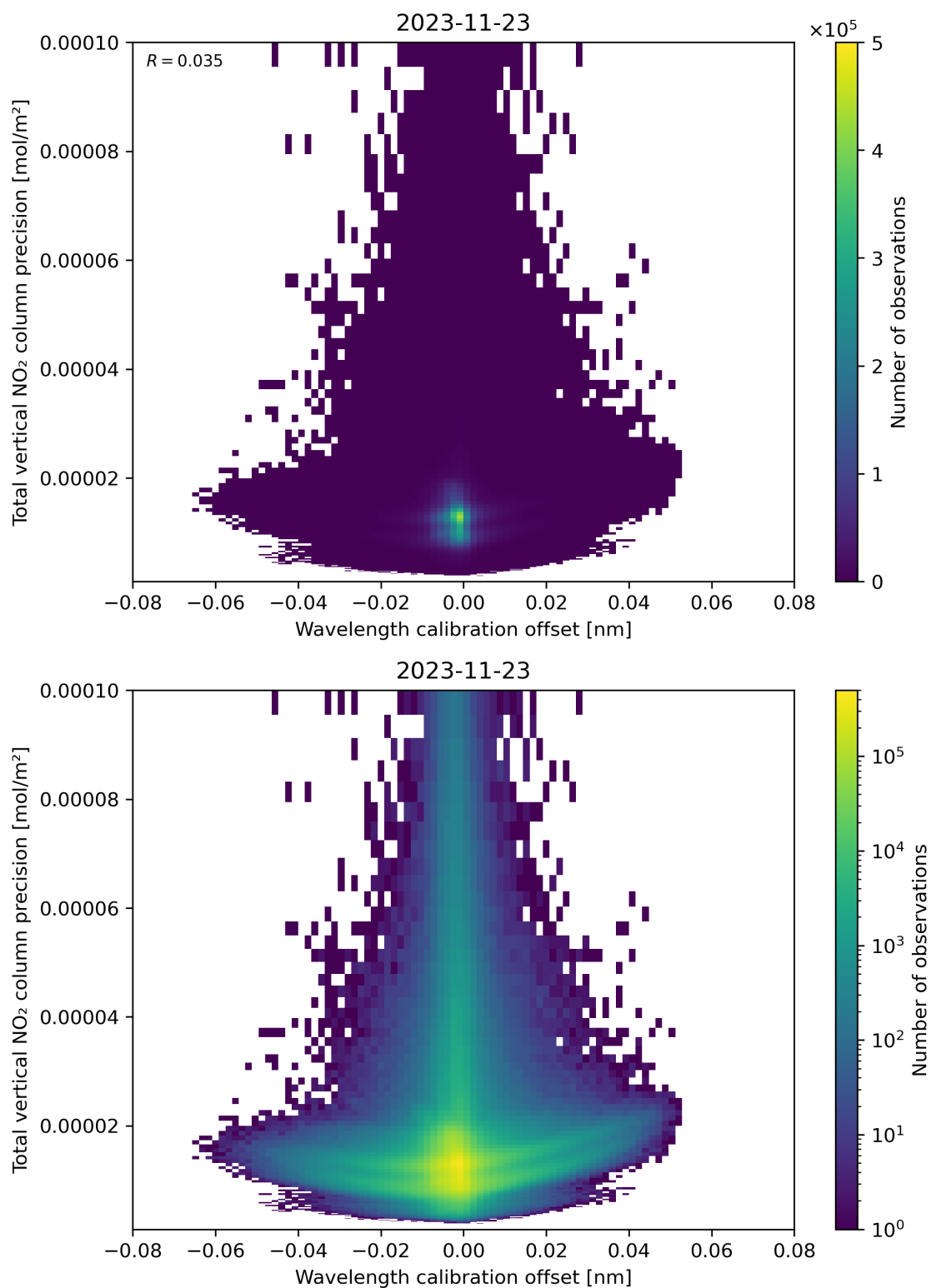
Figure 180: Scatter density plot of “Wavelength calibration offset” against “Total vertical NO 2 column precision” for 2023-11-23 to 2023-11-24.
