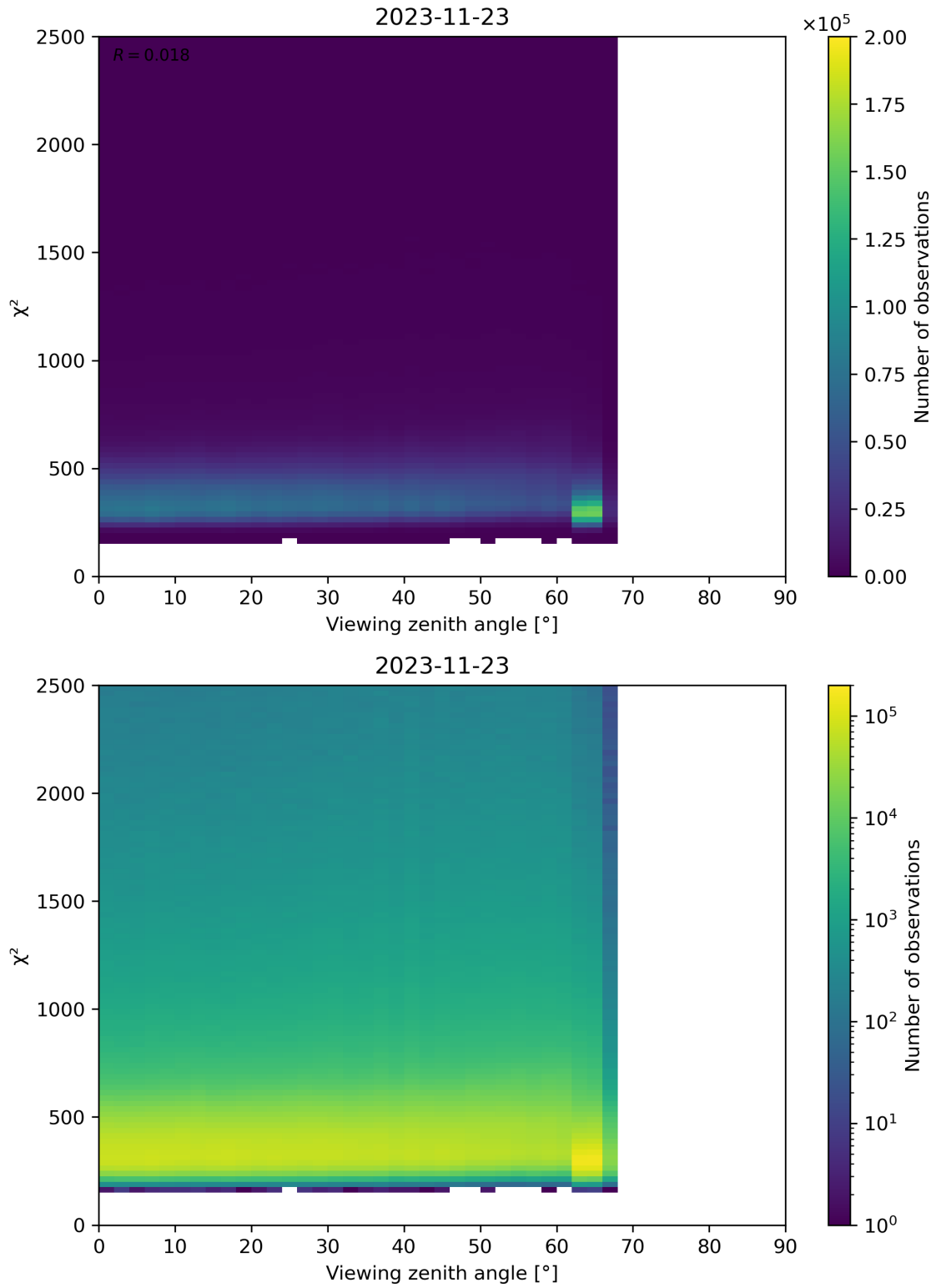
Figure 162: Scatter density plot of “Viewing zenith angle” against “ \chi^2 ” for 2023-11-23 to 2023-11-24.
