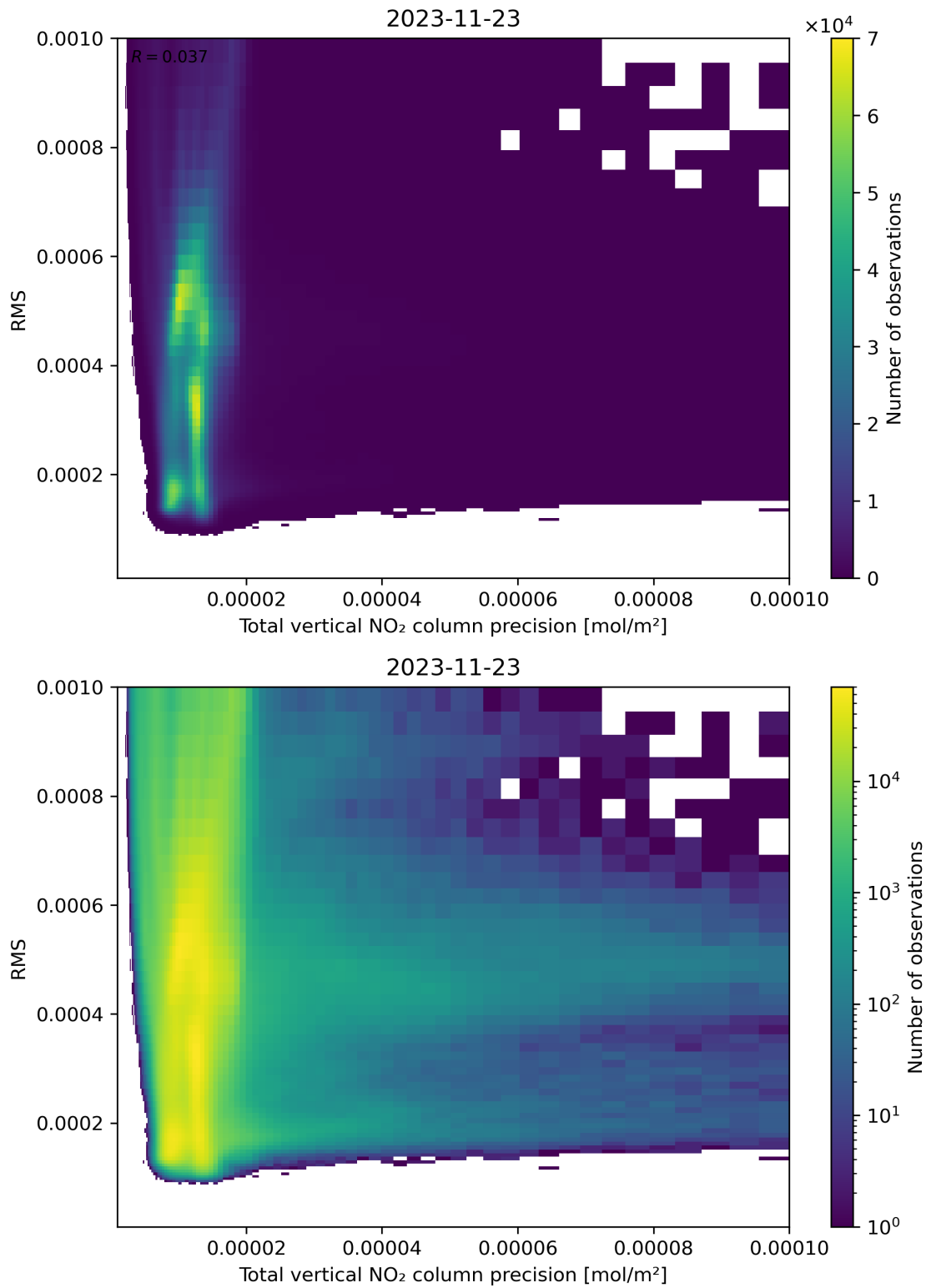
Figure 119: Scatter density plot of “Total vertical NO 2 column precision” against “RMS” for 2023-11-23 to 2023-11-24.
