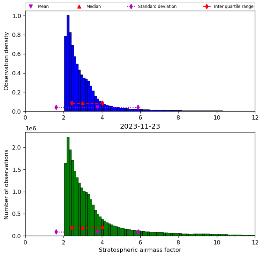
Figure 44: Histogram of “Stratospheric airmass factor” for 2023-11-23 to 2023-11-24
