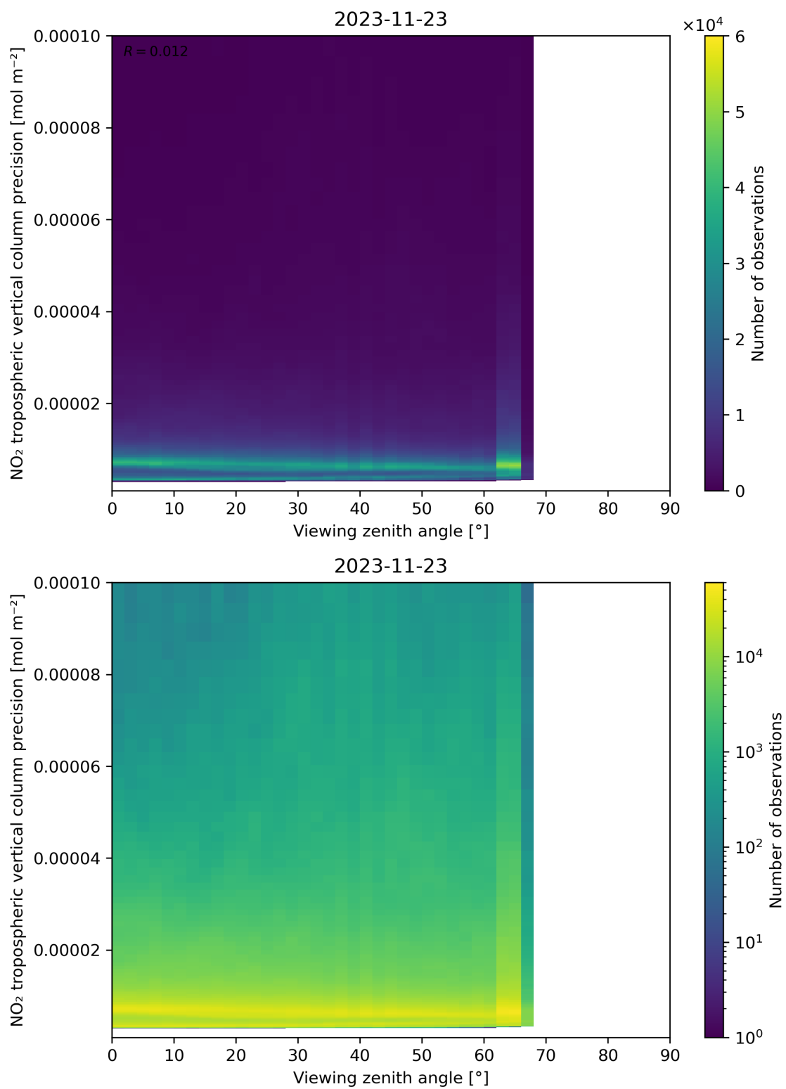
Figure 170: Scatter density plot of “Viewing zenith angle” against “NO 2 tropospheric vertical column precision” for 2023-11-23 to 2023-11-24.
