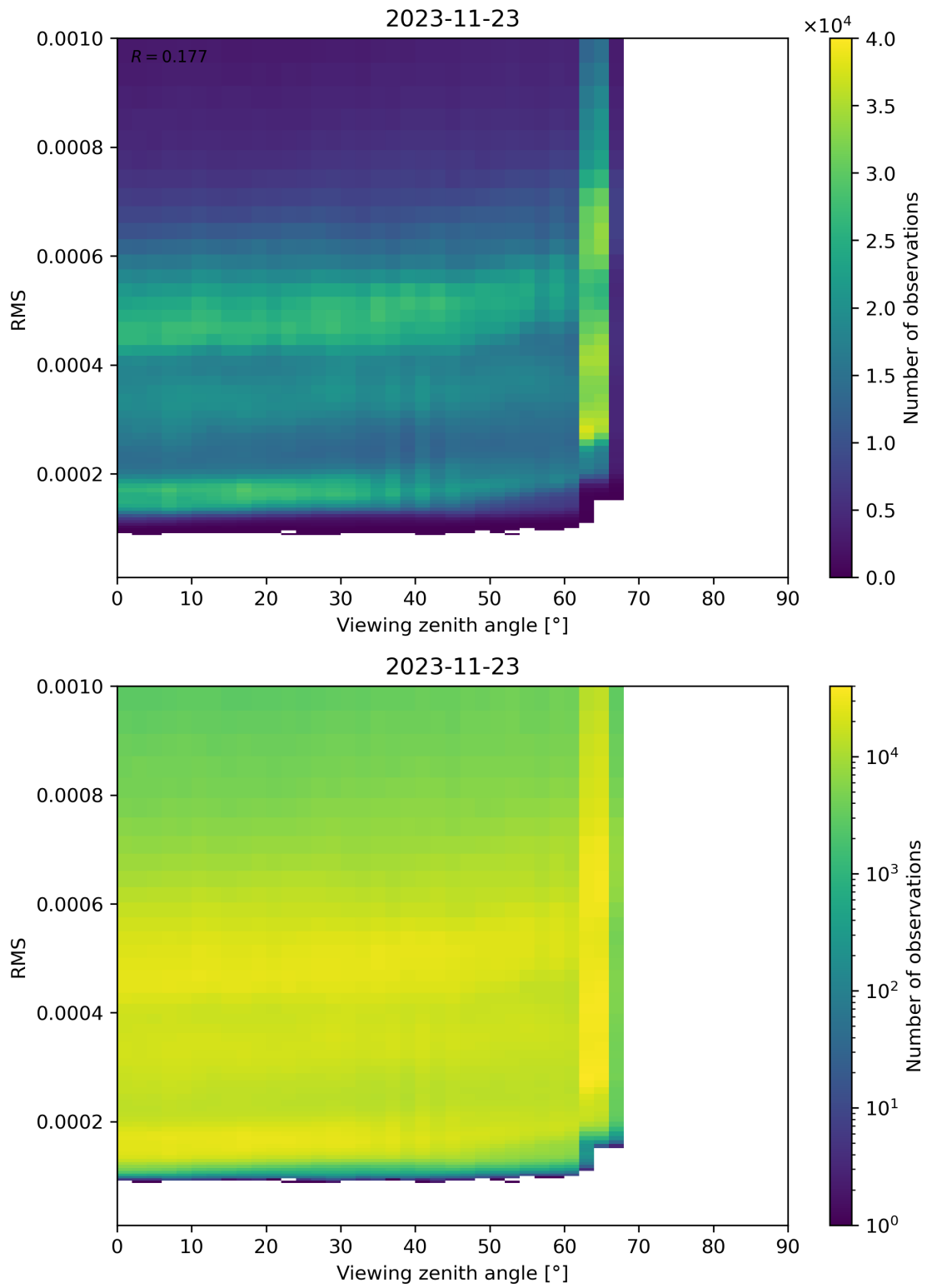
Figure 171: Scatter density plot of “Viewing zenith angle” against “RMS” for 2023-11-23 to 2023-11-24.
