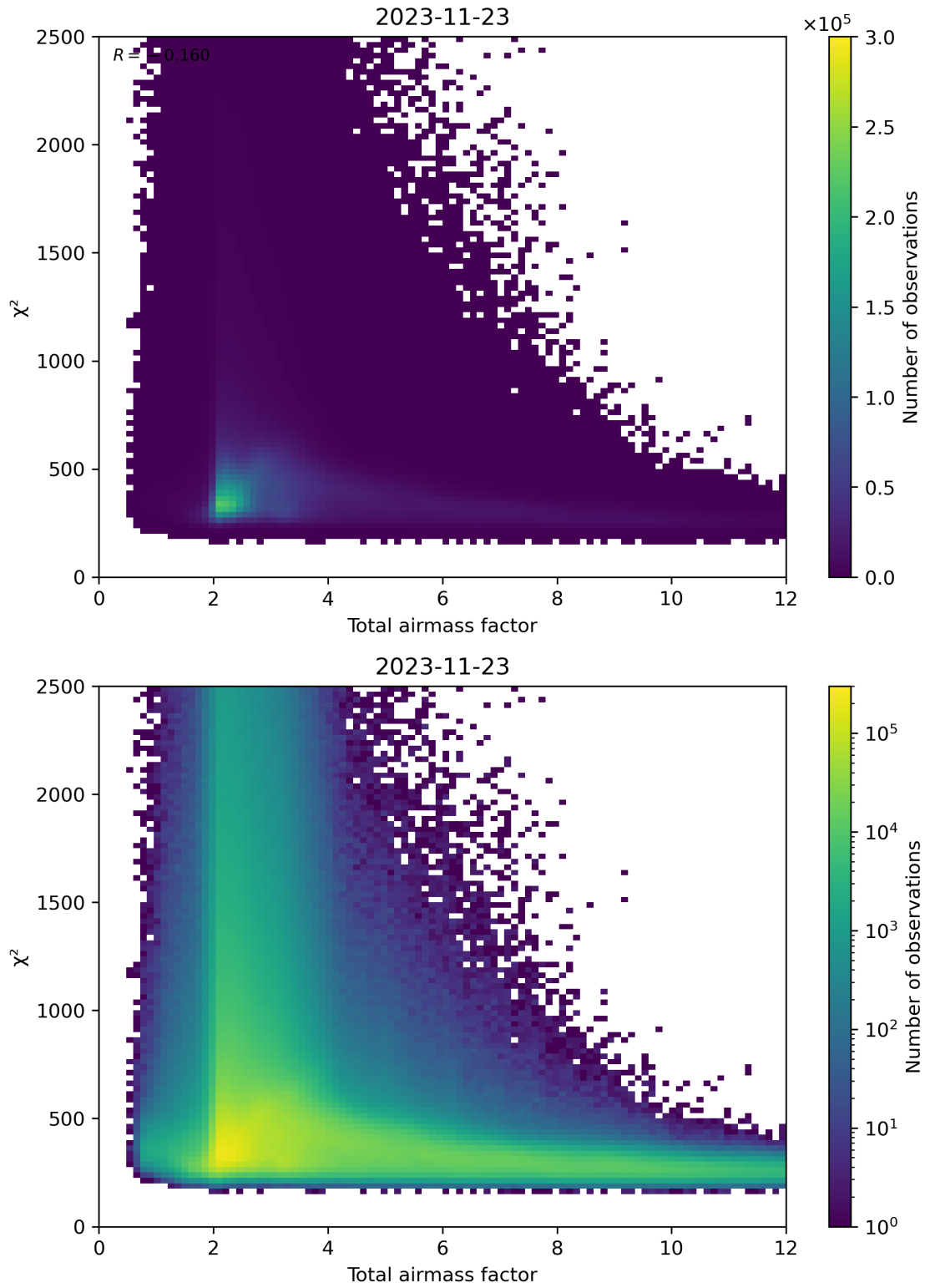
Figure 63: Scatter density plot of “Total airmass factor” against “ \chi^2 ” for 2023-11-23 to 2023-11-24.
