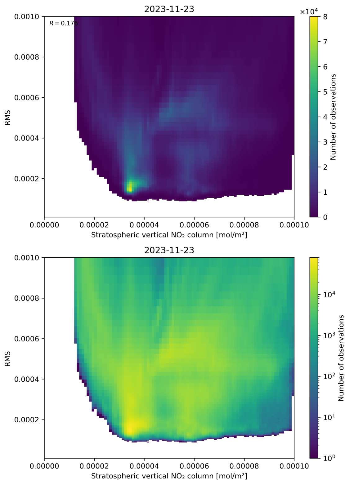
Figure 102: Scatter density plot of “Stratospheric vertical NO 2 column” against “RMS” for 2023-11-23 to 2023-11-24.
