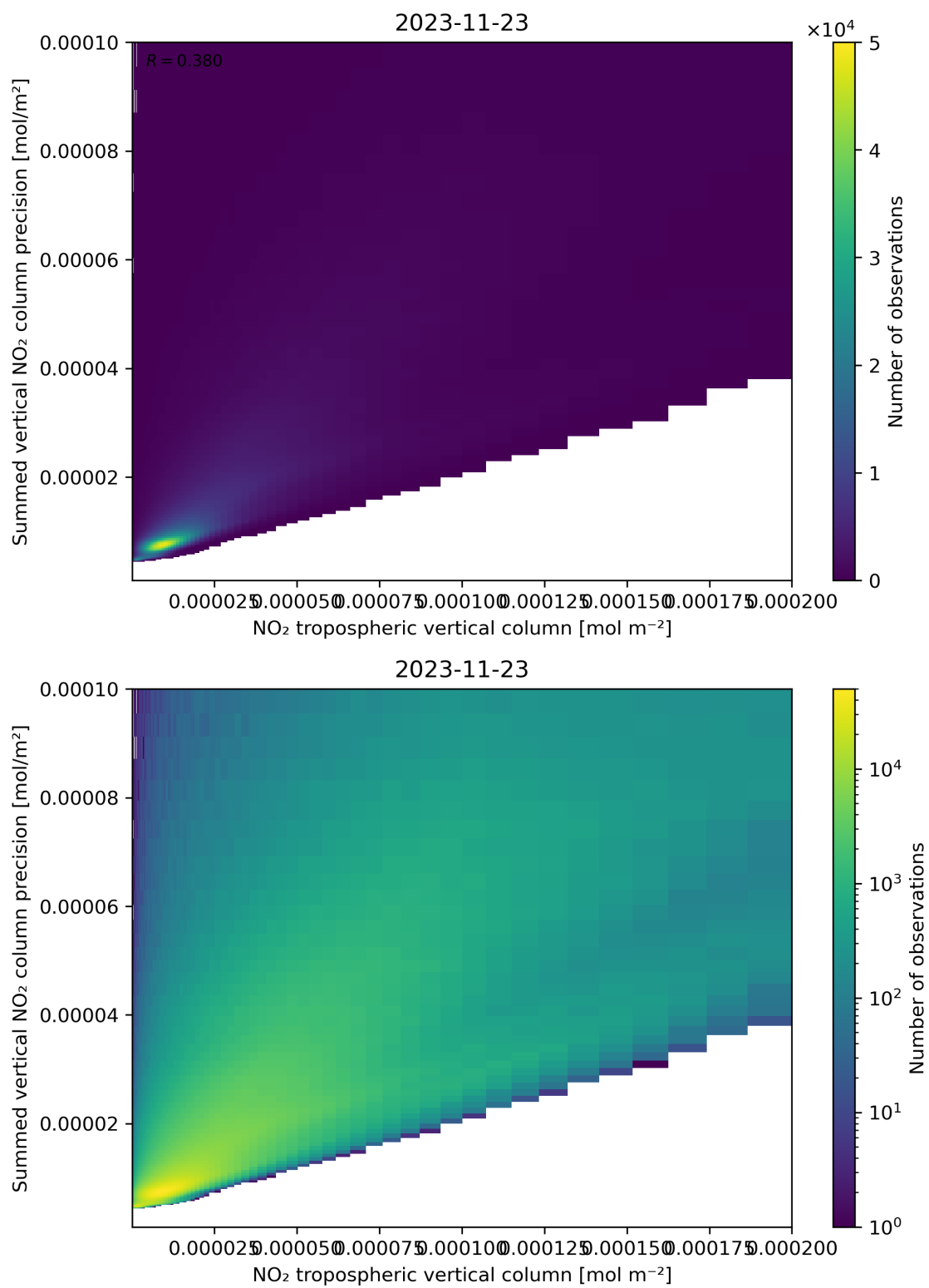
Figure 127: Scatter density plot of “NO 2 tropospheric vertical column” against “Summed vertical NO 2 column precision” for 2023-11-23 to 2023-11-24.
