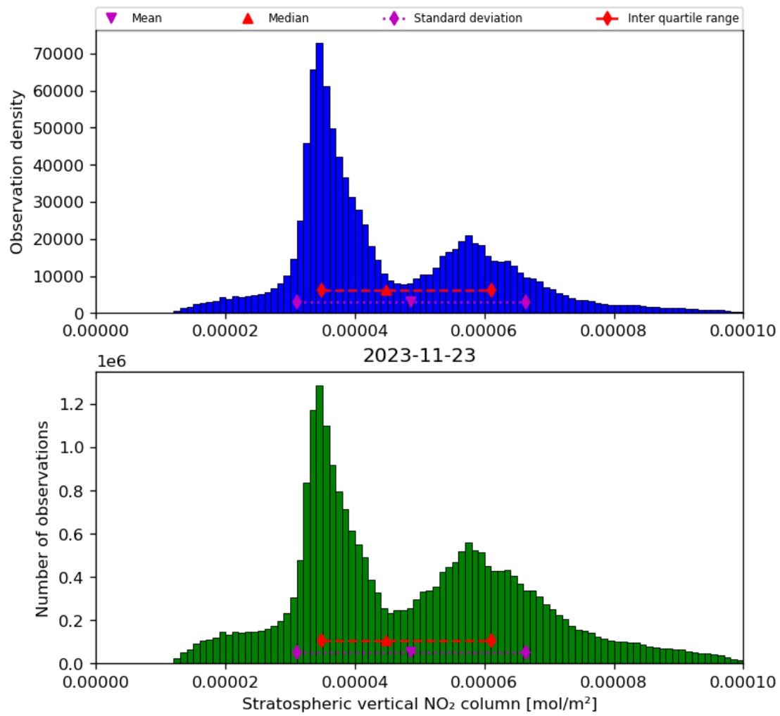
Figure 36: Histogram of “Stratospheric vertical NO 2 column” for 2023-11-23 to 2023-11-24
