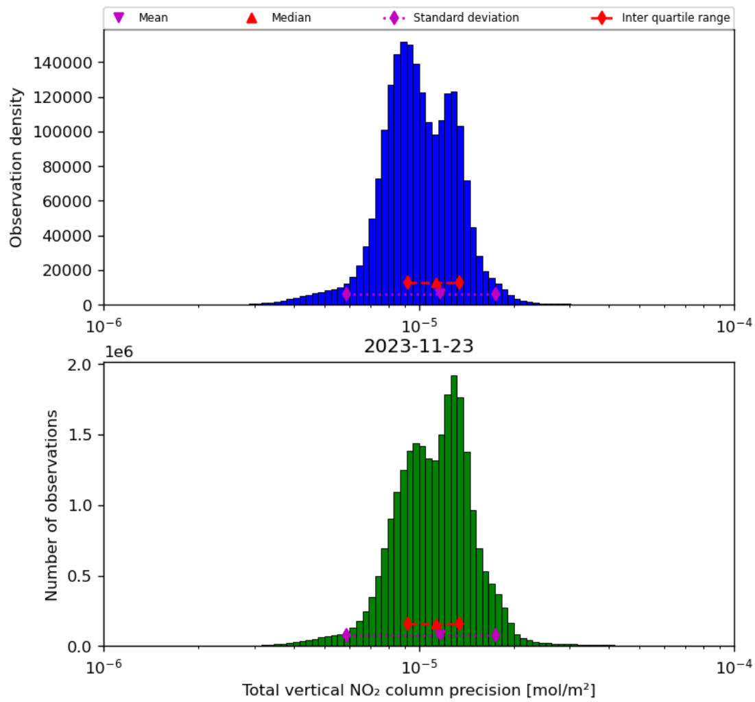
Figure 39: Histogram of “Total vertical NO 2 column precision” for 2023-11-23 to 2023-11-24
