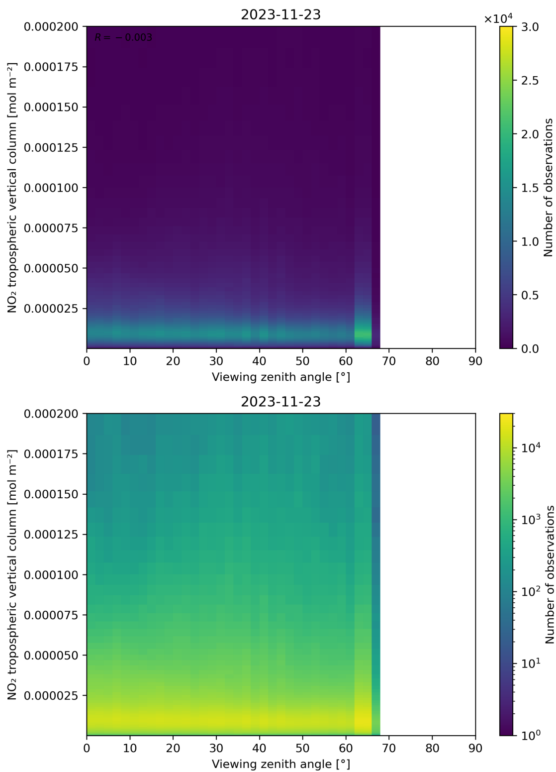
Figure 169: Scatter density plot of “Viewing zenith angle” against “NO 2 tropospheric vertical column” for 2023-11-23 to 2023-11-24.
