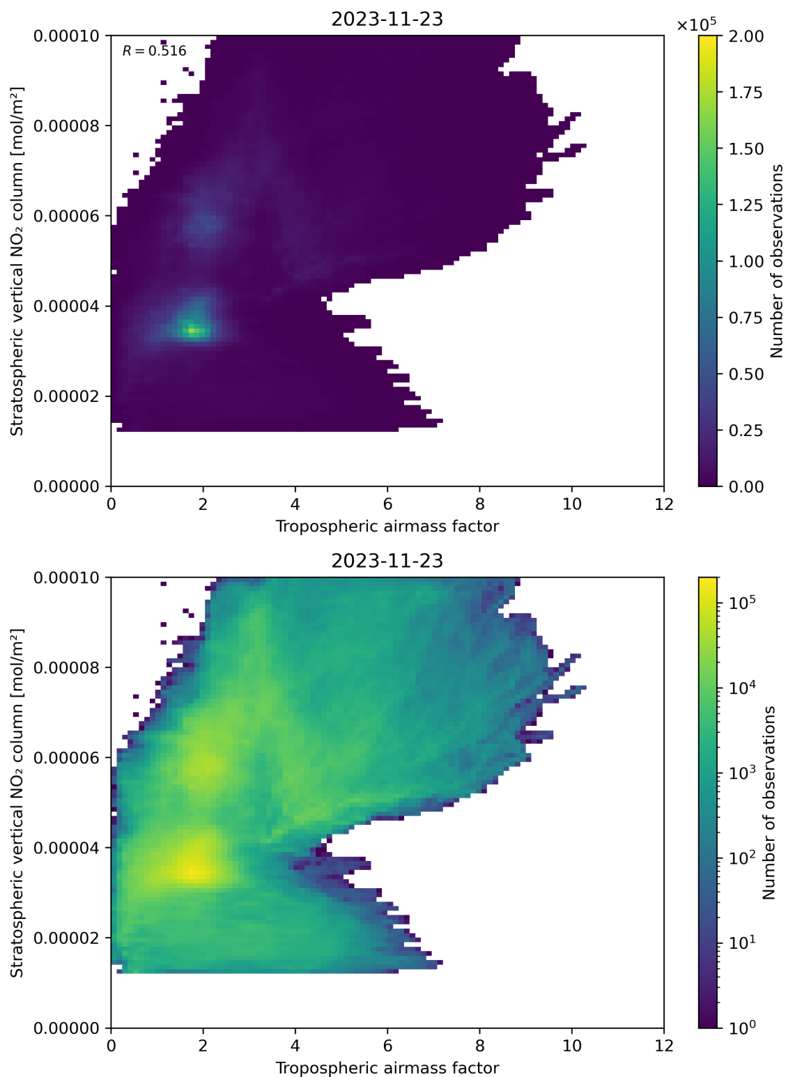
Figure 74: Scatter density plot of “Tropospheric air mass factor” against “Stratospheric vertical NO 2 column” for 2023-11-23 to 2023-11-24.
