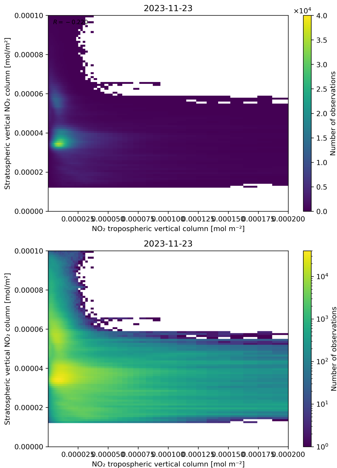
Figure 125: Scatter density plot of “NO 2 tropospheric vertical column” against “Stratospheric vertical NO 2 column” for 2023-11-23 to 2023-11-24.
