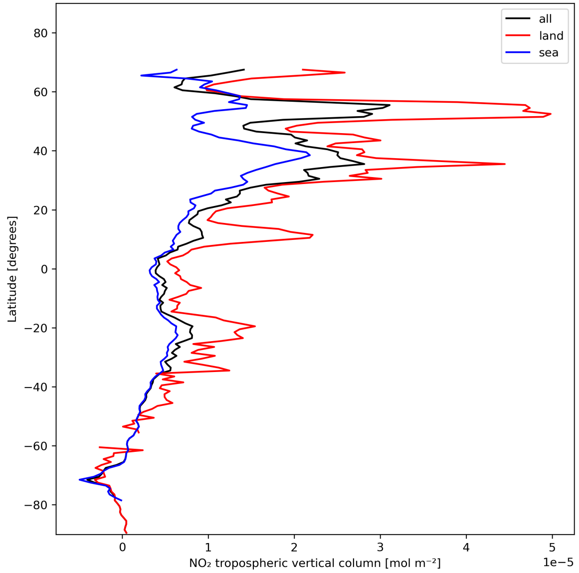
Figure 12: Zonal average of “NO 2 tropospheric vertical column” for 2023-11-23 to 2023-11-24.
