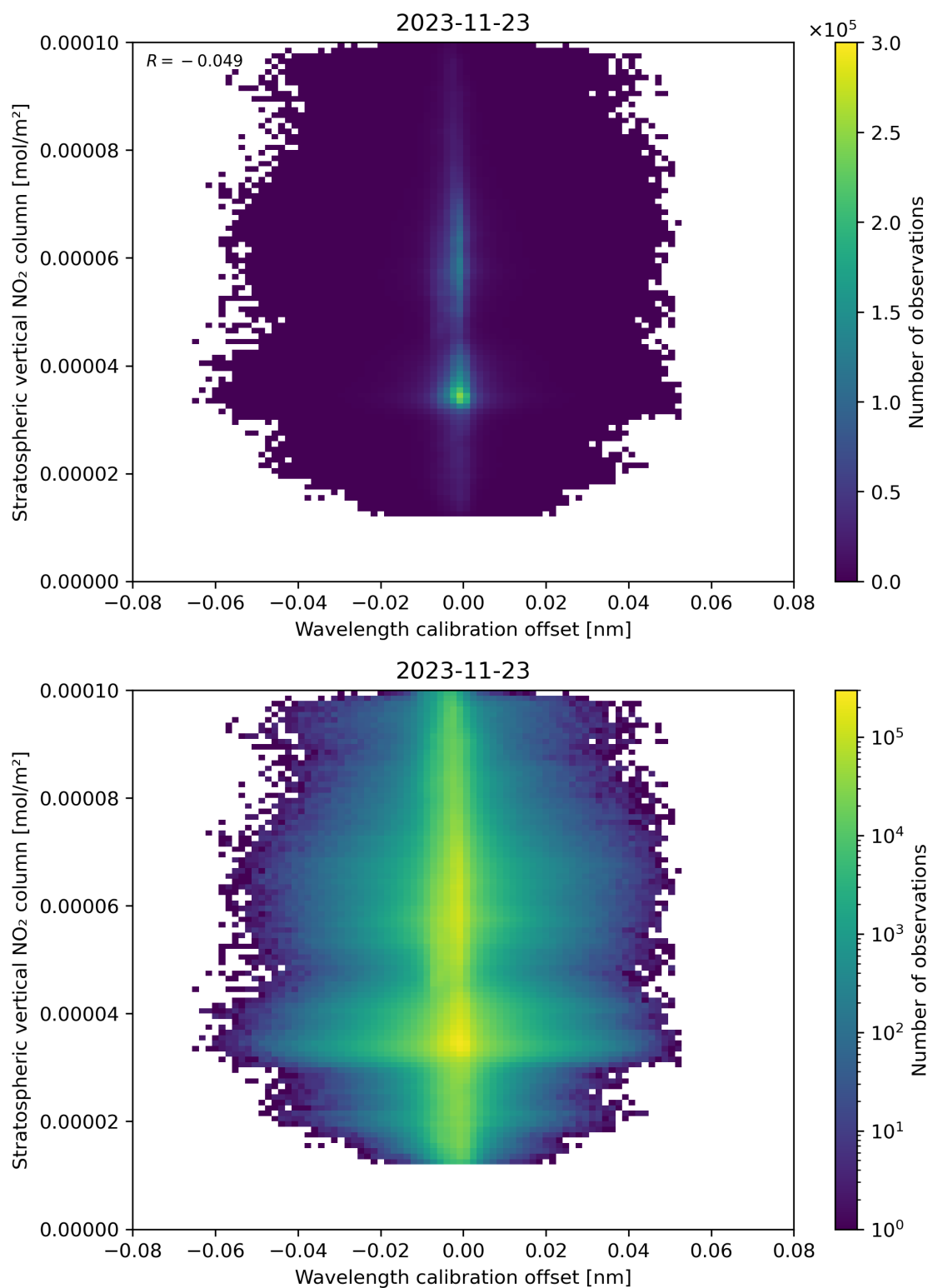
Figure 176: Scatter density plot of “Wavelength calibration offset” against “Stratospheric vertical NO 2 column” for 2023-11-23 to 2023-11-24.
