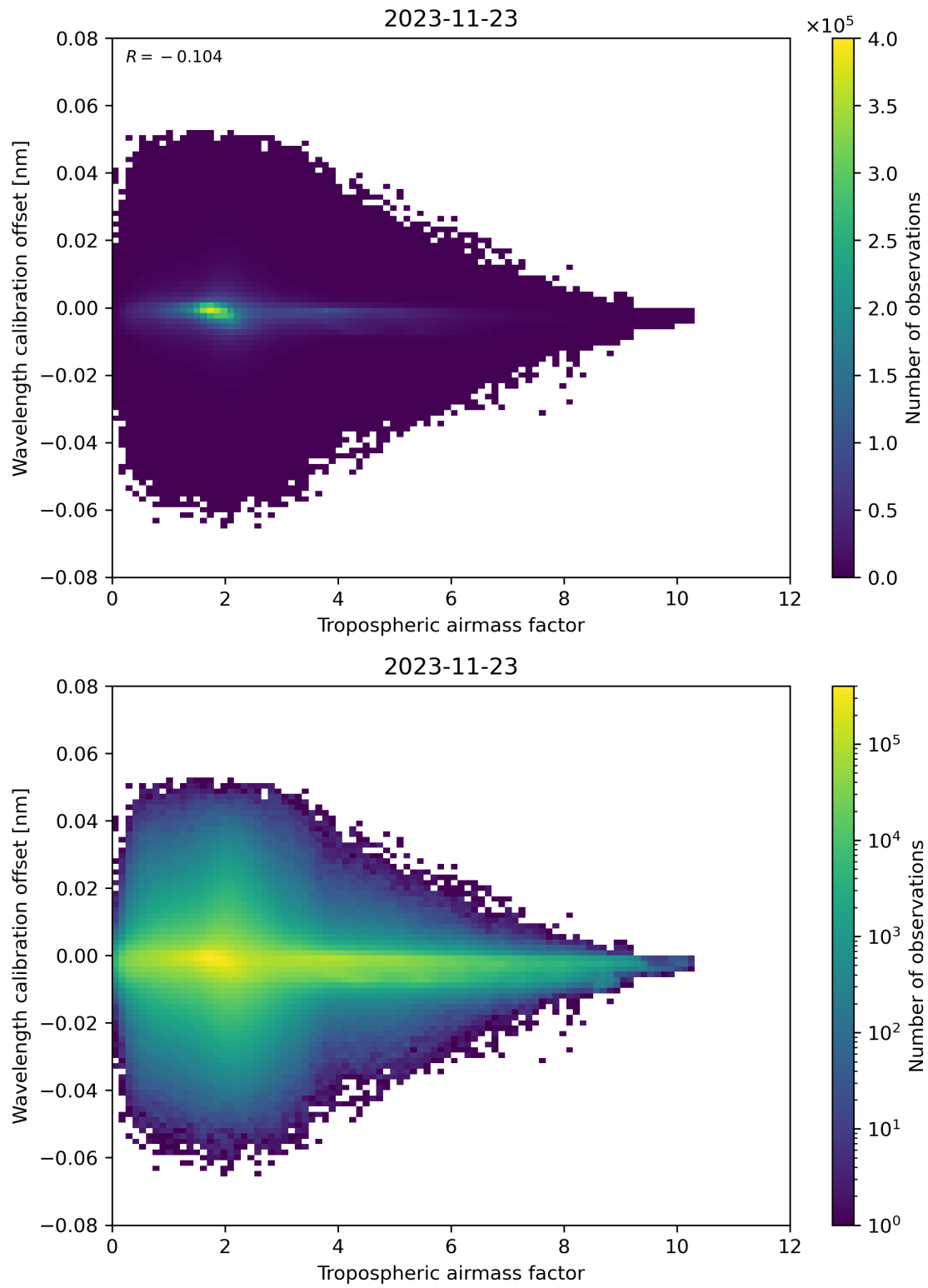
Figure 80: Scatter density plot of “Tropospheric air mass factor” against “Wavelength calibration offset” for 2023-11-23 to 2023-11-24.
