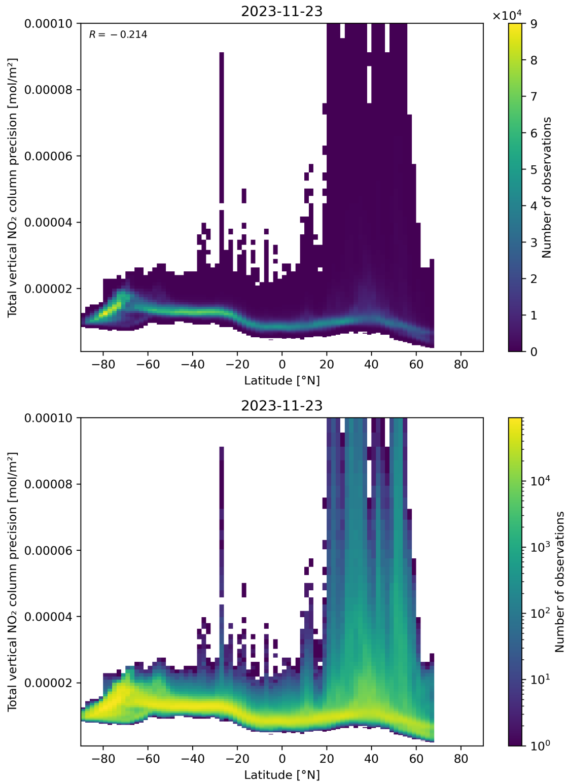
Figure 91: Scatter density plot of “Latitude” against “Total vertical NO 2 column precision” for 2023-11-23 to 2023-11-24.
