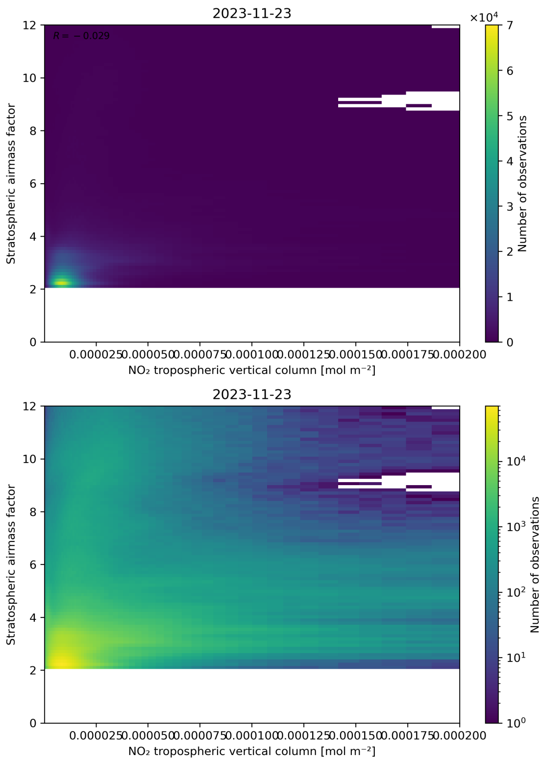
Figure 121: Scatter density plot of “NO 2 tropospheric vertical column” against “Stratospheric airmass factor” for 2023-11-23 to 2023-11-24.
