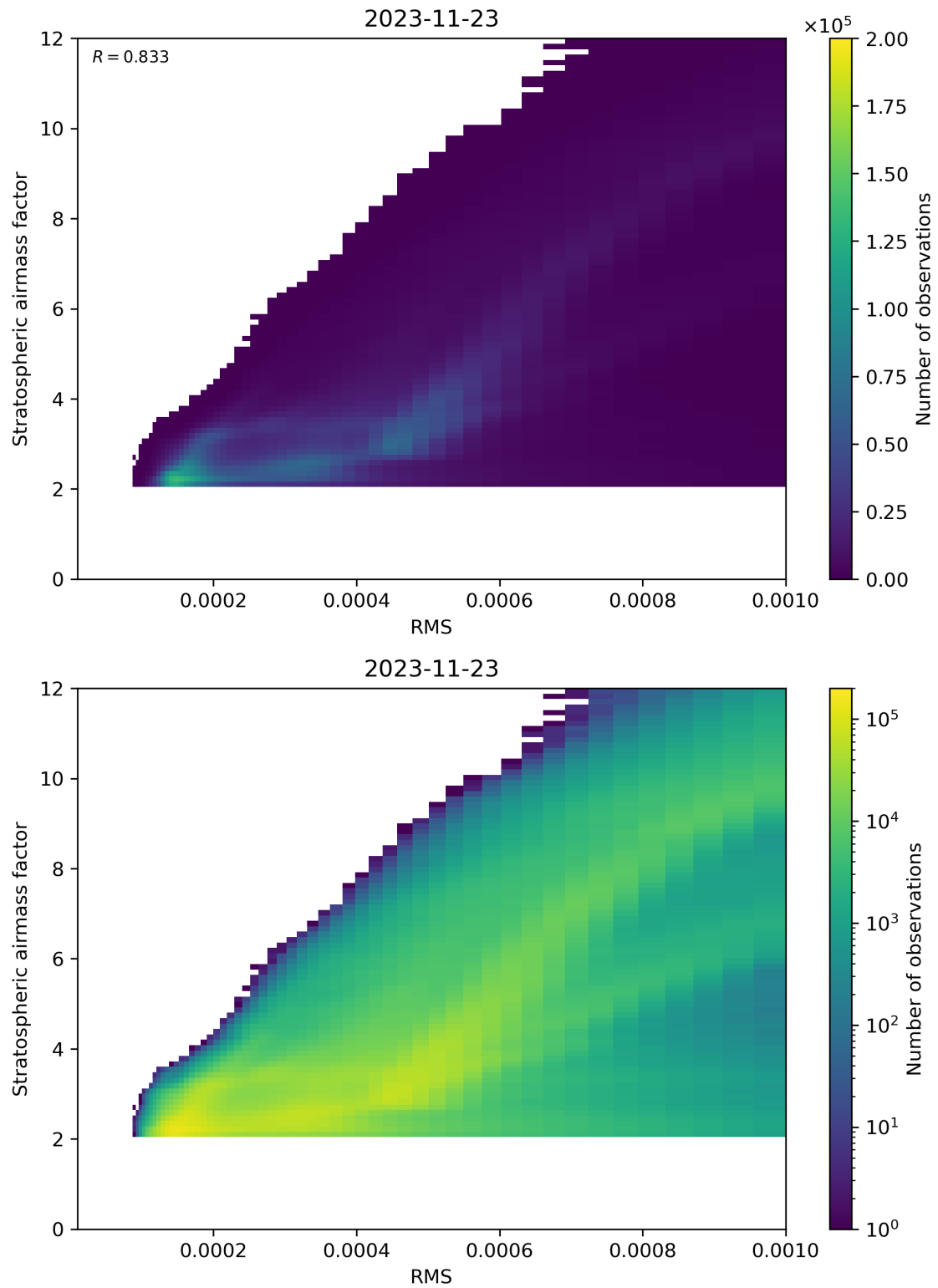
Figure 144: Scatter density plot of “RMS” against “Stratospheric airmass factor” for 2023-11-23 to 2023-11-24.
