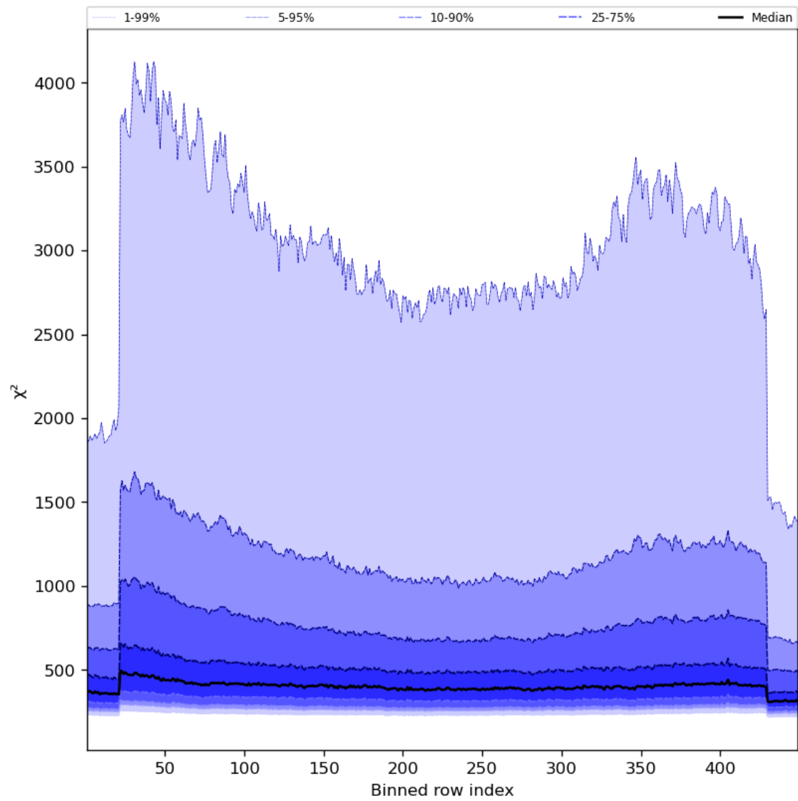
Figure 59: Along track statistics of “ \chi^2 ” for 2023-11-23 to 2023-11-24
