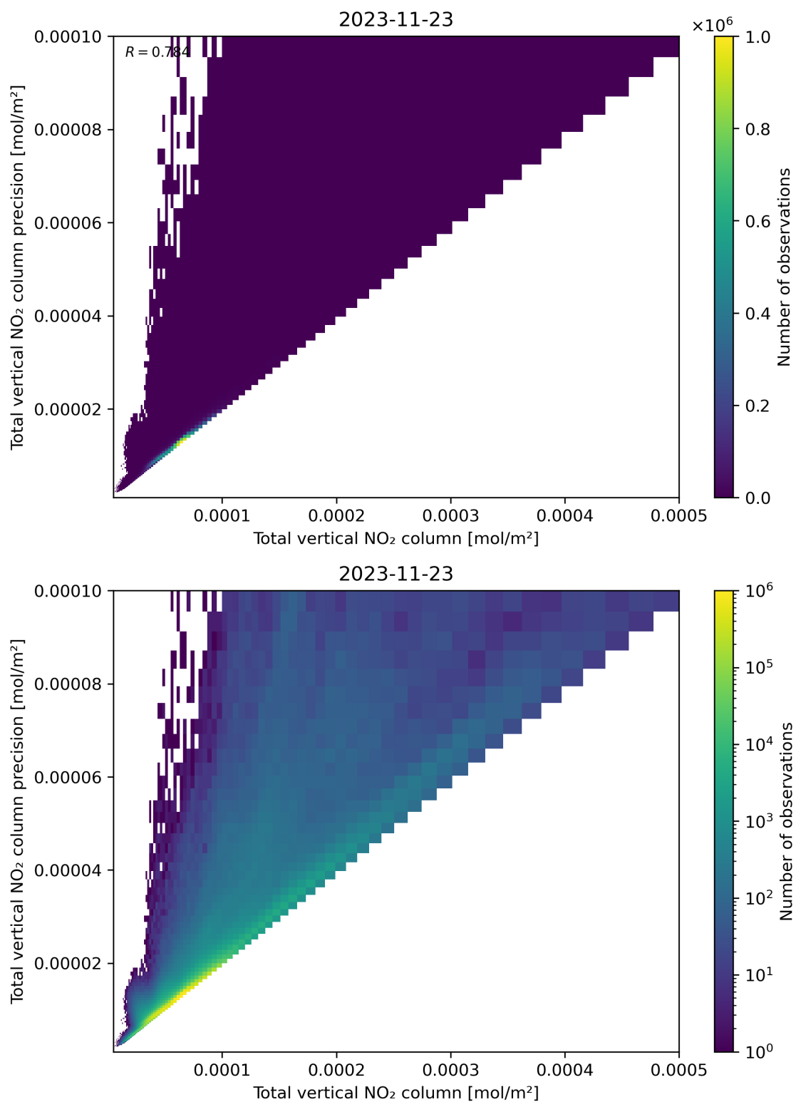
Figure 114: Scatter density plot of “Total vertical NO 2 column” against “Total vertical NO 2 column precision” for 2023-11-23 to 2023-11-24.
