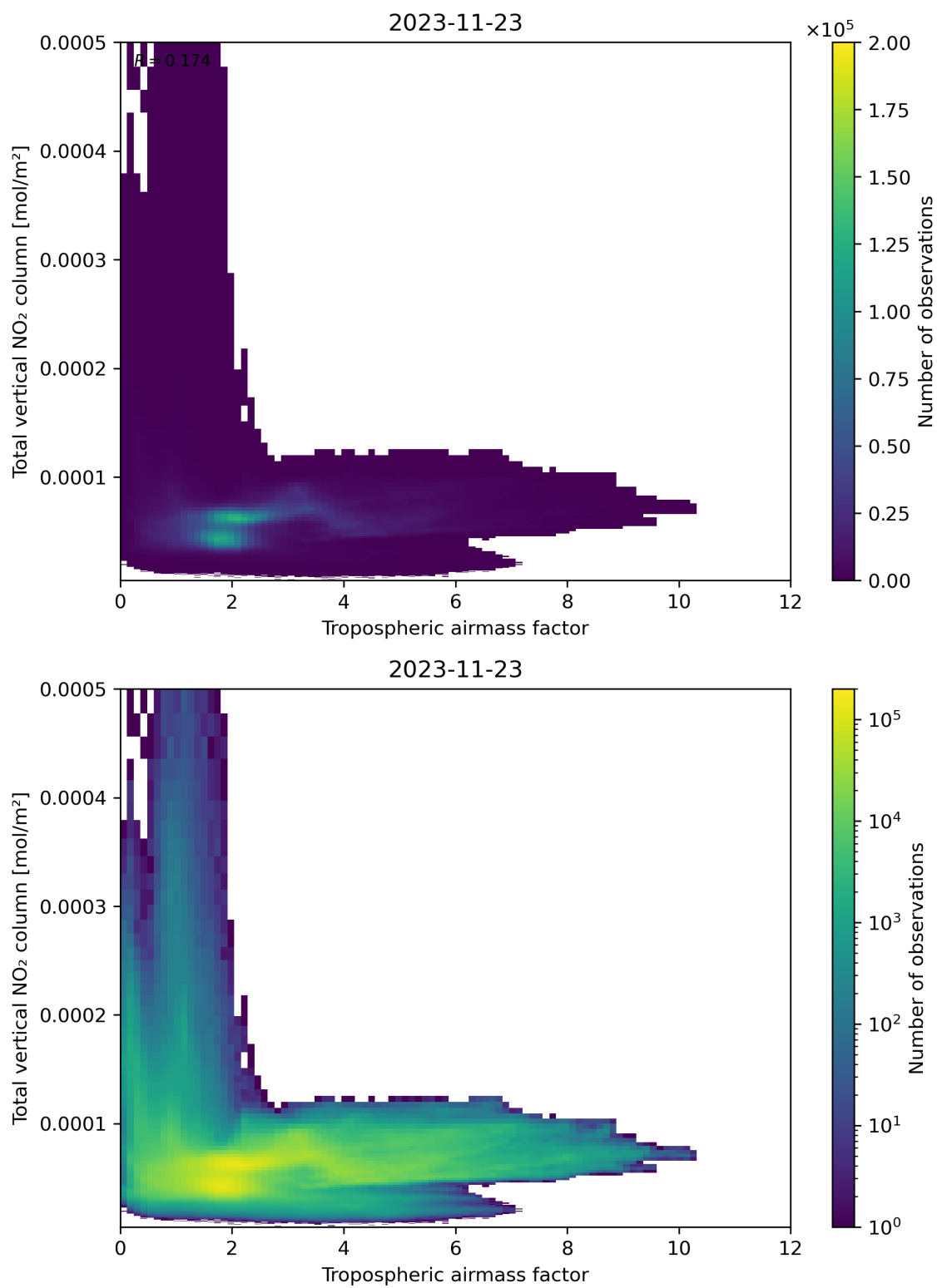
Figure 77: Scatter density plot of “Tropospheric airmass factor” against “Total vertical NO 2 column” for 2023-11-23 to 2023-11-24.
