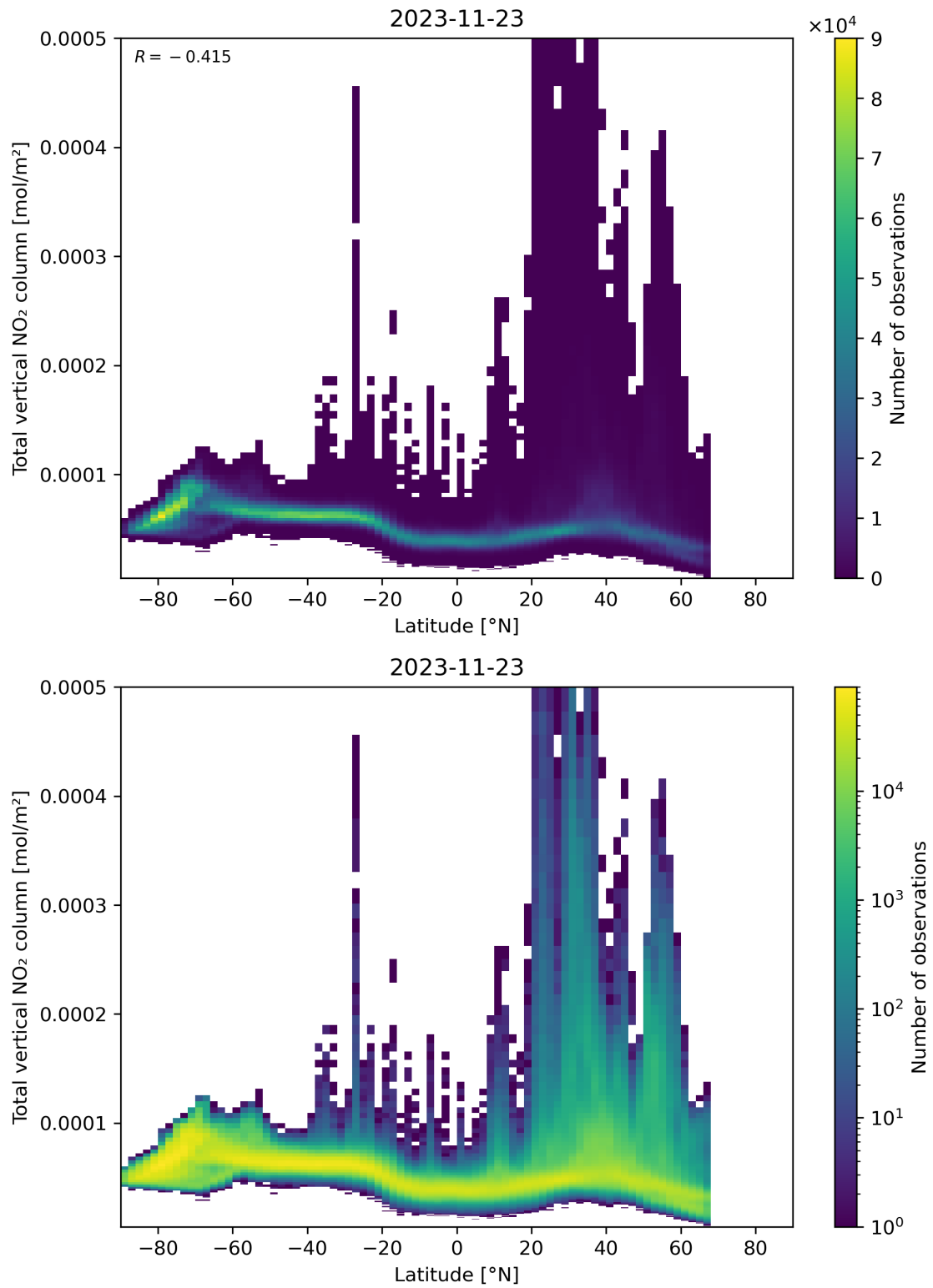
Figure 90: Scatter density plot of “Latitude” against “Total vertical NO 2 column” for 2023-11-23 to 2023-11-24.
