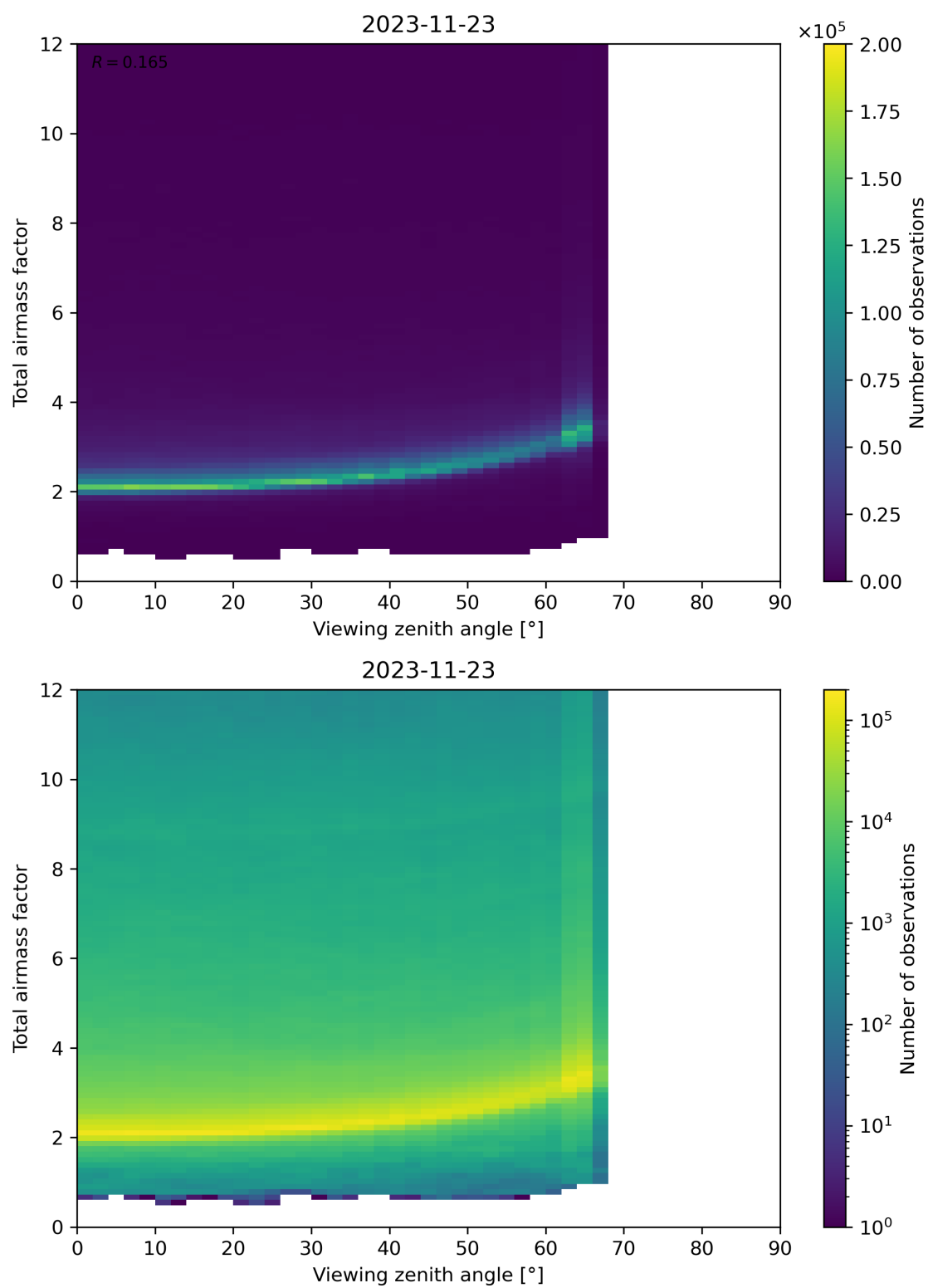
Figure 160: Scatter density plot of “Viewing zenith angle” against “Total airmass factor” for 2023-11-23 to 2023-11-24.
