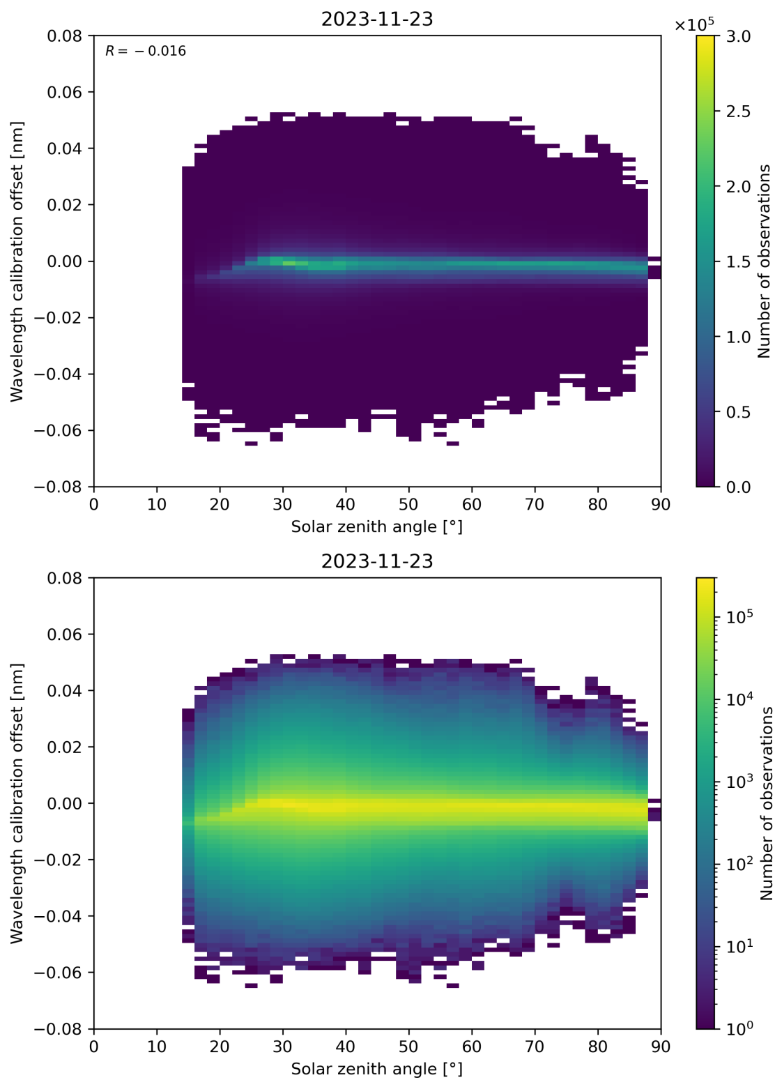
Figure 158: Scatter density plot of “Solar zenith angle” against “Wavelength calibration offset” for 2023-11-23 to 2023-11-24.
