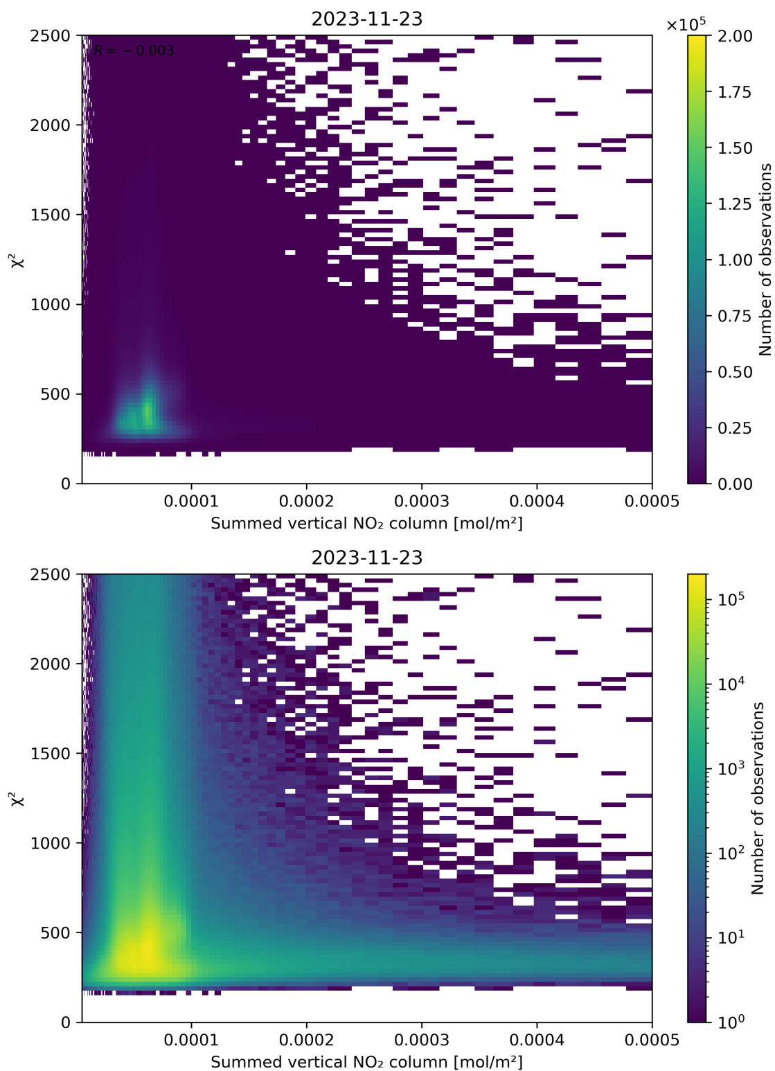
Figure 104: Scatter density plot of “Summed vertical NO 2 column” against “ \chi^2 ” for 2023-11-23 to 2023-11-24.
