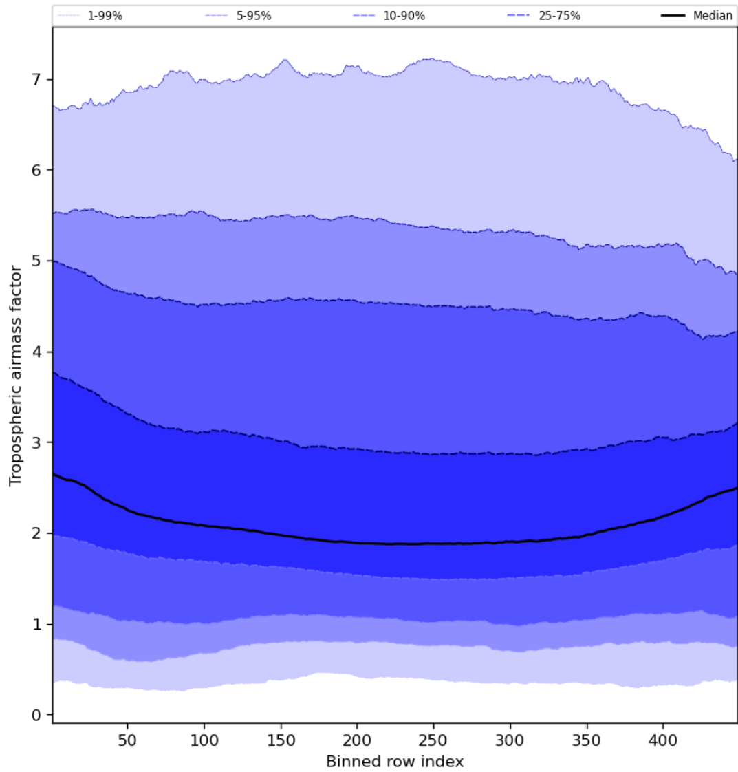
Figure 48: Along track statistics of “Tropospheric air mass factor” for 2023-11-23 to 2023-11-24
