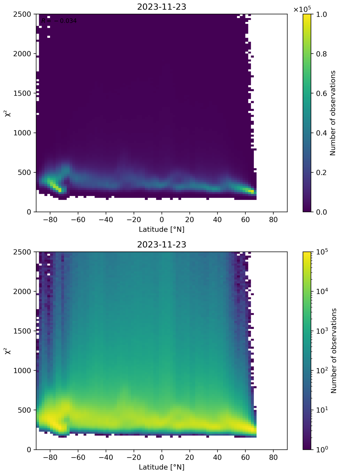
Figure 86: Scatter density plot of “Latitude” against “ \chi^2 ” for 2023-11-23 to 2023-11-24.
