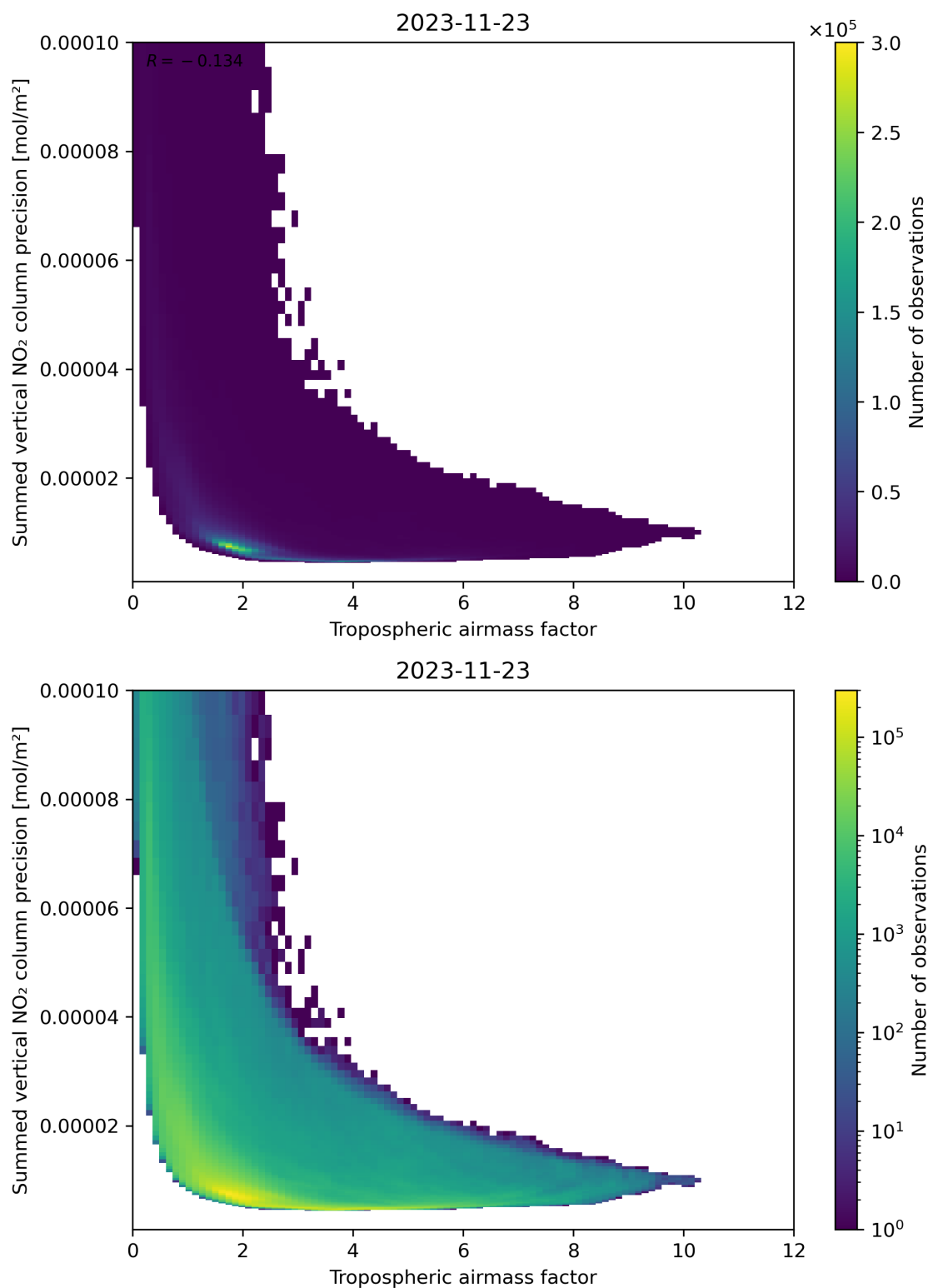
Figure 76: Scatter density plot of “Tropospheric air mass factor” against “Summed vertical NO 2 column precision” for 2023-11-23 to 2023-11-24.
