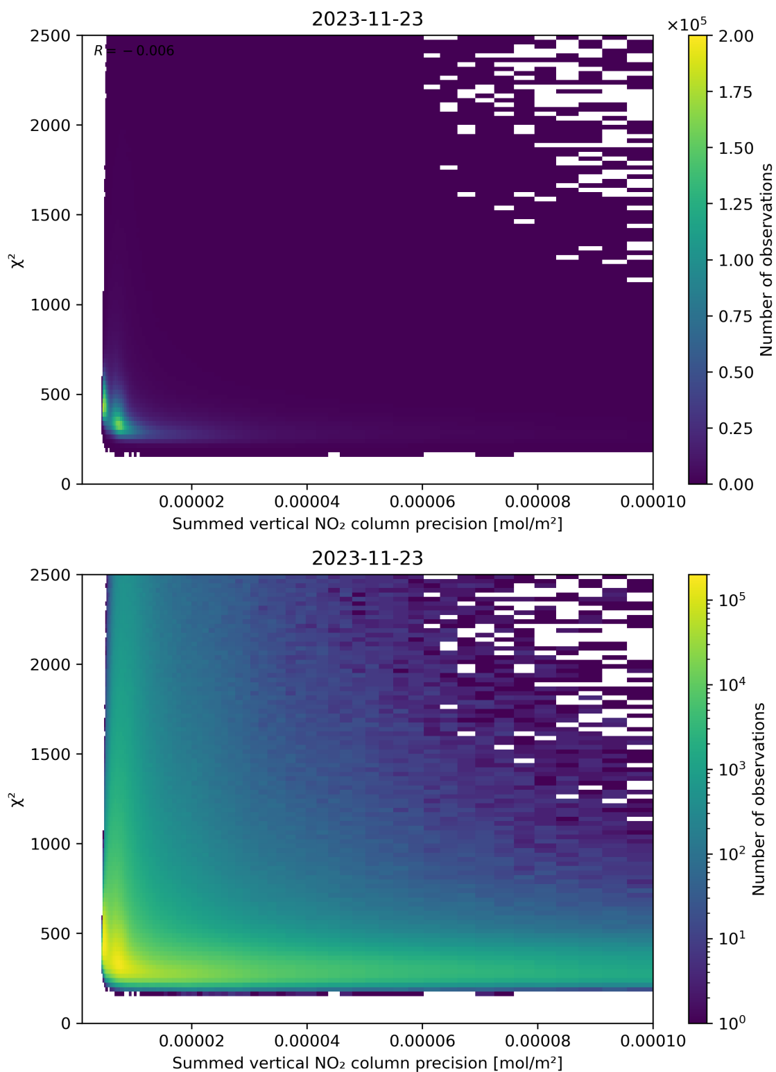
Figure 107: Scatter density plot of “Summed vertical NO 2 column precision” against “ \chi^2 ” for 2023-11-23 to 2023-11-24.
