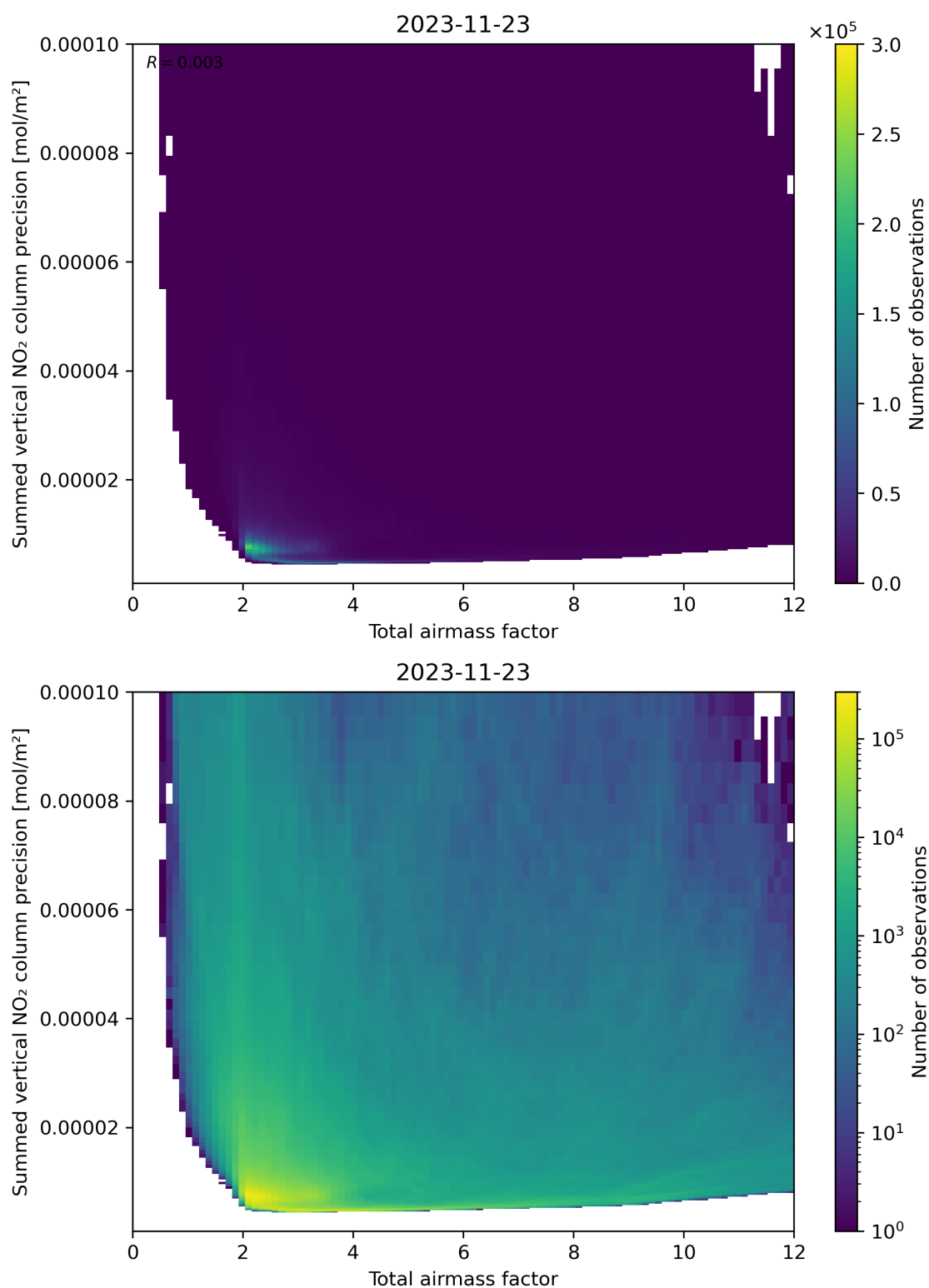
Figure 66: Scatter density plot of “Total airmass factor” against “Summed vertical NO 2 column precision” for 2023-11-23 to 2023-11-24.
