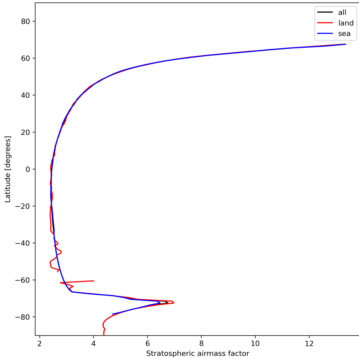
Figure 27: Zonal average of “Stratospheric airmass factor” for 2023-11-23 to 2023-11-24.
