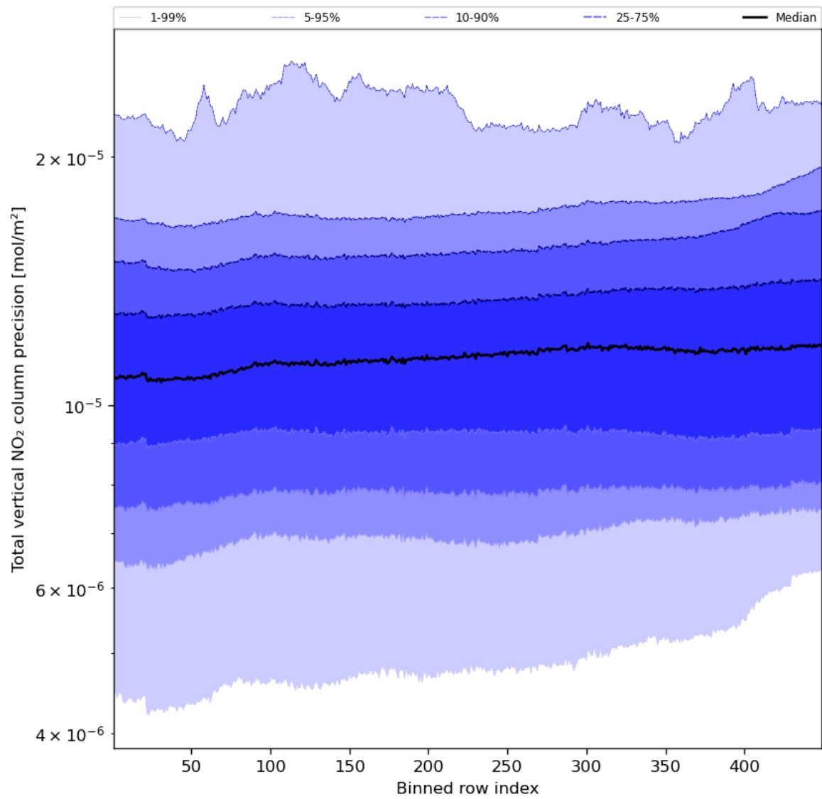
Figure 56: Along track statistics of “Total vertical NO 2 column precision” for 2023-11-23 to 2023-11-24
