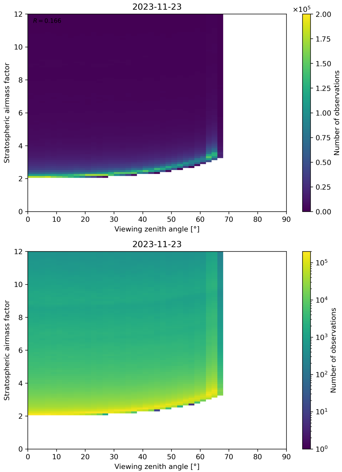
Figure 159: Scatter density plot of “Viewing zenith angle” against “Stratospheric airmass factor” for 2023-11-23 to 2023-11-24.
