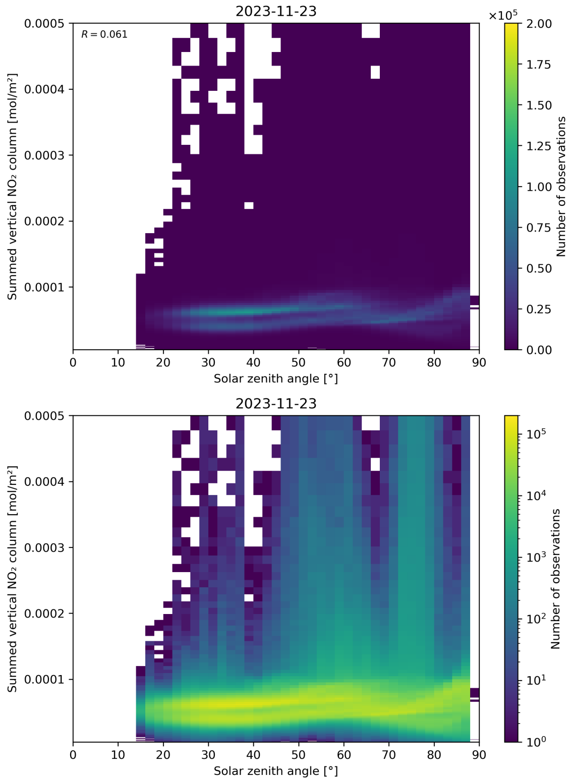
Figure 151: Scatter density plot of “Solar zenith angle” against “Summed vertical NO 2 column” for 2023-11-23 to 2023-11-24.
