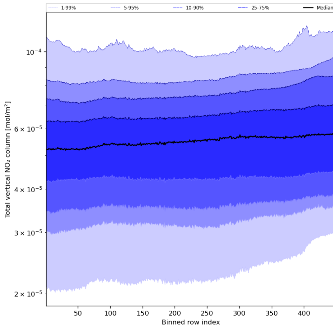
Figure 55: Along track statistics of “Total vertical NO 2 column” for 2023-11-23 to 2023-11-24
