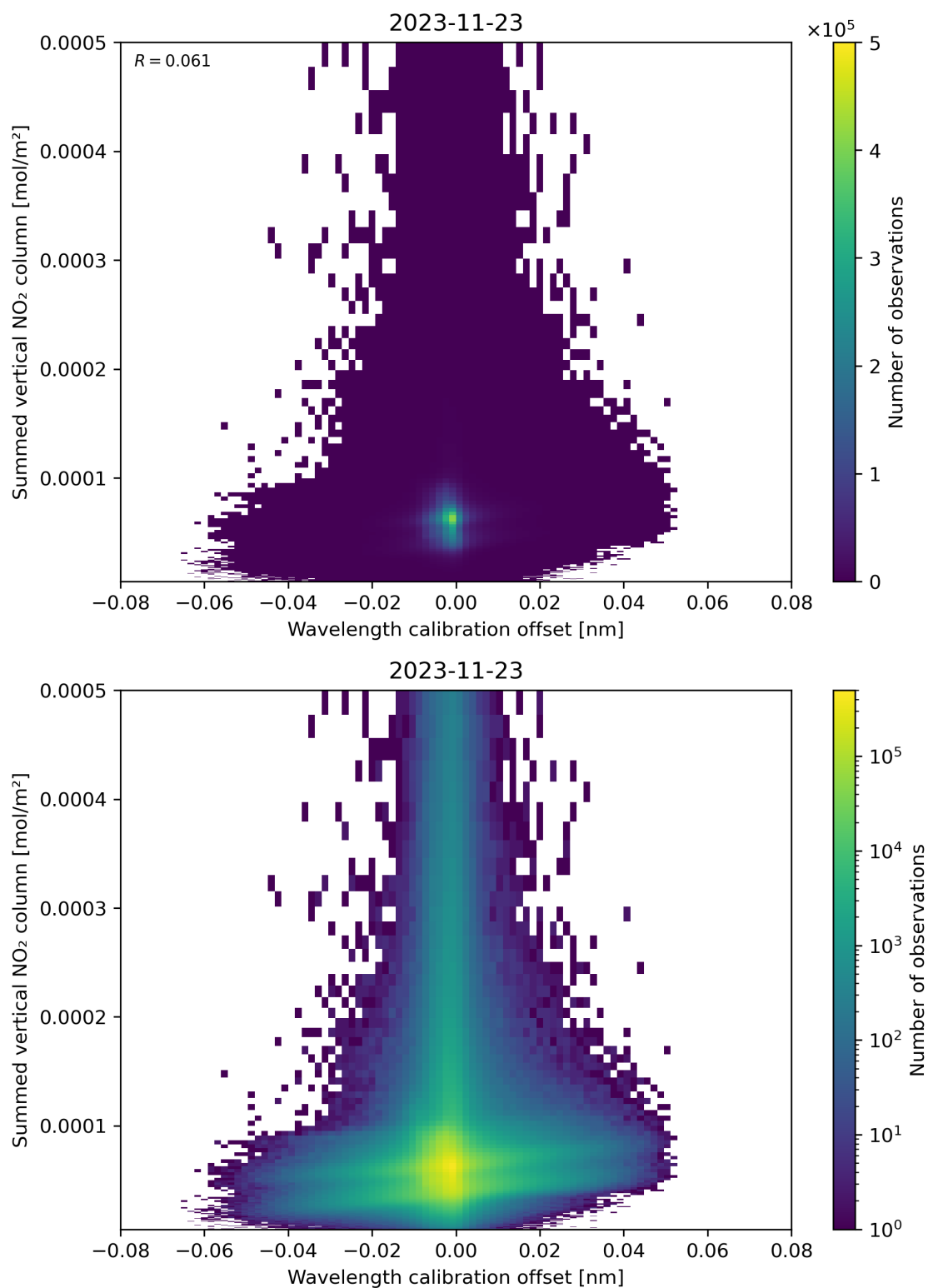
Figure 177: Scatter density plot of “Wavelength calibration offset” against “Summed vertical NO 2 column” for 2023-11-23 to 2023-11-24.
