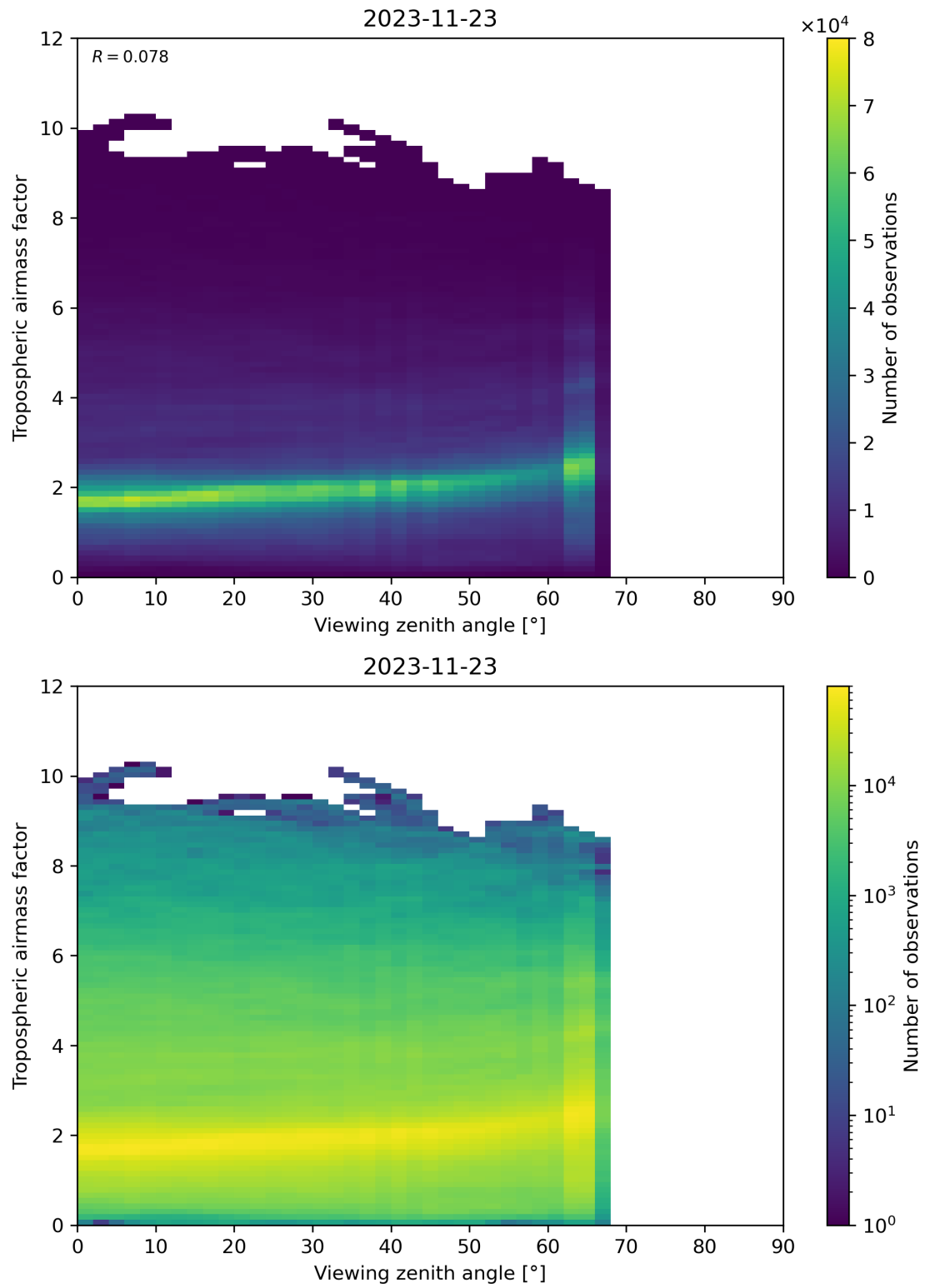
Figure 161: Scatter density plot of “Viewing zenith angle” against “Tropospheric airmass factor” for 2023-11-23 to 2023-11-24.
