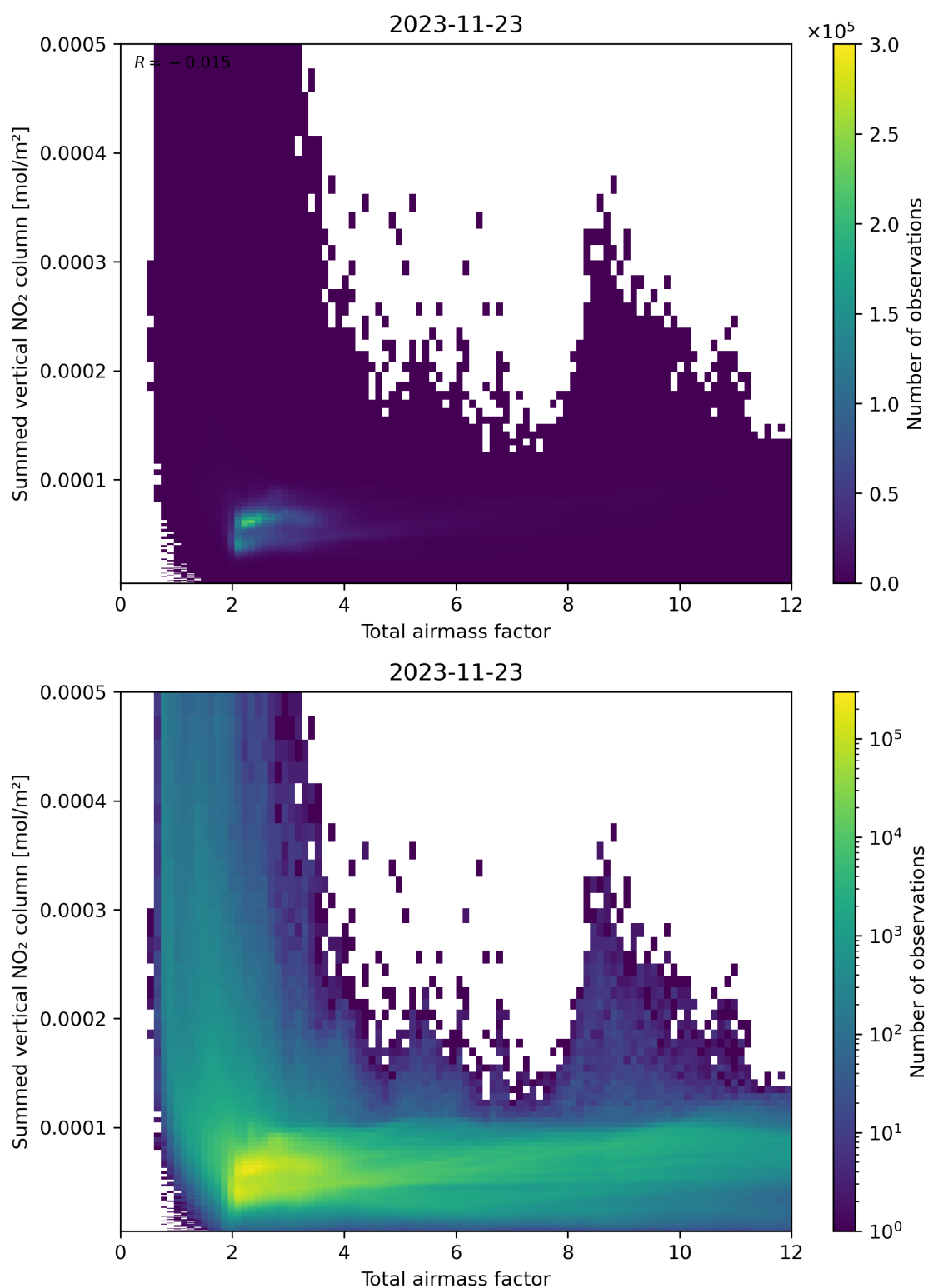
Figure 65: Scatter density plot of “Total airmass factor” against “Summed vertical NO 2 column” for 2023-11-23 to 2023-11-24.
