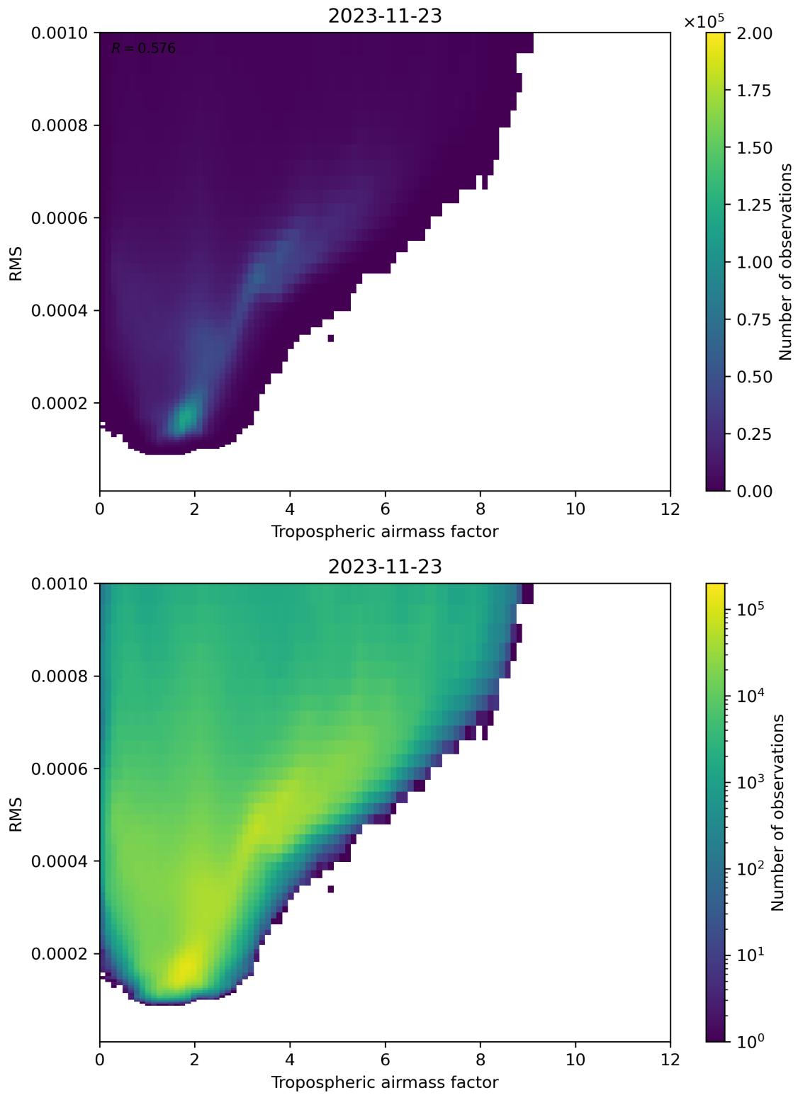
Figure 79: Scatter density plot of “Tropospheric airmass factor” against “RMS” for 2023-11-23 to 2023-11-24.
