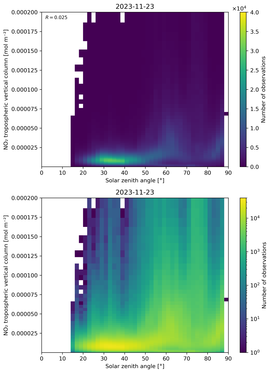
Figure 155: Scatter density plot of “Solar zenith angle” against “NO 2 tropospheric vertical column” for 2023-11-23 to 2023-11-24.
