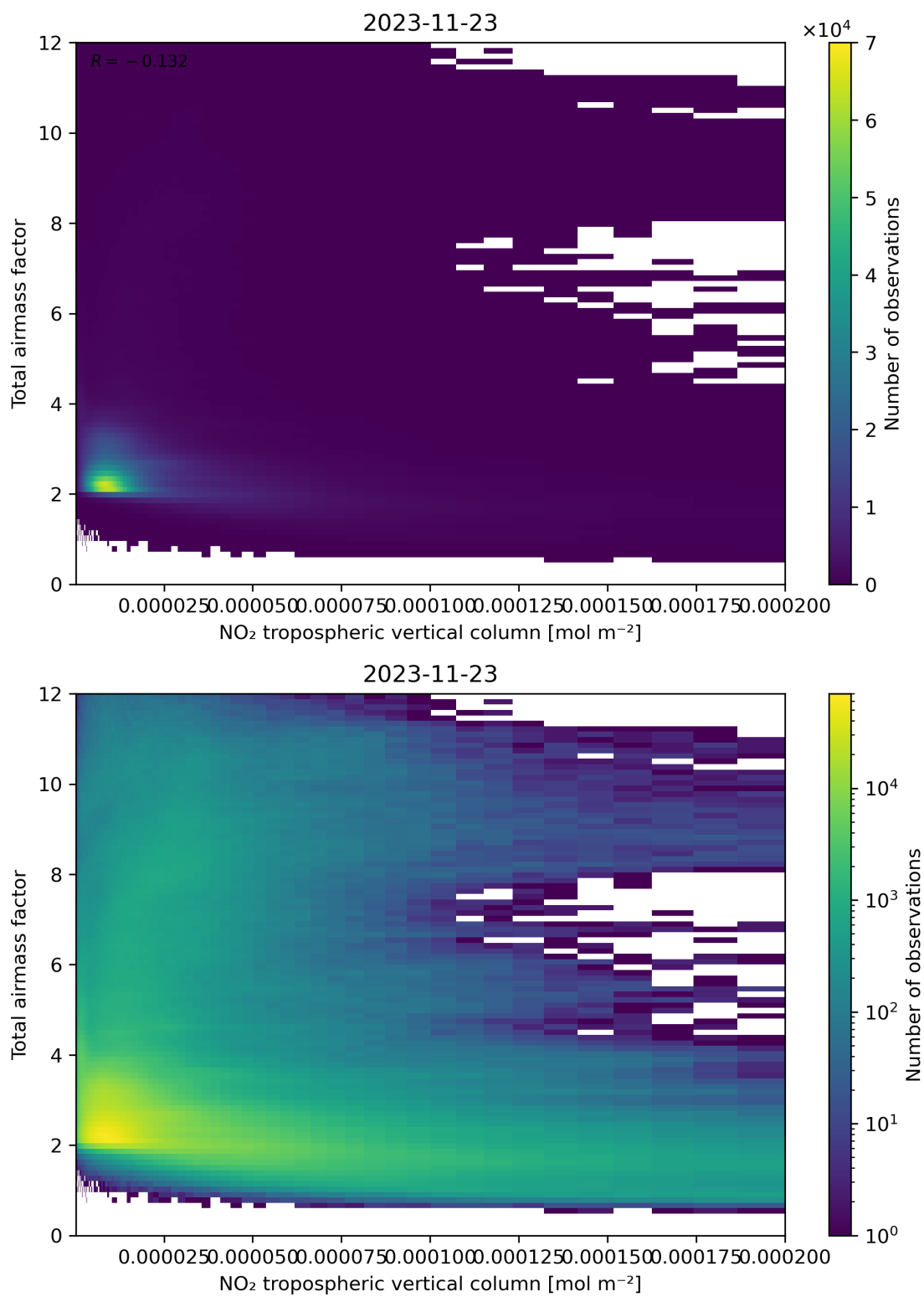
Figure 122: Scatter density plot of “NO 2 tropospheric vertical column” against “Total air mass factor” for 2023-11-23 to 2023-11-24.
