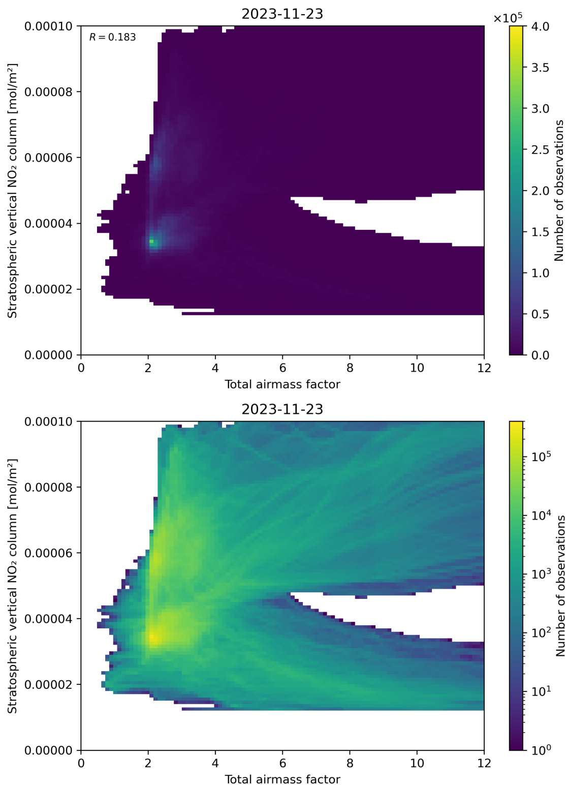
Figure 64: Scatter density plot of “Total airmass factor” against “Stratospheric vertical NO 2 column” for 2023-11-23 to 2023-11-24.
