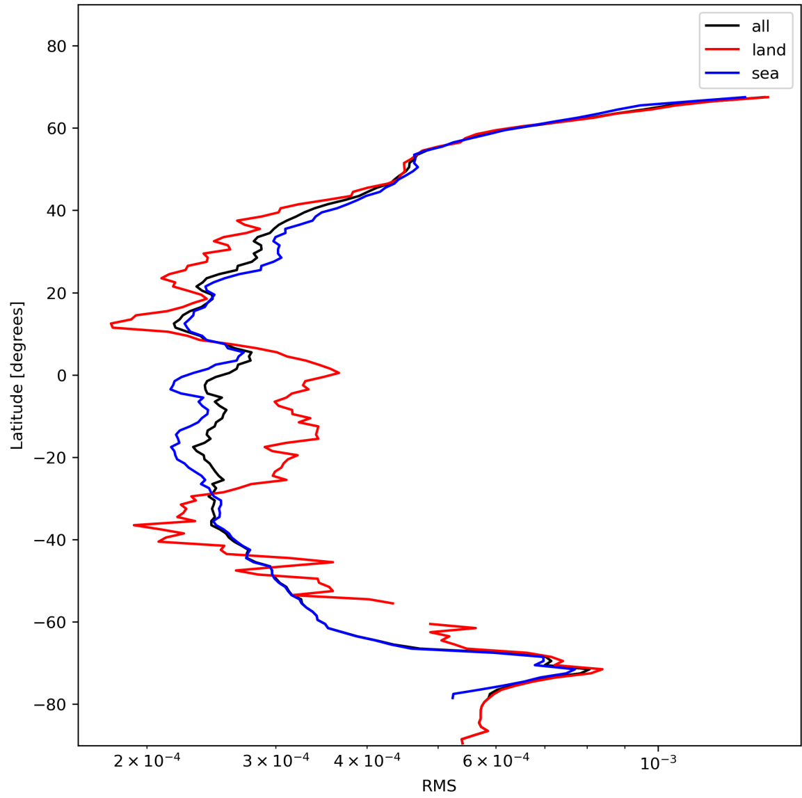
Figure 26: Zonal average of “RMS” for 2023-11-23 to 2023-11-24.
