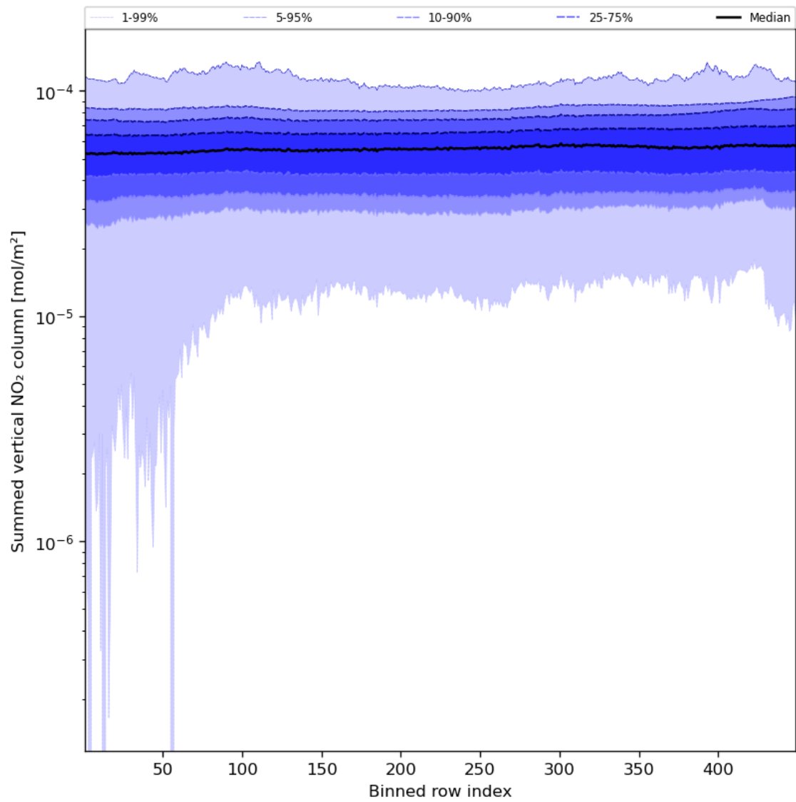
Figure 57: Along track statistics of “Summed vertical NO 2 column” for 2023-11-23 to 2023-11-24
