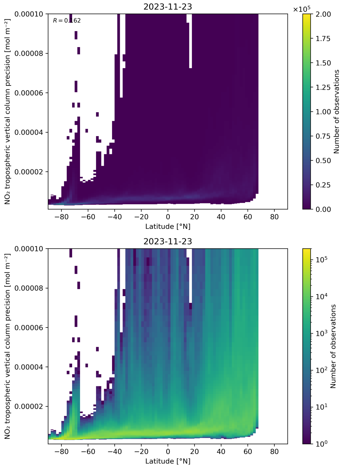
Figure 93: Scatter density plot of “Latitude” against “NO 2 tropospheric vertical column precision” for 2023-11-23 to 2023-11-24.
