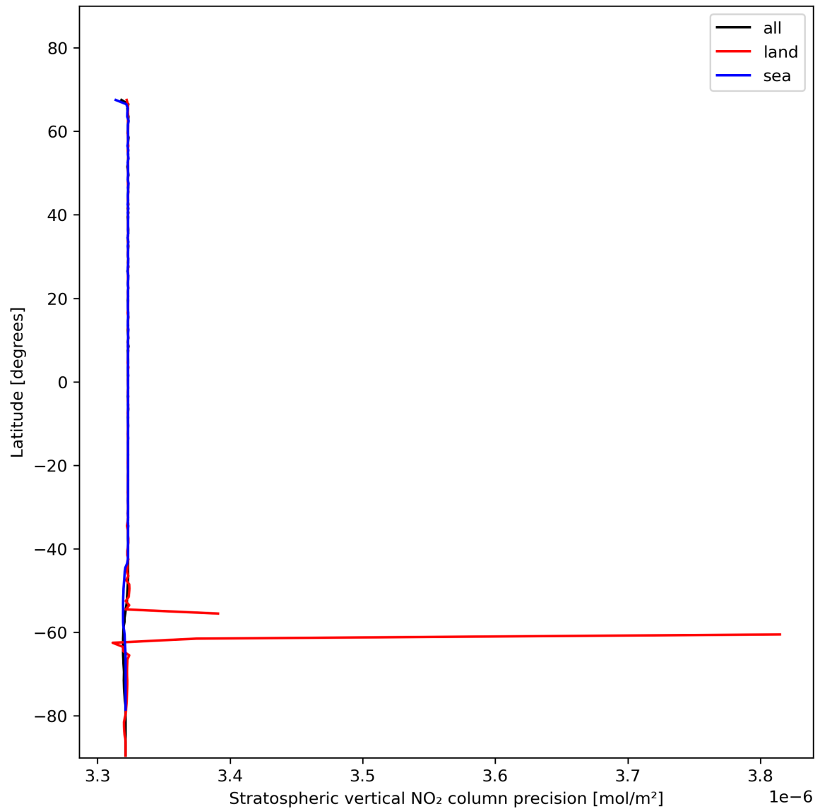
Figure 20: Zonal average of “Stratospheric vertical NO 2 column precision” for 2023-11-23 to 2023-11-24.
