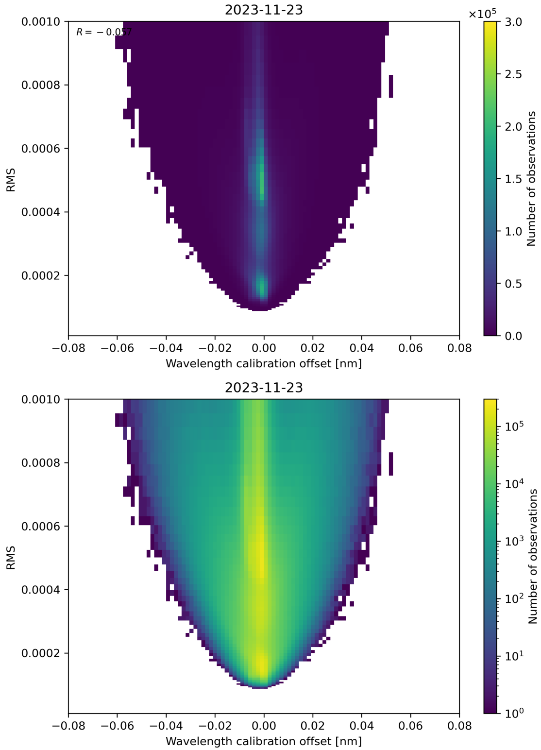
Figure 181: Scatter density plot of “Wavelength calibration offset” against “RMS” for 2023-11-23 to 2023-11-24.
