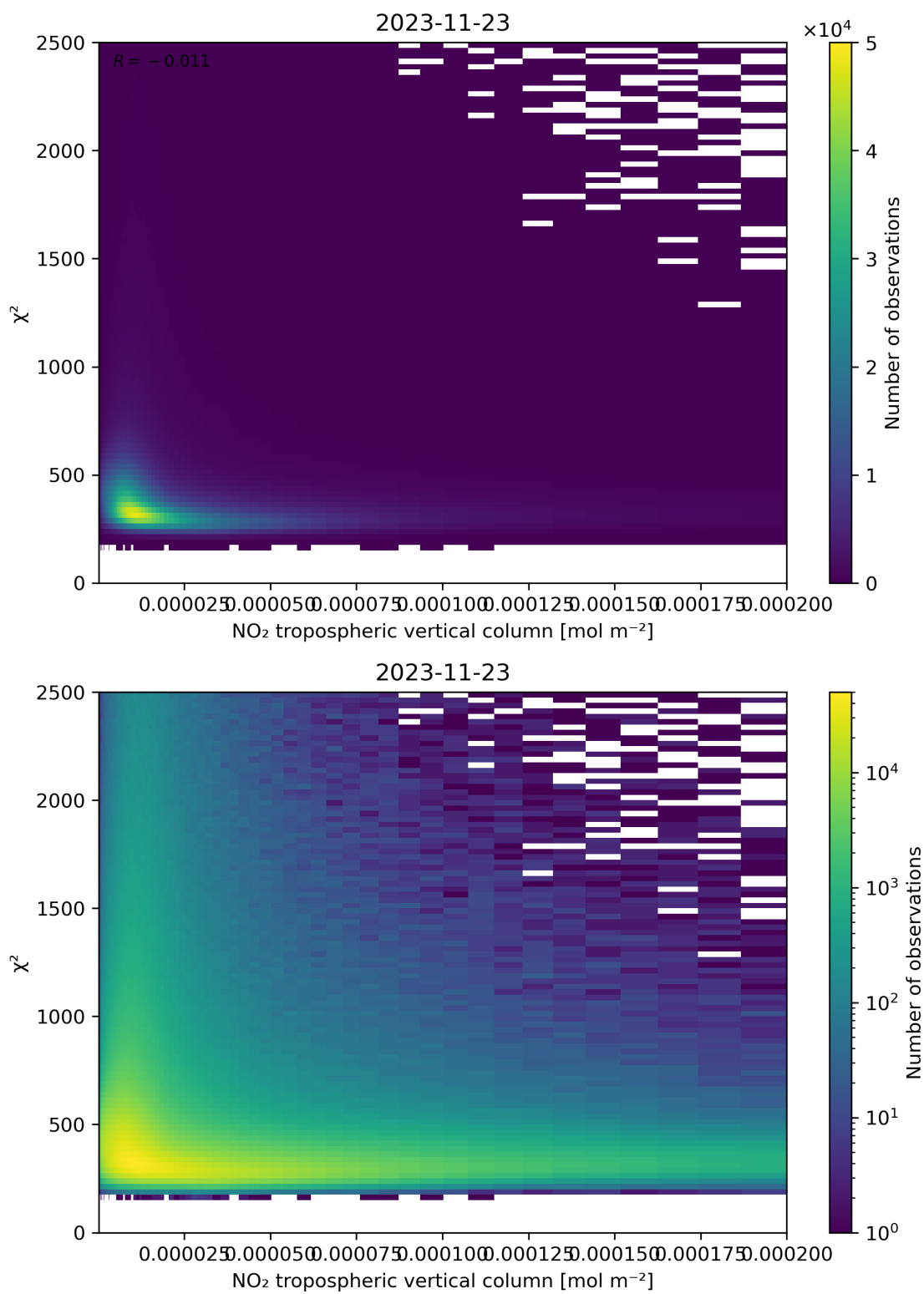
Figure 124: Scatter density plot of “NO 2 tropospheric vertical column” against “ \chi^2 ” for 2023-11-23 to 2023-11-24.
