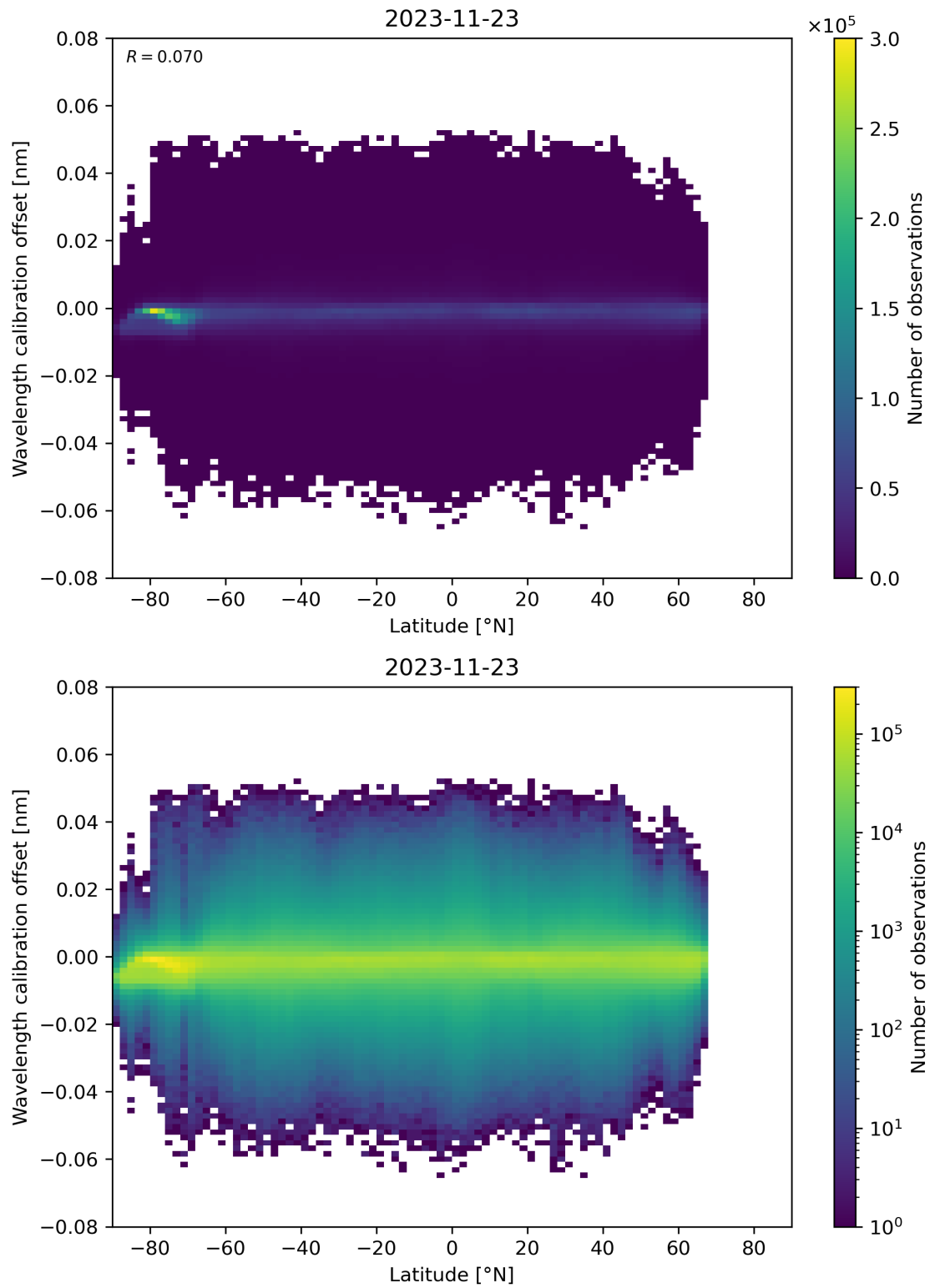
Figure 95: Scatter density plot of “Latitude” against “Wavelength calibration offset” for 2023-11-23 to 2023-11-24.
