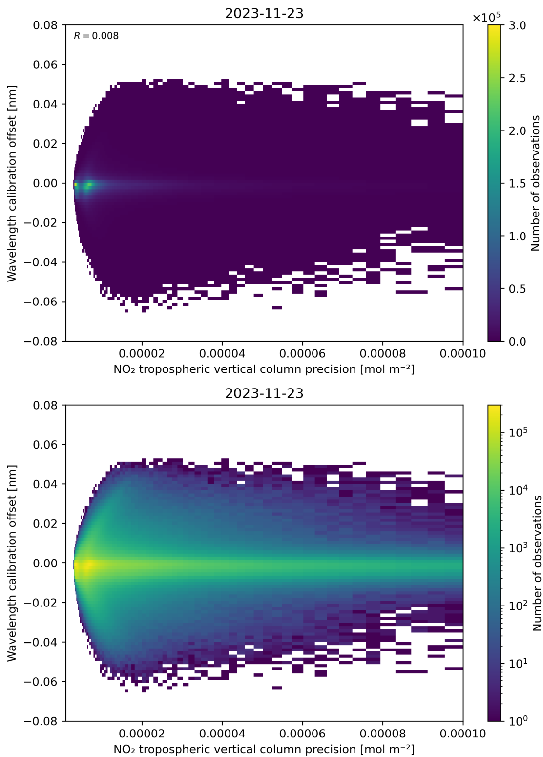
Figure 141: Scatter density plot of “NO 2 tropospheric vertical column precision” against “Wavelength calibration offset” for 2023-11-23 to 2023-11-24.
