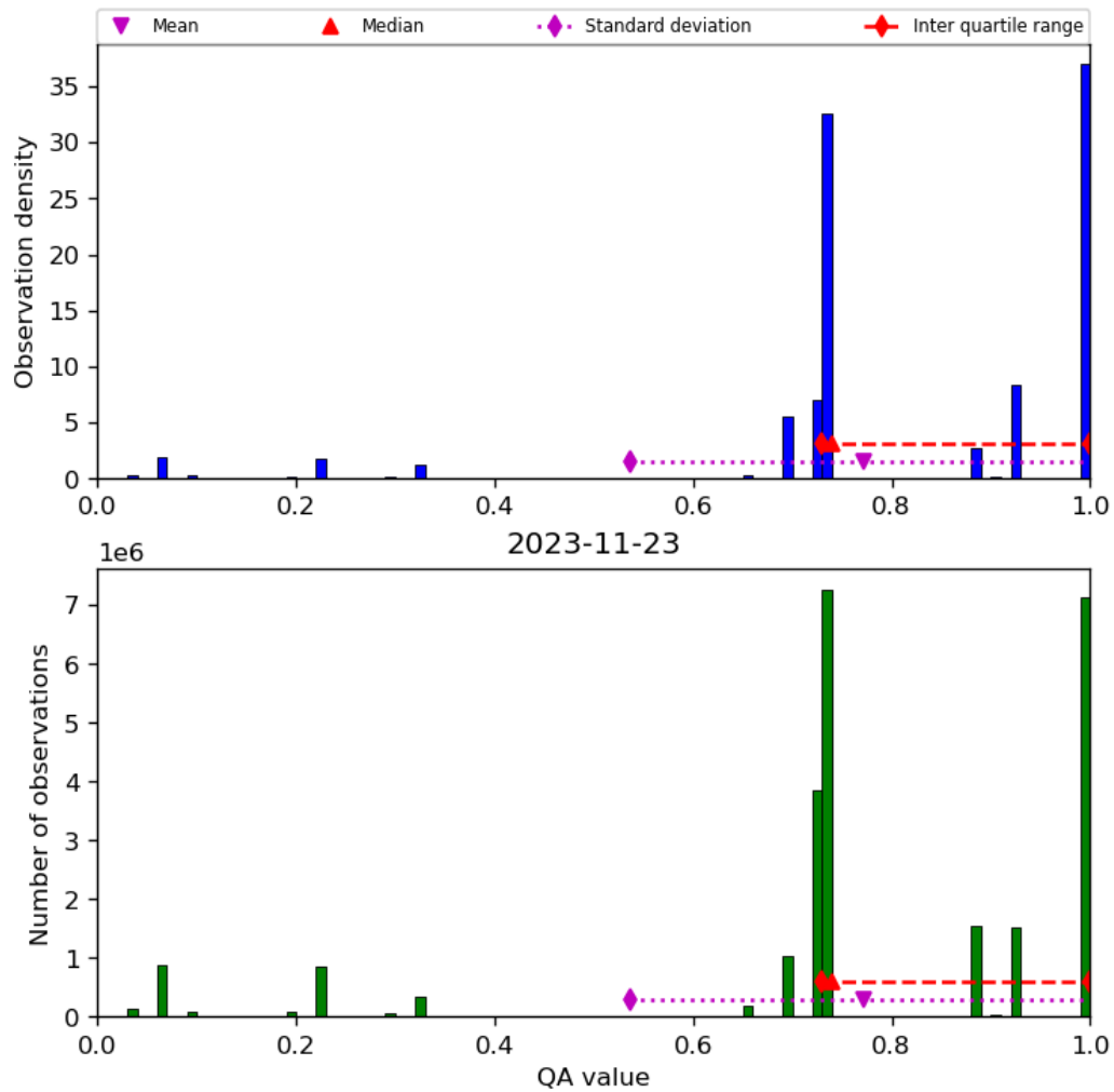
Figure 28: Histogram of “QA value” for 2023-11-23 to 2023-11-24
