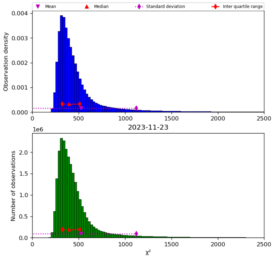
Figure 42: Histogram of “ \chi^2 ” for 2023-11-23 to 2023-11-24
