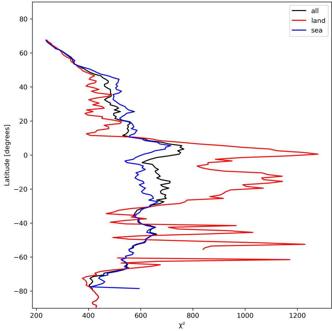
Figure 25: Zonal average of “ \chi^2 ” for 2023-11-23 to 2023-11-24.
