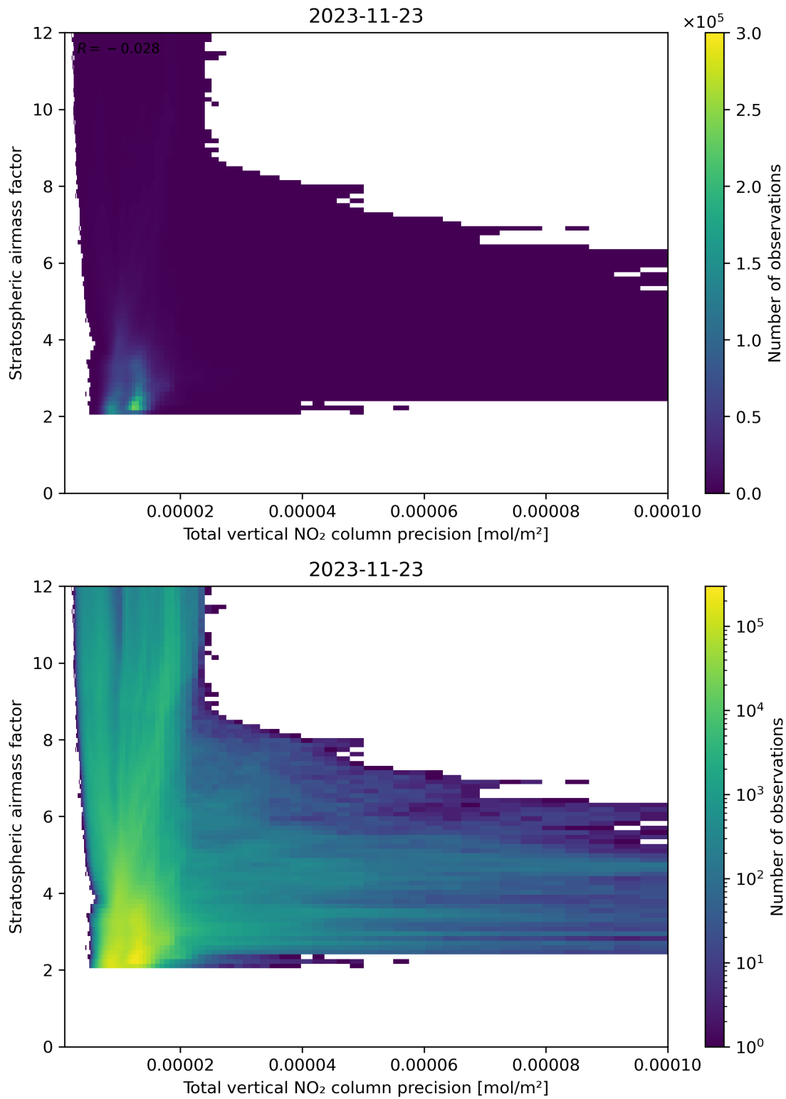
Figure 115: Scatter density plot of “Total vertical NO 2 column precision” against “Stratospheric air mass factor” for 2023-11-23 to 2023-11-24.
