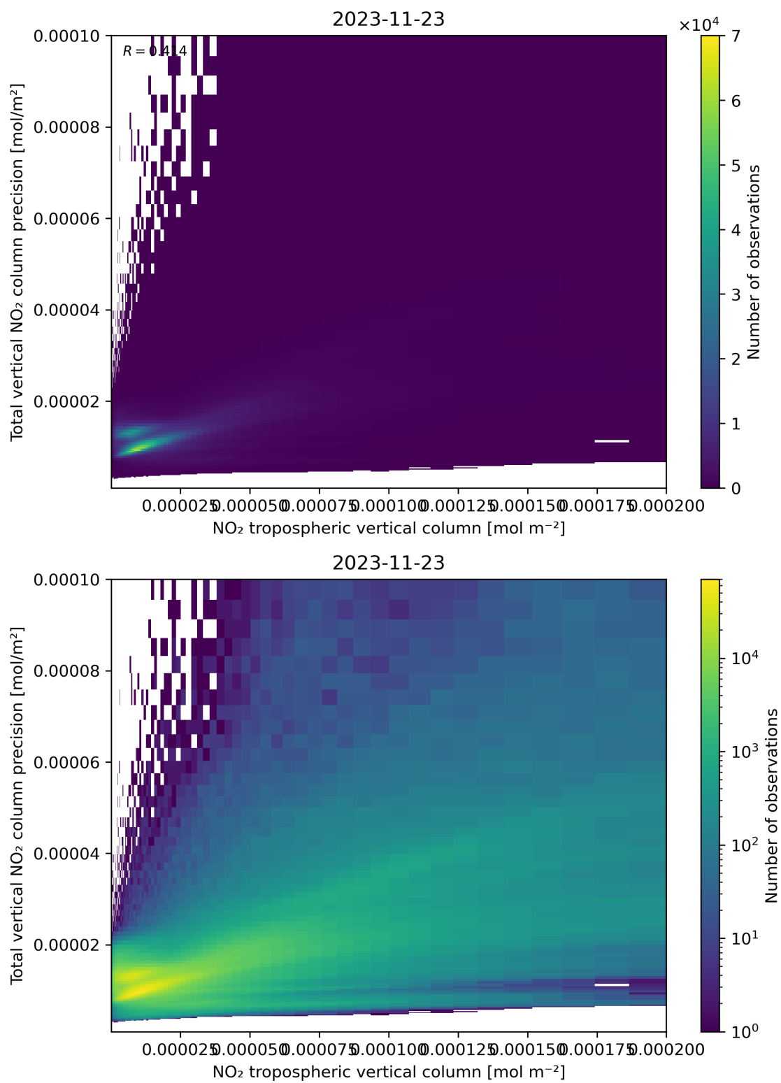
Figure 129: Scatter density plot of “NO 2 tropospheric vertical column” against “Total vertical NO 2 column precision” for 2023-11-23 to 2023-11-24.
