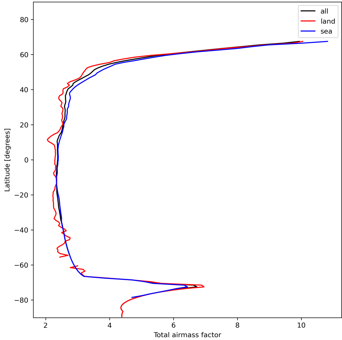
Figure 15: Zonal average of “Total airmass factor” for 2023-11-23 to 2023-11-24.
