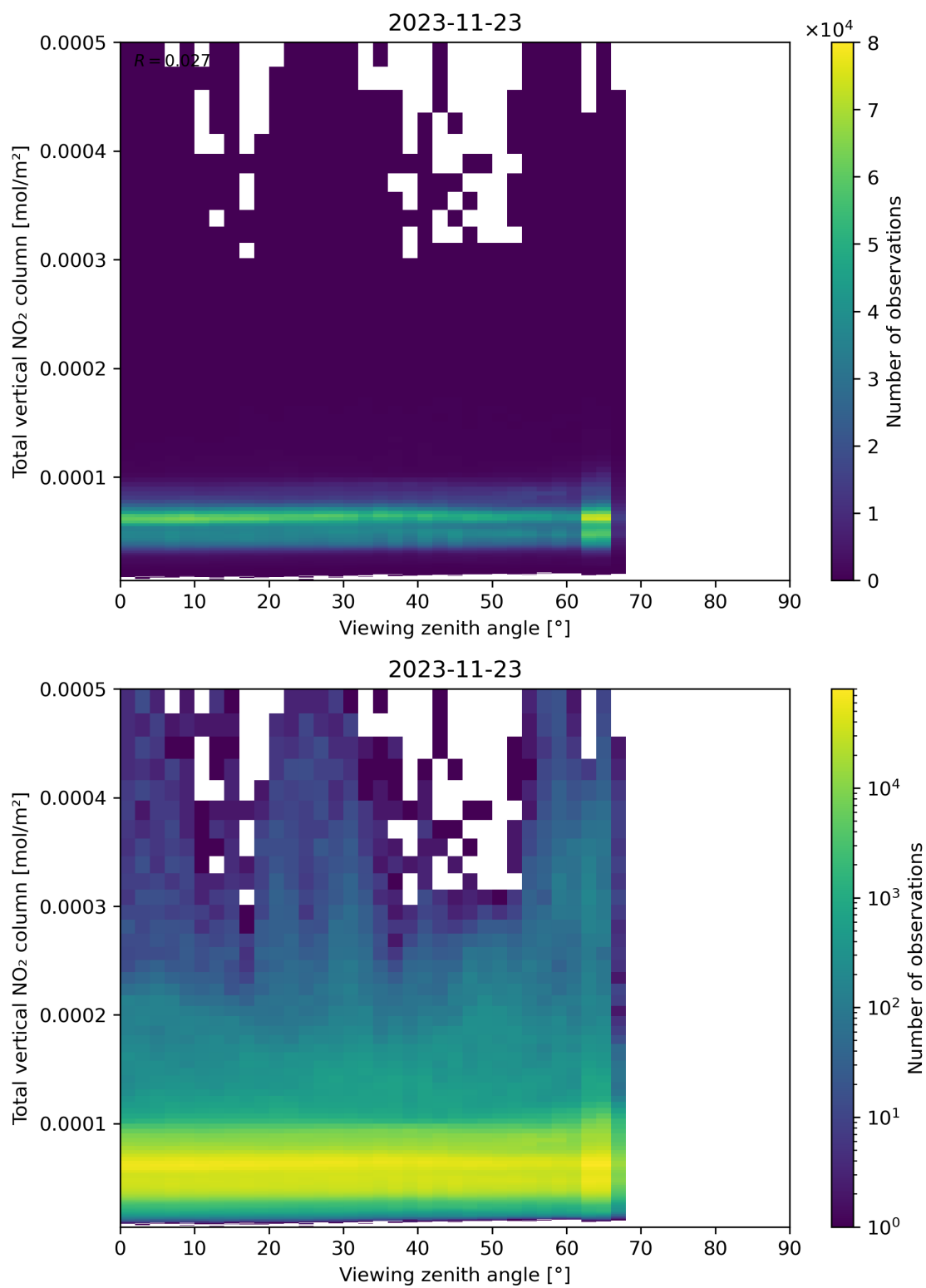
Figure 167: Scatter density plot of “Viewing zenith angle” against “Total vertical NO 2 column” for 2023-11-23 to 2023-11-24.
