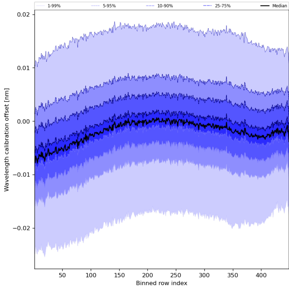
Figure 52: Along track statistics of “Wavelength calibration offset” for 2023-11-23 to 2023-11-24
