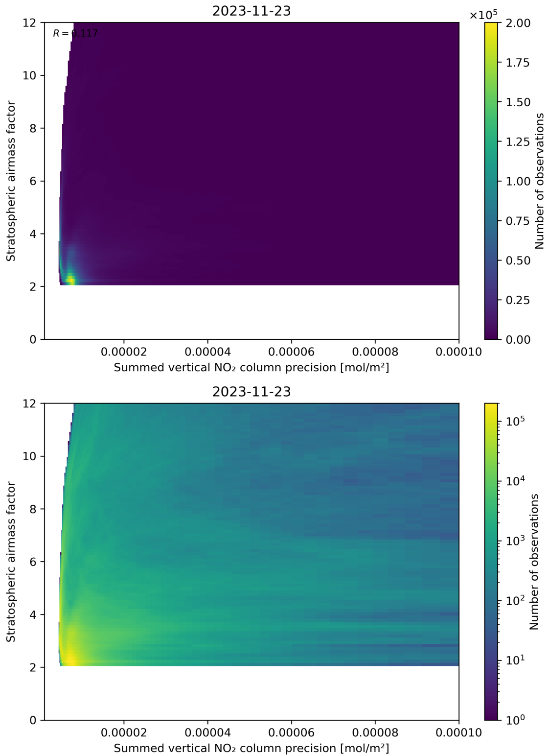
Figure 106: Scatter density plot of “Summed vertical NO 2 column precision” against “Stratospheric airmass factor” for 2023-11-23 to 2023-11-24.
