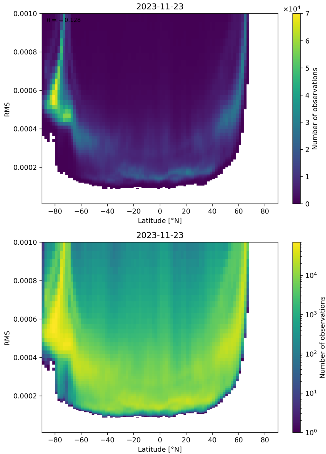
Figure 94: Scatter density plot of “Latitude” against “RMS” for 2023-11-23 to 2023-11-24.
