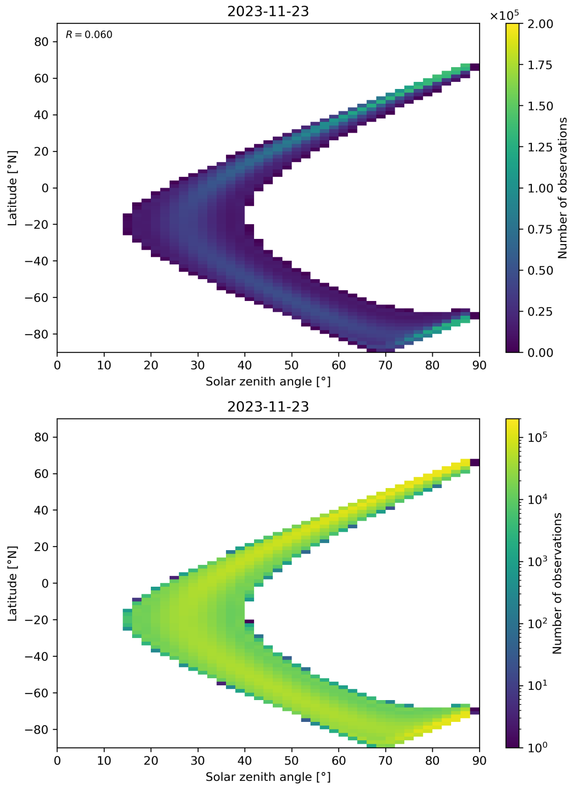
Figure 149: Scatter density plot of “Solar zenith angle” against “Latitude” for 2023-11-23 to 2023-11-24.
