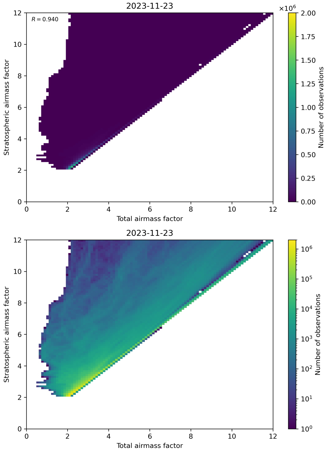
Figure 62: Scatter density plot of “Total airmass factor” against “Stratospheric airmass factor” for 2023-11-23 to 2023-11-24.
