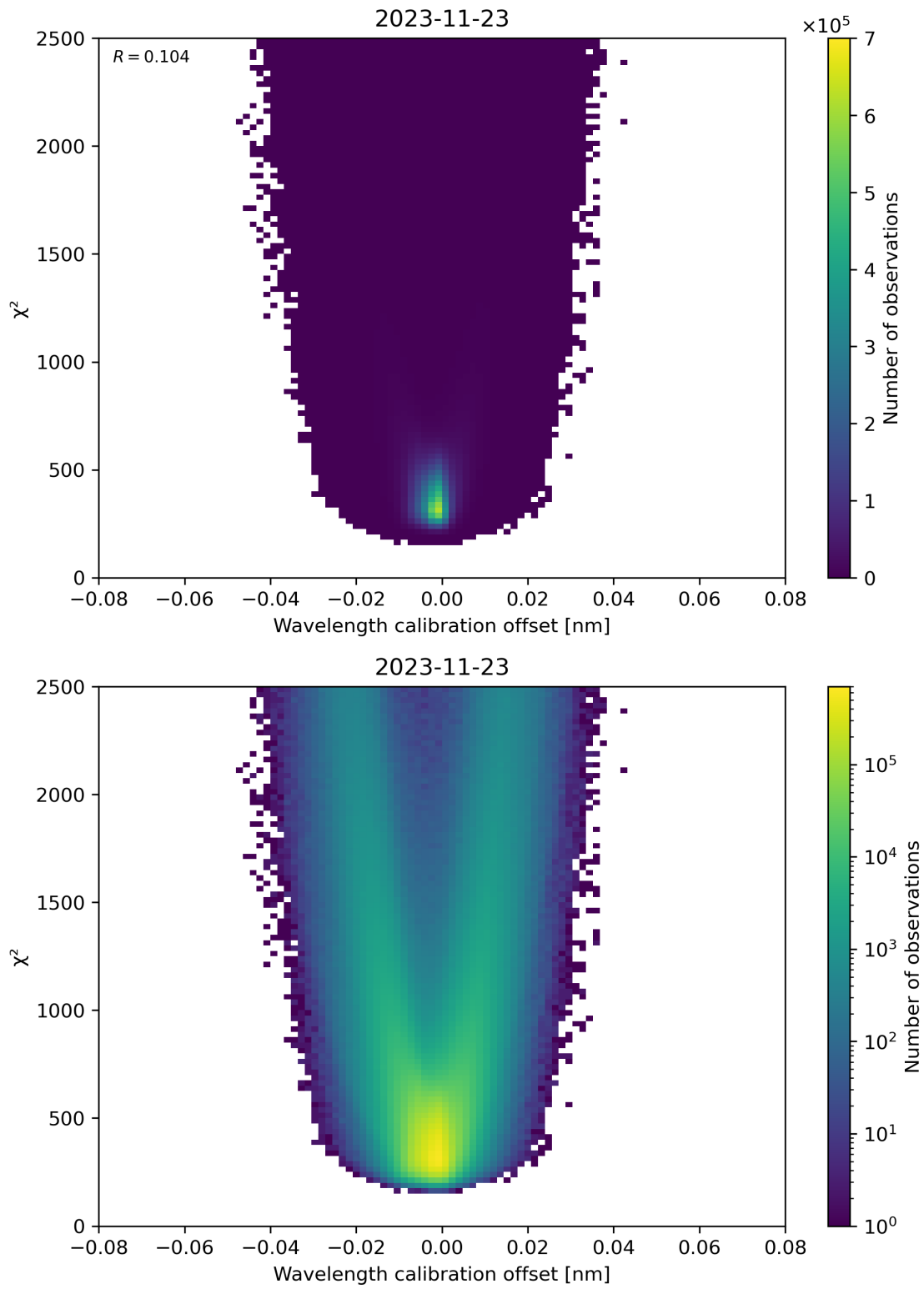
Figure 175: Scatter density plot of “Wavelength calibration offset” against “ \chi^2 ” for 2023-11-23 to 2023-11-24.
