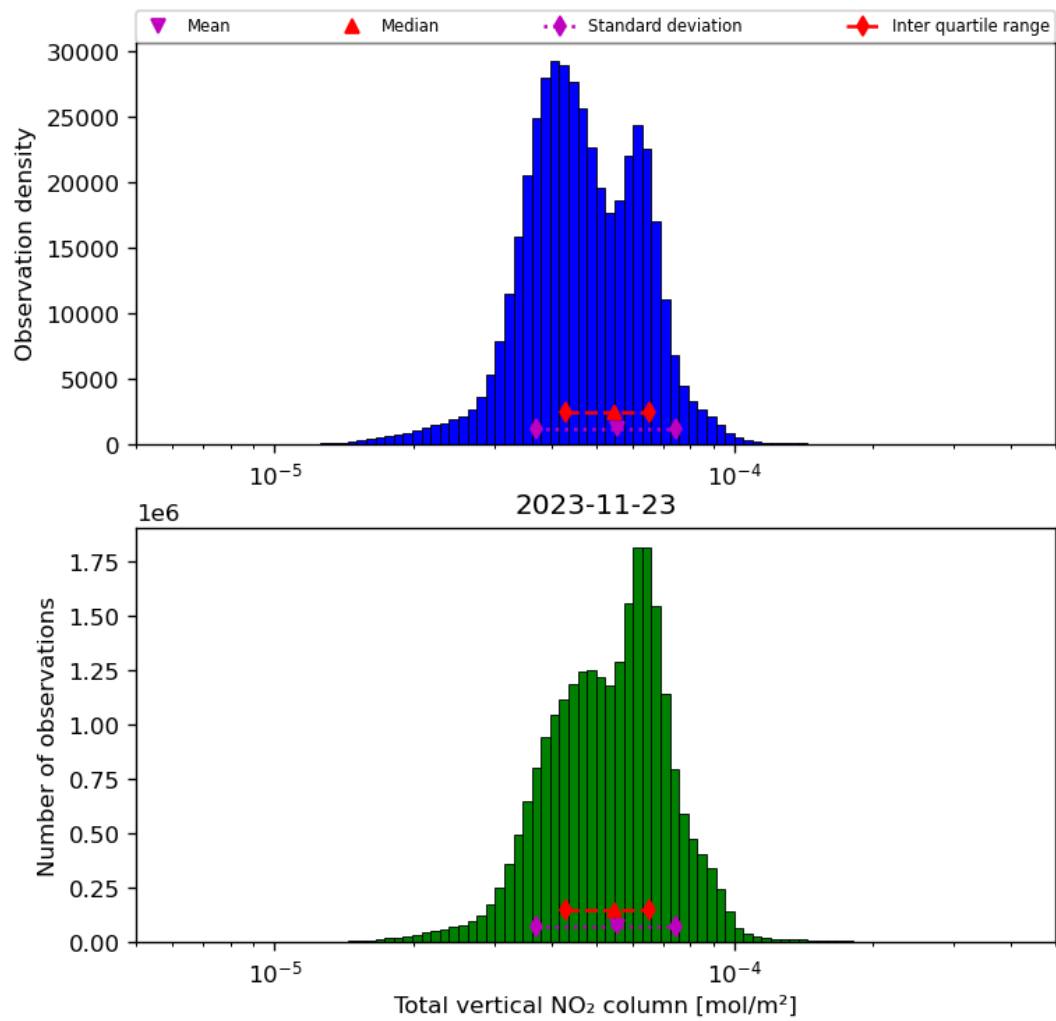
Figure 38: Histogram of “Total vertical NO 2 column” for 2023-11-23 to 2023-11-24
