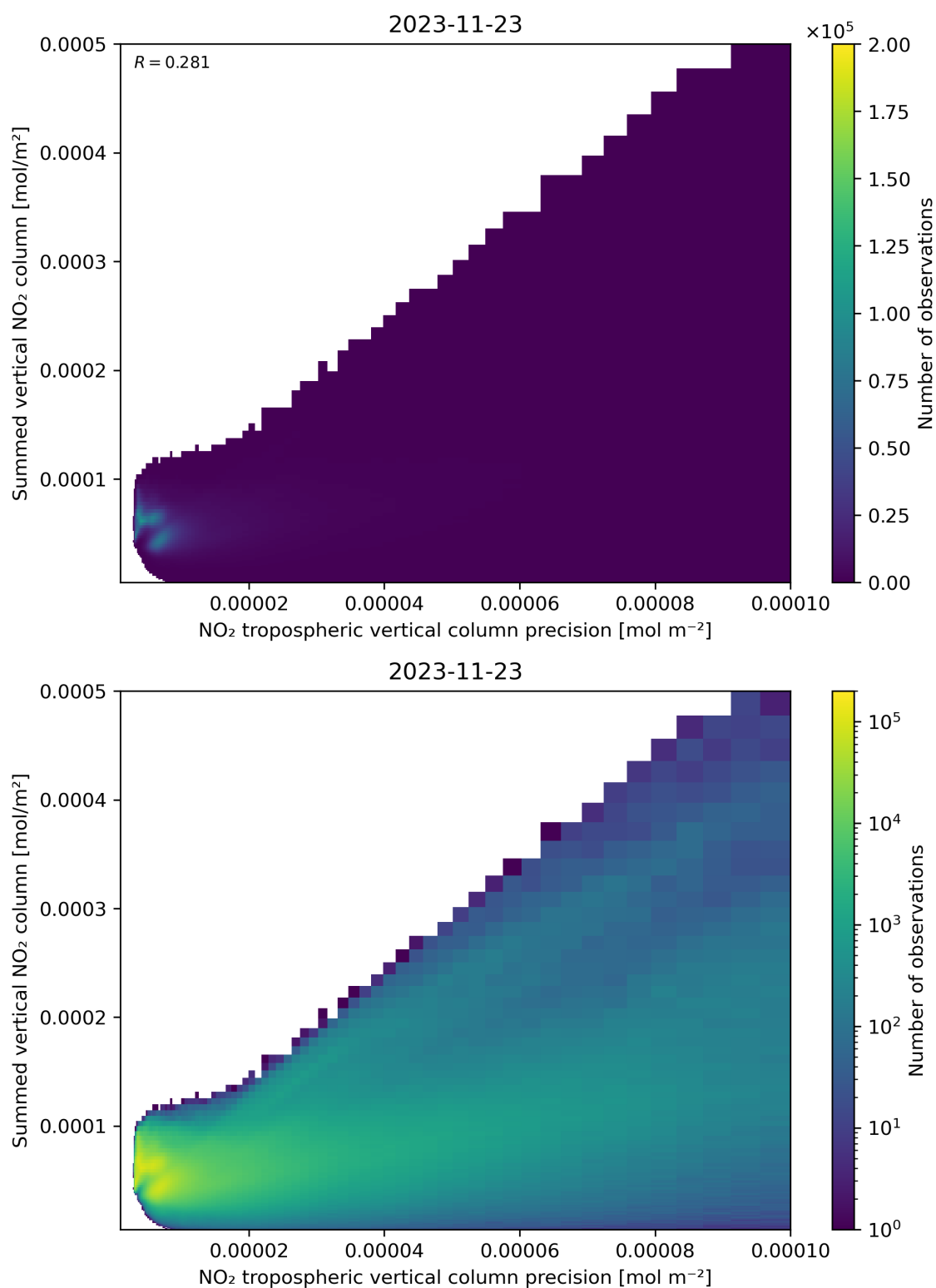
Figure 136: Scatter density plot of “NO 2 tropospheric vertical column precision” against “Summed vertical NO 2 column” for 2023-11-23 to 2023-11-24.
