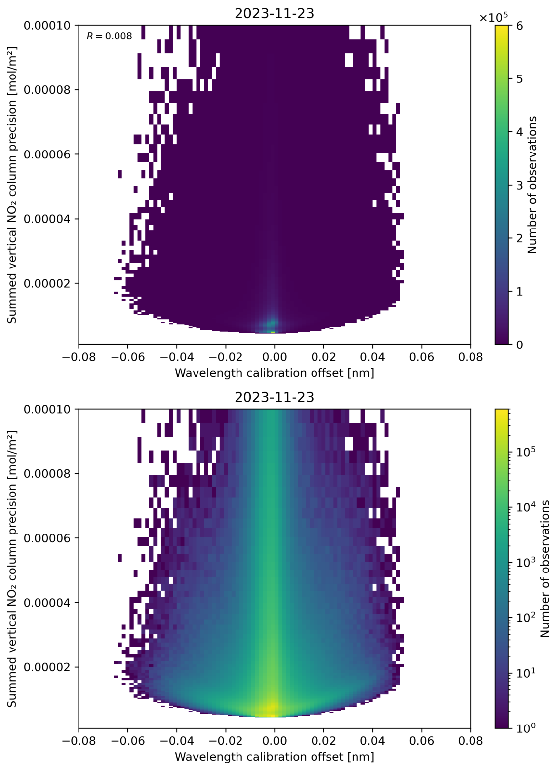
Figure 178: Scatter density plot of “Wavelength calibration offset” against “Summed vertical NO 2 column precision” for 2023-11-23 to 2023-11-24.
