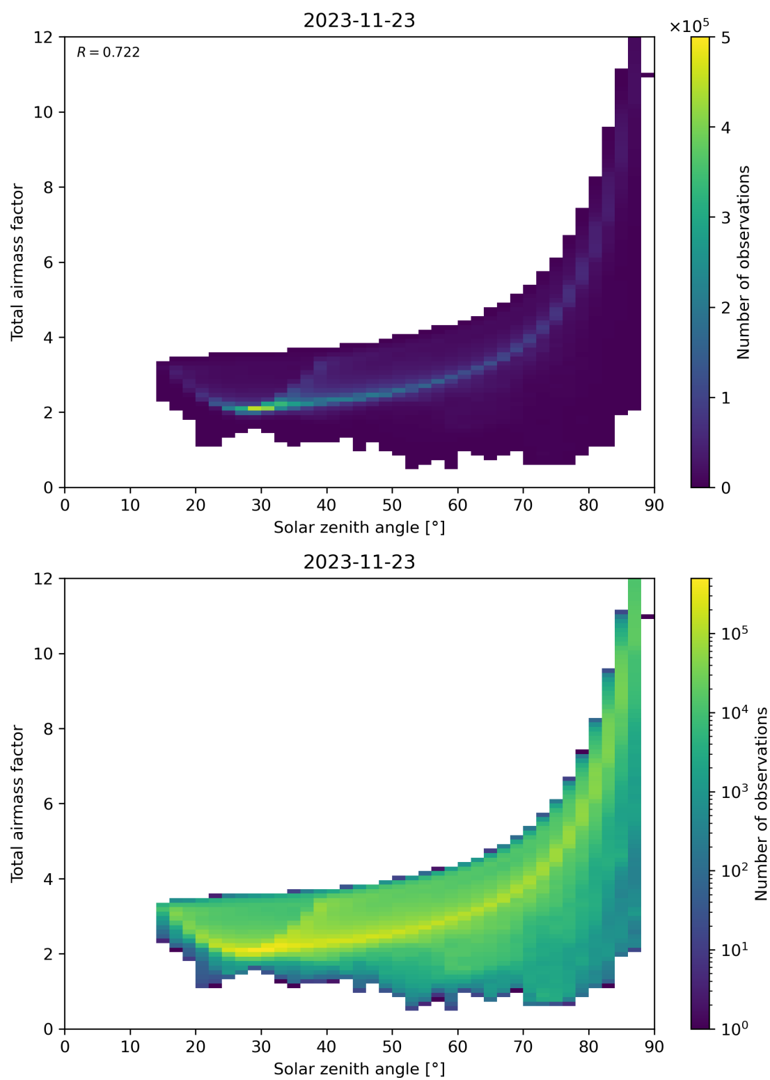
Figure 146: Scatter density plot of “Solar zenith angle” against “Total airmass factor” for 2023-11-23 to 2023-11-24.
