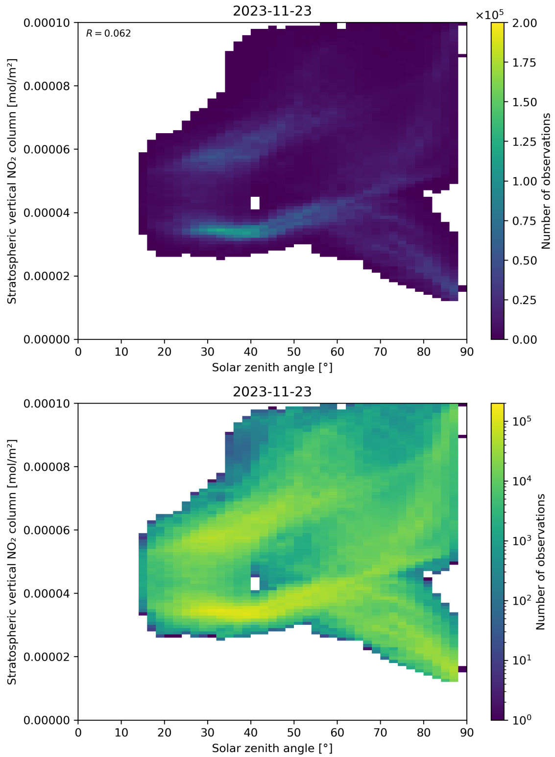
Figure 150: Scatter density plot of “Solar zenith angle” against “Stratospheric vertical NO 2 column” for 2023-11-23 to 2023-11-24.
