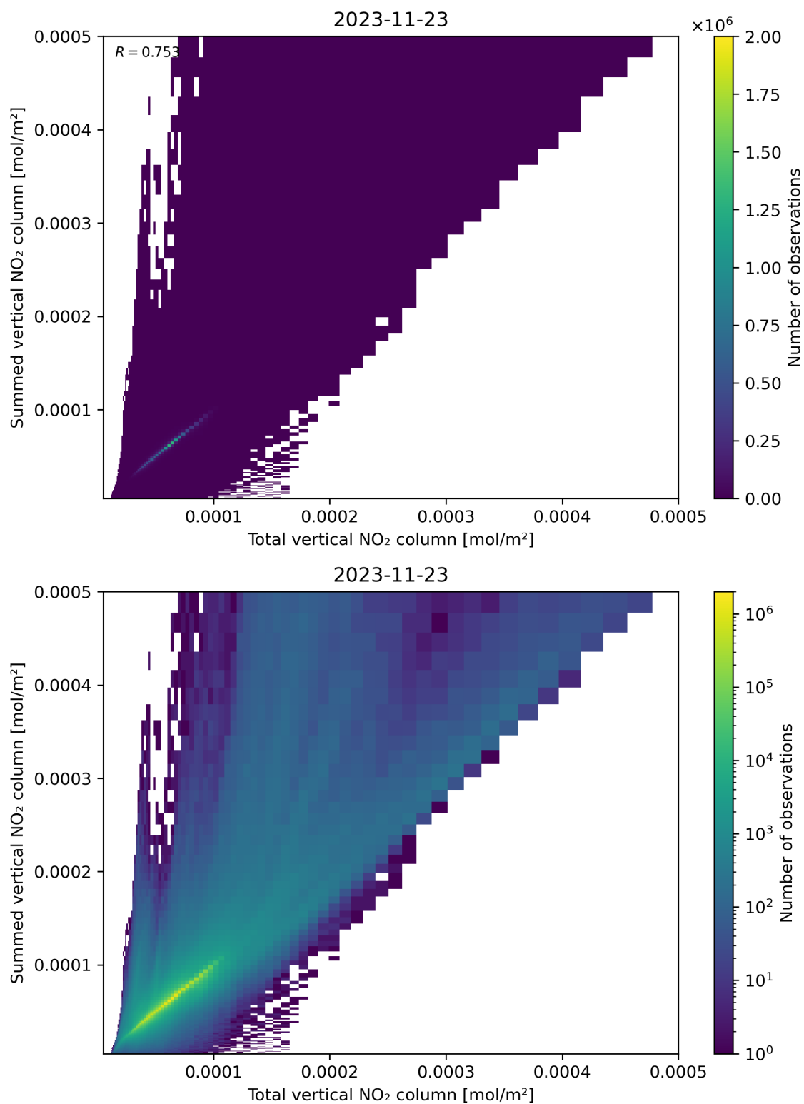
Figure 112: Scatter density plot of “Total vertical NO 2 column” against “Summed vertical NO 2 column” for 2023-11-23 to 2023-11-24.
