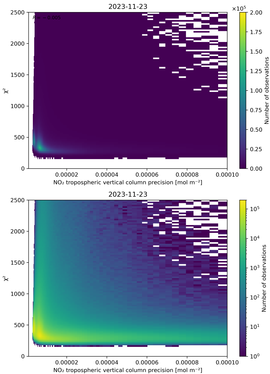
Figure 134: Scatter density plot of “NO 2 tropospheric vertical column precision” against “ \chi^2 ” for 2023-11-23 to 2023-11-24.
