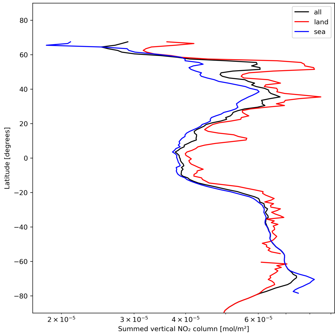
Figure 23: Zonal average of “Summed vertical NO 2 column” for 2023-11-23 to 2023-11-24.
