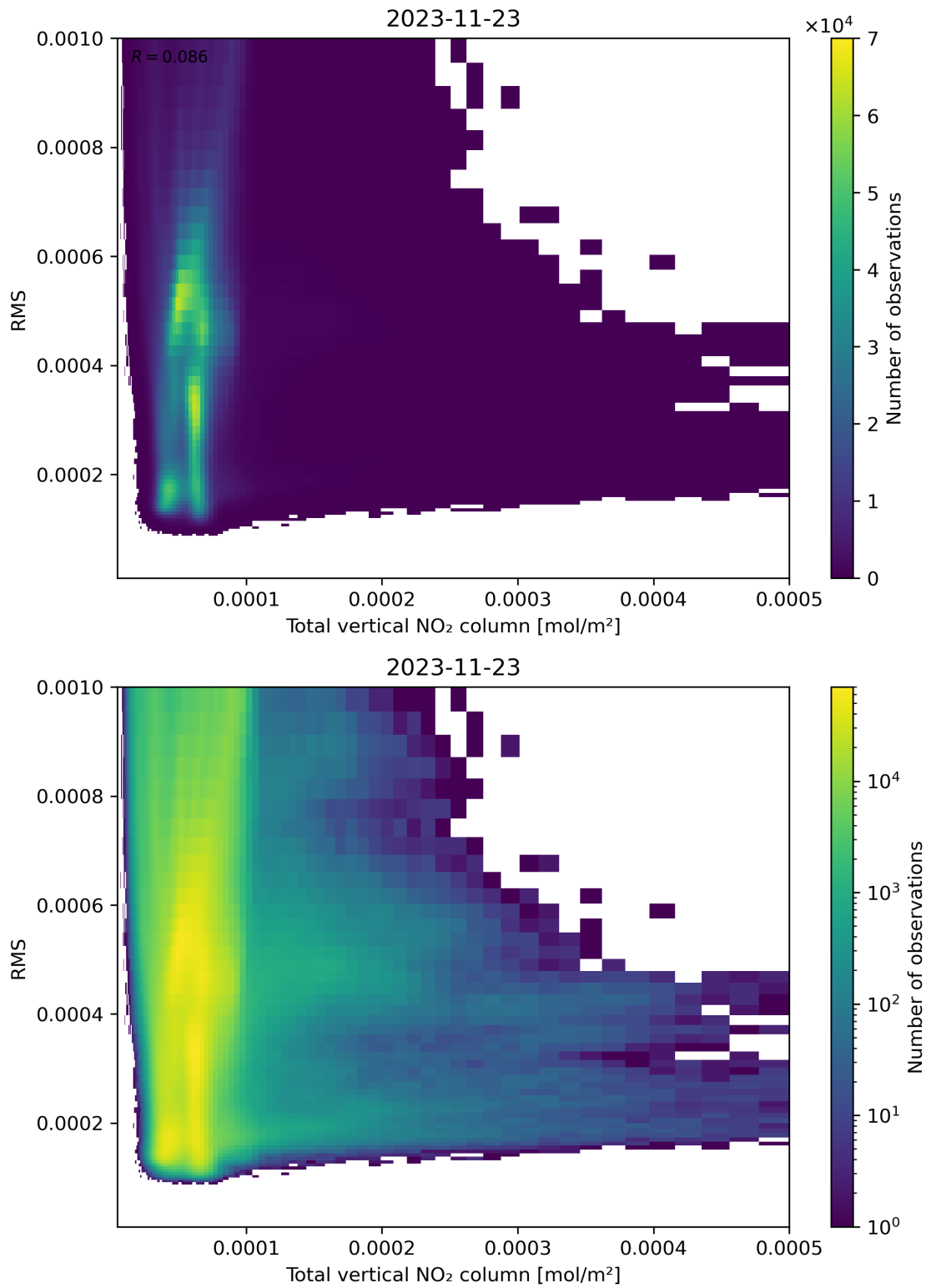
Figure 120: Scatter density plot of “Total vertical NO 2 column” against “RMS” for 2023-11-23 to 2023-11-24.
