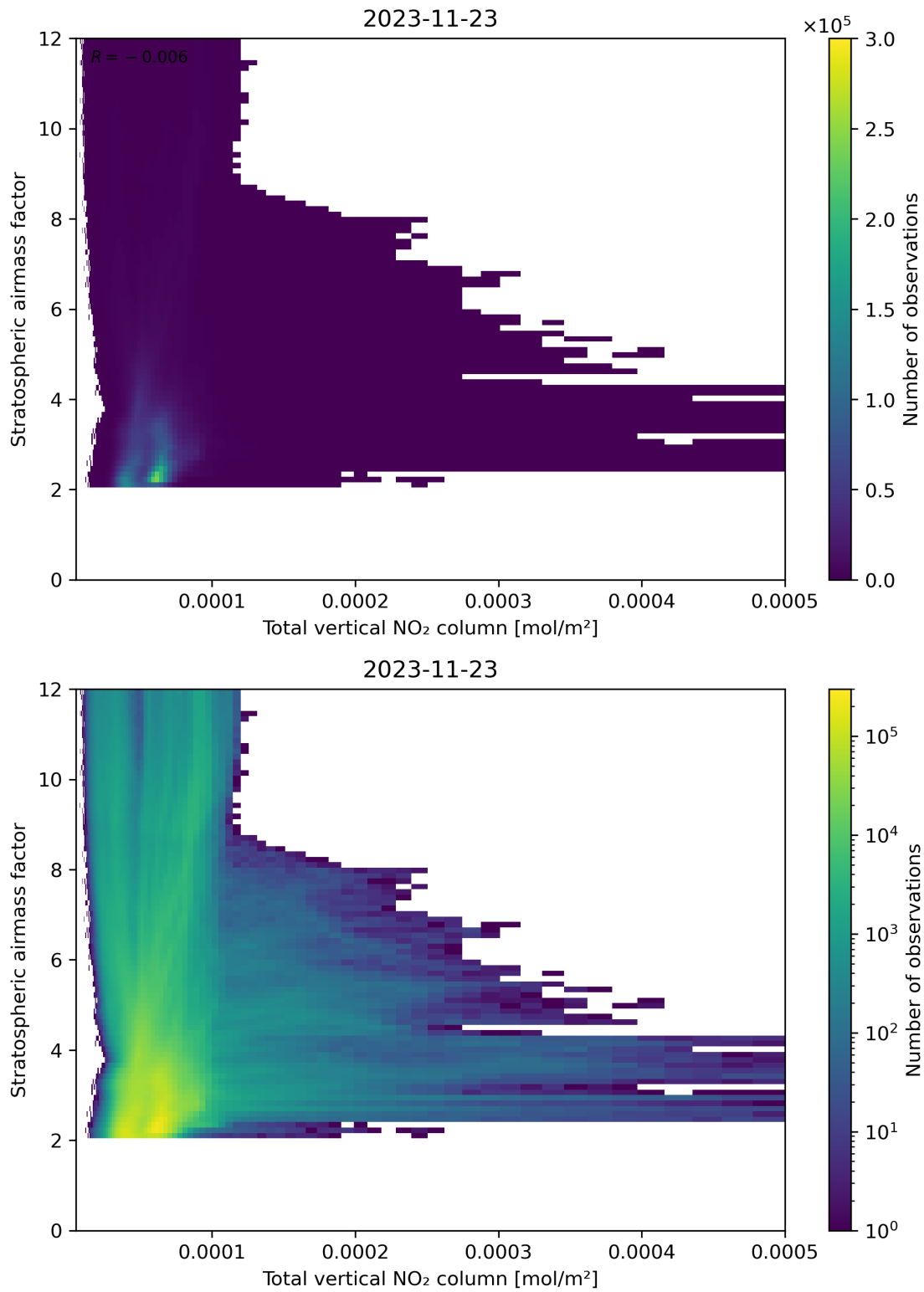
Figure 110: Scatter density plot of “Total vertical NO 2 column” against “Stratospheric airmass factor” for 2023-11-23 to 2023-11-24.
