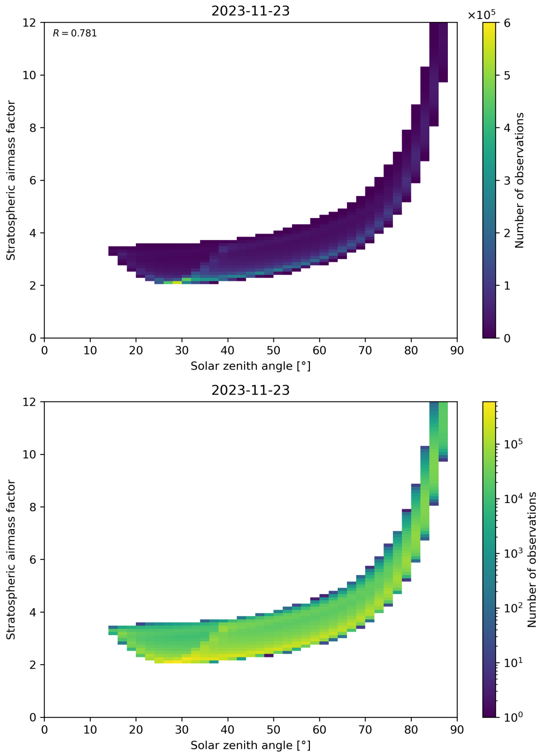
Figure 145: Scatter density plot of “Solar zenith angle” against “Stratospheric airmass factor” for 2023-11-23 to 2023-11-24.
