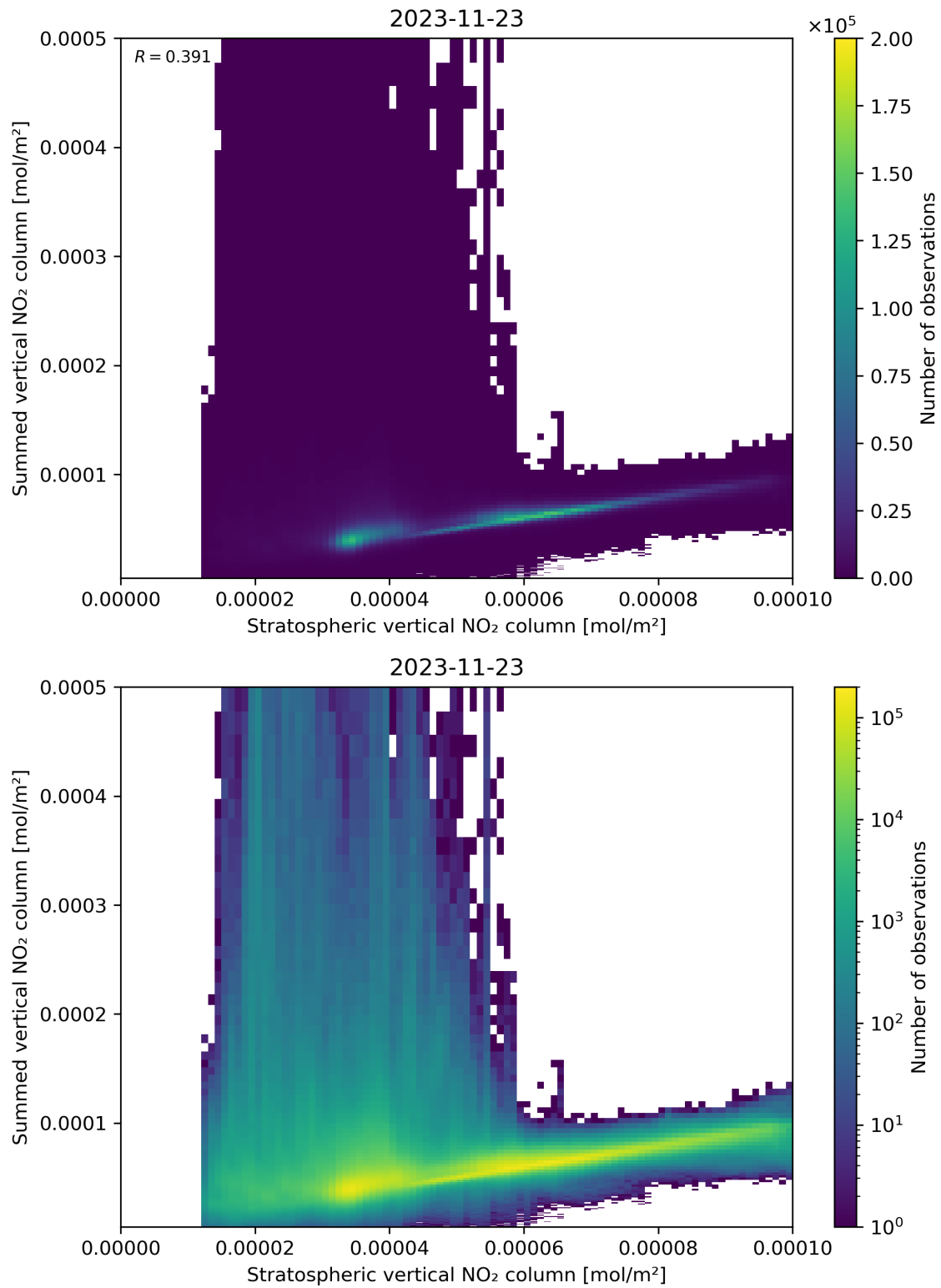
Figure 98: Scatter density plot of “Stratospheric vertical NO 2 column” against “Summed vertical NO 2 column” for 2023-11-23 to 2023-11-24.
