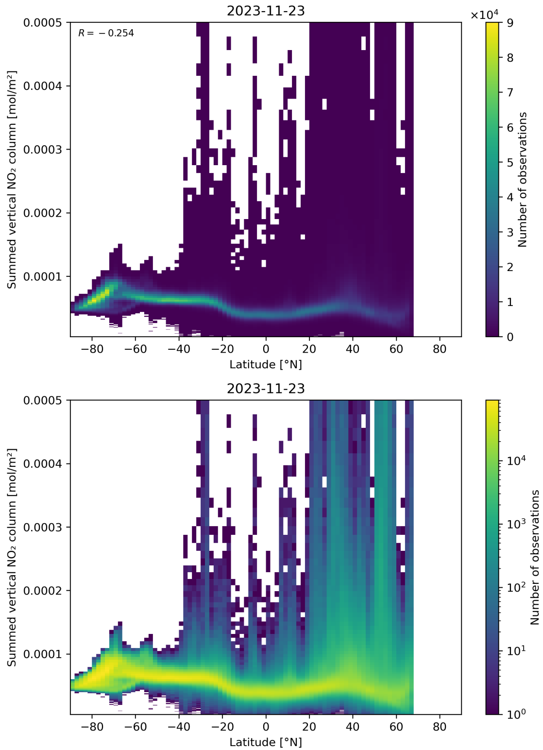
Figure 88: Scatter density plot of “Latitude” against “Summed vertical NO 2 column” for 2023-11-23 to 2023-11-24.
