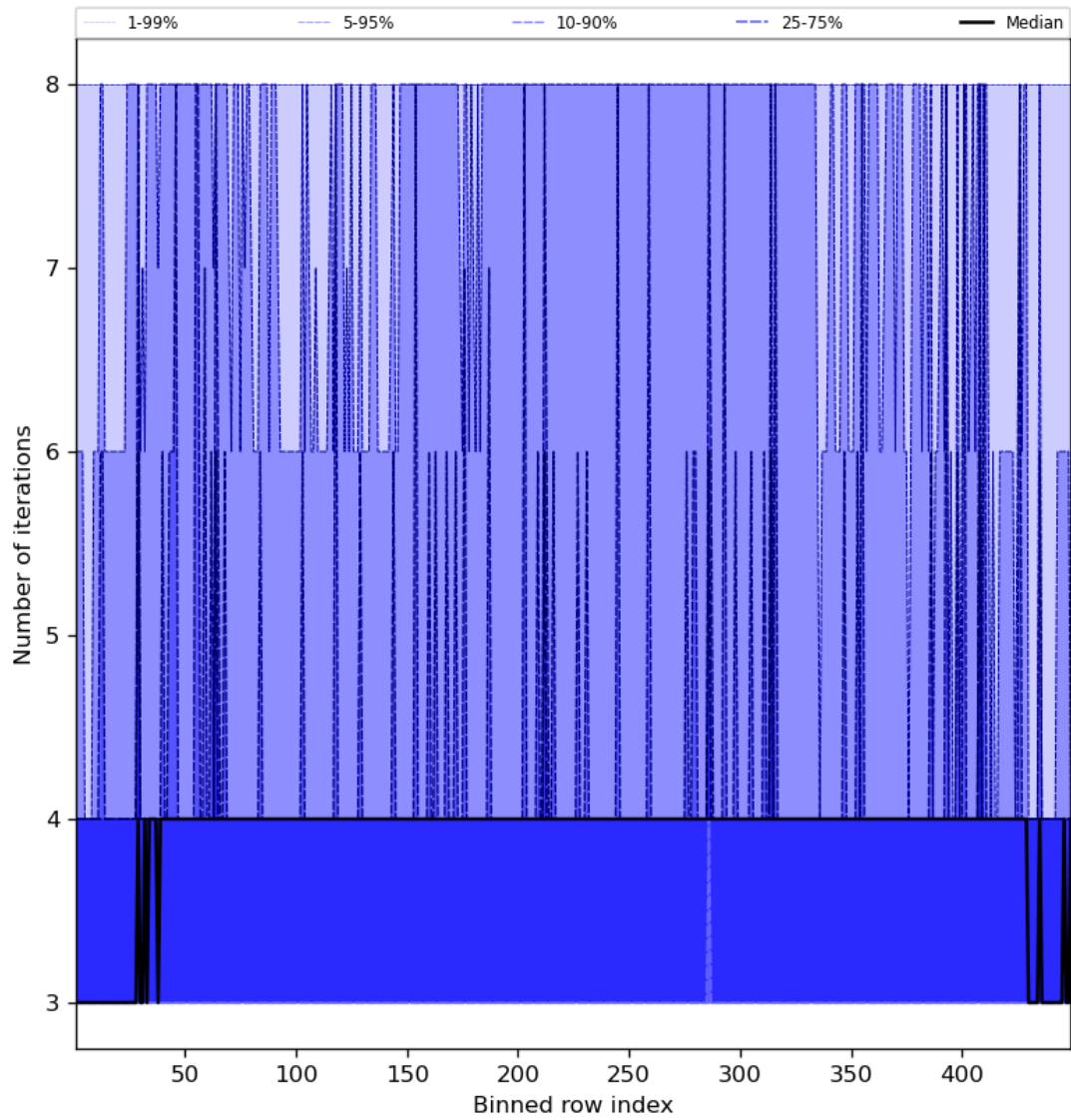
Figure 51: Along track statistics of “Number of iterations” for 2023-11-23 to 2023-11-24
