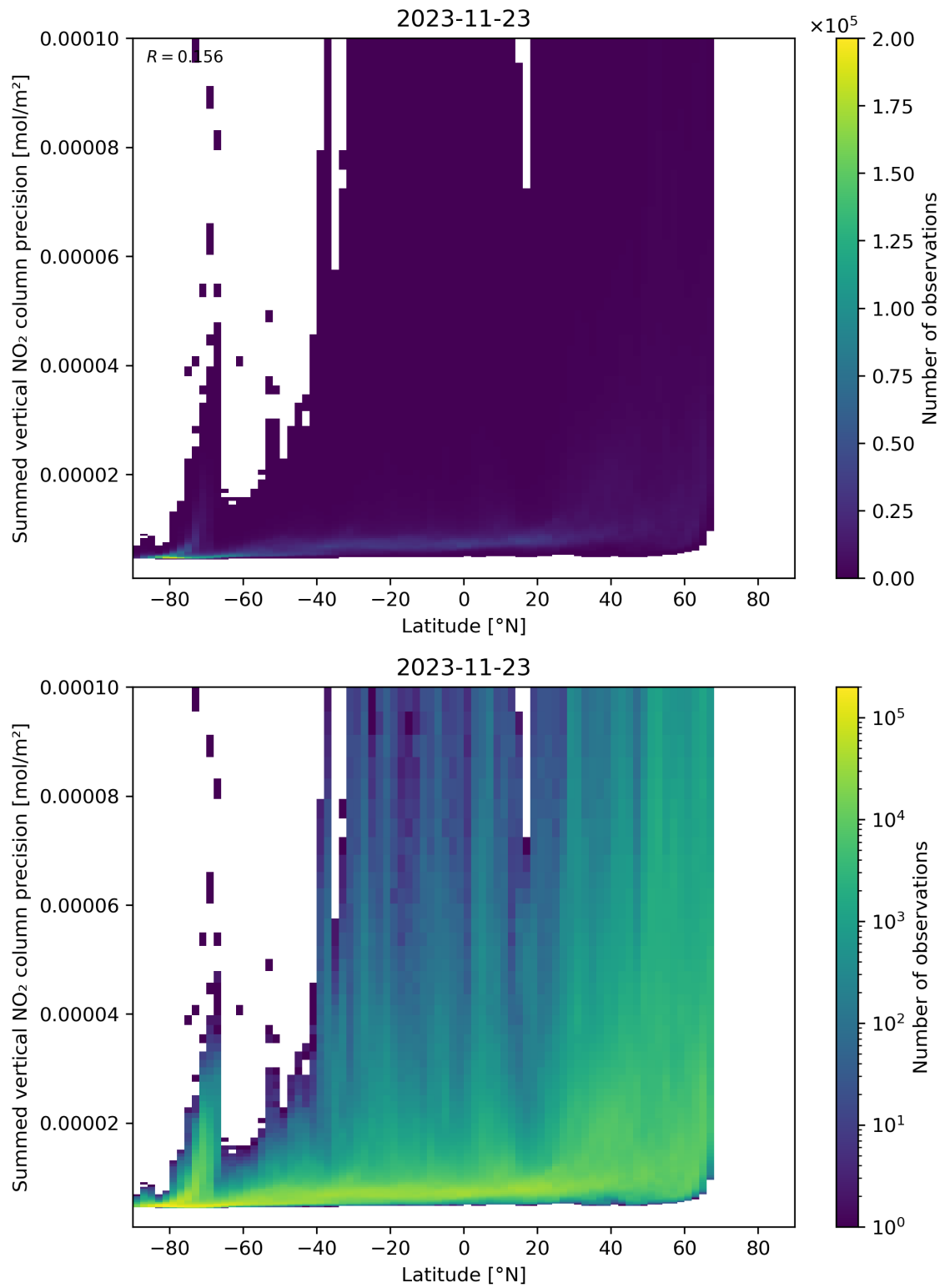
Figure 89: Scatter density plot of “Latitude” against “Summed vertical NO 2 column precision” for 2023-11-23 to 2023-11-24.
