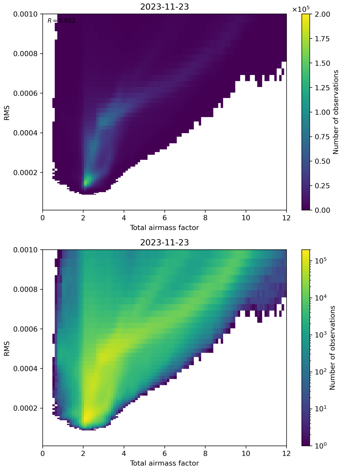
Figure 69: Scatter density plot of “Total airmass factor” against “RMS” for 2023-11-23 to 2023-11-24.
