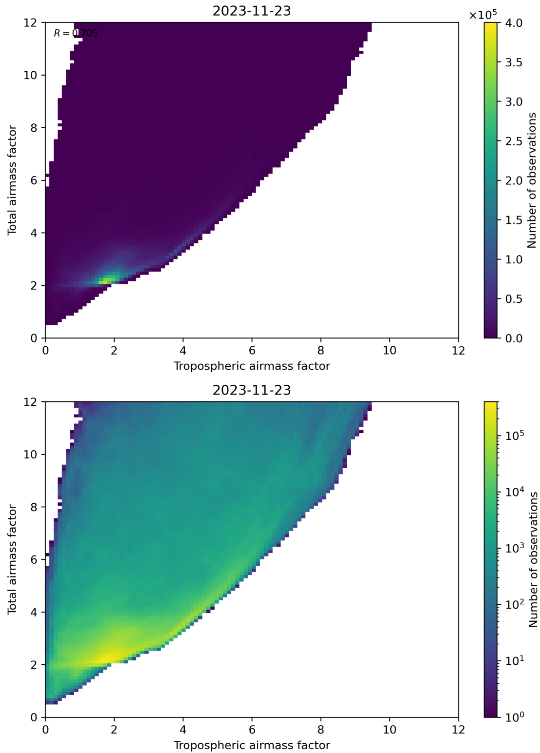
Figure 72: Scatter density plot of “Tropospheric airmass factor” against “Total airmass factor” for 2023-11-23 to 2023-11-24.
