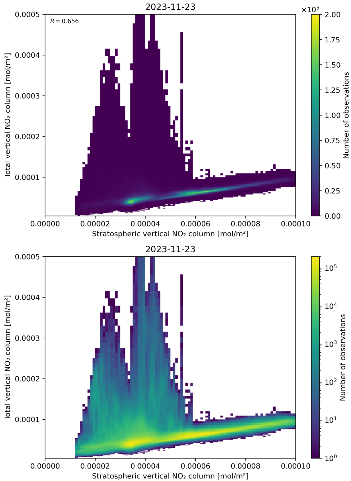
Figure 100: Scatter density plot of “Stratospheric vertical NO 2 column” against “Total vertical NO 2 column” for 2023-11-23 to 2023-11-24.
