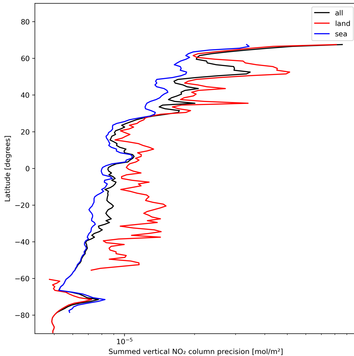
Figure 24: Zonal average of “Summed vertical NO 2 column precision” for 2023-11-23 to 2023-11-24.
