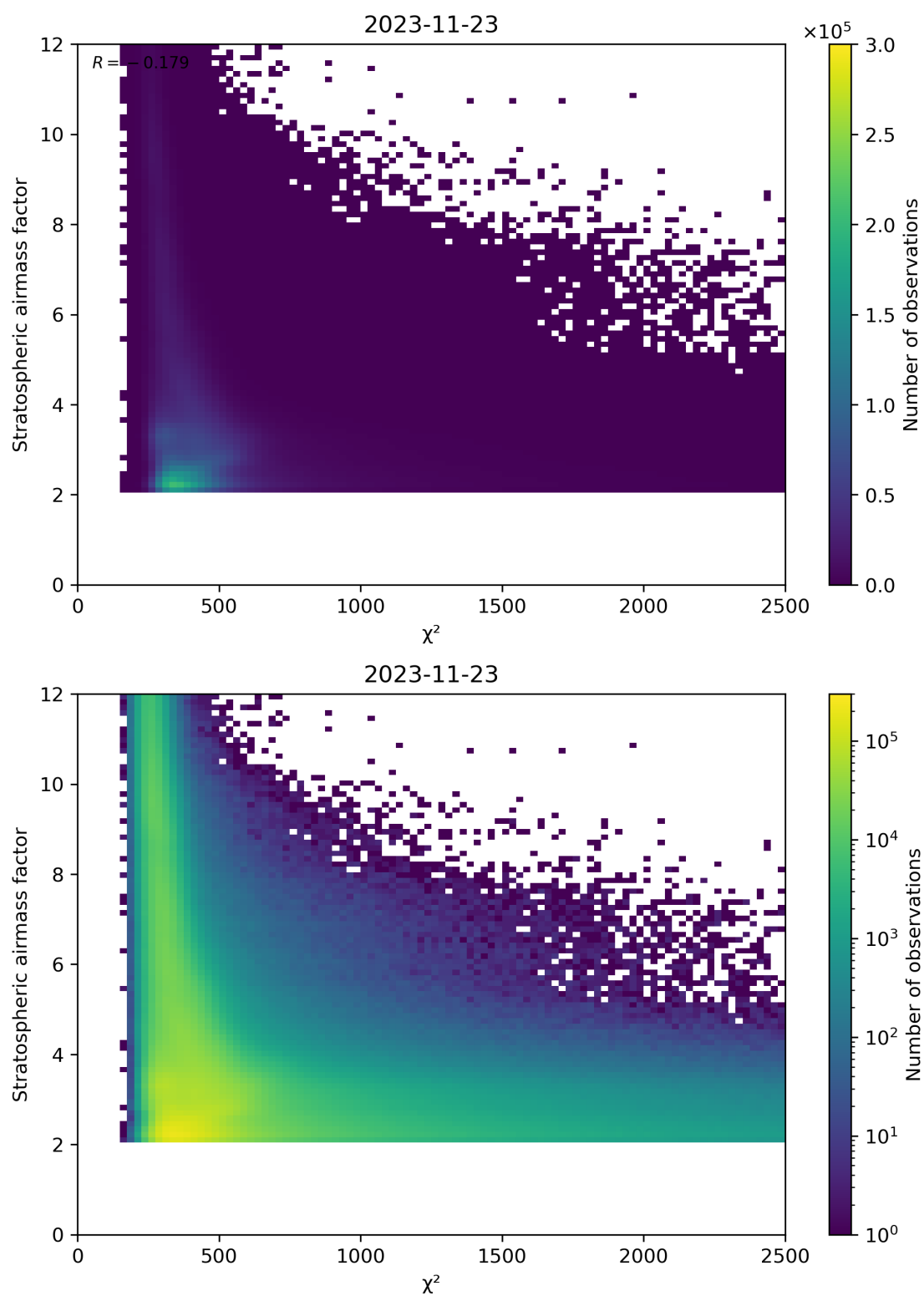
Figure 81: Scatter density plot of “ \chi^2 ” against “Stratospheric airmass factor” for 2023-11-23 to 2023-11-24.
