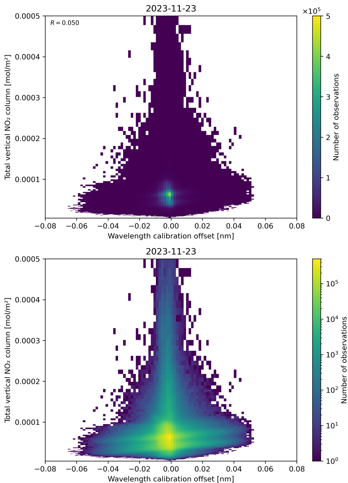
Figure 179: Scatter density plot of “Wavelength calibration offset” against “Total vertical NO 2 column” for 2023-11-23 to 2023-11-24.
