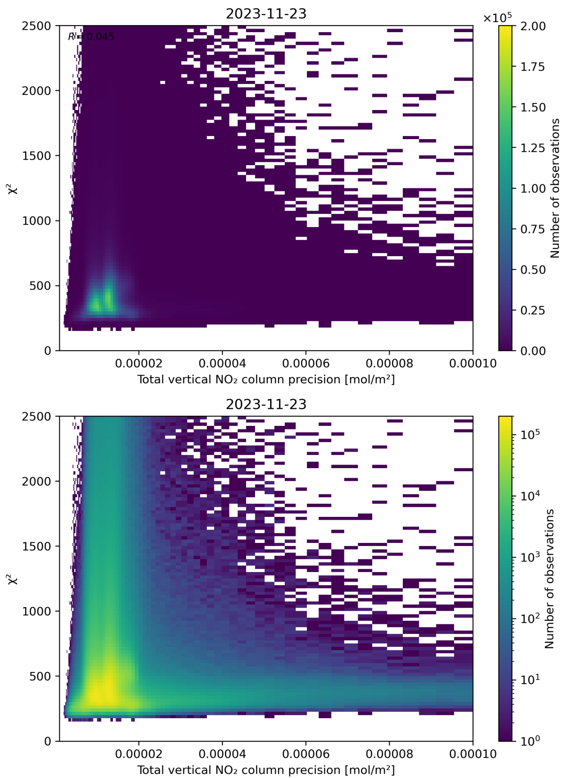
Figure 116: Scatter density plot of “Total vertical NO 2 column precision” against “ \chi^2 ” for 2023-11-23 to 2023-11-24.
