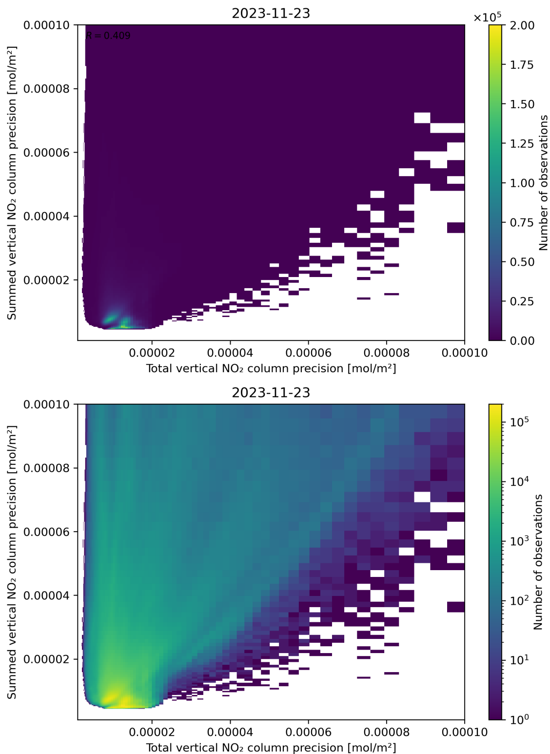
Figure 118: Scatter density plot of “Total vertical NO 2 column precision” against “Summed vertical NO 2 column precision” for 2023-11-23 to 2023-11-24.
