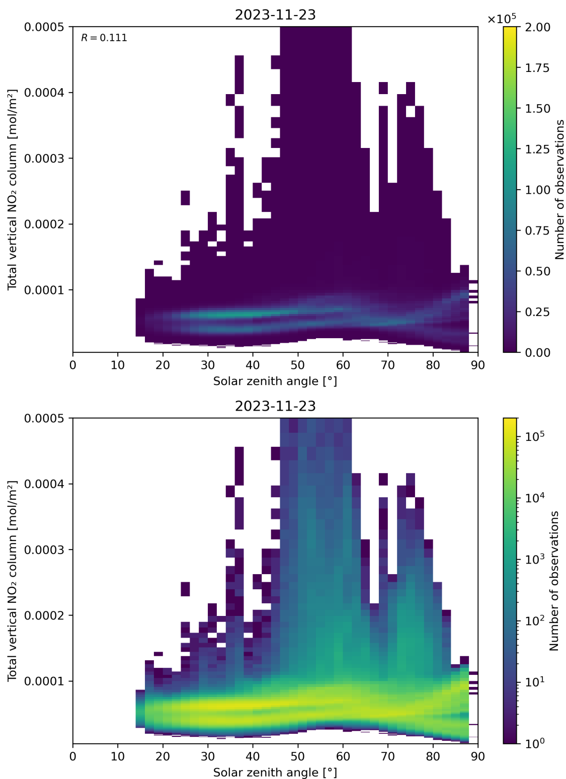
Figure 153: Scatter density plot of “Solar zenith angle” against “Total vertical NO 2 column” for 2023-11-23 to 2023-11-24.
