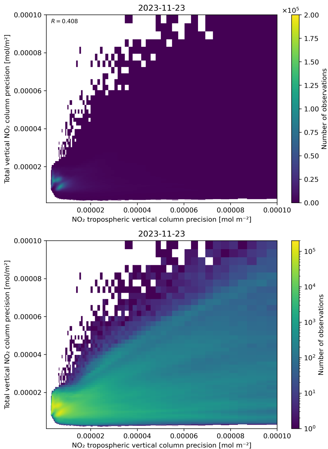
Figure 139: Scatter density plot of “NO 2 tropospheric vertical column precision” against “Total vertical NO 2 column precision” for 2023-11-23 to 2023-11-24.
