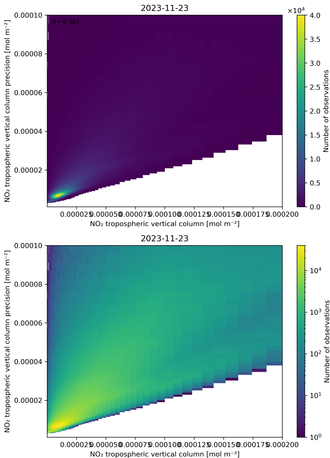
Figure 130: Scatter density plot of “NO 2 tropospheric vertical column” against “NO 2 tropospheric vertical column precision” for 2023-11-23 to 2023-11-24.
