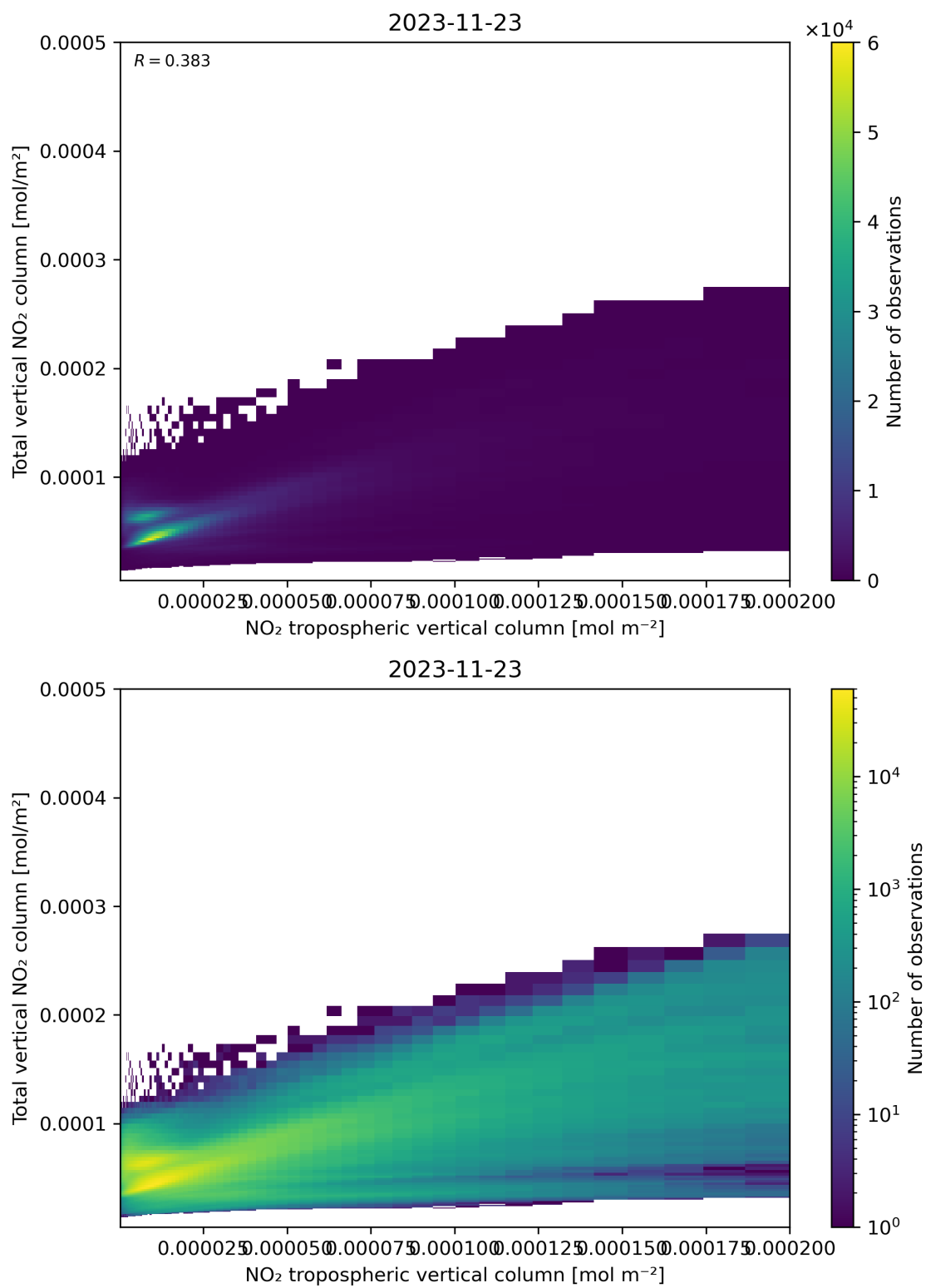
Figure 128: Scatter density plot of “NO 2 tropospheric vertical column” against “Total vertical NO 2 column” for 2023-11-23 to 2023-11-24.
