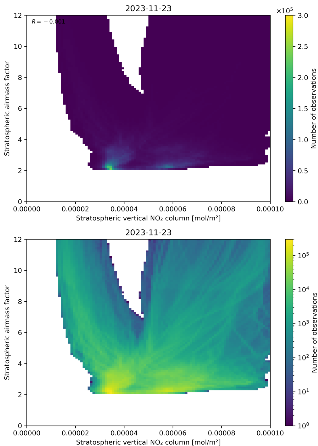
Figure 96: Scatter density plot of “Stratospheric vertical NO 2 column” against “Stratospheric airmass factor” for 2023-11-23 to 2023-11-24.
