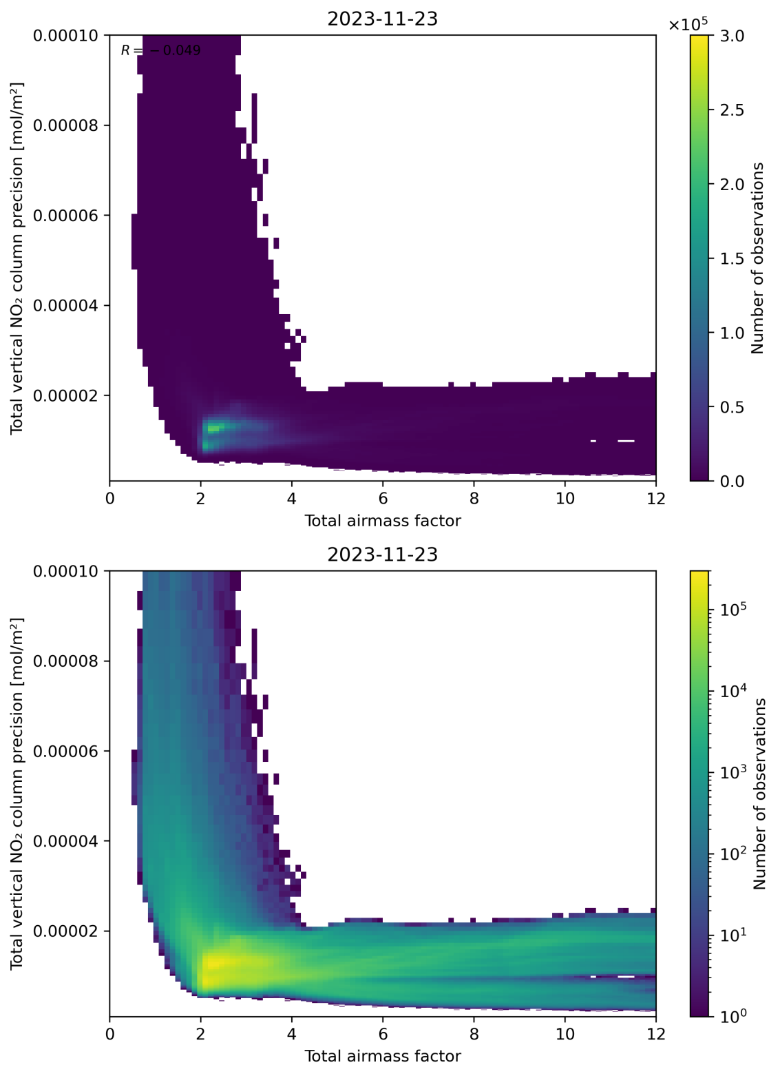
Figure 68: Scatter density plot of “Total airmass factor” against “Total vertical NO 2 column precision” for 2023-11-23 to 2023-11-24.
