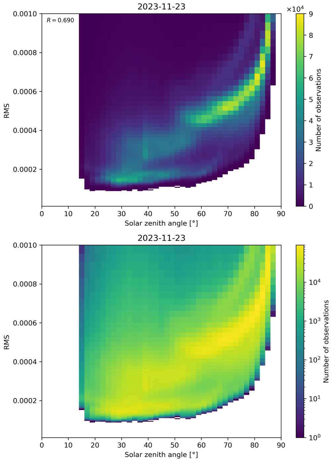
Figure 157: Scatter density plot of “Solar zenith angle” against “RMS” for 2023-11-23 to 2023-11-24.
