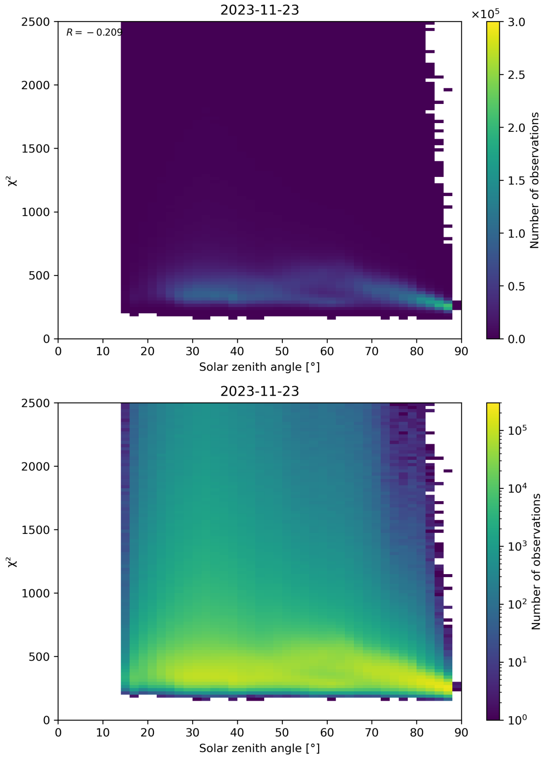
Figure 148: Scatter density plot of “Solar zenith angle” against “ \chi^2 ” for 2023-11-23 to 2023-11-24.
