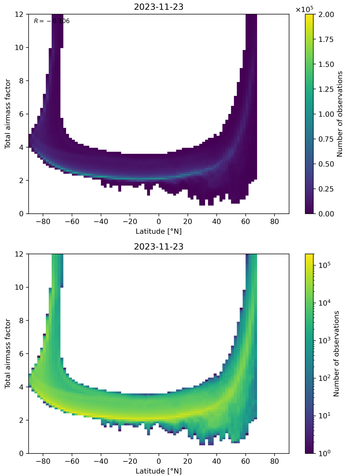
Figure 84: Scatter density plot of “Latitude” against “Total airmass factor” for 2023-11-23 to 2023-11-24.
