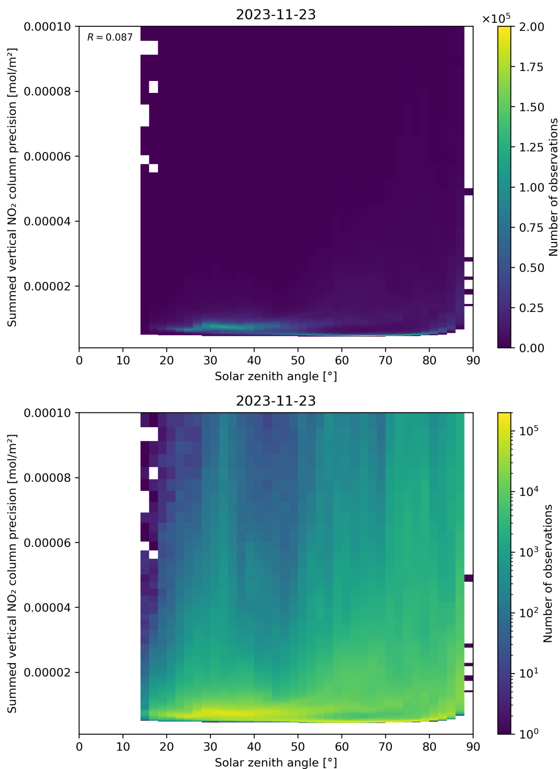
Figure 152: Scatter density plot of “Solar zenith angle” against “Summed vertical NO 2 column precision” for 2023-11-23 to 2023-11-24.
