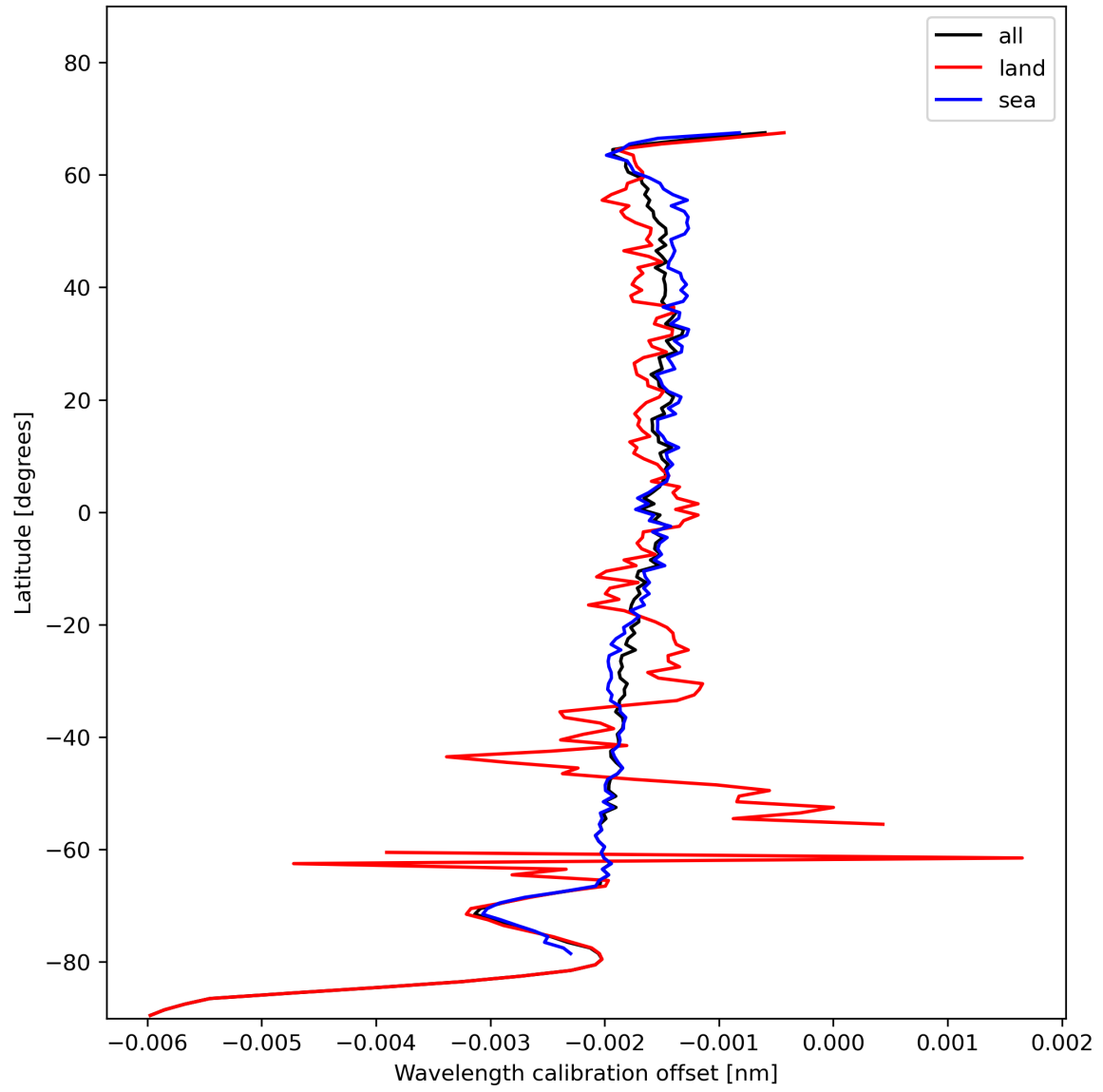
Figure 18: Zonal average of “Wavelength calibration offset” for 2023-11-23 to 2023-11-24.
