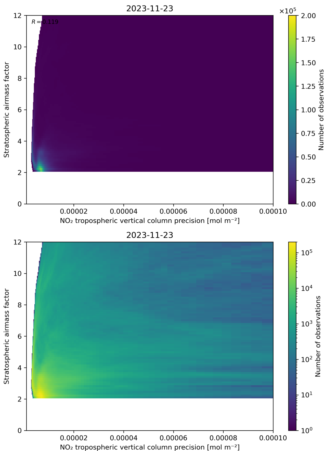
Figure 131: Scatter density plot of “NO 2 tropospheric vertical column precision” against “Stratospheric airmass factor” for 2023-11-23 to 2023-11-24.
