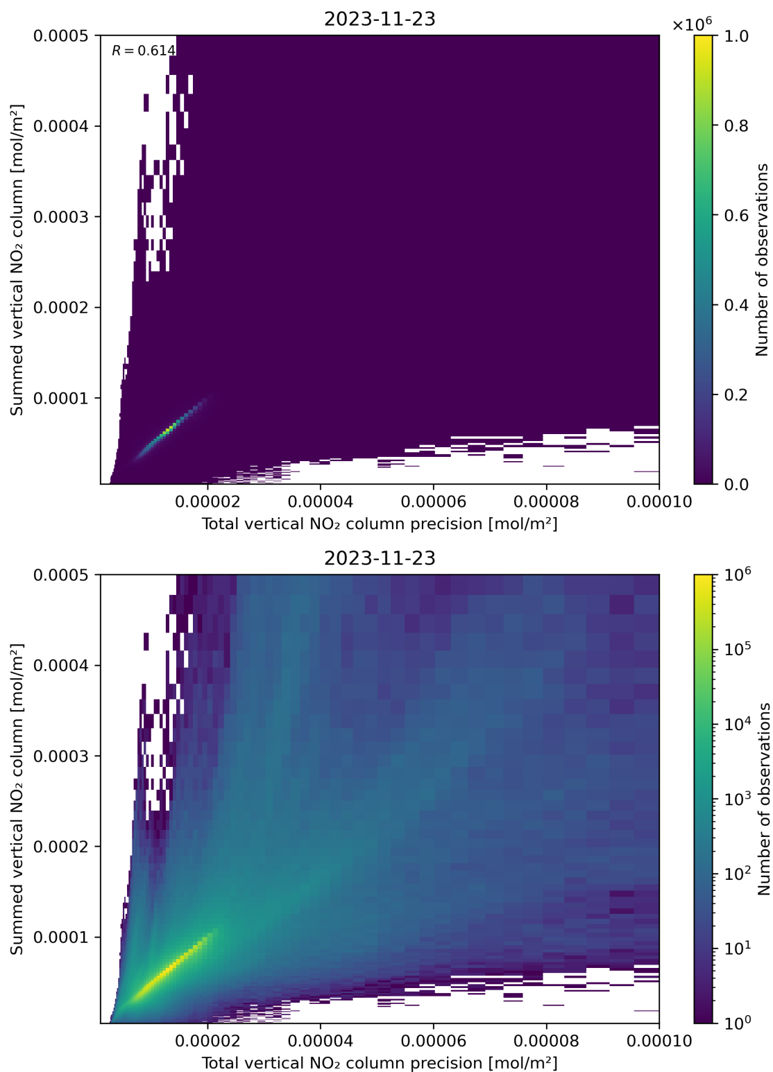
Figure 117: Scatter density plot of “Total vertical NO 2 column precision” against “Summed vertical NO 2 column” for 2023-11-23 to 2023-11-24.
