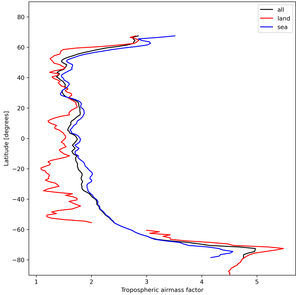
Figure 14: Zonal average of “Tropospheric airmass factor” for 2023-11-23 to 2023-11-24.
