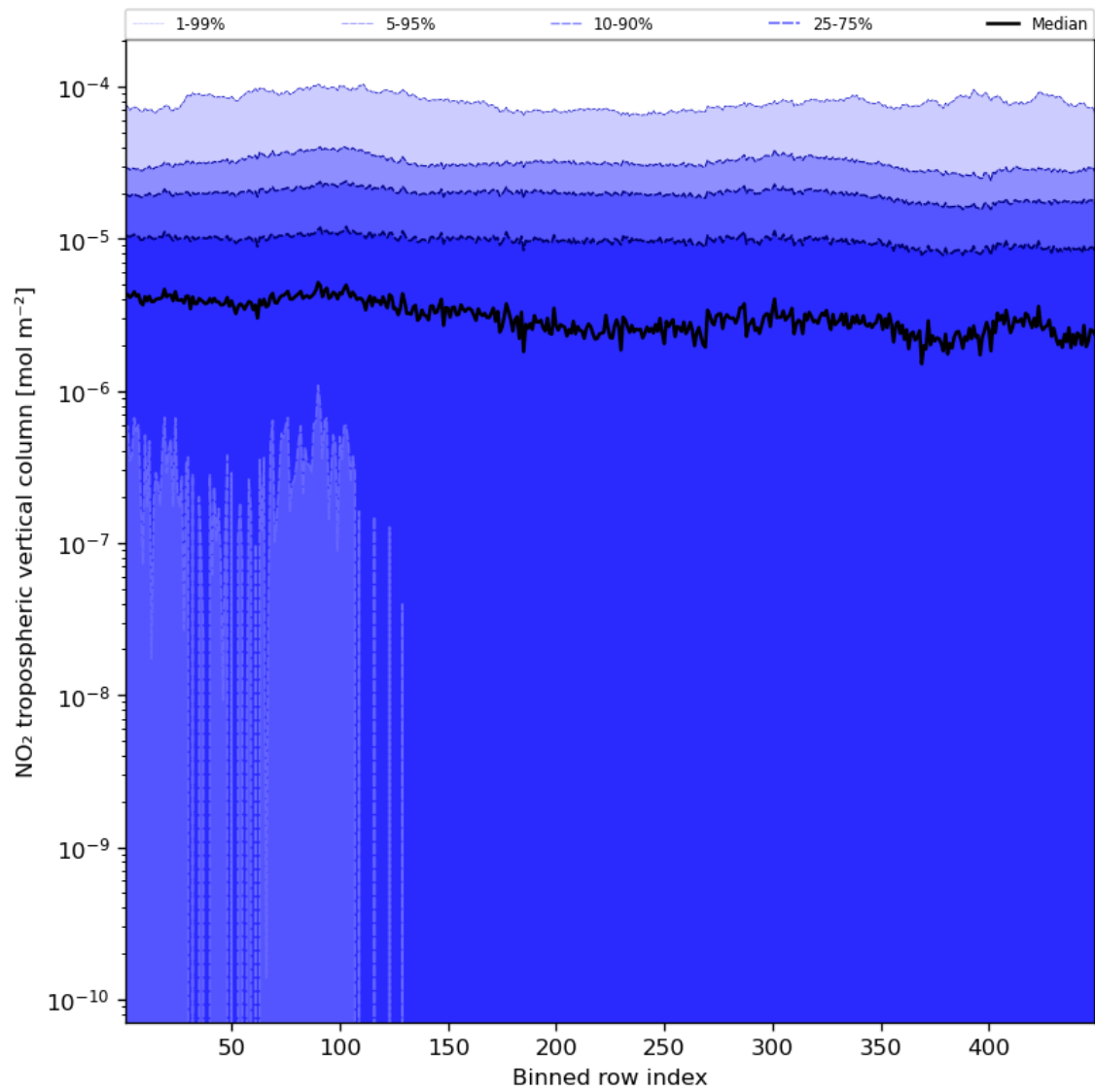
Figure 46: Along track statistics of “NO 2 tropospheric vertical column” for 2023-11-23 to 2023-11-24
