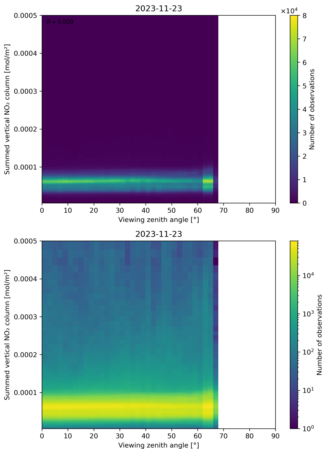
Figure 165: Scatter density plot of “Viewing zenith angle” against “Summed vertical NO 2 column” for 2023-11-23 to 2023-11-24.
