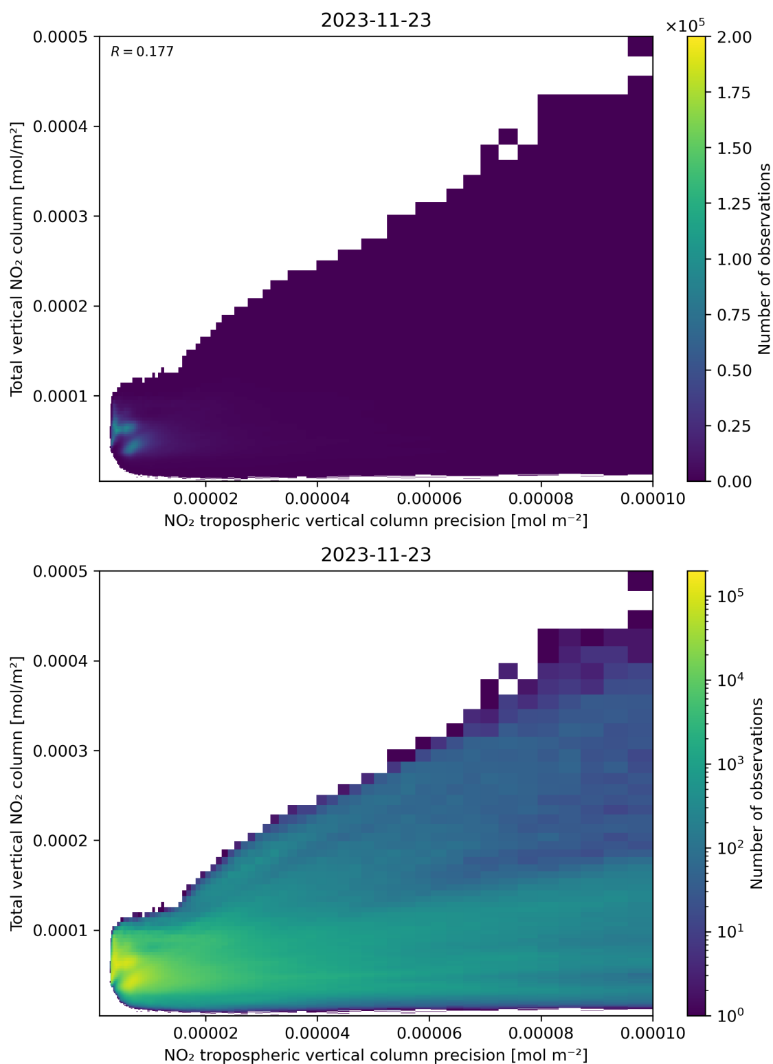
Figure 138: Scatter density plot of “NO 2 tropospheric vertical column precision” against “Total vertical NO 2 column” for 2023-11-23 to 2023-11-24.
