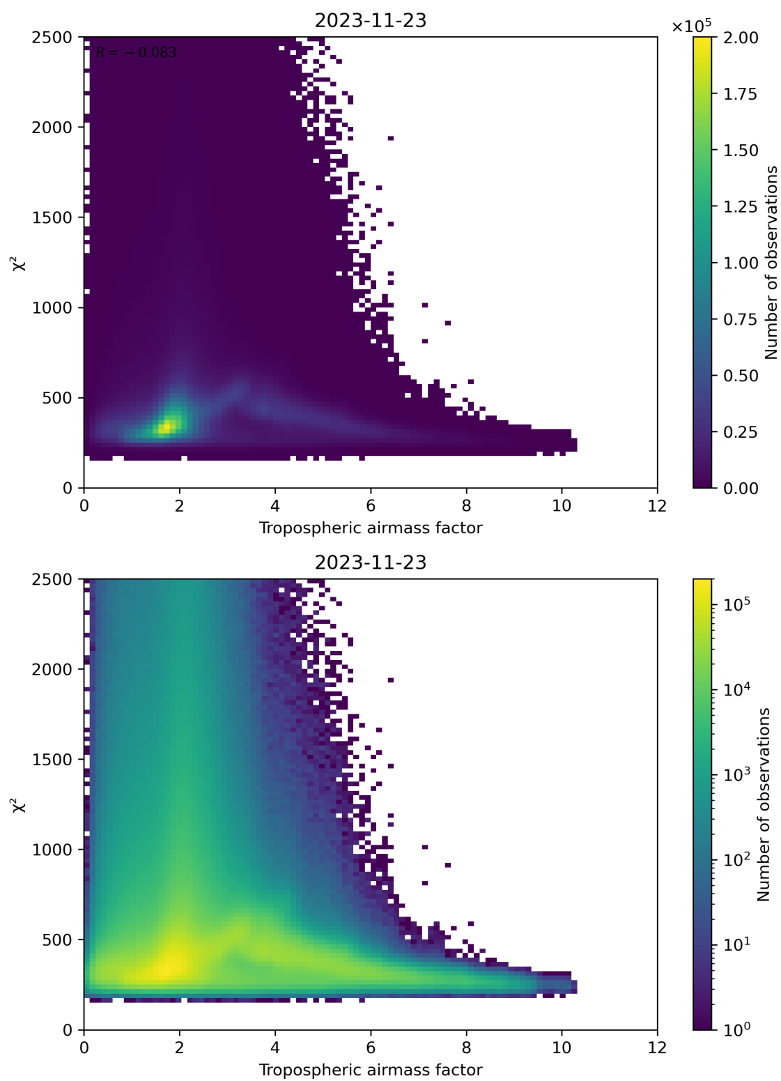
Figure 73: Scatter density plot of “Tropospheric airmass factor” against “ \chi^2 ” for 2023-11-23 to 2023-11-24.
