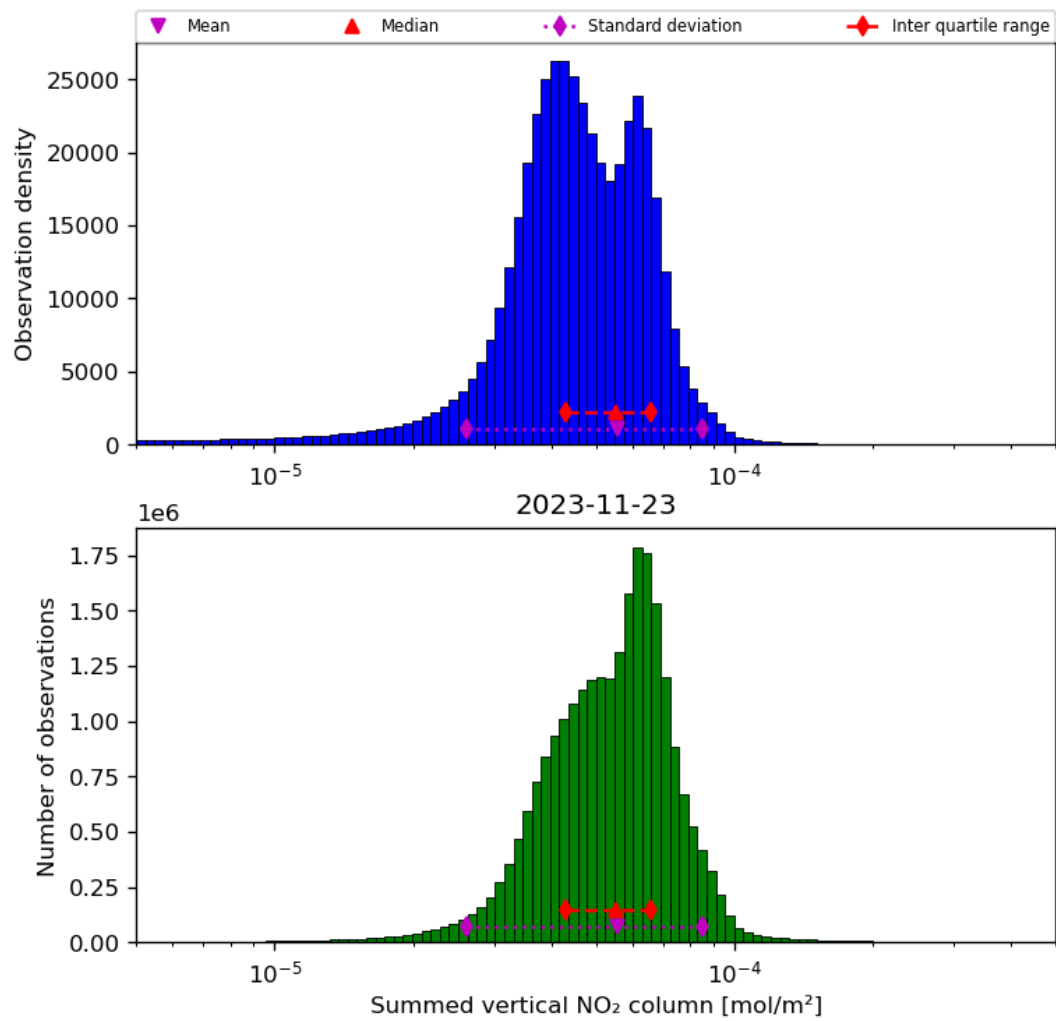
Figure 40: Histogram of “Summed vertical NO 2 column” for 2023-11-23 to 2023-11-24
