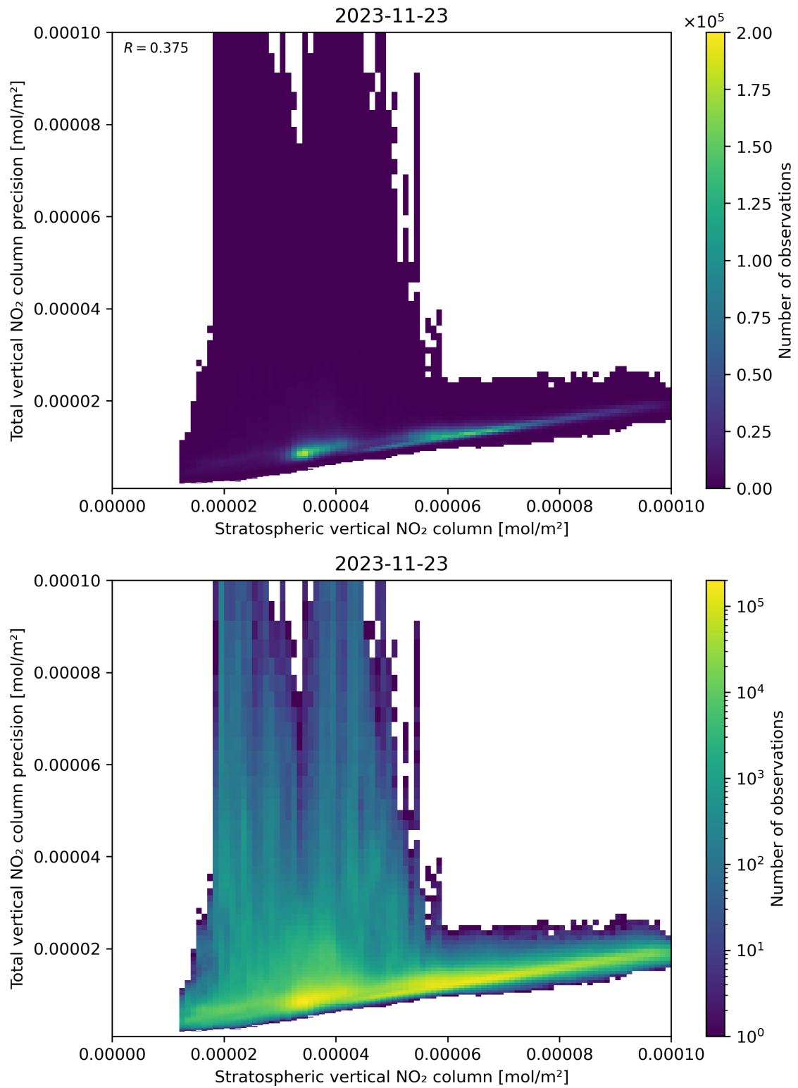
Figure 101: Scatter density plot of “Stratospheric vertical NO 2 column” against “Total vertical NO 2 column precision” for 2023-11-23 to 2023-11-24.
