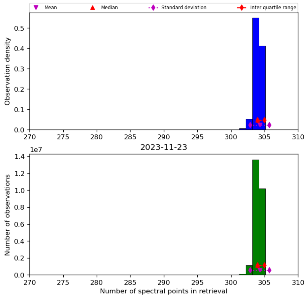
Figure 33: Histogram of “Number of spectral points in retrieval” for 2023-11-23 to 2023-11-24
