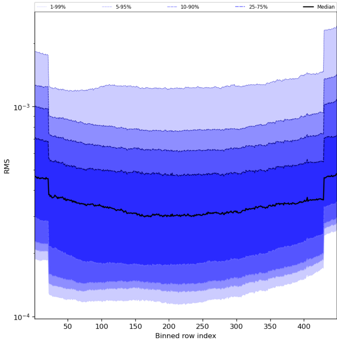
Figure 60: Along track statistics of “RMS” for 2023-11-23 to 2023-11-24
