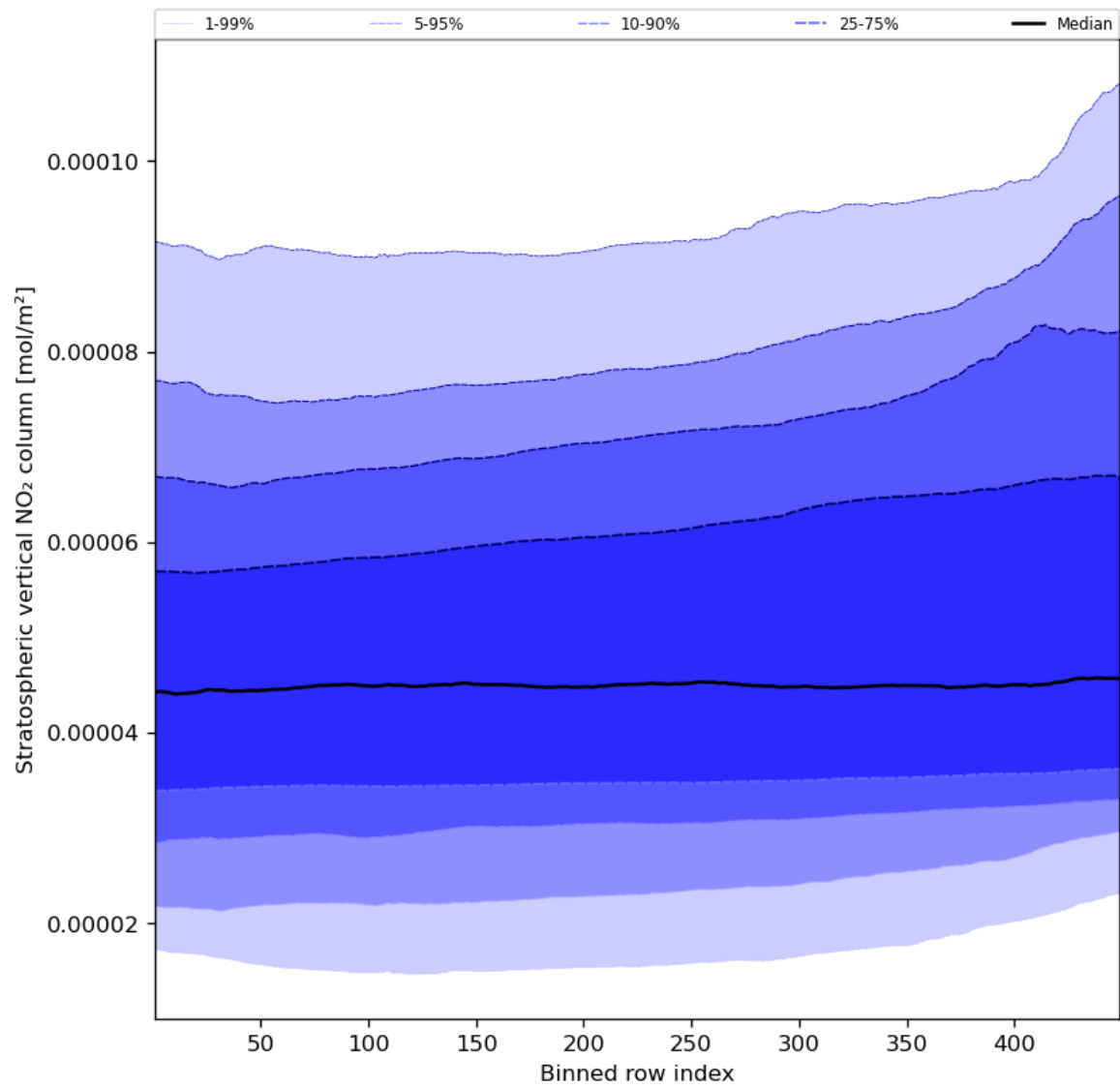
Figure 53: Along track statistics of “Stratospheric vertical NO 2 column” for 2023-11-23 to 2023-11-24
