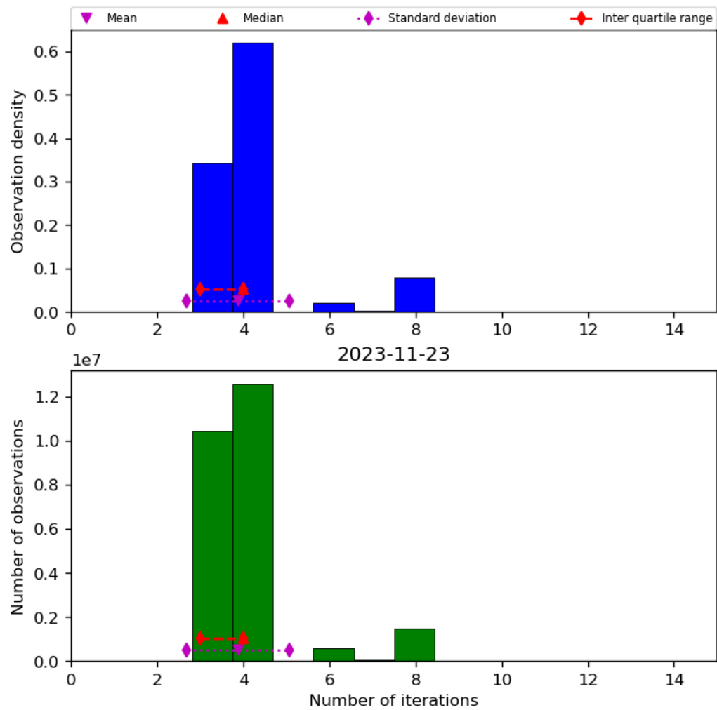
Figure 34: Histogram of “Number of iterations” for 2023-11-23 to 2023-11-24
