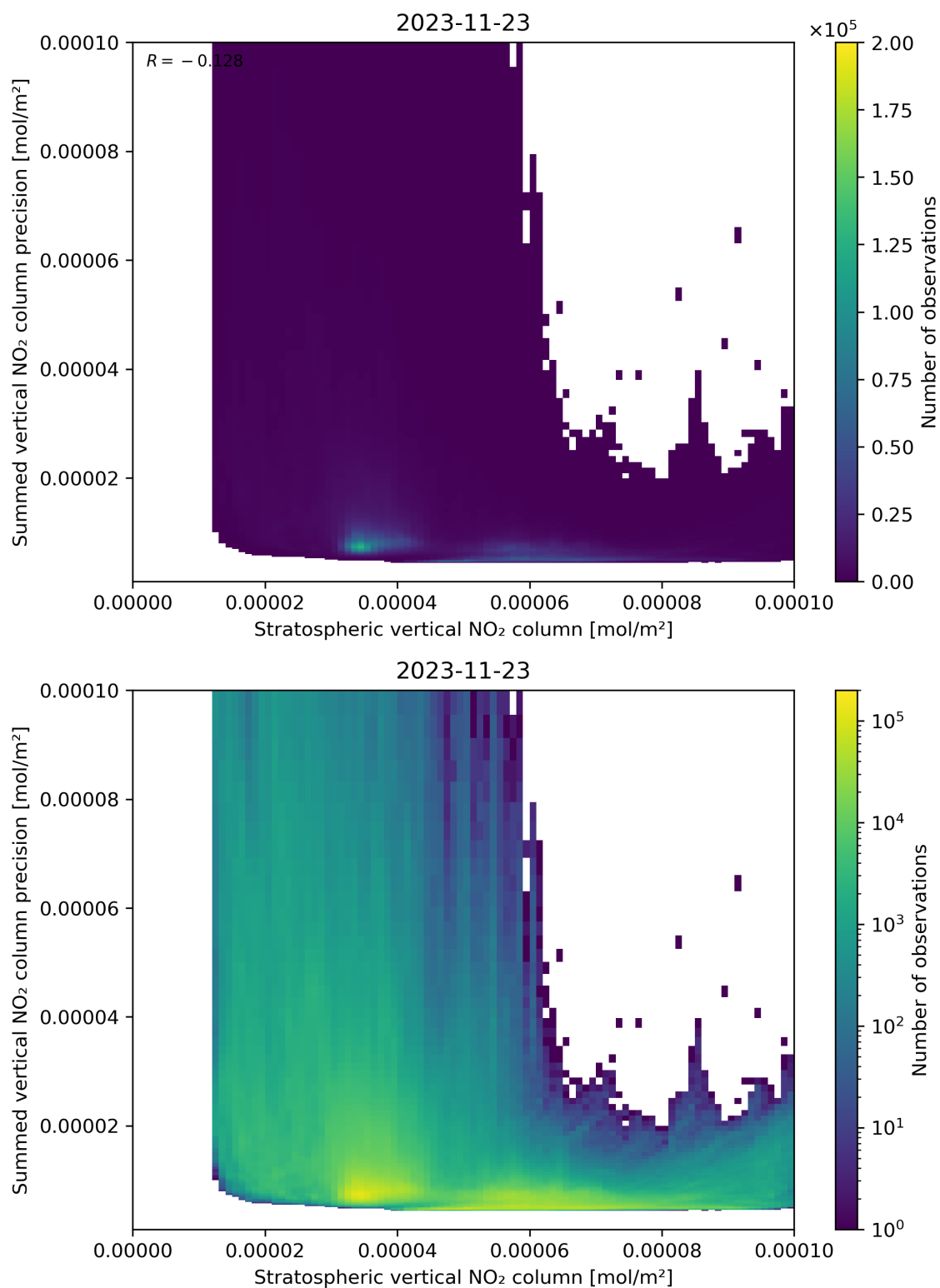
Figure 99: Scatter density plot of “Stratospheric vertical NO 2 column” against “Summed vertical NO 2 column precision” for 2023-11-23 to 2023-11-24.
