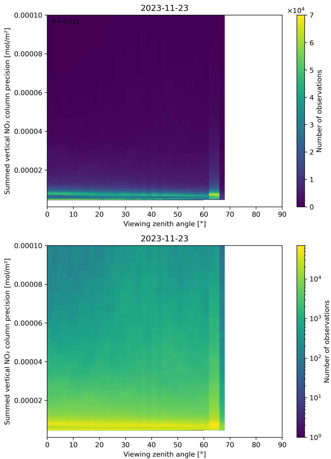
Figure 166: Scatter density plot of “Viewing zenith angle” against “Summed vertical NO 2 column precision” for 2023-11-23 to 2023-11-24.
