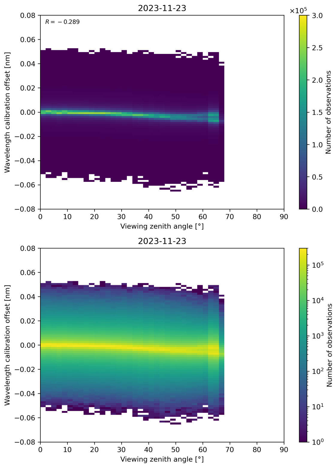
Figure 173: Scatter density plot of “Viewing zenith angle” against “Wavelength calibration offset” for 2023-11-23 to 2023-11-24.
