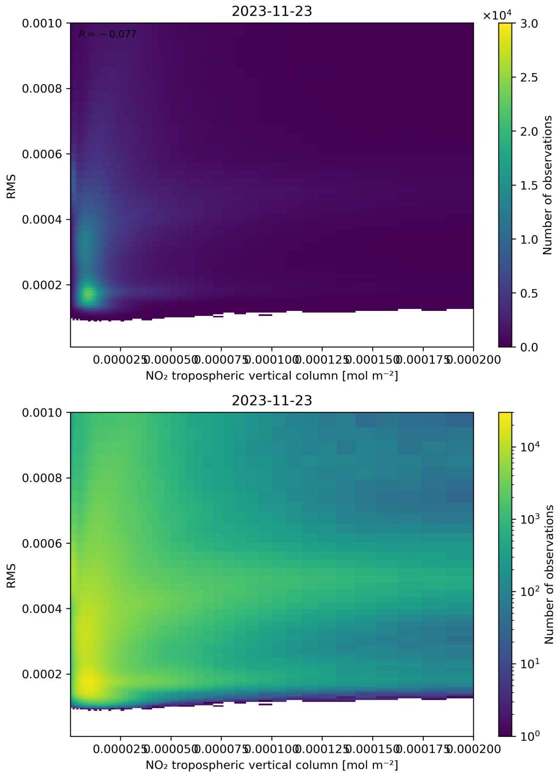
Figure 142: Scatter density plot of “NO 2 tropospheric vertical column” against “RMS” for 2023-11-23 to 2023-11-24.
