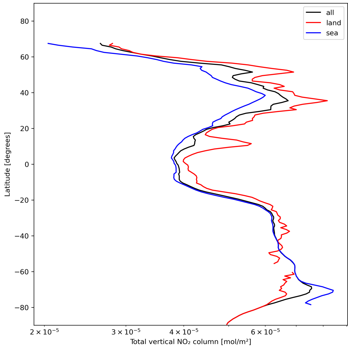
Figure 21: Zonal average of “Total vertical NO 2 column” for 2023-11-23 to 2023-11-24.
