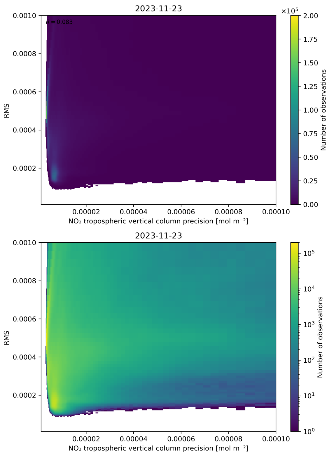
Figure 140: Scatter density plot of “NO 2 tropospheric vertical column precision” against “RMS” for 2023-11-23 to 2023-11-24.
