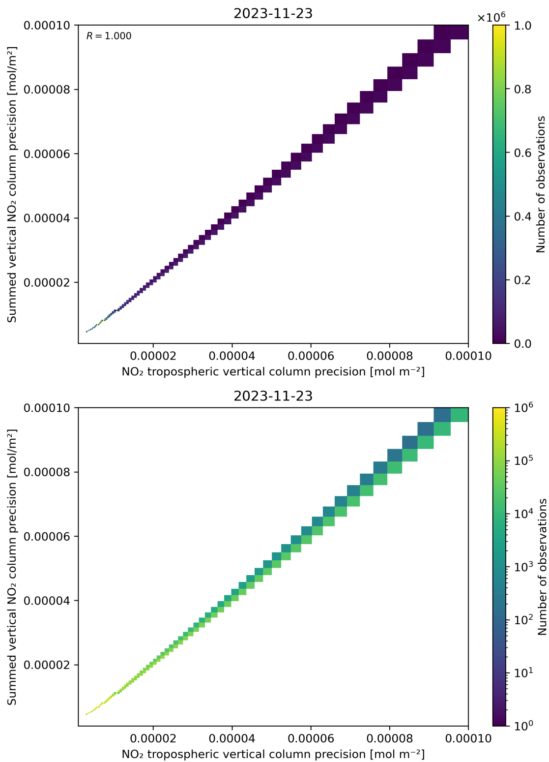
Figure 137: Scatter density plot of “NO 2 tropospheric vertical column precision” against “Summed vertical NO 2 column precision” for 2023-11-23 to 2023-11-24.
