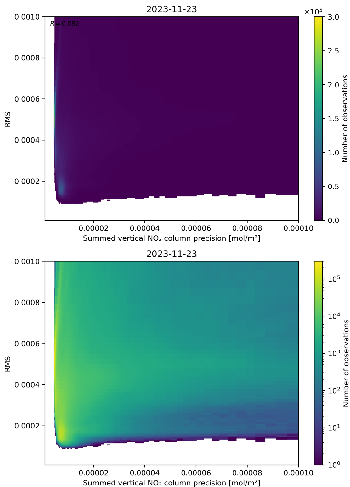
Figure 108: Scatter density plot of “Summed vertical NO 2 column precision” against “RMS” for 2023-11-23 to 2023-11-24.
