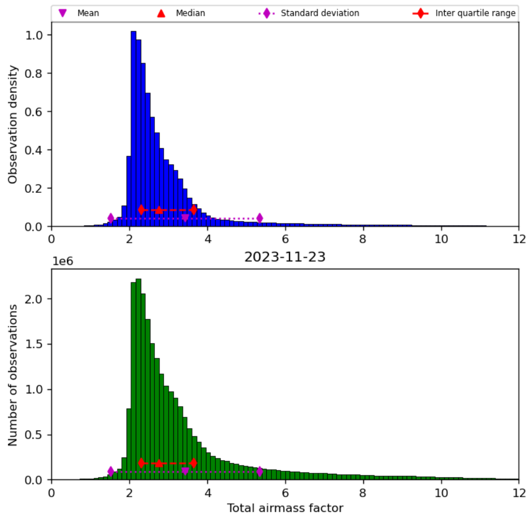
Figure 32: Histogram of “Total airmass factor” for 2023-11-23 to 2023-11-24
