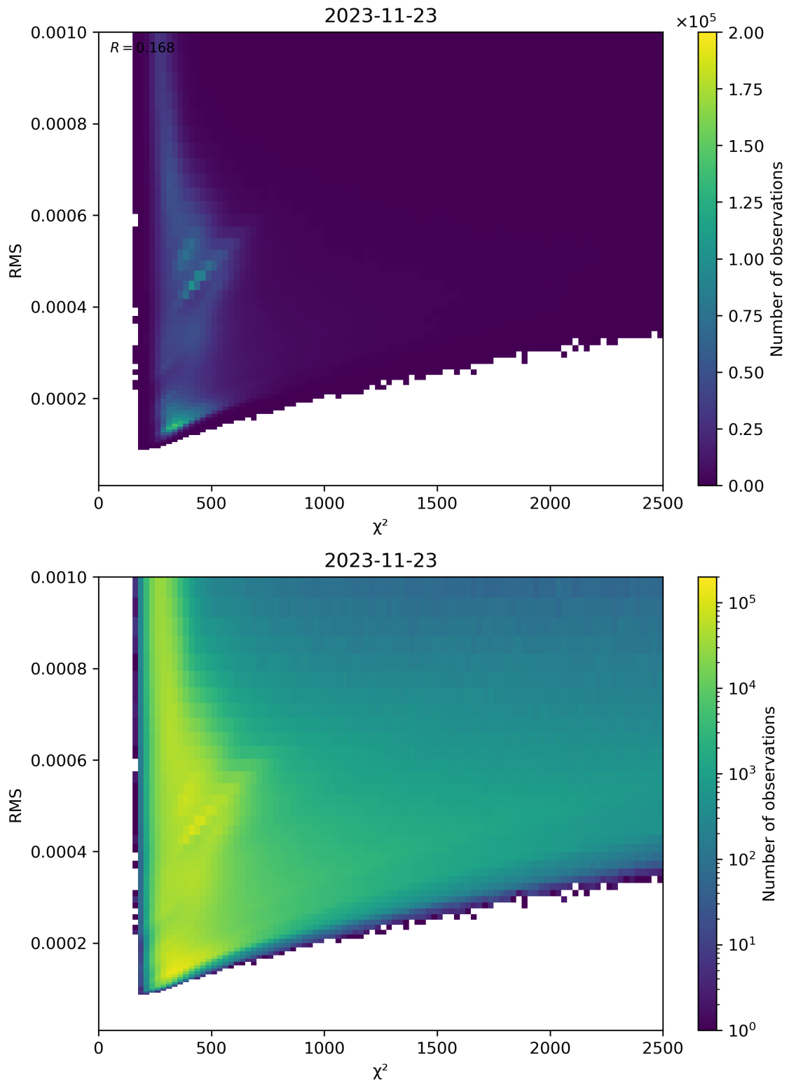
Figure 82: Scatter density plot of “ \chi^2 ” against “RMS” for 2023-11-23 to 2023-11-24.
