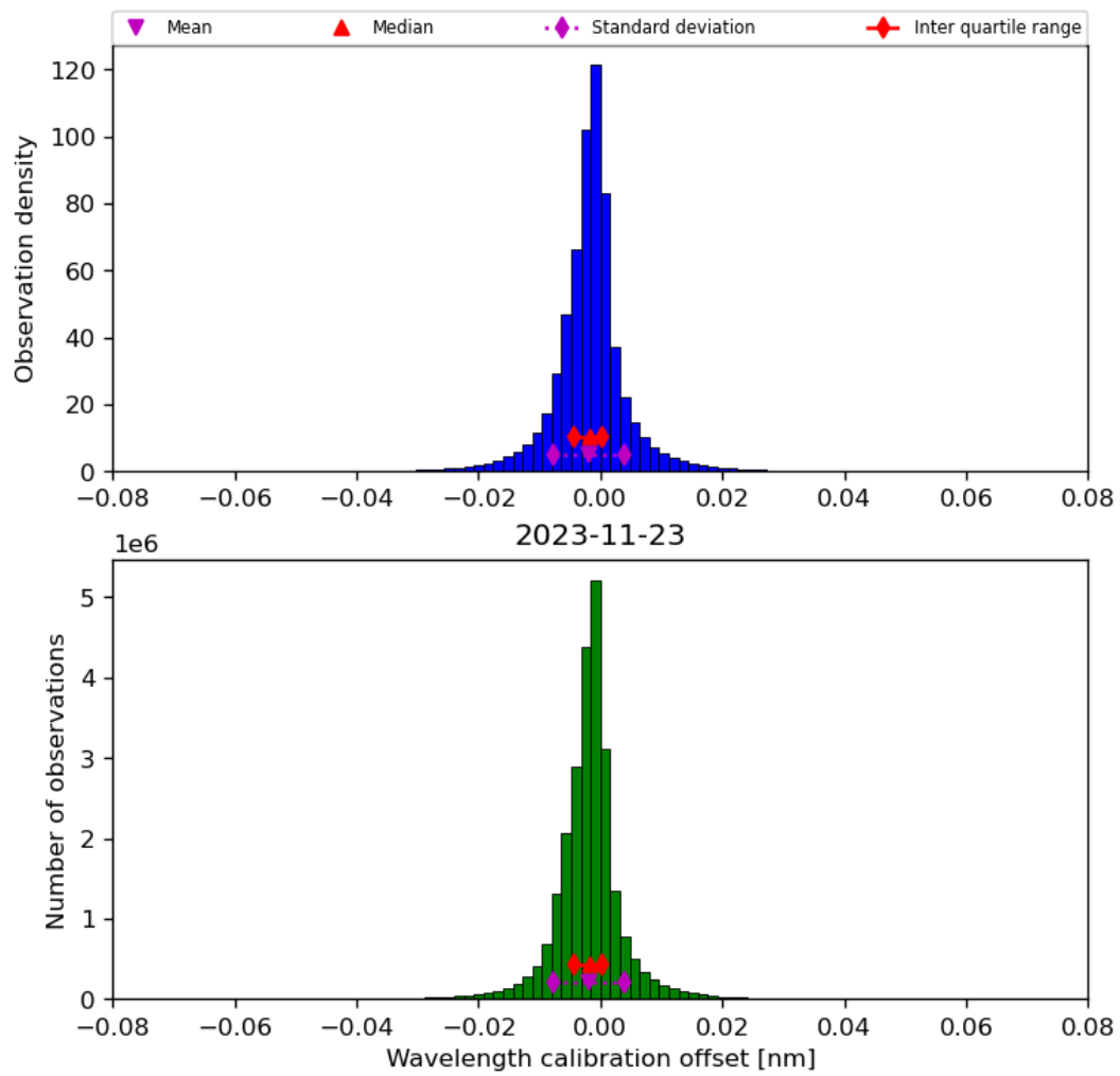
Figure 35: Histogram of “Wavelength calibration offset” for 2023-11-23 to 2023-11-24
