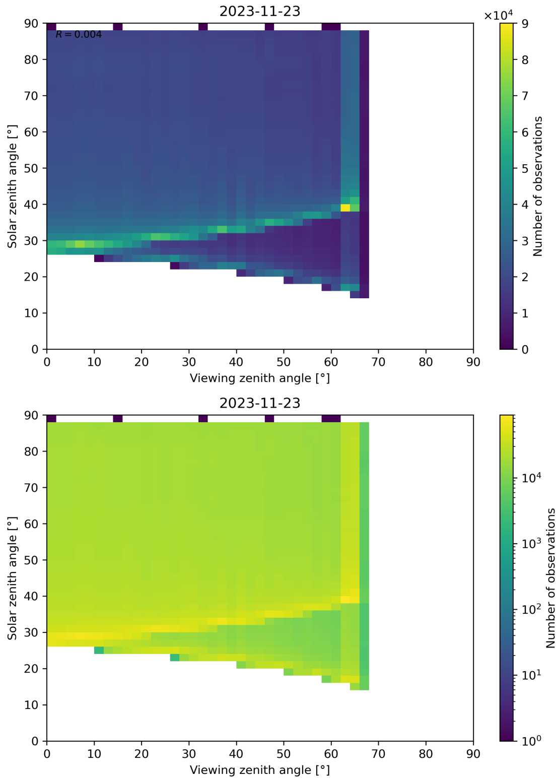
Figure 172: Scatter density plot of “Viewing zenith angle” against “Solar zenith angle” for 2023-11-23 to 2023-11-24.
