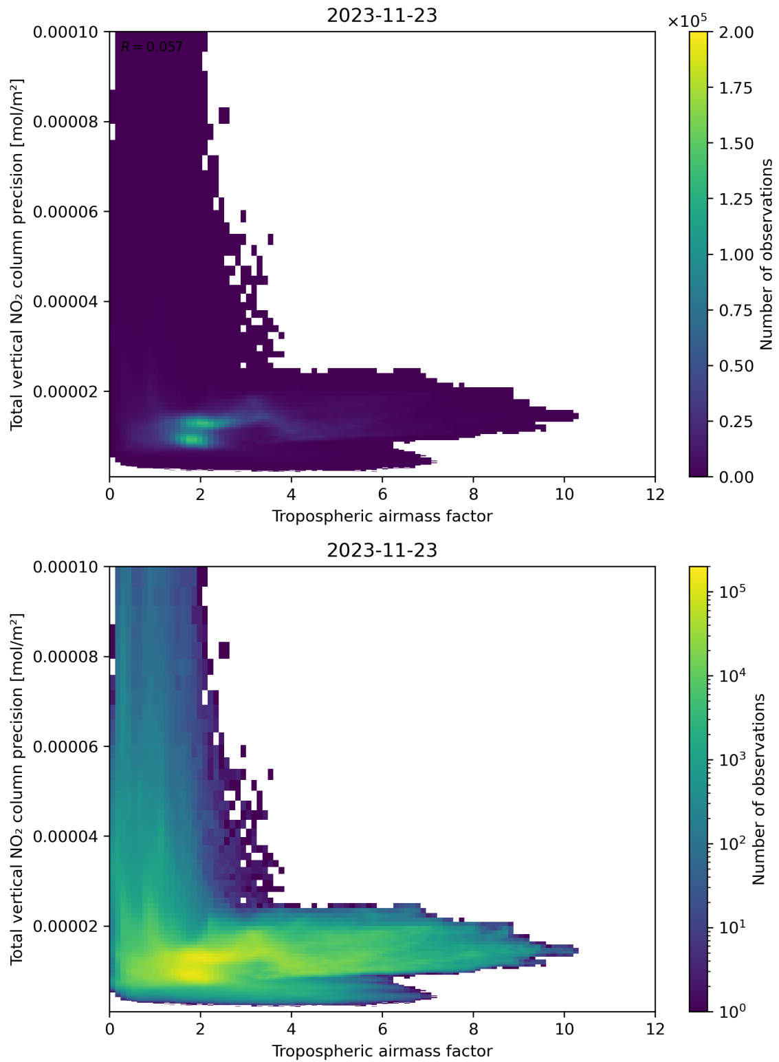
Figure 78: Scatter density plot of “Tropospheric air mass factor” against “Total vertical NO 2 column precision” for 2023-11-23 to 2023-11-24.
