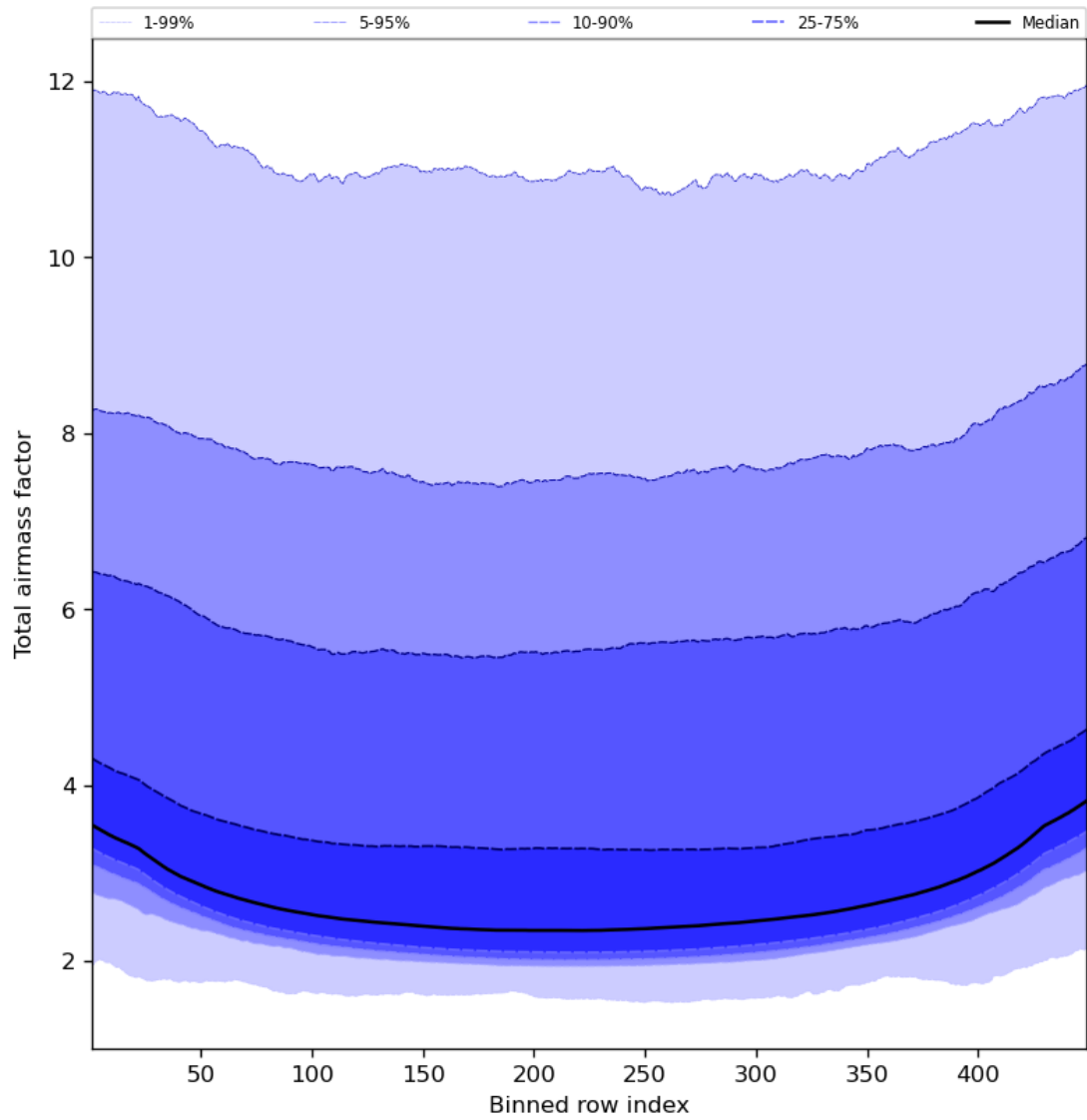
Figure 49: Along track statistics of “Total airmass factor” for 2023-11-23 to 2023-11-24
