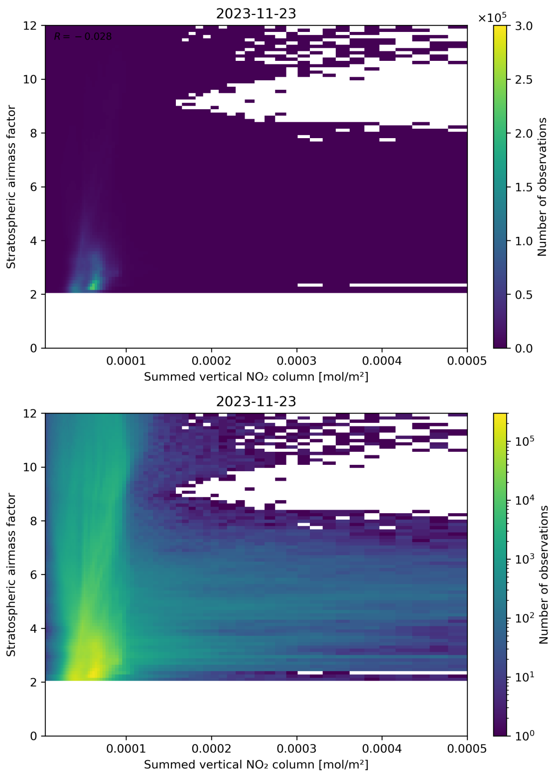
Figure 103: Scatter density plot of “Summed vertical NO 2 column” against “Stratospheric airmass factor” for 2023-11-23 to 2023-11-24.
