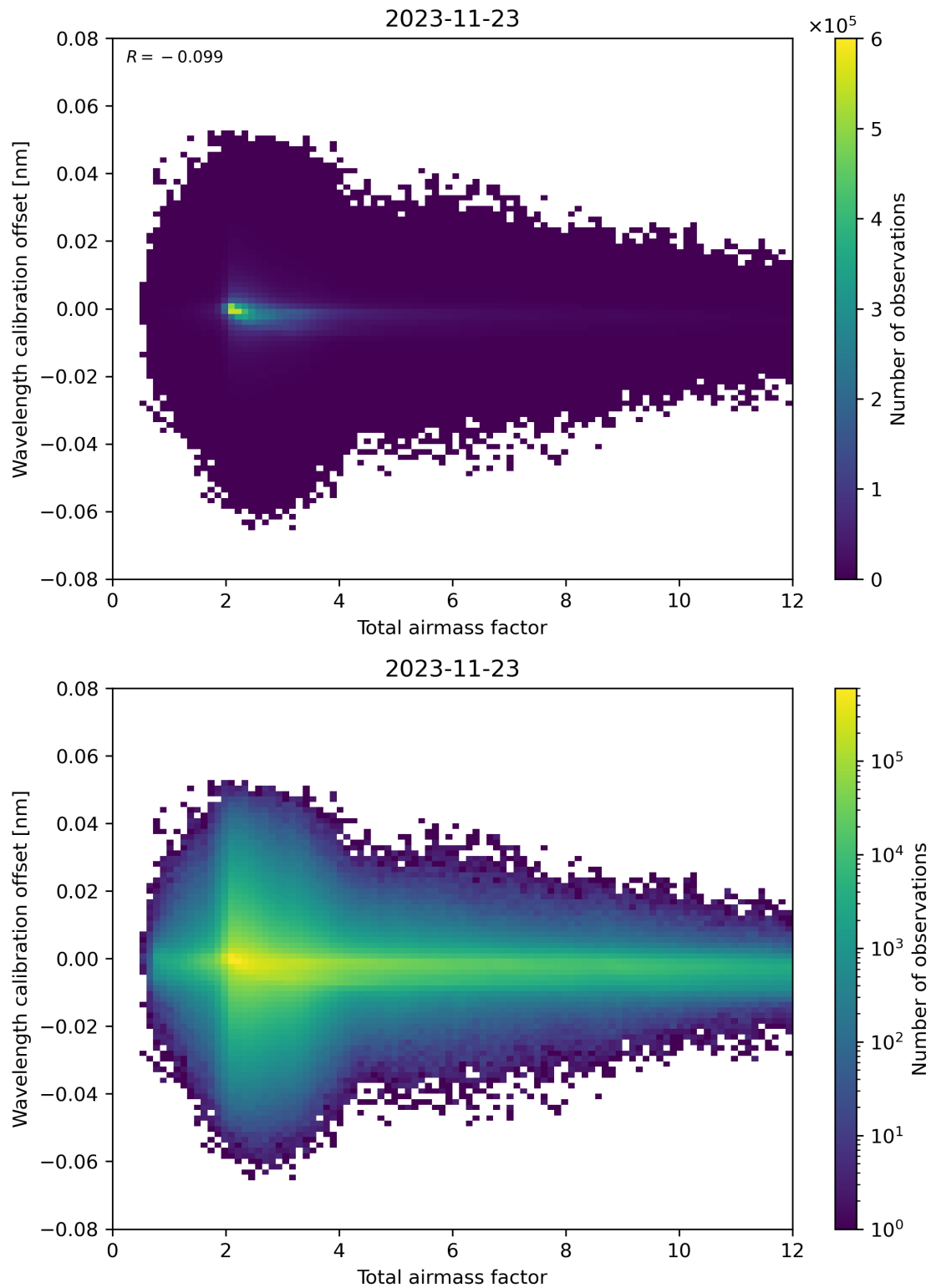
Figure 70: Scatter density plot of “Total airmass factor” against “Wavelength calibration offset” for 2023-11-23 to 2023-11-24.
