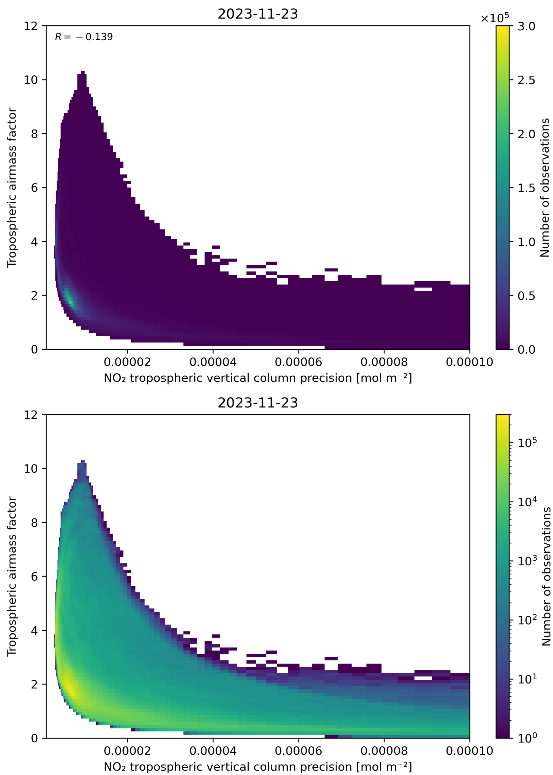
Figure 133: Scatter density plot of “NO 2 tropospheric vertical column precision” against “Tropospheric air mass factor” for 2023-11-23 to 2023-11-24.
