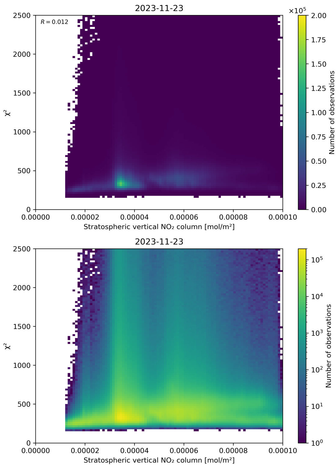
Figure 97: Scatter density plot of “Stratospheric vertical NO 2 column” against “ \chi^2 ” for 2023-11-23 to 2023-11-24.
