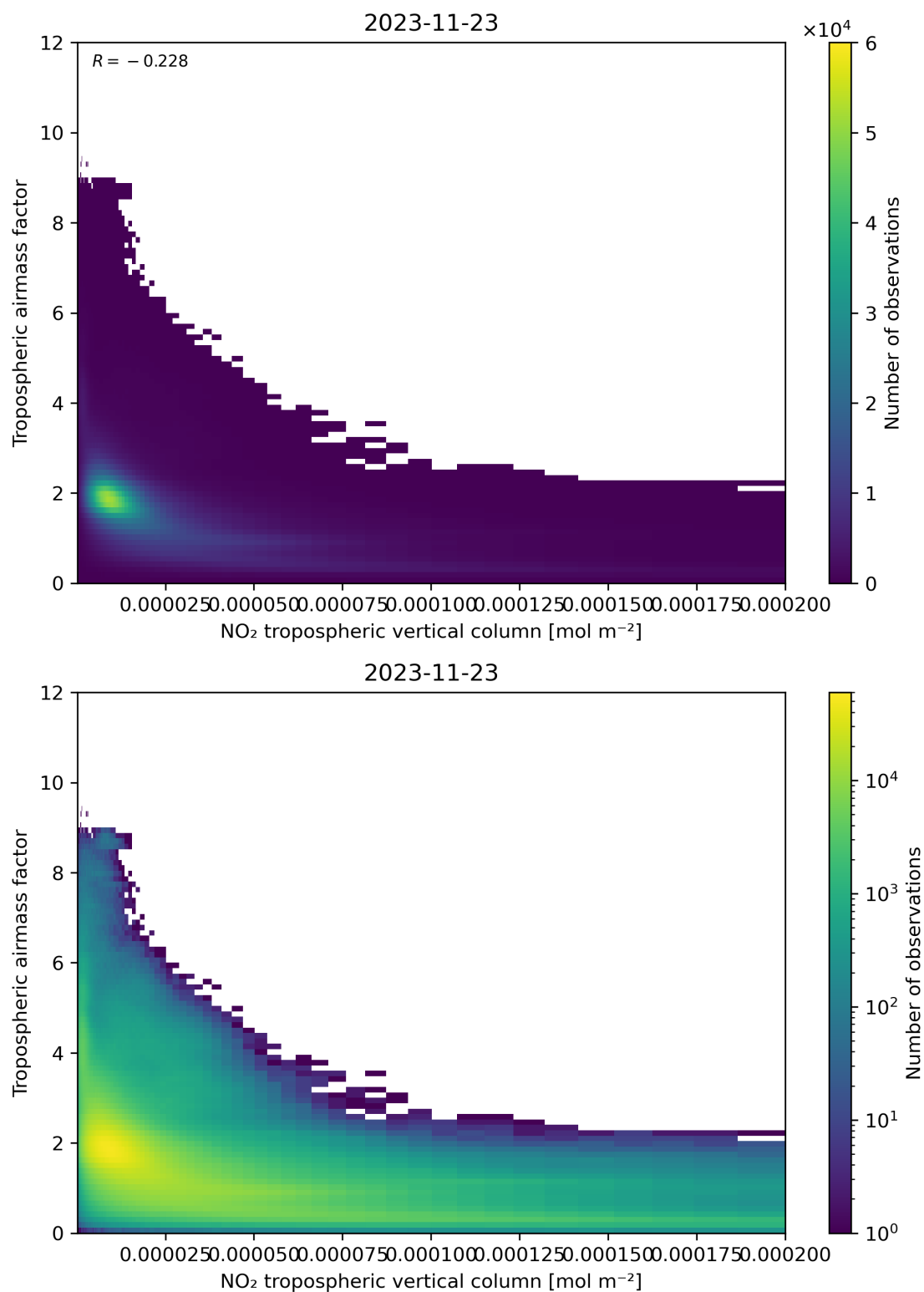
Figure 123: Scatter density plot of “NO 2 tropospheric vertical column” against “Tropospheric airmass factor” for 2023-11-23 to 2023-11-24.
