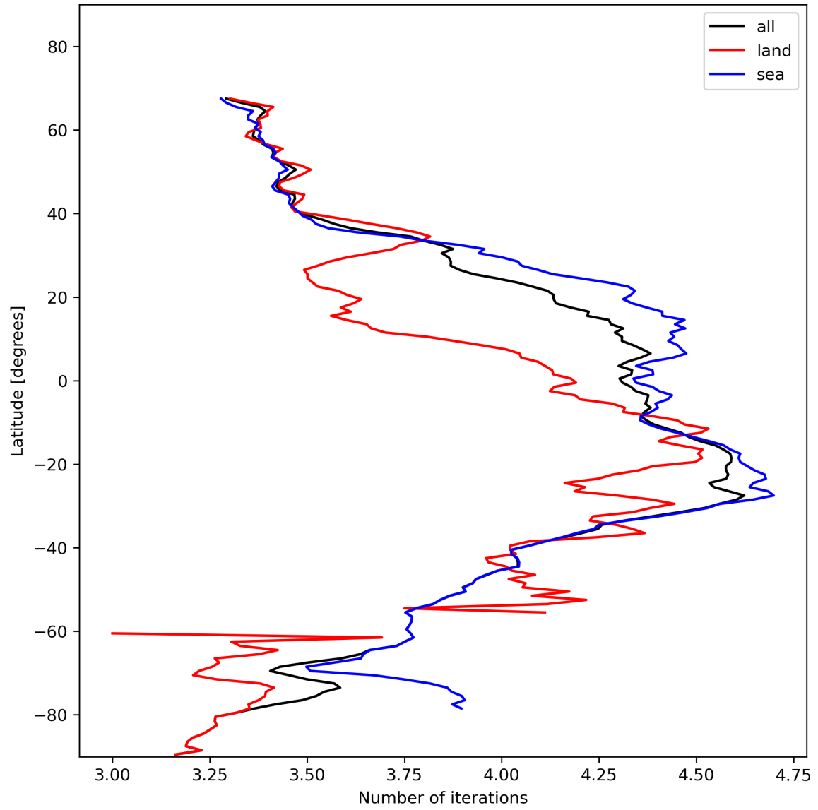
Figure 17: Zonal average of “Number of iterations” for 2023-11-23 to 2023-11-24.
