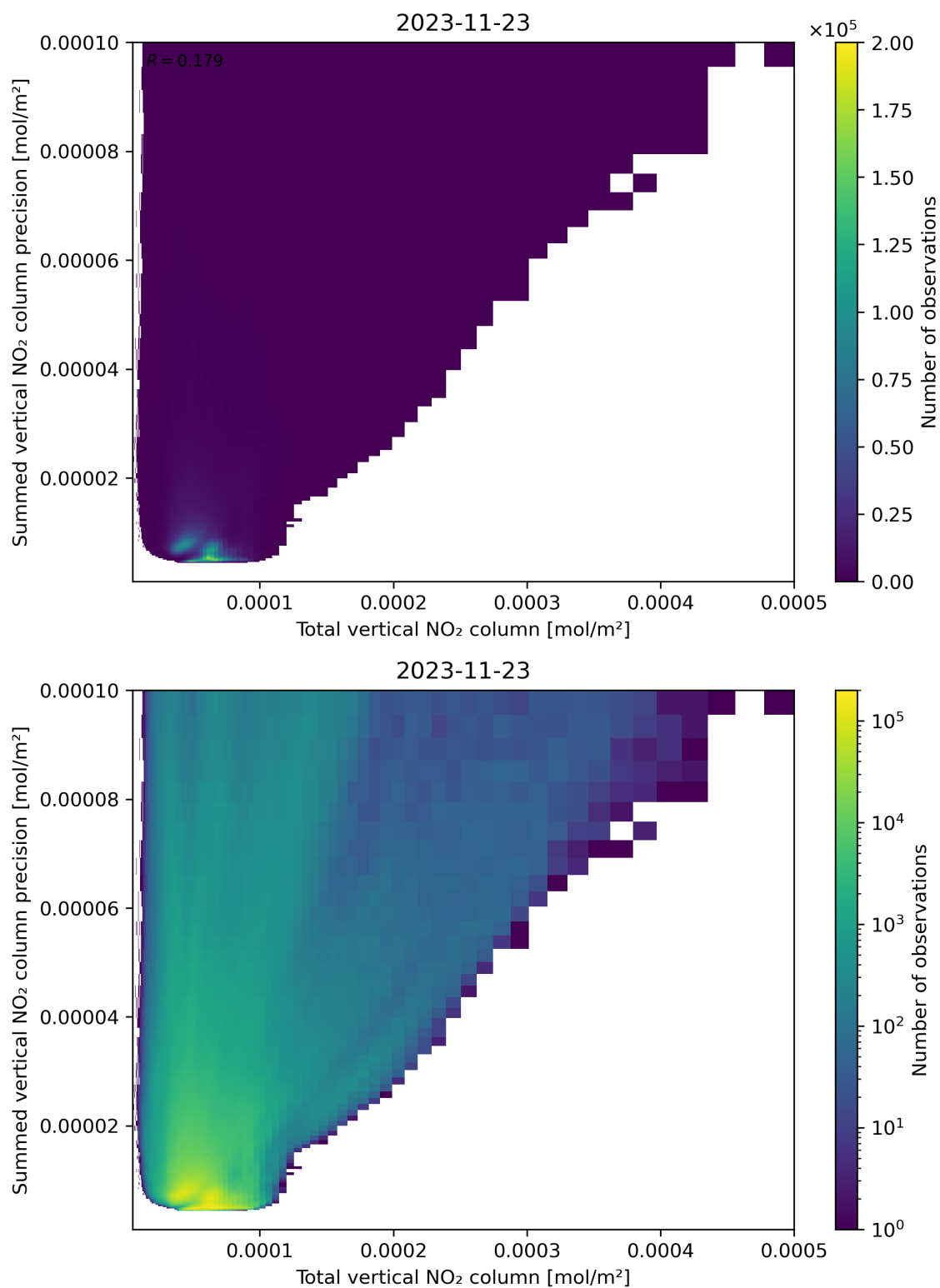
Figure 113: Scatter density plot of “Total vertical NO 2 column” against “Summed vertical NO 2 column precision” for 2023-11-23 to 2023-11-24.
