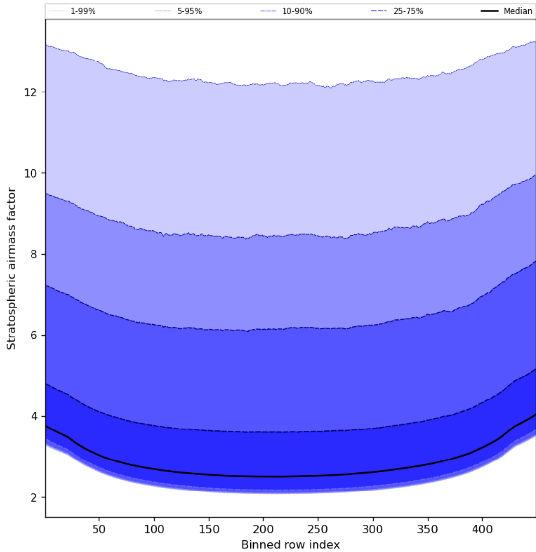
Figure 61: Along track statistics of “Stratospheric airmass factor” for 2023-11-23 to 2023-11-24
