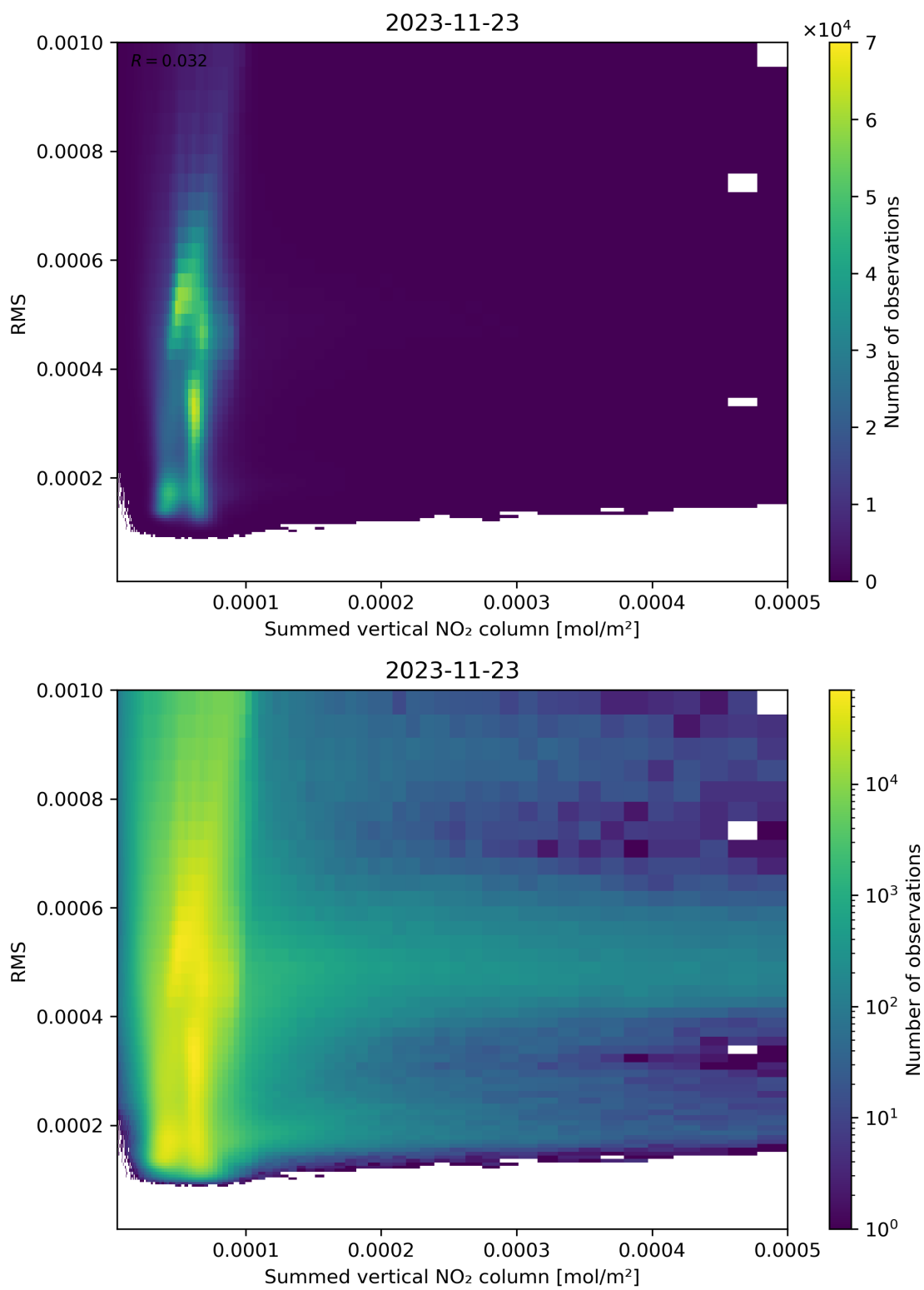
Figure 109: Scatter density plot of “Summed vertical NO 2 column” against “RMS” for 2023-11-23 to 2023-11-24.
