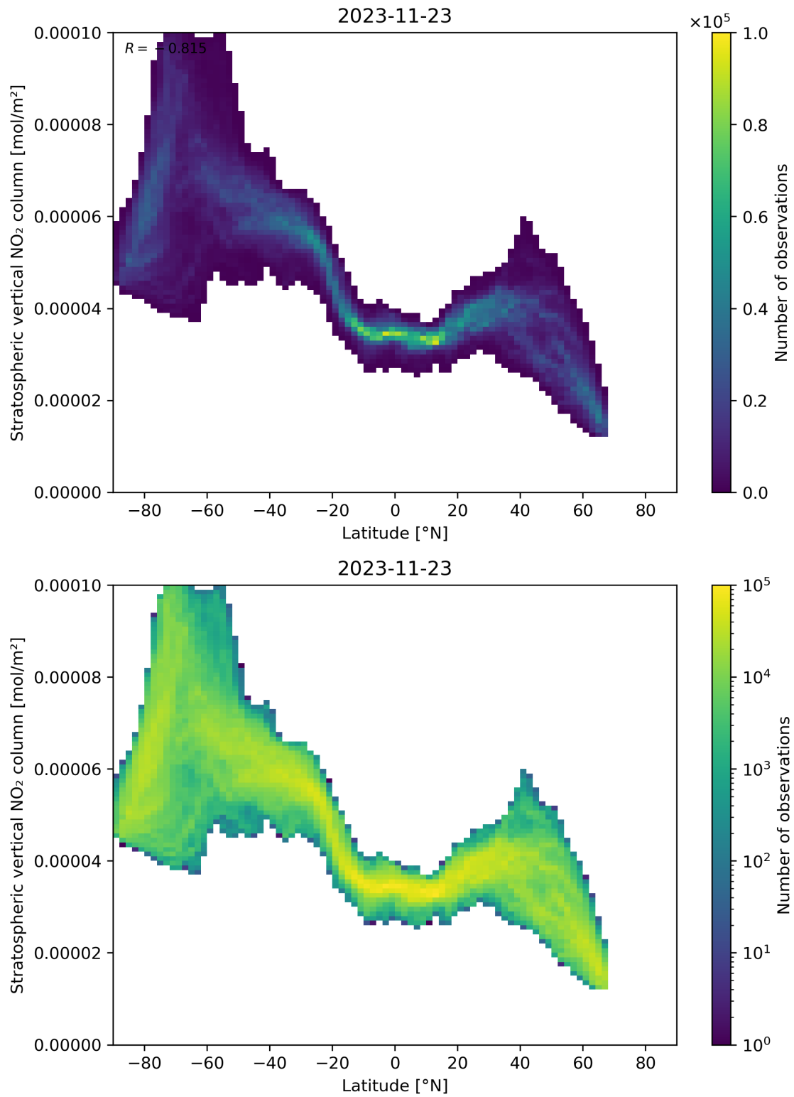
Figure 87: Scatter density plot of “Latitude” against “Stratospheric vertical NO 2 column” for 2023-11-23 to 2023-11-24.
