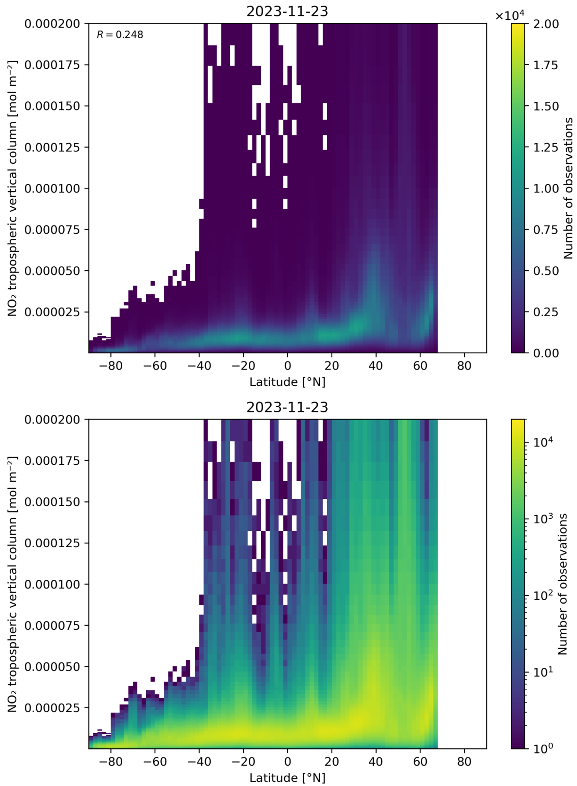
Figure 92: Scatter density plot of “Latitude” against “NO 2 tropospheric vertical column” for 2023-11-23 to 2023-11-24.
