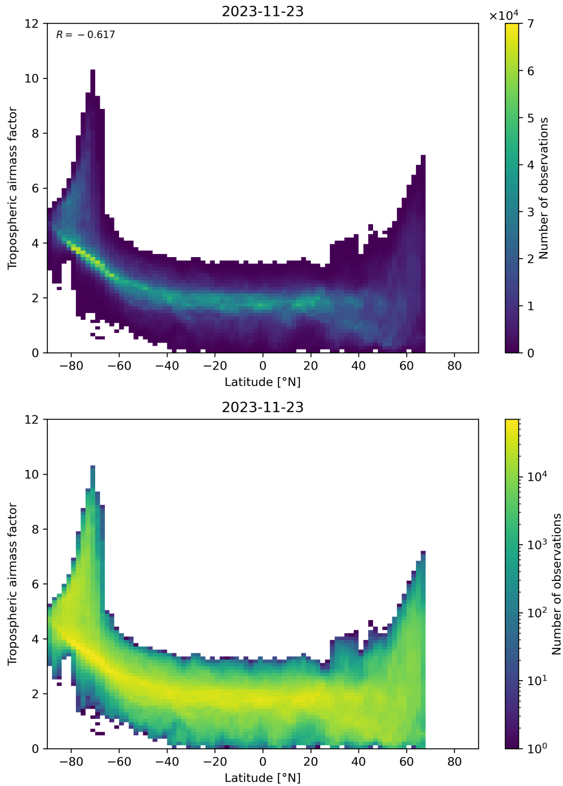
Figure 85: Scatter density plot of “Latitude” against “Tropospheric airmass factor” for 2023-11-23 to 2023-11-24.
