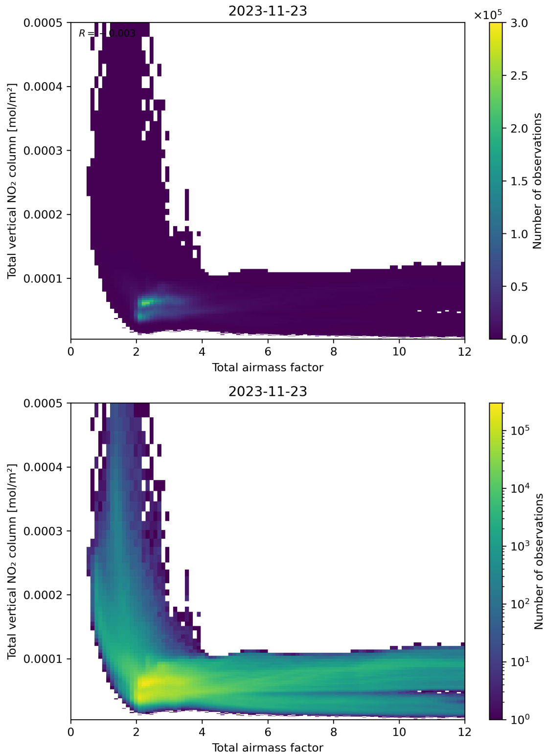
Figure 67: Scatter density plot of “Total airmass factor” against “Total vertical NO 2 column” for 2023-11-23 to 2023-11-24.
