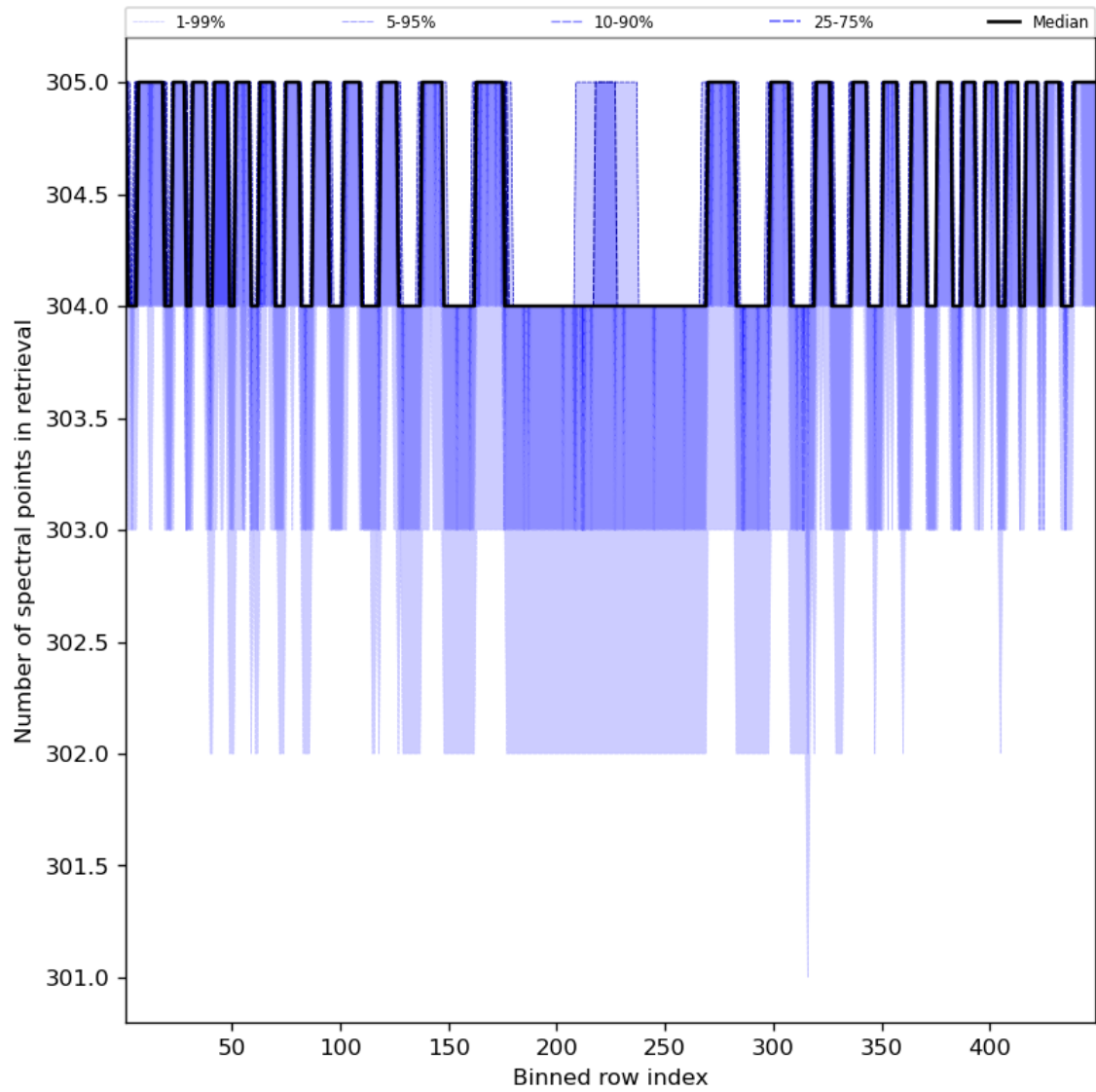
Figure 50: Along track statistics of “Number of spectral points in retrieval” for 2023-11-23 to 2023-11-24
