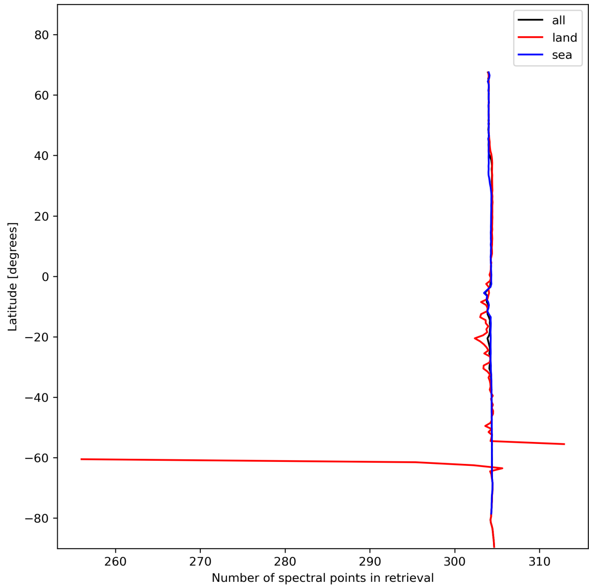
Figure 16: Zonal average of “Number of spectral points in retrieval” for 2023-11-23 to 2023-11-24.
