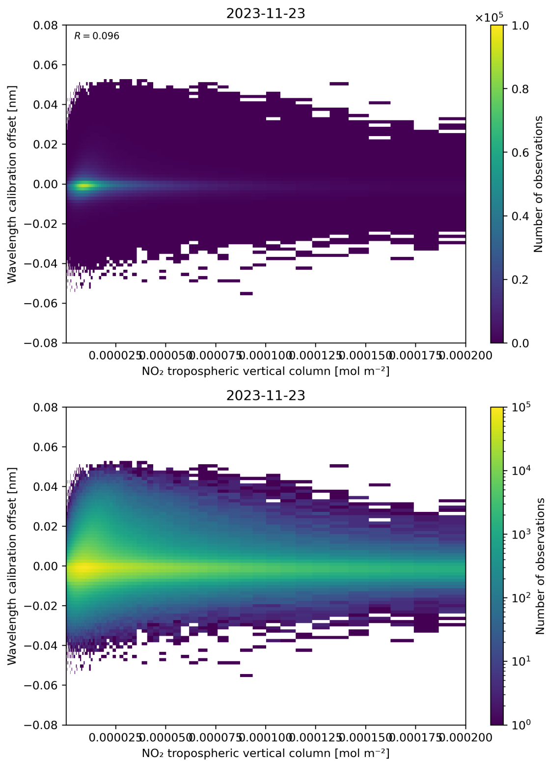
Figure 143: Scatter density plot of “NO 2 tropospheric vertical column” against “Wavelength calibration offset” for 2023-11-23 to 2023-11-24.
