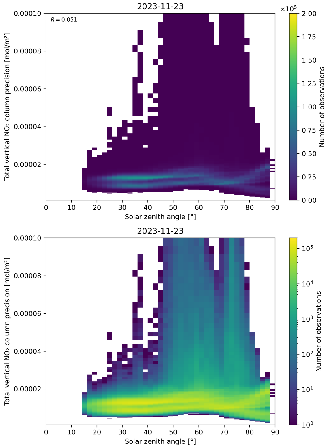
Figure 154: Scatter density plot of “Solar zenith angle” against “Total vertical NO 2 column precision” for 2023-11-23 to 2023-11-24.
