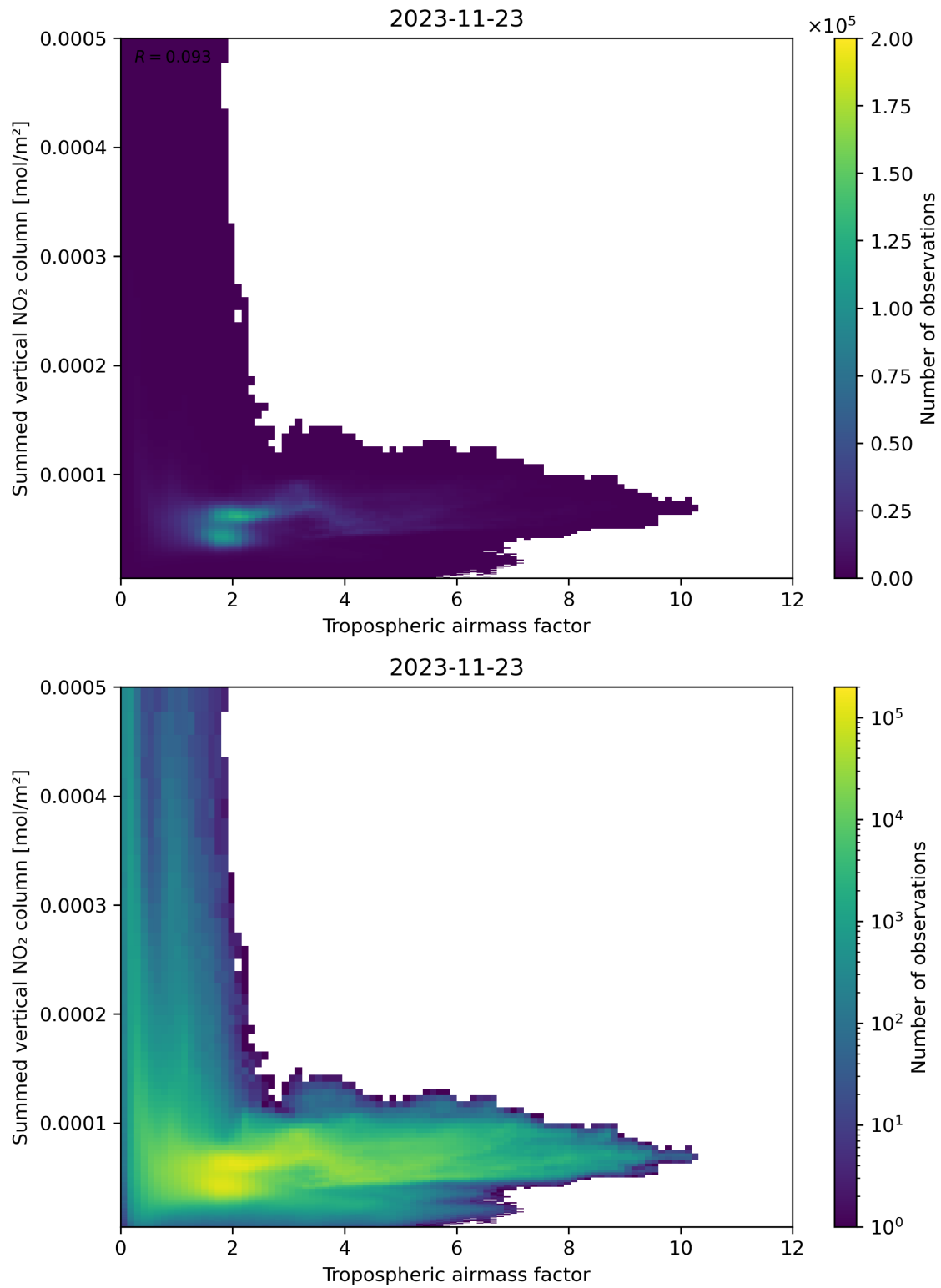
Figure 75: Scatter density plot of “Tropospheric airmass factor” against “Summed vertical NO 2 column” for 2023-11-23 to 2023-11-24.
