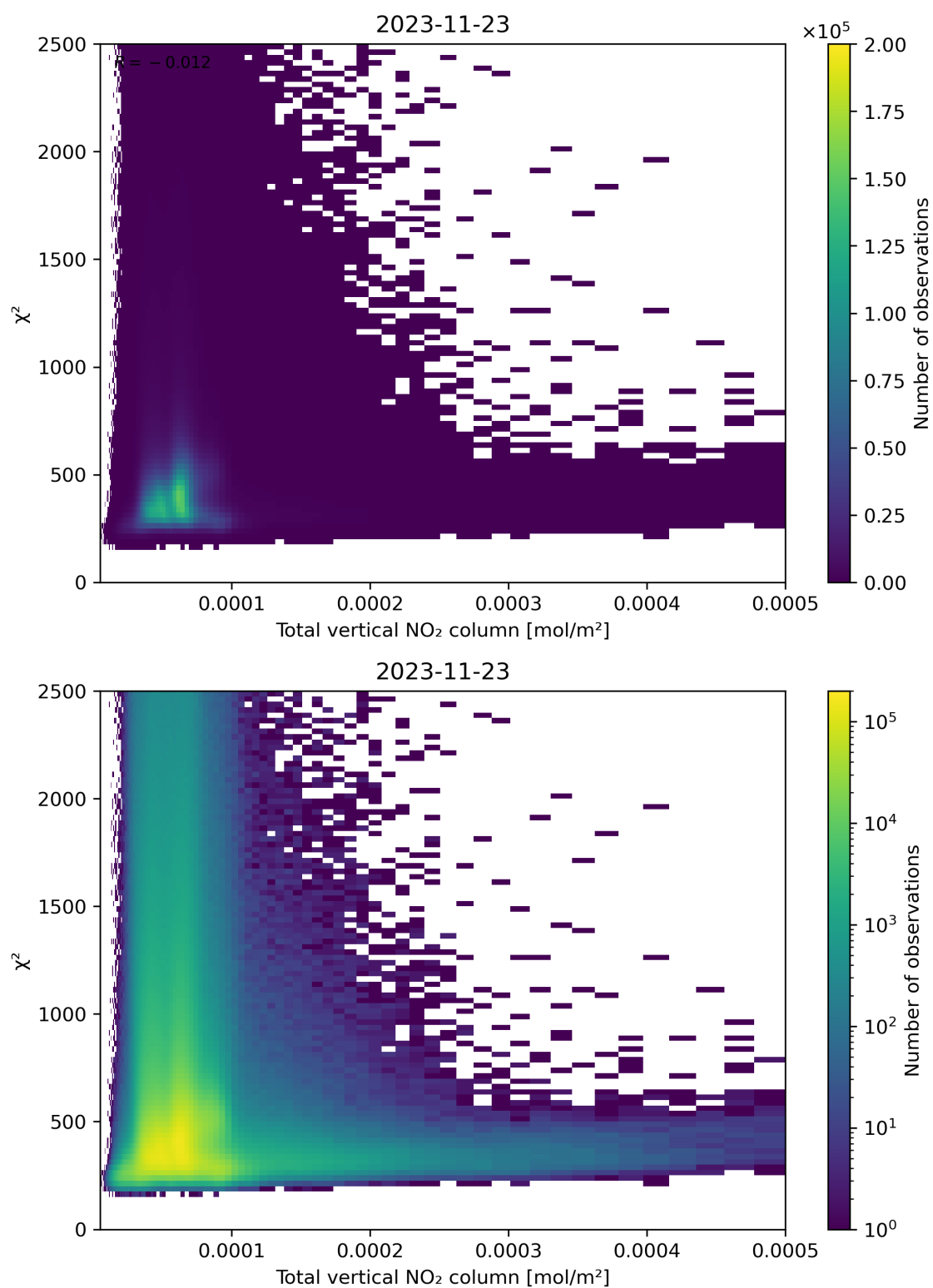
Figure 111: Scatter density plot of “Total vertical NO 2 column” against “ \chi^2 ” for 2023-11-23 to 2023-11-24.
