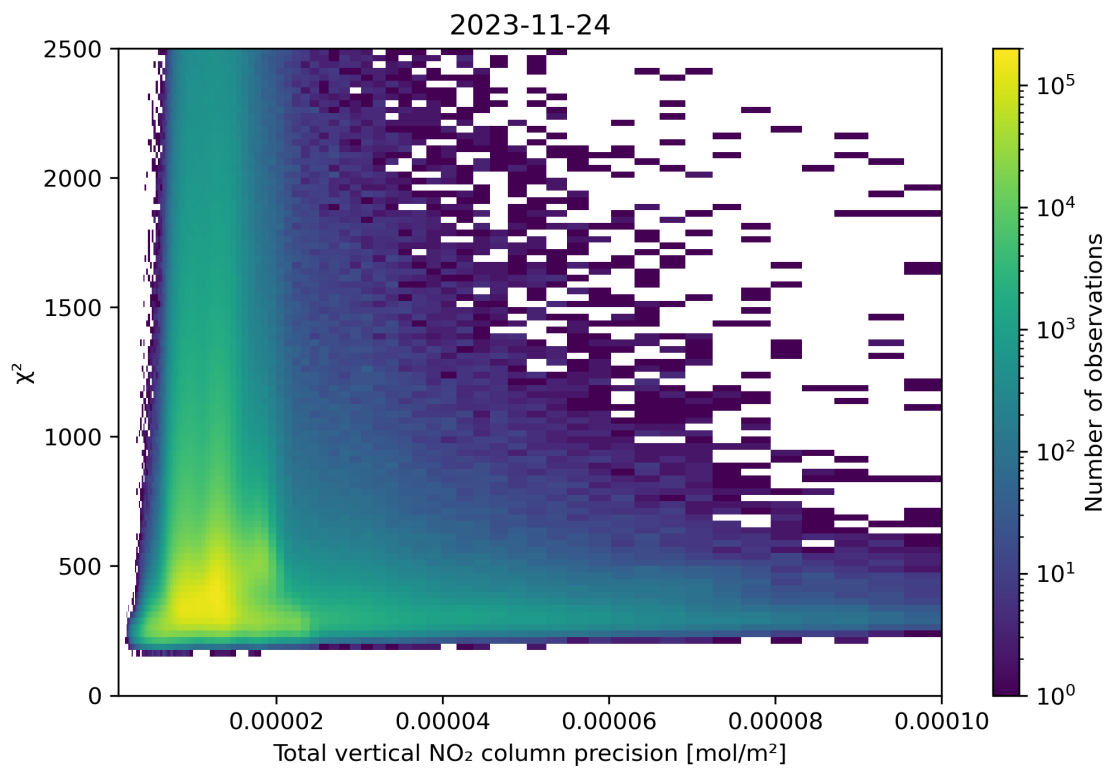
Figure 116: Scatter density plot of “Total vertical NO 2 column precision” against “ \chi^2 ” for 2023-11-23 to 2023-11-25.
