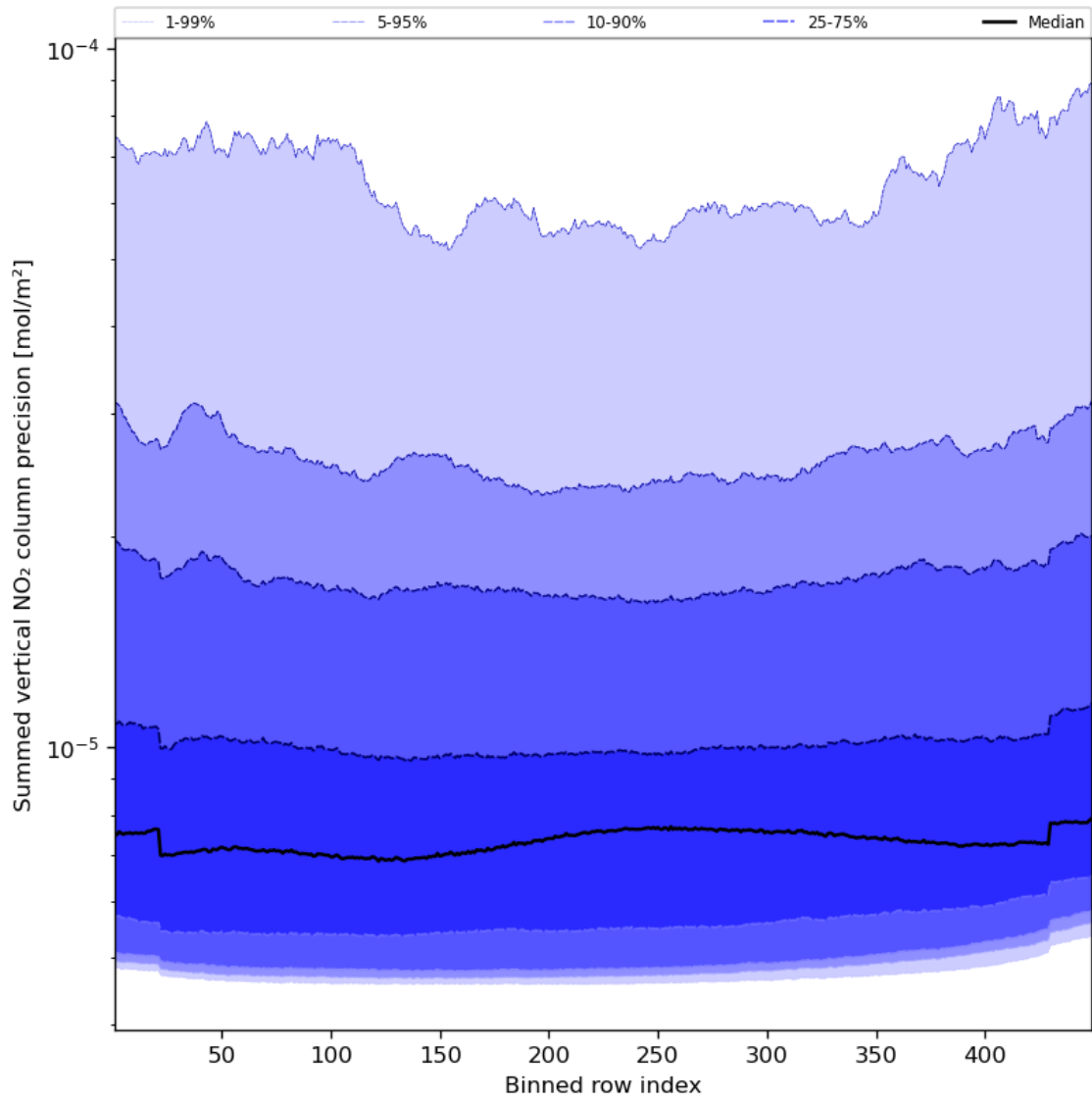
Figure 58: Along track statistics of “Summed vertical NO 2 column precision” for 2023-11-23 to 2023-11-25
