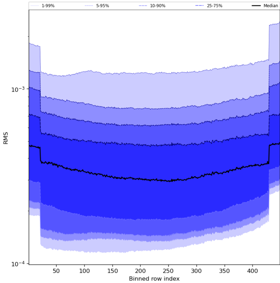
Figure 60: Along track statistics of “RMS” for 2023-11-23 to 2023-11-25
