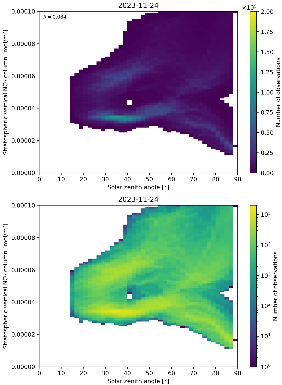
Figure 150: Scatter density plot of “Solar zenith angle” against “Stratospheric vertical NO 2 column” for 2023-11-23 to 2023-11-25.
