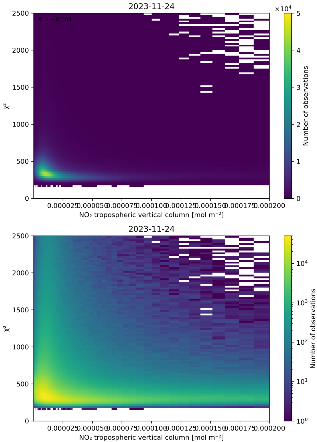
Figure 124: Scatter density plot of “NO 2 tropospheric vertical column” against “ \chi^2 ” for 2023-11-23 to 2023-11-25.
