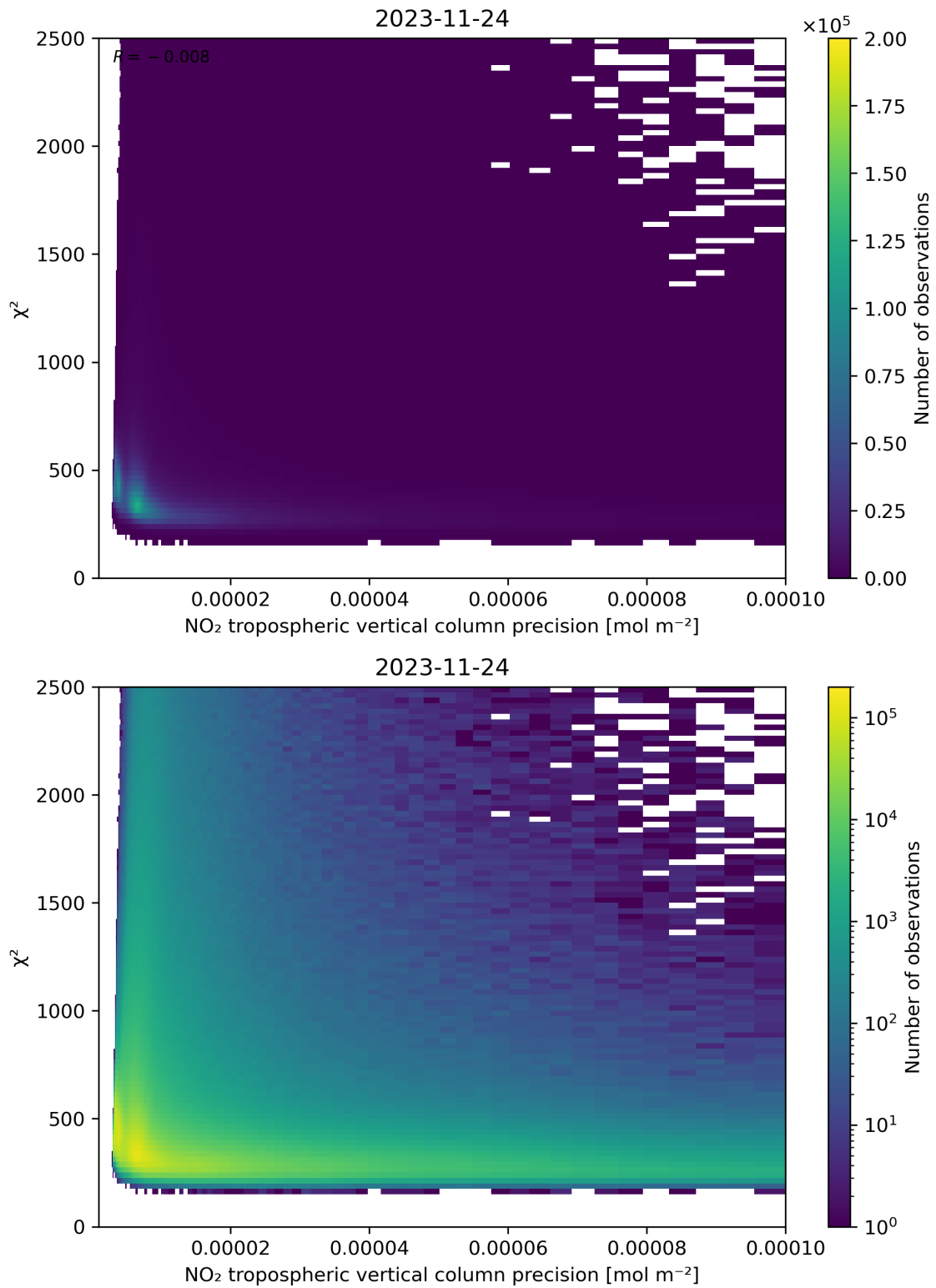
Figure 134: Scatter density plot of “NO 2 tropospheric vertical column precision” against “ \chi^2 ” for 2023-11-23 to 2023-11-25.
