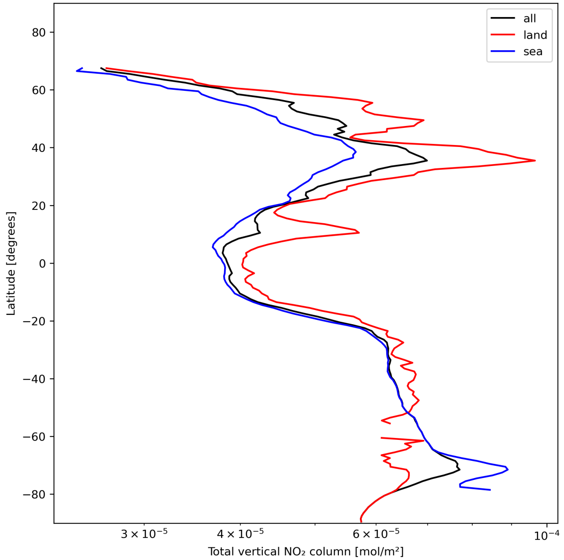
Figure 21: Zonal average of “Total vertical NO 2 column” for 2023-11-23 to 2023-11-25.
