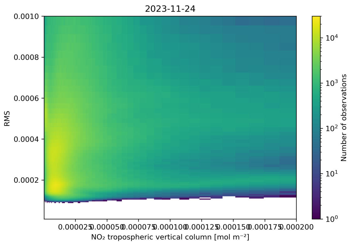
Figure 142: Scatter density plot of “NO 2 tropospheric vertical column” against “RMS” for 2023-11-23 to 2023-11-25.
