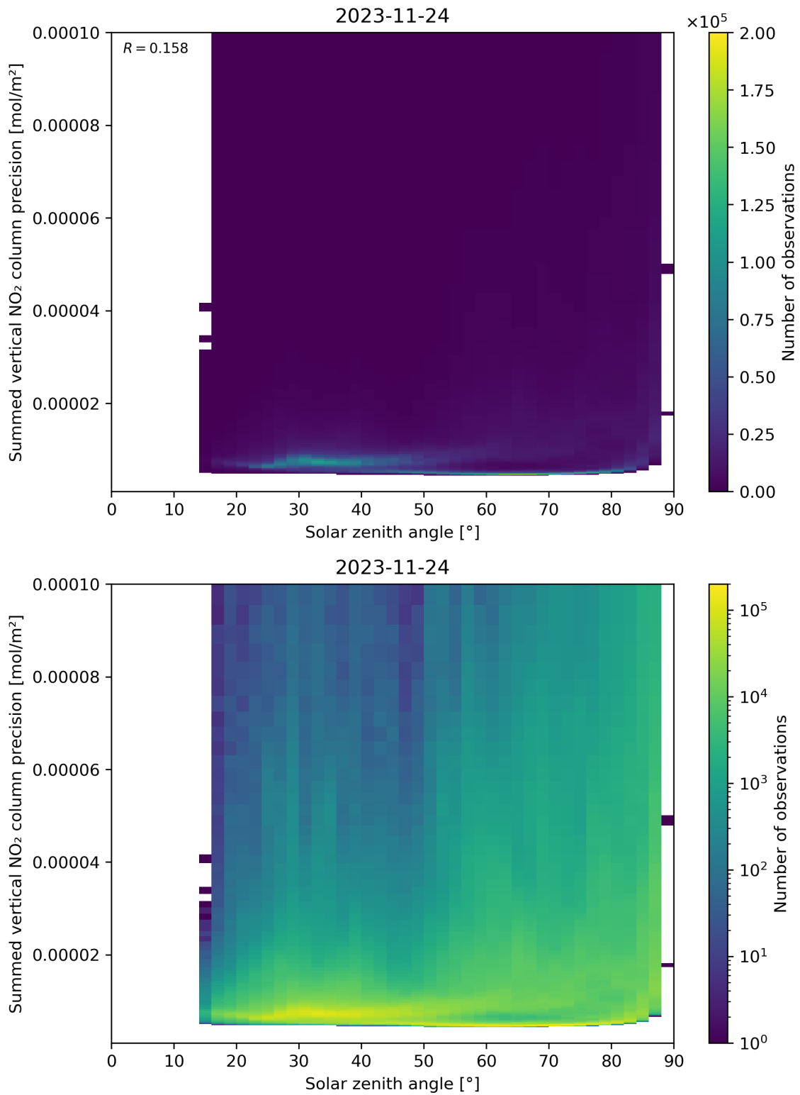
Figure 152: Scatter density plot of “Solar zenith angle” against “Summed vertical NO 2 column precision” for 2023-11-23 to 2023-11-25.
