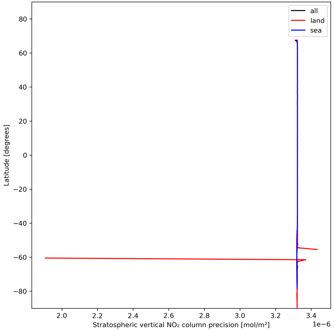
Figure 20: Zonal average of “Stratospheric vertical NO 2 column precision” for 2023-11-23 to 2023-11-25.
