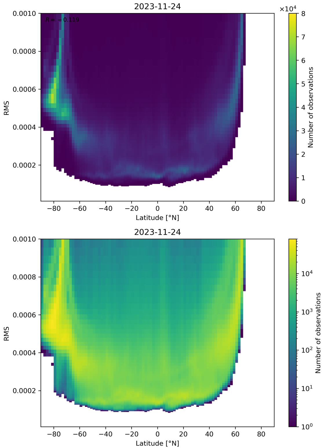
Figure 94: Scatter density plot of “Latitude” against “RMS” for 2023-11-23 to 2023-11-25.
