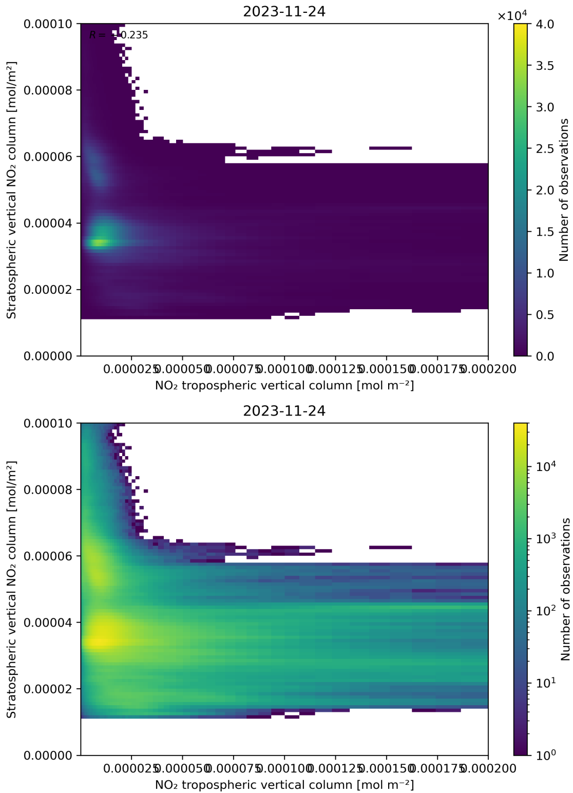
Figure 125: Scatter density plot of “NO 2 tropospheric vertical column” against “Stratospheric vertical NO 2 column” for 2023-11-23 to 2023-11-25.
