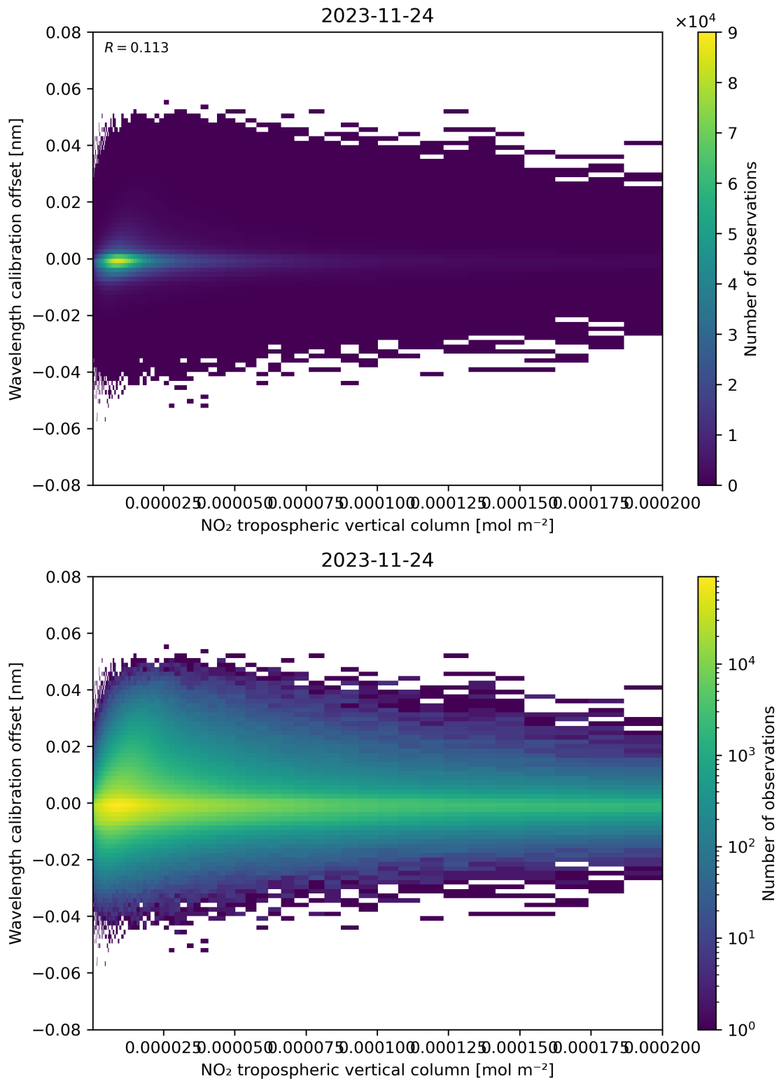
Figure 143: Scatter density plot of “NO 2 tropospheric vertical column” against “Wavelength calibration offset” for 2023-11-23 to 2023-11-25.
