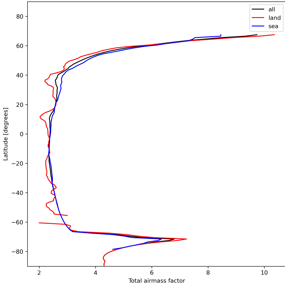
Figure 15: Zonal average of “Total air mass factor” for 2023-11-23 to 2023-11-25.
