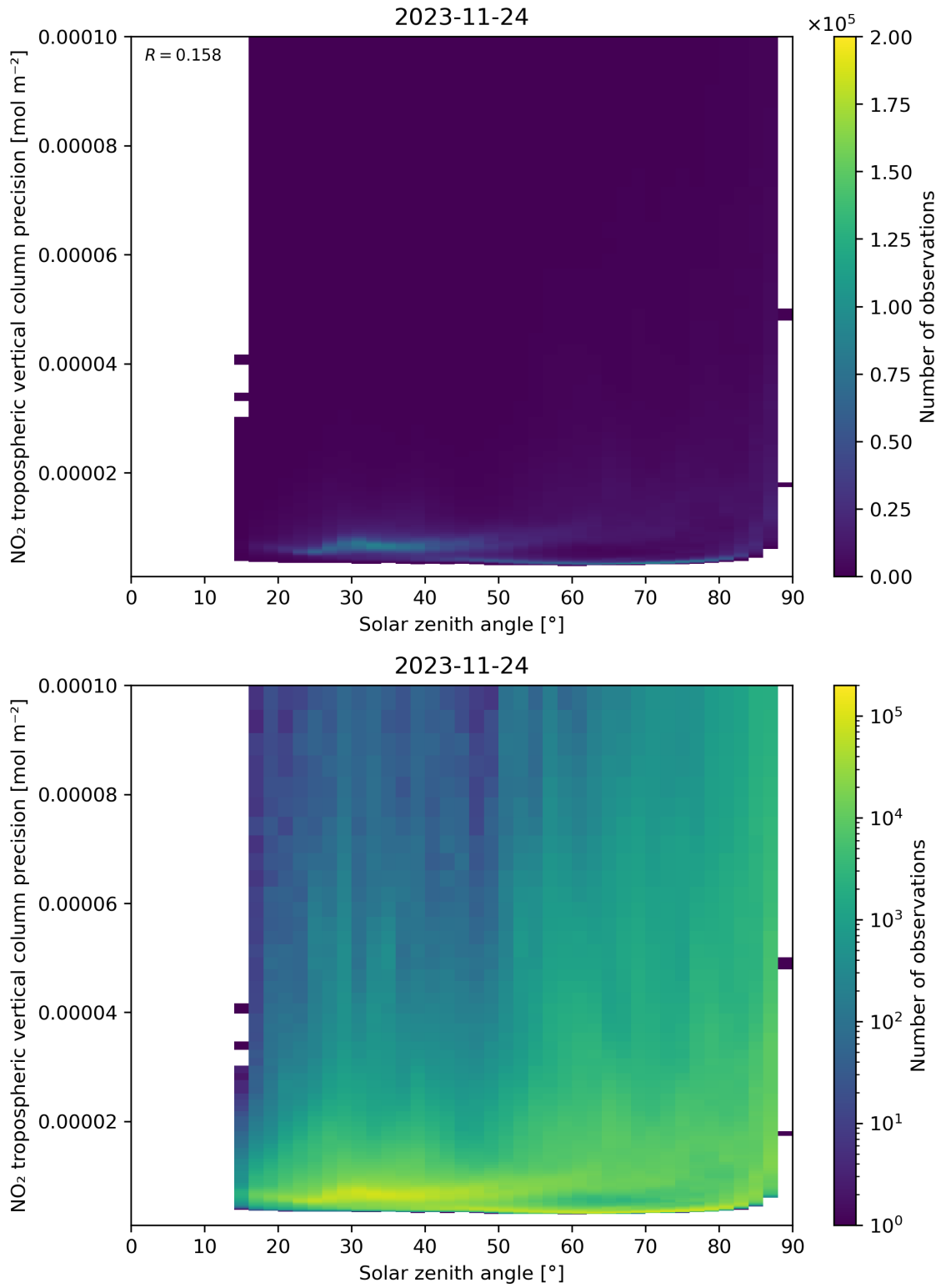
Figure 156: Scatter density plot of “Solar zenith angle” against “NO 2 tropospheric vertical column precision” for 2023-11-23 to 2023-11-25.
