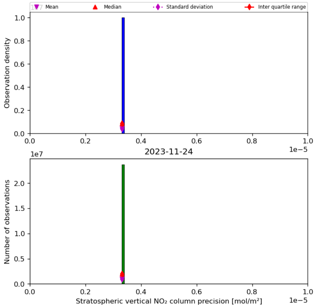
Figure 37: Histogram of “Stratospheric vertical NO 2 column precision” for 2023-11-23 to 2023-11-25
