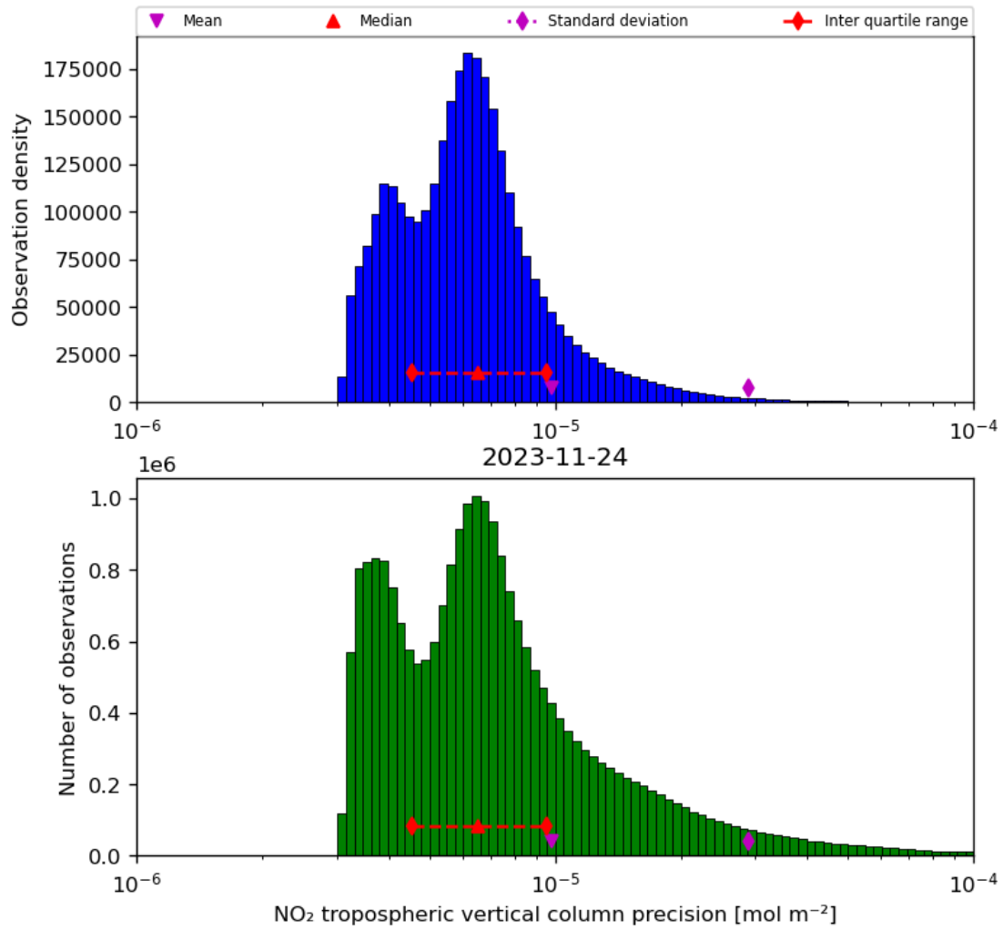
Figure 30: Histogram of “NO 2 tropospheric vertical column precision” for 2023-11-23 to 2023-11-25
