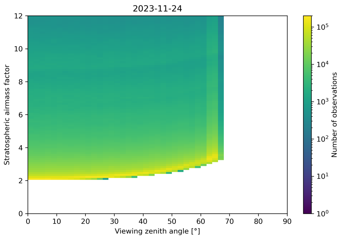
Figure 159: Scatter density plot of “Viewing zenith angle” against “Stratospheric airmass factor” for 2023-11-23 to 2023-11-25.
