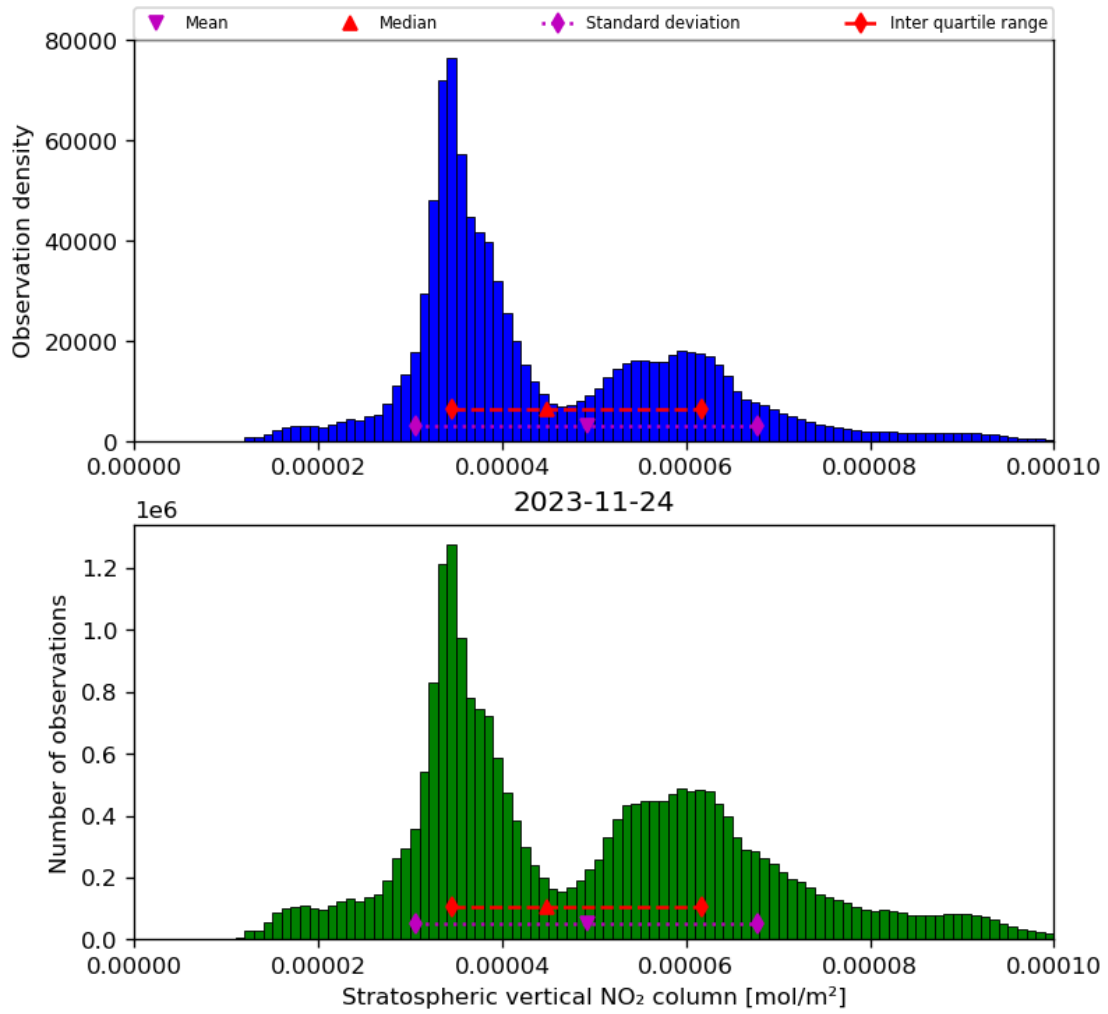
Figure 36: Histogram of “Stratospheric vertical NO 2 column” for 2023-11-23 to 2023-11-25
