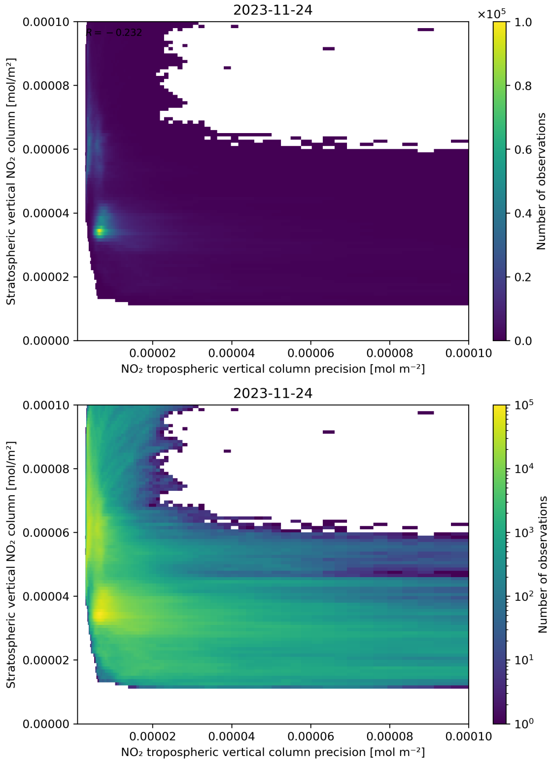
Figure 135: Scatter density plot of “NO 2 tropospheric vertical column precision” against “Stratospheric vertical NO 2 column” for 2023-11-23 to 2023-11-25.
