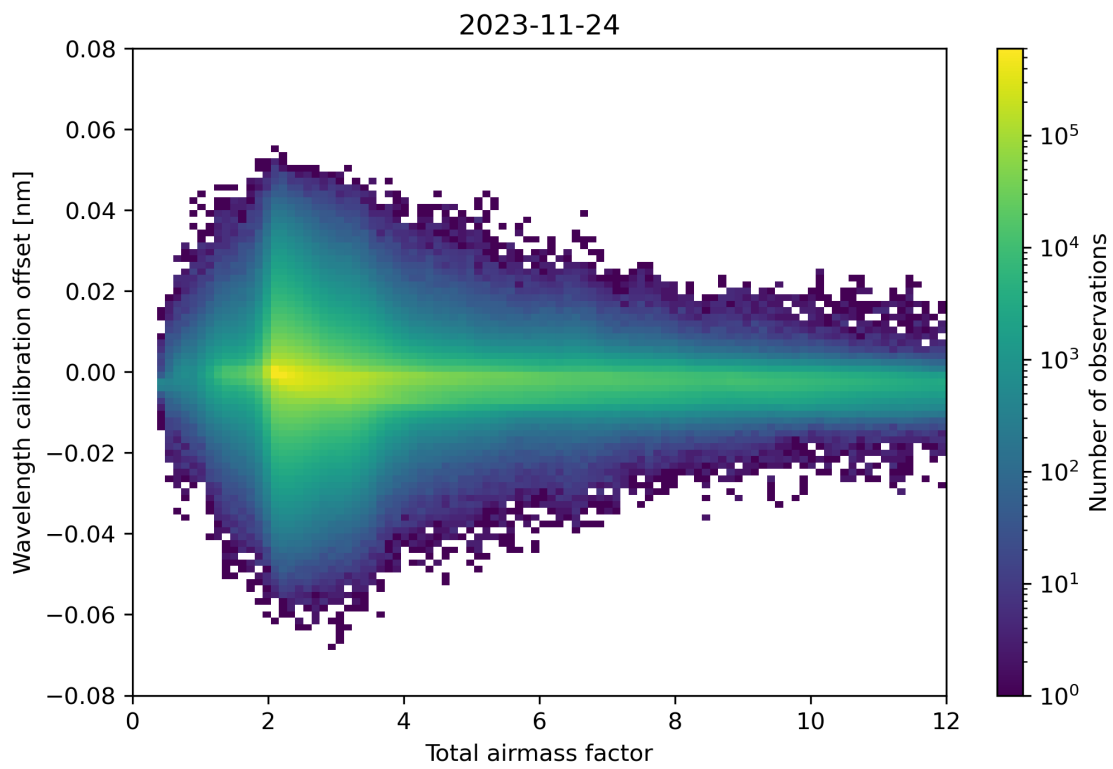
Figure 70: Scatter density plot of “Total airmass factor” against “Wavelength calibration offset” for 2023-11-23 to 2023-11-25.
