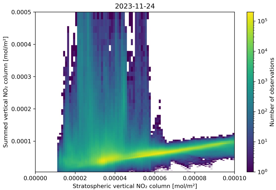
Figure 98: Scatter density plot of “Stratospheric vertical NO 2 column” against “Summed vertical NO 2 column” for 2023-11-23 to 2023-11-25.
