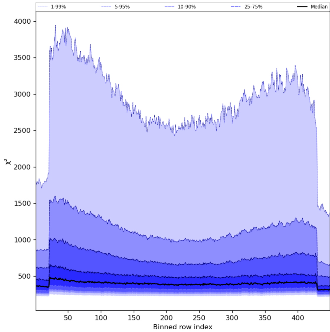
Figure 59: Along track statistics of “ \chi^2 ” for 2023-11-23 to 2023-11-25
