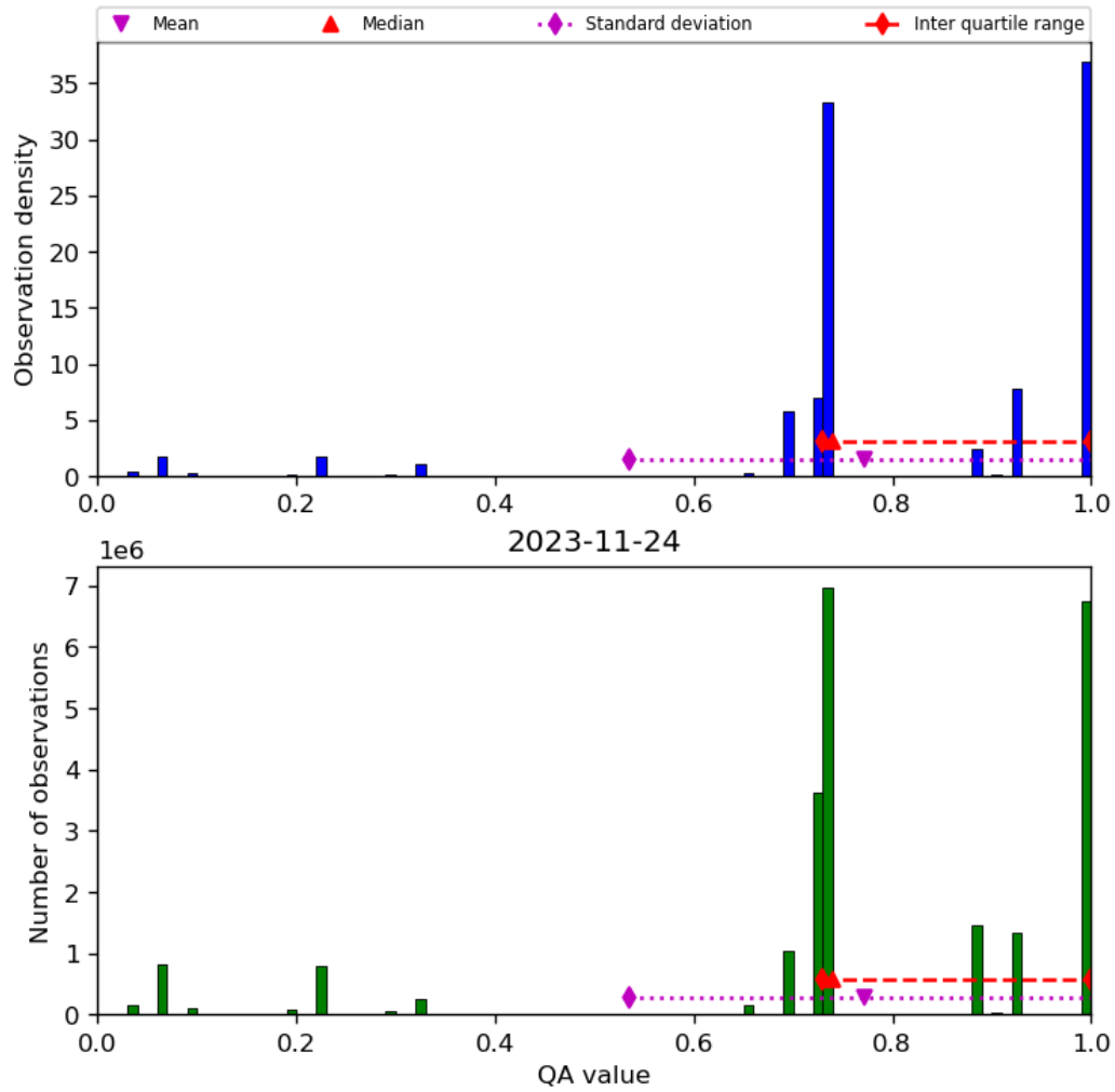
Figure 28: Histogram of “QA value” for 2023-11-23 to 2023-11-25
