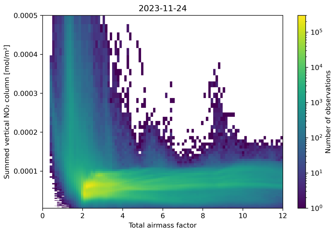
Figure 65: Scatter density plot of “Total airmass factor” against “Summed vertical NO 2 column” for 2023-11-23 to 2023-11-25.
