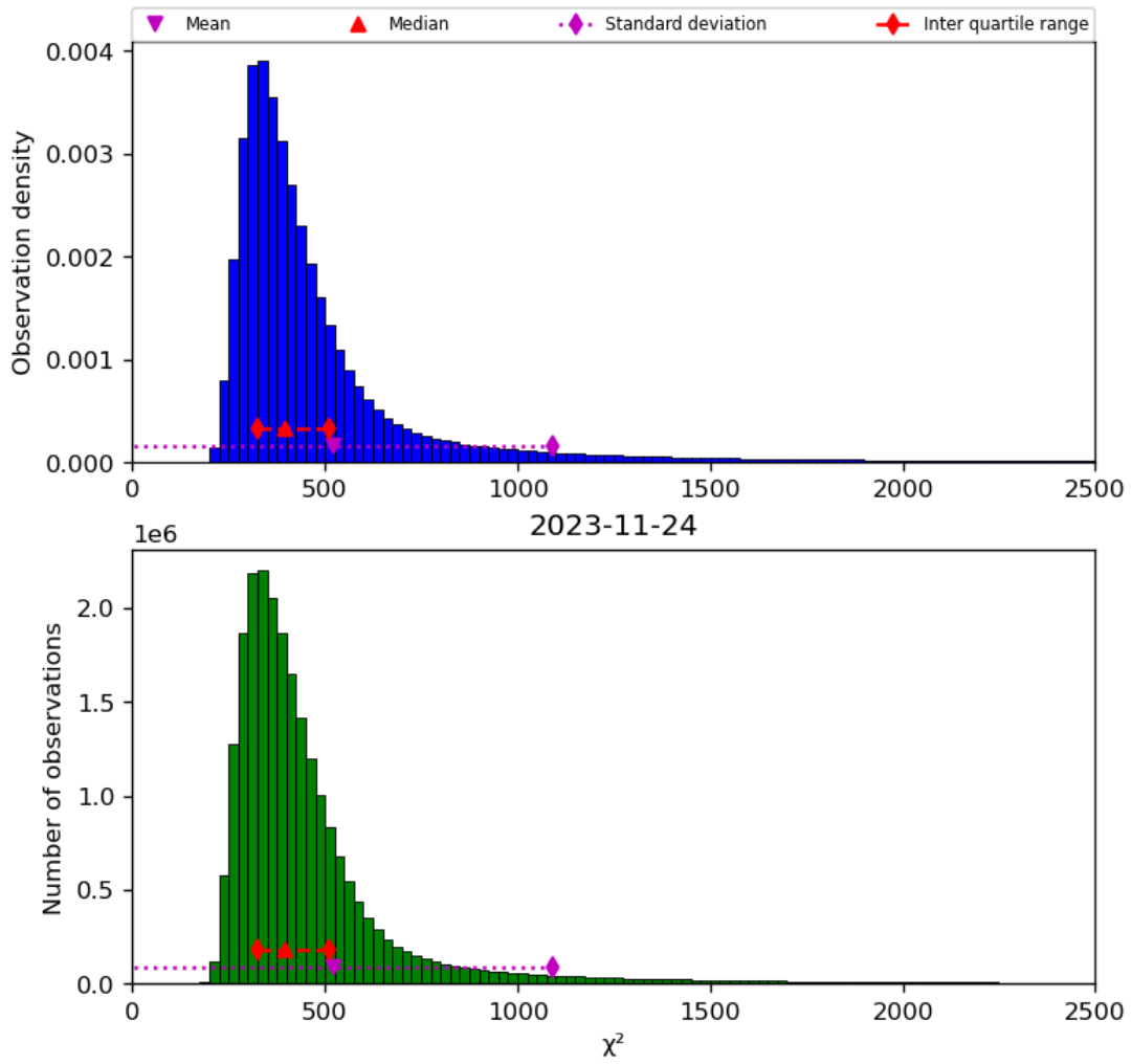
Figure 42: Histogram of “ \chi^2 ” for 2023-11-23 to 2023-11-25
