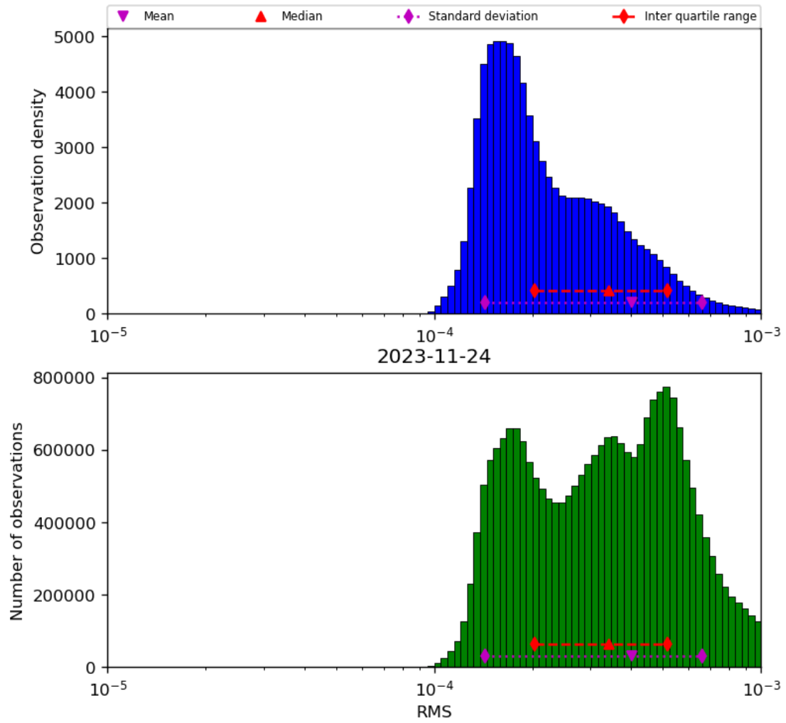
Figure 43: Histogram of “RMS” for 2023-11-23 to 2023-11-25
