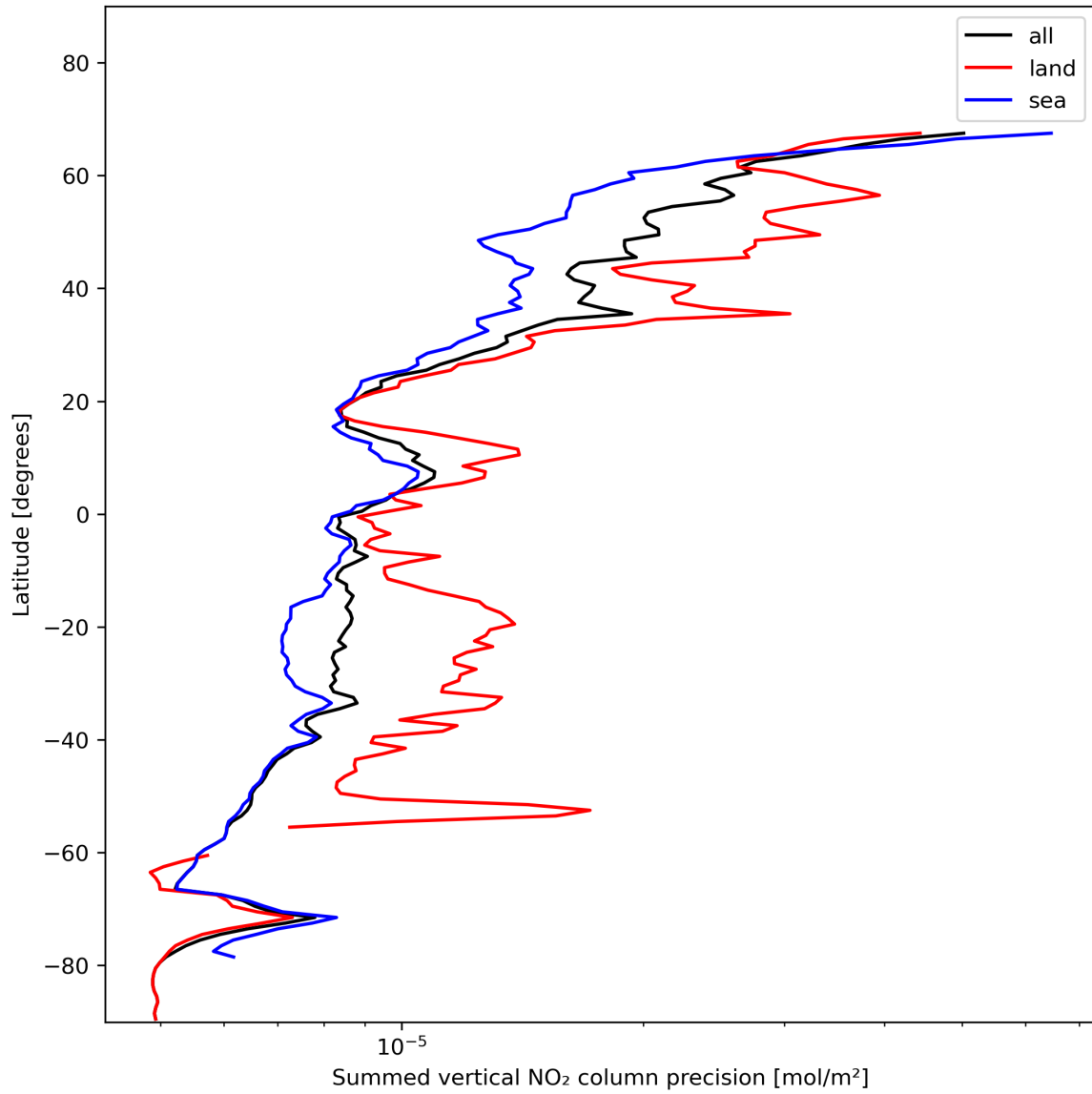
Figure 24: Zonal average of “Summed vertical NO 2 column precision” for 2023-11-23 to 2023-11-25.
