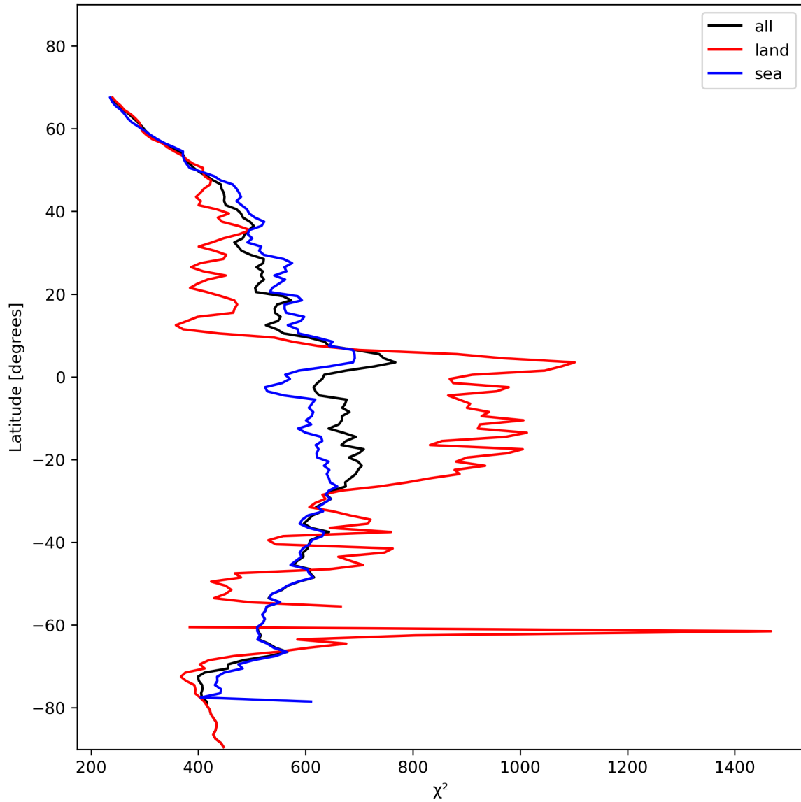
Figure 25: Zonal average of " \chi^2 " for 2023-11-23 to 2023-11-25.
