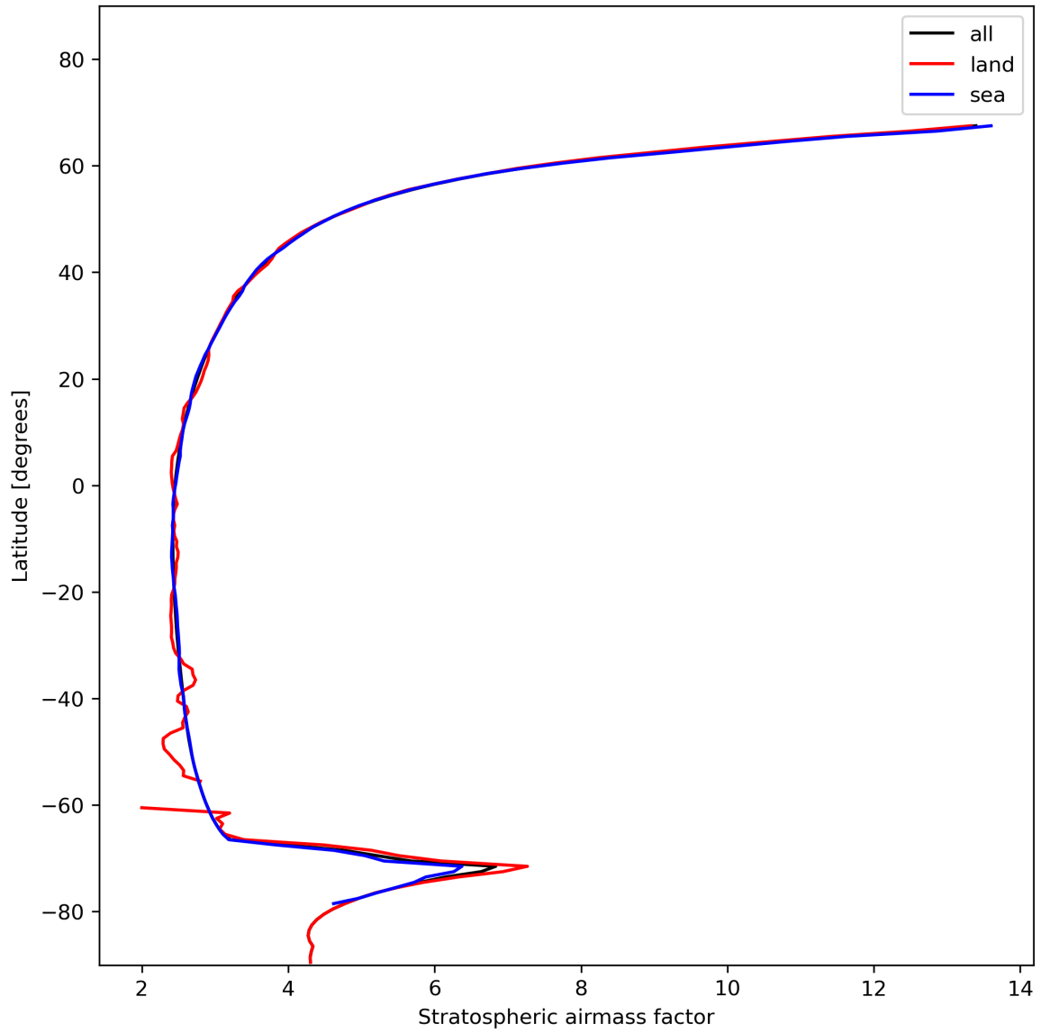
Figure 27: Zonal average of “Stratospheric air mass factor” for 2023-11-23 to 2023-11-25.
