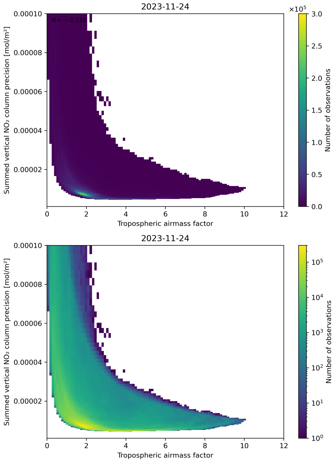
Figure 76: Scatter density plot of “Tropospheric airmass factor” against “Summed vertical NO 2 column precision” for 2023-11-23 to 2023-11-25.
