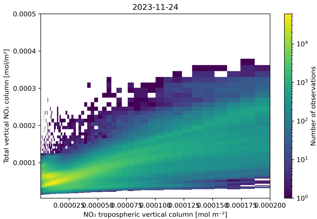
Figure 128: Scatter density plot of “NO 2 tropospheric vertical column” against “Total vertical NO 2 column” for 2023-11-23 to 2023-11-25.
