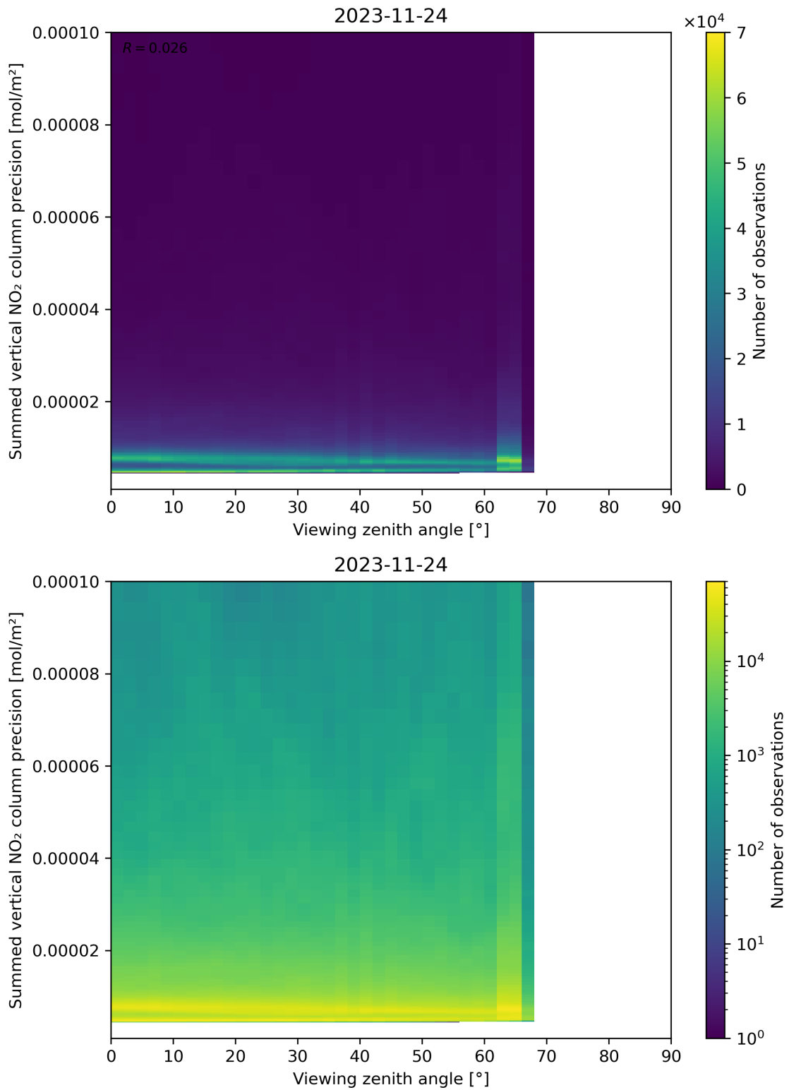
Figure 166: Scatter density plot of “Viewing zenith angle” against “Summed vertical NO 2 column precision” for 2023-11-23 to 2023-11-25.
