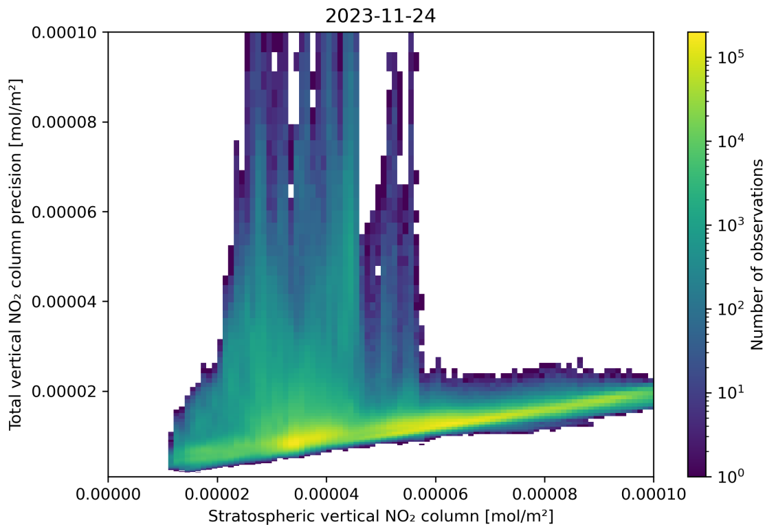
Figure 101: Scatter density plot of “Stratospheric vertical NO 2 column” against “Total vertical NO 2 column precision” for 2023-11-23 to 2023-11-25.
