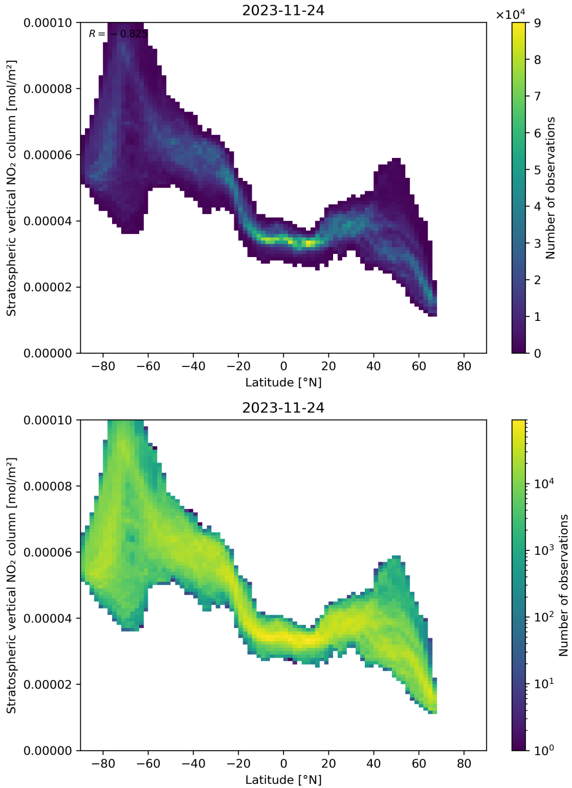
Figure 87: Scatter density plot of “Latitude” against “Stratospheric vertical NO 2 column” for 2023-11-23 to 2023-11-25.
