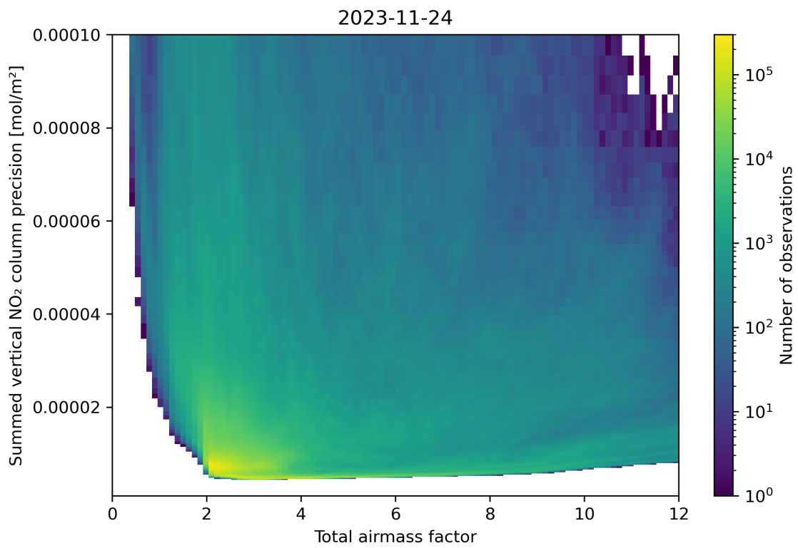
Figure 66: Scatter density plot of “Total airmass factor” against “Summed vertical NO 2 column precision” for 2023-11-23 to 2023-11-25.
