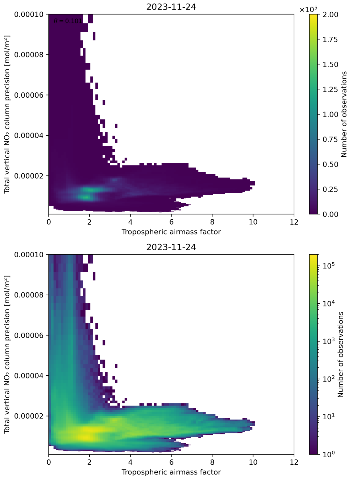
Figure 78: Scatter density plot of “Tropospheric airmass factor” against “Total vertical NO 2 column precision” for 2023-11-23 to 2023-11-25.
