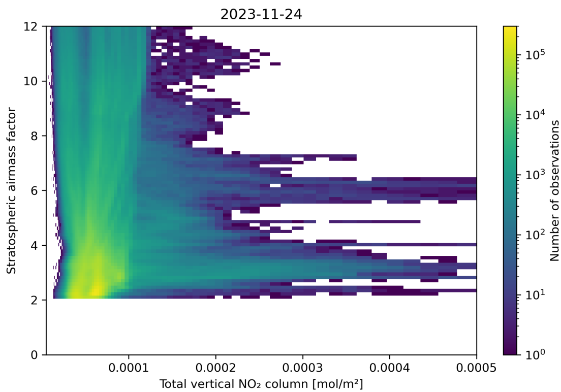
Figure 110: Scatter density plot of “Total vertical NO 2 column” against “Stratospheric airmass factor” for 2023-11-23 to 2023-11-25.
