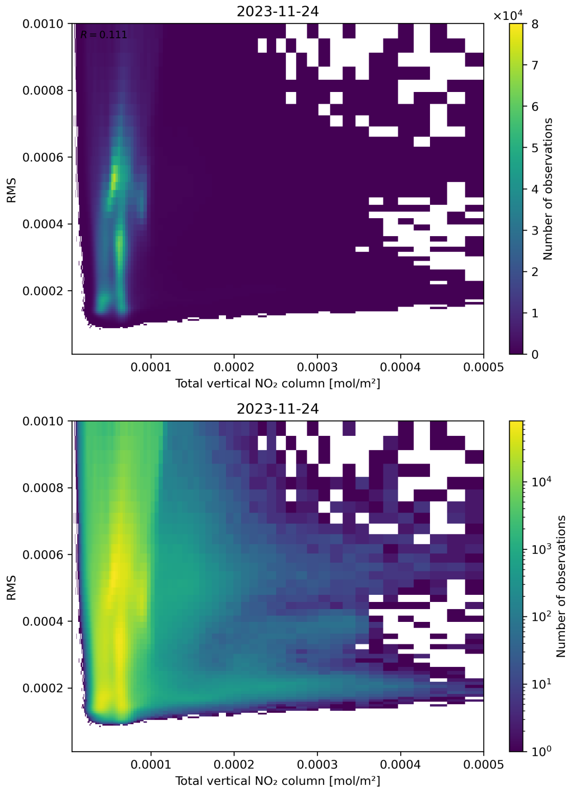
Figure 120: Scatter density plot of “Total vertical NO 2 column” against “RMS” for 2023-11-23 to 2023-11-25.
