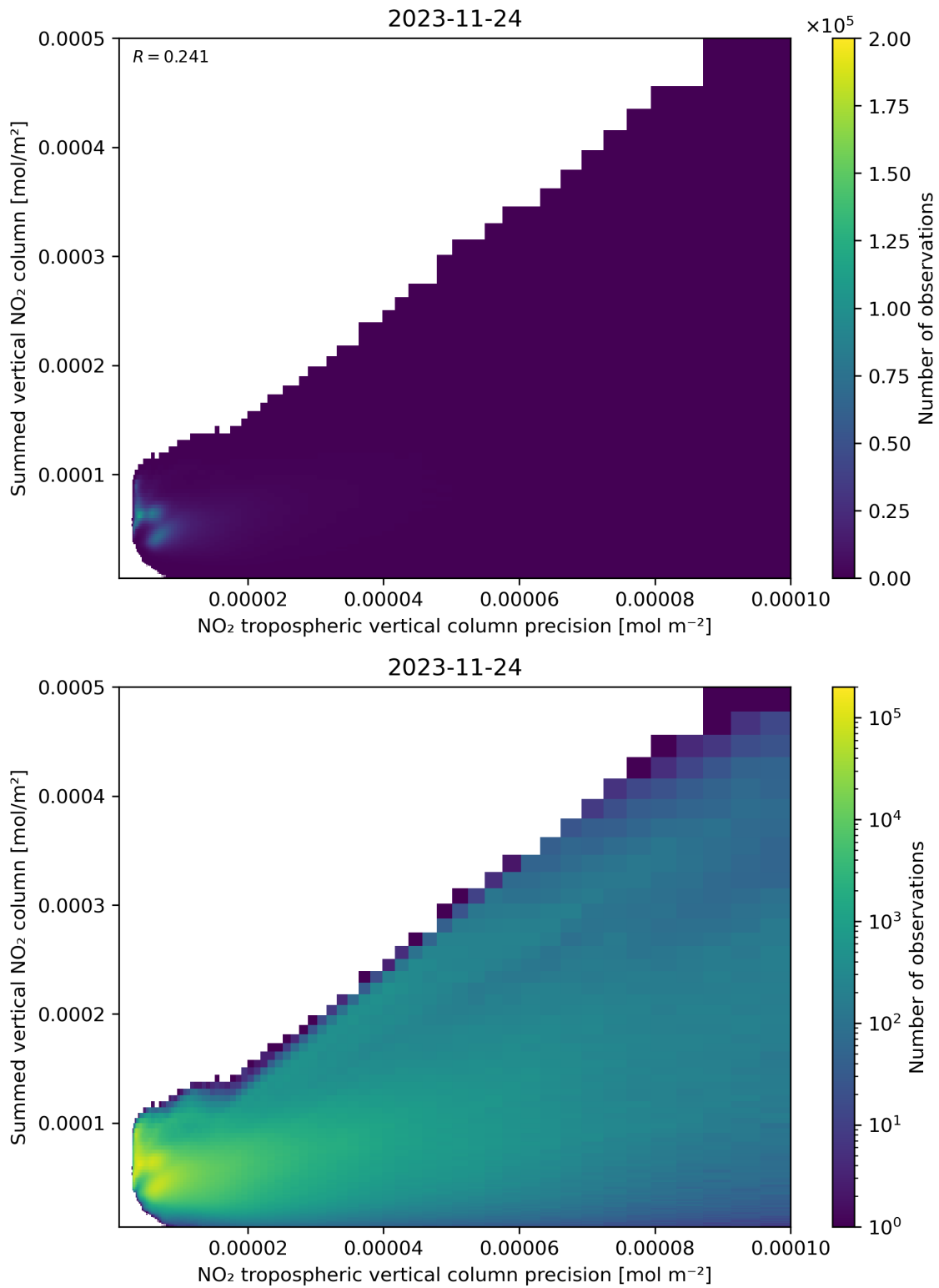
Figure 136: Scatter density plot of “NO 2 tropospheric vertical column precision” against “Summed vertical NO 2 column” for 2023-11-23 to 2023-11-25.
