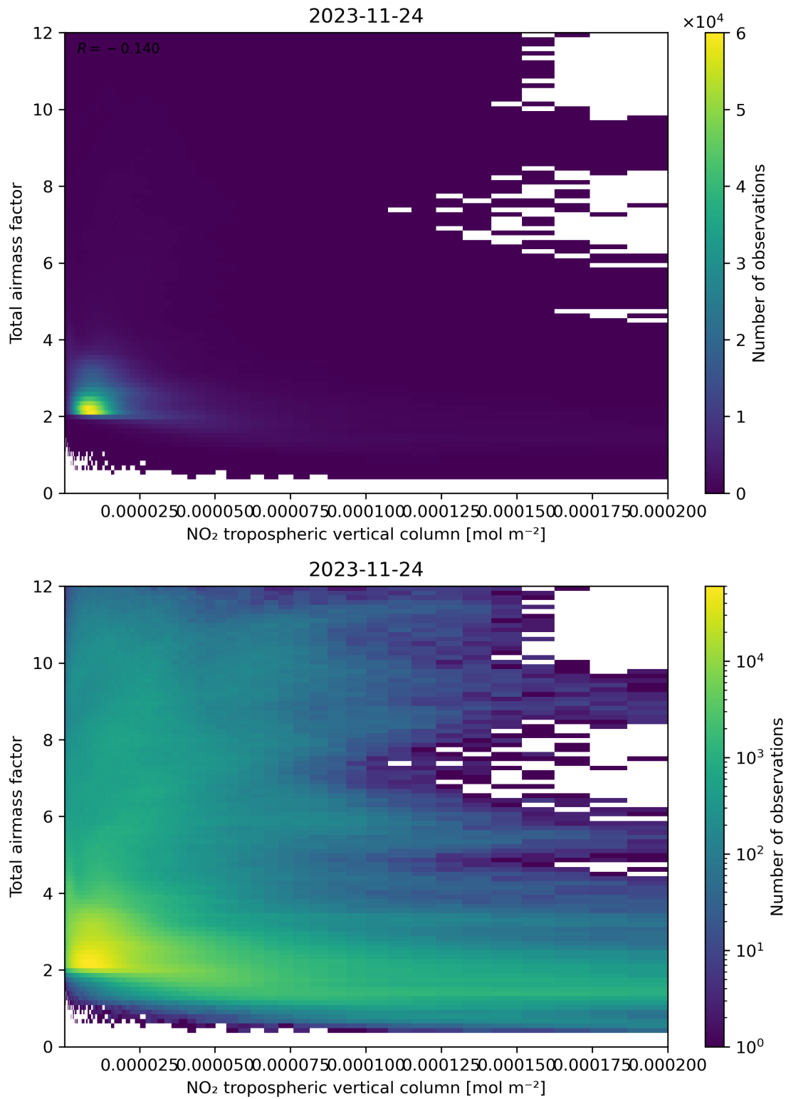
Figure 122: Scatter density plot of “NO 2 tropospheric vertical column” against “Total airmass factor” for 2023-11-23 to 2023-11-25.
