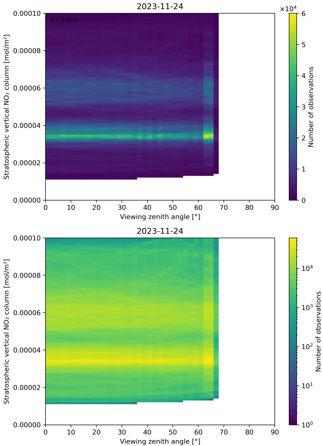
Figure 164: Scatter density plot of “Viewing zenith angle” against “Stratospheric vertical NO 2 column” for 2023-11-23 to 2023-11-25.
