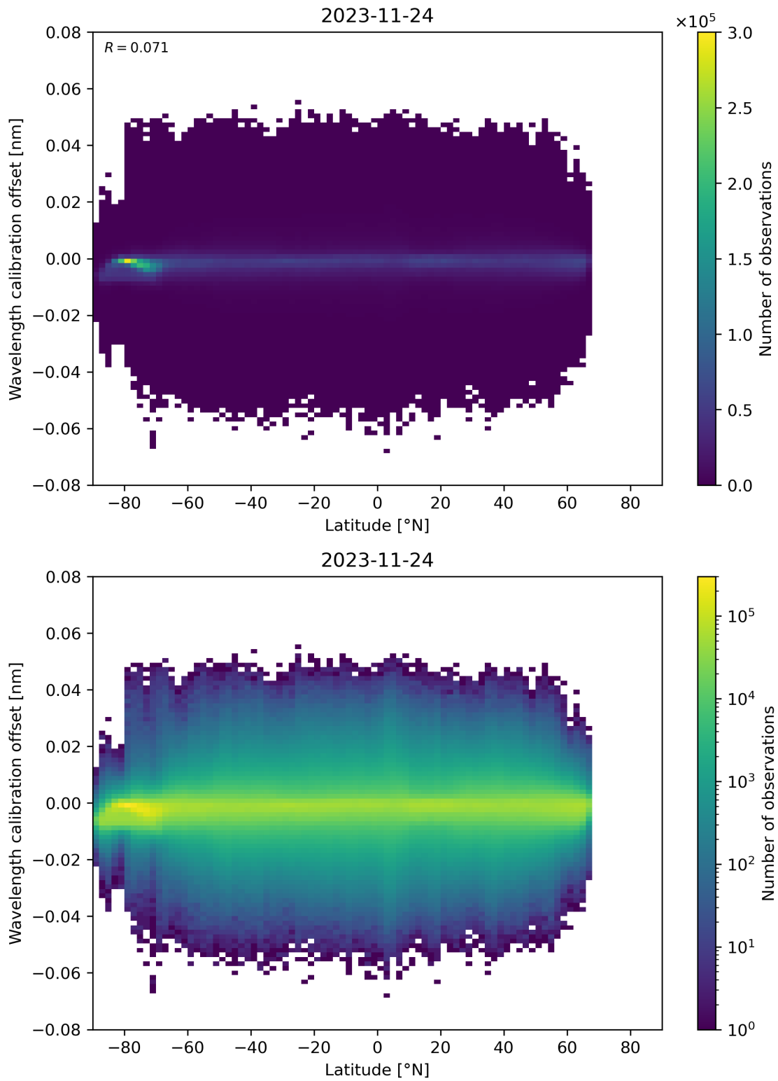
Figure 95: Scatter density plot of “Latitude” against “Wavelength calibration offset” for 2023-11-23 to 2023-11-25.
