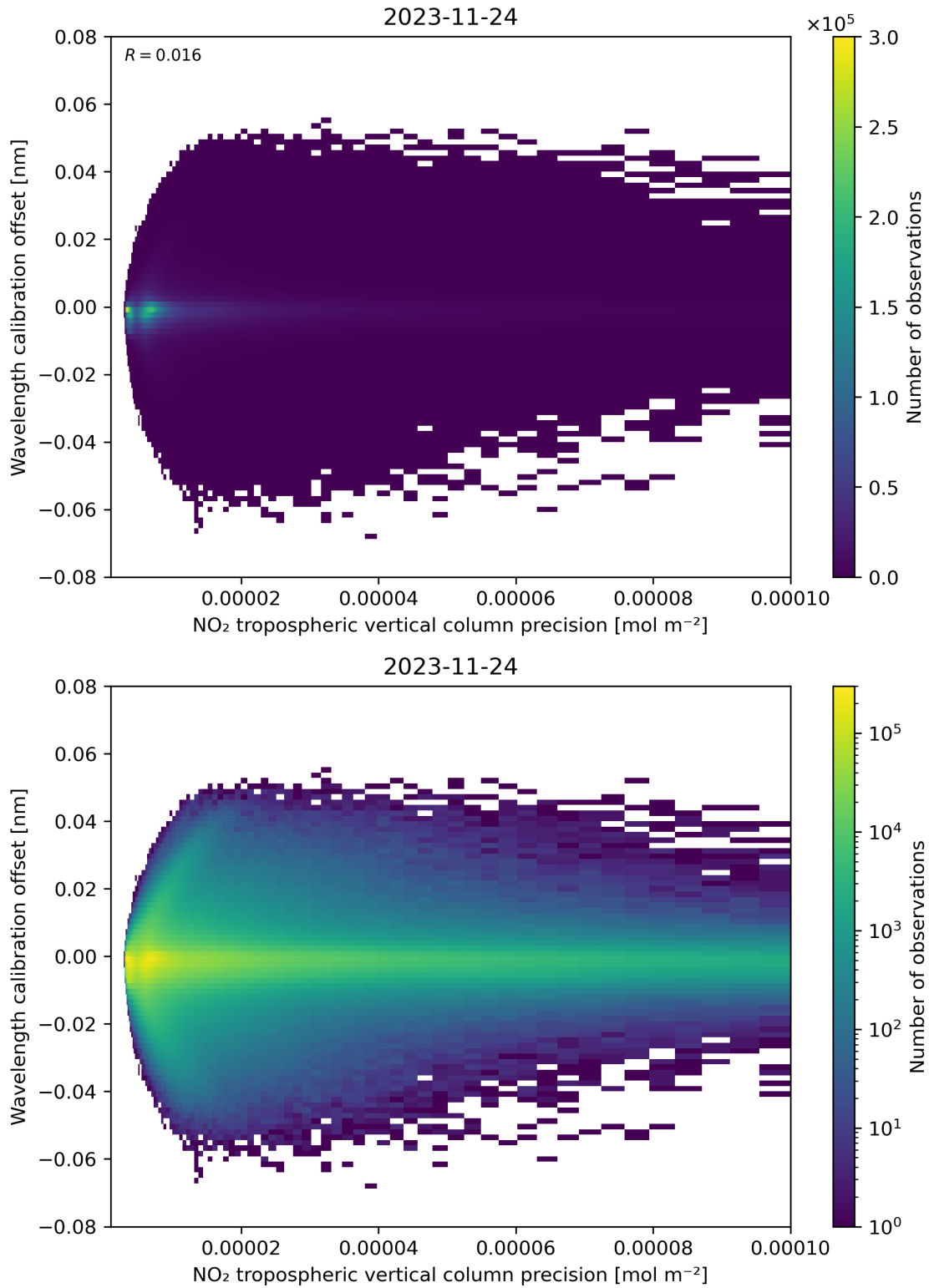
Figure 141: Scatter density plot of “NO 2 tropospheric vertical column precision” against “Wavelength calibration offset” for 2023-11-23 to 2023-11-25.
