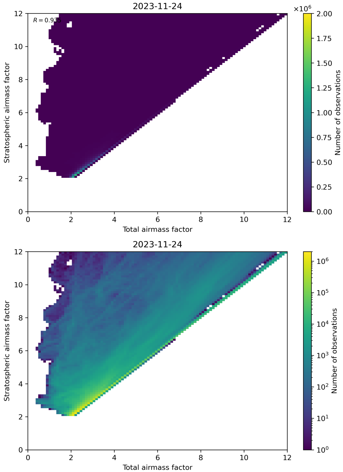
Figure 62: Scatter density plot of “Total airmass factor” against “Stratospheric airmass factor” for 2023-11-23 to 2023-11-25.
