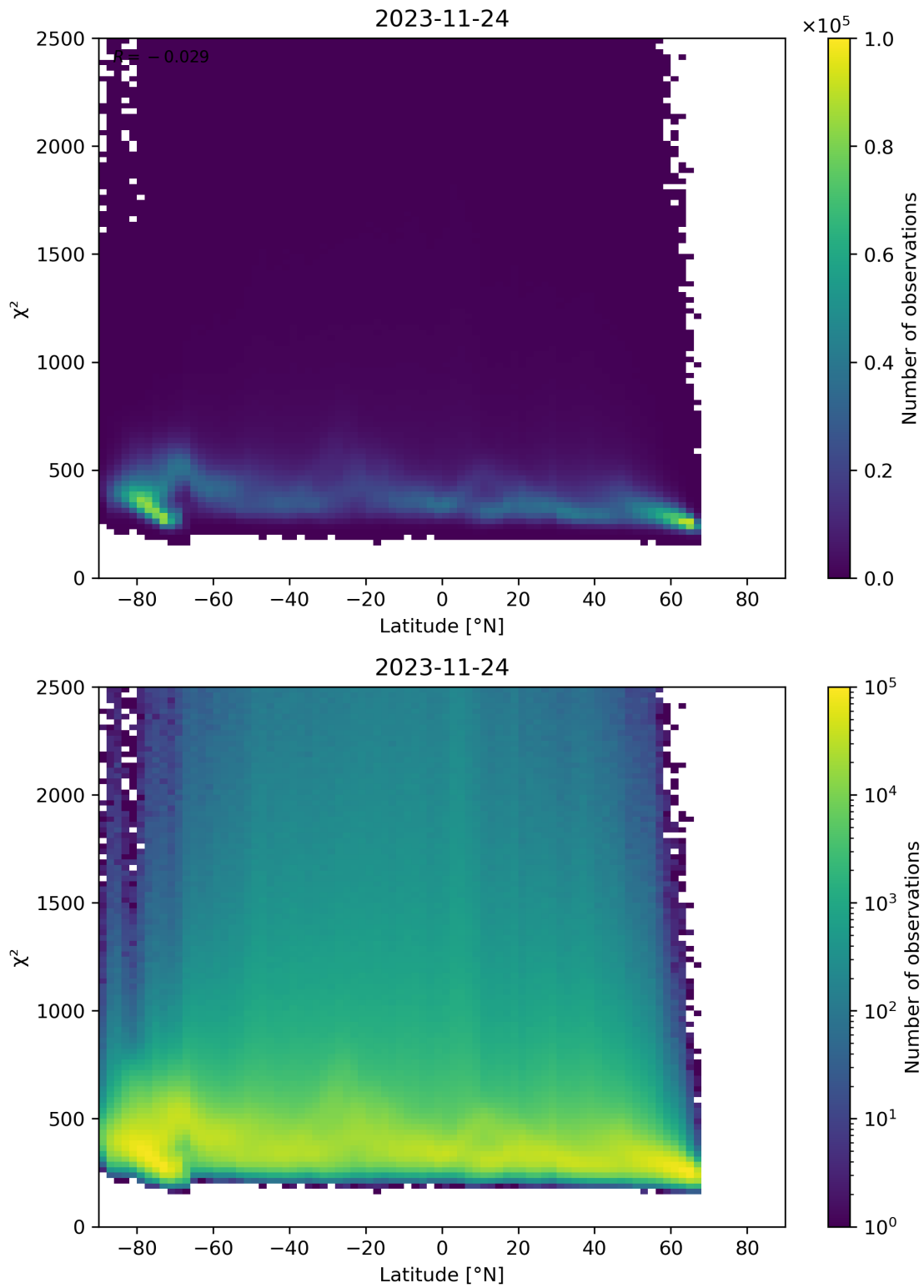
Figure 86: Scatter density plot of “Latitude” against “ \chi^2 ” for 2023-11-23 to 2023-11-25.
