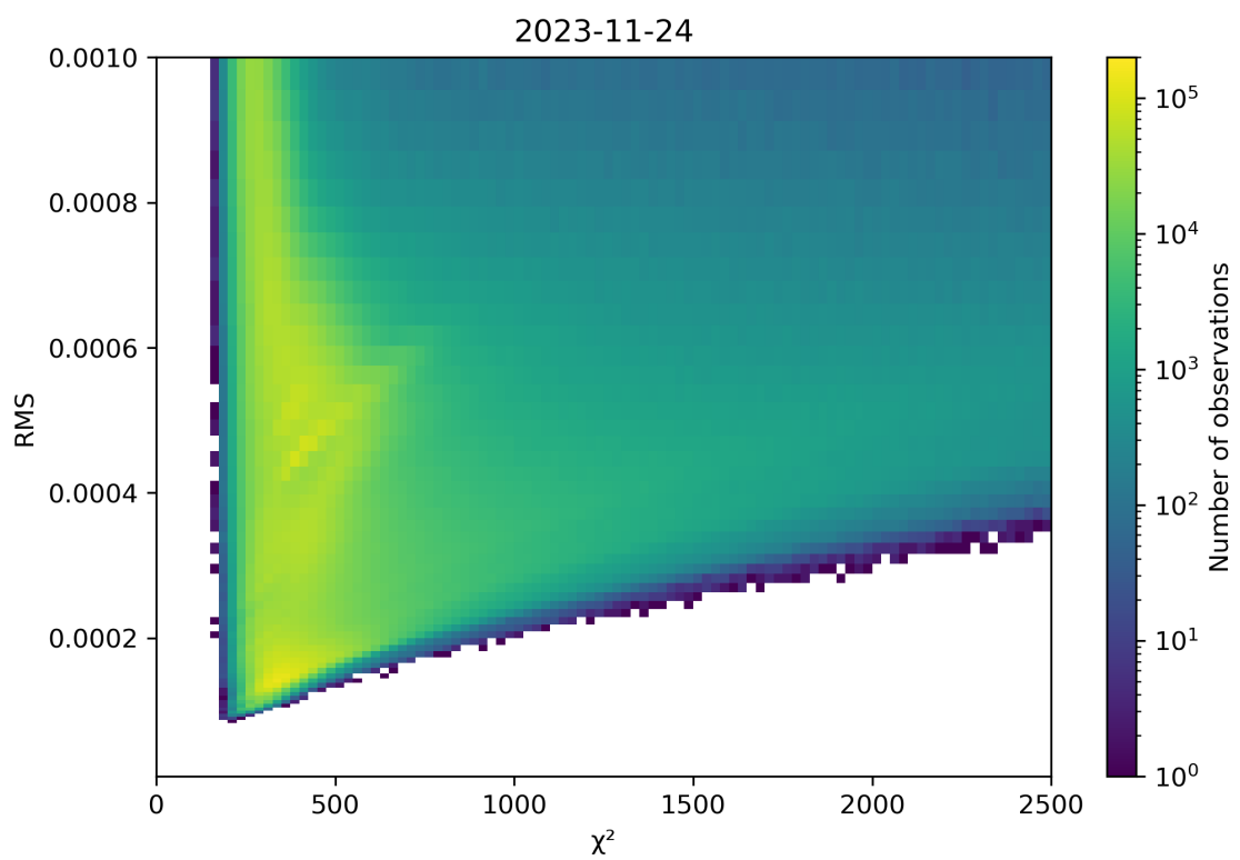
Figure 82: Scatter density plot of " \chi^2 " against "RMS" for 2023-11-23 to 2023-11-25.
