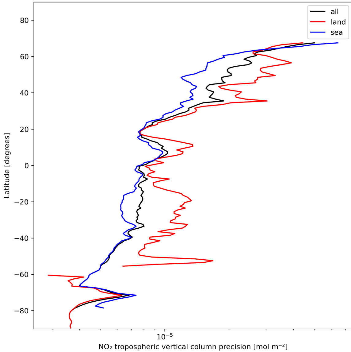
Figure 13: Zonal average of “NO 2 tropospheric vertical column precision” for 2023-11-23 to 2023-11-25.
