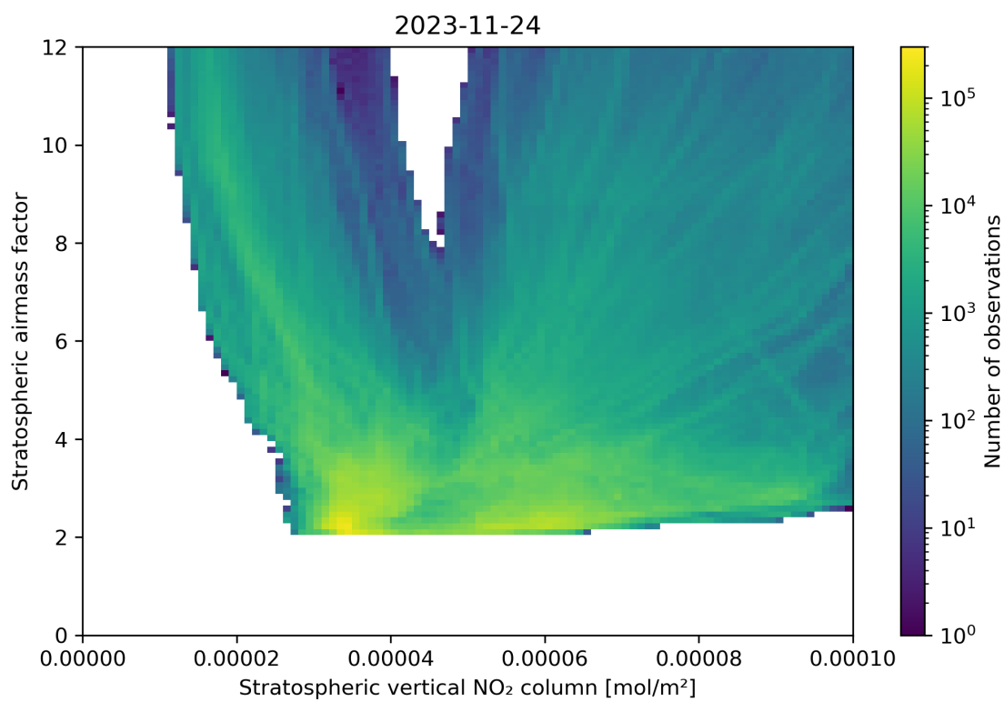
Figure 96: Scatter density plot of “Stratospheric vertical NO 2 column” against “Stratospheric airmass factor” for 2023-11-23 to 2023-11-25.
