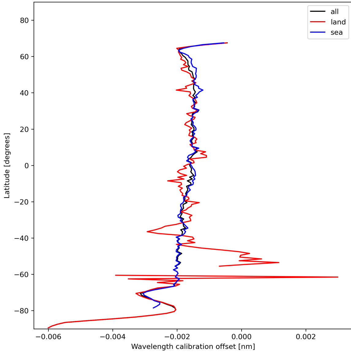
Figure 18: Zonal average of “Wavelength calibration offset” for 2023-11-23 to 2023-11-25.
