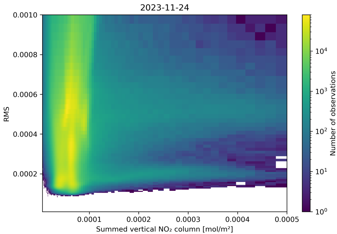
Figure 109: Scatter density plot of “Summed vertical NO 2 column” against “RMS” for 2023-11-23 to 2023-11-25.
