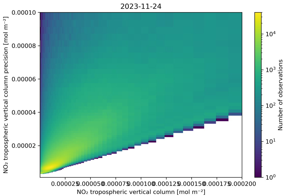
Figure 130: Scatter density plot of “NO 2 tropospheric vertical column” against “NO 2 tropospheric vertical column precision” for 2023-11-23 to 2023-11-25.
