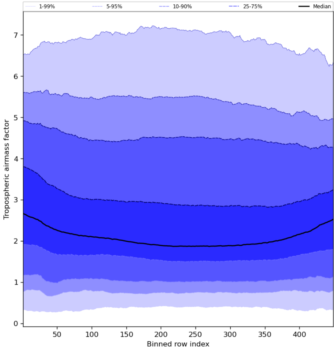
Figure 48: Along track statistics of “Tropospheric airmass factor” for 2023-11-23 to 2023-11-25
