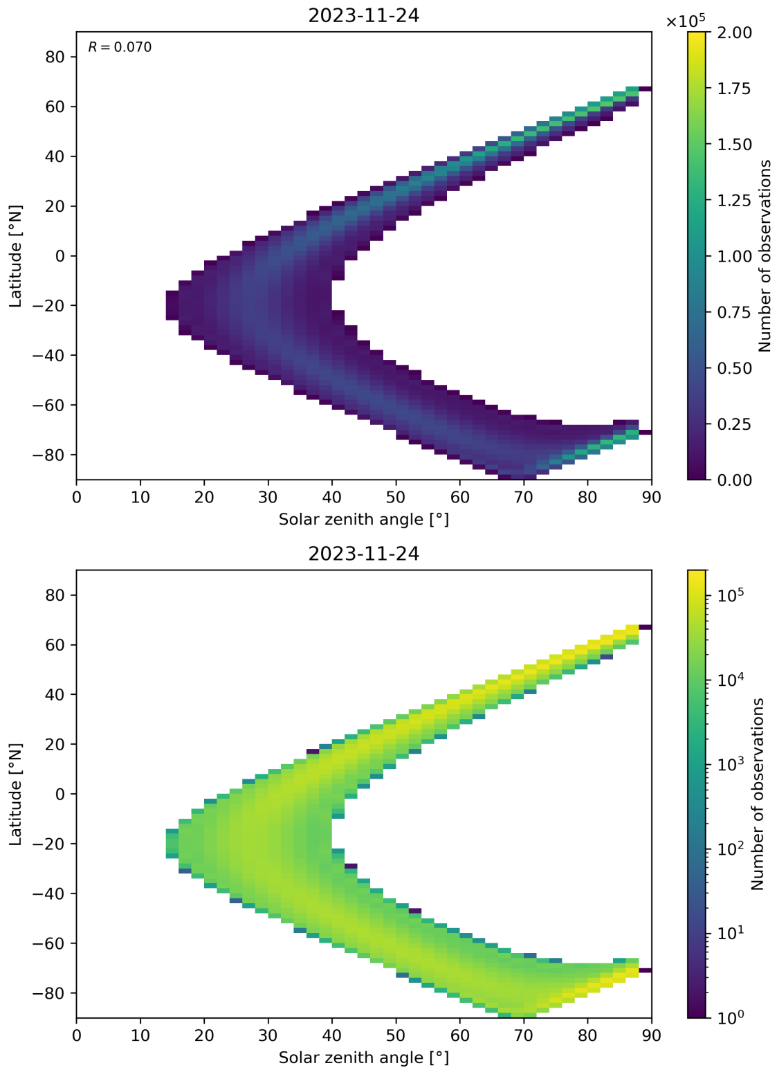
Figure 149: Scatter density plot of “Solar zenith angle” against “Latitude” for 2023-11-23 to 2023-11-25.
