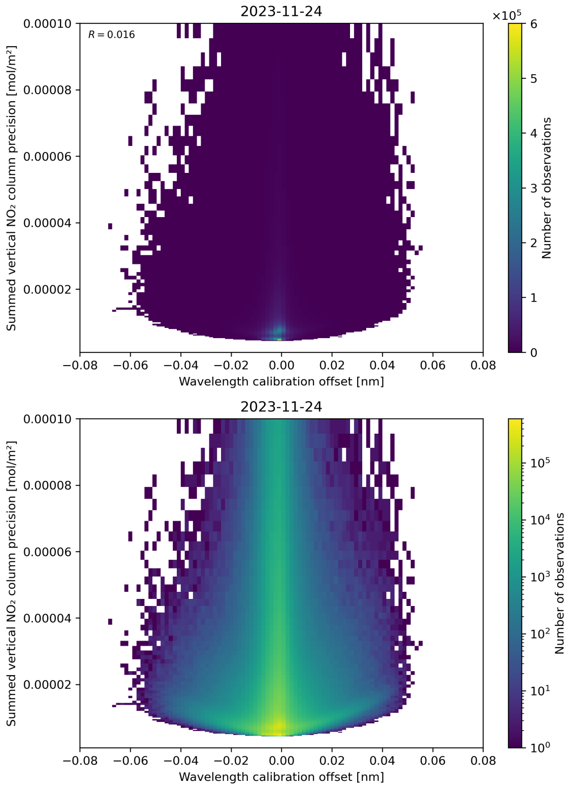
Figure 178: Scatter density plot of “Wavelength calibration offset” against “Summed vertical NO 2 column precision” for 2023-11-23 to 2023-11-25.
