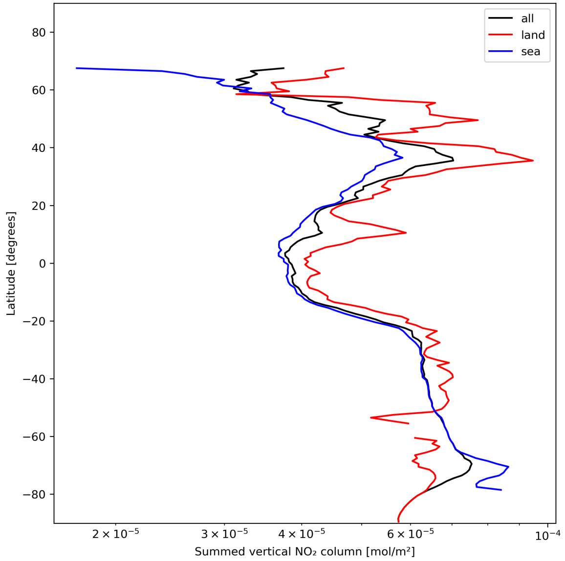
Figure 23: Zonal average of “Summed vertical NO 2 column” for 2023-11-23 to 2023-11-25.
