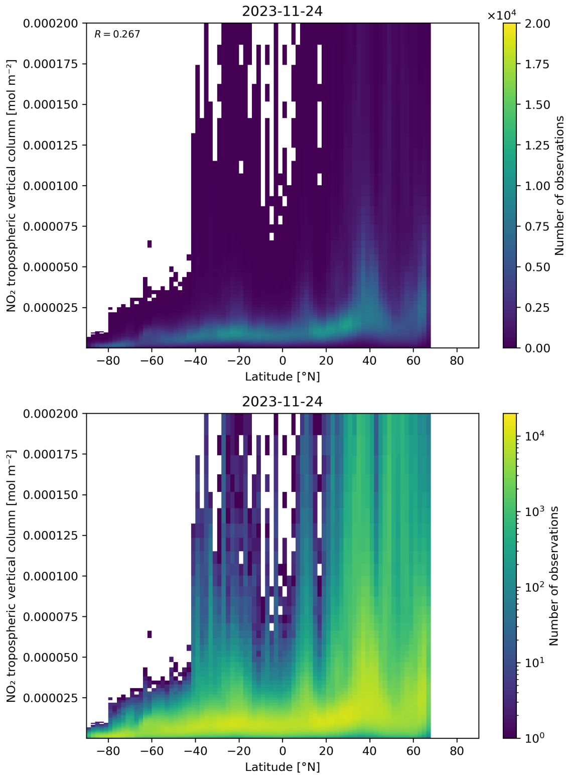
Figure 92: Scatter density plot of “Latitude” against “NO 2 tropospheric vertical column” for 2023-11-23 to 2023-11-25.
