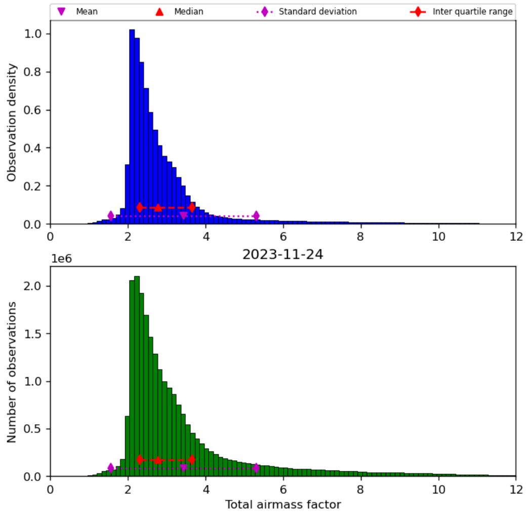
Figure 32: Histogram of “Total air mass factor” for 2023-11-23 to 2023-11-25
