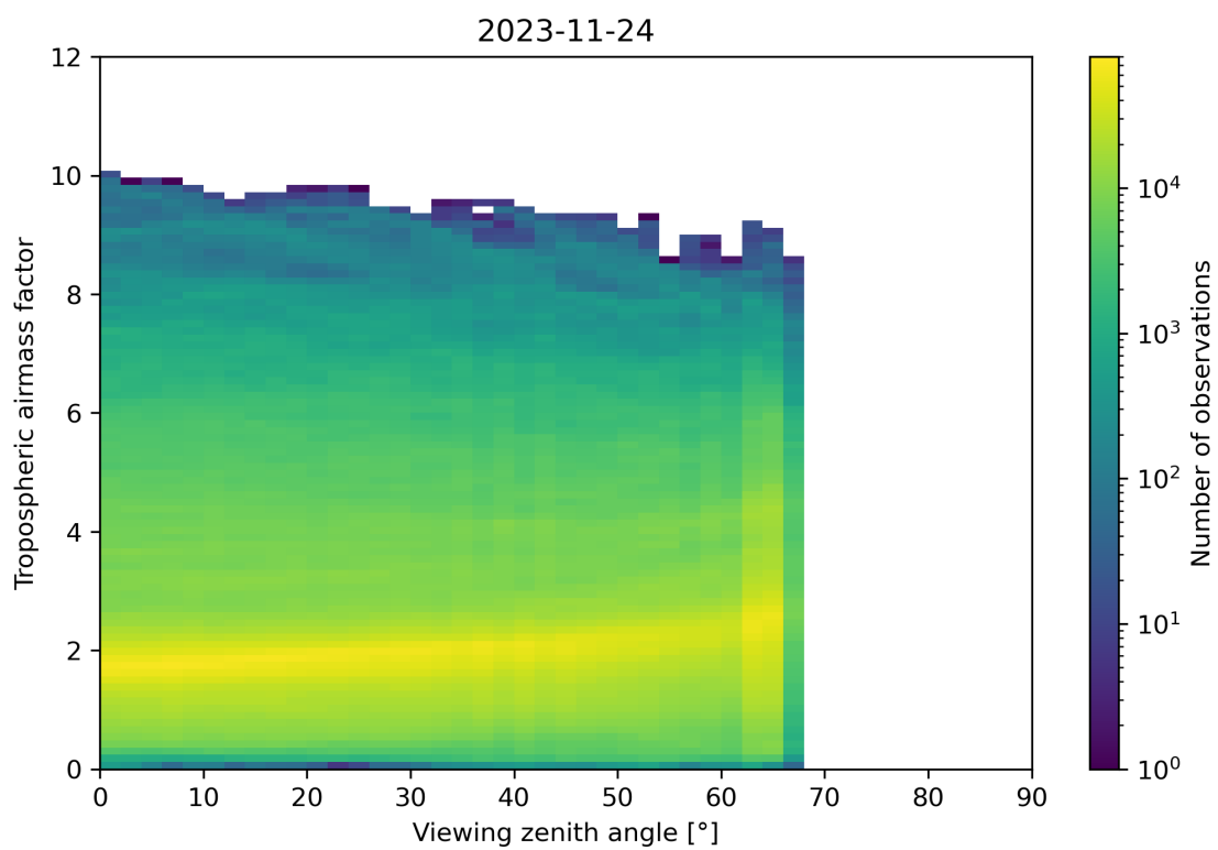
Figure 161: Scatter density plot of “Viewing zenith angle” against “Tropospheric airmass factor” for 2023-11-23 to 2023-11-25.
