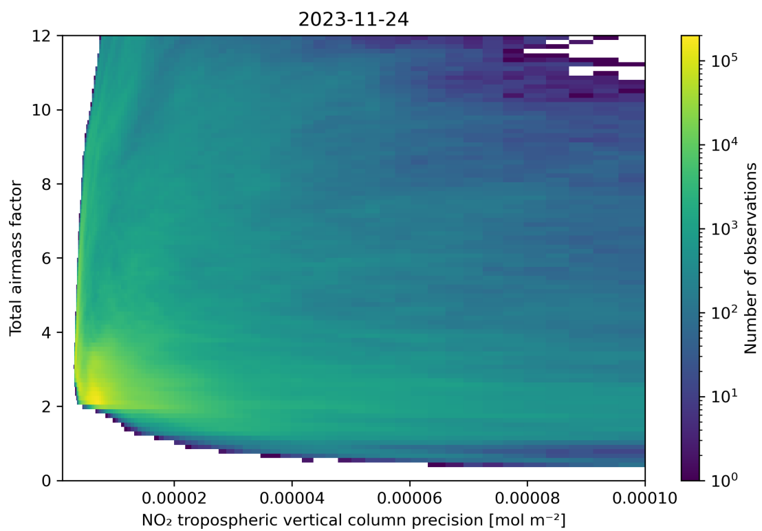
Figure 132: Scatter density plot of “NO 2 tropospheric vertical column precision” against “Total airmass factor” for 2023-11-23 to 2023-11-25.
