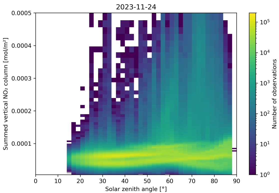
Figure 151: Scatter density plot of “Solar zenith angle” against “Summed vertical NO 2 column” for 2023-11-23 to 2023-11-25.
