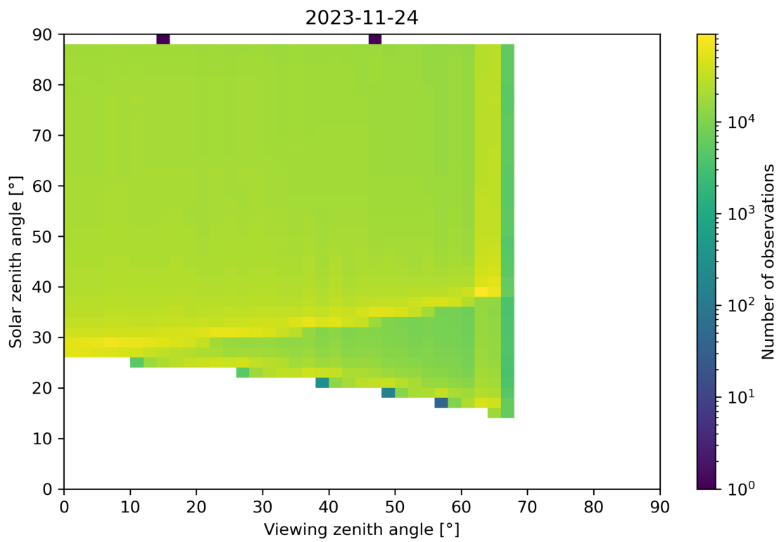
Figure 172: Scatter density plot of “Viewing zenith angle” against “Solar zenith angle” for 2023-11-23 to 2023-11-25.
