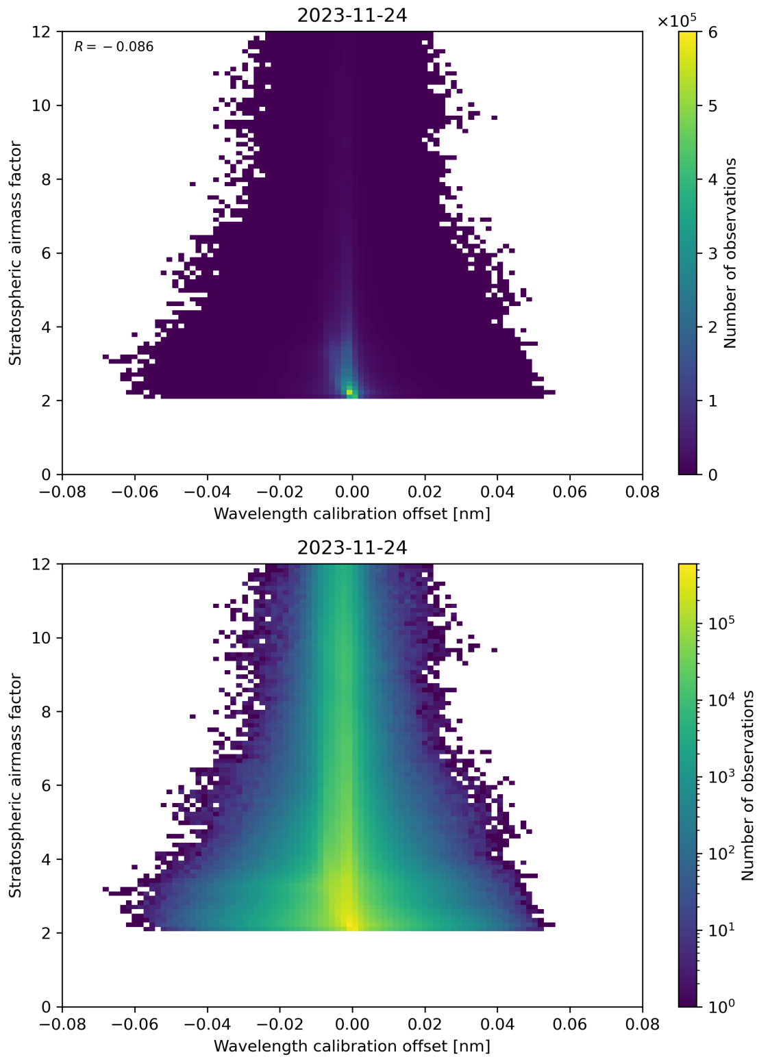
Figure 174: Scatter density plot of “Wavelength calibration offset” against “Stratospheric airmass factor” for 2023-11-23 to 2023-11-25.
