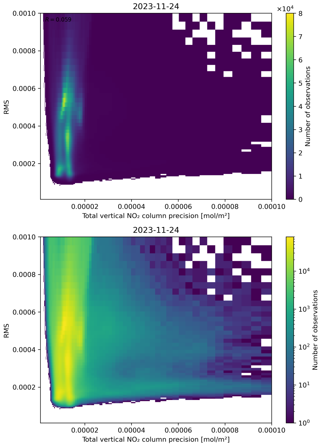
Figure 119: Scatter density plot of “Total vertical NO 2 column precision” against “RMS” for 2023-11-23 to 2023-11-25.
