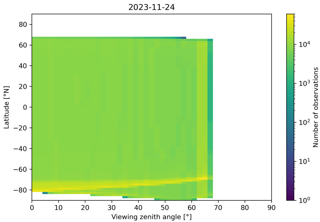
Figure 163: Scatter density plot of “Viewing zenith angle” against “Latitude” for 2023-11-23 to 2023-11-25.
