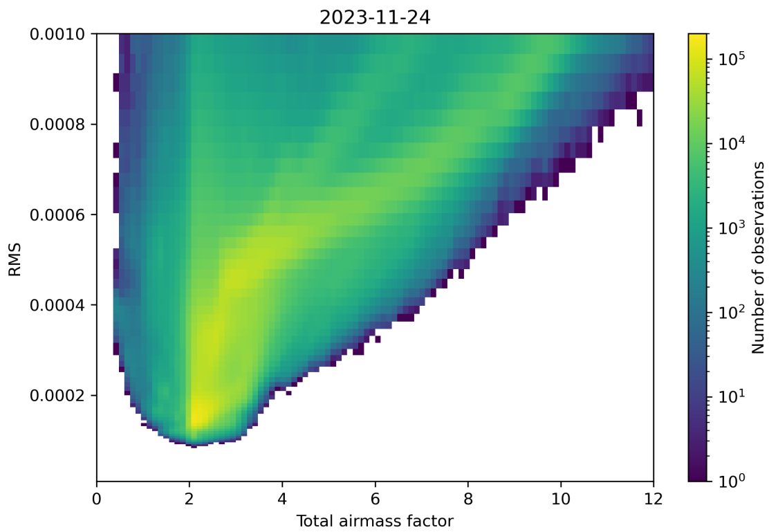
Figure 69: Scatter density plot of “Total airmass factor” against “RMS” for 2023-11-23 to 2023-11-25.
