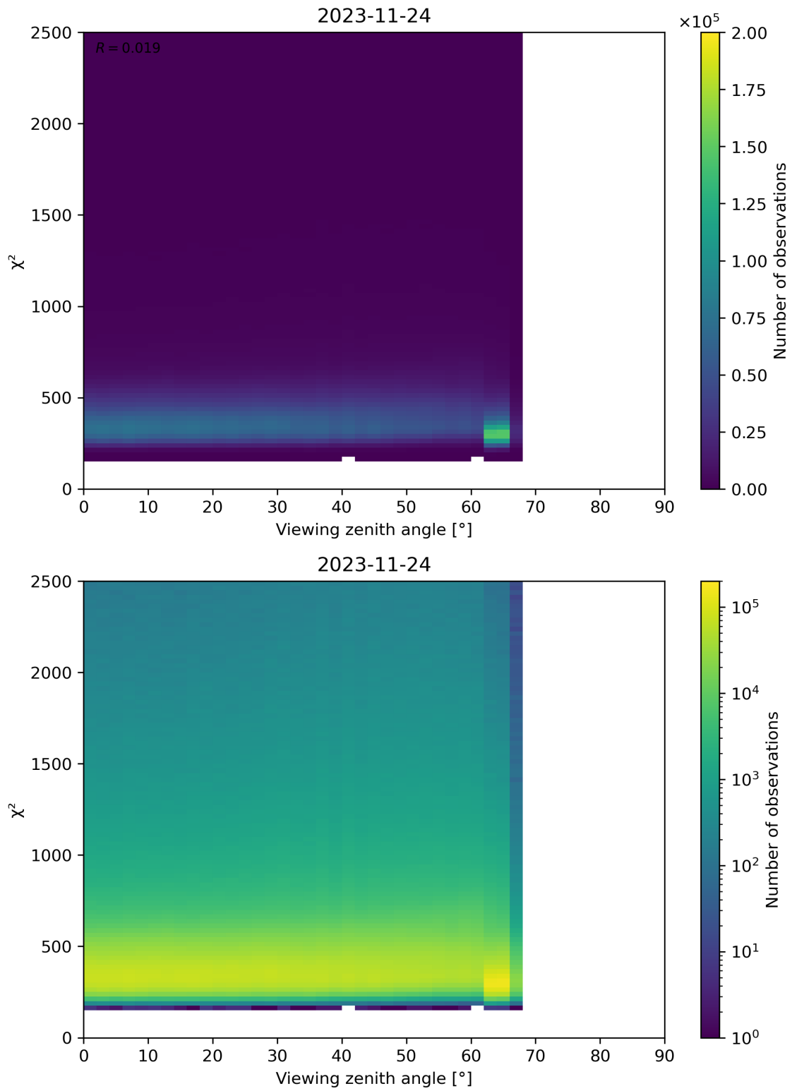
Figure 162: Scatter density plot of “Viewing zenith angle” against “ \chi^2 ” for 2023-11-23 to 2023-11-25.
