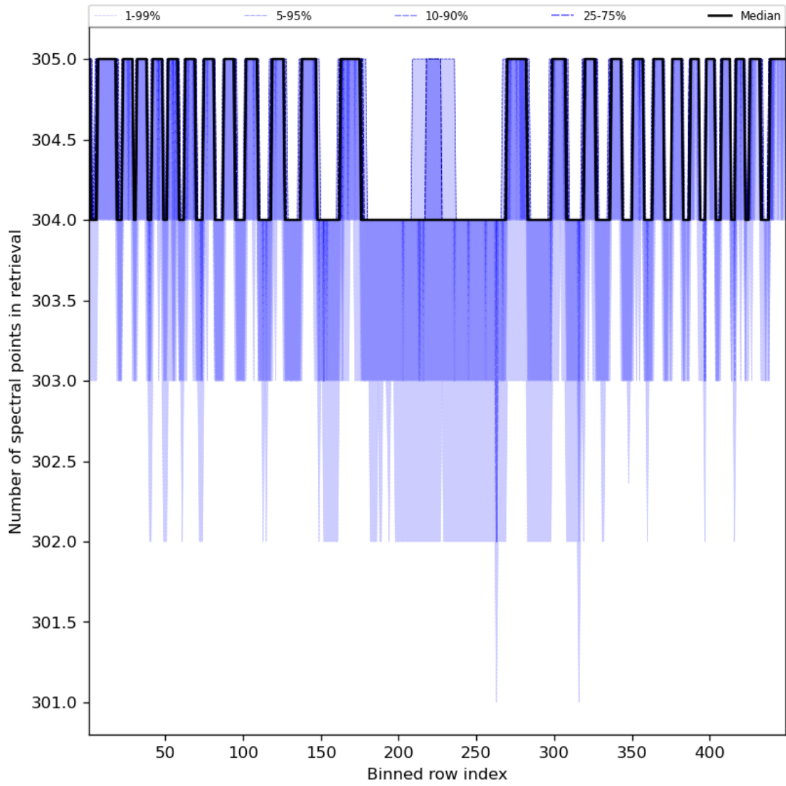
Figure 50: Along track statistics of “Number of spectral points in retrieval” for 2023-11-23 to 2023-11-25
