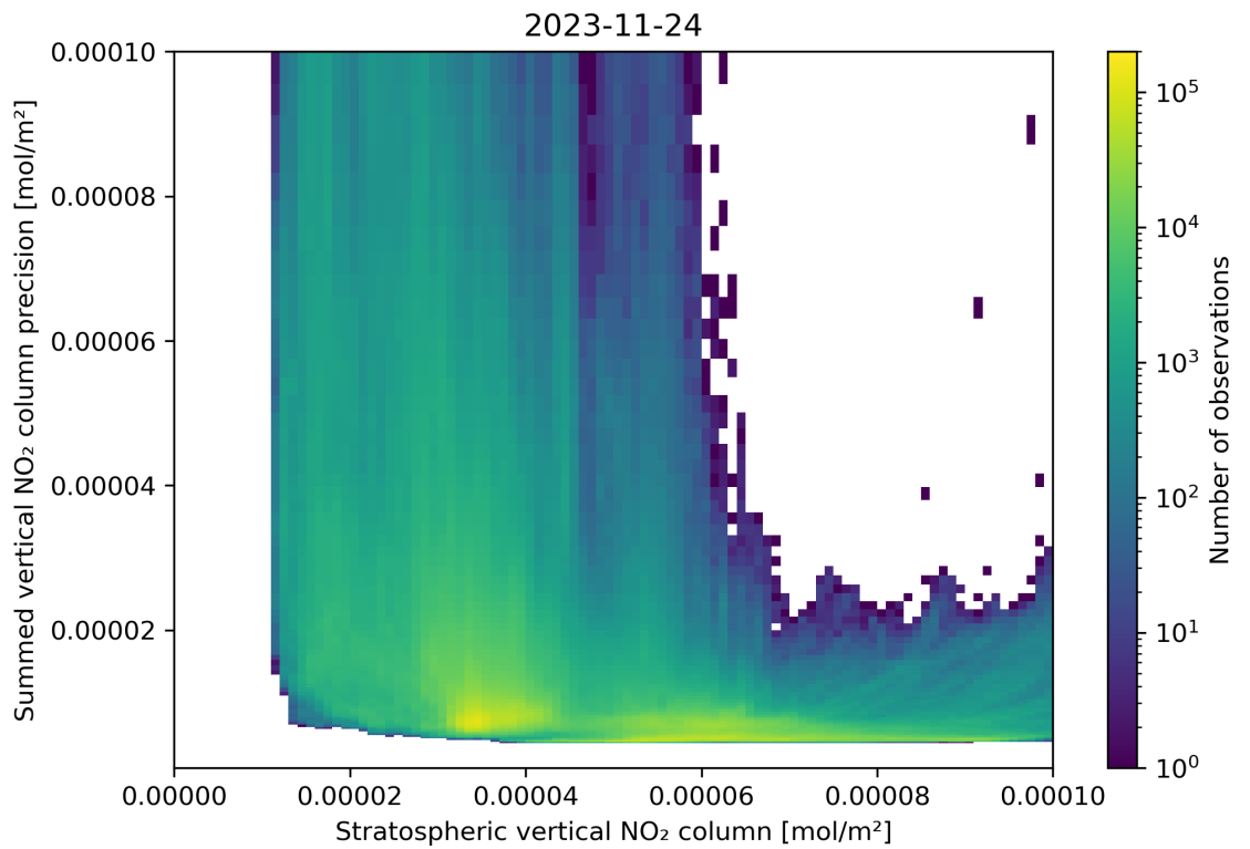
Figure 99: Scatter density plot of “Stratospheric vertical NO 2 column” against “Summed vertical NO 2 column precision” for 2023-11-23 to 2023-11-25.
