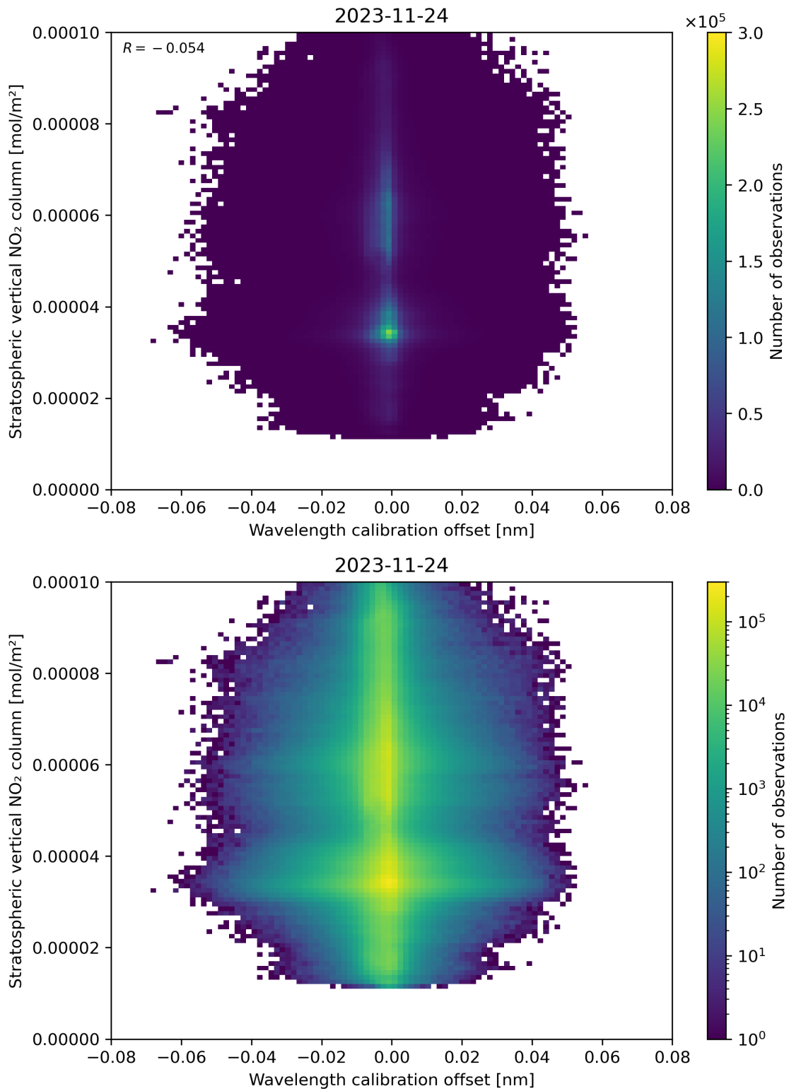
Figure 176: Scatter density plot of “Wavelength calibration offset” against “Stratospheric vertical NO 2 column” for 2023-11-23 to 2023-11-25.
