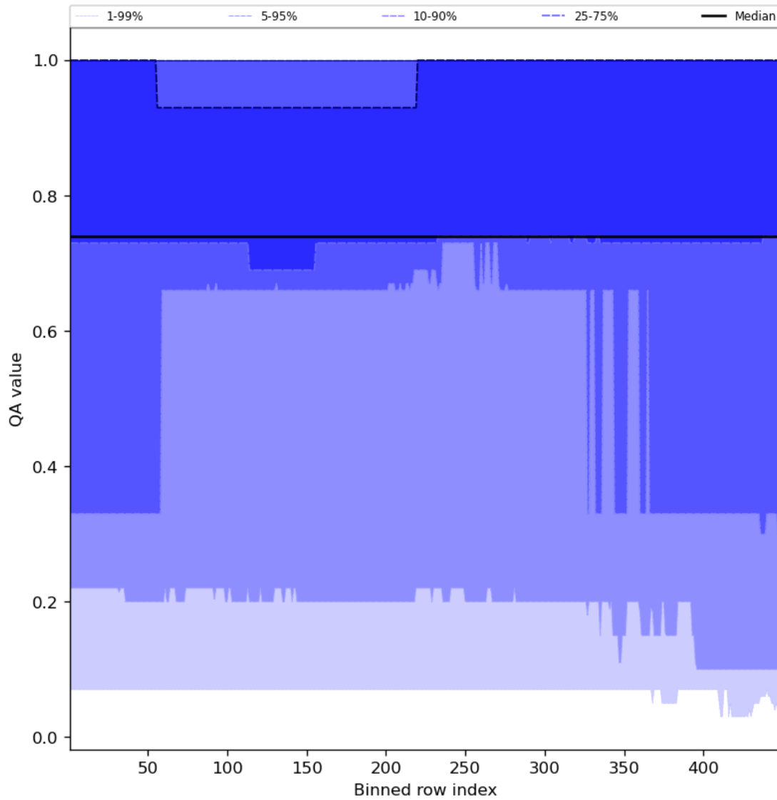
Figure 45: Along track statistics of "QA value" for 2023-11-23 to 2023-11-25
