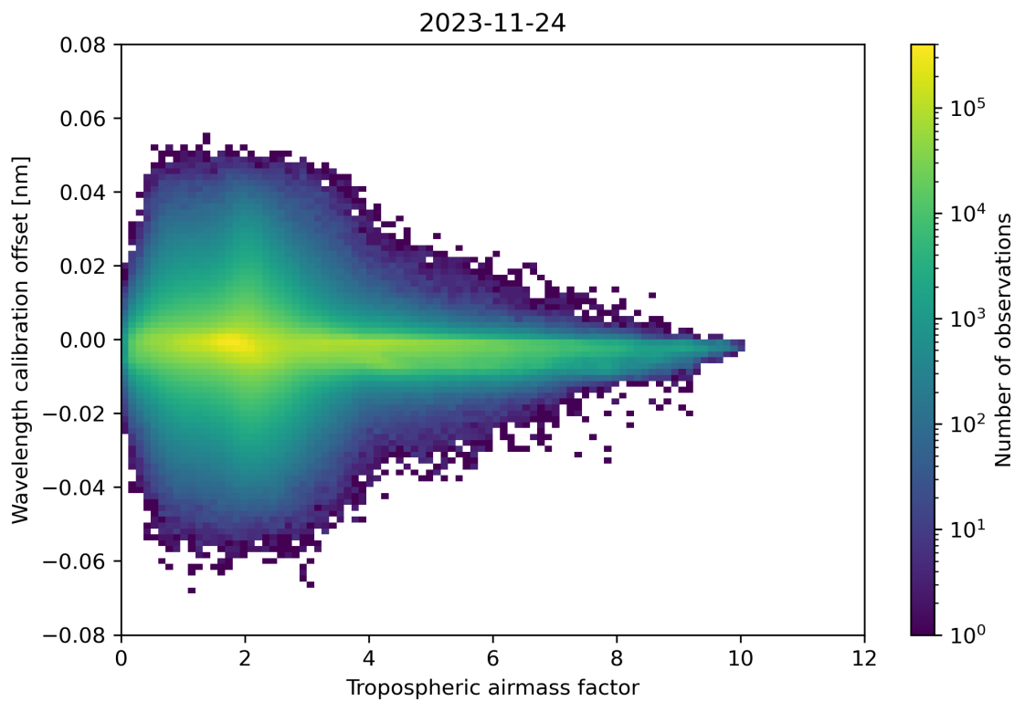
Figure 80: Scatter density plot of “Tropospheric airmass factor” against “Wavelength calibration offset” for 2023-11-23 to 2023-11-25.
