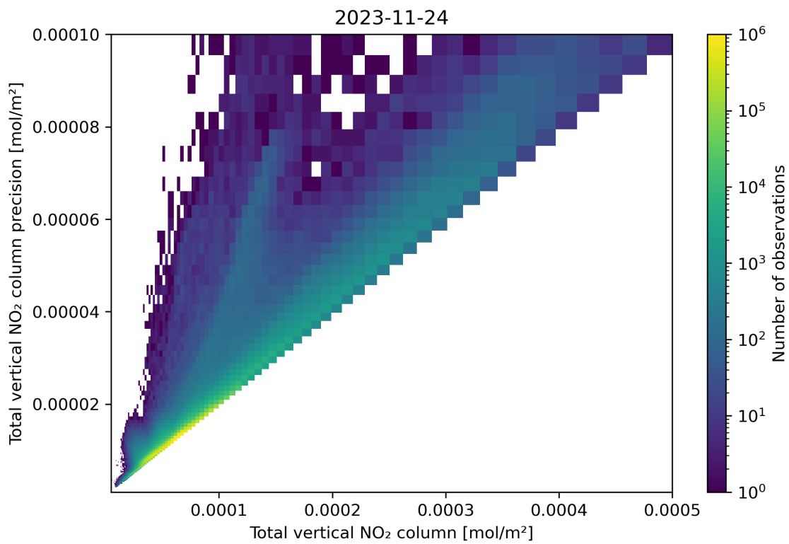
Figure 114: Scatter density plot of “Total vertical NO 2 column” against “Total vertical NO 2 column precision” for 2023-11-23 to 2023-11-25.
