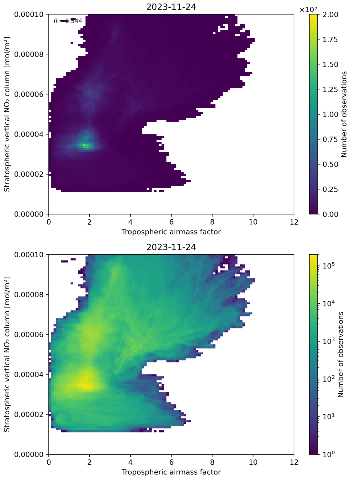
Figure 74: Scatter density plot of “Tropospheric airmass factor” against “Stratospheric vertical NO 2 column” for 2023-11-23 to 2023-11-25.
