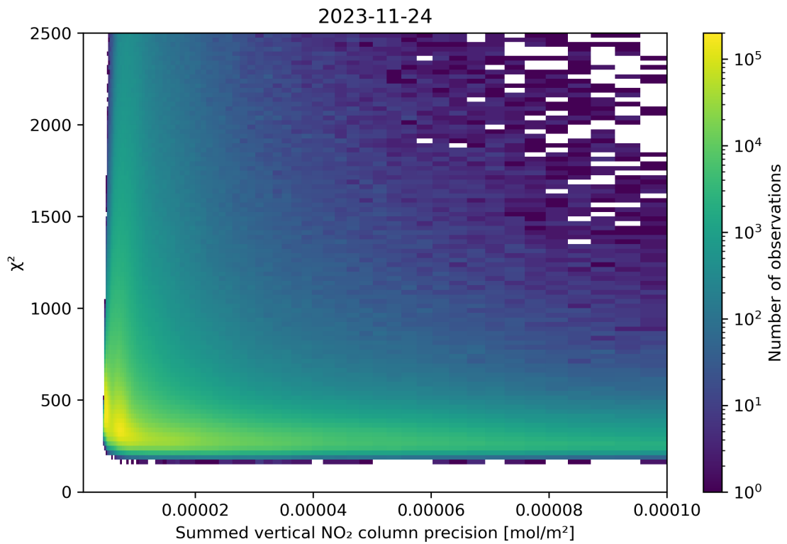
Figure 107: Scatter density plot of “Summed vertical NO 2 column precision” against “ \chi^2 ” for 2023-11-23 to 2023-11-25.
