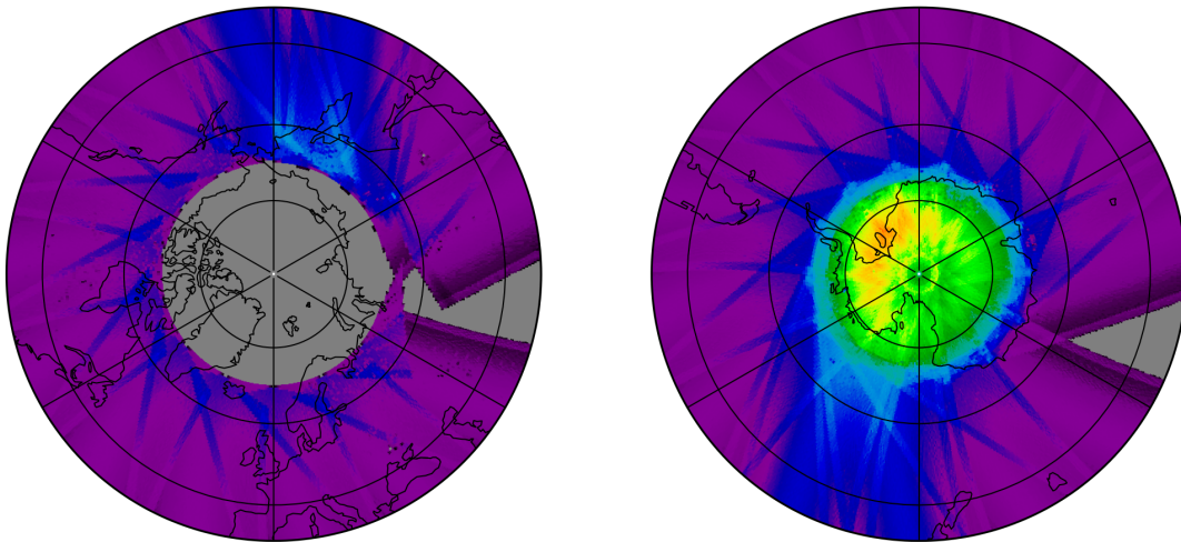
Figure 10: Map of the number of observations for 2023-11-23 to 2023-11-25
