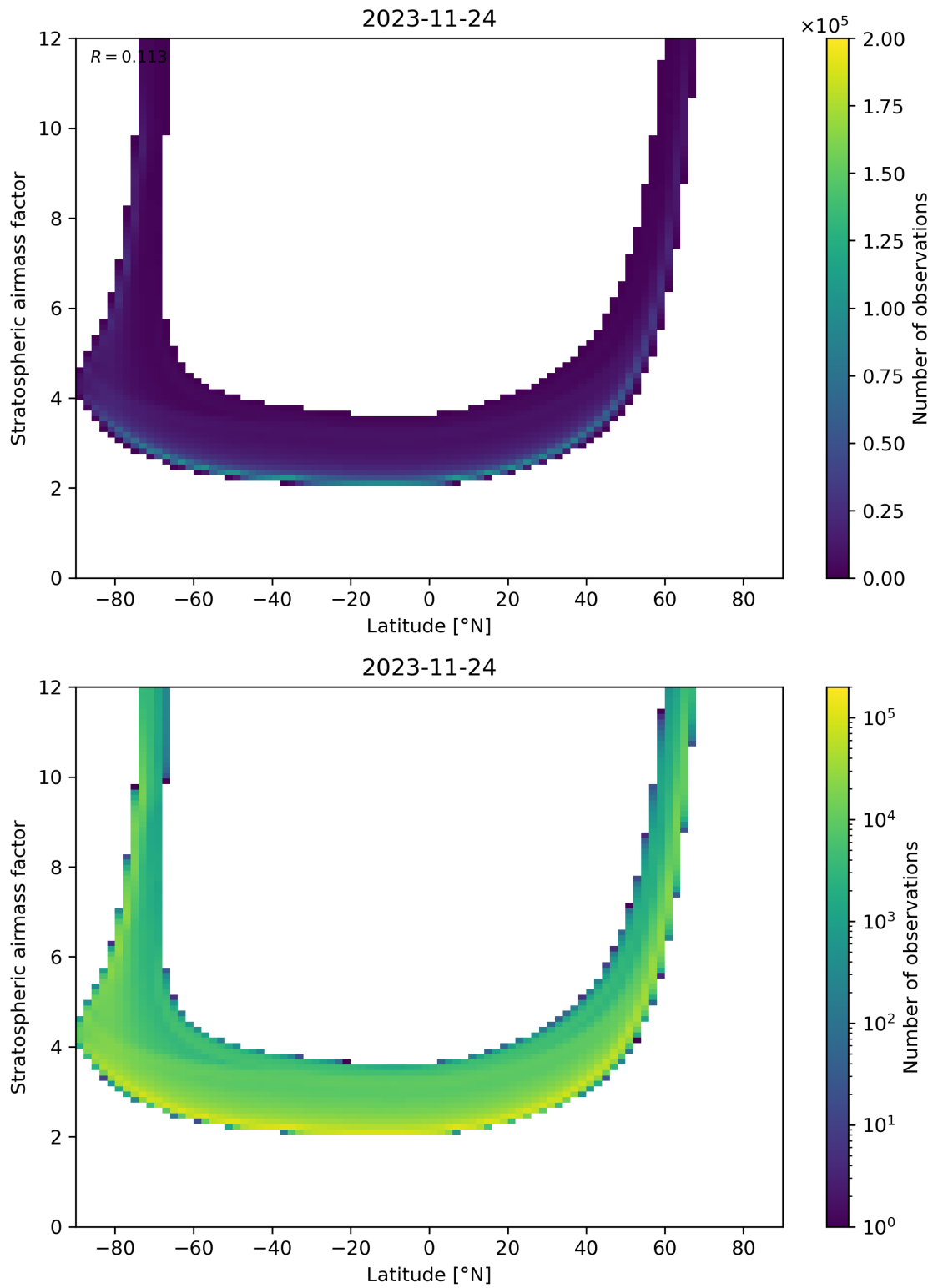
Figure 83: Scatter density plot of “Latitude” against “Stratospheric airmass factor” for 2023-11-23 to 2023-11-25.
