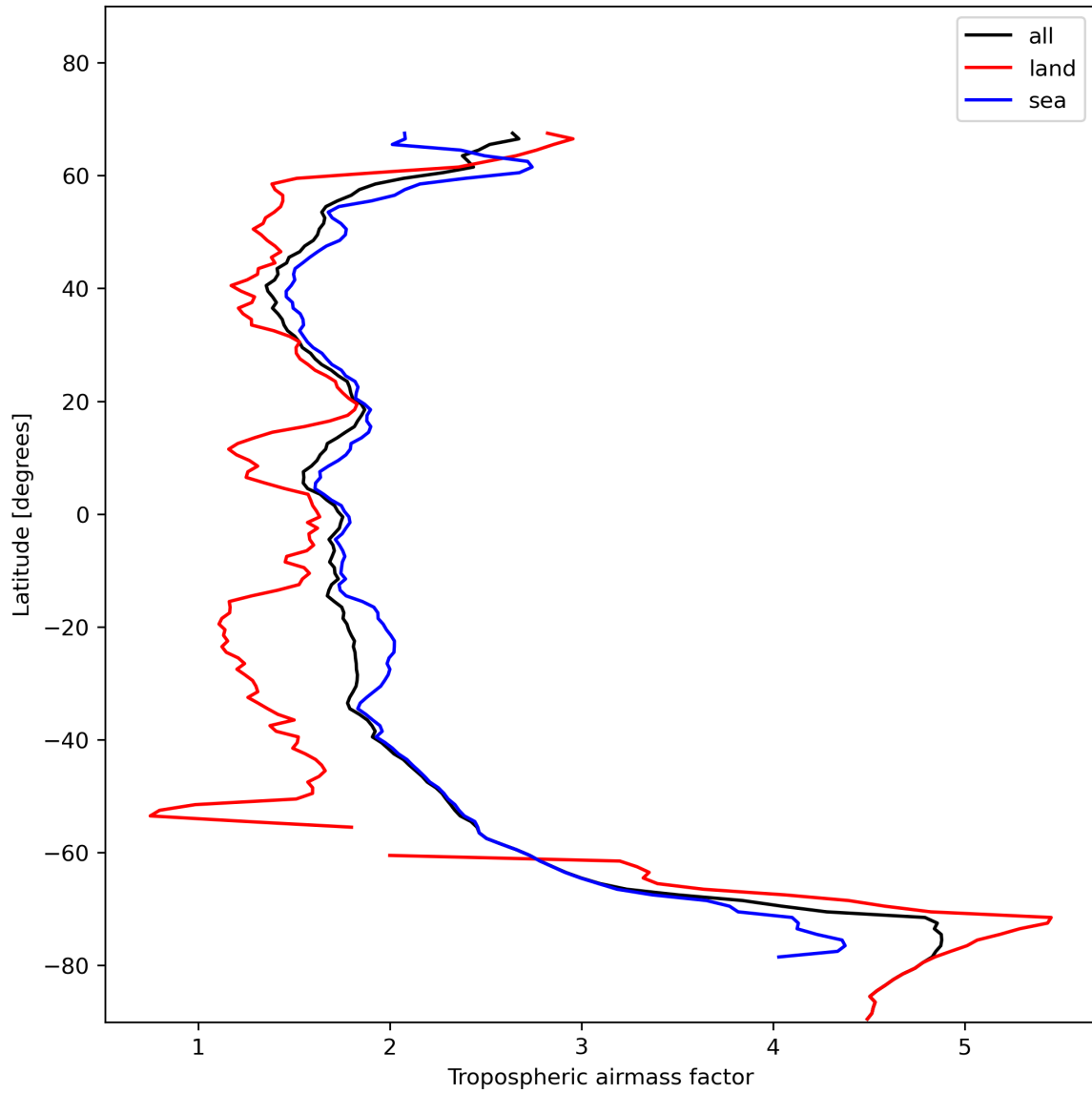
Figure 14: Zonal average of “Tropospheric airmass factor” for 2023-11-23 to 2023-11-25.
