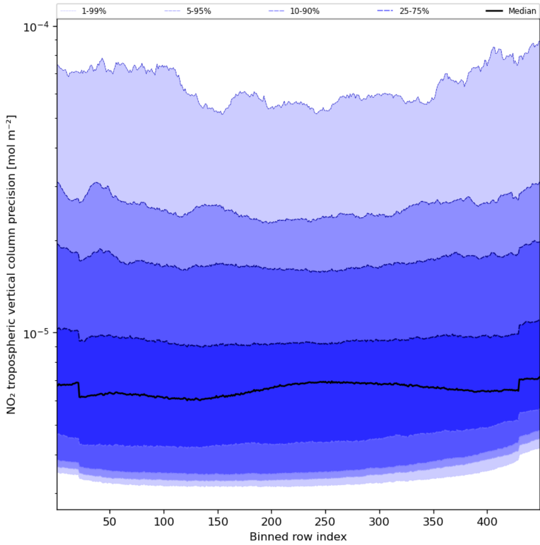
Figure 47: Along track statistics of “NO 2 tropospheric vertical column precision” for 2023-11-23 to 2023-11-25
