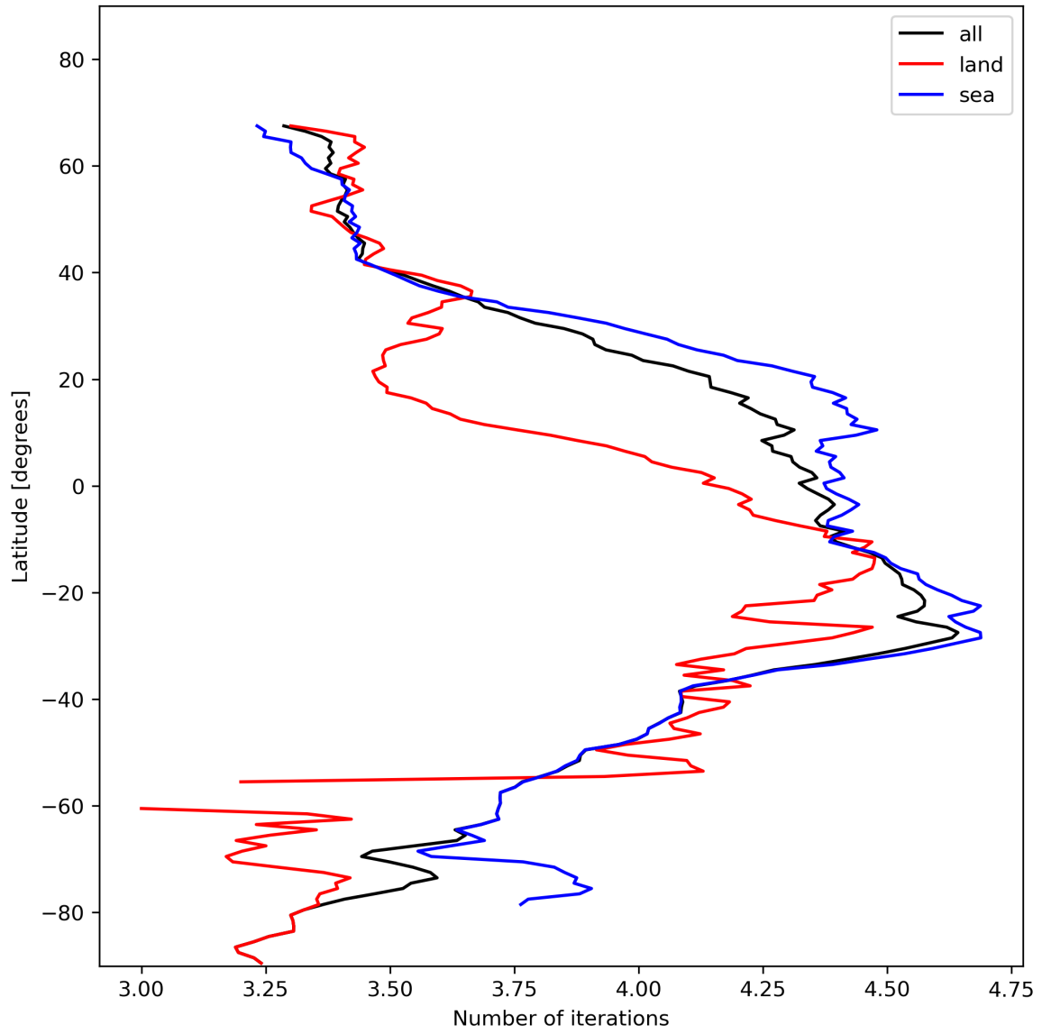
Figure 17: Zonal average of “Number of iterations” for 2023-11-23 to 2023-11-25.
