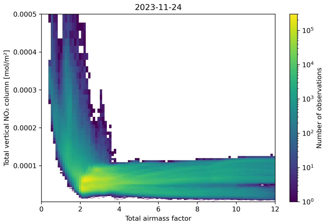
Figure 67: Scatter density plot of “Total airmass factor” against “Total vertical NO 2 column” for 2023-11-23 to 2023-11-25.
