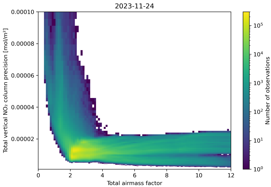
Figure 68: Scatter density plot of “Total airmass factor” against “Total vertical NO 2 column precision” for 2023-11-23 to 2023-11-25.
