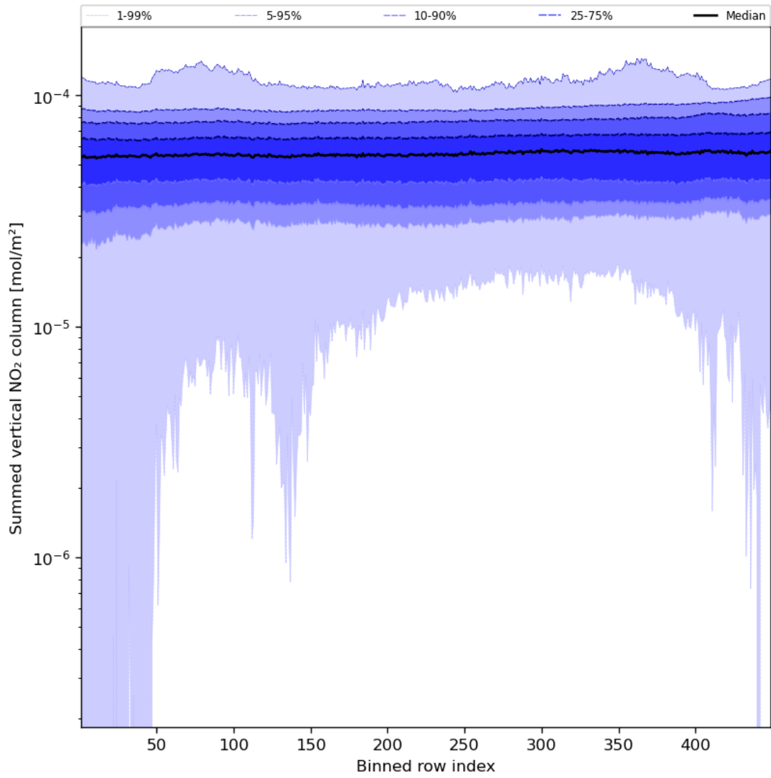
Figure 57: Along track statistics of “Summed vertical NO 2 column” for 2023-11-23 to 2023-11-25
