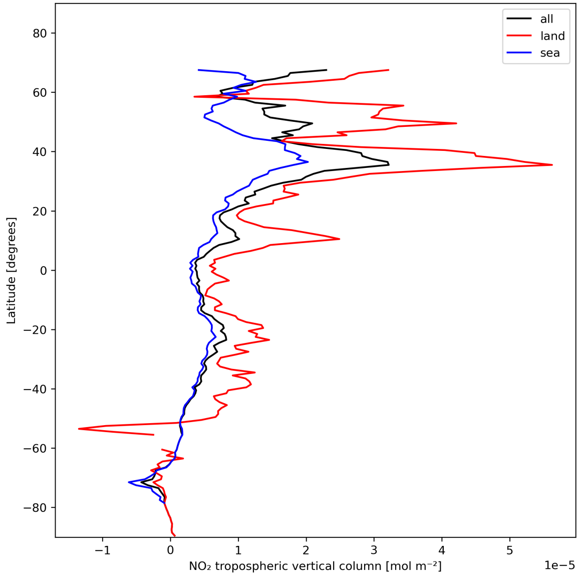
Figure 12: Zonal average of “NO 2 tropospheric vertical column” for 2023-11-23 to 2023-11-25.
