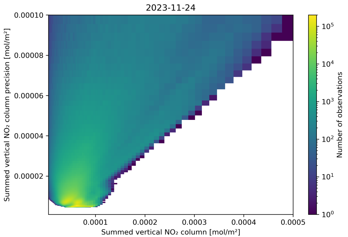
Figure 105: Scatter density plot of “Summed vertical NO 2 column” against “Summed vertical NO 2 column precision” for 2023-11-23 to 2023-11-25.
