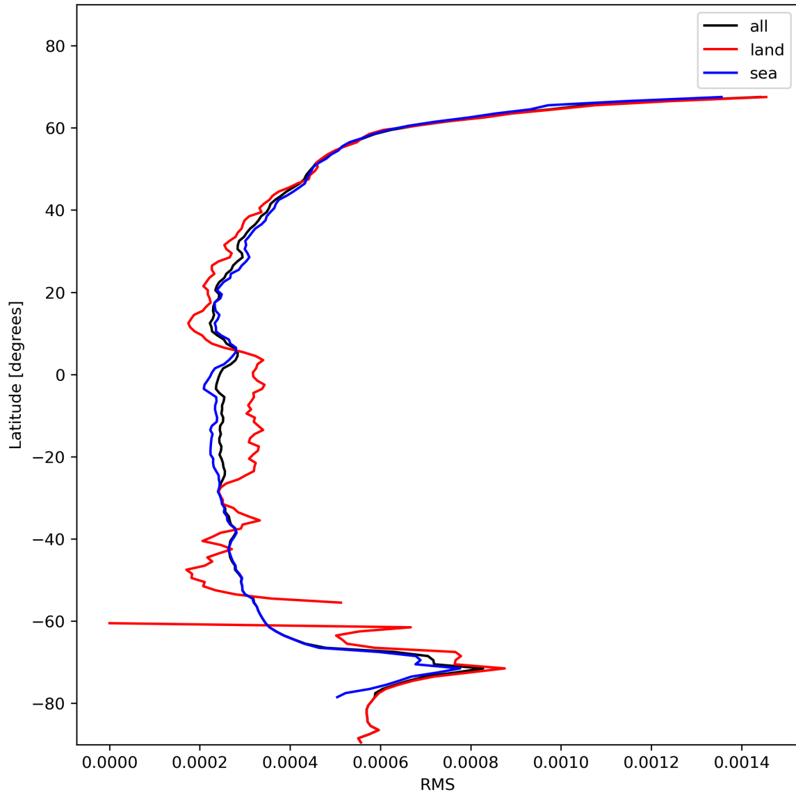
Figure 26: Zonal average of “RMS” for 2023-11-23 to 2023-11-25.
