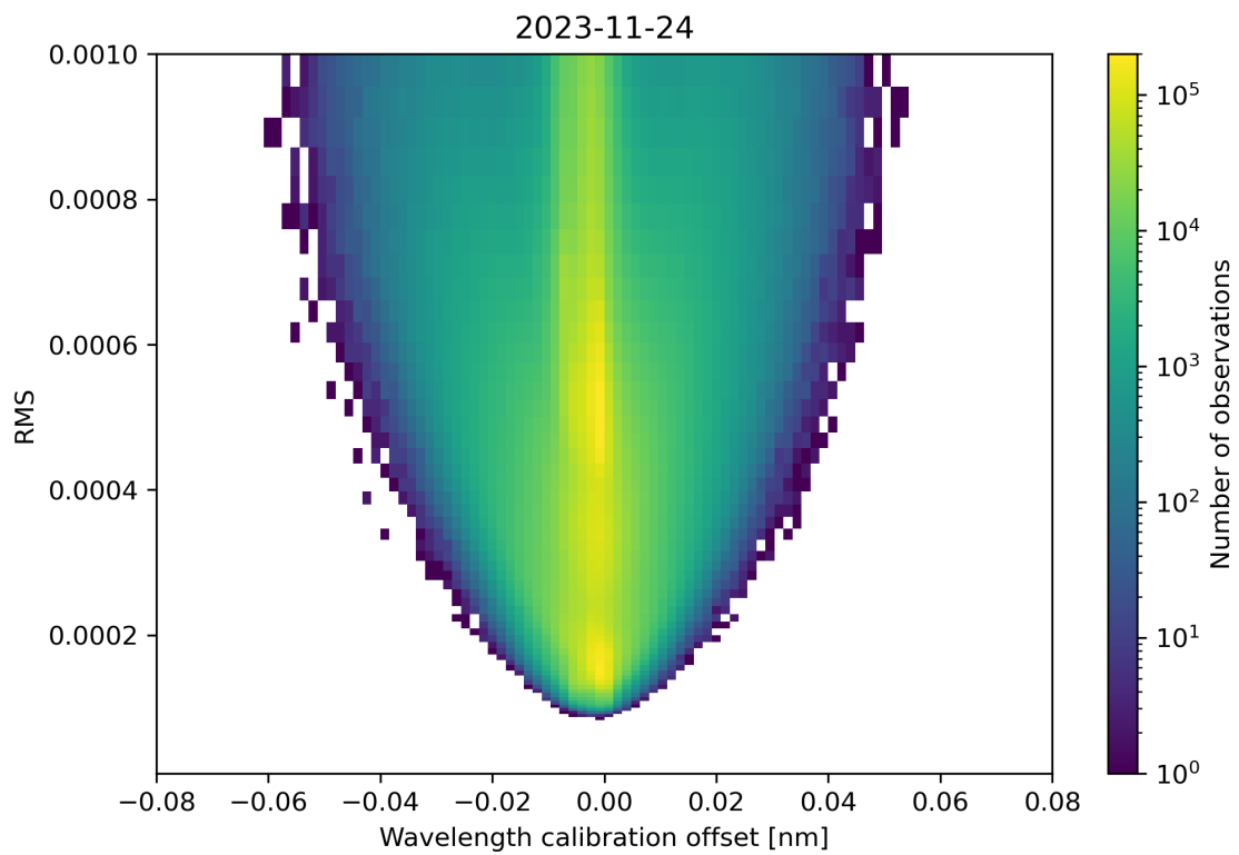
Figure 181: Scatter density plot of “Wavelength calibration offset” against “RMS” for 2023-11-23 to 2023-11-25.
