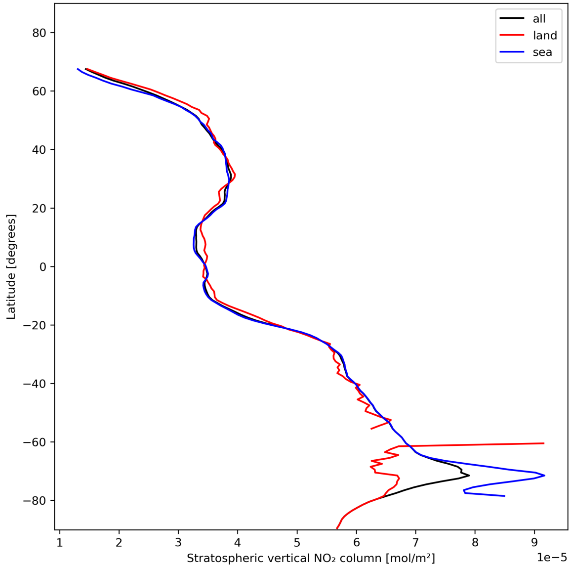
Figure 19: Zonal average of “Stratospheric vertical NO 2 column” for 2023-11-23 to 2023-11-25.
