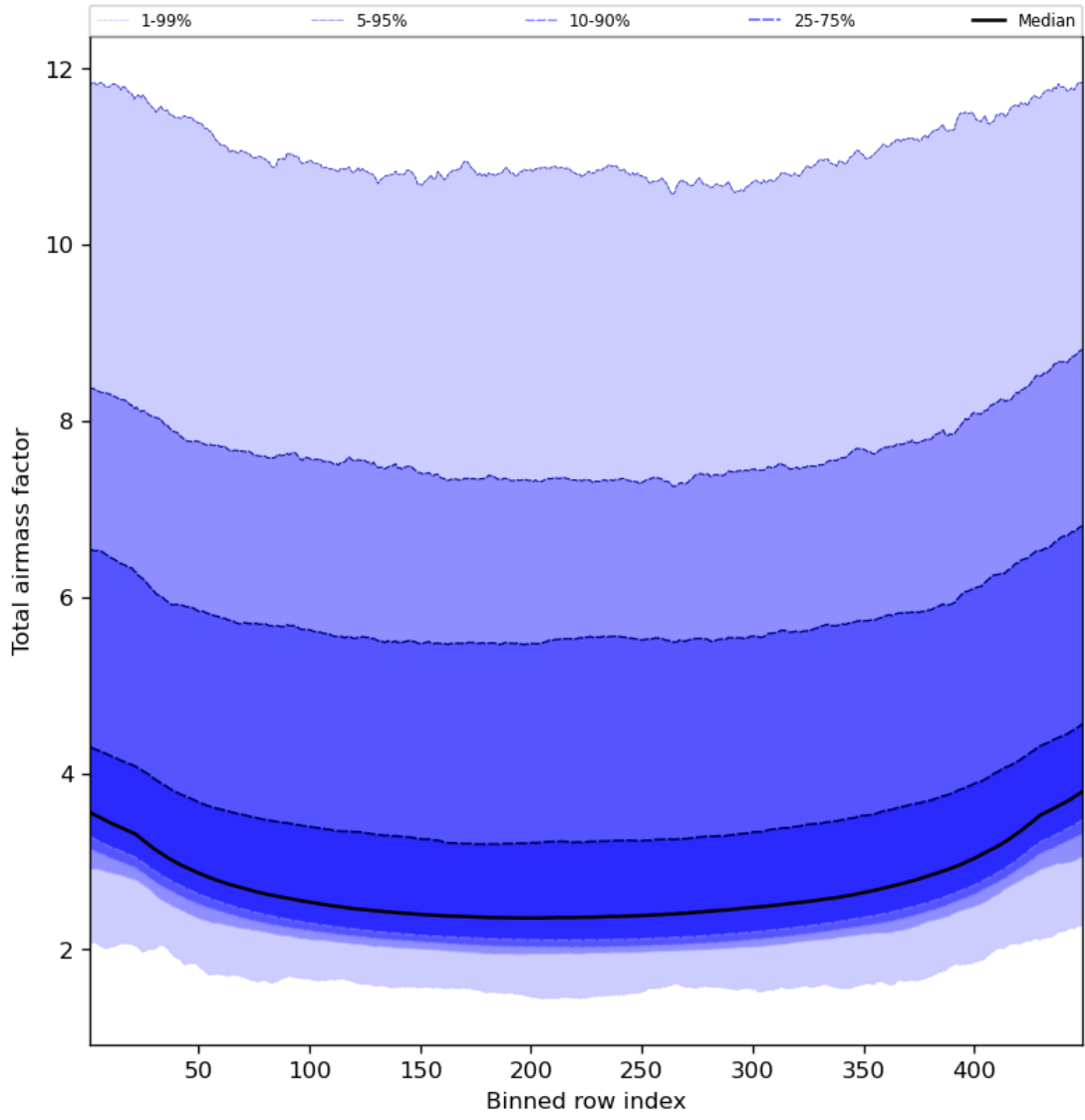
Figure 49: Along track statistics of “Total airmass factor” for 2023-11-23 to 2023-11-25
