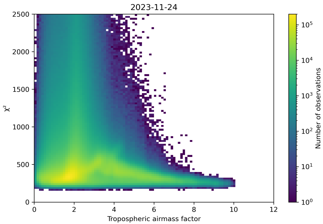
Figure 73: Scatter density plot of “Tropospheric airmass factor” against “ \chi^2 ” for 2023-11-23 to 2023-11-25.
