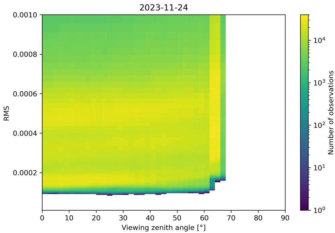
Figure 171: Scatter density plot of “Viewing zenith angle” against “RMS” for 2023-11-23 to 2023-11-25.
