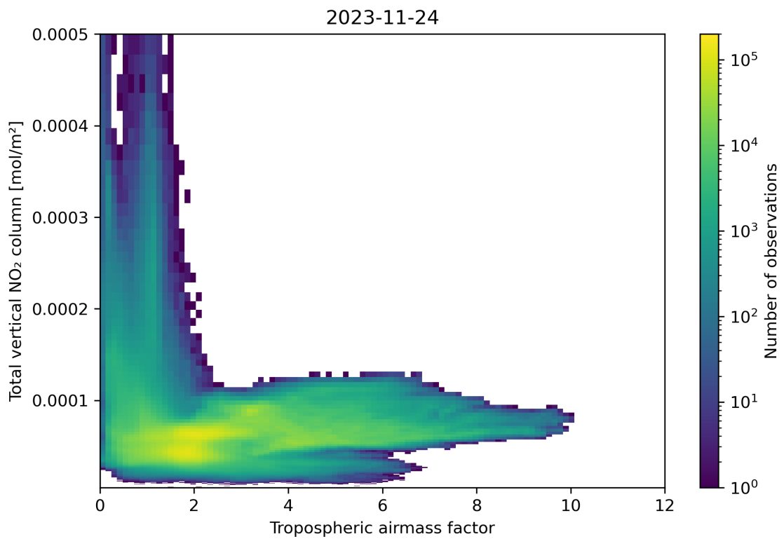
Figure 77: Scatter density plot of “Tropospheric airmass factor” against “Total vertical NO 2 column” for 2023-11-23 to 2023-11-25.
