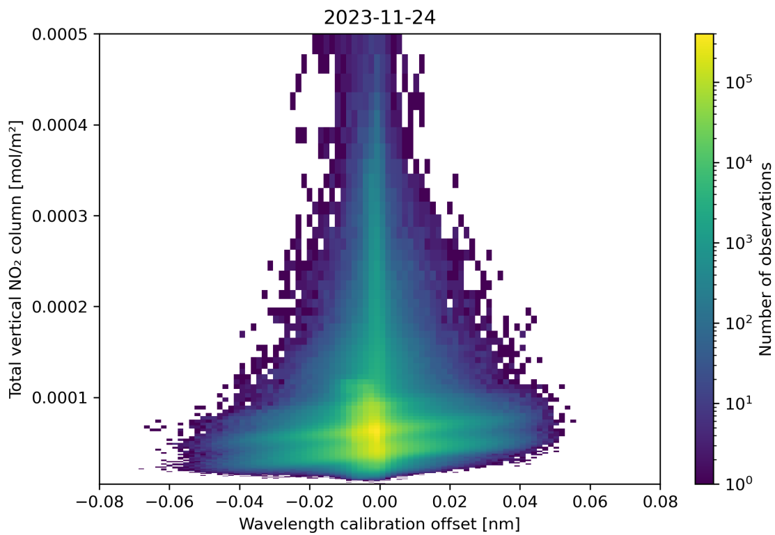
Figure 179: Scatter density plot of “Wavelength calibration offset” against “Total vertical NO 2 column” for 2023-11-23 to 2023-11-25.
