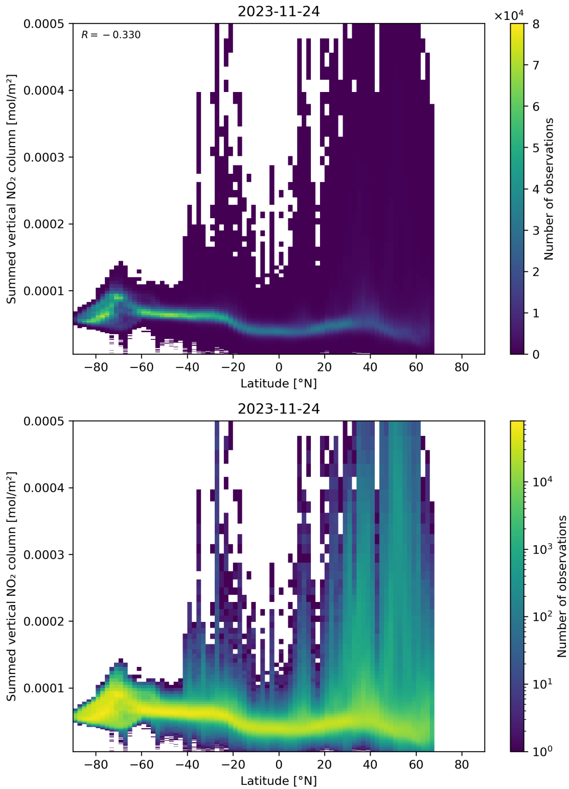
Figure 88: Scatter density plot of “Latitude” against “Summed vertical NO 2 column” for 2023-11-23 to 2023-11-25.
