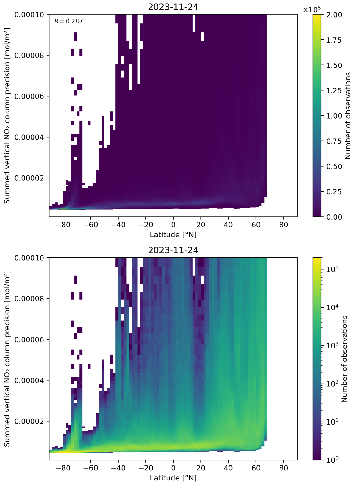
Figure 89: Scatter density plot of “Latitude” against “Summed vertical NO 2 column precision” for 2023-11-23 to 2023-11-25.
