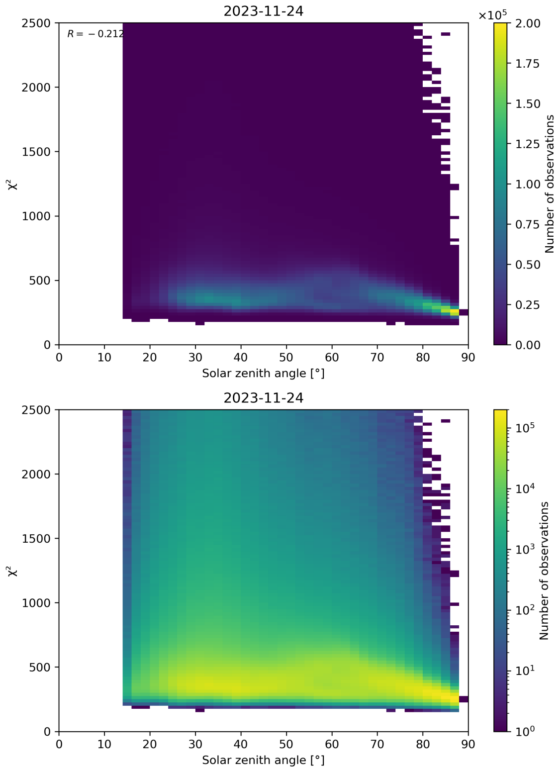
Figure 148: Scatter density plot of “Solar zenith angle” against “ \chi^2 ” for 2023-11-23 to 2023-11-25.
