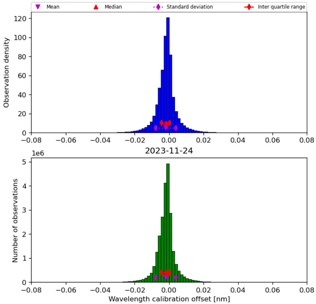
Figure 35: Histogram of “Wavelength calibration offset” for 2023-11-23 to 2023-11-25
