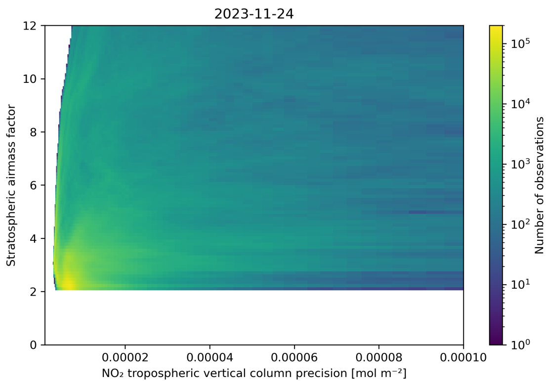
Figure 131: Scatter density plot of “NO 2 tropospheric vertical column precision” against “Stratospheric airmass factor” for 2023-11-23 to 2023-11-25.
