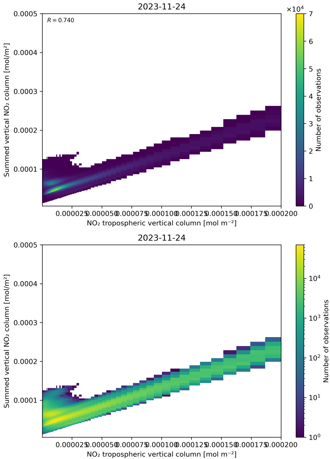
Figure 126: Scatter density plot of “NO 2 tropospheric vertical column” against “Summed vertical NO 2 column” for 2023-11-23 to 2023-11-25.
