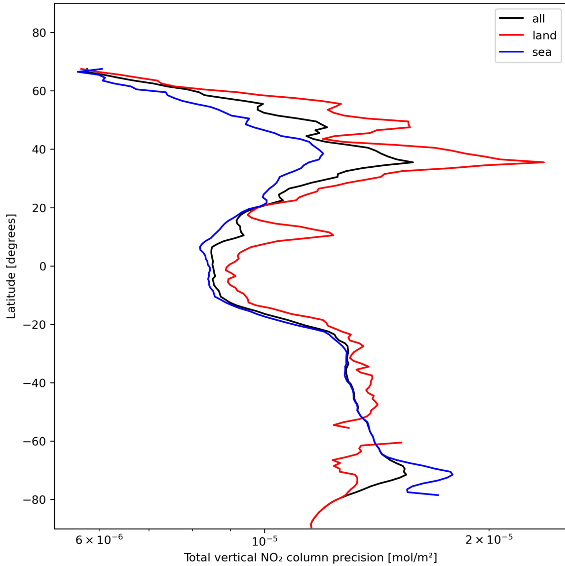
Figure 22: Zonal average of “Total vertical NO 2 column precision” for 2023-11-23 to 2023-11-25.
