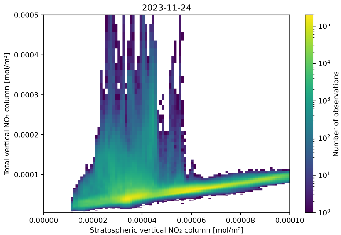
Figure 100: Scatter density plot of “Stratospheric vertical NO 2 column” against “Total vertical NO 2 column” for 2023-11-23 to 2023-11-25.
