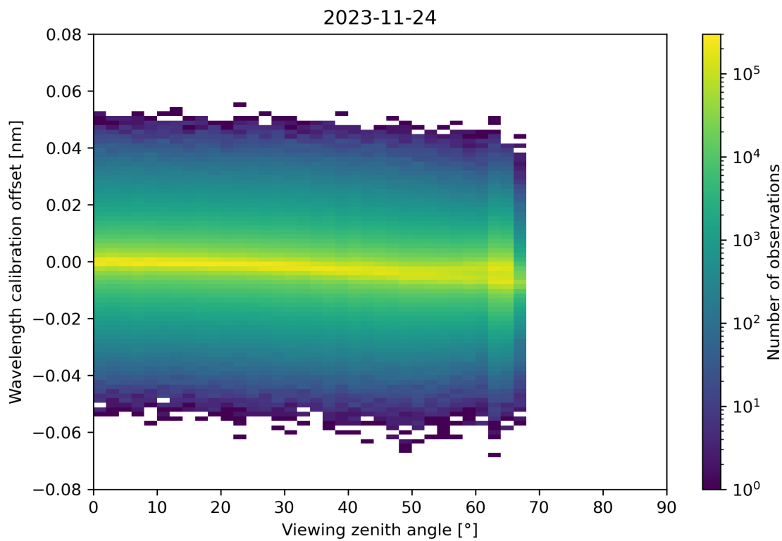
Figure 173: Scatter density plot of “Viewing zenith angle” against “Wavelength calibration offset” for 2023-11-23 to 2023-11-25.
