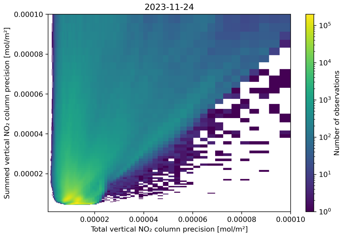
Figure 118: Scatter density plot of “Total vertical NO 2 column precision” against “Summed vertical NO 2 column precision” for 2023-11-23 to 2023-11-25.
