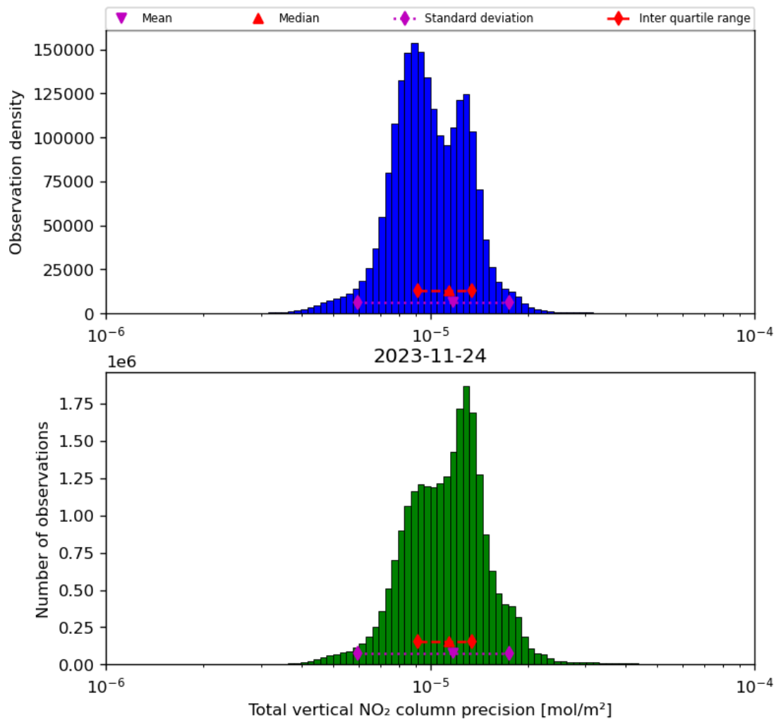
Figure 39: Histogram of “Total vertical NO 2 column precision” for 2023-11-23 to 2023-11-25
