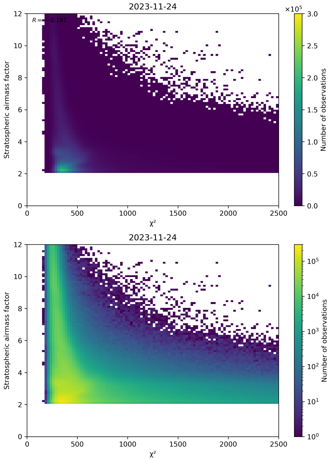
Figure 81: Scatter density plot of “ \chi^2 ” against “Stratospheric airmass factor” for 2023-11-23 to 2023-11-25.
