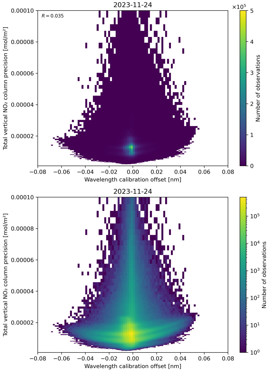
Figure 180: Scatter density plot of “Wavelength calibration offset” against “Total vertical NO 2 column precision” for 2023-11-23 to 2023-11-25.
