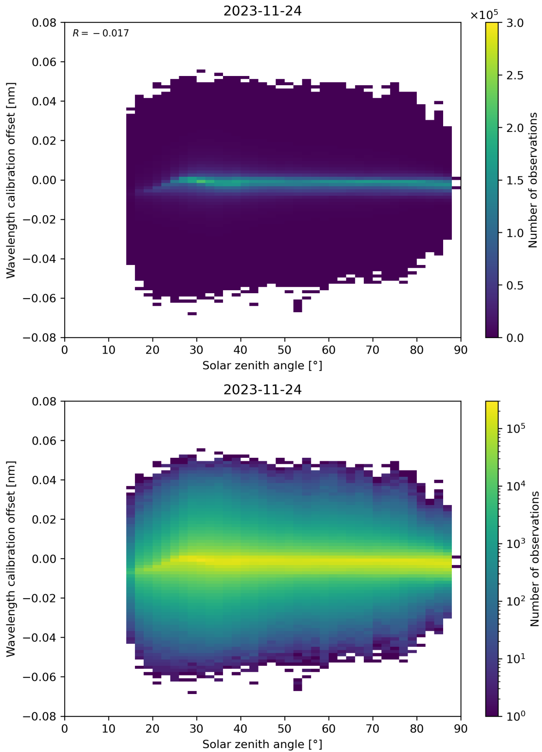
Figure 158: Scatter density plot of “Solar zenith angle” against “Wavelength calibration offset” for 2023-11-23 to 2023-11-25.
