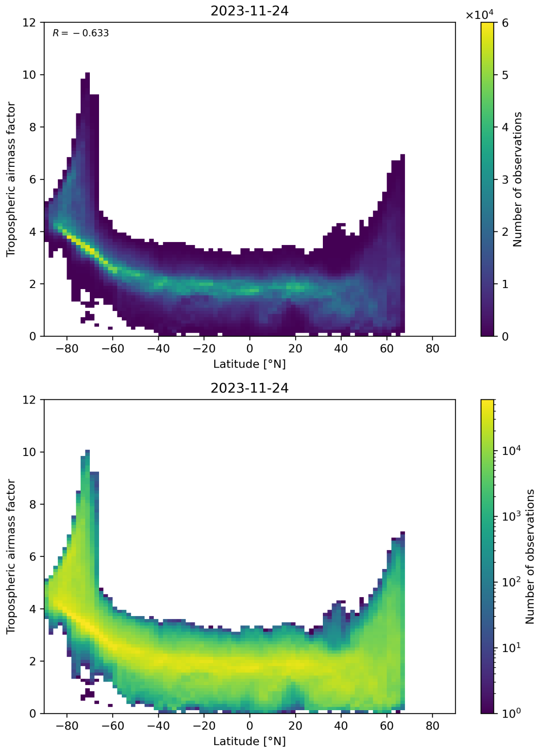
Figure 85: Scatter density plot of “Latitude” against “Tropospheric airmass factor” for 2023-11-23 to 2023-11-25.
