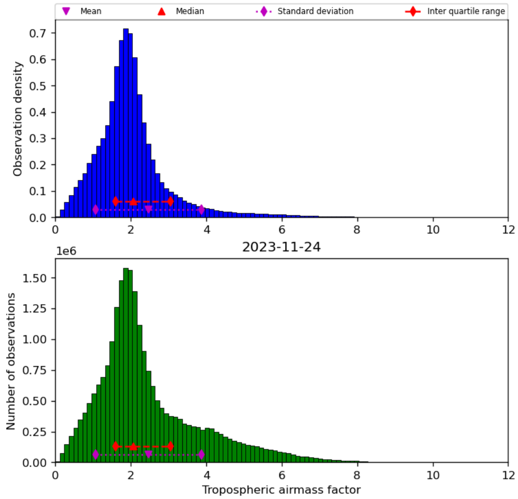
Figure 31: Histogram of “Tropospheric airmass factor” for 2023-11-23 to 2023-11-25
