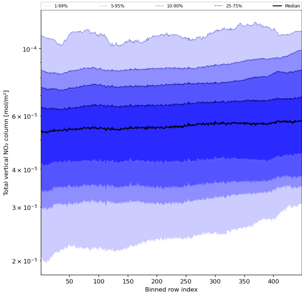
Figure 55: Along track statistics of “Total vertical NO 2 column” for 2023-11-23 to 2023-11-25
