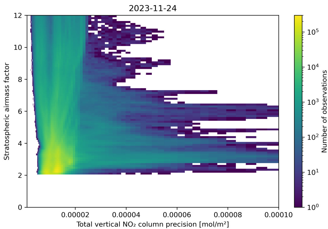
Figure 115: Scatter density plot of “Total vertical NO 2 column precision” against “Stratospheric airmass factor” for 2023-11-23 to 2023-11-25.
