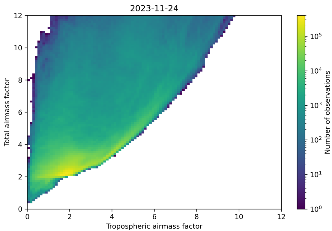
Figure 72: Scatter density plot of “Tropospheric airmass factor” against “Total airmass factor” for 2023-11-23 to 2023-11-25.
