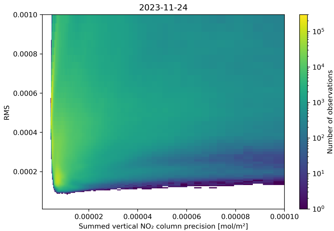
Figure 108: Scatter density plot of “Summed vertical NO 2 column precision” against “RMS” for 2023-11-23 to 2023-11-25.
