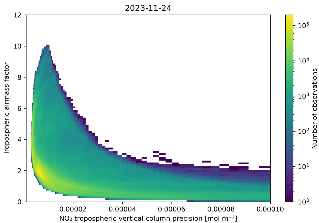
Figure 133: Scatter density plot of “NO 2 tropospheric vertical column precision” against “Tropospheric airmass factor” for 2023-11-23 to 2023-11-25.
