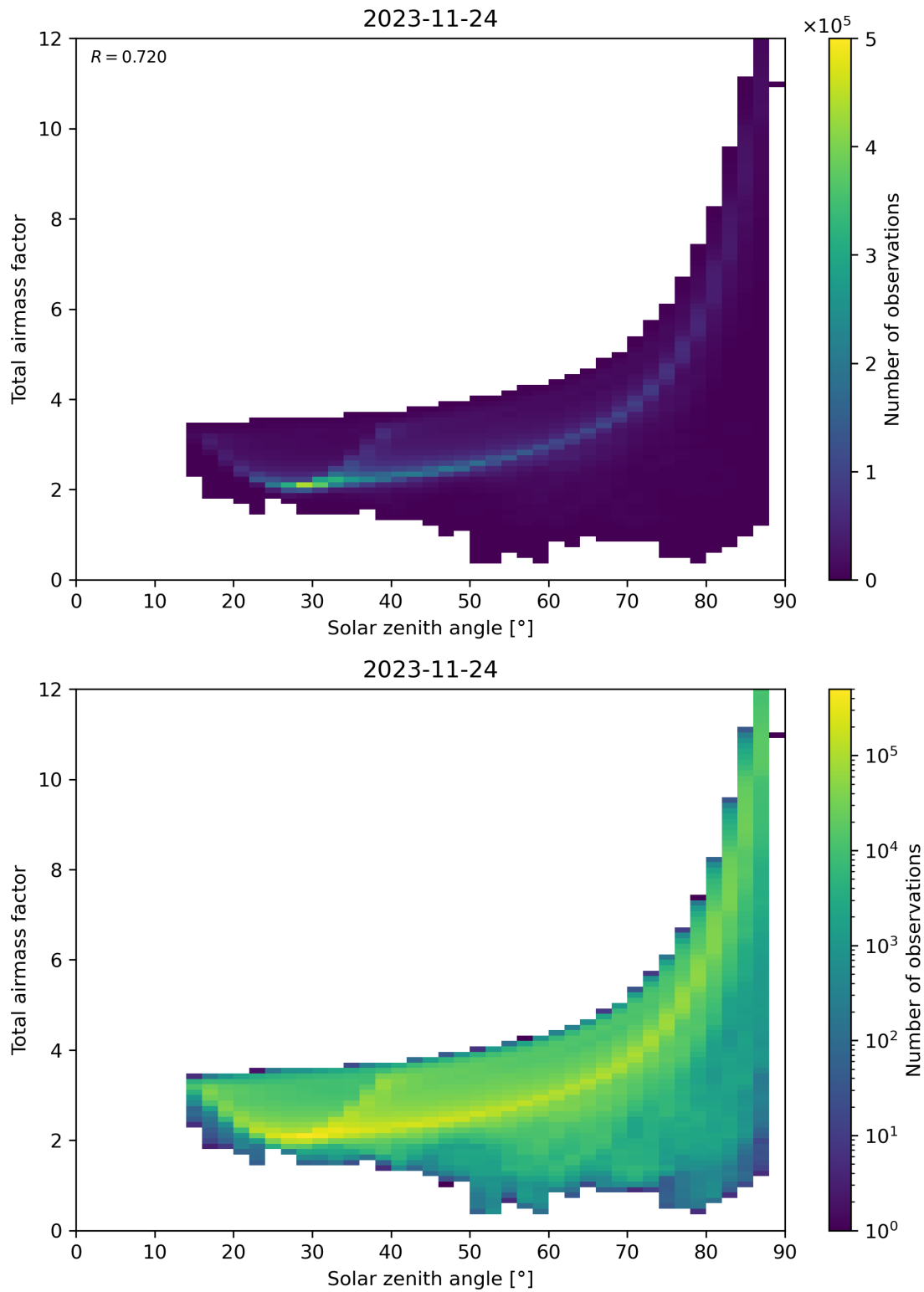
Figure 146: Scatter density plot of “Solar zenith angle” against “Total airmass factor” for 2023-11-23 to 2023-11-25.
