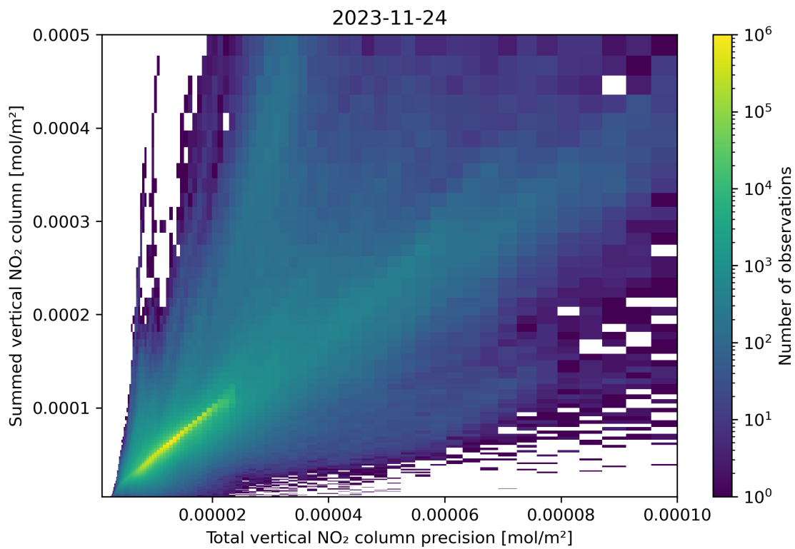
Figure 117: Scatter density plot of “Total vertical NO 2 column precision” against “Summed vertical NO 2 column” for 2023-11-23 to 2023-11-25.
