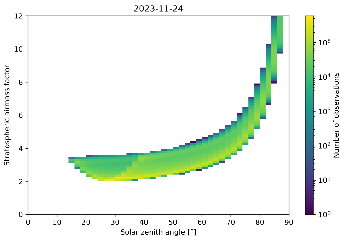
Figure 145: Scatter density plot of “Solar zenith angle” against “Stratospheric airmass factor” for 2023-11-23 to 2023-11-25.
