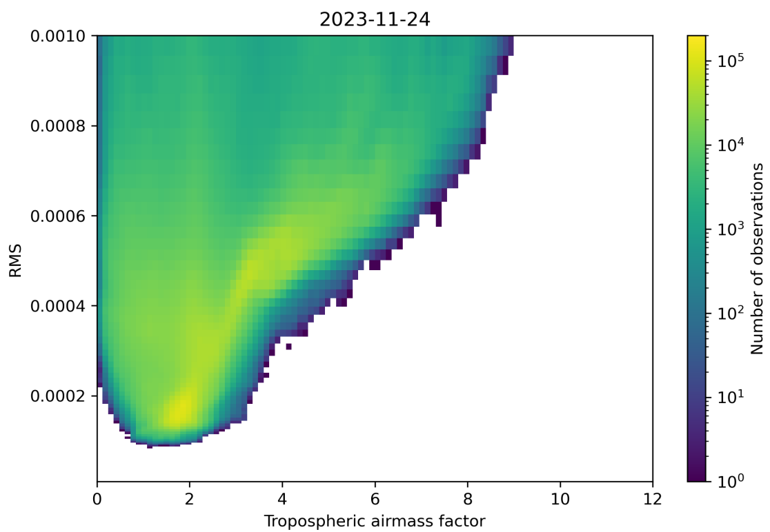
Figure 79: Scatter density plot of “Tropospheric airmass factor” against “RMS” for 2023-11-23 to 2023-11-25.
