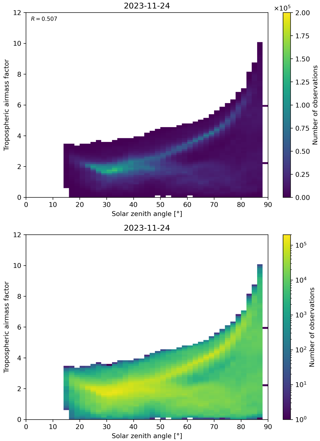
Figure 147: Scatter density plot of “Solar zenith angle” against “Tropospheric airmass factor” for 2023-11-23 to 2023-11-25.
