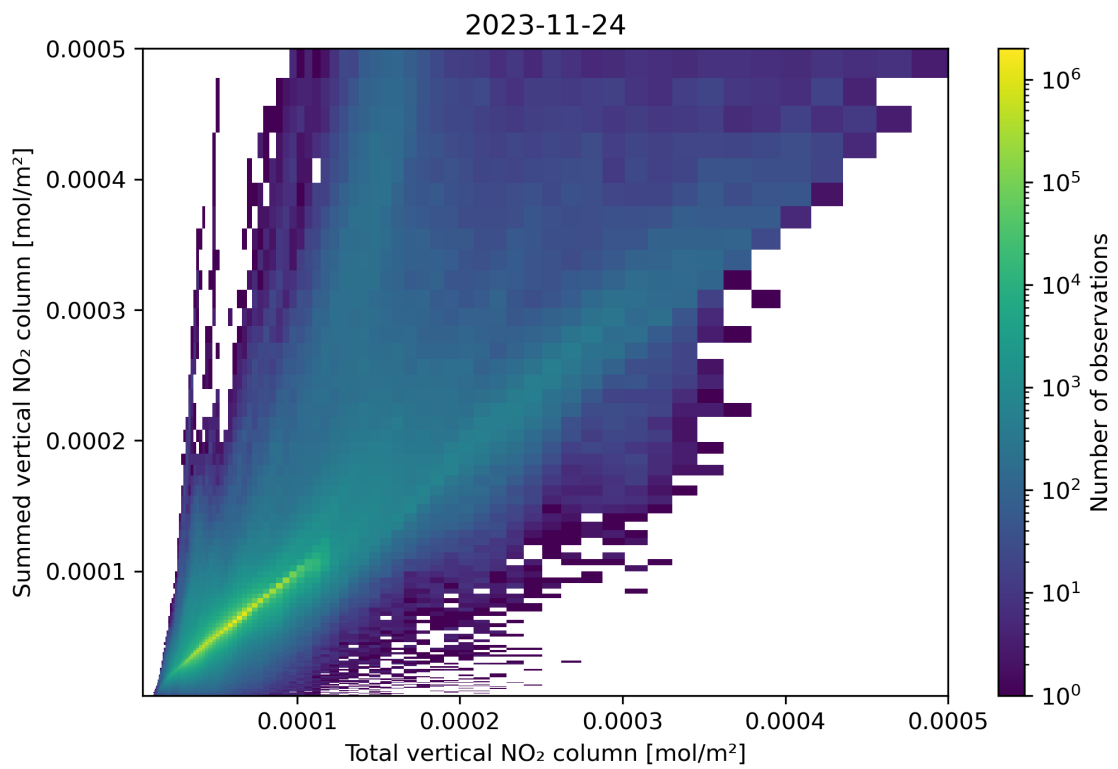
Figure 112: Scatter density plot of “Total vertical NO 2 column” against “Summed vertical NO 2 column” for 2023-11-23 to 2023-11-25.
