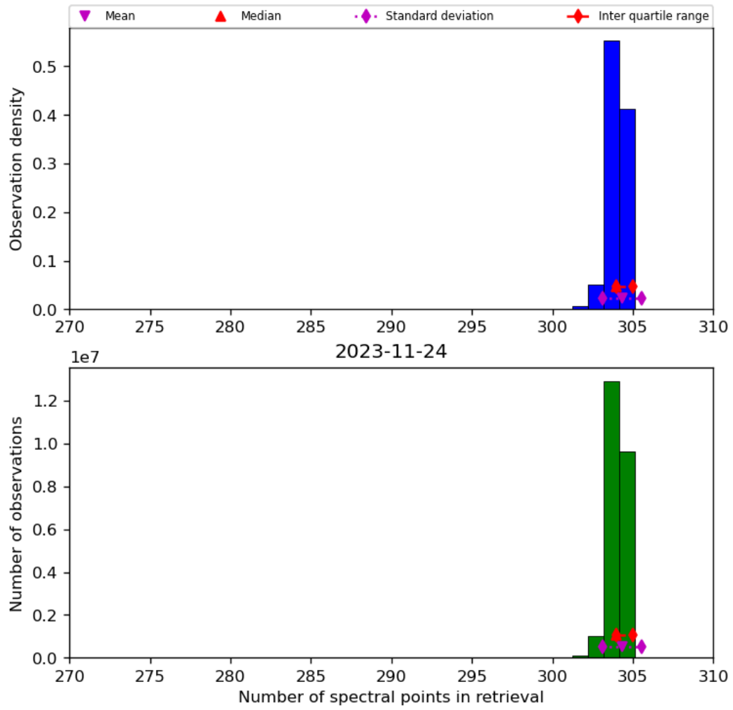
Figure 33: Histogram of “Number of spectral points in retrieval” for 2023-11-23 to 2023-11-25
