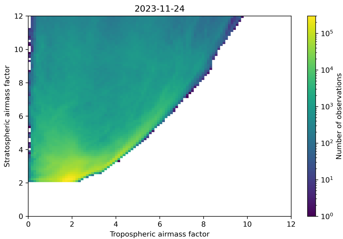
Figure 71: Scatter density plot of “Tropospheric airmass factor” against “Stratospheric airmass factor” for 2023-11-23 to 2023-11-25.
