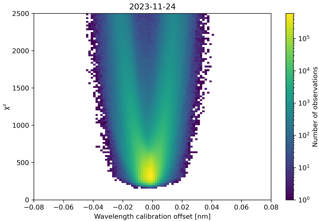
Figure 175: Scatter density plot of “Wavelength calibration offset” against “ \chi^2 ” for 2023-11-23 to 2023-11-25.
