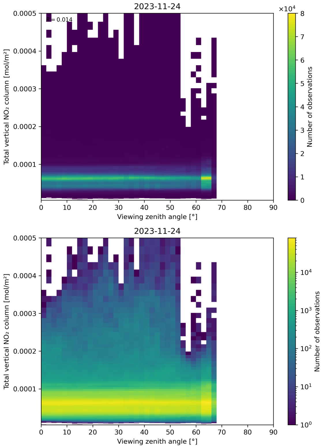
Figure 167: Scatter density plot of “Viewing zenith angle” against “Total vertical NO 2 column” for 2023-11-23 to 2023-11-25.
