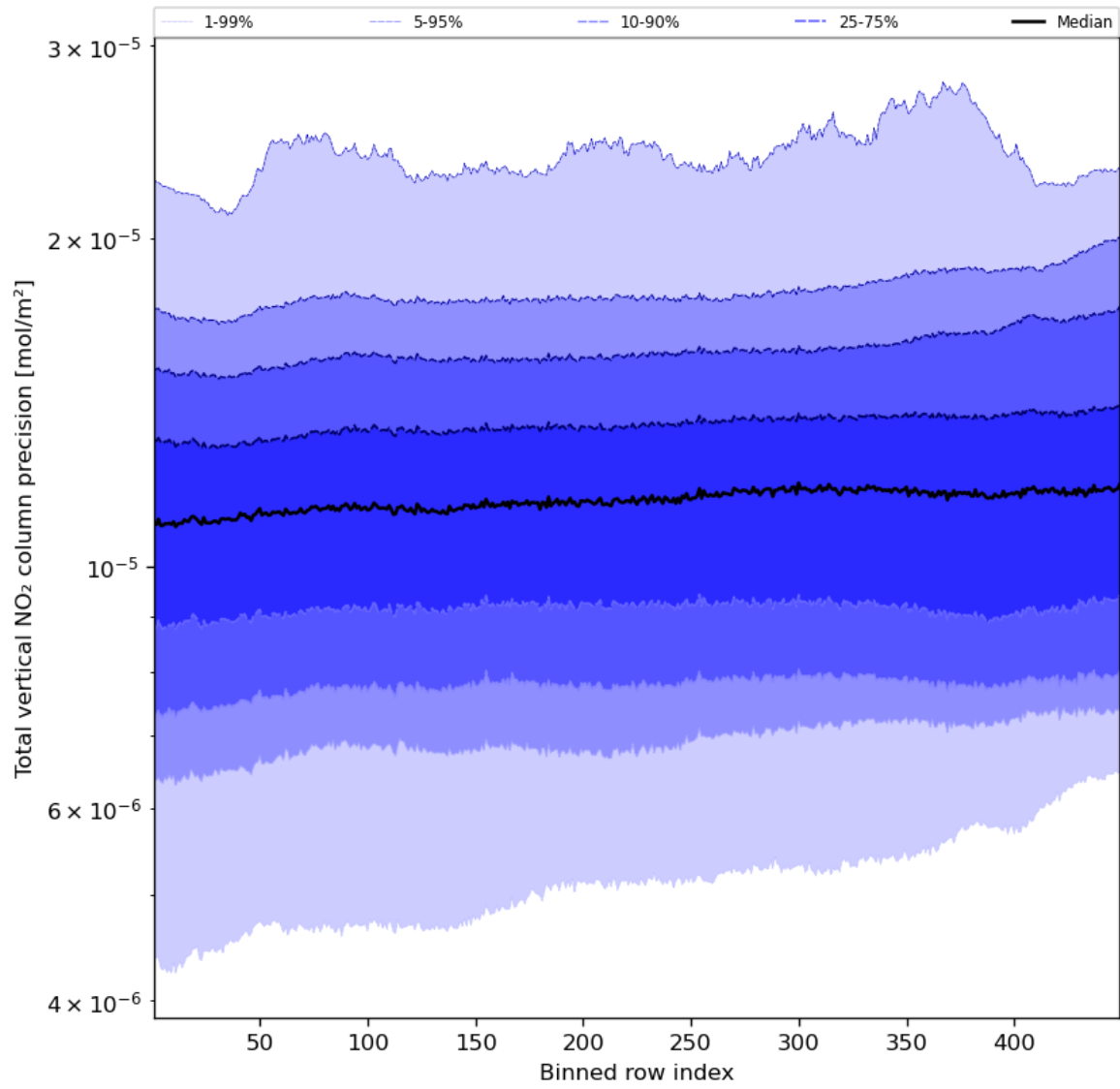
Figure 56: Along track statistics of “Total vertical NO 2 column precision” for 2023-11-23 to 2023-11-25
