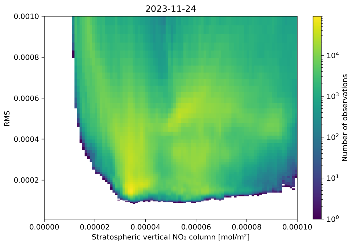
Figure 102: Scatter density plot of “Stratospheric vertical NO 2 column” against “RMS” for 2023-11-23 to 2023-11-25.
