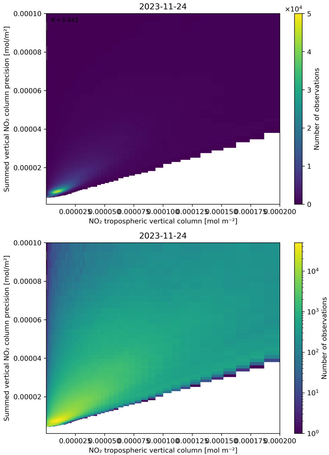
Figure 127: Scatter density plot of “NO 2 tropospheric vertical column” against “Summed vertical NO 2 column precision” for 2023-11-23 to 2023-11-25.
