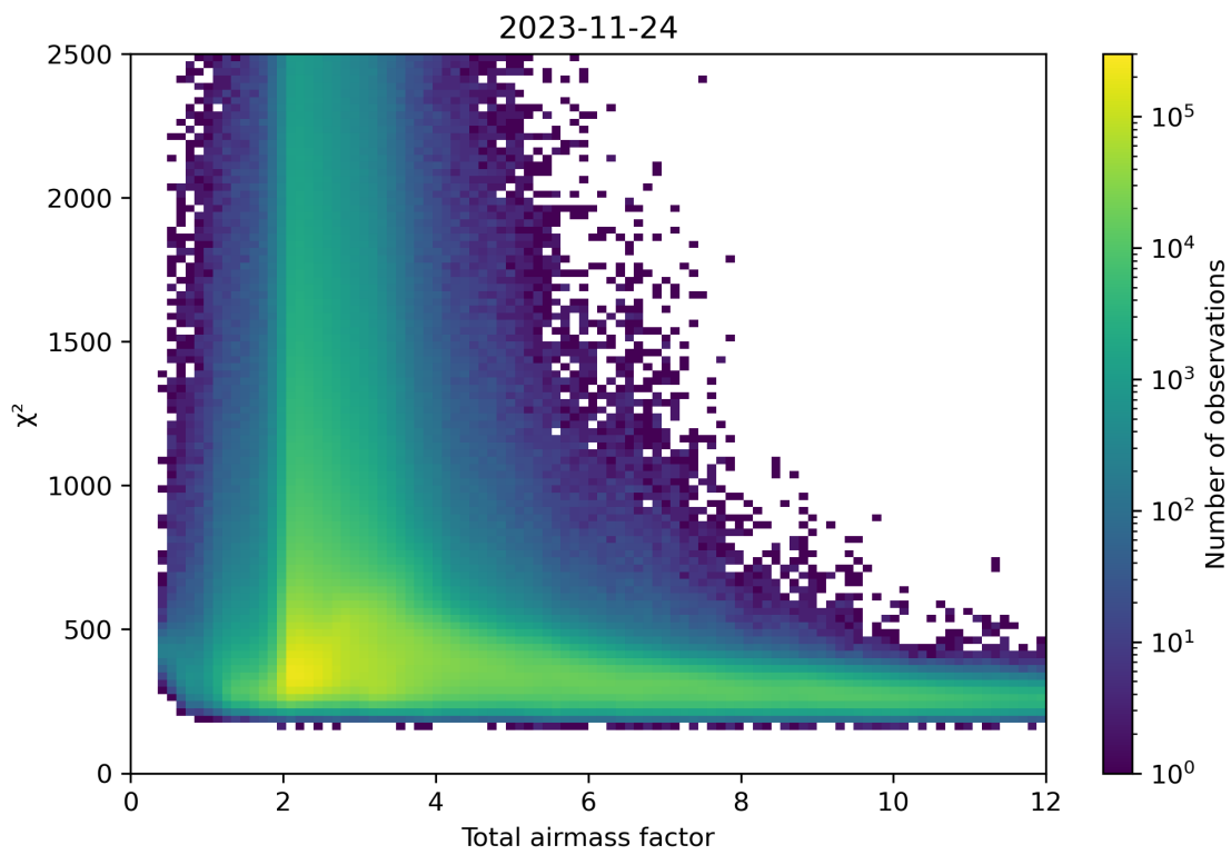
Figure 63: Scatter density plot of “Total airmass factor” against “ \chi^2 ” for 2023-11-23 to 2023-11-25.
