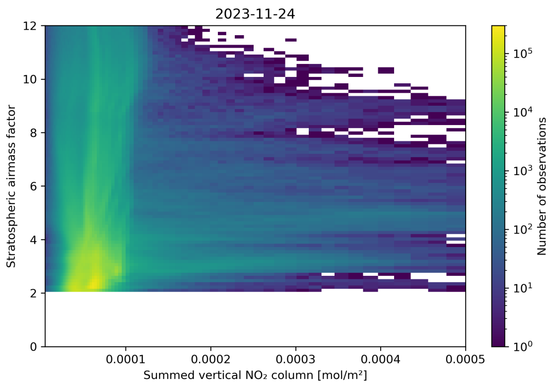
Figure 103: Scatter density plot of “Summed vertical NO 2 column” against “Stratospheric airmass factor” for 2023-11-23 to 2023-11-25.
