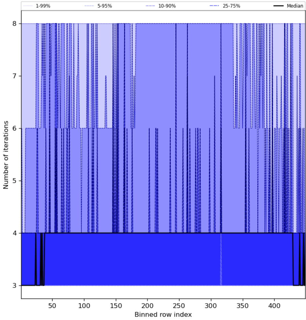
Figure 51: Along track statistics of “Number of iterations” for 2023-11-23 to 2023-11-25
