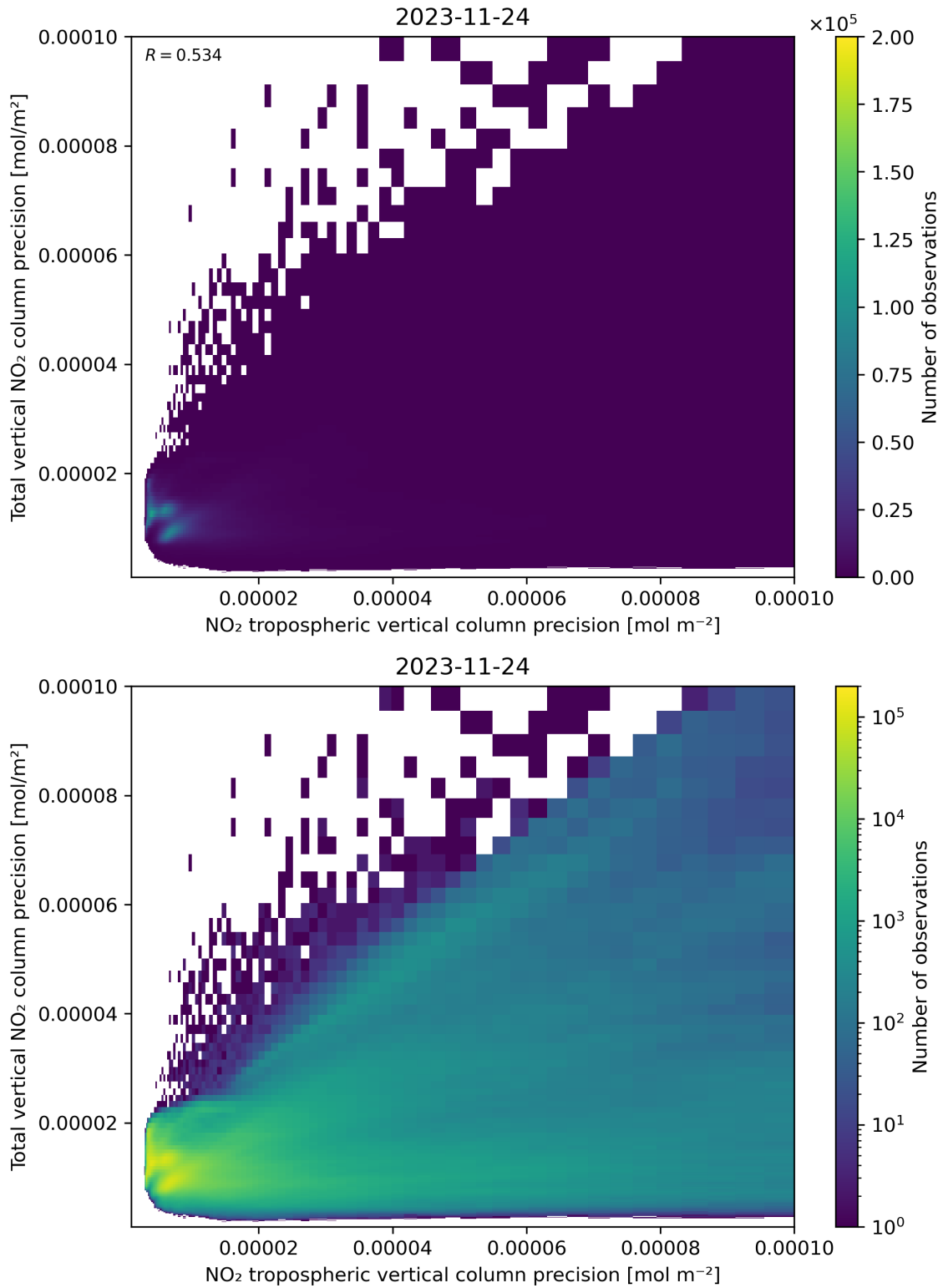
Figure 139: Scatter density plot of “NO 2 tropospheric vertical column precision” against “Total vertical NO 2 column precision” for 2023-11-23 to 2023-11-25.
