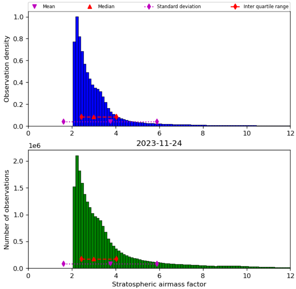
Figure 44: Histogram of “Stratospheric airmass factor” for 2023-11-23 to 2023-11-25
