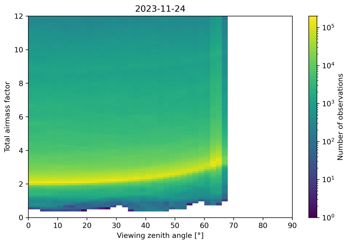
Figure 160: Scatter density plot of “Viewing zenith angle” against “Total airmass factor” for 2023-11-23 to 2023-11-25.
