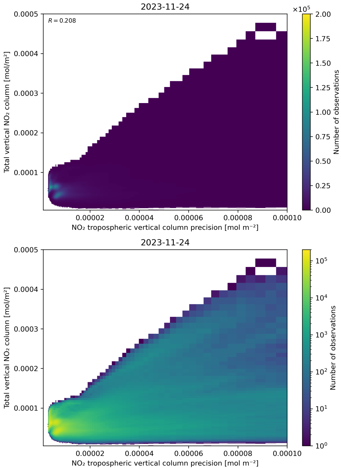
Figure 138: Scatter density plot of “NO 2 tropospheric vertical column precision” against “Total vertical NO 2 column” for 2023-11-23 to 2023-11-25.
