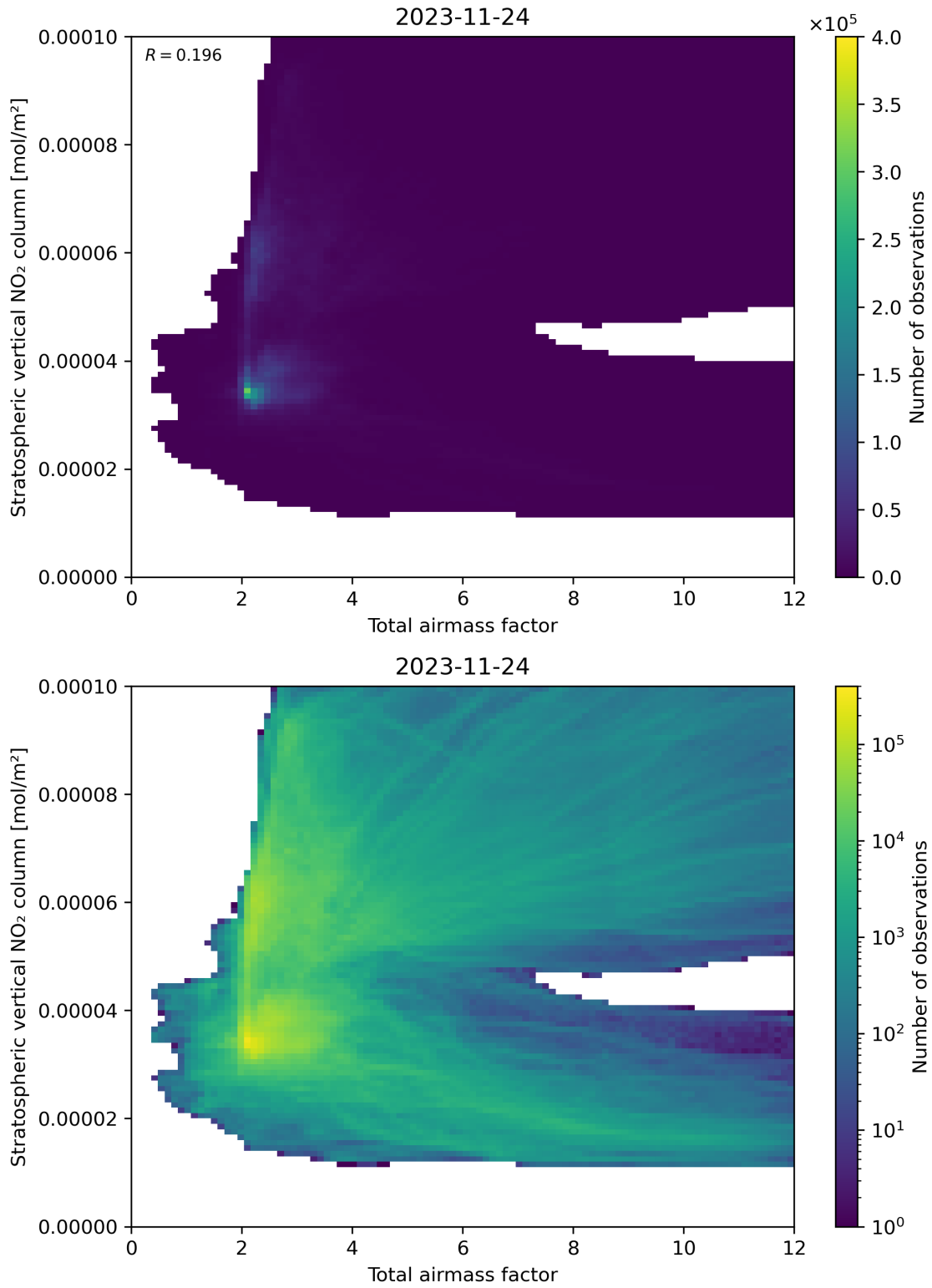
Figure 64: Scatter density plot of “Total airmass factor” against “Stratospheric vertical NO 2 column” for 2023-11-23 to 2023-11-25.
