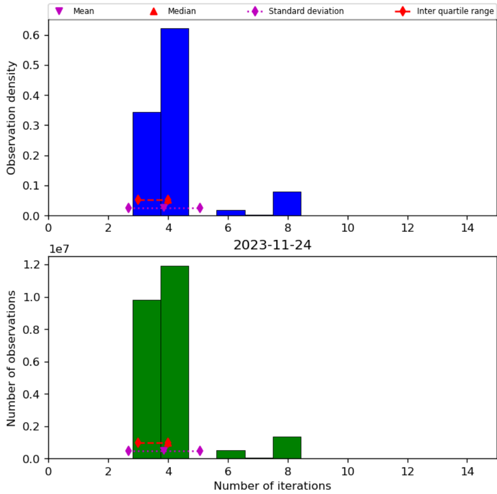
Figure 34: Histogram of “Number of iterations” for 2023-11-23 to 2023-11-25
