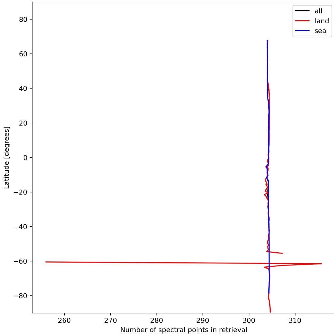
Figure 16: Zonal average of “Number of spectral points in retrieval” for 2023-11-23 to 2023-11-25.
