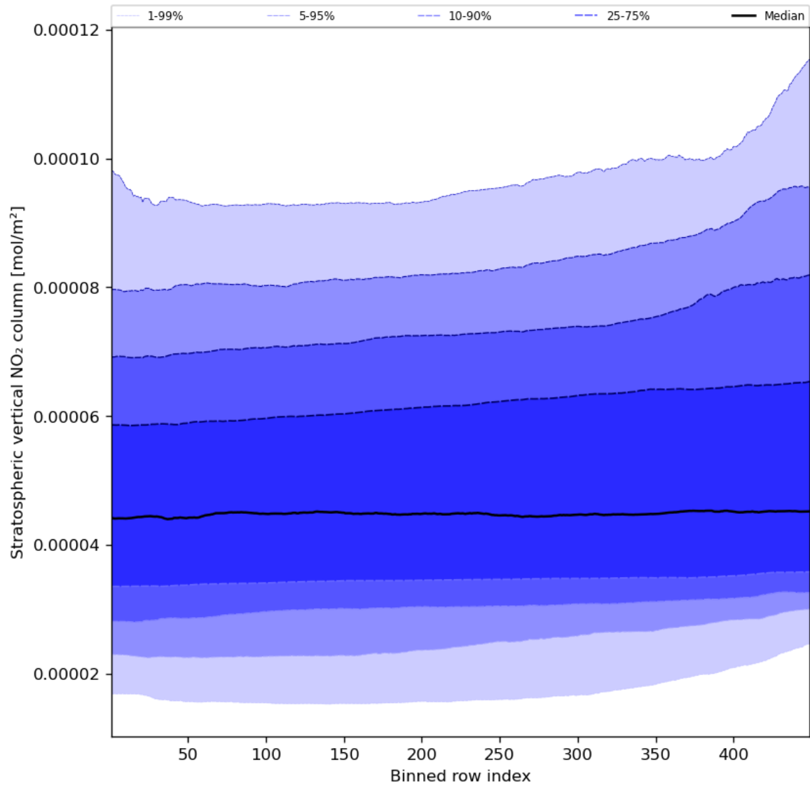
Figure 53: Along track statistics of “Stratospheric vertical NO 2 column” for 2023-11-23 to 2023-11-25
