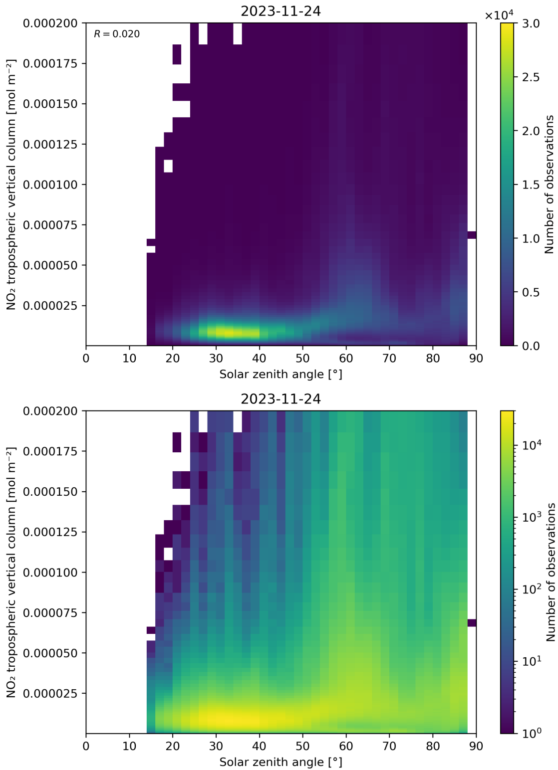
Figure 155: Scatter density plot of “Solar zenith angle” against “NO 2 tropospheric vertical column” for 2023-11-23 to 2023-11-25.
