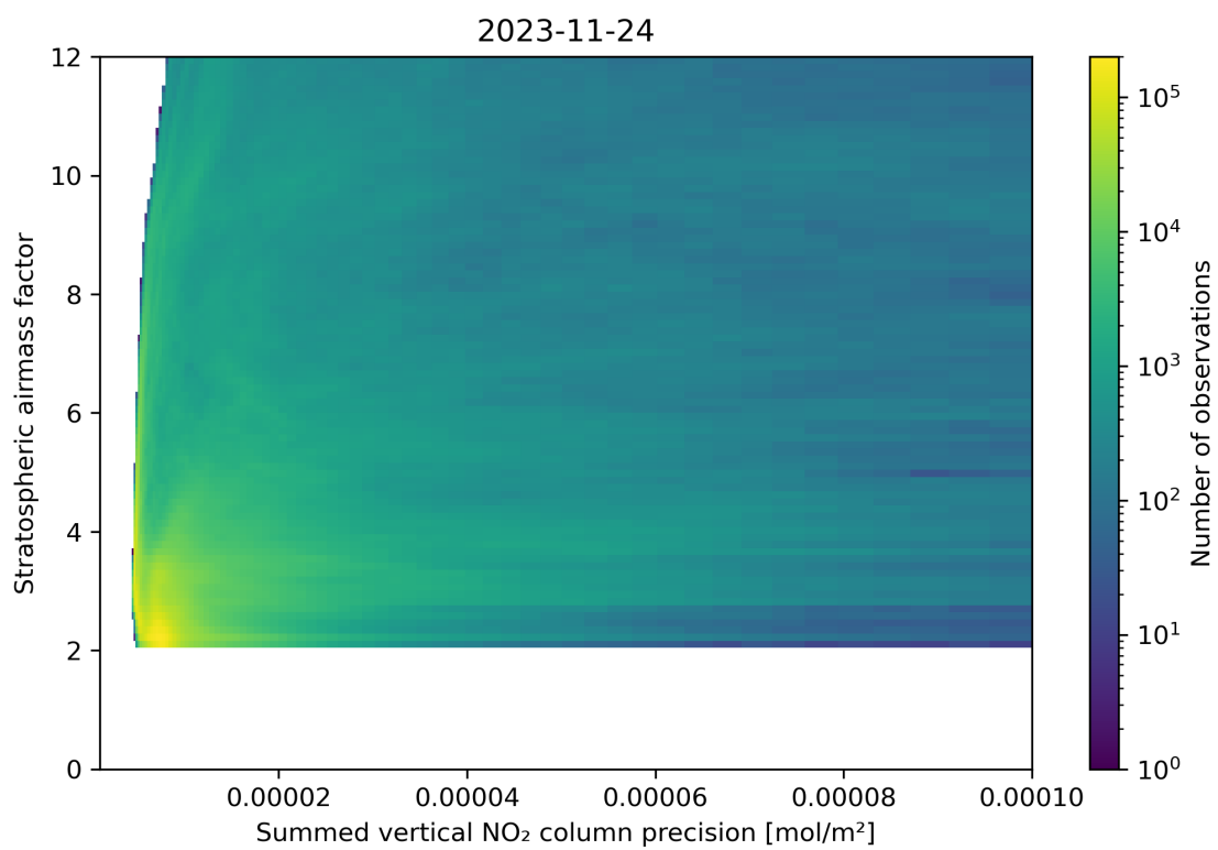
Figure 106: Scatter density plot of “Summed vertical NO 2 column precision” against “Stratospheric airmass factor” for 2023-11-23 to 2023-11-25.
