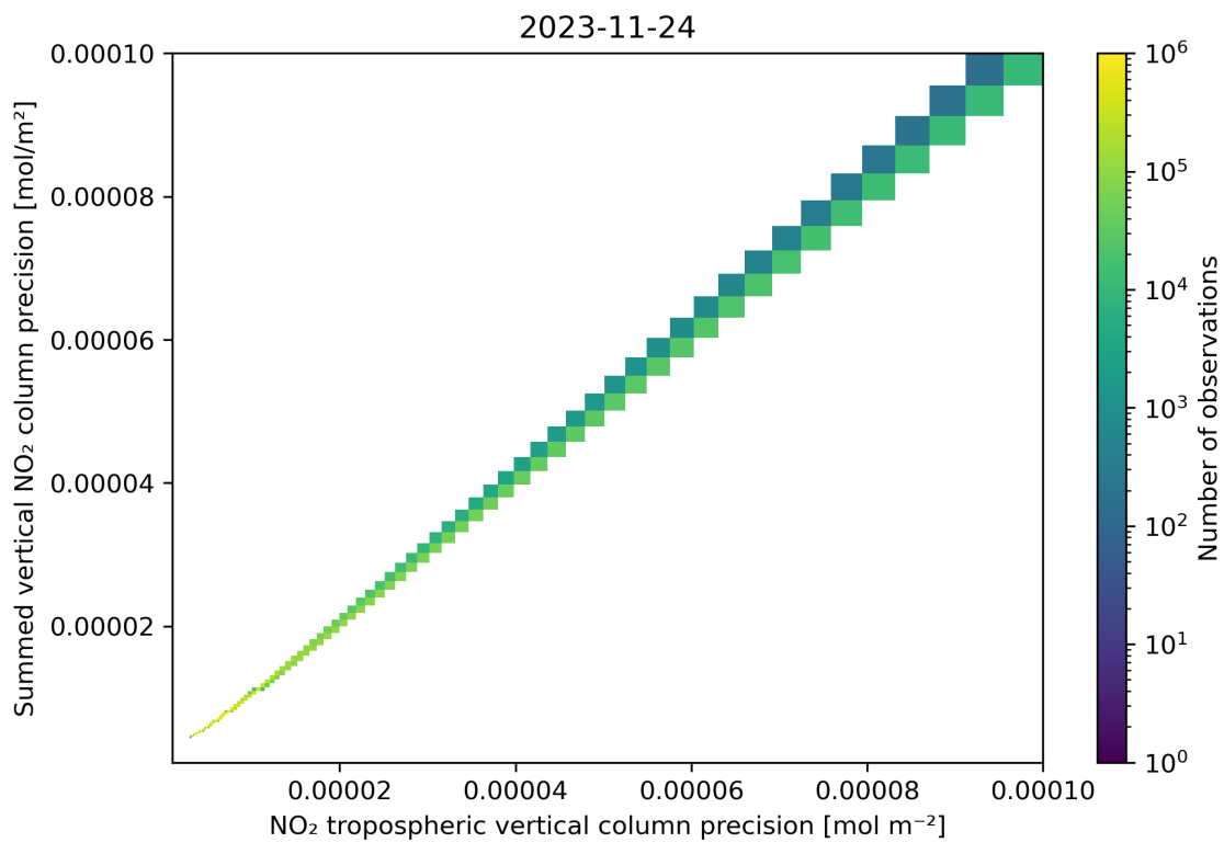
Figure 137: Scatter density plot of “NO 2 tropospheric vertical column precision” against “Summed vertical NO 2 column precision” for 2023-11-23 to 2023-11-25.
