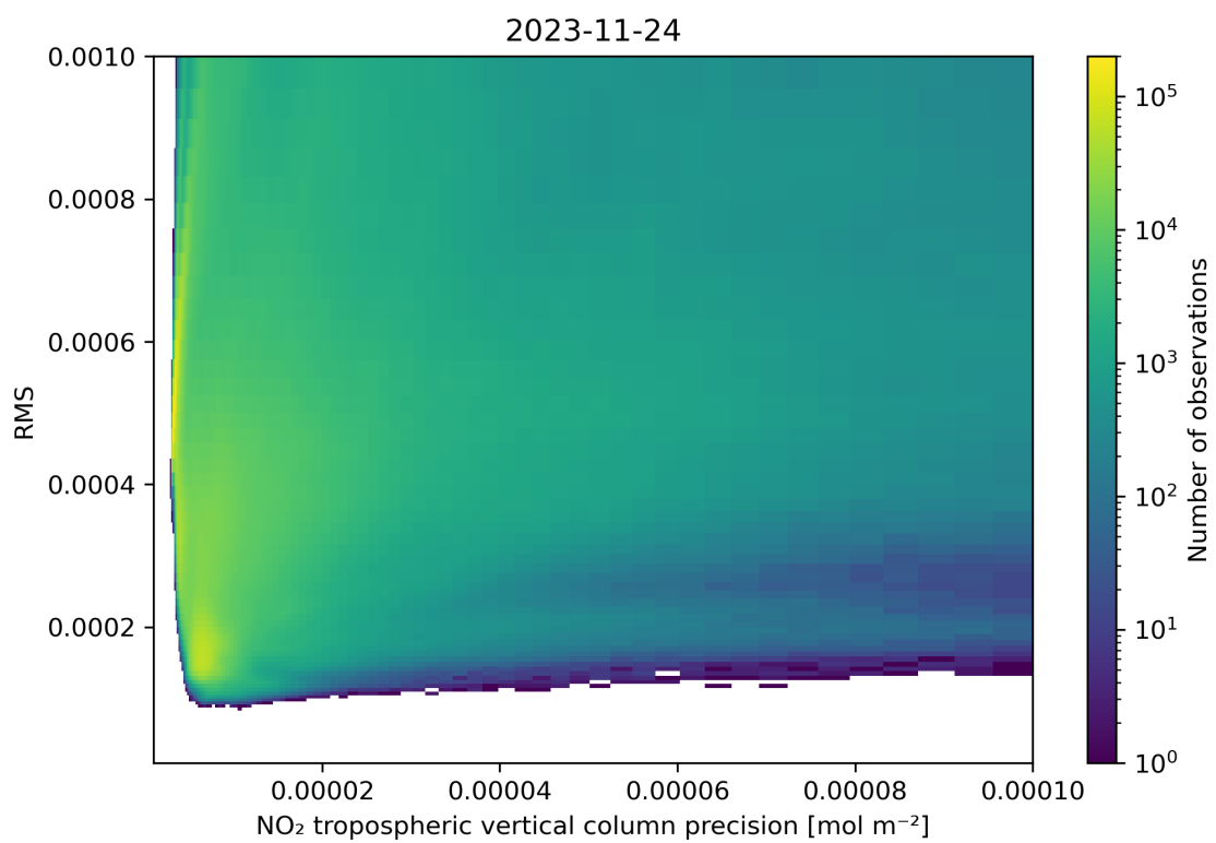
Figure 140: Scatter density plot of “NO 2 tropospheric vertical column precision” against “RMS” for 2023-11-23 to 2023-11-25.
