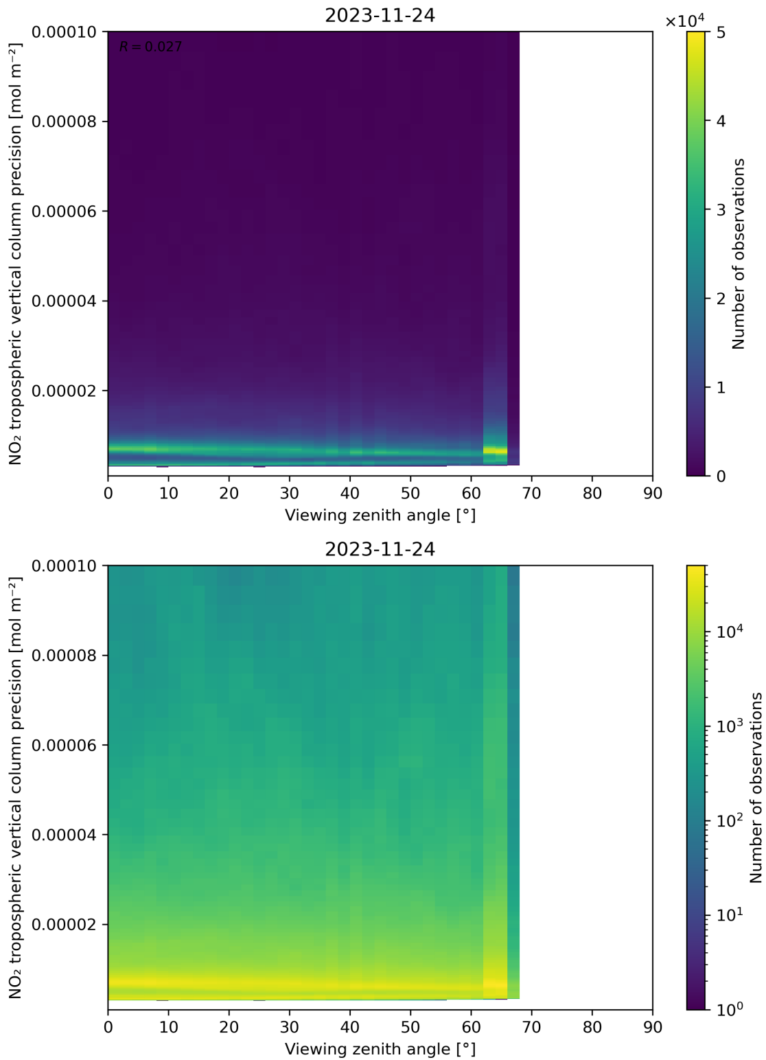
Figure 170: Scatter density plot of “Viewing zenith angle” against “NO 2 tropospheric vertical column precision” for 2023-11-23 to 2023-11-25.
