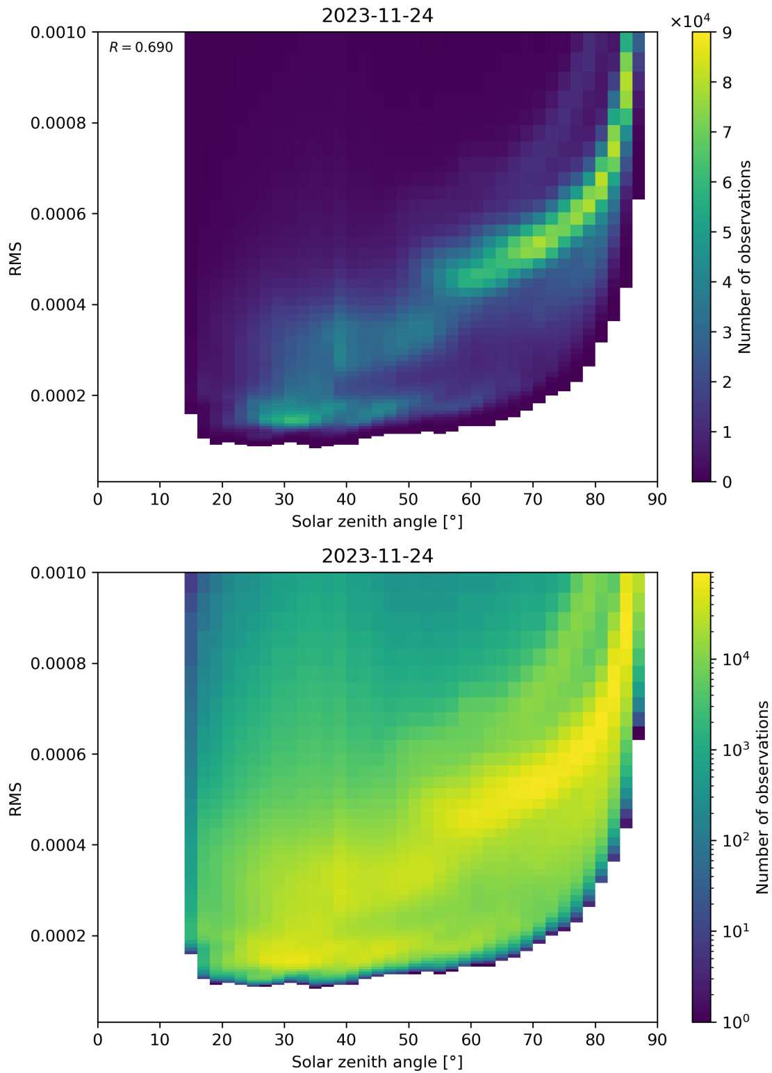
Figure 157: Scatter density plot of “Solar zenith angle” against “RMS” for 2023-11-23 to 2023-11-25.
