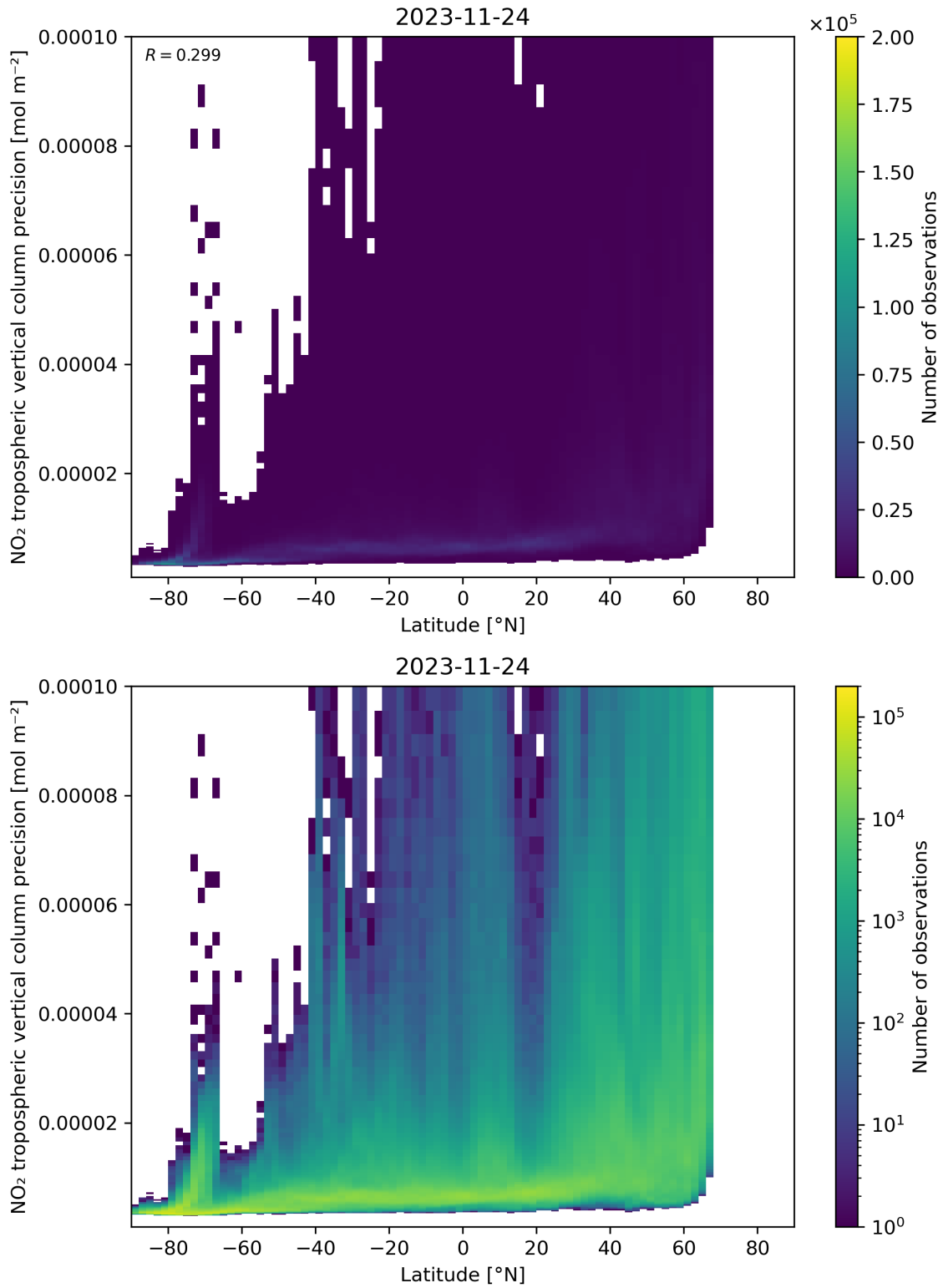
Figure 93: Scatter density plot of “Latitude” against “NO 2 tropospheric vertical column precision” for 2023-11-23 to 2023-11-25.
