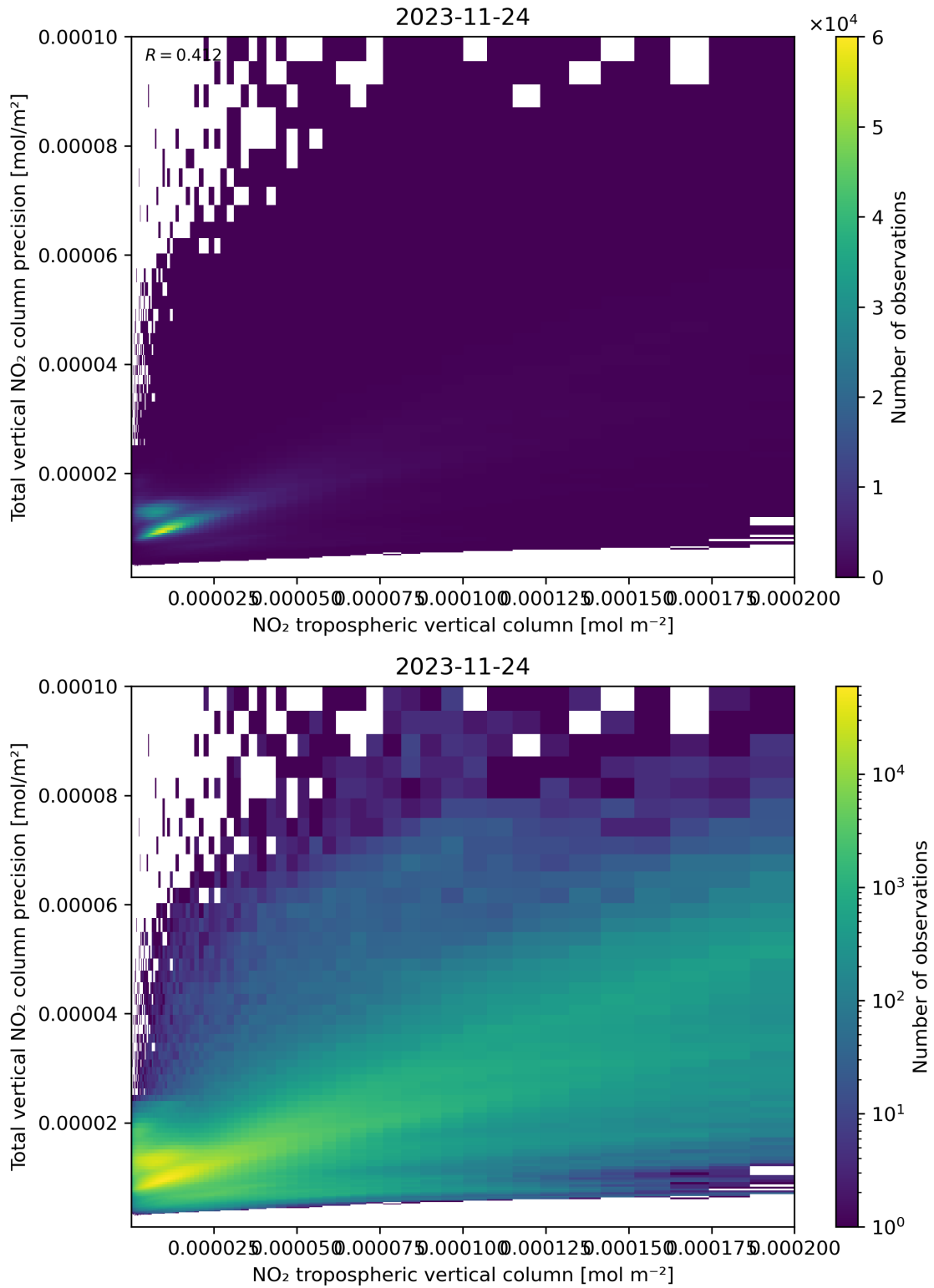
Figure 129: Scatter density plot of “NO 2 tropospheric vertical column” against “Total vertical NO 2 column precision” for 2023-11-23 to 2023-11-25.
