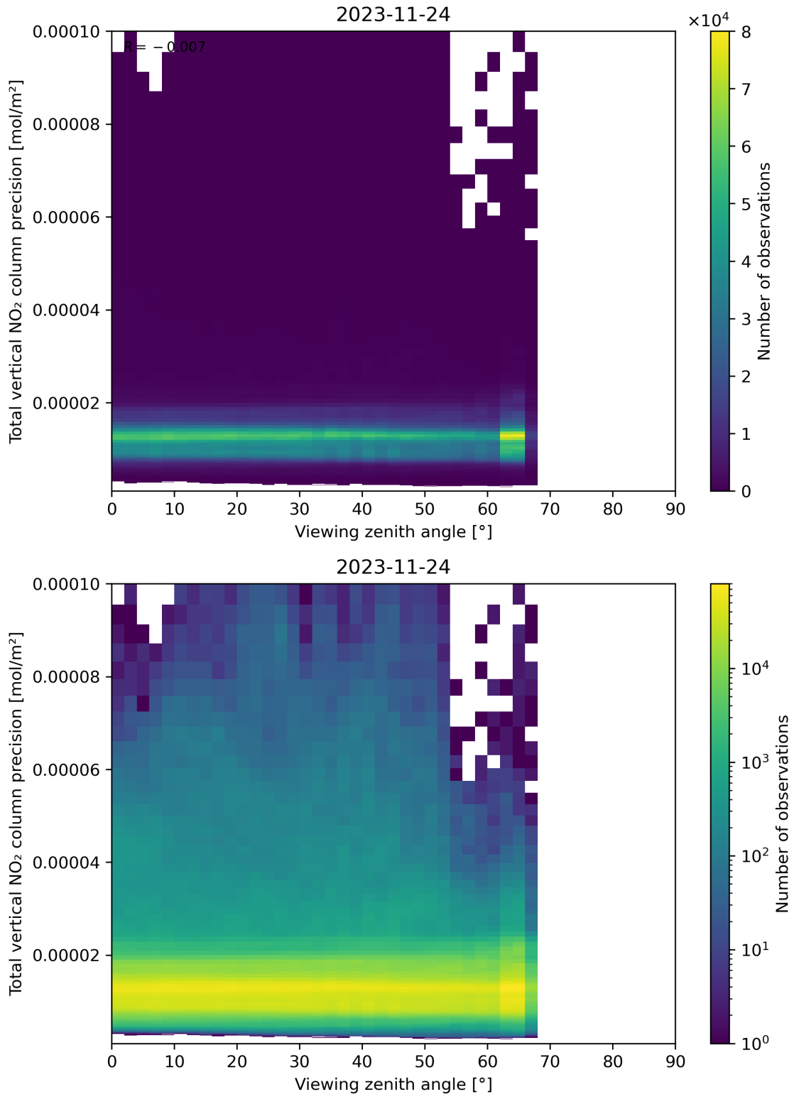
Figure 168: Scatter density plot of “Viewing zenith angle” against “Total vertical NO 2 column precision” for 2023-11-23 to 2023-11-25.
