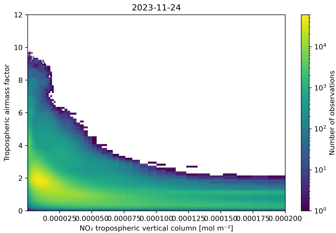
Figure 123: Scatter density plot of “NO 2 tropospheric vertical column” against “Tropospheric airmass factor” for 2023-11-23 to 2023-11-25.
