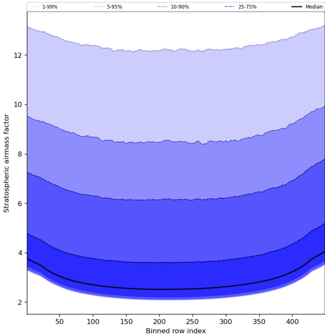
Figure 61: Along track statistics of “Stratospheric airmass factor” for 2023-11-23 to 2023-11-25
