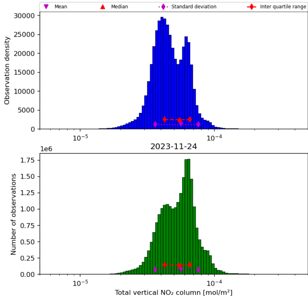
Figure 38: Histogram of “Total vertical NO 2 column” for 2023-11-23 to 2023-11-25
