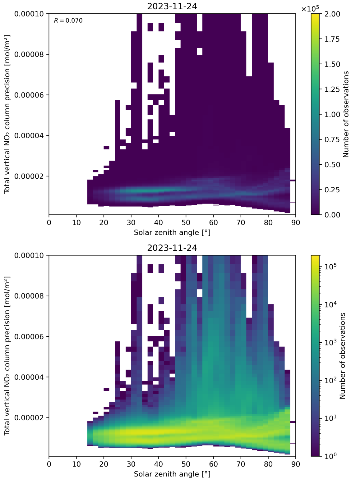
Figure 154: Scatter density plot of “Solar zenith angle” against “Total vertical NO 2 column precision” for 2023-11-23 to 2023-11-25.
