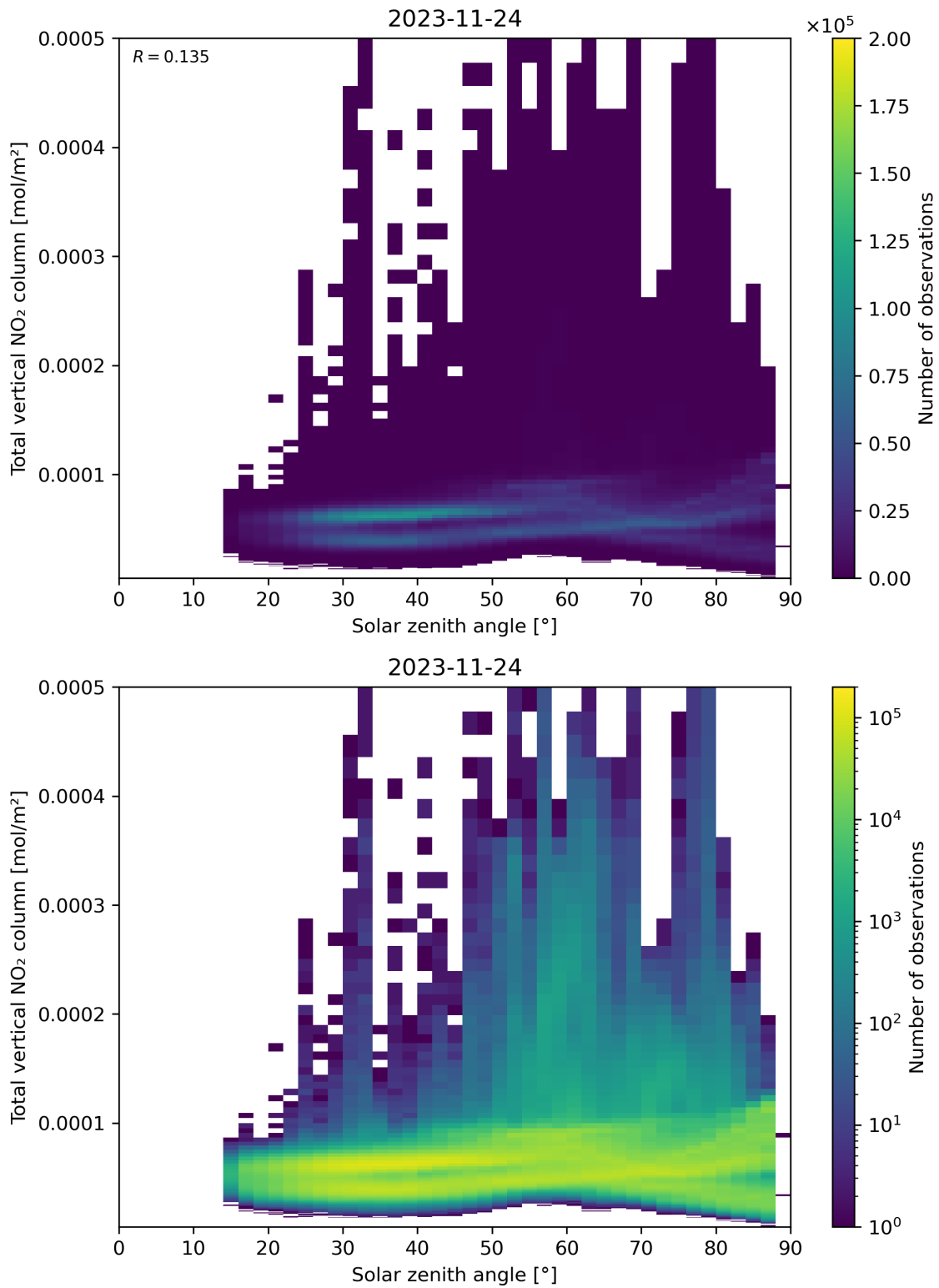
Figure 153: Scatter density plot of “Solar zenith angle” against “Total vertical NO 2 column” for 2023-11-23 to 2023-11-25.
