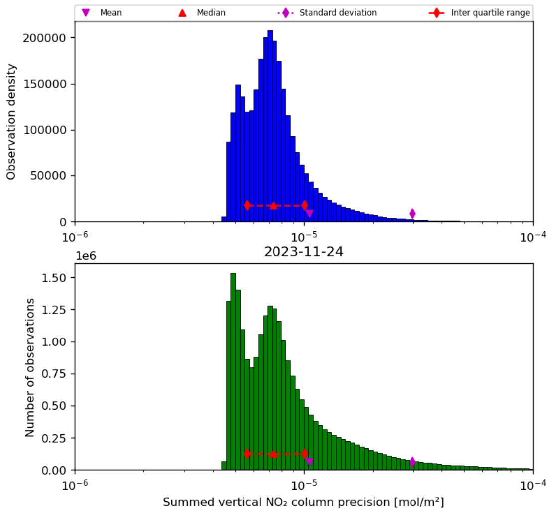
Figure 41: Histogram of “Summed vertical NO 2 column precision” for 2023-11-23 to 2023-11-25
