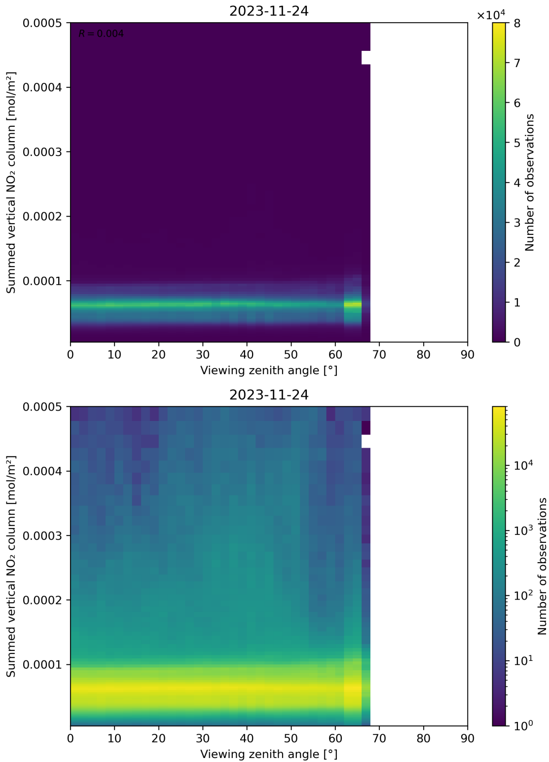
Figure 165: Scatter density plot of “Viewing zenith angle” against “Summed vertical NO 2 column” for 2023-11-23 to 2023-11-25.
