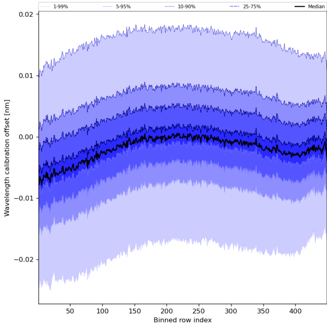
Figure 52: Along track statistics of “Wavelength calibration offset” for 2023-11-23 to 2023-11-25
