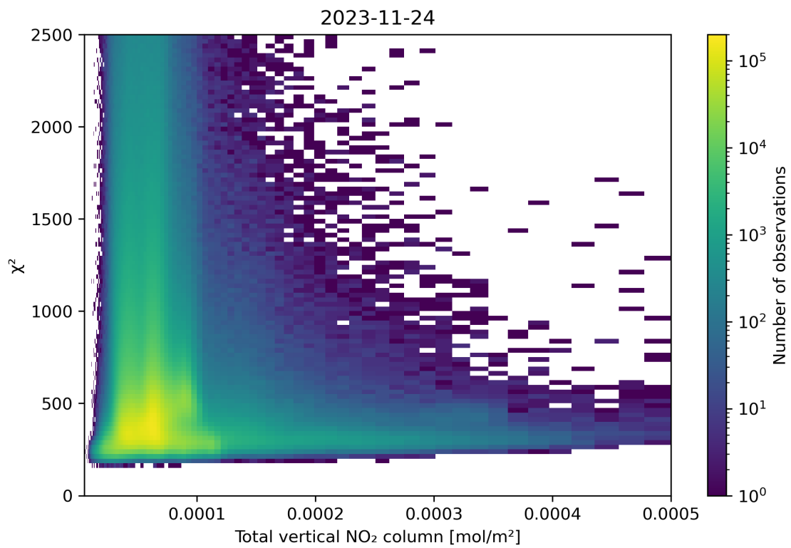
Figure 111: Scatter density plot of “Total vertical NO 2 column” against “ \chi^2 ” for 2023-11-23 to 2023-11-25.
