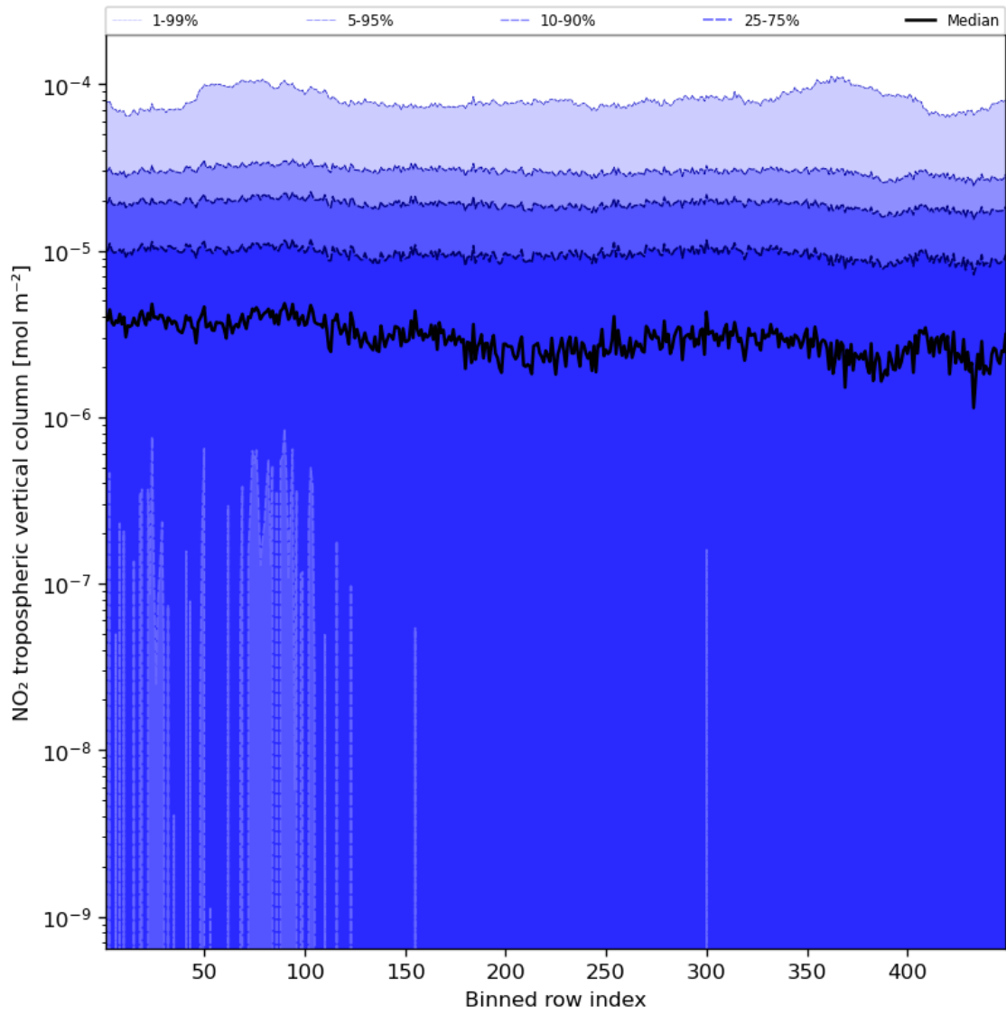
Figure 46: Along track statistics of “NO 2 tropospheric vertical column” for 2023-11-23 to 2023-11-25
