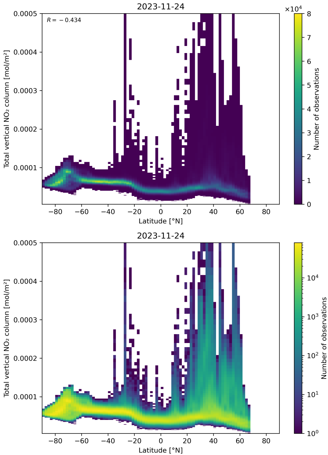
Figure 90: Scatter density plot of “Latitude” against “Total vertical NO 2 column” for 2023-11-23 to 2023-11-25.
