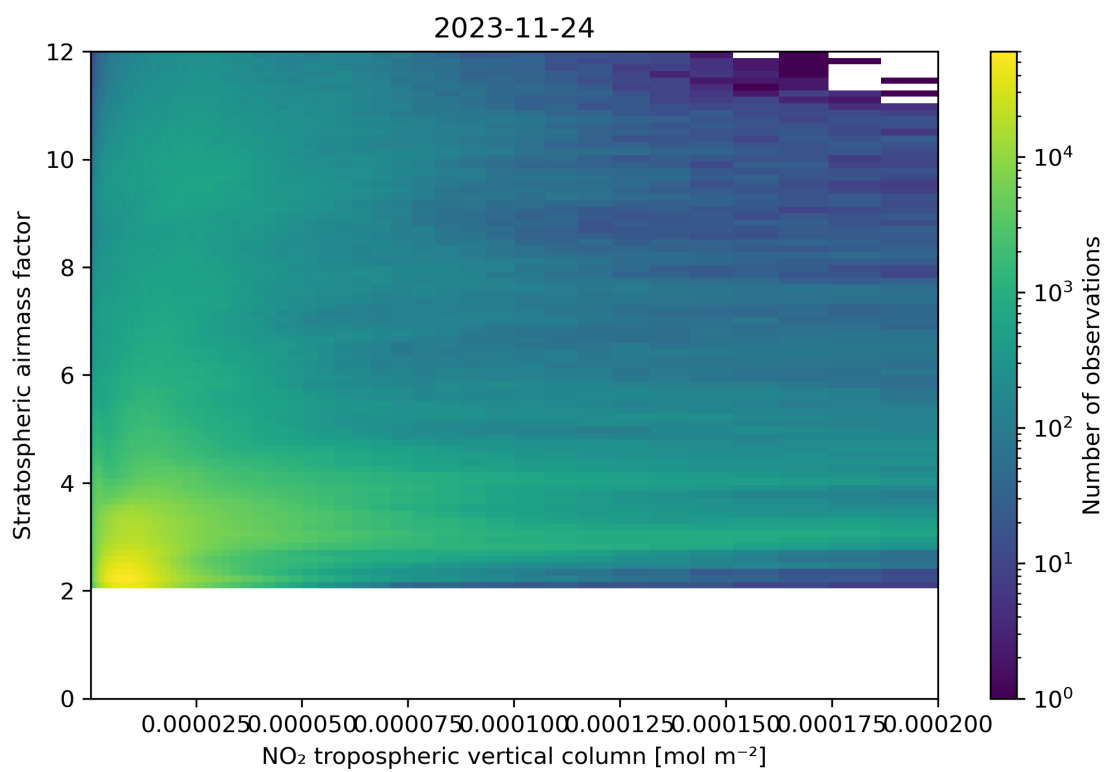
Figure 121: Scatter density plot of “NO 2 tropospheric vertical column” against “Stratospheric airmass factor” for 2023-11-23 to 2023-11-25.
