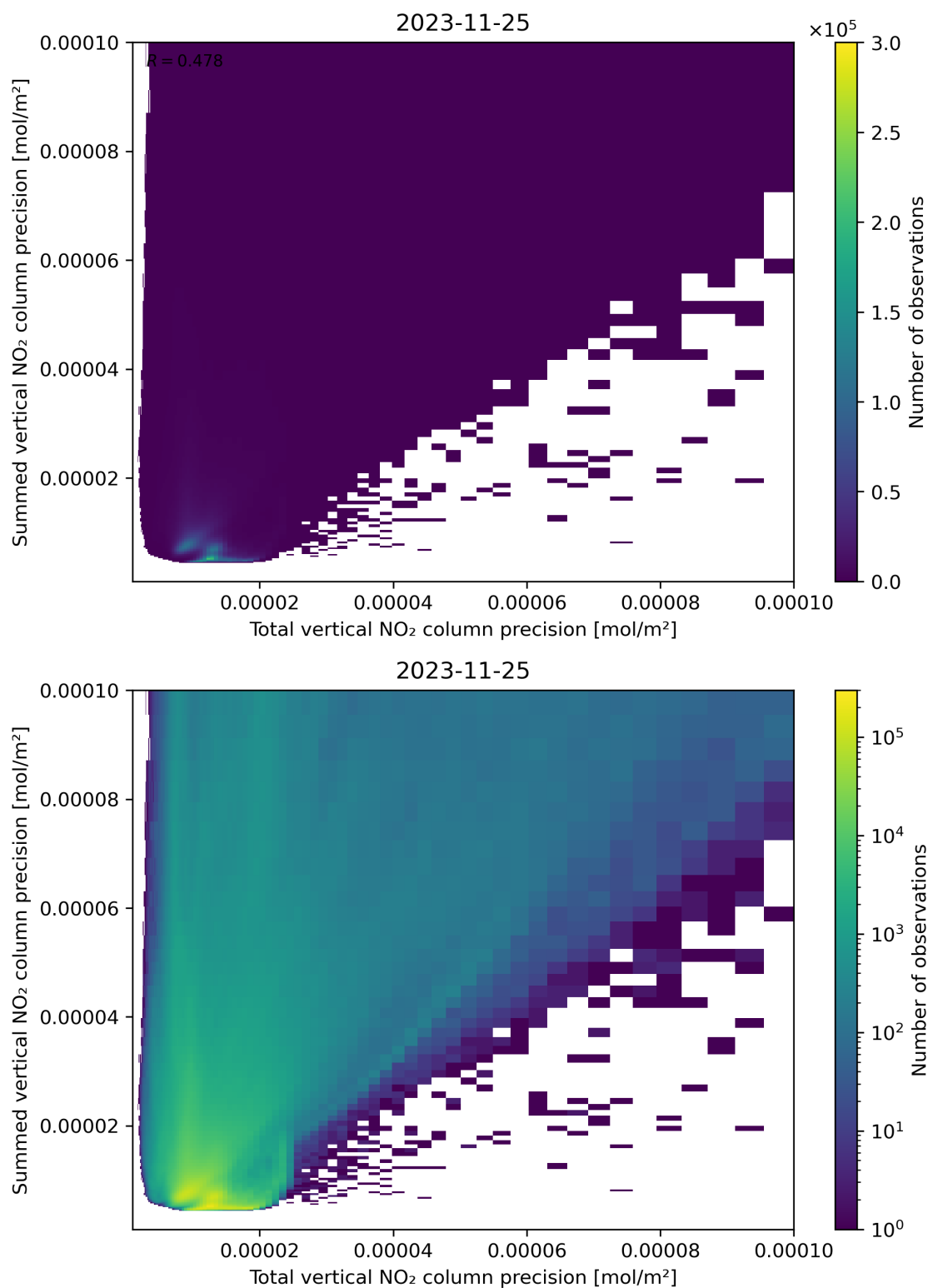
Figure 118: Scatter density plot of “Total vertical NO 2 column precision” against “Summed vertical NO 2 column precision” for 2023-11-24 to 2023-11-26.
