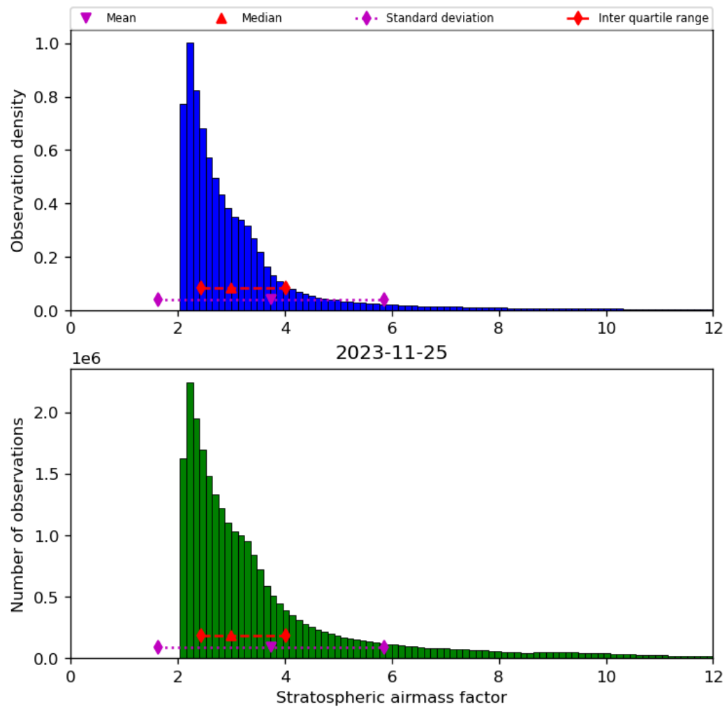
Figure 44: Histogram of “Stratospheric airmass factor” for 2023-11-24 to 2023-11-26
