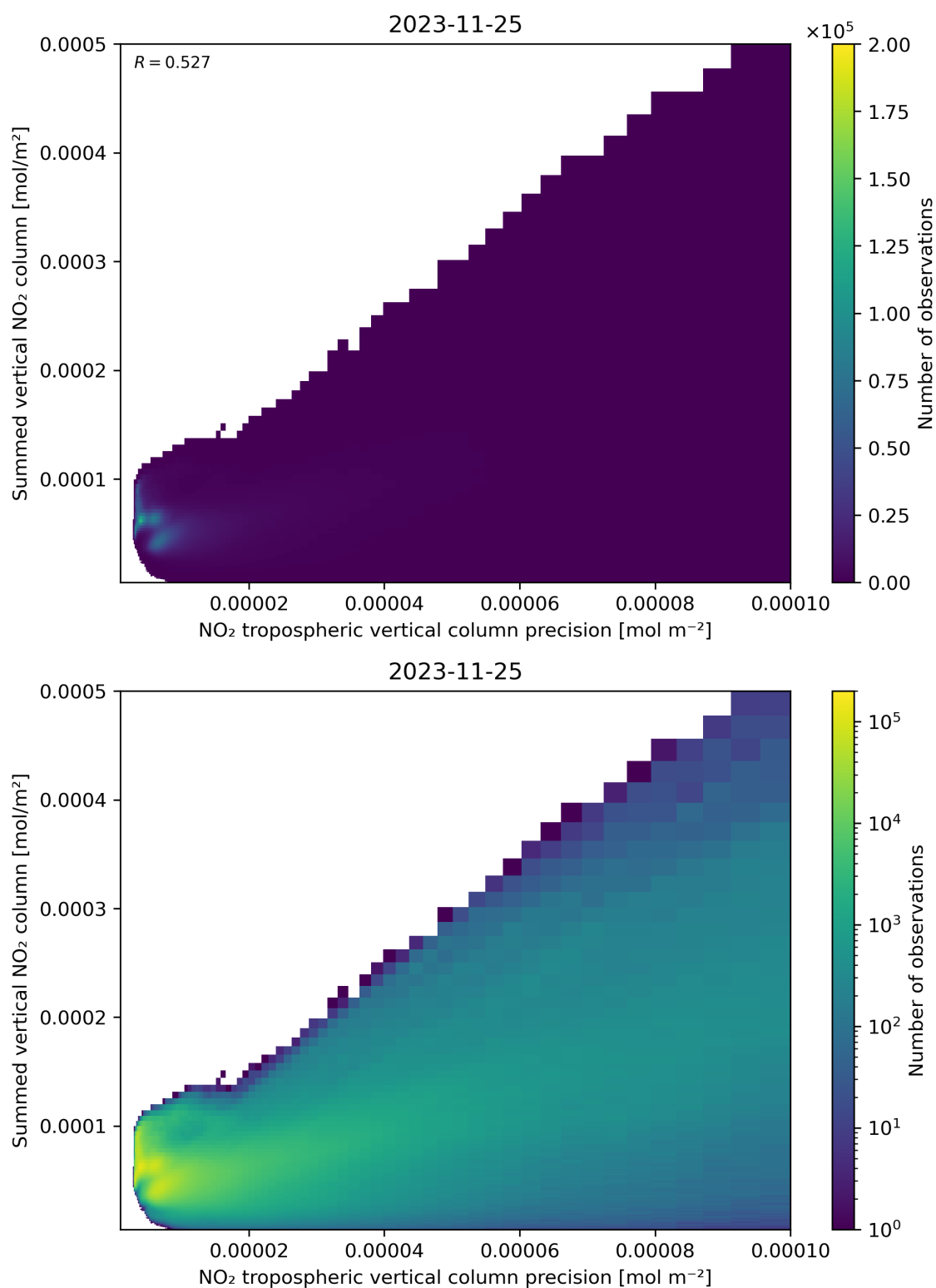
Figure 136: Scatter density plot of “NO 2 tropospheric vertical column precision” against “Summed vertical NO 2 column” for 2023-11-24 to 2023-11-26.
