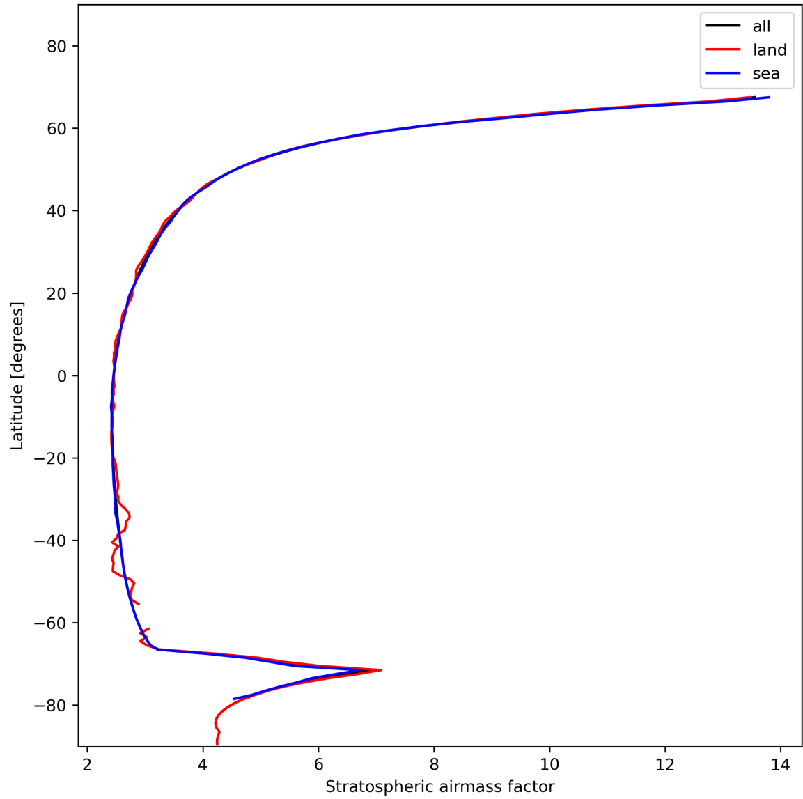
Figure 27: Zonal average of “Stratospheric airmass factor” for 2023-11-24 to 2023-11-26.
