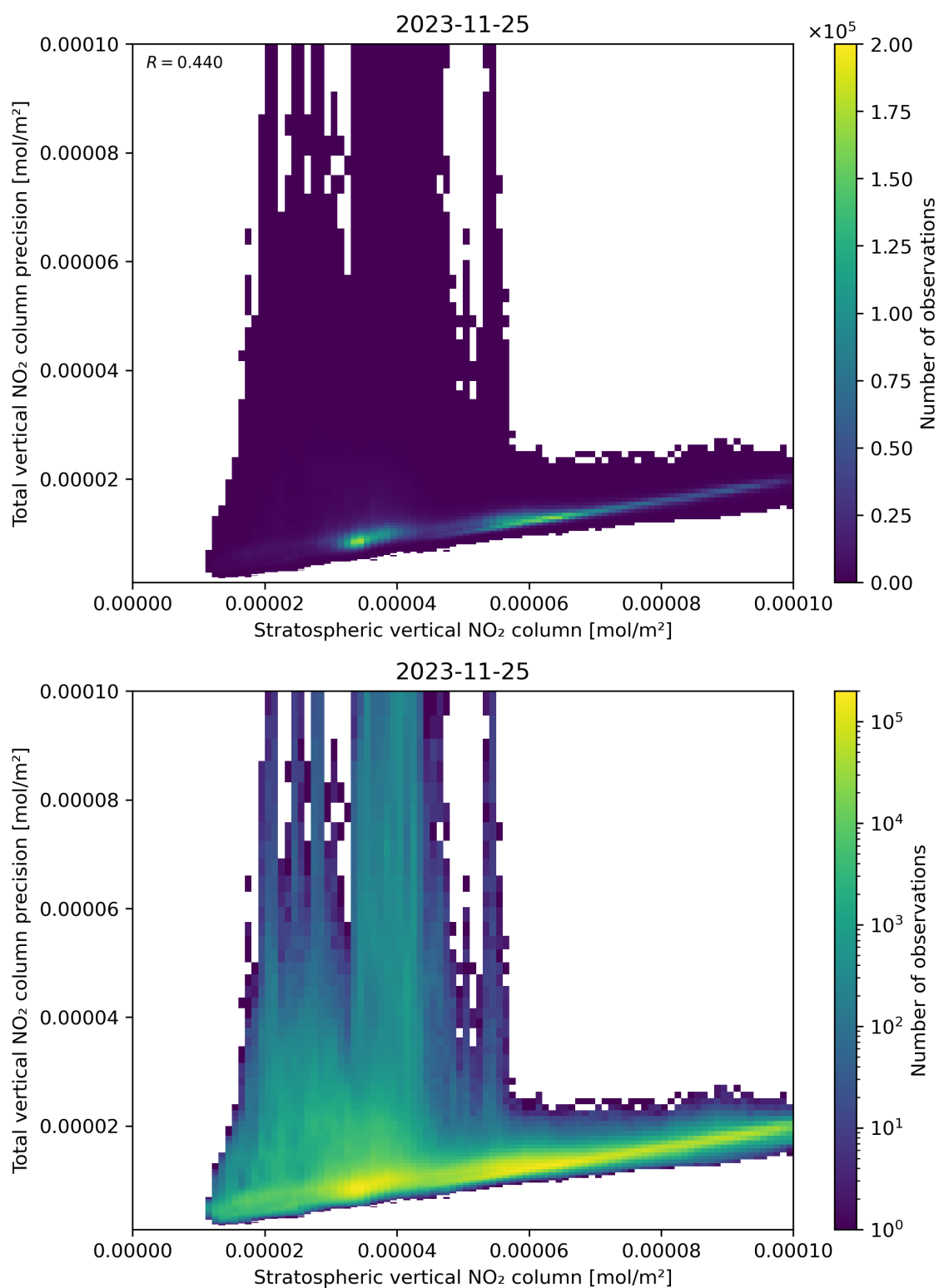
Figure 101: Scatter density plot of “Stratospheric vertical NO 2 column” against “Total vertical NO 2 column precision” for 2023-11-24 to 2023-11-26.
