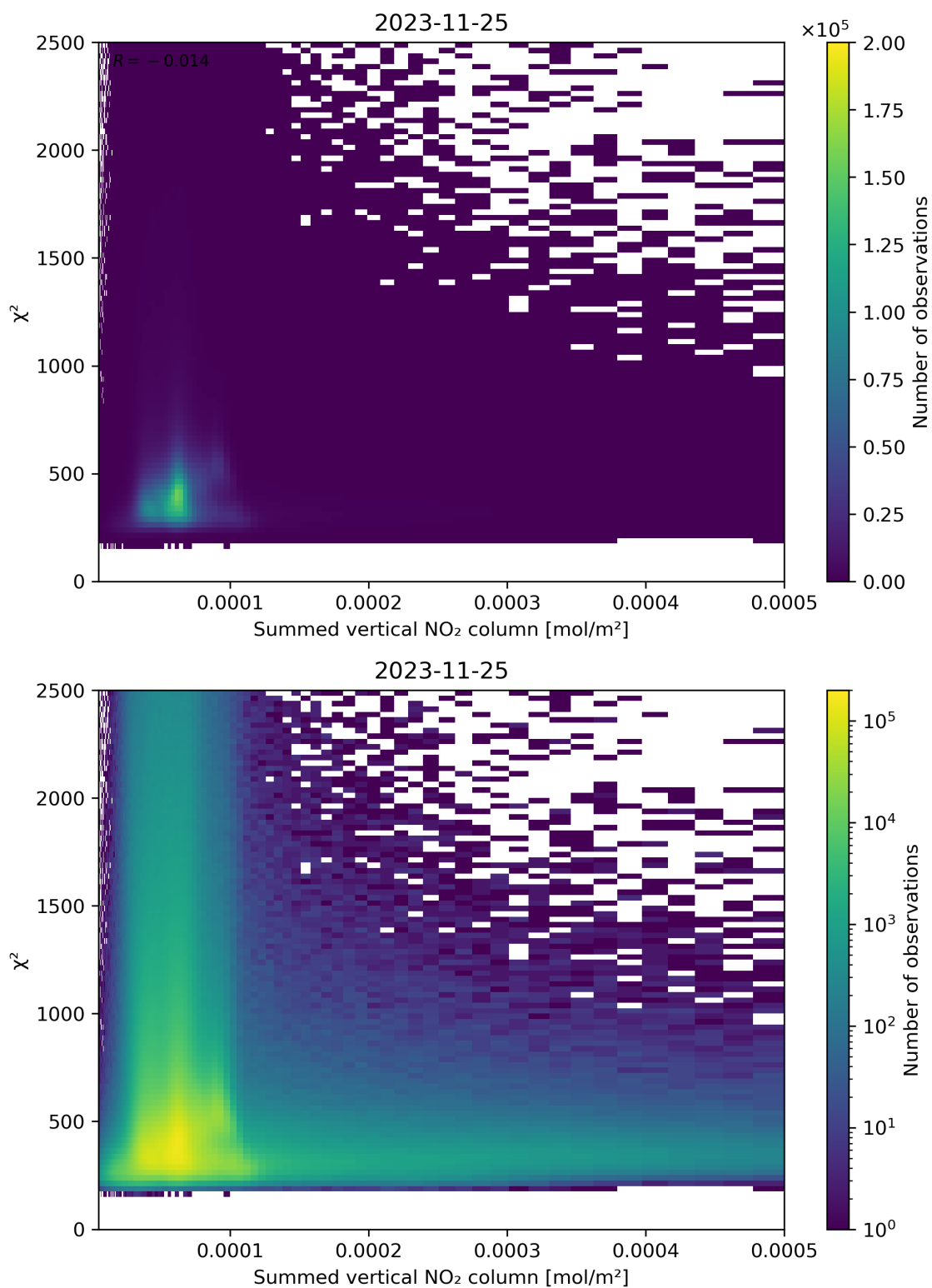
Figure 104: Scatter density plot of “Summed vertical NO 2 column” against “ \chi^2 ” for 2023-11-24 to 2023-11-26.
