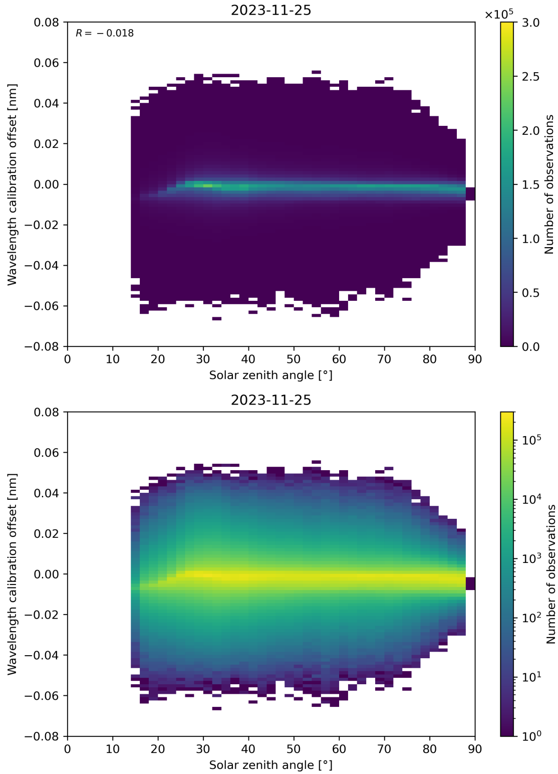
Figure 158: Scatter density plot of “Solar zenith angle” against “Wavelength calibration offset” for 2023-11-24 to 2023-11-26.
