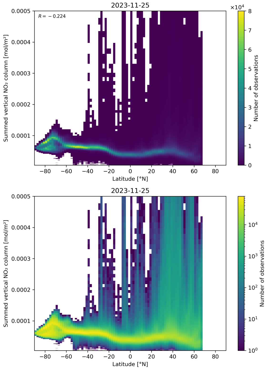
Figure 88: Scatter density plot of “Latitude” against “Summed vertical NO 2 column” for 2023-11-24 to 2023-11-26.
