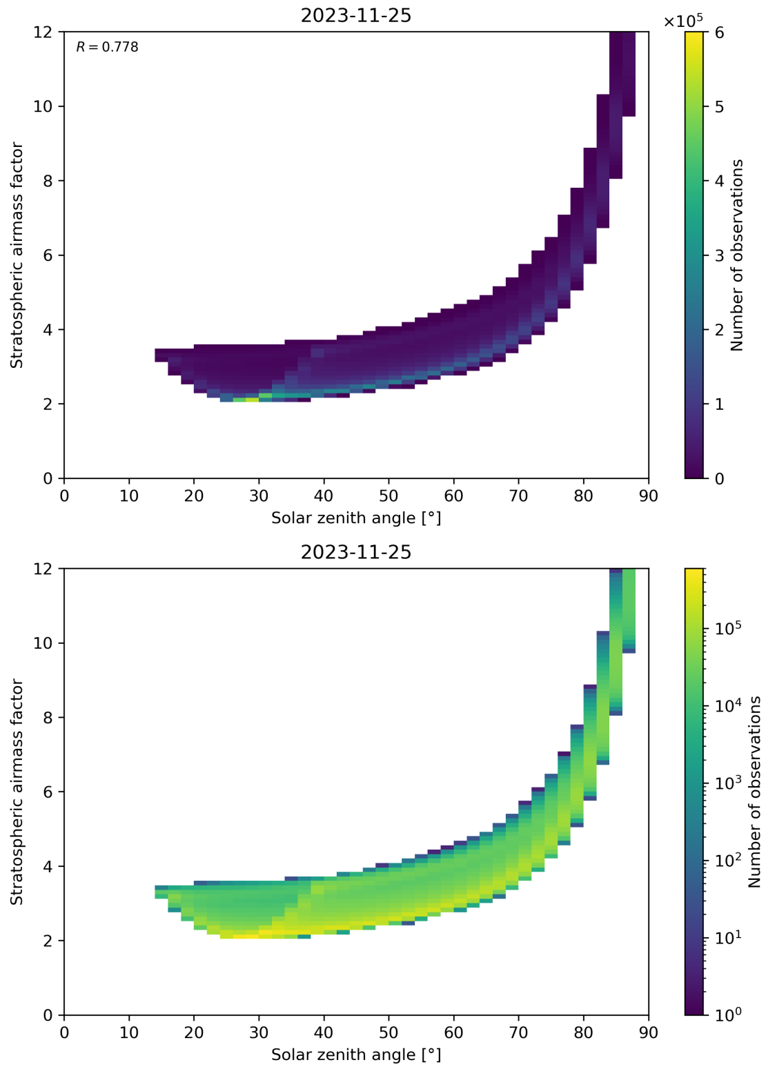
Figure 145: Scatter density plot of “Solar zenith angle” against “Stratospheric airmass factor” for 2023-11-24 to 2023-11-26.
