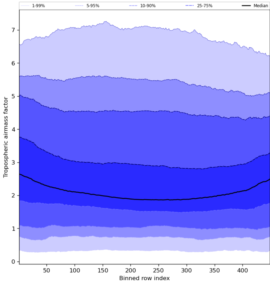
Figure 48: Along track statistics of “Tropospheric airmass factor” for 2023-11-24 to 2023-11-26
