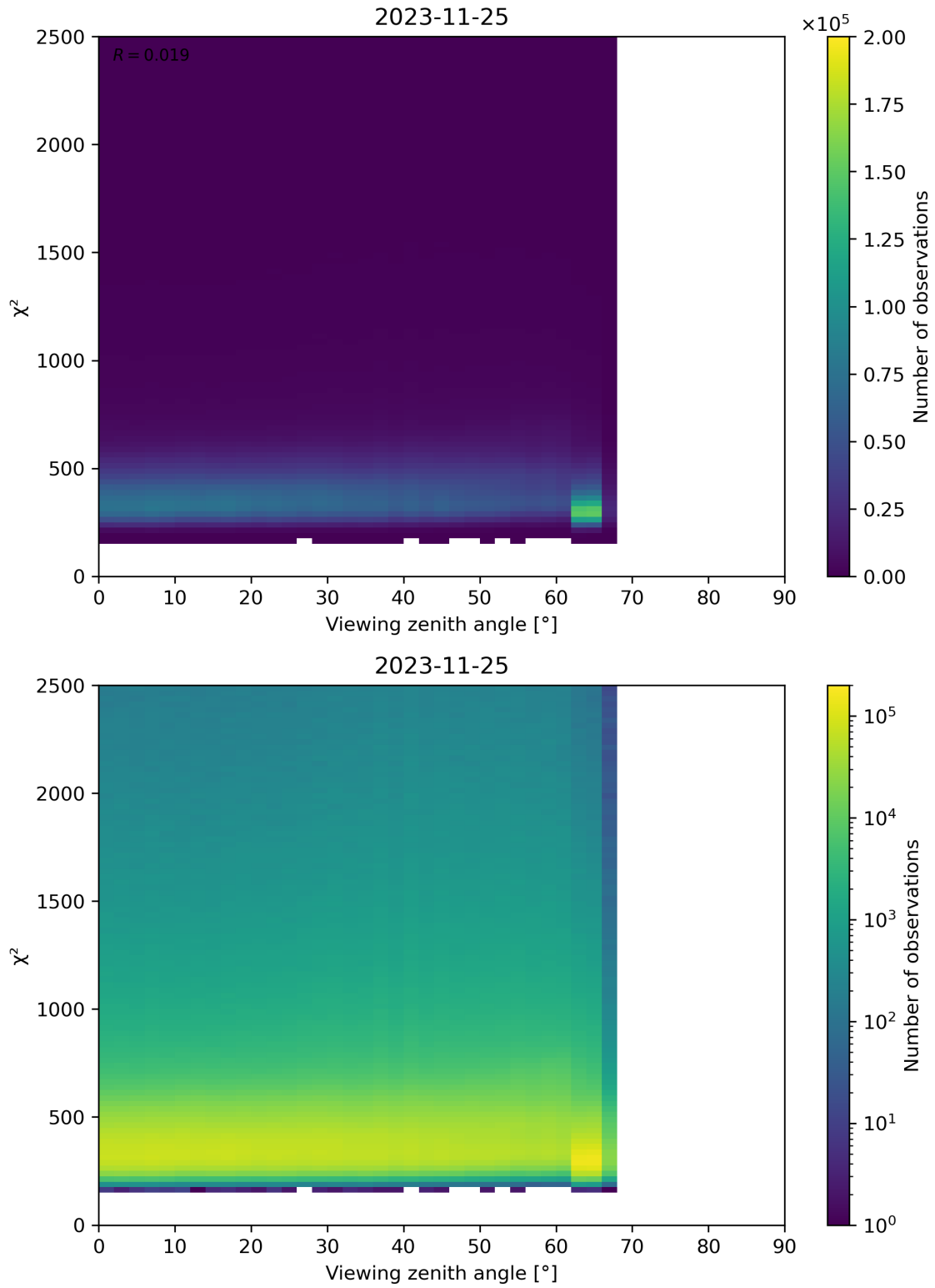
Figure 162: Scatter density plot of “Viewing zenith angle” against “ \chi^2 ” for 2023-11-24 to 2023-11-26.
