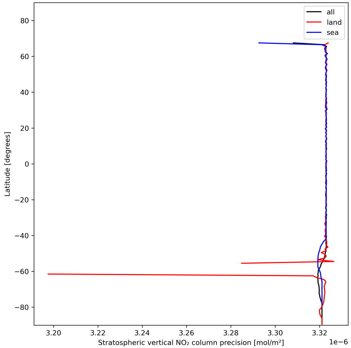
Figure 20: Zonal average of “Stratospheric vertical NO 2 column precision” for 2023-11-24 to 2023-11-26.
