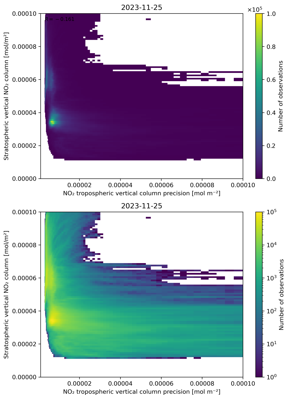
Figure 135: Scatter density plot of “NO 2 tropospheric vertical column precision” against “Stratospheric vertical NO 2 column” for 2023-11-24 to 2023-11-26.
