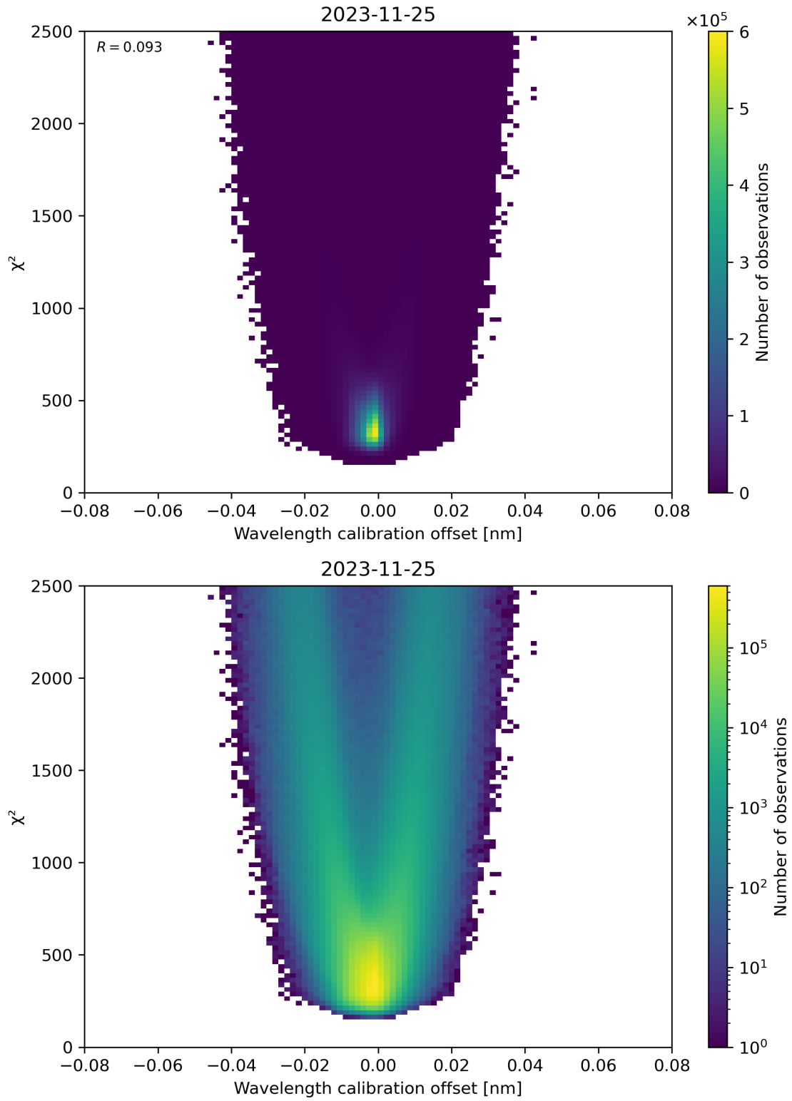
Figure 175: Scatter density plot of “Wavelength calibration offset” against “ \chi^2 ” for 2023-11-24 to 2023-11-26.
