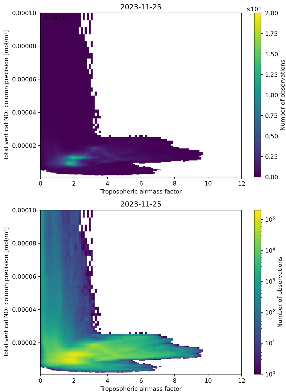
Figure 78: Scatter density plot of “Tropospheric air mass factor” against “Total vertical NO 2 column precision” for 2023-11-24 to 2023-11-26.
