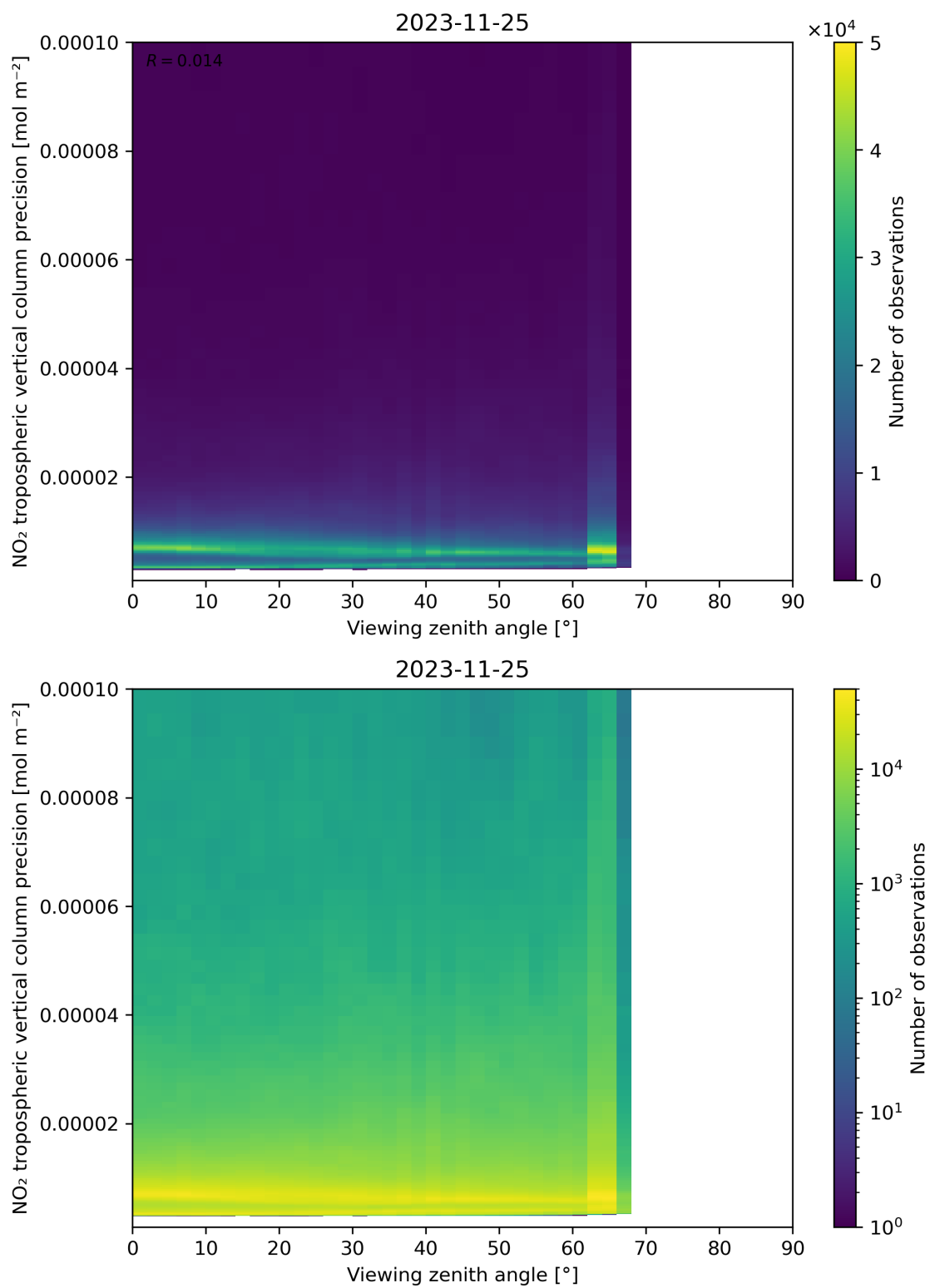
Figure 170: Scatter density plot of “Viewing zenith angle” against “NO 2 tropospheric vertical column precision” for 2023-11-24 to 2023-11-26.
