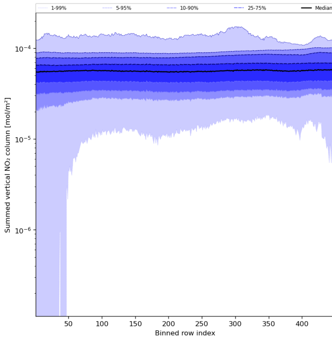
Figure 57: Along track statistics of “Summed vertical NO 2 column” for 2023-11-24 to 2023-11-26
