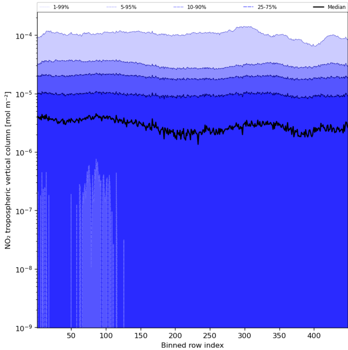
Figure 46: Along track statistics of “NO 2 tropospheric vertical column” for 2023-11-24 to 2023-11-26
