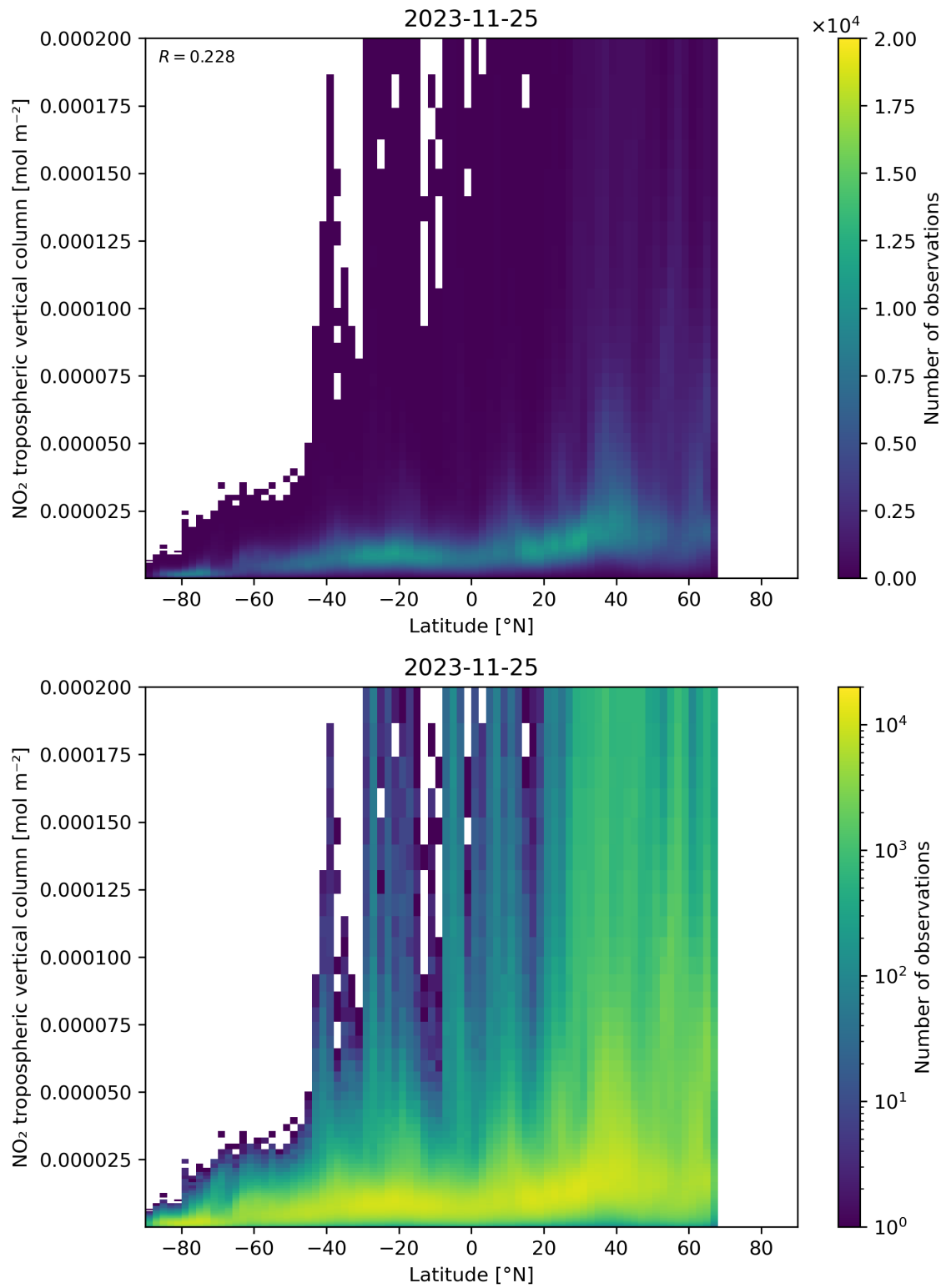
Figure 92: Scatter density plot of “Latitude” against “NO 2 tropospheric vertical column” for 2023-11-24 to 2023-11-26.
