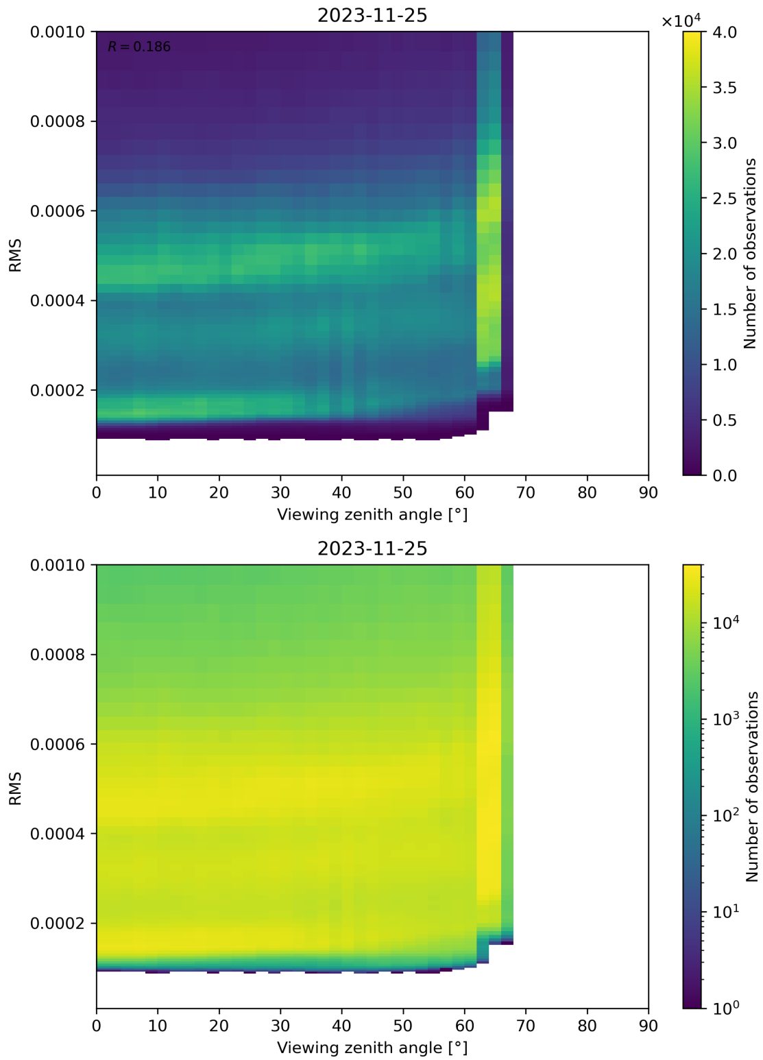
Figure 171: Scatter density plot of “Viewing zenith angle” against “RMS” for 2023-11-24 to 2023-11-26.
