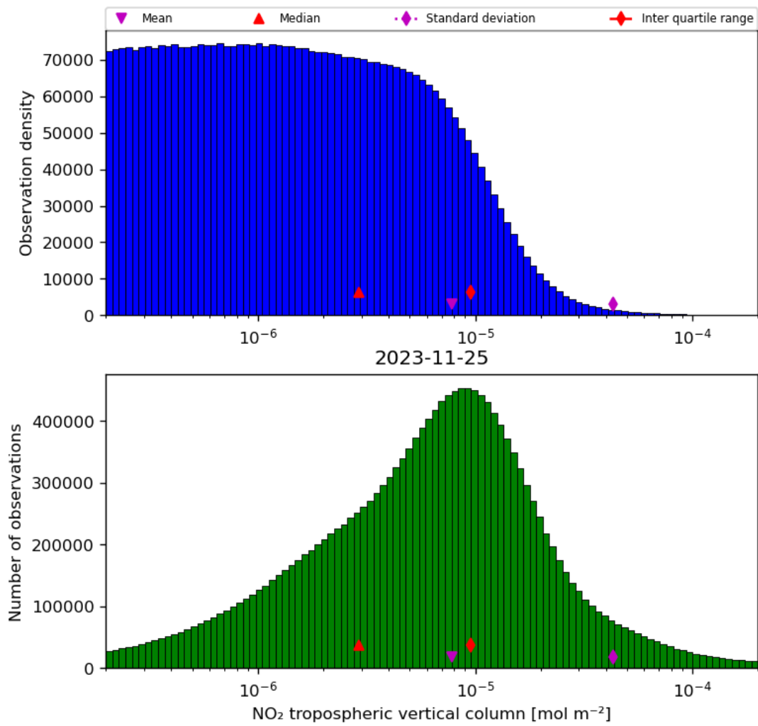
Figure 29: Histogram of “NO 2 tropospheric vertical column” for 2023-11-24 to 2023-11-26
