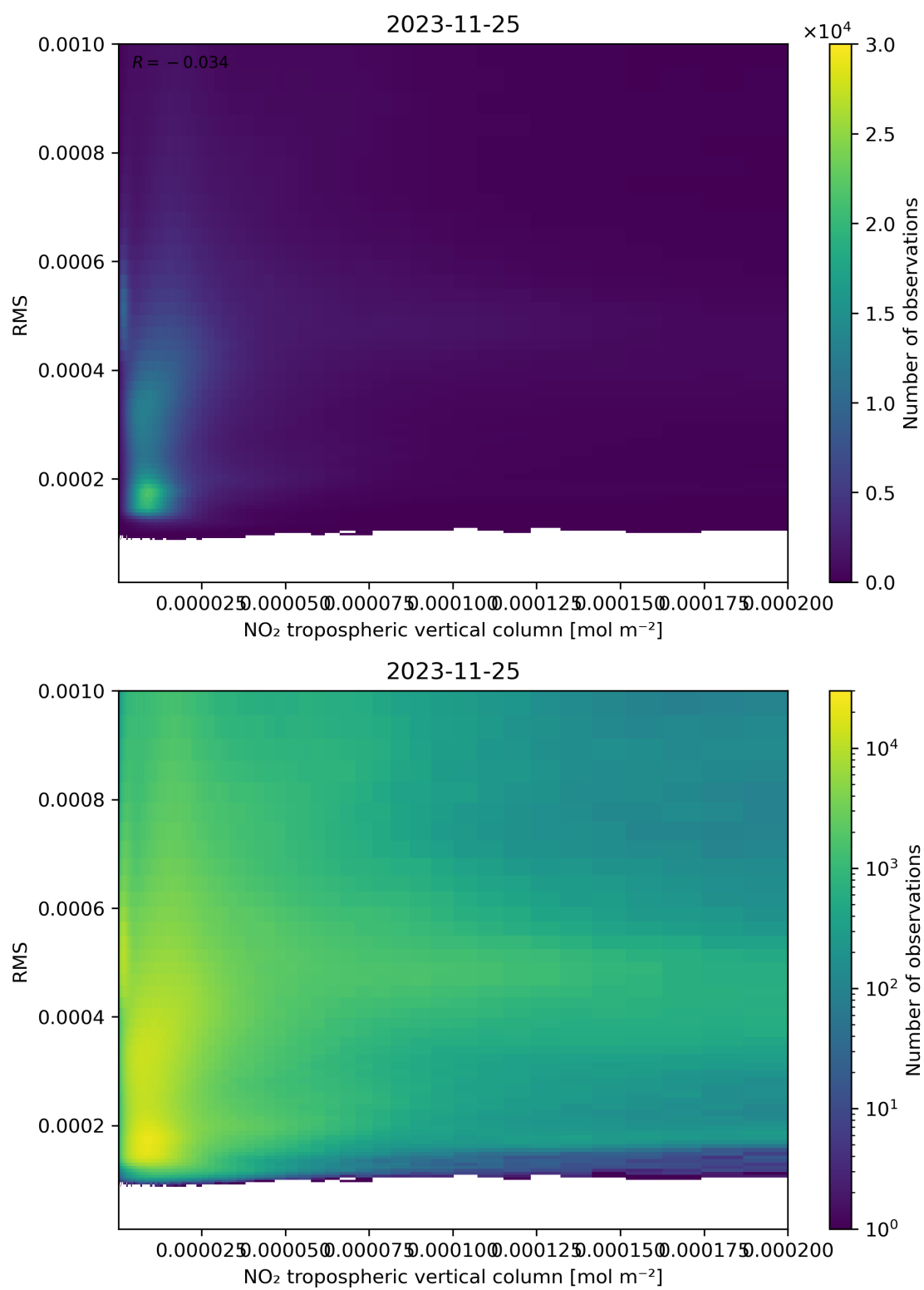
Figure 142: Scatter density plot of “NO 2 tropospheric vertical column” against “RMS” for 2023-11-24 to 2023-11-26.
