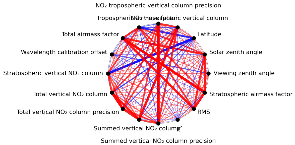
Figure 1: Map of correlation graph for 2023-11-24 to 2023-11-26.
