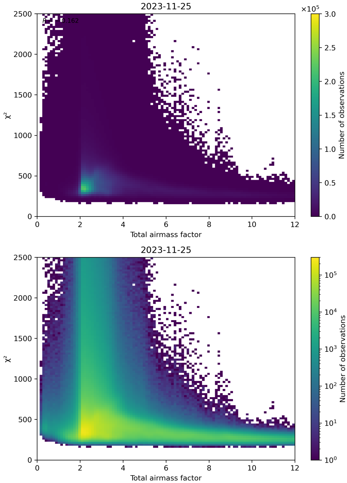
Figure 63: Scatter density plot of “Total airmass factor” against “ \chi^2 ” for 2023-11-24 to 2023-11-26.
