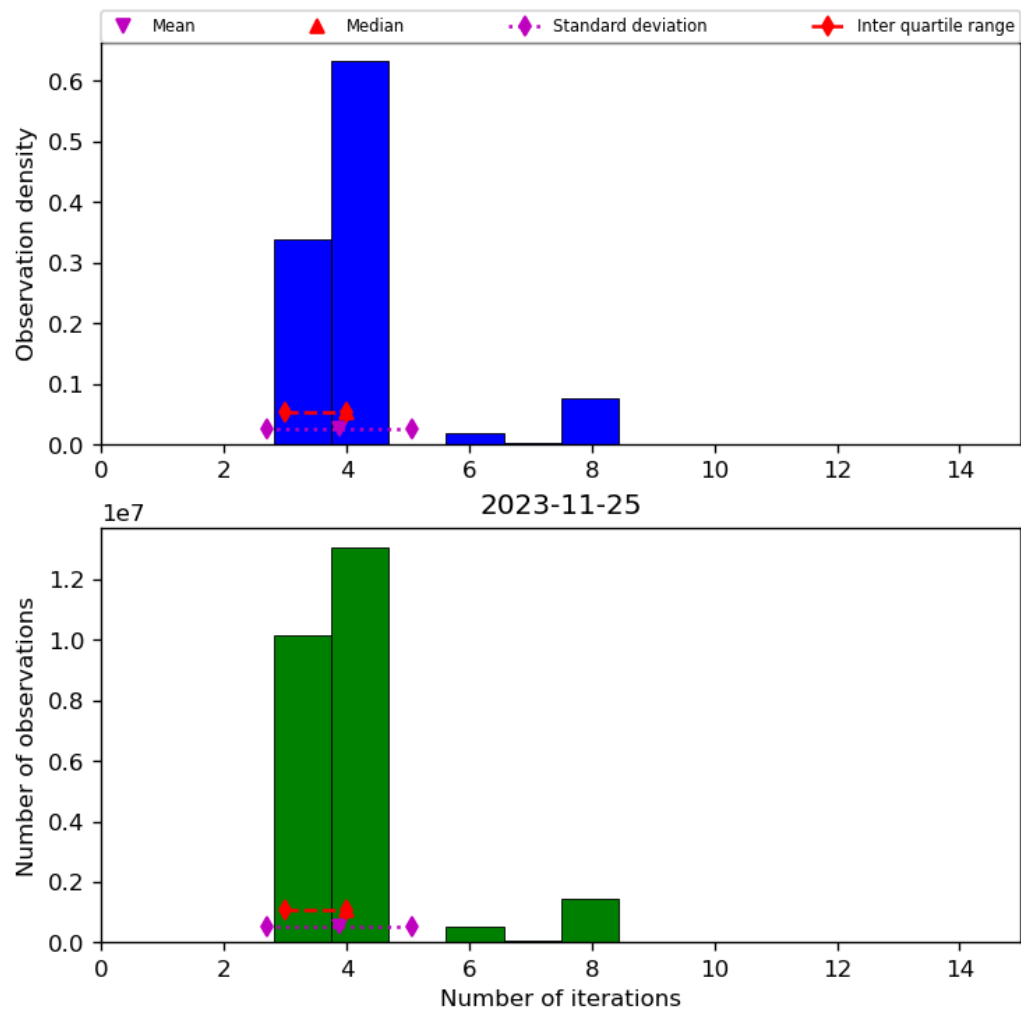
Figure 34: Histogram of “Number of iterations” for 2023-11-24 to 2023-11-26
