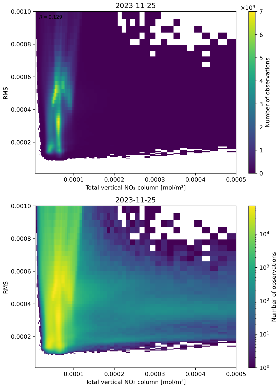
Figure 120: Scatter density plot of “Total vertical NO 2 column” against “RMS” for 2023-11-24 to 2023-11-26.
