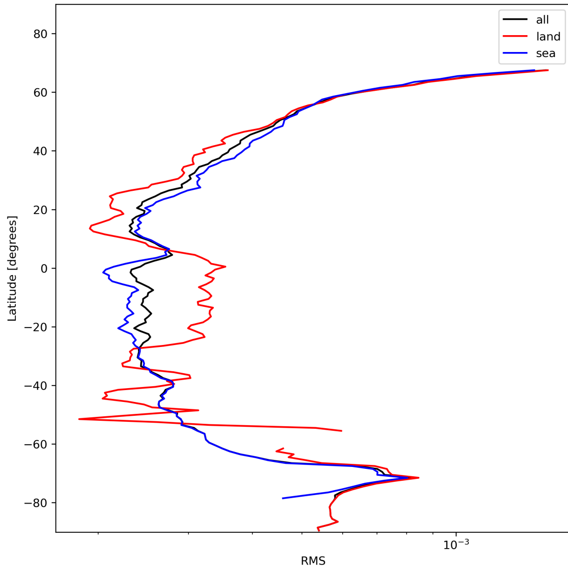
Figure 26: Zonal average of “RMS” for 2023-11-24 to 2023-11-26.
