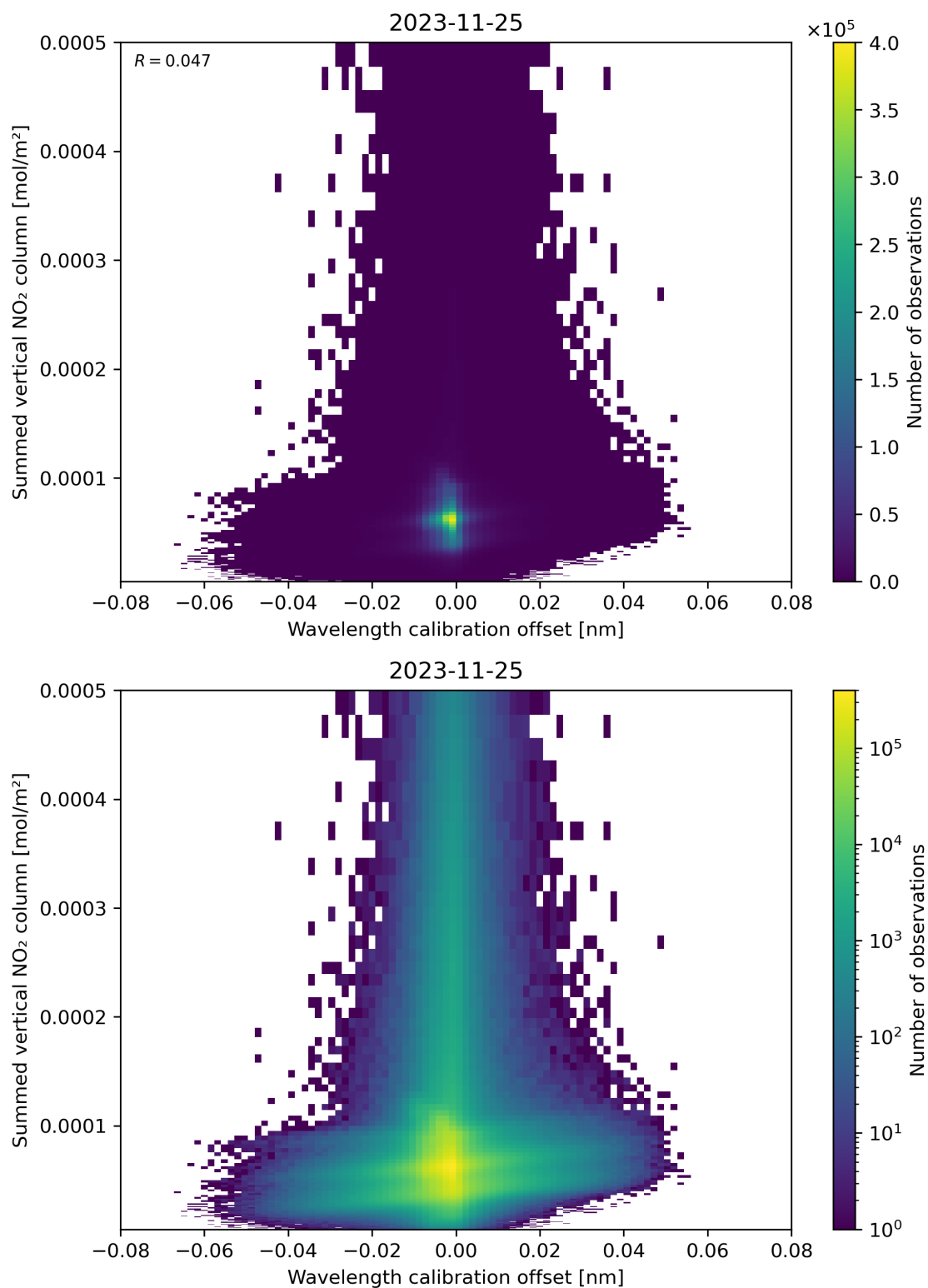
Figure 177: Scatter density plot of “Wavelength calibration offset” against “Summed vertical NO 2 column” for 2023-11-24 to 2023-11-26.
