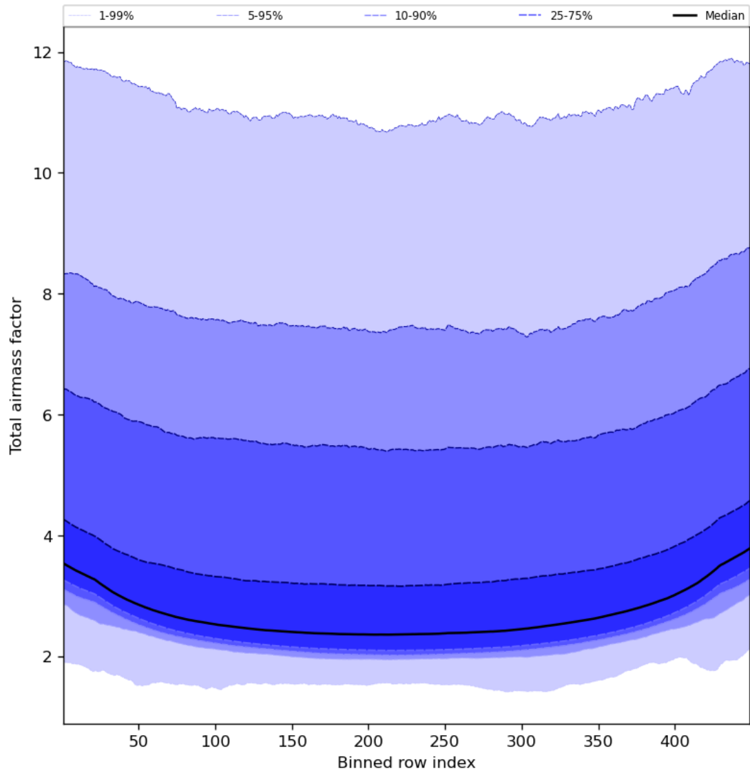
Figure 49: Along track statistics of “Total airmass factor” for 2023-11-24 to 2023-11-26
