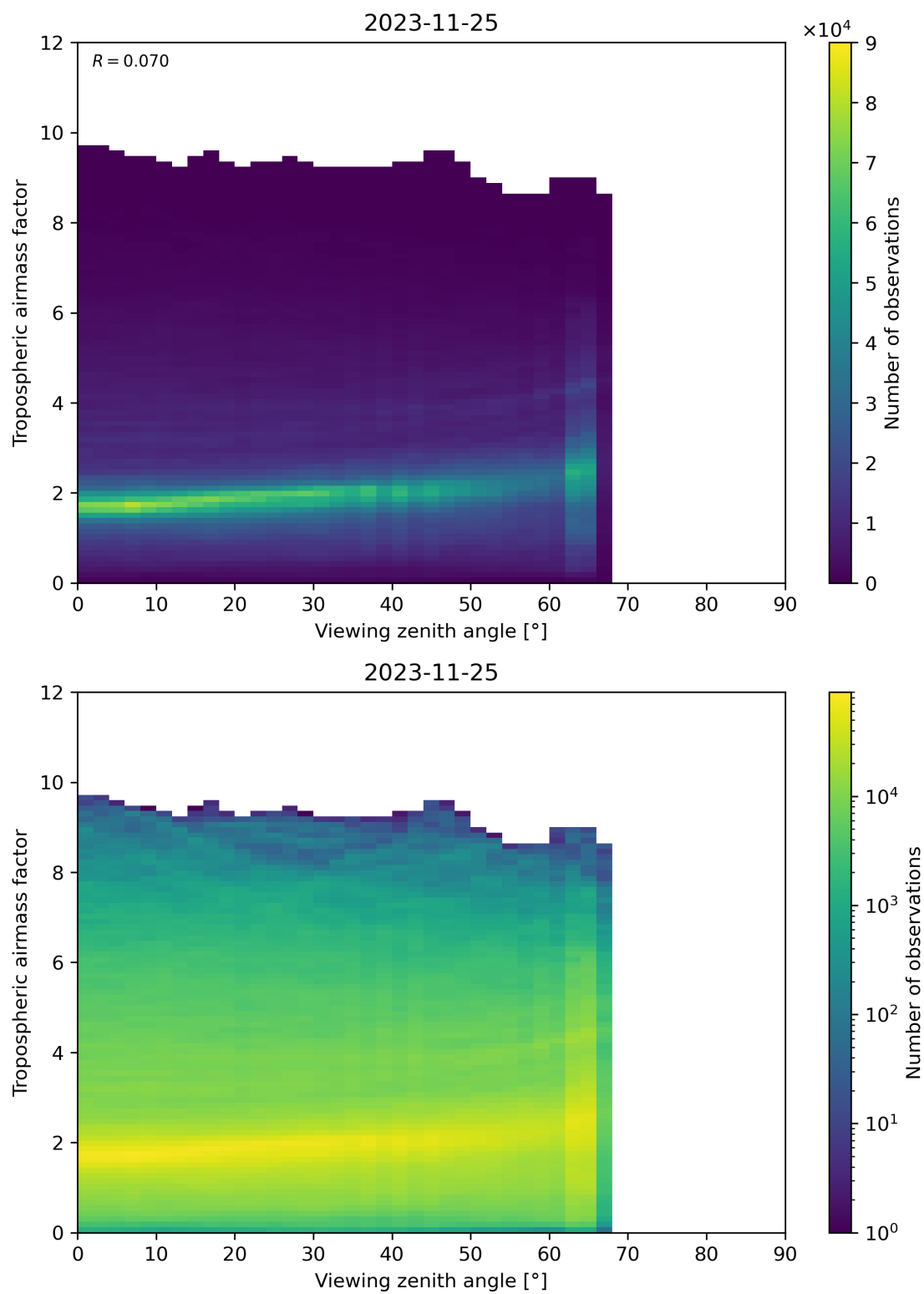
Figure 161: Scatter density plot of “Viewing zenith angle” against “Tropospheric airmass factor” for 2023-11-24 to 2023-11-26.
