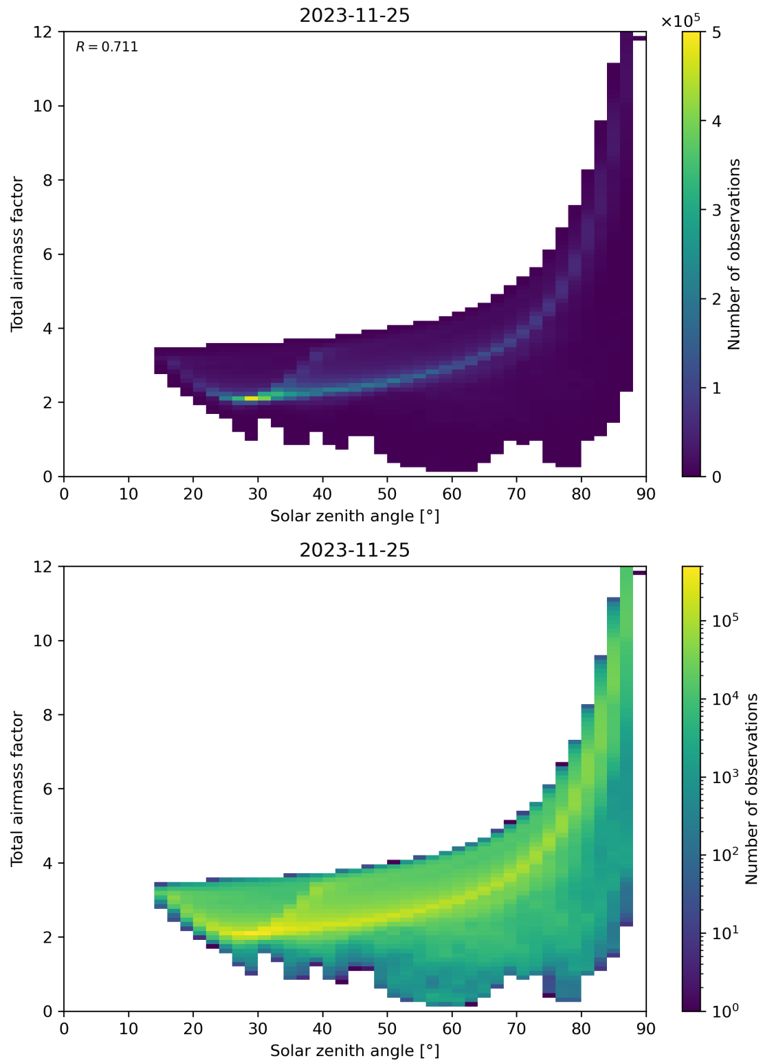
Figure 146: Scatter density plot of “Solar zenith angle” against “Total air mass factor” for 2023-11-24 to 2023-11-26.
