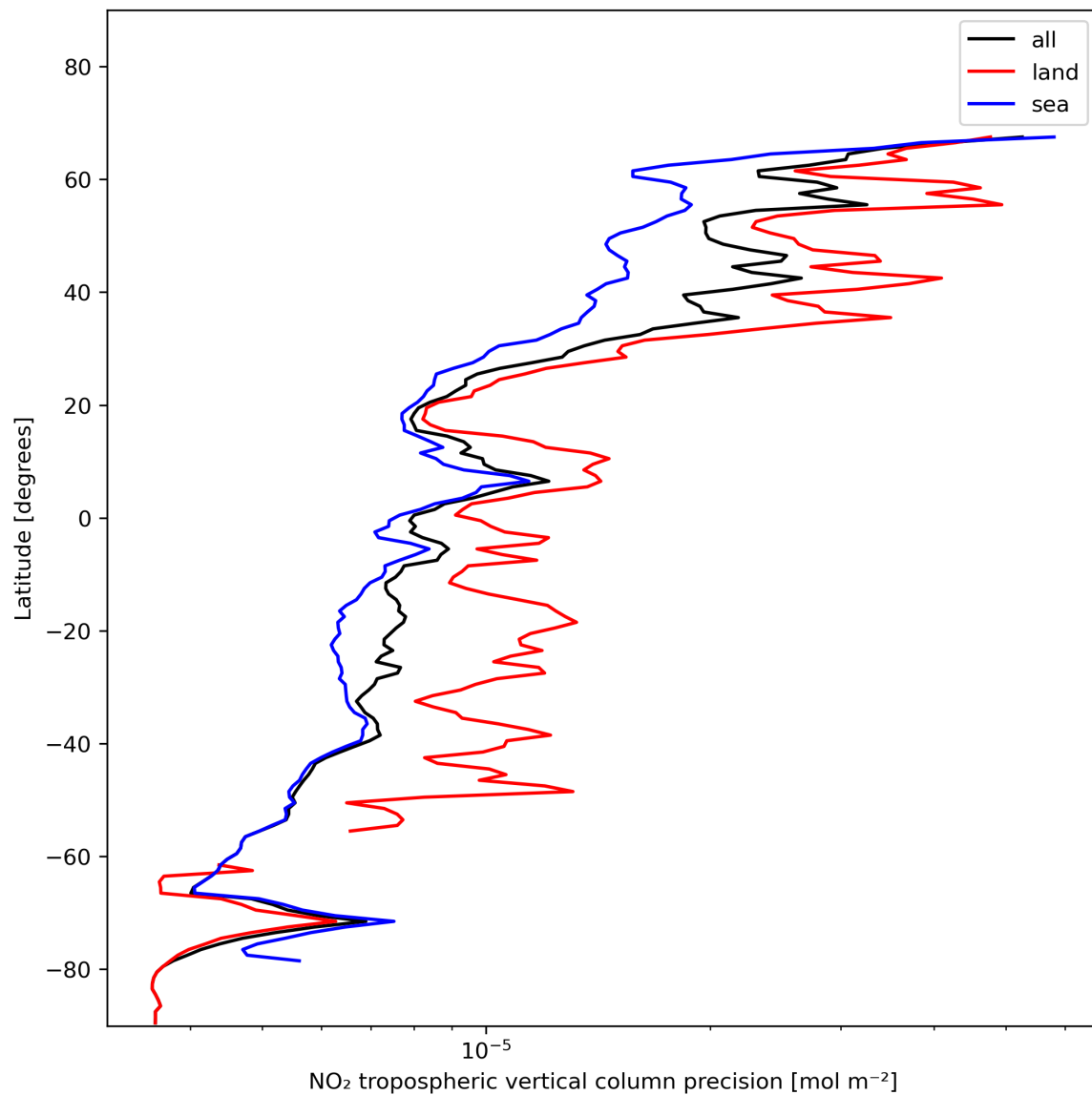
Figure 13: Zonal average of “NO 2 tropospheric vertical column precision” for 2023-11-24 to 2023-11-26.
