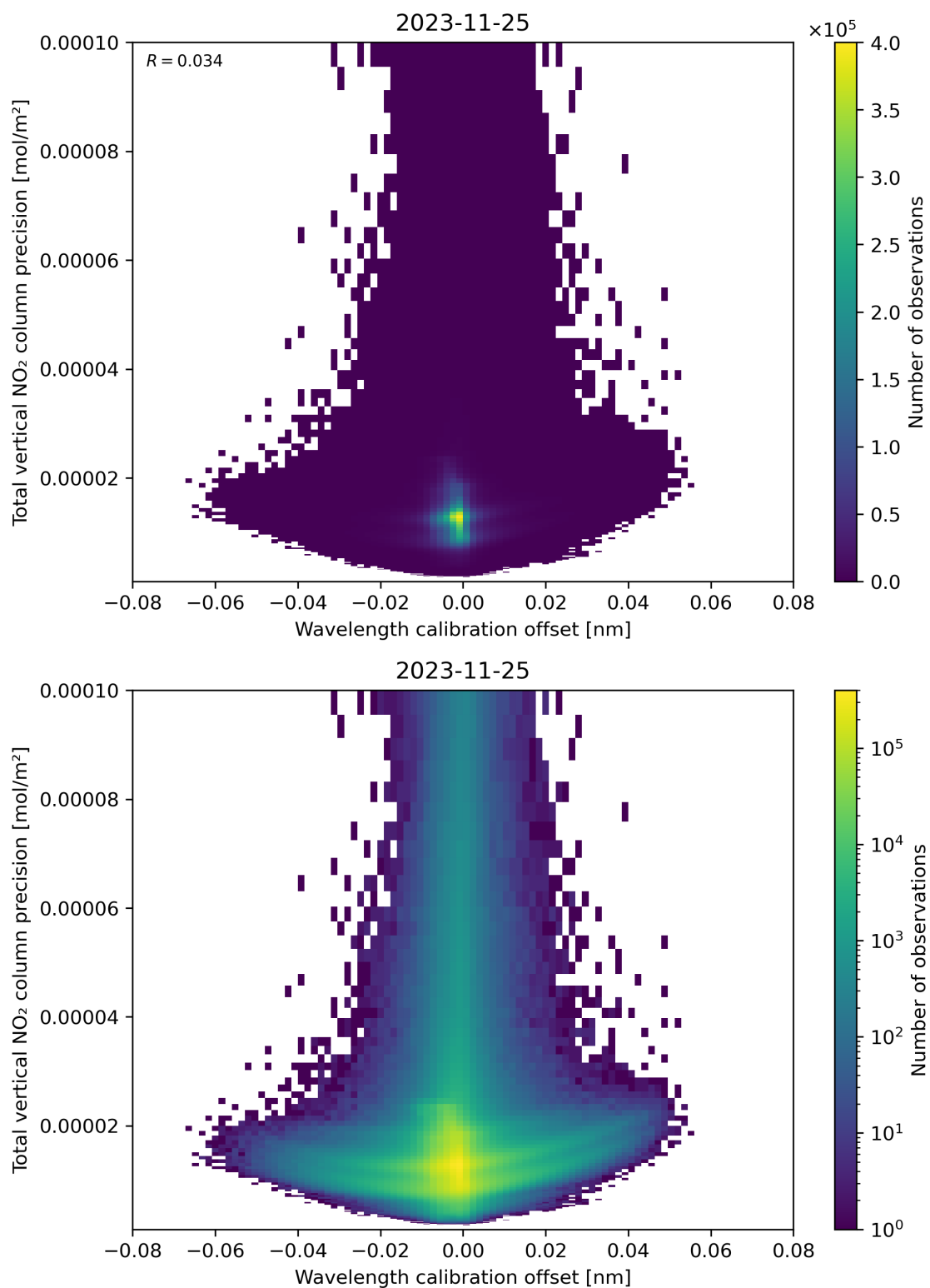
Figure 180: Scatter density plot of “Wavelength calibration offset” against “Total vertical NO 2 column precision” for 2023-11-24 to 2023-11-26.
