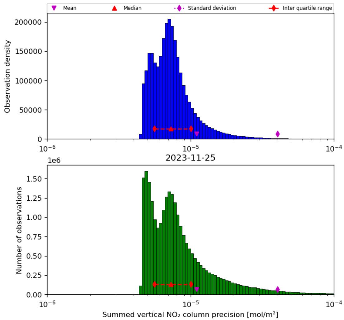
Figure 41: Histogram of "Summed vertical NO 2 column precision" for 2023-11-24 to 2023-11-26
