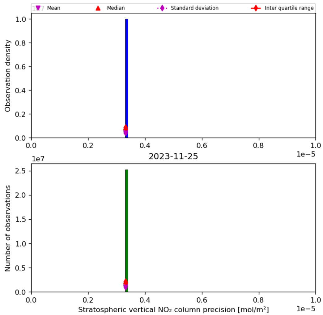
Figure 37: Histogram of “Stratospheric vertical NO 2 column precision” for 2023-11-24 to 2023-11-26
