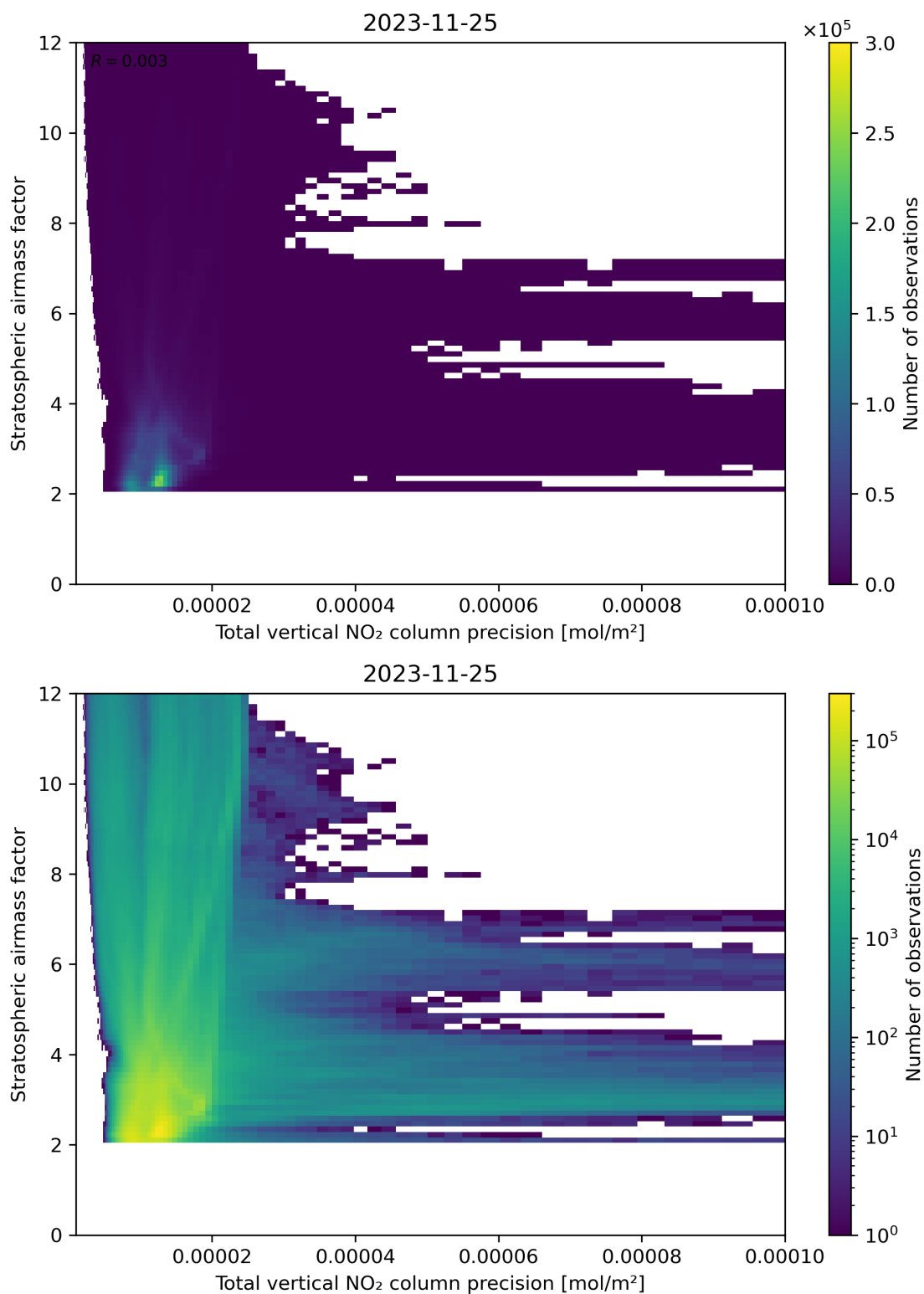
Figure 115: Scatter density plot of “Total vertical NO 2 column precision” against “Stratospheric air mass factor” for 2023-11-24 to 2023-11-26.
