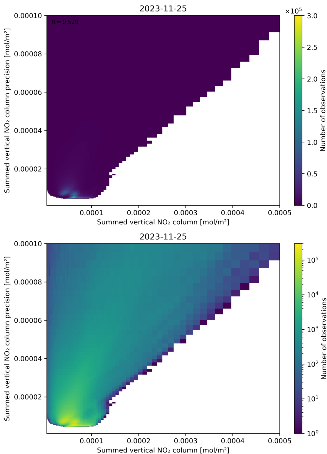
Figure 105: Scatter density plot of “Summed vertical NO 2 column” against “Summed vertical NO 2 column precision” for 2023-11-24 to 2023-11-26.
