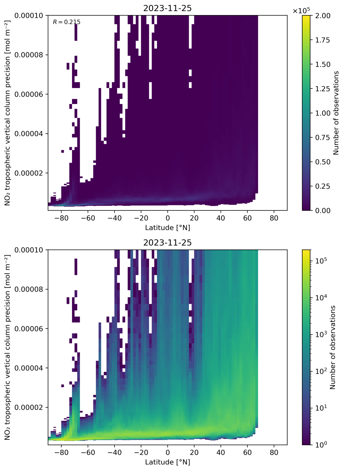
Figure 93: Scatter density plot of “Latitude” against “NO 2 tropospheric vertical column precision” for 2023-11-24 to 2023-11-26.
