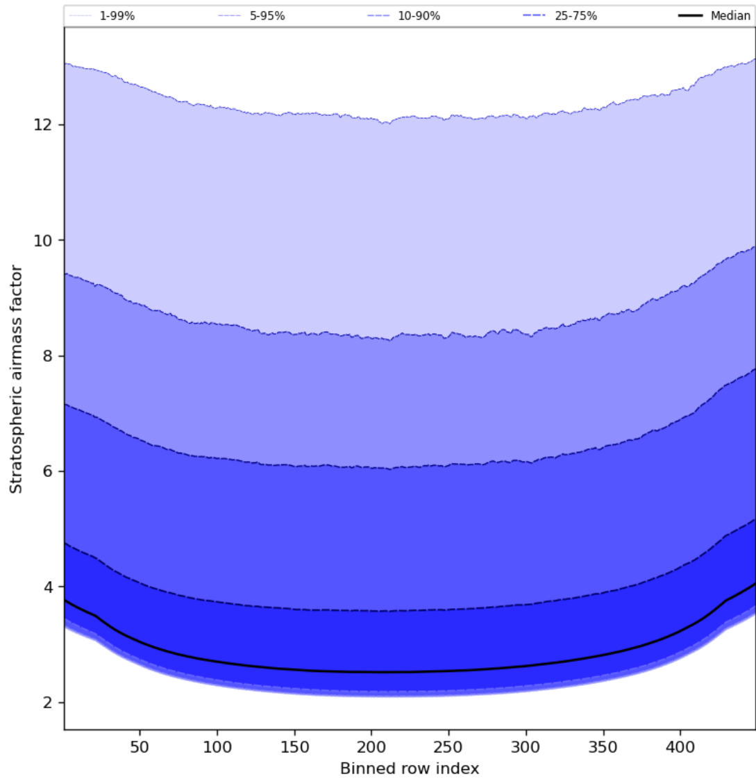
Figure 61: Along track statistics of “Stratospheric airmass factor” for 2023-11-24 to 2023-11-26
