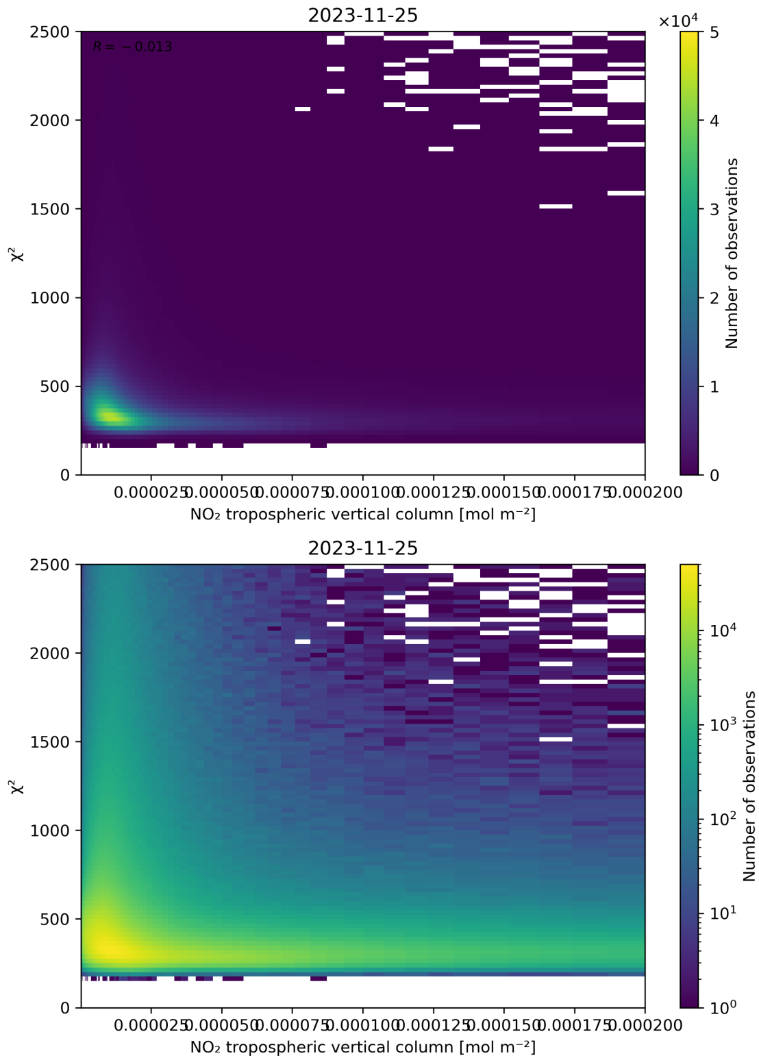
Figure 124: Scatter density plot of “NO 2 tropospheric vertical column” against “ \chi^2 ” for 2023-11-24 to 2023-11-26.
