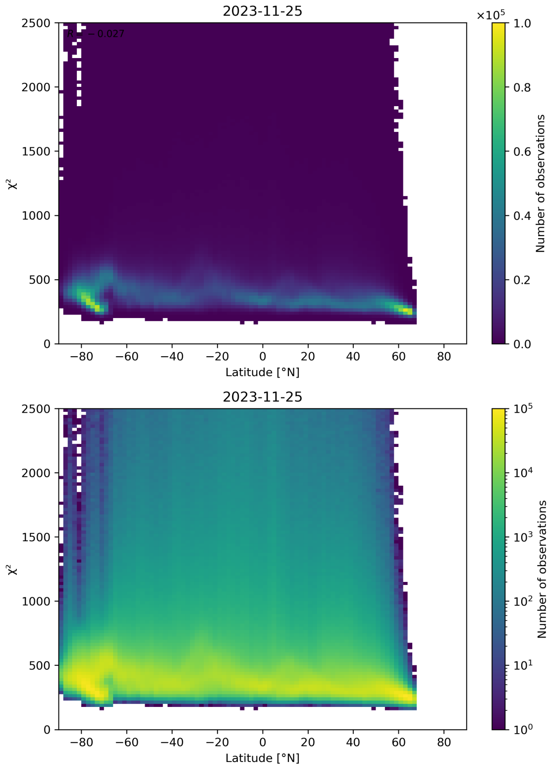
Figure 86: Scatter density plot of “Latitude” against “ \chi^2 ” for 2023-11-24 to 2023-11-26.
