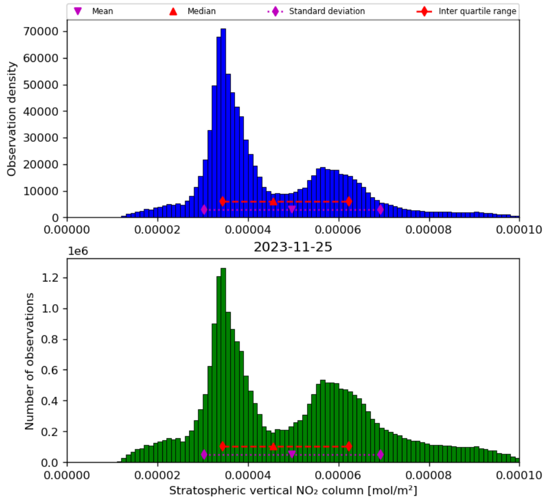
Figure 36: Histogram of “Stratospheric vertical NO 2 column” for 2023-11-24 to 2023-11-26
