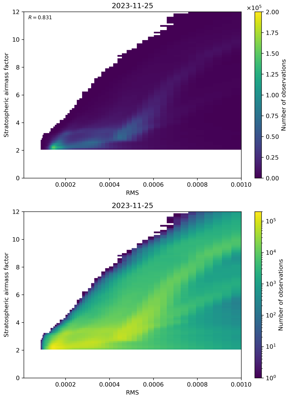
Figure 144: Scatter density plot of “RMS” against “Stratospheric airmass factor” for 2023-11-24 to 2023-11-26.
