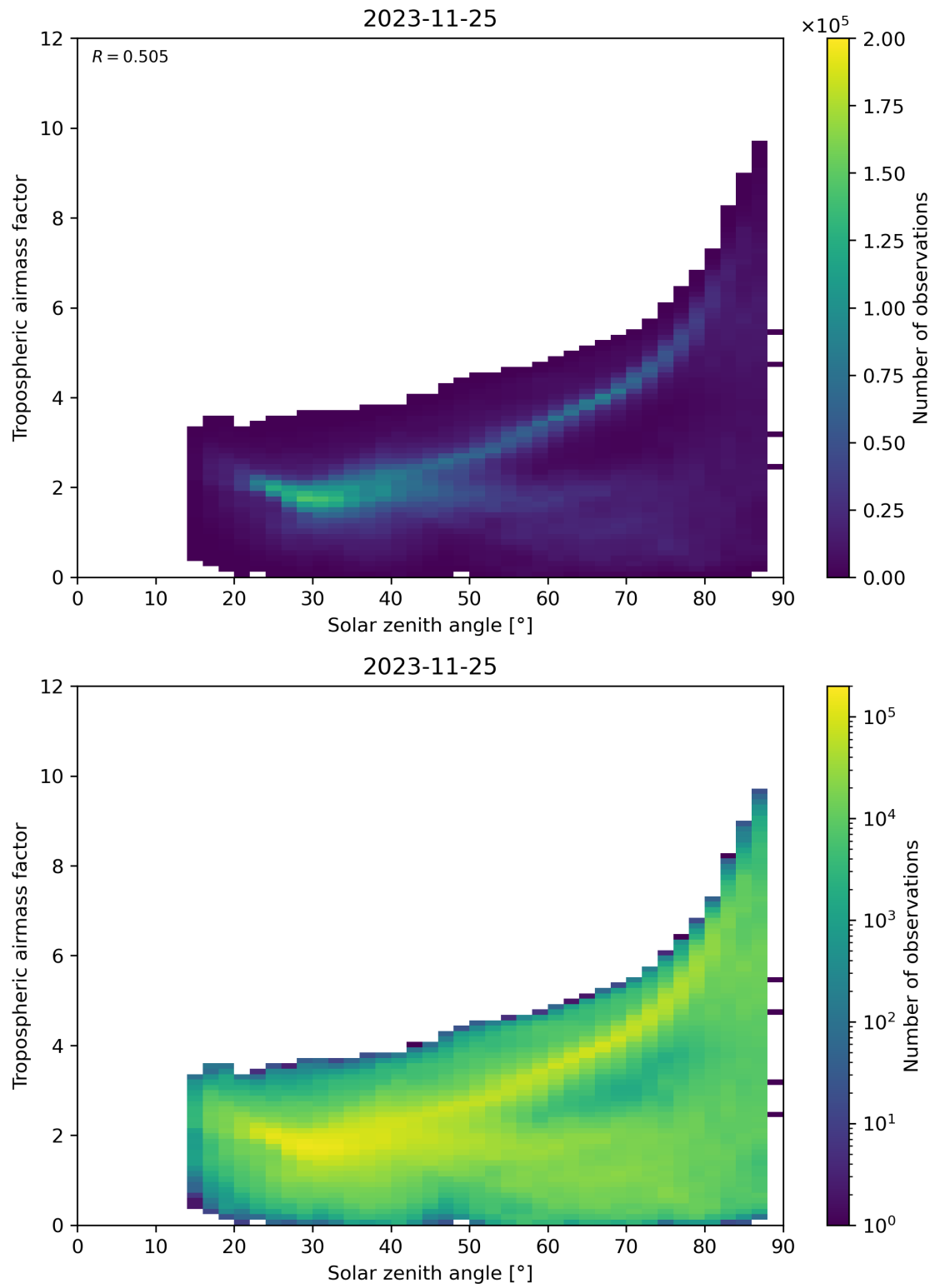
Figure 147: Scatter density plot of “Solar zenith angle” against “Tropospheric airmass factor” for 2023-11-24 to 2023-11-26.
