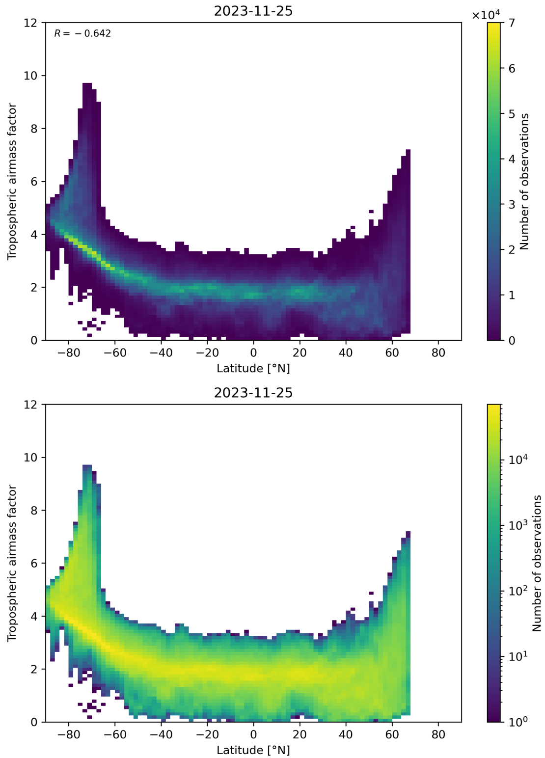
Figure 85: Scatter density plot of “Latitude” against “Tropospheric airmass factor” for 2023-11-24 to 2023-11-26.
