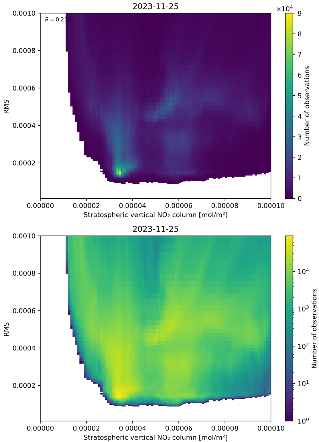
Figure 102: Scatter density plot of “Stratospheric vertical NO 2 column” against “RMS” for 2023-11-24 to 2023-11-26.
