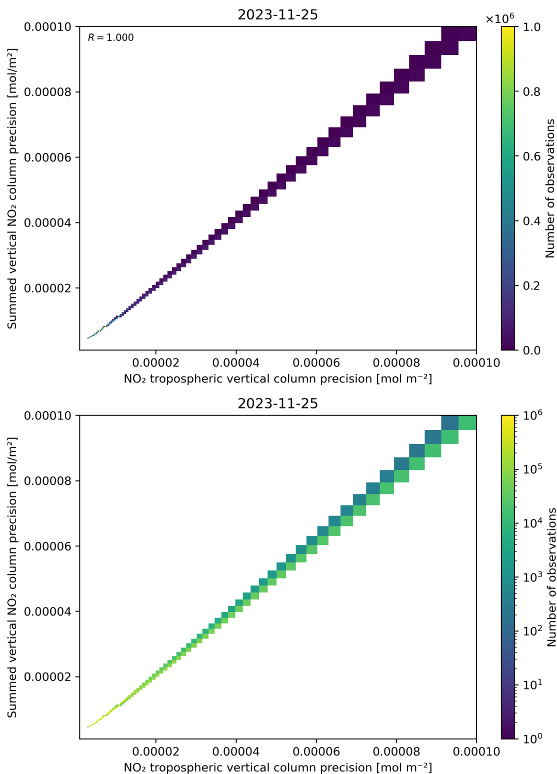
Figure 137: Scatter density plot of “NO 2 tropospheric vertical column precision” against “Summed vertical NO 2 column precision” for 2023-11-24 to 2023-11-26.
