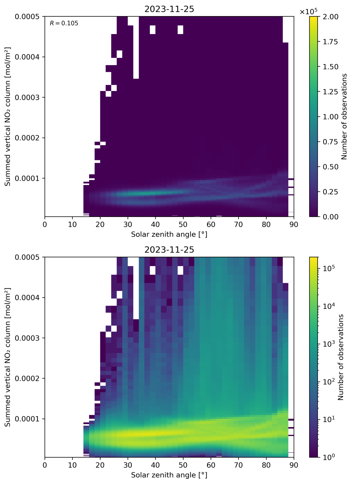
Figure 151: Scatter density plot of “Solar zenith angle” against “Summed vertical NO 2 column” for 2023-11-24 to 2023-11-26.
