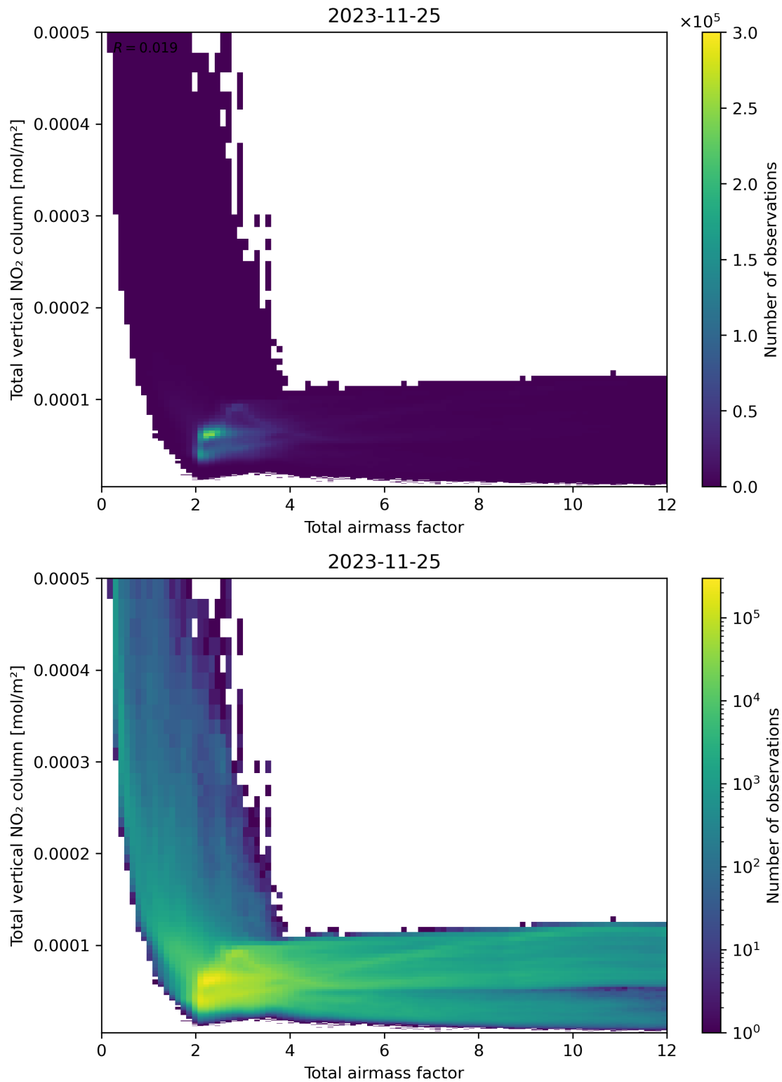
Figure 67: Scatter density plot of “Total airmass factor” against “Total vertical NO 2 column” for 2023-11-24 to 2023-11-26.
