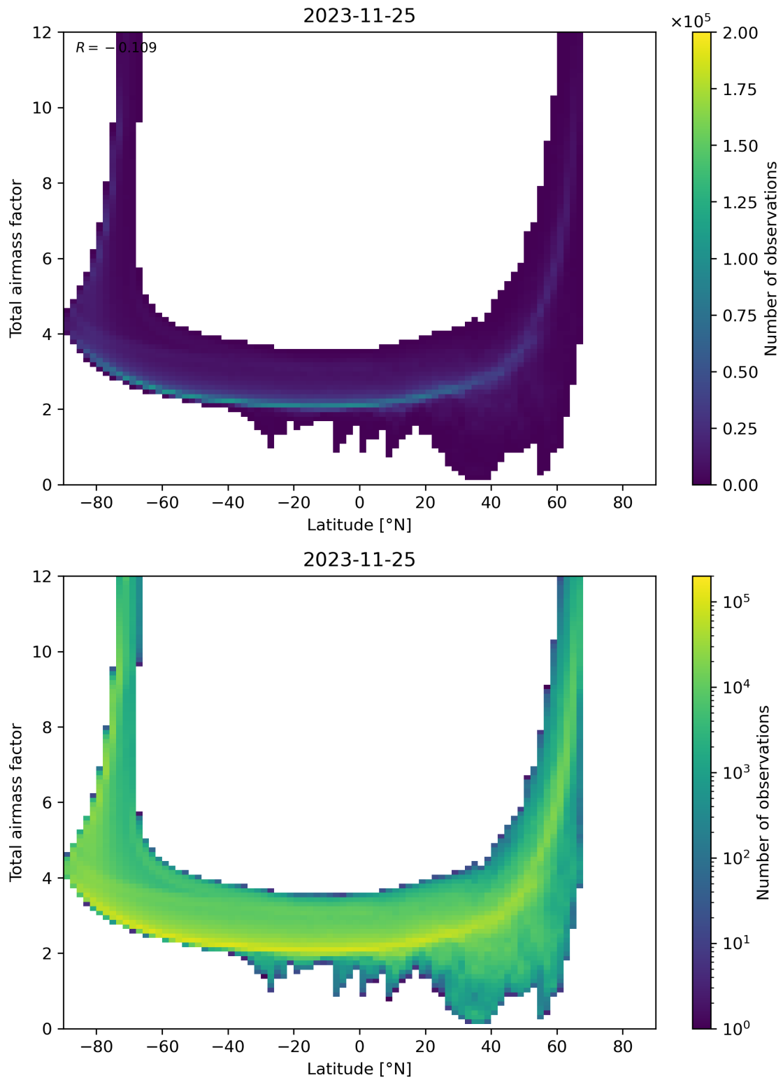
Figure 84: Scatter density plot of “Latitude” against “Total airmass factor” for 2023-11-24 to 2023-11-26.
