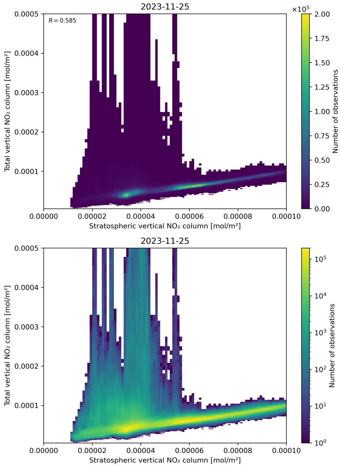
Figure 100: Scatter density plot of “Stratospheric vertical NO 2 column” against “Total vertical NO 2 column” for 2023-11-24 to 2023-11-26.
