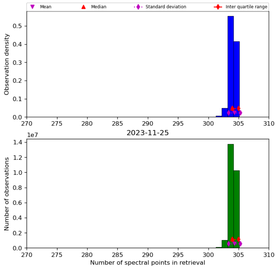
Figure 33: Histogram of “Number of spectral points in retrieval” for 2023-11-24 to 2023-11-26
