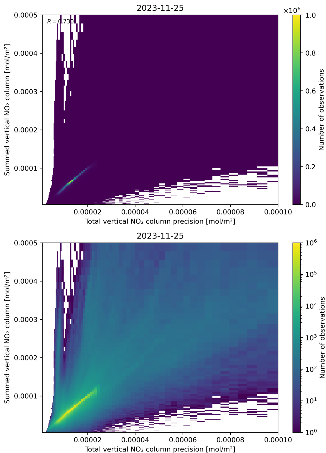
Figure 117: Scatter density plot of “Total vertical NO 2 column precision” against “Summed vertical NO 2 column” for 2023-11-24 to 2023-11-26.
