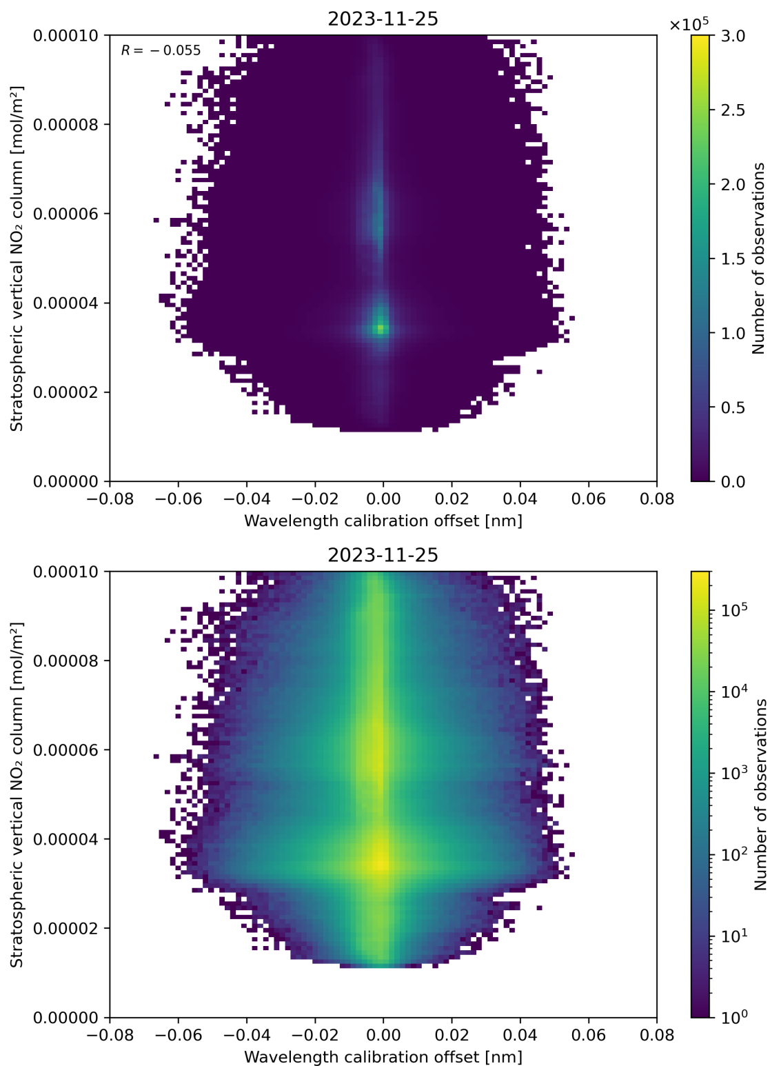
Figure 176: Scatter density plot of “Wavelength calibration offset” against “Stratospheric vertical NO 2 column” for 2023-11-24 to 2023-11-26.
