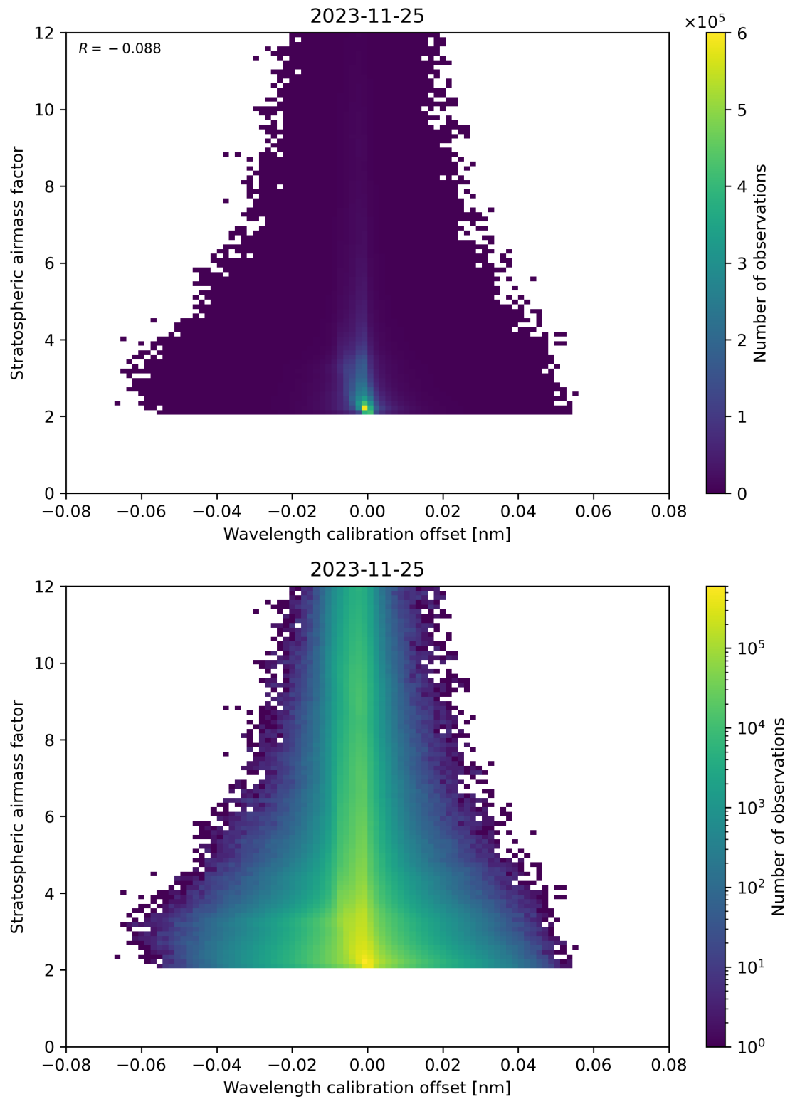
Figure 174: Scatter density plot of “Wavelength calibration offset” against “Stratospheric airmass factor” for 2023-11-24 to 2023-11-26.
