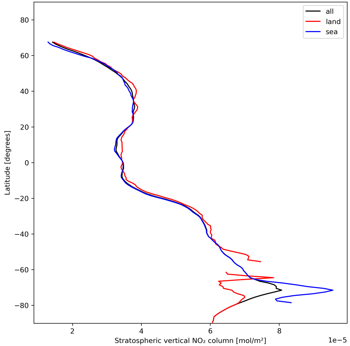
Figure 19: Zonal average of “Stratospheric vertical NO 2 column” for 2023-11-24 to 2023-11-26.
