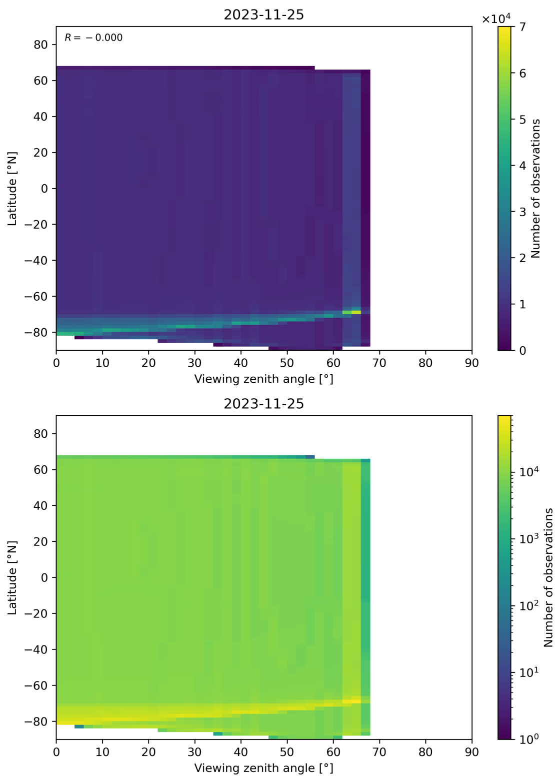
Figure 163: Scatter density plot of “Viewing zenith angle” against “Latitude” for 2023-11-24 to 2023-11-26.
