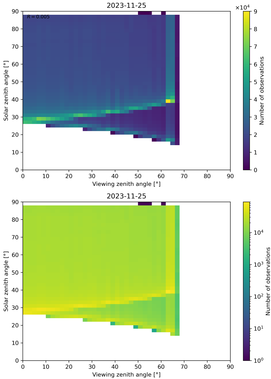
Figure 172: Scatter density plot of “Viewing zenith angle” against “Solar zenith angle” for 2023-11-24 to 2023-11-26.
