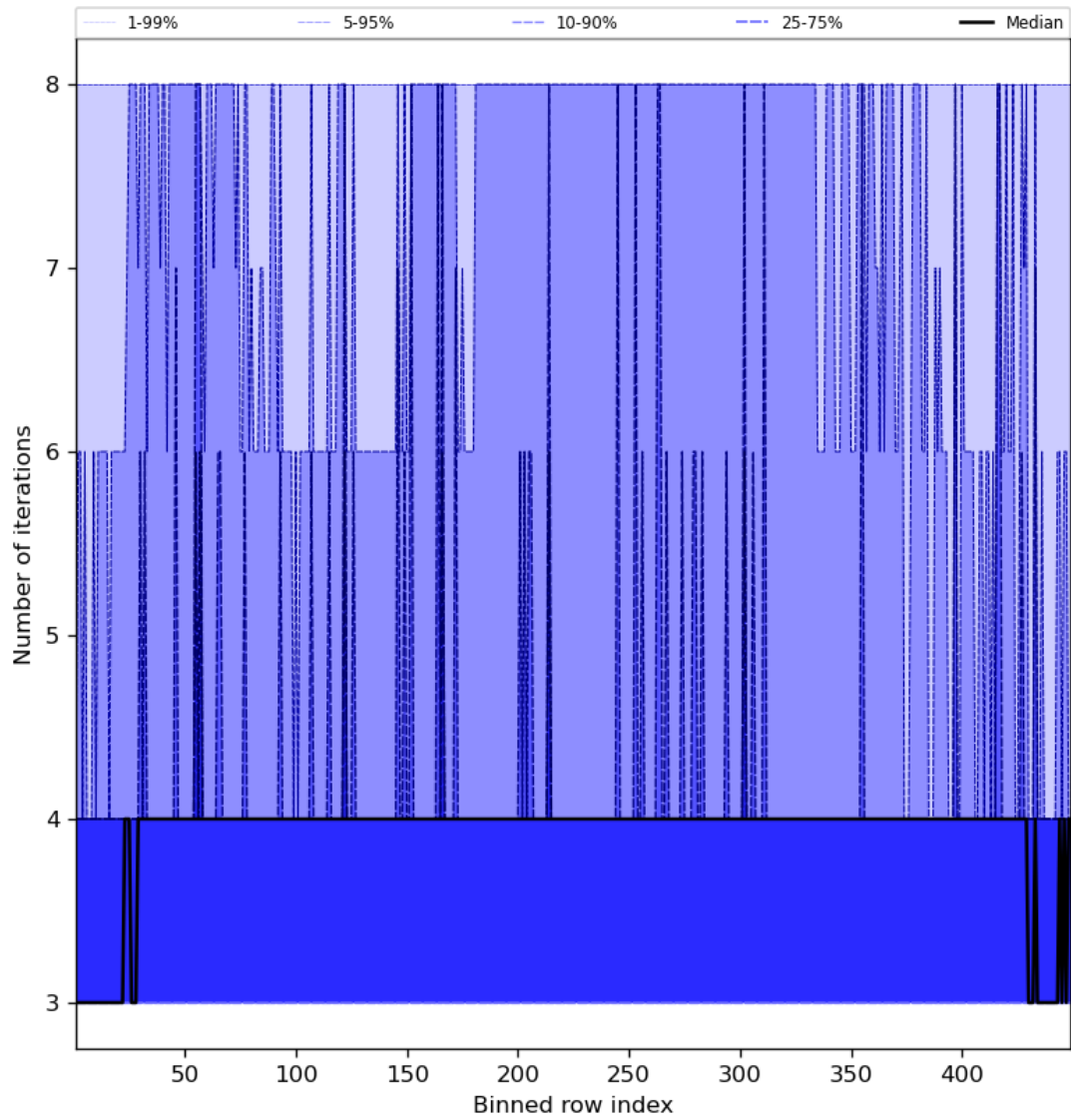
Figure 51: Along track statistics of “Number of iterations” for 2023-11-24 to 2023-11-26
