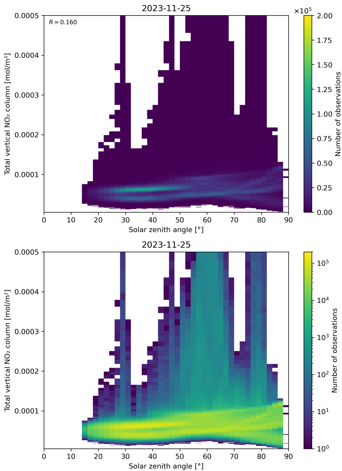
Figure 153: Scatter density plot of “Solar zenith angle” against “Total vertical NO 2 column” for 2023-11-24 to 2023-11-26.
