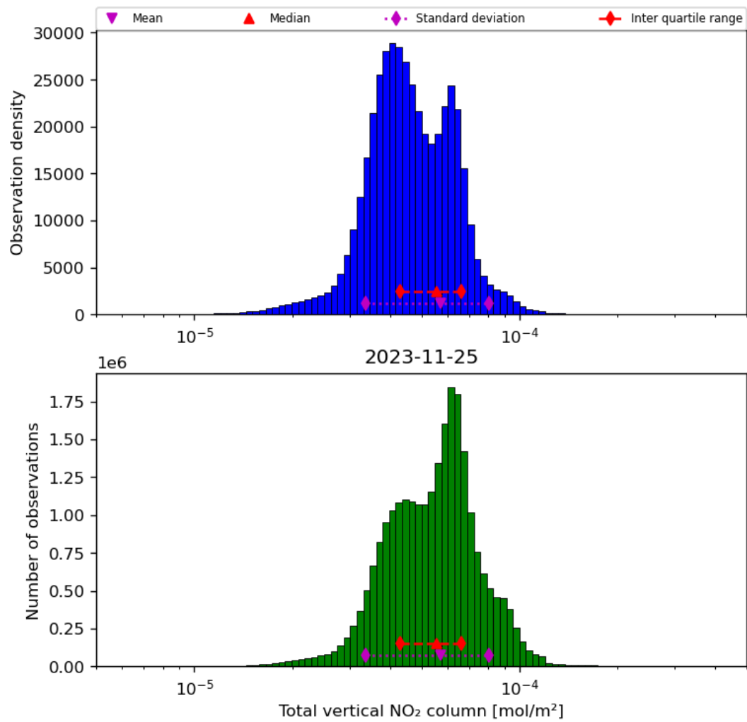
Figure 38: Histogram of “Total vertical NO 2 column” for 2023-11-24 to 2023-11-26
