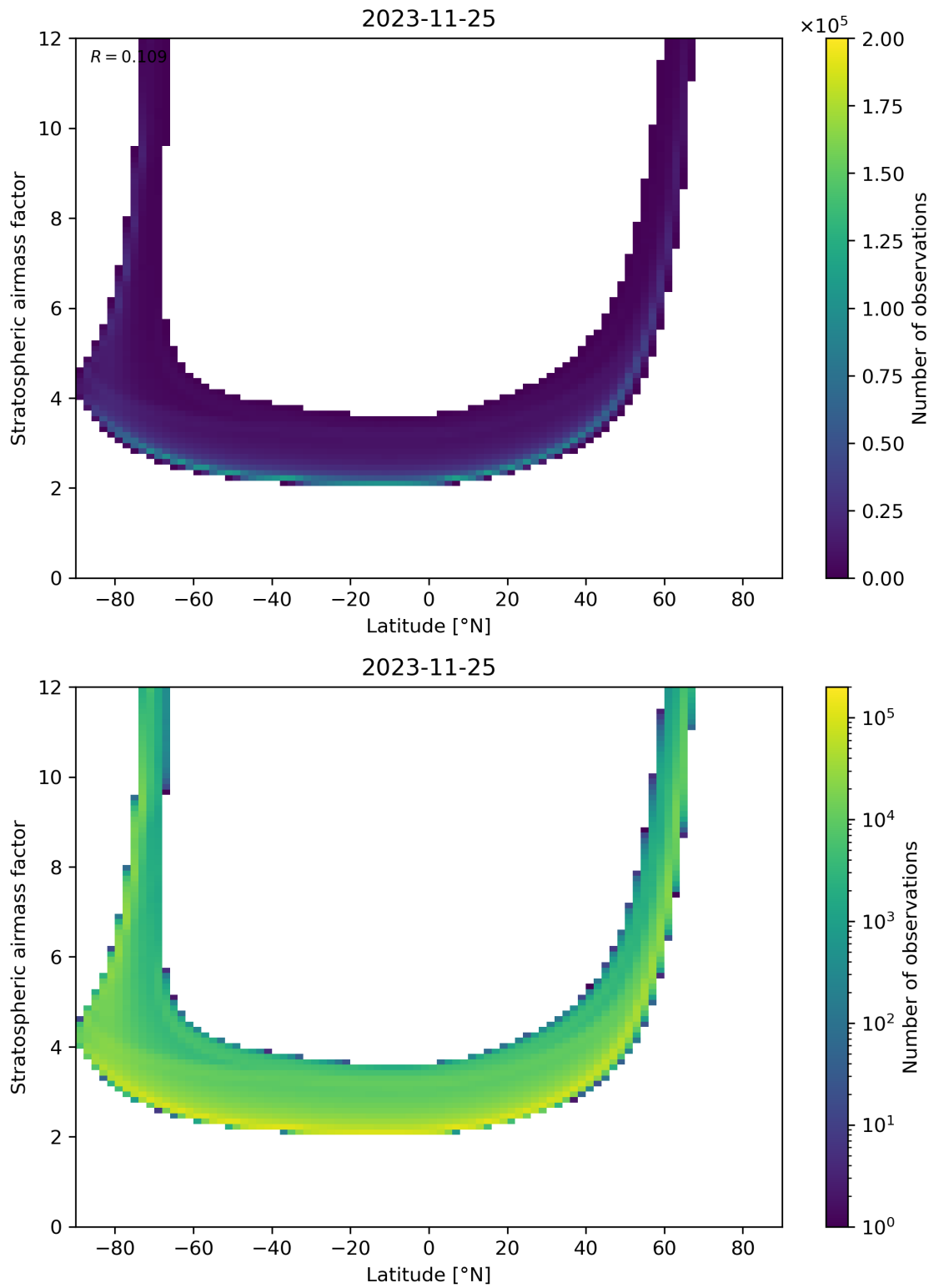
Figure 83: Scatter density plot of “Latitude” against “Stratospheric air mass factor” for 2023-11-24 to 2023-11-26.
