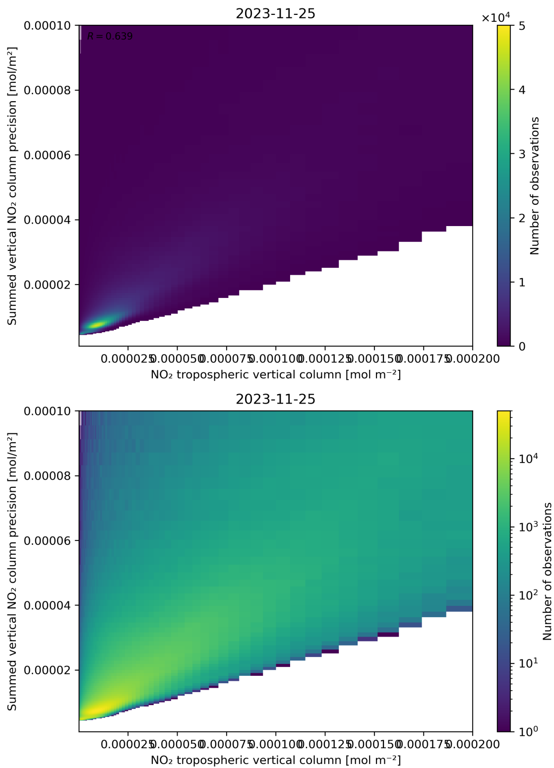
Figure 127: Scatter density plot of “NO 2 tropospheric vertical column” against “Summed vertical NO 2 column precision” for 2023-11-24 to 2023-11-26.
