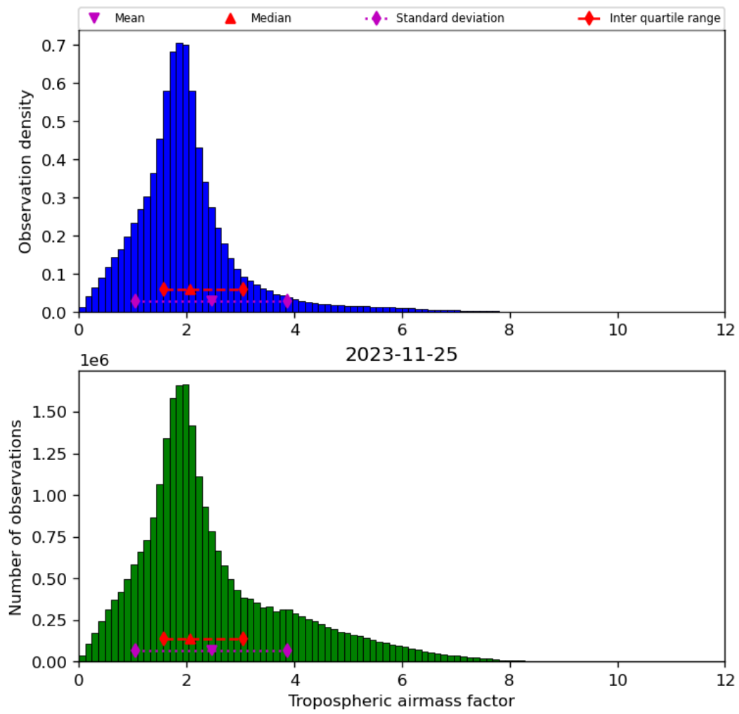
Figure 31: Histogram of “Tropospheric airmass factor” for 2023-11-24 to 2023-11-26
