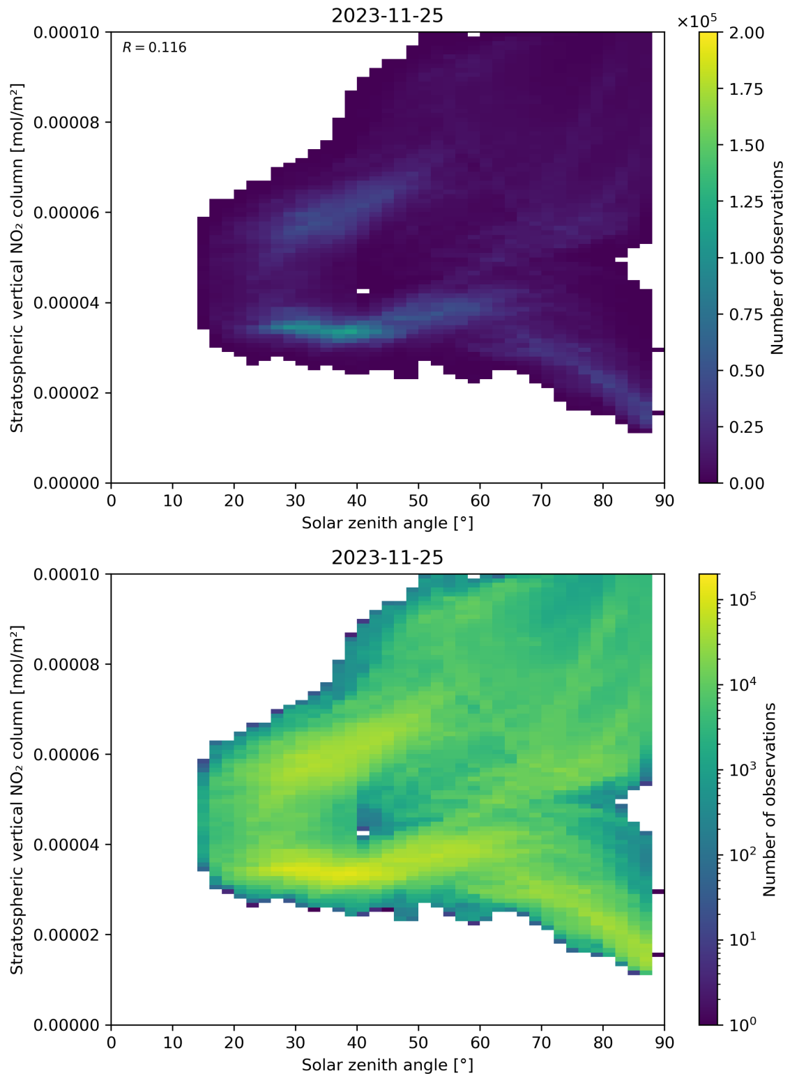
Figure 150: Scatter density plot of “Solar zenith angle” against “Stratospheric vertical NO 2 column” for 2023-11-24 to 2023-11-26.
