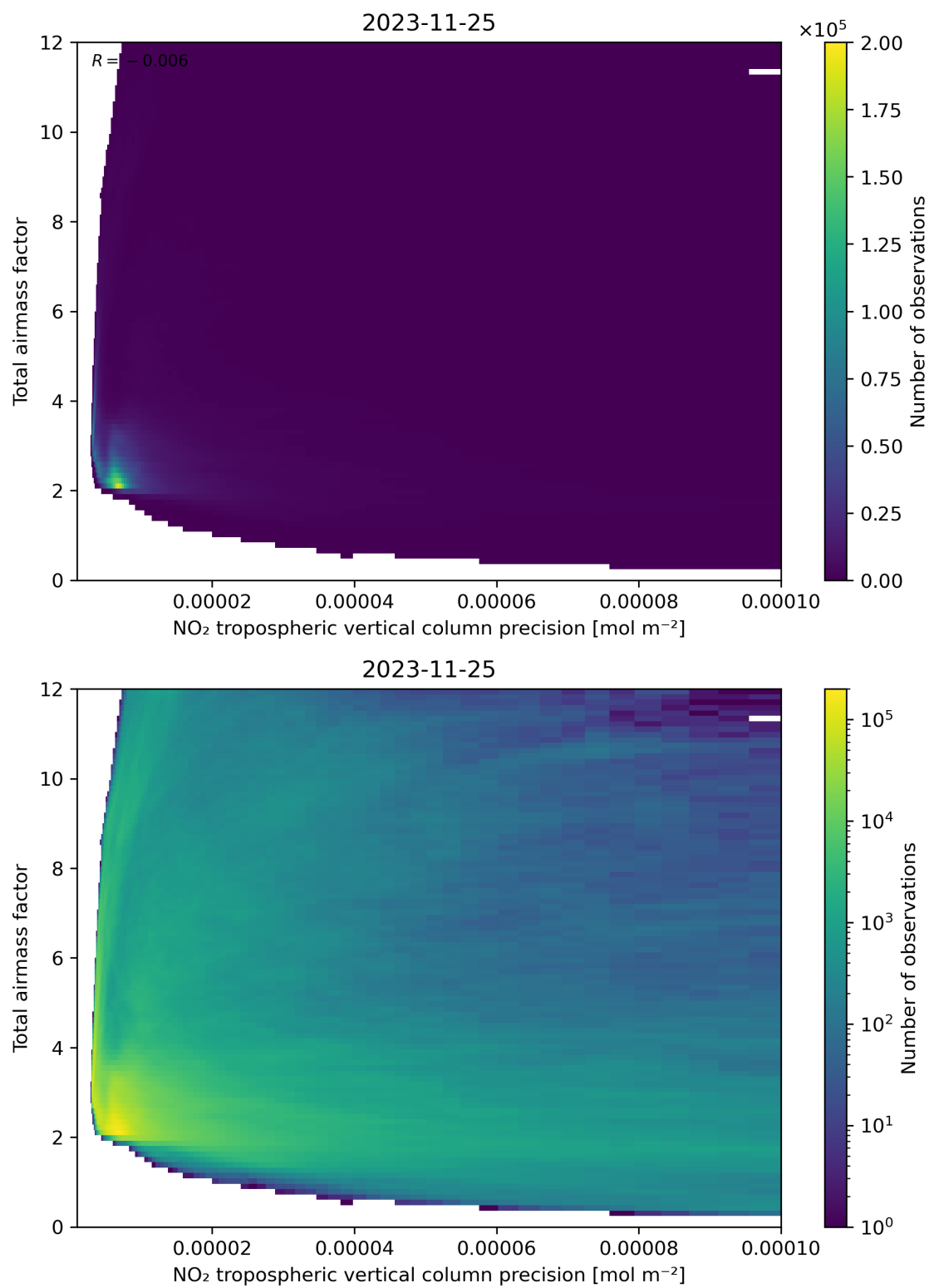
Figure 132: Scatter density plot of “NO 2 tropospheric vertical column precision” against “Total air mass factor” for 2023-11-24 to 2023-11-26.
