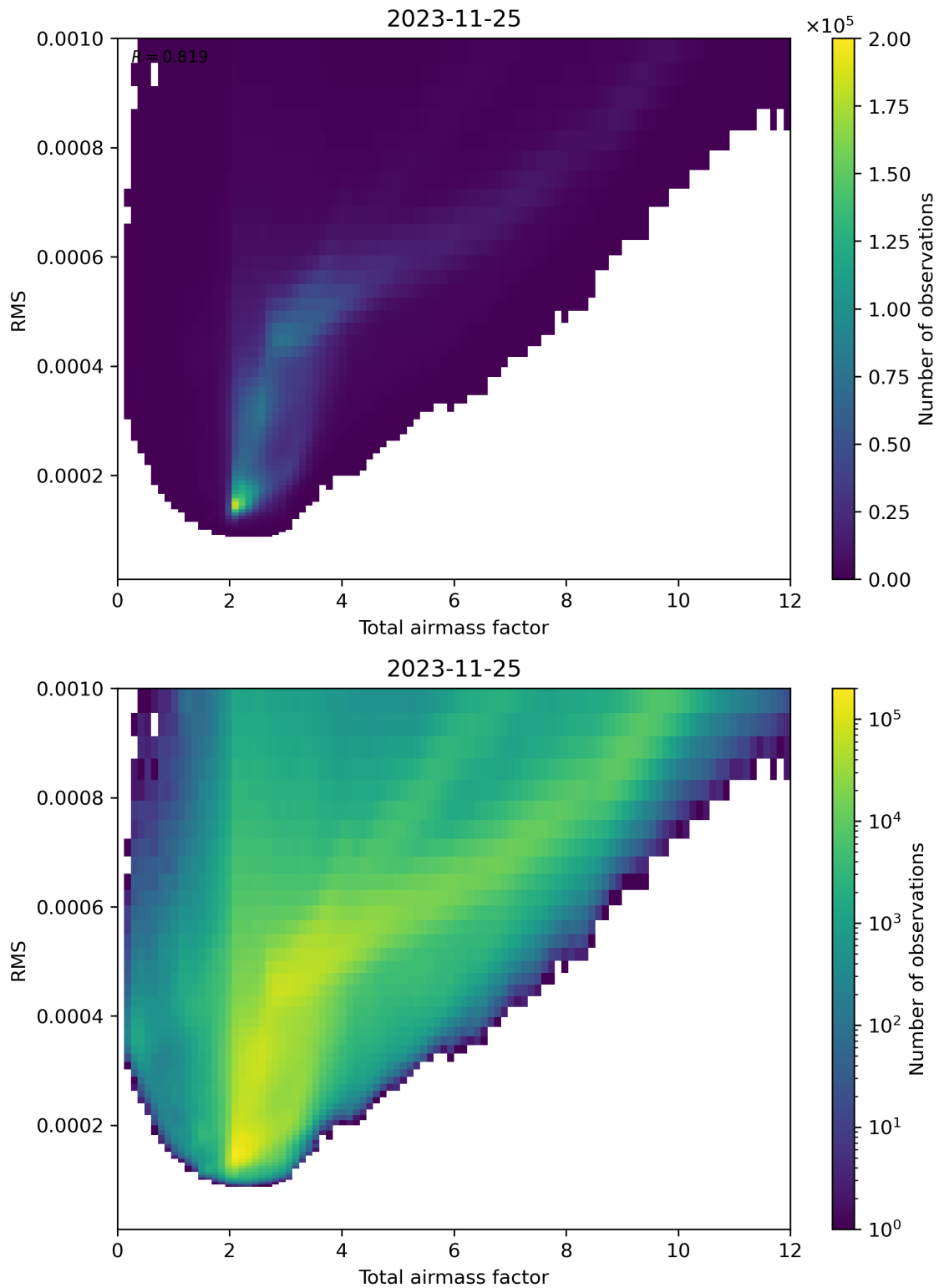
Figure 69: Scatter density plot of “Total airmass factor” against “RMS” for 2023-11-24 to 2023-11-26.
