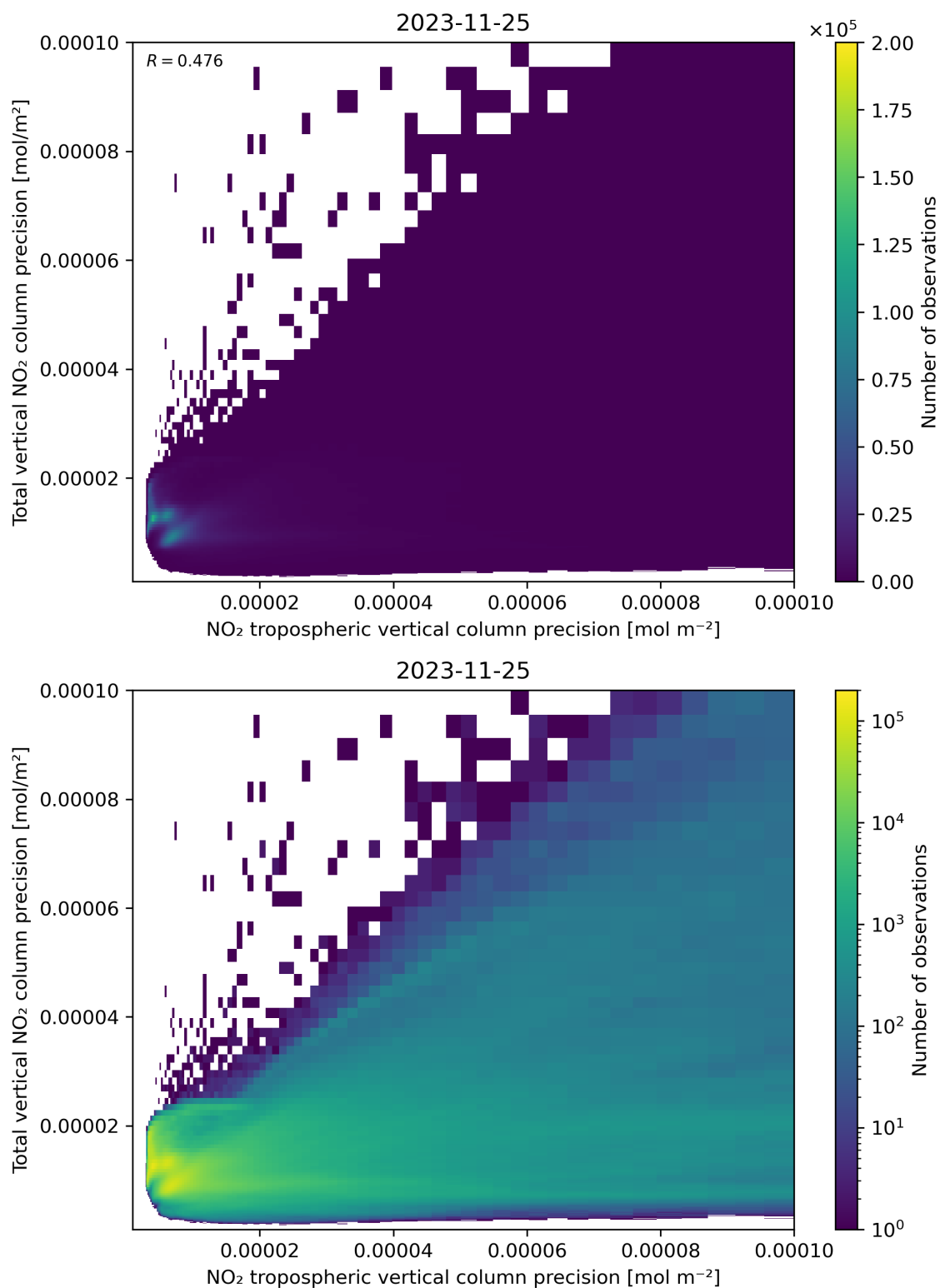
Figure 139: Scatter density plot of “NO 2 tropospheric vertical column precision” against “Total vertical NO 2 column precision” for 2023-11-24 to 2023-11-26.
