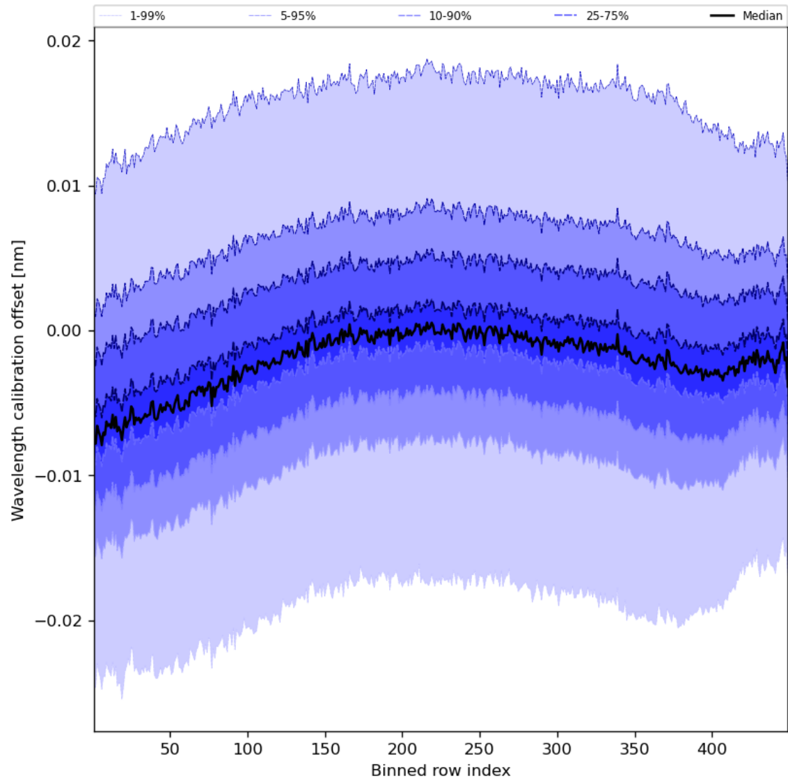
Figure 52: Along track statistics of “Wavelength calibration offset” for 2023-11-24 to 2023-11-26
