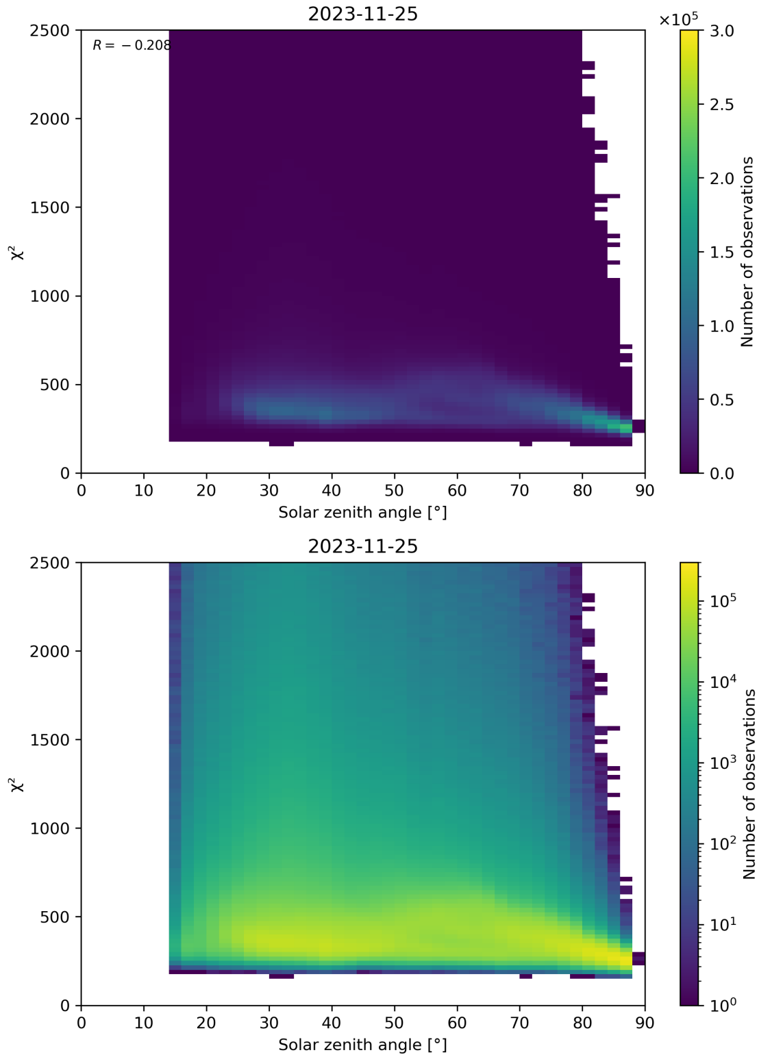
Figure 148: Scatter density plot of “Solar zenith angle” against “ \chi^2 ” for 2023-11-24 to 2023-11-26.
