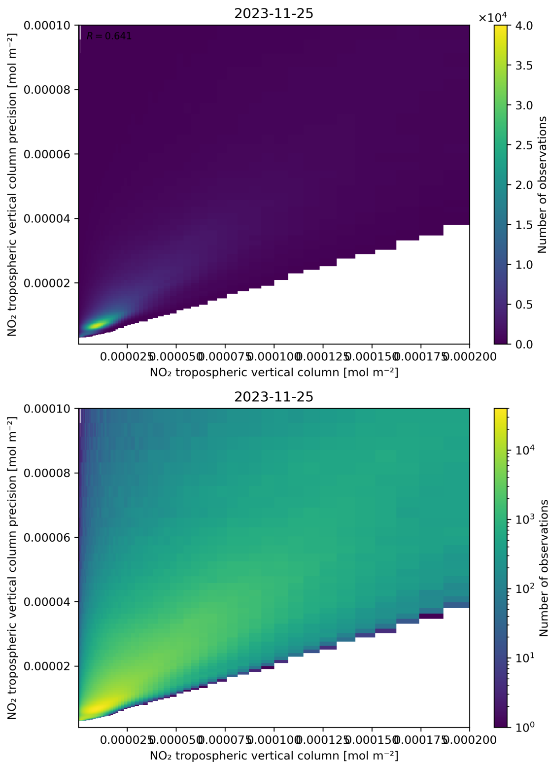
Figure 130: Scatter density plot of “NO 2 tropospheric vertical column” against “NO 2 tropospheric vertical column precision” for 2023-11-24 to 2023-11-26.
