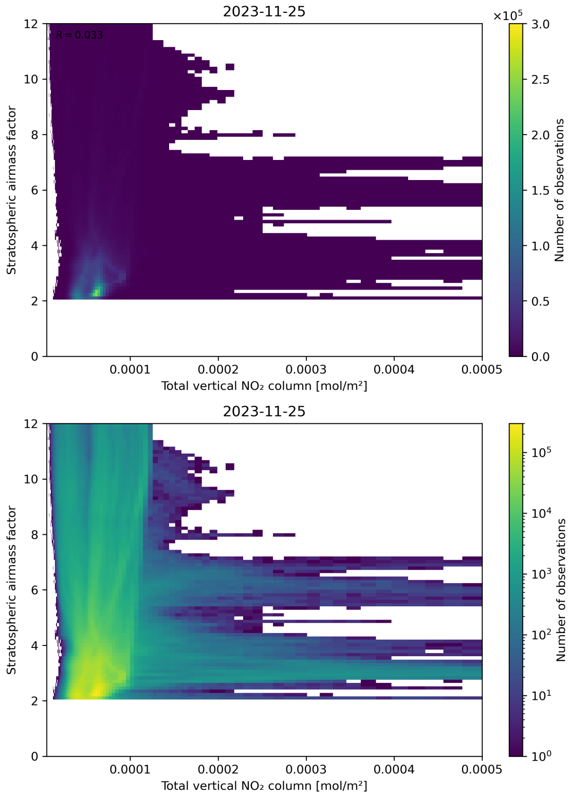
Figure 110: Scatter density plot of “Total vertical NO 2 column” against “Stratospheric airmass factor” for 2023-11-24 to 2023-11-26.
