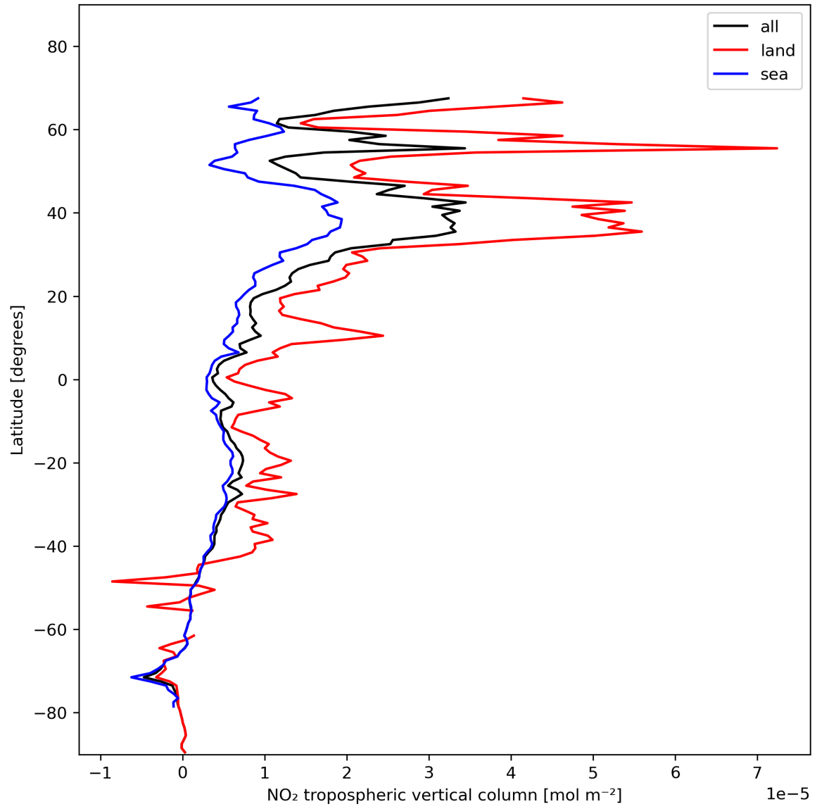
Figure 12: Zonal average of “NO 2 tropospheric vertical column” for 2023-11-24 to 2023-11-26.
