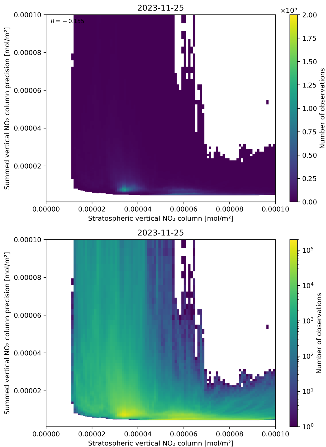
Figure 99: Scatter density plot of “Stratospheric vertical NO 2 column” against “Summed vertical NO 2 column precision” for 2023-11-24 to 2023-11-26.
