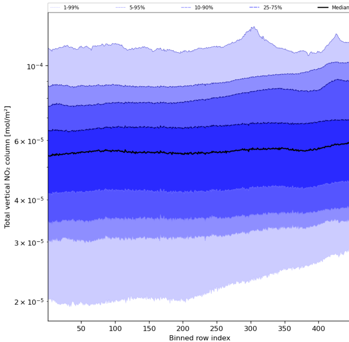
Figure 55: Along track statistics of “Total vertical NO 2 column” for 2023-11-24 to 2023-11-26
