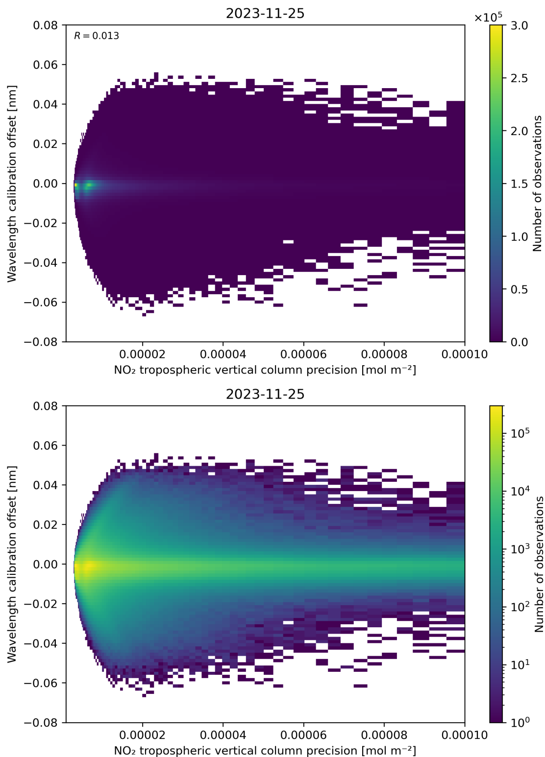
Figure 141: Scatter density plot of “NO 2 tropospheric vertical column precision” against “Wavelength calibration offset” for 2023-11-24 to 2023-11-26.
