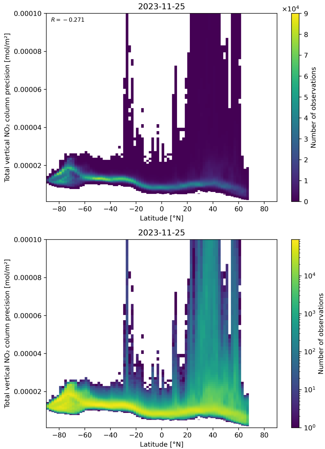
Figure 91: Scatter density plot of “Latitude” against “Total vertical NO 2 column precision” for 2023-11-24 to 2023-11-26.
