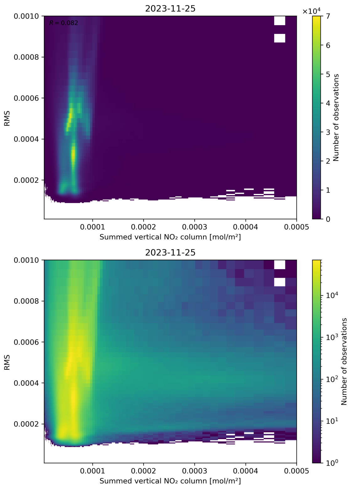
Figure 109: Scatter density plot of “Summed vertical NO 2 column” against “RMS” for 2023-11-24 to 2023-11-26.
