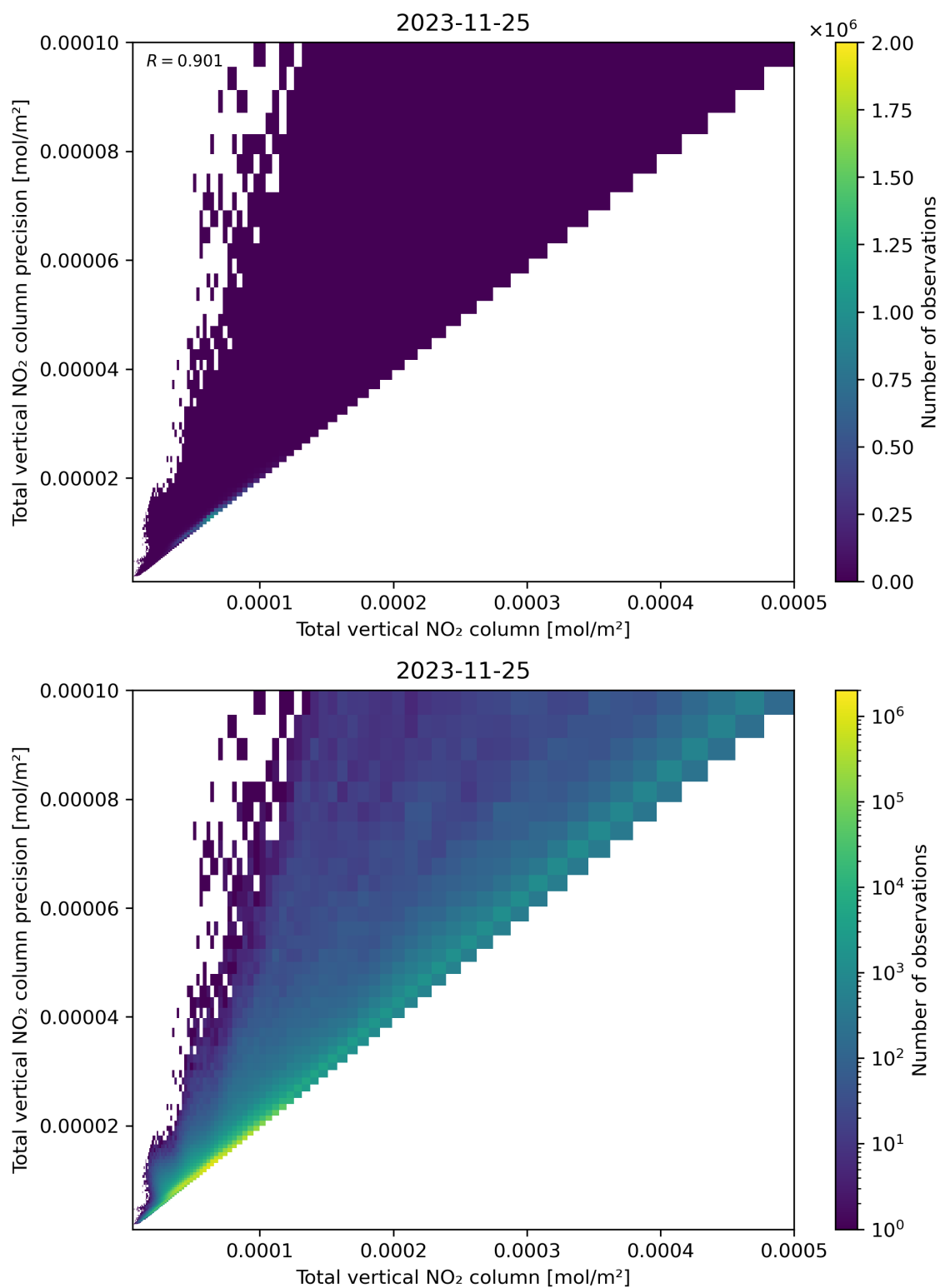
Figure 114: Scatter density plot of “Total vertical NO 2 column” against “Total vertical NO 2 column precision” for 2023-11-24 to 2023-11-26.
