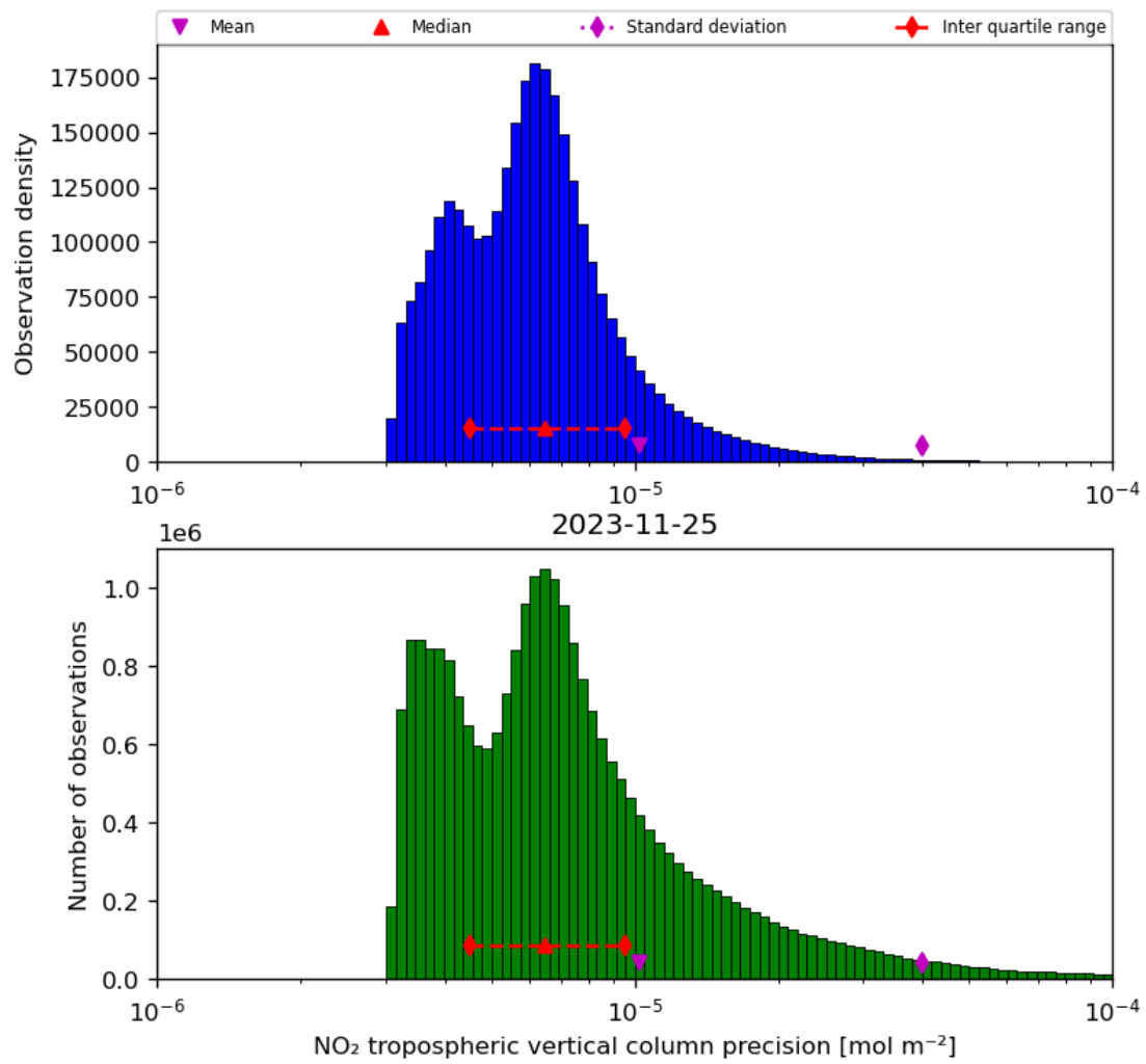
Figure 30: Histogram of “NO 2 tropospheric vertical column precision” for 2023-11-24 to 2023-11-26
