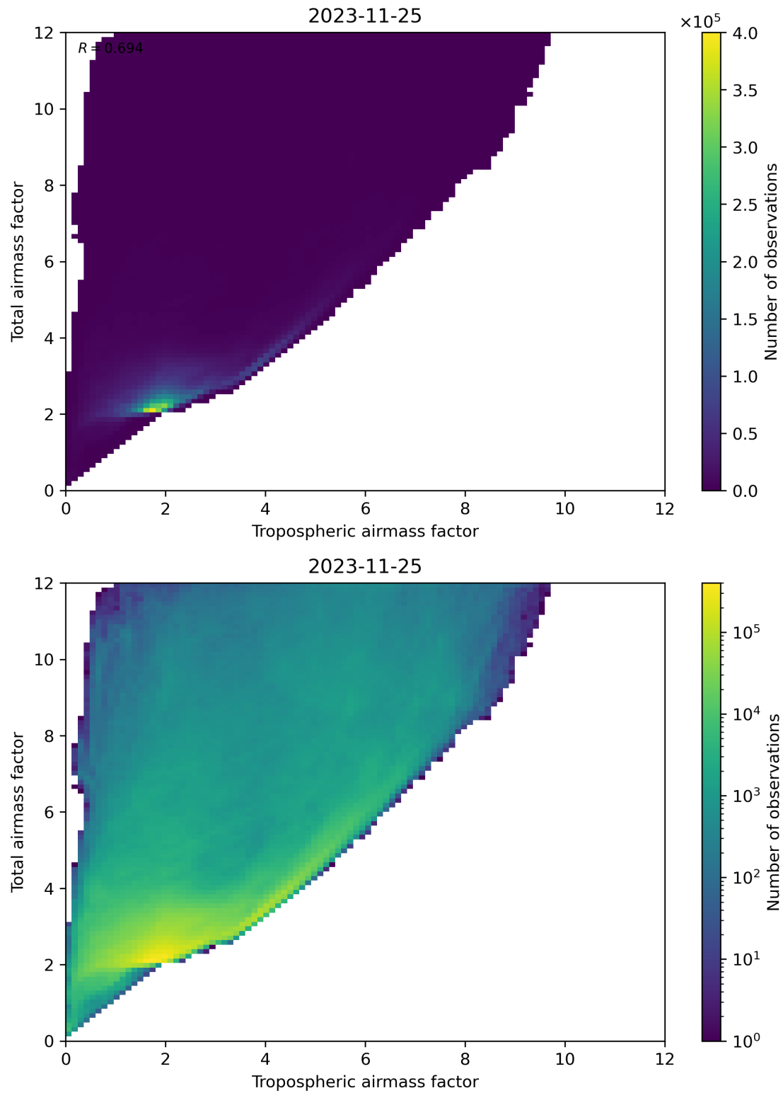
Figure 72: Scatter density plot of “Tropospheric airmass factor” against “Total airmass factor” for 2023-11-24 to 2023-11-26.
