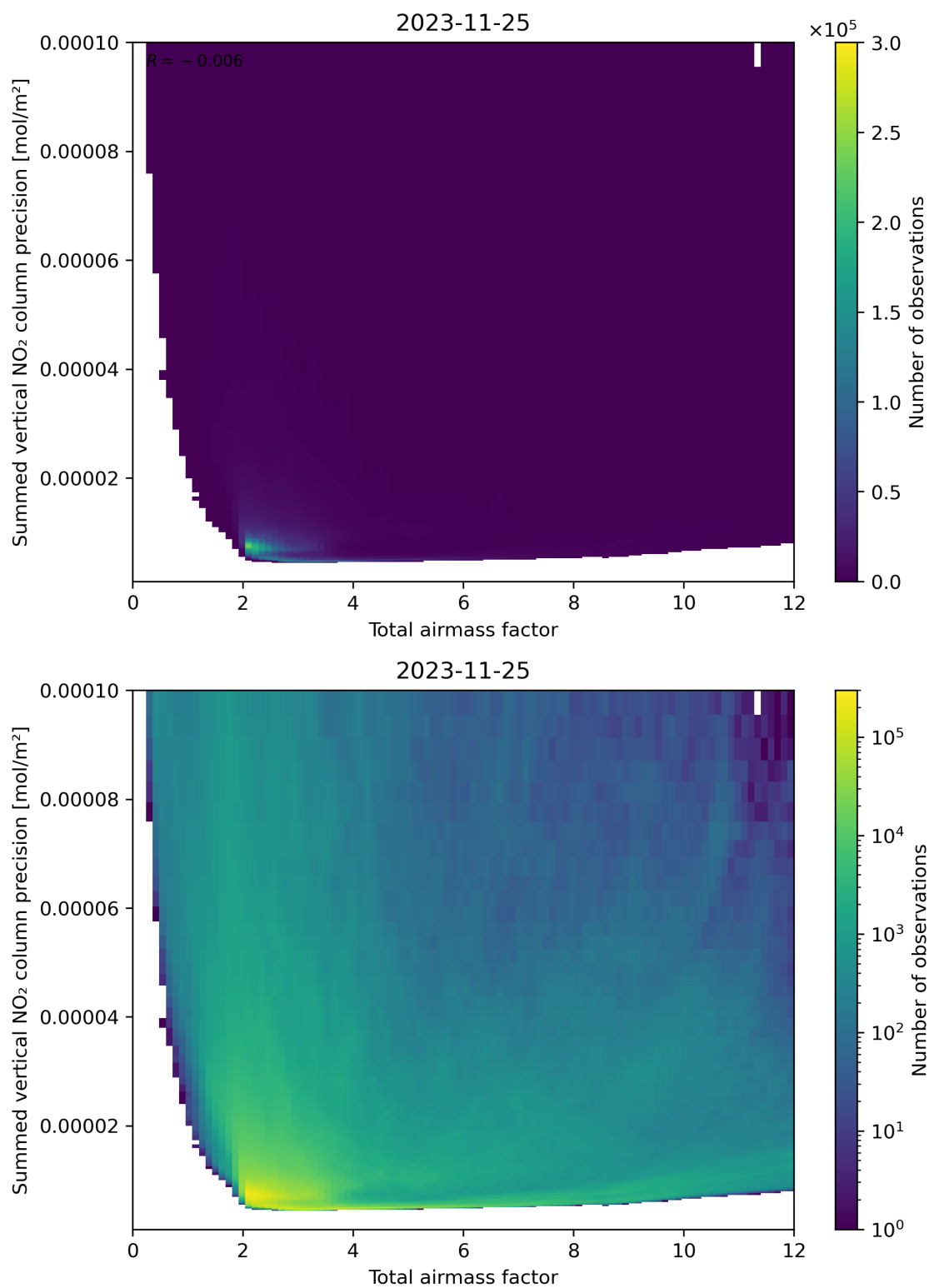
Figure 66: Scatter density plot of “Total airmass factor” against “Summed vertical NO 2 column precision” for 2023-11-24 to 2023-11-26.
