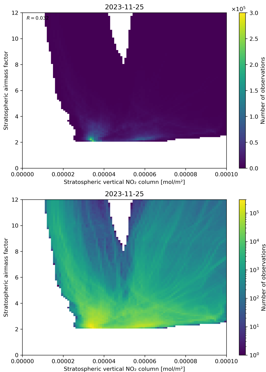
Figure 96: Scatter density plot of “Stratospheric vertical NO 2 column” against “Stratospheric airmass factor” for 2023-11-24 to 2023-11-26.
