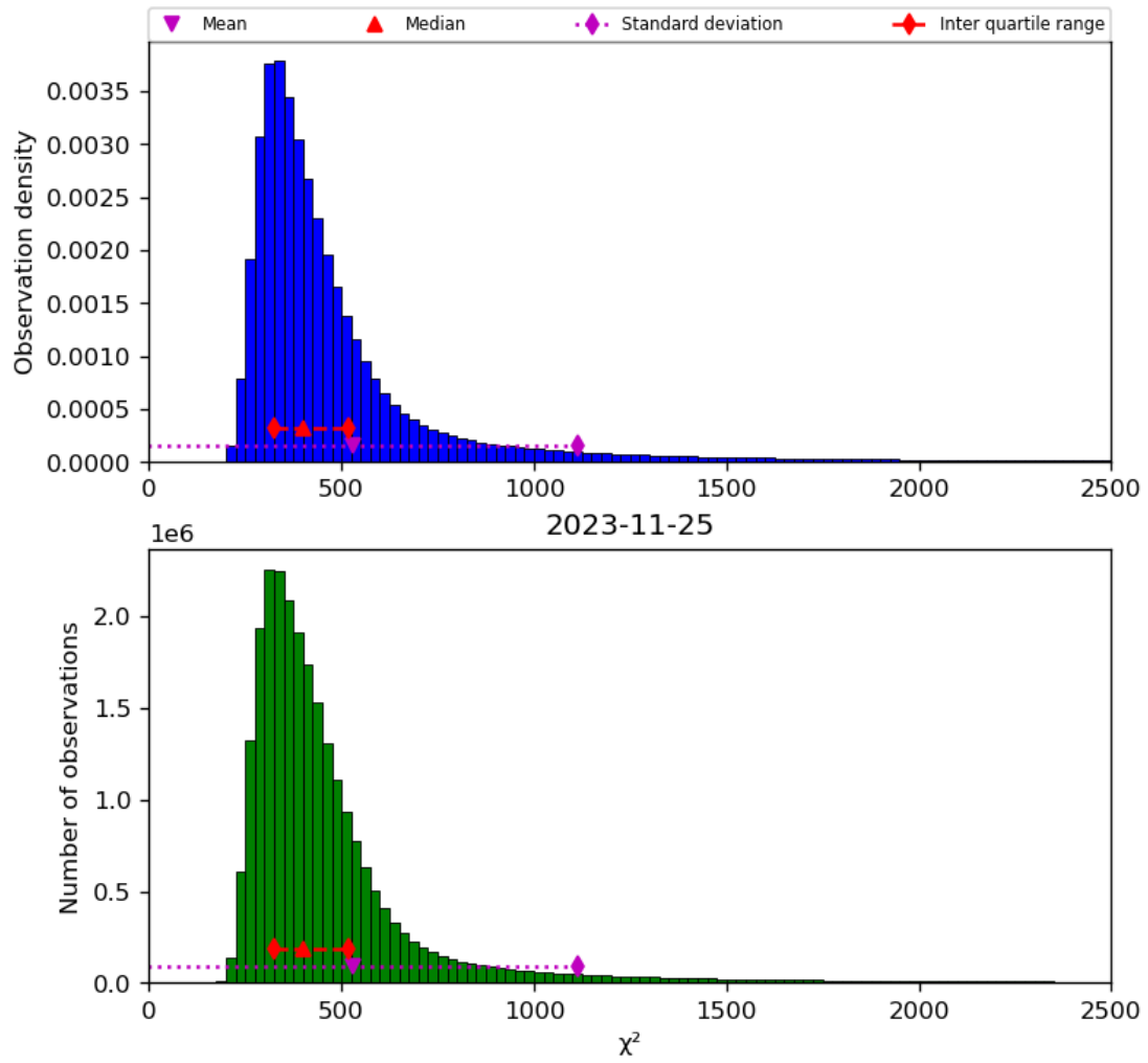
Figure 42: Histogram of “ \chi^2 ” for 2023-11-24 to 2023-11-26
