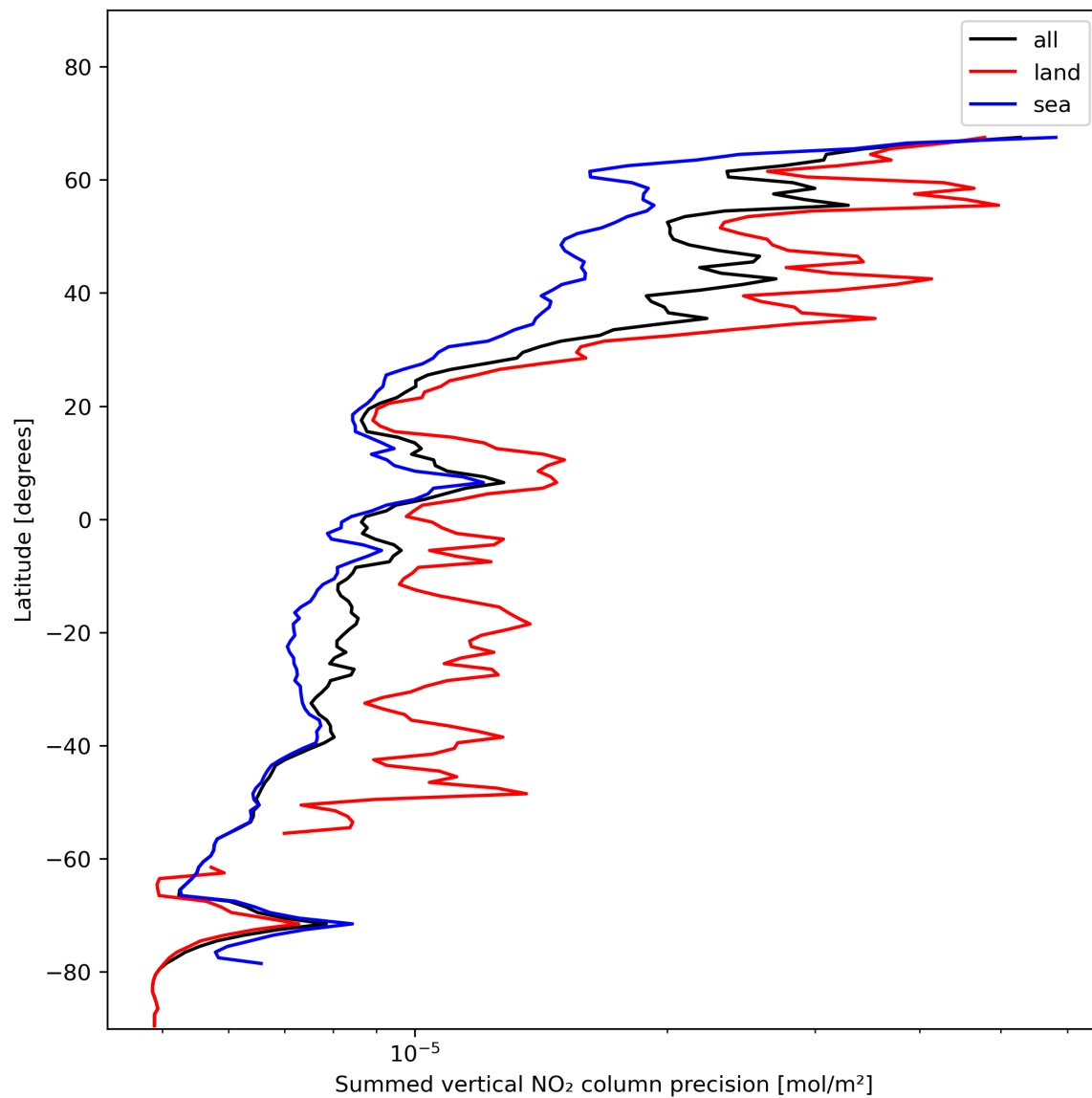
Figure 24: Zonal average of “Summed vertical NO 2 column precision” for 2023-11-24 to 2023-11-26.
