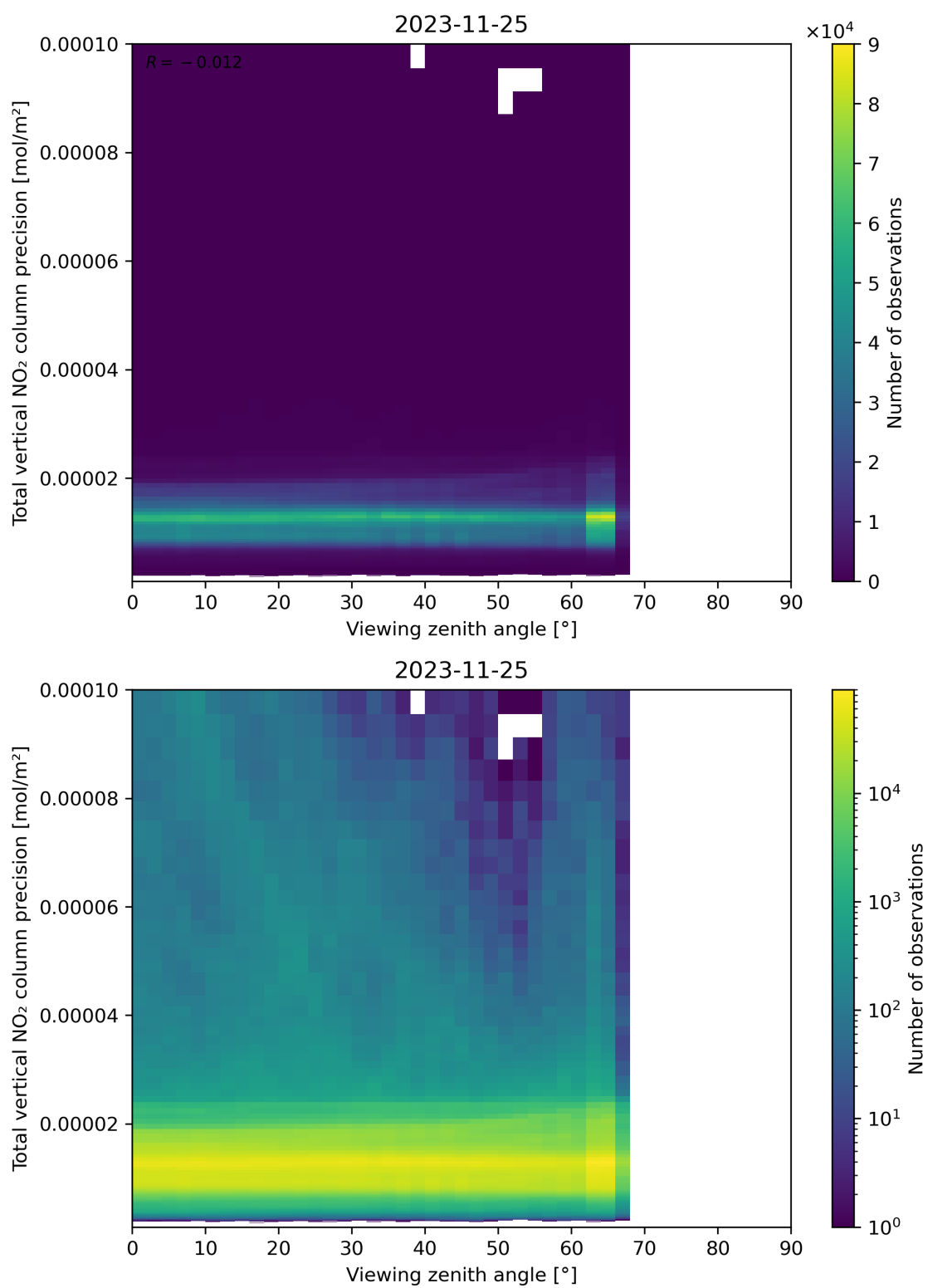
Figure 168: Scatter density plot of “Viewing zenith angle” against “Total vertical NO 2 column precision” for 2023-11-24 to 2023-11-26.
