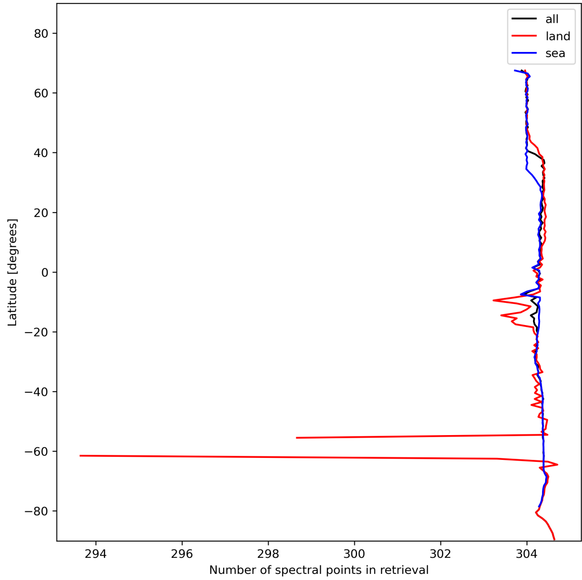
Figure 16: Zonal average of “Number of spectral points in retrieval” for 2023-11-24 to 2023-11-26.
