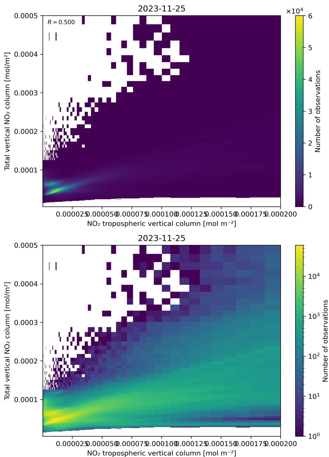
Figure 128: Scatter density plot of “NO 2 tropospheric vertical column” against “Total vertical NO 2 column” for 2023-11-24 to 2023-11-26.
