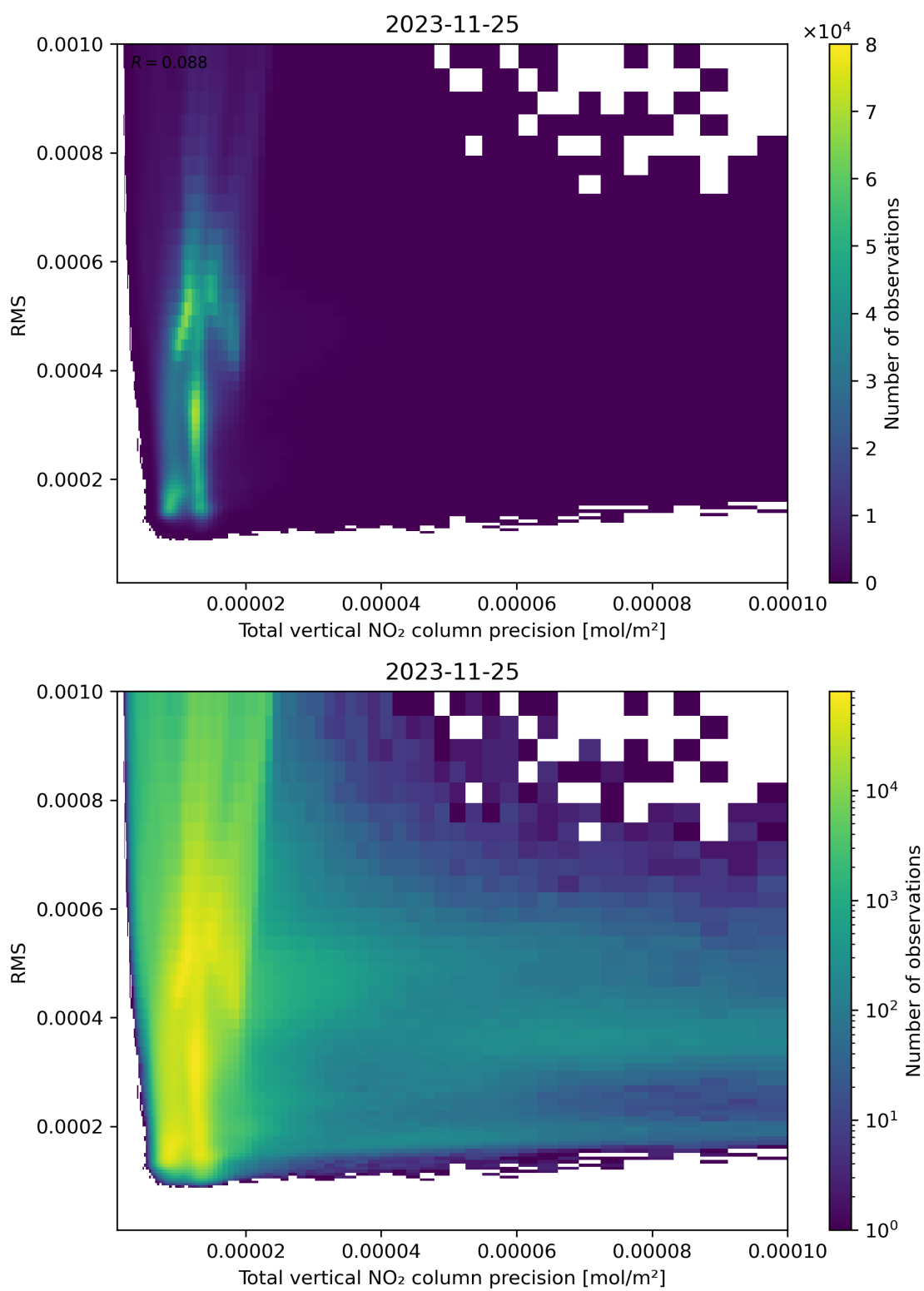
Figure 119: Scatter density plot of “Total vertical NO 2 column precision” against “RMS” for 2023-11-24 to 2023-11-26.
