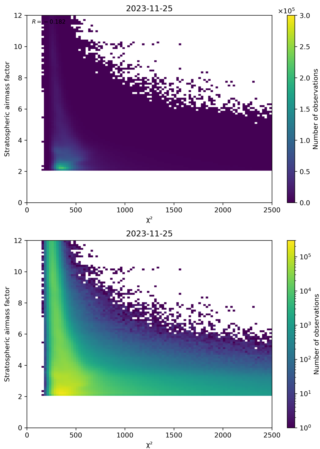
Figure 81: Scatter density plot of “ \chi^2 ” against “Stratospheric airmass factor” for 2023-11-24 to 2023-11-26.
