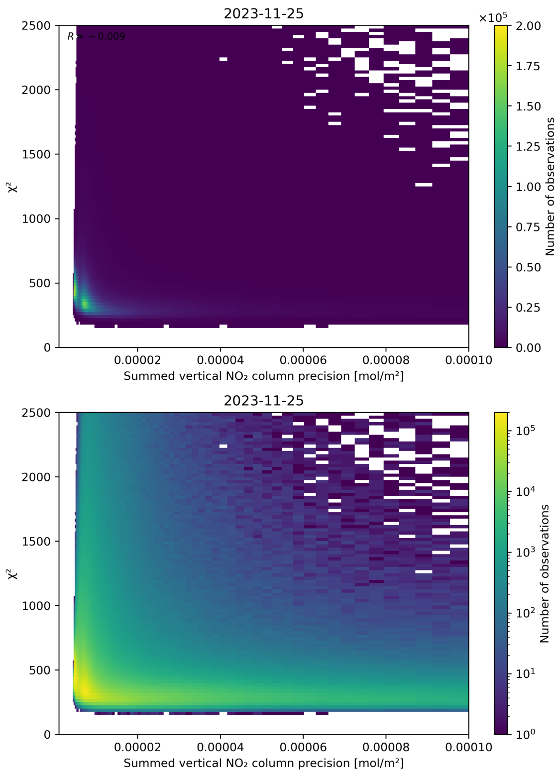
Figure 107: Scatter density plot of “Summed vertical NO 2 column precision” against “ \chi^2 ” for 2023-11-24 to 2023-11-26.
