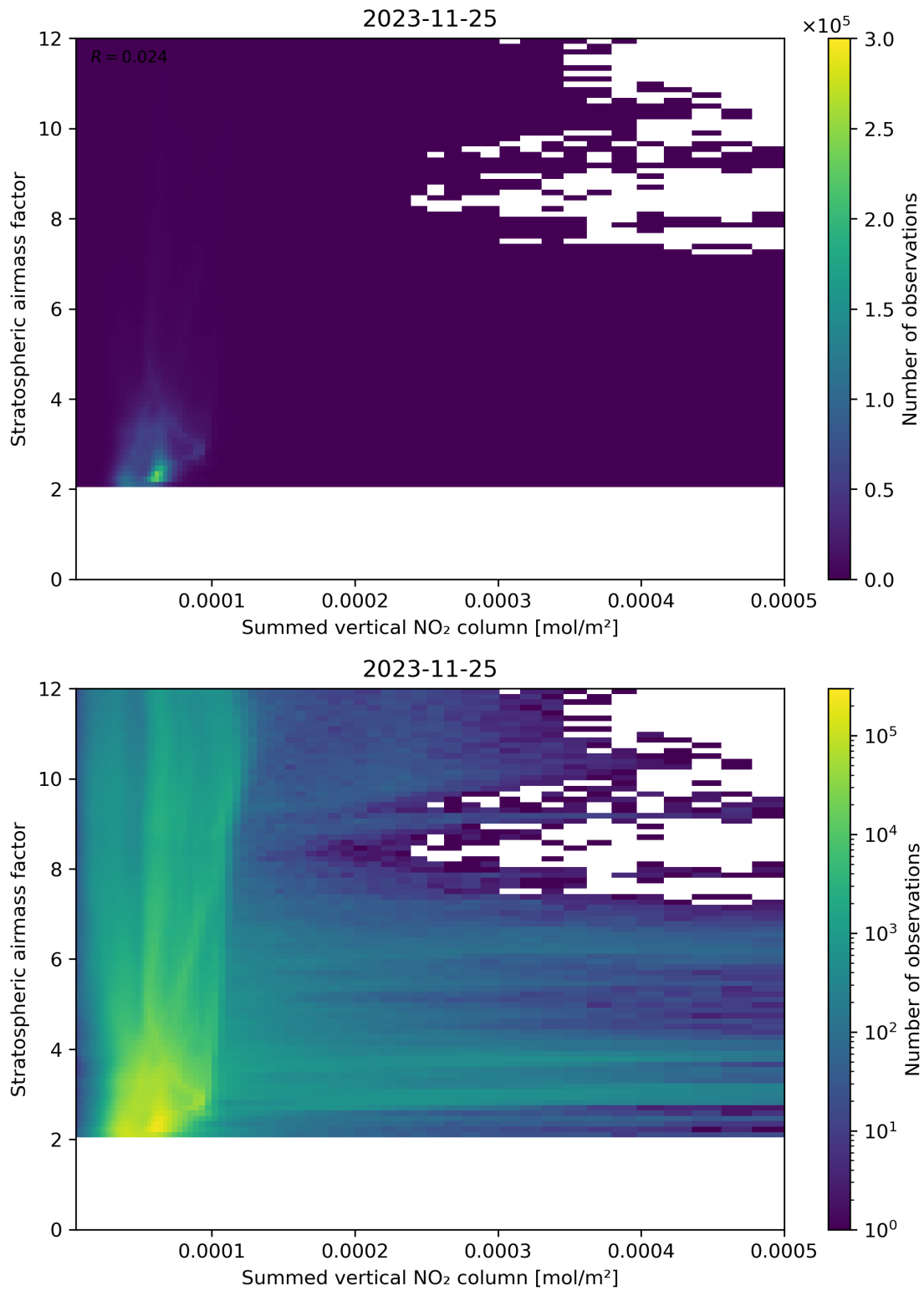
Figure 103: Scatter density plot of “Summed vertical NO 2 column” against “Stratospheric air mass factor” for 2023-11-24 to 2023-11-26.
