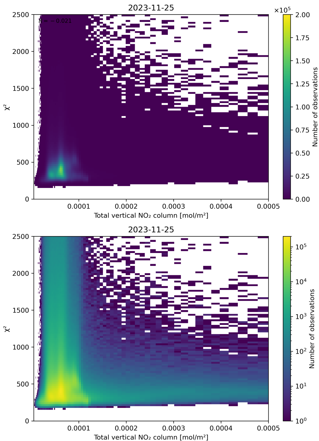
Figure 111: Scatter density plot of “Total vertical NO 2 column” against “ \chi^2 ” for 2023-11-24 to 2023-11-26.
