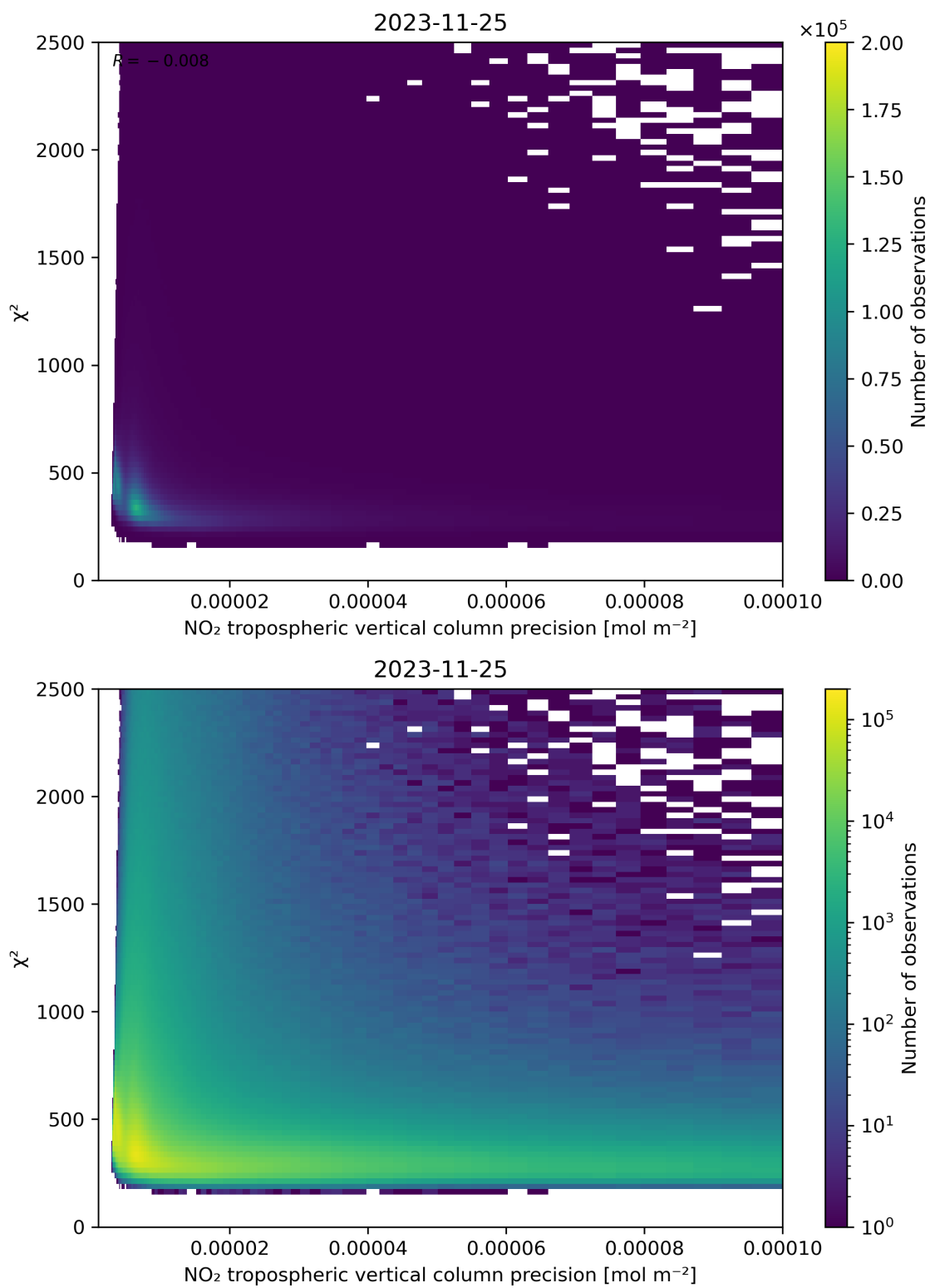
Figure 134: Scatter density plot of “NO 2 tropospheric vertical column precision” against “ \chi^2 ” for 2023-11-24 to 2023-11-26.
