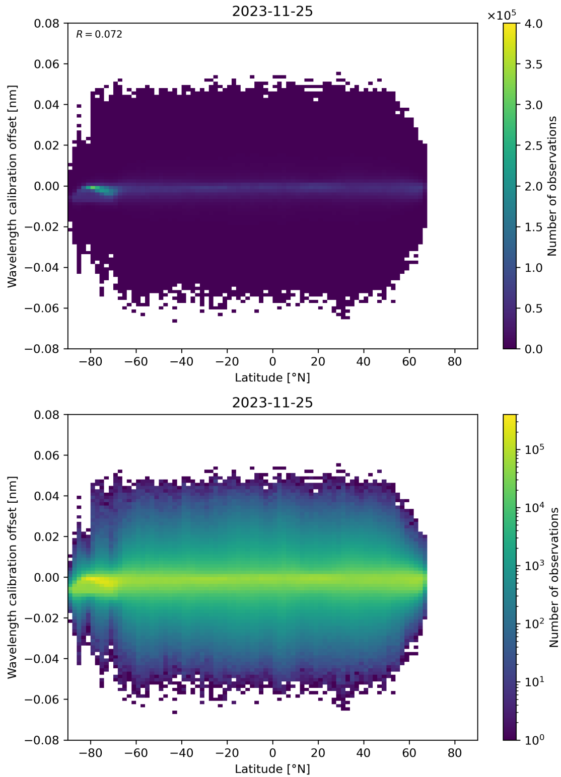
Figure 95: Scatter density plot of “Latitude” against “Wavelength calibration offset” for 2023-11-24 to 2023-11-26.
