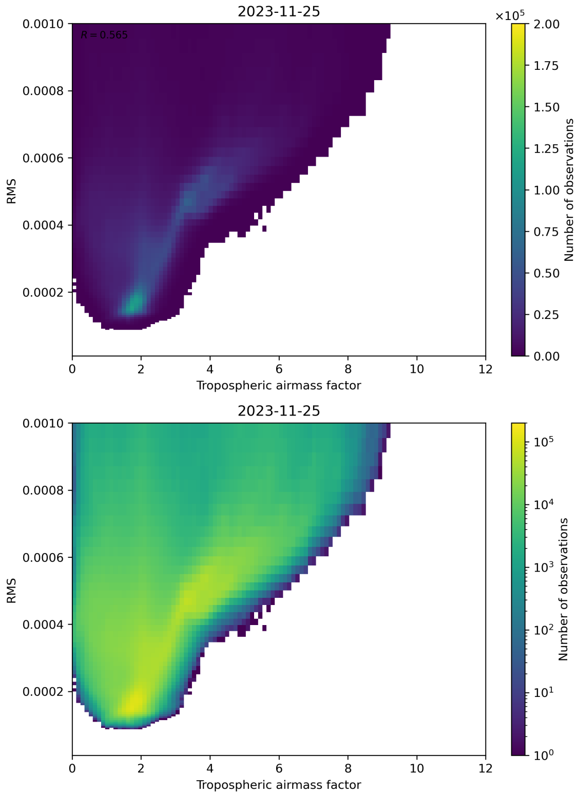
Figure 79: Scatter density plot of “Tropospheric airmass factor” against “RMS” for 2023-11-24 to 2023-11-26.
