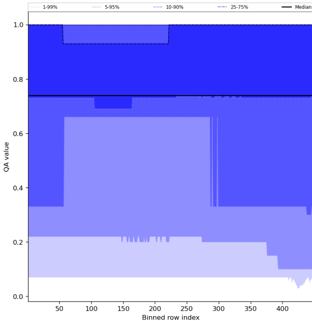
Figure 45: Along track statistics of “QA value” for 2023-11-24 to 2023-11-26
