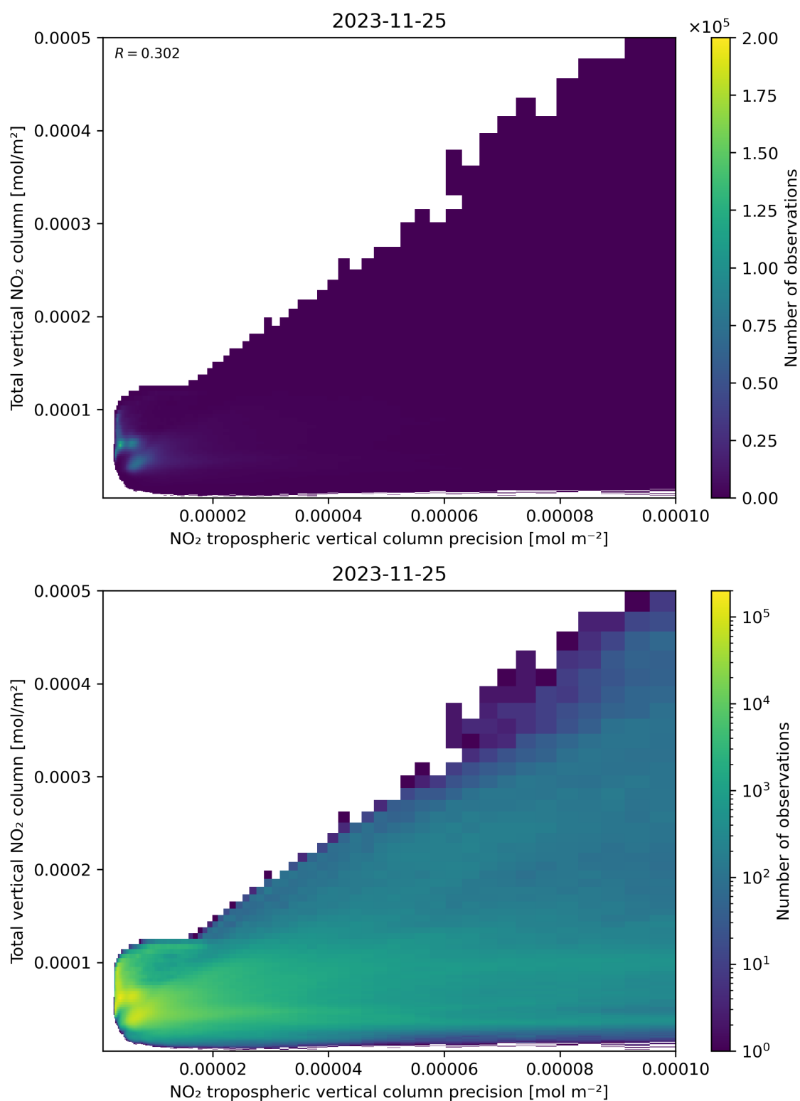
Figure 138: Scatter density plot of “NO 2 tropospheric vertical column precision” against “Total vertical NO 2 column” for 2023-11-24 to 2023-11-26.
