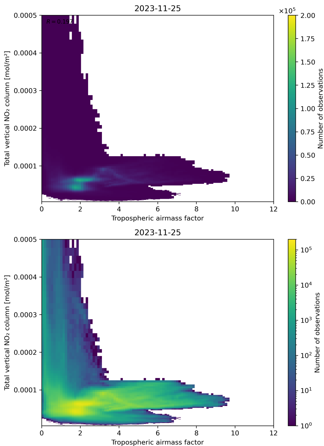
Figure 77: Scatter density plot of “Tropospheric airmass factor” against “Total vertical NO 2 column” for 2023-11-24 to 2023-11-26.
