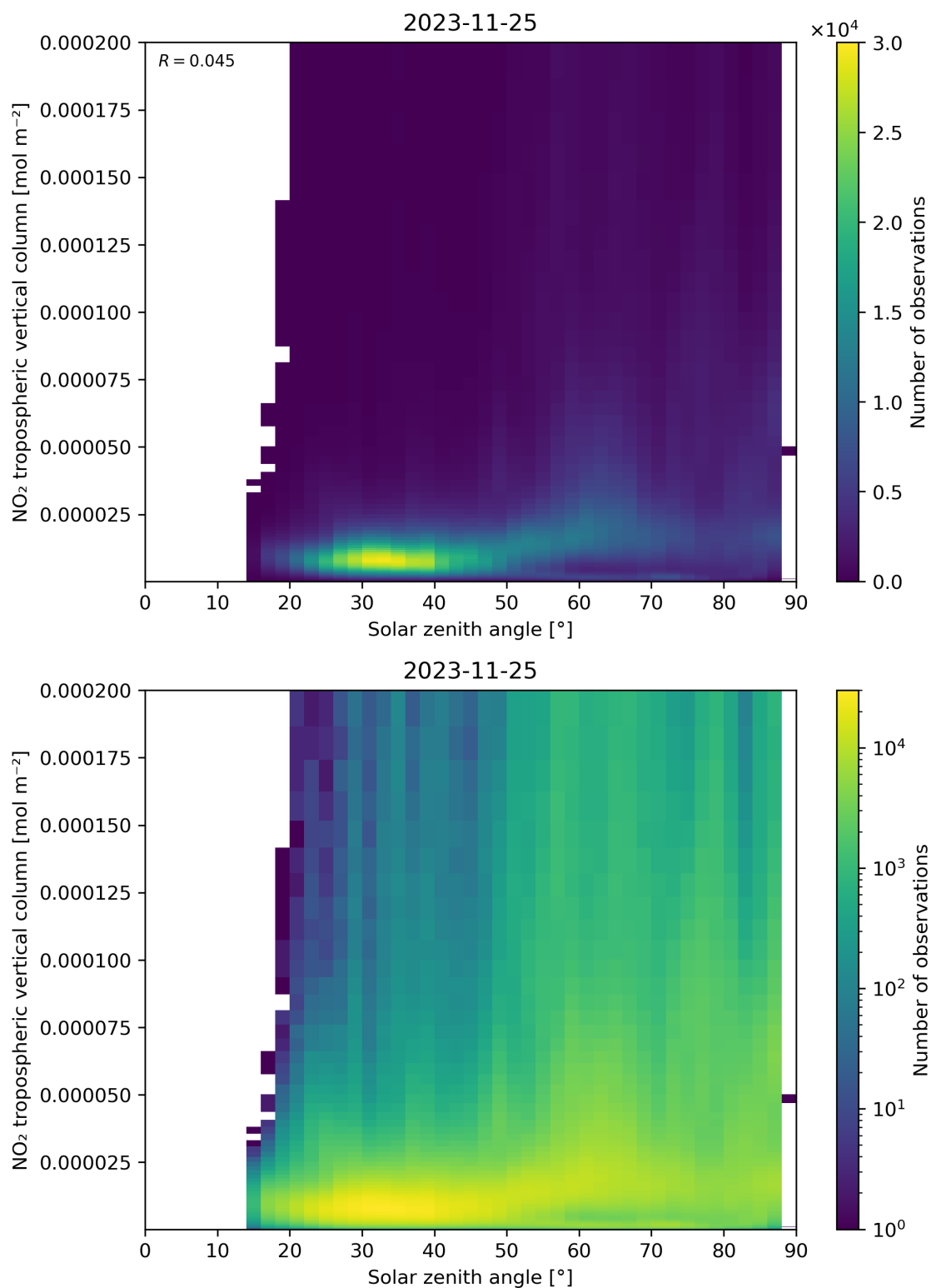
Figure 155: Scatter density plot of “Solar zenith angle” against “NO 2 tropospheric vertical column” for 2023-11-24 to 2023-11-26.
