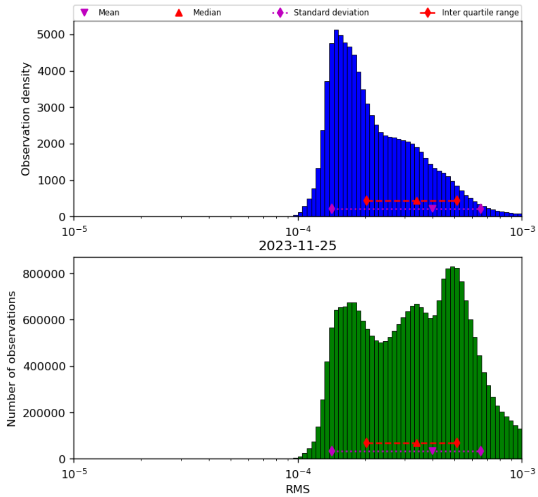
Figure 43: Histogram of “RMS” for 2023-11-24 to 2023-11-26
