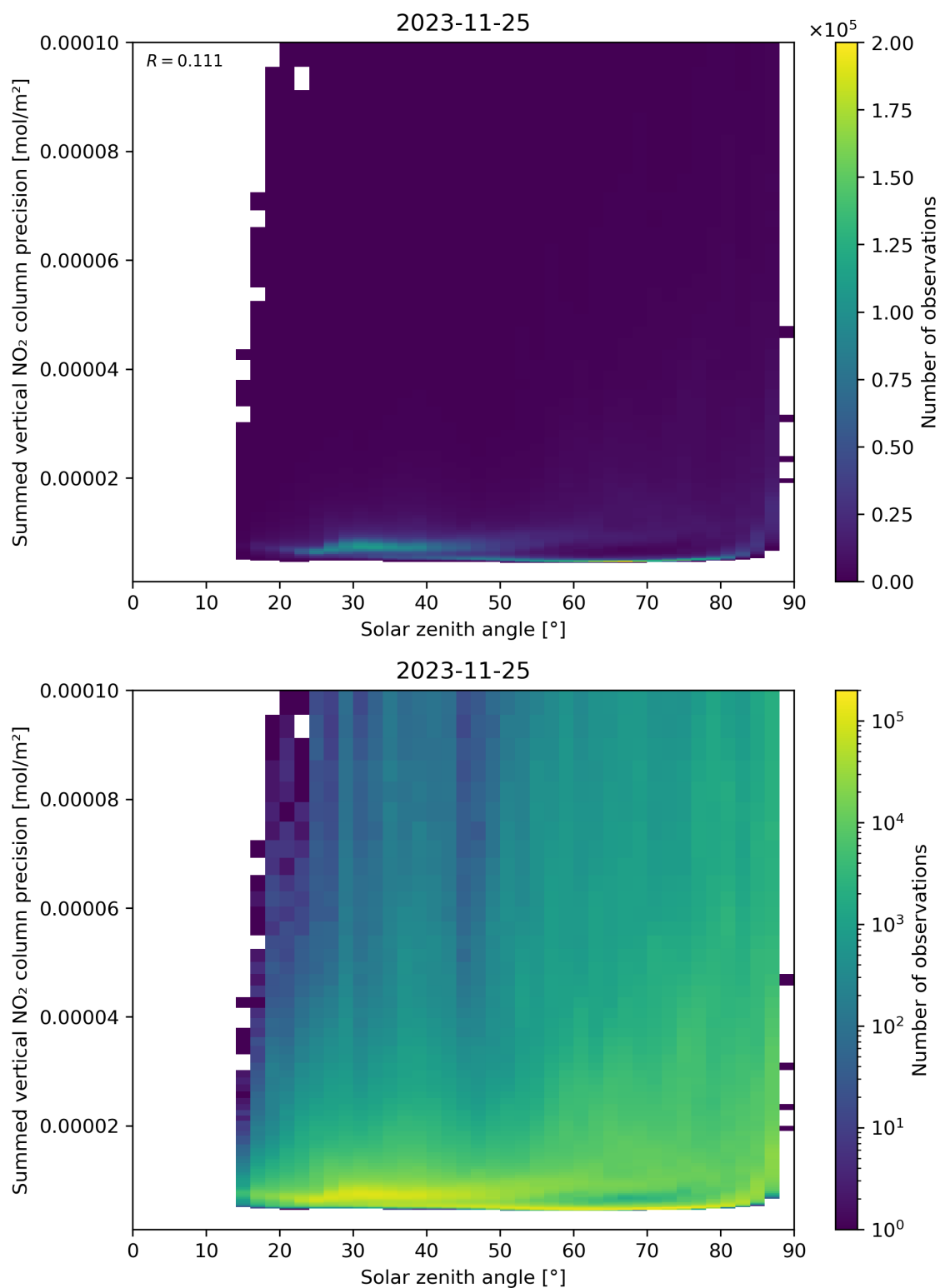
Figure 152: Scatter density plot of “Solar zenith angle” against “Summed vertical NO 2 column precision” for 2023-11-24 to 2023-11-26.
