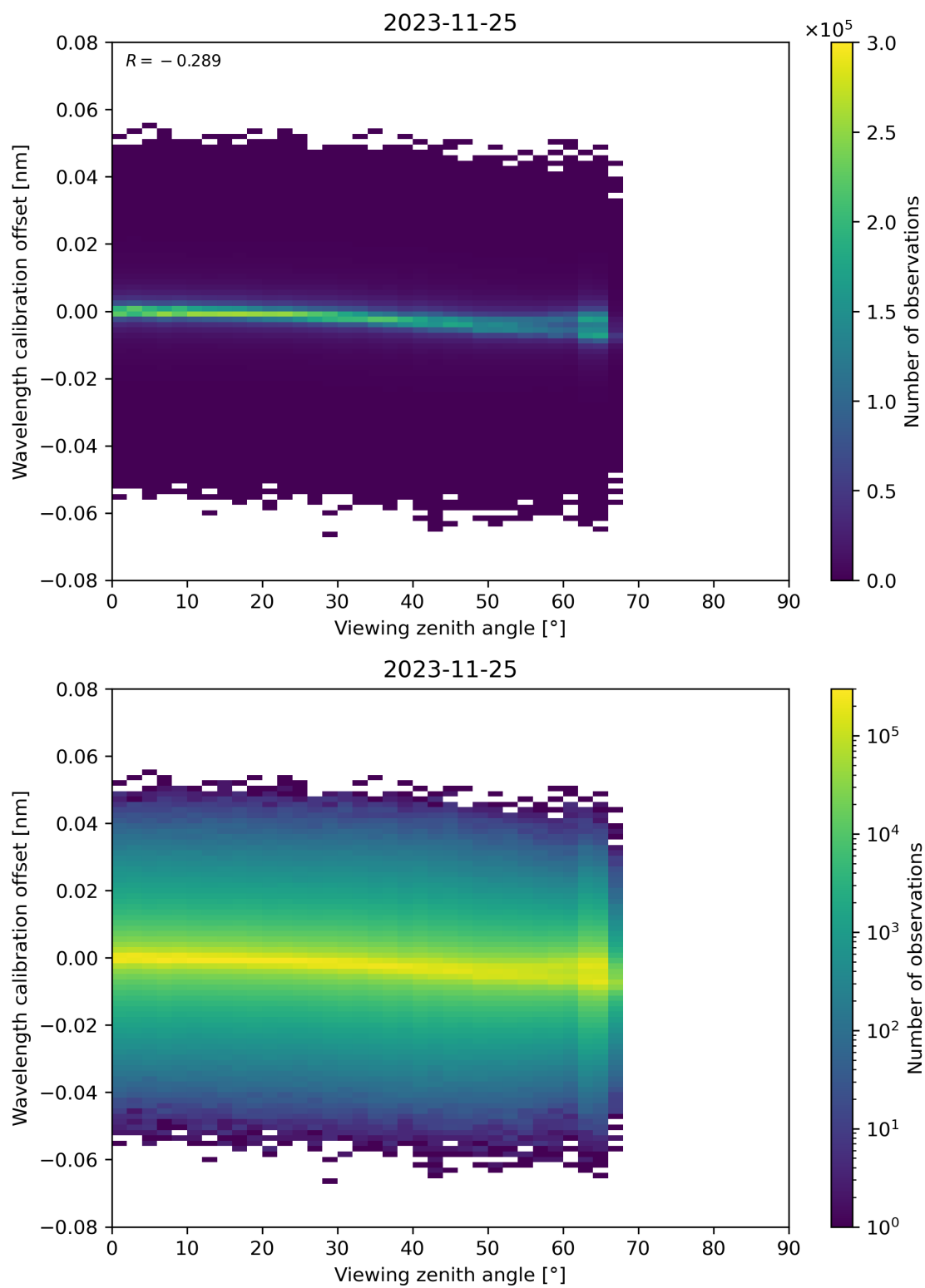
Figure 173: Scatter density plot of “Viewing zenith angle” against “Wavelength calibration offset” for 2023-11-24 to 2023-11-26.
