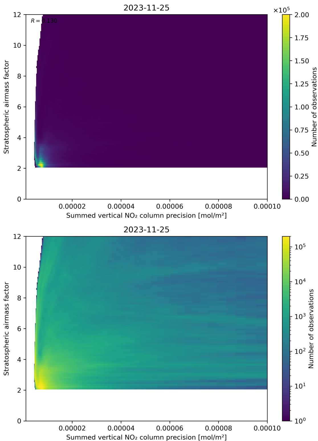
Figure 106: Scatter density plot of “Summed vertical NO 2 column precision” against “Stratospheric airmass factor” for 2023-11-24 to 2023-11-26.
