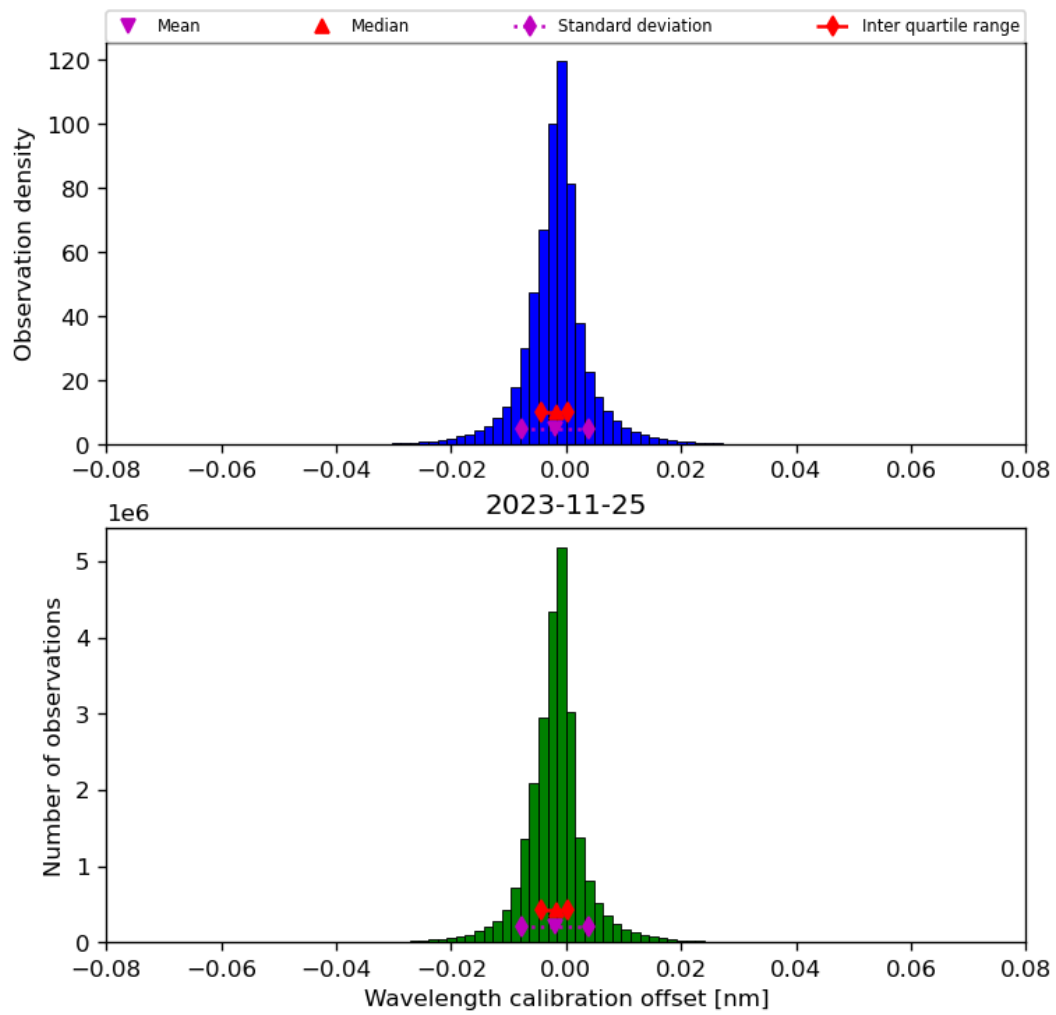
Figure 35: Histogram of “Wavelength calibration offset” for 2023-11-24 to 2023-11-26
