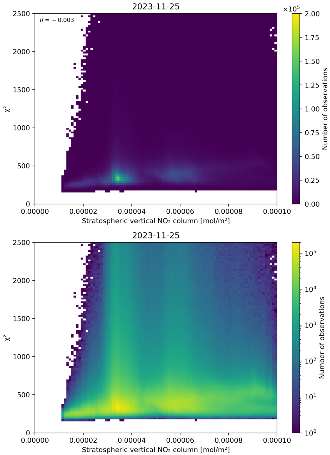
Figure 97: Scatter density plot of “Stratospheric vertical NO 2 column” against “ \chi^2 ” for 2023-11-24 to 2023-11-26.
