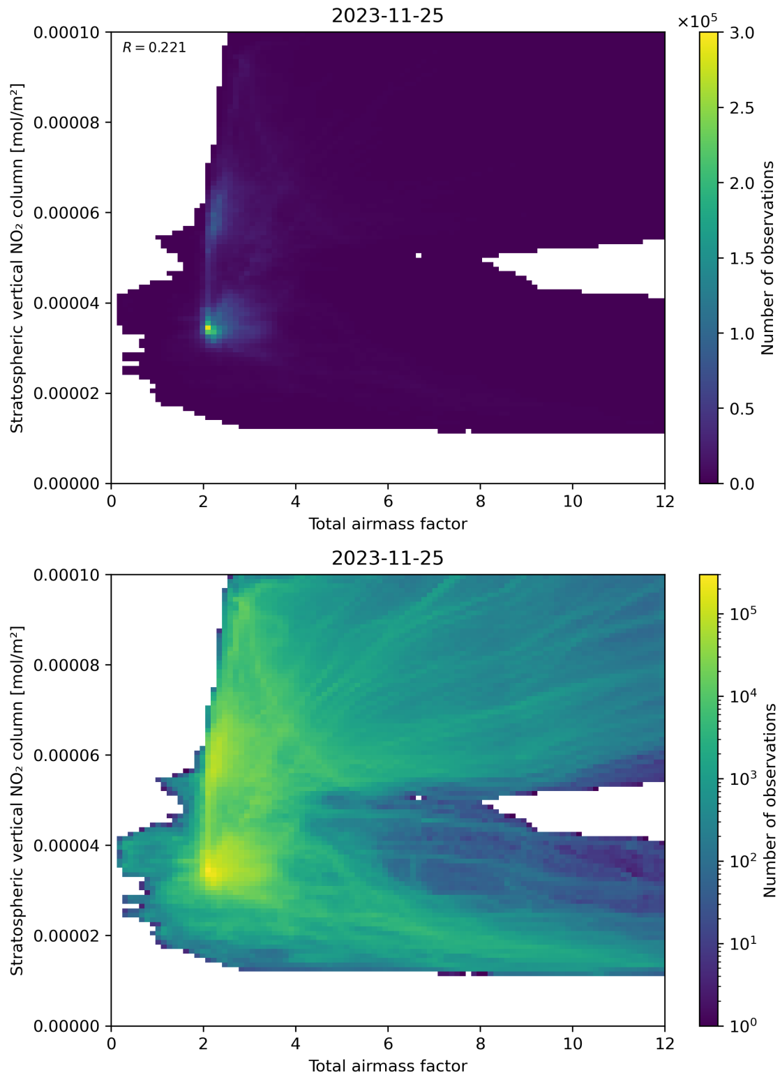
Figure 64: Scatter density plot of “Total airmass factor” against “Stratospheric vertical NO 2 column” for 2023-11-24 to 2023-11-26.
