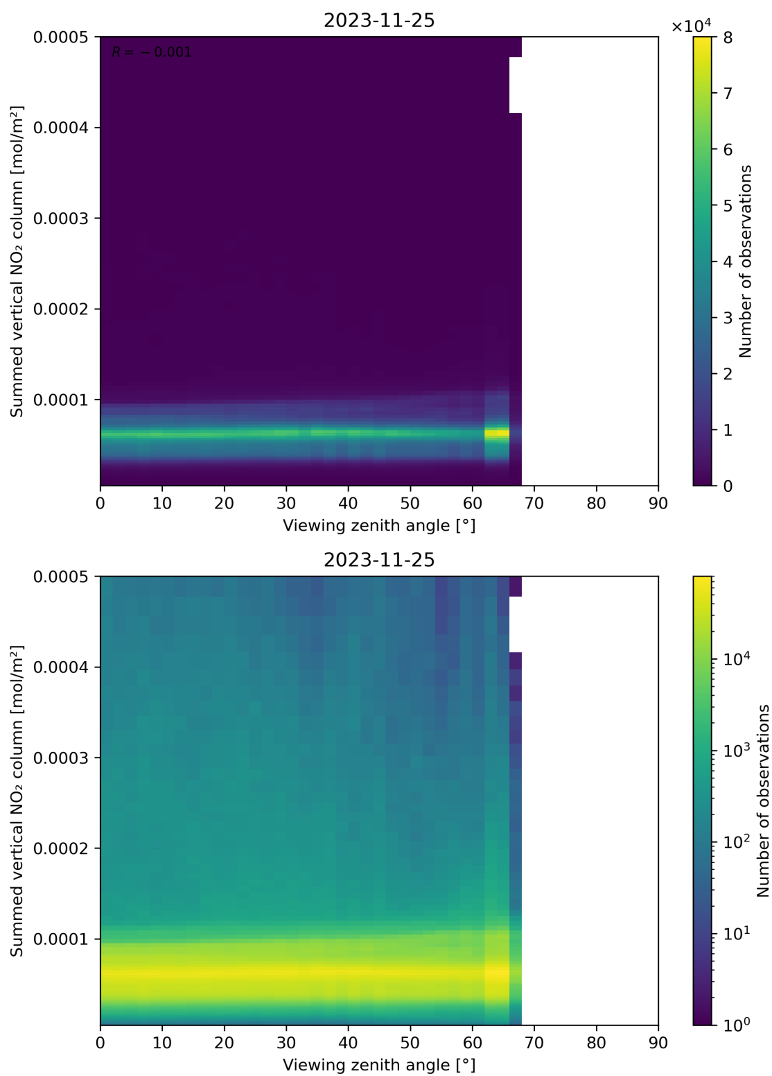
Figure 165: Scatter density plot of “Viewing zenith angle” against “Summed vertical NO 2 column” for 2023-11-24 to 2023-11-26.
