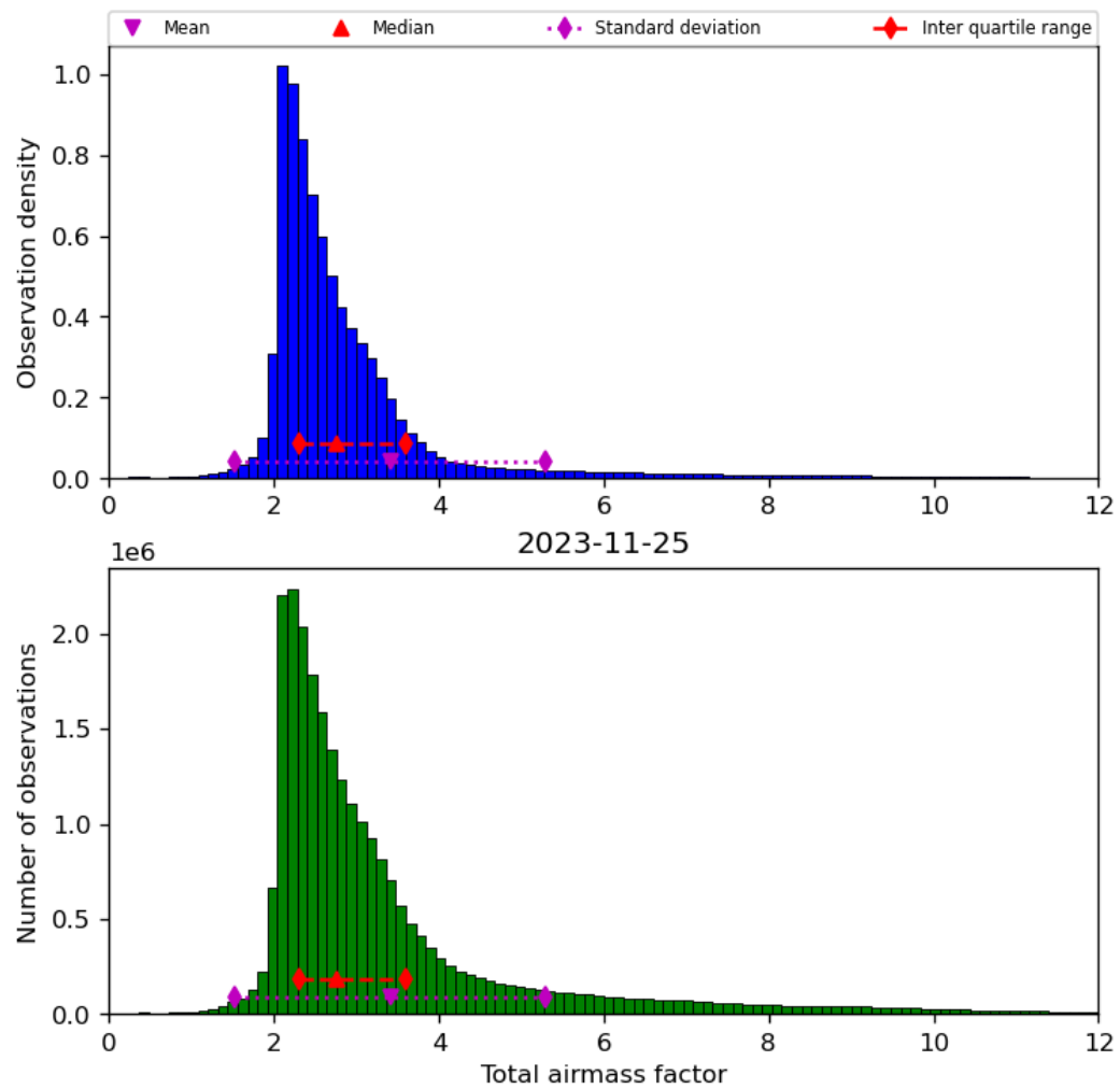
Figure 32: Histogram of “Total airmass factor” for 2023-11-24 to 2023-11-26
