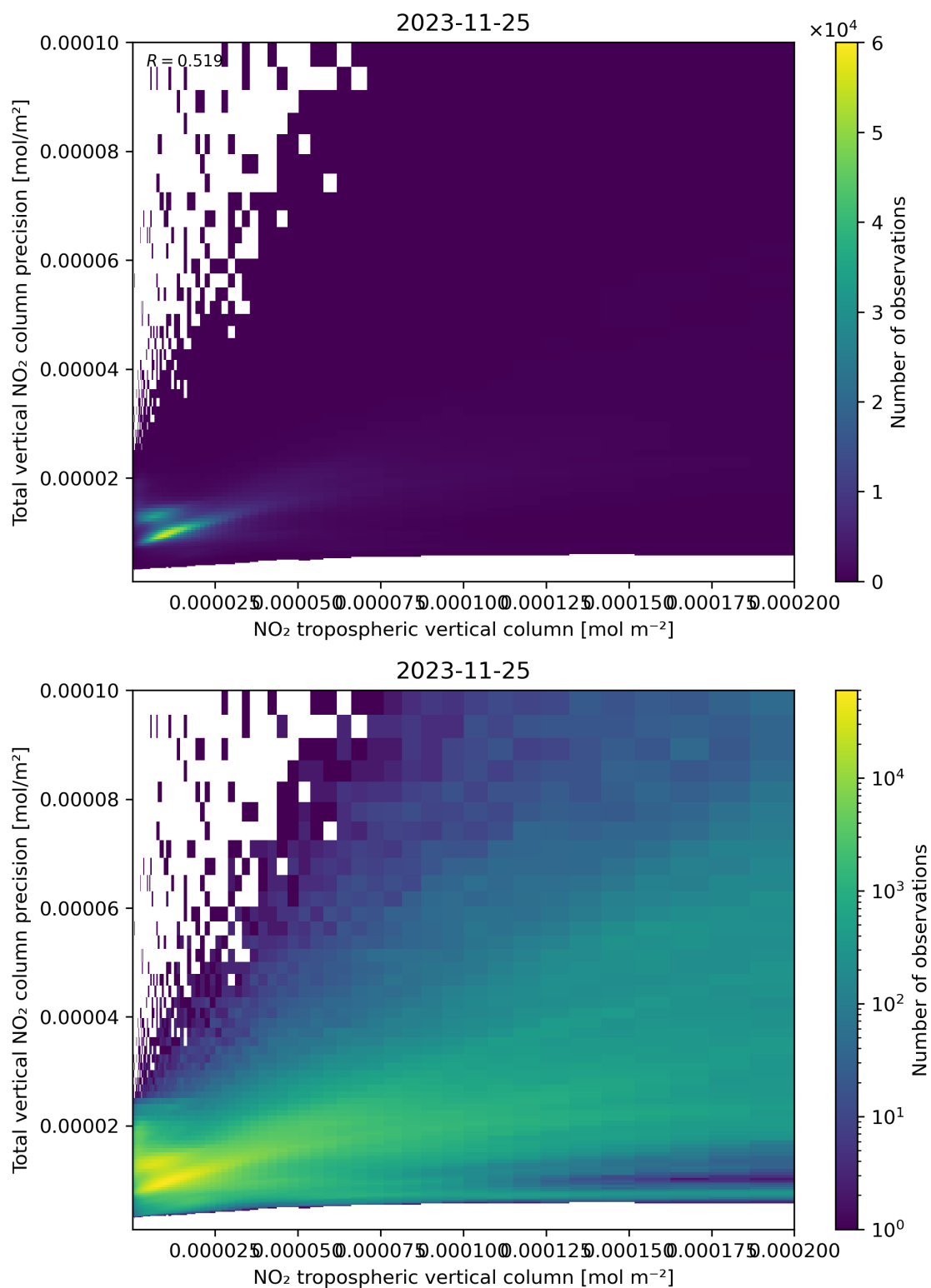
Figure 129: Scatter density plot of “NO 2 tropospheric vertical column” against “Total vertical NO 2 column precision” for 2023-11-24 to 2023-11-26.
