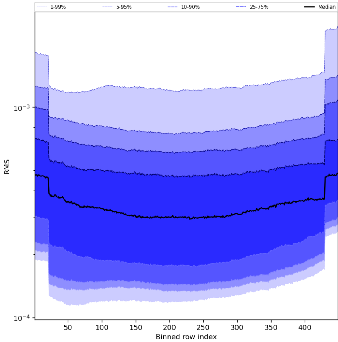
Figure 60: Along track statistics of “RMS” for 2023-11-24 to 2023-11-26
