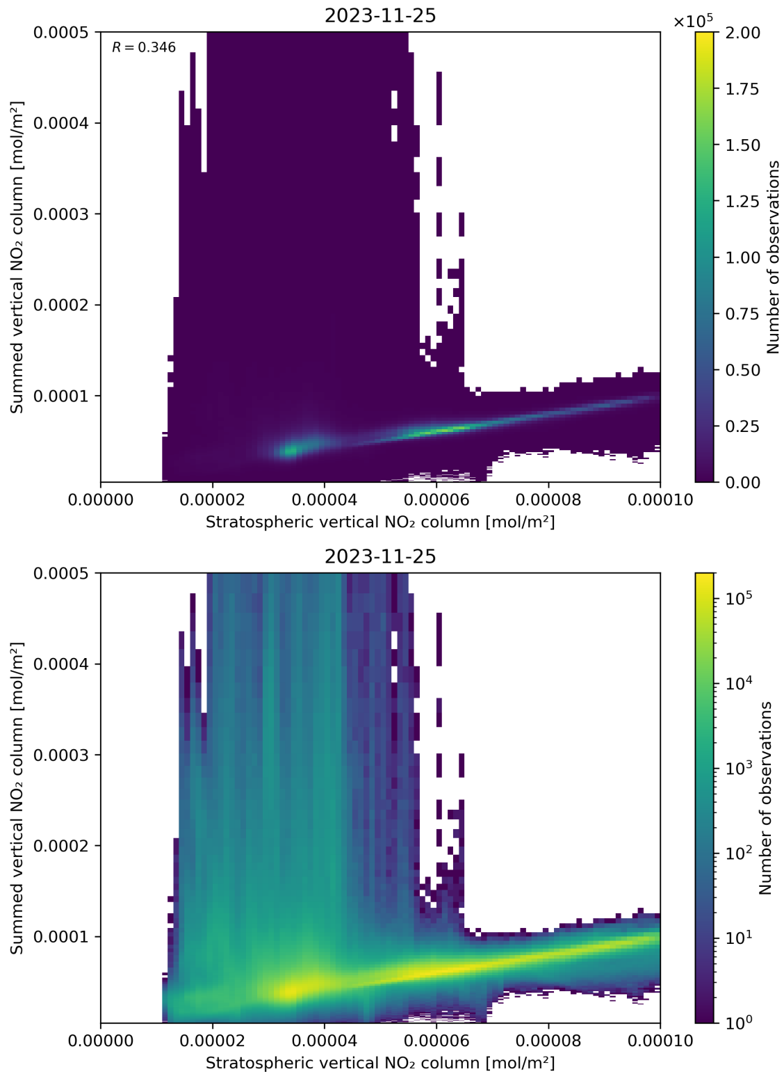
Figure 98: Scatter density plot of “Stratospheric vertical NO 2 column” against “Summed vertical NO 2 column” for 2023-11-24 to 2023-11-26.
