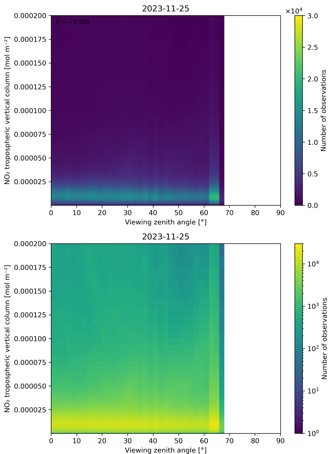
Figure 169: Scatter density plot of “Viewing zenith angle” against “NO 2 tropospheric vertical column” for 2023-11-24 to 2023-11-26.
