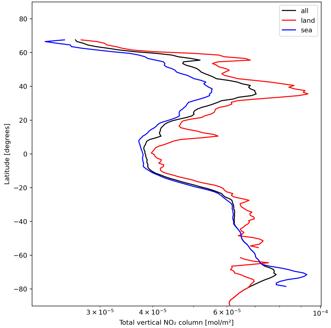
Figure 21: Zonal average of “Total vertical NO 2 column” for 2023-11-24 to 2023-11-26.
