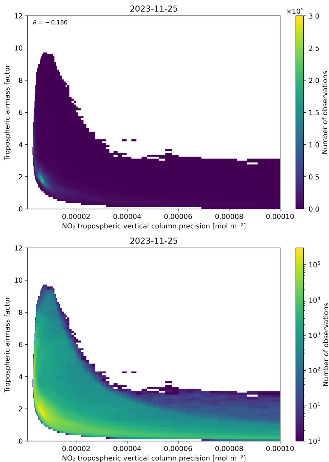
Figure 133: Scatter density plot of “NO 2 tropospheric vertical column precision” against “Tropospheric airmass factor” for 2023-11-24 to 2023-11-26.
