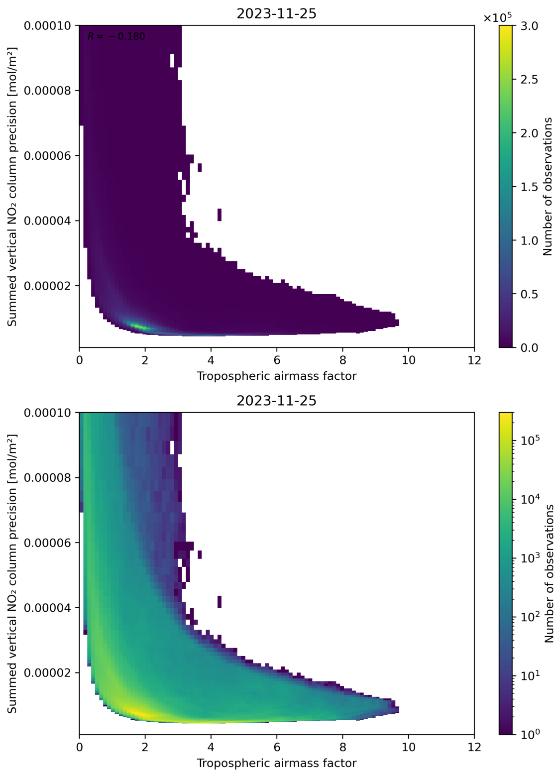
Figure 76: Scatter density plot of “Tropospheric air mass factor” against “Summed vertical NO 2 column precision” for 2023-11-24 to 2023-11-26.
