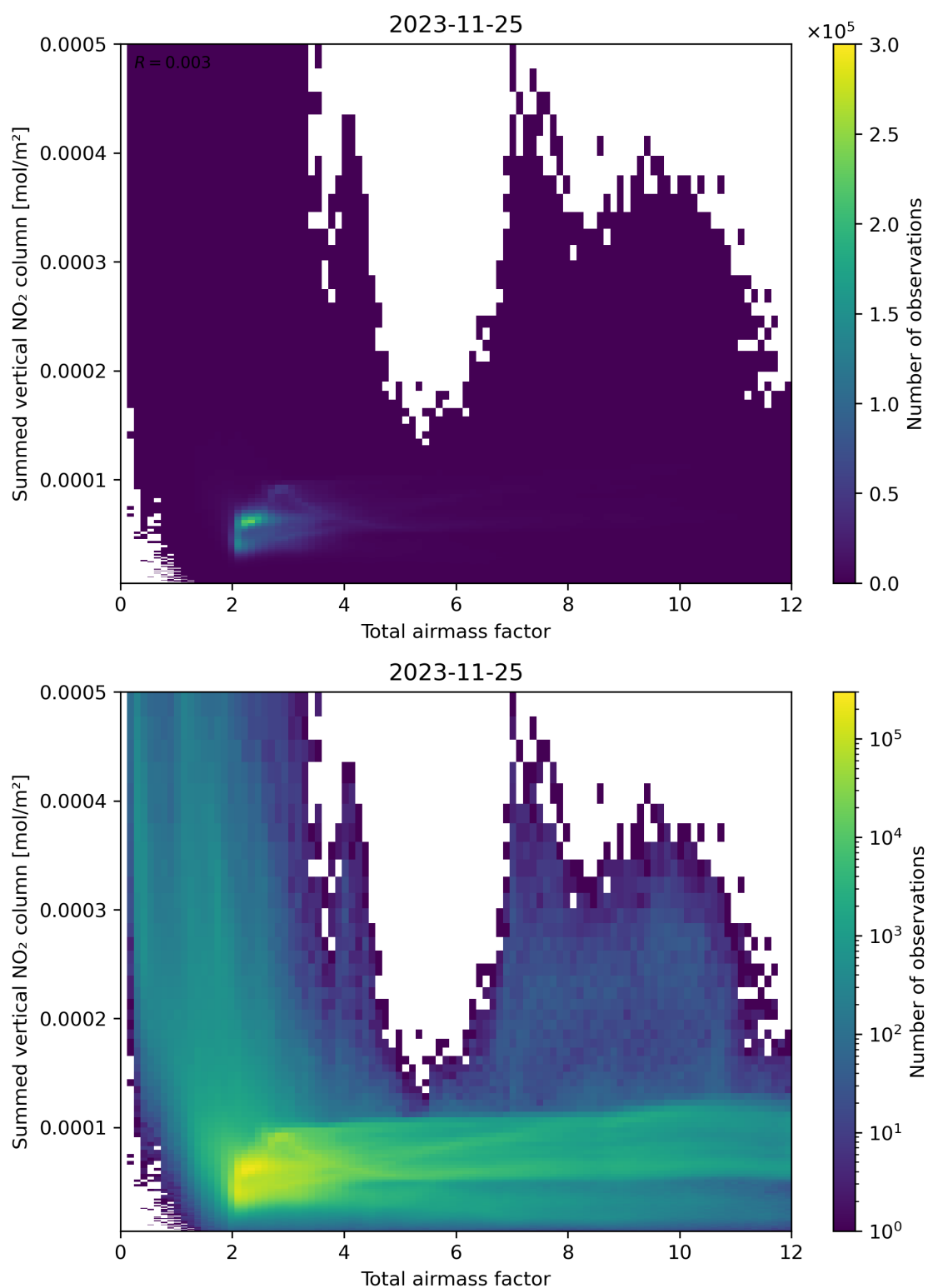
Figure 65: Scatter density plot of “Total airmass factor” against “Summed vertical NO 2 column” for 2023-11-24 to 2023-11-26.
