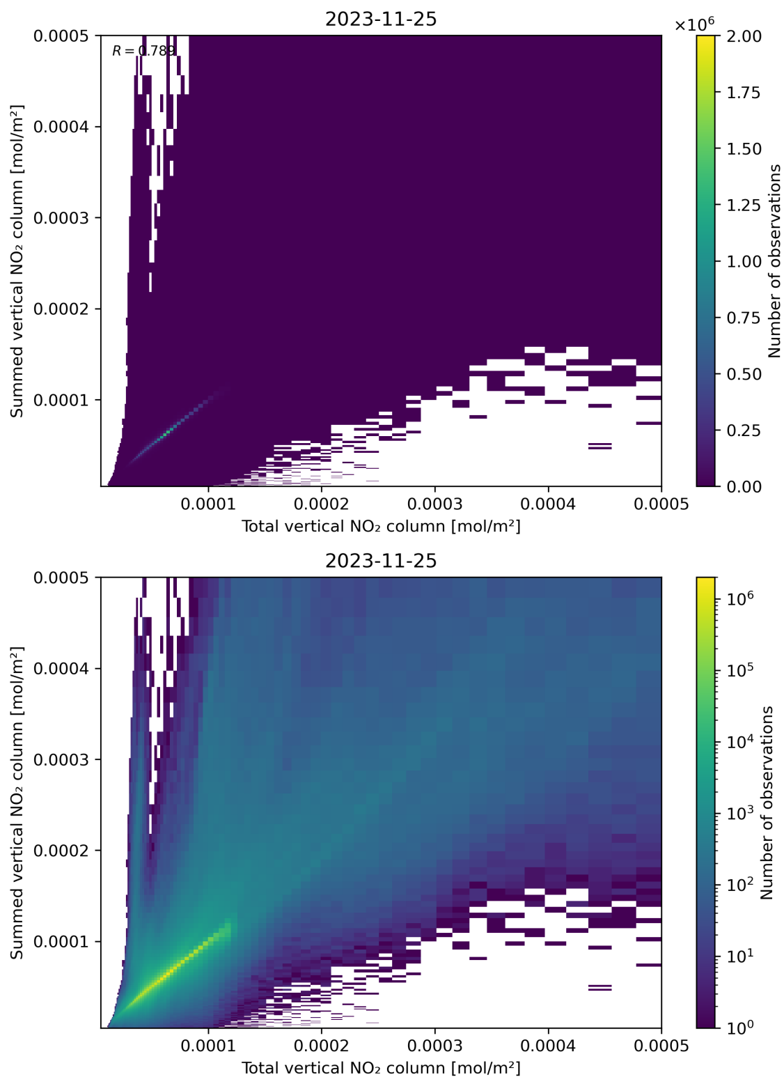
Figure 112: Scatter density plot of “Total vertical NO 2 column” against “Summed vertical NO 2 column” for 2023-11-24 to 2023-11-26.
