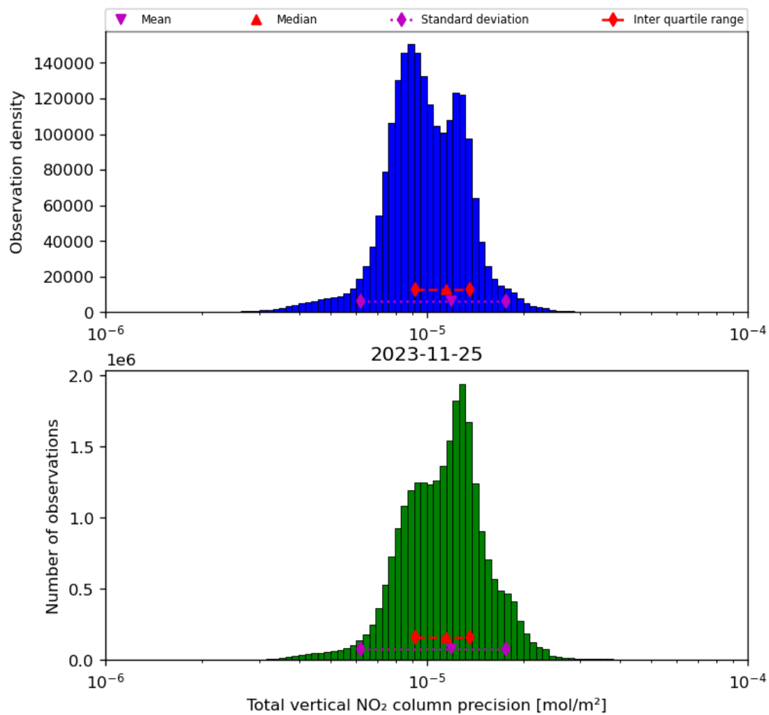
Figure 39: Histogram of “Total vertical NO 2 column precision” for 2023-11-24 to 2023-11-26
