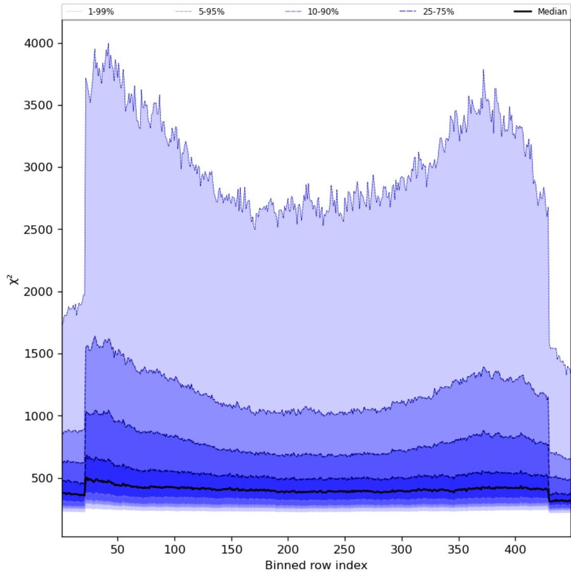
Figure 59: Along track statistics of “ \chi^2 ” for 2023-11-24 to 2023-11-26
