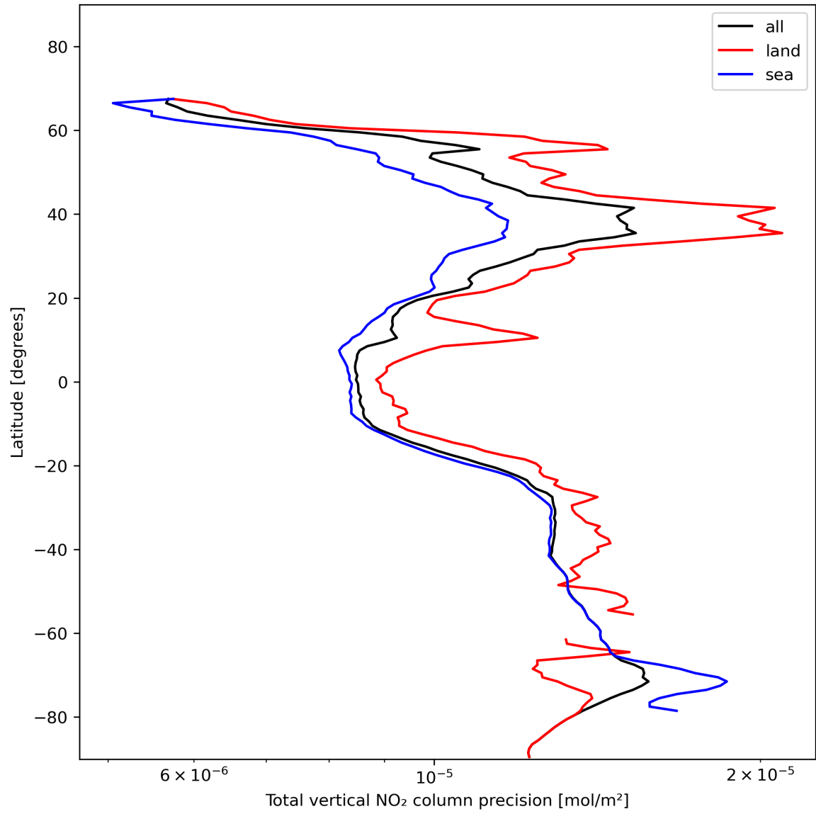
Figure 22: Zonal average of “Total vertical NO 2 column precision” for 2023-11-24 to 2023-11-26.
