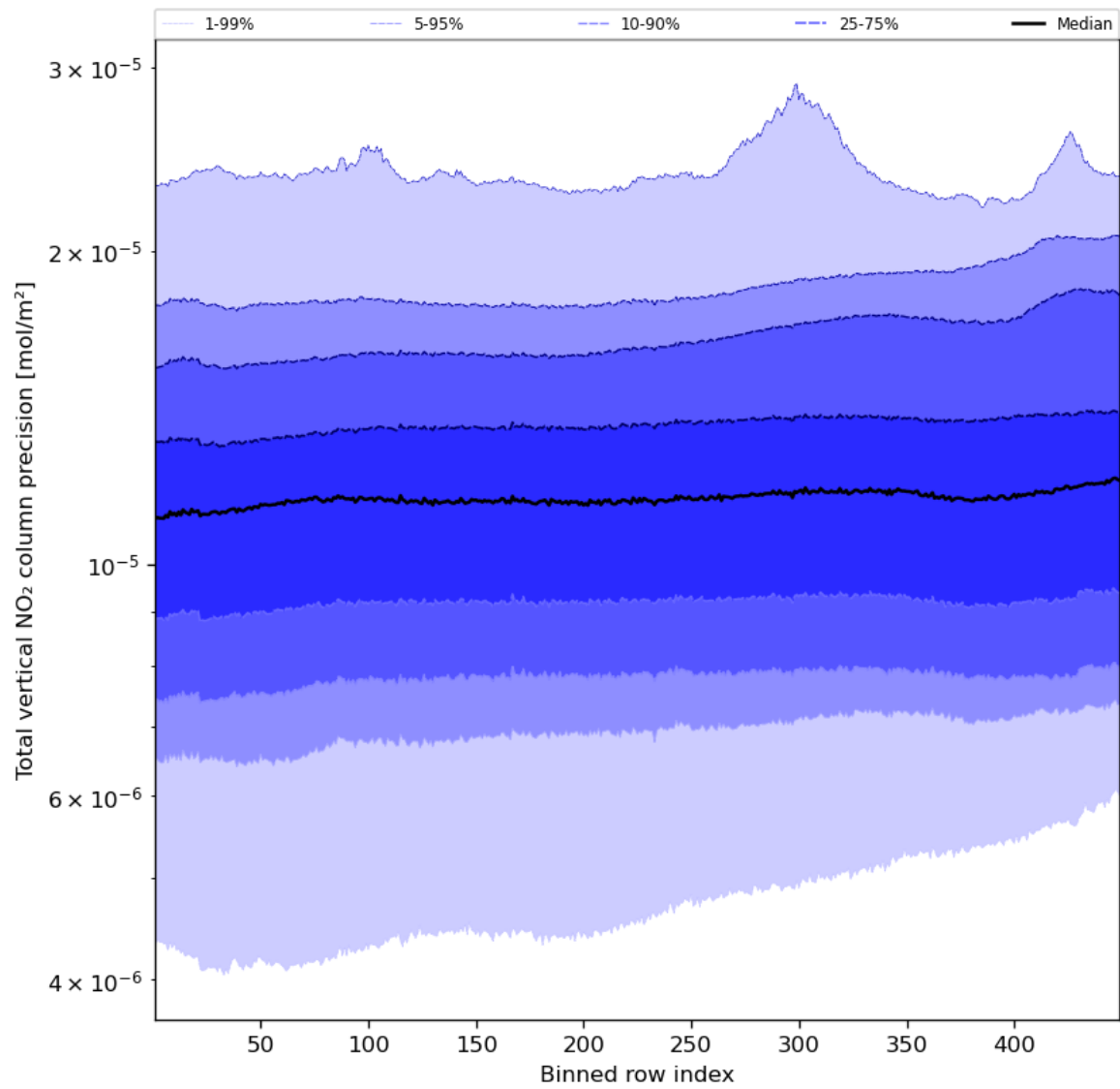
Figure 56: Along track statistics of "Total vertical NO 2 column precision" for 2023-11-24 to 2023-11-26
