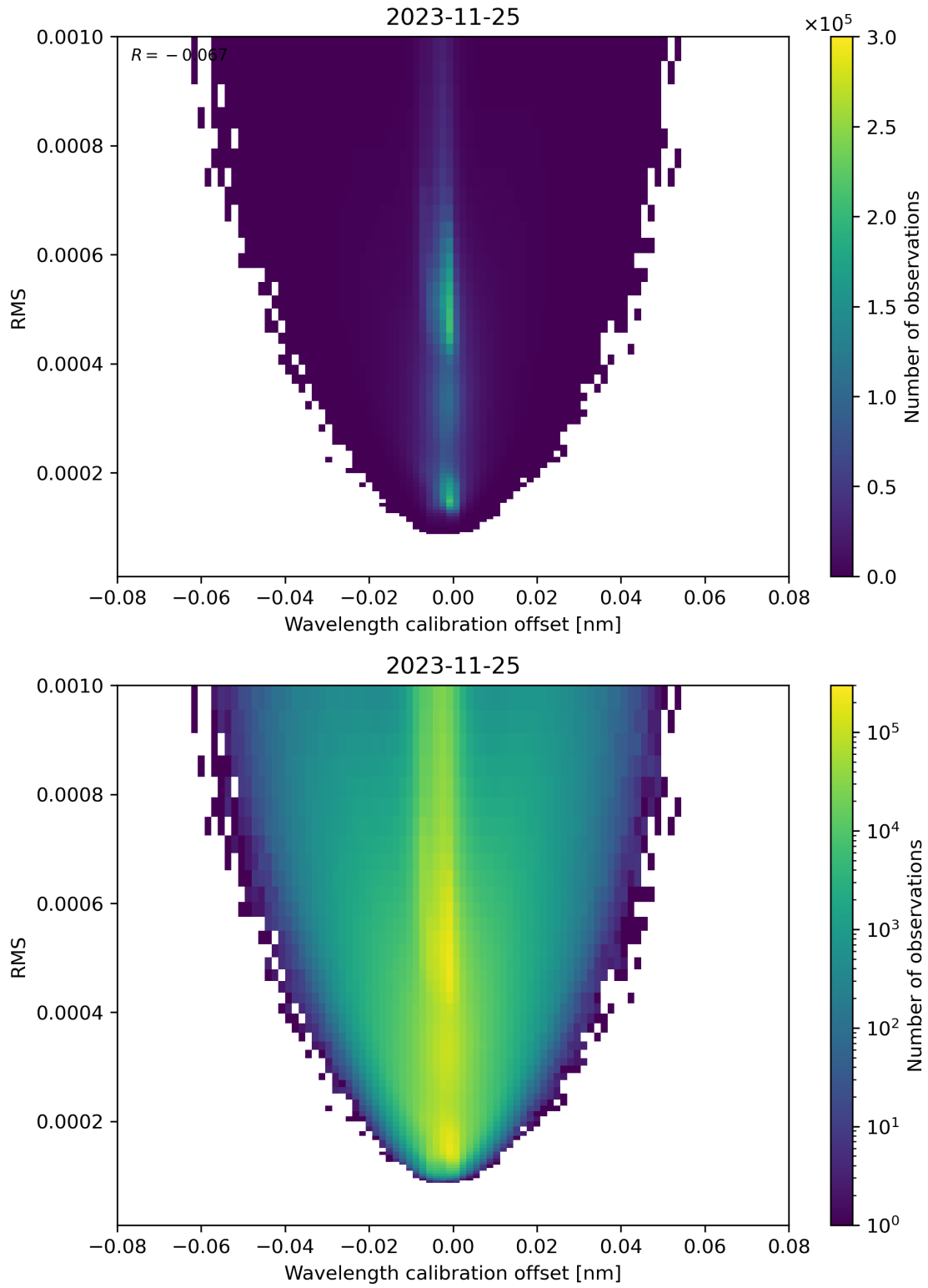
Figure 181: Scatter density plot of “Wavelength calibration offset” against “RMS” for 2023-11-24 to 2023-11-26.
