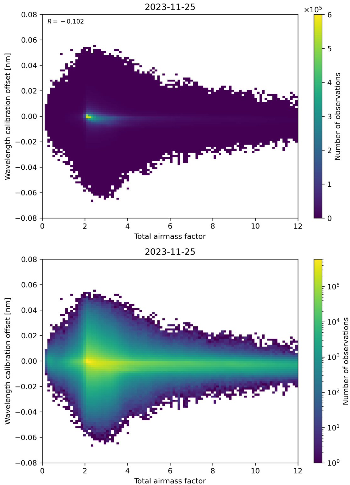
Figure 70: Scatter density plot of “Total airmass factor” against “Wavelength calibration offset” for 2023-11-24 to 2023-11-26.
