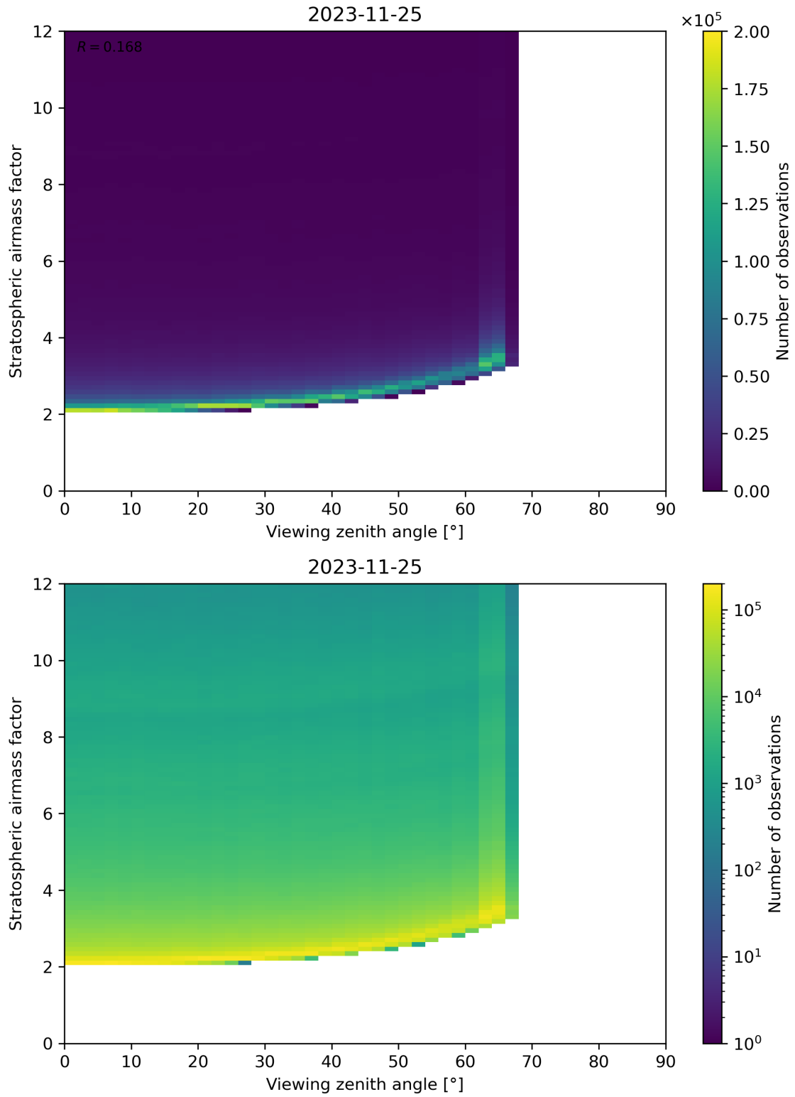
Figure 159: Scatter density plot of “Viewing zenith angle” against “Stratospheric airmass factor” for 2023-11-24 to 2023-11-26.
