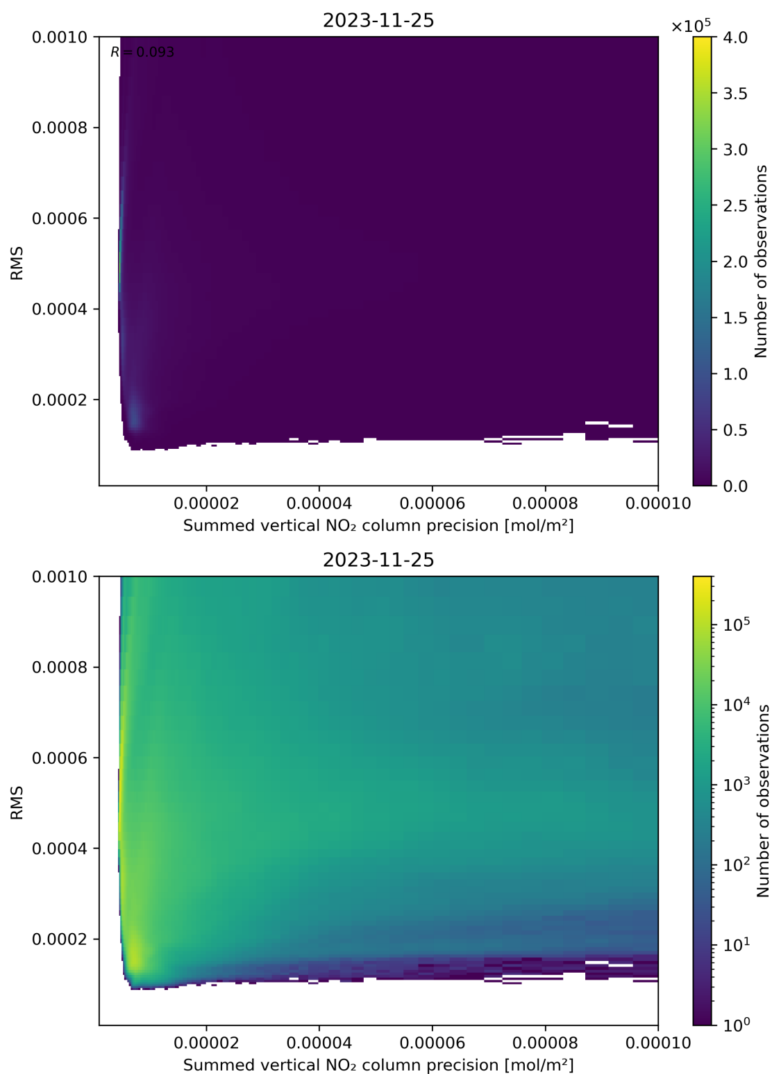
Figure 108: Scatter density plot of “Summed vertical NO 2 column precision” against “RMS” for 2023-11-24 to 2023-11-26.
