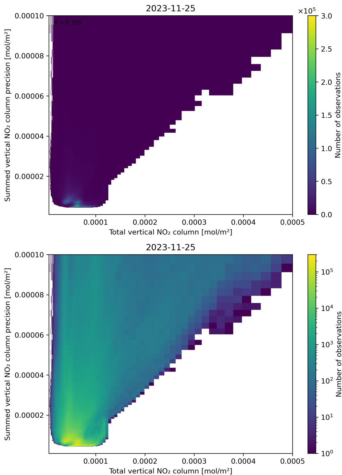
Figure 113: Scatter density plot of “Total vertical NO 2 column” against “Summed vertical NO 2 column precision” for 2023-11-24 to 2023-11-26.
