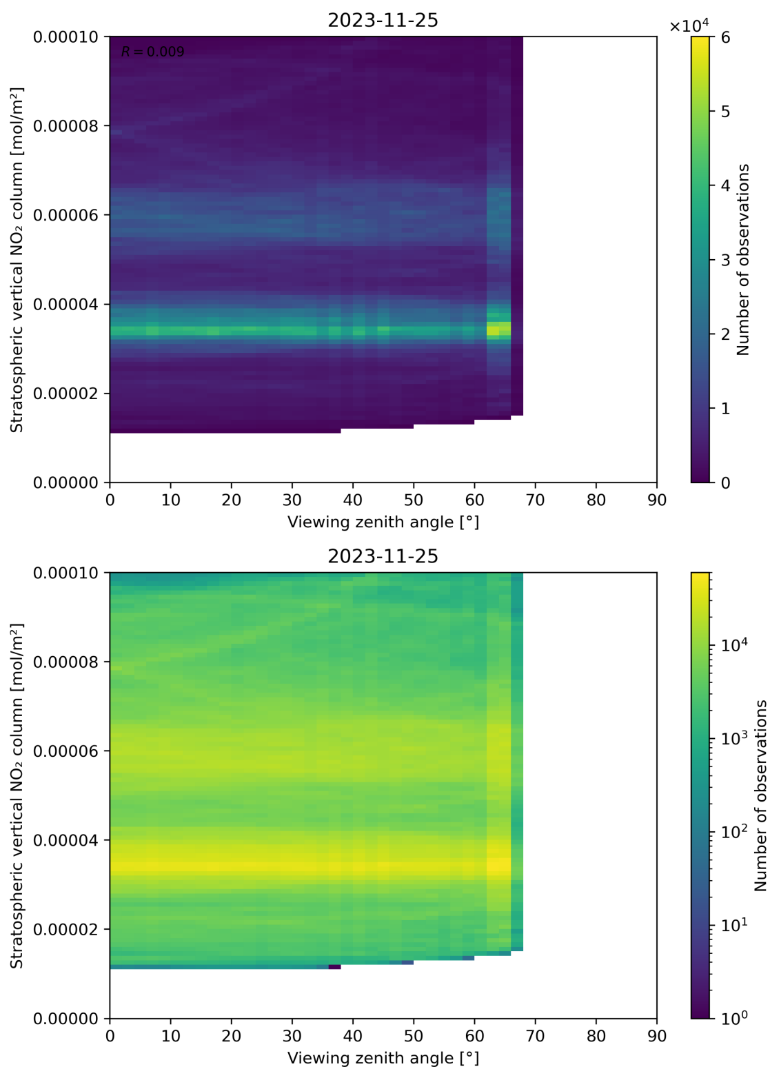
Figure 164: Scatter density plot of “Viewing zenith angle” against “Stratospheric vertical NO 2 column” for 2023-11-24 to 2023-11-26.
