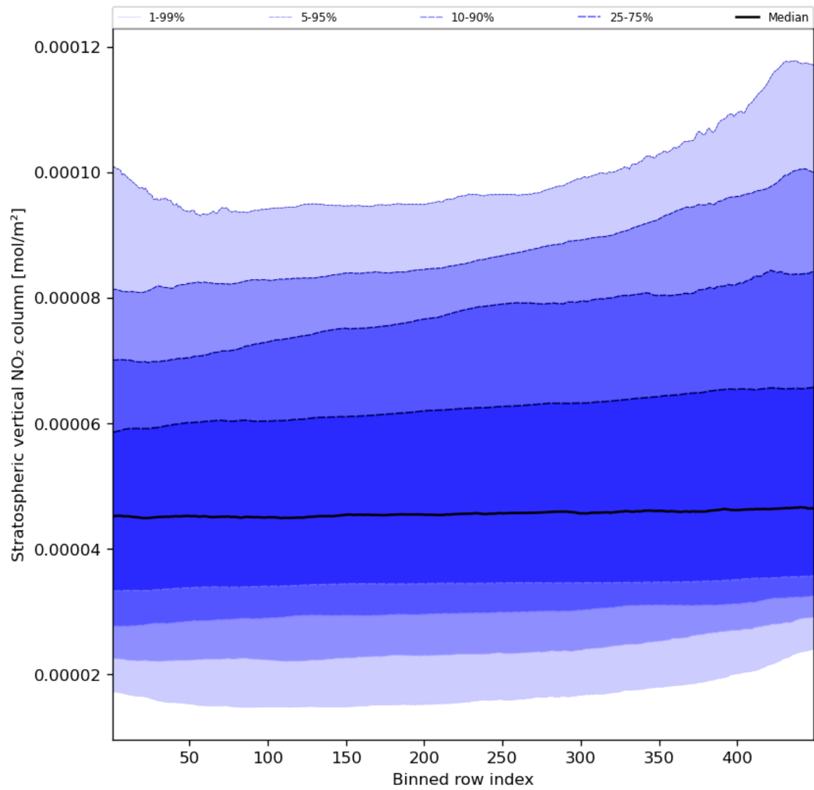
Figure 53: Along track statistics of “Stratospheric vertical NO 2 column” for 2023-11-24 to 2023-11-26
