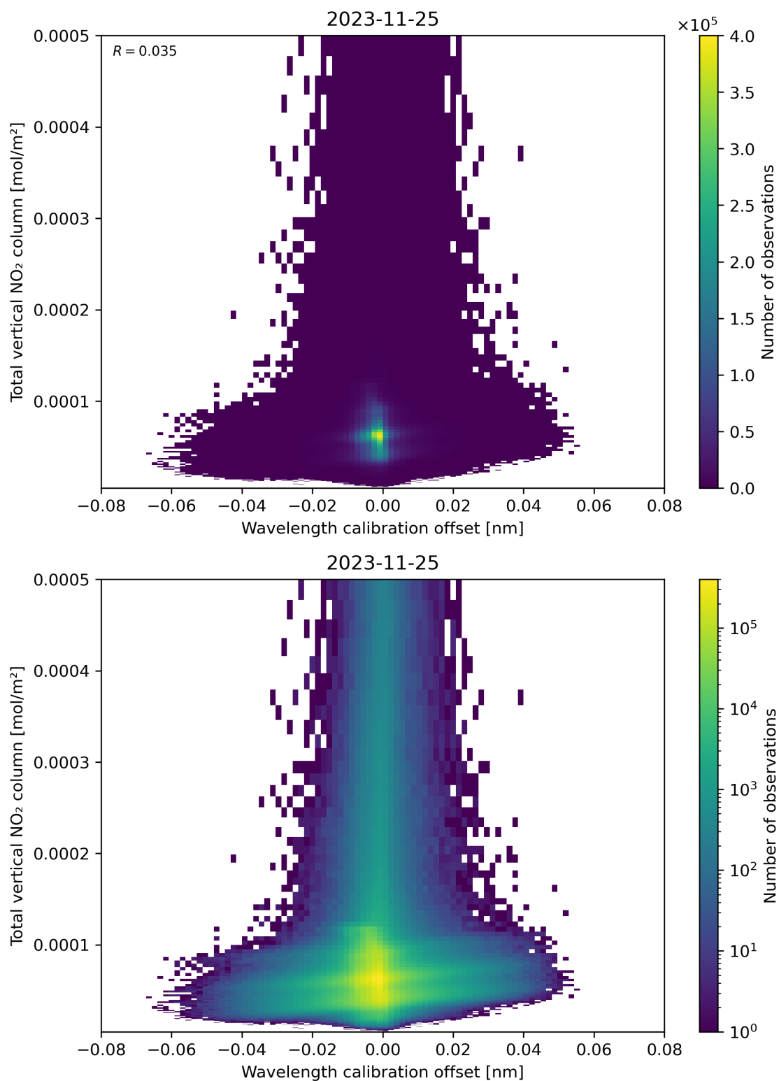
Figure 179: Scatter density plot of “Wavelength calibration offset” against “Total vertical NO 2 column” for 2023-11-24 to 2023-11-26.
