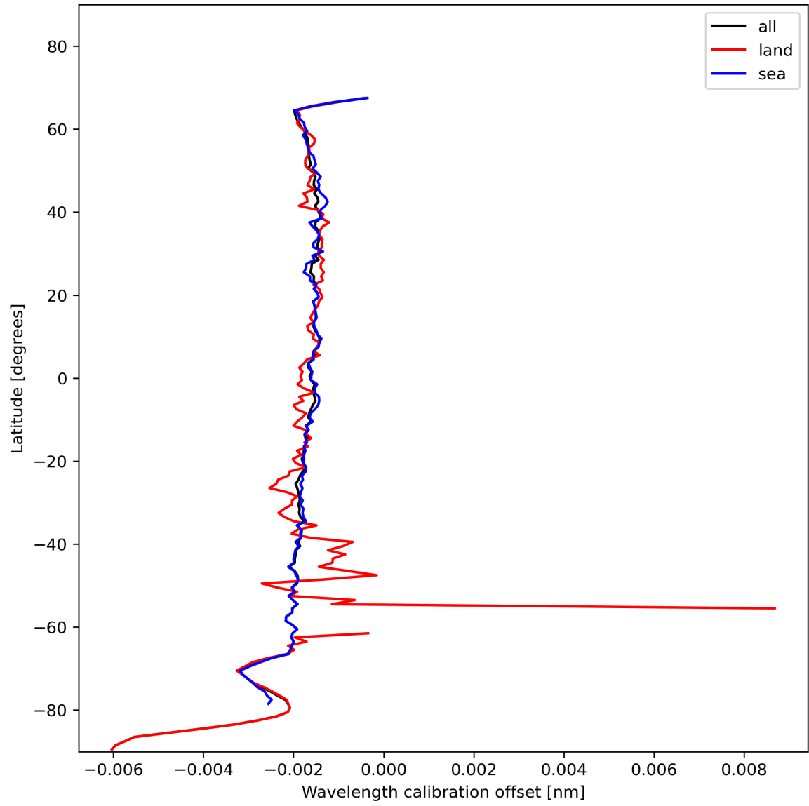
Figure 18: Zonal average of “Wavelength calibration offset” for 2023-11-24 to 2023-11-26.
