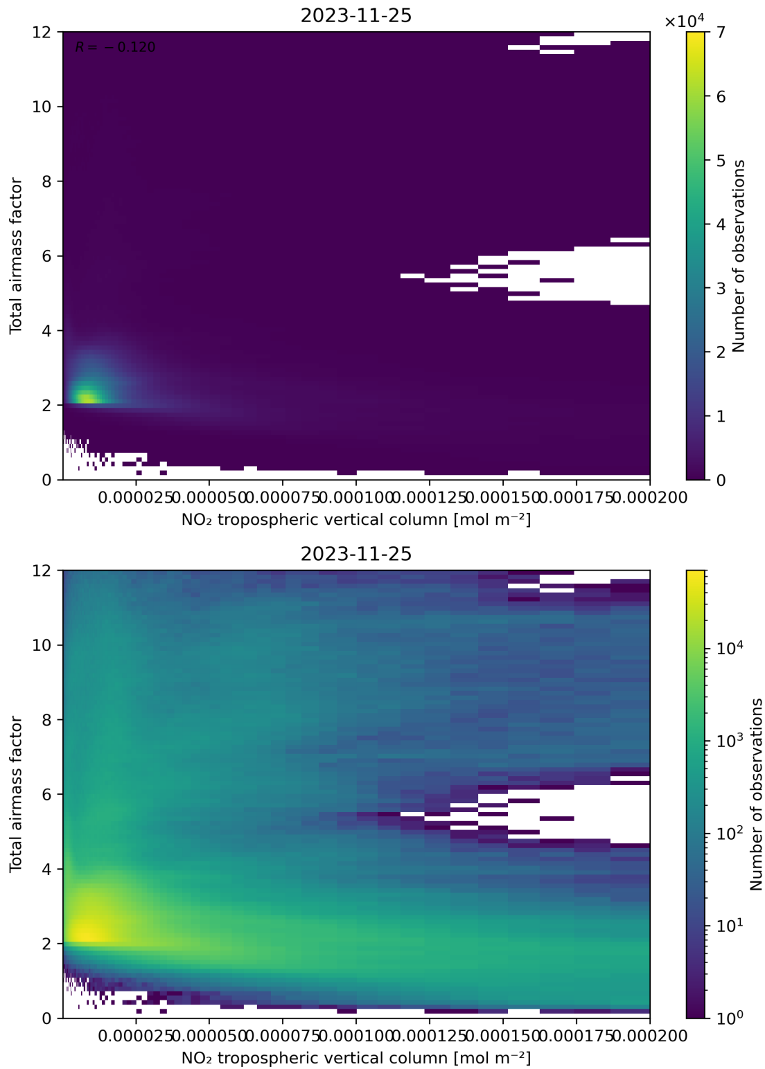
Figure 122: Scatter density plot of “NO 2 tropospheric vertical column” against “Total air mass factor” for 2023-11-24 to 2023-11-26.
