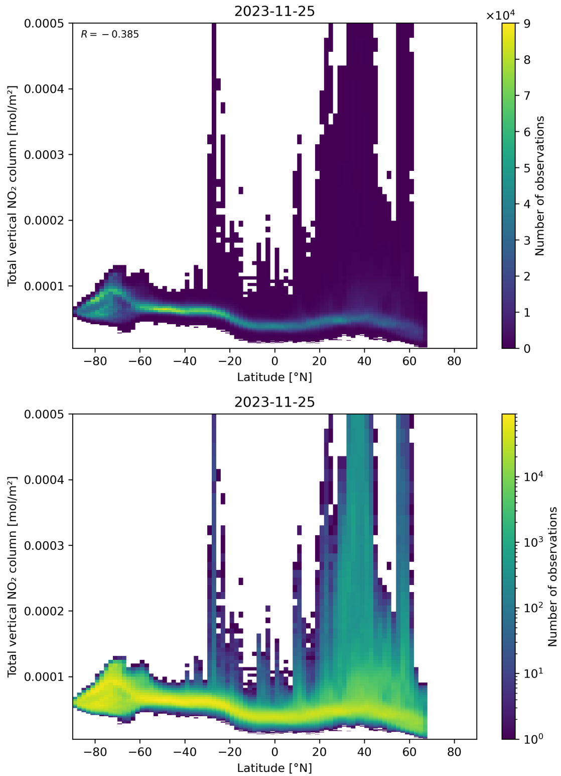
Figure 90: Scatter density plot of “Latitude” against “Total vertical NO 2 column” for 2023-11-24 to 2023-11-26.
