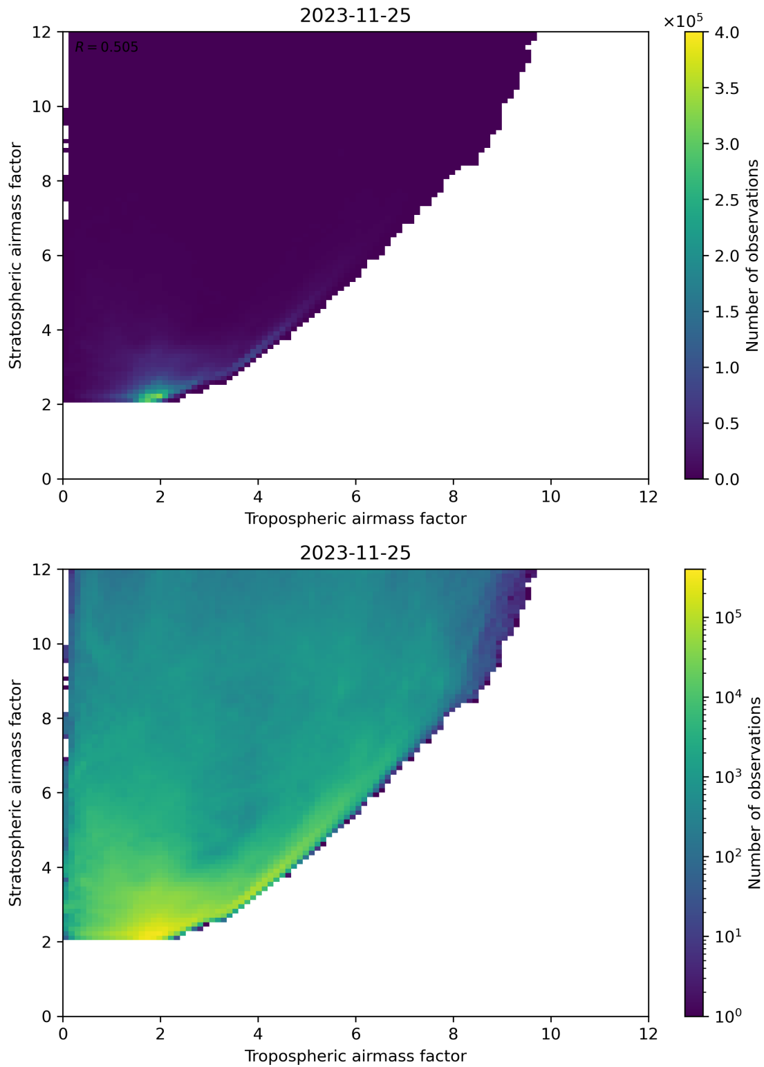
Figure 71: Scatter density plot of “Tropospheric airmass factor” against “Stratospheric airmass factor” for 2023-11-24 to 2023-11-26.
