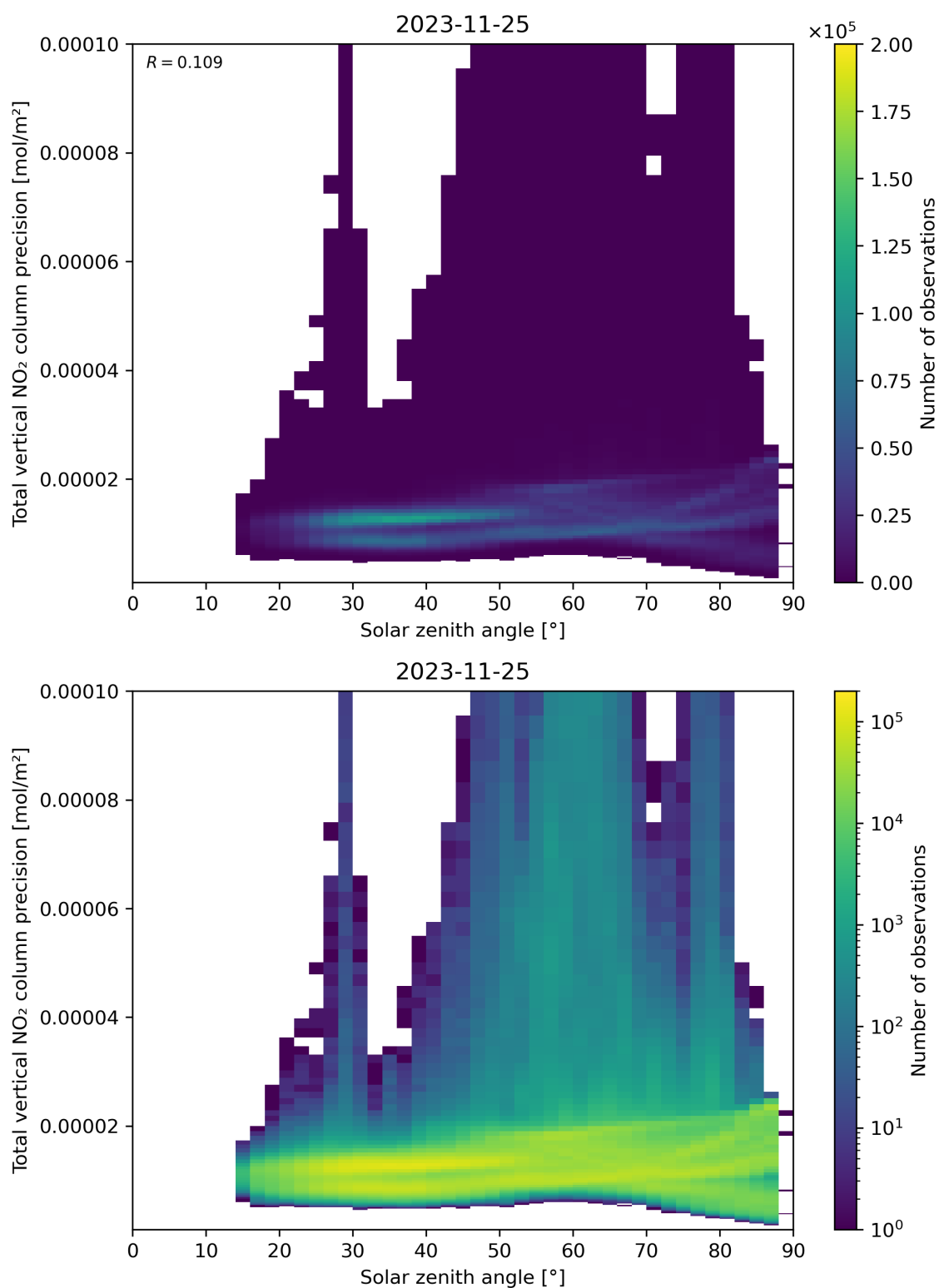
Figure 154: Scatter density plot of “Solar zenith angle” against “Total vertical NO 2 column precision” for 2023-11-24 to 2023-11-26.
