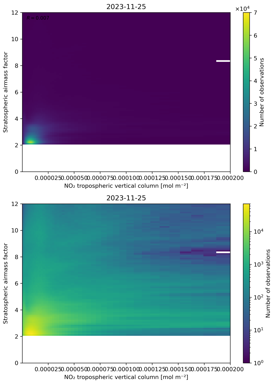
Figure 121: Scatter density plot of “NO 2 tropospheric vertical column” against “Stratospheric airmass factor” for 2023-11-24 to 2023-11-26.
