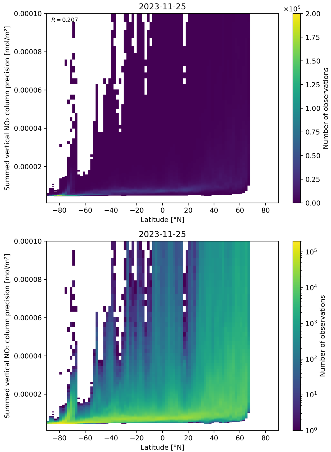
Figure 89: Scatter density plot of “Latitude” against “Summed vertical NO 2 column precision” for 2023-11-24 to 2023-11-26.
