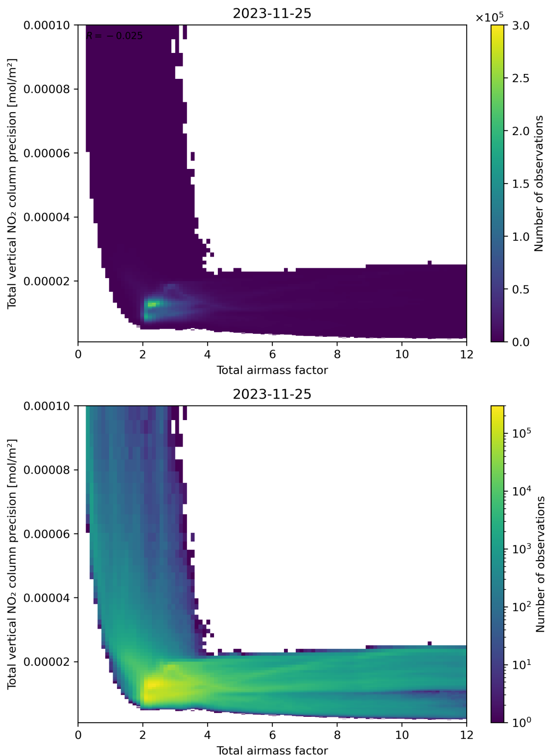
Figure 68: Scatter density plot of “Total airmass factor” against “Total vertical NO 2 column precision” for 2023-11-24 to 2023-11-26.
