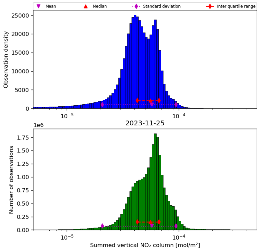
Figure 40: Histogram of “Summed vertical NO 2 column” for 2023-11-24 to 2023-11-26
