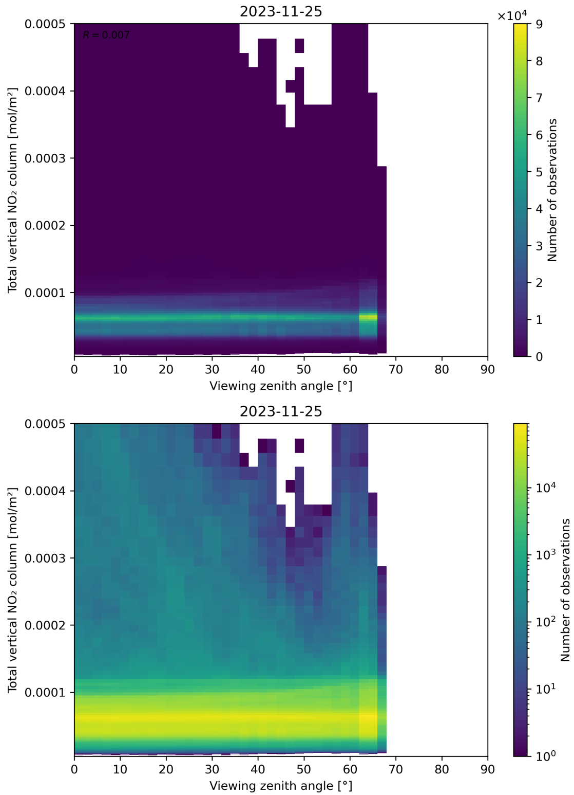
Figure 167: Scatter density plot of “Viewing zenith angle” against “Total vertical NO 2 column” for 2023-11-24 to 2023-11-26.
