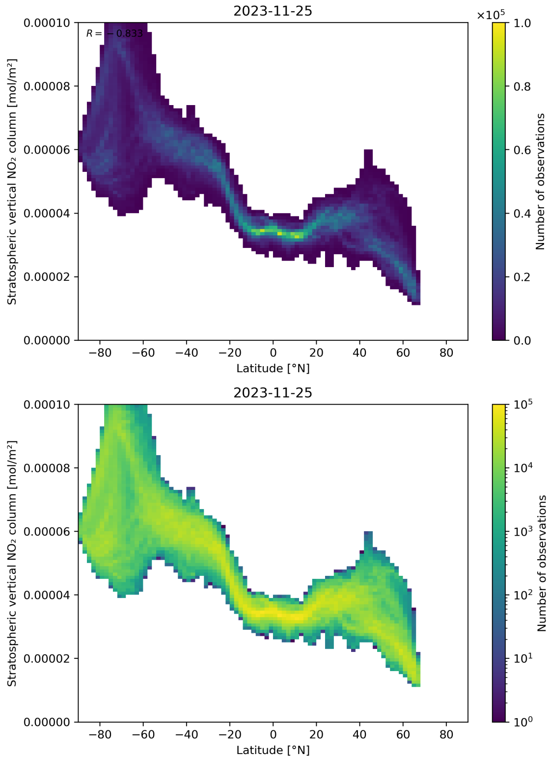
Figure 87: Scatter density plot of “Latitude” against “Stratospheric vertical NO 2 column” for 2023-11-24 to 2023-11-26.
