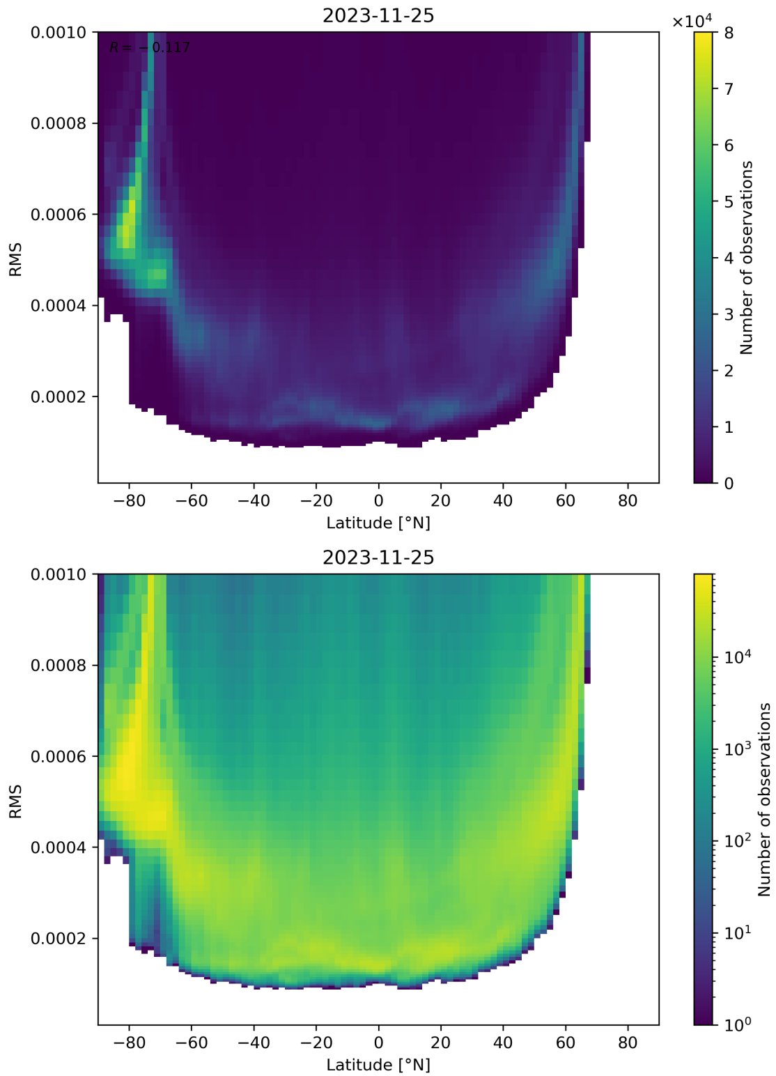
Figure 94: Scatter density plot of “Latitude” against “RMS” for 2023-11-24 to 2023-11-26.
