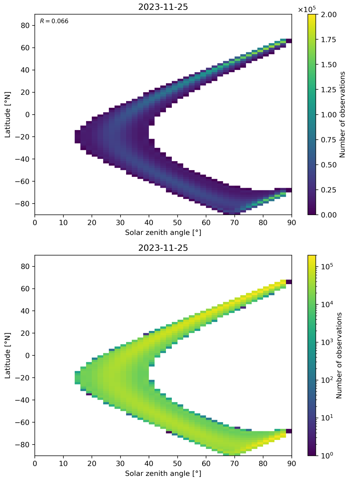
Figure 149: Scatter density plot of “Solar zenith angle” against “Latitude” for 2023-11-24 to 2023-11-26.
