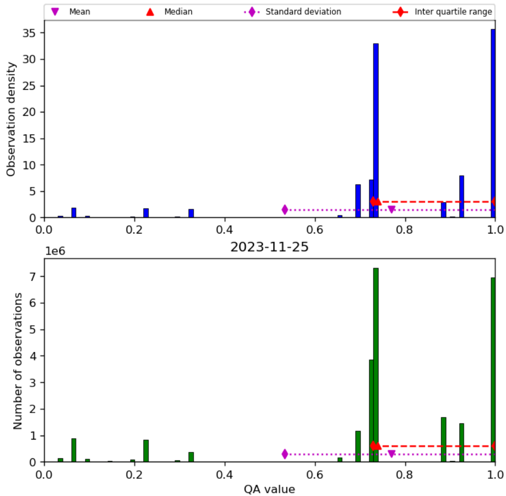
Figure 28: Histogram of “QA value” for 2023-11-24 to 2023-11-26
