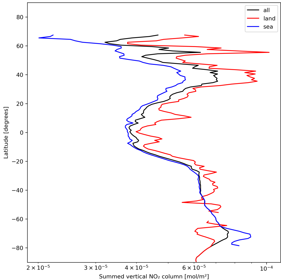
Figure 23: Zonal average of “Summed vertical NO 2 column” for 2023-11-24 to 2023-11-26.
