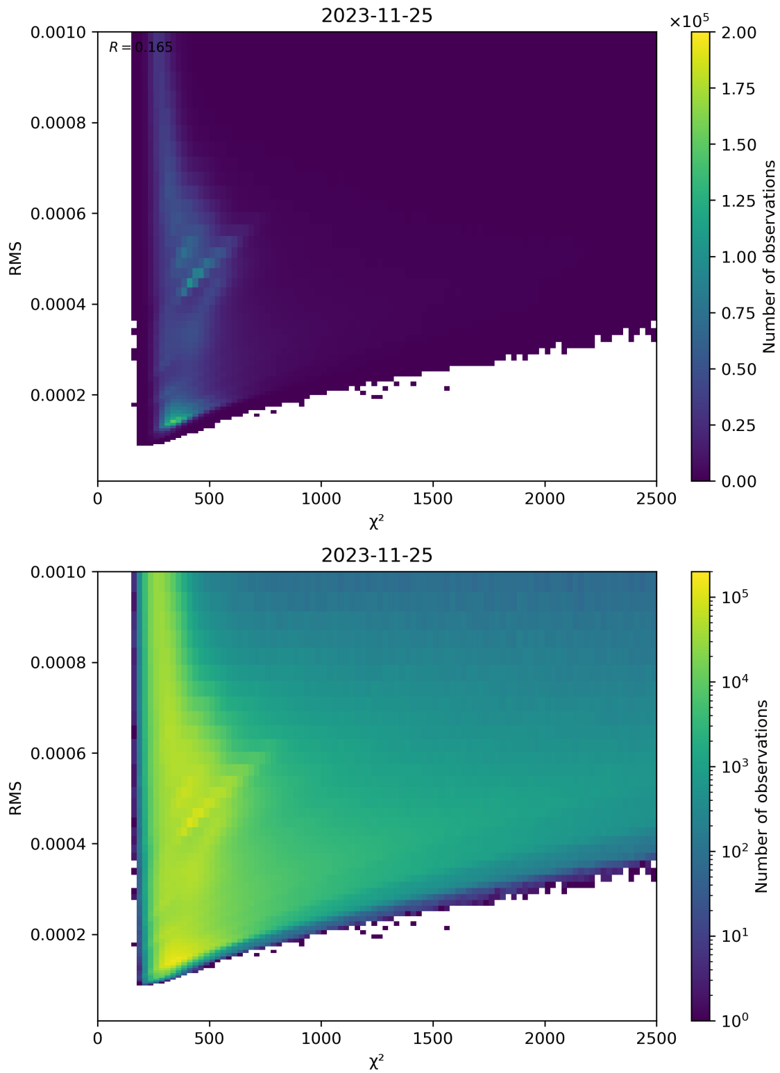
Figure 82: Scatter density plot of “ \chi^2 ” against “RMS” for 2023-11-24 to 2023-11-26.
