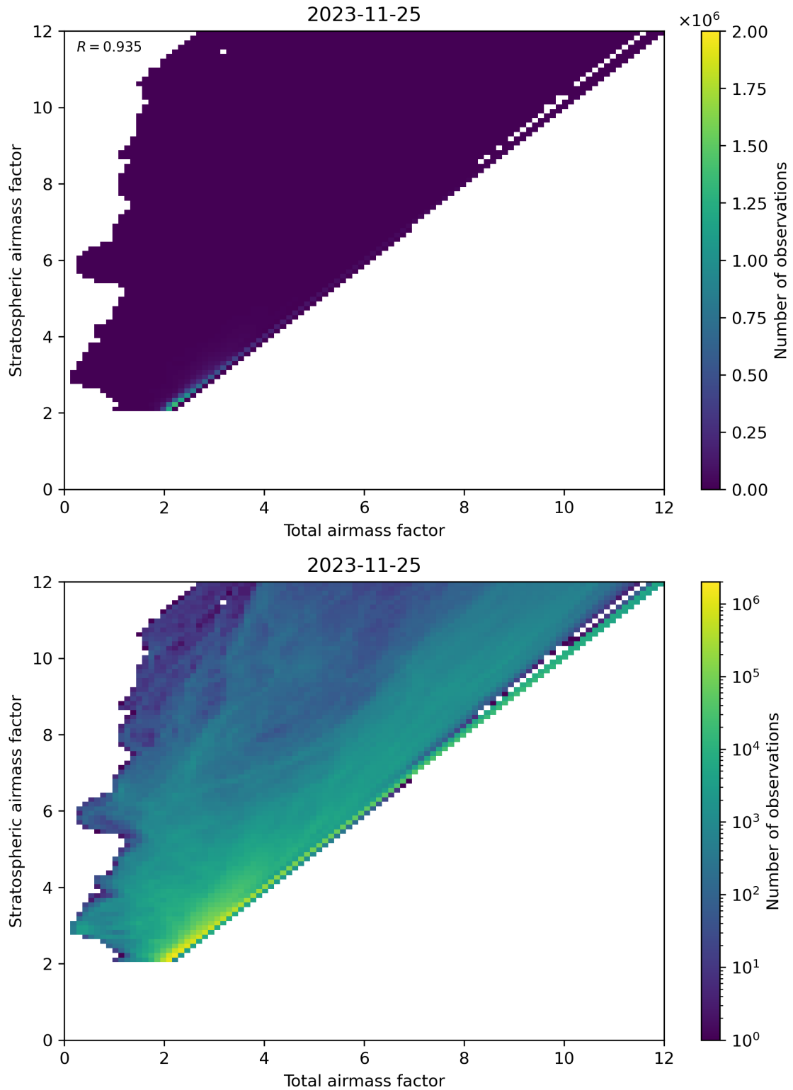
Figure 62: Scatter density plot of “Total airmass factor” against “Stratospheric airmass factor” for 2023-11-24 to 2023-11-26.
