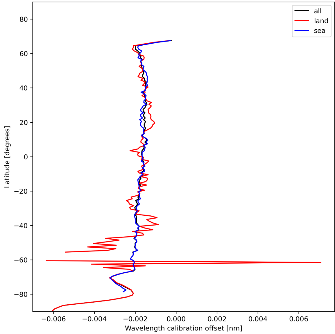
Figure 18: Zonal average of “Wavelength calibration offset” for 2023-11-25 to 2023-11-27.
