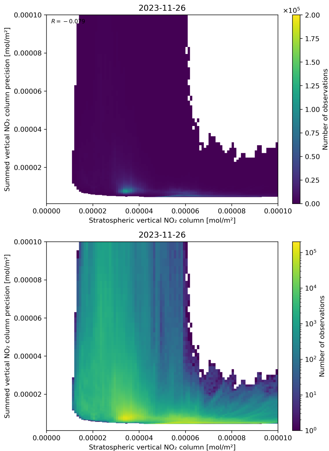
Figure 99: Scatter density plot of “Stratospheric vertical NO 2 column” against “Summed vertical NO 2 column precision” for 2023-11-25 to 2023-11-27.
