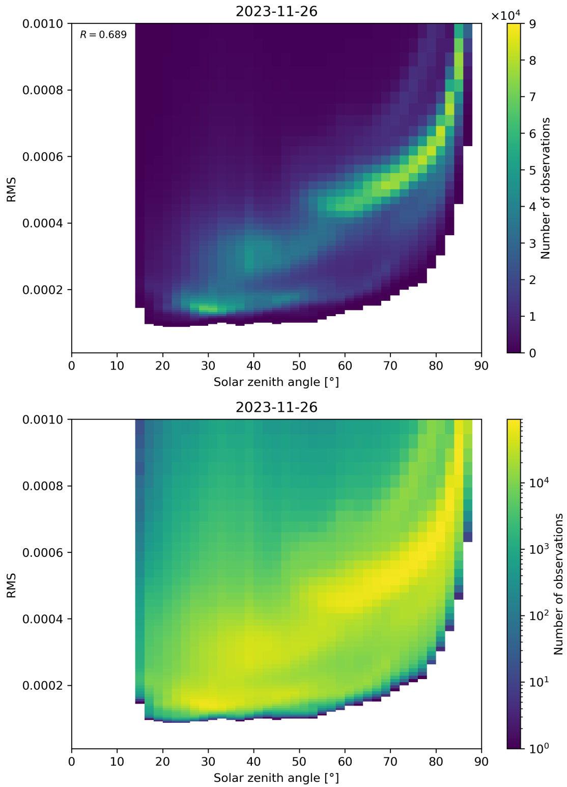
Figure 157: Scatter density plot of “Solar zenith angle” against “RMS” for 2023-11-25 to 2023-11-27.
