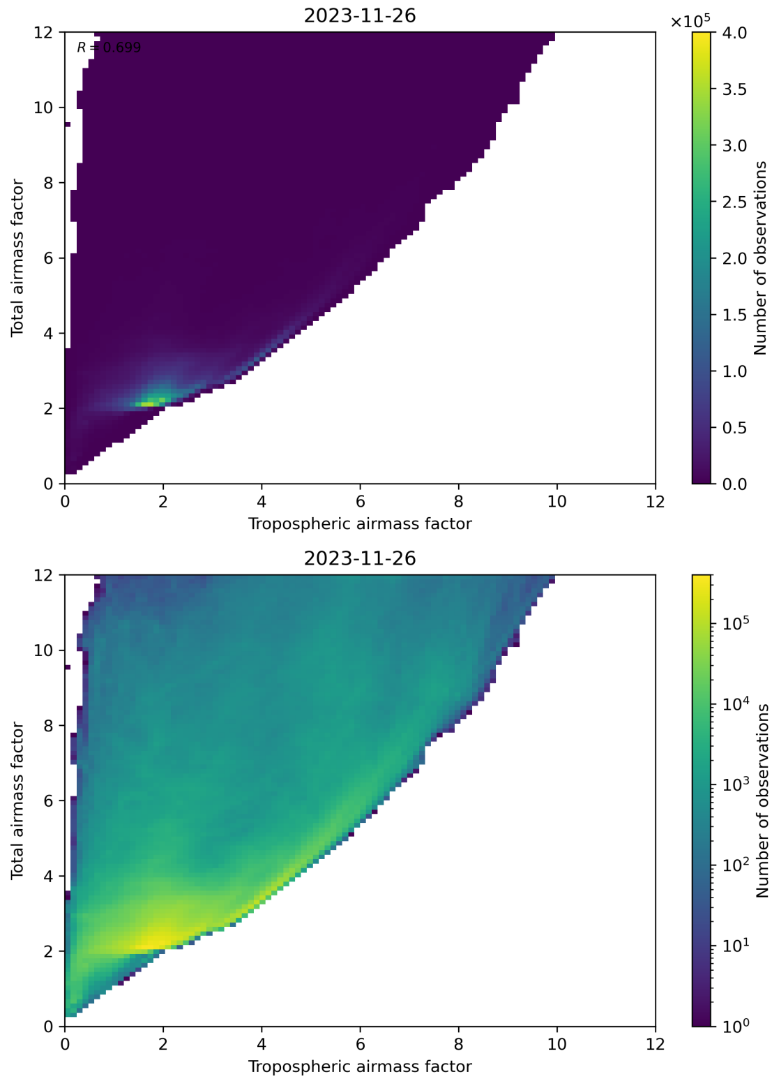
Figure 72: Scatter density plot of “Tropospheric airmass factor” against “Total airmass factor” for 2023-11-25 to 2023-11-27.
