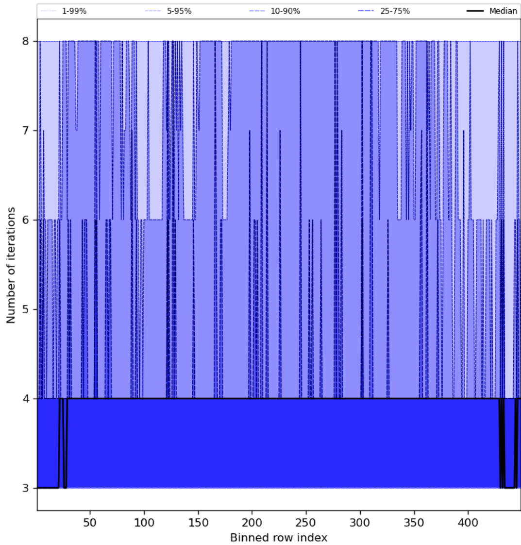
Figure 51: Along track statistics of “Number of iterations” for 2023-11-25 to 2023-11-27
