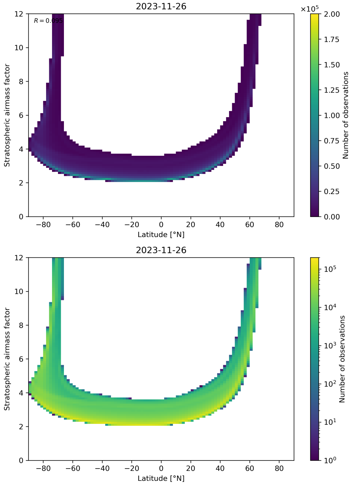
Figure 83: Scatter density plot of “Latitude” against “Stratospheric airmass factor” for 2023-11-25 to 2023-11-27.
