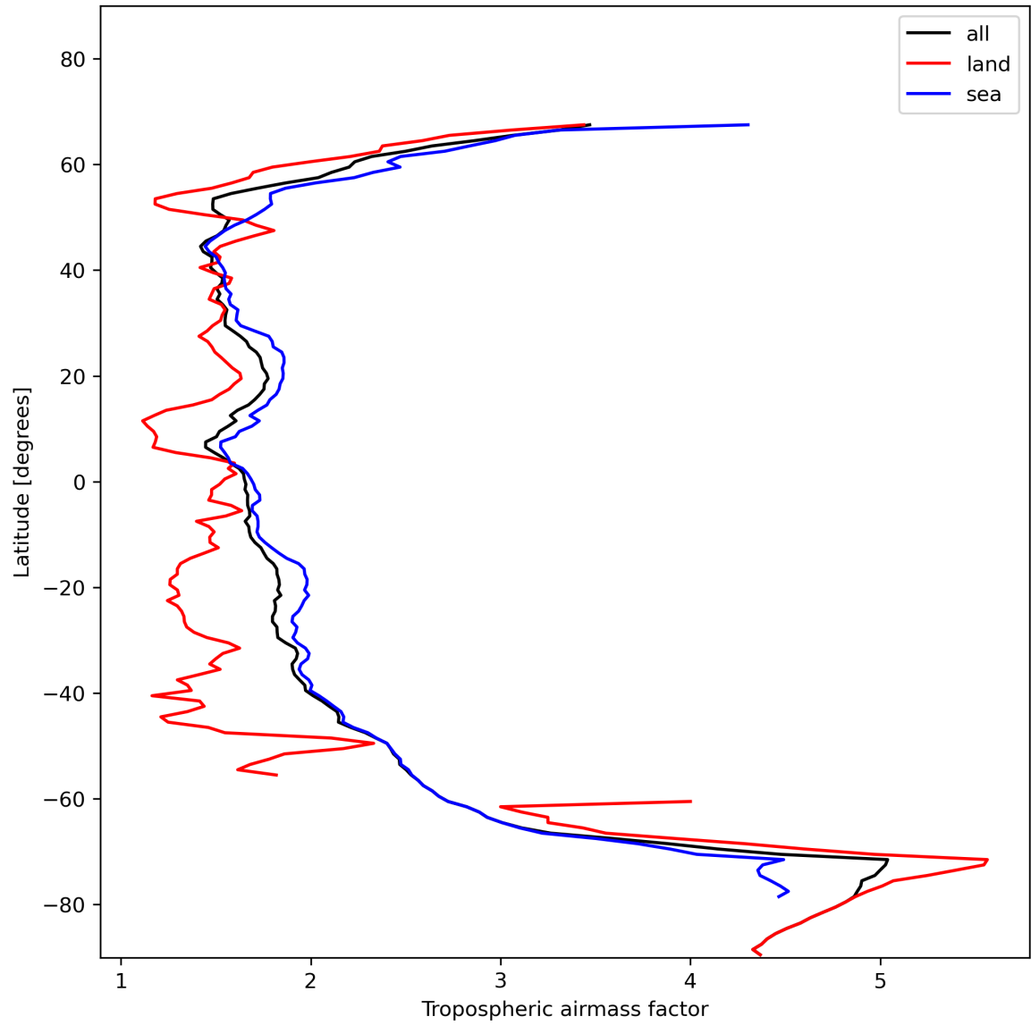
Figure 14: Zonal average of “Tropospheric airmass factor” for 2023-11-25 to 2023-11-27.
