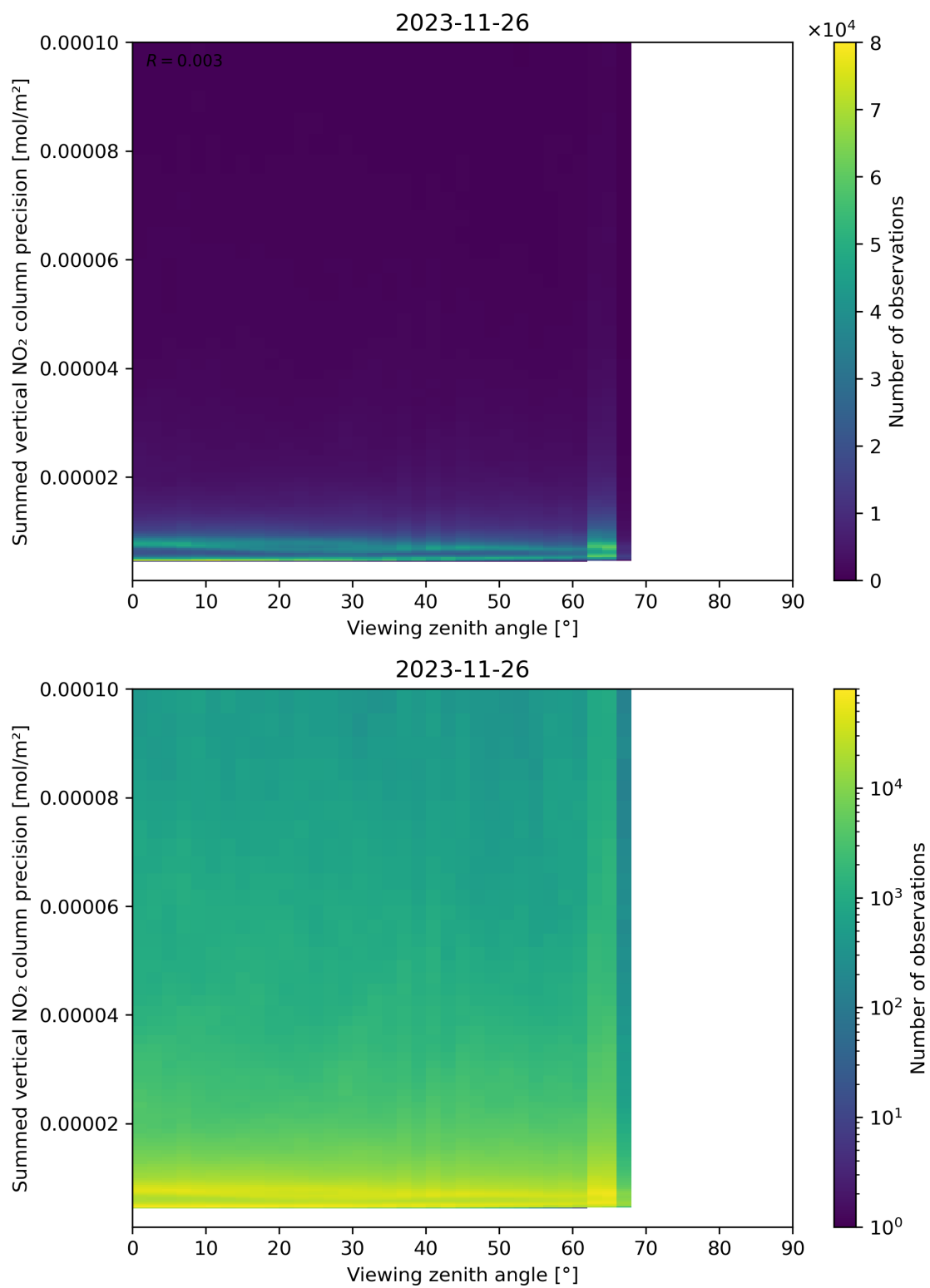
Figure 166: Scatter density plot of “Viewing zenith angle” against “Summed vertical NO 2 column precision” for 2023-11-25 to 2023-11-27.
