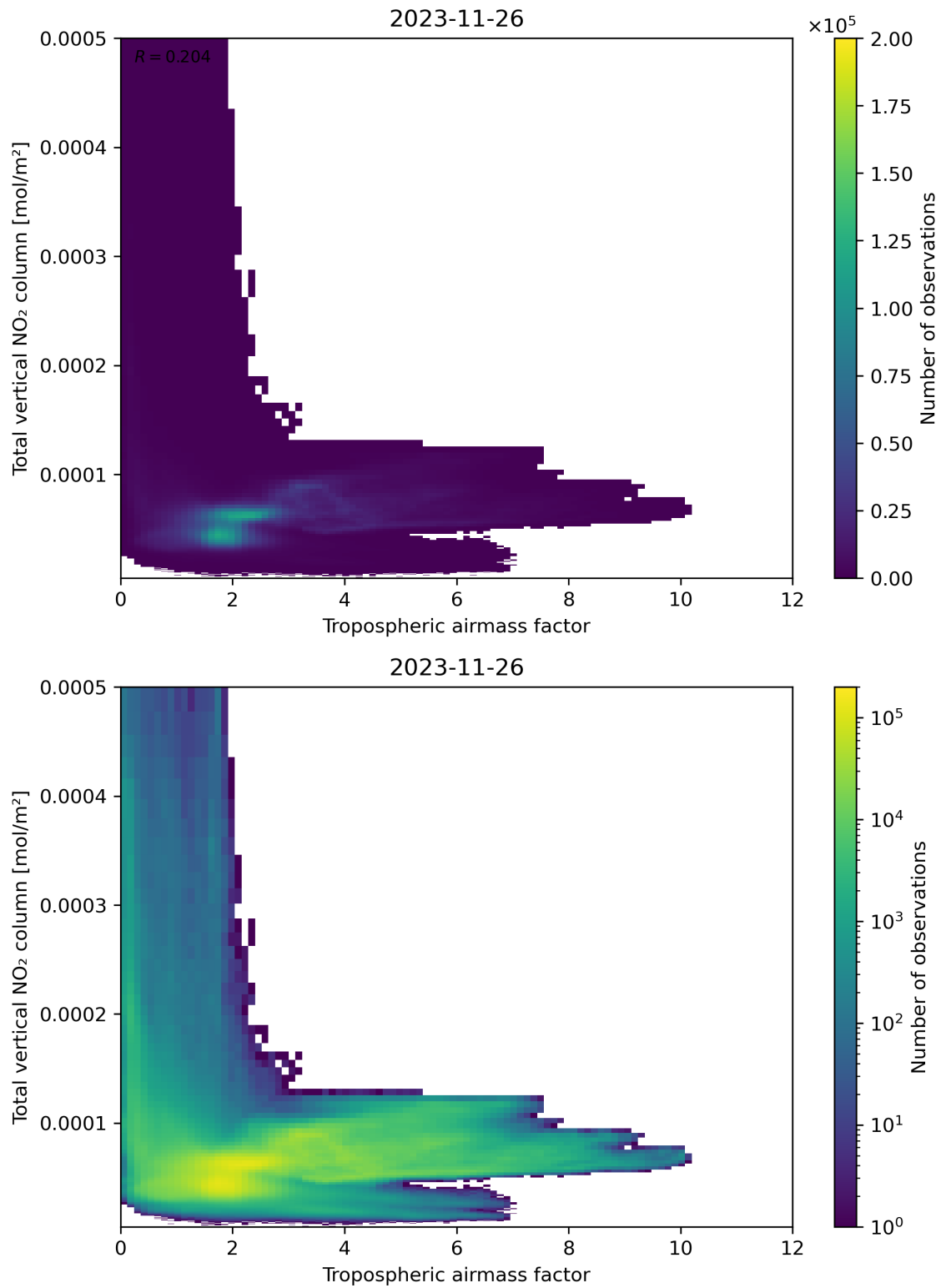
Figure 77: Scatter density plot of “Tropospheric airmass factor” against “Total vertical \text{NO}_2 column” for 2023-11-25 to 2023-11-27.
