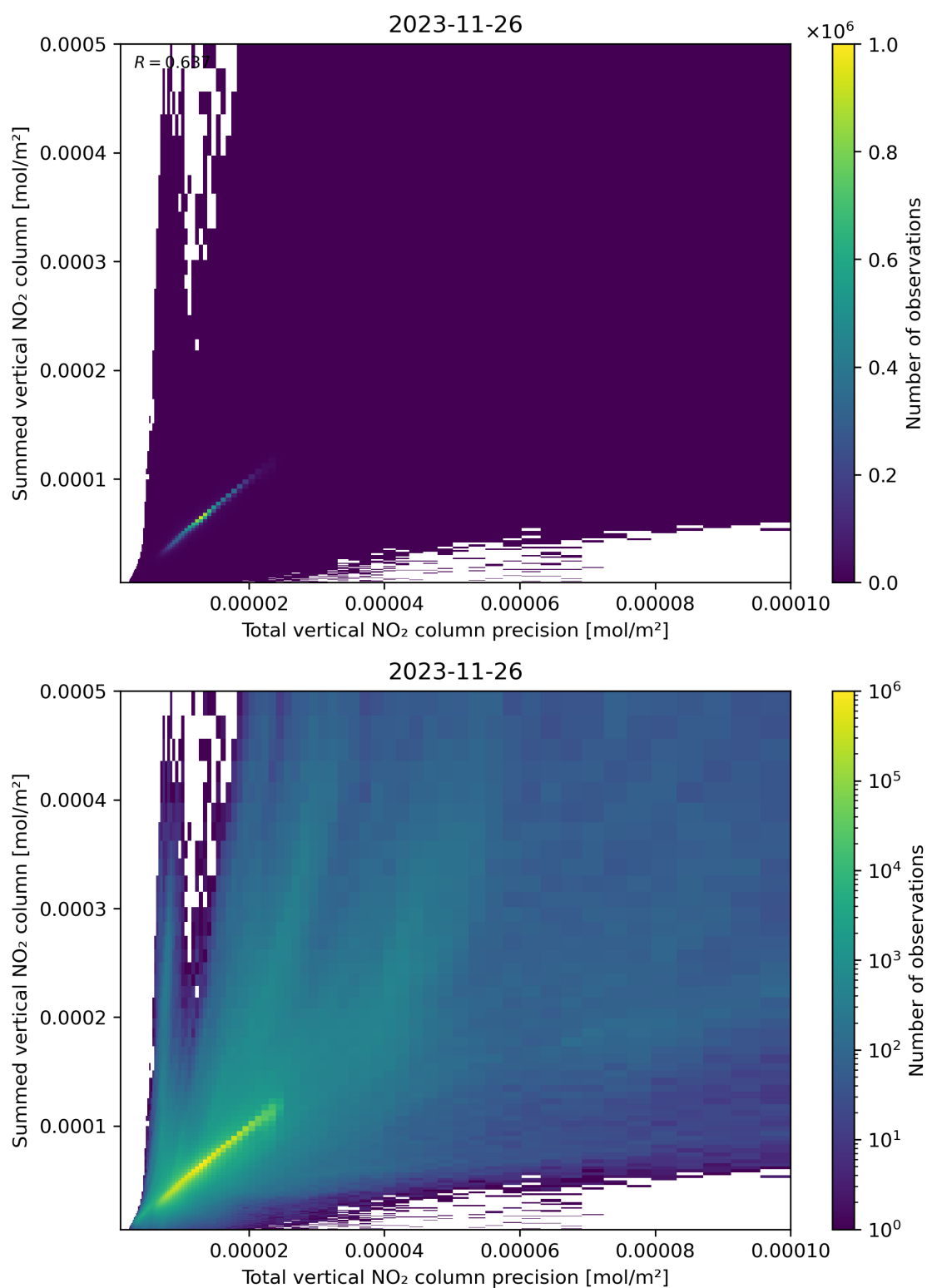
Figure 117: Scatter density plot of “Total vertical NO 2 column precision” against “Summed vertical NO 2 column” for 2023-11-25 to 2023-11-27.
