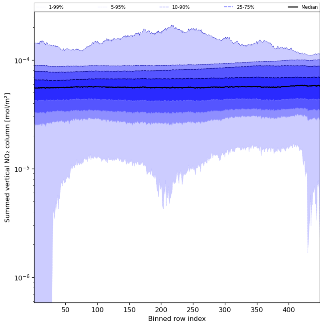
Figure 57: Along track statistics of “Summed vertical NO 2 column” for 2023-11-25 to 2023-11-27
