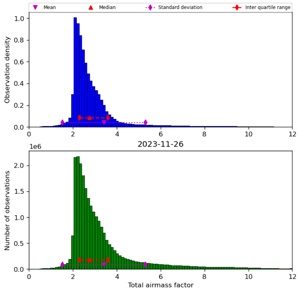
Figure 32: Histogram of “Total airmass factor” for 2023-11-25 to 2023-11-27
