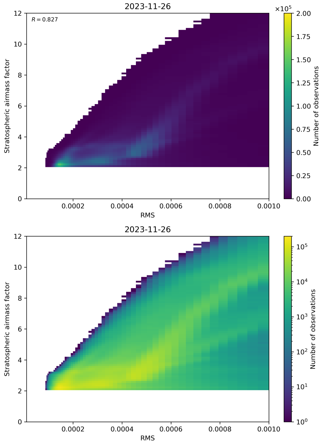
Figure 144: Scatter density plot of “RMS” against “Stratospheric airmass factor” for 2023-11-25 to 2023-11-27.
