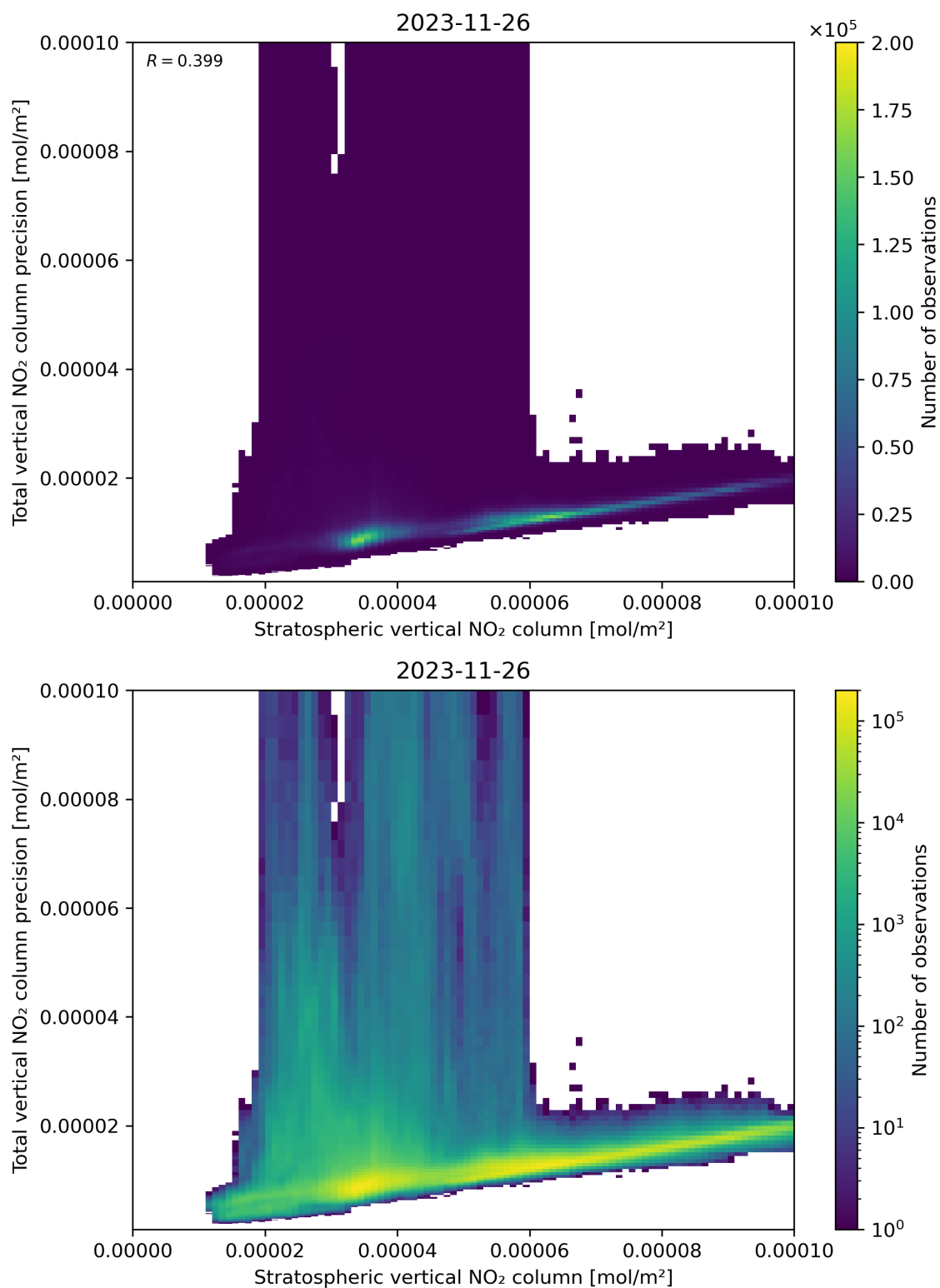
Figure 101: Scatter density plot of “Stratospheric vertical NO 2 column” against “Total vertical NO 2 column precision” for 2023-11-25 to 2023-11-27.
