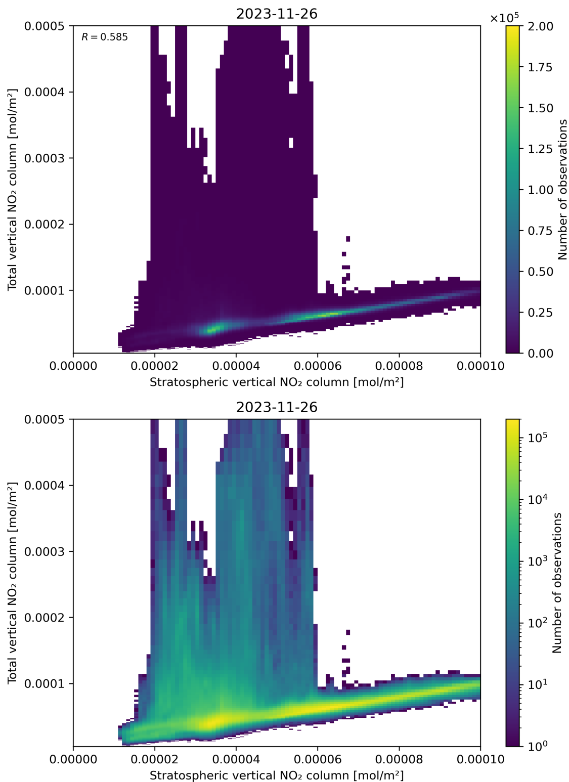
Figure 100: Scatter density plot of “Stratospheric vertical NO 2 column” against “Total vertical NO 2 column” for 2023-11-25 to 2023-11-27.
