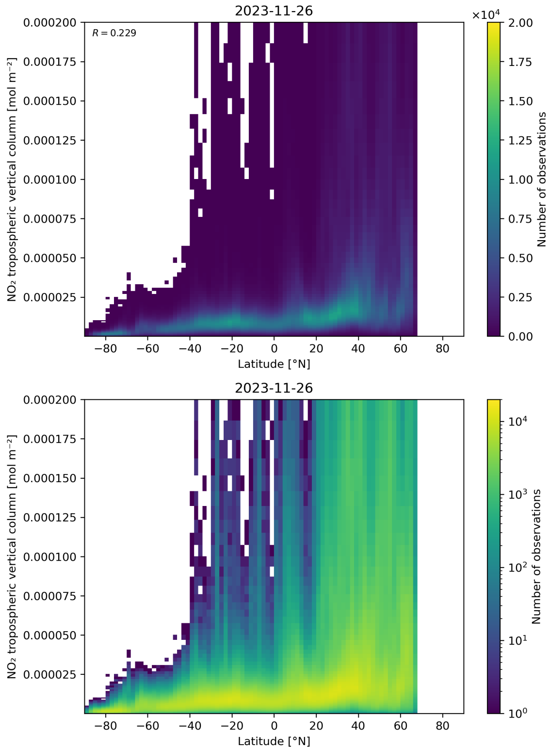
Figure 92: Scatter density plot of “Latitude” against “NO 2 tropospheric vertical column” for 2023-11-25 to 2023-11-27.
