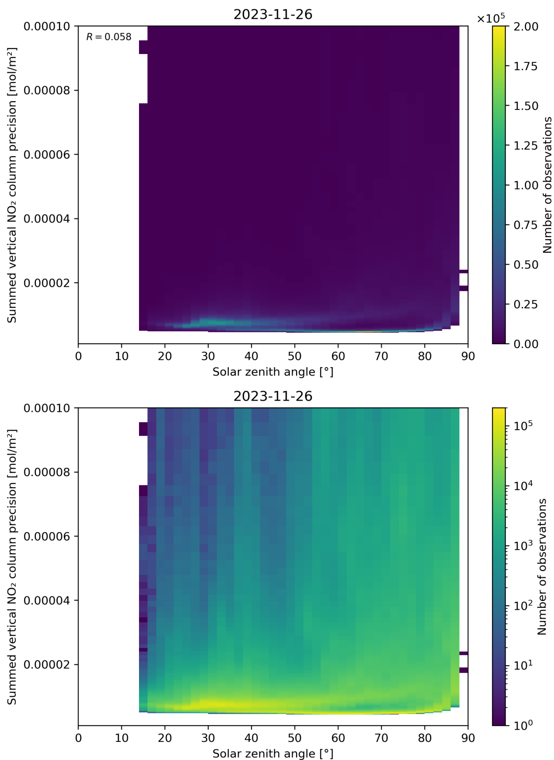
Figure 152: Scatter density plot of “Solar zenith angle” against “Summed vertical NO 2 column precision” for 2023-11-25 to 2023-11-27.
