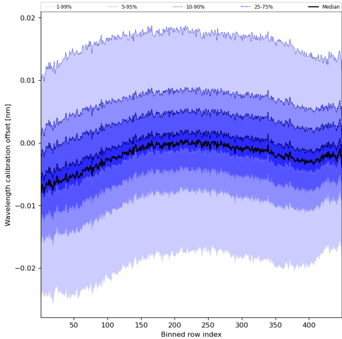
Figure 52: Along track statistics of “Wavelength calibration offset” for 2023-11-25 to 2023-11-27
