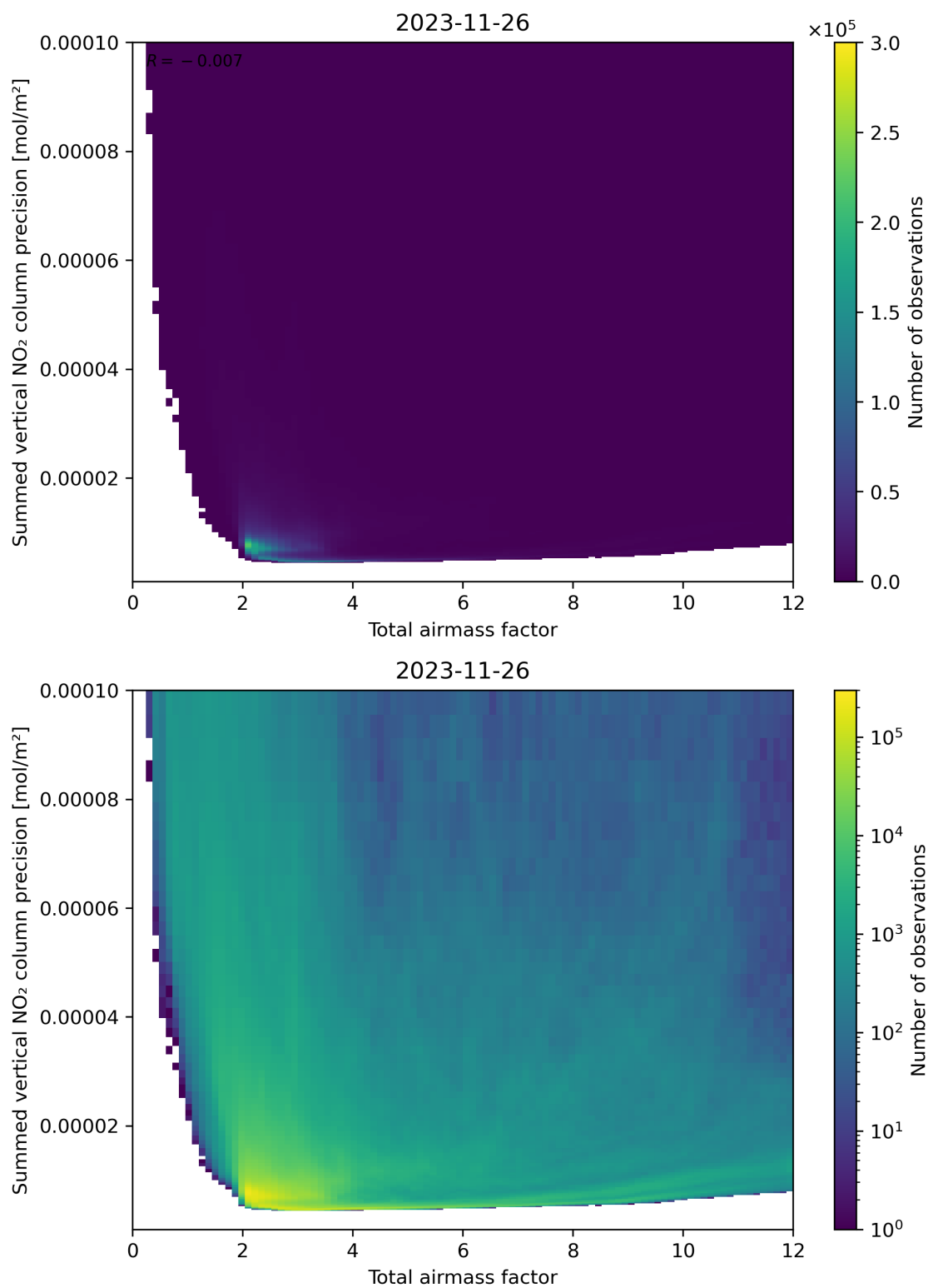
Figure 66: Scatter density plot of “Total airmass factor” against “Summed vertical NO 2 column precision” for 2023-11-25 to 2023-11-27.
