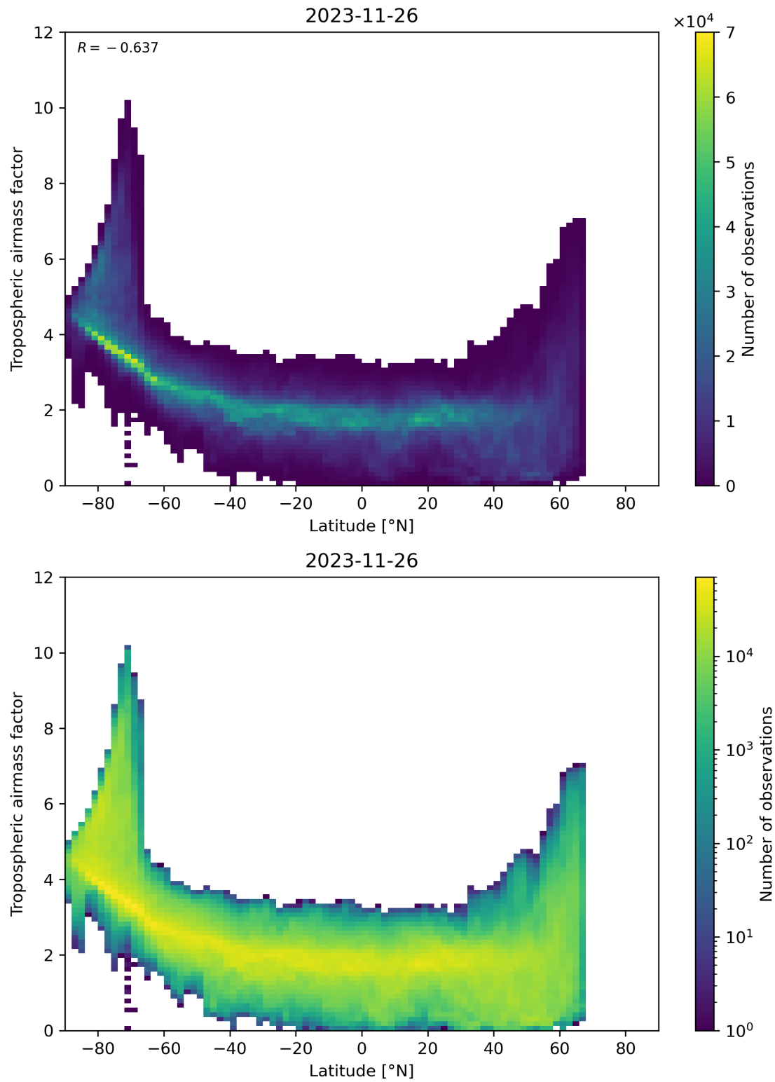
Figure 85: Scatter density plot of “Latitude” against “Tropospheric airmass factor” for 2023-11-25 to 2023-11-27.
