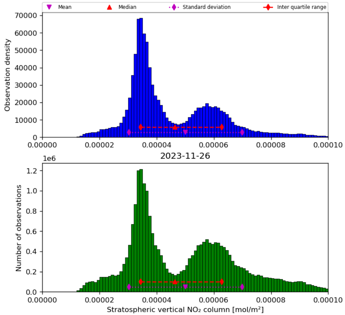
Figure 36: Histogram of “Stratospheric vertical NO 2 column” for 2023-11-25 to 2023-11-27
