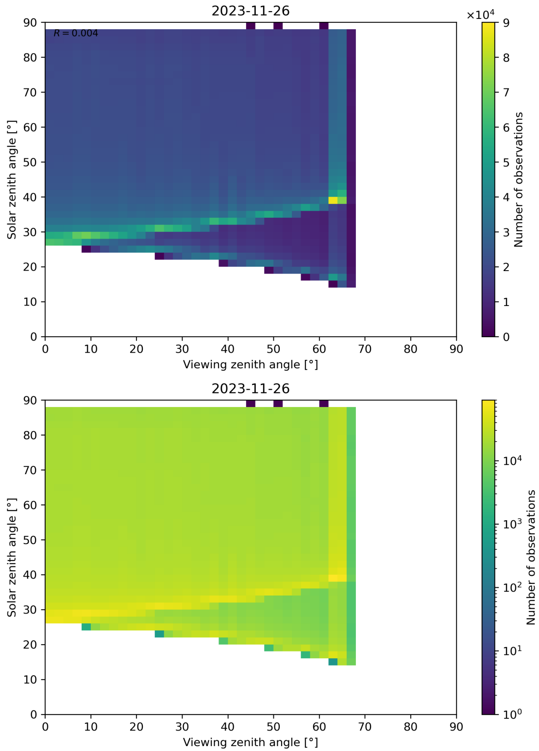
Figure 172: Scatter density plot of “Viewing zenith angle” against “Solar zenith angle” for 2023-11-25 to 2023-11-27.
