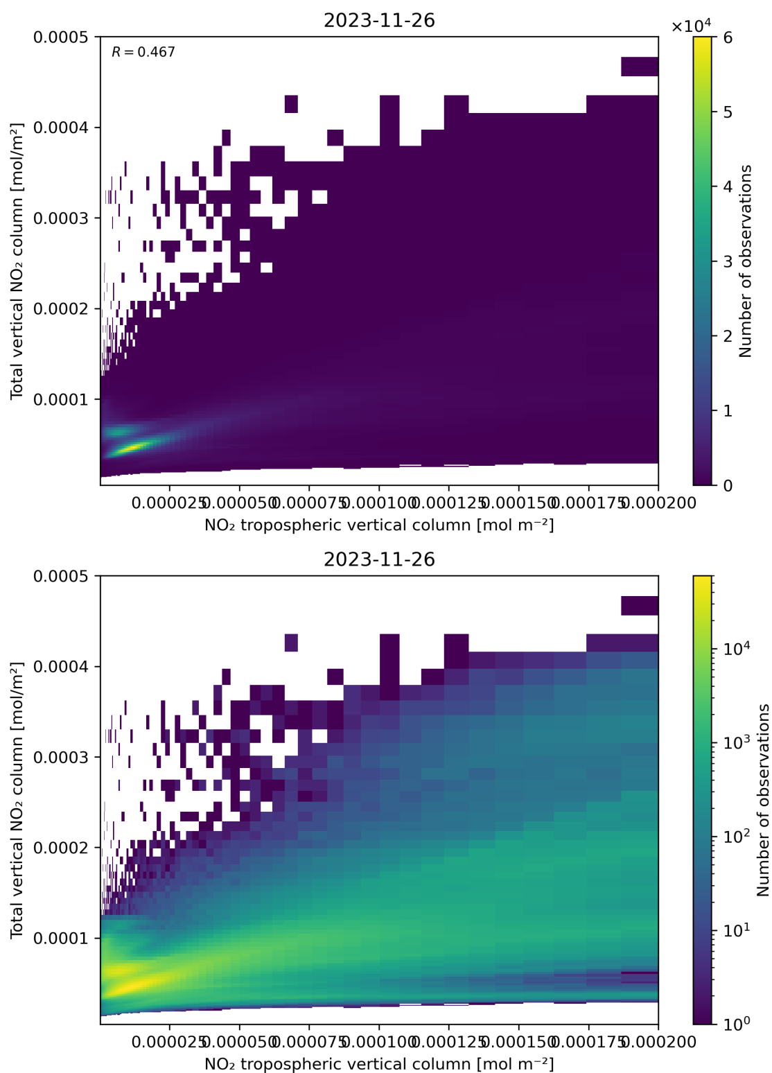
Figure 128: Scatter density plot of “NO 2 tropospheric vertical column” against “Total vertical NO 2 column” for 2023-11-25 to 2023-11-27.
