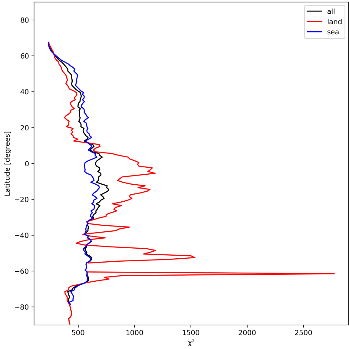
Figure 25: Zonal average of “ \chi^2 ” for 2023-11-25 to 2023-11-27.
