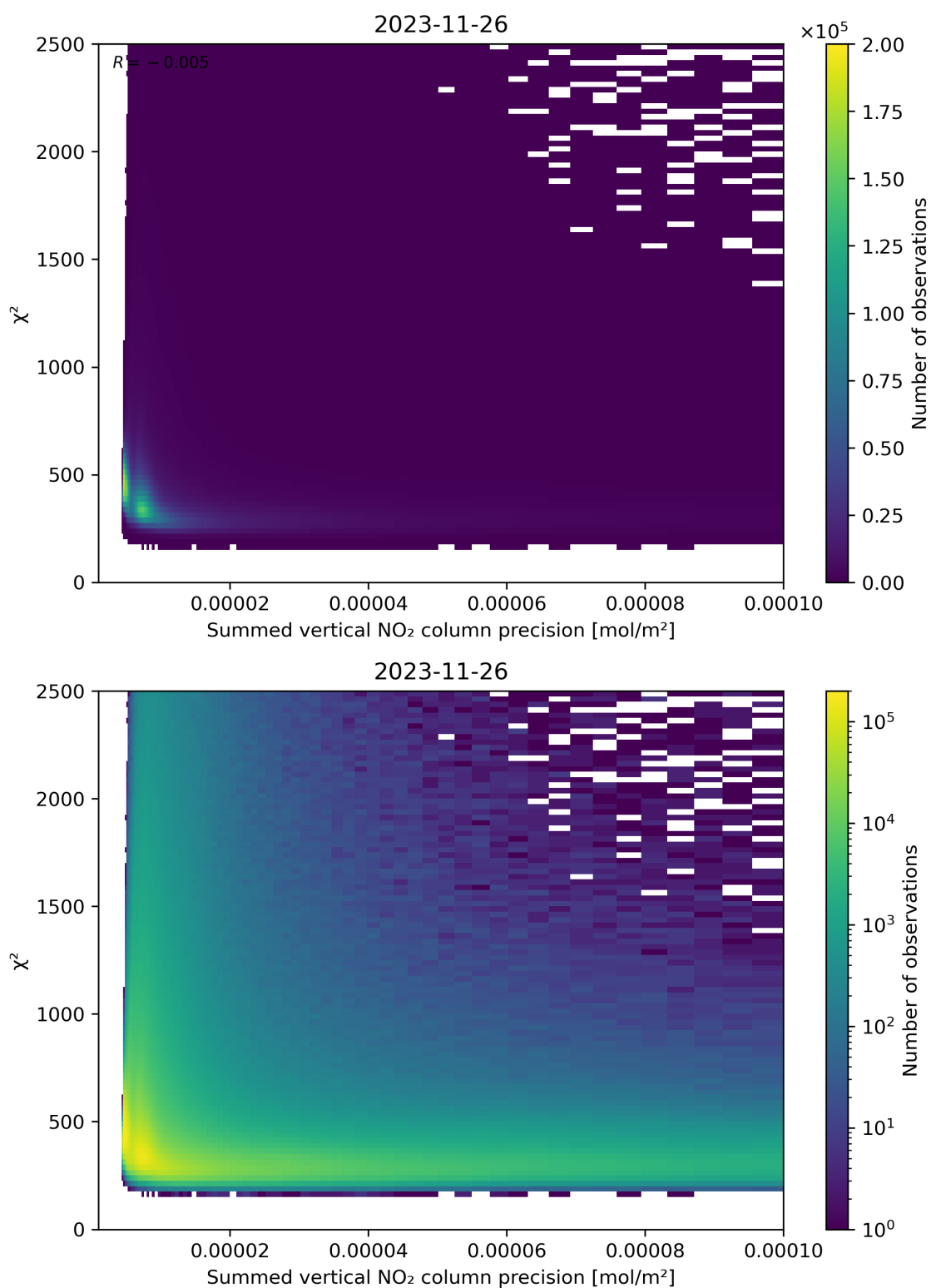
Figure 107: Scatter density plot of “Summed vertical NO 2 column precision” against “ \chi^2 ” for 2023-11-25 to 2023-11-27.
