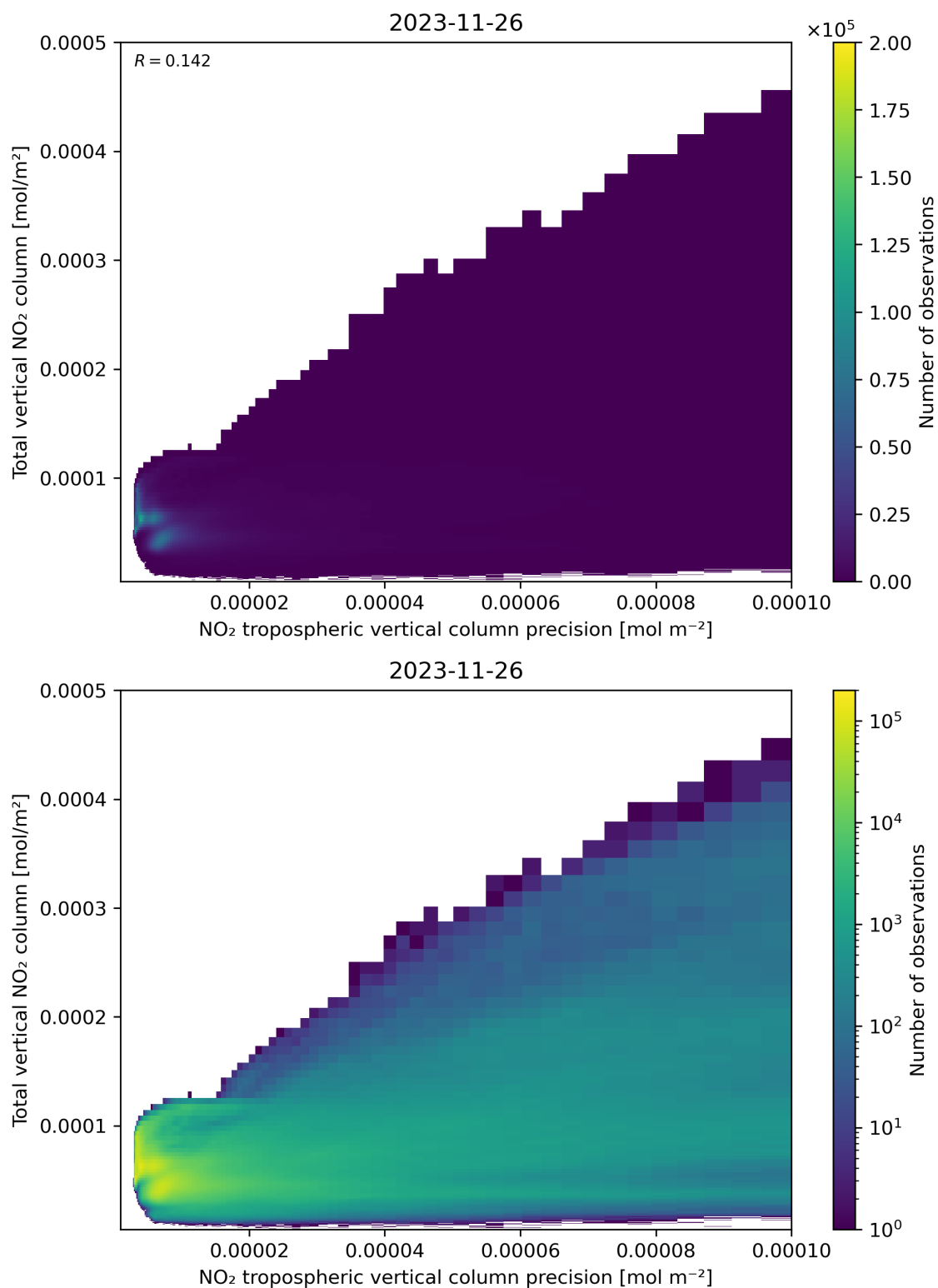
Figure 138: Scatter density plot of “NO 2 tropospheric vertical column precision” against “Total vertical NO 2 column” for 2023-11-25 to 2023-11-27.
