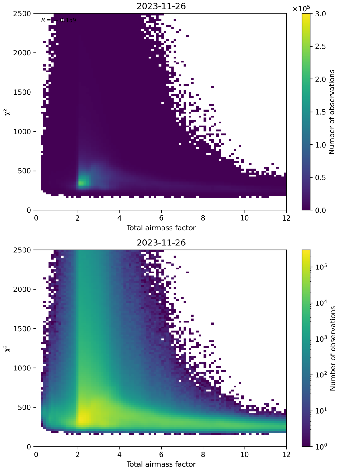
Figure 63: Scatter density plot of “Total airmass factor” against “ \chi^2 ” for 2023-11-25 to 2023-11-27.
