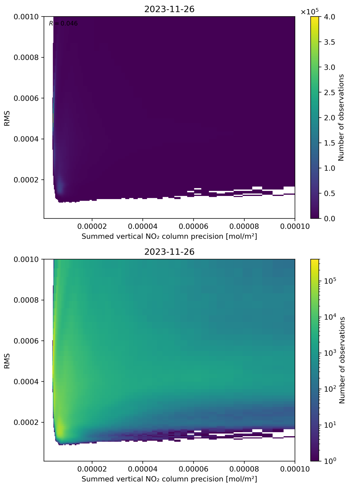
Figure 108: Scatter density plot of “Summed vertical NO 2 column precision” against “RMS” for 2023-11-25 to 2023-11-27.
