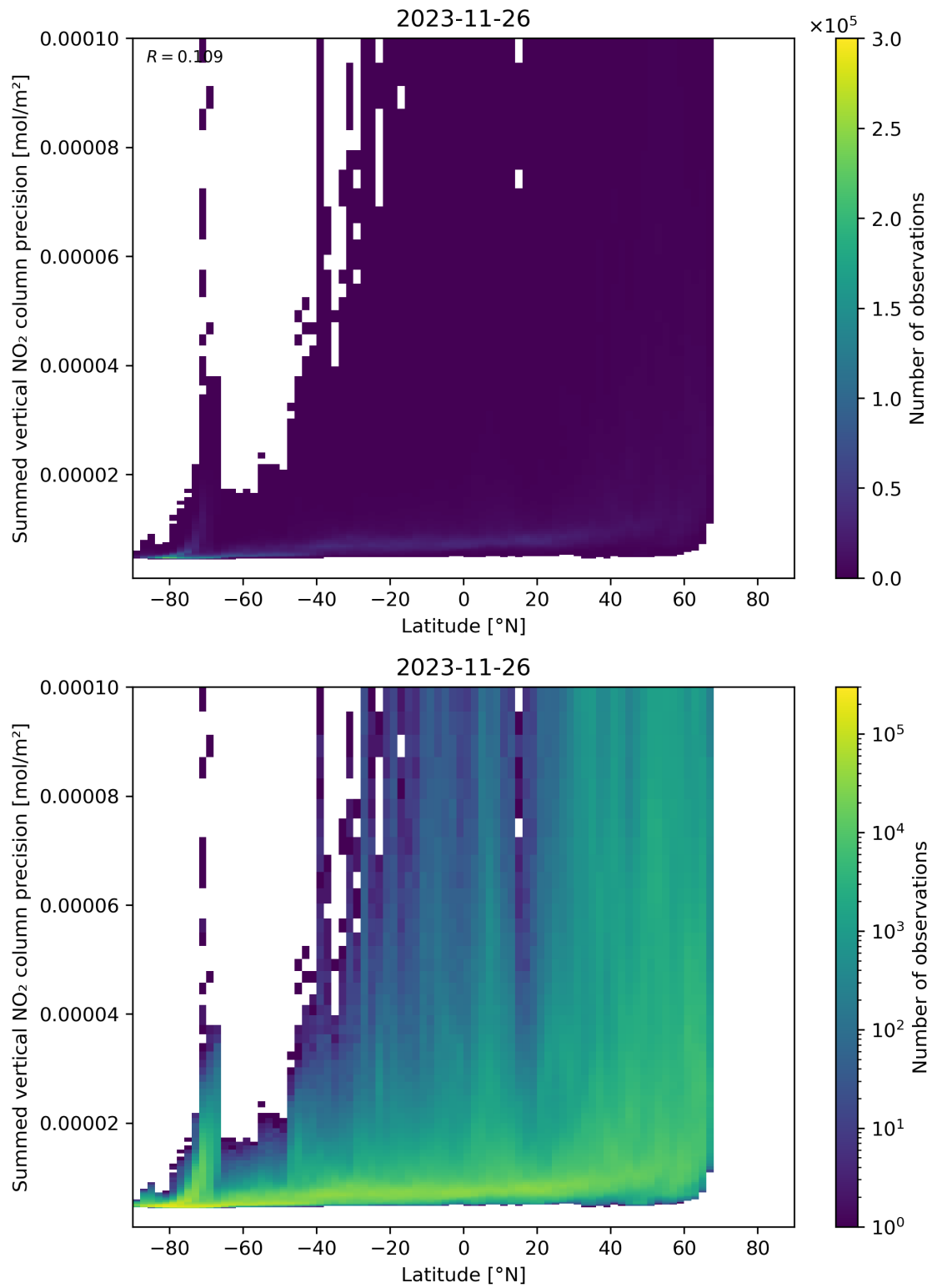
Figure 89: Scatter density plot of “Latitude” against “Summed vertical NO 2 column precision” for 2023-11-25 to 2023-11-27.
