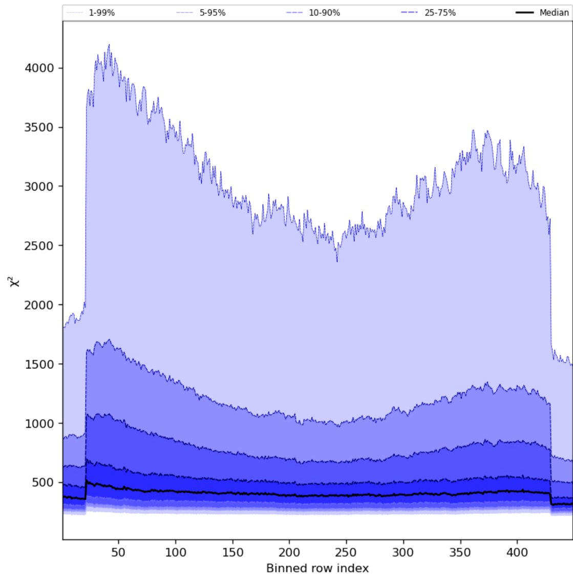
Figure 59: Along track statistics of “ \chi^2 ” for 2023-11-25 to 2023-11-27
