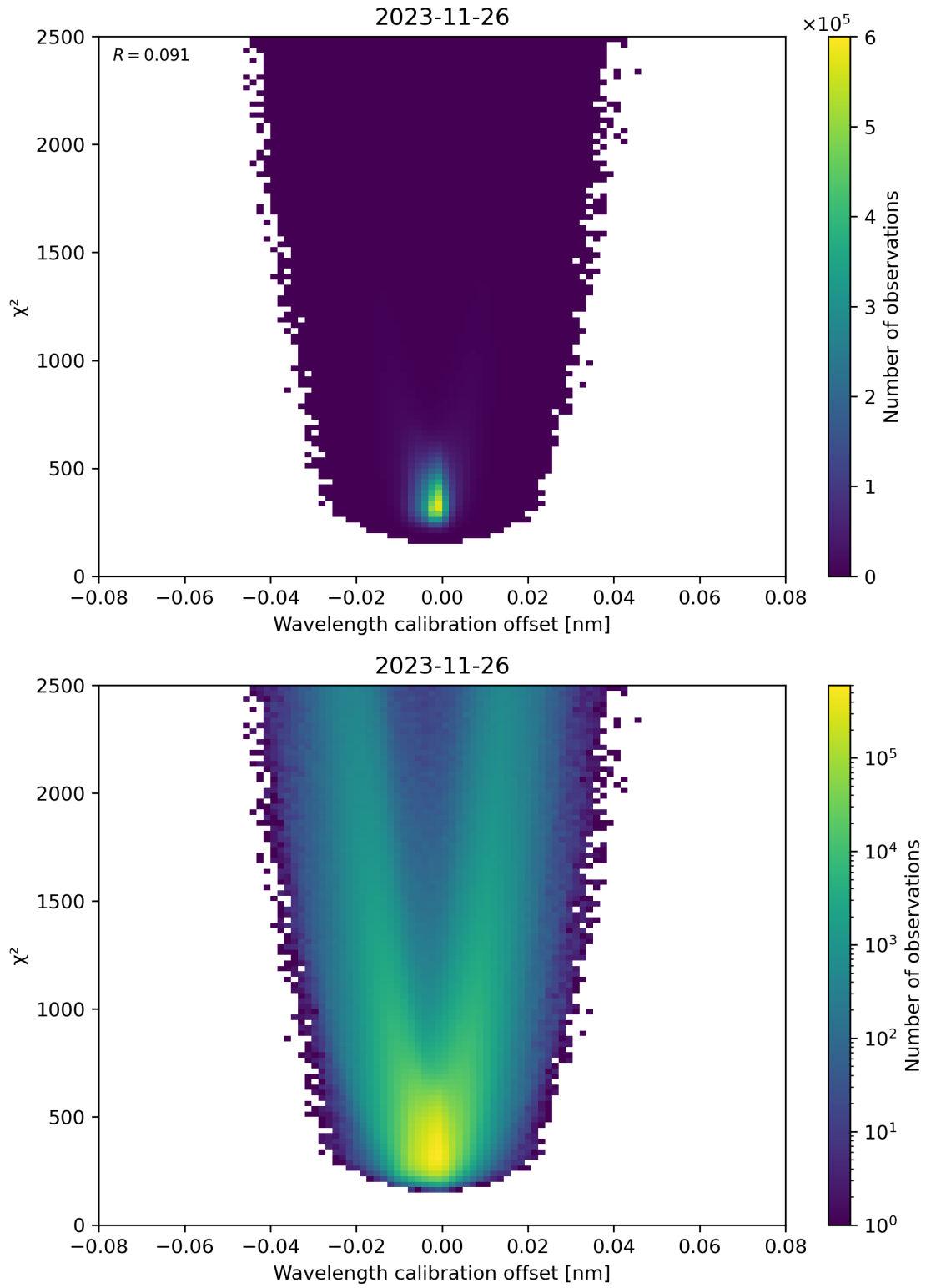
Figure 175: Scatter density plot of “Wavelength calibration offset” against “ \chi^2 ” for 2023-11-25 to 2023-11-27.
