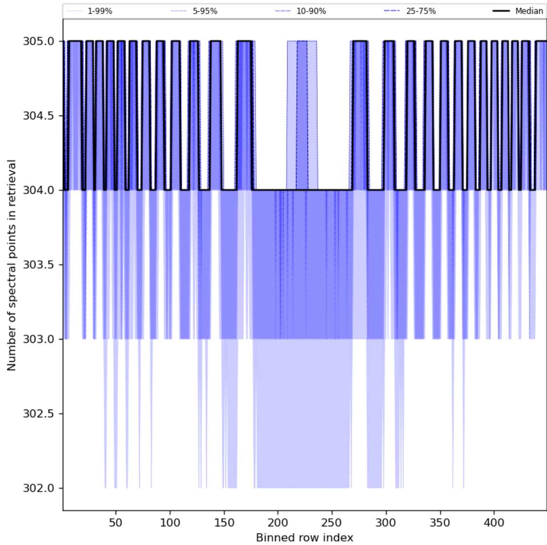
Figure 50: Along track statistics of “Number of spectral points in retrieval” for 2023-11-25 to 2023-11-27
