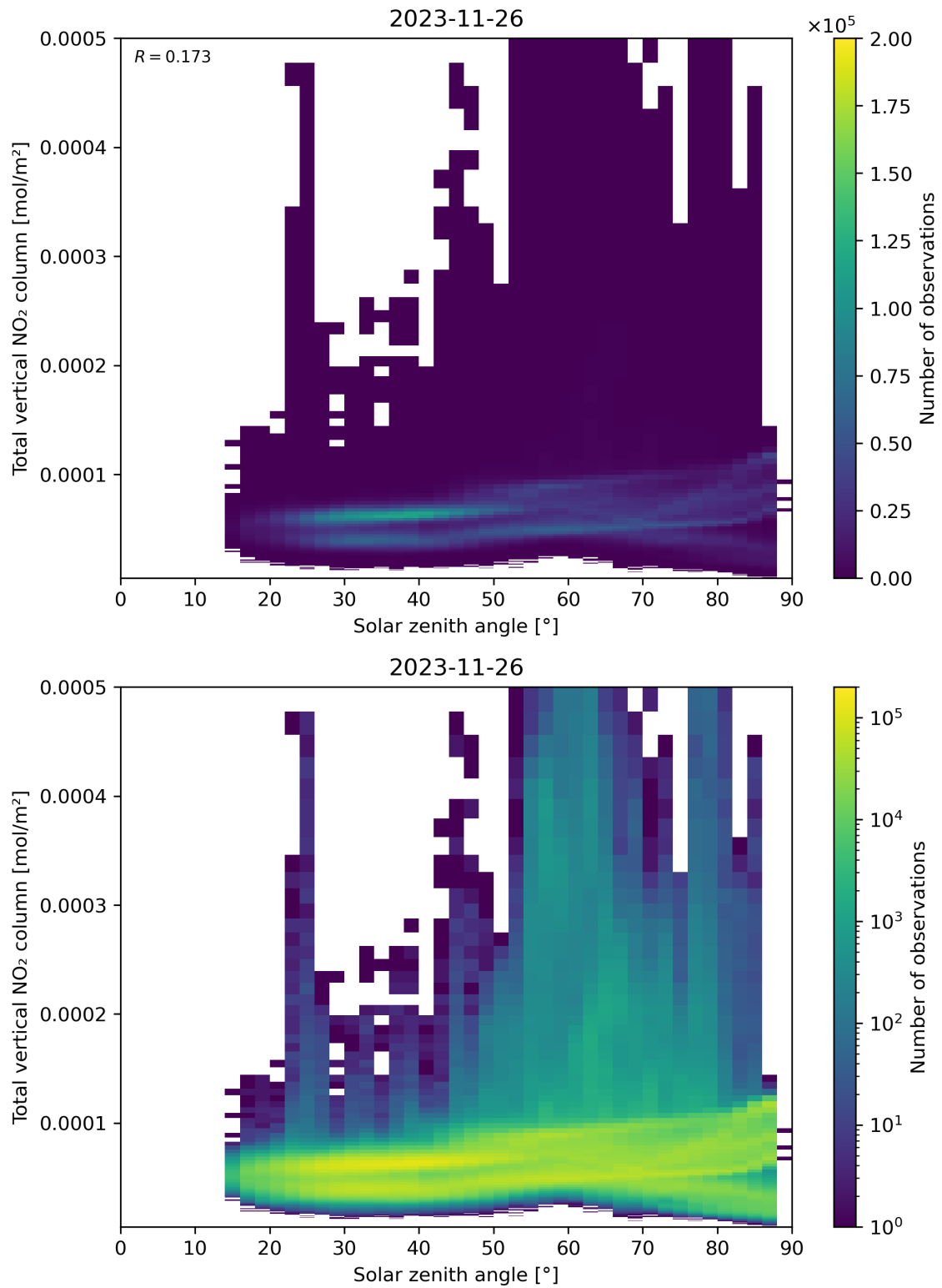
Figure 153: Scatter density plot of “Solar zenith angle” against “Total vertical NO 2 column” for 2023-11-25 to 2023-11-27.
