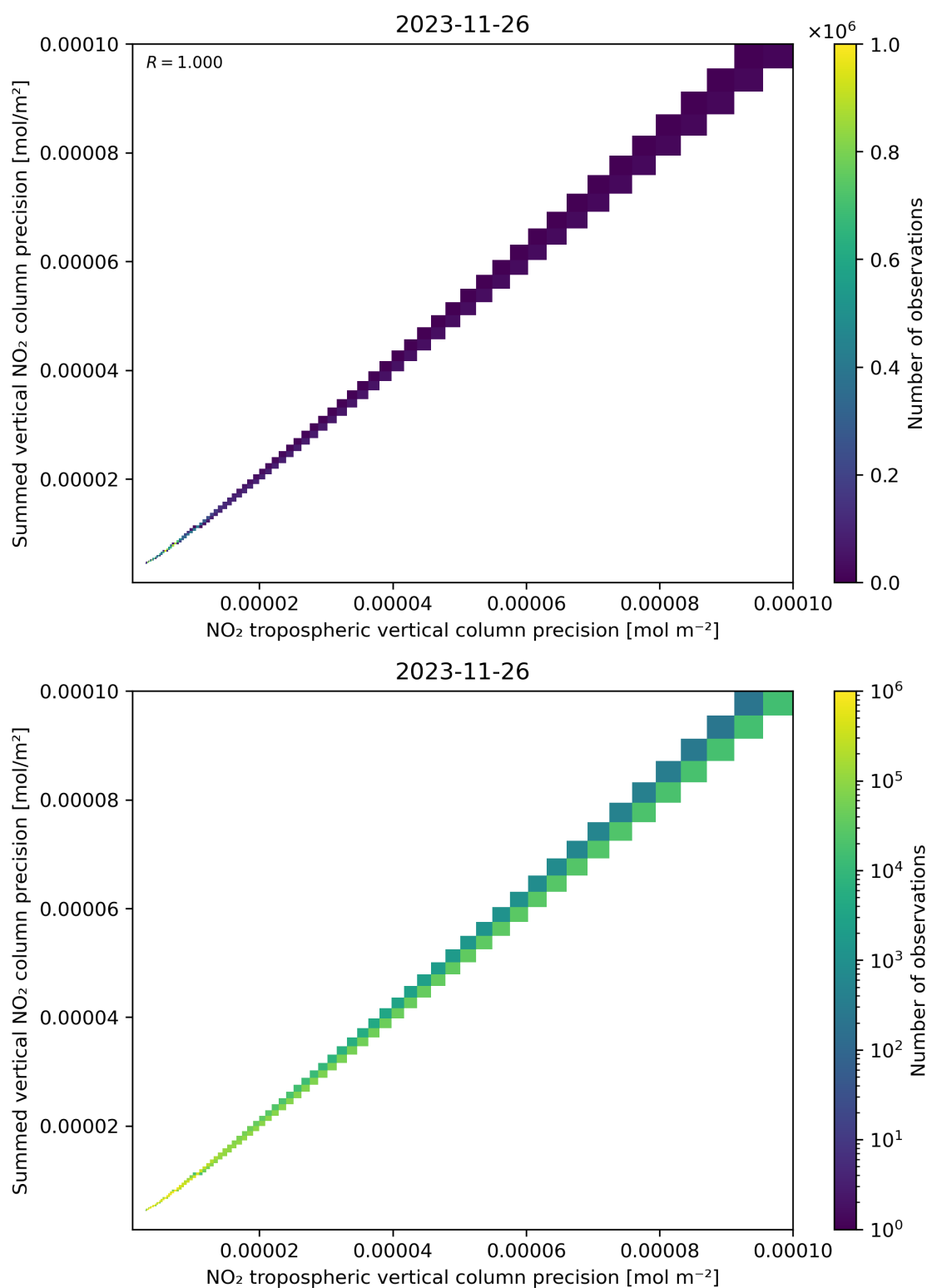
Figure 137: Scatter density plot of “NO 2 tropospheric vertical column precision” against “Summed vertical NO 2 column precision” for 2023-11-25 to 2023-11-27.
