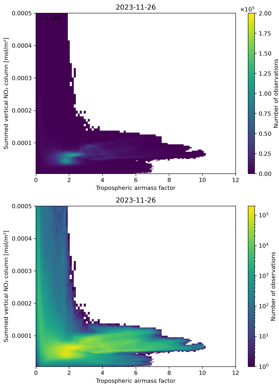
Figure 75: Scatter density plot of “Tropospheric airmass factor” against “Summed vertical NO 2 column” for 2023-11-25 to 2023-11-27.
