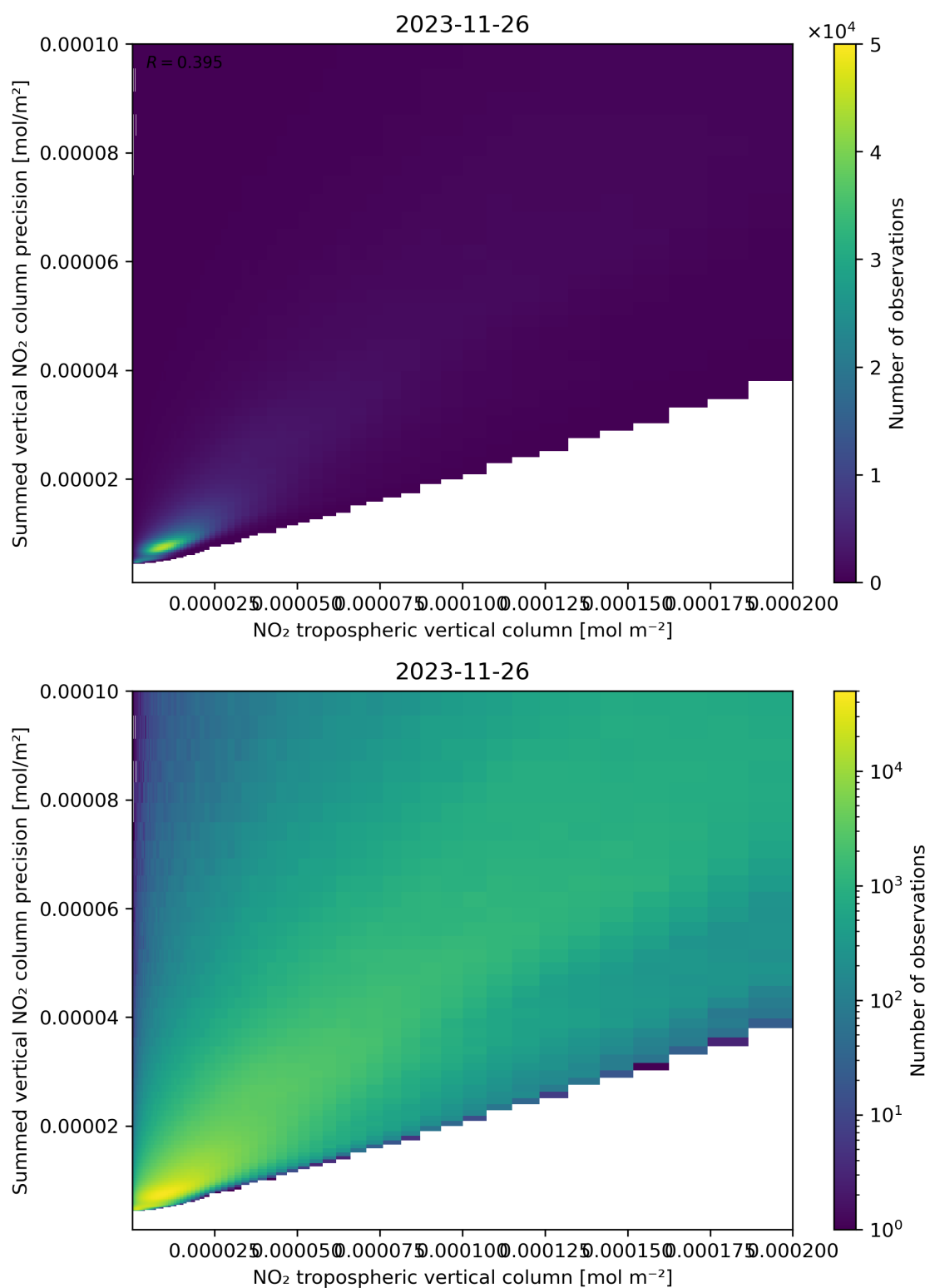
Figure 127: Scatter density plot of “NO 2 tropospheric vertical column” against “Summed vertical NO 2 column precision” for 2023-11-25 to 2023-11-27.
