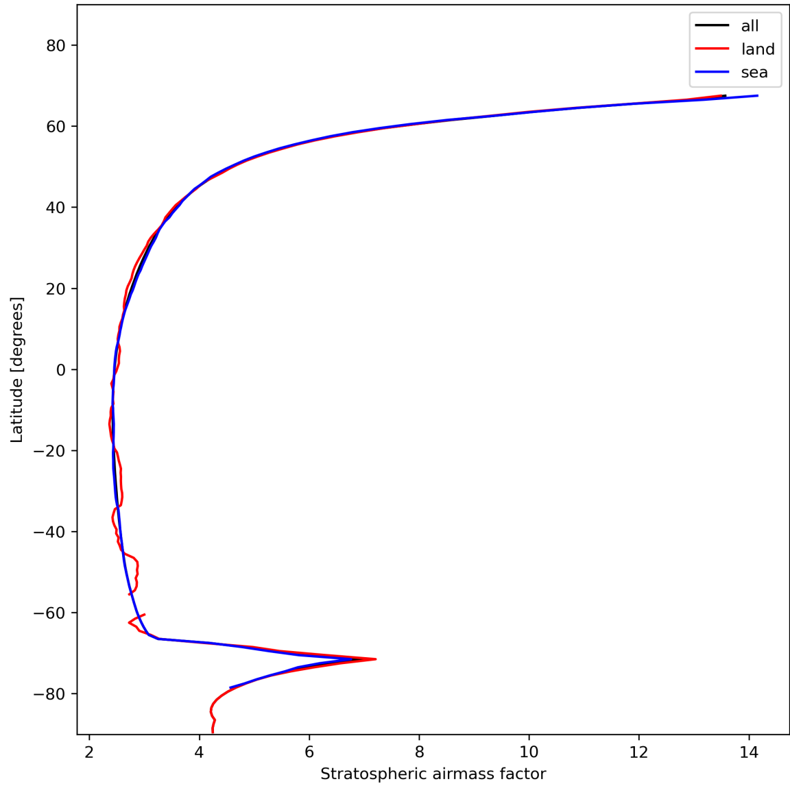
Figure 27: Zonal average of “Stratospheric air mass factor” for 2023-11-25 to 2023-11-27.
