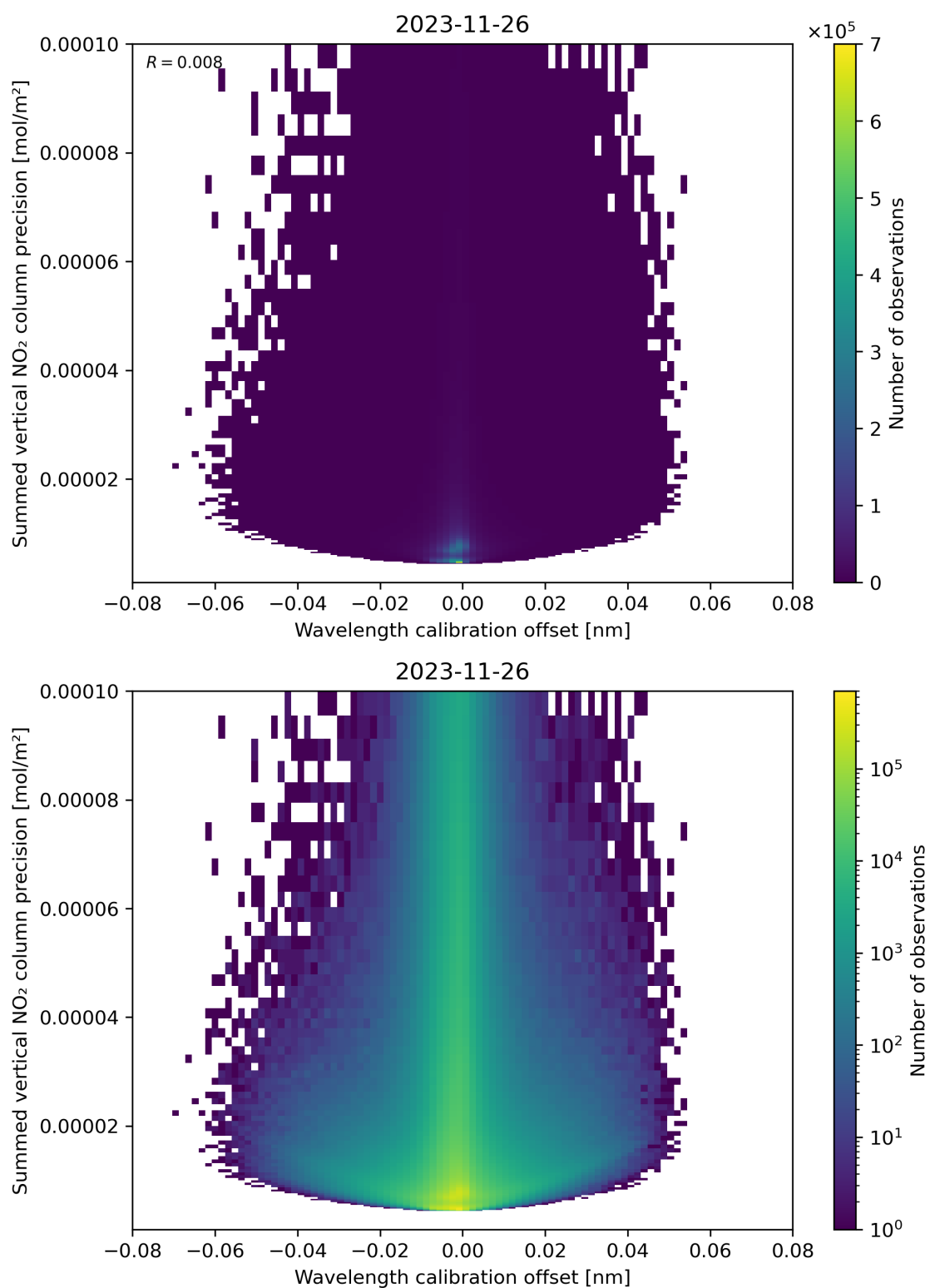
Figure 178: Scatter density plot of “Wavelength calibration offset” against “Summed vertical NO 2 column precision” for 2023-11-25 to 2023-11-27.
