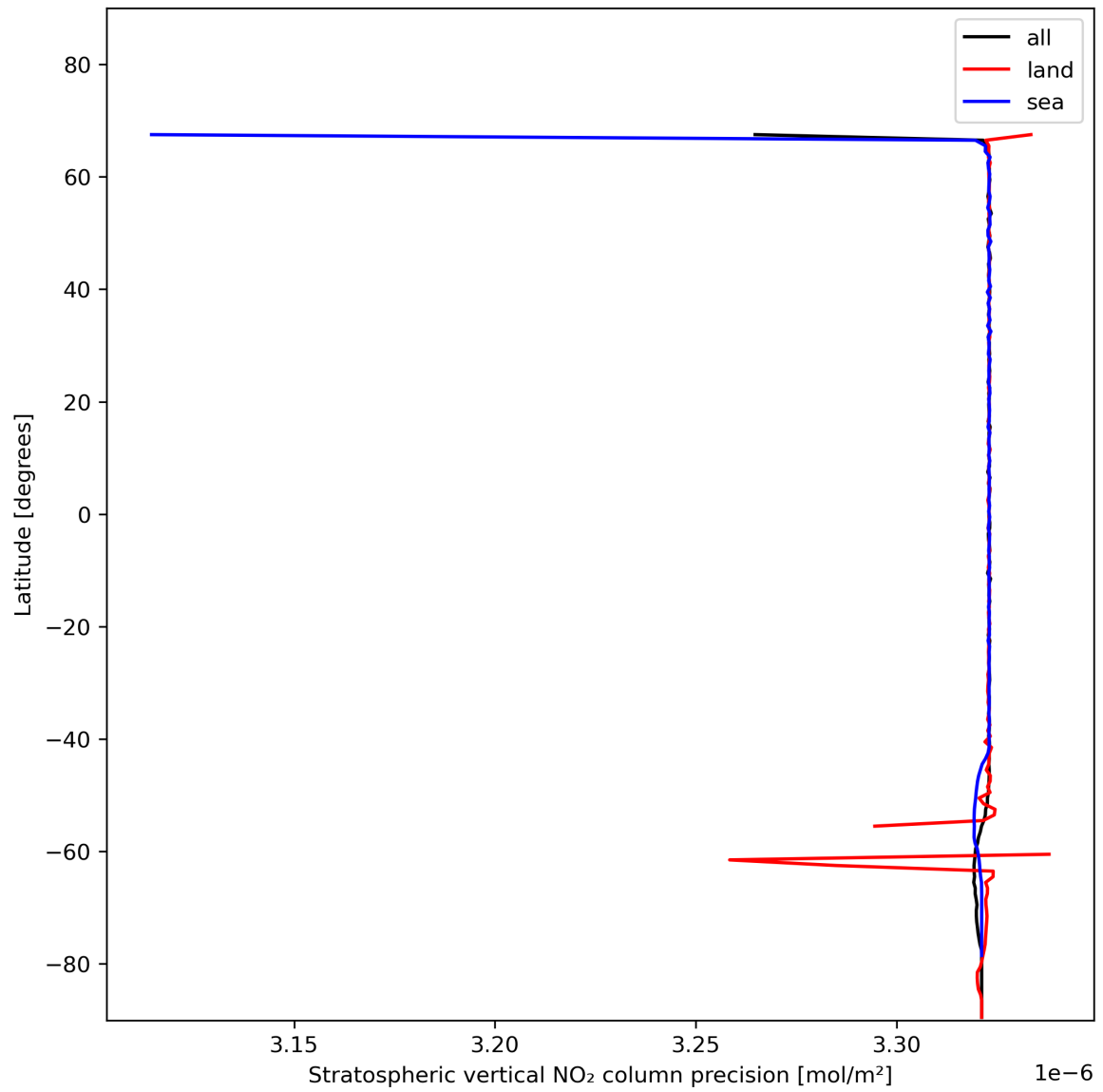
Figure 20: Zonal average of “Stratospheric vertical NO 2 column precision” for 2023-11-25 to 2023-11-27.
