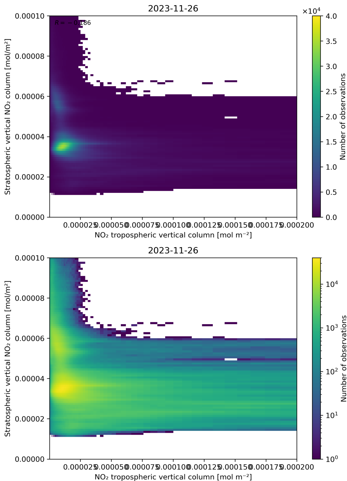
Figure 125: Scatter density plot of “NO 2 tropospheric vertical column” against “Stratospheric vertical NO 2 column” for 2023-11-25 to 2023-11-27.
