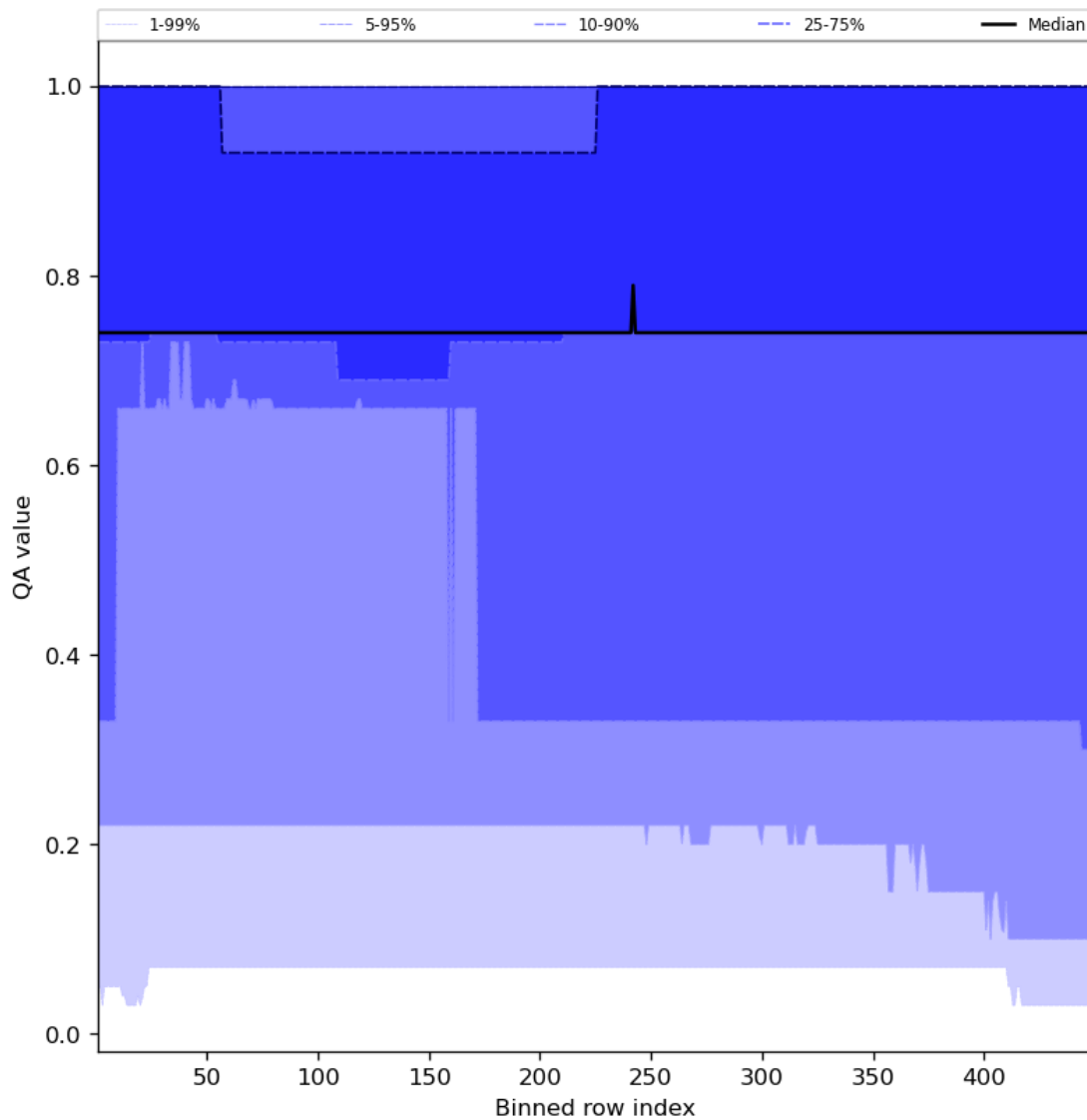
Figure 45: Along track statistics of “QA value” for 2023-11-25 to 2023-11-27
