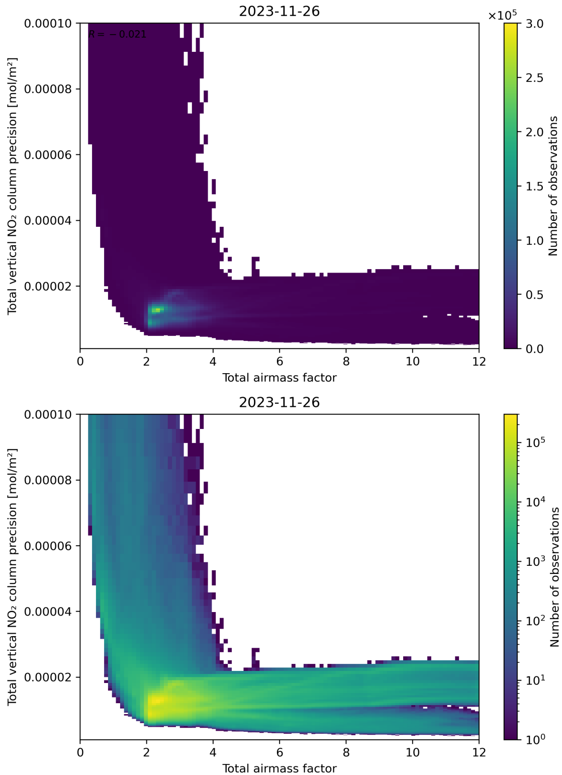
Figure 68: Scatter density plot of “Total airmass factor” against “Total vertical NO 2 column precision” for 2023-11-25 to 2023-11-27.
