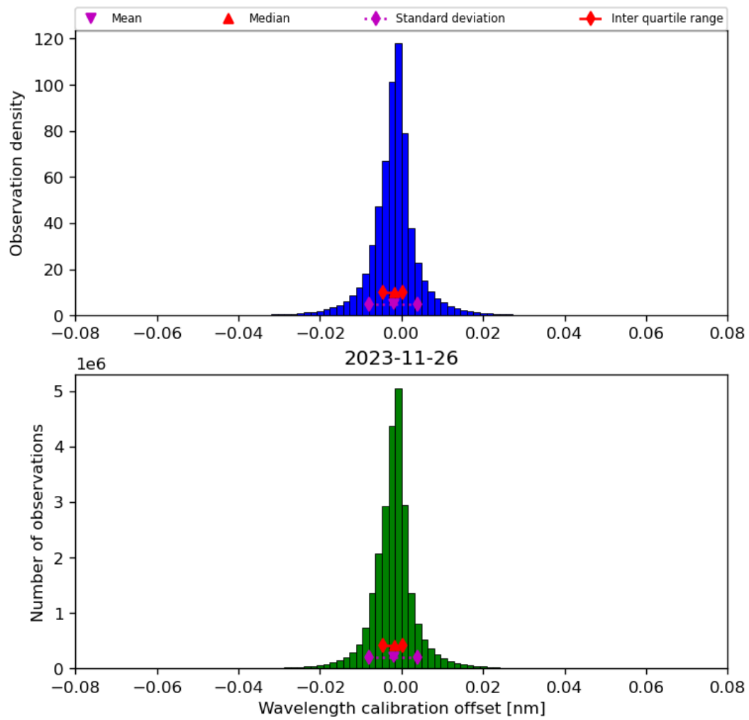
Figure 35: Histogram of “Wavelength calibration offset” for 2023-11-25 to 2023-11-27
