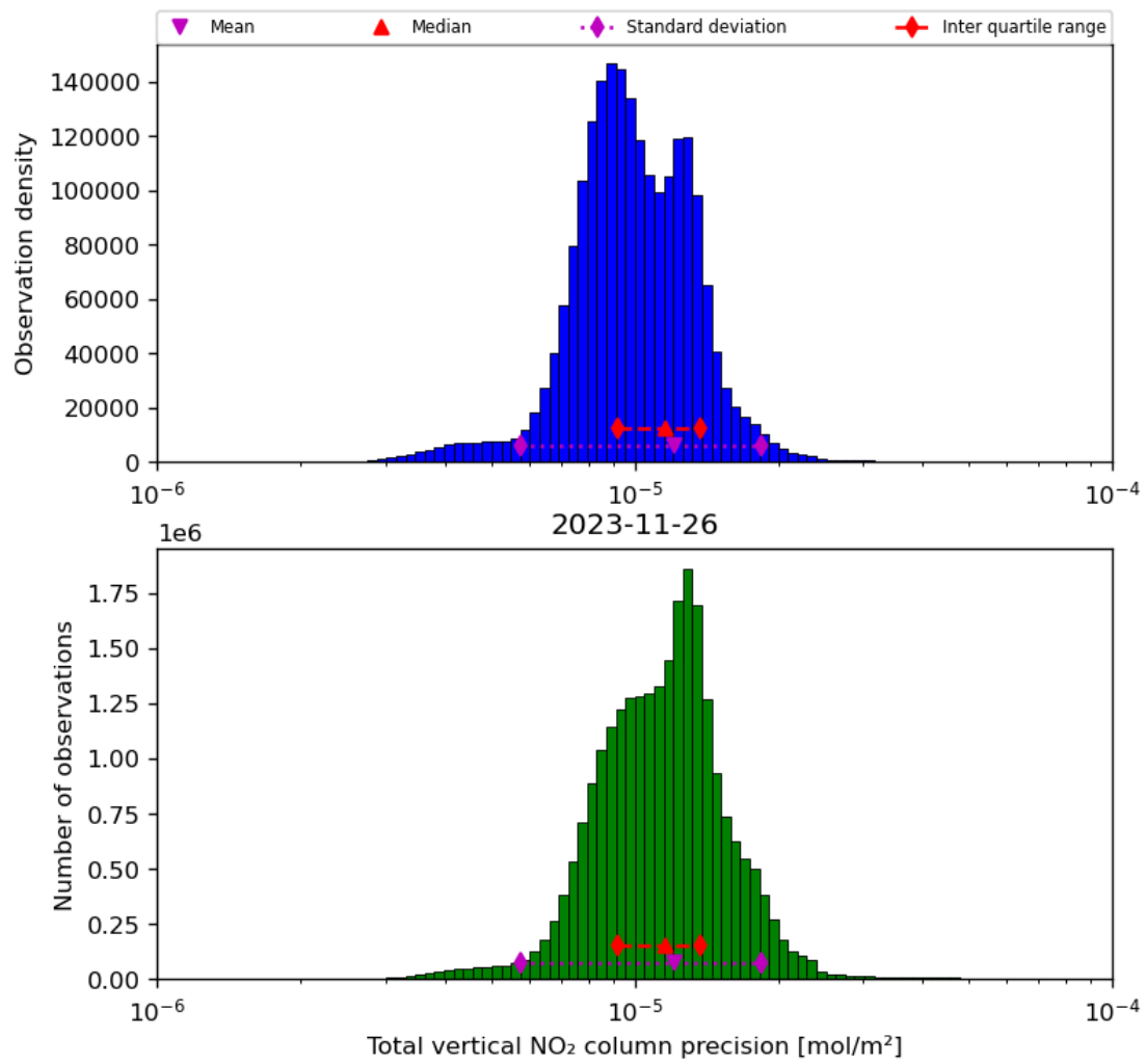
Figure 39: Histogram of “Total vertical NO 2 column precision” for 2023-11-25 to 2023-11-27
