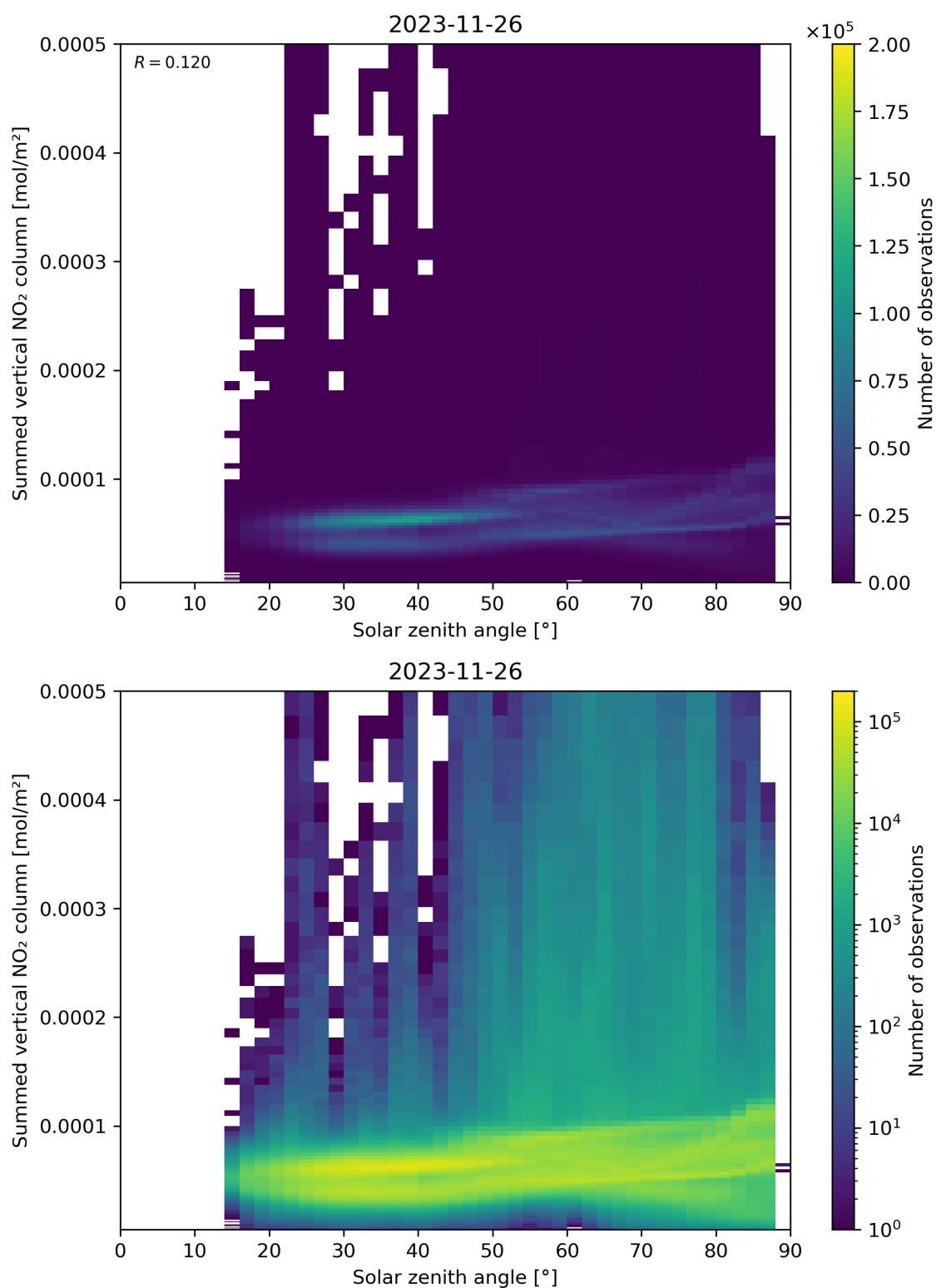
Figure 151: Scatter density plot of “Solar zenith angle” against “Summed vertical NO 2 column” for 2023-11-25 to 2023-11-27.
