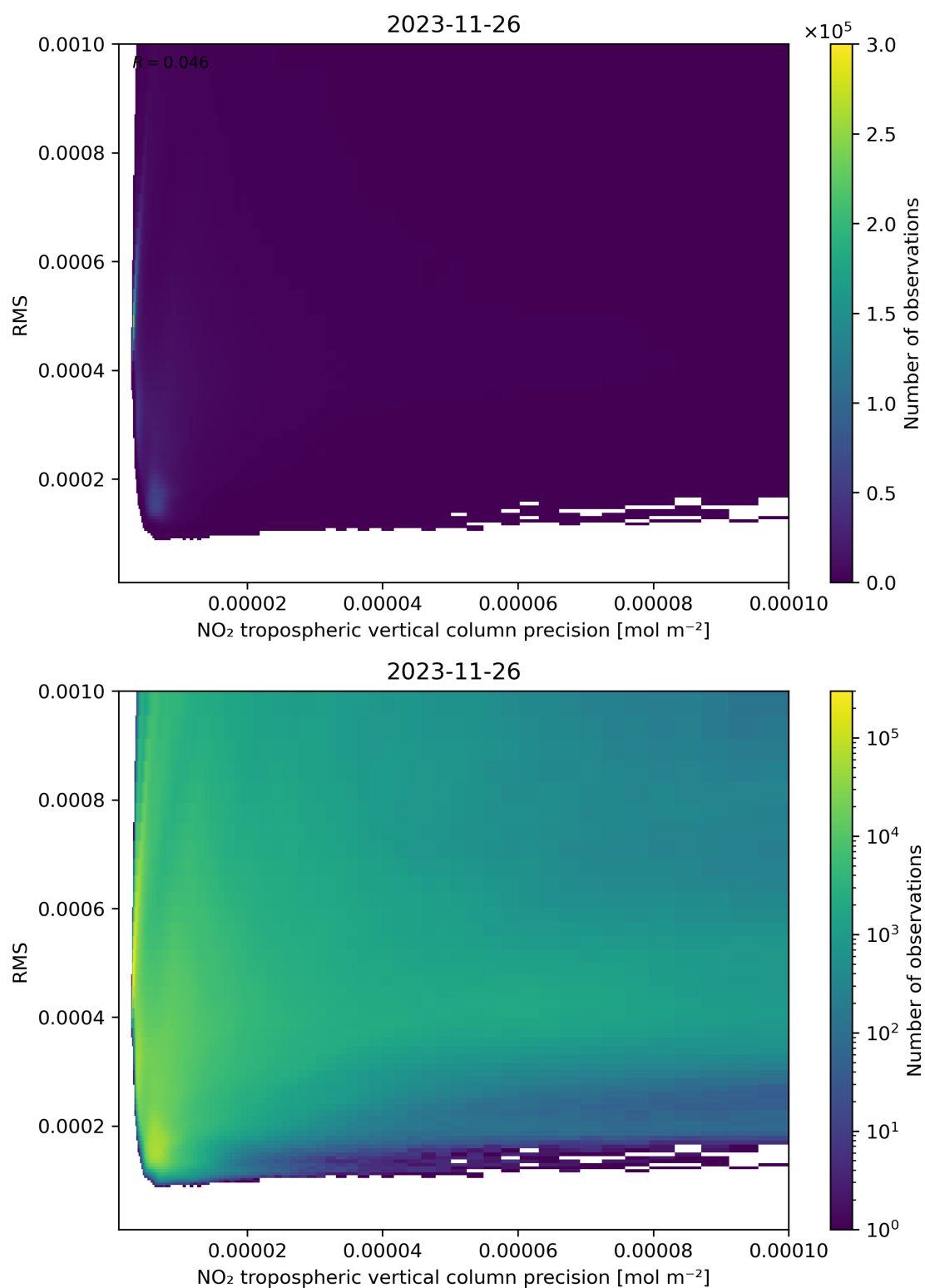
Figure 140: Scatter density plot of “NO 2 tropospheric vertical column precision” against “RMS” for 2023-11-25 to 2023-11-27.
