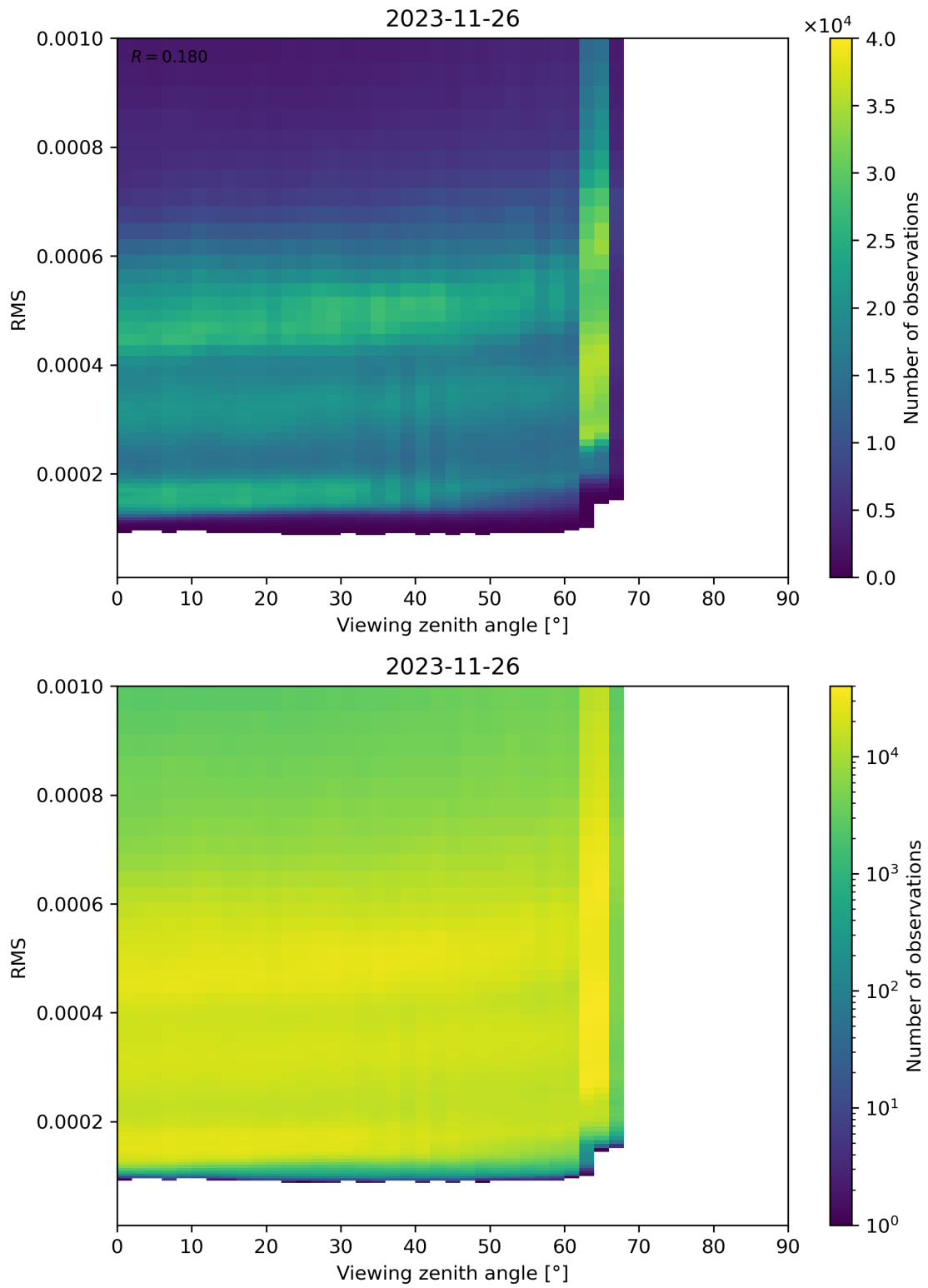
Figure 171: Scatter density plot of “Viewing zenith angle” against “RMS” for 2023-11-25 to 2023-11-27.
