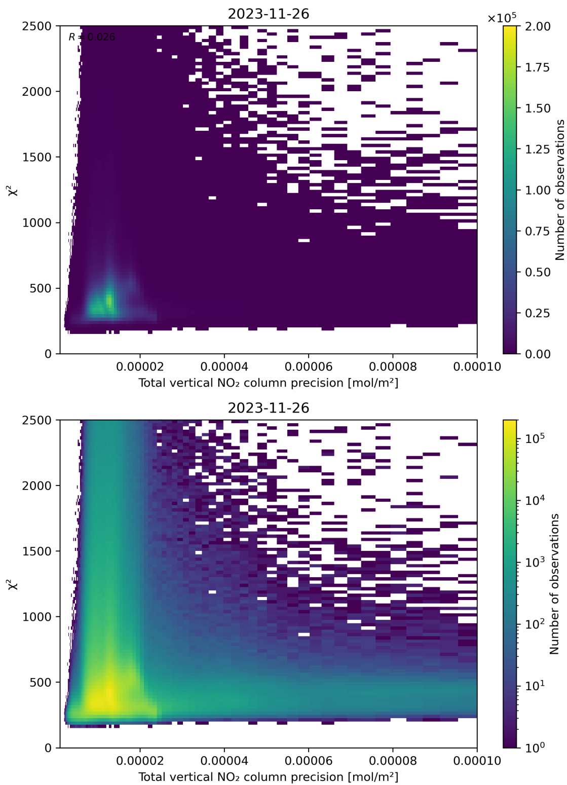
Figure 116: Scatter density plot of “Total vertical NO 2 column precision” against “ \chi^2 ” for 2023-11-25 to 2023-11-27.
