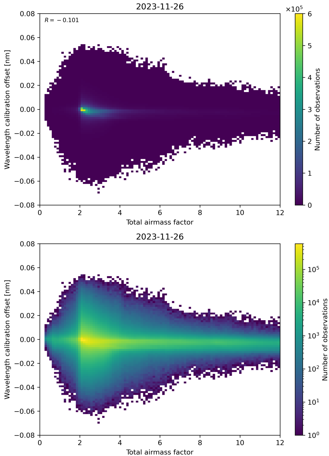
Figure 70: Scatter density plot of “Total airmass factor” against “Wavelength calibration offset” for 2023-11-25 to 2023-11-27.
