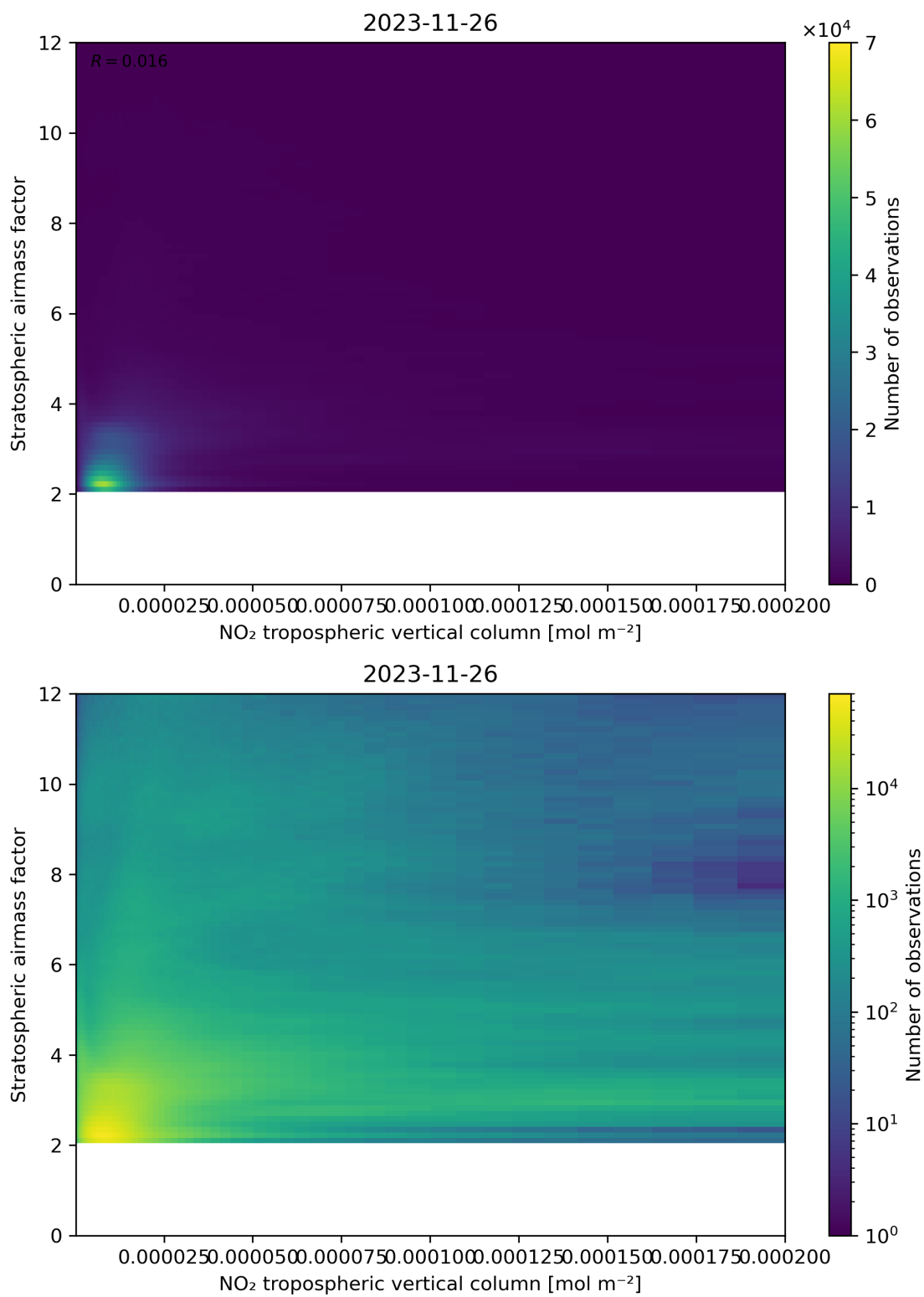
Figure 121: Scatter density plot of “NO 2 tropospheric vertical column” against “Stratospheric airmass factor” for 2023-11-25 to 2023-11-27.
