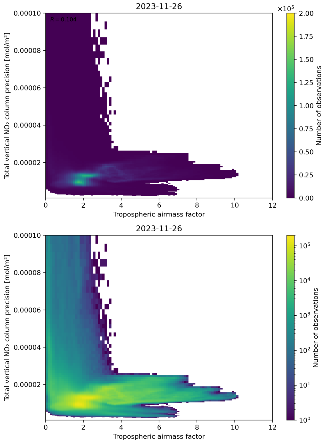
Figure 78: Scatter density plot of “Tropospheric air mass factor” against “Total vertical NO 2 column precision” for 2023-11-25 to 2023-11-27.
