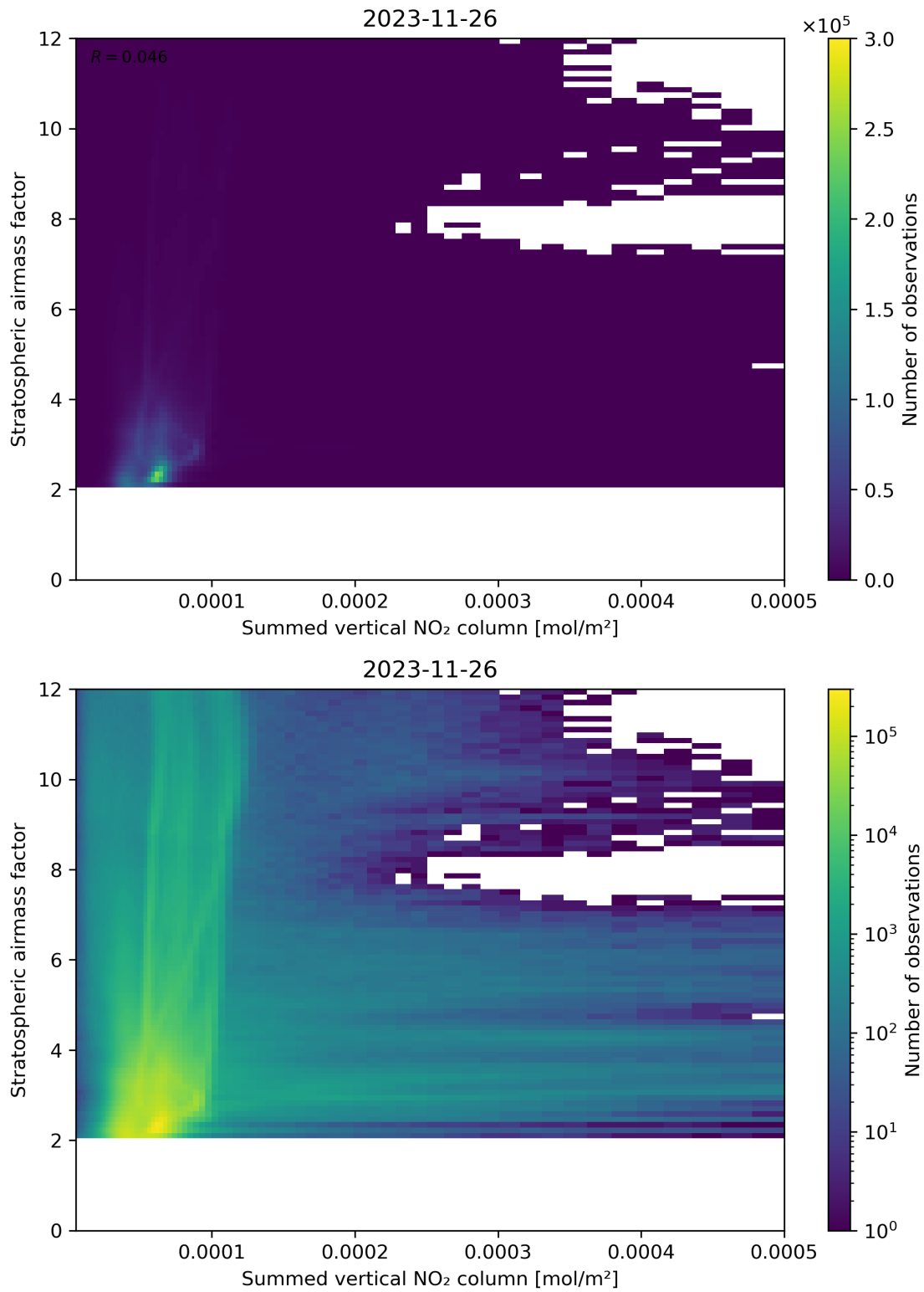
Figure 103: Scatter density plot of “Summed vertical NO 2 column” against “Stratospheric airmass factor” for 2023-11-25 to 2023-11-27.
