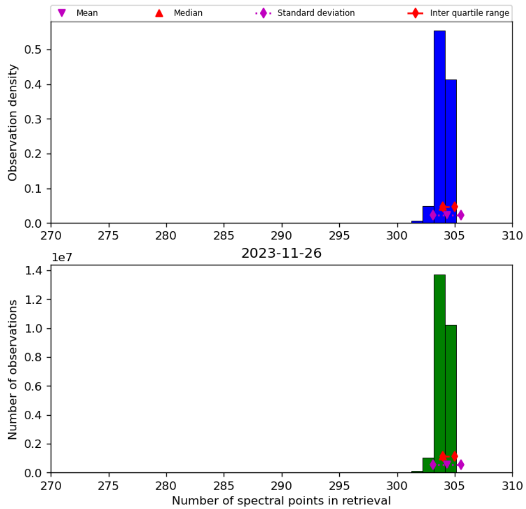
Figure 33: Histogram of “Number of spectral points in retrieval” for 2023-11-25 to 2023-11-27
