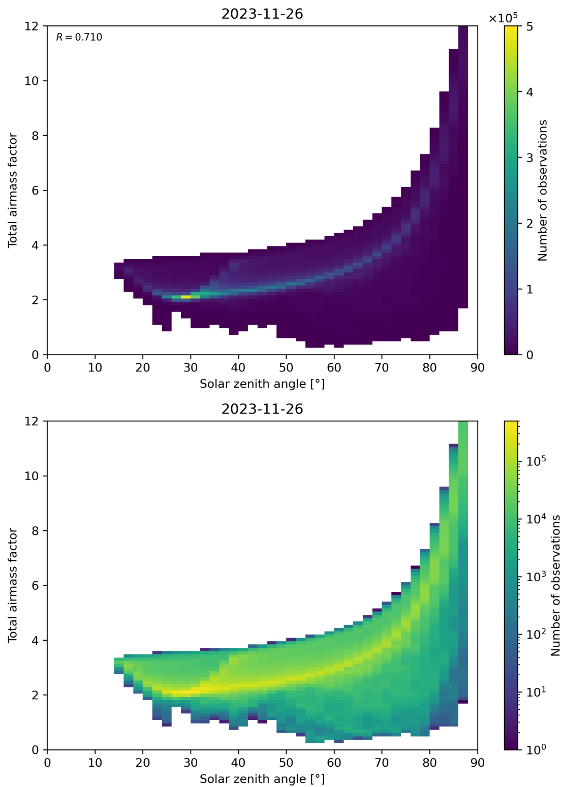
Figure 146: Scatter density plot of “Solar zenith angle” against “Total air mass factor” for 2023-11-25 to 2023-11-27.
