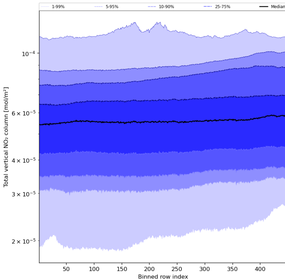
Figure 55: Along track statistics of “Total vertical NO 2 column” for 2023-11-25 to 2023-11-27
