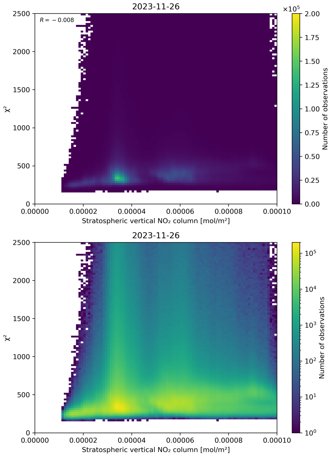
Figure 97: Scatter density plot of “Stratospheric vertical NO 2 column” against “ \chi^2 ” for 2023-11-25 to 2023-11-27.
