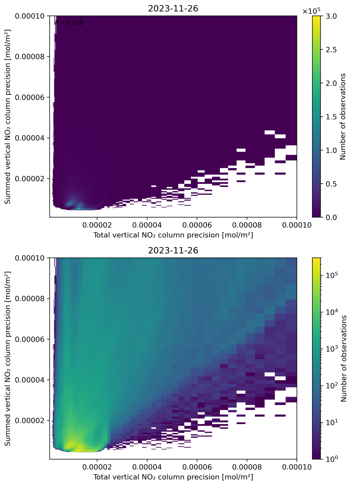
Figure 118: Scatter density plot of “Total vertical NO 2 column precision” against “Summed vertical NO 2 column precision” for 2023-11-25 to 2023-11-27.
