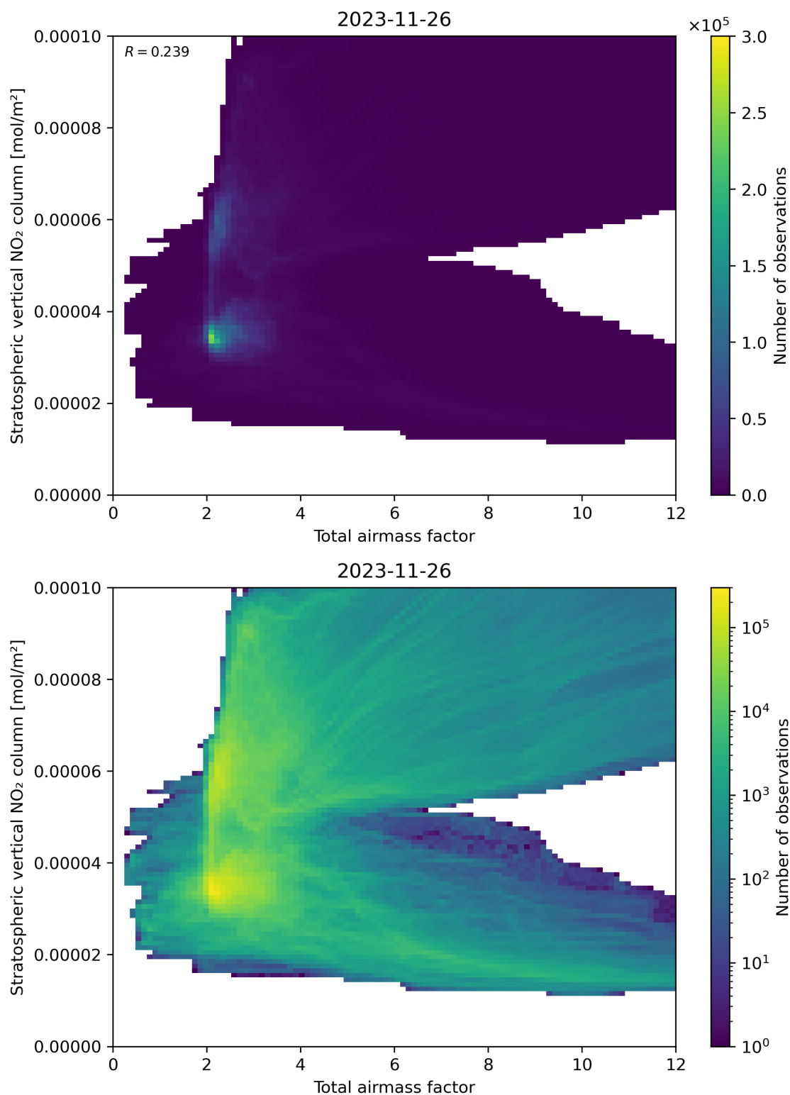
Figure 64: Scatter density plot of “Total airmass factor” against “Stratospheric vertical NO 2 column” for 2023-11-25 to 2023-11-27.
