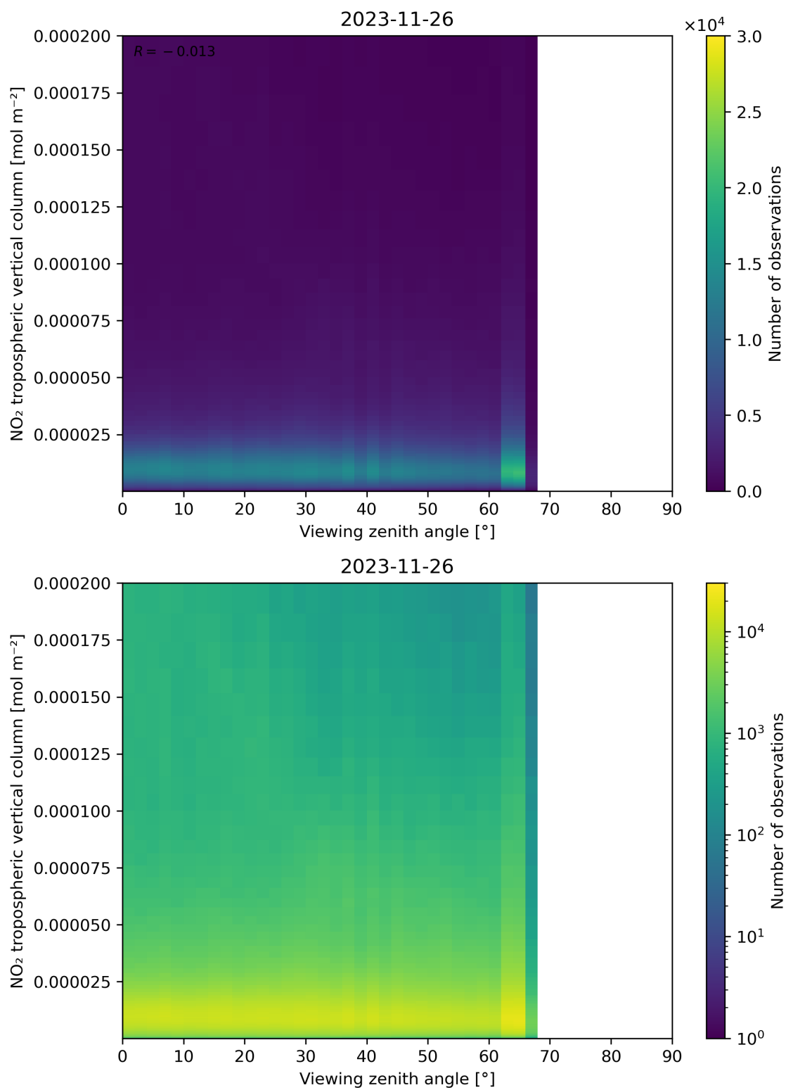
Figure 169: Scatter density plot of “Viewing zenith angle” against “NO 2 tropospheric vertical column” for 2023-11-25 to 2023-11-27.
