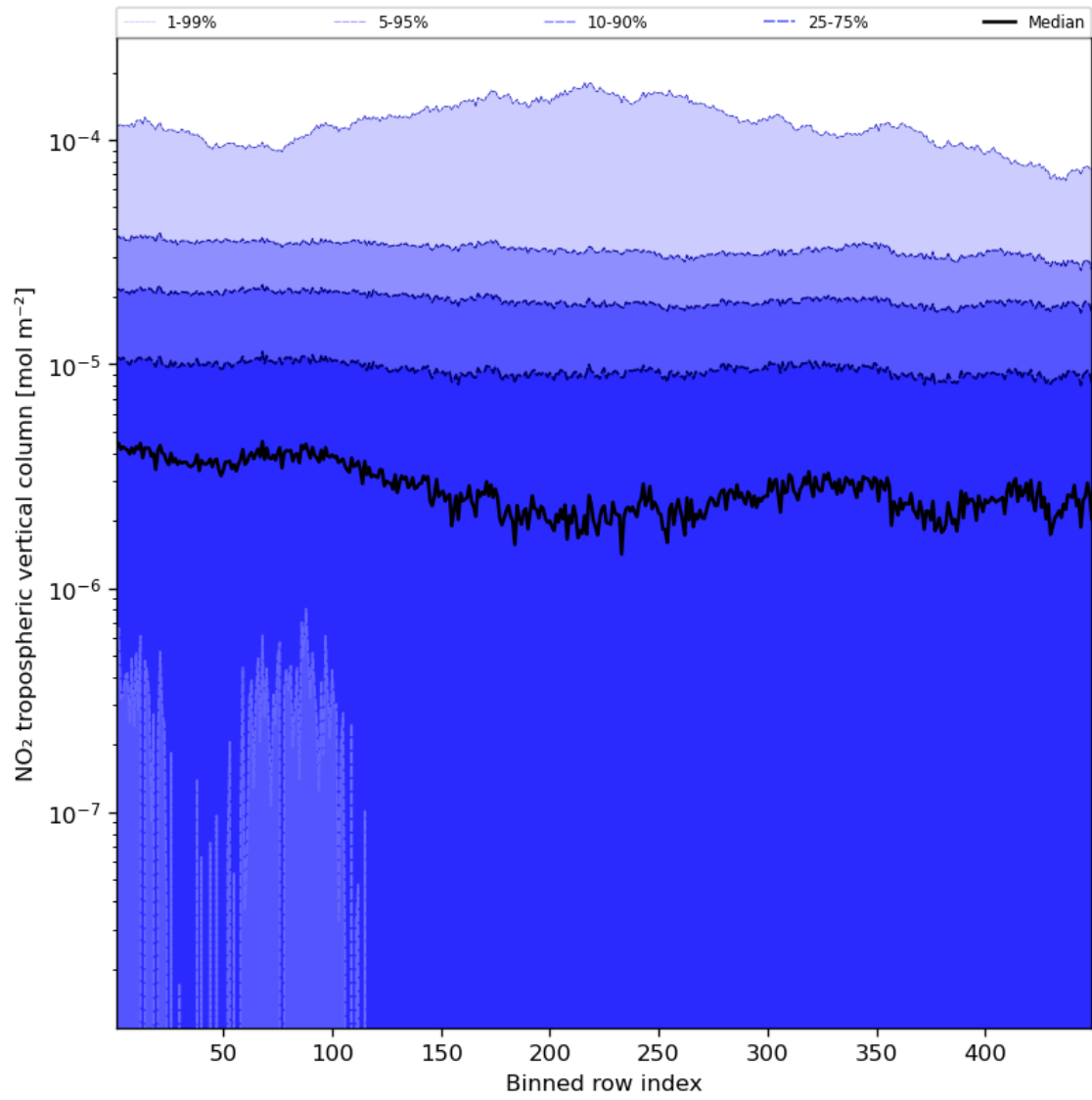
Figure 46: Along track statistics of “NO 2 tropospheric vertical column” for 2023-11-25 to 2023-11-27
