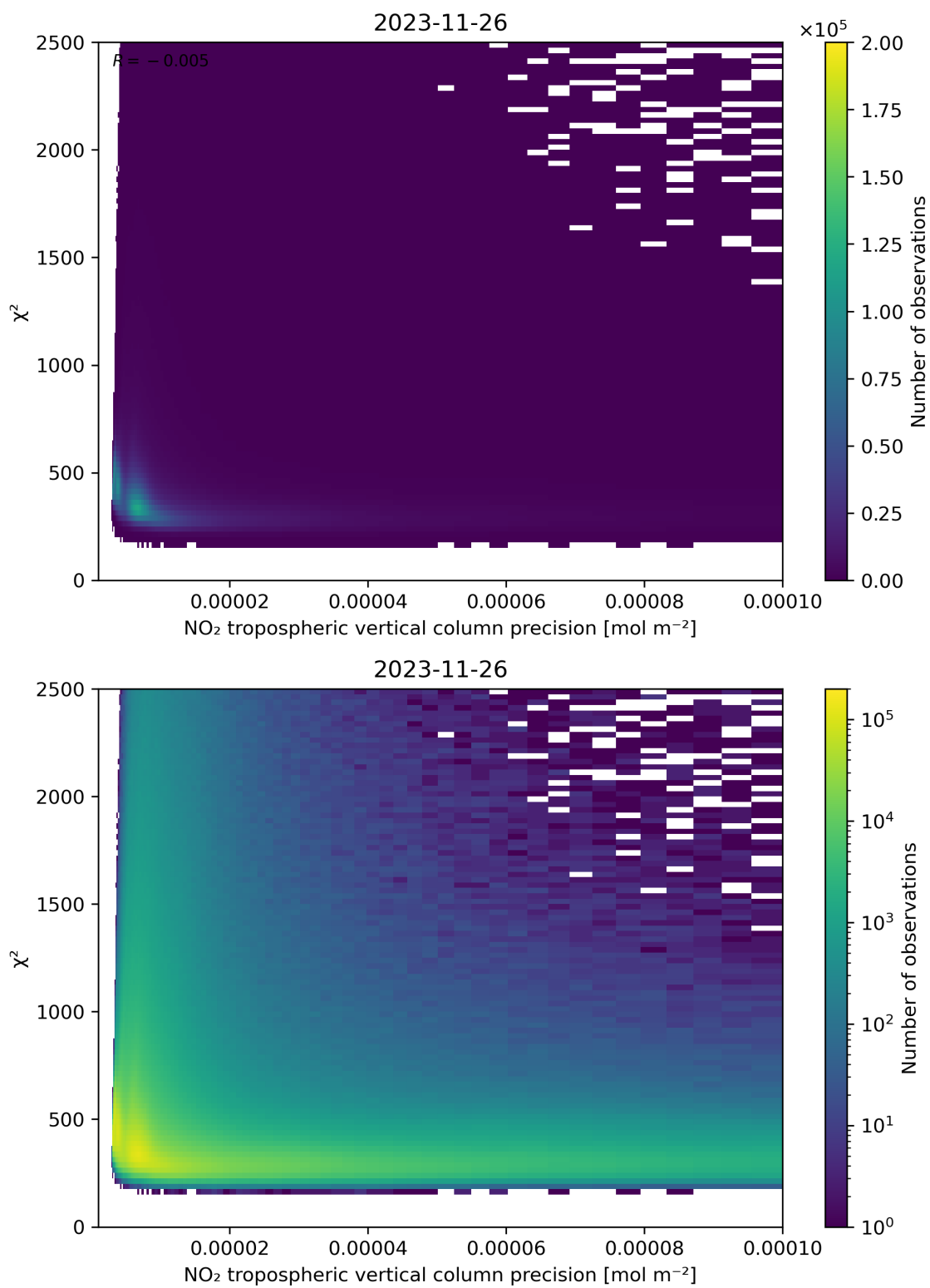
Figure 134: Scatter density plot of “NO 2 tropospheric vertical column precision” against “ \chi^2 ” for 2023-11-25 to 2023-11-27.
