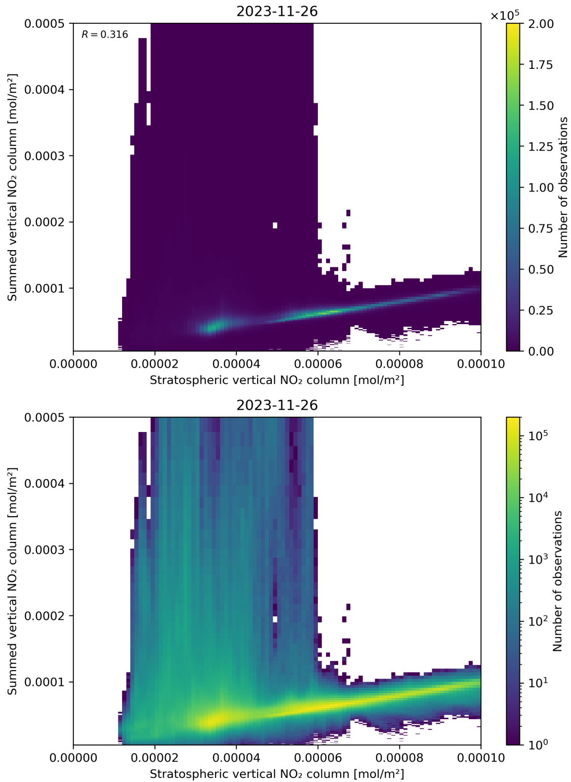
Figure 98: Scatter density plot of “Stratospheric vertical NO 2 column” against “Summed vertical NO 2 column” for 2023-11-25 to 2023-11-27.
