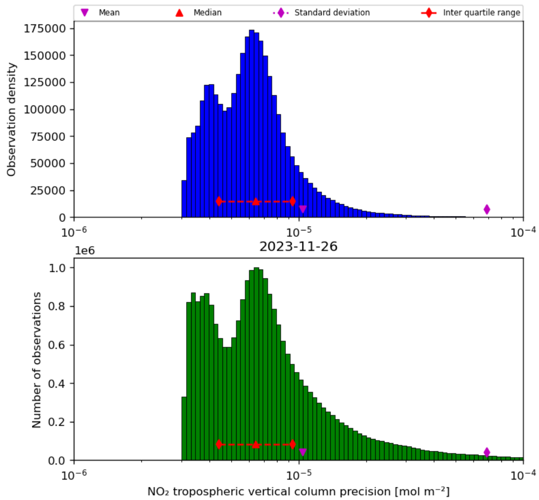
Figure 30: Histogram of “NO 2 tropospheric vertical column precision” for 2023-11-25 to 2023-11-27
