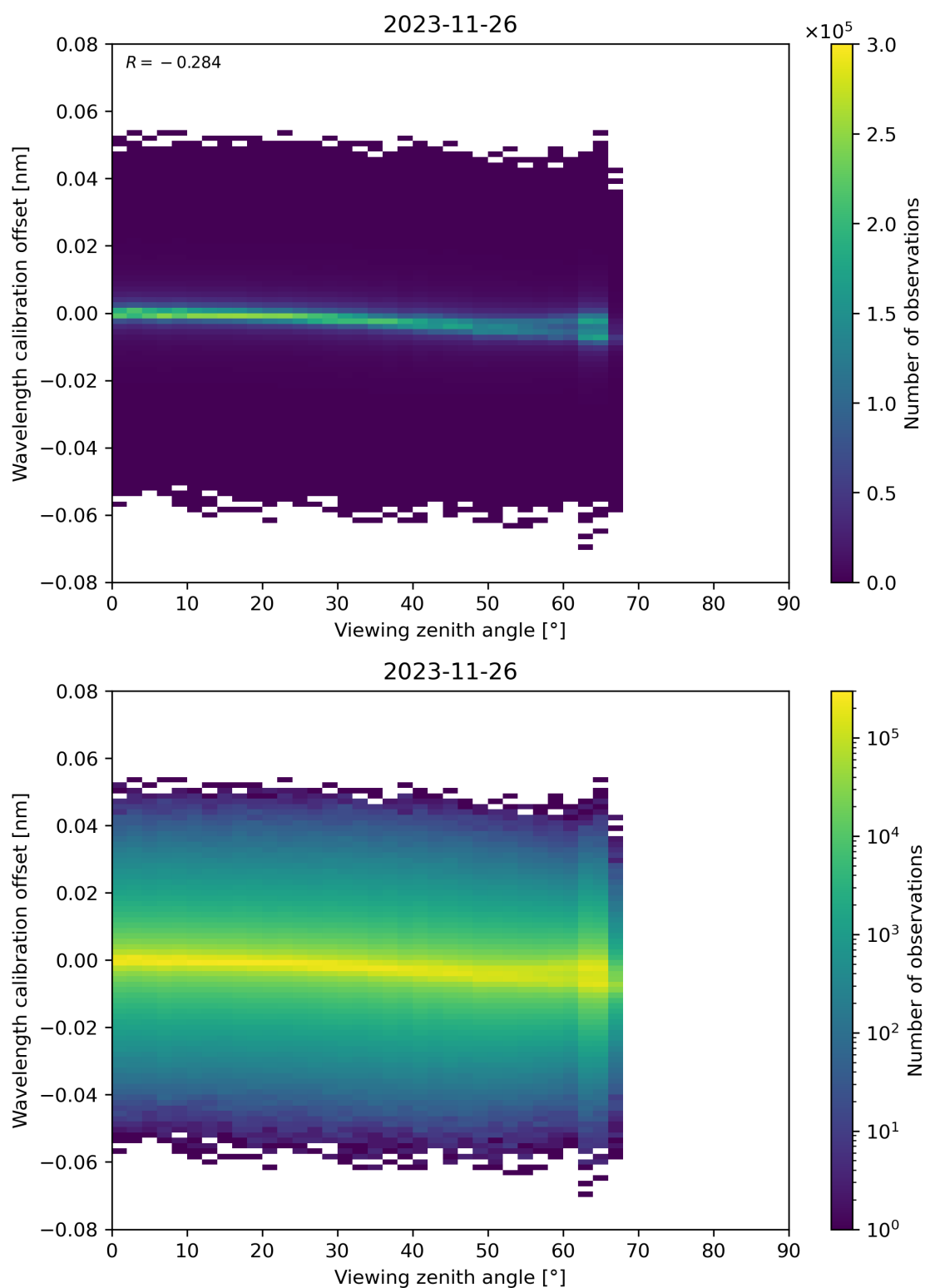
Figure 173: Scatter density plot of “Viewing zenith angle” against “Wavelength calibration offset” for 2023-11-25 to 2023-11-27.
