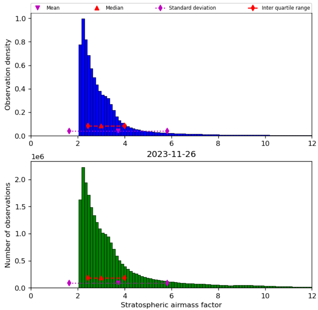
Figure 44: Histogram of “Stratospheric airmass factor” for 2023-11-25 to 2023-11-27
