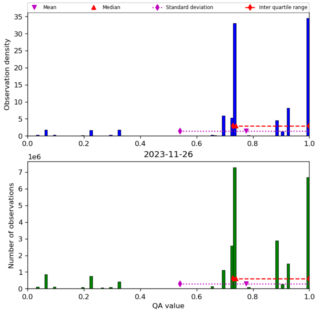
Figure 28: Histogram of “QA value” for 2023-11-25 to 2023-11-27
