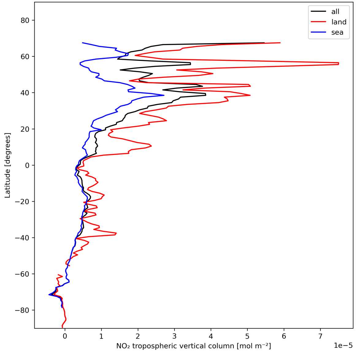
Figure 12: Zonal average of “NO 2 tropospheric vertical column” for 2023-11-25 to 2023-11-27.
