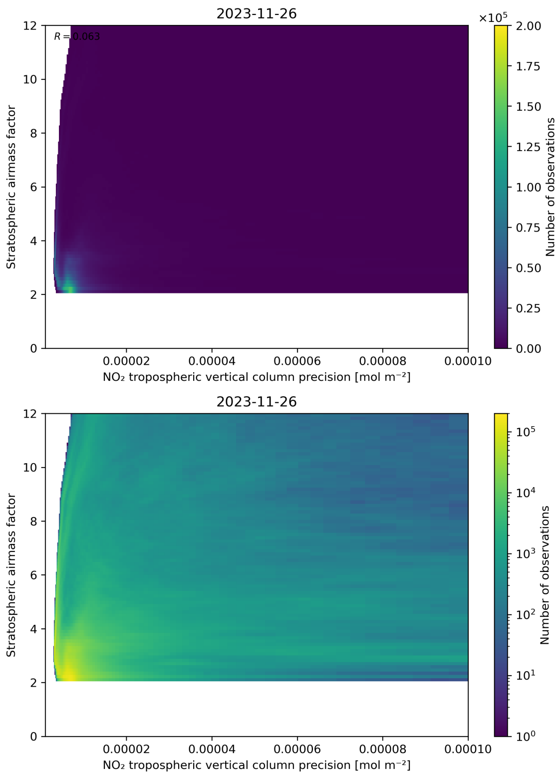
Figure 131: Scatter density plot of “NO 2 tropospheric vertical column precision” against “Stratospheric airmass factor” for 2023-11-25 to 2023-11-27.
