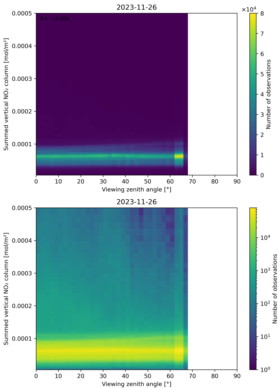
Figure 165: Scatter density plot of “Viewing zenith angle” against “Summed vertical NO 2 column” for 2023-11-25 to 2023-11-27.
