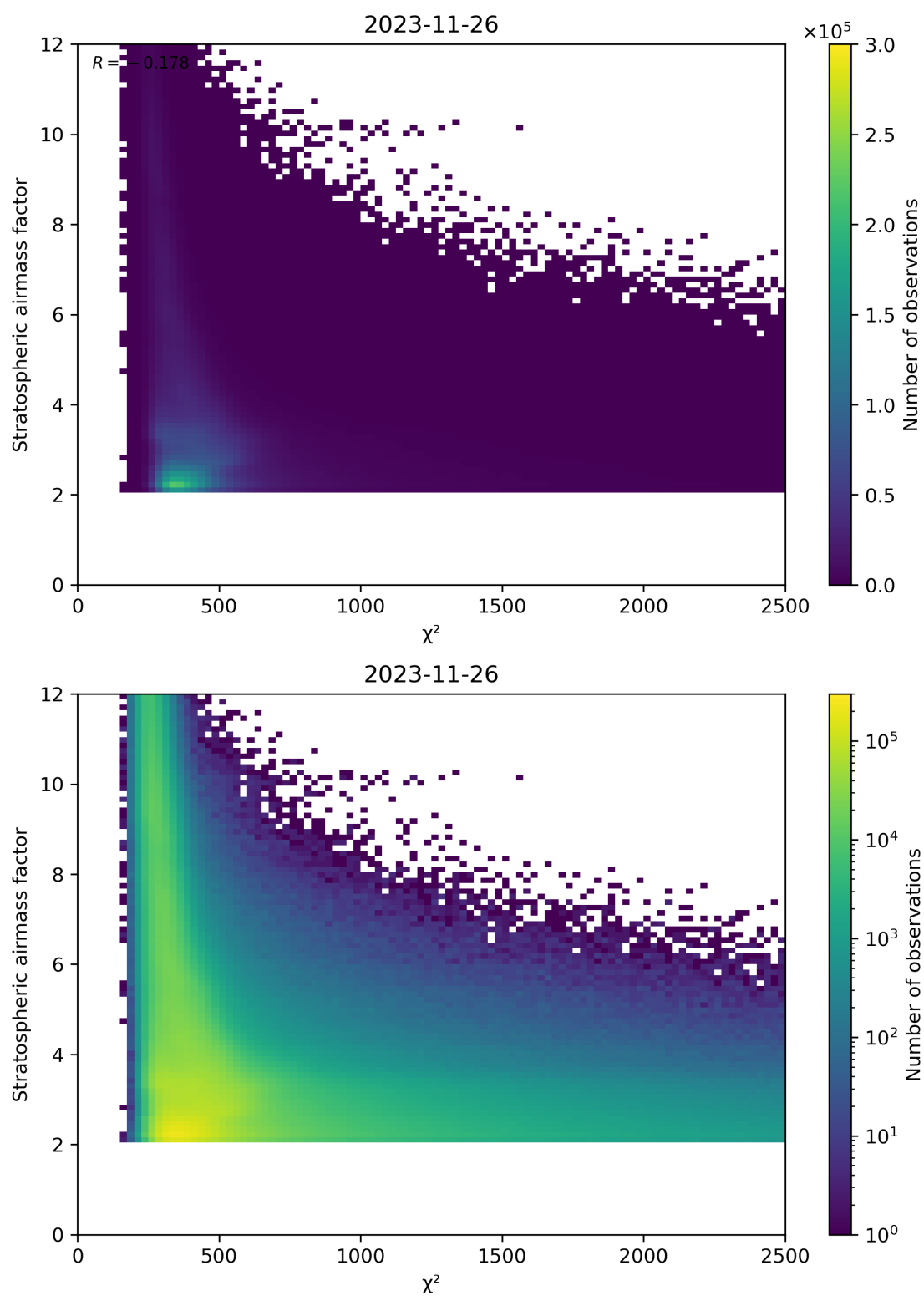
Figure 81: Scatter density plot of “ \chi^2 ” against “Stratospheric airmass factor” for 2023-11-25 to 2023-11-27.
