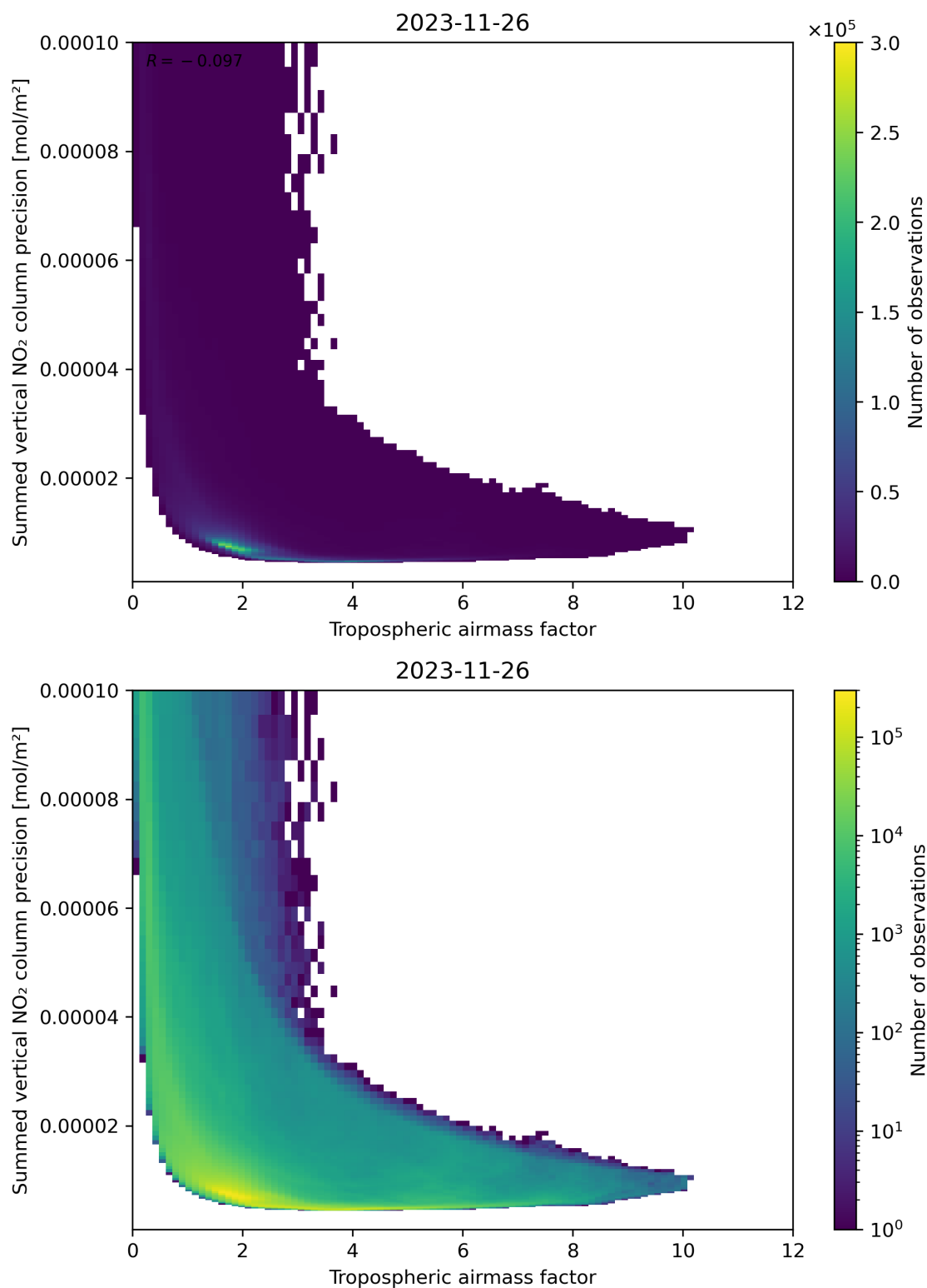
Figure 76: Scatter density plot of “Tropospheric air mass factor” against “Summed vertical NO 2 column precision” for 2023-11-25 to 2023-11-27.
