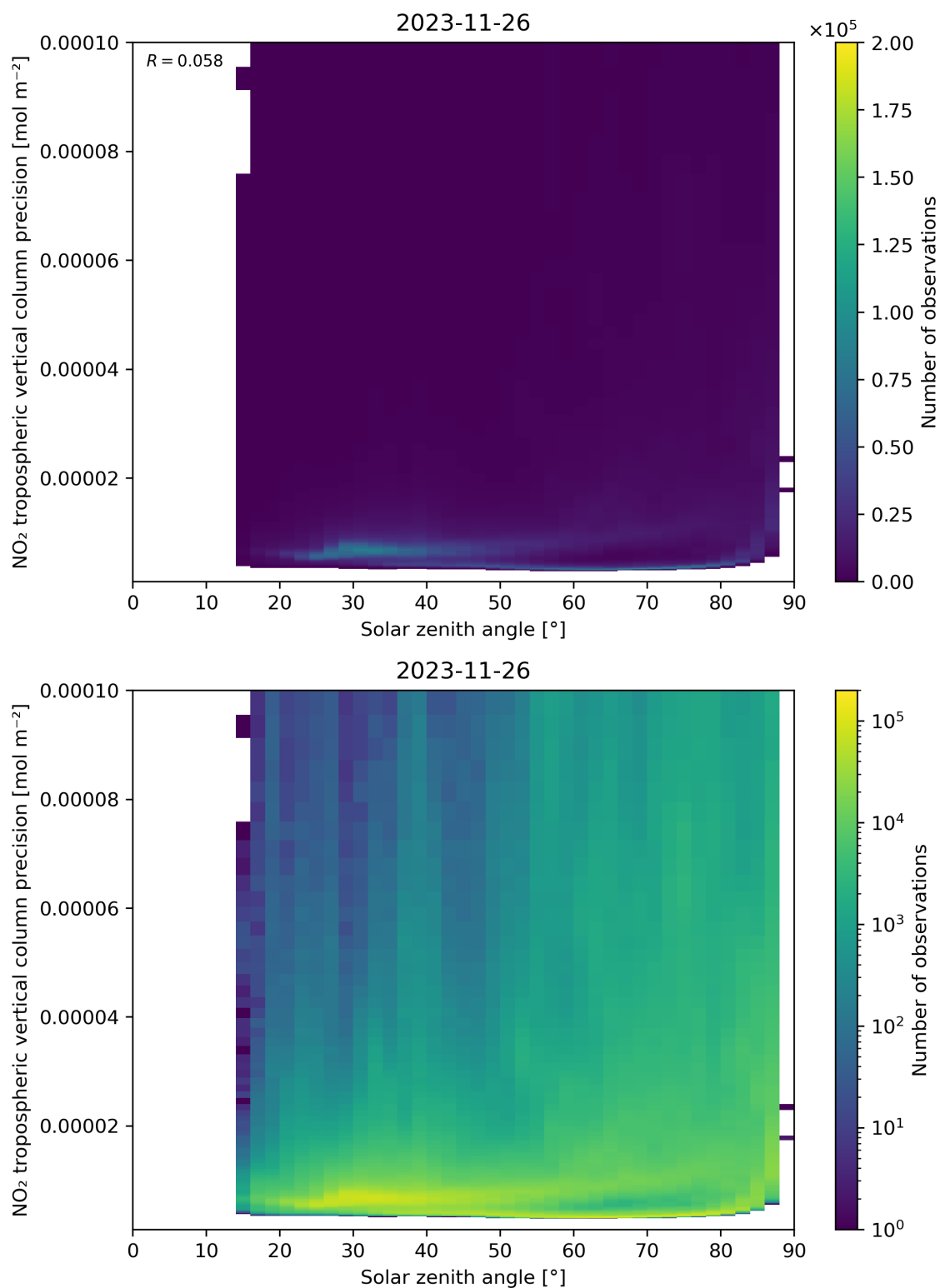
Figure 156: Scatter density plot of “Solar zenith angle” against “NO 2 tropospheric vertical column precision” for 2023-11-25 to 2023-11-27.
