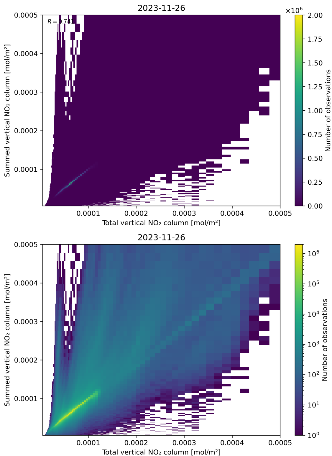
Figure 112: Scatter density plot of “Total vertical NO 2 column” against “Summed vertical NO 2 column” for 2023-11-25 to 2023-11-27.
