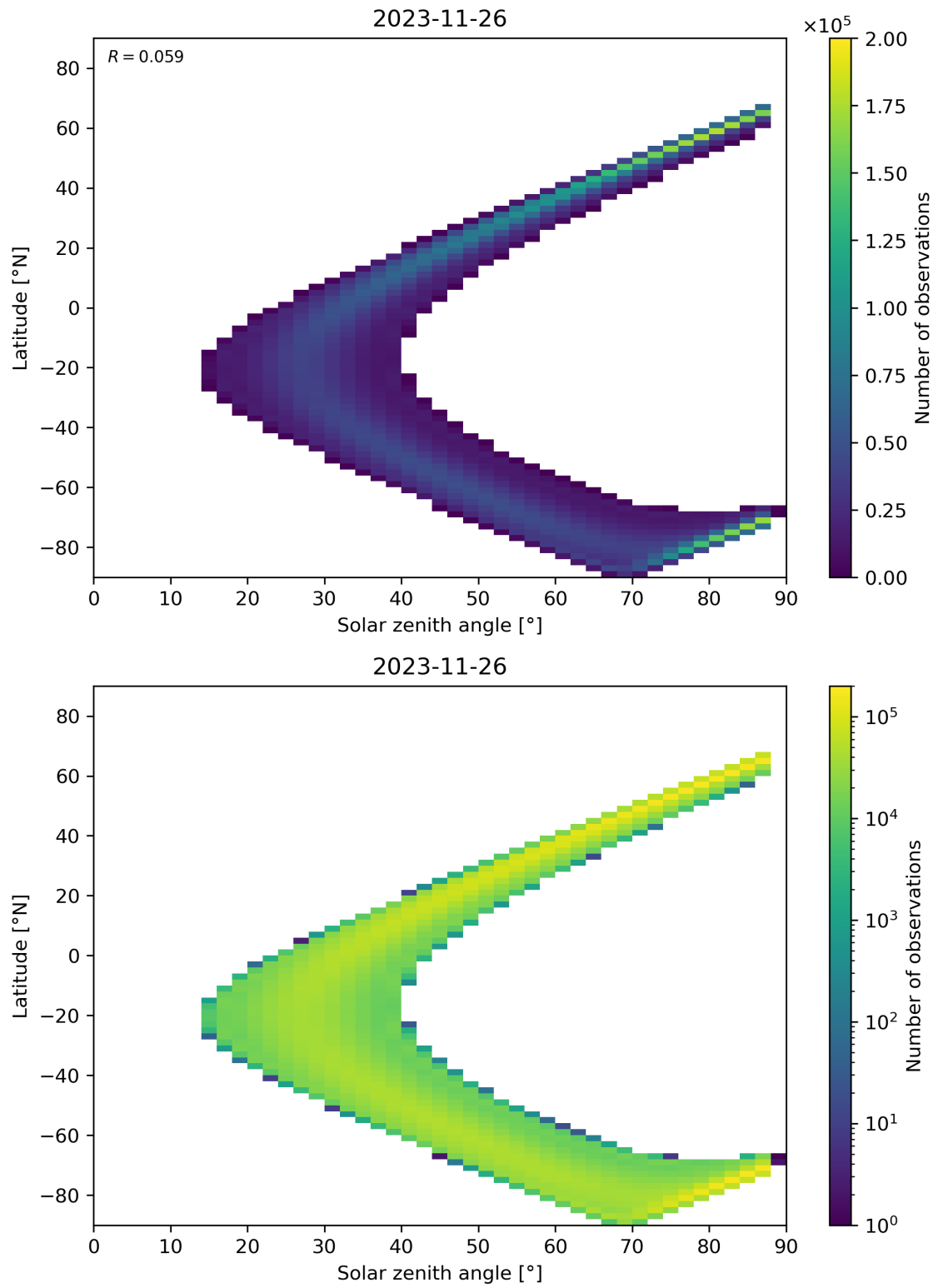
Figure 149: Scatter density plot of “Solar zenith angle” against “Latitude” for 2023-11-25 to 2023-11-27.
