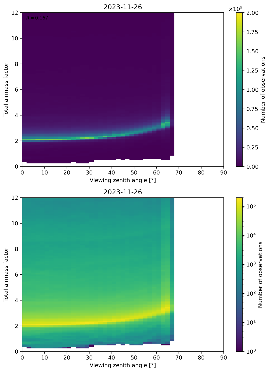
Figure 160: Scatter density plot of “Viewing zenith angle” against “Total airmass factor” for 2023-11-25 to 2023-11-27.
