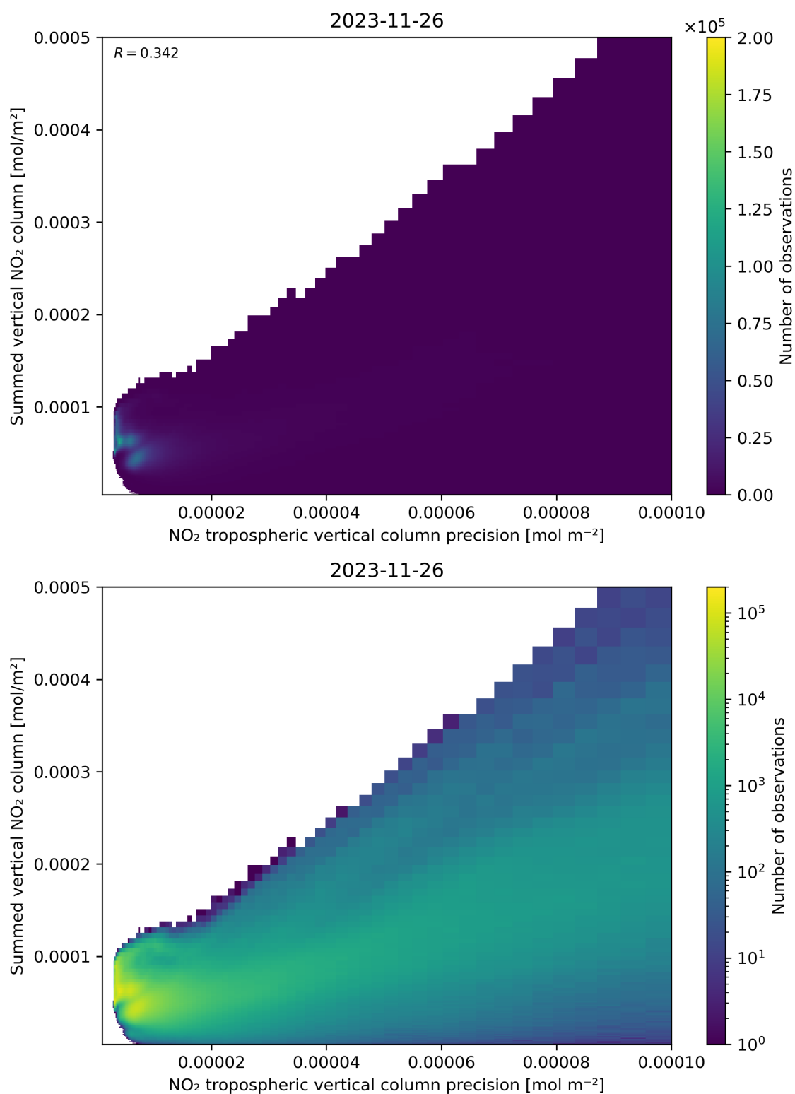
Figure 136: Scatter density plot of “NO 2 tropospheric vertical column precision” against “Summed vertical NO 2 column” for 2023-11-25 to 2023-11-27.
