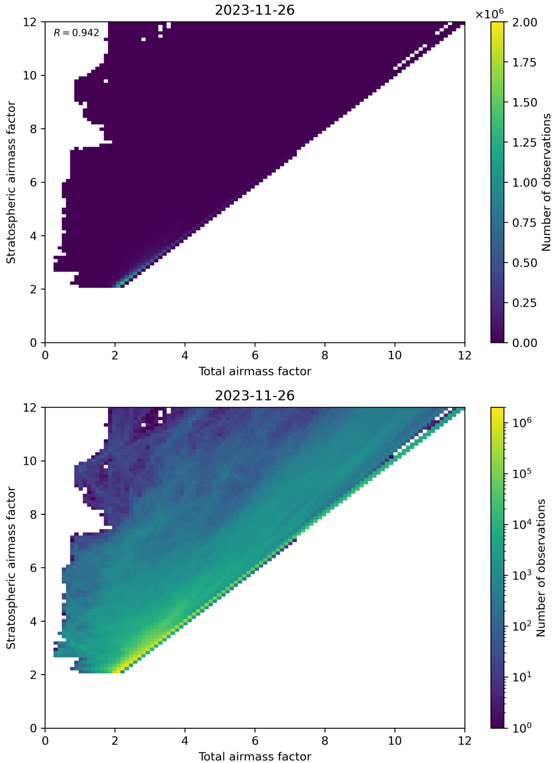
Figure 62: Scatter density plot of “Total airmass factor” against “Stratospheric airmass factor” for 2023-11-25 to 2023-11-27.
