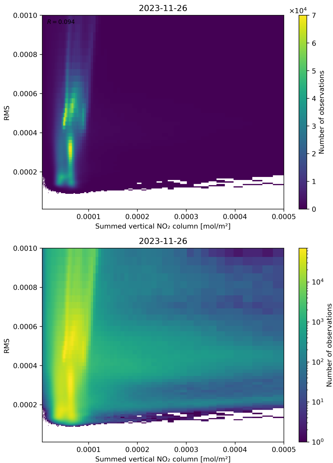
Figure 109: Scatter density plot of “Summed vertical NO 2 column” against “RMS” for 2023-11-25 to 2023-11-27.
