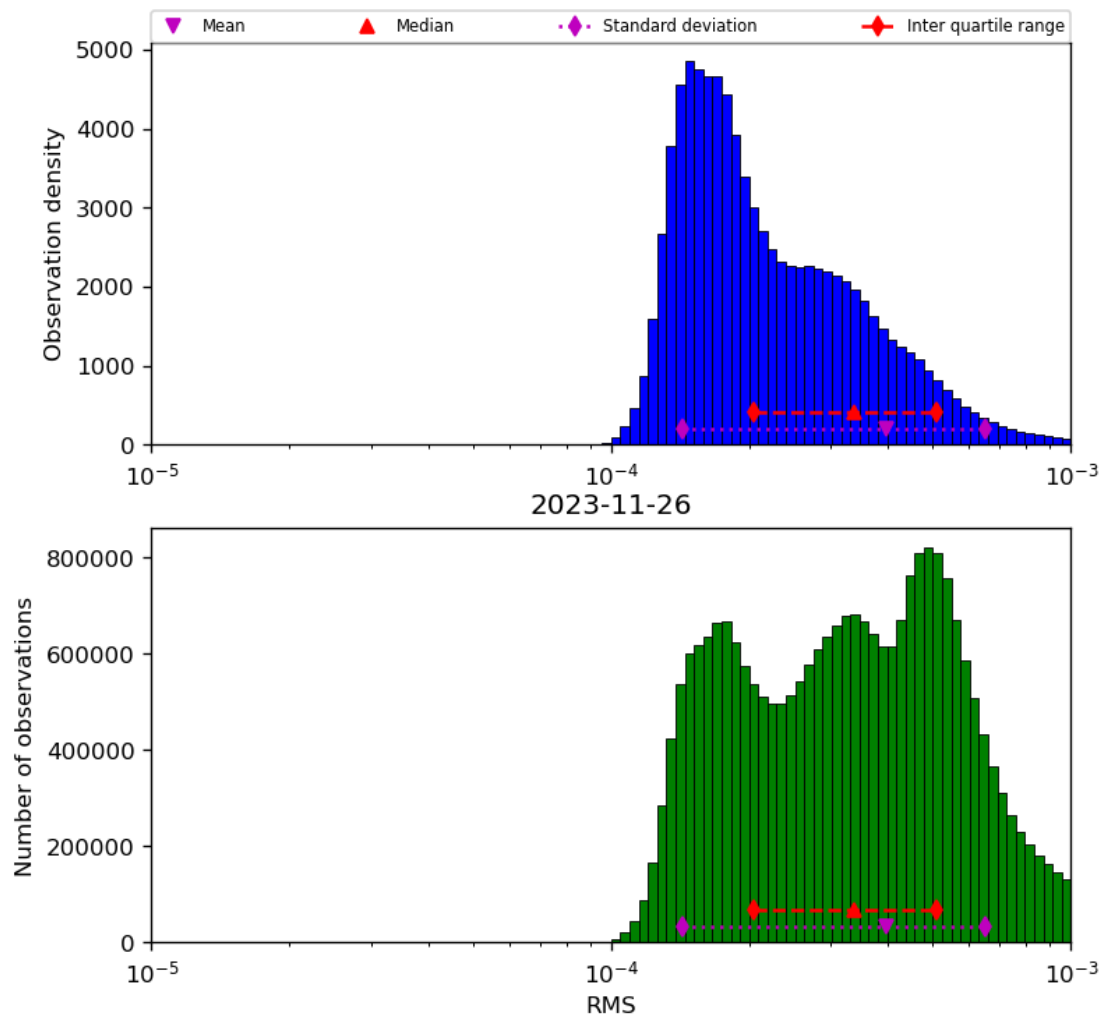
Figure 43: Histogram of “RMS” for 2023-11-25 to 2023-11-27
