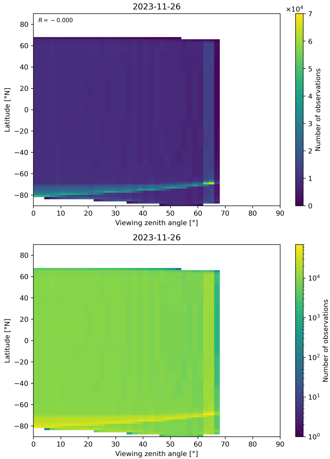
Figure 163: Scatter density plot of “Viewing zenith angle” against “Latitude” for 2023-11-25 to 2023-11-27.
