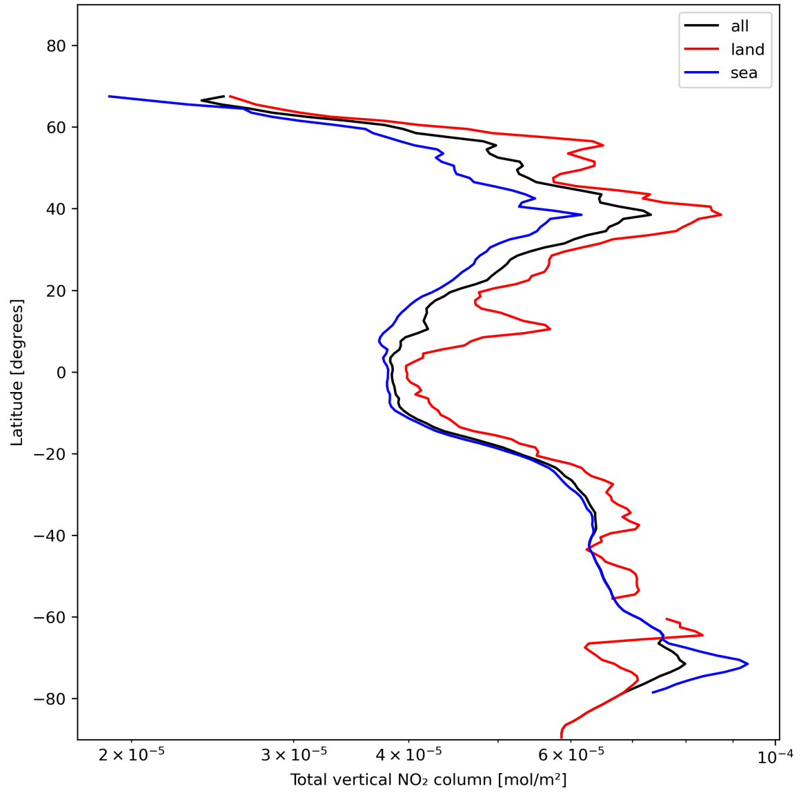
Figure 21: Zonal average of “Total vertical NO 2 column” for 2023-11-25 to 2023-11-27.
