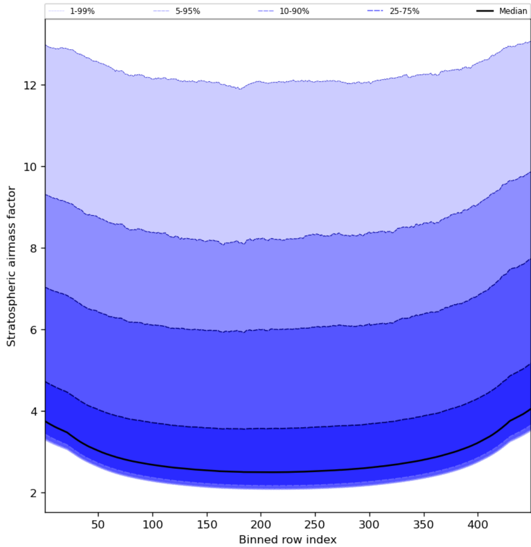
Figure 61: Along track statistics of “Stratospheric airmass factor” for 2023-11-25 to 2023-11-27
