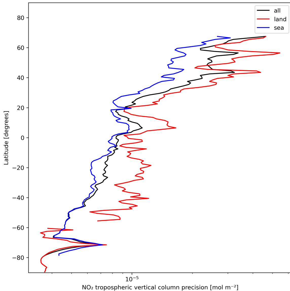
Figure 13: Zonal average of “NO 2 tropospheric vertical column precision” for 2023-11-25 to 2023-11-27.
