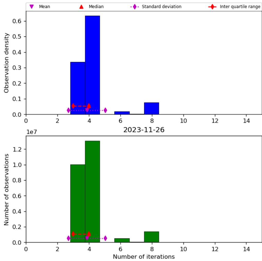
Figure 34: Histogram of “Number of iterations” for 2023-11-25 to 2023-11-27
