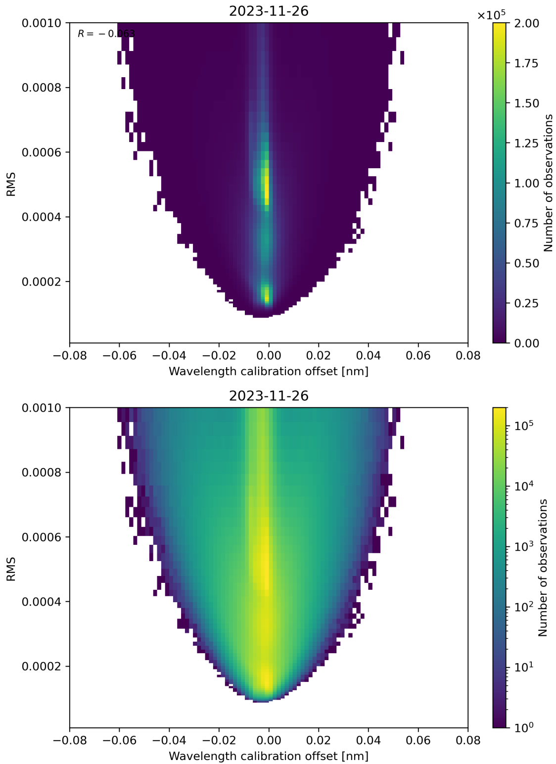
Figure 181: Scatter density plot of “Wavelength calibration offset” against “RMS” for 2023-11-25 to 2023-11-27.
