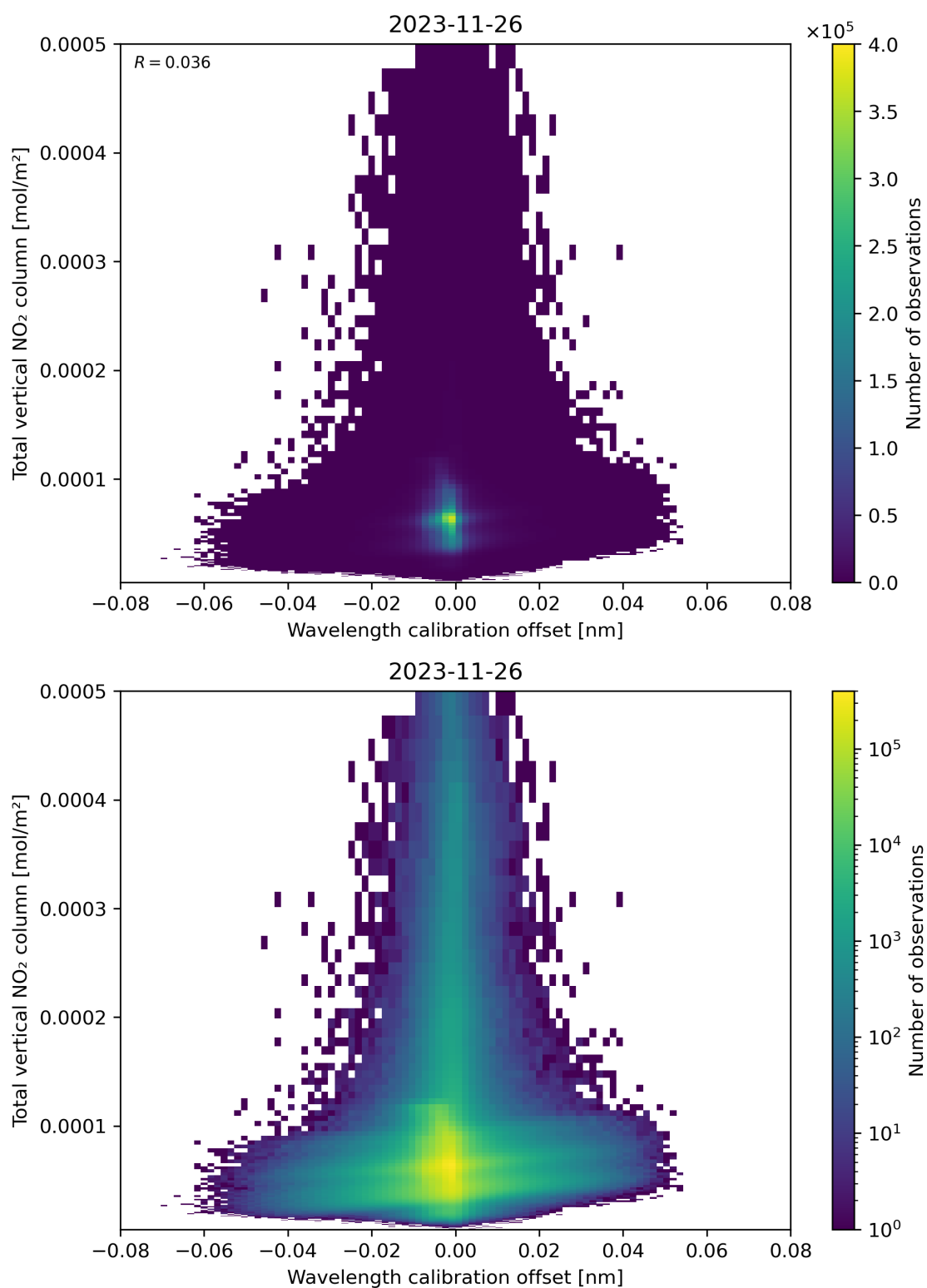
Figure 179: Scatter density plot of “Wavelength calibration offset” against “Total vertical NO 2 column” for 2023-11-25 to 2023-11-27.
