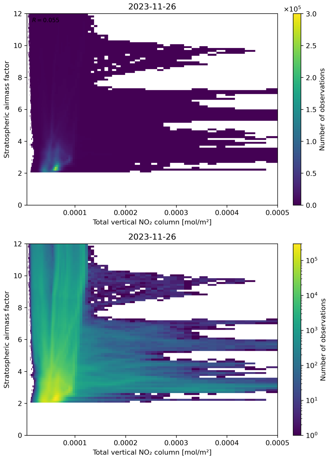
Figure 110: Scatter density plot of “Total vertical NO 2 column” against “Stratospheric air mass factor” for 2023-11-25 to 2023-11-27.
