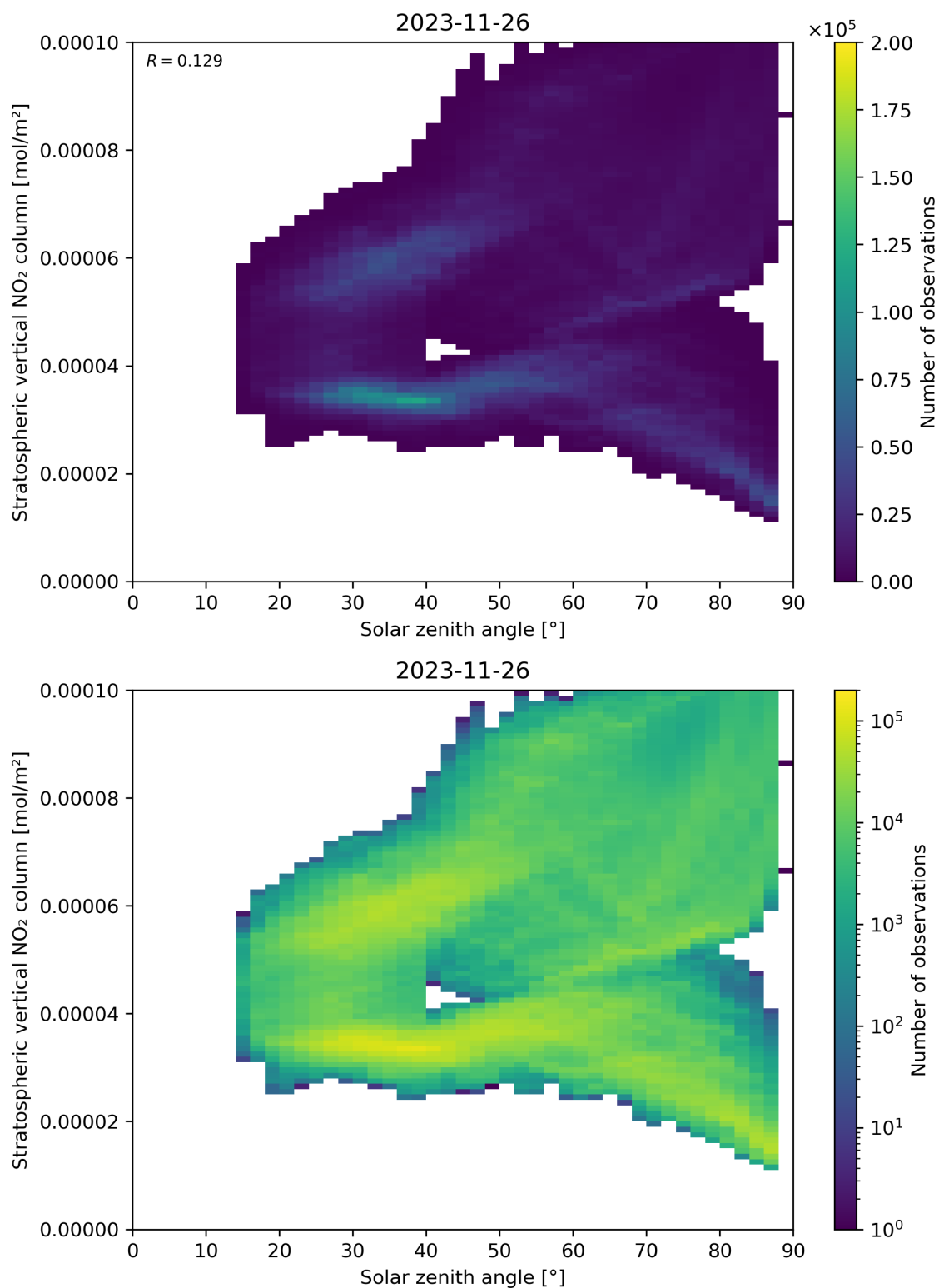
Figure 150: Scatter density plot of “Solar zenith angle” against “Stratospheric vertical NO 2 column” for 2023-11-25 to 2023-11-27.
