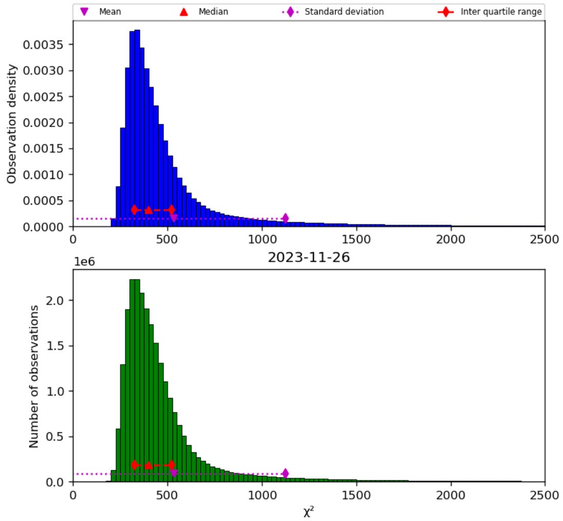
Figure 42: Histogram of “ \chi^2 ” for 2023-11-25 to 2023-11-27
