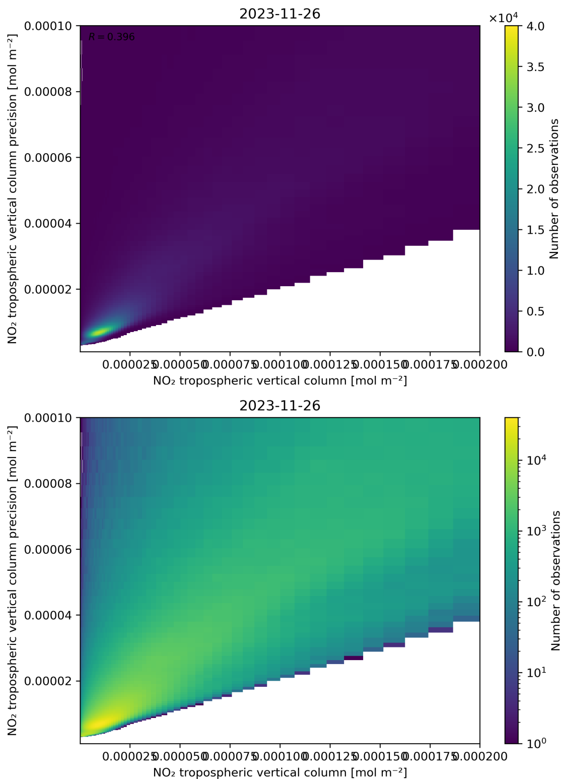
Figure 130: Scatter density plot of “NO 2 tropospheric vertical column” against “NO 2 tropospheric vertical column precision” for 2023-11-25 to 2023-11-27.
