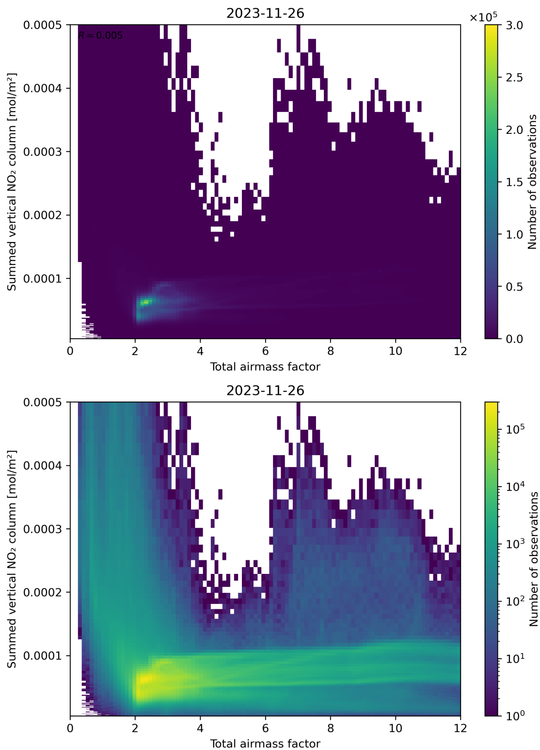
Figure 65: Scatter density plot of “Total airmass factor” against “Summed vertical NO 2 column” for 2023-11-25 to 2023-11-27.
