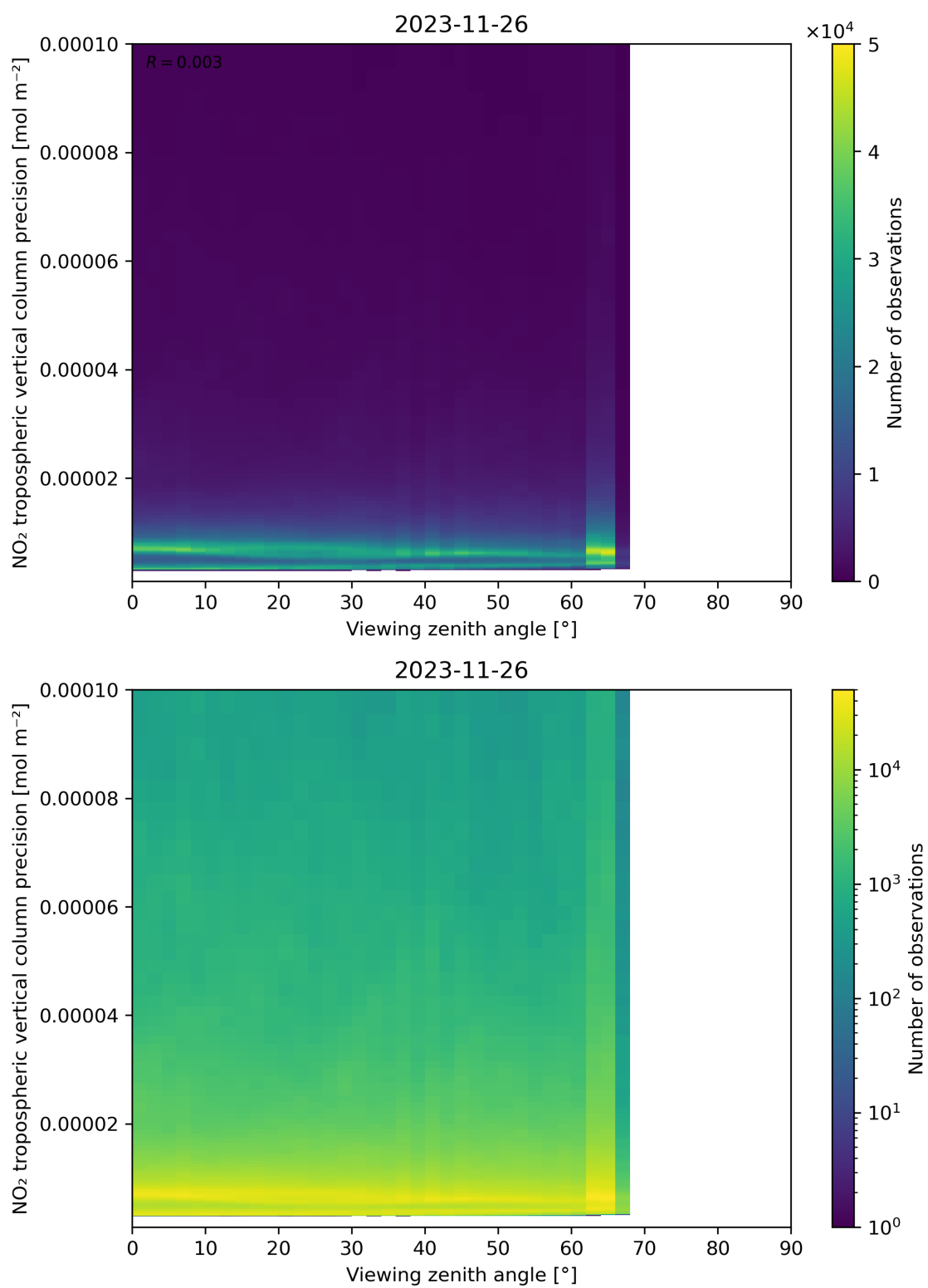
Figure 170: Scatter density plot of “Viewing zenith angle” against “NO 2 tropospheric vertical column precision” for 2023-11-25 to 2023-11-27.
