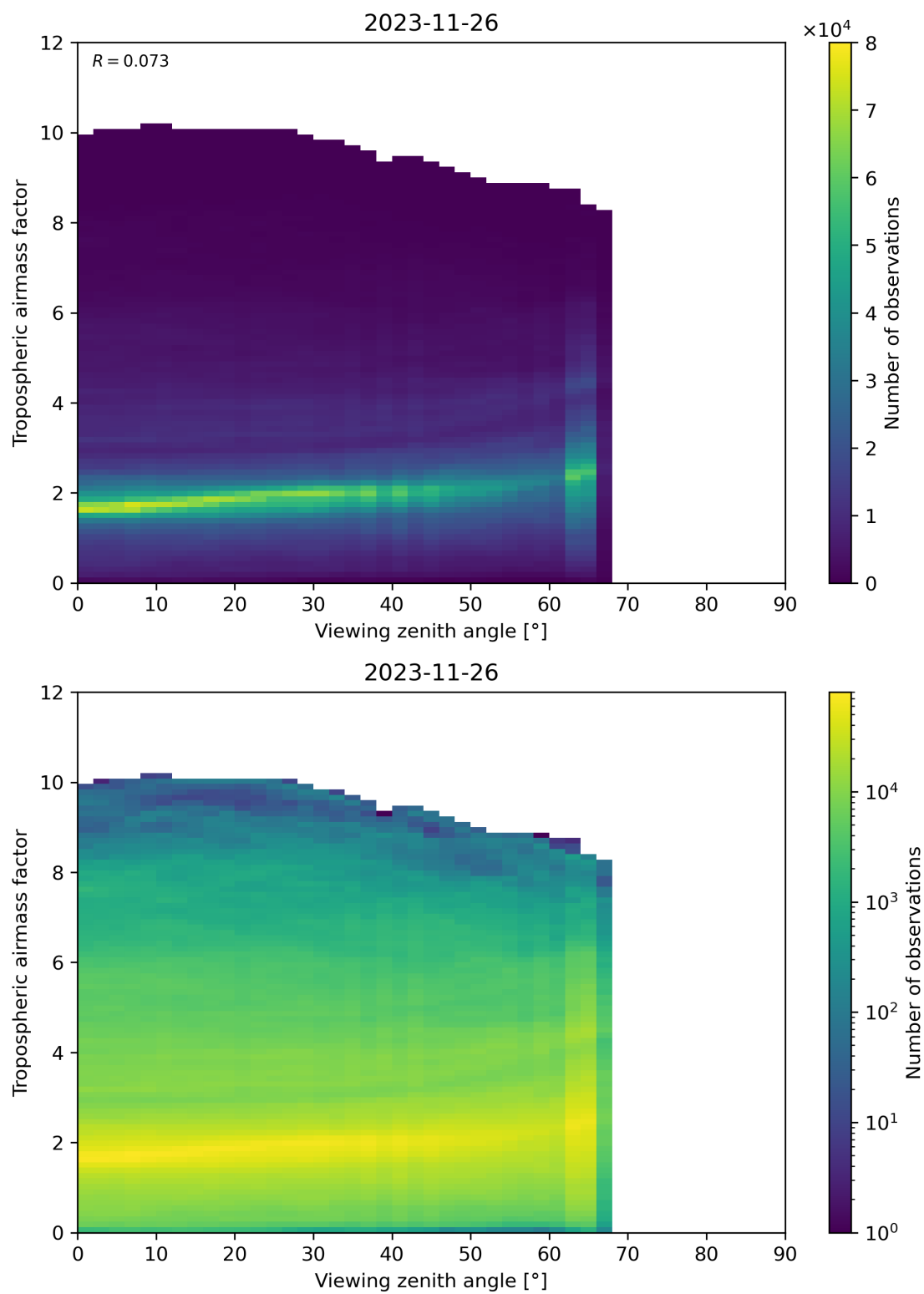
Figure 161: Scatter density plot of “Viewing zenith angle” against “Tropospheric airmass factor” for 2023-11-25 to 2023-11-27.
