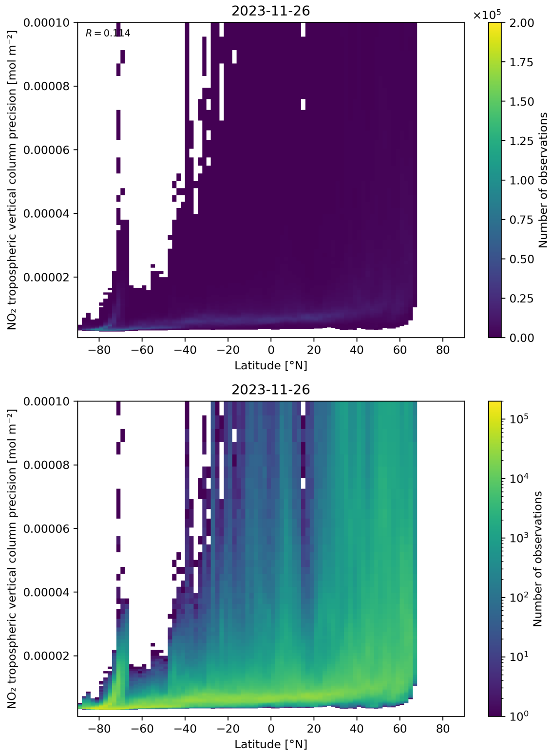
Figure 93: Scatter density plot of “Latitude” against “NO 2 tropospheric vertical column precision” for 2023-11-25 to 2023-11-27.
