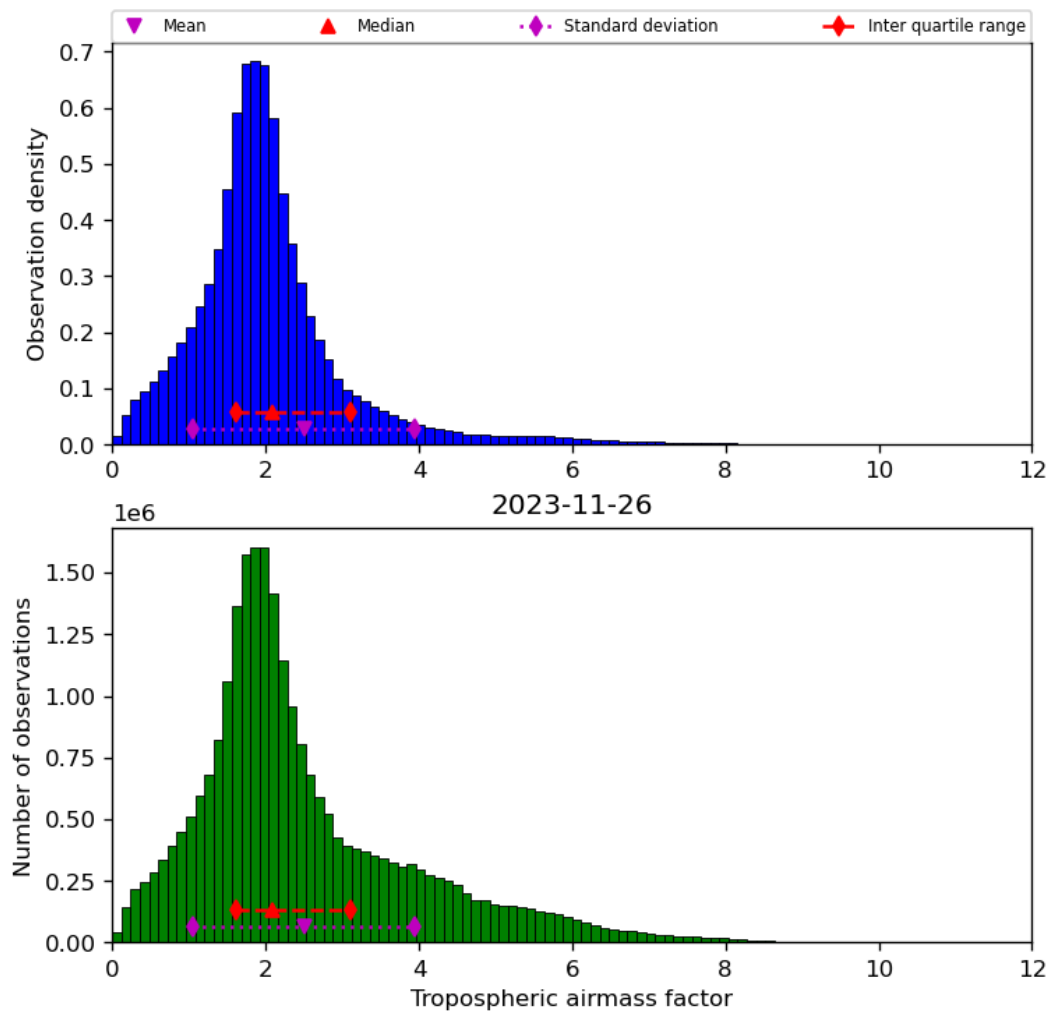
Figure 31: Histogram of “Tropospheric airmass factor” for 2023-11-25 to 2023-11-27
