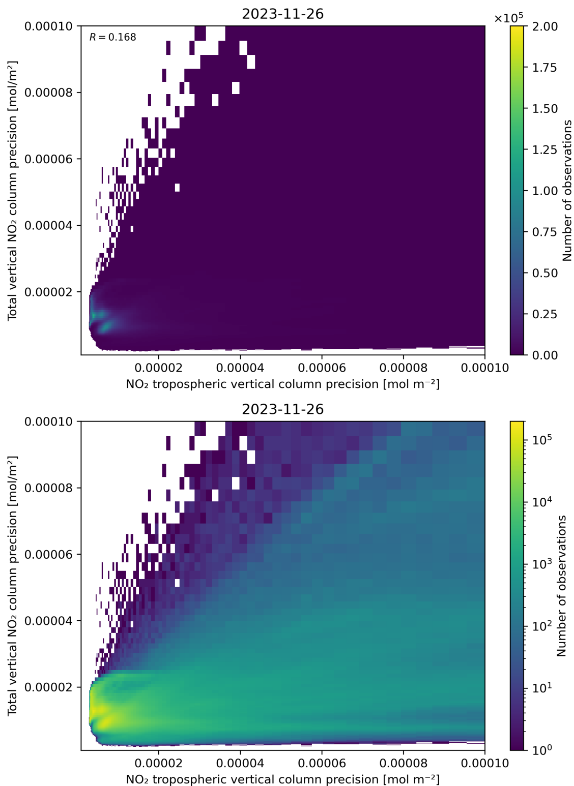
Figure 139: Scatter density plot of “NO 2 tropospheric vertical column precision” against “Total vertical NO 2 column precision” for 2023-11-25 to 2023-11-27.
