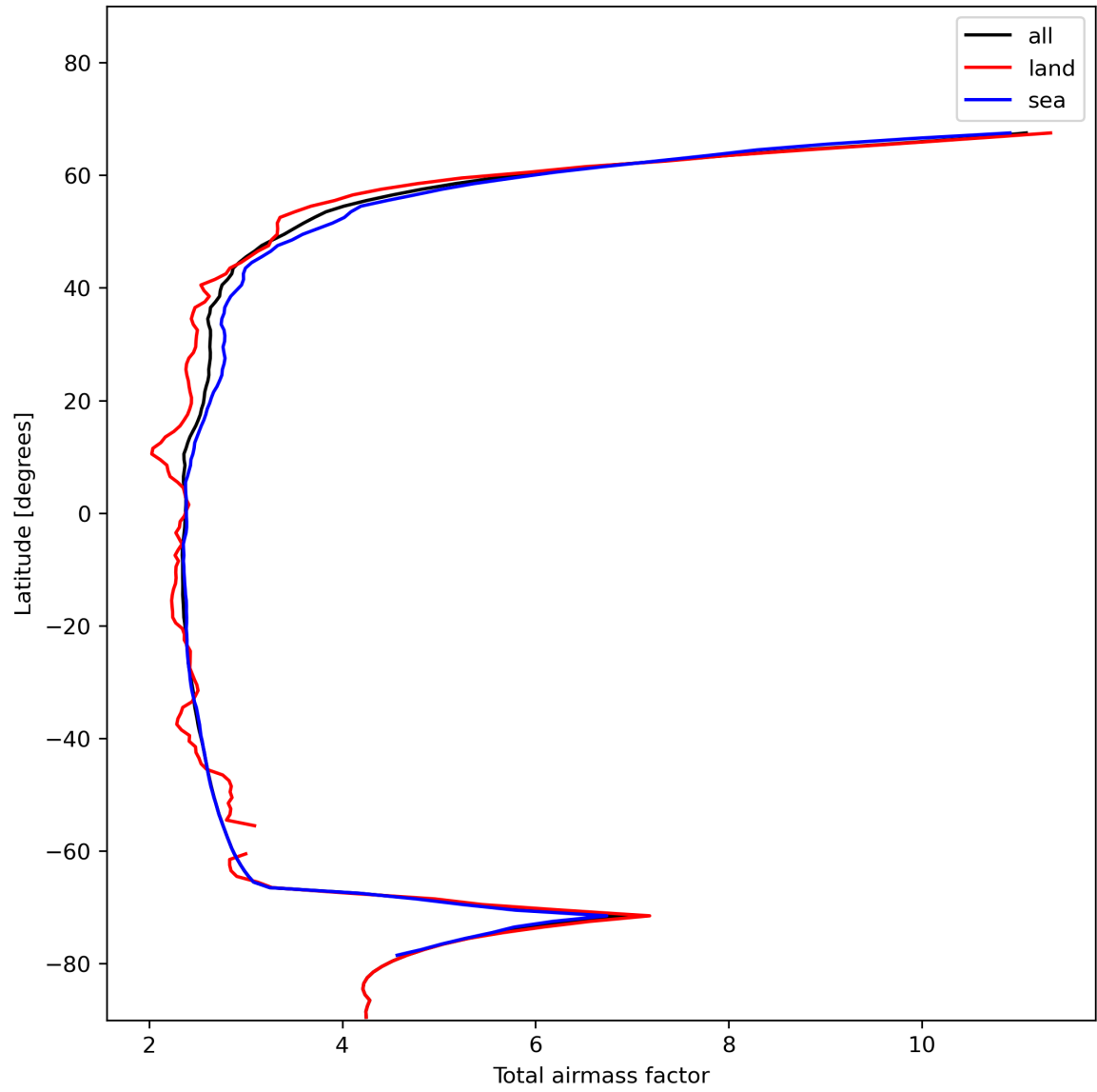
Figure 15: Zonal average of “Total airmass factor” for 2023-11-25 to 2023-11-27.
