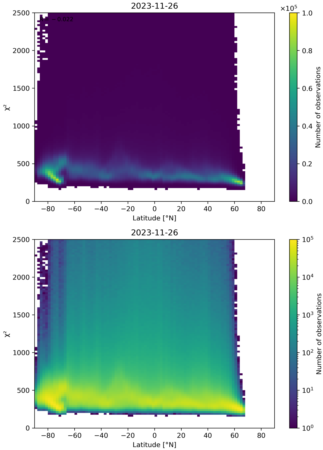
Figure 86: Scatter density plot of “Latitude” against “ \chi^2 ” for 2023-11-25 to 2023-11-27.
