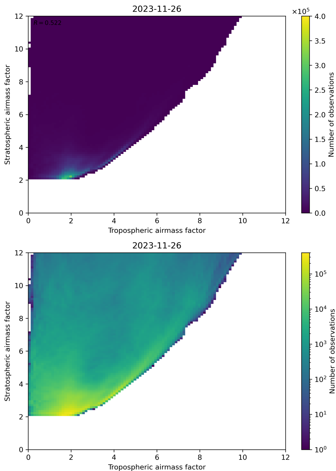
Figure 71: Scatter density plot of “Tropospheric airmass factor” against “Stratospheric airmass factor” for 2023-11-25 to 2023-11-27.
