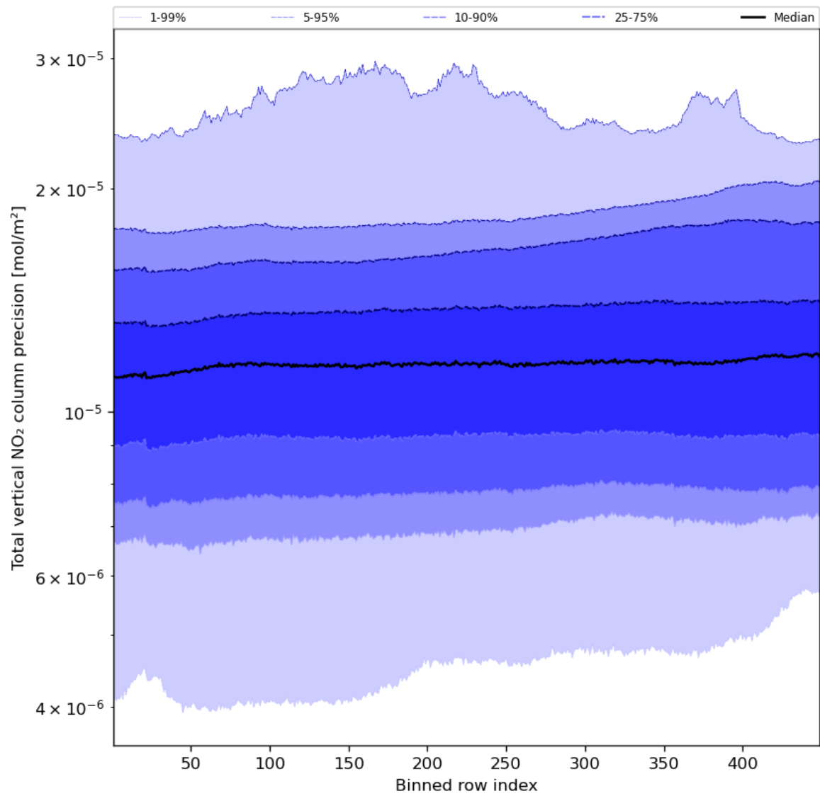
Figure 56: Along track statistics of “Total vertical NO 2 column precision” for 2023-11-25 to 2023-11-27
