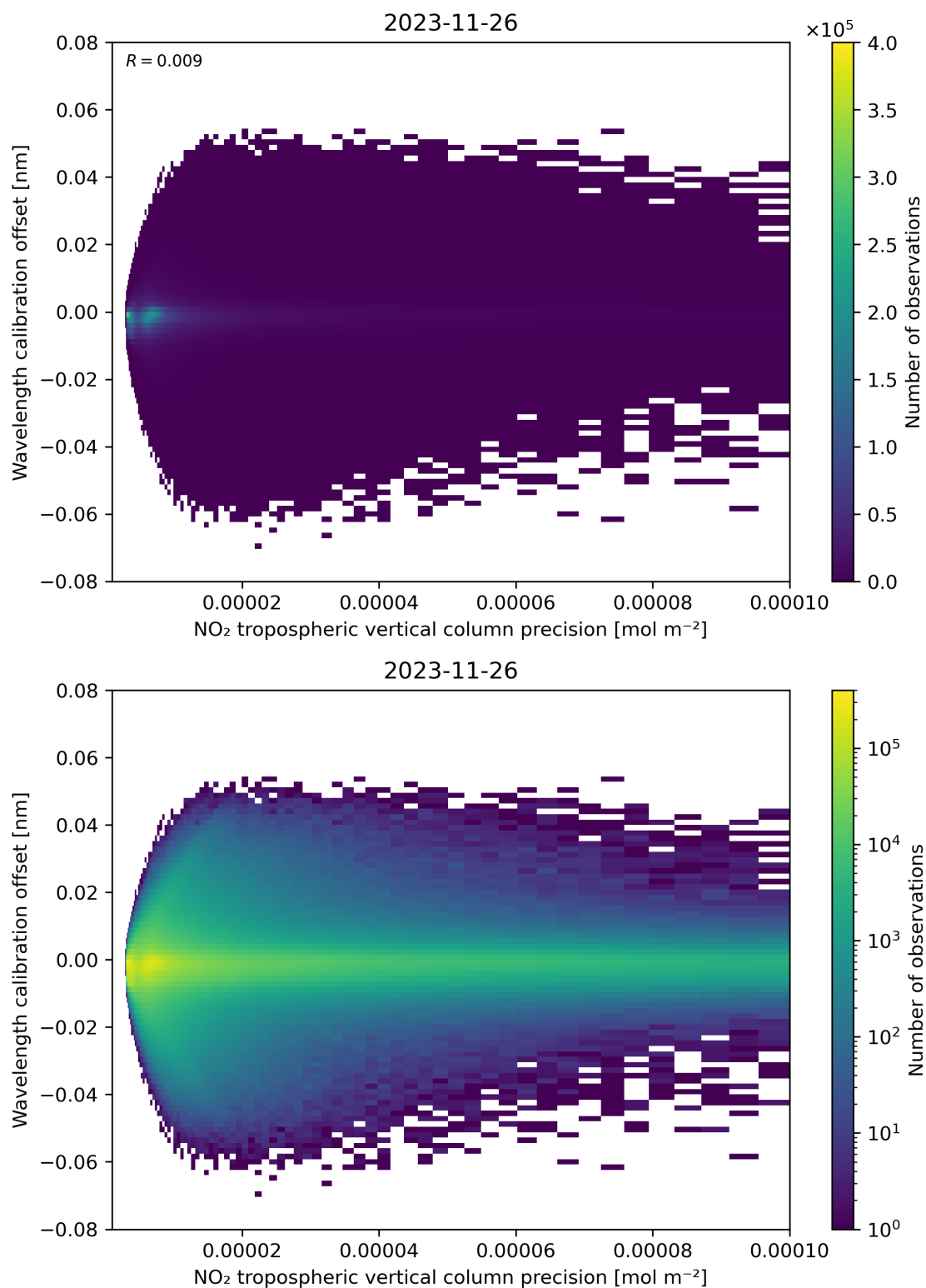
Figure 141: Scatter density plot of “NO 2 tropospheric vertical column precision” against “Wavelength calibration offset” for 2023-11-25 to 2023-11-27.
