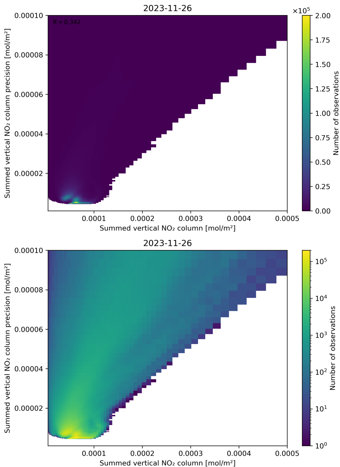
Figure 105: Scatter density plot of “Summed vertical NO 2 column” against “Summed vertical NO 2 column precision” for 2023-11-25 to 2023-11-27.
