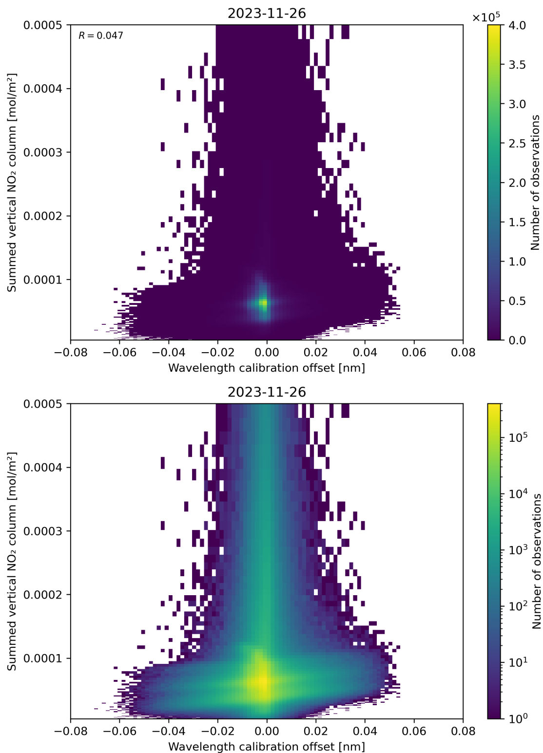
Figure 177: Scatter density plot of “Wavelength calibration offset” against “Summed vertical NO 2 column” for 2023-11-25 to 2023-11-27.
