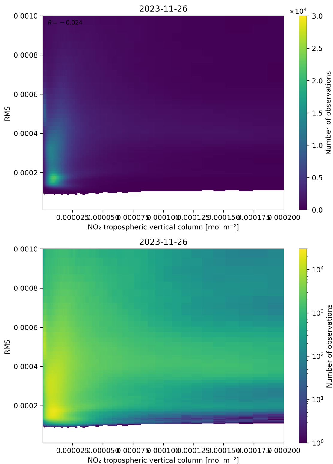
Figure 142: Scatter density plot of “NO 2 tropospheric vertical column” against “RMS” for 2023-11-25 to 2023-11-27.
