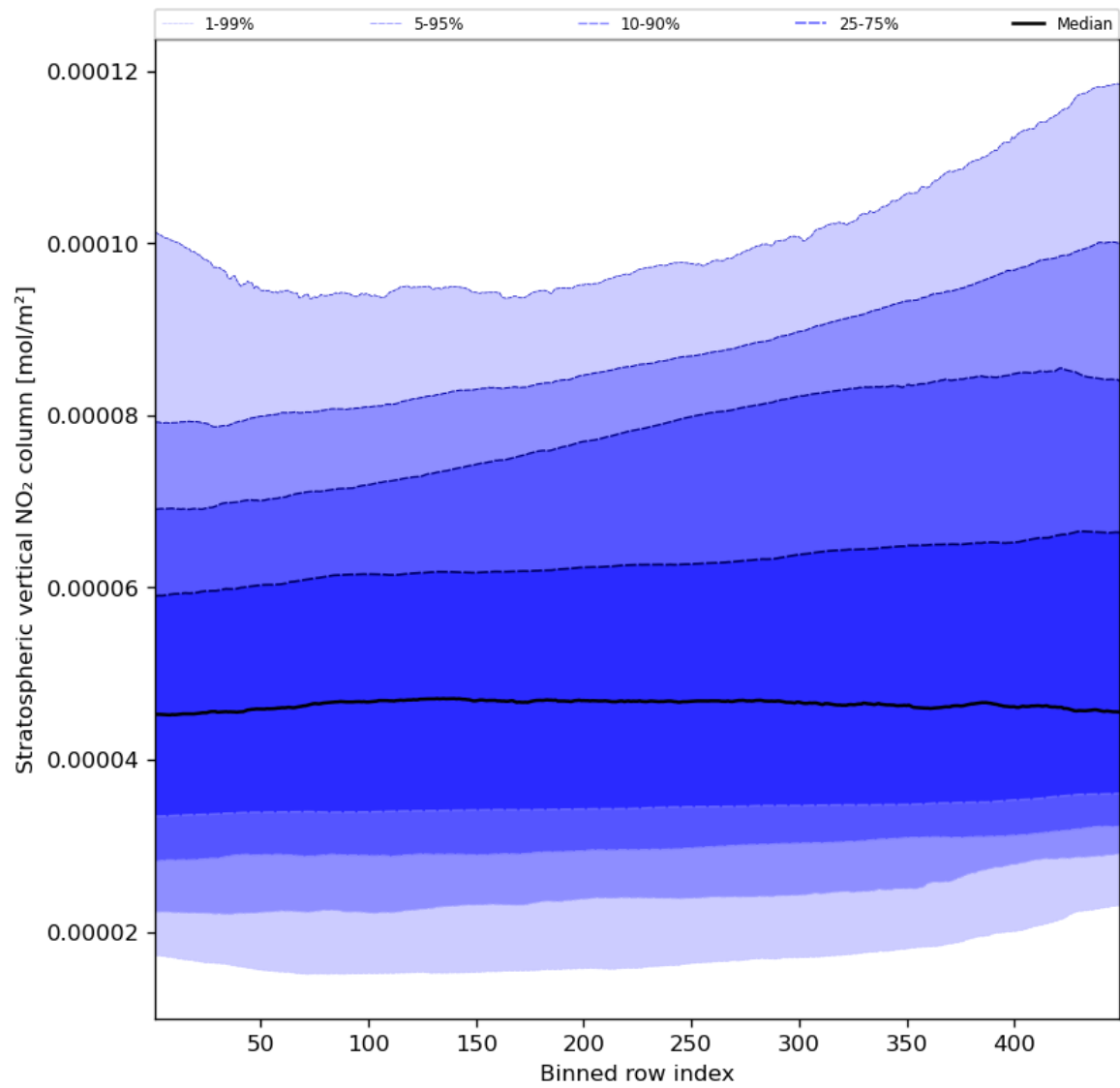
Figure 53: Along track statistics of “Stratospheric vertical NO 2 column” for 2023-11-25 to 2023-11-27
