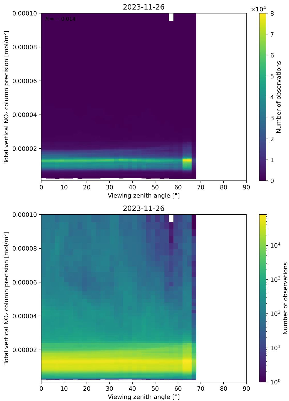
Figure 168: Scatter density plot of “Viewing zenith angle” against “Total vertical NO 2 column precision” for 2023-11-25 to 2023-11-27.
