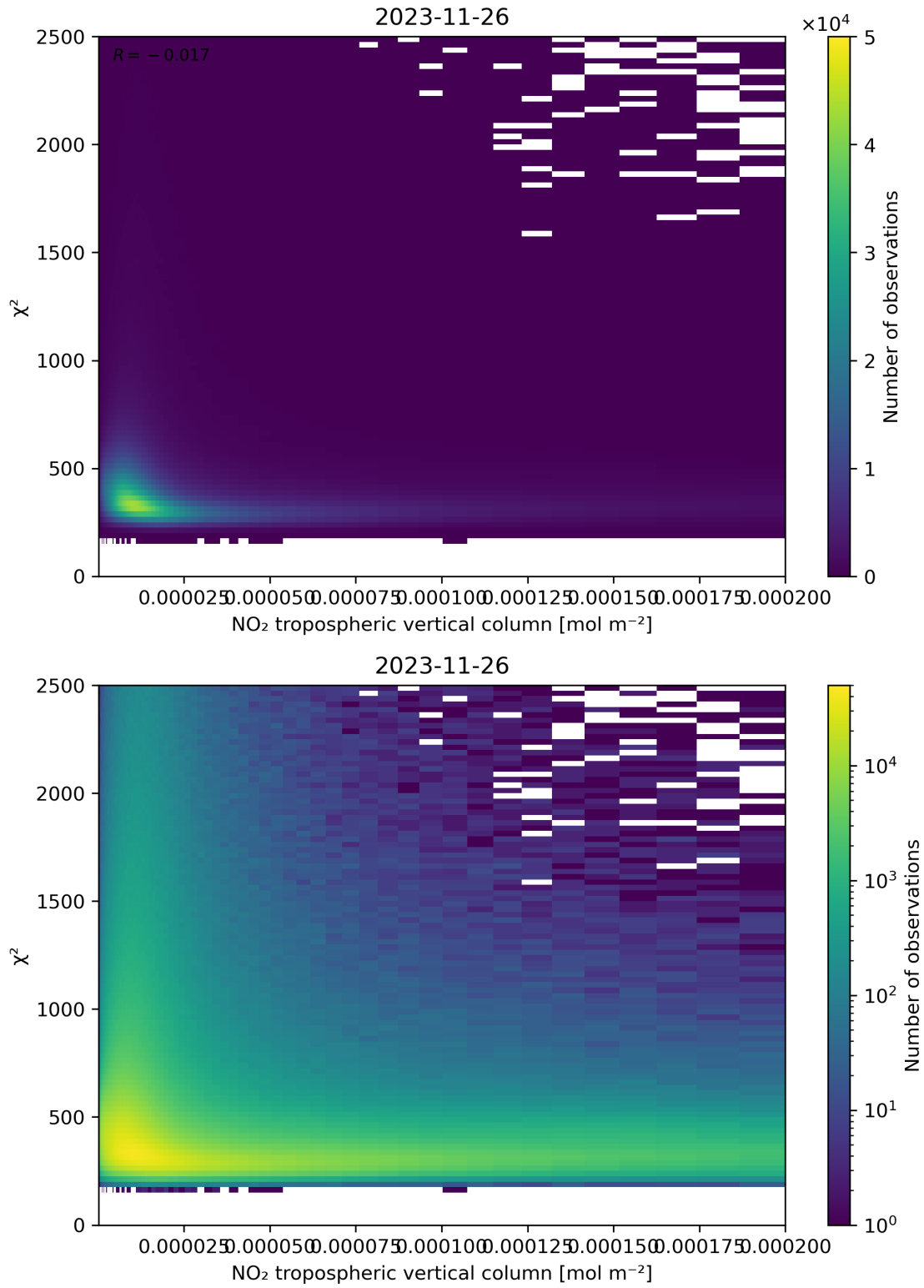
Figure 124: Scatter density plot of “NO 2 tropospheric vertical column” against “ \chi^2 ” for 2023-11-25 to 2023-11-27.
