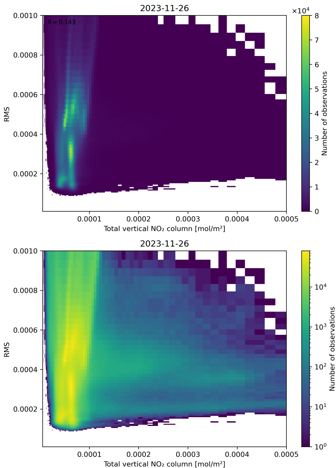
Figure 120: Scatter density plot of “Total vertical NO 2 column” against “RMS” for 2023-11-25 to 2023-11-27.
