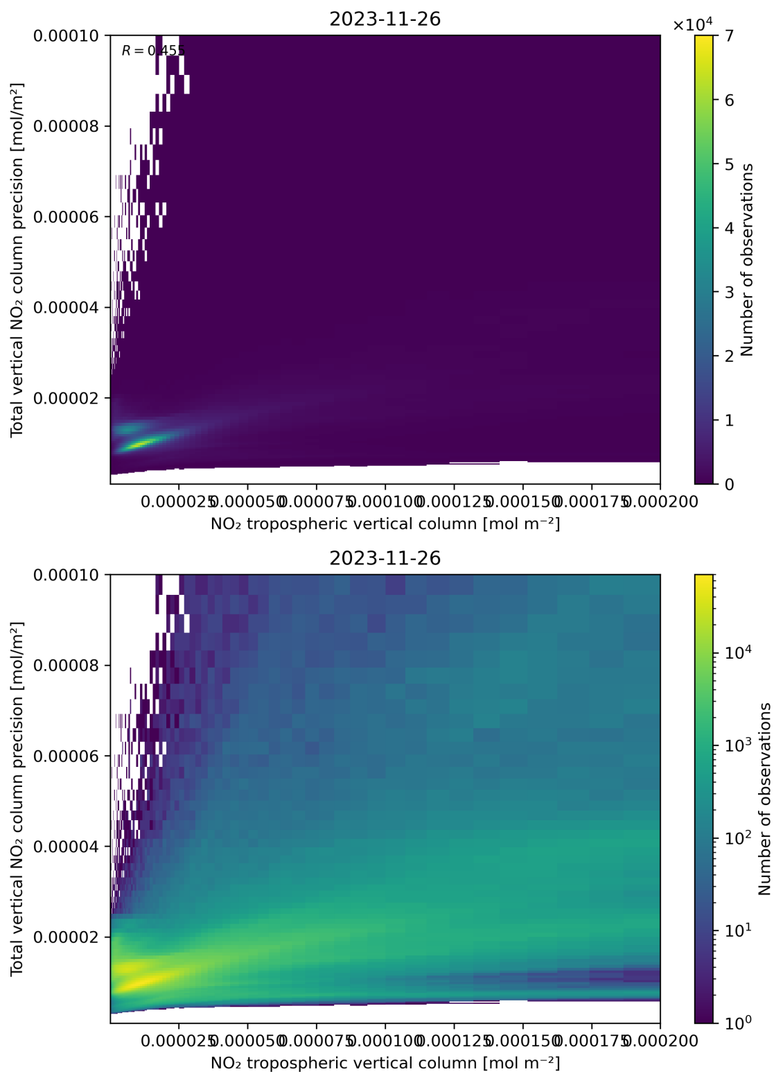
Figure 129: Scatter density plot of “NO 2 tropospheric vertical column” against “Total vertical NO 2 column precision” for 2023-11-25 to 2023-11-27.
