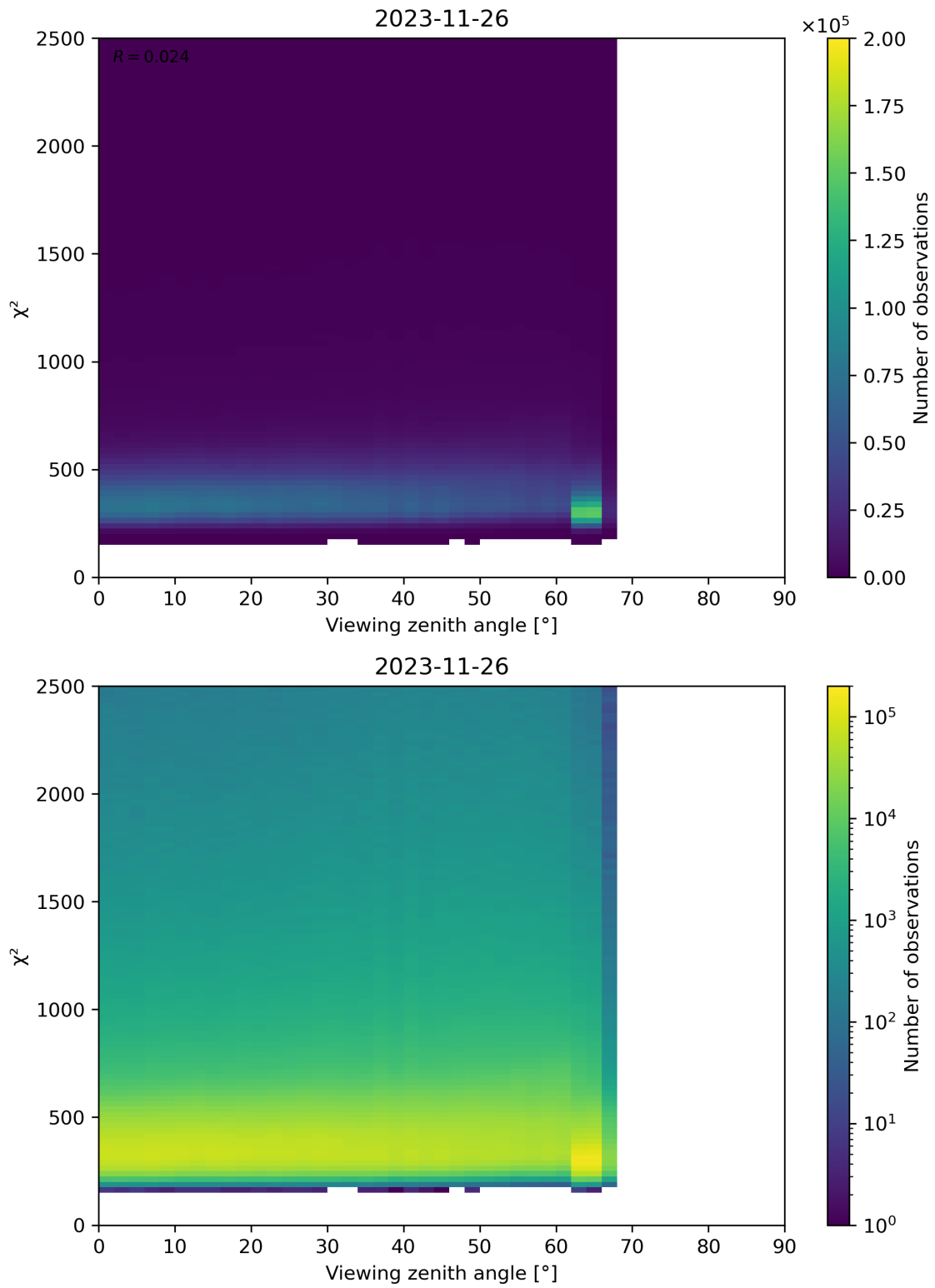
Figure 162: Scatter density plot of “Viewing zenith angle” against “ \chi^2 ” for 2023-11-25 to 2023-11-27.
