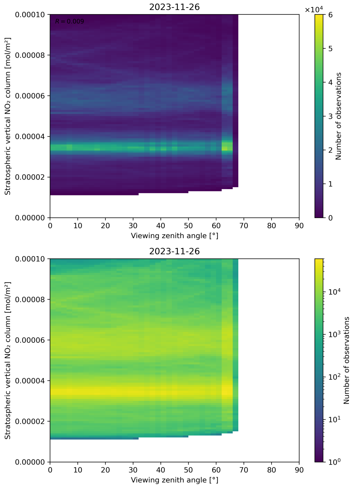
Figure 164: Scatter density plot of “Viewing zenith angle” against “Stratospheric vertical NO 2 column” for 2023-11-25 to 2023-11-27.
