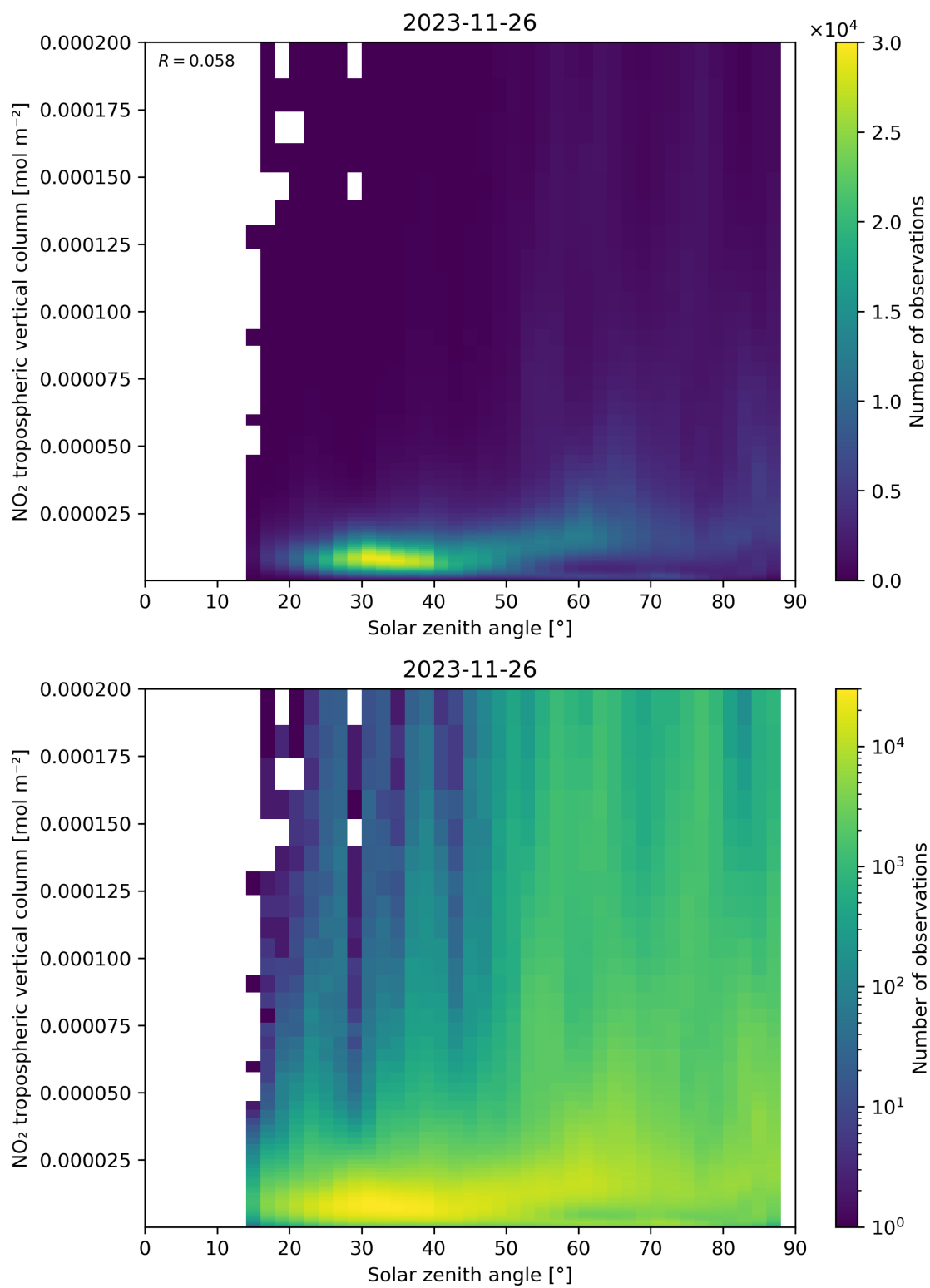
Figure 155: Scatter density plot of “Solar zenith angle” against “NO 2 tropospheric vertical column” for 2023-11-25 to 2023-11-27.
