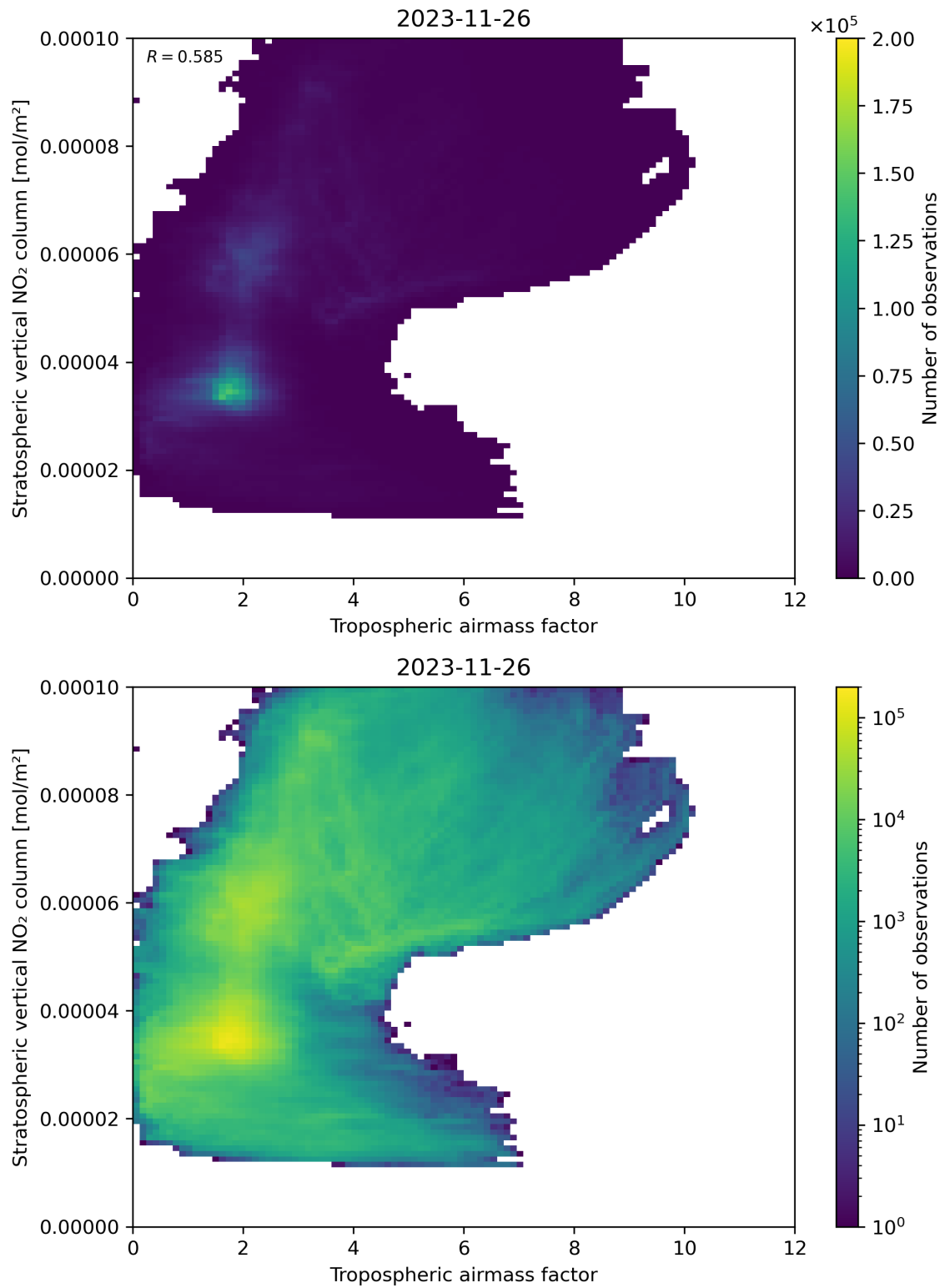
Figure 74: Scatter density plot of “Tropospheric air mass factor” against “Stratospheric vertical NO 2 column” for 2023-11-25 to 2023-11-27.
