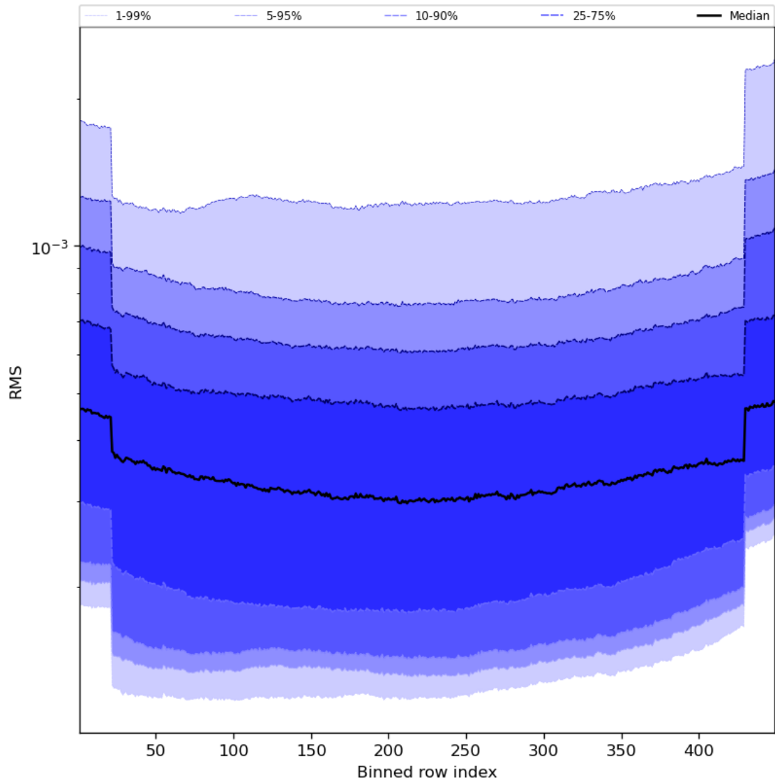
Figure 60: Along track statistics of “RMS” for 2023-11-25 to 2023-11-27
