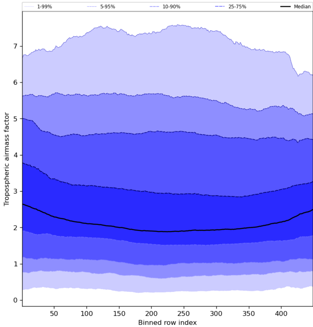
Figure 48: Along track statistics of “Tropospheric airmass factor” for 2023-11-25 to 2023-11-27
