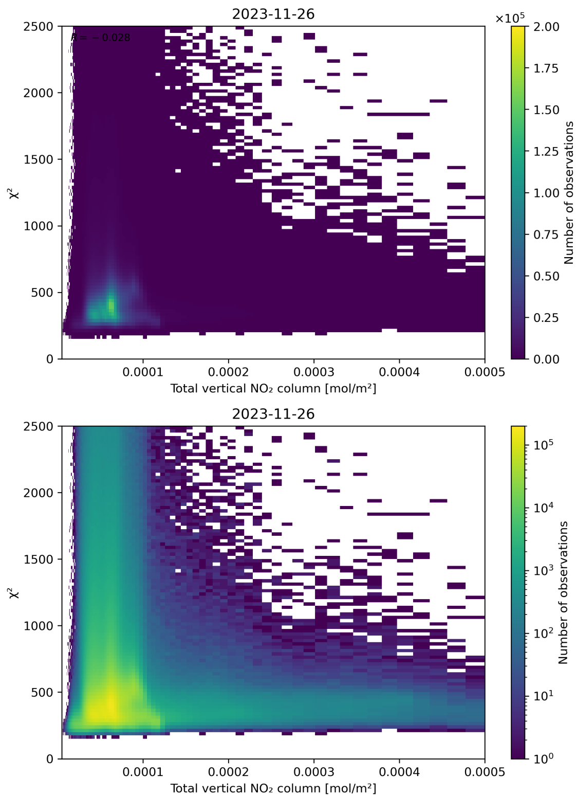
Figure 111: Scatter density plot of “Total vertical NO 2 column” against “ \chi^2 ” for 2023-11-25 to 2023-11-27.
