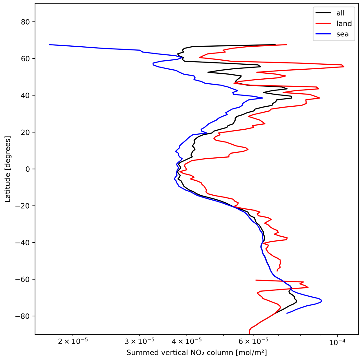
Figure 23: Zonal average of “Summed vertical NO 2 column” for 2023-11-25 to 2023-11-27.
