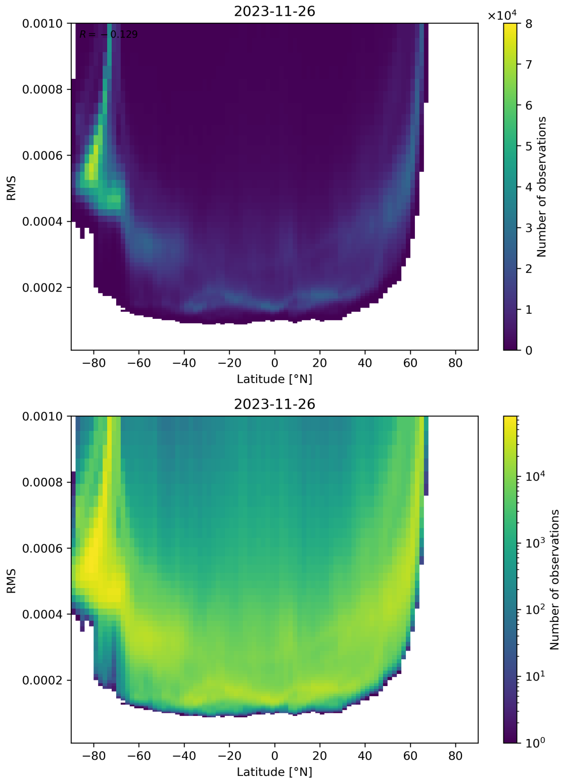
Figure 94: Scatter density plot of “Latitude” against “RMS” for 2023-11-25 to 2023-11-27.
