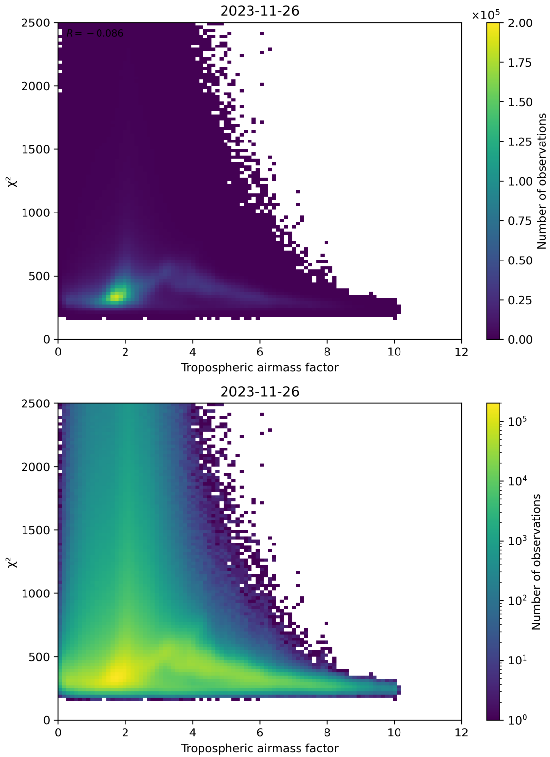
Figure 73: Scatter density plot of “Tropospheric airmass factor” against “ \chi^2 ” for 2023-11-25 to 2023-11-27.
