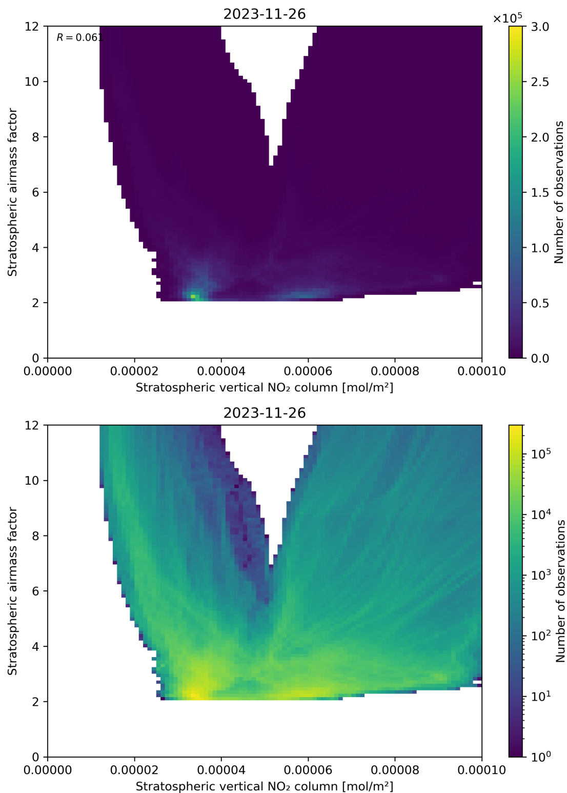
Figure 96: Scatter density plot of “Stratospheric vertical NO 2 column” against “Stratospheric airmass factor” for 2023-11-25 to 2023-11-27.
