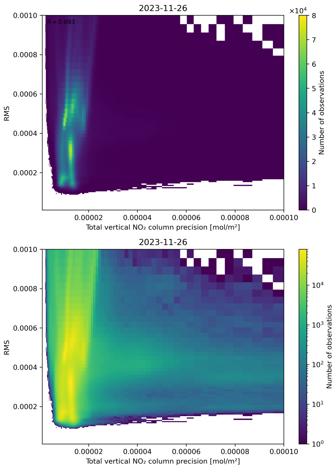
Figure 119: Scatter density plot of “Total vertical NO 2 column precision” against “RMS” for 2023-11-25 to 2023-11-27.
