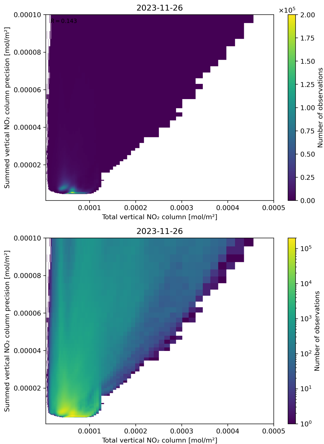
Figure 113: Scatter density plot of “Total vertical NO 2 column” against “Summed vertical NO 2 column precision” for 2023-11-25 to 2023-11-27.
