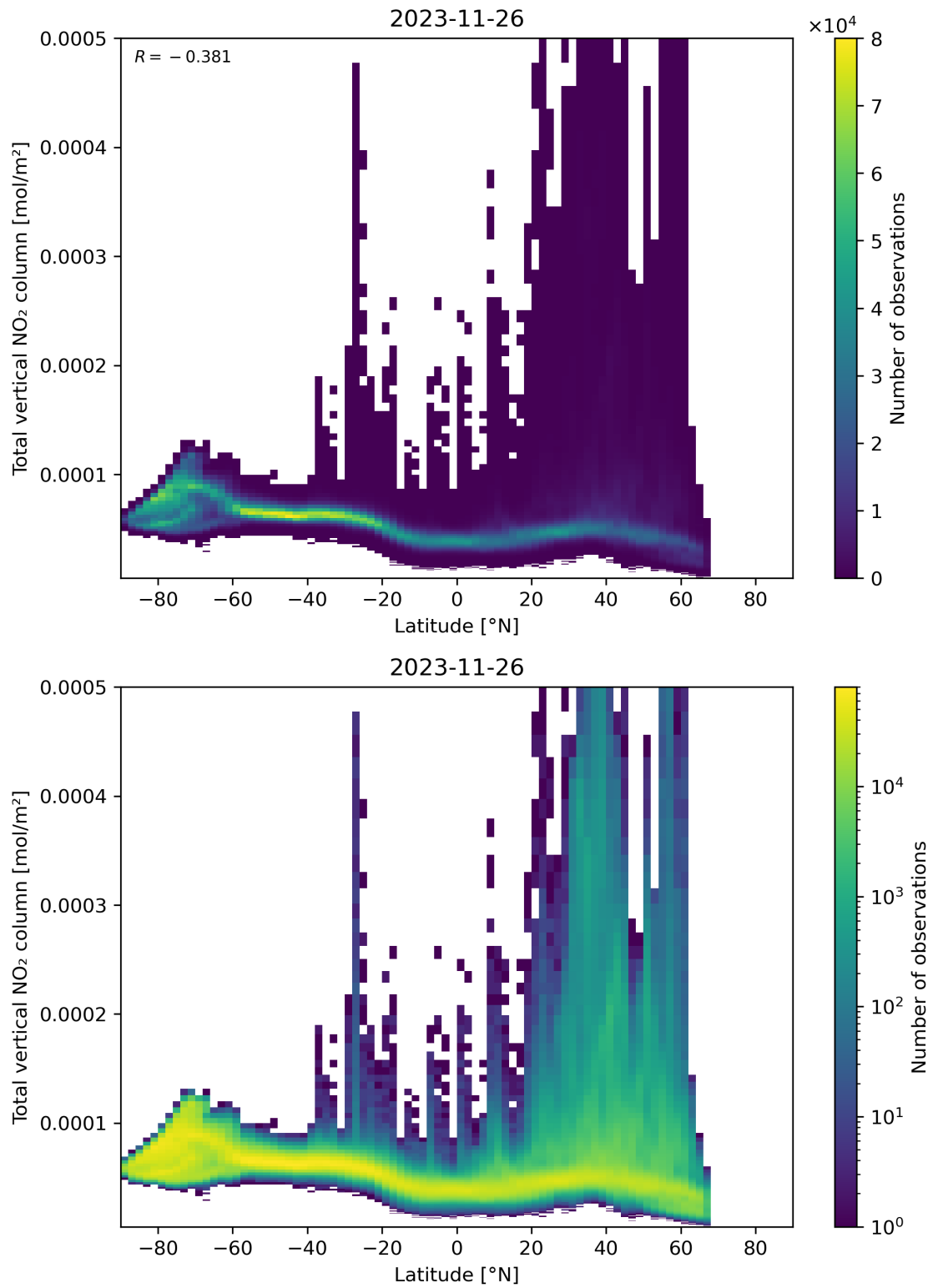
Figure 90: Scatter density plot of “Latitude” against “Total vertical NO 2 column” for 2023-11-25 to 2023-11-27.
