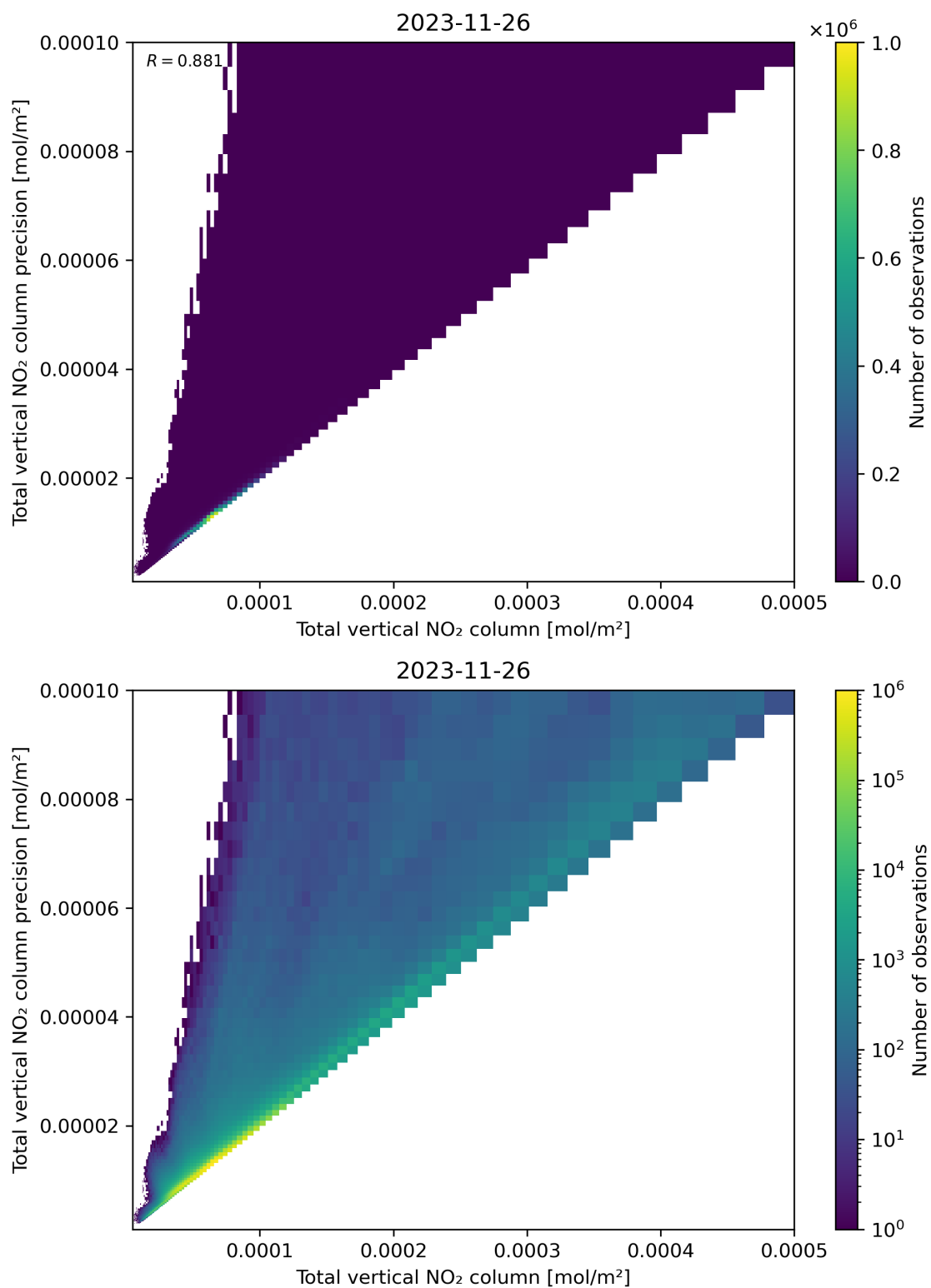
Figure 114: Scatter density plot of “Total vertical NO 2 column” against “Total vertical NO 2 column precision” for 2023-11-25 to 2023-11-27.
