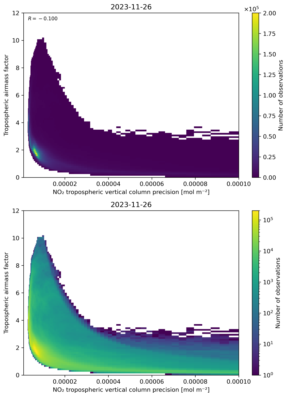
Figure 133: Scatter density plot of “NO 2 tropospheric vertical column precision” against “Tropospheric airmass factor” for 2023-11-25 to 2023-11-27.
