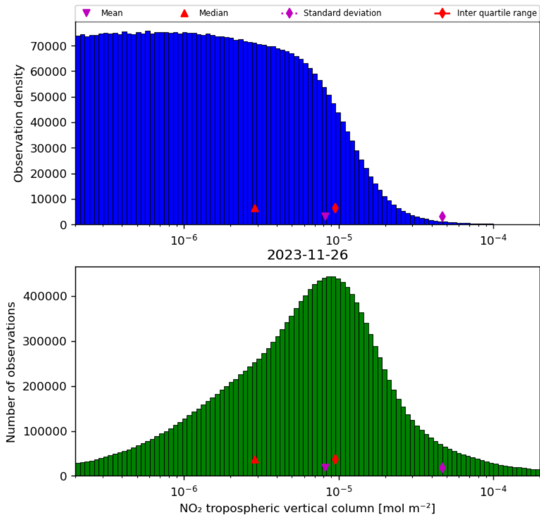
Figure 29: Histogram of “NO 2 tropospheric vertical column” for 2023-11-25 to 2023-11-27
