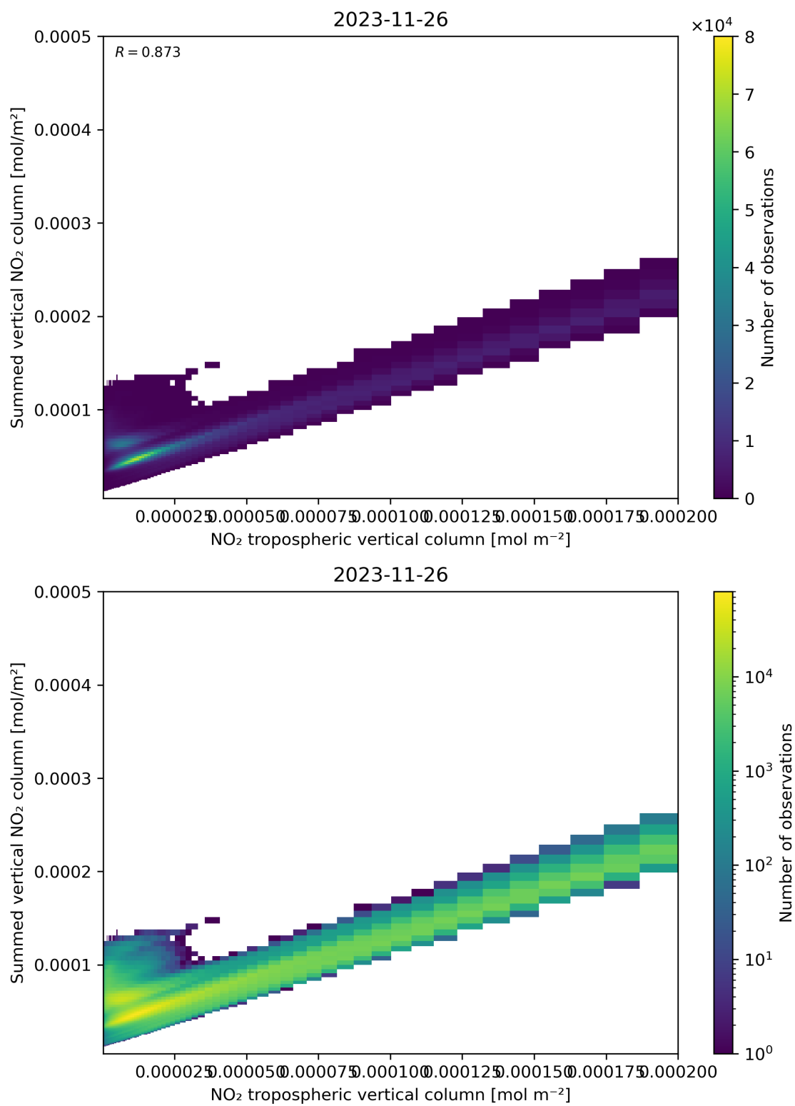
Figure 126: Scatter density plot of “NO 2 tropospheric vertical column” against “Summed vertical NO 2 column” for 2023-11-25 to 2023-11-27.
