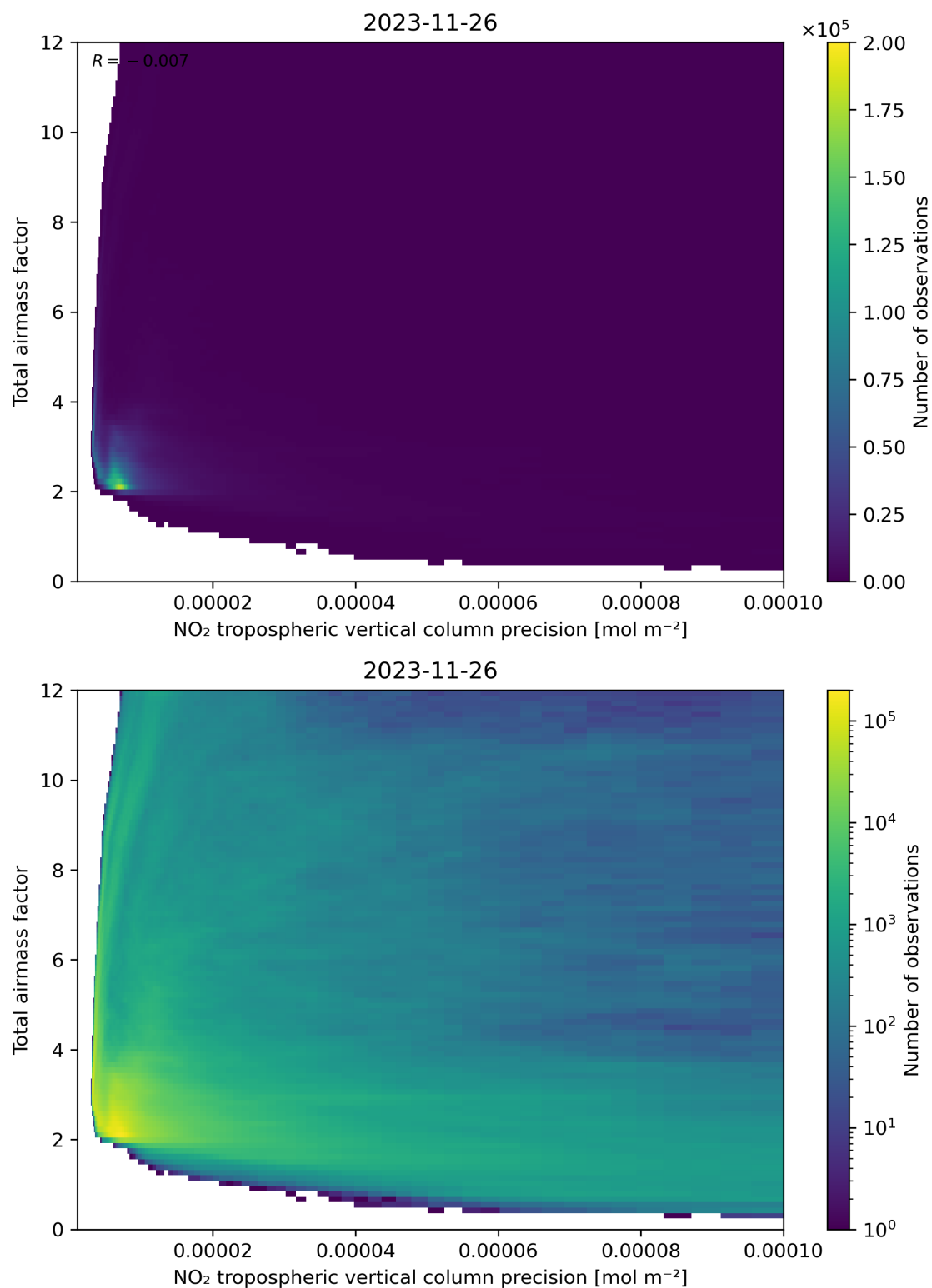
Figure 132: Scatter density plot of “NO 2 tropospheric vertical column precision” against “Total air mass factor” for 2023-11-25 to 2023-11-27.
