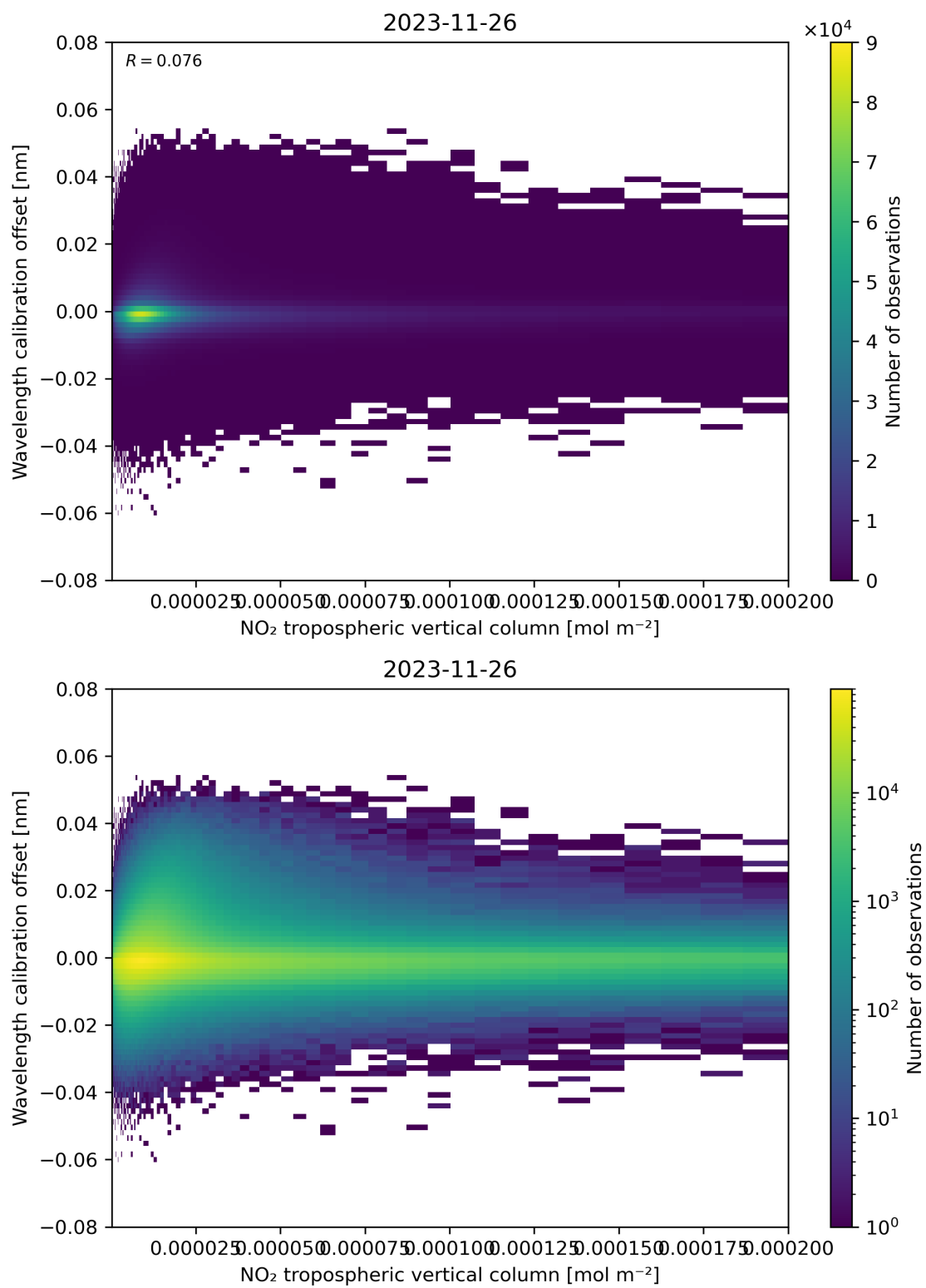
Figure 143: Scatter density plot of “NO 2 tropospheric vertical column” against “Wavelength calibration offset” for 2023-11-25 to 2023-11-27.
