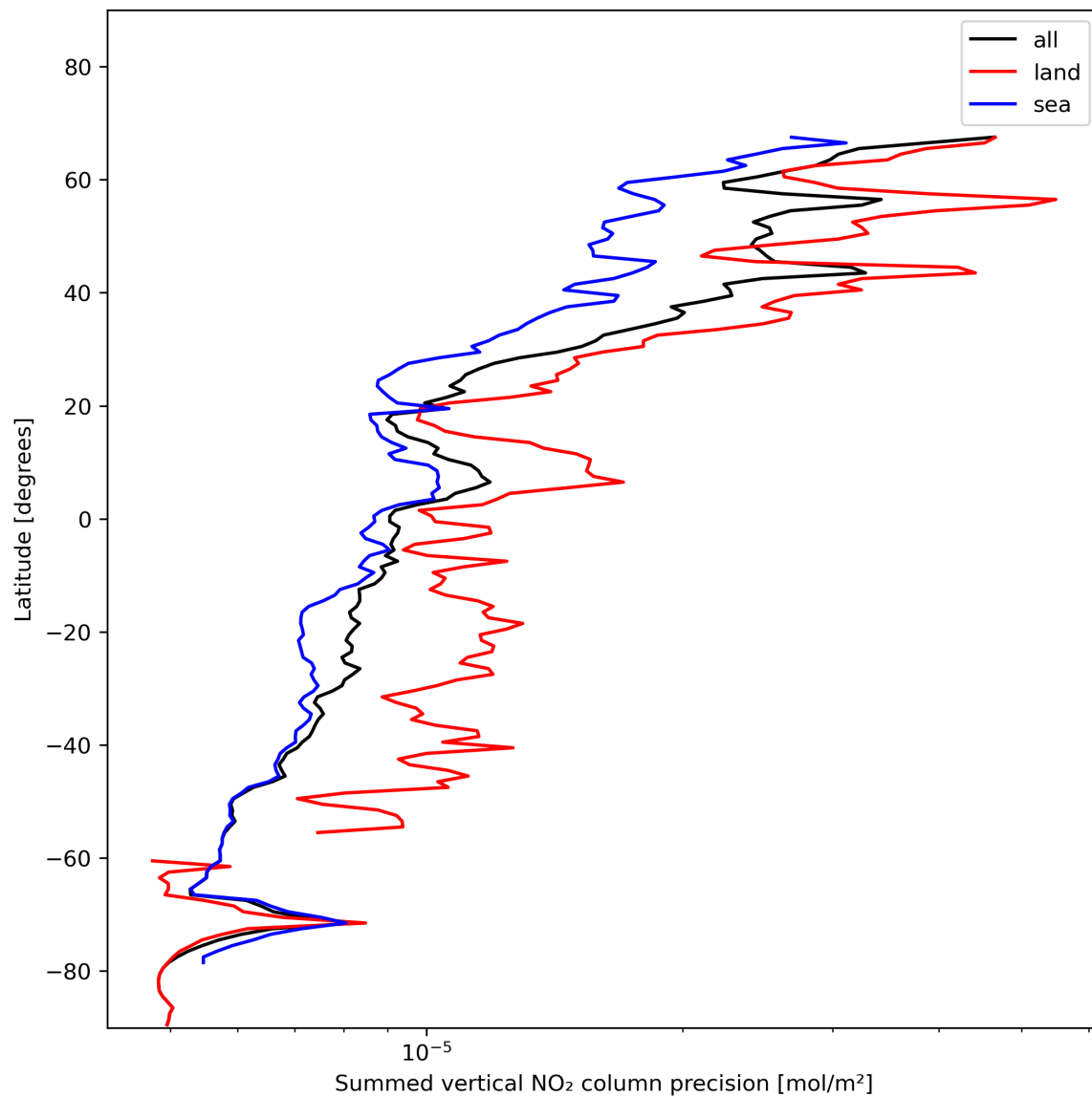
Figure 24: Zonal average of “Summed vertical NO 2 column precision” for 2023-11-25 to 2023-11-27.
