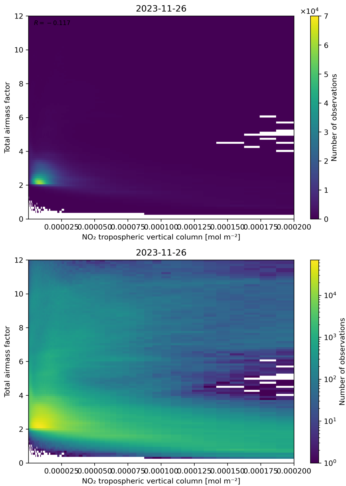
Figure 122: Scatter density plot of “NO 2 tropospheric vertical column” against “Total air mass factor” for 2023-11-25 to 2023-11-27.
