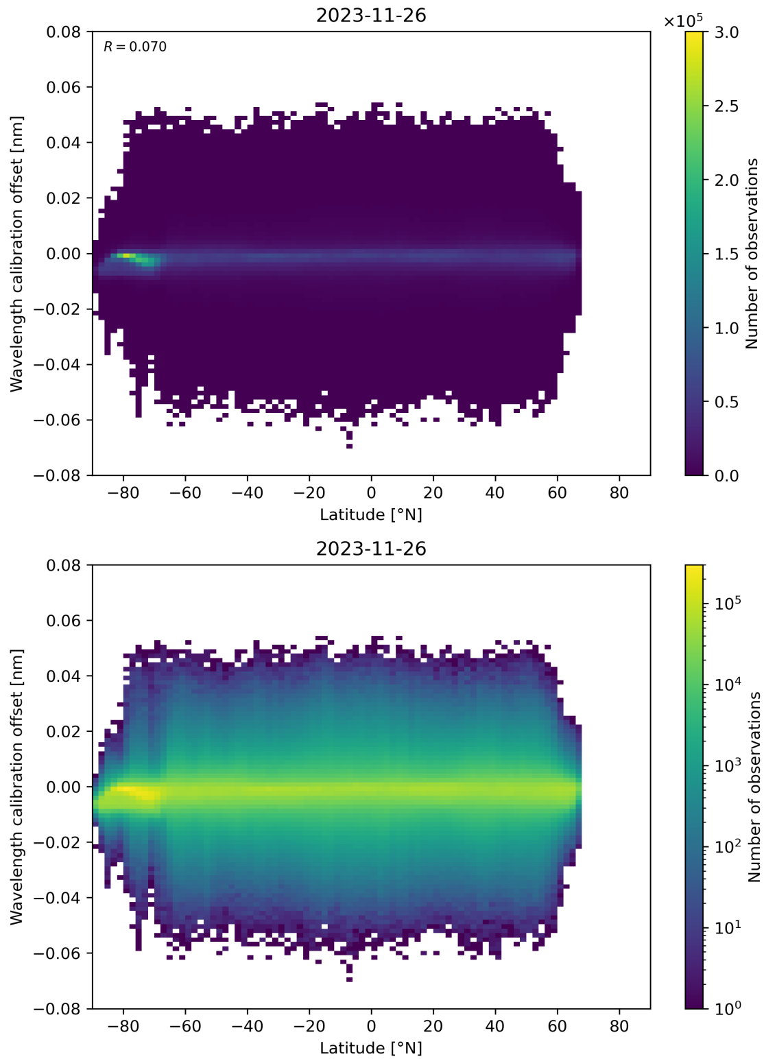
Figure 95: Scatter density plot of “Latitude” against “Wavelength calibration offset” for 2023-11-25 to 2023-11-27.
