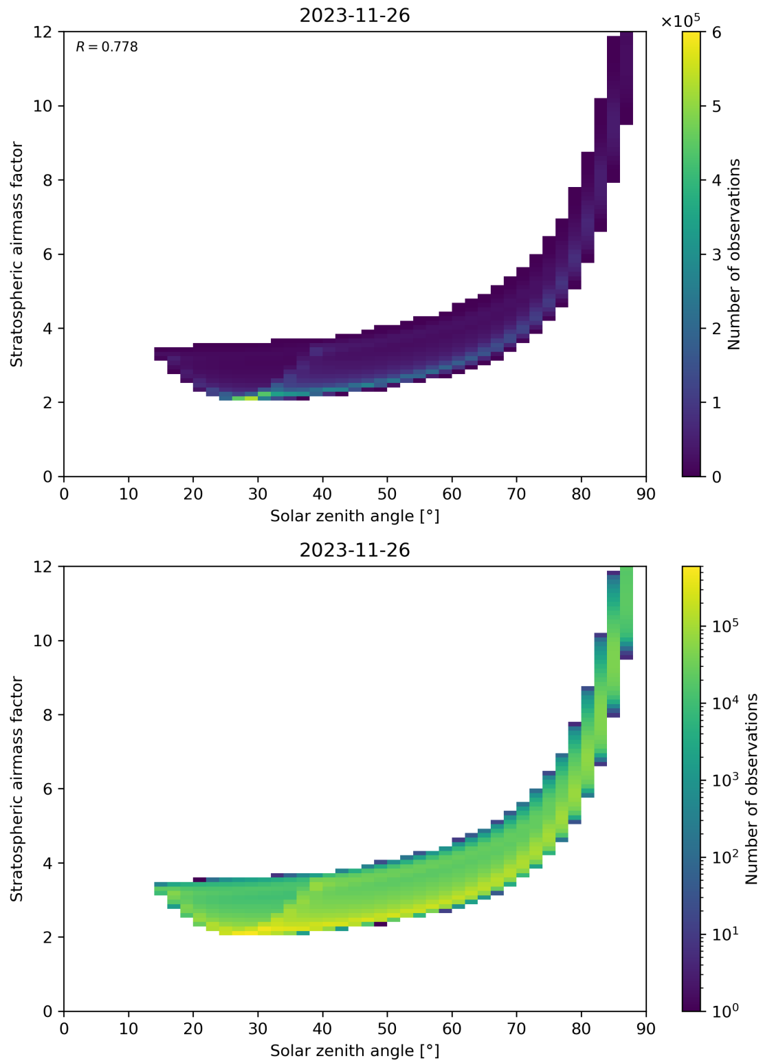
Figure 145: Scatter density plot of “Solar zenith angle” against “Stratospheric airmass factor” for 2023-11-25 to 2023-11-27.
