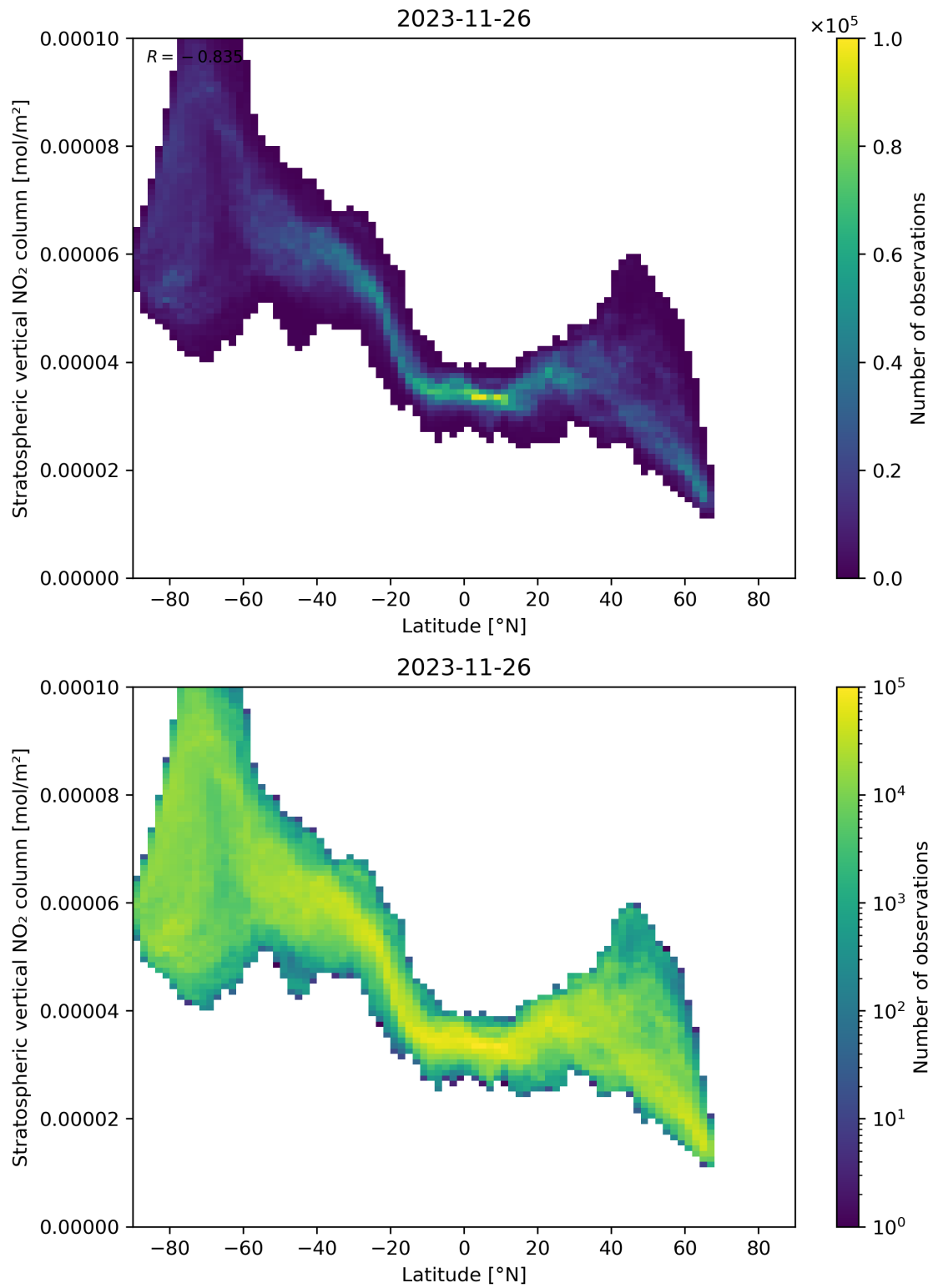
Figure 87: Scatter density plot of “Latitude” against “Stratospheric vertical NO 2 column” for 2023-11-25 to 2023-11-27.
