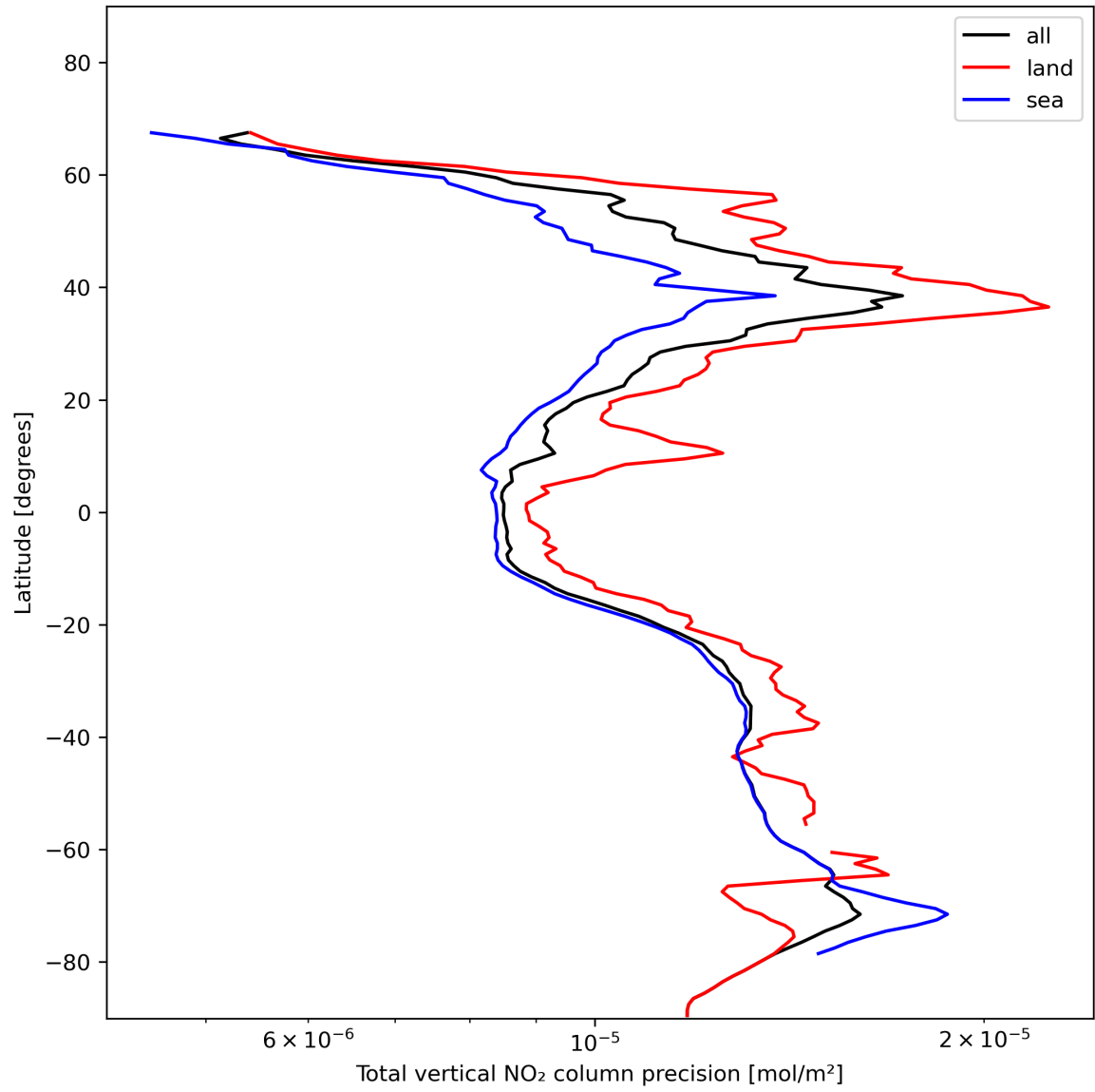
Figure 22: Zonal average of “Total vertical NO 2 column precision” for 2023-11-25 to 2023-11-27.
