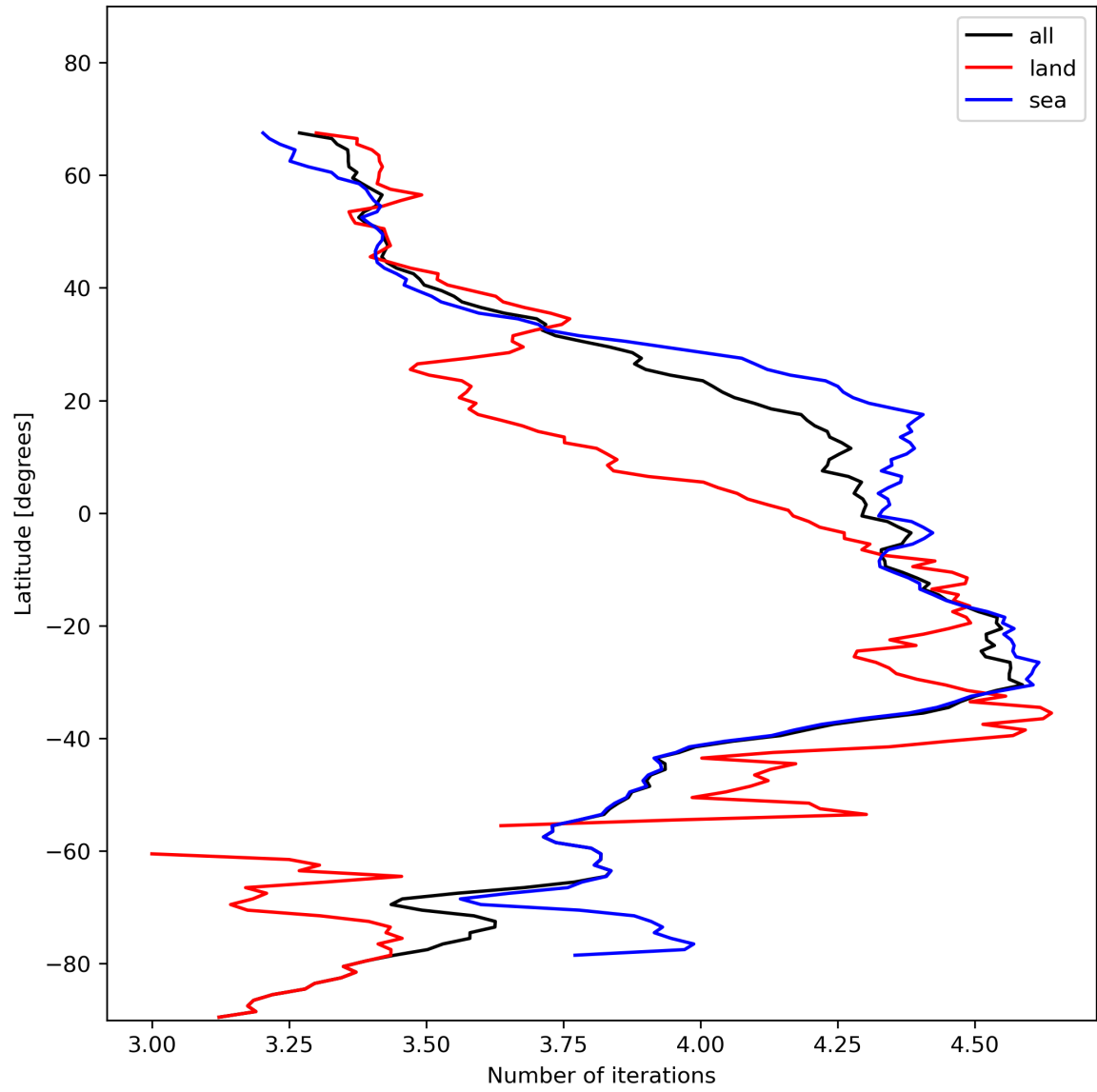
Figure 17: Zonal average of “Number of iterations” for 2023-11-25 to 2023-11-27.
