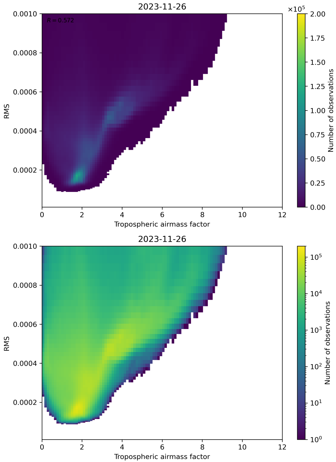
Figure 79: Scatter density plot of “Tropospheric airmass factor” against “RMS” for 2023-11-25 to 2023-11-27.
