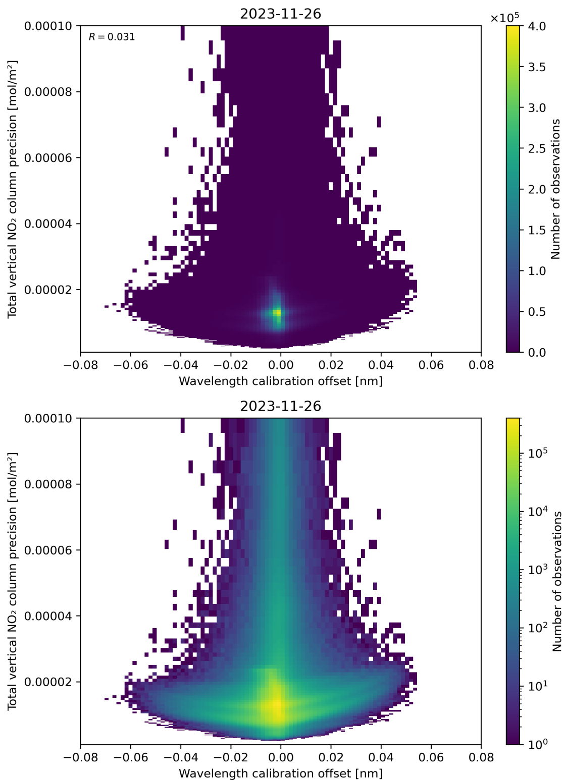
Figure 180: Scatter density plot of “Wavelength calibration offset” against “Total vertical NO 2 column precision” for 2023-11-25 to 2023-11-27.
