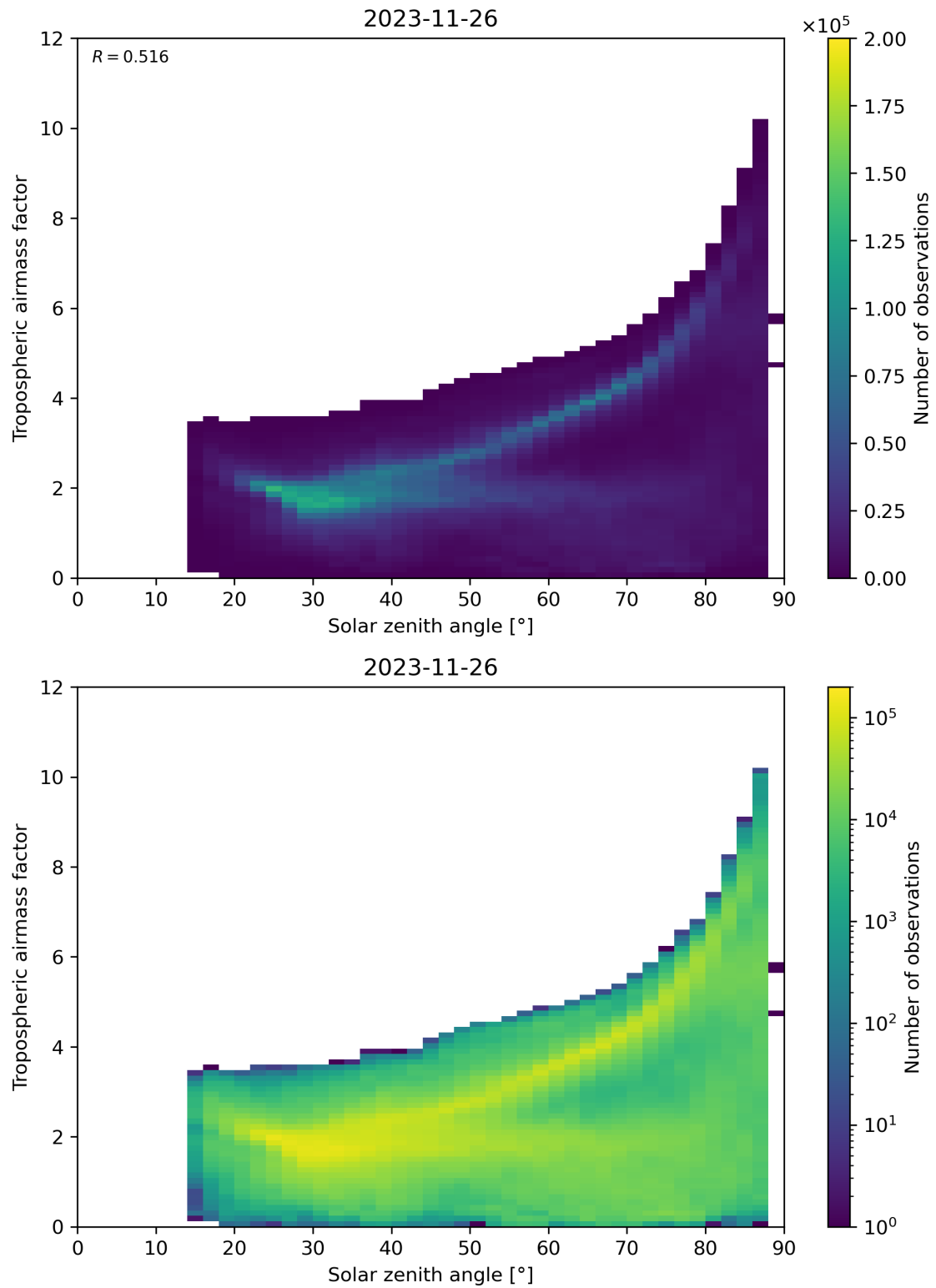
Figure 147: Scatter density plot of “Solar zenith angle” against “Tropospheric airmass factor” for 2023-11-25 to 2023-11-27.
