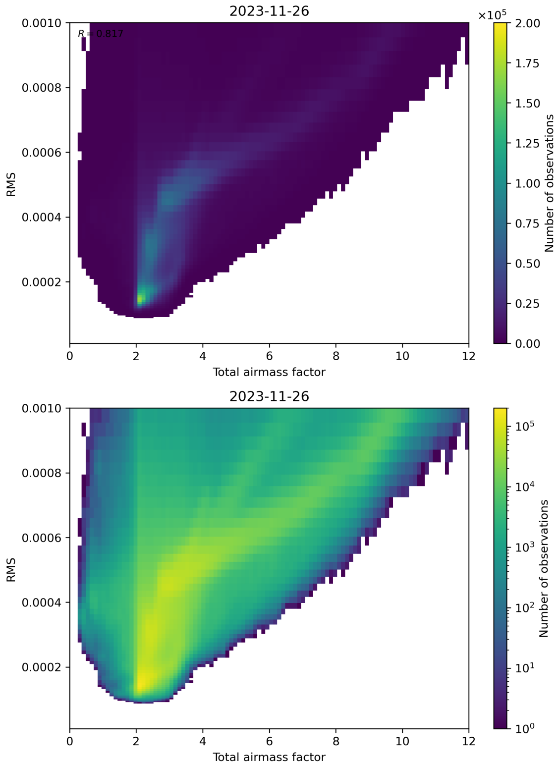
Figure 69: Scatter density plot of “Total airmass factor” against “RMS” for 2023-11-25 to 2023-11-27.
