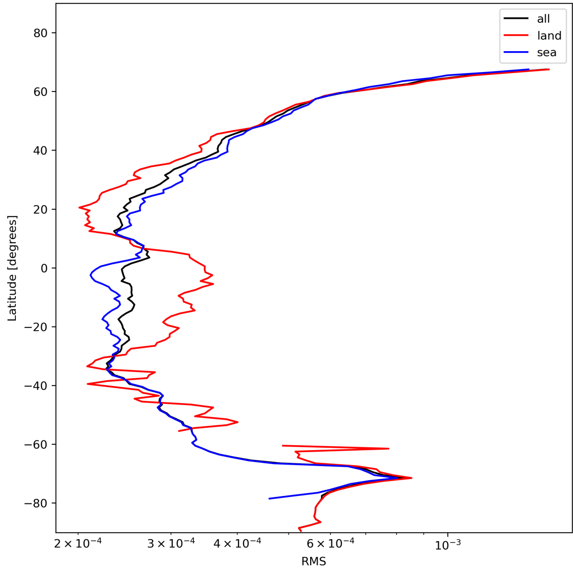
Figure 26: Zonal average of “RMS” for 2023-11-25 to 2023-11-27.
