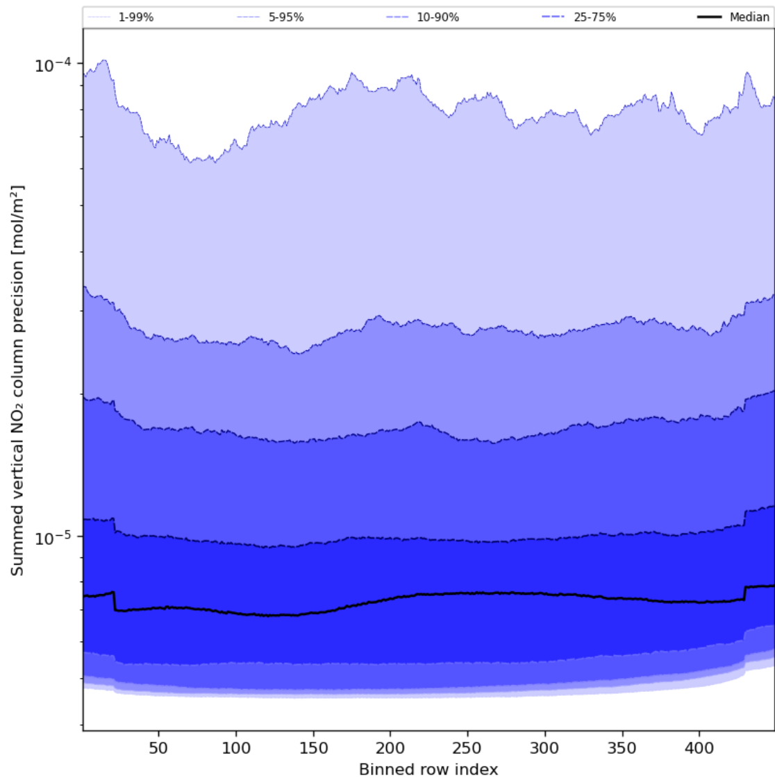
Figure 58: Along track statistics of “Summed vertical NO 2 column precision” for 2023-11-25 to 2023-11-27
