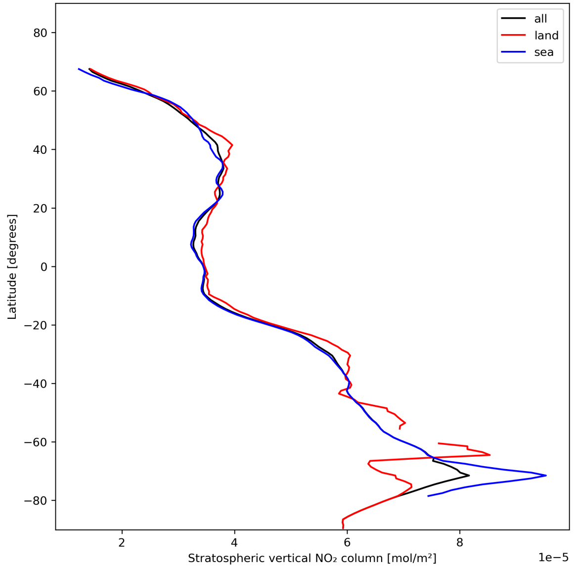
Figure 19: Zonal average of “Stratospheric vertical NO 2 column” for 2023-11-25 to 2023-11-27.
