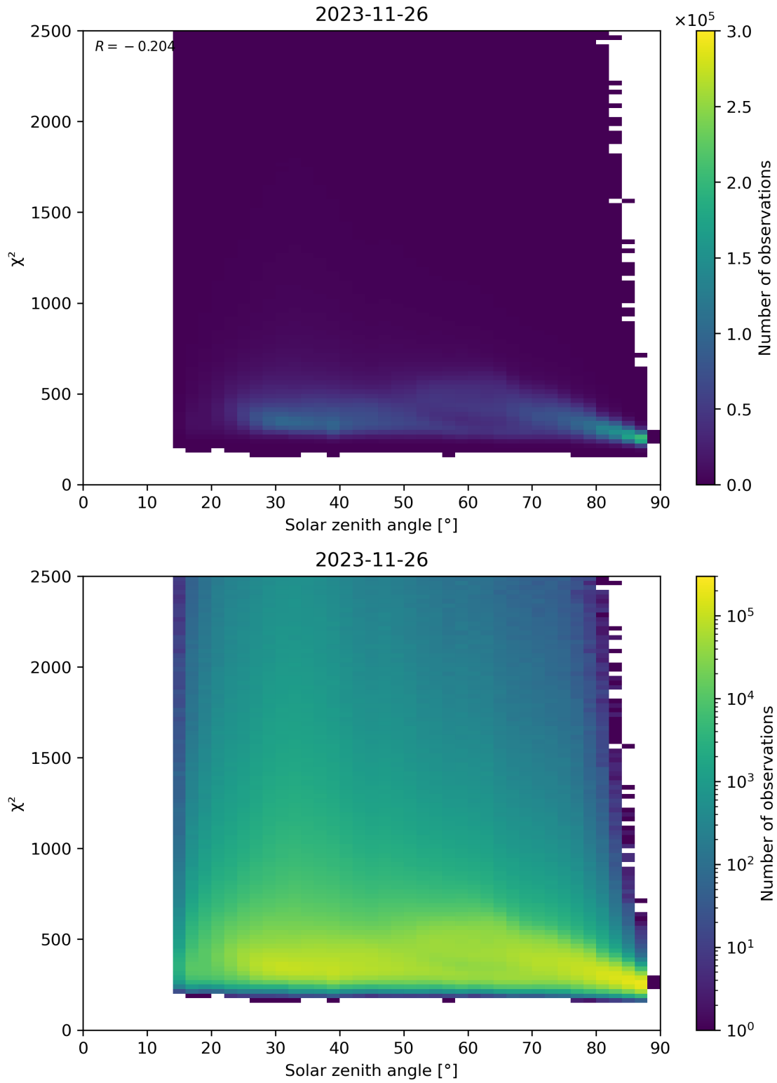
Figure 148: Scatter density plot of “Solar zenith angle” against “ \chi^2 ” for 2023-11-25 to 2023-11-27.
