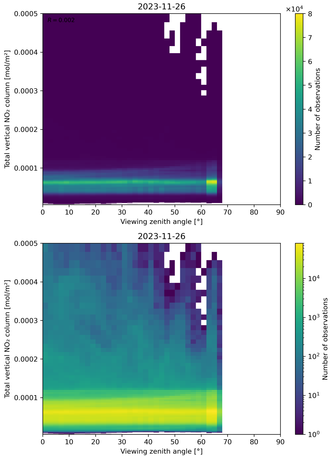
Figure 167: Scatter density plot of “Viewing zenith angle” against “Total vertical NO 2 column” for 2023-11-25 to 2023-11-27.
