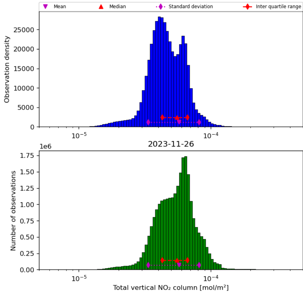
Figure 38: Histogram of “Total vertical NO 2 column” for 2023-11-25 to 2023-11-27
