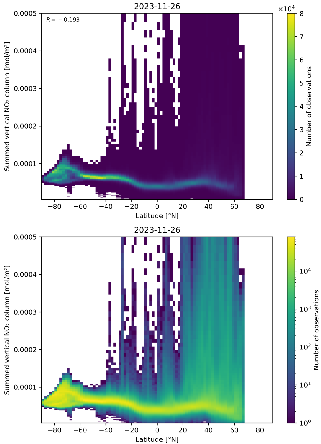
Figure 88: Scatter density plot of “Latitude” against “Summed vertical NO 2 column” for 2023-11-25 to 2023-11-27.
