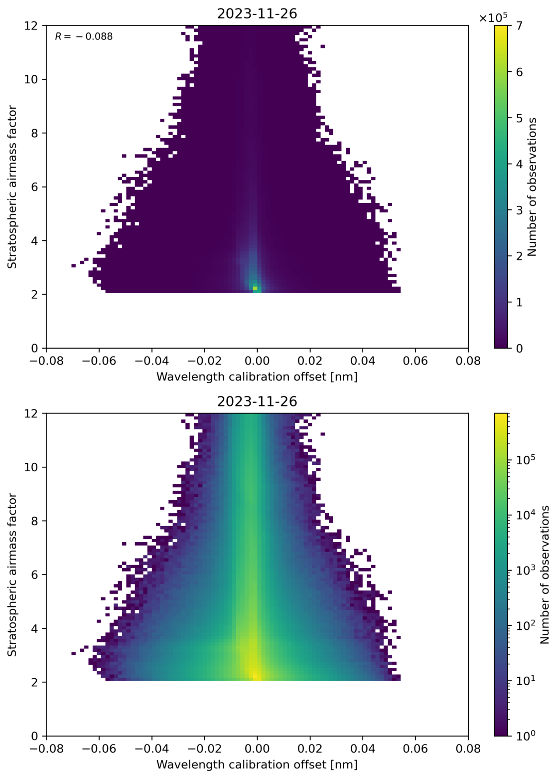
Figure 174: Scatter density plot of “Wavelength calibration offset” against “Stratospheric air mass factor” for 2023-11-25 to 2023-11-27.
