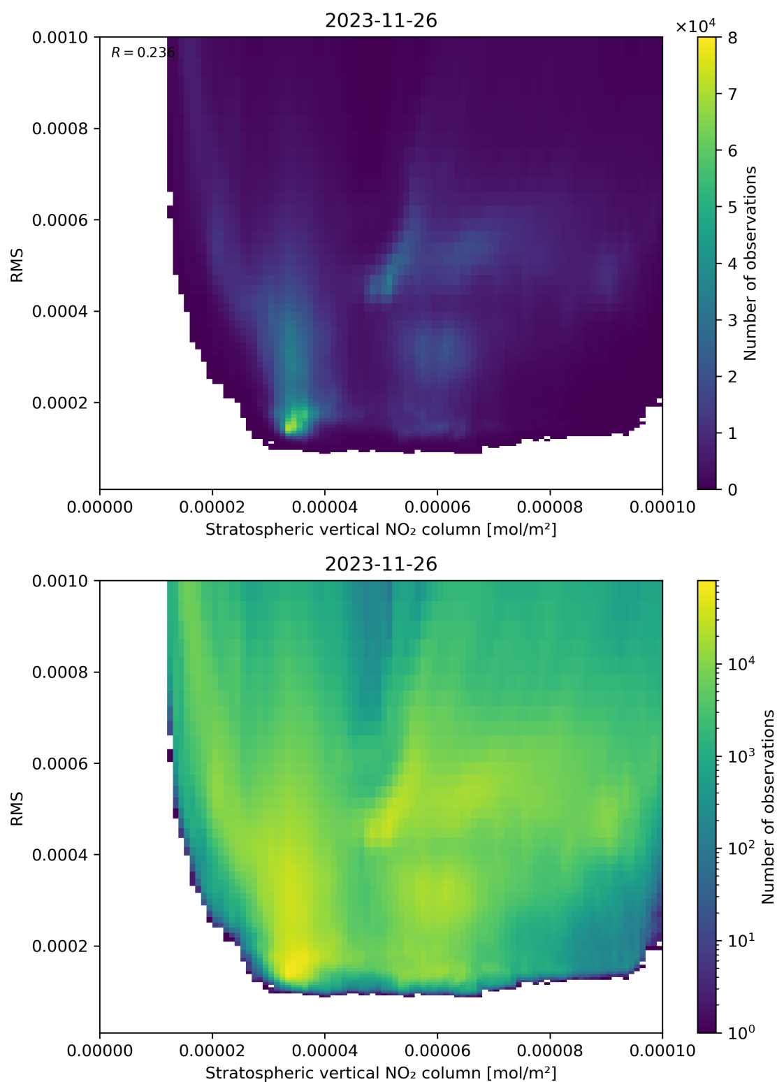
Figure 102: Scatter density plot of “Stratospheric vertical NO 2 column” against “RMS” for 2023-11-25 to 2023-11-27.
