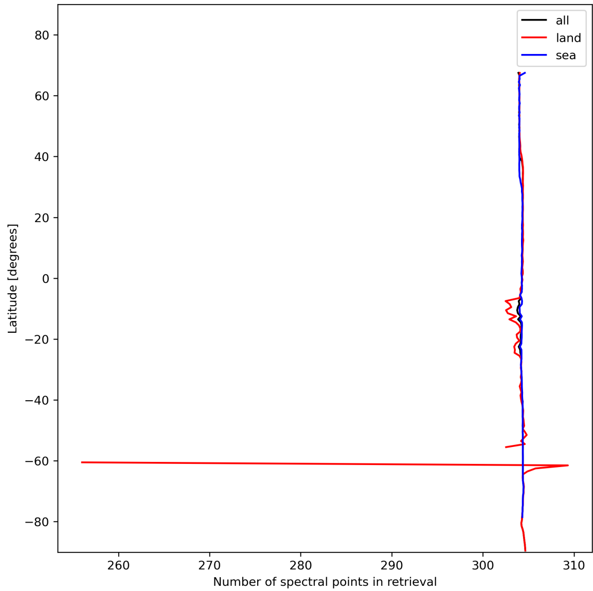
Figure 16: Zonal average of “Number of spectral points in retrieval” for 2023-11-25 to 2023-11-27.
