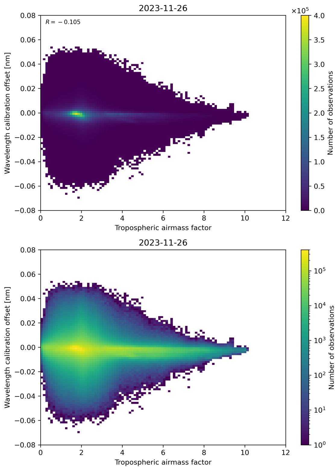
Figure 80: Scatter density plot of “Tropospheric airmass factor” against “Wavelength calibration offset” for 2023-11-25 to 2023-11-27.
