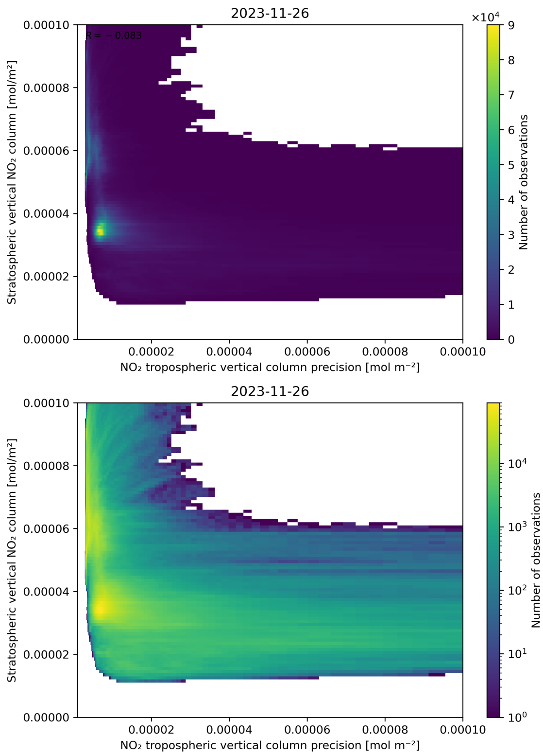
Figure 135: Scatter density plot of “NO 2 tropospheric vertical column precision” against “Stratospheric vertical NO 2 column” for 2023-11-25 to 2023-11-27.
