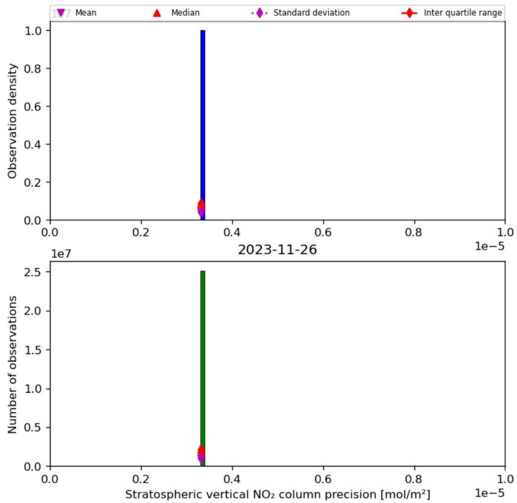
Figure 37: Histogram of “Stratospheric vertical NO 2 column precision” for 2023-11-25 to 2023-11-27
