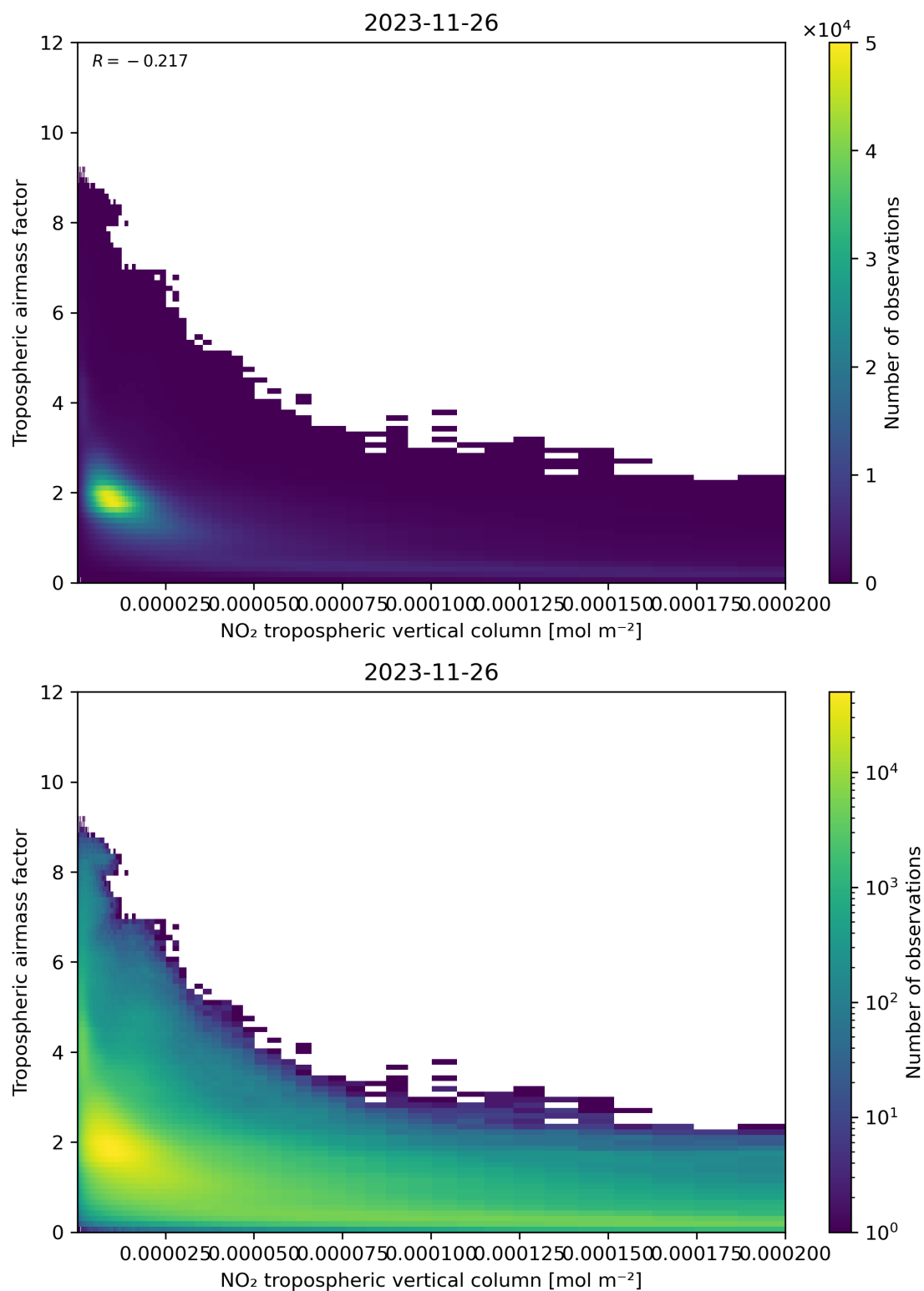
Figure 123: Scatter density plot of “NO 2 tropospheric vertical column” against “Tropospheric airmass factor” for 2023-11-25 to 2023-11-27.
