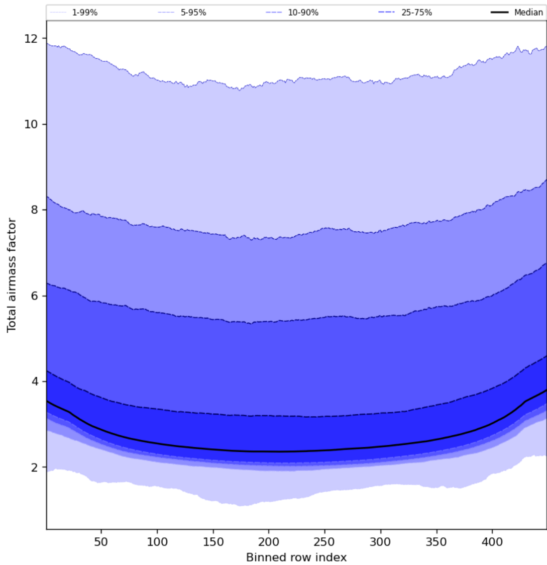
Figure 49: Along track statistics of “Total airmass factor” for 2023-11-25 to 2023-11-27
