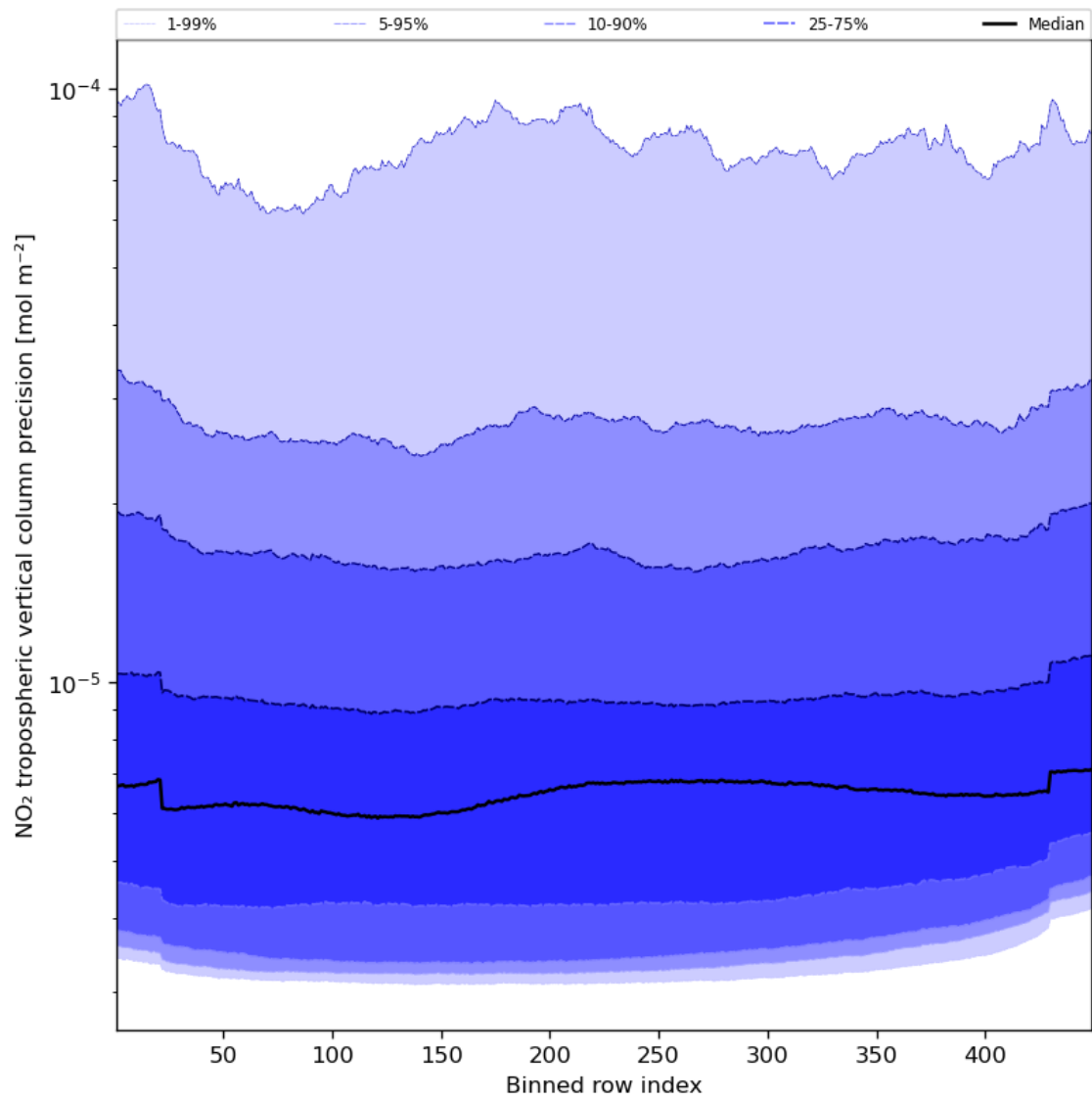
Figure 47: Along track statistics of “NO 2 tropospheric vertical column precision” for 2023-11-25 to 2023-11-27
