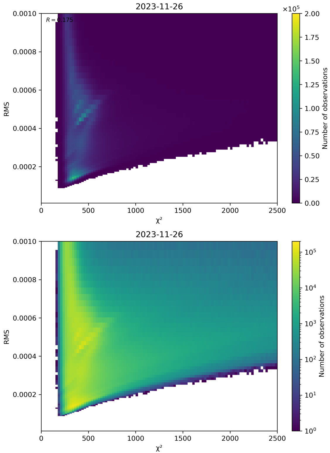
Figure 82: Scatter density plot of “ \chi^2 ” against “RMS” for 2023-11-25 to 2023-11-27.
