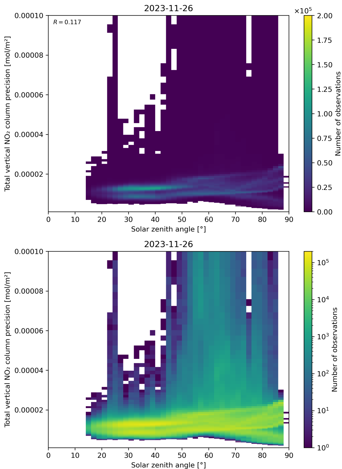
Figure 154: Scatter density plot of “Solar zenith angle” against “Total vertical NO 2 column precision” for 2023-11-25 to 2023-11-27.
