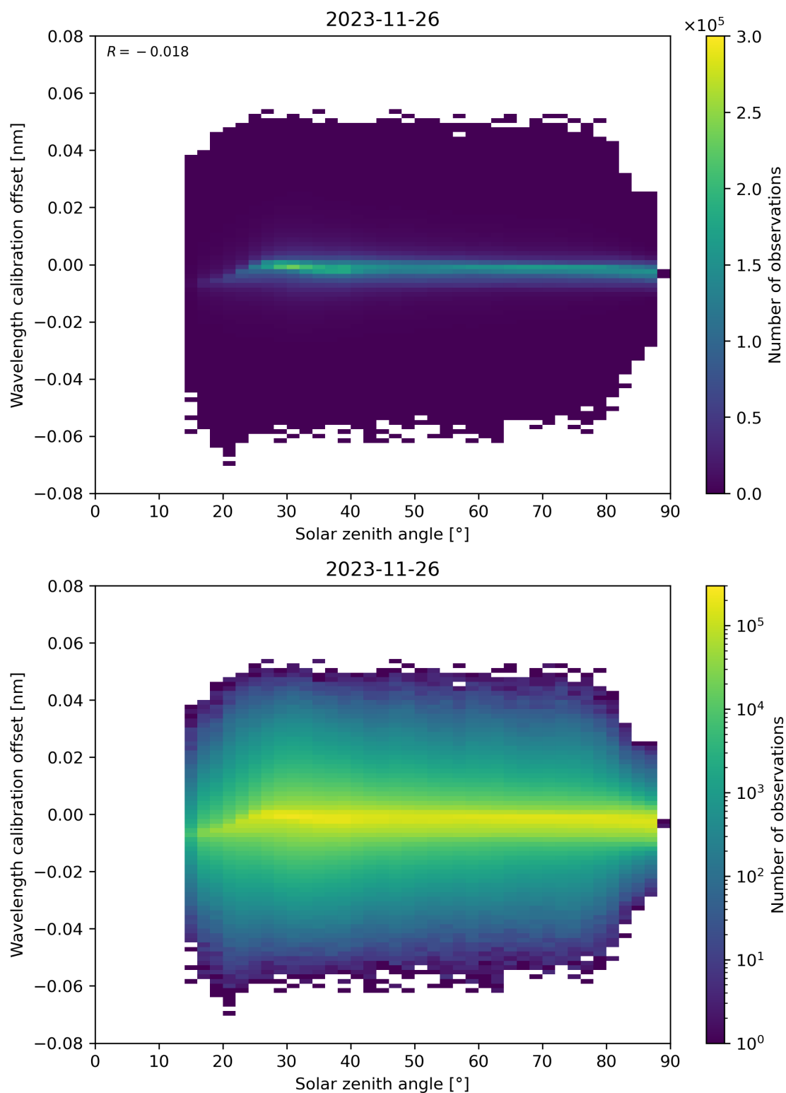
Figure 158: Scatter density plot of “Solar zenith angle” against “Wavelength calibration offset” for 2023-11-25 to 2023-11-27.
