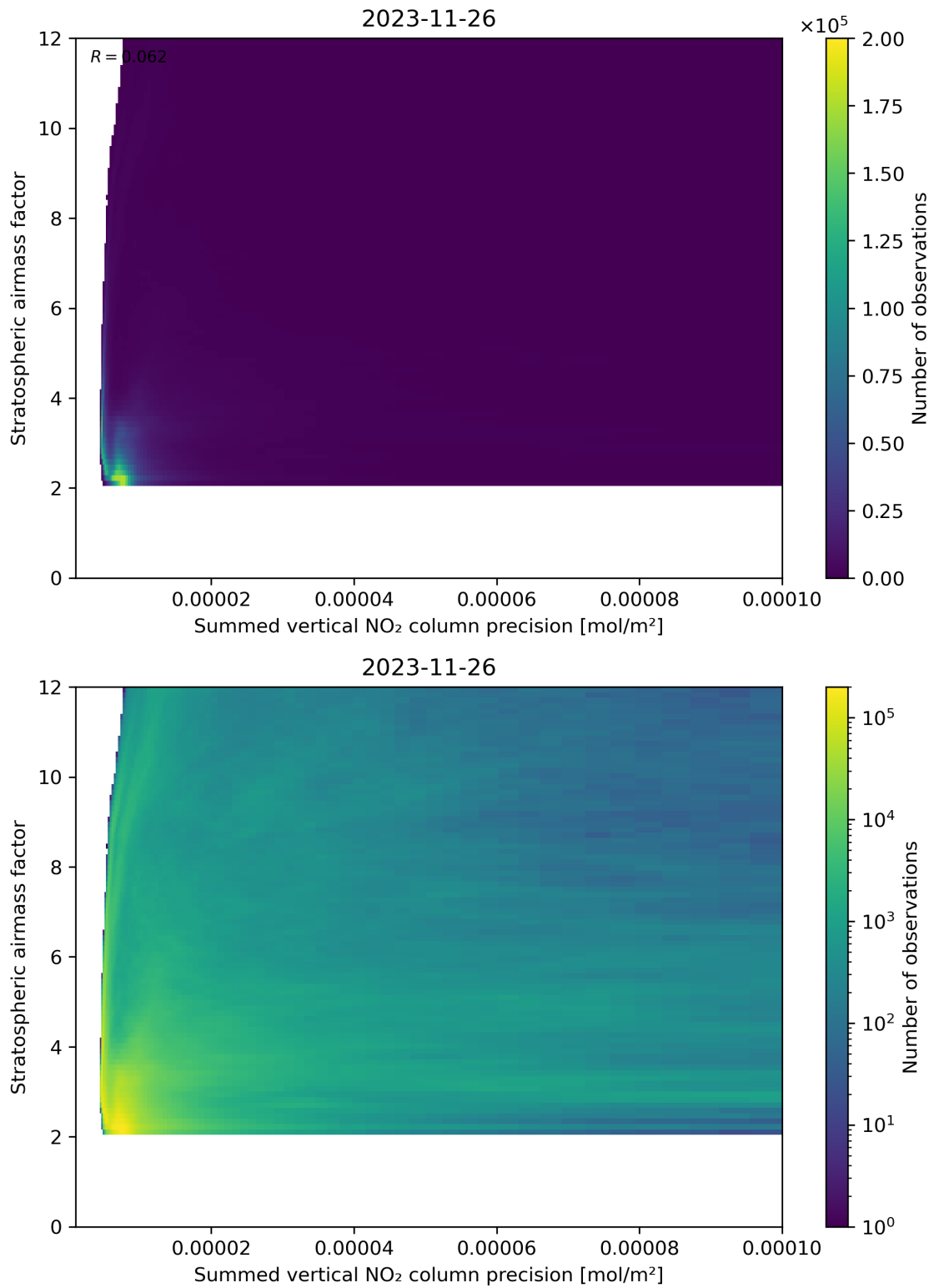
Figure 106: Scatter density plot of “Summed vertical NO 2 column precision” against “Stratospheric airmass factor” for 2023-11-25 to 2023-11-27.
