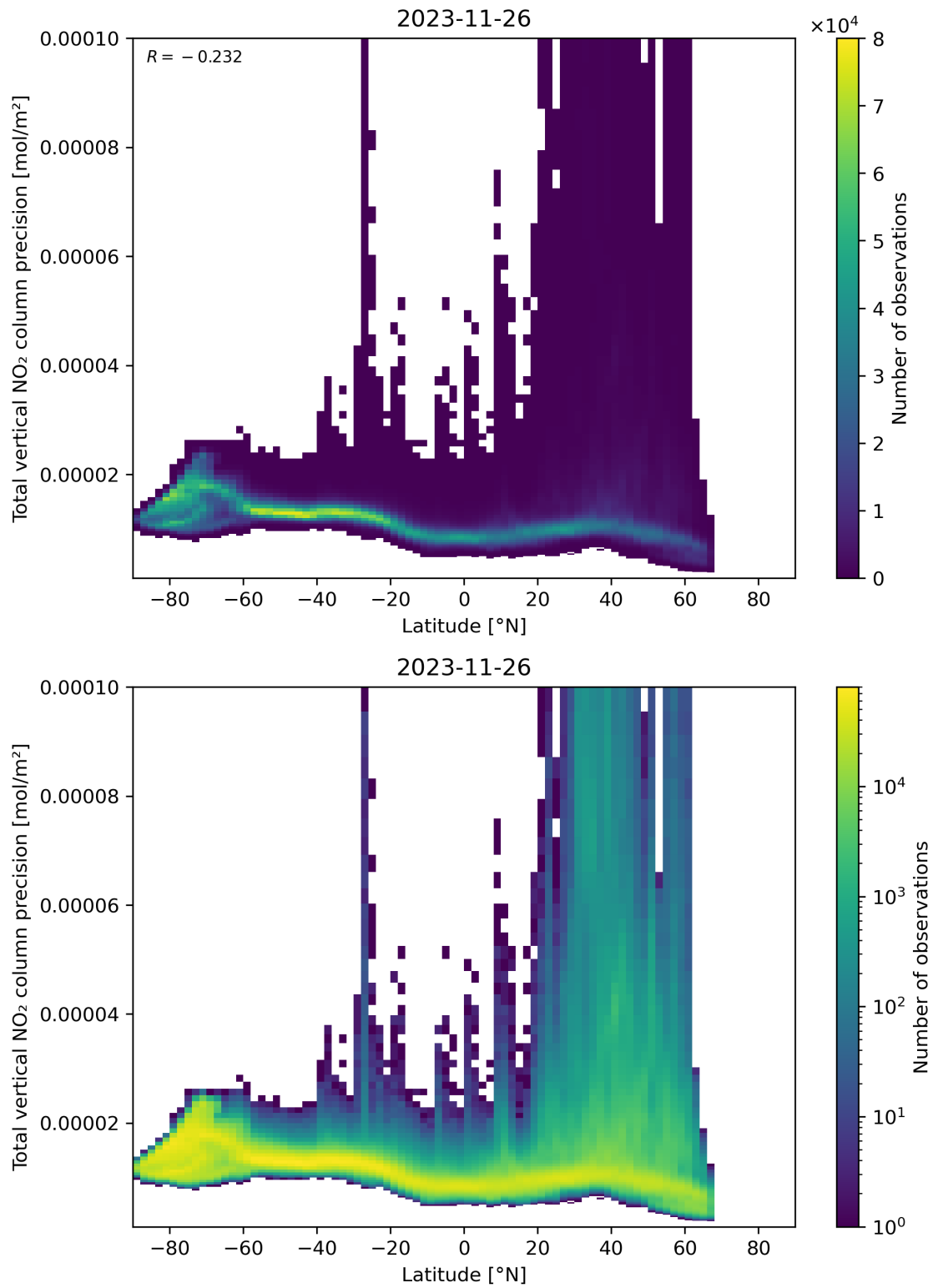
Figure 91: Scatter density plot of “Latitude” against “Total vertical NO 2 column precision” for 2023-11-25 to 2023-11-27.
