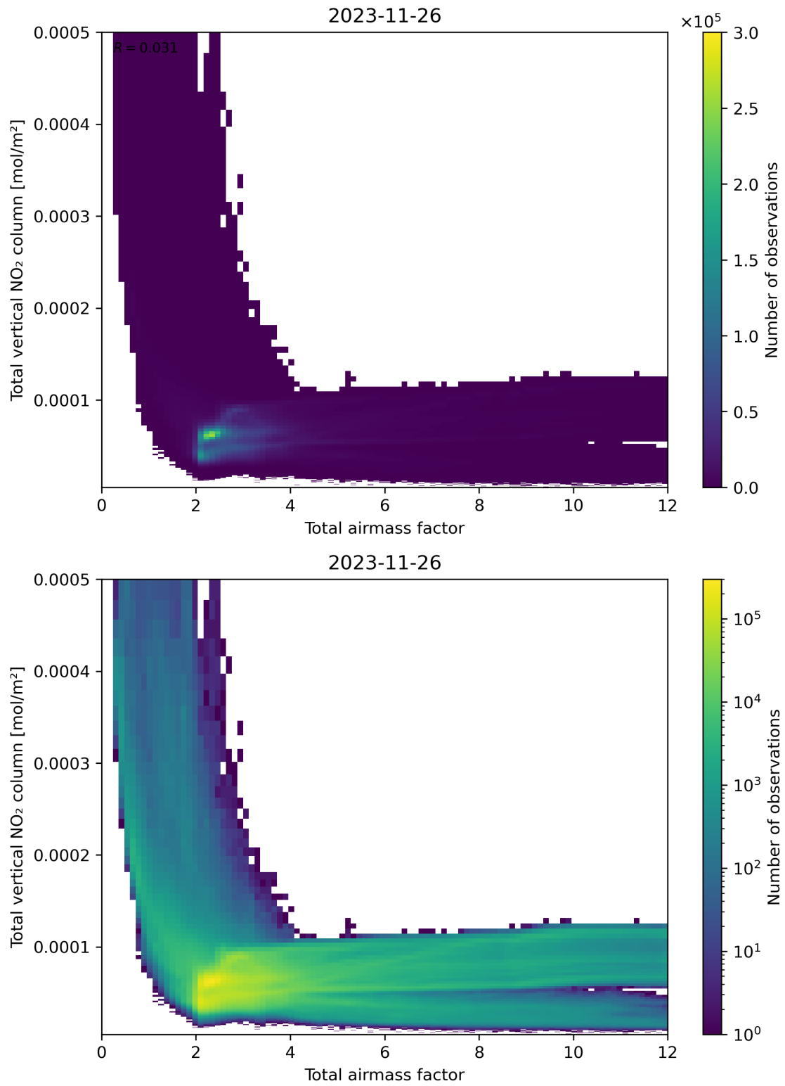
Figure 67: Scatter density plot of “Total airmass factor” against “Total vertical NO 2 column” for 2023-11-25 to 2023-11-27.
