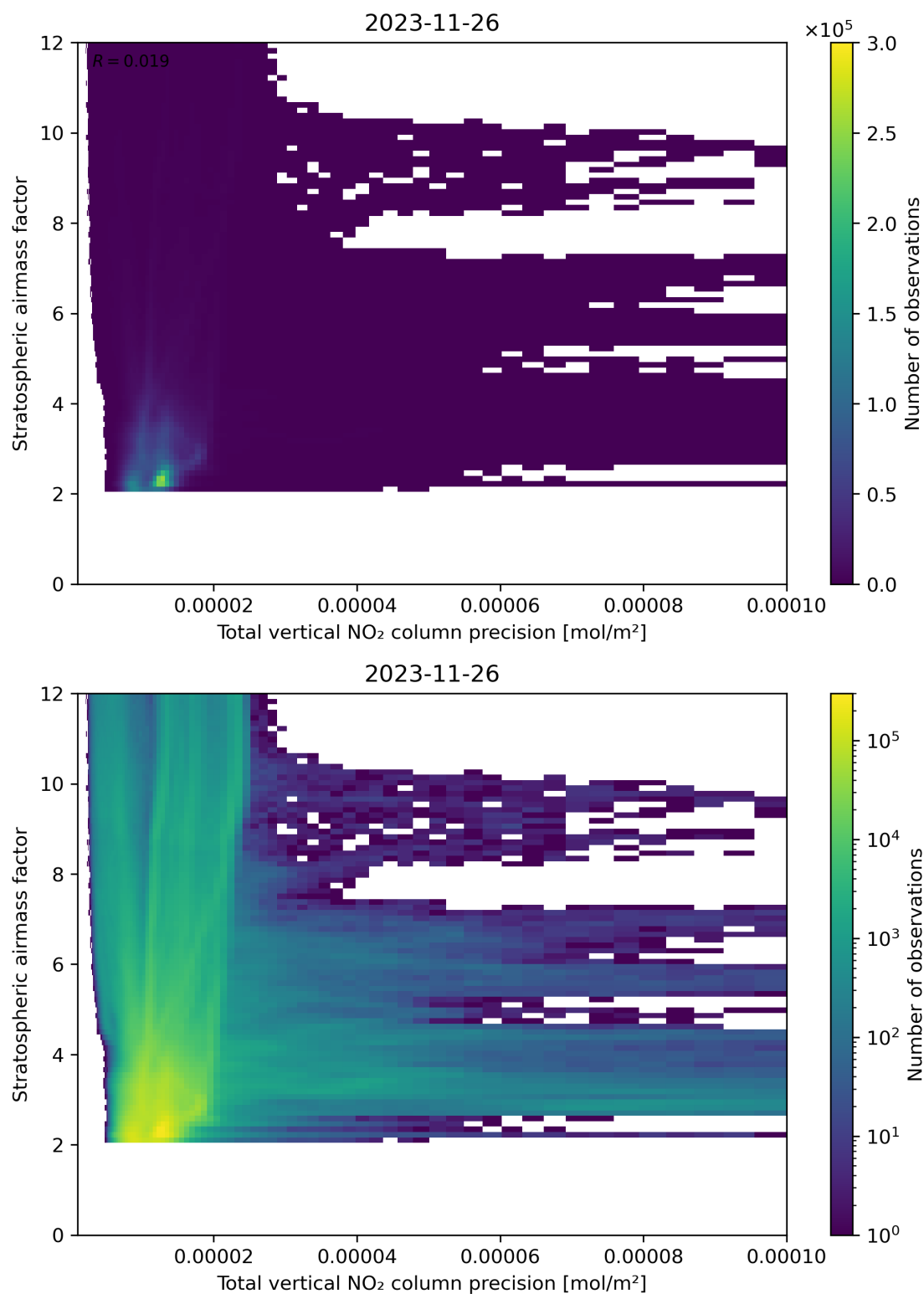
Figure 115: Scatter density plot of “Total vertical NO 2 column precision” against “Stratospheric air mass factor” for 2023-11-25 to 2023-11-27.
