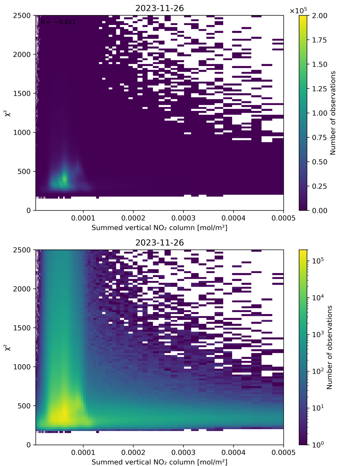
Figure 104: Scatter density plot of “Summed vertical NO 2 column” against “ \chi^2 ” for 2023-11-25 to 2023-11-27.
