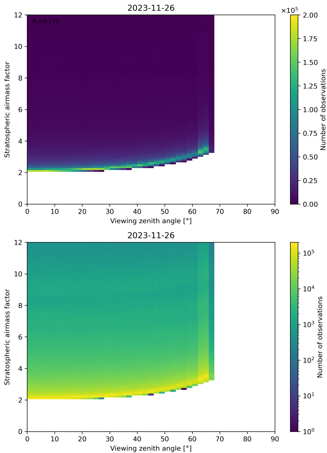
Figure 159: Scatter density plot of “Viewing zenith angle” against “Stratospheric airmass factor” for 2023-11-25 to 2023-11-27.
