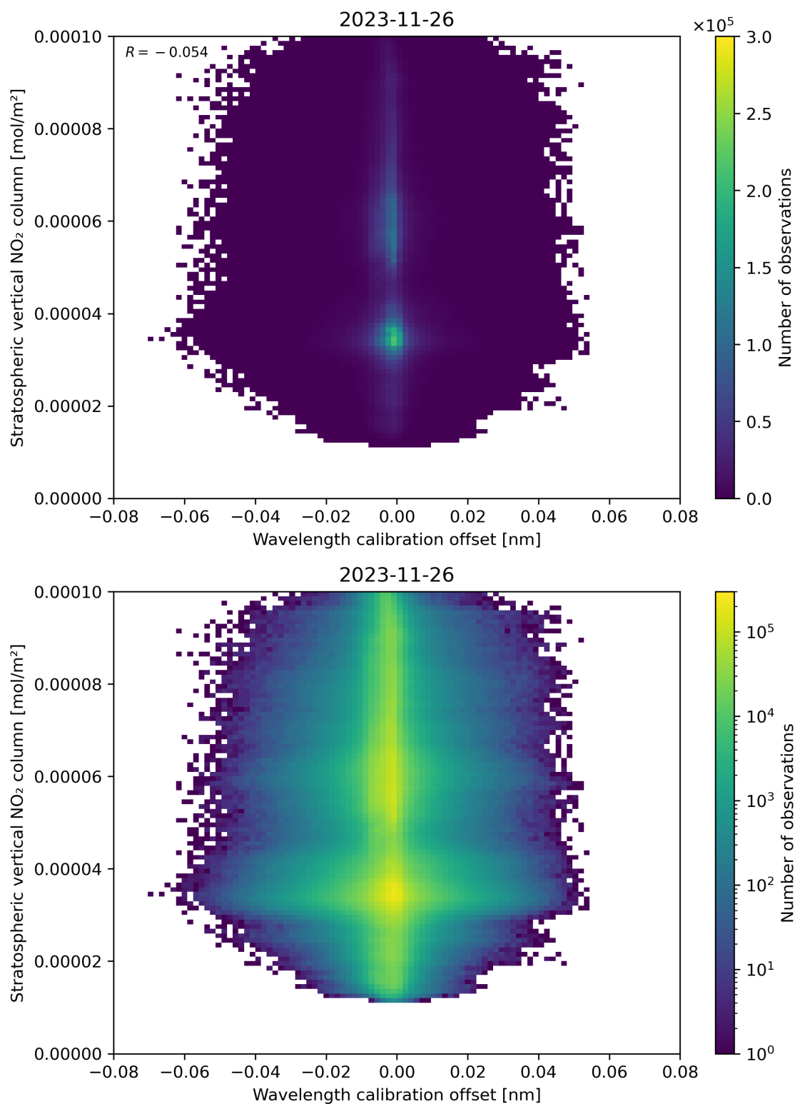
Figure 176: Scatter density plot of “Wavelength calibration offset” against “Stratospheric vertical NO 2 column” for 2023-11-25 to 2023-11-27.
