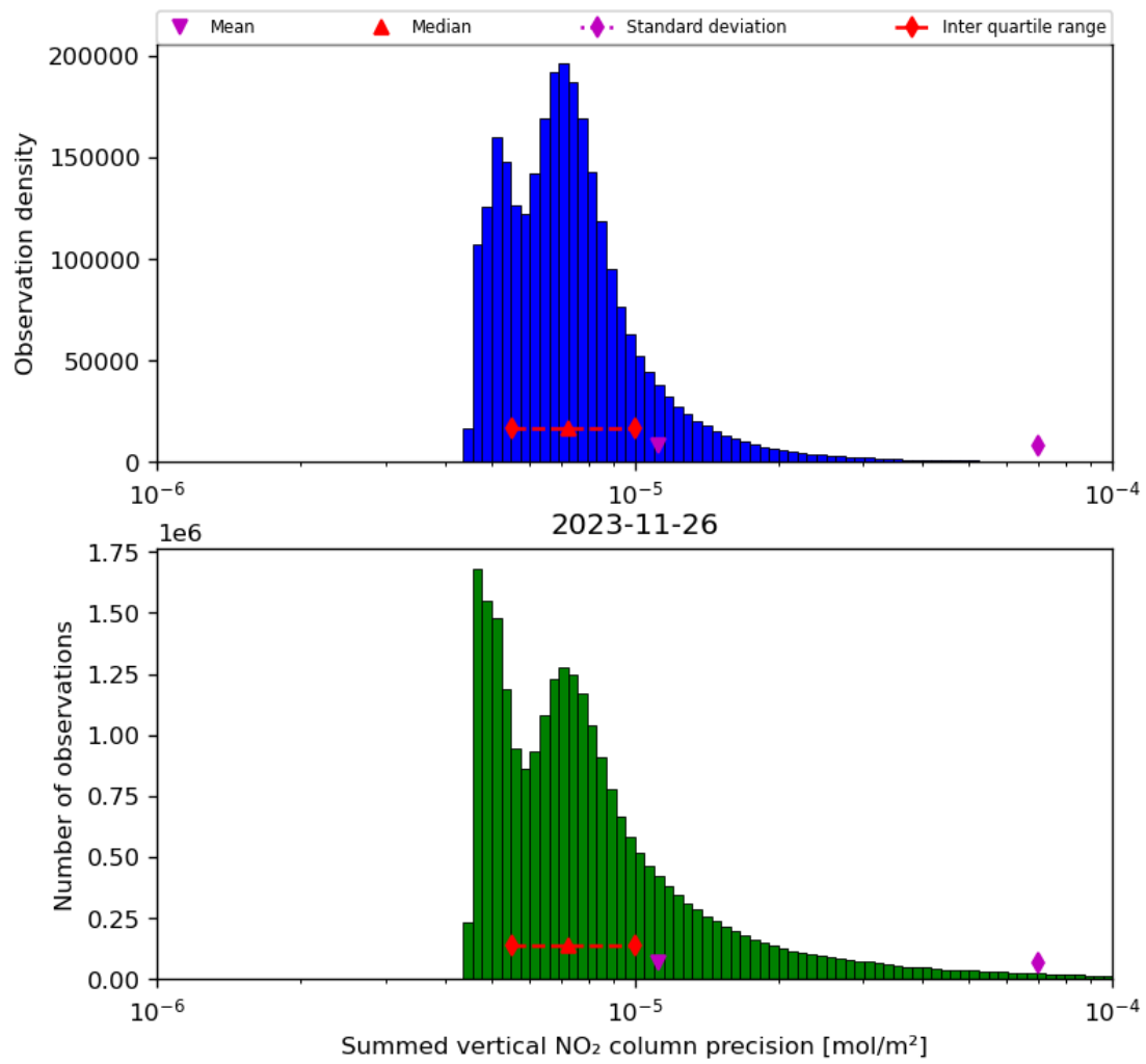
Figure 41: Histogram of "Summed vertical NO 2 column precision" for 2023-11-25 to 2023-11-27
