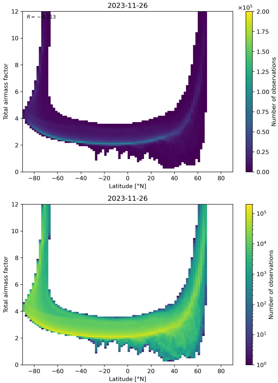
Figure 84: Scatter density plot of “Latitude” against “Total airmass factor” for 2023-11-25 to 2023-11-27.
