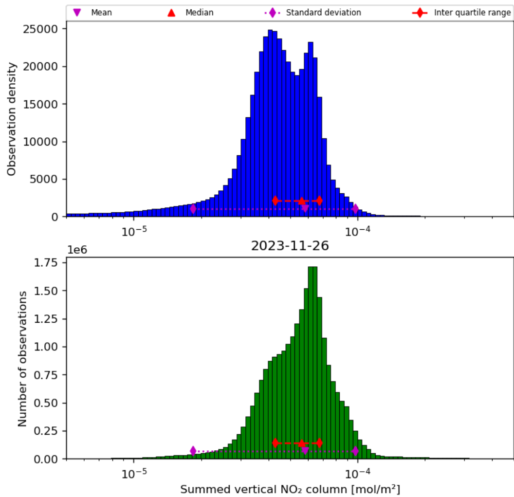
Figure 40: Histogram of “Summed vertical NO 2 column” for 2023-11-25 to 2023-11-27
