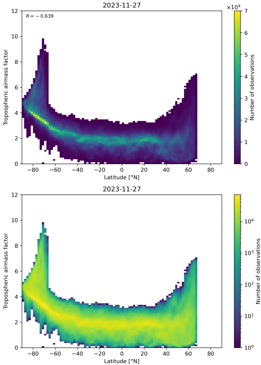
Figure 85: Scatter density plot of “Latitude” against “Tropospheric airmass factor” for 2023-11-26 to 2023-11-28.
