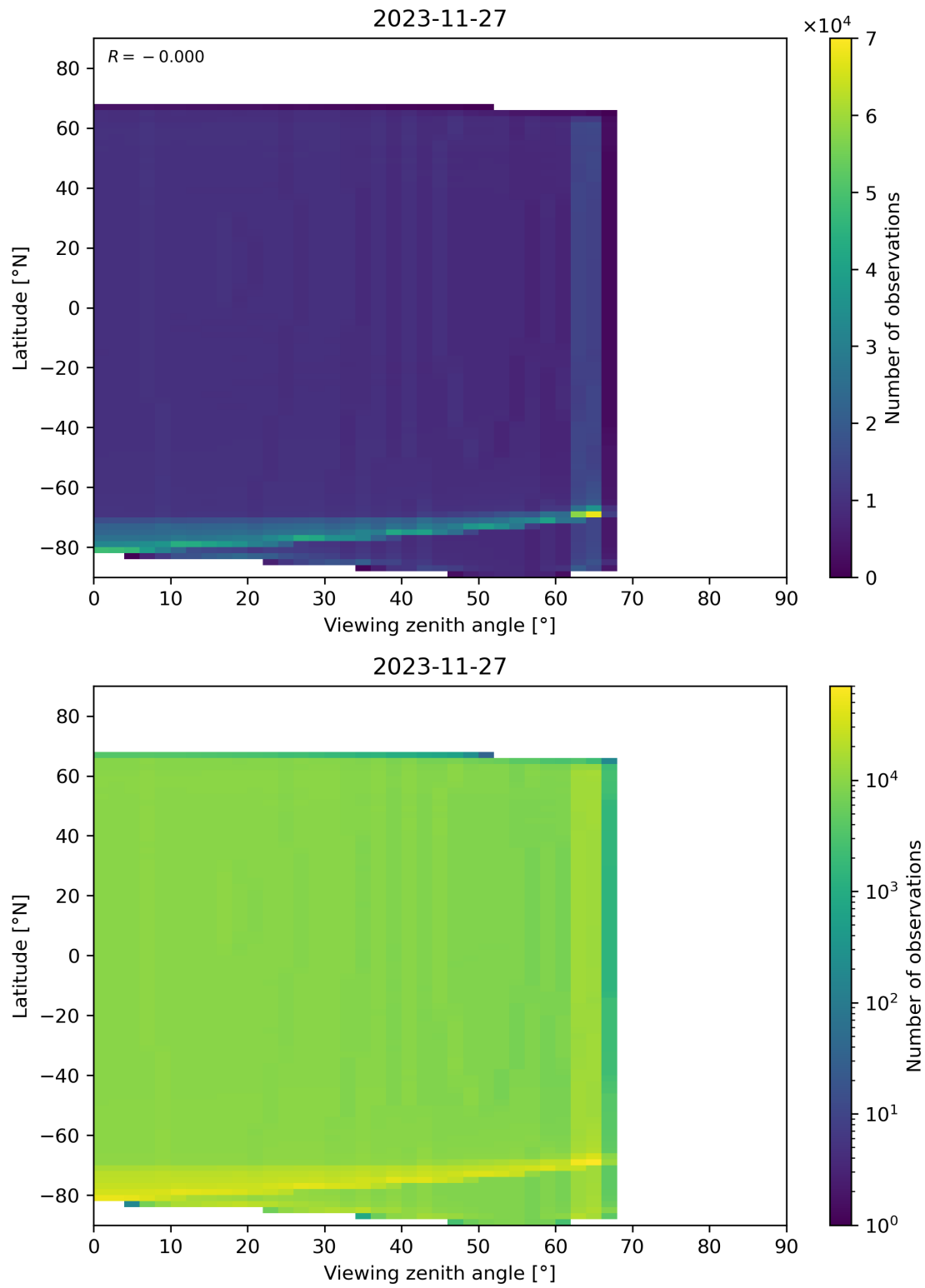
Figure 163: Scatter density plot of “Viewing zenith angle” against “Latitude” for 2023-11-26 to 2023-11-28.
