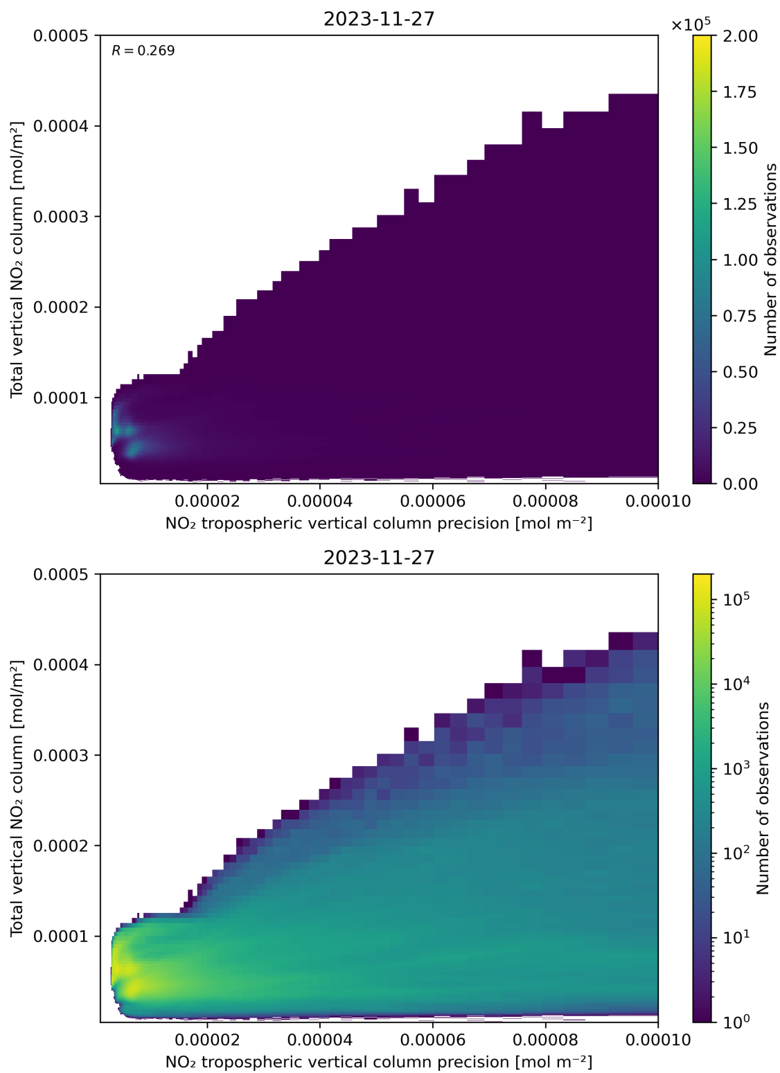
Figure 138: Scatter density plot of “NO 2 tropospheric vertical column precision” against “Total vertical NO 2 column” for 2023-11-26 to 2023-11-28.
