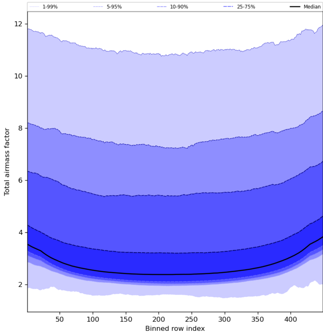
Figure 49: Along track statistics of “Total airmass factor” for 2023-11-26 to 2023-11-28
