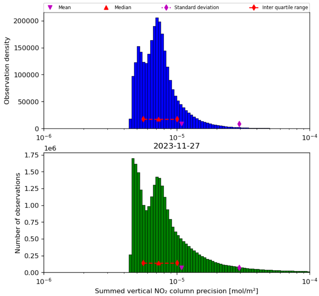
Figure 41: Histogram of "Summed vertical NO 2 column precision" for 2023-11-26 to 2023-11-28
