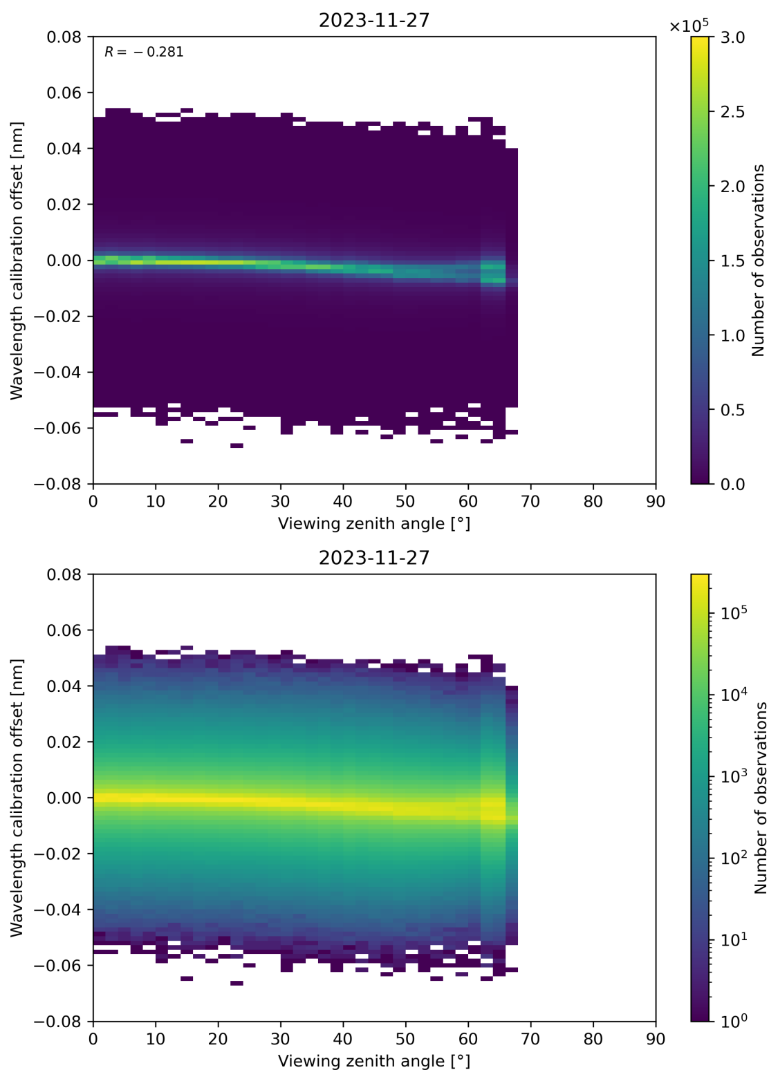
Figure 173: Scatter density plot of “Viewing zenith angle” against “Wavelength calibration offset” for 2023-11-26 to 2023-11-28.
