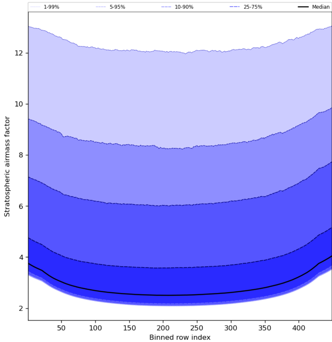
Figure 61: Along track statistics of “Stratospheric air mass factor” for 2023-11-26 to 2023-11-28
