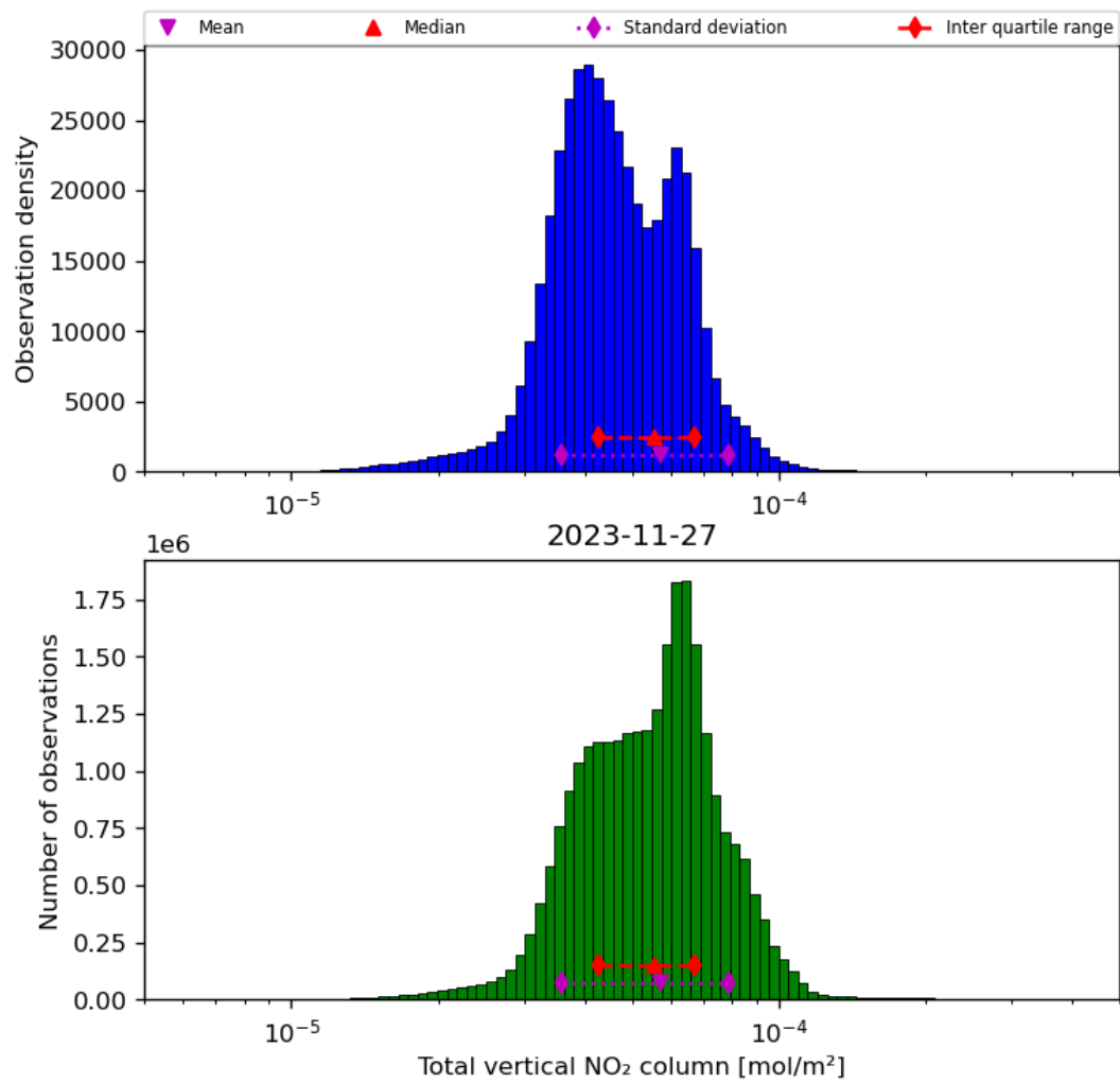
Figure 38: Histogram of “Total vertical NO 2 column” for 2023-11-26 to 2023-11-28
