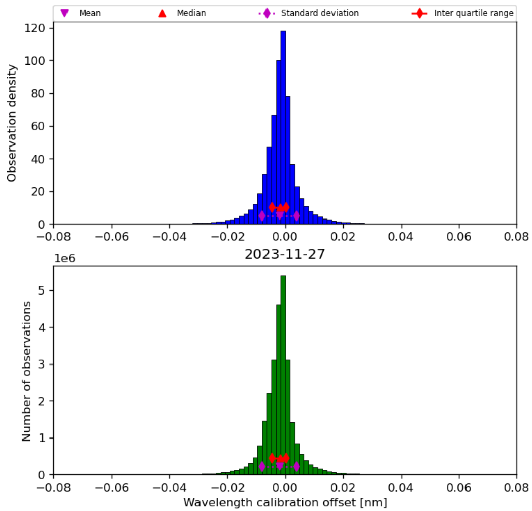
Figure 35: Histogram of “Wavelength calibration offset” for 2023-11-26 to 2023-11-28
