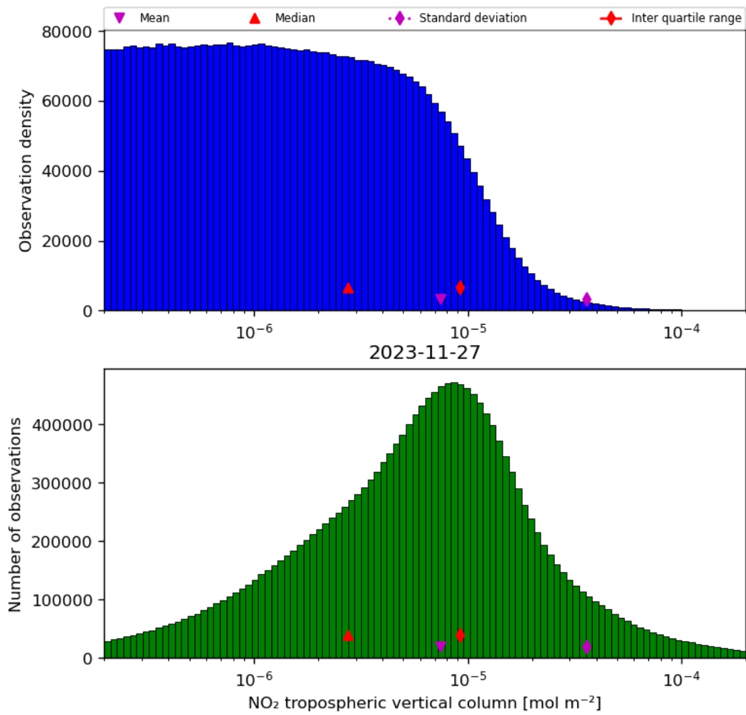
Figure 29: Histogram of “NO 2 tropospheric vertical column” for 2023-11-26 to 2023-11-28
