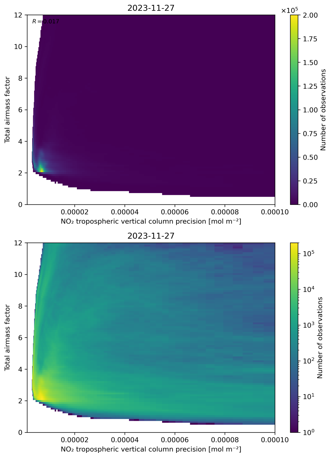
Figure 132: Scatter density plot of “NO 2 tropospheric vertical column precision” against “Total air mass factor” for 2023-11-26 to 2023-11-28.
