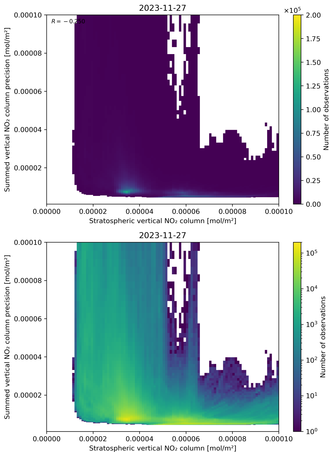
Figure 99: Scatter density plot of “Stratospheric vertical NO 2 column” against “Summed vertical NO 2 column precision” for 2023-11-26 to 2023-11-28.
