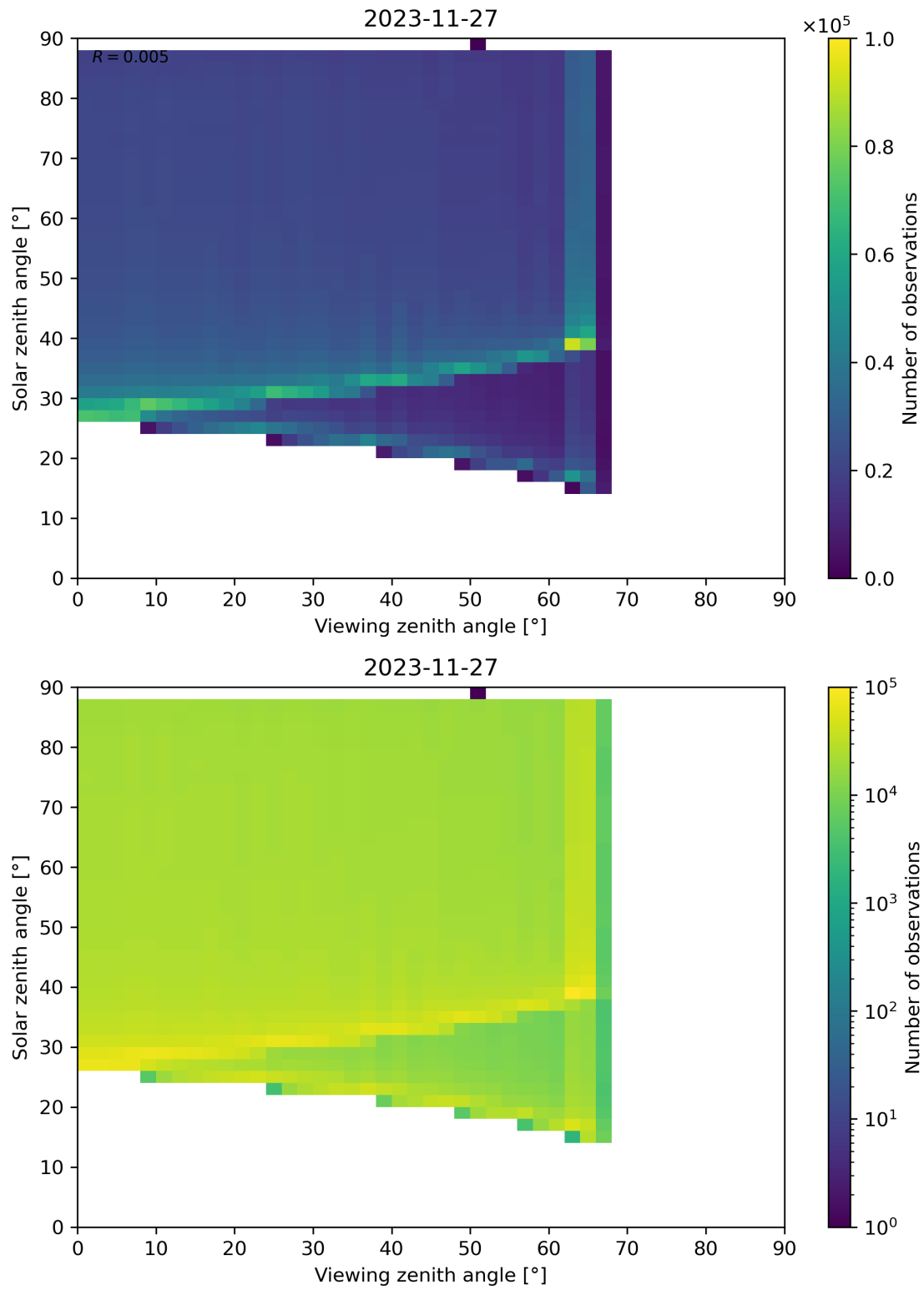
Figure 172: Scatter density plot of “Viewing zenith angle” against “Solar zenith angle” for 2023-11-26 to 2023-11-28.
