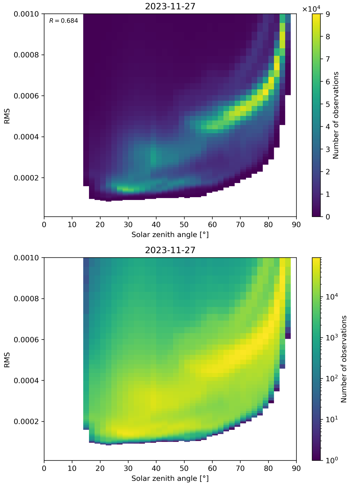
Figure 157: Scatter density plot of “Solar zenith angle” against “RMS” for 2023-11-26 to 2023-11-28.
