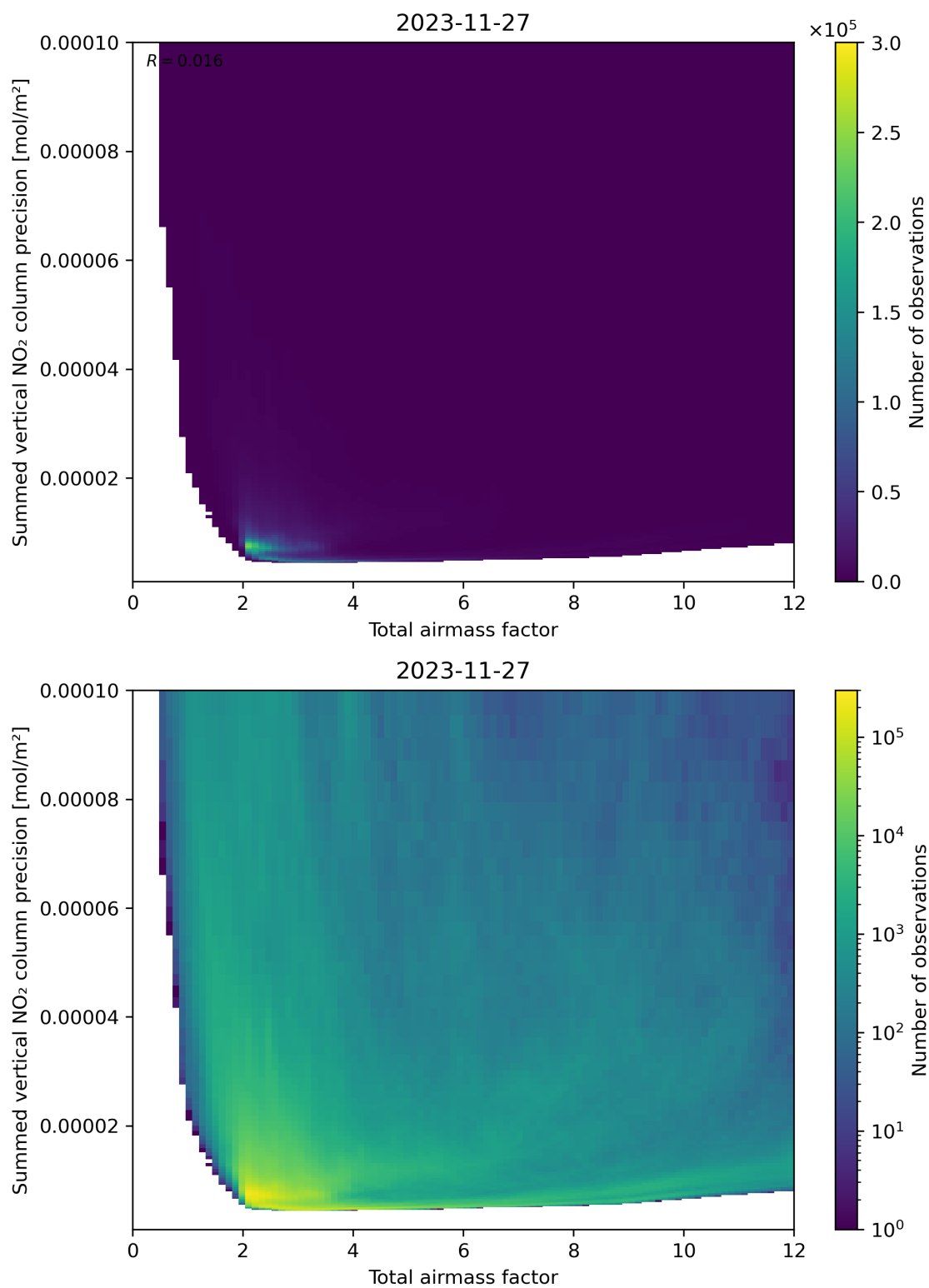
Figure 66: Scatter density plot of “Total airmass factor” against “Summed vertical NO 2 column precision” for 2023-11-26 to 2023-11-28.
