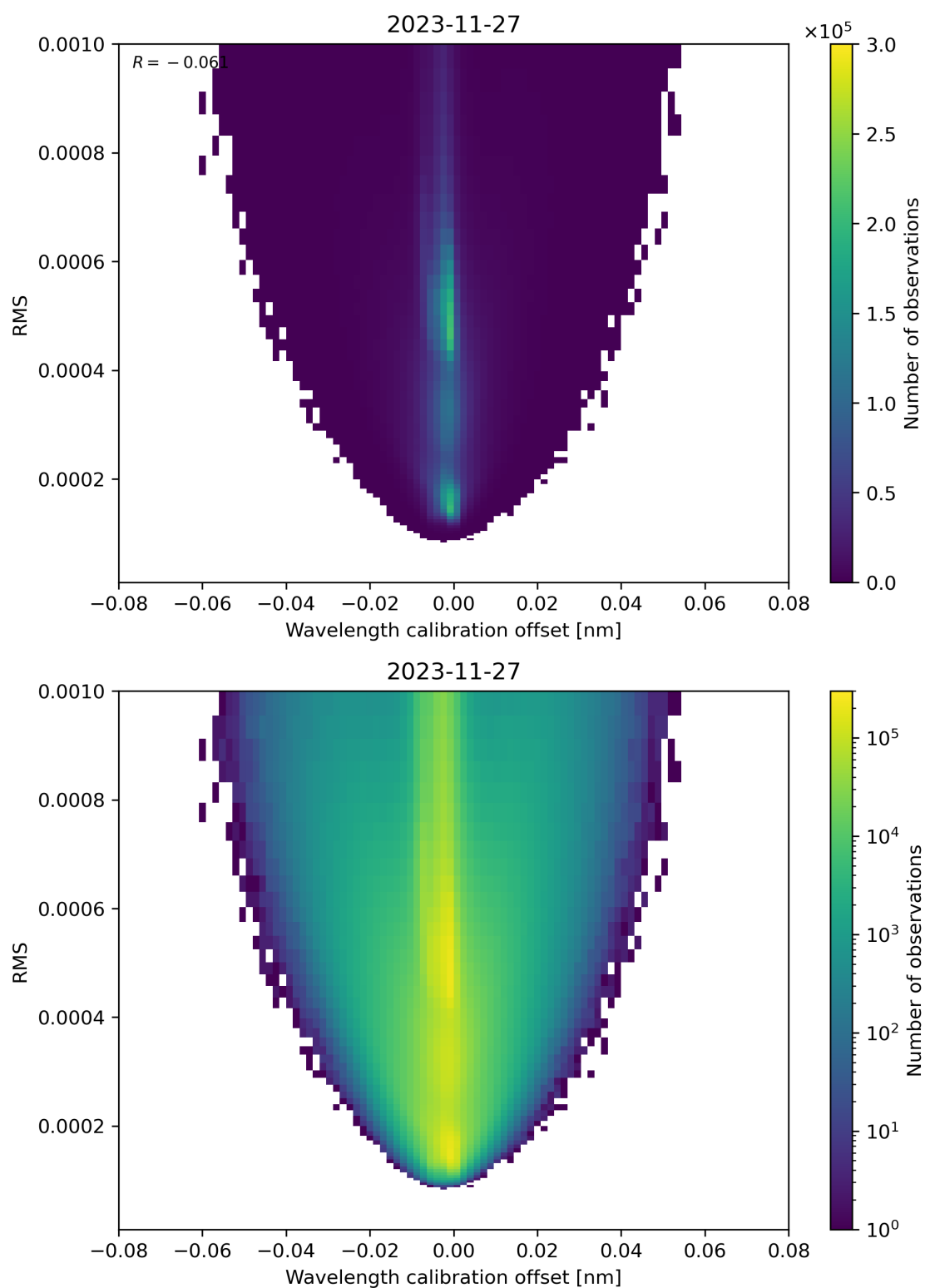
Figure 181: Scatter density plot of “Wavelength calibration offset” against “RMS” for 2023-11-26 to 2023-11-28.
