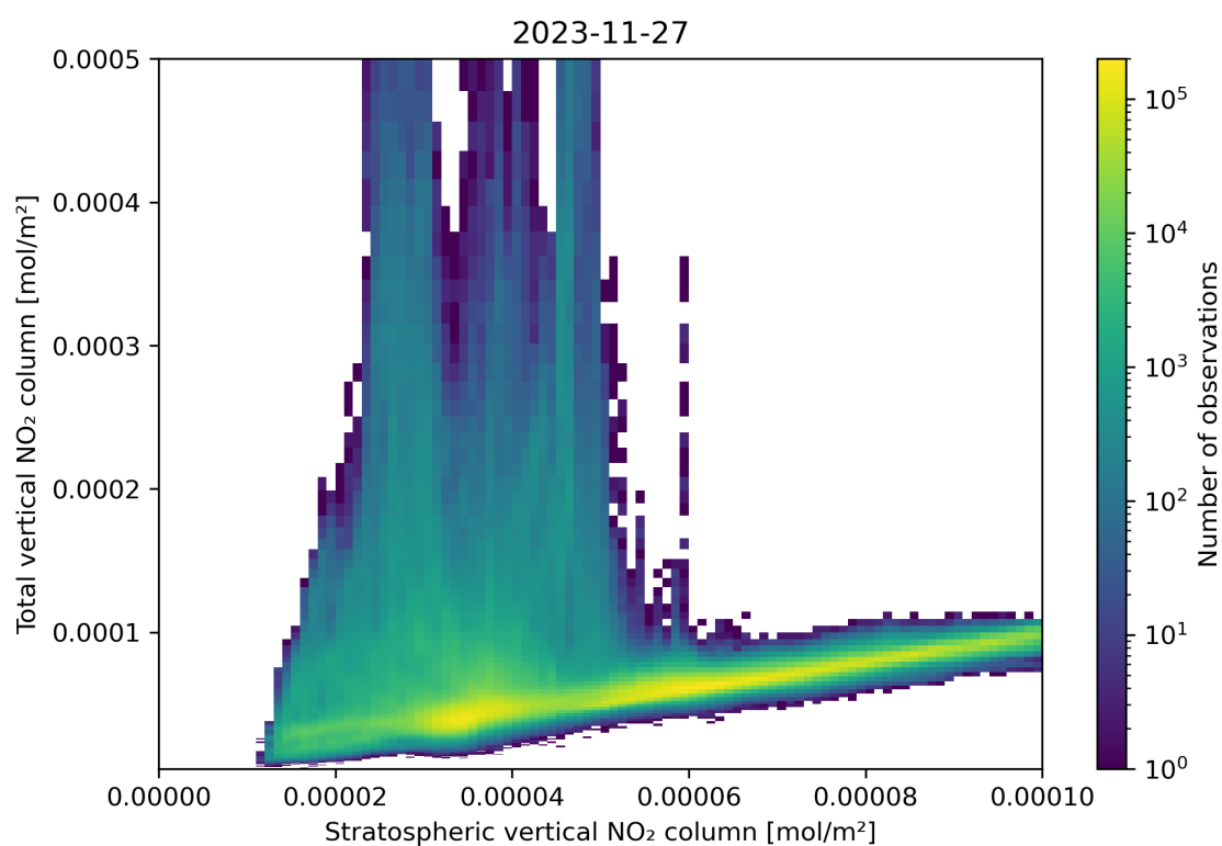
Figure 100: Scatter density plot of “Stratospheric vertical NO 2 column” against “Total vertical NO 2 column” for 2023-11-26 to 2023-11-28.
