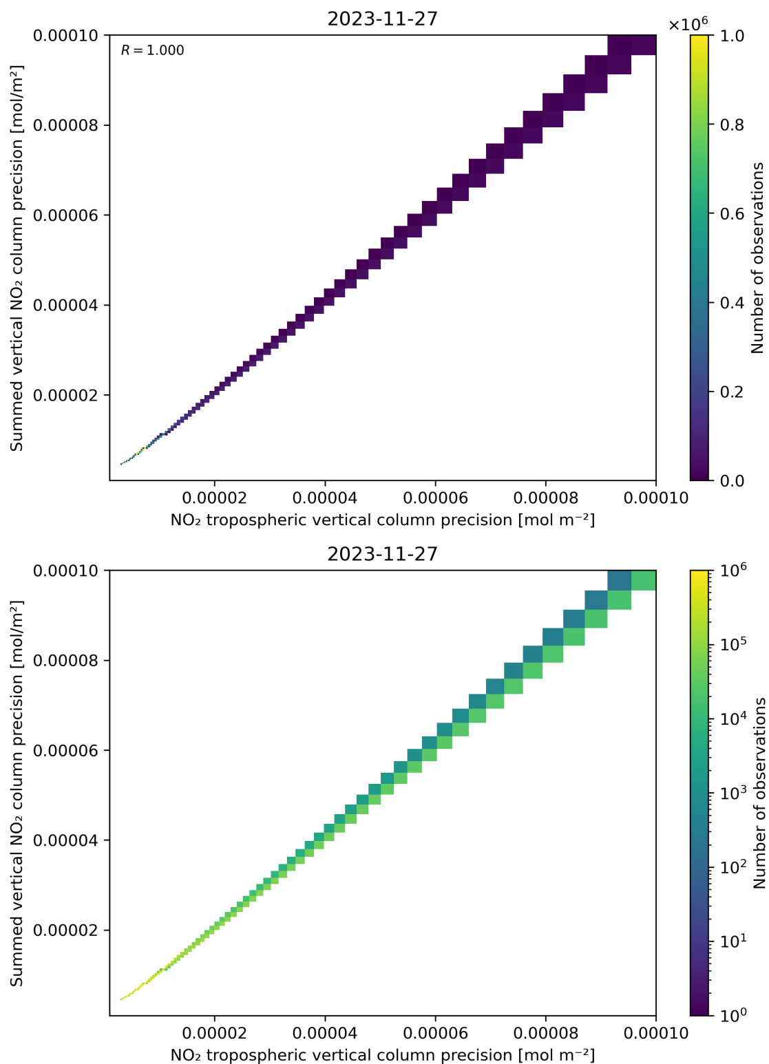
Figure 137: Scatter density plot of “NO 2 tropospheric vertical column precision” against “Summed vertical NO 2 column precision” for 2023-11-26 to 2023-11-28.
