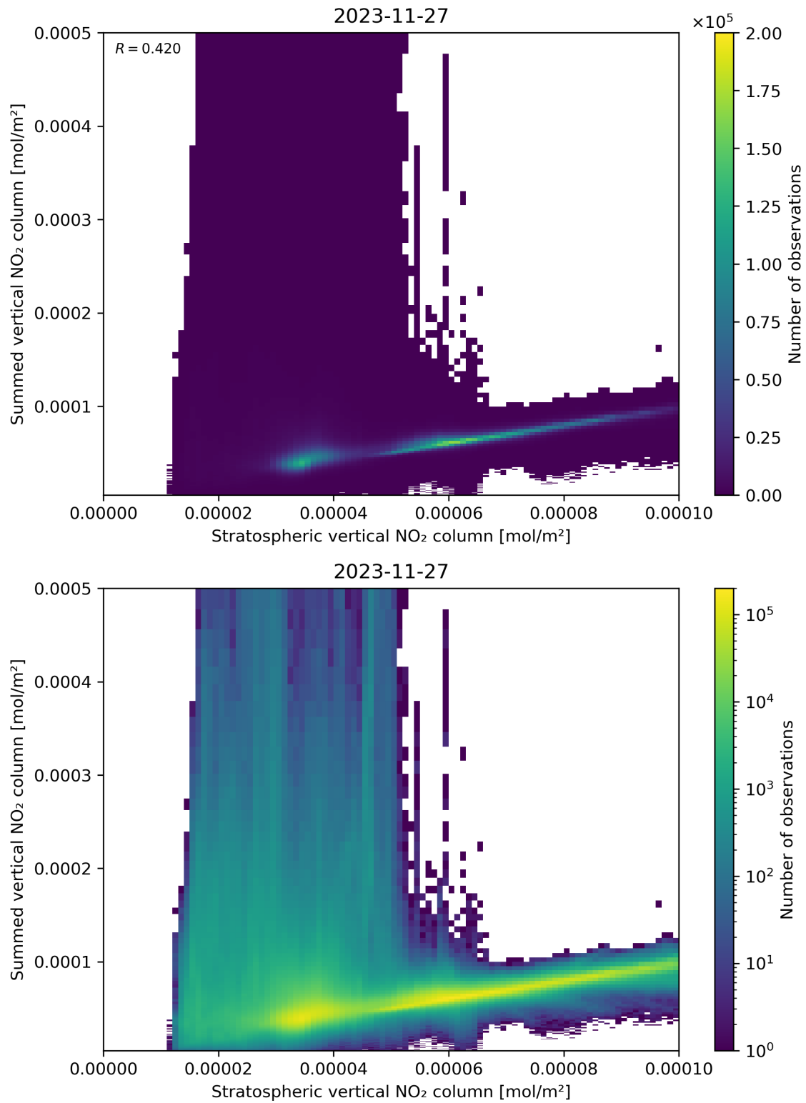
Figure 98: Scatter density plot of “Stratospheric vertical NO 2 column” against “Summed vertical NO 2 column” for 2023-11-26 to 2023-11-28.
