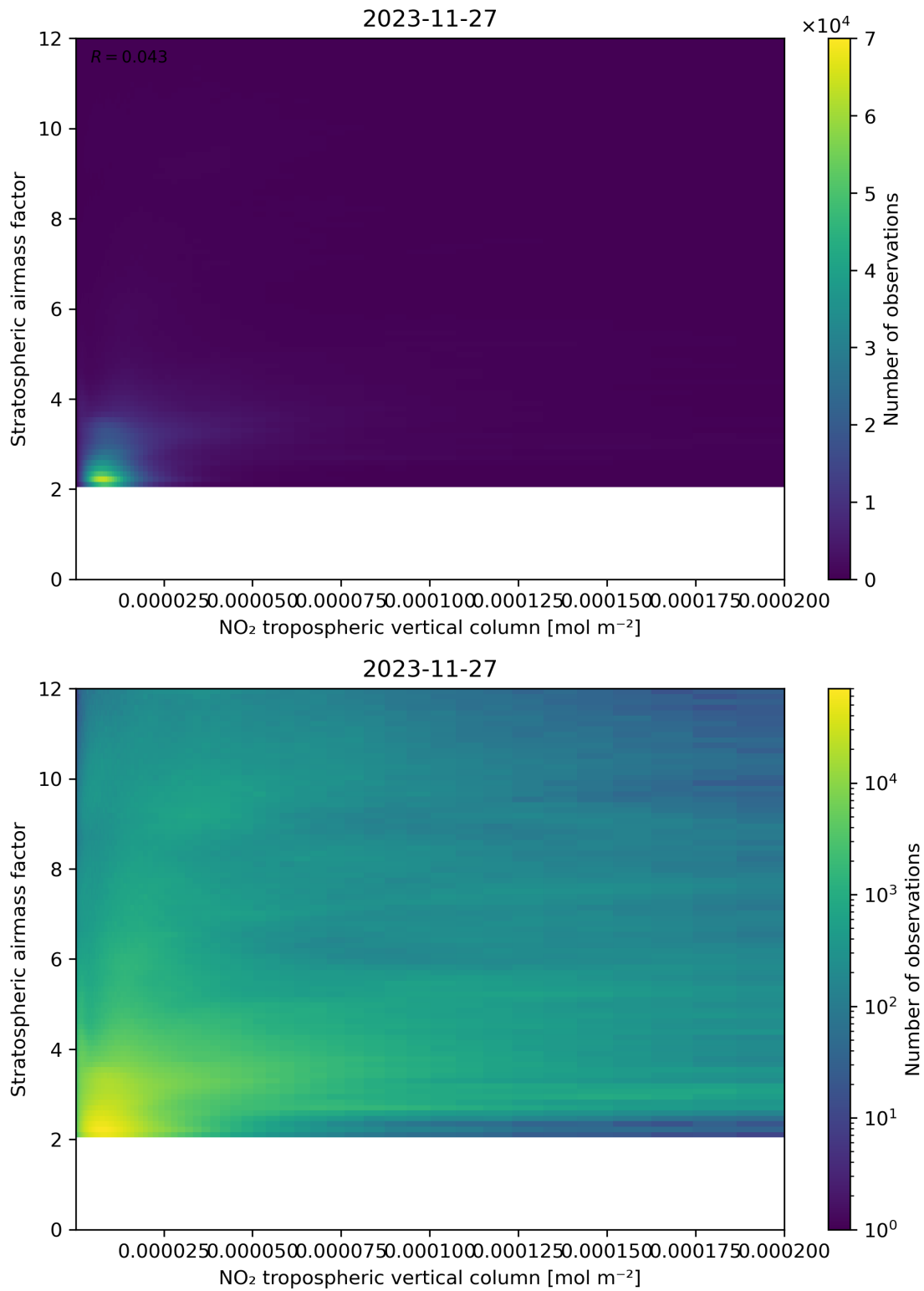
Figure 121: Scatter density plot of “NO 2 tropospheric vertical column” against “Stratospheric airmass factor” for 2023-11-26 to 2023-11-28.
