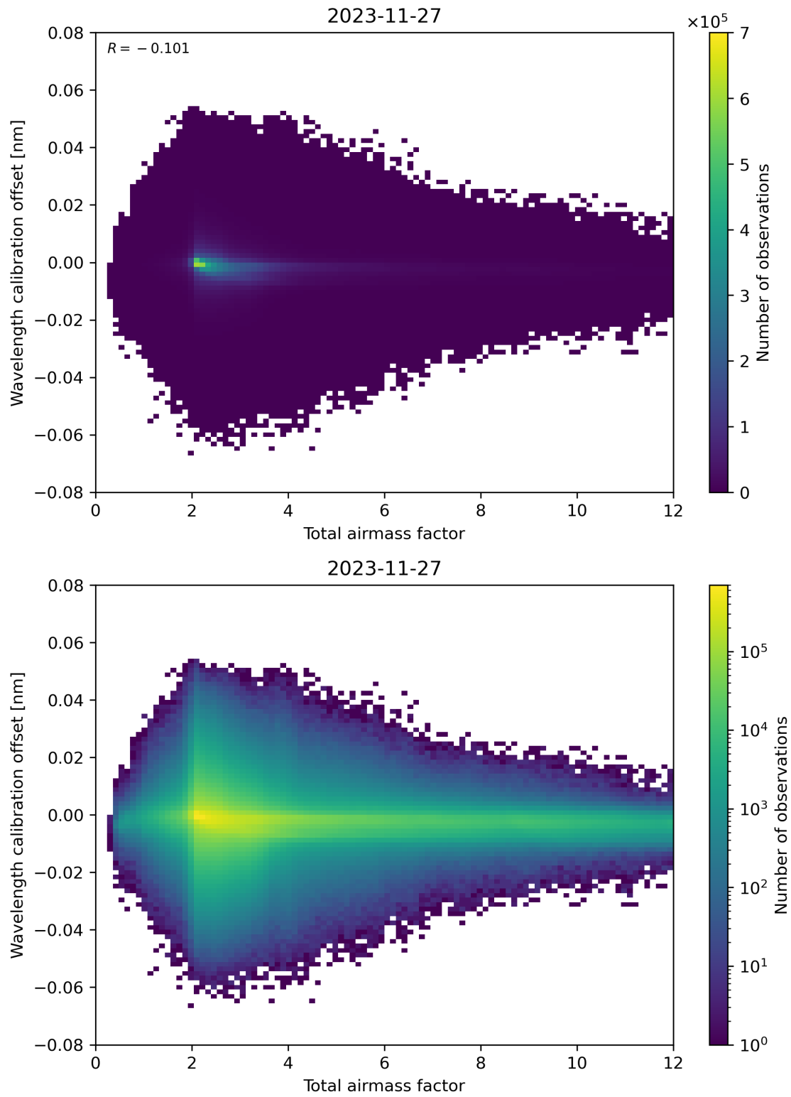
Figure 70: Scatter density plot of “Total airmass factor” against “Wavelength calibration offset” for 2023-11-26 to 2023-11-28.
