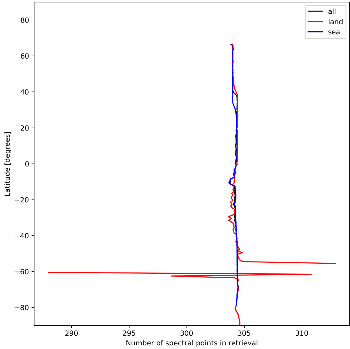
Figure 16: Zonal average of “Number of spectral points in retrieval” for 2023-11-26 to 2023-11-28.
