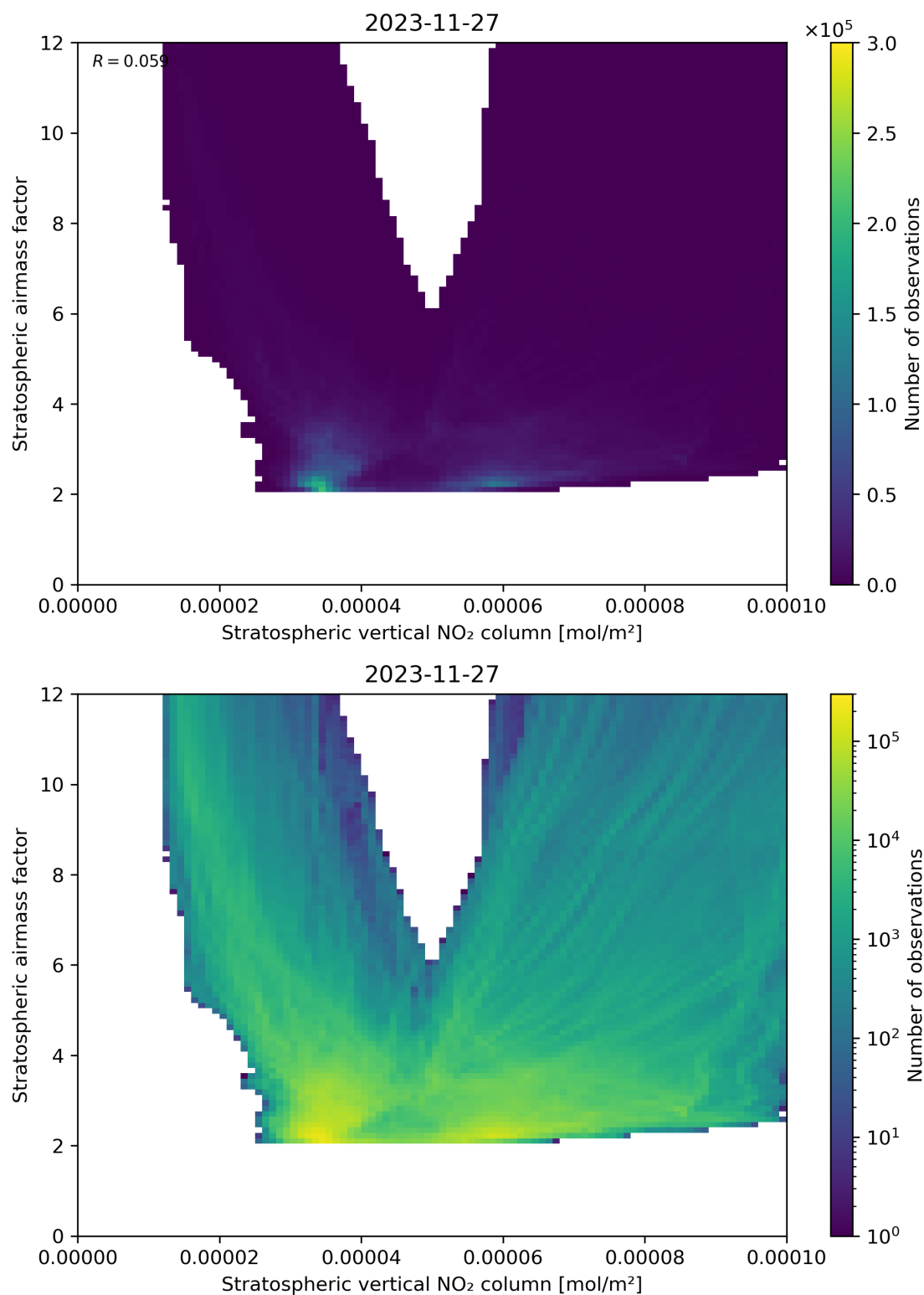
Figure 96: Scatter density plot of “Stratospheric vertical NO 2 column” against “Stratospheric airmass factor” for 2023-11-26 to 2023-11-28.
