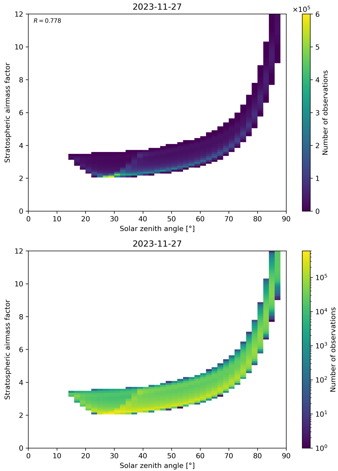
Figure 145: Scatter density plot of “Solar zenith angle” against “Stratospheric airmass factor” for 2023-11-26 to 2023-11-28.
