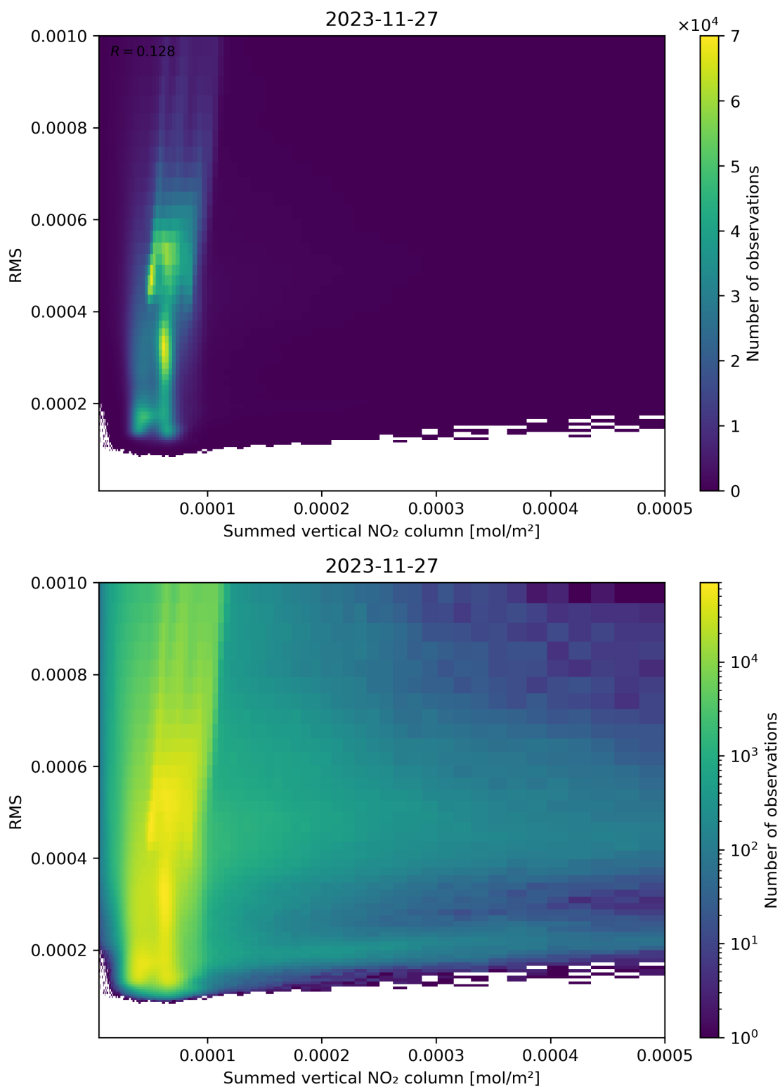
Figure 109: Scatter density plot of “Summed vertical NO 2 column” against “RMS” for 2023-11-26 to 2023-11-28.
