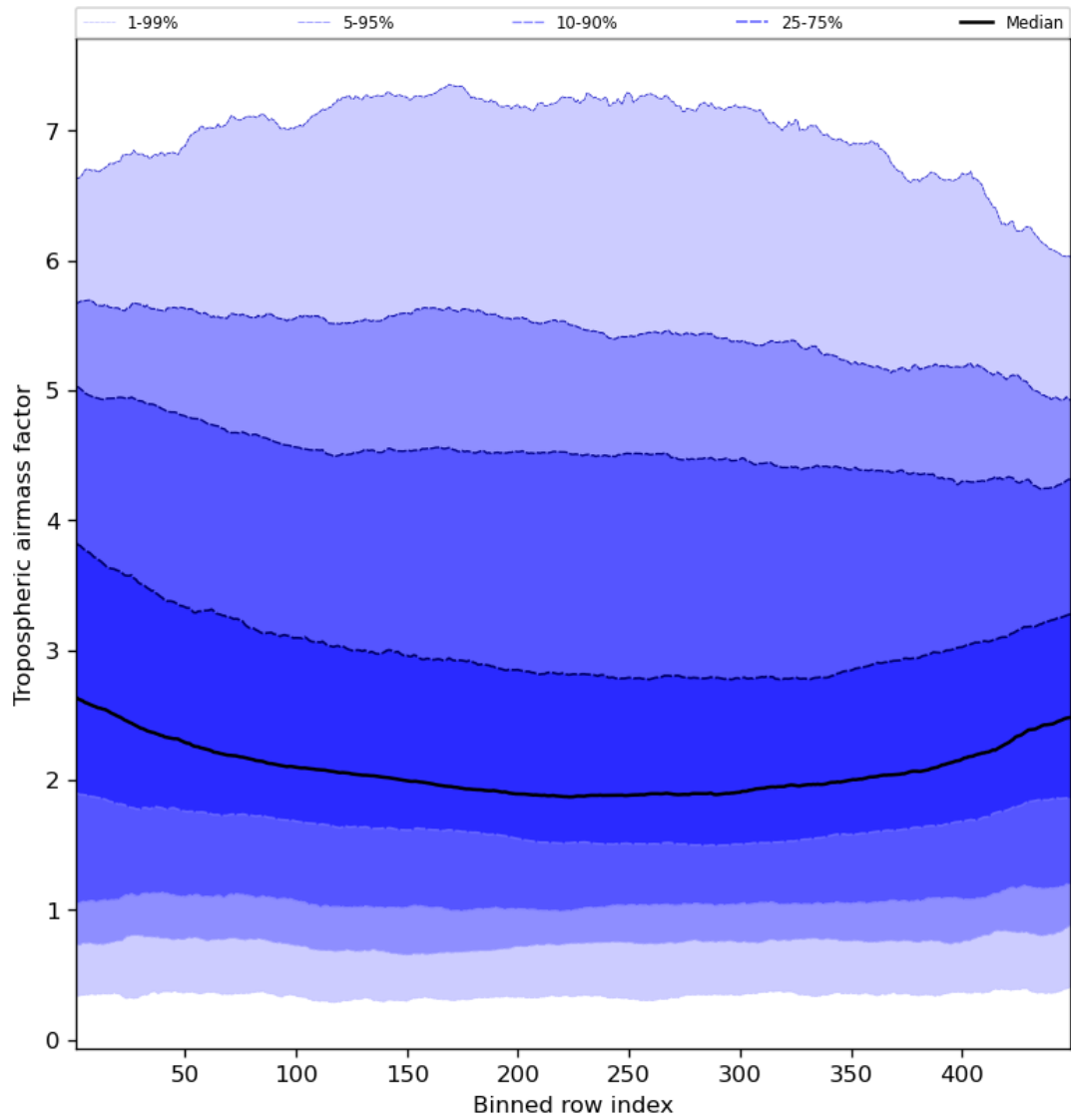
Figure 48: Along track statistics of “Tropospheric air mass factor” for 2023-11-26 to 2023-11-28
