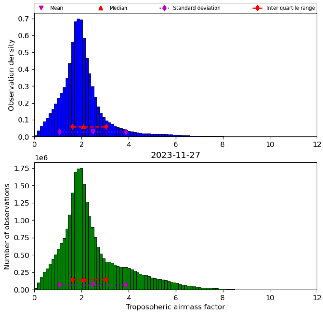
Figure 31: Histogram of “Tropospheric airmass factor” for 2023-11-26 to 2023-11-28
