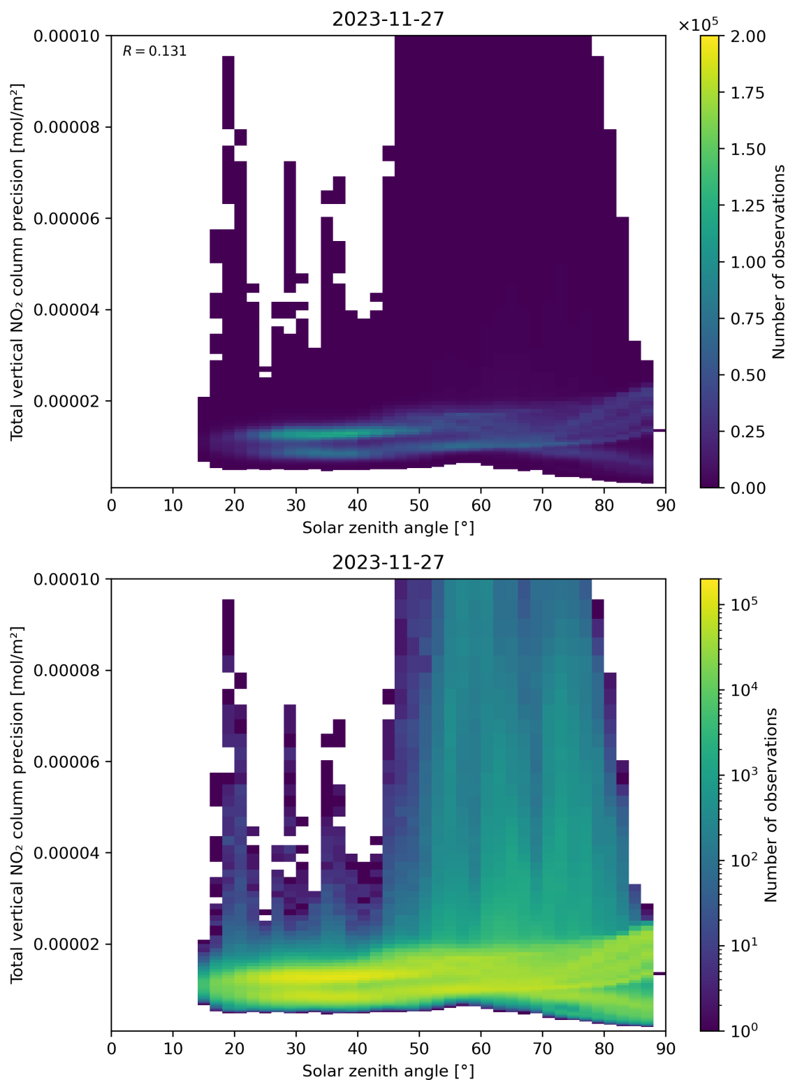
Figure 154: Scatter density plot of “Solar zenith angle” against “Total vertical NO 2 column precision” for 2023-11-26 to 2023-11-28.
