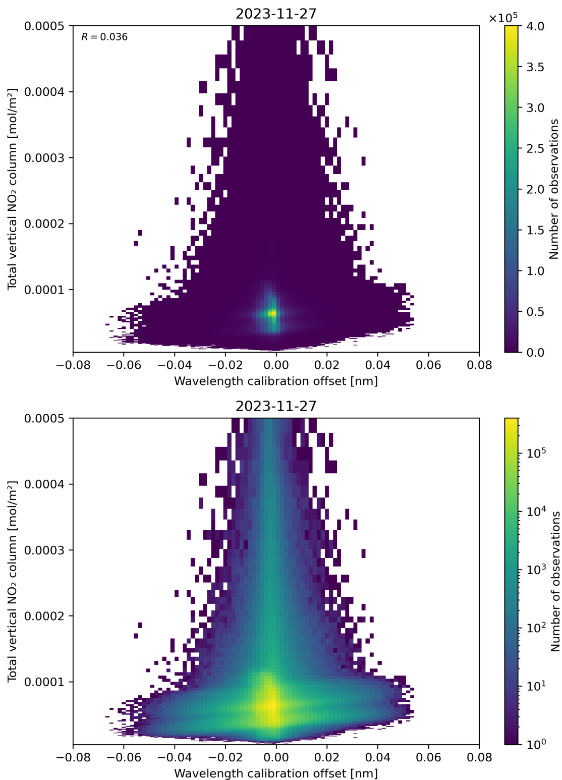
Figure 179: Scatter density plot of “Wavelength calibration offset” against “Total vertical NO 2 column” for 2023-11-26 to 2023-11-28.
