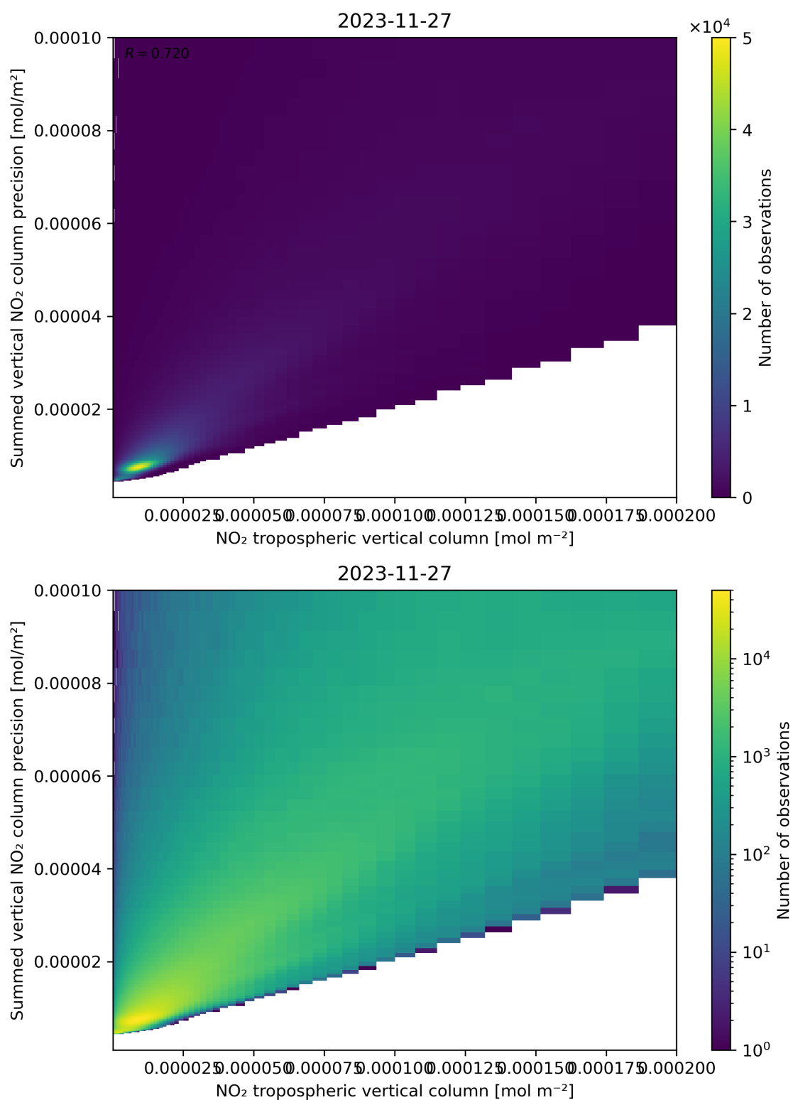
Figure 127: Scatter density plot of “NO 2 tropospheric vertical column” against “Summed vertical NO 2 column precision” for 2023-11-26 to 2023-11-28.
