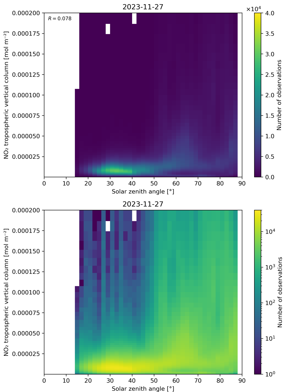
Figure 155: Scatter density plot of “Solar zenith angle” against “NO 2 tropospheric vertical column” for 2023-11-26 to 2023-11-28.
