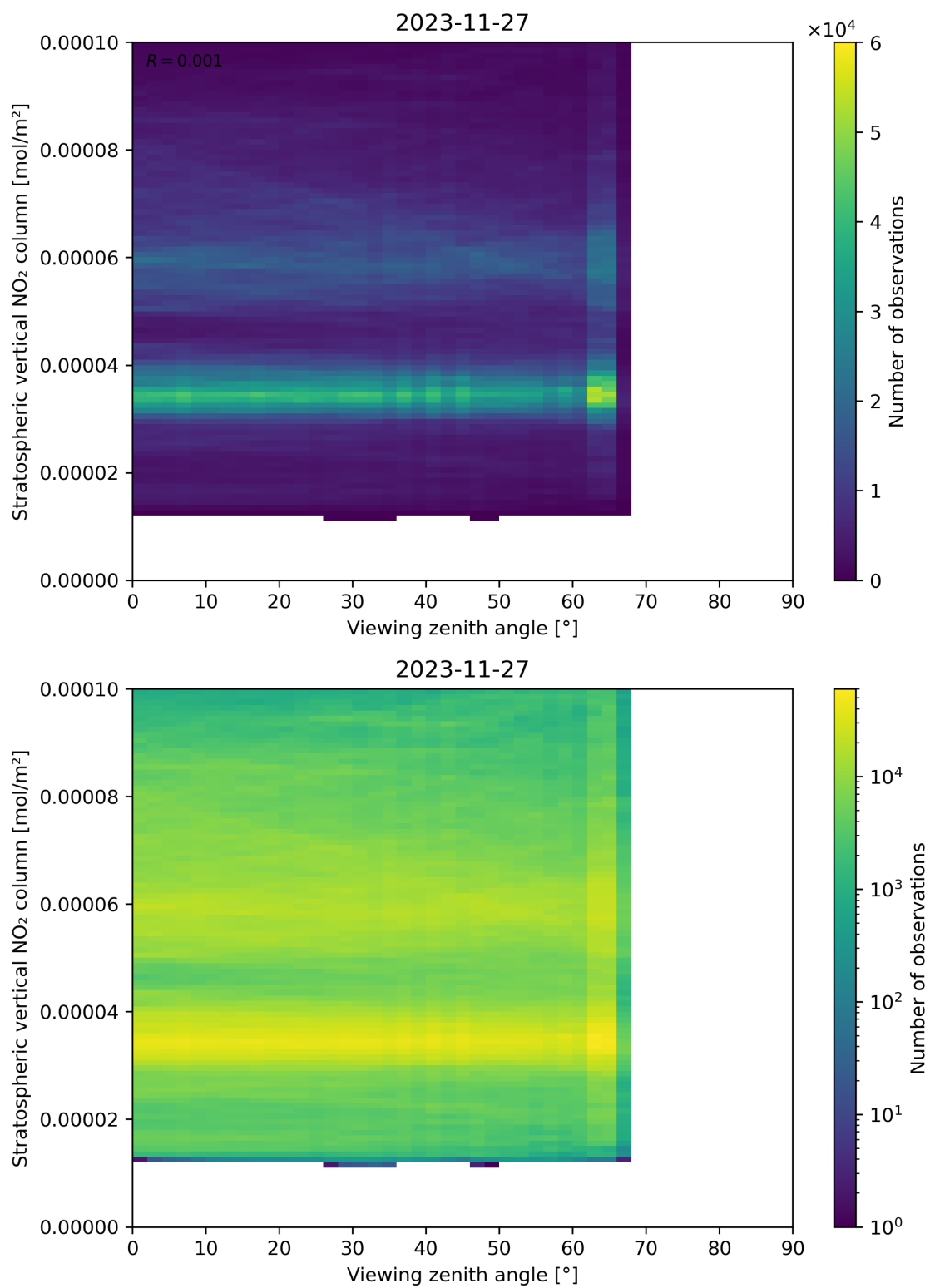
Figure 164: Scatter density plot of “Viewing zenith angle” against “Stratospheric vertical NO 2 column” for 2023-11-26 to 2023-11-28.
