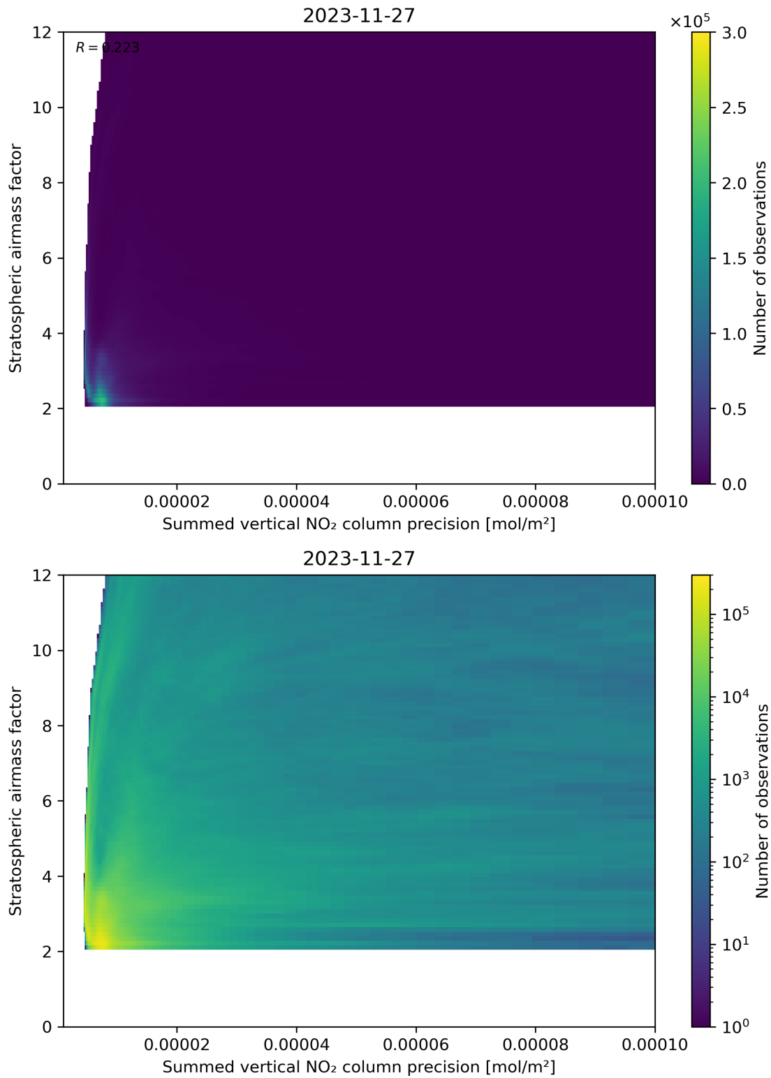
Figure 106: Scatter density plot of “Summed vertical NO 2 column precision” against “Stratospheric airmass factor” for 2023-11-26 to 2023-11-28.
