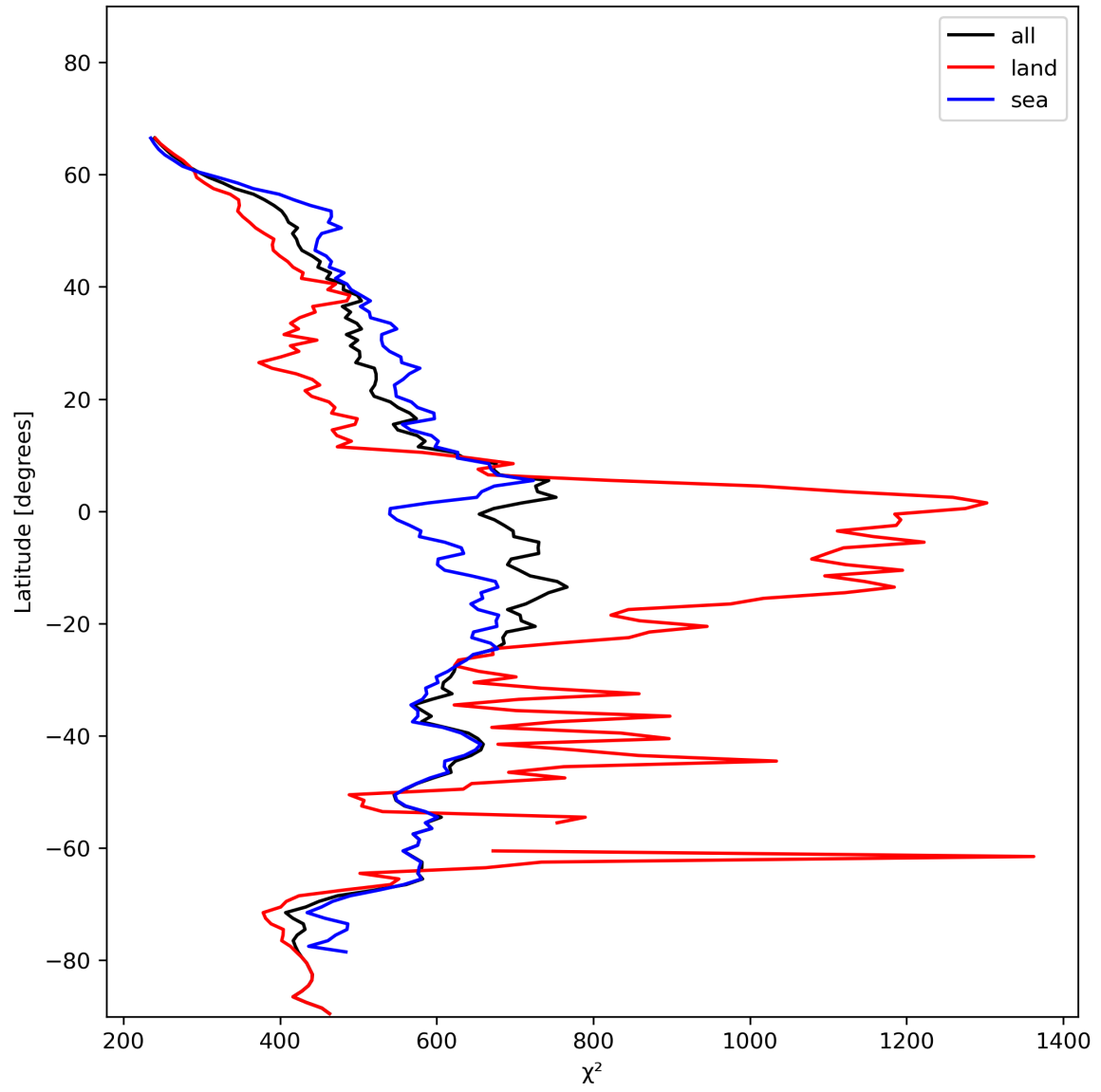
Figure 25: Zonal average of “ \chi^2 ” for 2023-11-26 to 2023-11-28.
