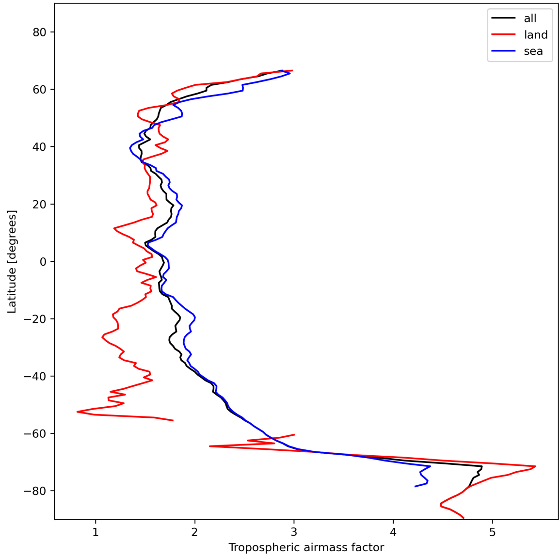
Figure 14: Zonal average of “Tropospheric air mass factor” for 2023-11-26 to 2023-11-28.
