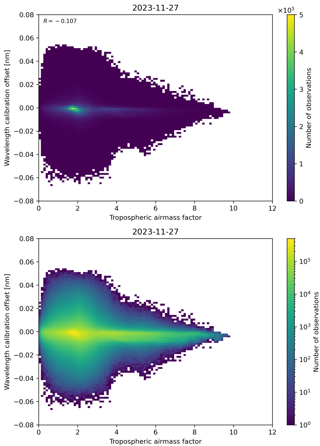
Figure 80: Scatter density plot of “Tropospheric air mass factor” against “Wavelength calibration offset” for 2023-11-26 to 2023-11-28.
