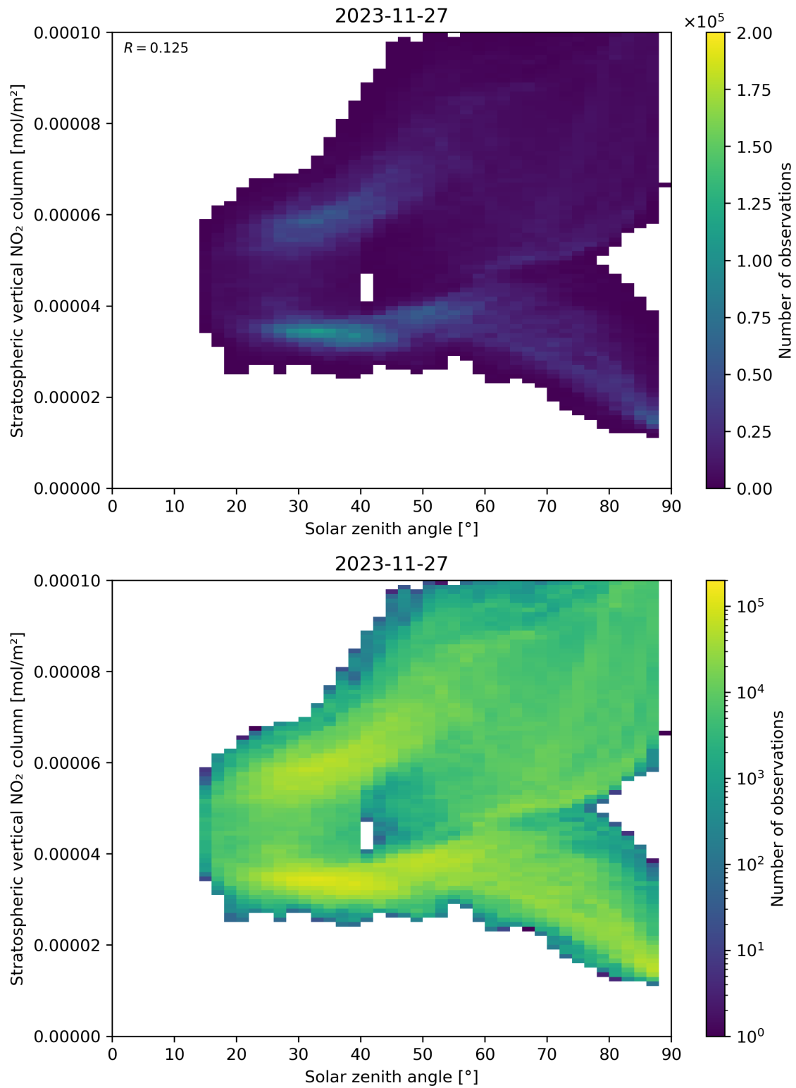
Figure 150: Scatter density plot of “Solar zenith angle” against “Stratospheric vertical NO 2 column” for 2023-11-26 to 2023-11-28.
