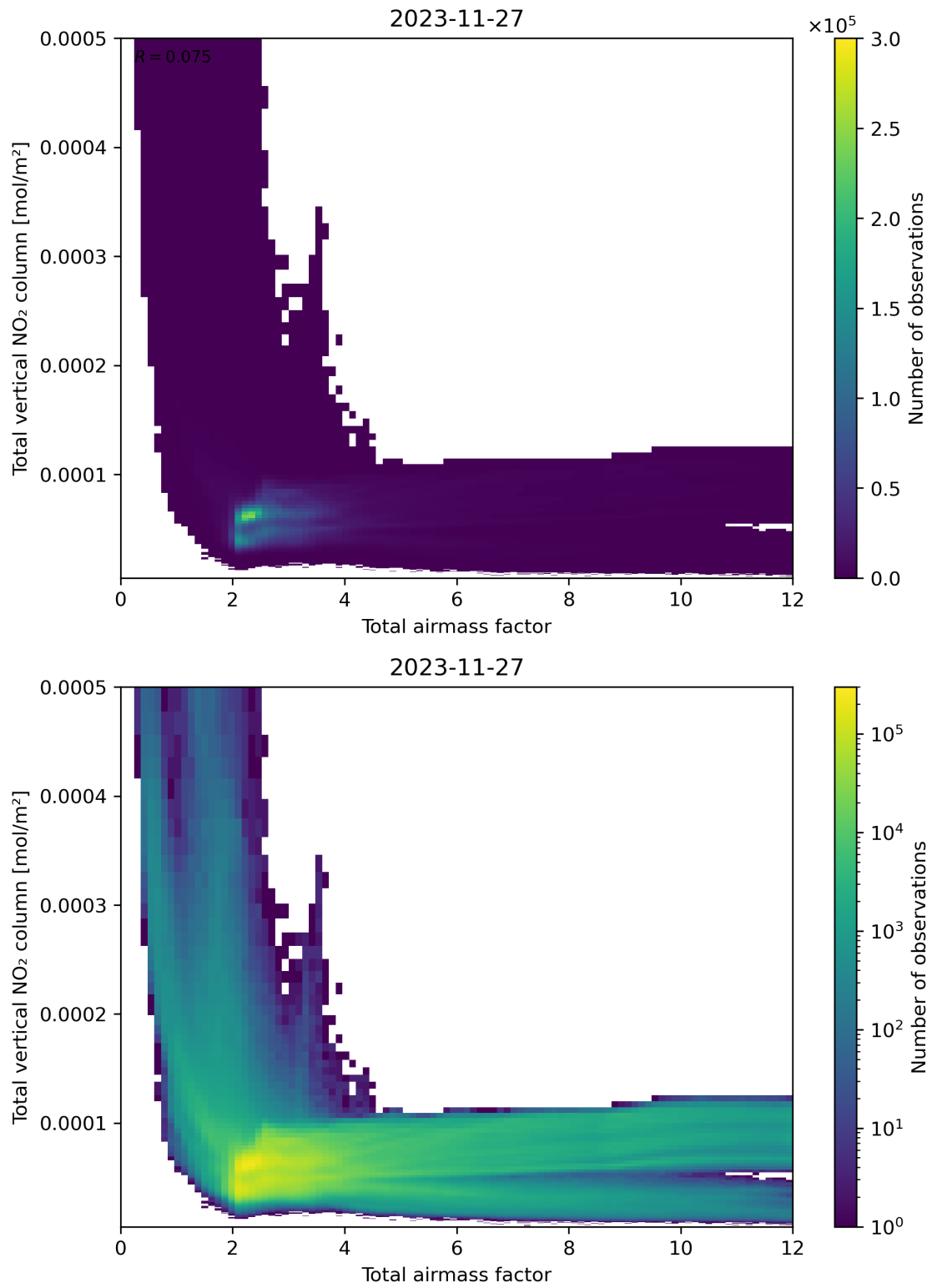
Figure 67: Scatter density plot of “Total airmass factor” against “Total vertical NO 2 column” for 2023-11-26 to 2023-11-28.
