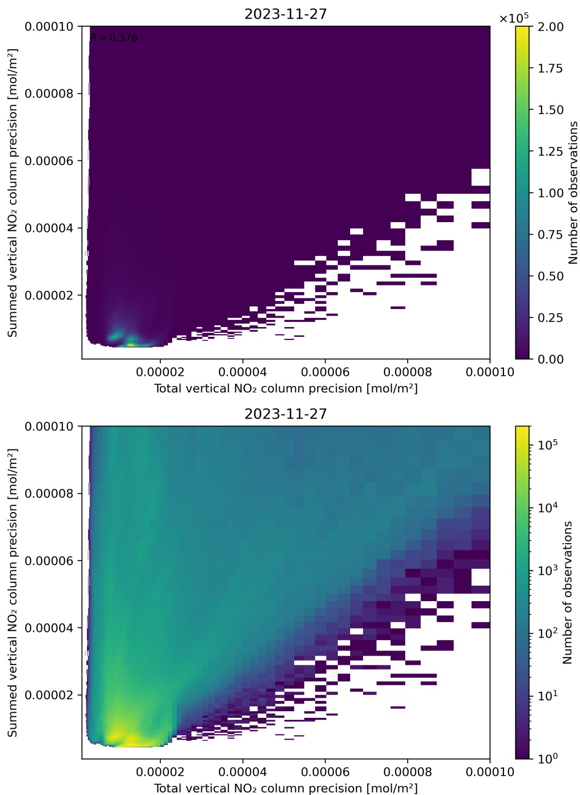
Figure 118: Scatter density plot of “Total vertical NO 2 column precision” against “Summed vertical NO 2 column precision” for 2023-11-26 to 2023-11-28.
