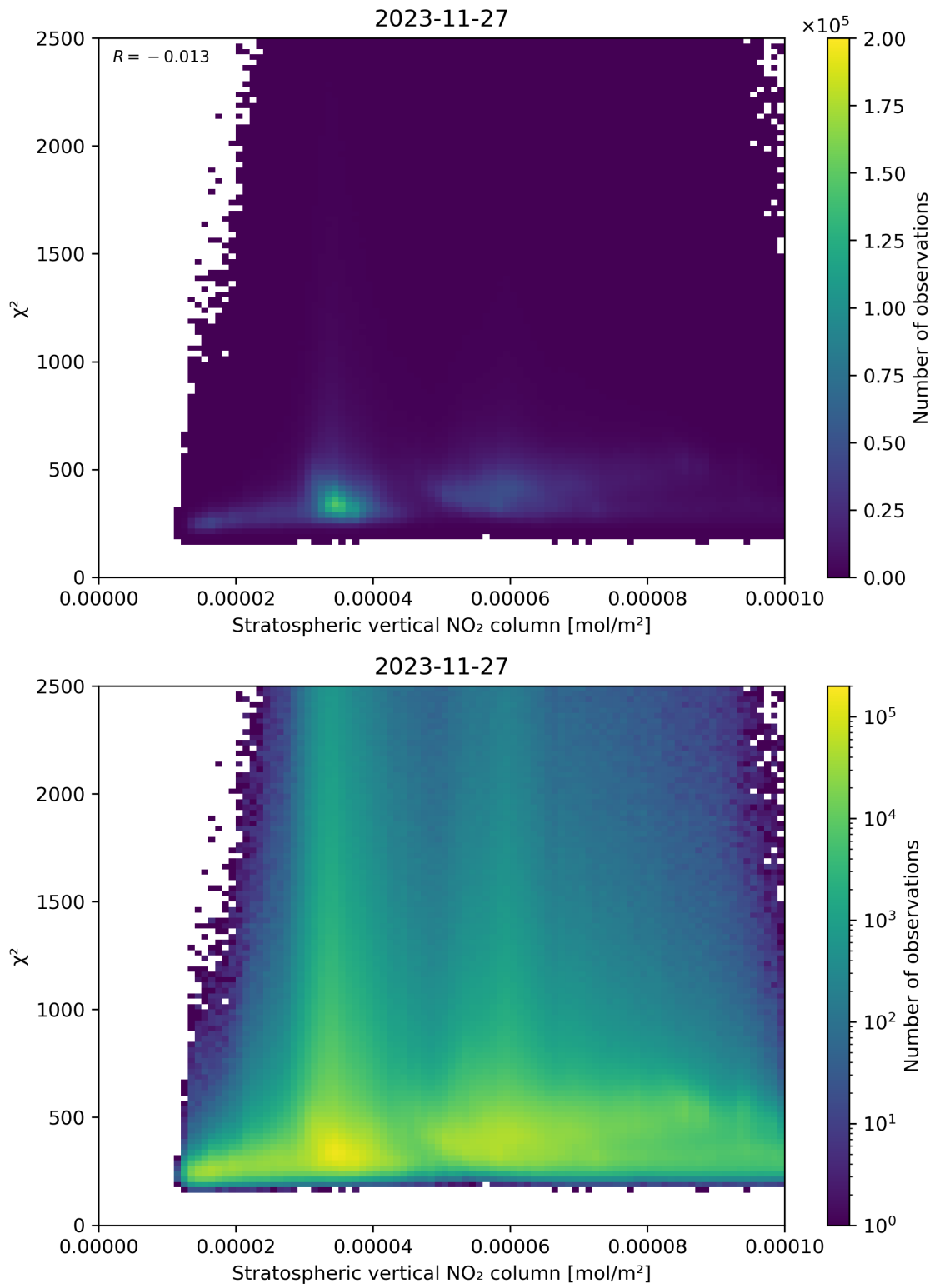
Figure 97: Scatter density plot of “Stratospheric vertical NO 2 column” against “ \chi^2 ” for 2023-11-26 to 2023-11-28.
