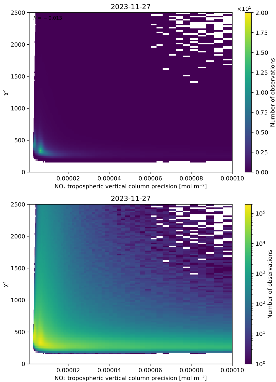
Figure 134: Scatter density plot of “NO 2 tropospheric vertical column precision” against “ \chi^2 ” for 2023-11-26 to 2023-11-28.
