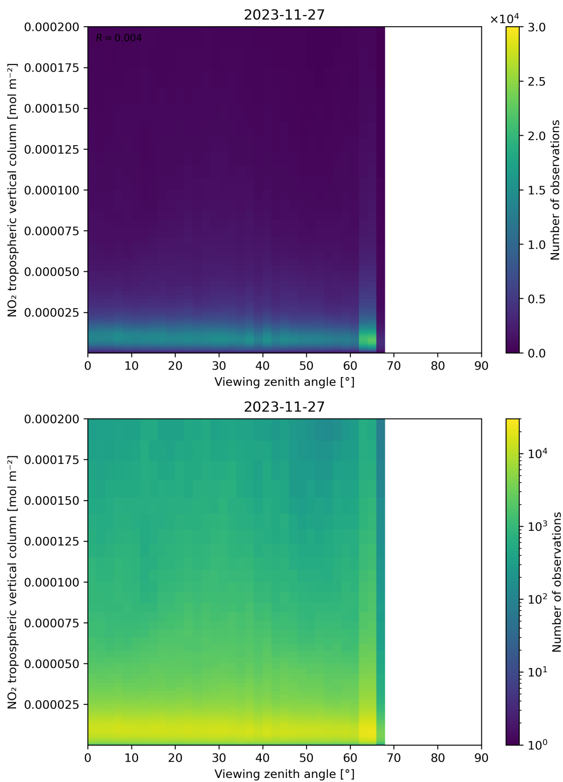
Figure 169: Scatter density plot of “Viewing zenith angle” against “NO 2 tropospheric vertical column” for 2023-11-26 to 2023-11-28.
