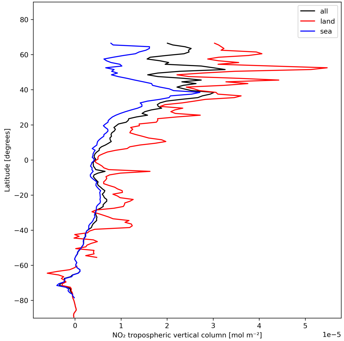
Figure 12: Zonal average of “NO 2 tropospheric vertical column” for 2023-11-26 to 2023-11-28.
