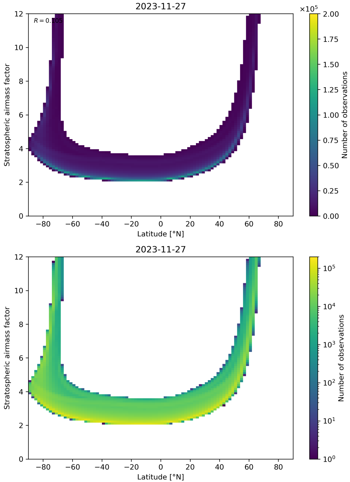
Figure 83: Scatter density plot of “Latitude” against “Stratospheric air mass factor” for 2023-11-26 to 2023-11-28.
