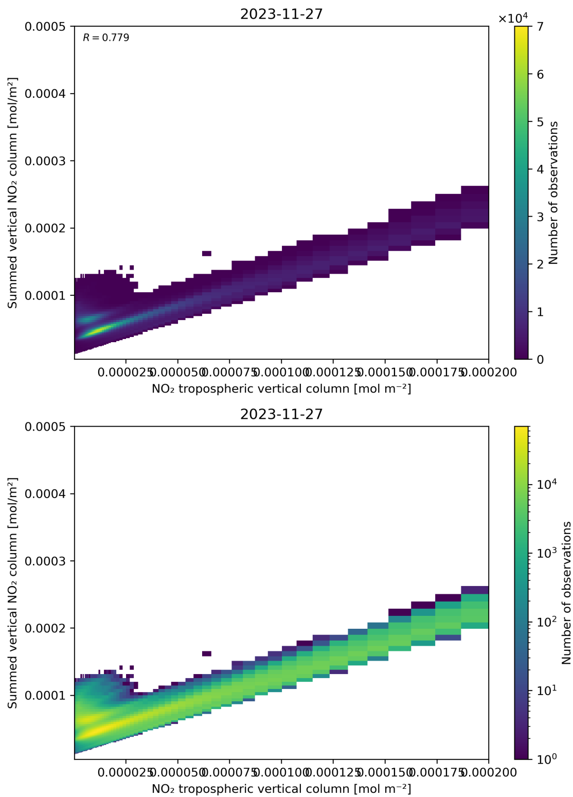
Figure 126: Scatter density plot of “NO 2 tropospheric vertical column” against “Summed vertical NO 2 column” for 2023-11-26 to 2023-11-28.
