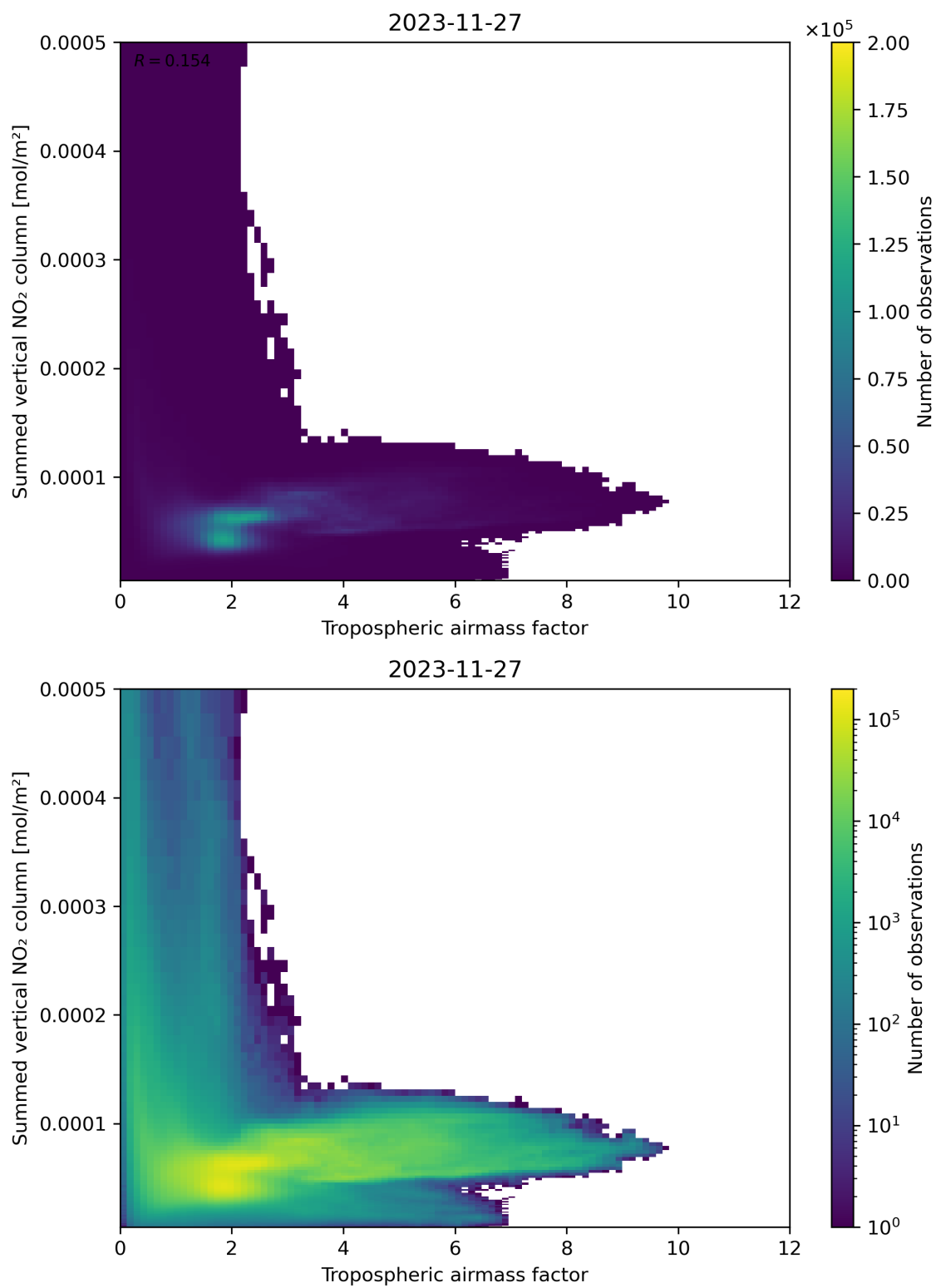
Figure 75: Scatter density plot of “Tropospheric airmass factor” against “Summed vertical NO 2 column” for 2023-11-26 to 2023-11-28.
