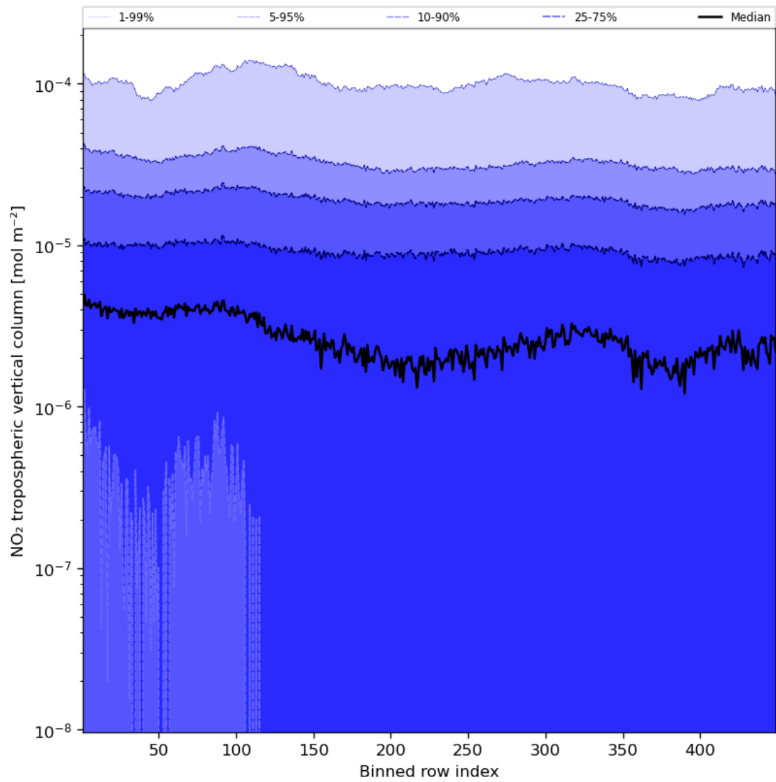
Figure 46: Along track statistics of “NO 2 tropospheric vertical column” for 2023-11-26 to 2023-11-28
