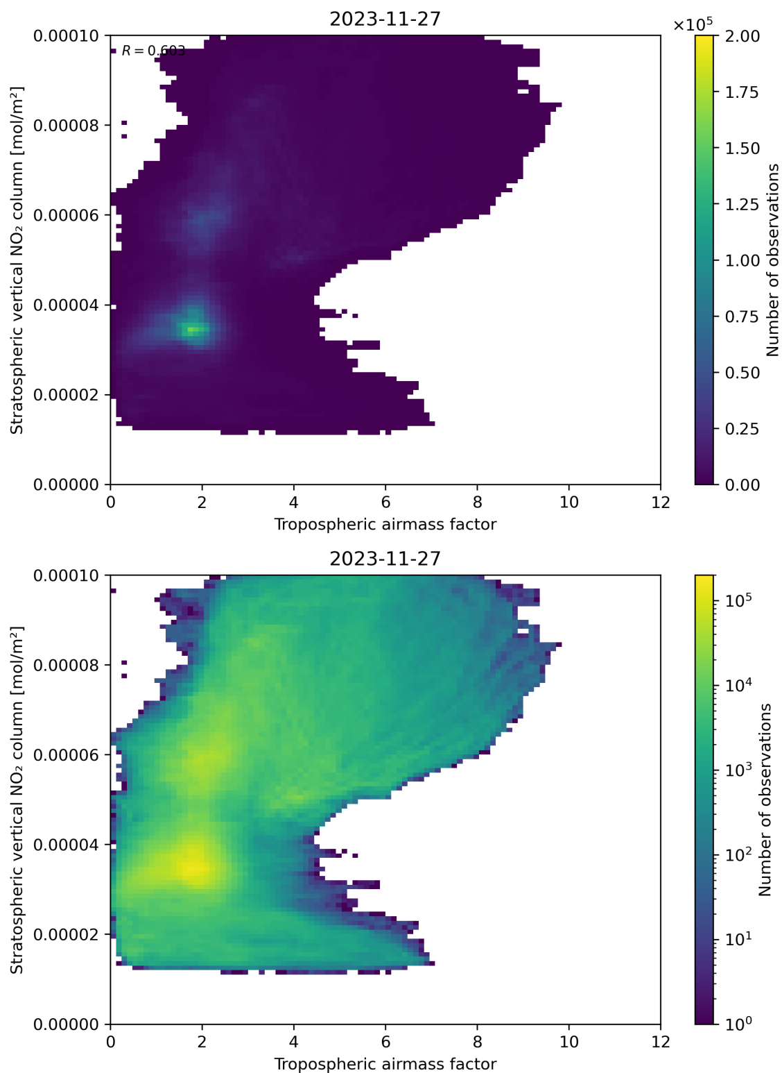
Figure 74: Scatter density plot of “Tropospheric air mass factor” against “Stratospheric vertical NO 2 column” for 2023-11-26 to 2023-11-28.
