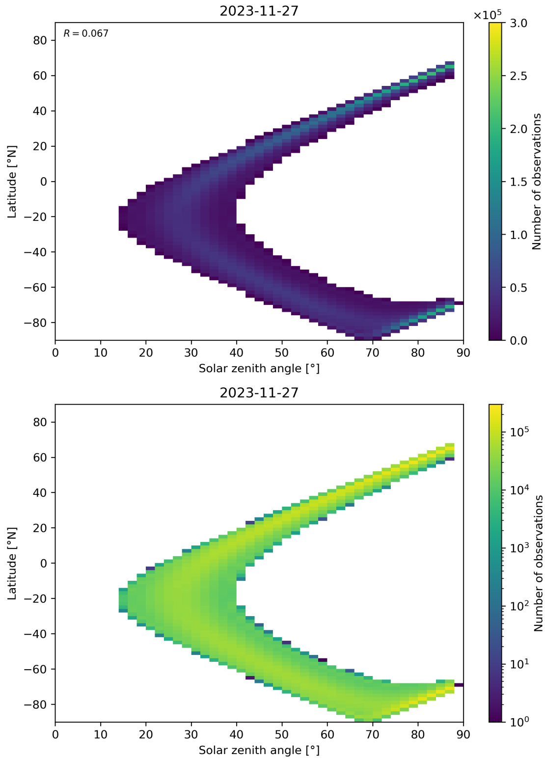
Figure 149: Scatter density plot of “Solar zenith angle” against “Latitude” for 2023-11-26 to 2023-11-28.
