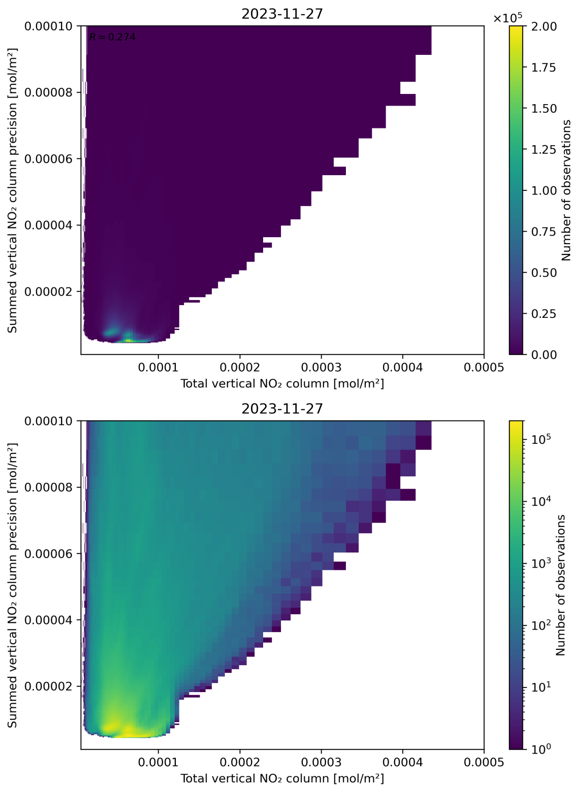
Figure 113: Scatter density plot of “Total vertical NO 2 column” against “Summed vertical NO 2 column precision” for 2023-11-26 to 2023-11-28.
