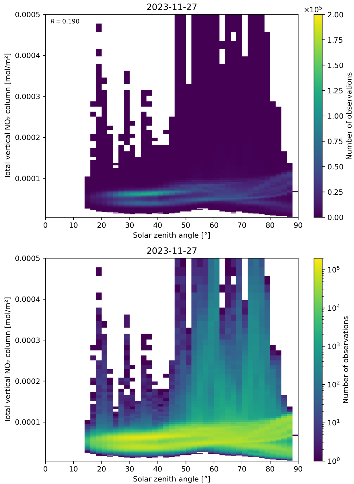
Figure 153: Scatter density plot of “Solar zenith angle” against “Total vertical NO 2 column” for 2023-11-26 to 2023-11-28.
