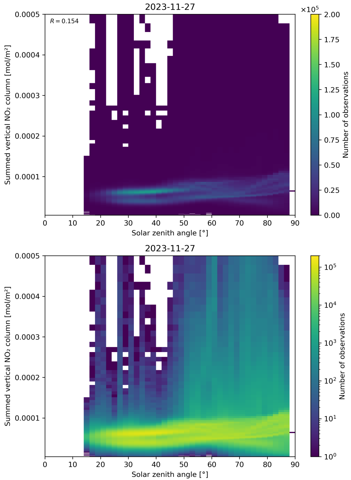
Figure 151: Scatter density plot of “Solar zenith angle” against “Summed vertical NO 2 column” for 2023-11-26 to 2023-11-28.
