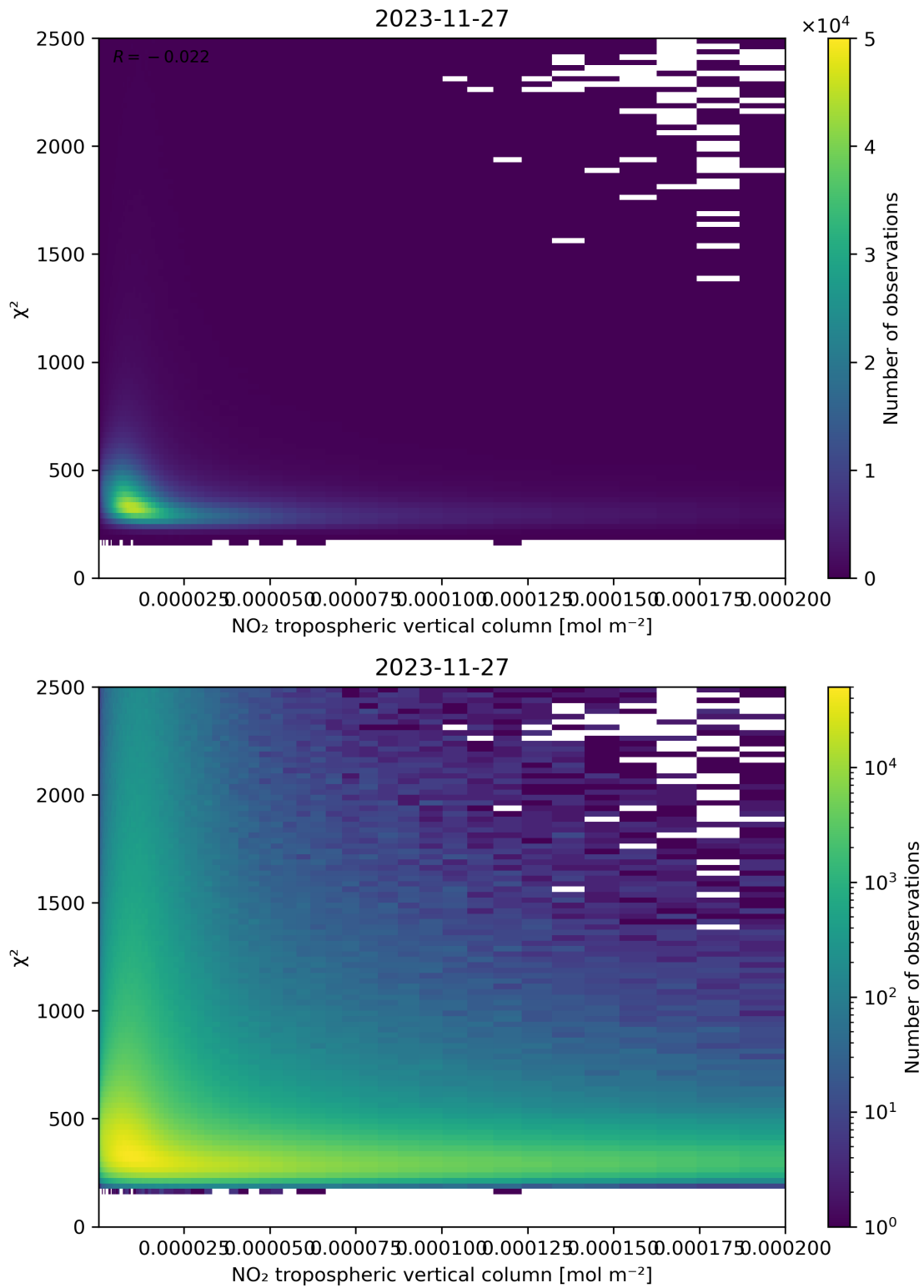
Figure 124: Scatter density plot of “NO 2 tropospheric vertical column” against “ \chi^2 ” for 2023-11-26 to 2023-11-28.
