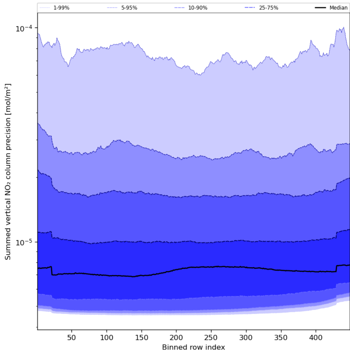
Figure 58: Along track statistics of “Summed vertical NO 2 column precision” for 2023-11-26 to 2023-11-28
