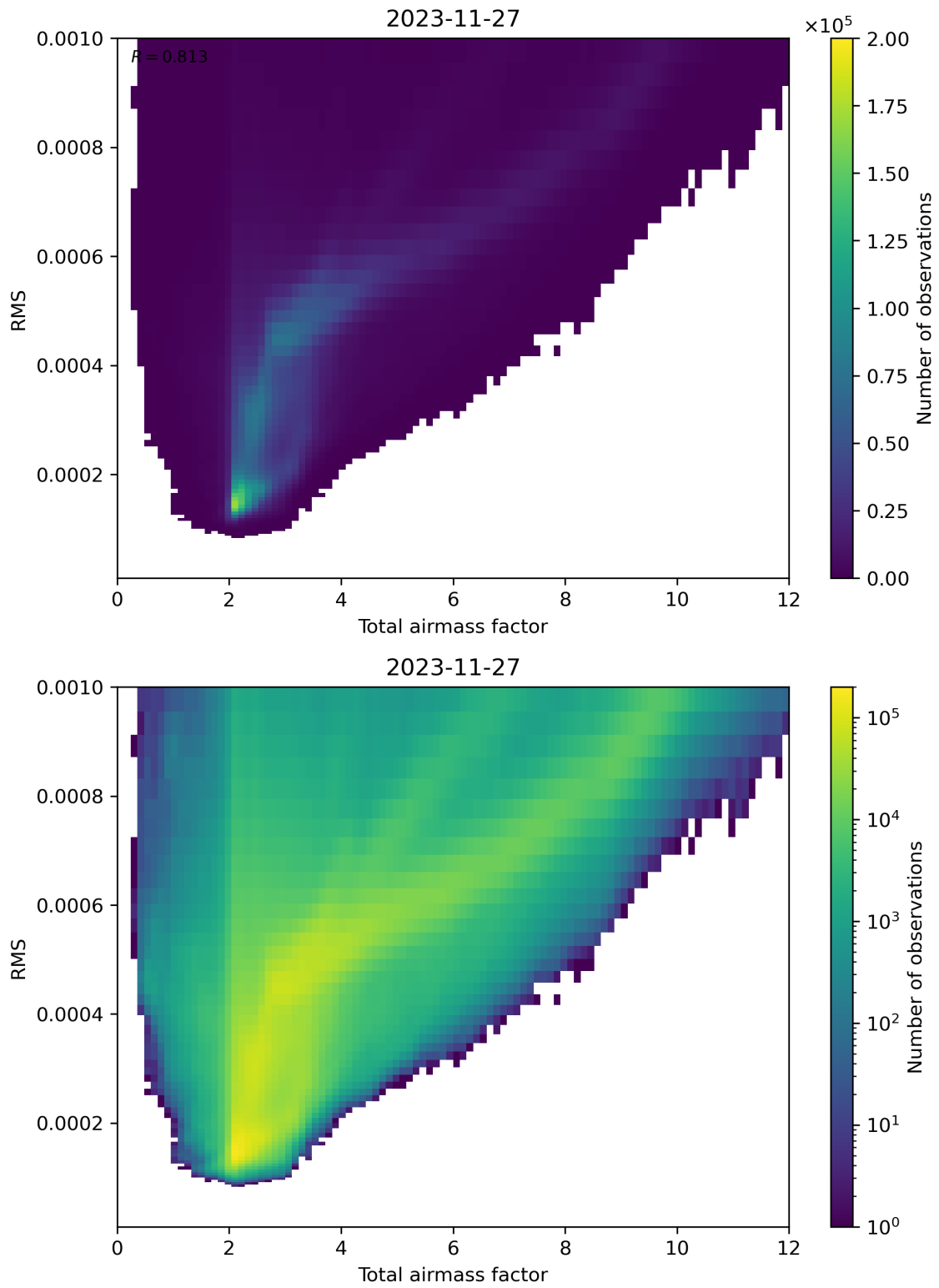
Figure 69: Scatter density plot of “Total airmass factor” against “RMS” for 2023-11-26 to 2023-11-28.
