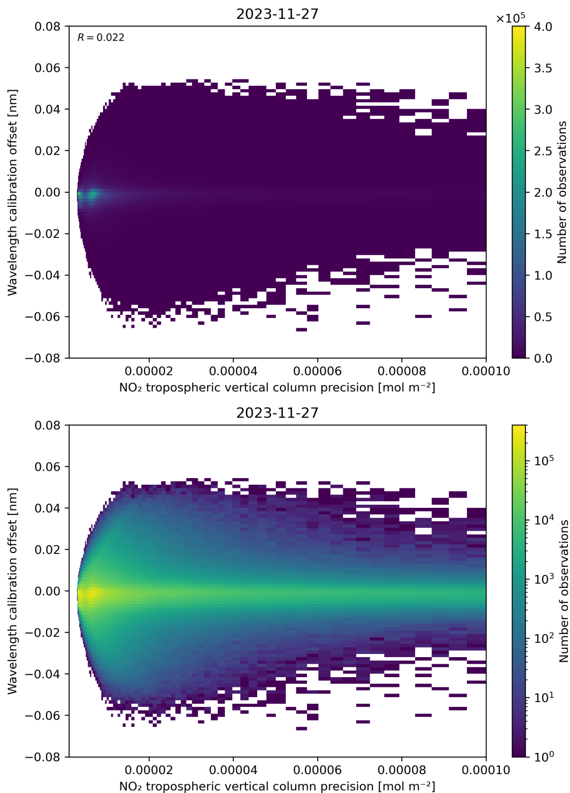
Figure 141: Scatter density plot of “NO 2 tropospheric vertical column precision” against “Wavelength calibration offset” for 2023-11-26 to 2023-11-28.
