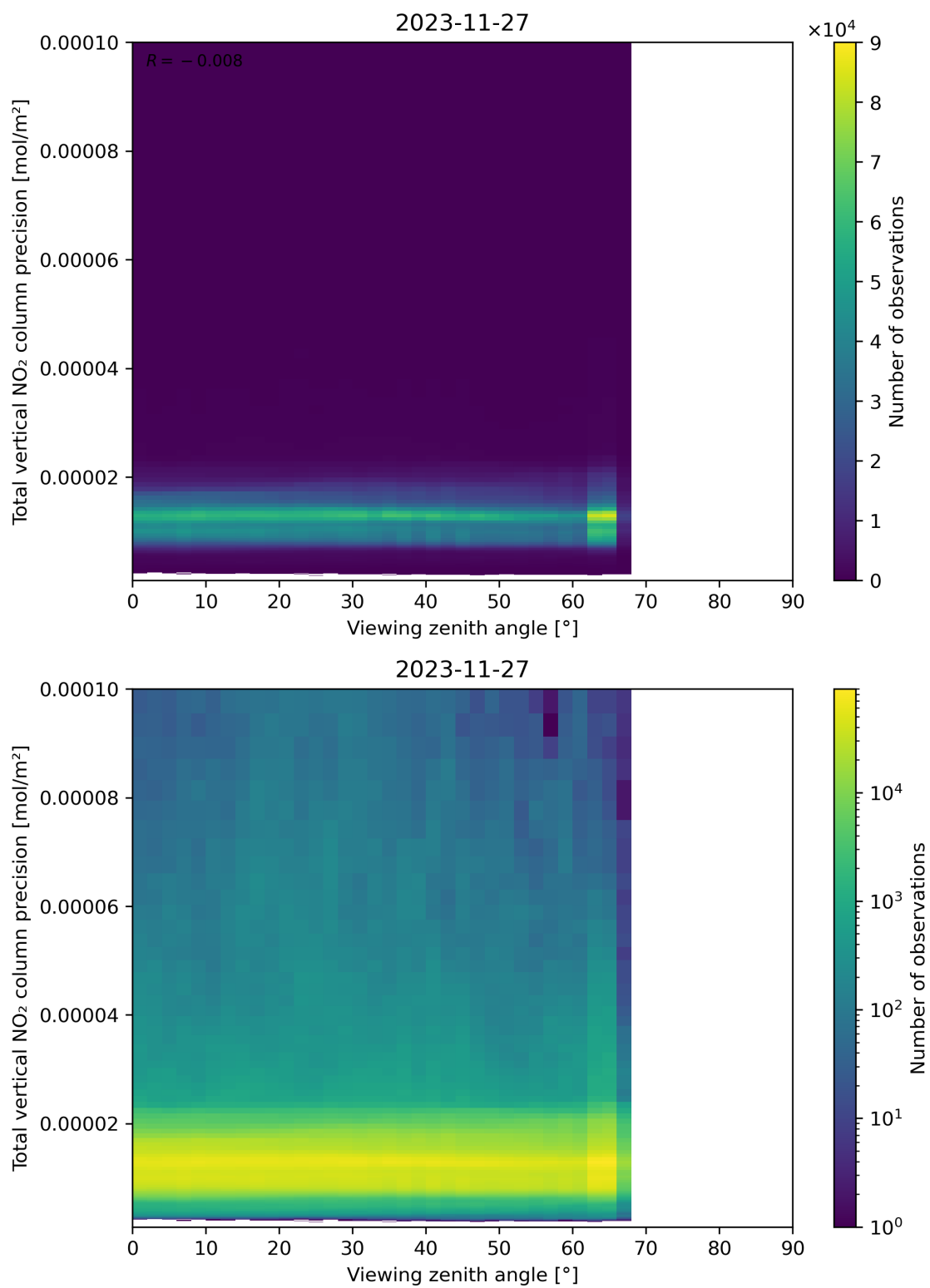
Figure 168: Scatter density plot of “Viewing zenith angle” against “Total vertical NO 2 column precision” for 2023-11-26 to 2023-11-28.
