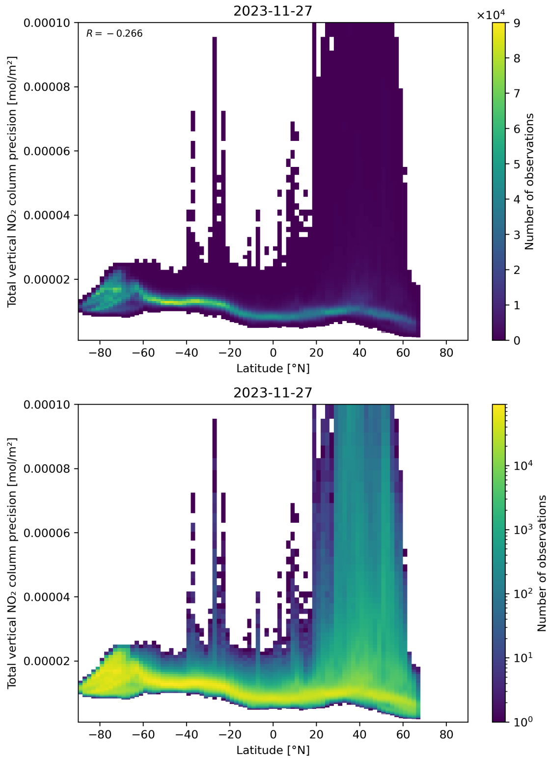
Figure 91: Scatter density plot of “Latitude” against “Total vertical NO 2 column precision” for 2023-11-26 to 2023-11-28.
