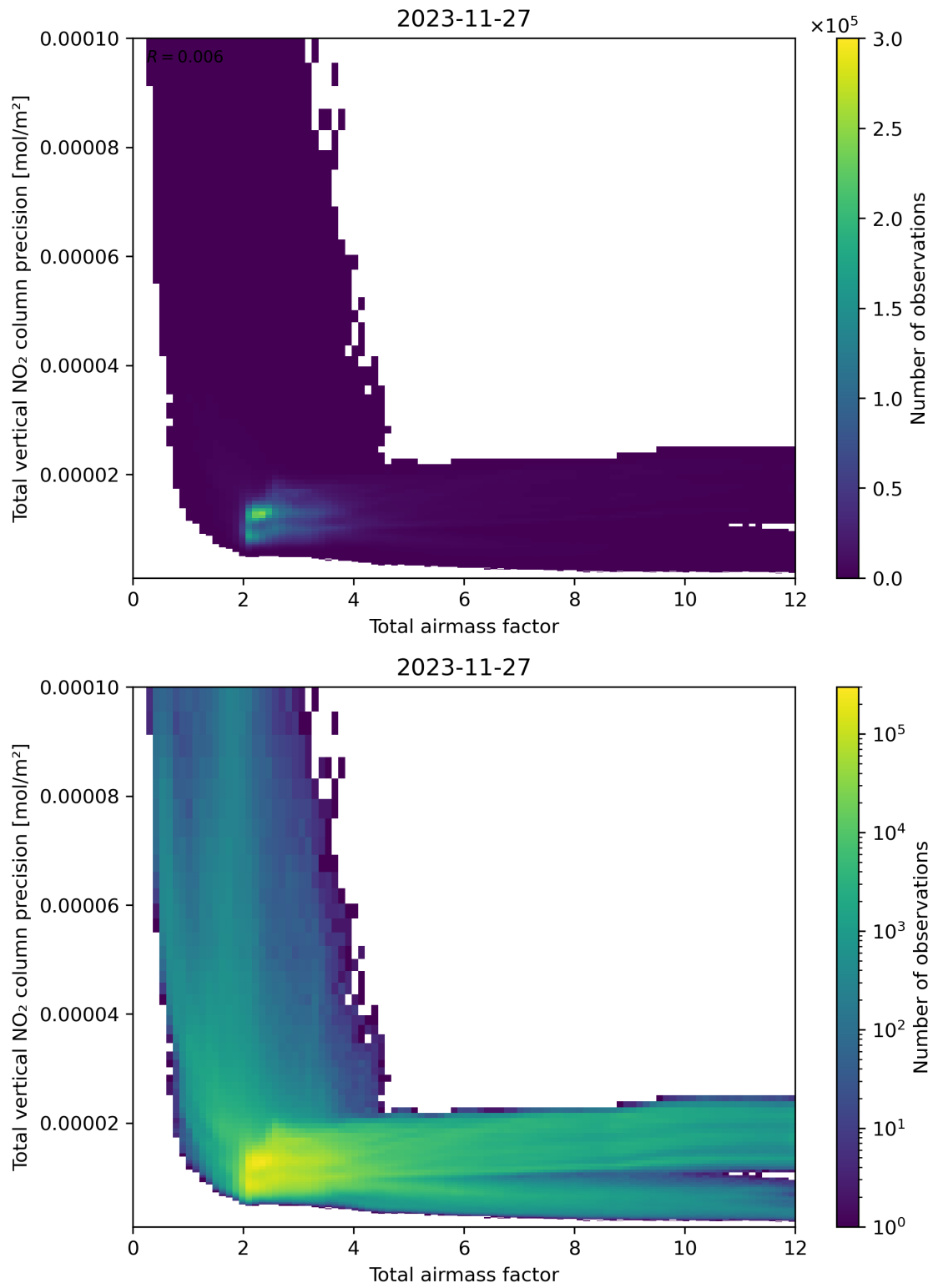
Figure 68: Scatter density plot of “Total airmass factor” against “Total vertical NO 2 column precision” for 2023-11-26 to 2023-11-28.
