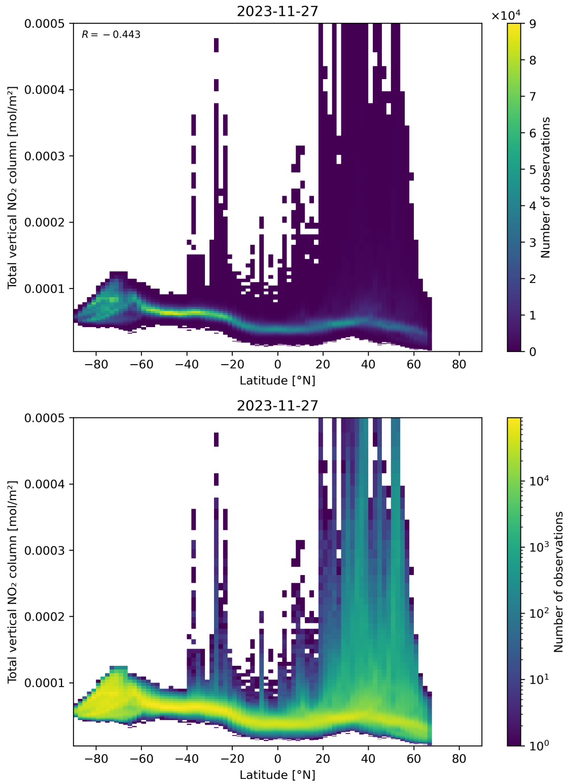
Figure 90: Scatter density plot of “Latitude” against “Total vertical NO 2 column” for 2023-11-26 to 2023-11-28.
