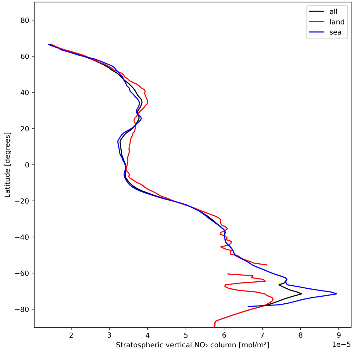
Figure 19: Zonal average of “Stratospheric vertical NO 2 column” for 2023-11-26 to 2023-11-28.
