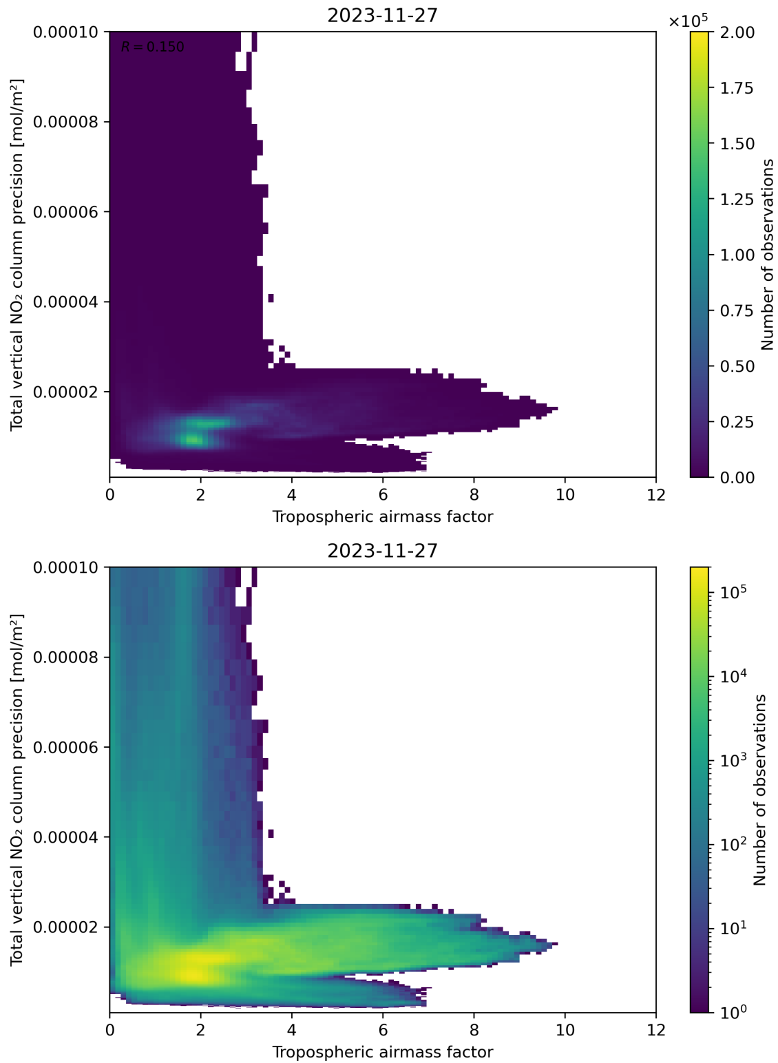
Figure 78: Scatter density plot of “Tropospheric air mass factor” against “Total vertical NO 2 column precision” for 2023-11-26 to 2023-11-28.
