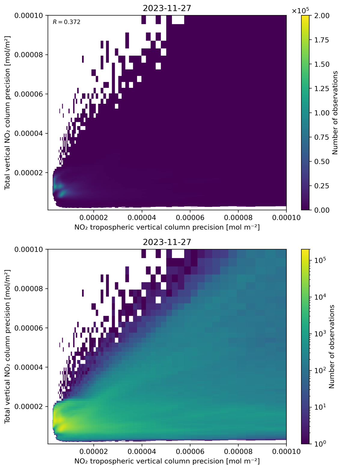
Figure 139: Scatter density plot of “NO 2 tropospheric vertical column precision” against “Total vertical NO 2 column precision” for 2023-11-26 to 2023-11-28.
