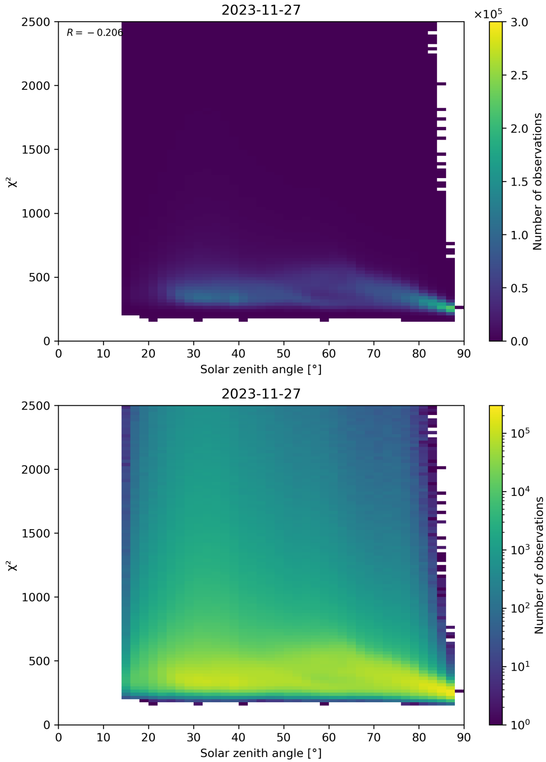
Figure 148: Scatter density plot of “Solar zenith angle” against “ \chi^2 ” for 2023-11-26 to 2023-11-28.
