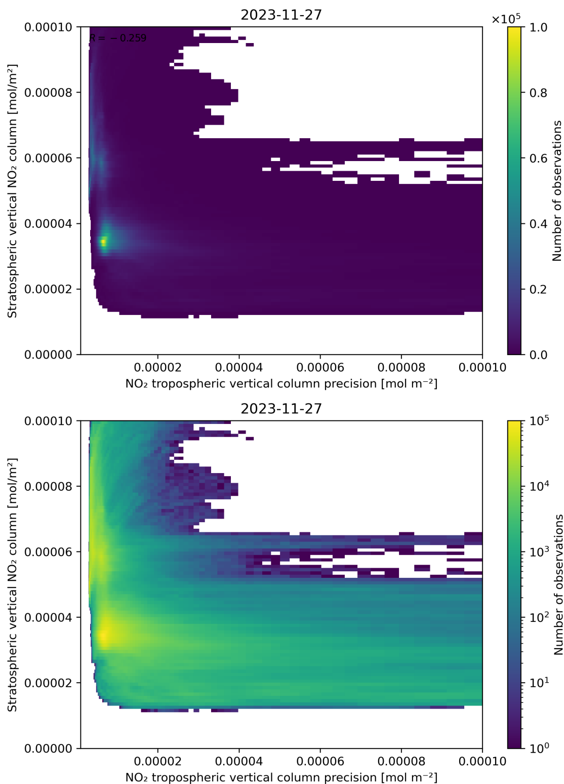
Figure 135: Scatter density plot of “NO 2 tropospheric vertical column precision” against “Stratospheric vertical NO 2 column” for 2023-11-26 to 2023-11-28.
