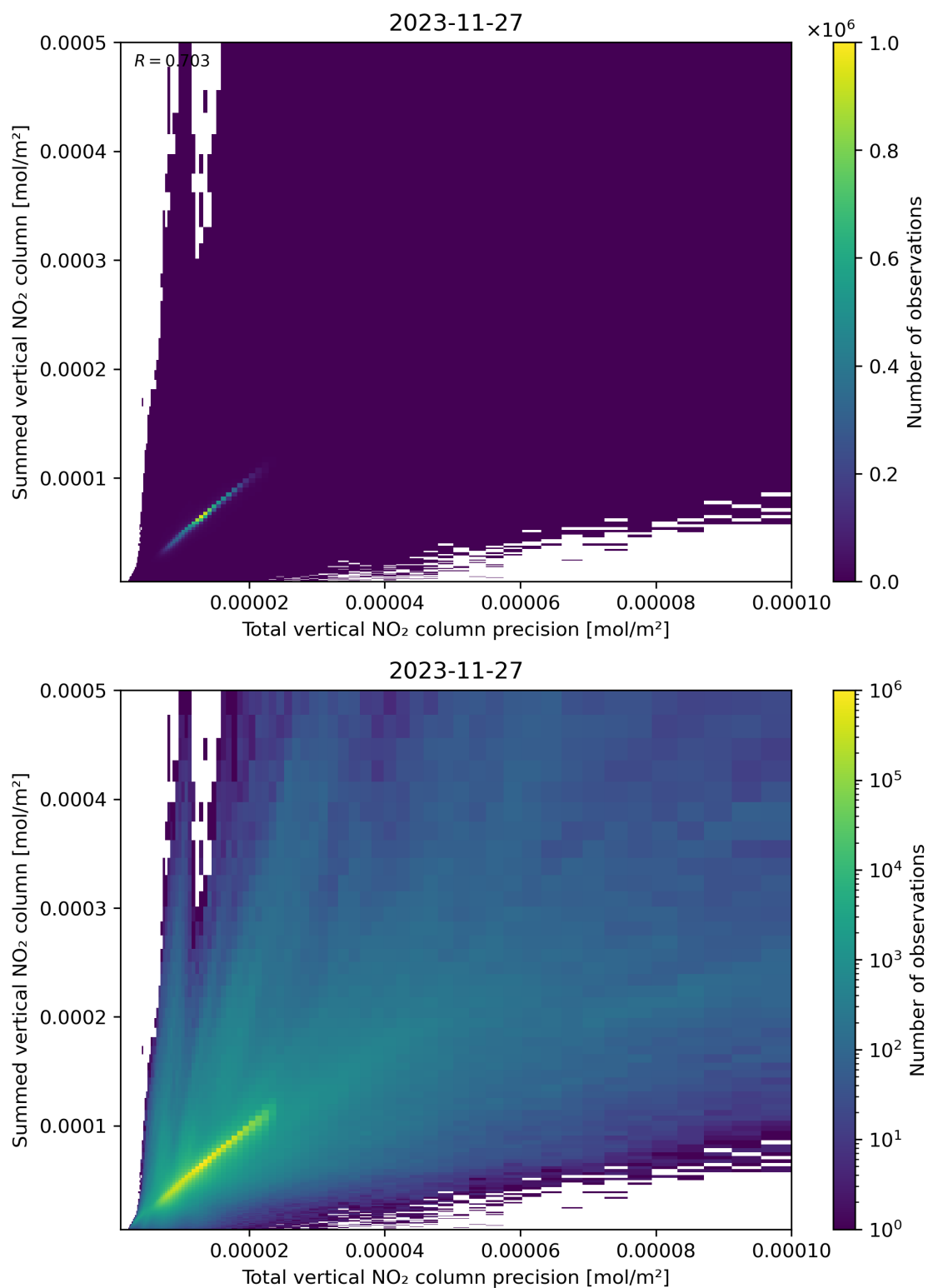
Figure 117: Scatter density plot of “Total vertical NO 2 column precision” against “Summed vertical NO 2 column” for 2023-11-26 to 2023-11-28.
