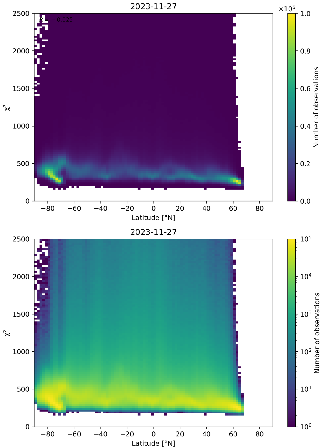
Figure 86: Scatter density plot of “Latitude” against “ \chi^2 ” for 2023-11-26 to 2023-11-28.
