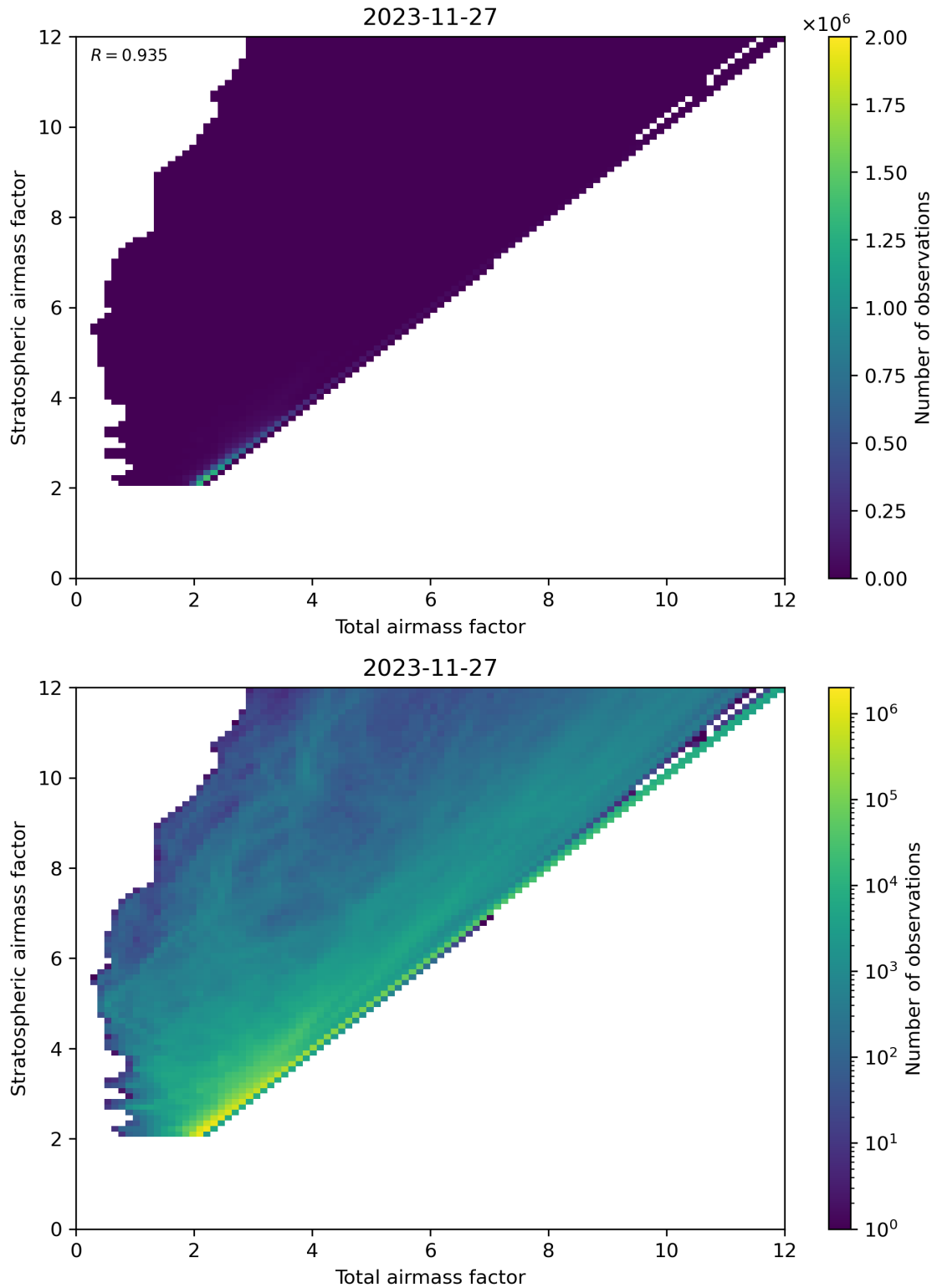
Figure 62: Scatter density plot of “Total airmass factor” against “Stratospheric airmass factor” for 2023-11-26 to 2023-11-28.
