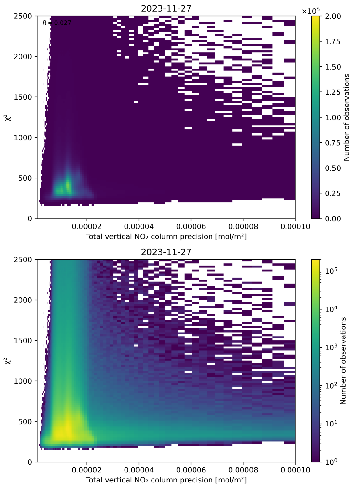
Figure 116: Scatter density plot of “Total vertical NO 2 column precision” against “ \chi^2 ” for 2023-11-26 to 2023-11-28.
