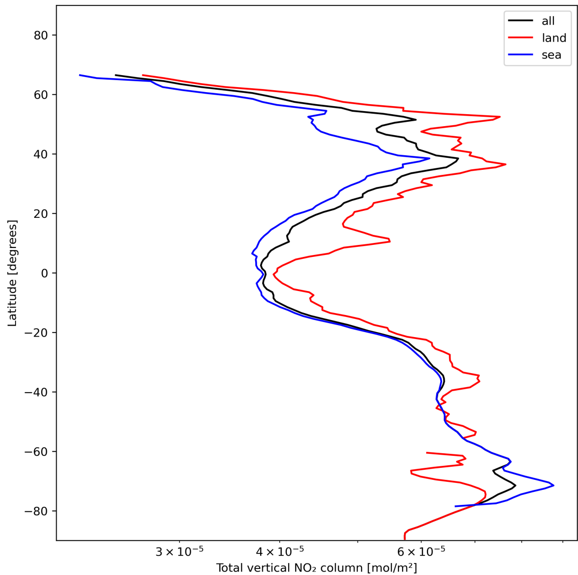
Figure 21: Zonal average of “Total vertical NO 2 column” for 2023-11-26 to 2023-11-28.
