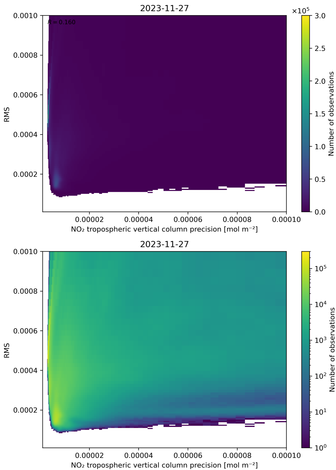
Figure 140: Scatter density plot of “NO 2 tropospheric vertical column precision” against “RMS” for 2023-11-26 to 2023-11-28.
