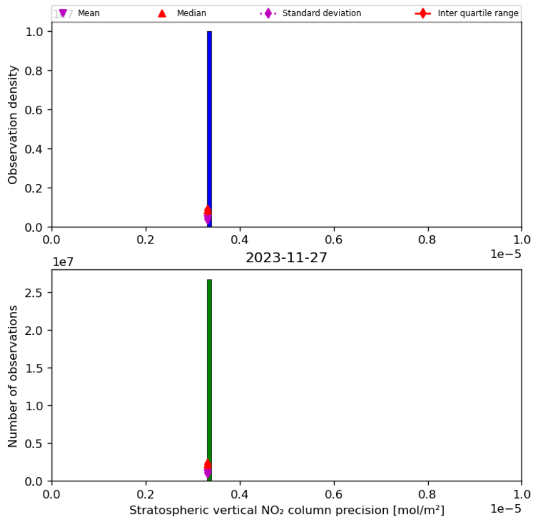
Figure 37: Histogram of “Stratospheric vertical NO 2 column precision” for 2023-11-26 to 2023-11-28
