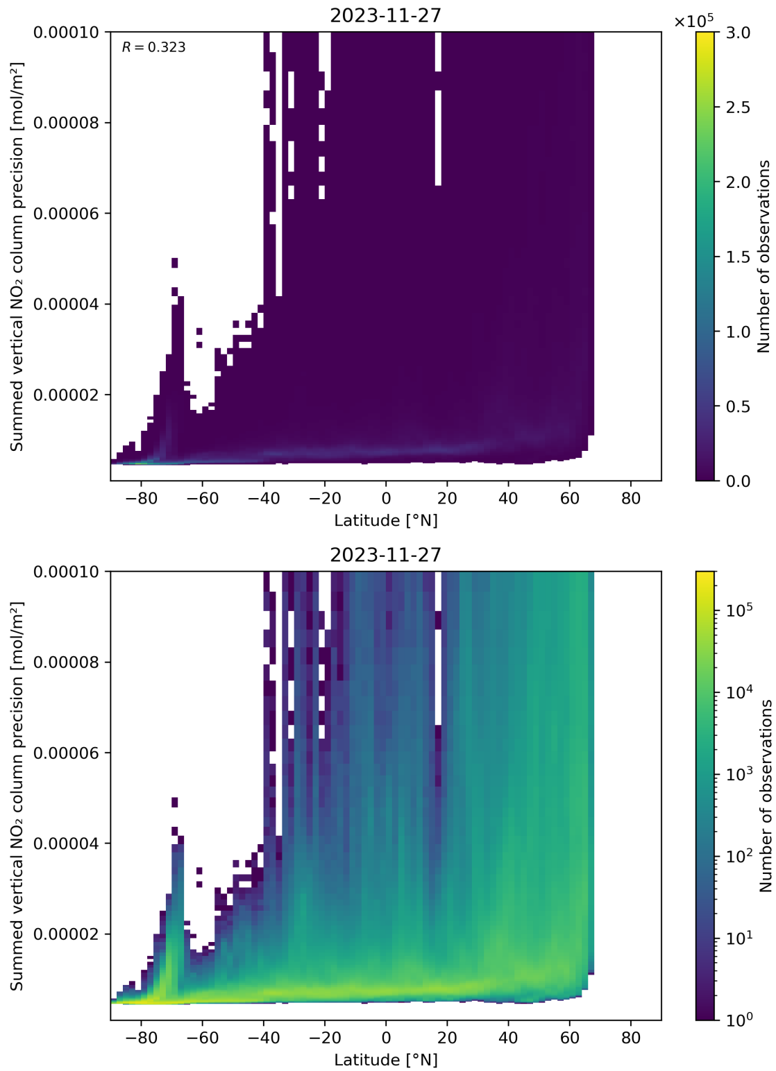
Figure 89: Scatter density plot of “Latitude” against “Summed vertical NO 2 column precision” for 2023-11-26 to 2023-11-28.
