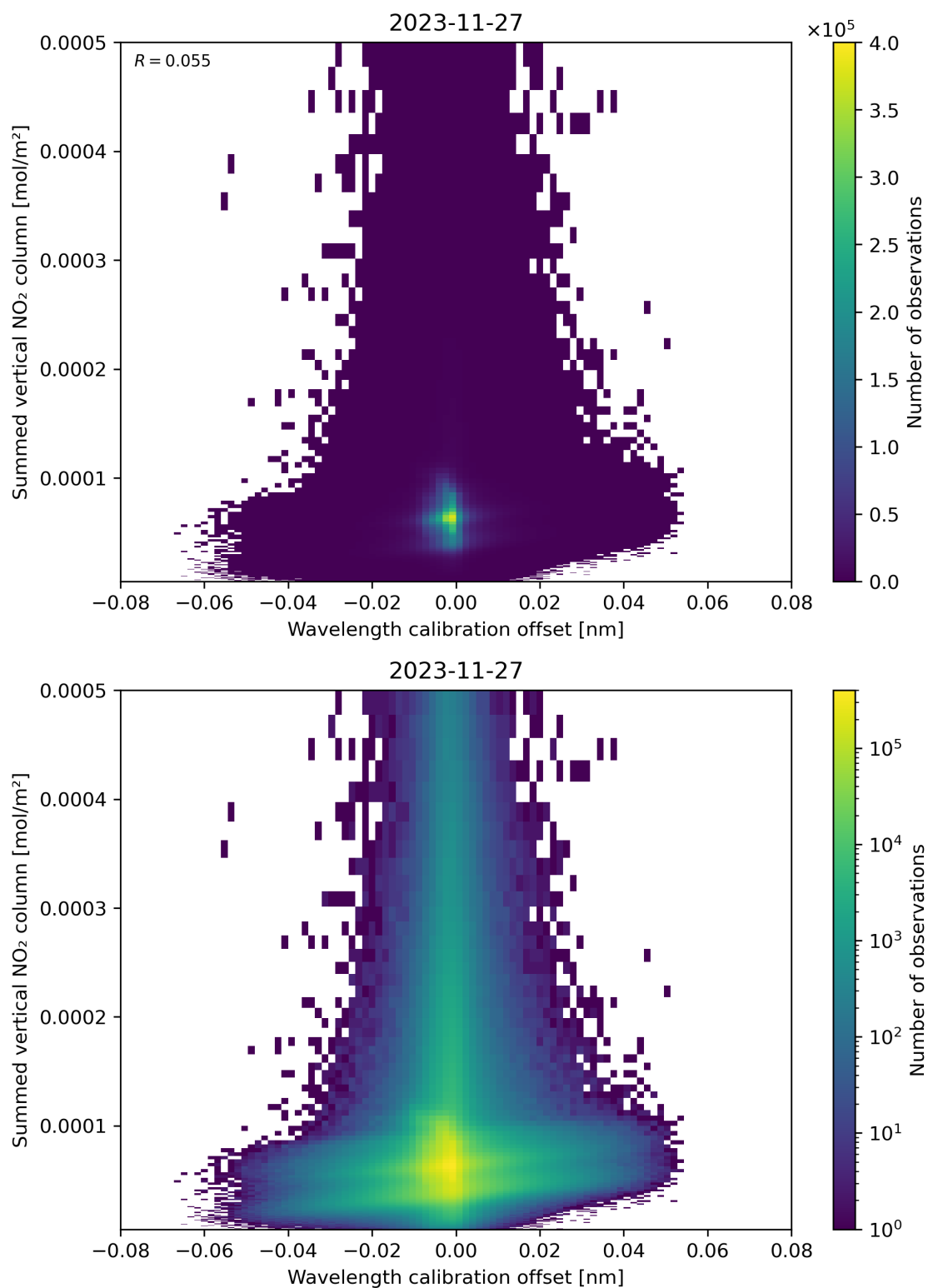
Figure 177: Scatter density plot of “Wavelength calibration offset” against “Summed vertical NO 2 column” for 2023-11-26 to 2023-11-28.
