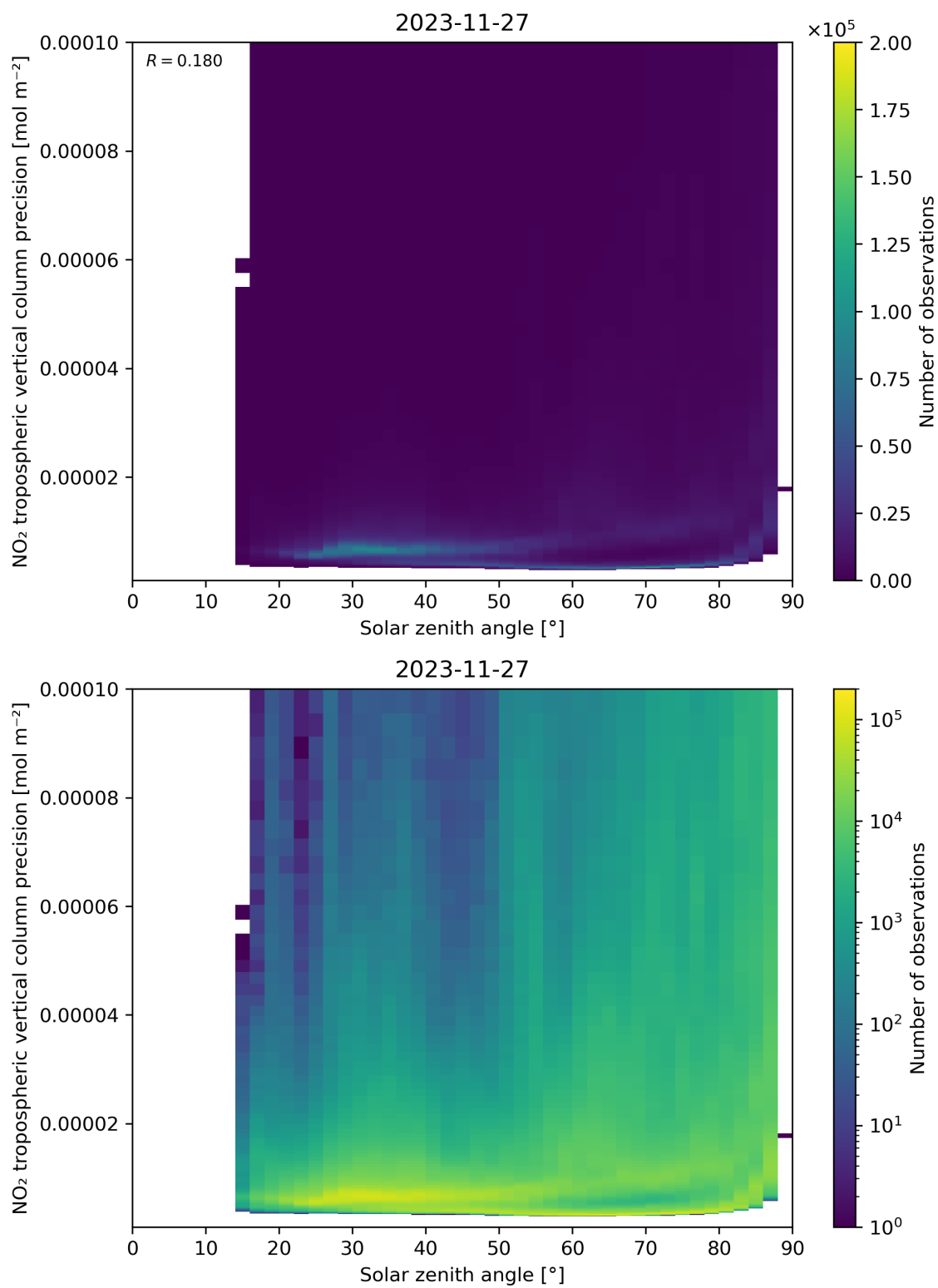
Figure 156: Scatter density plot of “Solar zenith angle” against “NO 2 tropospheric vertical column precision” for 2023-11-26 to 2023-11-28.
