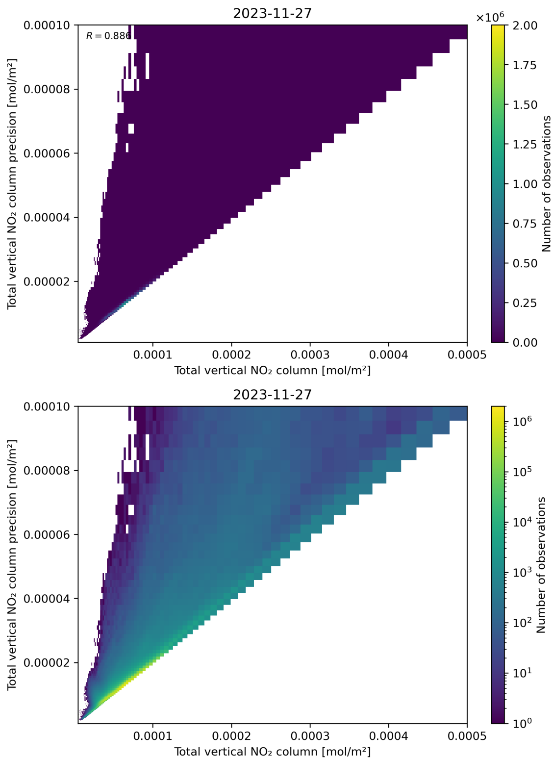
Figure 114: Scatter density plot of “Total vertical NO 2 column” against “Total vertical NO 2 column precision” for 2023-11-26 to 2023-11-28.
