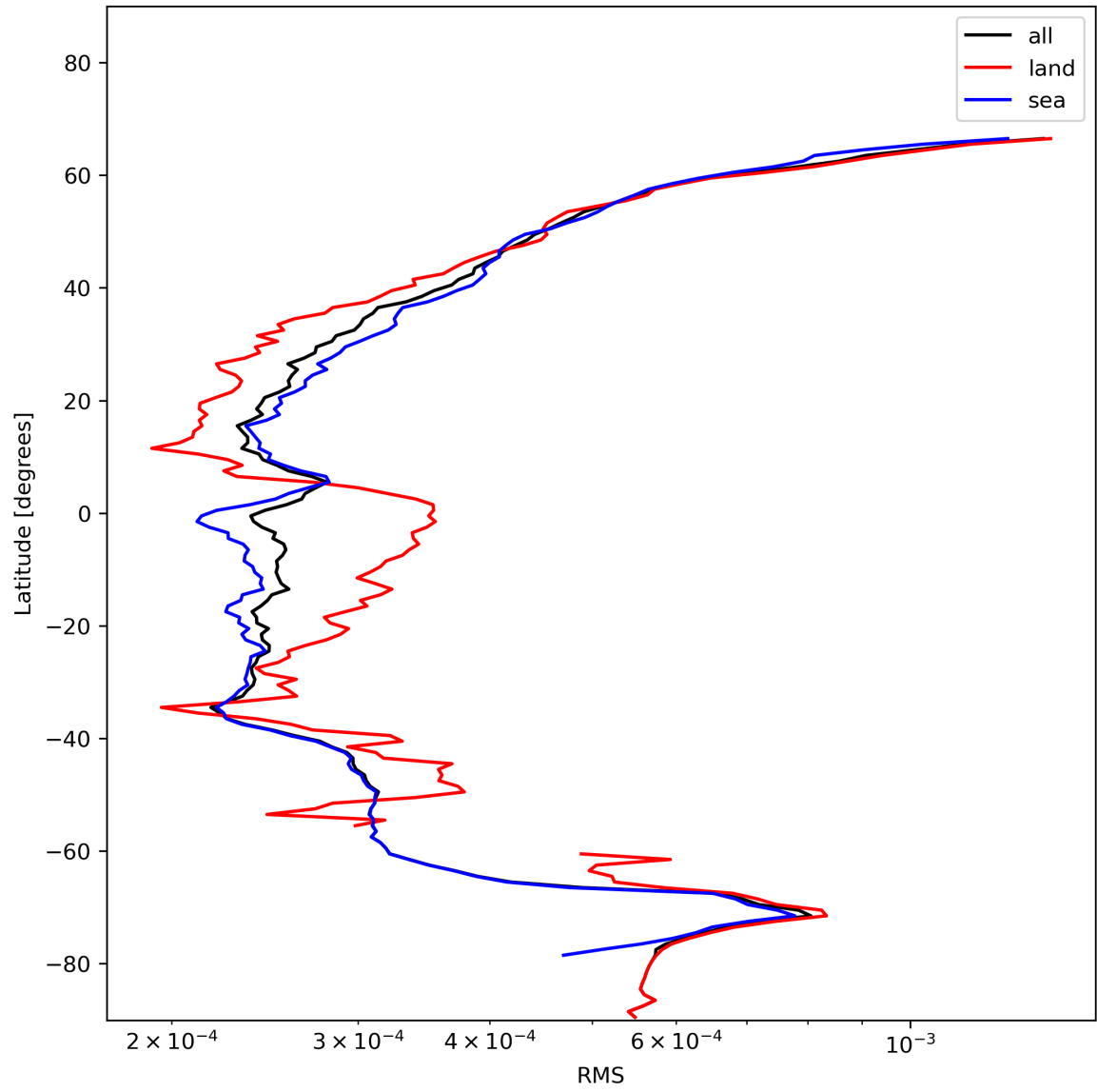
Figure 26: Zonal average of “RMS” for 2023-11-26 to 2023-11-28.
