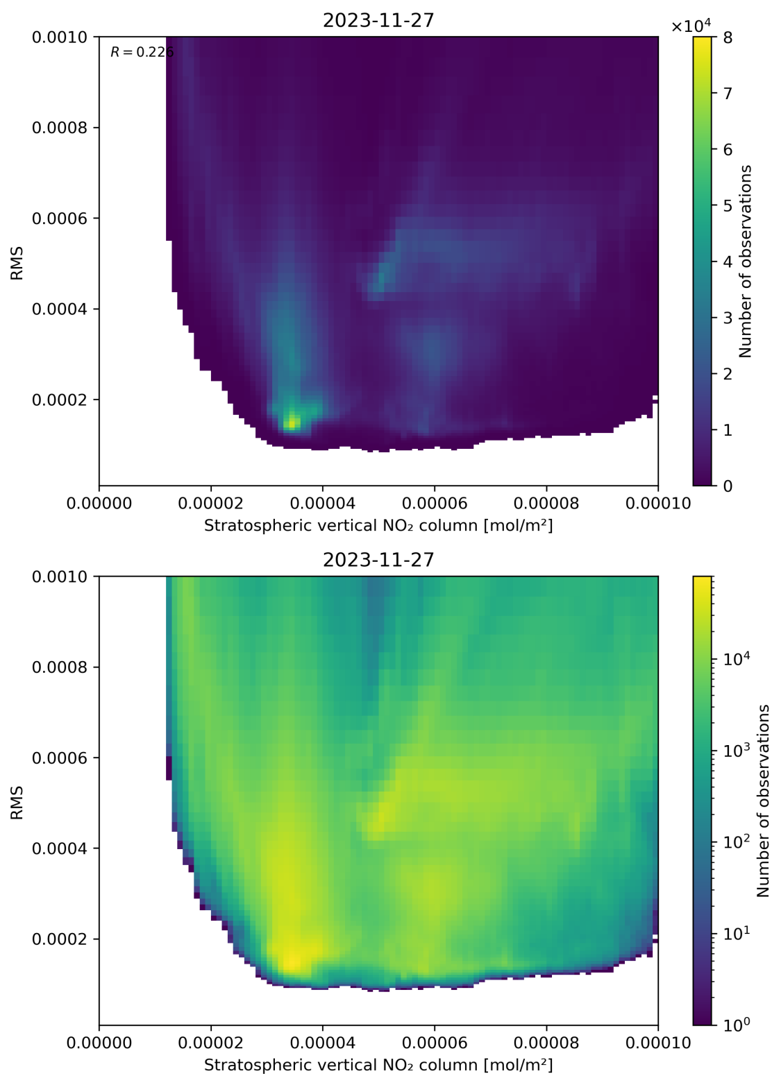
Figure 102: Scatter density plot of “Stratospheric vertical NO 2 column” against “RMS” for 2023-11-26 to 2023-11-28.
