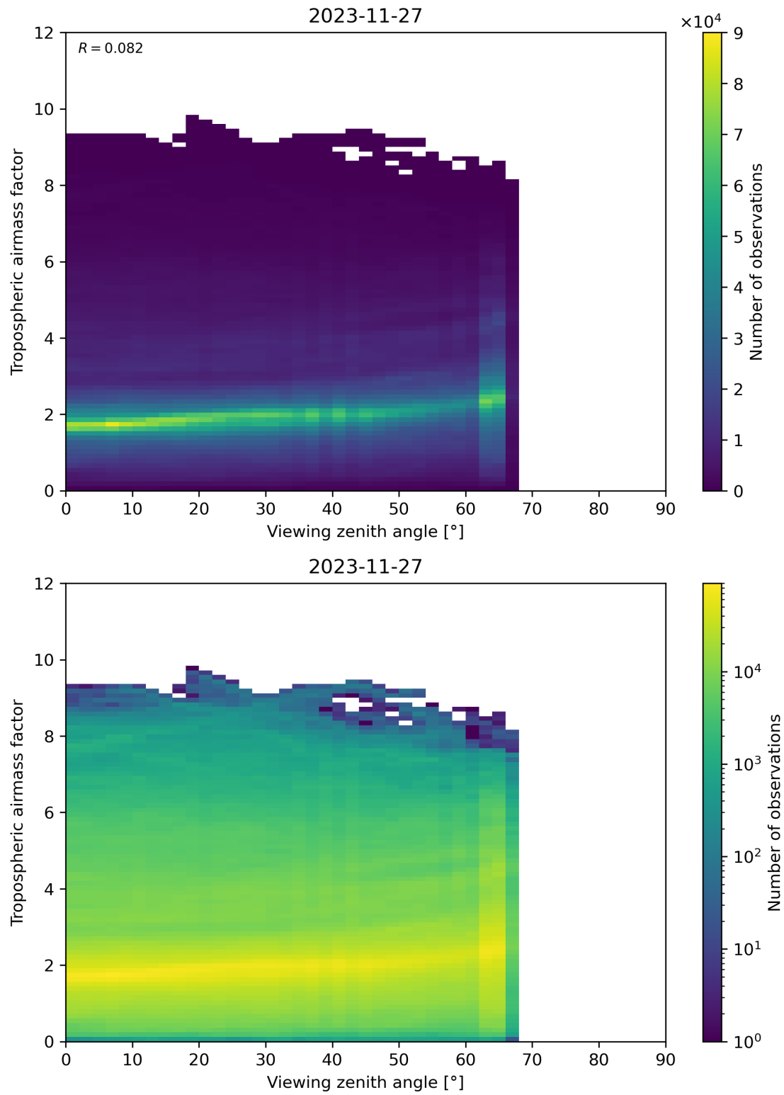
Figure 161: Scatter density plot of “Viewing zenith angle” against “Tropospheric airmass factor” for 2023-11-26 to 2023-11-28.
