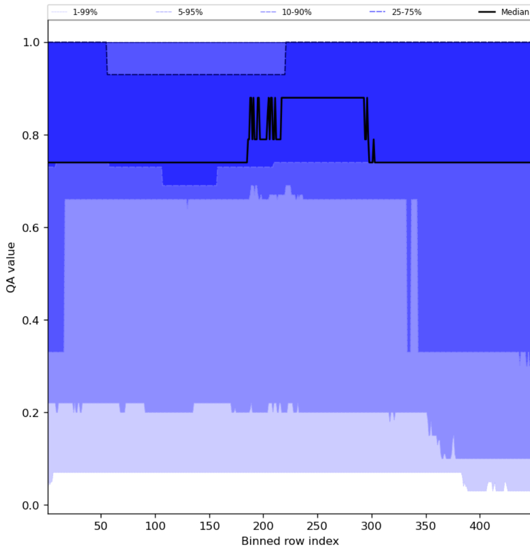
Figure 45: Along track statistics of “QA value” for 2023-11-26 to 2023-11-28
