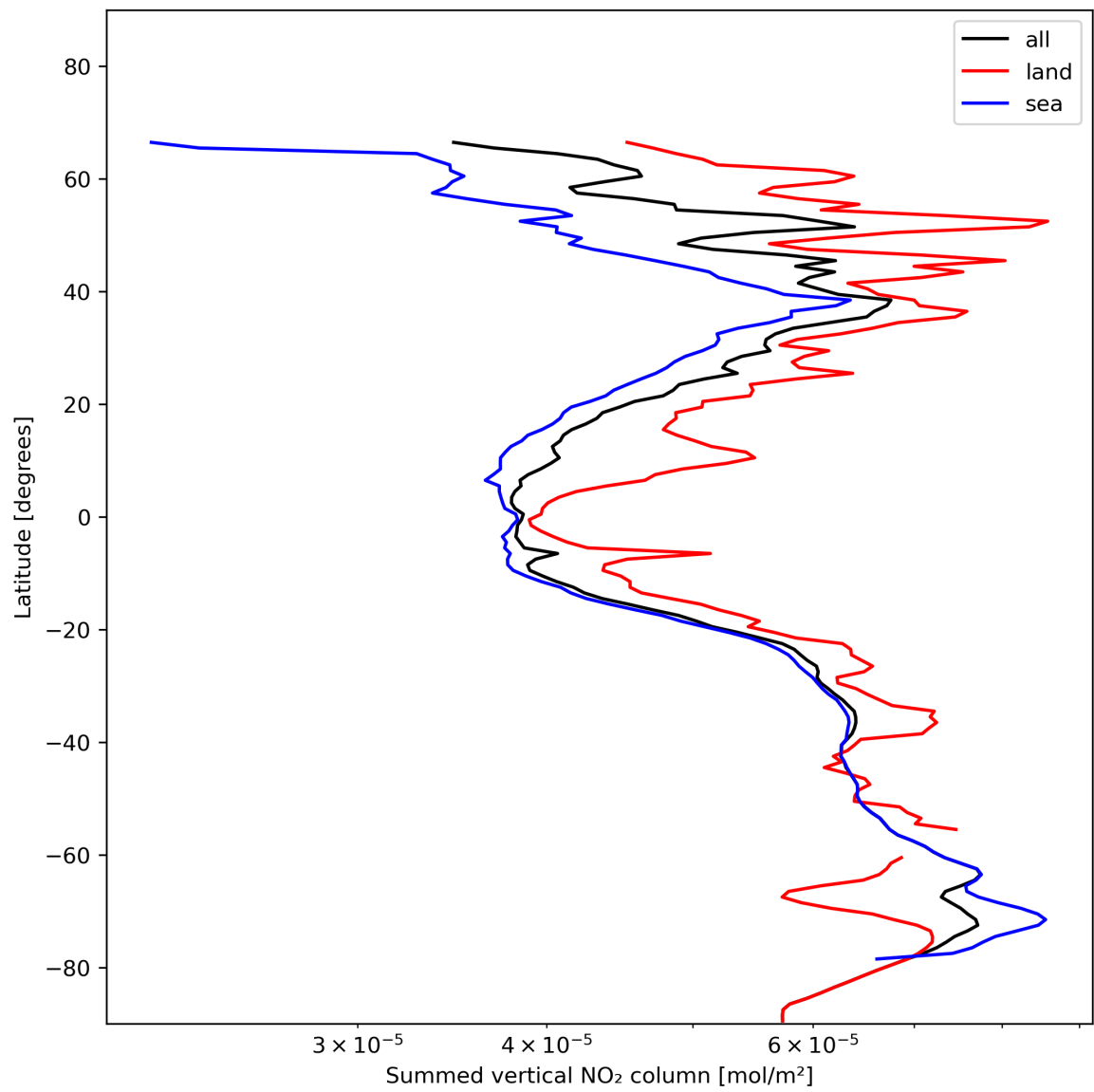
Figure 23: Zonal average of “Summed vertical NO 2 column” for 2023-11-26 to 2023-11-28.
