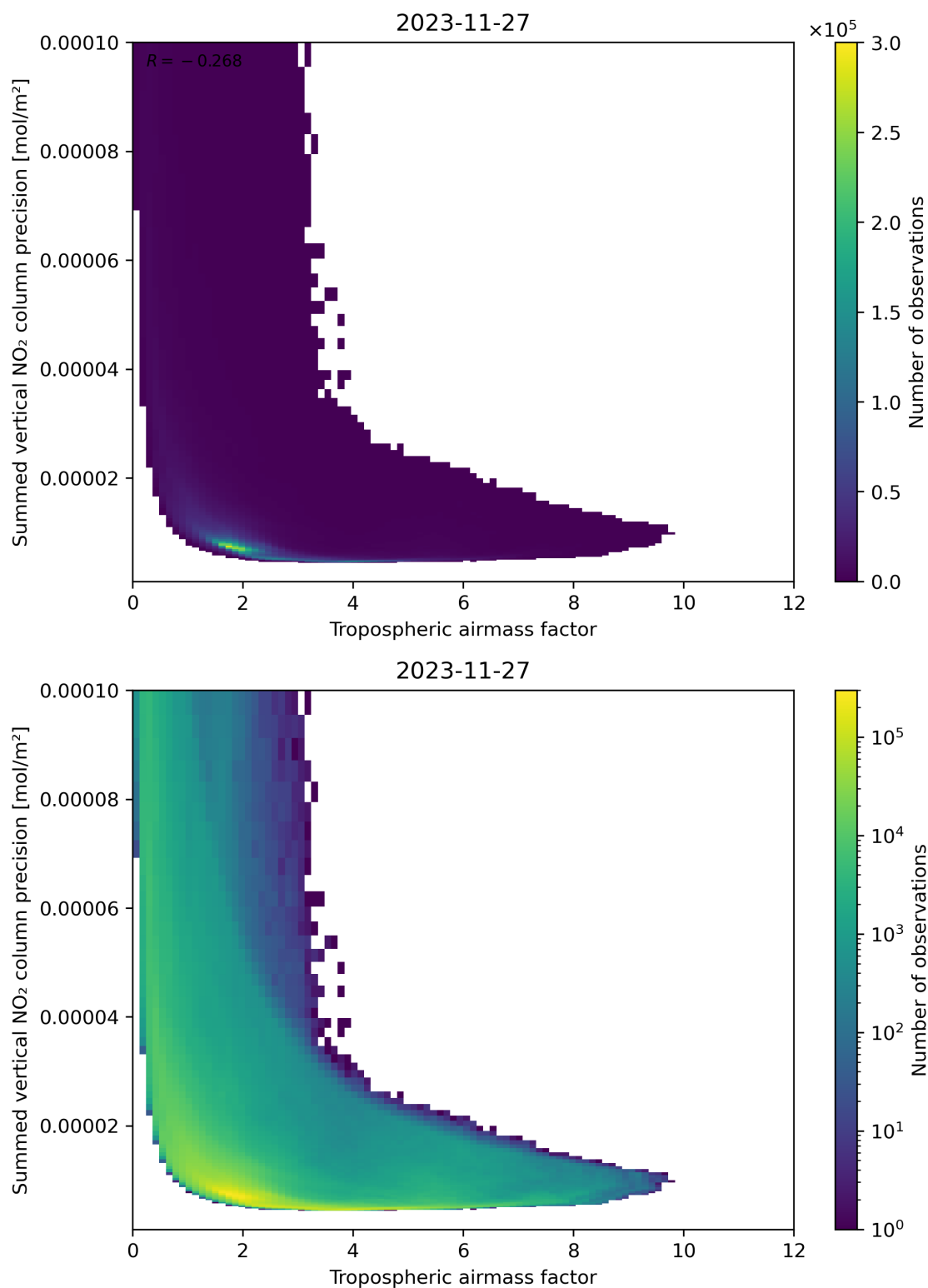
Figure 76: Scatter density plot of “Tropospheric air mass factor” against “Summed vertical NO 2 column precision” for 2023-11-26 to 2023-11-28.
