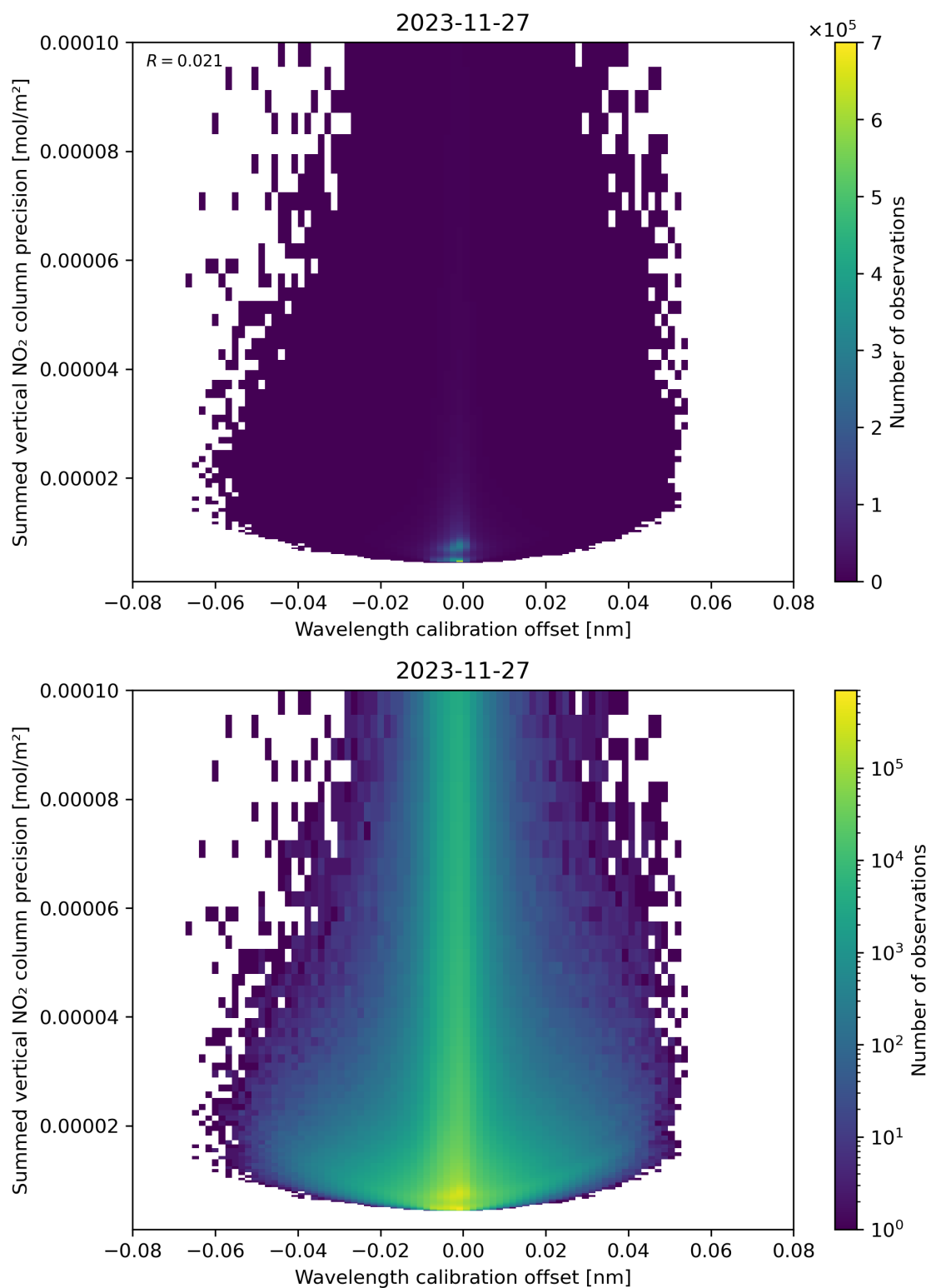
Figure 178: Scatter density plot of “Wavelength calibration offset” against “Summed vertical NO 2 column precision” for 2023-11-26 to 2023-11-28.
