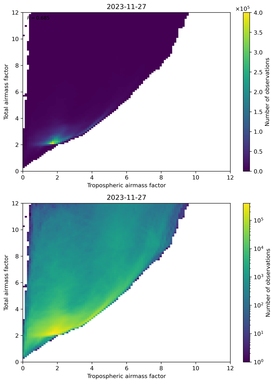
Figure 72: Scatter density plot of “Tropospheric airmass factor” against “Total airmass factor” for 2023-11-26 to 2023-11-28.
