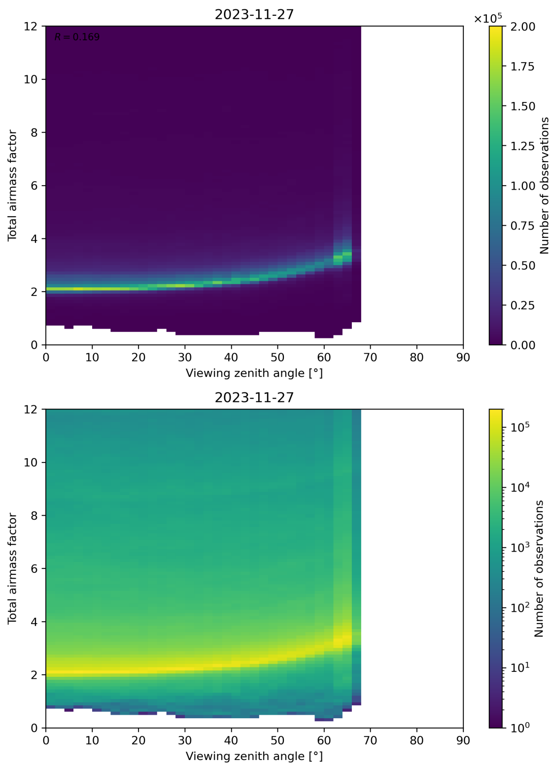
Figure 160: Scatter density plot of “Viewing zenith angle” against “Total airmass factor” for 2023-11-26 to 2023-11-28.
