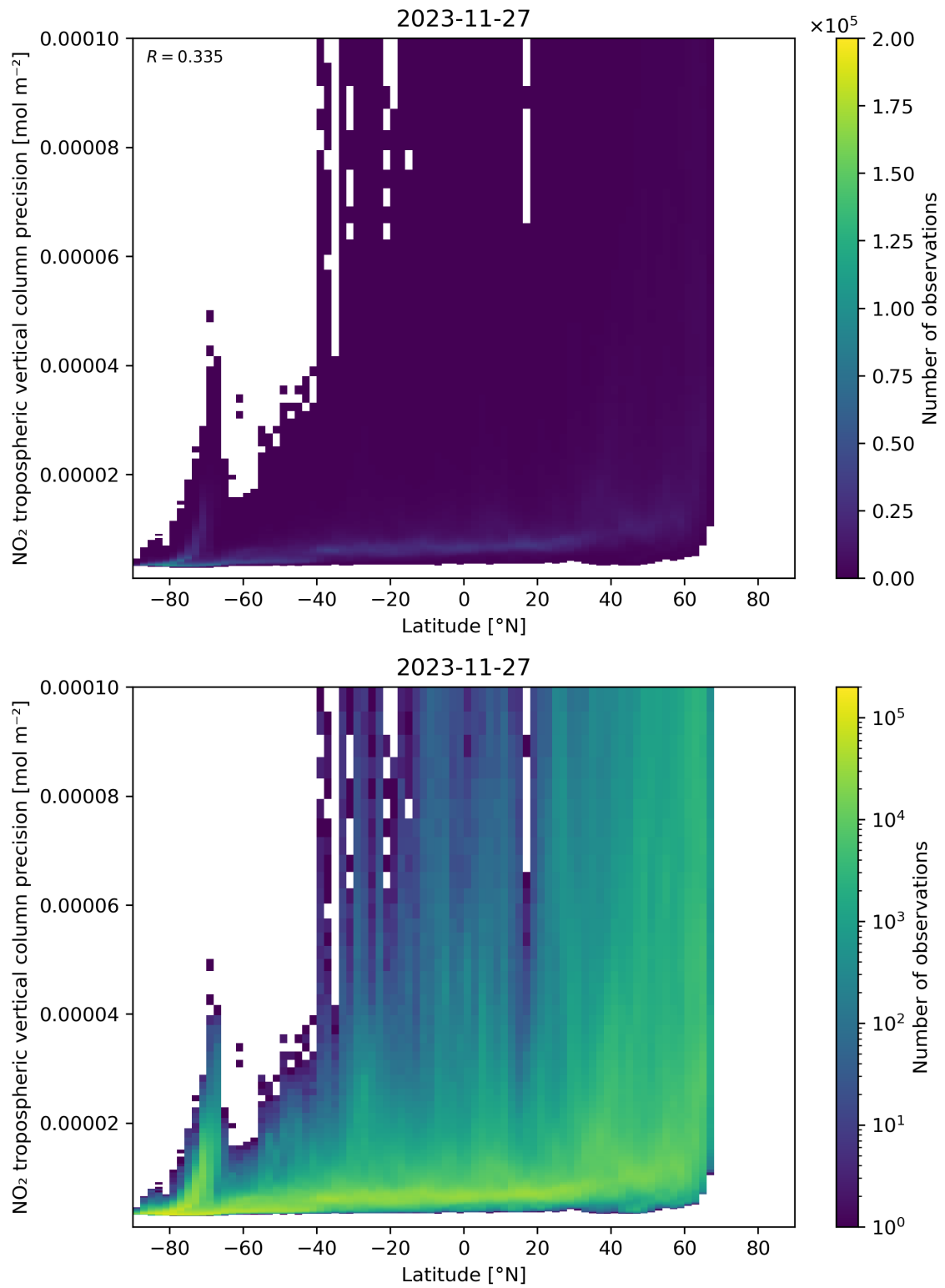
Figure 93: Scatter density plot of “Latitude” against “NO 2 tropospheric vertical column precision” for 2023-11-26 to 2023-11-28.
