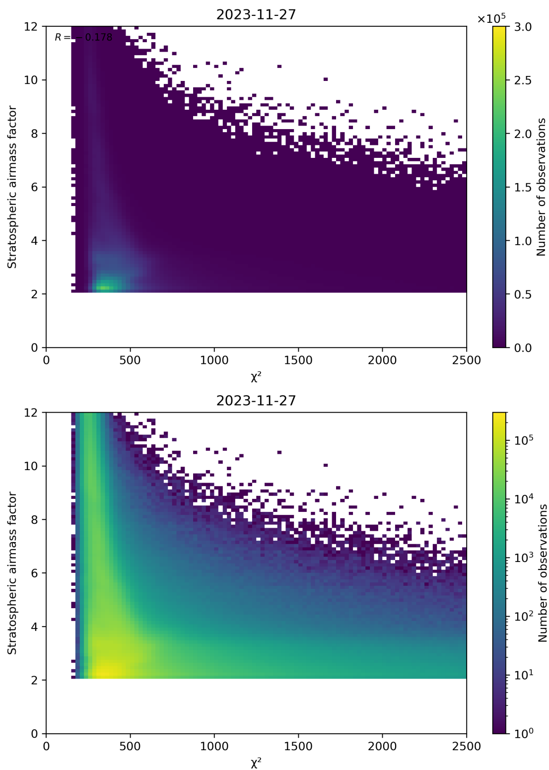
Figure 81: Scatter density plot of “ \chi^2 ” against “Stratospheric airmass factor” for 2023-11-26 to 2023-11-28.
