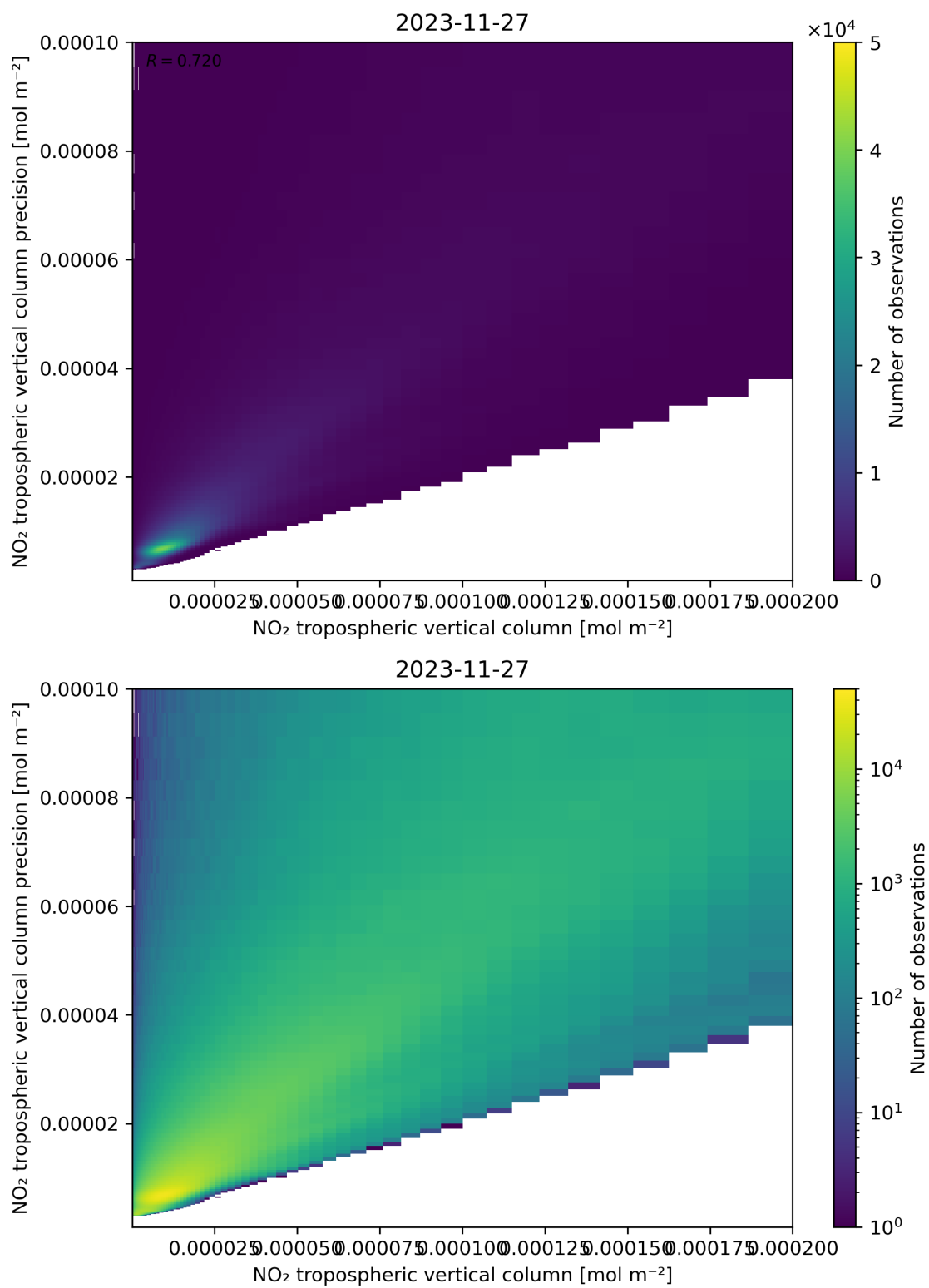
Figure 130: Scatter density plot of “NO 2 tropospheric vertical column” against “NO 2 tropospheric vertical column precision” for 2023-11-26 to 2023-11-28.
