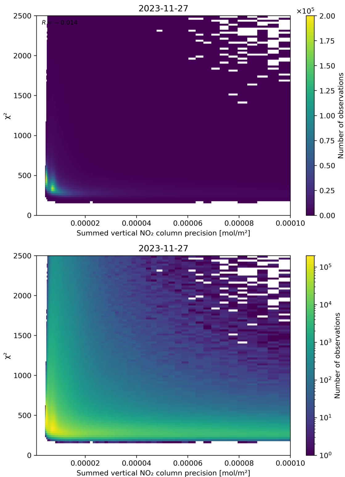
Figure 107: Scatter density plot of “Summed vertical NO 2 column precision” against “ \chi^2 ” for 2023-11-26 to 2023-11-28.
