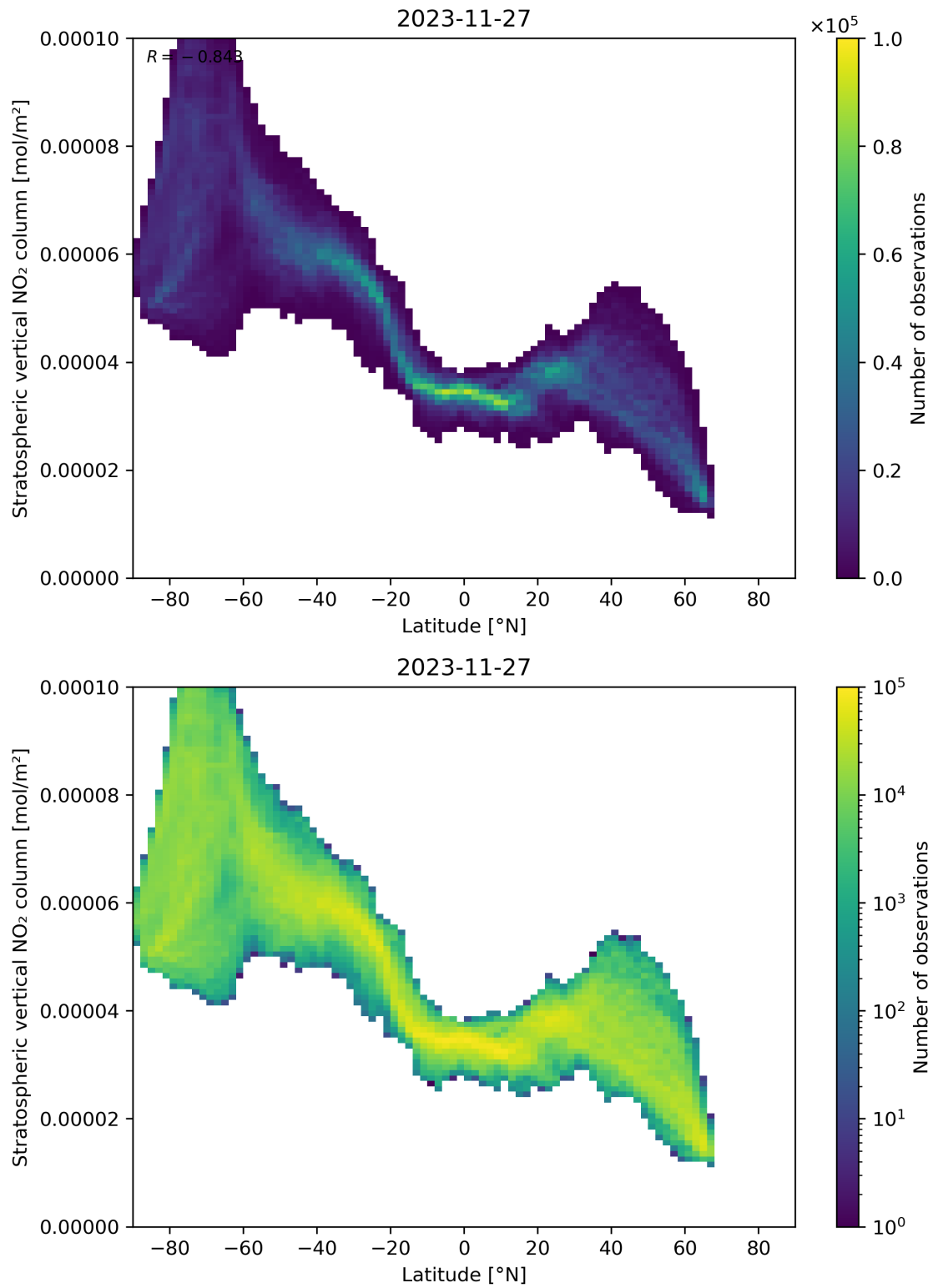
Figure 87: Scatter density plot of “Latitude” against “Stratospheric vertical NO 2 column” for 2023-11-26 to 2023-11-28.
