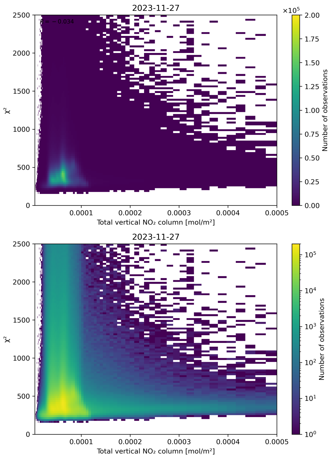
Figure 111: Scatter density plot of “Total vertical NO 2 column” against “ \chi^2 ” for 2023-11-26 to 2023-11-28.
