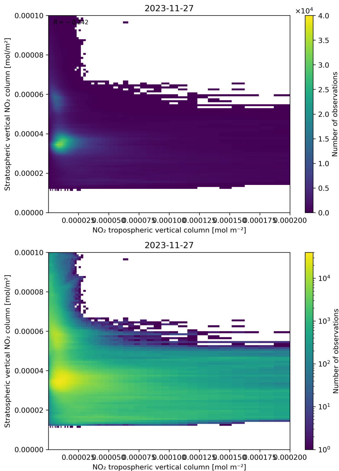
Figure 125: Scatter density plot of “NO 2 tropospheric vertical column” against “Stratospheric vertical NO 2 column” for 2023-11-26 to 2023-11-28.
