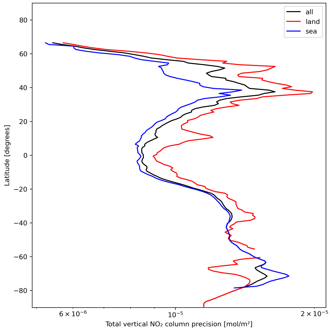
Figure 22: Zonal average of “Total vertical NO 2 column precision” for 2023-11-26 to 2023-11-28.
