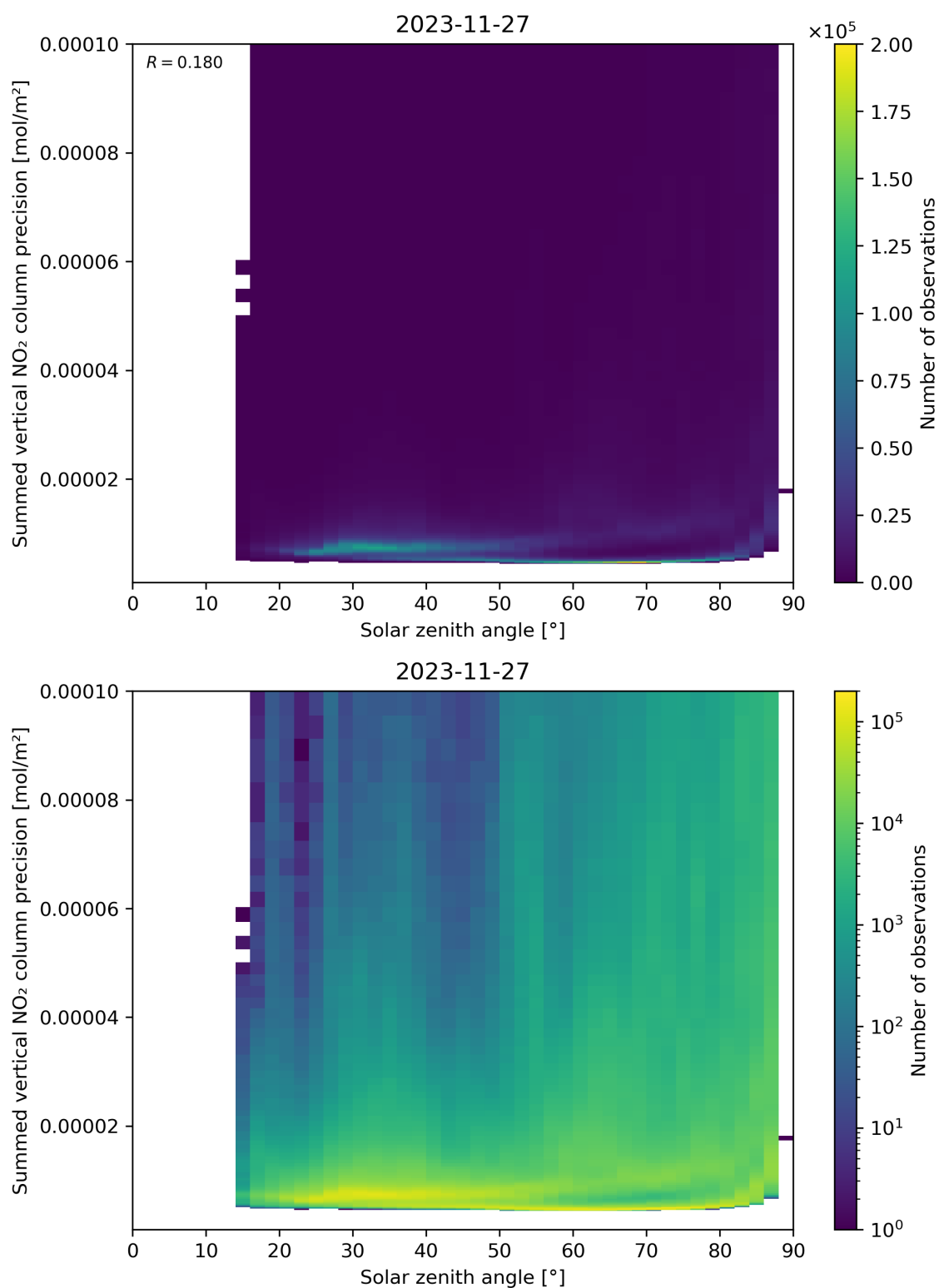
Figure 152: Scatter density plot of “Solar zenith angle” against “Summed vertical NO 2 column precision” for 2023-11-26 to 2023-11-28.
