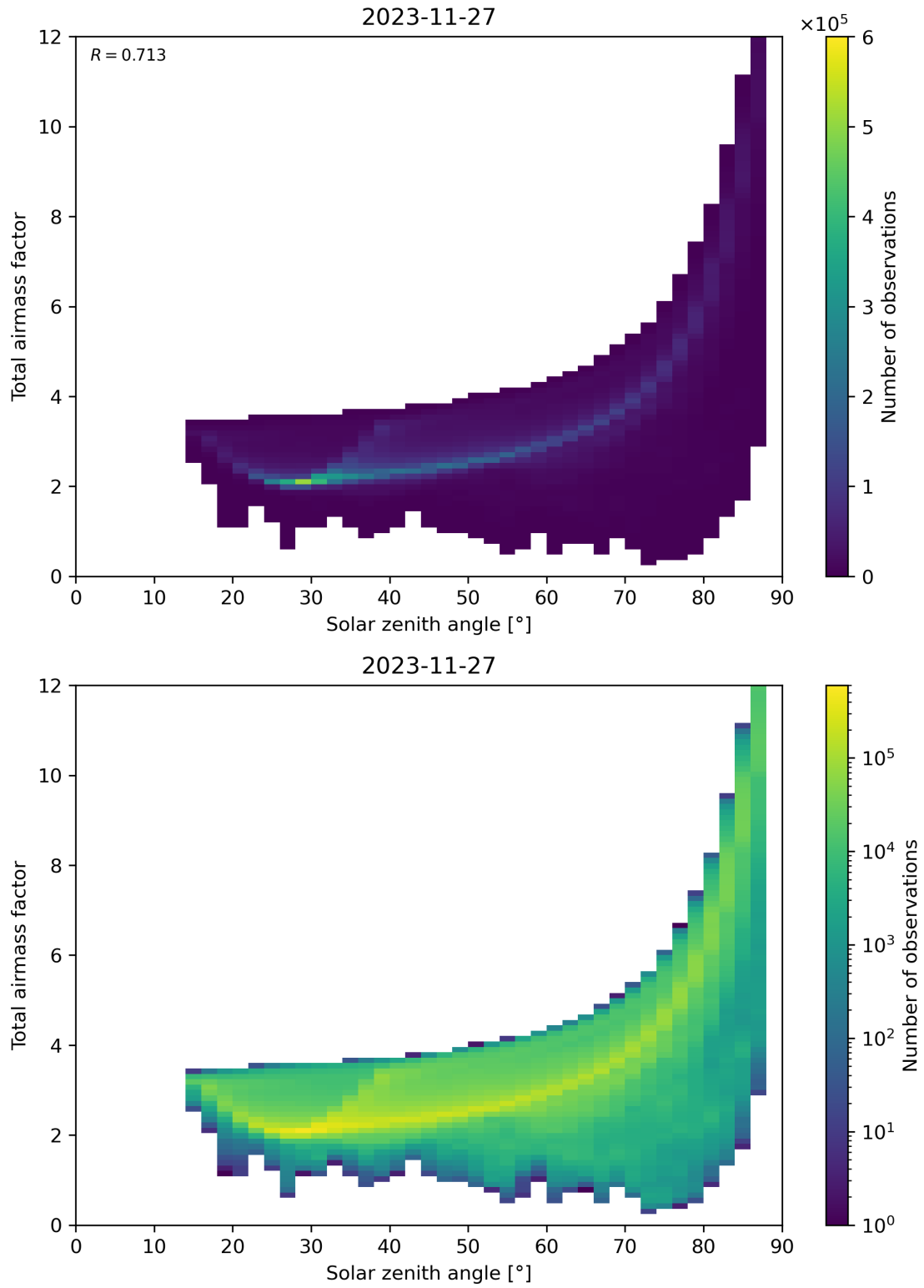
Figure 146: Scatter density plot of “Solar zenith angle” against “Total airmass factor” for 2023-11-26 to 2023-11-28.
