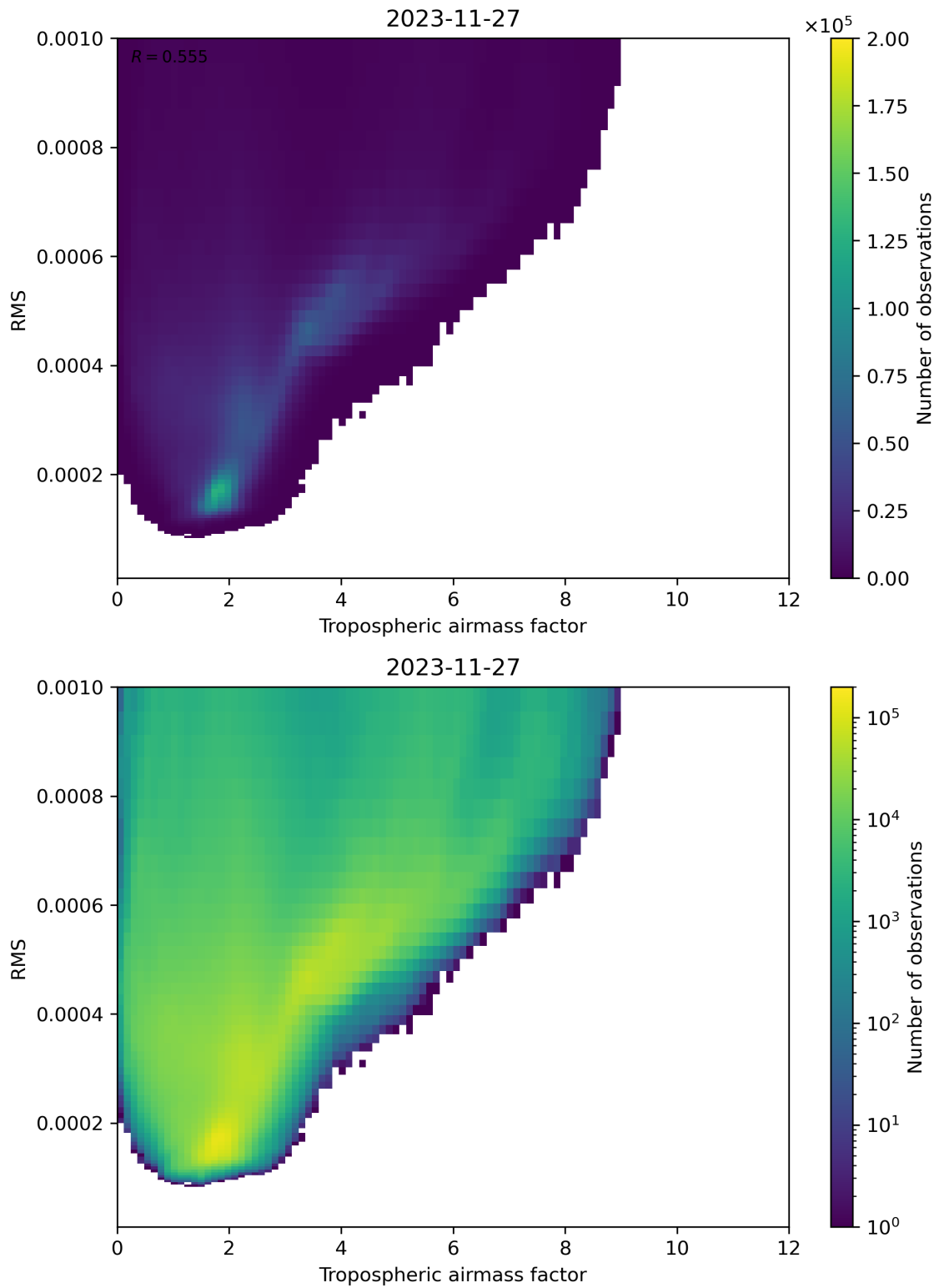
Figure 79: Scatter density plot of “Tropospheric airmass factor” against “RMS” for 2023-11-26 to 2023-11-28.
