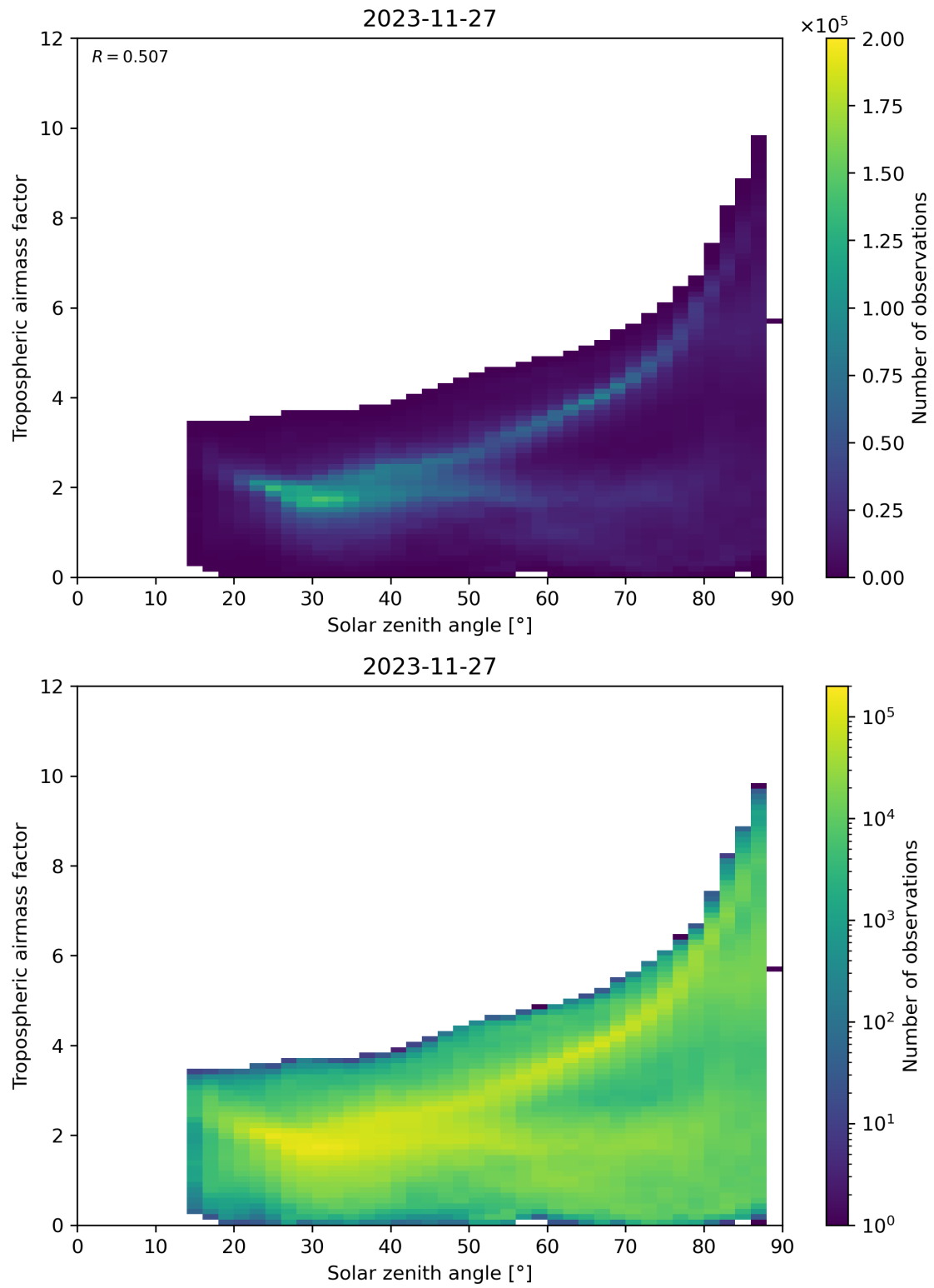
Figure 147: Scatter density plot of “Solar zenith angle” against “Tropospheric airmass factor” for 2023-11-26 to 2023-11-28.
