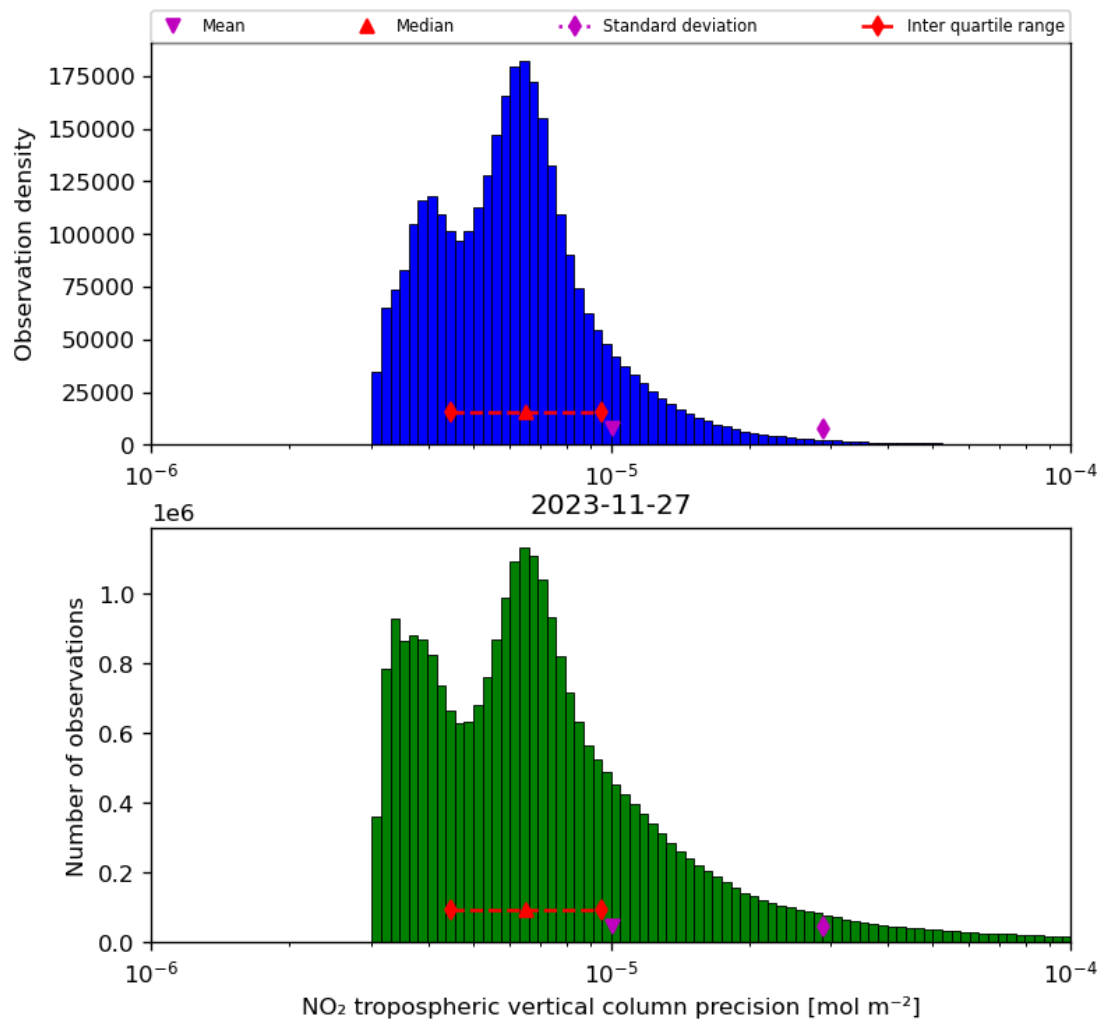
Figure 30: Histogram of “NO 2 tropospheric vertical column precision” for 2023-11-26 to 2023-11-28
