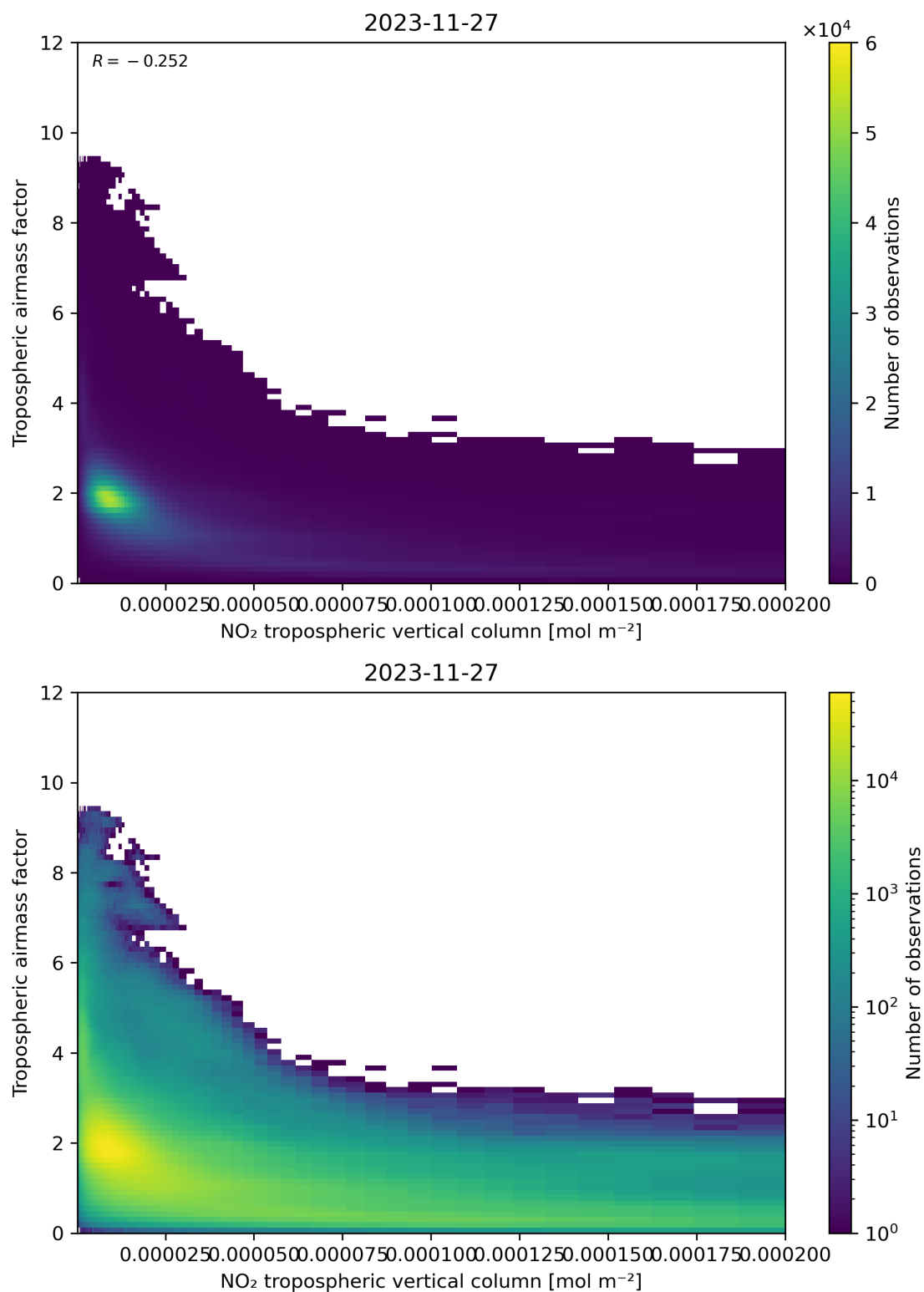
Figure 123: Scatter density plot of “NO 2 tropospheric vertical column” against “Tropospheric airmass factor” for 2023-11-26 to 2023-11-28.
