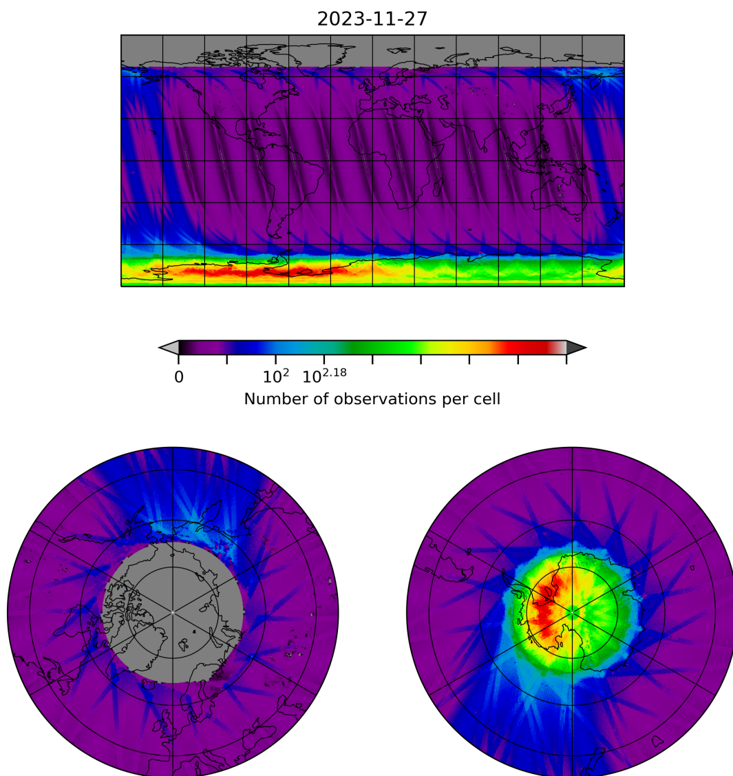
Figure 10: Map of the number of observations for 2023-11-26 to 2023-11-28
