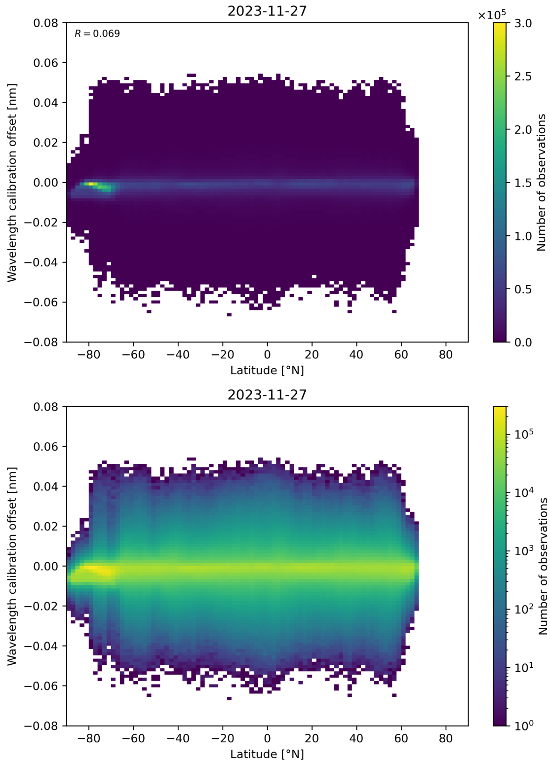
Figure 95: Scatter density plot of “Latitude” against “Wavelength calibration offset” for 2023-11-26 to 2023-11-28.
