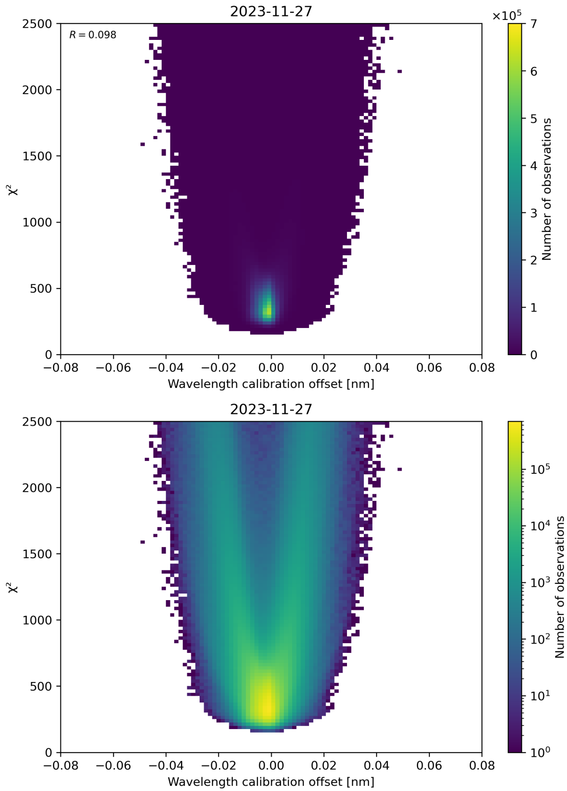
Figure 175: Scatter density plot of “Wavelength calibration offset” against “ \chi^2 ” for 2023-11-26 to 2023-11-28.
