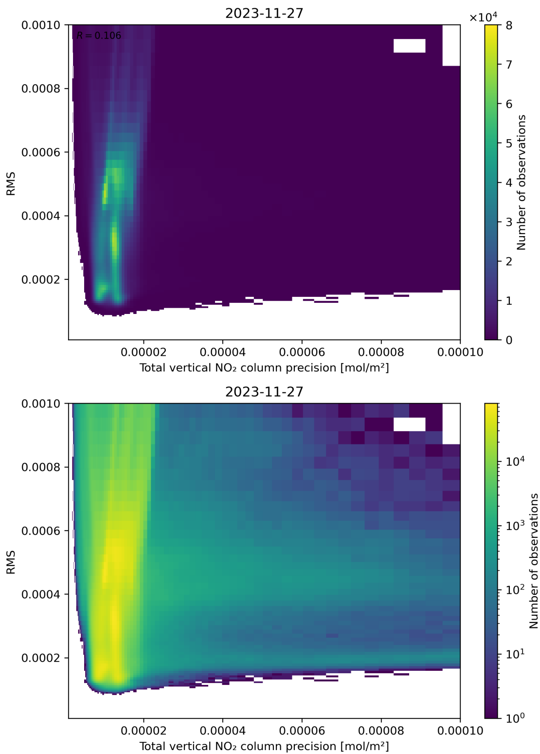
Figure 119: Scatter density plot of “Total vertical NO 2 column precision” against “RMS” for 2023-11-26 to 2023-11-28.
