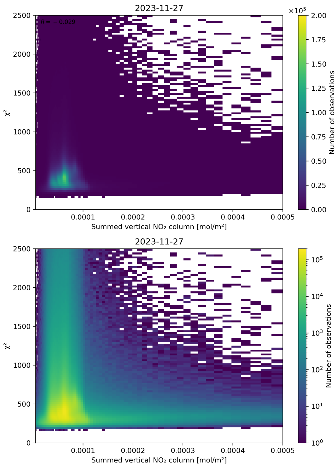
Figure 104: Scatter density plot of “Summed vertical NO 2 column” against “ \chi^2 ” for 2023-11-26 to 2023-11-28.
