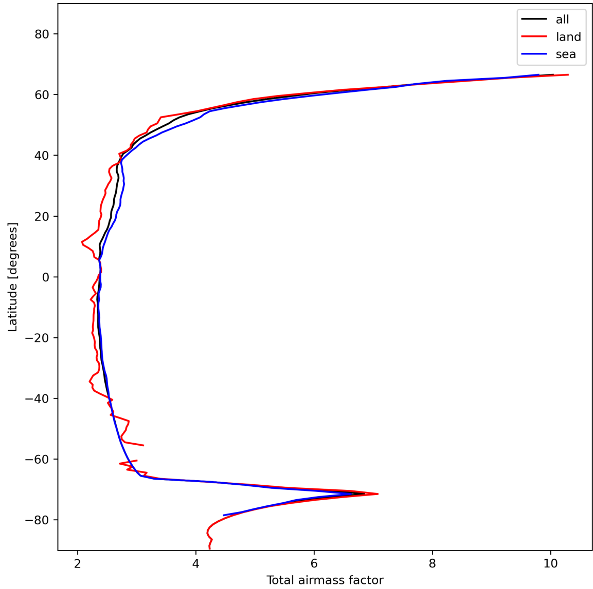
Figure 15: Zonal average of “Total airmass factor” for 2023-11-26 to 2023-11-28.
