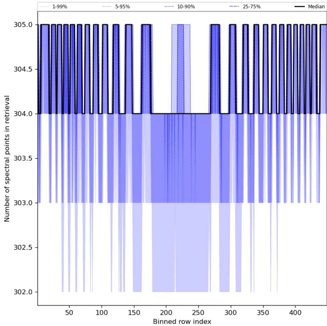
Figure 50: Along track statistics of “Number of spectral points in retrieval” for 2023-11-26 to 2023-11-28
