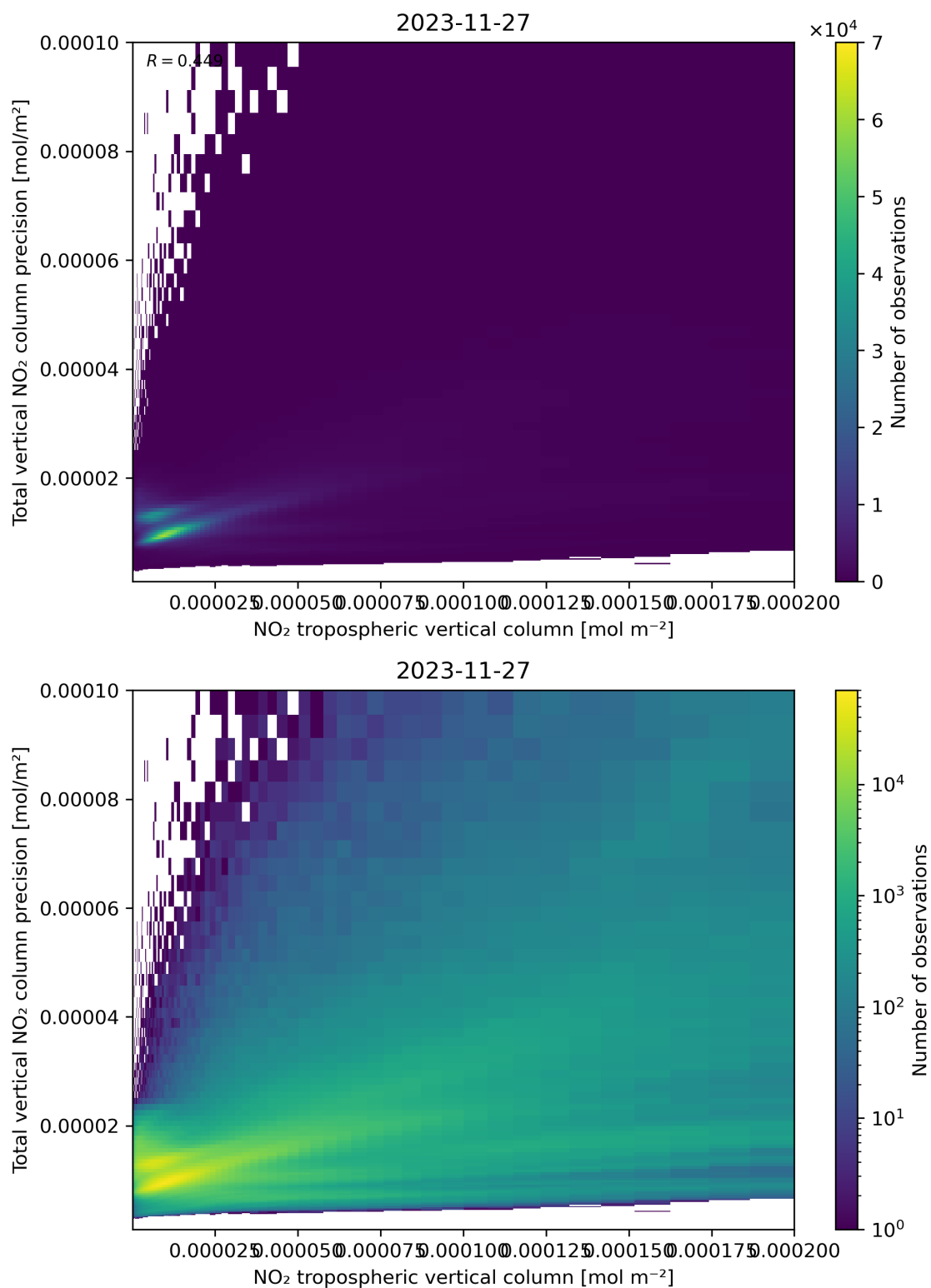
Figure 129: Scatter density plot of “NO 2 tropospheric vertical column” against “Total vertical NO 2 column precision” for 2023-11-26 to 2023-11-28.
