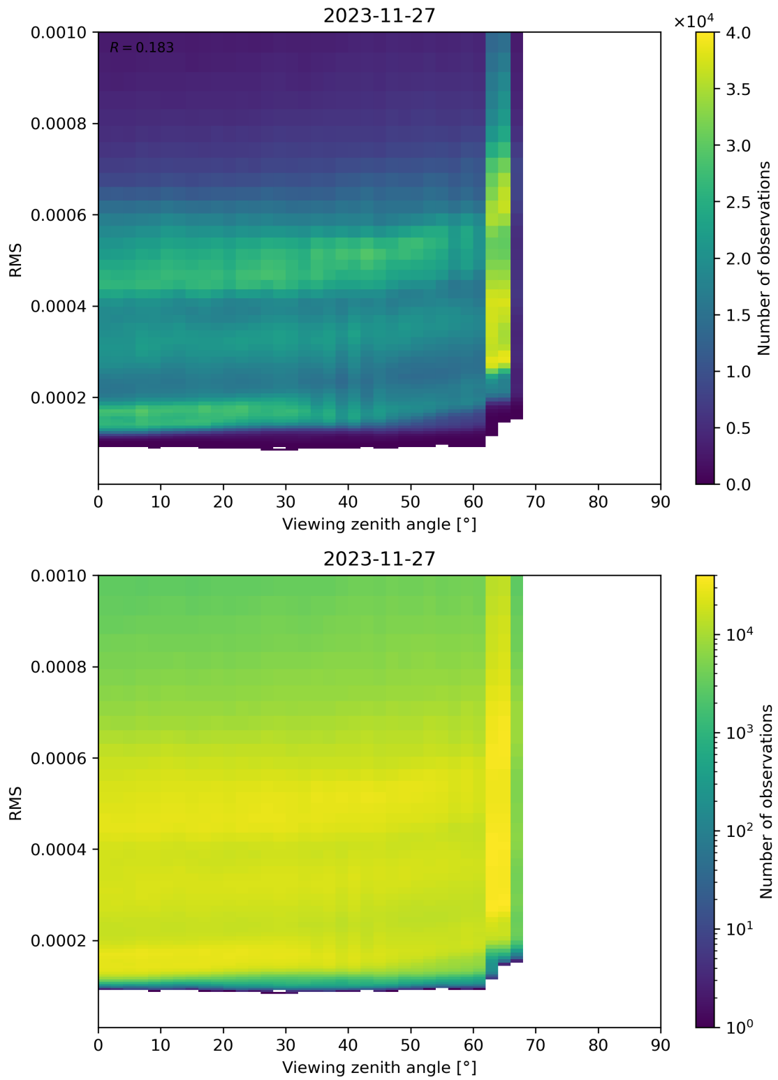
Figure 171: Scatter density plot of “Viewing zenith angle” against “RMS” for 2023-11-26 to 2023-11-28.
