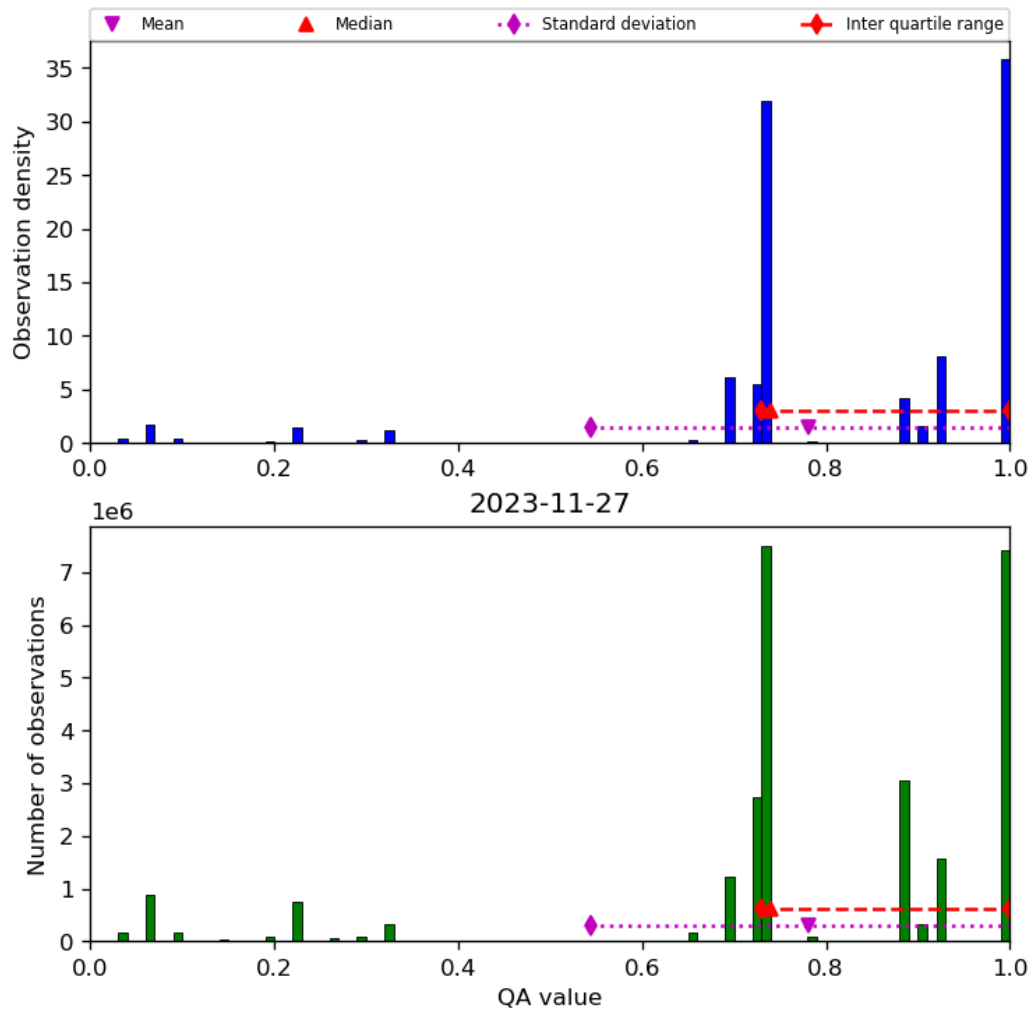
Figure 28: Histogram of “QA value” for 2023-11-26 to 2023-11-28
