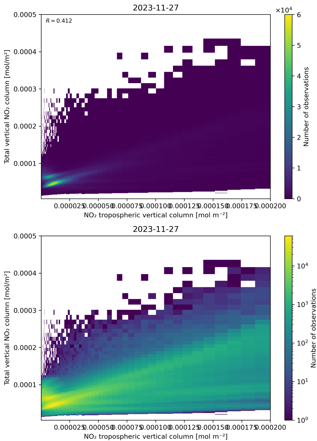
Figure 128: Scatter density plot of “NO 2 tropospheric vertical column” against “Total vertical NO 2 column” for 2023-11-26 to 2023-11-28.
