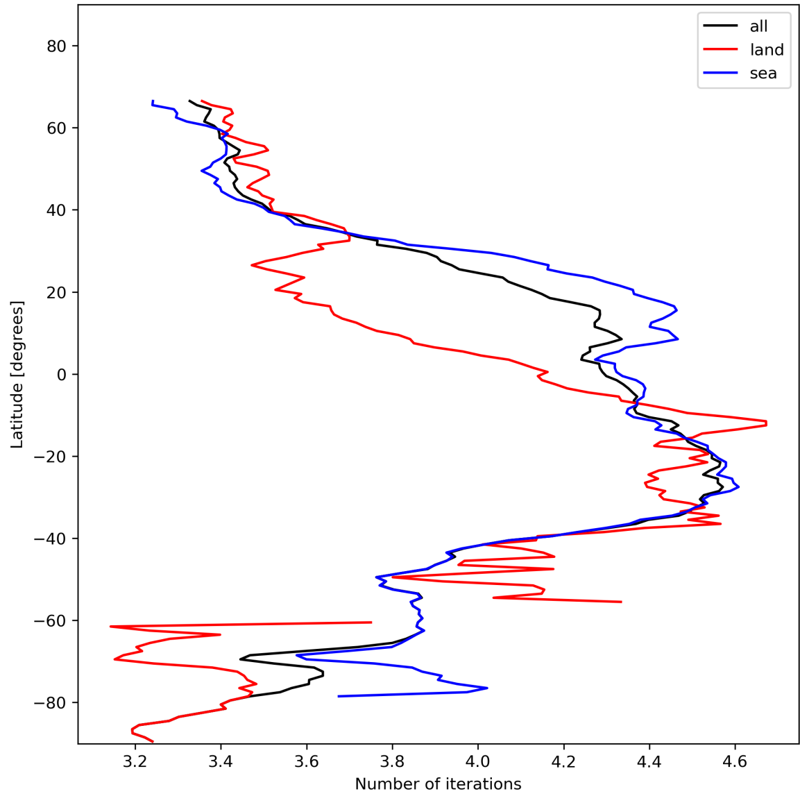
Figure 17: Zonal average of “Number of iterations” for 2023-11-26 to 2023-11-28.
