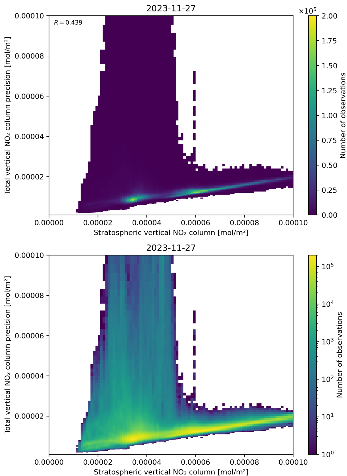
Figure 101: Scatter density plot of “Stratospheric vertical NO 2 column” against “Total vertical NO 2 column precision” for 2023-11-26 to 2023-11-28.
