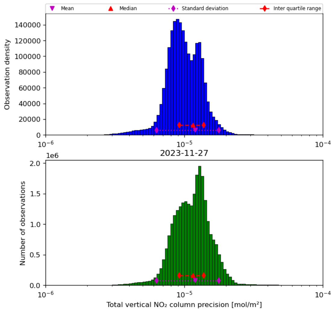
Figure 39: Histogram of “Total vertical NO 2 column precision” for 2023-11-26 to 2023-11-28
