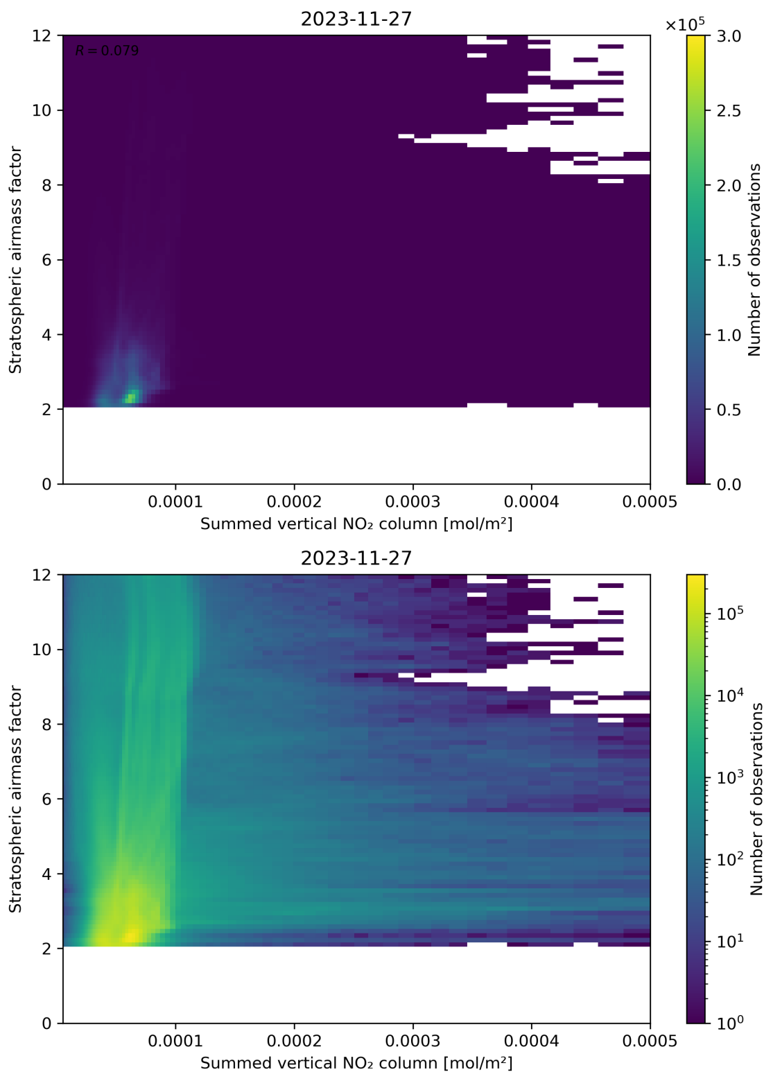
Figure 103: Scatter density plot of “Summed vertical NO 2 column” against “Stratospheric airmass factor” for 2023-11-26 to 2023-11-28.
