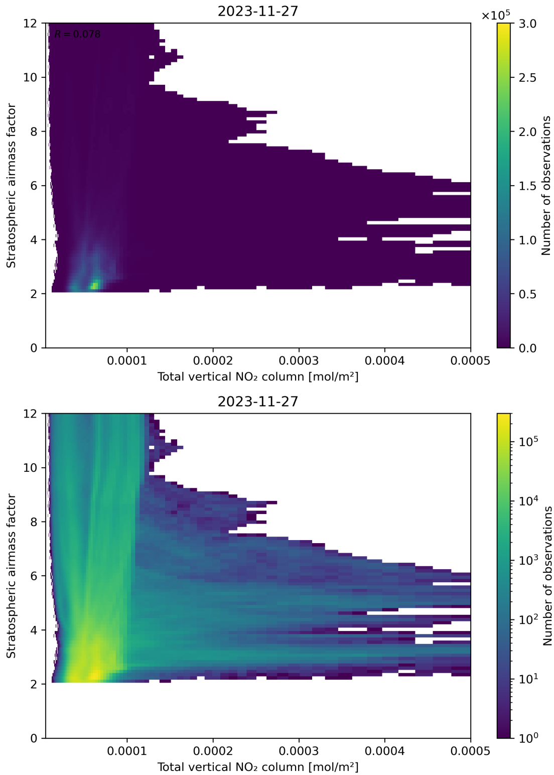
Figure 110: Scatter density plot of “Total vertical NO 2 column” against “Stratospheric airmass factor” for 2023-11-26 to 2023-11-28.
