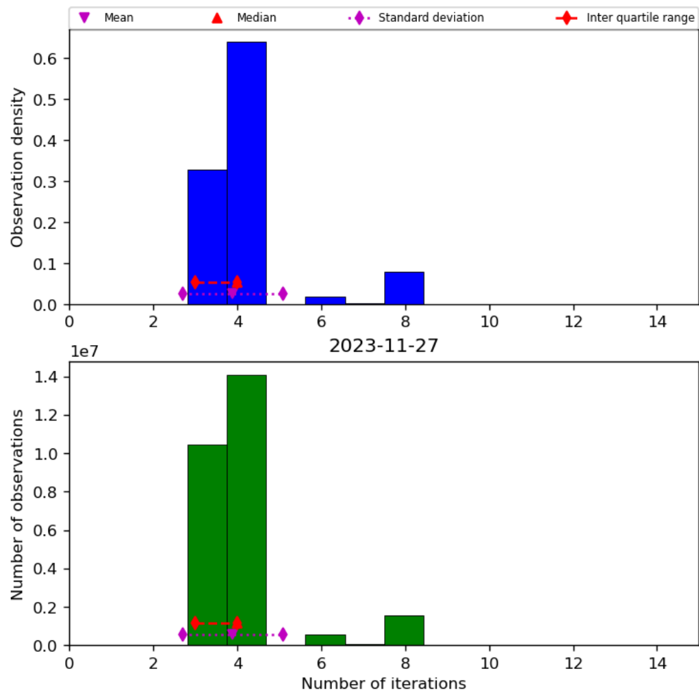
Figure 34: Histogram of “Number of iterations” for 2023-11-26 to 2023-11-28
