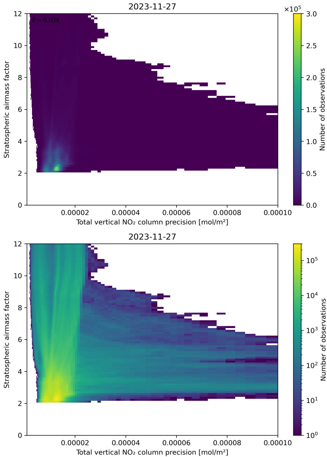
Figure 115: Scatter density plot of “Total vertical NO 2 column precision” against “Stratospheric airmass factor” for 2023-11-26 to 2023-11-28.
