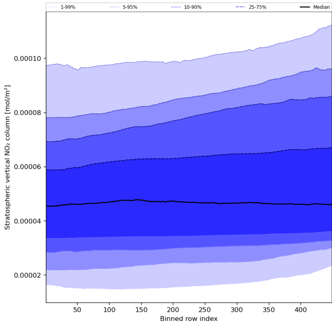
Figure 53: Along track statistics of “Stratospheric vertical NO 2 column” for 2023-11-26 to 2023-11-28
