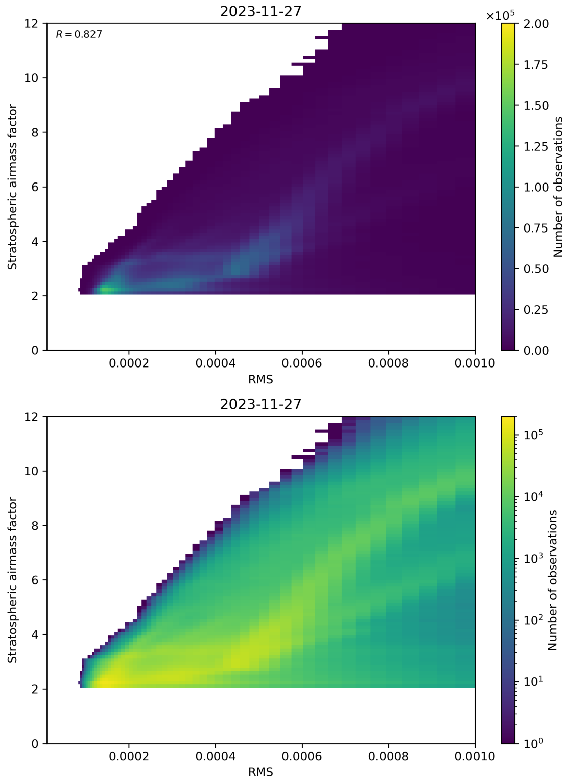
Figure 144: Scatter density plot of “RMS” against “Stratospheric airmass factor” for 2023-11-26 to 2023-11-28.
