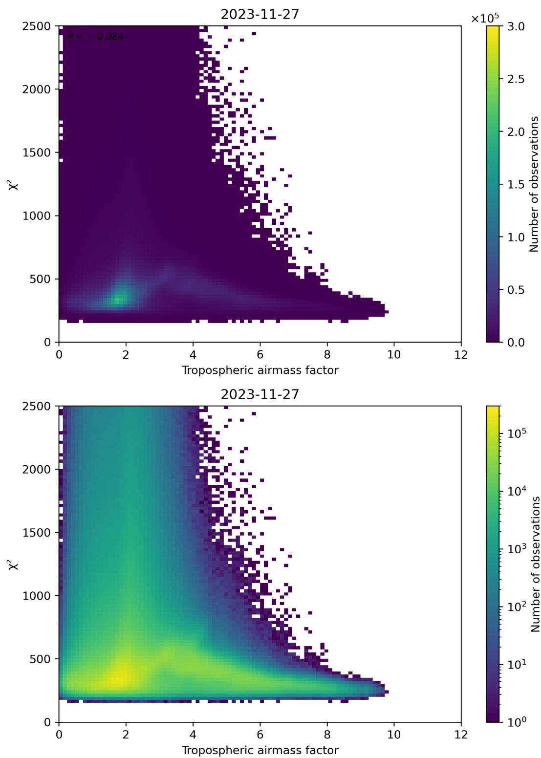
Figure 73: Scatter density plot of “Tropospheric airmass factor” against “ \chi^2 ” for 2023-11-26 to 2023-11-28.
