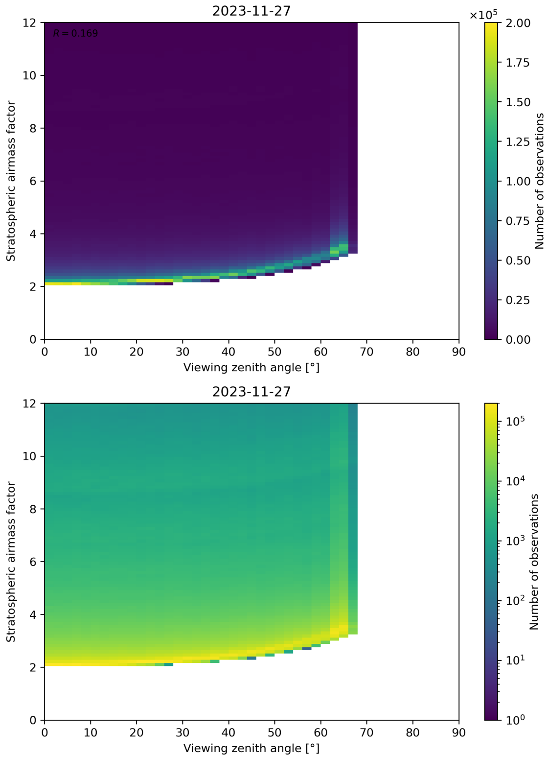
Figure 159: Scatter density plot of “Viewing zenith angle” against “Stratospheric airmass factor” for 2023-11-26 to 2023-11-28.
