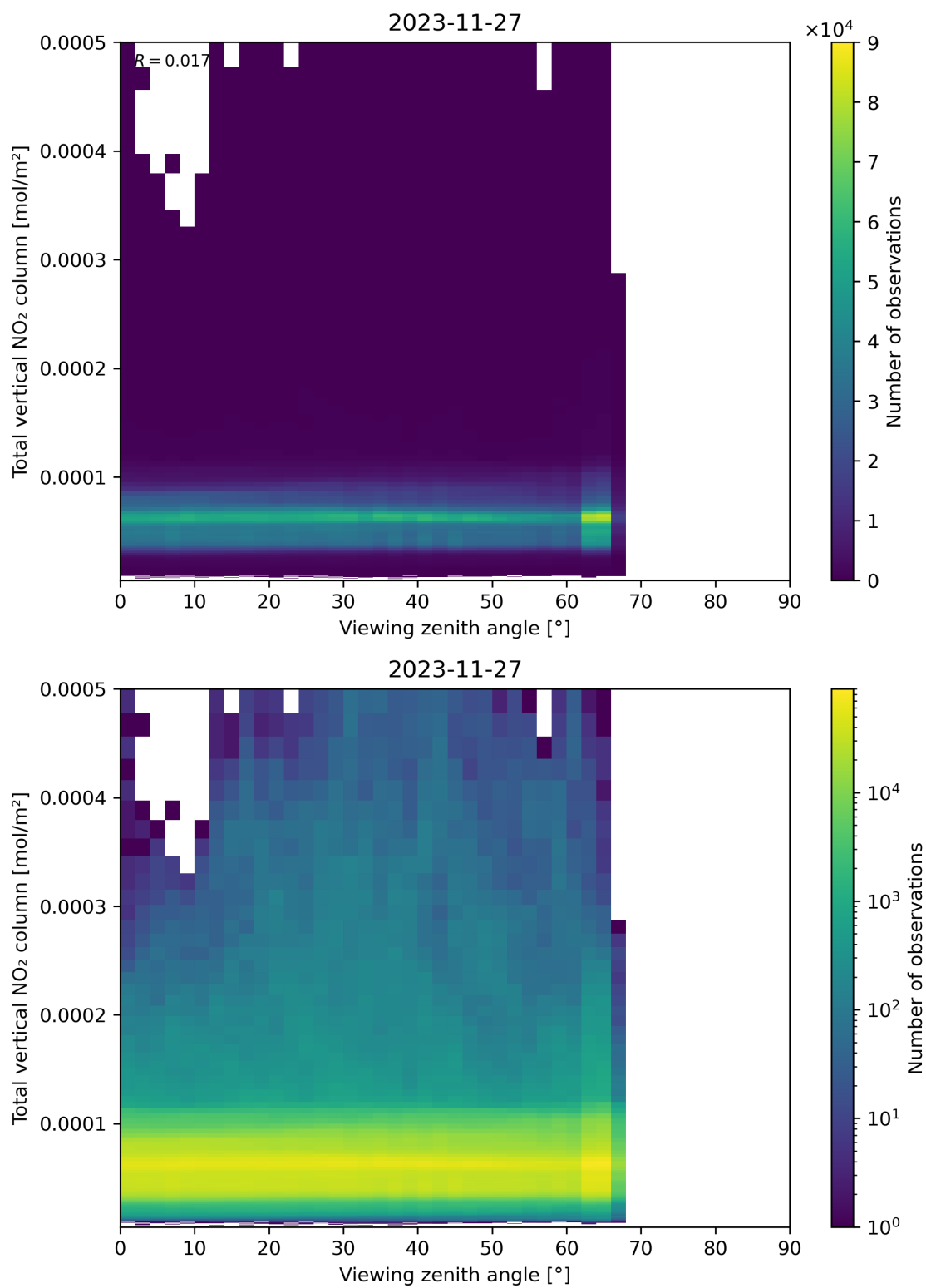
Figure 167: Scatter density plot of “Viewing zenith angle” against “Total vertical NO 2 column” for 2023-11-26 to 2023-11-28.
