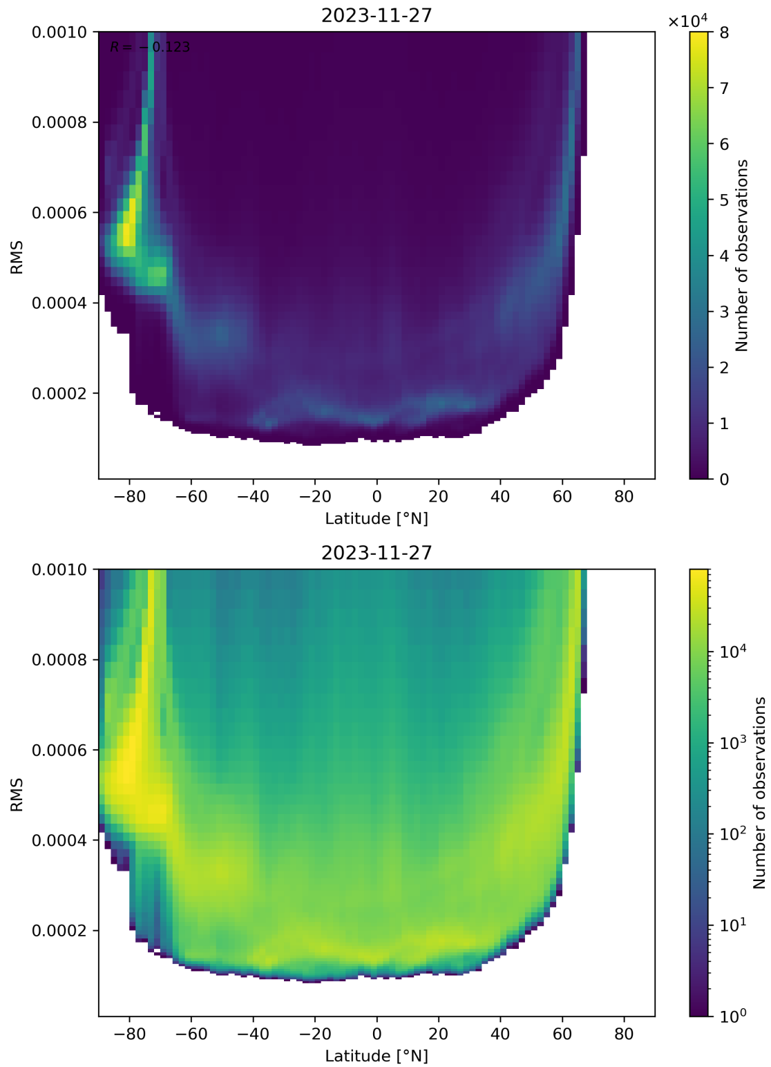
Figure 94: Scatter density plot of “Latitude” against “RMS” for 2023-11-26 to 2023-11-28.
