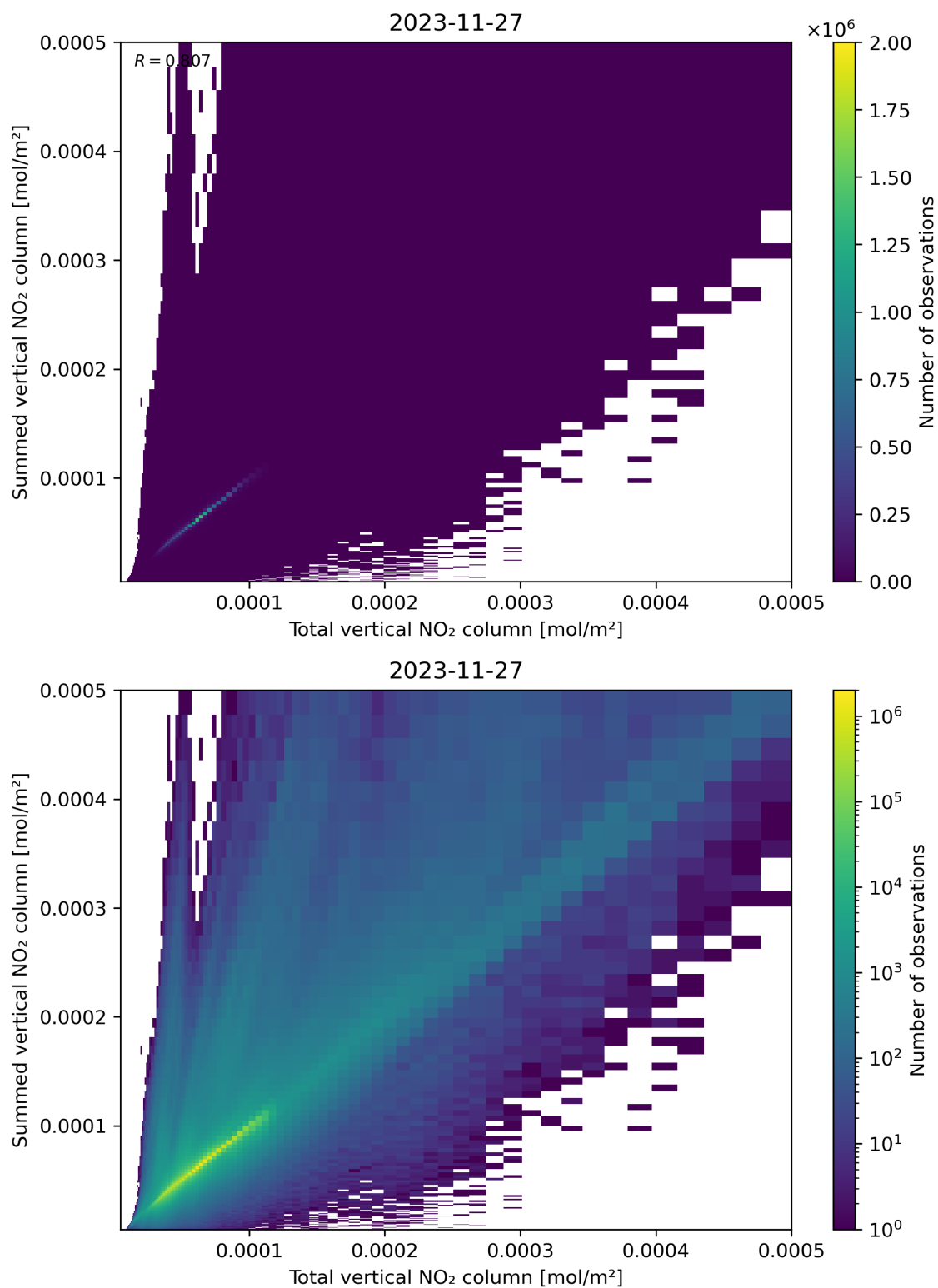
Figure 112: Scatter density plot of “Total vertical NO 2 column” against “Summed vertical NO 2 column” for 2023-11-26 to 2023-11-28.
