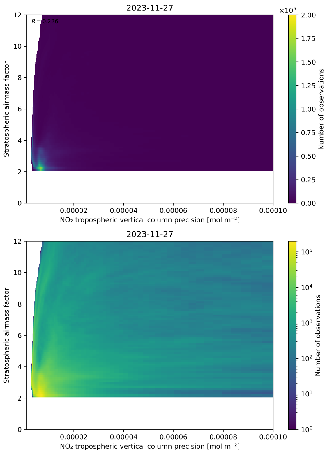
Figure 131: Scatter density plot of “NO 2 tropospheric vertical column precision” against “Stratospheric airmass factor” for 2023-11-26 to 2023-11-28.
