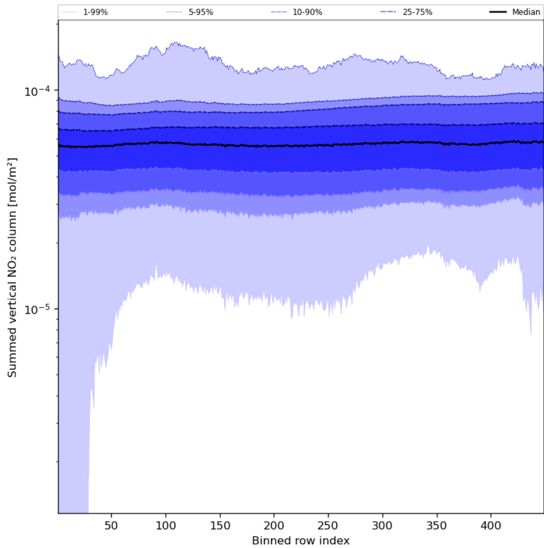
Figure 57: Along track statistics of “Summed vertical NO 2 column” for 2023-11-26 to 2023-11-28
