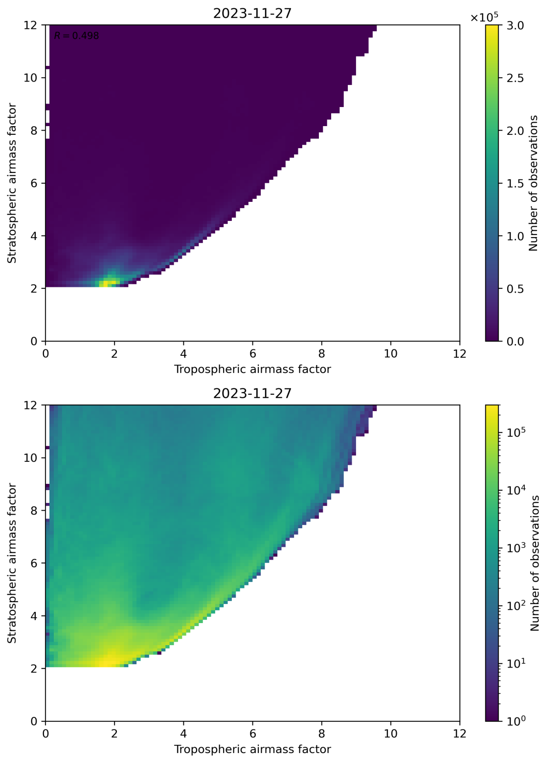
Figure 71: Scatter density plot of “Tropospheric airmass factor” against “Stratospheric airmass factor” for 2023-11-26 to 2023-11-28.
