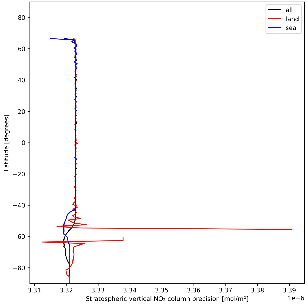
Figure 20: Zonal average of "Stratospheric vertical NO 2 column precision" for 2023-11-26 to 2023-11-28.
