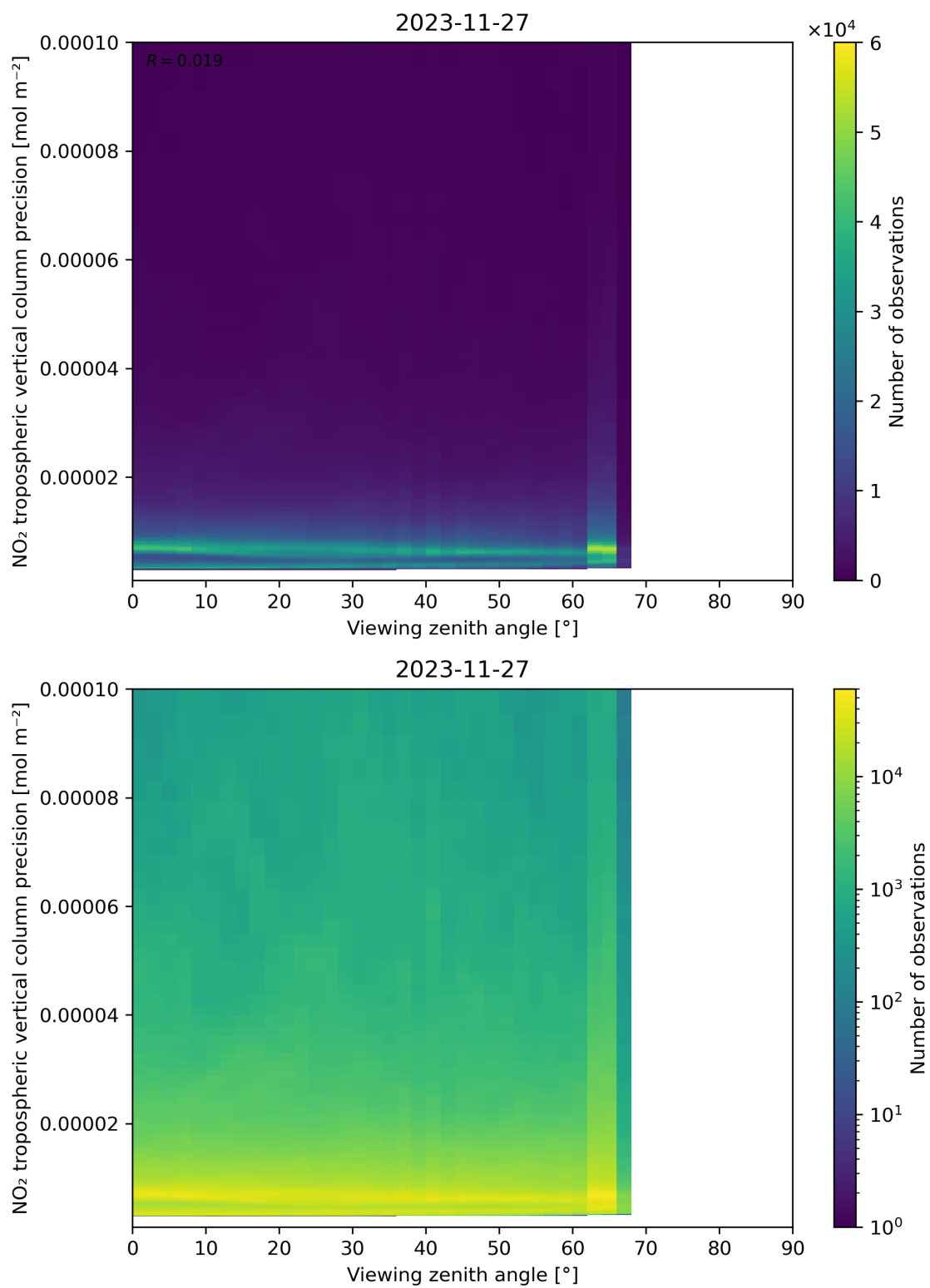
Figure 170: Scatter density plot of “Viewing zenith angle” against “NO 2 tropospheric vertical column precision” for 2023-11-26 to 2023-11-28.
