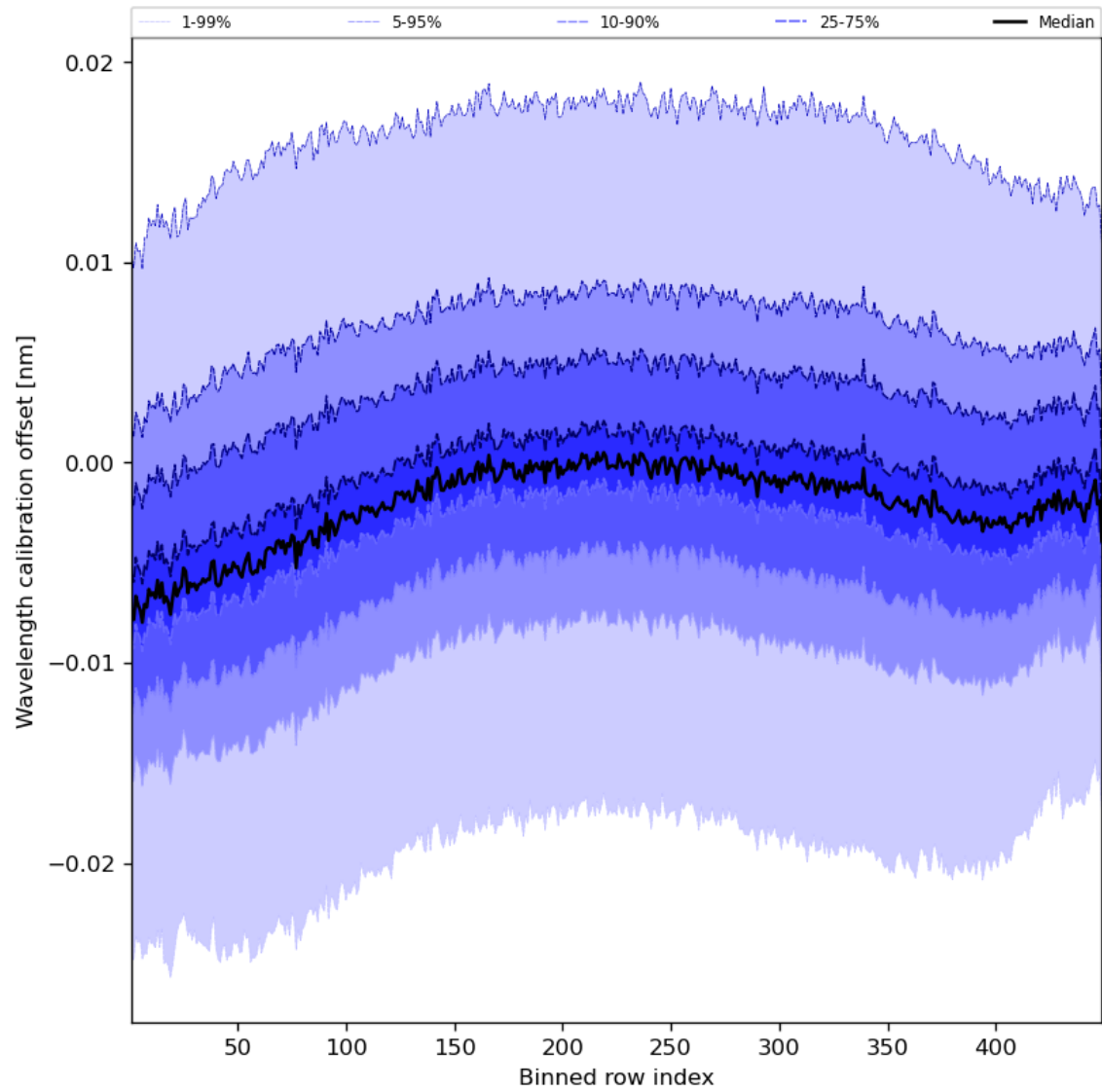
Figure 52: Along track statistics of “Wavelength calibration offset” for 2023-11-26 to 2023-11-28
