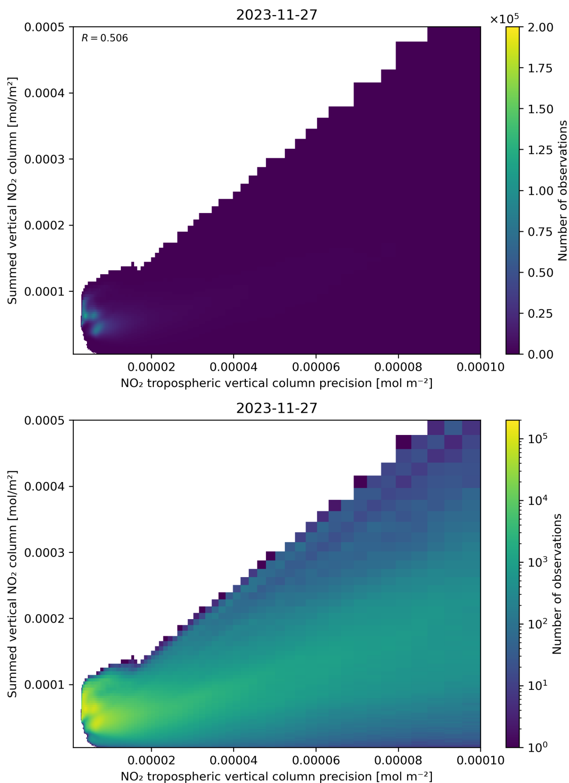
Figure 136: Scatter density plot of “NO 2 tropospheric vertical column precision” against “Summed vertical NO 2 column” for 2023-11-26 to 2023-11-28.
