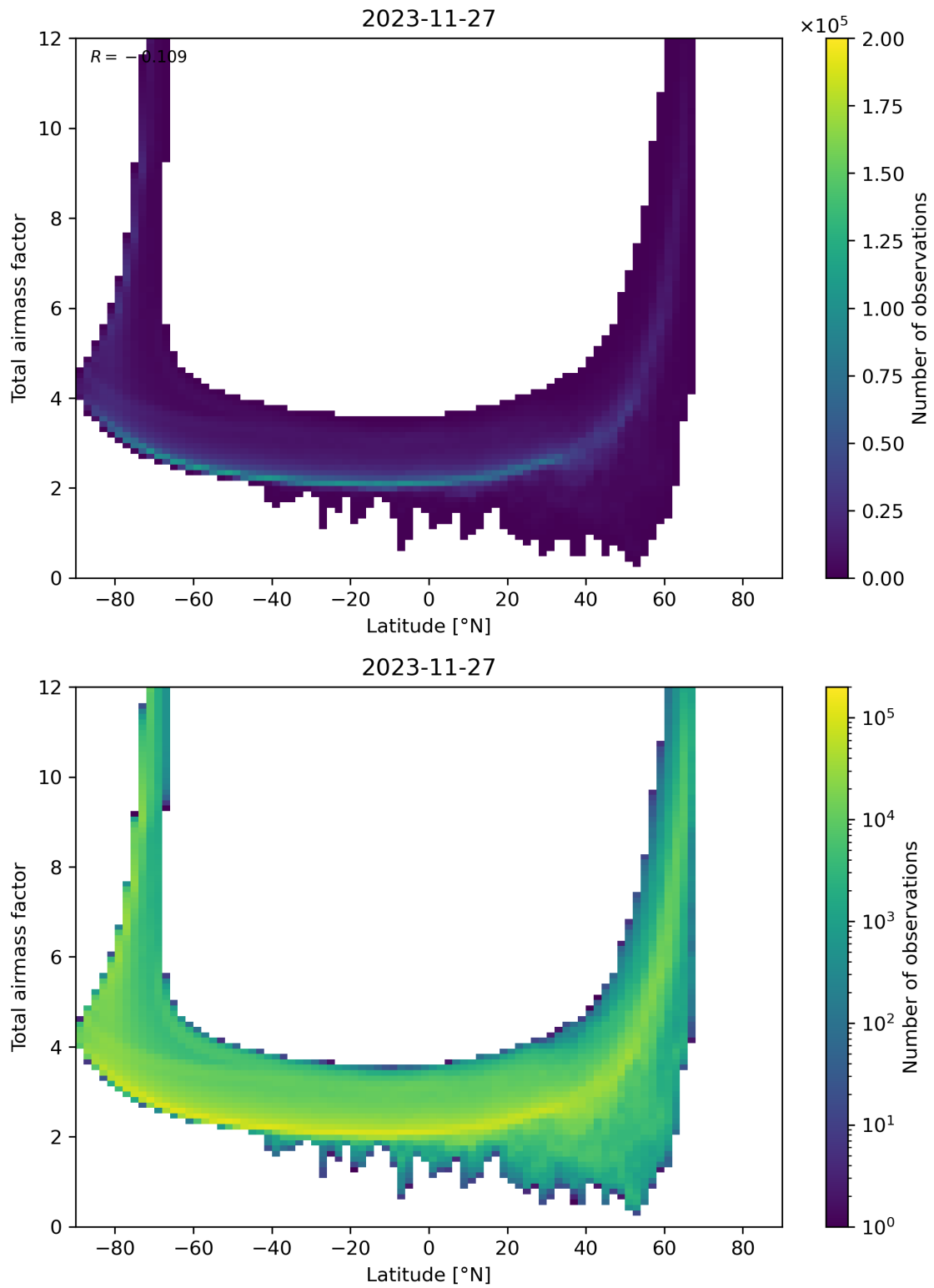
Figure 84: Scatter density plot of “Latitude” against “Total airmass factor” for 2023-11-26 to 2023-11-28.
