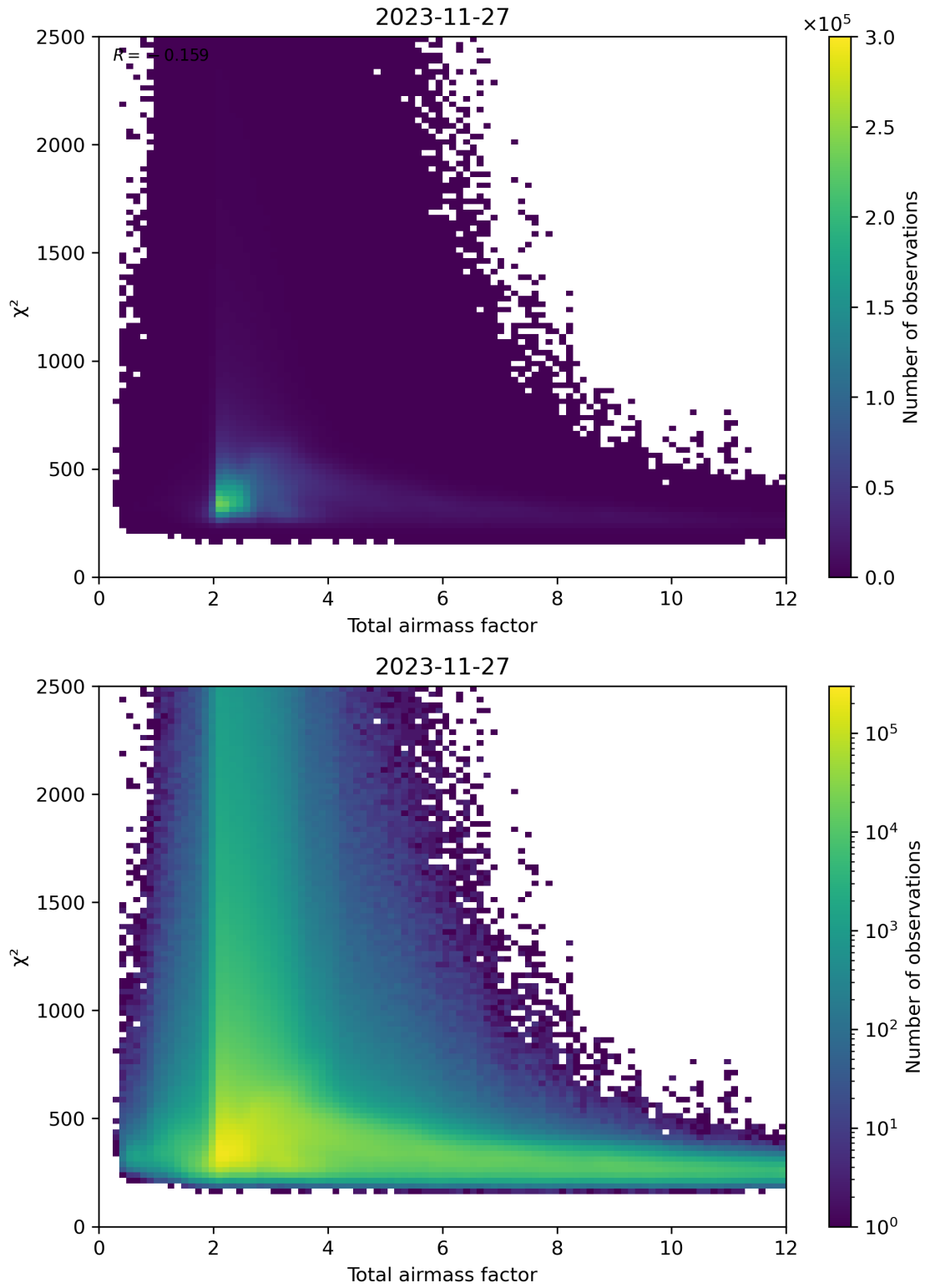
Figure 63: Scatter density plot of “Total airmass factor” against “ \chi^2 ” for 2023-11-26 to 2023-11-28.
