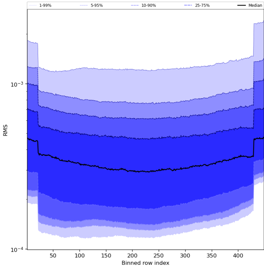
Figure 60: Along track statistics of “RMS” for 2023-11-26 to 2023-11-28
