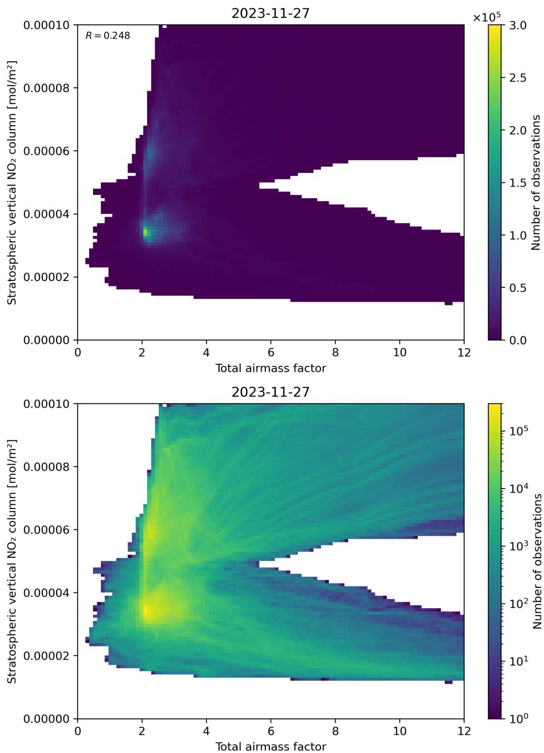
Figure 64: Scatter density plot of “Total airmass factor” against “Stratospheric vertical NO 2 column” for 2023-11-26 to 2023-11-28.
