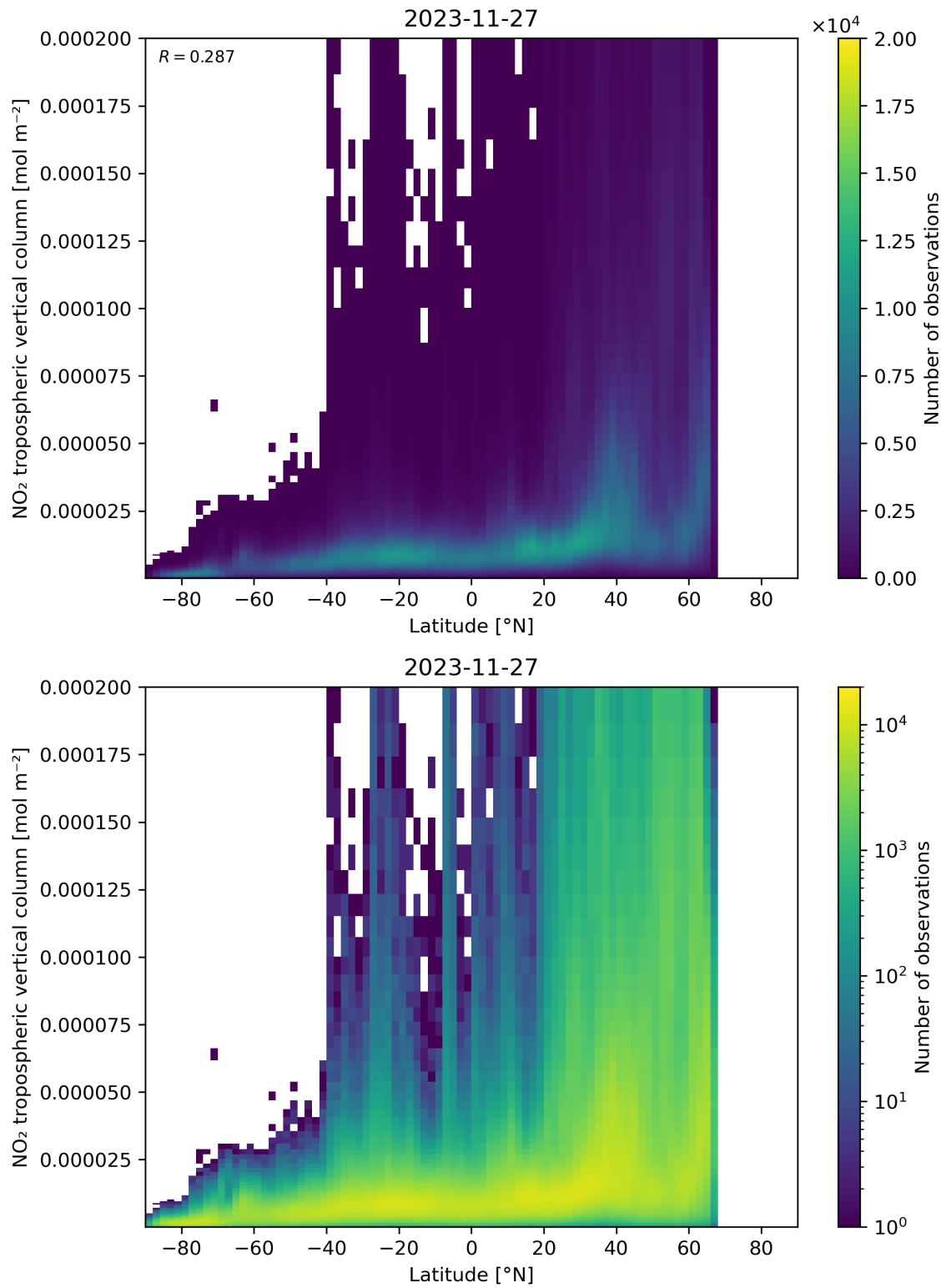
Figure 92: Scatter density plot of “Latitude” against “NO 2 tropospheric vertical column” for 2023-11-26 to 2023-11-28.
