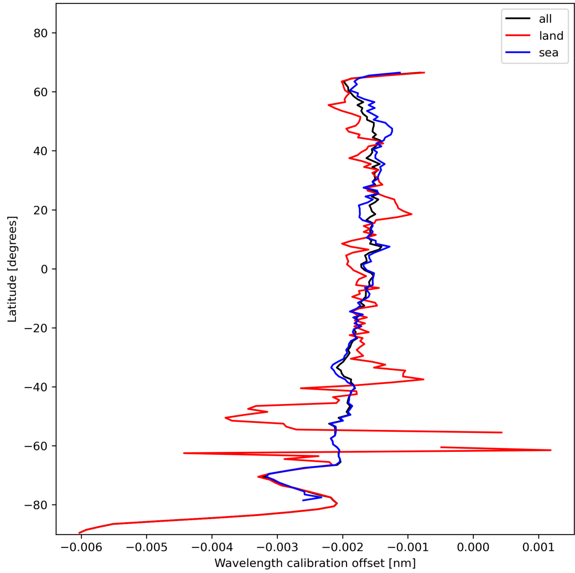
Figure 18: Zonal average of “Wavelength calibration offset” for 2023-11-26 to 2023-11-28.
