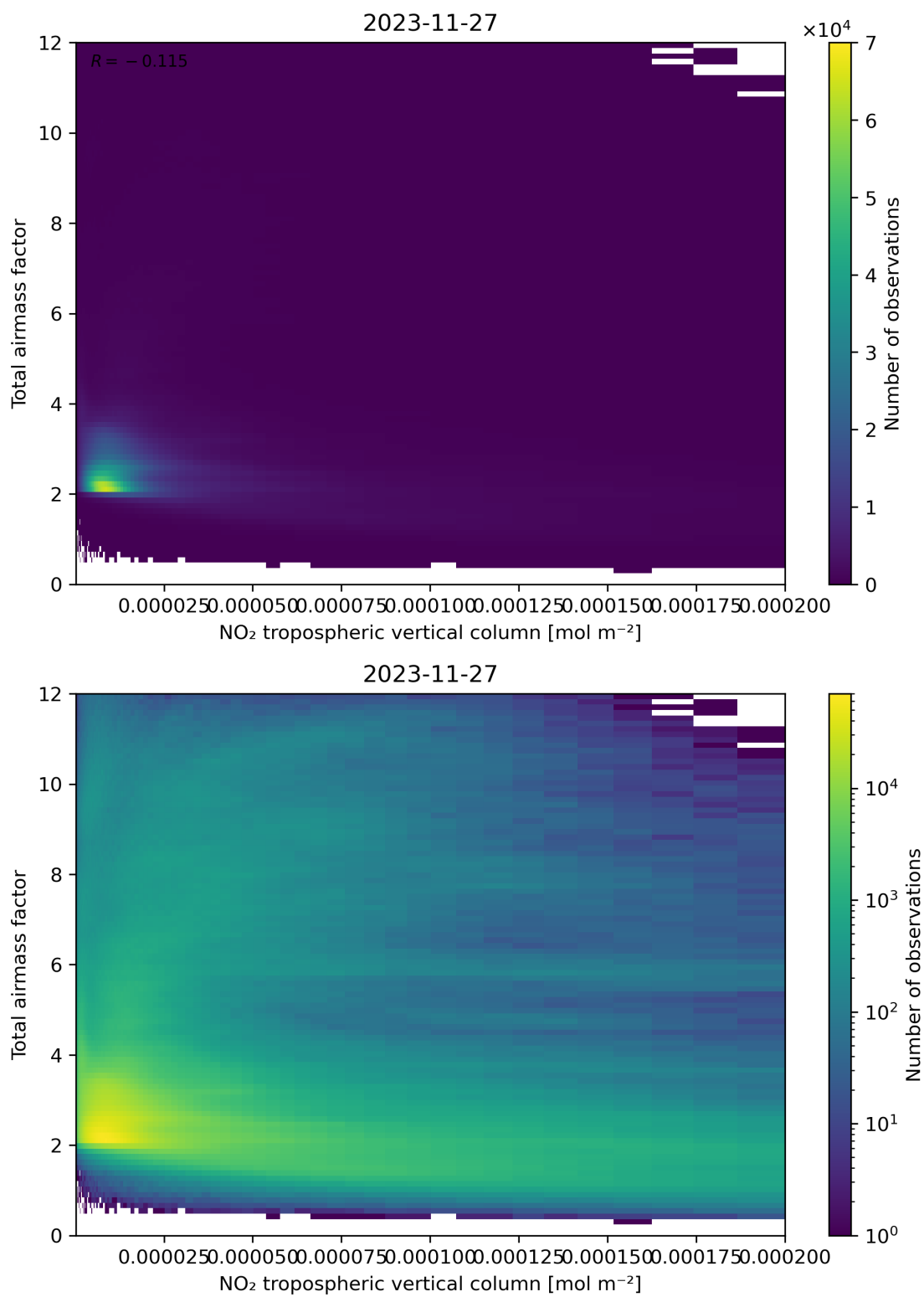
Figure 122: Scatter density plot of “NO 2 tropospheric vertical column” against “Total air mass factor” for 2023-11-26 to 2023-11-28.
