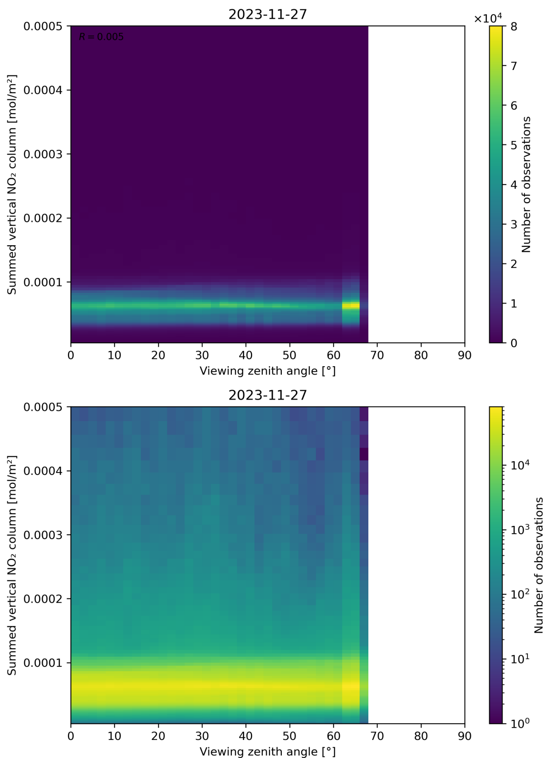
Figure 165: Scatter density plot of “Viewing zenith angle” against “Summed vertical NO 2 column” for 2023-11-26 to 2023-11-28.
