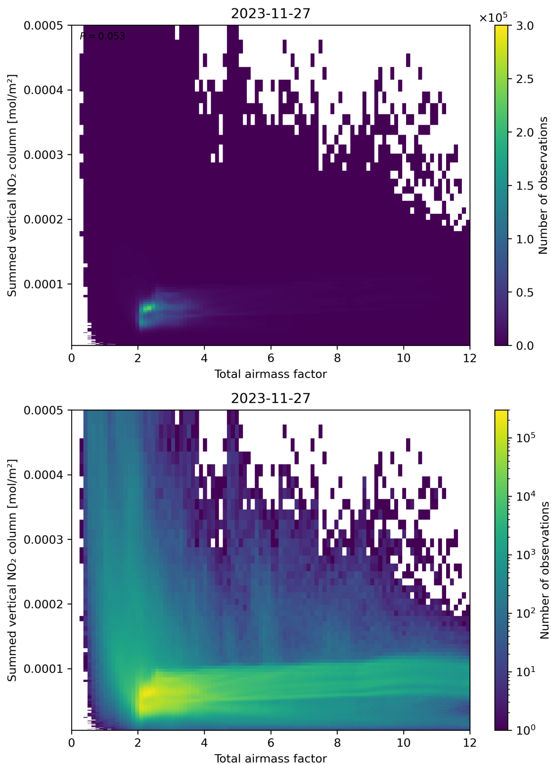
Figure 65: Scatter density plot of “Total airmass factor” against “Summed vertical NO 2 column” for 2023-11-26 to 2023-11-28.
