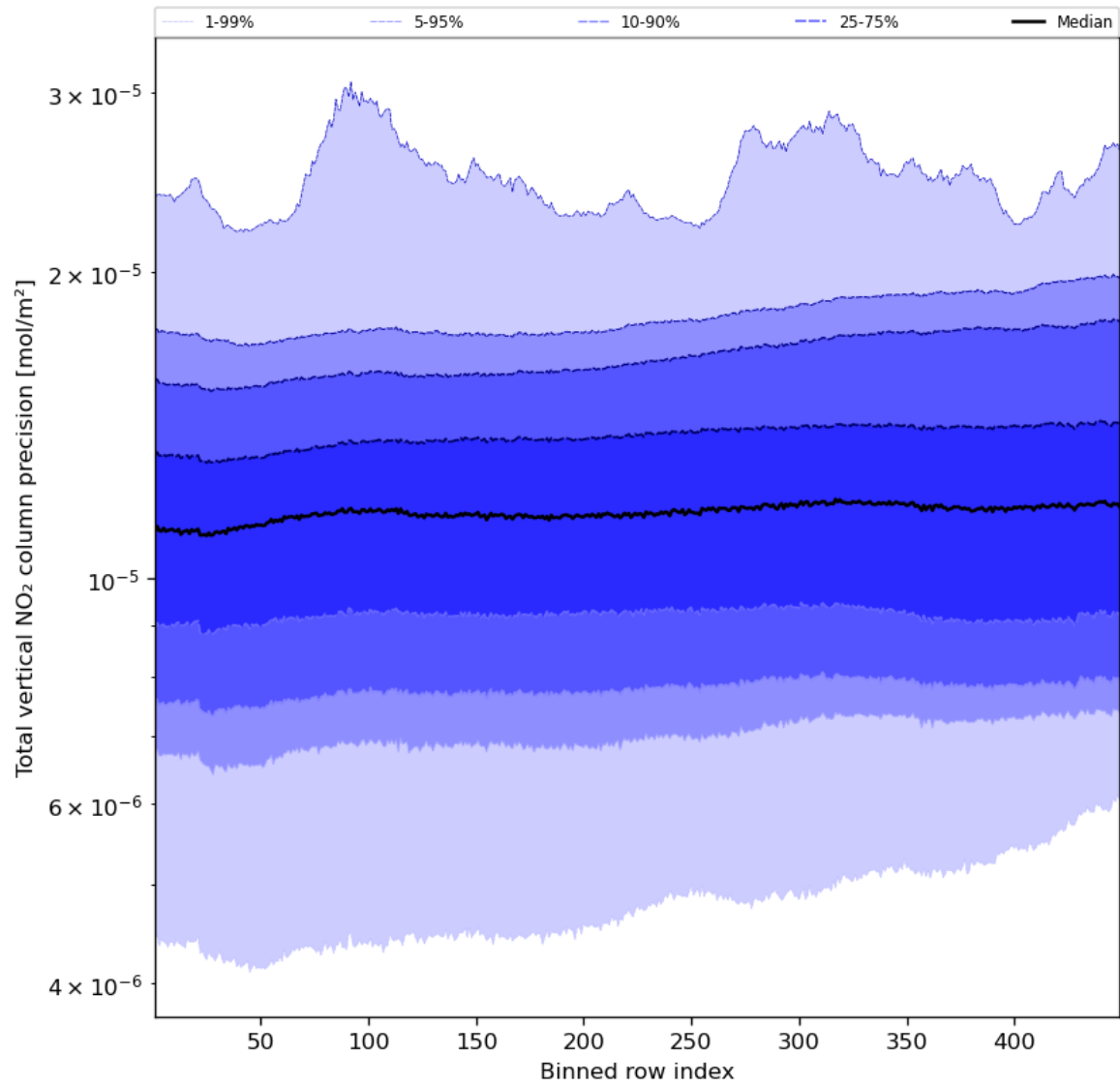
Figure 56: Along track statistics of "Total vertical NO 2 column precision" for 2023-11-26 to 2023-11-28
