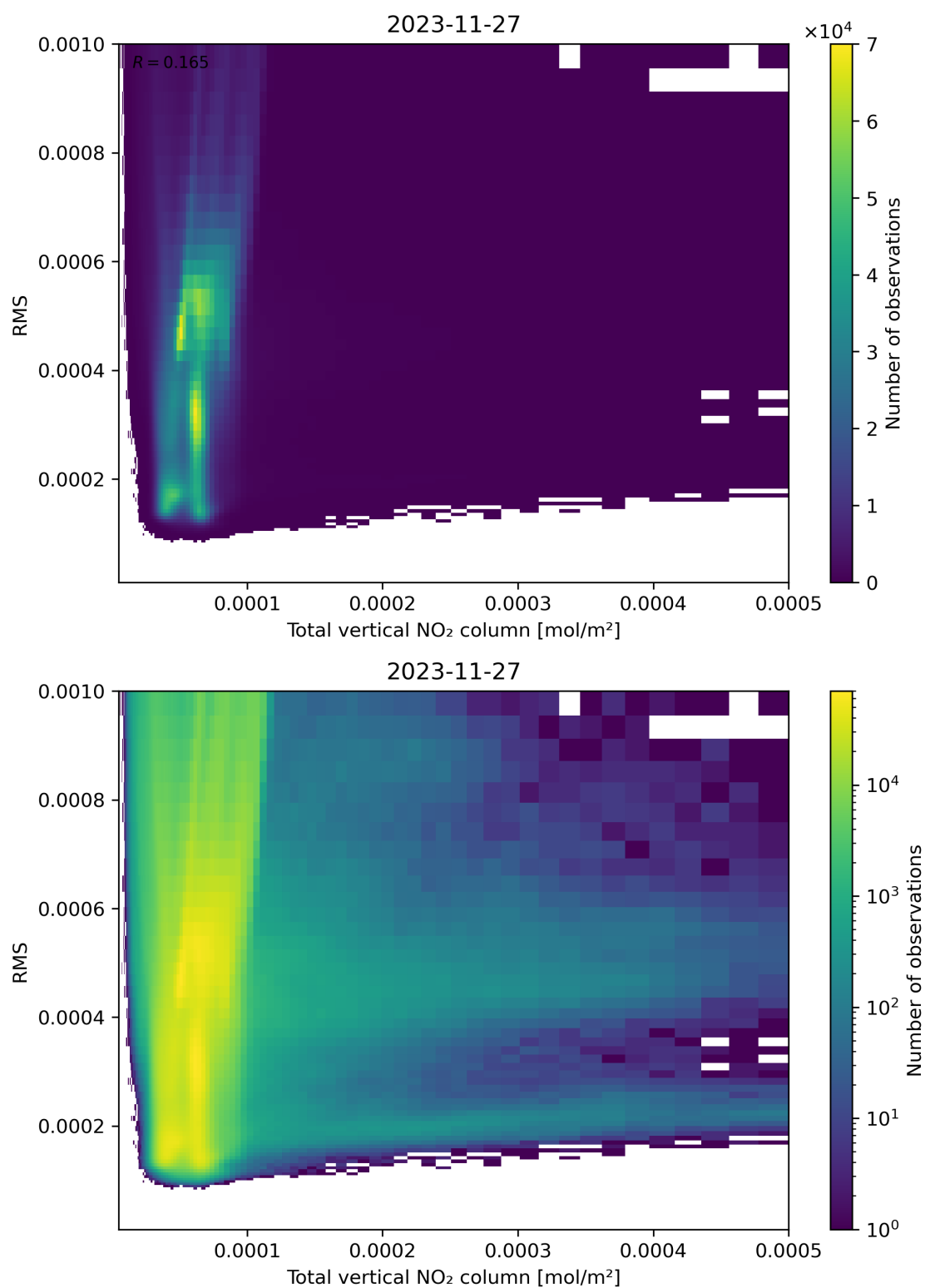
Figure 120: Scatter density plot of “Total vertical NO 2 column” against “RMS” for 2023-11-26 to 2023-11-28.
