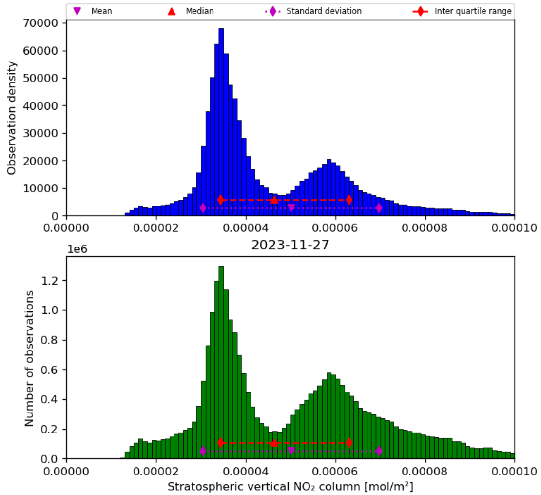
Figure 36: Histogram of “Stratospheric vertical NO 2 column” for 2023-11-26 to 2023-11-28
