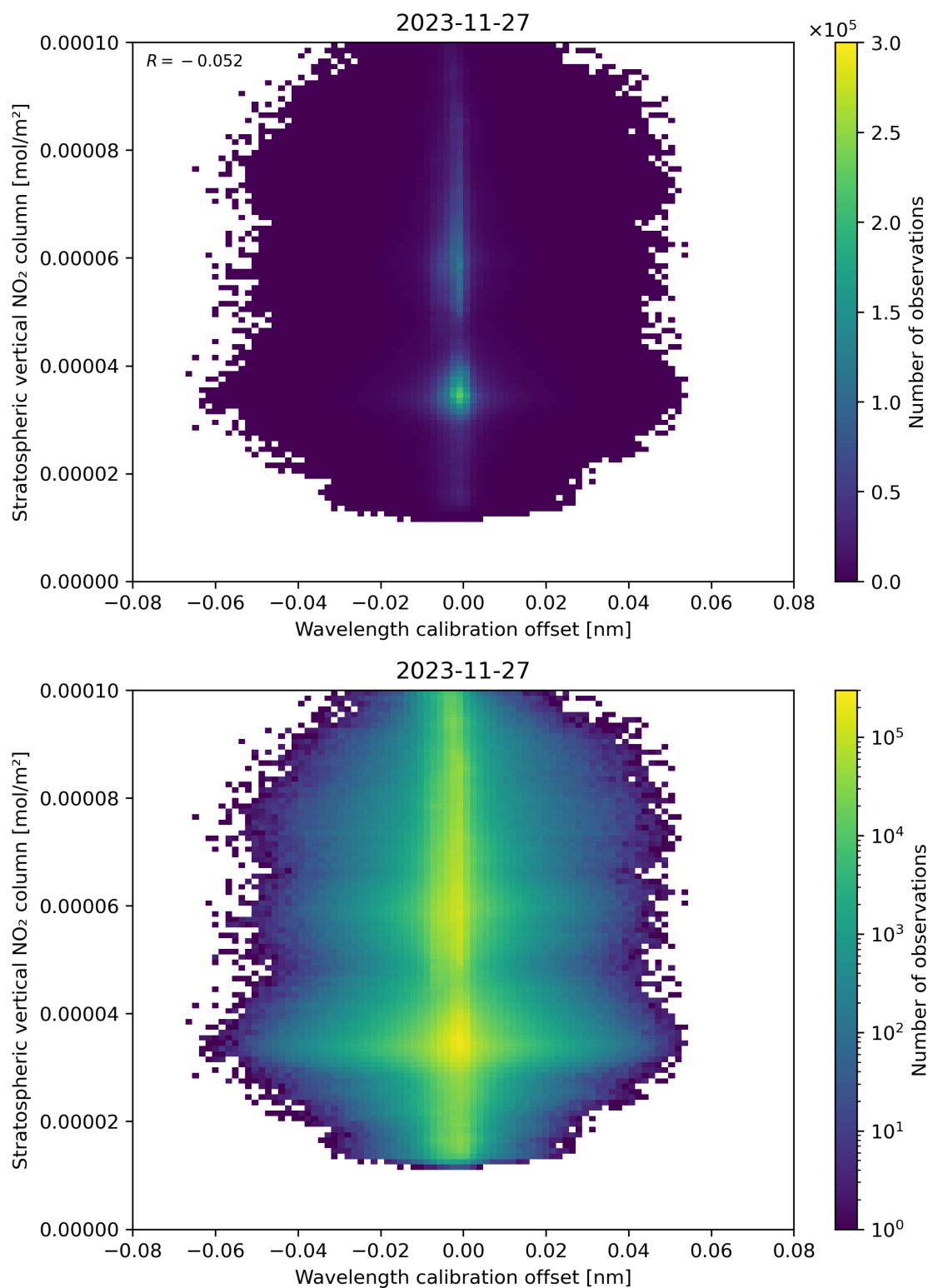
Figure 176: Scatter density plot of “Wavelength calibration offset” against “Stratospheric vertical NO 2 column” for 2023-11-26 to 2023-11-28.
