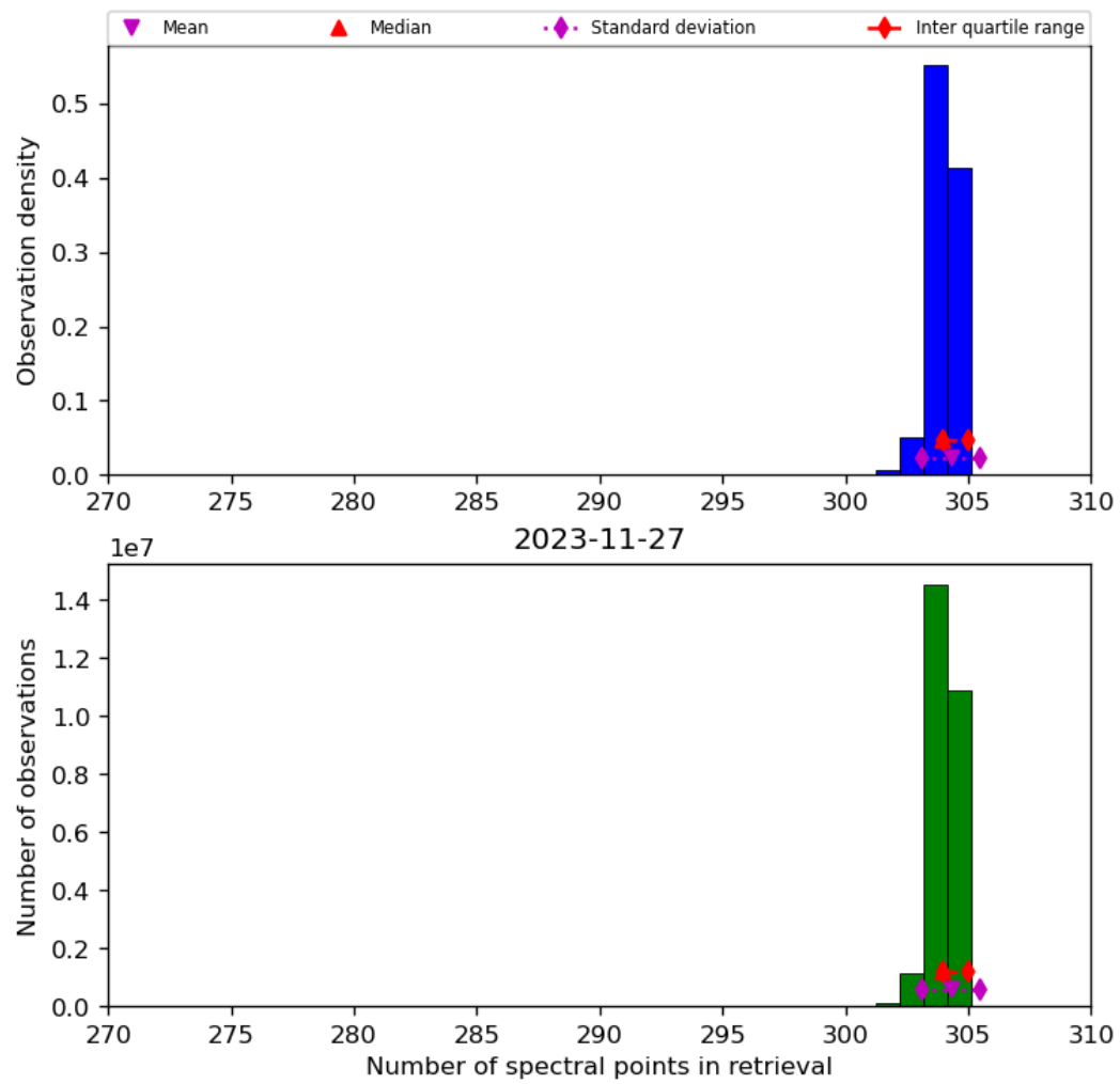
Figure 33: Histogram of “Number of spectral points in retrieval” for 2023-11-26 to 2023-11-28
