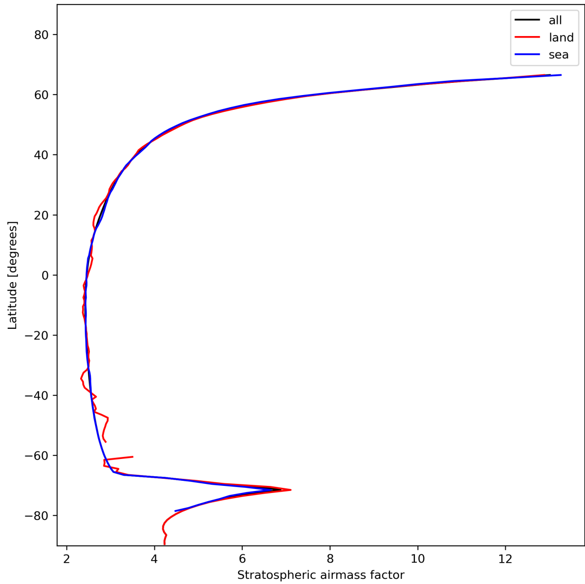
Figure 27: Zonal average of “Stratospheric airmass factor” for 2023-11-26 to 2023-11-28.
