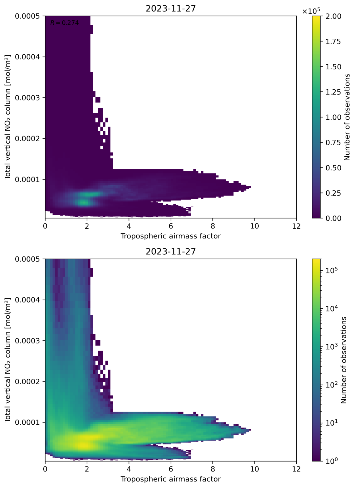
Figure 77: Scatter density plot of “Tropospheric airmass factor” against “Total vertical NO 2 column” for 2023-11-26 to 2023-11-28.
