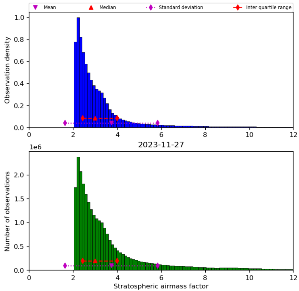
Figure 44: Histogram of “Stratospheric airmass factor” for 2023-11-26 to 2023-11-28
