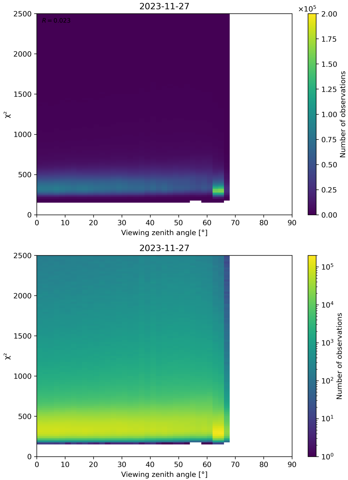
Figure 162: Scatter density plot of “Viewing zenith angle” against “ \chi^2 ” for 2023-11-26 to 2023-11-28.
