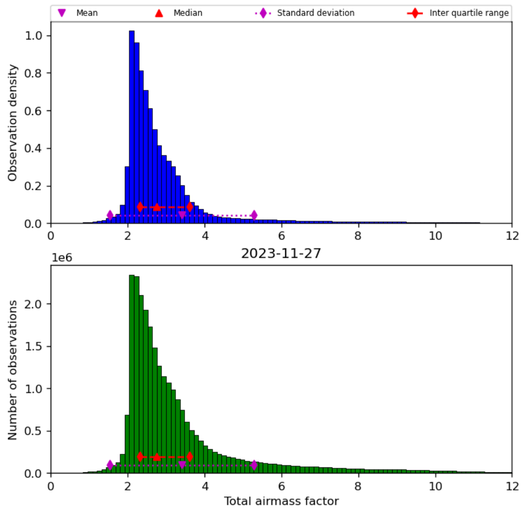
Figure 32: Histogram of “Total airmass factor” for 2023-11-26 to 2023-11-28
