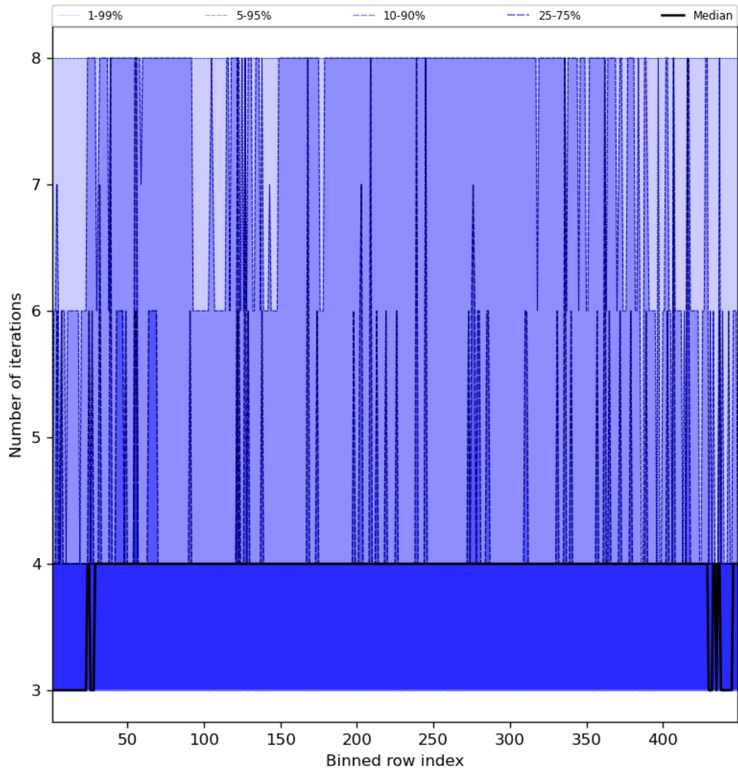
Figure 51: Along track statistics of “Number of iterations” for 2023-11-26 to 2023-11-28
