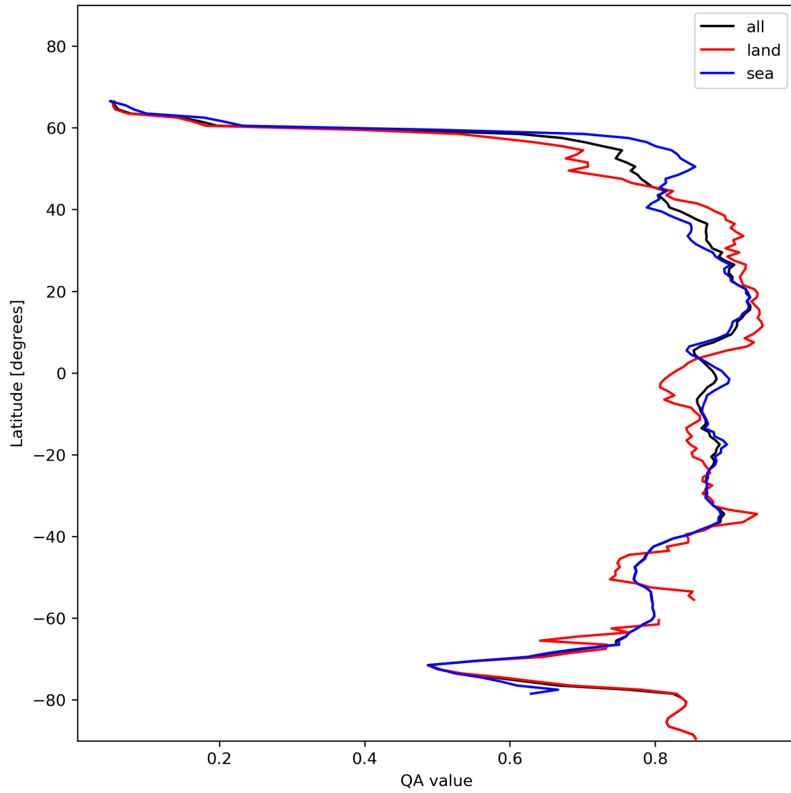
Figure 11: Zonal average of “QA value” for 2023-11-26 to 2023-11-28.
