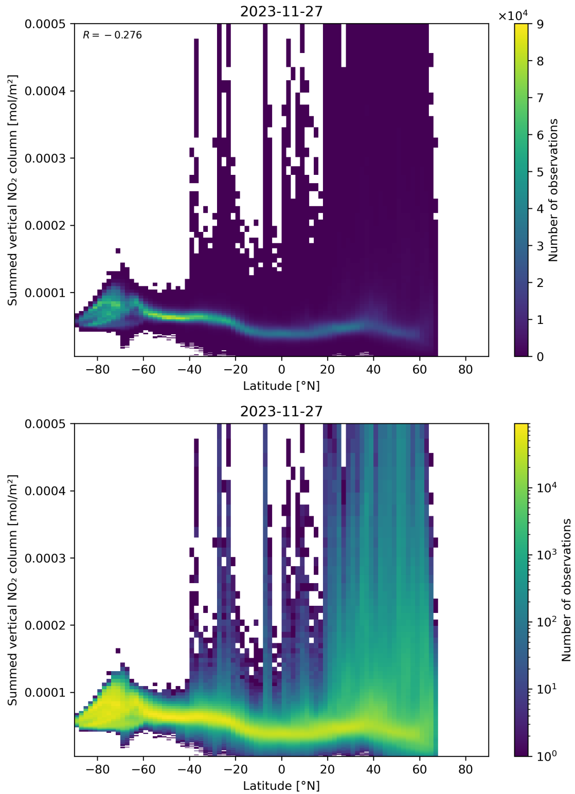
Figure 88: Scatter density plot of “Latitude” against “Summed vertical NO 2 column” for 2023-11-26 to 2023-11-28.
