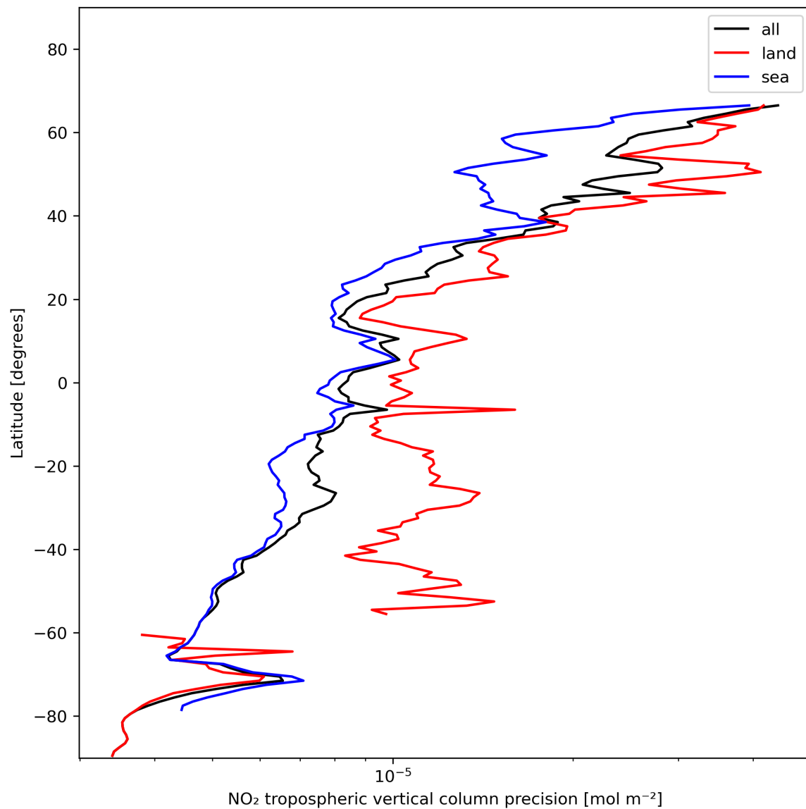
Figure 13: Zonal average of “NO 2 tropospheric vertical column precision” for 2023-11-26 to 2023-11-28.
