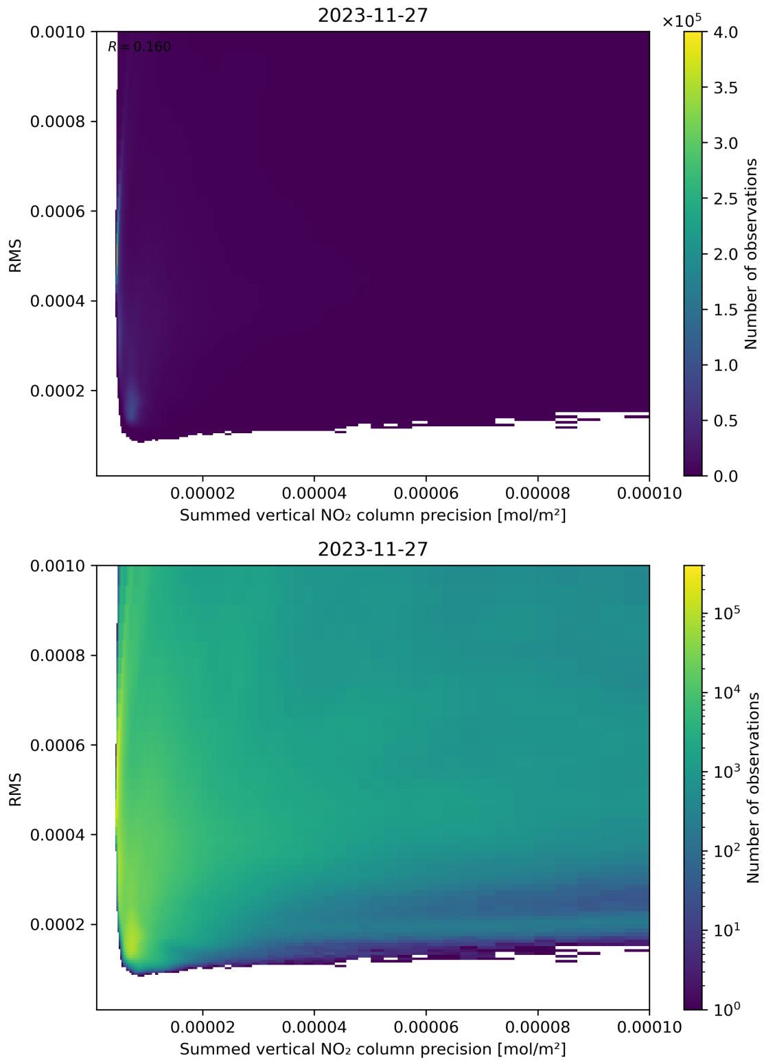
Figure 108: Scatter density plot of “Summed vertical NO 2 column precision” against “RMS” for 2023-11-26 to 2023-11-28.
