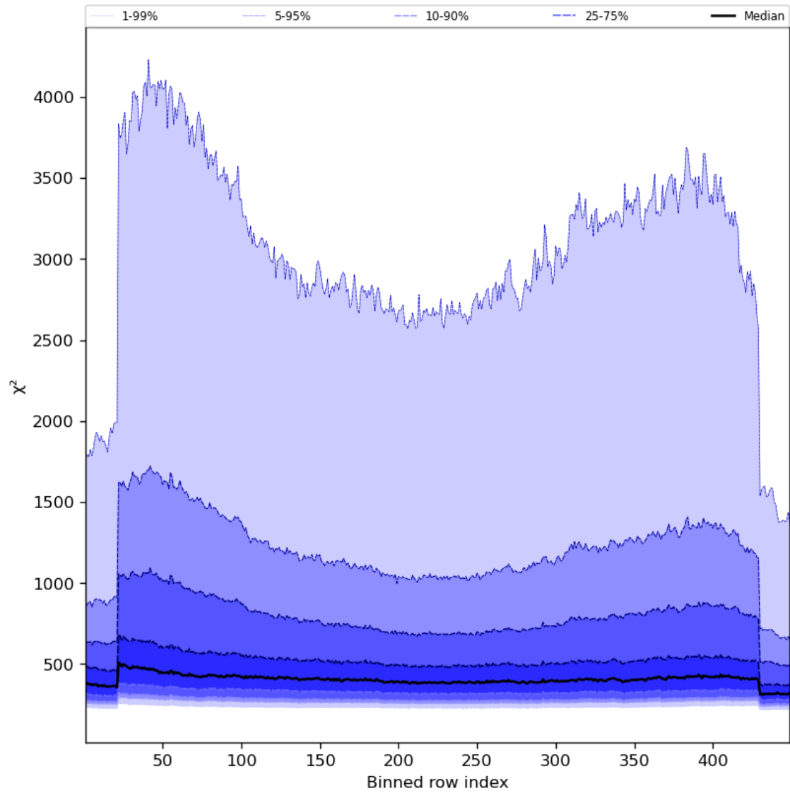
Figure 59: Along track statistics of “ \chi^2 ” for 2023-11-26 to 2023-11-28
