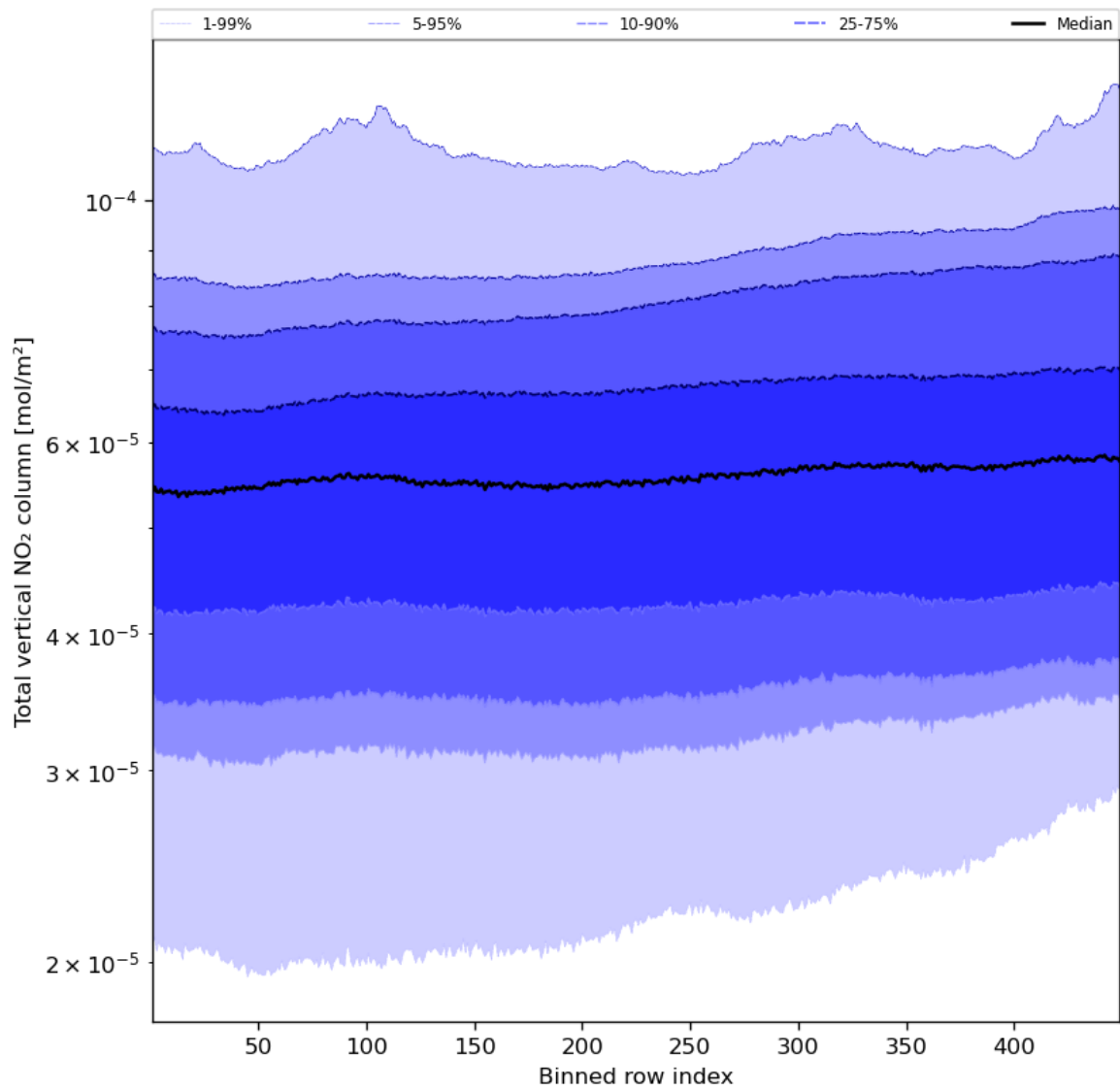
Figure 55: Along track statistics of “Total vertical NO 2 column” for 2023-11-26 to 2023-11-28
