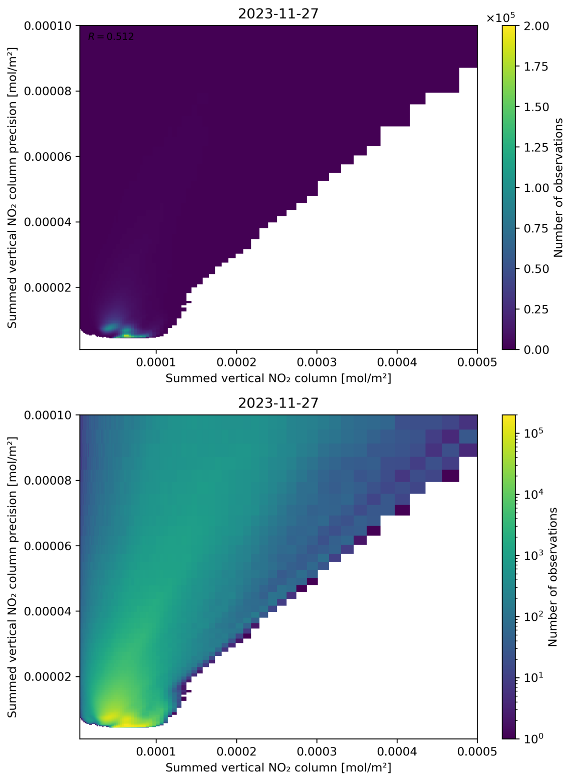
Figure 105: Scatter density plot of “Summed vertical NO 2 column” against “Summed vertical NO 2 column precision” for 2023-11-26 to 2023-11-28.
