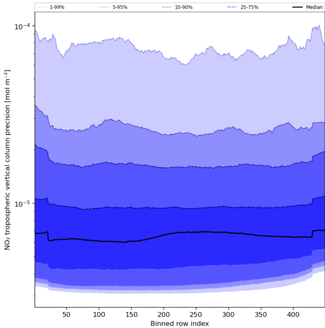
Figure 47: Along track statistics of “NO 2 tropospheric vertical column precision” for 2023-11-26 to 2023-11-28
