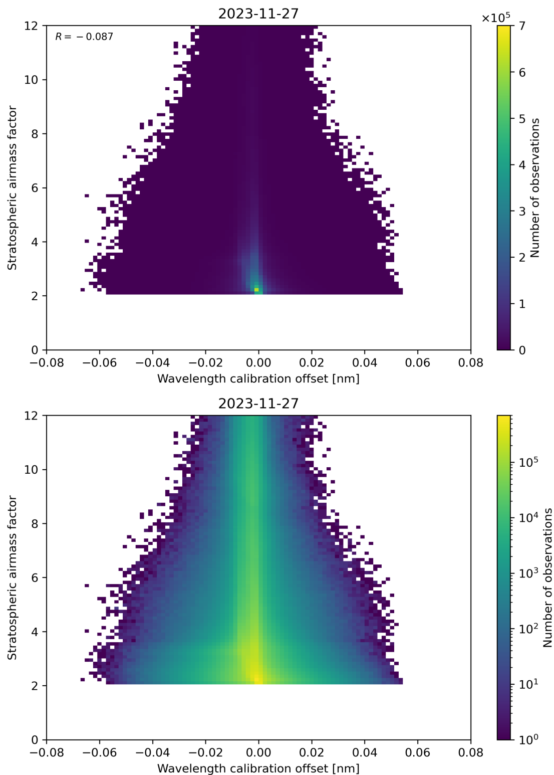
Figure 174: Scatter density plot of “Wavelength calibration offset” against “Stratospheric air mass factor” for 2023-11-26 to 2023-11-28.
