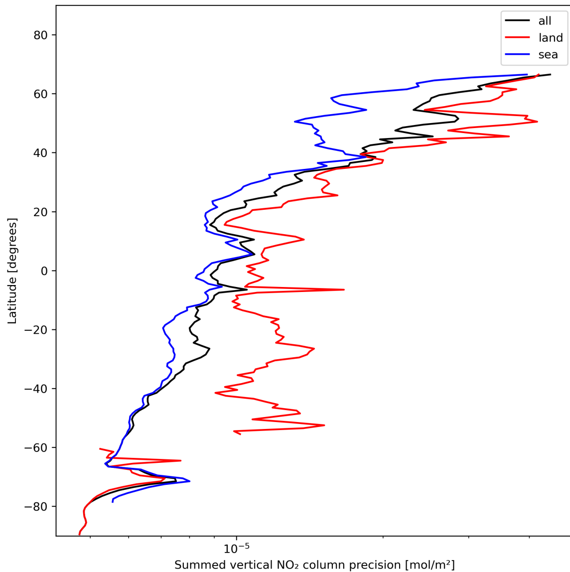
Figure 24: Zonal average of “Summed vertical NO 2 column precision” for 2023-11-26 to 2023-11-28.
