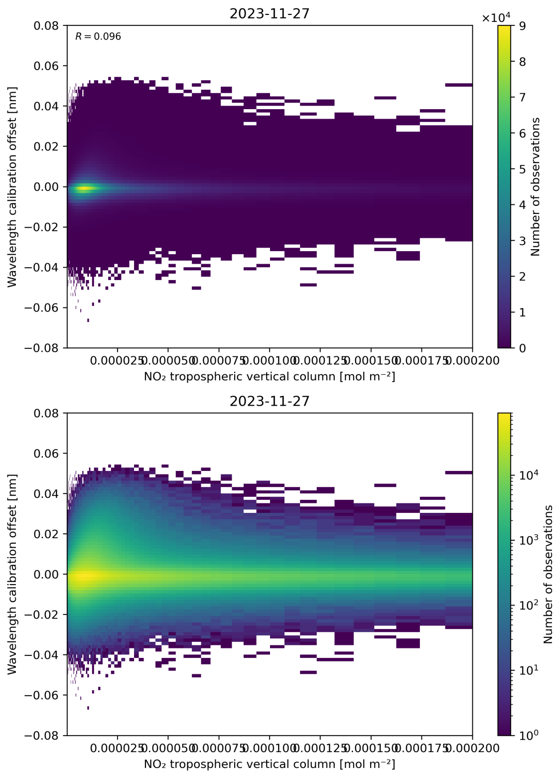
Figure 143: Scatter density plot of “NO 2 tropospheric vertical column” against “Wavelength calibration offset” for 2023-11-26 to 2023-11-28.
