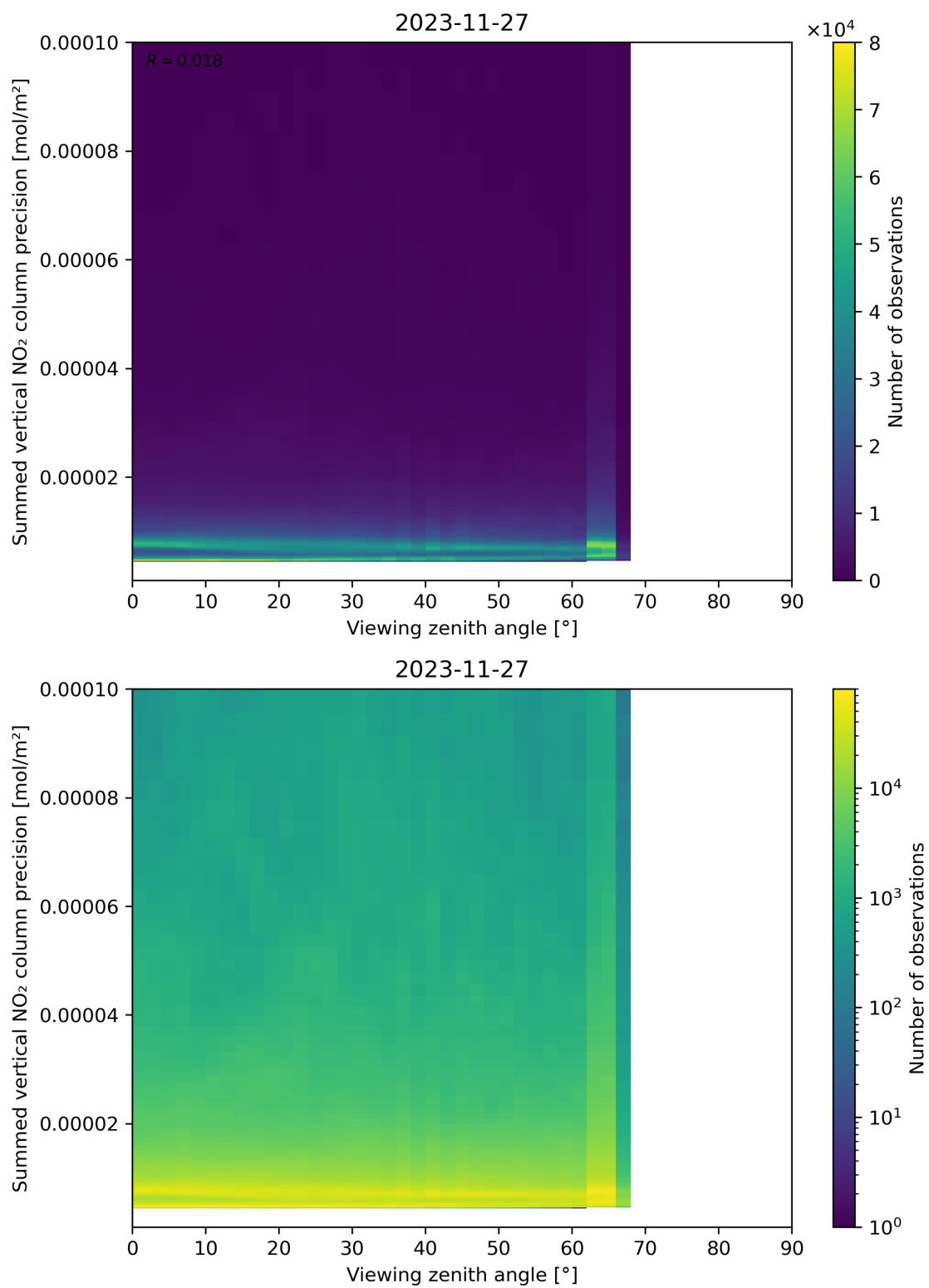
Figure 166: Scatter density plot of “Viewing zenith angle” against “Summed vertical NO 2 column precision” for 2023-11-26 to 2023-11-28.
