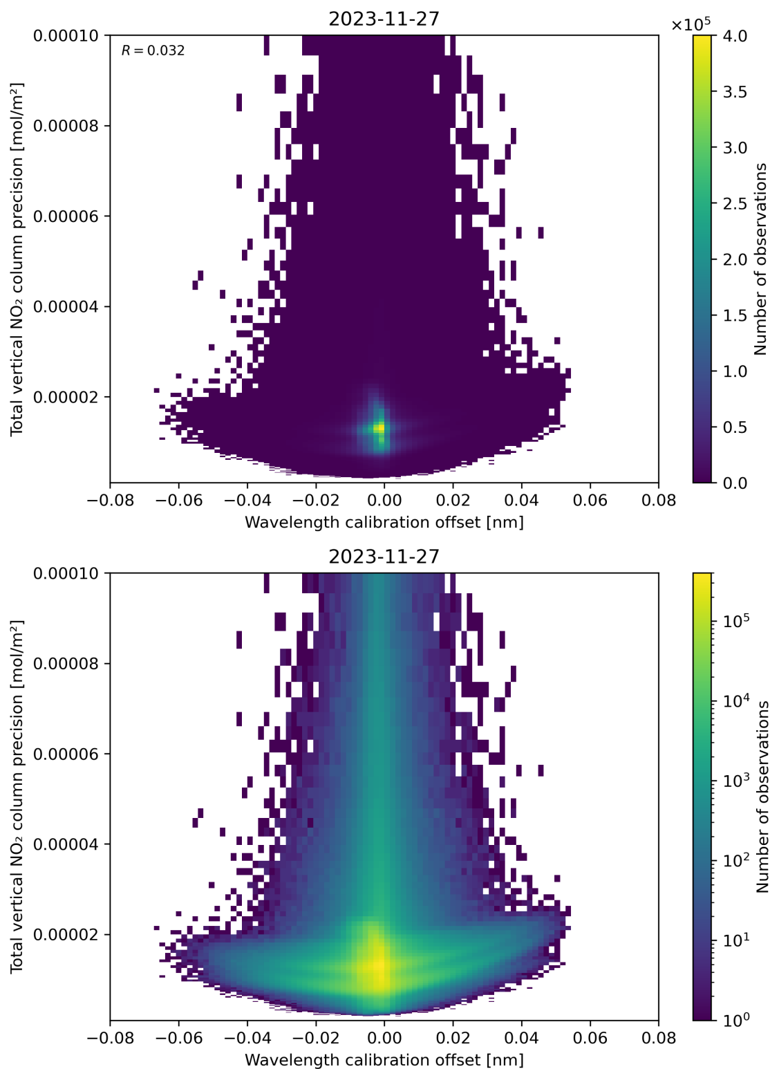
Figure 180: Scatter density plot of “Wavelength calibration offset” against “Total vertical NO 2 column precision” for 2023-11-26 to 2023-11-28.
