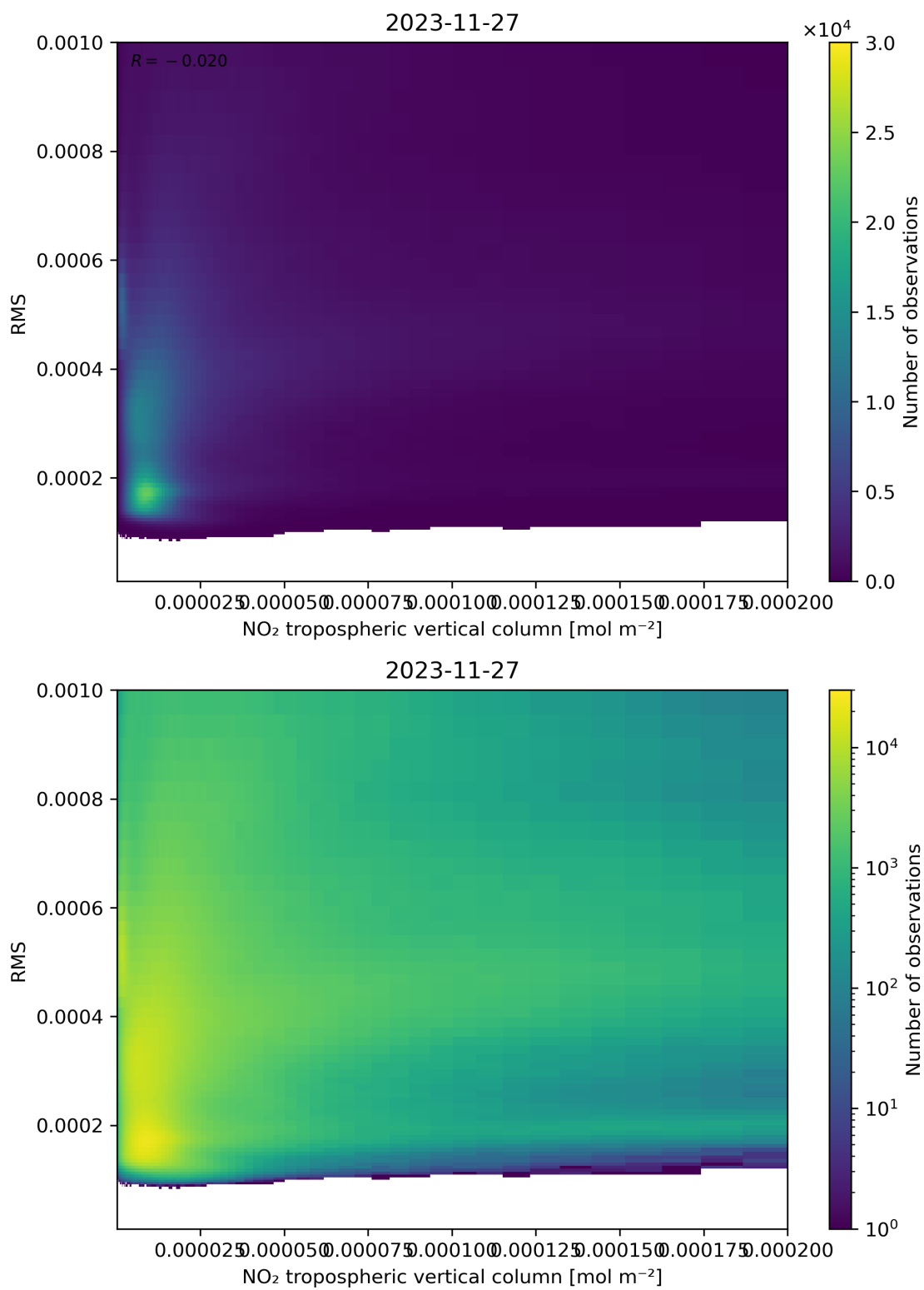
Figure 142: Scatter density plot of “NO 2 tropospheric vertical column” against “RMS” for 2023-11-26 to 2023-11-28.
