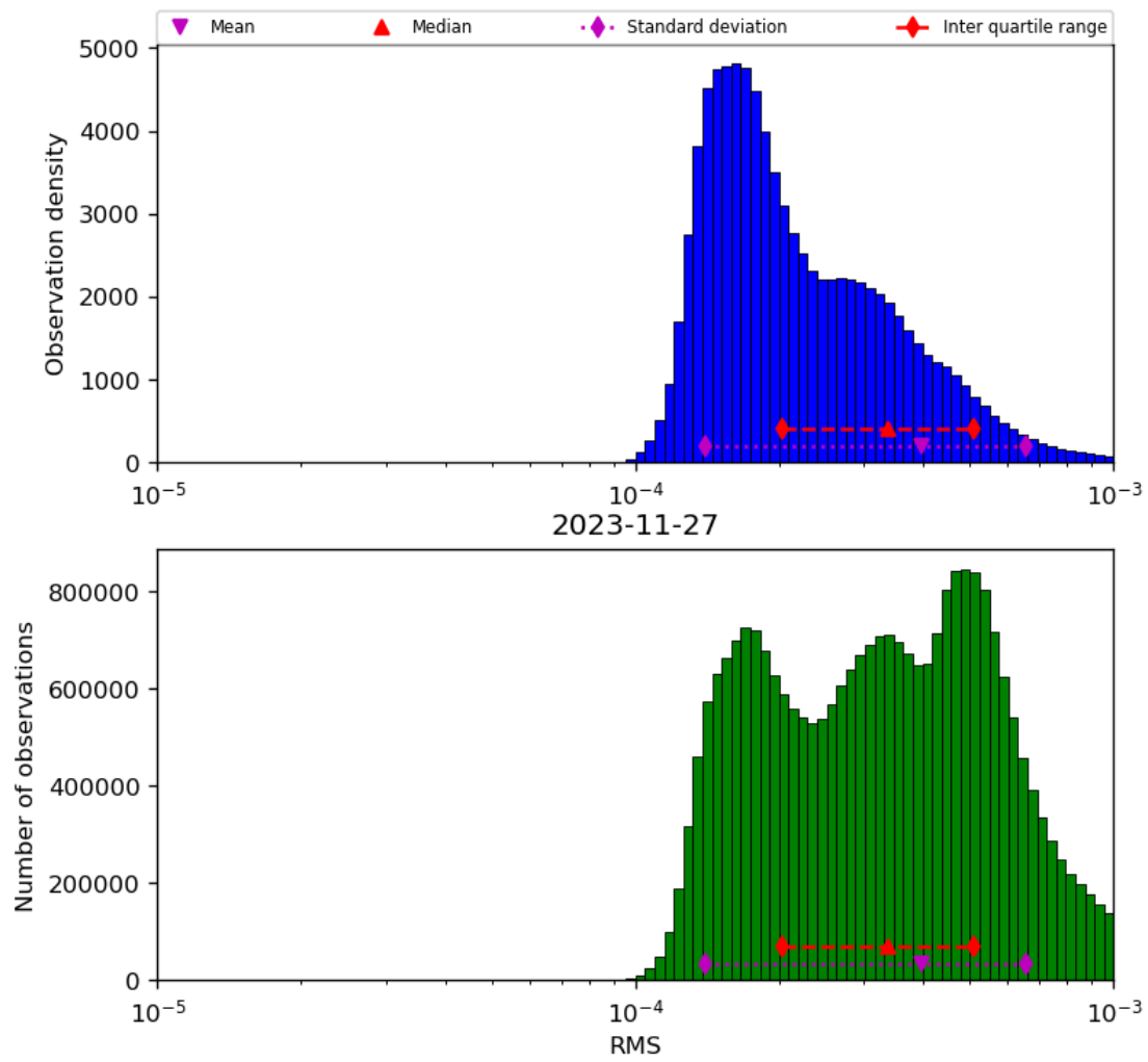
Figure 43: Histogram of “RMS” for 2023-11-26 to 2023-11-28
