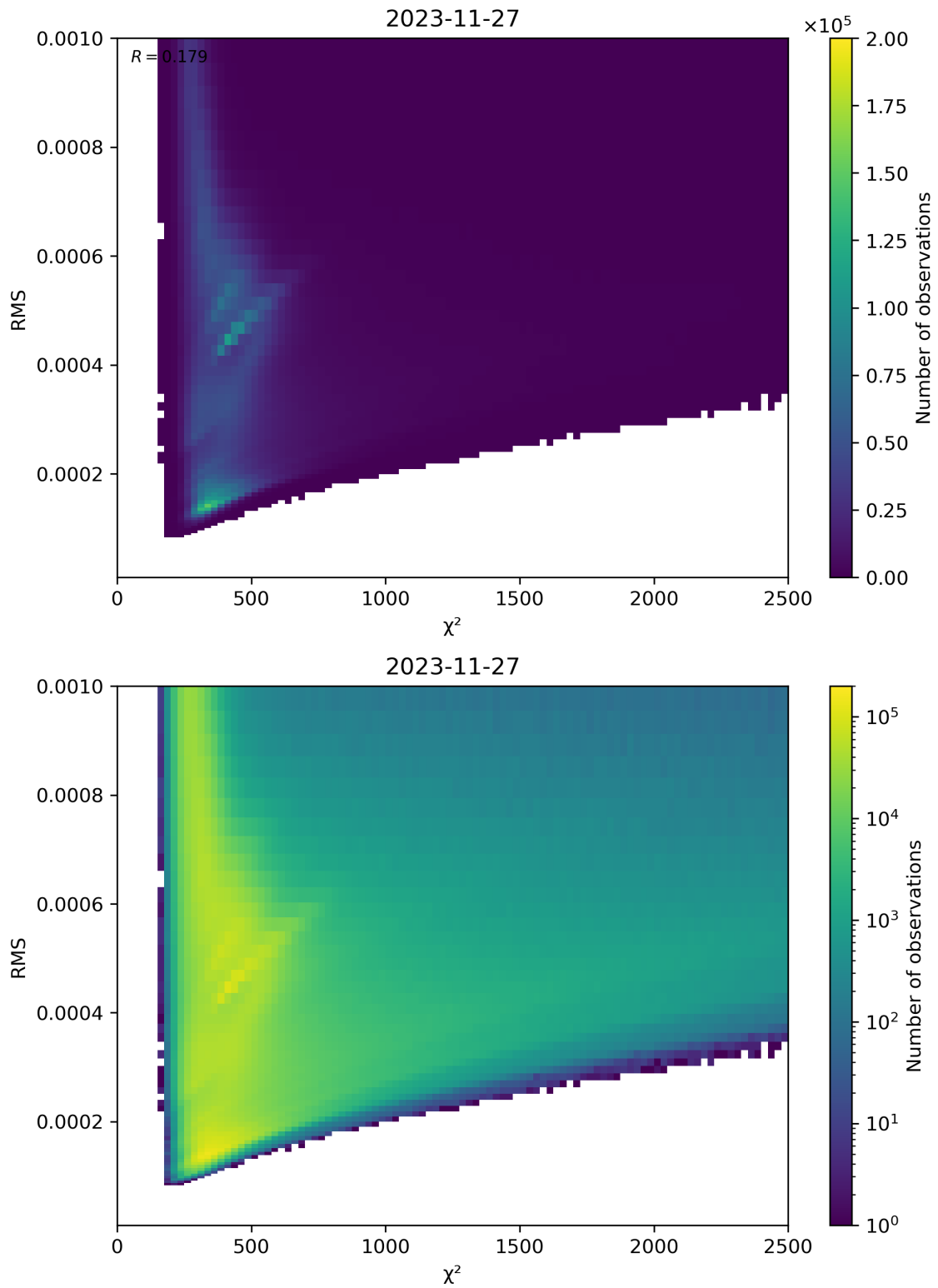
Figure 82: Scatter density plot of “ \chi^2 ” against “RMS” for 2023-11-26 to 2023-11-28.
