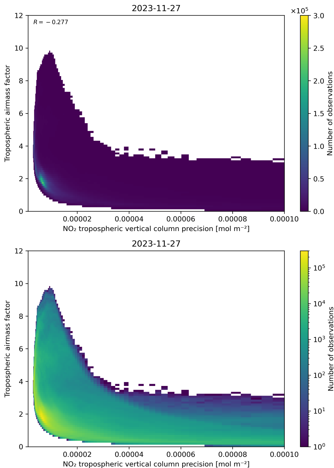
Figure 133: Scatter density plot of “NO 2 tropospheric vertical column precision” against “Tropospheric airmass factor” for 2023-11-26 to 2023-11-28.
