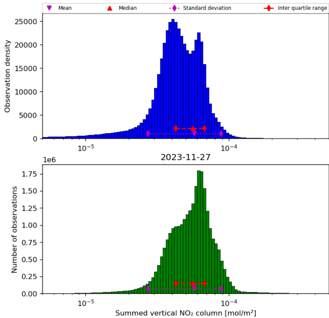
Figure 40: Histogram of “Summed vertical NO 2 column” for 2023-11-26 to 2023-11-28
