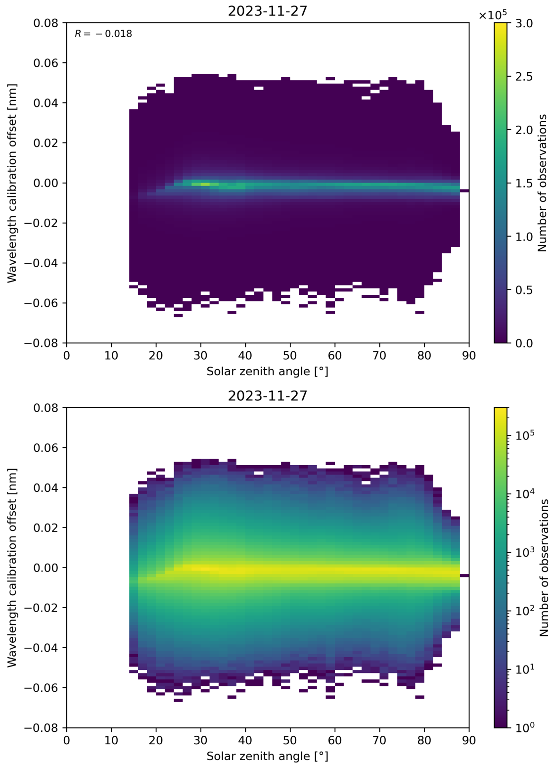
Figure 158: Scatter density plot of “Solar zenith angle” against “Wavelength calibration offset” for 2023-11-26 to 2023-11-28.
