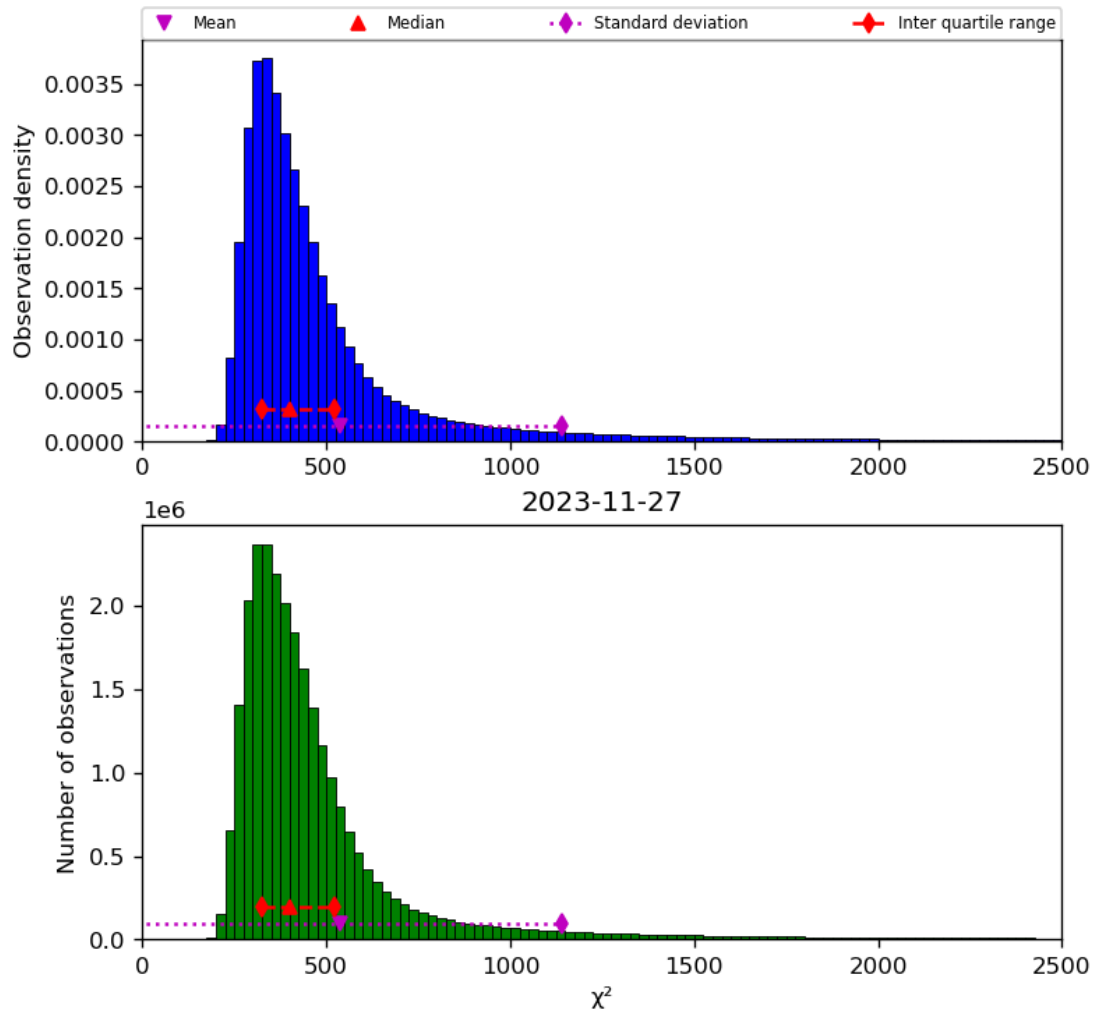
Figure 42: Histogram of “ \chi^2 ” for 2023-11-26 to 2023-11-28
