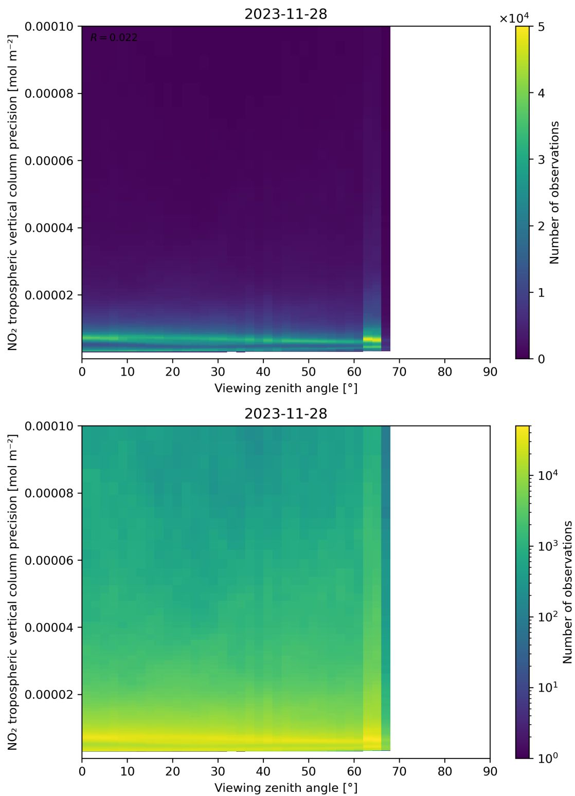
Figure 170: Scatter density plot of “Viewing zenith angle” against “NO 2 tropospheric vertical column precision” for 2023-11-28 to 2023-11-29.
