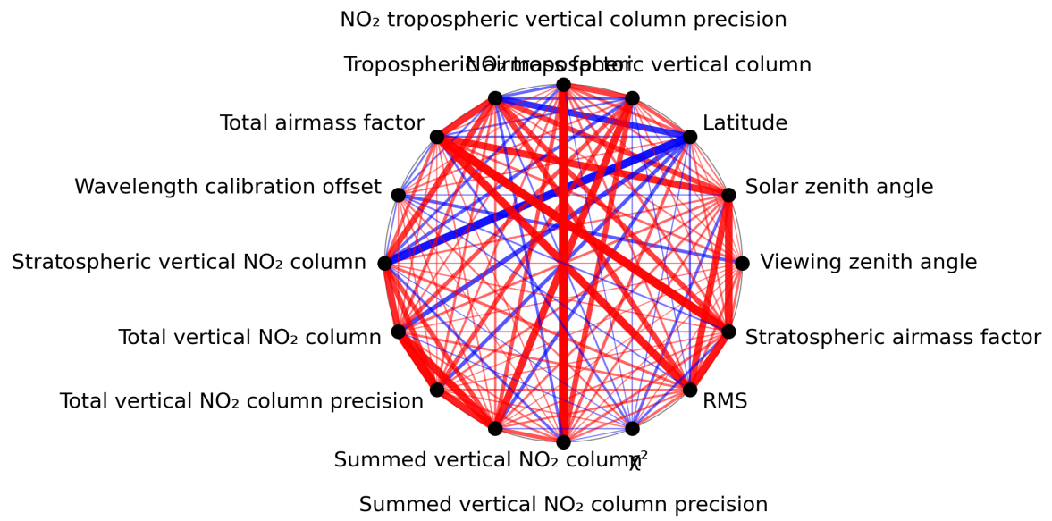
Figure 1: Map of correlation graph for 2023-11-28 to 2023-11-29.
