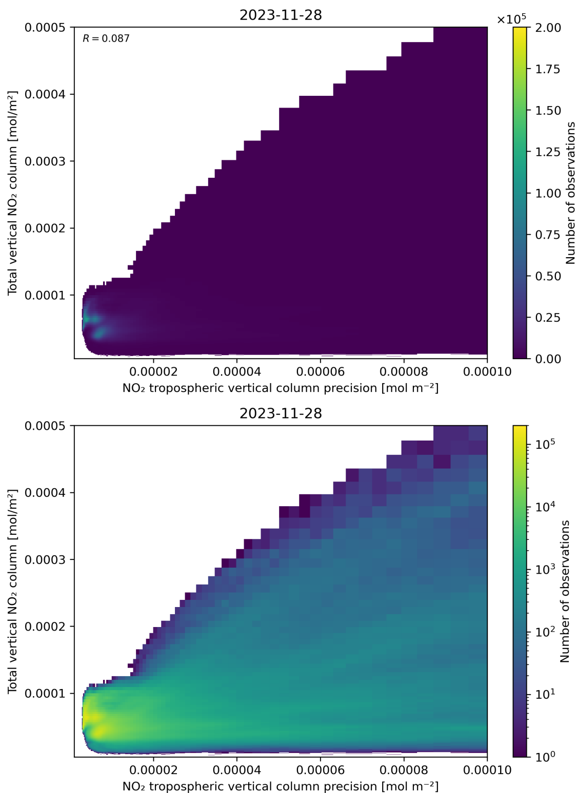
Figure 138: Scatter density plot of “NO 2 tropospheric vertical column precision” against “Total vertical NO 2 column” for 2023-11-28 to 2023-11-29.
