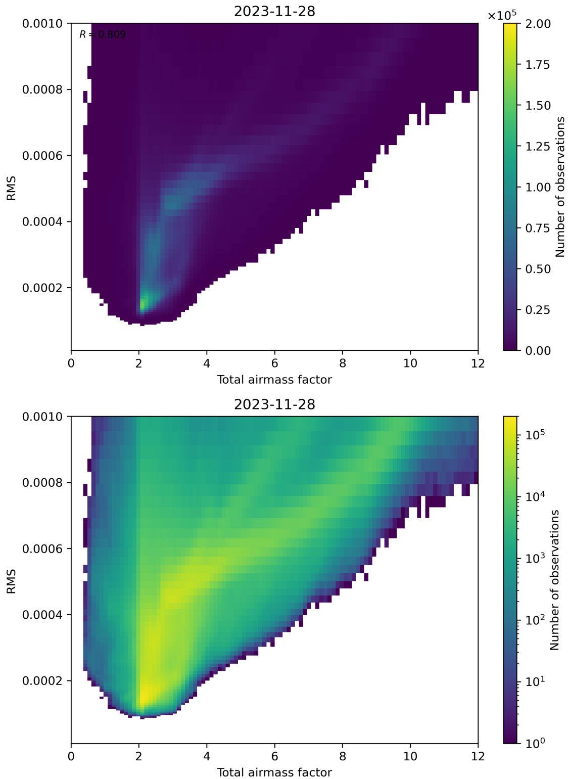
Figure 69: Scatter density plot of “Total airmass factor” against “RMS” for 2023-11-28 to 2023-11-29.
