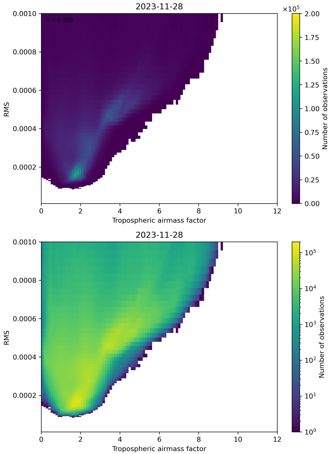
Figure 79: Scatter density plot of “Tropospheric airmass factor” against “RMS” for 2023-11-28 to 2023-11-29.
