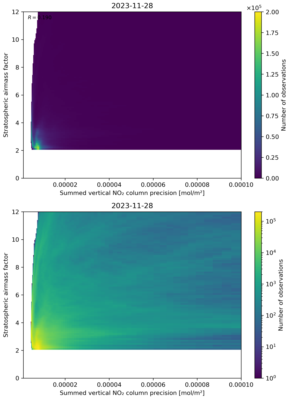
Figure 106: Scatter density plot of “Summed vertical NO 2 column precision” against “Stratospheric airmass factor” for 2023-11-28 to 2023-11-29.
