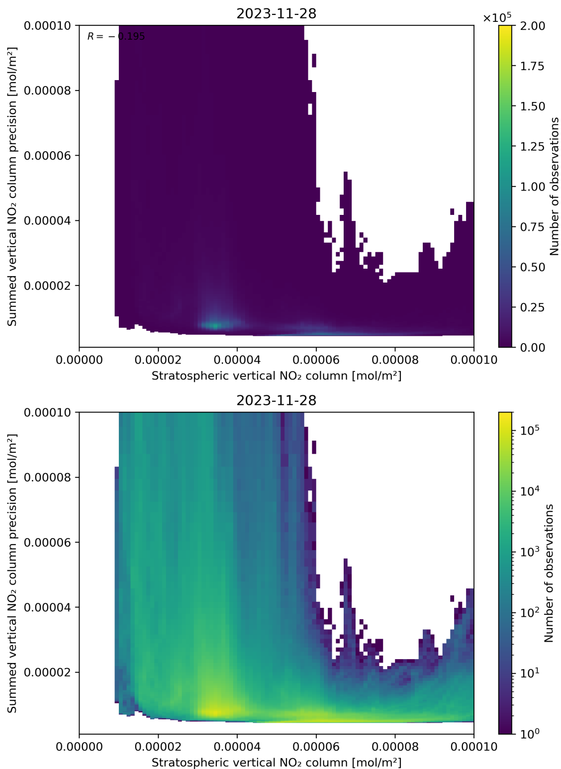
Figure 99: Scatter density plot of “Stratospheric vertical NO 2 column” against “Summed vertical NO 2 column precision” for 2023-11-28 to 2023-11-29.
