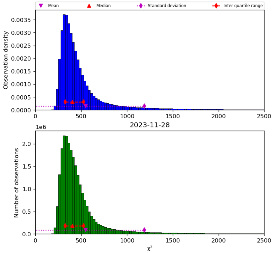
Figure 42: Histogram of “ \chi^2 ” for 2023-11-28 to 2023-11-29
