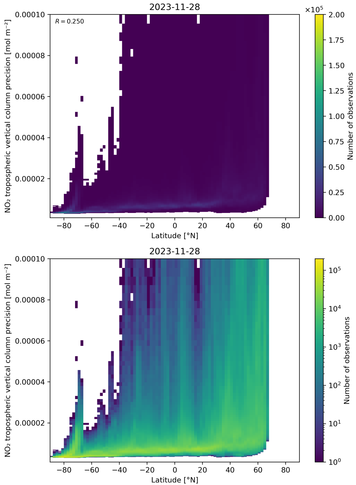
Figure 93: Scatter density plot of “Latitude” against “NO 2 tropospheric vertical column precision” for 2023-11-28 to 2023-11-29.
