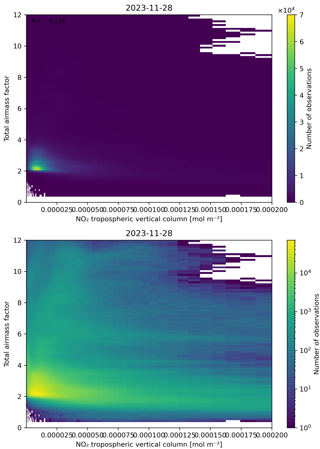
Figure 122: Scatter density plot of “NO 2 tropospheric vertical column” against “Total air mass factor” for 2023-11-28 to 2023-11-29.
