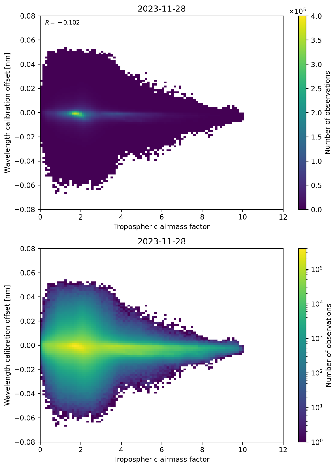
Figure 80: Scatter density plot of “Tropospheric airmass factor” against “Wavelength calibration offset” for 2023-11-28 to 2023-11-29.
