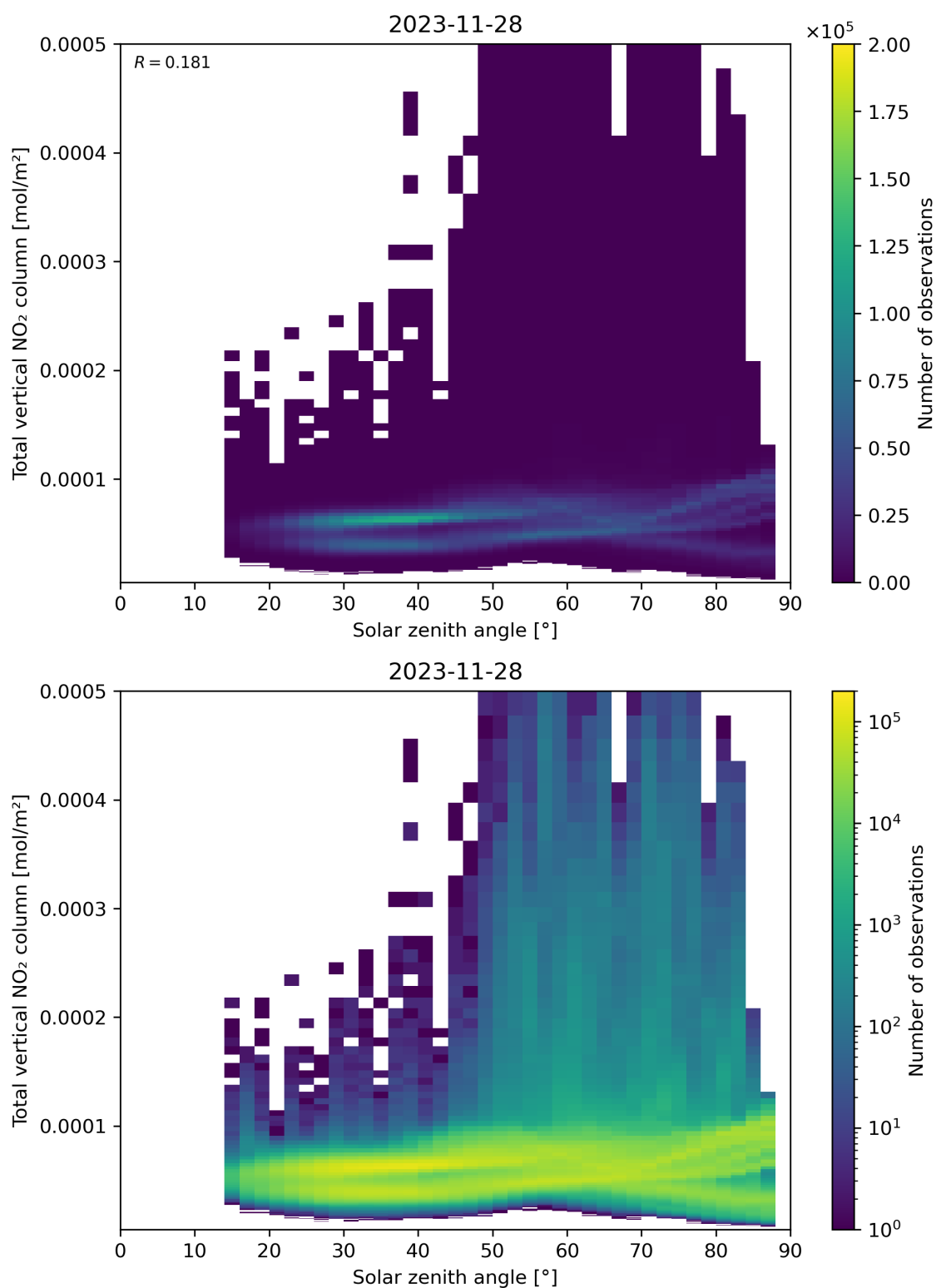
Figure 153: Scatter density plot of “Solar zenith angle” against “Total vertical NO 2 column” for 2023-11-28 to 2023-11-29.
