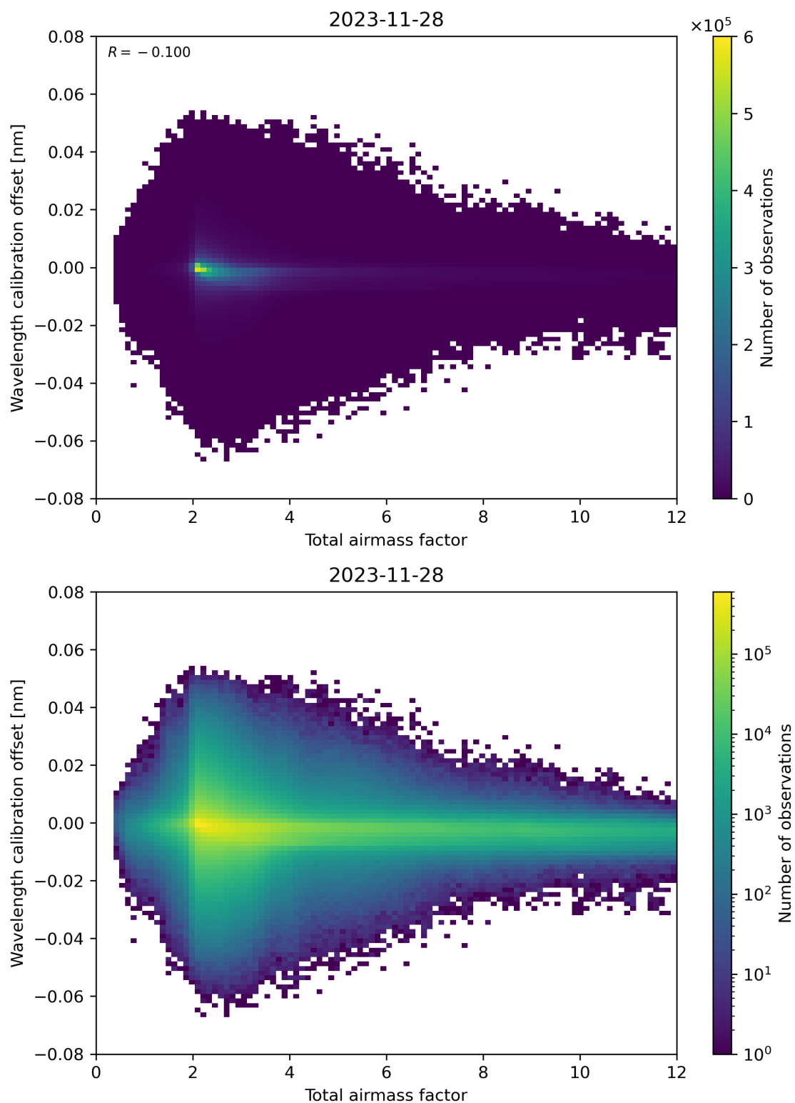
Figure 70: Scatter density plot of “Total airmass factor” against “Wavelength calibration offset” for 2023-11-28 to 2023-11-29.
