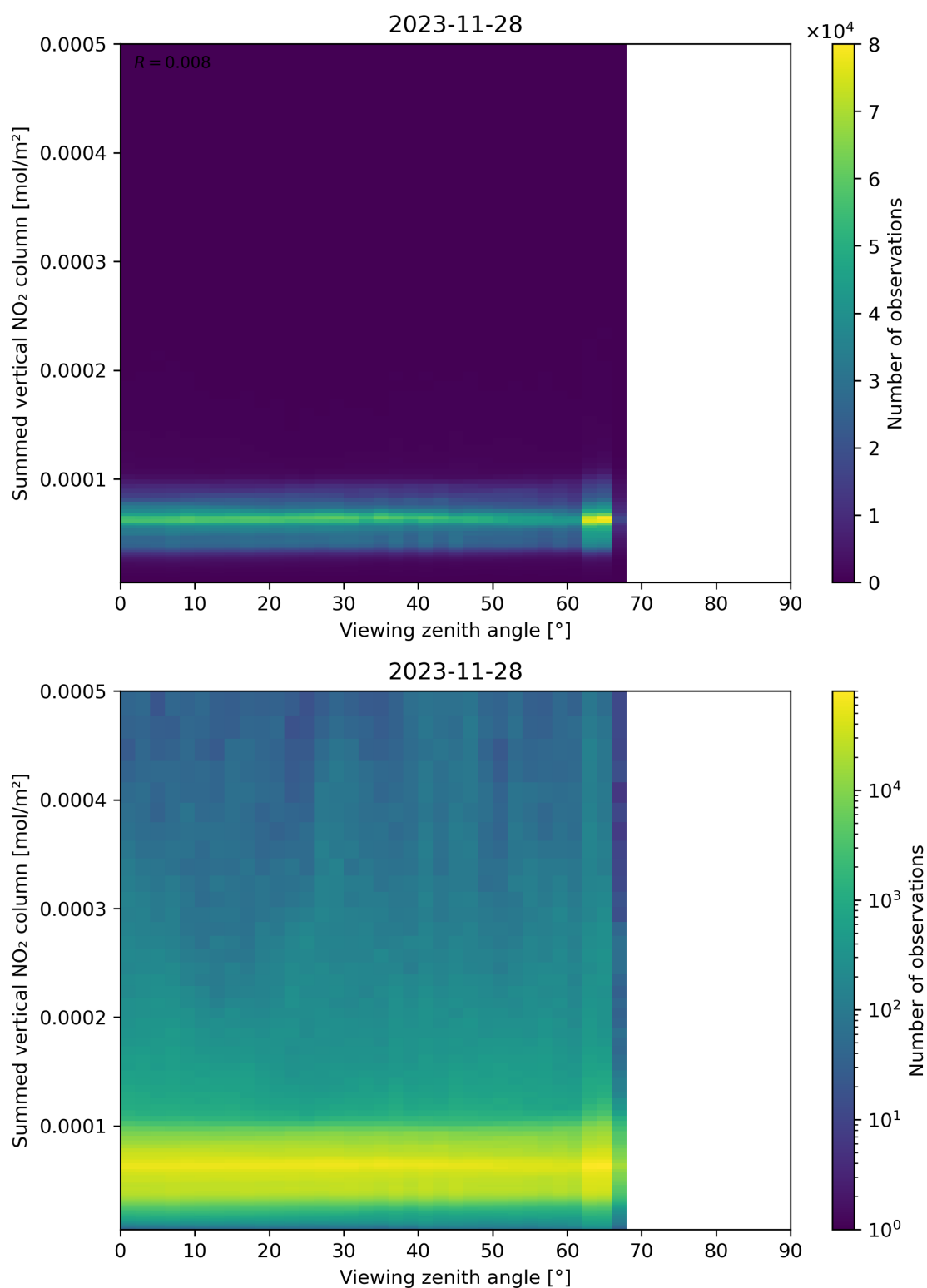
Figure 165: Scatter density plot of “Viewing zenith angle” against “Summed vertical NO 2 column” for 2023-11-28 to 2023-11-29.
