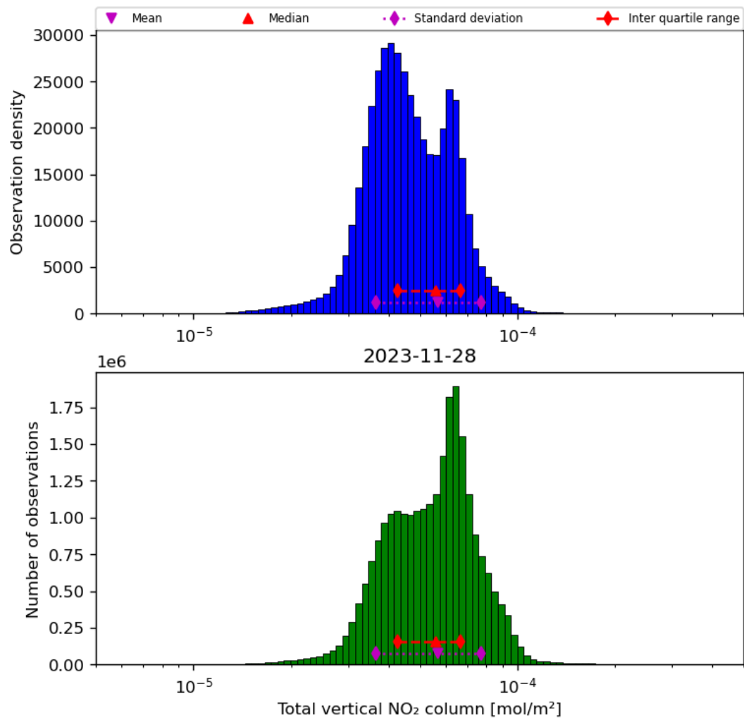
Figure 38: Histogram of “Total vertical NO 2 column” for 2023-11-28 to 2023-11-29
