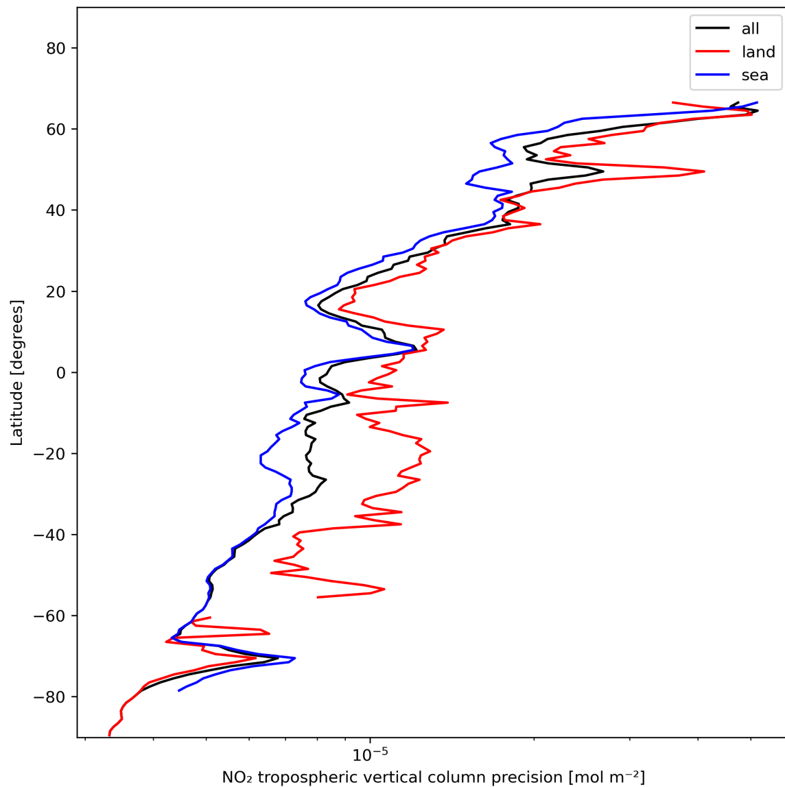
Figure 13: Zonal average of “NO 2 tropospheric vertical column precision” for 2023-11-28 to 2023-11-29.
