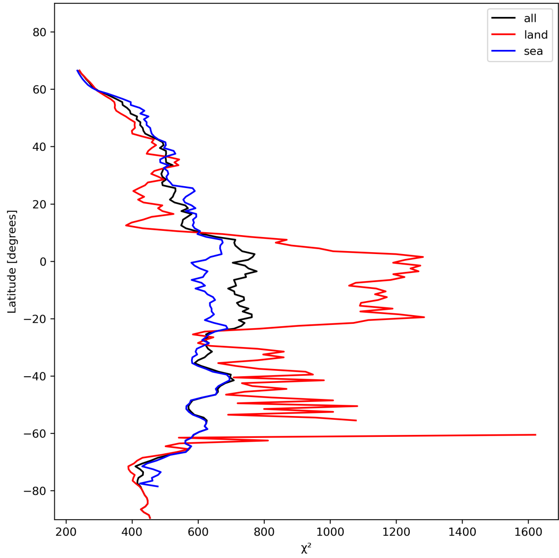
Figure 25: Zonal average of “ \chi^2 ” for 2023-11-28 to 2023-11-29.
