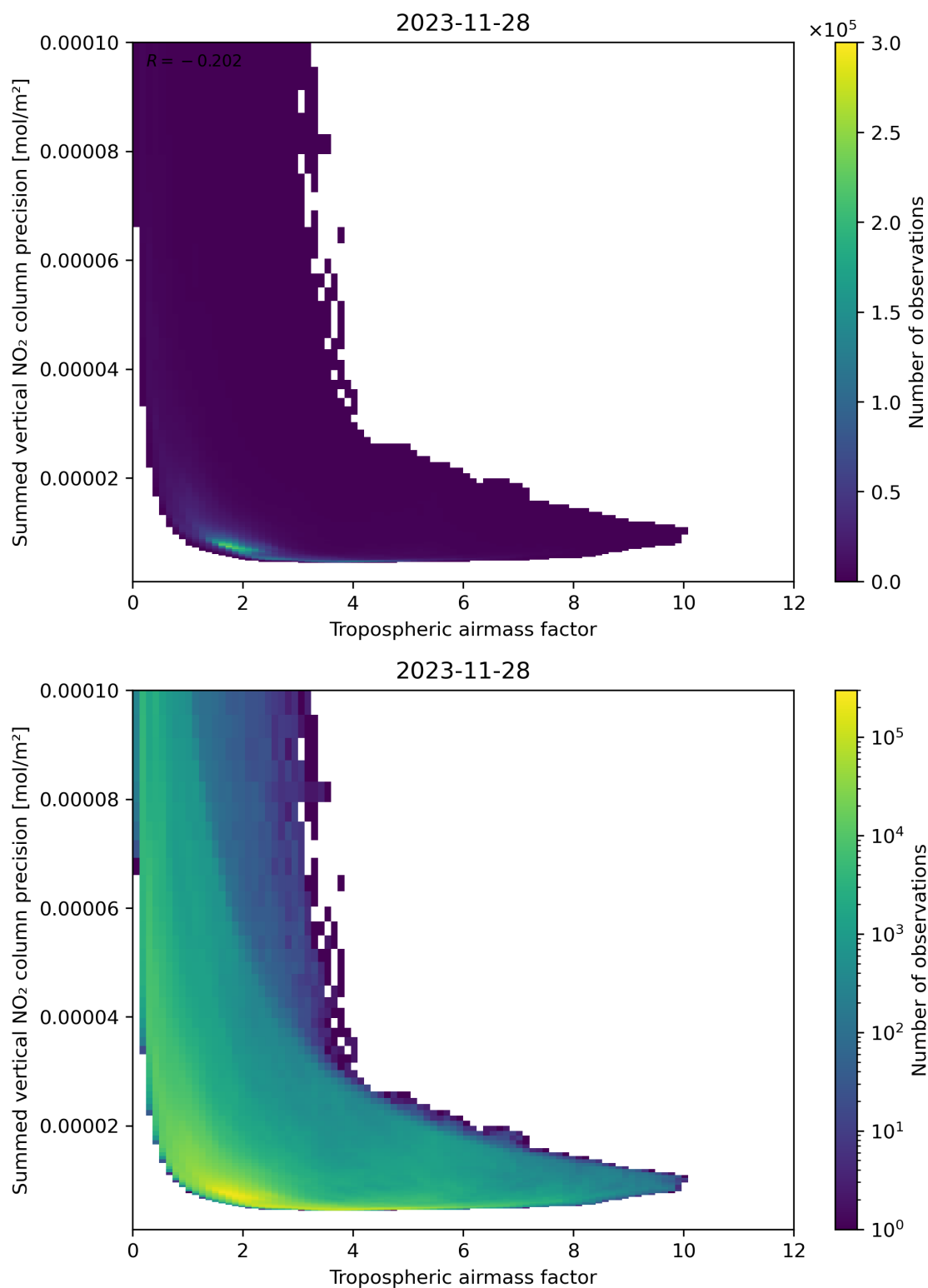
Figure 76: Scatter density plot of “Tropospheric air mass factor” against “Summed vertical NO 2 column precision” for 2023-11-28 to 2023-11-29.
