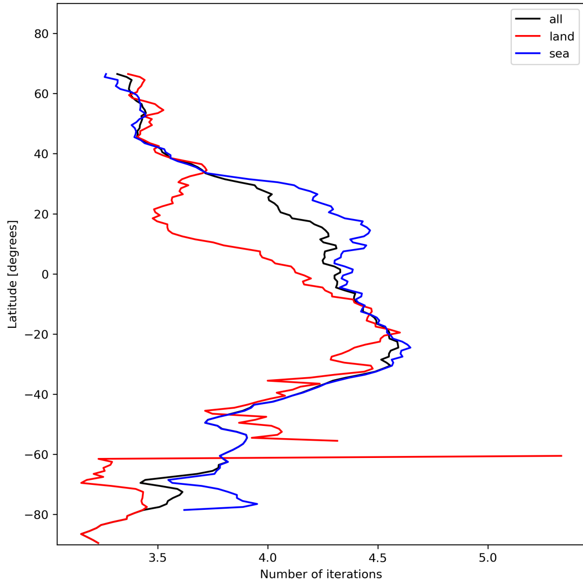
Figure 17: Zonal average of “Number of iterations” for 2023-11-28 to 2023-11-29.
