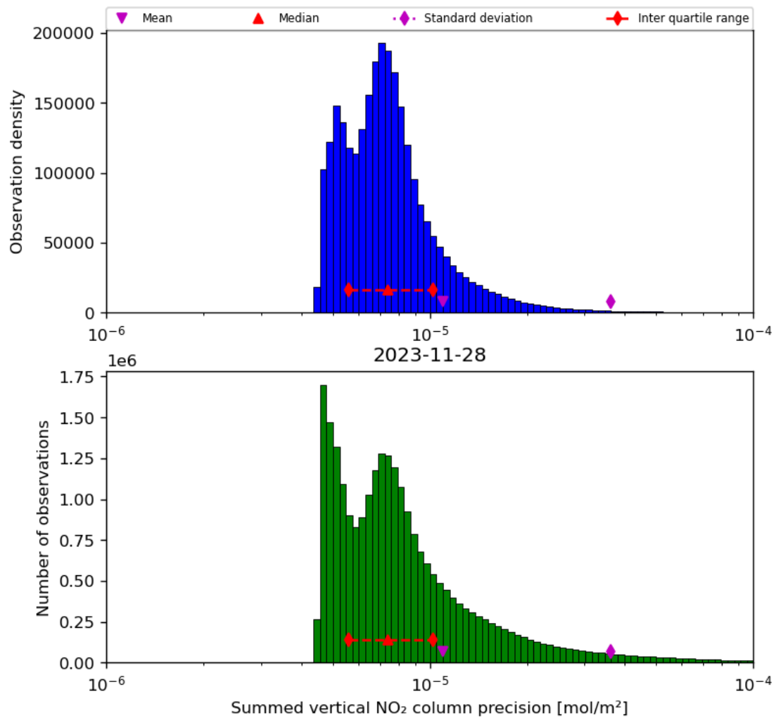
Figure 41: Histogram of “Summed vertical NO 2 column precision” for 2023-11-28 to 2023-11-29
