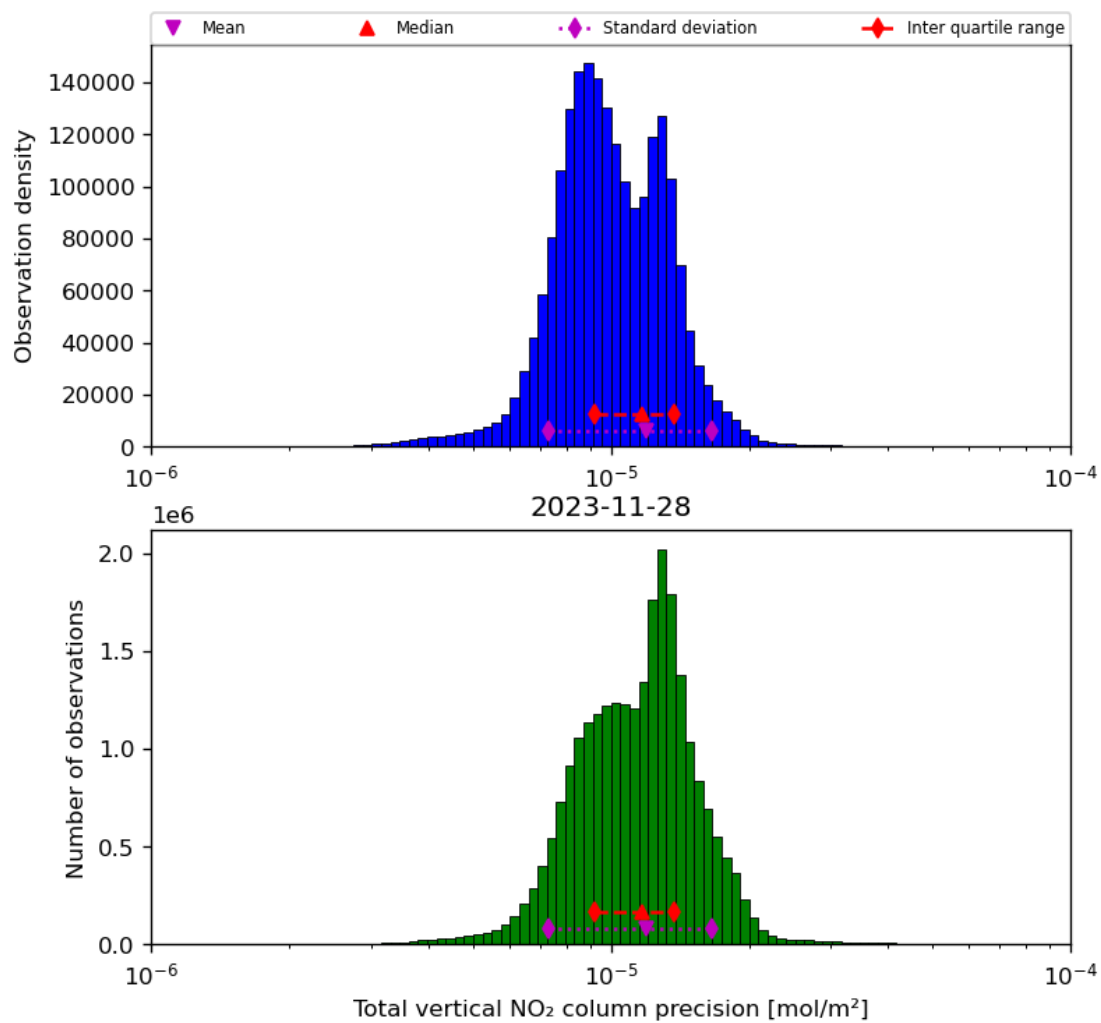
Figure 39: Histogram of “Total vertical NO 2 column precision” for 2023-11-28 to 2023-11-29
