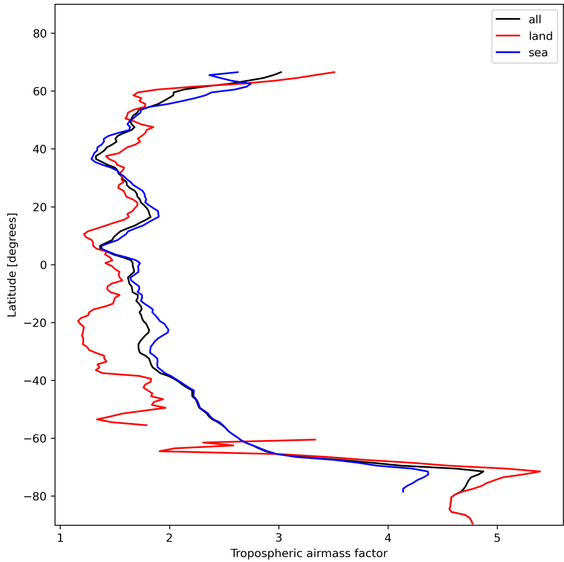
Figure 14: Zonal average of “Tropospheric airmass factor” for 2023-11-28 to 2023-11-29.
