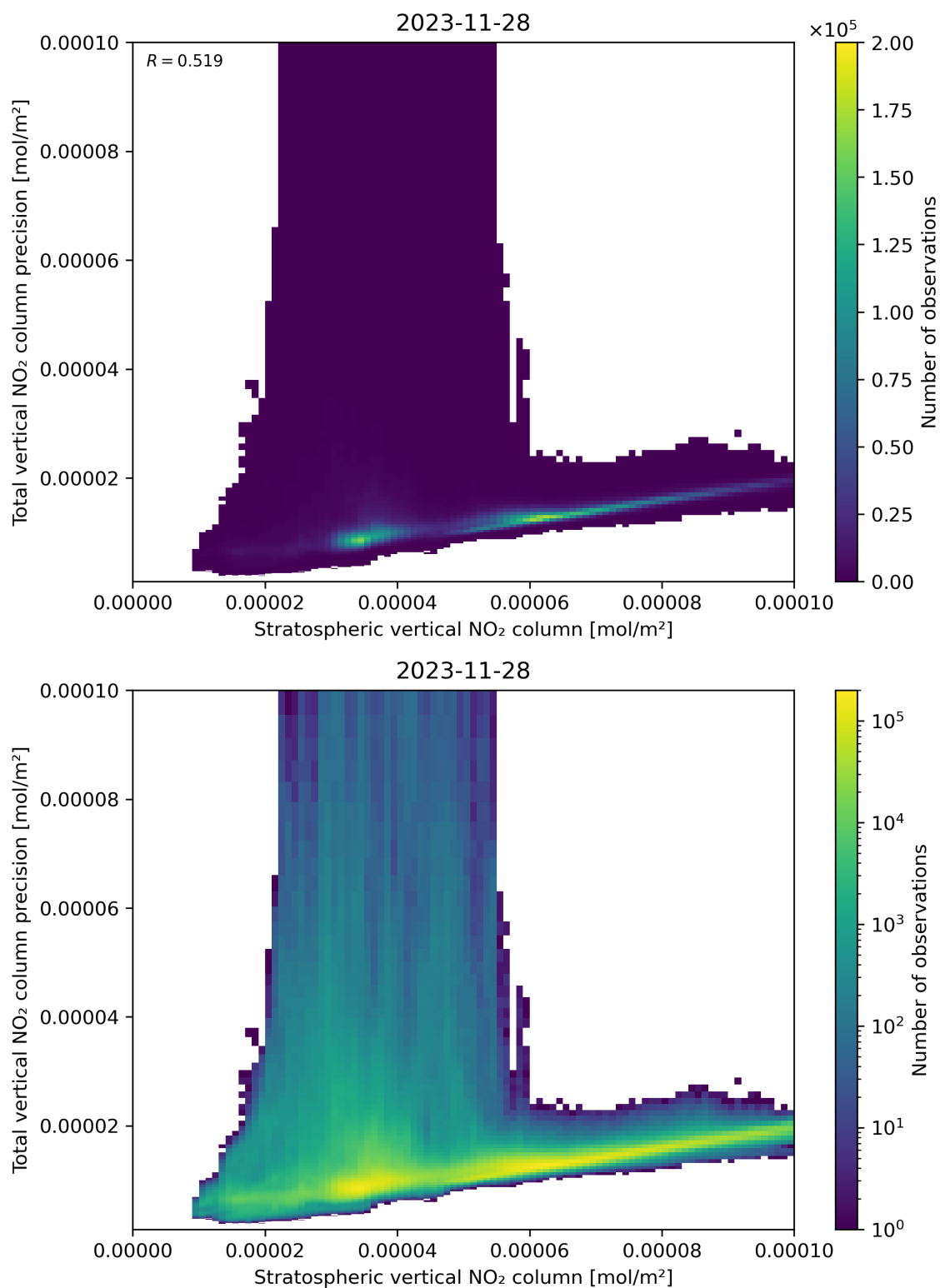
Figure 101: Scatter density plot of “Stratospheric vertical NO 2 column” against “Total vertical NO 2 column precision” for 2023-11-28 to 2023-11-29.
