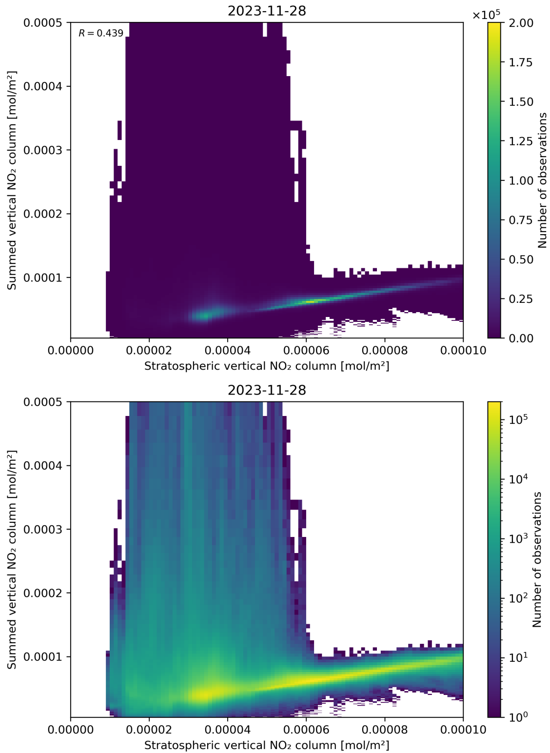
Figure 98: Scatter density plot of “Stratospheric vertical NO 2 column” against “Summed vertical NO 2 column” for 2023-11-28 to 2023-11-29.
