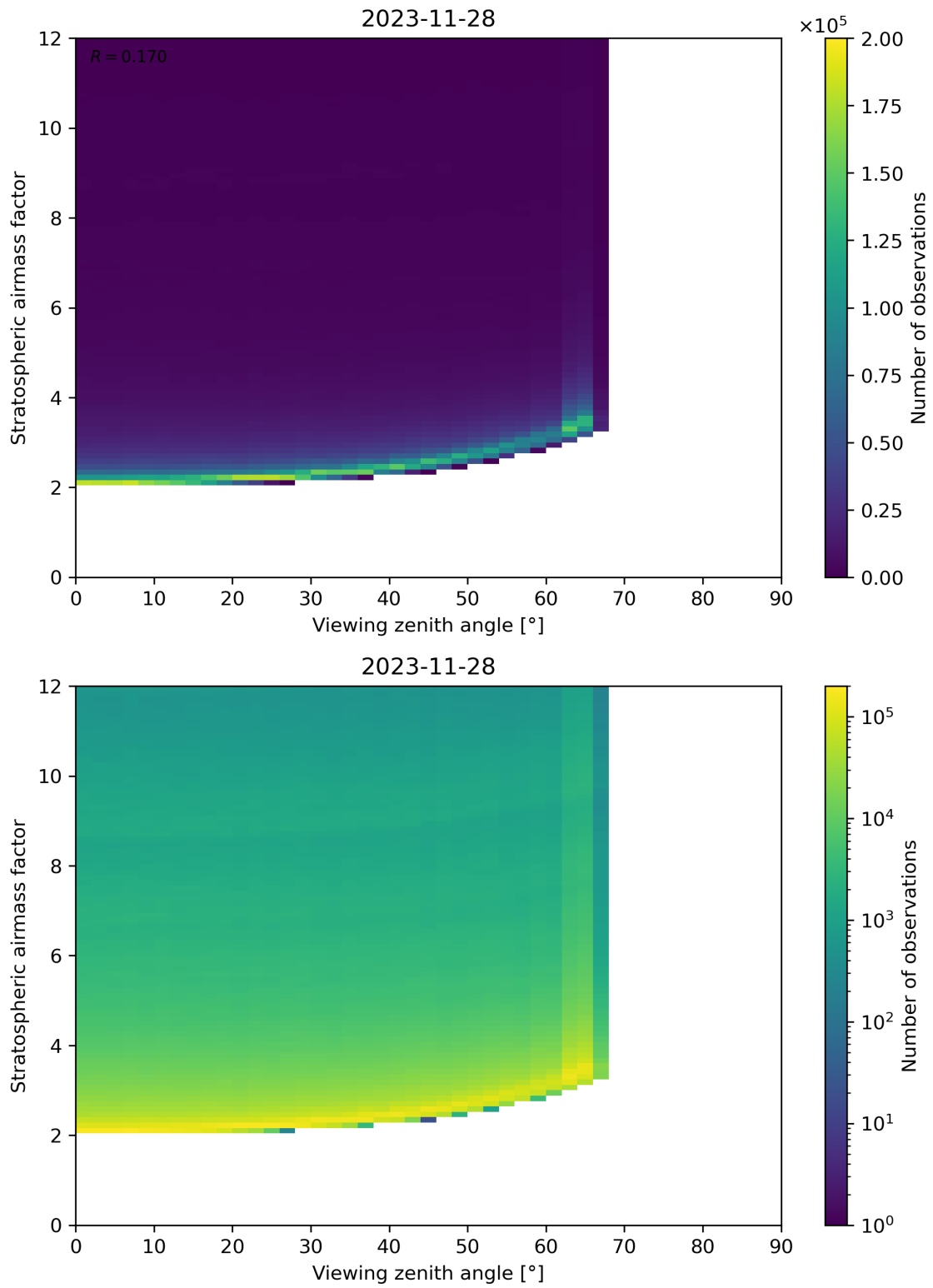
Figure 159: Scatter density plot of “Viewing zenith angle” against “Stratospheric airmass factor” for 2023-11-28 to 2023-11-29.
