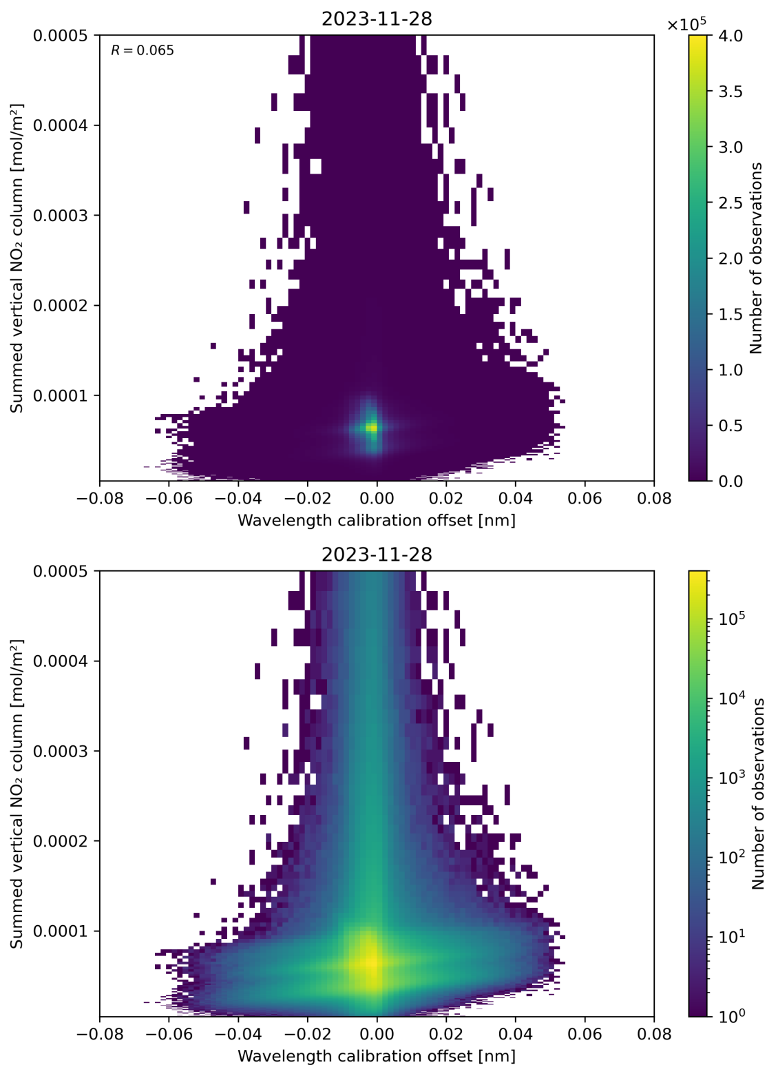
Figure 177: Scatter density plot of “Wavelength calibration offset” against “Summed vertical NO 2 column” for 2023-11-28 to 2023-11-29.
