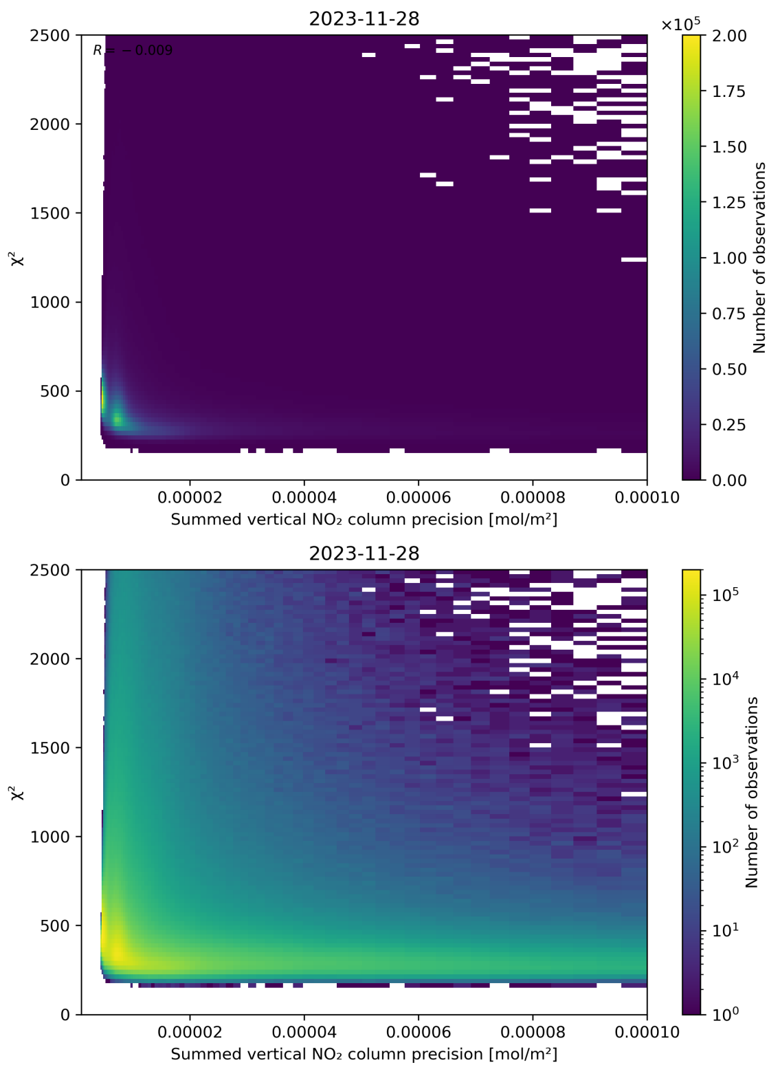
Figure 107: Scatter density plot of “Summed vertical NO 2 column precision” against “ \chi^2 ” for 2023-11-28 to 2023-11-29.
