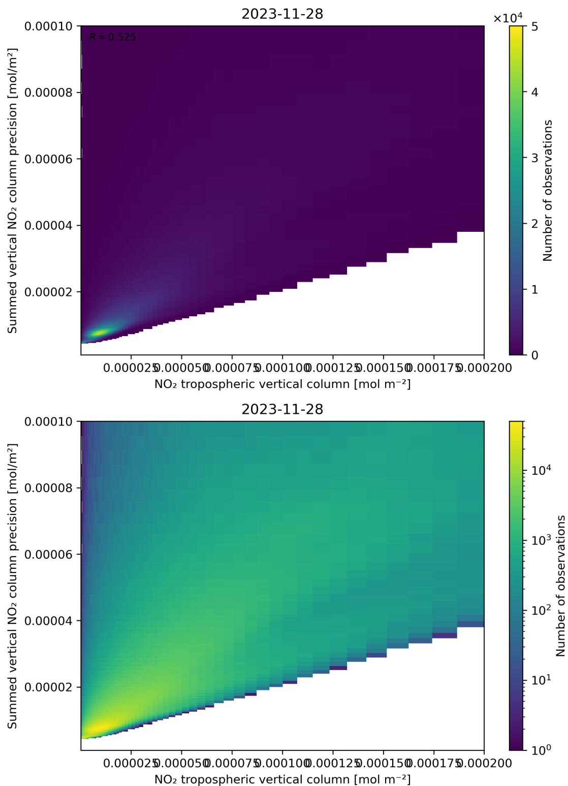
Figure 127: Scatter density plot of “NO 2 tropospheric vertical column” against “Summed vertical NO 2 column precision” for 2023-11-28 to 2023-11-29.
