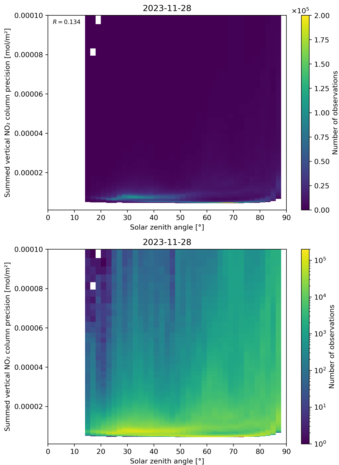
Figure 152: Scatter density plot of “Solar zenith angle” against “Summed vertical NO 2 column precision” for 2023-11-28 to 2023-11-29.
