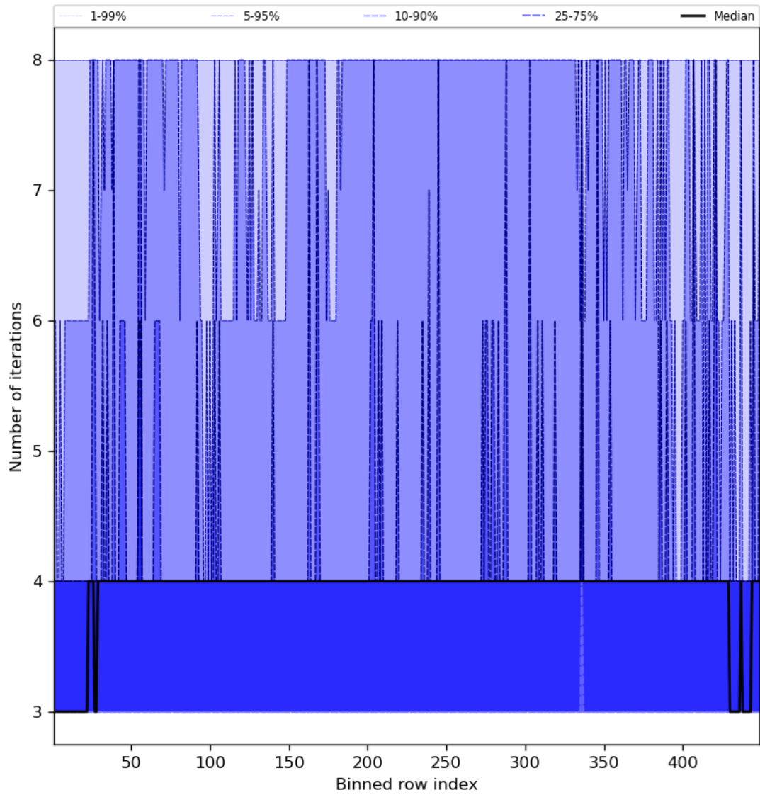
Figure 51: Along track statistics of “Number of iterations” for 2023-11-28 to 2023-11-29
