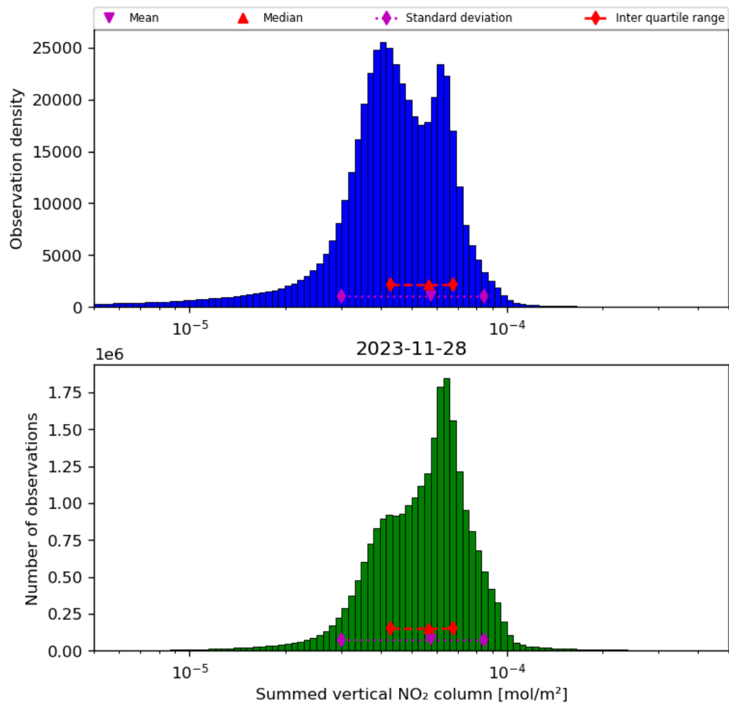
Figure 40: Histogram of “Summed vertical NO 2 column” for 2023-11-28 to 2023-11-29
