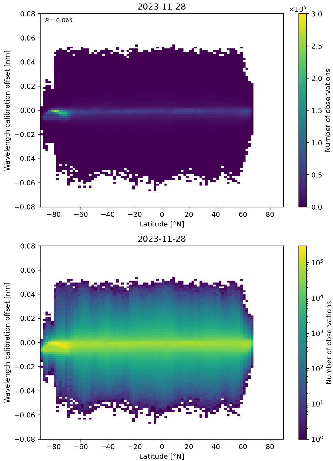
Figure 95: Scatter density plot of “Latitude” against “Wavelength calibration offset” for 2023-11-28 to 2023-11-29.
