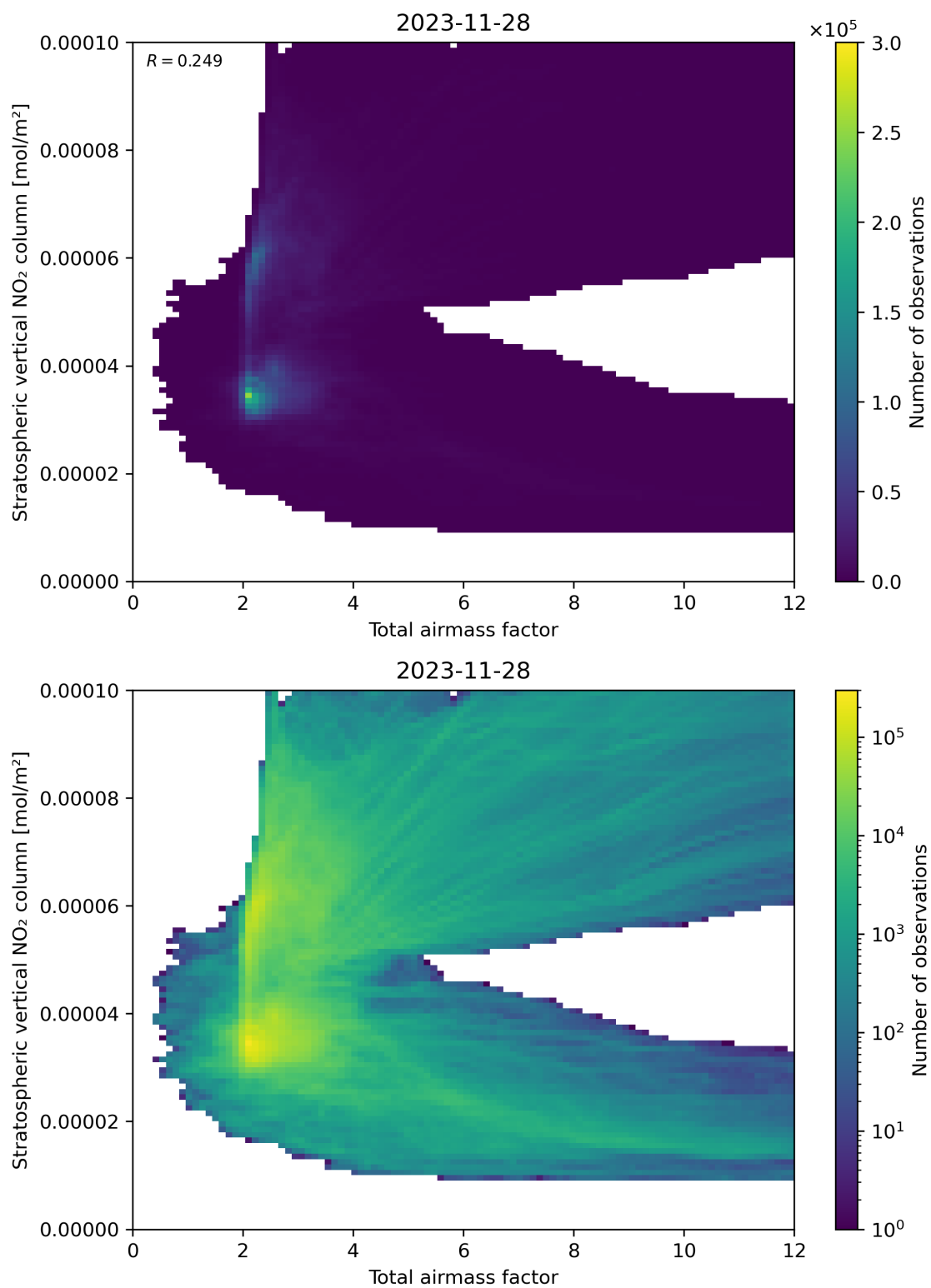
Figure 64: Scatter density plot of “Total airmass factor” against “Stratospheric vertical NO 2 column” for 2023-11-28 to 2023-11-29.
