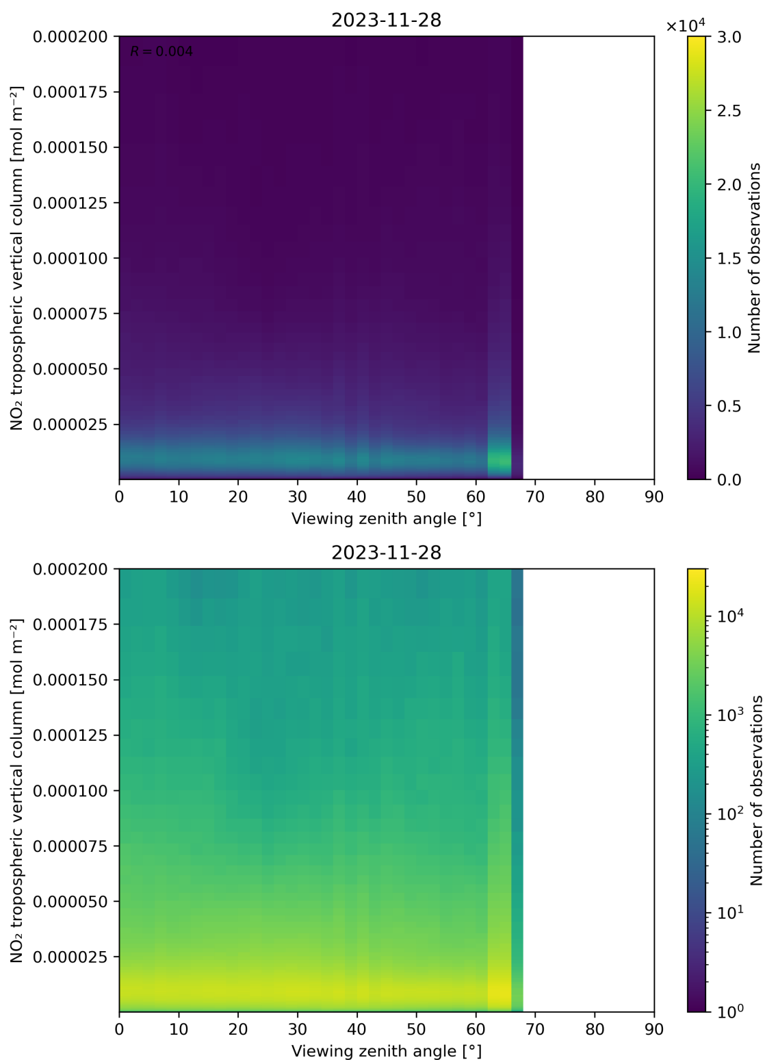
Figure 169: Scatter density plot of “Viewing zenith angle” against “NO 2 tropospheric vertical column” for 2023-11-28 to 2023-11-29.
