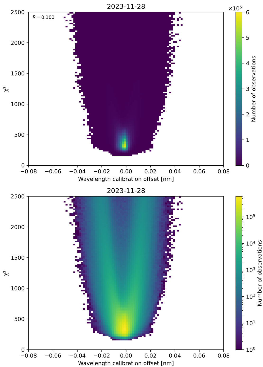
Figure 175: Scatter density plot of “Wavelength calibration offset” against “ \chi^2 ” for 2023-11-28 to 2023-11-29.
