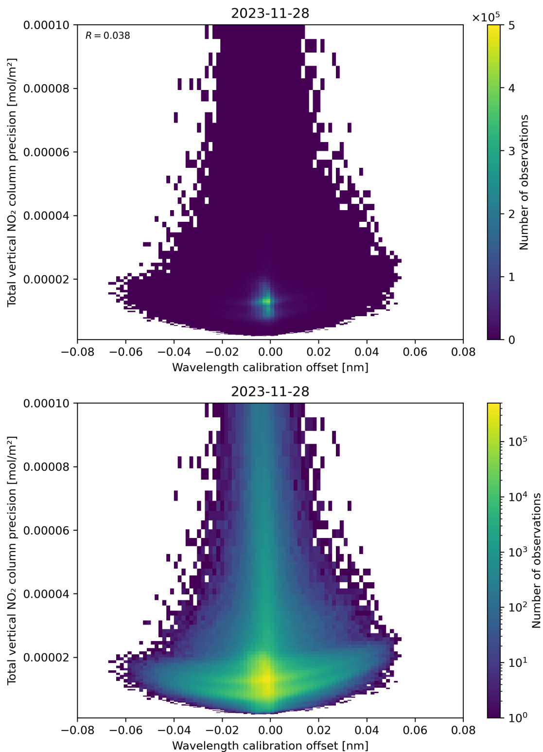
Figure 180: Scatter density plot of “Wavelength calibration offset” against “Total vertical NO 2 column precision” for 2023-11-28 to 2023-11-29.
