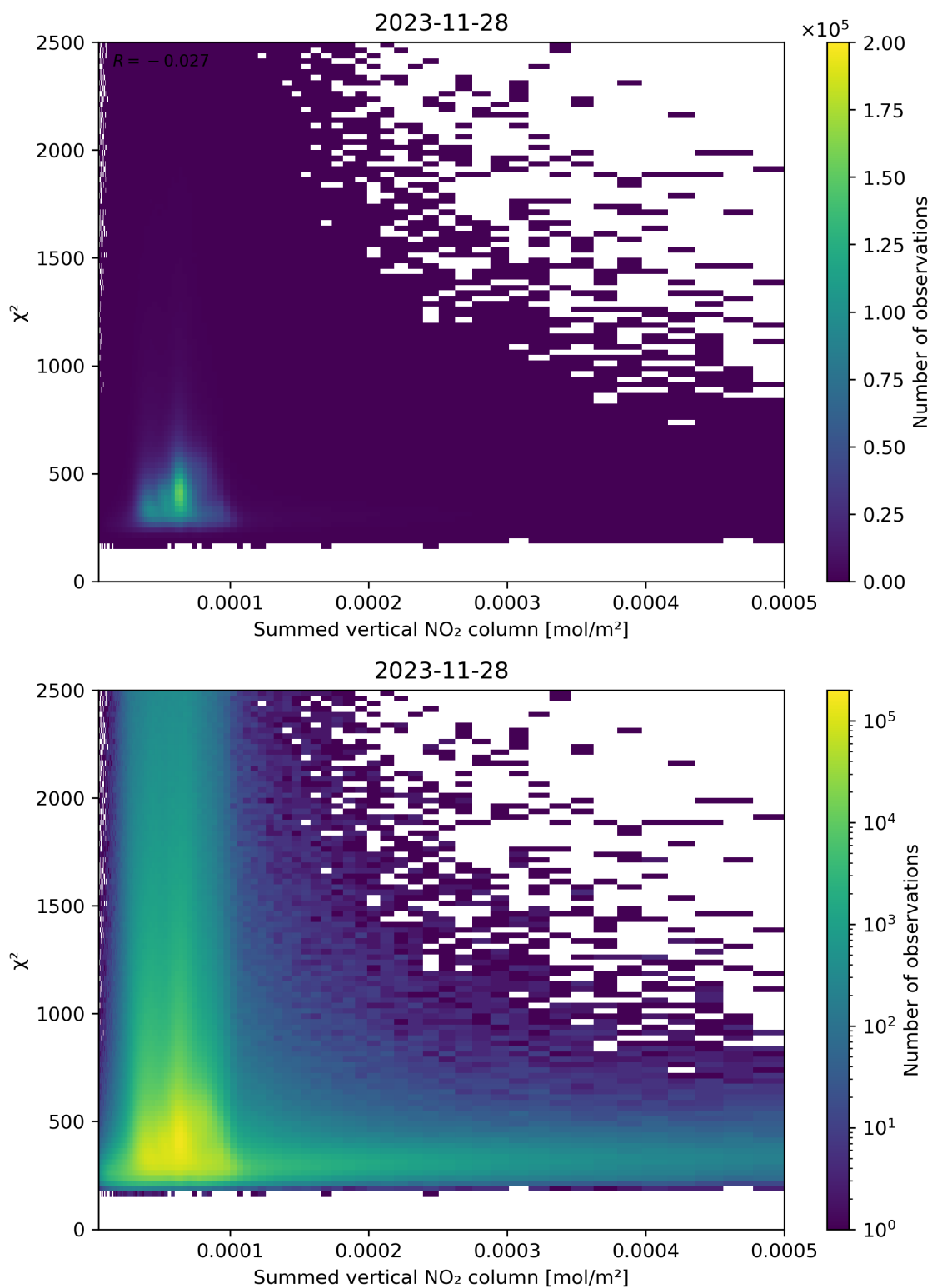
Figure 104: Scatter density plot of “Summed vertical NO 2 column” against “ \chi^2 ” for 2023-11-28 to 2023-11-29.
