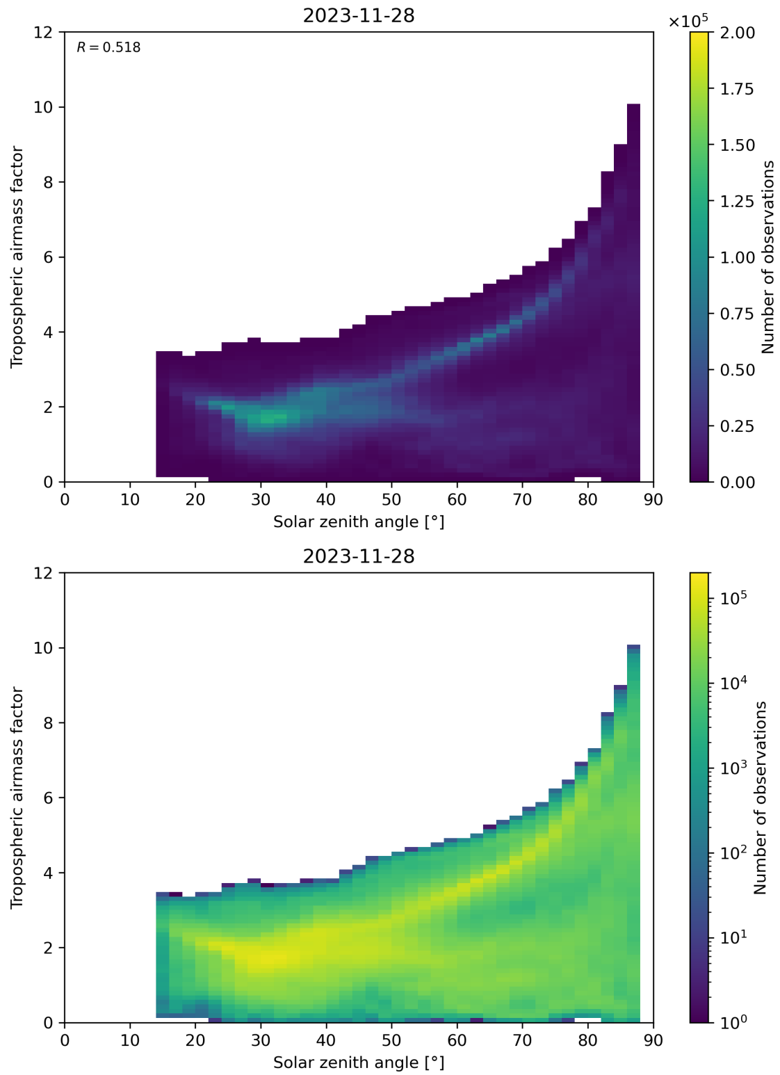
Figure 147: Scatter density plot of “Solar zenith angle” against “Tropospheric airmass factor” for 2023-11-28 to 2023-11-29.
