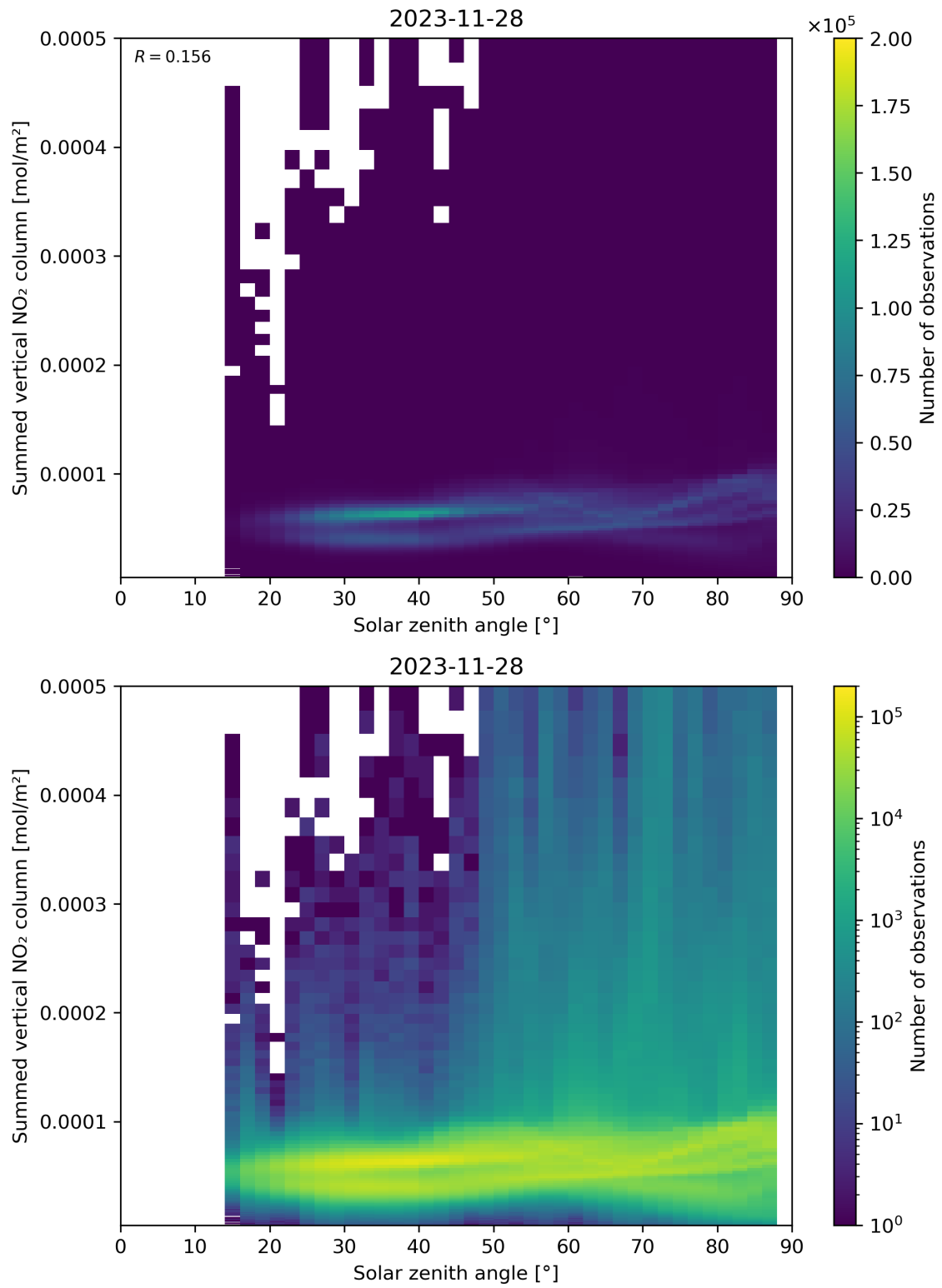
Figure 151: Scatter density plot of “Solar zenith angle” against “Summed vertical NO 2 column” for 2023-11-28 to 2023-11-29.
