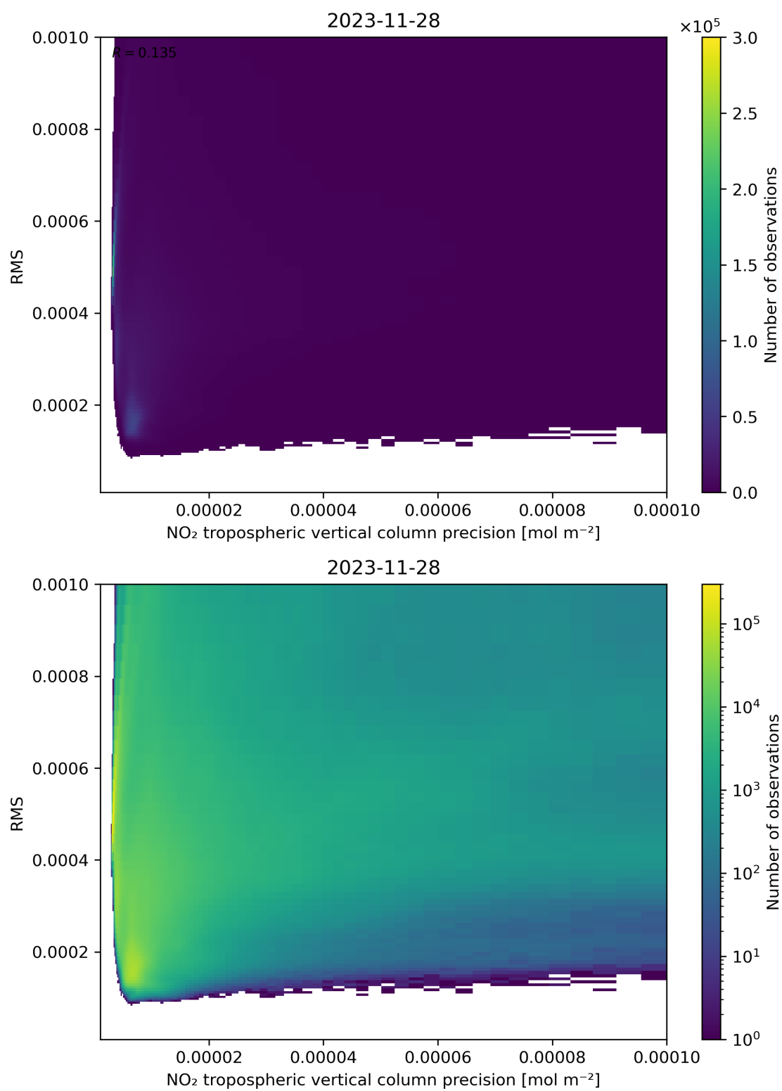
Figure 140: Scatter density plot of “NO 2 tropospheric vertical column precision” against “RMS” for 2023-11-28 to 2023-11-29.
