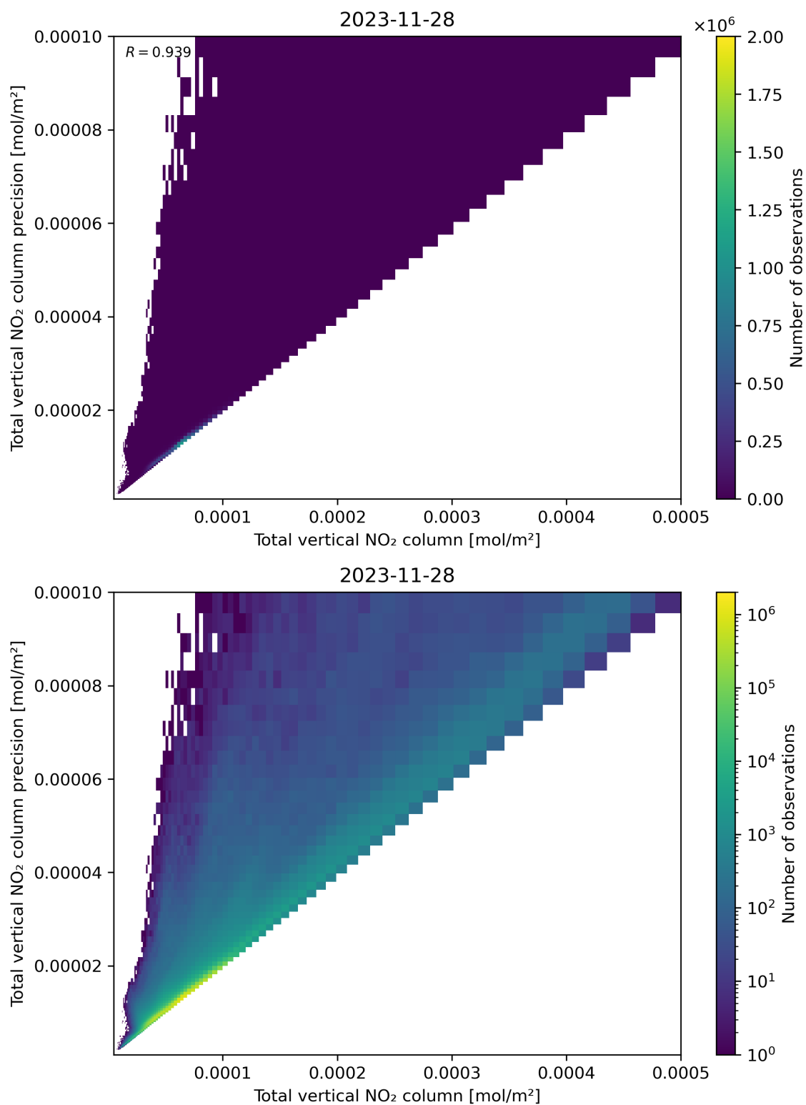
Figure 114: Scatter density plot of “Total vertical NO 2 column” against “Total vertical NO 2 column precision” for 2023-11-28 to 2023-11-29.
