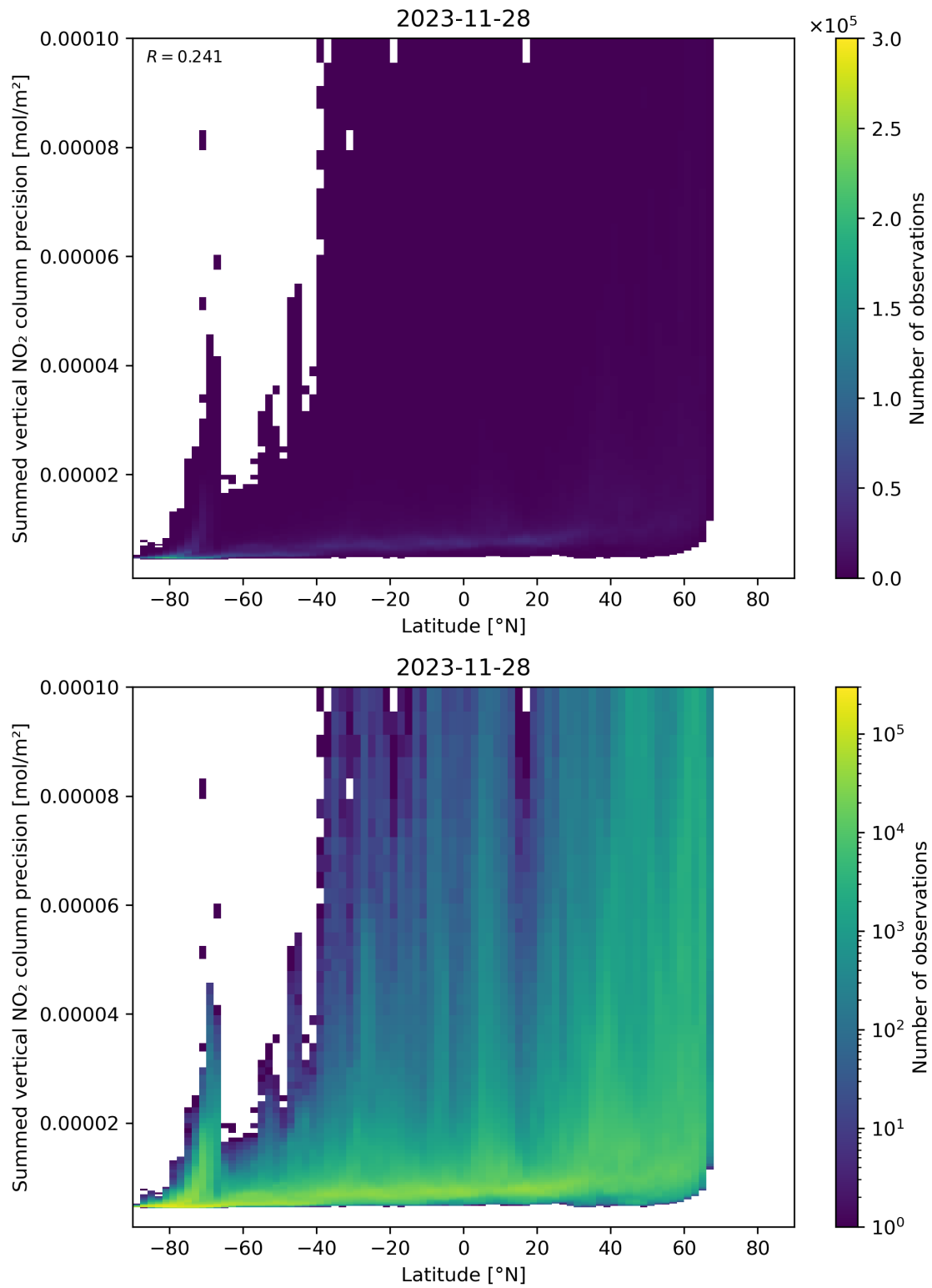
Figure 89: Scatter density plot of “Latitude” against “Summed vertical NO 2 column precision” for 2023-11-28 to 2023-11-29.
