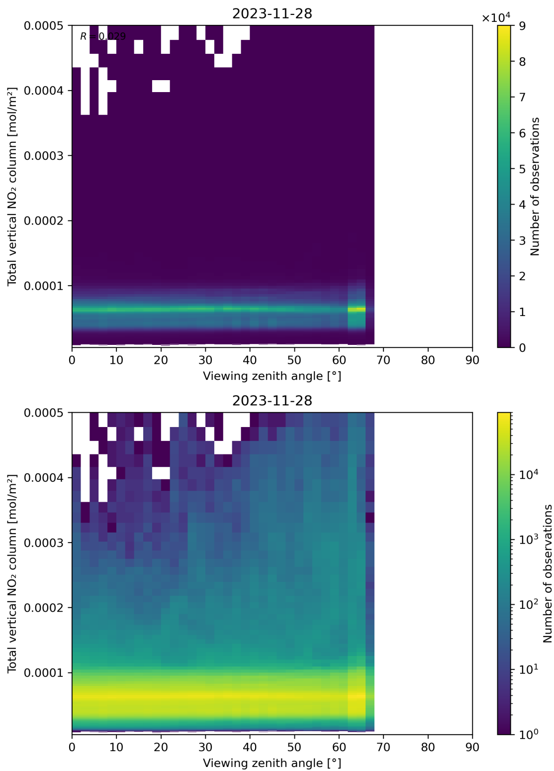
Figure 167: Scatter density plot of “Viewing zenith angle” against “Total vertical NO 2 column” for 2023-11-28 to 2023-11-29.
