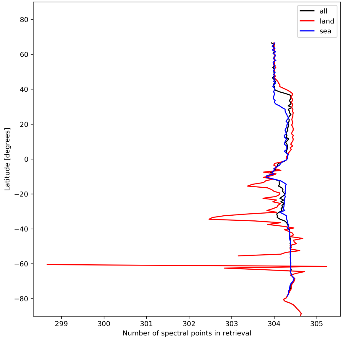
Figure 16: Zonal average of “Number of spectral points in retrieval” for 2023-11-28 to 2023-11-29.
