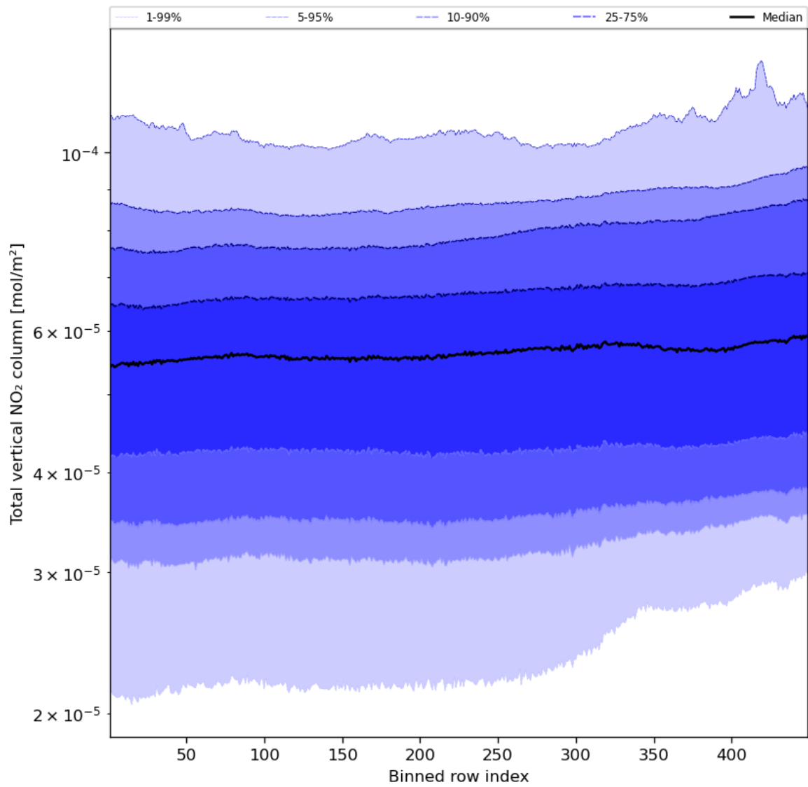
Figure 55: Along track statistics of “Total vertical NO 2 column” for 2023-11-28 to 2023-11-29
