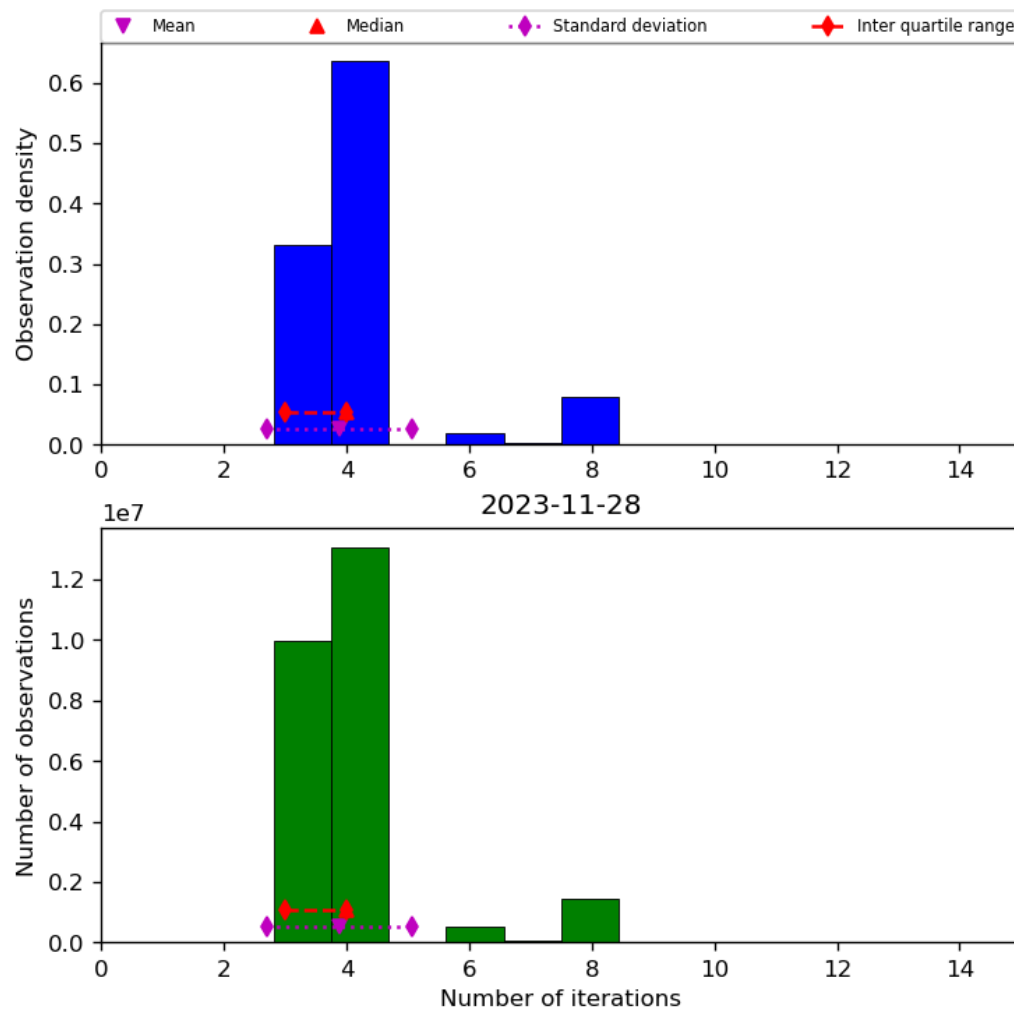
Figure 34: Histogram of “Number of iterations” for 2023-11-28 to 2023-11-29
