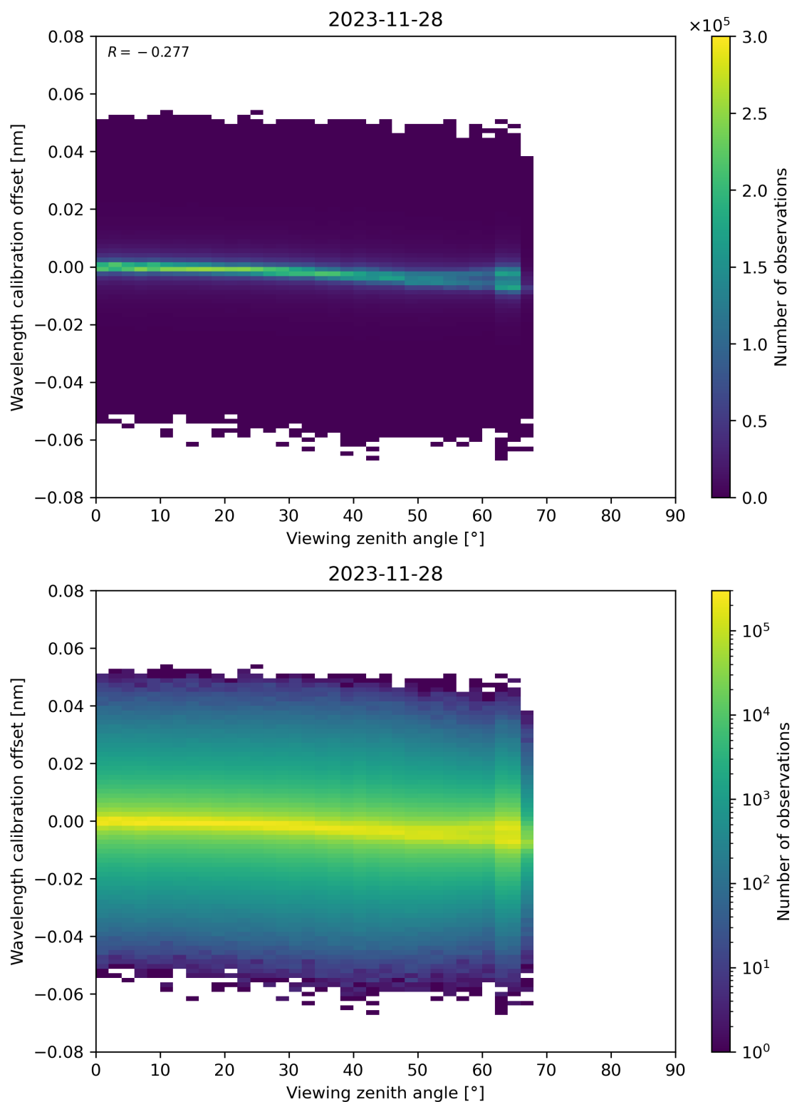
Figure 173: Scatter density plot of “Viewing zenith angle” against “Wavelength calibration offset” for 2023-11-28 to 2023-11-29.
