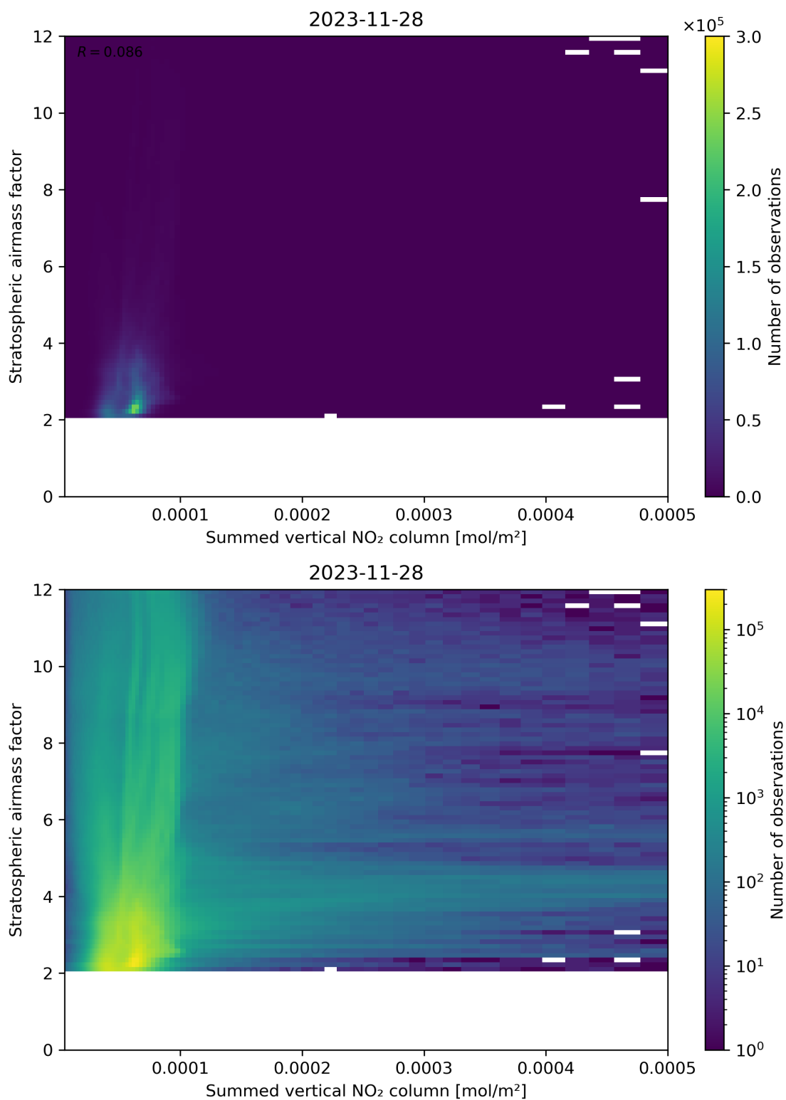
Figure 103: Scatter density plot of “Summed vertical NO 2 column” against “Stratospheric airmass factor” for 2023-11-28 to 2023-11-29.
