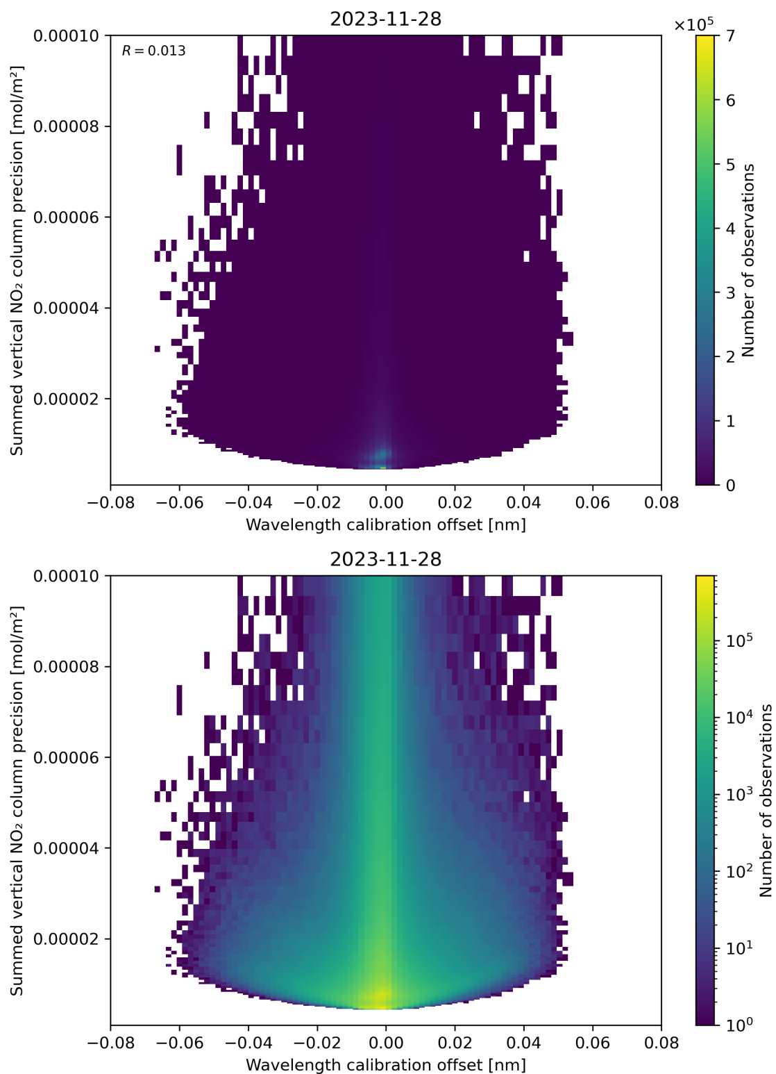
Figure 178: Scatter density plot of “Wavelength calibration offset” against “Summed vertical NO 2 column precision” for 2023-11-28 to 2023-11-29.
