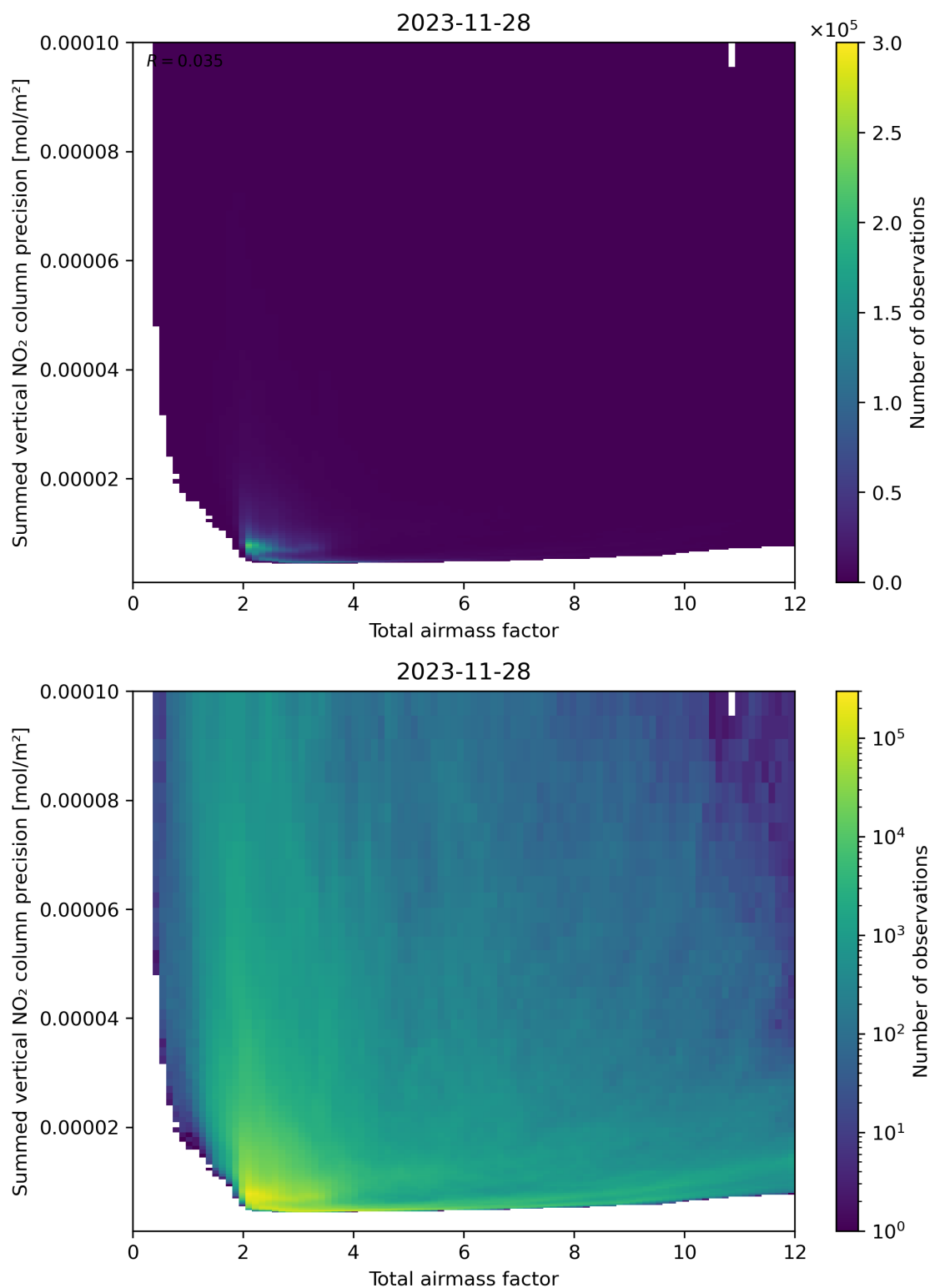
Figure 66: Scatter density plot of “Total airmass factor” against “Summed vertical NO 2 column precision” for 2023-11-28 to 2023-11-29.
