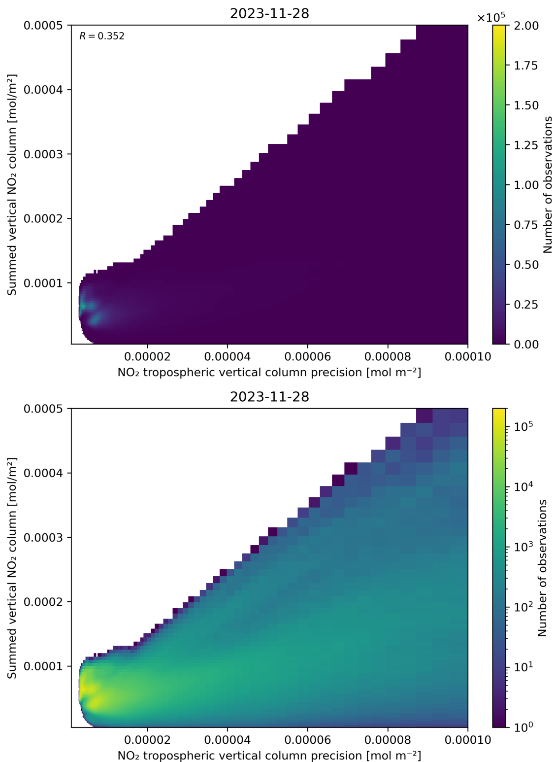
Figure 136: Scatter density plot of “NO 2 tropospheric vertical column precision” against “Summed vertical NO 2 column” for 2023-11-28 to 2023-11-29.
