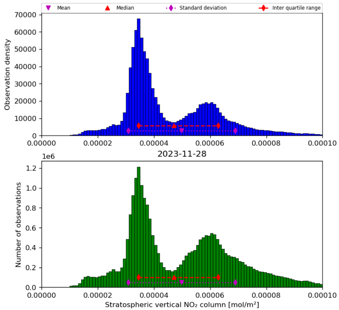
Figure 36: Histogram of “Stratospheric vertical NO 2 column” for 2023-11-28 to 2023-11-29
