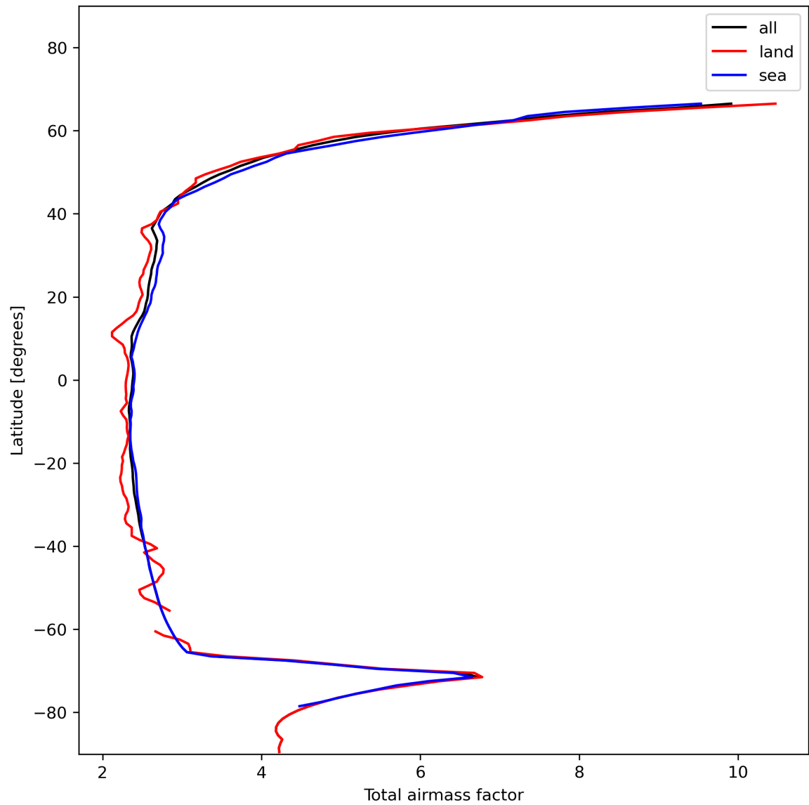
Figure 15: Zonal average of “Total airmass factor” for 2023-11-28 to 2023-11-29.
