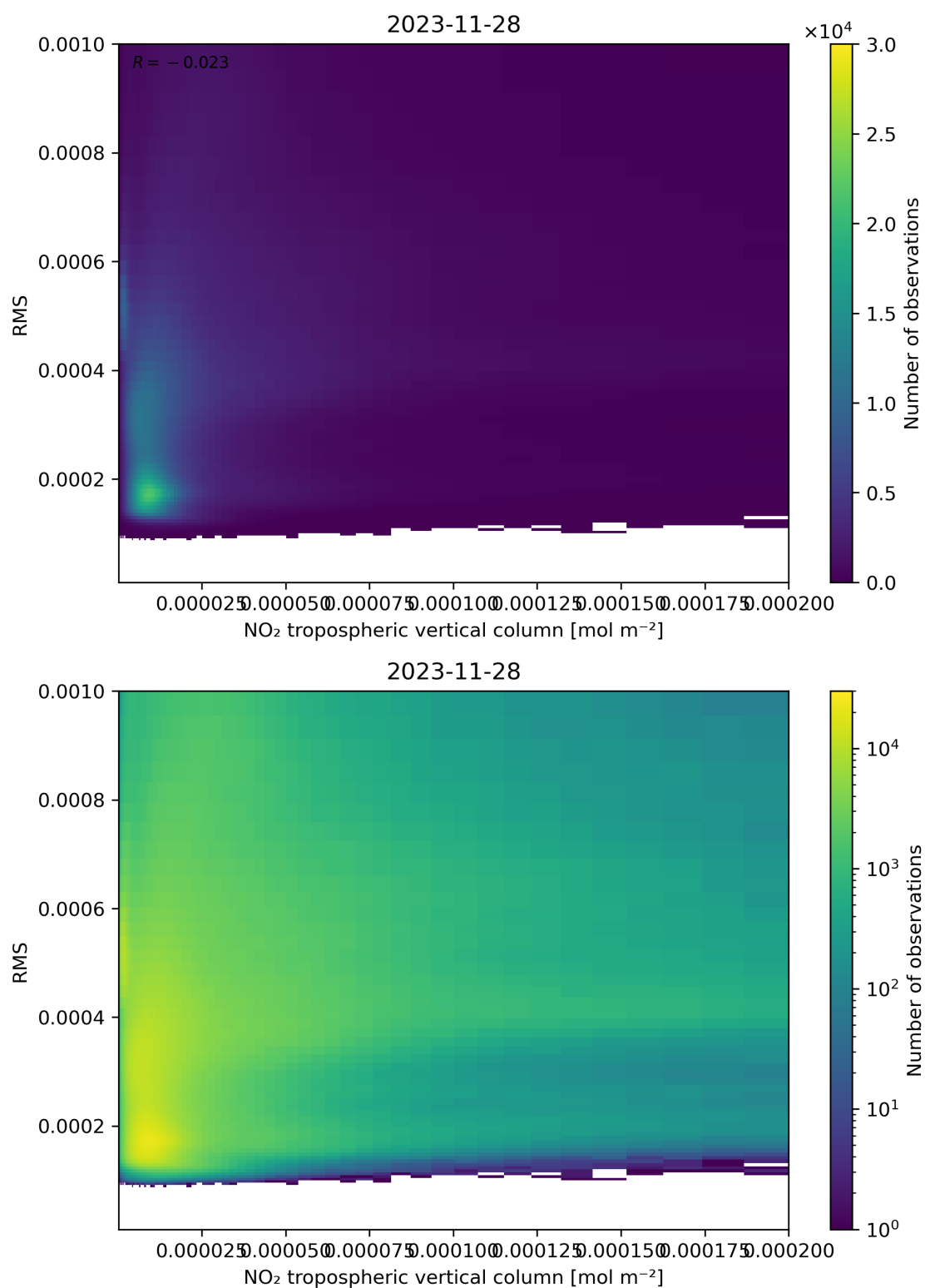
Figure 142: Scatter density plot of “NO 2 tropospheric vertical column” against “RMS” for 2023-11-28 to 2023-11-29.
