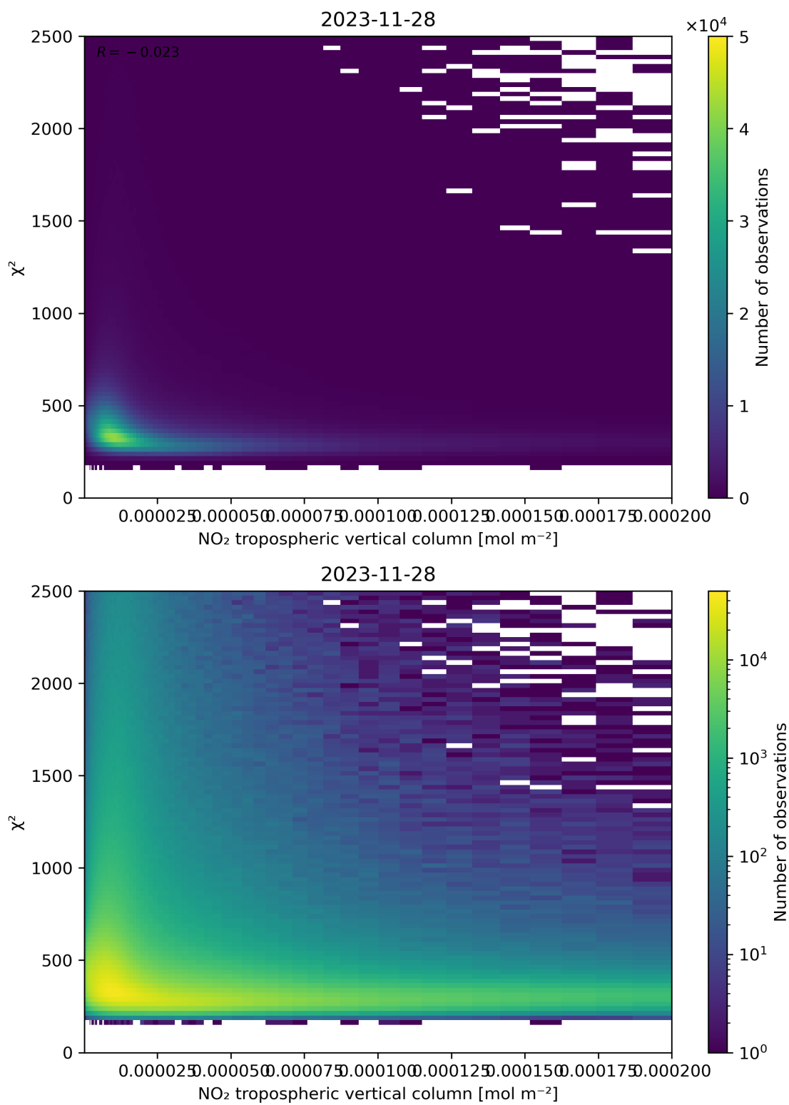
Figure 124: Scatter density plot of “NO 2 tropospheric vertical column” against “ \chi^2 ” for 2023-11-28 to 2023-11-29.
