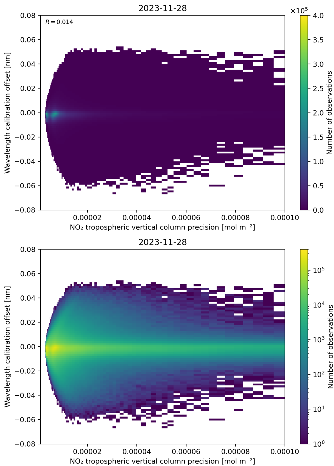
Figure 141: Scatter density plot of “NO 2 tropospheric vertical column precision” against “Wavelength calibration offset” for 2023-11-28 to 2023-11-29.
