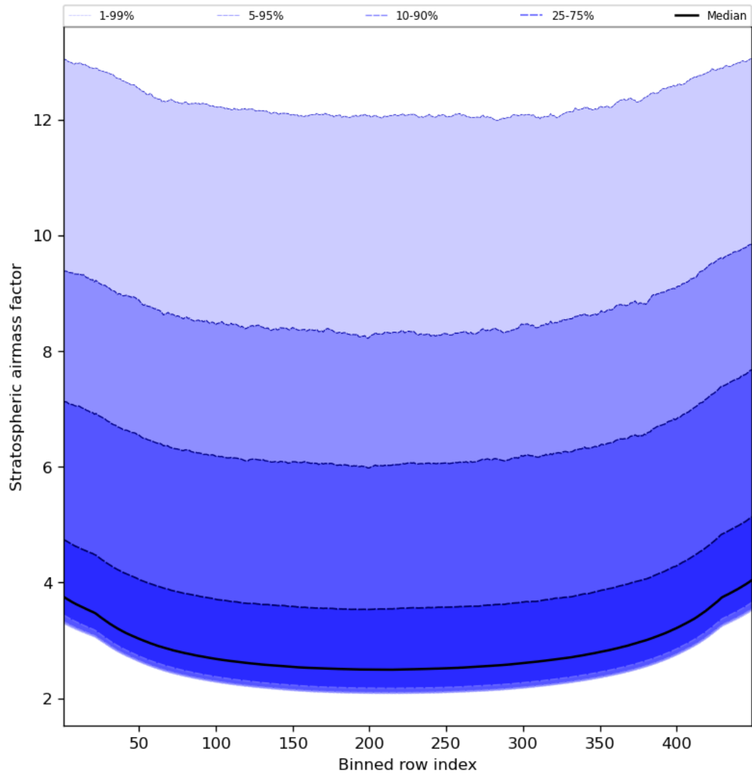
Figure 61: Along track statistics of “Stratospheric air mass factor” for 2023-11-28 to 2023-11-29
