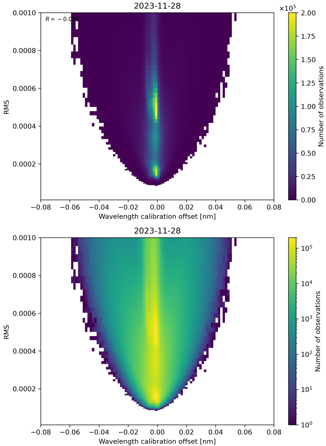
Figure 181: Scatter density plot of “Wavelength calibration offset” against “RMS” for 2023-11-28 to 2023-11-29.
