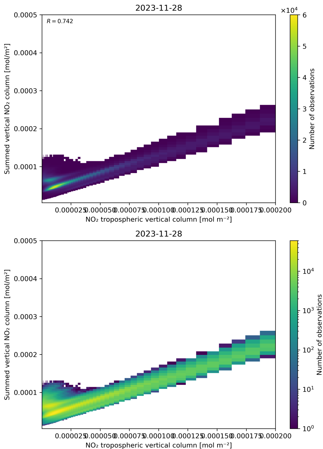
Figure 126: Scatter density plot of “NO 2 tropospheric vertical column” against “Summed vertical NO 2 column” for 2023-11-28 to 2023-11-29.
