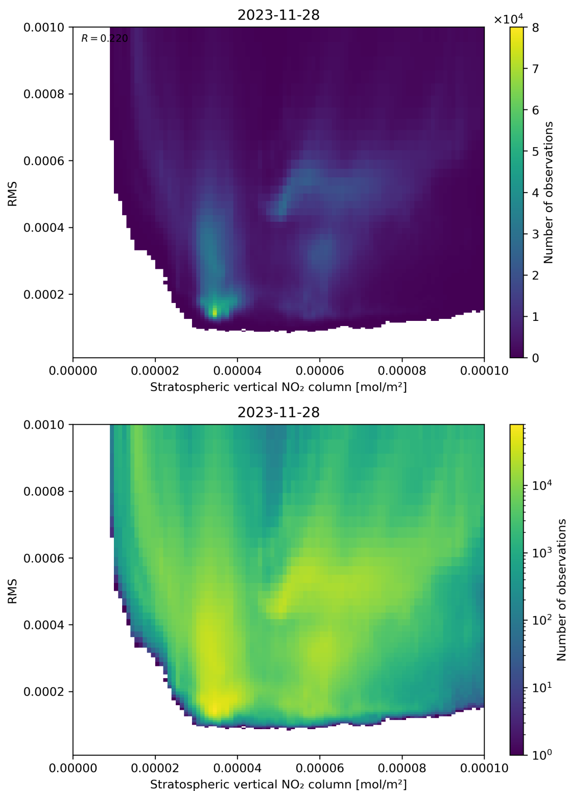
Figure 102: Scatter density plot of “Stratospheric vertical NO 2 column” against “RMS” for 2023-11-28 to 2023-11-29.
