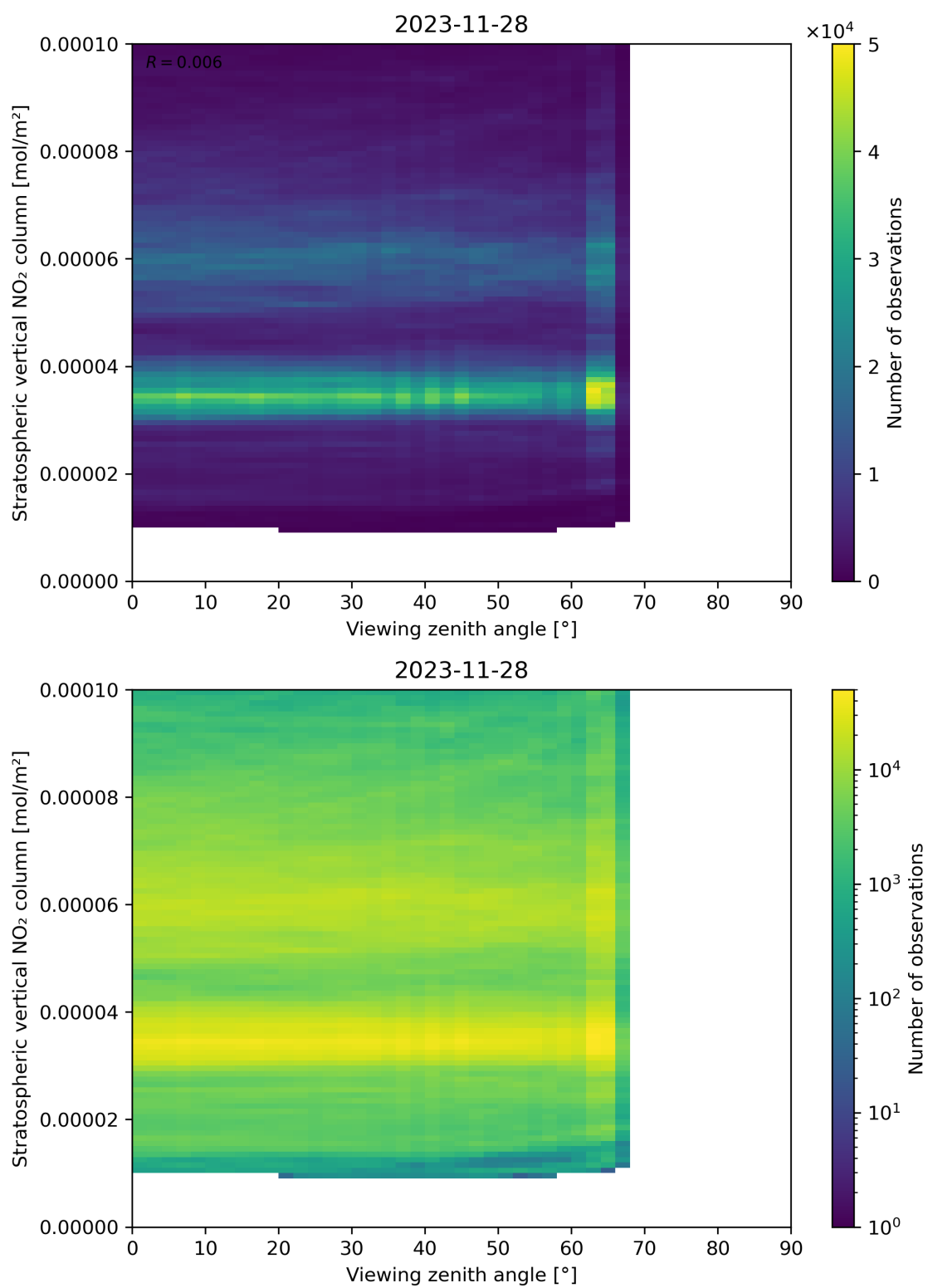
Figure 164: Scatter density plot of “Viewing zenith angle” against “Stratospheric vertical NO 2 column” for 2023-11-28 to 2023-11-29.
