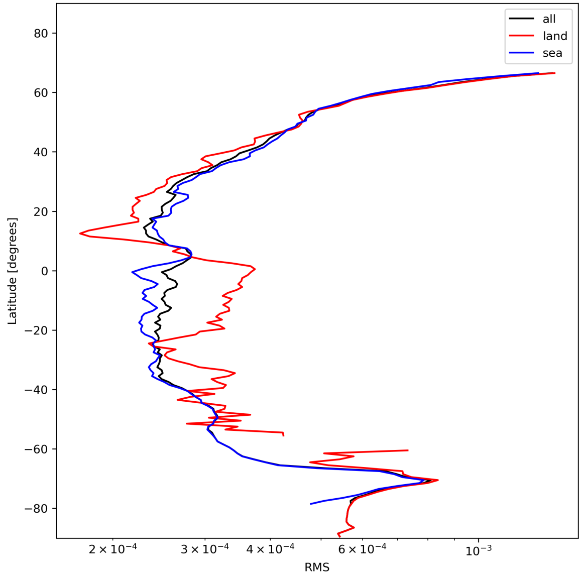
Figure 26: Zonal average of “RMS” for 2023-11-28 to 2023-11-29.
