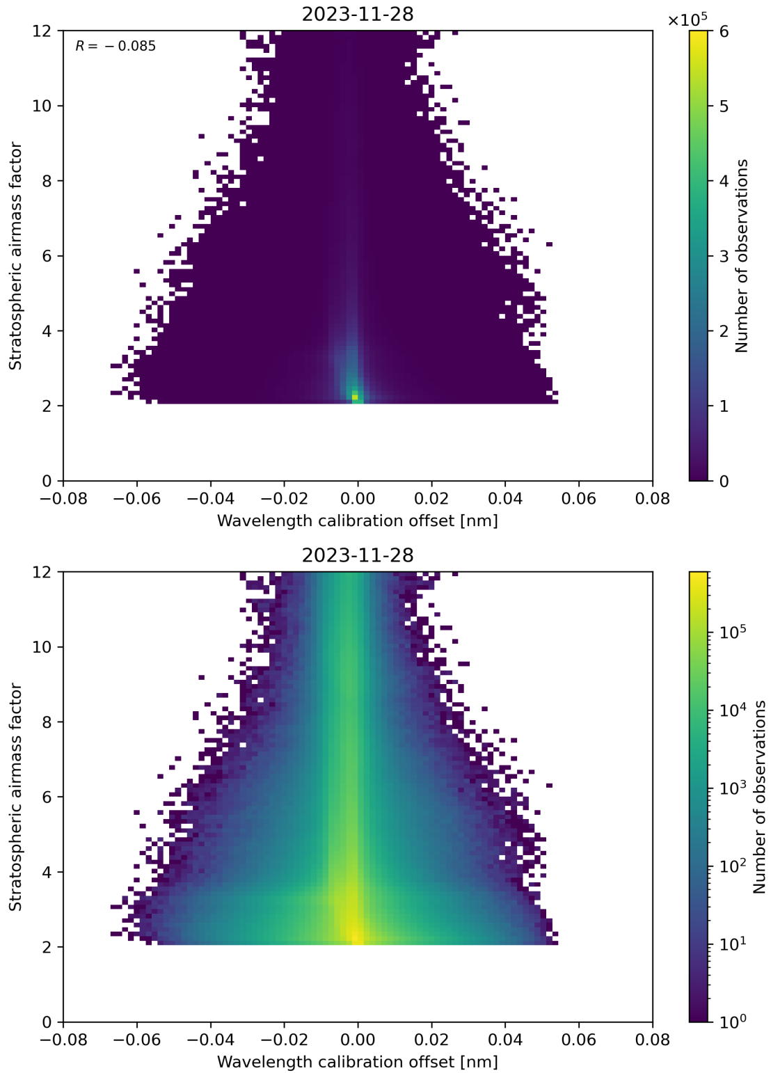
Figure 174: Scatter density plot of “Wavelength calibration offset” against “Stratospheric airmass factor” for 2023-11-28 to 2023-11-29.
