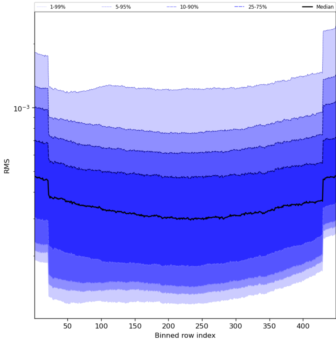
Figure 60: Along track statistics of “RMS” for 2023-11-28 to 2023-11-29
