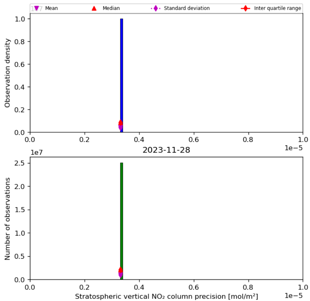
Figure 37: Histogram of “Stratospheric vertical NO 2 column precision” for 2023-11-28 to 2023-11-29
