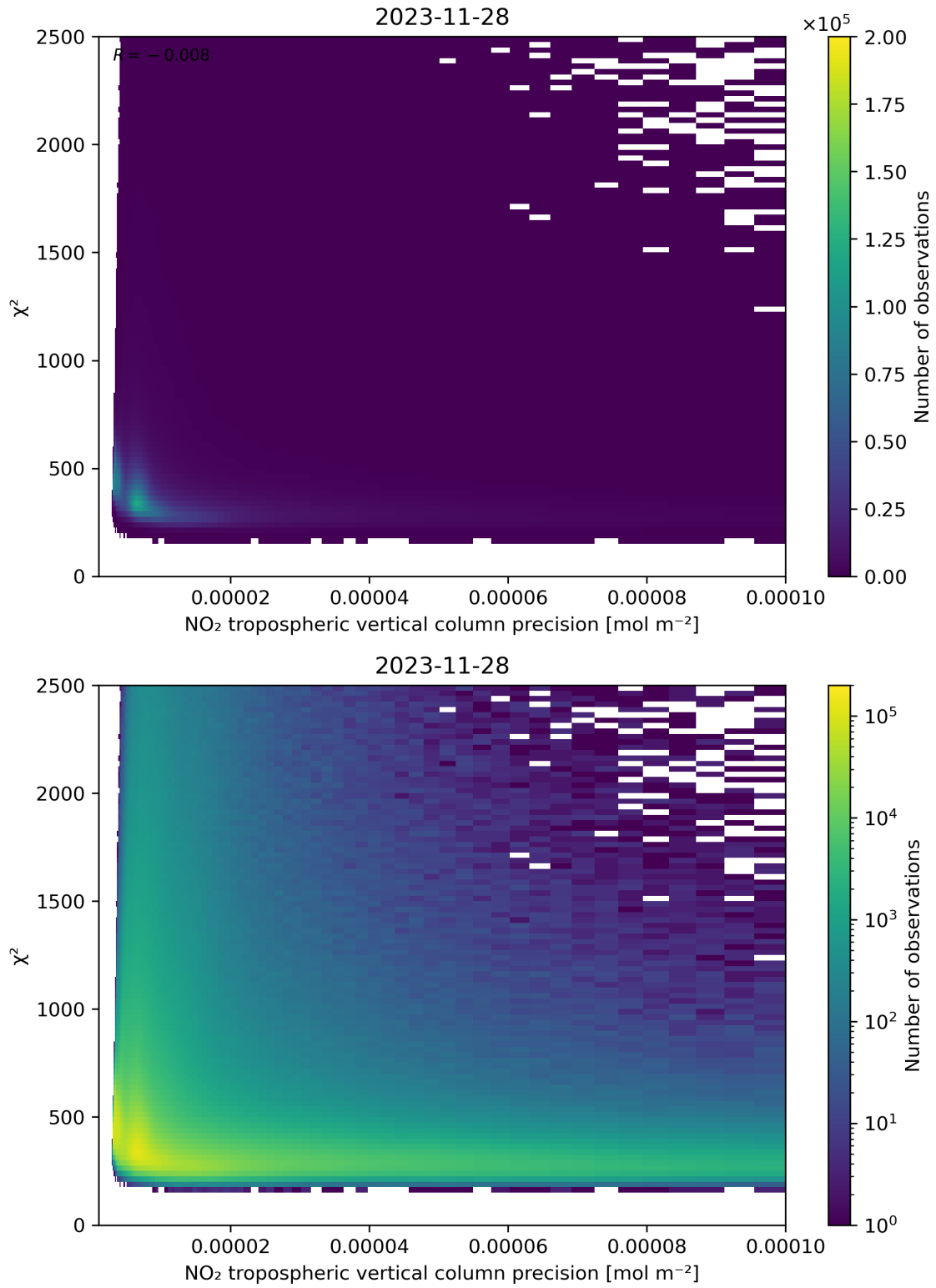
Figure 134: Scatter density plot of “NO 2 tropospheric vertical column precision” against “ \chi^2 ” for 2023-11-28 to 2023-11-29.
