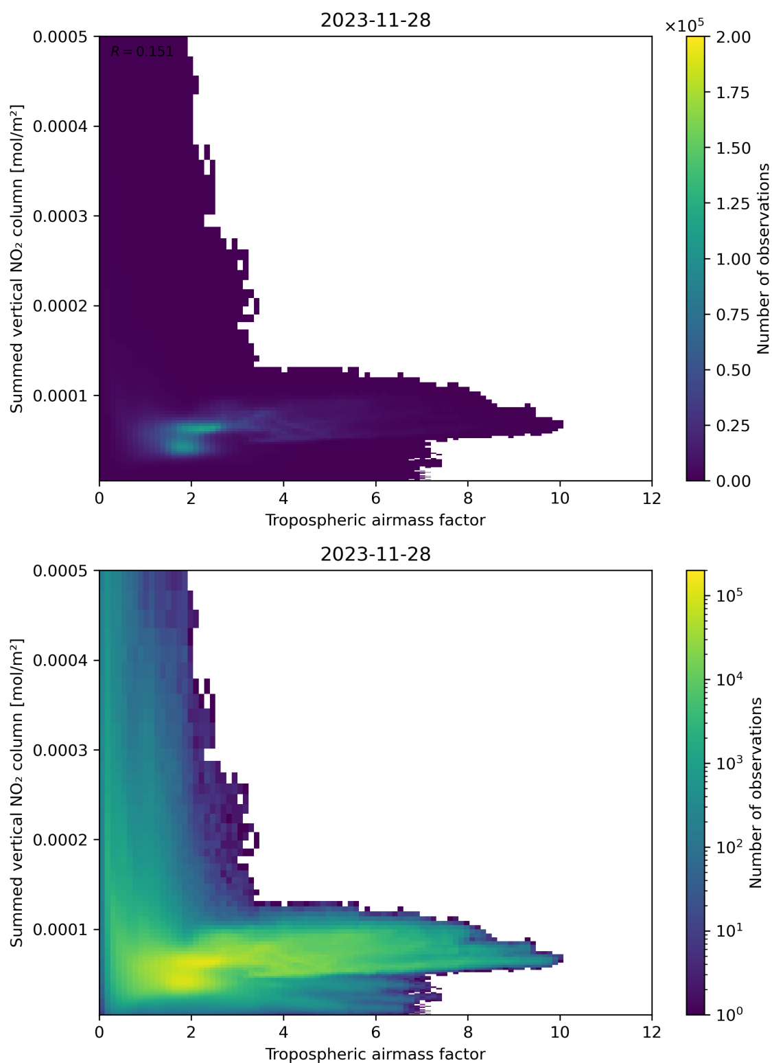
Figure 75: Scatter density plot of “Tropospheric airmass factor” against “Summed vertical NO 2 column” for 2023-11-28 to 2023-11-29.
