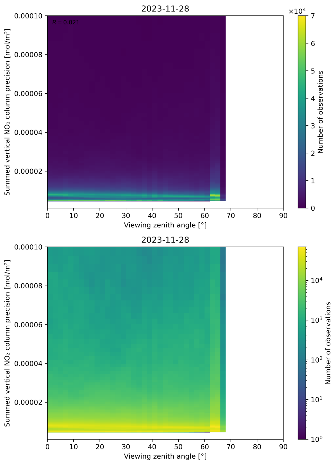
Figure 166: Scatter density plot of “Viewing zenith angle” against “Summed vertical NO 2 column precision” for 2023-11-28 to 2023-11-29.
