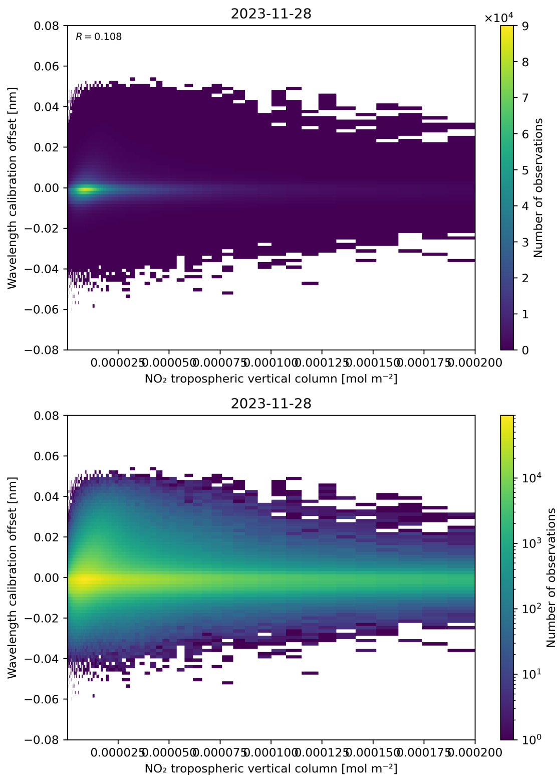
Figure 143: Scatter density plot of “NO 2 tropospheric vertical column” against “Wavelength calibration offset” for 2023-11-28 to 2023-11-29.
