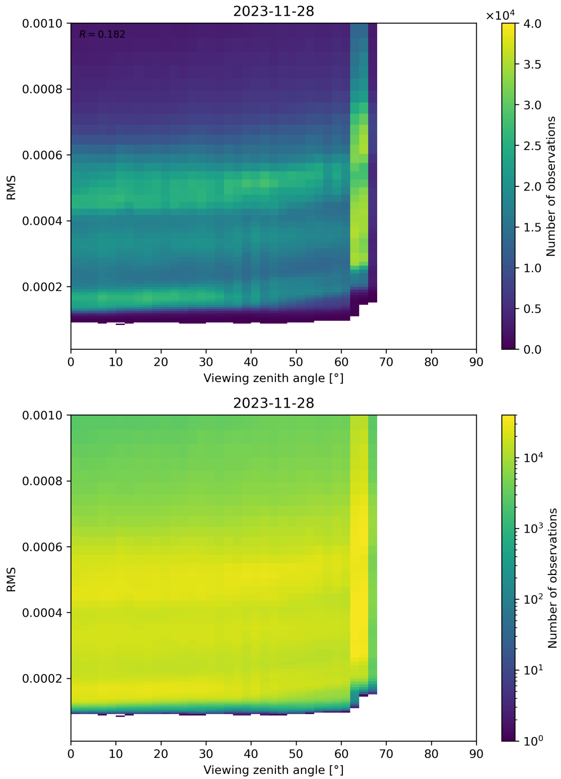
Figure 171: Scatter density plot of “Viewing zenith angle” against “RMS” for 2023-11-28 to 2023-11-29.
