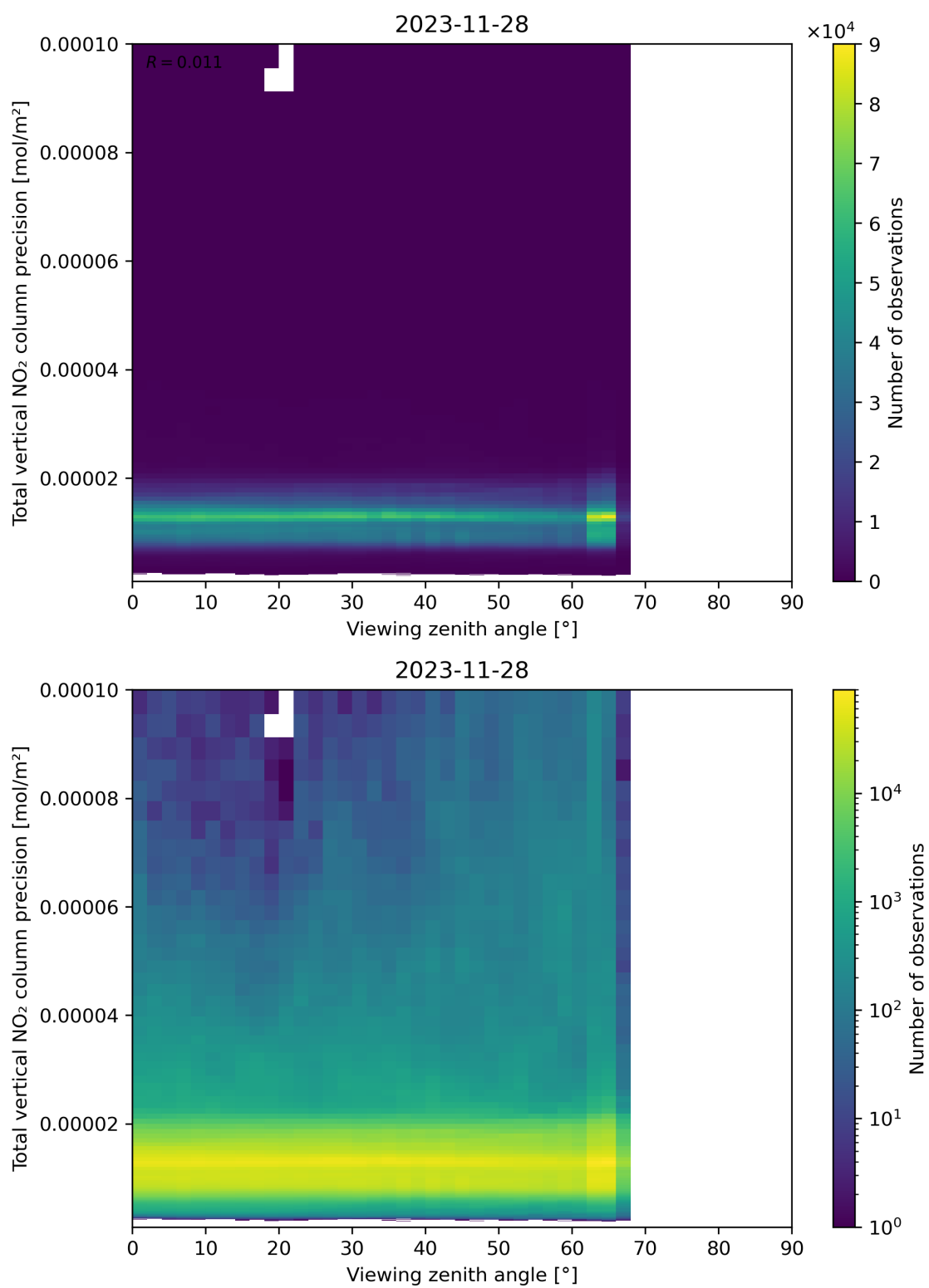
Figure 168: Scatter density plot of “Viewing zenith angle” against “Total vertical NO 2 column precision” for 2023-11-28 to 2023-11-29.
