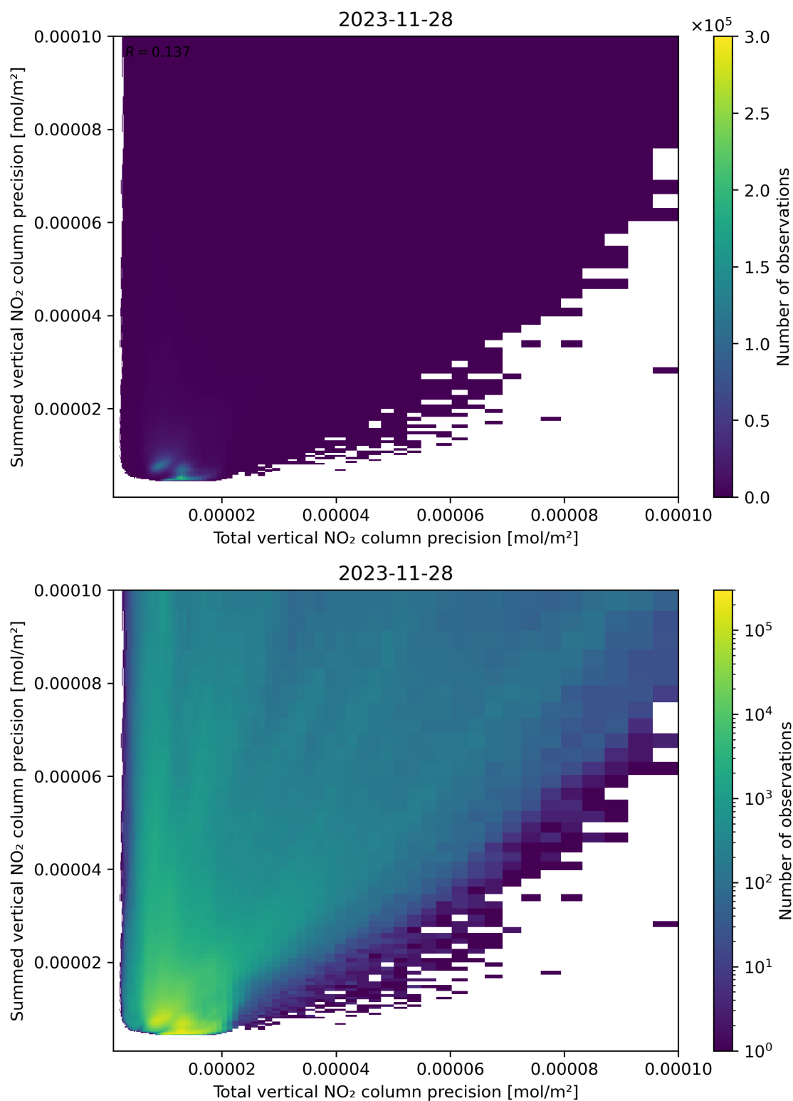
Figure 118: Scatter density plot of “Total vertical NO 2 column precision” against “Summed vertical NO 2 column precision” for 2023-11-28 to 2023-11-29.
