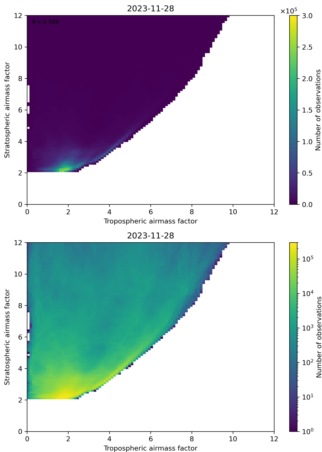
Figure 71: Scatter density plot of “Tropospheric airmass factor” against “Stratospheric airmass factor” for 2023-11-28 to 2023-11-29.
