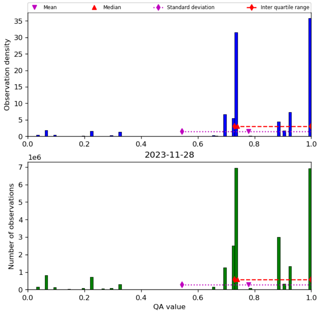
Figure 28: Histogram of “QA value” for 2023-11-28 to 2023-11-29
