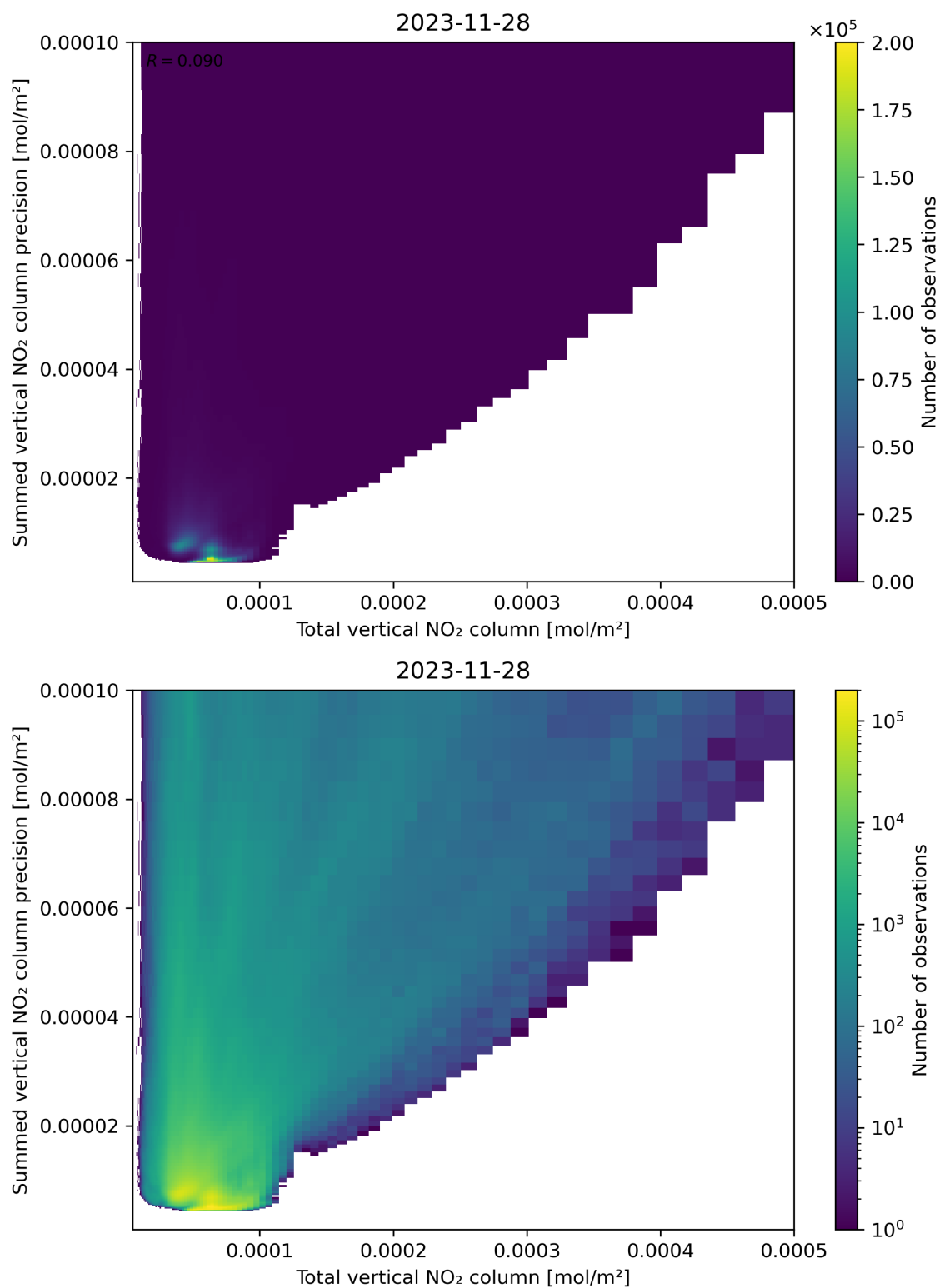
Figure 113: Scatter density plot of “Total vertical NO 2 column” against “Summed vertical NO 2 column precision” for 2023-11-28 to 2023-11-29.
