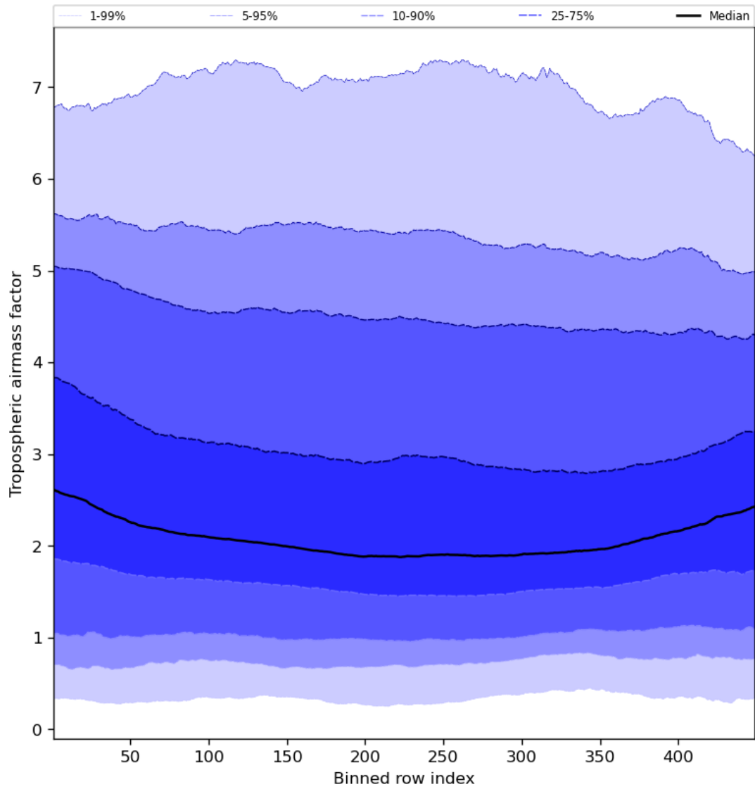
Figure 48: Along track statistics of “Tropospheric airmass factor” for 2023-11-28 to 2023-11-29
