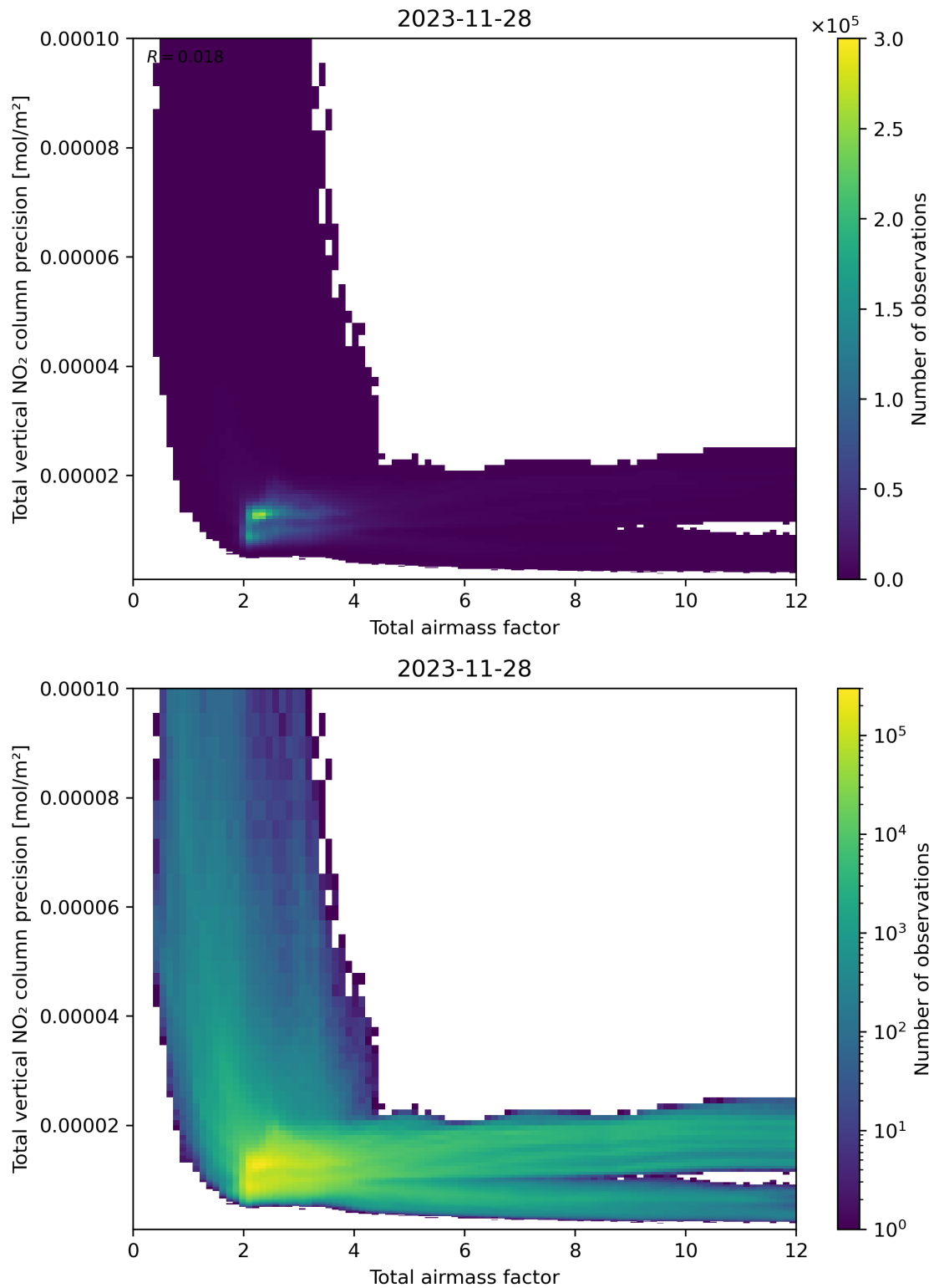
Figure 68: Scatter density plot of “Total airmass factor” against “Total vertical NO 2 column precision” for 2023-11-28 to 2023-11-29.
