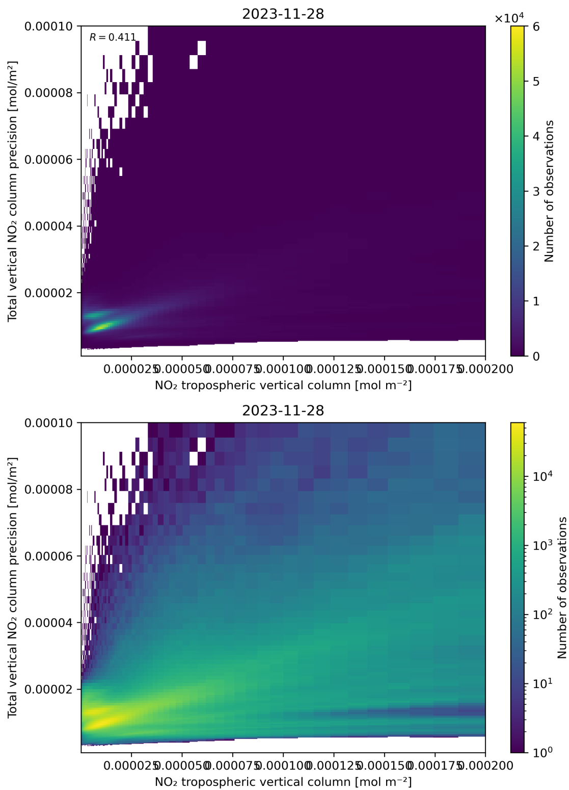
Figure 129: Scatter density plot of “NO 2 tropospheric vertical column” against “Total vertical NO 2 column precision” for 2023-11-28 to 2023-11-29.
