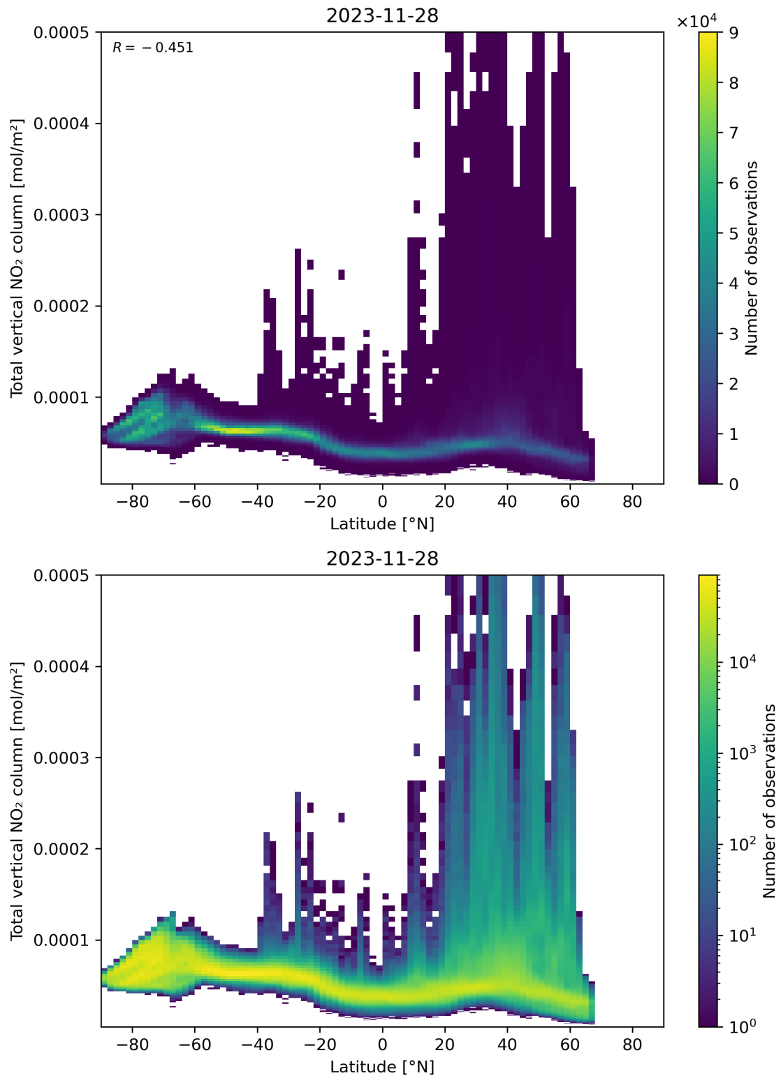
Figure 90: Scatter density plot of “Latitude” against “Total vertical NO 2 column” for 2023-11-28 to 2023-11-29.
