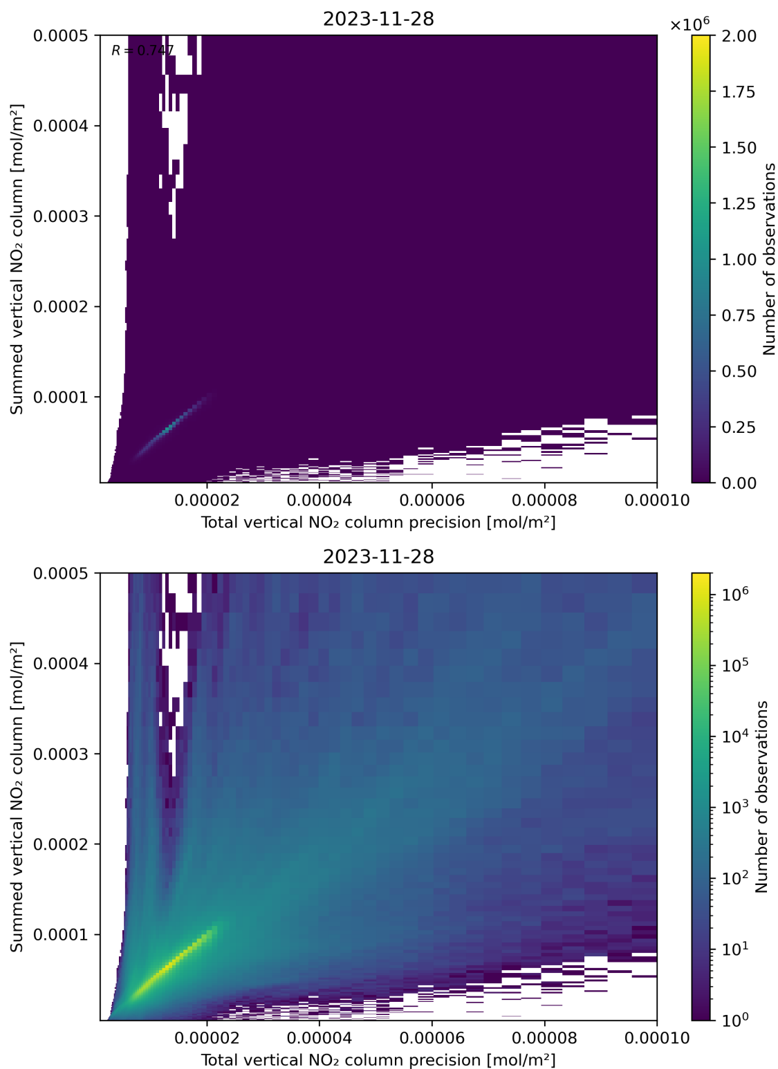
Figure 117: Scatter density plot of “Total vertical NO 2 column precision” against “Summed vertical NO 2 column” for 2023-11-28 to 2023-11-29.
