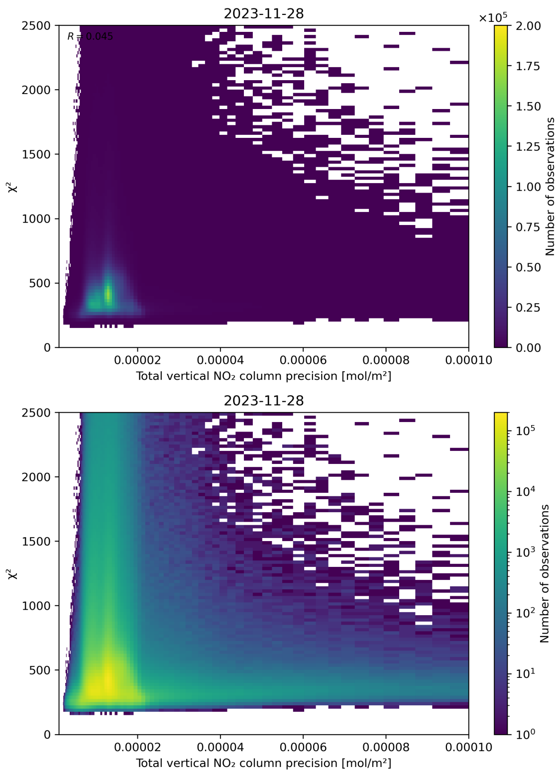
Figure 116: Scatter density plot of “Total vertical NO 2 column precision” against “ \chi^2 ” for 2023-11-28 to 2023-11-29.
