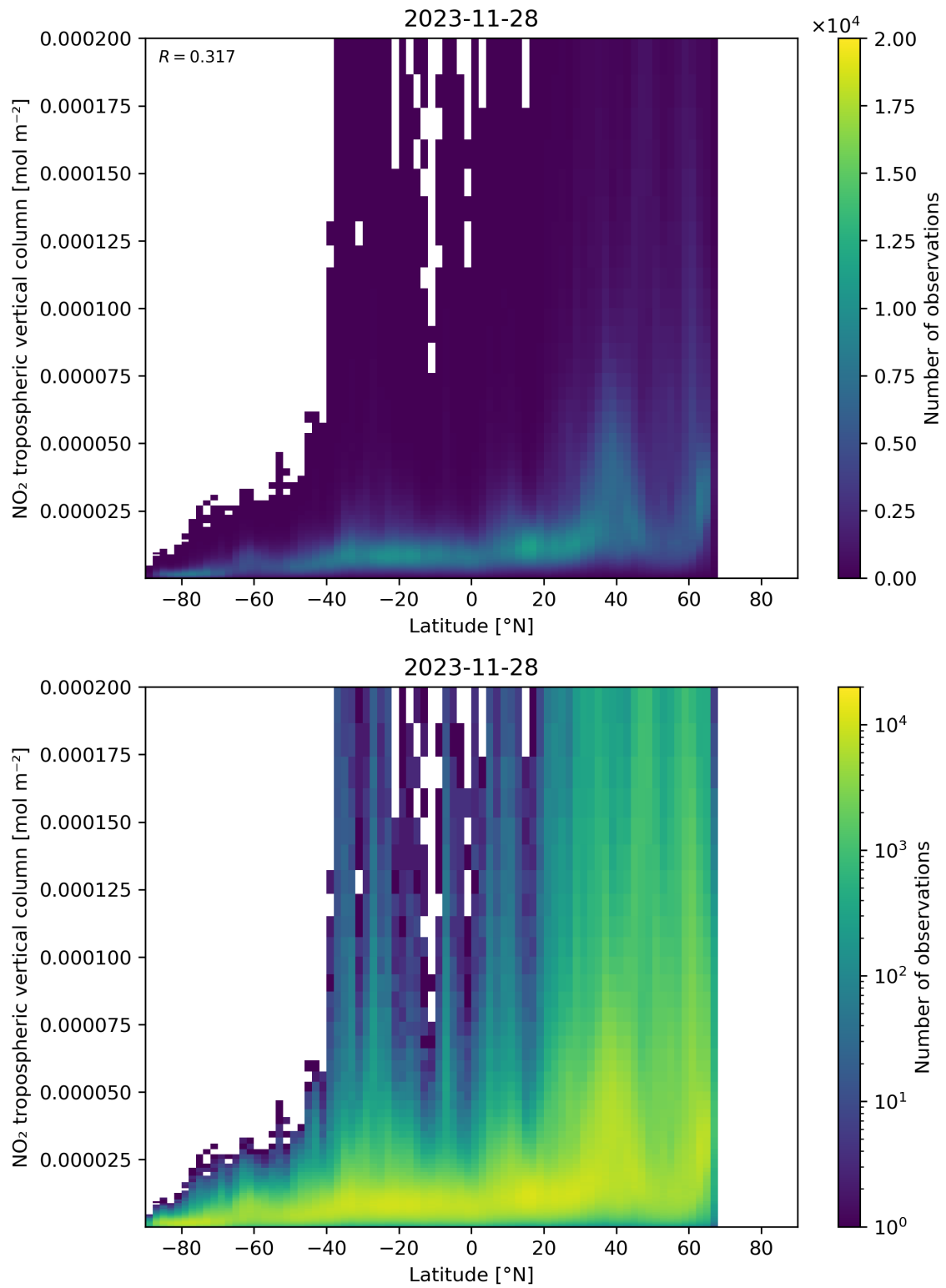
Figure 92: Scatter density plot of “Latitude” against “NO 2 tropospheric vertical column” for 2023-11-28 to 2023-11-29.
