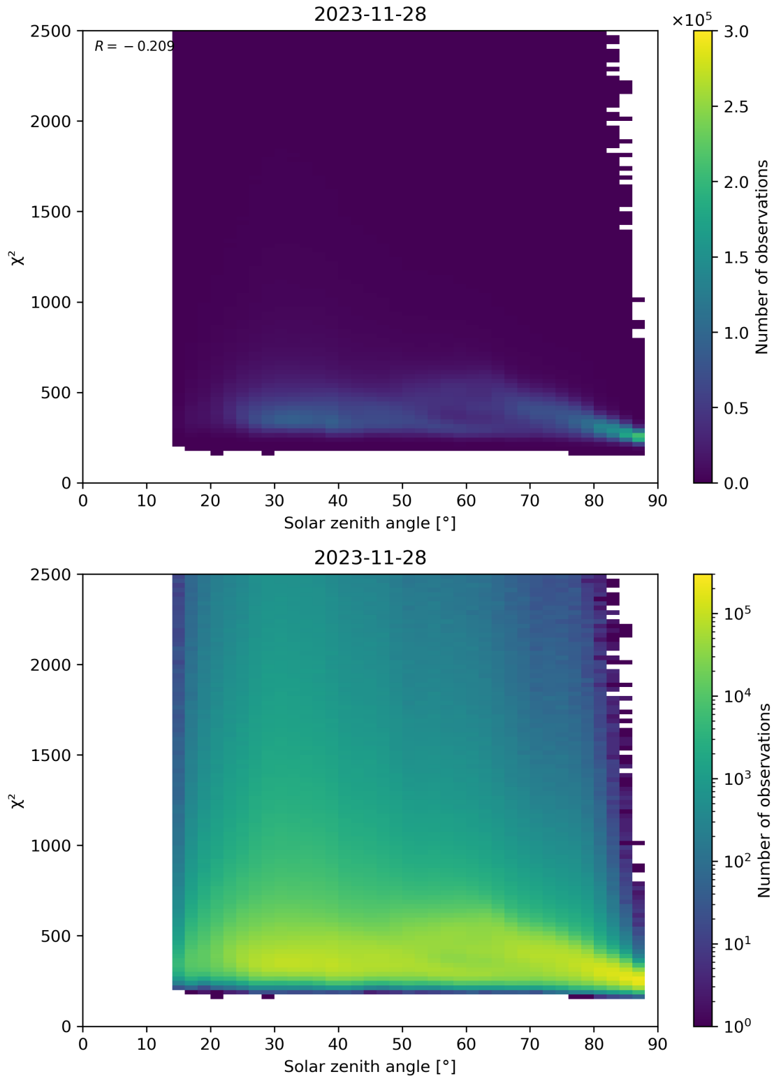
Figure 148: Scatter density plot of “Solar zenith angle” against “ \chi^2 ” for 2023-11-28 to 2023-11-29.
