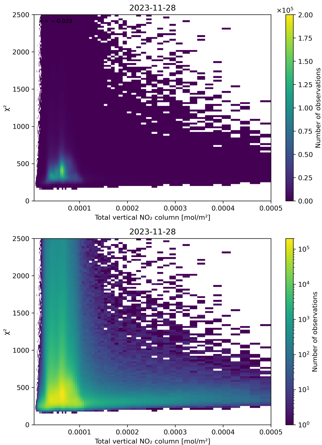
Figure 111: Scatter density plot of “Total vertical NO 2 column” against “ \chi^2 ” for 2023-11-28 to 2023-11-29.
