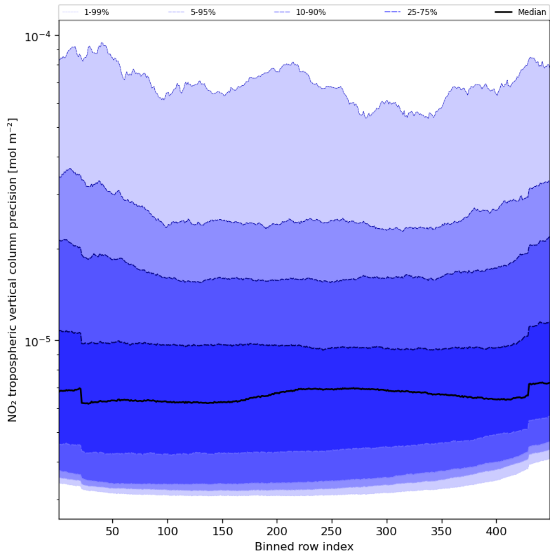
Figure 47: Along track statistics of “NO 2 tropospheric vertical column precision” for 2023-11-28 to 2023-11-29
