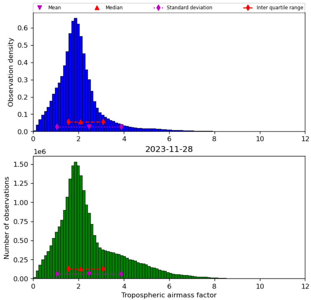
Figure 31: Histogram of “Tropospheric airmass factor” for 2023-11-28 to 2023-11-29
