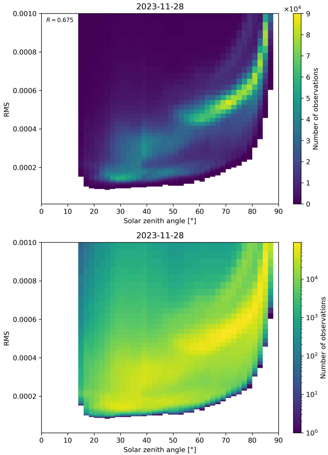
Figure 157: Scatter density plot of “Solar zenith angle” against “RMS” for 2023-11-28 to 2023-11-29.
