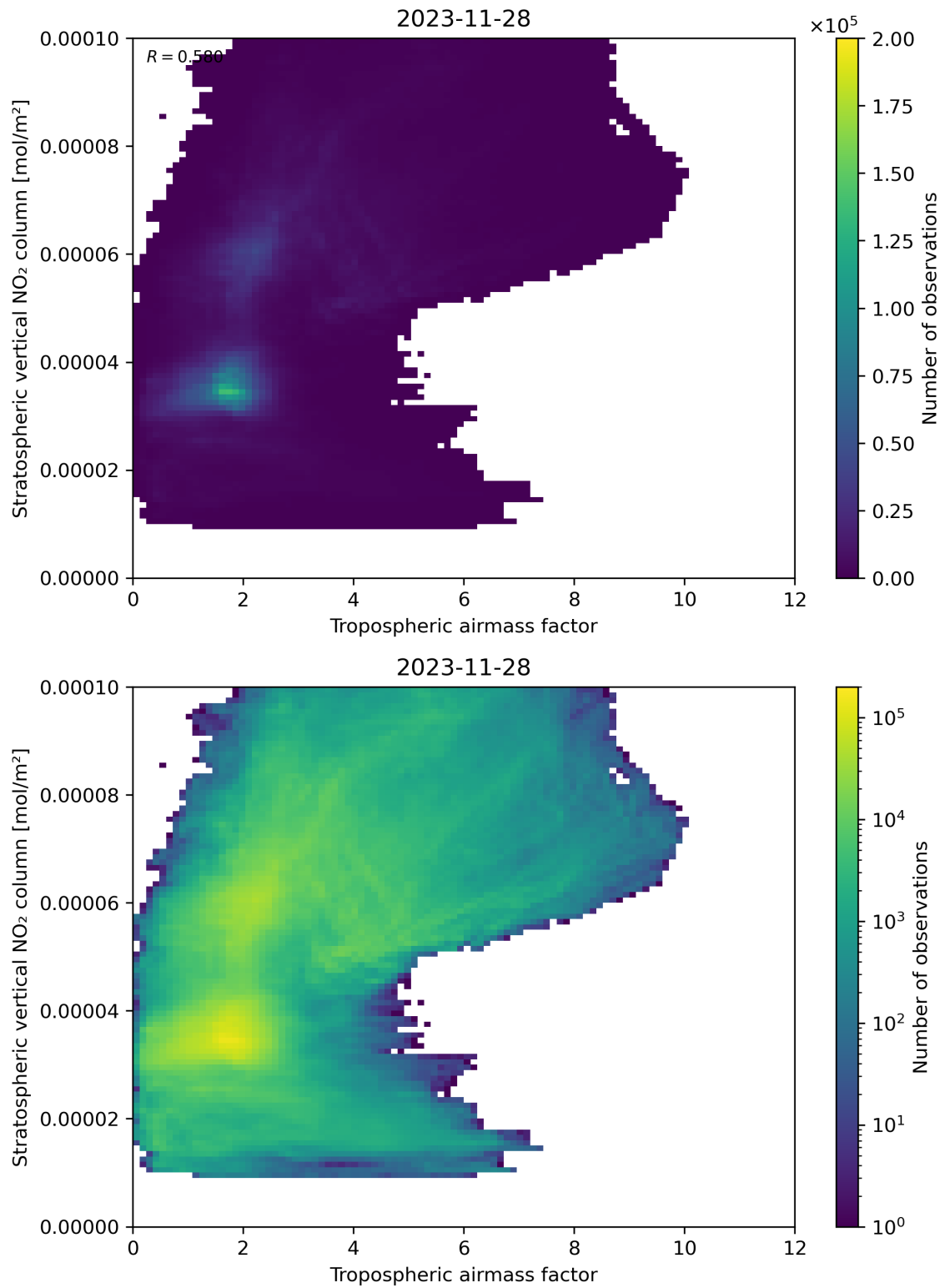
Figure 74: Scatter density plot of “Tropospheric air mass factor” against “Stratospheric vertical NO 2 column” for 2023-11-28 to 2023-11-29.
