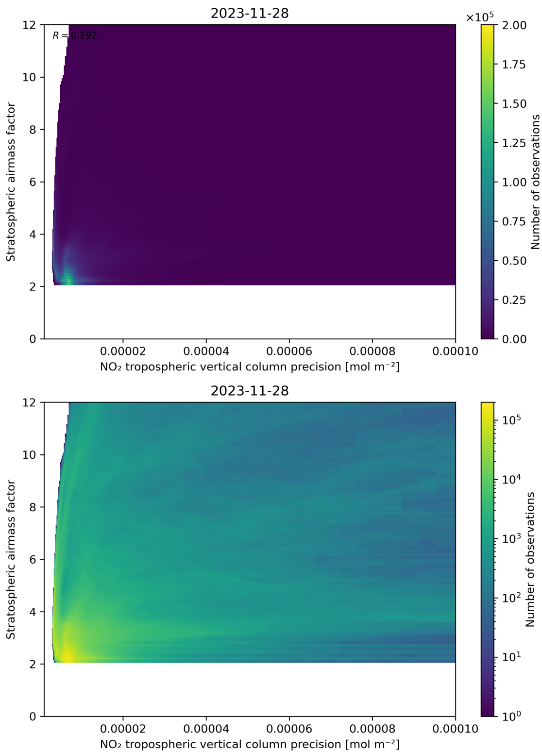
Figure 131: Scatter density plot of “NO 2 tropospheric vertical column precision” against “Stratospheric airmass factor” for 2023-11-28 to 2023-11-29.
