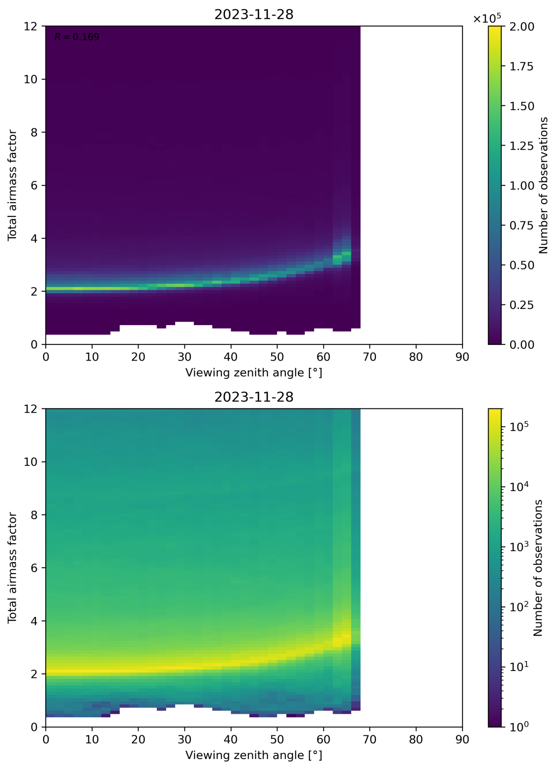
Figure 160: Scatter density plot of “Viewing zenith angle” against “Total airmass factor” for 2023-11-28 to 2023-11-29.
