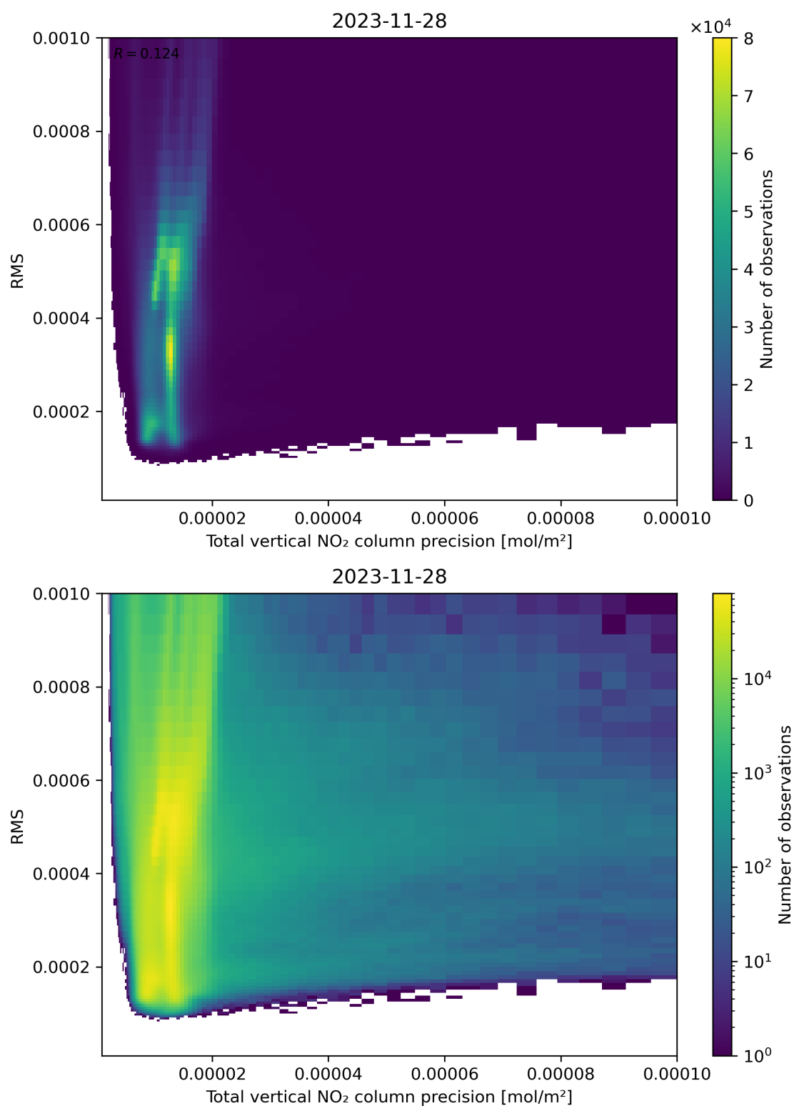
Figure 119: Scatter density plot of “Total vertical NO 2 column precision” against “RMS” for 2023-11-28 to 2023-11-29.
