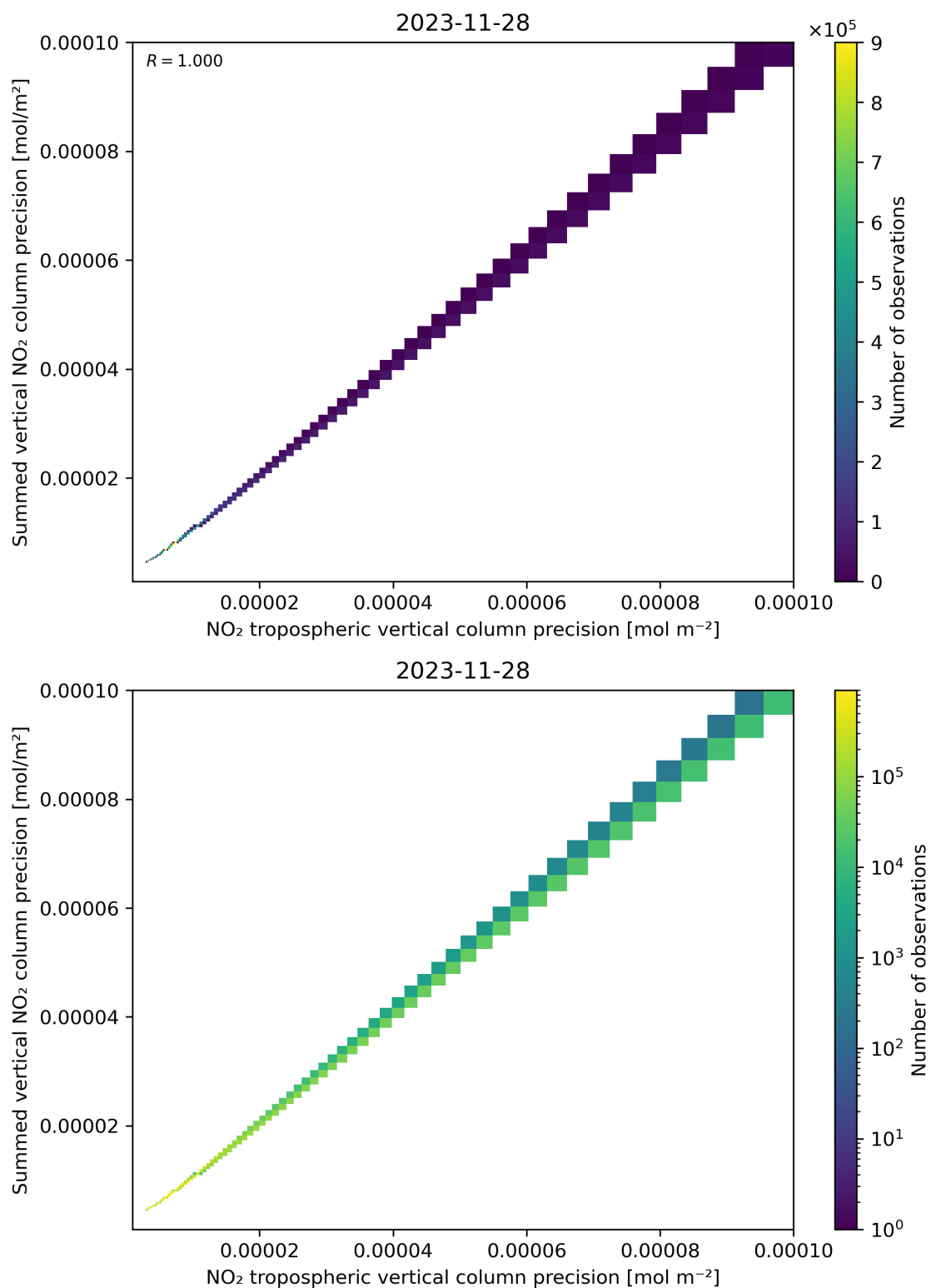
Figure 137: Scatter density plot of “NO 2 tropospheric vertical column precision” against “Summed vertical NO 2 column precision” for 2023-11-28 to 2023-11-29.
