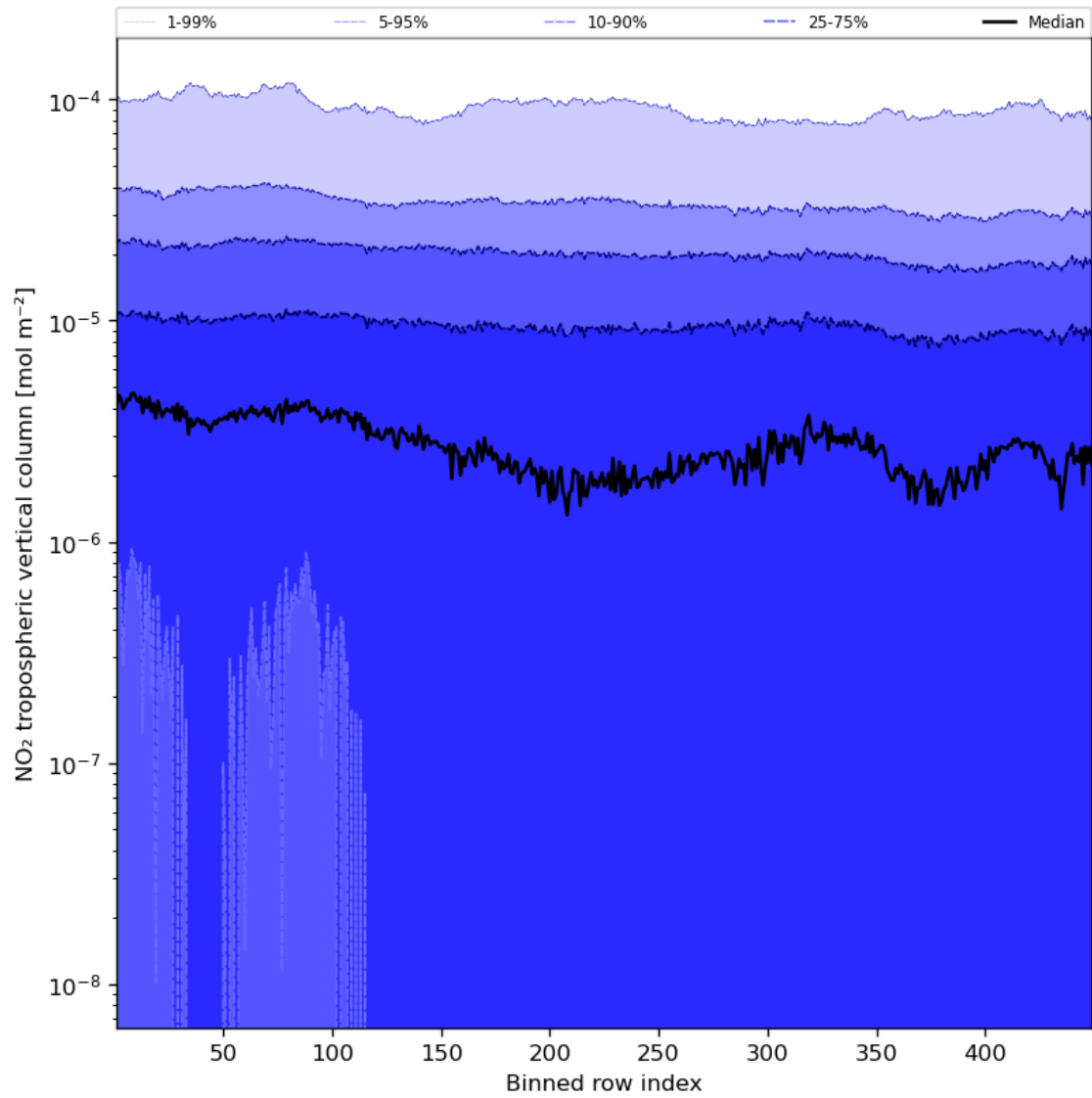
Figure 46: Along track statistics of “NO 2 tropospheric vertical column” for 2023-11-28 to 2023-11-29
