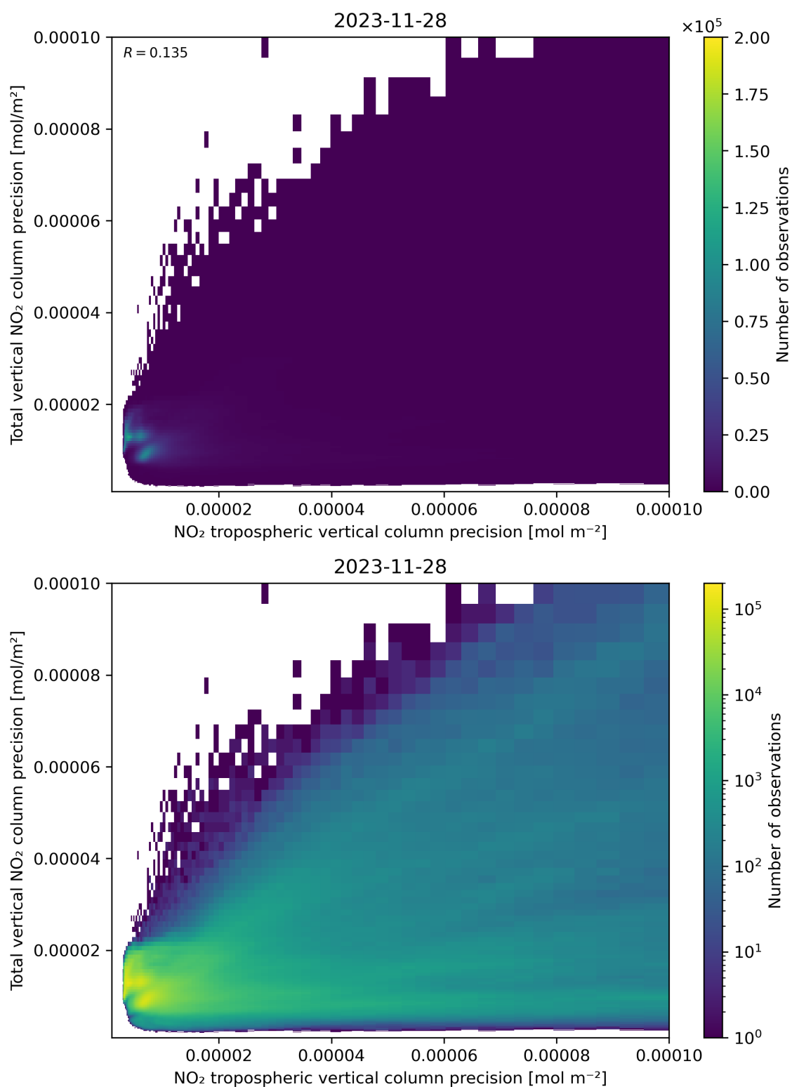
Figure 139: Scatter density plot of “NO 2 tropospheric vertical column precision” against “Total vertical NO 2 column precision” for 2023-11-28 to 2023-11-29.
