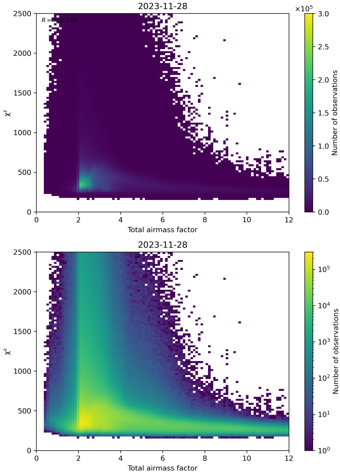
Figure 63: Scatter density plot of “Total airmass factor” against “ \chi^2 ” for 2023-11-28 to 2023-11-29.
