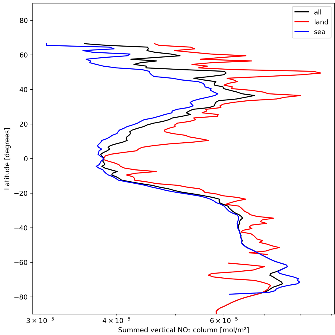
Figure 23: Zonal average of “Summed vertical NO 2 column” for 2023-11-28 to 2023-11-29.
