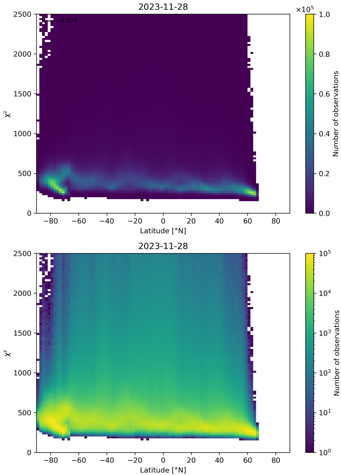
Figure 86: Scatter density plot of “Latitude” against “ \chi^2 ” for 2023-11-28 to 2023-11-29.
