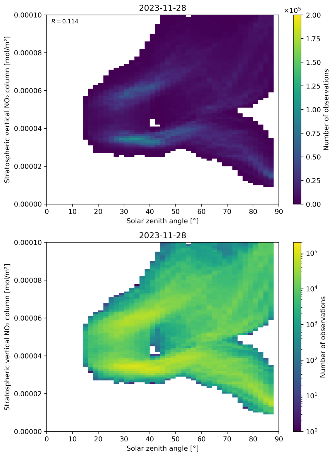
Figure 150: Scatter density plot of “Solar zenith angle” against “Stratospheric vertical NO 2 column” for 2023-11-28 to 2023-11-29.
