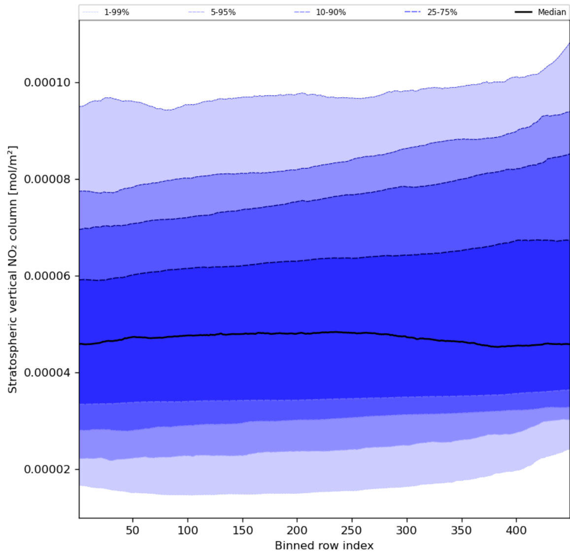
Figure 53: Along track statistics of “Stratospheric vertical NO 2 column” for 2023-11-28 to 2023-11-29
