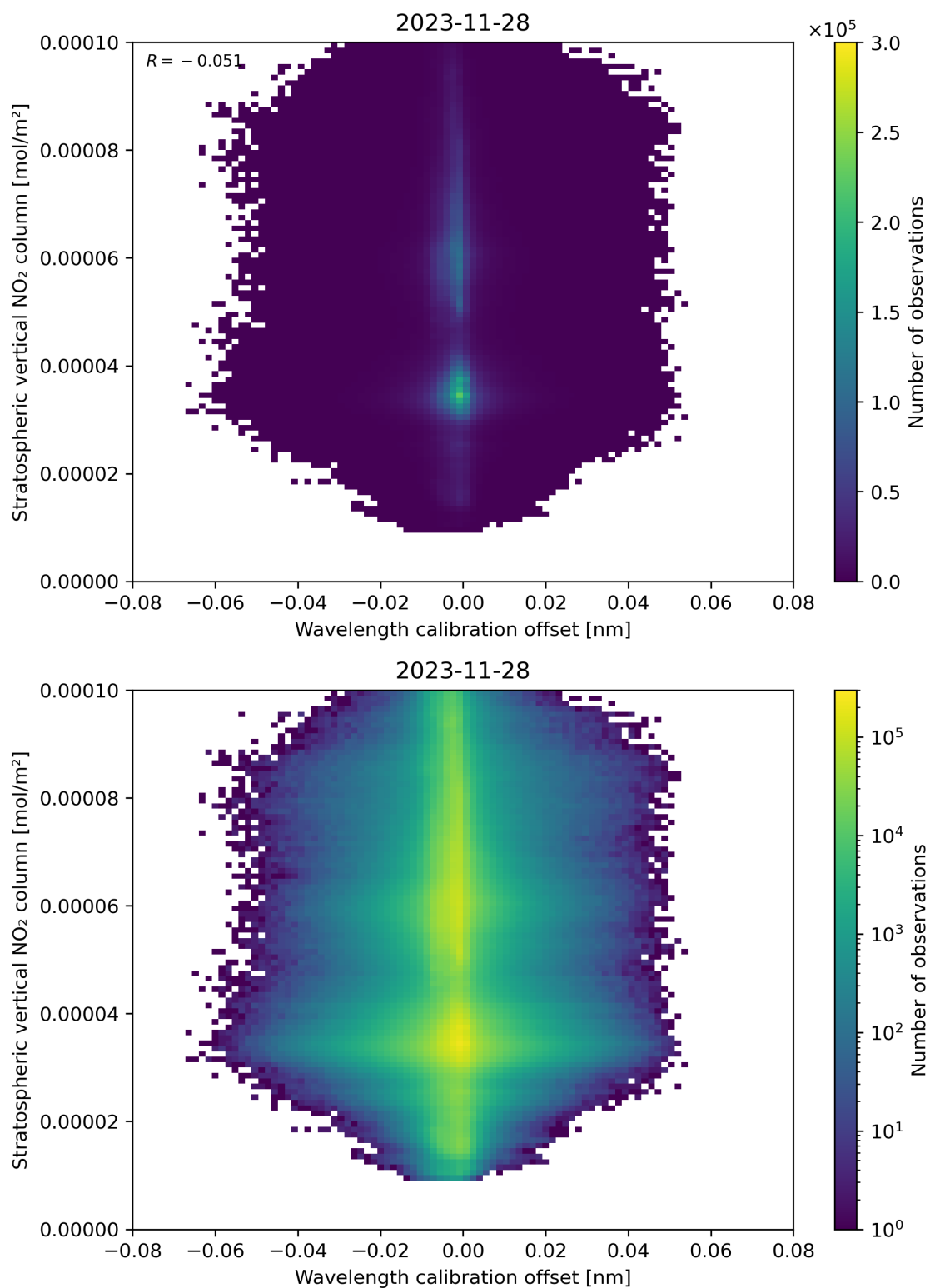
Figure 176: Scatter density plot of “Wavelength calibration offset” against “Stratospheric vertical NO 2 column” for 2023-11-28 to 2023-11-29.
