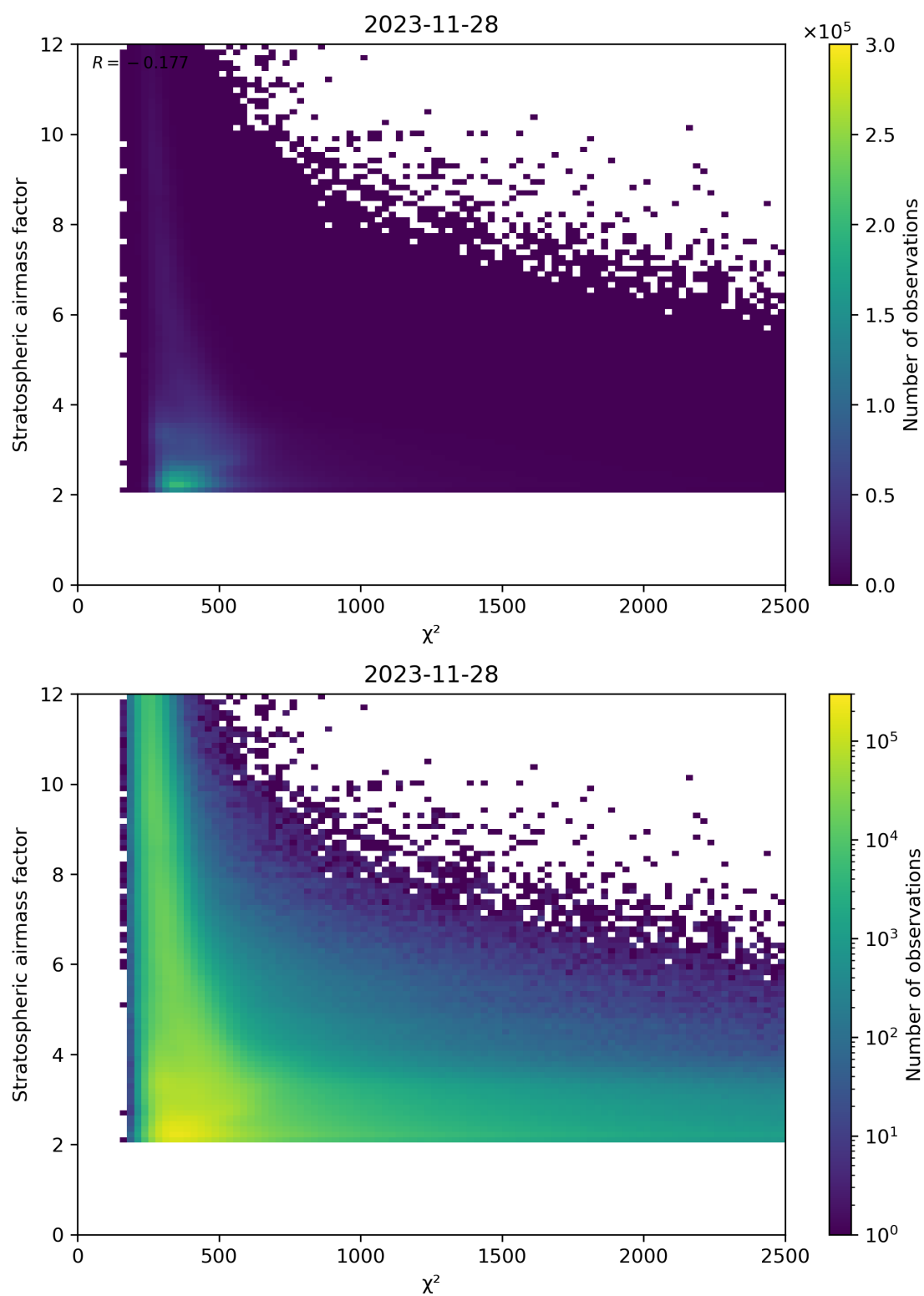
Figure 81: Scatter density plot of " \chi^2 " against "Stratospheric airmass factor" for 2023-11-28 to 2023-11-29.
