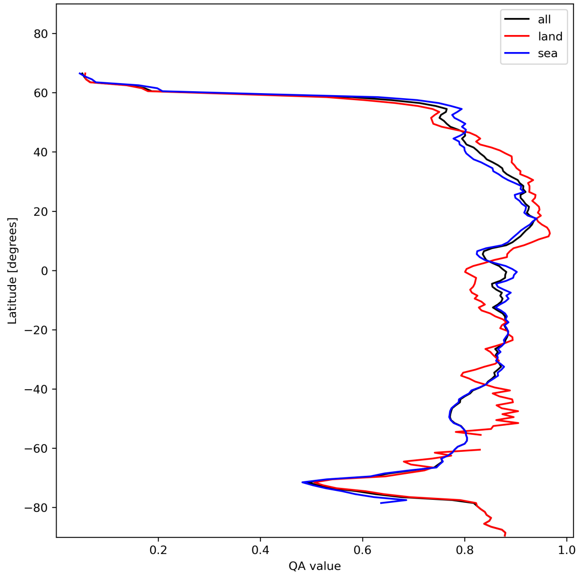
Figure 11: Zonal average of “QA value” for 2023-11-28 to 2023-11-29.
