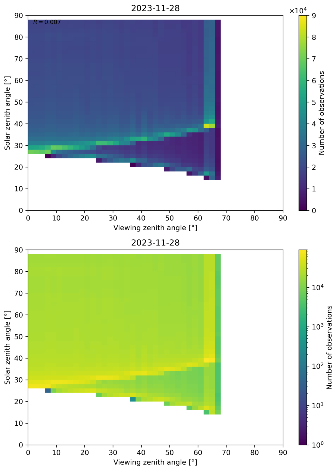
Figure 172: Scatter density plot of “Viewing zenith angle” against “Solar zenith angle” for 2023-11-28 to 2023-11-29.
