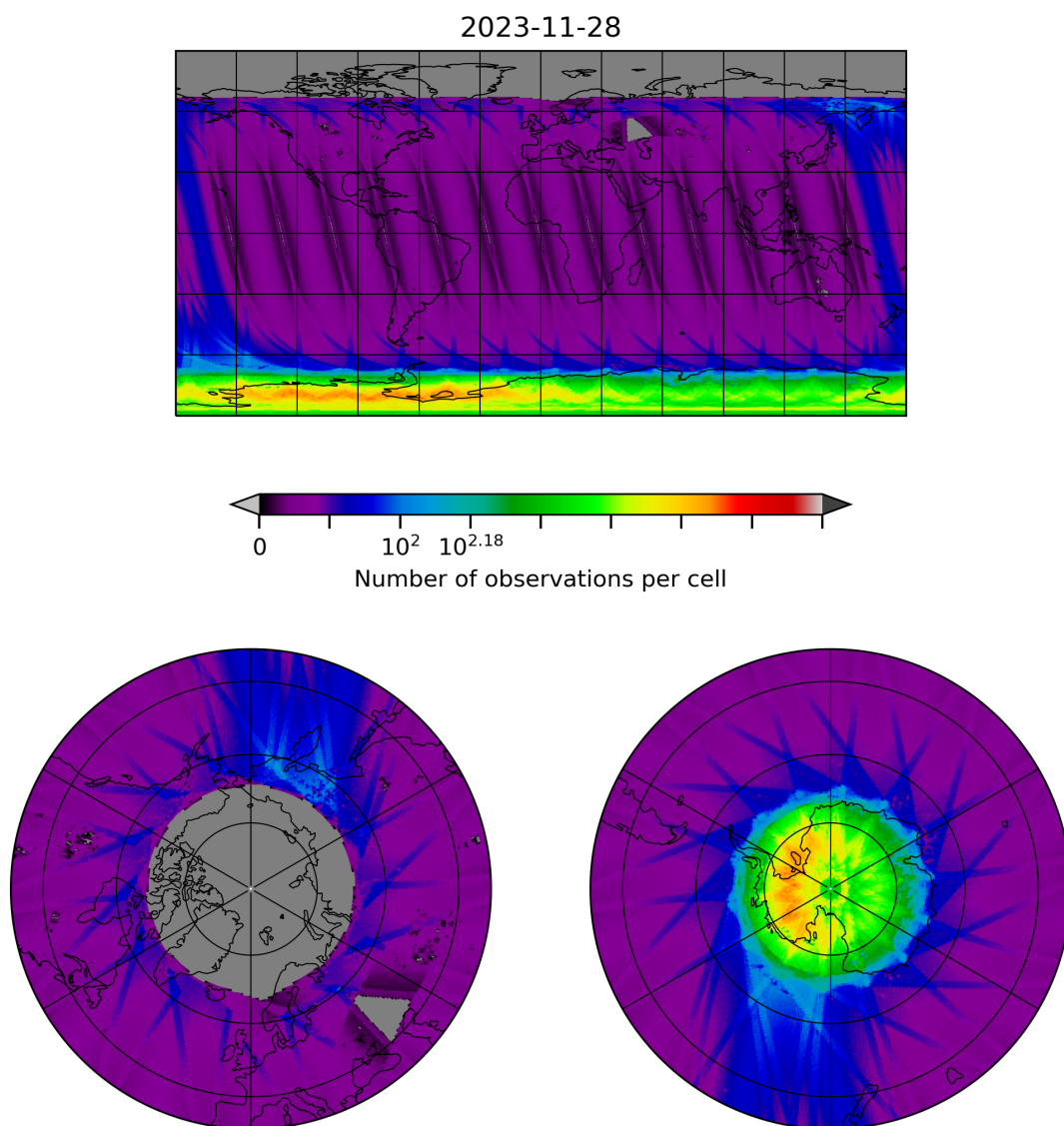
Figure 10: Map of the number of observations for 2023-11-28 to 2023-11-29
