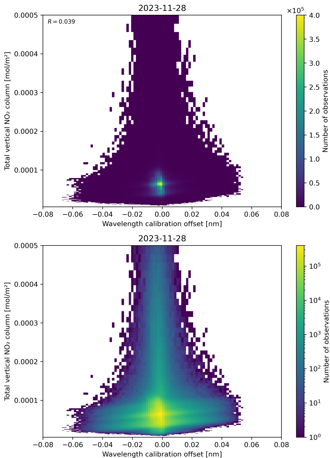
Figure 179: Scatter density plot of “Wavelength calibration offset” against “Total vertical NO 2 column” for 2023-11-28 to 2023-11-29.
