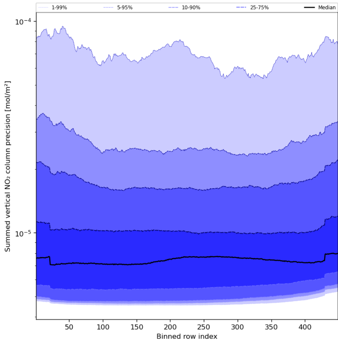
Figure 58: Along track statistics of “Summed vertical NO 2 column precision” for 2023-11-28 to 2023-11-29
