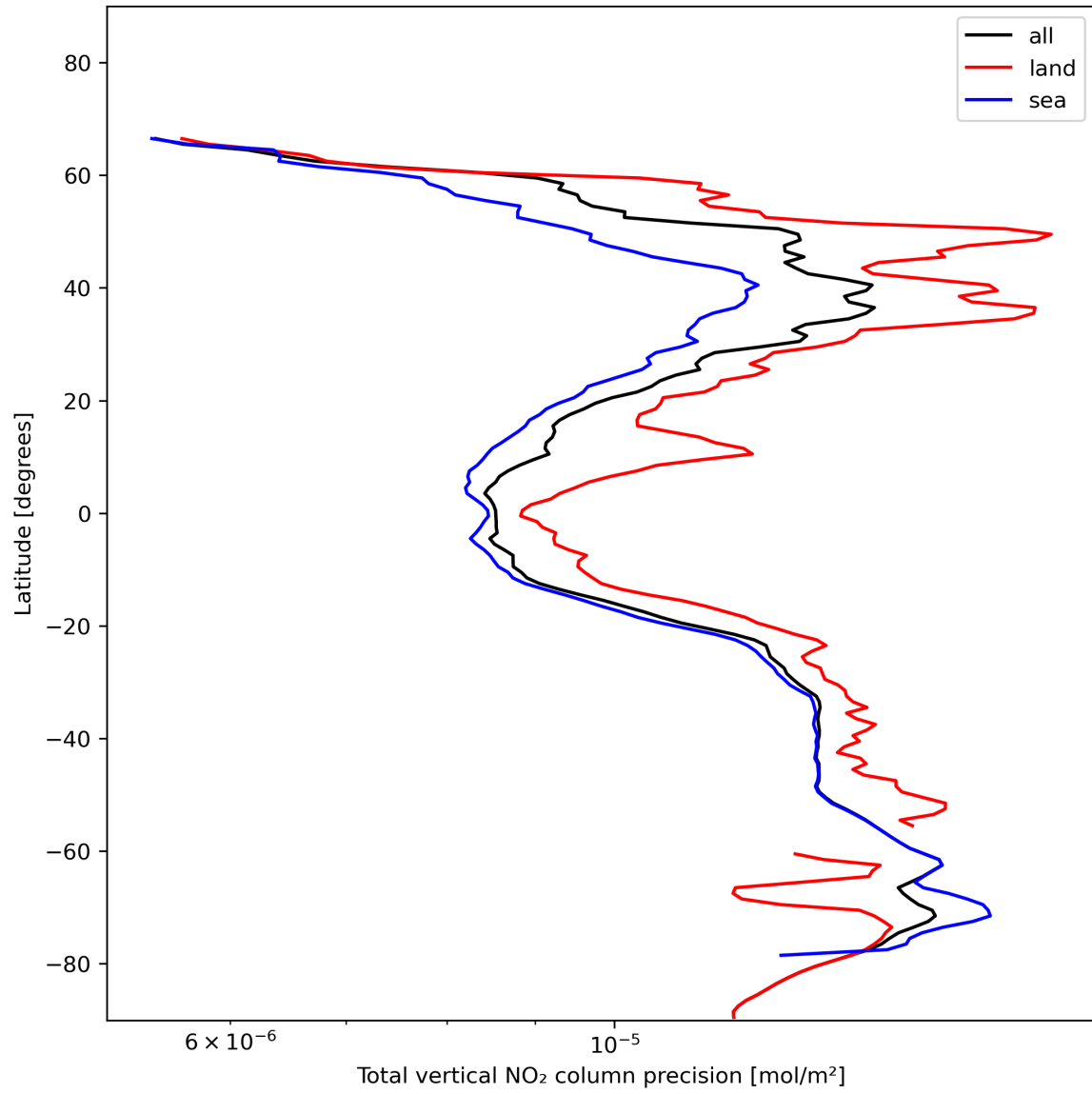
Figure 22: Zonal average of “Total vertical NO 2 column precision” for 2023-11-28 to 2023-11-29.
