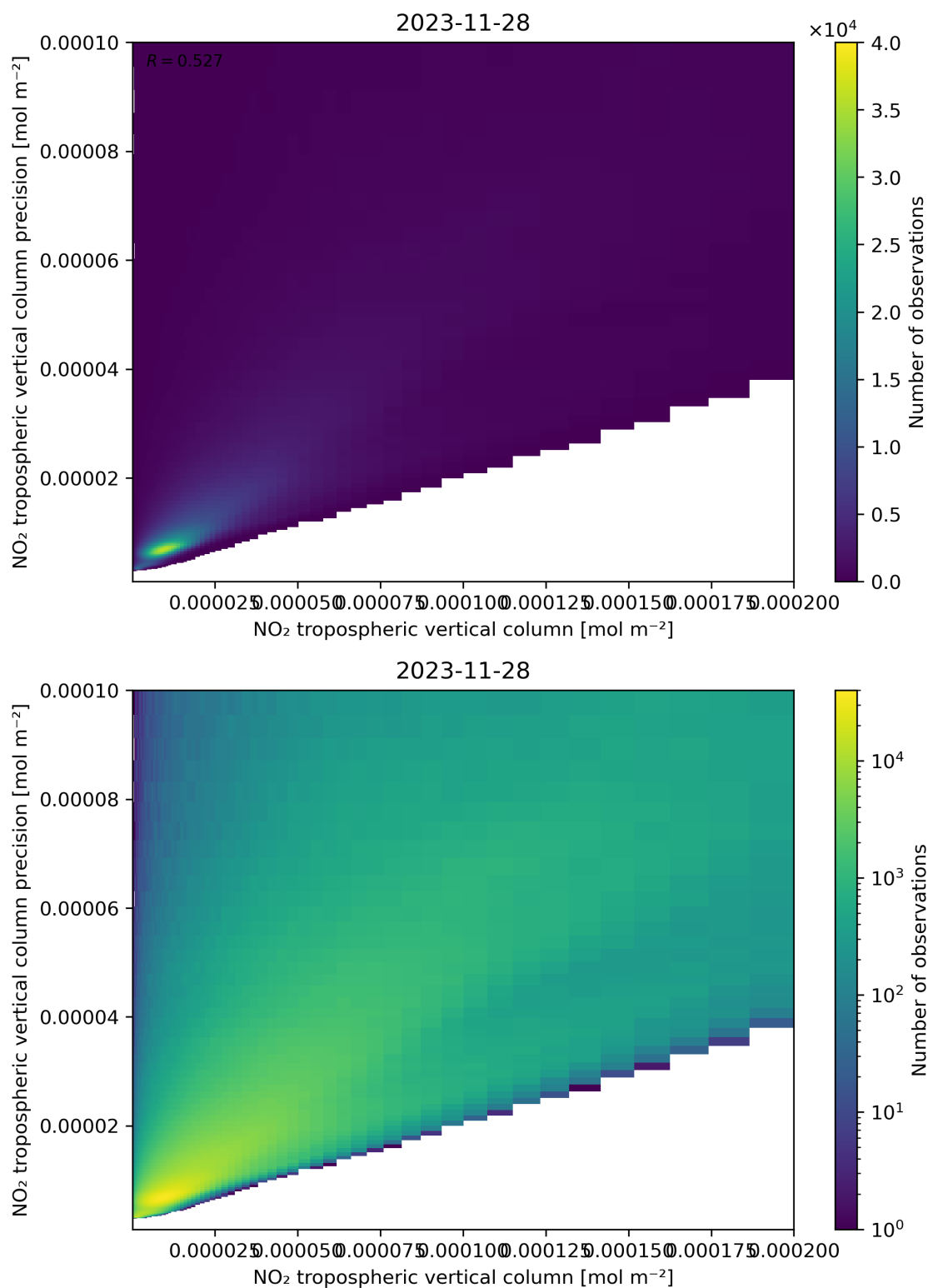
Figure 130: Scatter density plot of “NO 2 tropospheric vertical column” against “NO 2 tropospheric vertical column precision” for 2023-11-28 to 2023-11-29.
