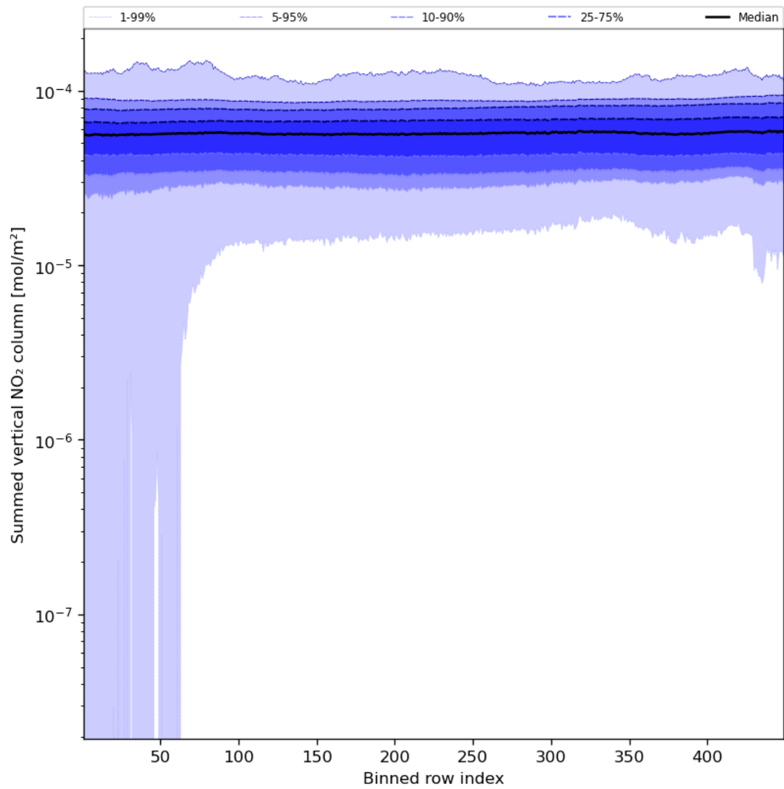
Figure 57: Along track statistics of “Summed vertical NO 2 column” for 2023-11-28 to 2023-11-29
