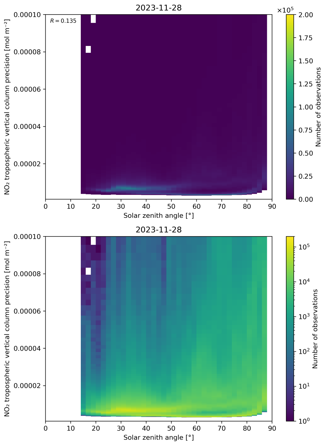
Figure 156: Scatter density plot of “Solar zenith angle” against “NO 2 tropospheric vertical column precision” for 2023-11-28 to 2023-11-29.
