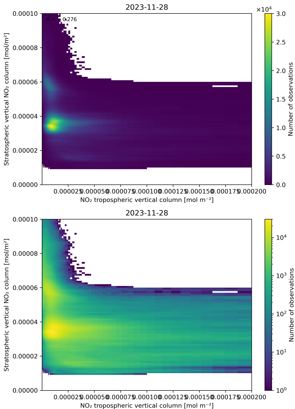
Figure 125: Scatter density plot of “NO 2 tropospheric vertical column” against “Stratospheric vertical NO 2 column” for 2023-11-28 to 2023-11-29.
