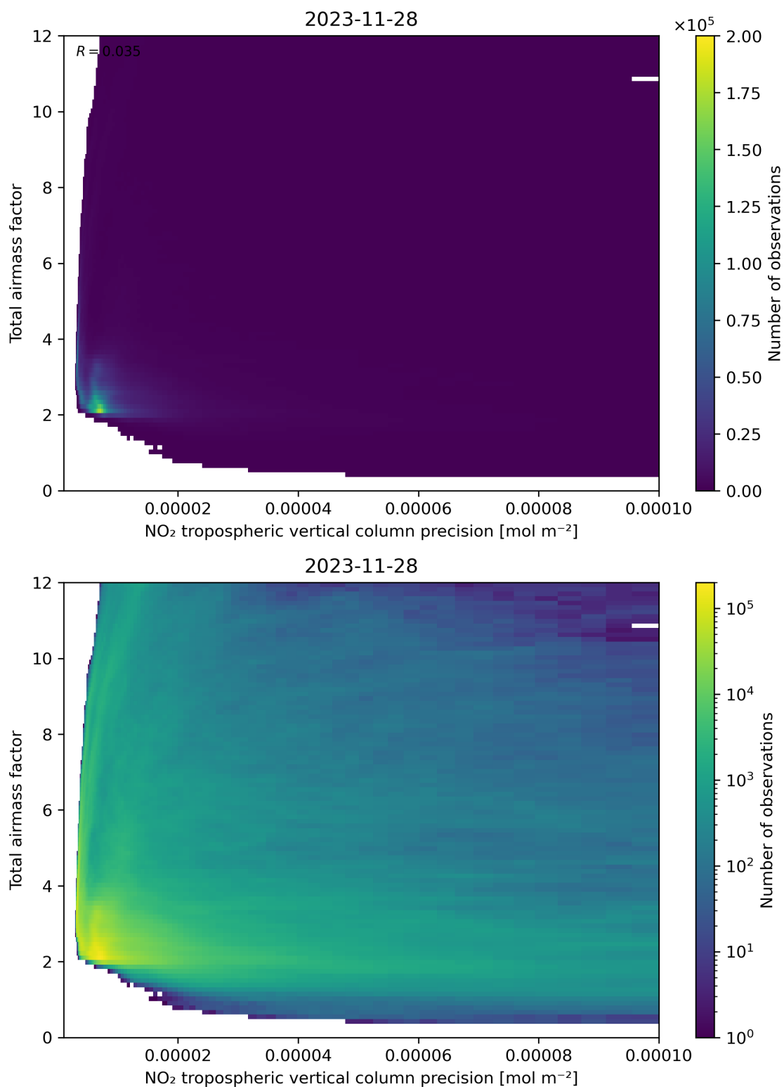
Figure 132: Scatter density plot of “NO 2 tropospheric vertical column precision” against “Total air mass factor” for 2023-11-28 to 2023-11-29.
