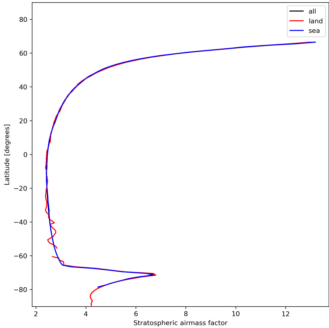
Figure 27: Zonal average of “Stratospheric airmass factor” for 2023-11-28 to 2023-11-29.
