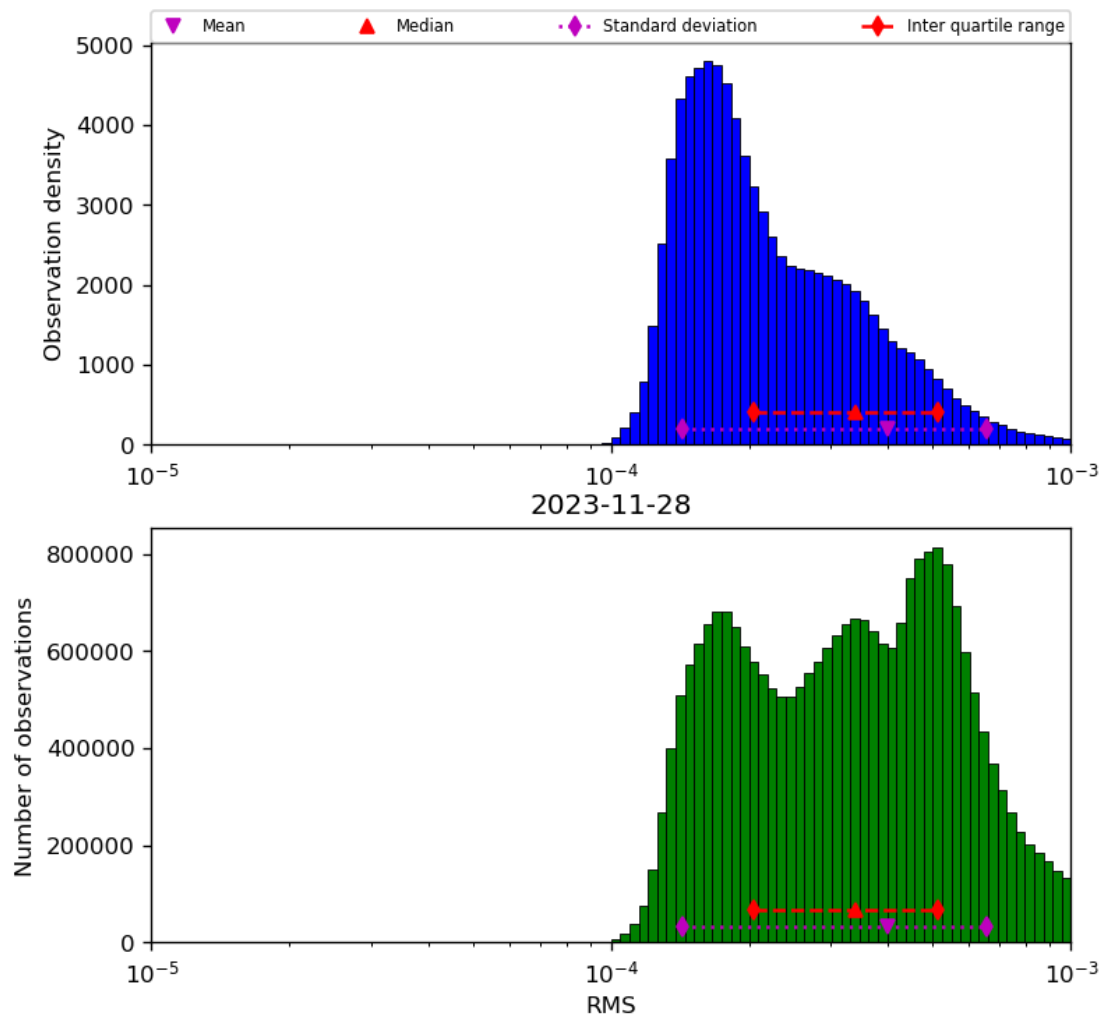
Figure 43: Histogram of “RMS” for 2023-11-28 to 2023-11-29
