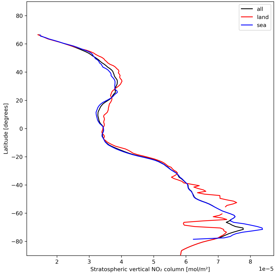
Figure 19: Zonal average of “Stratospheric vertical NO 2 column” for 2023-11-28 to 2023-11-29.
