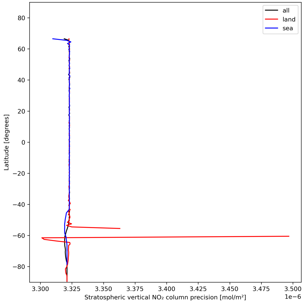
Figure 20: Zonal average of “Stratospheric vertical NO 2 column precision” for 2023-11-28 to 2023-11-29.
