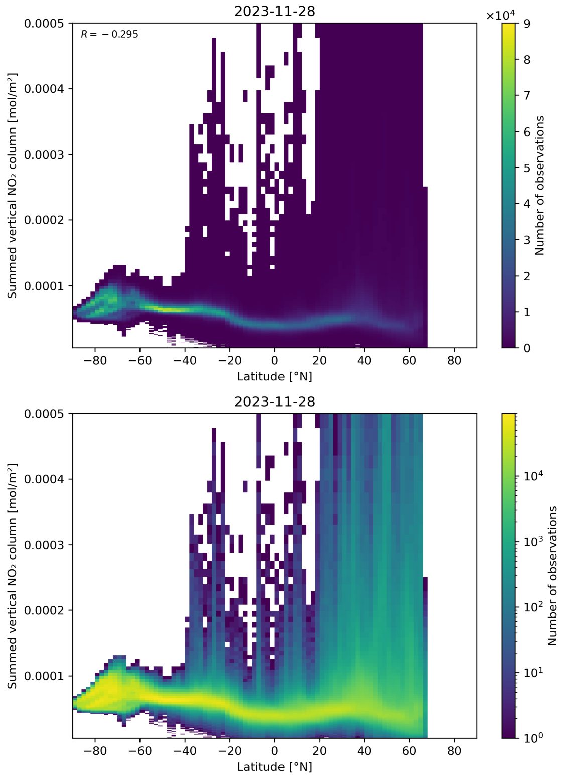
Figure 88: Scatter density plot of “Latitude” against “Summed vertical NO 2 column” for 2023-11-28 to 2023-11-29.
