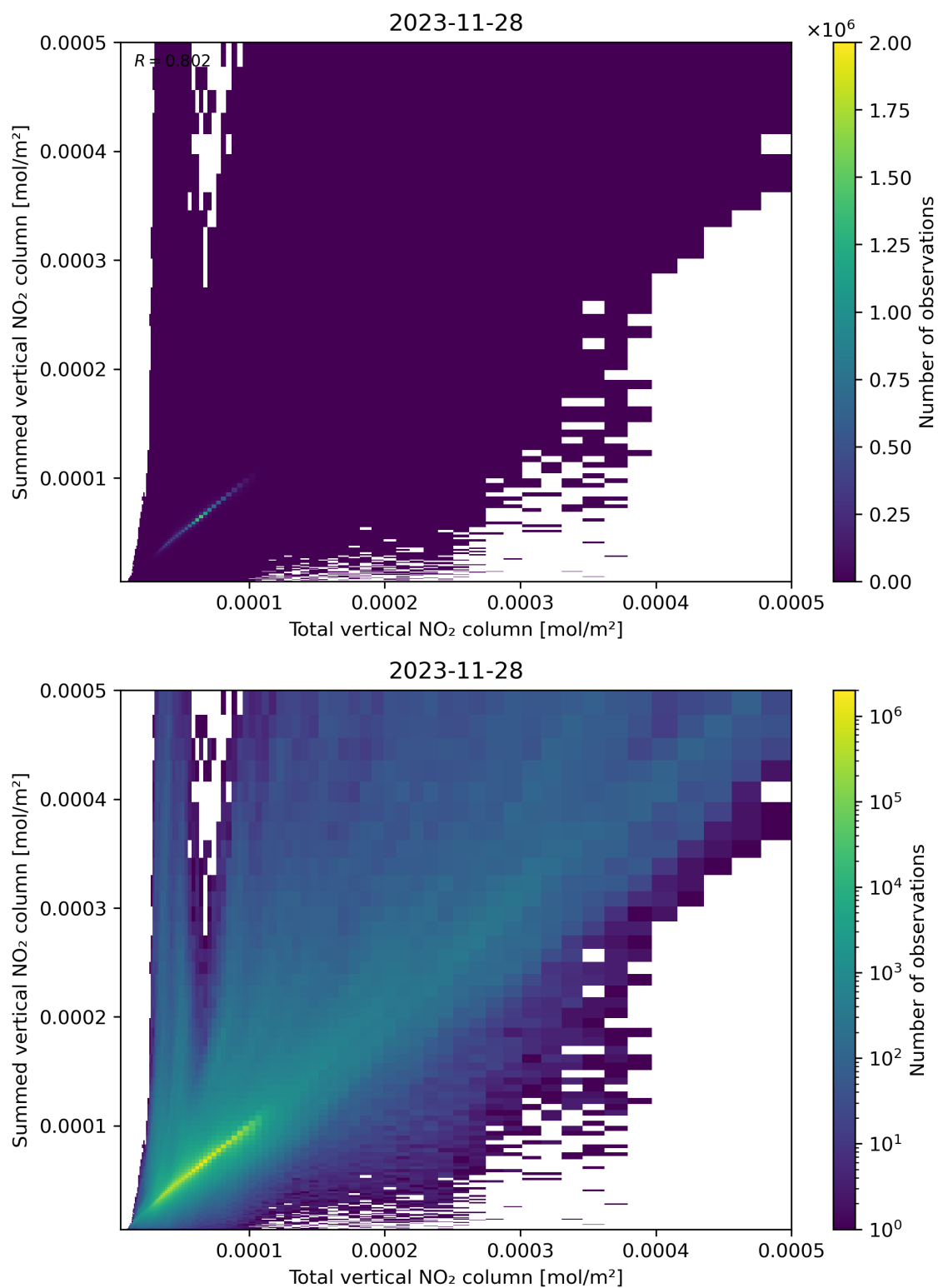
Figure 112: Scatter density plot of “Total vertical NO 2 column” against “Summed vertical NO 2 column” for 2023-11-28 to 2023-11-29.
