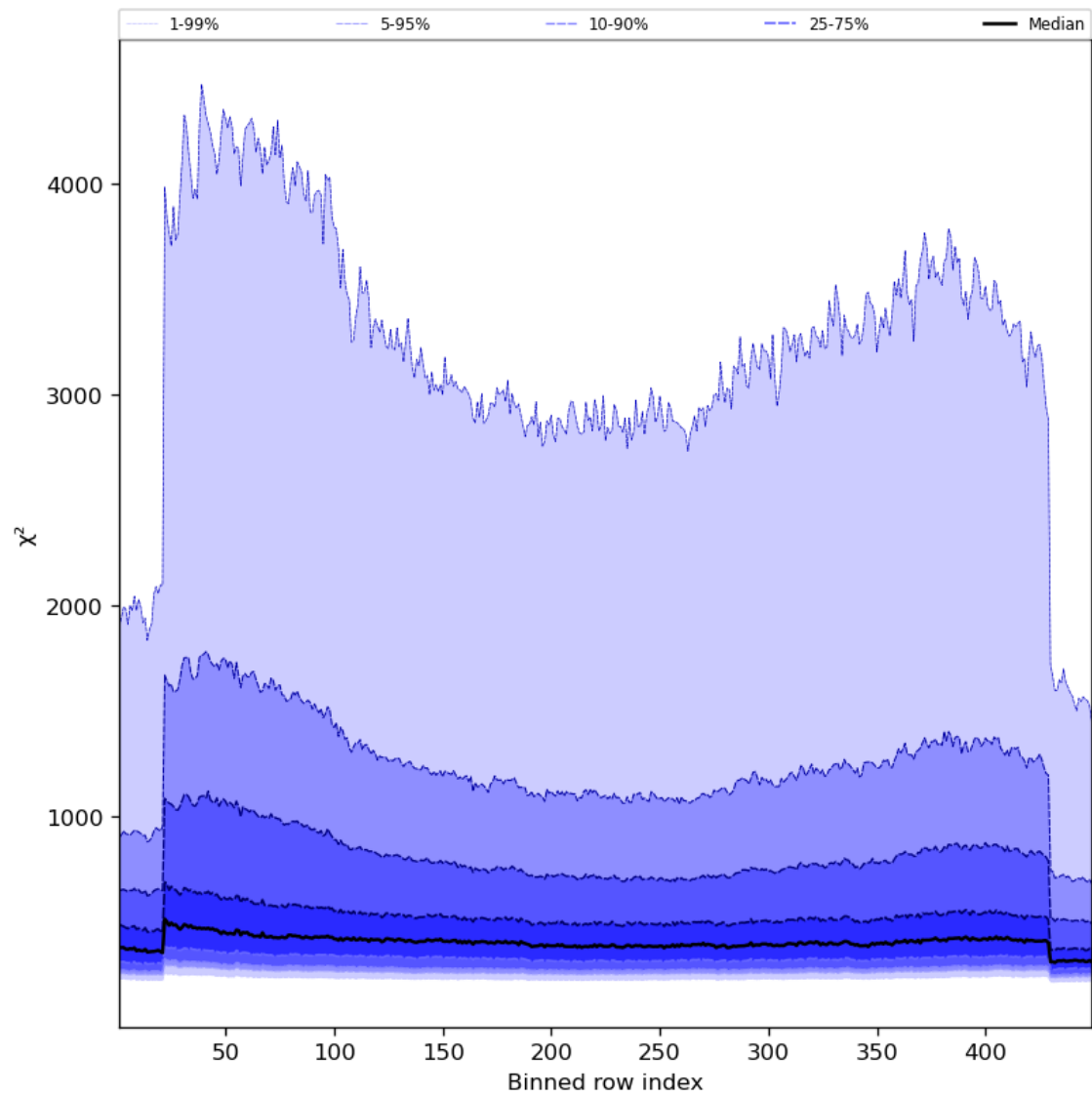
Figure 59: Along track statistics of “ \chi^2 ” for 2023-11-28 to 2023-11-29
