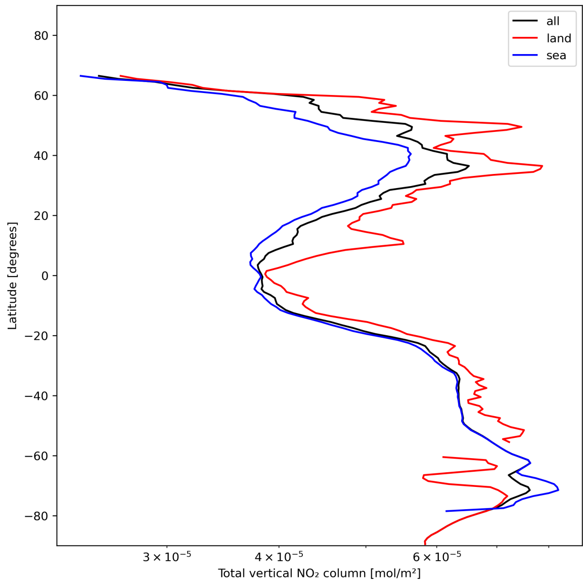
Figure 21: Zonal average of “Total vertical NO 2 column” for 2023-11-28 to 2023-11-29.
