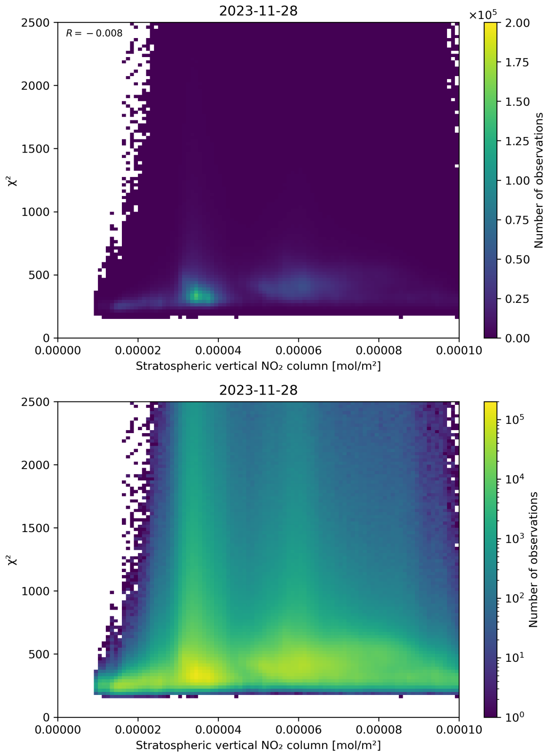
Figure 97: Scatter density plot of “Stratospheric vertical NO 2 column” against “ \chi^2 ” for 2023-11-28 to 2023-11-29.
