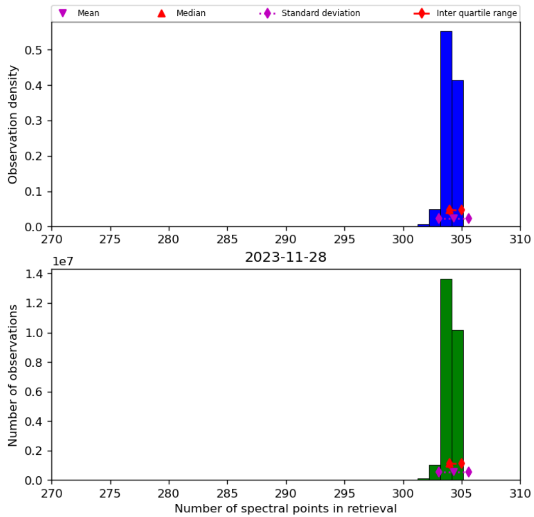
Figure 33: Histogram of “Number of spectral points in retrieval” for 2023-11-28 to 2023-11-29
