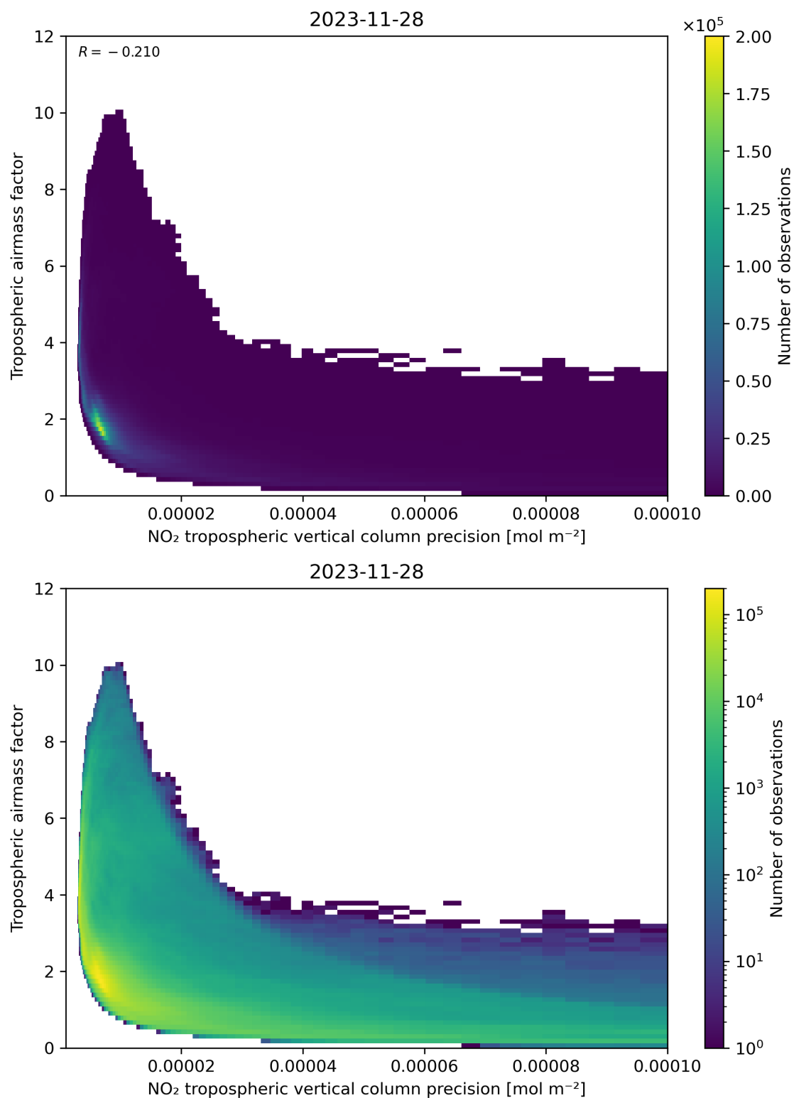
Figure 133: Scatter density plot of “NO 2 tropospheric vertical column precision” against “Tropospheric airmass factor” for 2023-11-28 to 2023-11-29.
