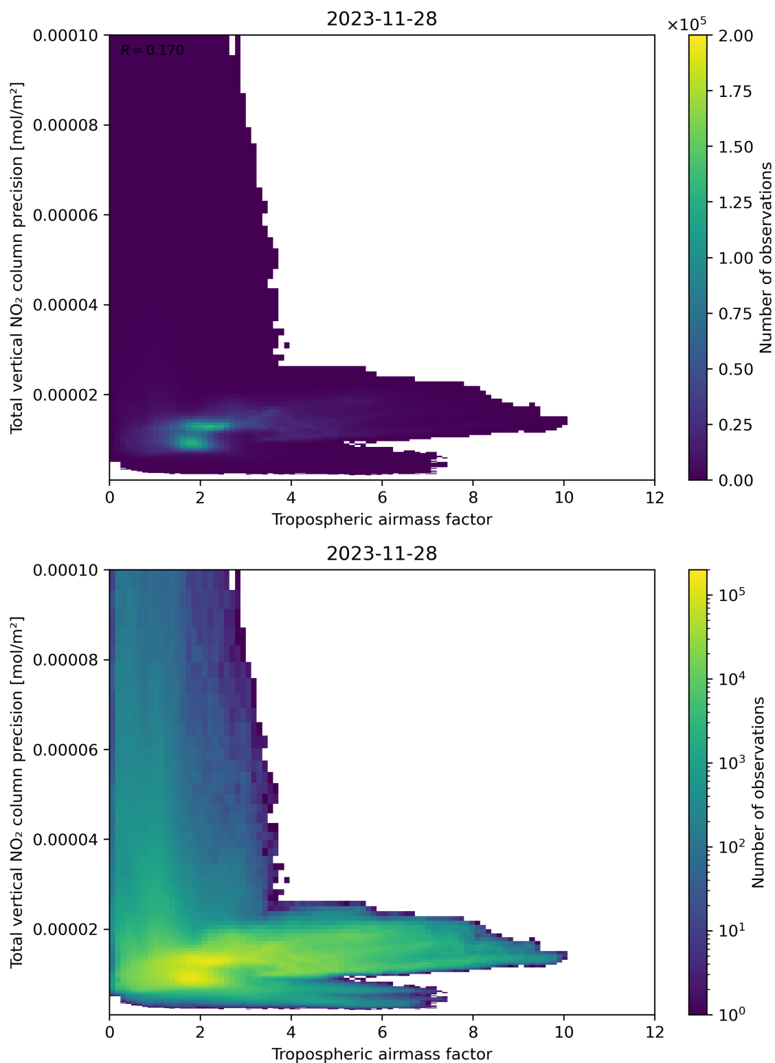
Figure 78: Scatter density plot of “Tropospheric air mass factor” against “Total vertical NO 2 column precision” for 2023-11-28 to 2023-11-29.
