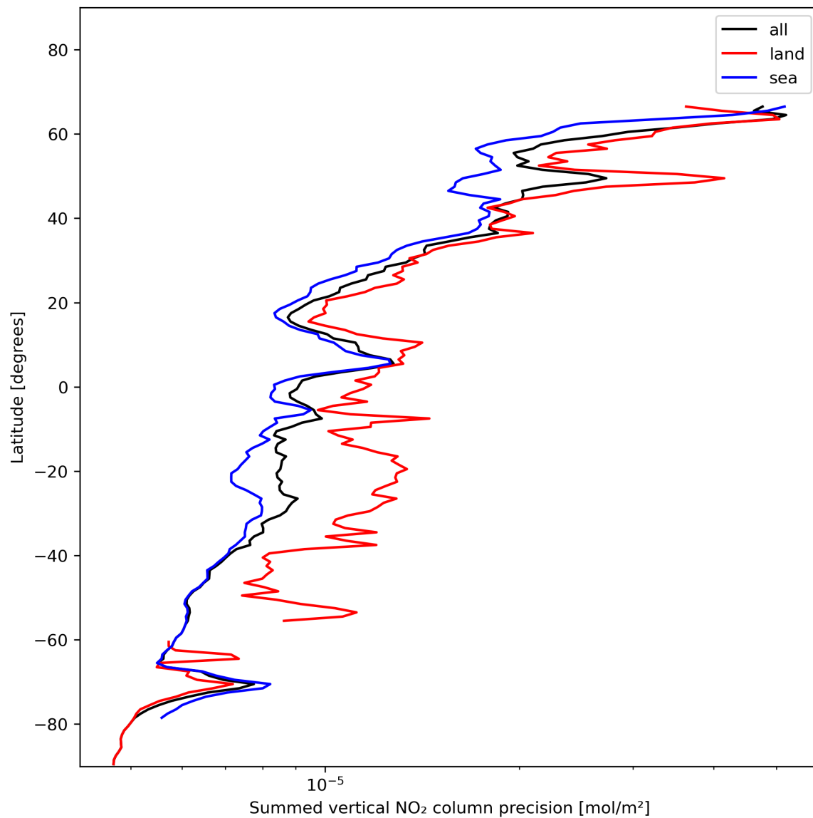
Figure 24: Zonal average of “Summed vertical NO 2 column precision” for 2023-11-28 to 2023-11-29.
