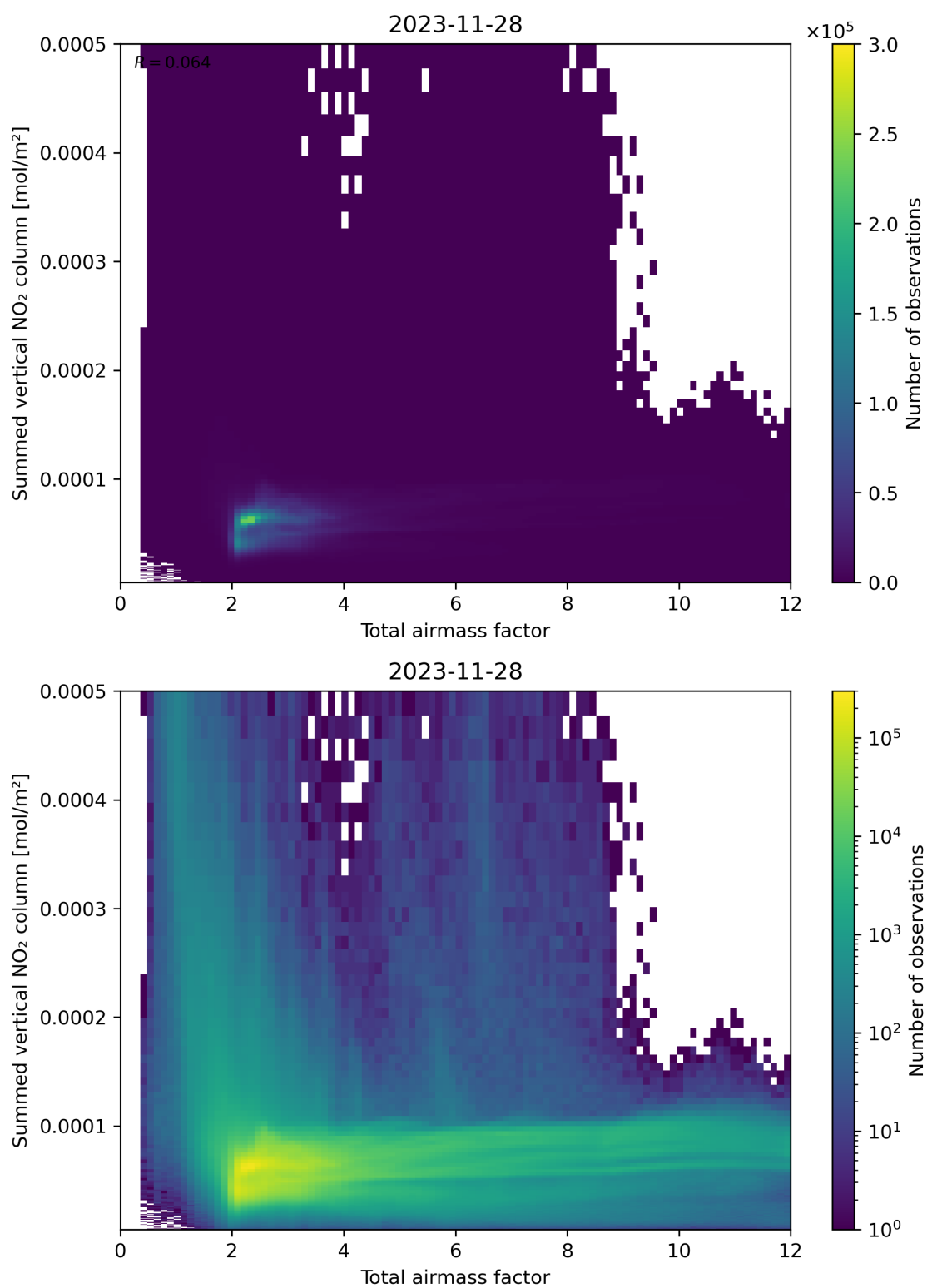
Figure 65: Scatter density plot of “Total airmass factor” against “Summed vertical NO 2 column” for 2023-11-28 to 2023-11-29.
