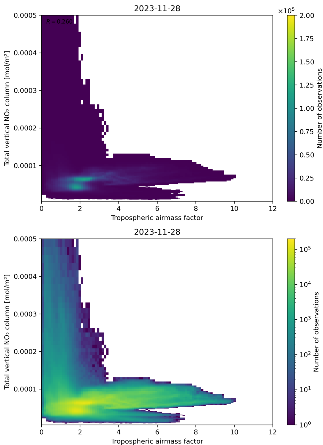
Figure 77: Scatter density plot of “Tropospheric airmass factor” against “Total vertical NO 2 column” for 2023-11-28 to 2023-11-29.
