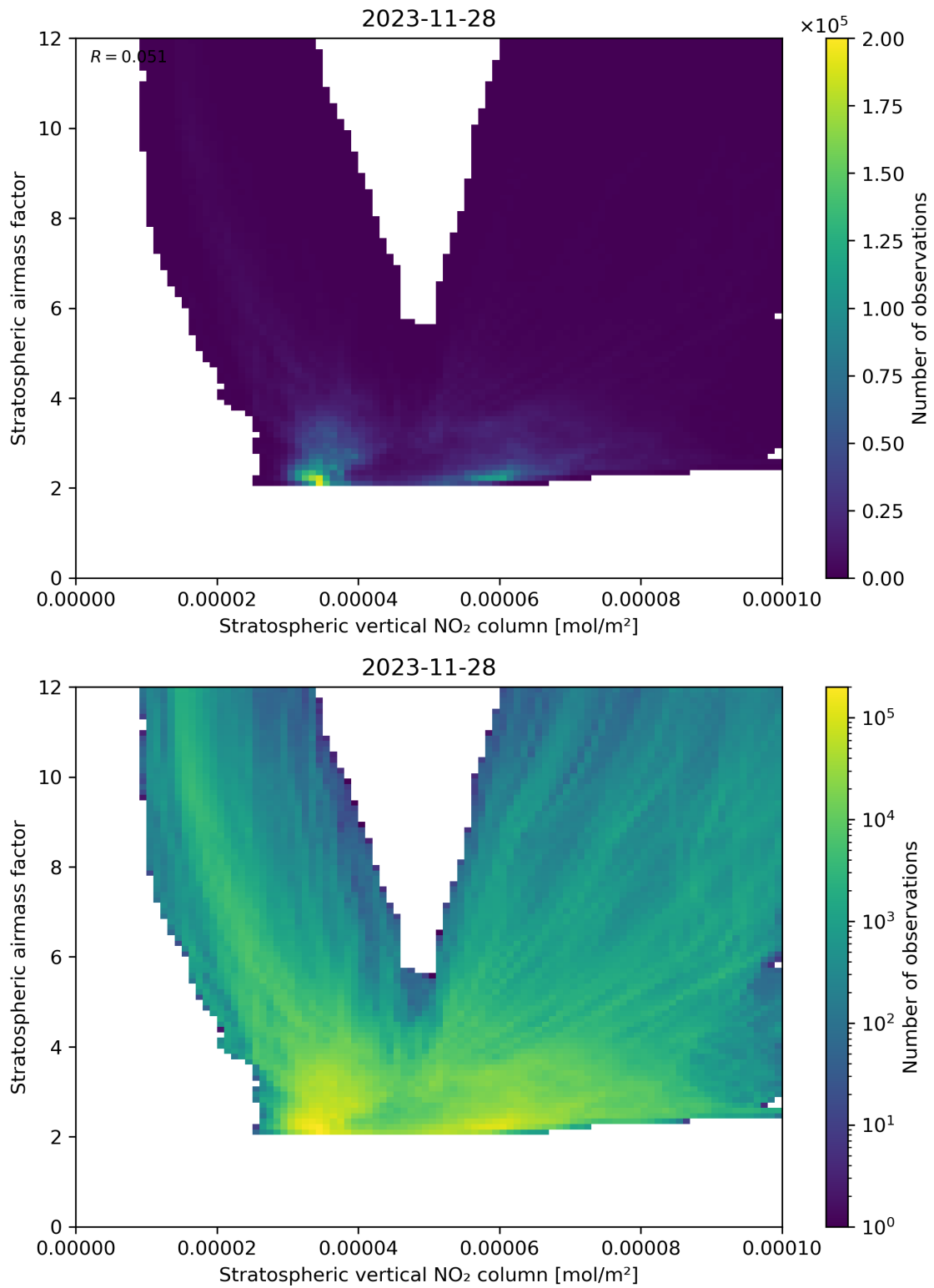
Figure 96: Scatter density plot of “Stratospheric vertical NO 2 column” against “Stratospheric airmass factor” for 2023-11-28 to 2023-11-29.
