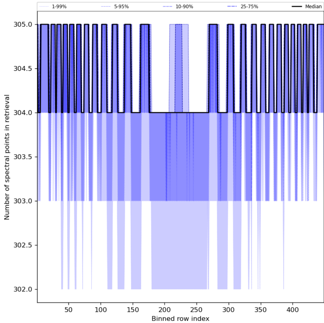
Figure 50: Along track statistics of “Number of spectral points in retrieval” for 2023-11-28 to 2023-11-29
