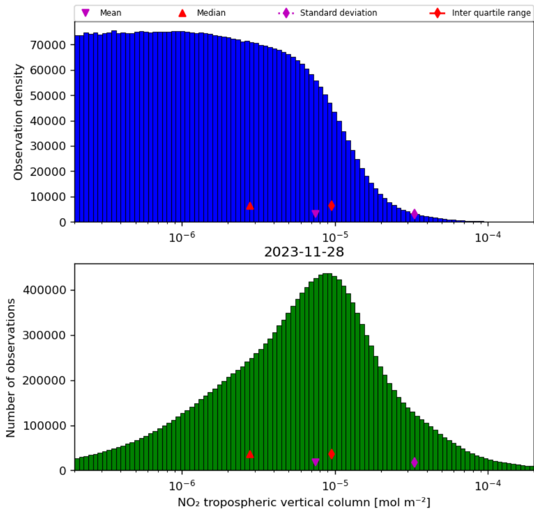
Figure 29: Histogram of “NO 2 tropospheric vertical column” for 2023-11-28 to 2023-11-29
