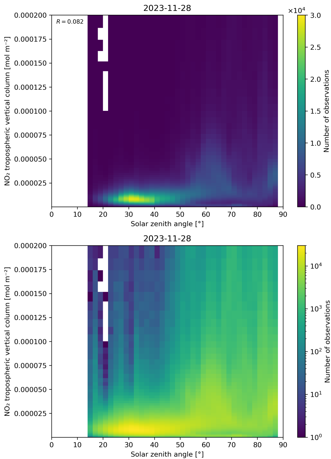
Figure 155: Scatter density plot of “Solar zenith angle” against “NO 2 tropospheric vertical column” for 2023-11-28 to 2023-11-29.
