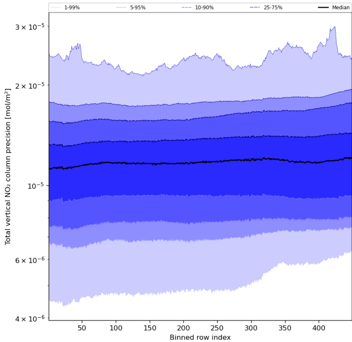
Figure 56: Along track statistics of “Total vertical NO 2 column precision” for 2023-11-28 to 2023-11-29
