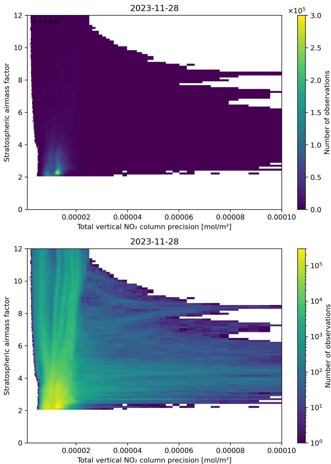
Figure 115: Scatter density plot of “Total vertical NO 2 column precision” against “Stratospheric air mass factor” for 2023-11-28 to 2023-11-29.
