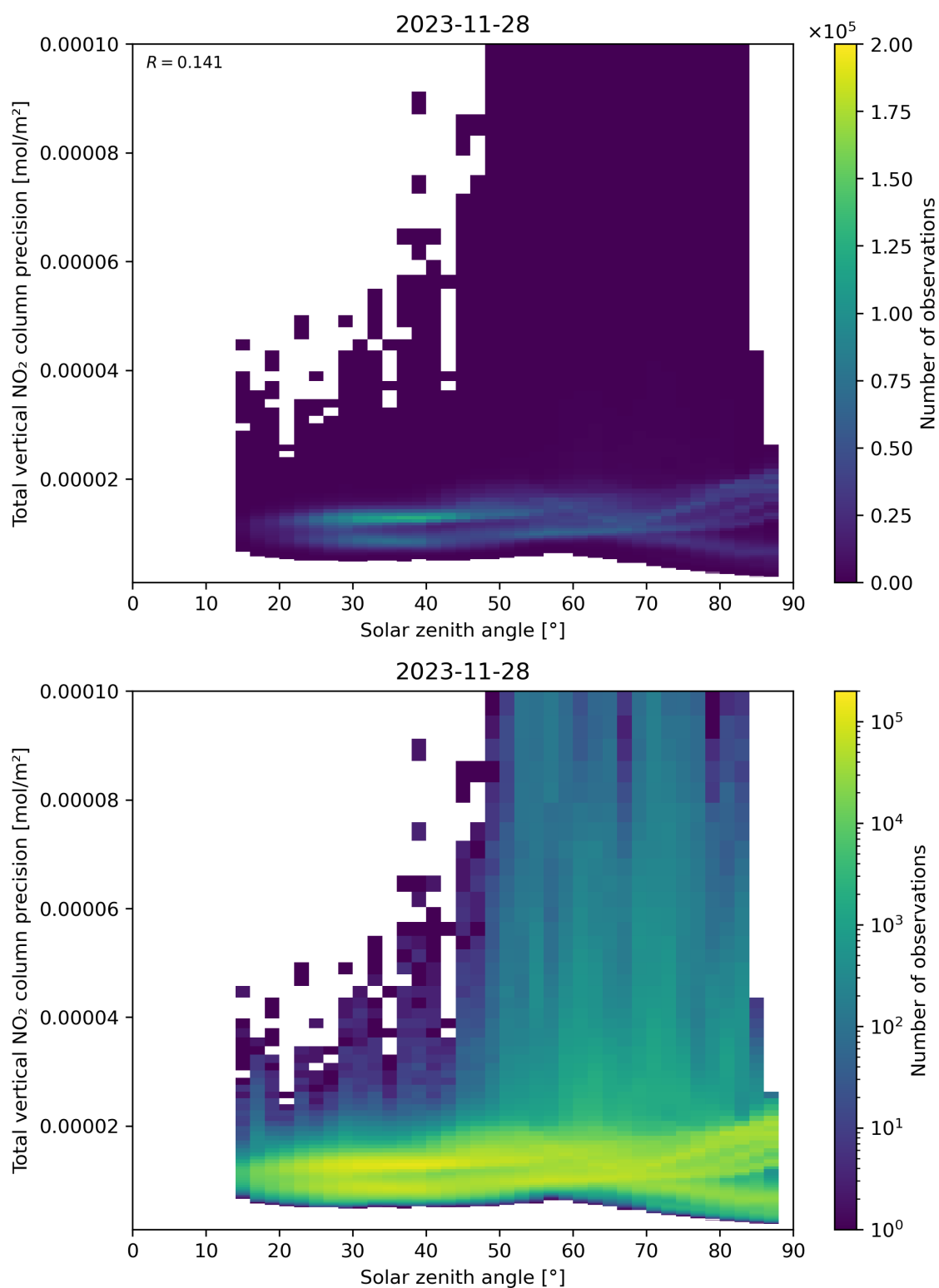
Figure 154: Scatter density plot of “Solar zenith angle” against “Total vertical NO 2 column precision” for 2023-11-28 to 2023-11-29.
