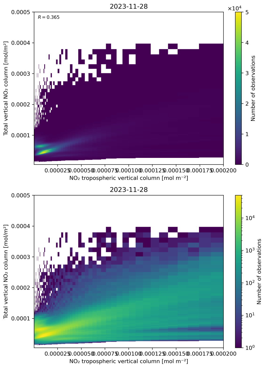
Figure 128: Scatter density plot of “NO 2 tropospheric vertical column” against “Total vertical NO 2 column” for 2023-11-28 to 2023-11-29.
