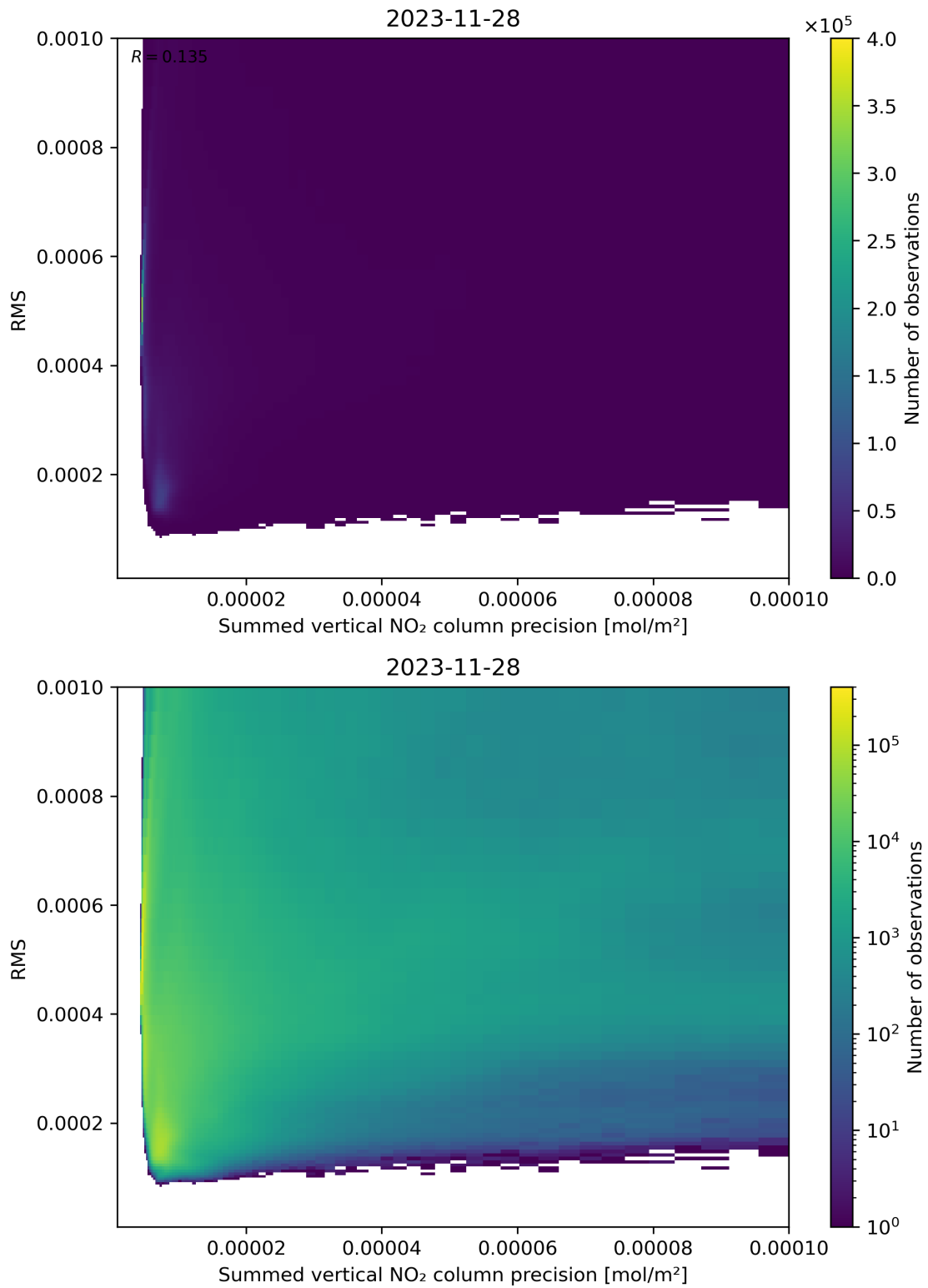
Figure 108: Scatter density plot of “Summed vertical NO 2 column precision” against “RMS” for 2023-11-28 to 2023-11-29.
