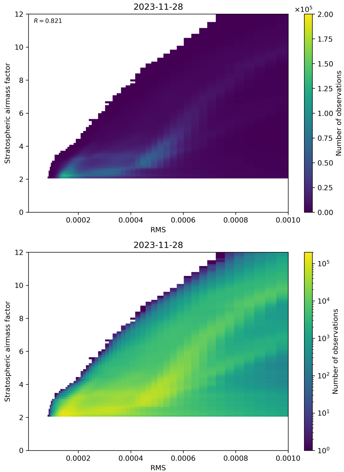
Figure 144: Scatter density plot of “RMS” against “Stratospheric airmass factor” for 2023-11-28 to 2023-11-29.
