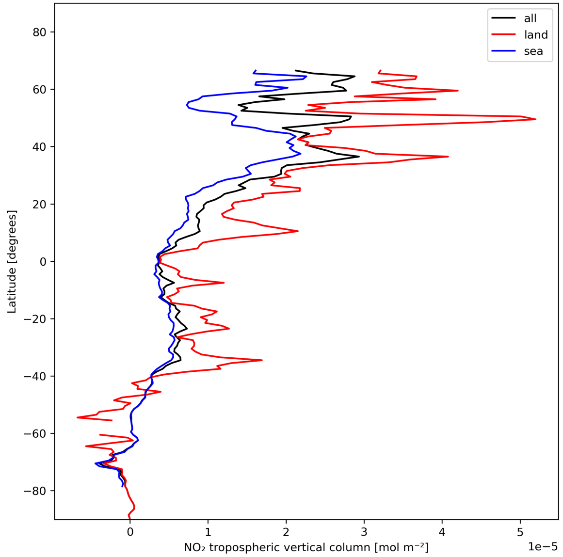
Figure 12: Zonal average of “NO 2 tropospheric vertical column” for 2023-11-28 to 2023-11-29.
