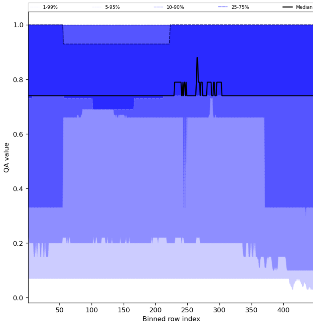
Figure 45: Along track statistics of “QA value” for 2023-11-28 to 2023-11-29
