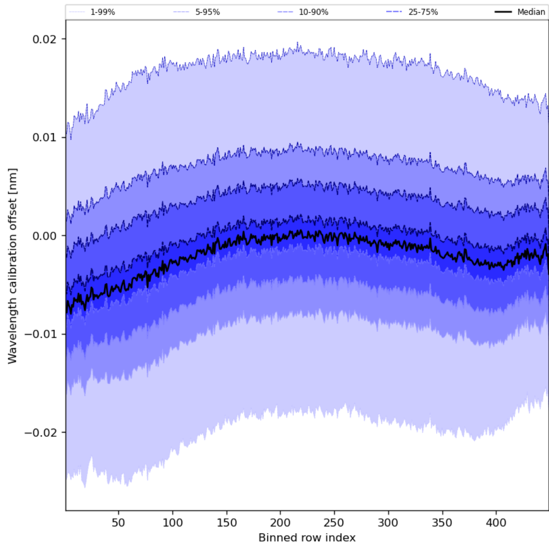
Figure 52: Along track statistics of “Wavelength calibration offset” for 2023-11-28 to 2023-11-29
