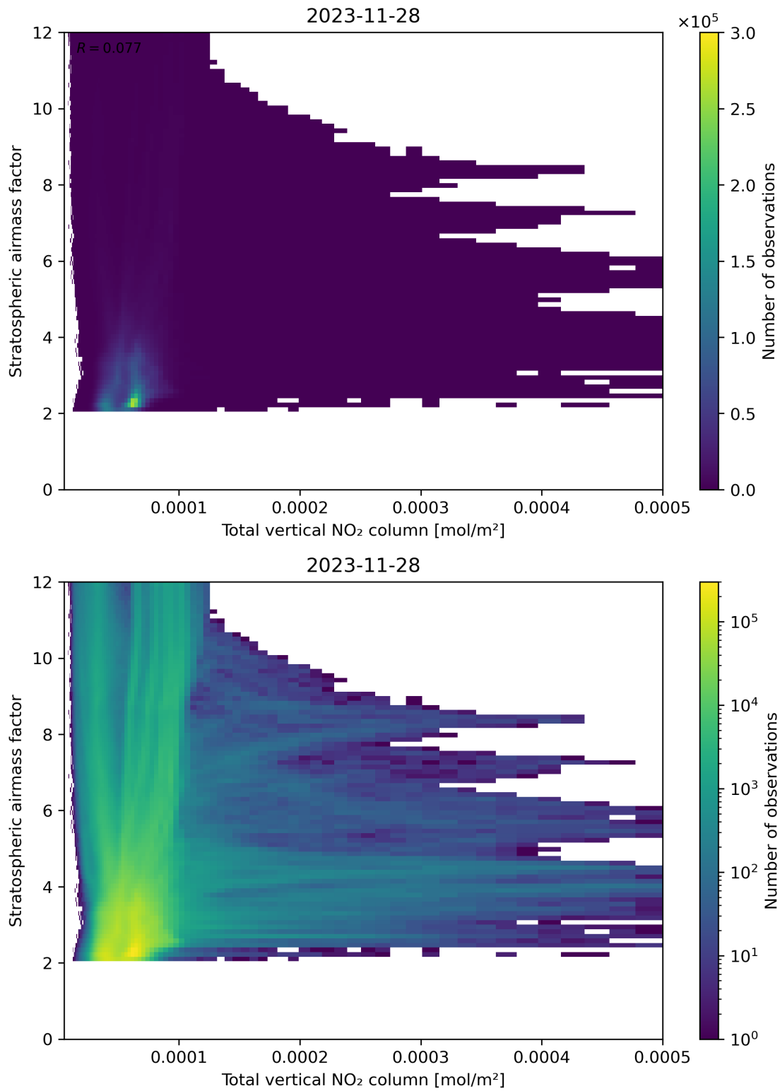
Figure 110: Scatter density plot of “Total vertical NO 2 column” against “Stratospheric airmass factor” for 2023-11-28 to 2023-11-29.
