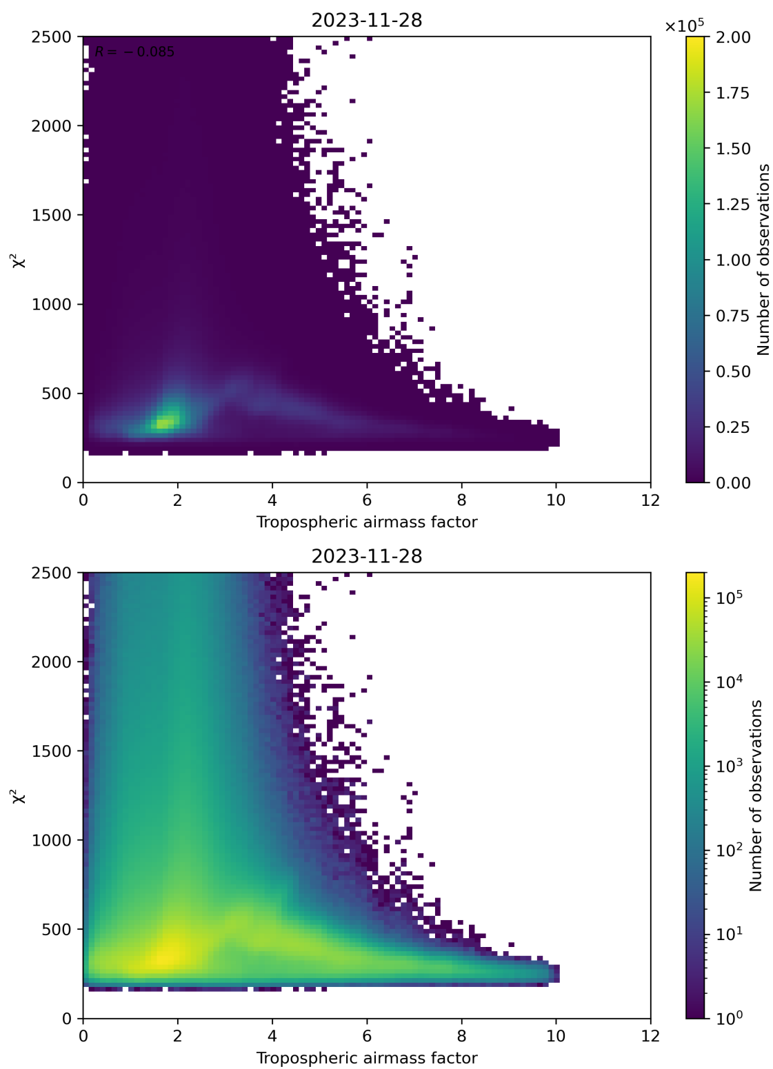
Figure 73: Scatter density plot of “Tropospheric airmass factor” against “ \chi^2 ” for 2023-11-28 to 2023-11-29.
