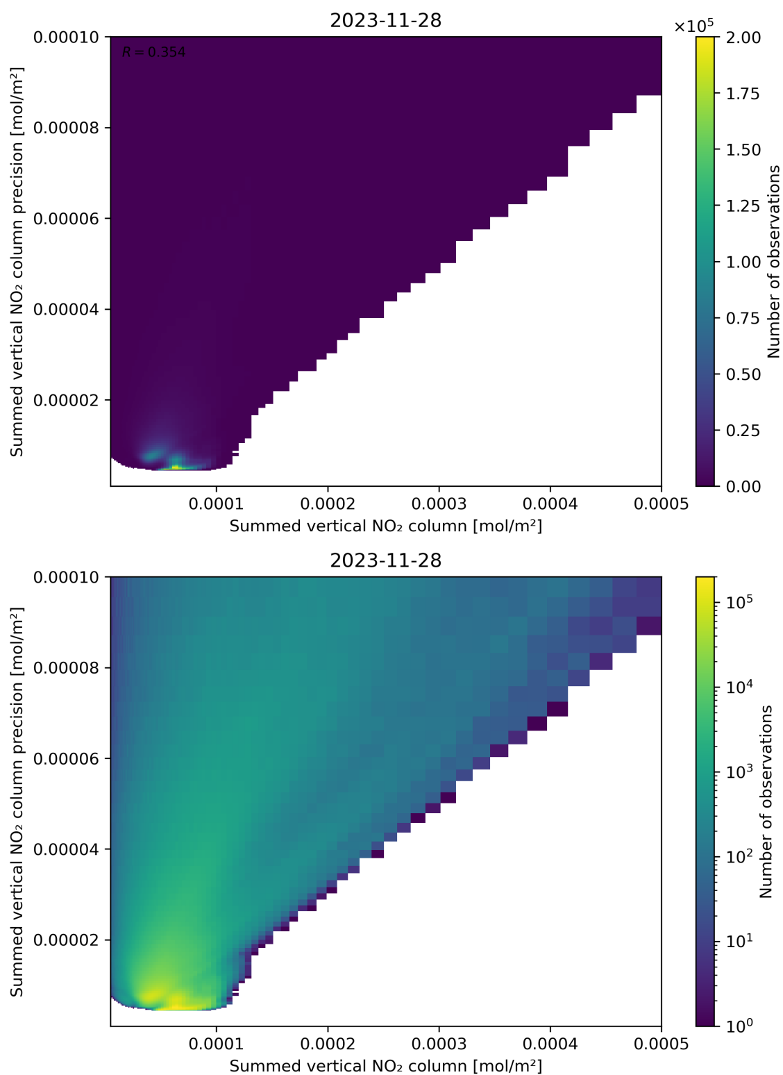
Figure 105: Scatter density plot of “Summed vertical NO 2 column” against “Summed vertical NO 2 column precision” for 2023-11-28 to 2023-11-29.
