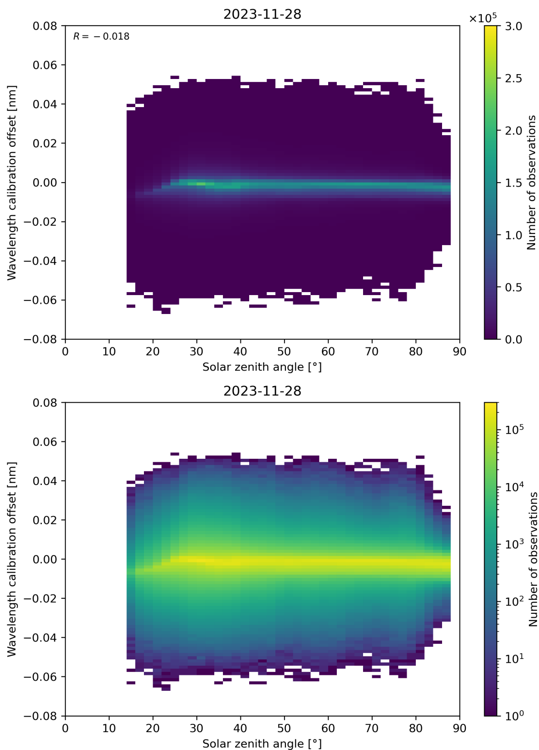
Figure 158: Scatter density plot of “Solar zenith angle” against “Wavelength calibration offset” for 2023-11-28 to 2023-11-29.
