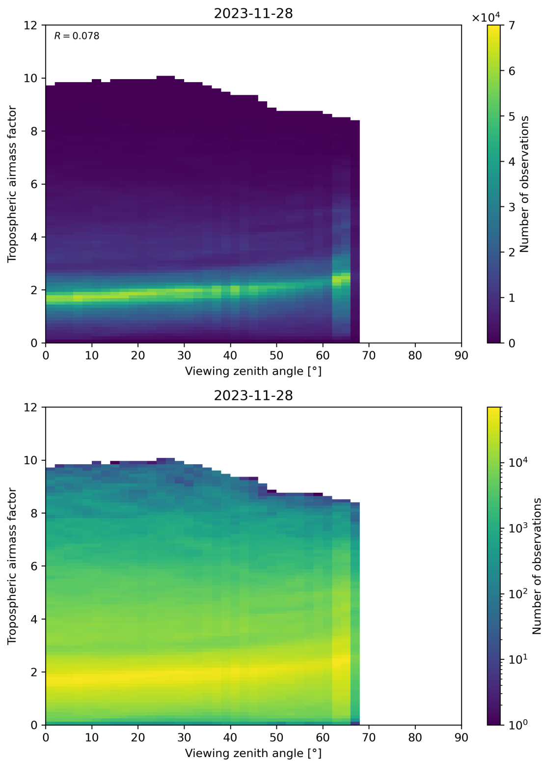
Figure 161: Scatter density plot of “Viewing zenith angle” against “Tropospheric airmass factor” for 2023-11-28 to 2023-11-29.
