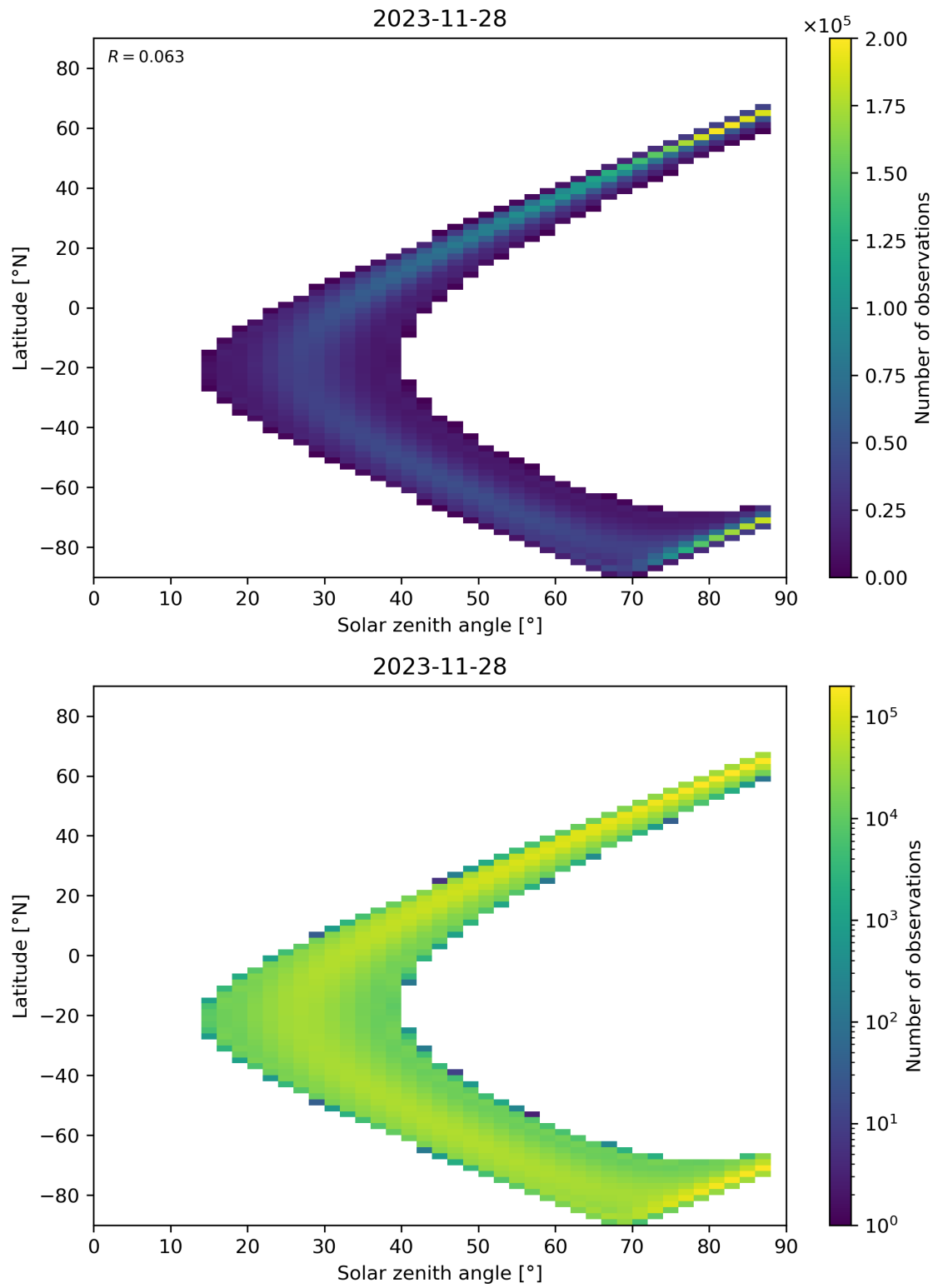
Figure 149: Scatter density plot of “Solar zenith angle” against “Latitude” for 2023-11-28 to 2023-11-29.
