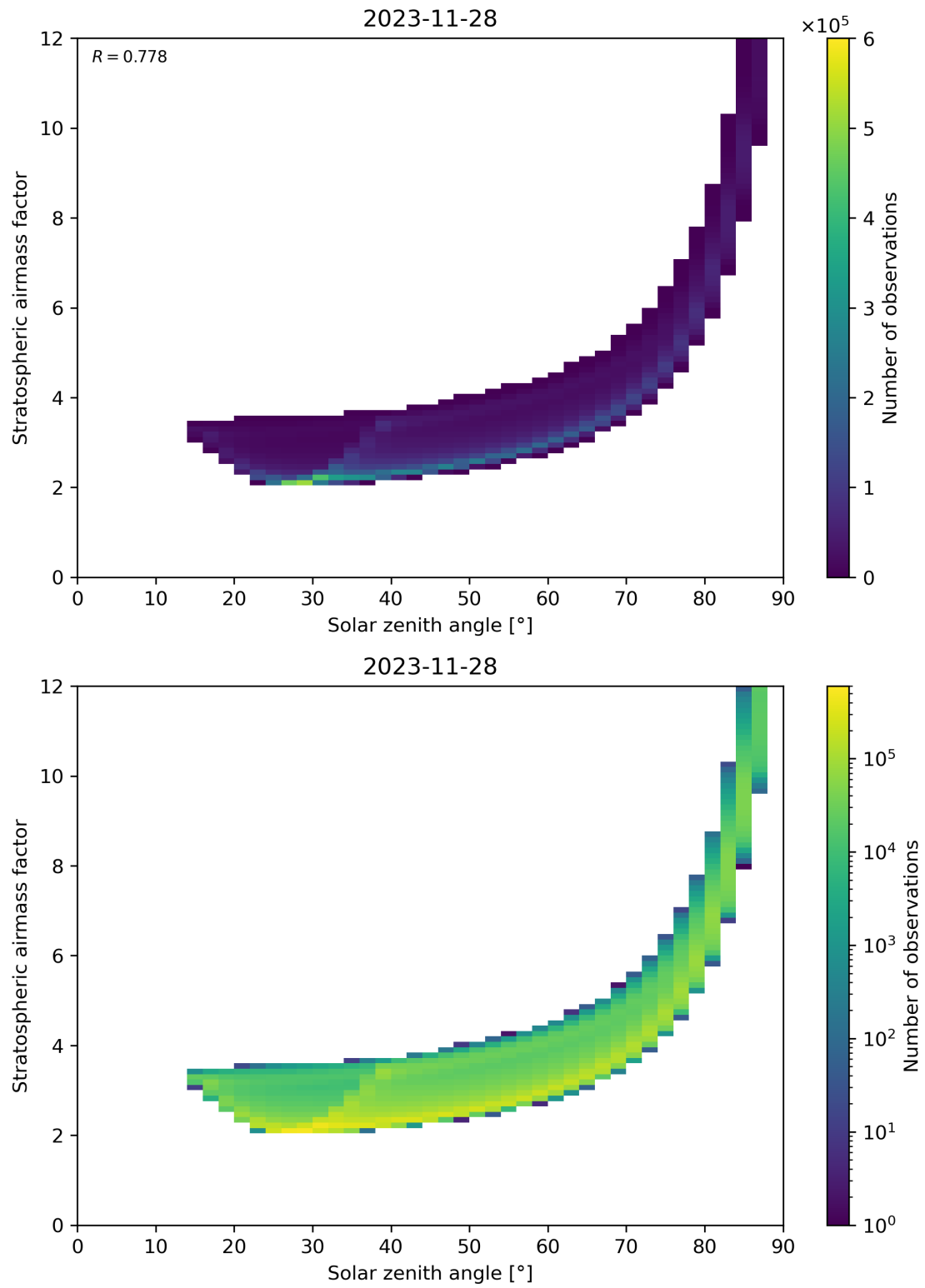
Figure 145: Scatter density plot of “Solar zenith angle” against “Stratospheric airmass factor” for 2023-11-28 to 2023-11-29.
