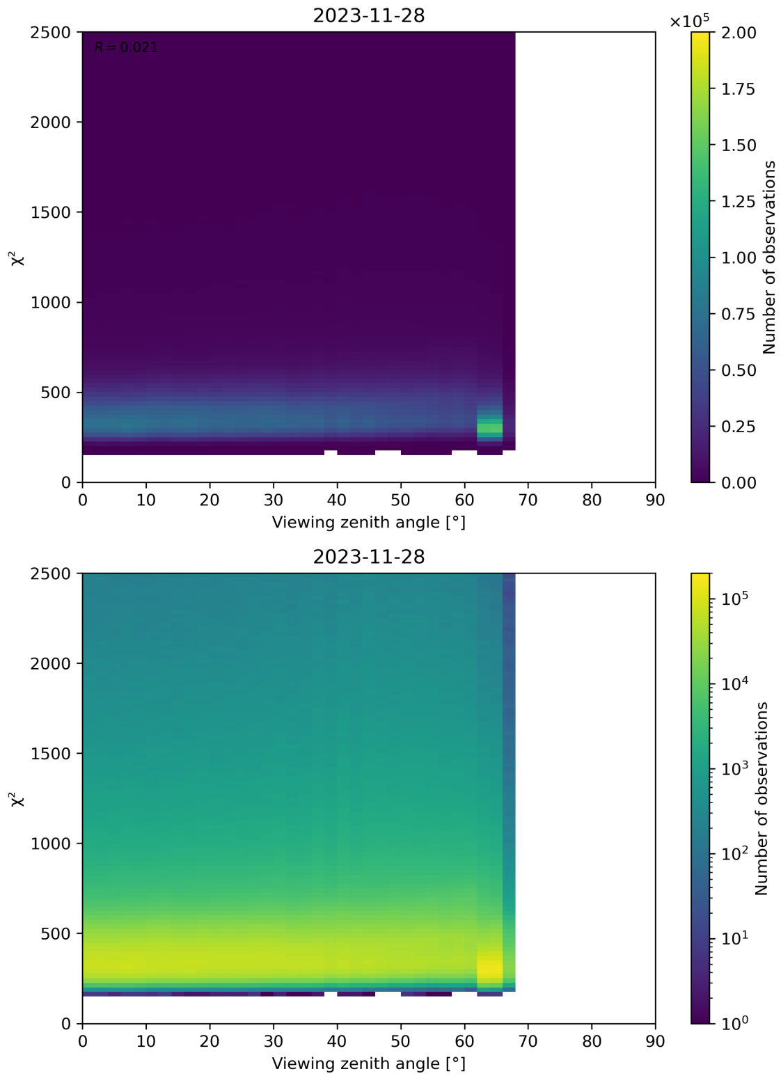
Figure 162: Scatter density plot of “Viewing zenith angle” against “ \chi^2 ” for 2023-11-28 to 2023-11-29.
