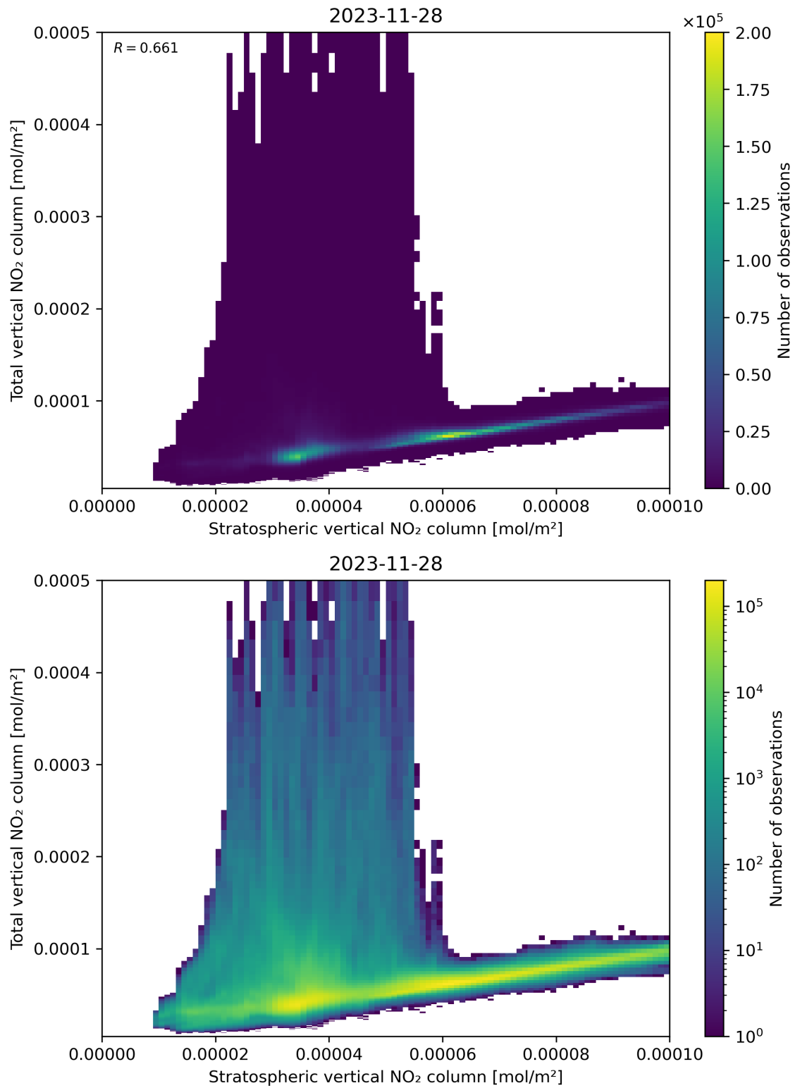
Figure 100: Scatter density plot of “Stratospheric vertical NO 2 column” against “Total vertical NO 2 column” for 2023-11-28 to 2023-11-29.
