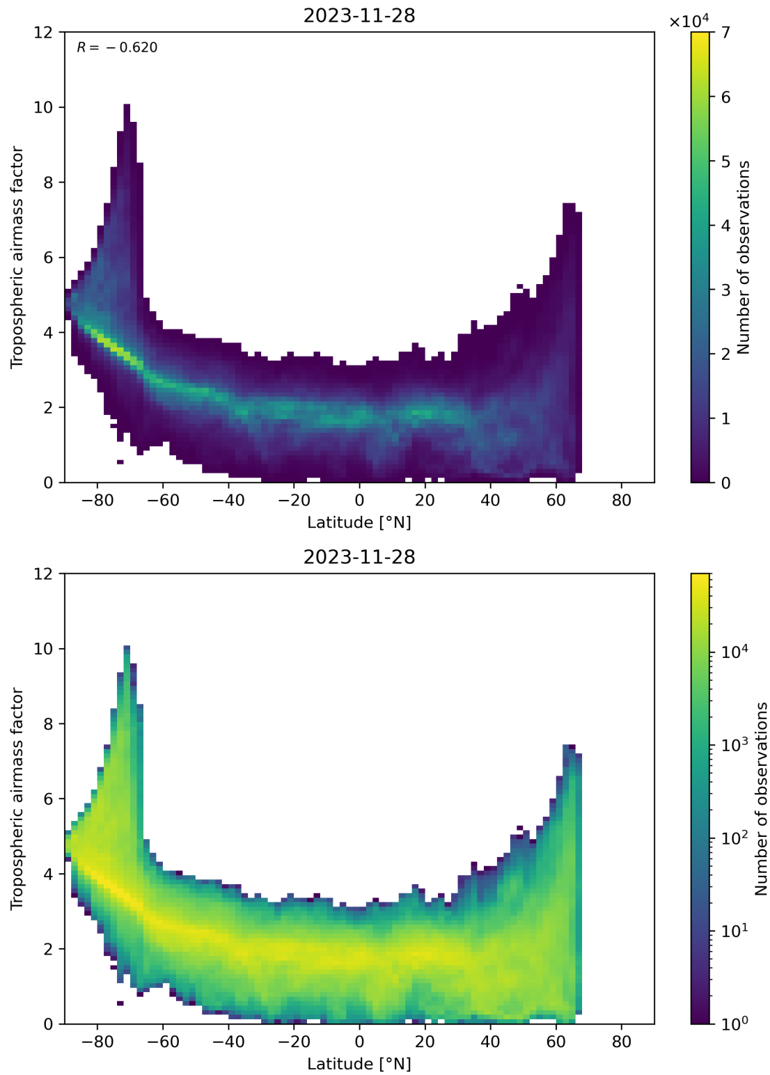
Figure 85: Scatter density plot of “Latitude” against “Tropospheric airmass factor” for 2023-11-28 to 2023-11-29.
