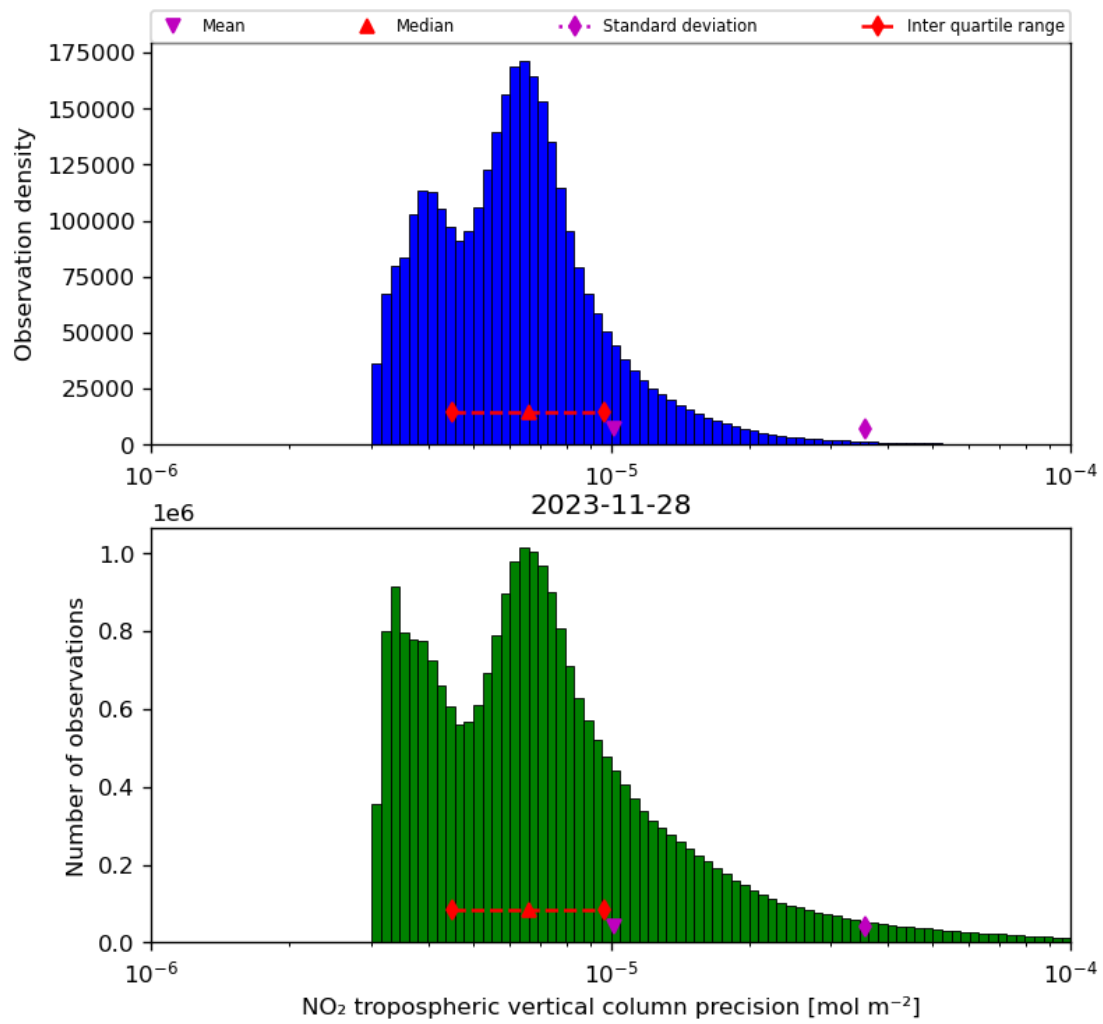
Figure 30: Histogram of “NO 2 tropospheric vertical column precision” for 2023-11-28 to 2023-11-29
