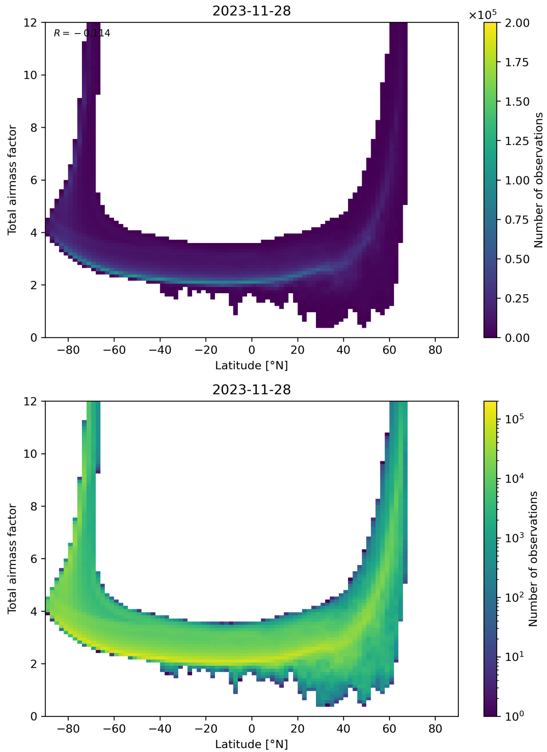
Figure 84: Scatter density plot of “Latitude” against “Total airmass factor” for 2023-11-28 to 2023-11-29.
