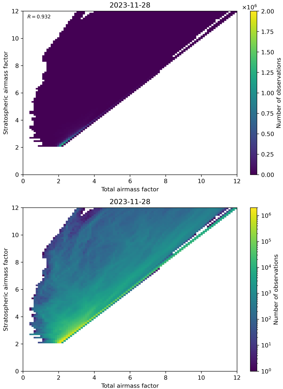
Figure 62: Scatter density plot of “Total airmass factor” against “Stratospheric airmass factor” for 2023-11-28 to 2023-11-29.
