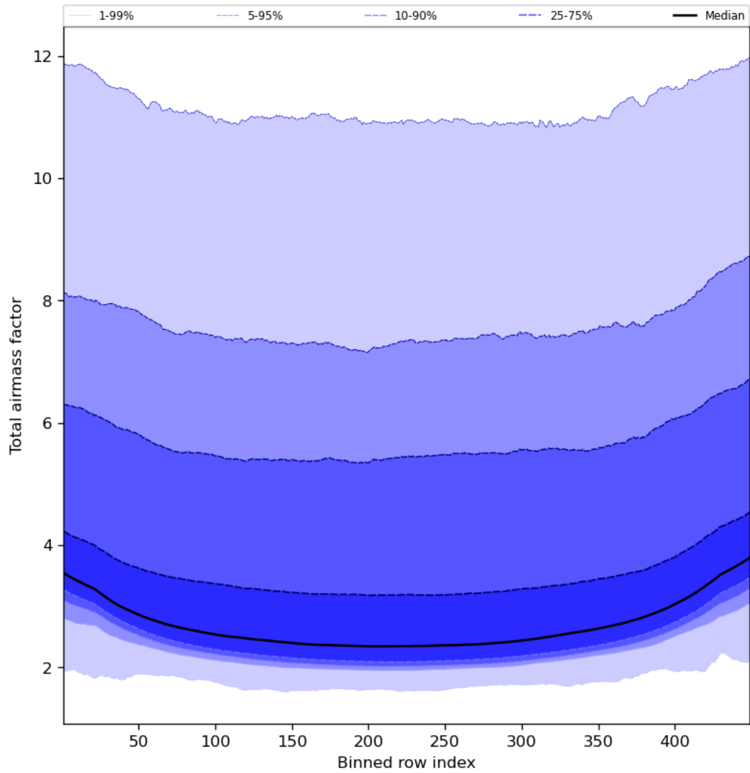
Figure 49: Along track statistics of “Total airmass factor” for 2023-11-28 to 2023-11-29
