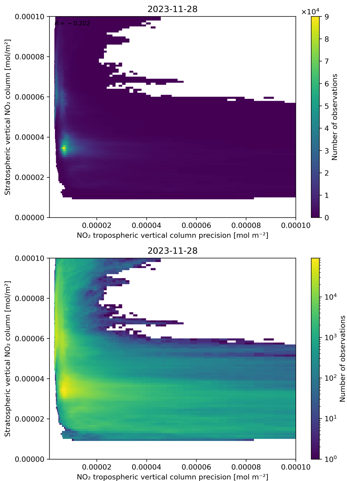
Figure 135: Scatter density plot of “NO 2 tropospheric vertical column precision” against “Stratospheric vertical NO 2 column” for 2023-11-28 to 2023-11-29.
