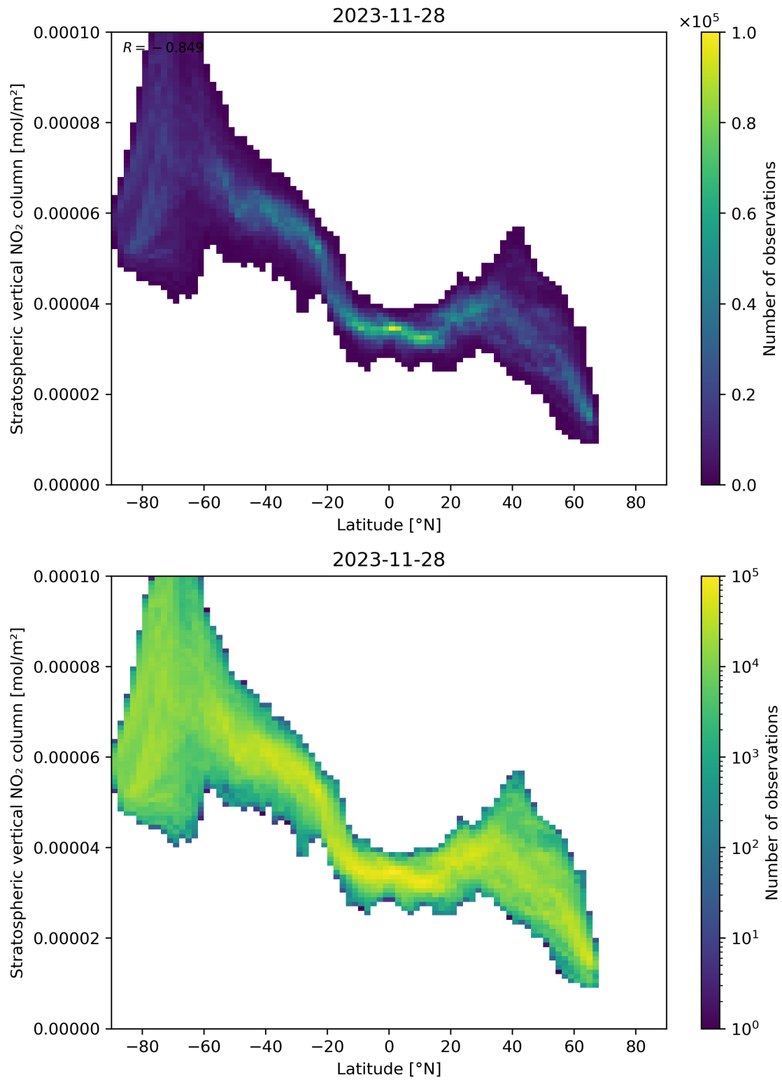
Figure 87: Scatter density plot of “Latitude” against “Stratospheric vertical NO 2 column” for 2023-11-28 to 2023-11-29.
