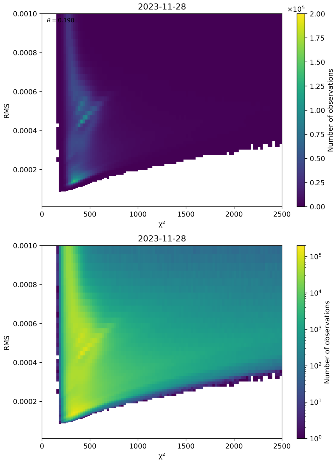
Figure 82: Scatter density plot of “ \chi^2 ” against “RMS” for 2023-11-28 to 2023-11-29.
