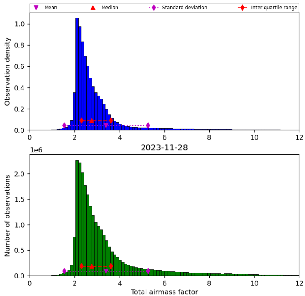
Figure 32: Histogram of “Total airmass factor” for 2023-11-28 to 2023-11-29
