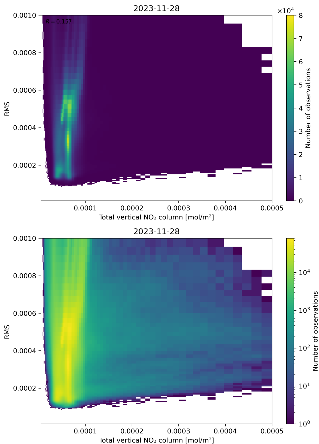
Figure 120: Scatter density plot of “Total vertical NO 2 column” against “RMS” for 2023-11-28 to 2023-11-29.
