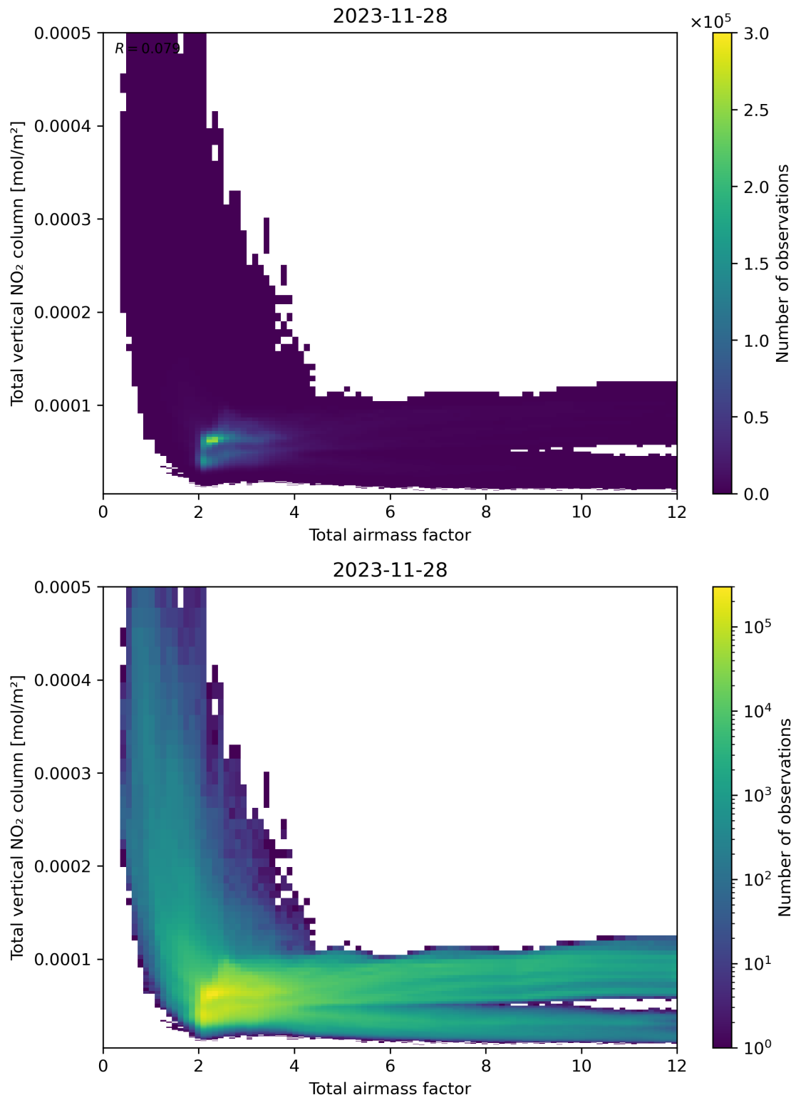
Figure 67: Scatter density plot of “Total airmass factor” against “Total vertical NO 2 column” for 2023-11-28 to 2023-11-29.
