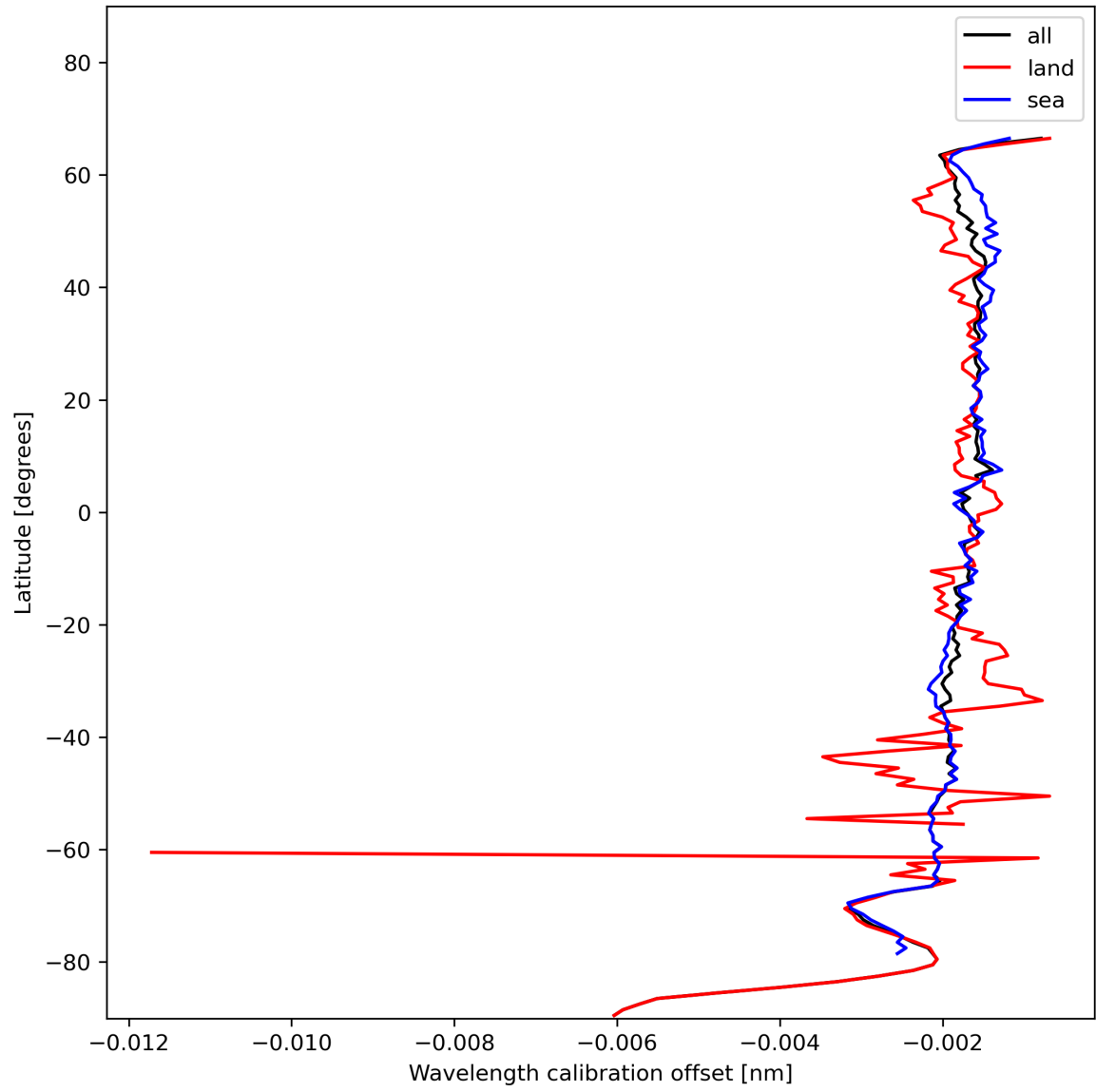
Figure 18: Zonal average of “Wavelength calibration offset” for 2023-11-28 to 2023-11-29.
