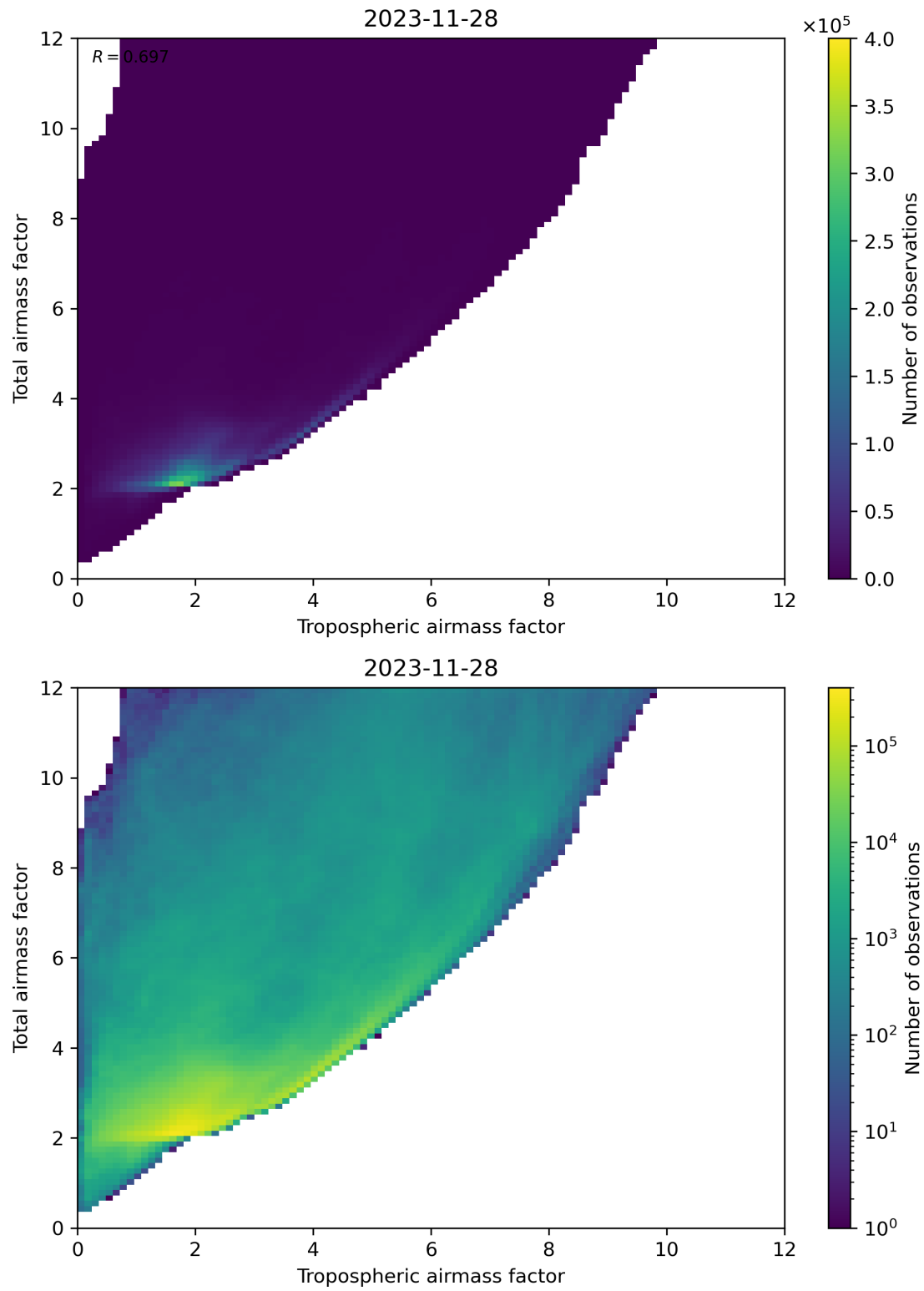
Figure 72: Scatter density plot of “Tropospheric airmass factor” against “Total airmass factor” for 2023-11-28 to 2023-11-29.
