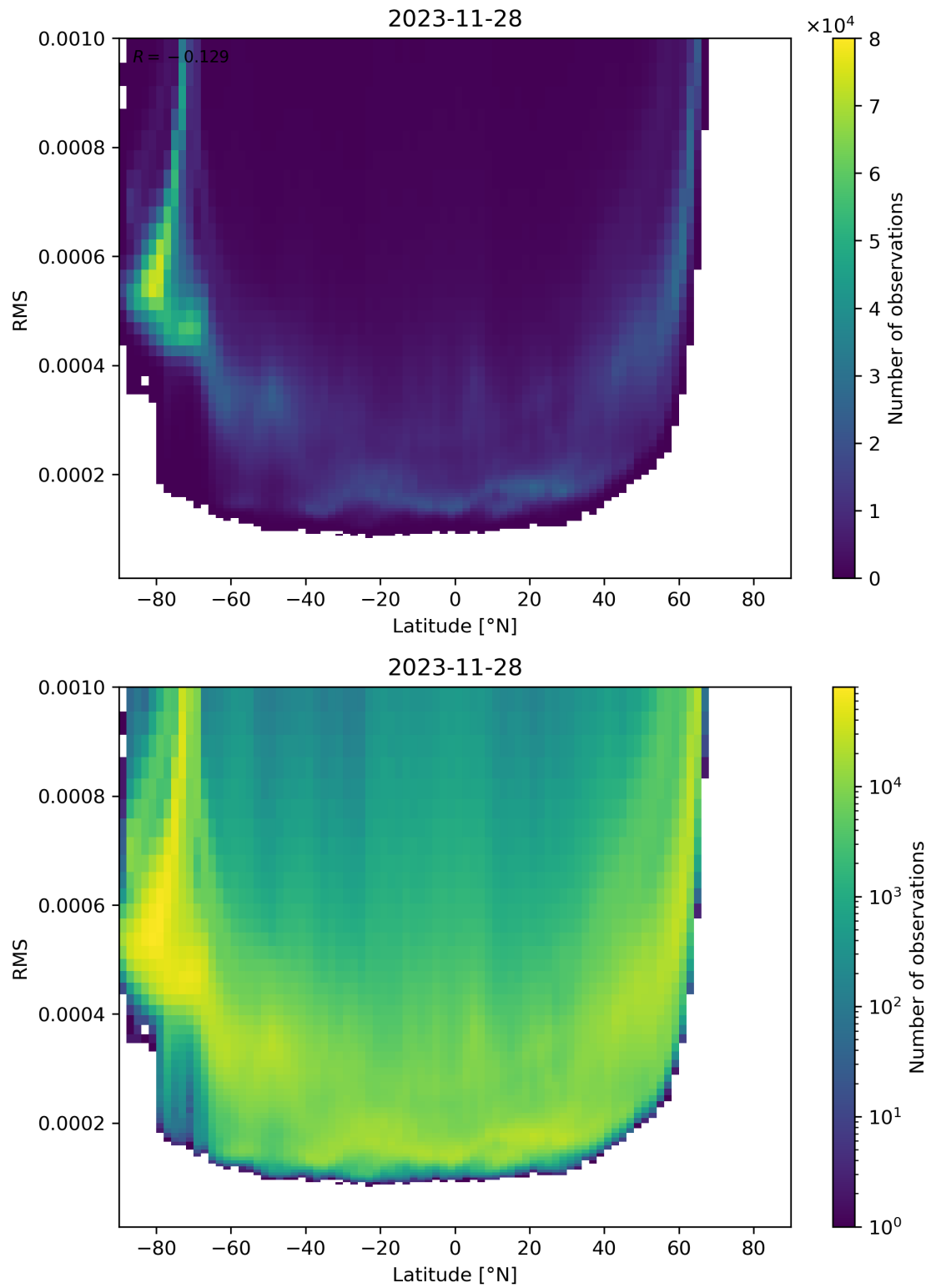
Figure 94: Scatter density plot of “Latitude” against “RMS” for 2023-11-28 to 2023-11-29.
