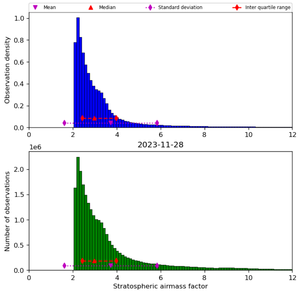
Figure 44: Histogram of “Stratospheric airmass factor” for 2023-11-28 to 2023-11-29
