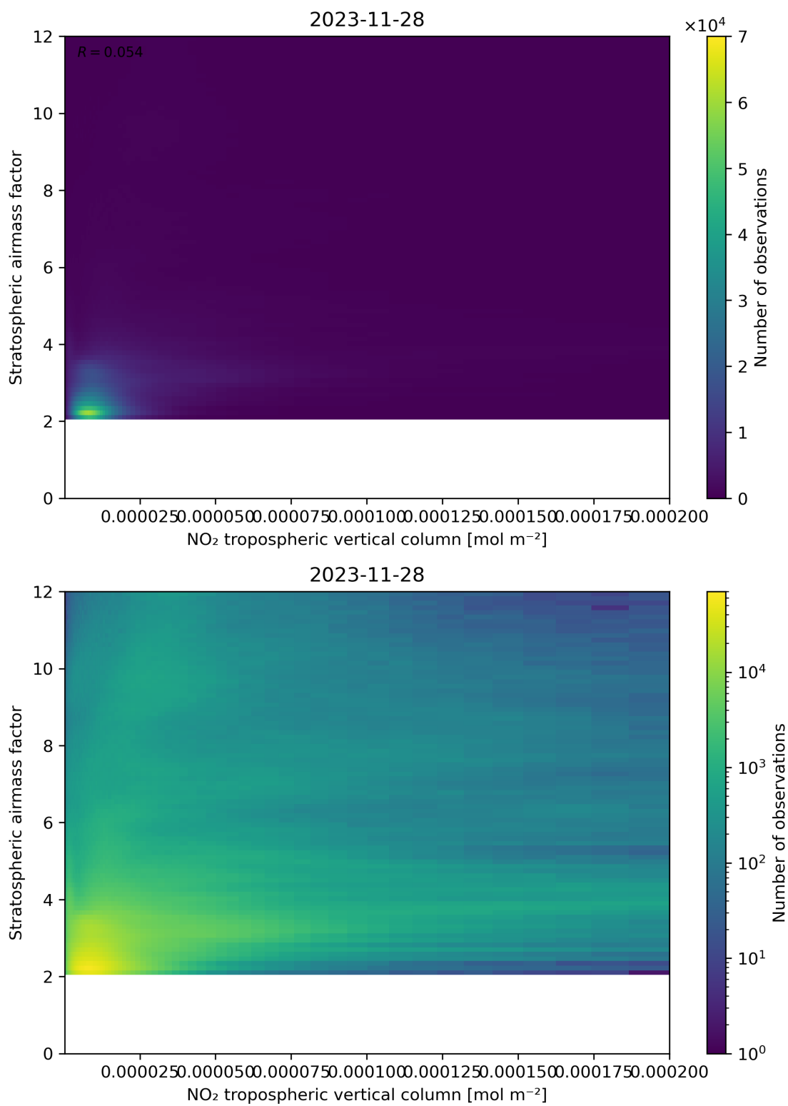
Figure 121: Scatter density plot of “NO 2 tropospheric vertical column” against “Stratospheric airmass factor” for 2023-11-28 to 2023-11-29.
