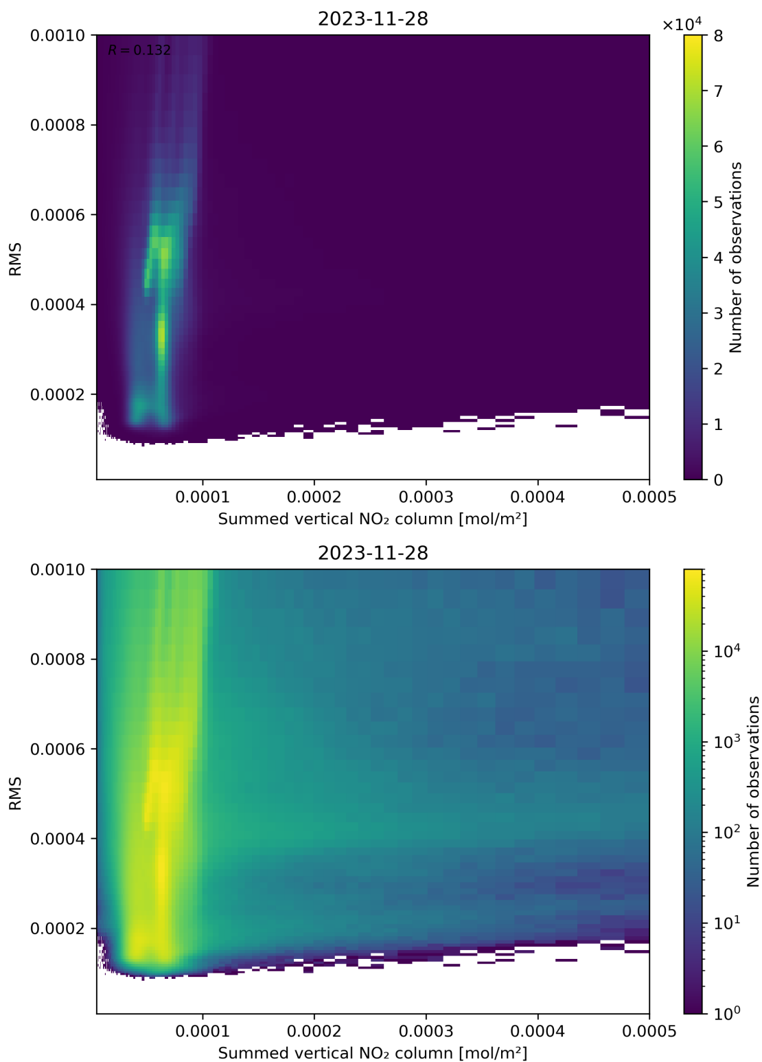
Figure 109: Scatter density plot of “Summed vertical NO 2 column” against “RMS” for 2023-11-28 to 2023-11-29.
