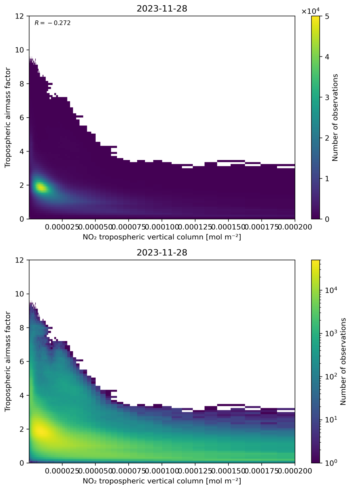
Figure 123: Scatter density plot of “NO 2 tropospheric vertical column” against “Tropospheric air mass factor” for 2023-11-28 to 2023-11-29.
