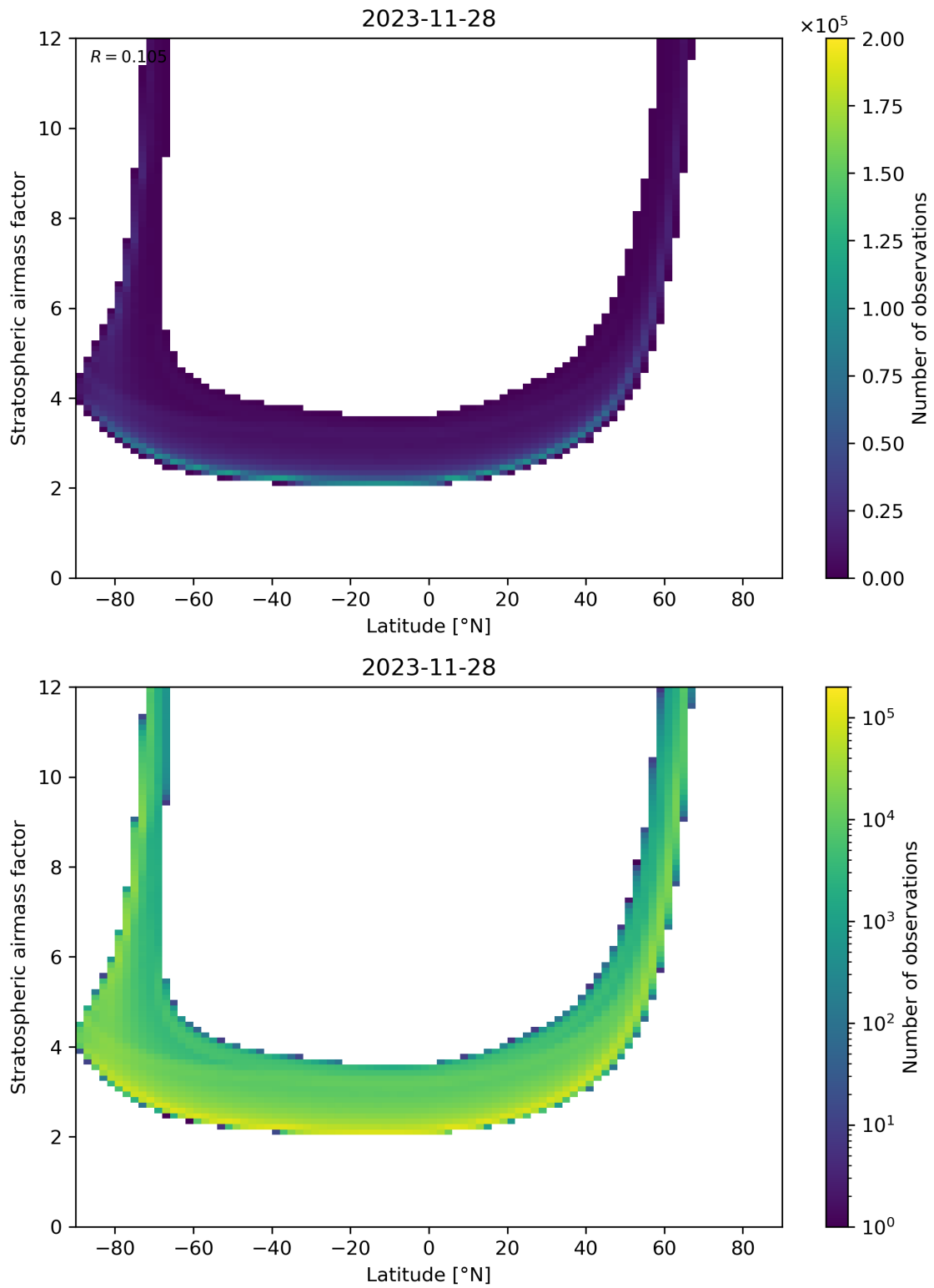
Figure 83: Scatter density plot of “Latitude” against “Stratospheric air mass factor” for 2023-11-28 to 2023-11-29.
