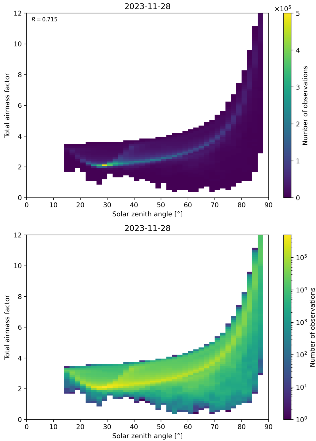
Figure 146: Scatter density plot of “Solar zenith angle” against “Total airmass factor” for 2023-11-28 to 2023-11-29.
