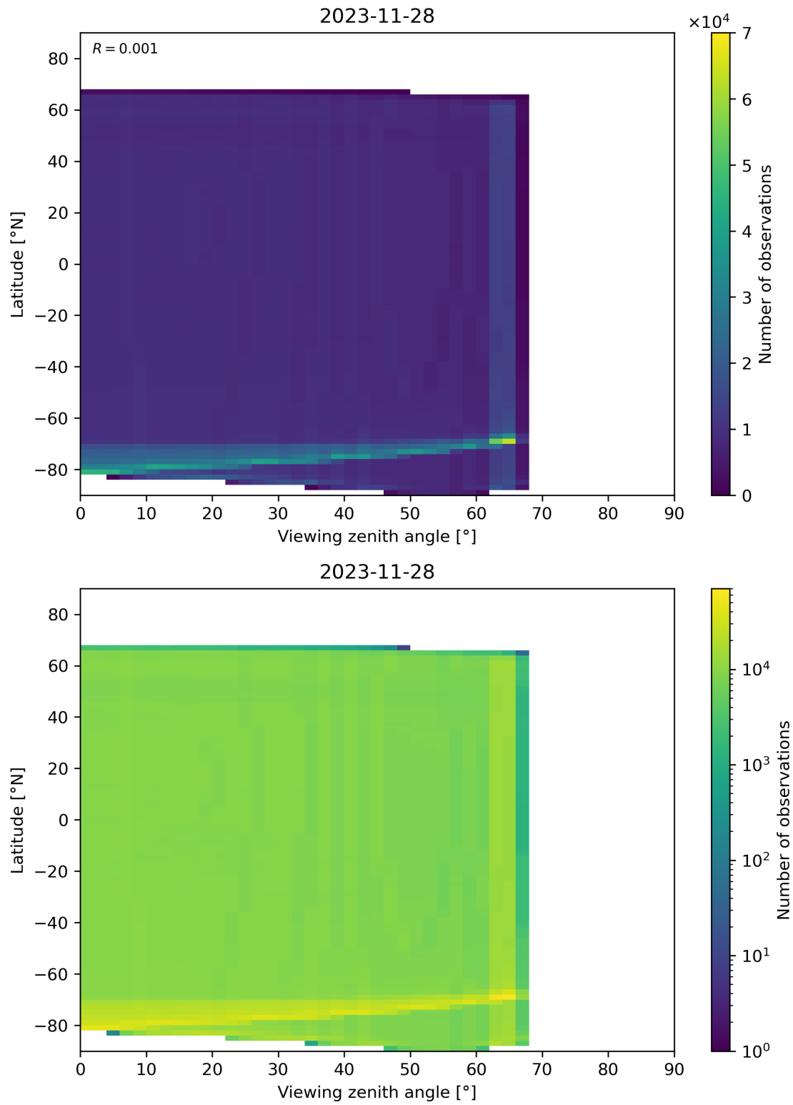
Figure 163: Scatter density plot of “Viewing zenith angle” against “Latitude” for 2023-11-28 to 2023-11-29.
