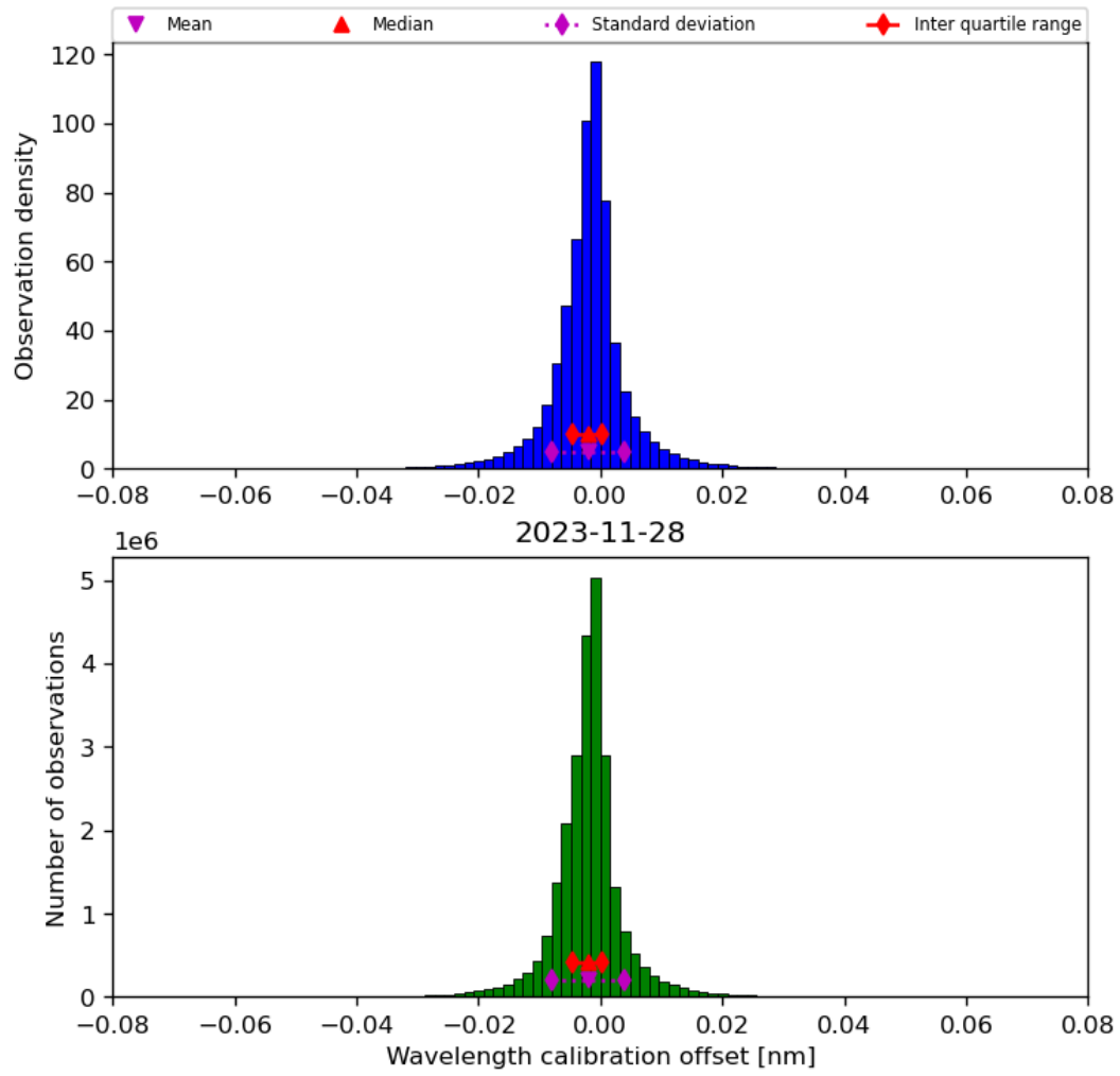
Figure 35: Histogram of “Wavelength calibration offset” for 2023-11-28 to 2023-11-29
