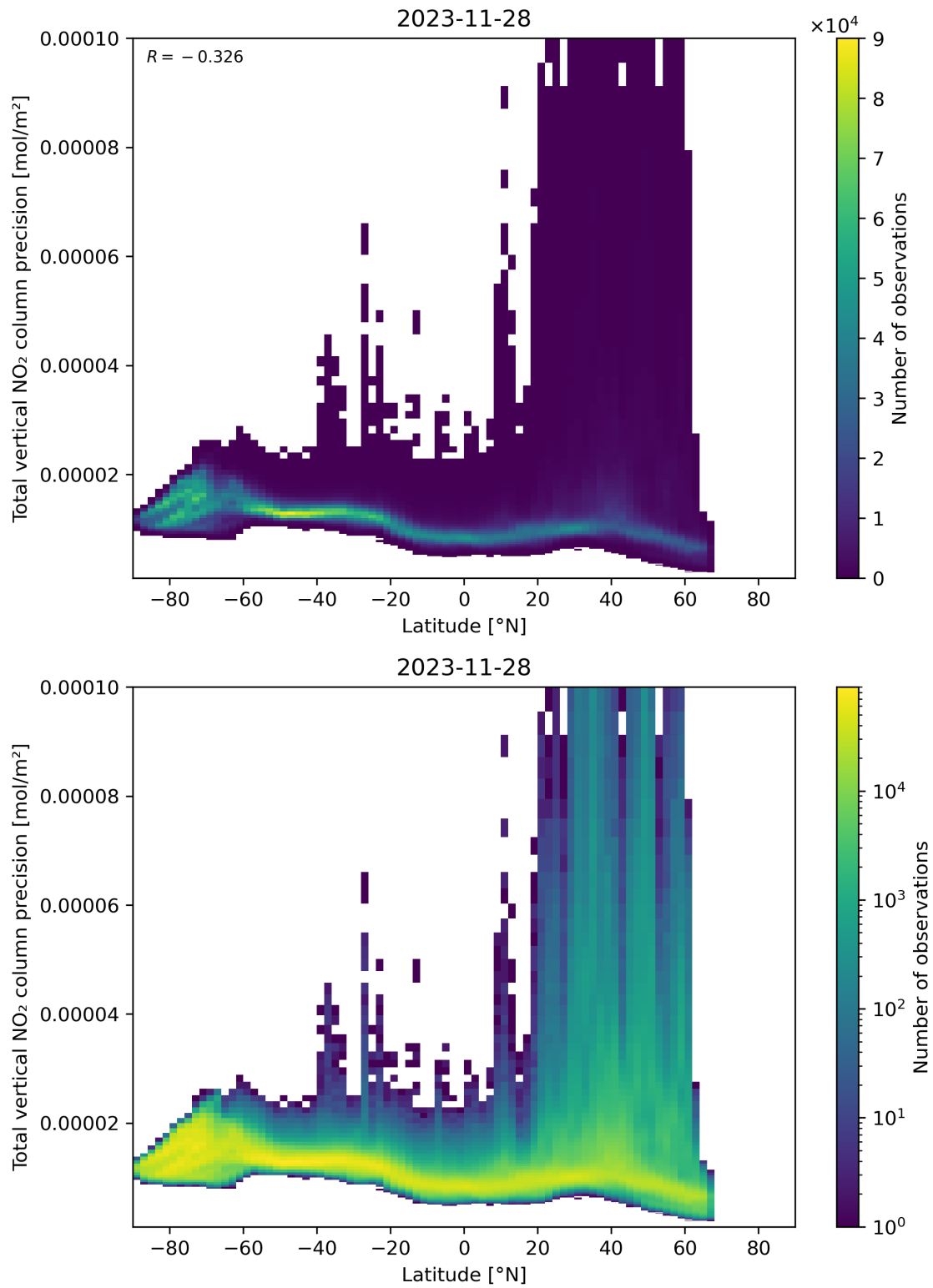
Figure 91: Scatter density plot of “Latitude” against “Total vertical NO 2 column precision” for 2023-11-28 to 2023-11-29.
