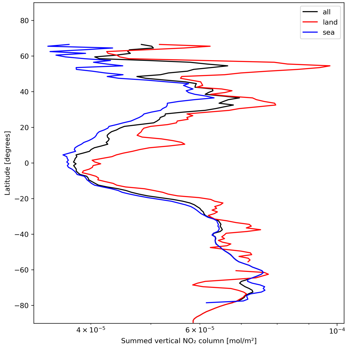
Figure 23: Zonal average of “Summed vertical NO 2 column” for 2023-11-28 to 2023-11-30.
