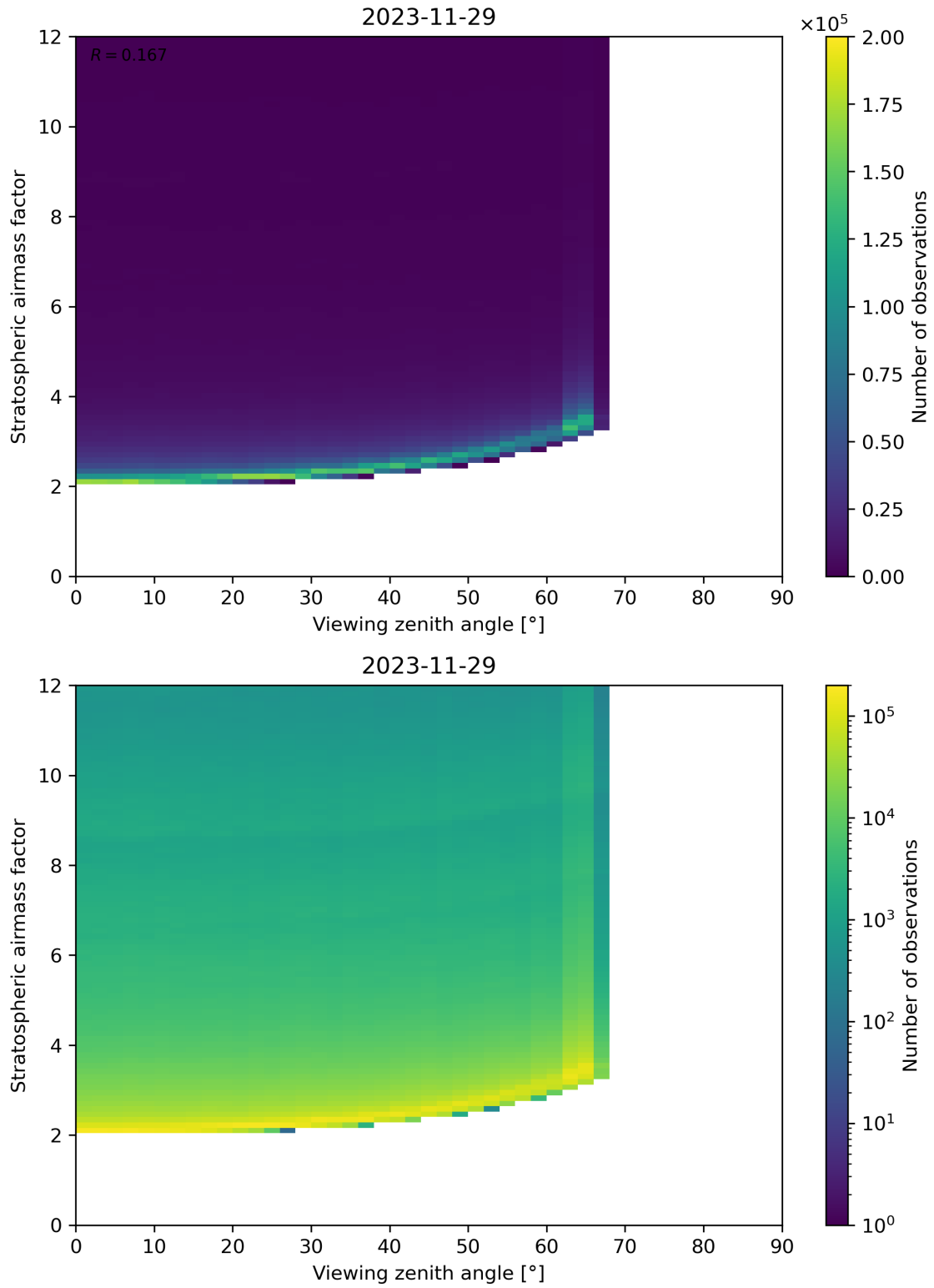
Figure 159: Scatter density plot of “Viewing zenith angle” against “Stratospheric airmass factor” for 2023-11-28 to 2023-11-30.
