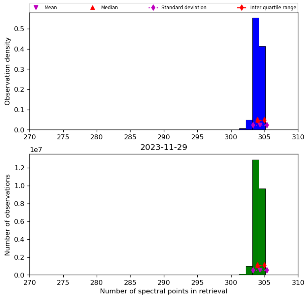
Figure 33: Histogram of “Number of spectral points in retrieval” for 2023-11-28 to 2023-11-30
