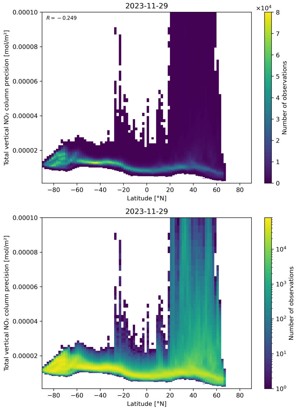
Figure 91: Scatter density plot of “Latitude” against “Total vertical NO 2 column precision” for 2023-11-28 to 2023-11-30.
