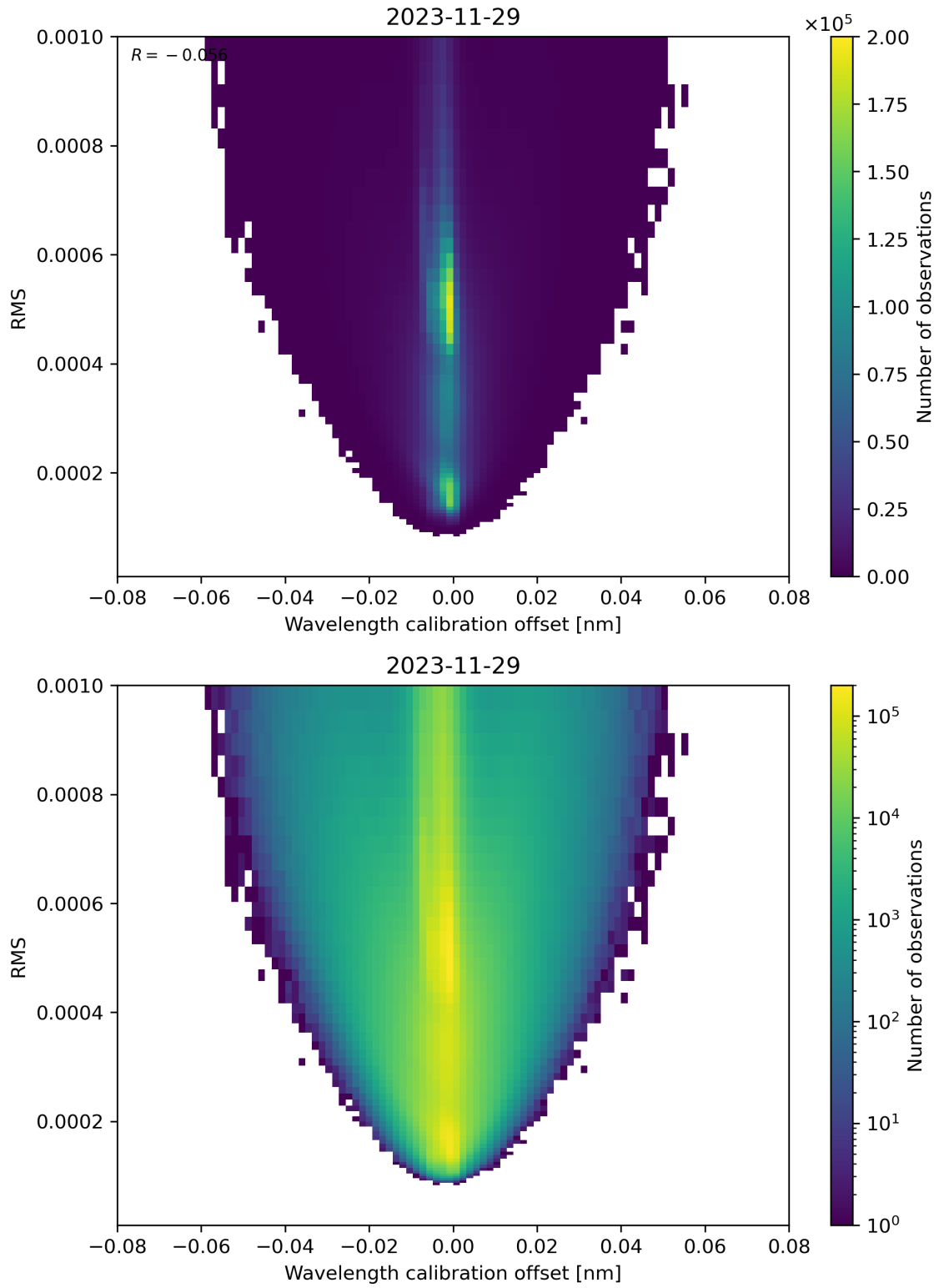
Figure 181: Scatter density plot of “Wavelength calibration offset” against “RMS” for 2023-11-28 to 2023-11-30.
