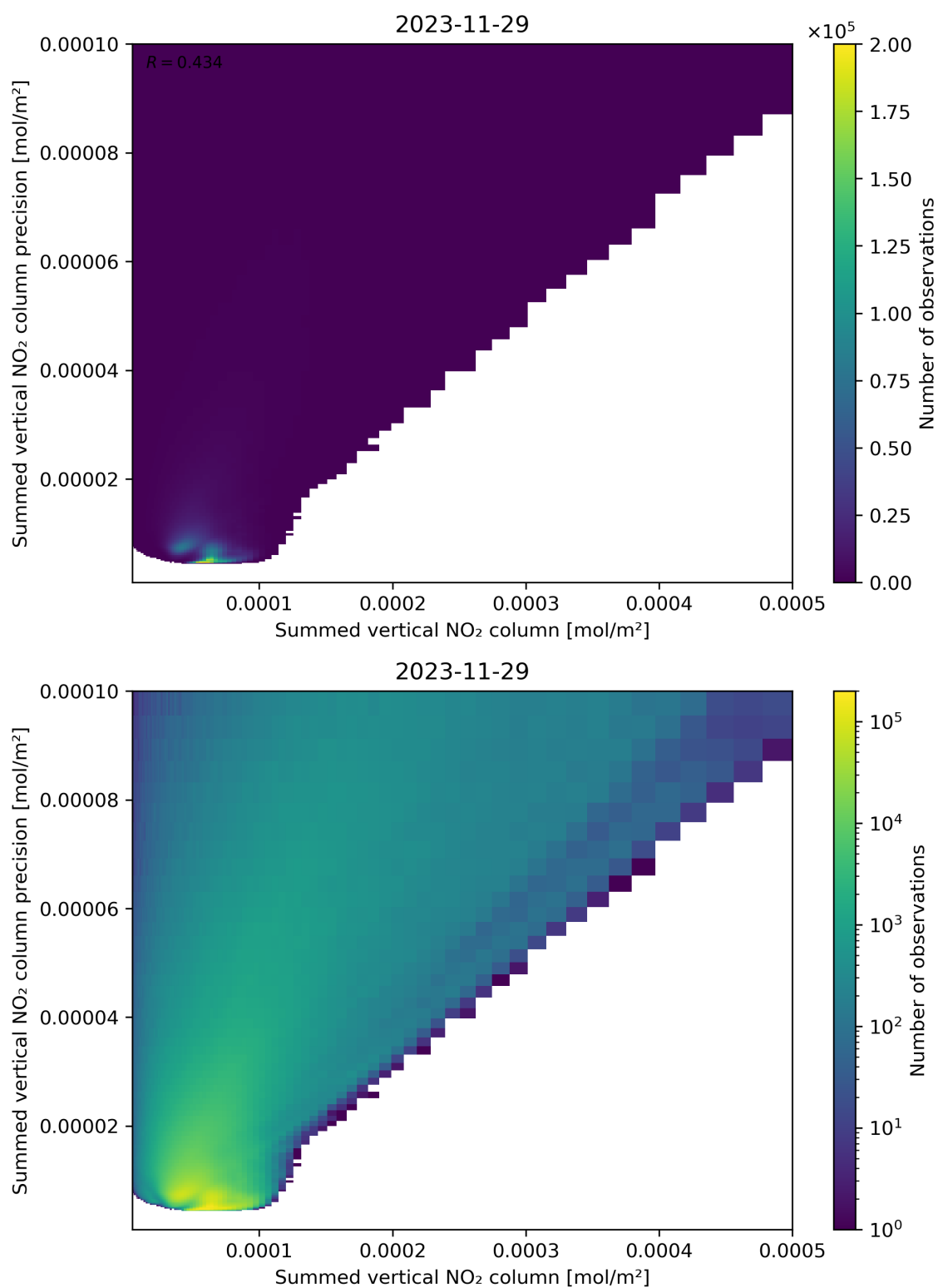
Figure 105: Scatter density plot of “Summed vertical NO 2 column” against “Summed vertical NO 2 column precision” for 2023-11-28 to 2023-11-30.
