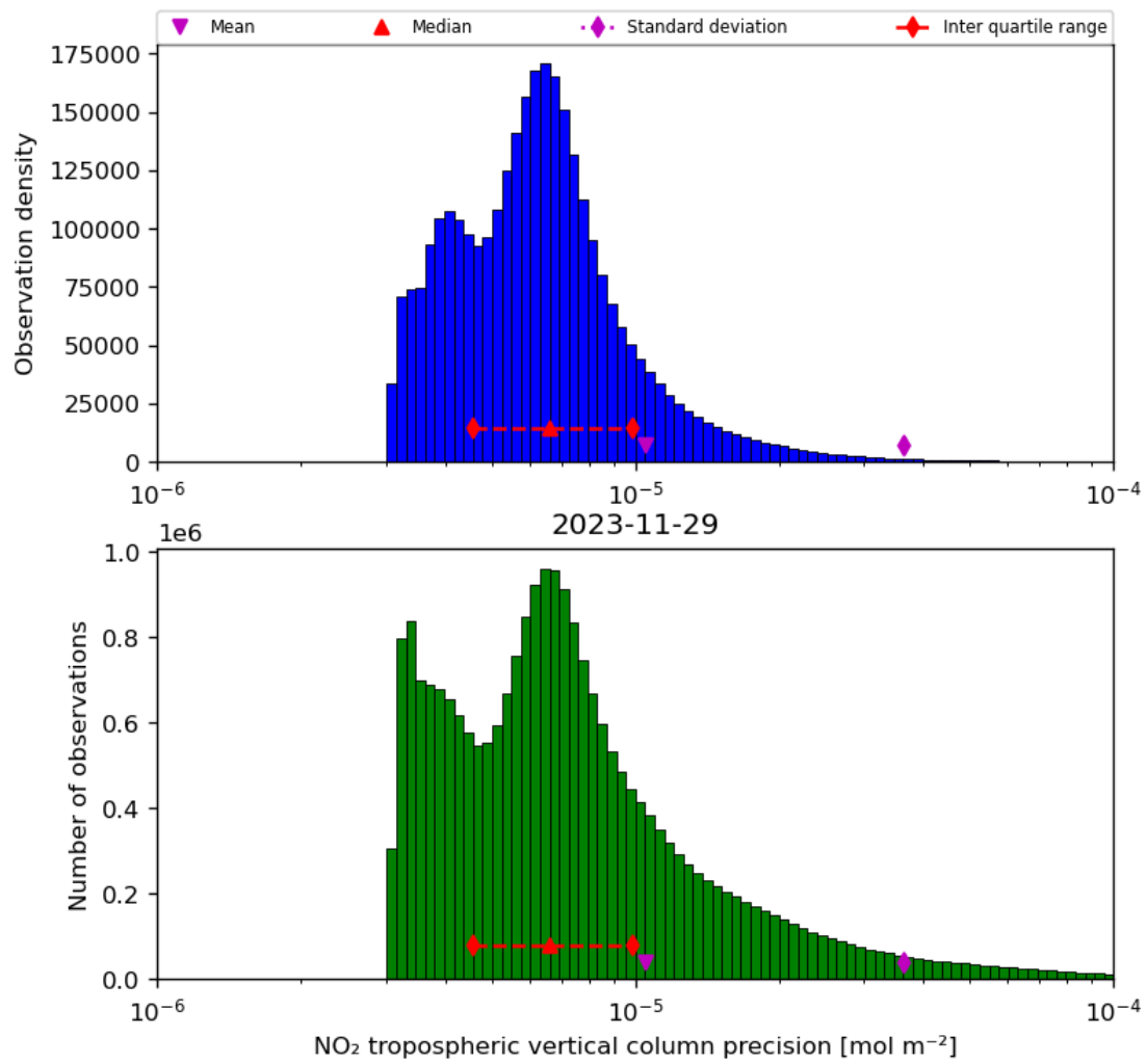
Figure 30: Histogram of “NO 2 tropospheric vertical column precision” for 2023-11-28 to 2023-11-30
