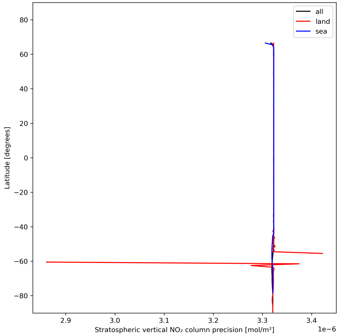
Figure 20: Zonal average of “Stratospheric vertical NO 2 column precision” for 2023-11-28 to 2023-11-30.
