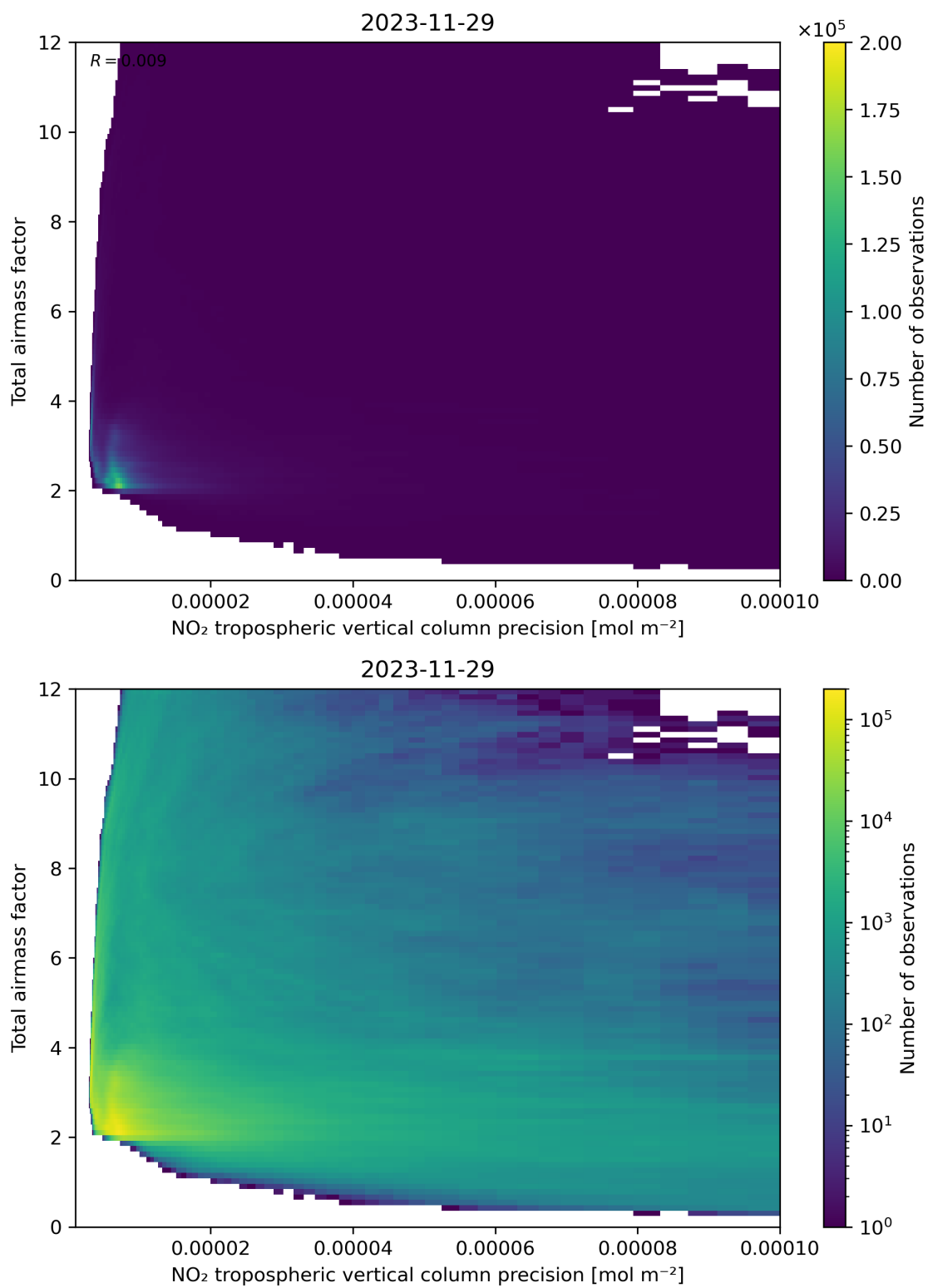
Figure 132: Scatter density plot of “NO 2 tropospheric vertical column precision” against “Total air mass factor” for 2023-11-28 to 2023-11-30.
