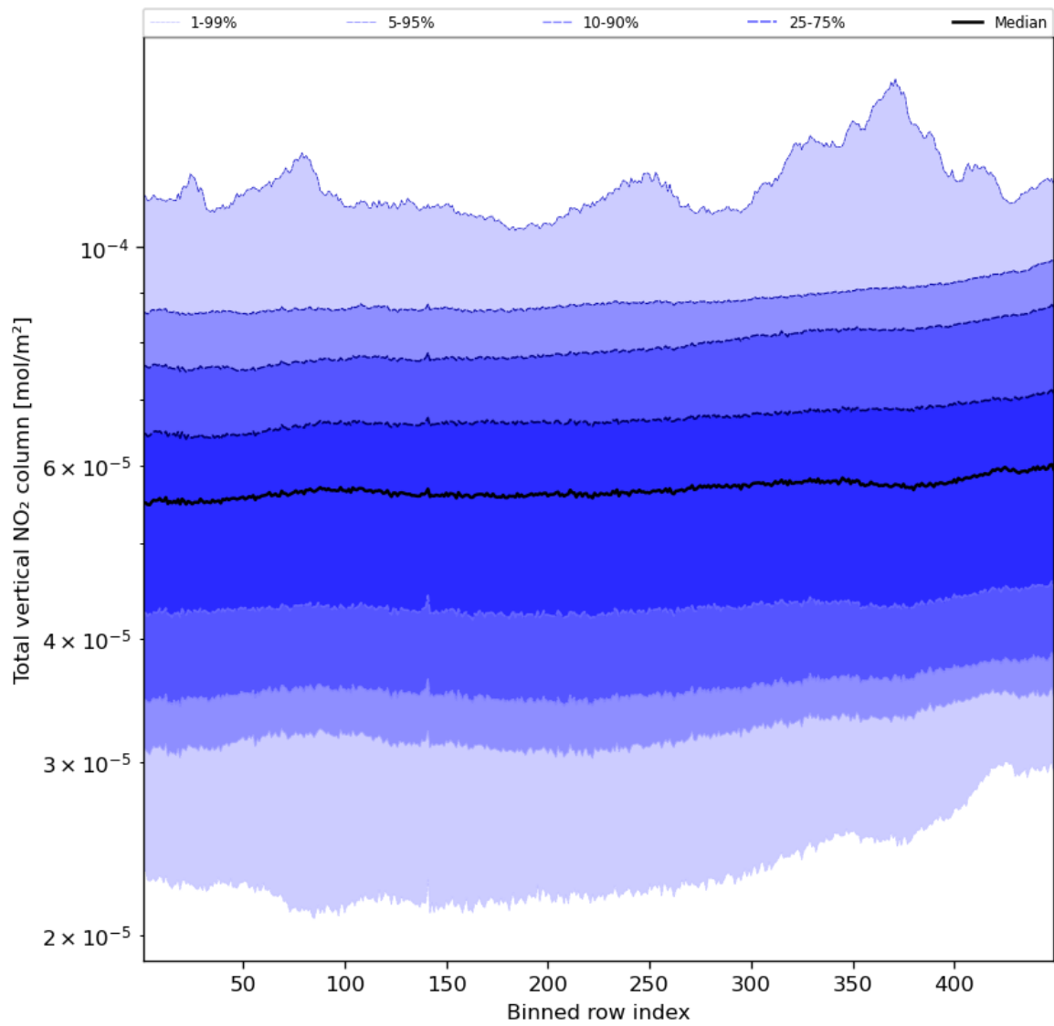
Figure 55: Along track statistics of “Total vertical NO 2 column” for 2023-11-28 to 2023-11-30
