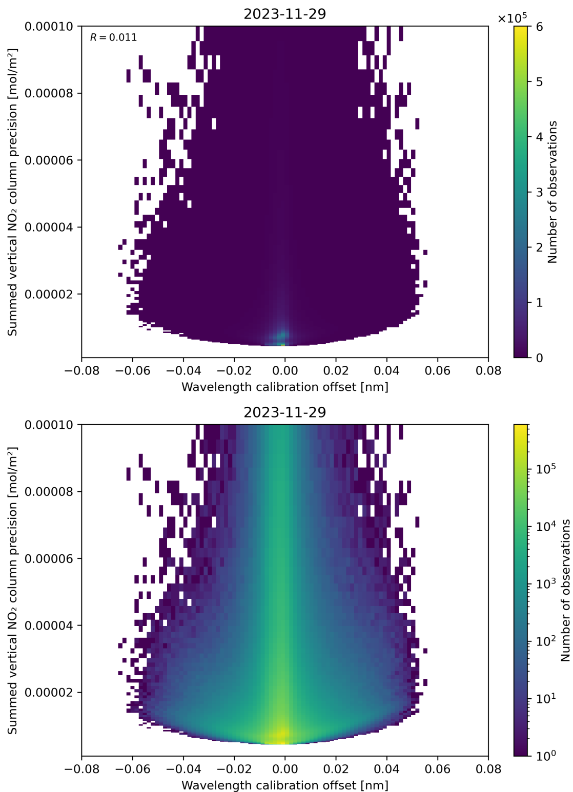
Figure 178: Scatter density plot of “Wavelength calibration offset” against “Summed vertical NO 2 column precision” for 2023-11-28 to 2023-11-30.
