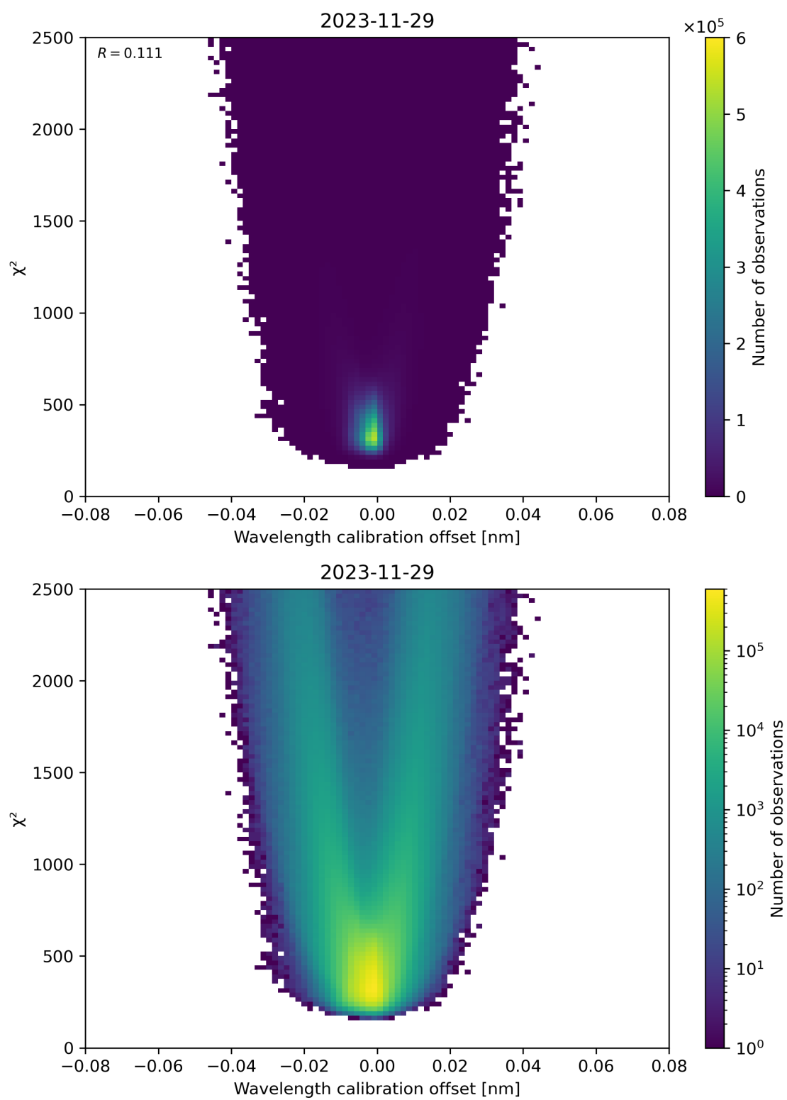
Figure 175: Scatter density plot of “Wavelength calibration offset” against “ \chi^2 ” for 2023-11-28 to 2023-11-30.
