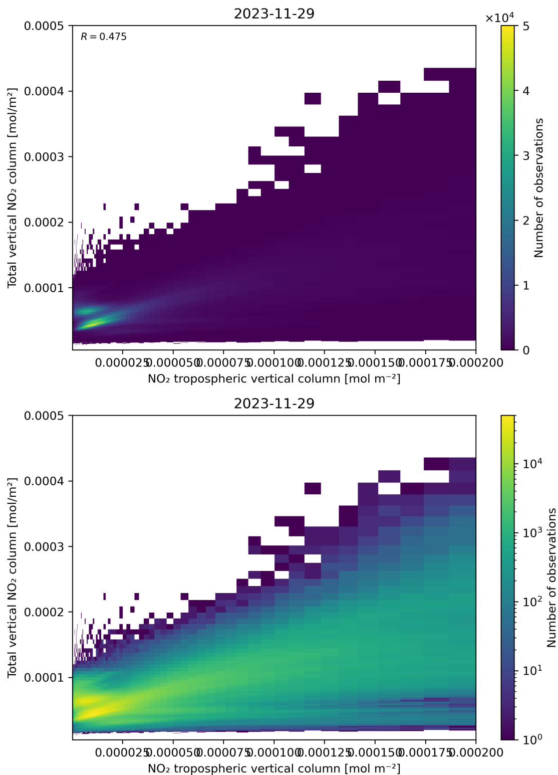
Figure 128: Scatter density plot of “NO 2 tropospheric vertical column” against “Total vertical NO 2 column” for 2023-11-28 to 2023-11-30.
