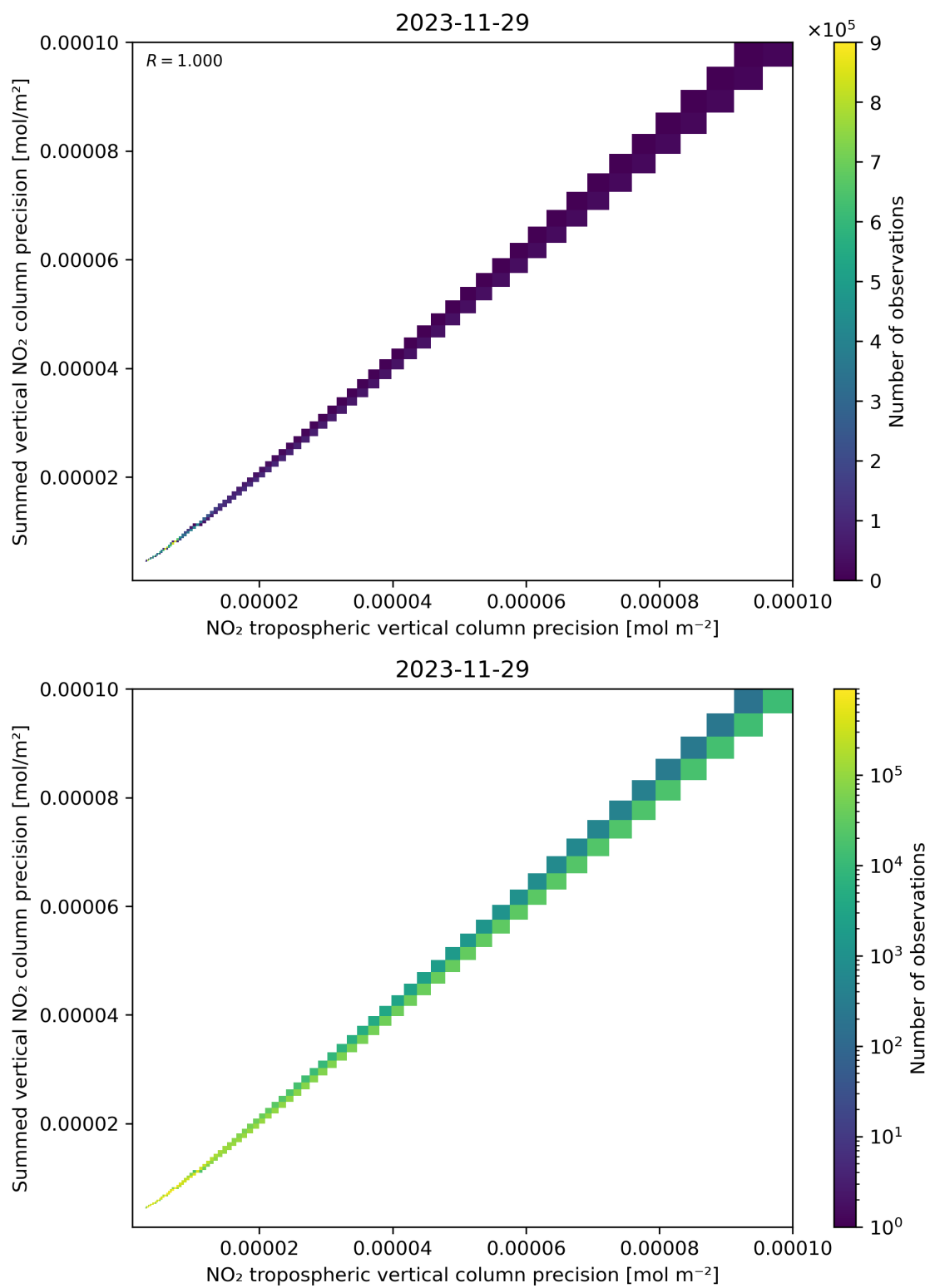
Figure 137: Scatter density plot of “NO 2 tropospheric vertical column precision” against “Summed vertical NO 2 column precision” for 2023-11-28 to 2023-11-30.
