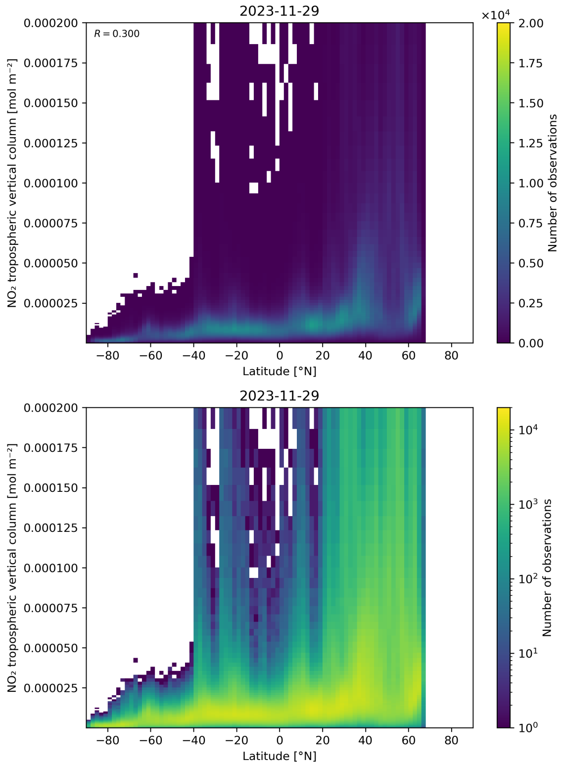
Figure 92: Scatter density plot of “Latitude” against “NO 2 tropospheric vertical column” for 2023-11-28 to 2023-11-30.
