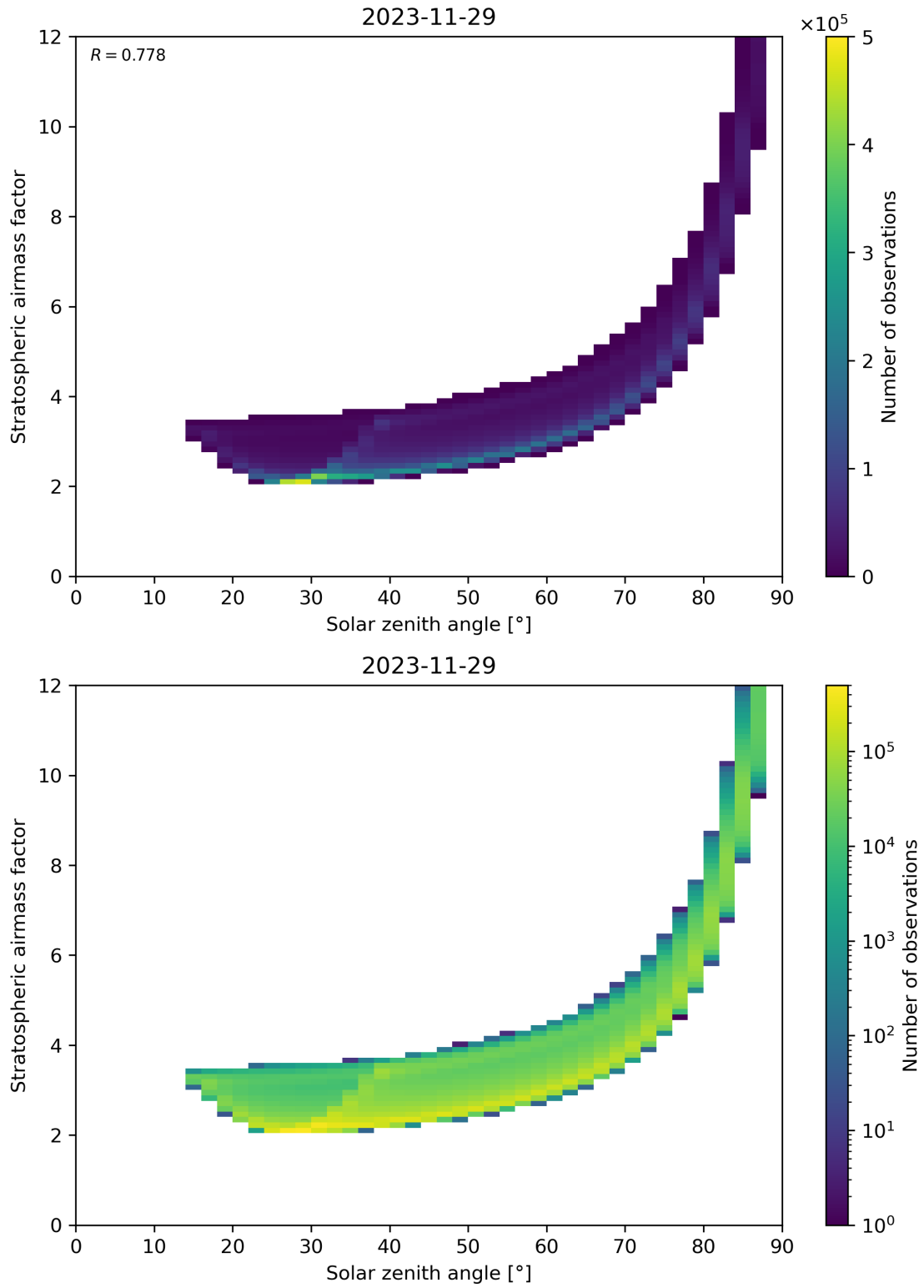
Figure 145: Scatter density plot of “Solar zenith angle” against “Stratospheric airmass factor” for 2023-11-28 to 2023-11-30.
