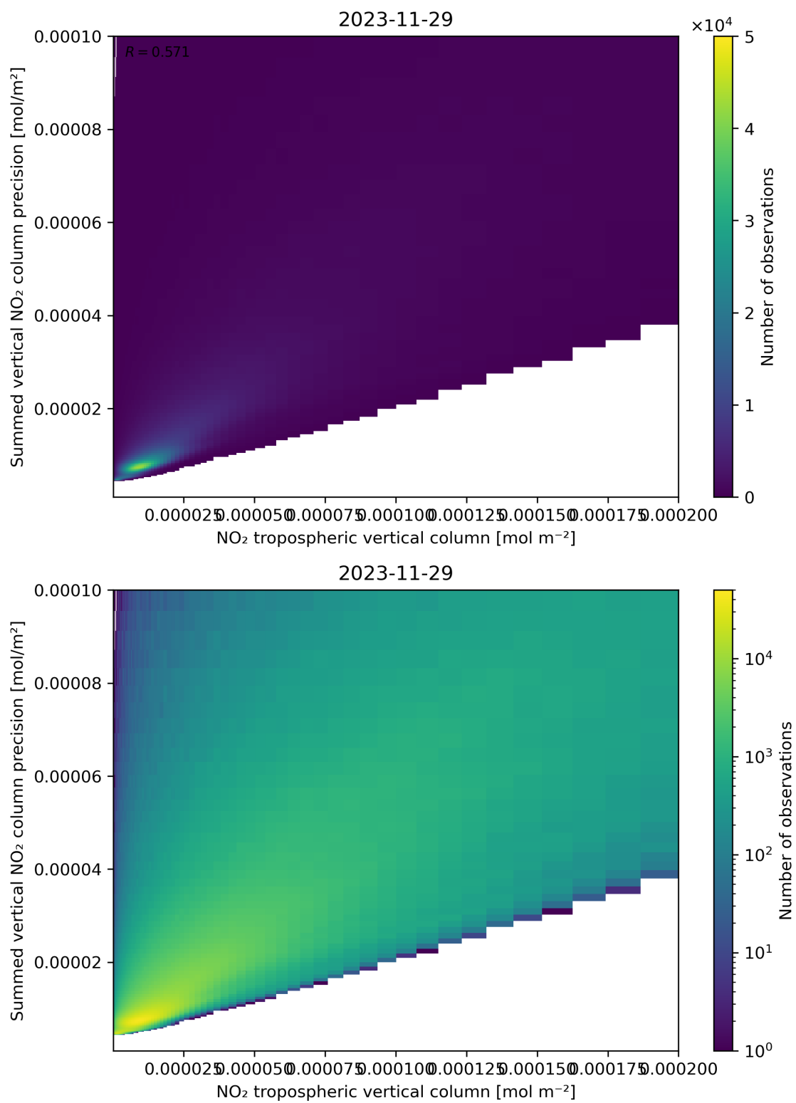
Figure 127: Scatter density plot of “NO 2 tropospheric vertical column” against “Summed vertical NO 2 column precision” for 2023-11-28 to 2023-11-30.
