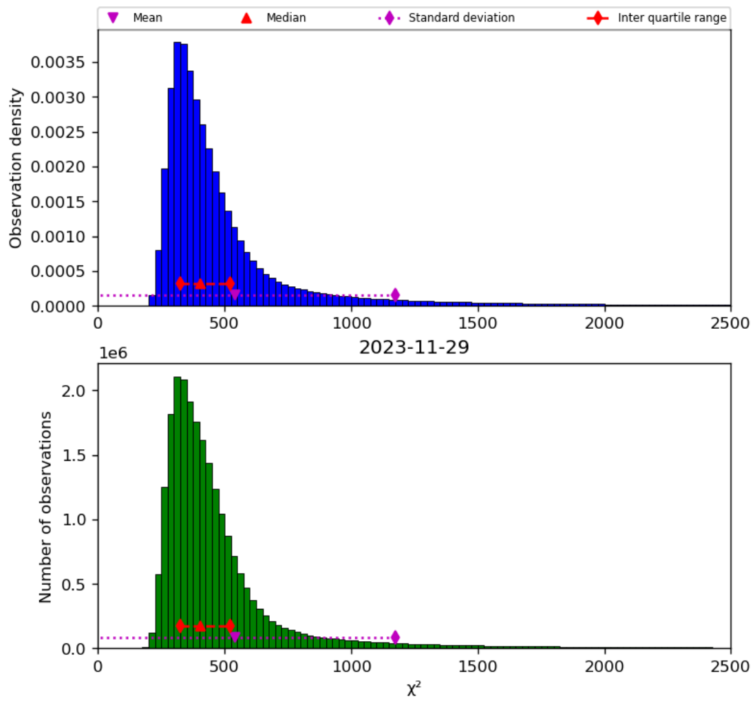
Figure 42: Histogram of “ \chi^2 ” for 2023-11-28 to 2023-11-30
