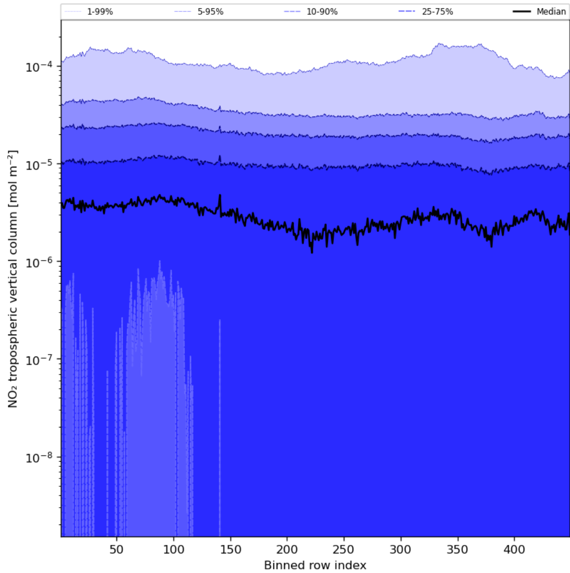
Figure 46: Along track statistics of “NO 2 tropospheric vertical column” for 2023-11-28 to 2023-11-30
