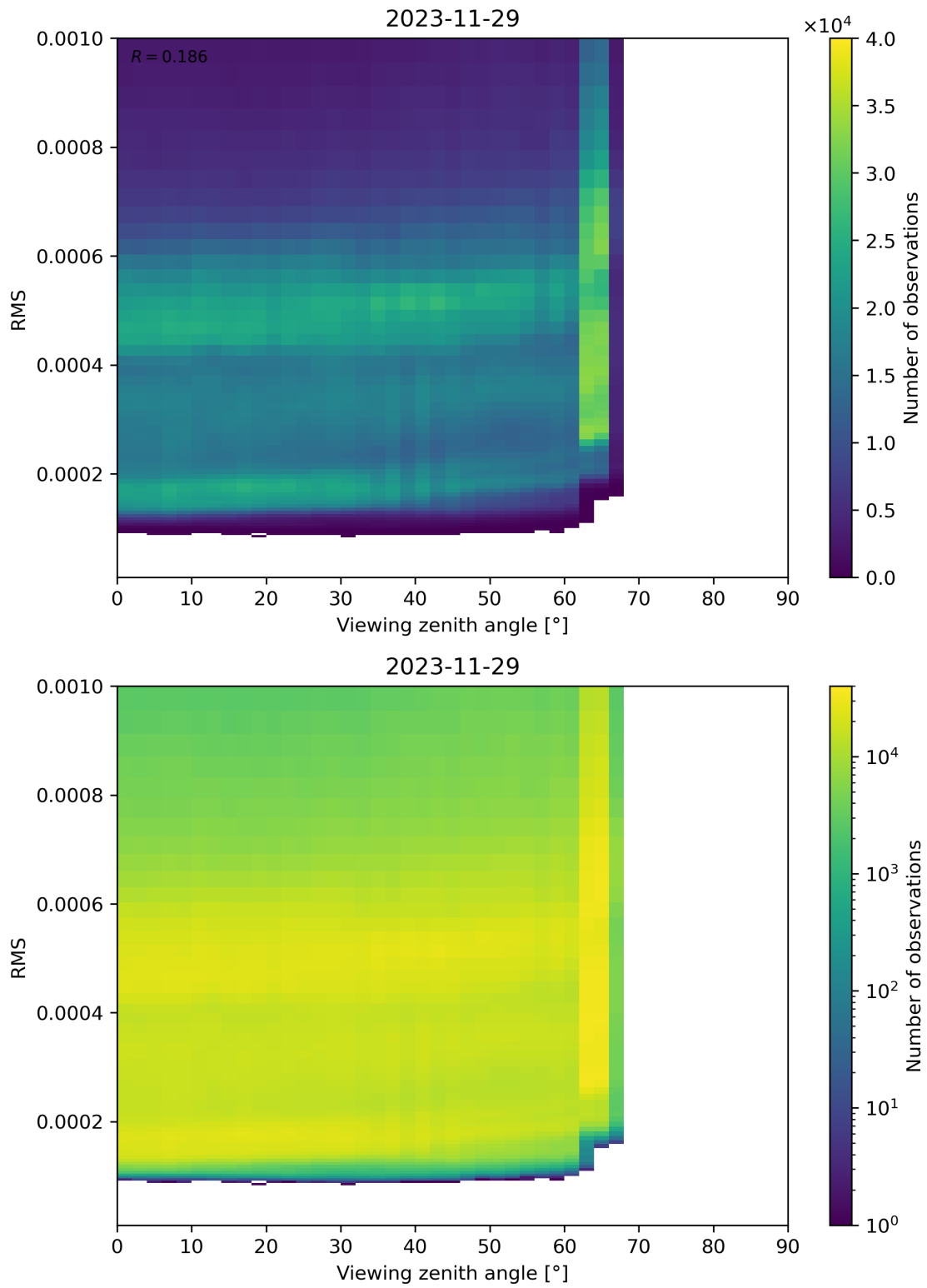
Figure 171: Scatter density plot of “Viewing zenith angle” against “RMS” for 2023-11-28 to 2023-11-30.
