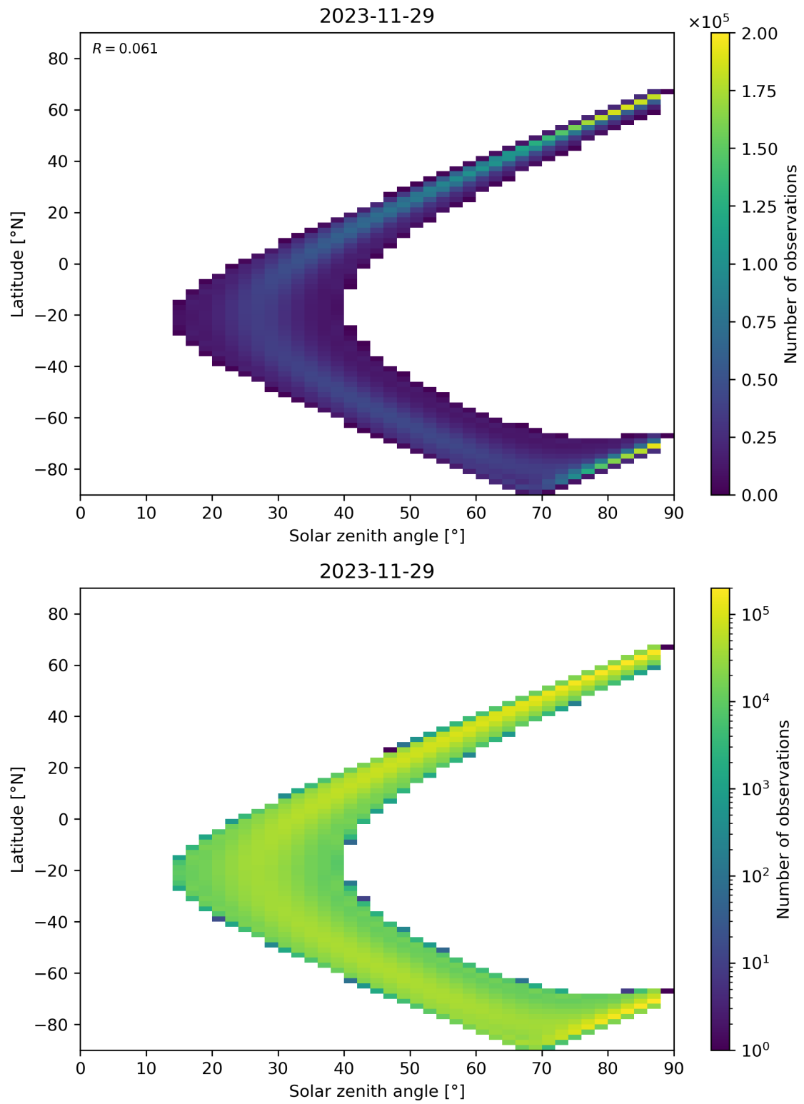
Figure 149: Scatter density plot of “Solar zenith angle” against “Latitude” for 2023-11-28 to 2023-11-30.
