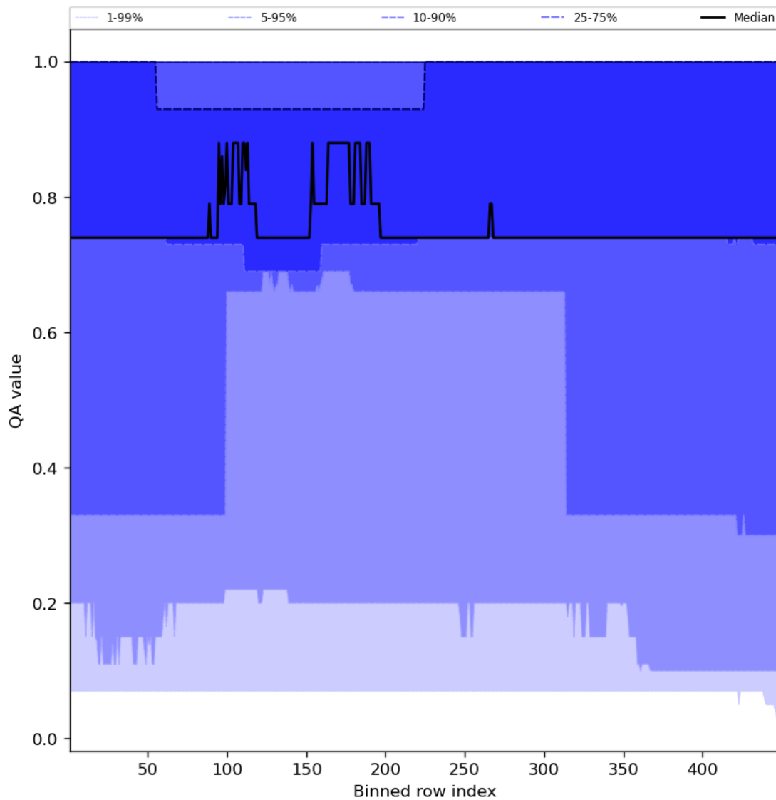
Figure 45: Along track statistics of “QA value” for 2023-11-28 to 2023-11-30
