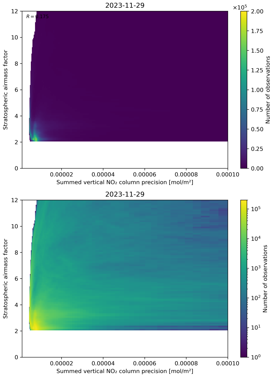
Figure 106: Scatter density plot of “Summed vertical NO 2 column precision” against “Stratospheric airmass factor” for 2023-11-28 to 2023-11-30.
