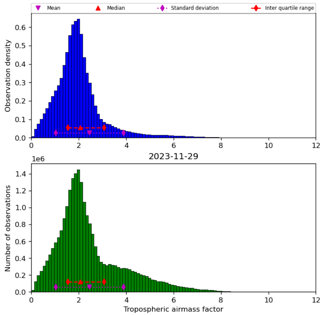
Figure 31: Histogram of “Tropospheric airmass factor” for 2023-11-28 to 2023-11-30
