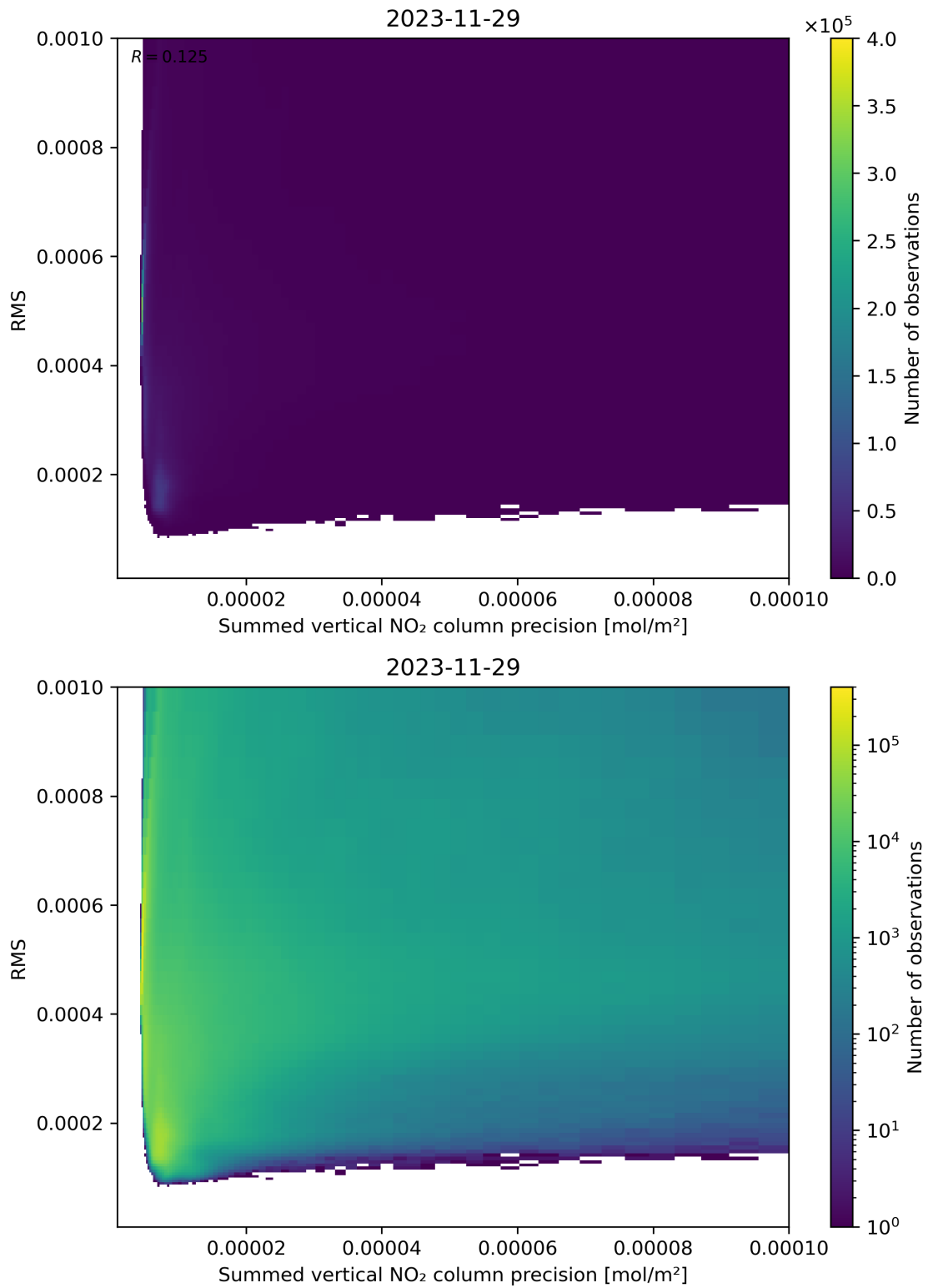
Figure 108: Scatter density plot of “Summed vertical NO 2 column precision” against “RMS” for 2023-11-28 to 2023-11-30.
