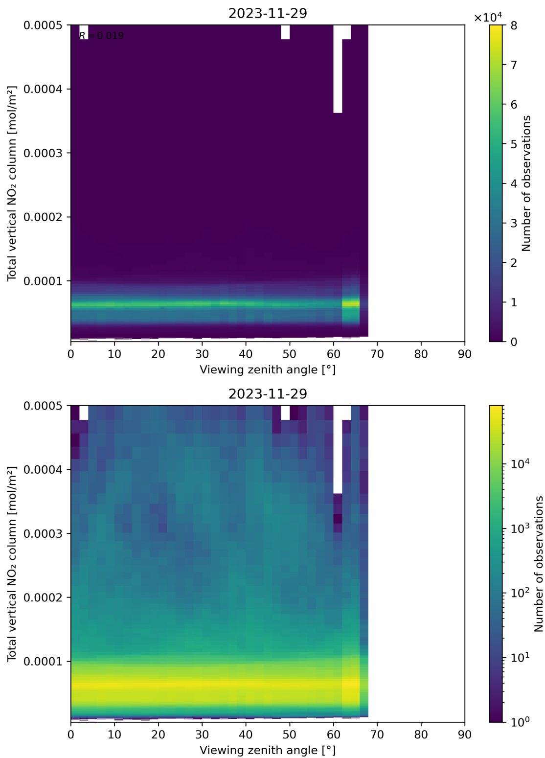
Figure 167: Scatter density plot of “Viewing zenith angle” against “Total vertical NO 2 column” for 2023-11-28 to 2023-11-30.
