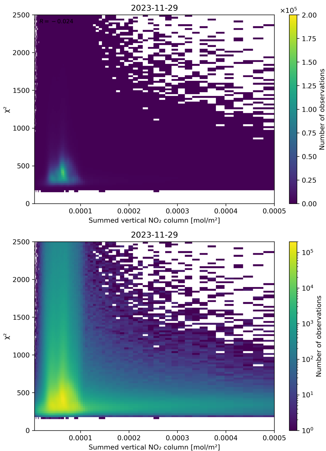
Figure 104: Scatter density plot of “Summed vertical NO 2 column” against “ \chi^2 ” for 2023-11-28 to 2023-11-30.
