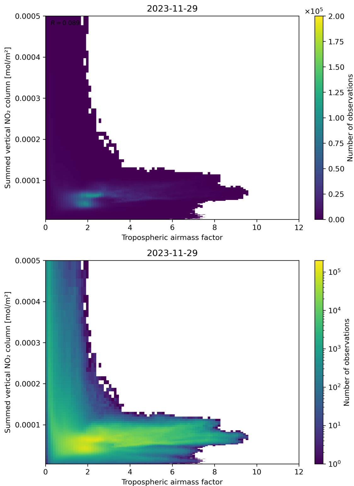
Figure 75: Scatter density plot of “Tropospheric airmass factor” against “Summed vertical NO 2 column” for 2023-11-28 to 2023-11-30.
