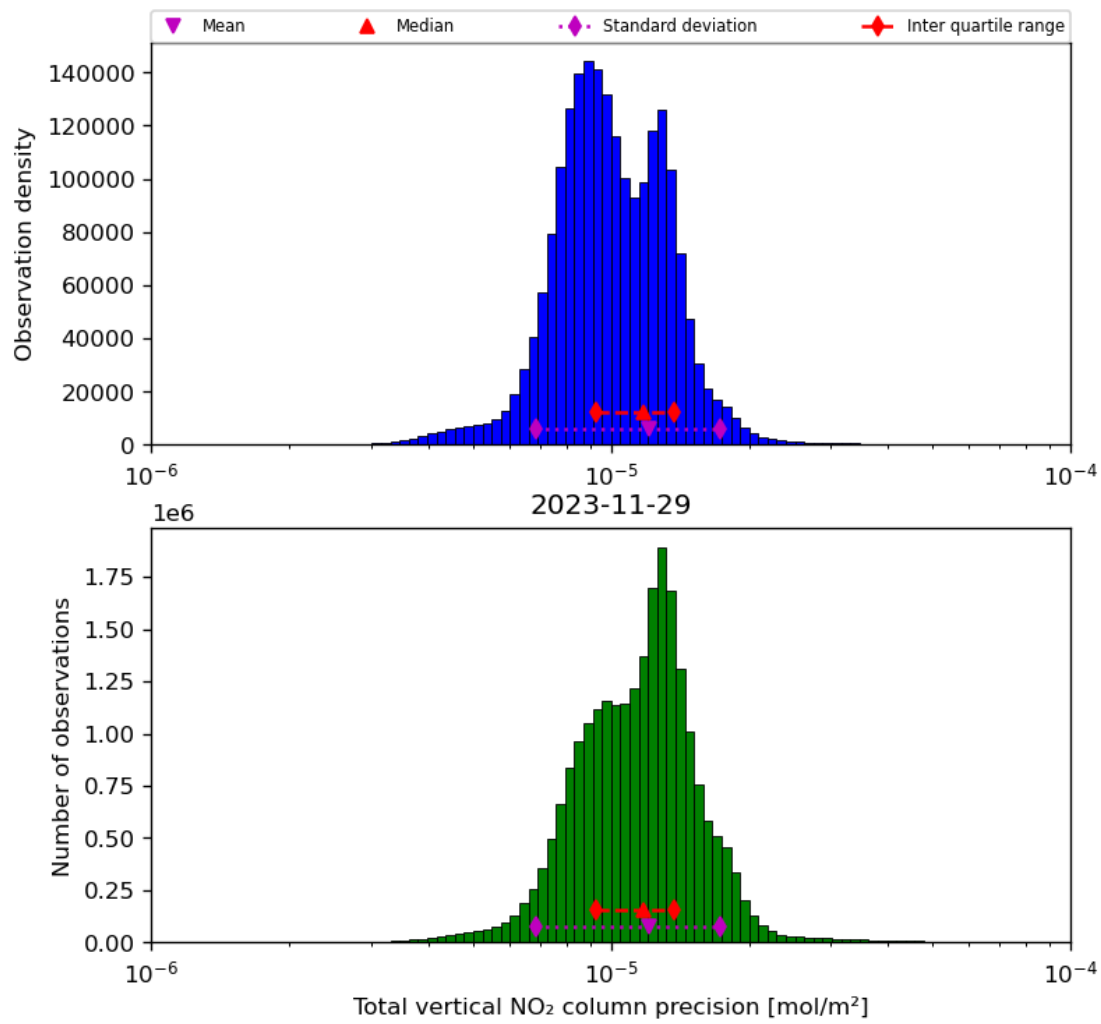
Figure 39: Histogram of "Total vertical NO 2 column precision" for 2023-11-28 to 2023-11-30
