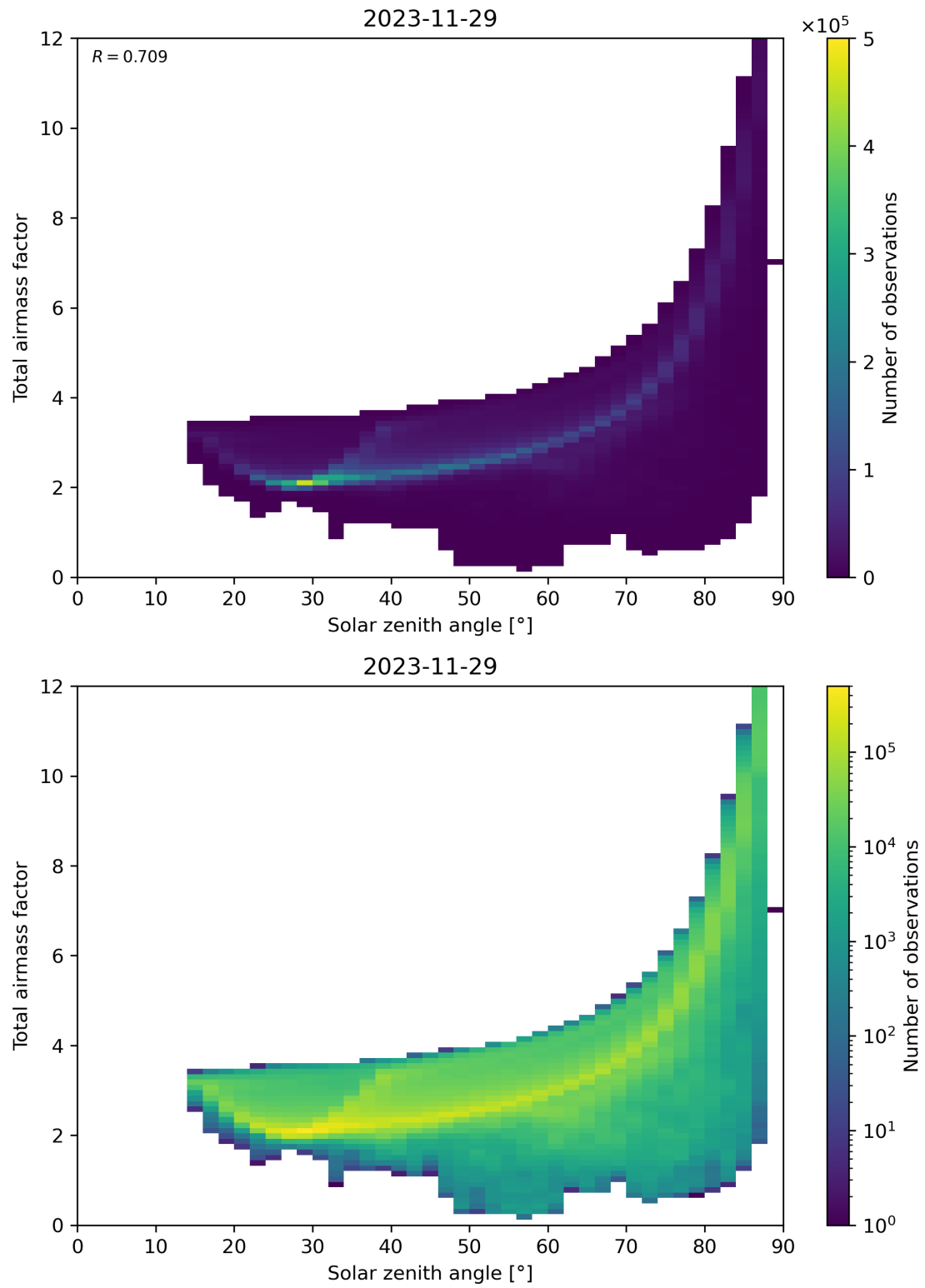
Figure 146: Scatter density plot of “Solar zenith angle” against “Total airmass factor” for 2023-11-28 to 2023-11-30.
