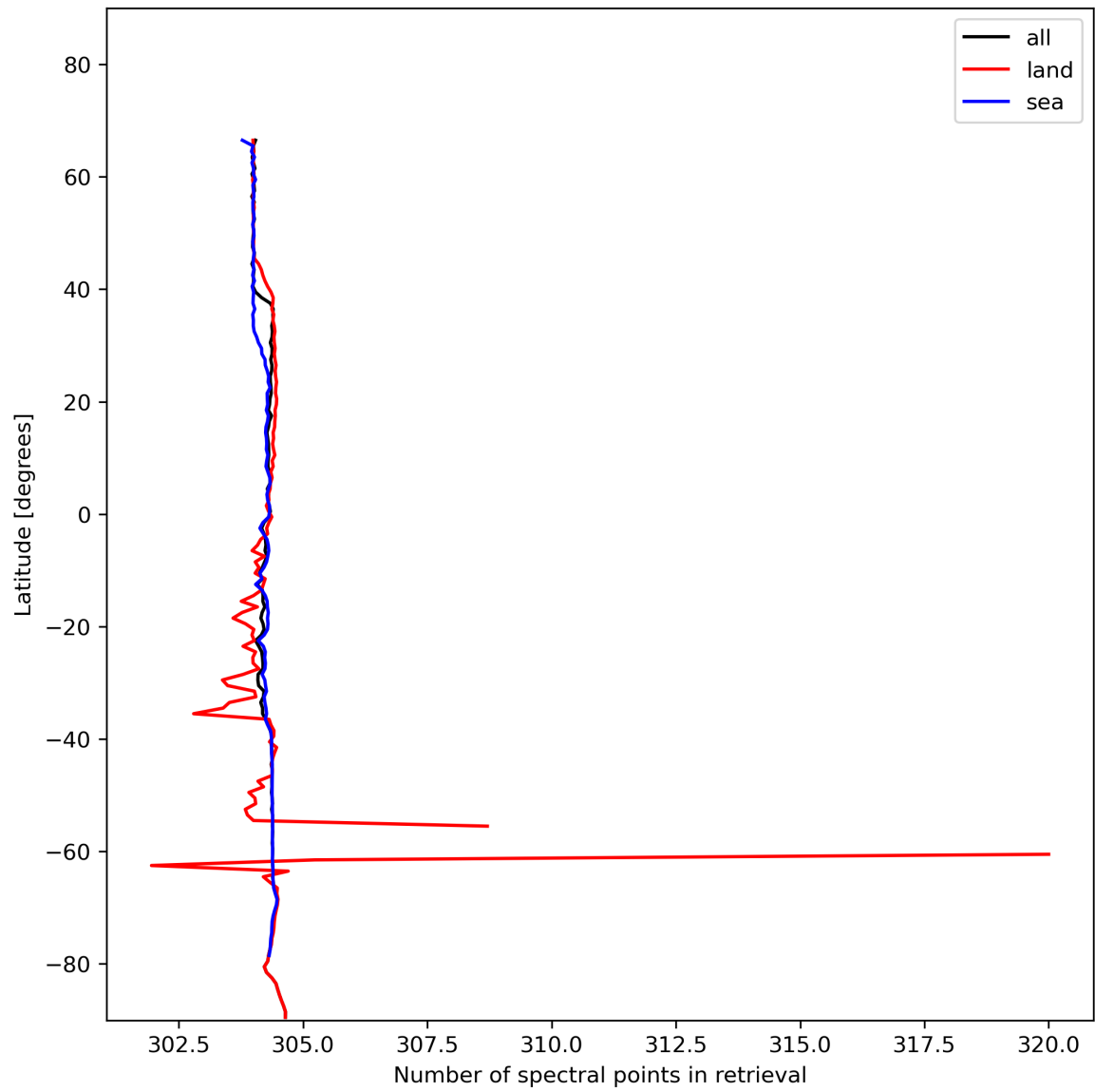
Figure 16: Zonal average of “Number of spectral points in retrieval” for 2023-11-28 to 2023-11-30.
