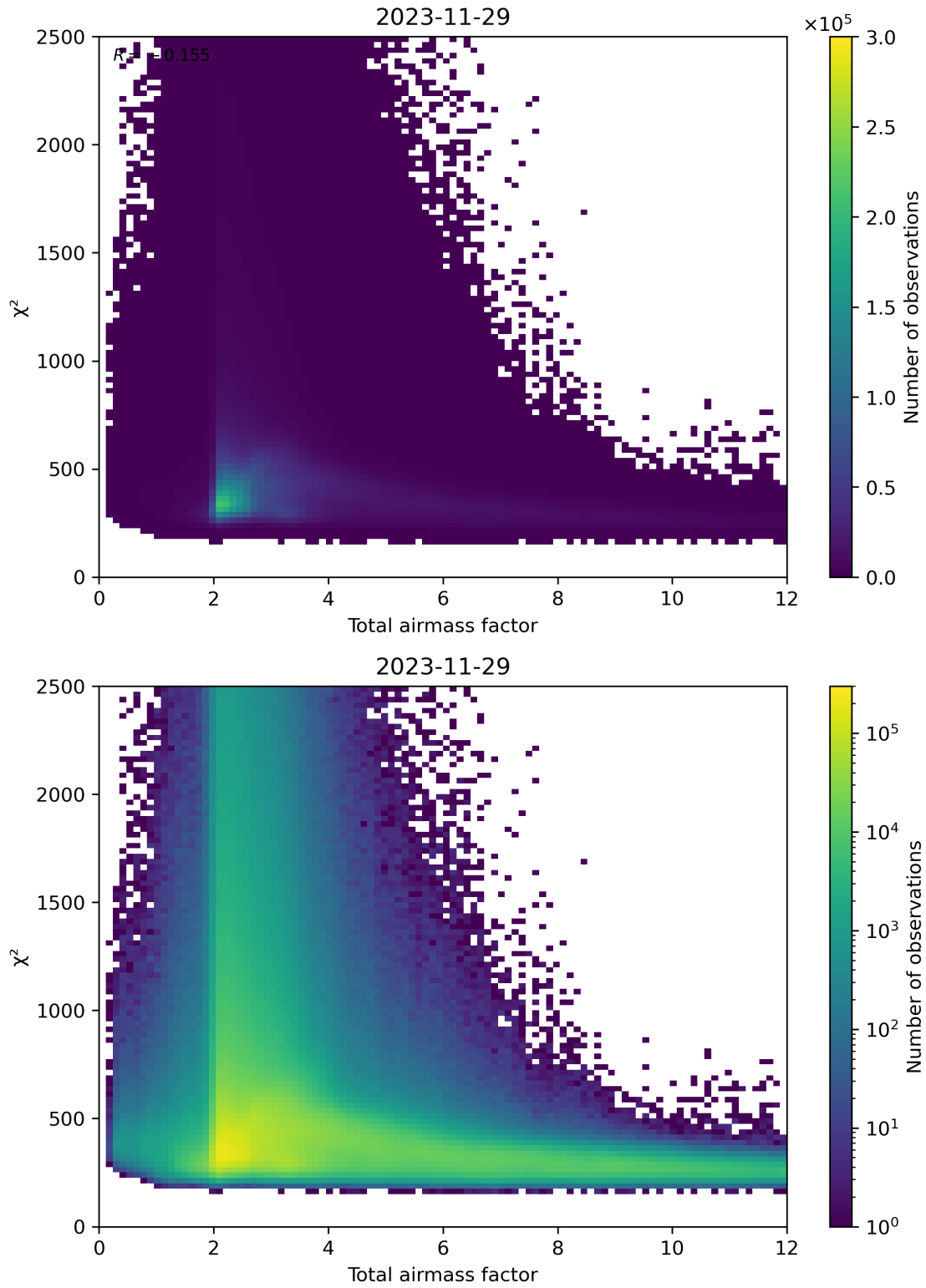
Figure 63: Scatter density plot of “Total airmass factor” against “ \chi^2 ” for 2023-11-28 to 2023-11-30.
