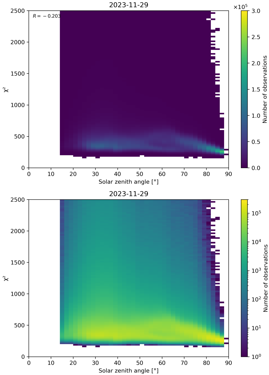
Figure 148: Scatter density plot of “Solar zenith angle” against “ \chi^2 ” for 2023-11-28 to 2023-11-30.
