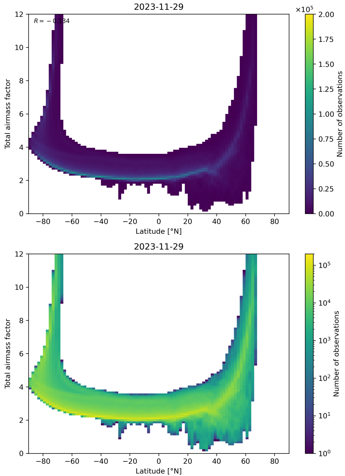
Figure 84: Scatter density plot of “Latitude” against “Total airmass factor” for 2023-11-28 to 2023-11-30.
