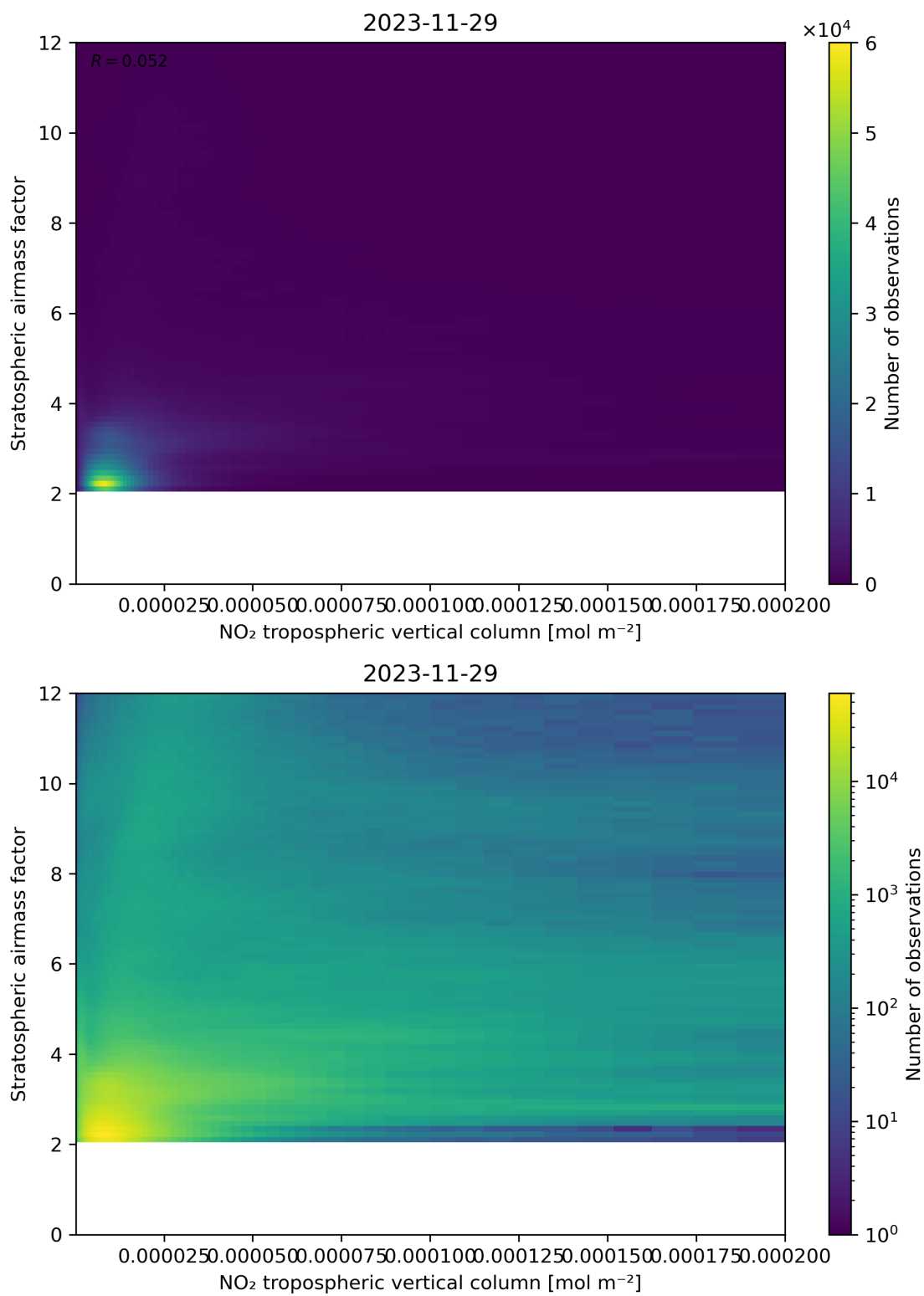
Figure 121: Scatter density plot of “NO 2 tropospheric vertical column” against “Stratospheric airmass factor” for 2023-11-28 to 2023-11-30.
