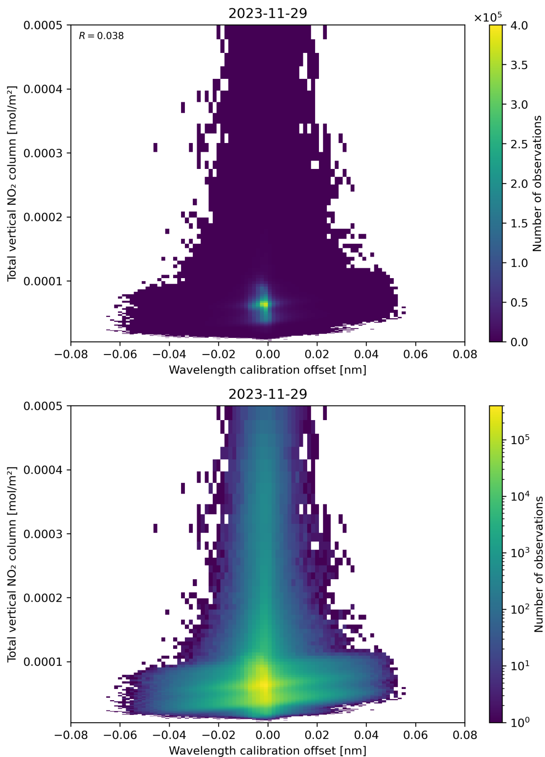
Figure 179: Scatter density plot of “Wavelength calibration offset” against “Total vertical NO 2 column” for 2023-11-28 to 2023-11-30.
