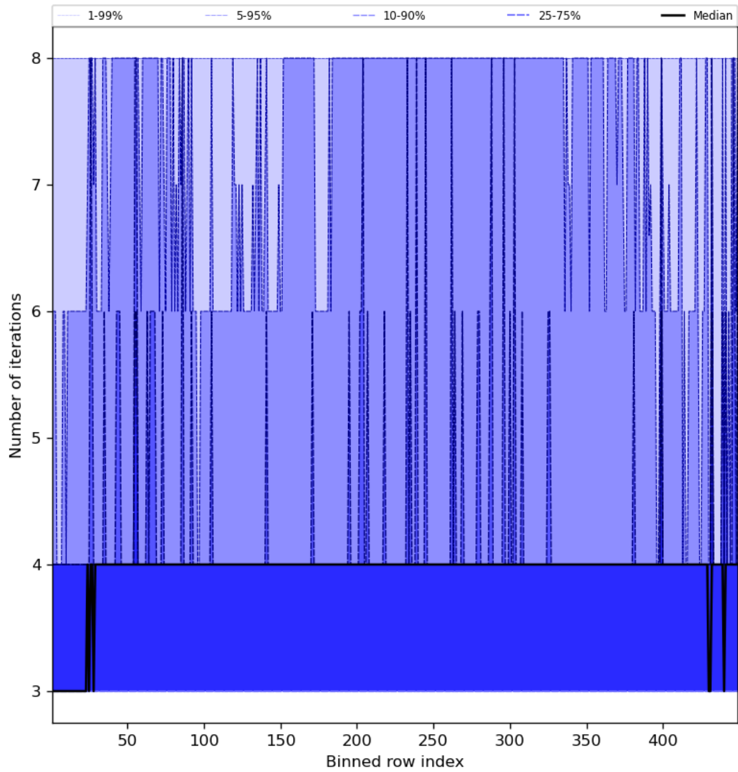
Figure 51: Along track statistics of “Number of iterations” for 2023-11-28 to 2023-11-30
