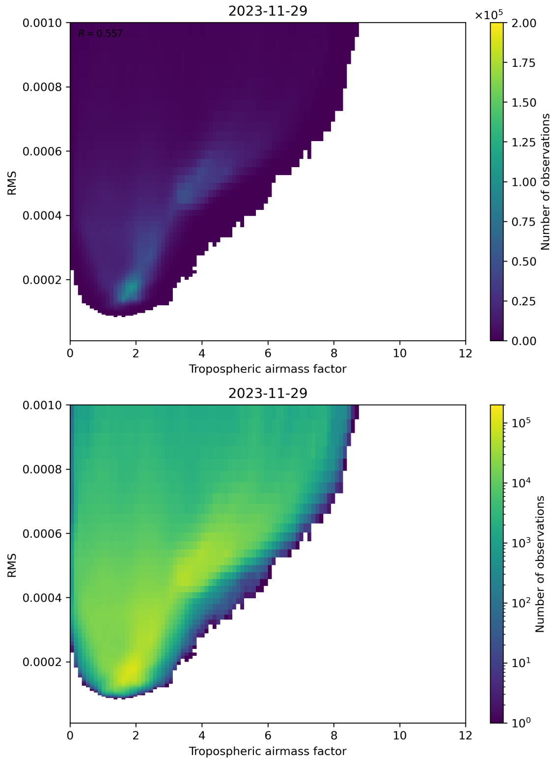
Figure 79: Scatter density plot of “Tropospheric airmass factor” against “RMS” for 2023-11-28 to 2023-11-30.
