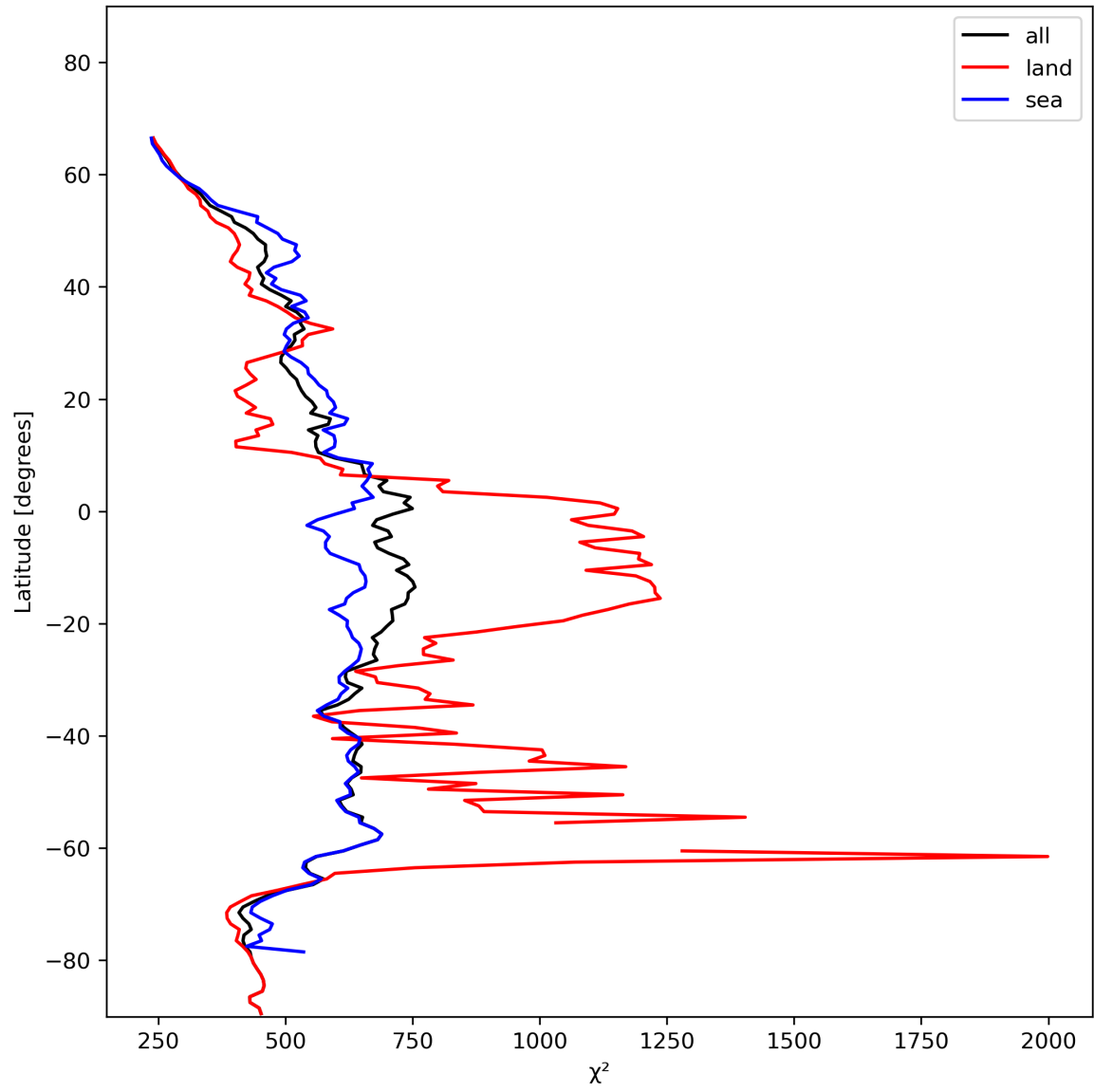
Figure 25: Zonal average of “ \chi^2 ” for 2023-11-28 to 2023-11-30.
