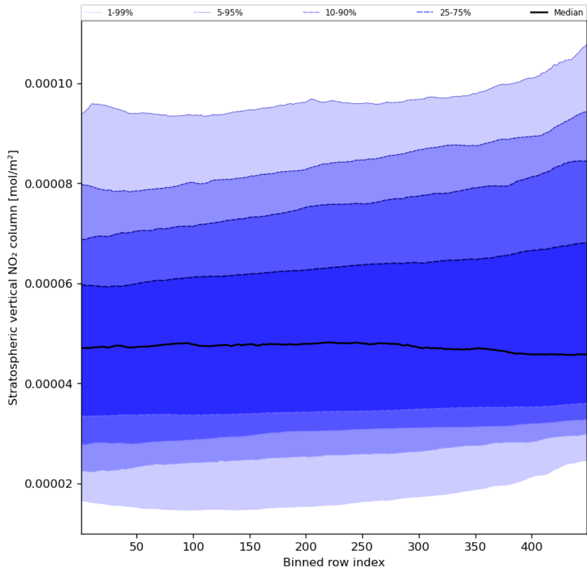
Figure 53: Along track statistics of “Stratospheric vertical NO 2 column” for 2023-11-28 to 2023-11-30
