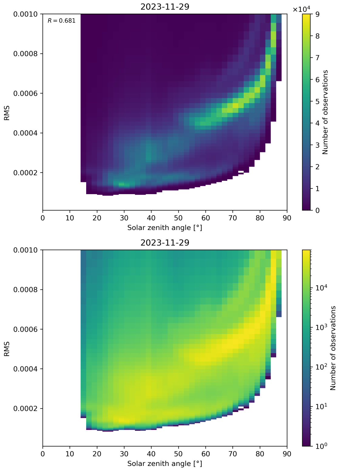
Figure 157: Scatter density plot of “Solar zenith angle” against “RMS” for 2023-11-28 to 2023-11-30.
