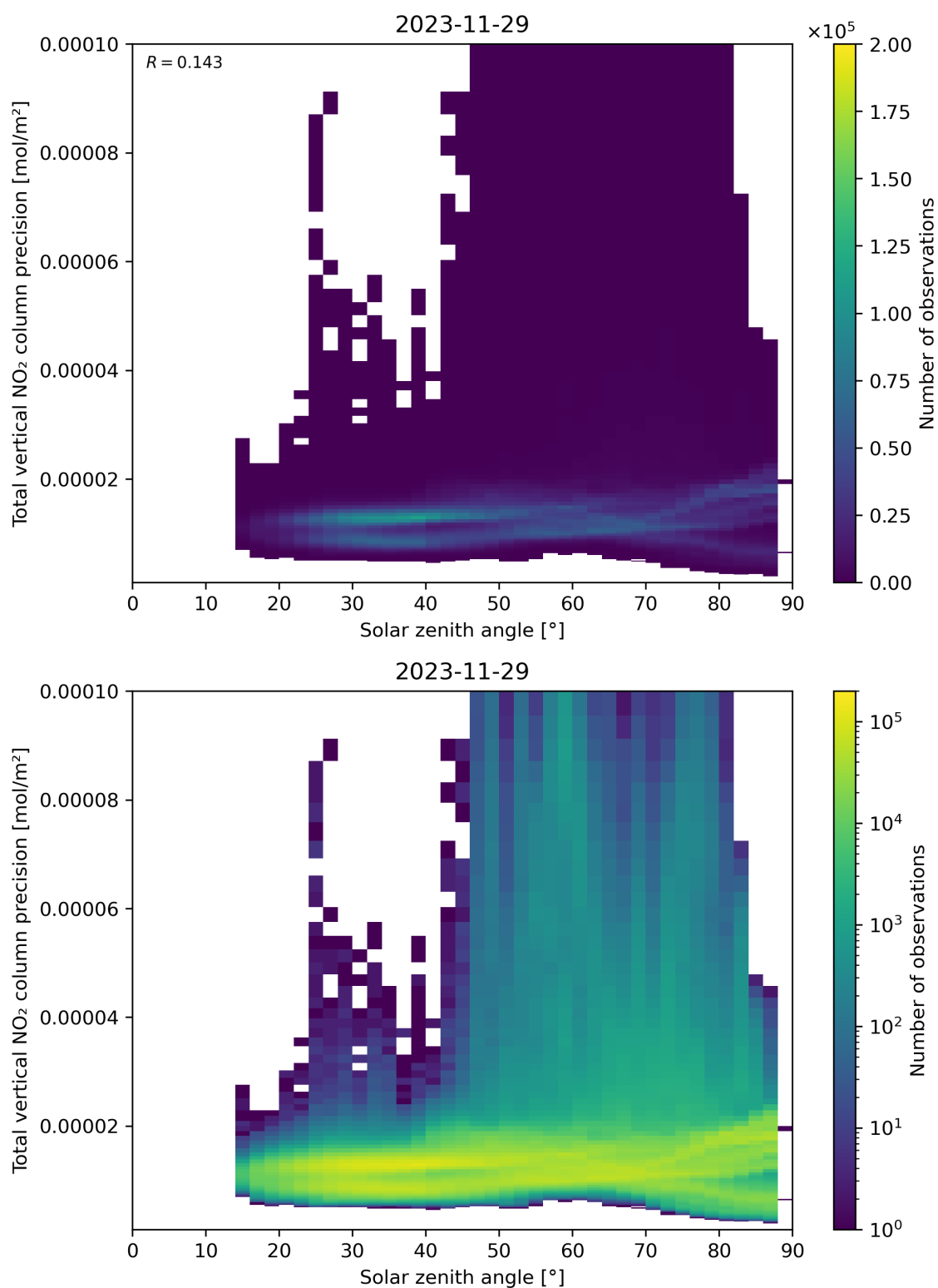
Figure 154: Scatter density plot of “Solar zenith angle” against “Total vertical NO 2 column precision” for 2023-11-28 to 2023-11-30.
