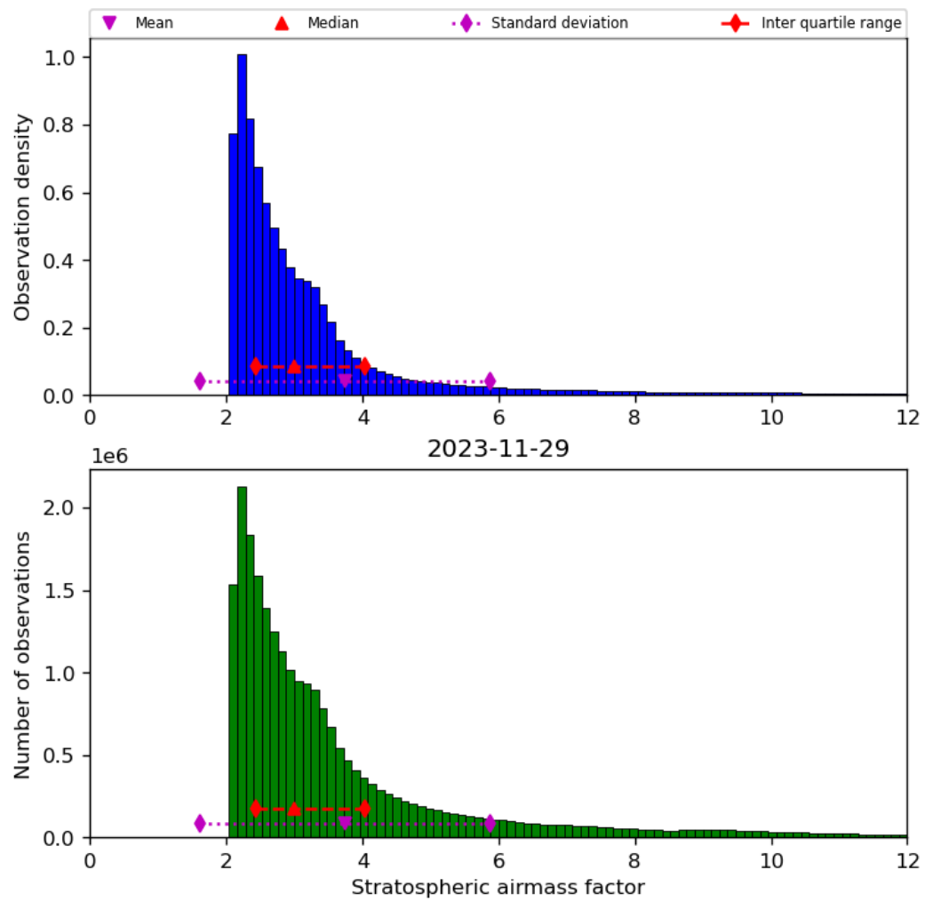
Figure 44: Histogram of “Stratospheric airmass factor” for 2023-11-28 to 2023-11-30
