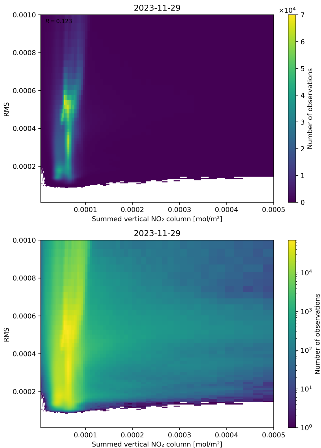
Figure 109: Scatter density plot of “Summed vertical NO 2 column” against “RMS” for 2023-11-28 to 2023-11-30.
