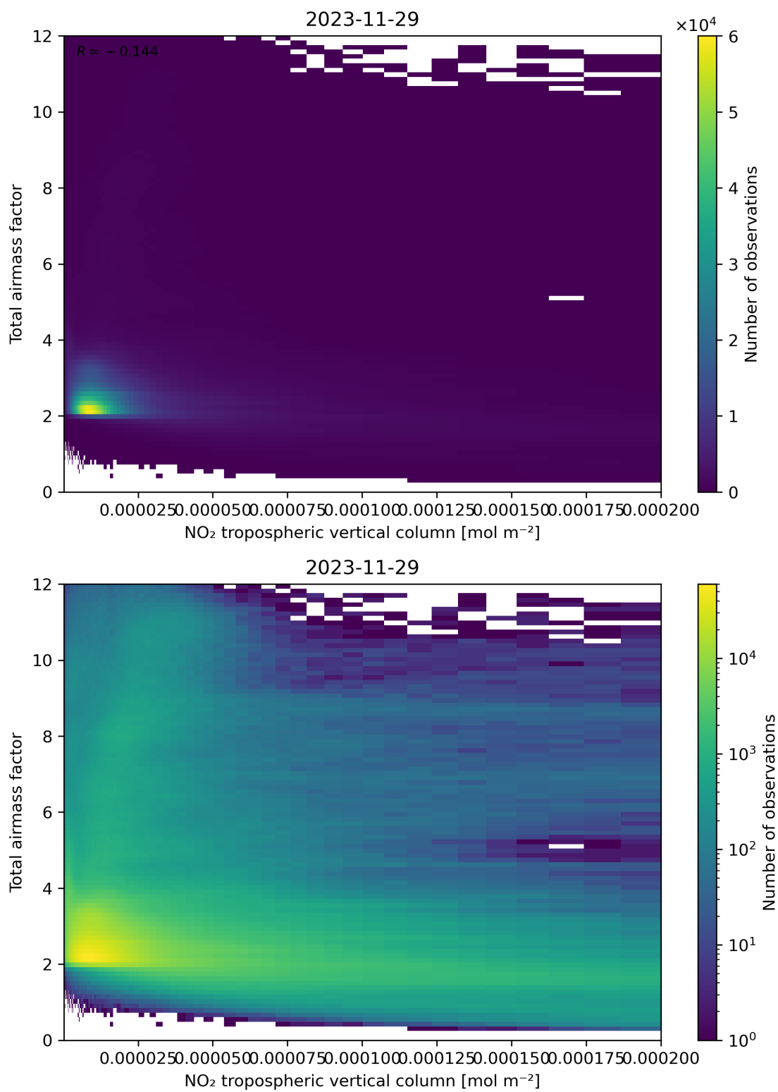
Figure 122: Scatter density plot of “NO 2 tropospheric vertical column” against “Total air mass factor” for 2023-11-28 to 2023-11-30.
