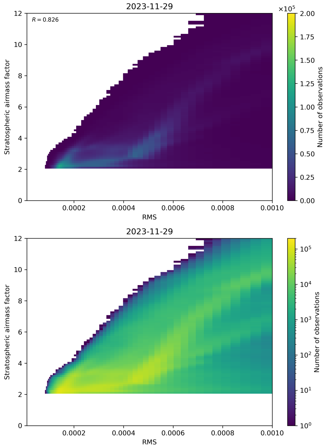
Figure 144: Scatter density plot of “RMS” against “Stratospheric airmass factor” for 2023-11-28 to 2023-11-30.
