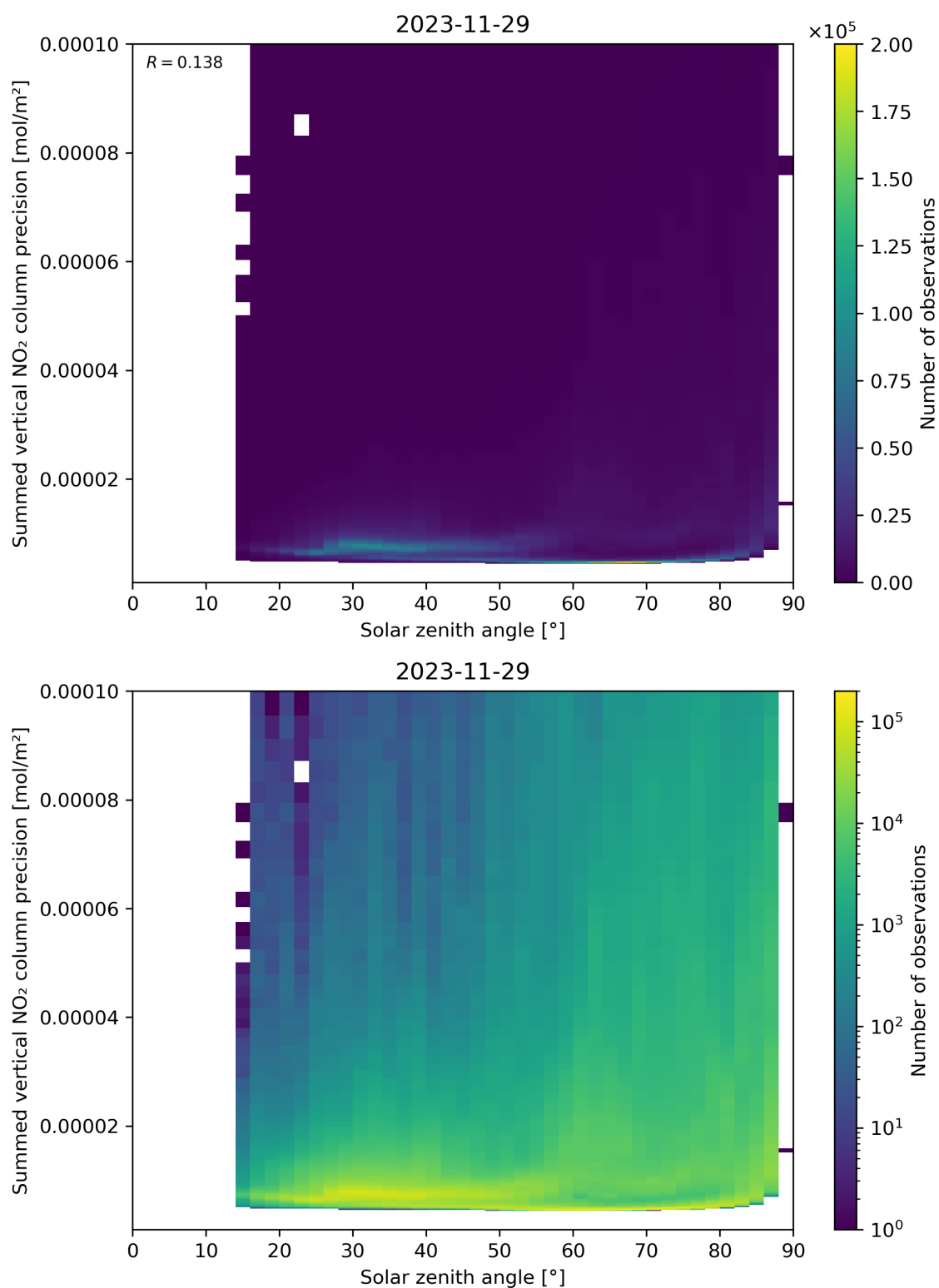
Figure 152: Scatter density plot of “Solar zenith angle” against “Summed vertical NO 2 column precision” for 2023-11-28 to 2023-11-30.
