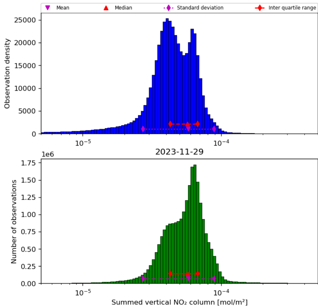
Figure 40: Histogram of “Summed vertical NO 2 column” for 2023-11-28 to 2023-11-30
