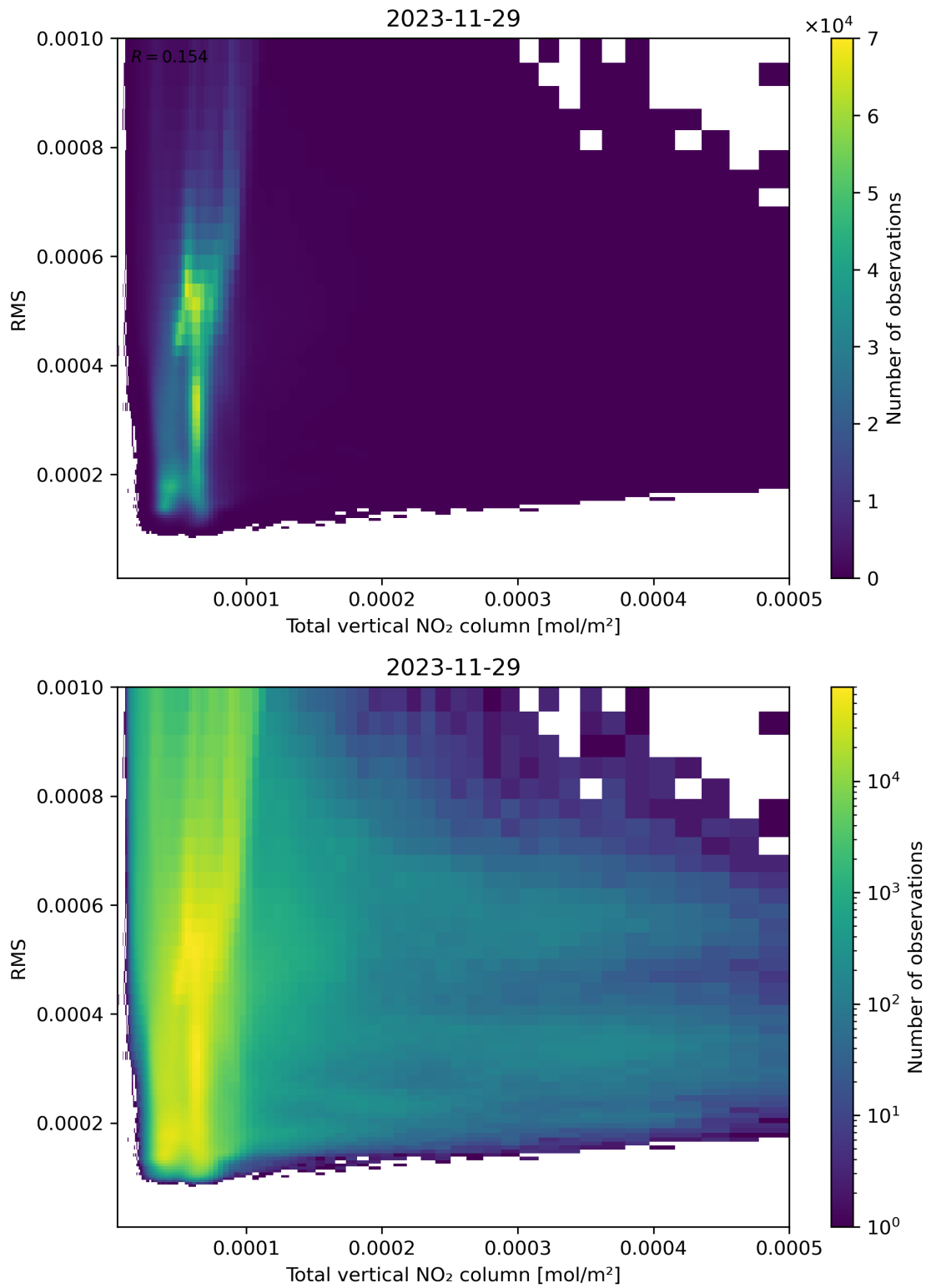
Figure 120: Scatter density plot of “Total vertical NO 2 column” against “RMS” for 2023-11-28 to 2023-11-30.
