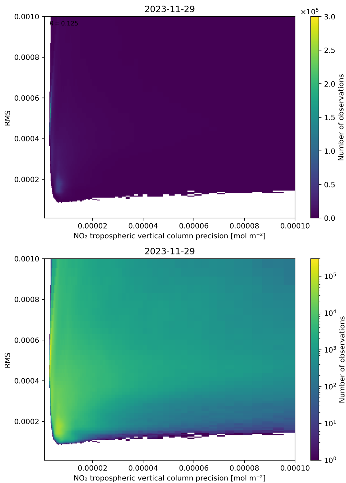
Figure 140: Scatter density plot of “NO 2 tropospheric vertical column precision” against “RMS” for 2023-11-28 to 2023-11-30.
