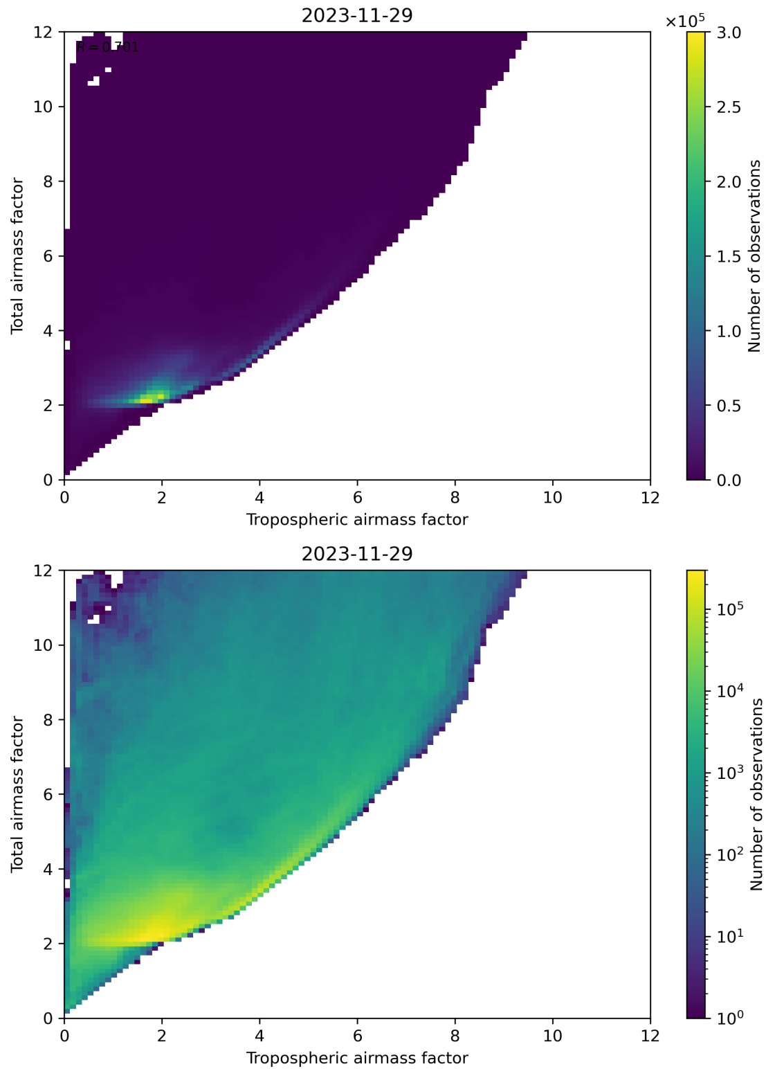
Figure 72: Scatter density plot of “Tropospheric airmass factor” against “Total airmass factor” for 2023-11-28 to 2023-11-30.
