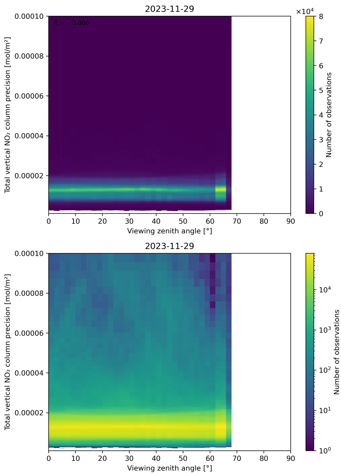
Figure 168: Scatter density plot of “Viewing zenith angle” against “Total vertical NO 2 column precision” for 2023-11-28 to 2023-11-30.
