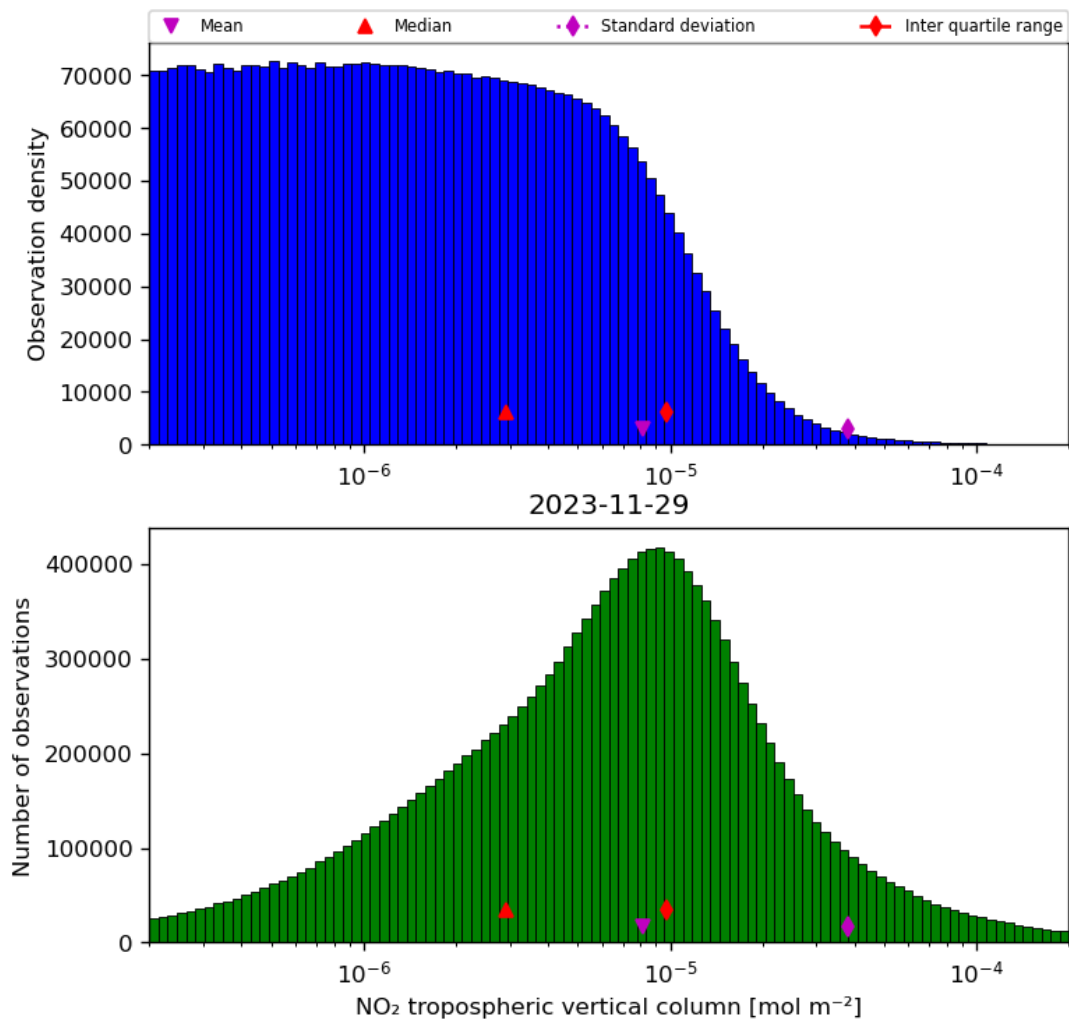
Figure 29: Histogram of “NO 2 tropospheric vertical column” for 2023-11-28 to 2023-11-30
