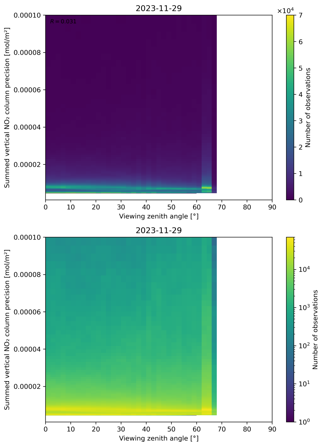
Figure 166: Scatter density plot of “Viewing zenith angle” against “Summed vertical NO 2 column precision” for 2023-11-28 to 2023-11-30.
