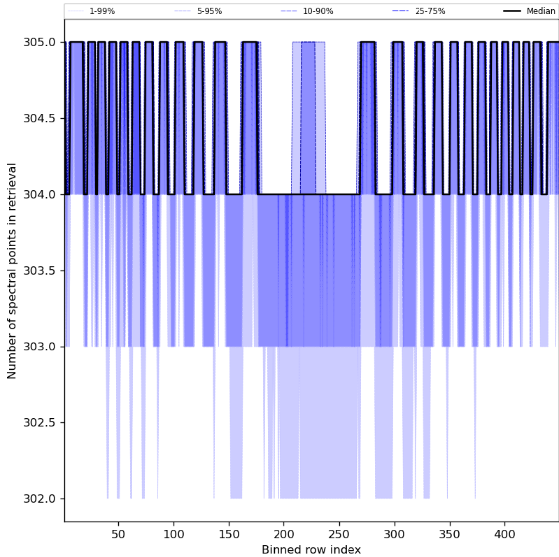
Figure 50: Along track statistics of “Number of spectral points in retrieval” for 2023-11-28 to 2023-11-30
