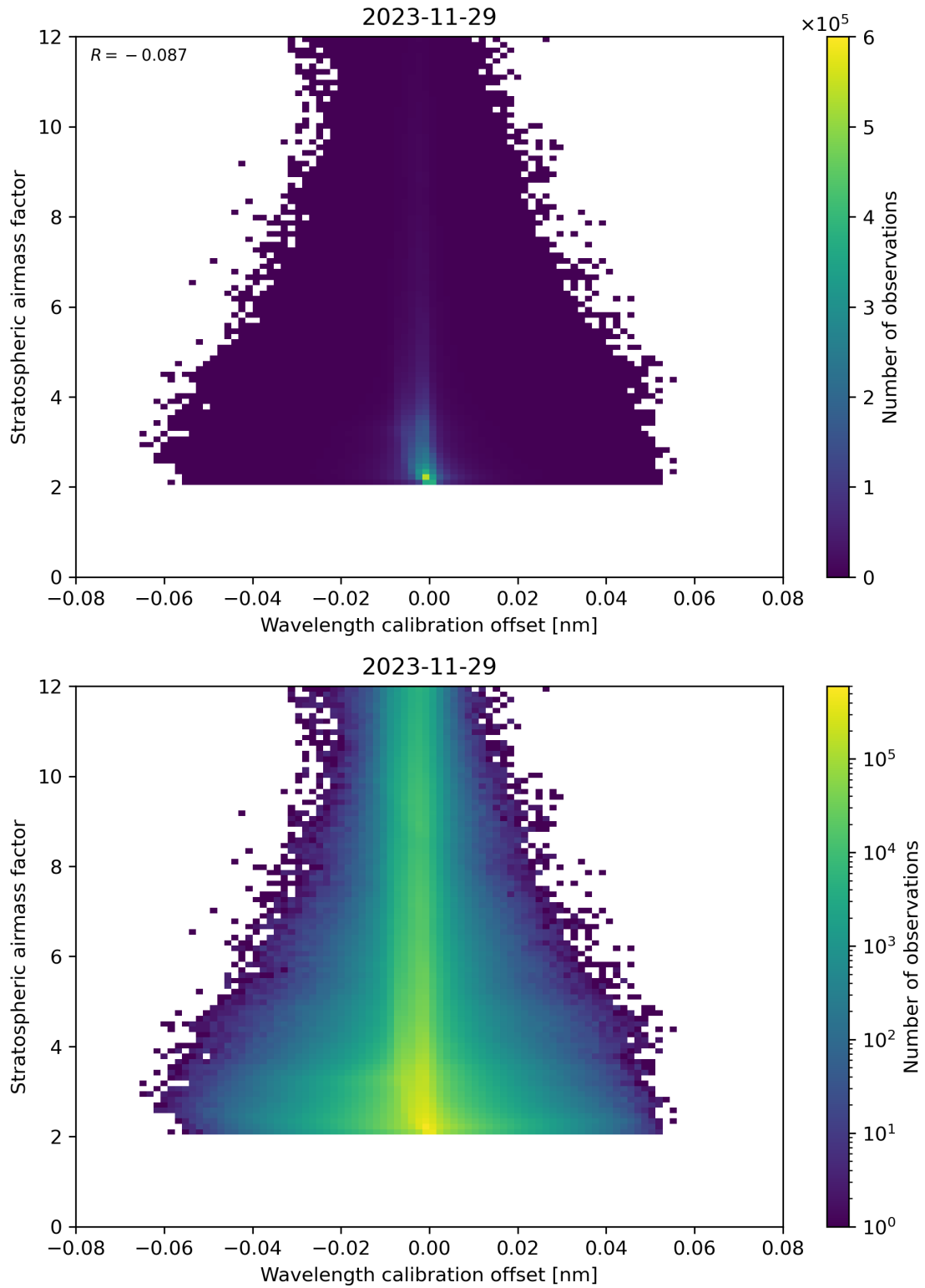
Figure 174: Scatter density plot of “Wavelength calibration offset” against “Stratospheric air mass factor” for 2023-11-28 to 2023-11-30.
