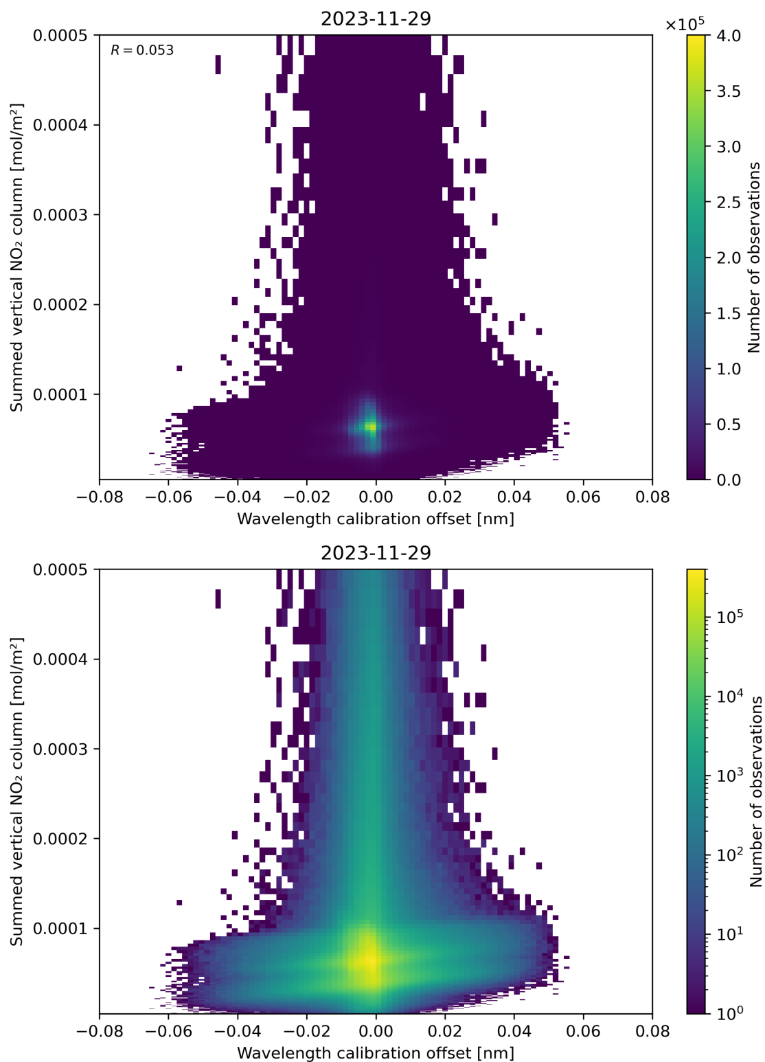
Figure 177: Scatter density plot of “Wavelength calibration offset” against “Summed vertical NO 2 column” for 2023-11-28 to 2023-11-30.
