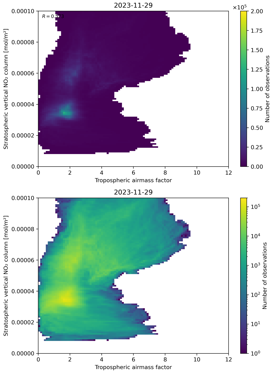
Figure 74: Scatter density plot of “Tropospheric air mass factor” against “Stratospheric vertical NO 2 column” for 2023-11-28 to 2023-11-30.
