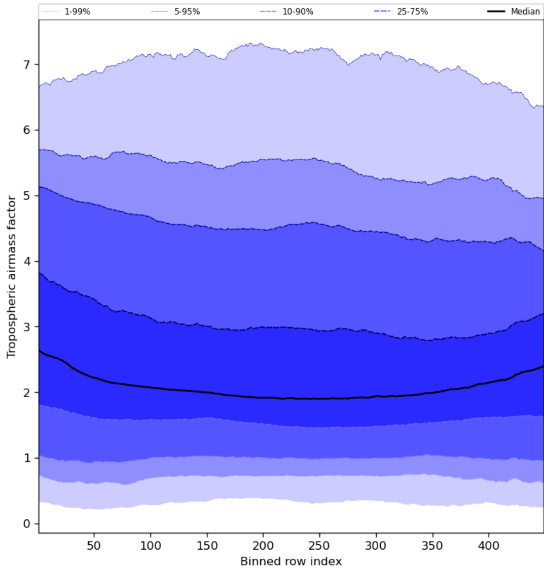
Figure 48: Along track statistics of “Tropospheric airmass factor” for 2023-11-28 to 2023-11-30
