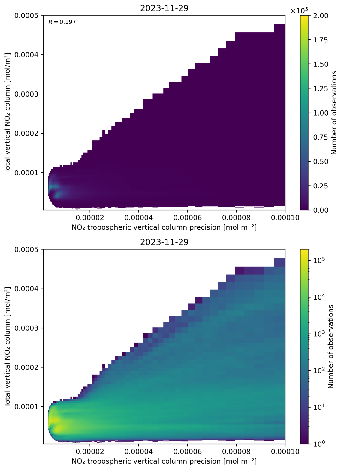
Figure 138: Scatter density plot of “NO 2 tropospheric vertical column precision” against “Total vertical NO 2 column” for 2023-11-28 to 2023-11-30.
