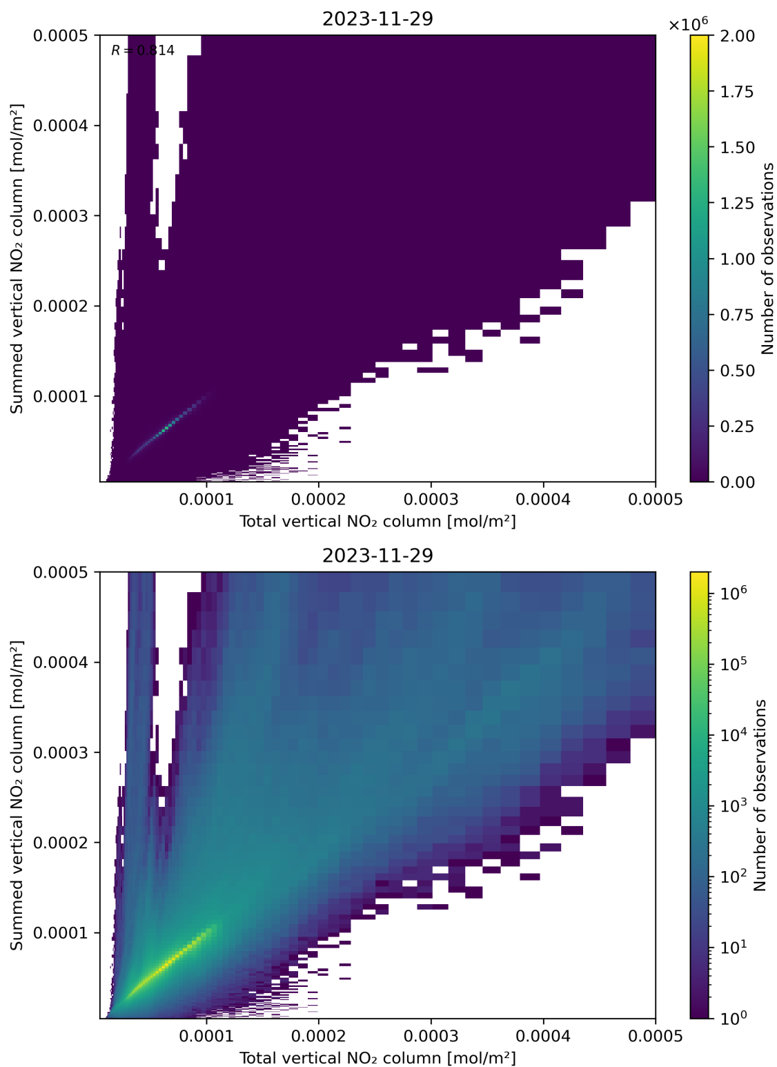
Figure 112: Scatter density plot of “Total vertical NO 2 column” against “Summed vertical NO 2 column” for 2023-11-28 to 2023-11-30.
