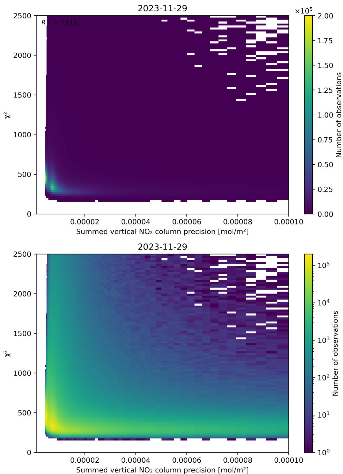
Figure 107: Scatter density plot of “Summed vertical NO 2 column precision” against “ \chi^2 ” for 2023-11-28 to 2023-11-30.
