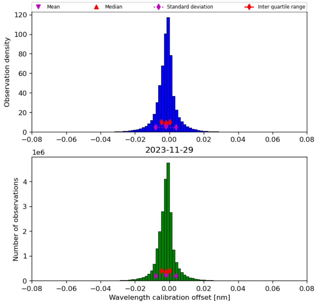
Figure 35: Histogram of “Wavelength calibration offset” for 2023-11-28 to 2023-11-30
