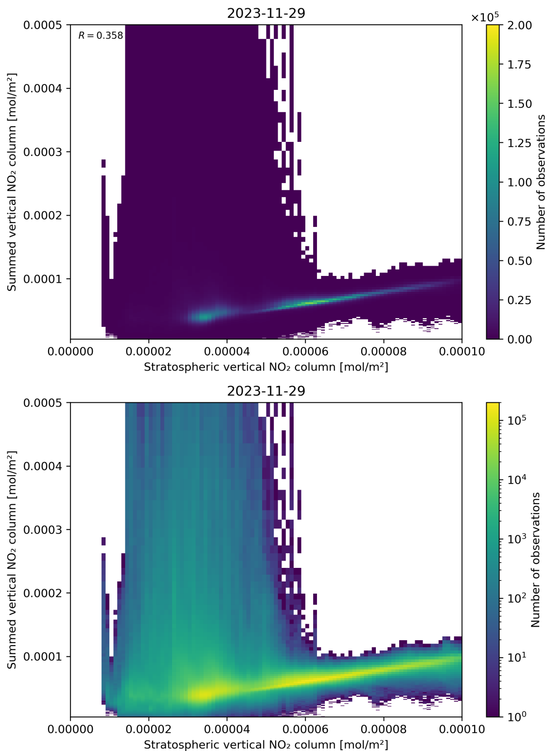
Figure 98: Scatter density plot of “Stratospheric vertical NO 2 column” against “Summed vertical NO 2 column” for 2023-11-28 to 2023-11-30.
