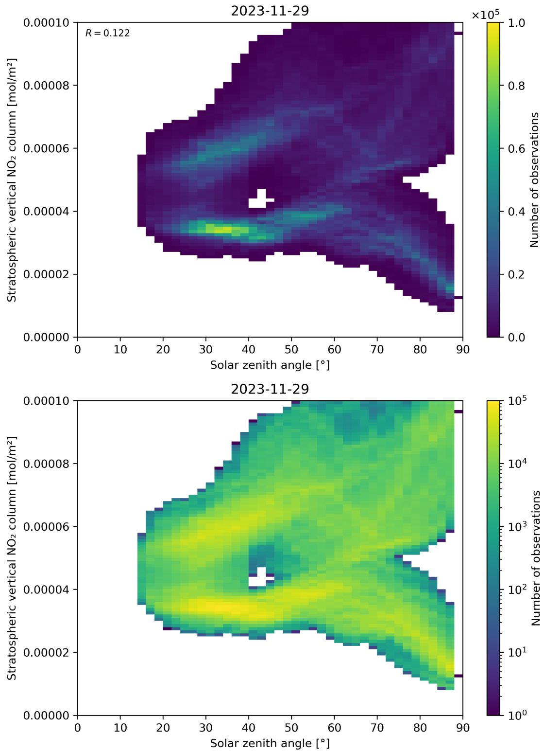
Figure 150: Scatter density plot of “Solar zenith angle” against “Stratospheric vertical NO 2 column” for 2023-11-28 to 2023-11-30.
