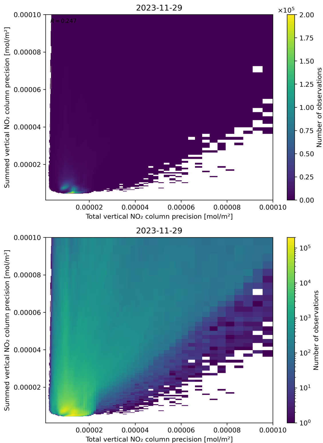
Figure 118: Scatter density plot of “Total vertical NO 2 column precision” against “Summed vertical NO 2 column precision” for 2023-11-28 to 2023-11-30.
