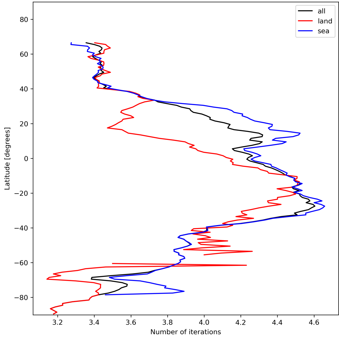
Figure 17: Zonal average of “Number of iterations” for 2023-11-28 to 2023-11-30.
