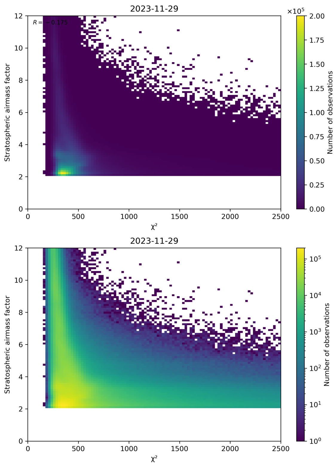
Figure 81: Scatter density plot of “ \chi^2 ” against “Stratospheric airmass factor” for 2023-11-28 to 2023-11-30.
