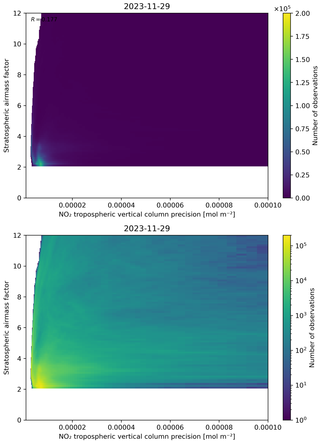
Figure 131: Scatter density plot of “NO 2 tropospheric vertical column precision” against “Stratospheric airmass factor” for 2023-11-28 to 2023-11-30.
