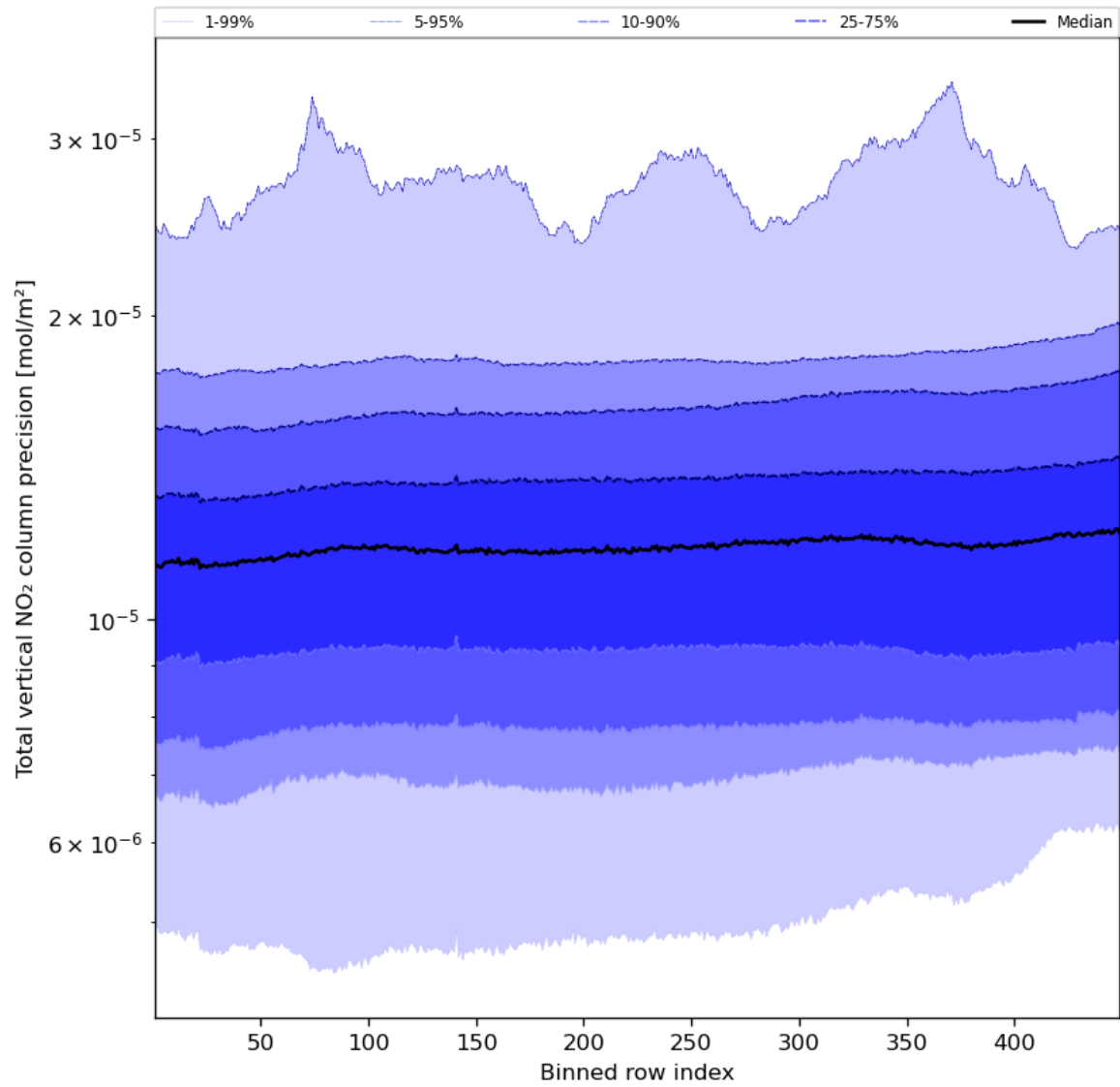
Figure 56: Along track statistics of “Total vertical NO 2 column precision” for 2023-11-28 to 2023-11-30
