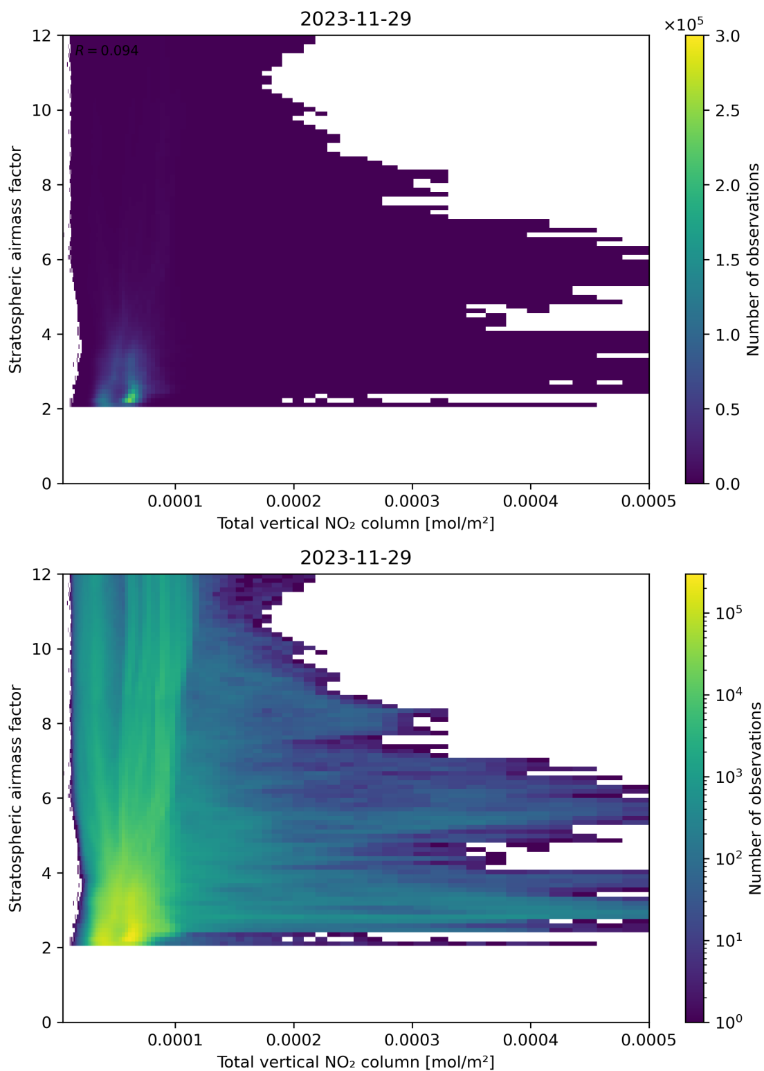
Figure 110: Scatter density plot of “Total vertical NO 2 column” against “Stratospheric air mass factor” for 2023-11-28 to 2023-11-30.
