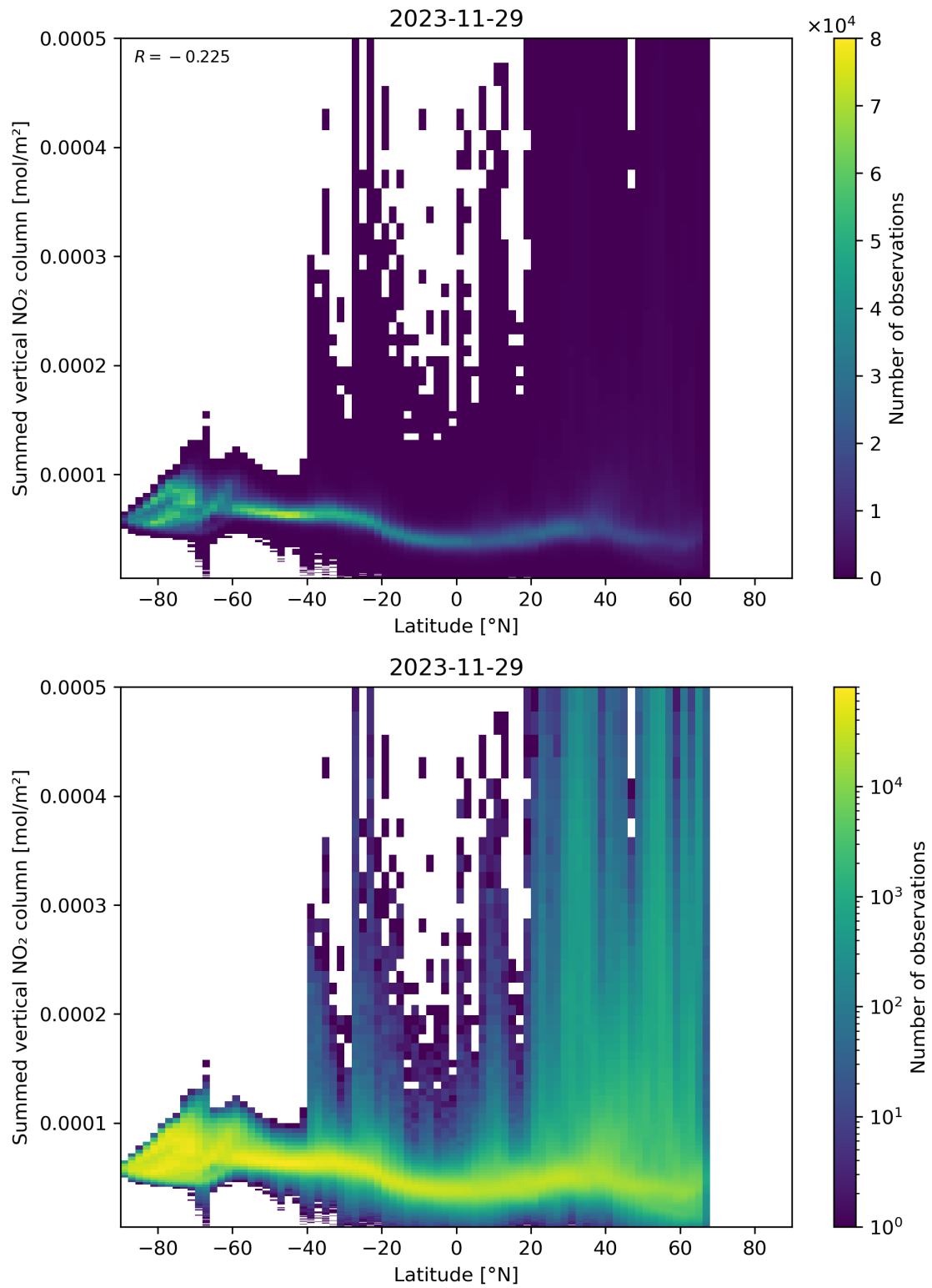
Figure 88: Scatter density plot of “Latitude” against “Summed vertical NO 2 column” for 2023-11-28 to 2023-11-30.
