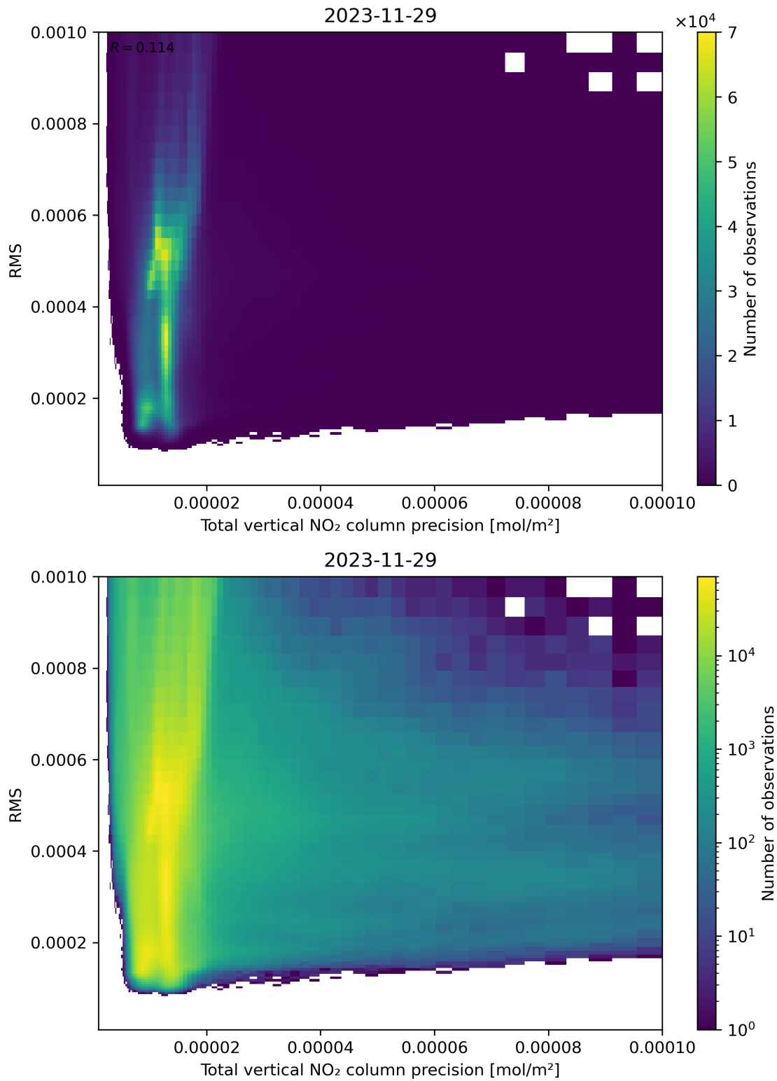
Figure 119: Scatter density plot of “Total vertical NO 2 column precision” against “RMS” for 2023-11-28 to 2023-11-30.
