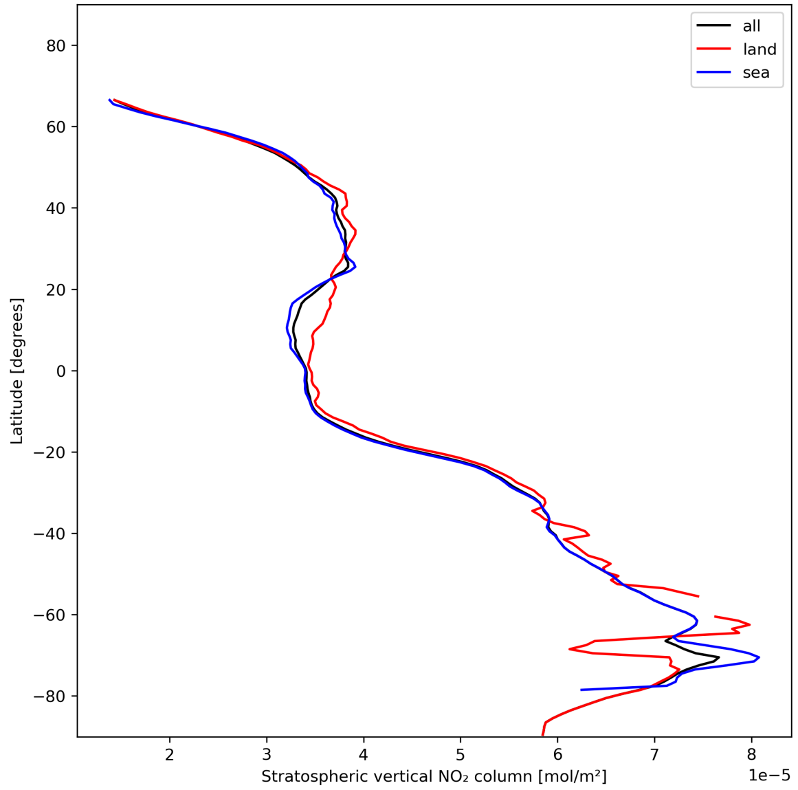
Figure 19: Zonal average of “Stratospheric vertical NO 2 column” for 2023-11-28 to 2023-11-30.
