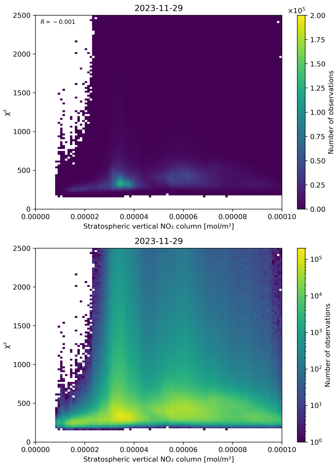
Figure 97: Scatter density plot of “Stratospheric vertical NO 2 column” against “ \chi^2 ” for 2023-11-28 to 2023-11-30.
