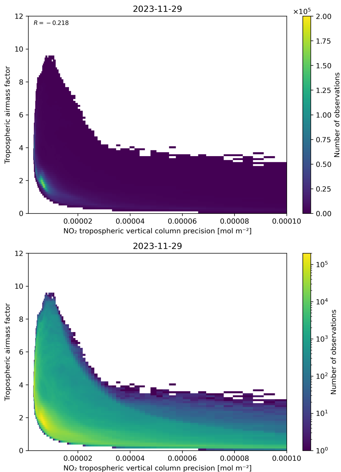
Figure 133: Scatter density plot of “NO 2 tropospheric vertical column precision” against “Tropospheric airmass factor” for 2023-11-28 to 2023-11-30.
