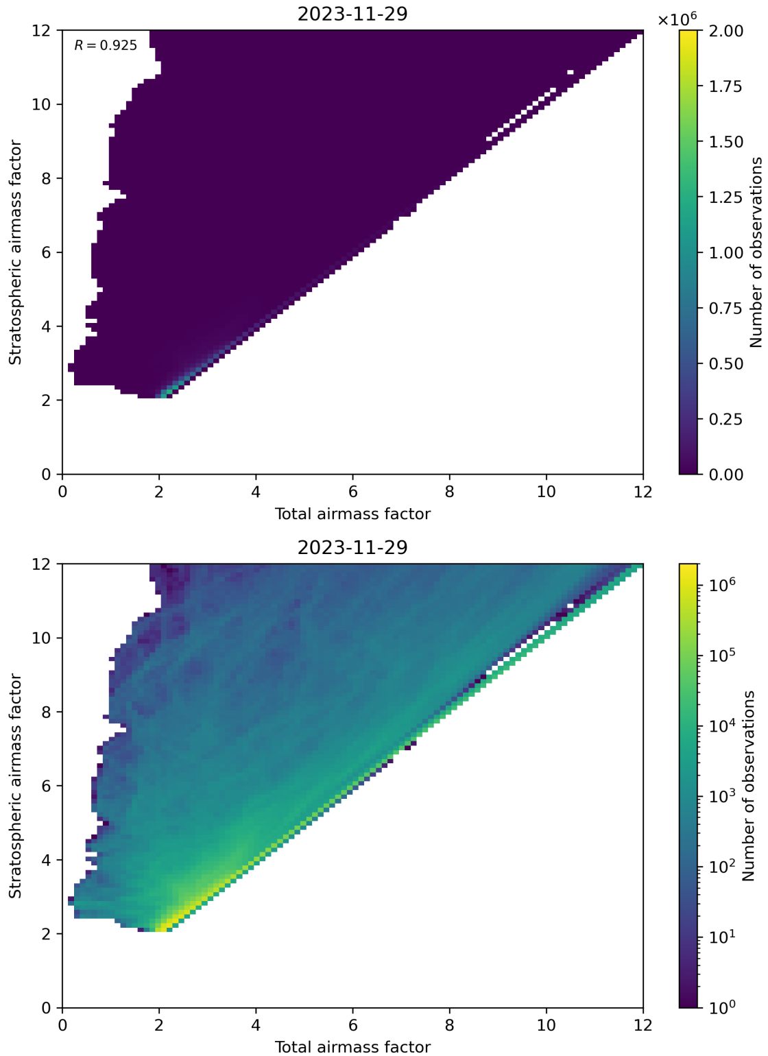
Figure 62: Scatter density plot of “Total airmass factor” against “Stratospheric airmass factor” for 2023-11-28 to 2023-11-30.
