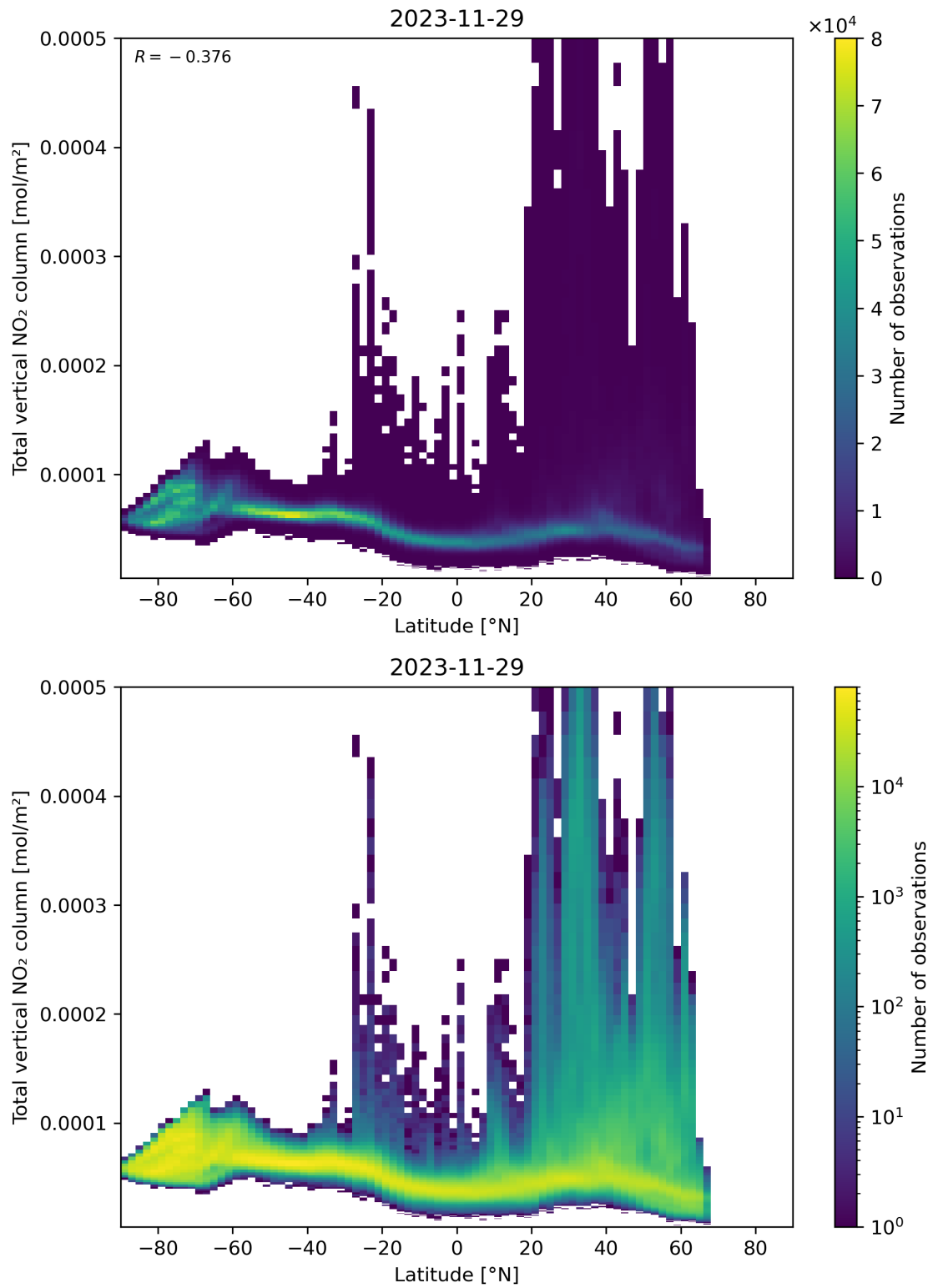
Figure 90: Scatter density plot of “Latitude” against “Total vertical NO 2 column” for 2023-11-28 to 2023-11-30.
