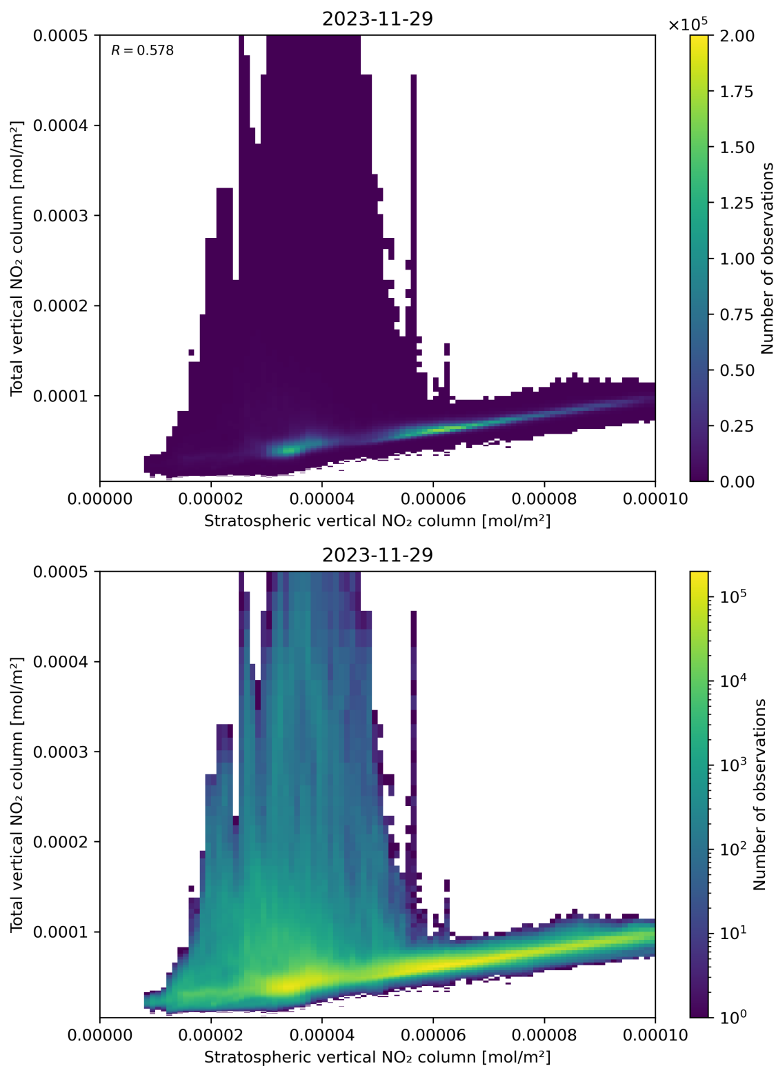
Figure 100: Scatter density plot of “Stratospheric vertical NO 2 column” against “Total vertical NO 2 column” for 2023-11-28 to 2023-11-30.
