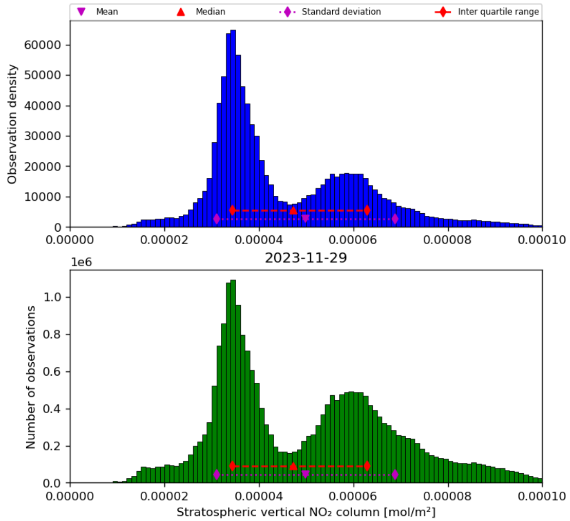
Figure 36: Histogram of “Stratospheric vertical NO 2 column” for 2023-11-28 to 2023-11-30
