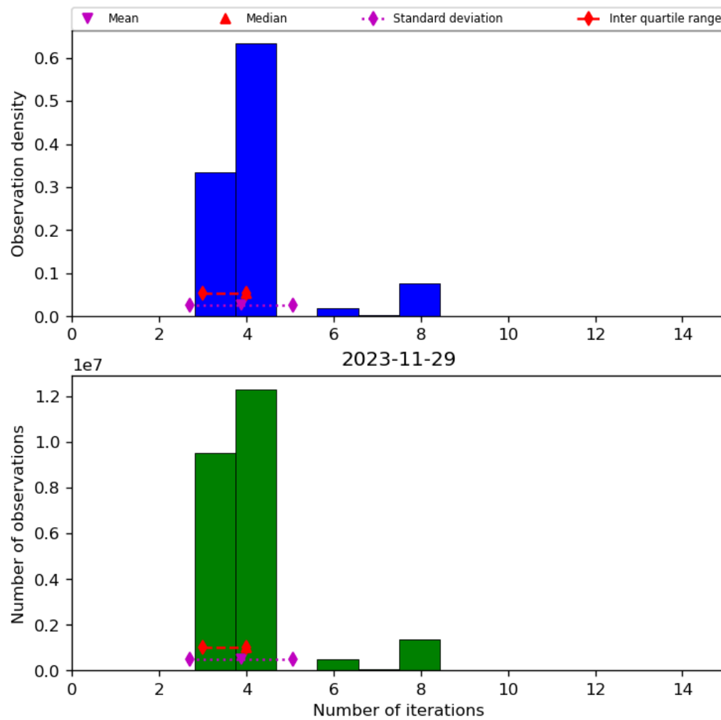
Figure 34: Histogram of “Number of iterations” for 2023-11-28 to 2023-11-30
