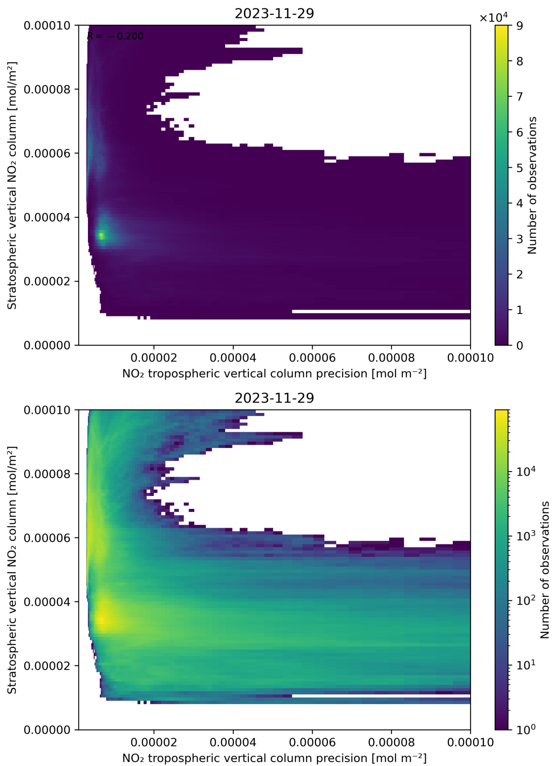
Figure 135: Scatter density plot of “NO 2 tropospheric vertical column precision” against “Stratospheric vertical NO 2 column” for 2023-11-28 to 2023-11-30.
