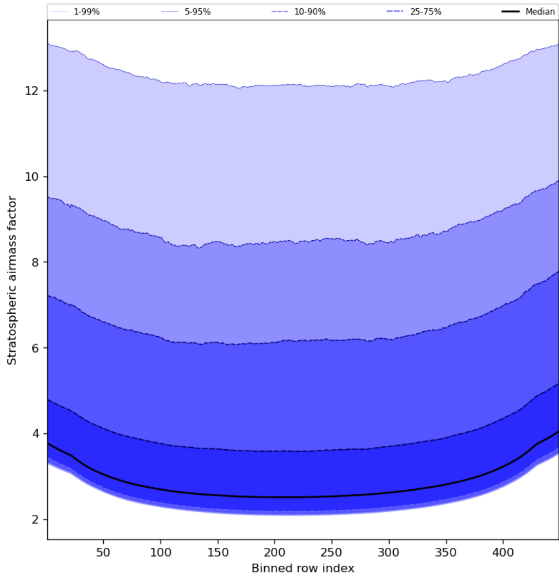
Figure 61: Along track statistics of “Stratospheric airmass factor” for 2023-11-28 to 2023-11-30
