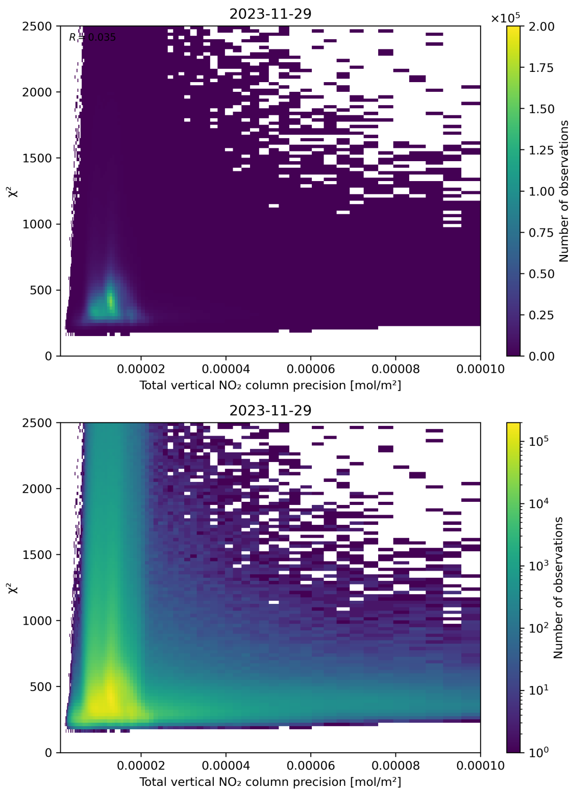
Figure 116: Scatter density plot of “Total vertical NO 2 column precision” against “ \chi^2 ” for 2023-11-28 to 2023-11-30.
