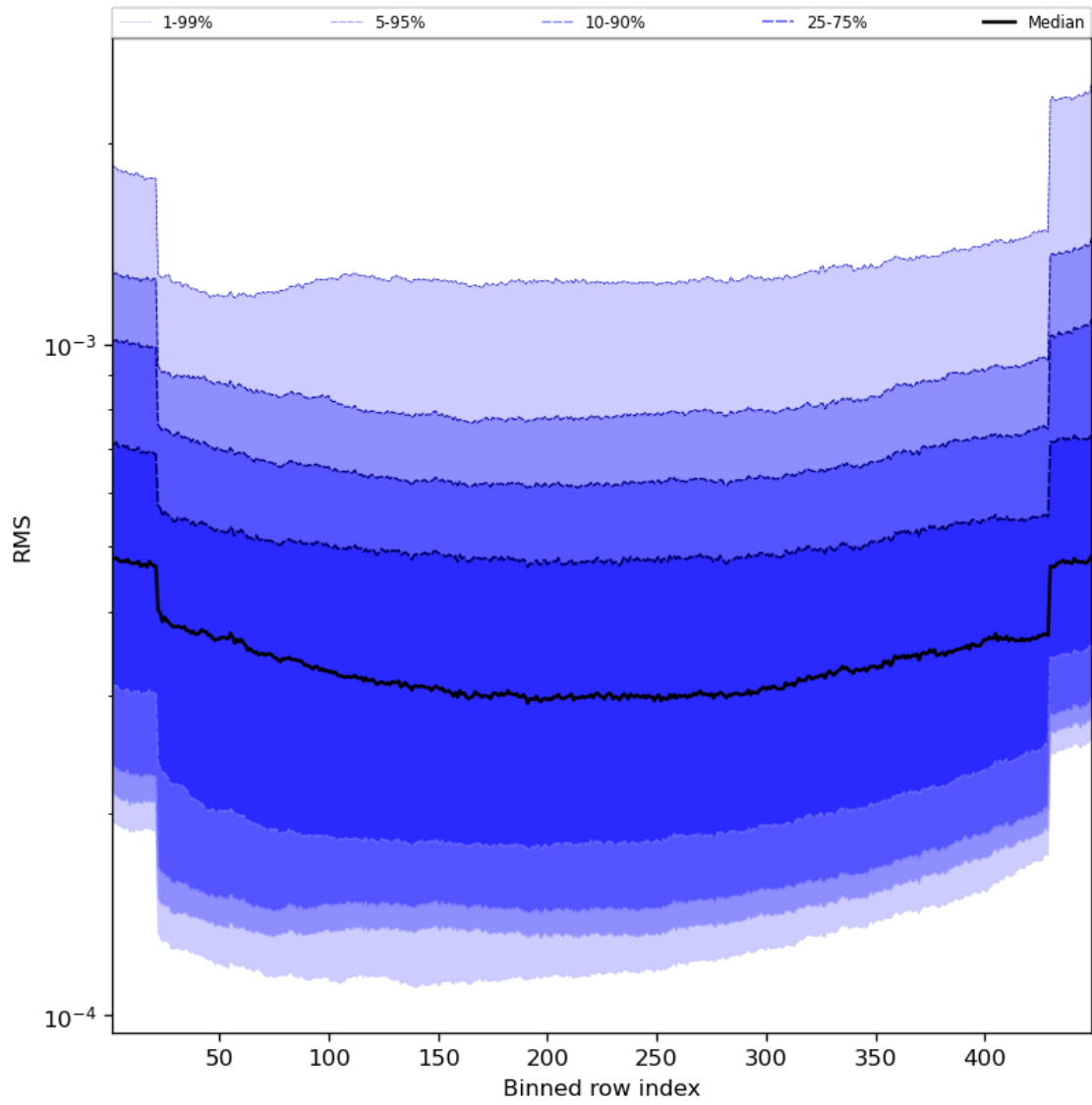
Figure 60: Along track statistics of “RMS” for 2023-11-28 to 2023-11-30
