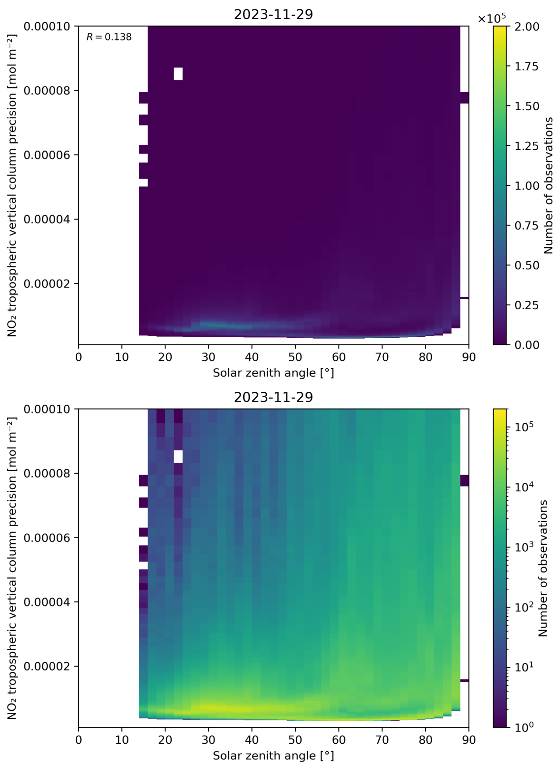
Figure 156: Scatter density plot of “Solar zenith angle” against “NO 2 tropospheric vertical column precision” for 2023-11-28 to 2023-11-30.
