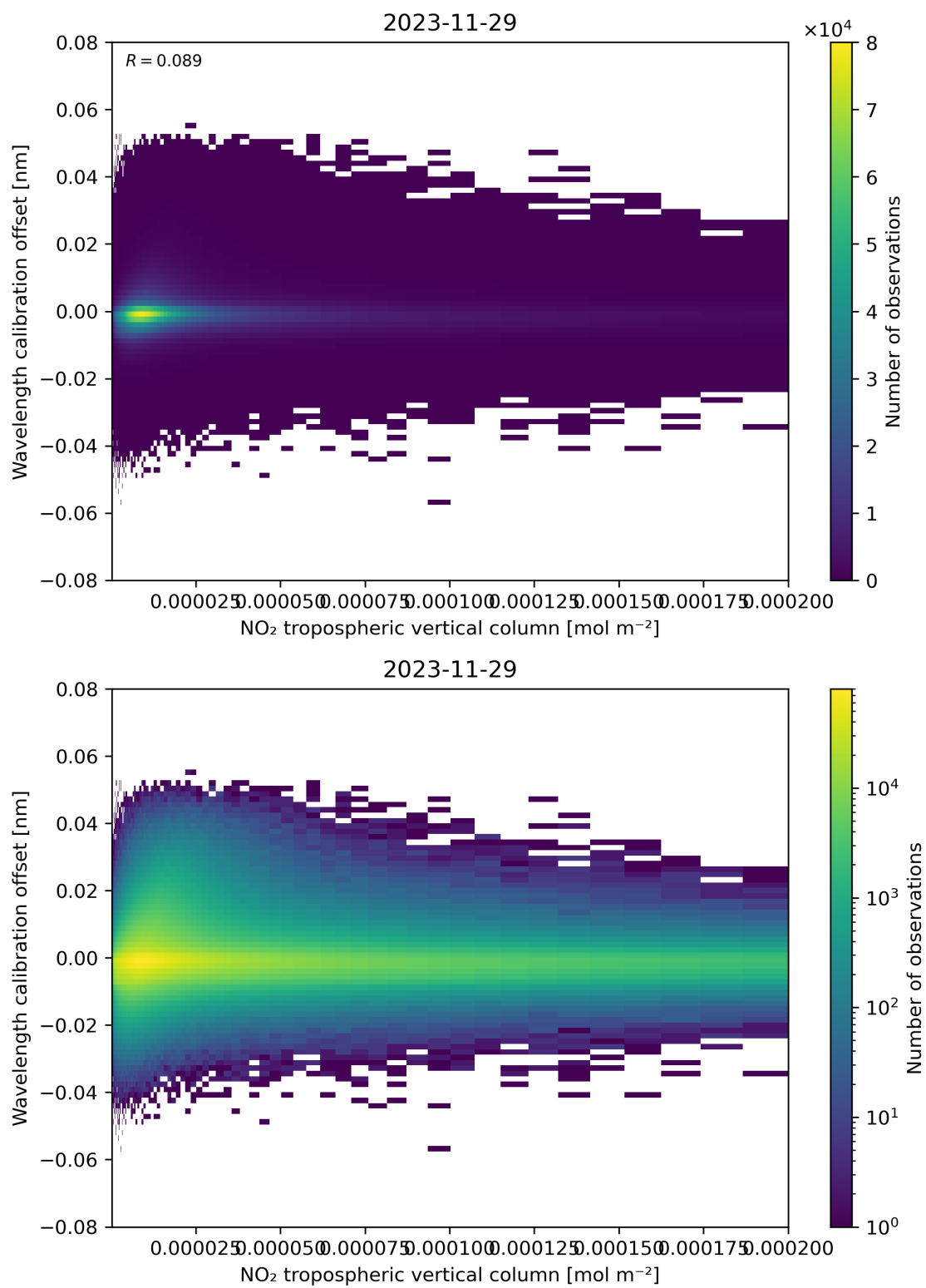
Figure 143: Scatter density plot of “NO 2 tropospheric vertical column” against “Wavelength calibration offset” for 2023-11-28 to 2023-11-30.
