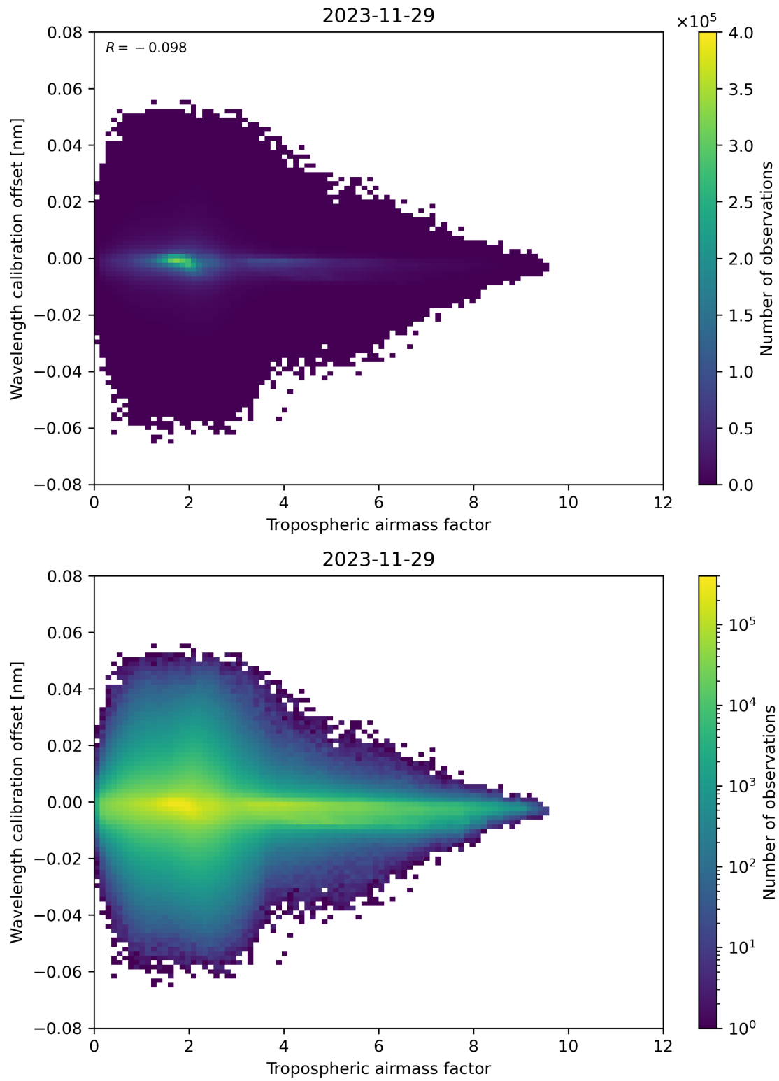
Figure 80: Scatter density plot of “Tropospheric airmass factor” against “Wavelength calibration offset” for 2023-11-28 to 2023-11-30.
