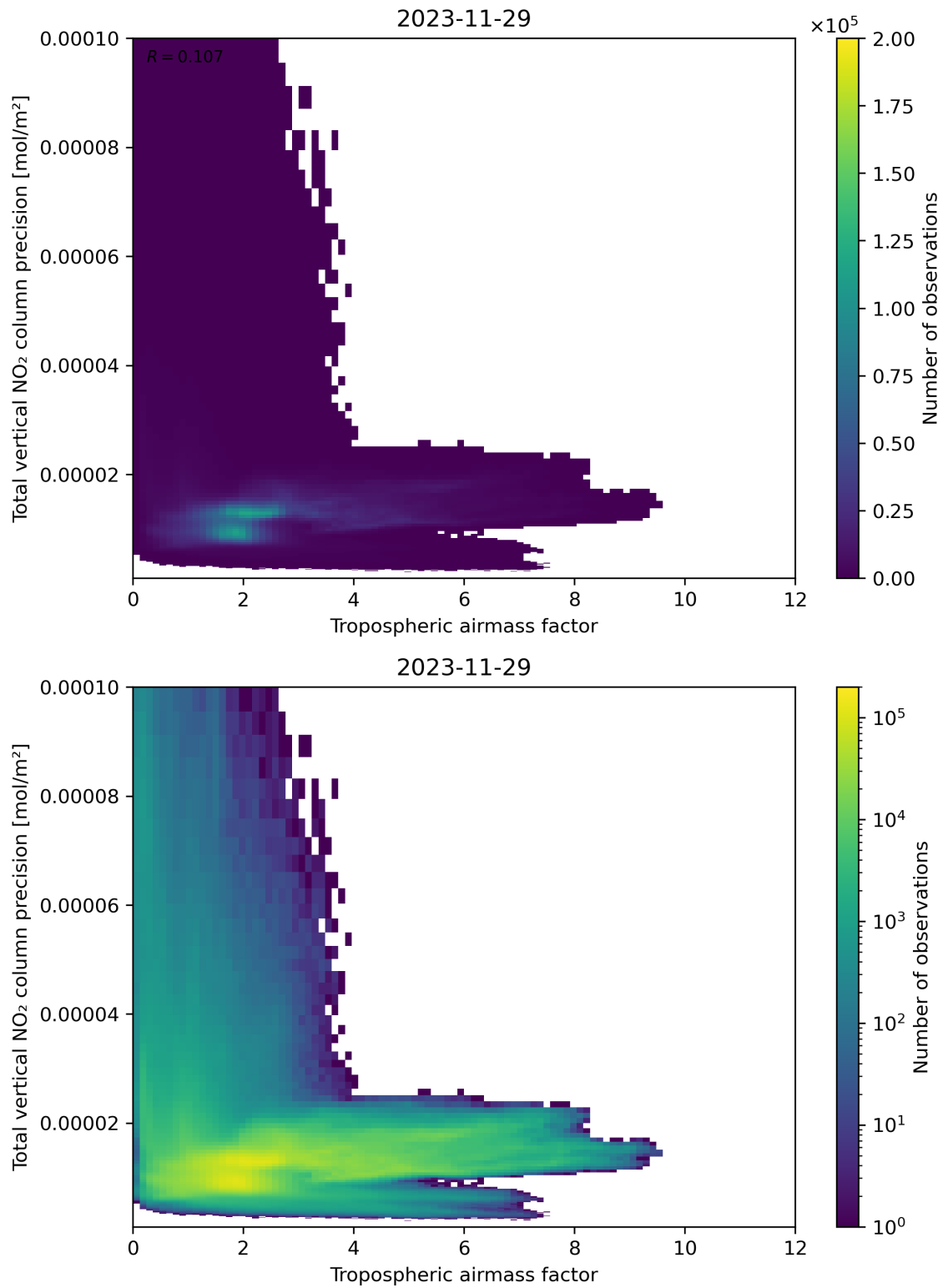
Figure 78: Scatter density plot of “Tropospheric air mass factor” against “Total vertical NO 2 column precision” for 2023-11-28 to 2023-11-30.
