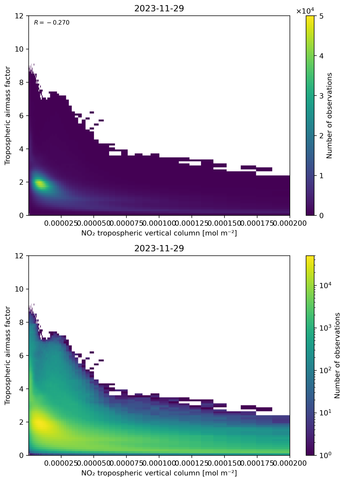
Figure 123: Scatter density plot of “NO 2 tropospheric vertical column” against “Tropospheric airmass factor” for 2023-11-28 to 2023-11-30.
