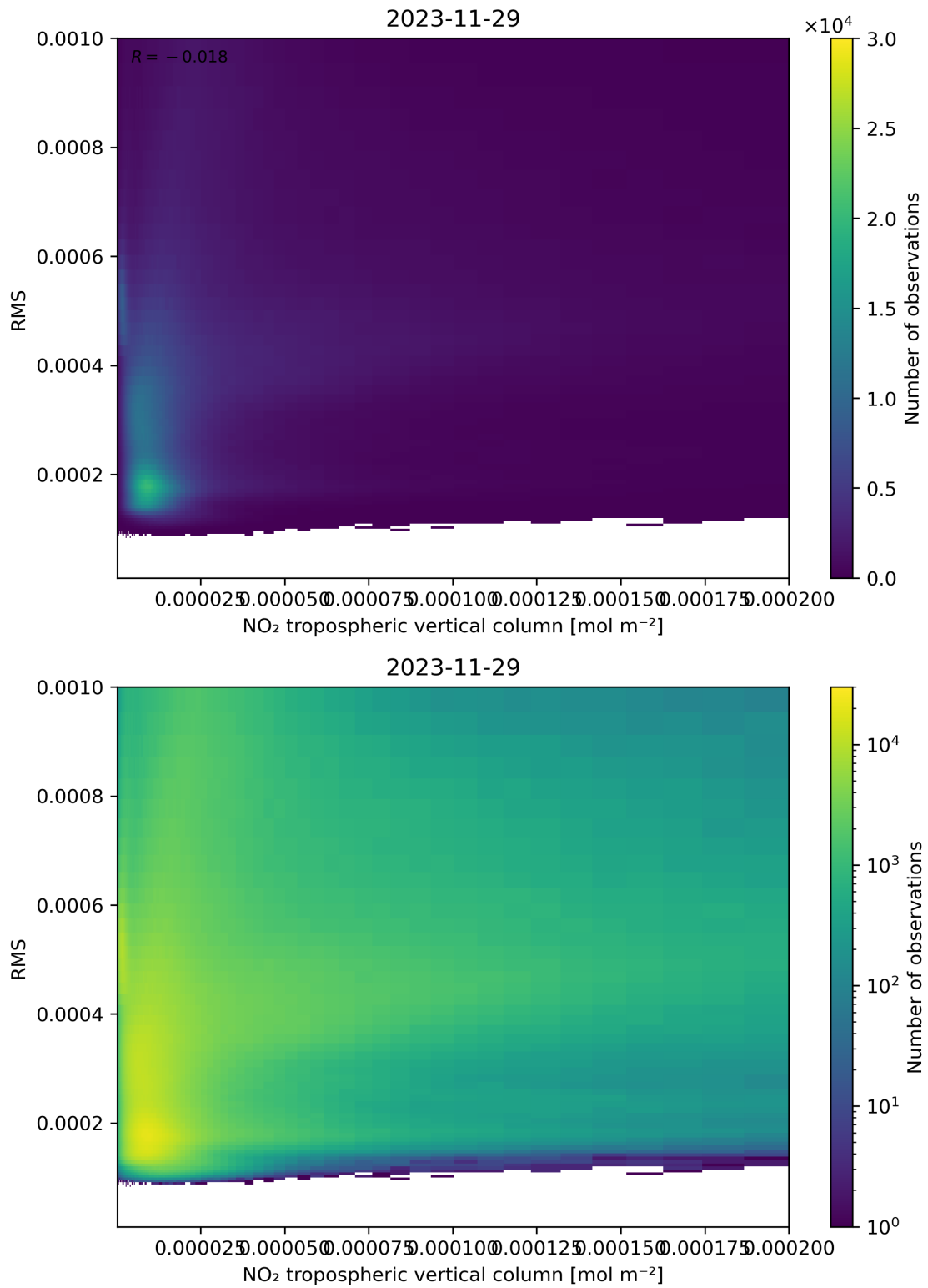
Figure 142: Scatter density plot of “NO 2 tropospheric vertical column” against “RMS” for 2023-11-28 to 2023-11-30.
