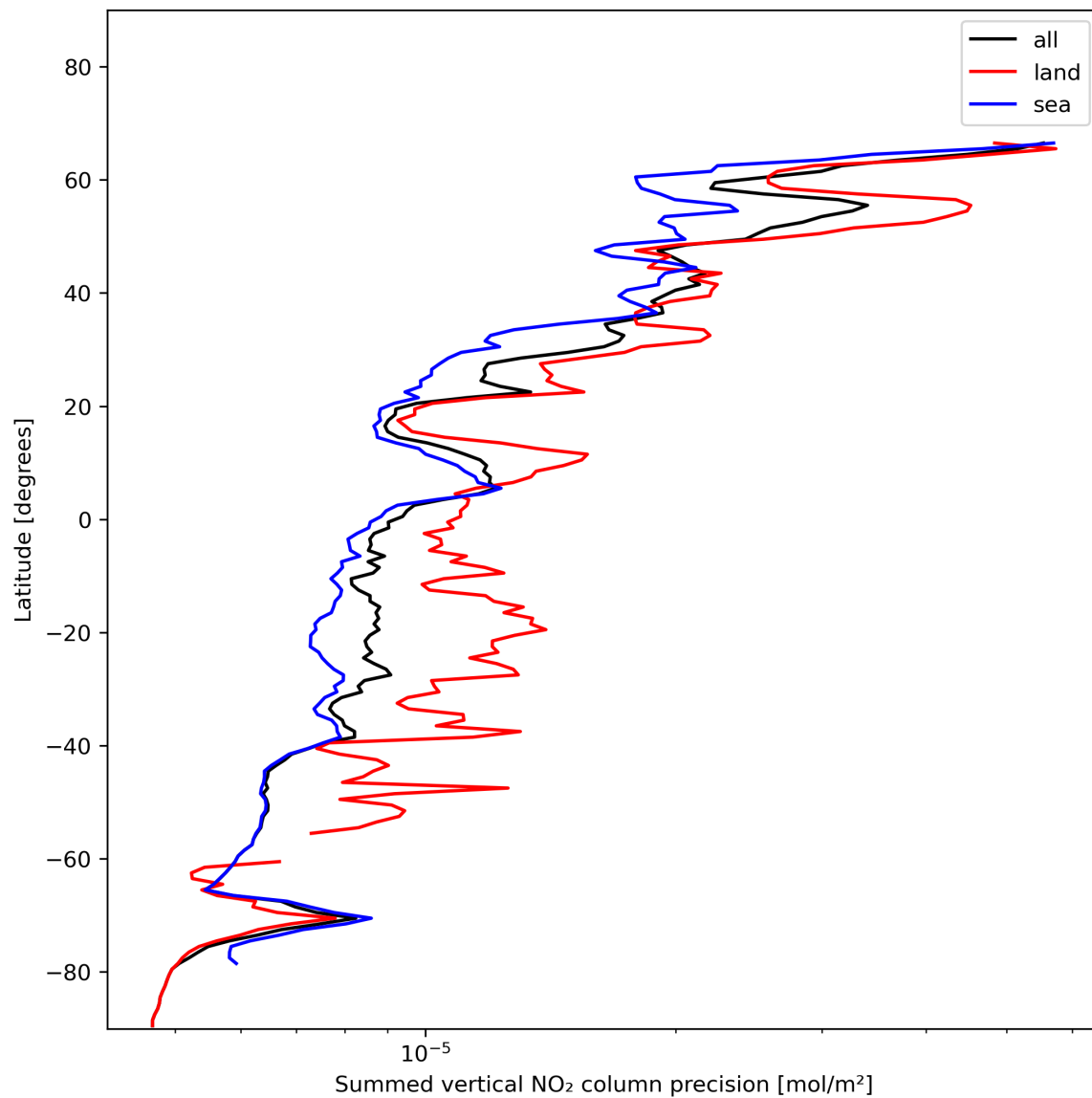
Figure 24: Zonal average of “Summed vertical NO 2 column precision” for 2023-11-28 to 2023-11-30.
