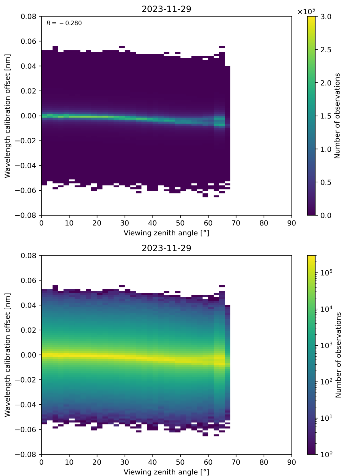
Figure 173: Scatter density plot of “Viewing zenith angle” against “Wavelength calibration offset” for 2023-11-28 to 2023-11-30.
