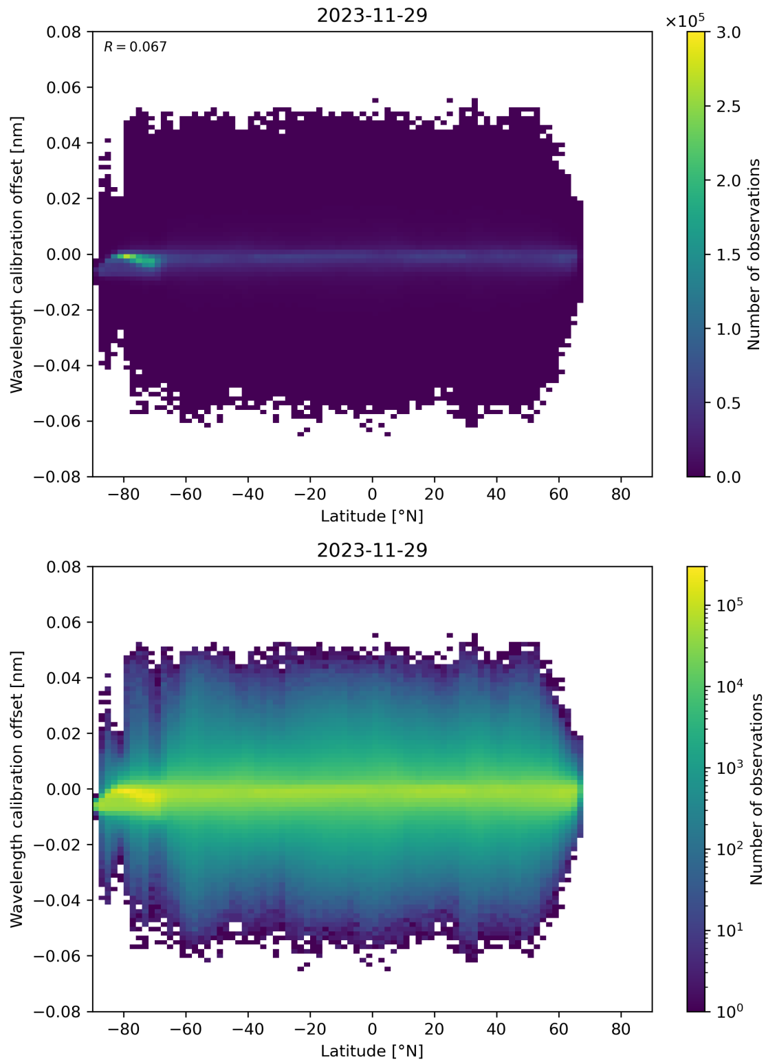
Figure 95: Scatter density plot of “Latitude” against “Wavelength calibration offset” for 2023-11-28 to 2023-11-30.
