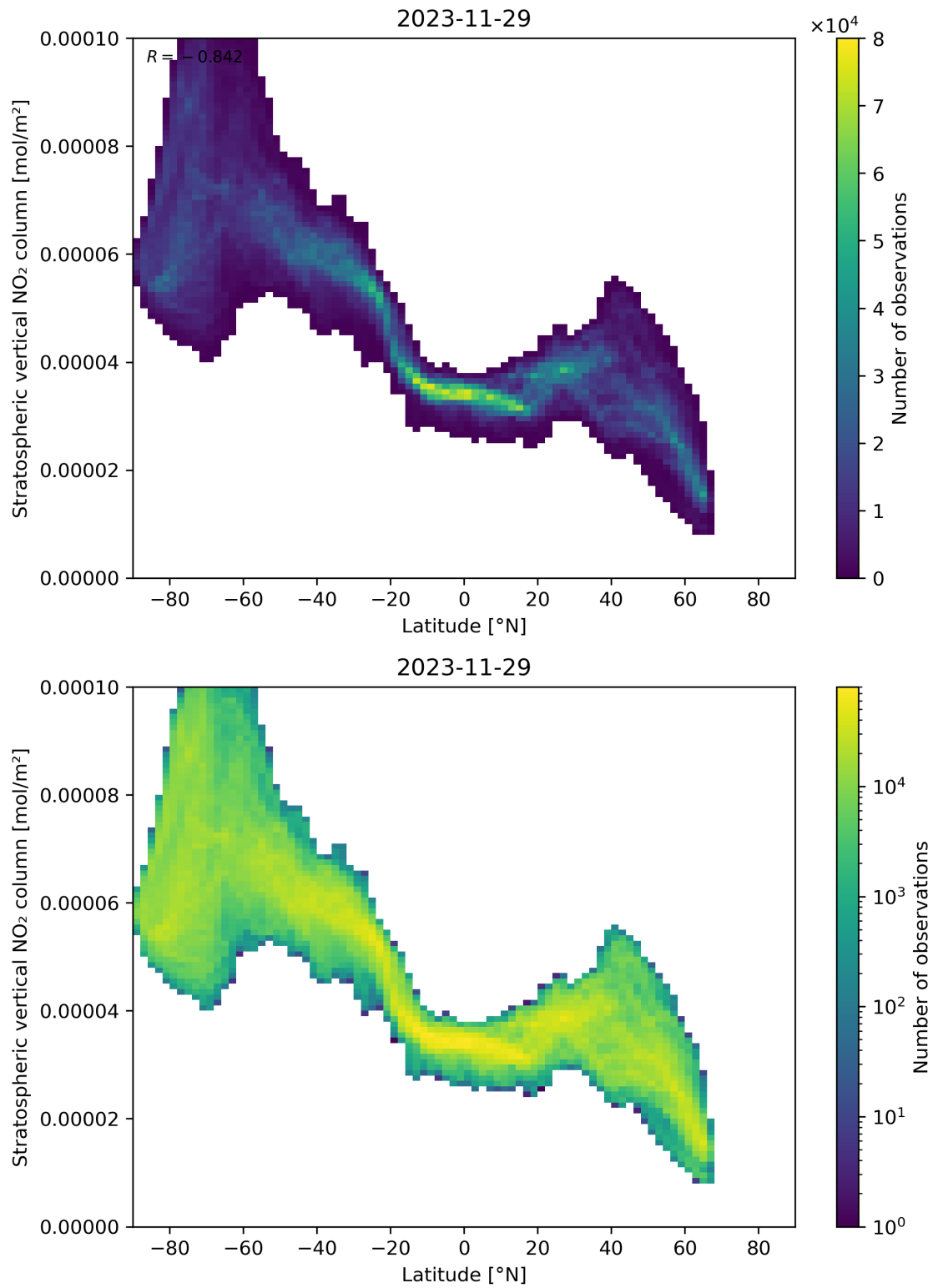
Figure 87: Scatter density plot of “Latitude” against “Stratospheric vertical NO 2 column” for 2023-11-28 to 2023-11-30.
