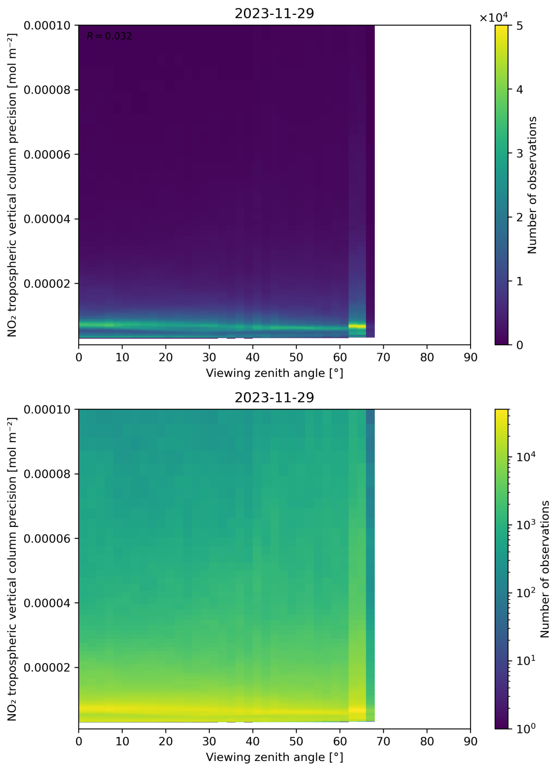
Figure 170: Scatter density plot of “Viewing zenith angle” against “NO 2 tropospheric vertical column precision” for 2023-11-28 to 2023-11-30.
