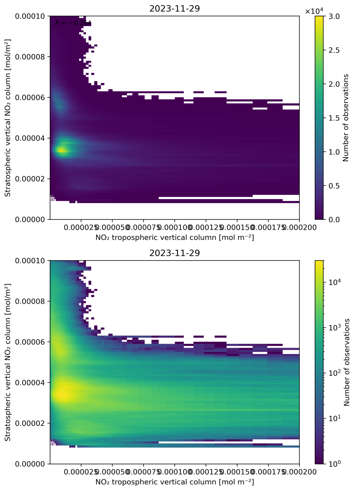
Figure 125: Scatter density plot of “NO 2 tropospheric vertical column” against “Stratospheric vertical NO 2 column” for 2023-11-28 to 2023-11-30.
