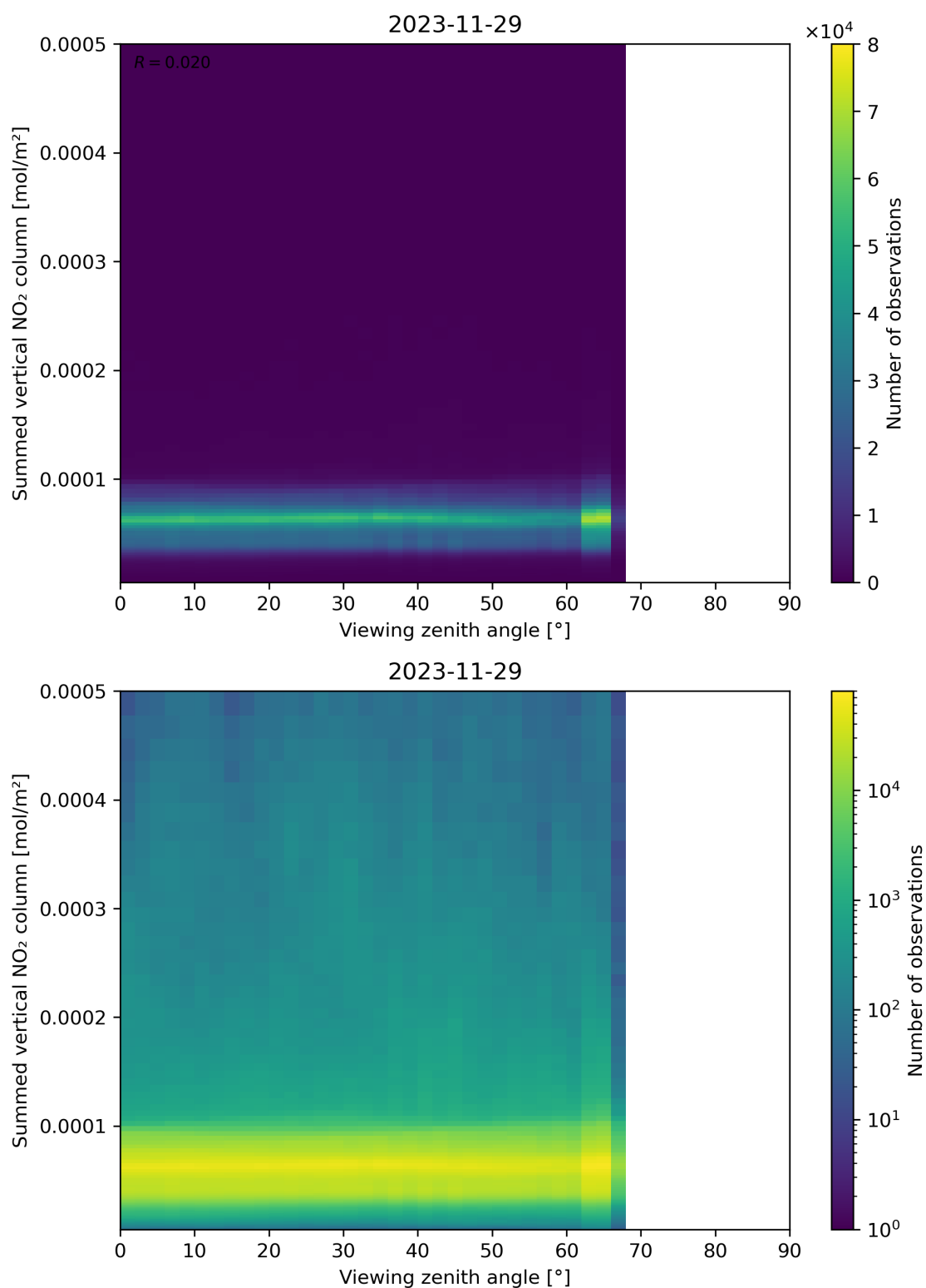
Figure 165: Scatter density plot of “Viewing zenith angle” against “Summed vertical NO 2 column” for 2023-11-28 to 2023-11-30.
