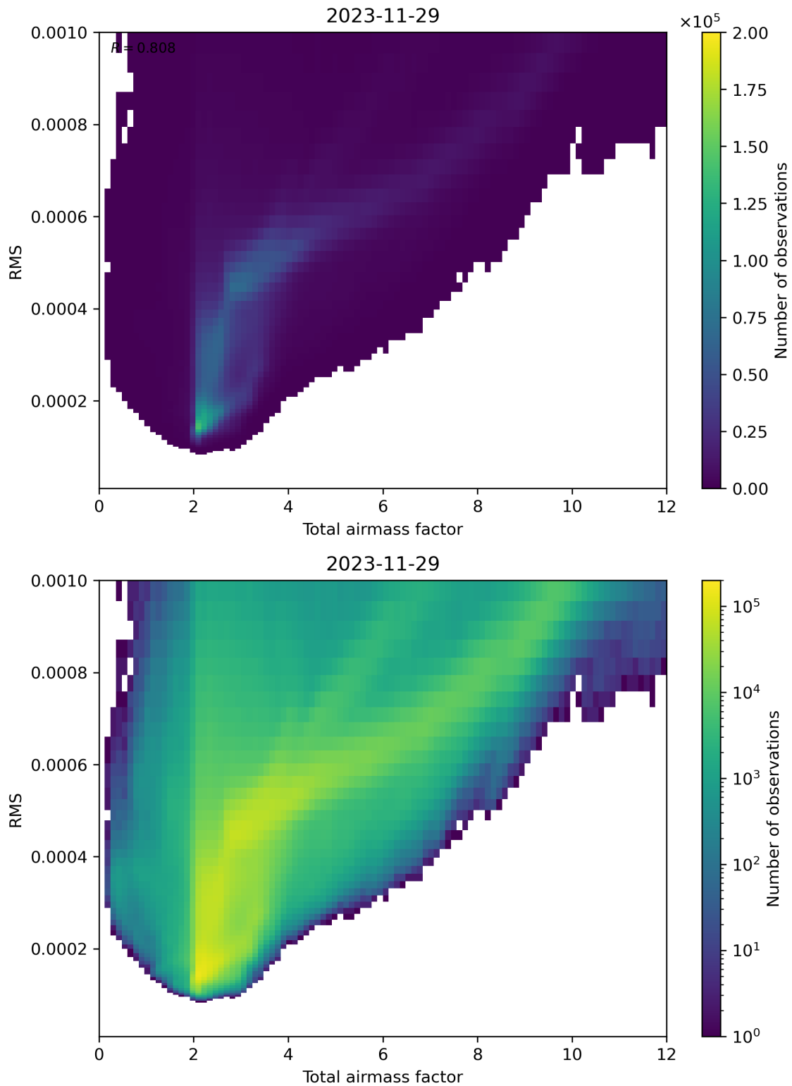
Figure 69: Scatter density plot of “Total airmass factor” against “RMS” for 2023-11-28 to 2023-11-30.
