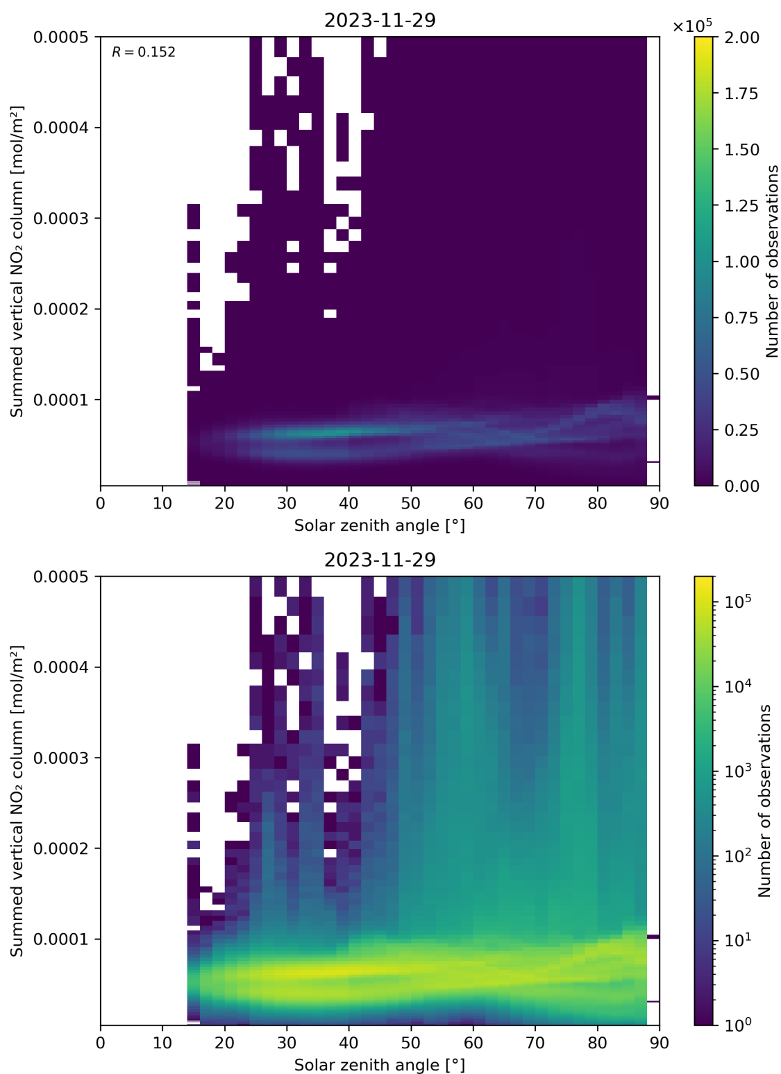
Figure 151: Scatter density plot of “Solar zenith angle” against “Summed vertical NO 2 column” for 2023-11-28 to 2023-11-30.
