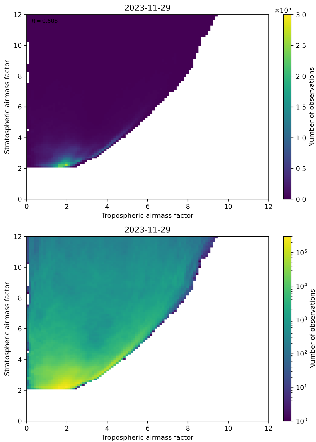
Figure 71: Scatter density plot of “Tropospheric airmass factor” against “Stratospheric airmass factor” for 2023-11-28 to 2023-11-30.
