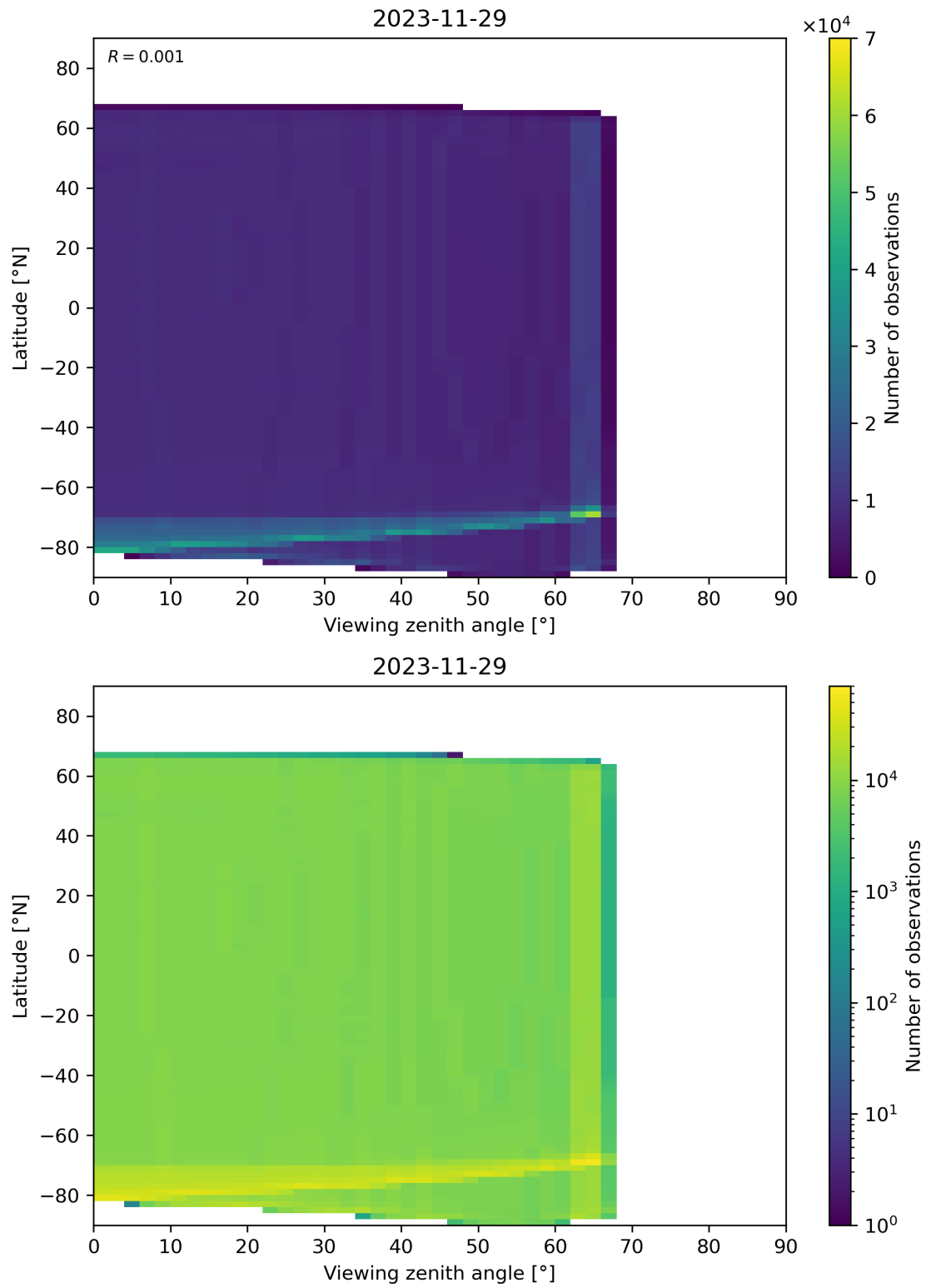
Figure 163: Scatter density plot of “Viewing zenith angle” against “Latitude” for 2023-11-28 to 2023-11-30.
