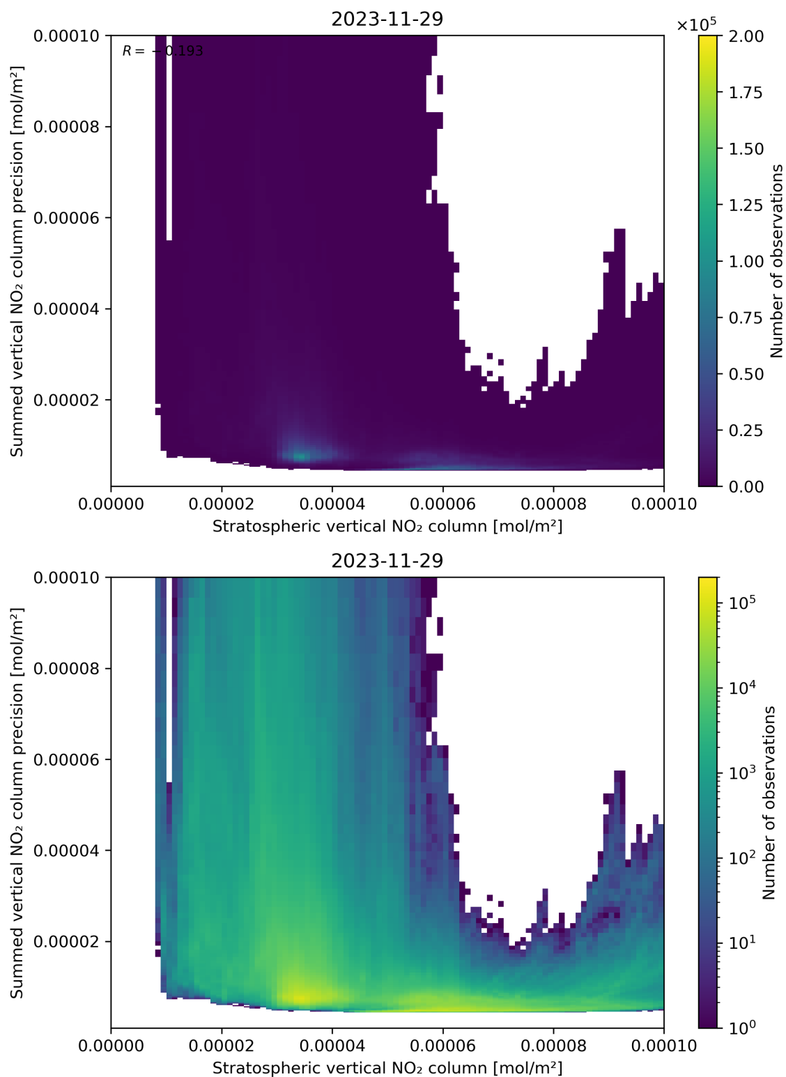
Figure 99: Scatter density plot of “Stratospheric vertical NO 2 column” against “Summed vertical NO 2 column precision” for 2023-11-28 to 2023-11-30.
