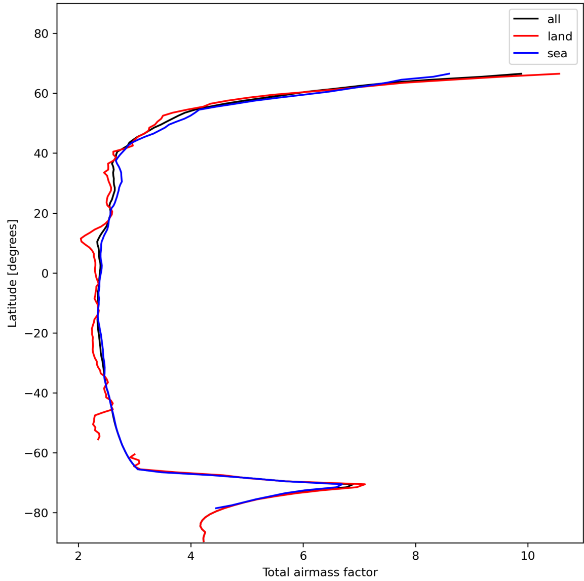
Figure 15: Zonal average of “Total airmass factor” for 2023-11-28 to 2023-11-30.
