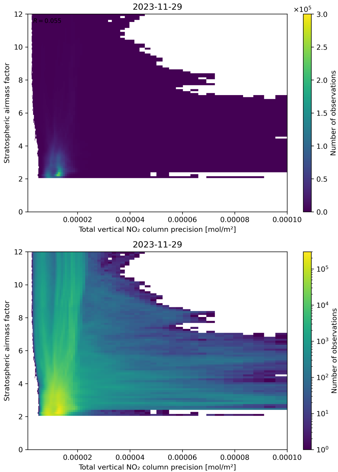
Figure 115: Scatter density plot of “Total vertical NO 2 column precision” against “Stratospheric air mass factor” for 2023-11-28 to 2023-11-30.
