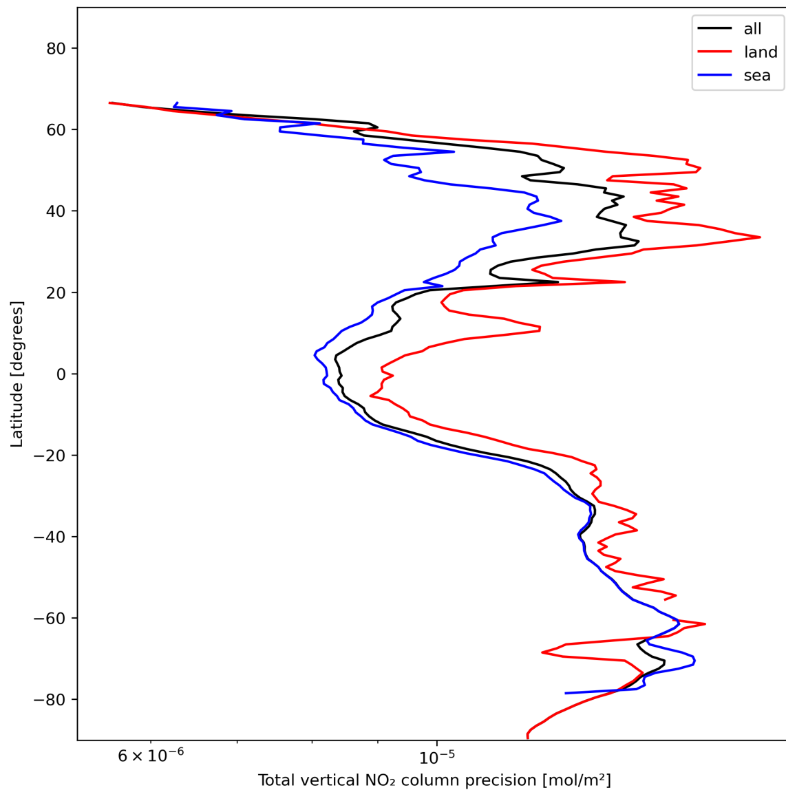
Figure 22: Zonal average of “Total vertical NO 2 column precision” for 2023-11-28 to 2023-11-30.
