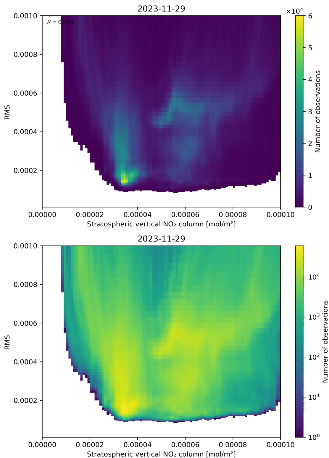
Figure 102: Scatter density plot of “Stratospheric vertical NO 2 column” against “RMS” for 2023-11-28 to 2023-11-30.
