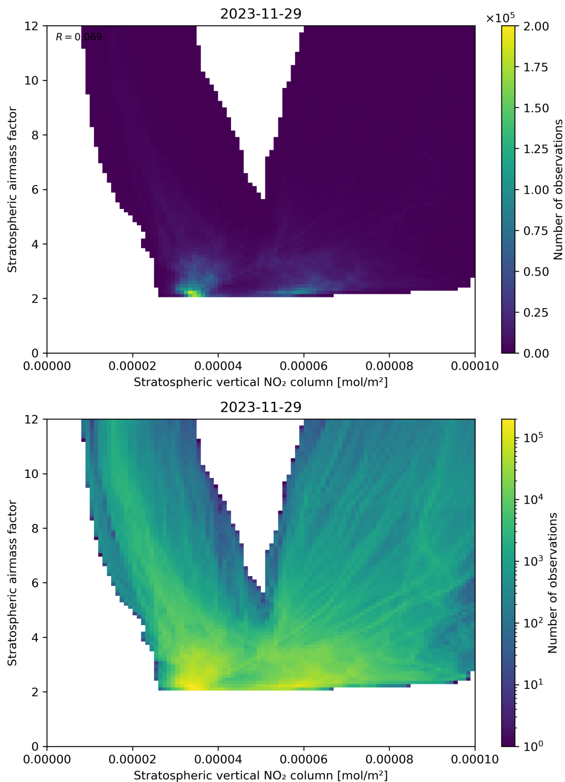
Figure 96: Scatter density plot of “Stratospheric vertical NO 2 column” against “Stratospheric airmass factor” for 2023-11-28 to 2023-11-30.
