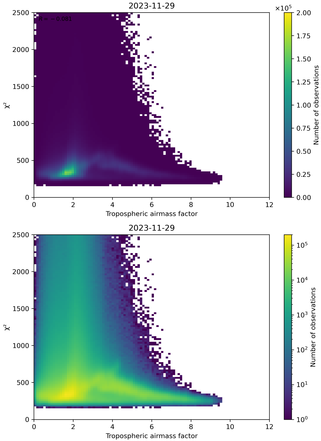
Figure 73: Scatter density plot of “Tropospheric airmass factor” against “ \chi^2 ” for 2023-11-28 to 2023-11-30.
