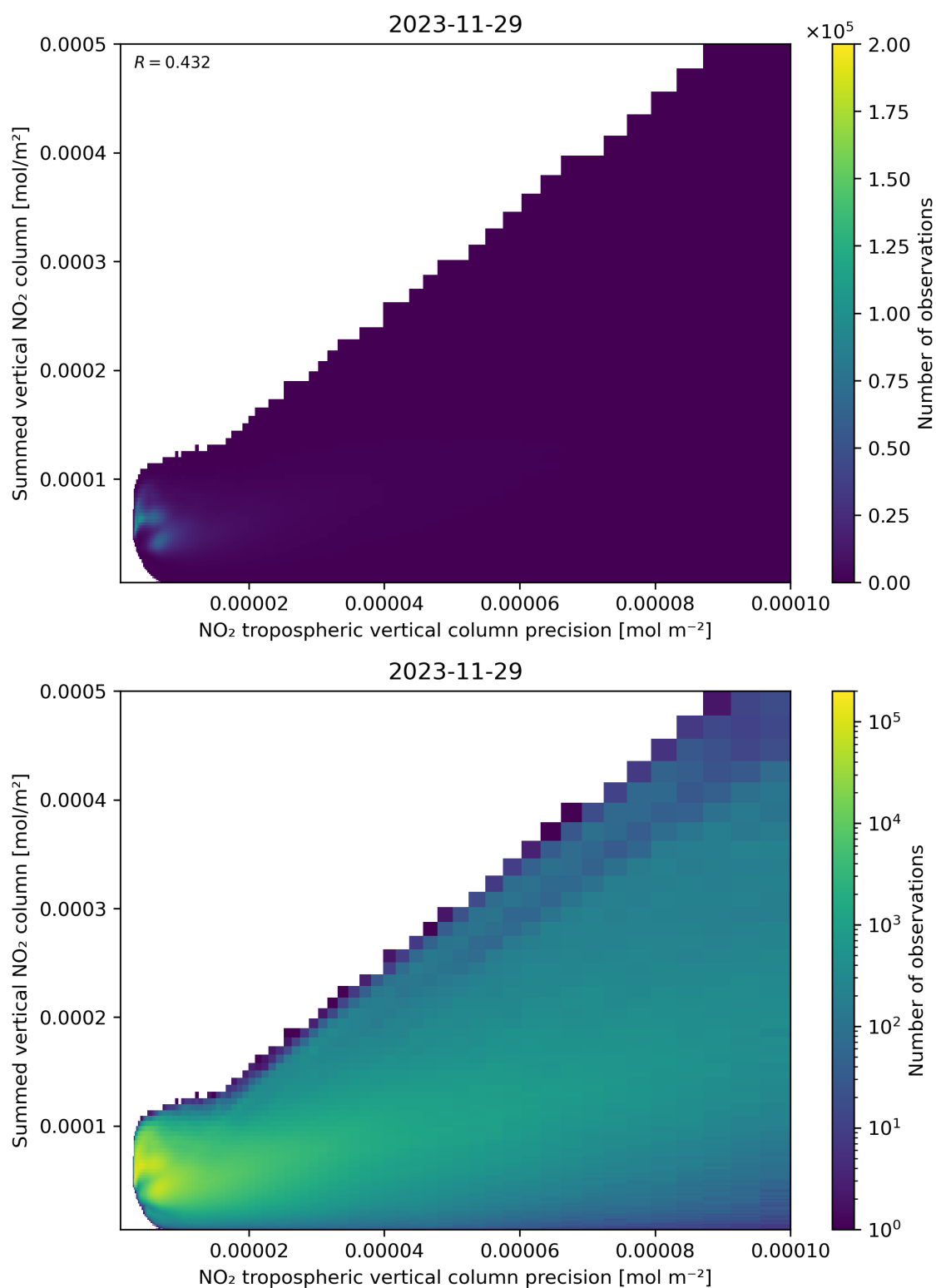
Figure 136: Scatter density plot of “NO 2 tropospheric vertical column precision” against “Summed vertical NO 2 column” for 2023-11-28 to 2023-11-30.
