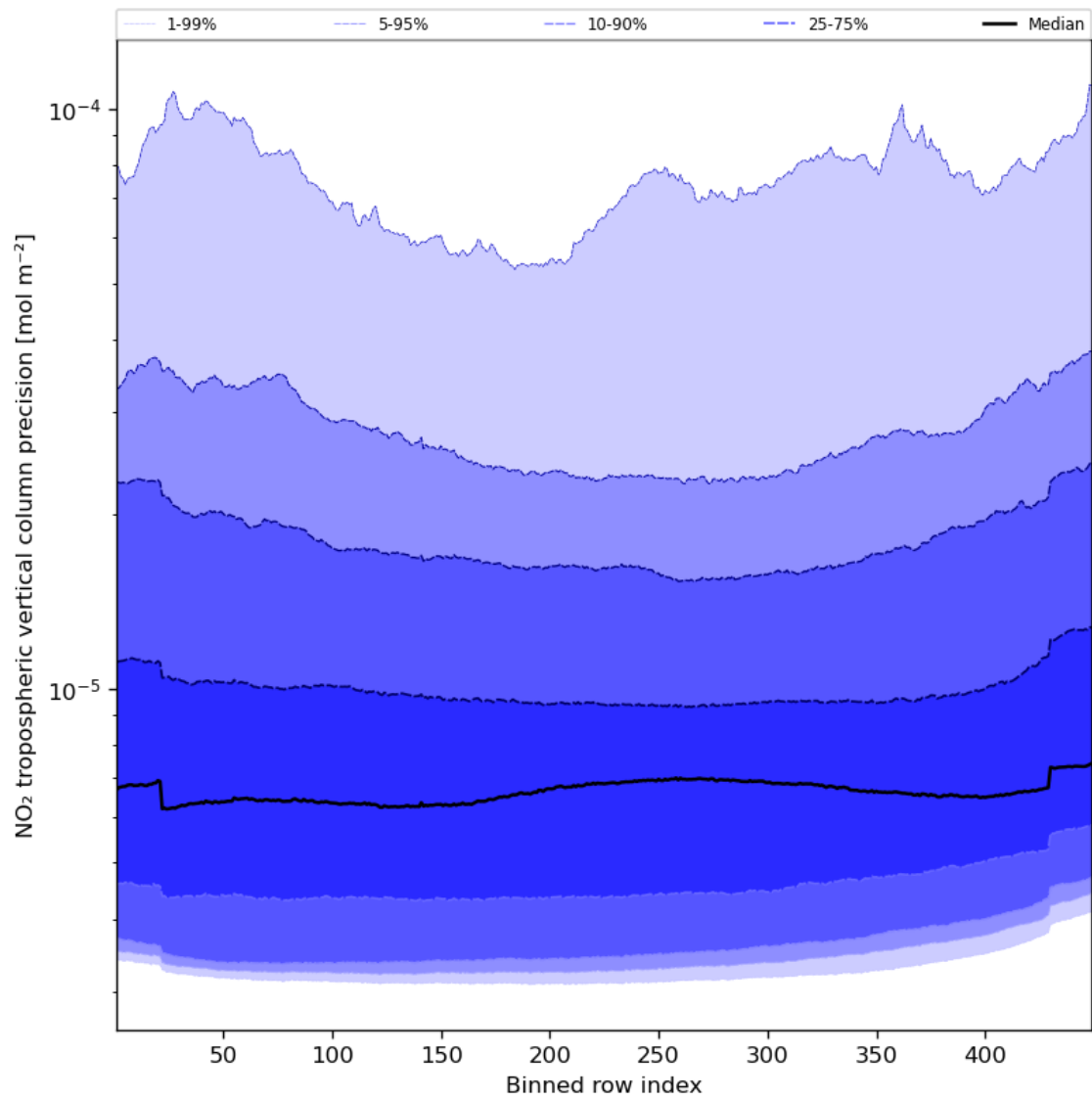
Figure 47: Along track statistics of “NO 2 tropospheric vertical column precision” for 2023-11-28 to 2023-11-30
