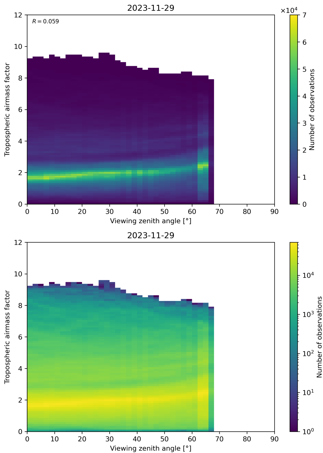
Figure 161: Scatter density plot of “Viewing zenith angle” against “Tropospheric airmass factor” for 2023-11-28 to 2023-11-30.
