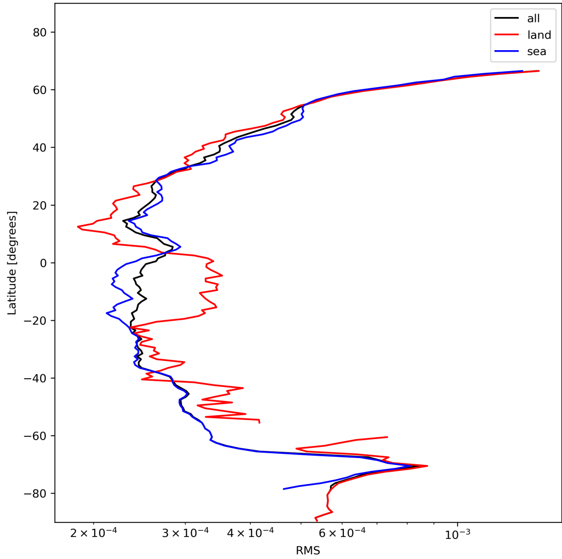
Figure 26: Zonal average of “RMS” for 2023-11-28 to 2023-11-30.
