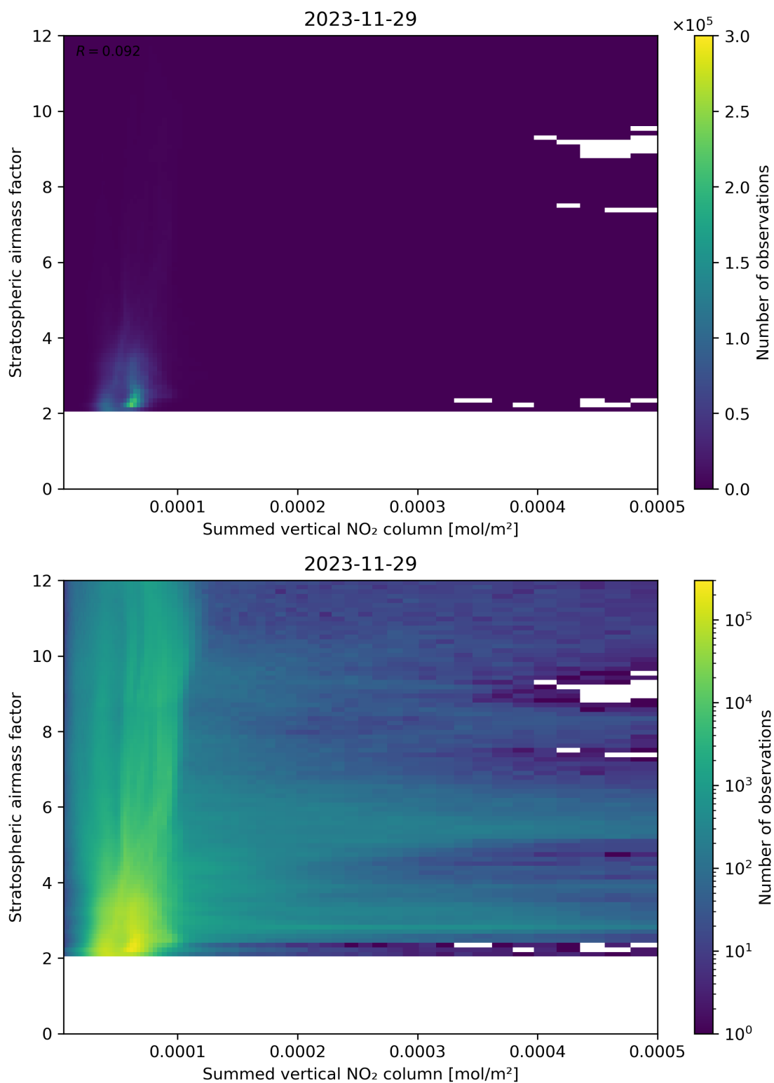
Figure 103: Scatter density plot of “Summed vertical NO 2 column” against “Stratospheric air mass factor” for 2023-11-28 to 2023-11-30.
