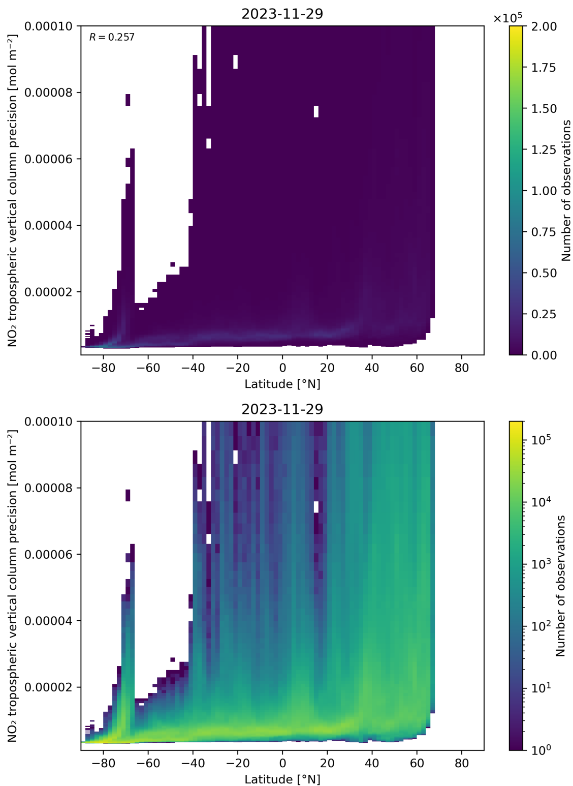
Figure 93: Scatter density plot of “Latitude” against “NO 2 tropospheric vertical column precision” for 2023-11-28 to 2023-11-30.
