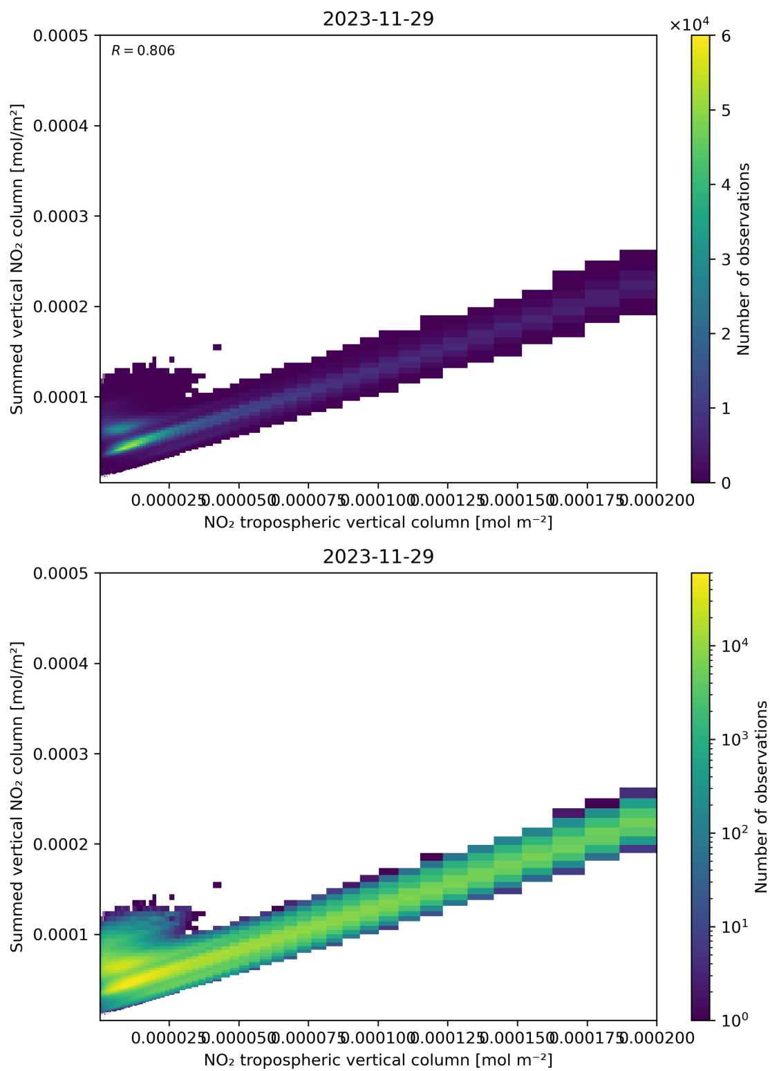
Figure 126: Scatter density plot of “NO 2 tropospheric vertical column” against “Summed vertical NO 2 column” for 2023-11-28 to 2023-11-30.
