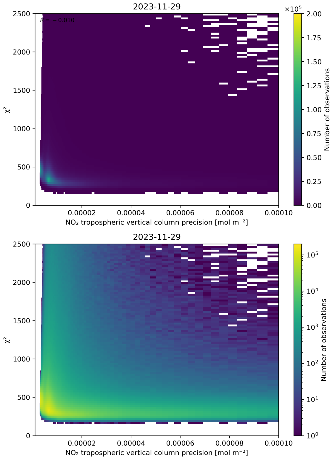
Figure 134: Scatter density plot of “NO 2 tropospheric vertical column precision” against “ \chi^2 ” for 2023-11-28 to 2023-11-30.
