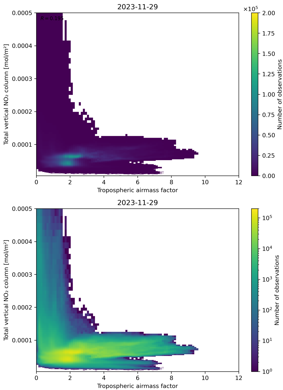
Figure 77: Scatter density plot of “Tropospheric airmass factor” against “Total vertical NO 2 column” for 2023-11-28 to 2023-11-30.
