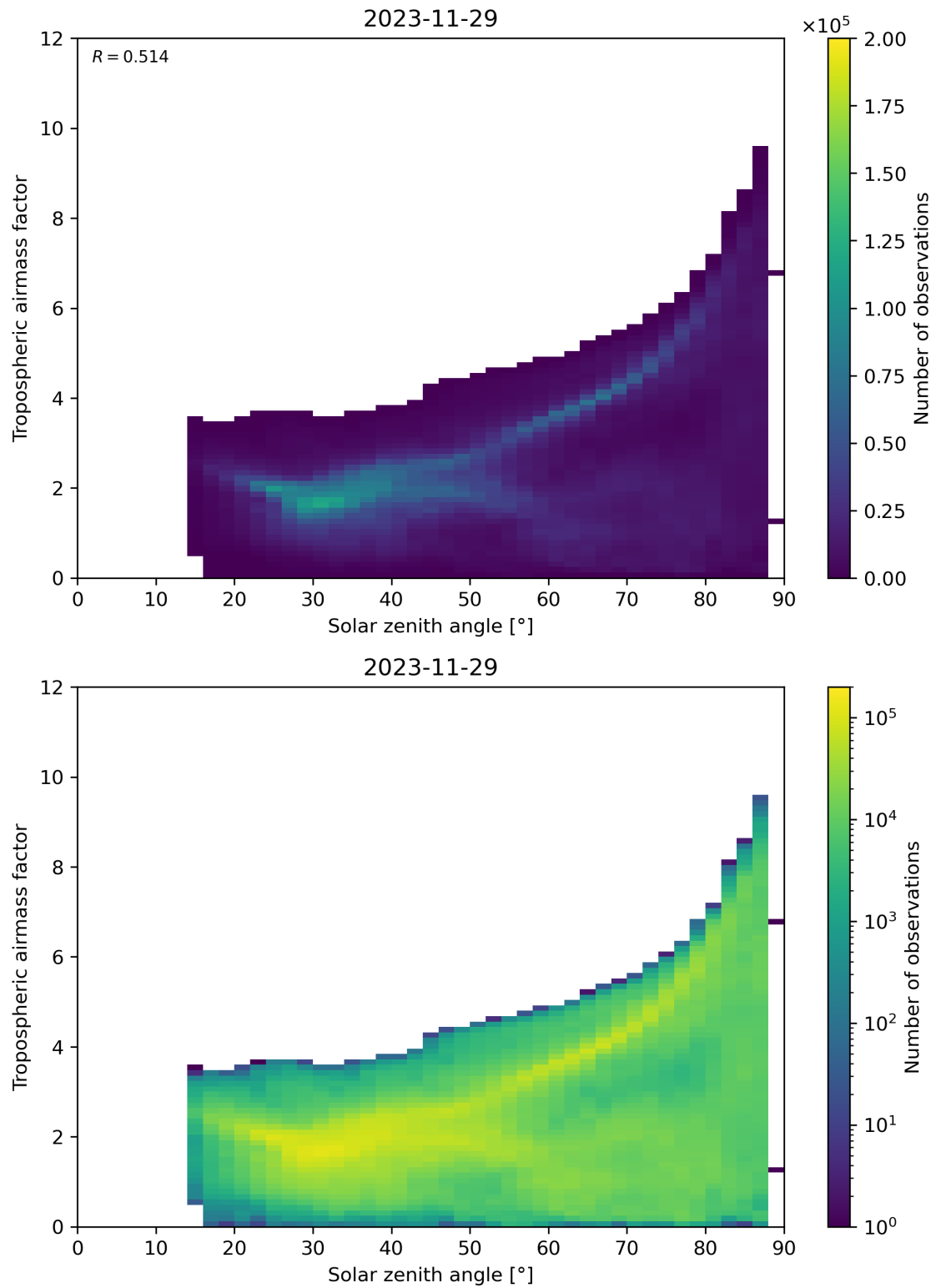
Figure 147: Scatter density plot of “Solar zenith angle” against “Tropospheric airmass factor” for 2023-11-28 to 2023-11-30.
