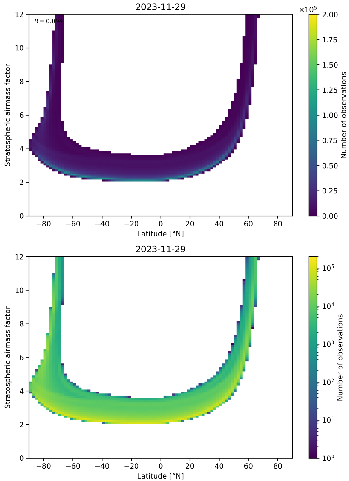
Figure 83: Scatter density plot of “Latitude” against “Stratospheric air mass factor” for 2023-11-28 to 2023-11-30.
