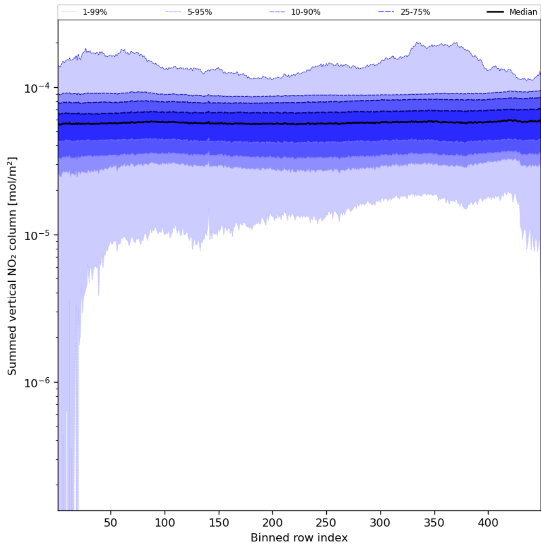
Figure 57: Along track statistics of “Summed vertical NO 2 column” for 2023-11-28 to 2023-11-30
