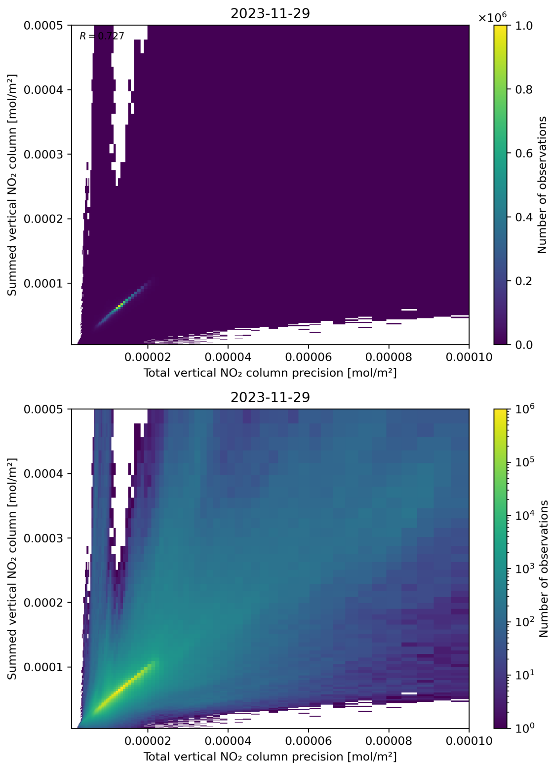
Figure 117: Scatter density plot of “Total vertical NO 2 column precision” against “Summed vertical NO 2 column” for 2023-11-28 to 2023-11-30.
