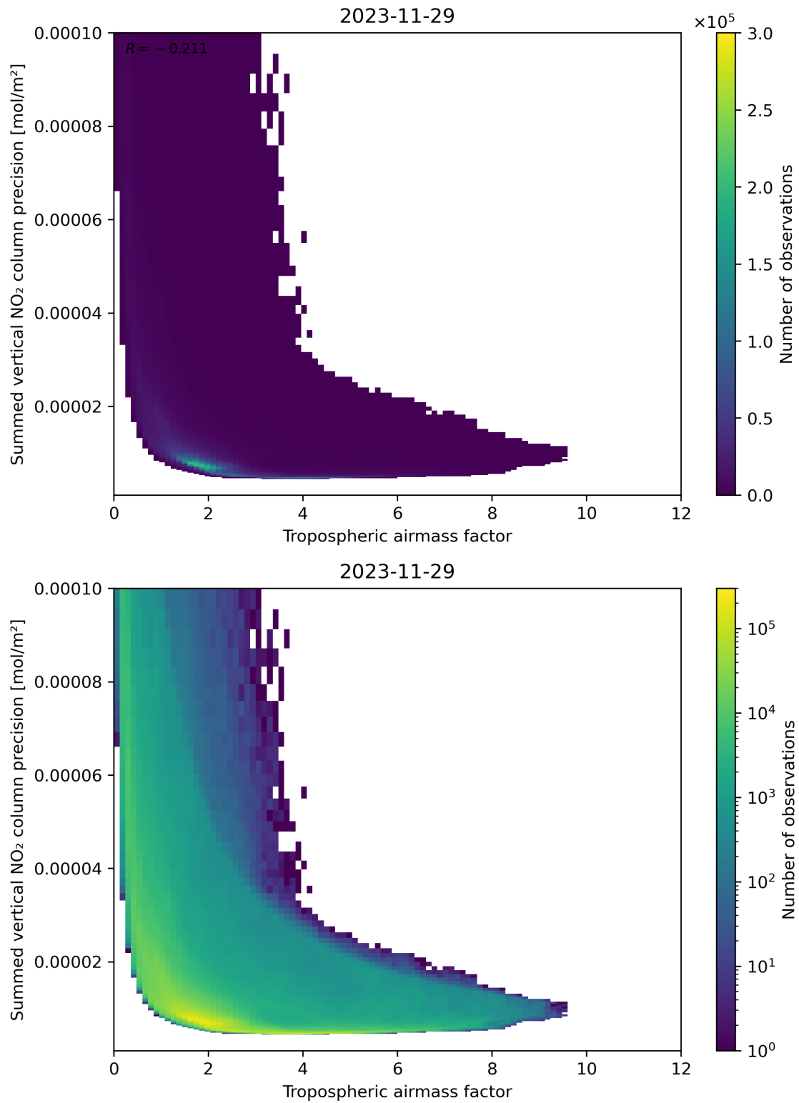
Figure 76: Scatter density plot of “Tropospheric air mass factor” against “Summed vertical NO 2 column precision” for 2023-11-28 to 2023-11-30.
