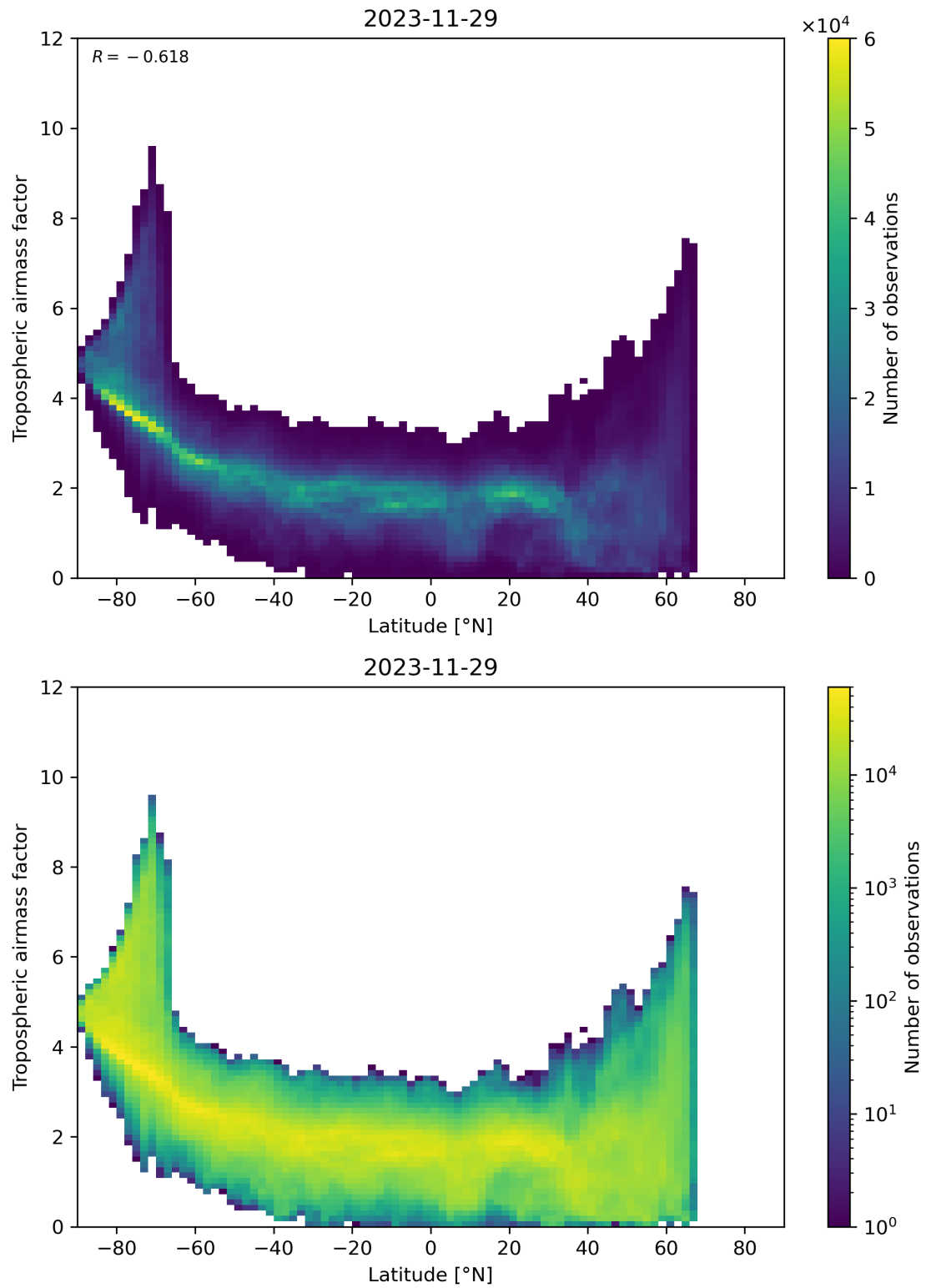
Figure 85: Scatter density plot of “Latitude” against “Tropospheric airmass factor” for 2023-11-28 to 2023-11-30.
