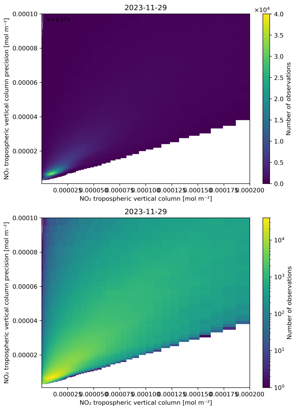
Figure 130: Scatter density plot of “NO 2 tropospheric vertical column” against “NO 2 tropospheric vertical column precision” for 2023-11-28 to 2023-11-30.
