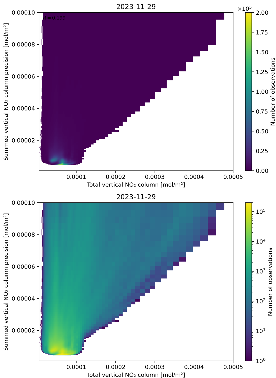
Figure 113: Scatter density plot of “Total vertical NO 2 column” against “Summed vertical NO 2 column precision” for 2023-11-28 to 2023-11-30.
