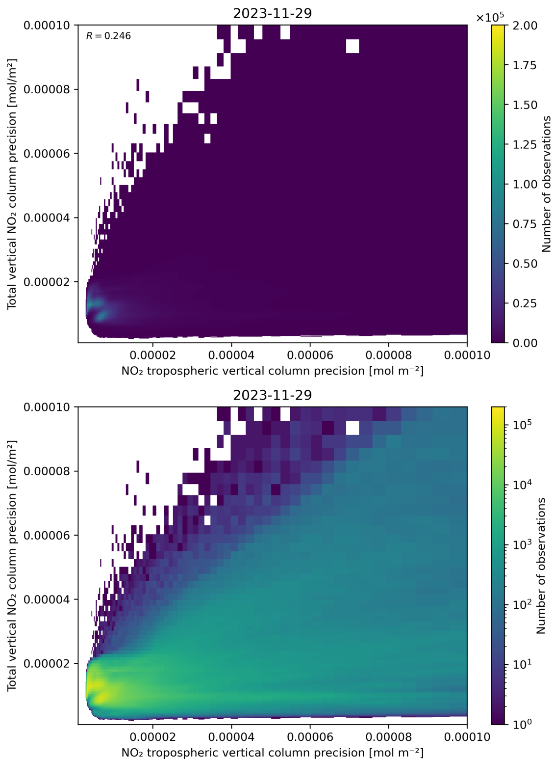
Figure 139: Scatter density plot of “NO 2 tropospheric vertical column precision” against “Total vertical NO 2 column precision” for 2023-11-28 to 2023-11-30.
