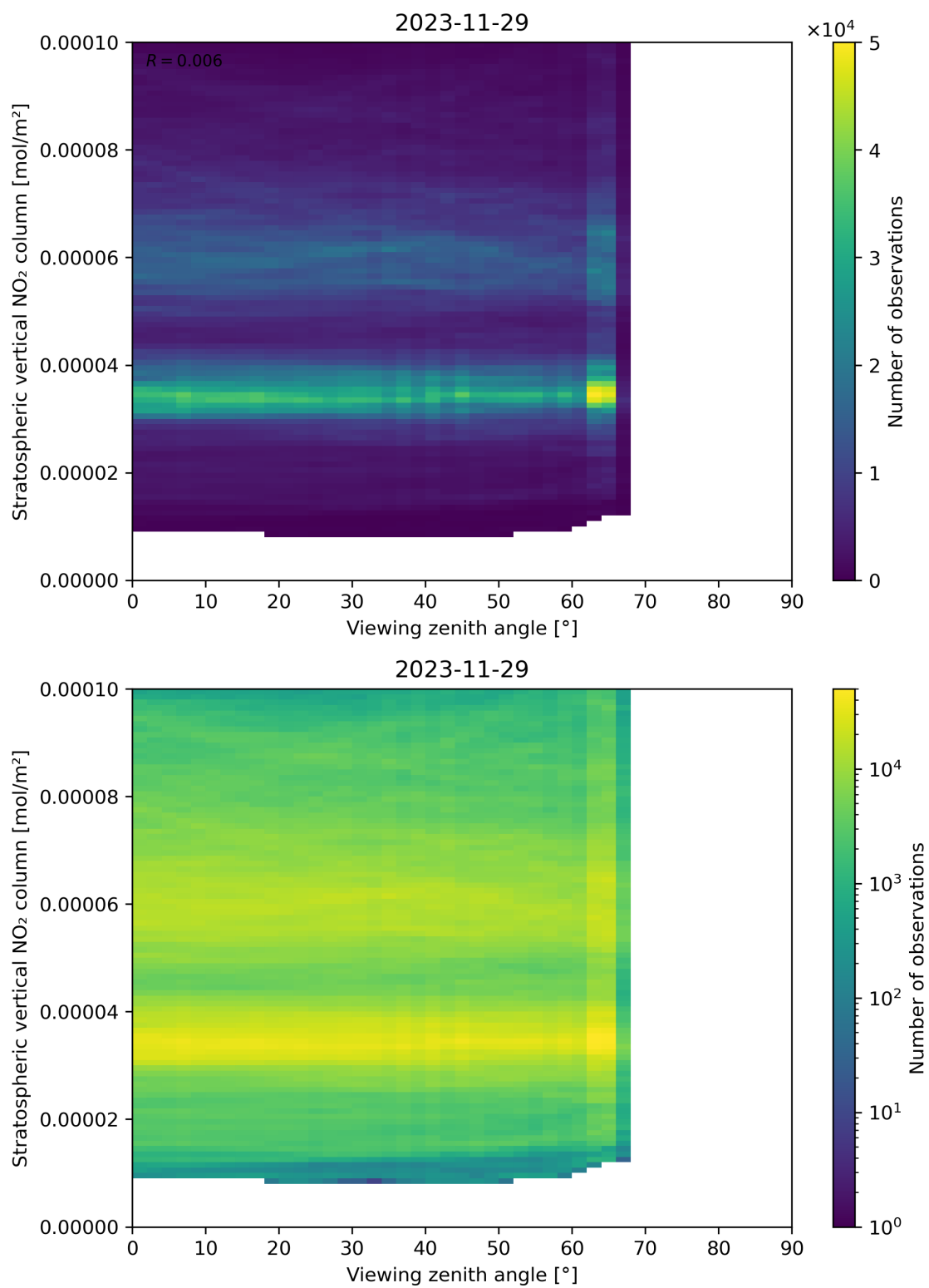
Figure 164: Scatter density plot of “Viewing zenith angle” against “Stratospheric vertical NO 2 column” for 2023-11-28 to 2023-11-30.
