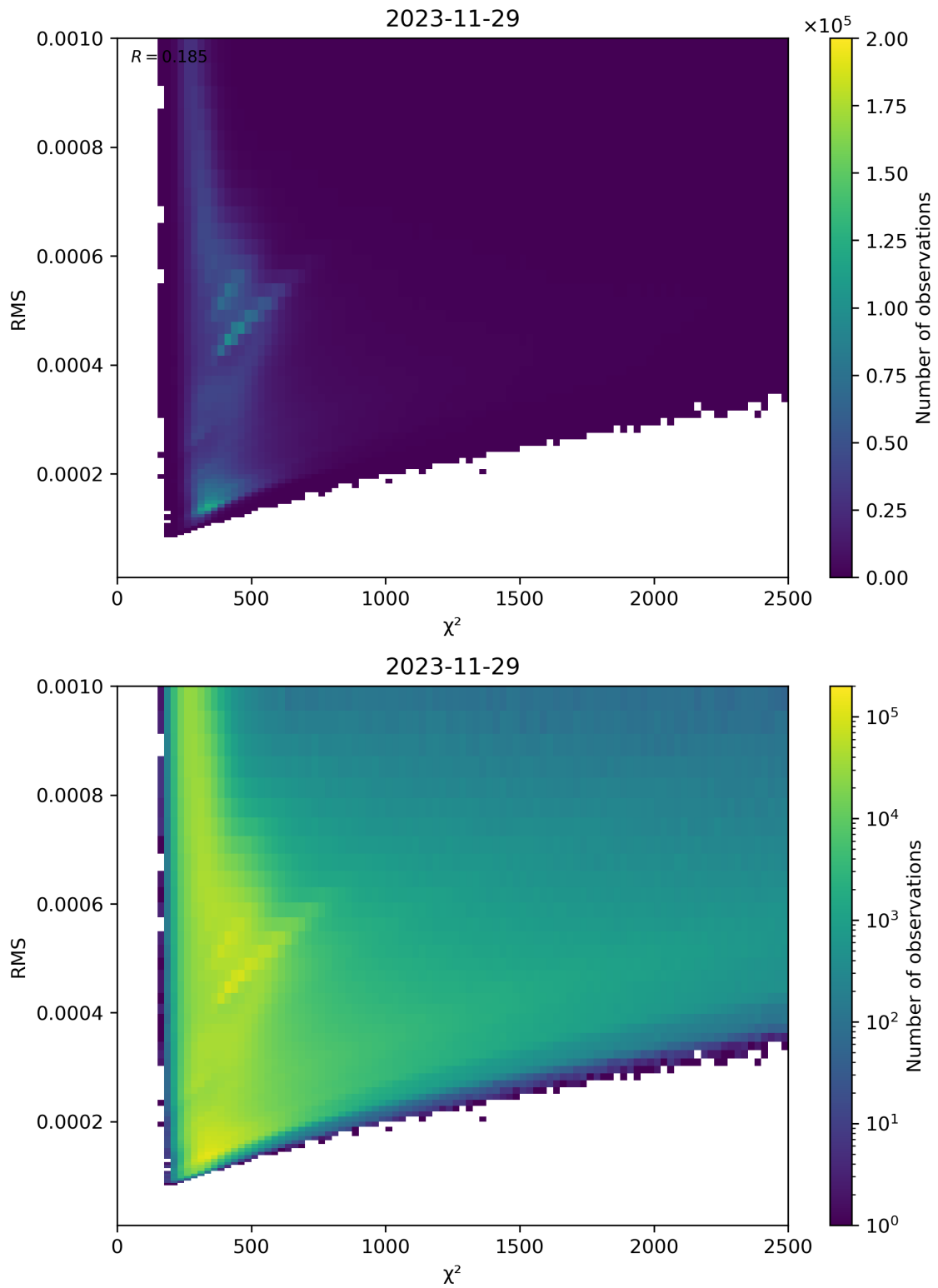
Figure 82: Scatter density plot of “ \chi^2 ” against “RMS” for 2023-11-28 to 2023-11-30.
