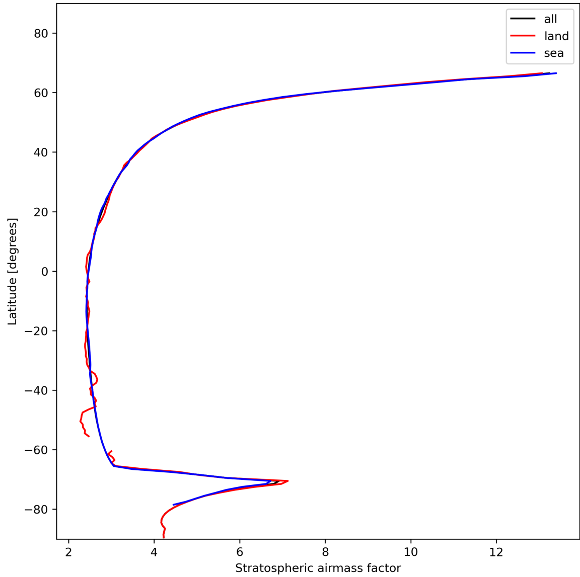
Figure 27: Zonal average of “Stratospheric air mass factor” for 2023-11-28 to 2023-11-30.
