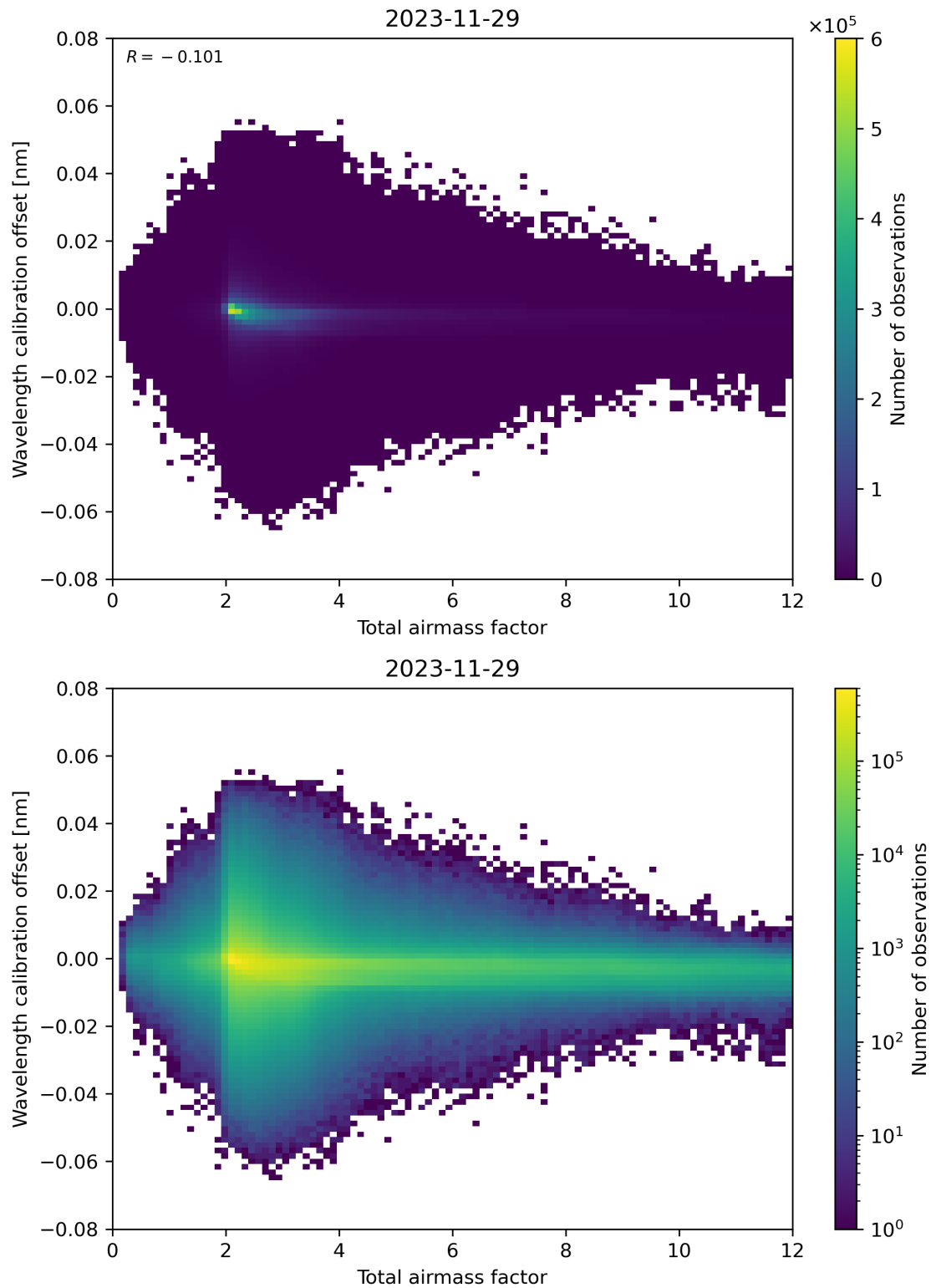
Figure 70: Scatter density plot of “Total airmass factor” against “Wavelength calibration offset” for 2023-11-28 to 2023-11-30.
