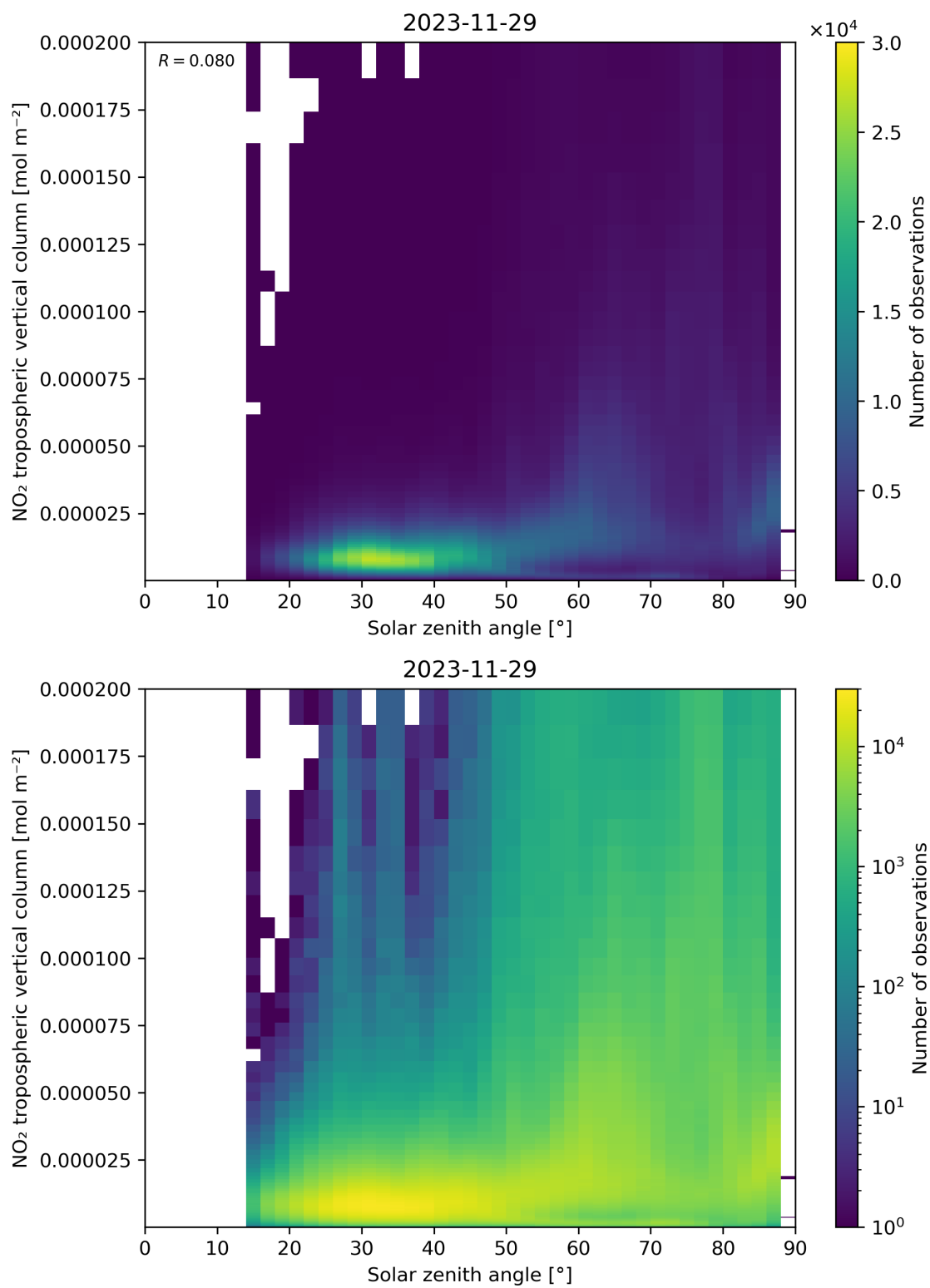
Figure 155: Scatter density plot of “Solar zenith angle” against “NO 2 tropospheric vertical column” for 2023-11-28 to 2023-11-30.
