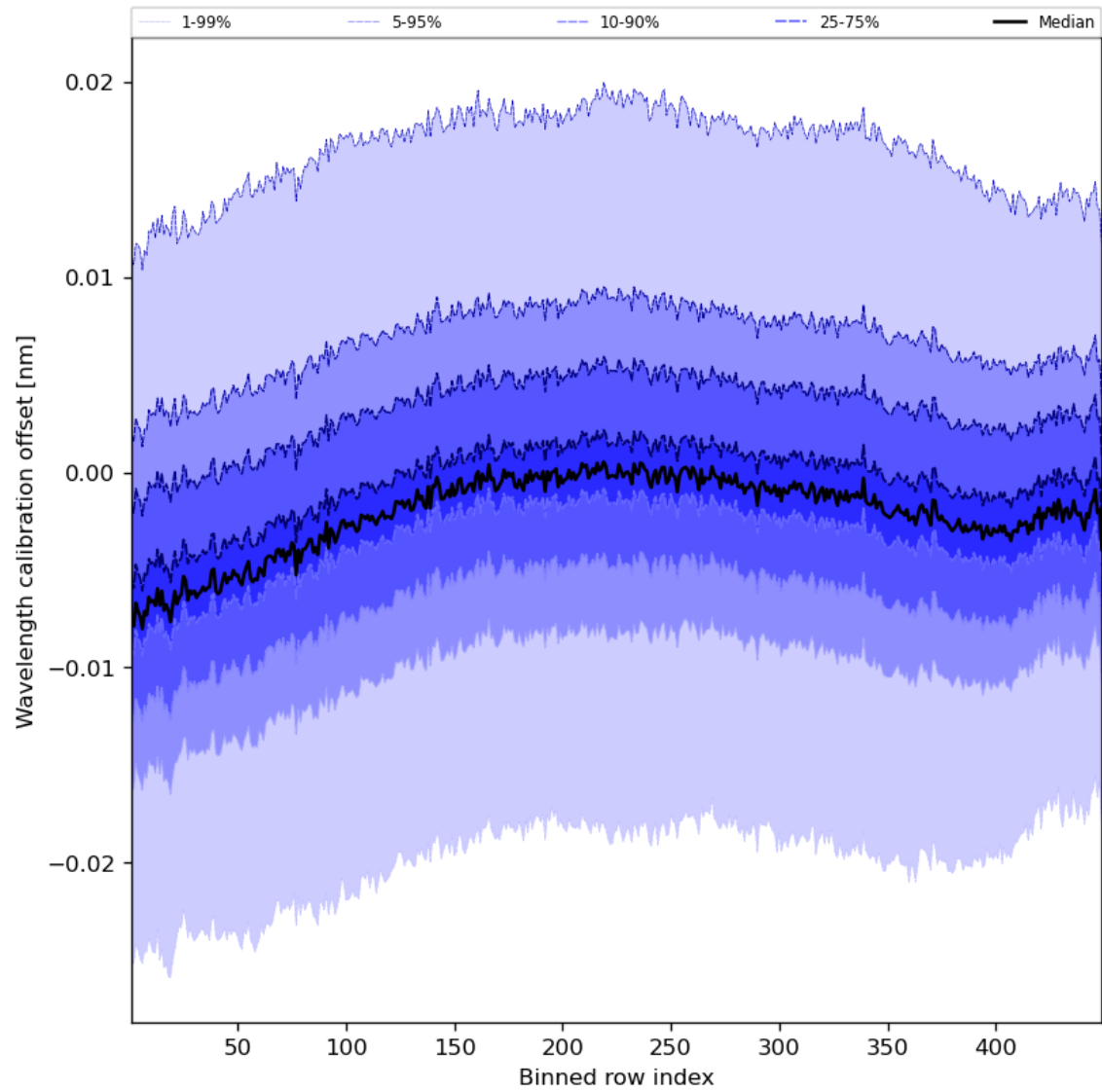
Figure 52: Along track statistics of “Wavelength calibration offset” for 2023-11-28 to 2023-11-30
