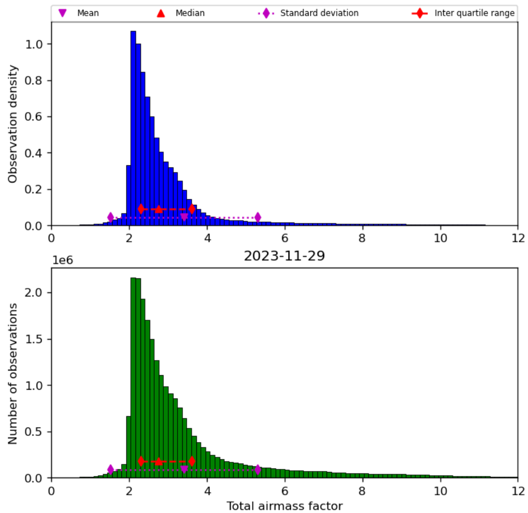
Figure 32: Histogram of “Total airmass factor” for 2023-11-28 to 2023-11-30
