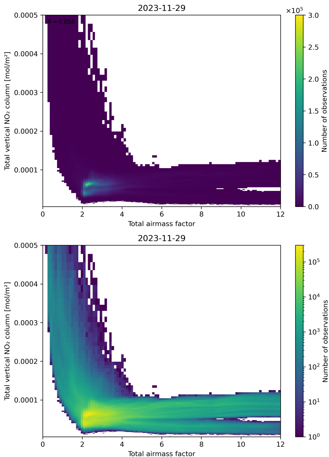
Figure 67: Scatter density plot of “Total airmass factor” against “Total vertical NO 2 column” for 2023-11-28 to 2023-11-30.
