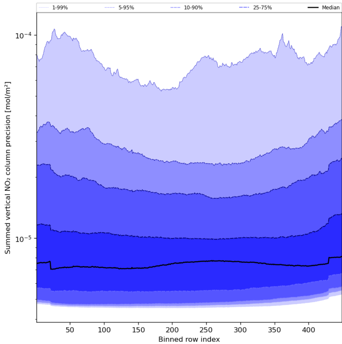
Figure 58: Along track statistics of “Summed vertical NO 2 column precision” for 2023-11-28 to 2023-11-30
