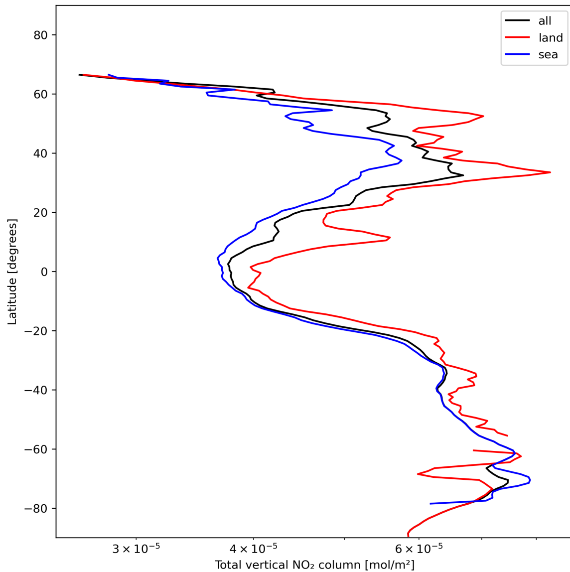
Figure 21: Zonal average of “Total vertical NO 2 column” for 2023-11-28 to 2023-11-30.
