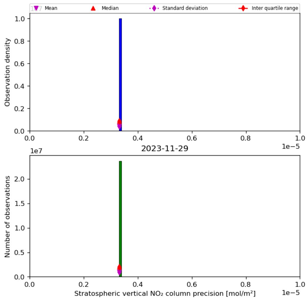
Figure 37: Histogram of “Stratospheric vertical NO 2 column precision” for 2023-11-28 to 2023-11-30
