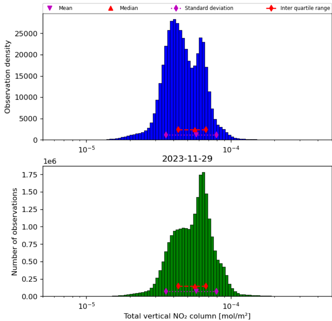
Figure 38: Histogram of “Total vertical NO 2 column” for 2023-11-28 to 2023-11-30
