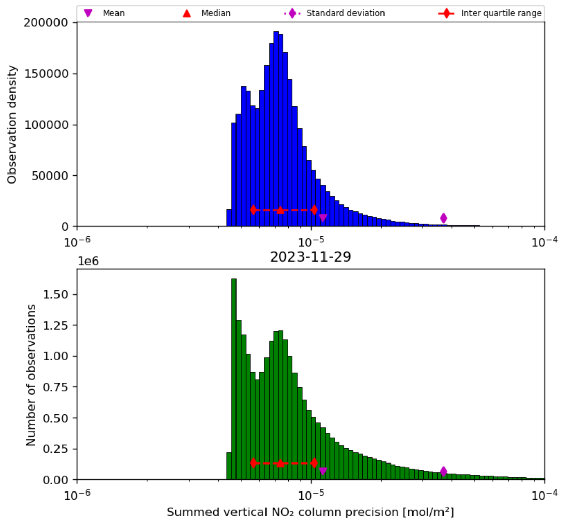
Figure 41: Histogram of “Summed vertical NO 2 column precision” for 2023-11-28 to 2023-11-30
