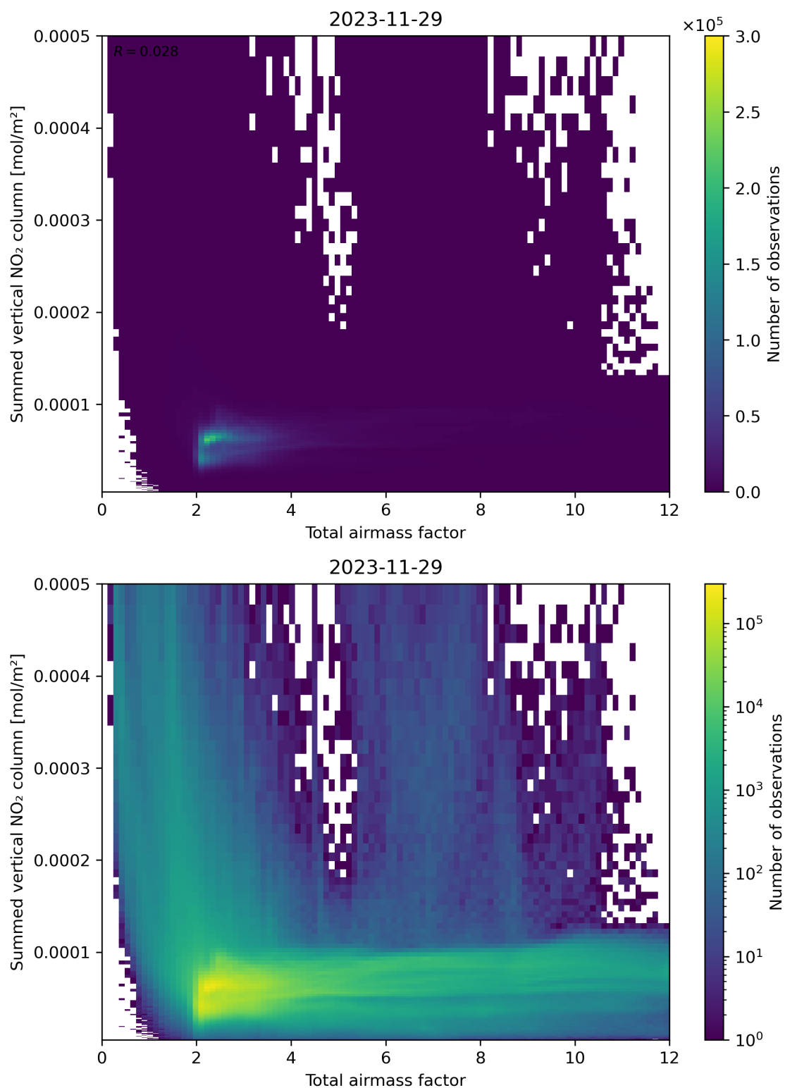
Figure 65: Scatter density plot of “Total airmass factor” against “Summed vertical NO 2 column” for 2023-11-28 to 2023-11-30.
