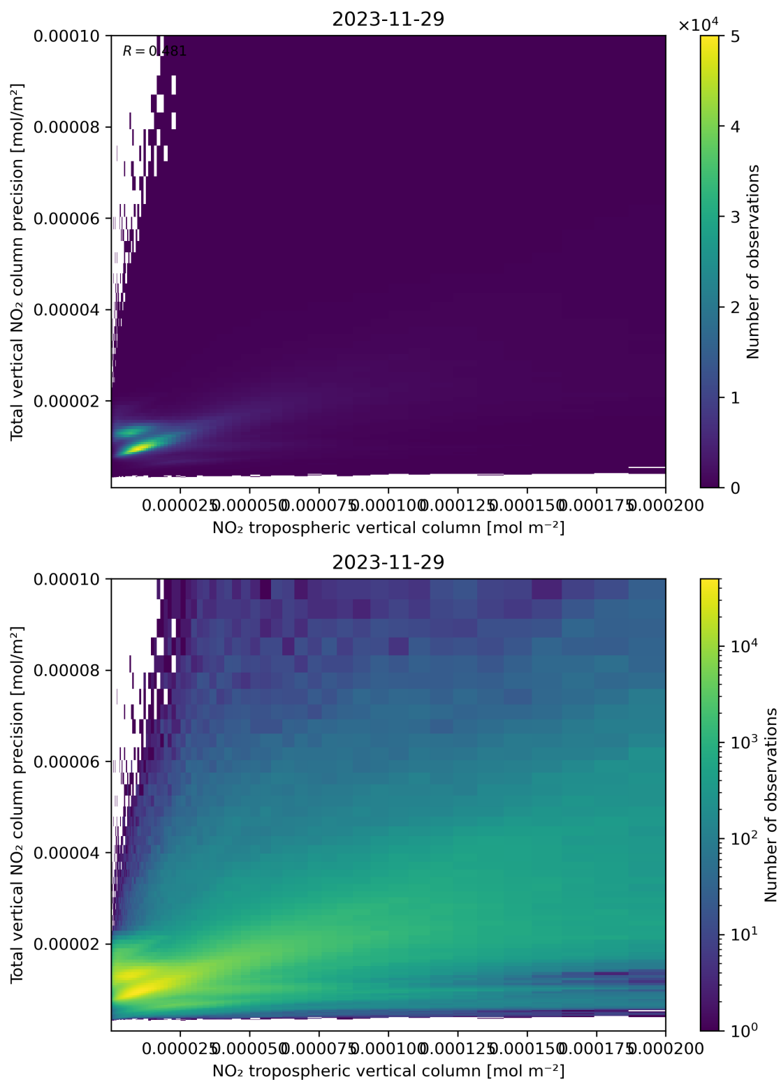
Figure 129: Scatter density plot of “NO 2 tropospheric vertical column” against “Total vertical NO 2 column precision” for 2023-11-28 to 2023-11-30.
