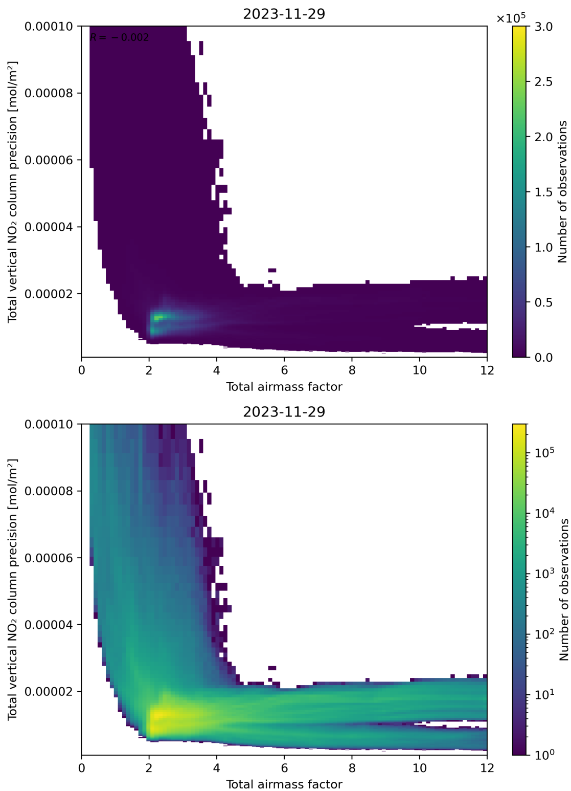
Figure 68: Scatter density plot of “Total airmass factor” against “Total vertical NO 2 column precision” for 2023-11-28 to 2023-11-30.
