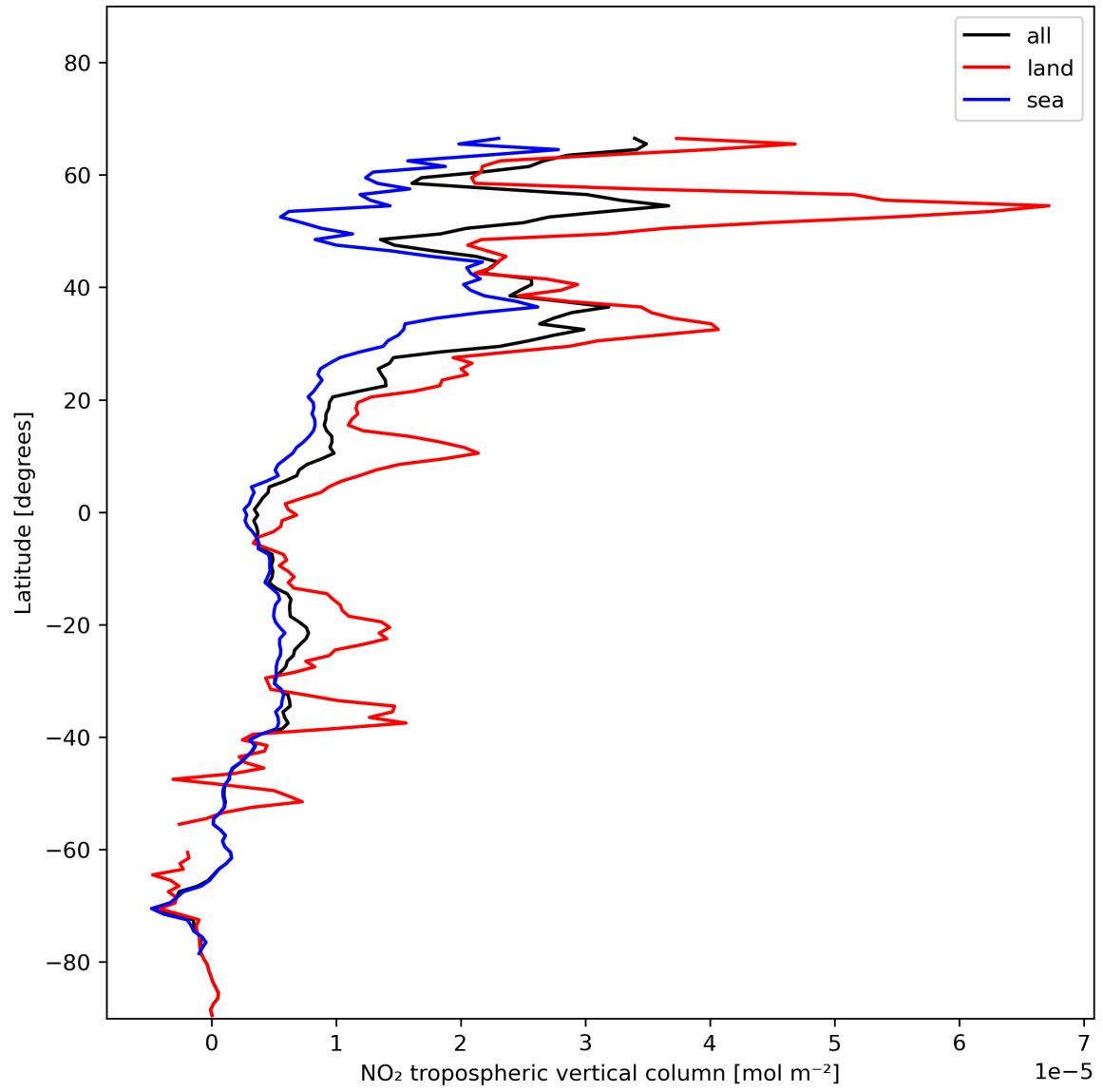
Figure 12: Zonal average of “NO 2 tropospheric vertical column” for 2023-11-28 to 2023-11-30.
