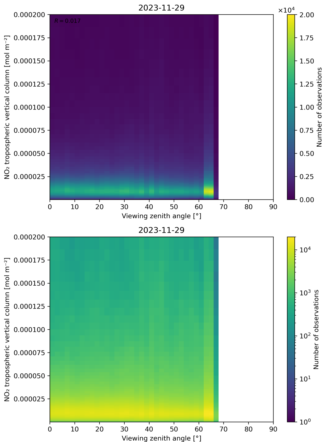
Figure 169: Scatter density plot of “Viewing zenith angle” against “NO 2 tropospheric vertical column” for 2023-11-28 to 2023-11-30.
