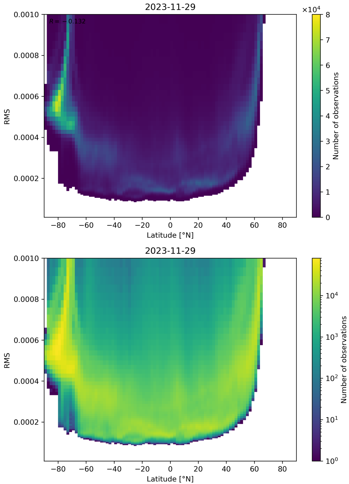
Figure 94: Scatter density plot of “Latitude” against “RMS” for 2023-11-28 to 2023-11-30.
