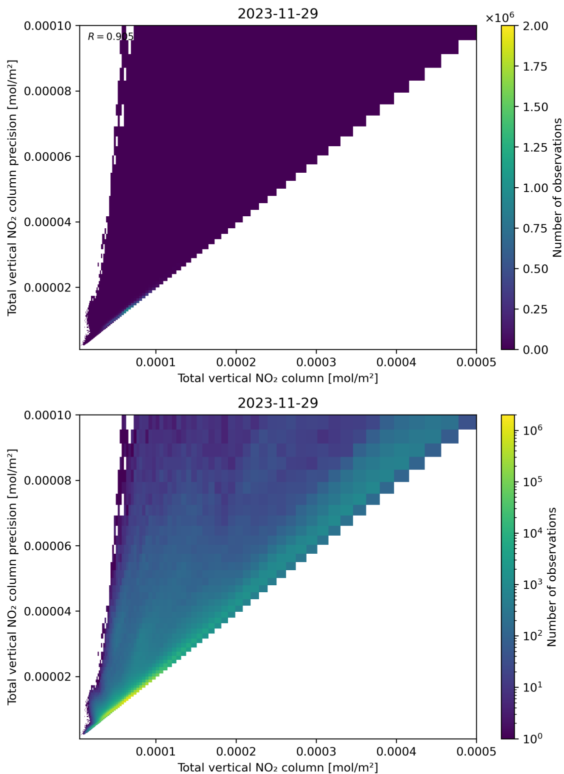
Figure 114: Scatter density plot of “Total vertical NO 2 column” against “Total vertical NO 2 column precision” for 2023-11-28 to 2023-11-30.
