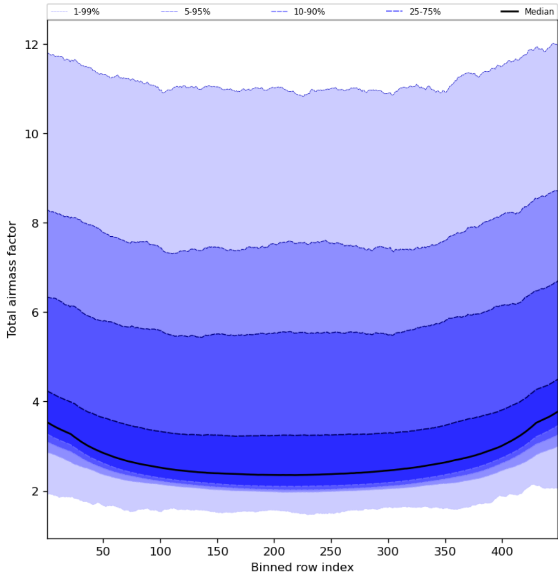
Figure 49: Along track statistics of “Total airmass factor” for 2023-11-28 to 2023-11-30
