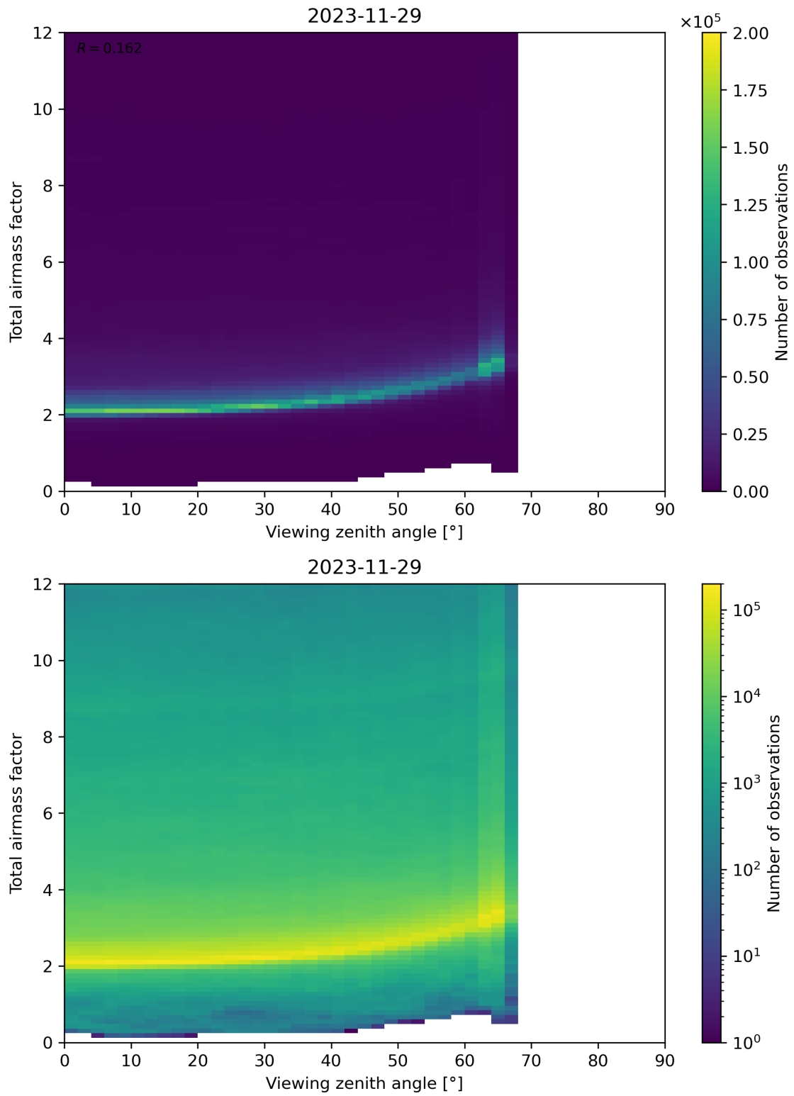
Figure 160: Scatter density plot of “Viewing zenith angle” against “Total airmass factor” for 2023-11-28 to 2023-11-30.
