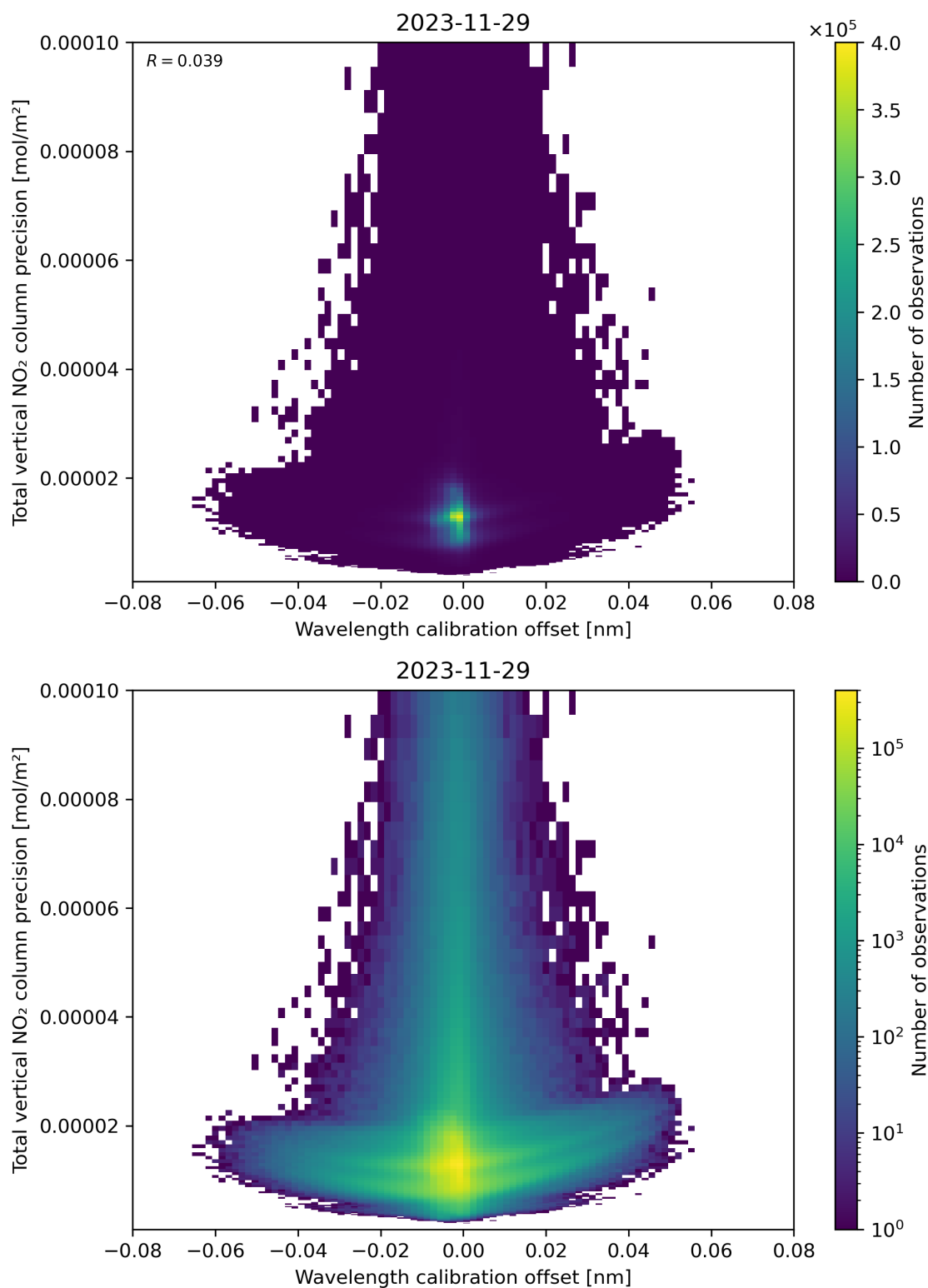
Figure 180: Scatter density plot of “Wavelength calibration offset” against “Total vertical NO 2 column precision” for 2023-11-28 to 2023-11-30.
