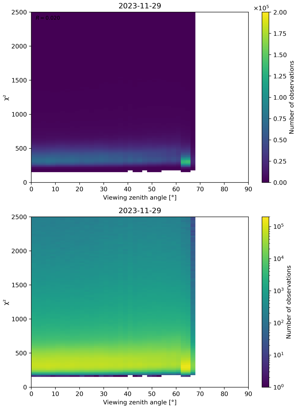
Figure 162: Scatter density plot of “Viewing zenith angle” against “ \chi^2 ” for 2023-11-28 to 2023-11-30.
