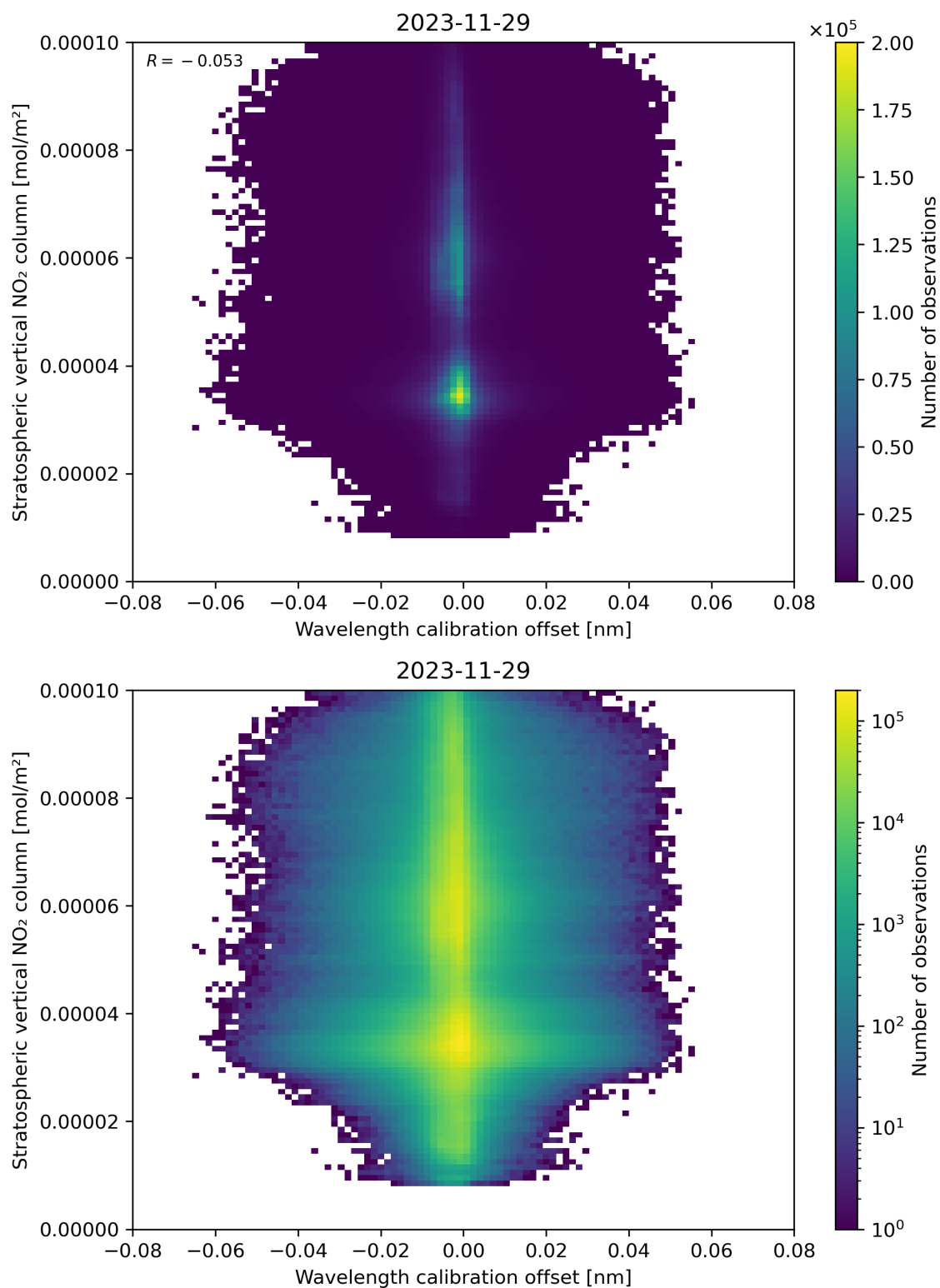
Figure 176: Scatter density plot of “Wavelength calibration offset” against “Stratospheric vertical NO 2 column” for 2023-11-28 to 2023-11-30.
