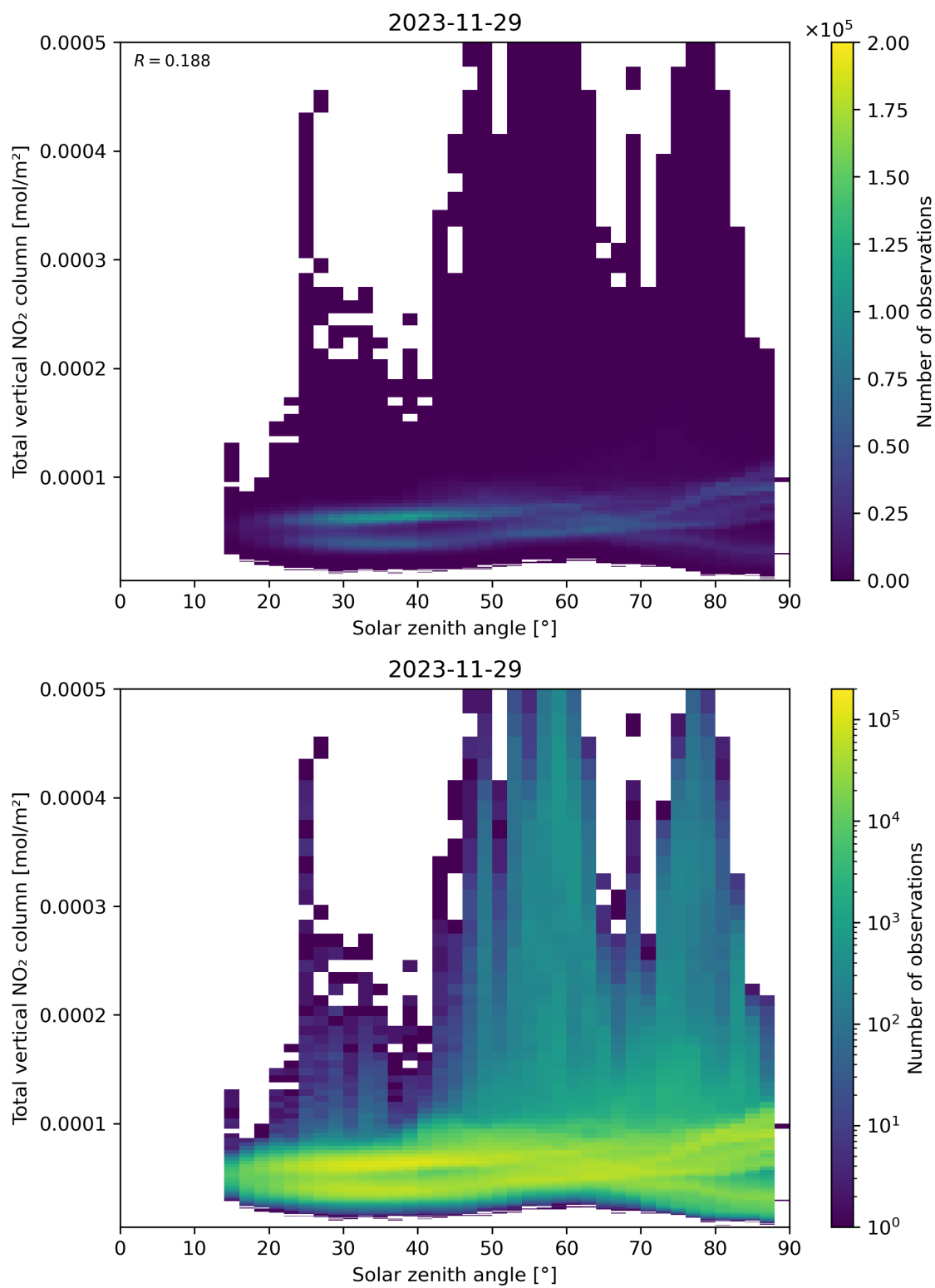
Figure 153: Scatter density plot of “Solar zenith angle” against “Total vertical NO 2 column” for 2023-11-28 to 2023-11-30.
