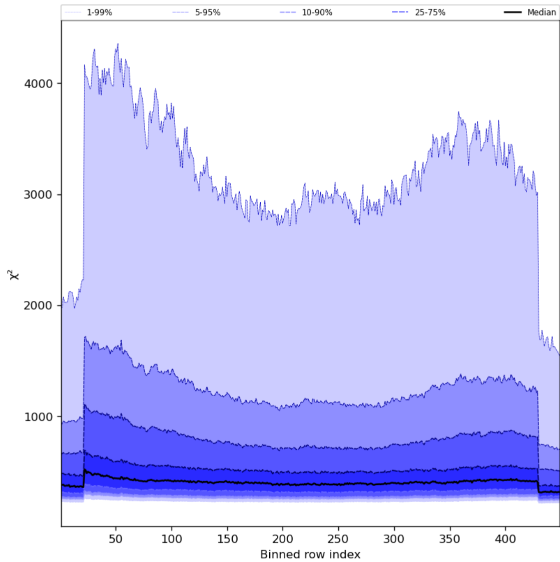
Figure 59: Along track statistics of “ \chi^2 ” for 2023-11-28 to 2023-11-30
