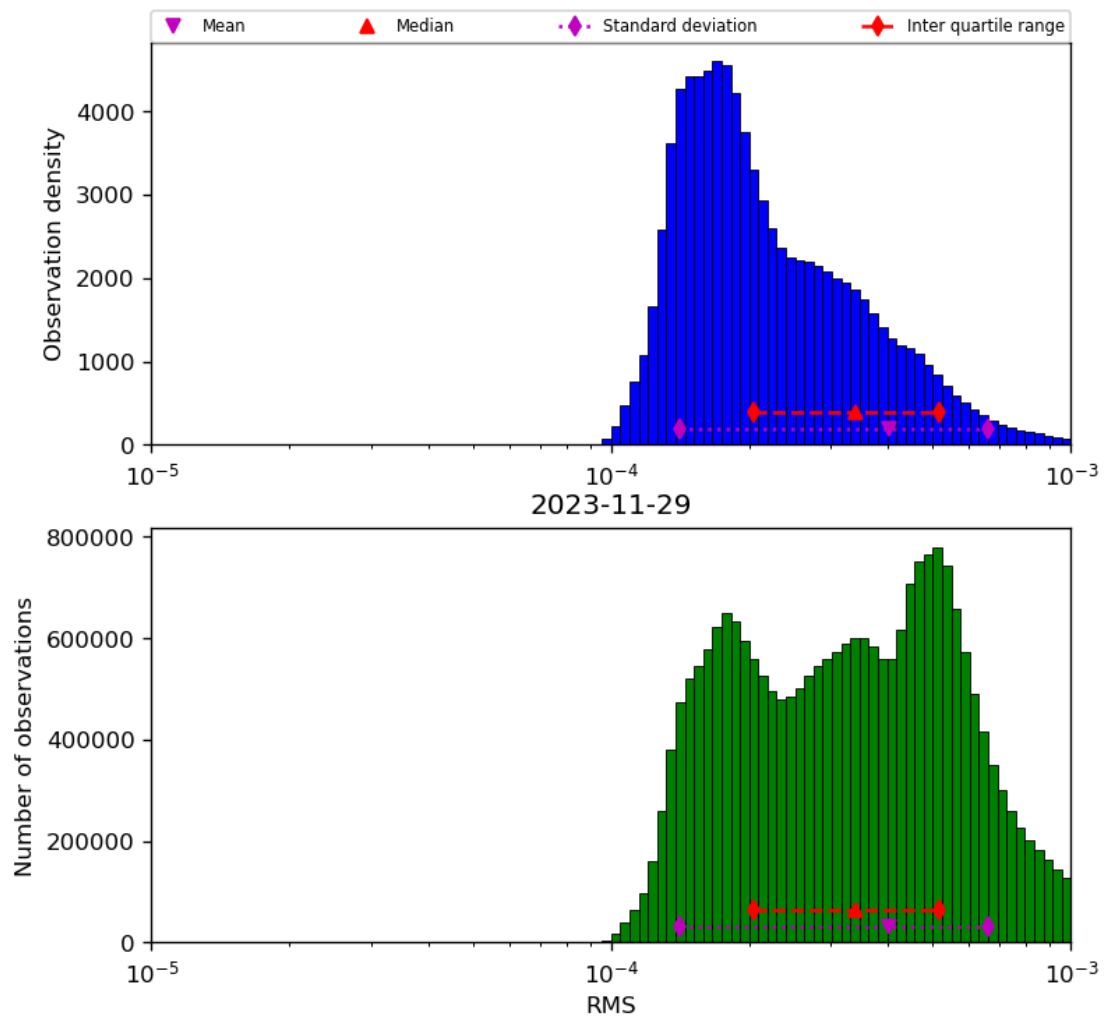
Figure 43: Histogram of “RMS” for 2023-11-28 to 2023-11-30
