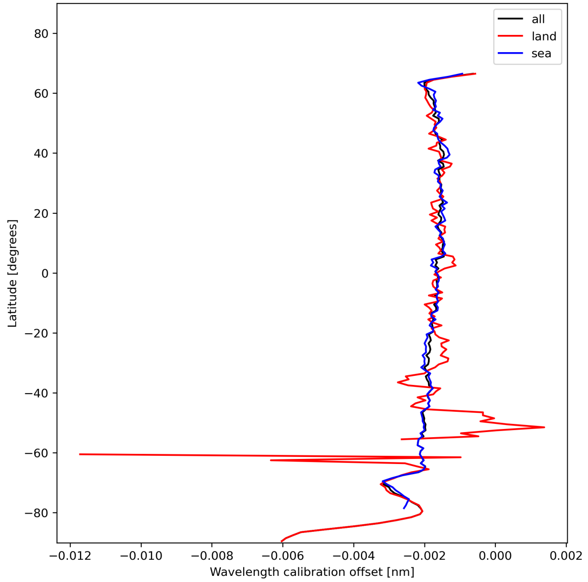
Figure 18: Zonal average of “Wavelength calibration offset” for 2023-11-28 to 2023-11-30.
