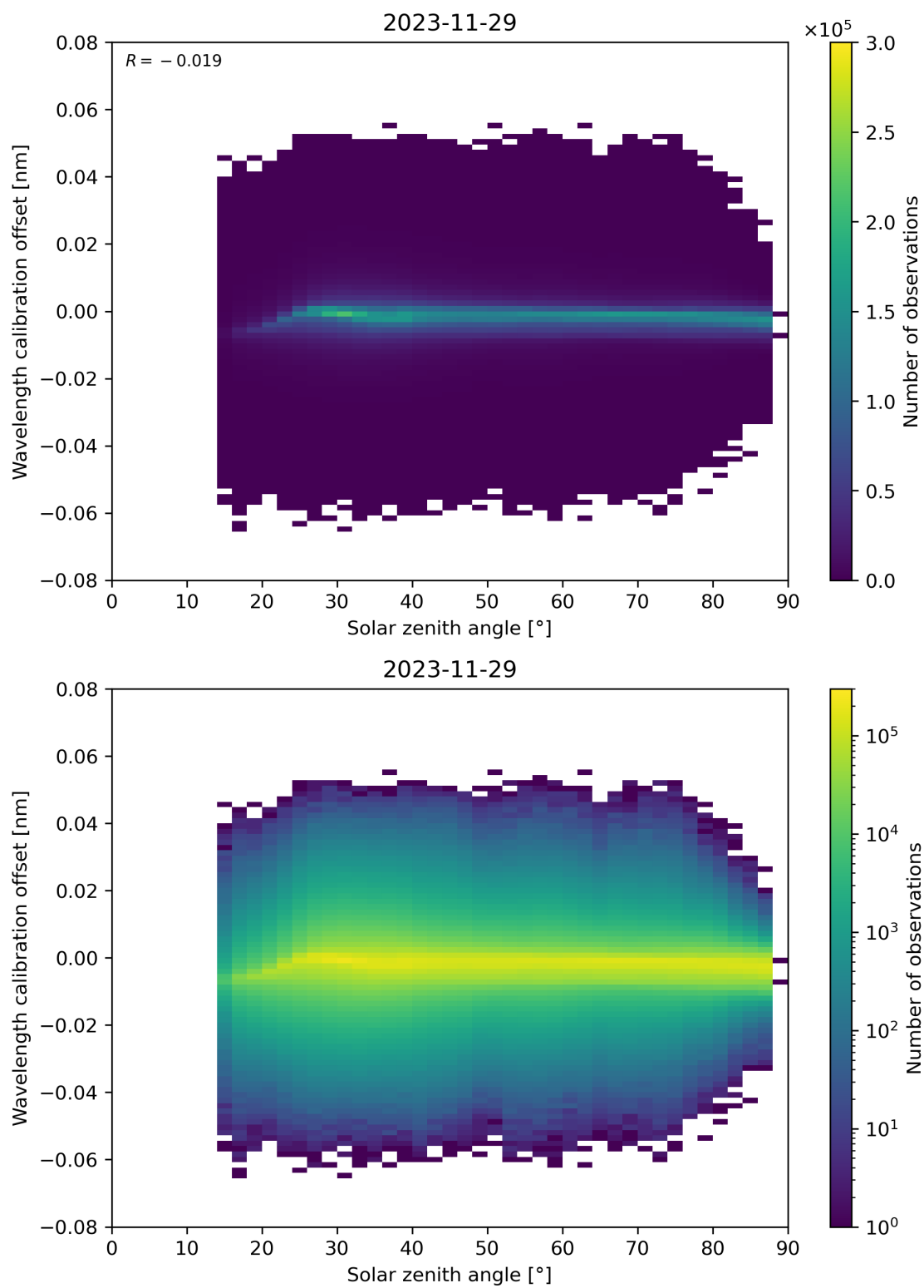
Figure 158: Scatter density plot of “Solar zenith angle” against “Wavelength calibration offset” for 2023-11-28 to 2023-11-30.
