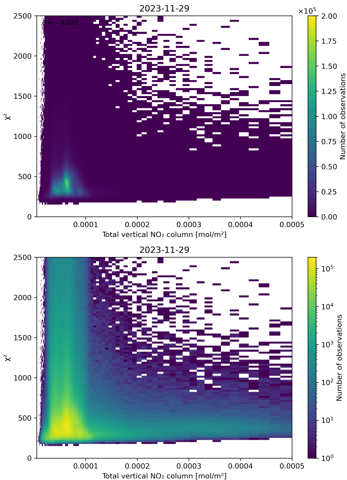
Figure 111: Scatter density plot of “Total vertical NO 2 column” against “ \chi^2 ” for 2023-11-28 to 2023-11-30.
