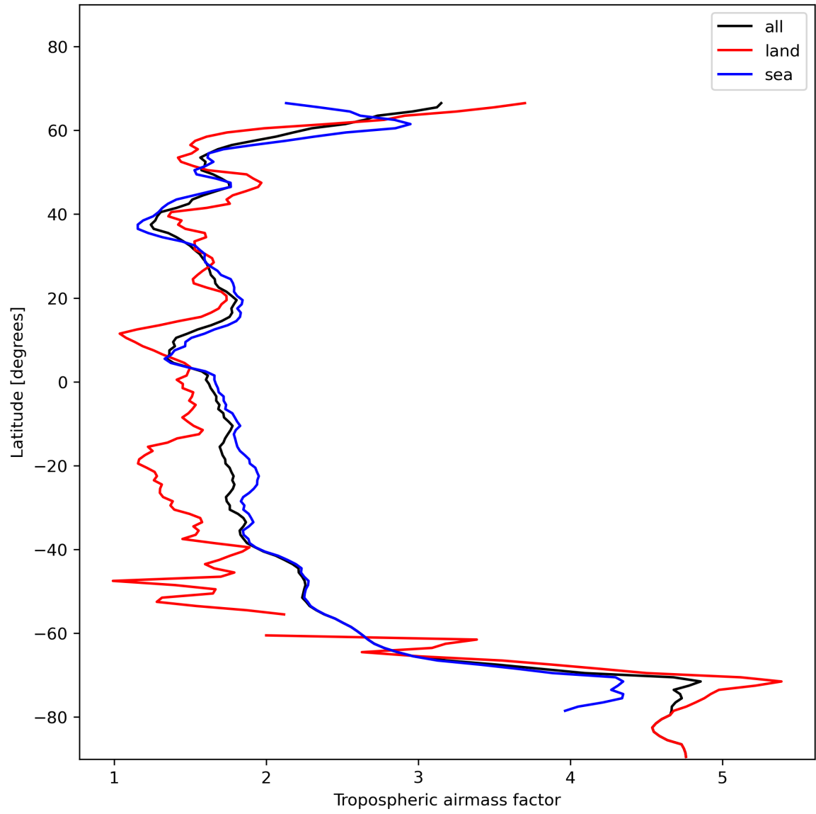
Figure 14: Zonal average of “Tropospheric airmass factor” for 2023-11-28 to 2023-11-30.
