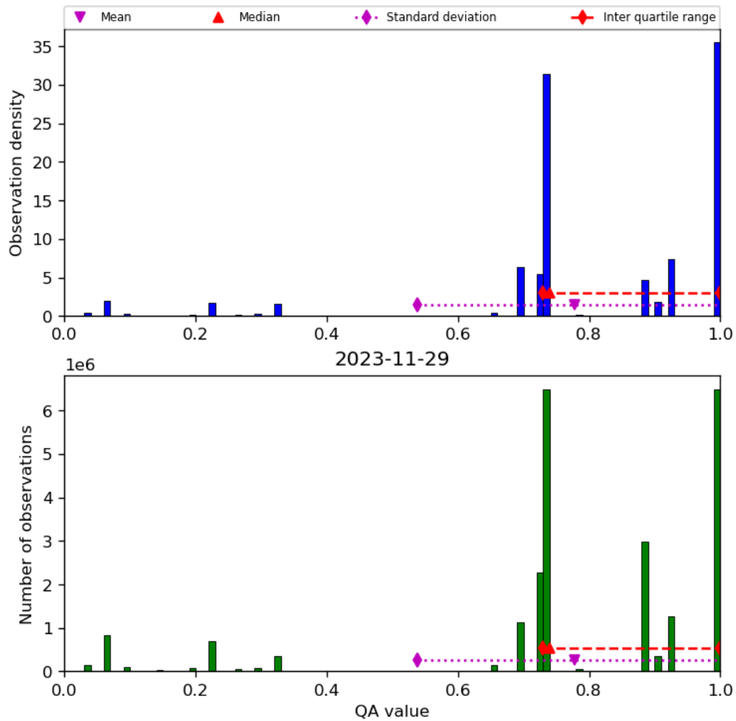
Figure 28: Histogram of “QA value” for 2023-11-28 to 2023-11-30
