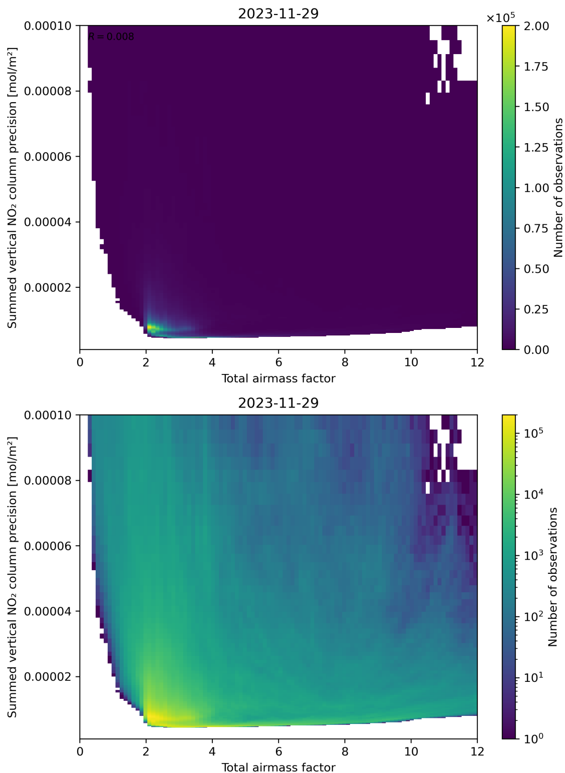
Figure 66: Scatter density plot of “Total airmass factor” against “Summed vertical NO 2 column precision” for 2023-11-28 to 2023-11-30.
