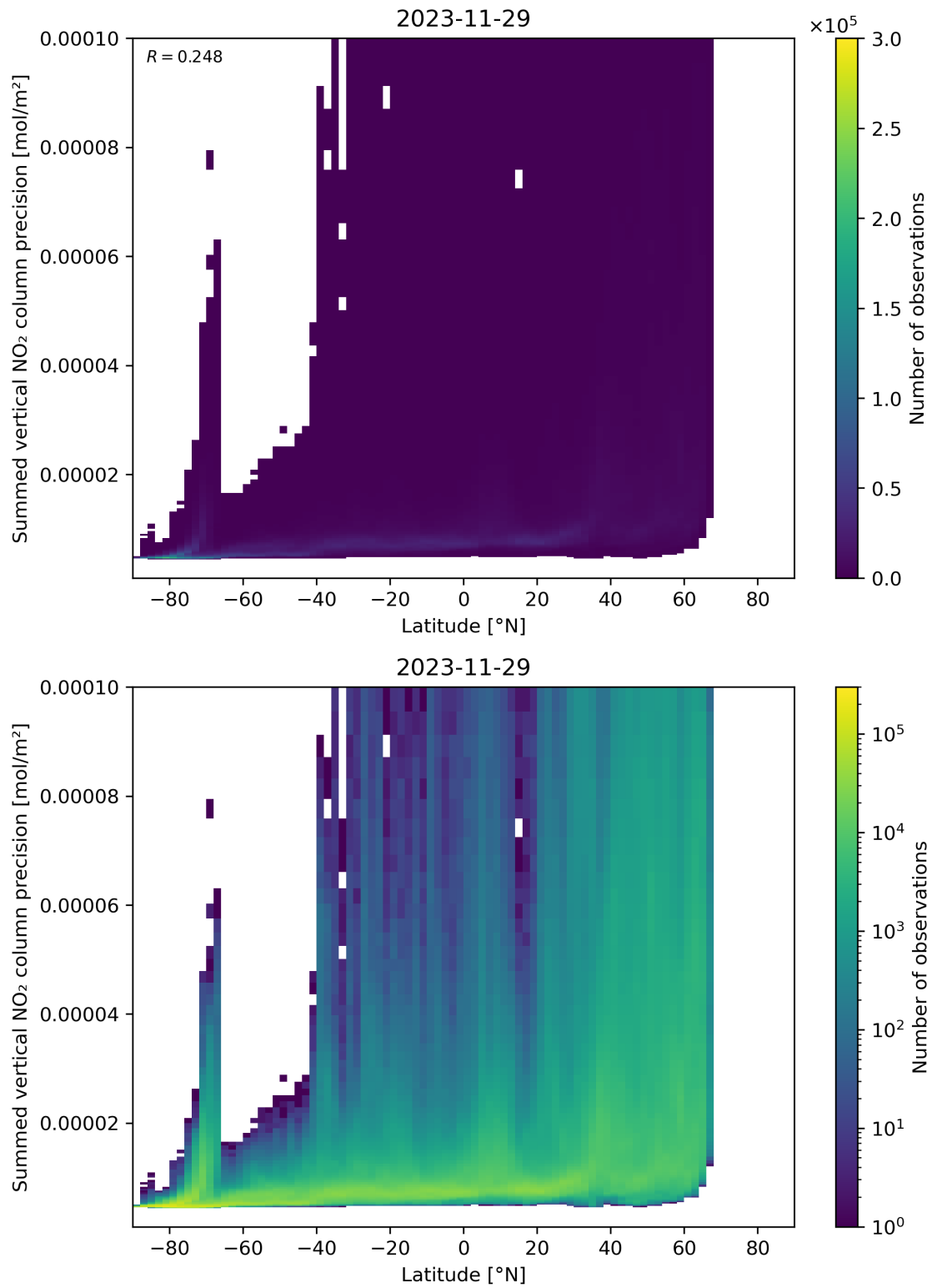
Figure 89: Scatter density plot of “Latitude” against “Summed vertical NO 2 column precision” for 2023-11-28 to 2023-11-30.
