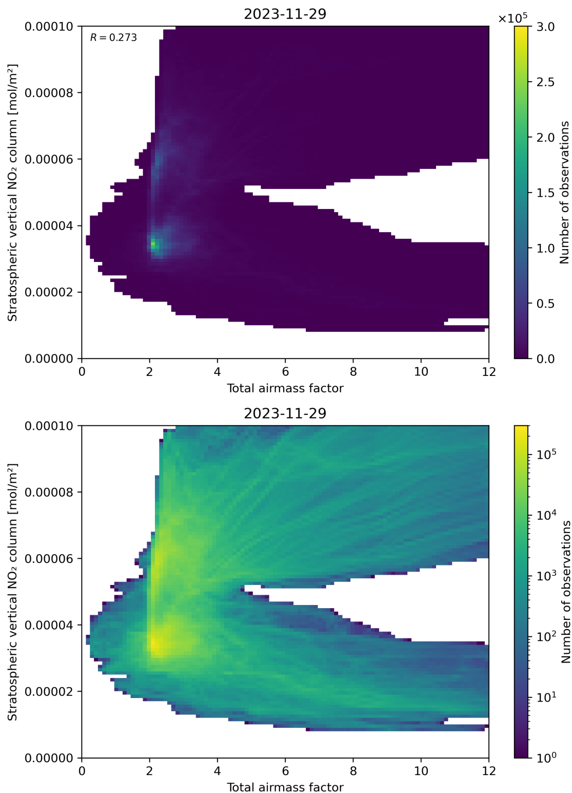
Figure 64: Scatter density plot of “Total airmass factor” against “Stratospheric vertical NO 2 column” for 2023-11-28 to 2023-11-30.
