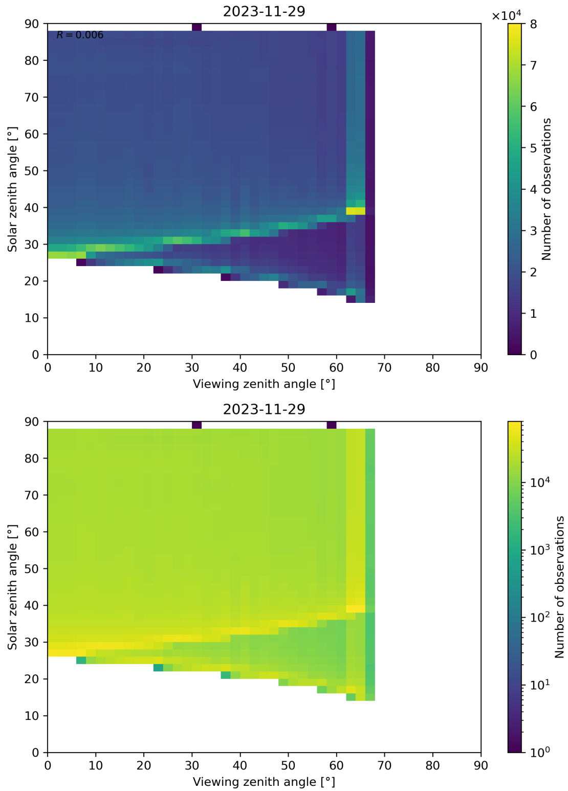
Figure 172: Scatter density plot of “Viewing zenith angle” against “Solar zenith angle” for 2023-11-28 to 2023-11-30.
