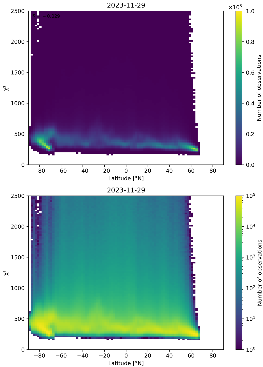
Figure 86: Scatter density plot of “Latitude” against “ \chi^2 ” for 2023-11-28 to 2023-11-30.
