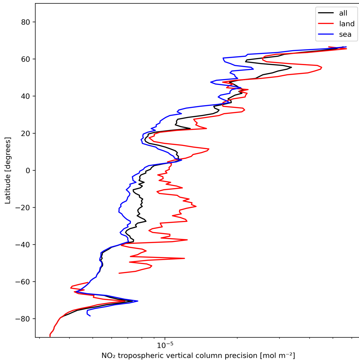
Figure 13: Zonal average of “NO 2 tropospheric vertical column precision” for 2023-11-28 to 2023-11-30.
