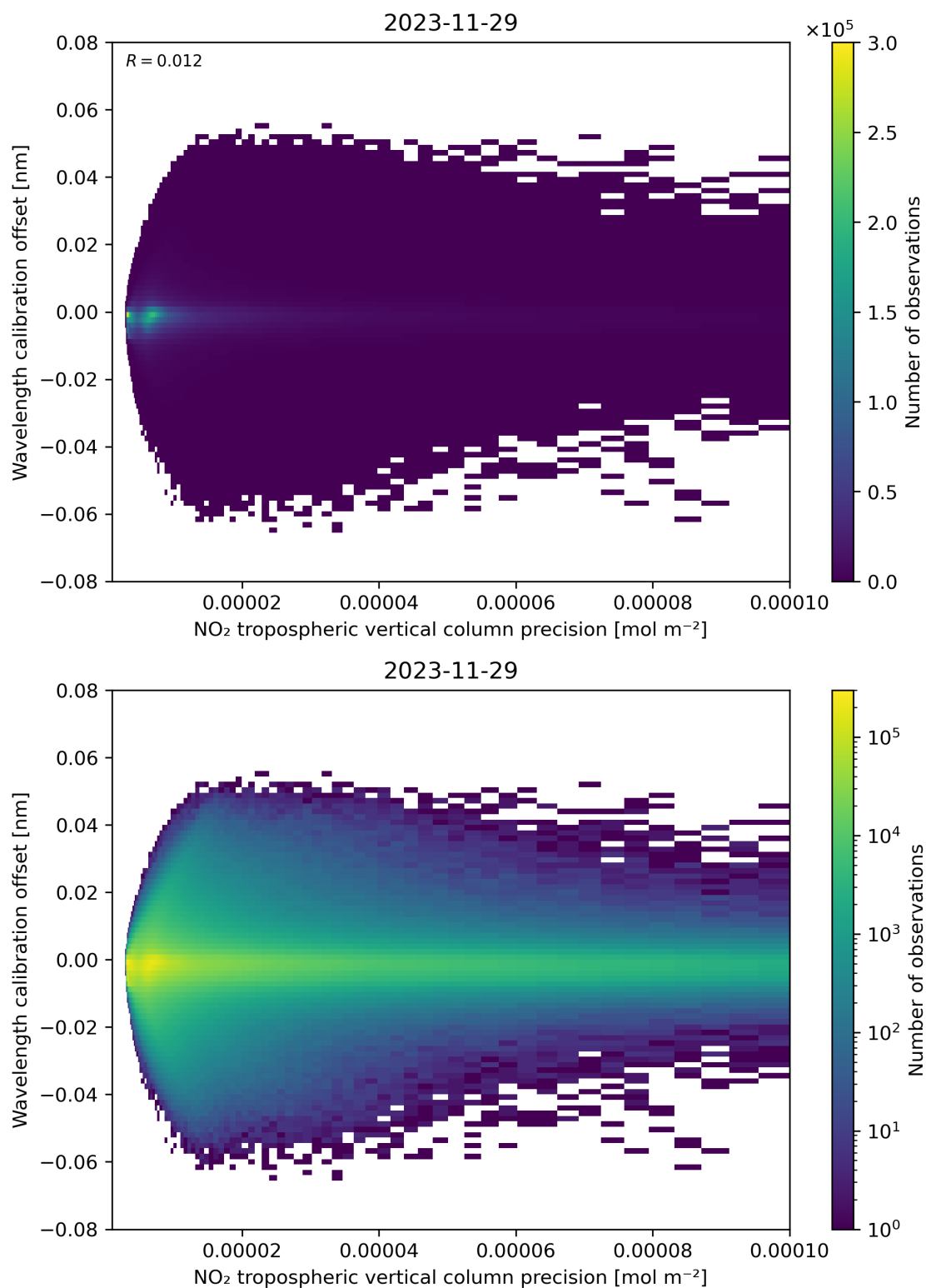
Figure 141: Scatter density plot of “NO 2 tropospheric vertical column precision” against “Wavelength calibration offset” for 2023-11-28 to 2023-11-30.
