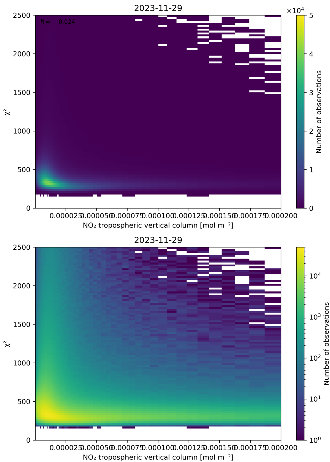
Figure 124: Scatter density plot of “NO 2 tropospheric vertical column” against “ \chi^2 ” for 2023-11-28 to 2023-11-30.
