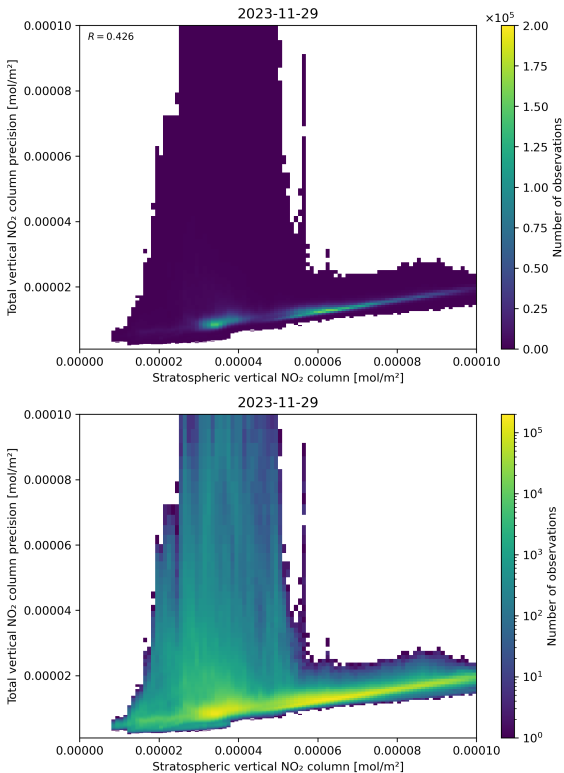
Figure 101: Scatter density plot of “Stratospheric vertical NO 2 column” against “Total vertical NO 2 column precision” for 2023-11-28 to 2023-11-30.
