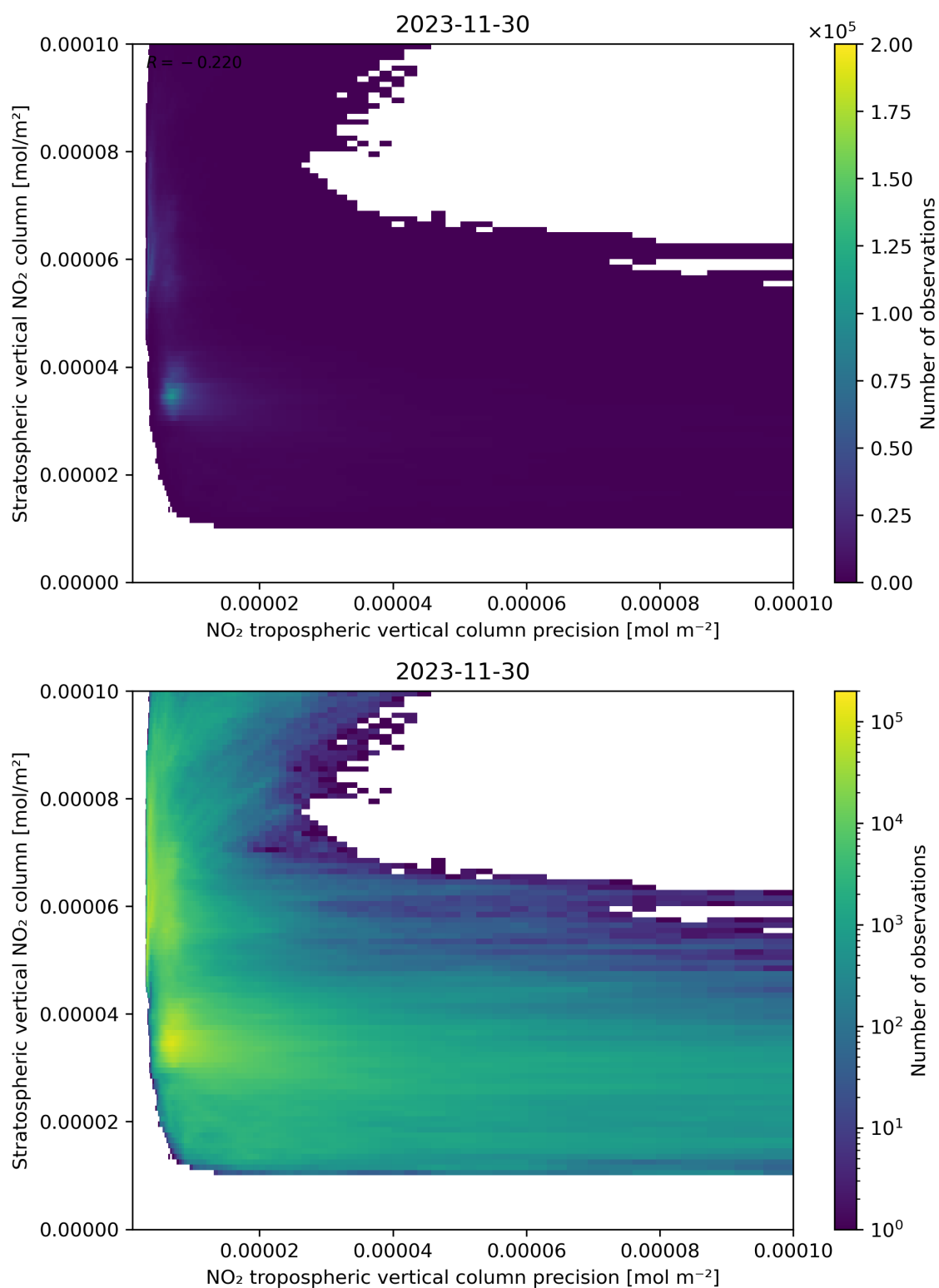
Figure 135: Scatter density plot of “NO 2 tropospheric vertical column precision” against “Stratospheric vertical NO 2 column” for 2023-11-29 to 2023-12-01.
