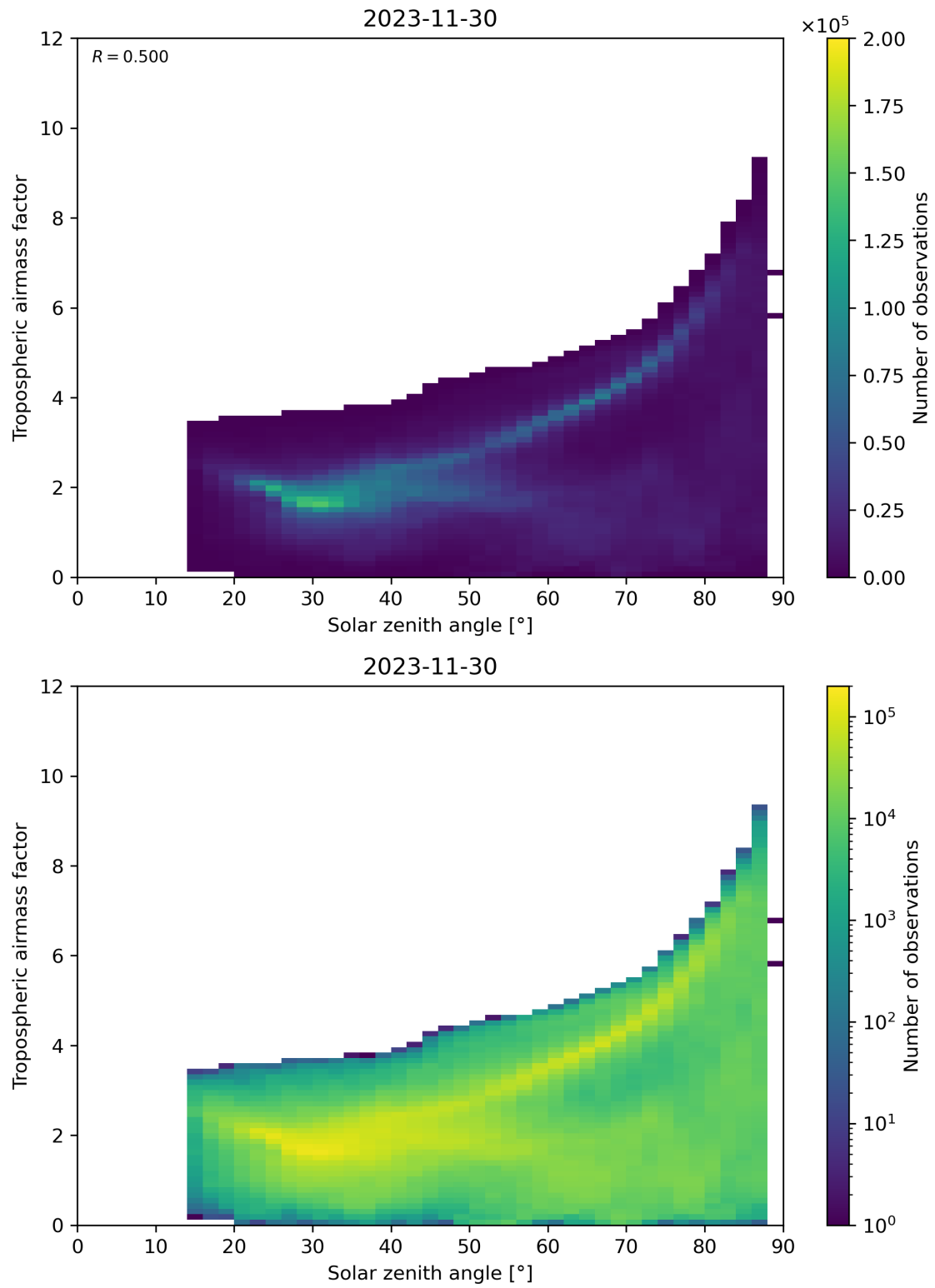
Figure 147: Scatter density plot of “Solar zenith angle” against “Tropospheric airmass factor” for 2023-11-29 to 2023-12-01.
