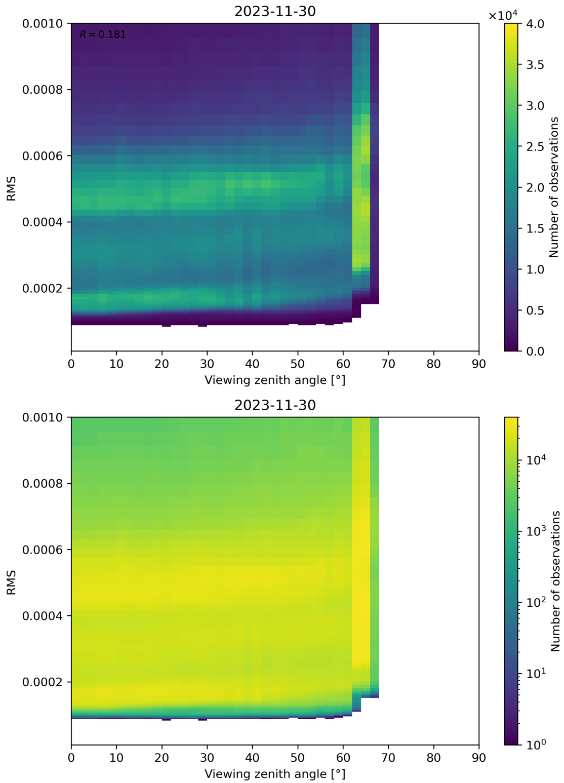
Figure 171: Scatter density plot of “Viewing zenith angle” against “RMS” for 2023-11-29 to 2023-12-01.
