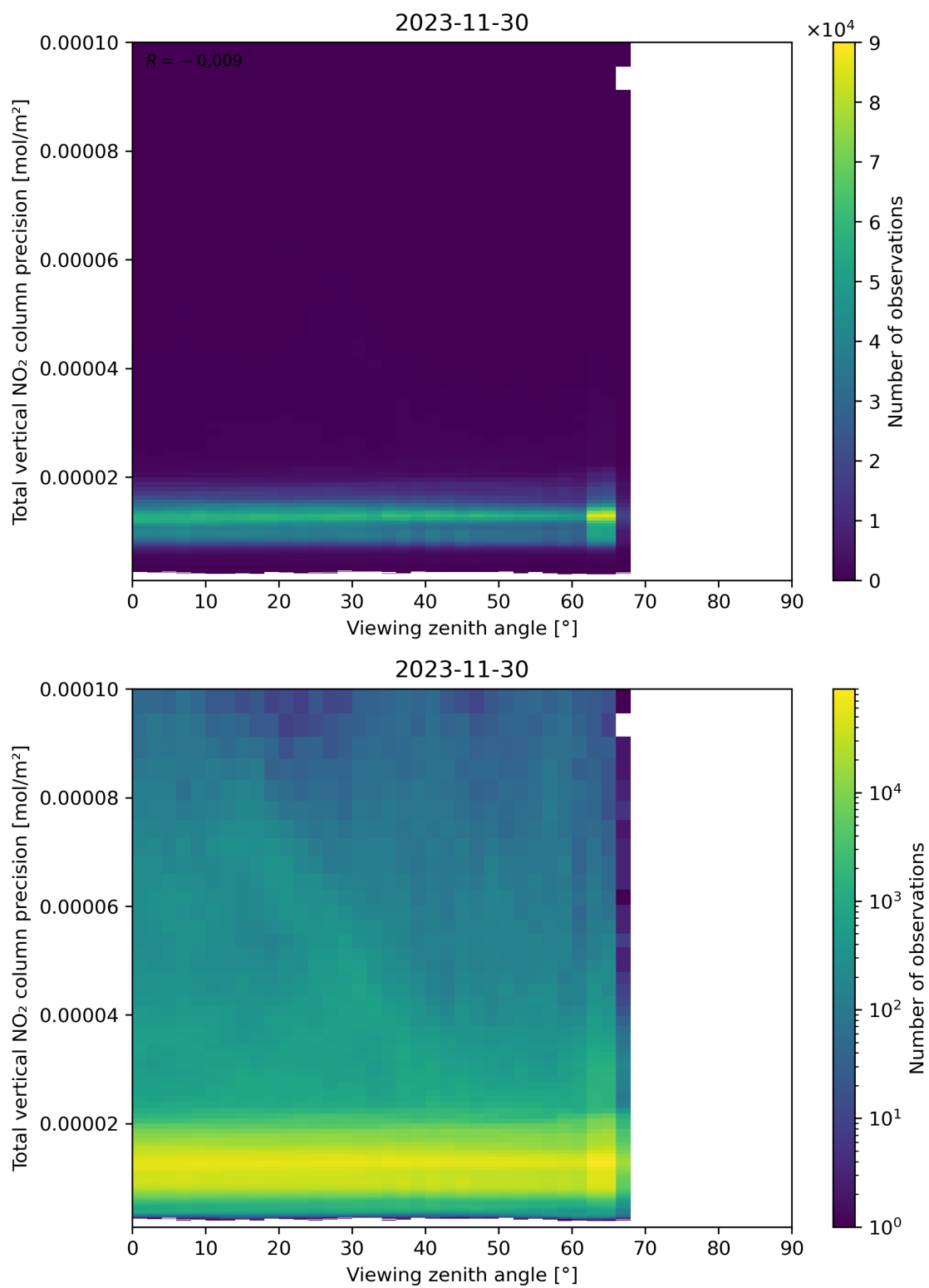
Figure 168: Scatter density plot of “Viewing zenith angle” against “Total vertical NO 2 column precision” for 2023-11-29 to 2023-12-01.
