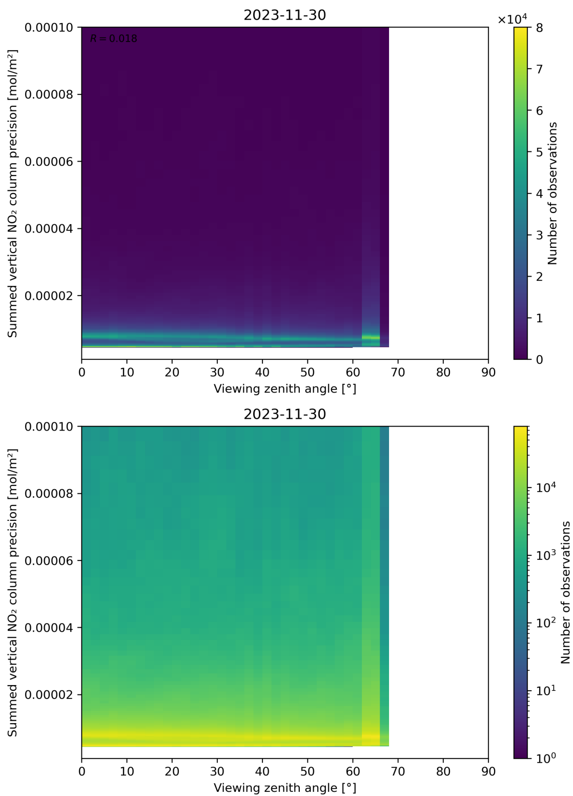
Figure 166: Scatter density plot of “Viewing zenith angle” against “Summed vertical NO 2 column precision” for 2023-11-29 to 2023-12-01.
