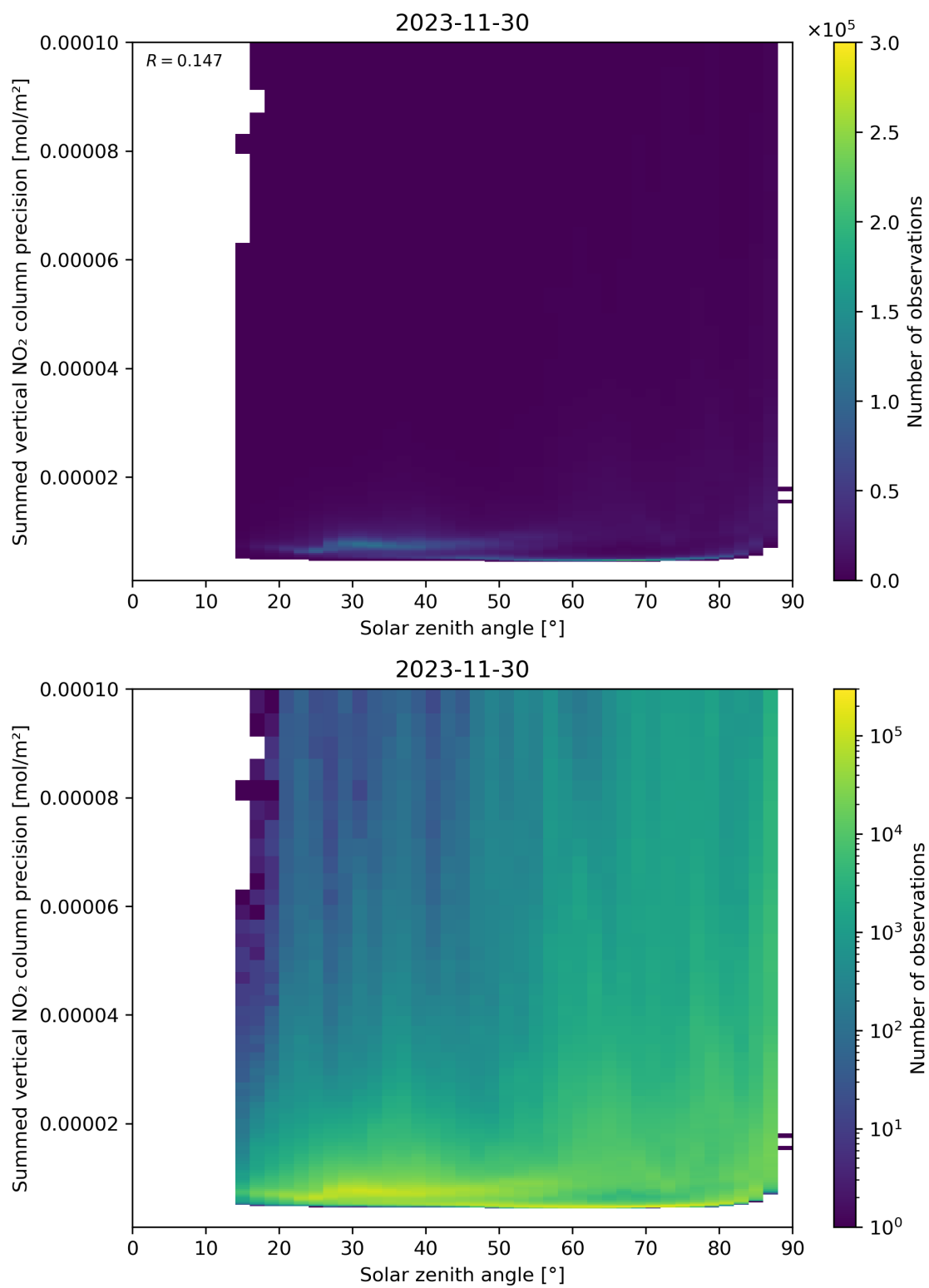
Figure 152: Scatter density plot of “Solar zenith angle” against “Summed vertical NO 2 column precision” for 2023-11-29 to 2023-12-01.
