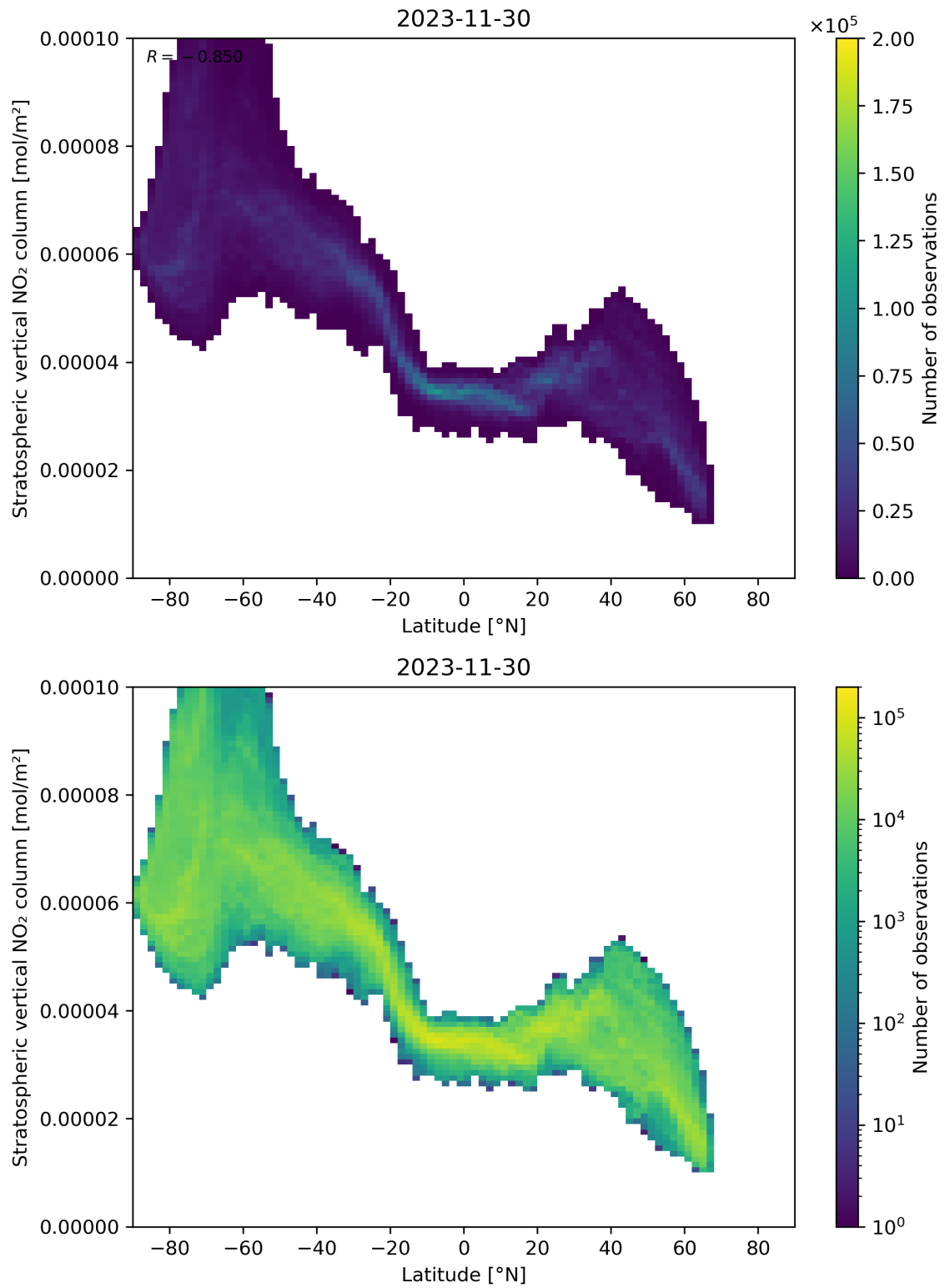
Figure 87: Scatter density plot of “Latitude” against “Stratospheric vertical NO 2 column” for 2023-11-29 to 2023-12-01.
