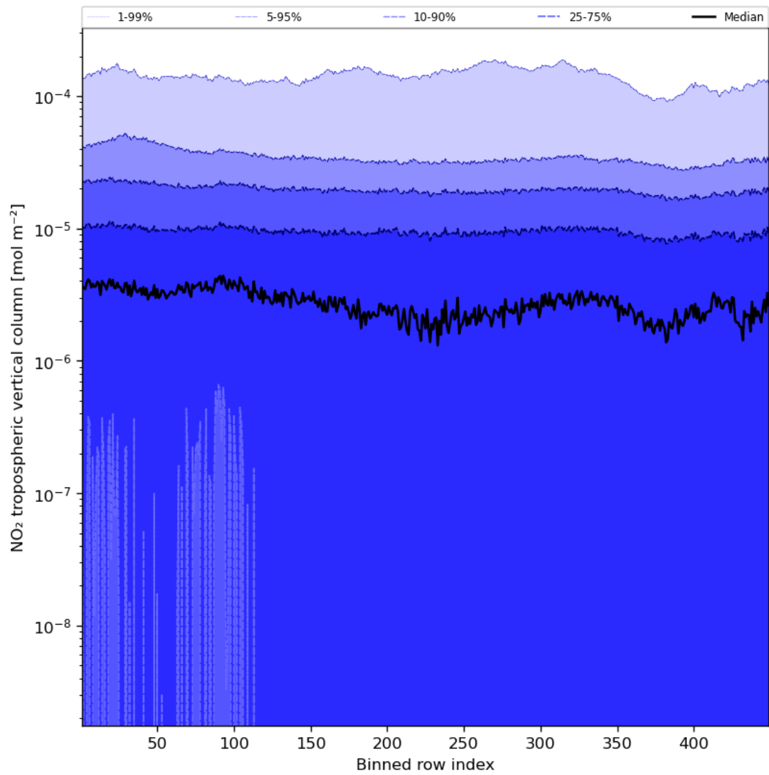
Figure 46: Along track statistics of “NO 2 tropospheric vertical column” for 2023-11-29 to 2023-12-01
