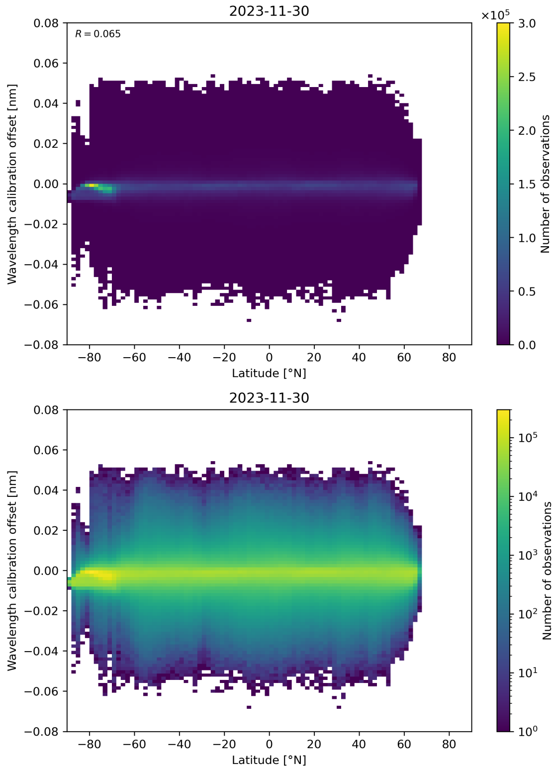
Figure 95: Scatter density plot of “Latitude” against “Wavelength calibration offset” for 2023-11-29 to 2023-12-01.
