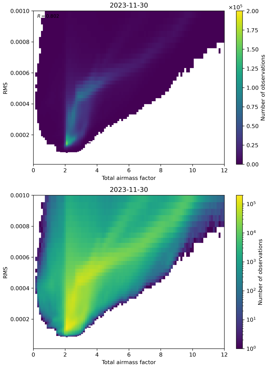
Figure 69: Scatter density plot of “Total airmass factor” against “RMS” for 2023-11-29 to 2023-12-01.
