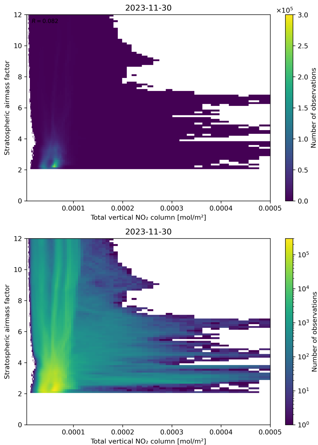
Figure 110: Scatter density plot of “Total vertical NO 2 column” against “Stratospheric airmass factor” for 2023-11-29 to 2023-12-01.
