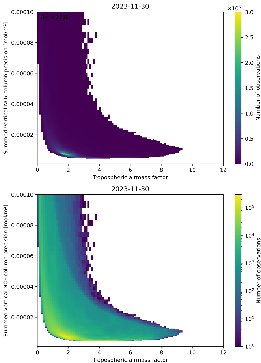
Figure 76: Scatter density plot of “Tropospheric air mass factor” against “Summed vertical NO 2 column precision” for 2023-11-29 to 2023-12-01.
