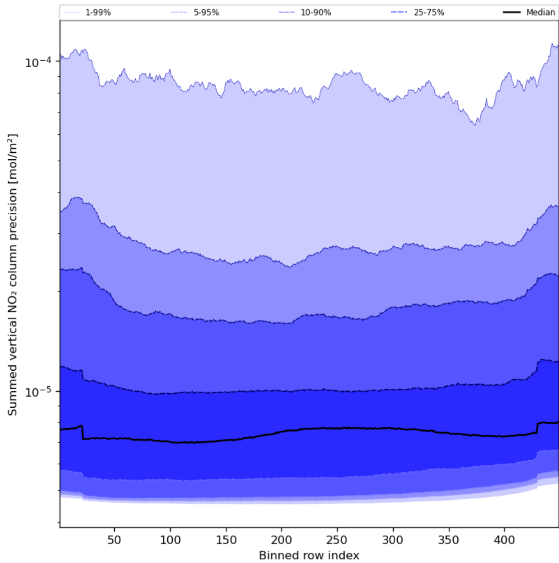
Figure 58: Along track statistics of “Summed vertical NO 2 column precision” for 2023-11-29 to 2023-12-01
