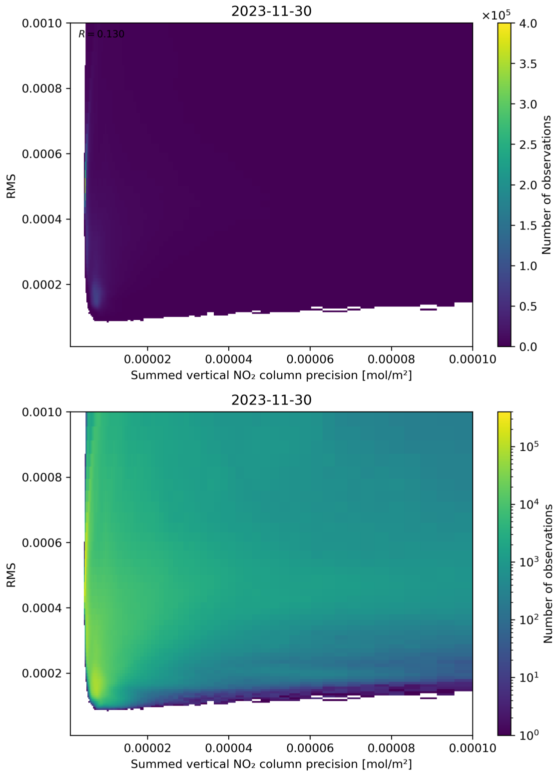
Figure 108: Scatter density plot of “Summed vertical NO 2 column precision” against “RMS” for 2023-11-29 to 2023-12-01.
