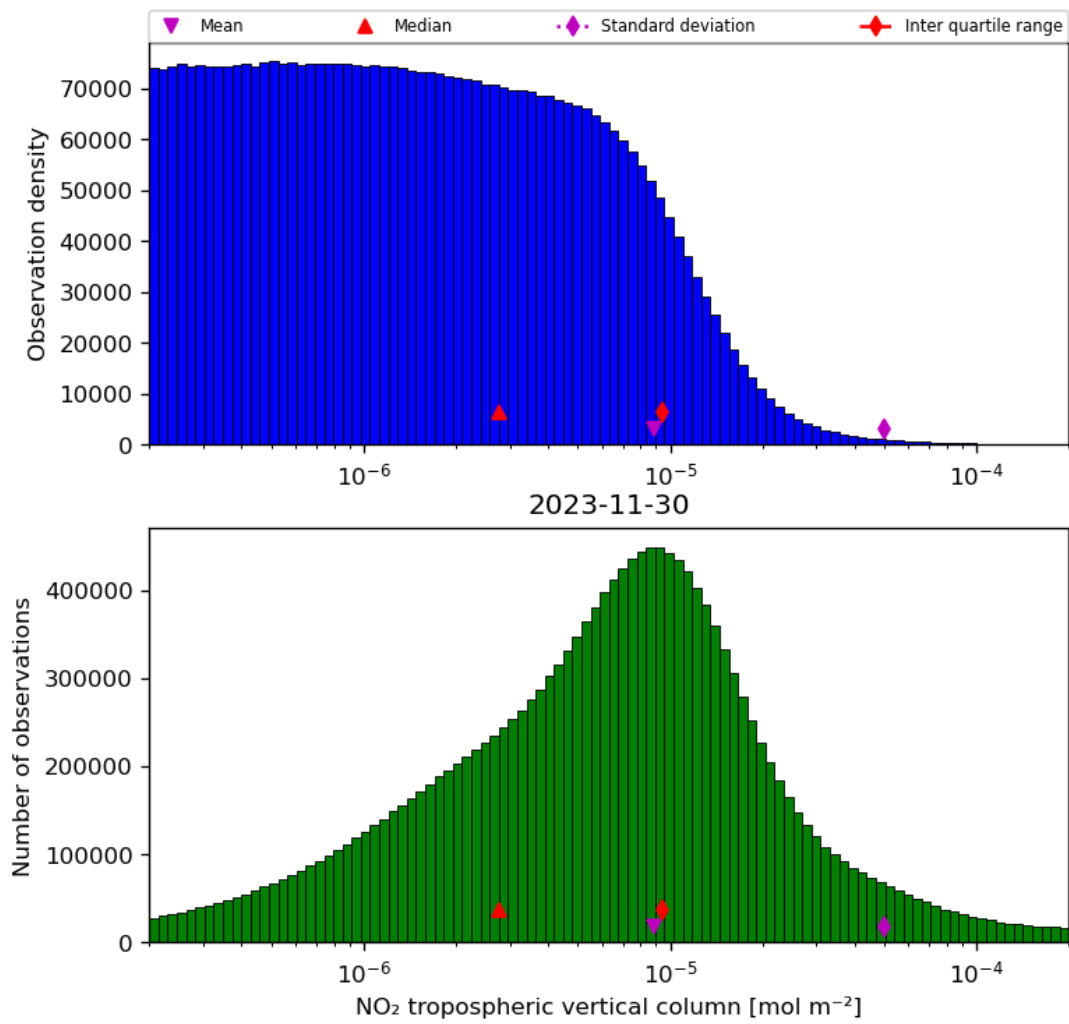
Figure 29: Histogram of “NO 2 tropospheric vertical column” for 2023-11-29 to 2023-12-01
