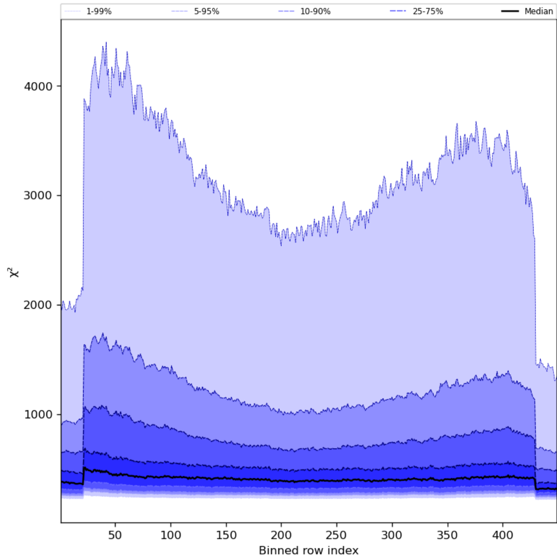
Figure 59: Along track statistics of “ \chi^2 ” for 2023-11-29 to 2023-12-01
