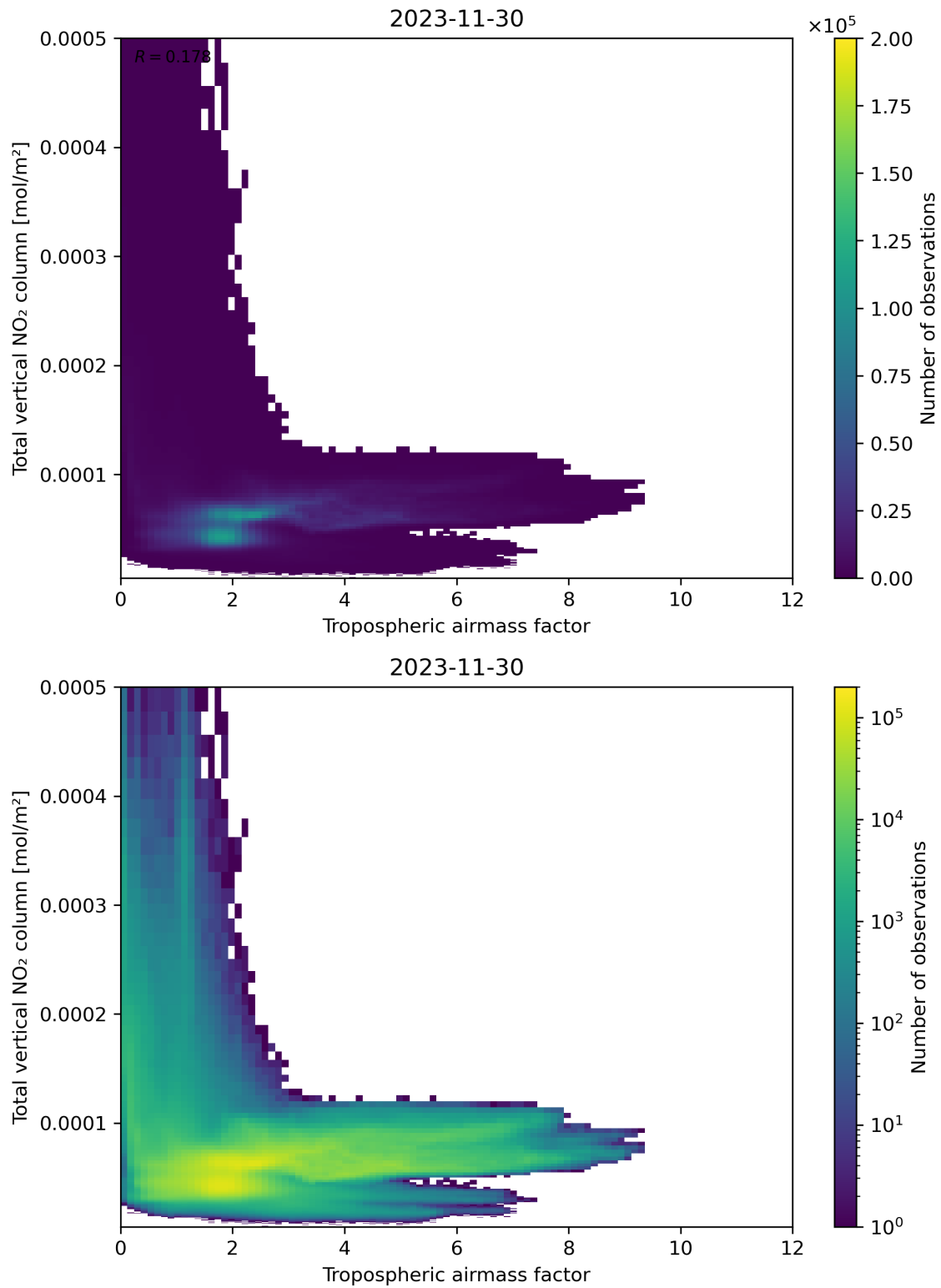
Figure 77: Scatter density plot of “Tropospheric airmass factor” against “Total vertical NO 2 column” for 2023-11-29 to 2023-12-01.
