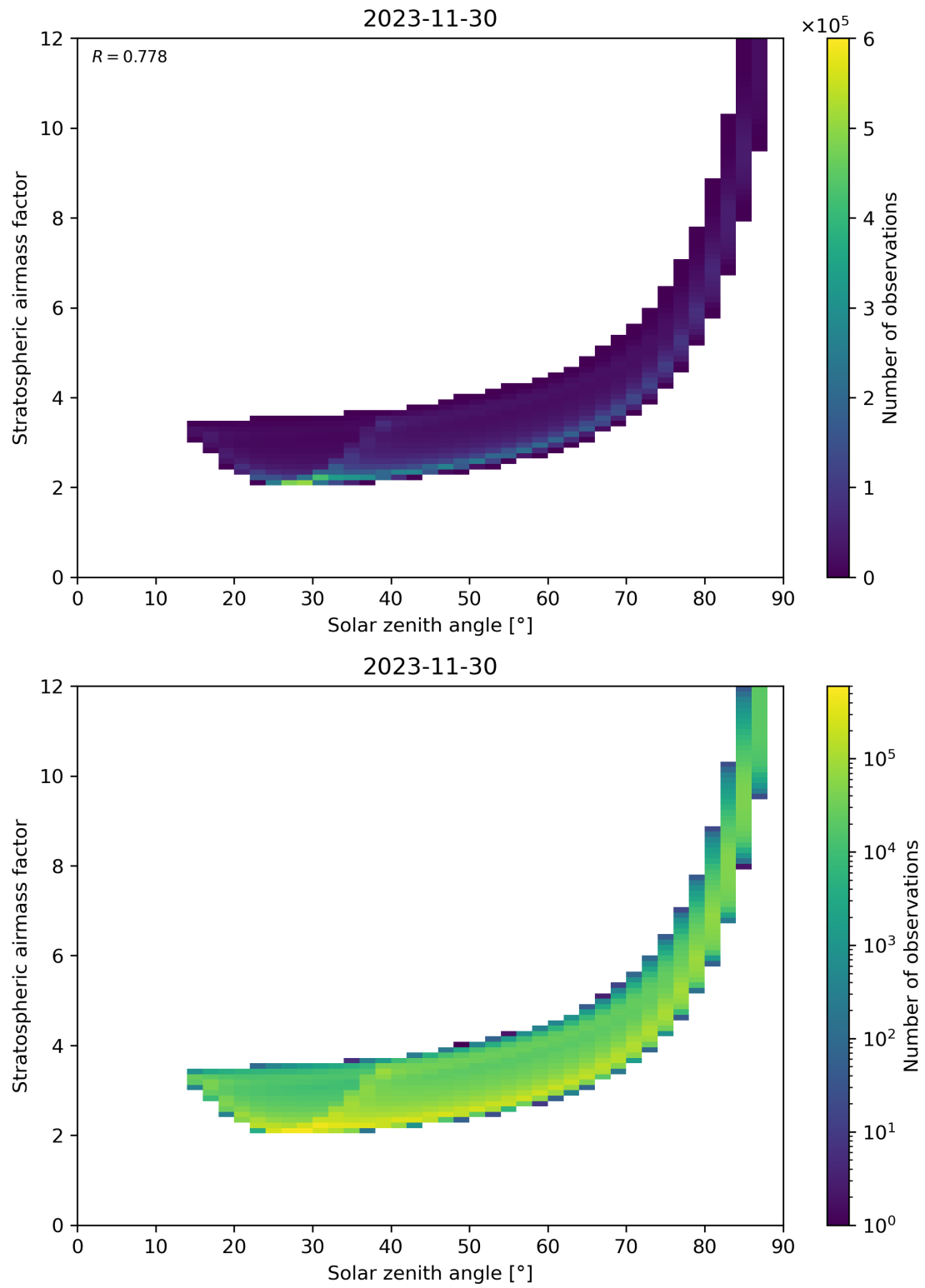
Figure 145: Scatter density plot of “Solar zenith angle” against “Stratospheric airmass factor” for 2023-11-29 to 2023-12-01.
