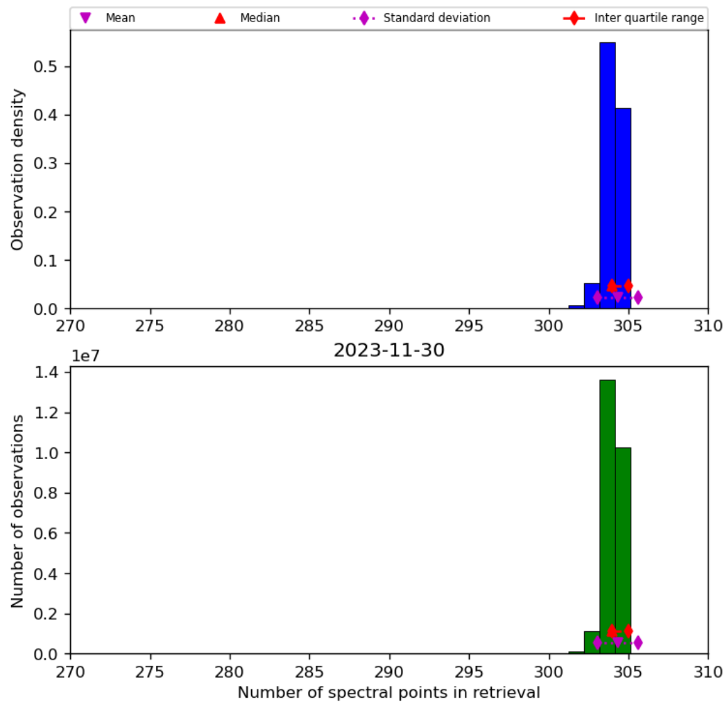
Figure 33: Histogram of “Number of spectral points in retrieval” for 2023-11-29 to 2023-12-01
