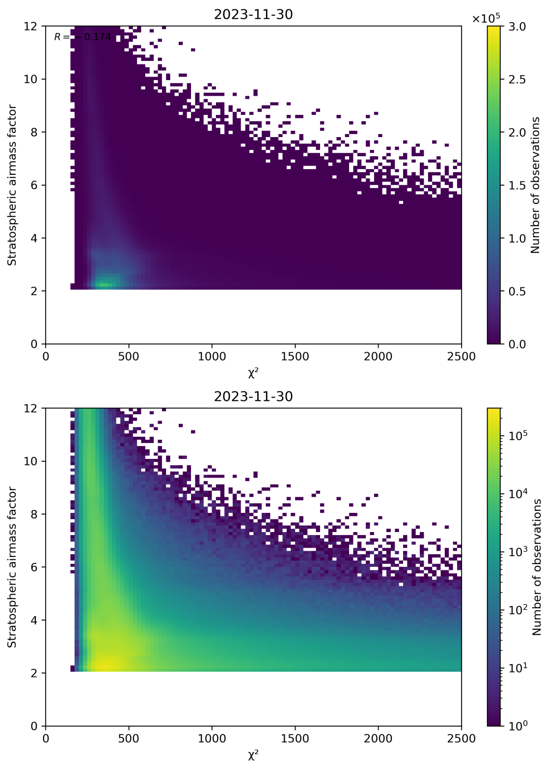
Figure 81: Scatter density plot of “ \chi^2 ” against “Stratospheric air mass factor” for 2023-11-29 to 2023-12-01.
