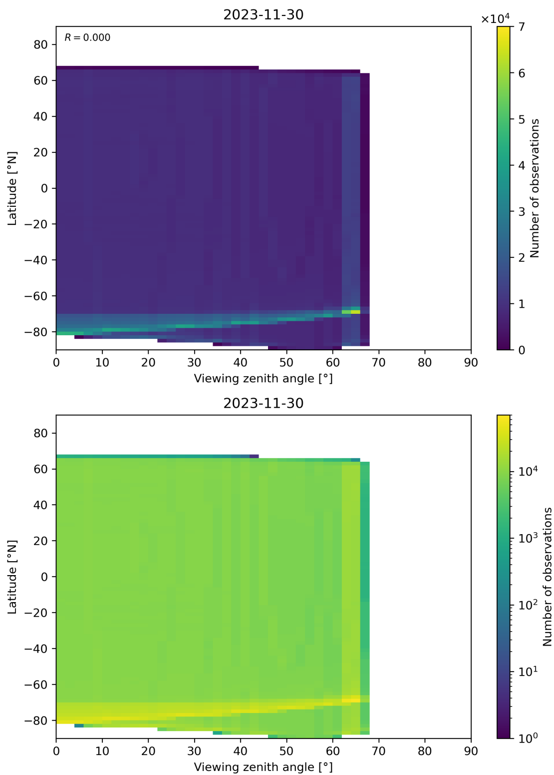
Figure 163: Scatter density plot of “Viewing zenith angle” against “Latitude” for 2023-11-29 to 2023-12-01.
