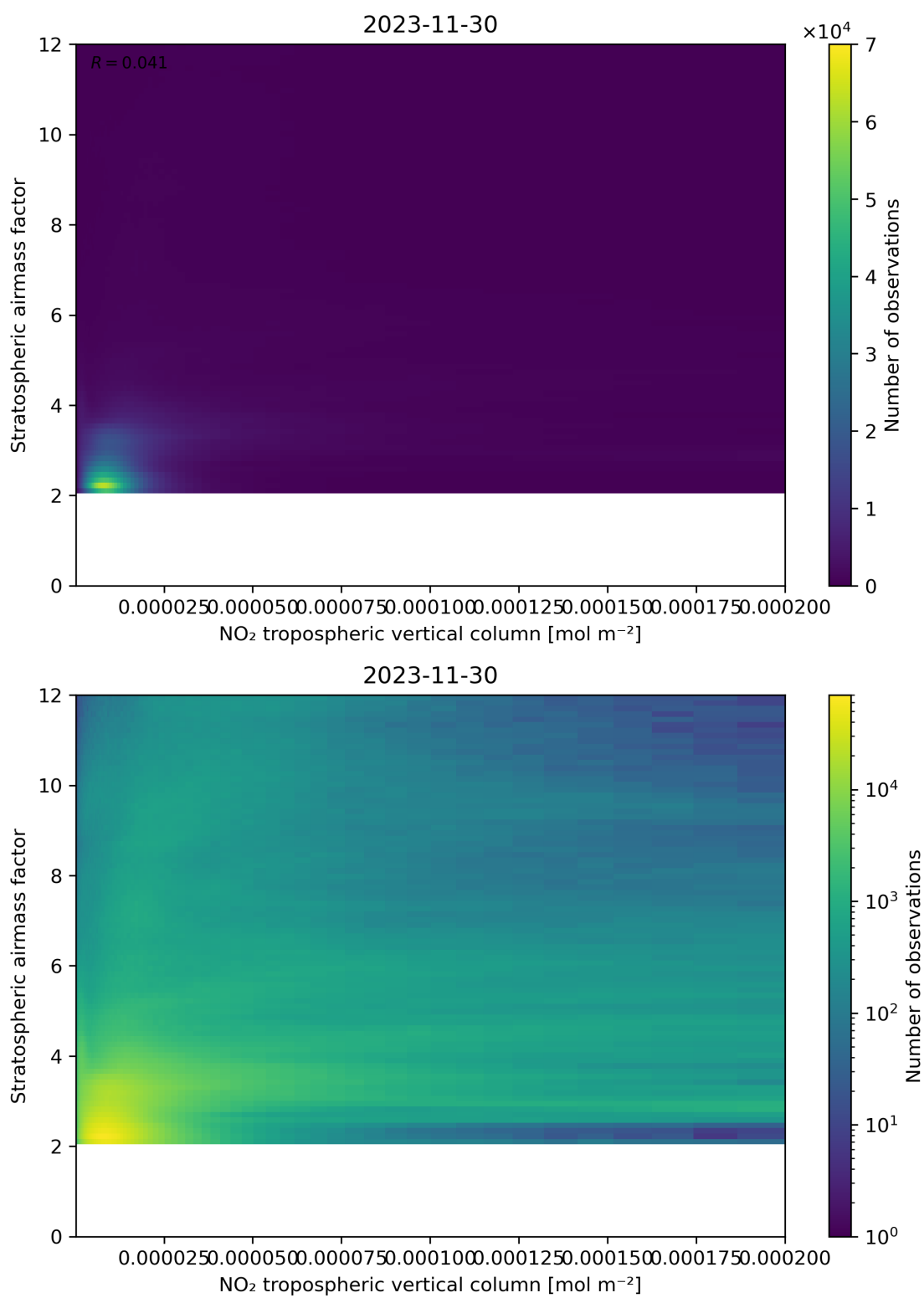
Figure 121: Scatter density plot of “NO 2 tropospheric vertical column” against “Stratospheric airmass factor” for 2023-11-29 to 2023-12-01.
