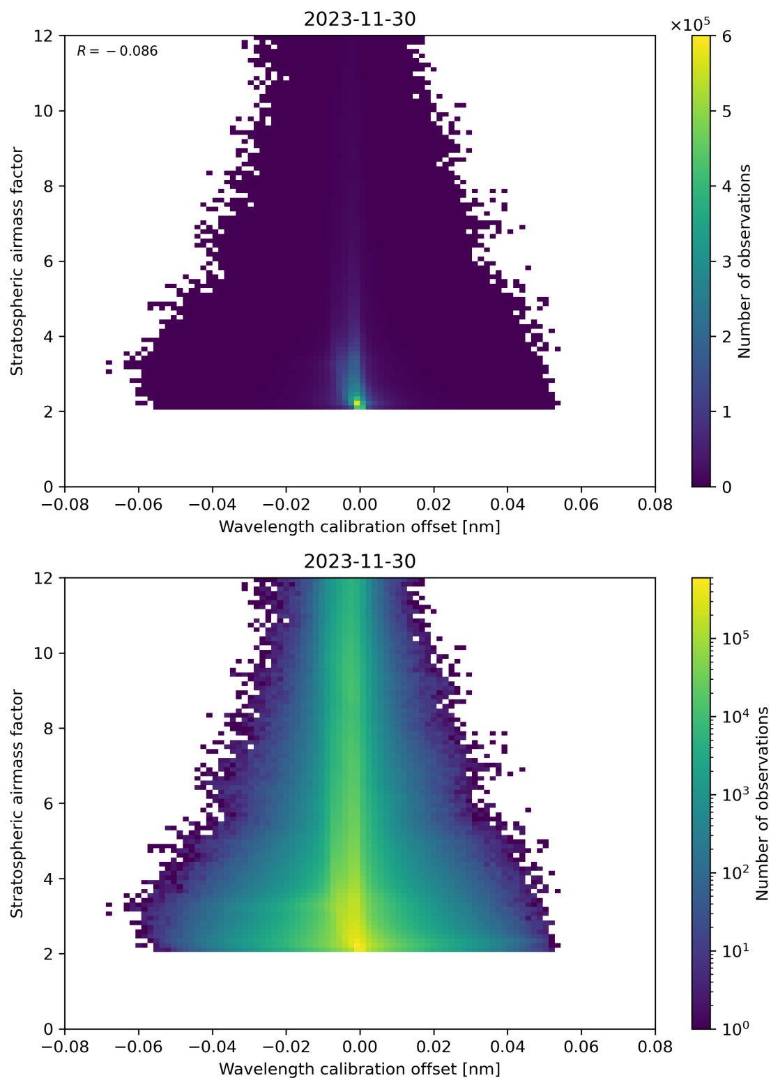
Figure 174: Scatter density plot of “Wavelength calibration offset” against “Stratospheric airmass factor” for 2023-11-29 to 2023-12-01.
