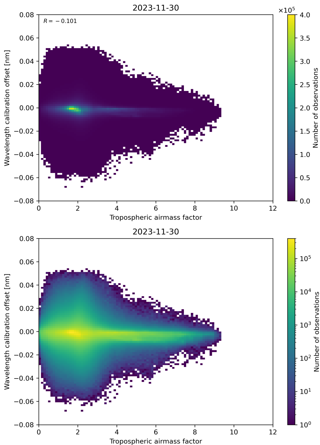
Figure 80: Scatter density plot of “Tropospheric air mass factor” against “Wavelength calibration offset” for 2023-11-29 to 2023-12-01.
