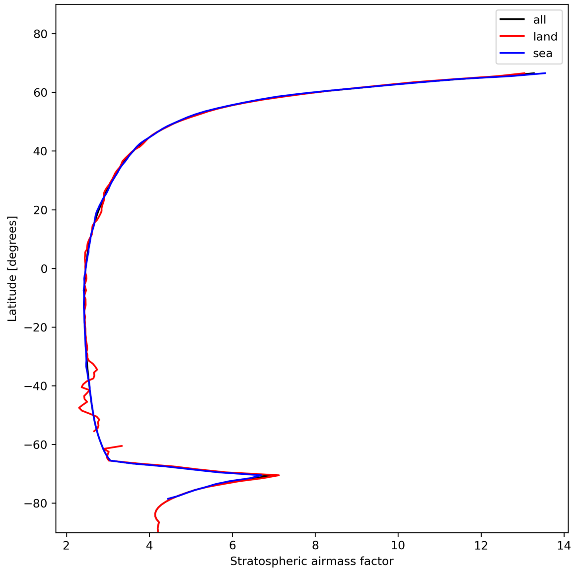
Figure 27: Zonal average of “Stratospheric airmass factor” for 2023-11-29 to 2023-12-01.
