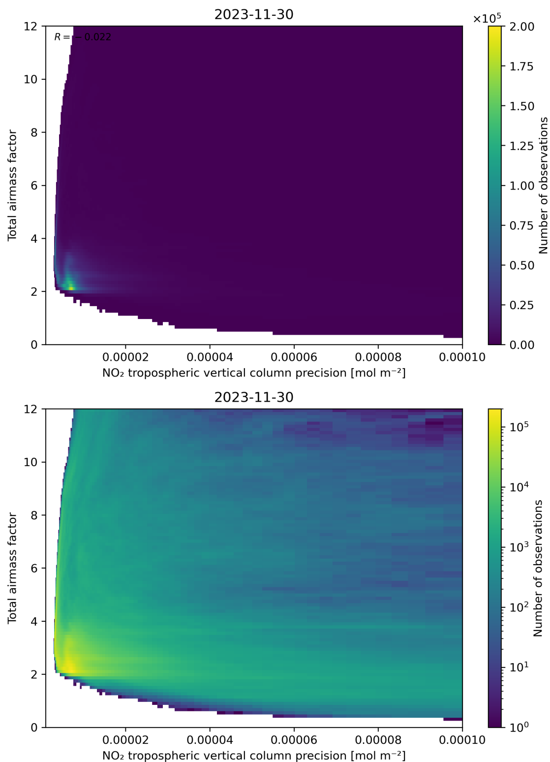
Figure 132: Scatter density plot of “NO 2 tropospheric vertical column precision” against “Total air mass factor” for 2023-11-29 to 2023-12-01.
