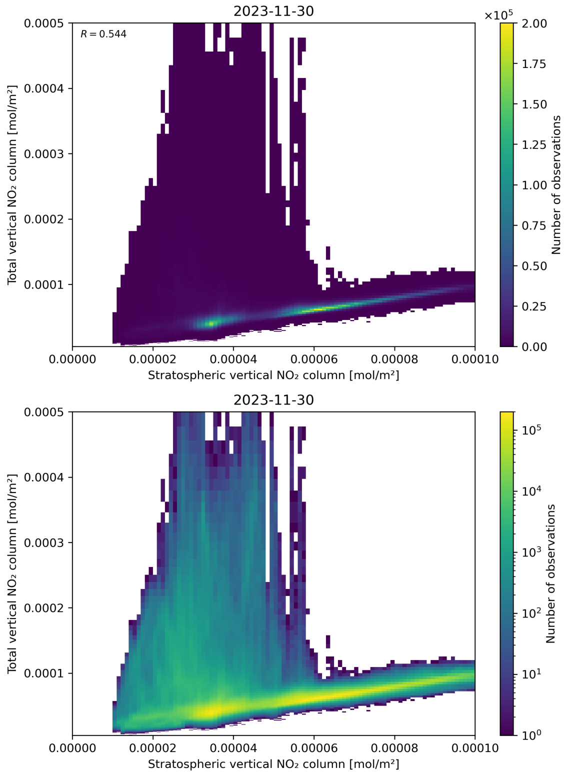
Figure 100: Scatter density plot of “Stratospheric vertical NO 2 column” against “Total vertical NO 2 column” for 2023-11-29 to 2023-12-01.
