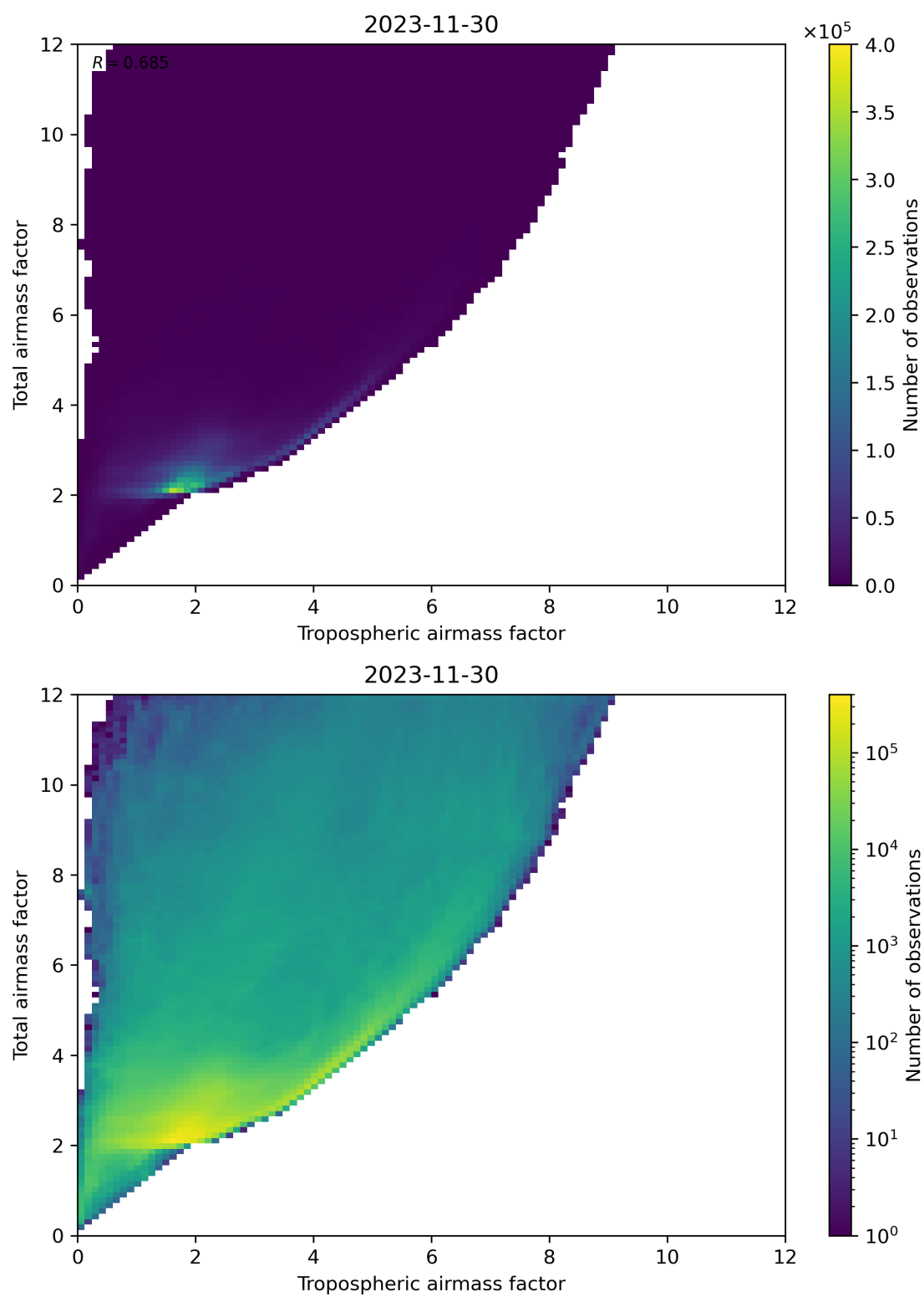
Figure 72: Scatter density plot of “Tropospheric airmass factor” against “Total airmass factor” for 2023-11-29 to 2023-12-01.
