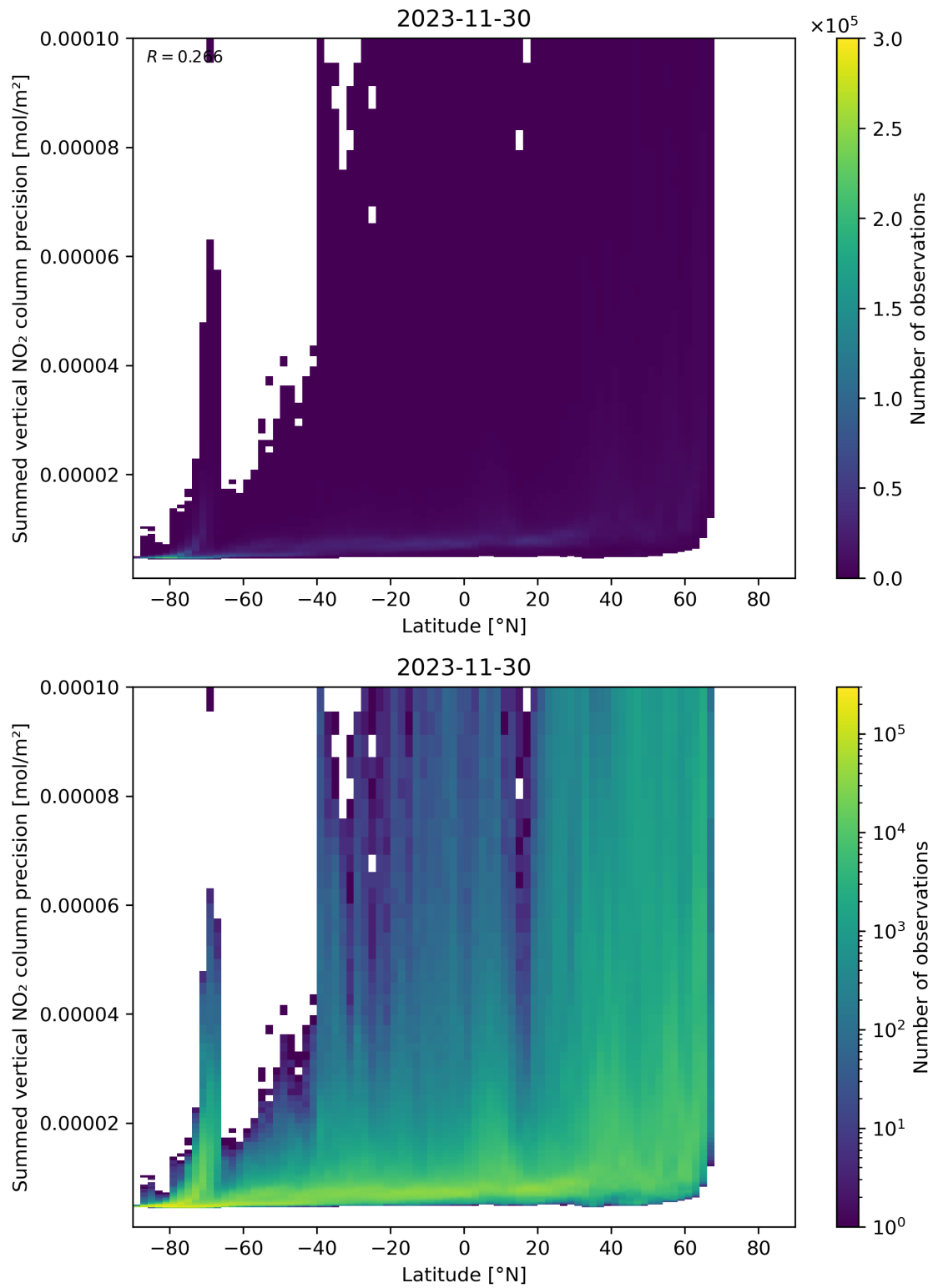
Figure 89: Scatter density plot of “Latitude” against “Summed vertical NO 2 column precision” for 2023-11-29 to 2023-12-01.
