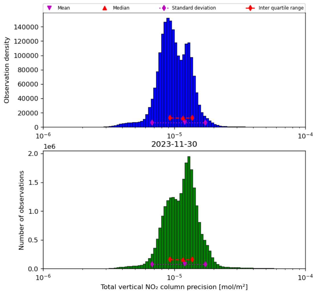
Figure 39: Histogram of “Total vertical NO 2 column precision” for 2023-11-29 to 2023-12-01
