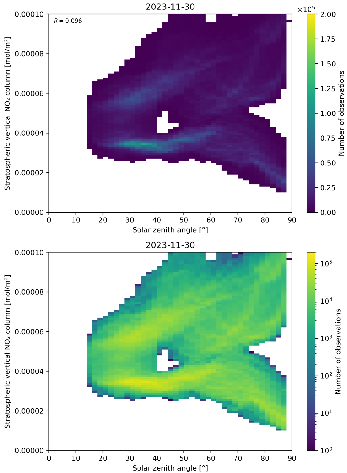
Figure 150: Scatter density plot of “Solar zenith angle” against “Stratospheric vertical NO 2 column” for 2023-11-29 to 2023-12-01.
