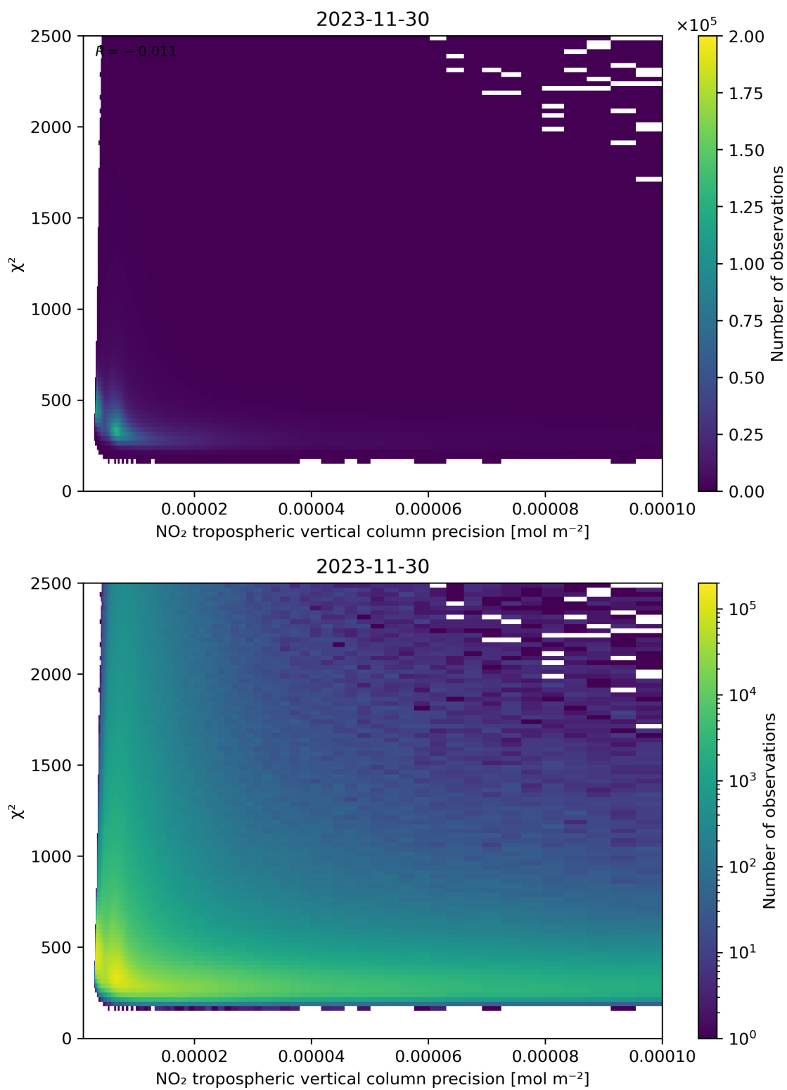
Figure 134: Scatter density plot of “NO 2 tropospheric vertical column precision” against “ \chi^2 ” for 2023-11-29 to 2023-12-01.
