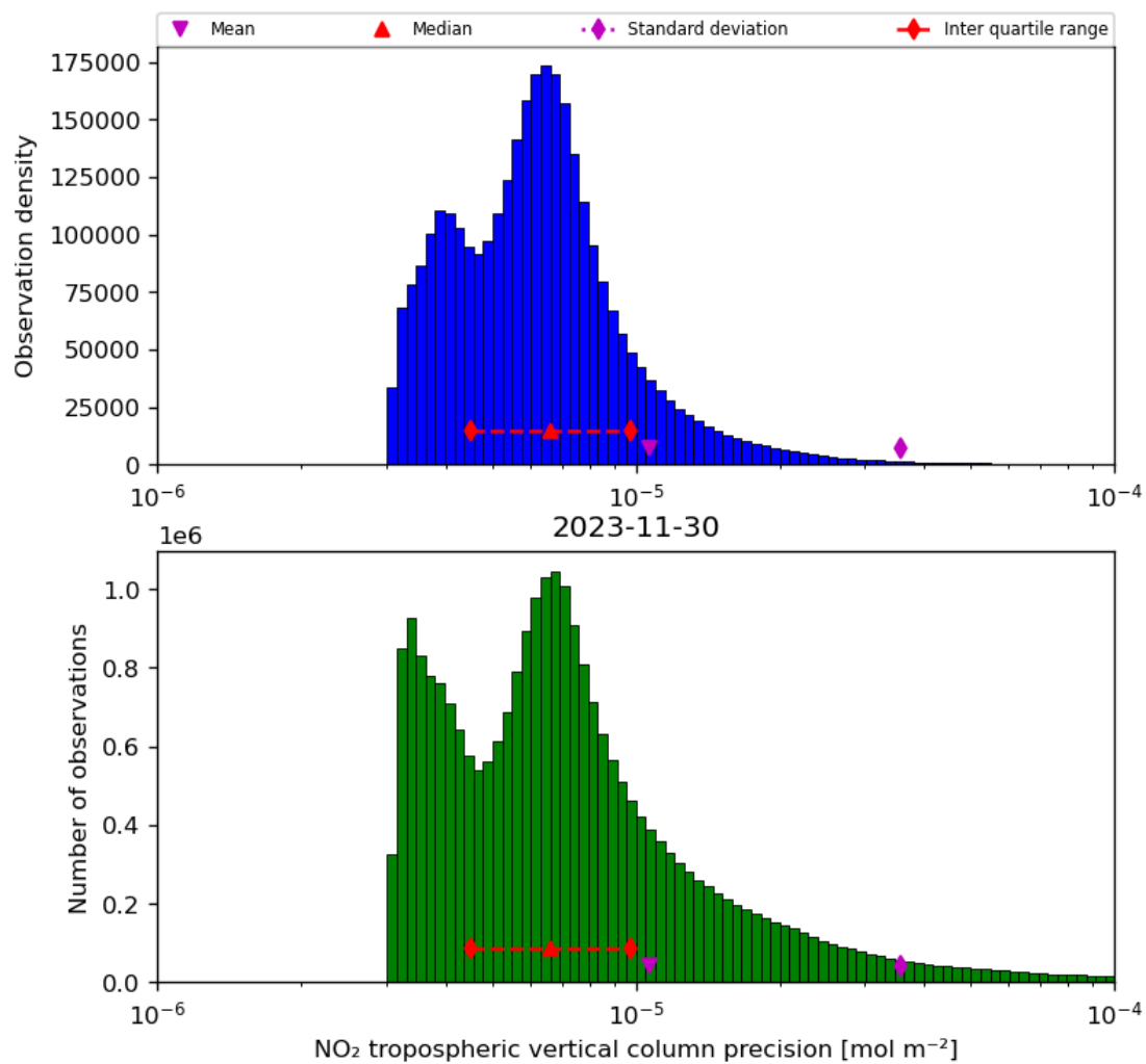
Figure 30: Histogram of “NO 2 tropospheric vertical column precision” for 2023-11-29 to 2023-12-01
