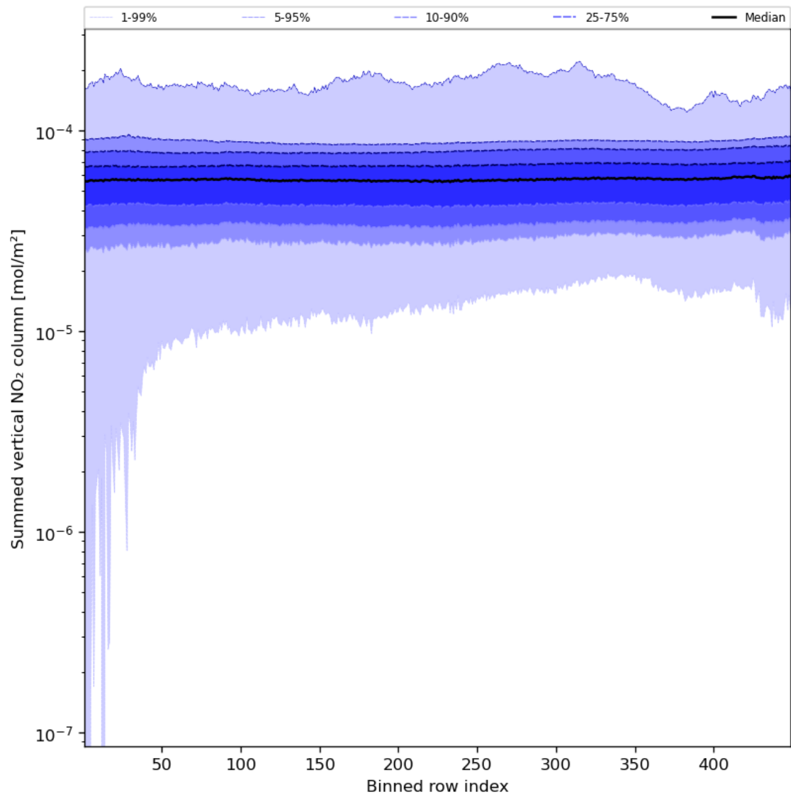
Figure 57: Along track statistics of “Summed vertical NO 2 column” for 2023-11-29 to 2023-12-01
