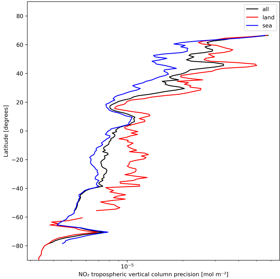
Figure 13: Zonal average of “NO 2 tropospheric vertical column precision” for 2023-11-29 to 2023-12-01.
