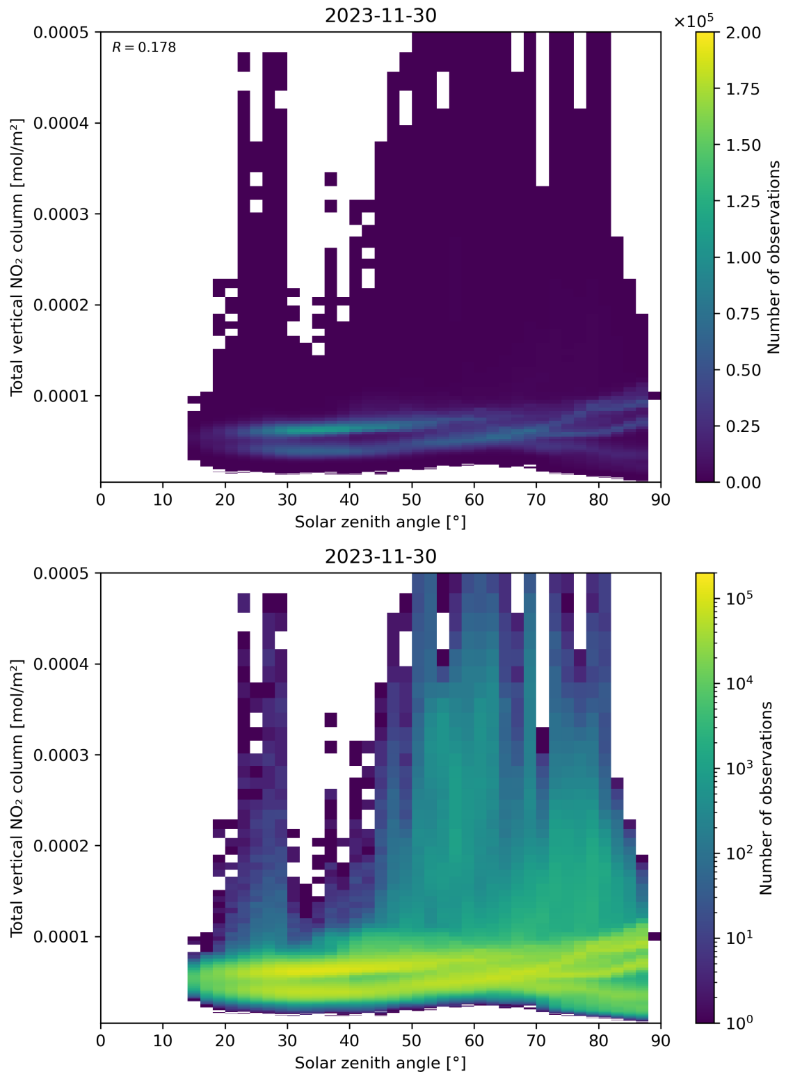
Figure 153: Scatter density plot of “Solar zenith angle” against “Total vertical \text{NO}_2 column” for 2023-11-29 to 2023-12-01.
