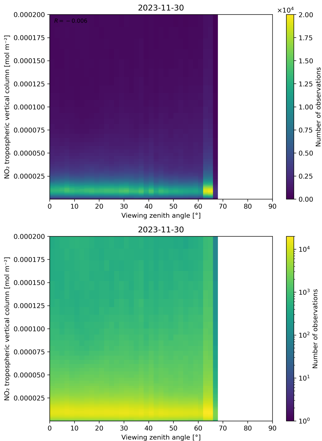
Figure 169: Scatter density plot of “Viewing zenith angle” against “NO 2 tropospheric vertical column” for 2023-11-29 to 2023-12-01.
