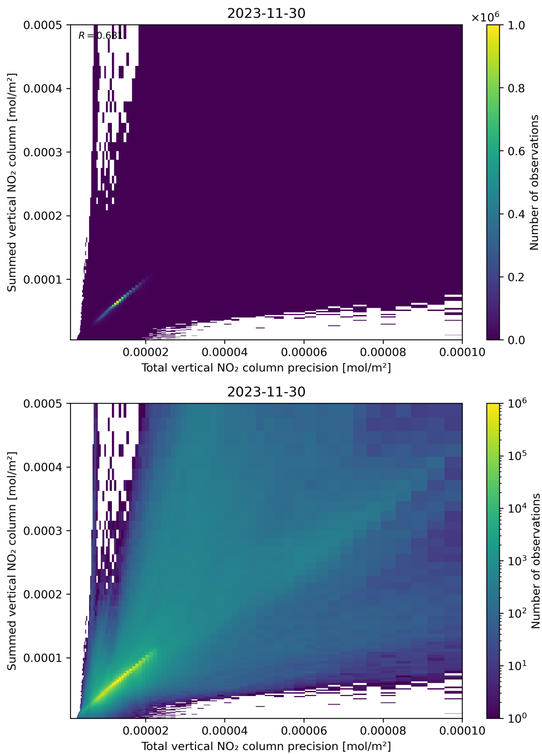
Figure 117: Scatter density plot of “Total vertical NO 2 column precision” against “Summed vertical NO 2 column” for 2023-11-29 to 2023-12-01.
