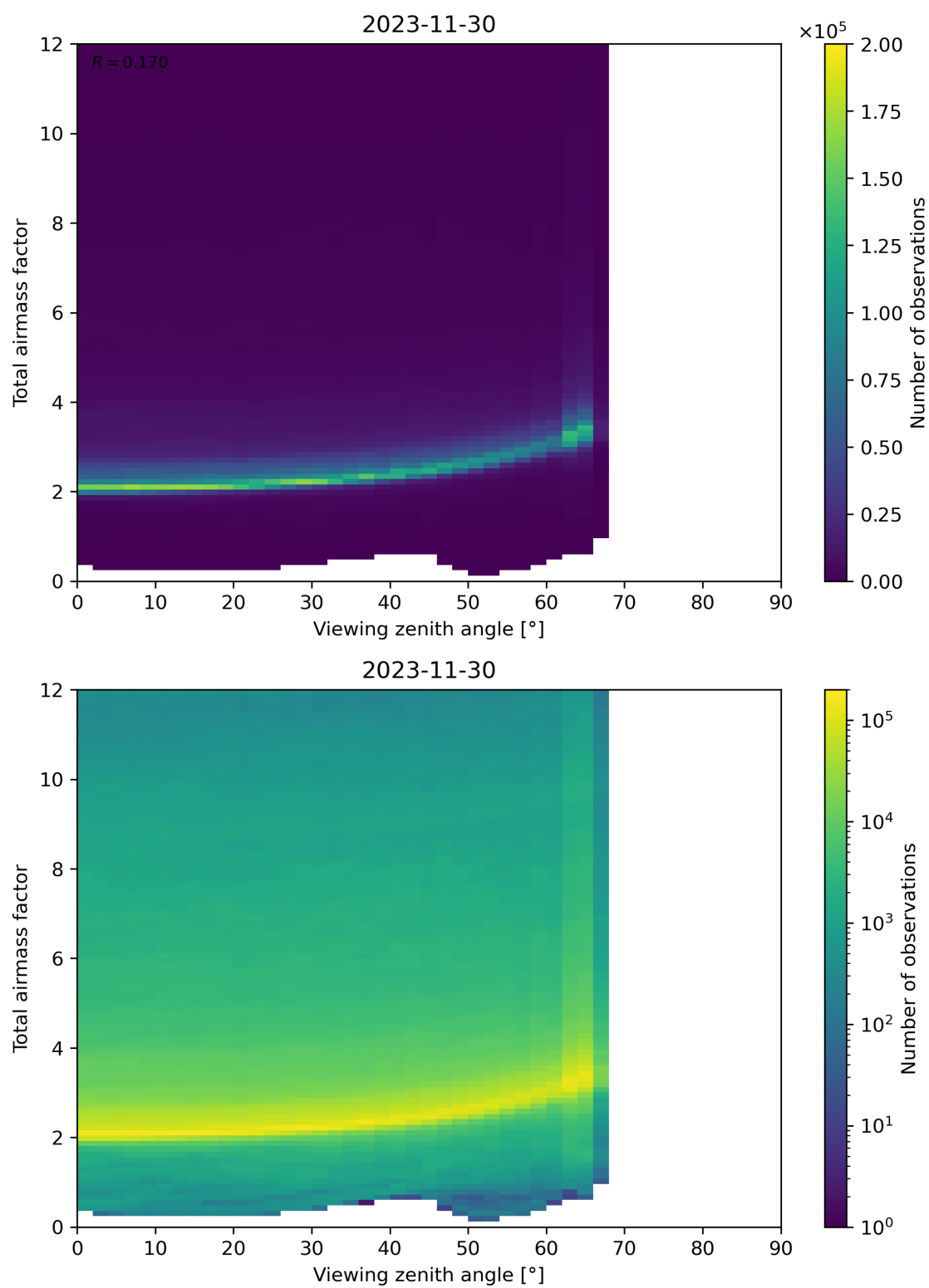
Figure 160: Scatter density plot of “Viewing zenith angle” against “Total airmass factor” for 2023-11-29 to 2023-12-01.
