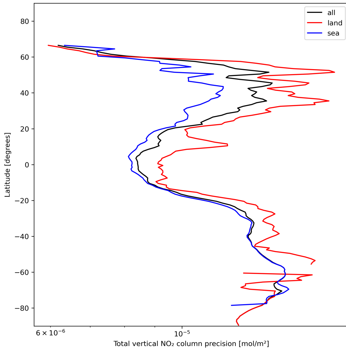
Figure 22: Zonal average of “Total vertical NO 2 column precision” for 2023-11-29 to 2023-12-01.
