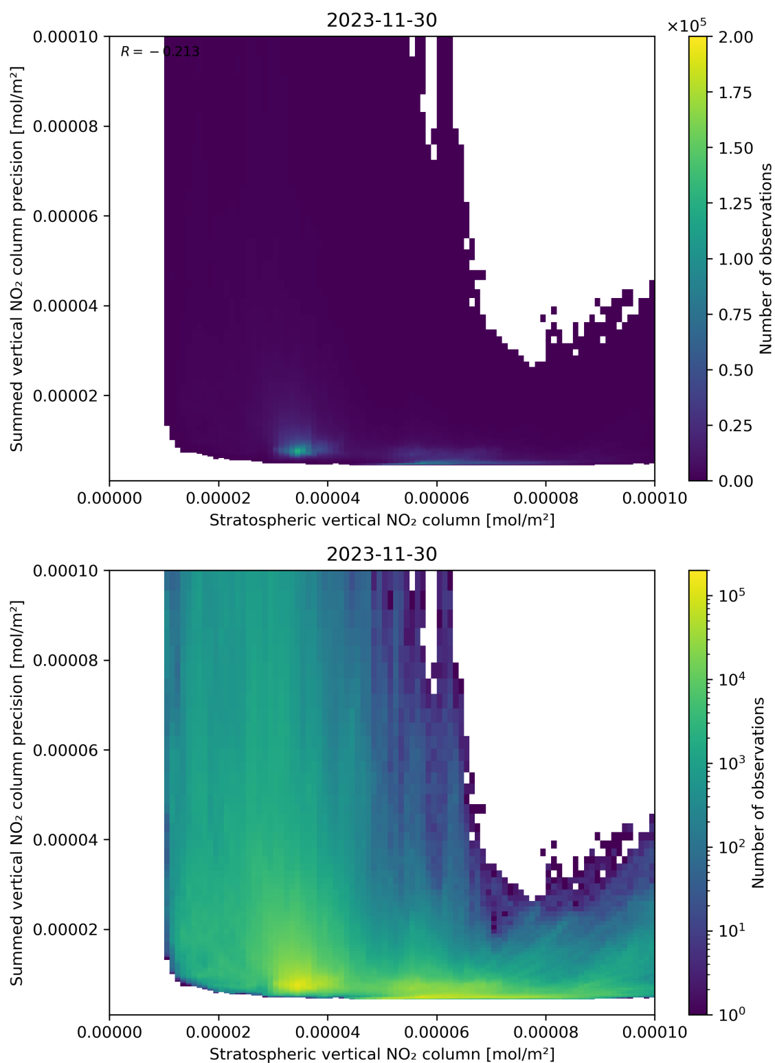
Figure 99: Scatter density plot of “Stratospheric vertical NO 2 column” against “Summed vertical NO 2 column precision” for 2023-11-29 to 2023-12-01.
