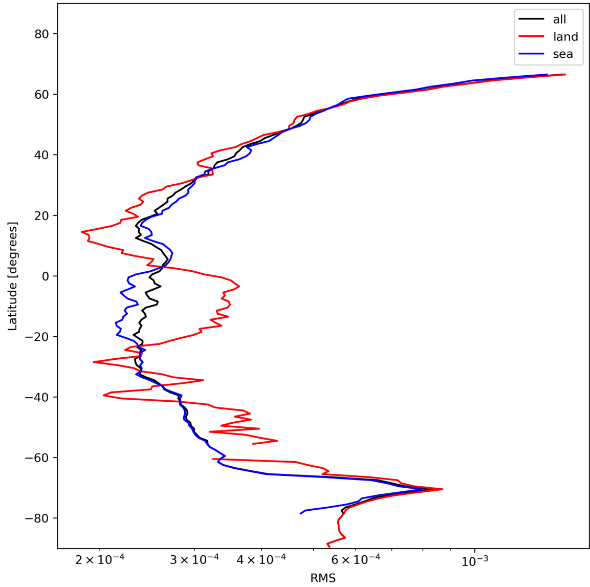
Figure 26: Zonal average of “RMS” for 2023-11-29 to 2023-12-01.
