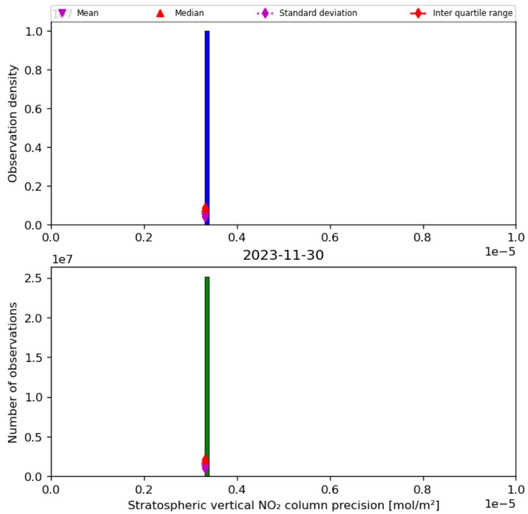
Figure 37: Histogram of “Stratospheric vertical NO 2 column precision” for 2023-11-29 to 2023-12-01
