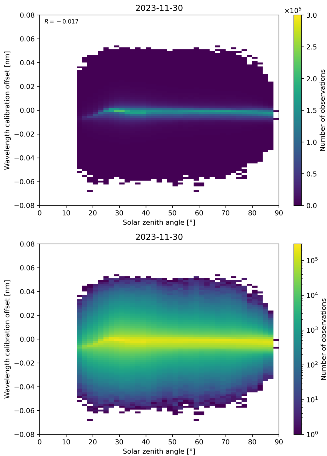
Figure 158: Scatter density plot of “Solar zenith angle” against “Wavelength calibration offset” for 2023-11-29 to 2023-12-01.
