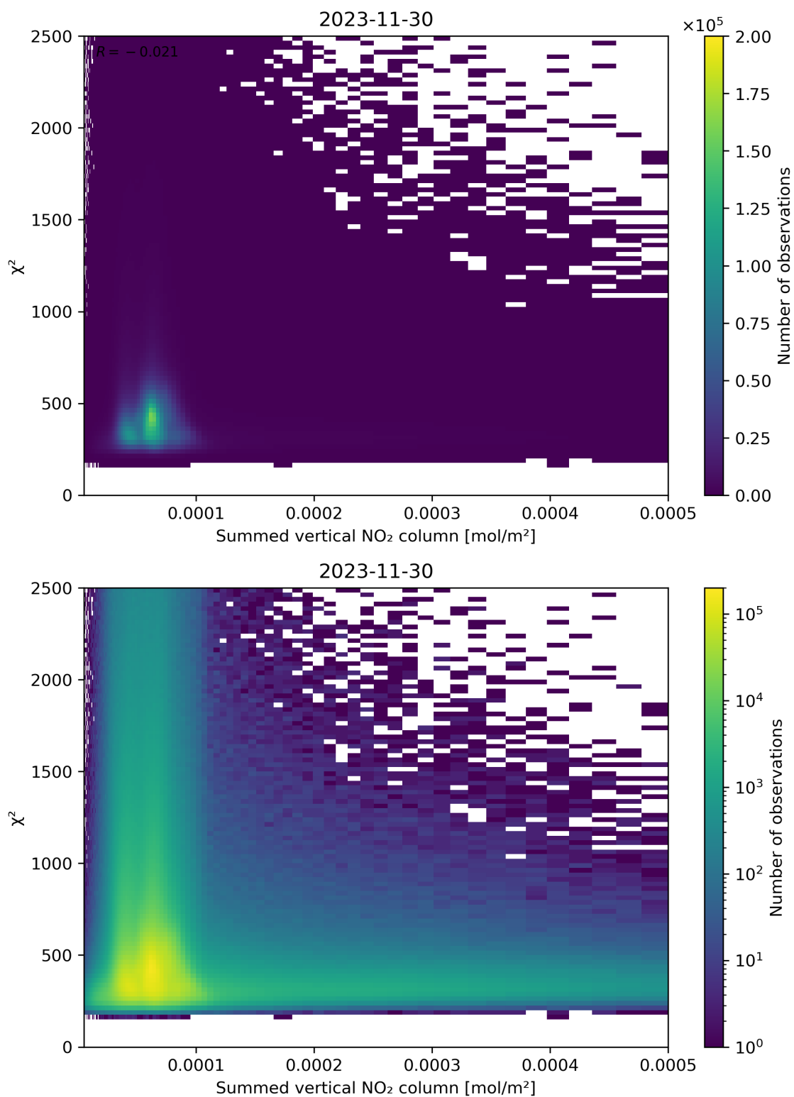
Figure 104: Scatter density plot of “Summed vertical NO 2 column” against “ \chi^2 ” for 2023-11-29 to 2023-12-01.
