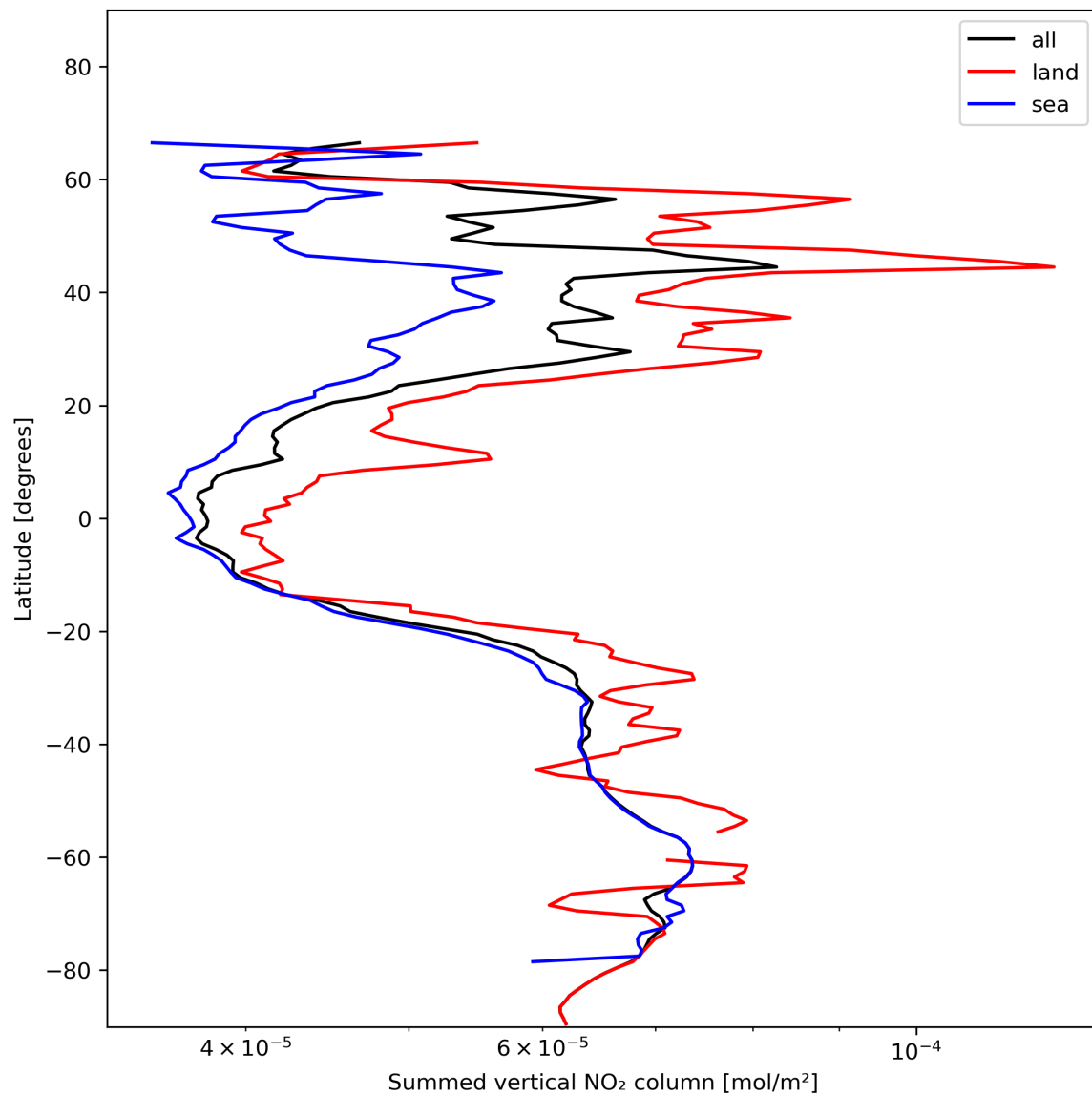
Figure 23: Zonal average of “Summed vertical NO 2 column” for 2023-11-29 to 2023-12-01.
