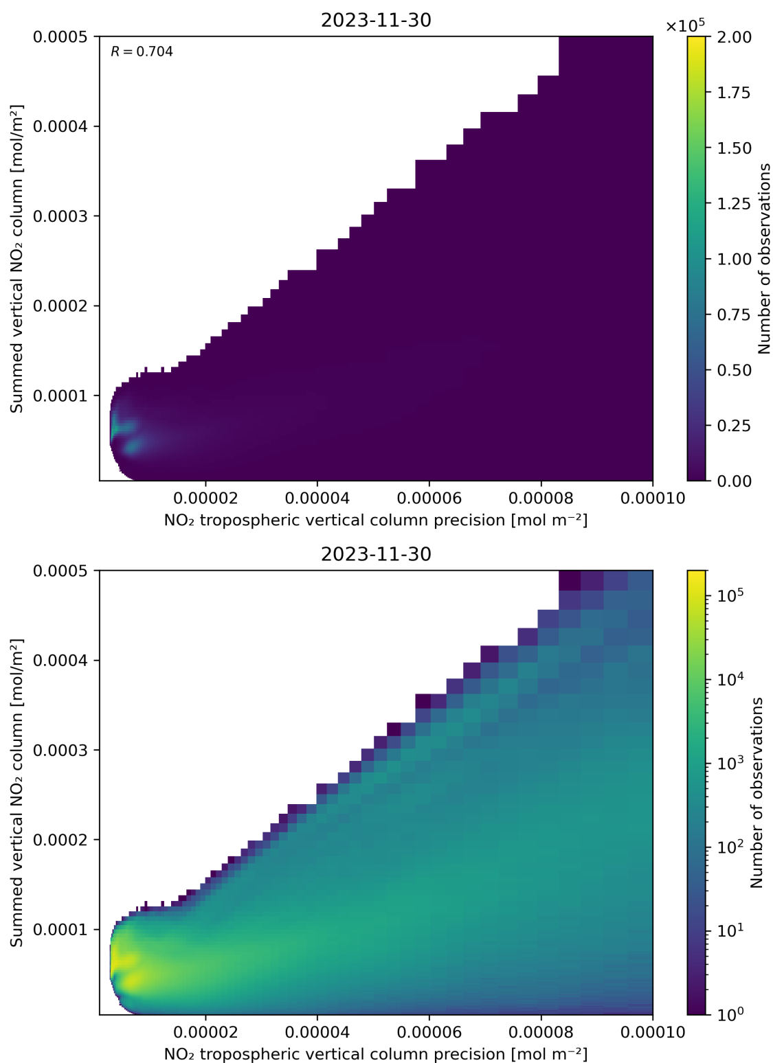
Figure 136: Scatter density plot of “NO 2 tropospheric vertical column precision” against “Summed vertical NO 2 column” for 2023-11-29 to 2023-12-01.
