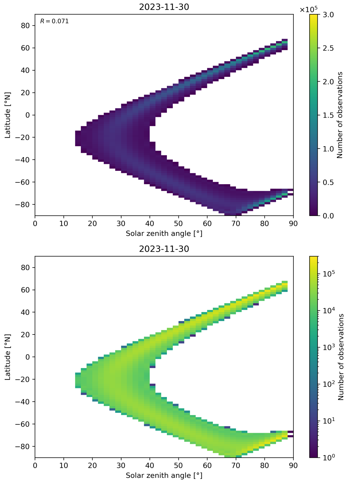
Figure 149: Scatter density plot of “Solar zenith angle” against “Latitude” for 2023-11-29 to 2023-12-01.
