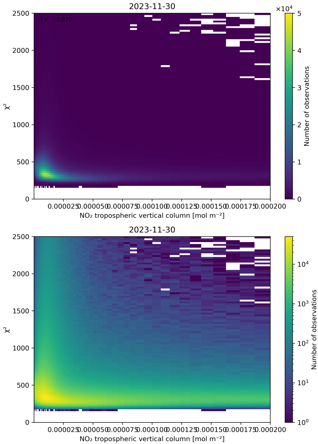
Figure 124: Scatter density plot of “NO 2 tropospheric vertical column” against “ \chi^2 ” for 2023-11-29 to 2023-12-01.
