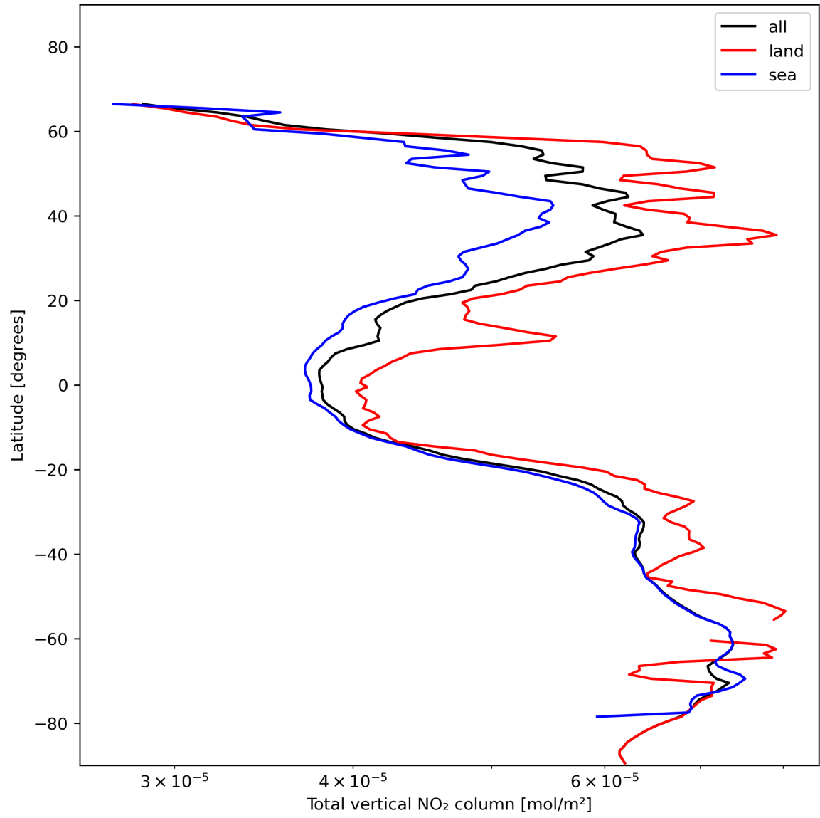
Figure 21: Zonal average of “Total vertical NO 2 column” for 2023-11-29 to 2023-12-01.
