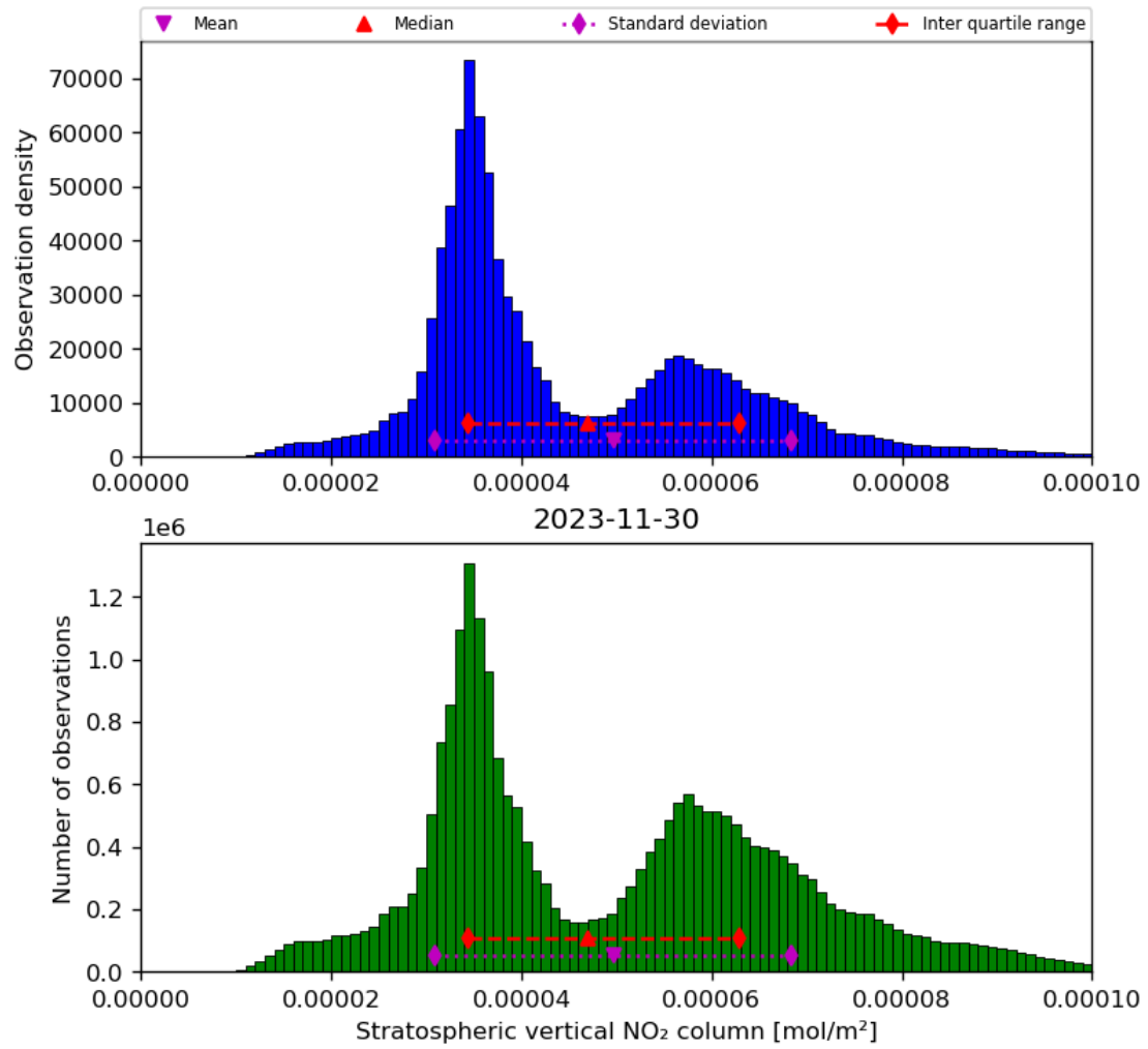
Figure 36: Histogram of “Stratospheric vertical NO 2 column” for 2023-11-29 to 2023-12-01
