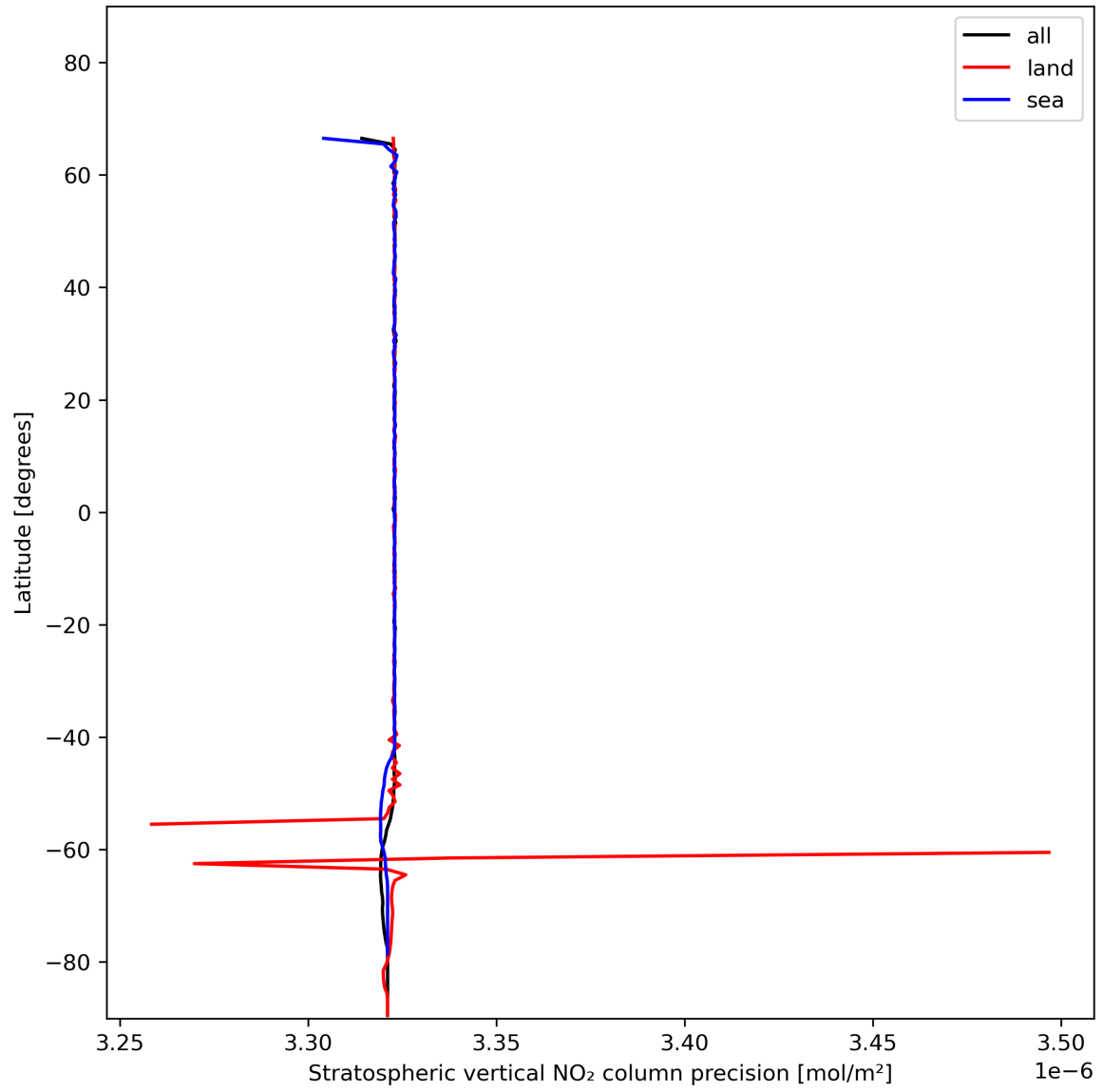
Figure 20: Zonal average of “Stratospheric vertical NO 2 column precision” for 2023-11-29 to 2023-12-01.
