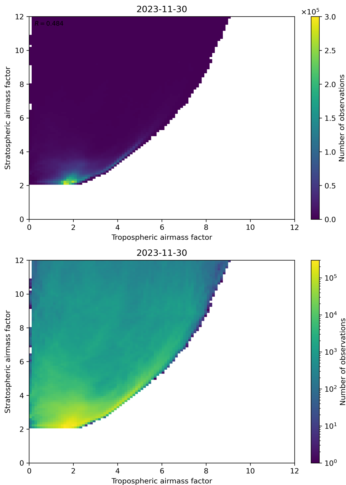
Figure 71: Scatter density plot of “Tropospheric airmass factor” against “Stratospheric airmass factor” for 2023-11-29 to 2023-12-01.
