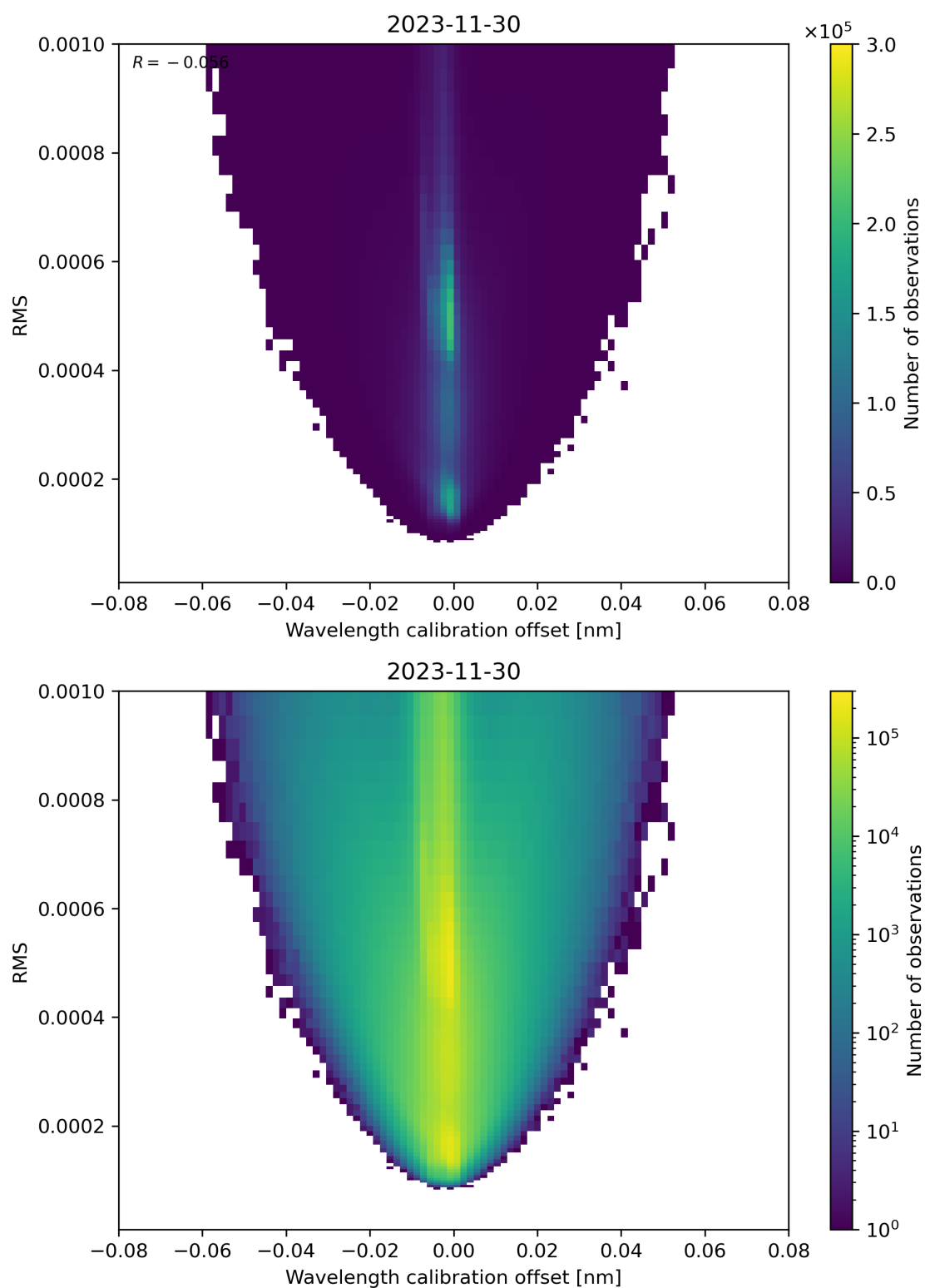
Figure 181: Scatter density plot of “Wavelength calibration offset” against “RMS” for 2023-11-29 to 2023-12-01.
