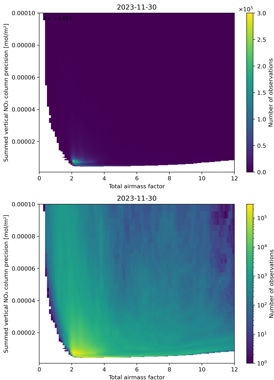
Figure 66: Scatter density plot of “Total airmass factor” against “Summed vertical NO 2 column precision” for 2023-11-29 to 2023-12-01.
