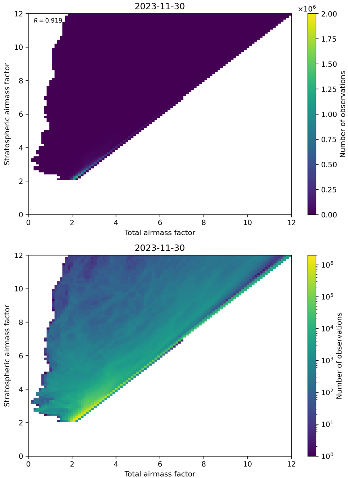
Figure 62: Scatter density plot of “Total airmass factor” against “Stratospheric airmass factor” for 2023-11-29 to 2023-12-01.
