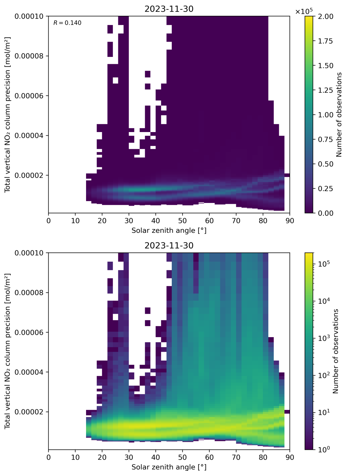
Figure 154: Scatter density plot of “Solar zenith angle” against “Total vertical NO 2 column precision” for 2023-11-29 to 2023-12-01.
