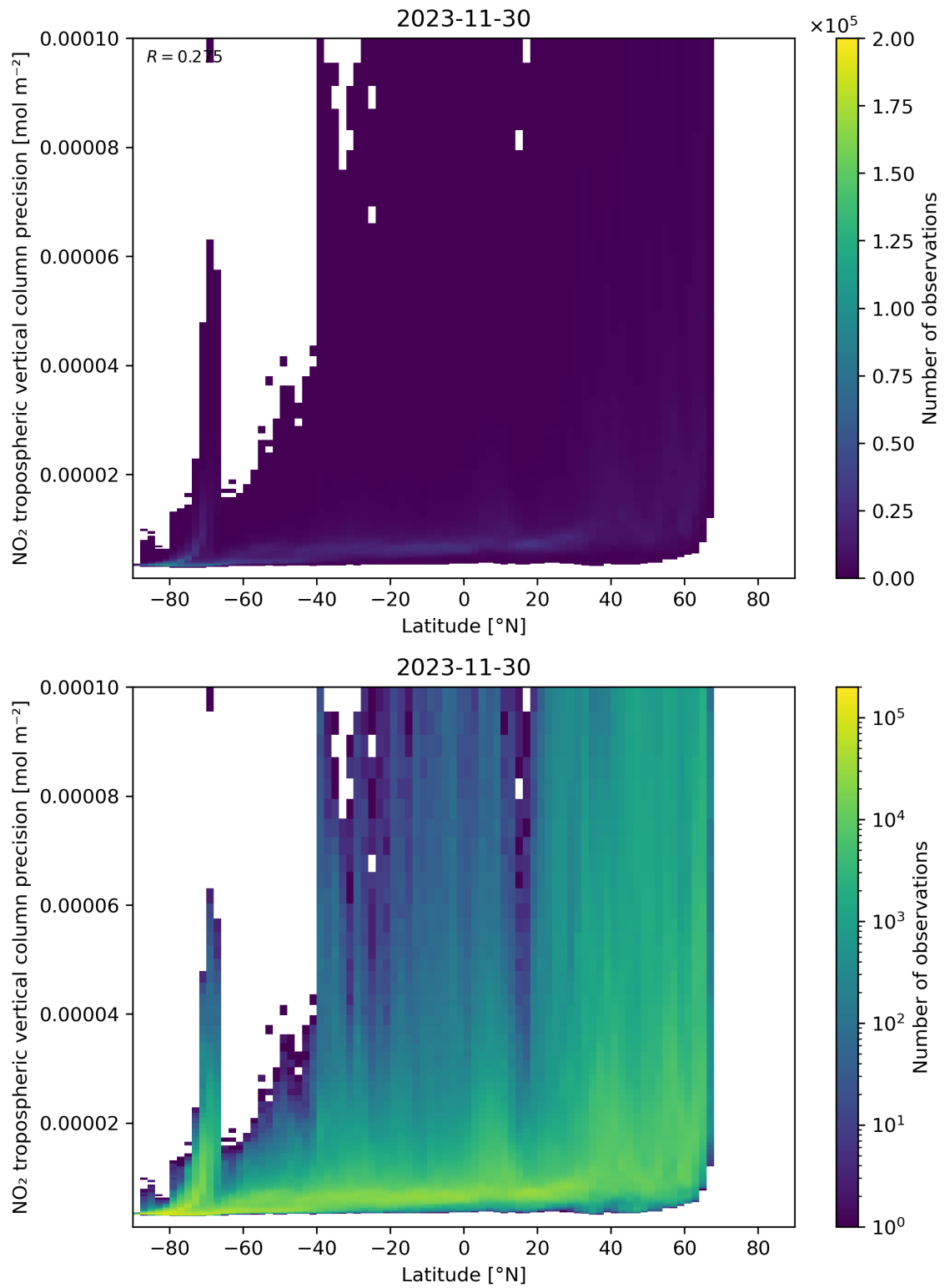
Figure 93: Scatter density plot of “Latitude” against “NO 2 tropospheric vertical column precision” for 2023-11-29 to 2023-12-01.
