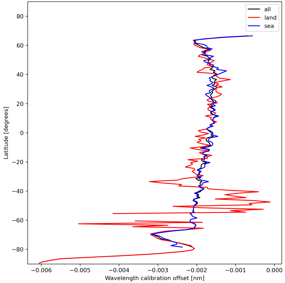
Figure 18: Zonal average of “Wavelength calibration offset” for 2023-11-29 to 2023-12-01.
