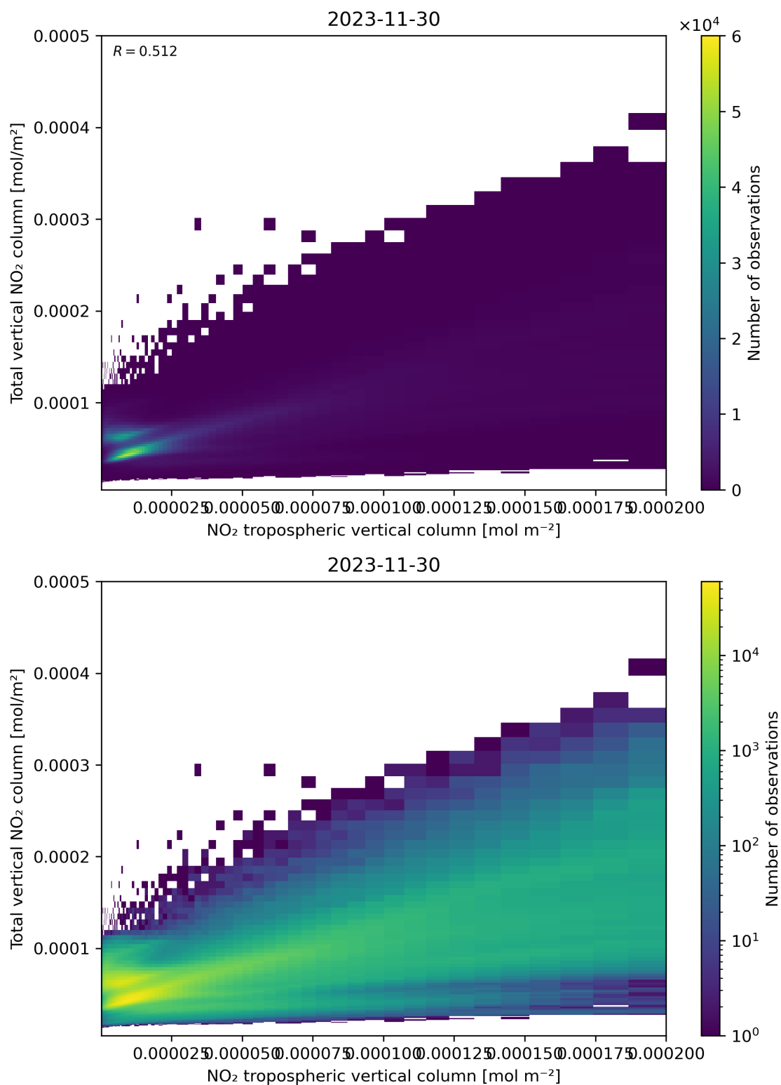
Figure 128: Scatter density plot of “NO 2 tropospheric vertical column” against “Total vertical NO 2 column” for 2023-11-29 to 2023-12-01.
