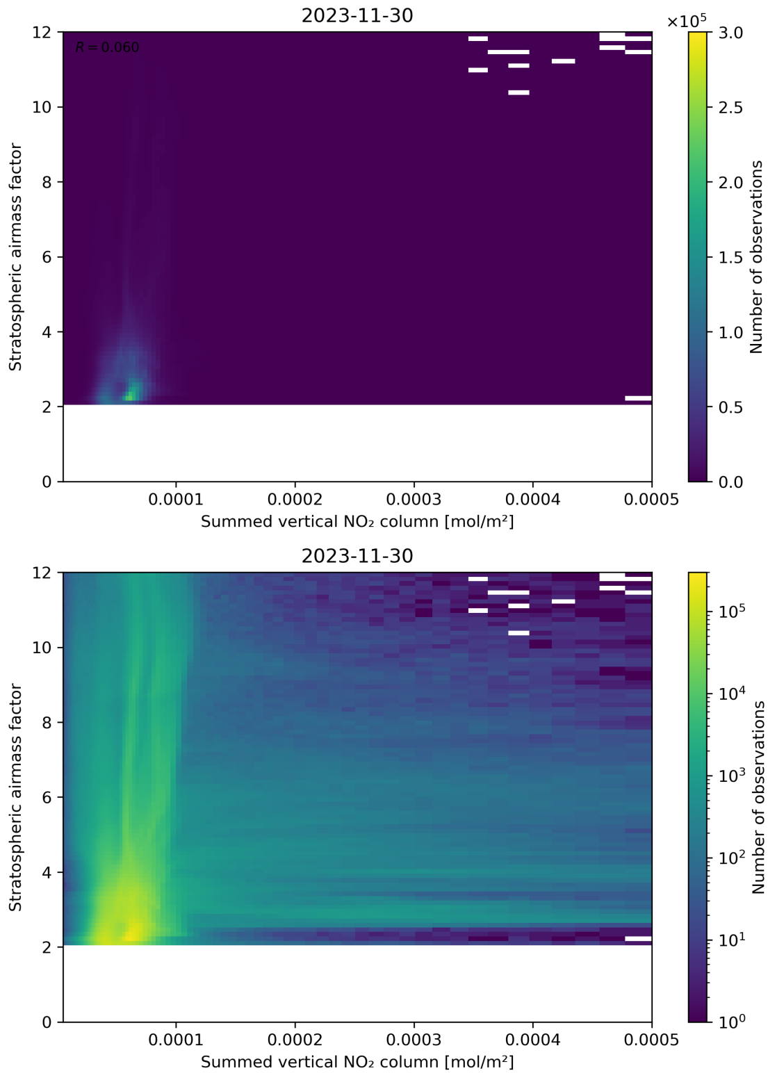
Figure 103: Scatter density plot of “Summed vertical NO 2 column” against “Stratospheric airmass factor” for 2023-11-29 to 2023-12-01.
