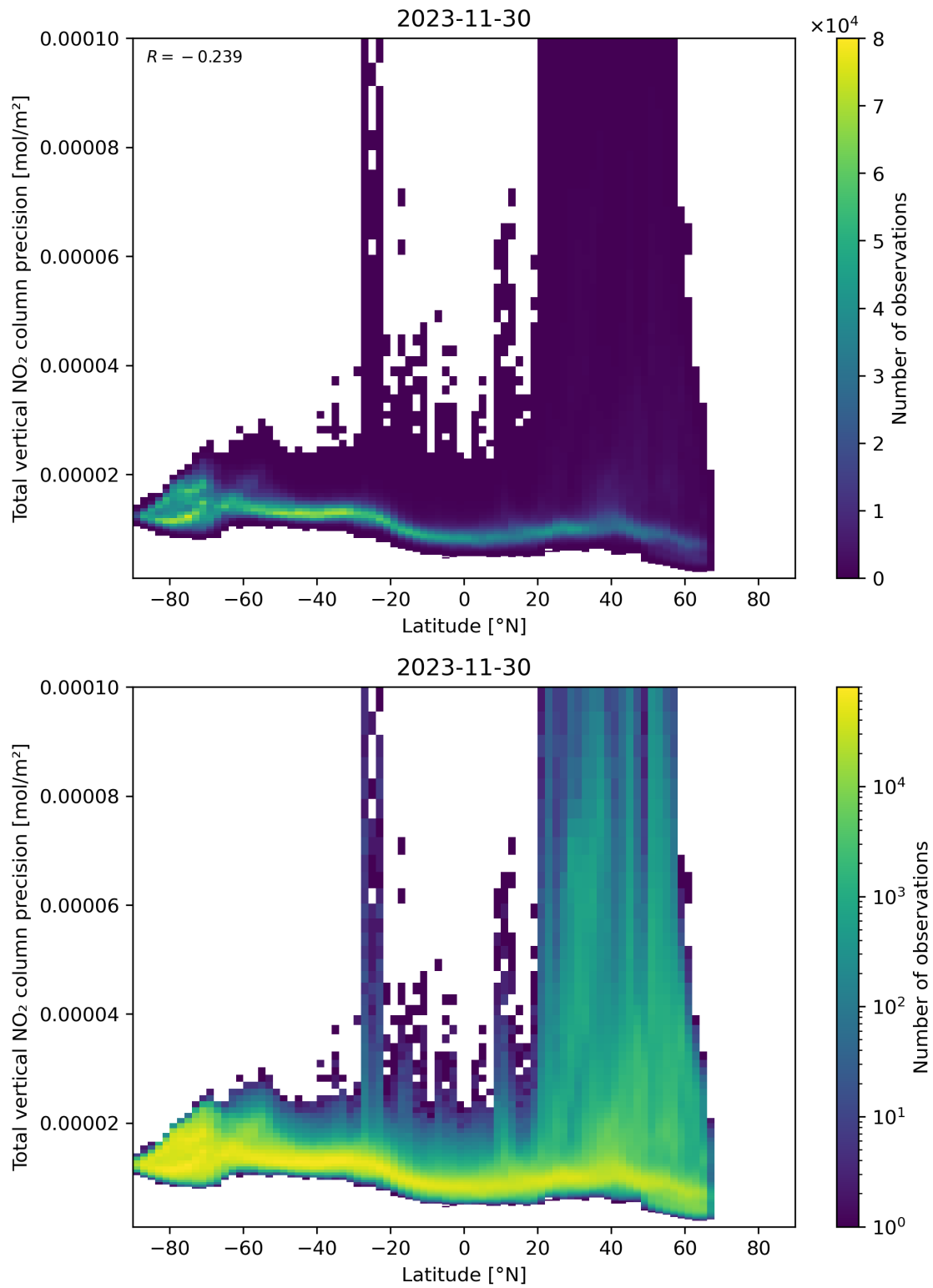
Figure 91: Scatter density plot of “Latitude” against “Total vertical NO 2 column precision” for 2023-11-29 to 2023-12-01.
