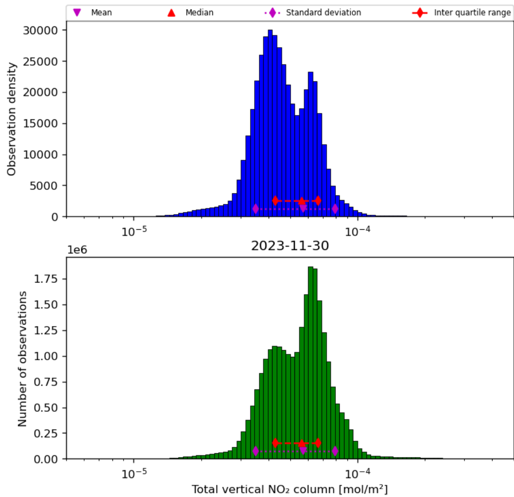
Figure 38: Histogram of “Total vertical NO 2 column” for 2023-11-29 to 2023-12-01
