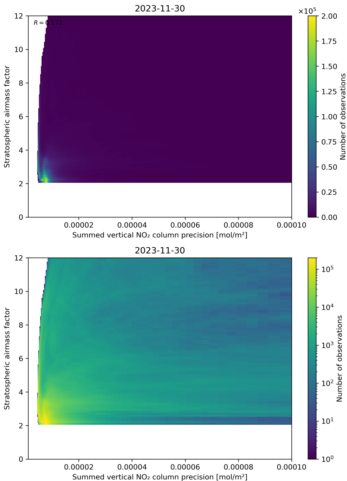
Figure 106: Scatter density plot of “Summed vertical NO 2 column precision” against “Stratospheric airmass factor” for 2023-11-29 to 2023-12-01.
