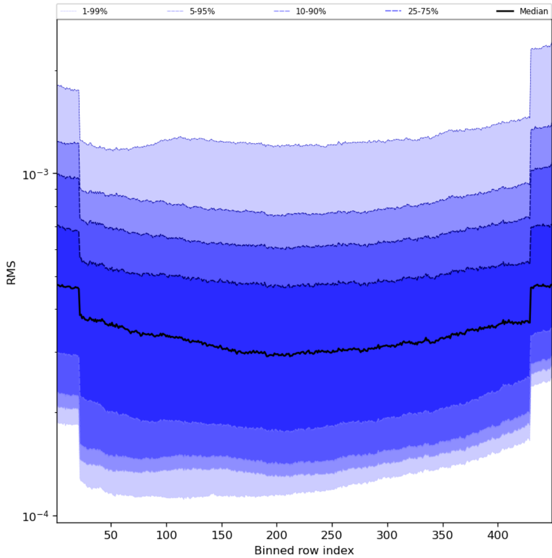
Figure 60: Along track statistics of “RMS” for 2023-11-29 to 2023-12-01
