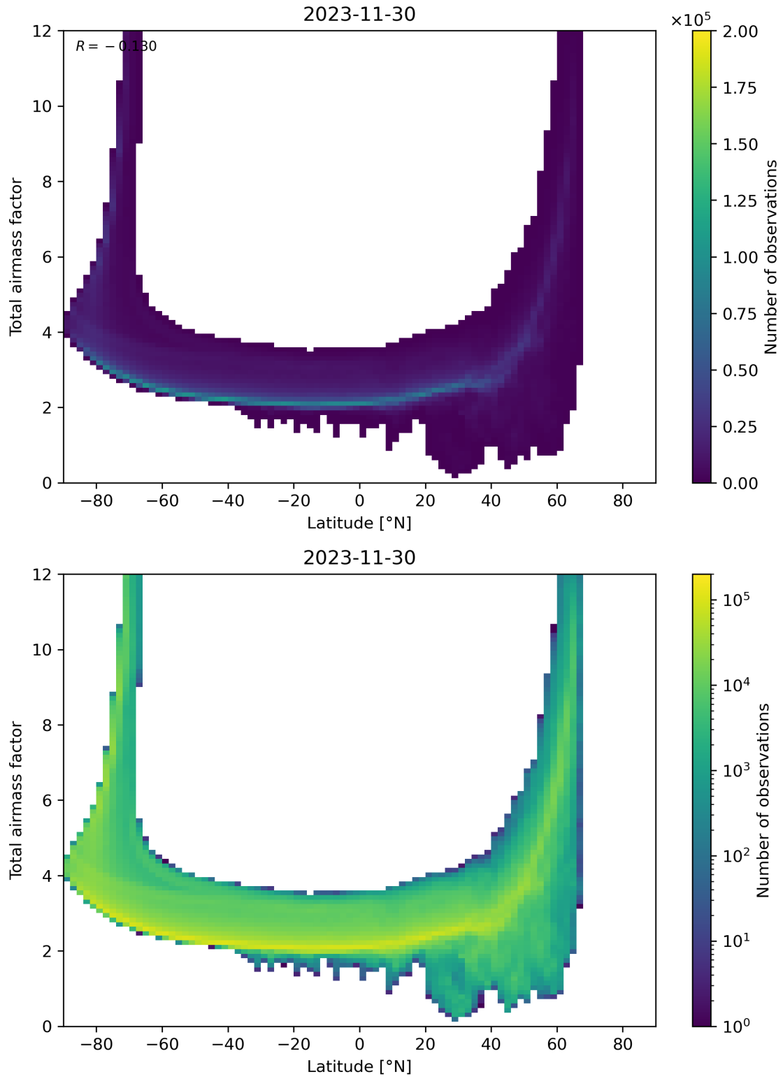
Figure 84: Scatter density plot of “Latitude” against “Total airmass factor” for 2023-11-29 to 2023-12-01.
