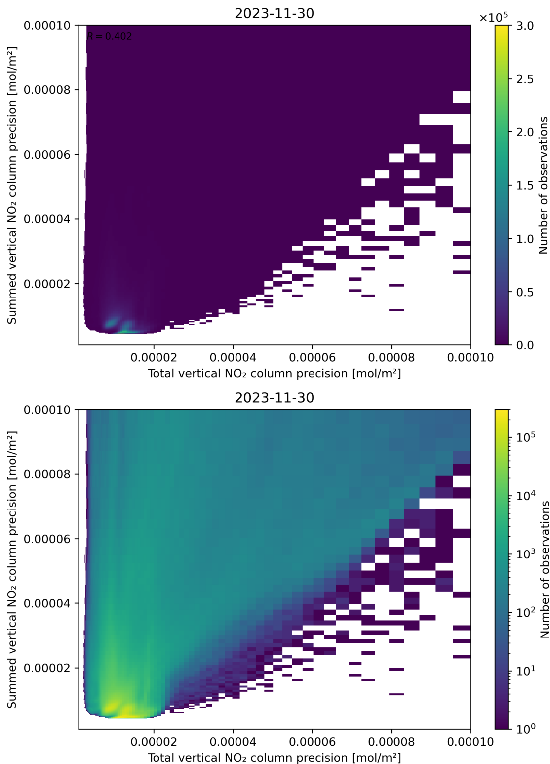
Figure 118: Scatter density plot of “Total vertical NO 2 column precision” against “Summed vertical NO 2 column precision” for 2023-11-29 to 2023-12-01.
