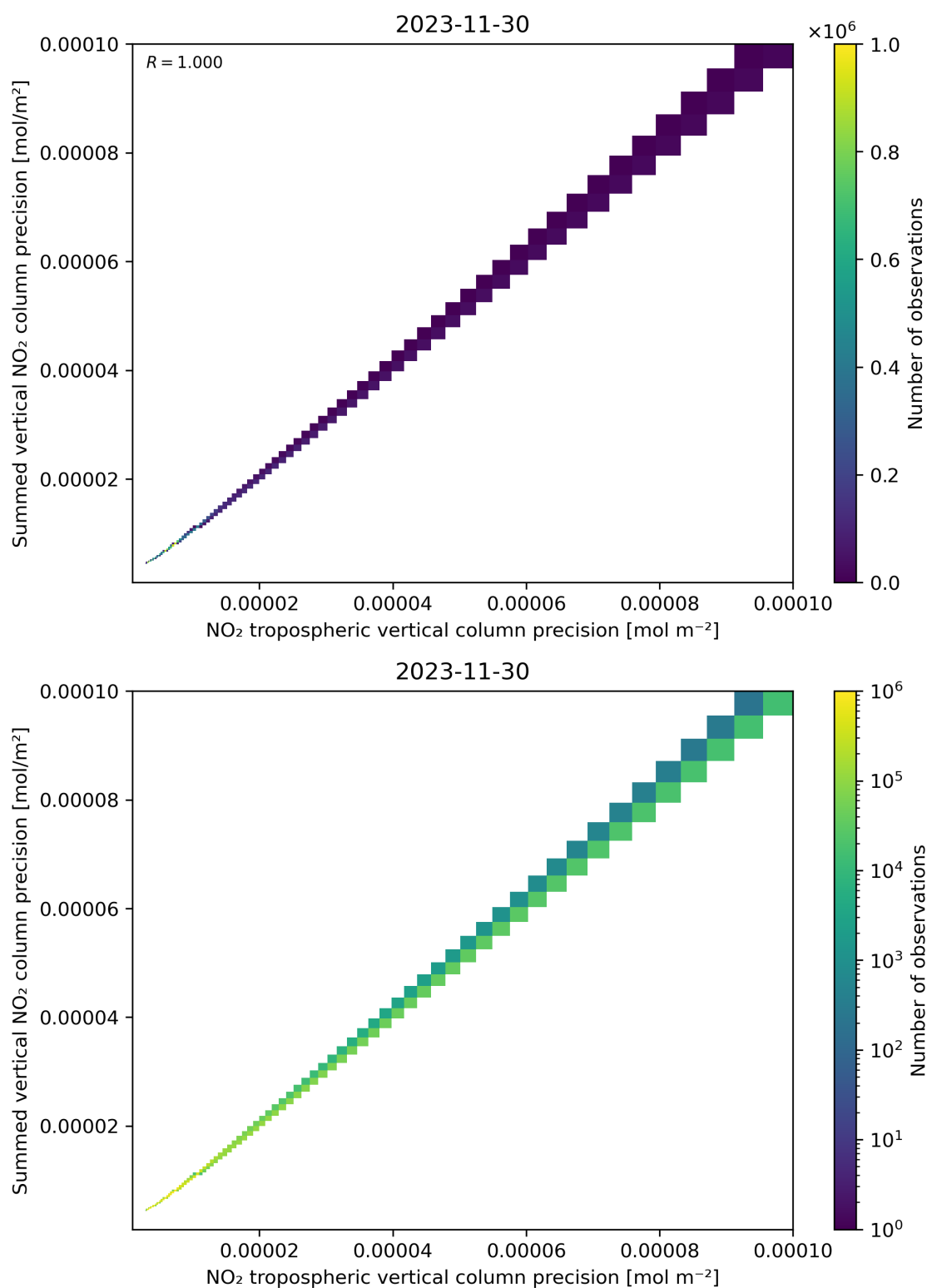
Figure 137: Scatter density plot of “NO 2 tropospheric vertical column precision” against “Summed vertical NO 2 column precision” for 2023-11-29 to 2023-12-01.
