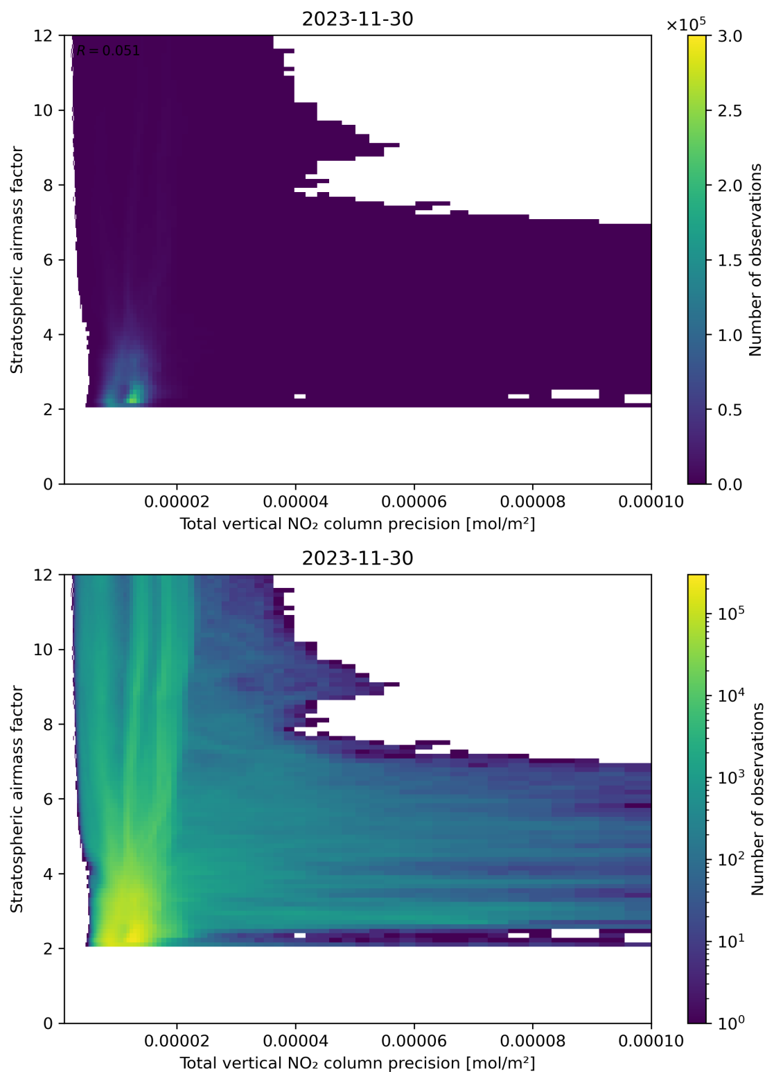
Figure 115: Scatter density plot of “Total vertical NO 2 column precision” against “Stratospheric air mass factor” for 2023-11-29 to 2023-12-01.
