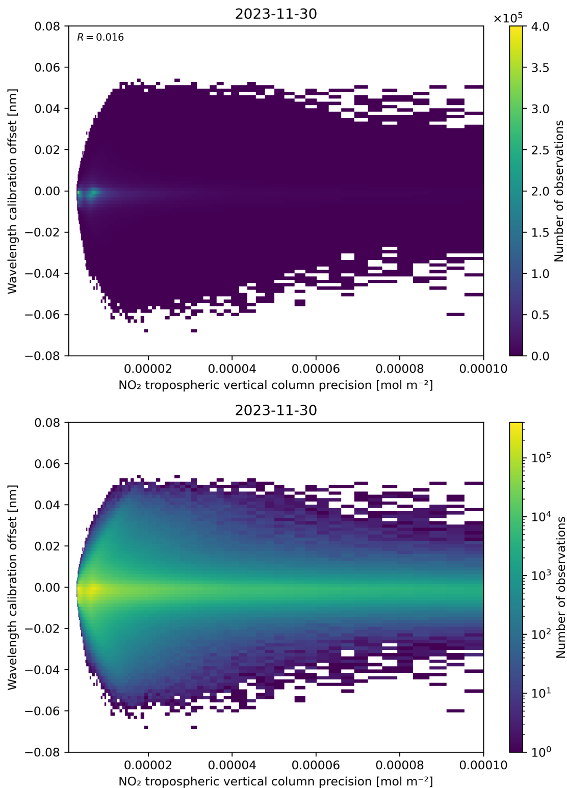
Figure 141: Scatter density plot of “NO 2 tropospheric vertical column precision” against “Wavelength calibration offset” for 2023-11-29 to 2023-12-01.
