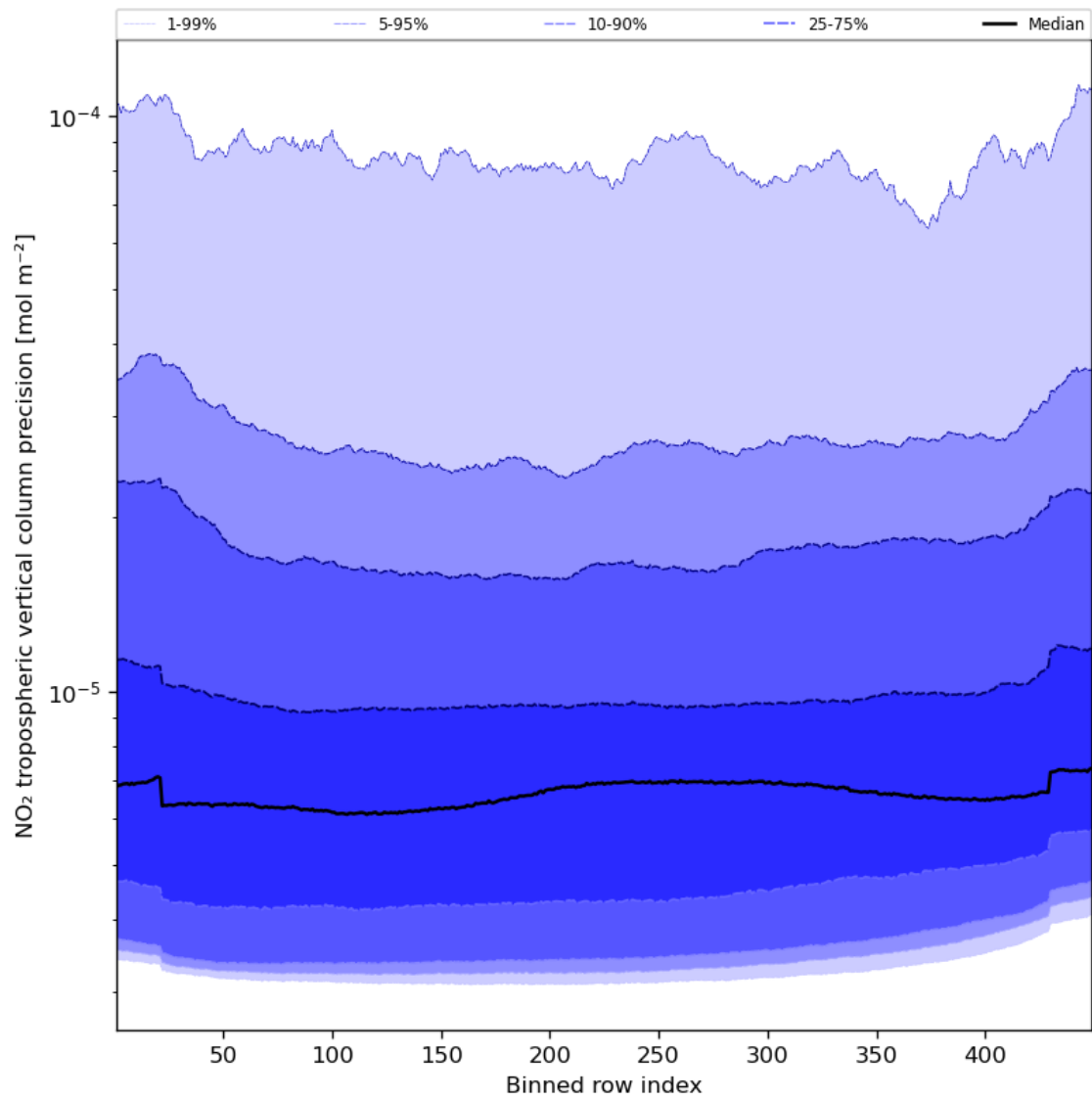
Figure 47: Along track statistics of “NO 2 tropospheric vertical column precision” for 2023-11-29 to 2023-12-01
