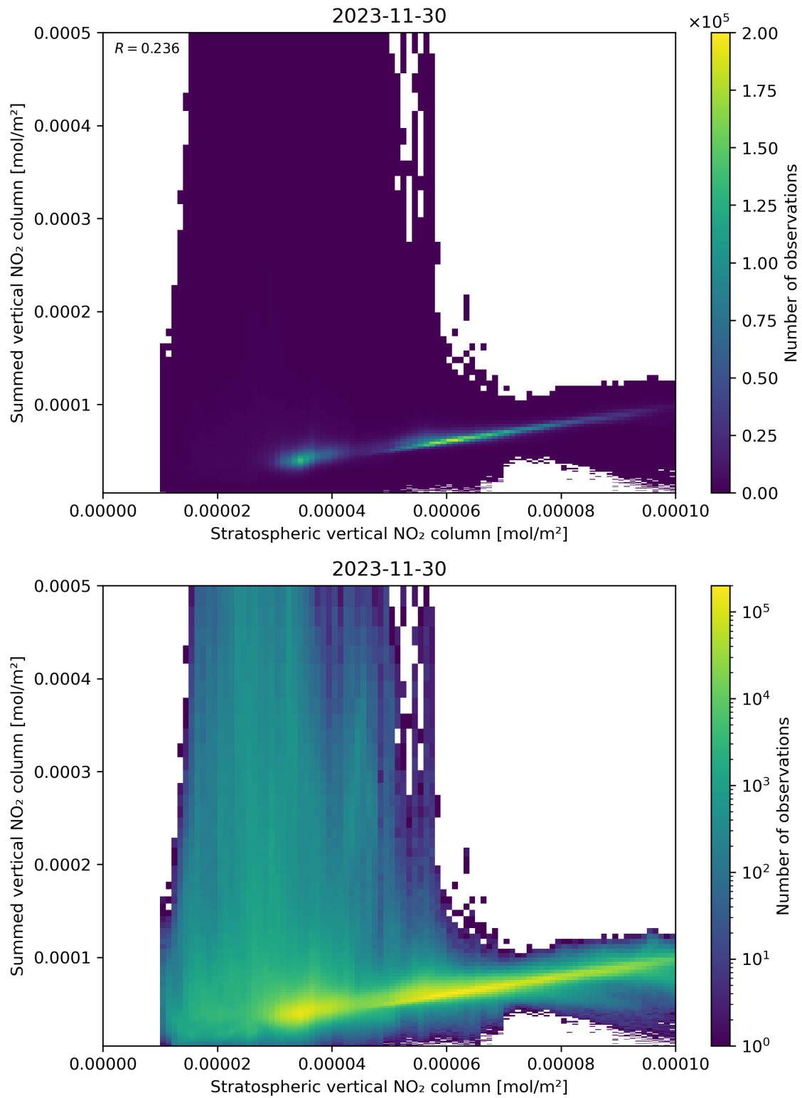
Figure 98: Scatter density plot of “Stratospheric vertical NO 2 column” against “Summed vertical NO 2 column” for 2023-11-29 to 2023-12-01.
