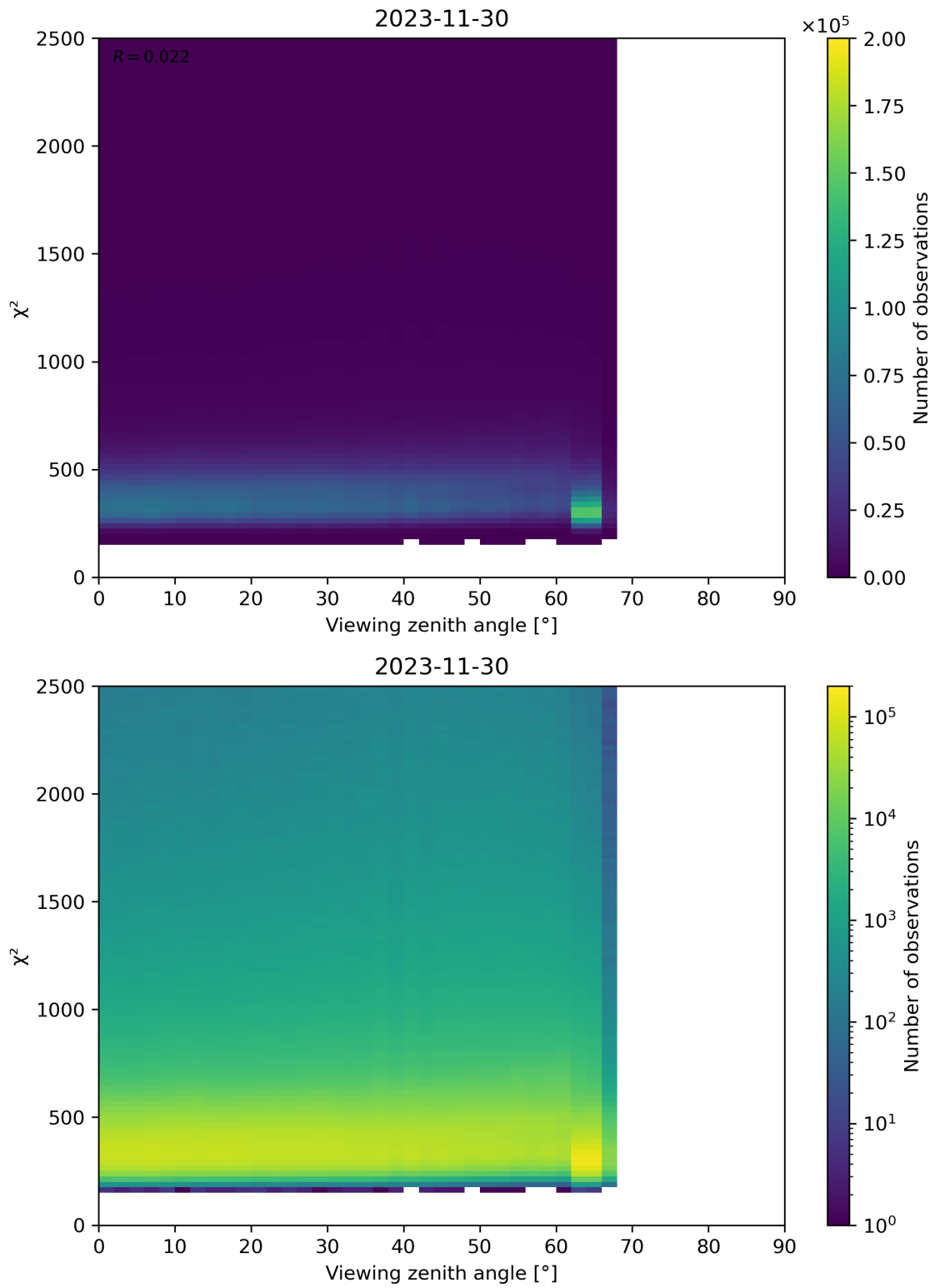
Figure 162: Scatter density plot of “Viewing zenith angle” against “ \chi^2 ” for 2023-11-29 to 2023-12-01.
