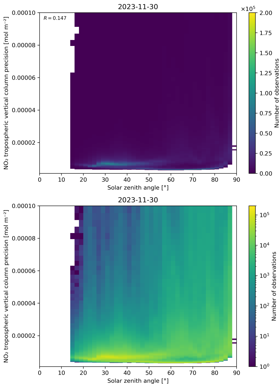
Figure 156: Scatter density plot of “Solar zenith angle” against “NO 2 tropospheric vertical column precision” for 2023-11-29 to 2023-12-01.
