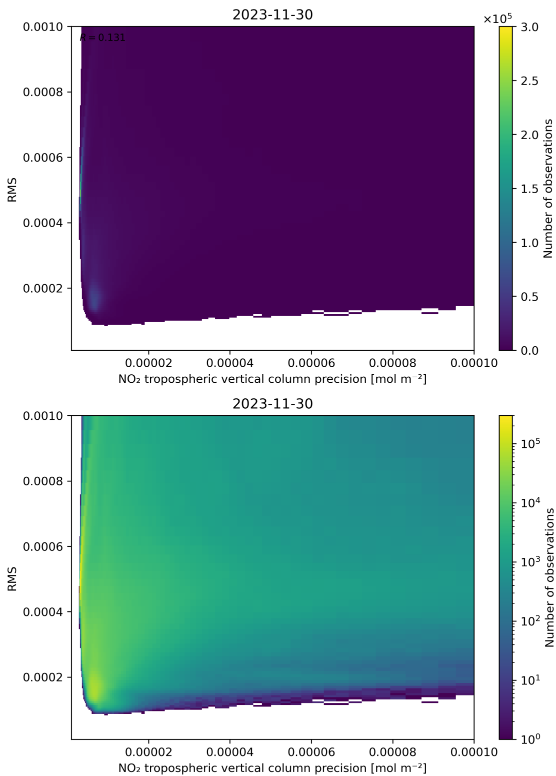
Figure 140: Scatter density plot of “NO 2 tropospheric vertical column precision” against “RMS” for 2023-11-29 to 2023-12-01.
