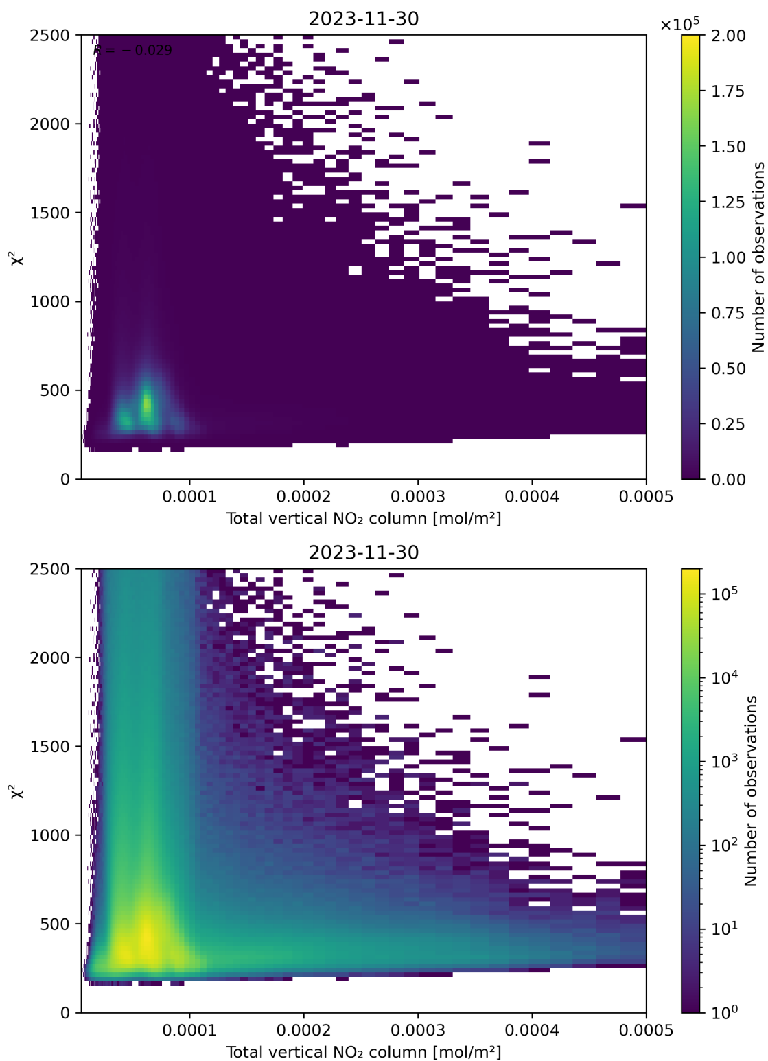
Figure 111: Scatter density plot of “Total vertical NO 2 column” against “ \chi^2 ” for 2023-11-29 to 2023-12-01.
