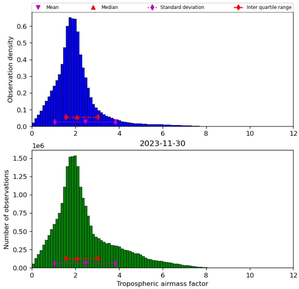
Figure 31: Histogram of “Tropospheric airmass factor” for 2023-11-29 to 2023-12-01
