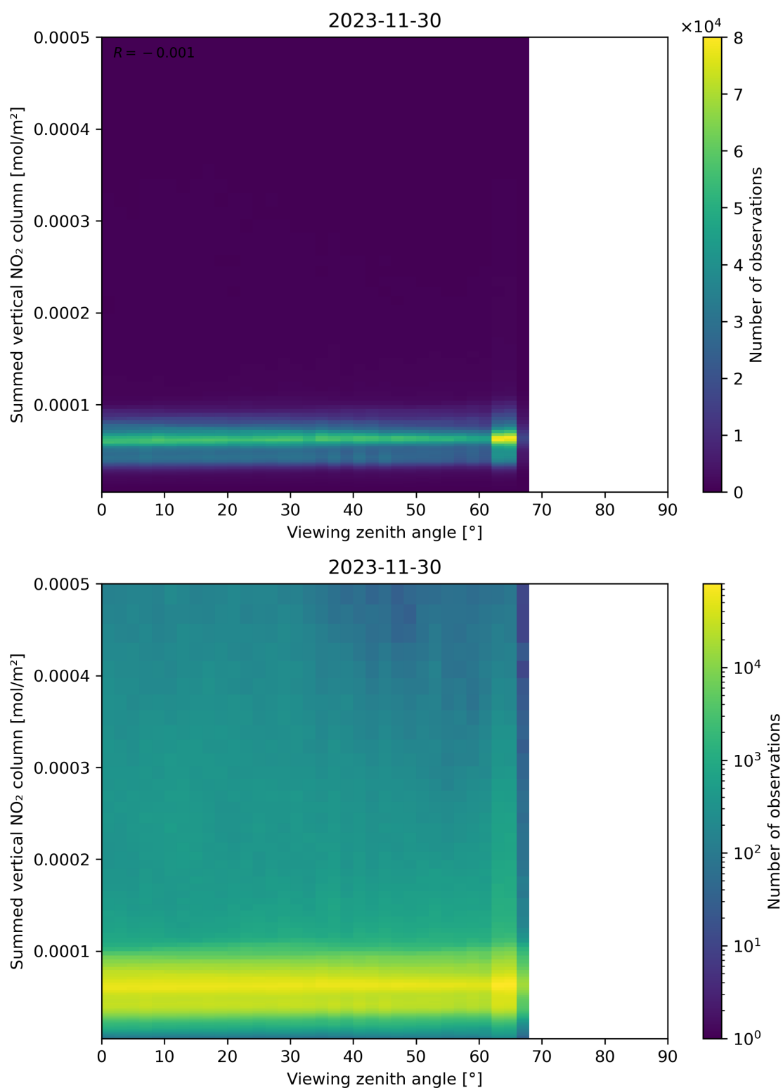
Figure 165: Scatter density plot of “Viewing zenith angle” against “Summed vertical NO 2 column” for 2023-11-29 to 2023-12-01.
