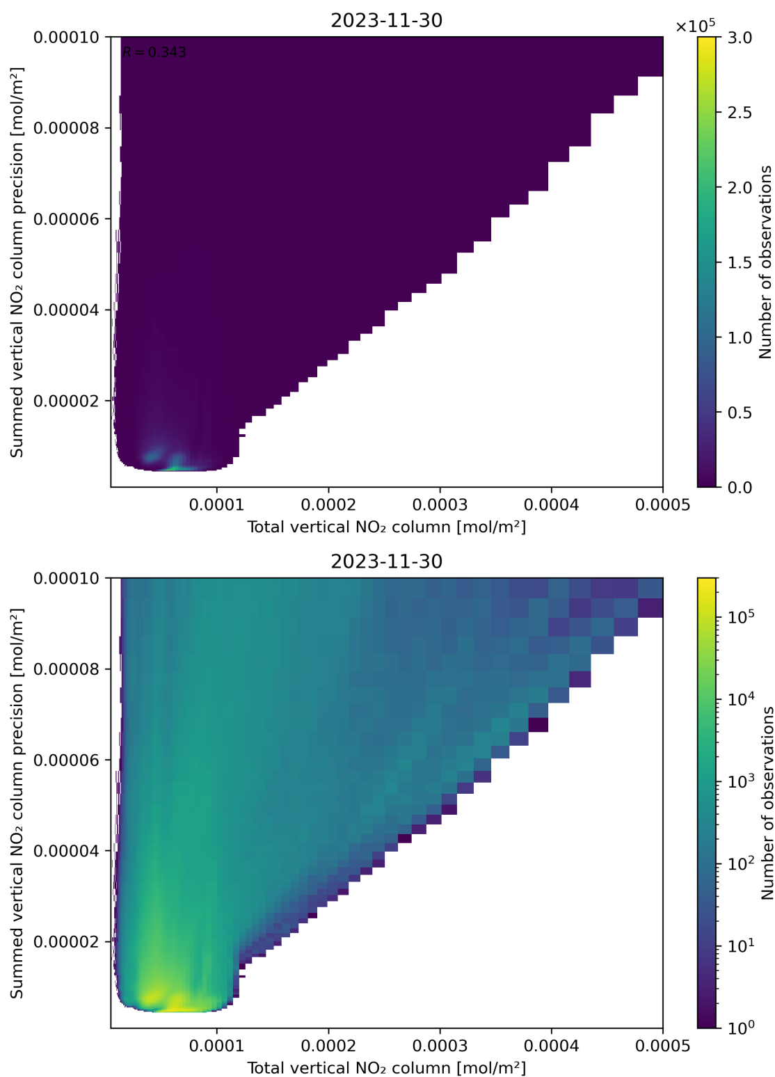
Figure 113: Scatter density plot of “Total vertical NO 2 column” against “Summed vertical NO 2 column precision” for 2023-11-29 to 2023-12-01.
