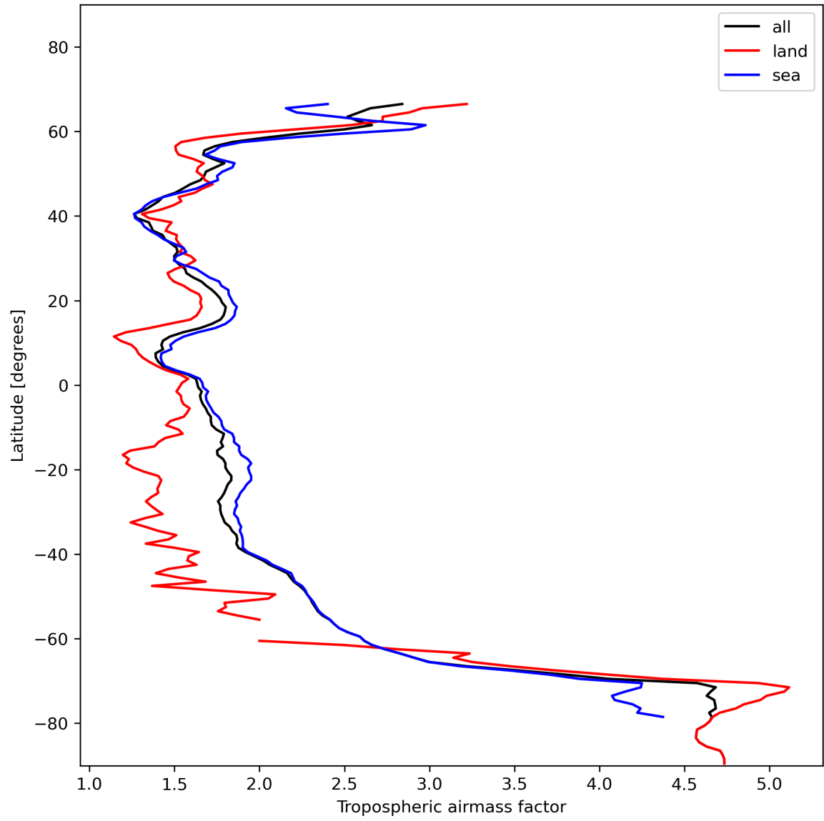
Figure 14: Zonal average of “Tropospheric airmass factor” for 2023-11-29 to 2023-12-01.
