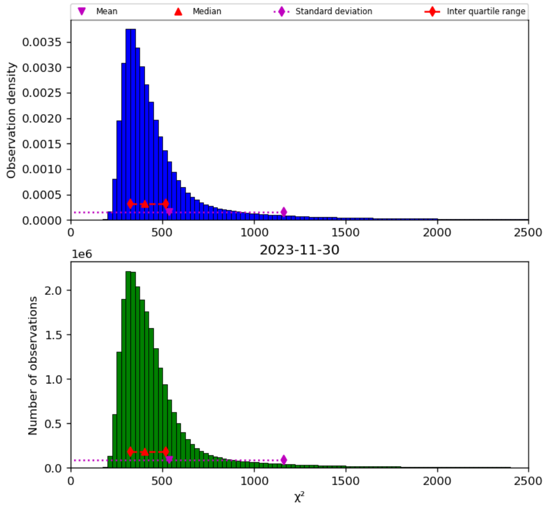
Figure 42: Histogram of " \chi^2 " for 2023-11-29 to 2023-12-01
