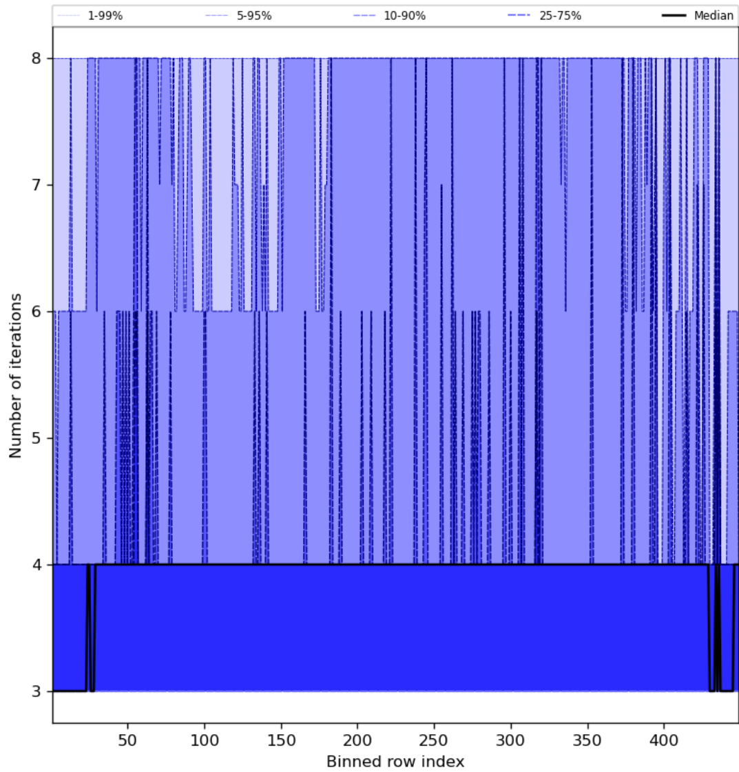
Figure 51: Along track statistics of “Number of iterations” for 2023-11-29 to 2023-12-01
