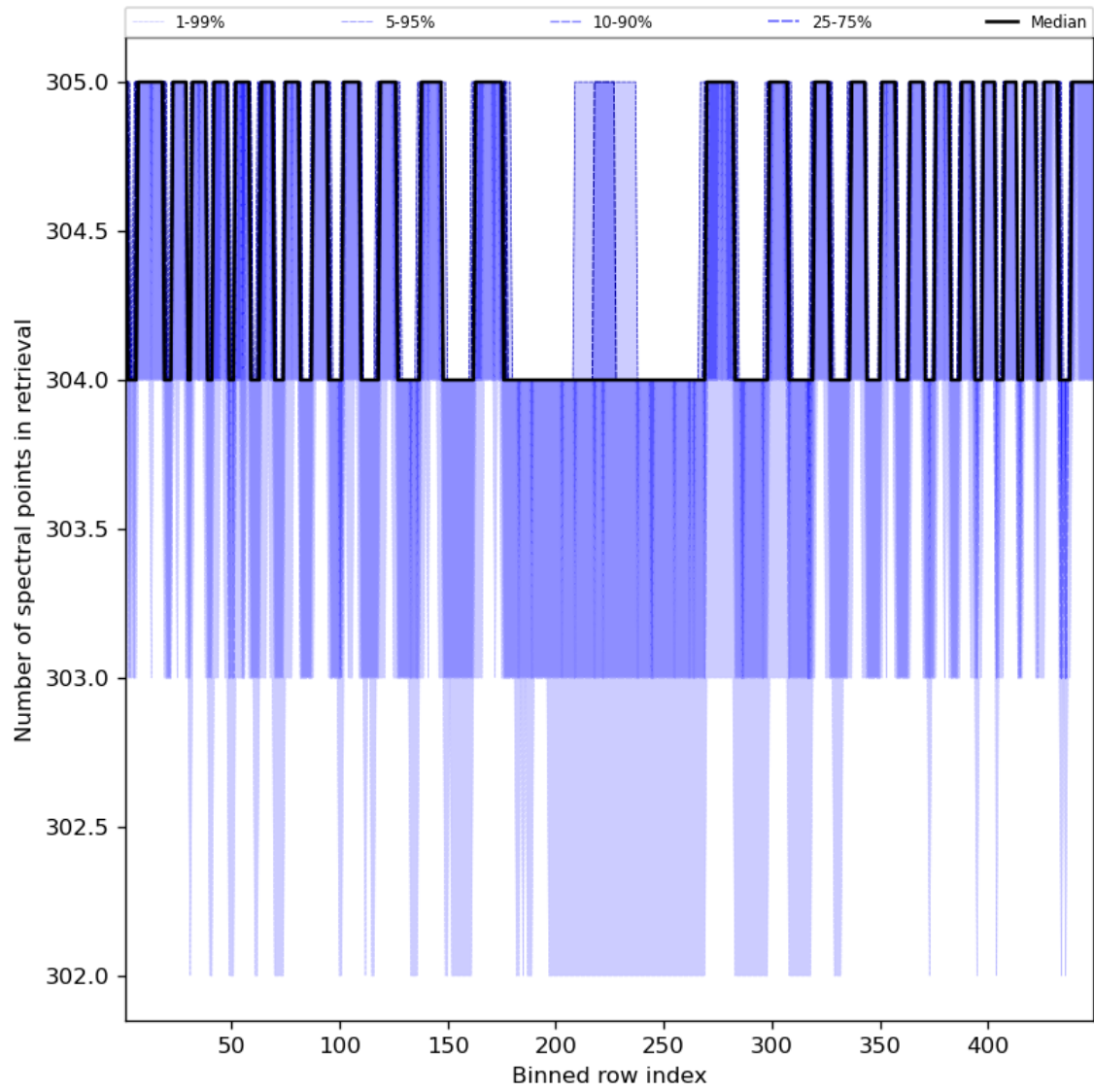
Figure 50: Along track statistics of “Number of spectral points in retrieval” for 2023-11-29 to 2023-12-01
