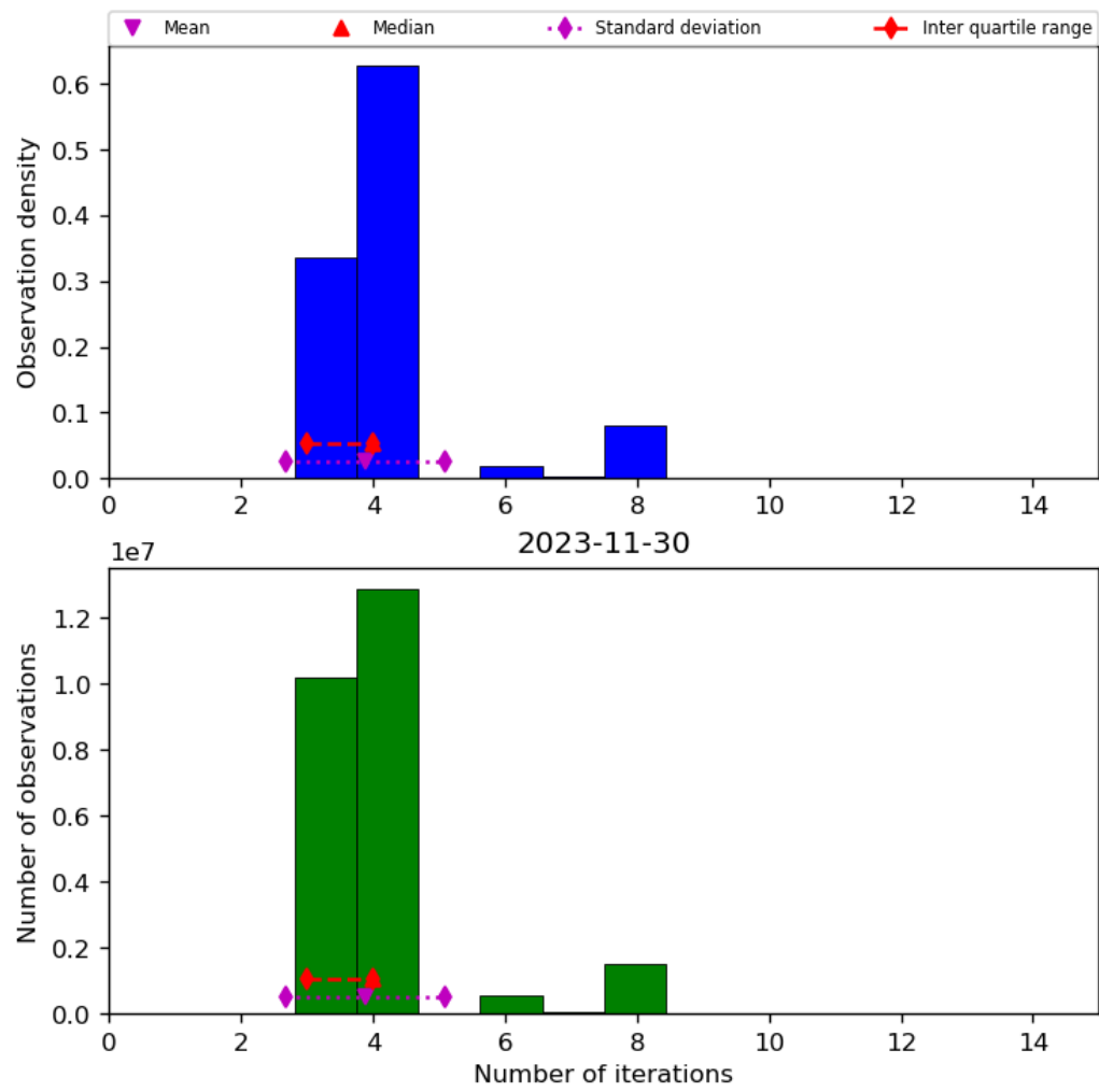
Figure 34: Histogram of “Number of iterations” for 2023-11-29 to 2023-12-01
