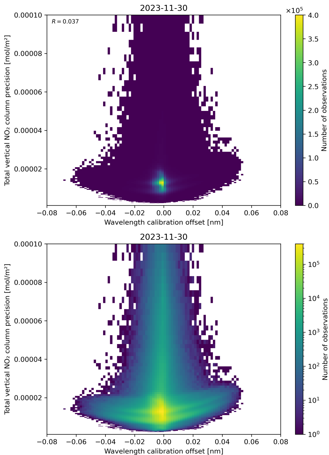
Figure 180: Scatter density plot of “Wavelength calibration offset” against “Total vertical NO 2 column precision” for 2023-11-29 to 2023-12-01.
