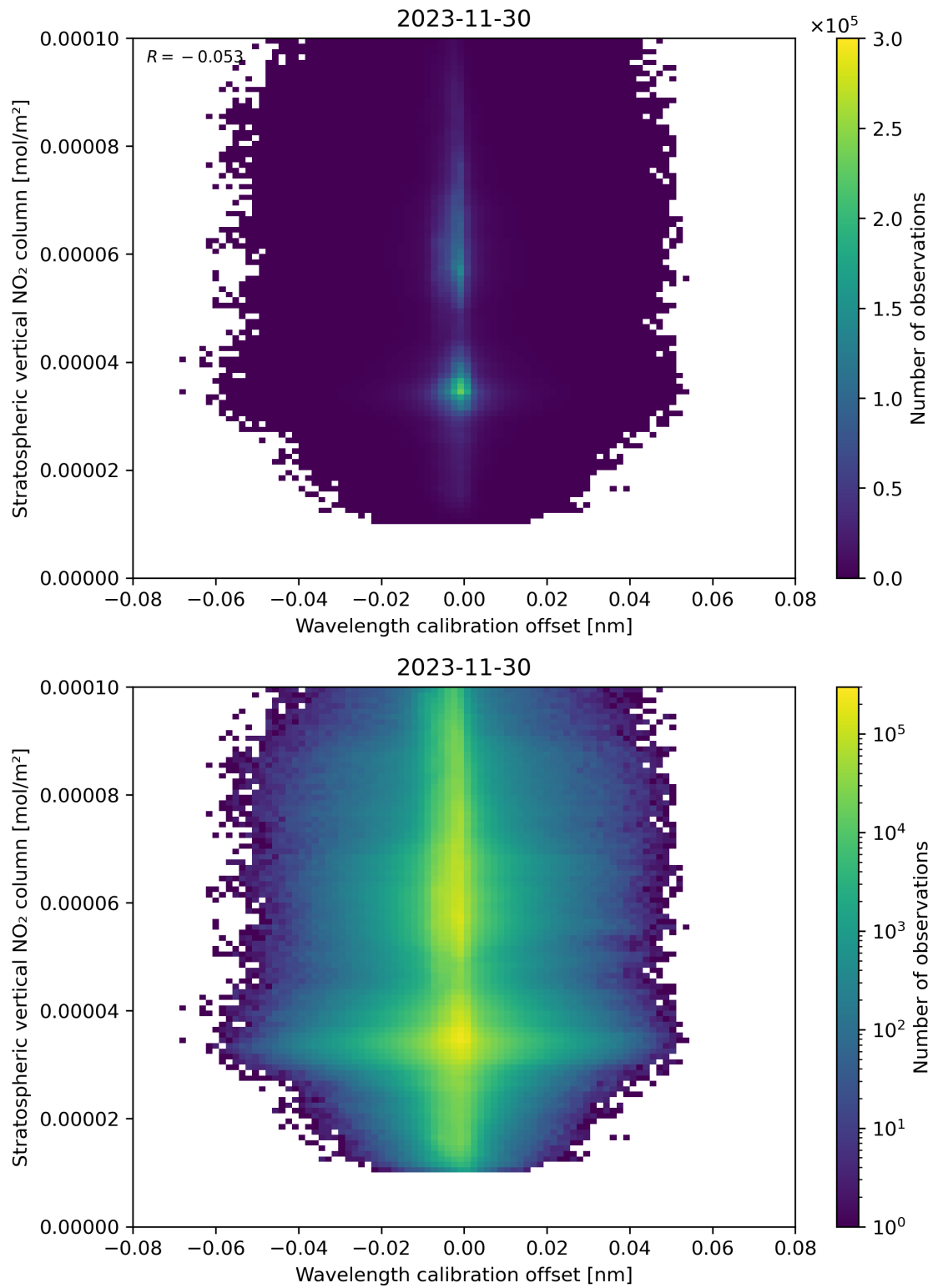
Figure 176: Scatter density plot of “Wavelength calibration offset” against “Stratospheric vertical NO 2 column” for 2023-11-29 to 2023-12-01.
