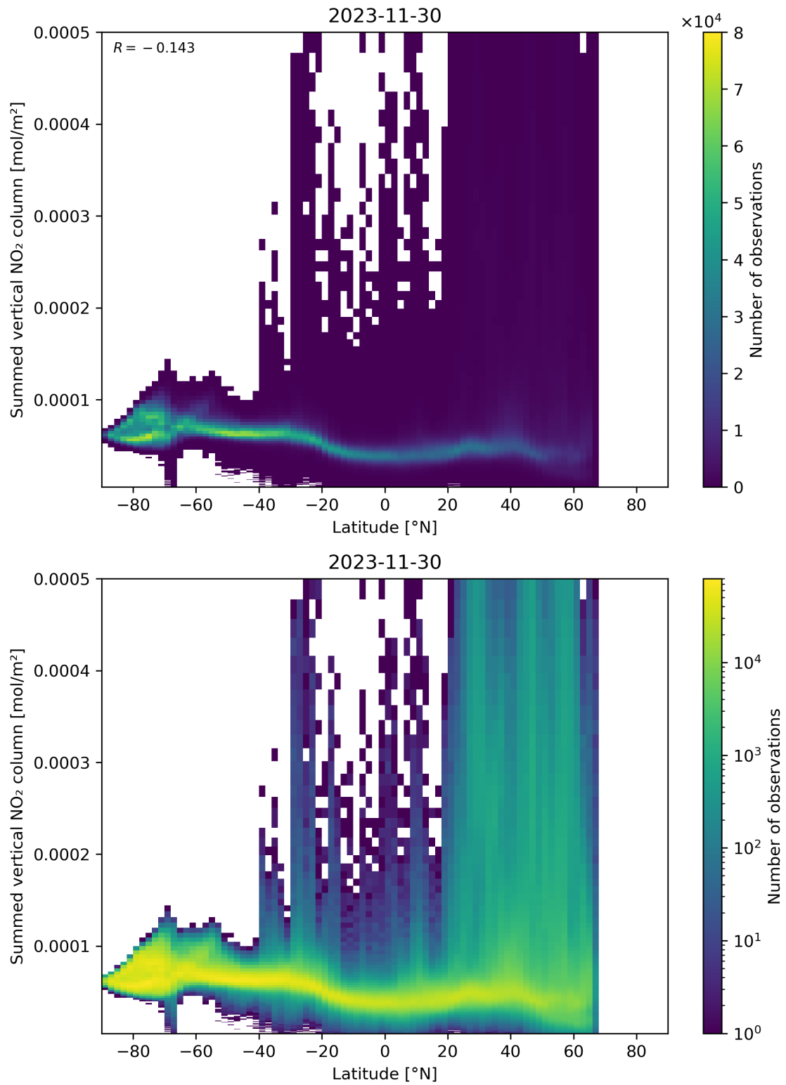
Figure 88: Scatter density plot of “Latitude” against “Summed vertical NO 2 column” for 2023-11-29 to 2023-12-01.
