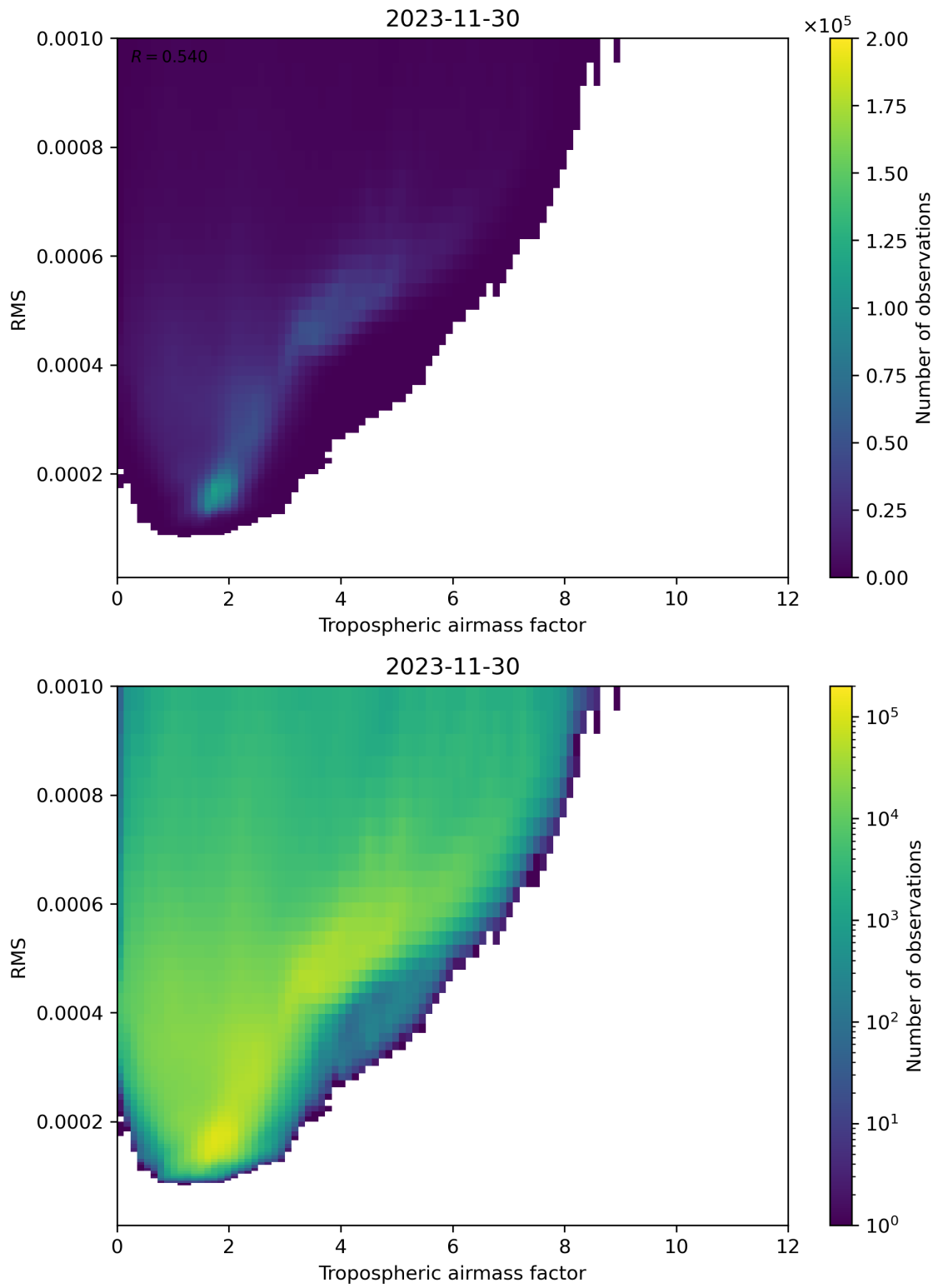
Figure 79: Scatter density plot of “Tropospheric airmass factor” against “RMS” for 2023-11-29 to 2023-12-01.
