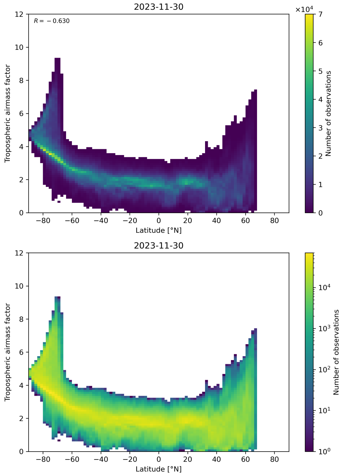
Figure 85: Scatter density plot of “Latitude” against “Tropospheric airmass factor” for 2023-11-29 to 2023-12-01.
