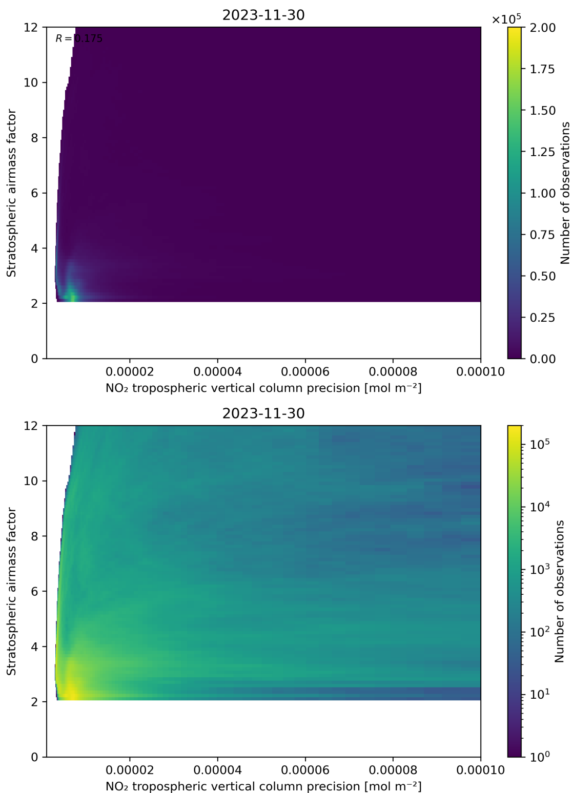
Figure 131: Scatter density plot of “NO 2 tropospheric vertical column precision” against “Stratospheric airmass factor” for 2023-11-29 to 2023-12-01.
