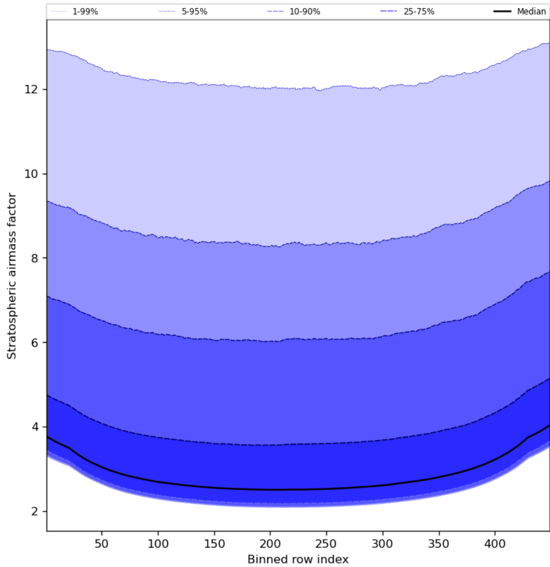
Figure 61: Along track statistics of “Stratospheric air mass factor” for 2023-11-29 to 2023-12-01
