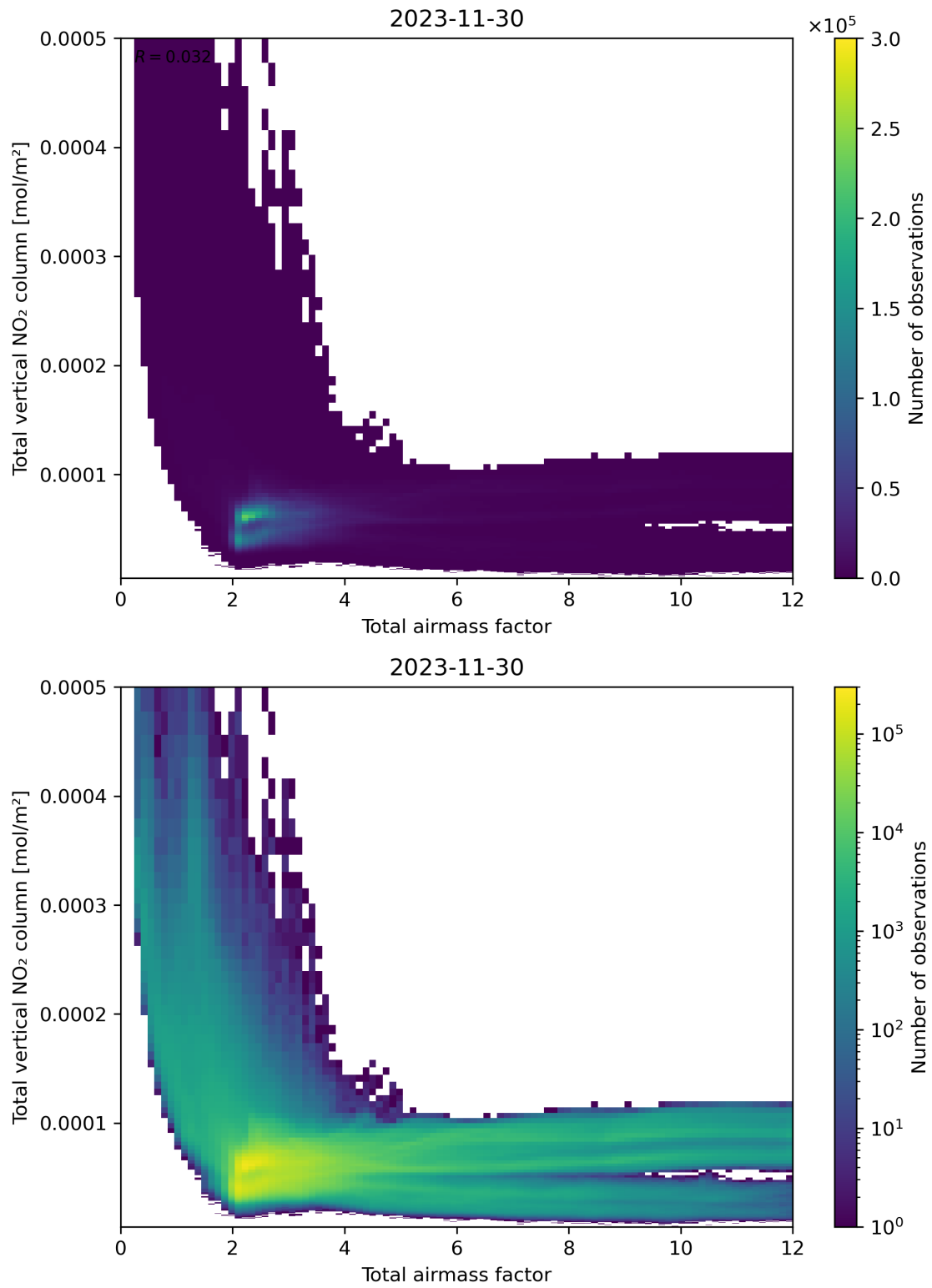
Figure 67: Scatter density plot of “Total airmass factor” against “Total vertical NO 2 column” for 2023-11-29 to 2023-12-01.
