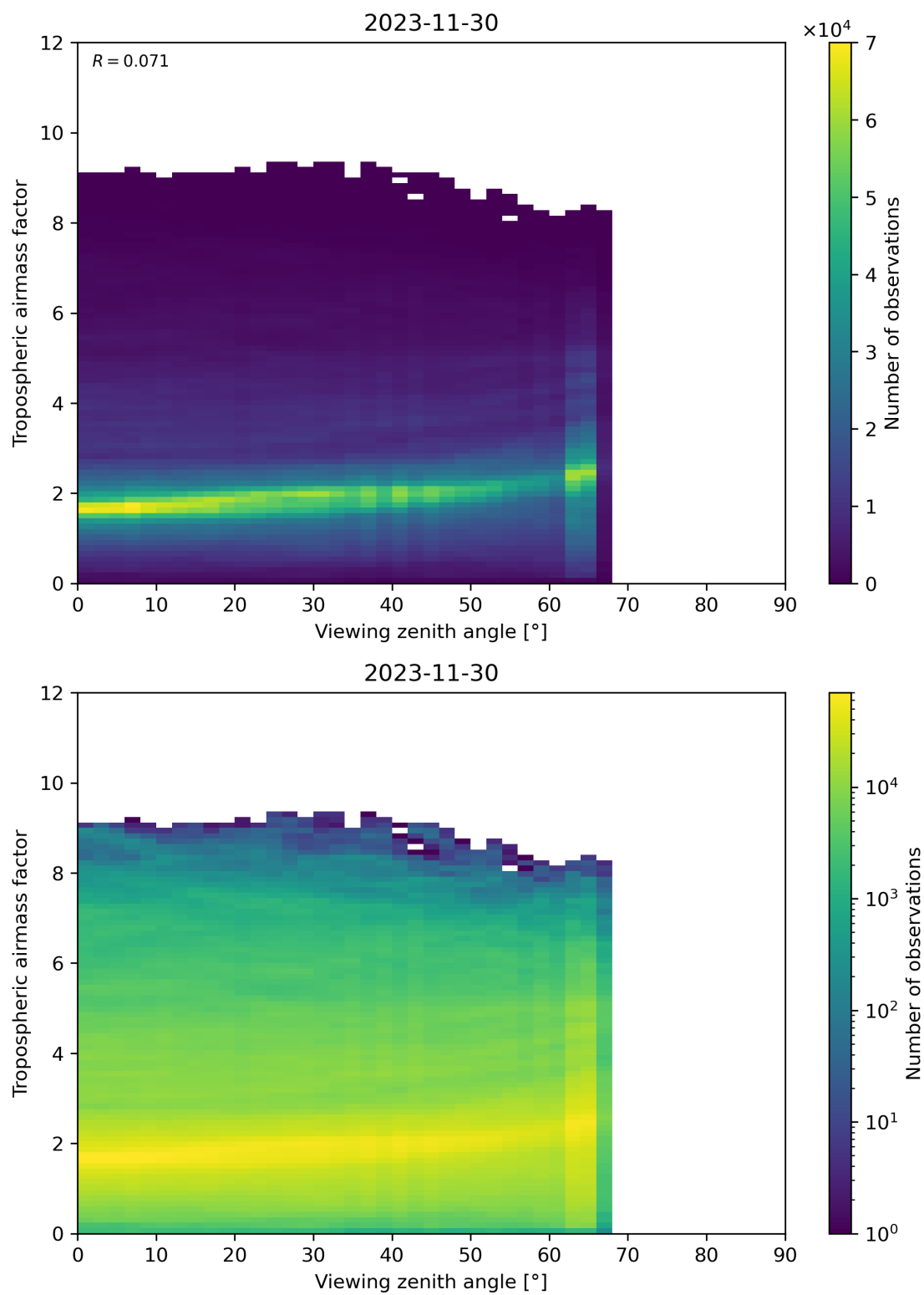
Figure 161: Scatter density plot of “Viewing zenith angle” against “Tropospheric airmass factor” for 2023-11-29 to 2023-12-01.
