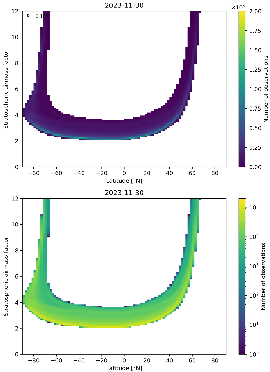
Figure 83: Scatter density plot of “Latitude” against “Stratospheric air mass factor” for 2023-11-29 to 2023-12-01.
