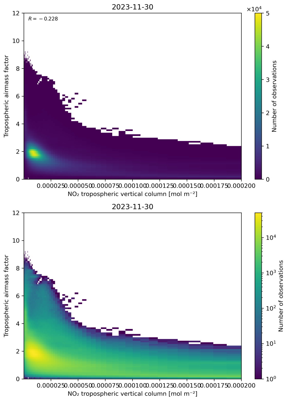
Figure 123: Scatter density plot of “NO 2 tropospheric vertical column” against “Tropospheric airmass factor” for 2023-11-29 to 2023-12-01.
