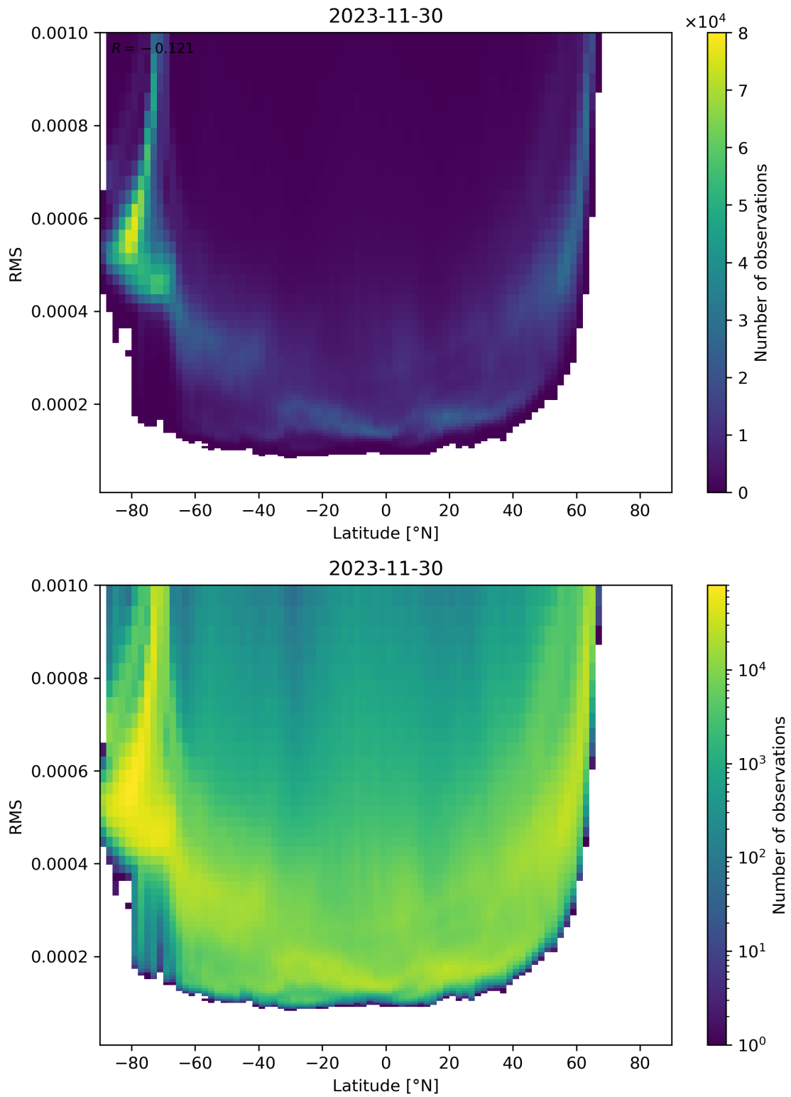
Figure 94: Scatter density plot of “Latitude” against “RMS” for 2023-11-29 to 2023-12-01.
