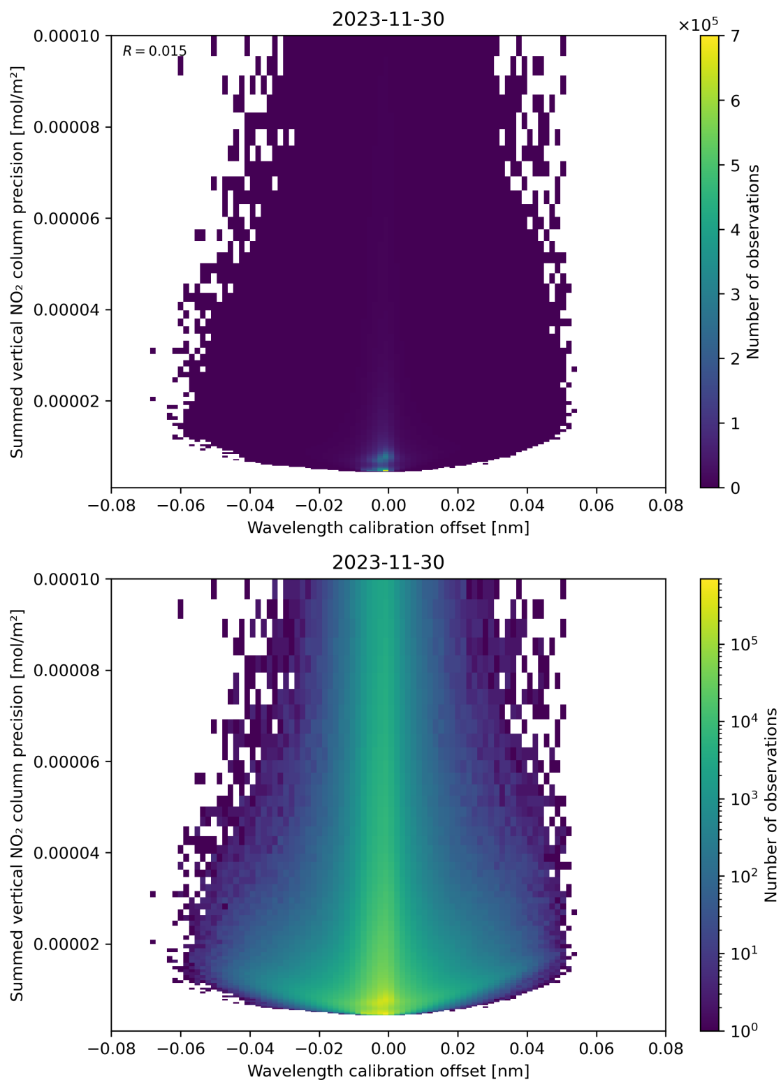
Figure 178: Scatter density plot of “Wavelength calibration offset” against “Summed vertical NO 2 column precision” for 2023-11-29 to 2023-12-01.
