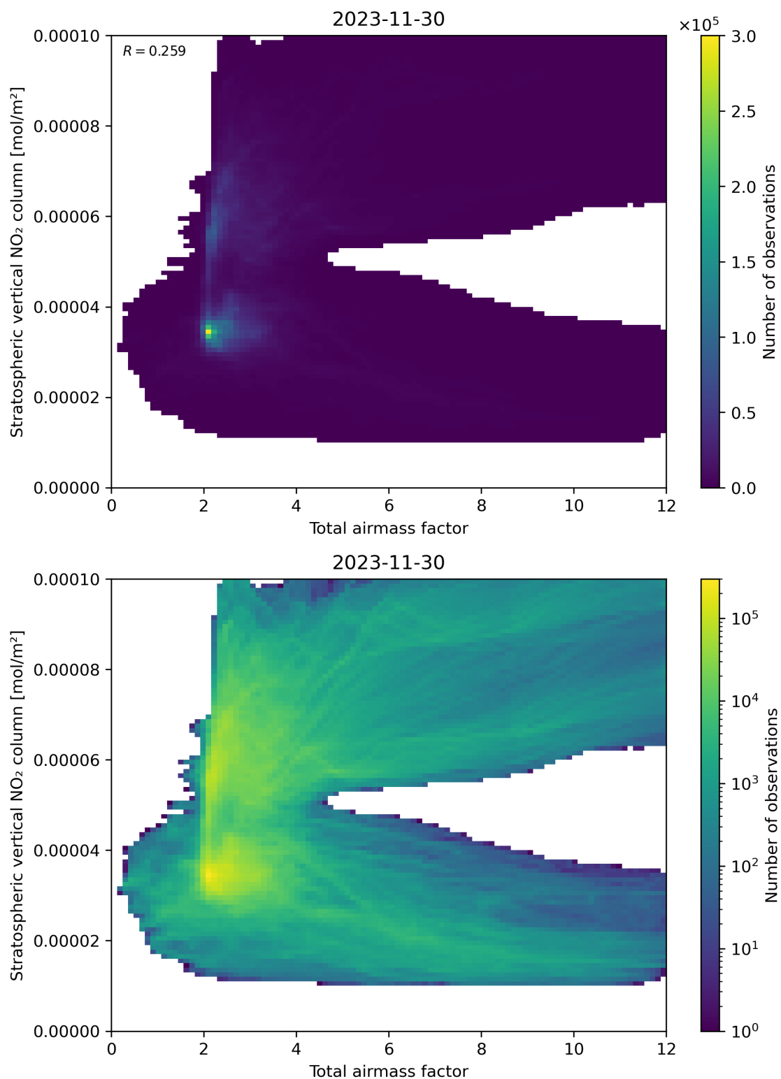
Figure 64: Scatter density plot of “Total airmass factor” against “Stratospheric vertical NO 2 column” for 2023-11-29 to 2023-12-01.
