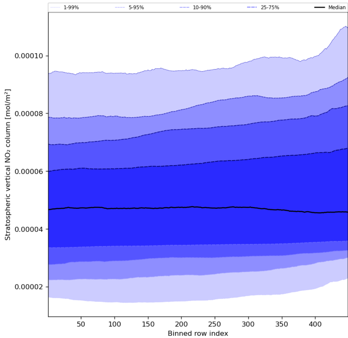
Figure 53: Along track statistics of “Stratospheric vertical NO 2 column” for 2023-11-29 to 2023-12-01
