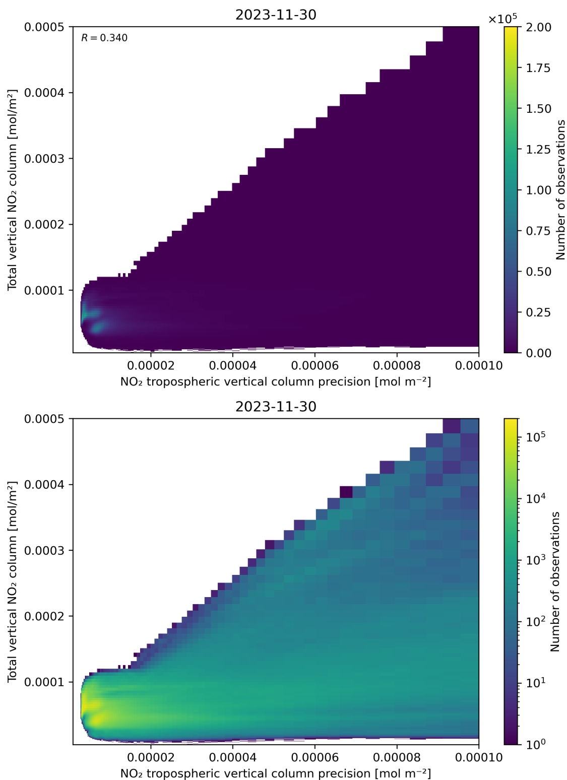
Figure 138: Scatter density plot of “NO 2 tropospheric vertical column precision” against “Total vertical NO 2 column” for 2023-11-29 to 2023-12-01.
