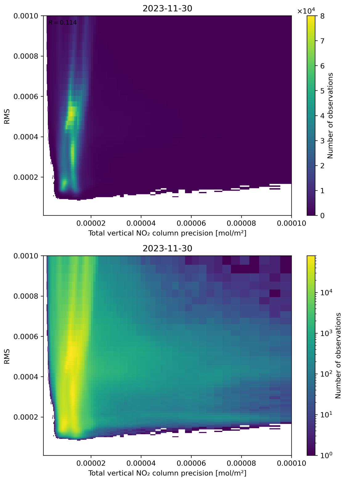
Figure 119: Scatter density plot of “Total vertical NO 2 column precision” against “RMS” for 2023-11-29 to 2023-12-01.
