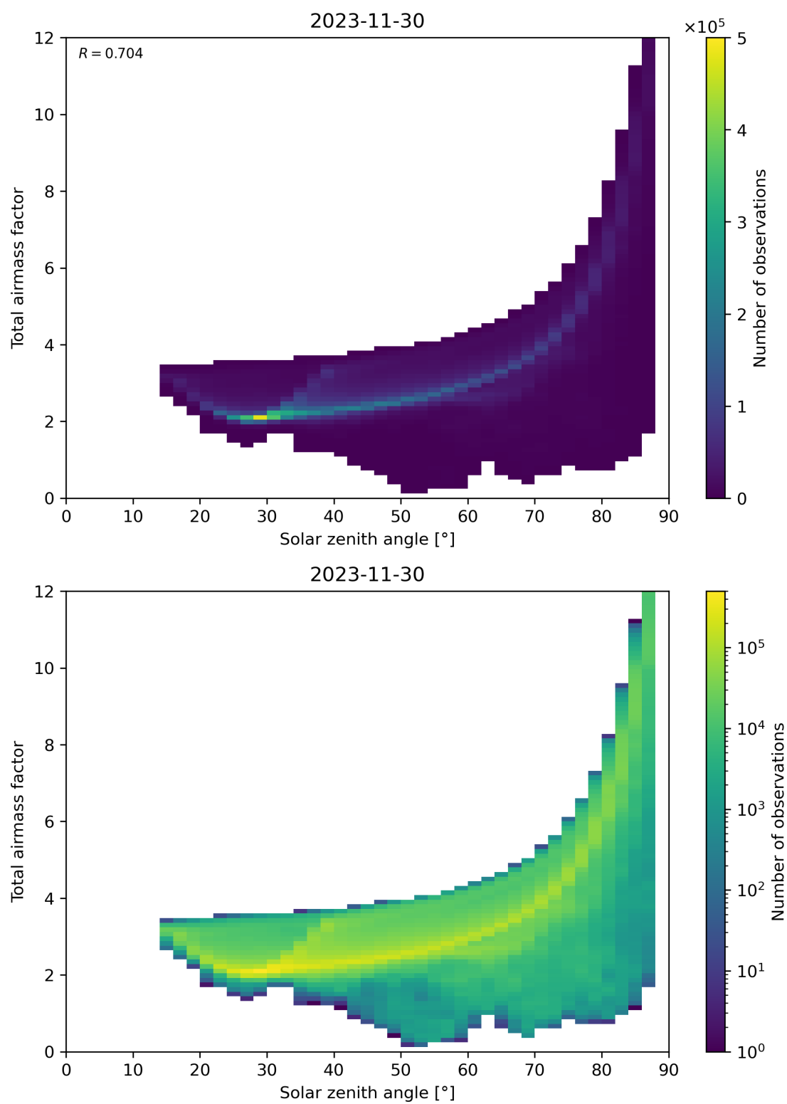
Figure 146: Scatter density plot of “Solar zenith angle” against “Total air mass factor” for 2023-11-29 to 2023-12-01.
