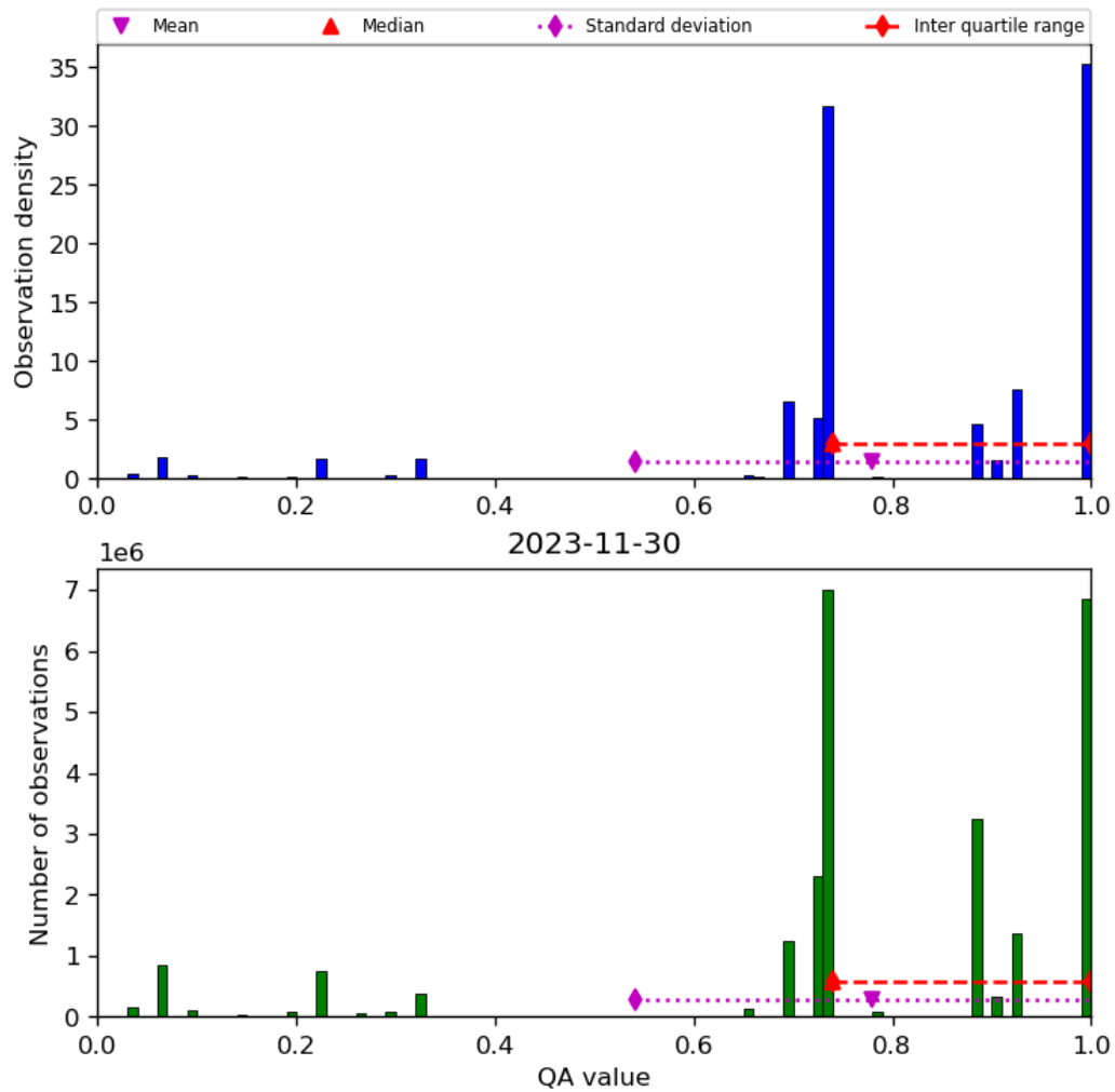
Figure 28: Histogram of “QA value” for 2023-11-29 to 2023-12-01
