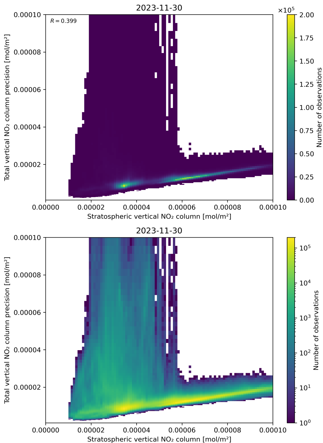
Figure 101: Scatter density plot of “Stratospheric vertical NO 2 column” against “Total vertical NO 2 column precision” for 2023-11-29 to 2023-12-01.
