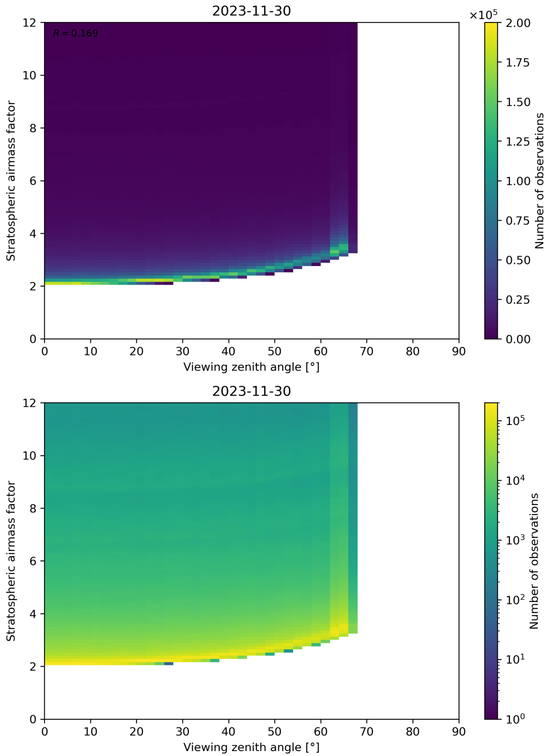
Figure 159: Scatter density plot of “Viewing zenith angle” against “Stratospheric airmass factor” for 2023-11-29 to 2023-12-01.
