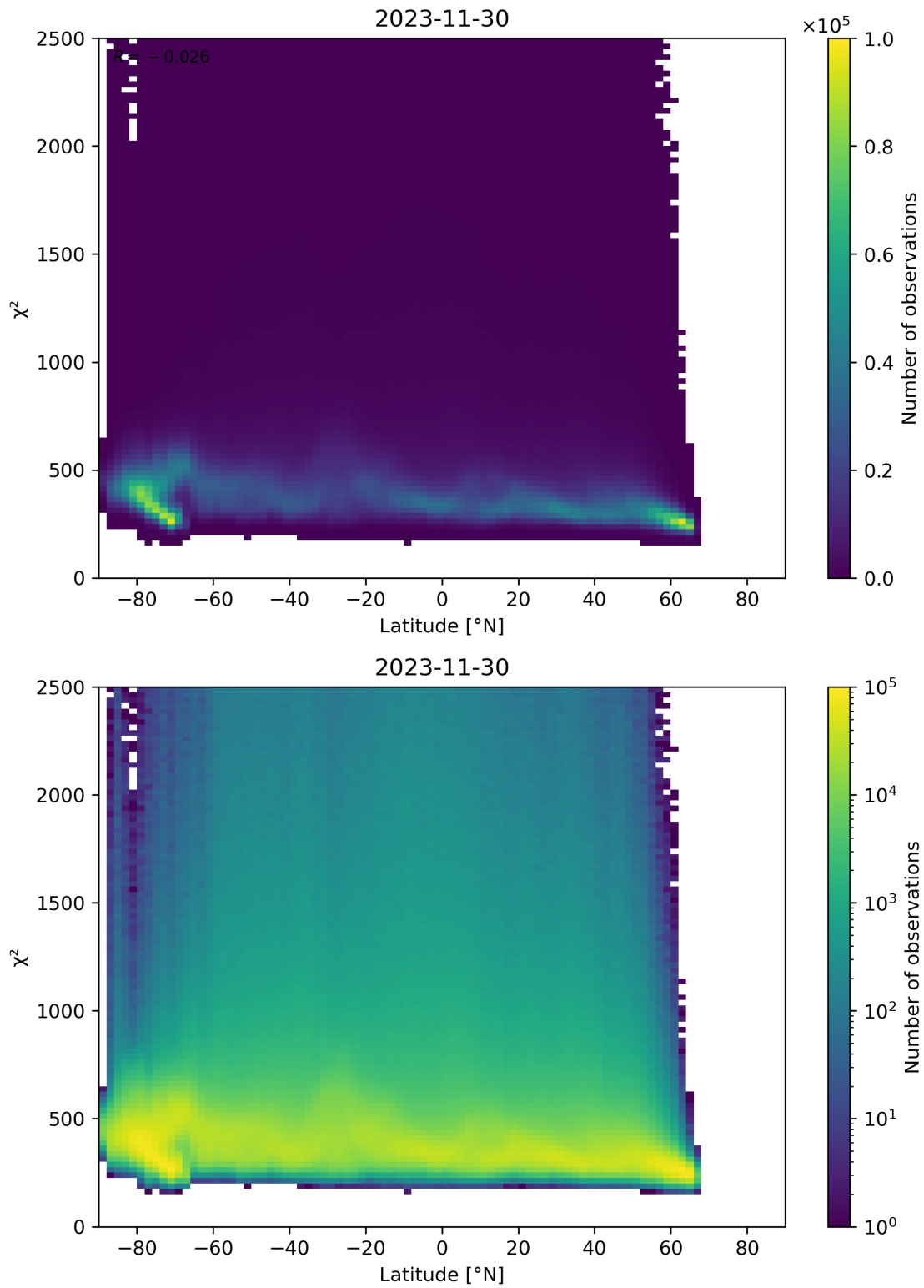
Figure 86: Scatter density plot of “Latitude” against “ \chi^2 ” for 2023-11-29 to 2023-12-01.
