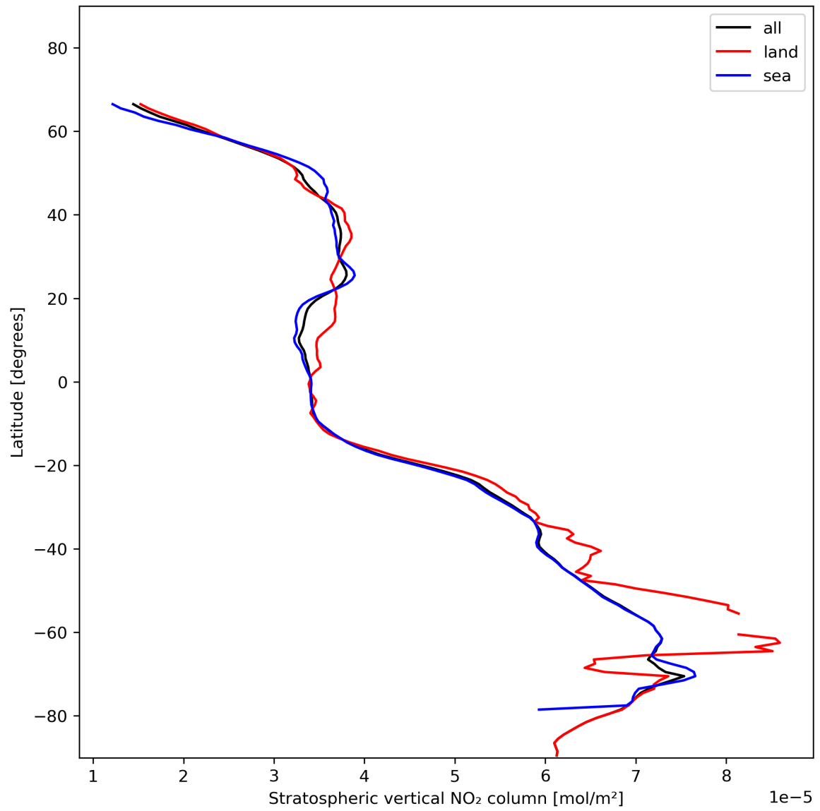
Figure 19: Zonal average of “Stratospheric vertical NO 2 column” for 2023-11-29 to 2023-12-01.
