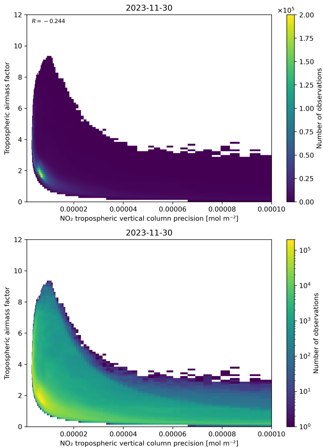
Figure 133: Scatter density plot of “NO 2 tropospheric vertical column precision” against “Tropospheric airmass factor” for 2023-11-29 to 2023-12-01.
