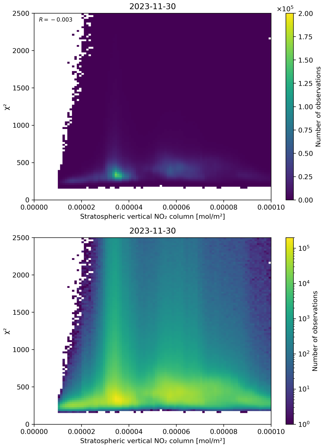
Figure 97: Scatter density plot of “Stratospheric vertical NO 2 column” against “ \chi^2 ” for 2023-11-29 to 2023-12-01.
