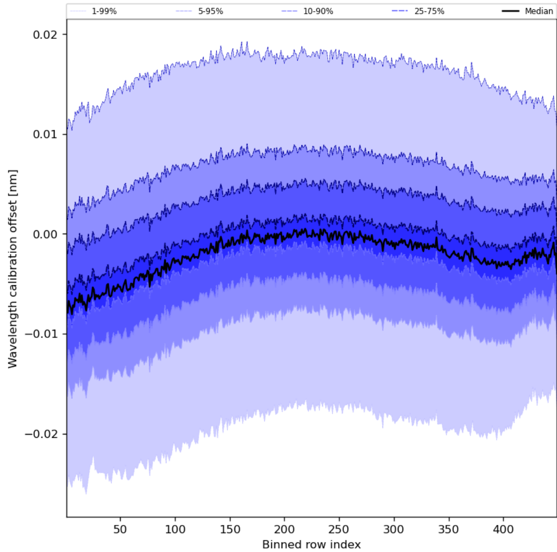
Figure 52: Along track statistics of “Wavelength calibration offset” for 2023-11-29 to 2023-12-01
