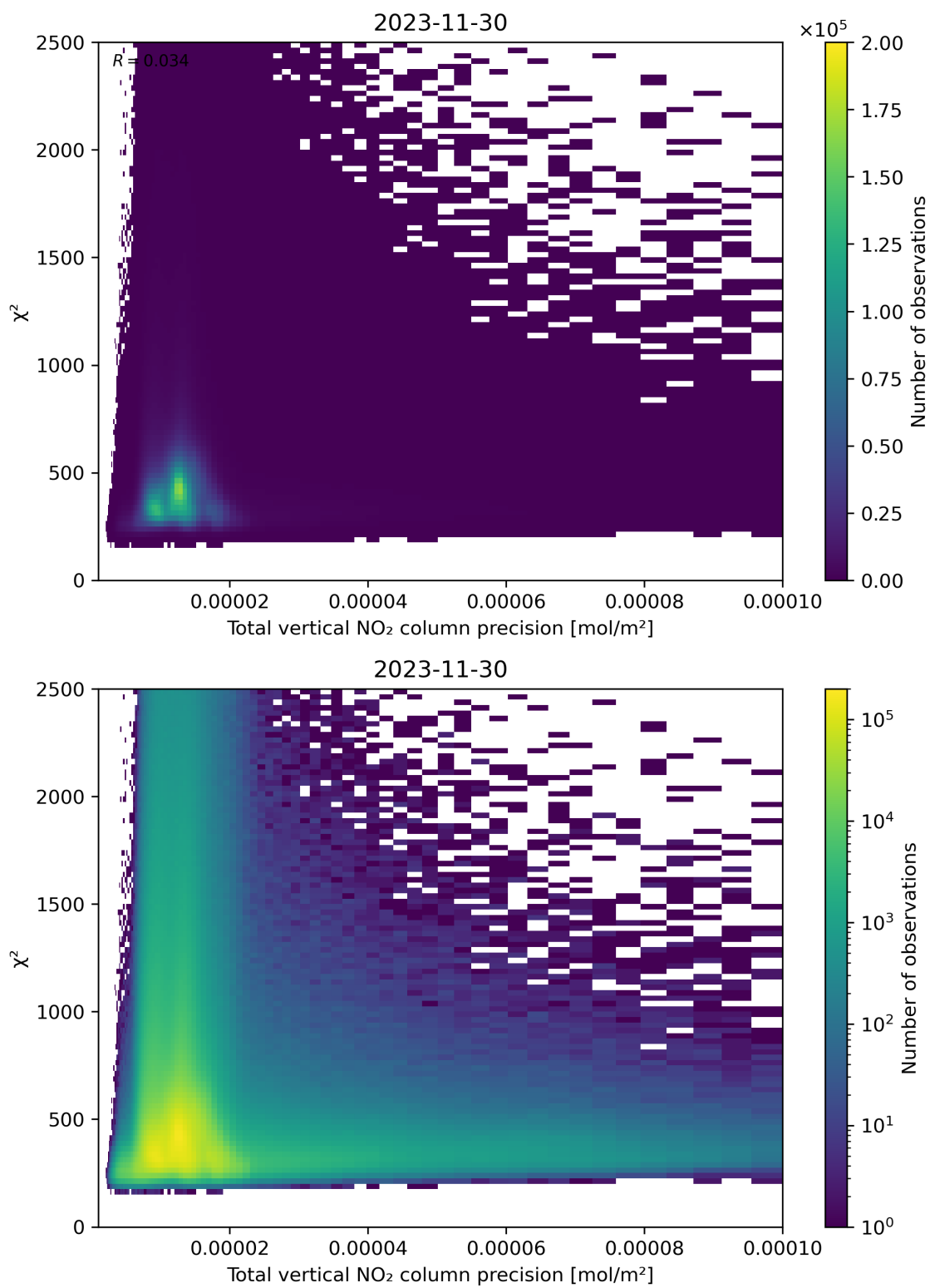
Figure 116: Scatter density plot of “Total vertical NO 2 column precision” against “ \chi^2 ” for 2023-11-29 to 2023-12-01.
