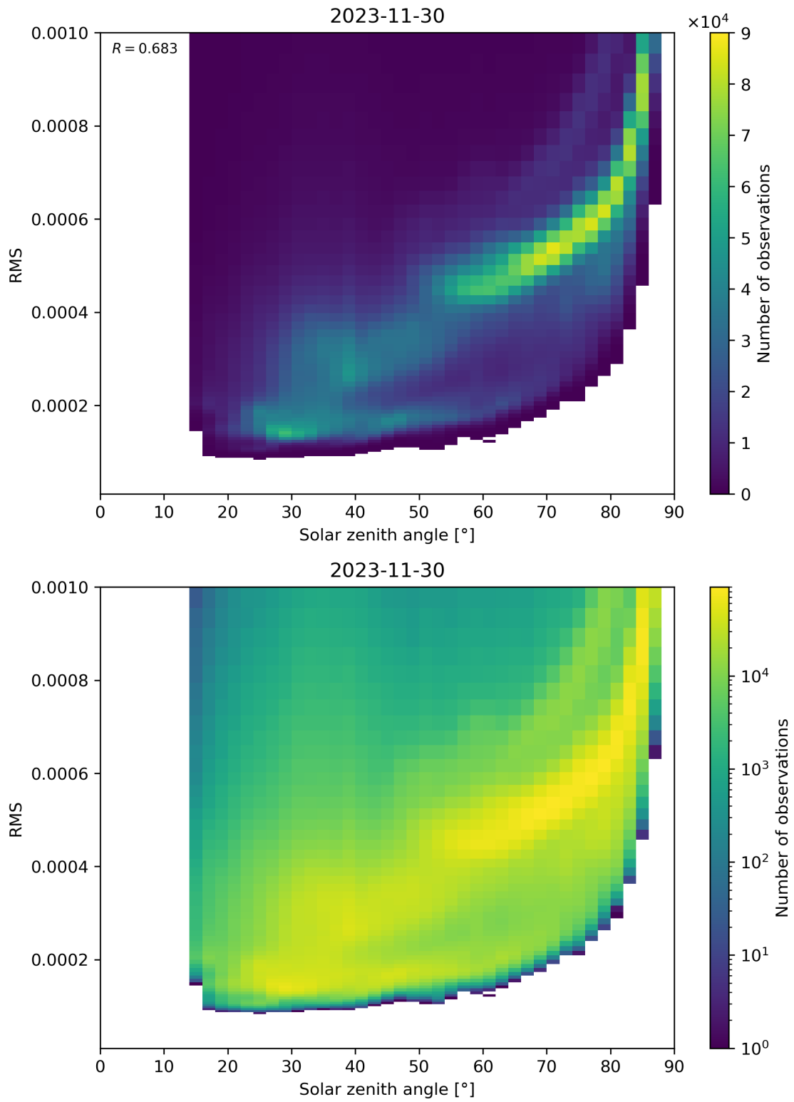
Figure 157: Scatter density plot of “Solar zenith angle” against “RMS” for 2023-11-29 to 2023-12-01.
