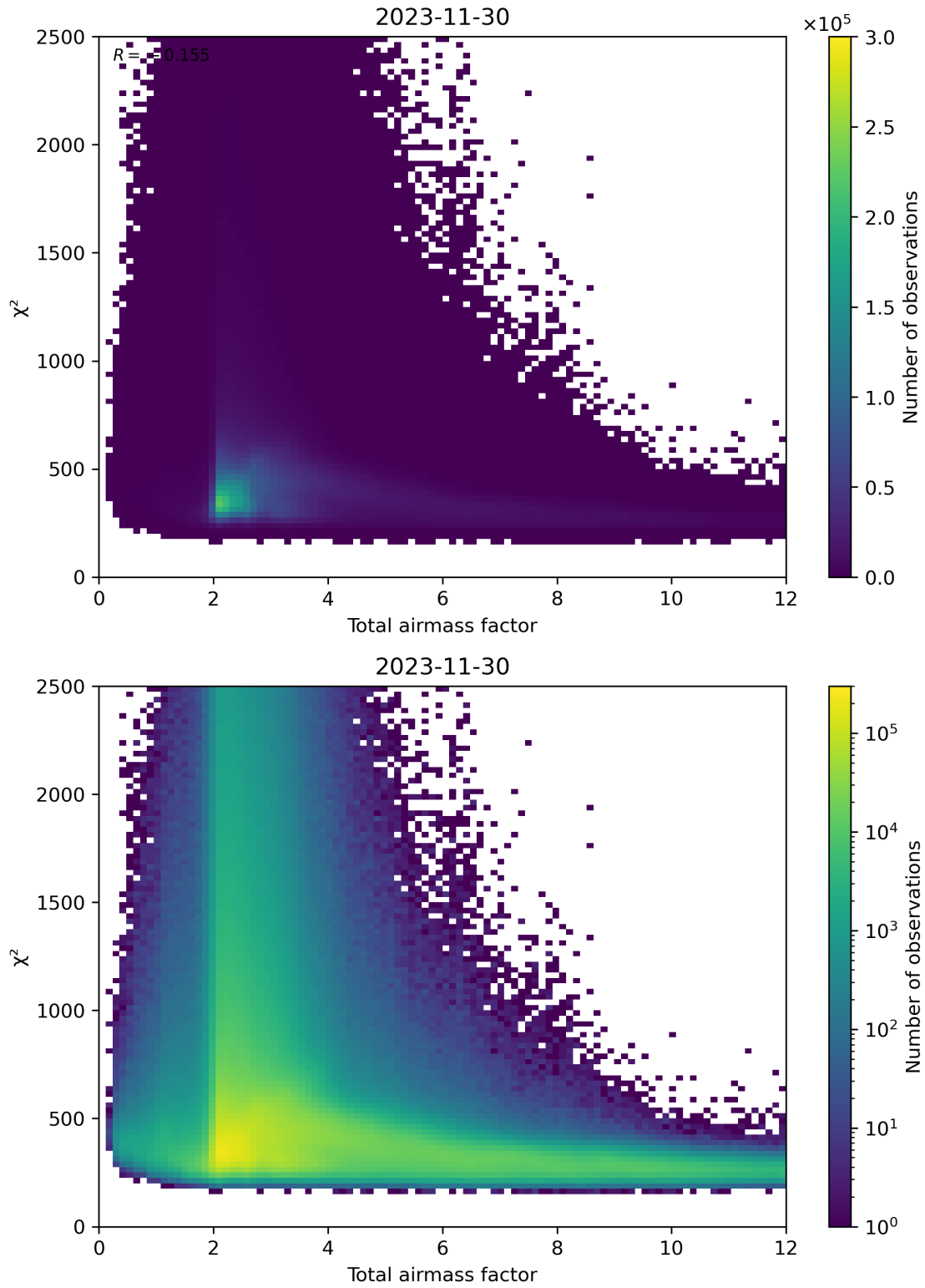
Figure 63: Scatter density plot of “Total airmass factor” against “ \chi^2 ” for 2023-11-29 to 2023-12-01.
