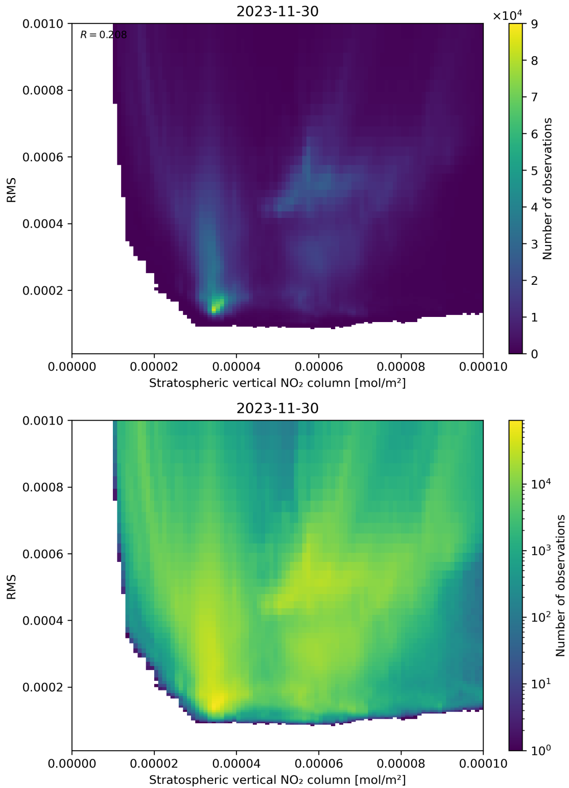
Figure 102: Scatter density plot of “Stratospheric vertical NO 2 column” against “RMS” for 2023-11-29 to 2023-12-01.
