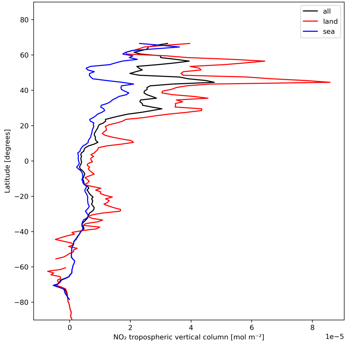
Figure 12: Zonal average of “NO 2 tropospheric vertical column” for 2023-11-29 to 2023-12-01.
