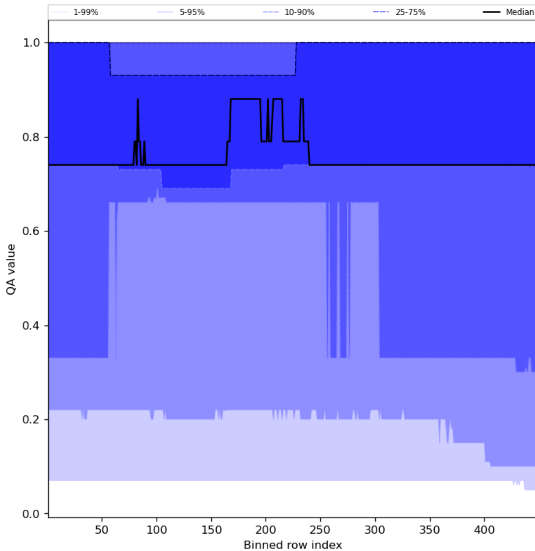
Figure 45: Along track statistics of “QA value” for 2023-11-29 to 2023-12-01
