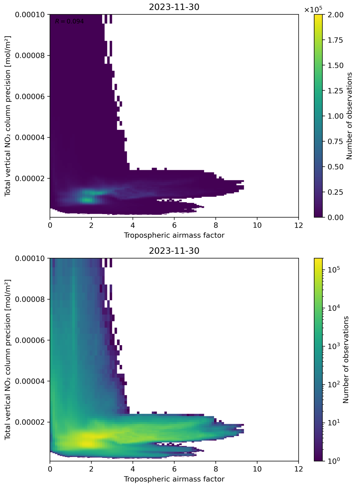
Figure 78: Scatter density plot of “Tropospheric air mass factor” against “Total vertical NO 2 column precision” for 2023-11-29 to 2023-12-01.
