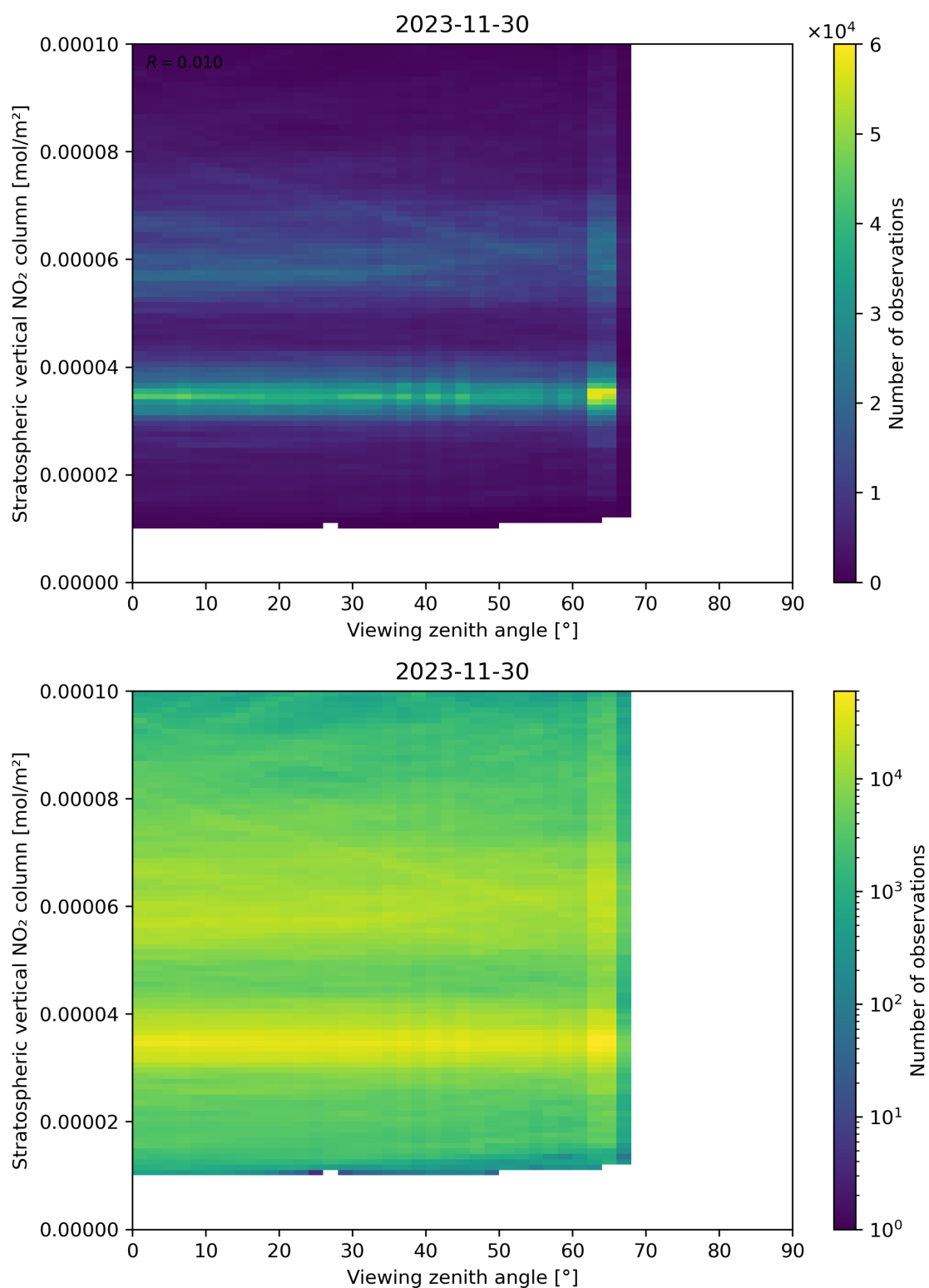
Figure 164: Scatter density plot of “Viewing zenith angle” against “Stratospheric vertical NO 2 column” for 2023-11-29 to 2023-12-01.
