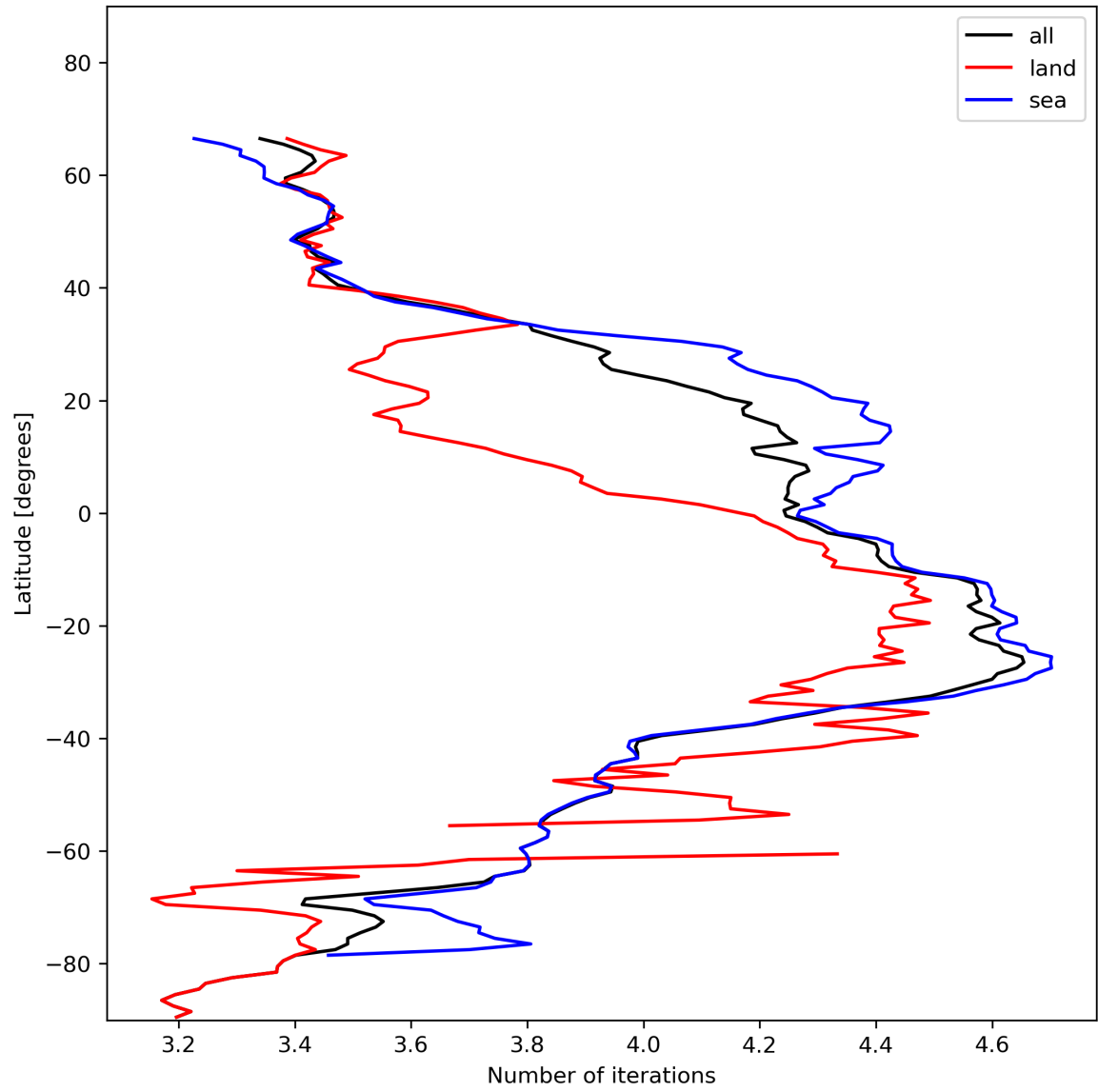
Figure 17: Zonal average of “Number of iterations” for 2023-11-29 to 2023-12-01.
