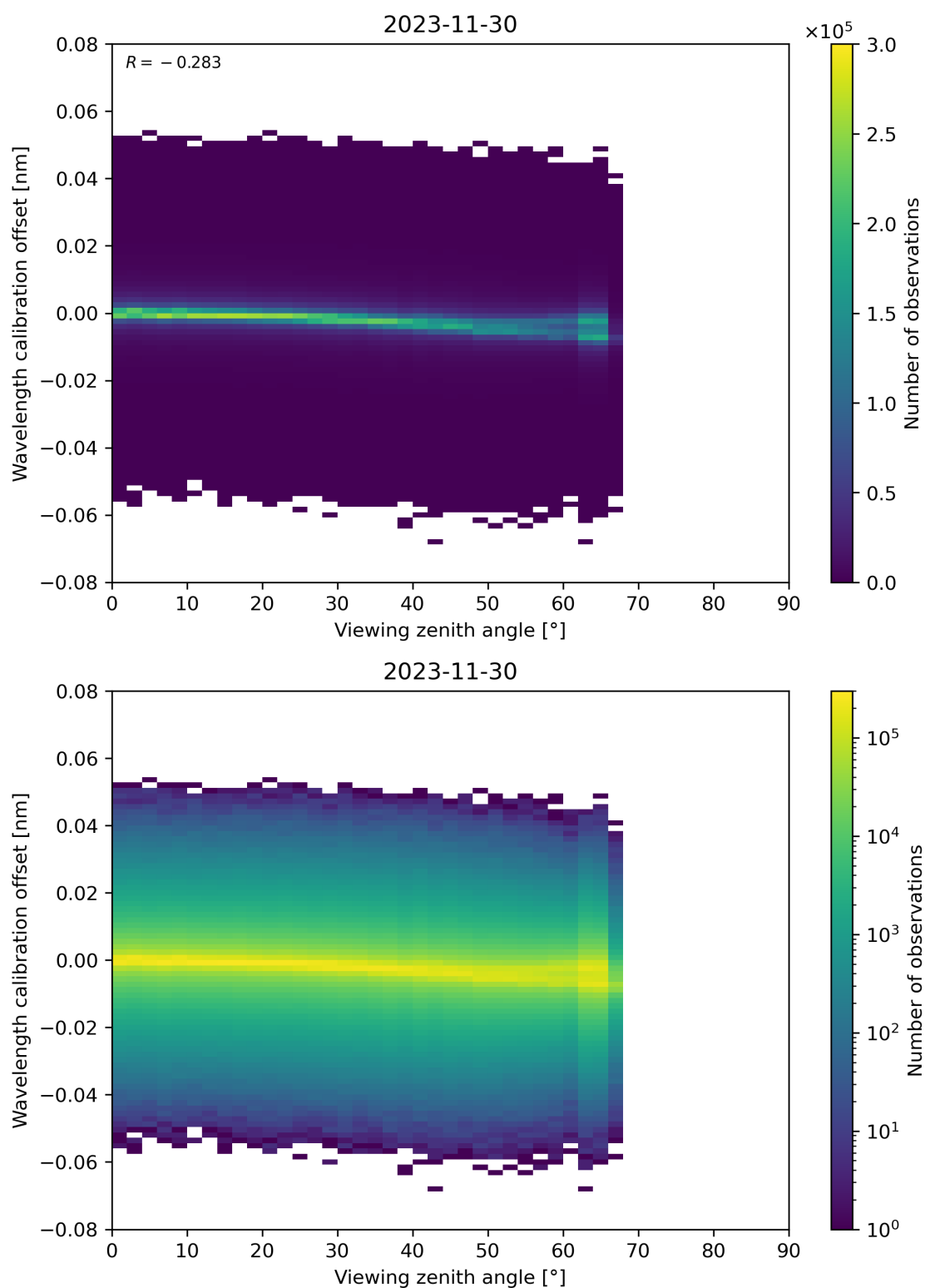
Figure 173: Scatter density plot of “Viewing zenith angle” against “Wavelength calibration offset” for 2023-11-29 to 2023-12-01.
