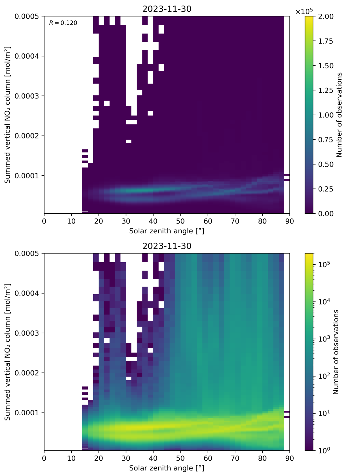
Figure 151: Scatter density plot of “Solar zenith angle” against “Summed vertical NO 2 column” for 2023-11-29 to 2023-12-01.
