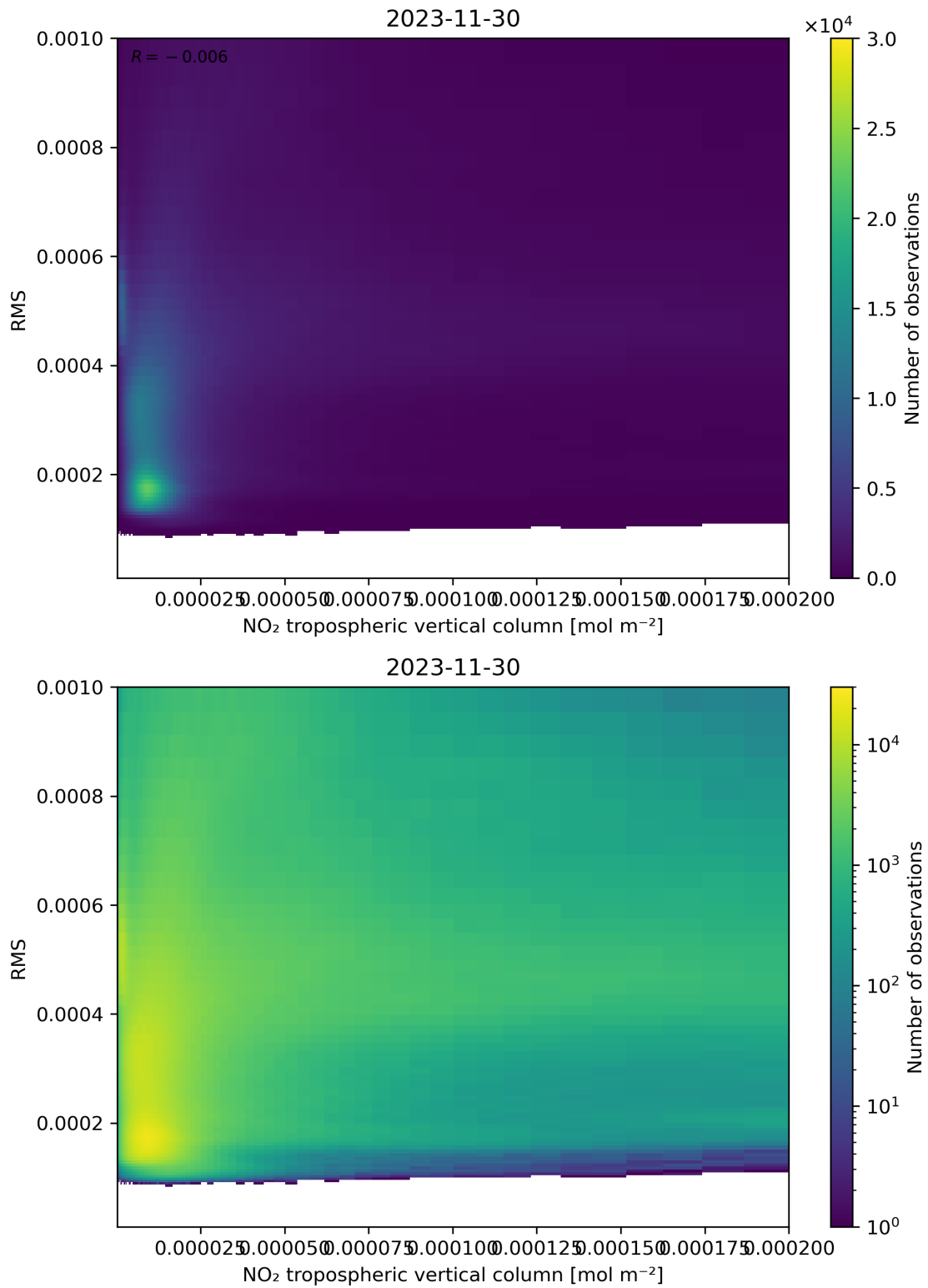
Figure 142: Scatter density plot of “NO 2 tropospheric vertical column” against “RMS” for 2023-11-29 to 2023-12-01.
