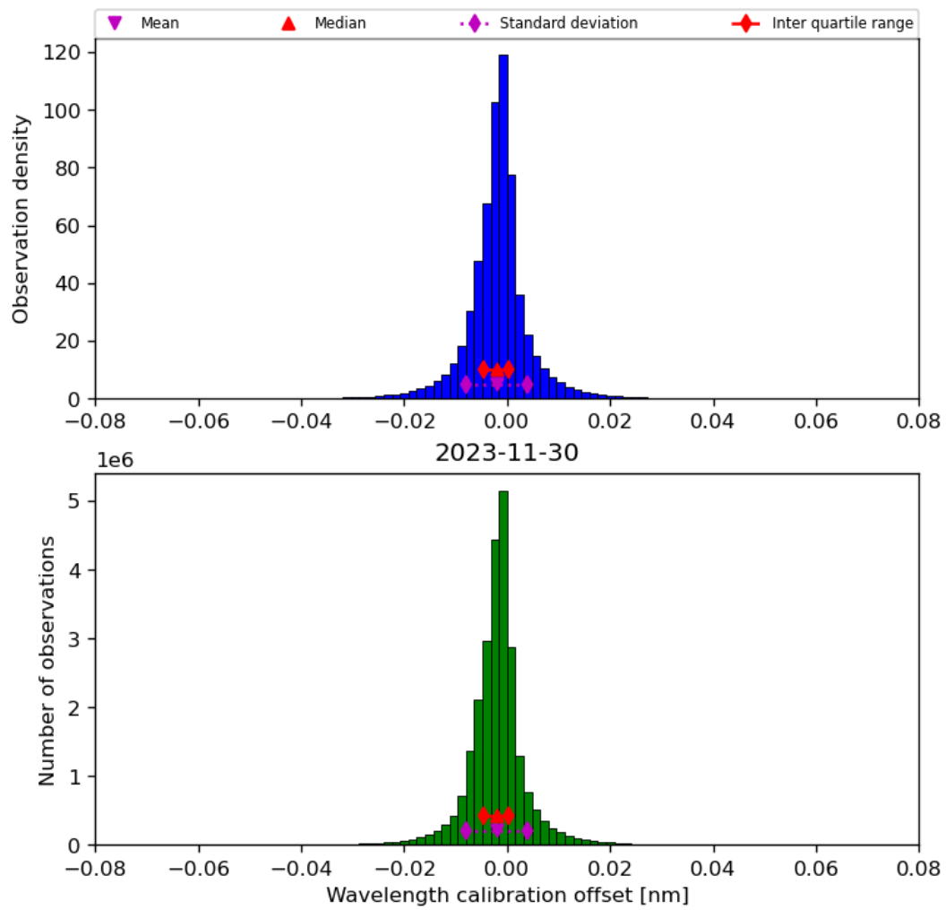
Figure 35: Histogram of “Wavelength calibration offset” for 2023-11-29 to 2023-12-01
