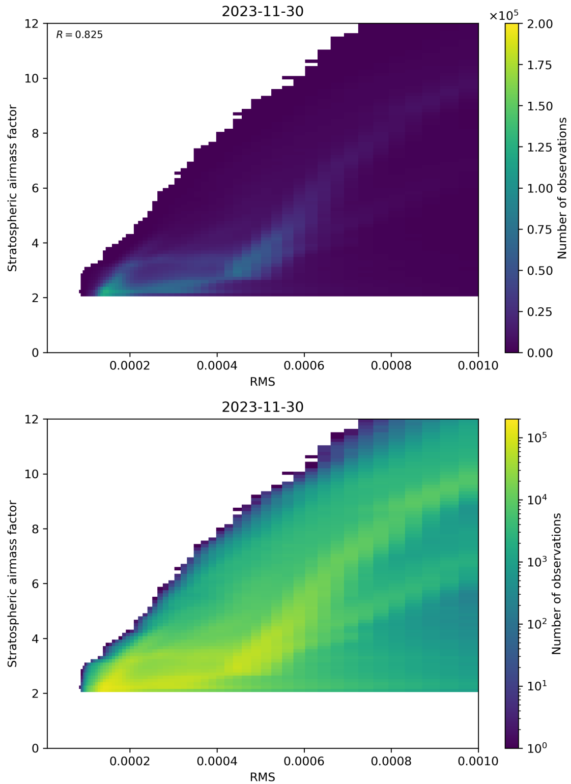
Figure 144: Scatter density plot of “RMS” against “Stratospheric airmass factor” for 2023-11-29 to 2023-12-01.
