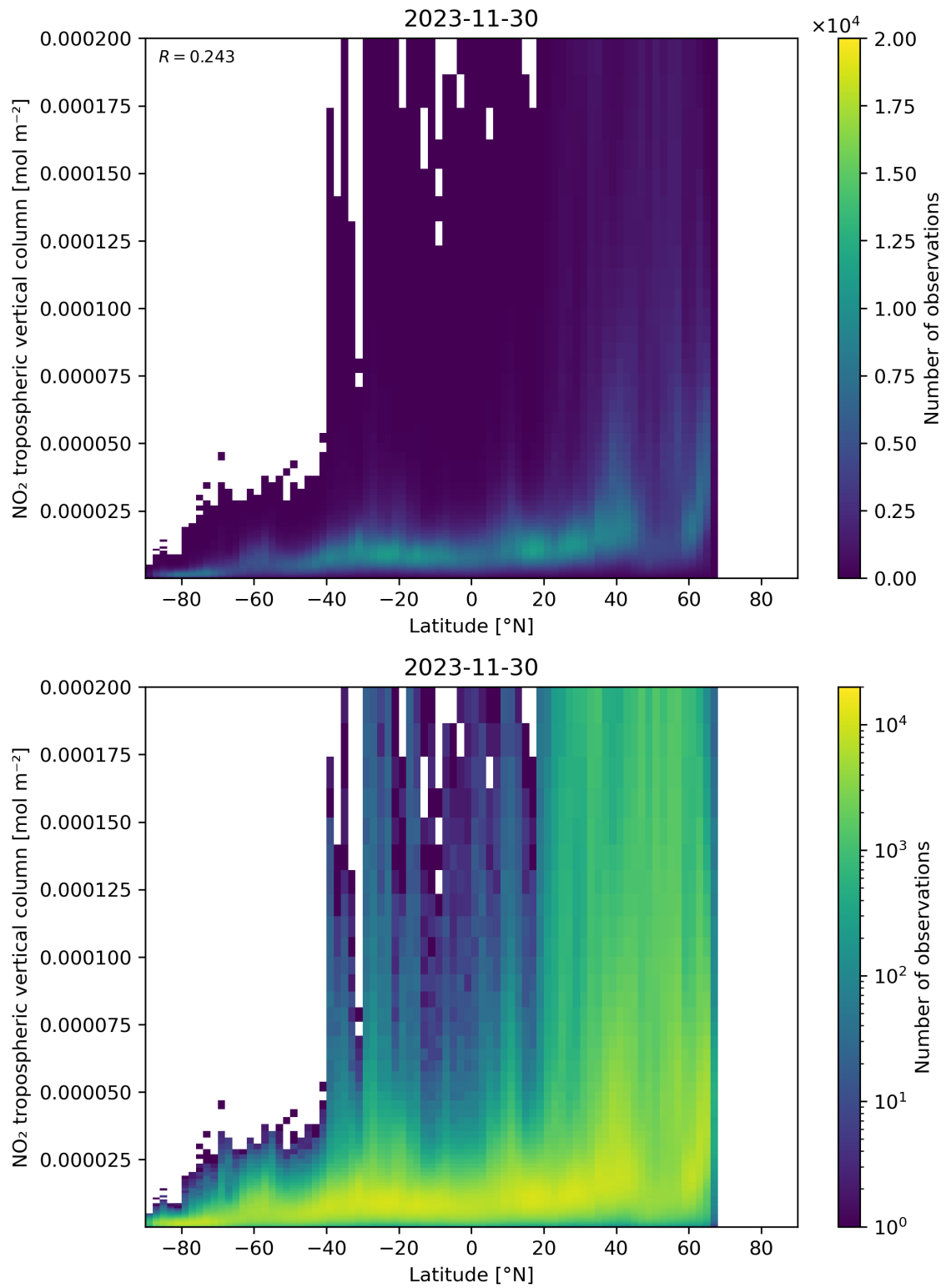
Figure 92: Scatter density plot of “Latitude” against “NO 2 tropospheric vertical column” for 2023-11-29 to 2023-12-01.
