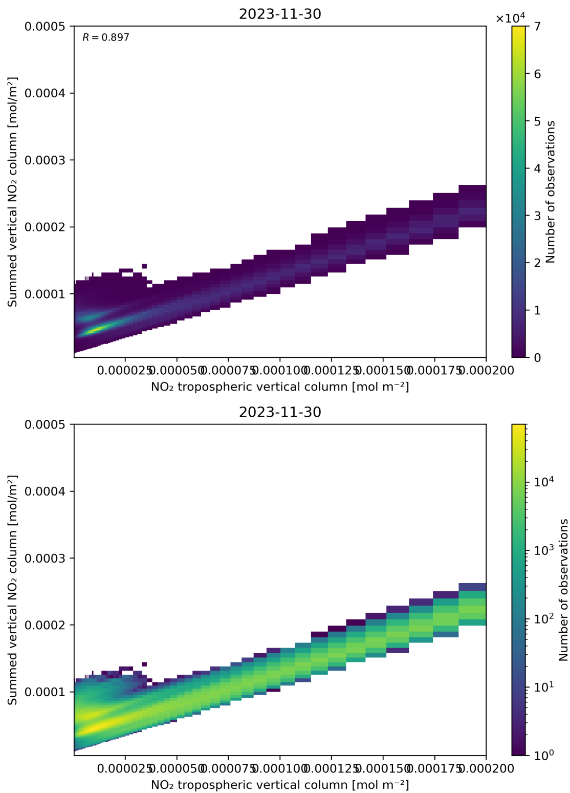
Figure 126: Scatter density plot of “NO 2 tropospheric vertical column” against “Summed vertical NO 2 column” for 2023-11-29 to 2023-12-01.
