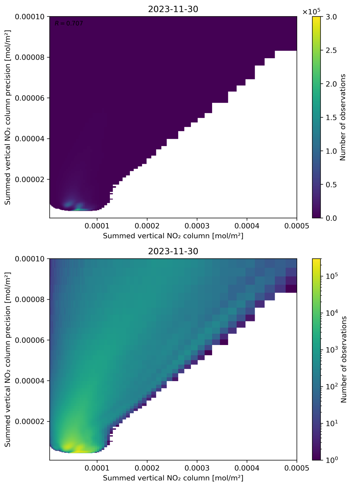
Figure 105: Scatter density plot of “Summed vertical NO 2 column” against “Summed vertical NO 2 column precision” for 2023-11-29 to 2023-12-01.
