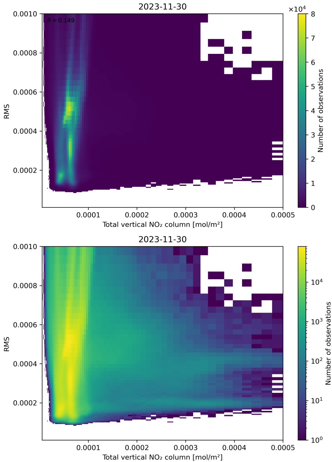
Figure 120: Scatter density plot of “Total vertical NO 2 column” against “RMS” for 2023-11-29 to 2023-12-01.
