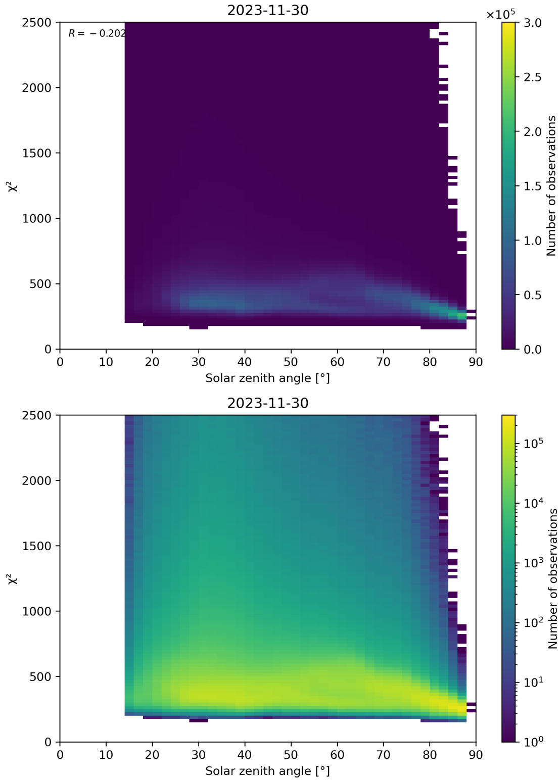
Figure 148: Scatter density plot of “Solar zenith angle” against “ \chi^2 ” for 2023-11-29 to 2023-12-01.
