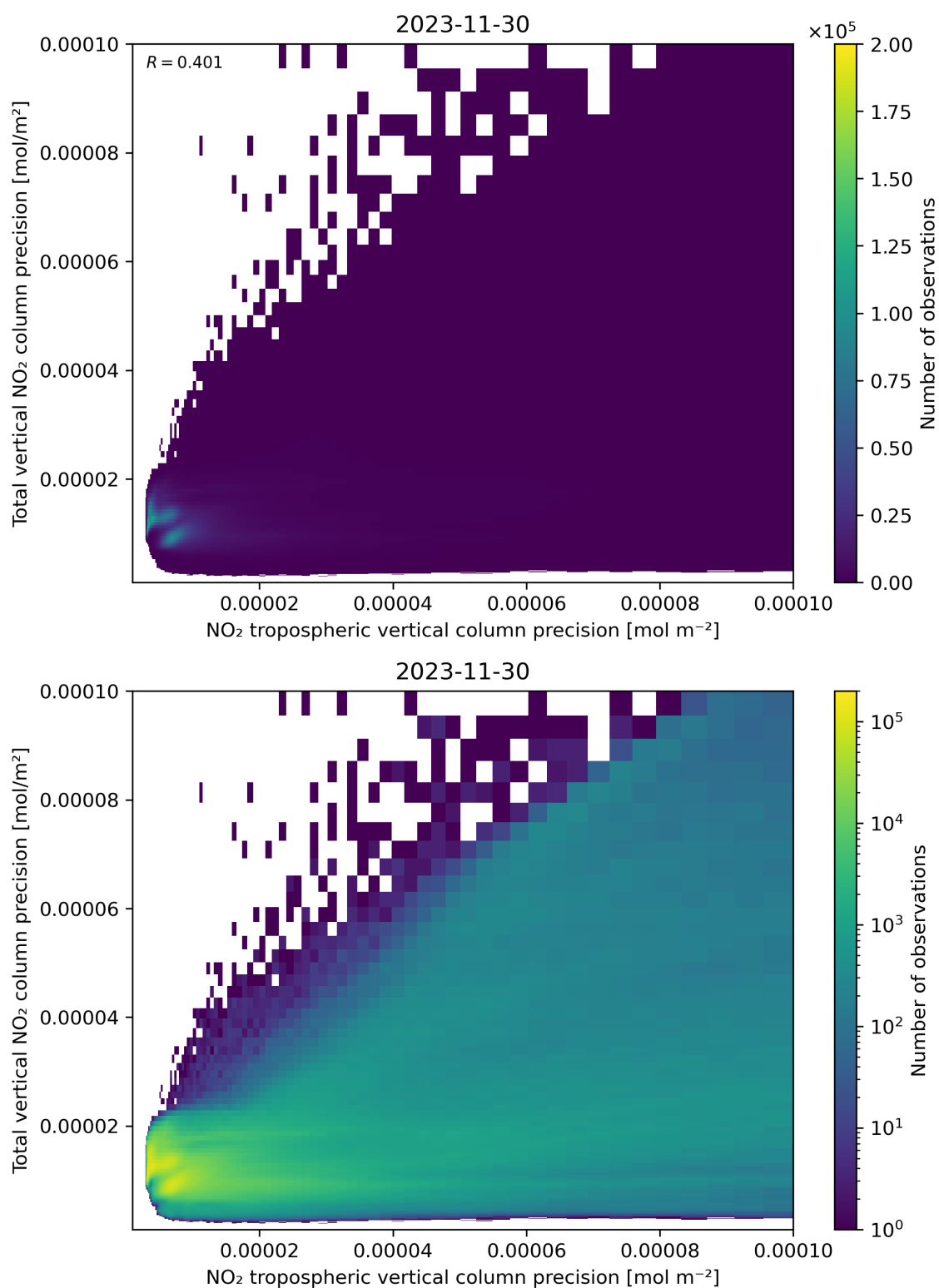
Figure 139: Scatter density plot of “NO 2 tropospheric vertical column precision” against “Total vertical NO 2 column precision” for 2023-11-29 to 2023-12-01.
