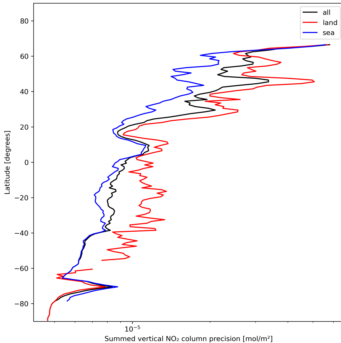
Figure 24: Zonal average of “Summed vertical NO 2 column precision” for 2023-11-29 to 2023-12-01.
