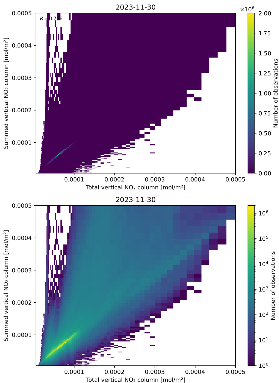
Figure 112: Scatter density plot of “Total vertical NO 2 column” against “Summed vertical NO 2 column” for 2023-11-29 to 2023-12-01.
