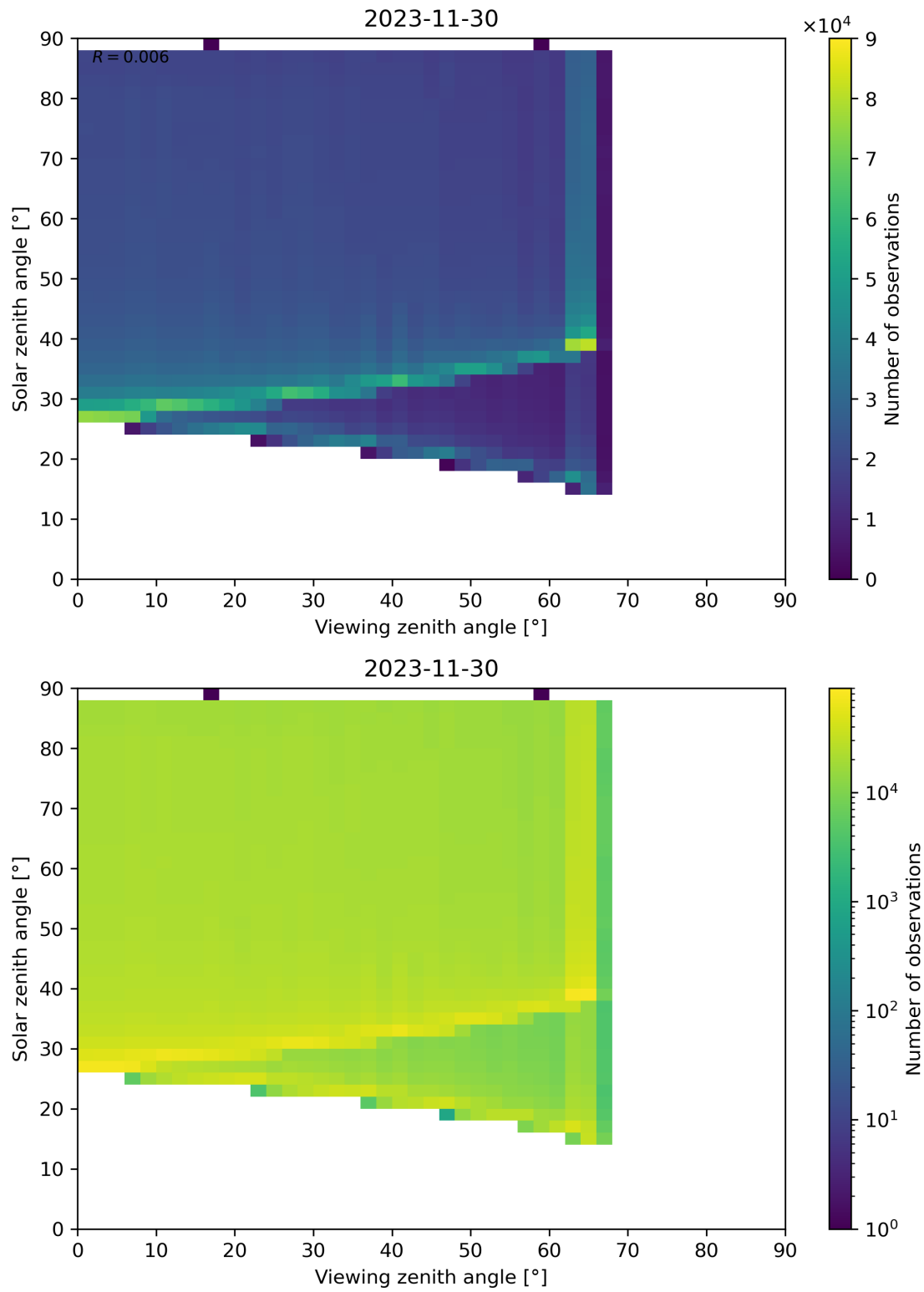
Figure 172: Scatter density plot of “Viewing zenith angle” against “Solar zenith angle” for 2023-11-29 to 2023-12-01.
