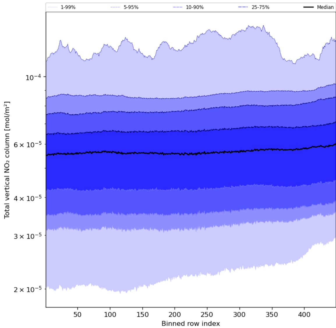
Figure 55: Along track statistics of “Total vertical NO 2 column” for 2023-11-29 to 2023-12-01
