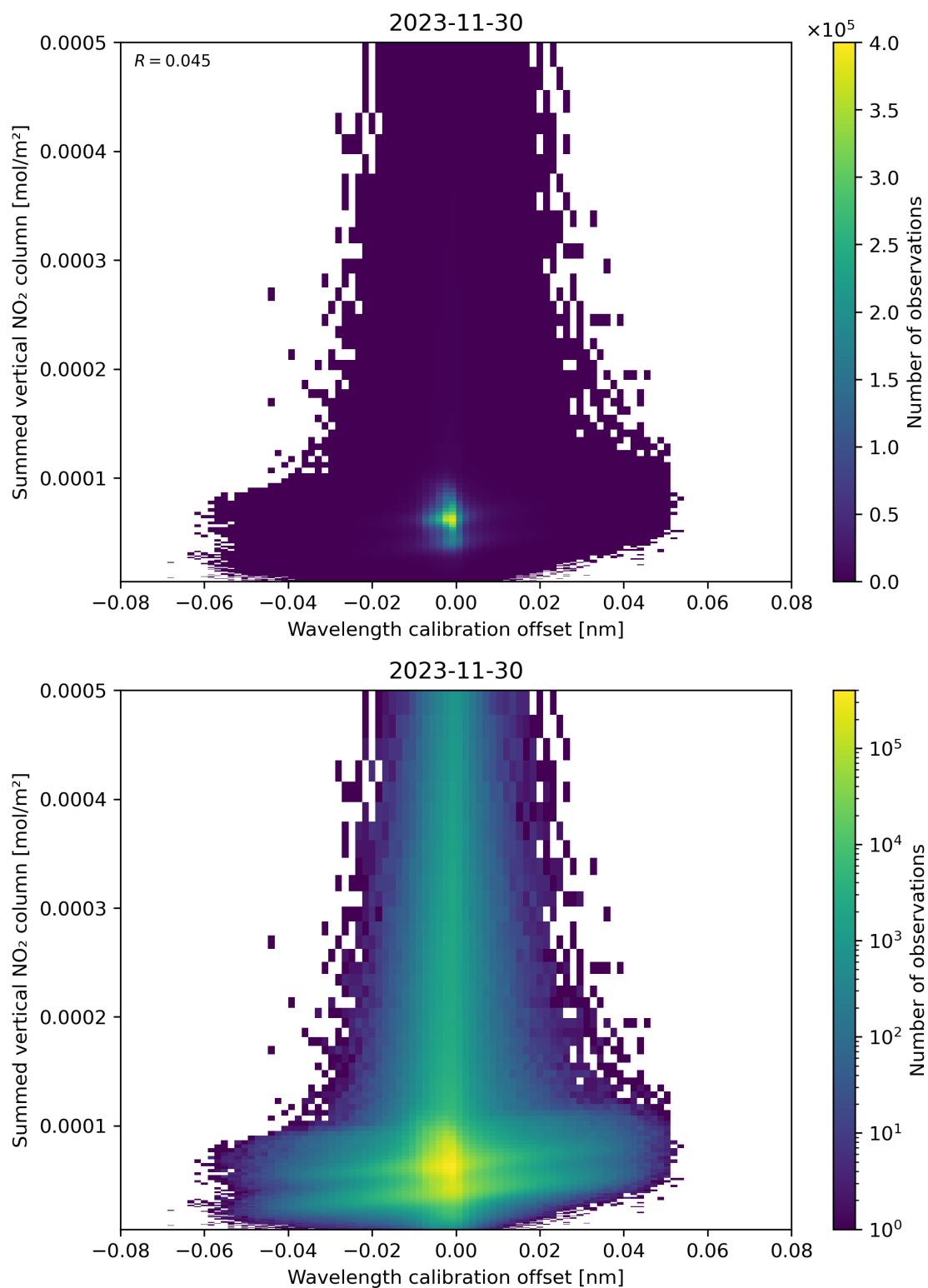
Figure 177: Scatter density plot of “Wavelength calibration offset” against “Summed vertical NO 2 column” for 2023-11-29 to 2023-12-01.
