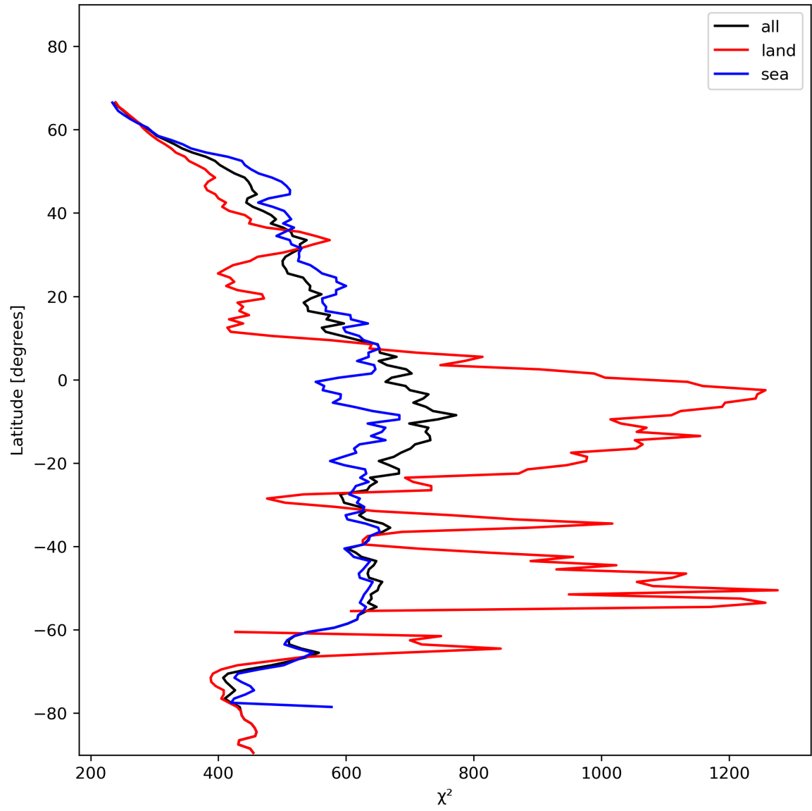
Figure 25: Zonal average of “ \chi^2 ” for 2023-11-29 to 2023-12-01.
