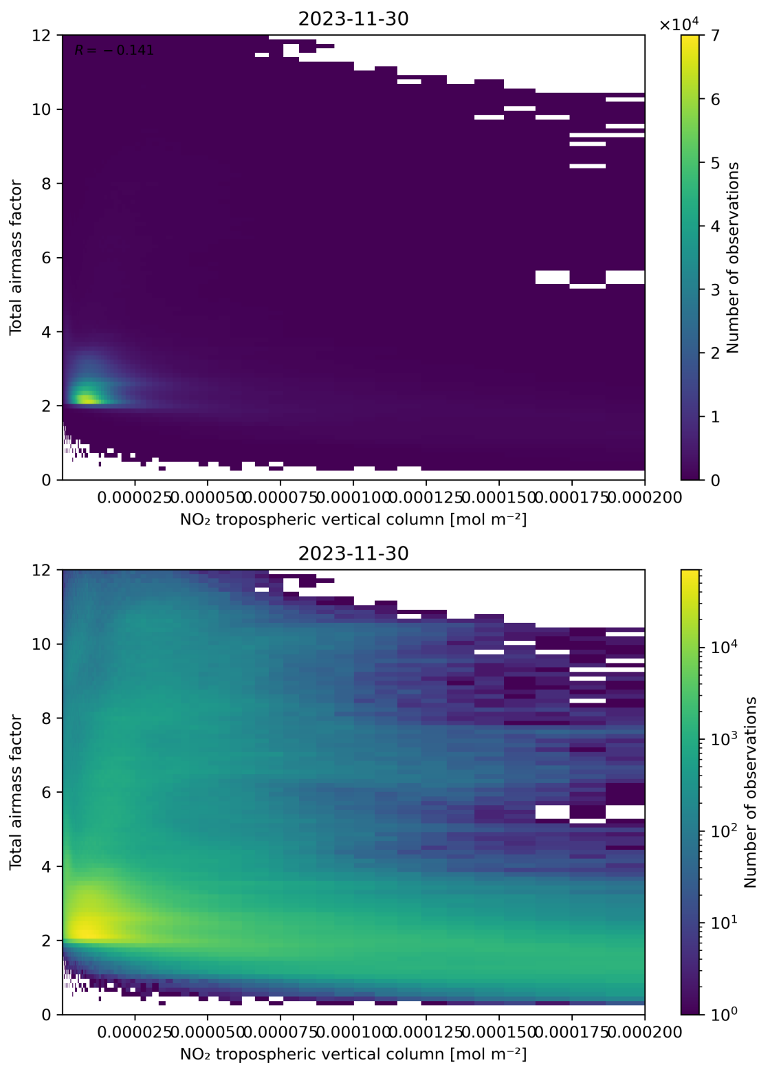
Figure 122: Scatter density plot of “NO 2 tropospheric vertical column” against “Total air mass factor” for 2023-11-29 to 2023-12-01.
