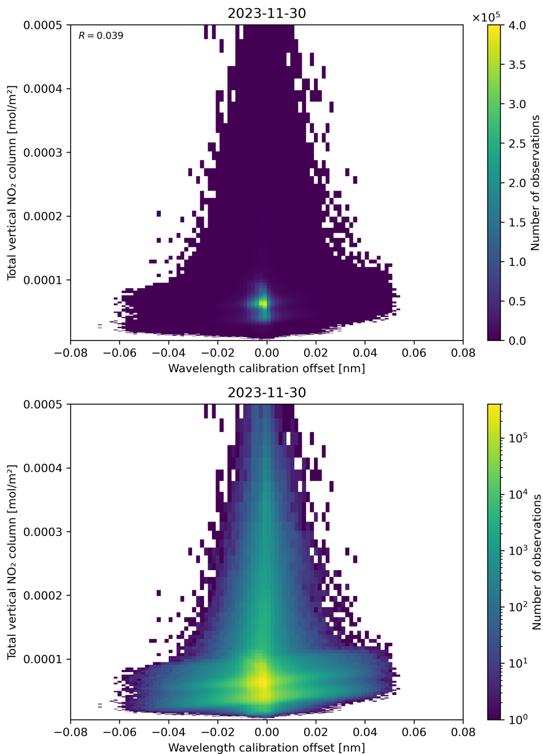
Figure 179: Scatter density plot of “Wavelength calibration offset” against “Total vertical NO 2 column” for 2023-11-29 to 2023-12-01.
