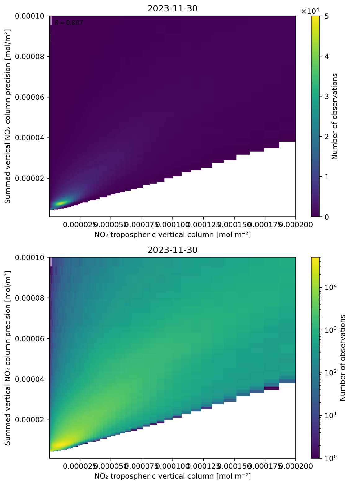
Figure 127: Scatter density plot of “NO 2 tropospheric vertical column” against “Summed vertical NO 2 column precision” for 2023-11-29 to 2023-12-01.
