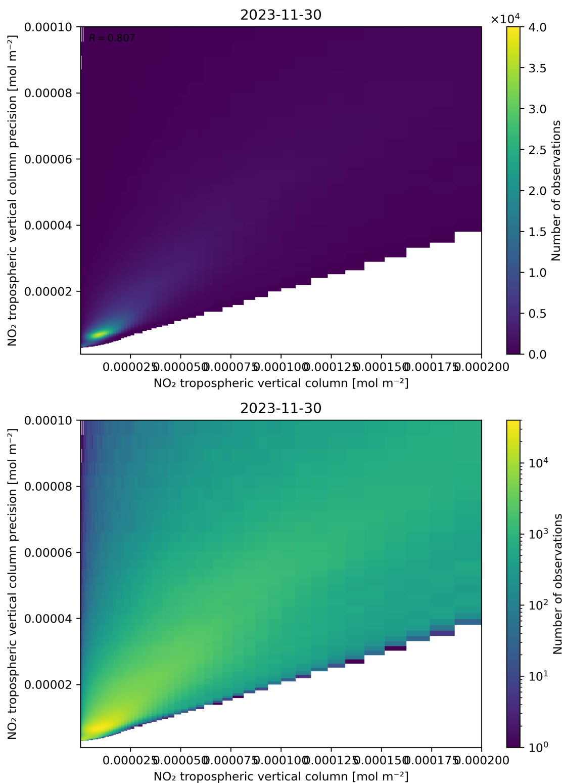
Figure 130: Scatter density plot of “NO 2 tropospheric vertical column” against “NO 2 tropospheric vertical column precision” for 2023-11-29 to 2023-12-01.
