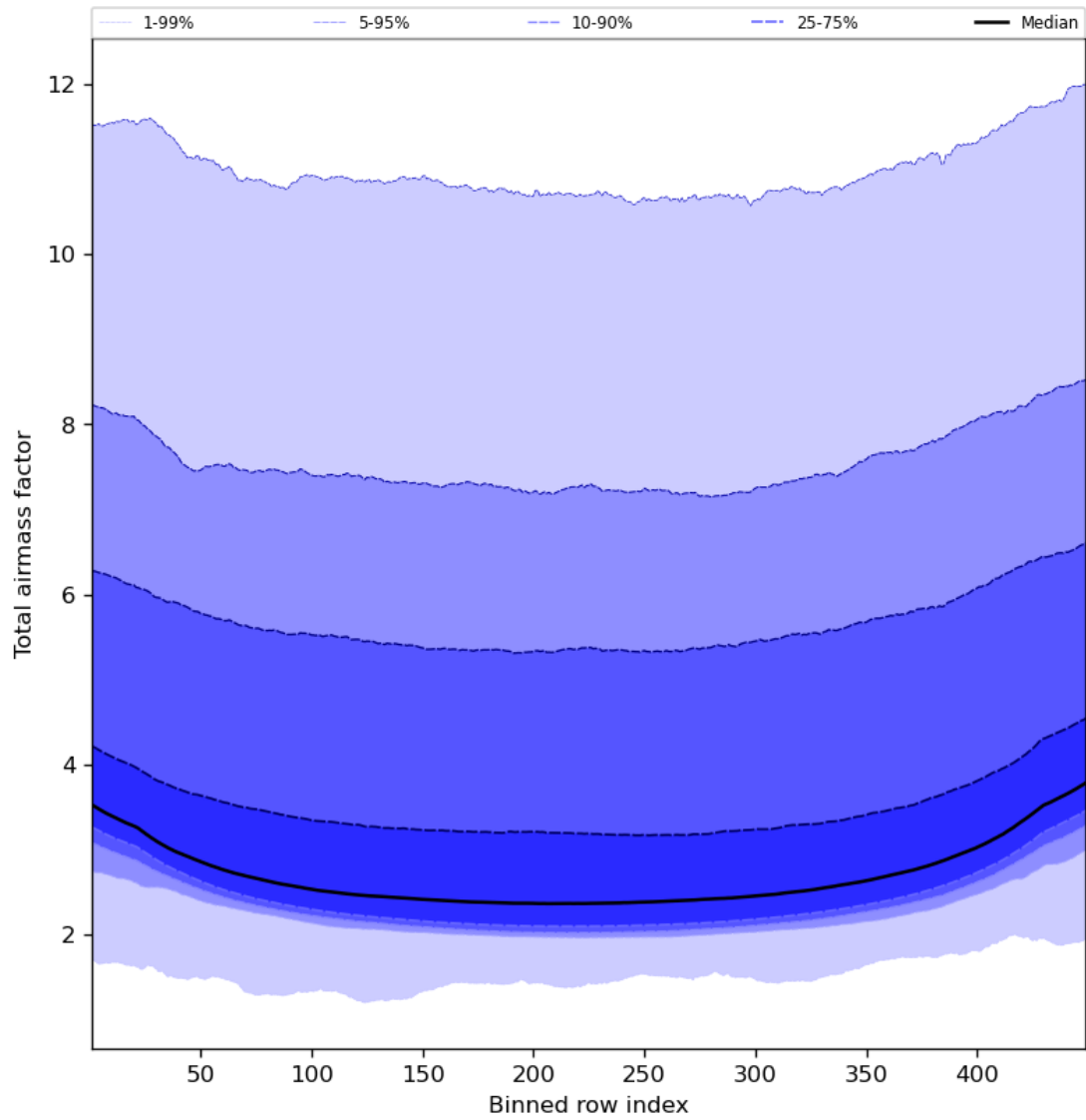
Figure 49: Along track statistics of “Total airmass factor” for 2023-11-29 to 2023-12-01
