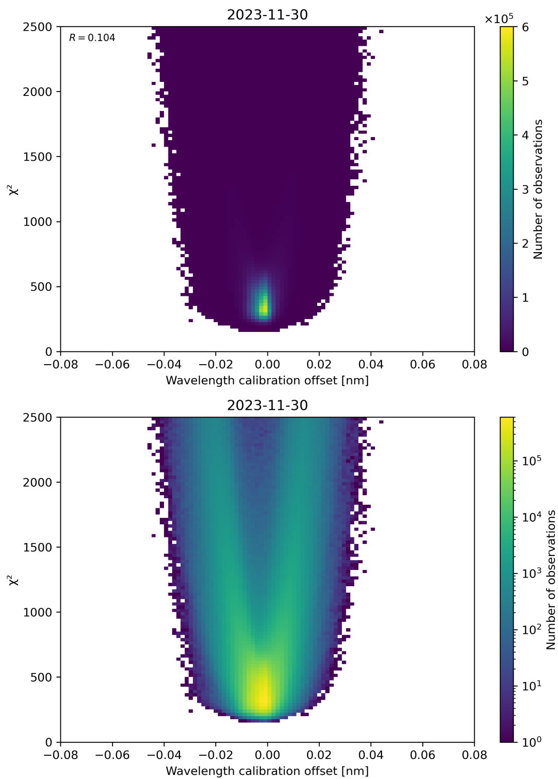
Figure 175: Scatter density plot of “Wavelength calibration offset” against “ \chi^2 ” for 2023-11-29 to 2023-12-01.
