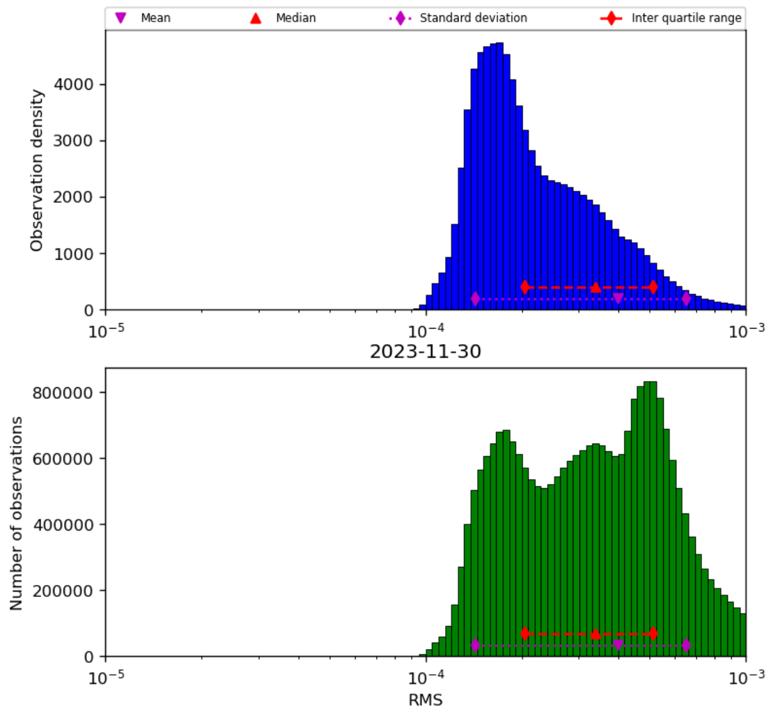
Figure 43: Histogram of “RMS” for 2023-11-29 to 2023-12-01
