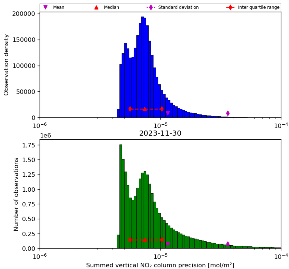
Figure 41: Histogram of "Summed vertical NO 2 column precision" for 2023-11-29 to 2023-12-01
