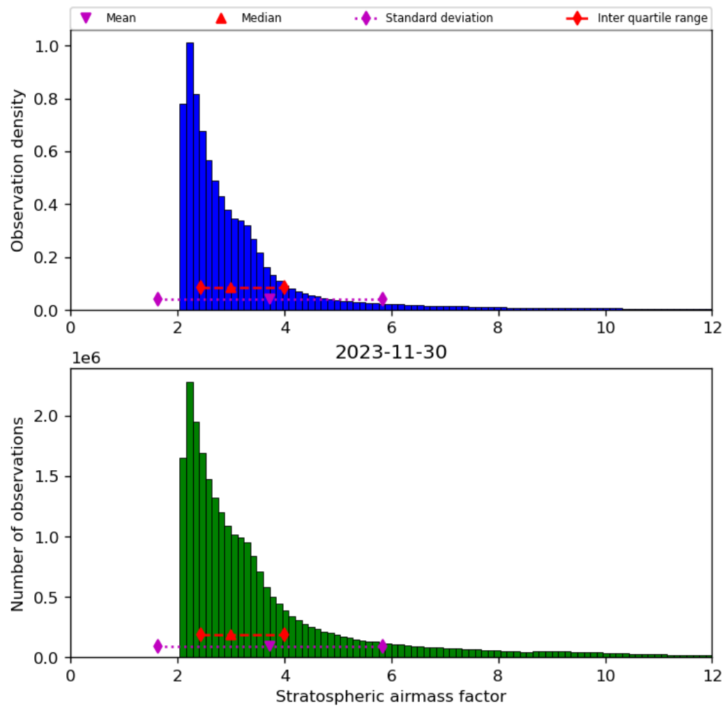
Figure 44: Histogram of “Stratospheric airmass factor” for 2023-11-29 to 2023-12-01
