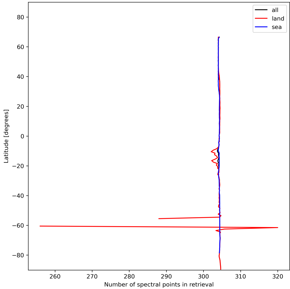
Figure 16: Zonal average of “Number of spectral points in retrieval” for 2023-11-29 to 2023-12-01.
