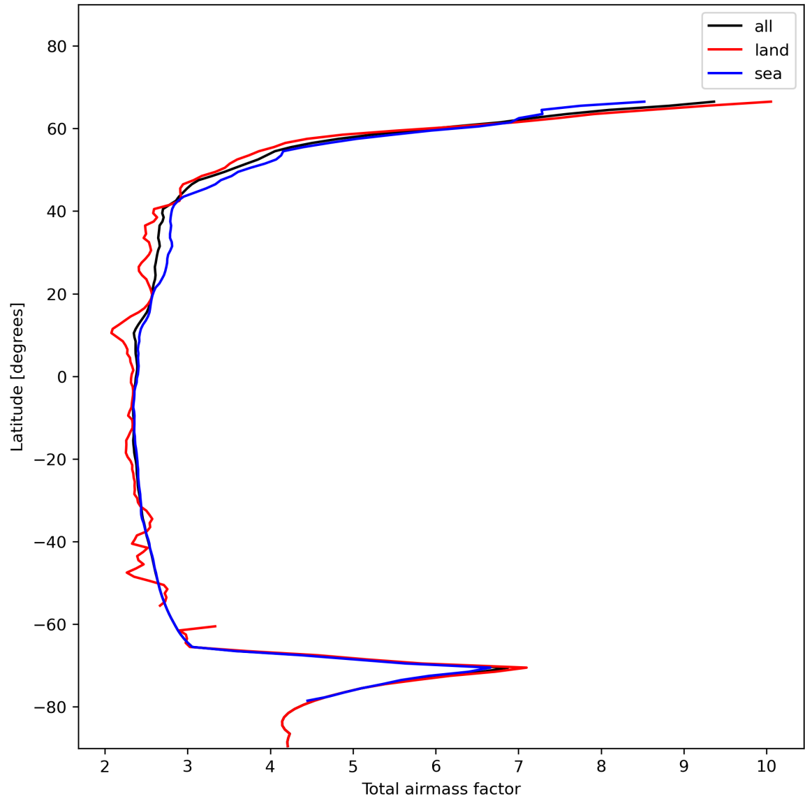
Figure 15: Zonal average of “Total airmass factor” for 2023-11-29 to 2023-12-01.
