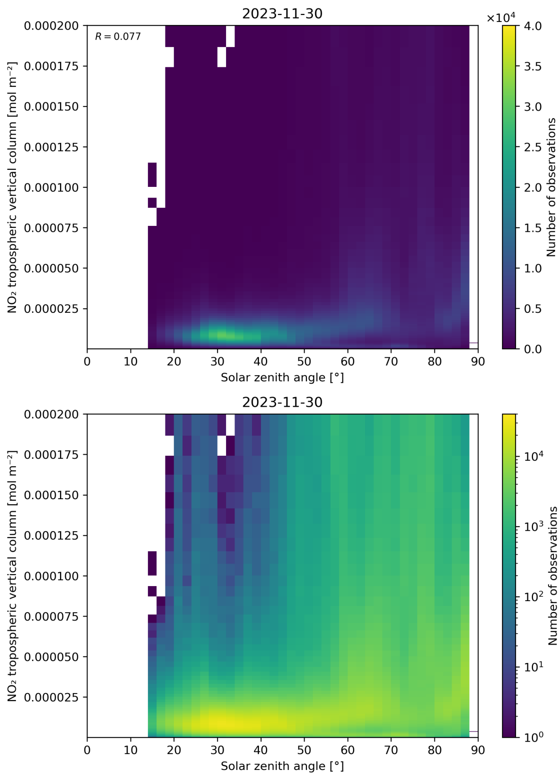
Figure 155: Scatter density plot of “Solar zenith angle” against “NO 2 tropospheric vertical column” for 2023-11-29 to 2023-12-01.
