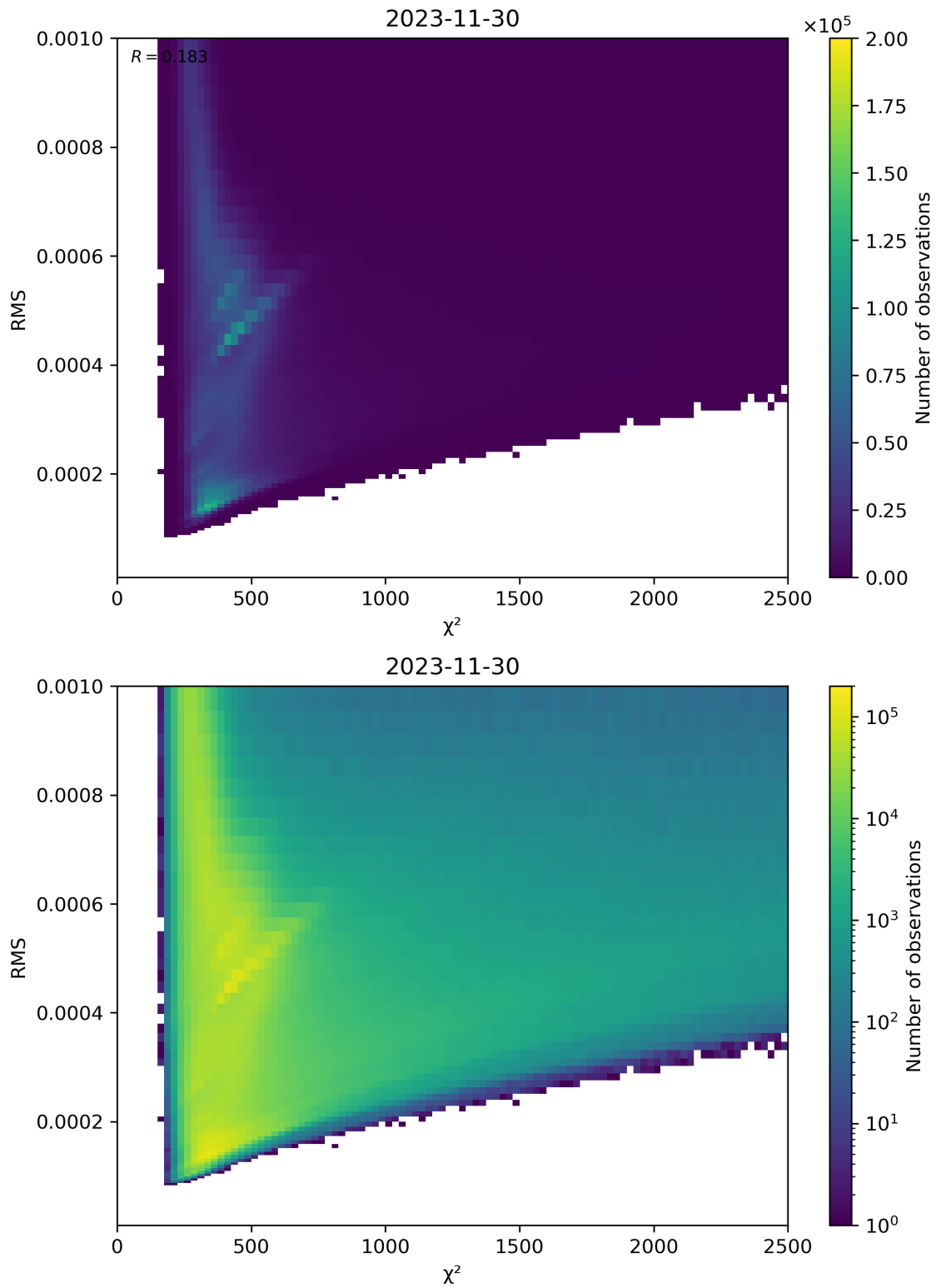
Figure 82: Scatter density plot of “ \chi^2 ” against “RMS” for 2023-11-29 to 2023-12-01.
