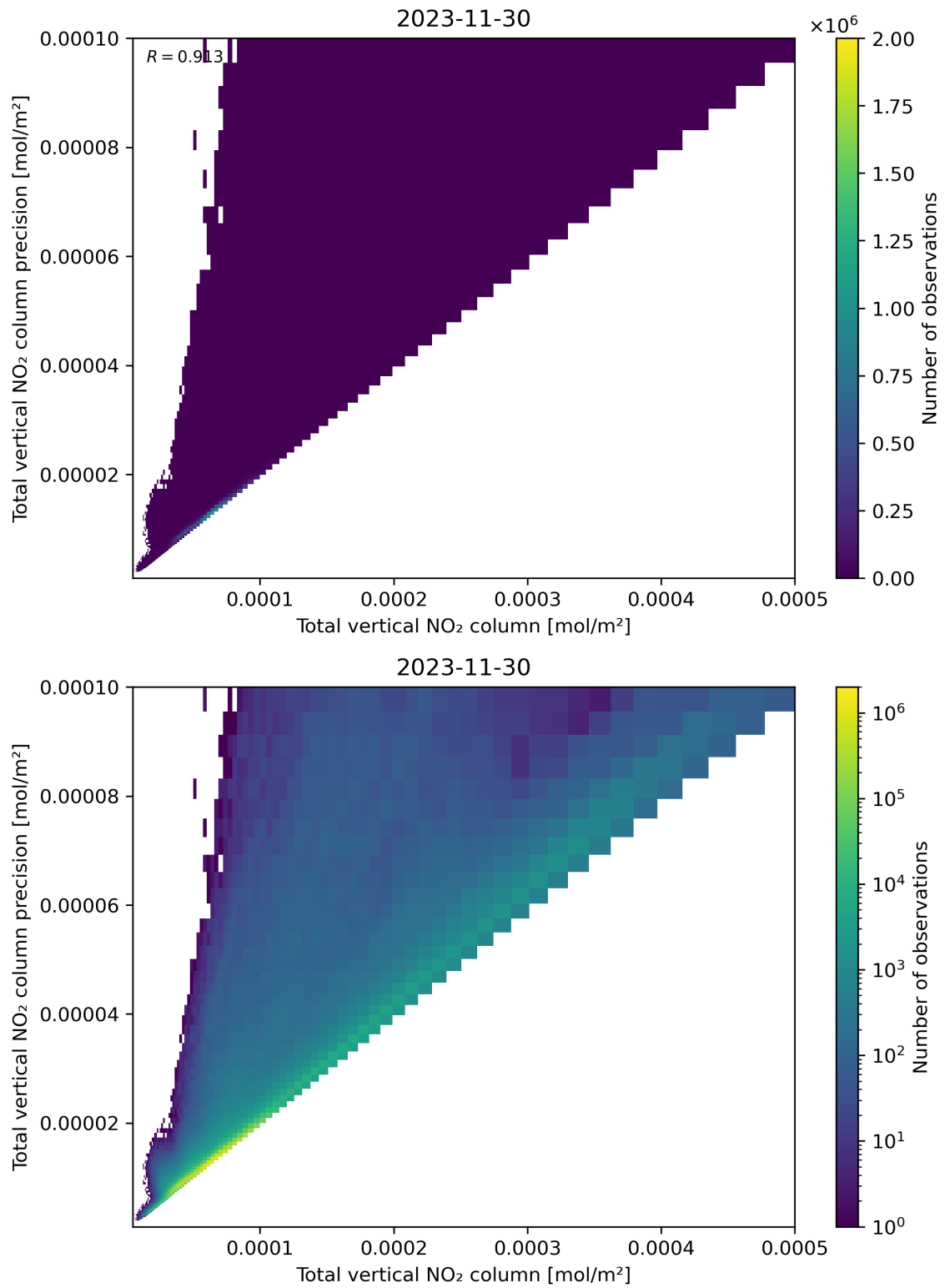
Figure 114: Scatter density plot of “Total vertical NO 2 column” against “Total vertical NO 2 column precision” for 2023-11-29 to 2023-12-01.
