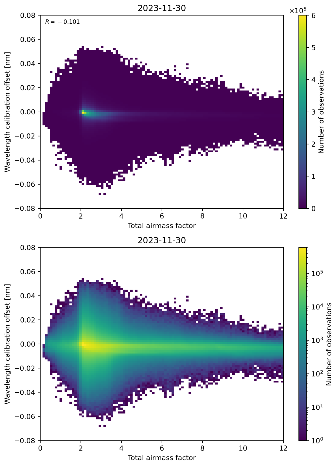
Figure 70: Scatter density plot of “Total airmass factor” against “Wavelength calibration offset” for 2023-11-29 to 2023-12-01.
