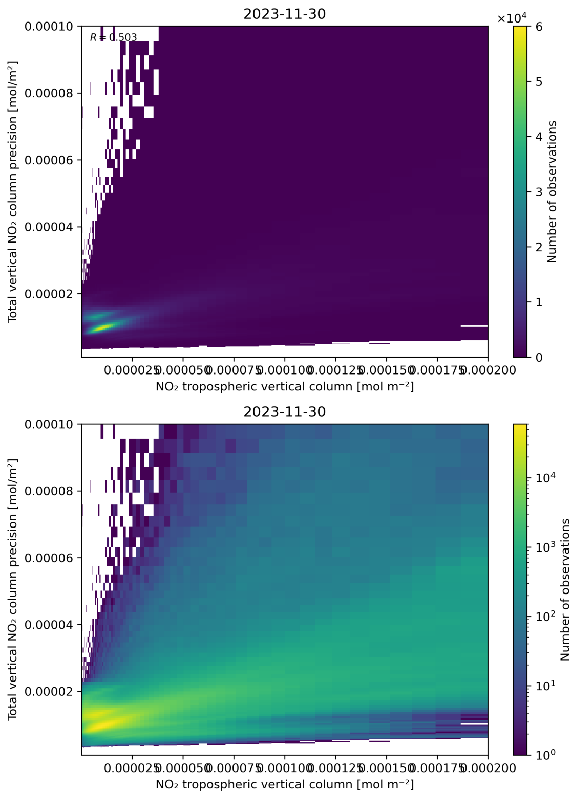
Figure 129: Scatter density plot of “NO 2 tropospheric vertical column” against “Total vertical NO 2 column precision” for 2023-11-29 to 2023-12-01.
