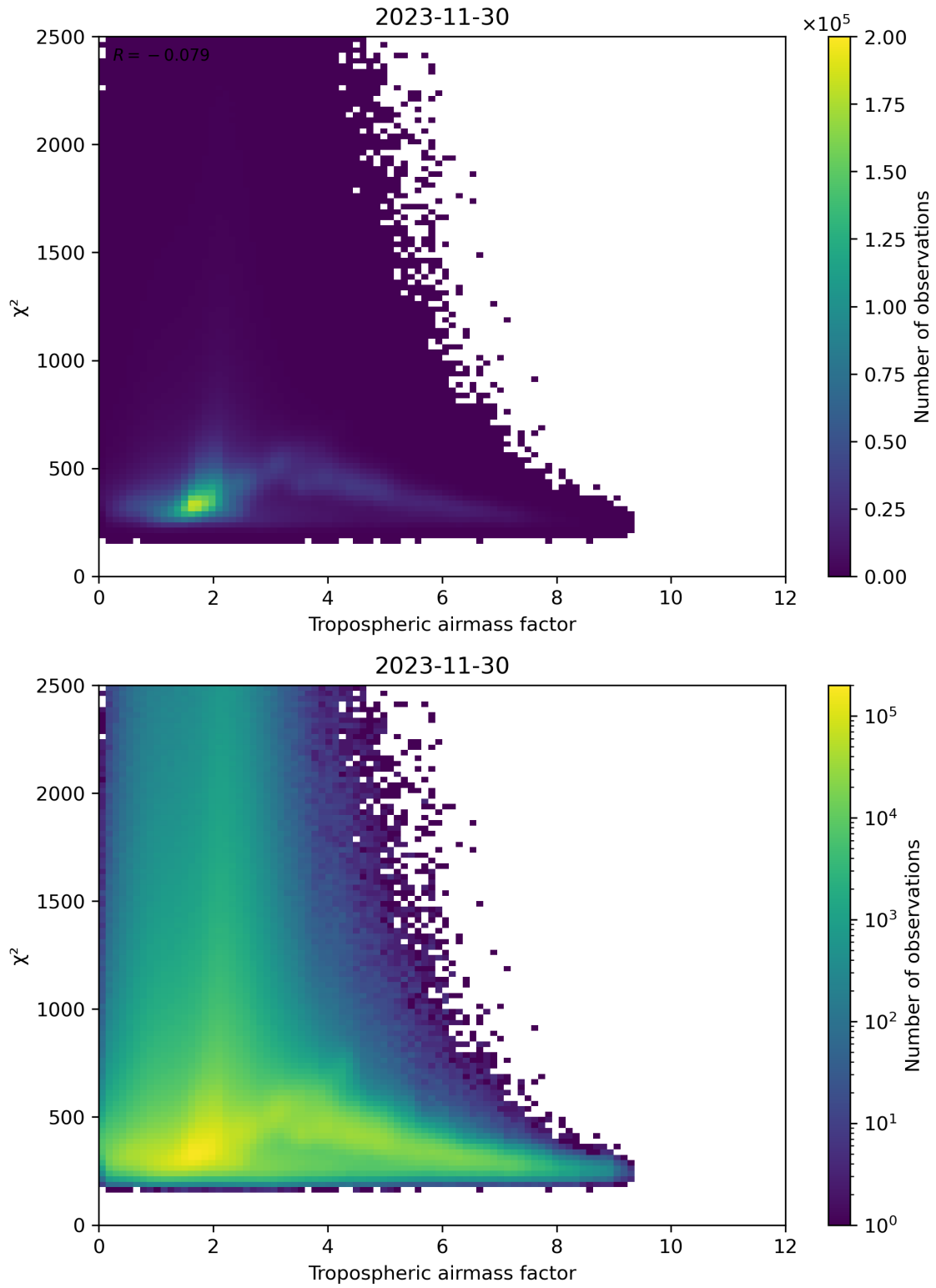
Figure 73: Scatter density plot of “Tropospheric airmass factor” against “ \chi^2 ” for 2023-11-29 to 2023-12-01.
