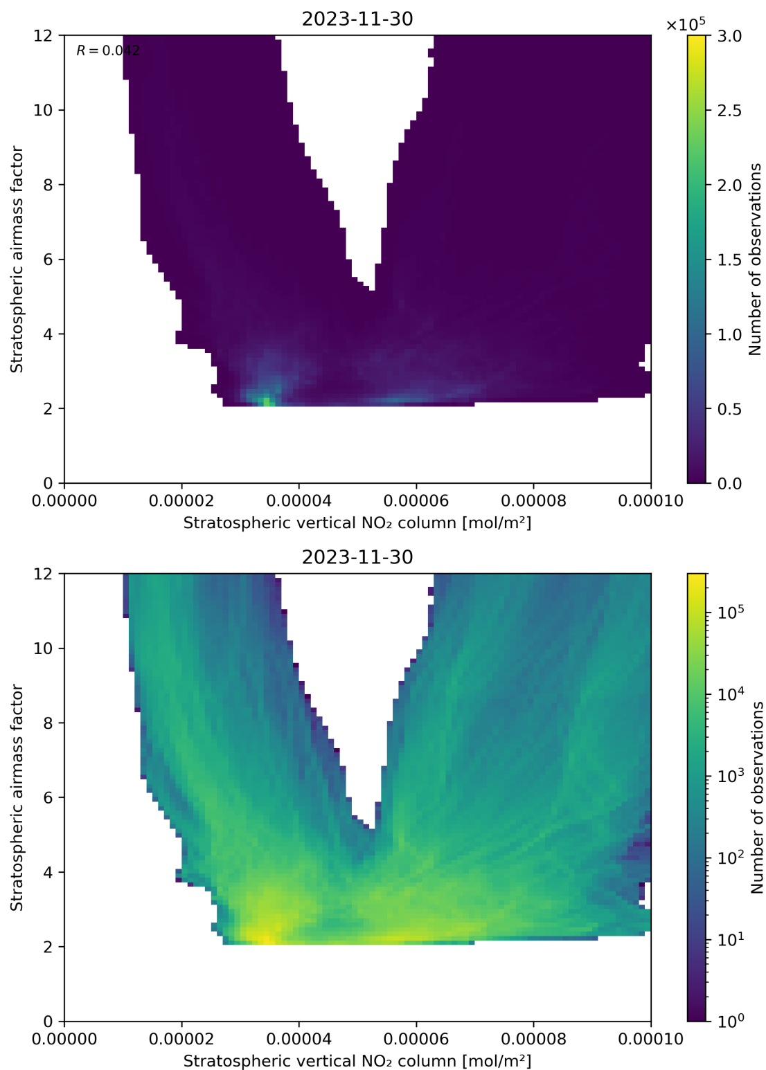
Figure 96: Scatter density plot of “Stratospheric vertical NO 2 column” against “Stratospheric airmass factor” for 2023-11-29 to 2023-12-01.
