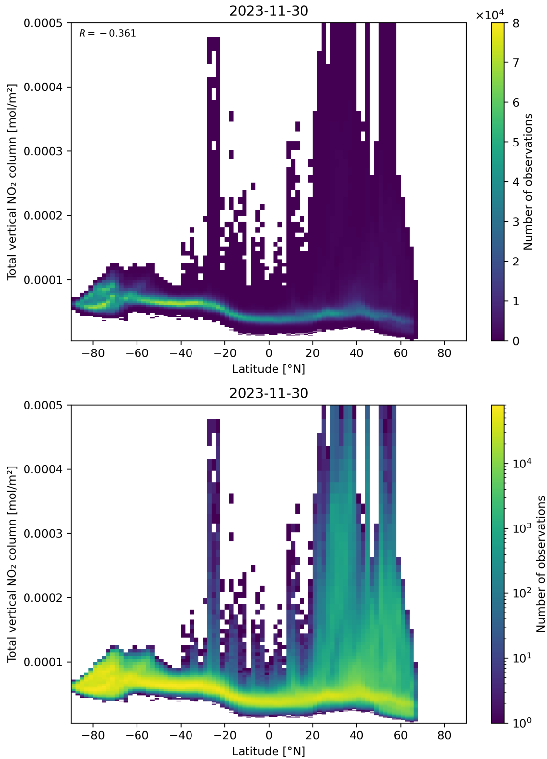
Figure 90: Scatter density plot of “Latitude” against “Total vertical NO 2 column” for 2023-11-29 to 2023-12-01.
