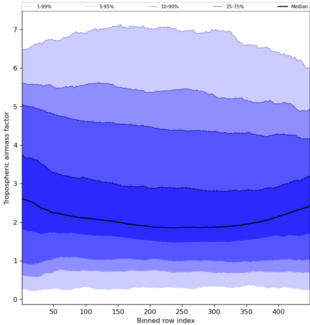
Figure 48: Along track statistics of “Tropospheric air mass factor” for 2023-11-29 to 2023-12-01
