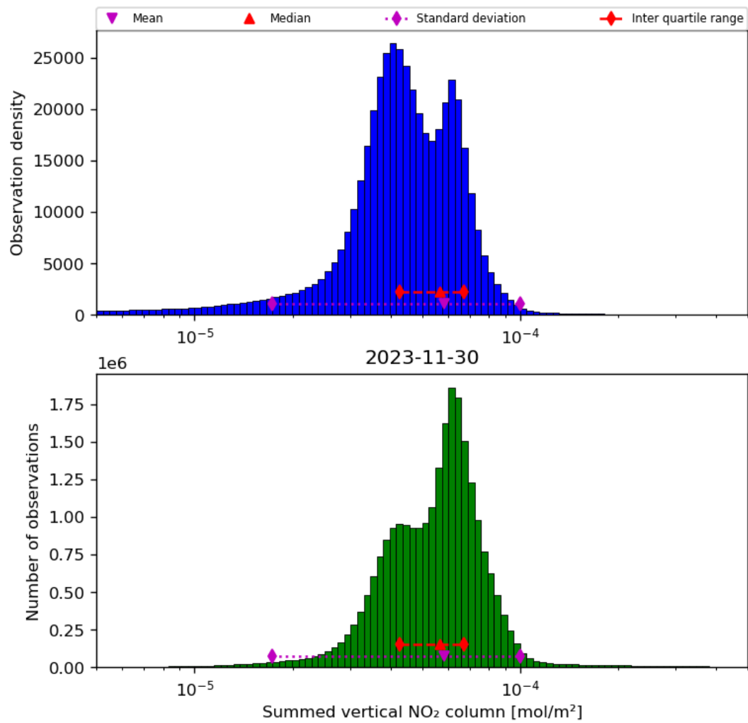
Figure 40: Histogram of “Summed vertical NO 2 column” for 2023-11-29 to 2023-12-01
