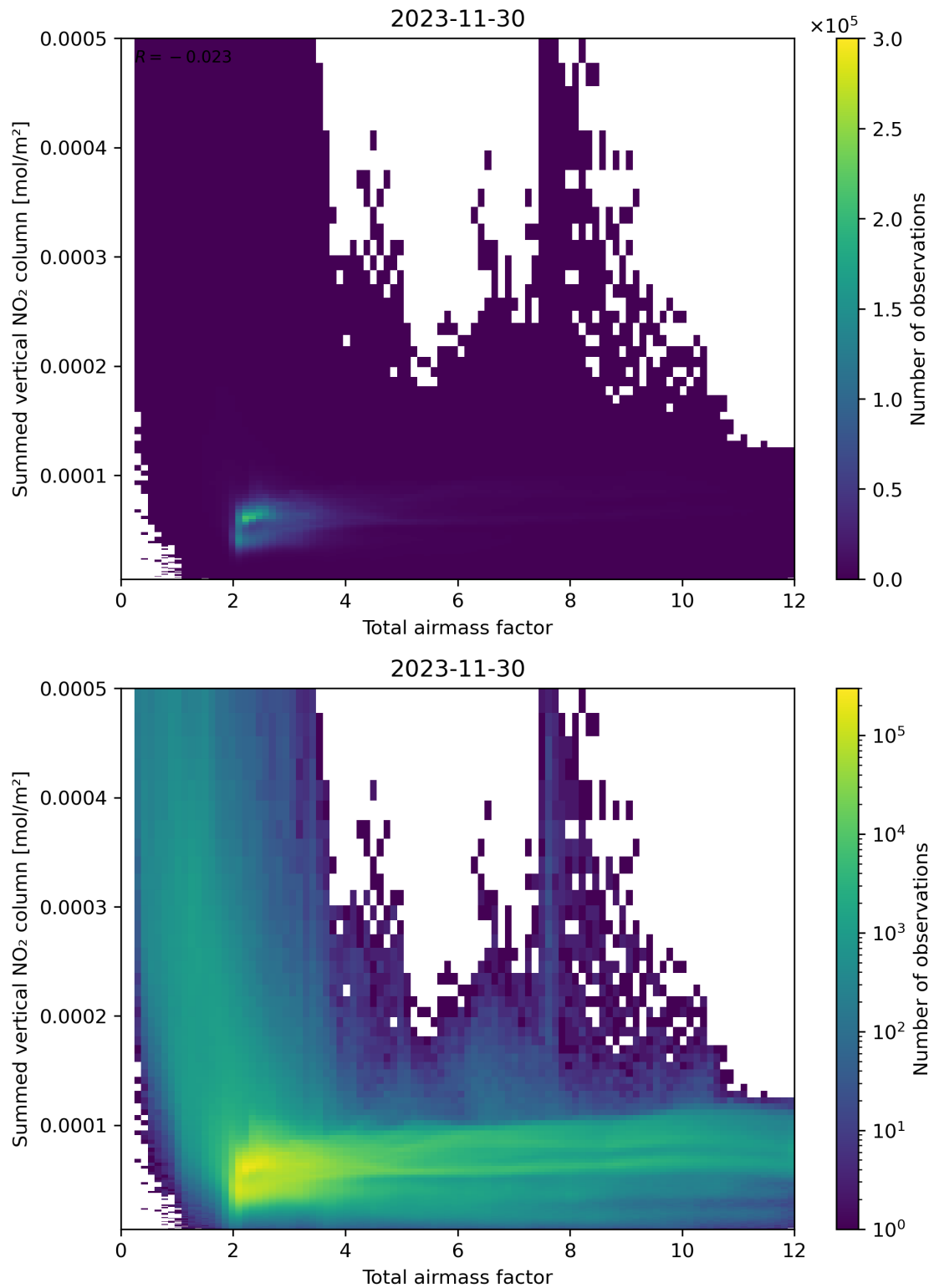
Figure 65: Scatter density plot of “Total airmass factor” against “Summed vertical NO 2 column” for 2023-11-29 to 2023-12-01.
