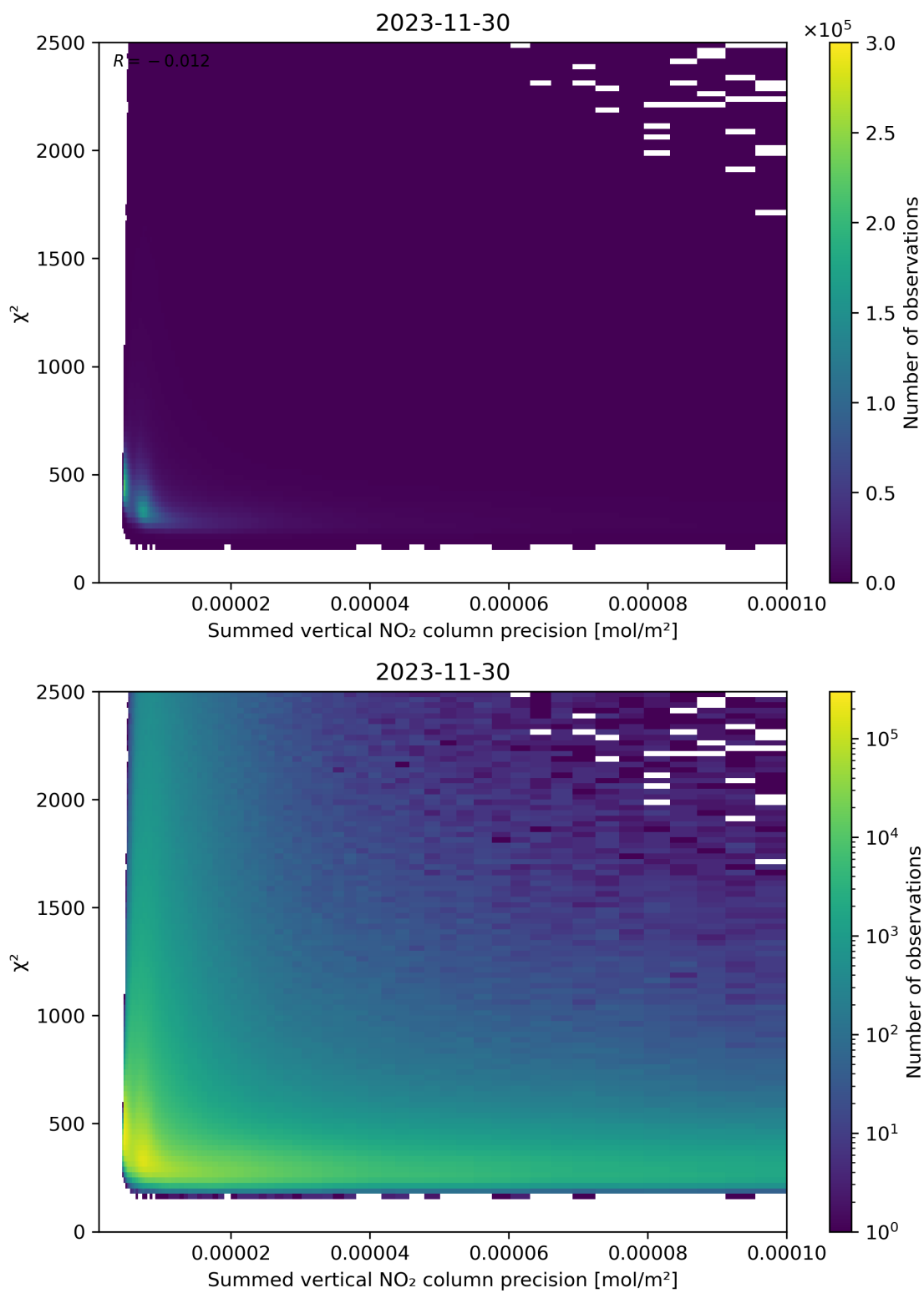
Figure 107: Scatter density plot of “Summed vertical NO 2 column precision” against “ \chi^2 ” for 2023-11-29 to 2023-12-01.
