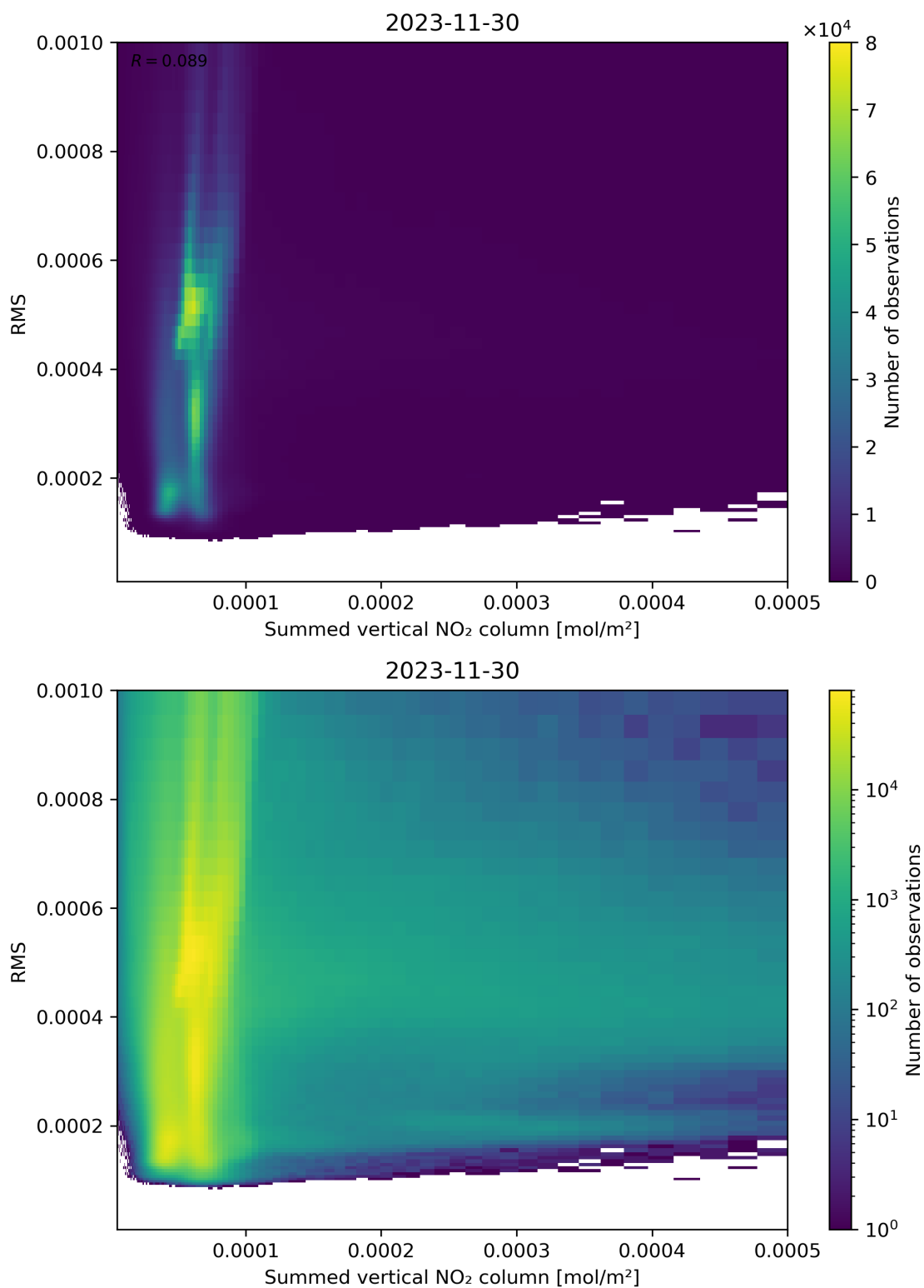
Figure 109: Scatter density plot of “Summed vertical NO 2 column” against “RMS” for 2023-11-29 to 2023-12-01.
