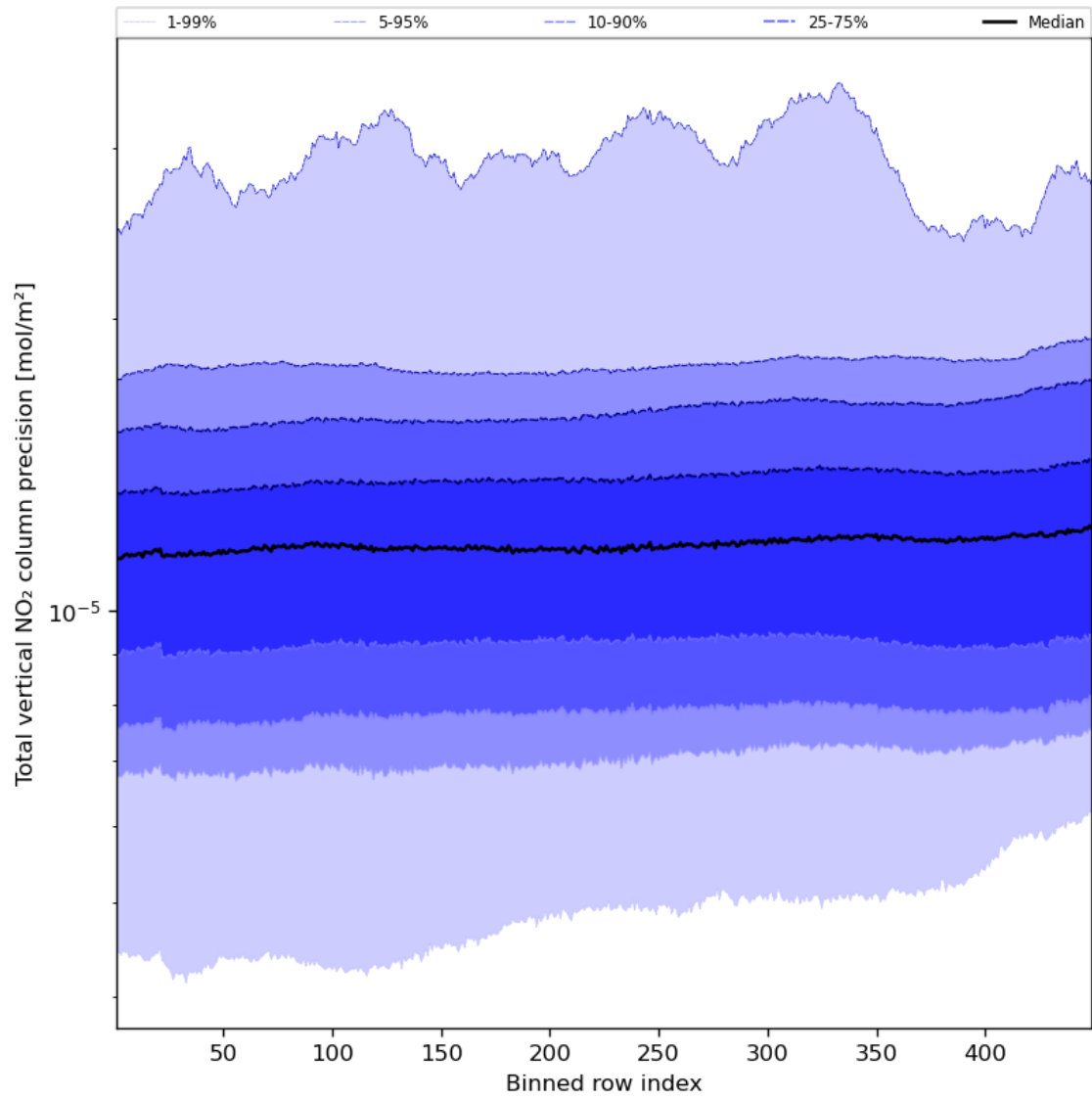
Figure 56: Along track statistics of “Total vertical NO 2 column precision” for 2023-11-29 to 2023-12-01
