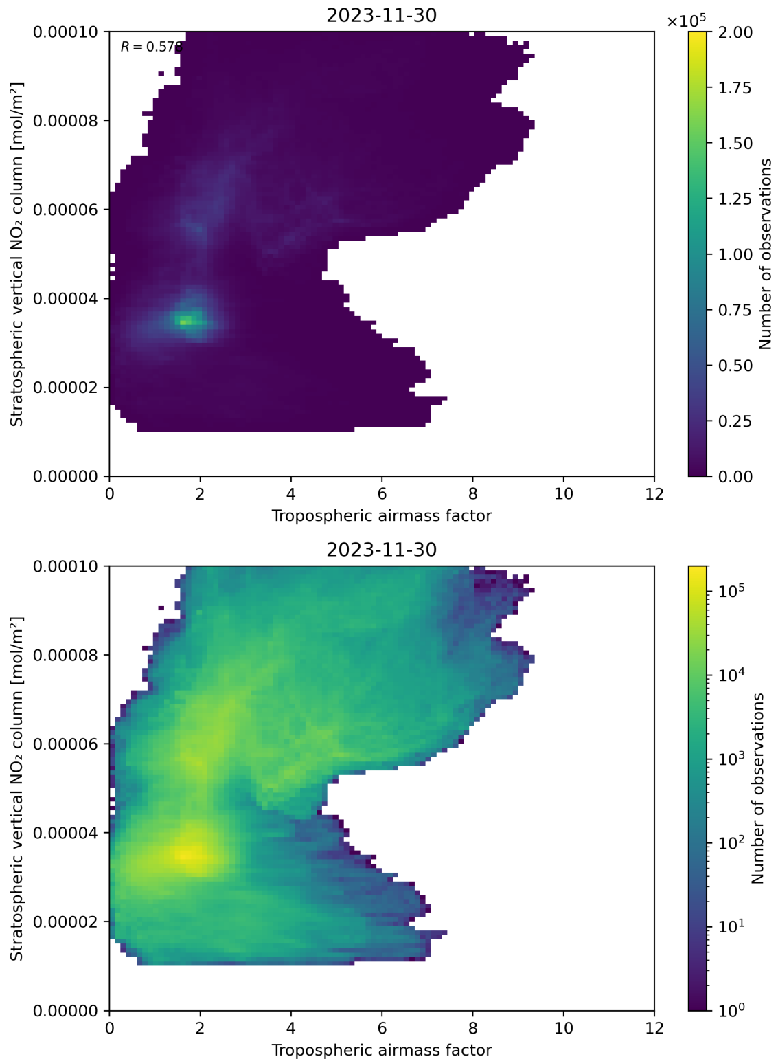
Figure 74: Scatter density plot of “Tropospheric air mass factor” against “Stratospheric vertical NO 2 column” for 2023-11-29 to 2023-12-01.
