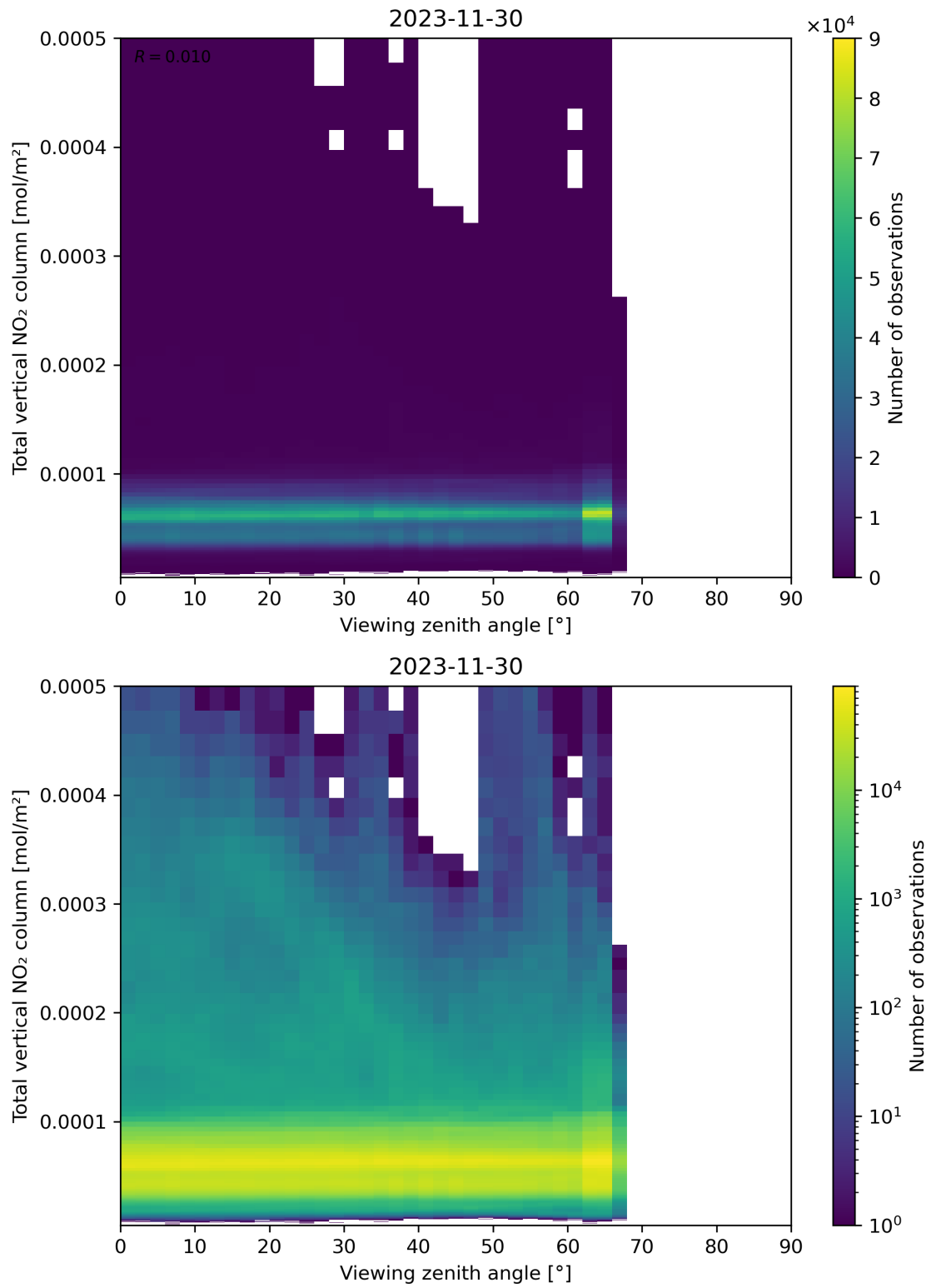
Figure 167: Scatter density plot of “Viewing zenith angle” against “Total vertical NO 2 column” for 2023-11-29 to 2023-12-01.
