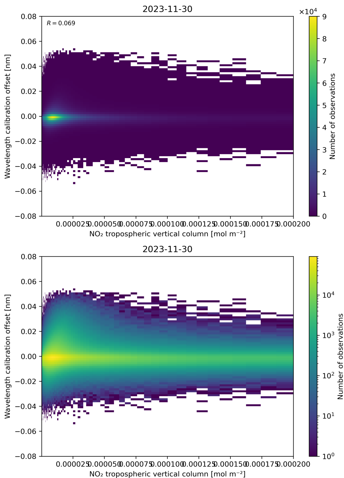
Figure 143: Scatter density plot of “NO 2 tropospheric vertical column” against “Wavelength calibration offset” for 2023-11-29 to 2023-12-01.
