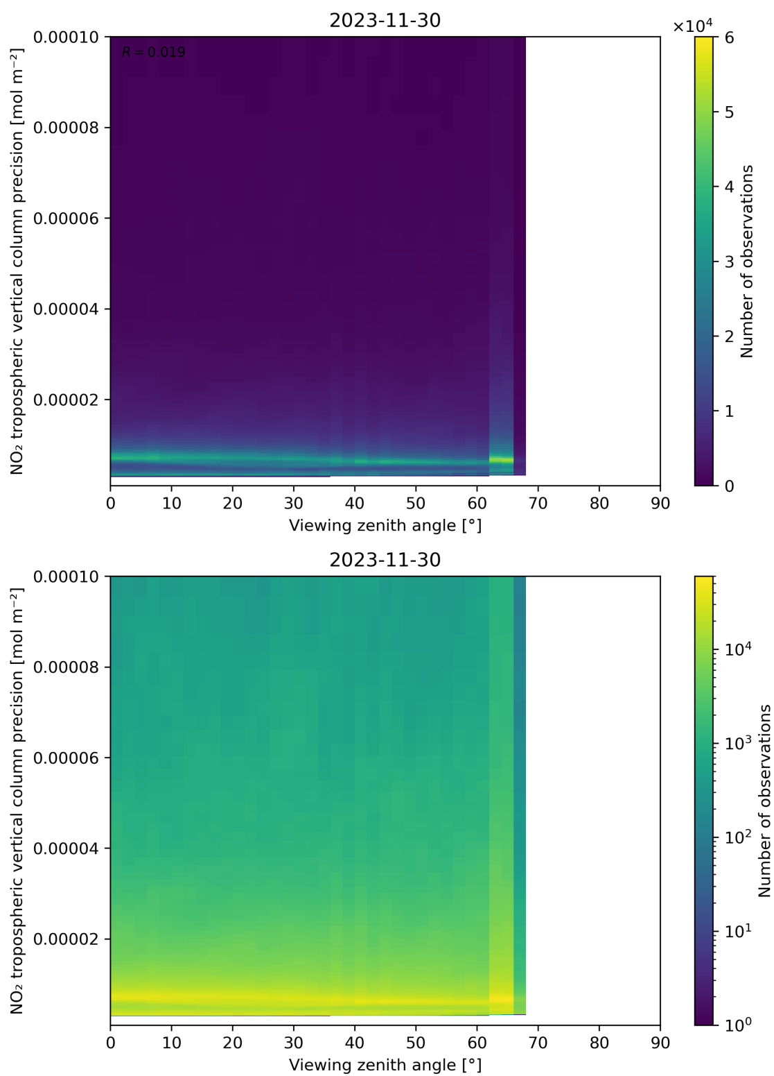
Figure 170: Scatter density plot of “Viewing zenith angle” against “NO 2 tropospheric vertical column precision” for 2023-11-29 to 2023-12-01.
