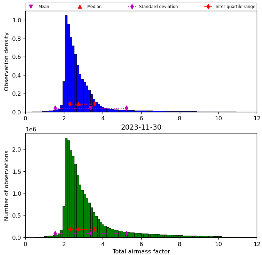
Figure 32: Histogram of “Total airmass factor” for 2023-11-29 to 2023-12-01
