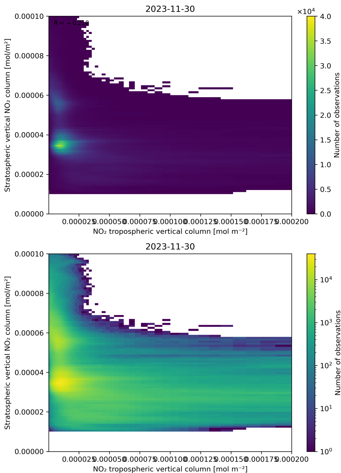
Figure 125: Scatter density plot of “NO 2 tropospheric vertical column” against “Stratospheric vertical NO 2 column” for 2023-11-29 to 2023-12-01.
