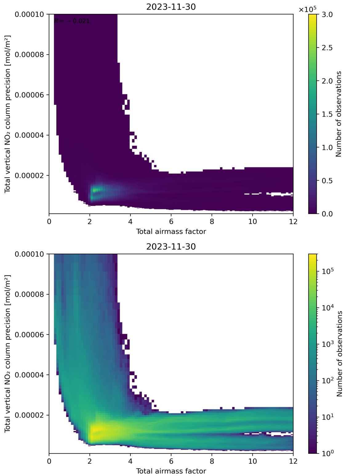
Figure 68: Scatter density plot of “Total airmass factor” against “Total vertical NO 2 column precision” for 2023-11-29 to 2023-12-01.
