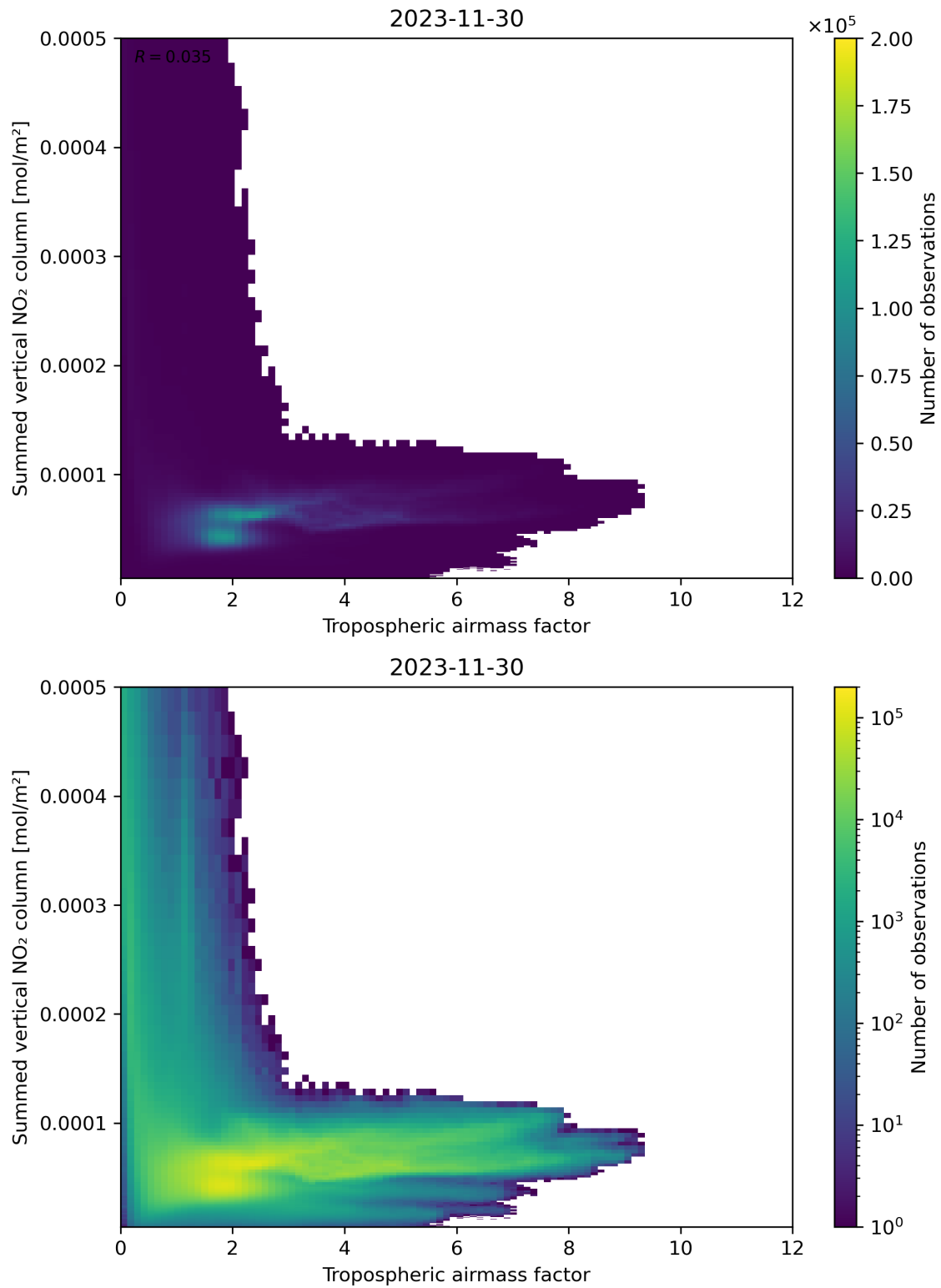
Figure 75: Scatter density plot of “Tropospheric air mass factor” against “Summed vertical NO 2 column” for 2023-11-29 to 2023-12-01.
