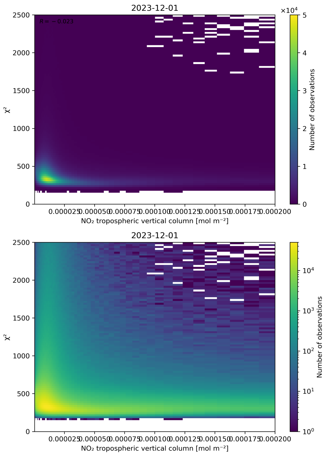
Figure 124: Scatter density plot of “NO 2 tropospheric vertical column” against “ \chi^2 ” for 2023-11-30 to 2023-12-02.
