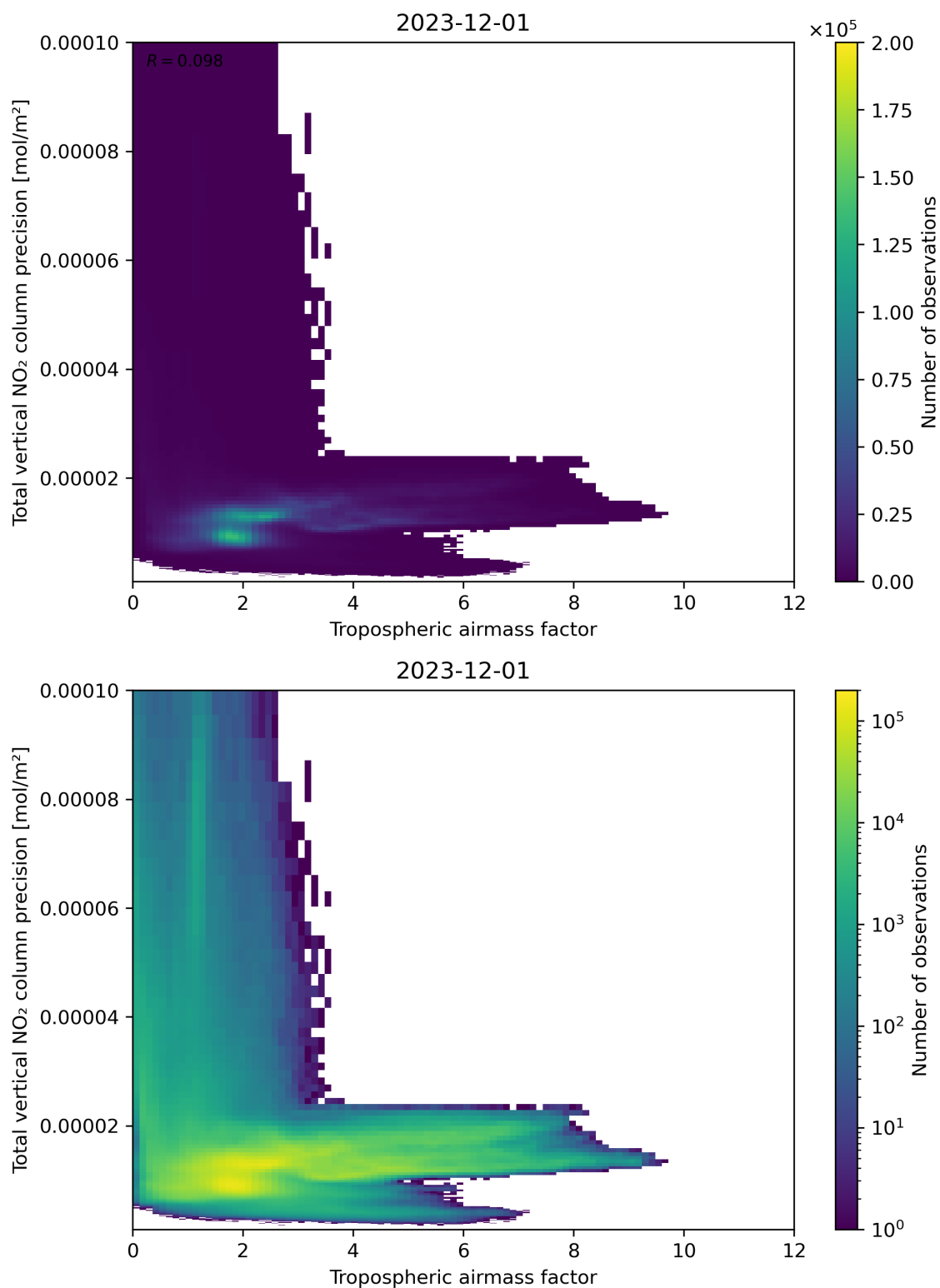
Figure 78: Scatter density plot of “Tropospheric air mass factor” against “Total vertical NO 2 column precision” for 2023-11-30 to 2023-12-02.
