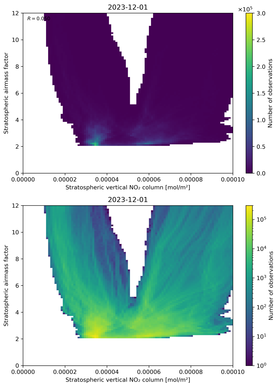
Figure 96: Scatter density plot of “Stratospheric vertical NO 2 column” against “Stratospheric airmass factor” for 2023-11-30 to 2023-12-02.
