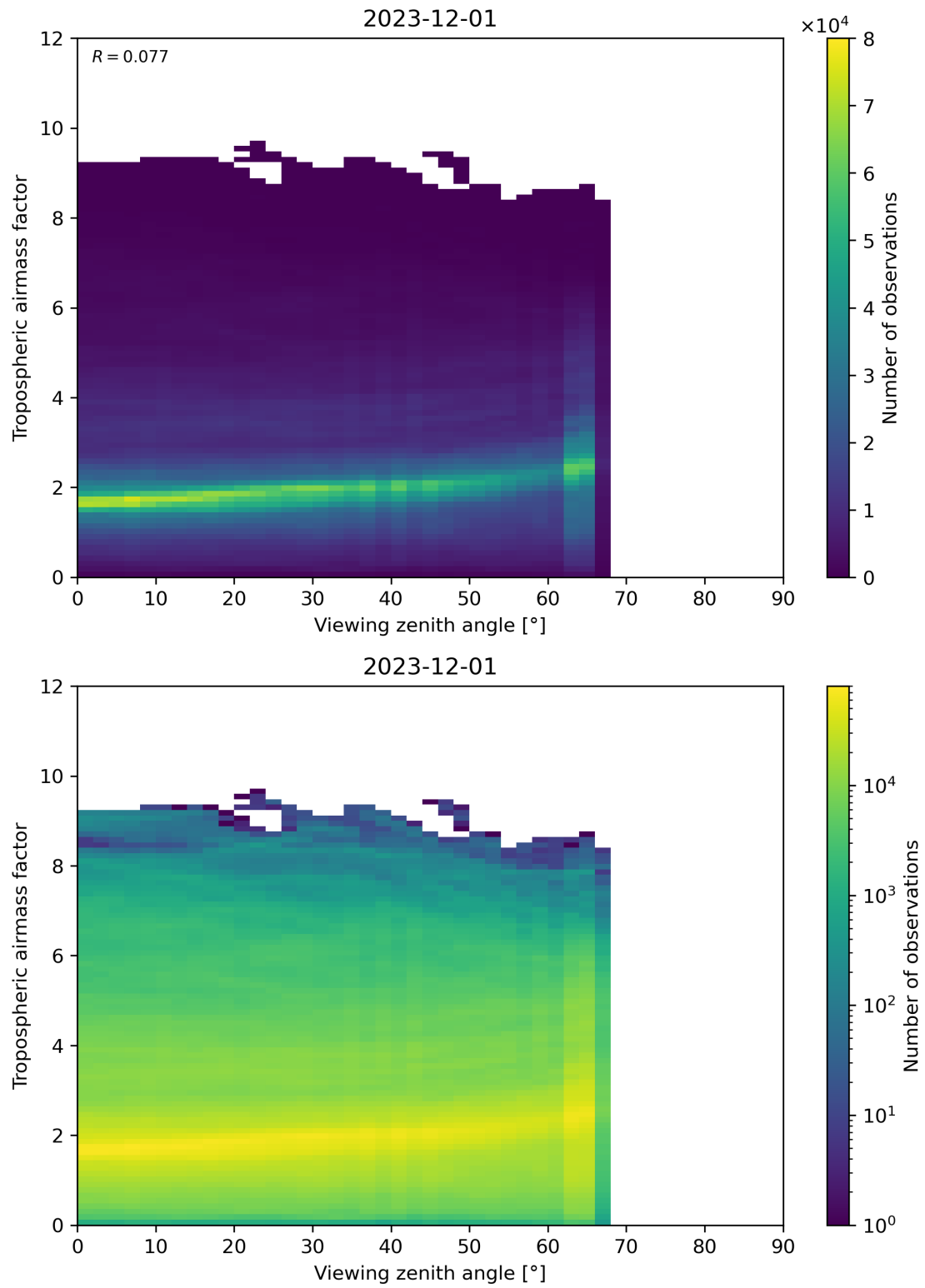
Figure 161: Scatter density plot of “Viewing zenith angle” against “Tropospheric airmass factor” for 2023-11-30 to 2023-12-02.
