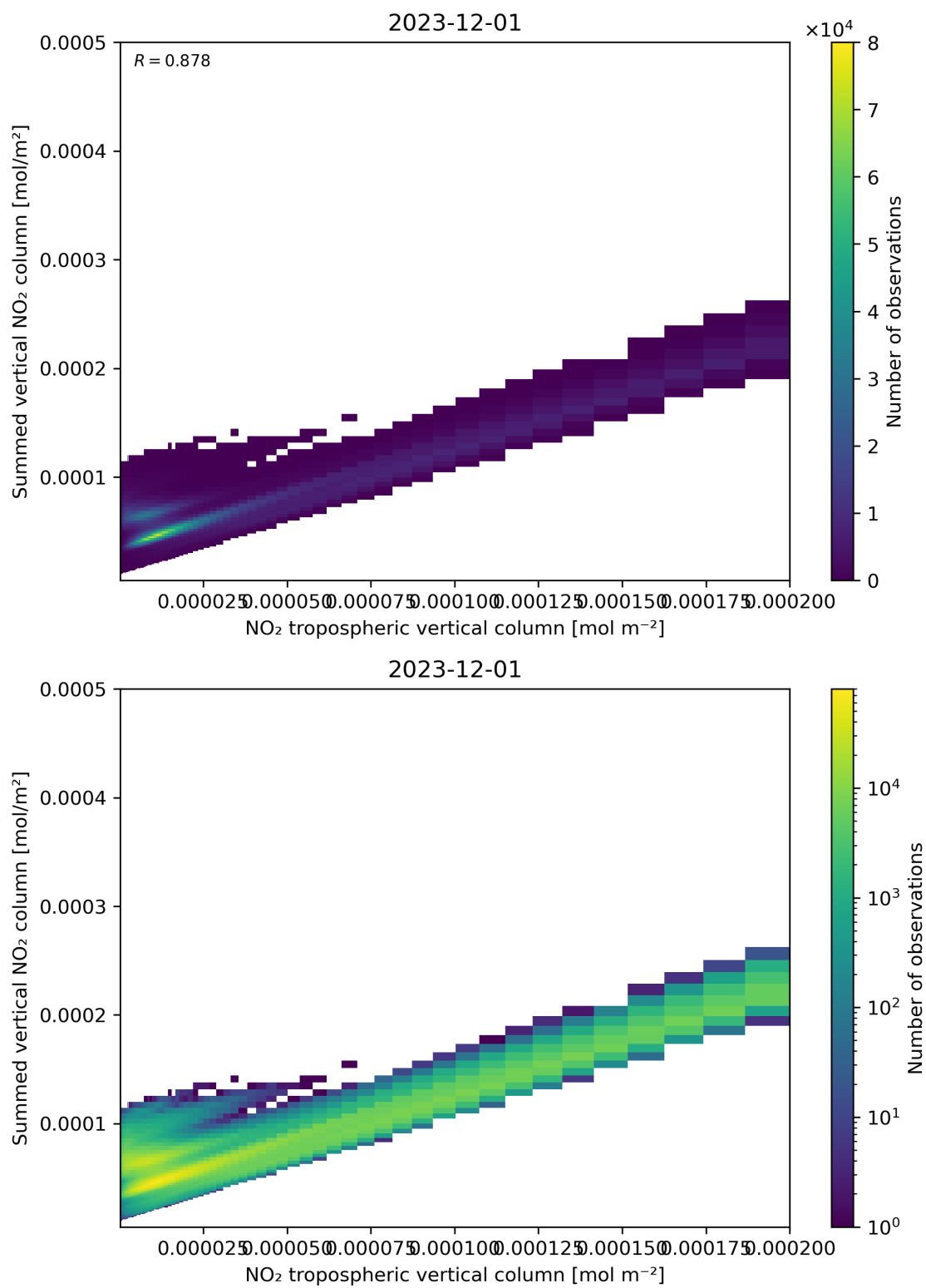
Figure 126: Scatter density plot of “NO 2 tropospheric vertical column” against “Summed vertical NO 2 column” for 2023-11-30 to 2023-12-02.
