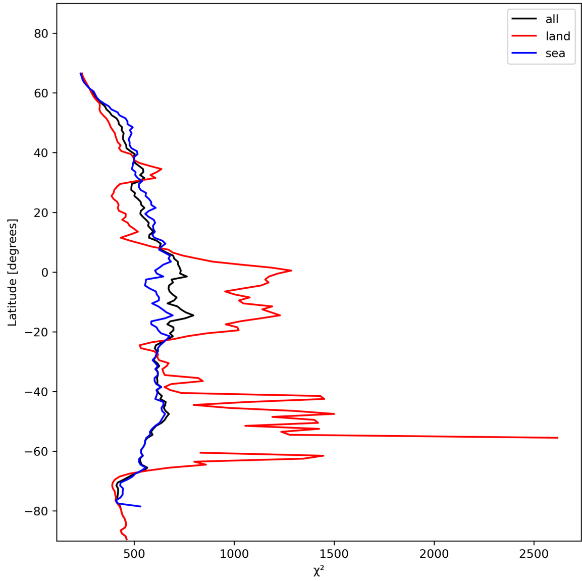
Figure 25: Zonal average of “ \chi^2 ” for 2023-11-30 to 2023-12-02.
