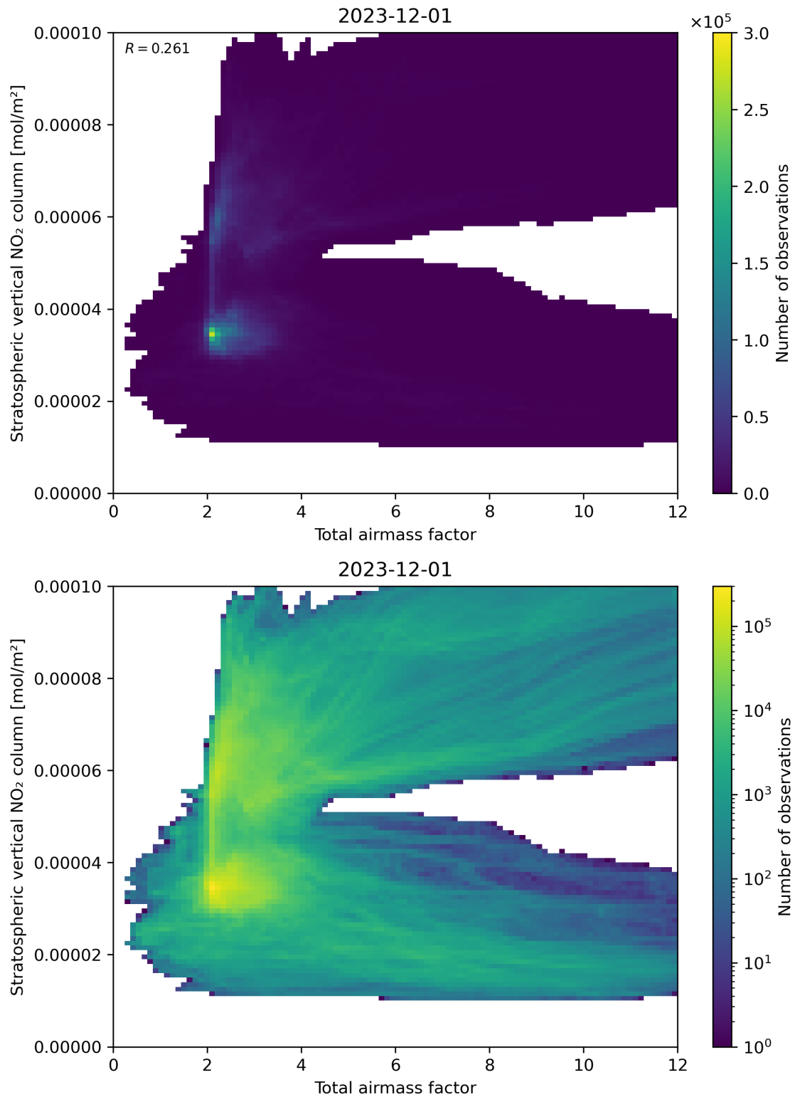
Figure 64: Scatter density plot of “Total airmass factor” against “Stratospheric vertical NO 2 column” for 2023-11-30 to 2023-12-02.
