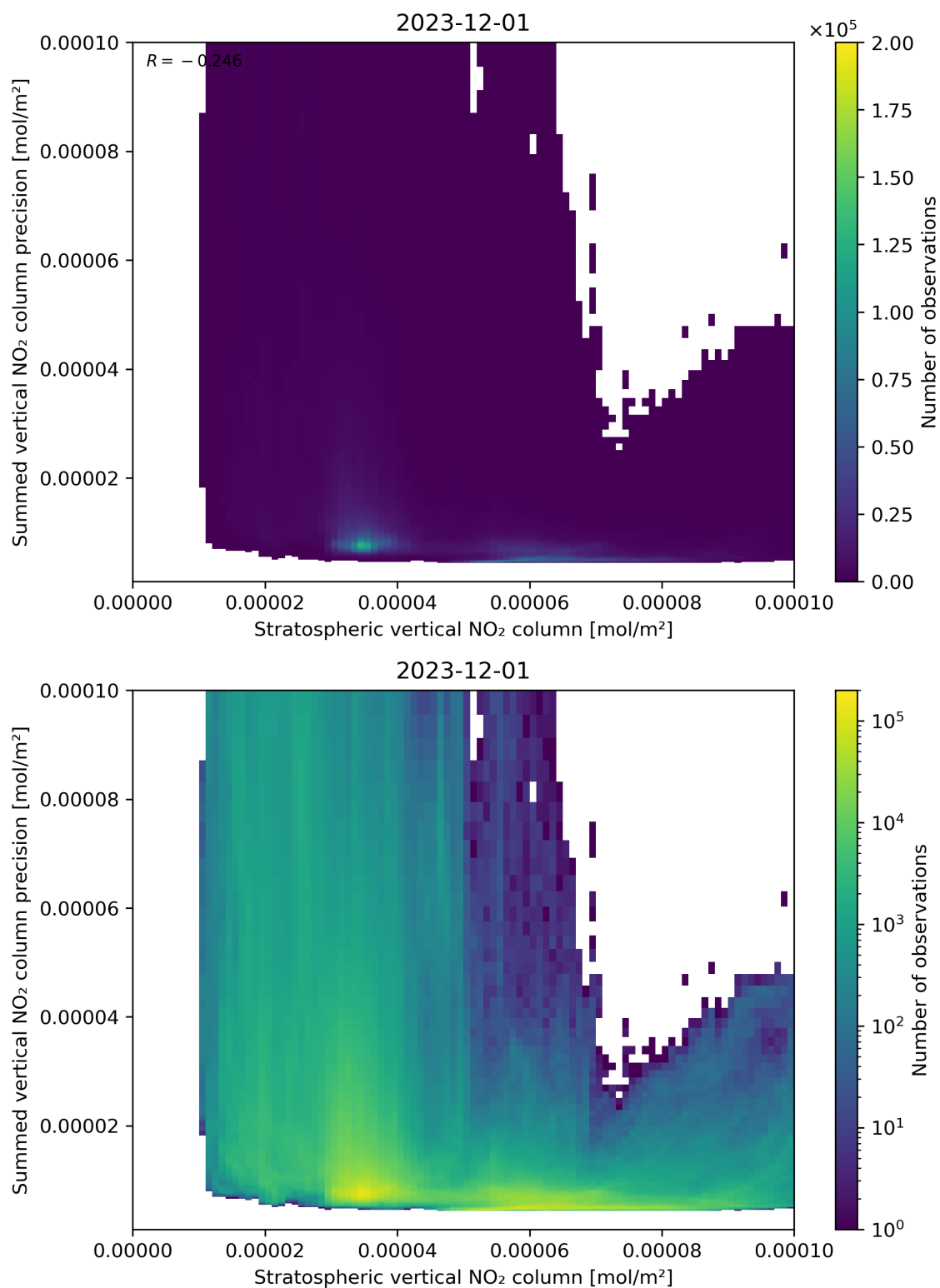
Figure 99: Scatter density plot of “Stratospheric vertical NO 2 column” against “Summed vertical NO 2 column precision” for 2023-11-30 to 2023-12-02.
