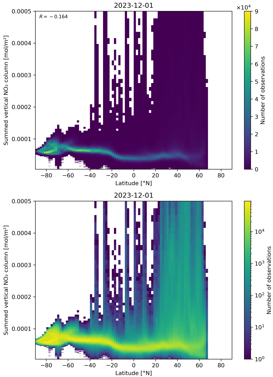
Figure 88: Scatter density plot of “Latitude” against “Summed vertical NO 2 column” for 2023-11-30 to 2023-12-02.
