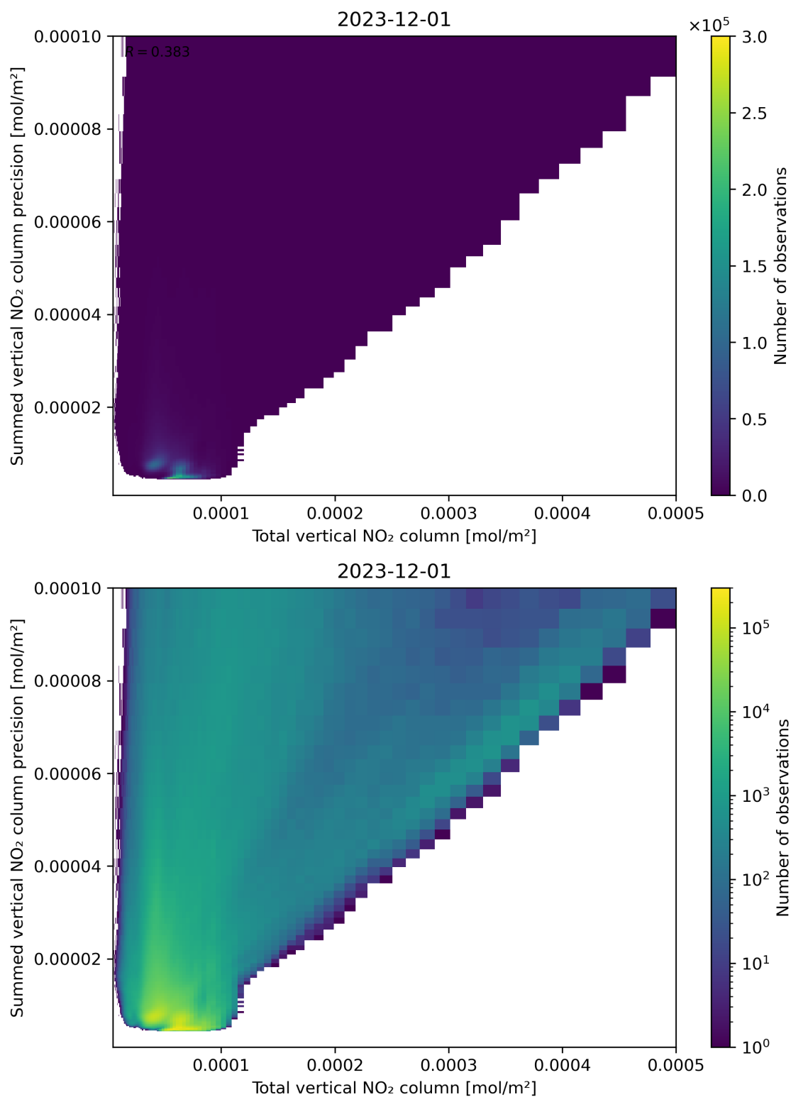
Figure 113: Scatter density plot of “Total vertical NO 2 column” against “Summed vertical NO 2 column precision” for 2023-11-30 to 2023-12-02.
