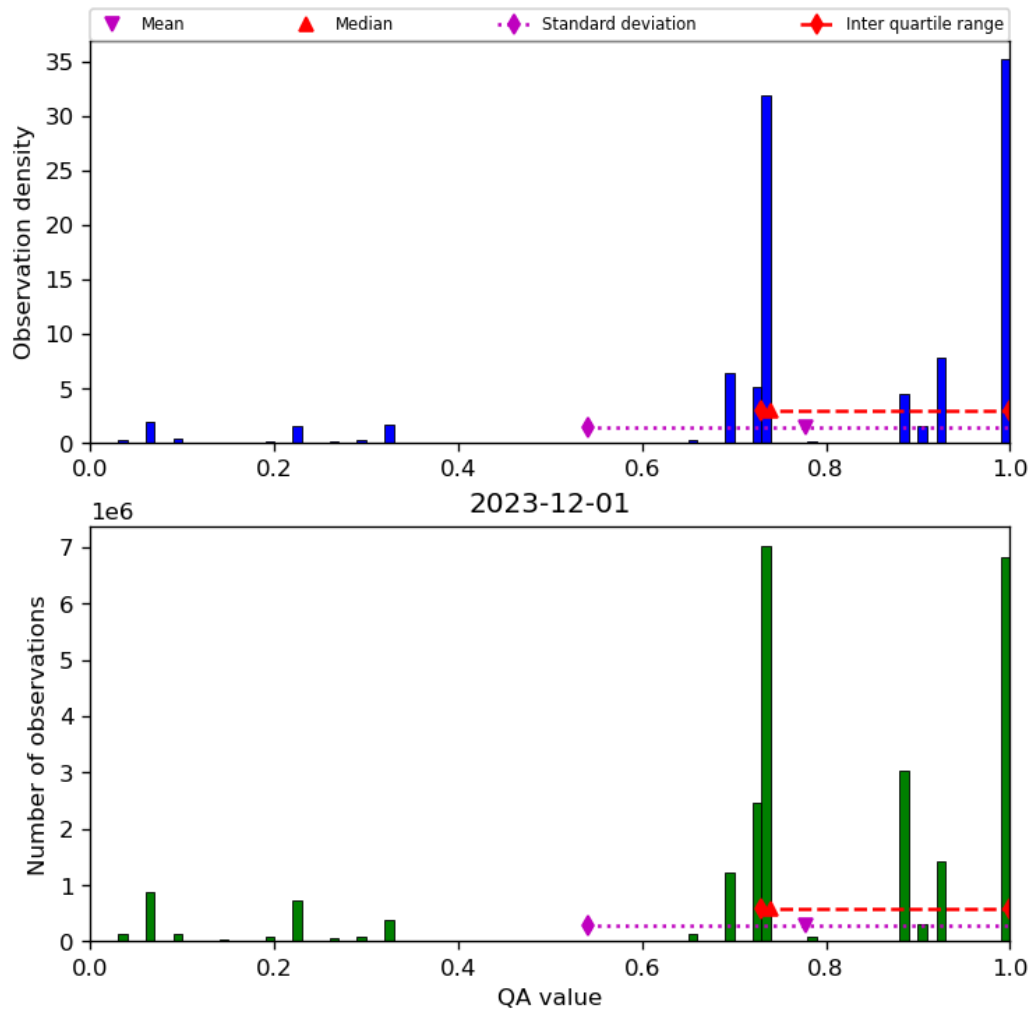
Figure 28: Histogram of “QA value” for 2023-11-30 to 2023-12-02
