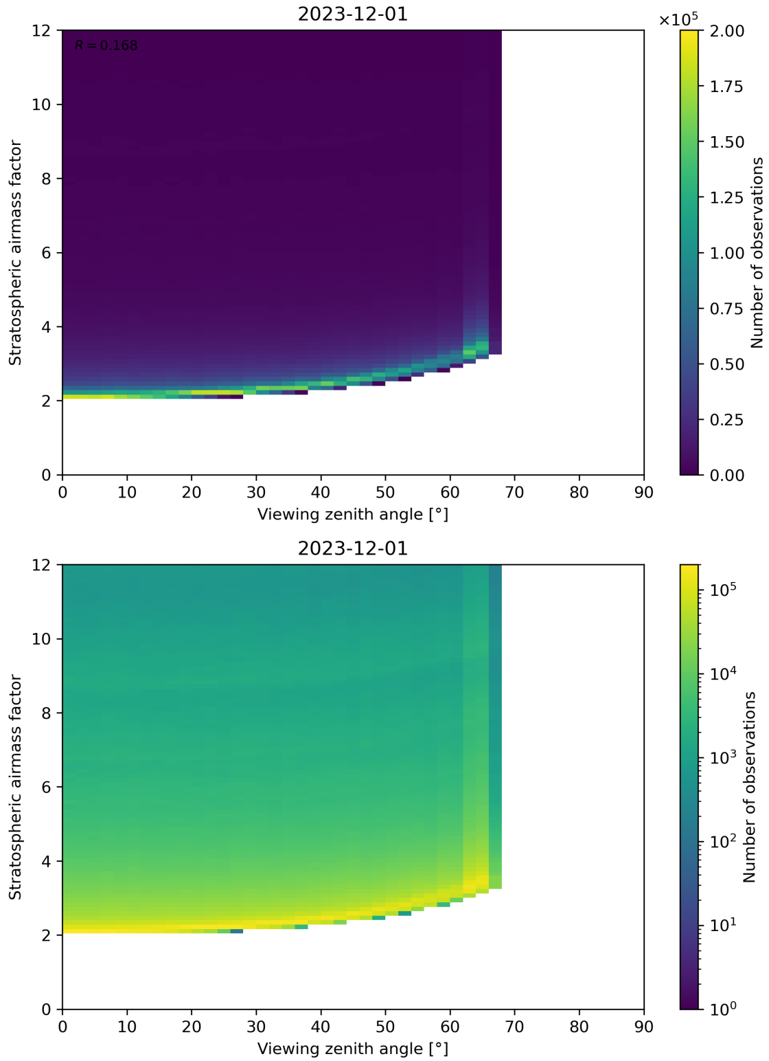
Figure 159: Scatter density plot of “Viewing zenith angle” against “Stratospheric airmass factor” for 2023-11-30 to 2023-12-02.
