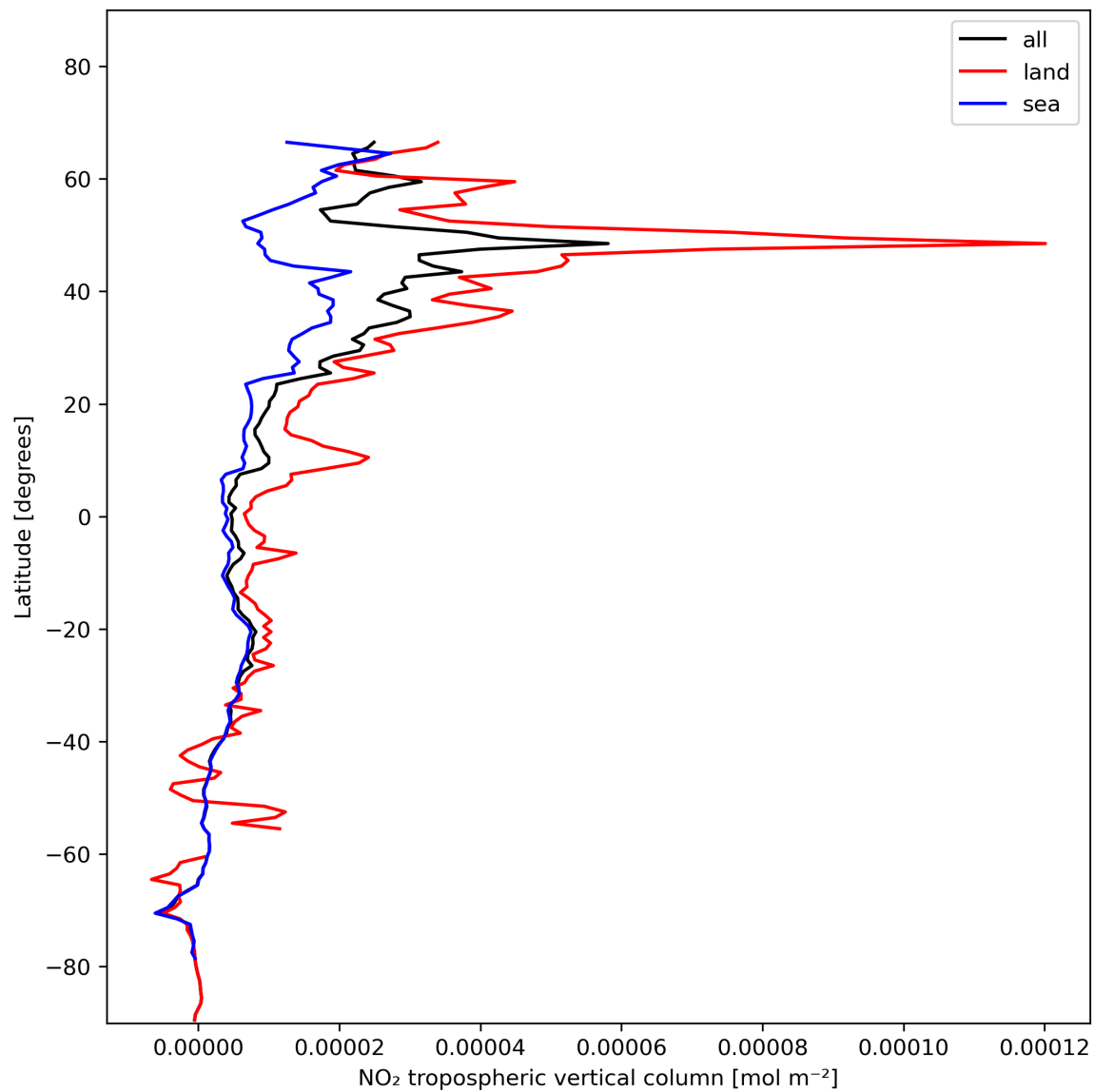
Figure 12: Zonal average of “NO 2 tropospheric vertical column” for 2023-11-30 to 2023-12-02.
