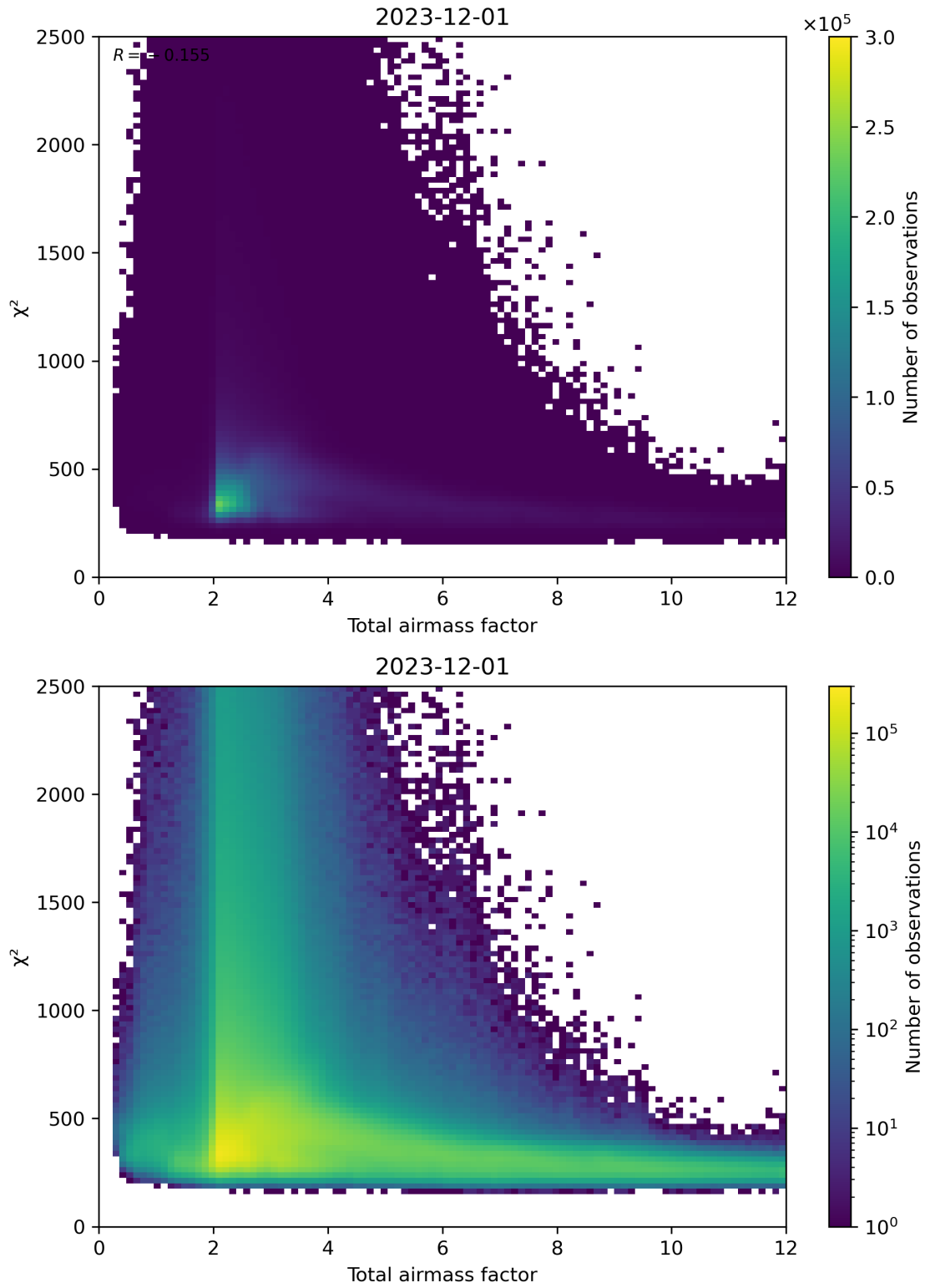
Figure 63: Scatter density plot of “Total airmass factor” against “ \chi^2 ” for 2023-11-30 to 2023-12-02.
