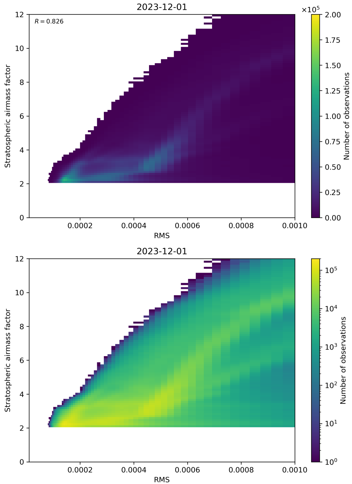
Figure 144: Scatter density plot of “RMS” against “Stratospheric airmass factor” for 2023-11-30 to 2023-12-02.
