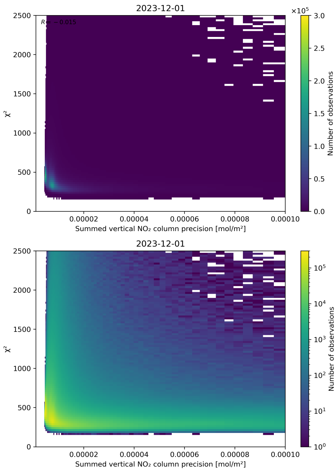
Figure 107: Scatter density plot of “Summed vertical NO 2 column precision” against “ \chi^2 ” for 2023-11-30 to 2023-12-02.
