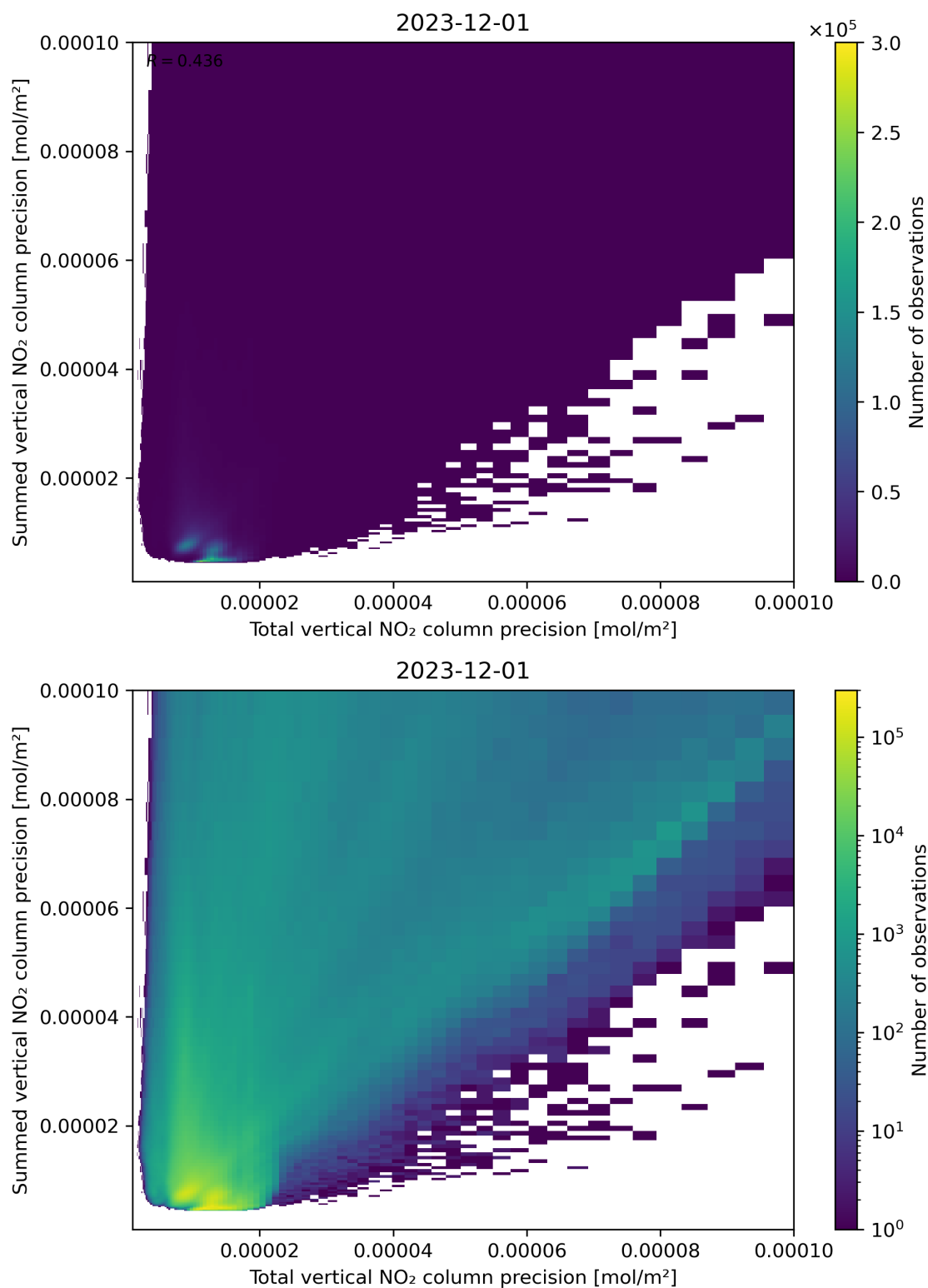
Figure 118: Scatter density plot of “Total vertical NO 2 column precision” against “Summed vertical NO 2 column precision” for 2023-11-30 to 2023-12-02.
