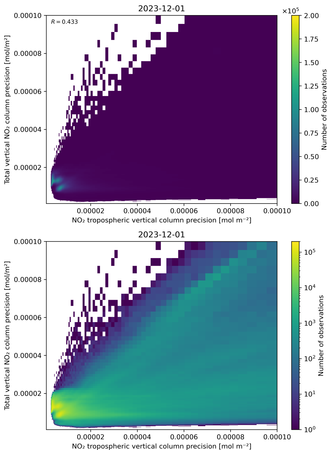
Figure 139: Scatter density plot of “NO 2 tropospheric vertical column precision” against “Total vertical NO 2 column precision” for 2023-11-30 to 2023-12-02.
