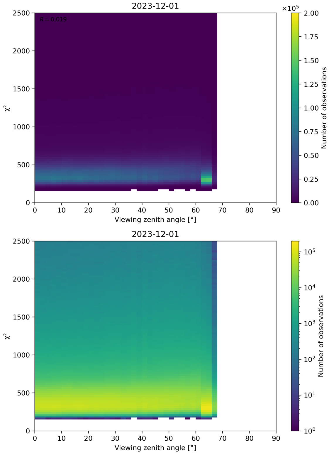
Figure 162: Scatter density plot of “Viewing zenith angle” against “ \chi^2 ” for 2023-11-30 to 2023-12-02.
