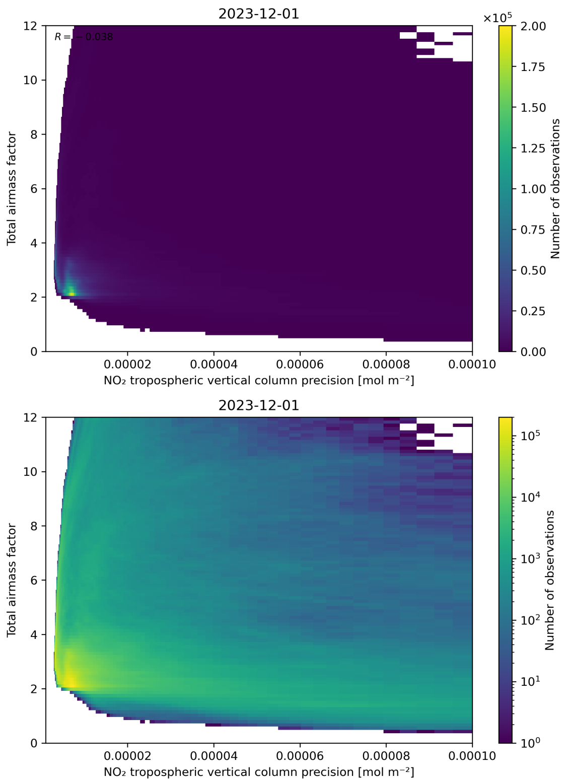
Figure 132: Scatter density plot of “NO 2 tropospheric vertical column precision” against “Total air mass factor” for 2023-11-30 to 2023-12-02.
