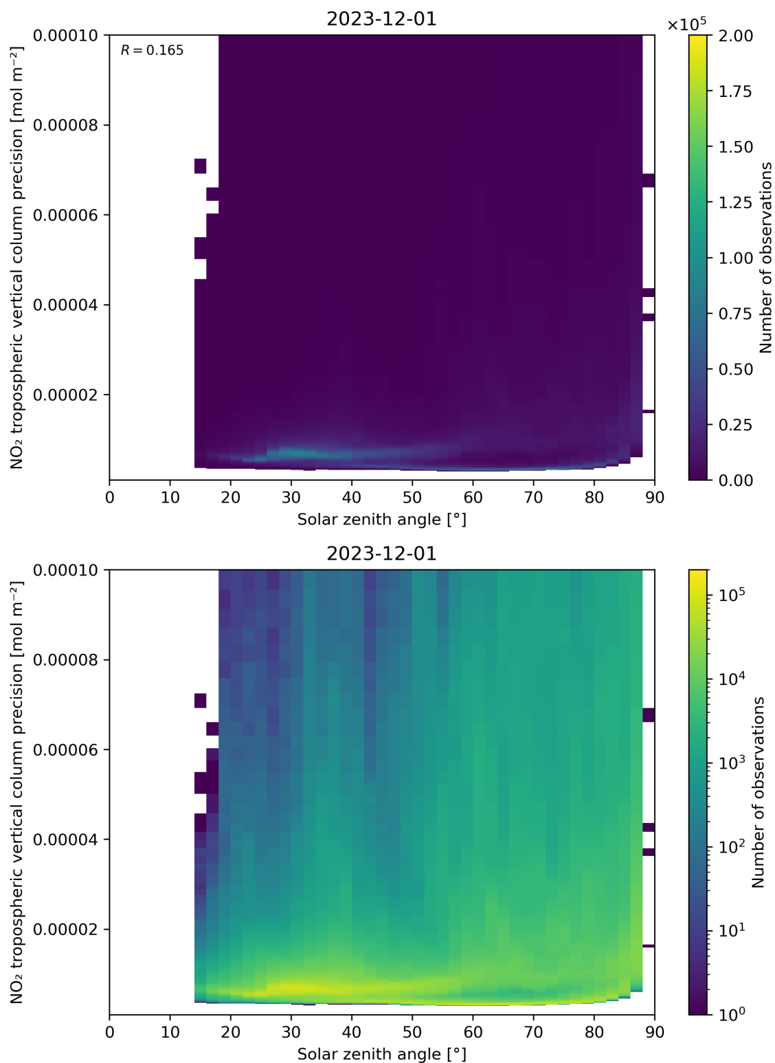
Figure 156: Scatter density plot of “Solar zenith angle” against “NO 2 tropospheric vertical column precision” for 2023-11-30 to 2023-12-02.
