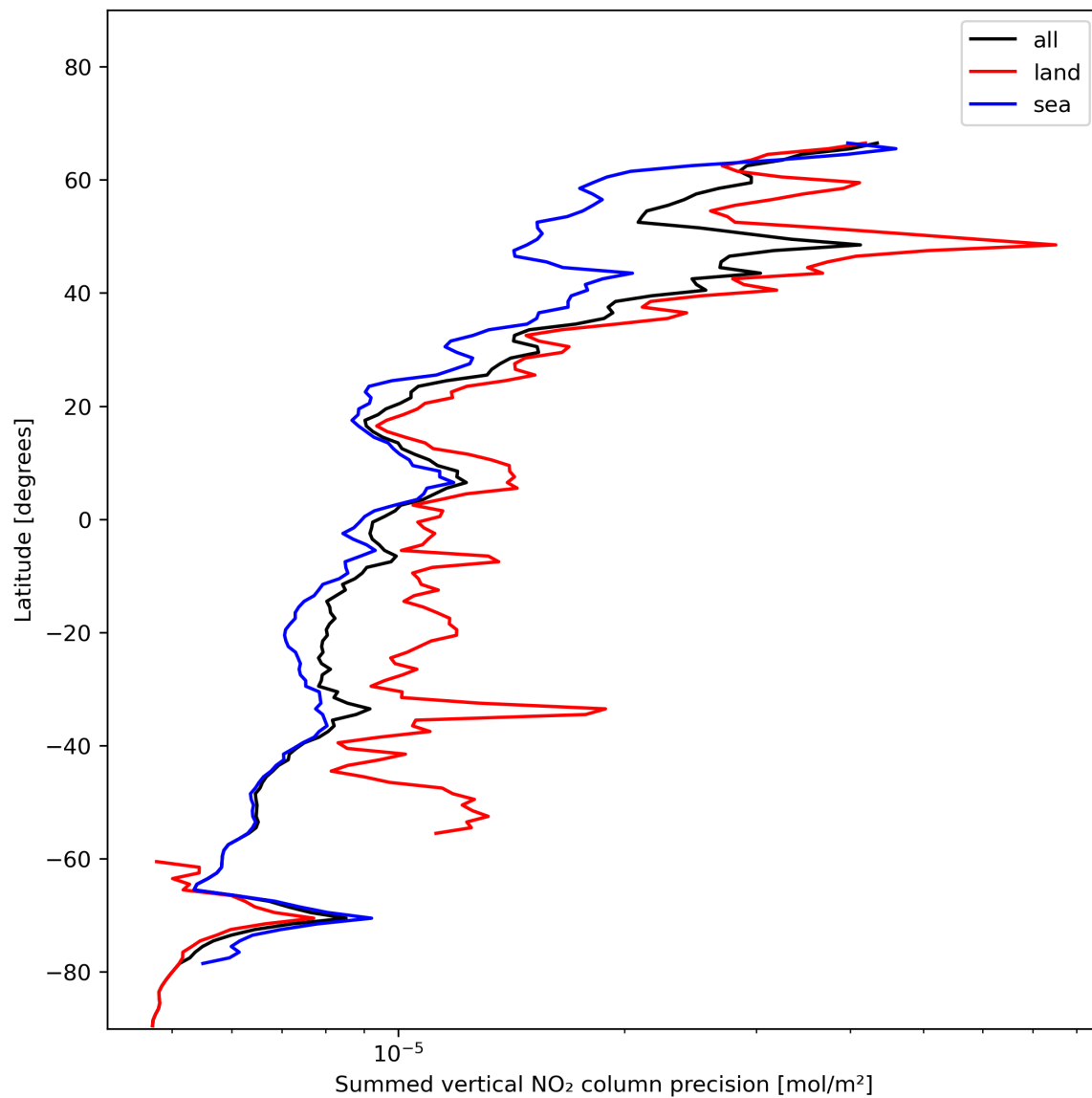
Figure 24: Zonal average of “Summed vertical NO 2 column precision” for 2023-11-30 to 2023-12-02.
