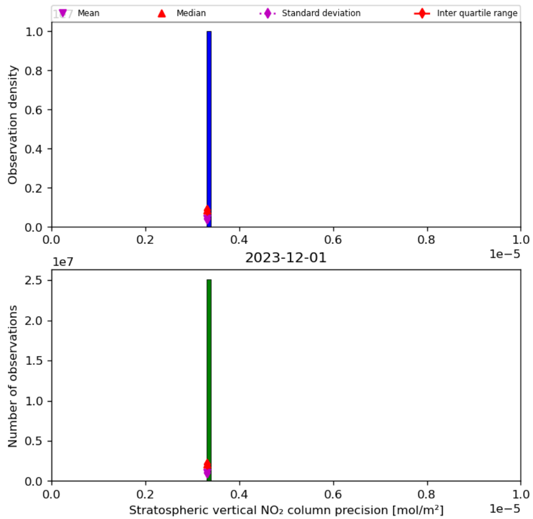
Figure 37: Histogram of “Stratospheric vertical NO 2 column precision” for 2023-11-30 to 2023-12-02
