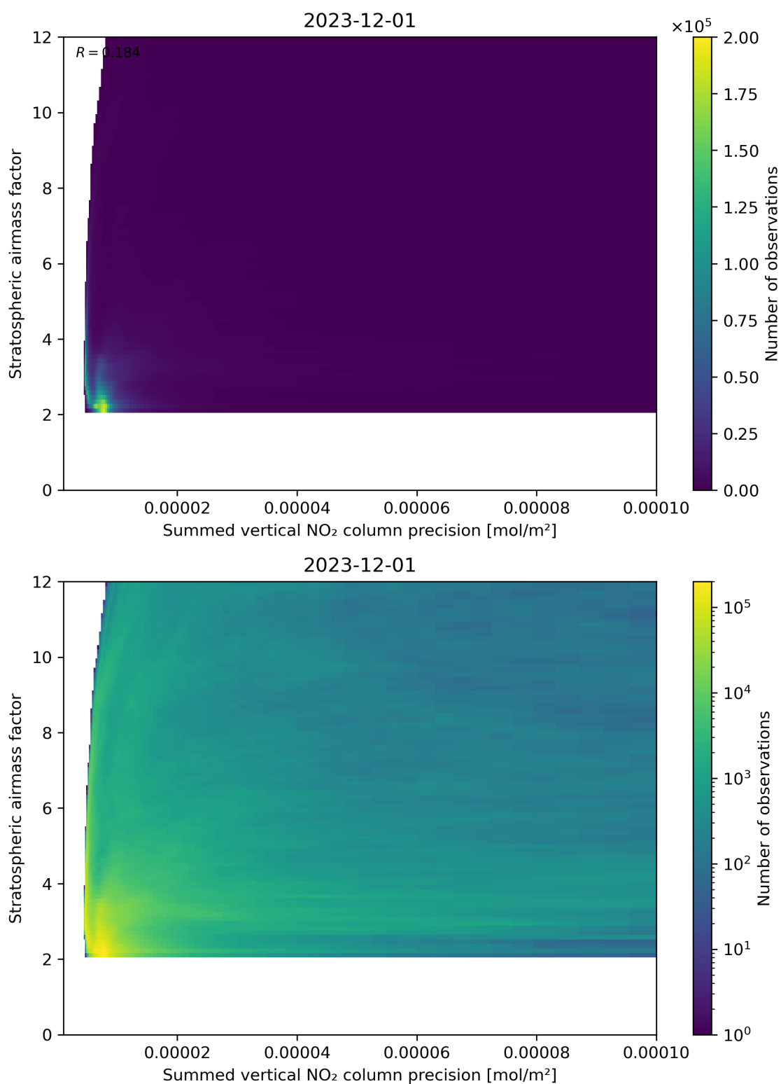
Figure 106: Scatter density plot of “Summed vertical NO 2 column precision” against “Stratospheric airmass factor” for 2023-11-30 to 2023-12-02.
