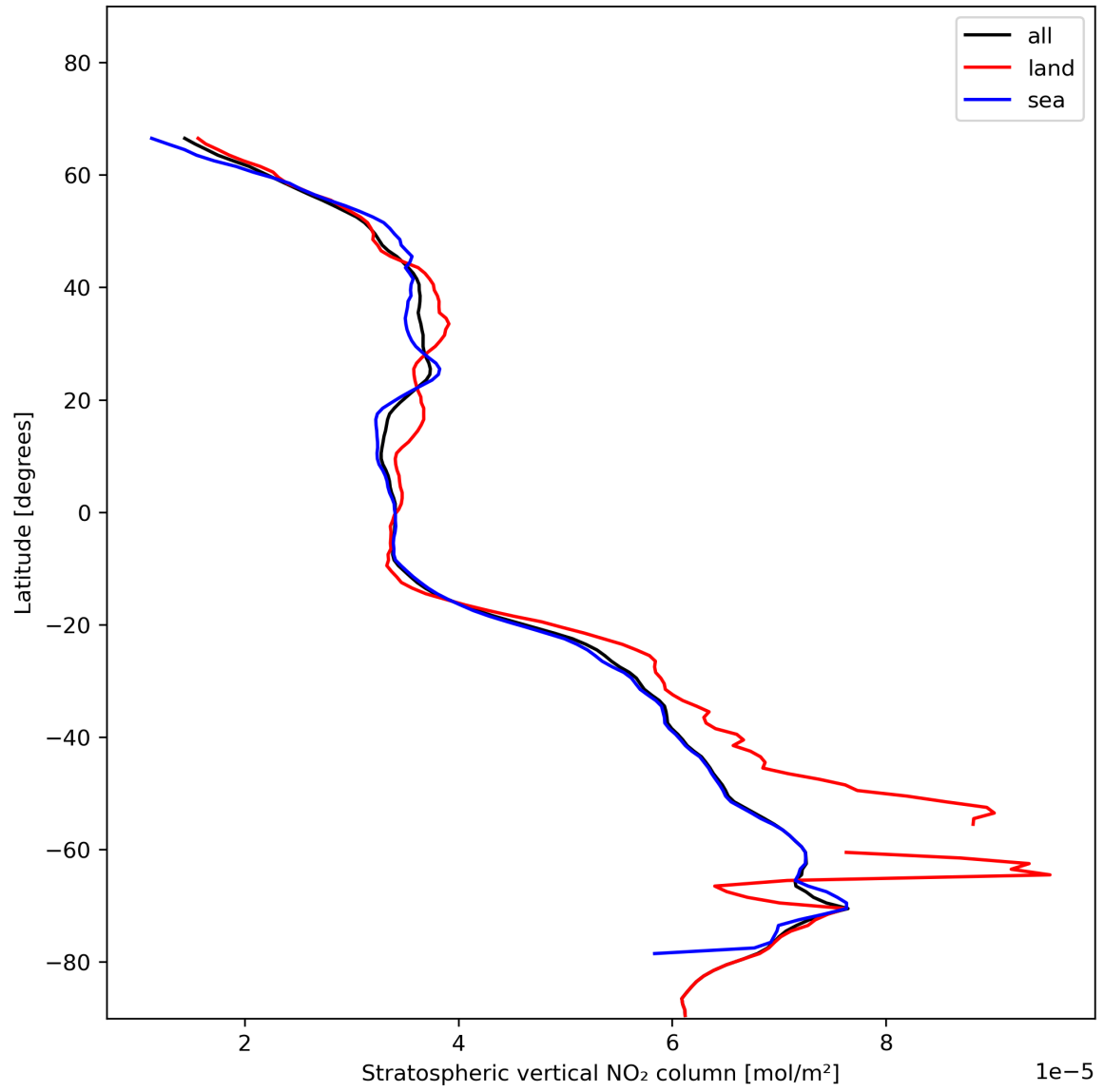
Figure 19: Zonal average of “Stratospheric vertical NO 2 column” for 2023-11-30 to 2023-12-02.
