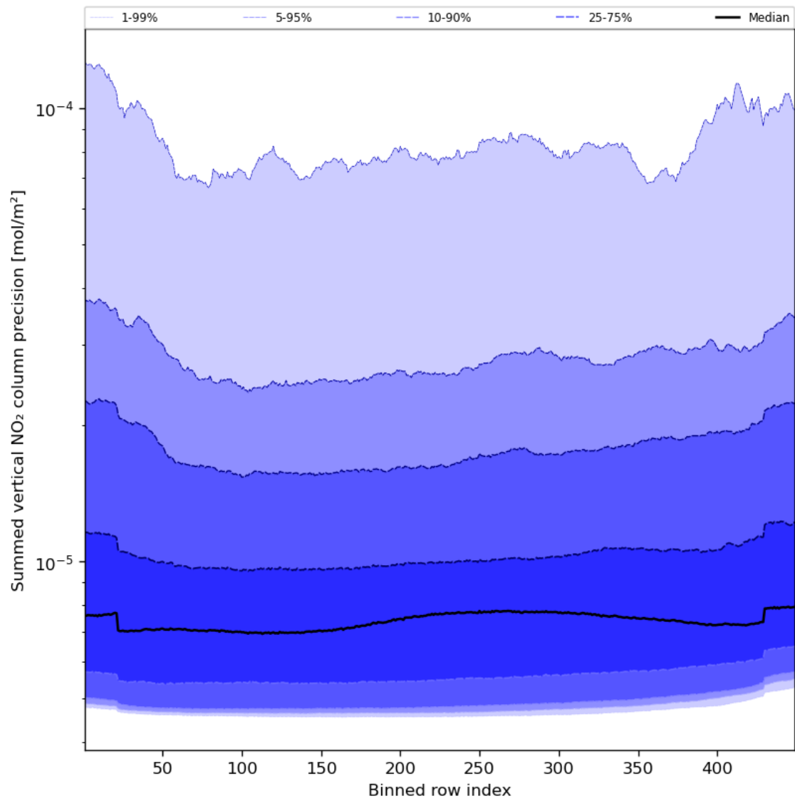
Figure 58: Along track statistics of “Summed vertical NO 2 column precision” for 2023-11-30 to 2023-12-02
