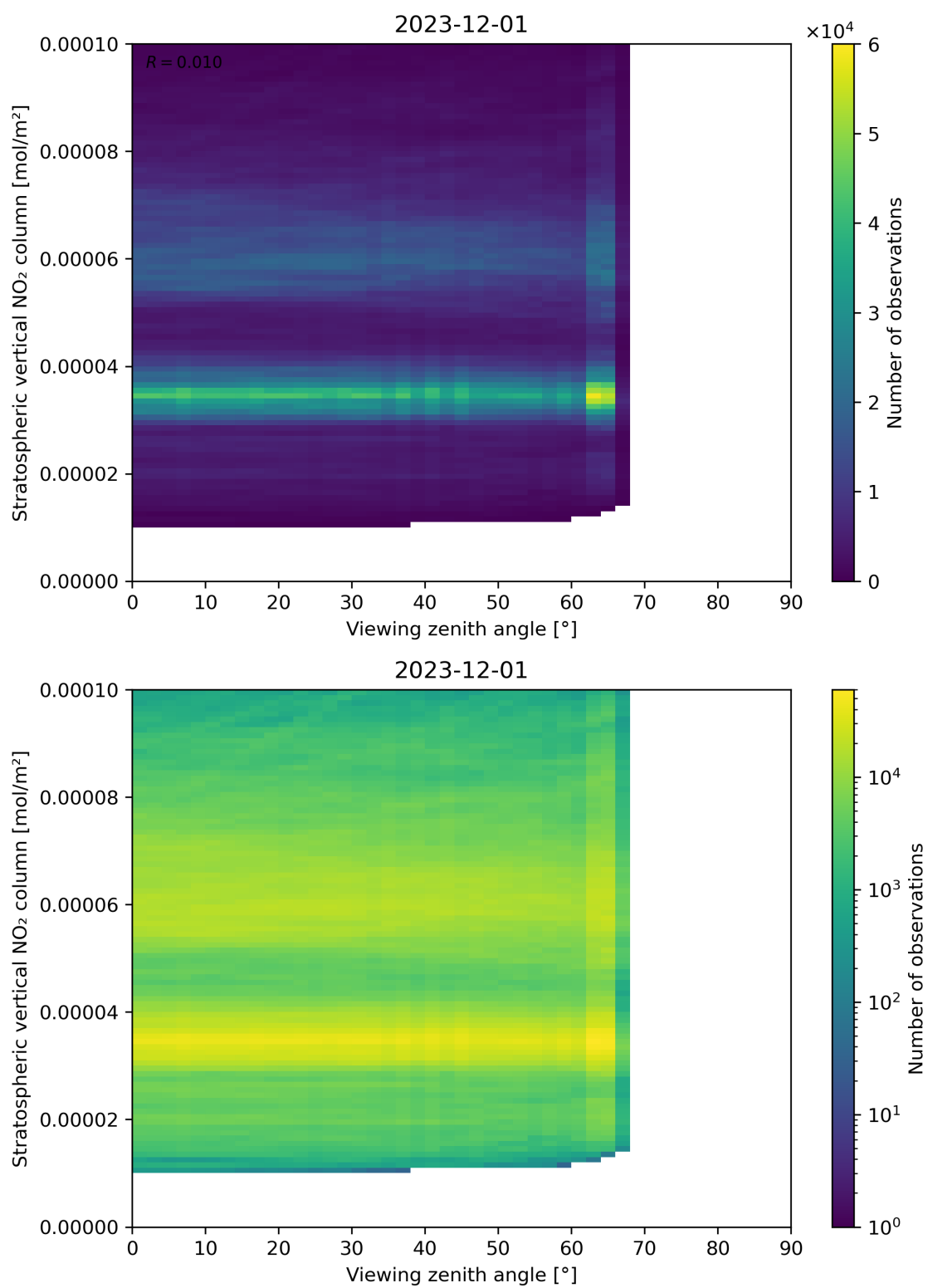
Figure 164: Scatter density plot of “Viewing zenith angle” against “Stratospheric vertical NO 2 column” for 2023-11-30 to 2023-12-02.
