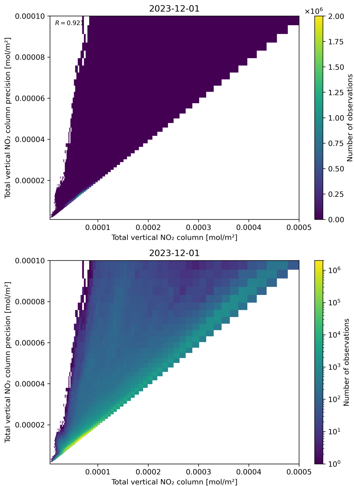
Figure 114: Scatter density plot of “Total vertical NO 2 column” against “Total vertical NO 2 column precision” for 2023-11-30 to 2023-12-02.
