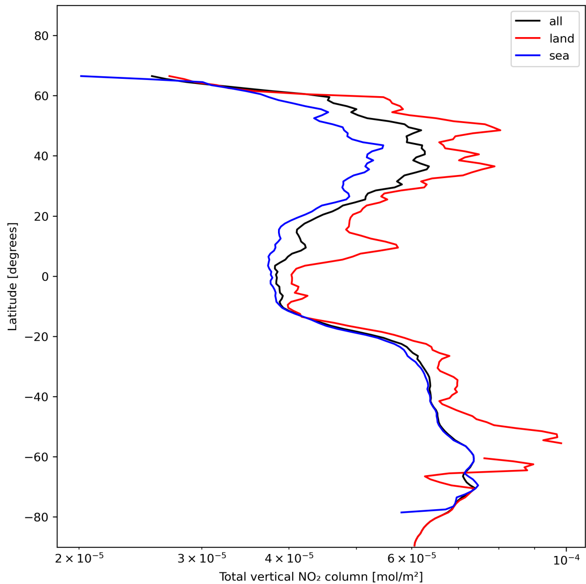
Figure 21: Zonal average of “Total vertical NO 2 column” for 2023-11-30 to 2023-12-02.
