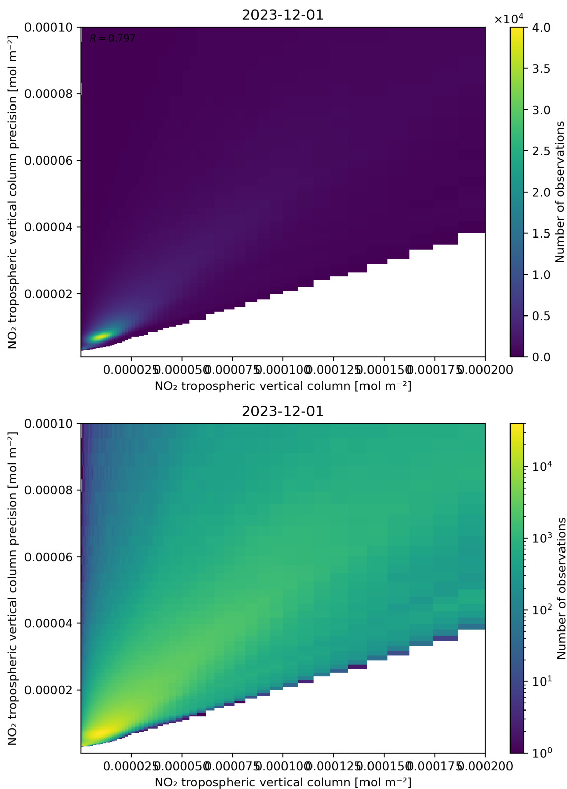
Figure 130: Scatter density plot of “NO 2 tropospheric vertical column” against “NO 2 tropospheric vertical column precision” for 2023-11-30 to 2023-12-02.
