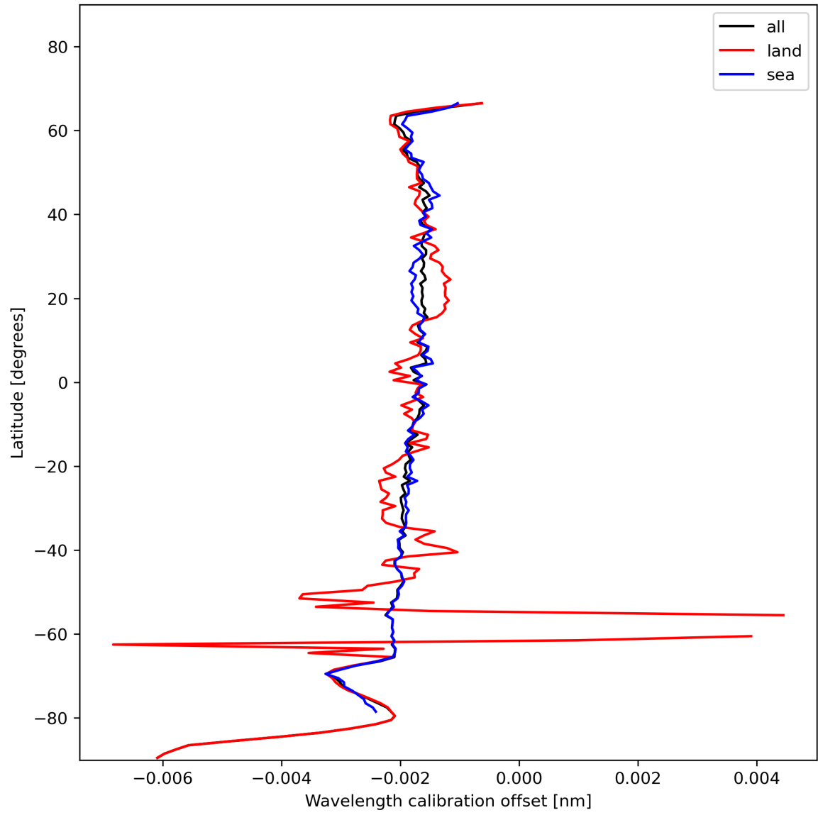
Figure 18: Zonal average of “Wavelength calibration offset” for 2023-11-30 to 2023-12-02.
