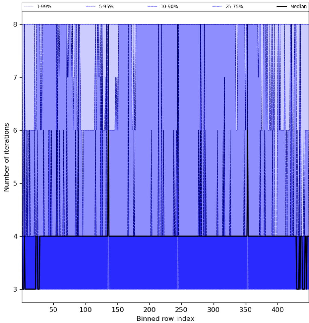
Figure 51: Along track statistics of “Number of iterations” for 2023-11-30 to 2023-12-02
