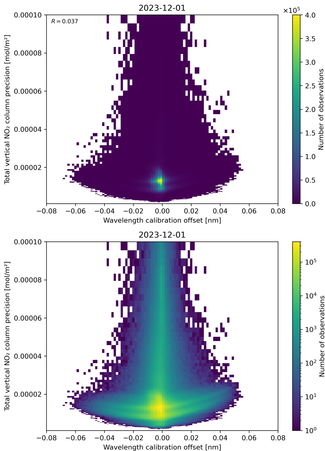
Figure 180: Scatter density plot of “Wavelength calibration offset” against “Total vertical NO 2 column precision” for 2023-11-30 to 2023-12-02.
