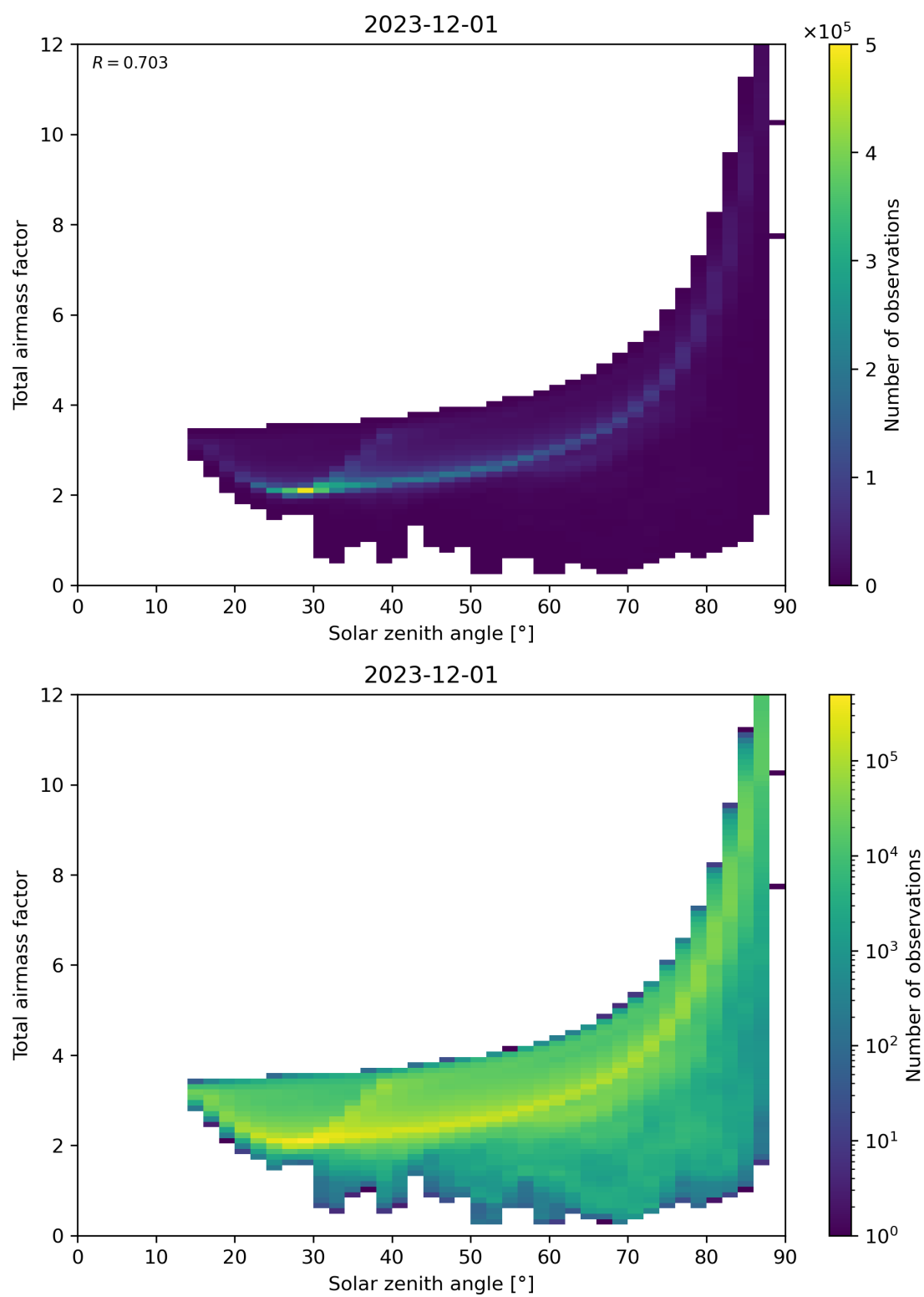
Figure 146: Scatter density plot of “Solar zenith angle” against “Total airmass factor” for 2023-11-30 to 2023-12-02.
