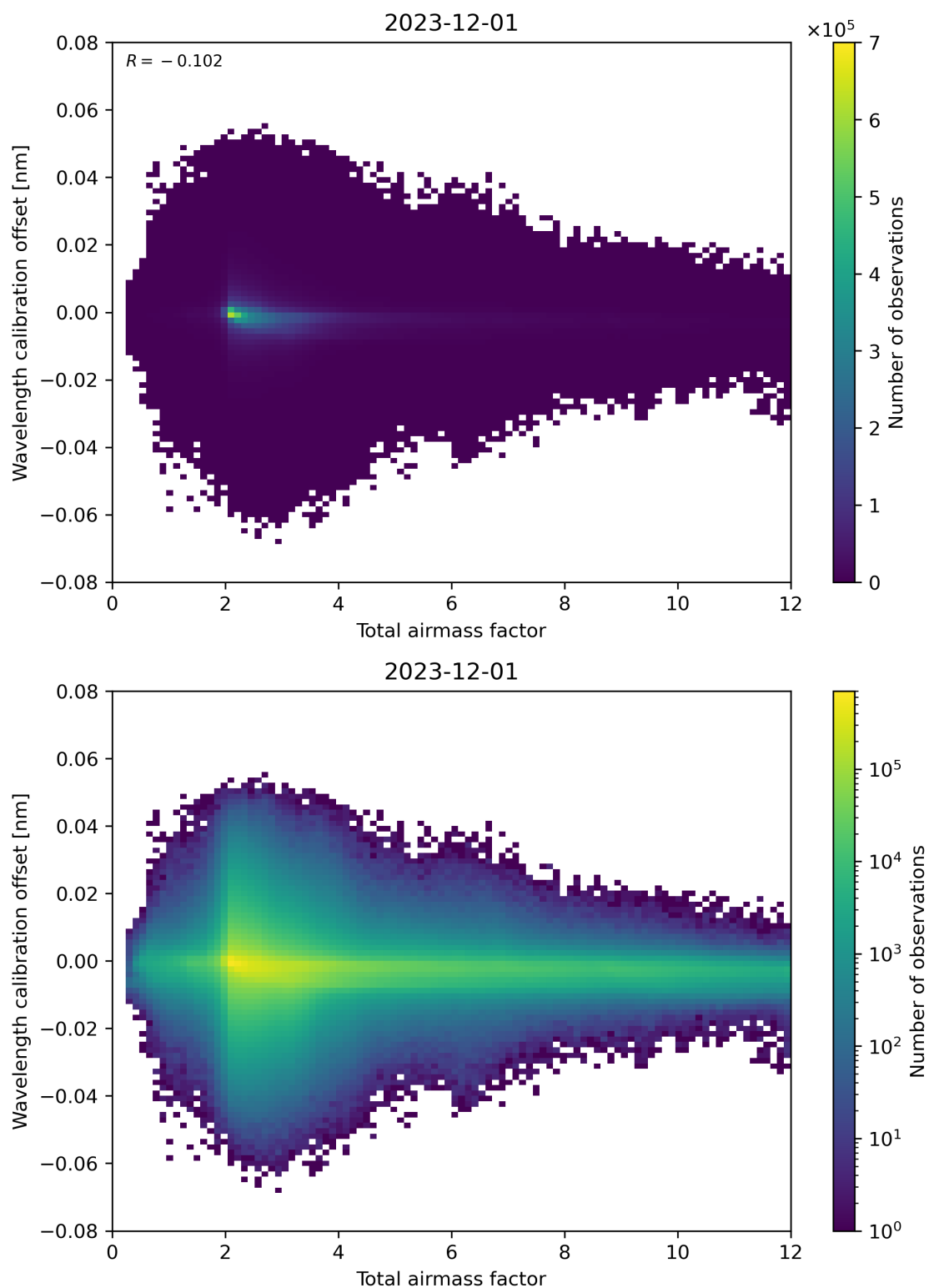
Figure 70: Scatter density plot of “Total airmass factor” against “Wavelength calibration offset” for 2023-11-30 to 2023-12-02.
