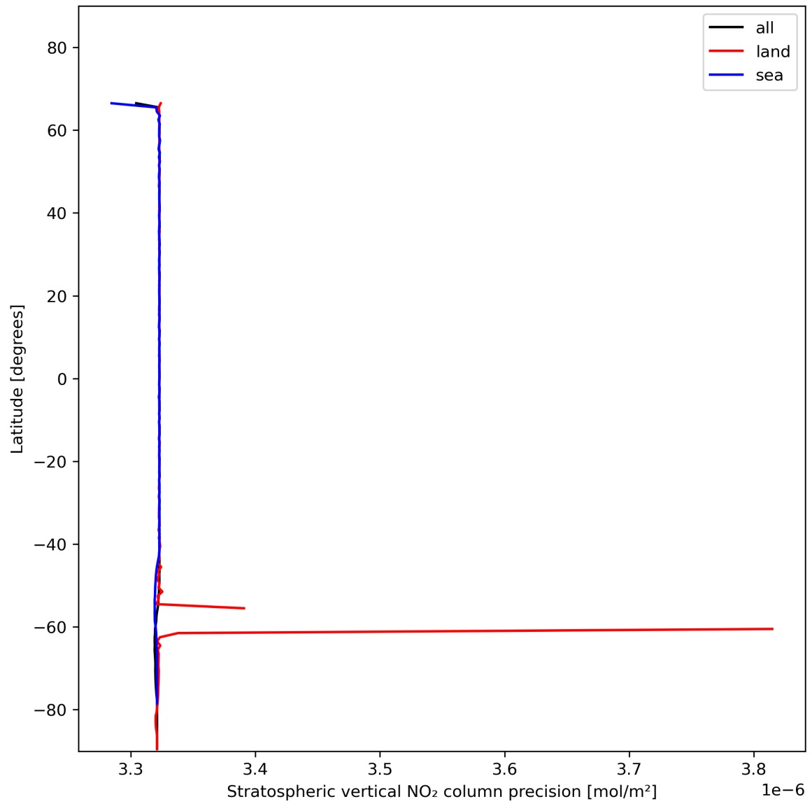
Figure 20: Zonal average of “Stratospheric vertical NO 2 column precision” for 2023-11-30 to 2023-12-02.
