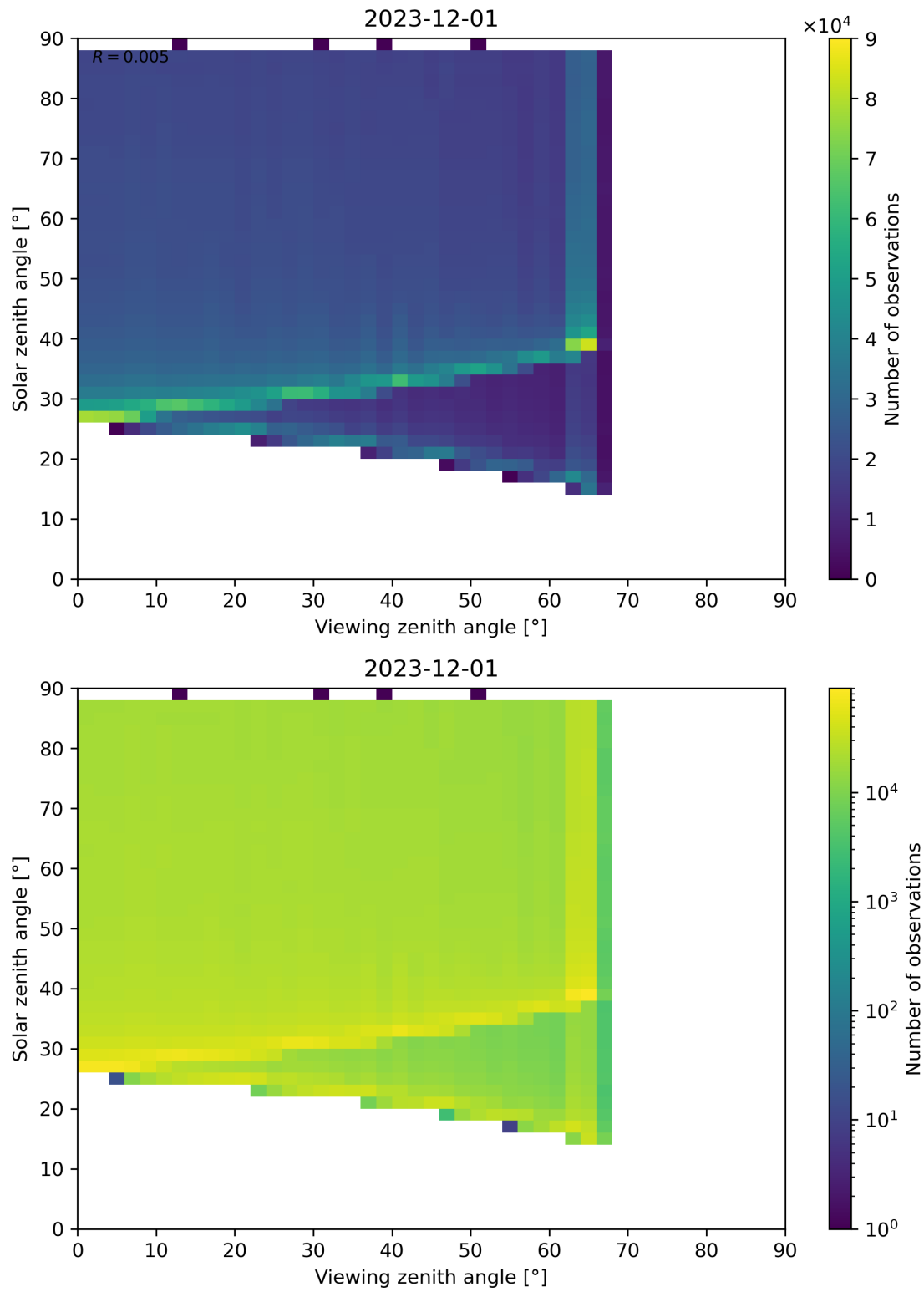
Figure 172: Scatter density plot of “Viewing zenith angle” against “Solar zenith angle” for 2023-11-30 to 2023-12-02.
