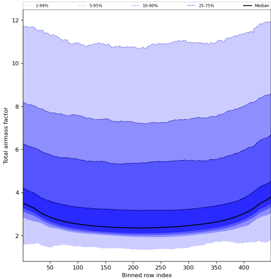
Figure 49: Along track statistics of “Total airmass factor” for 2023-11-30 to 2023-12-02
