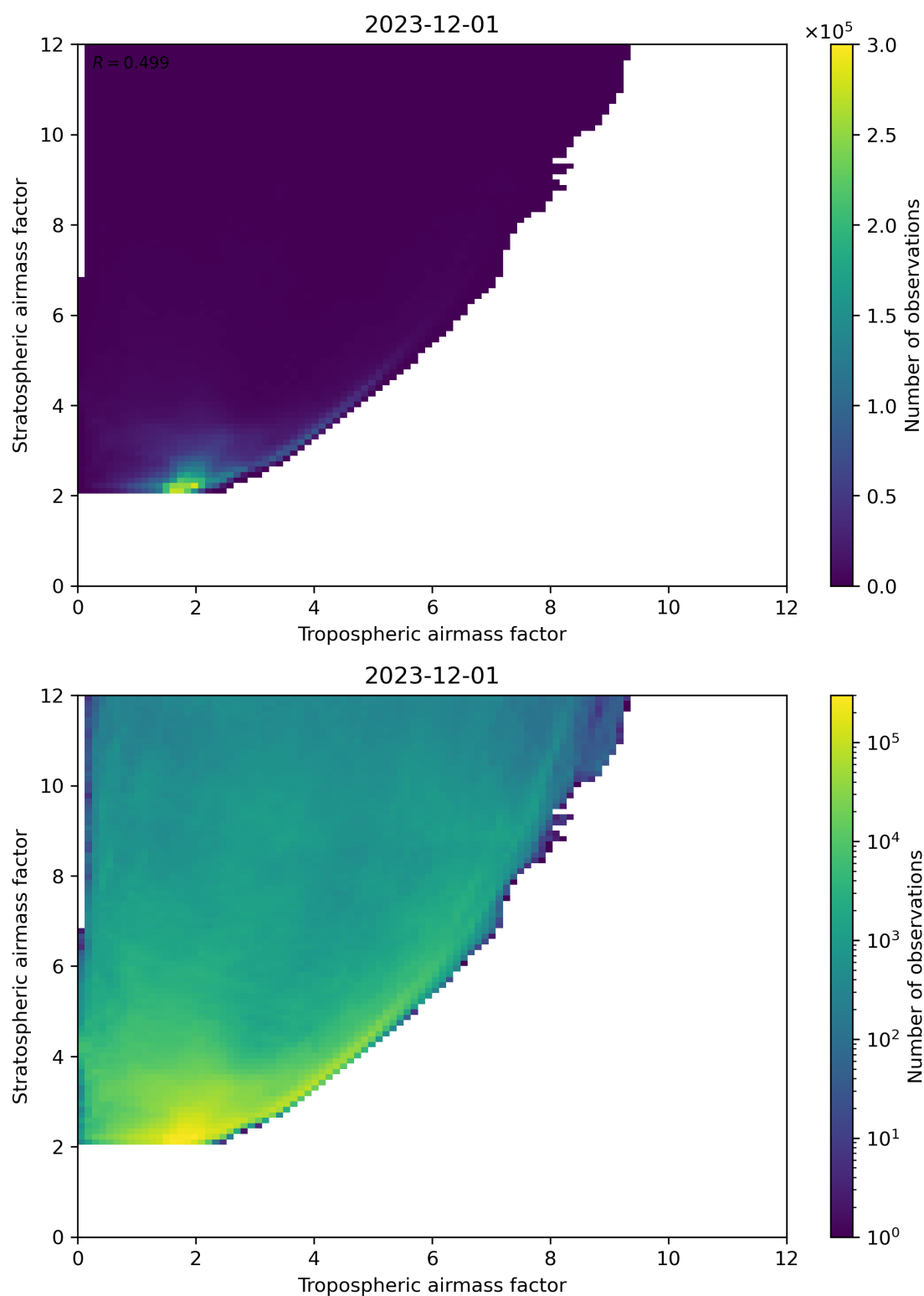
Figure 71: Scatter density plot of “Tropospheric airmass factor” against “Stratospheric airmass factor” for 2023-11-30 to 2023-12-02.
