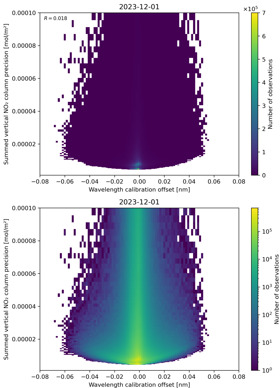
Figure 178: Scatter density plot of “Wavelength calibration offset” against “Summed vertical NO 2 column precision” for 2023-11-30 to 2023-12-02.
