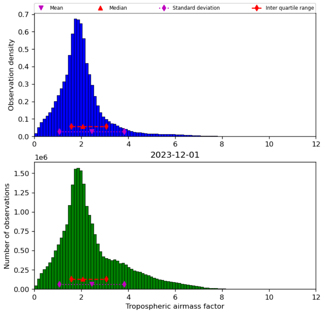
Figure 31: Histogram of “Tropospheric airmass factor” for 2023-11-30 to 2023-12-02
