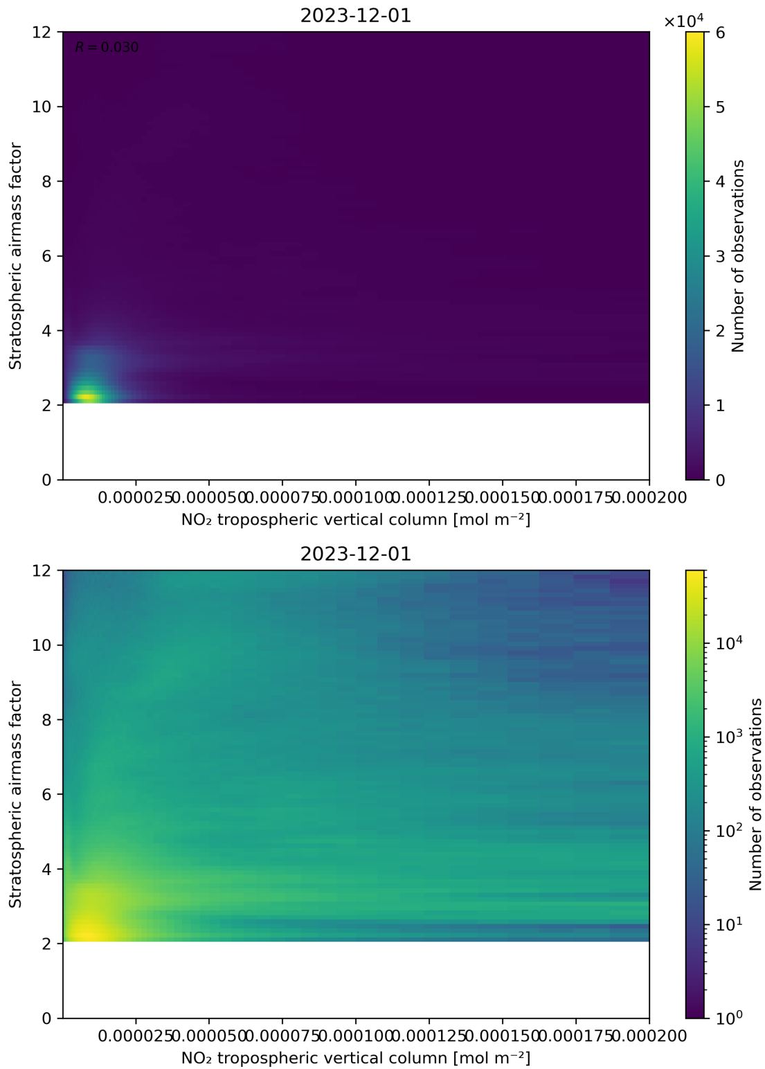
Figure 121: Scatter density plot of “NO 2 tropospheric vertical column” against “Stratospheric airmass factor” for 2023-11-30 to 2023-12-02.
