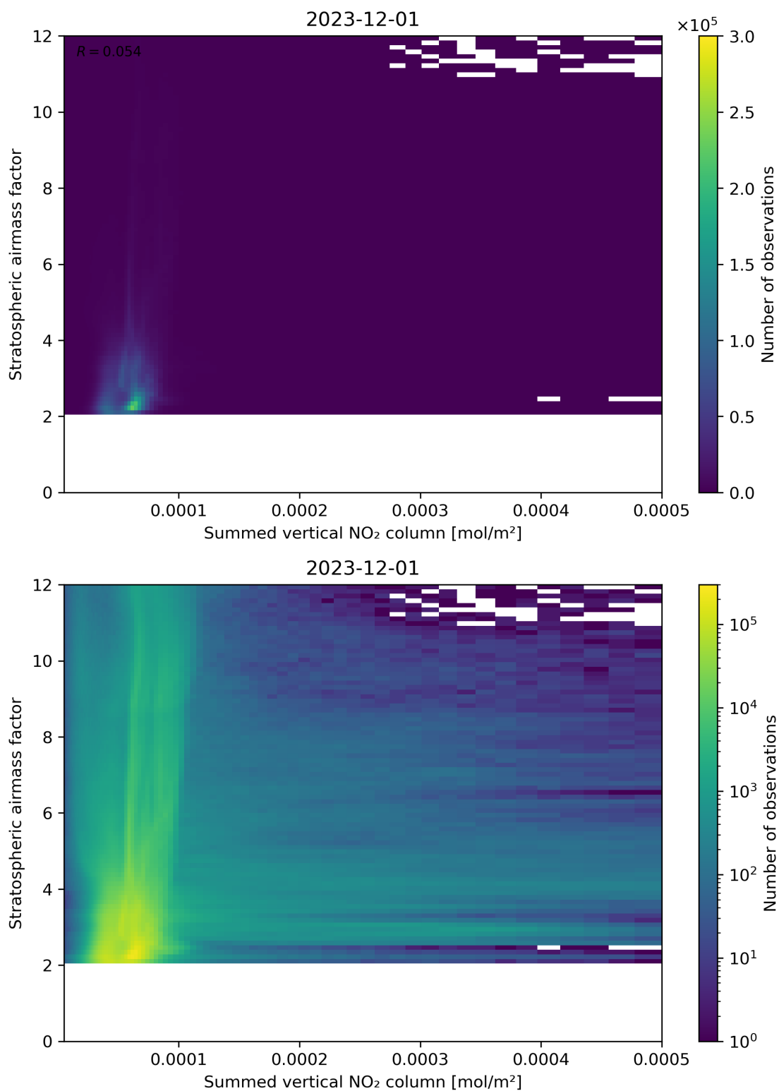
Figure 103: Scatter density plot of “Summed vertical NO 2 column” against “Stratospheric airmass factor” for 2023-11-30 to 2023-12-02.
