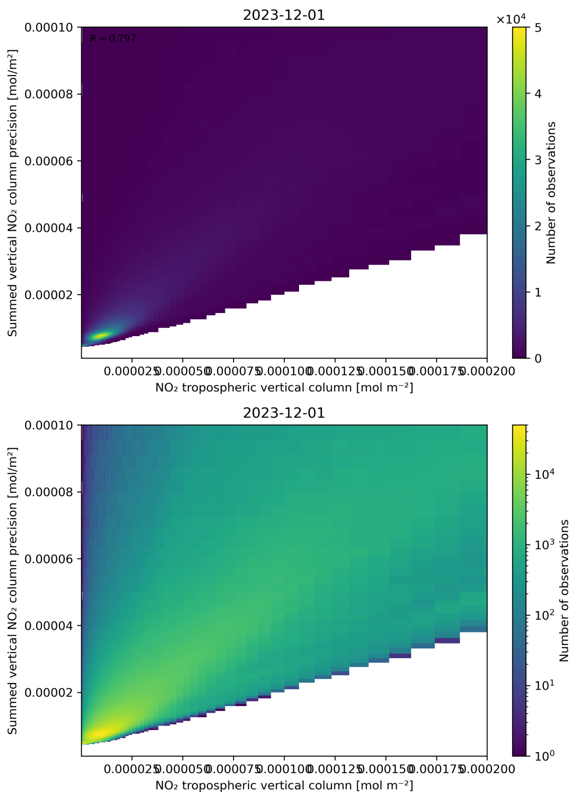
Figure 127: Scatter density plot of “NO 2 tropospheric vertical column” against “Summed vertical NO 2 column precision” for 2023-11-30 to 2023-12-02.
