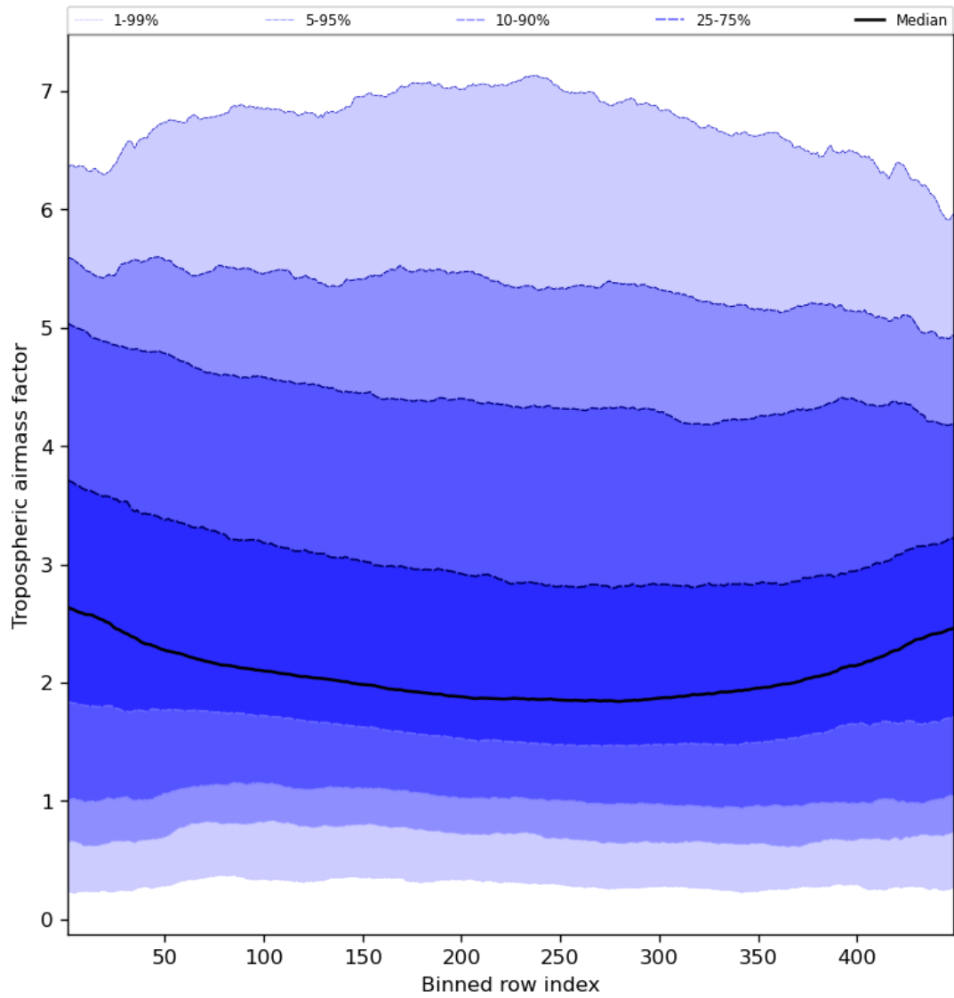
Figure 48: Along track statistics of “Tropospheric air mass factor” for 2023-11-30 to 2023-12-02
