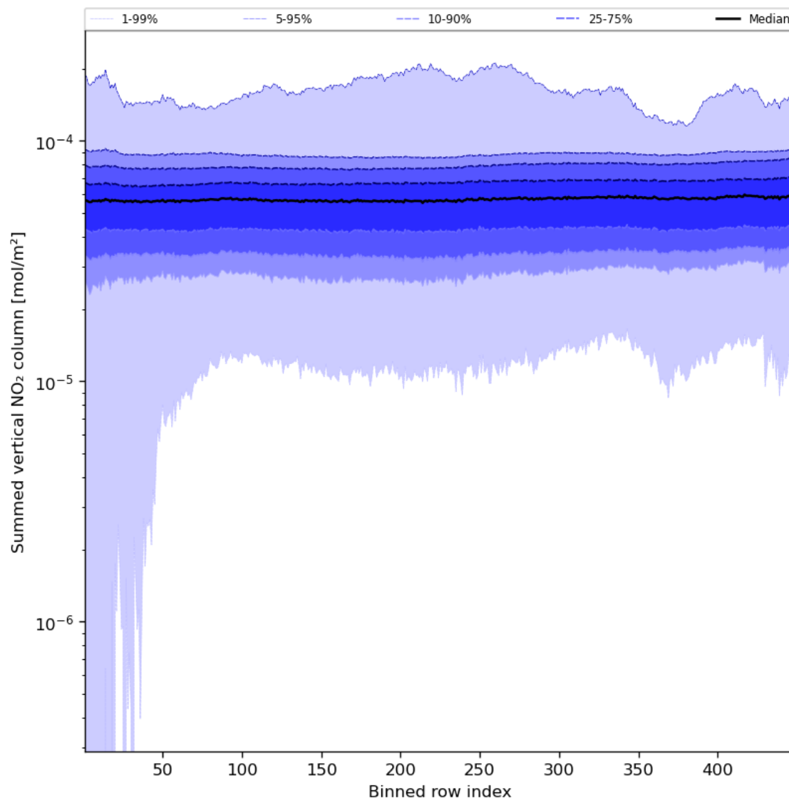
Figure 57: Along track statistics of “Summed vertical NO 2 column” for 2023-11-30 to 2023-12-02
