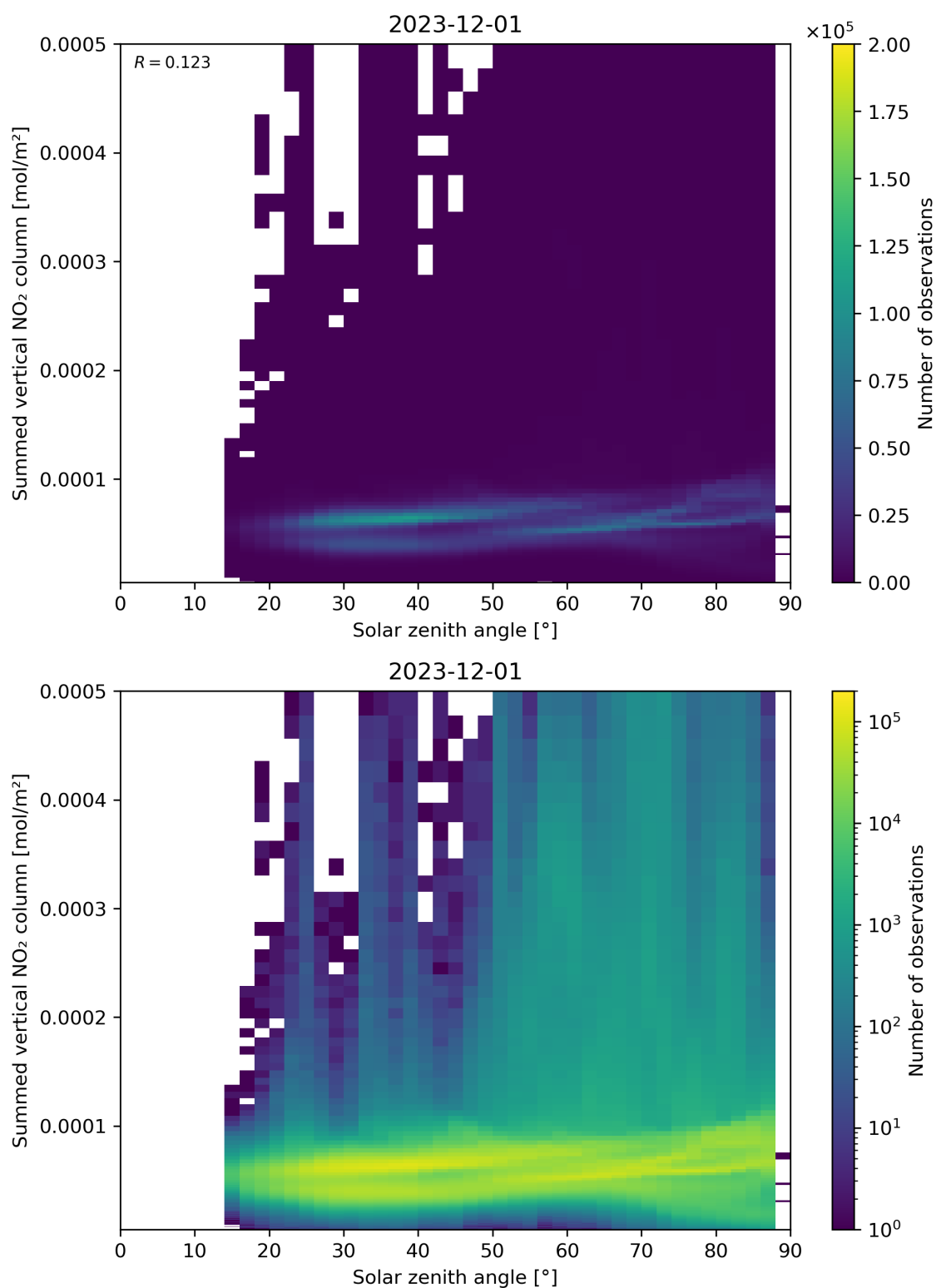
Figure 151: Scatter density plot of “Solar zenith angle” against “Summed vertical NO 2 column” for 2023-11-30 to 2023-12-02.
