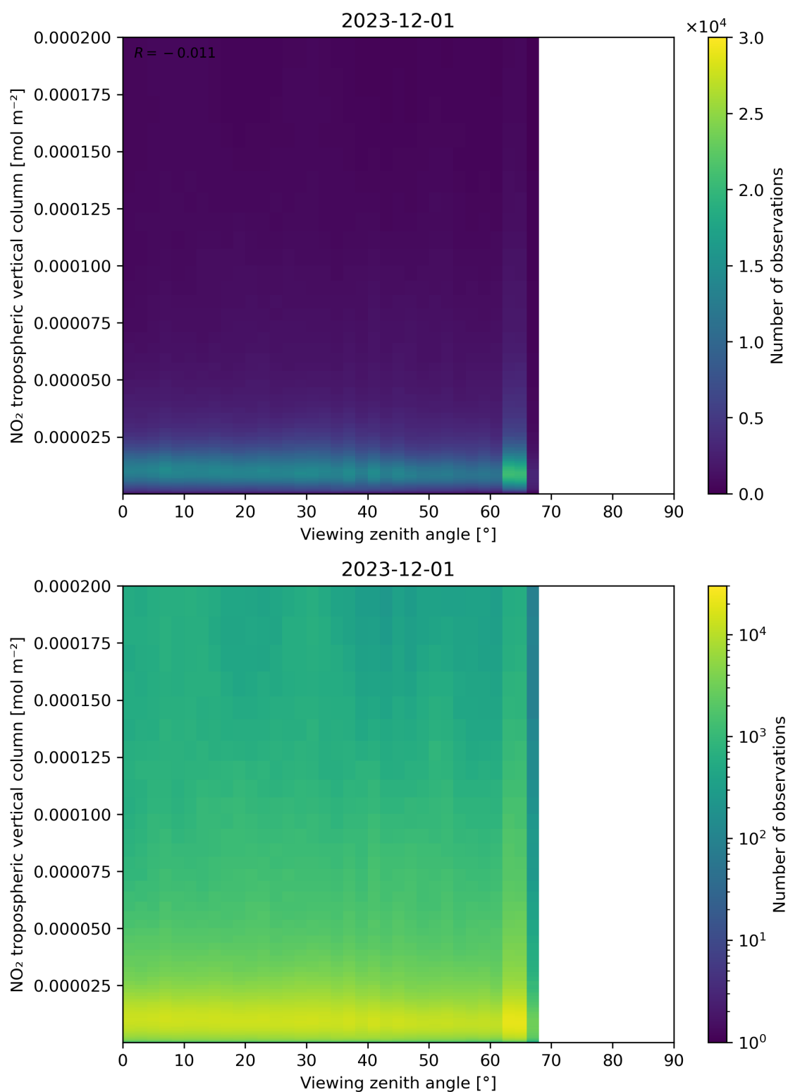
Figure 169: Scatter density plot of “Viewing zenith angle” against “NO 2 tropospheric vertical column” for 2023-11-30 to 2023-12-02.
