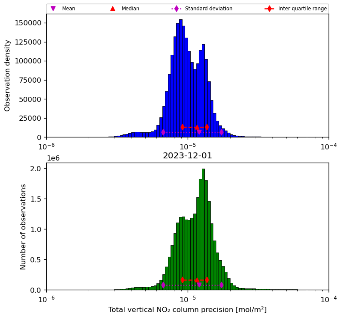
Figure 39: Histogram of “Total vertical NO 2 column precision” for 2023-11-30 to 2023-12-02
