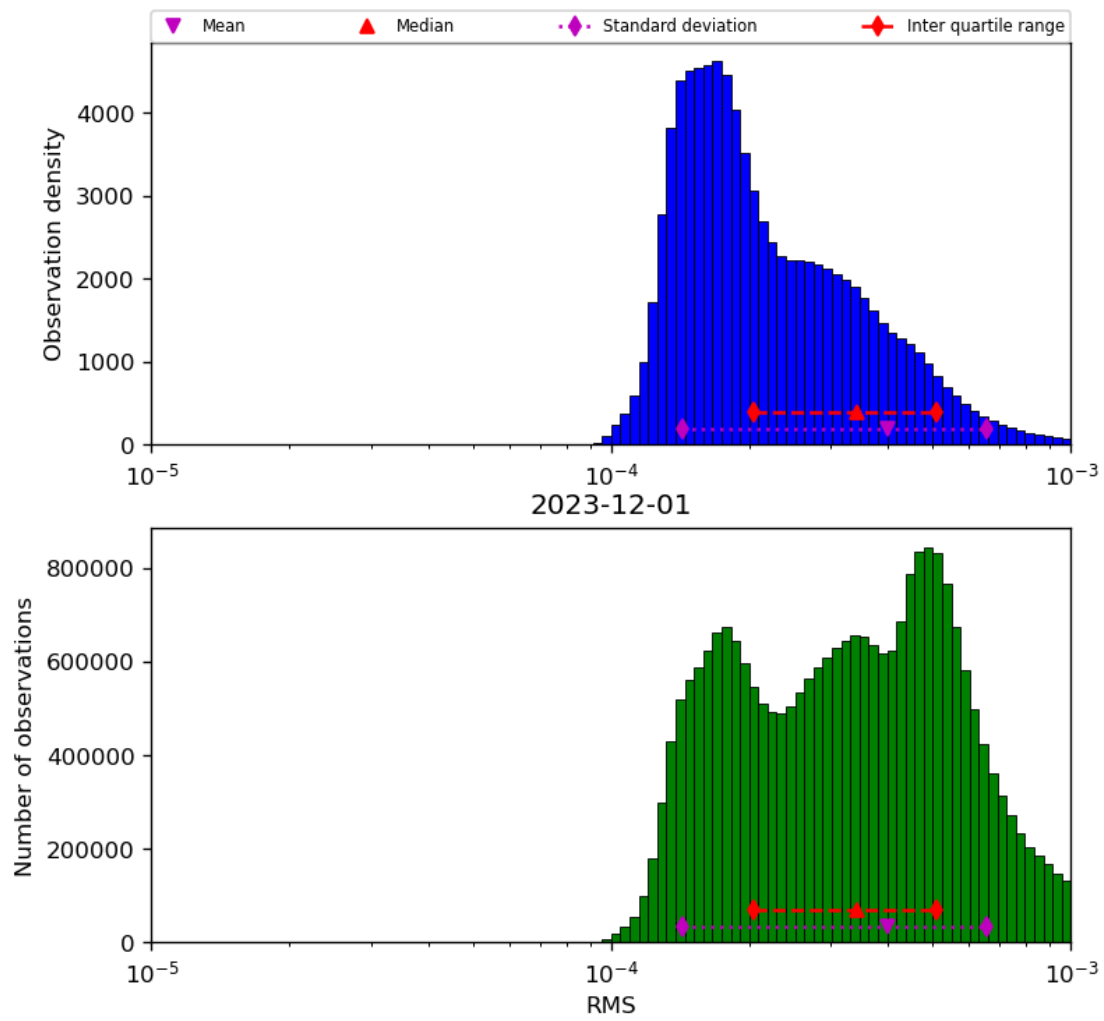
Figure 43: Histogram of “RMS” for 2023-11-30 to 2023-12-02
