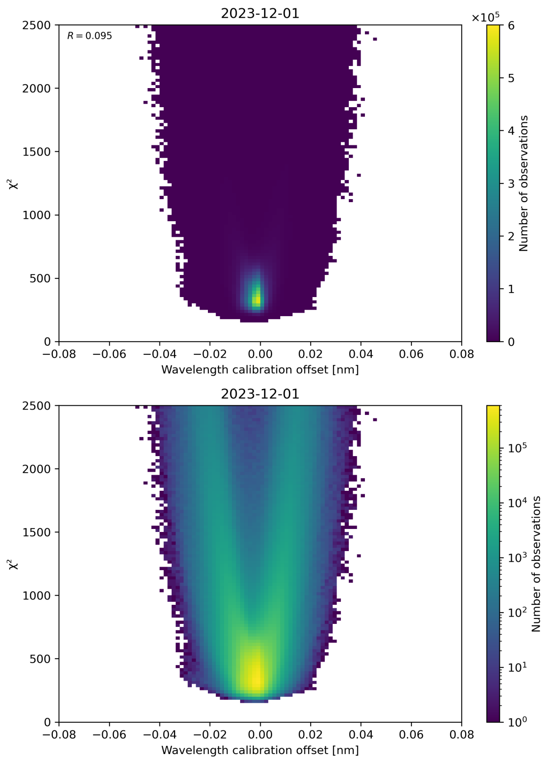
Figure 175: Scatter density plot of “Wavelength calibration offset” against “ \chi^2 ” for 2023-11-30 to 2023-12-02.
