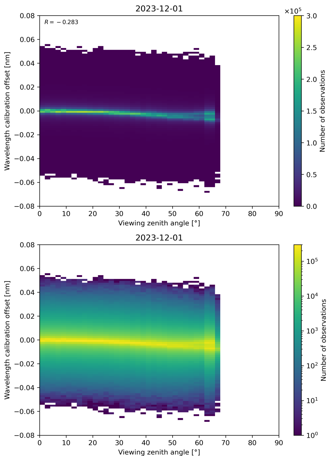
Figure 173: Scatter density plot of “Viewing zenith angle” against “Wavelength calibration offset” for 2023-11-30 to 2023-12-02.
