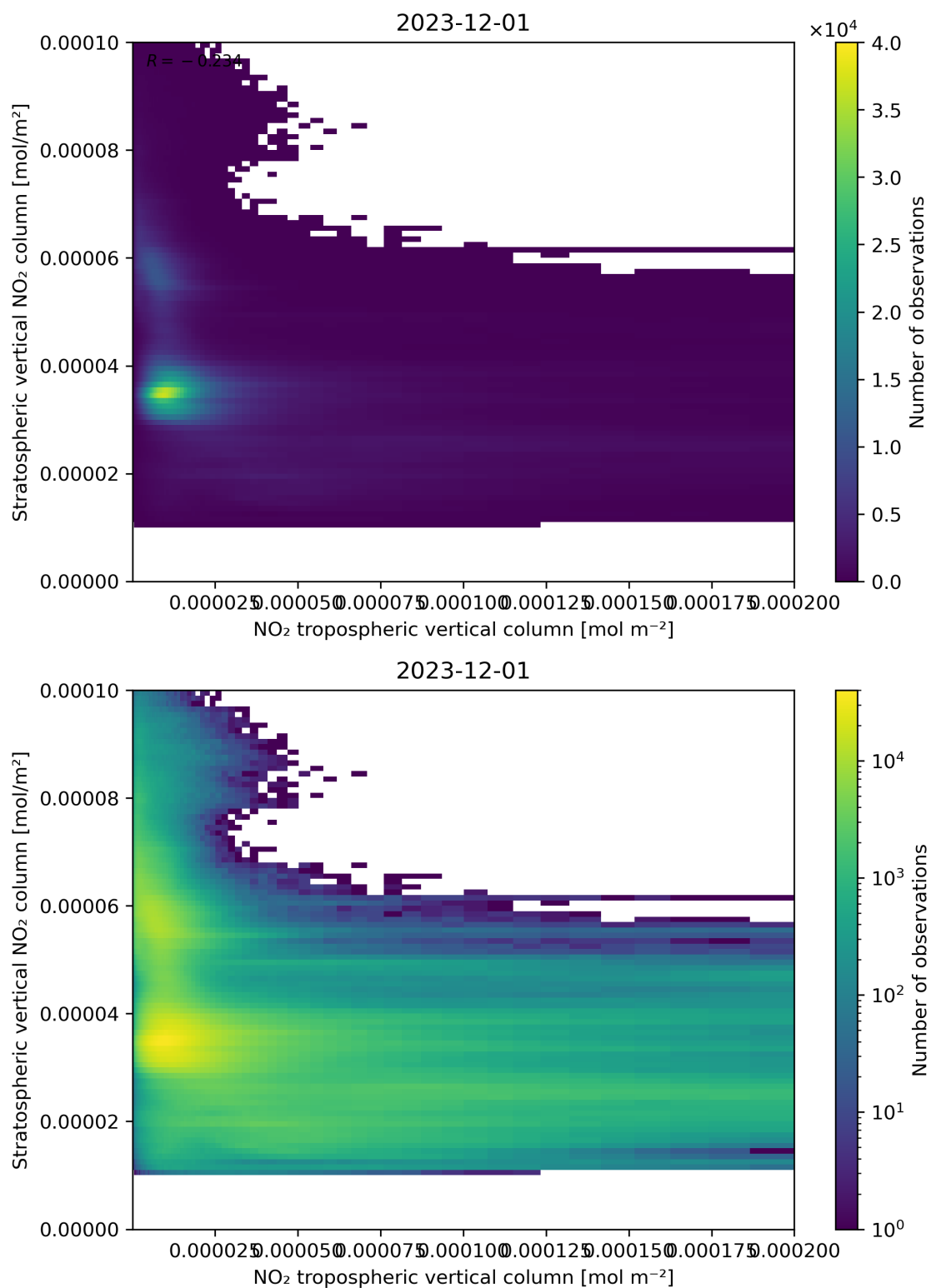
Figure 125: Scatter density plot of “NO 2 tropospheric vertical column” against “Stratospheric vertical NO 2 column” for 2023-11-30 to 2023-12-02.
