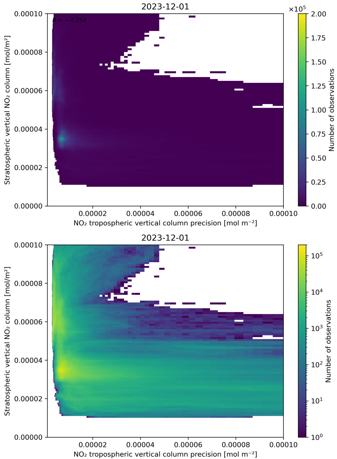
Figure 135: Scatter density plot of “NO 2 tropospheric vertical column precision” against “Stratospheric vertical NO 2 column” for 2023-11-30 to 2023-12-02.
