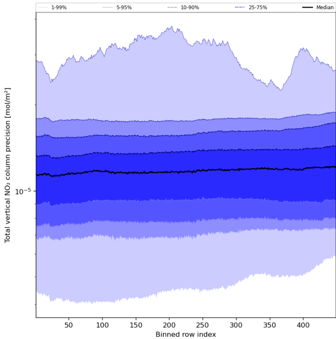
Figure 56: Along track statistics of “Total vertical NO 2 column precision” for 2023-11-30 to 2023-12-02
