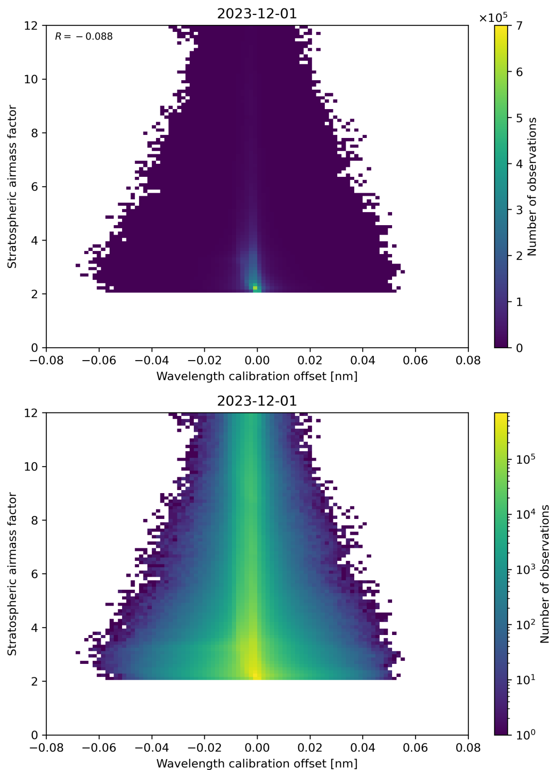
Figure 174: Scatter density plot of “Wavelength calibration offset” against “Stratospheric air mass factor” for 2023-11-30 to 2023-12-02.
