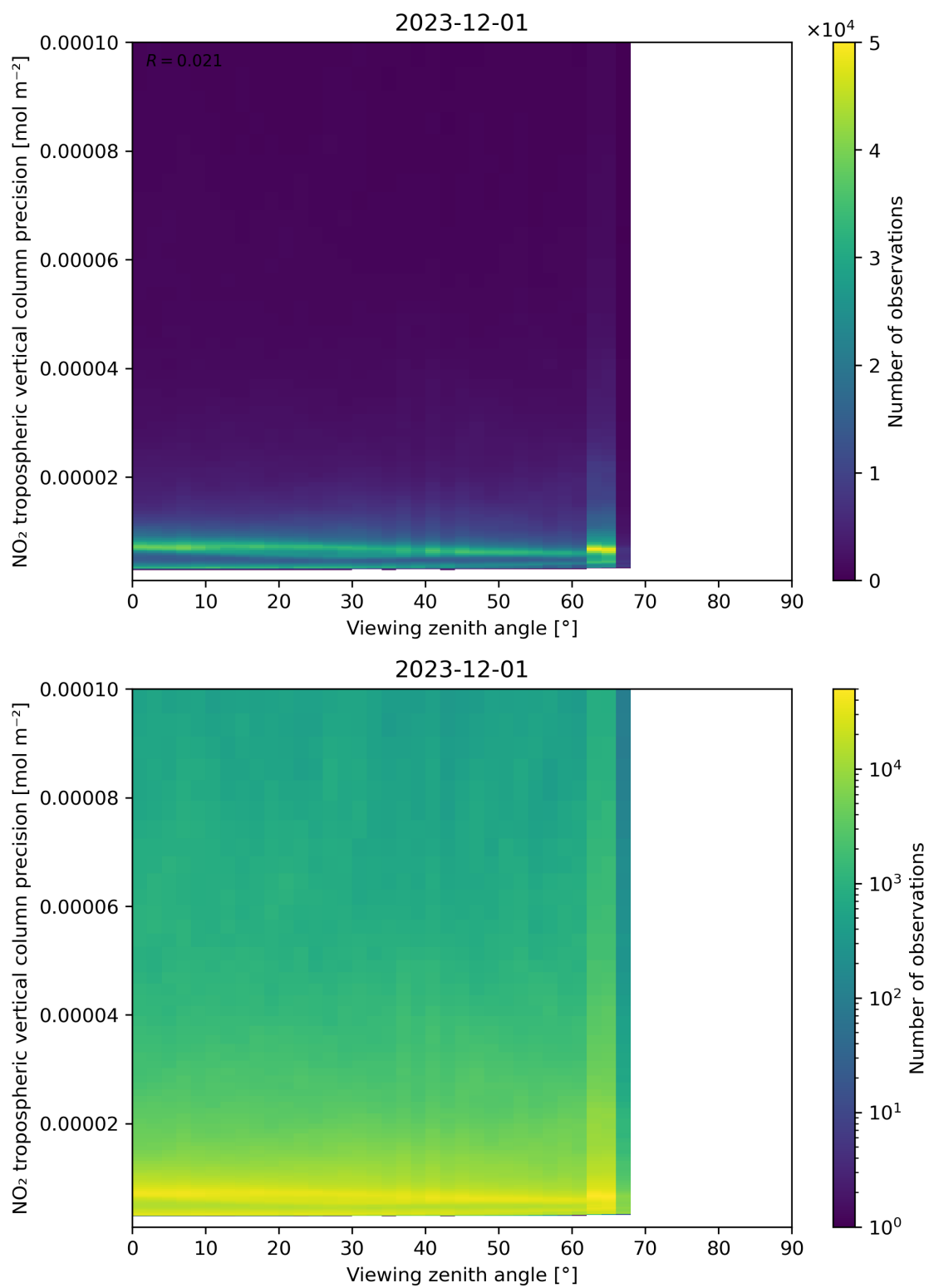
Figure 170: Scatter density plot of “Viewing zenith angle” against “NO 2 tropospheric vertical column precision” for 2023-11-30 to 2023-12-02.
