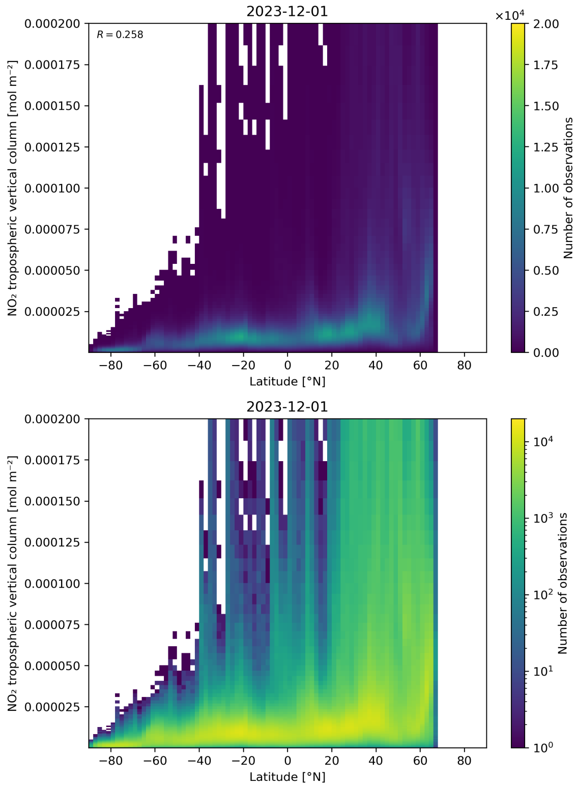
Figure 92: Scatter density plot of “Latitude” against “NO 2 tropospheric vertical column” for 2023-11-30 to 2023-12-02.
