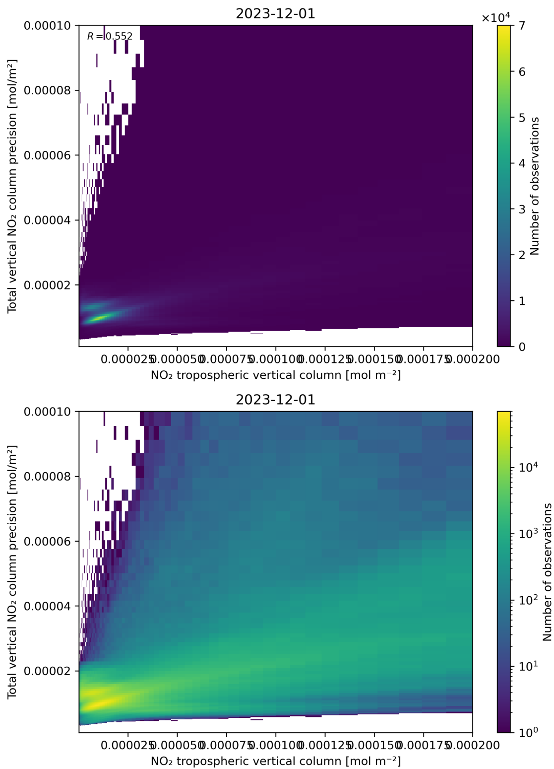
Figure 129: Scatter density plot of “NO 2 tropospheric vertical column” against “Total vertical NO 2 column precision” for 2023-11-30 to 2023-12-02.
