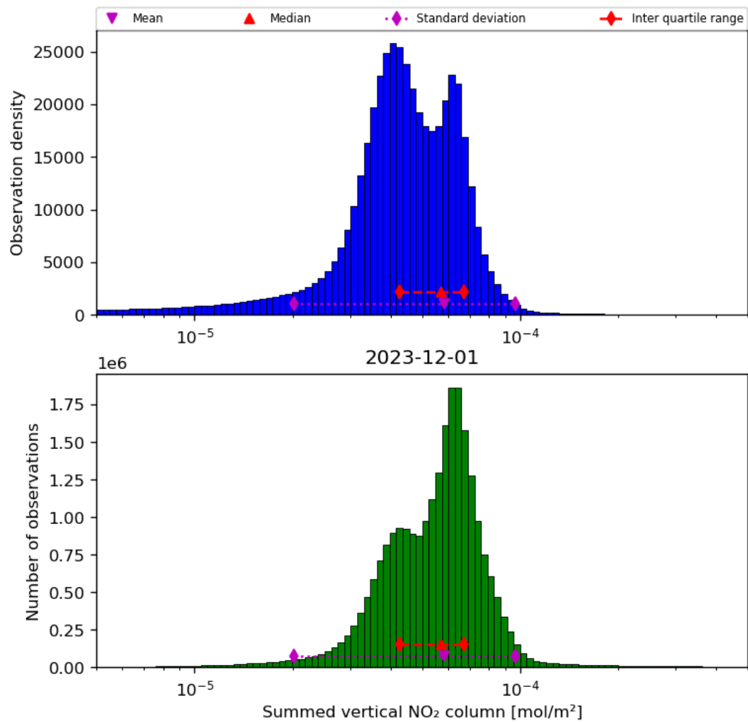
Figure 40: Histogram of “Summed vertical NO 2 column” for 2023-11-30 to 2023-12-02
