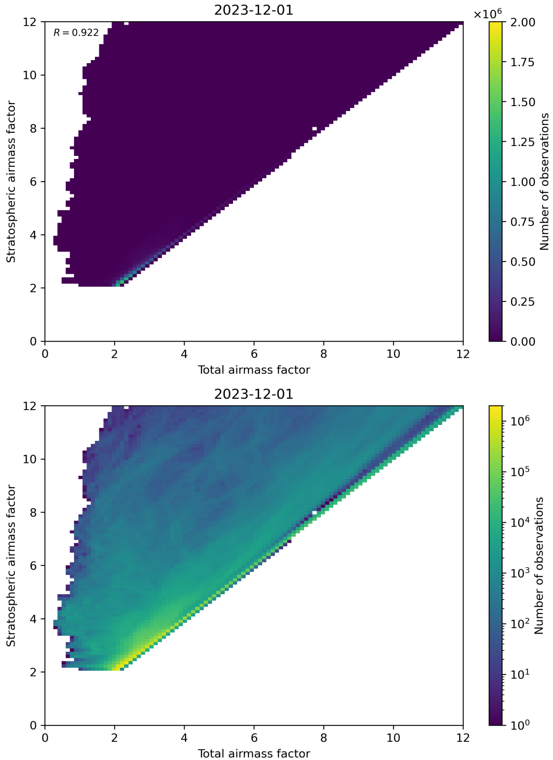
Figure 62: Scatter density plot of “Total airmass factor” against “Stratospheric airmass factor” for 2023-11-30 to 2023-12-02.
