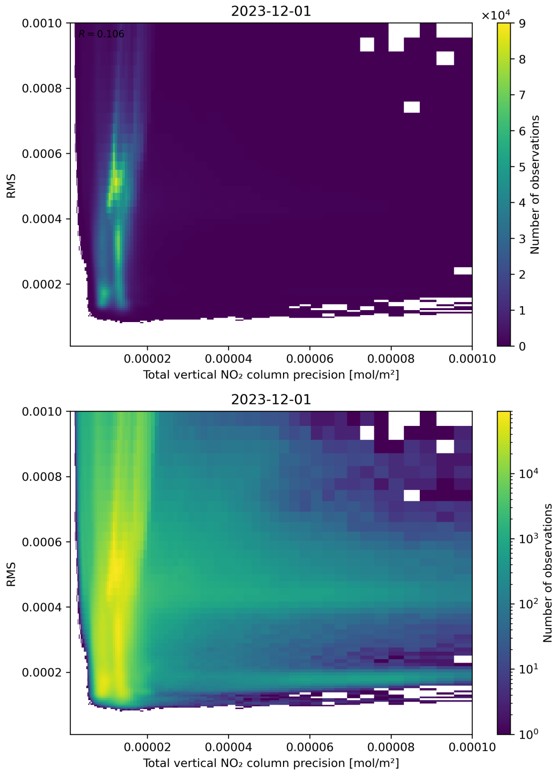
Figure 119: Scatter density plot of “Total vertical NO 2 column precision” against “RMS” for 2023-11-30 to 2023-12-02.
