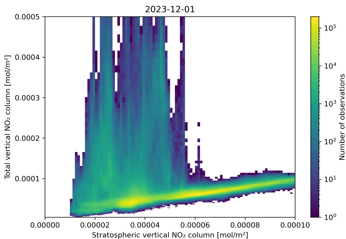
Figure 100: Scatter density plot of “Stratospheric vertical NO 2 column” against “Total vertical NO 2 column” for 2023-11-30 to 2023-12-02.
