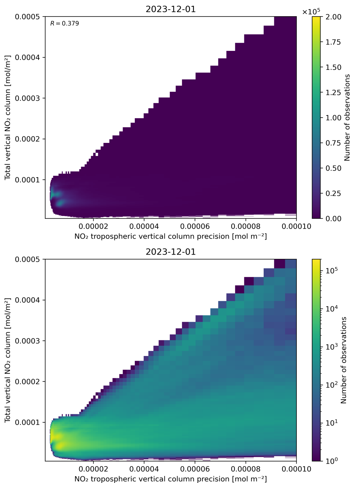
Figure 138: Scatter density plot of “NO 2 tropospheric vertical column precision” against “Total vertical NO 2 column” for 2023-11-30 to 2023-12-02.
