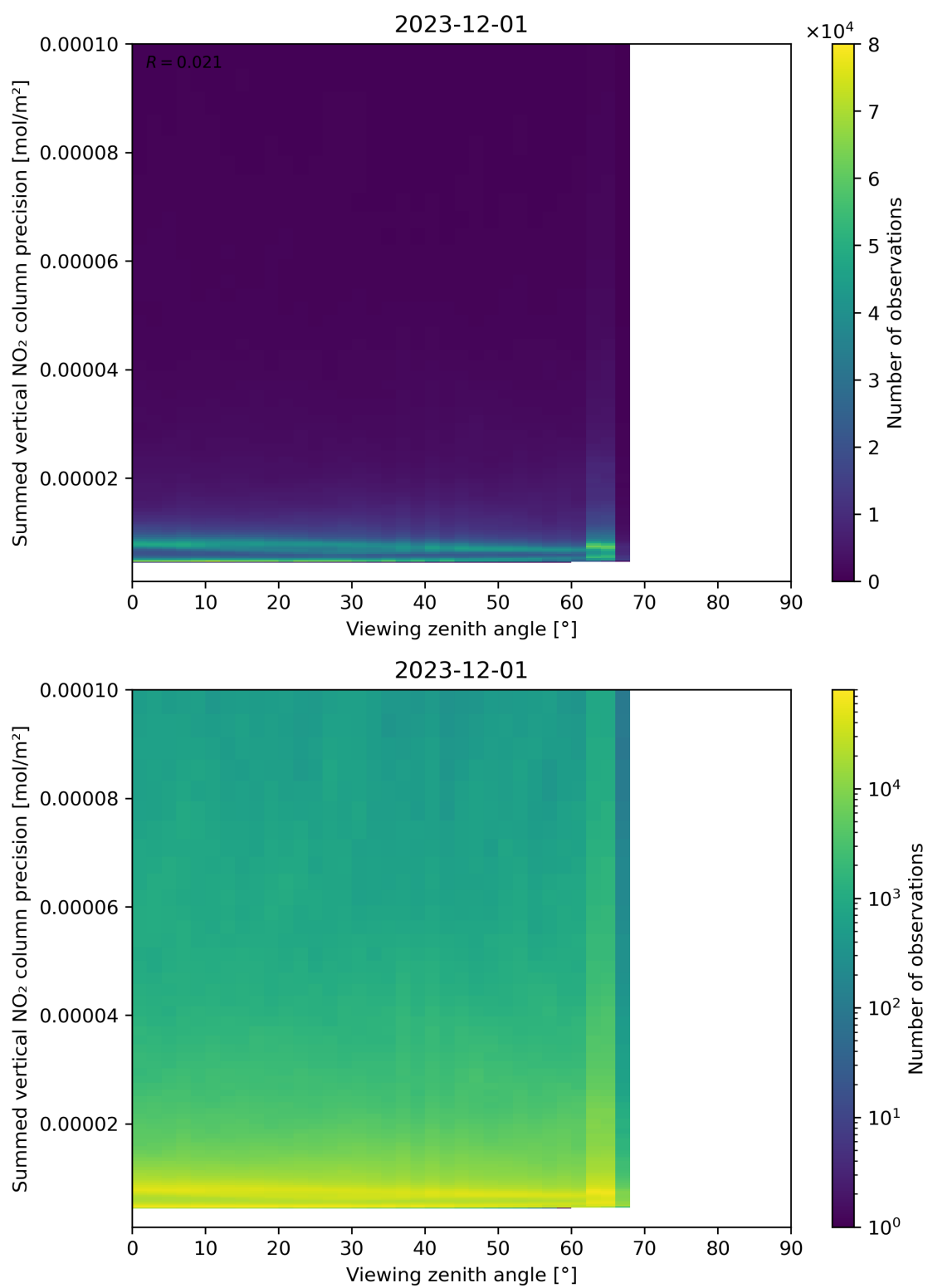
Figure 166: Scatter density plot of “Viewing zenith angle” against “Summed vertical NO 2 column precision” for 2023-11-30 to 2023-12-02.
