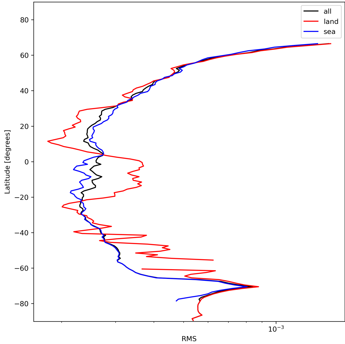
Figure 26: Zonal average of “RMS” for 2023-11-30 to 2023-12-02.
