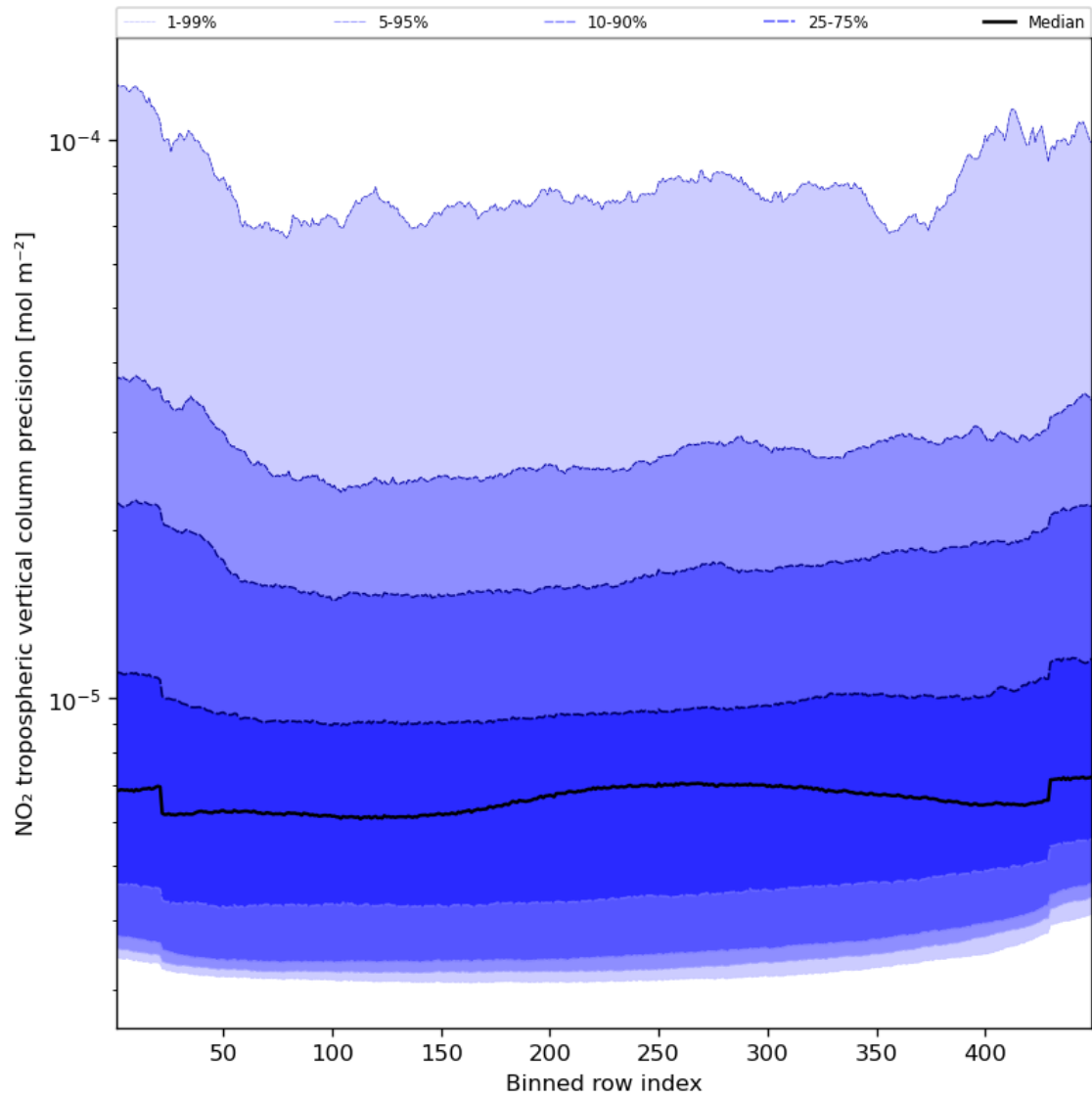
Figure 47: Along track statistics of “NO 2 tropospheric vertical column precision” for 2023-11-30 to 2023-12-02
