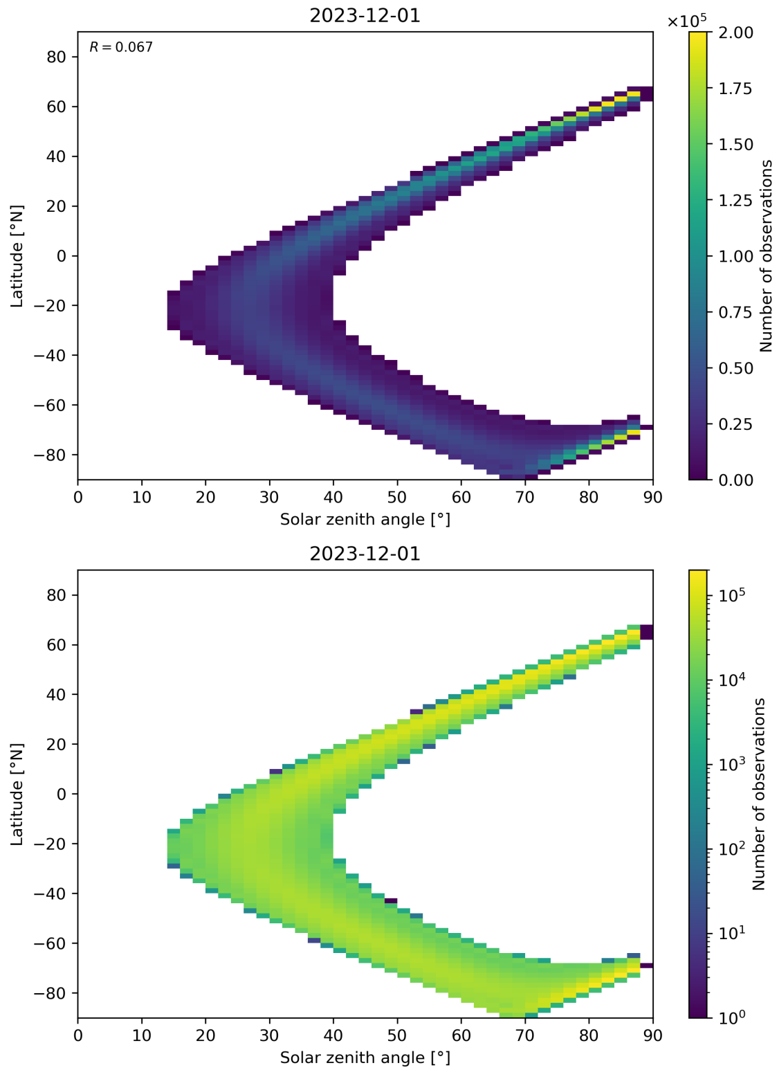
Figure 149: Scatter density plot of “Solar zenith angle” against “Latitude” for 2023-11-30 to 2023-12-02.
