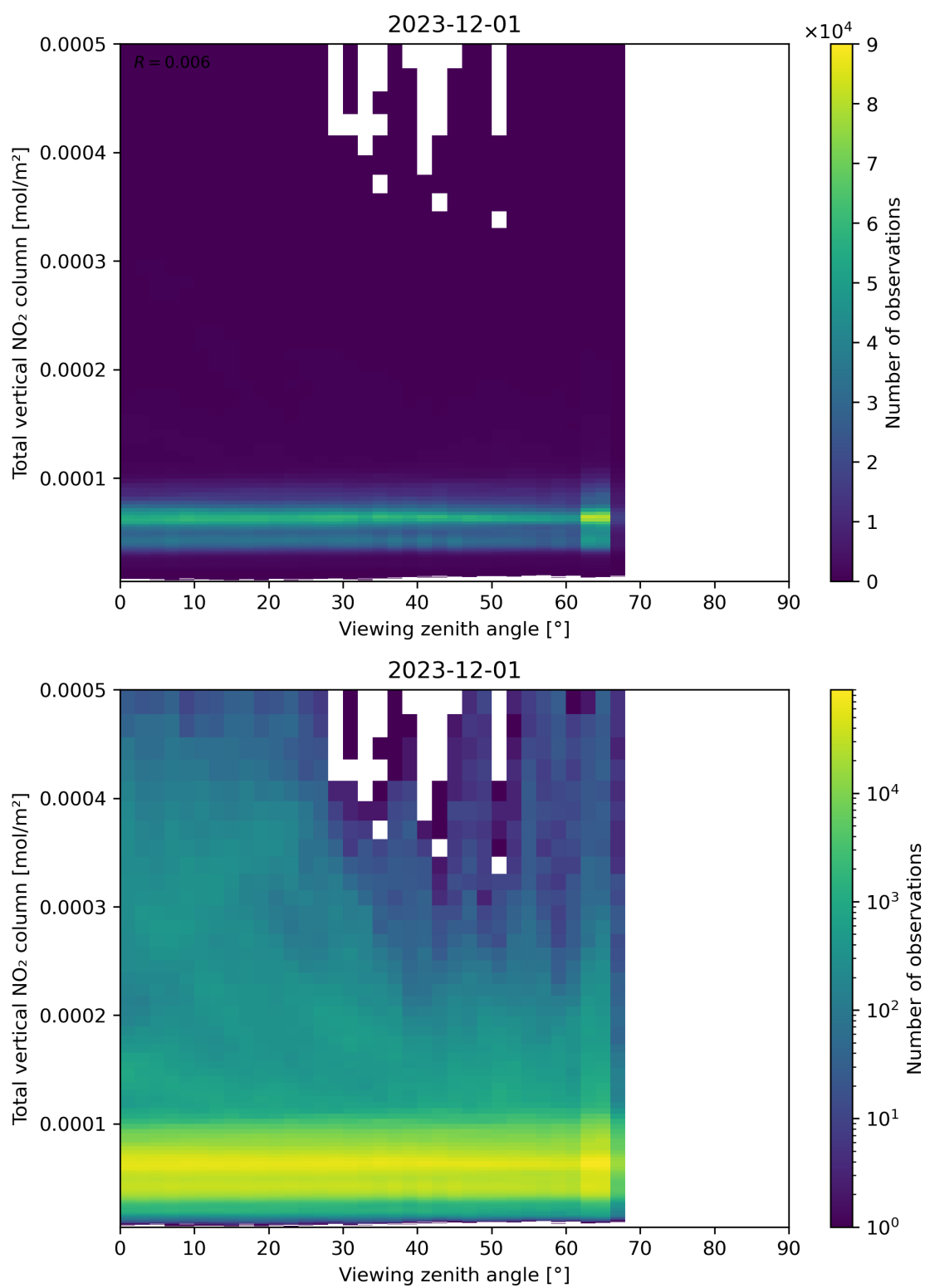
Figure 167: Scatter density plot of “Viewing zenith angle” against “Total vertical NO 2 column” for 2023-11-30 to 2023-12-02.
