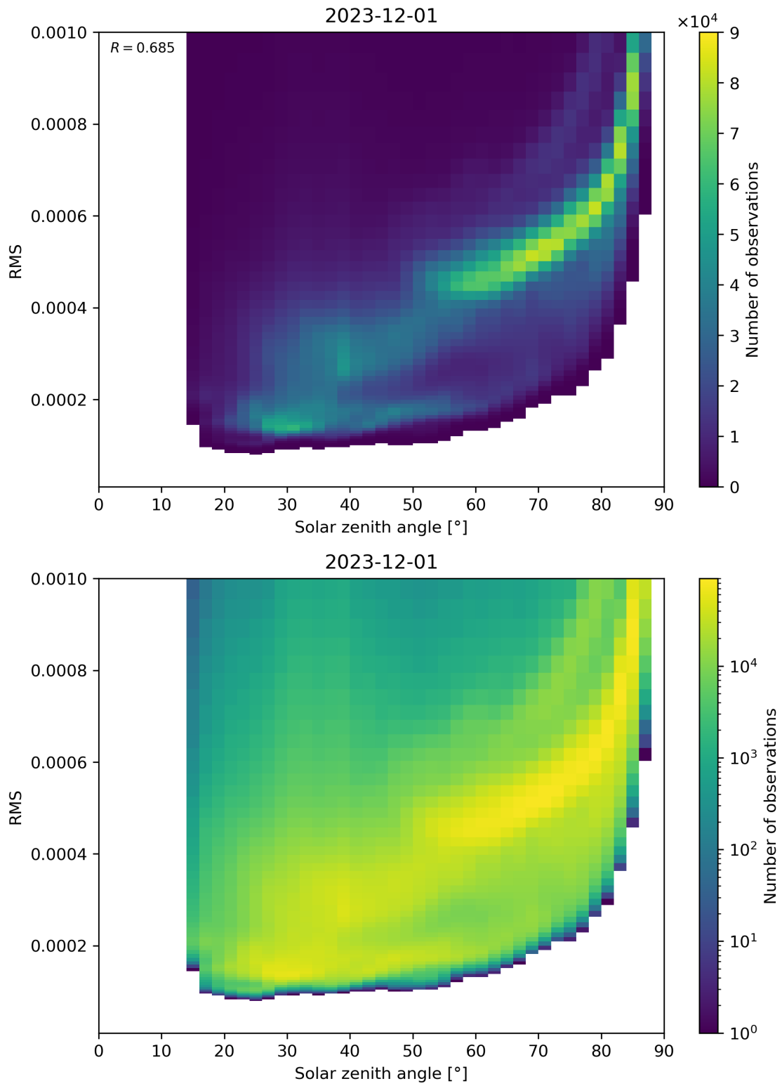
Figure 157: Scatter density plot of “Solar zenith angle” against “RMS” for 2023-11-30 to 2023-12-02.
