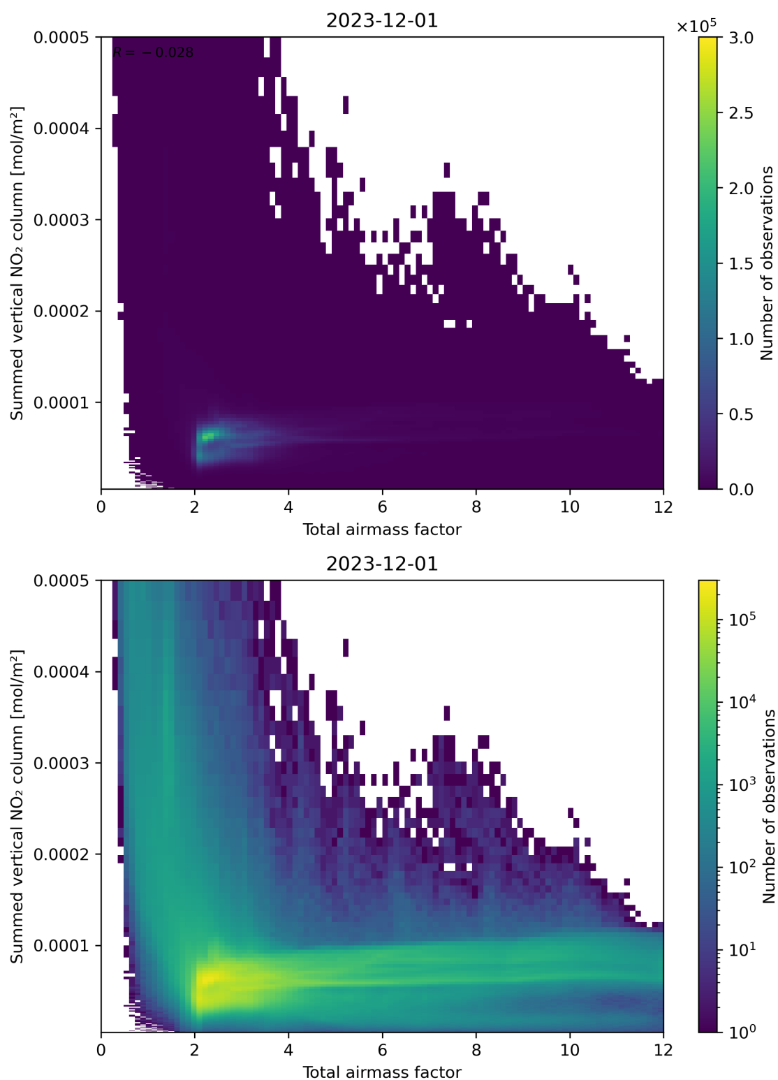
Figure 65: Scatter density plot of “Total airmass factor” against “Summed vertical NO 2 column” for 2023-11-30 to 2023-12-02.
