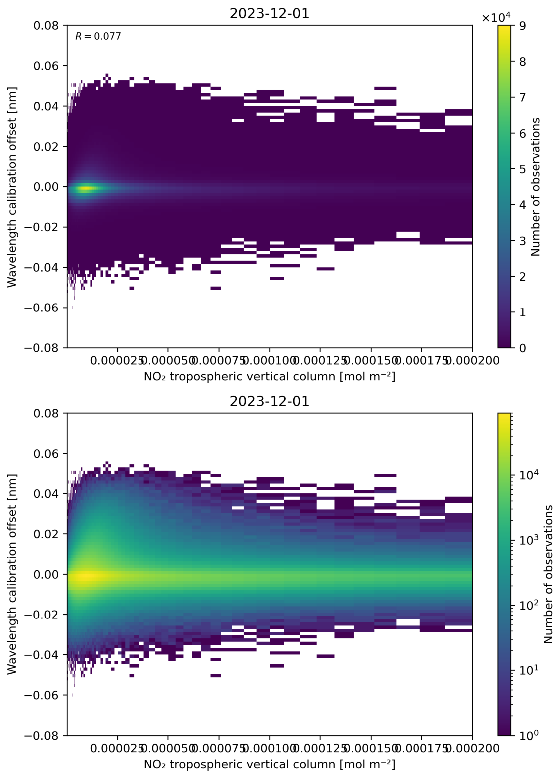
Figure 143: Scatter density plot of “NO 2 tropospheric vertical column” against “Wavelength calibration offset” for 2023-11-30 to 2023-12-02.
