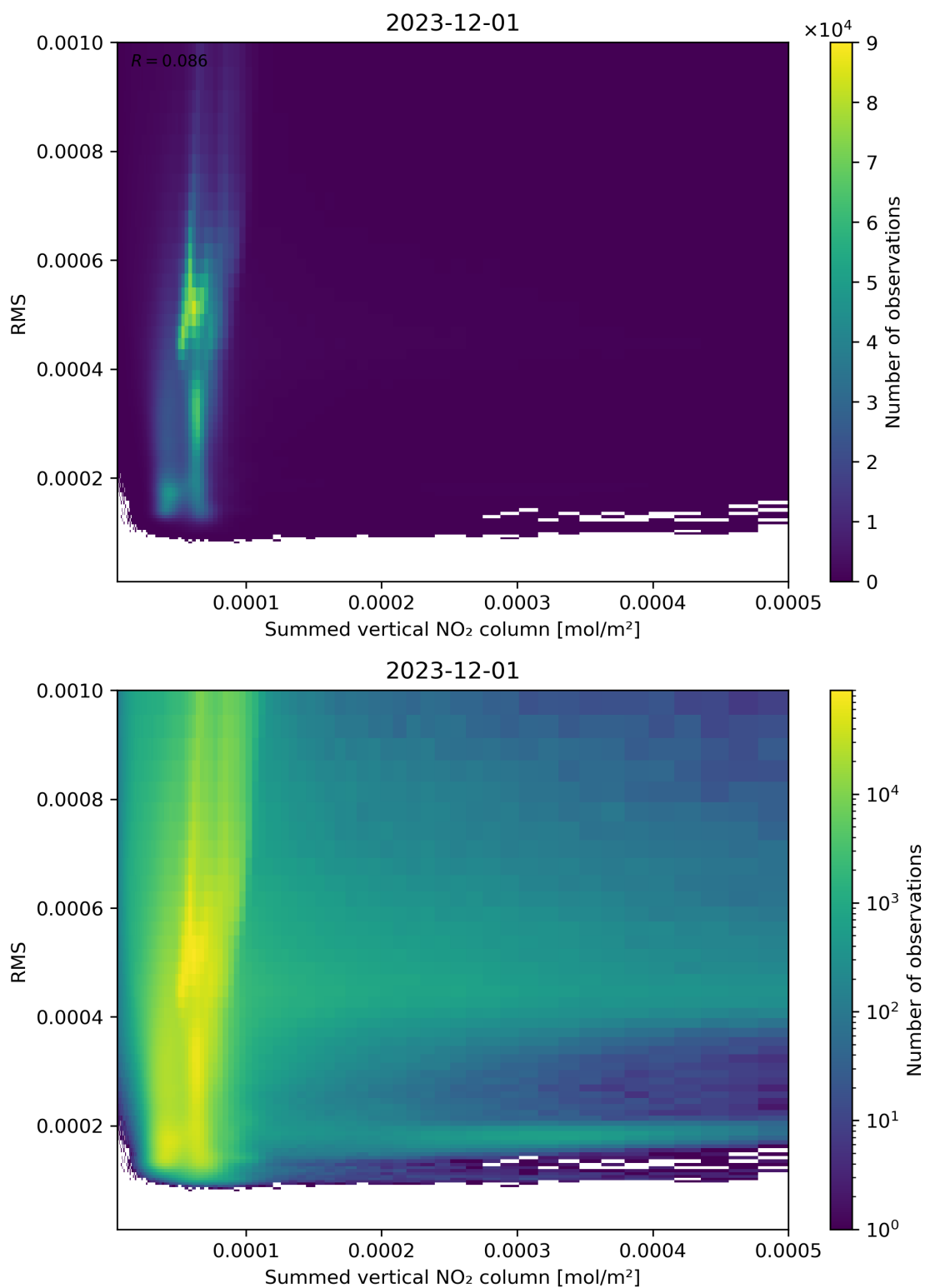
Figure 109: Scatter density plot of “Summed vertical NO 2 column” against “RMS” for 2023-11-30 to 2023-12-02.
