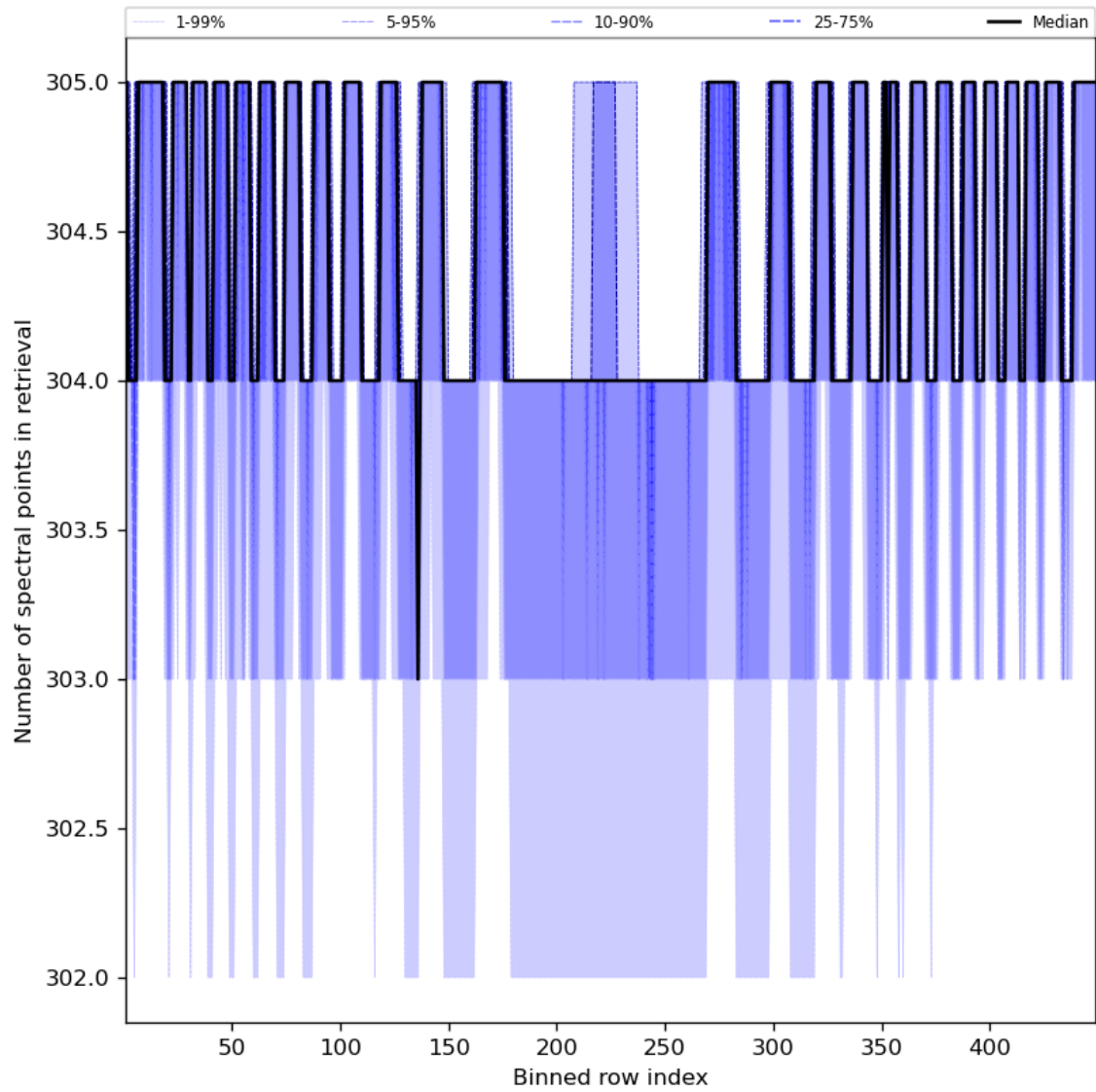
Figure 50: Along track statistics of “Number of spectral points in retrieval” for 2023-11-30 to 2023-12-02
