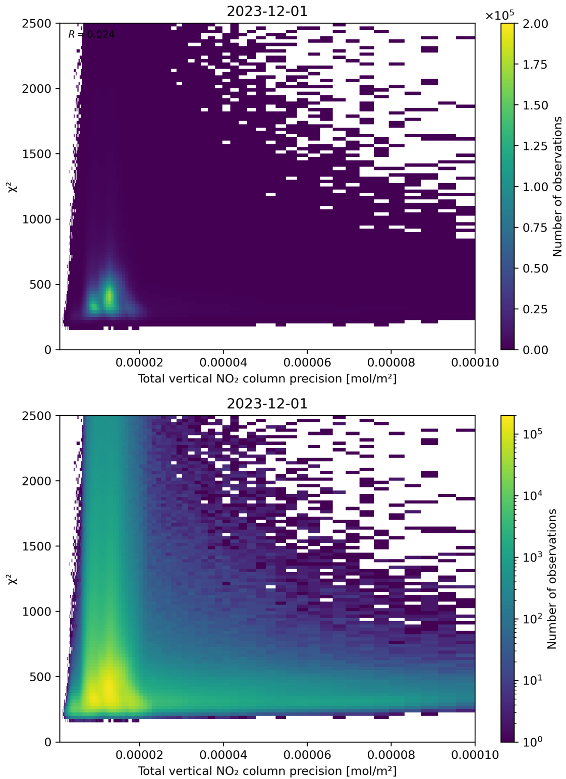
Figure 116: Scatter density plot of “Total vertical NO 2 column precision” against “ \chi^2 ” for 2023-11-30 to 2023-12-02.
