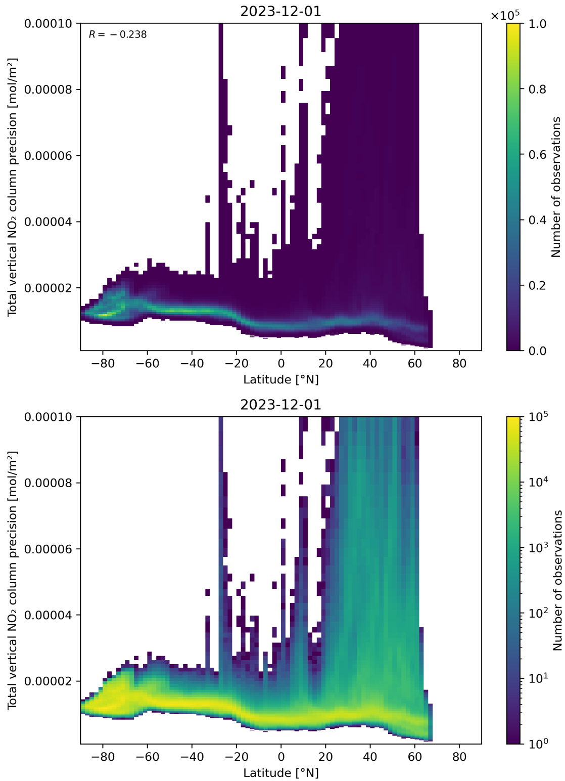
Figure 91: Scatter density plot of “Latitude” against “Total vertical NO 2 column precision” for 2023-11-30 to 2023-12-02.
