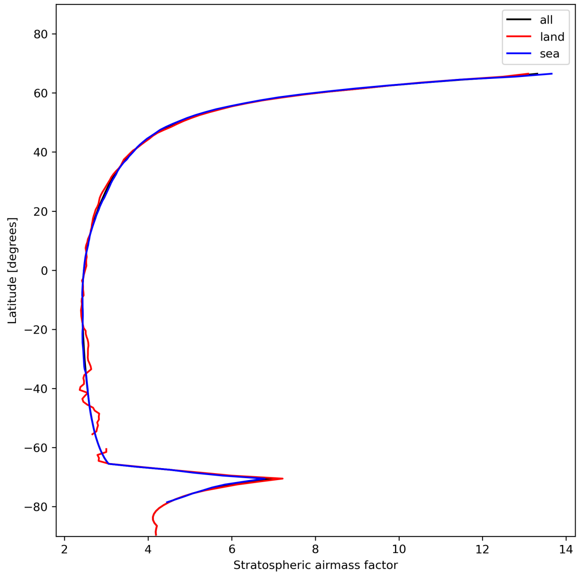
Figure 27: Zonal average of “Stratospheric air mass factor” for 2023-11-30 to 2023-12-02.
