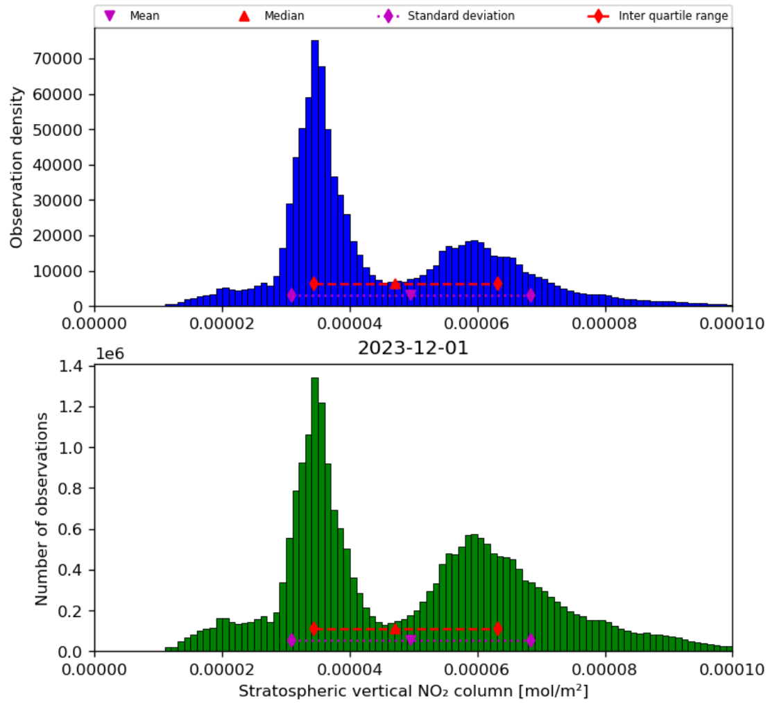
Figure 36: Histogram of “Stratospheric vertical NO 2 column” for 2023-11-30 to 2023-12-02
