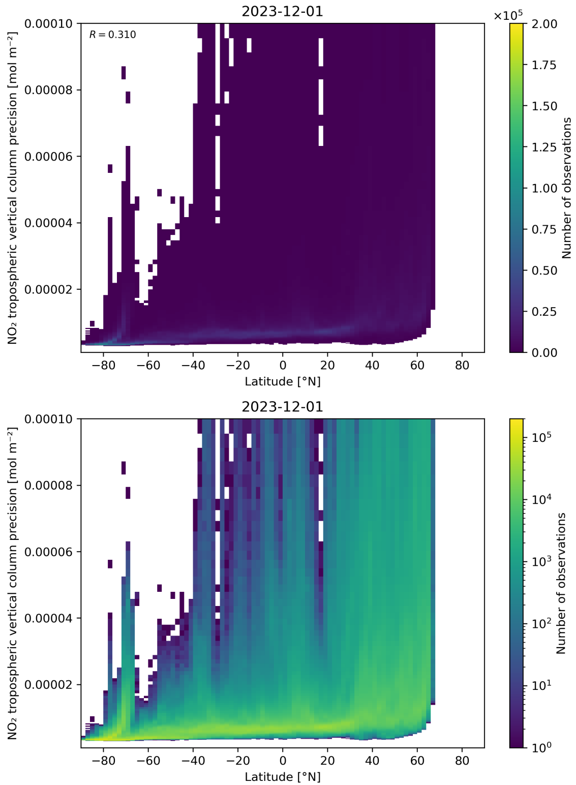
Figure 93: Scatter density plot of “Latitude” against “NO 2 tropospheric vertical column precision” for 2023-11-30 to 2023-12-02.
