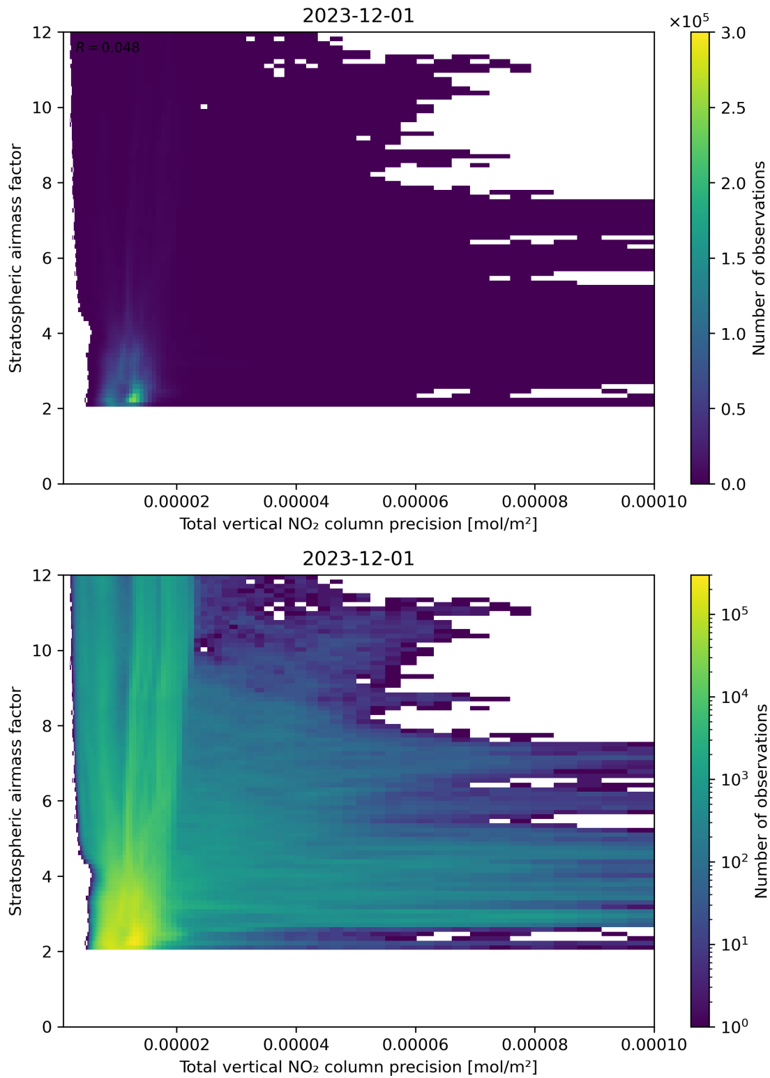
Figure 115: Scatter density plot of “Total vertical NO 2 column precision” against “Stratospheric air mass factor” for 2023-11-30 to 2023-12-02.
