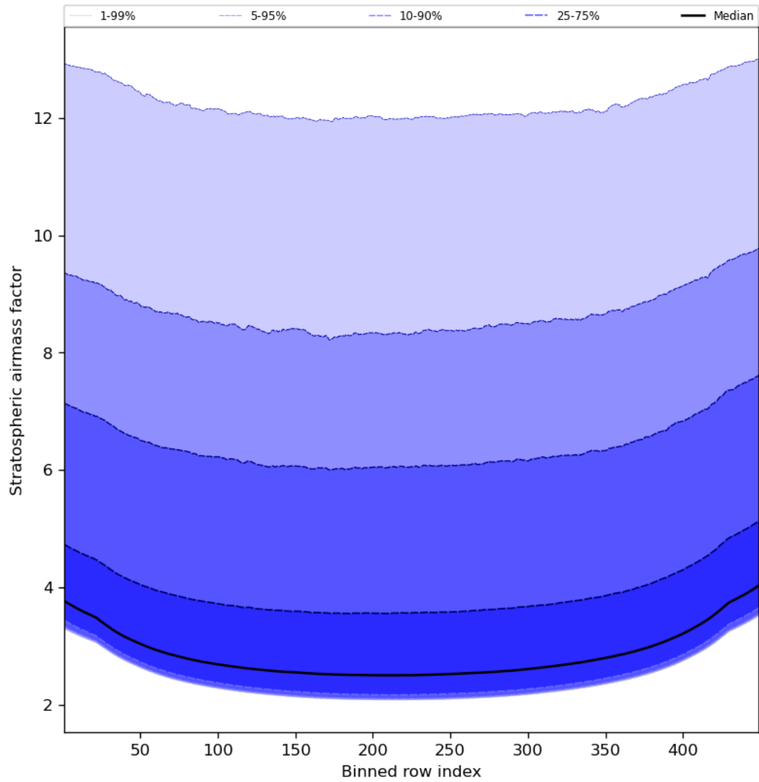
Figure 61: Along track statistics of “Stratospheric air mass factor” for 2023-11-30 to 2023-12-02
