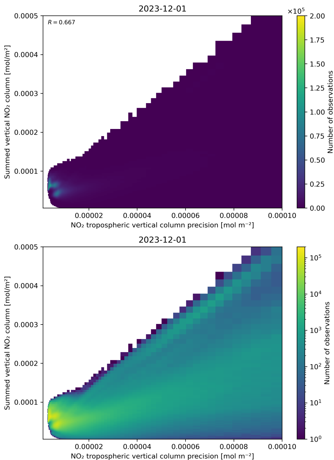
Figure 136: Scatter density plot of “NO 2 tropospheric vertical column precision” against “Summed vertical NO 2 column” for 2023-11-30 to 2023-12-02.
