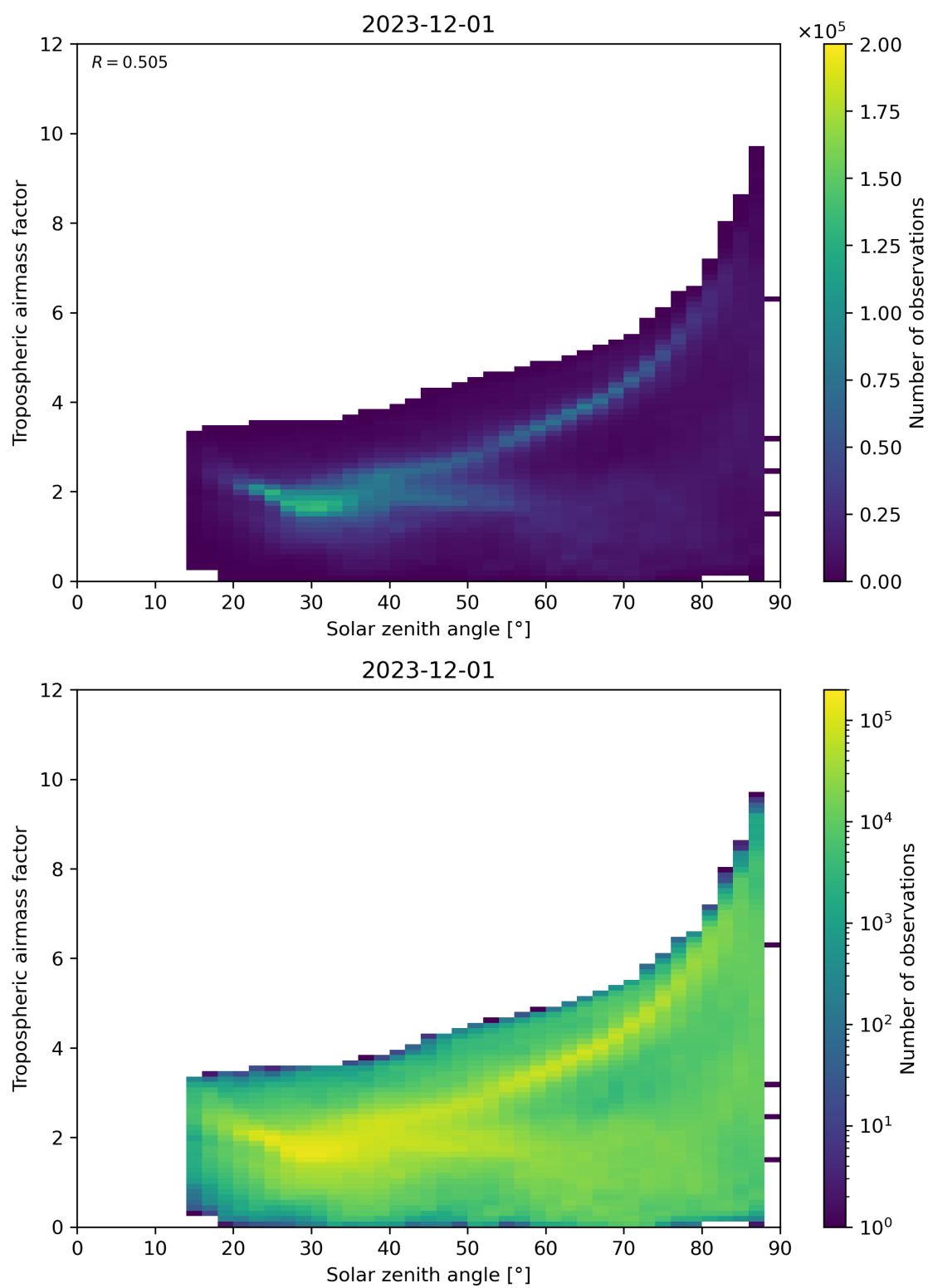
Figure 147: Scatter density plot of “Solar zenith angle” against “Tropospheric airmass factor” for 2023-11-30 to 2023-12-02.
