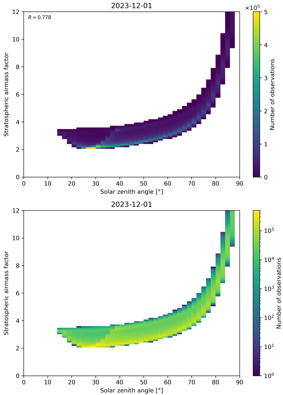
Figure 145: Scatter density plot of “Solar zenith angle” against “Stratospheric airmass factor” for 2023-11-30 to 2023-12-02.
