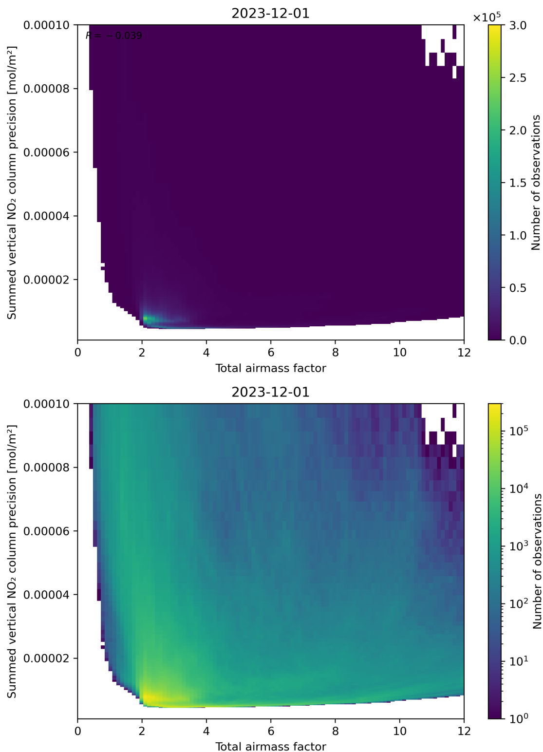
Figure 66: Scatter density plot of “Total airmass factor” against “Summed vertical NO 2 column precision” for 2023-11-30 to 2023-12-02.
