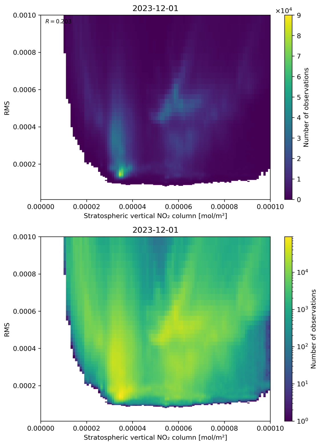
Figure 102: Scatter density plot of “Stratospheric vertical NO 2 column” against “RMS” for 2023-11-30 to 2023-12-02.
