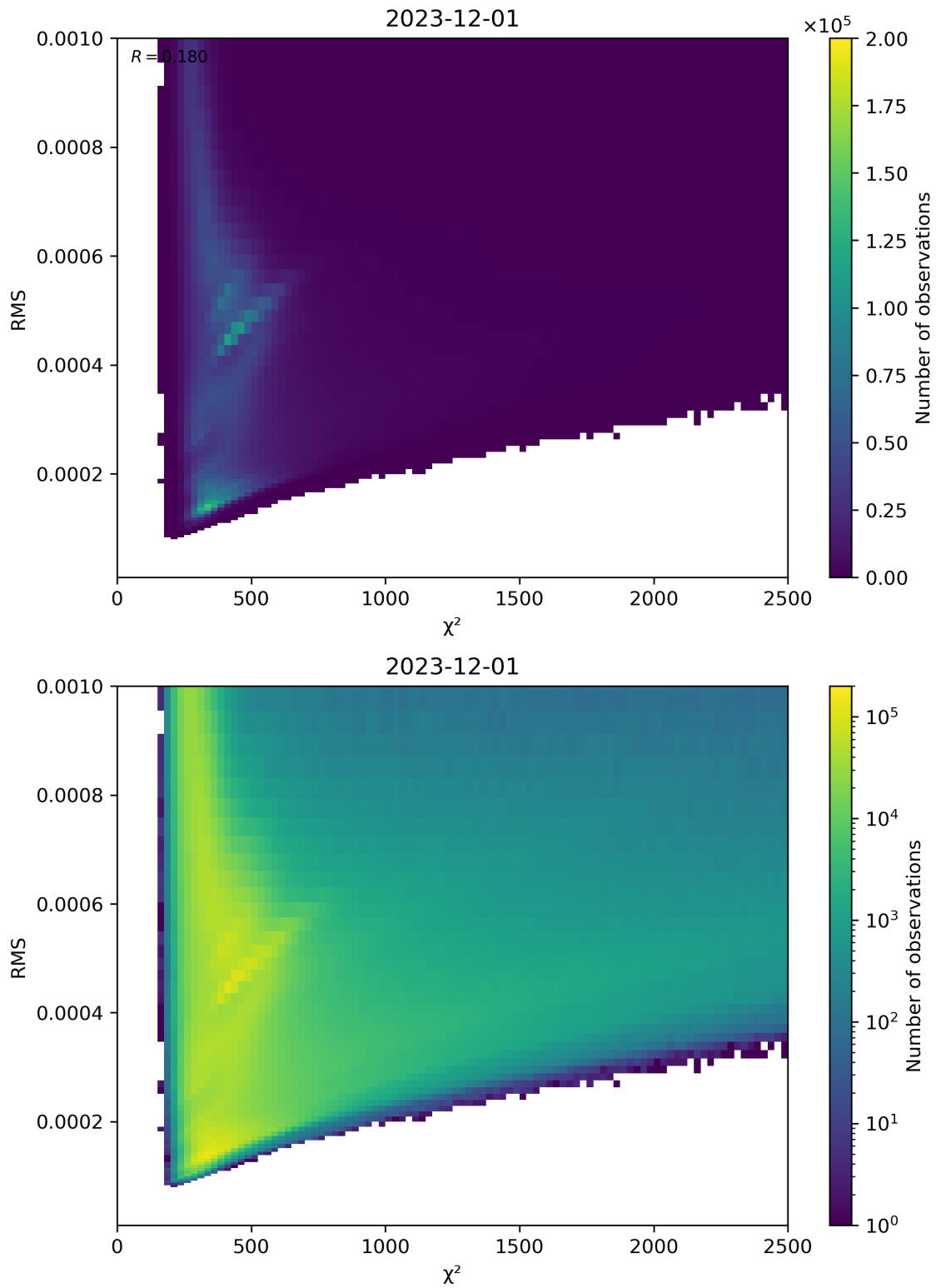
Figure 82: Scatter density plot of “ \chi^2 ” against “RMS” for 2023-11-30 to 2023-12-02.
