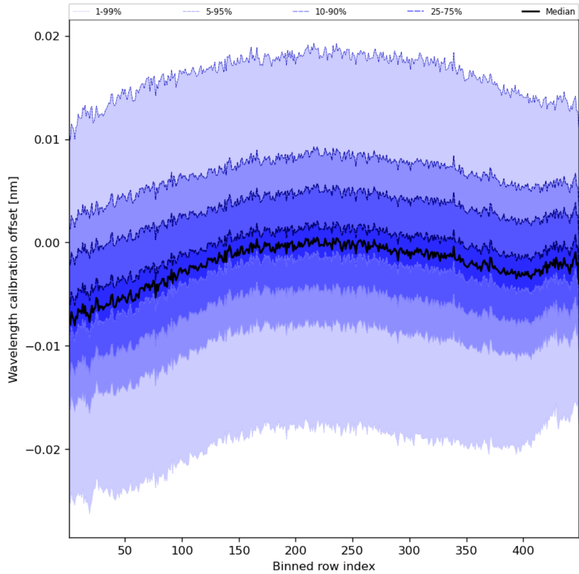
Figure 52: Along track statistics of “Wavelength calibration offset” for 2023-11-30 to 2023-12-02
