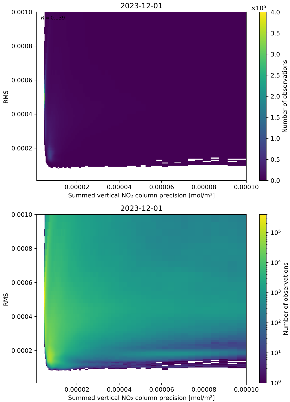
Figure 108: Scatter density plot of “Summed vertical NO 2 column precision” against “RMS” for 2023-11-30 to 2023-12-02.
