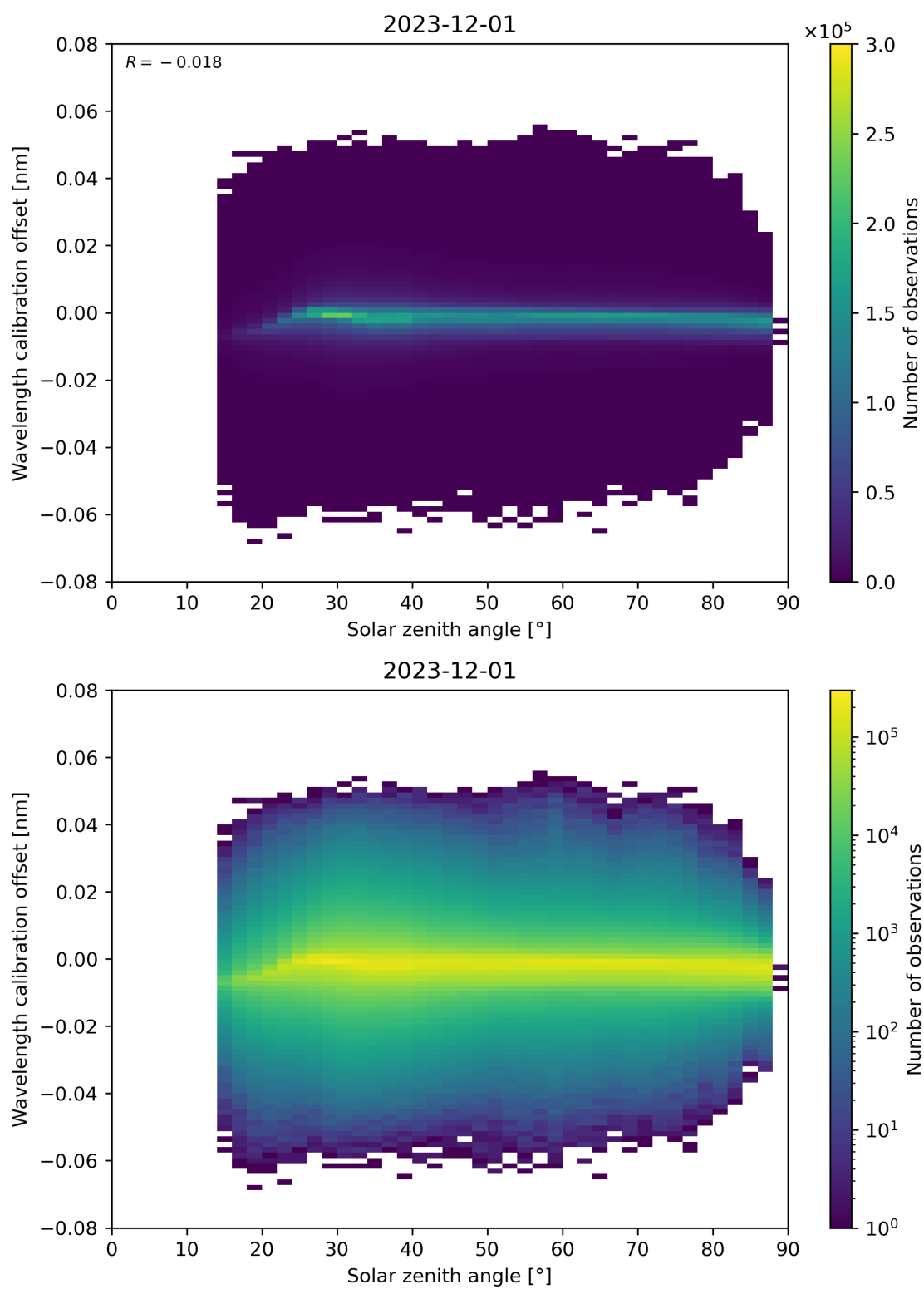
Figure 158: Scatter density plot of “Solar zenith angle” against “Wavelength calibration offset” for 2023-11-30 to 2023-12-02.
