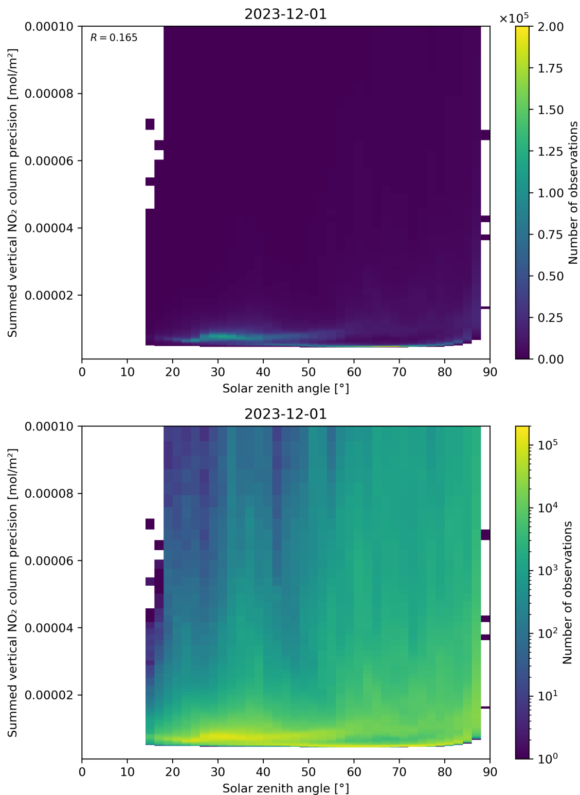
Figure 152: Scatter density plot of “Solar zenith angle” against “Summed vertical NO 2 column precision” for 2023-11-30 to 2023-12-02.
