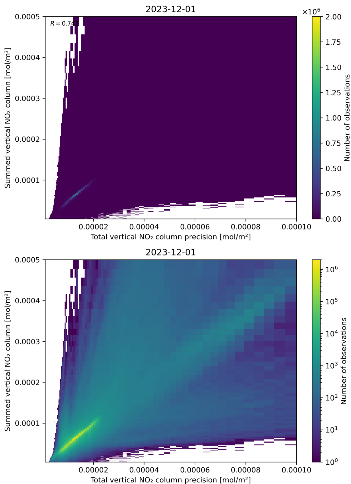
Figure 117: Scatter density plot of “Total vertical NO 2 column precision” against “Summed vertical NO 2 column” for 2023-11-30 to 2023-12-02.
