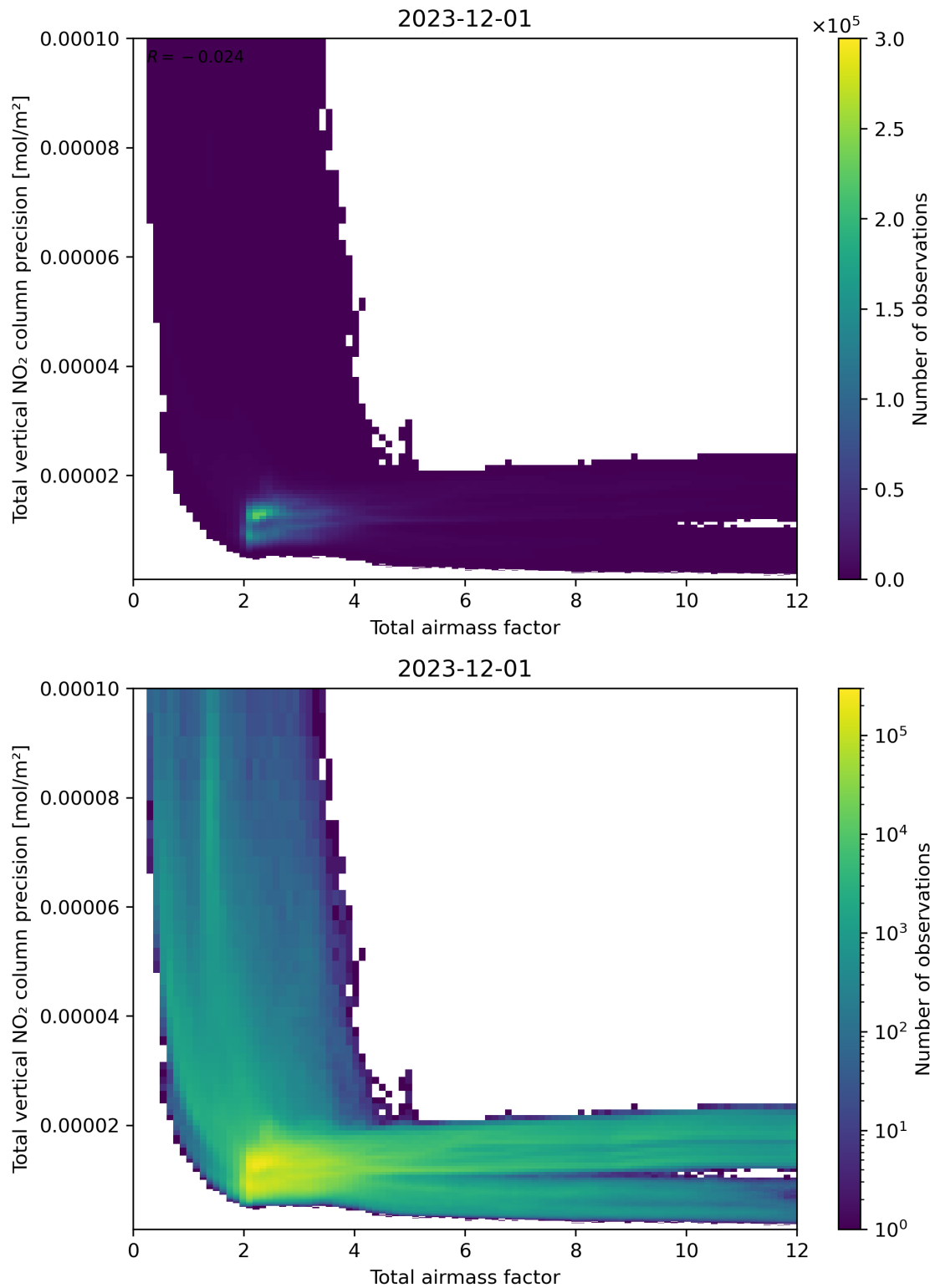
Figure 68: Scatter density plot of “Total airmass factor” against “Total vertical NO 2 column precision” for 2023-11-30 to 2023-12-02.
