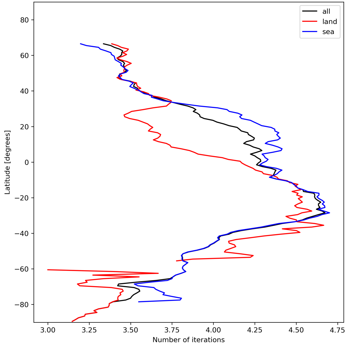
Figure 17: Zonal average of “Number of iterations” for 2023-11-30 to 2023-12-02.
