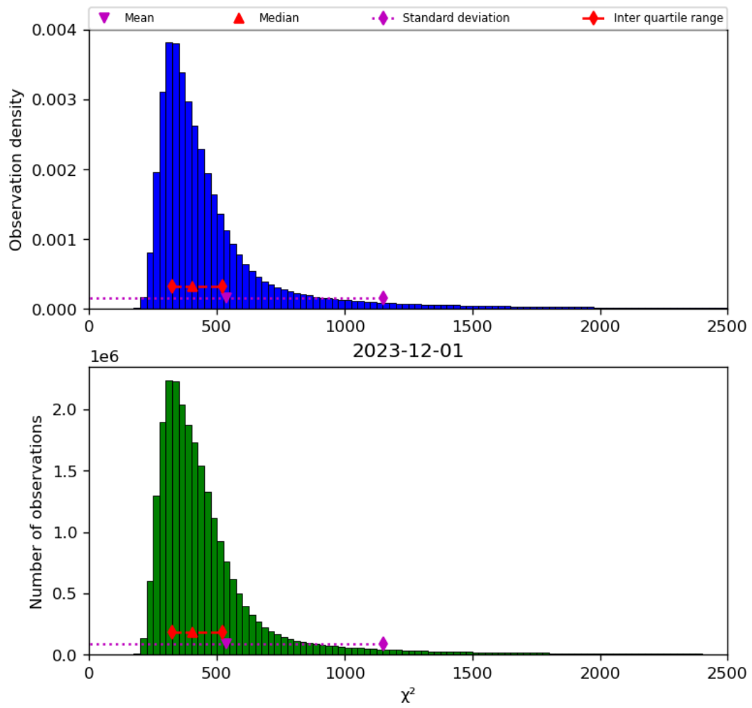
Figure 42: Histogram of “ \chi^2 ” for 2023-11-30 to 2023-12-02
