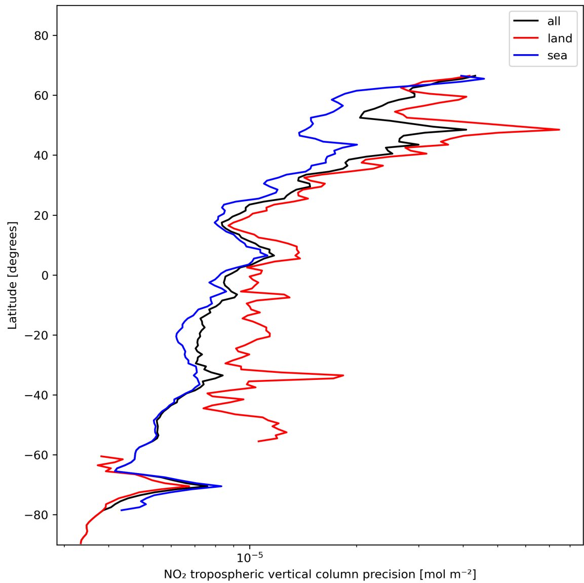
Figure 13: Zonal average of “NO 2 tropospheric vertical column precision” for 2023-11-30 to 2023-12-02.
