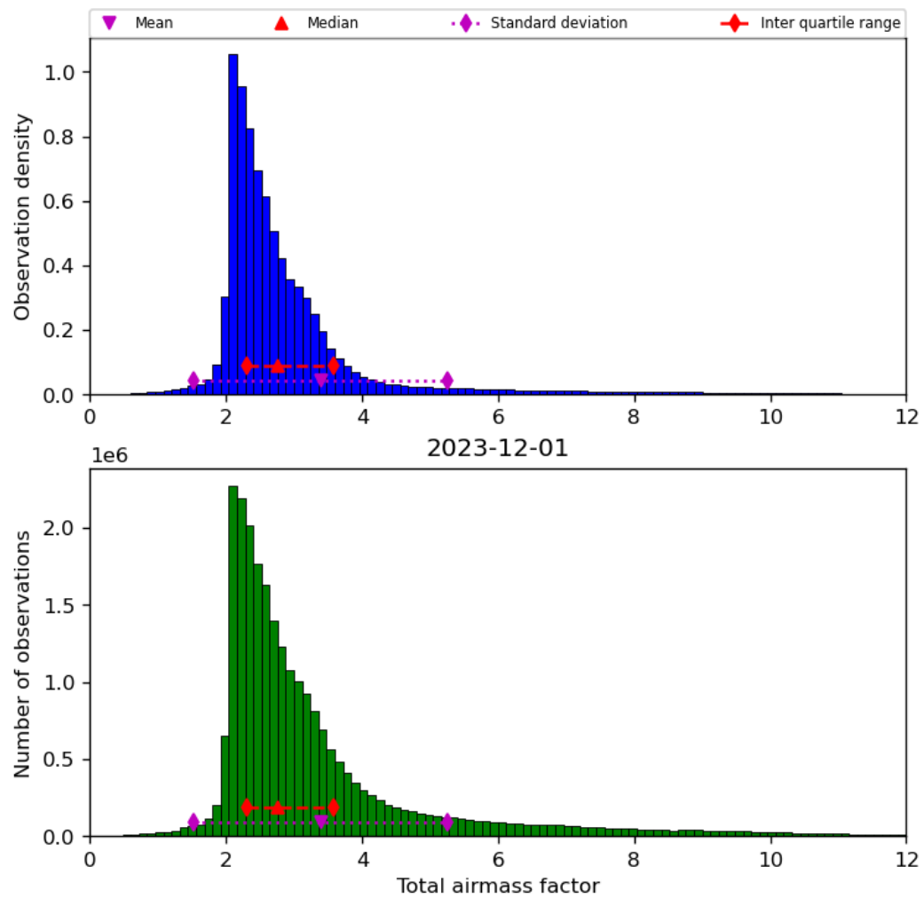
Figure 32: Histogram of “Total airmass factor” for 2023-11-30 to 2023-12-02
