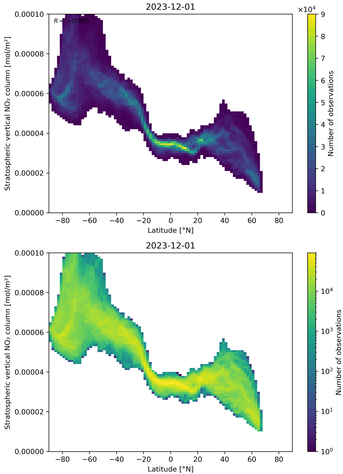
Figure 87: Scatter density plot of “Latitude” against “Stratospheric vertical NO 2 column” for 2023-11-30 to 2023-12-02.
