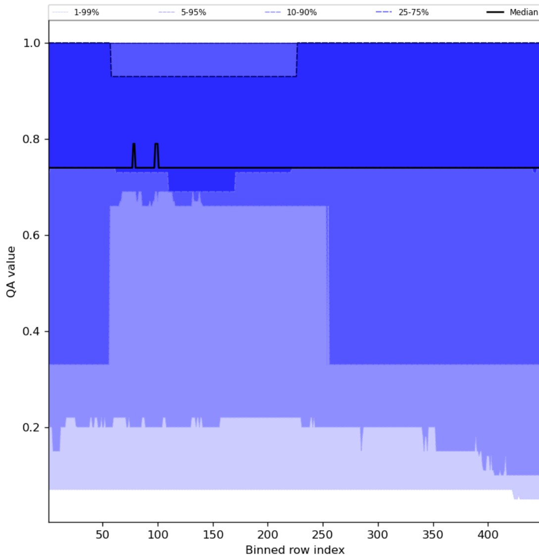
Figure 45: Along track statistics of “QA value” for 2023-11-30 to 2023-12-02
