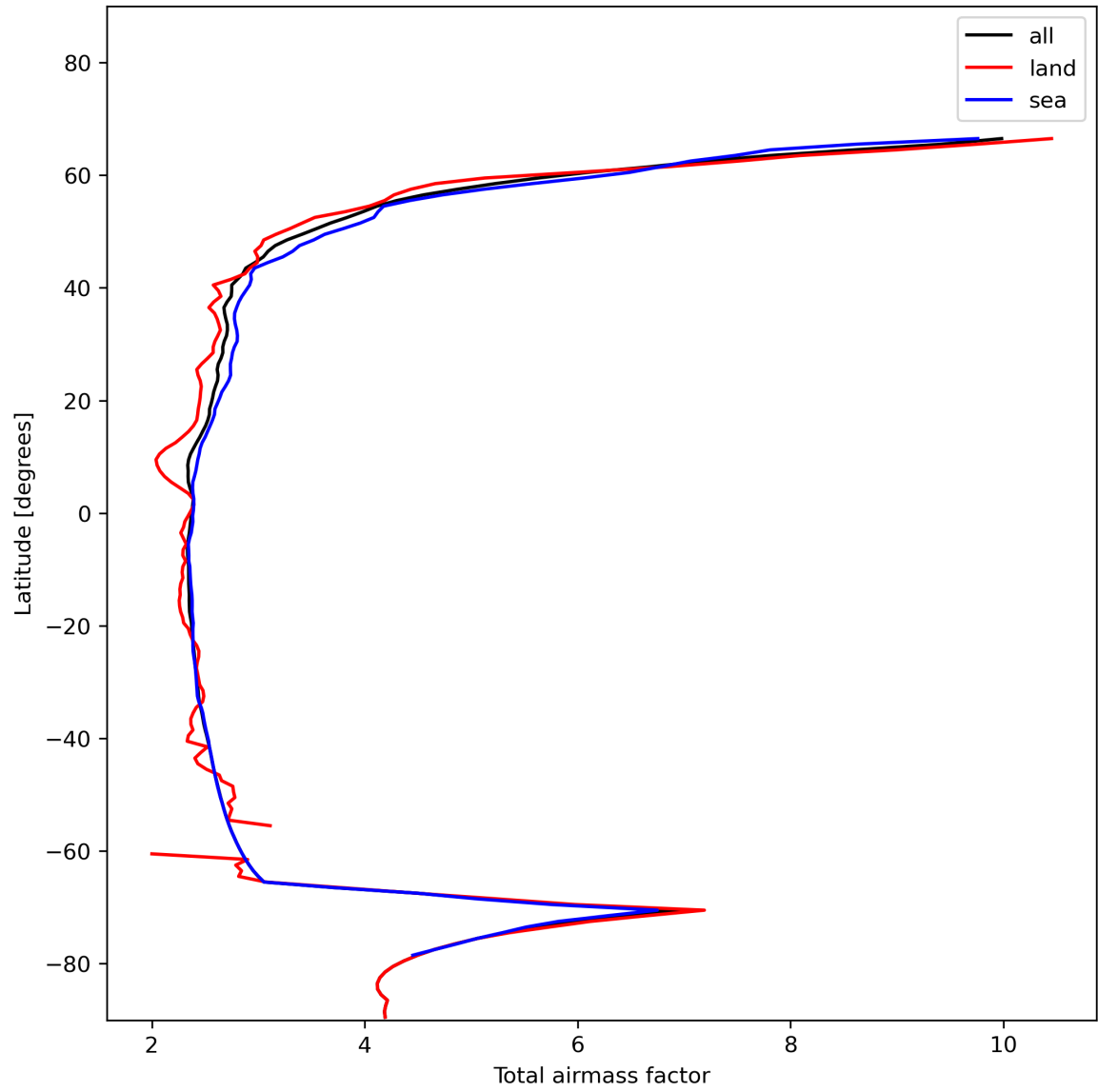
Figure 15: Zonal average of “Total airmass factor” for 2023-11-30 to 2023-12-02.
