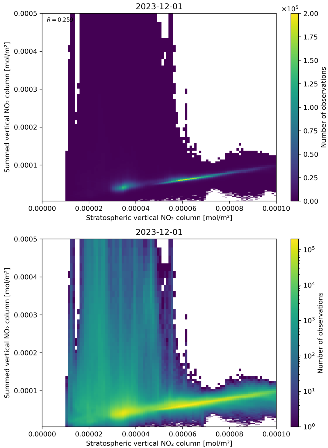
Figure 98: Scatter density plot of “Stratospheric vertical NO 2 column” against “Summed vertical NO 2 column” for 2023-11-30 to 2023-12-02.
