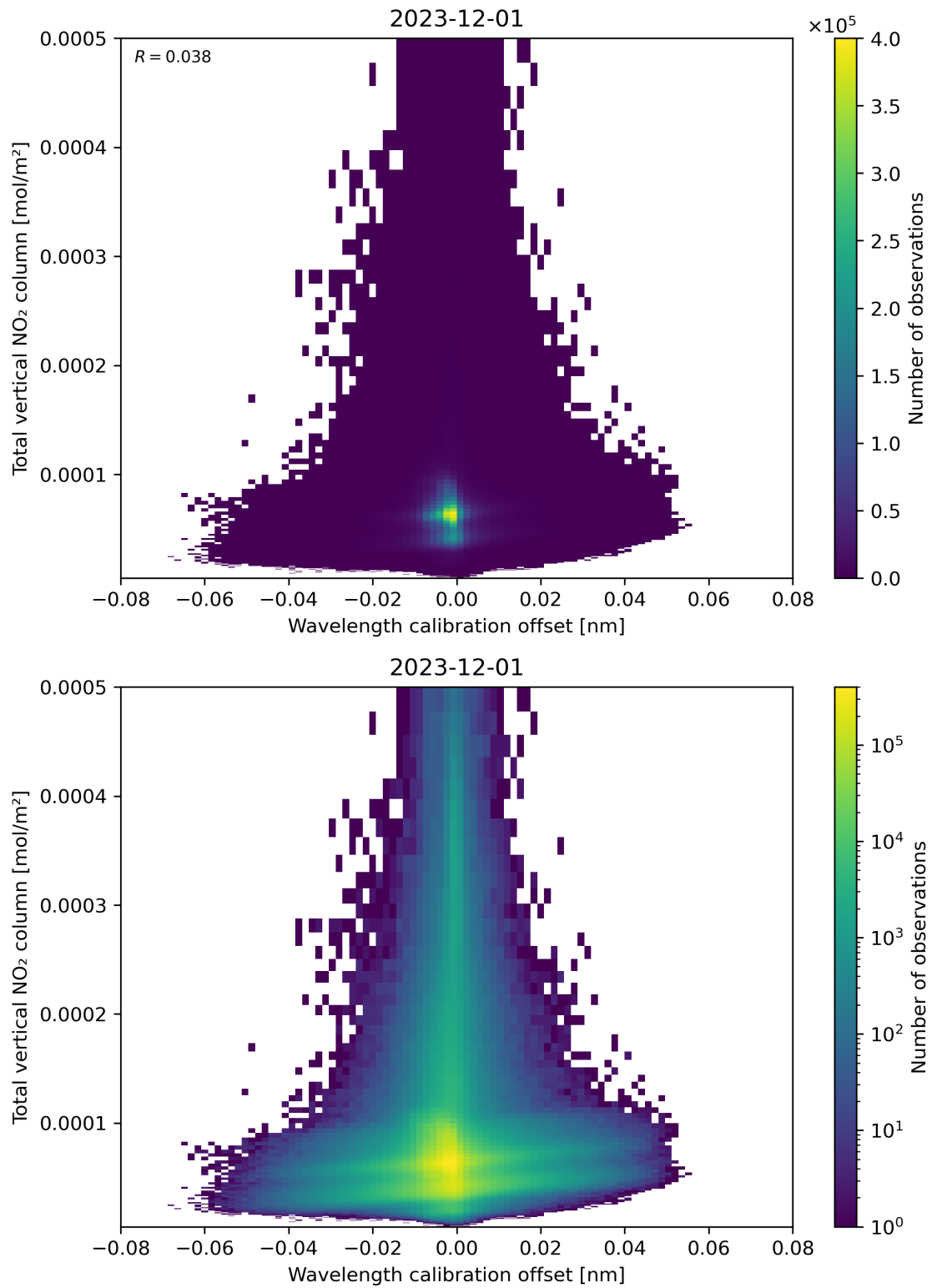
Figure 179: Scatter density plot of “Wavelength calibration offset” against “Total vertical NO 2 column” for 2023-11-30 to 2023-12-02.
