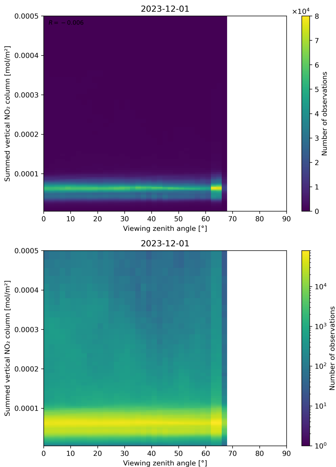
Figure 165: Scatter density plot of “Viewing zenith angle” against “Summed vertical NO 2 column” for 2023-11-30 to 2023-12-02.
