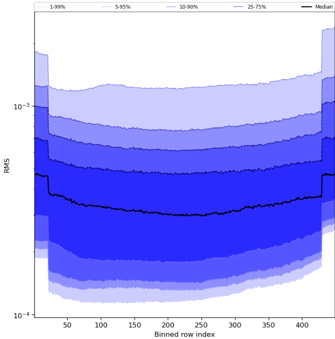
Figure 60: Along track statistics of “RMS” for 2023-11-30 to 2023-12-02
