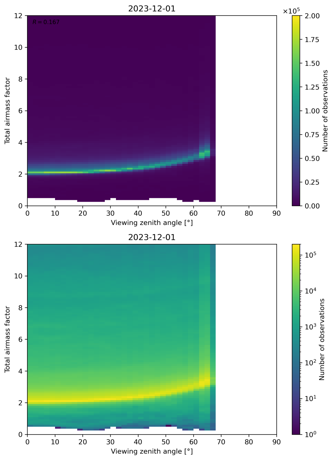
Figure 160: Scatter density plot of “Viewing zenith angle” against “Total airmass factor” for 2023-11-30 to 2023-12-02.
