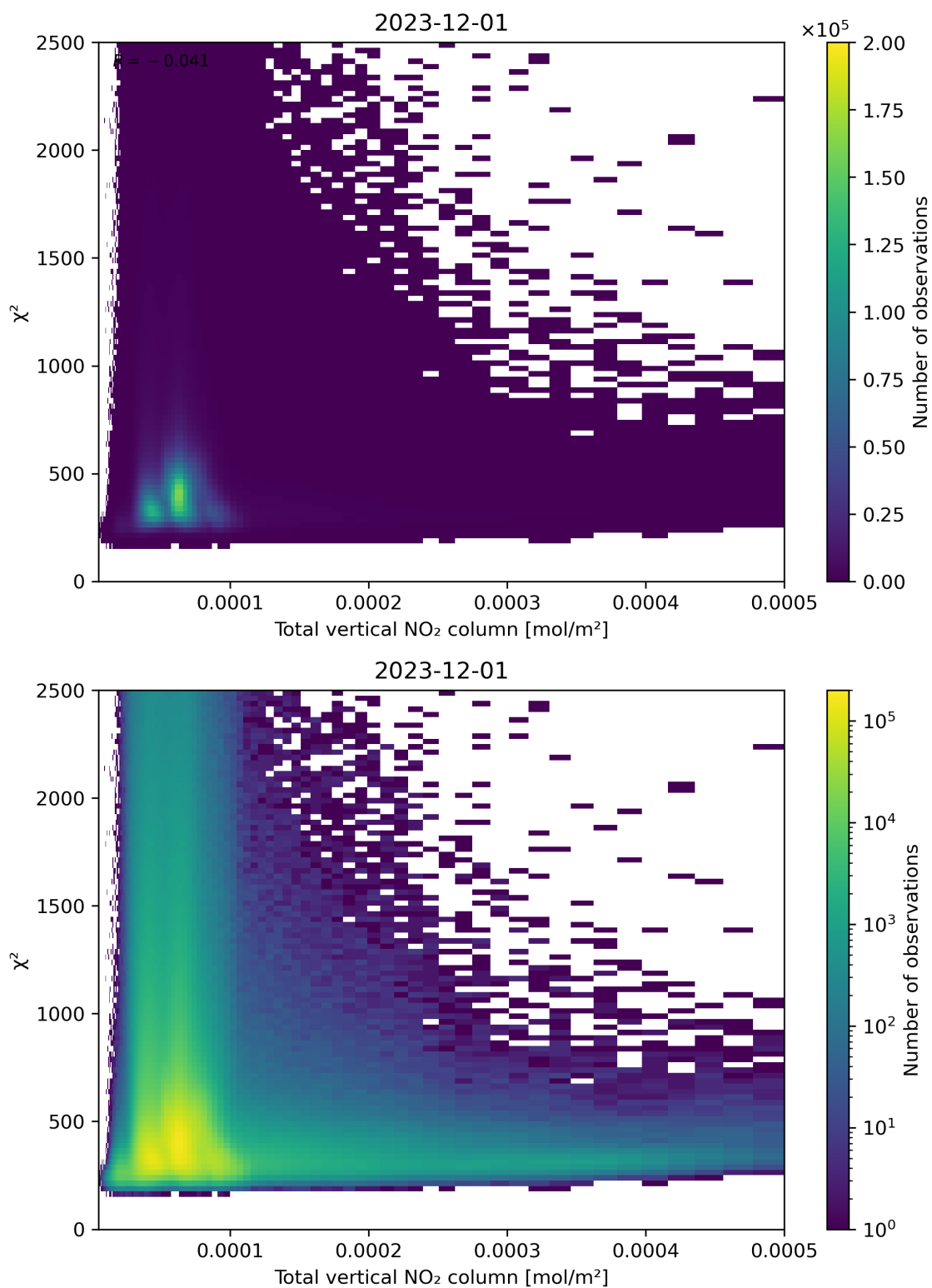
Figure 111: Scatter density plot of “Total vertical NO 2 column” against “ \chi^2 ” for 2023-11-30 to 2023-12-02.
