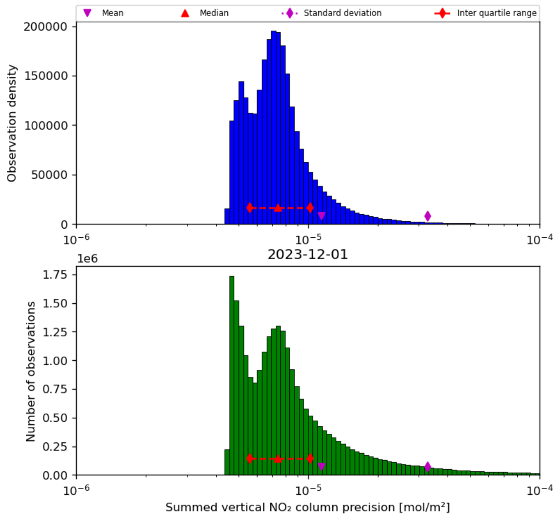
Figure 41: Histogram of "Summed vertical NO 2 column precision" for 2023-11-30 to 2023-12-02
