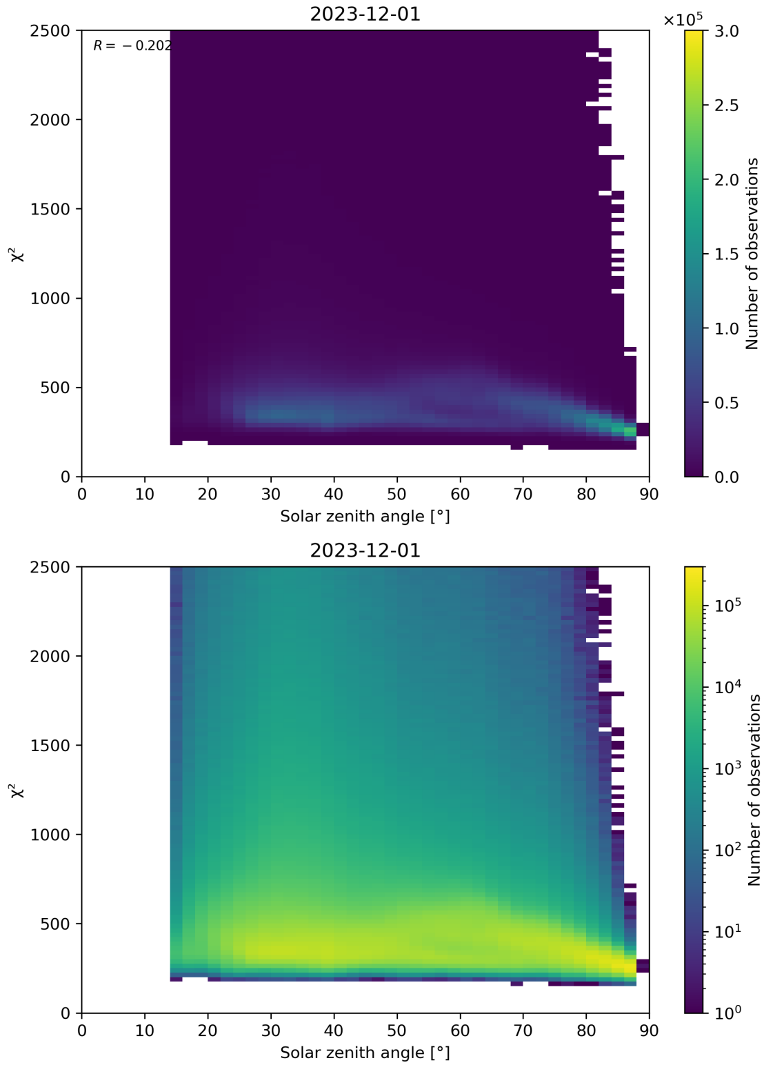
Figure 148: Scatter density plot of “Solar zenith angle” against “ \chi^2 ” for 2023-11-30 to 2023-12-02.
