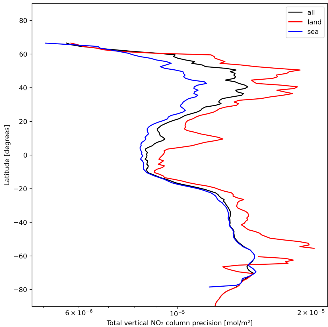
Figure 22: Zonal average of “Total vertical NO 2 column precision” for 2023-11-30 to 2023-12-02.
