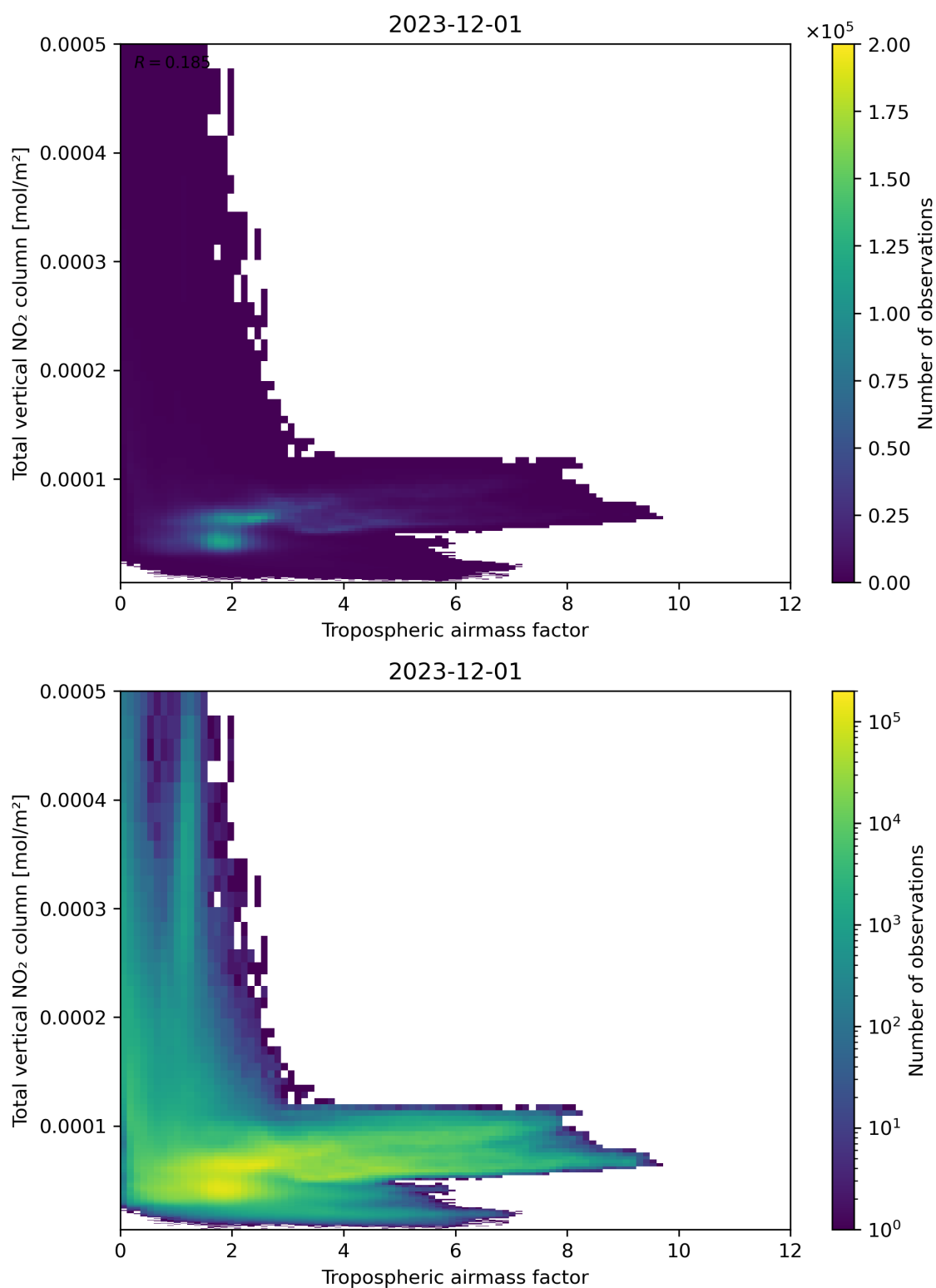
Figure 77: Scatter density plot of “Tropospheric airmass factor” against “Total vertical NO 2 column” for 2023-11-30 to 2023-12-02.
