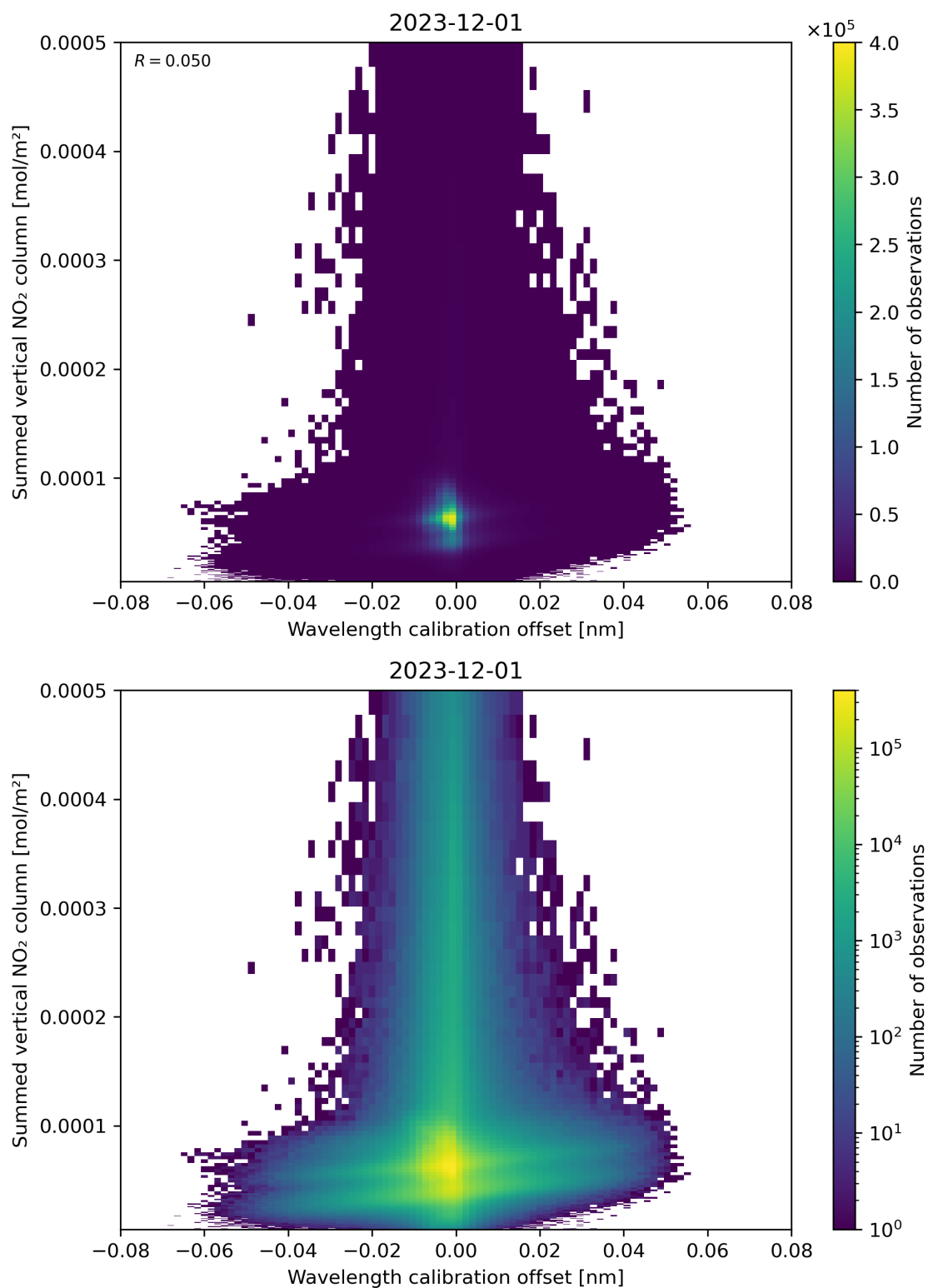
Figure 177: Scatter density plot of “Wavelength calibration offset” against “Summed vertical NO 2 column” for 2023-11-30 to 2023-12-02.
