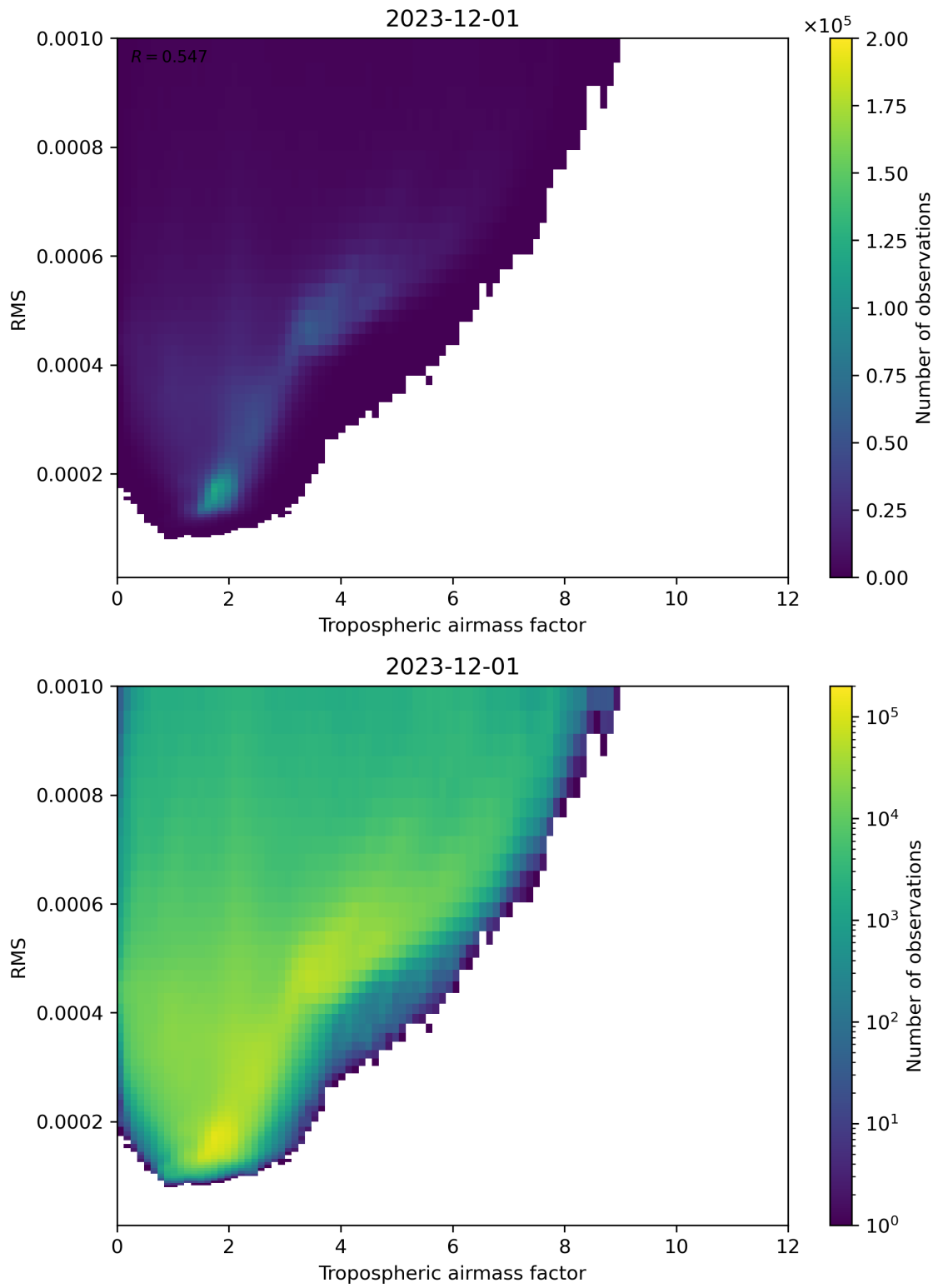
Figure 79: Scatter density plot of “Tropospheric airmass factor” against “RMS” for 2023-11-30 to 2023-12-02.
