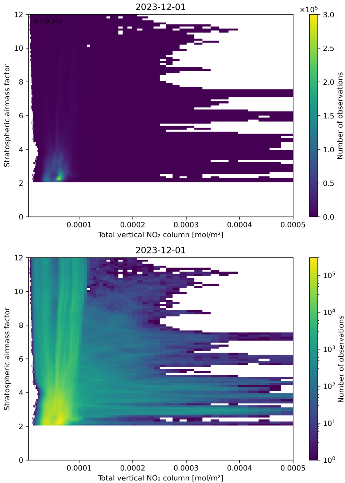
Figure 110: Scatter density plot of “Total vertical NO 2 column” against “Stratospheric airmass factor” for 2023-11-30 to 2023-12-02.
