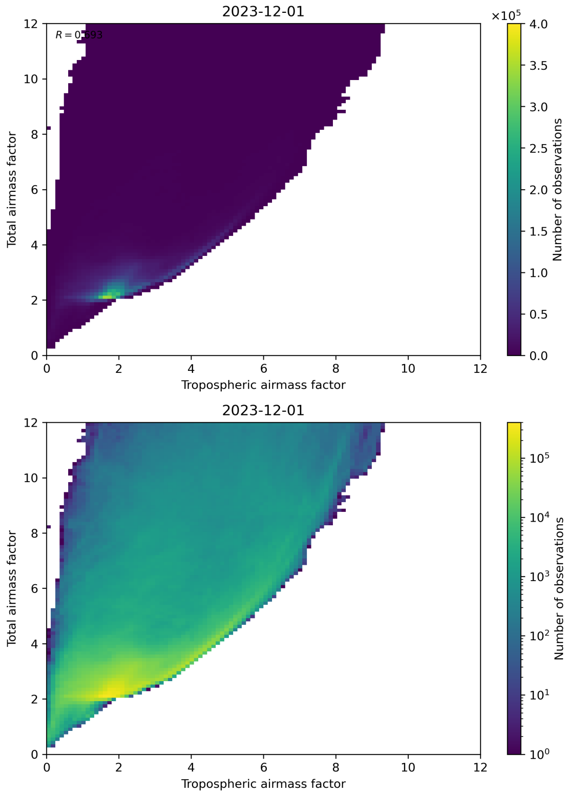
Figure 72: Scatter density plot of “Tropospheric airmass factor” against “Total airmass factor” for 2023-11-30 to 2023-12-02.
