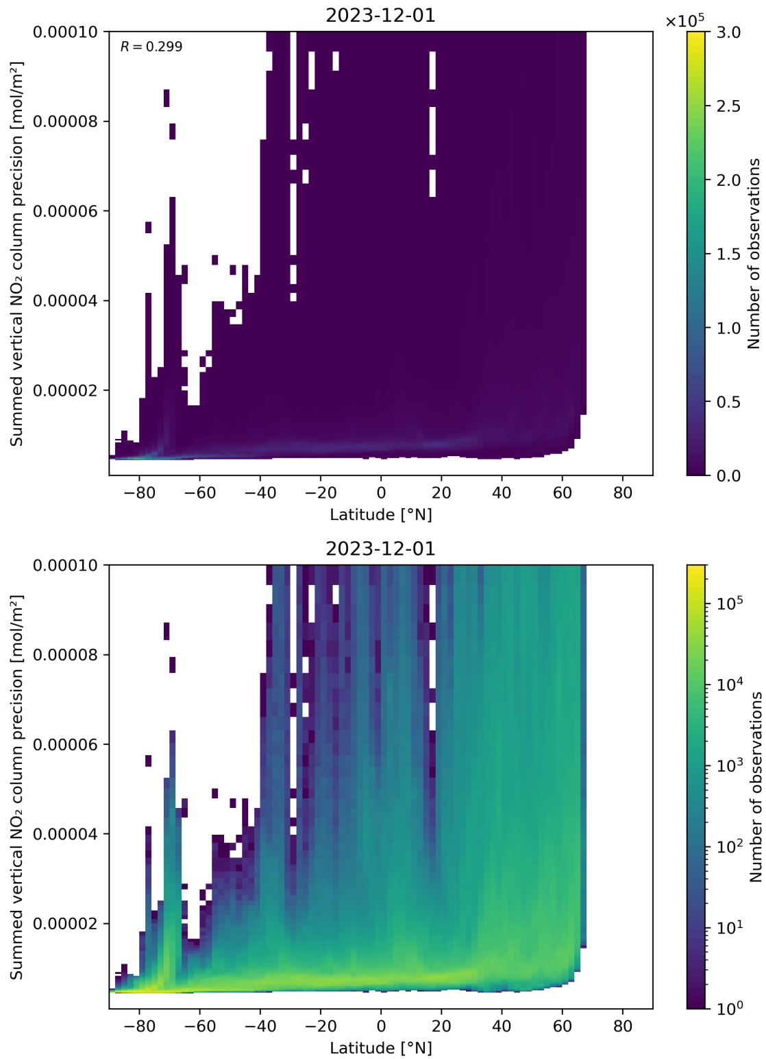
Figure 89: Scatter density plot of “Latitude” against “Summed vertical NO 2 column precision” for 2023-11-30 to 2023-12-02.
