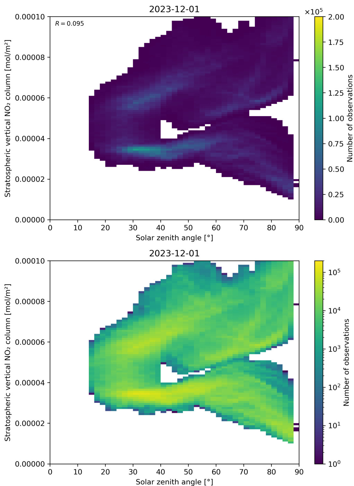
Figure 150: Scatter density plot of “Solar zenith angle” against “Stratospheric vertical NO 2 column” for 2023-11-30 to 2023-12-02.
