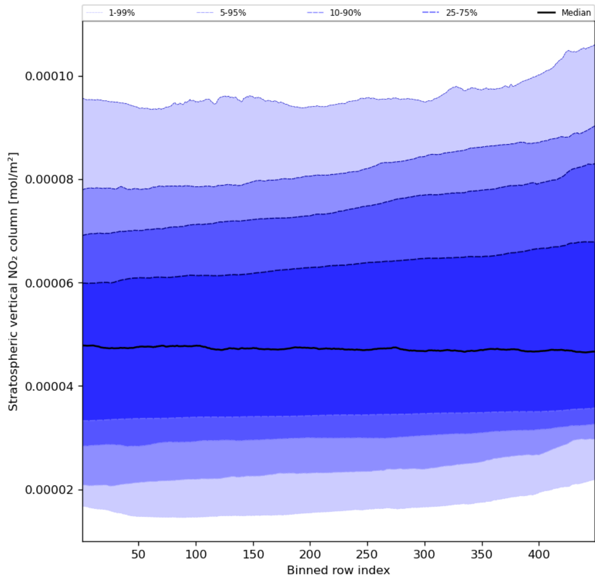
Figure 53: Along track statistics of “Stratospheric vertical NO 2 column” for 2023-11-30 to 2023-12-02
