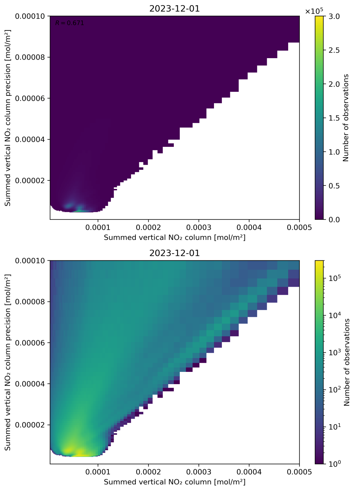
Figure 105: Scatter density plot of “Summed vertical NO 2 column” against “Summed vertical NO 2 column precision” for 2023-11-30 to 2023-12-02.
