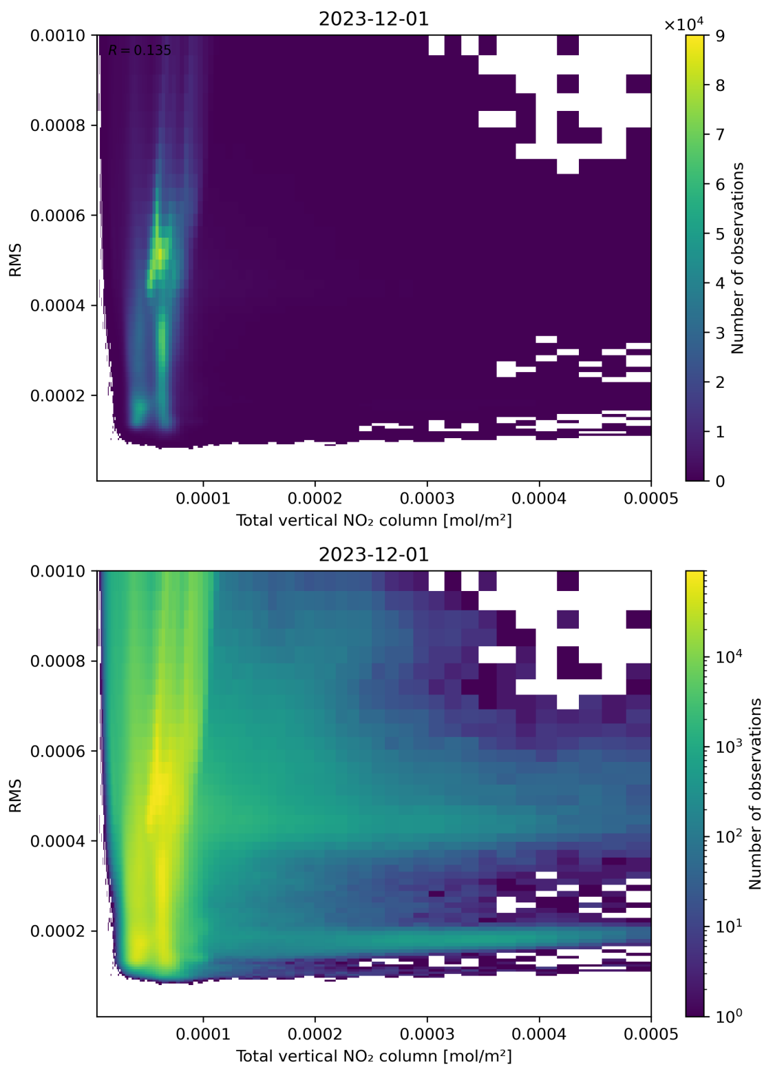
Figure 120: Scatter density plot of “Total vertical NO 2 column” against “RMS” for 2023-11-30 to 2023-12-02.
