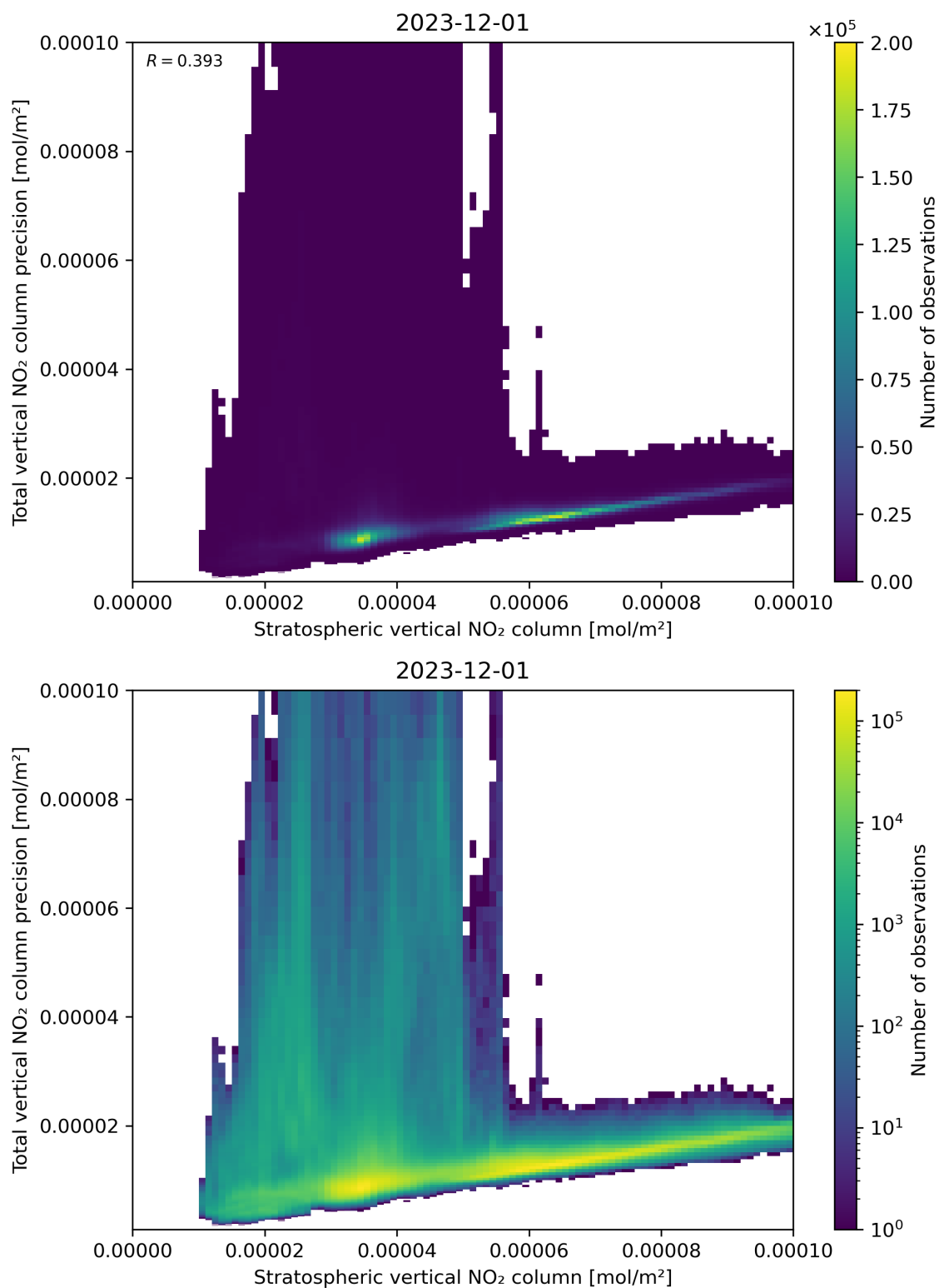
Figure 101: Scatter density plot of “Stratospheric vertical NO 2 column” against “Total vertical NO 2 column precision” for 2023-11-30 to 2023-12-02.
