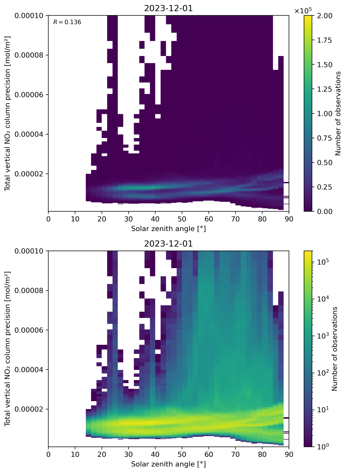
Figure 154: Scatter density plot of “Solar zenith angle” against “Total vertical NO 2 column precision” for 2023-11-30 to 2023-12-02.
