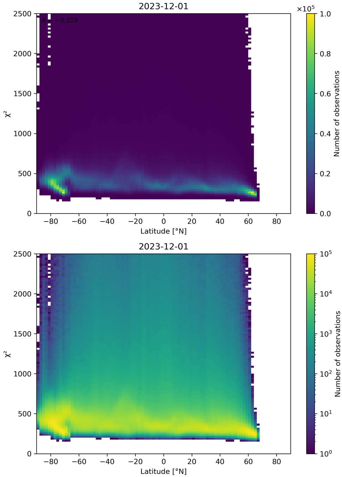
Figure 86: Scatter density plot of “Latitude” against “ \chi^2 ” for 2023-11-30 to 2023-12-02.
