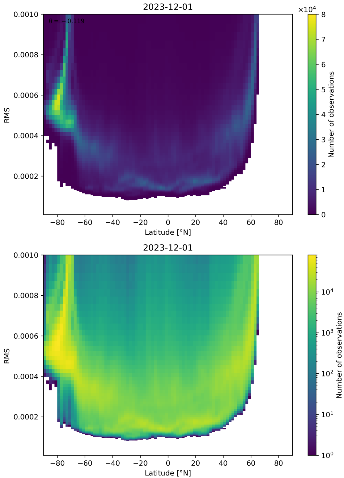
Figure 94: Scatter density plot of “Latitude” against “RMS” for 2023-11-30 to 2023-12-02.
