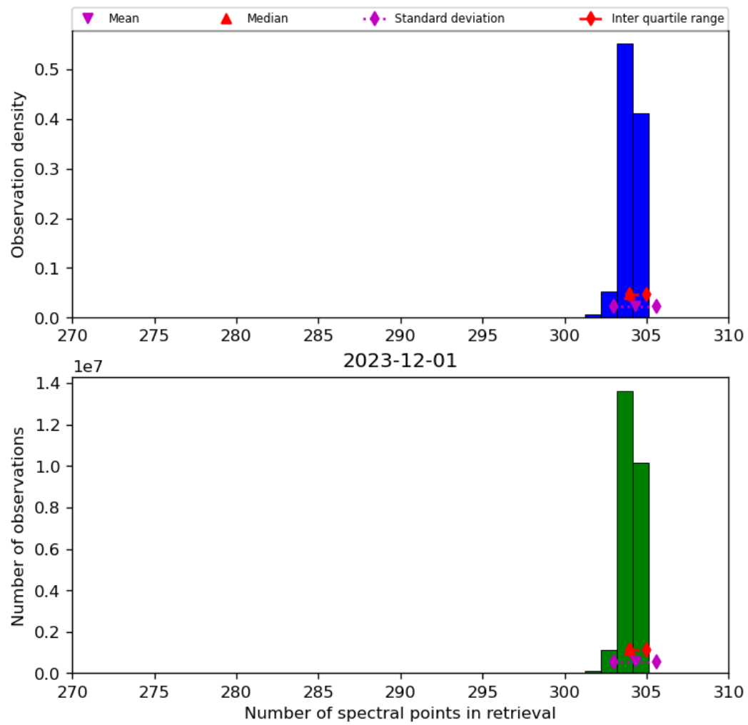
Figure 33: Histogram of “Number of spectral points in retrieval” for 2023-11-30 to 2023-12-02
