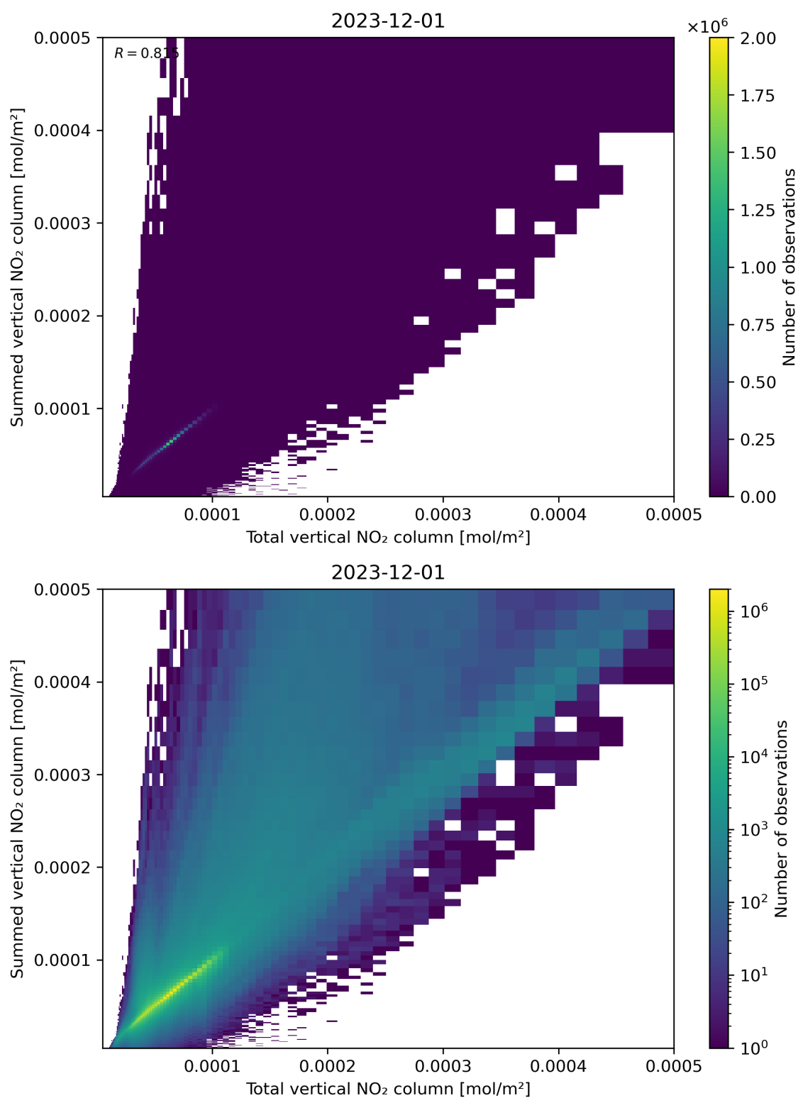
Figure 112: Scatter density plot of “Total vertical NO 2 column” against “Summed vertical NO 2 column” for 2023-11-30 to 2023-12-02.
