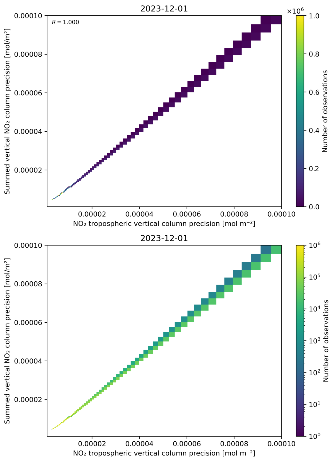
Figure 137: Scatter density plot of “NO 2 tropospheric vertical column precision” against “Summed vertical NO 2 column precision” for 2023-11-30 to 2023-12-02.
