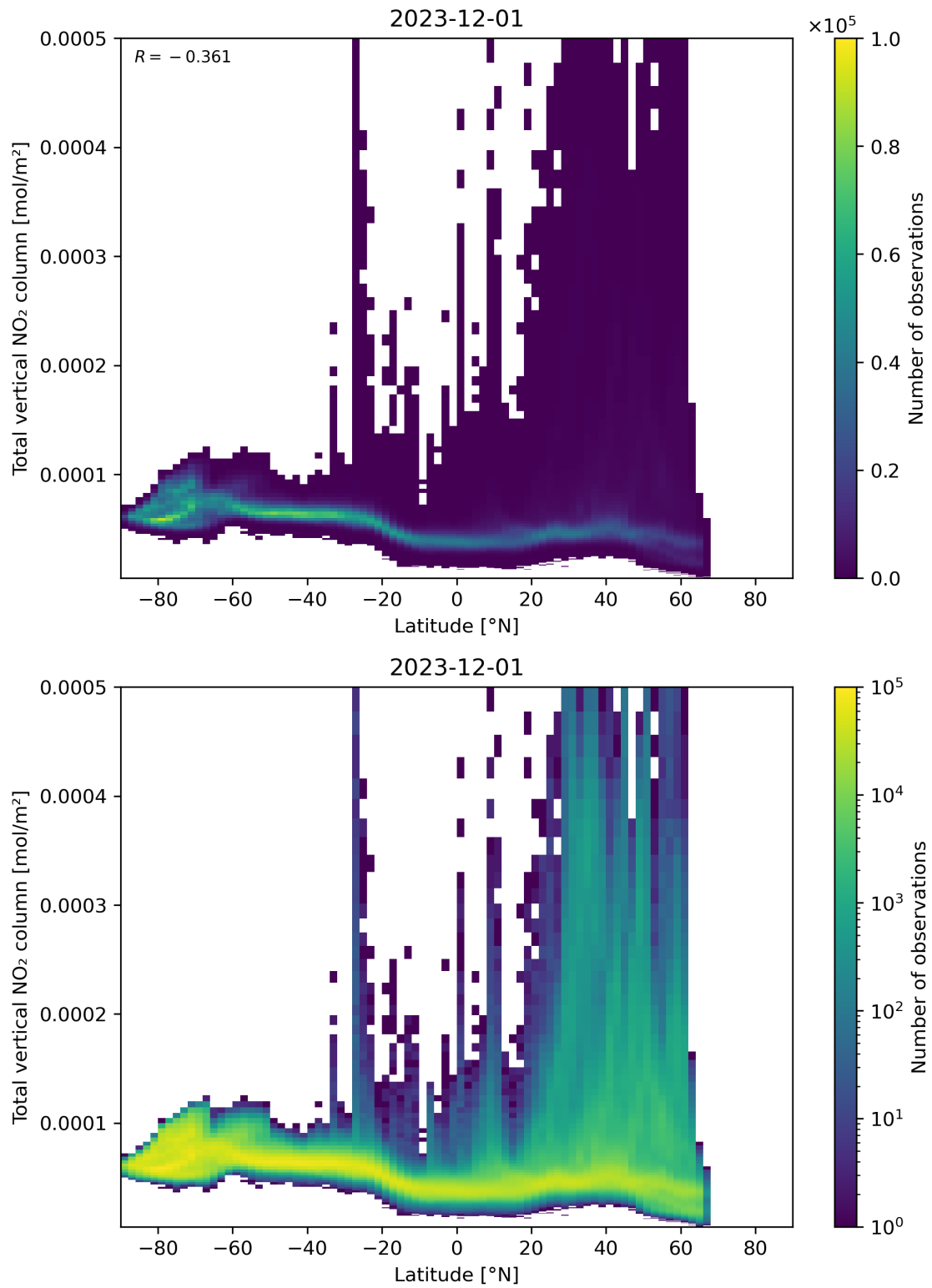
Figure 90: Scatter density plot of “Latitude” against “Total vertical NO 2 column” for 2023-11-30 to 2023-12-02.
