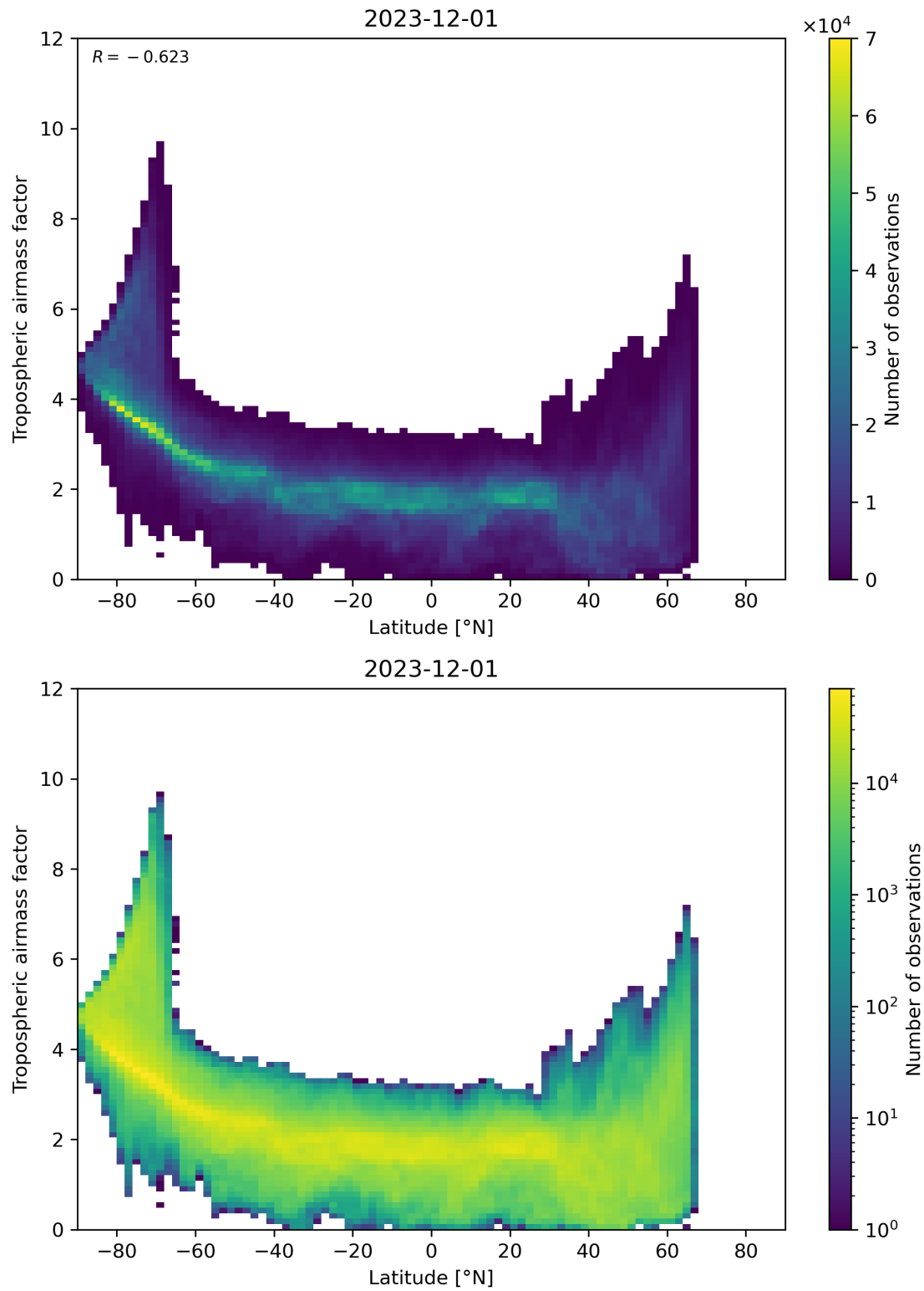
Figure 85: Scatter density plot of “Latitude” against “Tropospheric air mass factor” for 2023-11-30 to 2023-12-02.
