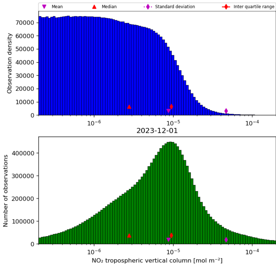
Figure 29: Histogram of “NO 2 tropospheric vertical column” for 2023-11-30 to 2023-12-02
