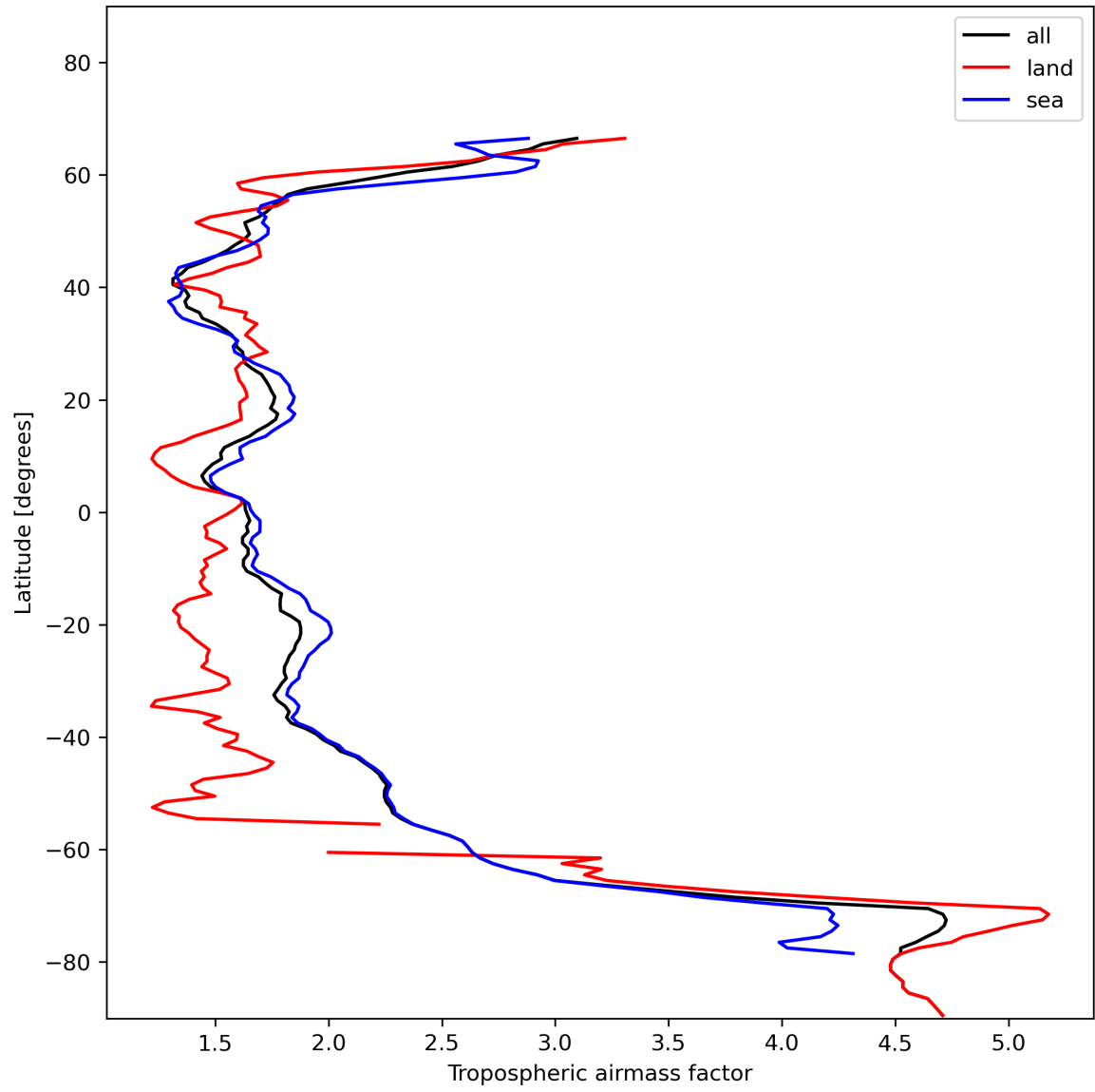
Figure 14: Zonal average of “Tropospheric airmass factor” for 2023-11-30 to 2023-12-02.
