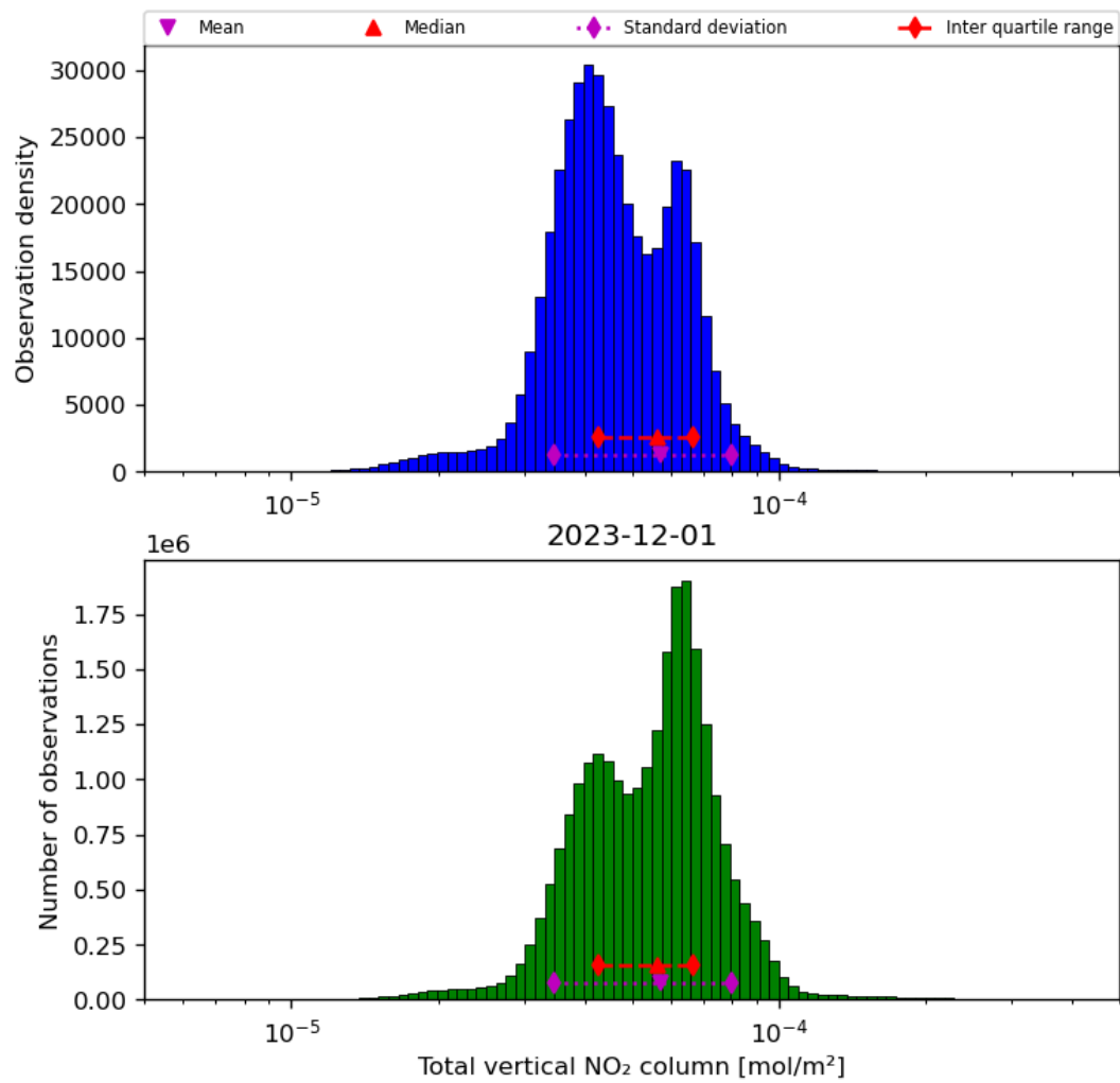
Figure 38: Histogram of “Total vertical NO 2 column” for 2023-11-30 to 2023-12-02
