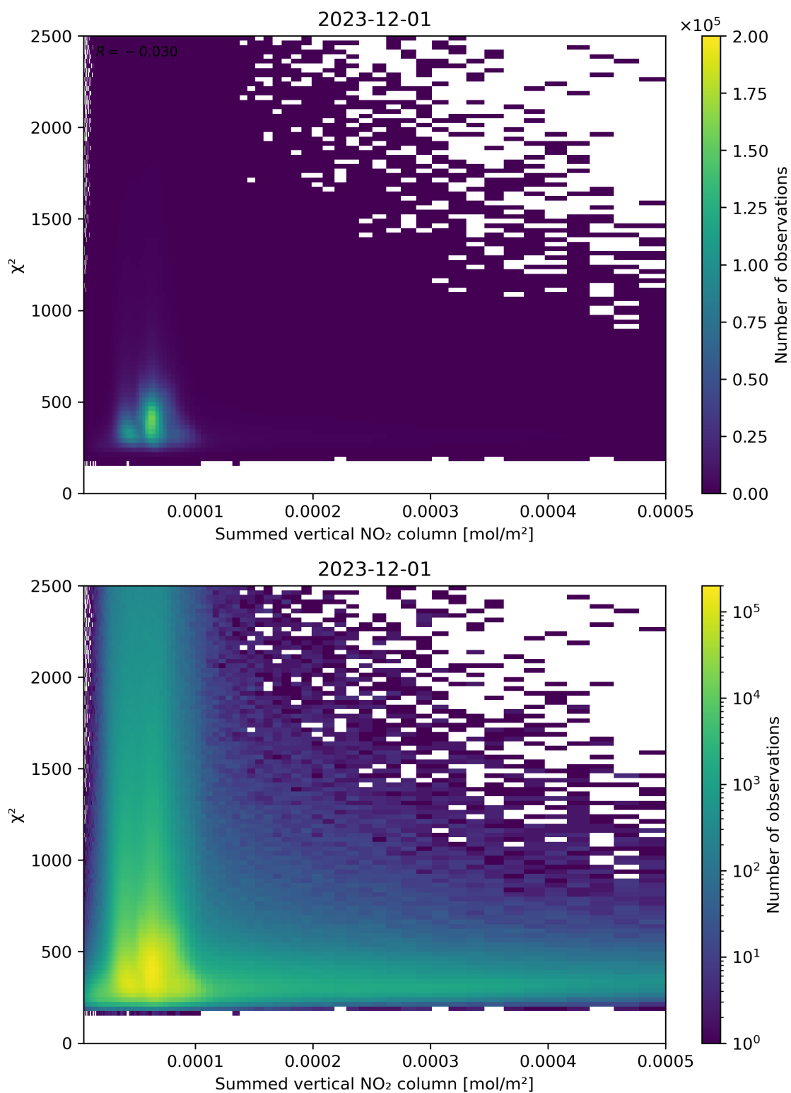
Figure 104: Scatter density plot of “Summed vertical NO 2 column” against “ \chi^2 ” for 2023-11-30 to 2023-12-02.
