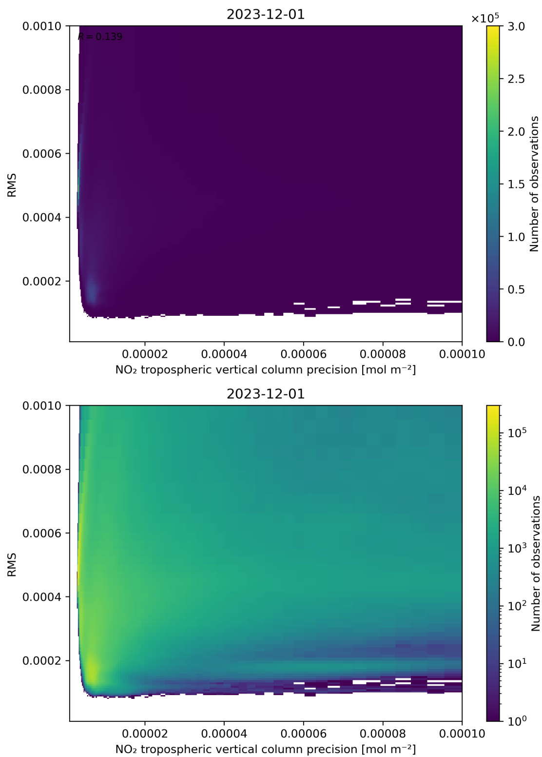
Figure 140: Scatter density plot of “NO 2 tropospheric vertical column precision” against “RMS” for 2023-11-30 to 2023-12-02.
