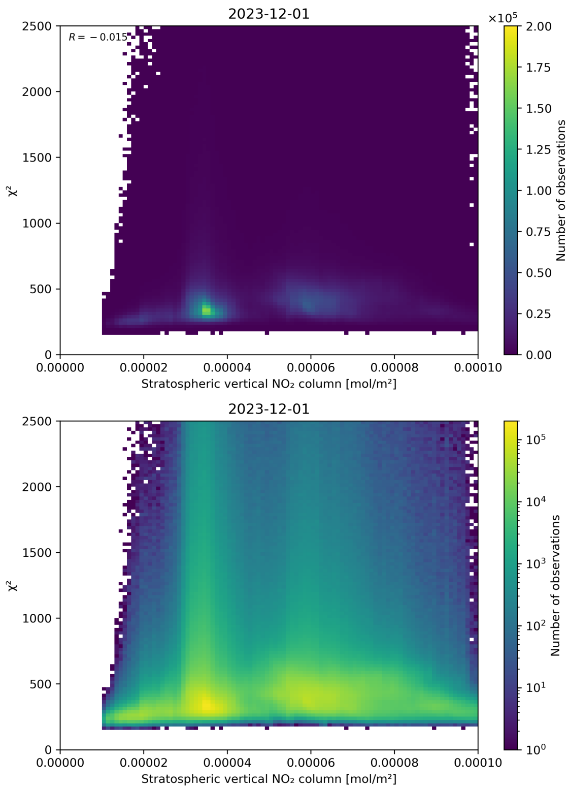
Figure 97: Scatter density plot of “Stratospheric vertical NO 2 column” against “ \chi^2 ” for 2023-11-30 to 2023-12-02.
