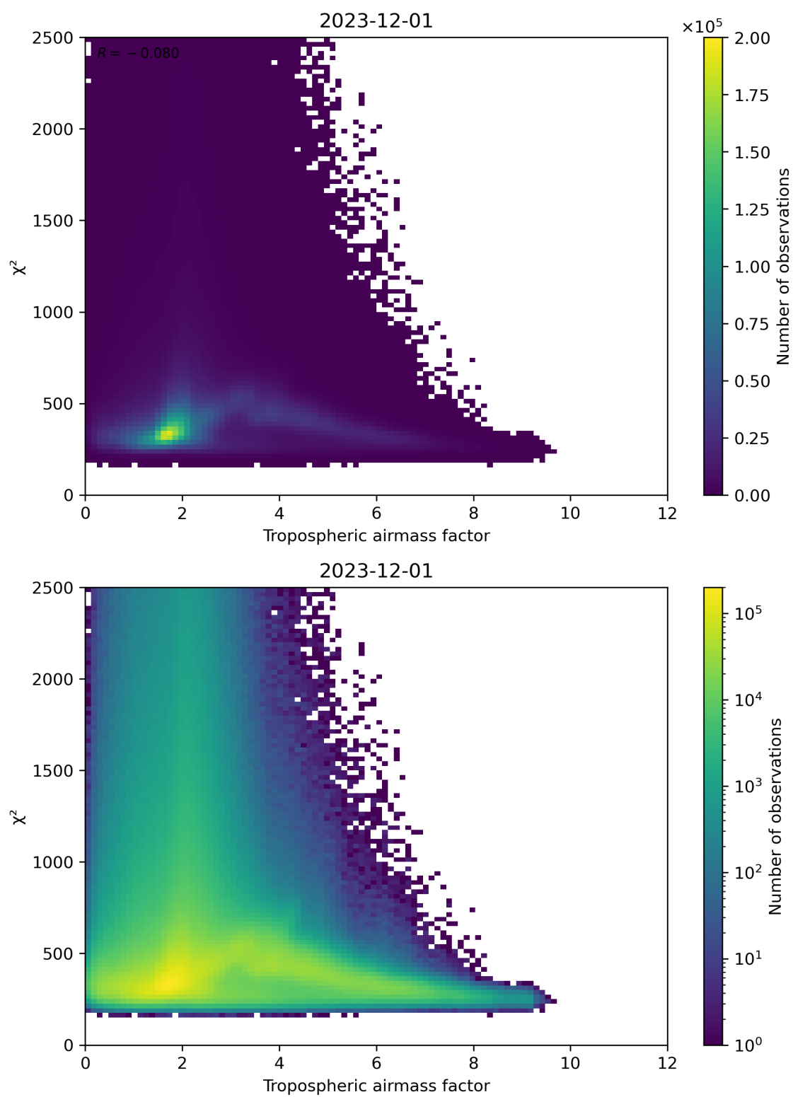
Figure 73: Scatter density plot of “Tropospheric airmass factor” against “ \chi^2 ” for 2023-11-30 to 2023-12-02.
