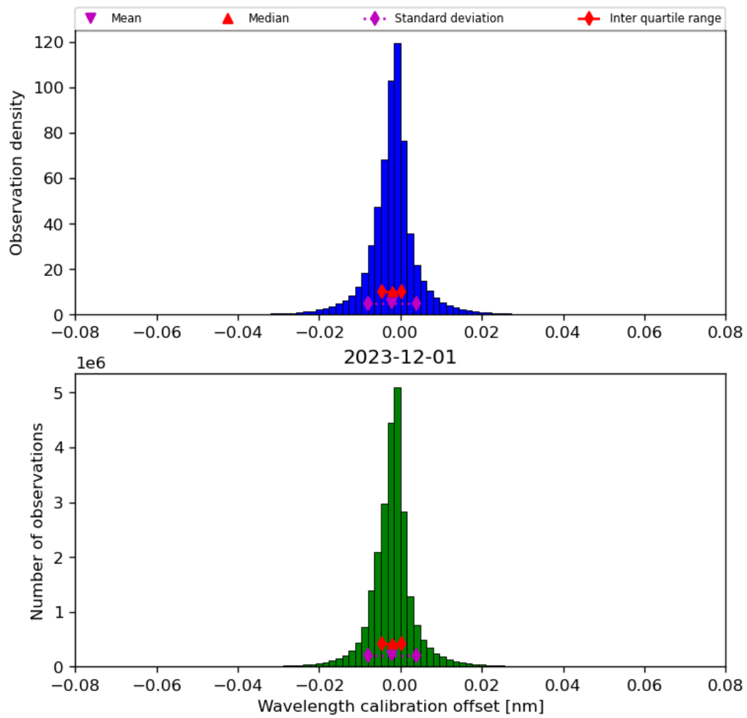
Figure 35: Histogram of “Wavelength calibration offset” for 2023-11-30 to 2023-12-02
