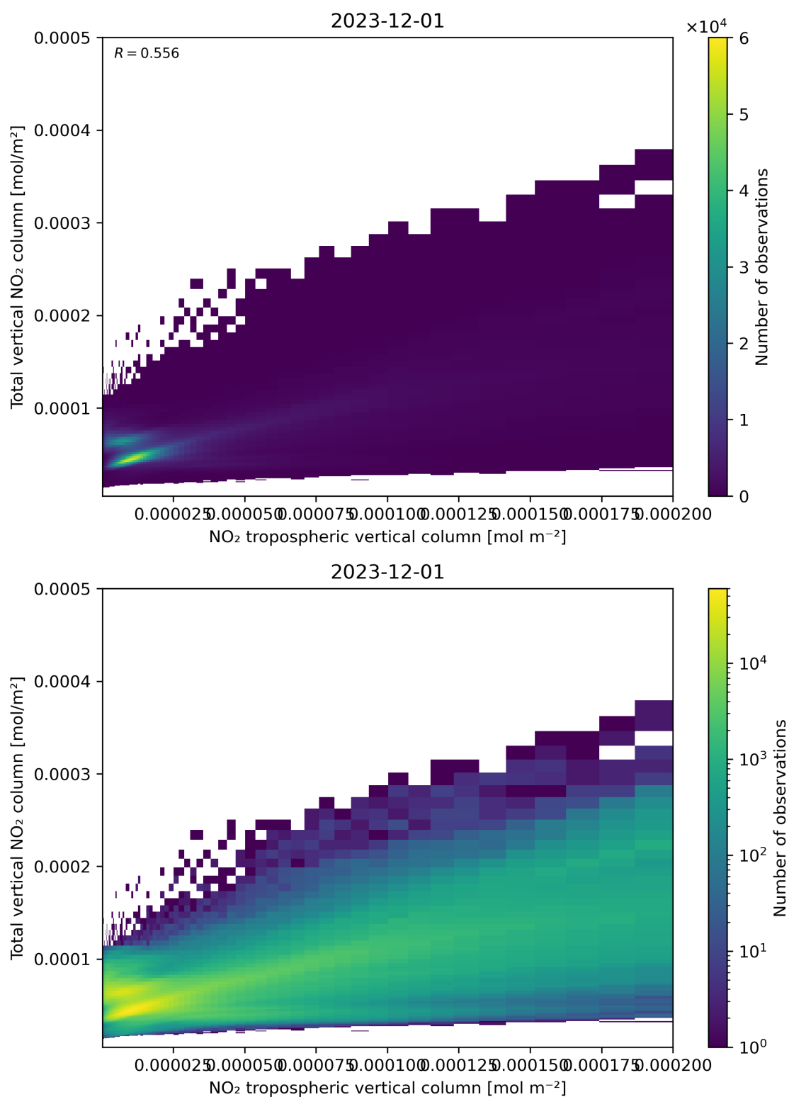
Figure 128: Scatter density plot of “NO 2 tropospheric vertical column” against “Total vertical NO 2 column” for 2023-11-30 to 2023-12-02.
