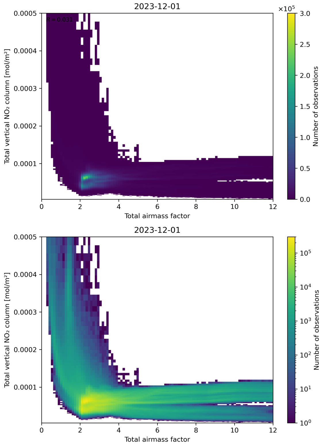
Figure 67: Scatter density plot of “Total airmass factor” against “Total vertical NO 2 column” for 2023-11-30 to 2023-12-02.
