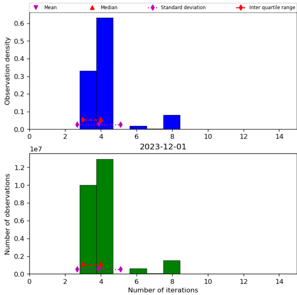
Figure 34: Histogram of “Number of iterations” for 2023-11-30 to 2023-12-02
