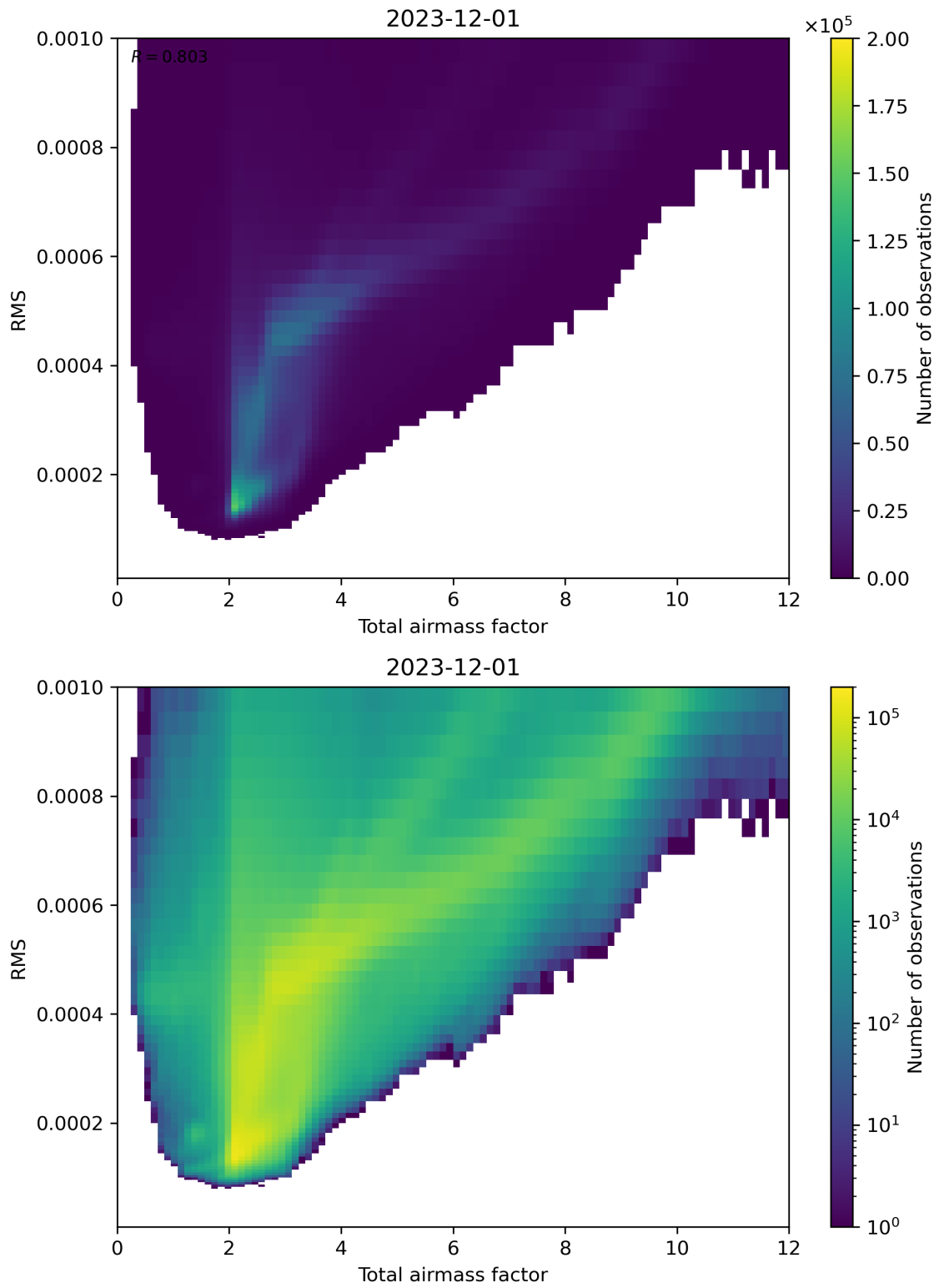
Figure 69: Scatter density plot of “Total airmass factor” against “RMS” for 2023-11-30 to 2023-12-02.
