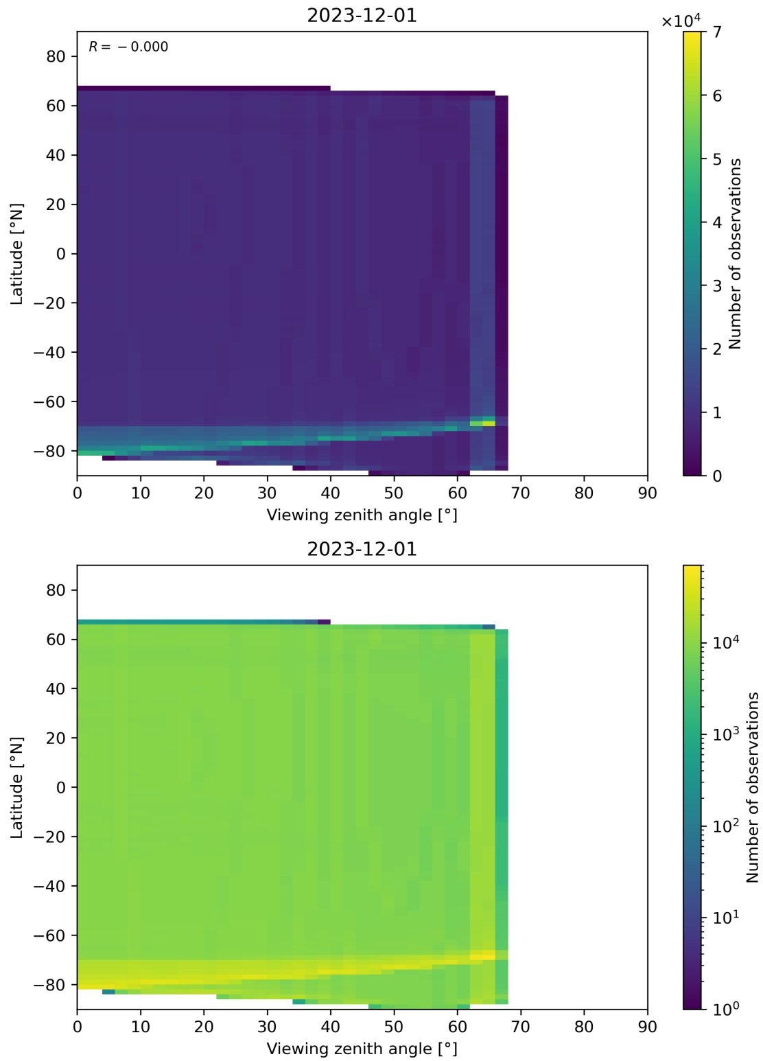
Figure 163: Scatter density plot of “Viewing zenith angle” against “Latitude” for 2023-11-30 to 2023-12-02.
