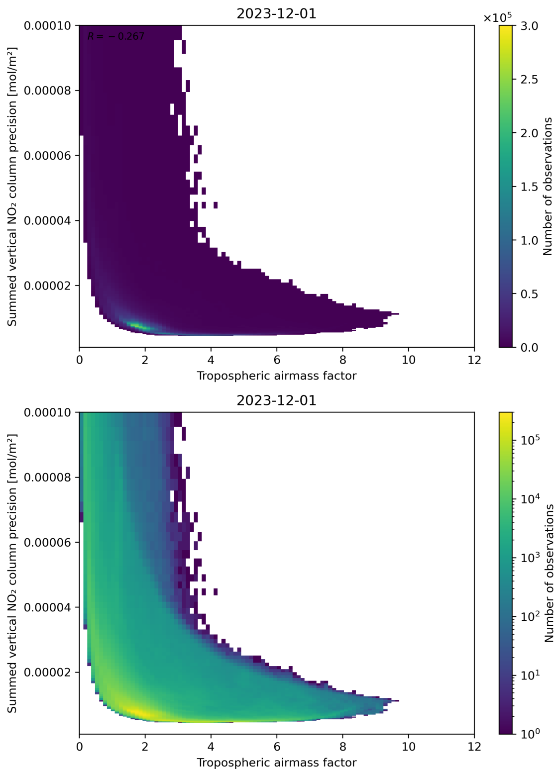
Figure 76: Scatter density plot of “Tropospheric air mass factor” against “Summed vertical NO 2 column precision” for 2023-11-30 to 2023-12-02.
