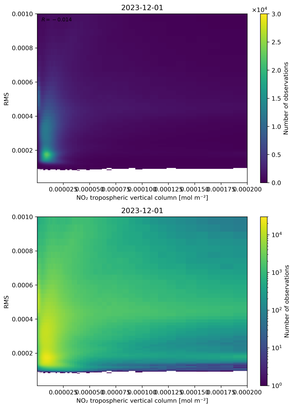
Figure 142: Scatter density plot of “NO 2 tropospheric vertical column” against “RMS” for 2023-11-30 to 2023-12-02.
