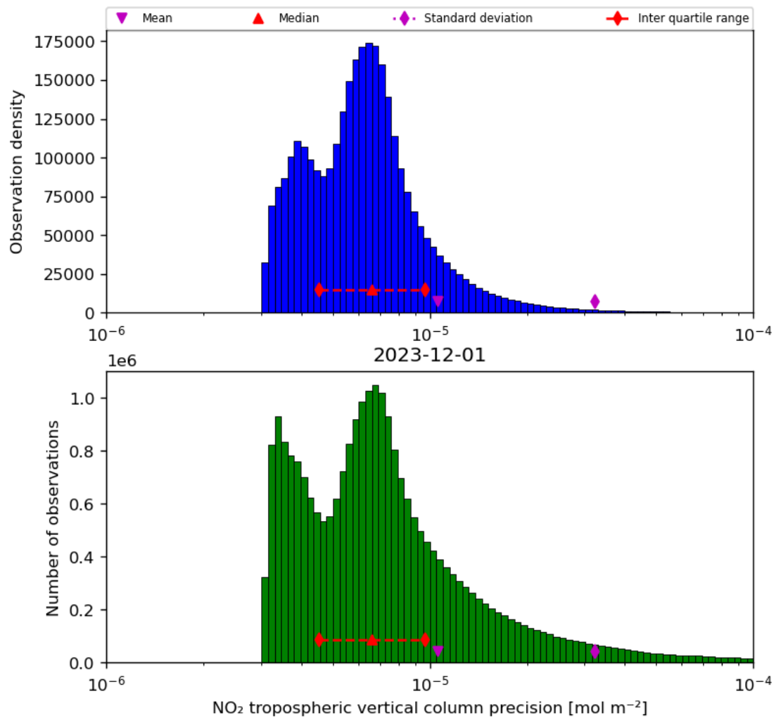
Figure 30: Histogram of “NO 2 tropospheric vertical column precision” for 2023-11-30 to 2023-12-02
