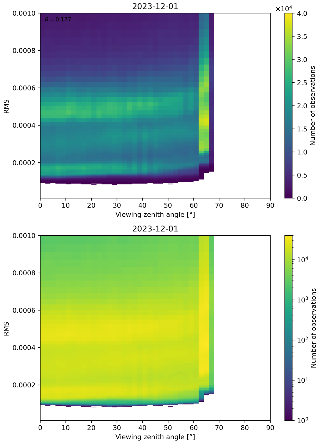
Figure 171: Scatter density plot of “Viewing zenith angle” against “RMS” for 2023-11-30 to 2023-12-02.
