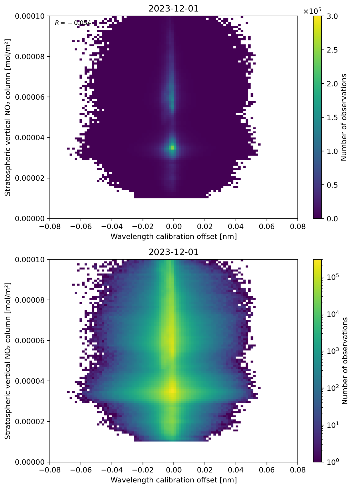
Figure 176: Scatter density plot of “Wavelength calibration offset” against “Stratospheric vertical NO 2 column” for 2023-11-30 to 2023-12-02.
