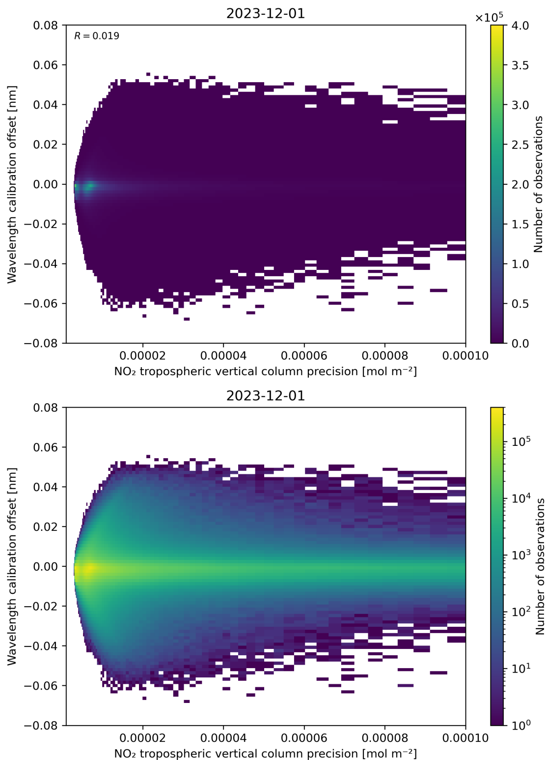
Figure 141: Scatter density plot of “NO 2 tropospheric vertical column precision” against “Wavelength calibration offset” for 2023-11-30 to 2023-12-02.
