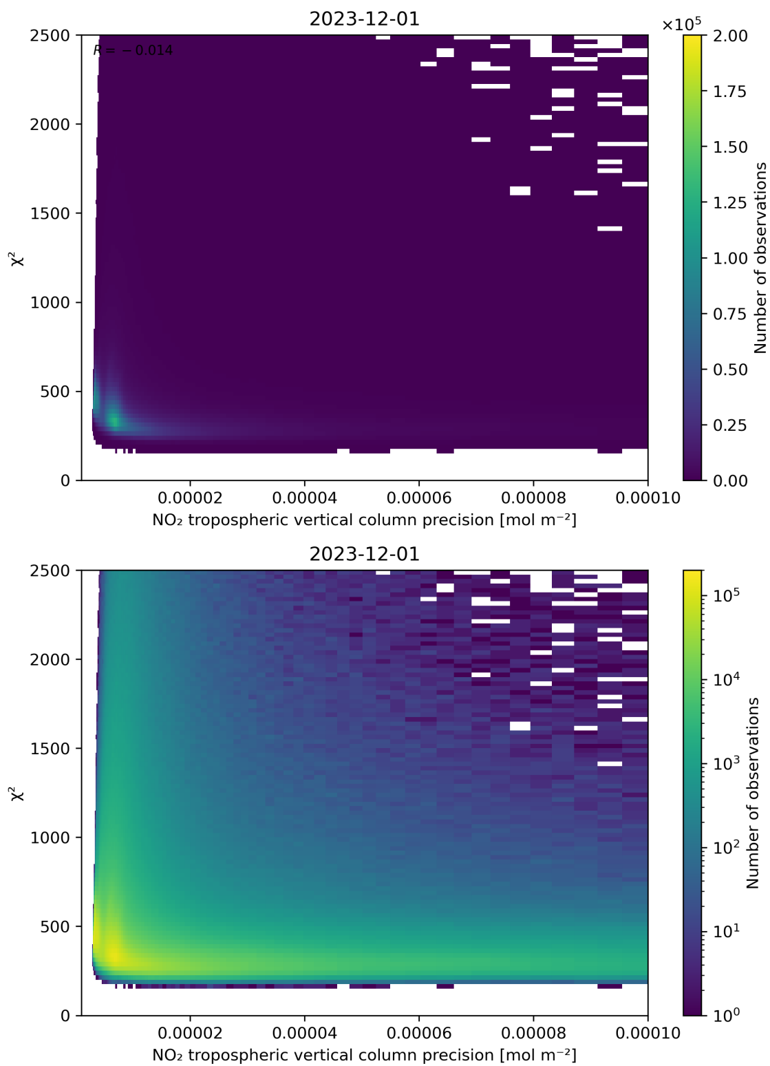
Figure 134: Scatter density plot of “NO 2 tropospheric vertical column precision” against “ \chi^2 ” for 2023-11-30 to 2023-12-02.
