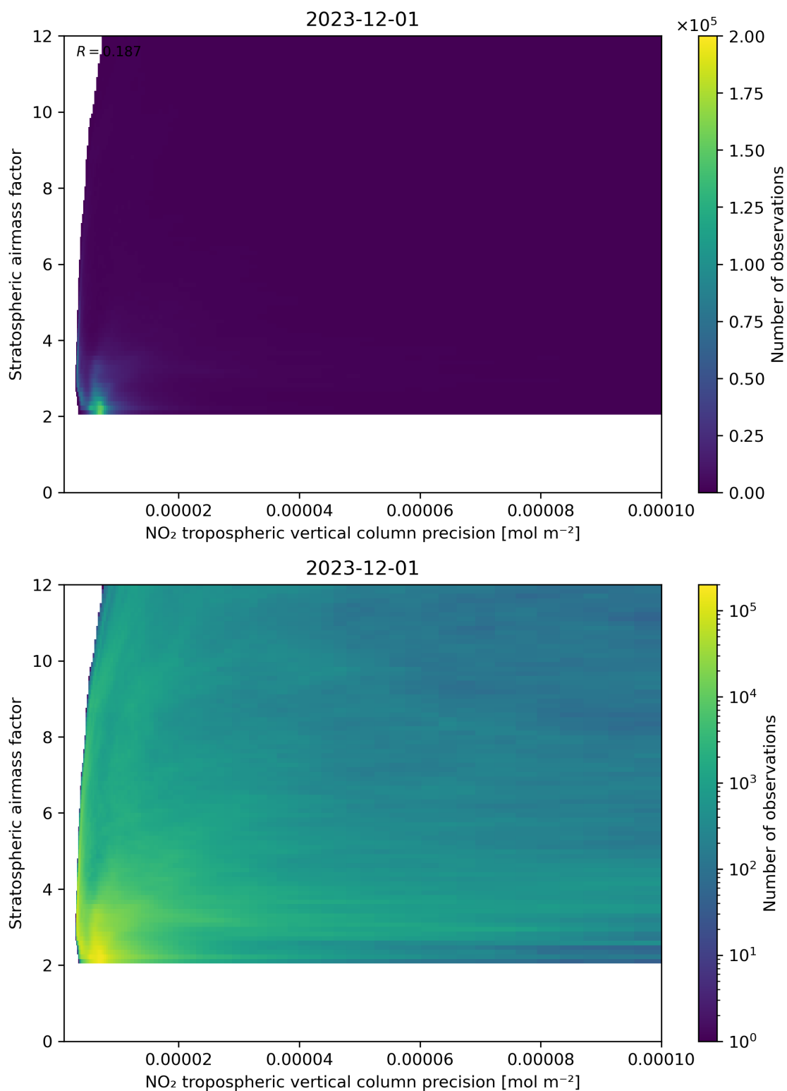
Figure 131: Scatter density plot of “NO 2 tropospheric vertical column precision” against “Stratospheric airmass factor” for 2023-11-30 to 2023-12-02.
