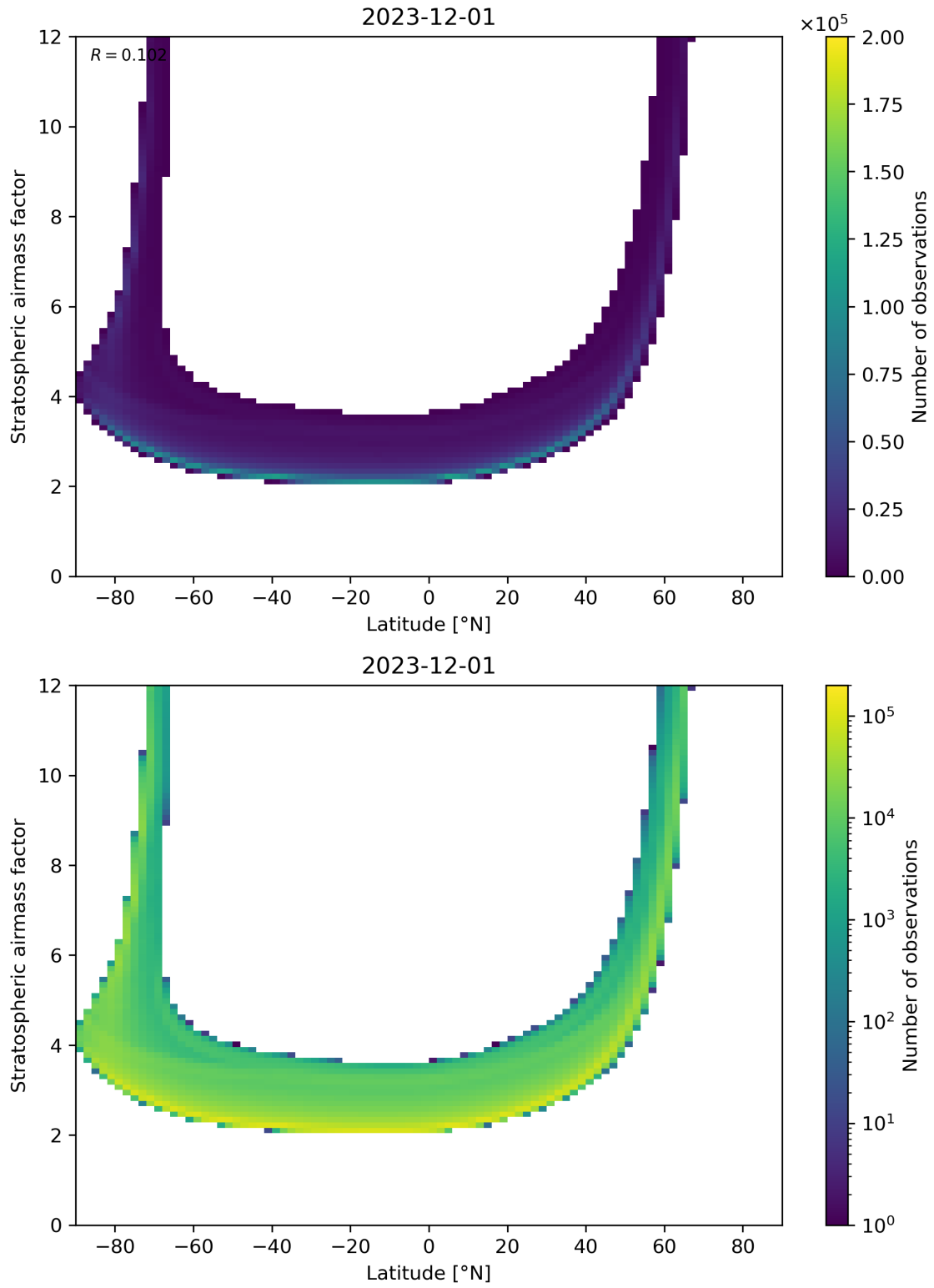
Figure 83: Scatter density plot of “Latitude” against “Stratospheric airmass factor” for 2023-11-30 to 2023-12-02.
