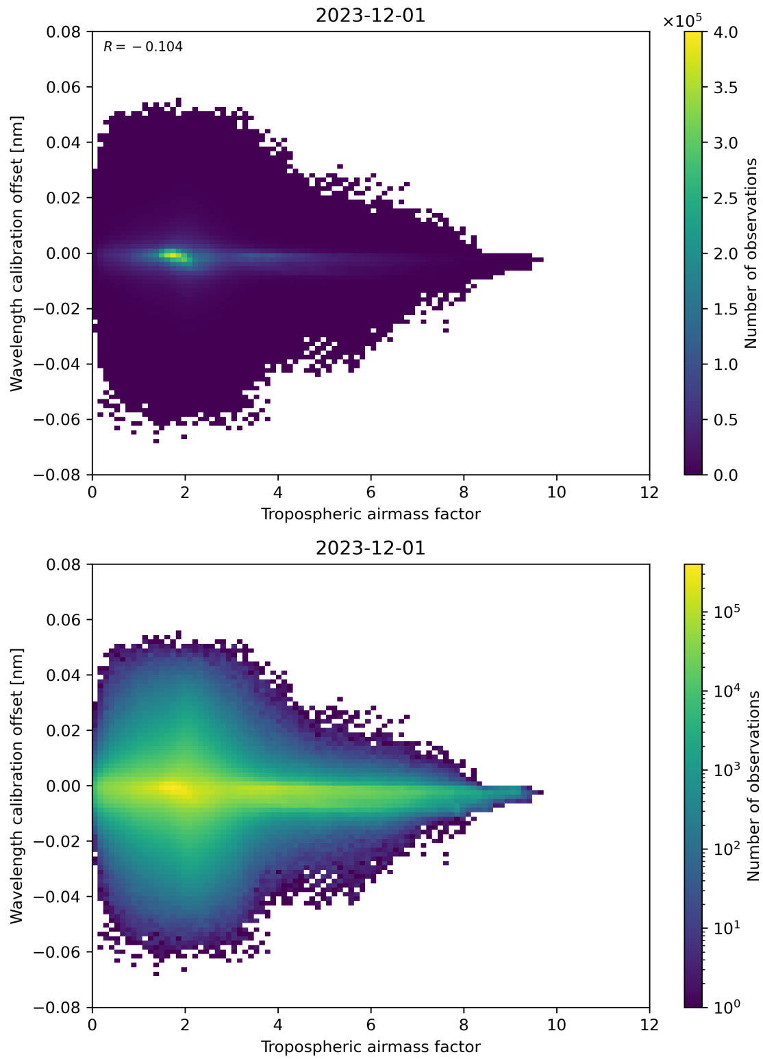
Figure 80: Scatter density plot of “Tropospheric airmass factor” against “Wavelength calibration offset” for 2023-11-30 to 2023-12-02.
