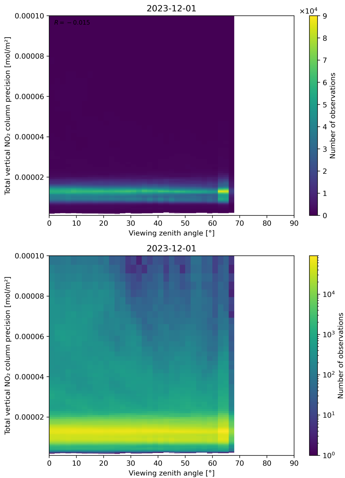
Figure 168: Scatter density plot of “Viewing zenith angle” against “Total vertical NO 2 column precision” for 2023-11-30 to 2023-12-02.
