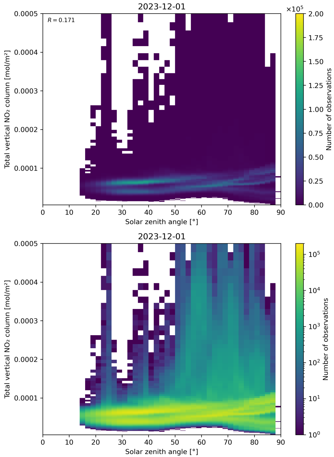
Figure 153: Scatter density plot of “Solar zenith angle” against “Total vertical NO 2 column” for 2023-11-30 to 2023-12-02.
