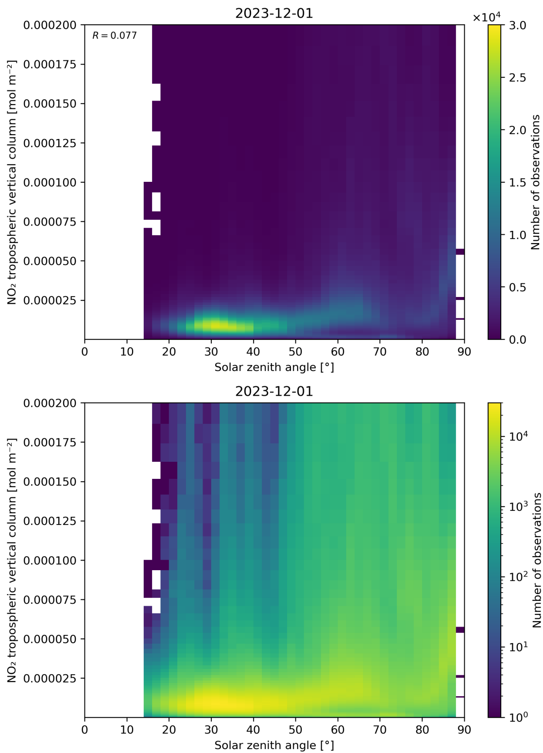
Figure 155: Scatter density plot of “Solar zenith angle” against “NO 2 tropospheric vertical column” for 2023-11-30 to 2023-12-02.
