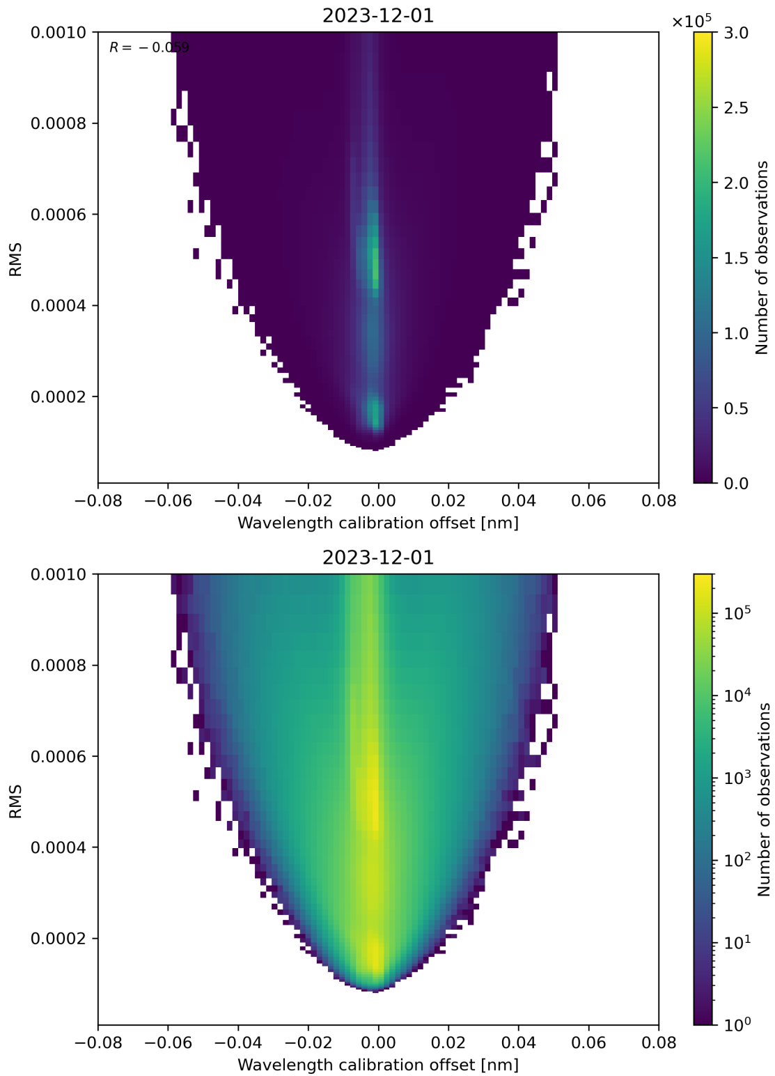
Figure 181: Scatter density plot of “Wavelength calibration offset” against “RMS” for 2023-11-30 to 2023-12-02.
