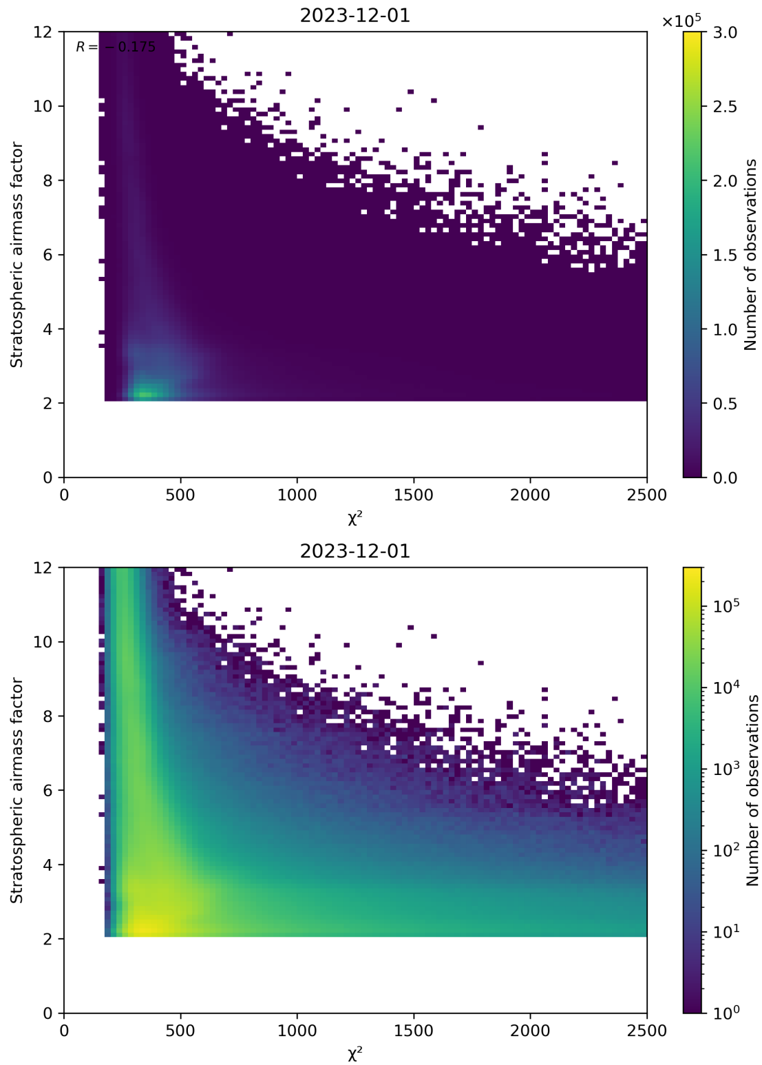
Figure 81: Scatter density plot of “ \chi^2 ” against “Stratospheric airmass factor” for 2023-11-30 to 2023-12-02.
