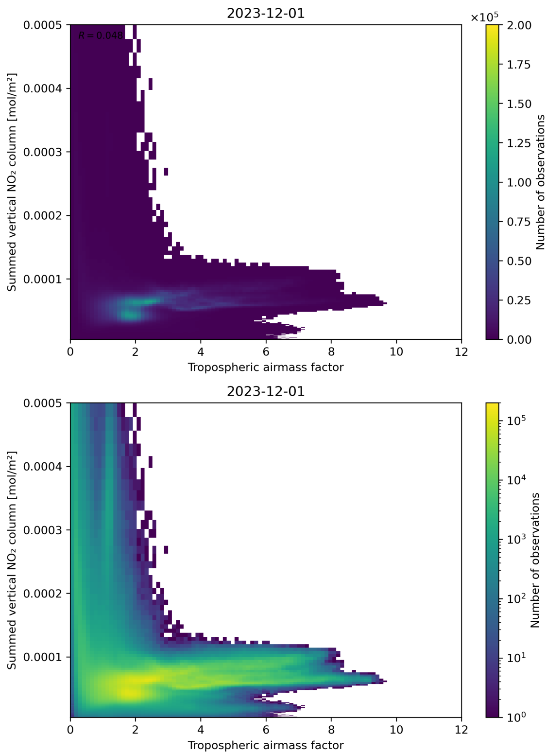
Figure 75: Scatter density plot of “Tropospheric airmass factor” against “Summed vertical NO 2 column” for 2023-11-30 to 2023-12-02.
