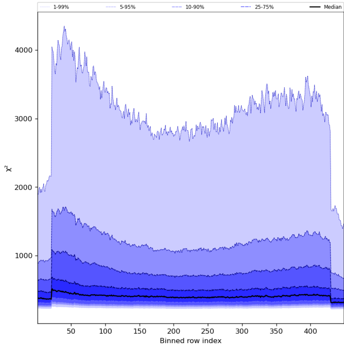
Figure 59: Along track statistics of “ \chi^2 ” for 2023-11-30 to 2023-12-02
