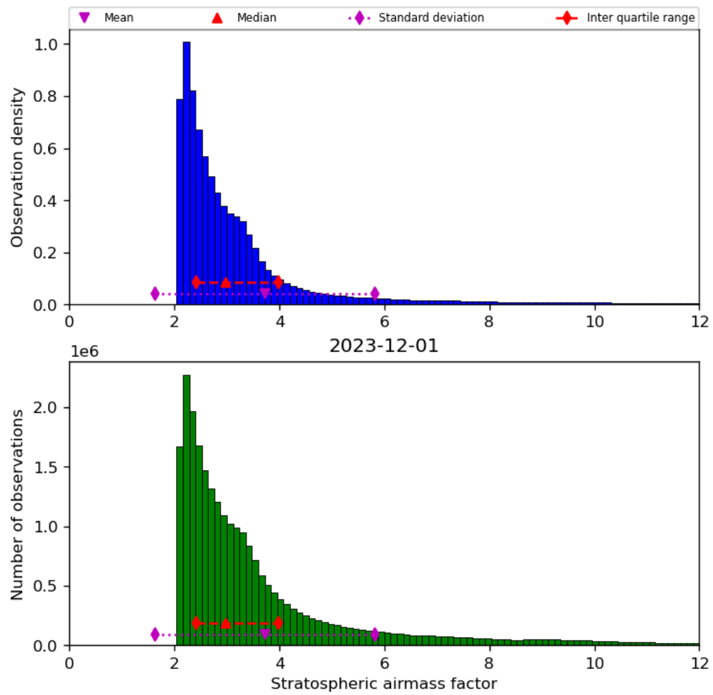
Figure 44: Histogram of “Stratospheric airmass factor” for 2023-11-30 to 2023-12-02
