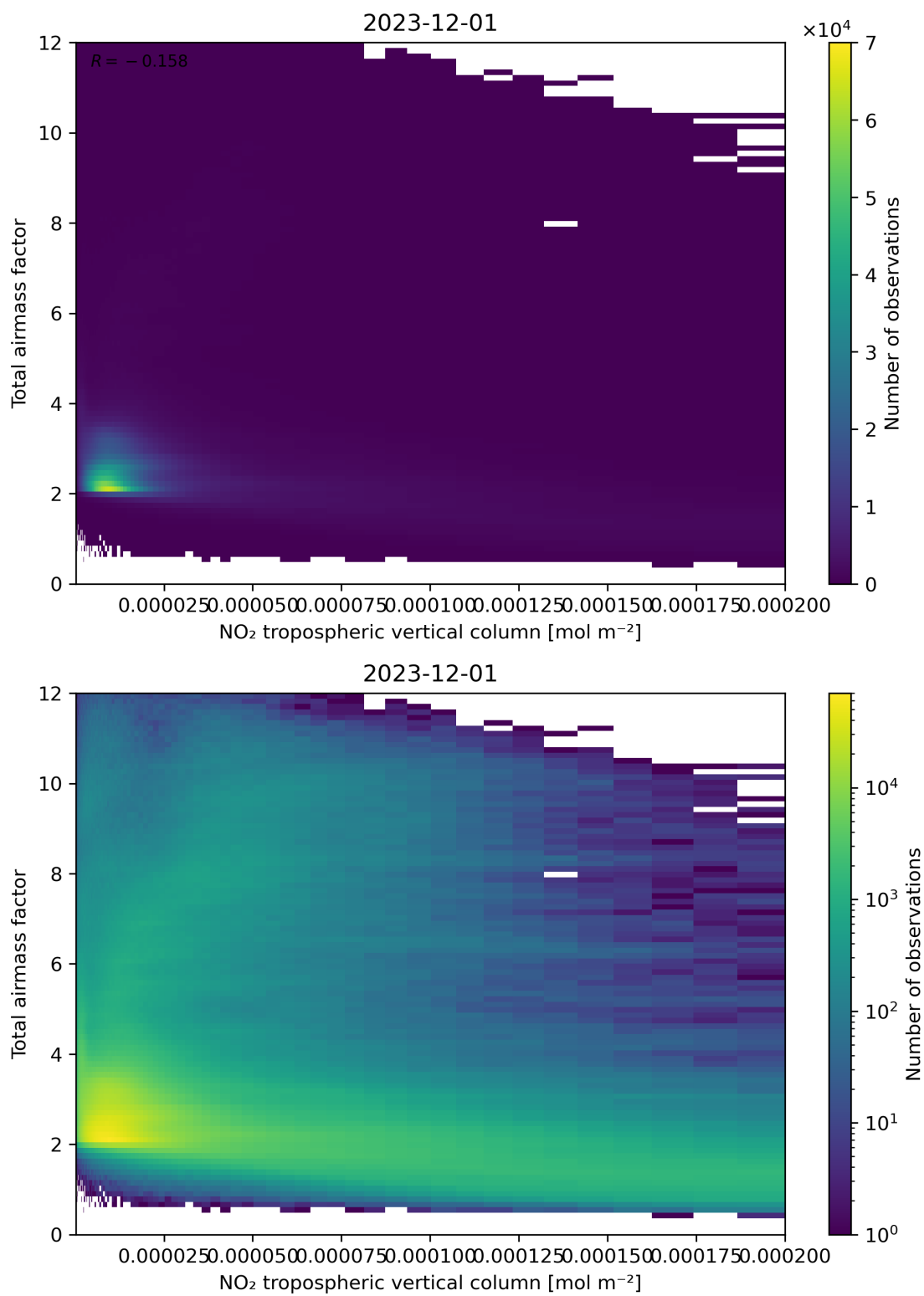
Figure 122: Scatter density plot of “NO 2 tropospheric vertical column” against “Total air mass factor” for 2023-11-30 to 2023-12-02.
