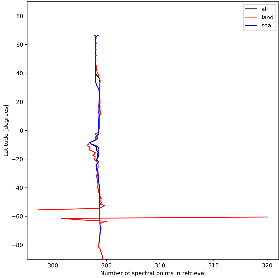
Figure 16: Zonal average of “Number of spectral points in retrieval” for 2023-11-30 to 2023-12-02.
