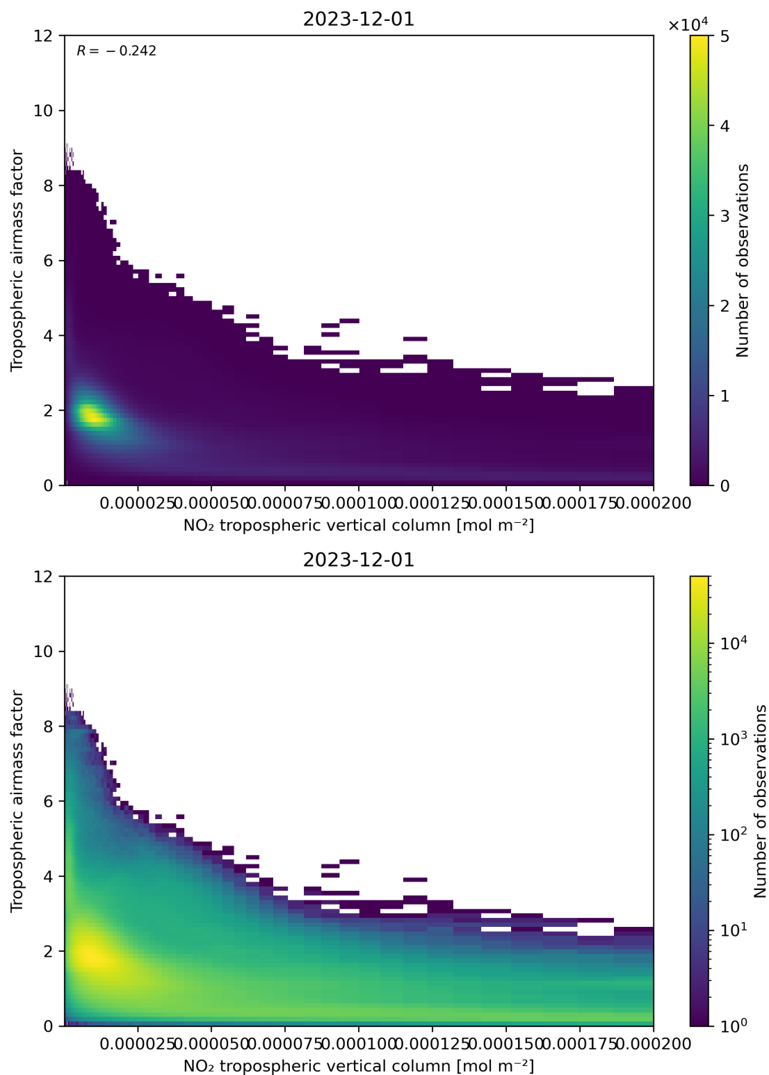
Figure 123: Scatter density plot of “NO 2 tropospheric vertical column” against “Tropospheric air mass factor” for 2023-11-30 to 2023-12-02.
