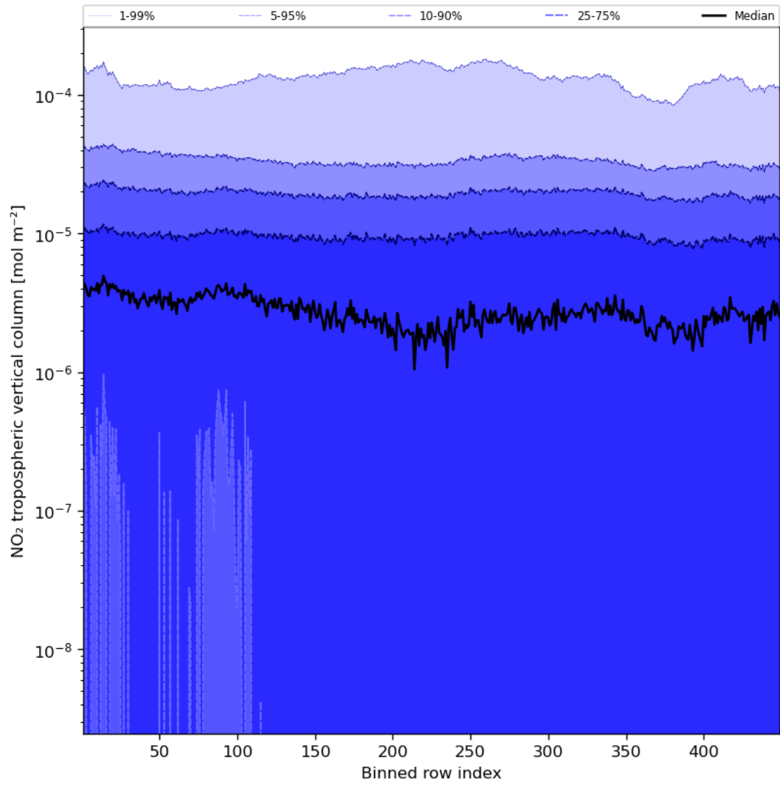
Figure 46: Along track statistics of “NO 2 tropospheric vertical column” for 2023-11-30 to 2023-12-02
