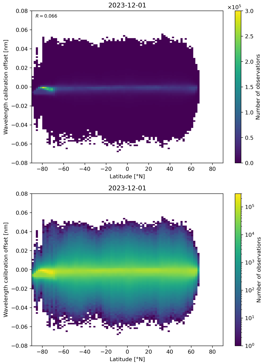
Figure 95: Scatter density plot of “Latitude” against “Wavelength calibration offset” for 2023-11-30 to 2023-12-02.
