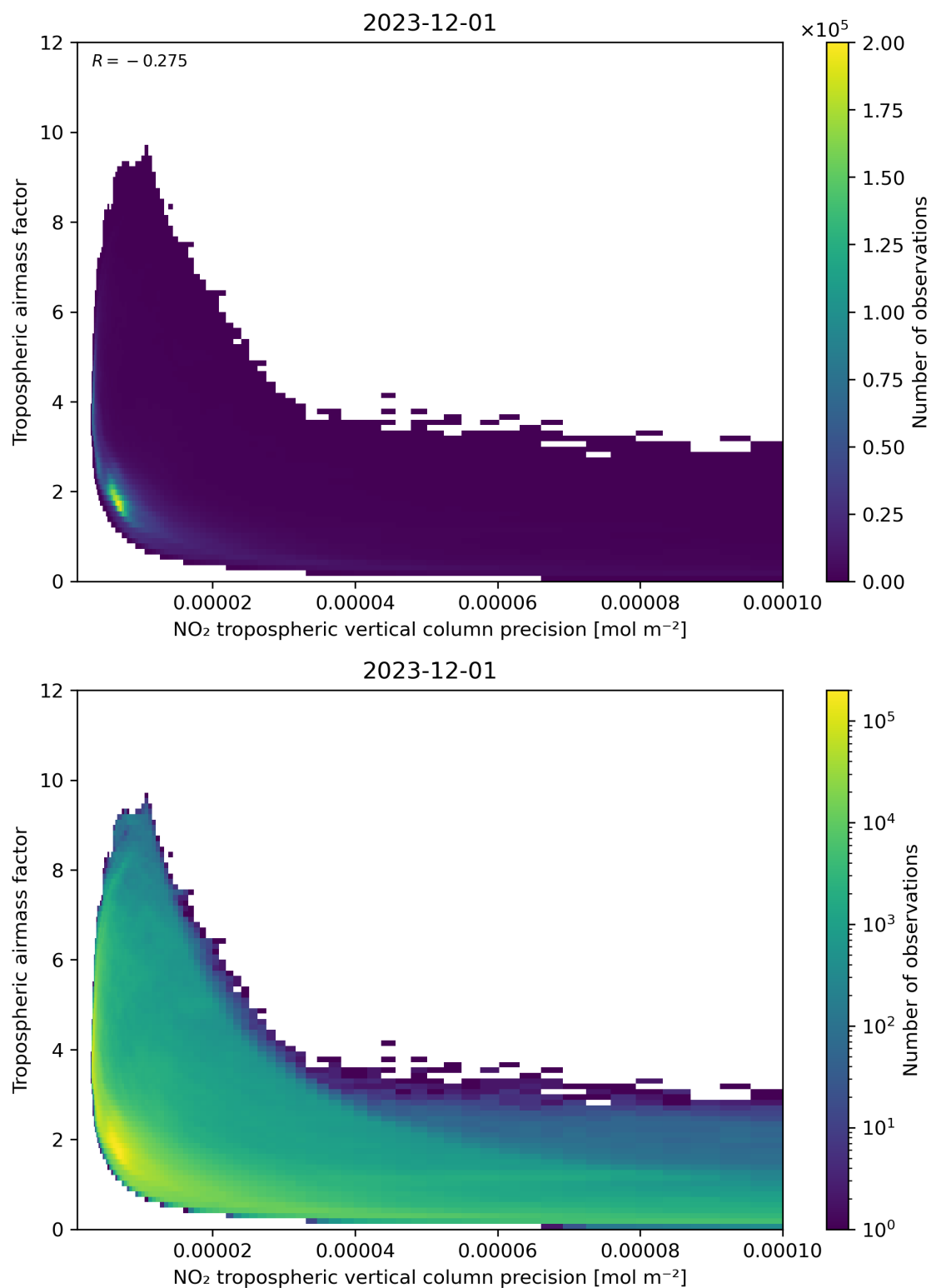
Figure 133: Scatter density plot of “NO 2 tropospheric vertical column precision” against “Tropospheric airmass factor” for 2023-11-30 to 2023-12-02.
