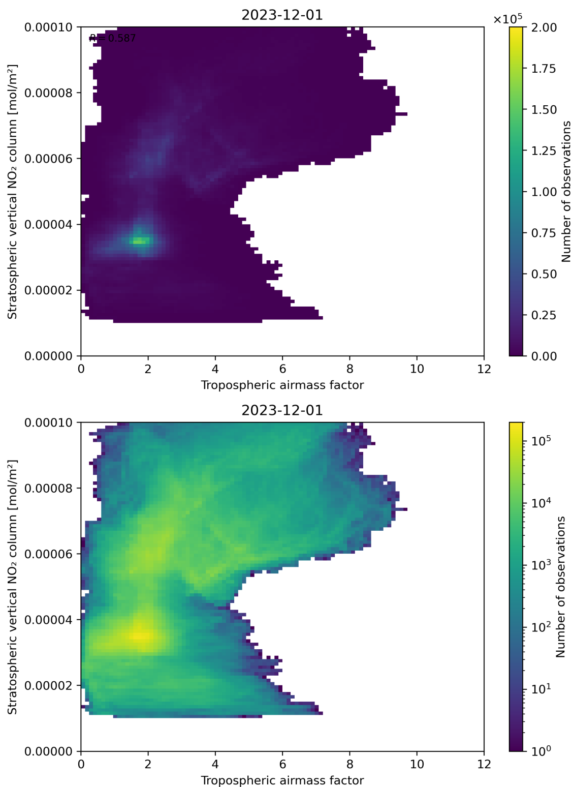
Figure 74: Scatter density plot of “Tropospheric air mass factor” against “Stratospheric vertical NO 2 column” for 2023-11-30 to 2023-12-02.
