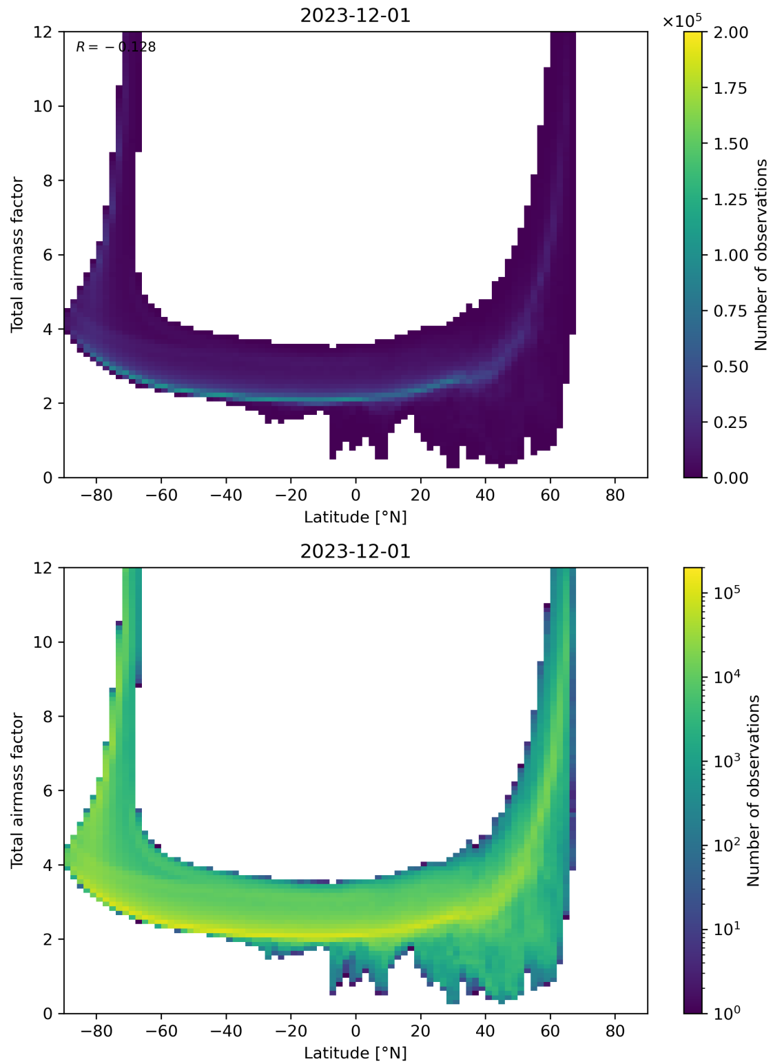
Figure 84: Scatter density plot of “Latitude” against “Total airmass factor” for 2023-11-30 to 2023-12-02.
