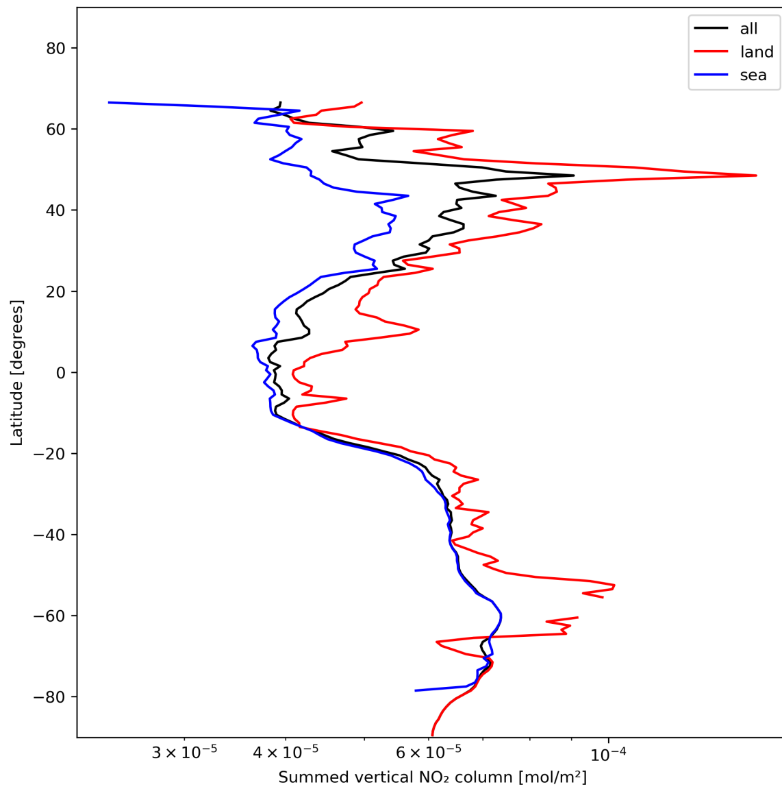
Figure 23: Zonal average of “Summed vertical NO 2 column” for 2023-11-30 to 2023-12-02.
