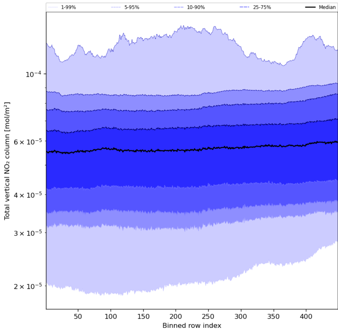
Figure 55: Along track statistics of “Total vertical NO 2 column” for 2023-11-30 to 2023-12-02
