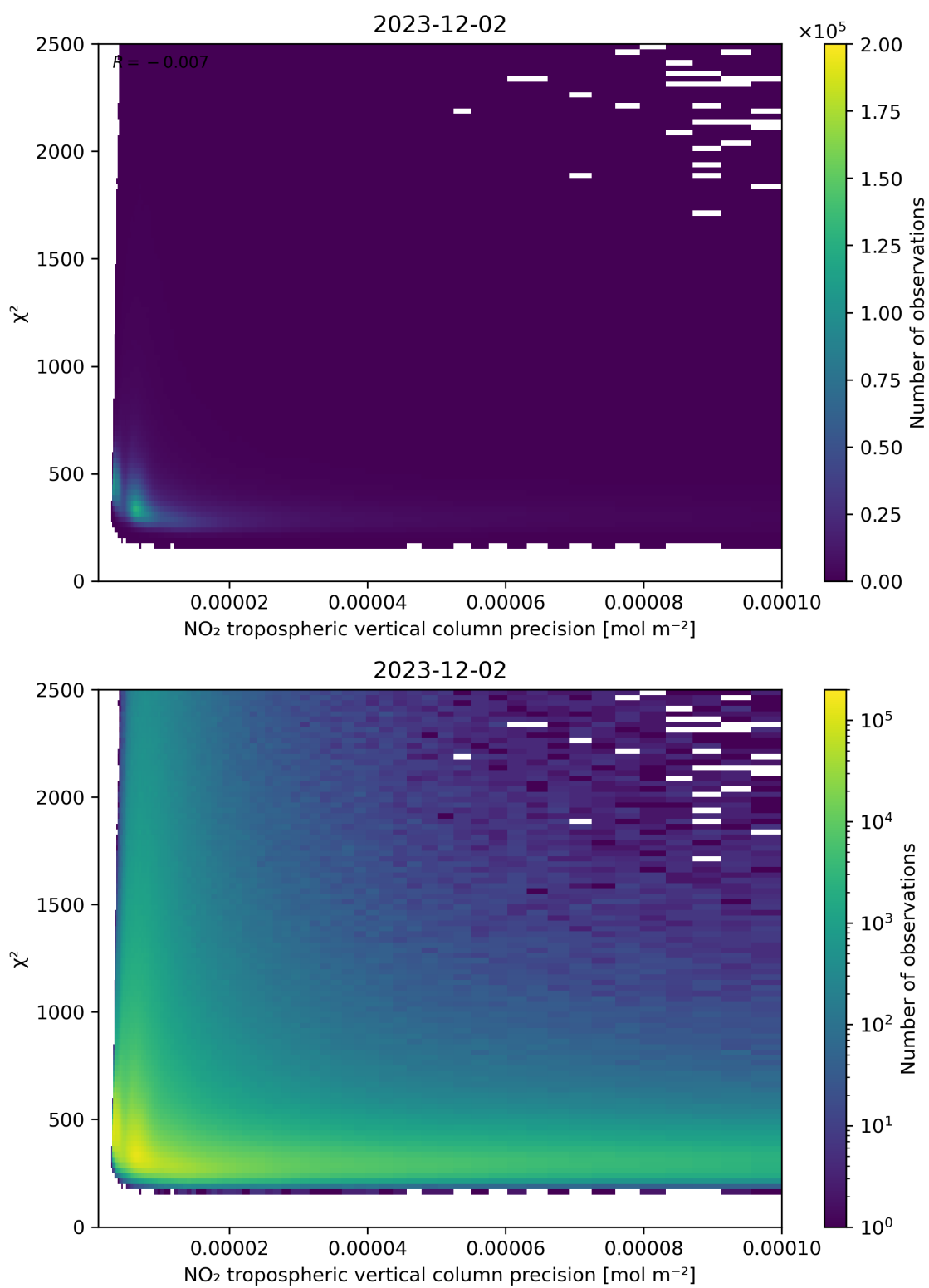
Figure 134: Scatter density plot of “NO 2 tropospheric vertical column precision” against “ \chi^2 ” for 2023-12-01 to 2023-12-03.
