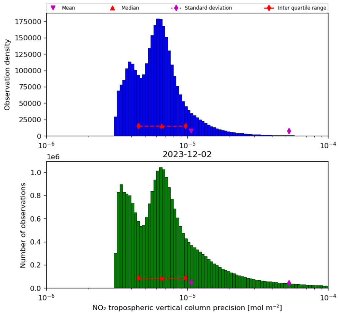
Figure 30: Histogram of “NO 2 tropospheric vertical column precision” for 2023-12-01 to 2023-12-03
