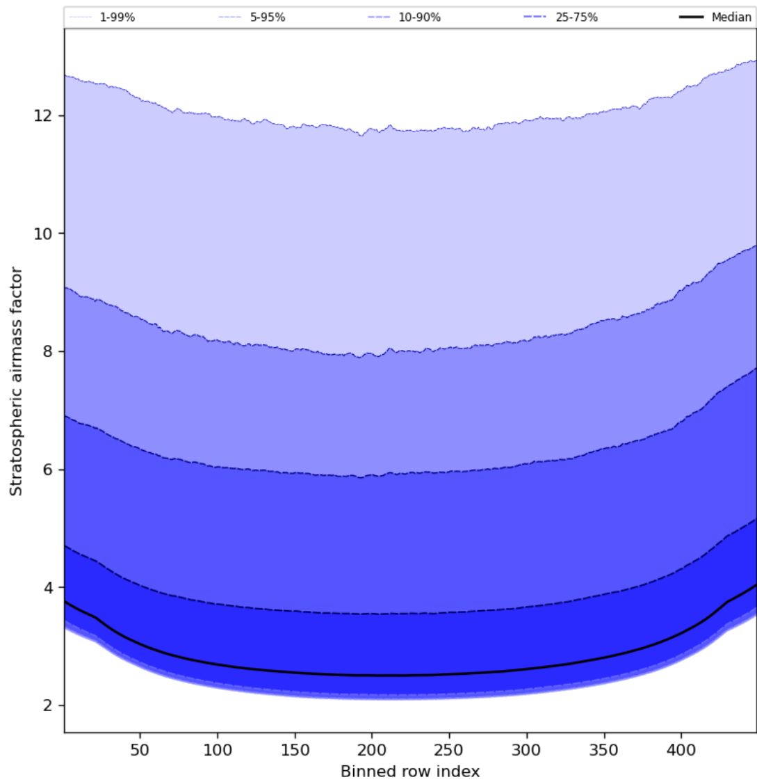
Figure 61: Along track statistics of “Stratospheric airmass factor” for 2023-12-01 to 2023-12-03
