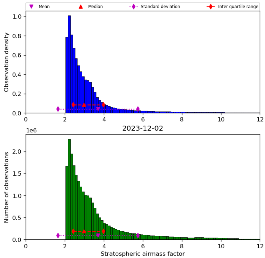
Figure 44: Histogram of “Stratospheric airmass factor” for 2023-12-01 to 2023-12-03
