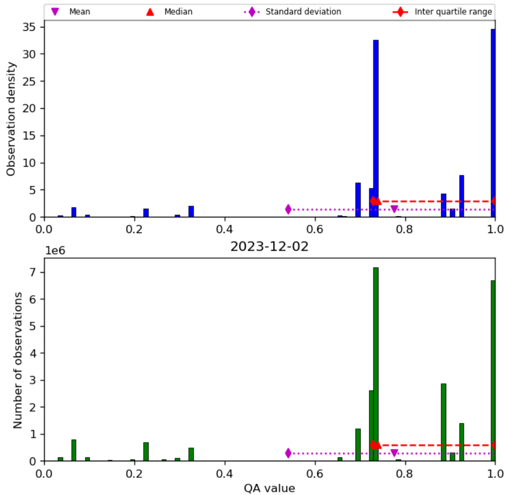
Figure 28: Histogram of “QA value” for 2023-12-01 to 2023-12-03
