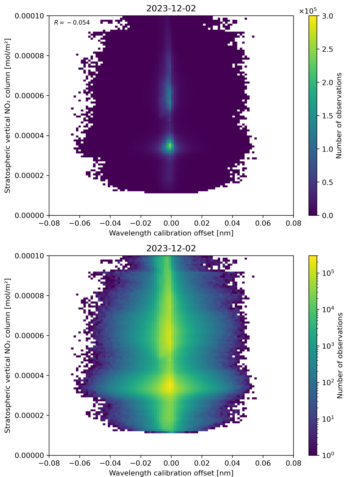
Figure 176: Scatter density plot of “Wavelength calibration offset” against “Stratospheric vertical NO 2 column” for 2023-12-01 to 2023-12-03.
