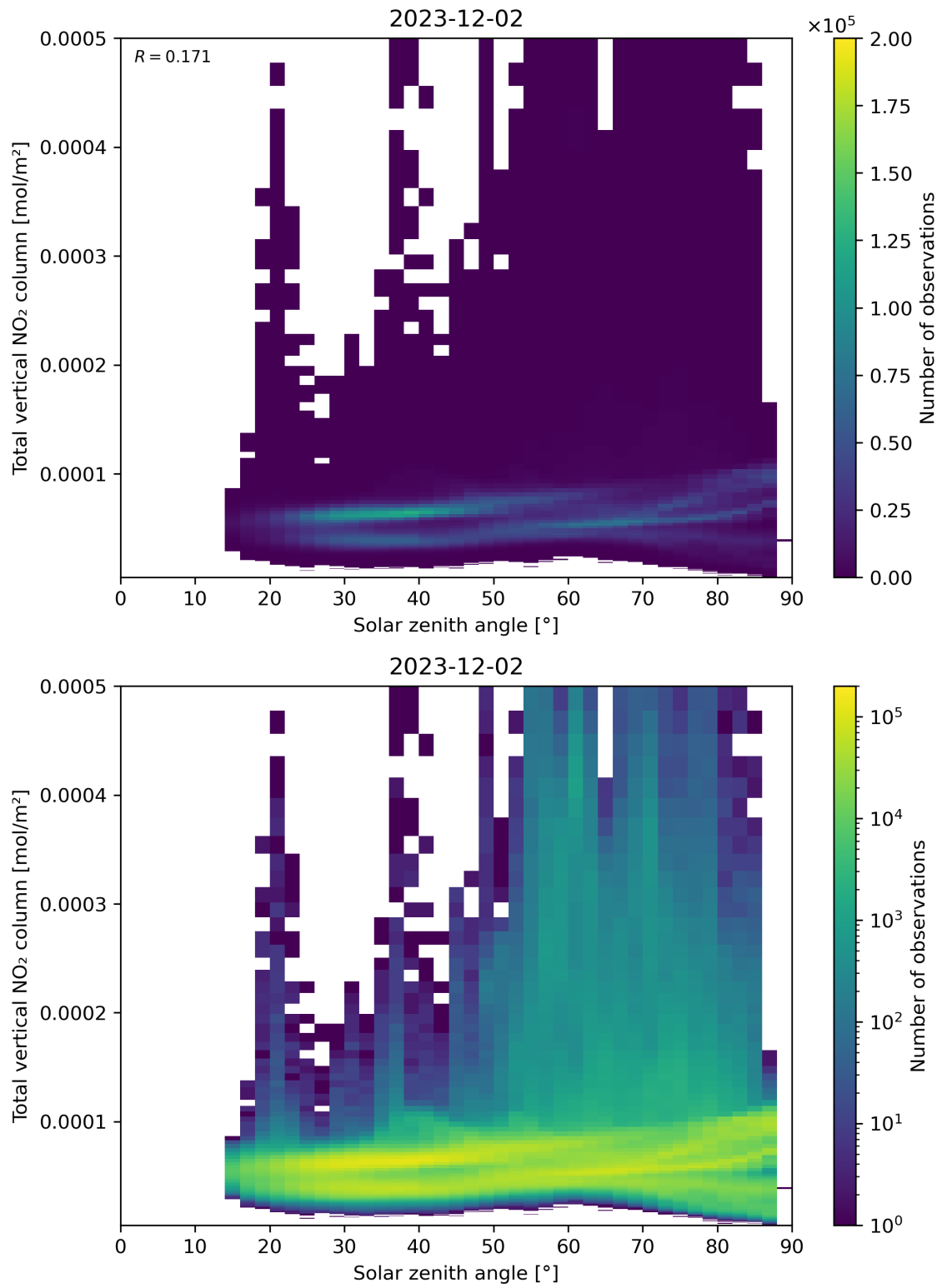
Figure 153: Scatter density plot of “Solar zenith angle” against “Total vertical NO 2 column” for 2023-12-01 to 2023-12-03.
