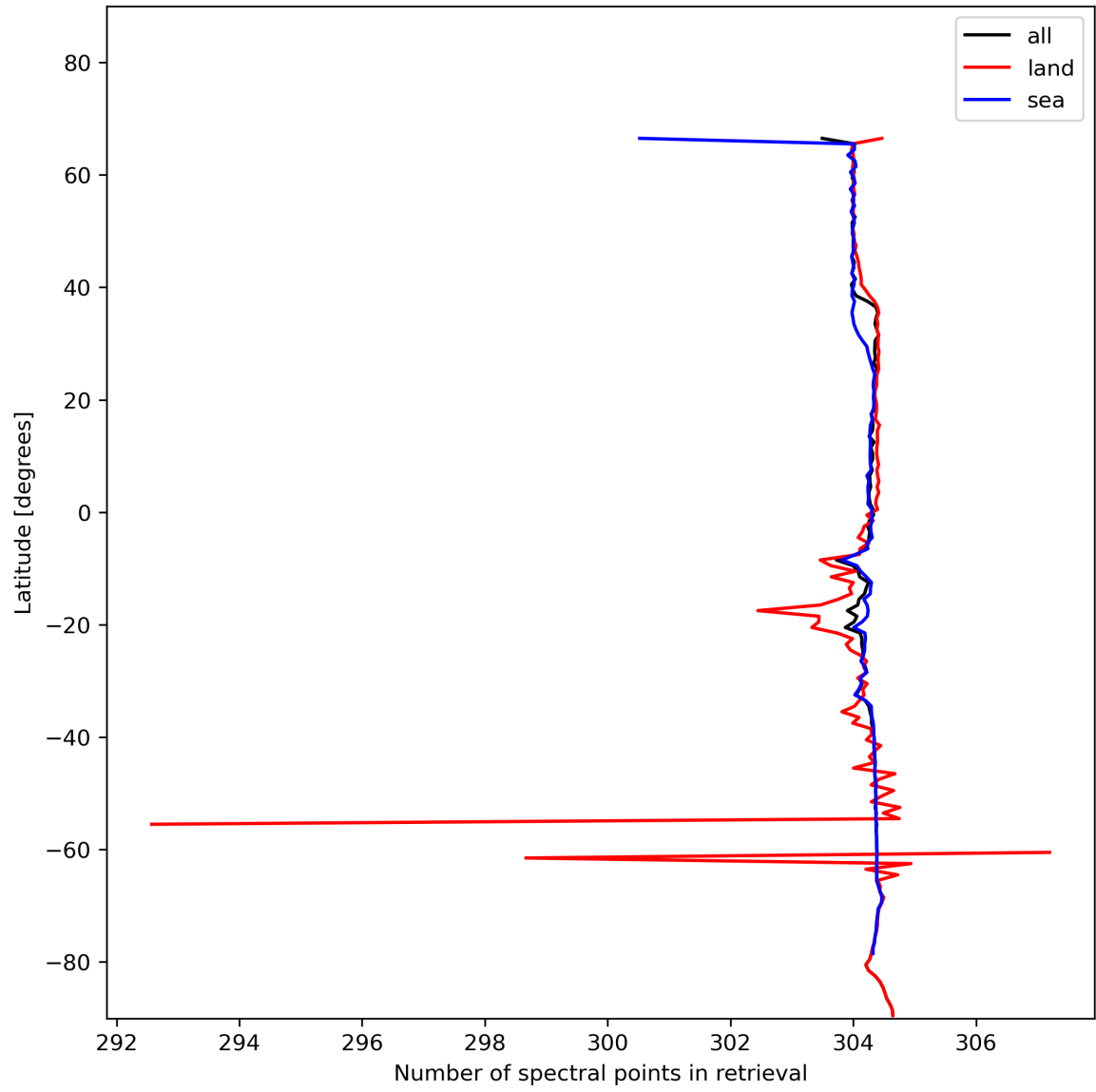
Figure 16: Zonal average of “Number of spectral points in retrieval” for 2023-12-01 to 2023-12-03.
