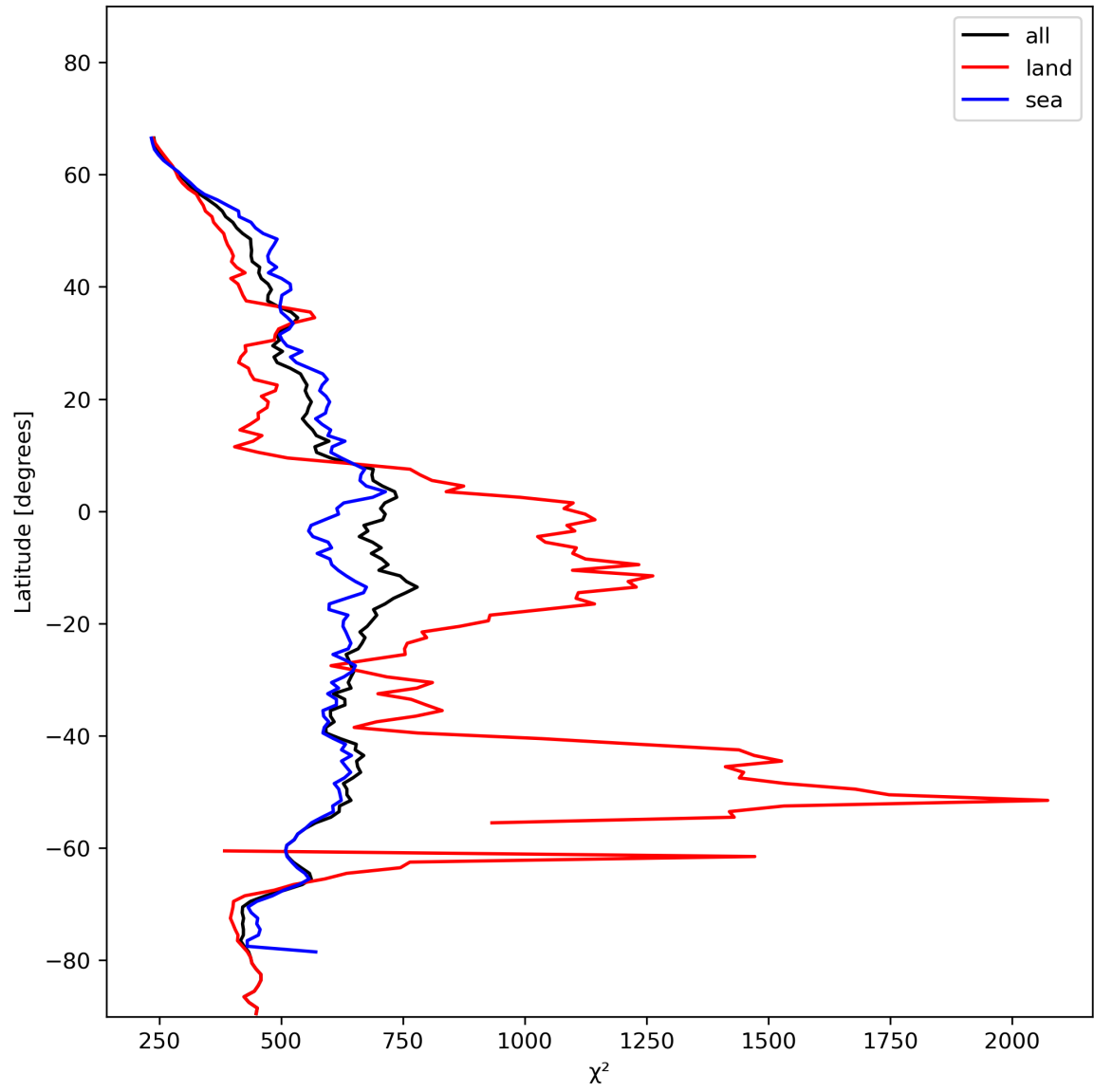
Figure 25: Zonal average of “ \chi^2 ” for 2023-12-01 to 2023-12-03.
