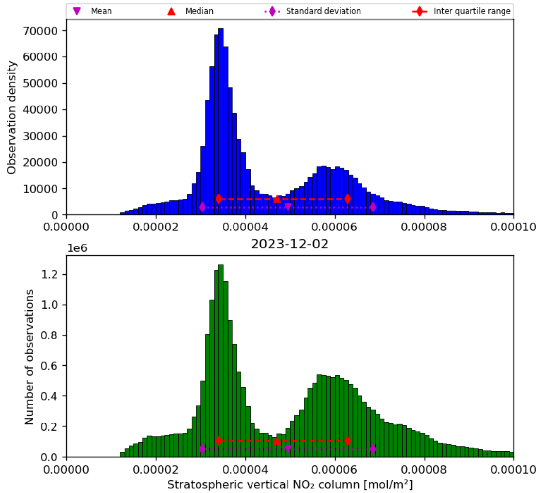
Figure 36: Histogram of “Stratospheric vertical NO 2 column” for 2023-12-01 to 2023-12-03
