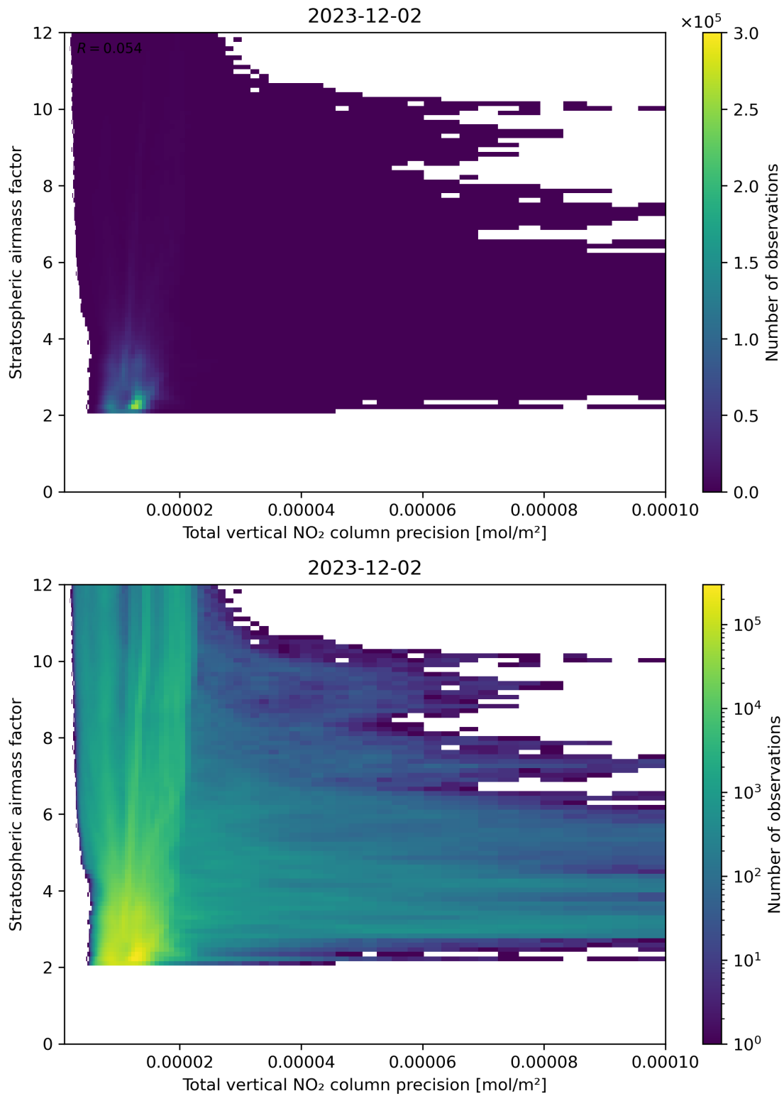
Figure 115: Scatter density plot of “Total vertical NO 2 column precision” against “Stratospheric air mass factor” for 2023-12-01 to 2023-12-03.
