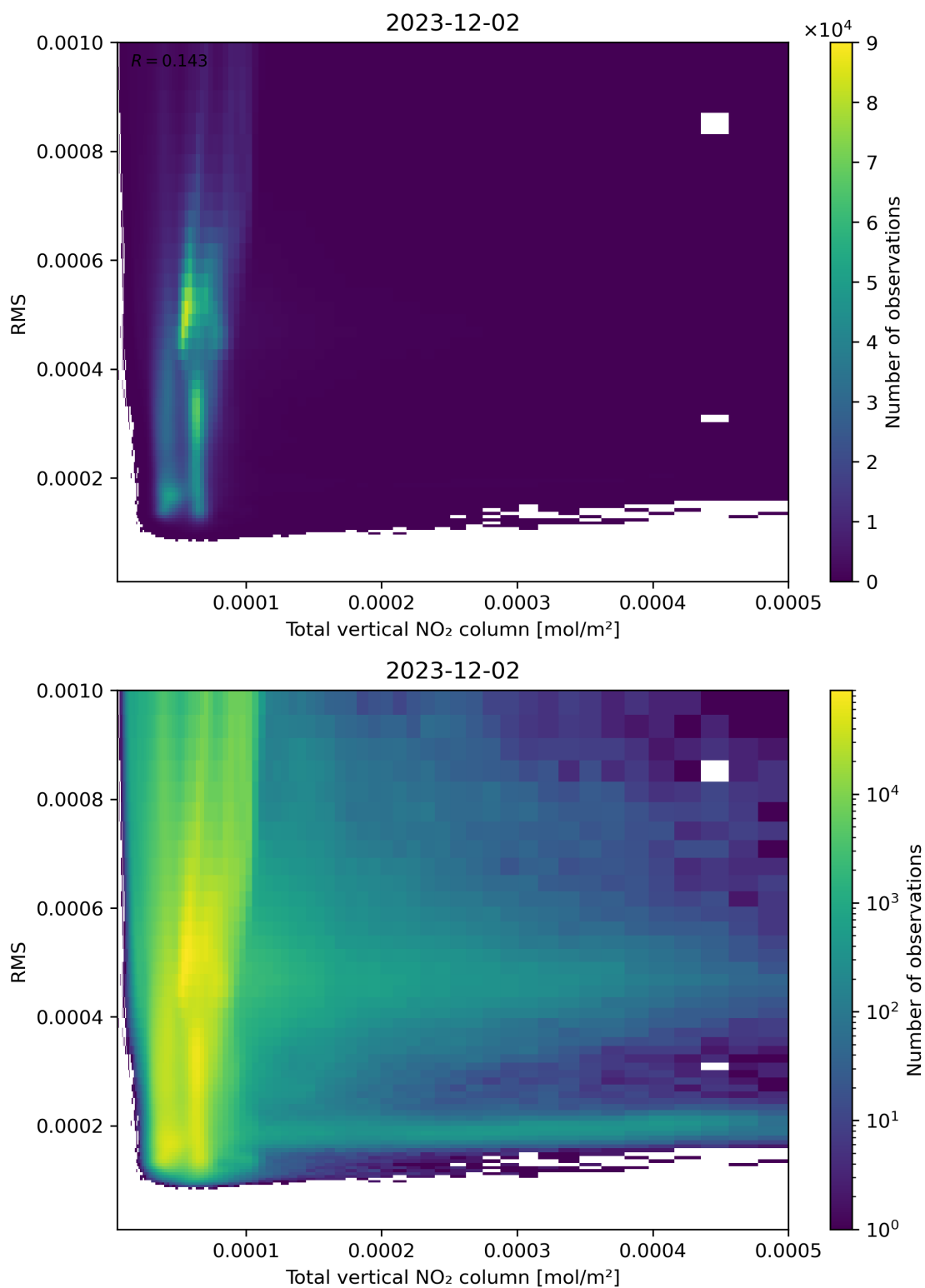
Figure 120: Scatter density plot of “Total vertical NO 2 column” against “RMS” for 2023-12-01 to 2023-12-03.
