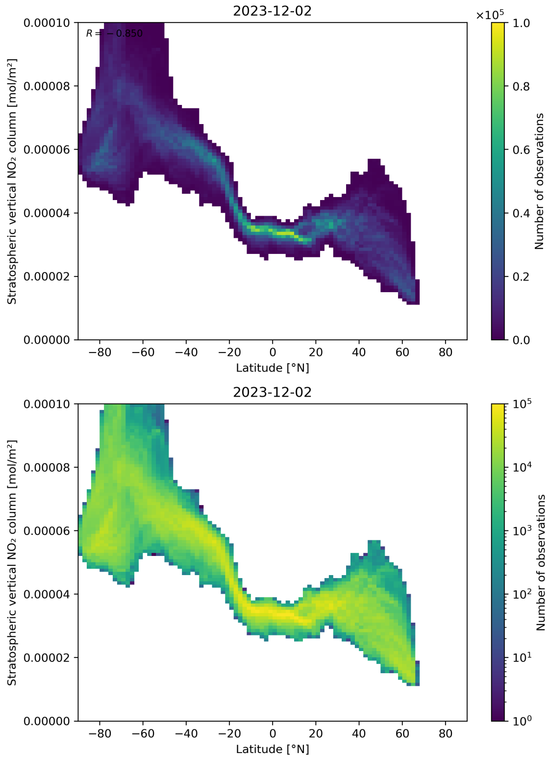
Figure 87: Scatter density plot of “Latitude” against “Stratospheric vertical NO 2 column” for 2023-12-01 to 2023-12-03.
