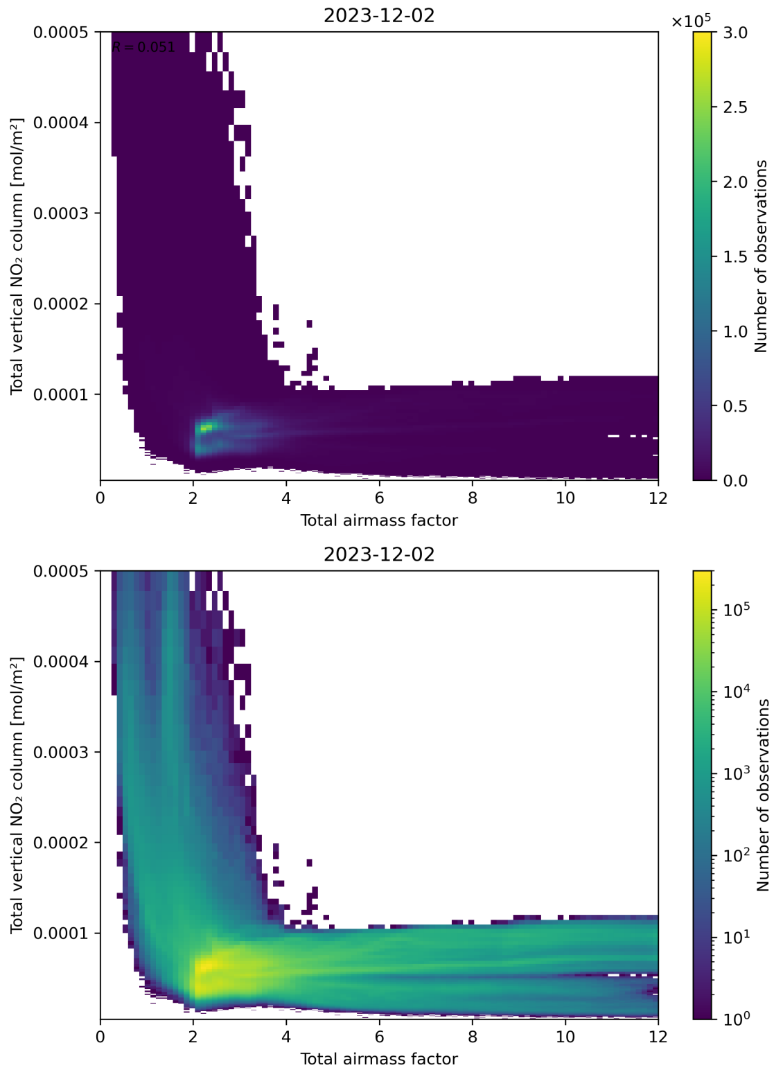
Figure 67: Scatter density plot of “Total airmass factor” against “Total vertical NO 2 column” for 2023-12-01 to 2023-12-03.
