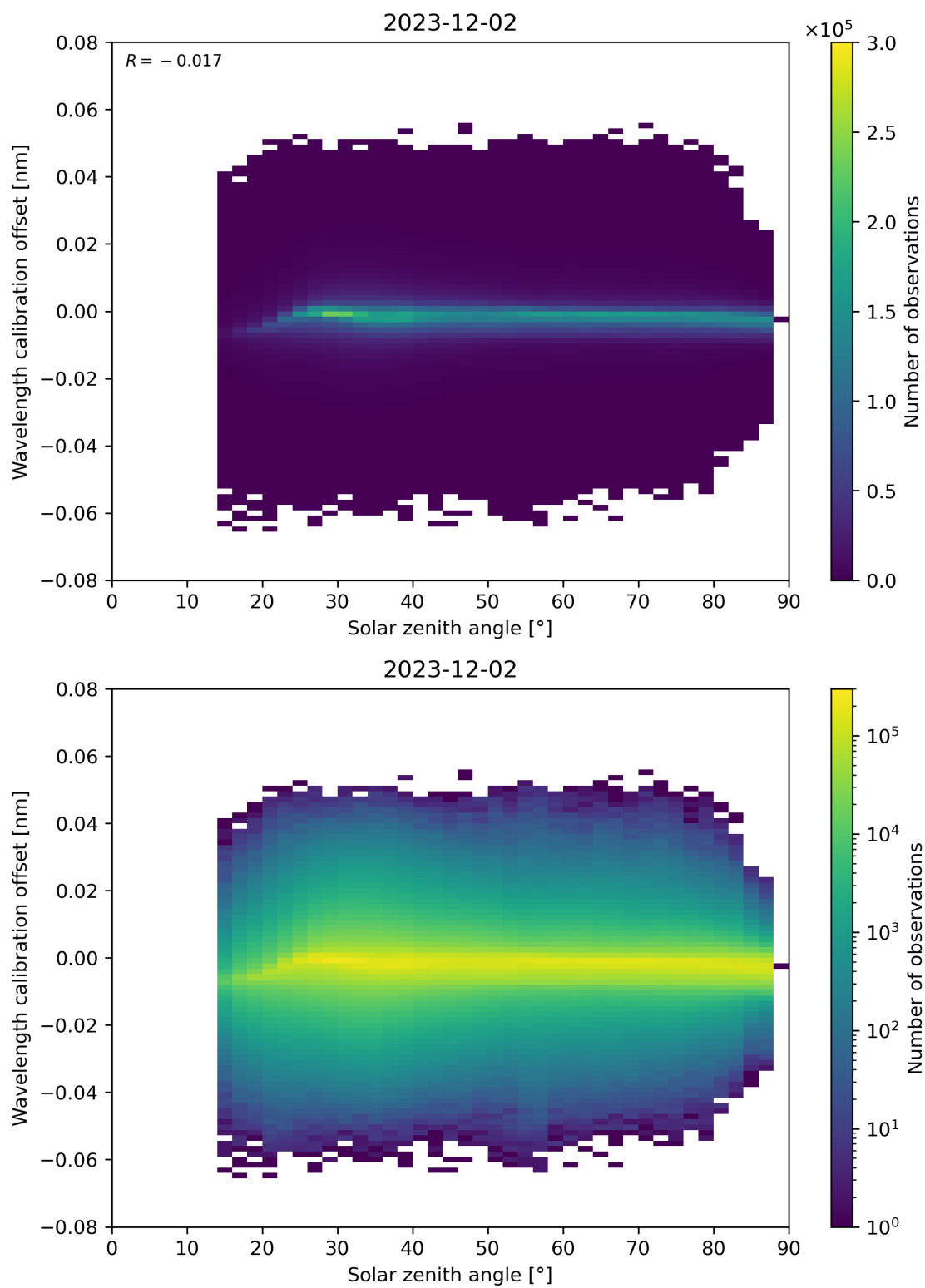
Figure 158: Scatter density plot of “Solar zenith angle” against “Wavelength calibration offset” for 2023-12-01 to 2023-12-03.
