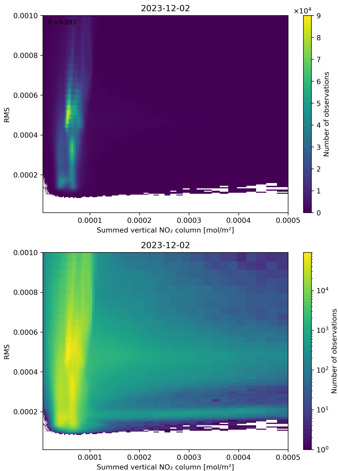
Figure 109: Scatter density plot of “Summed vertical NO 2 column” against “RMS” for 2023-12-01 to 2023-12-03.
