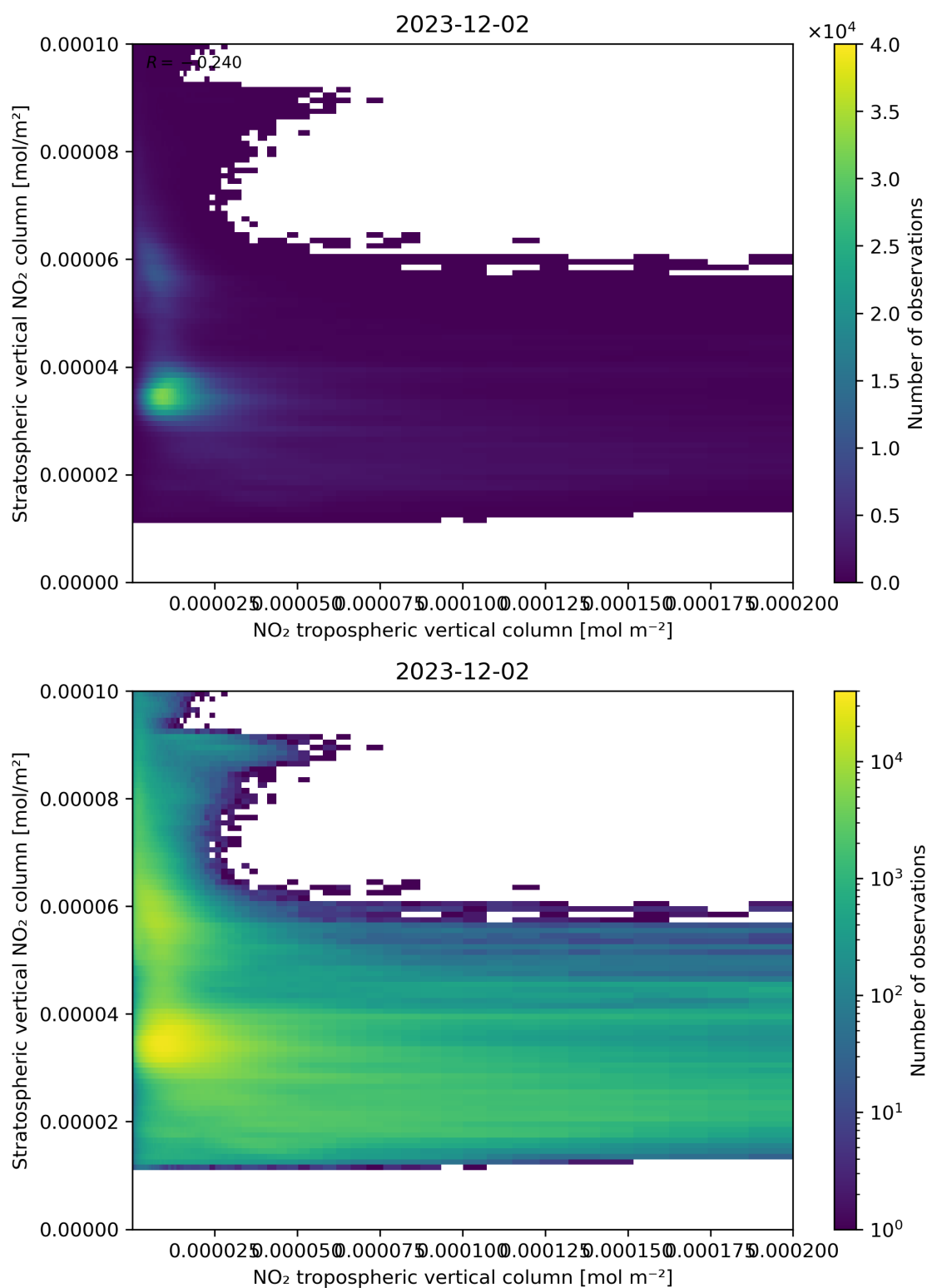
Figure 125: Scatter density plot of “NO 2 tropospheric vertical column” against “Stratospheric vertical NO 2 column” for 2023-12-01 to 2023-12-03.
