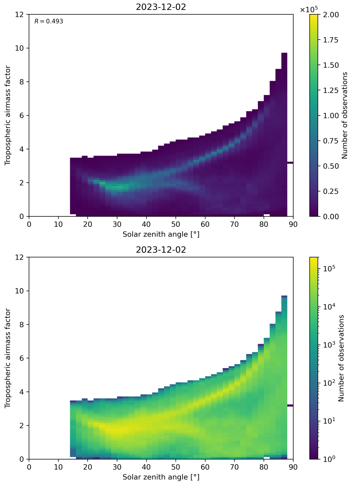
Figure 147: Scatter density plot of “Solar zenith angle” against “Tropospheric airmass factor” for 2023-12-01 to 2023-12-03.
