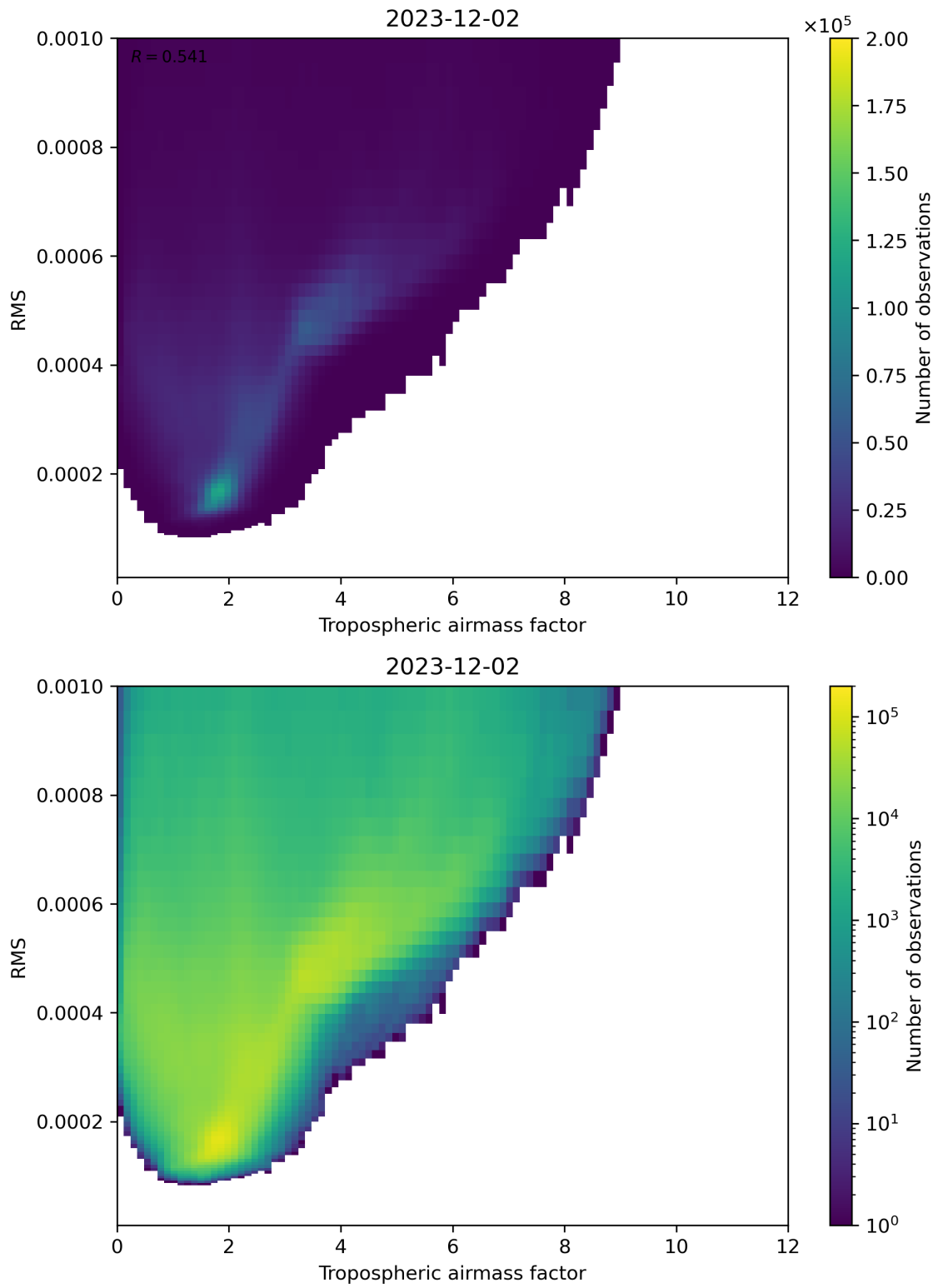
Figure 79: Scatter density plot of “Tropospheric airmass factor” against “RMS” for 2023-12-01 to 2023-12-03.
