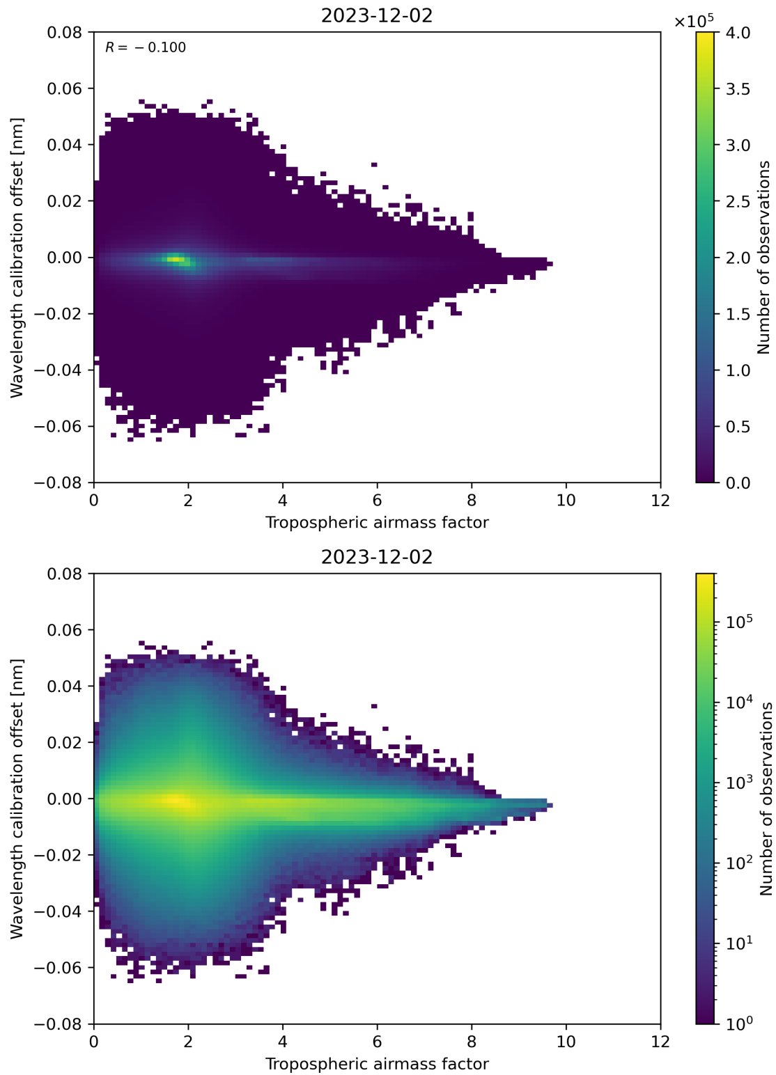
Figure 80: Scatter density plot of “Tropospheric airmass factor” against “Wavelength calibration offset” for 2023-12-01 to 2023-12-03.
