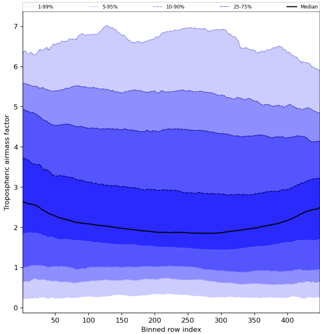
Figure 48: Along track statistics of “Tropospheric airmass factor” for 2023-12-01 to 2023-12-03
