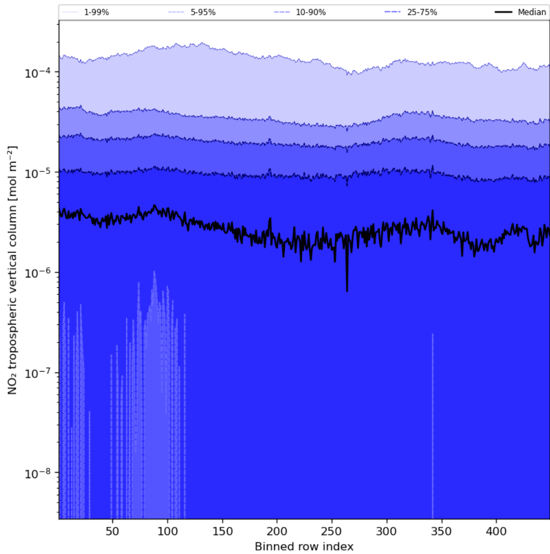
Figure 46: Along track statistics of “NO 2 tropospheric vertical column” for 2023-12-01 to 2023-12-03
