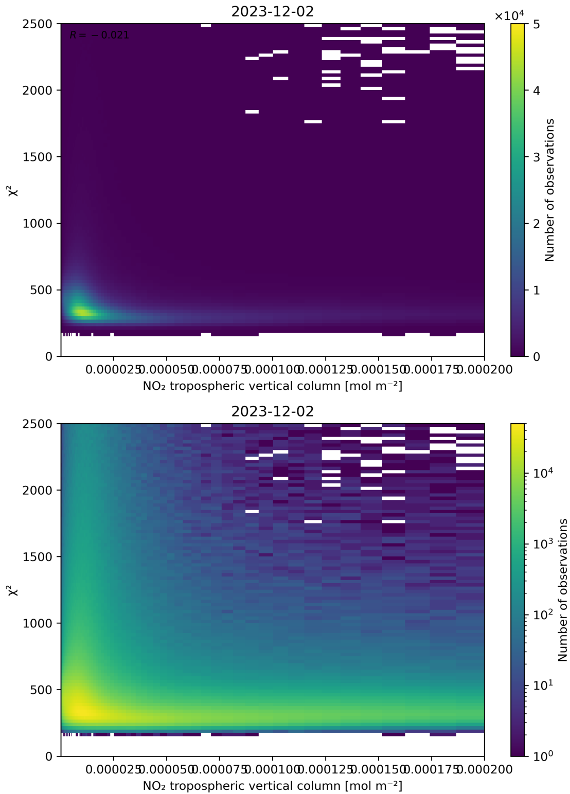
Figure 124: Scatter density plot of “NO 2 tropospheric vertical column” against “ \chi^2 ” for 2023-12-01 to 2023-12-03.
