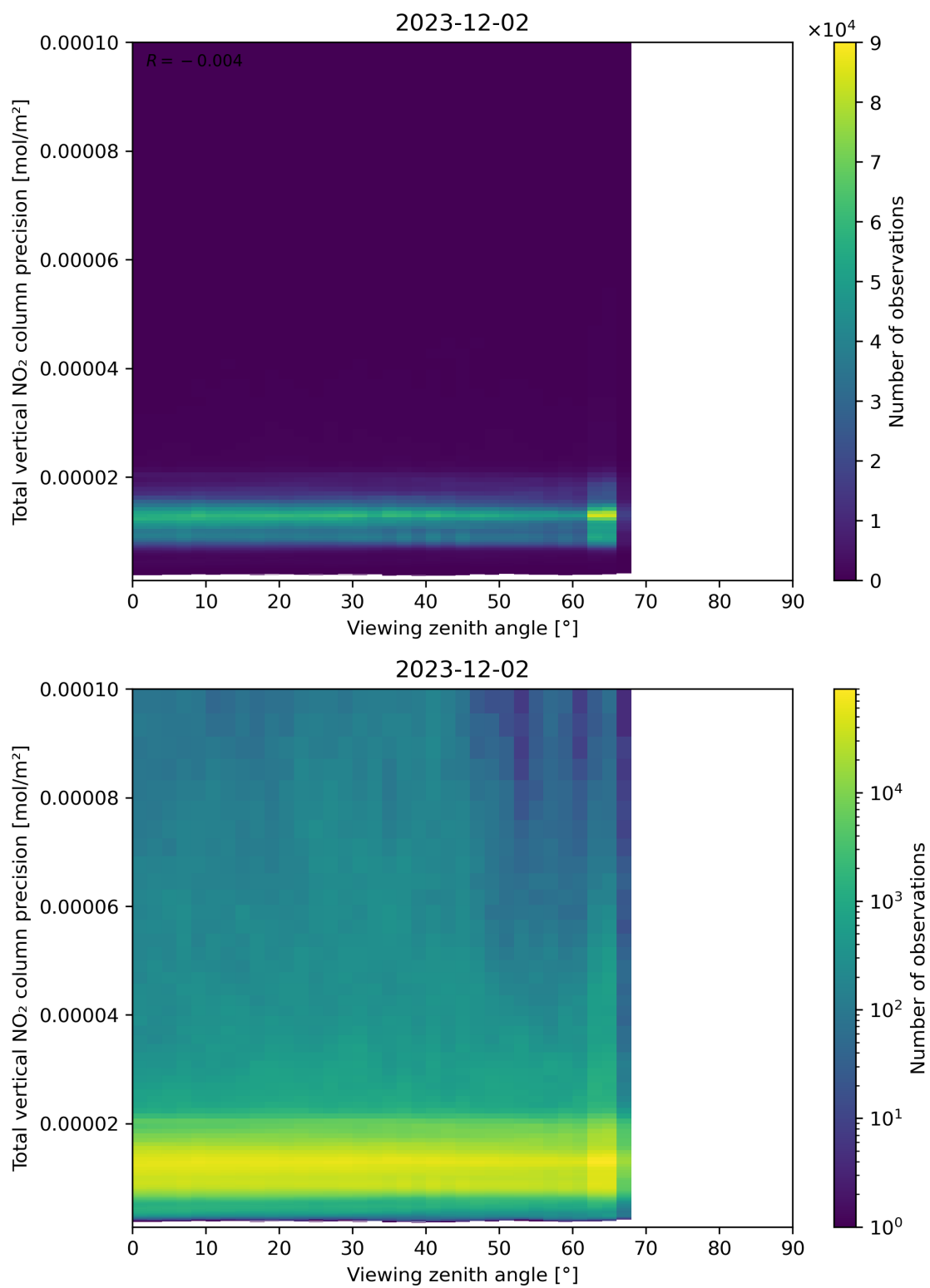
Figure 168: Scatter density plot of “Viewing zenith angle” against “Total vertical NO 2 column precision” for 2023-12-01 to 2023-12-03.
