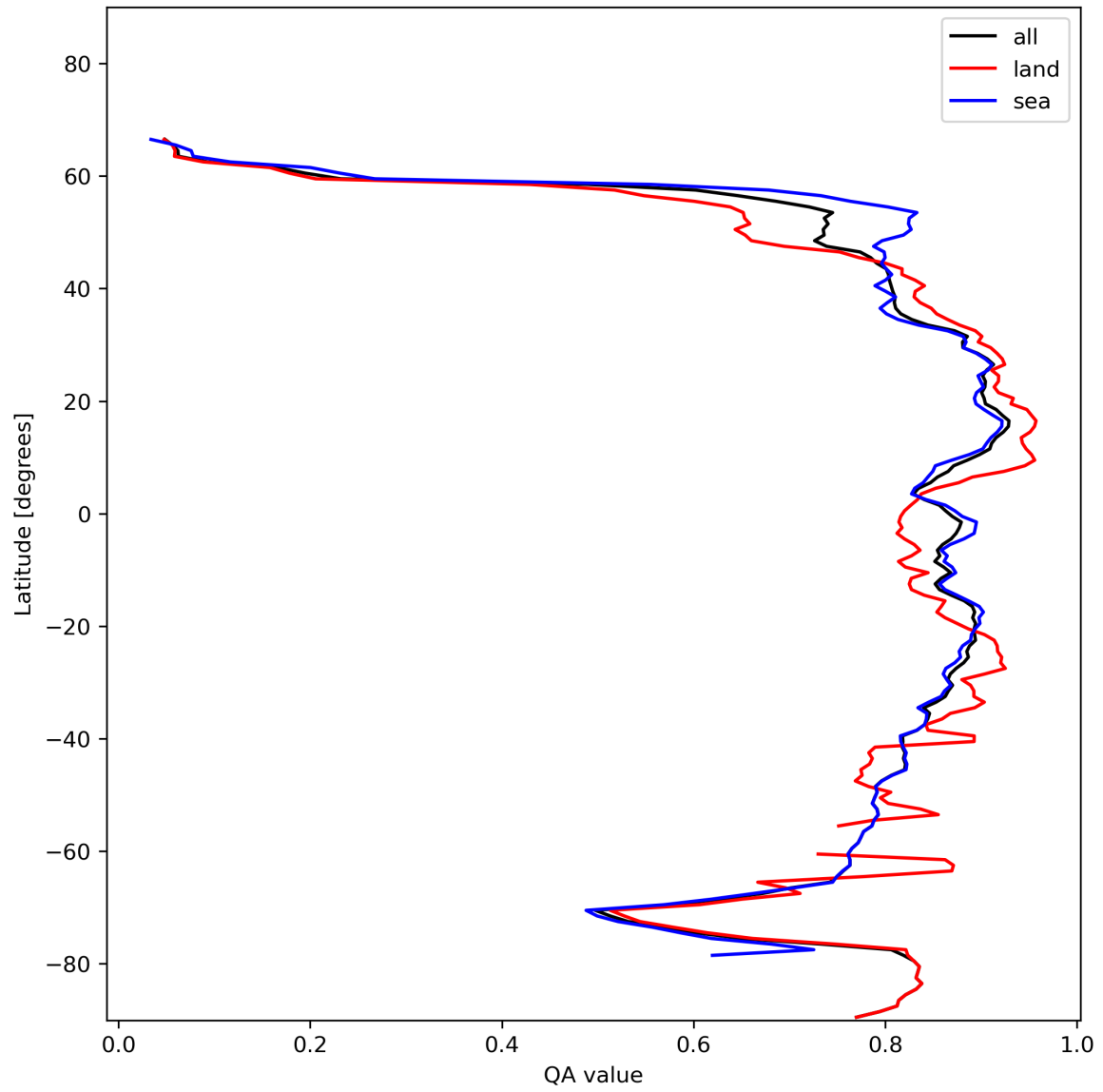
Figure 11: Zonal average of “QA value” for 2023-12-01 to 2023-12-03.
