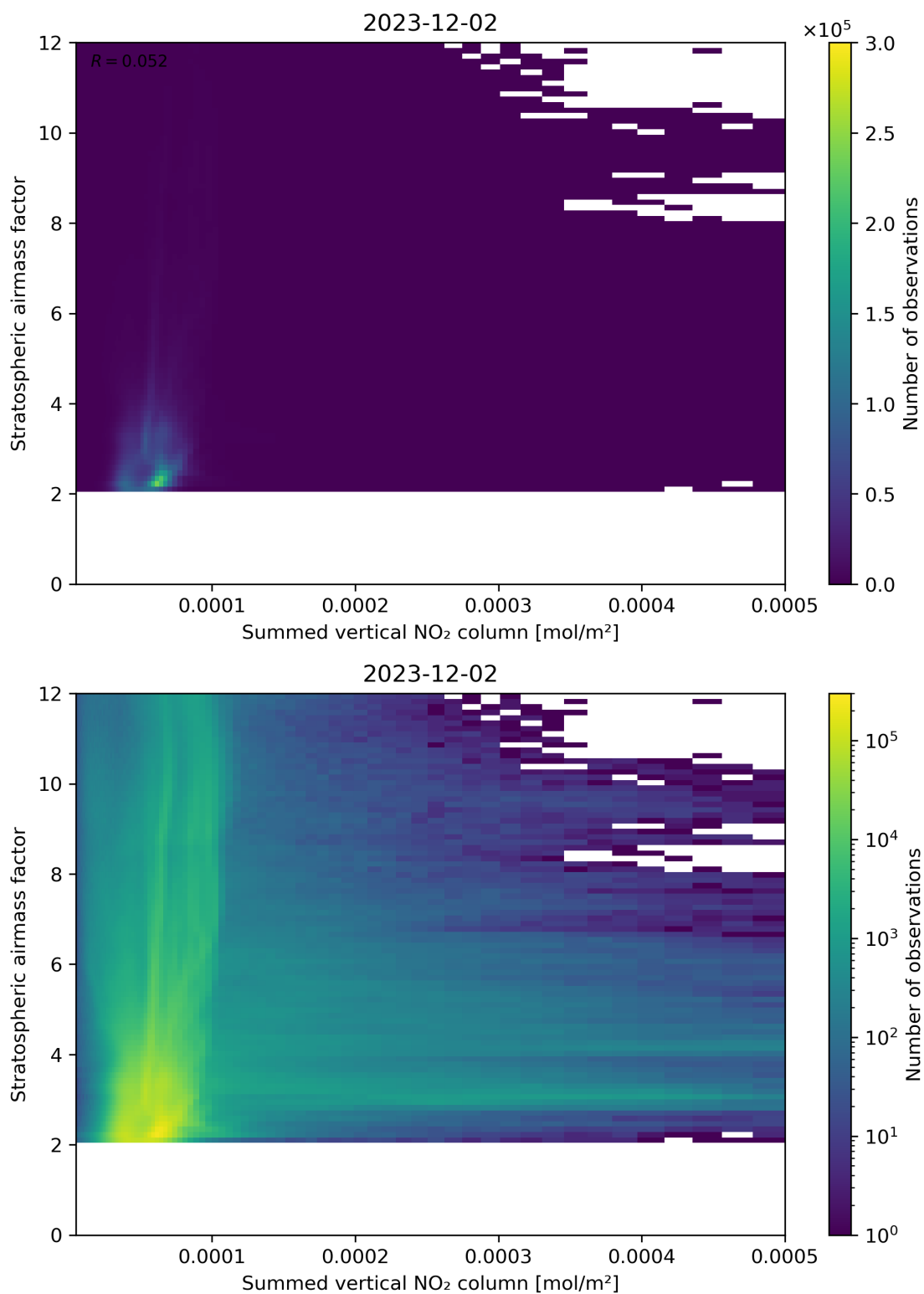
Figure 103: Scatter density plot of “Summed vertical NO 2 column” against “Stratospheric air mass factor” for 2023-12-01 to 2023-12-03.
