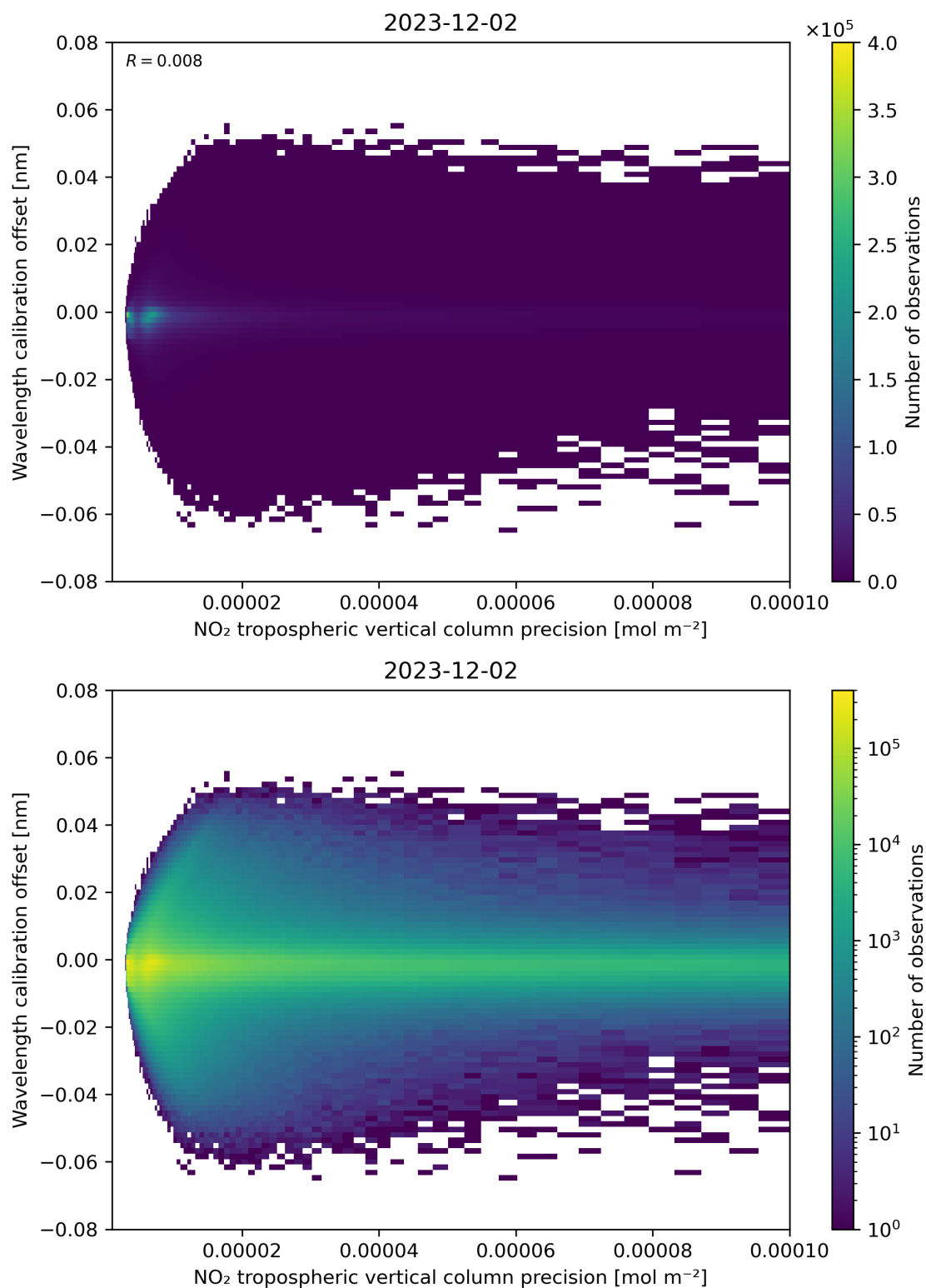
Figure 141: Scatter density plot of “NO 2 tropospheric vertical column precision” against “Wavelength calibration offset” for 2023-12-01 to 2023-12-03.
