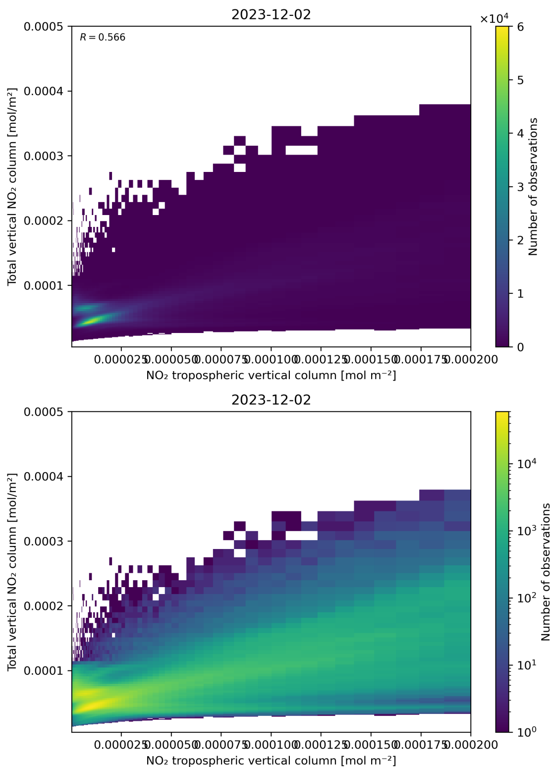
Figure 128: Scatter density plot of “NO 2 tropospheric vertical column” against “Total vertical NO 2 column” for 2023-12-01 to 2023-12-03.
