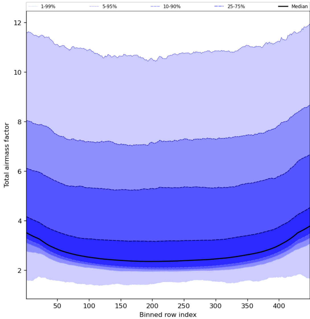
Figure 49: Along track statistics of “Total airmass factor” for 2023-12-01 to 2023-12-03
