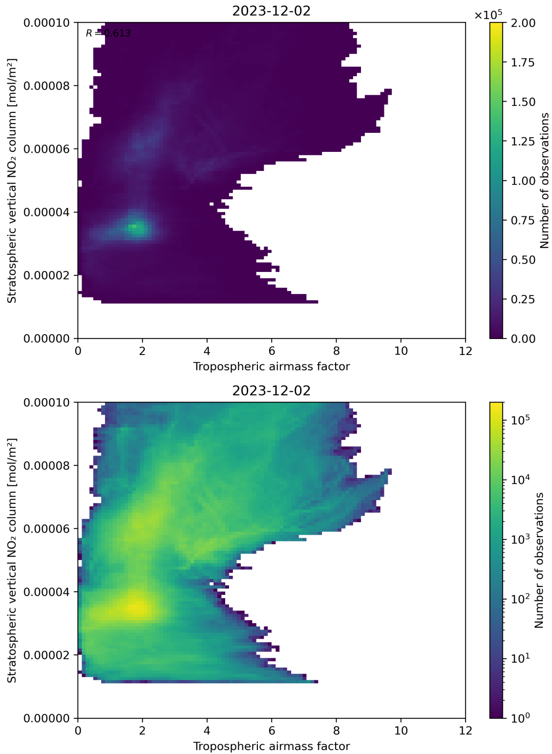
Figure 74: Scatter density plot of “Tropospheric air mass factor” against “Stratospheric vertical NO 2 column” for 2023-12-01 to 2023-12-03.
