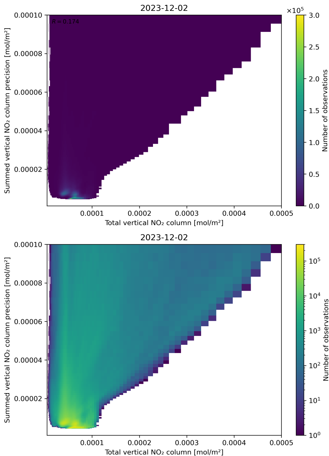
Figure 113: Scatter density plot of “Total vertical NO 2 column” against “Summed vertical NO 2 column precision” for 2023-12-01 to 2023-12-03.
