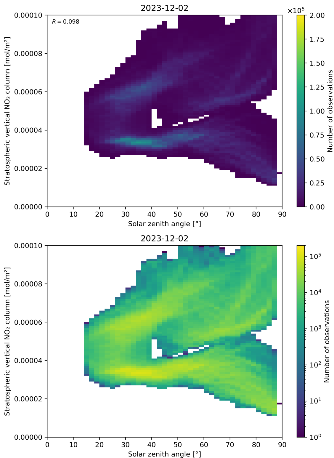
Figure 150: Scatter density plot of “Solar zenith angle” against “Stratospheric vertical NO 2 column” for 2023-12-01 to 2023-12-03.
