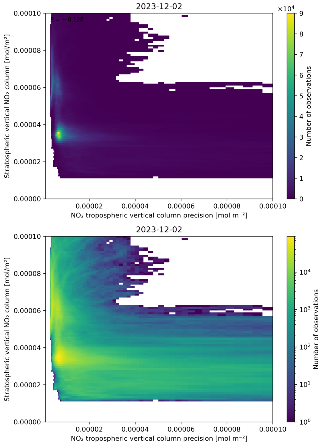
Figure 135: Scatter density plot of “NO 2 tropospheric vertical column precision” against “Stratospheric vertical NO 2 column” for 2023-12-01 to 2023-12-03.
