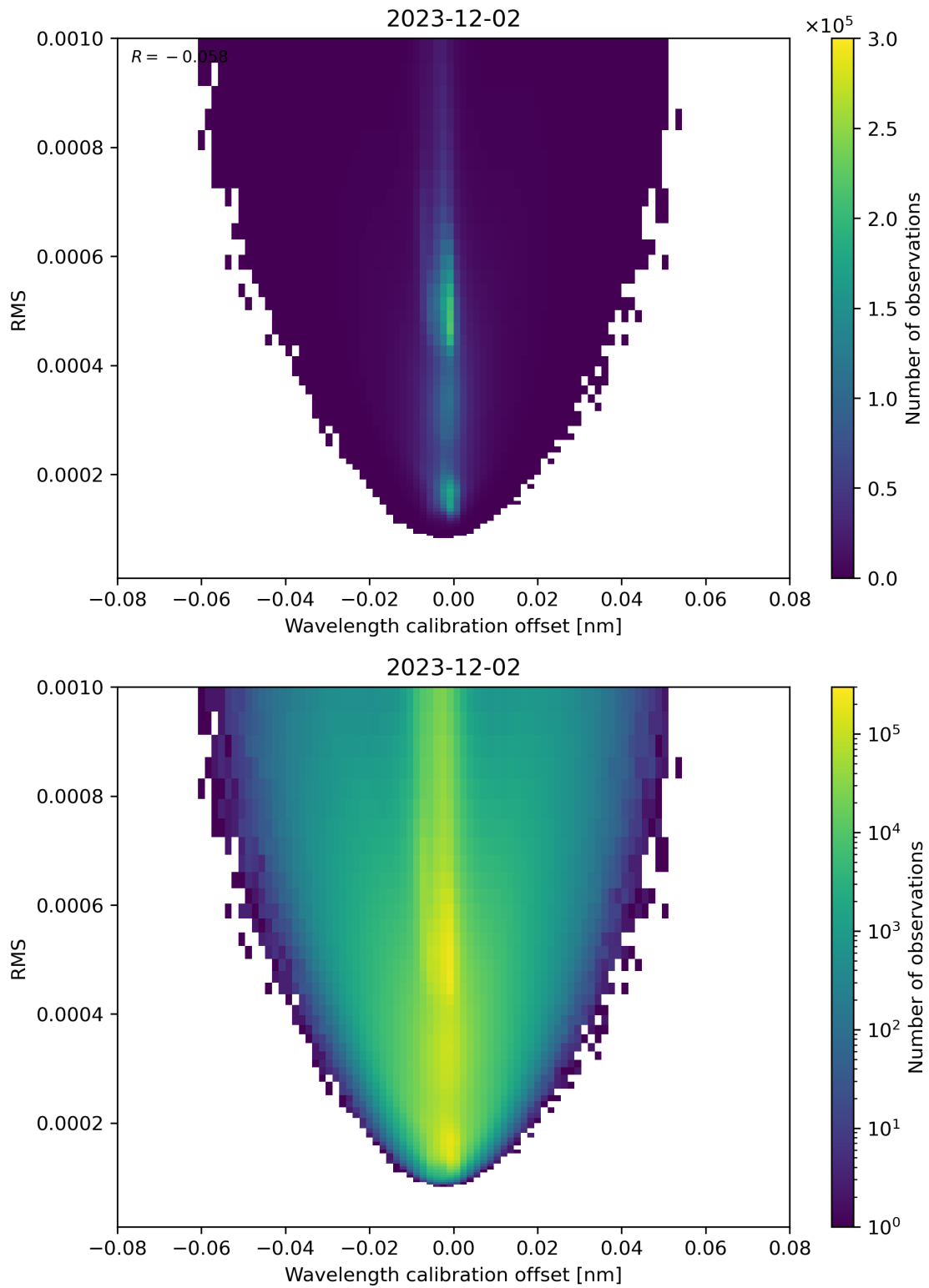
Figure 181: Scatter density plot of “Wavelength calibration offset” against “RMS” for 2023-12-01 to 2023-12-03.
