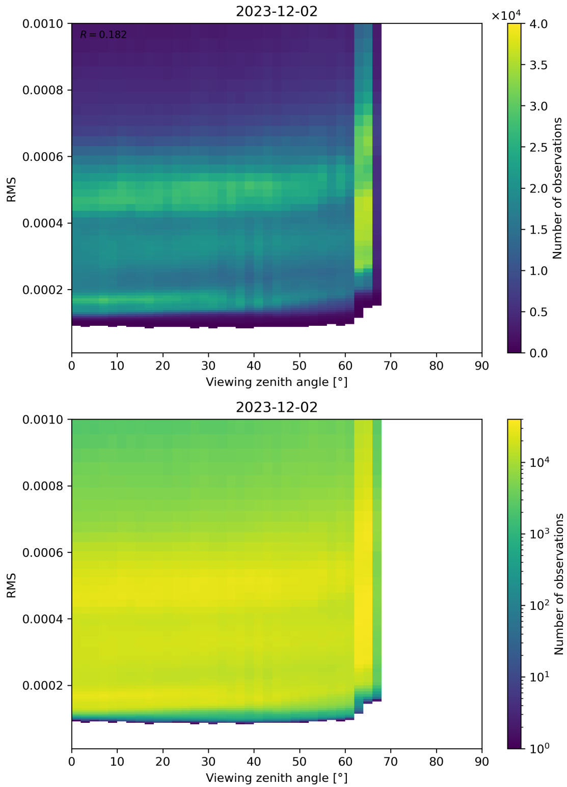
Figure 171: Scatter density plot of “Viewing zenith angle” against “RMS” for 2023-12-01 to 2023-12-03.
