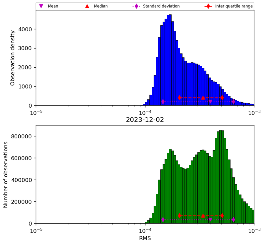
Figure 43: Histogram of “RMS” for 2023-12-01 to 2023-12-03
