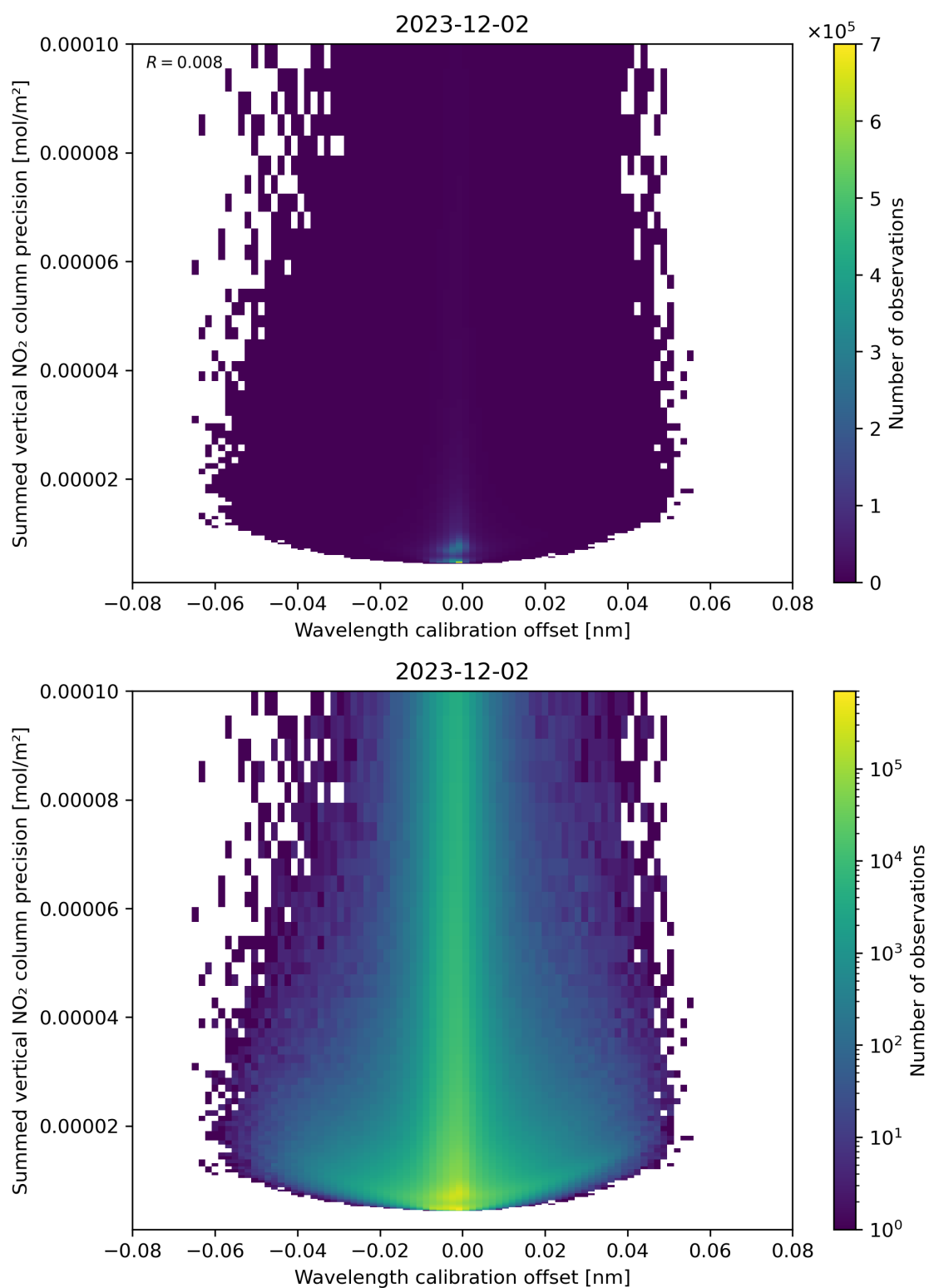
Figure 178: Scatter density plot of “Wavelength calibration offset” against “Summed vertical NO 2 column precision” for 2023-12-01 to 2023-12-03.
