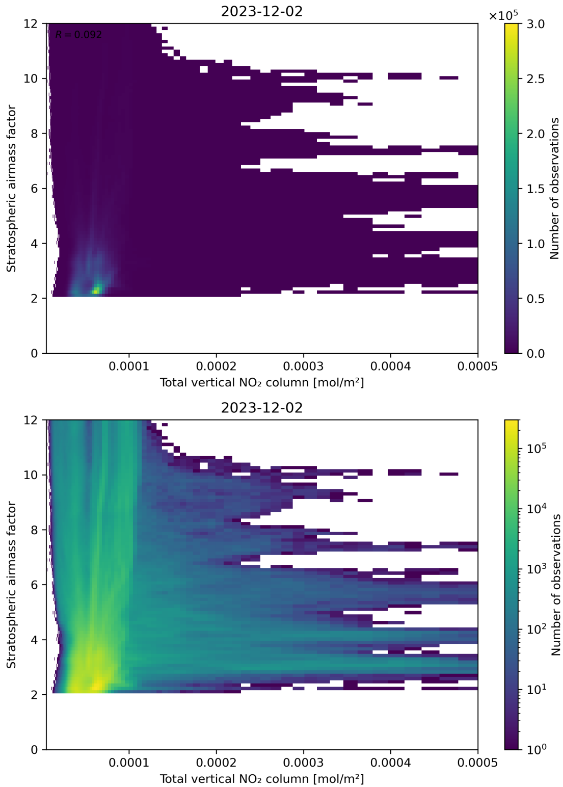
Figure 110: Scatter density plot of “Total vertical NO 2 column” against “Stratospheric airmass factor” for 2023-12-01 to 2023-12-03.
