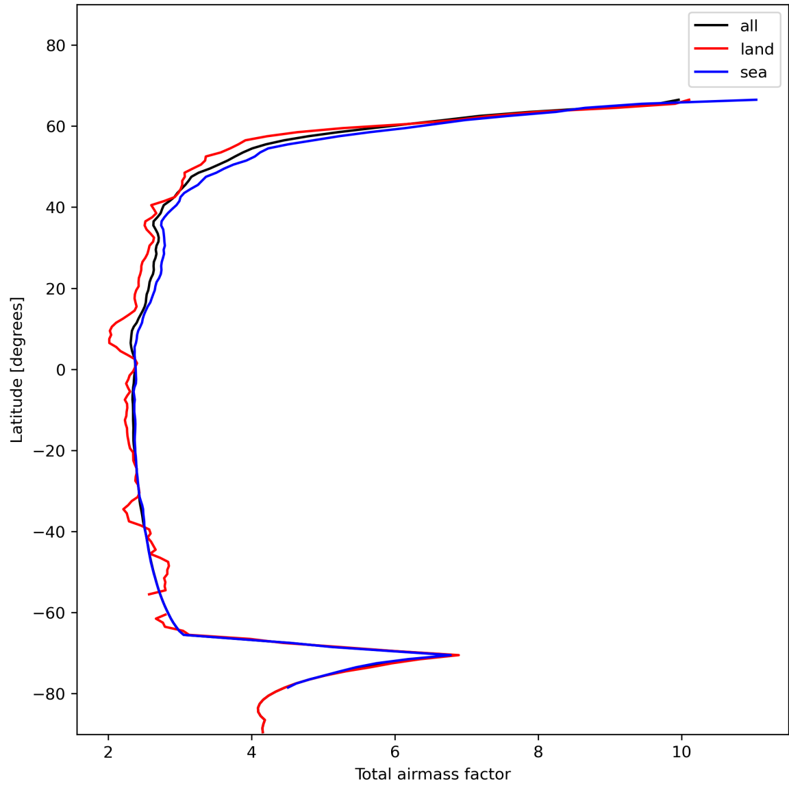
Figure 15: Zonal average of “Total airmass factor” for 2023-12-01 to 2023-12-03.
