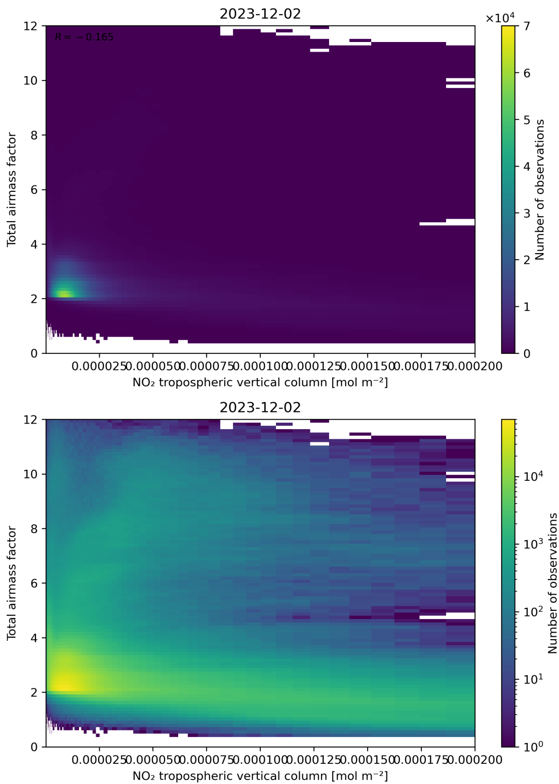
Figure 122: Scatter density plot of “NO 2 tropospheric vertical column” against “Total air mass factor” for 2023-12-01 to 2023-12-03.
