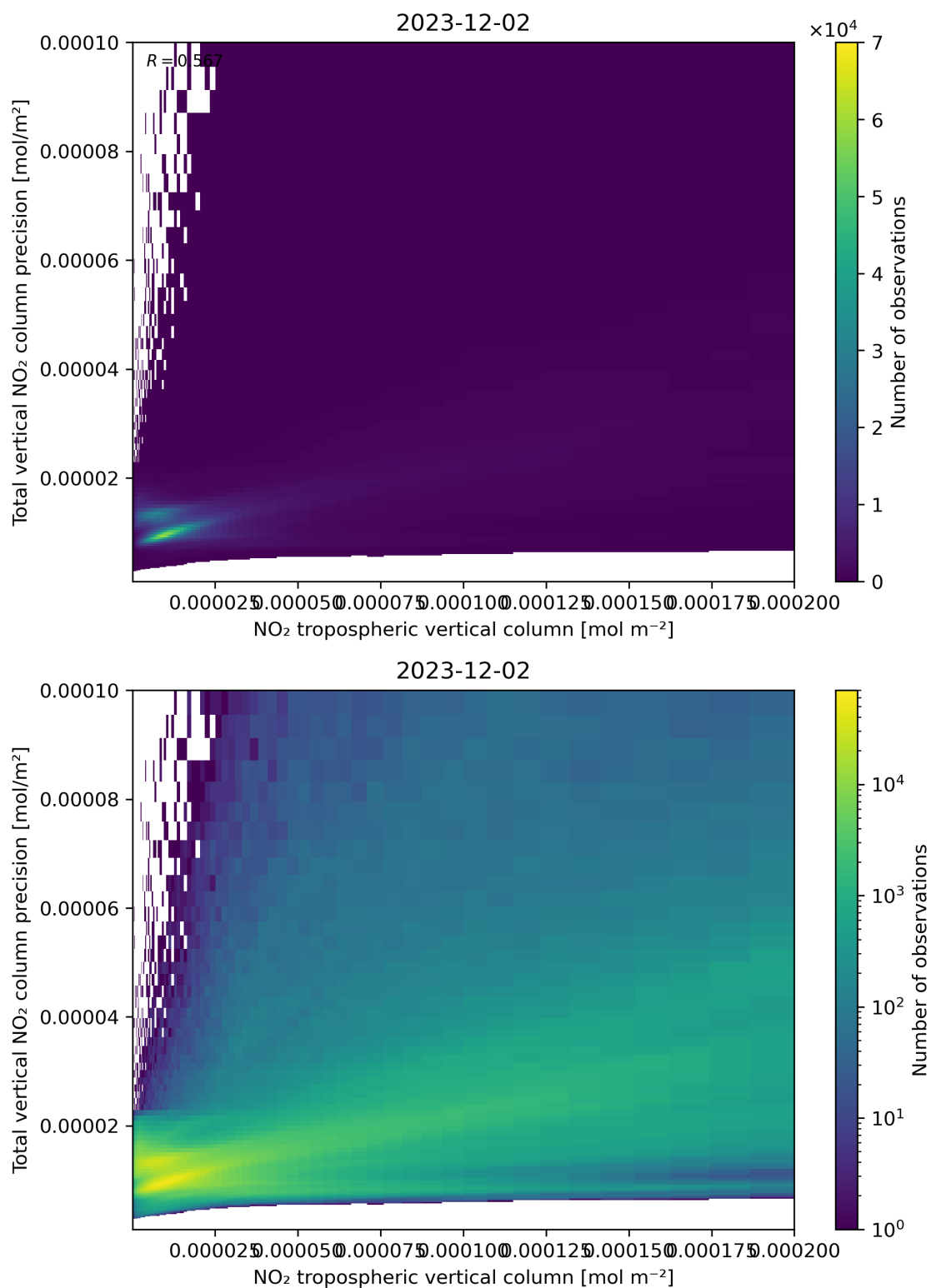
Figure 129: Scatter density plot of “NO 2 tropospheric vertical column” against “Total vertical NO 2 column precision” for 2023-12-01 to 2023-12-03.
