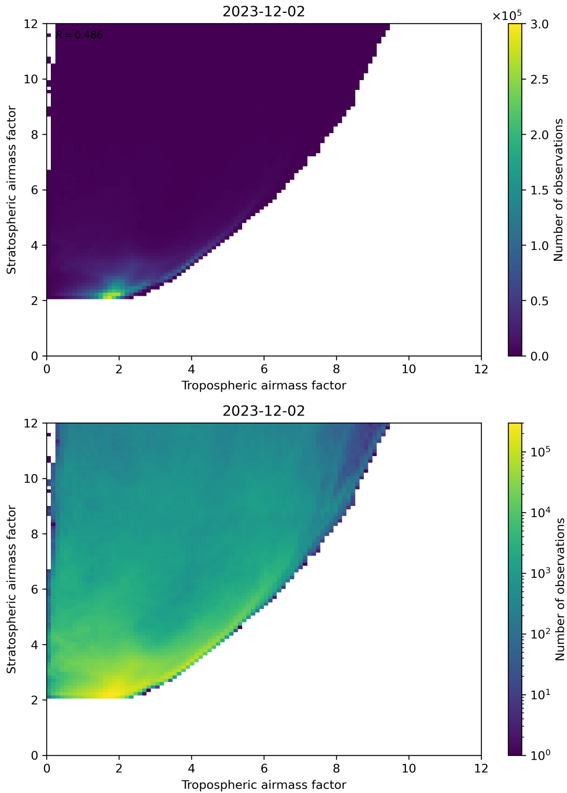
Figure 71: Scatter density plot of “Tropospheric airmass factor” against “Stratospheric airmass factor” for 2023-12-01 to 2023-12-03.
