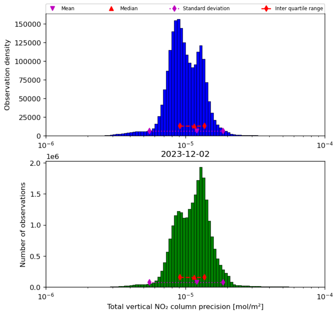
Figure 39: Histogram of “Total vertical NO 2 column precision” for 2023-12-01 to 2023-12-03
