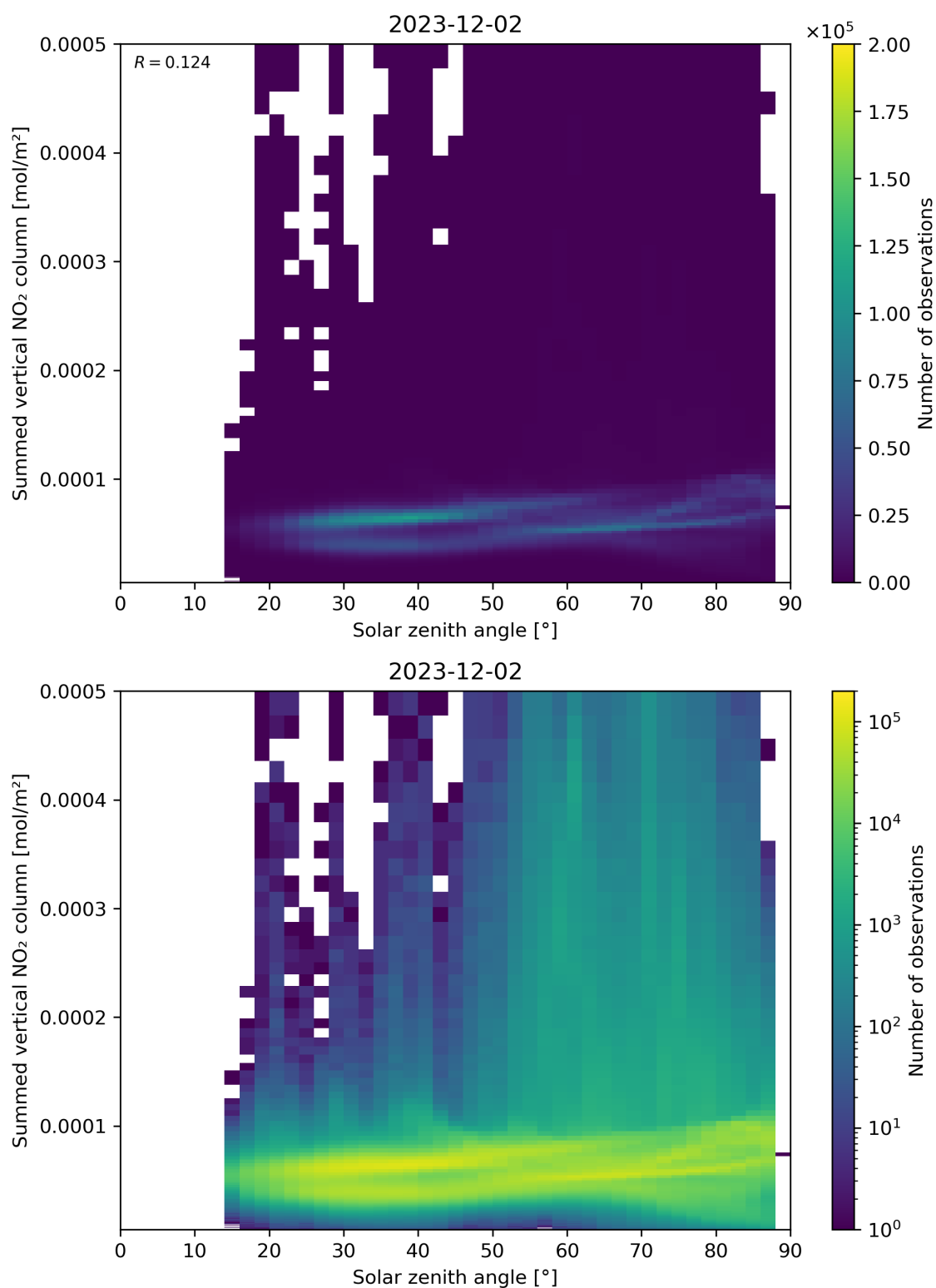
Figure 151: Scatter density plot of “Solar zenith angle” against “Summed vertical NO 2 column” for 2023-12-01 to 2023-12-03.
