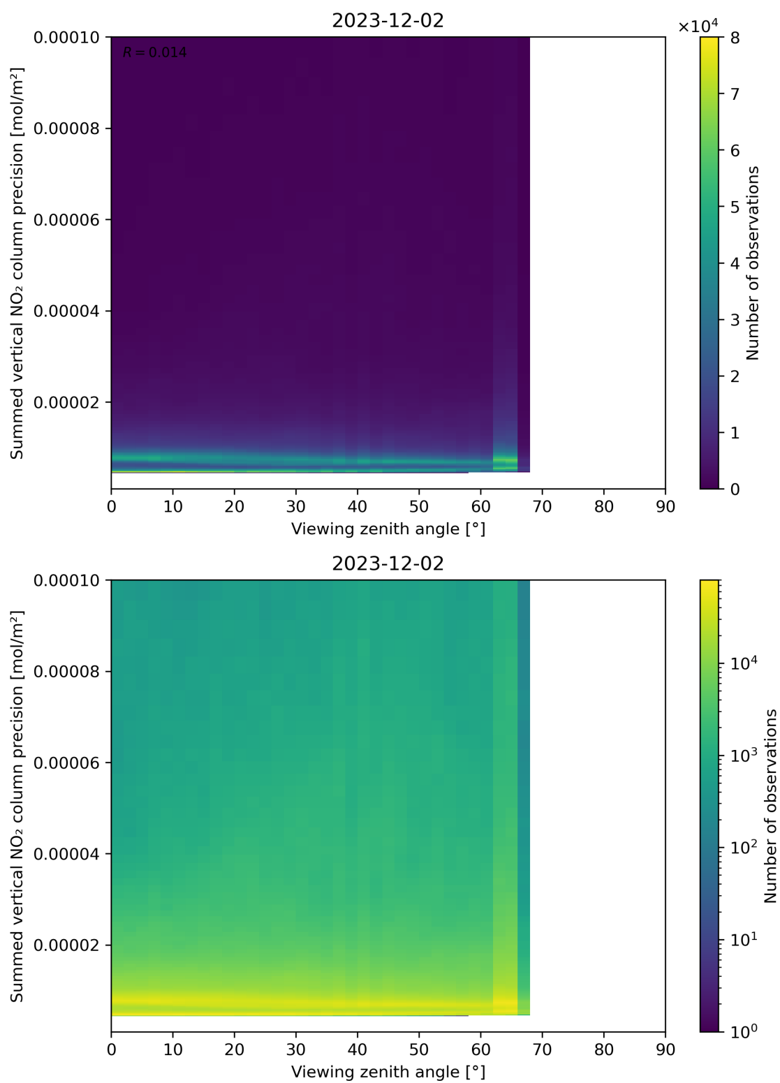
Figure 166: Scatter density plot of “Viewing zenith angle” against “Summed vertical NO 2 column precision” for 2023-12-01 to 2023-12-03.
