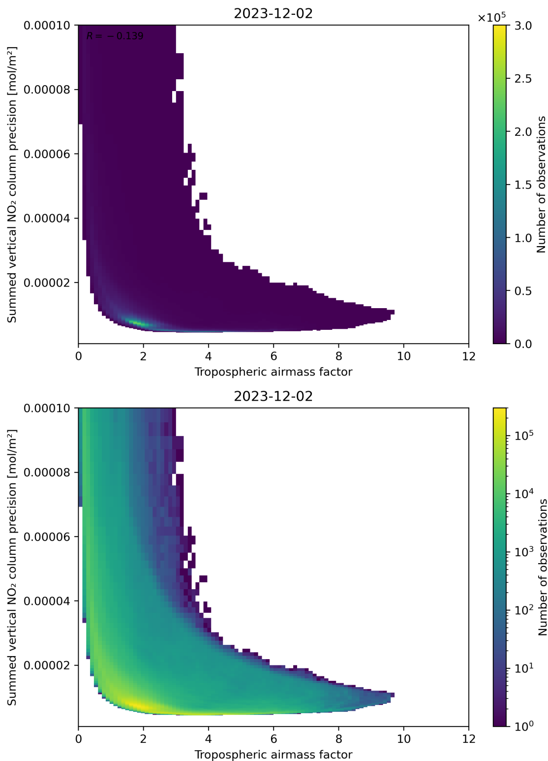
Figure 76: Scatter density plot of “Tropospheric air mass factor” against “Summed vertical NO 2 column precision” for 2023-12-01 to 2023-12-03.
