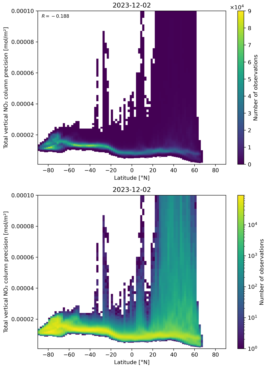
Figure 91: Scatter density plot of “Latitude” against “Total vertical NO 2 column precision” for 2023-12-01 to 2023-12-03.
