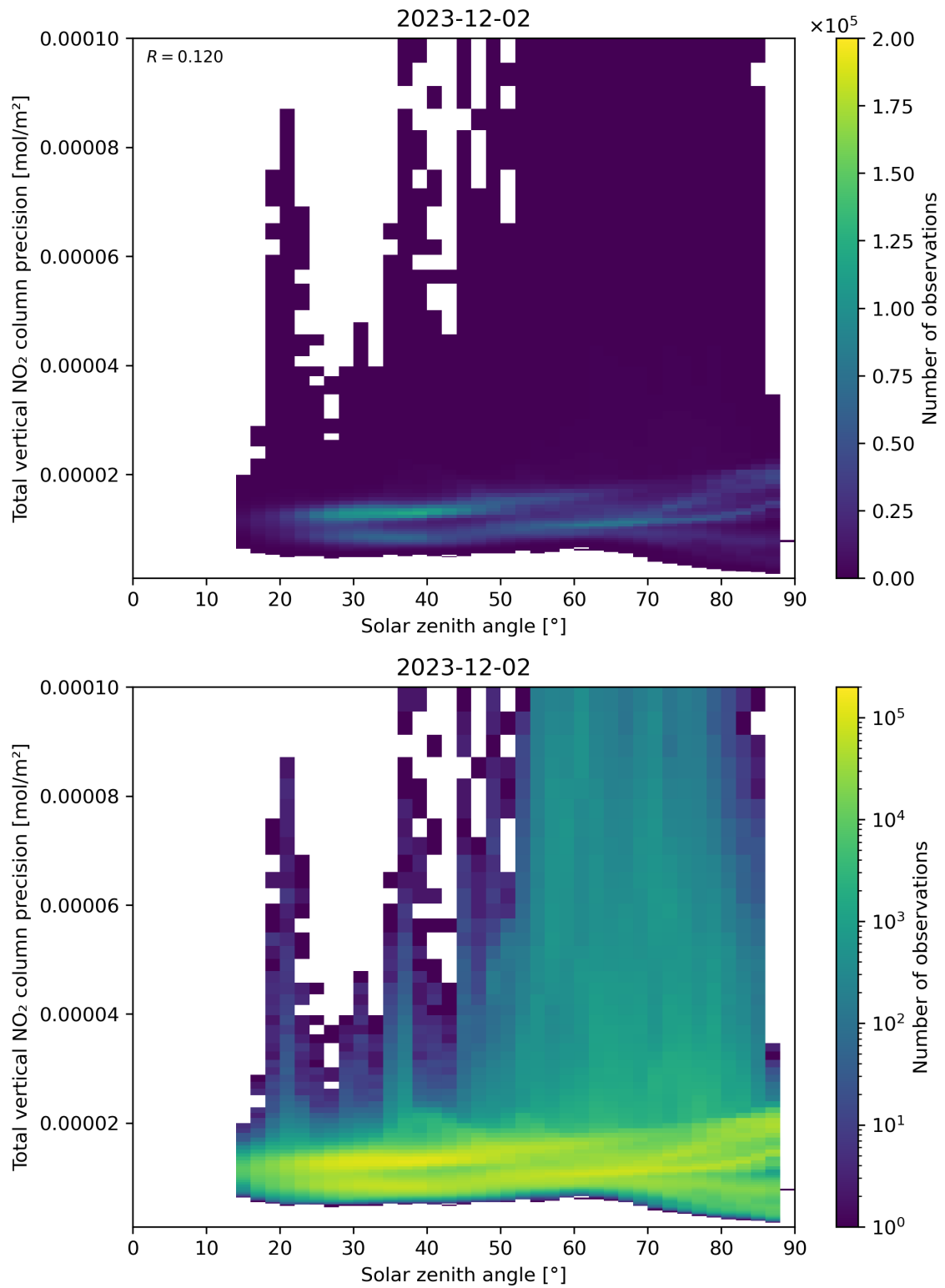
Figure 154: Scatter density plot of “Solar zenith angle” against “Total vertical NO 2 column precision” for 2023-12-01 to 2023-12-03.
