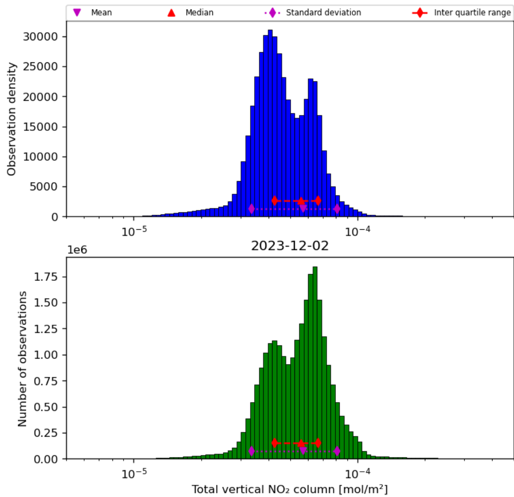
Figure 38: Histogram of “Total vertical NO 2 column” for 2023-12-01 to 2023-12-03
