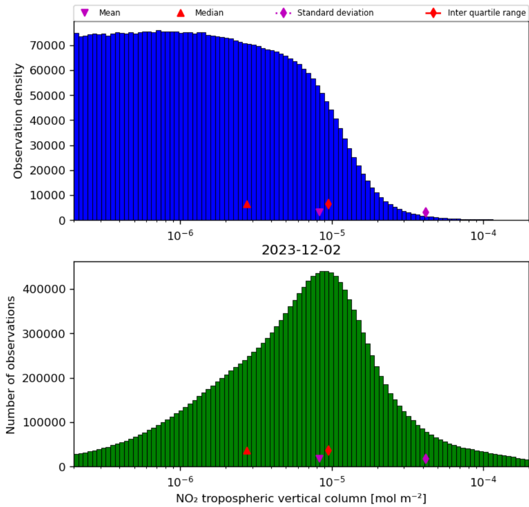
Figure 29: Histogram of “NO 2 tropospheric vertical column” for 2023-12-01 to 2023-12-03
