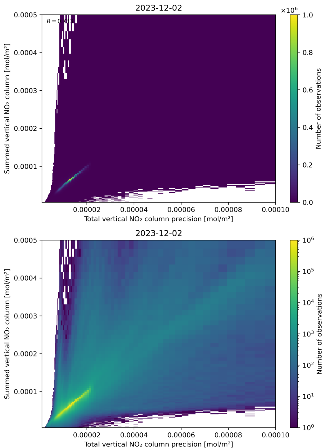
Figure 117: Scatter density plot of “Total vertical NO 2 column precision” against “Summed vertical NO 2 column” for 2023-12-01 to 2023-12-03.
