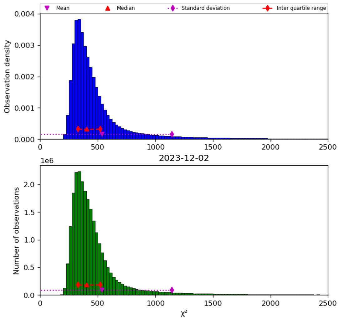
Figure 42: Histogram of “ \chi^2 ” for 2023-12-01 to 2023-12-03
