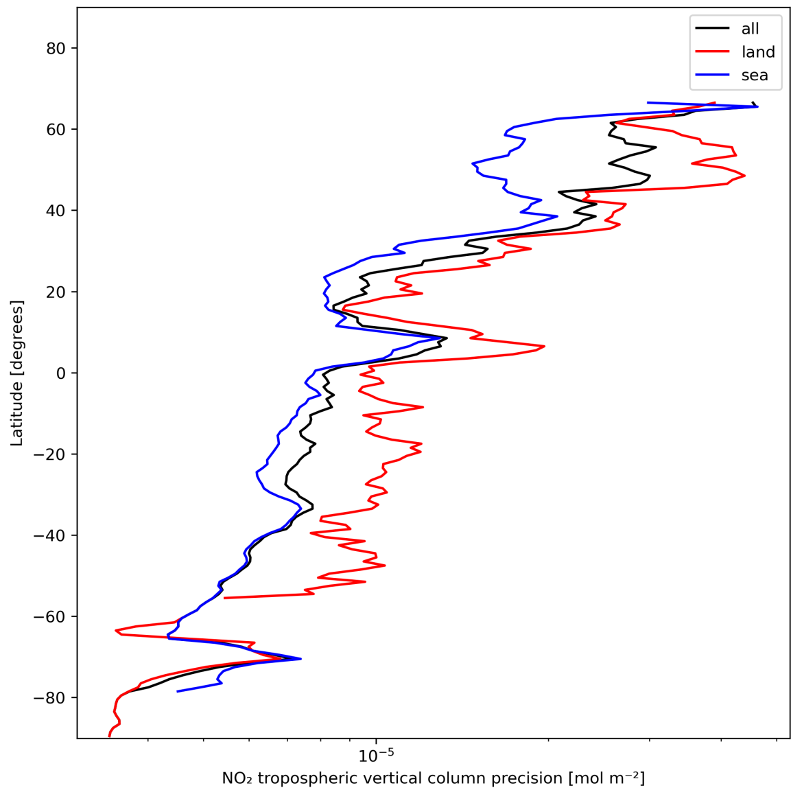
Figure 13: Zonal average of “NO 2 tropospheric vertical column precision” for 2023-12-01 to 2023-12-03.
