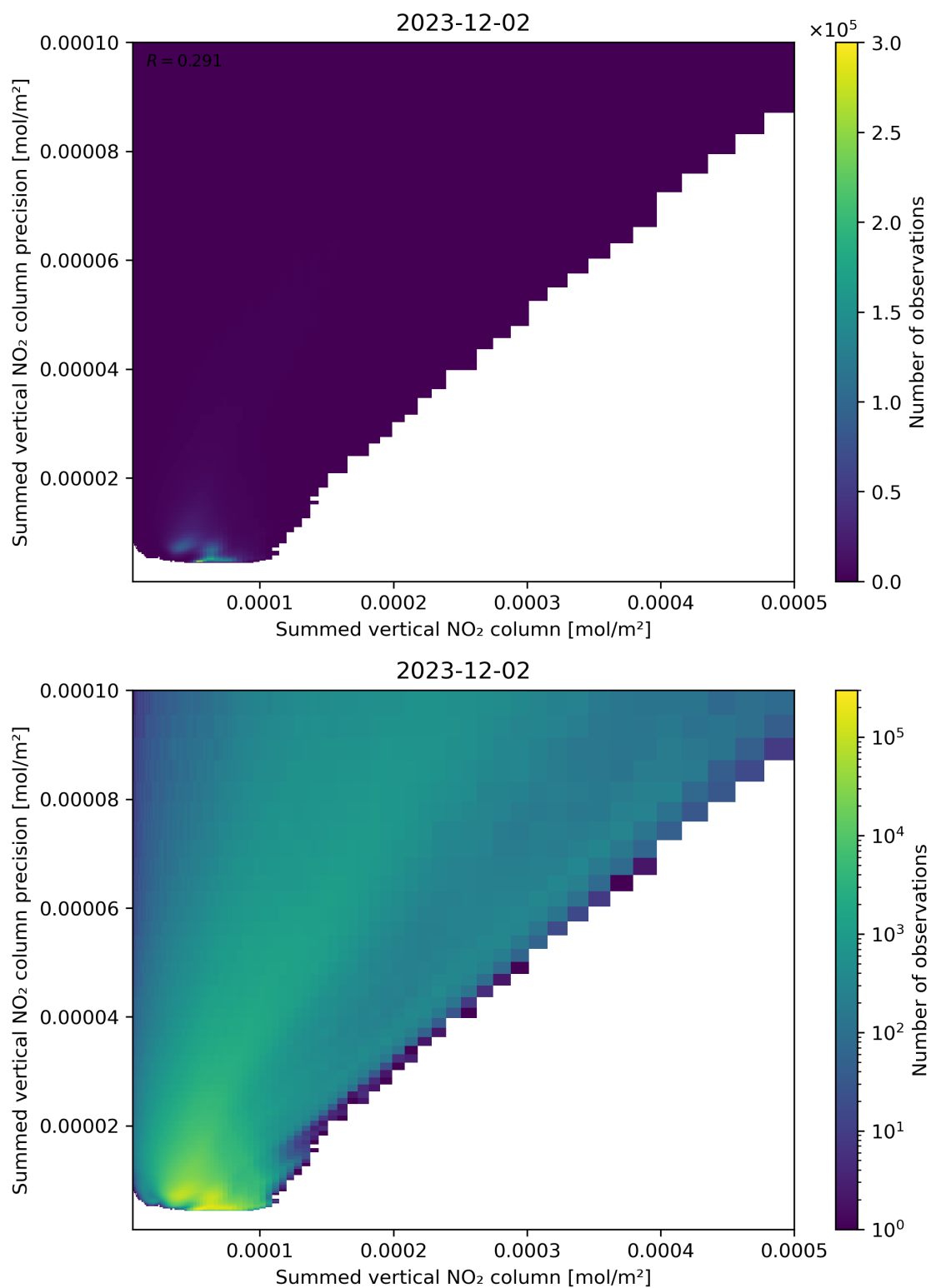
Figure 105: Scatter density plot of “Summed vertical NO 2 column” against “Summed vertical NO 2 column precision” for 2023-12-01 to 2023-12-03.
