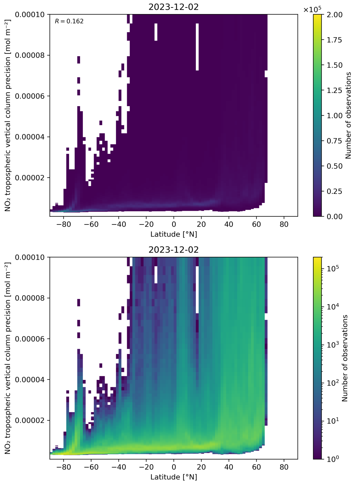
Figure 93: Scatter density plot of “Latitude” against “NO 2 tropospheric vertical column precision” for 2023-12-01 to 2023-12-03.
