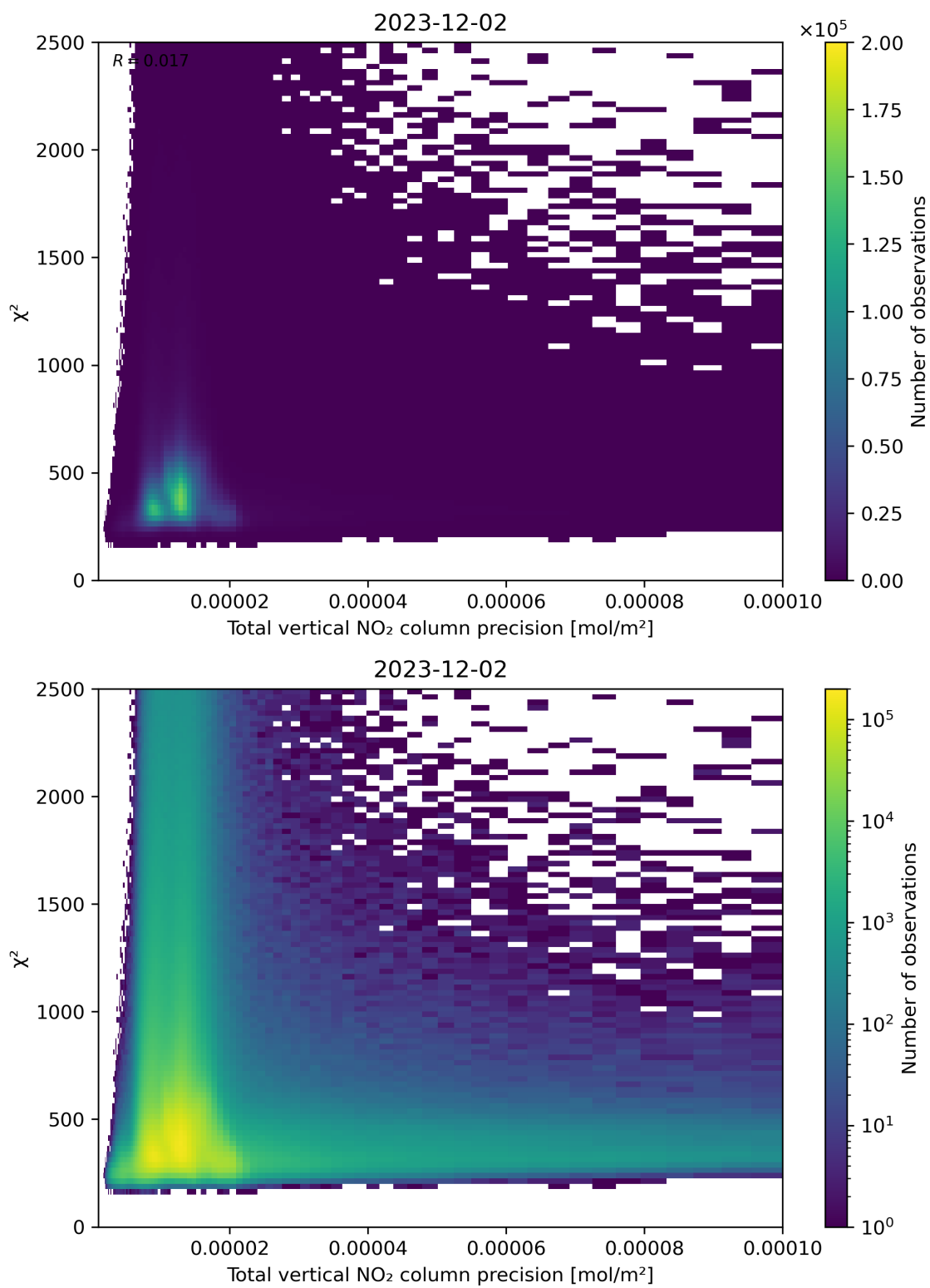
Figure 116: Scatter density plot of “Total vertical NO 2 column precision” against “ \chi^2 ” for 2023-12-01 to 2023-12-03.
