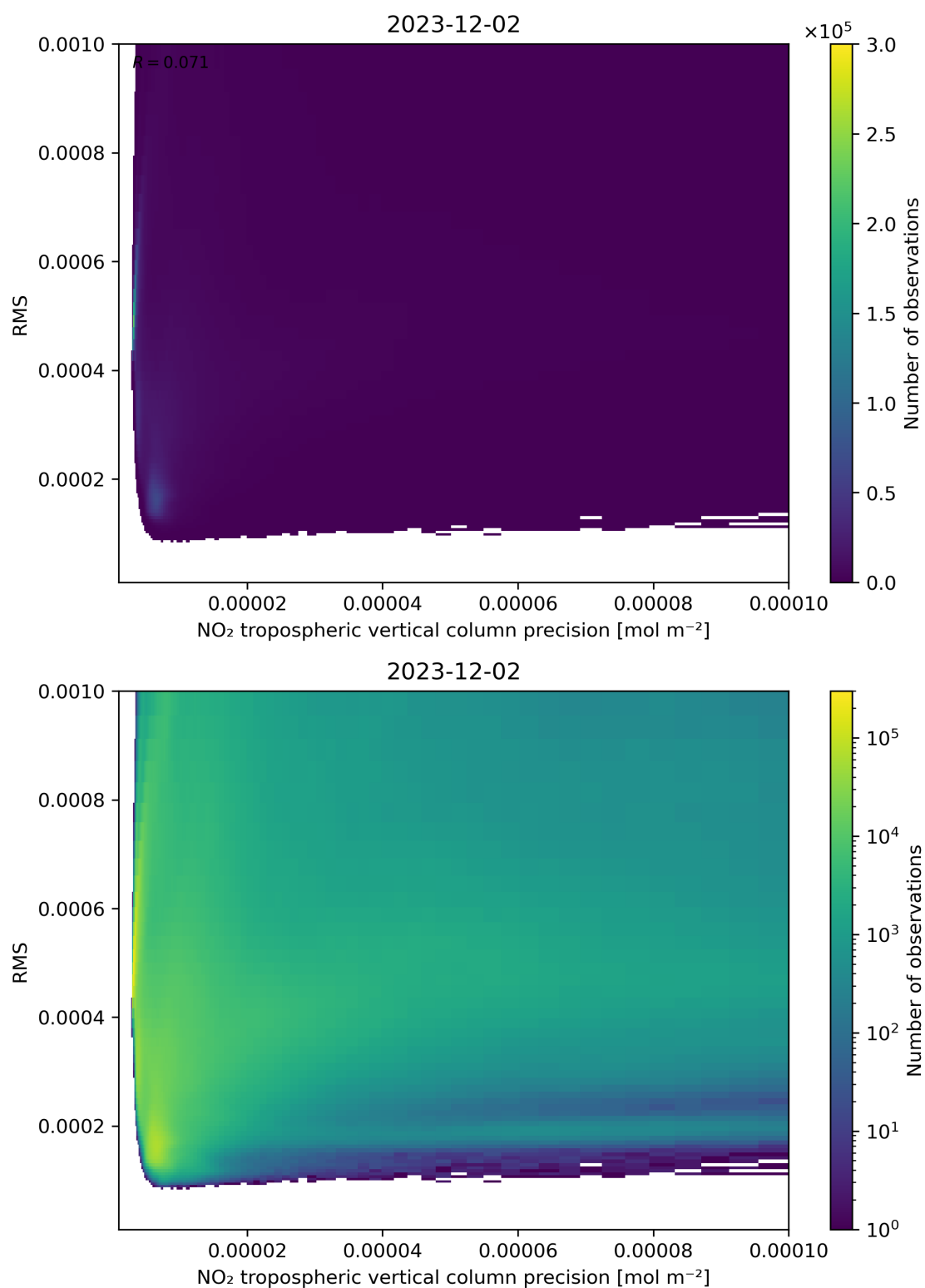
Figure 140: Scatter density plot of “NO 2 tropospheric vertical column precision” against “RMS” for 2023-12-01 to 2023-12-03.
