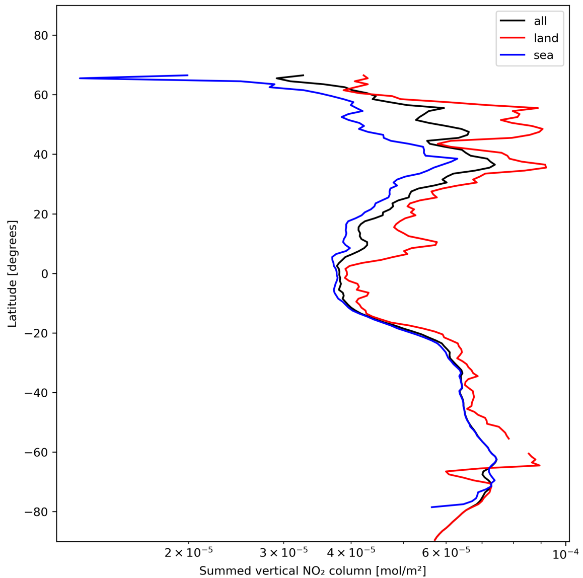
Figure 23: Zonal average of “Summed vertical NO 2 column” for 2023-12-01 to 2023-12-03.
