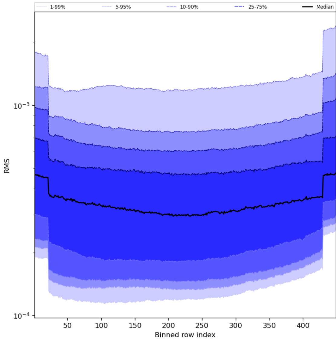
Figure 60: Along track statistics of “RMS” for 2023-12-01 to 2023-12-03
