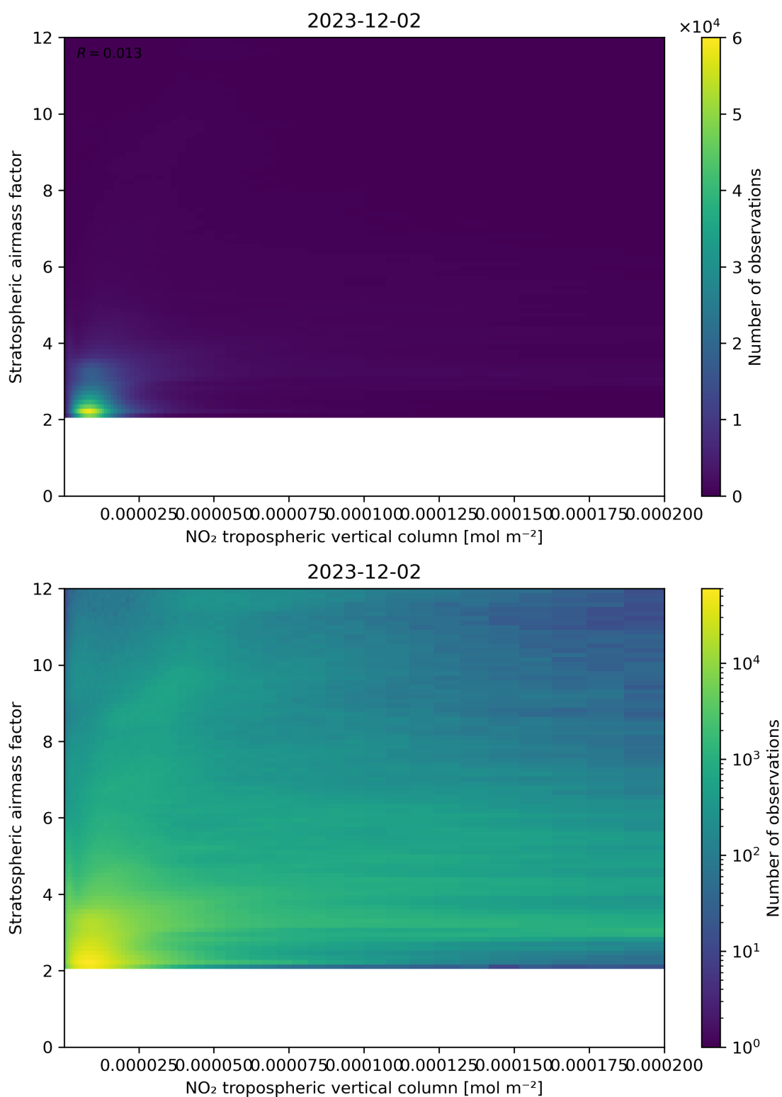
Figure 121: Scatter density plot of “NO 2 tropospheric vertical column” against “Stratospheric airmass factor” for 2023-12-01 to 2023-12-03.
