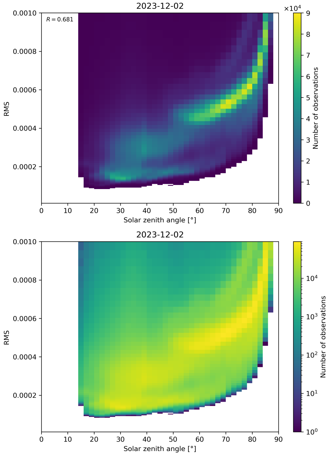
Figure 157: Scatter density plot of “Solar zenith angle” against “RMS” for 2023-12-01 to 2023-12-03.
