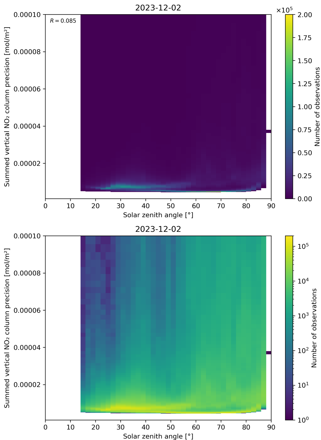
Figure 152: Scatter density plot of “Solar zenith angle” against “Summed vertical NO 2 column precision” for 2023-12-01 to 2023-12-03.
