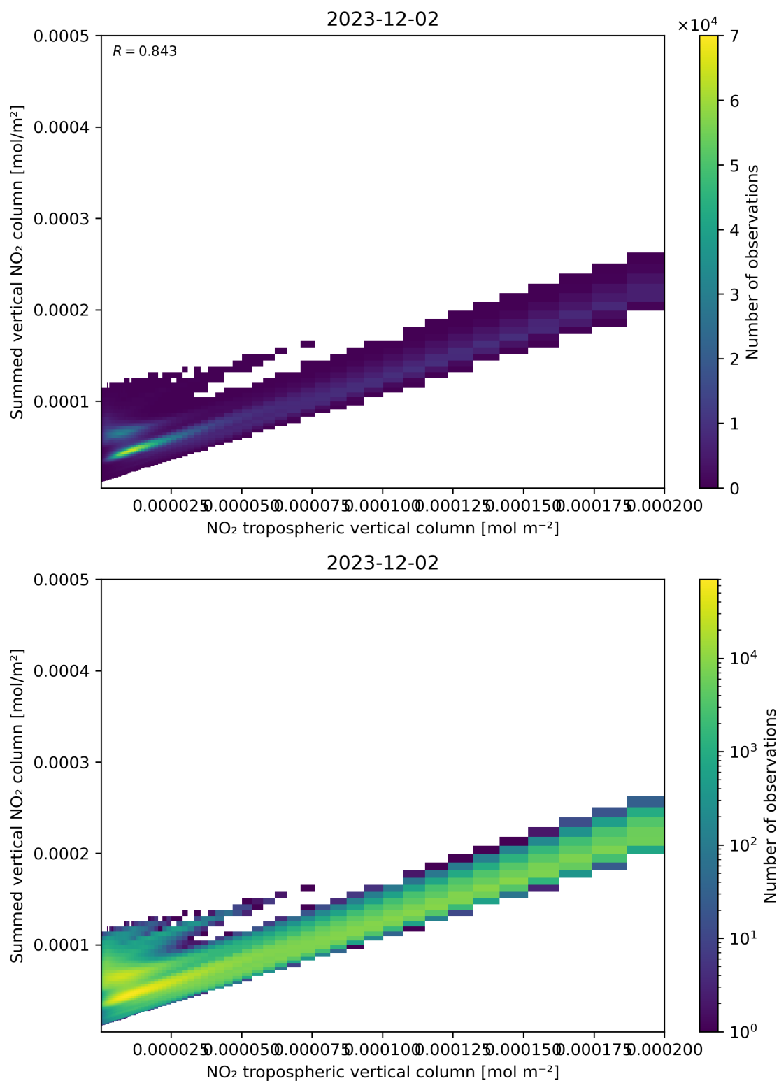
Figure 126: Scatter density plot of “NO 2 tropospheric vertical column” against “Summed vertical NO 2 column” for 2023-12-01 to 2023-12-03.
