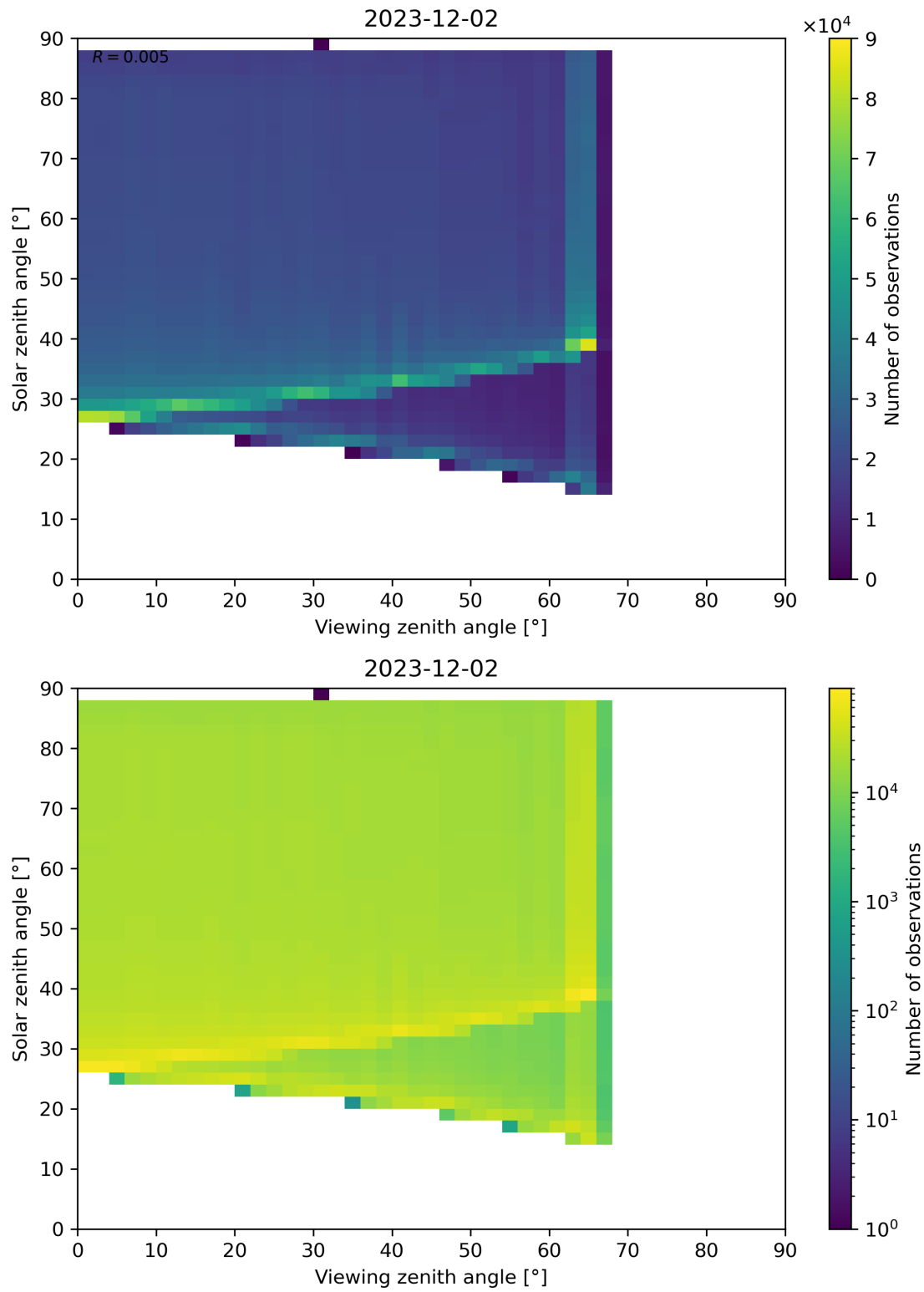
Figure 172: Scatter density plot of “Viewing zenith angle” against “Solar zenith angle” for 2023-12-01 to 2023-12-03.
