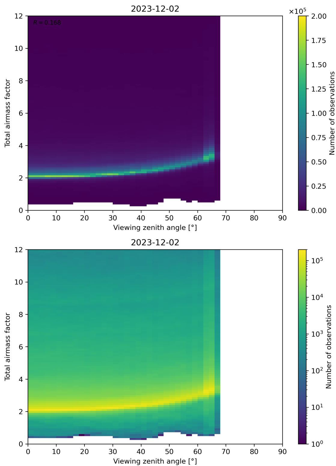
Figure 160: Scatter density plot of “Viewing zenith angle” against “Total airmass factor” for 2023-12-01 to 2023-12-03.
