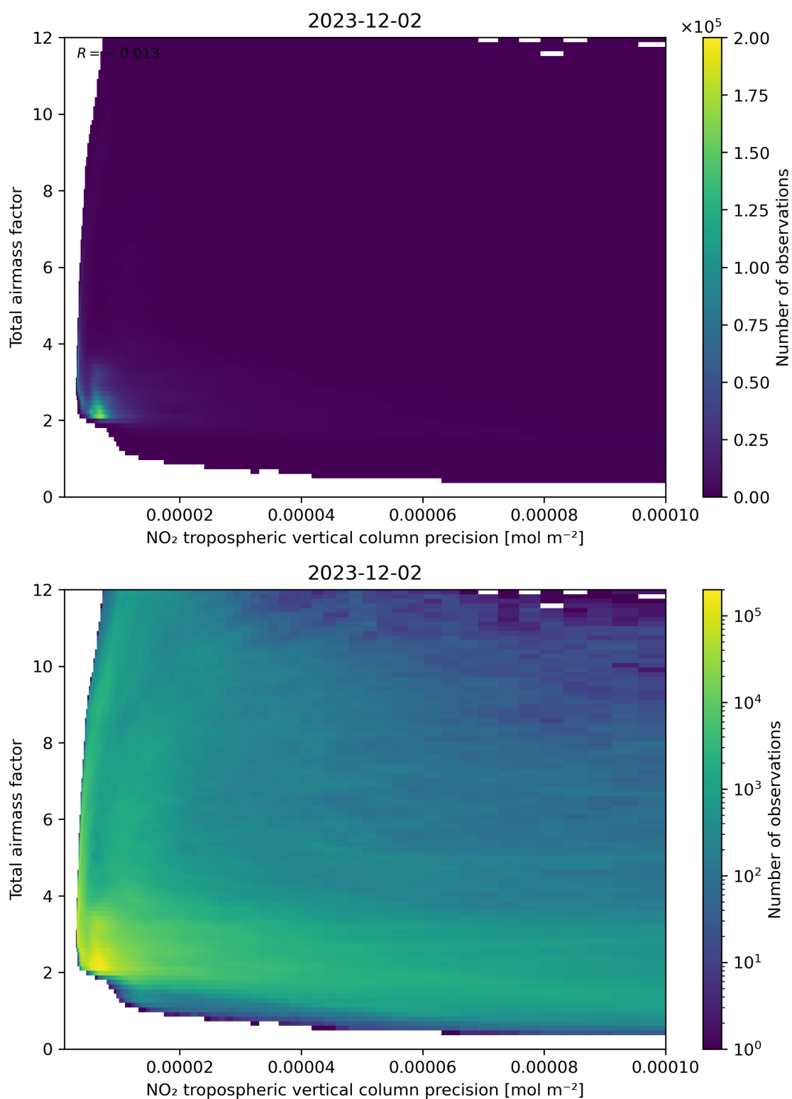
Figure 132: Scatter density plot of “NO 2 tropospheric vertical column precision” against “Total air mass factor” for 2023-12-01 to 2023-12-03.
