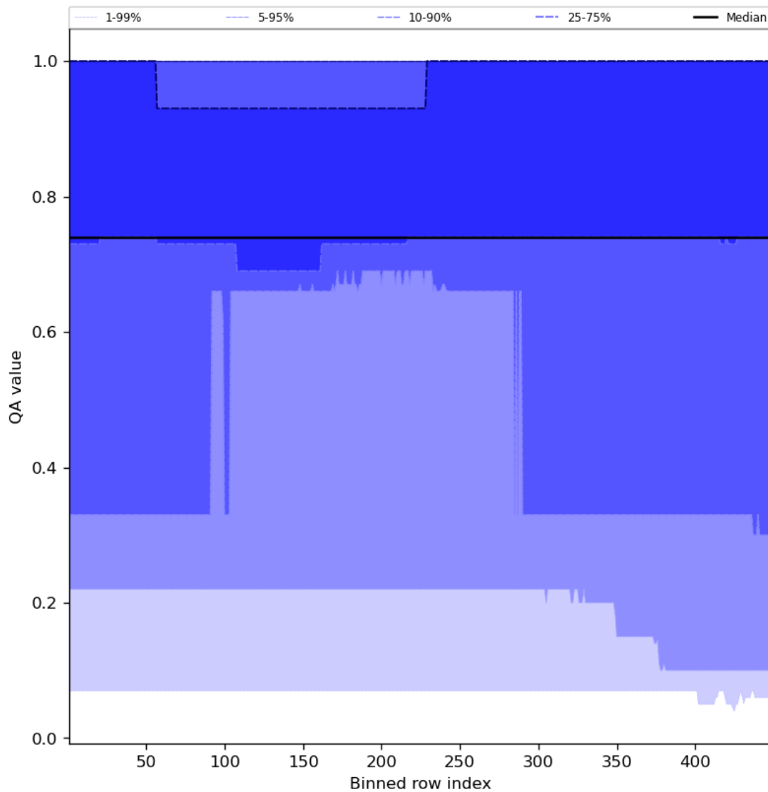
Figure 45: Along track statistics of “QA value” for 2023-12-01 to 2023-12-03
