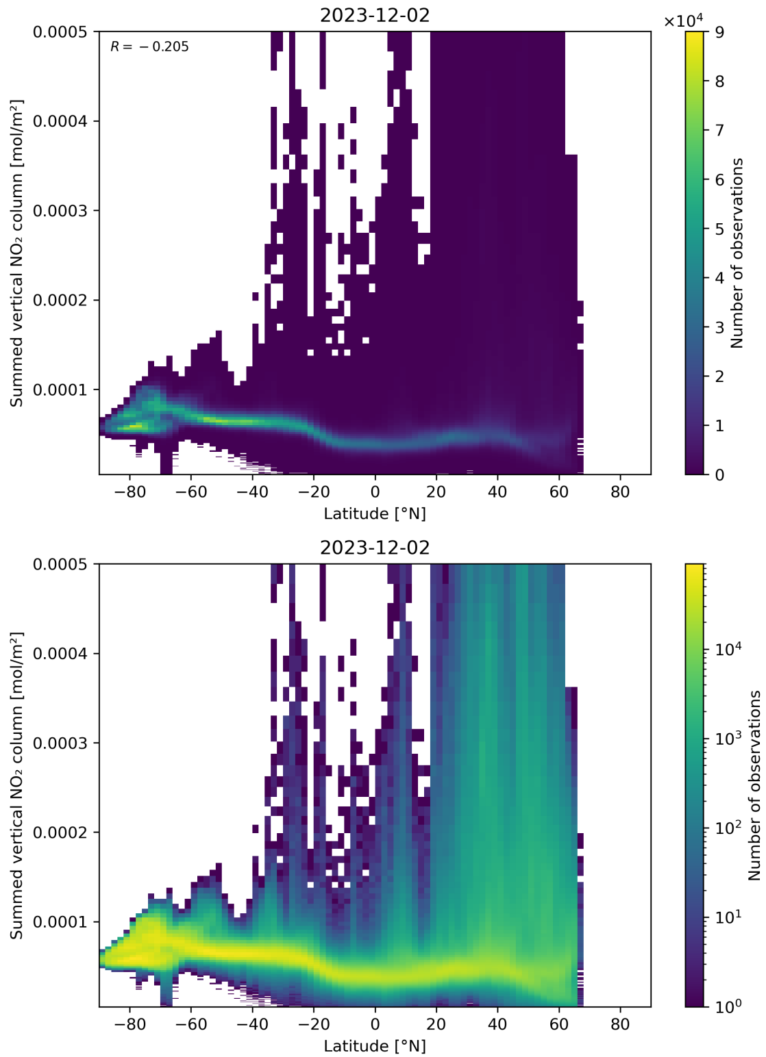
Figure 88: Scatter density plot of “Latitude” against “Summed vertical NO 2 column” for 2023-12-01 to 2023-12-03.
