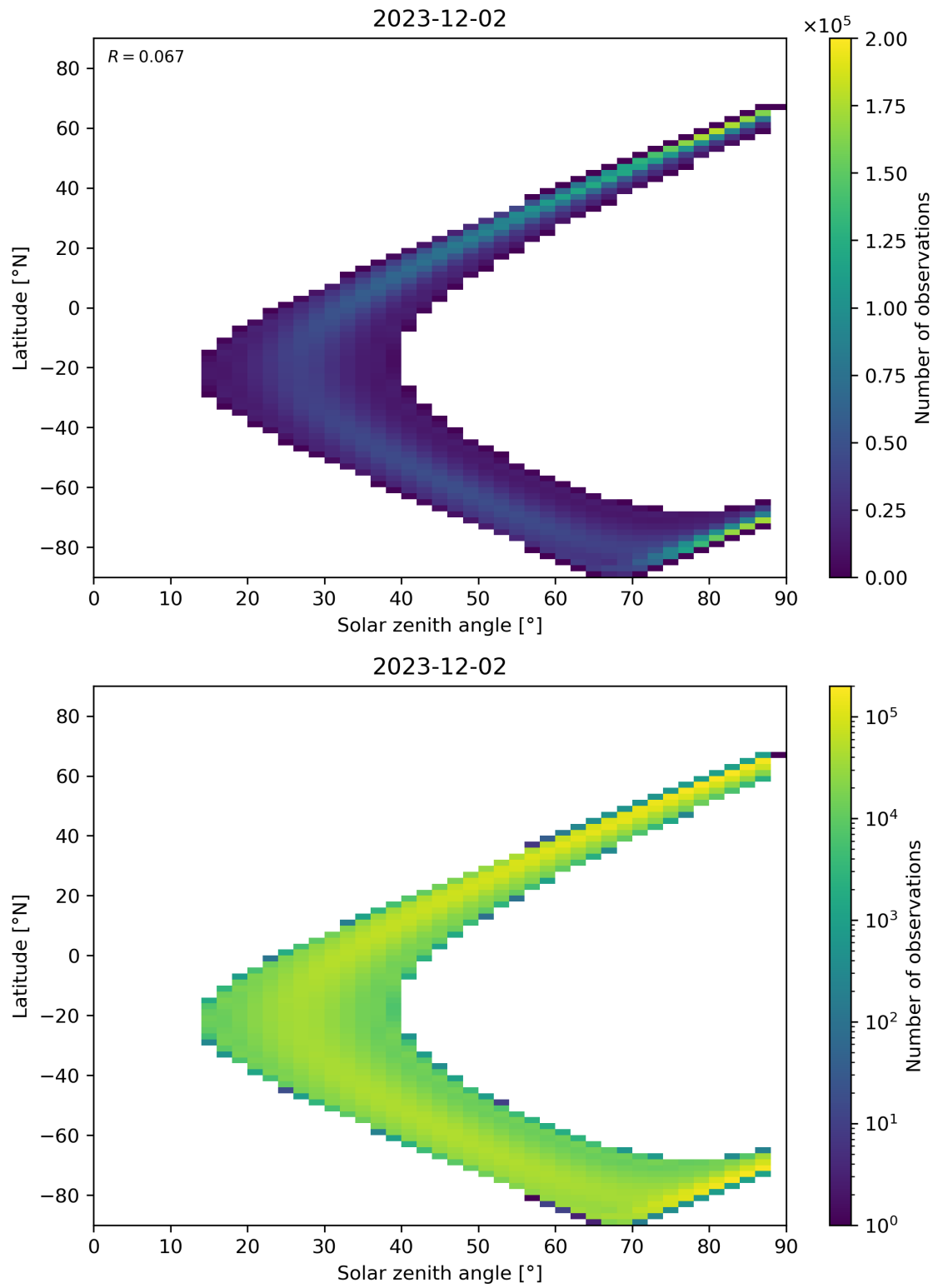
Figure 149: Scatter density plot of “Solar zenith angle” against “Latitude” for 2023-12-01 to 2023-12-03.
