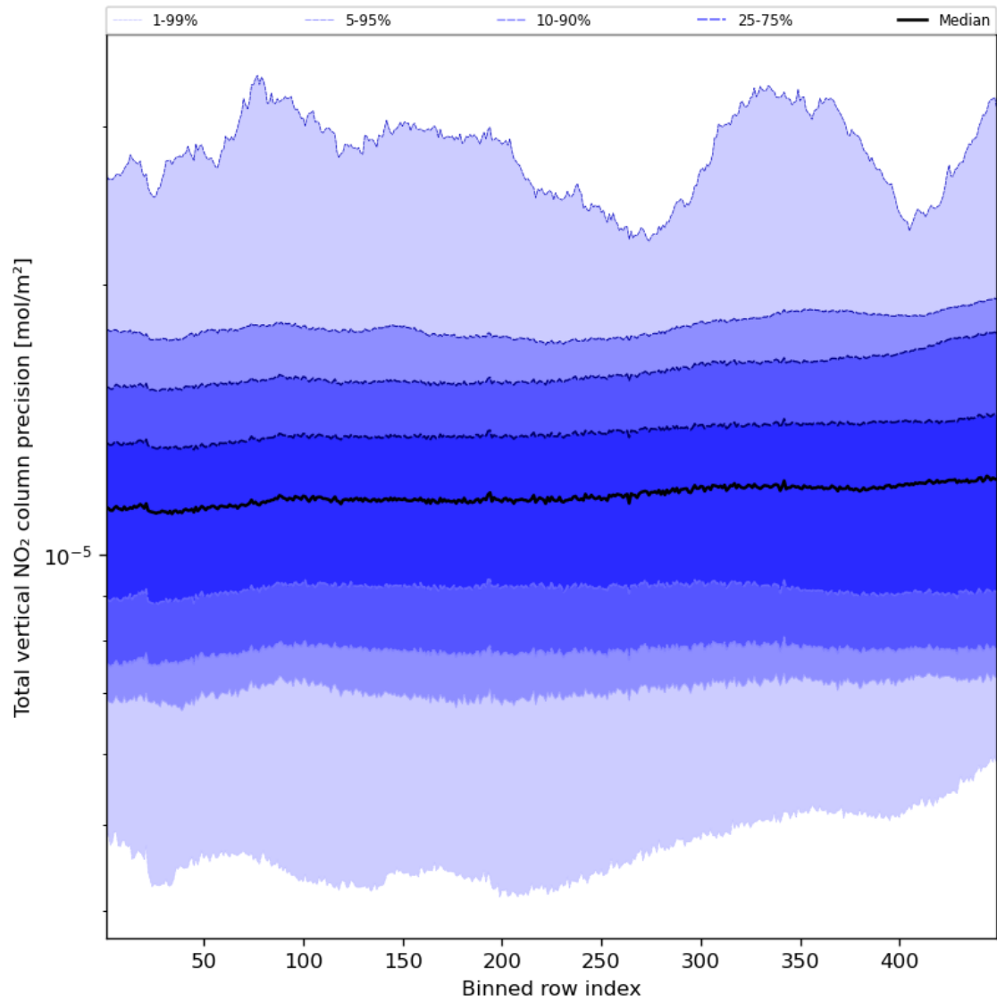
Figure 56: Along track statistics of “Total vertical NO 2 column precision” for 2023-12-01 to 2023-12-03
