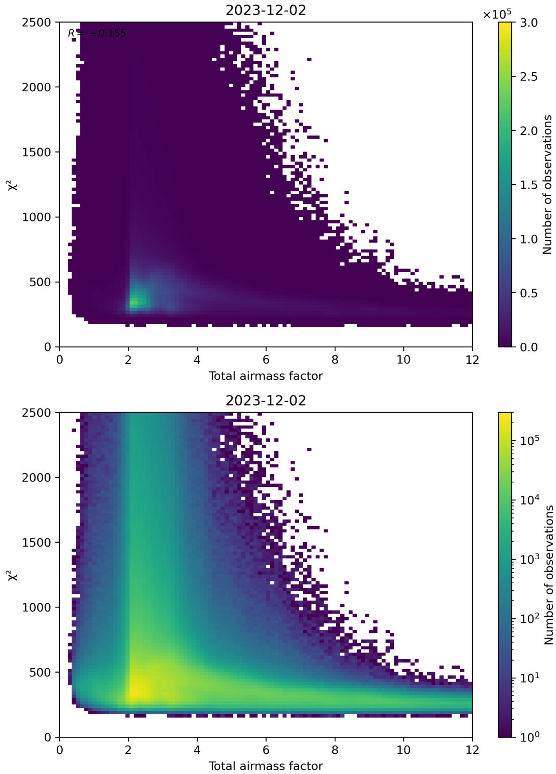
Figure 63: Scatter density plot of “Total airmass factor” against “ \chi^2 ” for 2023-12-01 to 2023-12-03.
