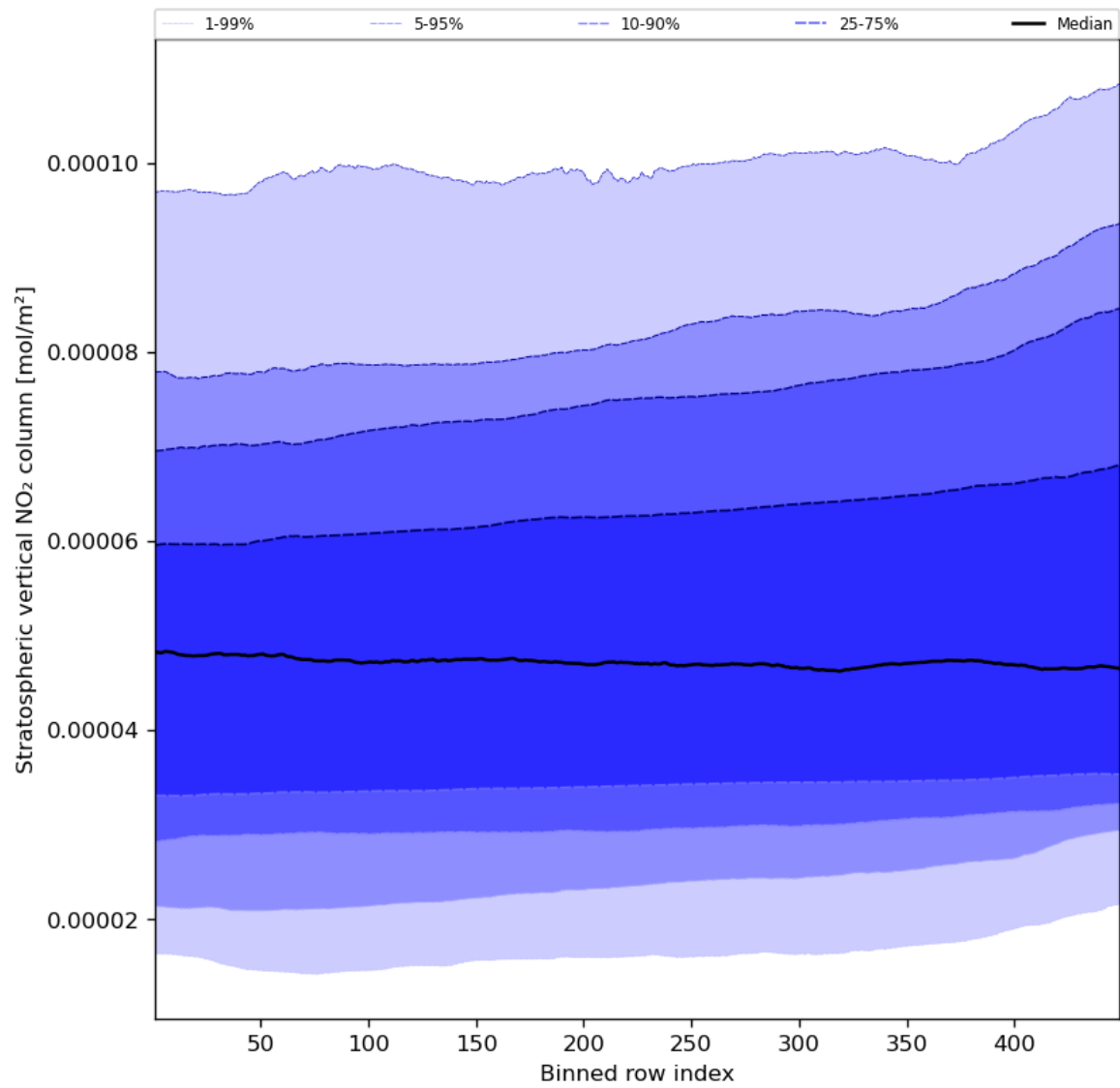
Figure 53: Along track statistics of “Stratospheric vertical NO 2 column” for 2023-12-01 to 2023-12-03
