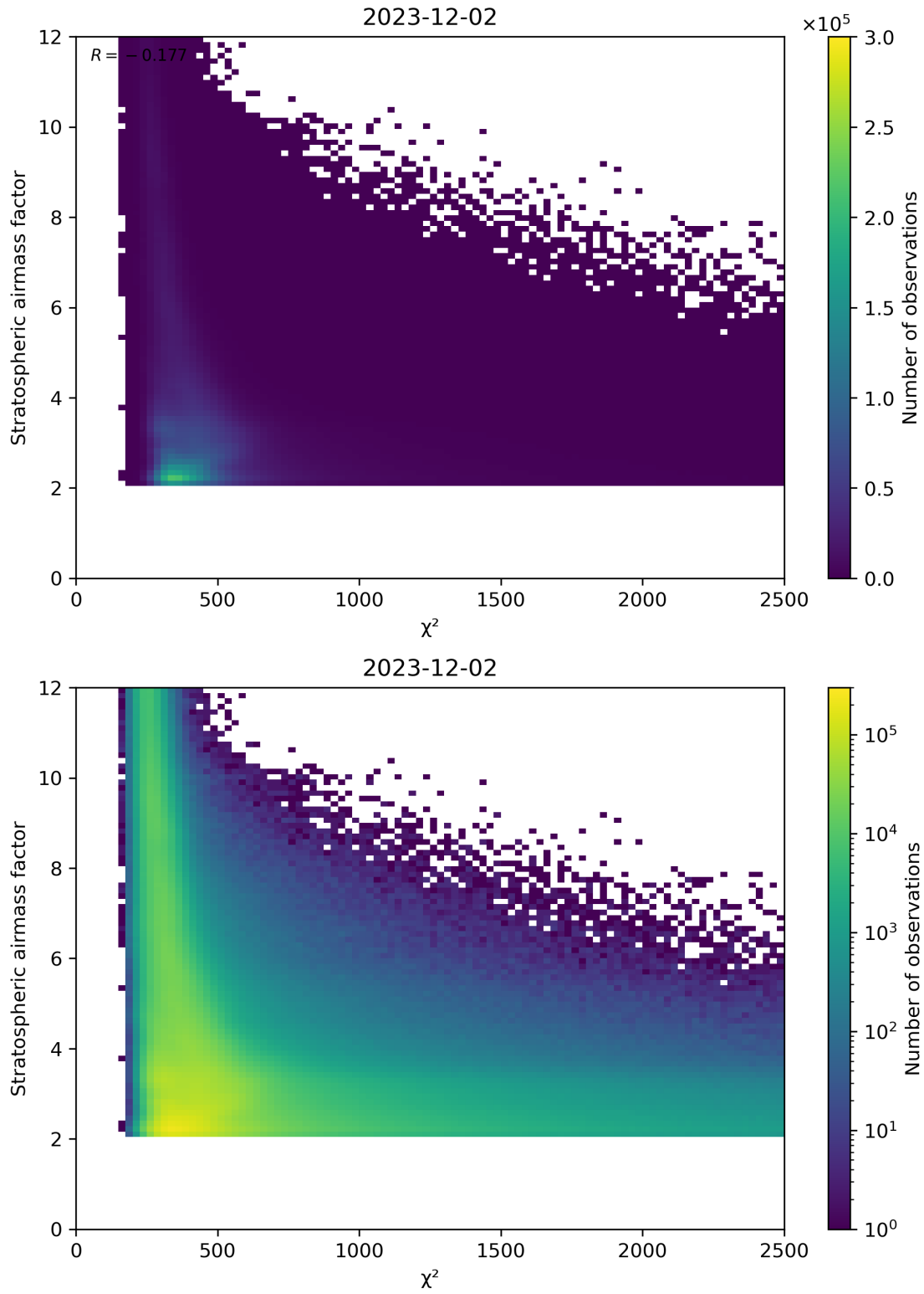
Figure 81: Scatter density plot of “ \chi^2 ” against “Stratospheric airmass factor” for 2023-12-01 to 2023-12-03.
