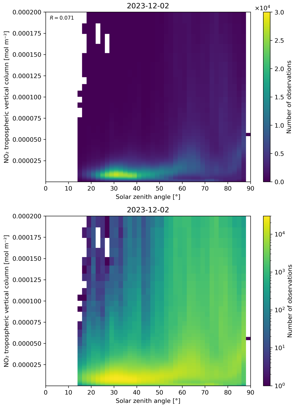
Figure 155: Scatter density plot of “Solar zenith angle” against “NO 2 tropospheric vertical column” for 2023-12-01 to 2023-12-03.
