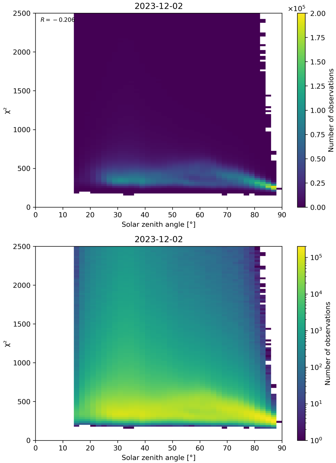
Figure 148: Scatter density plot of “Solar zenith angle” against “ \chi^2 ” for 2023-12-01 to 2023-12-03.
