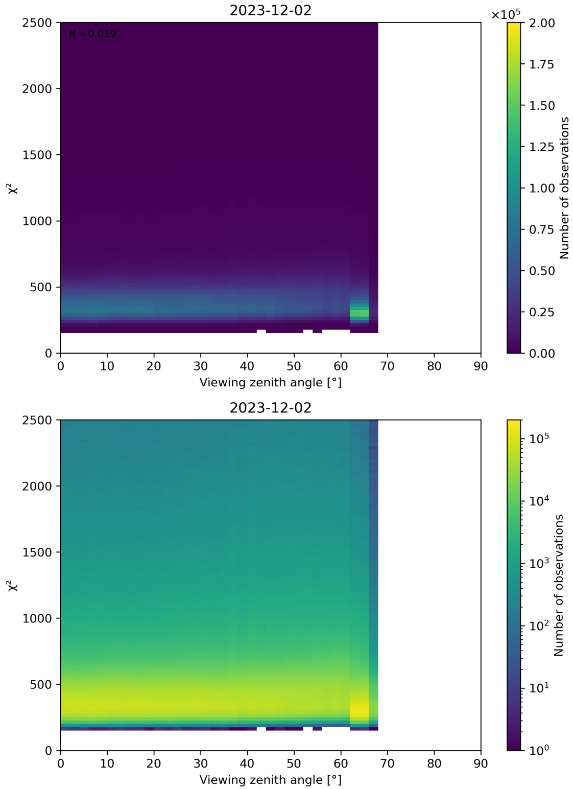
Figure 162: Scatter density plot of “Viewing zenith angle” against “ \chi^2 ” for 2023-12-01 to 2023-12-03.
