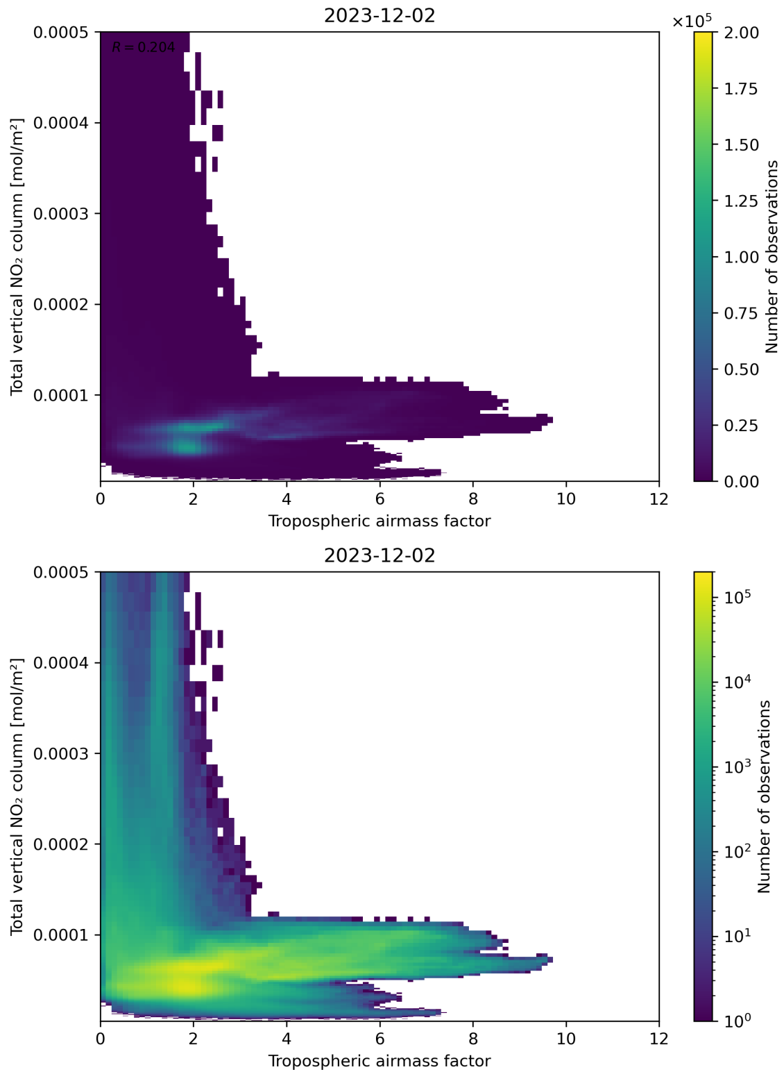
Figure 77: Scatter density plot of “Tropospheric airmass factor” against “Total vertical NO 2 column” for 2023-12-01 to 2023-12-03.
