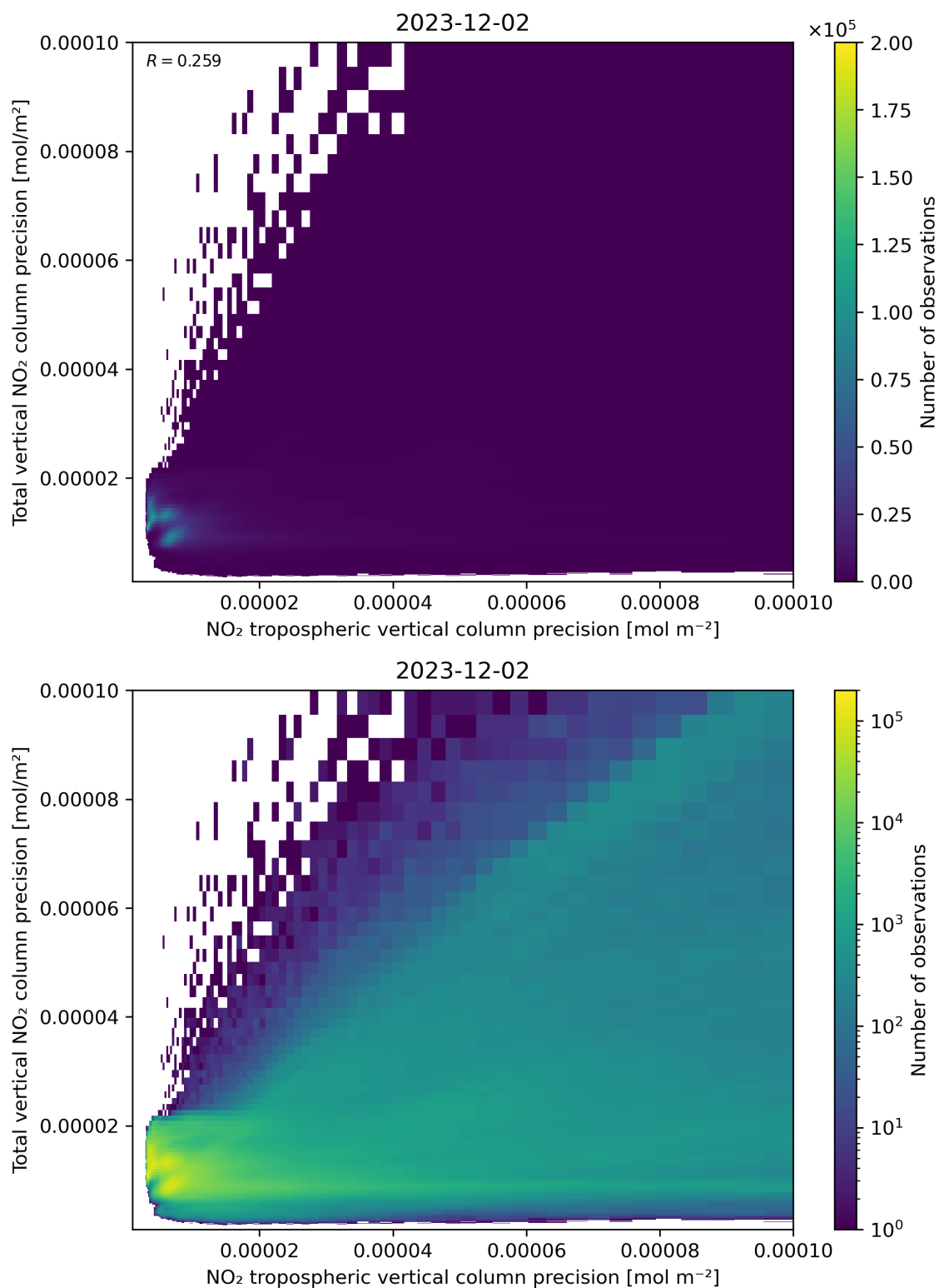
Figure 139: Scatter density plot of “NO 2 tropospheric vertical column precision” against “Total vertical NO 2 column precision” for 2023-12-01 to 2023-12-03.
