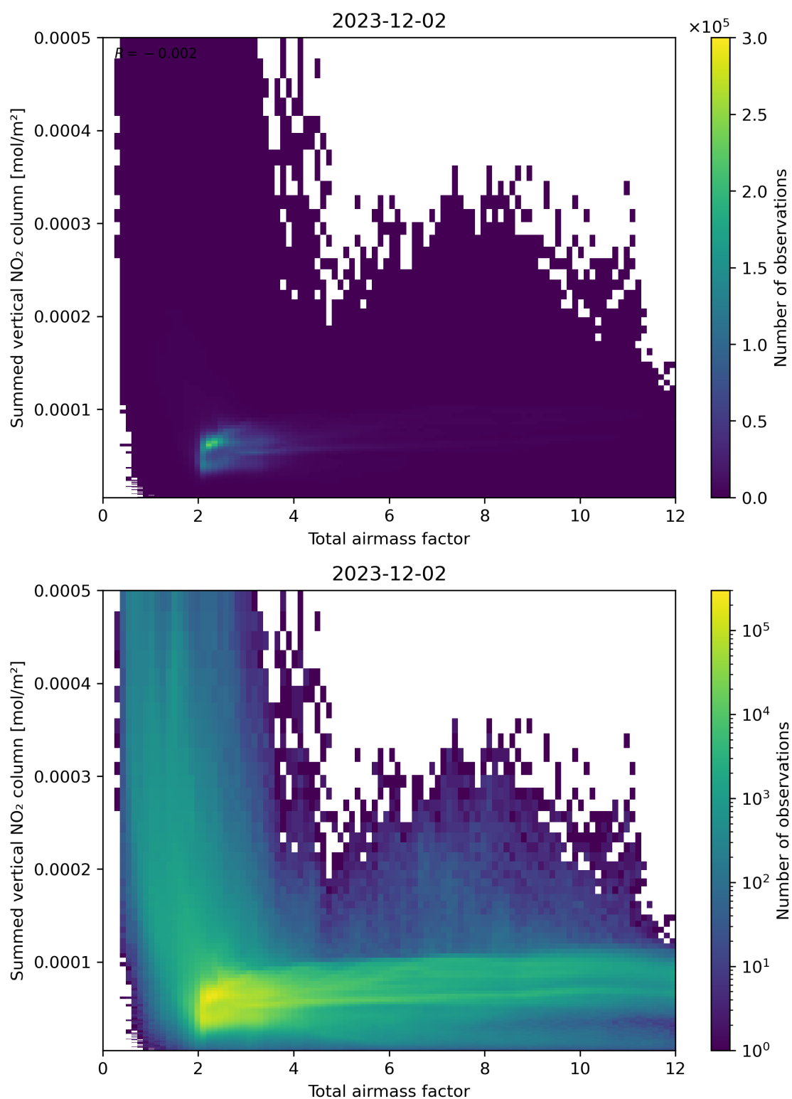
Figure 65: Scatter density plot of “Total airmass factor” against “Summed vertical NO 2 column” for 2023-12-01 to 2023-12-03.
