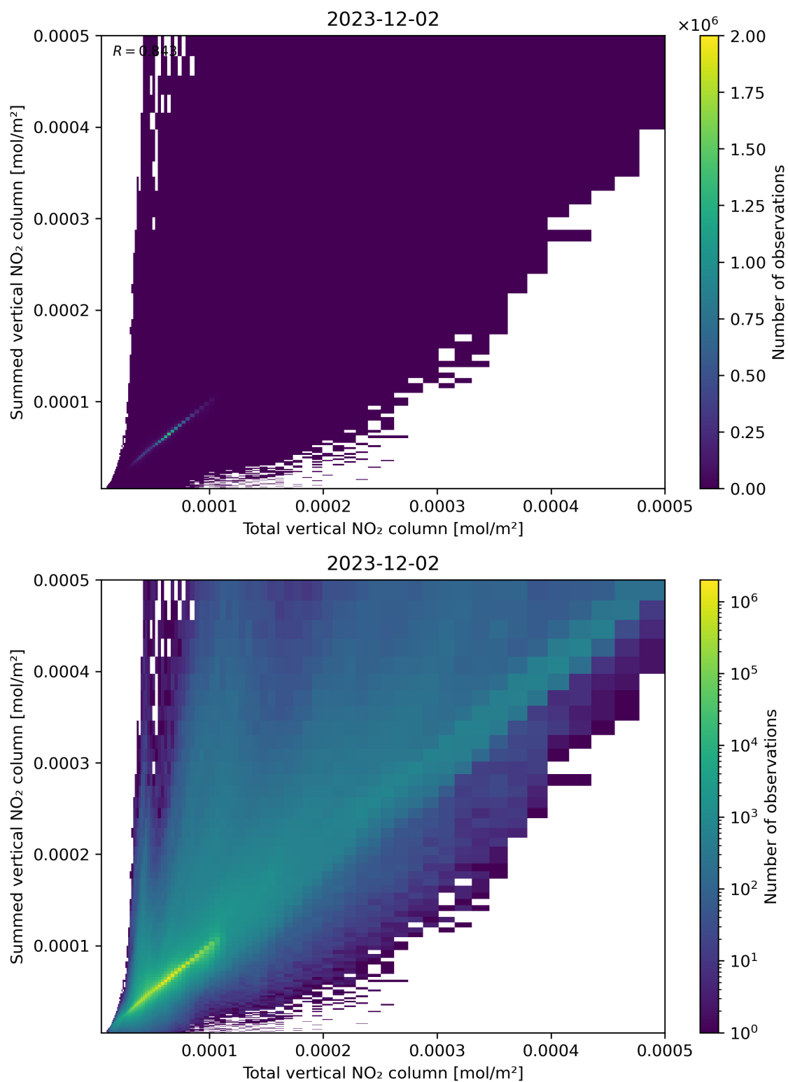
Figure 112: Scatter density plot of “Total vertical NO 2 column” against “Summed vertical NO 2 column” for 2023-12-01 to 2023-12-03.
