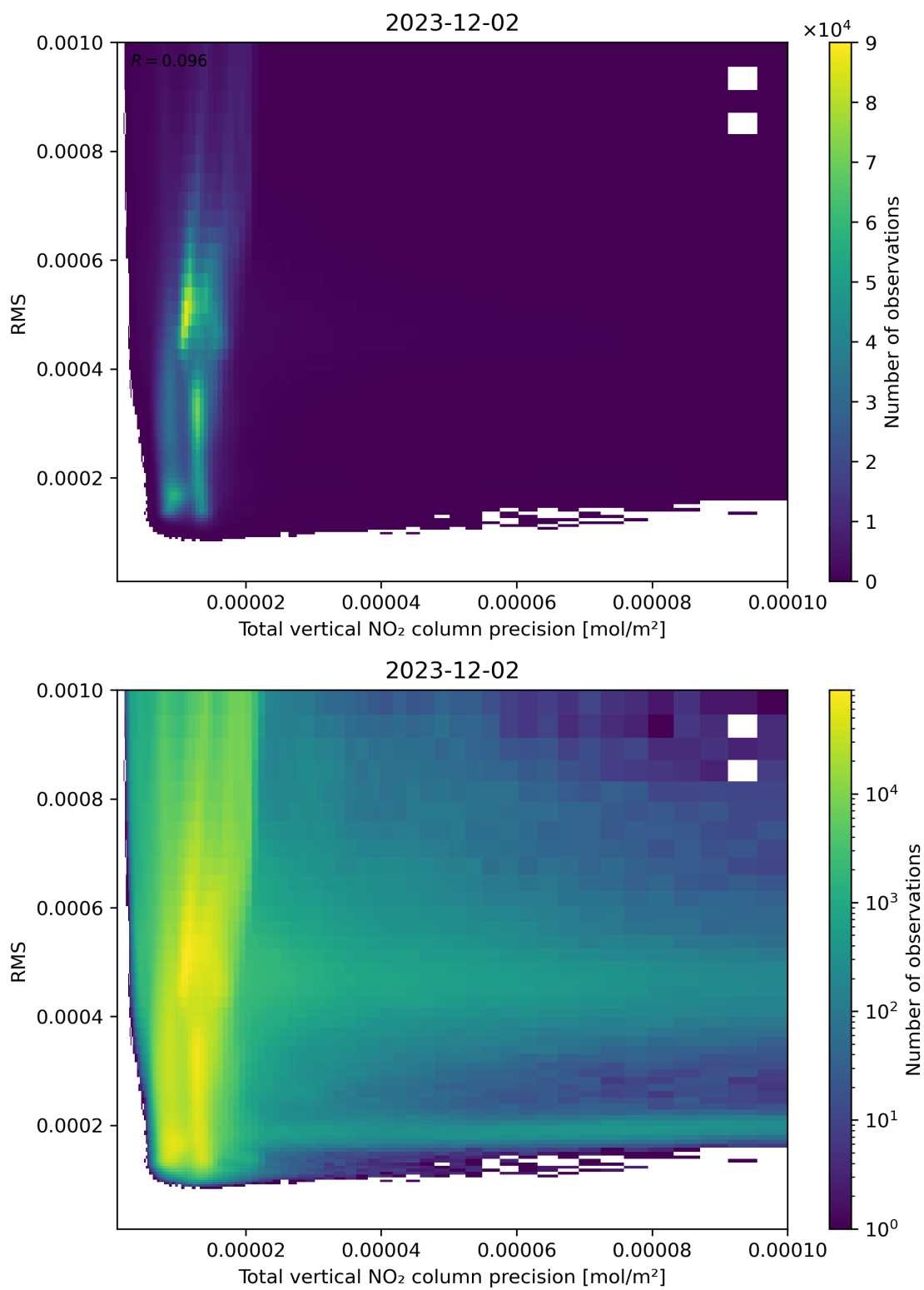
Figure 119: Scatter density plot of “Total vertical NO 2 column precision” against “RMS” for 2023-12-01 to 2023-12-03.
