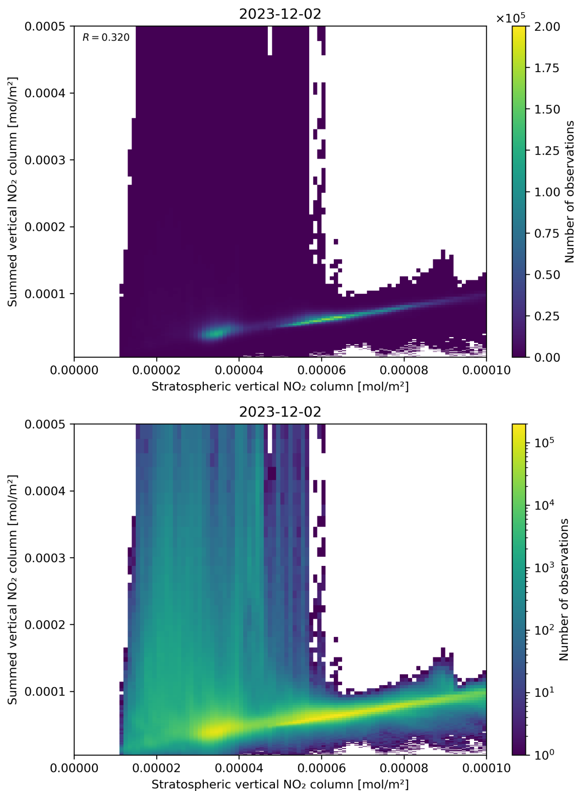
Figure 98: Scatter density plot of “Stratospheric vertical NO 2 column” against “Summed vertical NO 2 column” for 2023-12-01 to 2023-12-03.
