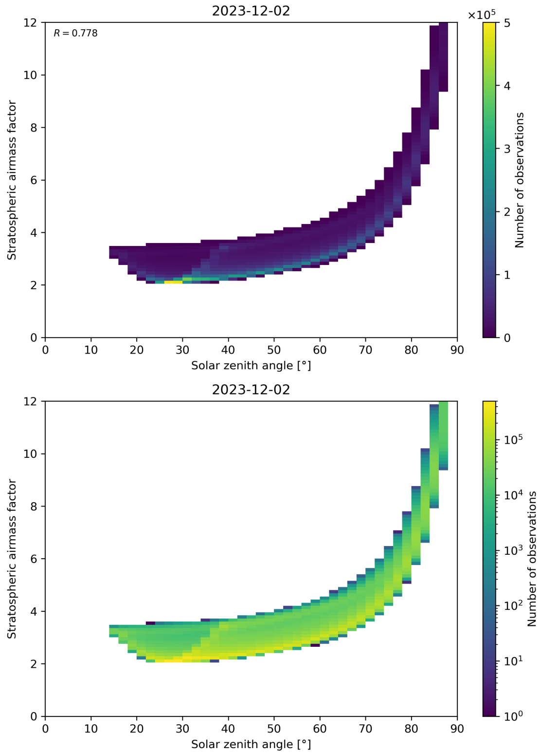
Figure 145: Scatter density plot of “Solar zenith angle” against “Stratospheric airmass factor” for 2023-12-01 to 2023-12-03.
