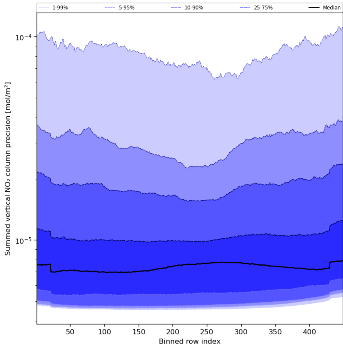
Figure 58: Along track statistics of “Summed vertical NO 2 column precision” for 2023-12-01 to 2023-12-03
