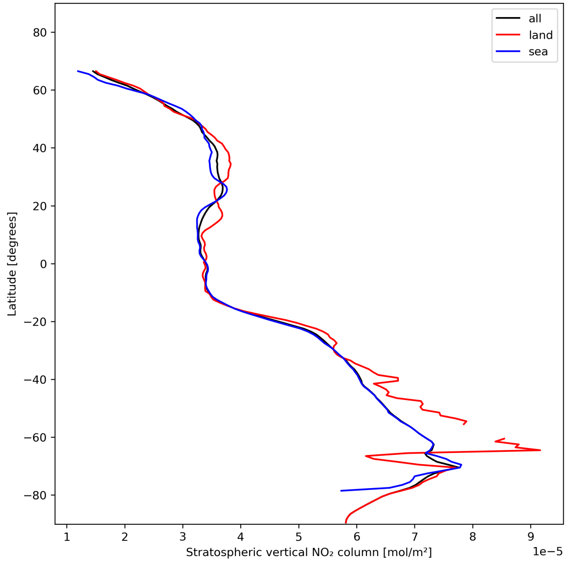
Figure 19: Zonal average of “Stratospheric vertical NO 2 column” for 2023-12-01 to 2023-12-03.
