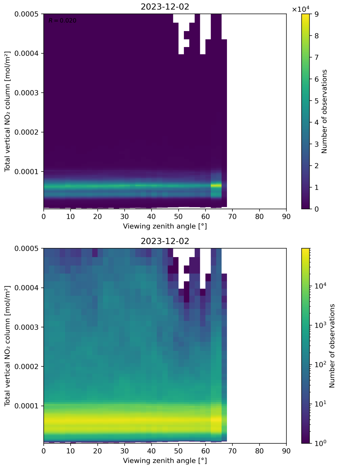
Figure 167: Scatter density plot of “Viewing zenith angle” against “Total vertical NO 2 column” for 2023-12-01 to 2023-12-03.
