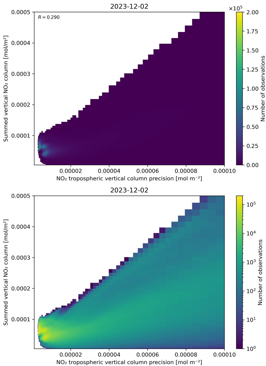
Figure 136: Scatter density plot of “NO 2 tropospheric vertical column precision” against “Summed vertical NO 2 column” for 2023-12-01 to 2023-12-03.
