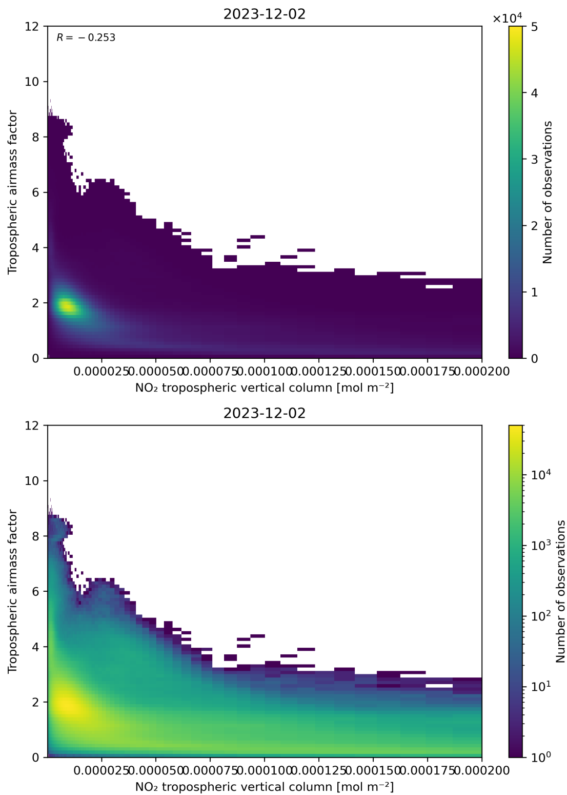
Figure 123: Scatter density plot of “NO 2 tropospheric vertical column” against “Tropospheric air mass factor” for 2023-12-01 to 2023-12-03.
