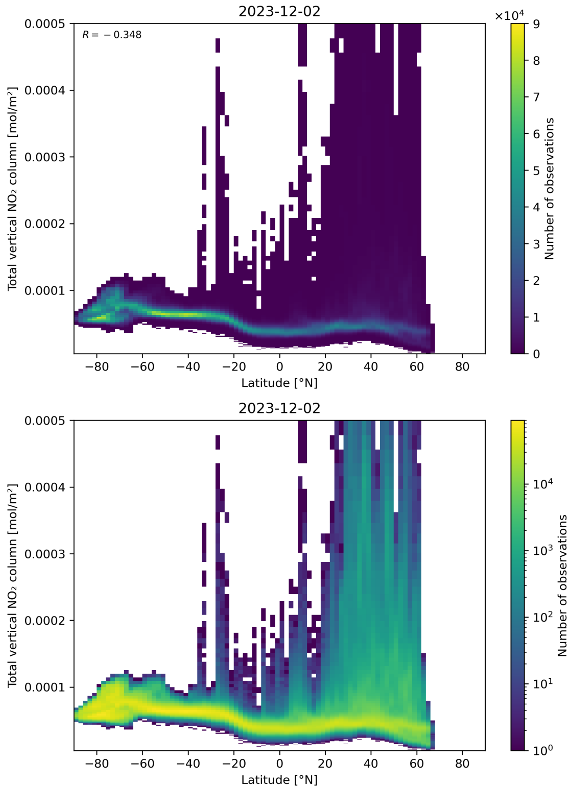
Figure 90: Scatter density plot of “Latitude” against “Total vertical NO 2 column” for 2023-12-01 to 2023-12-03.
