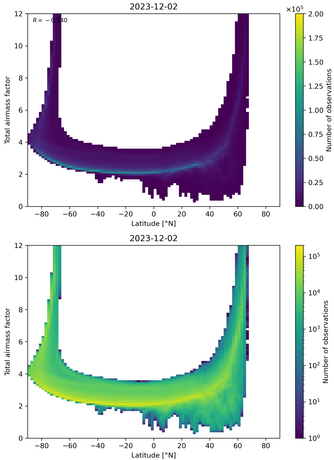
Figure 84: Scatter density plot of “Latitude” against “Total airmass factor” for 2023-12-01 to 2023-12-03.
