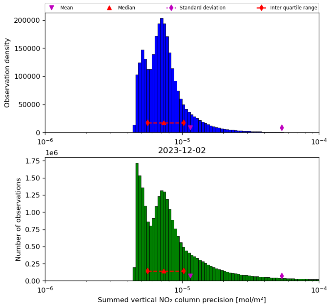
Figure 41: Histogram of “Summed vertical NO 2 column precision” for 2023-12-01 to 2023-12-03
