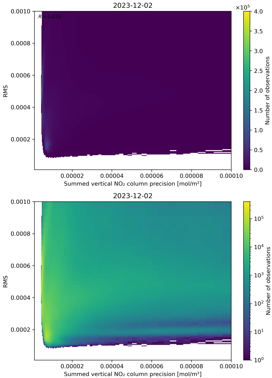
Figure 108: Scatter density plot of “Summed vertical NO 2 column precision” against “RMS” for 2023-12-01 to 2023-12-03.
