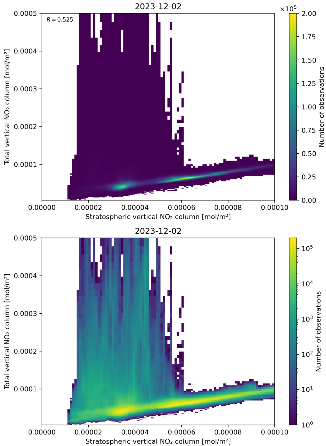
Figure 100: Scatter density plot of “Stratospheric vertical NO 2 column” against “Total vertical NO 2 column” for 2023-12-01 to 2023-12-03.
