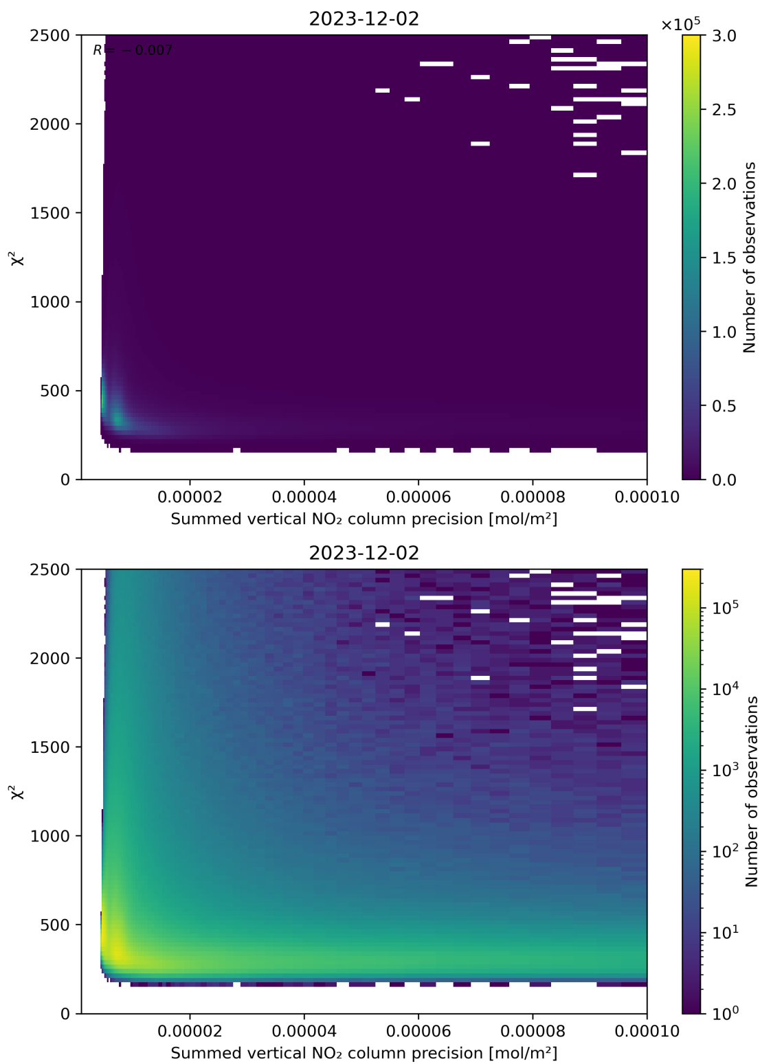
Figure 107: Scatter density plot of “Summed vertical NO 2 column precision” against “ \chi^2 ” for 2023-12-01 to 2023-12-03.
