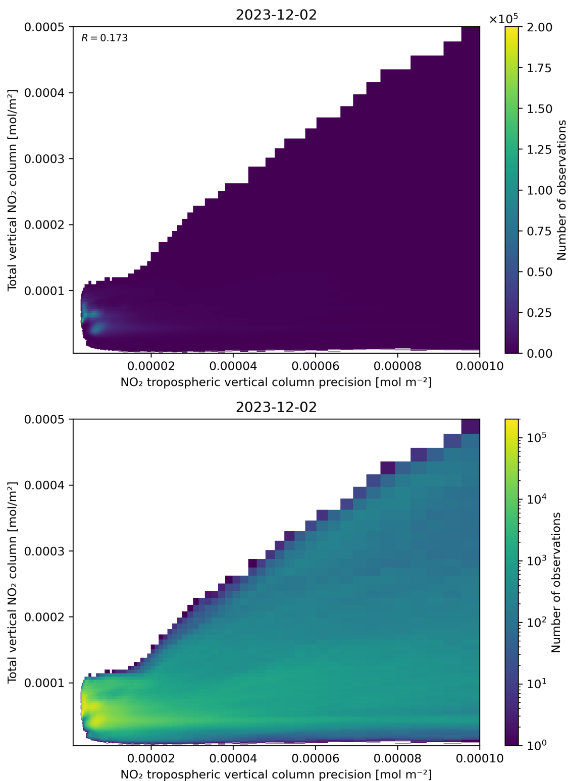
Figure 138: Scatter density plot of “NO 2 tropospheric vertical column precision” against “Total vertical NO 2 column” for 2023-12-01 to 2023-12-03.
