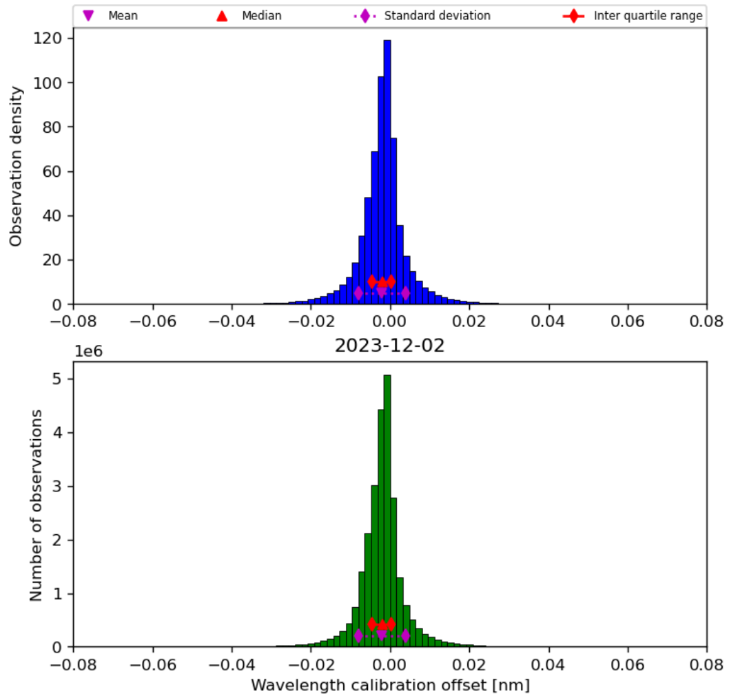
Figure 35: Histogram of “Wavelength calibration offset” for 2023-12-01 to 2023-12-03
