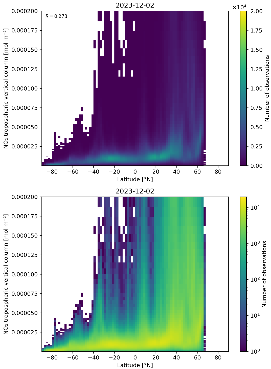
Figure 92: Scatter density plot of “Latitude” against “NO 2 tropospheric vertical column” for 2023-12-01 to 2023-12-03.
