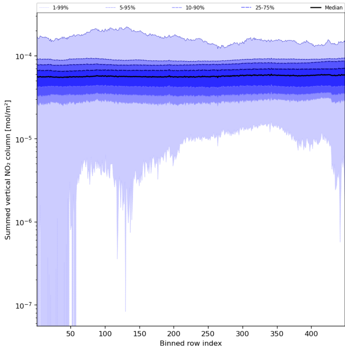
Figure 57: Along track statistics of “Summed vertical NO 2 column” for 2023-12-01 to 2023-12-03
