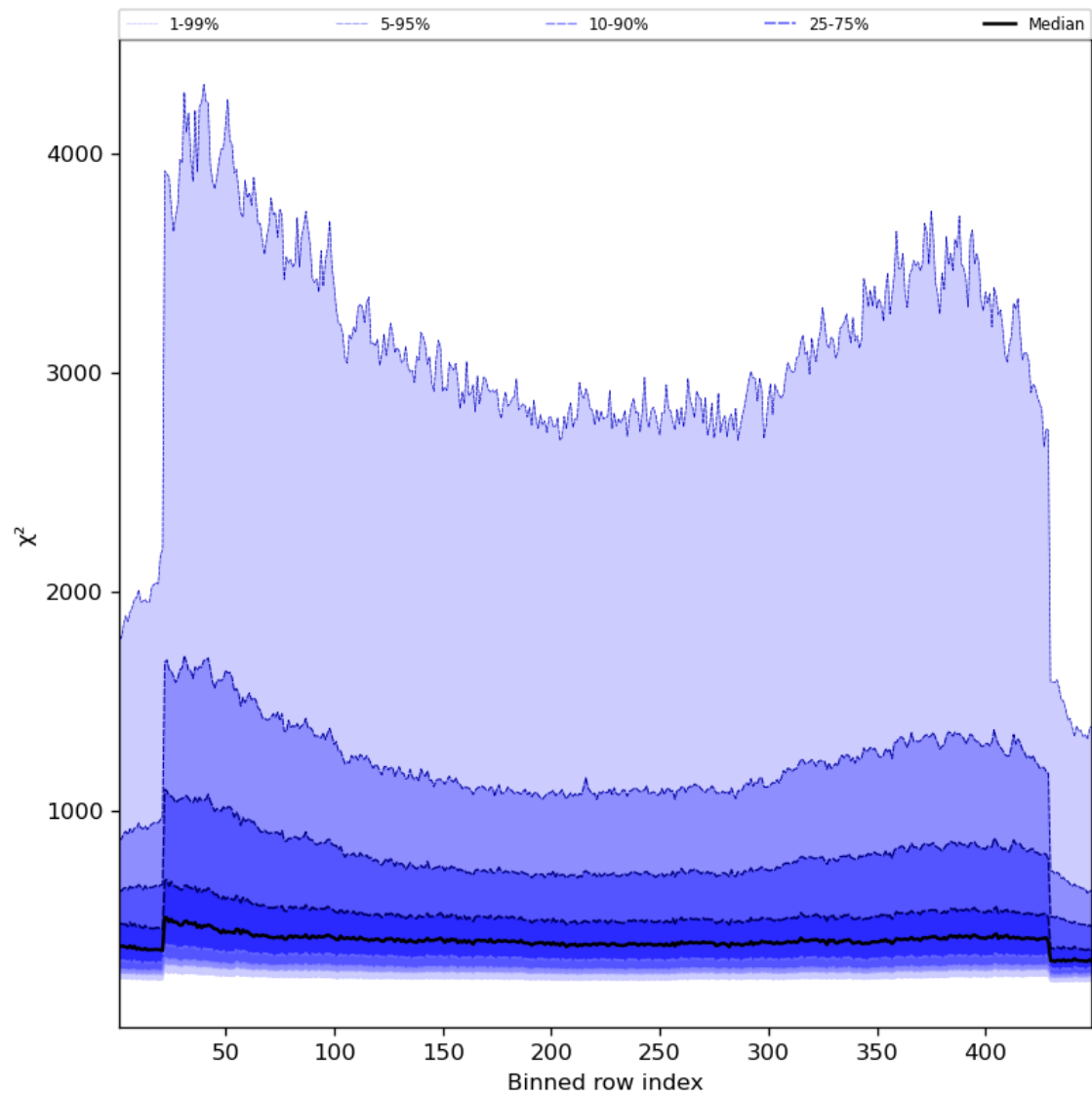
Figure 59: Along track statistics of “ \chi^2 ” for 2023-12-01 to 2023-12-03
