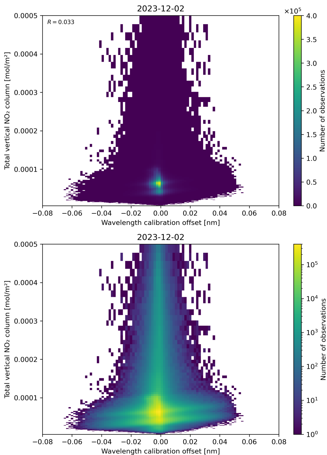
Figure 179: Scatter density plot of “Wavelength calibration offset” against “Total vertical NO 2 column” for 2023-12-01 to 2023-12-03.
