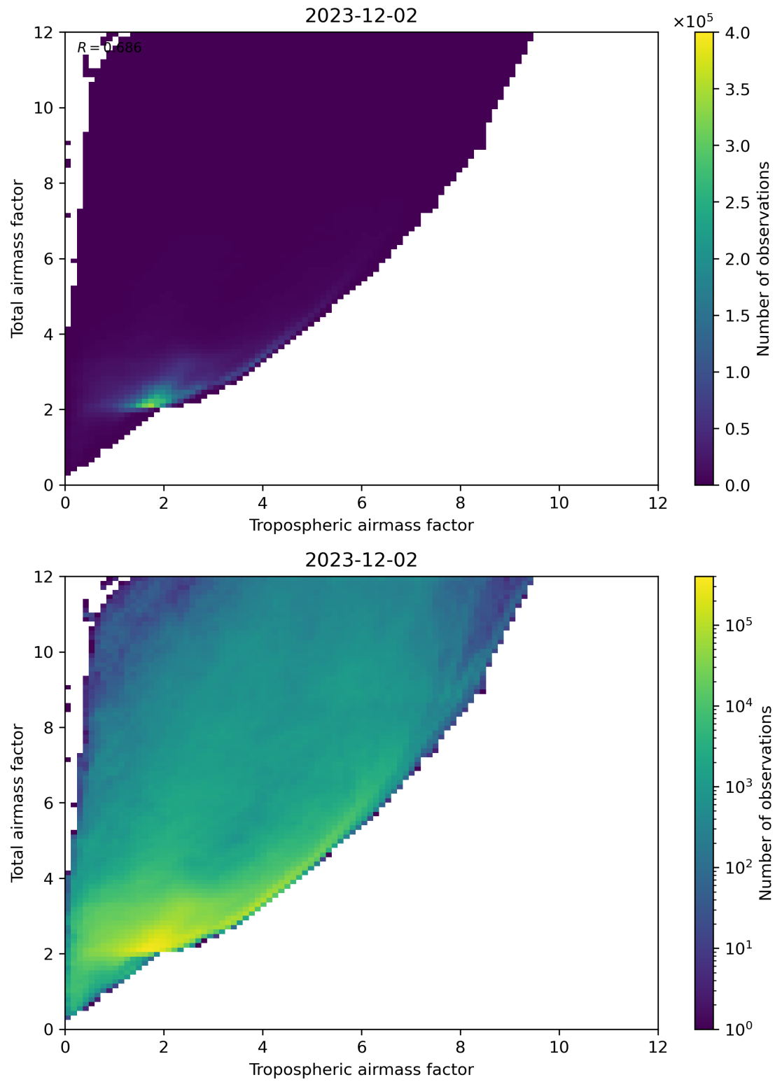
Figure 72: Scatter density plot of “Tropospheric airmass factor” against “Total airmass factor” for 2023-12-01 to 2023-12-03.
