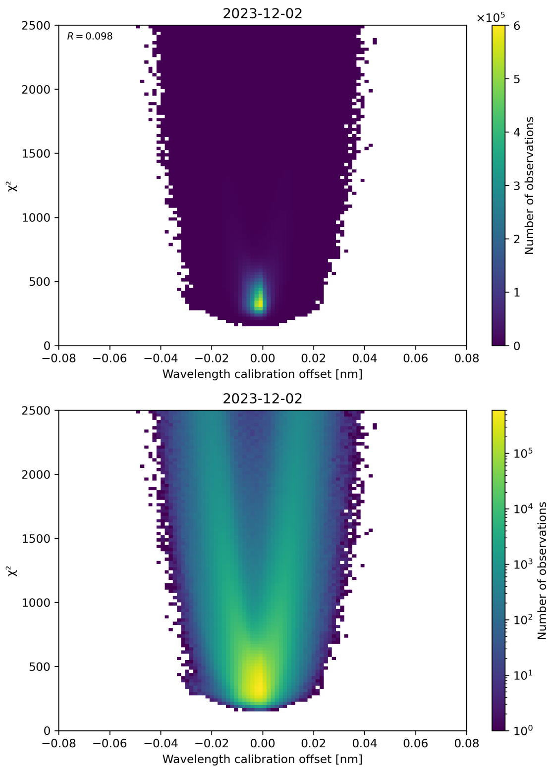
Figure 175: Scatter density plot of “Wavelength calibration offset” against “ \chi^2 ” for 2023-12-01 to 2023-12-03.
