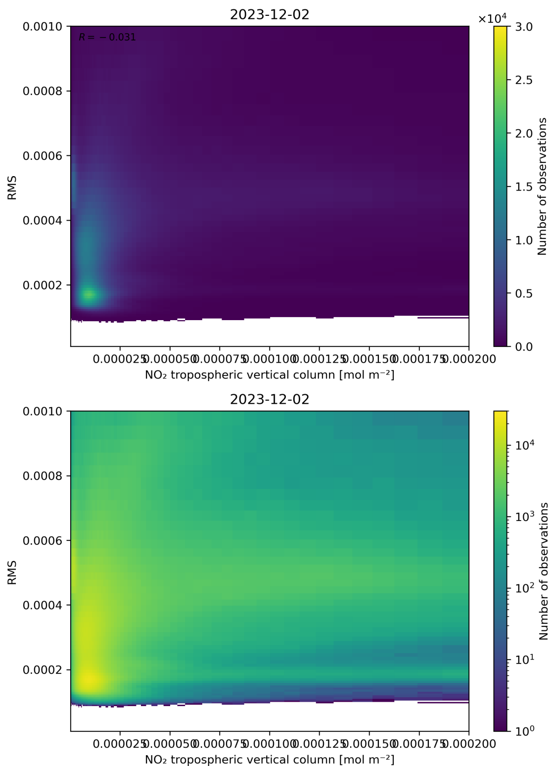
Figure 142: Scatter density plot of “NO 2 tropospheric vertical column” against “RMS” for 2023-12-01 to 2023-12-03.
