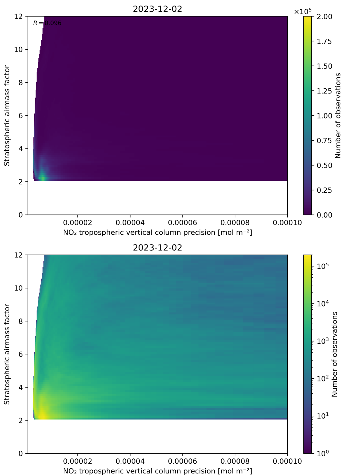
Figure 131: Scatter density plot of “NO 2 tropospheric vertical column precision” against “Stratospheric airmass factor” for 2023-12-01 to 2023-12-03.
