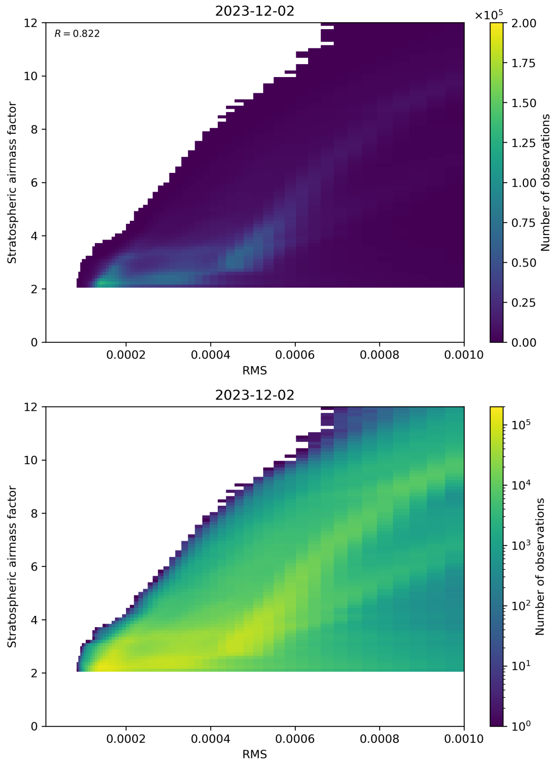
Figure 144: Scatter density plot of “RMS” against “Stratospheric airmass factor” for 2023-12-01 to 2023-12-03.
