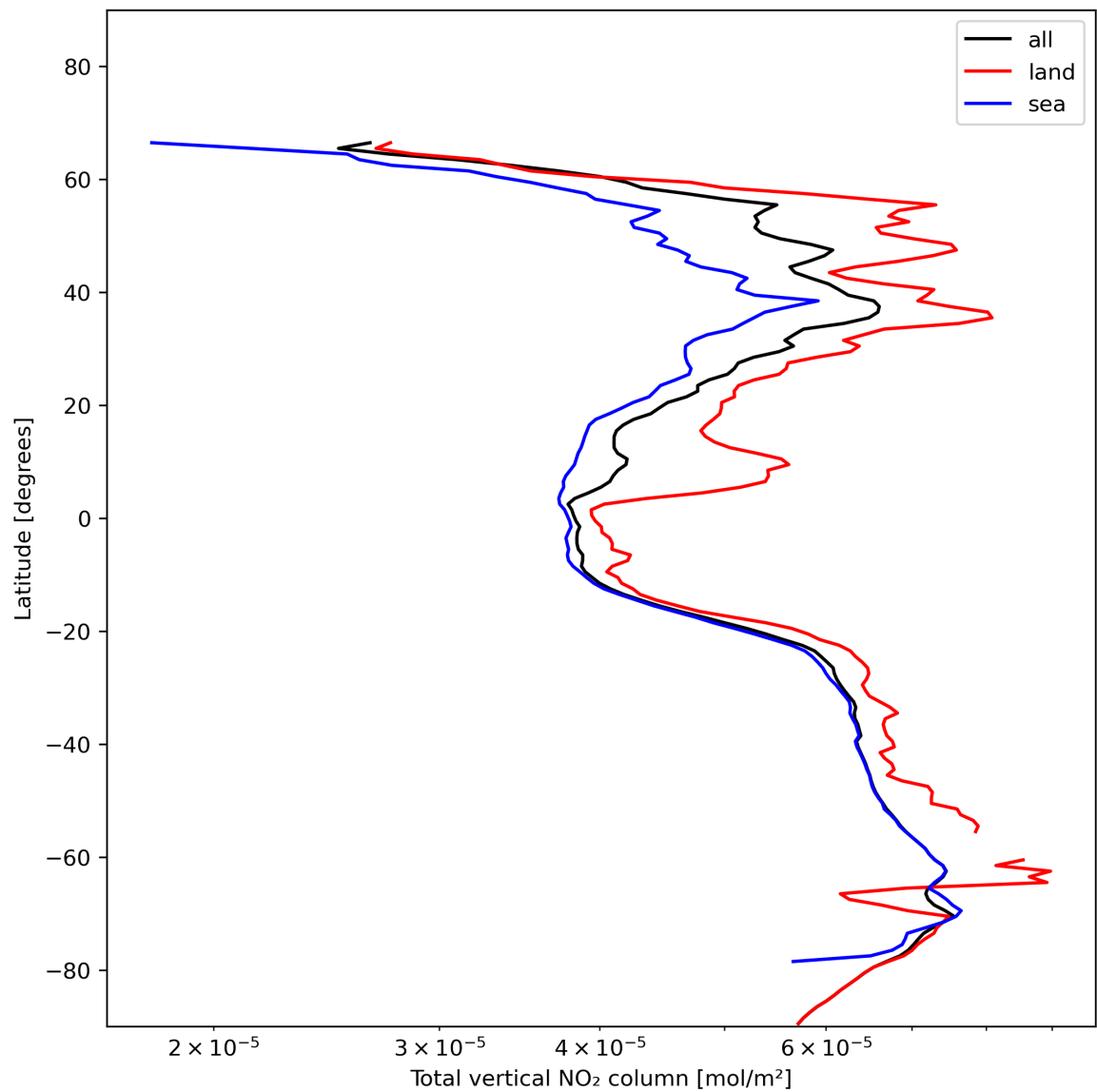
Figure 21: Zonal average of “Total vertical NO 2 column” for 2023-12-01 to 2023-12-03.
