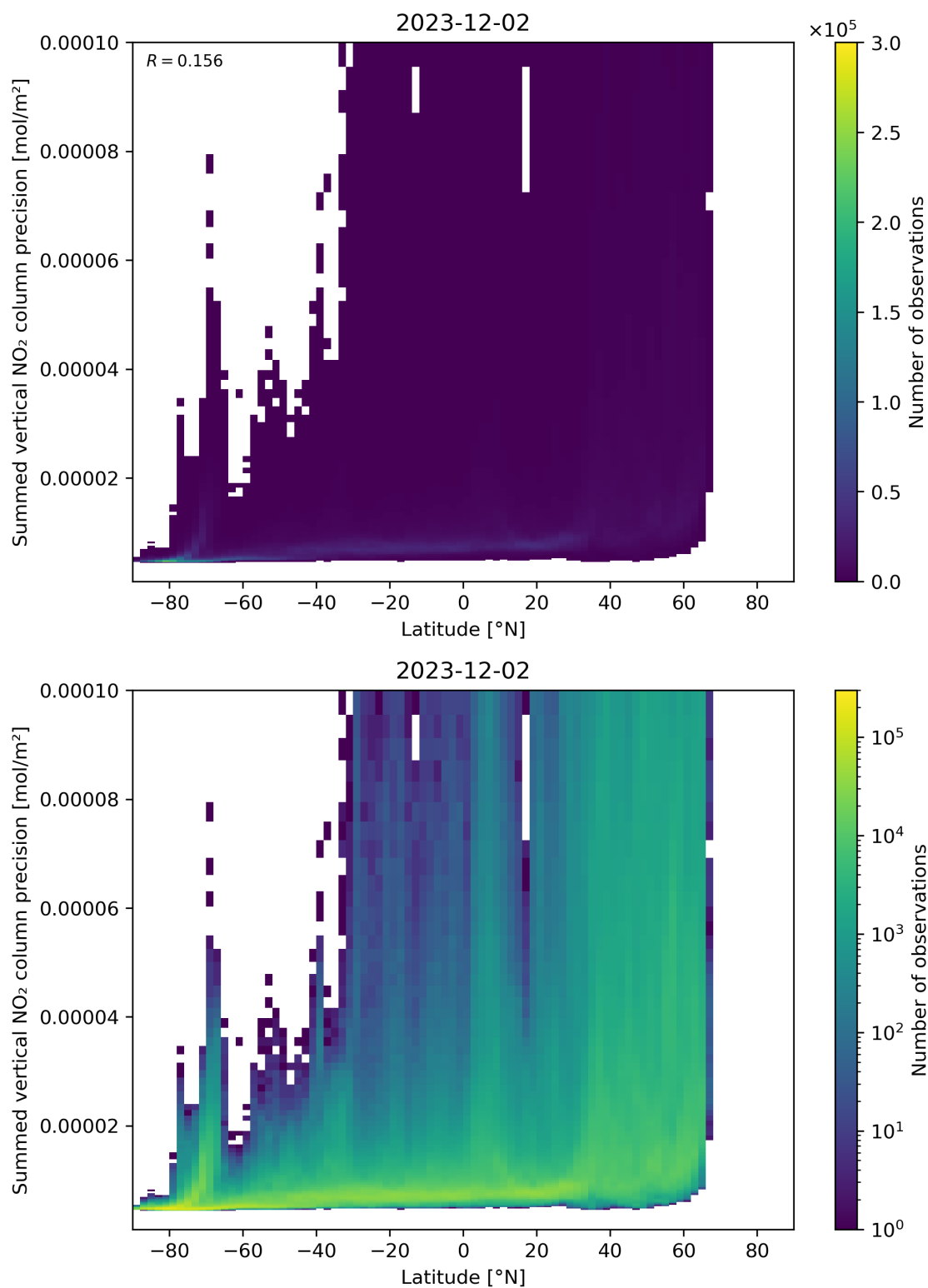
Figure 89: Scatter density plot of “Latitude” against “Summed vertical NO 2 column precision” for 2023-12-01 to 2023-12-03.
