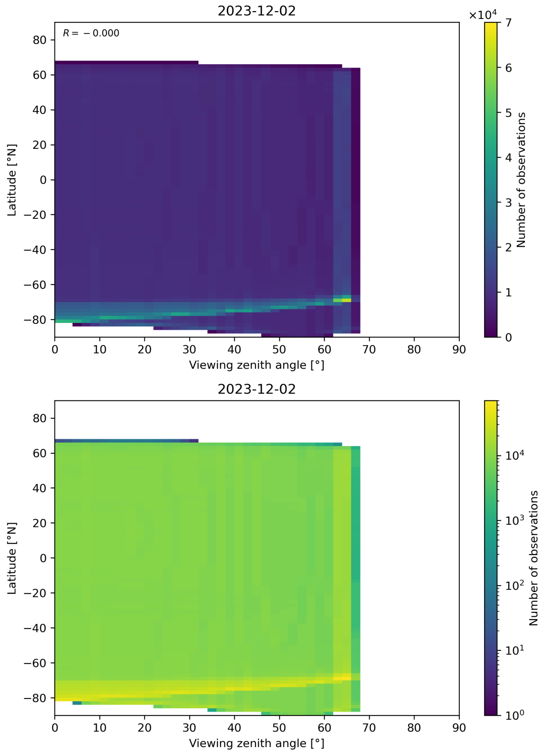
Figure 163: Scatter density plot of “Viewing zenith angle” against “Latitude” for 2023-12-01 to 2023-12-03.
