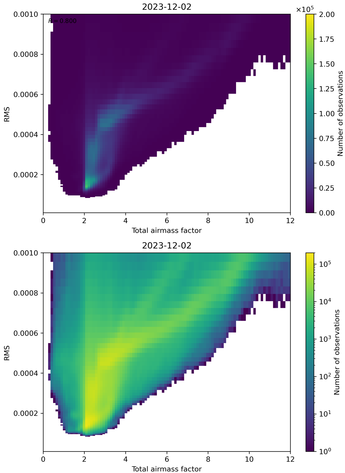
Figure 69: Scatter density plot of “Total airmass factor” against “RMS” for 2023-12-01 to 2023-12-03.
