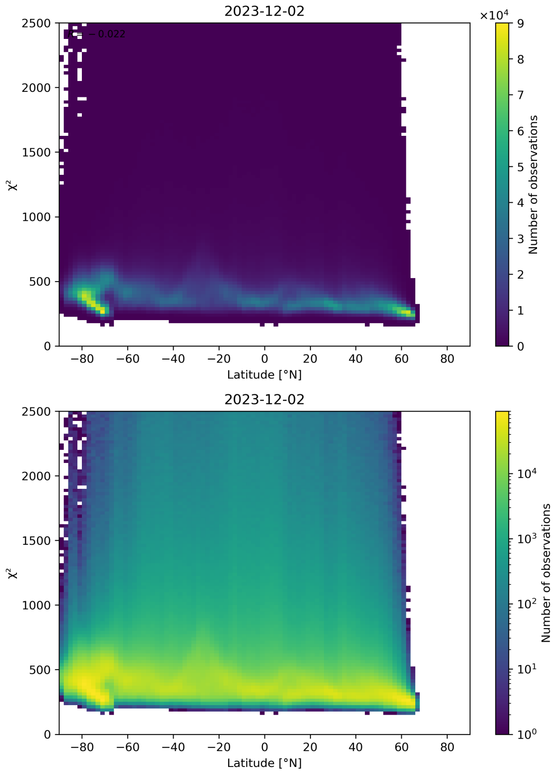
Figure 86: Scatter density plot of “Latitude” against “ \chi^2 ” for 2023-12-01 to 2023-12-03.
