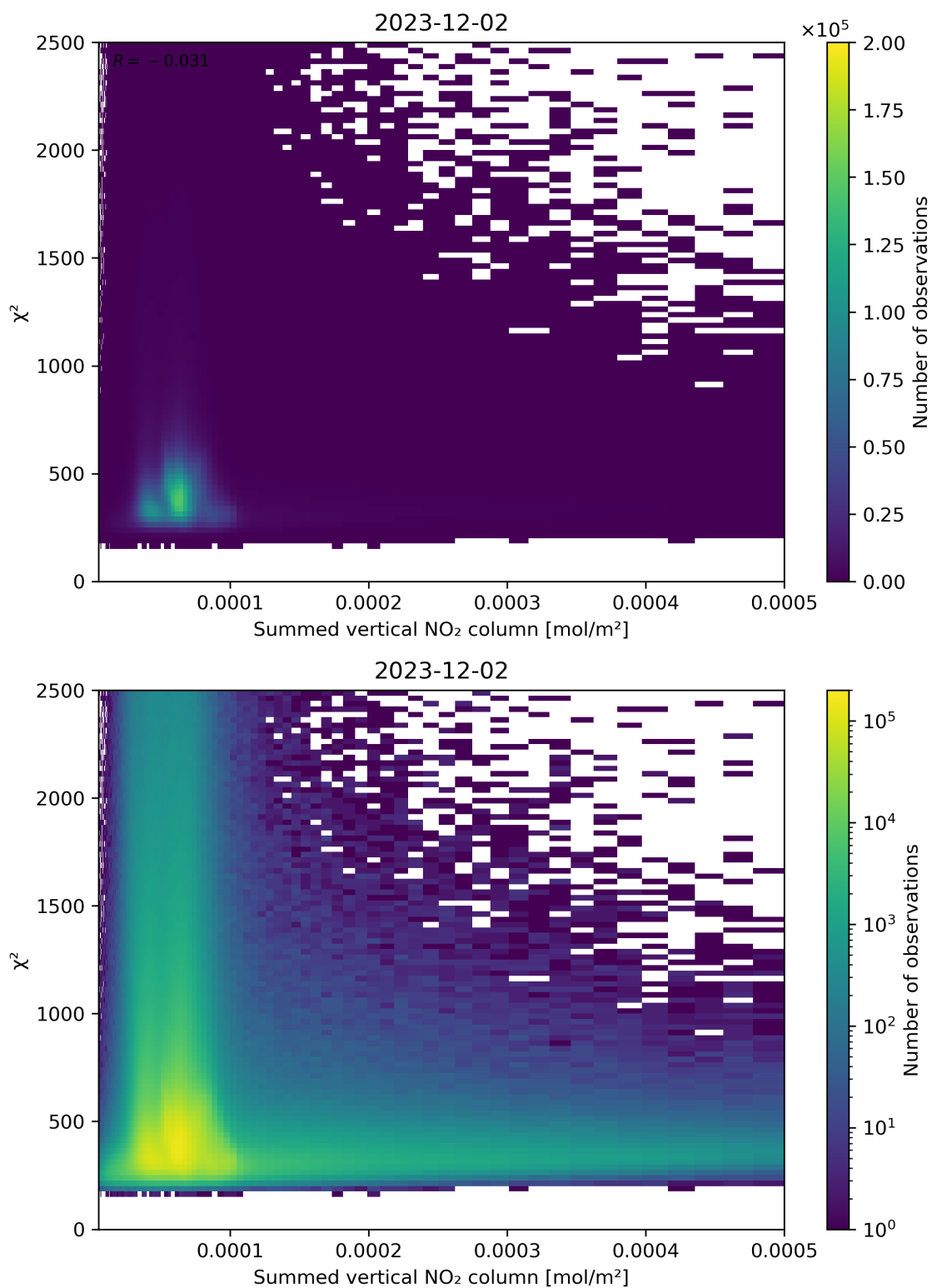
Figure 104: Scatter density plot of “Summed vertical NO 2 column” against “ \chi^2 ” for 2023-12-01 to 2023-12-03.
