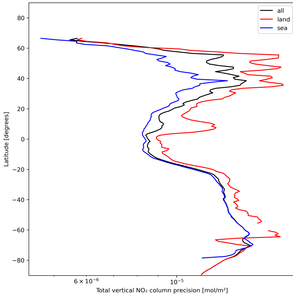
Figure 22: Zonal average of “Total vertical NO 2 column precision” for 2023-12-01 to 2023-12-03.
