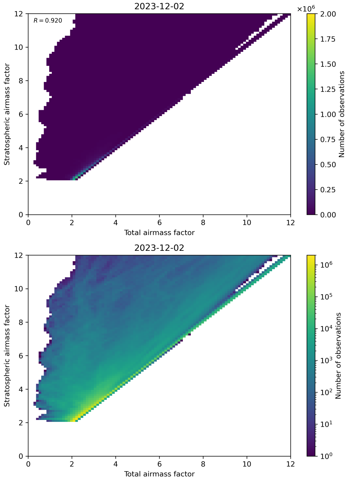
Figure 62: Scatter density plot of “Total airmass factor” against “Stratospheric airmass factor” for 2023-12-01 to 2023-12-03.
