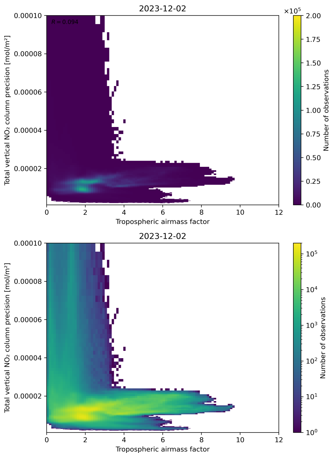
Figure 78: Scatter density plot of “Tropospheric air mass factor” against “Total vertical NO 2 column precision” for 2023-12-01 to 2023-12-03.
