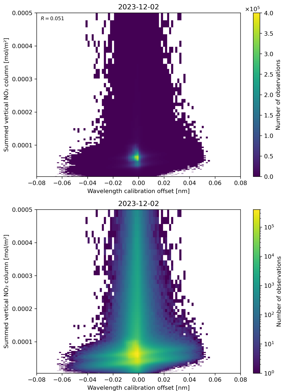
Figure 177: Scatter density plot of “Wavelength calibration offset” against “Summed vertical NO 2 column” for 2023-12-01 to 2023-12-03.
