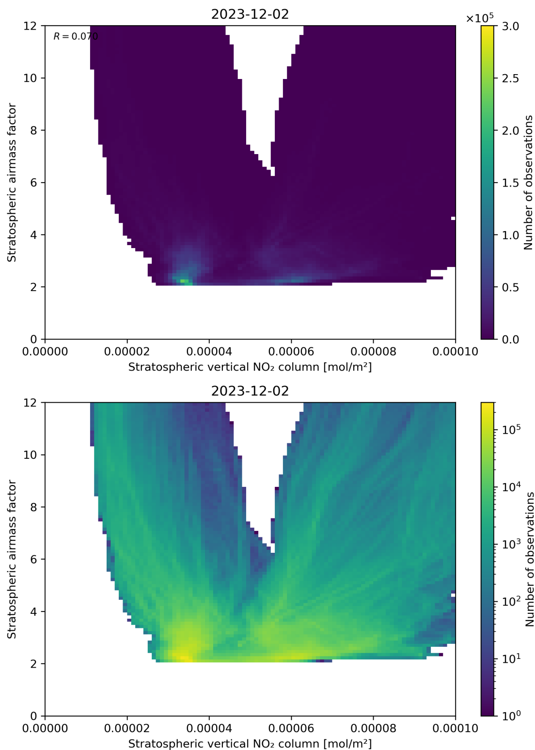
Figure 96: Scatter density plot of “Stratospheric vertical NO 2 column” against “Stratospheric airmass factor” for 2023-12-01 to 2023-12-03.
