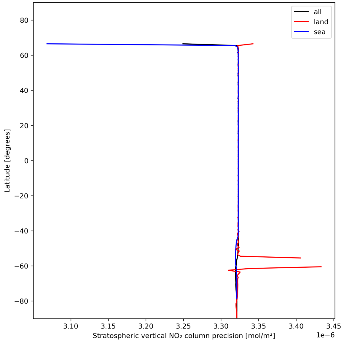
Figure 20: Zonal average of “Stratospheric vertical NO 2 column precision” for 2023-12-01 to 2023-12-03.
