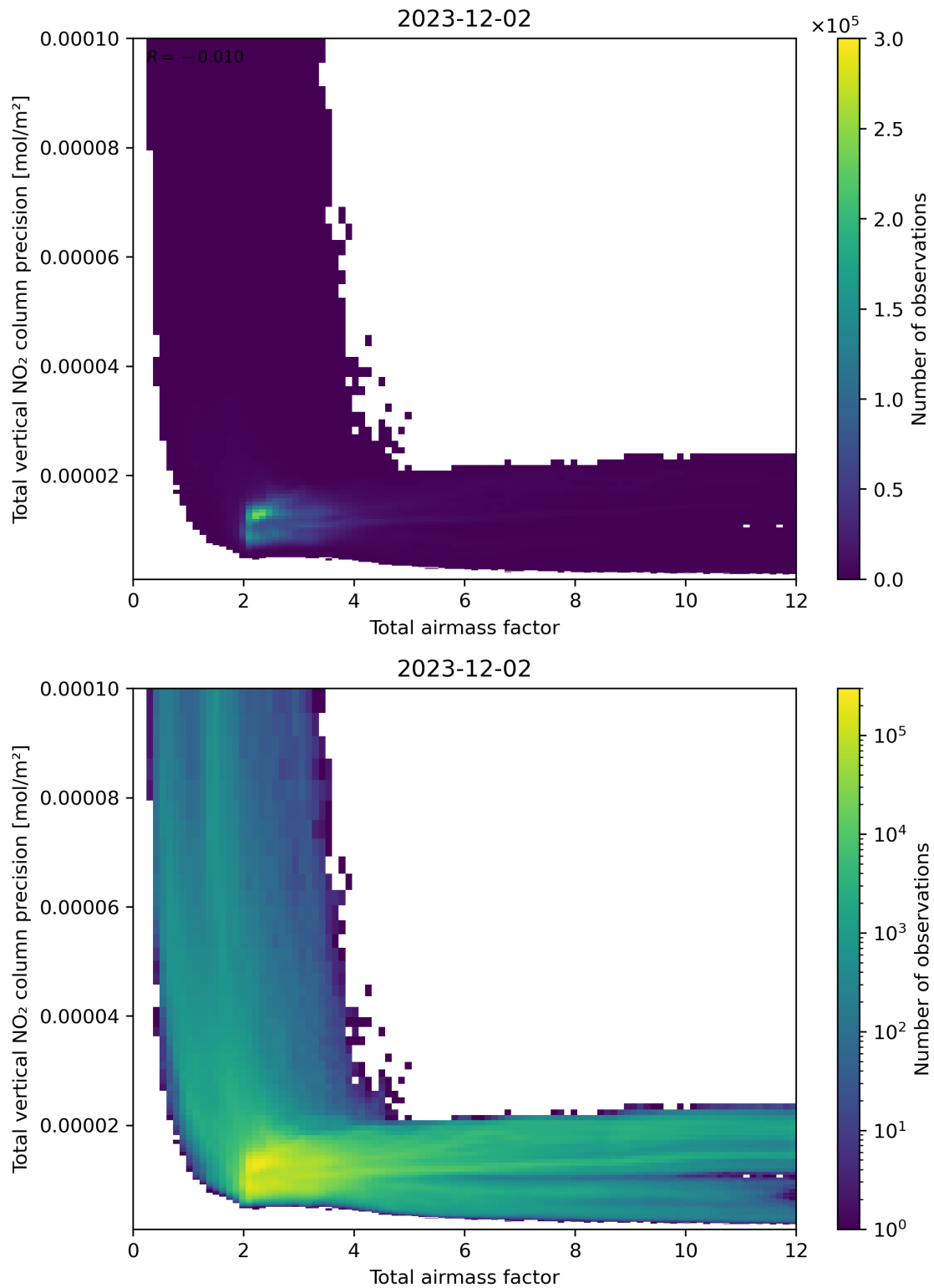
Figure 68: Scatter density plot of “Total airmass factor” against “Total vertical NO 2 column precision” for 2023-12-01 to 2023-12-03.
