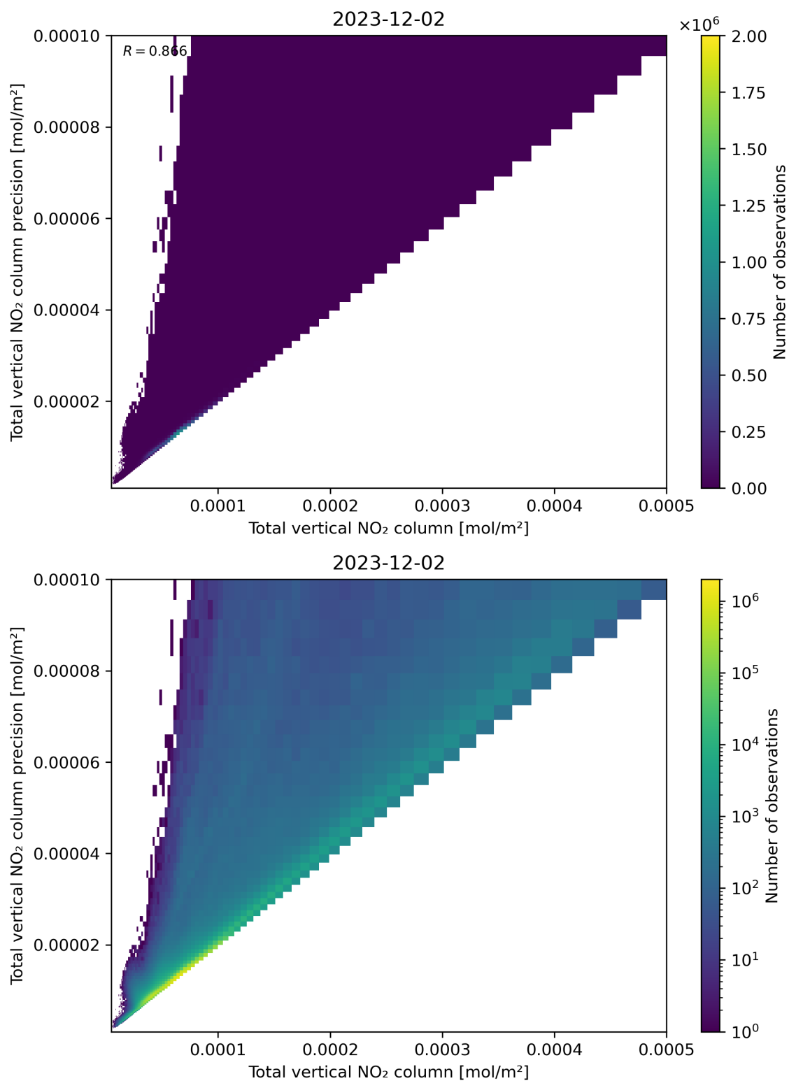
Figure 114: Scatter density plot of “Total vertical NO 2 column” against “Total vertical NO 2 column precision” for 2023-12-01 to 2023-12-03.
