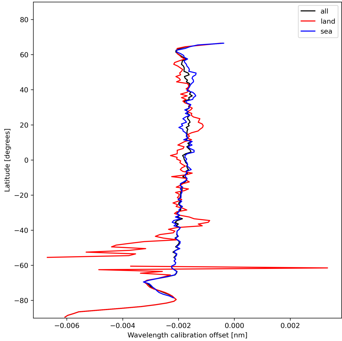
Figure 18: Zonal average of “Wavelength calibration offset” for 2023-12-01 to 2023-12-03.
