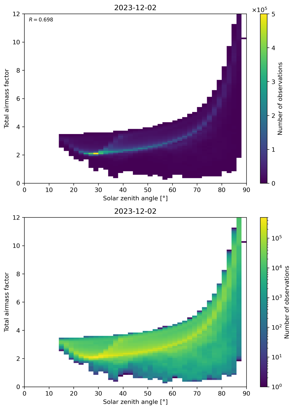
Figure 146: Scatter density plot of “Solar zenith angle” against “Total air mass factor” for 2023-12-01 to 2023-12-03.
