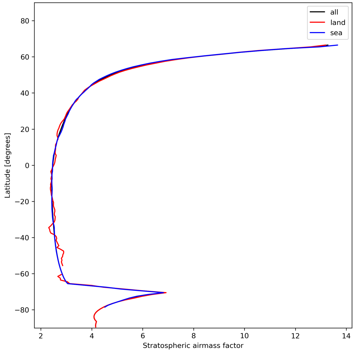
Figure 27: Zonal average of “Stratospheric air mass factor” for 2023-12-01 to 2023-12-03.
