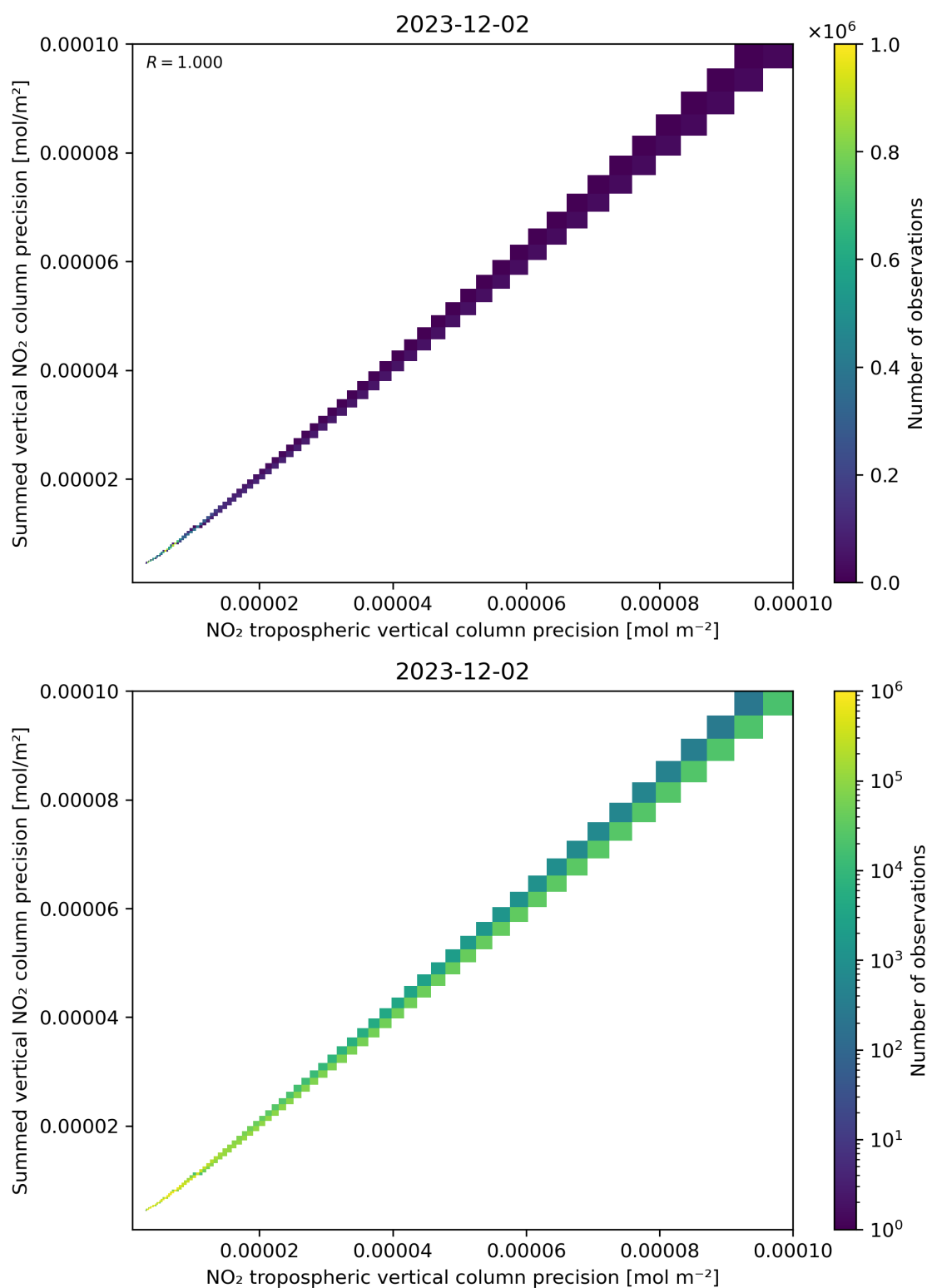
Figure 137: Scatter density plot of “NO 2 tropospheric vertical column precision” against “Summed vertical NO 2 column precision” for 2023-12-01 to 2023-12-03.
