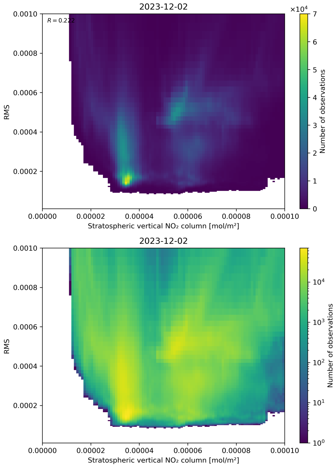
Figure 102: Scatter density plot of “Stratospheric vertical NO 2 column” against “RMS” for 2023-12-01 to 2023-12-03.
