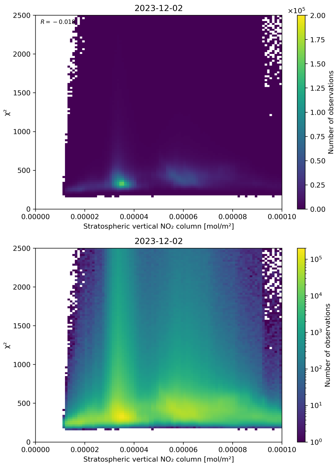
Figure 97: Scatter density plot of “Stratospheric vertical NO 2 column” against “ \chi^2 ” for 2023-12-01 to 2023-12-03.
