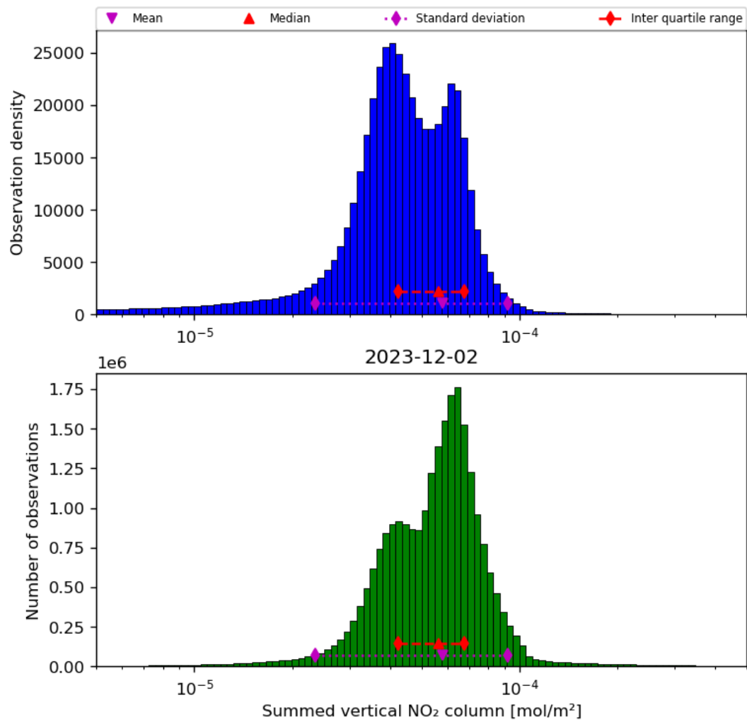
Figure 40: Histogram of “Summed vertical NO 2 column” for 2023-12-01 to 2023-12-03
