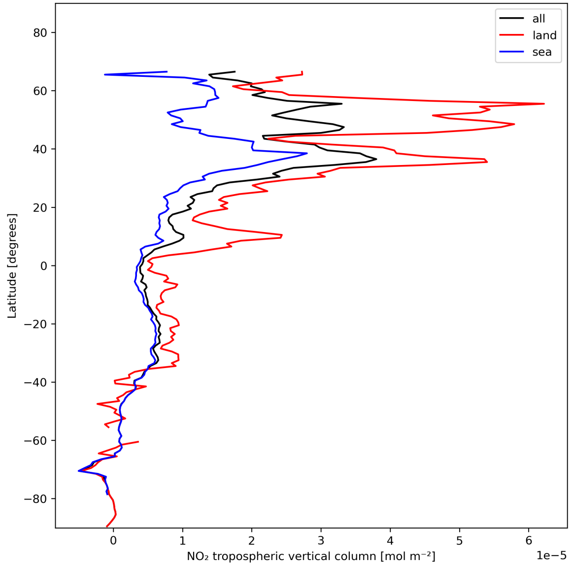
Figure 12: Zonal average of “NO 2 tropospheric vertical column” for 2023-12-01 to 2023-12-03.
