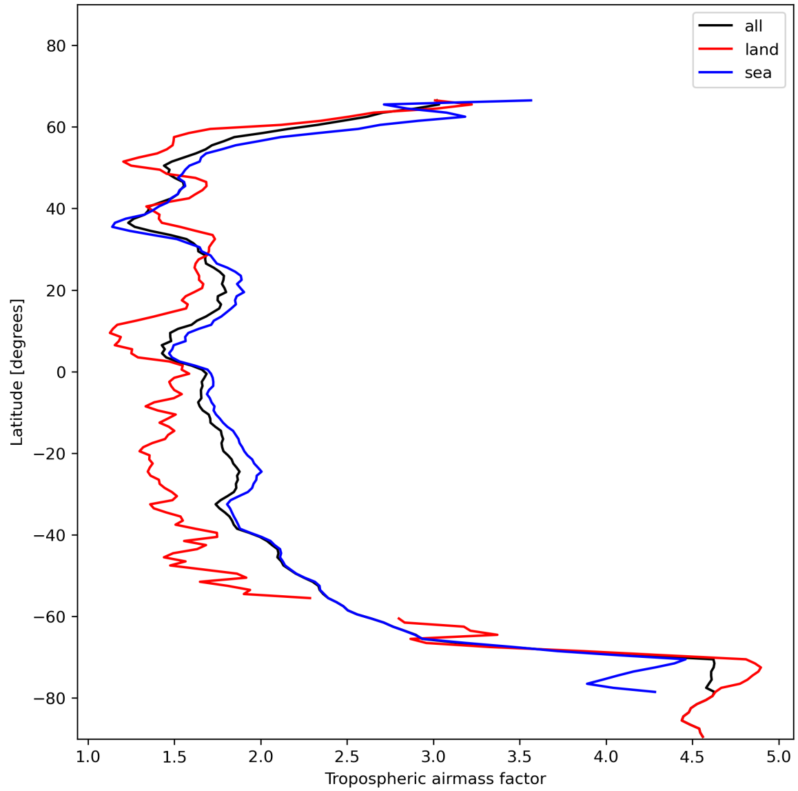
Figure 14: Zonal average of “Tropospheric airmass factor” for 2023-12-01 to 2023-12-03.
