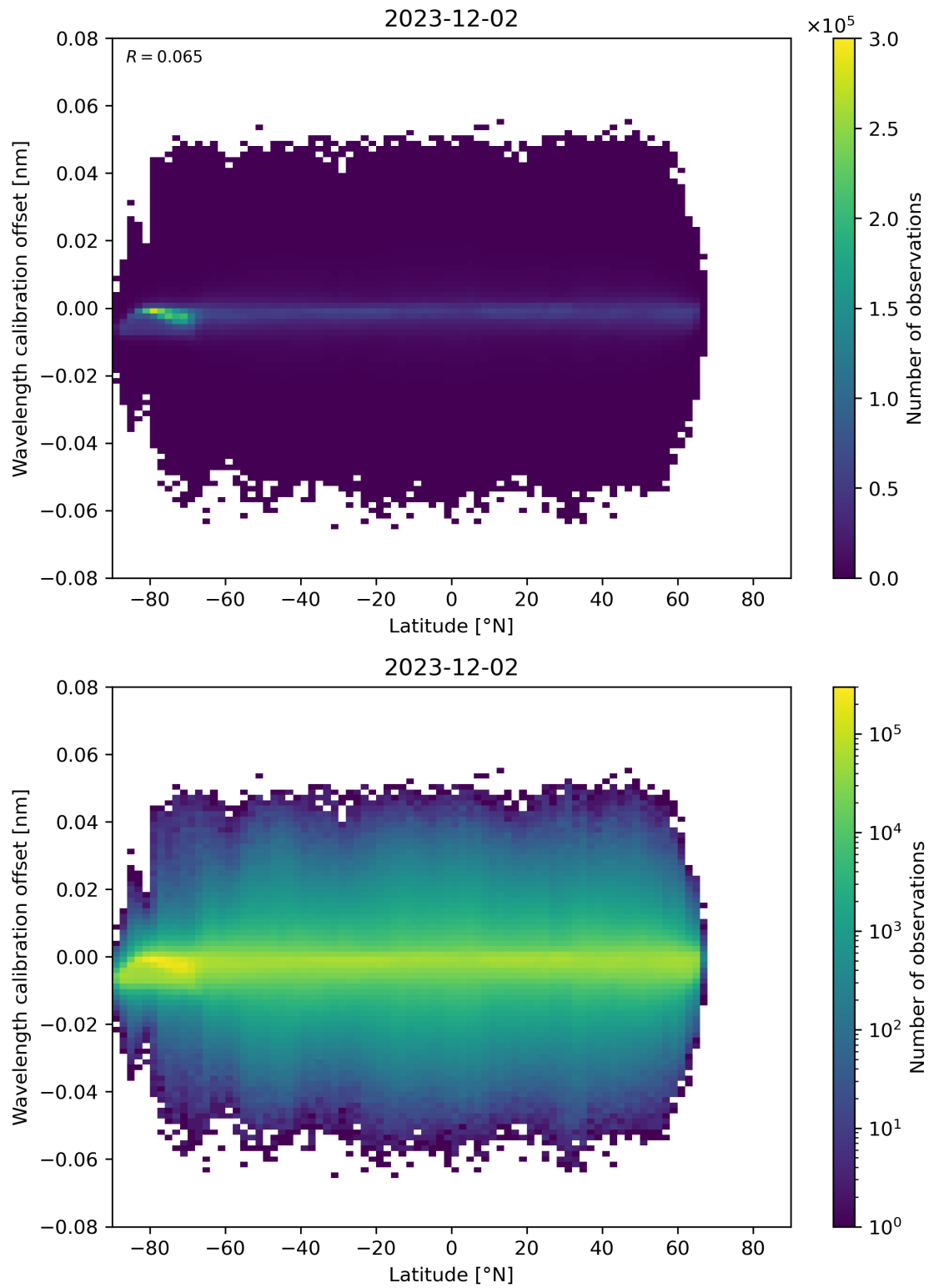
Figure 95: Scatter density plot of “Latitude” against “Wavelength calibration offset” for 2023-12-01 to 2023-12-03.
