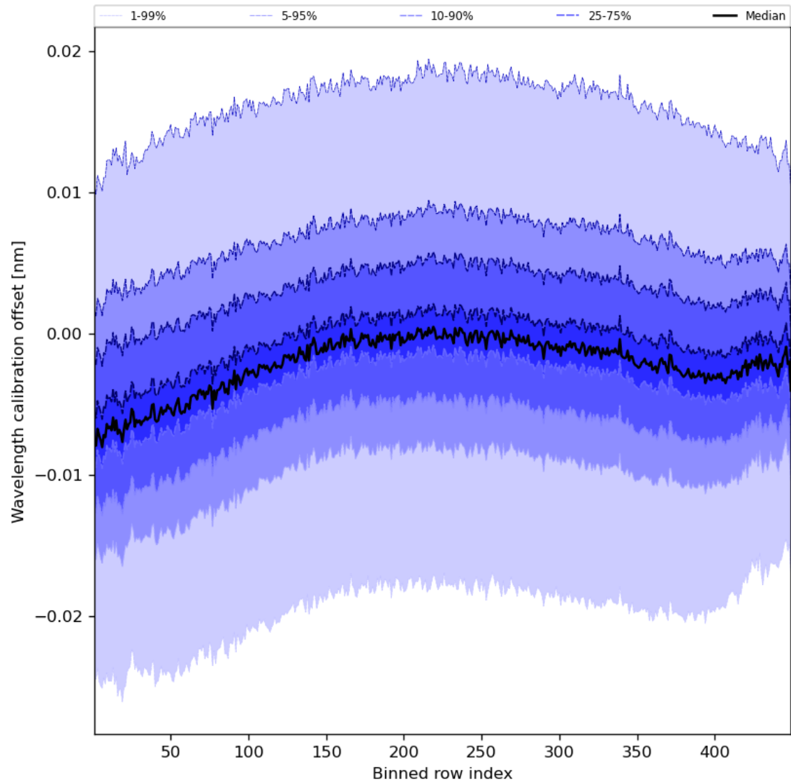
Figure 52: Along track statistics of “Wavelength calibration offset” for 2023-12-01 to 2023-12-03
