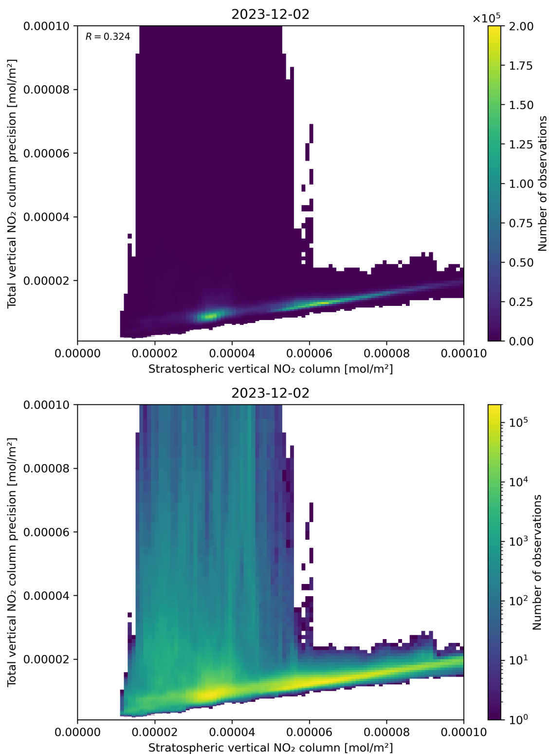
Figure 101: Scatter density plot of “Stratospheric vertical NO 2 column” against “Total vertical NO 2 column precision” for 2023-12-01 to 2023-12-03.
