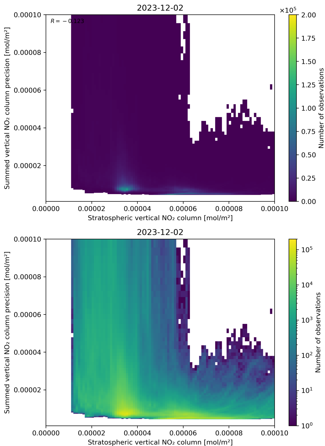
Figure 99: Scatter density plot of “Stratospheric vertical NO 2 column” against “Summed vertical NO 2 column precision” for 2023-12-01 to 2023-12-03.
