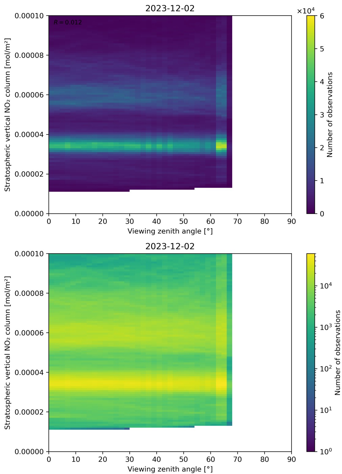
Figure 164: Scatter density plot of “Viewing zenith angle” against “Stratospheric vertical NO 2 column” for 2023-12-01 to 2023-12-03.
