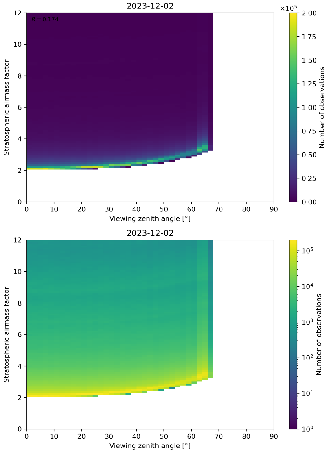
Figure 159: Scatter density plot of “Viewing zenith angle” against “Stratospheric airmass factor” for 2023-12-01 to 2023-12-03.
