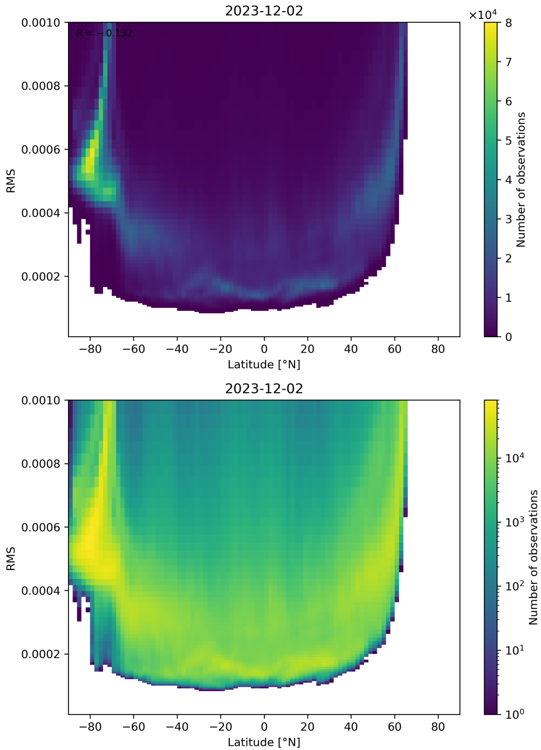
Figure 94: Scatter density plot of “Latitude” against “RMS” for 2023-12-01 to 2023-12-03.
