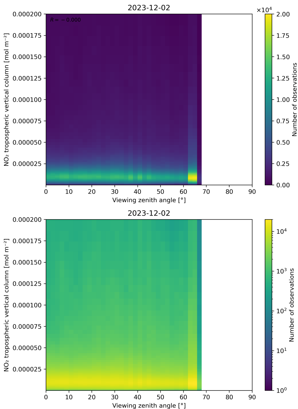
Figure 169: Scatter density plot of “Viewing zenith angle” against “NO 2 tropospheric vertical column” for 2023-12-01 to 2023-12-03.
