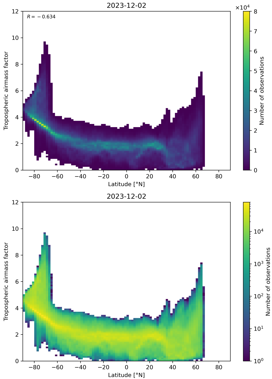
Figure 85: Scatter density plot of “Latitude” against “Tropospheric airmass factor” for 2023-12-01 to 2023-12-03.
