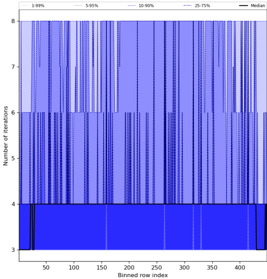
Figure 51: Along track statistics of “Number of iterations” for 2023-12-01 to 2023-12-03
