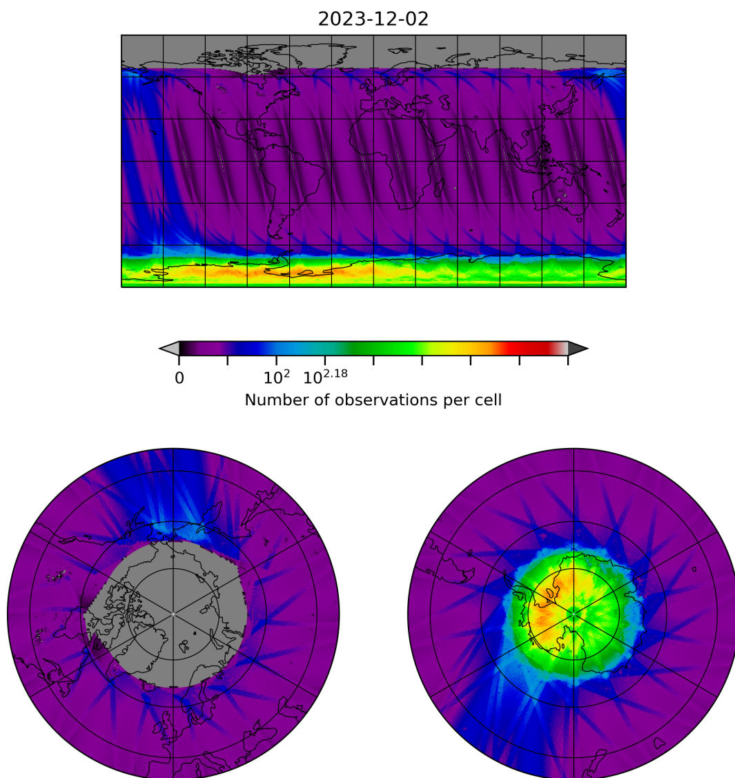
Figure 10: Map of the number of observations for 2023-12-01 to 2023-12-03
