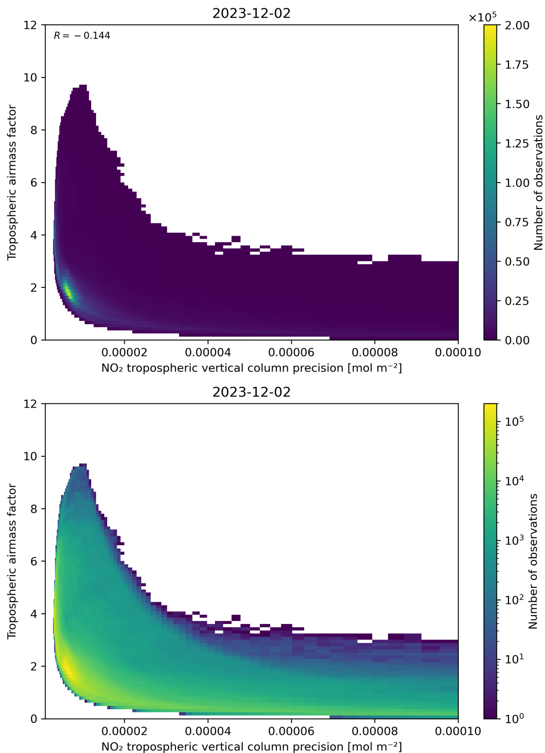
Figure 133: Scatter density plot of “NO 2 tropospheric vertical column precision” against “Tropospheric airmass factor” for 2023-12-01 to 2023-12-03.
