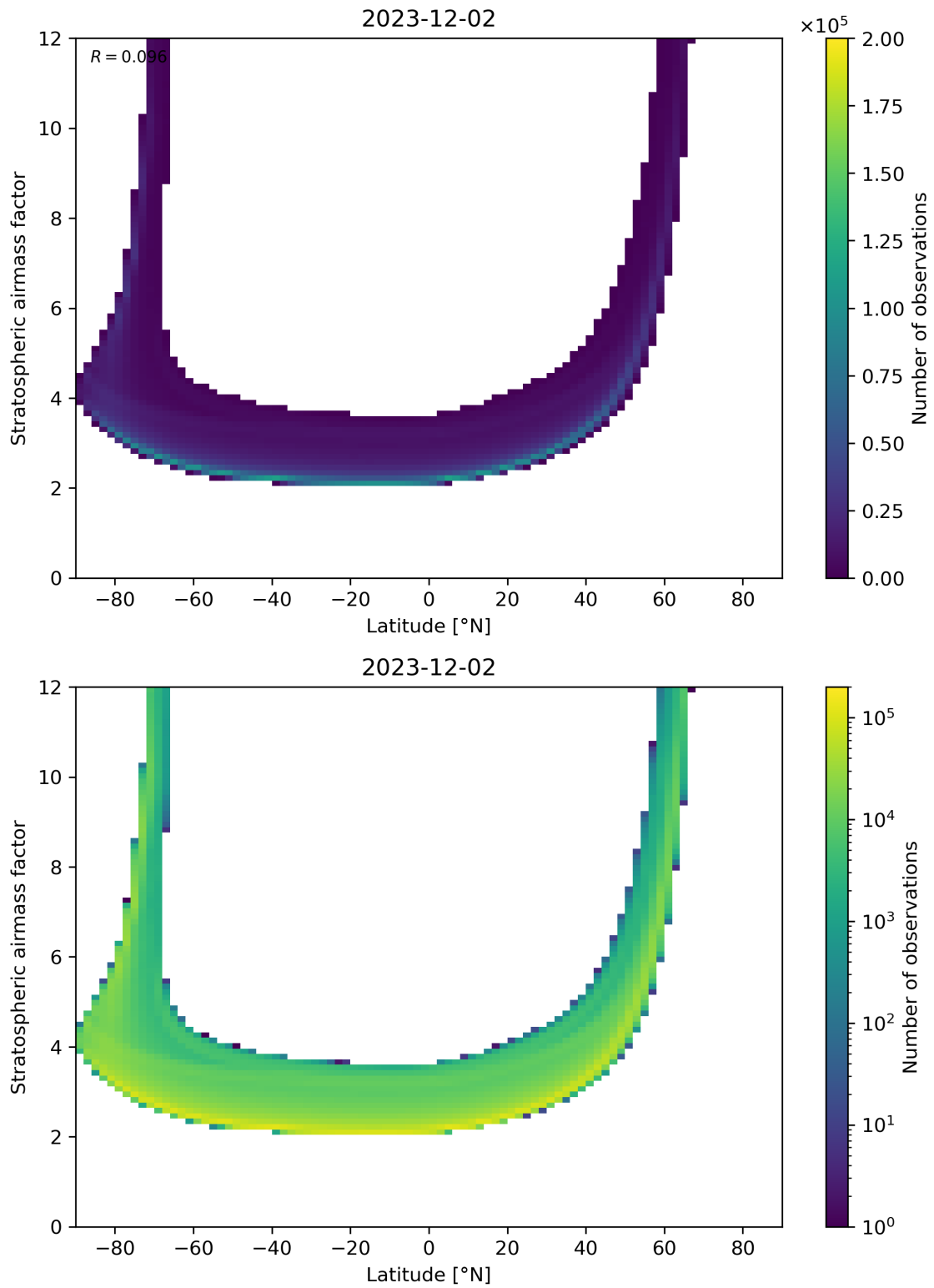
Figure 83: Scatter density plot of “Latitude” against “Stratospheric air mass factor” for 2023-12-01 to 2023-12-03.
