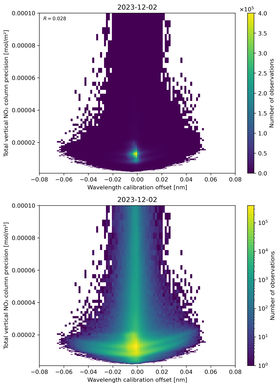
Figure 180: Scatter density plot of “Wavelength calibration offset” against “Total vertical NO 2 column precision” for 2023-12-01 to 2023-12-03.
