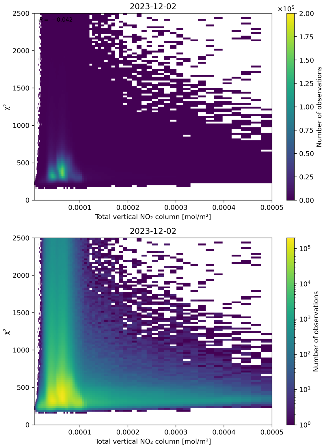
Figure 111: Scatter density plot of “Total vertical NO 2 column” against “ \chi^2 ” for 2023-12-01 to 2023-12-03.
