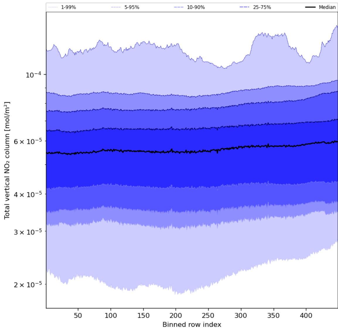
Figure 55: Along track statistics of “Total vertical NO 2 column” for 2023-12-01 to 2023-12-03
