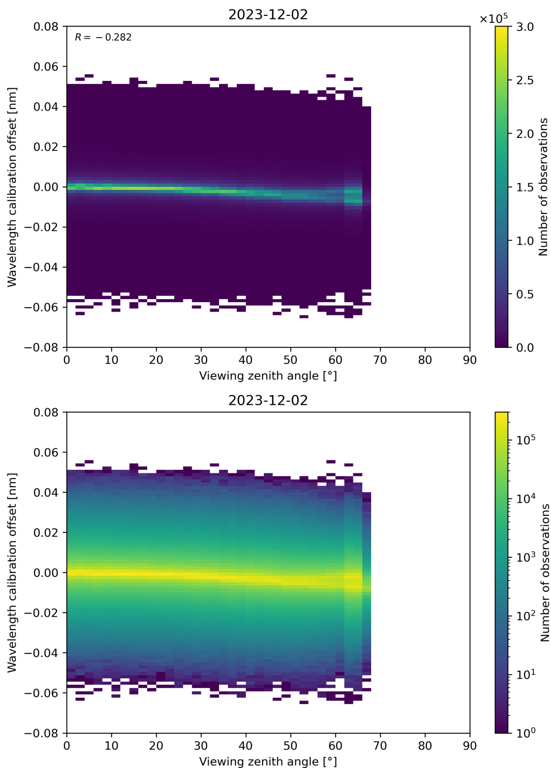
Figure 173: Scatter density plot of “Viewing zenith angle” against “Wavelength calibration offset” for 2023-12-01 to 2023-12-03.
