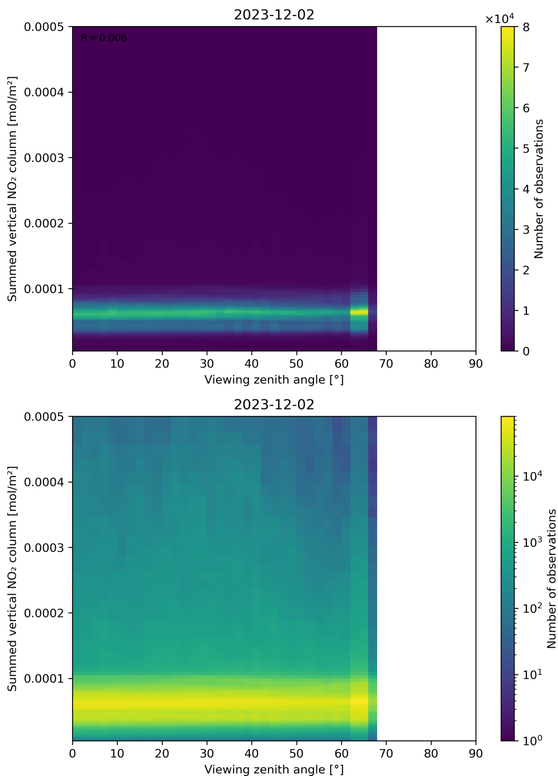
Figure 165: Scatter density plot of “Viewing zenith angle” against “Summed vertical NO 2 column” for 2023-12-01 to 2023-12-03.
