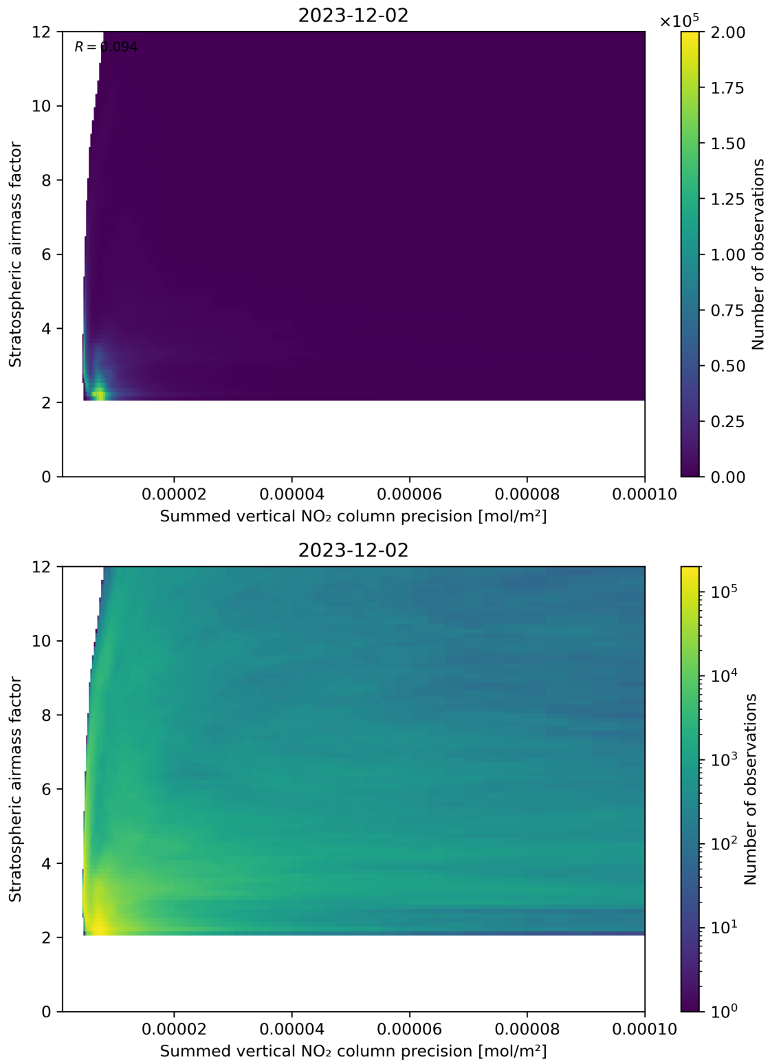
Figure 106: Scatter density plot of “Summed vertical NO 2 column precision” against “Stratospheric airmass factor” for 2023-12-01 to 2023-12-03.
