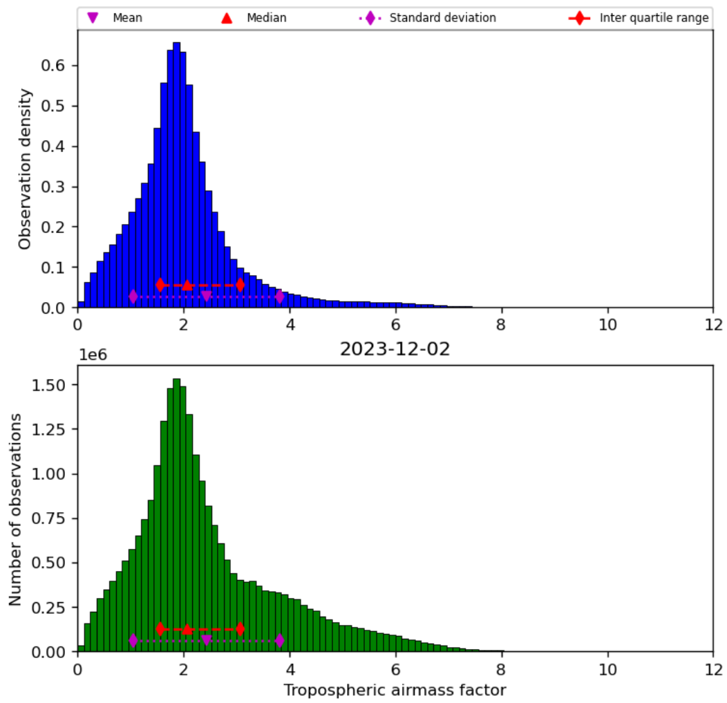
Figure 31: Histogram of “Tropospheric airmass factor” for 2023-12-01 to 2023-12-03
