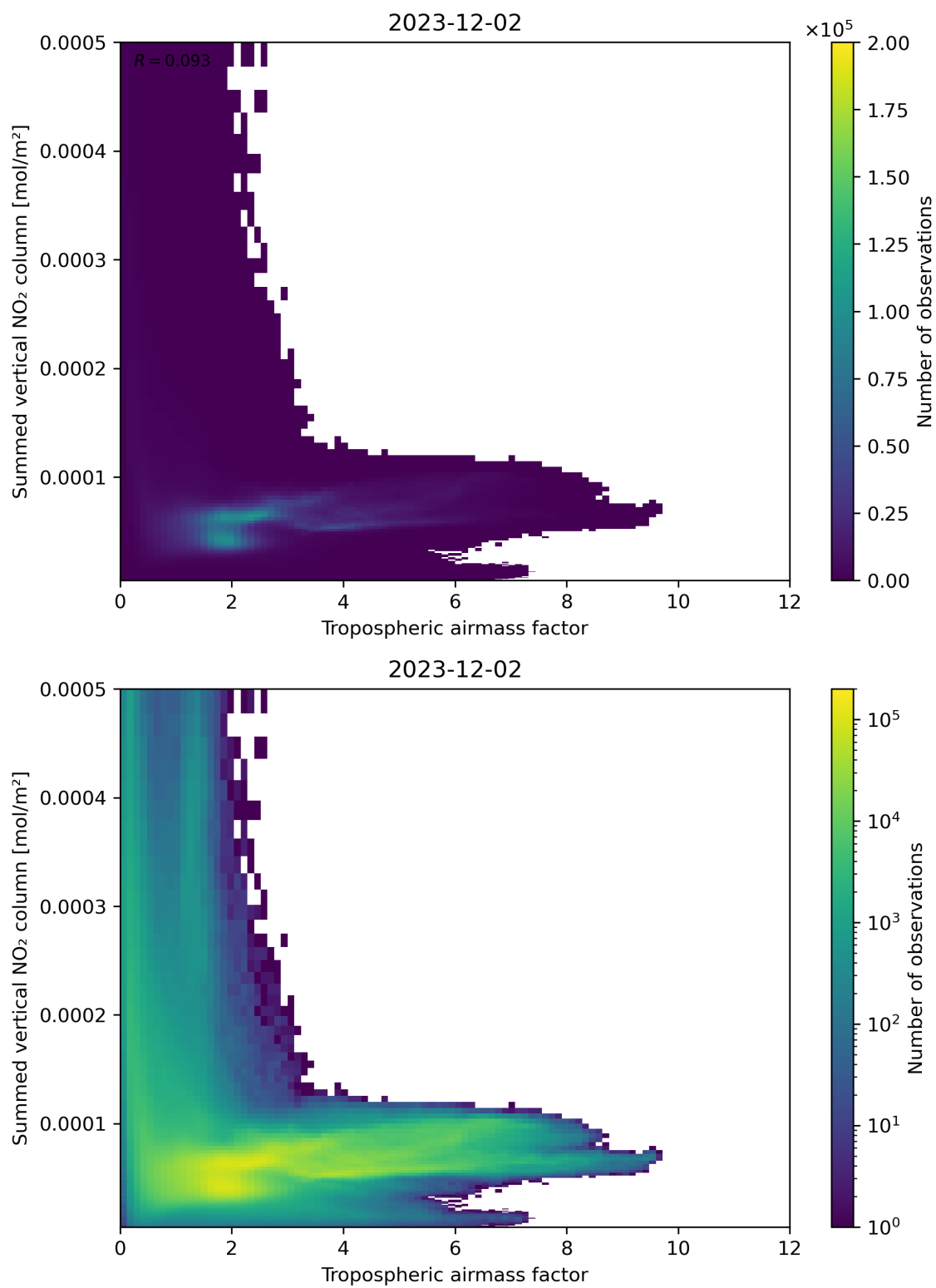
Figure 75: Scatter density plot of “Tropospheric airmass factor” against “Summed vertical NO 2 column” for 2023-12-01 to 2023-12-03.
