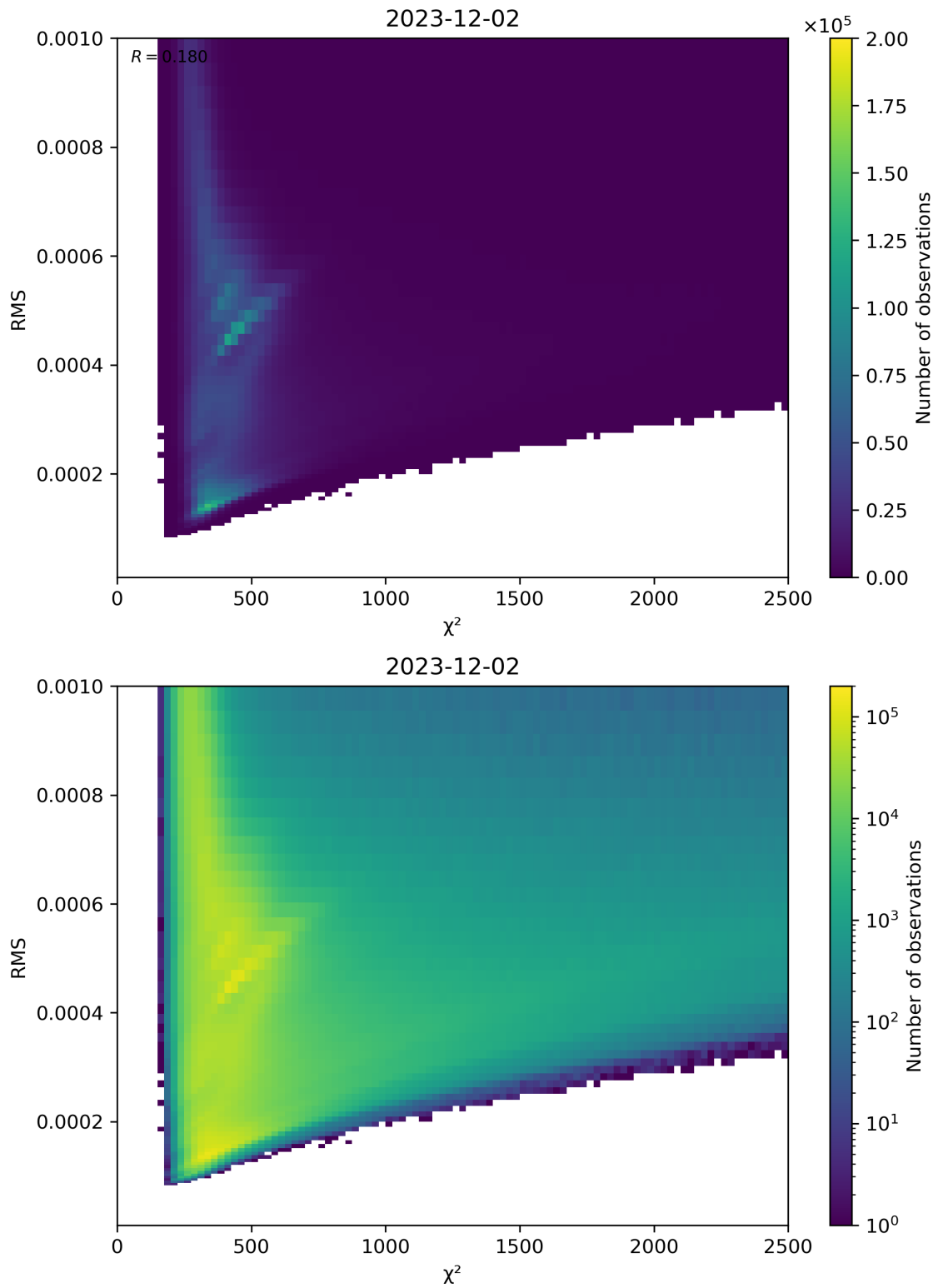
Figure 82: Scatter density plot of “ \chi^2 ” against “RMS” for 2023-12-01 to 2023-12-03.
