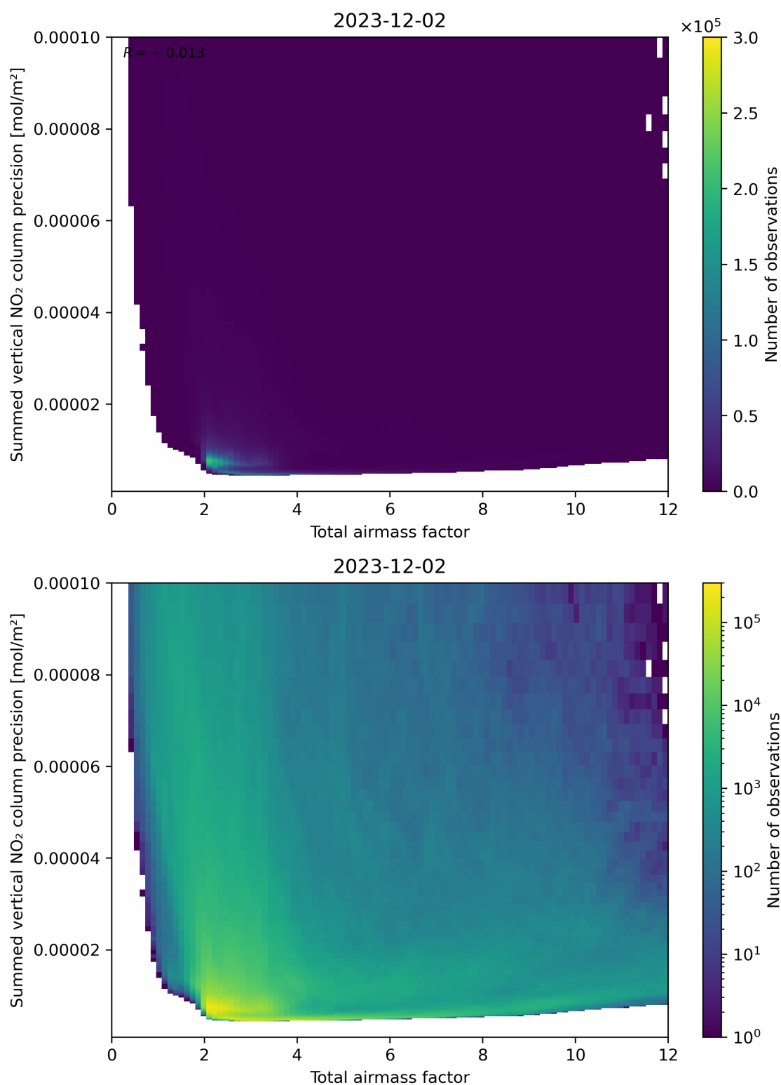
Figure 66: Scatter density plot of “Total airmass factor” against “Summed vertical NO 2 column precision” for 2023-12-01 to 2023-12-03.
