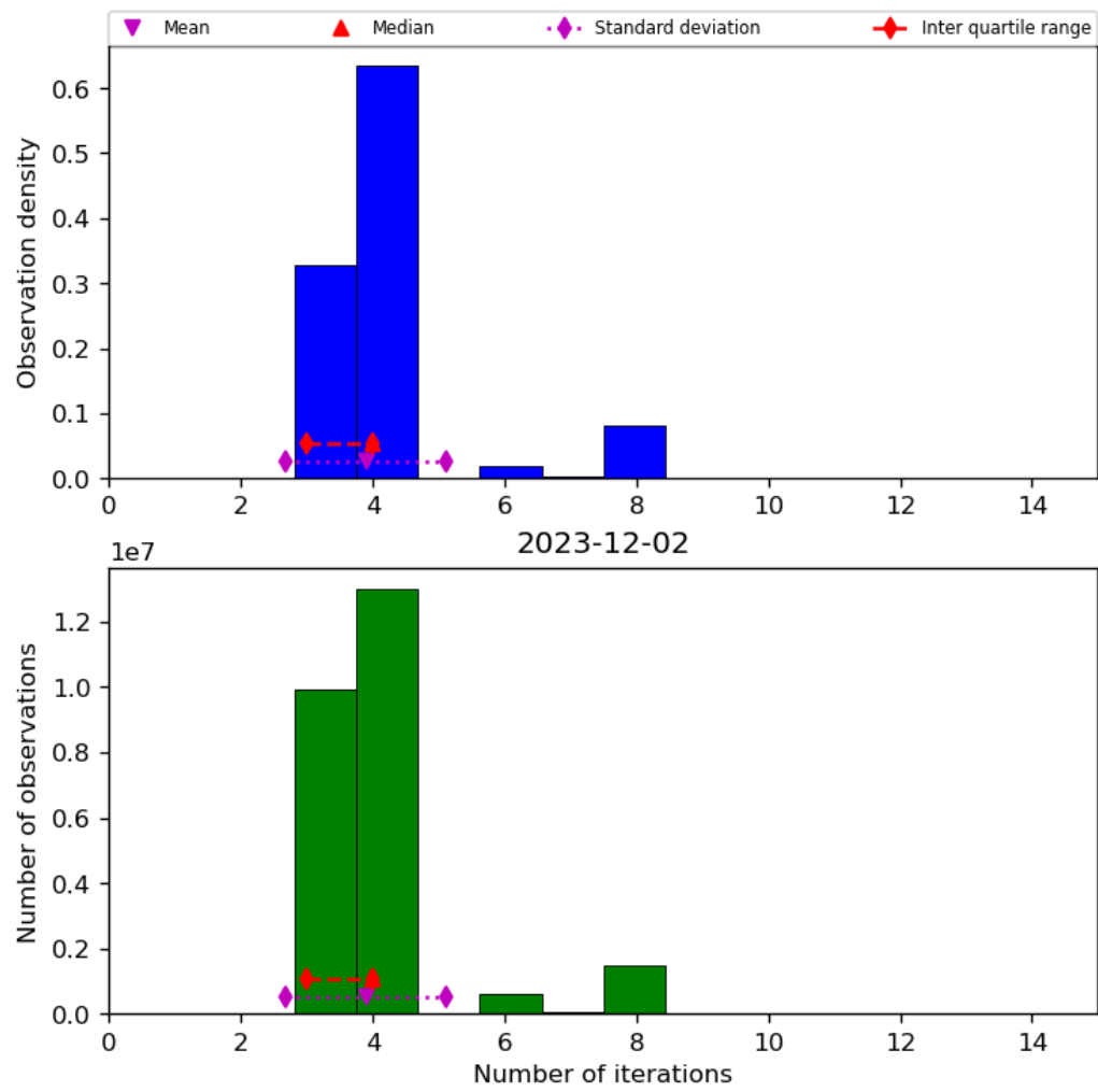
Figure 34: Histogram of “Number of iterations” for 2023-12-01 to 2023-12-03
