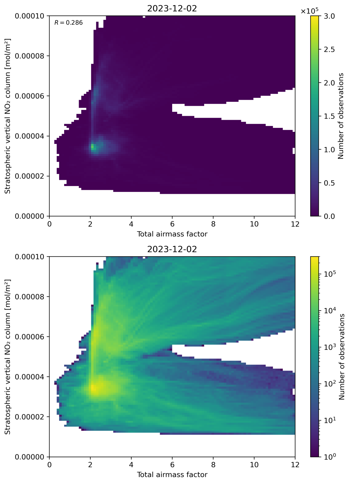
Figure 64: Scatter density plot of “Total airmass factor” against “Stratospheric vertical \text{NO}_2 column” for 2023-12-01 to 2023-12-03.
