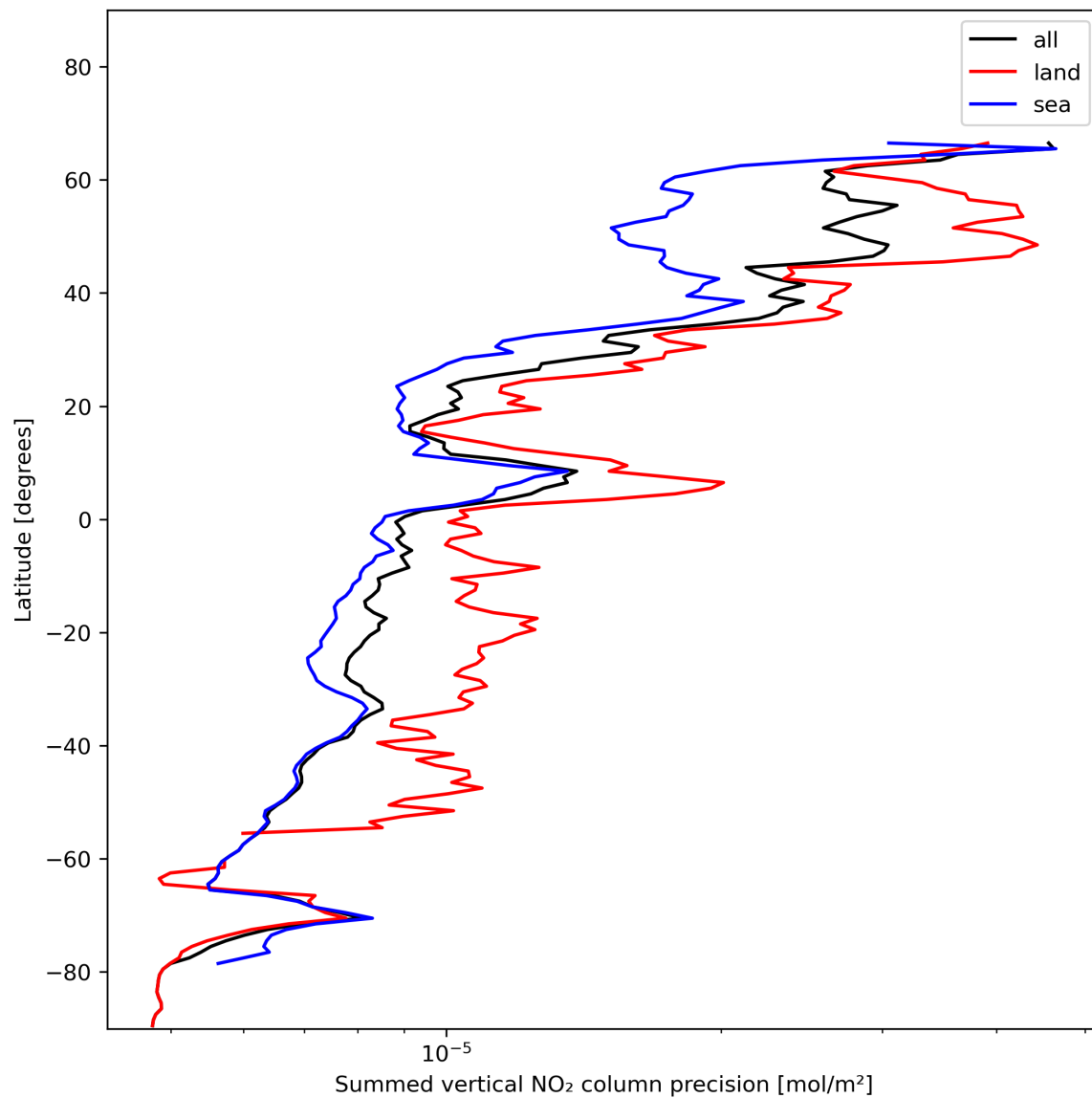
Figure 24: Zonal average of “Summed vertical NO 2 column precision” for 2023-12-01 to 2023-12-03.
