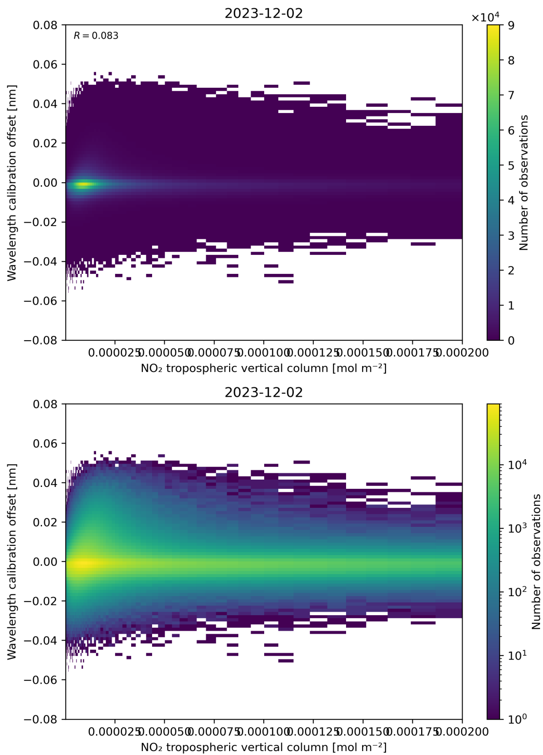
Figure 143: Scatter density plot of “NO 2 tropospheric vertical column” against “Wavelength calibration offset” for 2023-12-01 to 2023-12-03.
