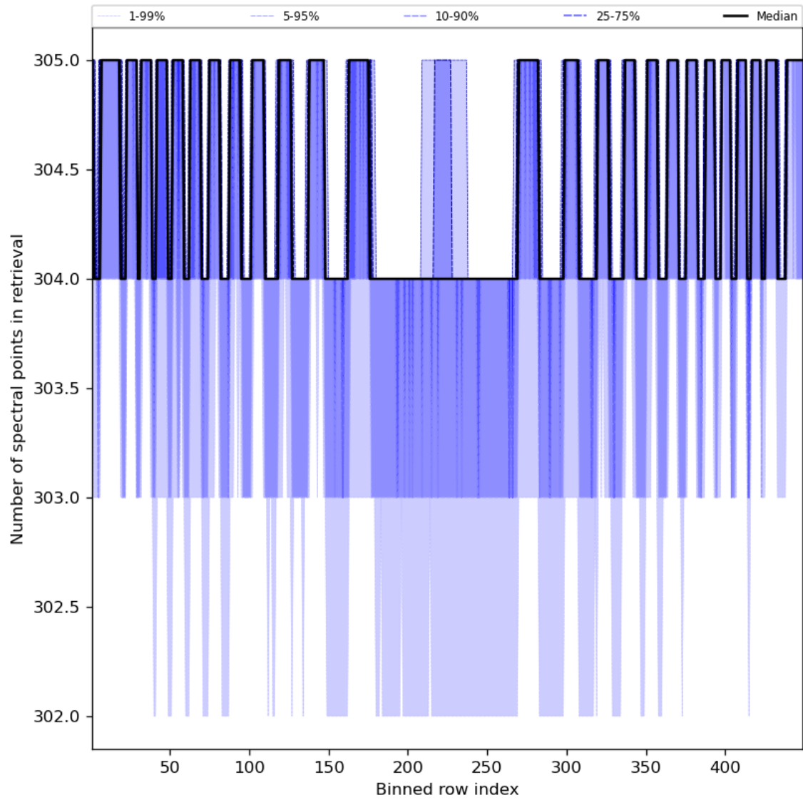
Figure 50: Along track statistics of “Number of spectral points in retrieval” for 2023-12-01 to 2023-12-03
