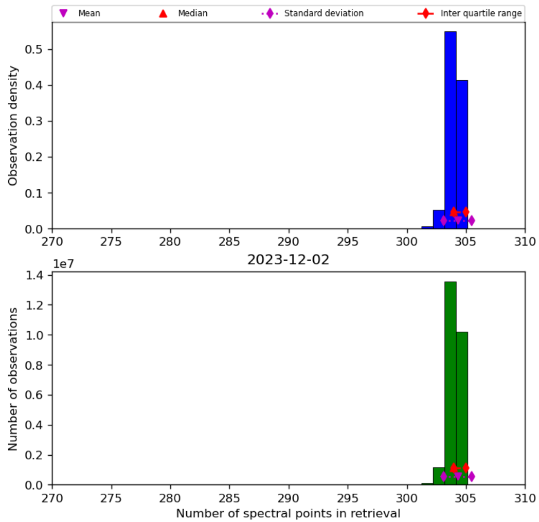
Figure 33: Histogram of “Number of spectral points in retrieval” for 2023-12-01 to 2023-12-03
