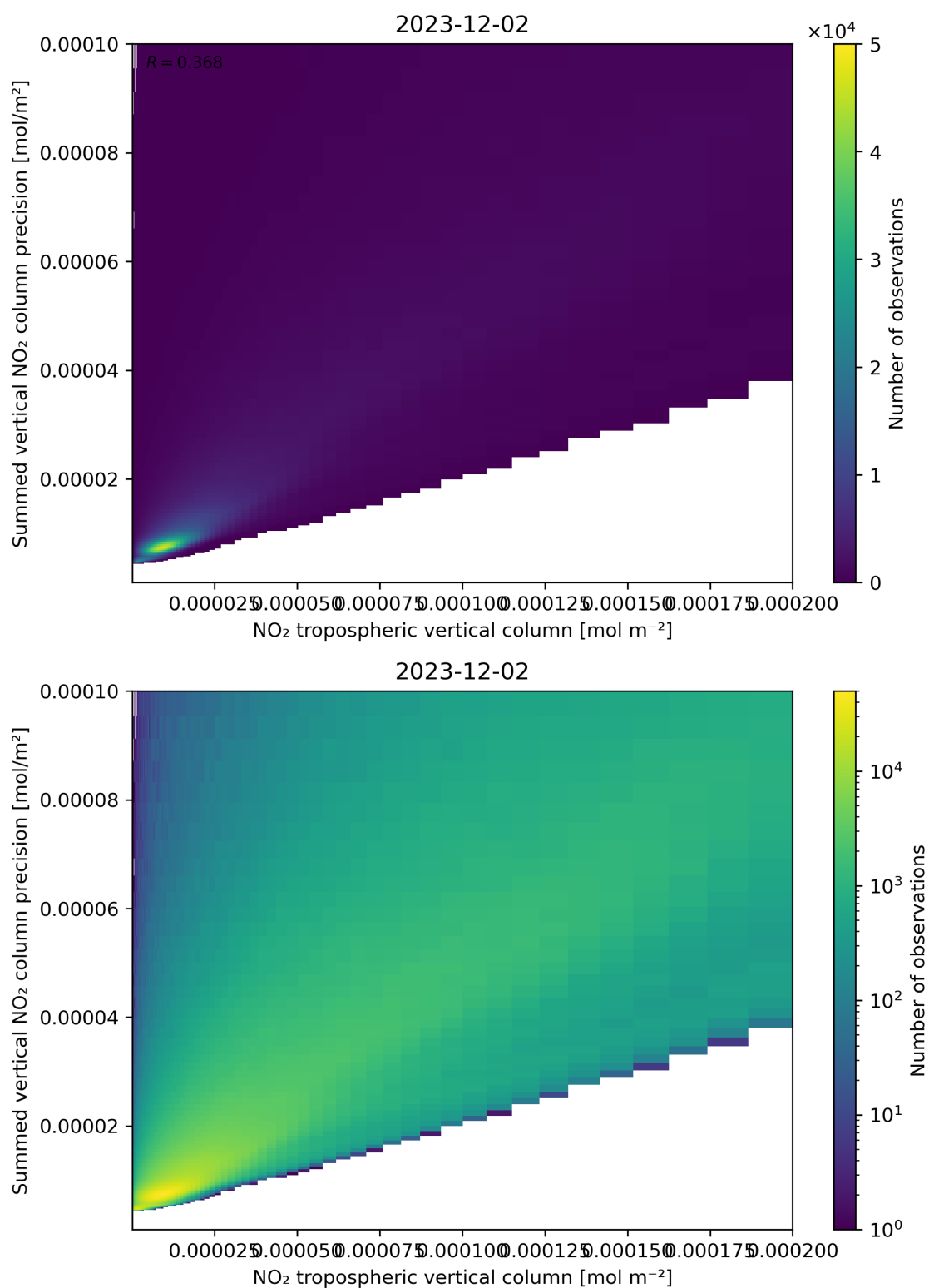
Figure 127: Scatter density plot of “NO 2 tropospheric vertical column” against “Summed vertical NO 2 column precision” for 2023-12-01 to 2023-12-03.
