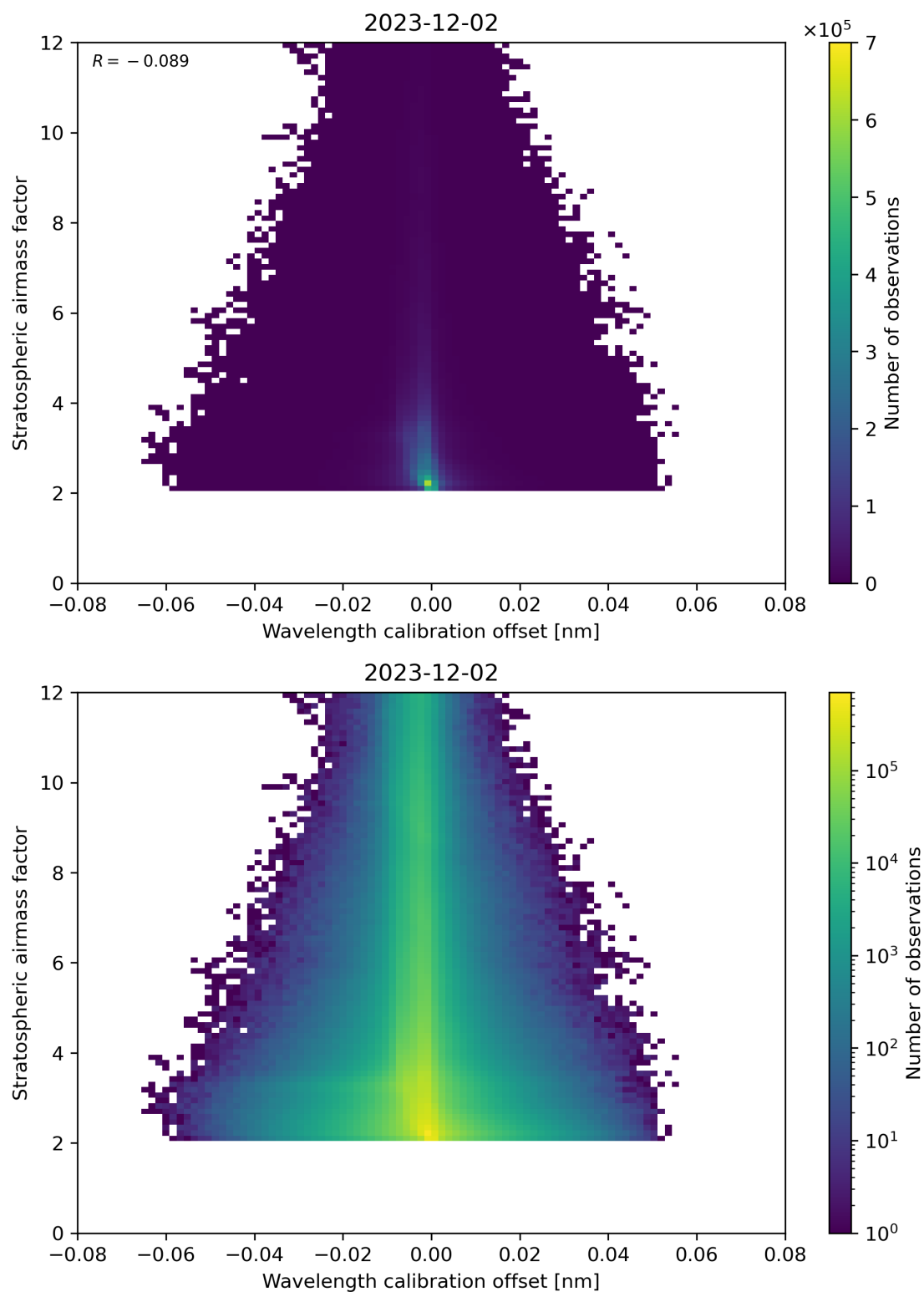
Figure 174: Scatter density plot of “Wavelength calibration offset” against “Stratospheric airmass factor” for 2023-12-01 to 2023-12-03.
