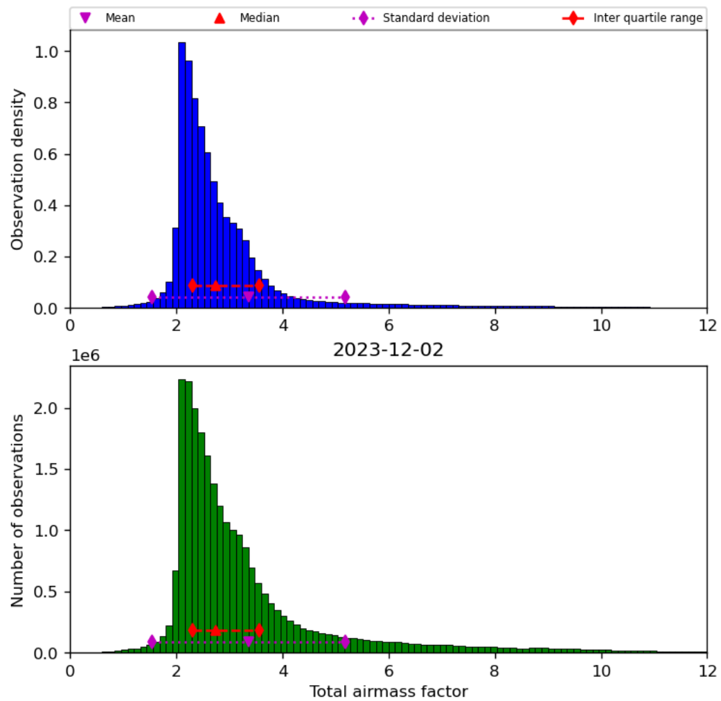
Figure 32: Histogram of “Total airmass factor” for 2023-12-01 to 2023-12-03
