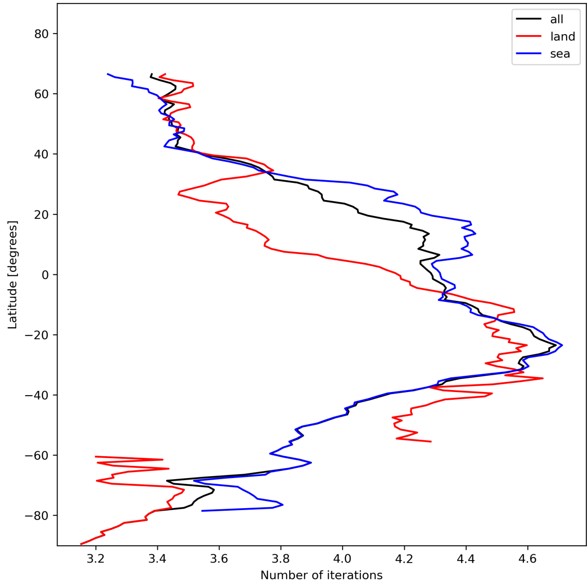
Figure 17: Zonal average of “Number of iterations” for 2023-12-01 to 2023-12-03.
