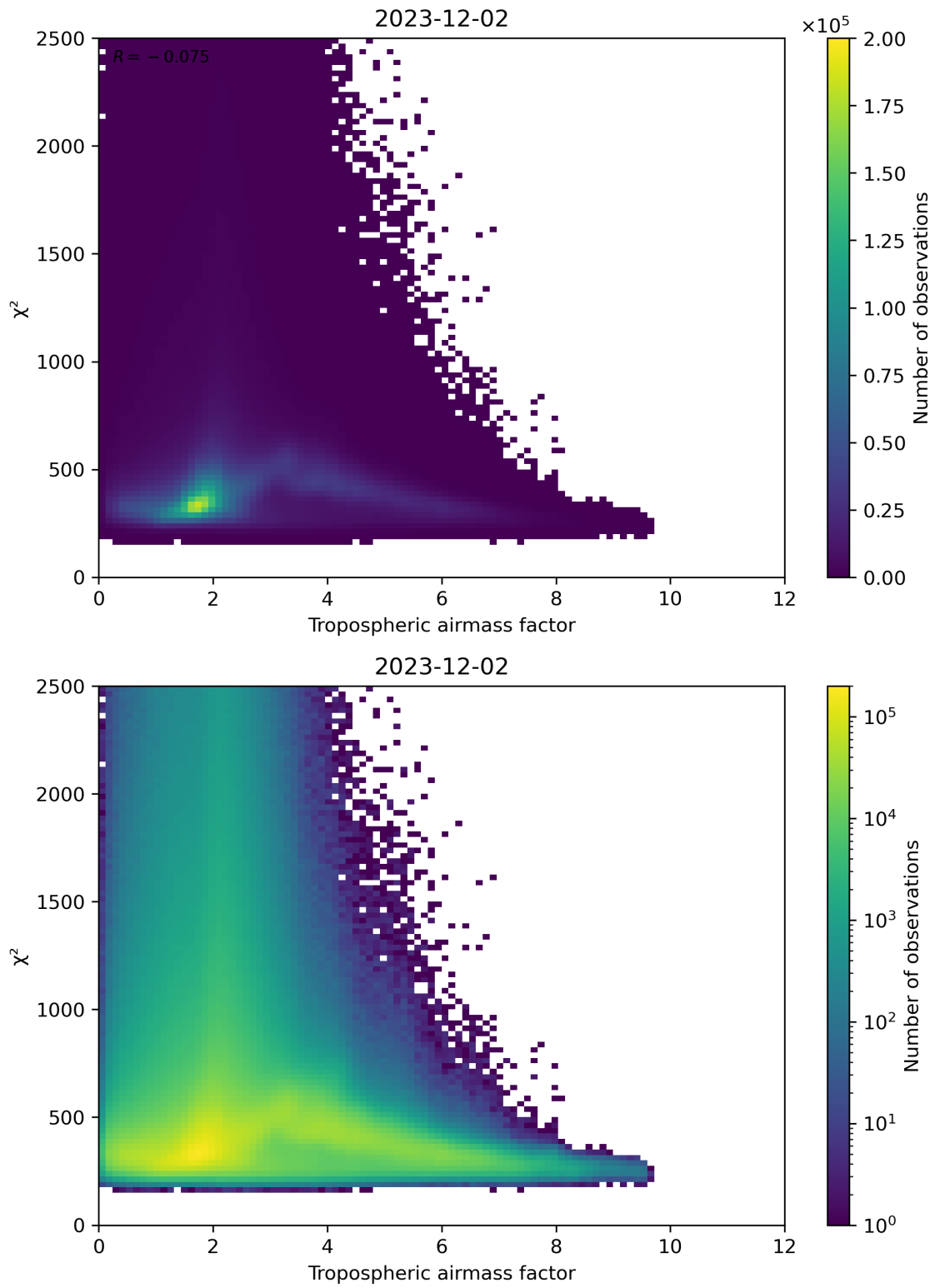
Figure 73: Scatter density plot of “Tropospheric airmass factor” against “ \chi^2 ” for 2023-12-01 to 2023-12-03.
