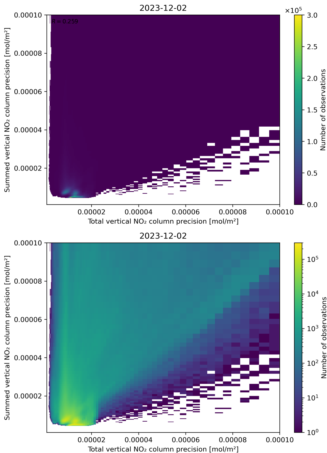
Figure 118: Scatter density plot of “Total vertical NO 2 column precision” against “Summed vertical NO 2 column precision” for 2023-12-01 to 2023-12-03.
