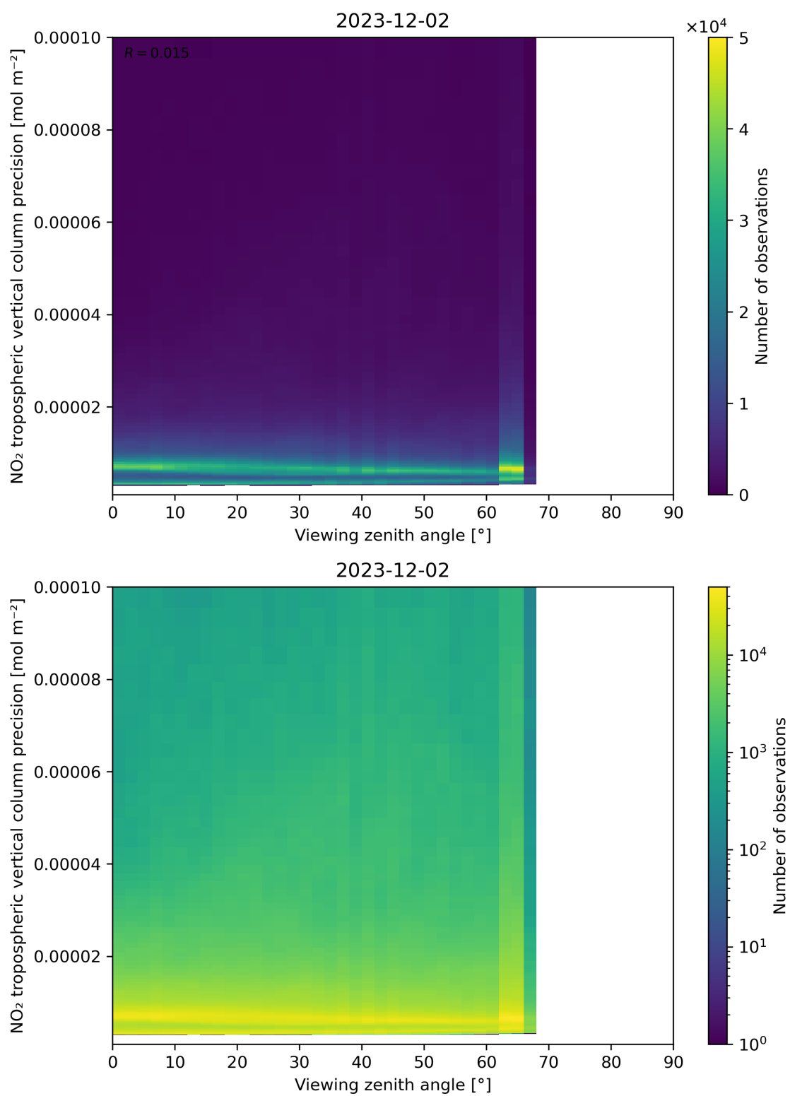
Figure 170: Scatter density plot of “Viewing zenith angle” against “NO 2 tropospheric vertical column precision” for 2023-12-01 to 2023-12-03.
