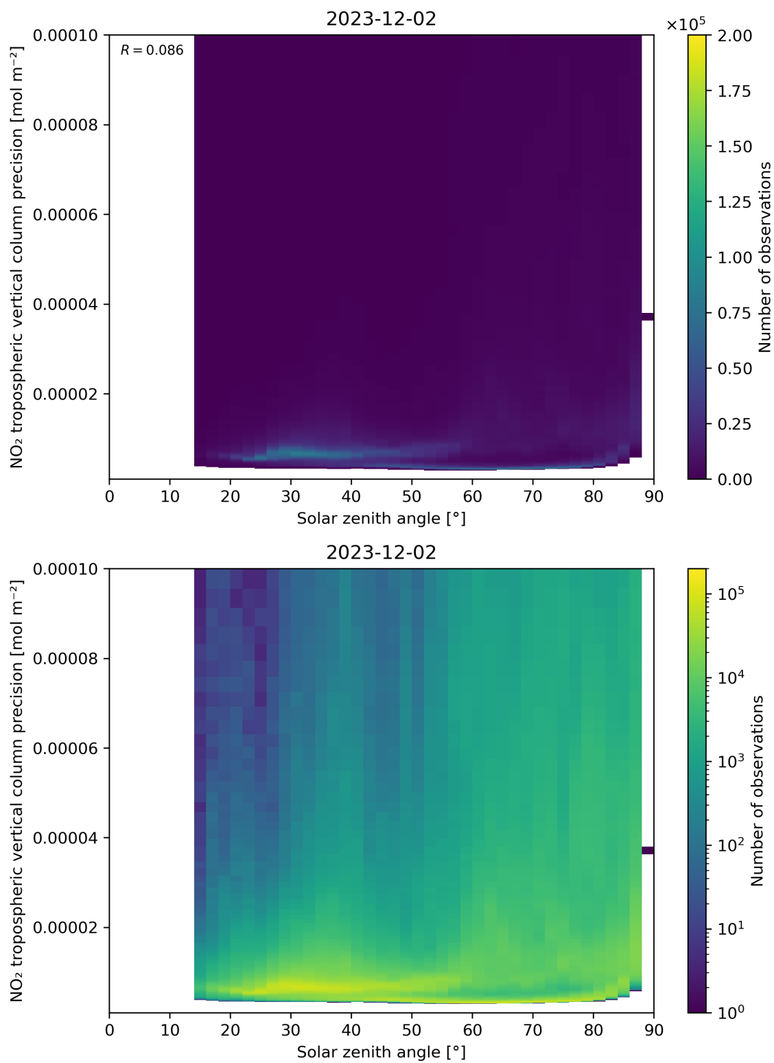
Figure 156: Scatter density plot of “Solar zenith angle” against “NO 2 tropospheric vertical column precision” for 2023-12-01 to 2023-12-03.
