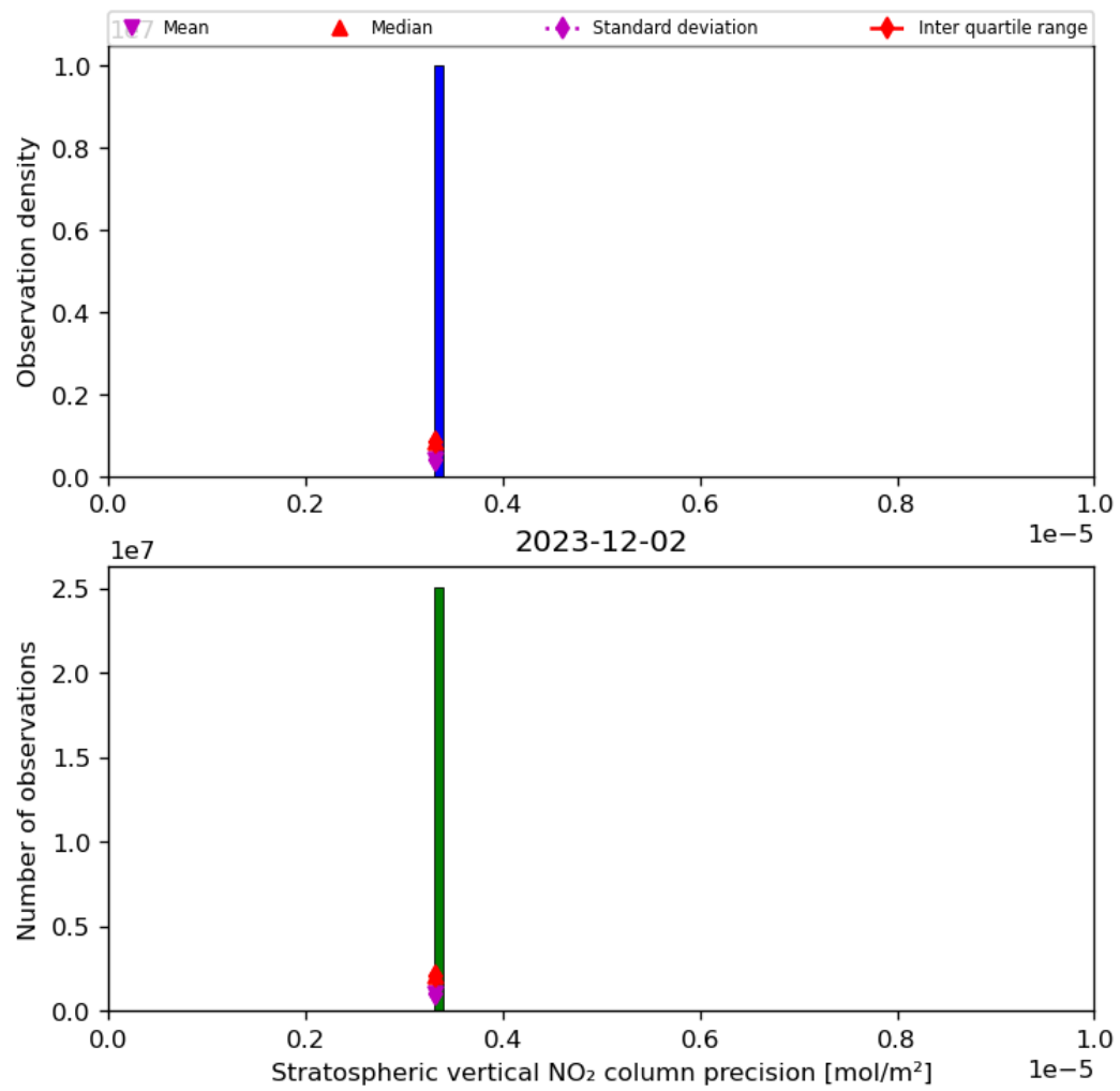
Figure 37: Histogram of “Stratospheric vertical NO 2 column precision” for 2023-12-01 to 2023-12-03
