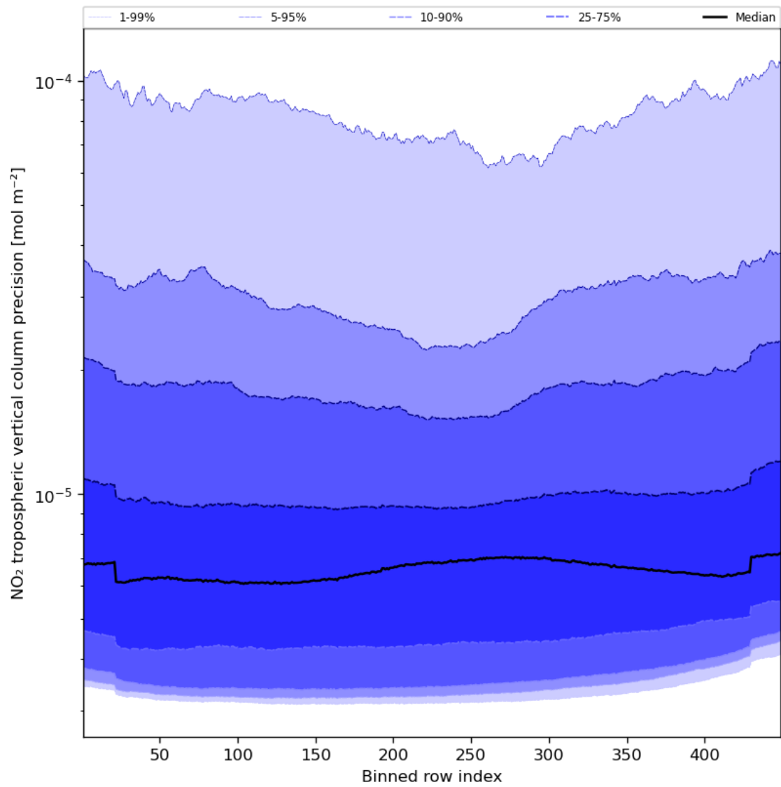
Figure 47: Along track statistics of “NO 2 tropospheric vertical column precision” for 2023-12-01 to 2023-12-03
