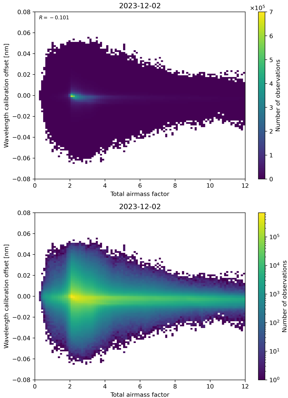
Figure 70: Scatter density plot of “Total airmass factor” against “Wavelength calibration offset” for 2023-12-01 to 2023-12-03.
