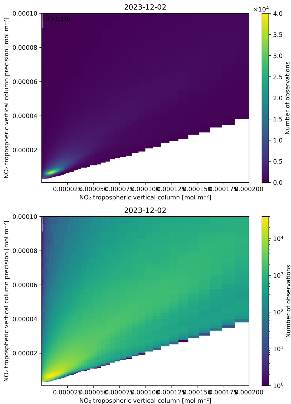
Figure 130: Scatter density plot of “NO 2 tropospheric vertical column” against “NO 2 tropospheric vertical column precision” for 2023-12-01 to 2023-12-03.
