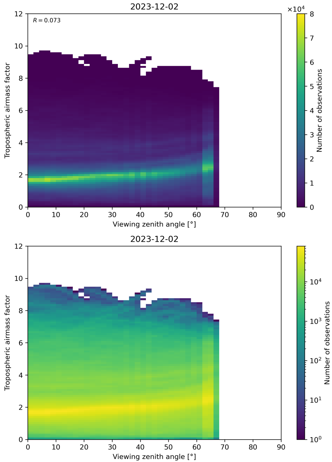
Figure 161: Scatter density plot of “Viewing zenith angle” against “Tropospheric airmass factor” for 2023-12-01 to 2023-12-03.
