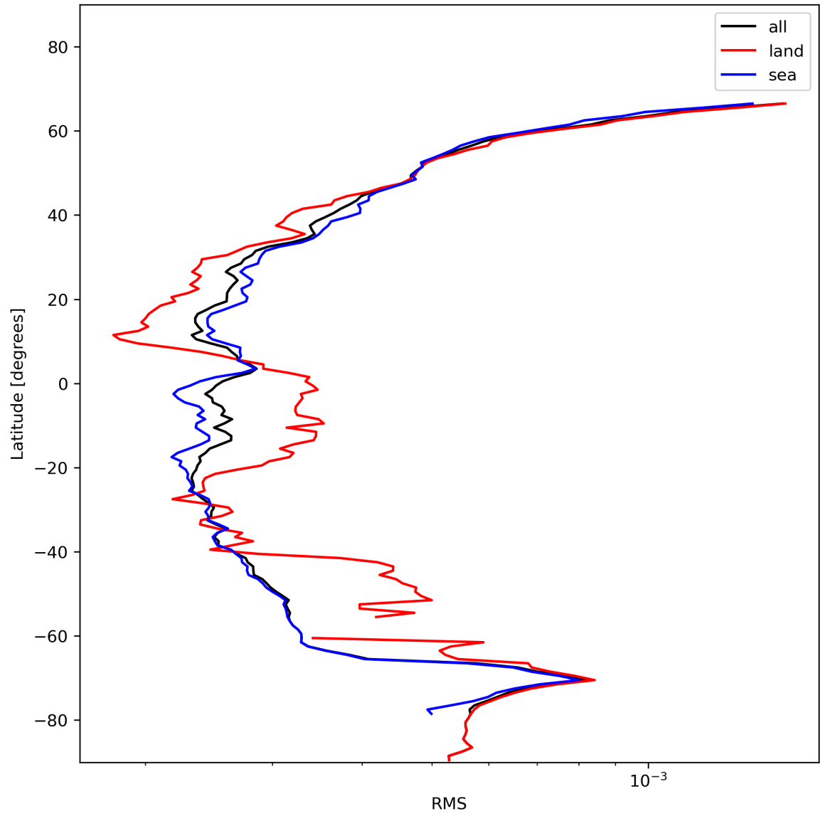
Figure 26: Zonal average of “RMS” for 2023-12-01 to 2023-12-03.
