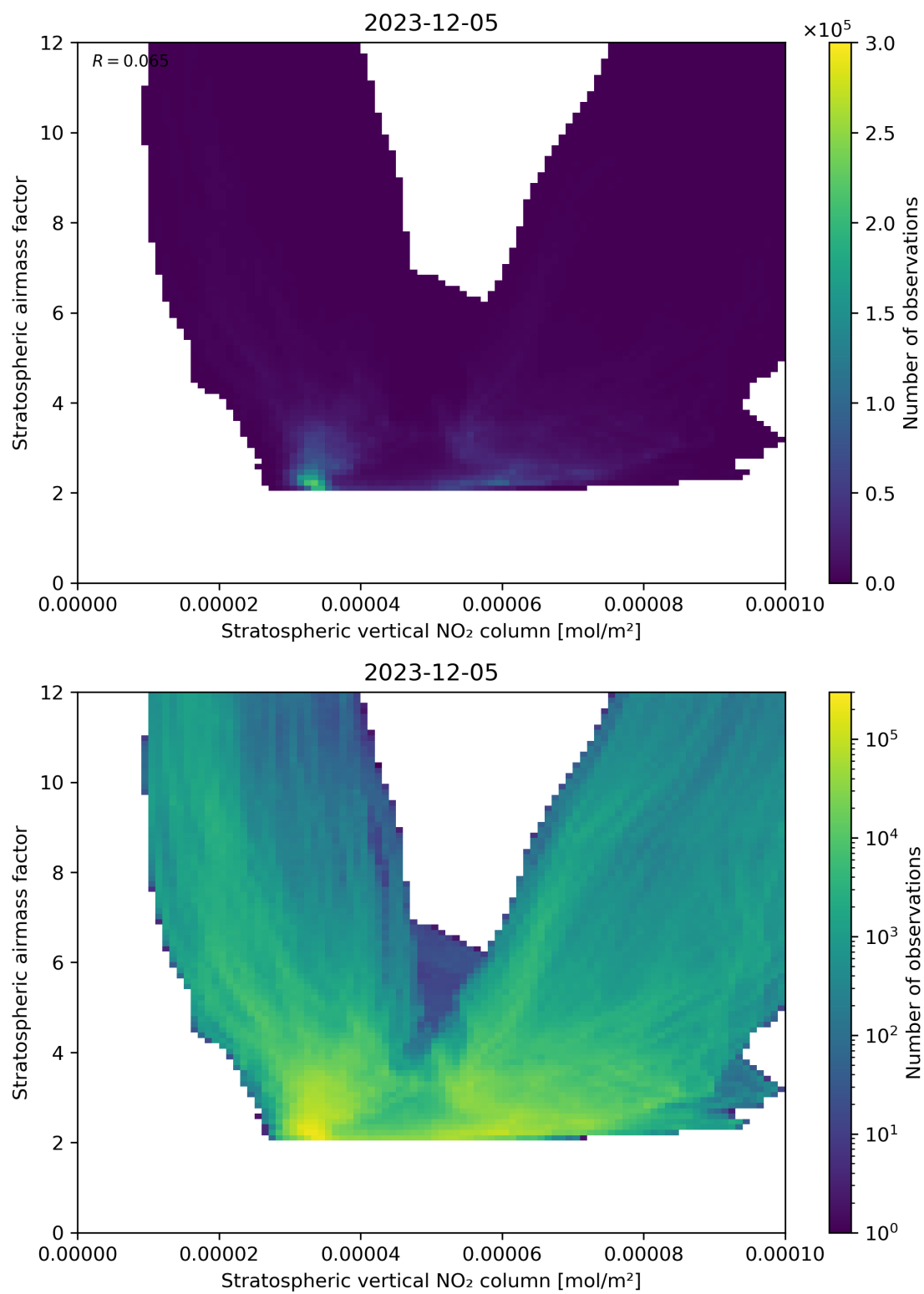
Figure 96: Scatter density plot of “Stratospheric vertical NO 2 column” against “Stratospheric airmass factor” for 2023-12-04 to 2023-12-06.
