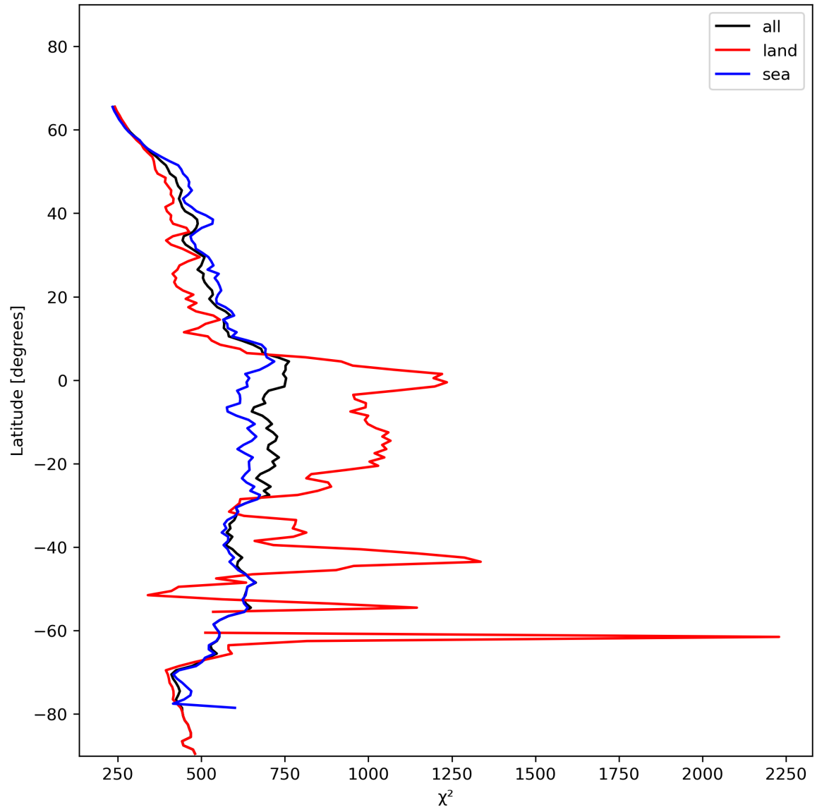
Figure 25: Zonal average of “ \chi^2 ” for 2023-12-04 to 2023-12-06.
