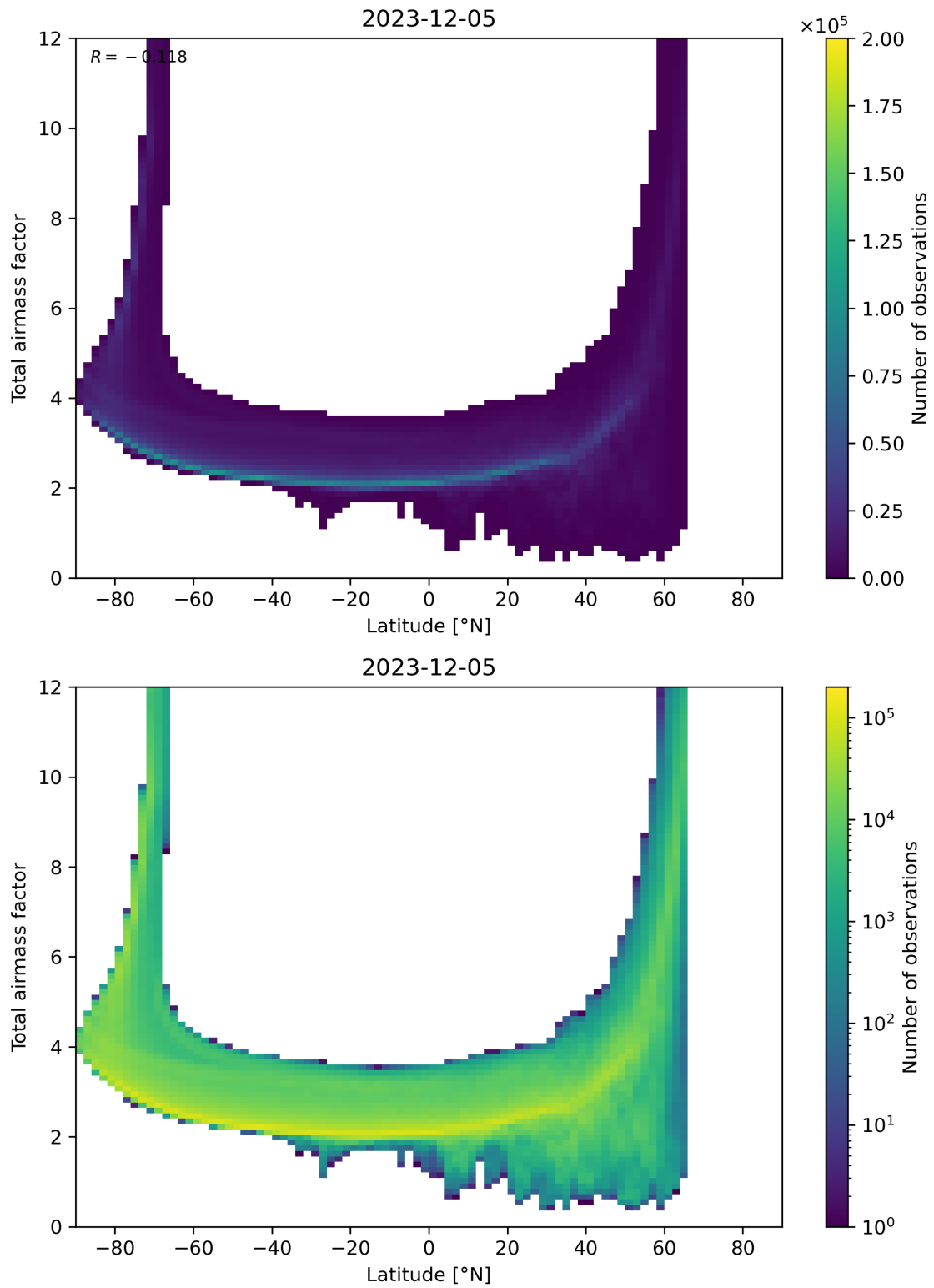
Figure 84: Scatter density plot of “Latitude” against “Total airmass factor” for 2023-12-04 to 2023-12-06.
