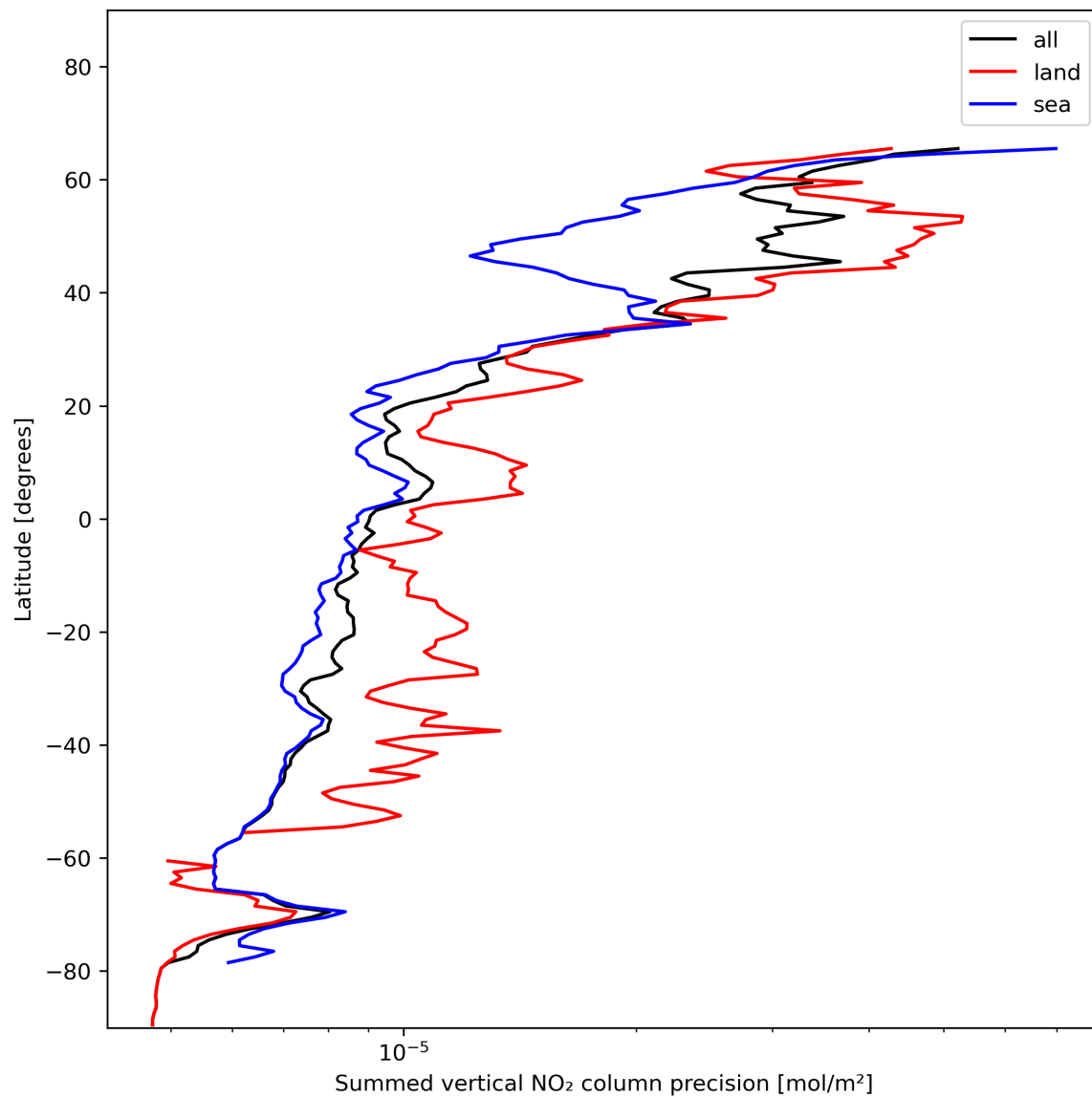
Figure 24: Zonal average of “Summed vertical NO 2 column precision” for 2023-12-04 to 2023-12-06.
