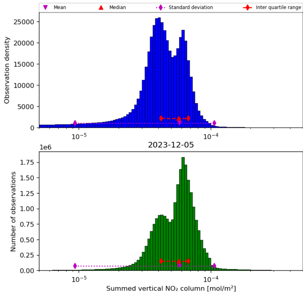
Figure 40: Histogram of “Summed vertical NO 2 column” for 2023-12-04 to 2023-12-06
