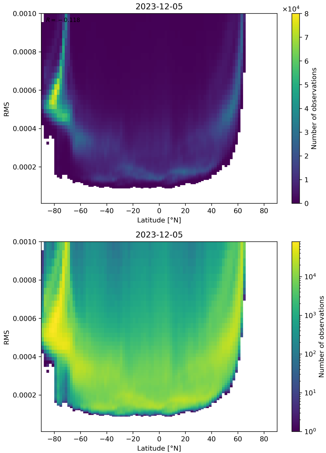
Figure 94: Scatter density plot of “Latitude” against “RMS” for 2023-12-04 to 2023-12-06.
