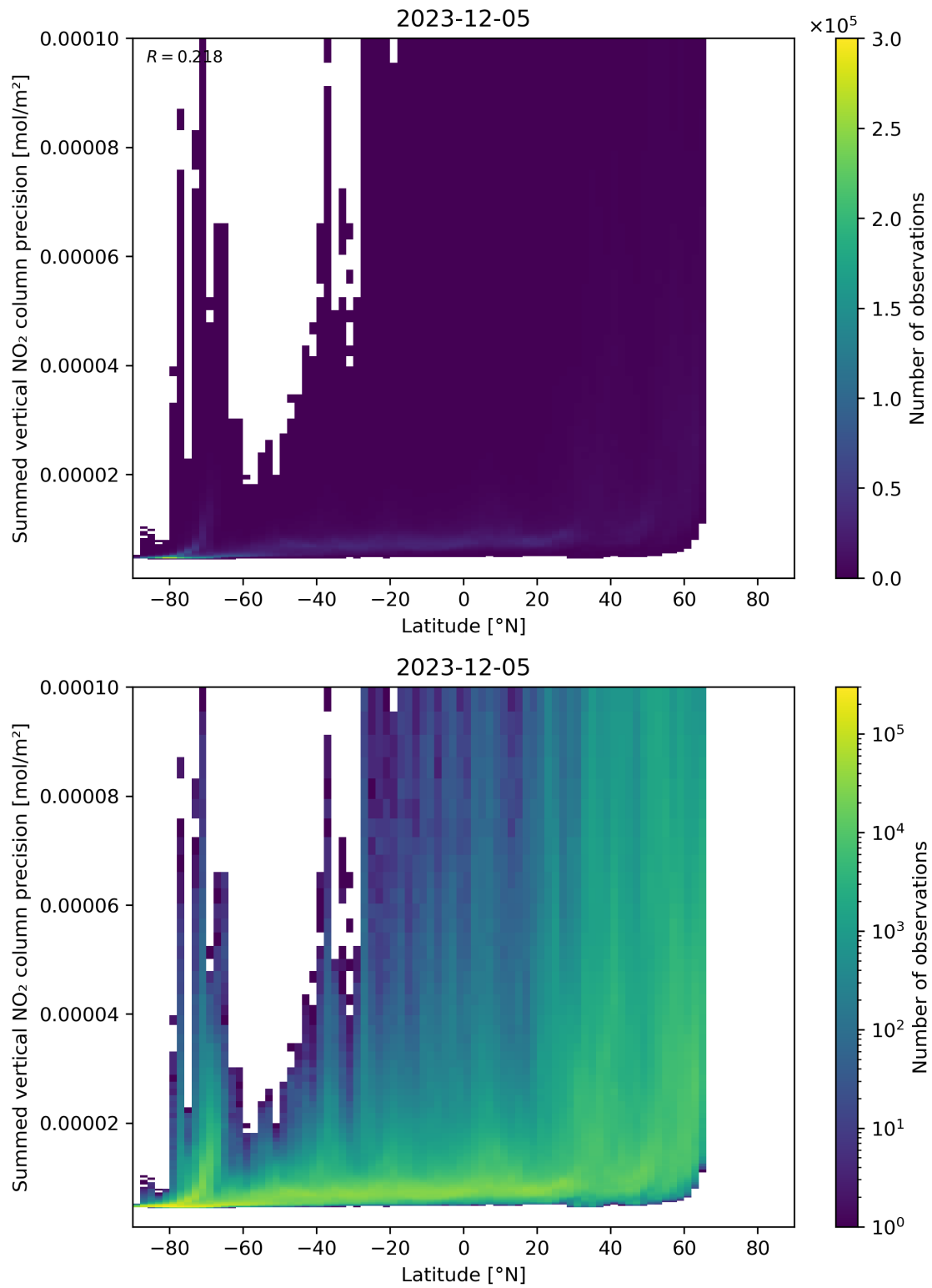
Figure 89: Scatter density plot of “Latitude” against “Summed vertical NO 2 column precision” for 2023-12-04 to 2023-12-06.
