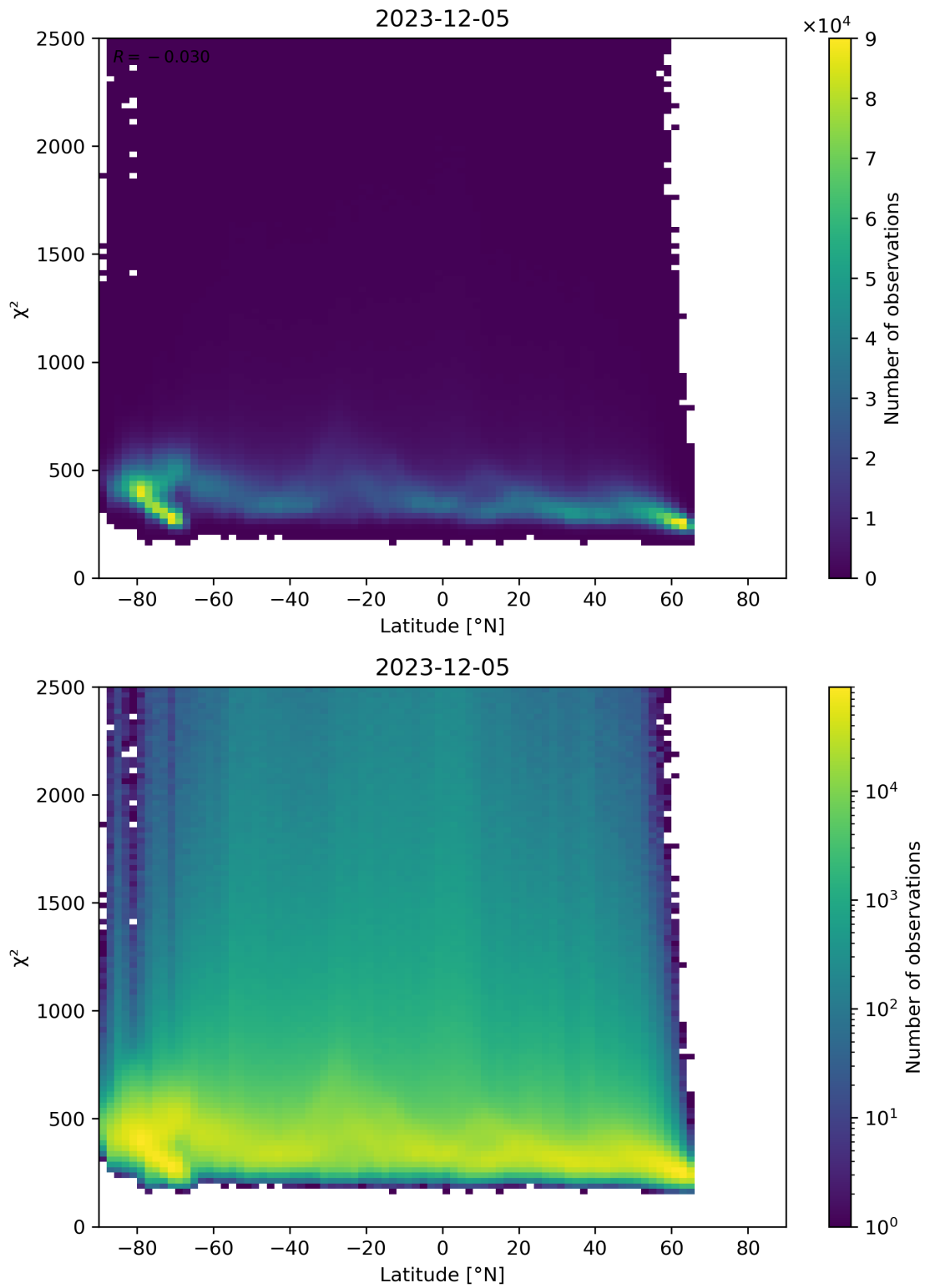
Figure 86: Scatter density plot of “Latitude” against “ \chi^2 ” for 2023-12-04 to 2023-12-06.
