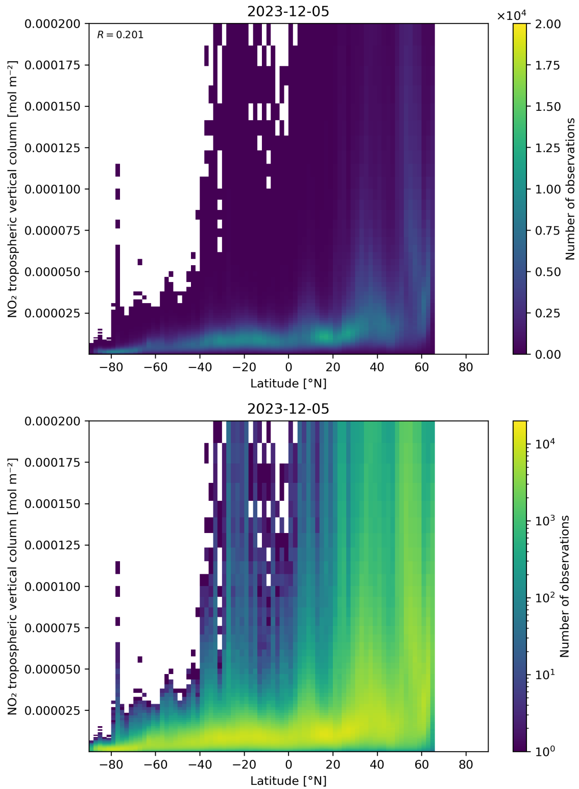
Figure 92: Scatter density plot of “Latitude” against “NO 2 tropospheric vertical column” for 2023-12-04 to 2023-12-06.
