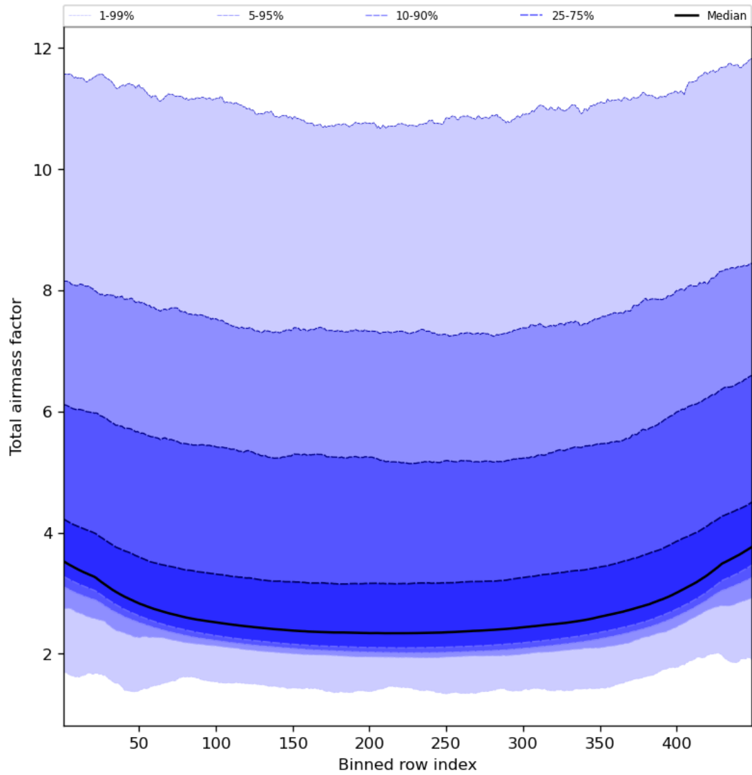
Figure 49: Along track statistics of “Total airmass factor” for 2023-12-04 to 2023-12-06
