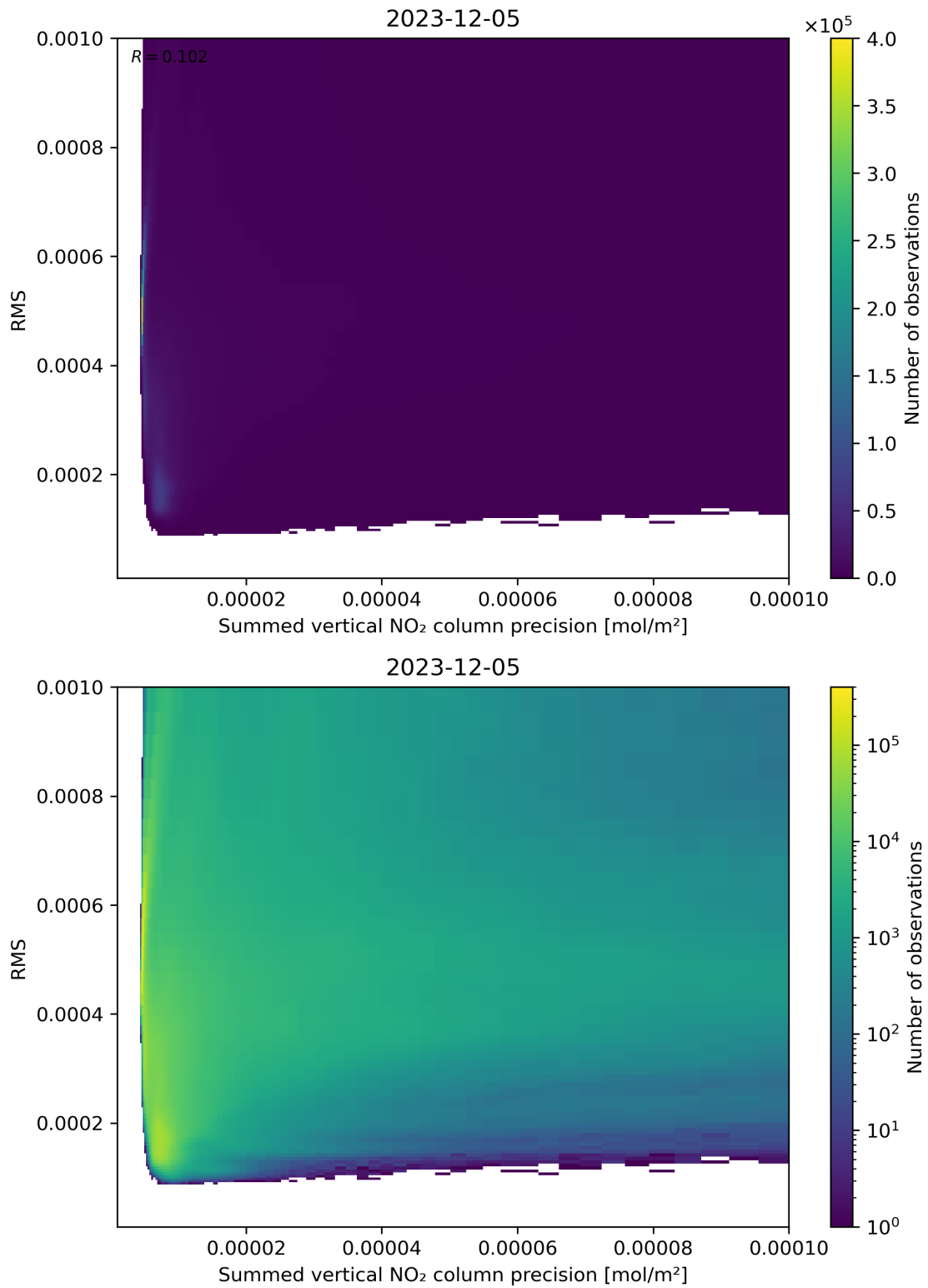
Figure 108: Scatter density plot of “Summed vertical NO 2 column precision” against “RMS” for 2023-12-04 to 2023-12-06.
