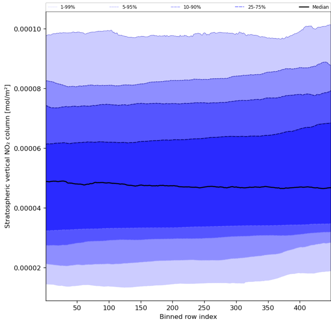
Figure 53: Along track statistics of “Stratospheric vertical NO 2 column” for 2023-12-04 to 2023-12-06
