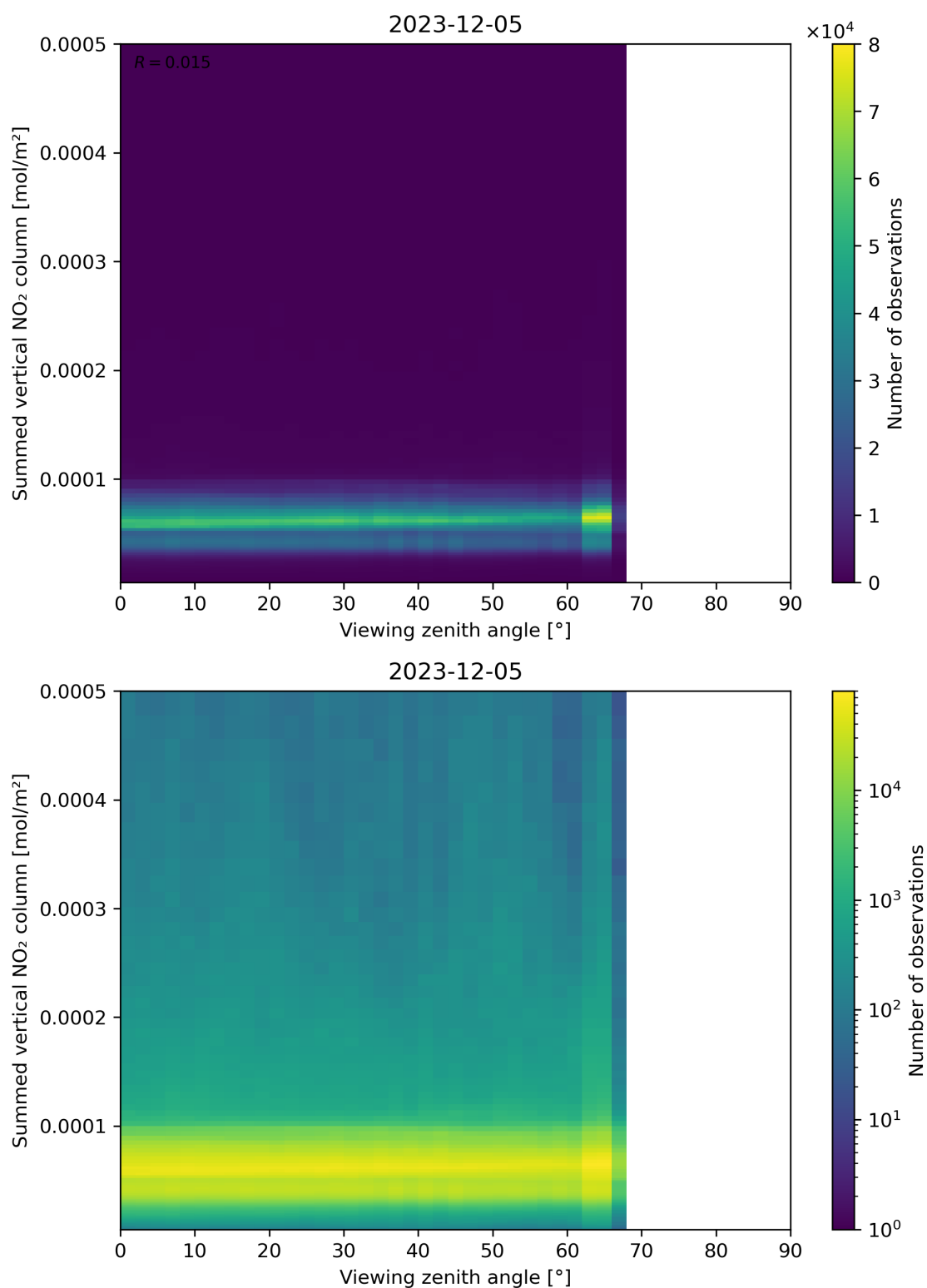
Figure 165: Scatter density plot of “Viewing zenith angle” against “Summed vertical NO 2 column” for 2023-12-04 to 2023-12-06.
