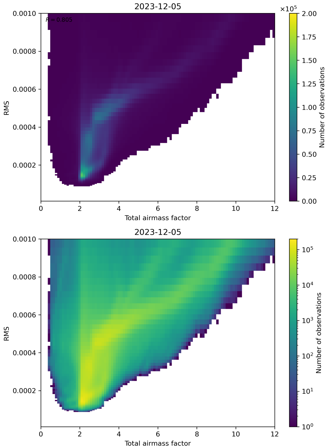
Figure 69: Scatter density plot of “Total airmass factor” against “RMS” for 2023-12-04 to 2023-12-06.
