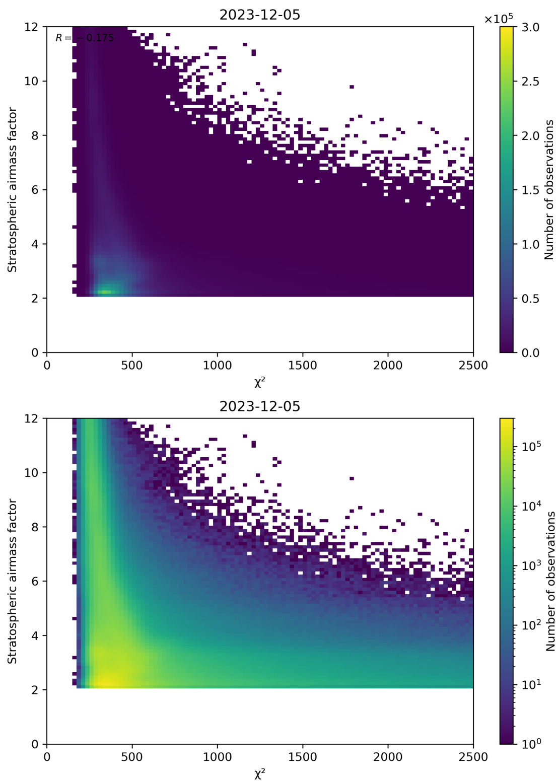
Figure 81: Scatter density plot of “ \chi^2 ” against “Stratospheric airmass factor” for 2023-12-04 to 2023-12-06.
