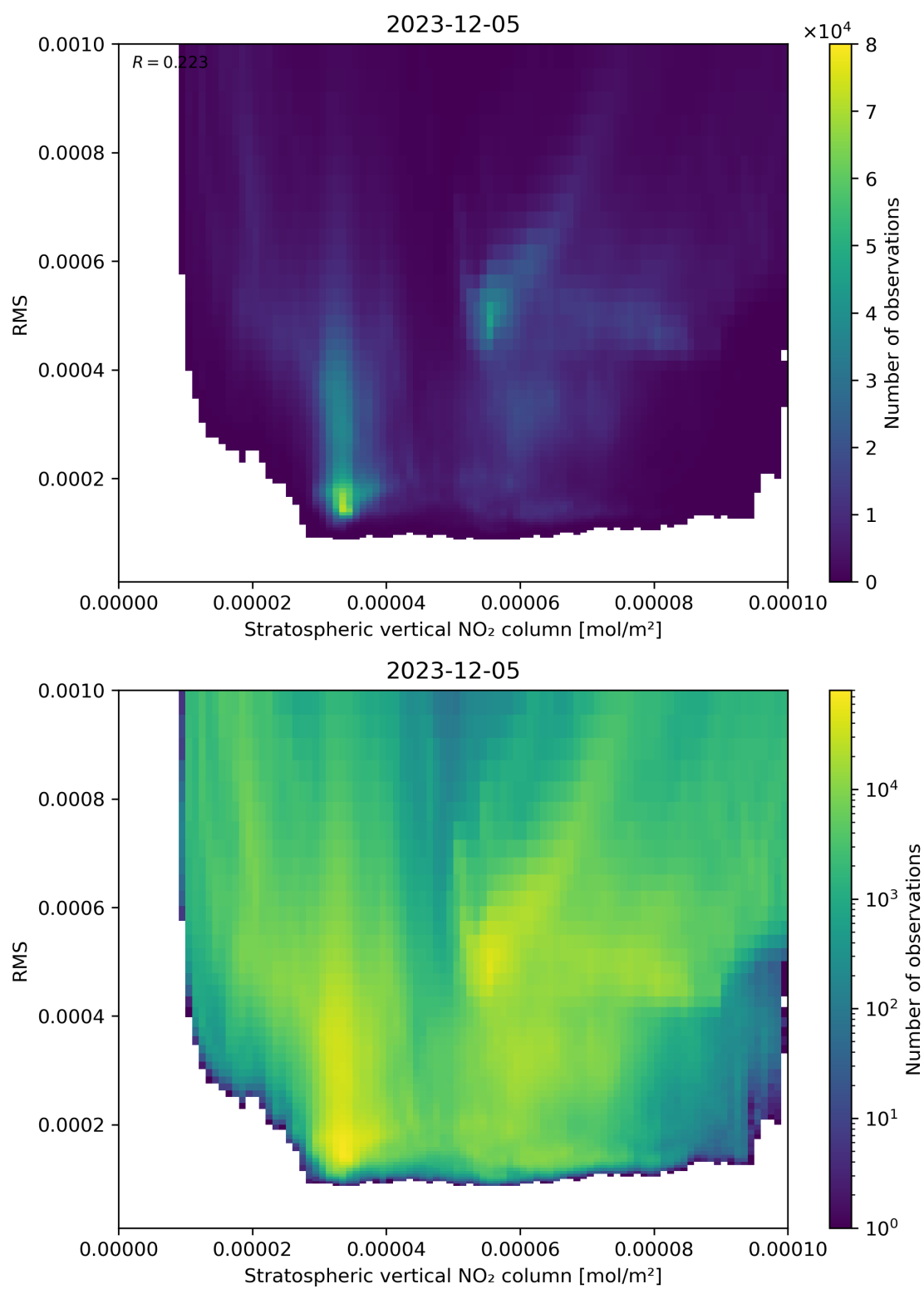
Figure 102: Scatter density plot of “Stratospheric vertical NO 2 column” against “RMS” for 2023-12-04 to 2023-12-06.
