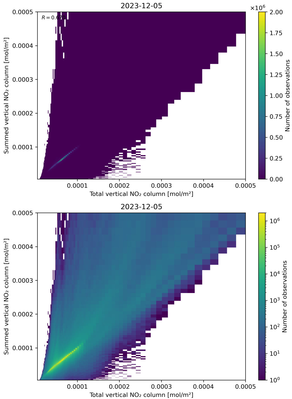
Figure 112: Scatter density plot of “Total vertical NO 2 column” against “Summed vertical NO 2 column” for 2023-12-04 to 2023-12-06.
