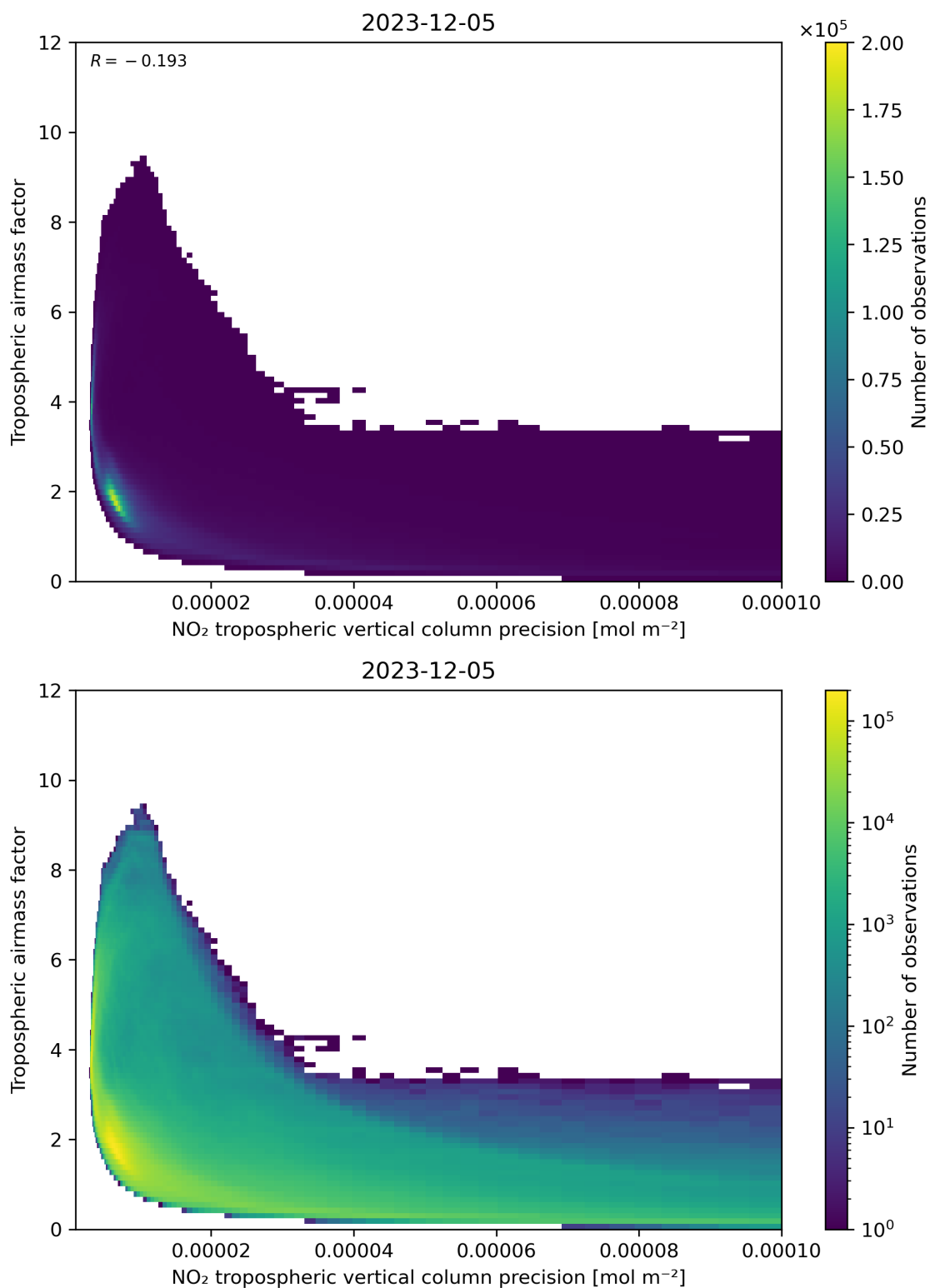
Figure 133: Scatter density plot of “NO 2 tropospheric vertical column precision” against “Tropospheric airmass factor” for 2023-12-04 to 2023-12-06.
