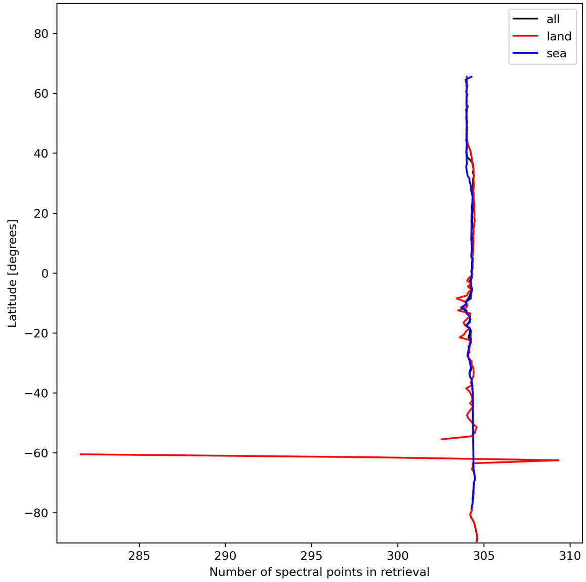
Figure 16: Zonal average of “Number of spectral points in retrieval” for 2023-12-04 to 2023-12-06.
