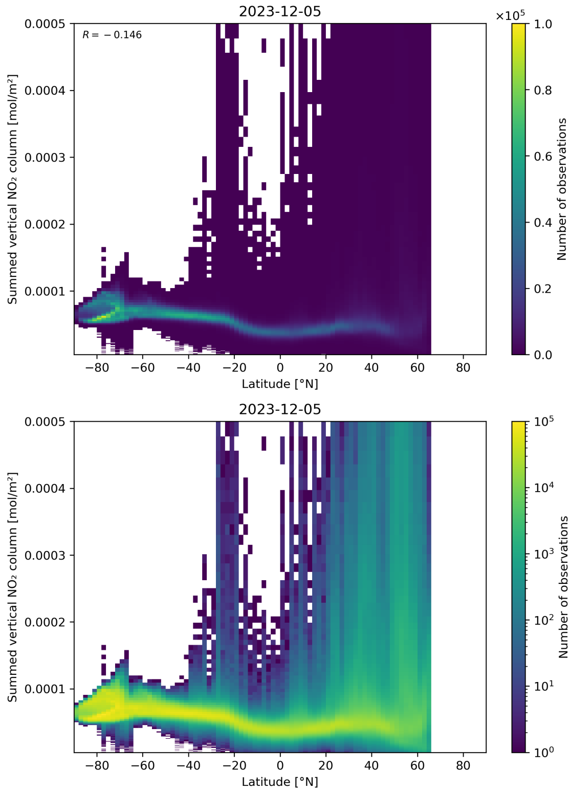
Figure 88: Scatter density plot of “Latitude” against “Summed vertical NO 2 column” for 2023-12-04 to 2023-12-06.
