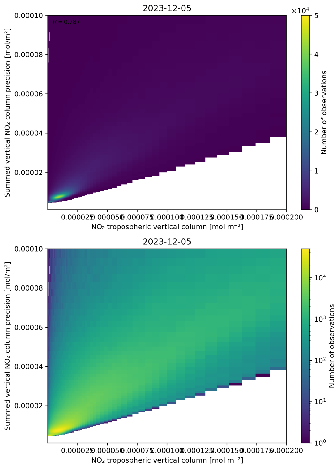
Figure 127: Scatter density plot of “NO 2 tropospheric vertical column” against “Summed vertical NO 2 column precision” for 2023-12-04 to 2023-12-06.
