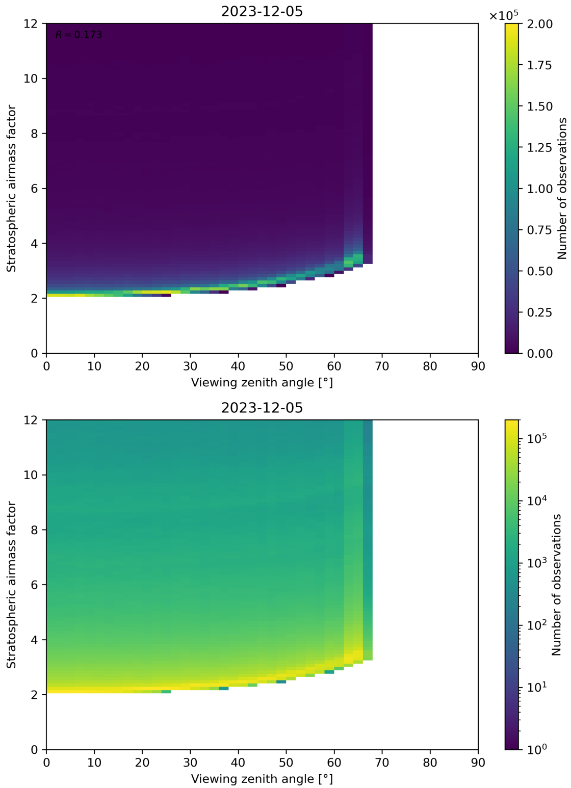
Figure 159: Scatter density plot of “Viewing zenith angle” against “Stratospheric airmass factor” for 2023-12-04 to 2023-12-06.
