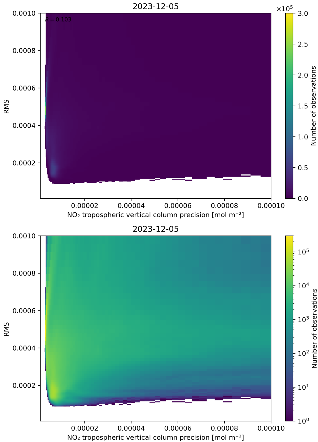
Figure 140: Scatter density plot of “NO 2 tropospheric vertical column precision” against “RMS” for 2023-12-04 to 2023-12-06.
