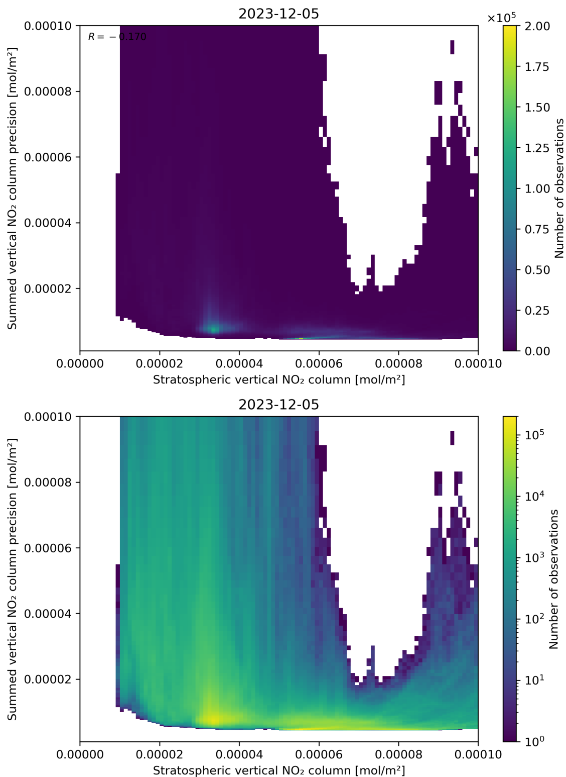
Figure 99: Scatter density plot of “Stratospheric vertical NO 2 column” against “Summed vertical NO 2 column precision” for 2023-12-04 to 2023-12-06.
