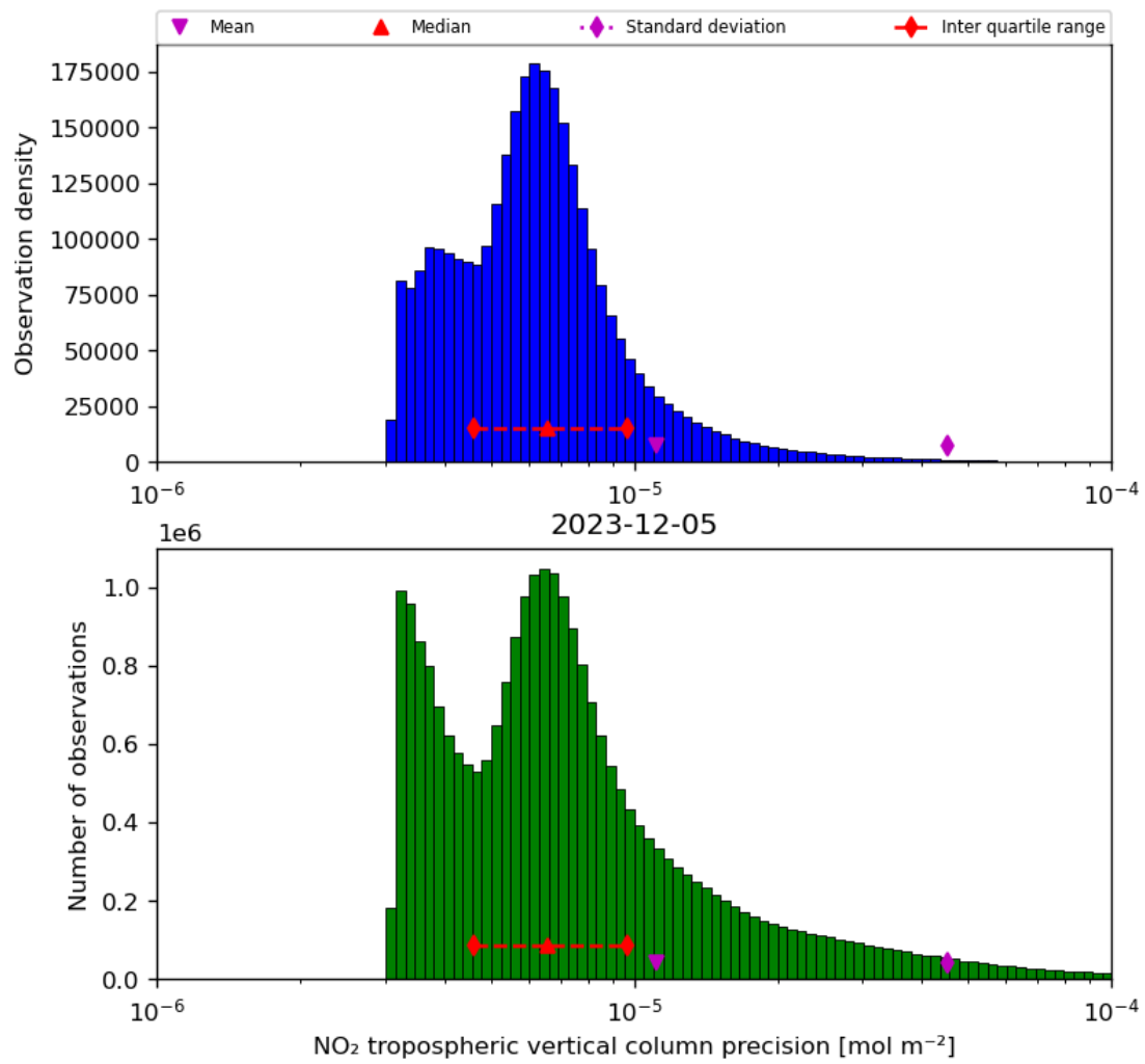
Figure 30: Histogram of “NO 2 tropospheric vertical column precision” for 2023-12-04 to 2023-12-06
