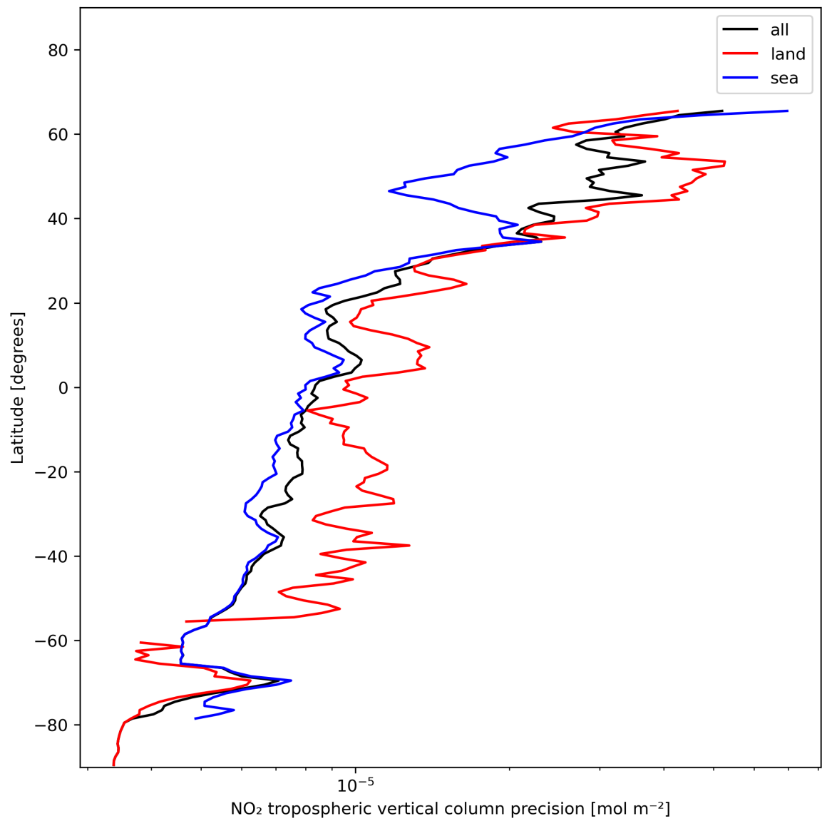
Figure 13: Zonal average of “NO 2 tropospheric vertical column precision” for 2023-12-04 to 2023-12-06.
