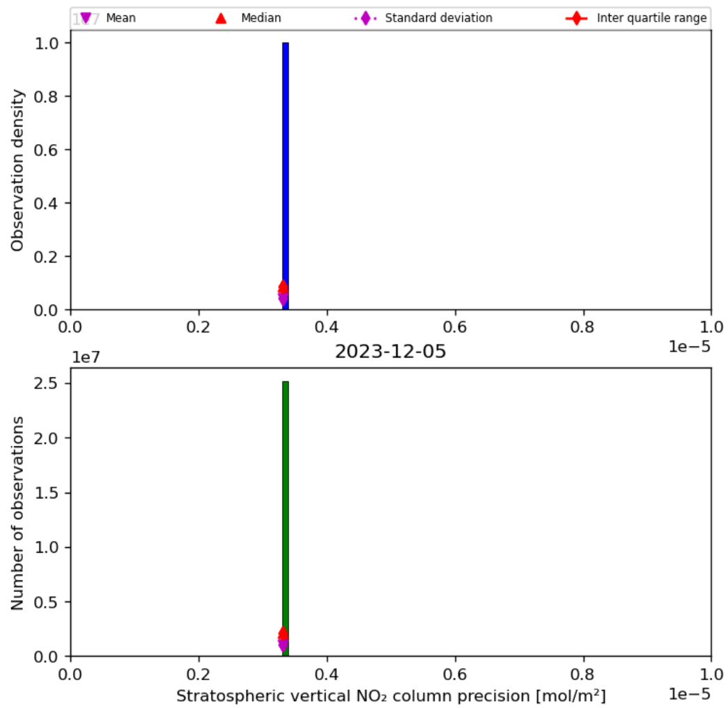
Figure 37: Histogram of “Stratospheric vertical NO 2 column precision” for 2023-12-04 to 2023-12-06
