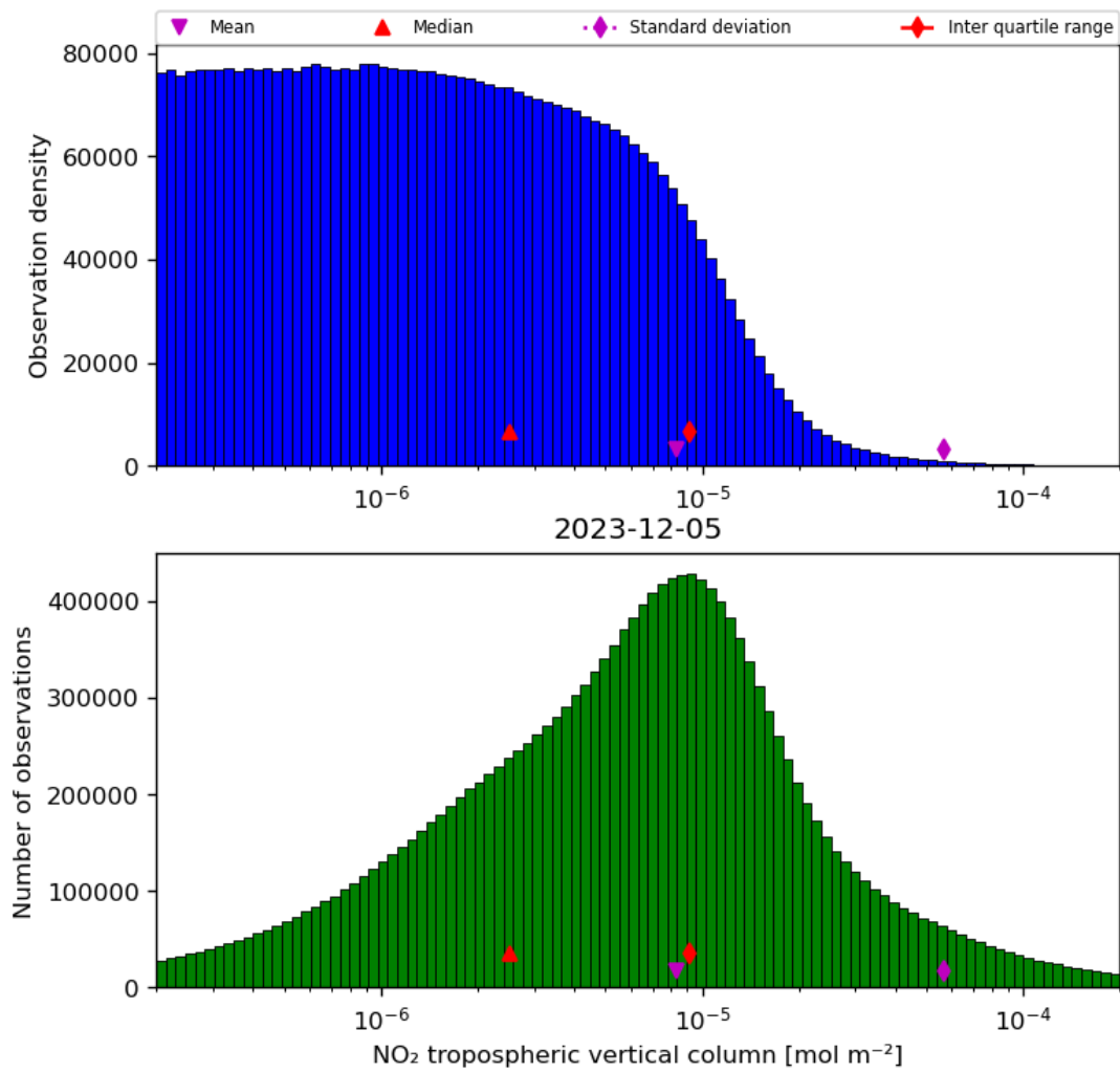
Figure 29: Histogram of “NO 2 tropospheric vertical column” for 2023-12-04 to 2023-12-06
