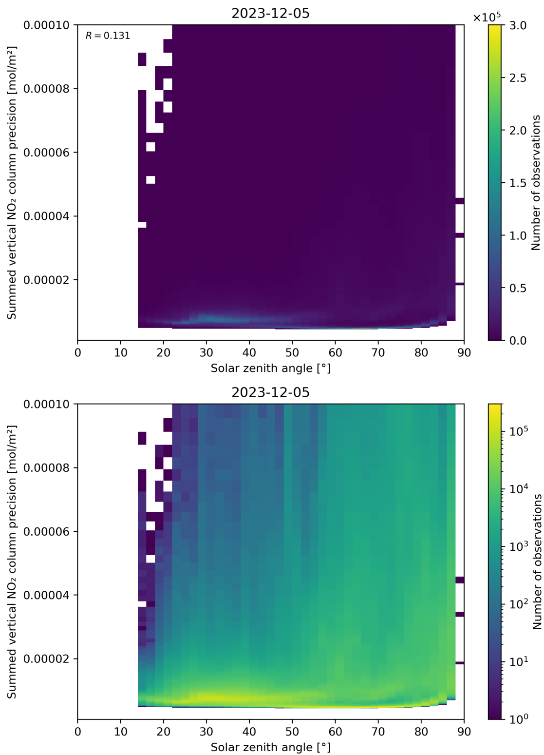
Figure 152: Scatter density plot of “Solar zenith angle” against “Summed vertical NO 2 column precision” for 2023-12-04 to 2023-12-06.
