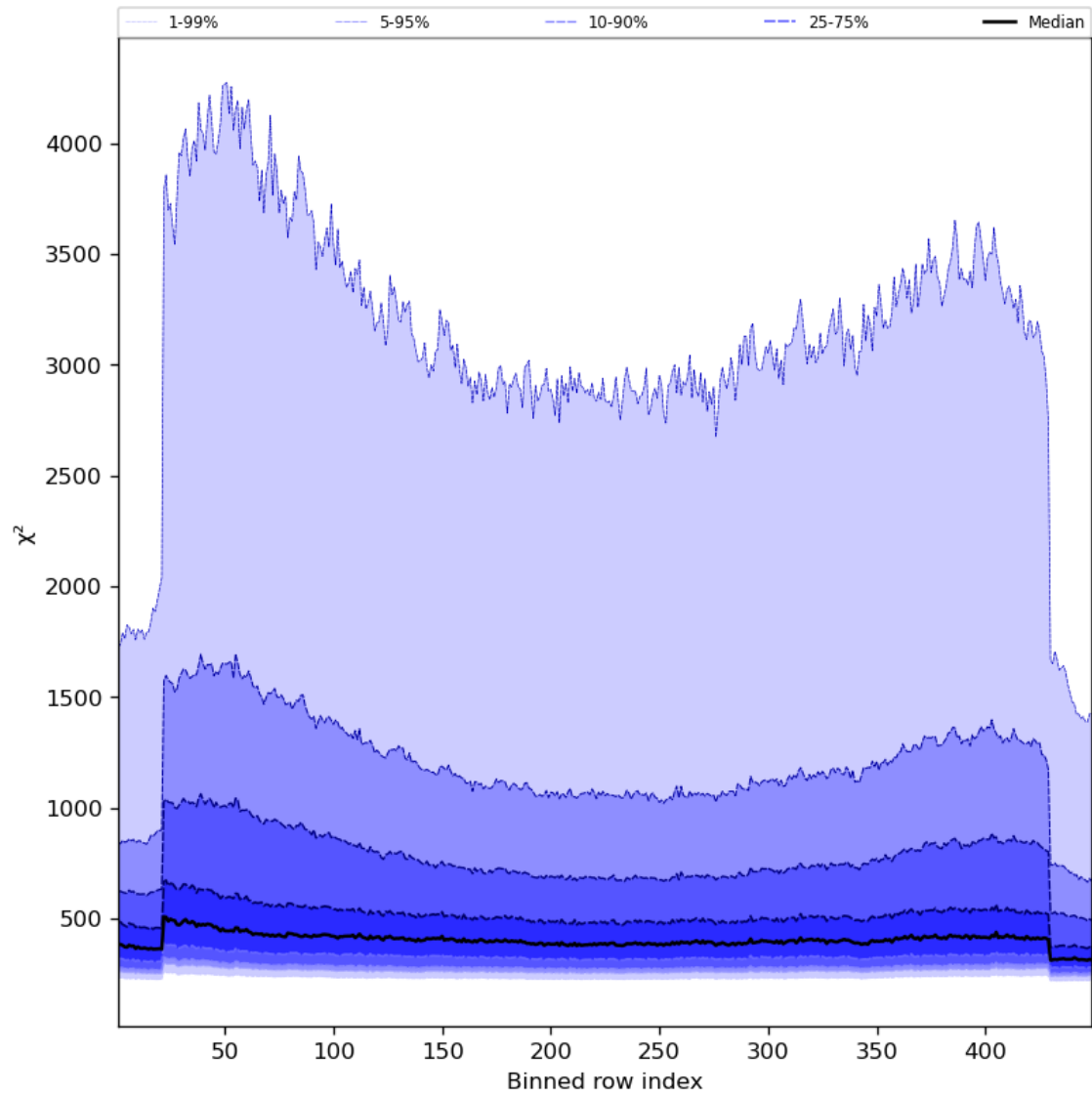
Figure 59: Along track statistics of “ \chi^2 ” for 2023-12-04 to 2023-12-06
