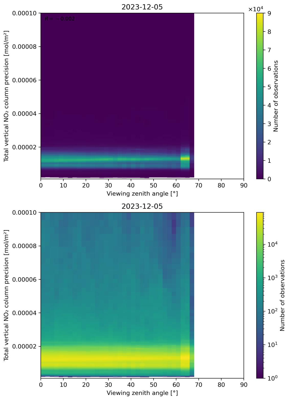
Figure 168: Scatter density plot of “Viewing zenith angle” against “Total vertical NO 2 column precision” for 2023-12-04 to 2023-12-06.
