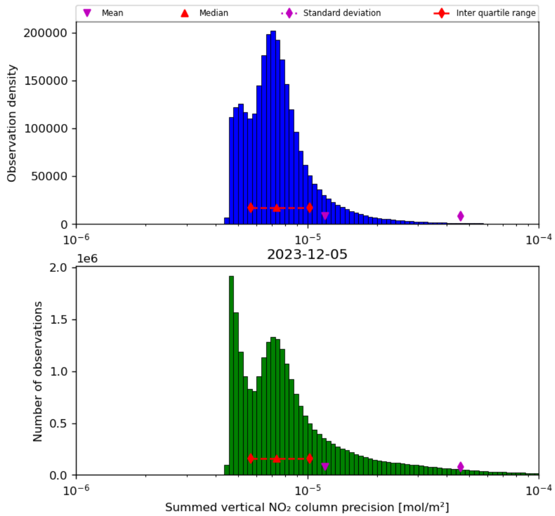
Figure 41: Histogram of “Summed vertical NO 2 column precision” for 2023-12-04 to 2023-12-06
