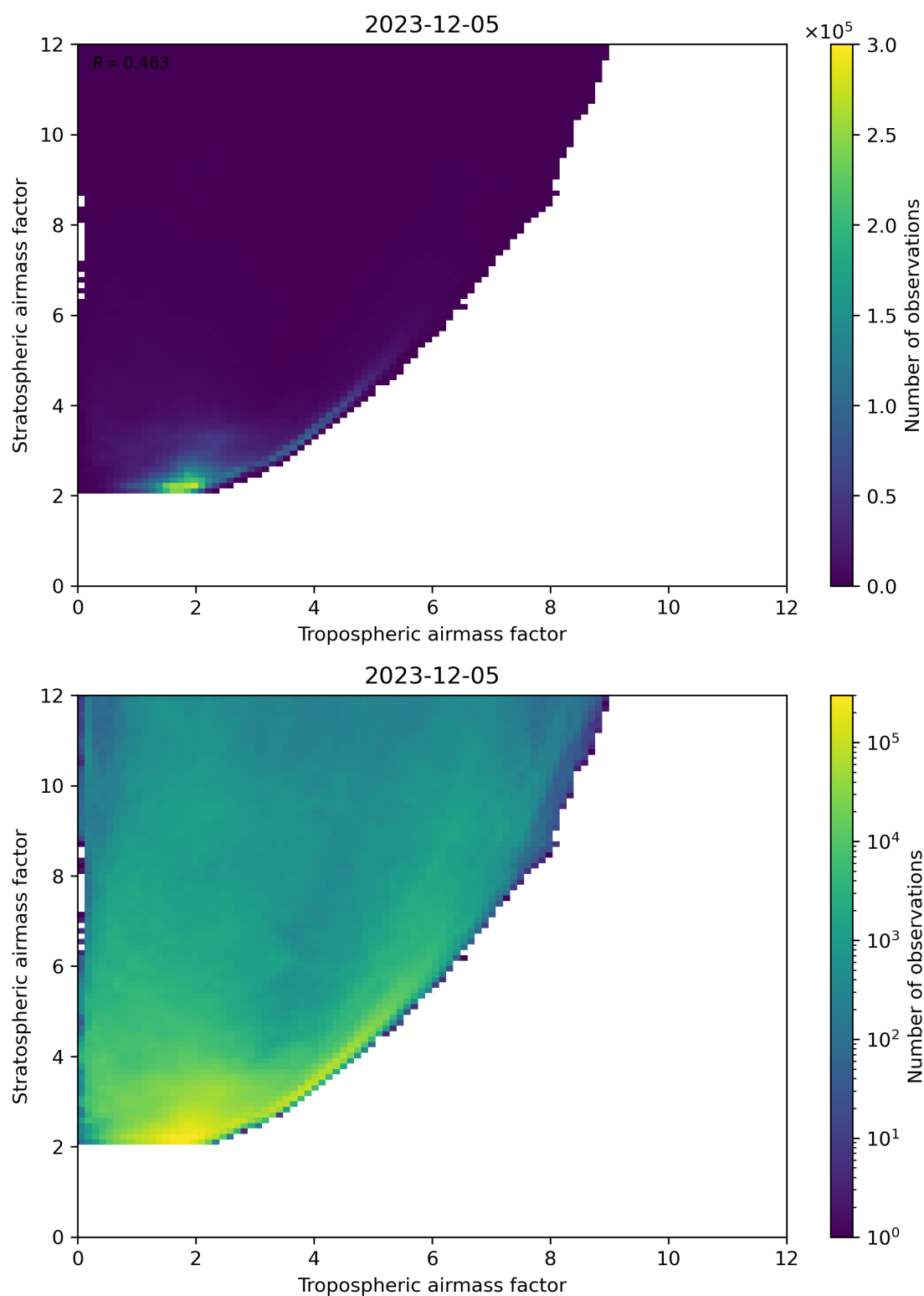
Figure 71: Scatter density plot of “Tropospheric airmass factor” against “Stratospheric airmass factor” for 2023-12-04 to 2023-12-06.
