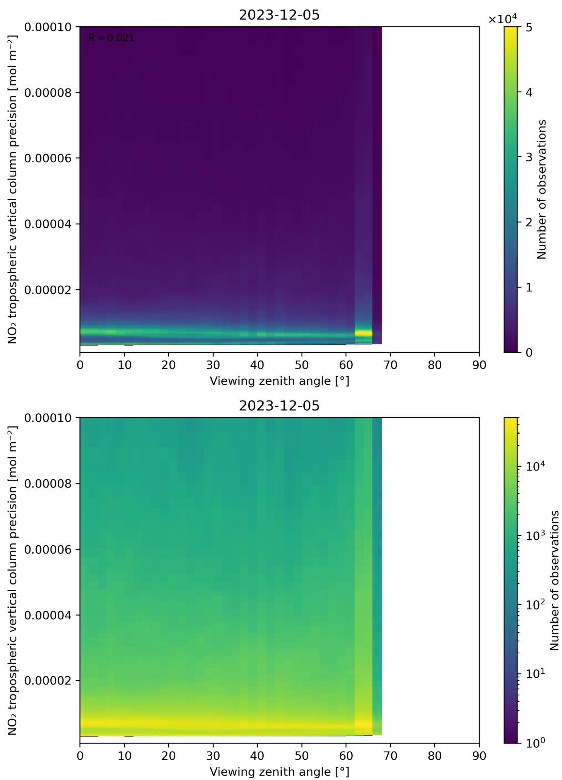
Figure 170: Scatter density plot of “Viewing zenith angle” against “NO 2 tropospheric vertical column precision” for 2023-12-04 to 2023-12-06.
