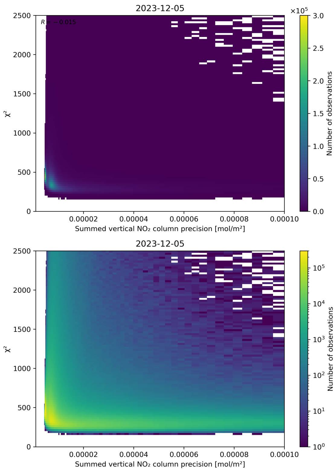
Figure 107: Scatter density plot of “Summed vertical NO 2 column precision” against “ \chi^2 ” for 2023-12-04 to 2023-12-06.
