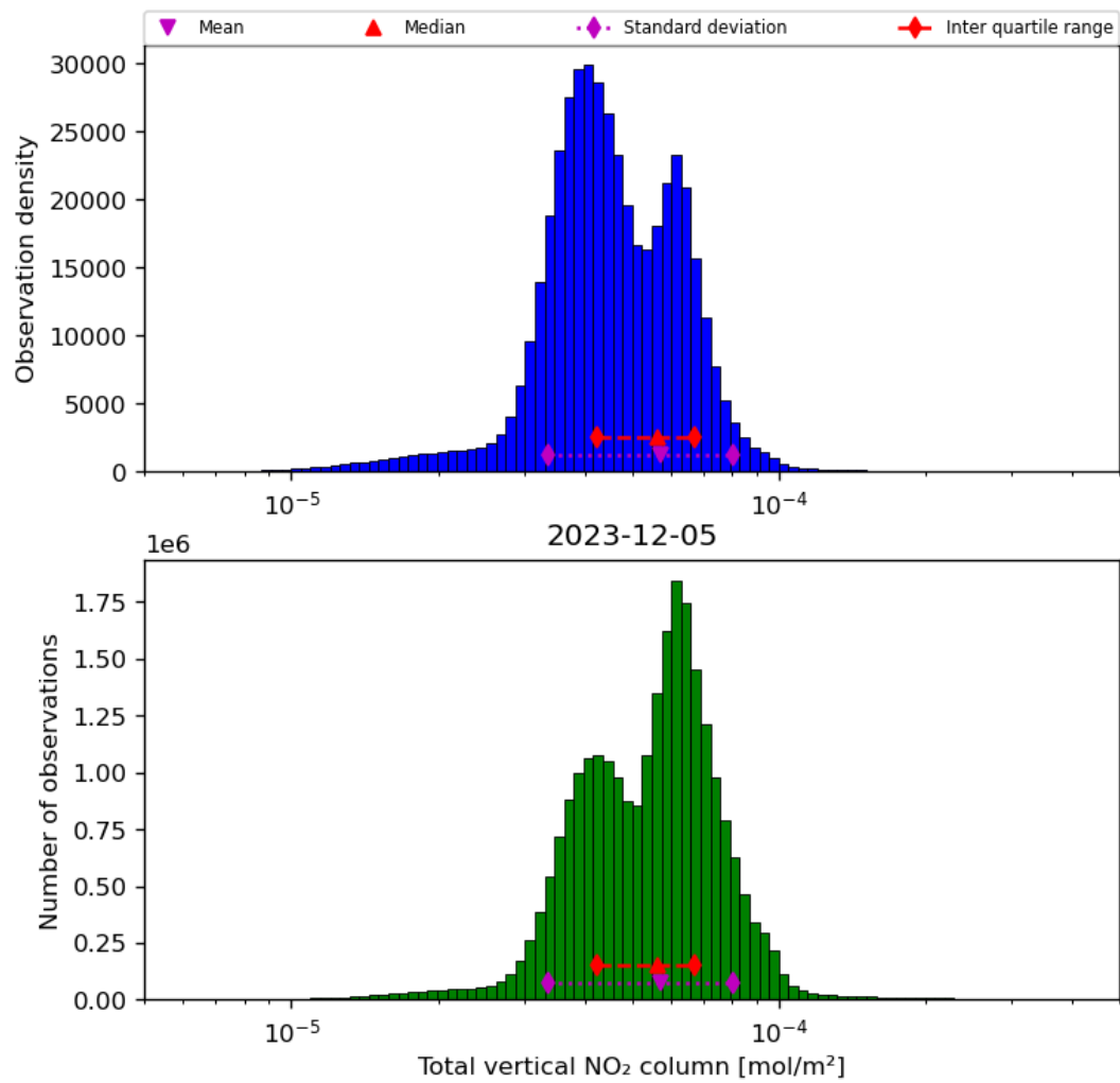
Figure 38: Histogram of “Total vertical NO 2 column” for 2023-12-04 to 2023-12-06
