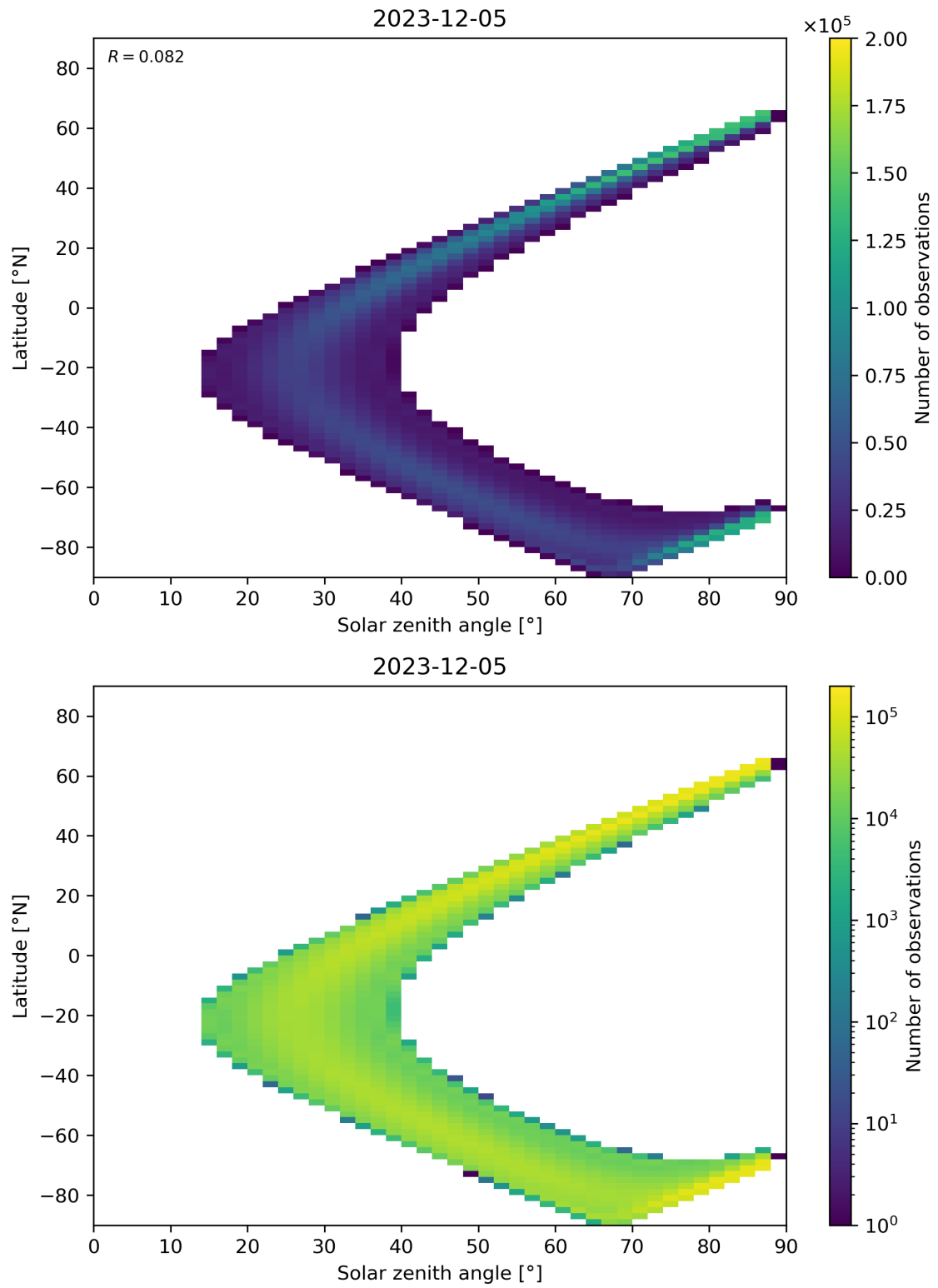
Figure 149: Scatter density plot of “Solar zenith angle” against “Latitude” for 2023-12-04 to 2023-12-06.
