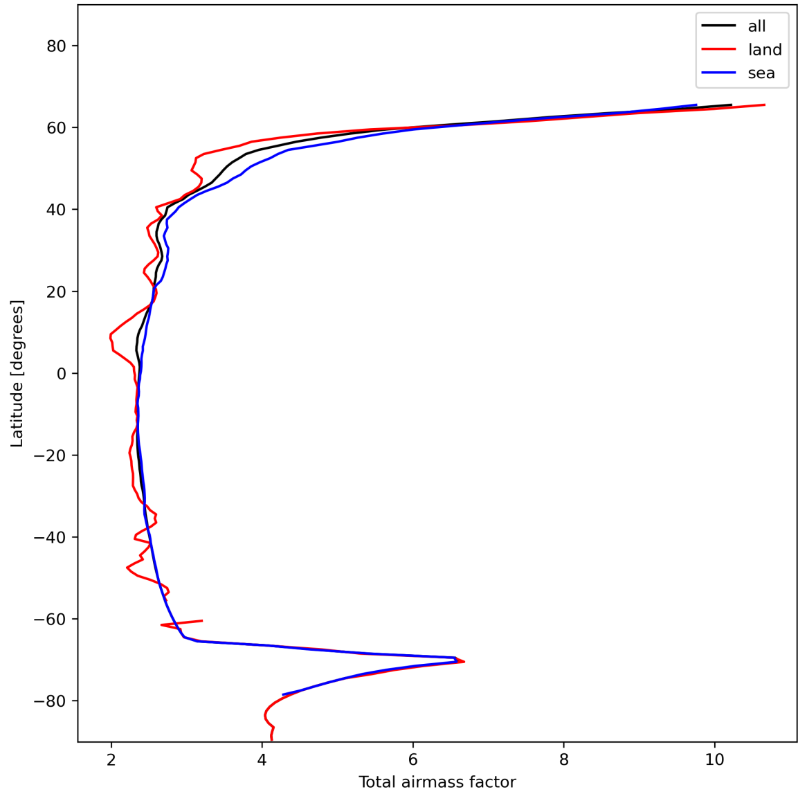
Figure 15: Zonal average of “Total airmass factor” for 2023-12-04 to 2023-12-06.
