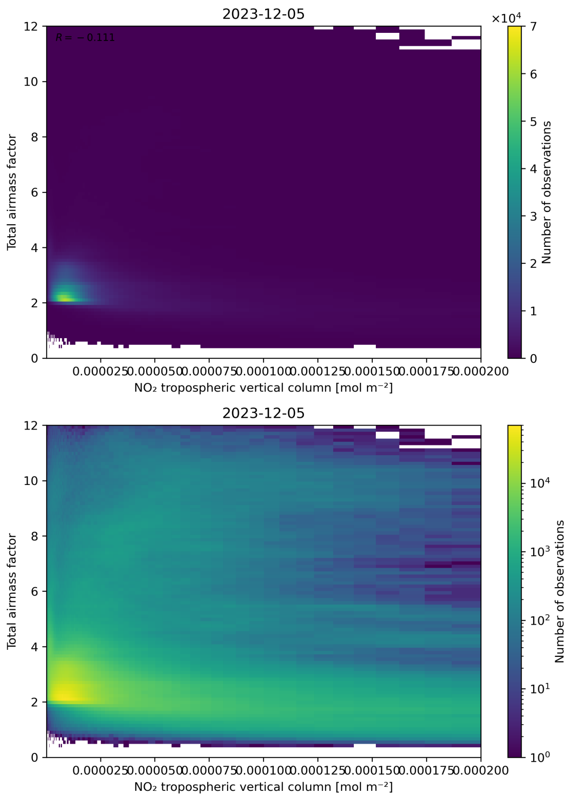
Figure 122: Scatter density plot of “NO 2 tropospheric vertical column” against “Total air mass factor” for 2023-12-04 to 2023-12-06.
