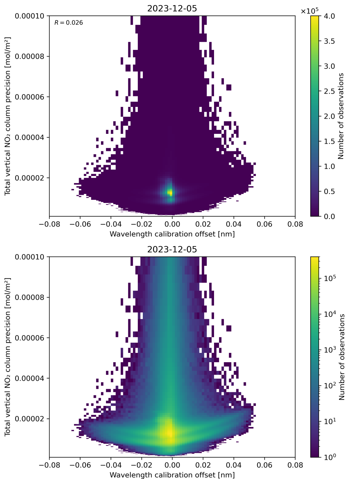
Figure 180: Scatter density plot of “Wavelength calibration offset” against “Total vertical NO 2 column precision” for 2023-12-04 to 2023-12-06.
