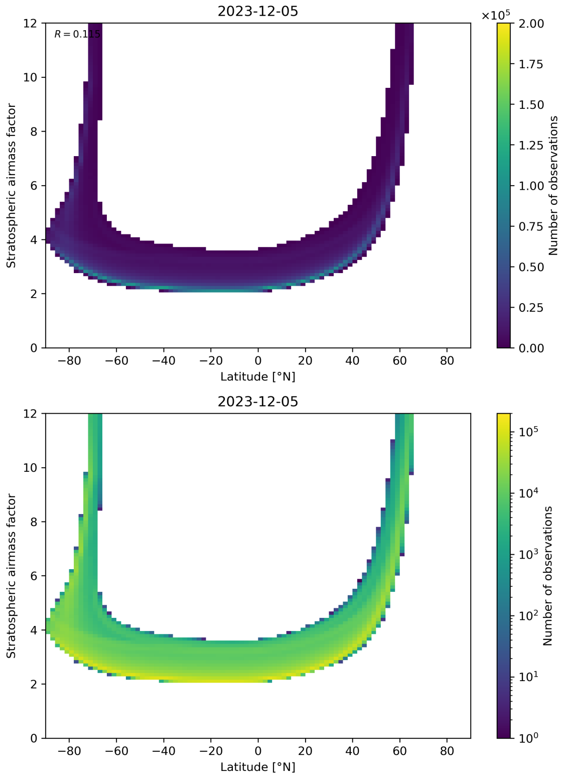
Figure 83: Scatter density plot of “Latitude” against “Stratospheric airmass factor” for 2023-12-04 to 2023-12-06.
