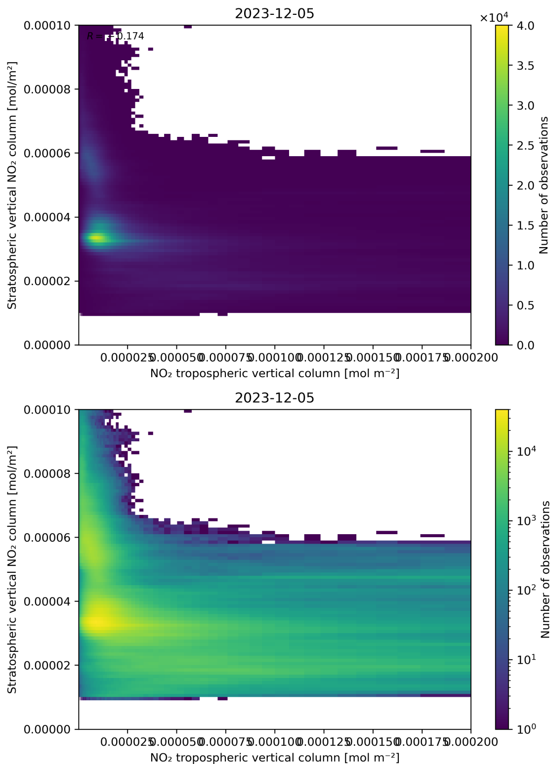
Figure 125: Scatter density plot of “NO 2 tropospheric vertical column” against “Stratospheric vertical NO 2 column” for 2023-12-04 to 2023-12-06.
