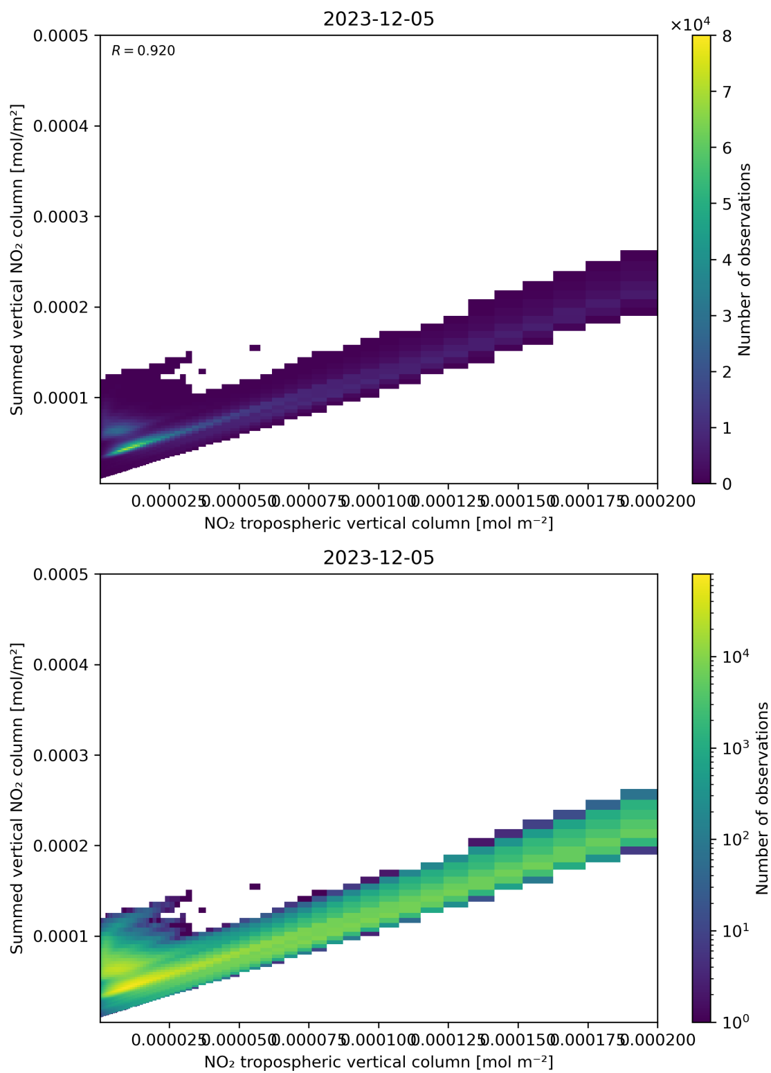
Figure 126: Scatter density plot of “NO 2 tropospheric vertical column” against “Summed vertical NO 2 column” for 2023-12-04 to 2023-12-06.
