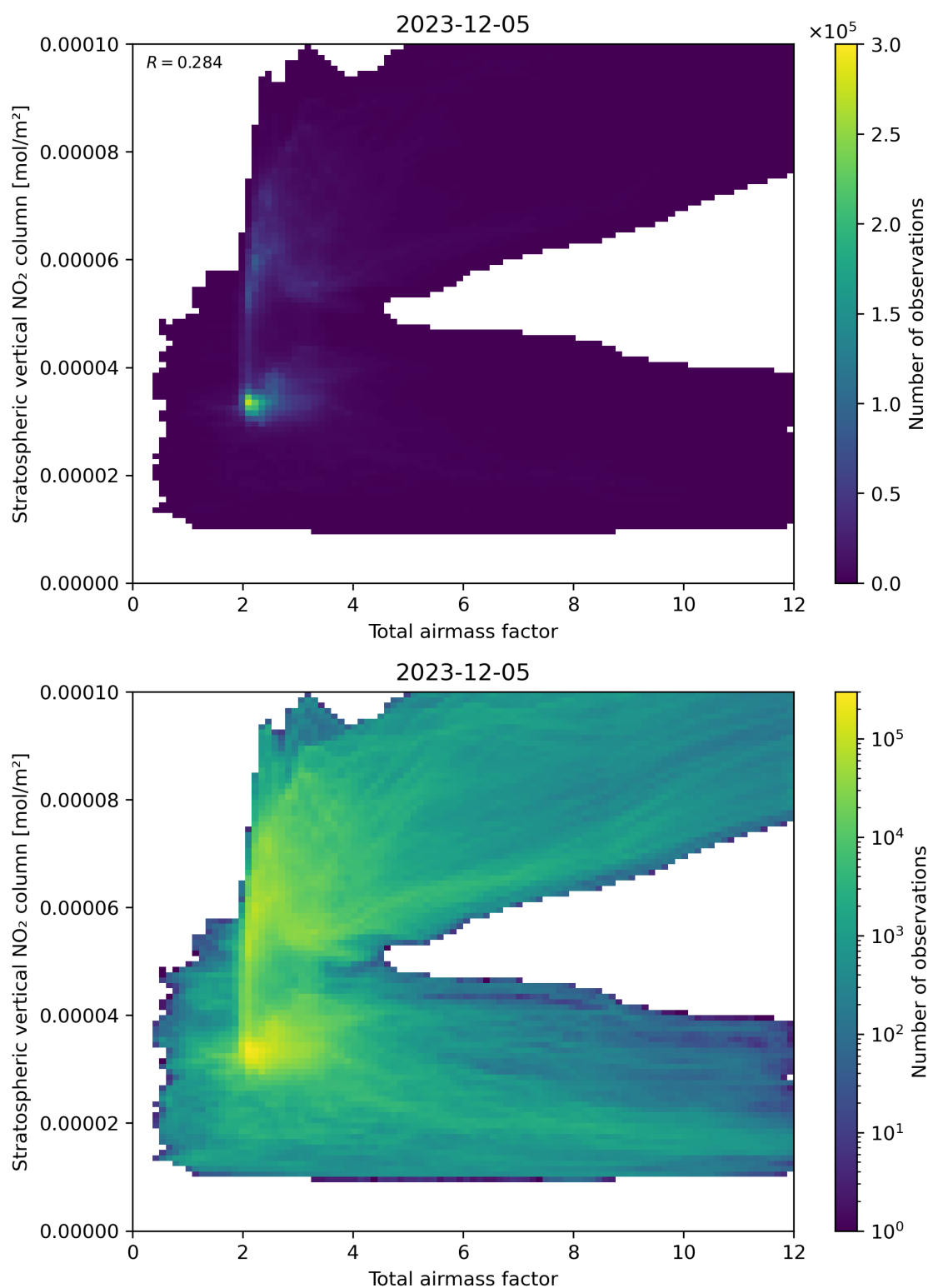
Figure 64: Scatter density plot of “Total airmass factor” against “Stratospheric vertical NO 2 column” for 2023-12-04 to 2023-12-06.
