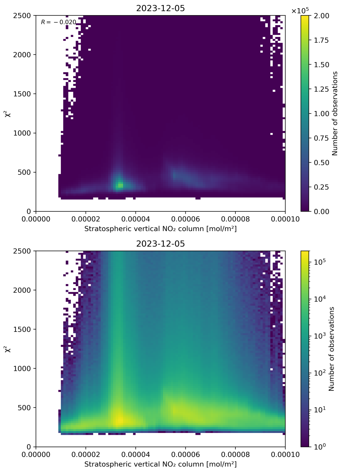
Figure 97: Scatter density plot of “Stratospheric vertical NO 2 column” against “ \chi^2 ” for 2023-12-04 to 2023-12-06.
