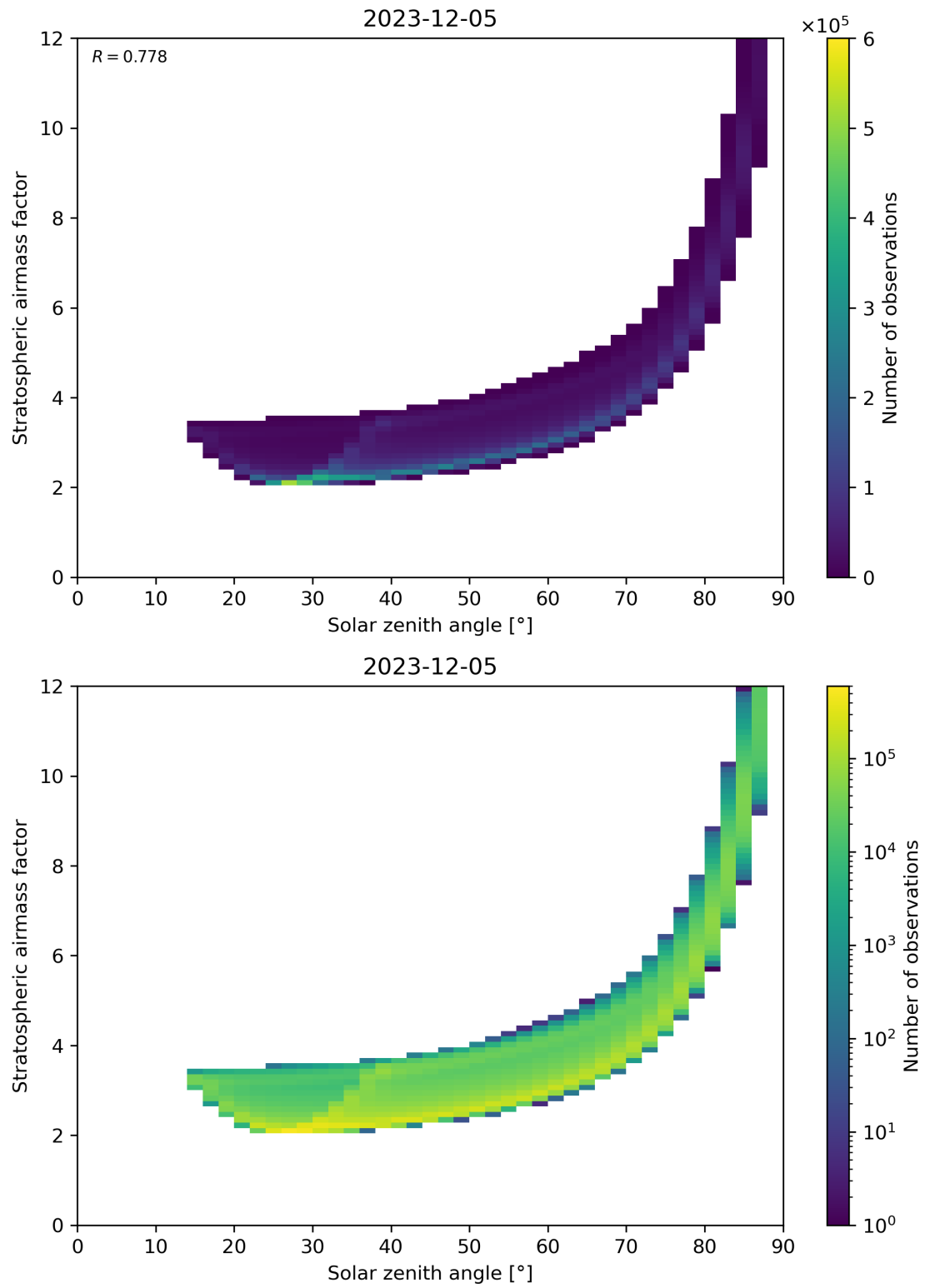
Figure 145: Scatter density plot of “Solar zenith angle” against “Stratospheric airmass factor” for 2023-12-04 to 2023-12-06.
