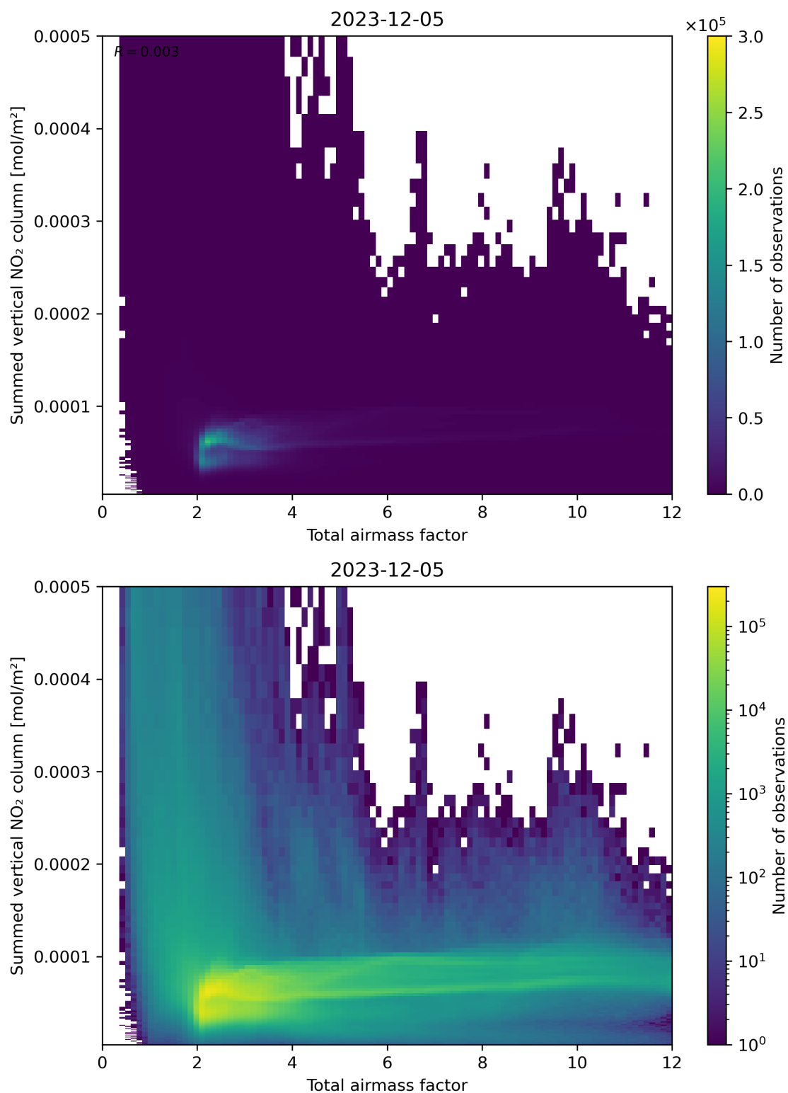
Figure 65: Scatter density plot of “Total air mass factor” against “Summed vertical NO 2 column” for 2023-12-04 to 2023-12-06.
