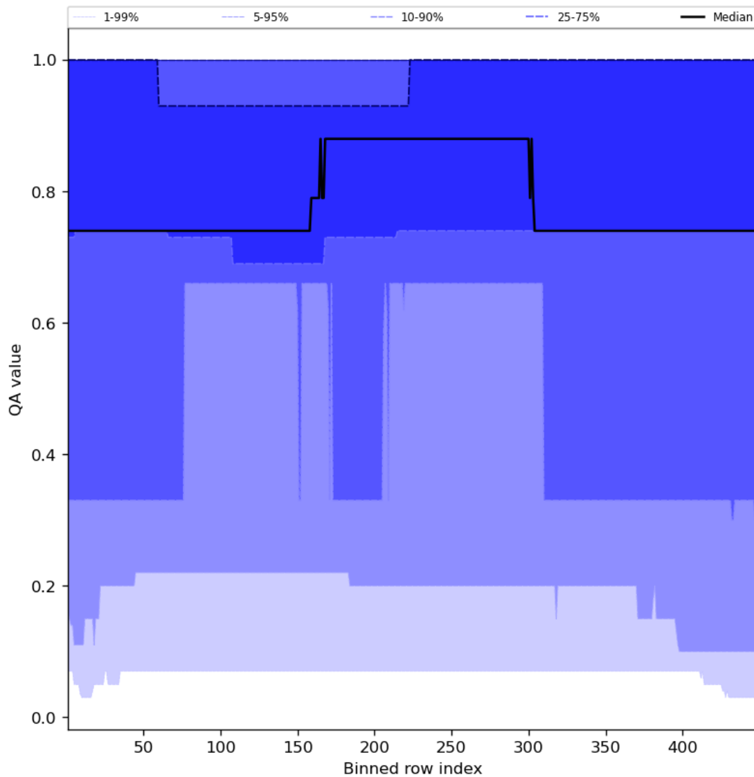
Figure 45: Along track statistics of “QA value” for 2023-12-04 to 2023-12-06
