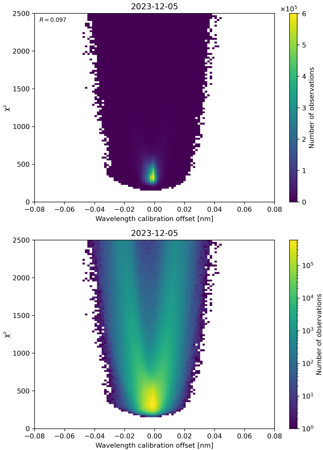
Figure 175: Scatter density plot of “Wavelength calibration offset” against “ \chi^2 ” for 2023-12-04 to 2023-12-06.
