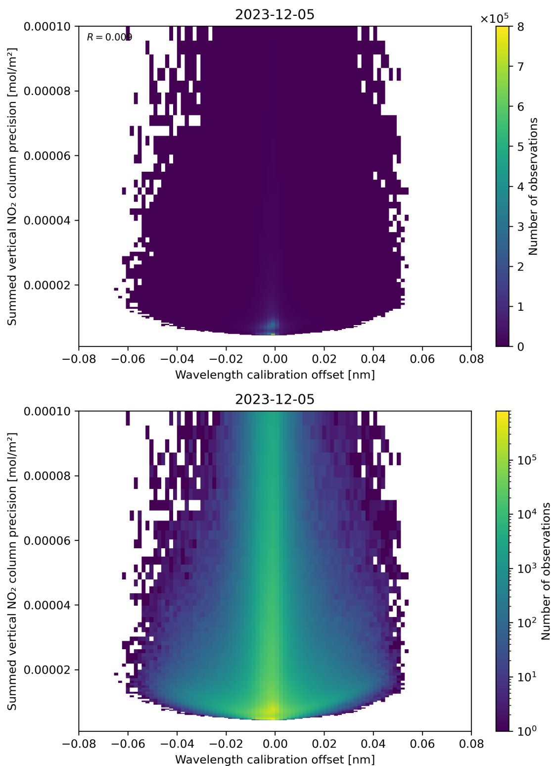
Figure 178: Scatter density plot of “Wavelength calibration offset” against “Summed vertical NO 2 column precision” for 2023-12-04 to 2023-12-06.
