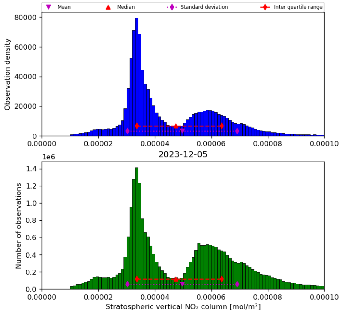
Figure 36: Histogram of “Stratospheric vertical NO 2 column” for 2023-12-04 to 2023-12-06
