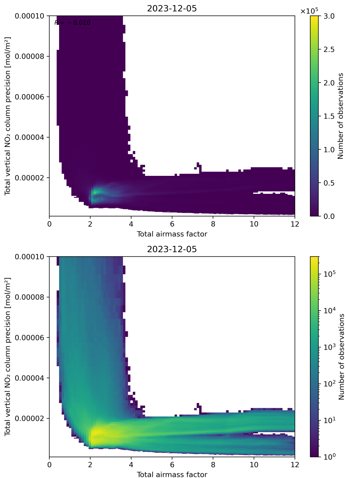
Figure 68: Scatter density plot of “Total airmass factor” against “Total vertical NO 2 column precision” for 2023-12-04 to 2023-12-06.
