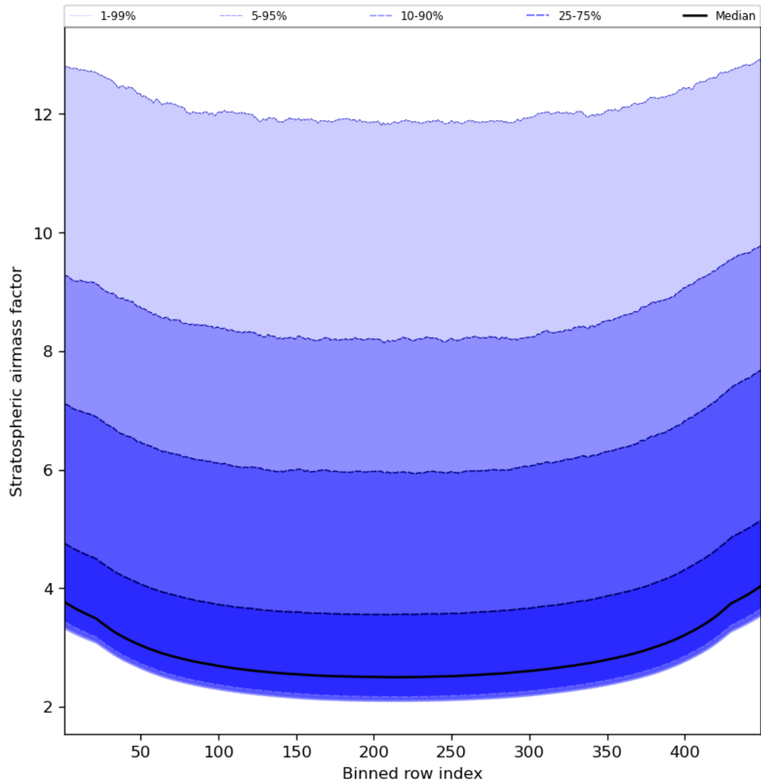
Figure 61: Along track statistics of “Stratospheric airmass factor” for 2023-12-04 to 2023-12-06
