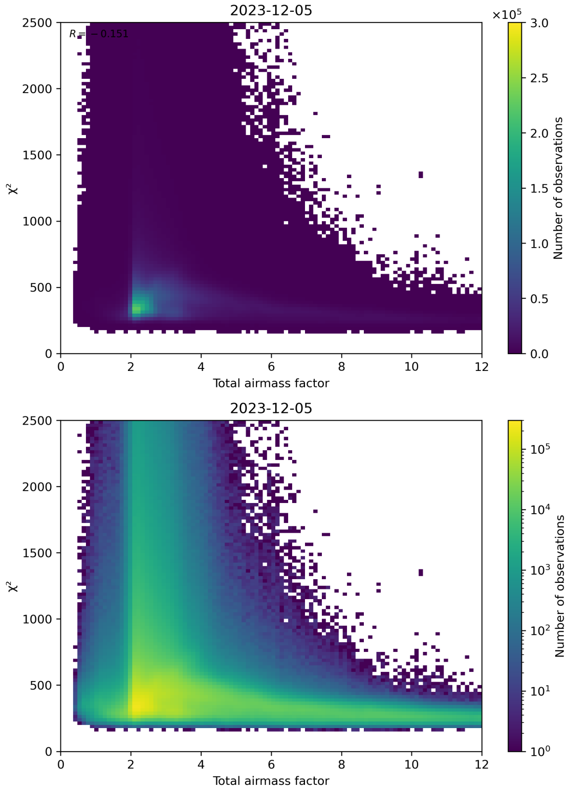
Figure 63: Scatter density plot of “Total airmass factor” against “ \chi^2 ” for 2023-12-04 to 2023-12-06.
