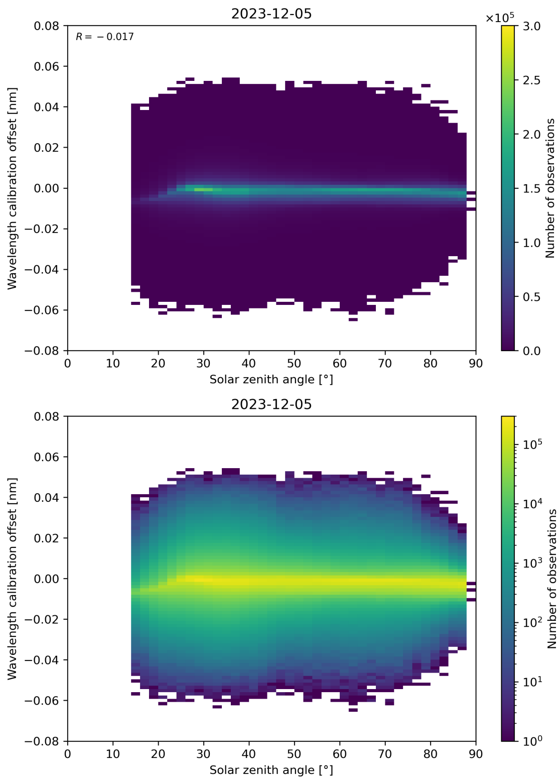
Figure 158: Scatter density plot of “Solar zenith angle” against “Wavelength calibration offset” for 2023-12-04 to 2023-12-06.
