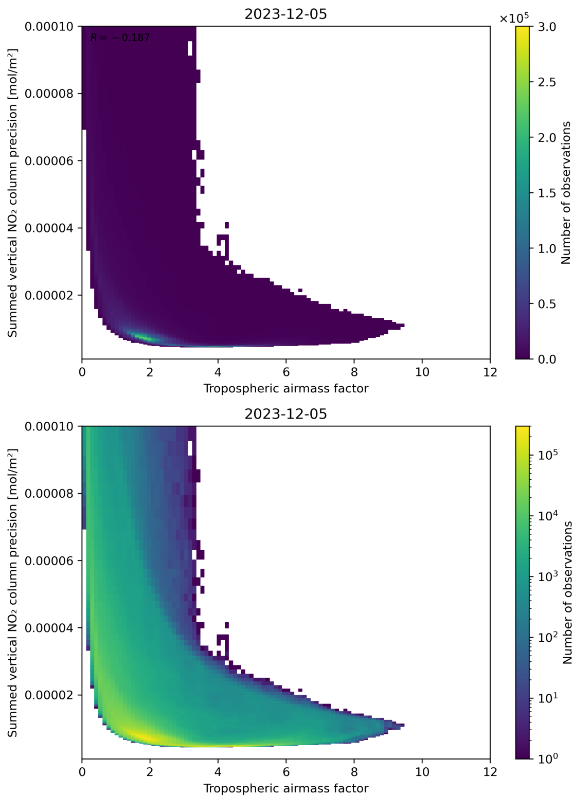
Figure 76: Scatter density plot of “Tropospheric air mass factor” against “Summed vertical NO 2 column precision” for 2023-12-04 to 2023-12-06.
