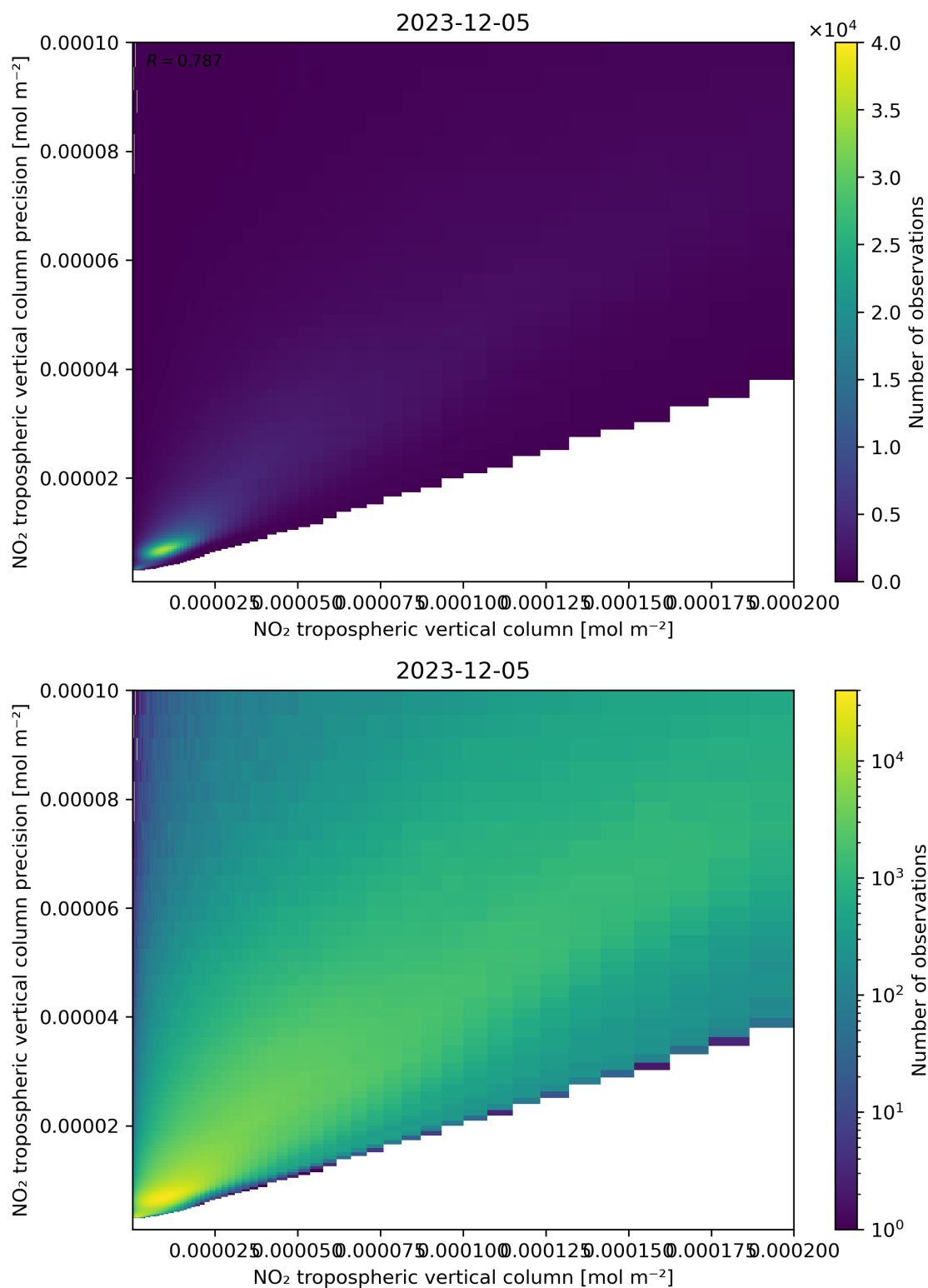
Figure 130: Scatter density plot of “NO 2 tropospheric vertical column” against “NO 2 tropospheric vertical column precision” for 2023-12-04 to 2023-12-06.
