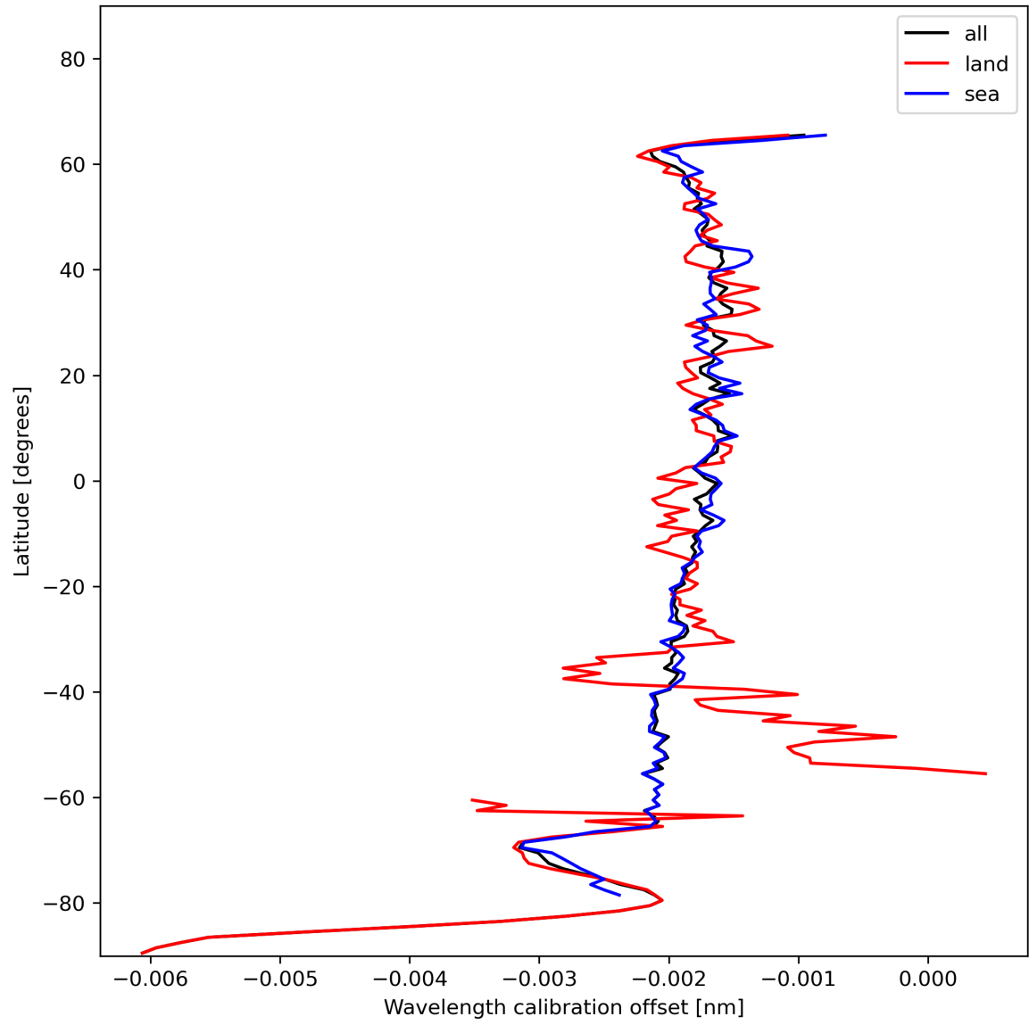
Figure 18: Zonal average of “Wavelength calibration offset” for 2023-12-04 to 2023-12-06.
