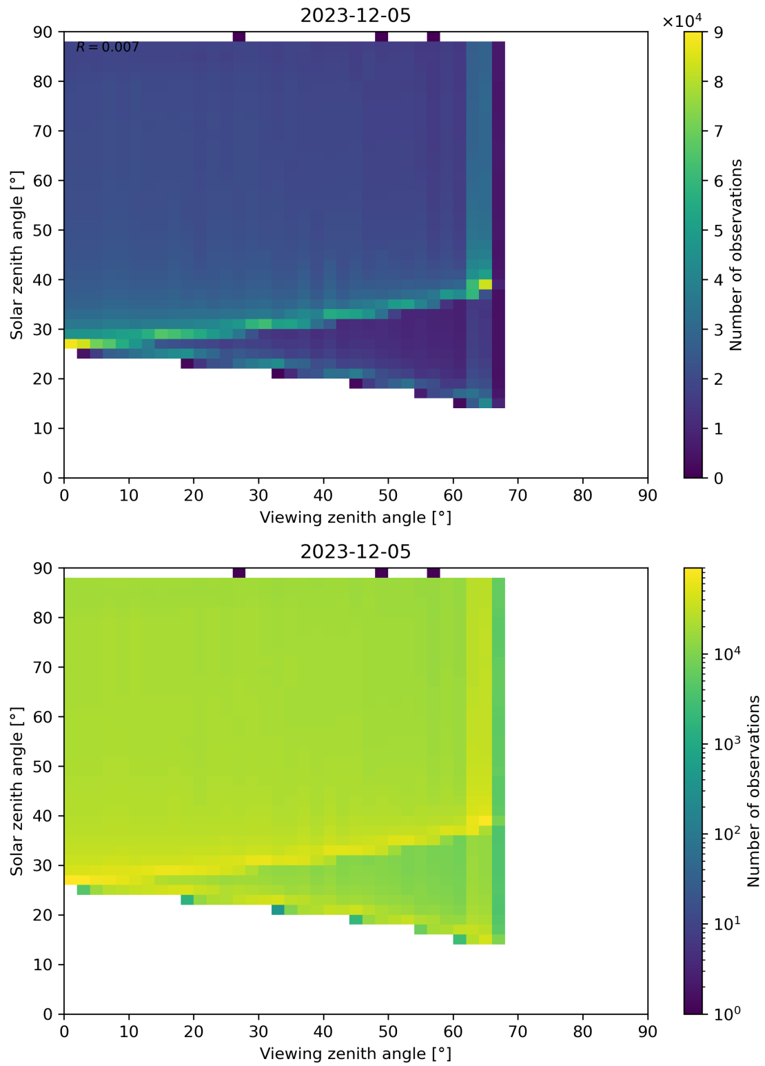
Figure 172: Scatter density plot of “Viewing zenith angle” against “Solar zenith angle” for 2023-12-04 to 2023-12-06.
