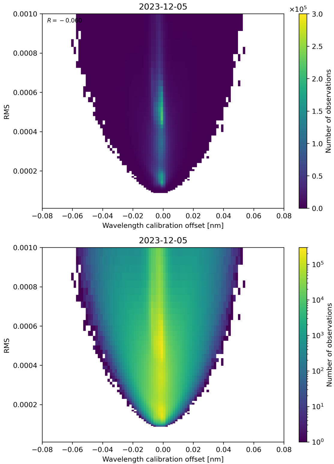
Figure 181: Scatter density plot of “Wavelength calibration offset” against “RMS” for 2023-12-04 to 2023-12-06.
