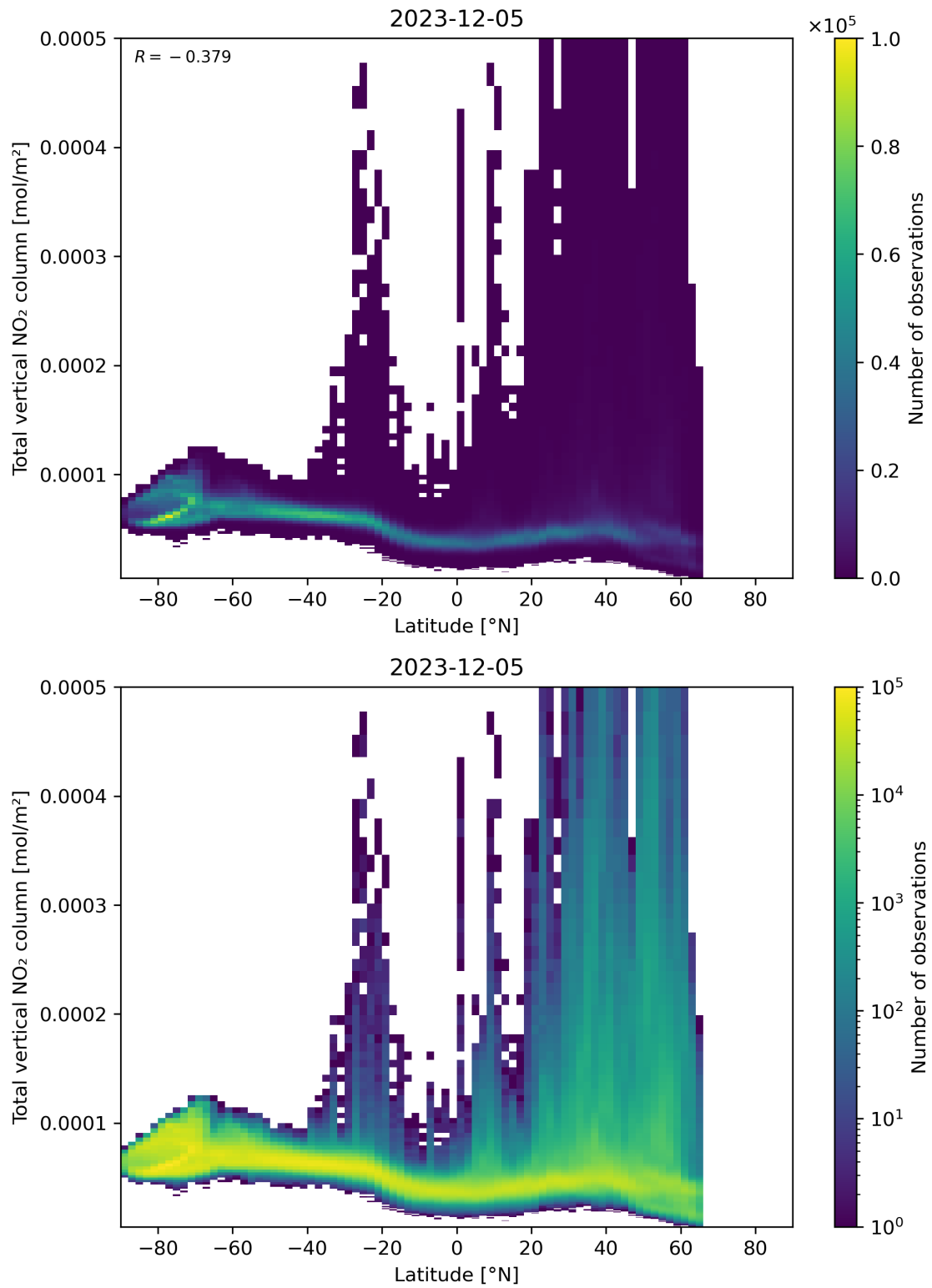
Figure 90: Scatter density plot of “Latitude” against “Total vertical NO 2 column” for 2023-12-04 to 2023-12-06.
