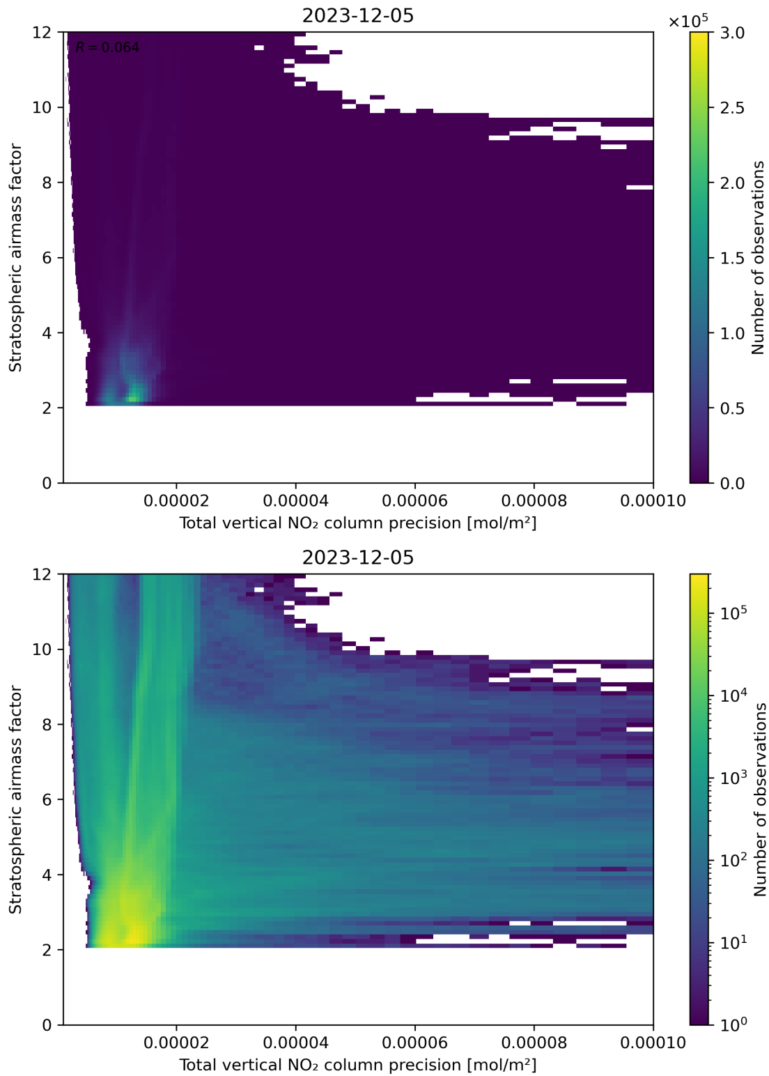
Figure 115: Scatter density plot of “Total vertical NO 2 column precision” against “Stratospheric airmass factor” for 2023-12-04 to 2023-12-06.
