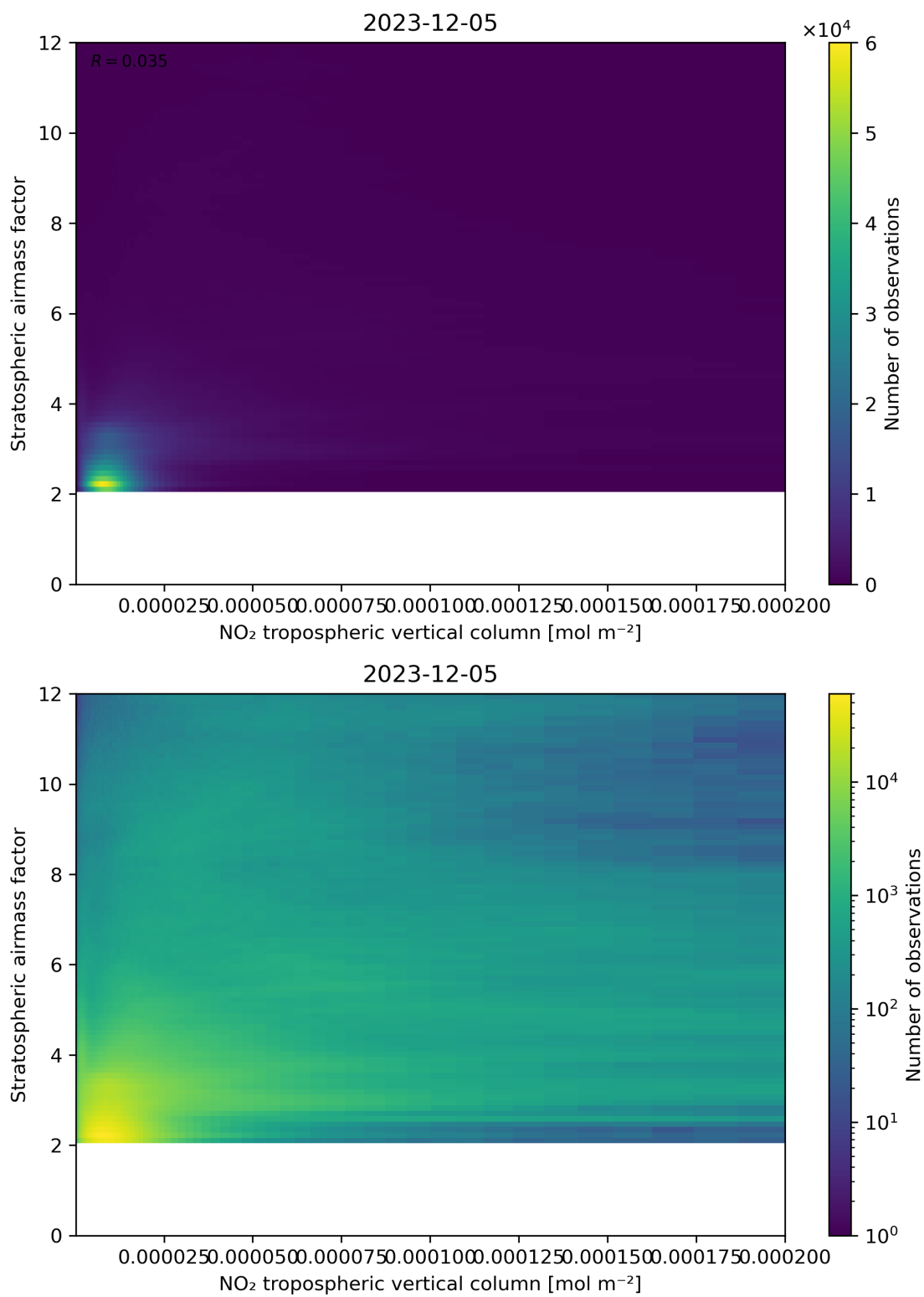
Figure 121: Scatter density plot of “NO 2 tropospheric vertical column” against “Stratospheric airmass factor” for 2023-12-04 to 2023-12-06.
