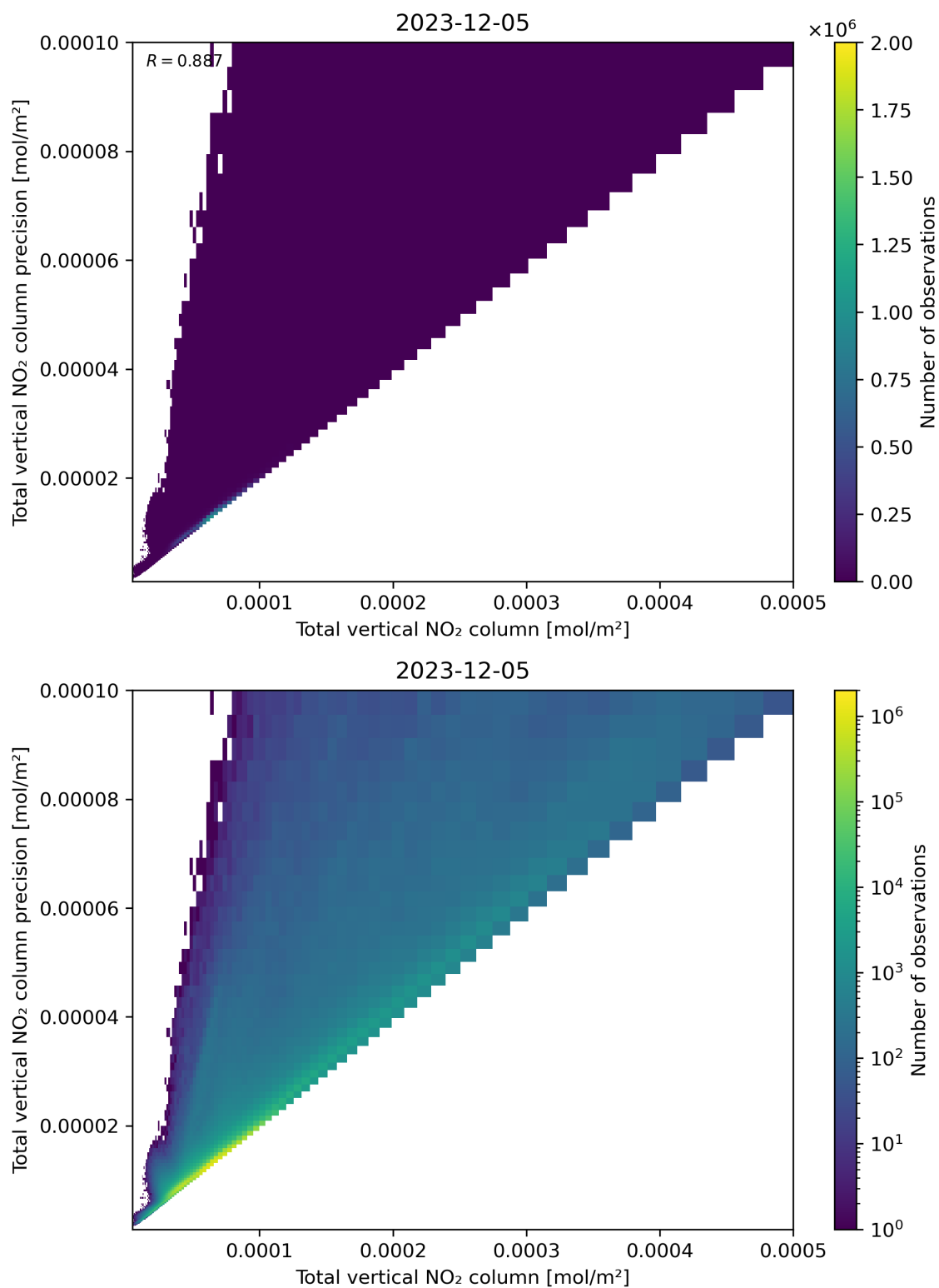
Figure 114: Scatter density plot of “Total vertical NO 2 column” against “Total vertical NO 2 column precision” for 2023-12-04 to 2023-12-06.
