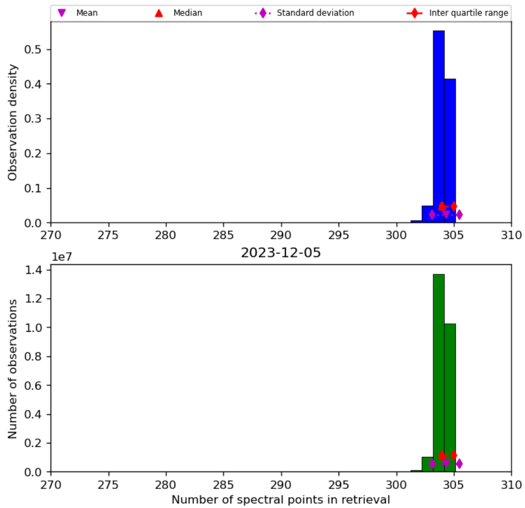
Figure 33: Histogram of “Number of spectral points in retrieval” for 2023-12-04 to 2023-12-06
