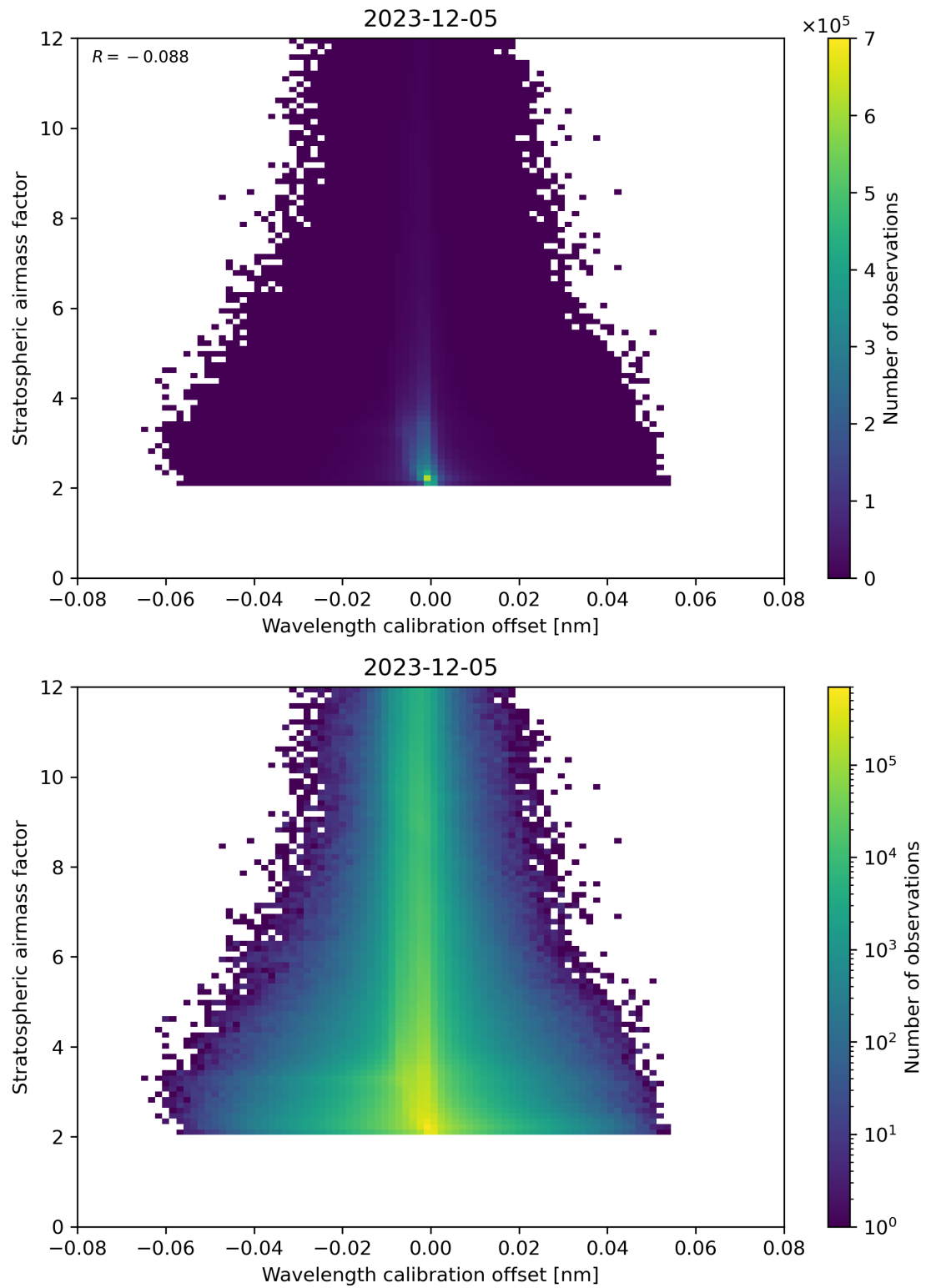
Figure 174: Scatter density plot of “Wavelength calibration offset” against “Stratospheric airmass factor” for 2023-12-04 to 2023-12-06.
