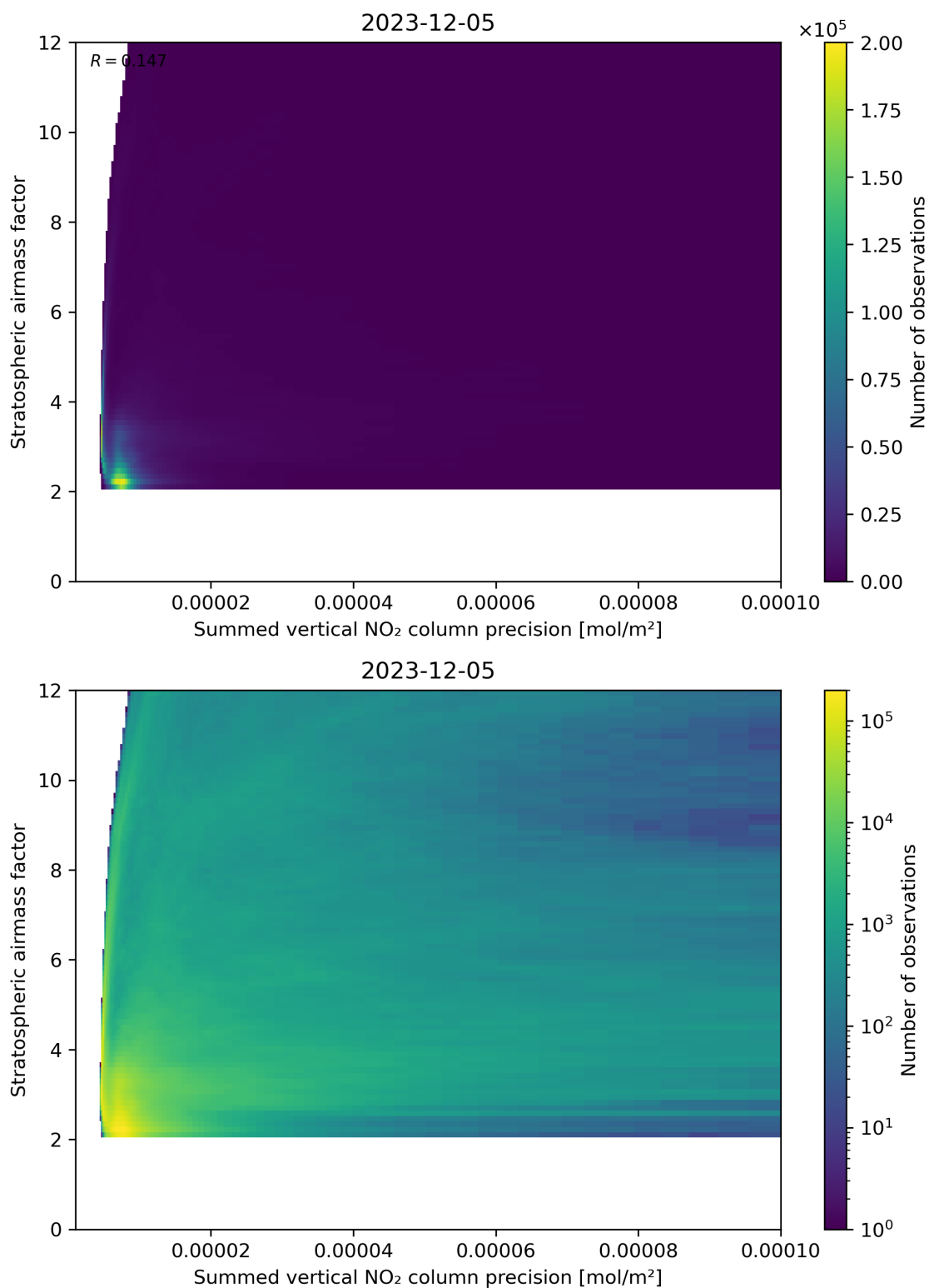
Figure 106: Scatter density plot of “Summed vertical NO 2 column precision” against “Stratospheric airmass factor” for 2023-12-04 to 2023-12-06.
