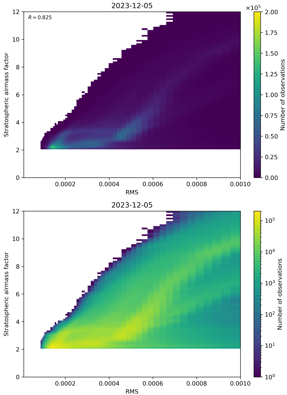
Figure 144: Scatter density plot of “RMS” against “Stratospheric airmass factor” for 2023-12-04 to 2023-12-06.
