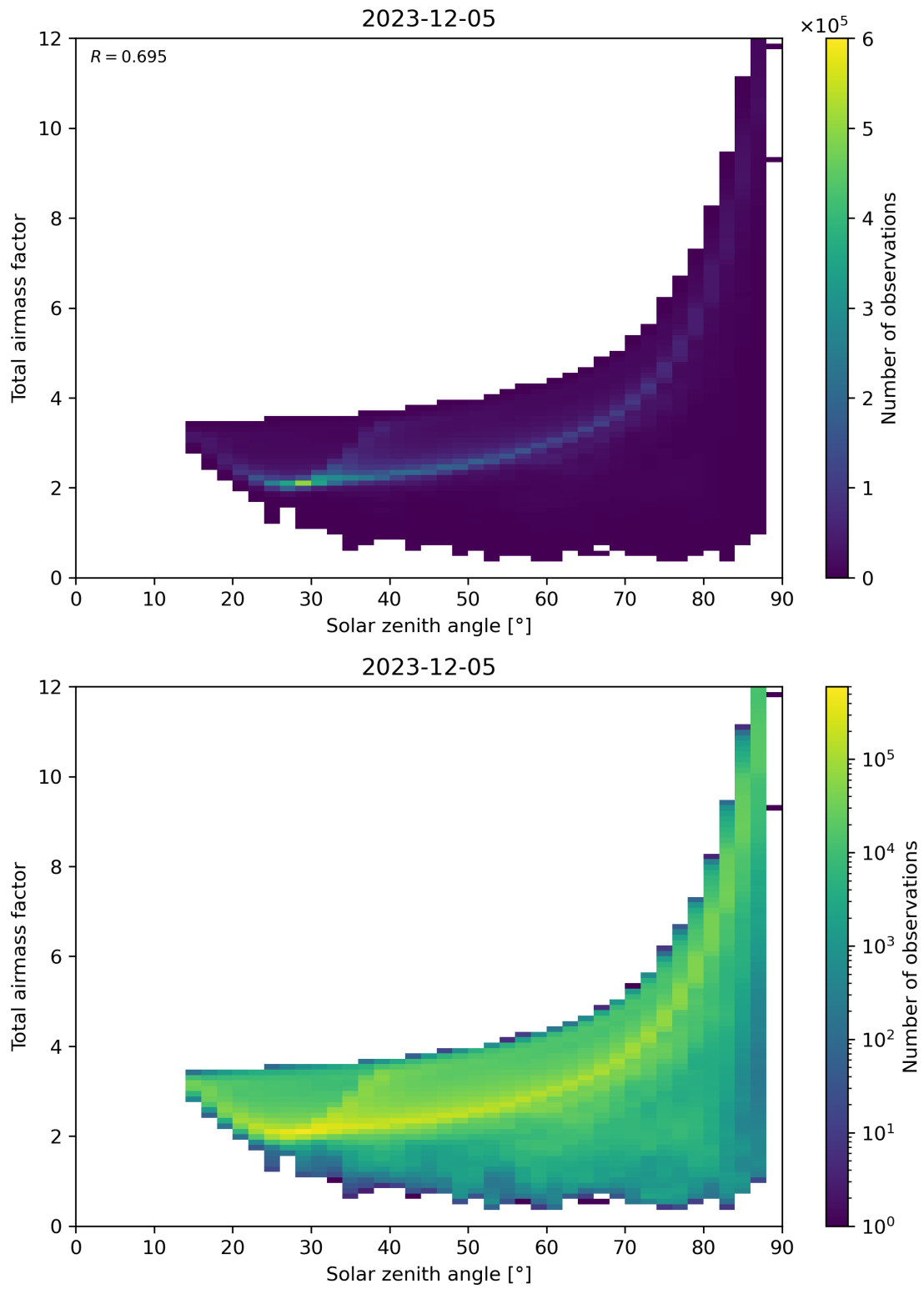
Figure 146: Scatter density plot of “Solar zenith angle” against “Total air mass factor” for 2023-12-04 to 2023-12-06.
