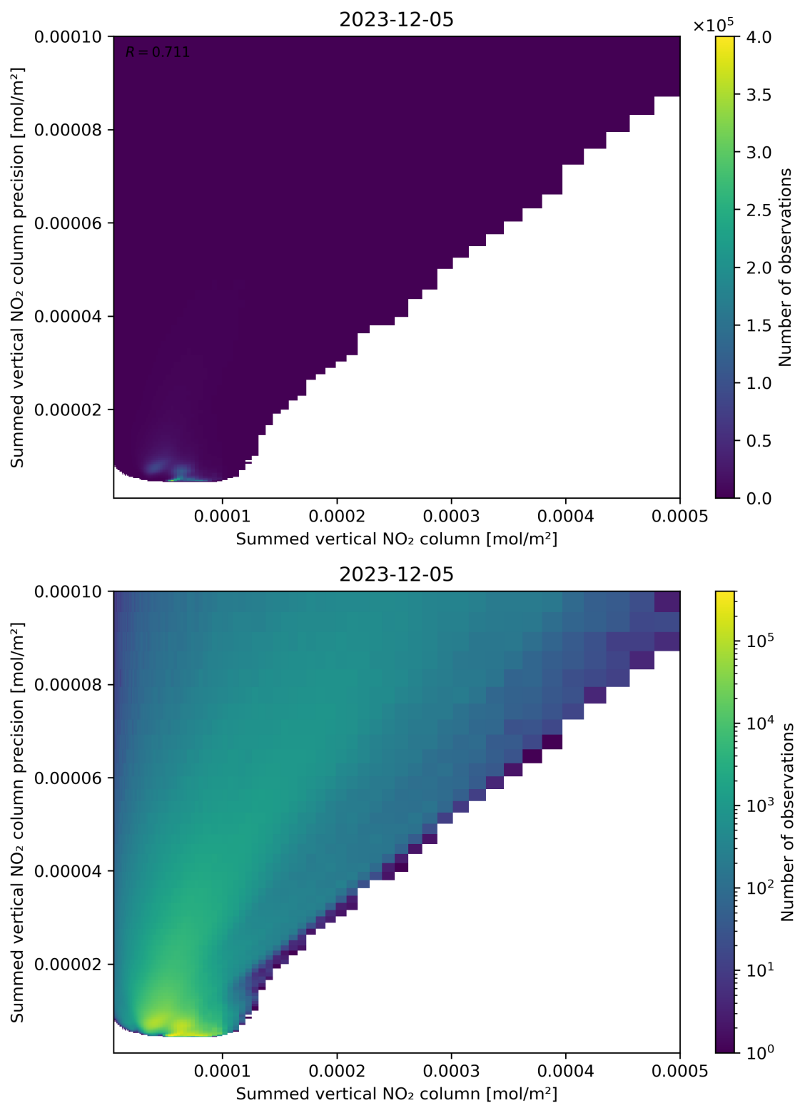
Figure 105: Scatter density plot of “Summed vertical NO 2 column” against “Summed vertical NO 2 column precision” for 2023-12-04 to 2023-12-06.
