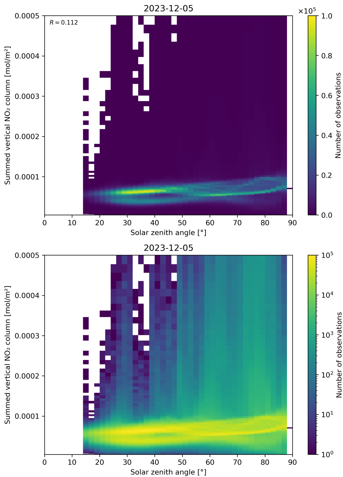
Figure 151: Scatter density plot of “Solar zenith angle” against “Summed vertical NO 2 column” for 2023-12-04 to 2023-12-06.
