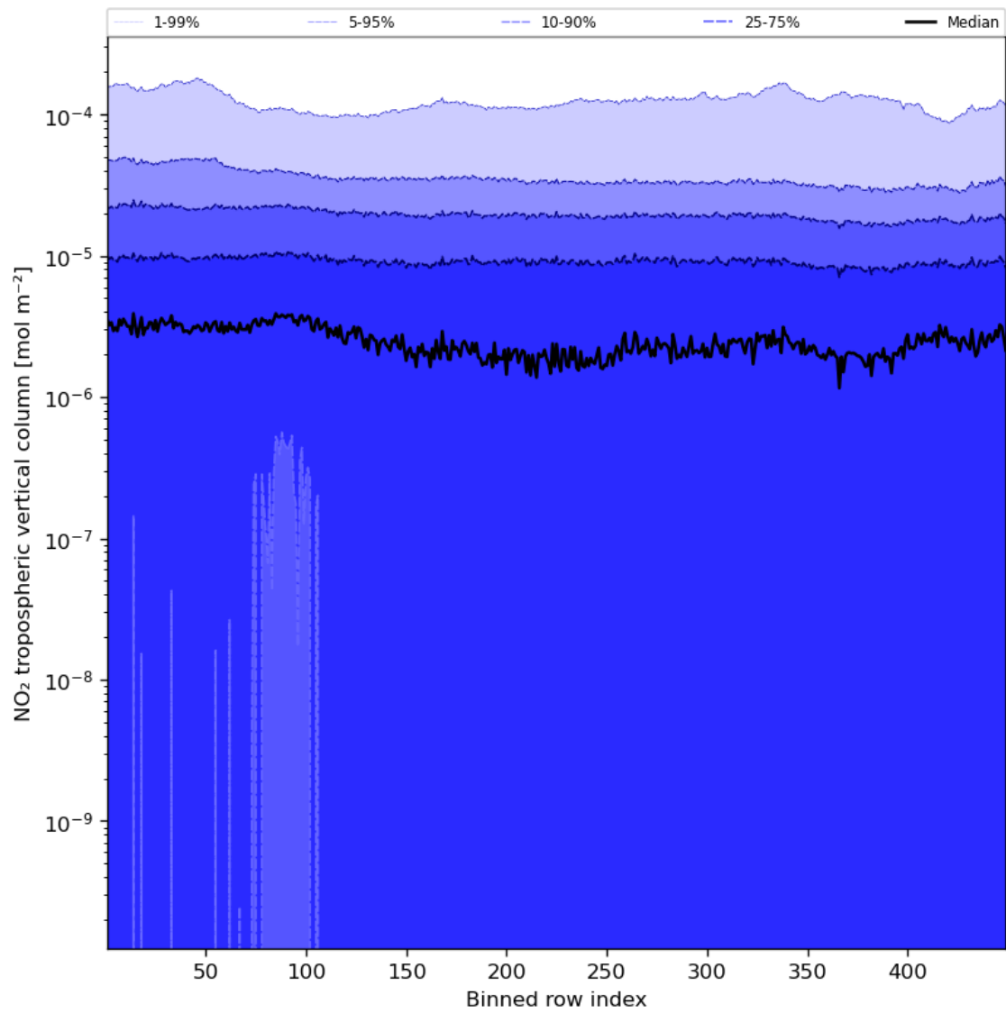
Figure 46: Along track statistics of “NO 2 tropospheric vertical column” for 2023-12-04 to 2023-12-06
