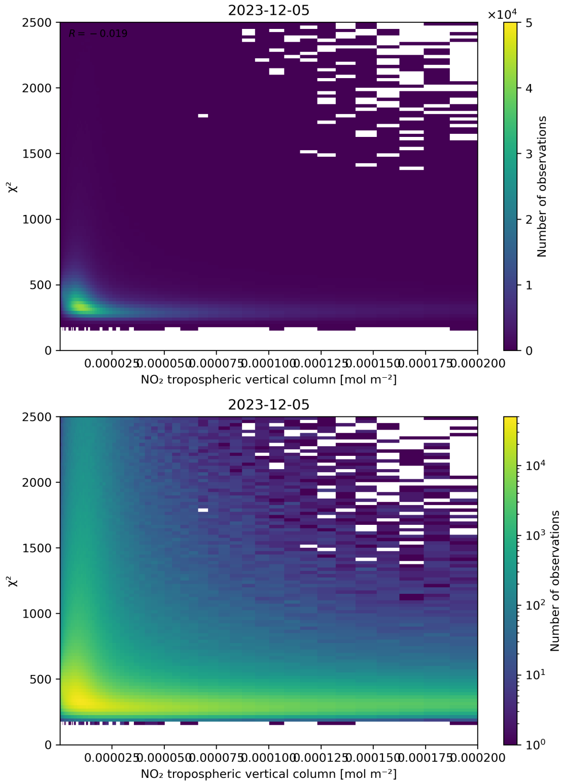
Figure 124: Scatter density plot of “NO 2 tropospheric vertical column” against “ \chi^2 ” for 2023-12-04 to 2023-12-06.
