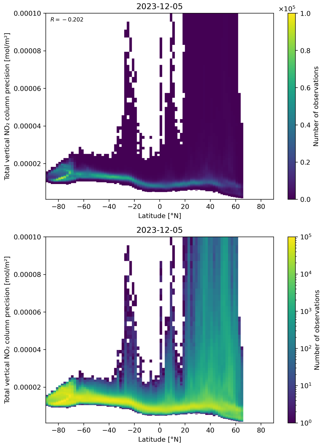
Figure 91: Scatter density plot of “Latitude” against “Total vertical NO 2 column precision” for 2023-12-04 to 2023-12-06.
