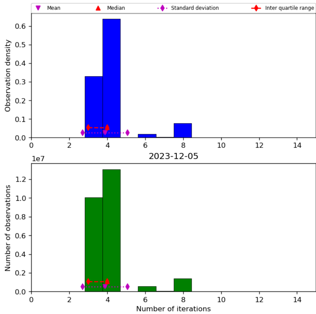
Figure 34: Histogram of “Number of iterations” for 2023-12-04 to 2023-12-06
