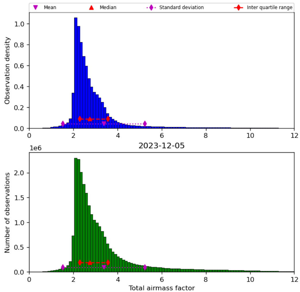
Figure 32: Histogram of “Total airmass factor” for 2023-12-04 to 2023-12-06
