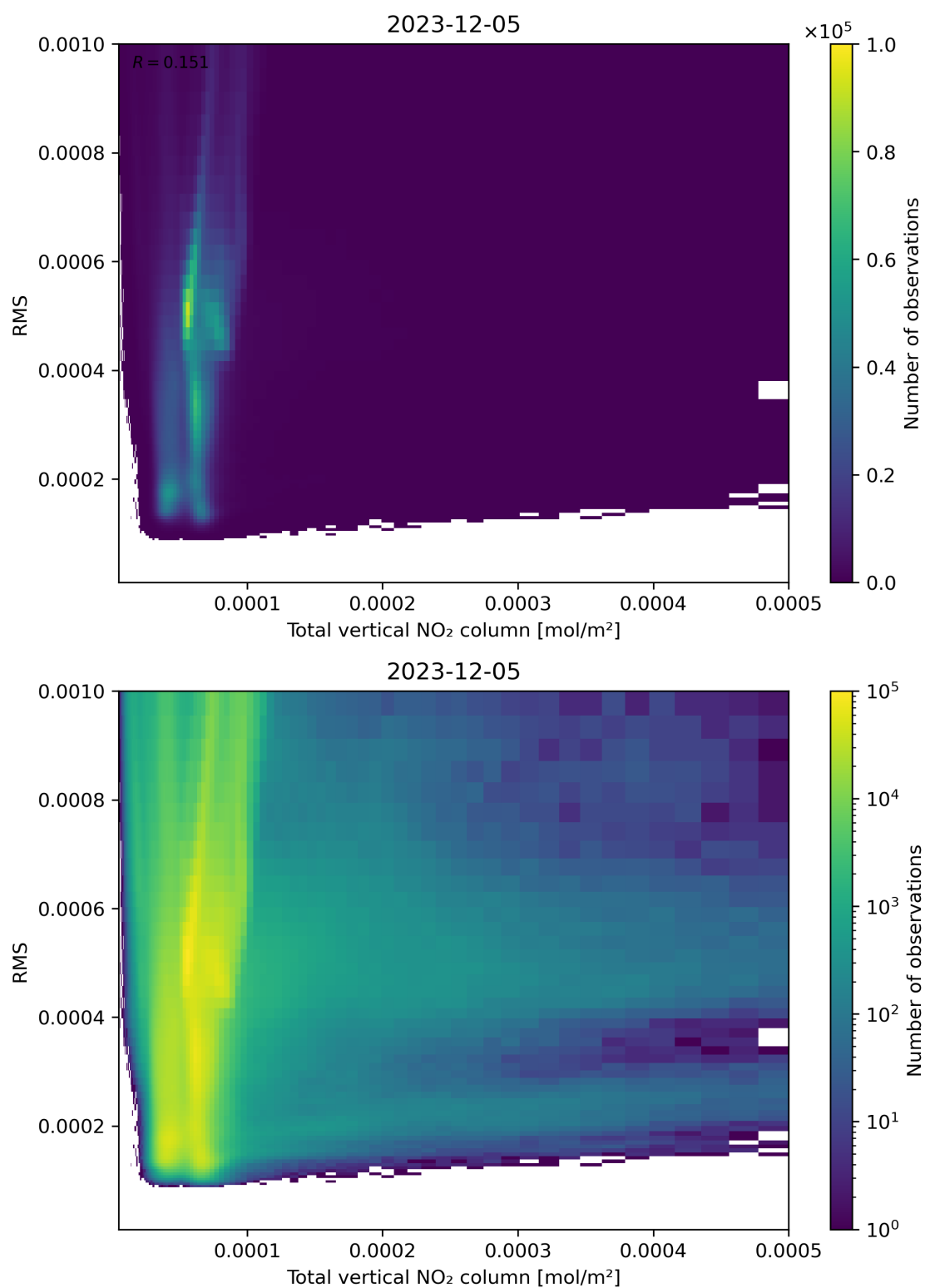
Figure 120: Scatter density plot of “Total vertical NO 2 column” against “RMS” for 2023-12-04 to 2023-12-06.
