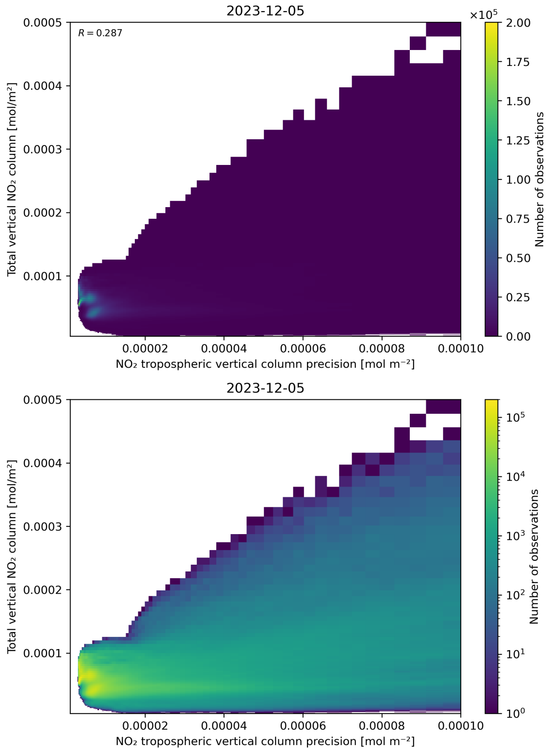
Figure 138: Scatter density plot of “NO 2 tropospheric vertical column precision” against “Total vertical NO 2 column” for 2023-12-04 to 2023-12-06.
