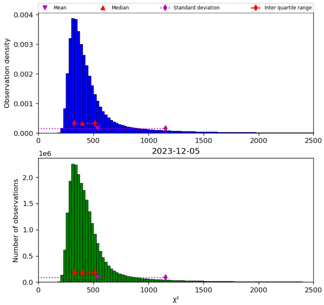
Figure 42: Histogram of “ \chi^2 ” for 2023-12-04 to 2023-12-06
