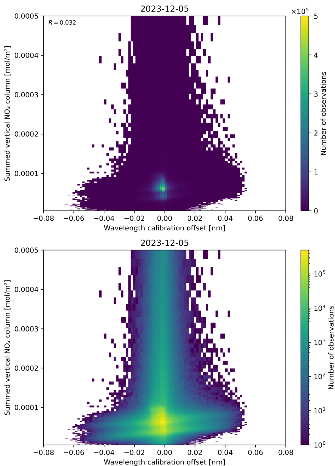
Figure 177: Scatter density plot of “Wavelength calibration offset” against “Summed vertical NO 2 column” for 2023-12-04 to 2023-12-06.
