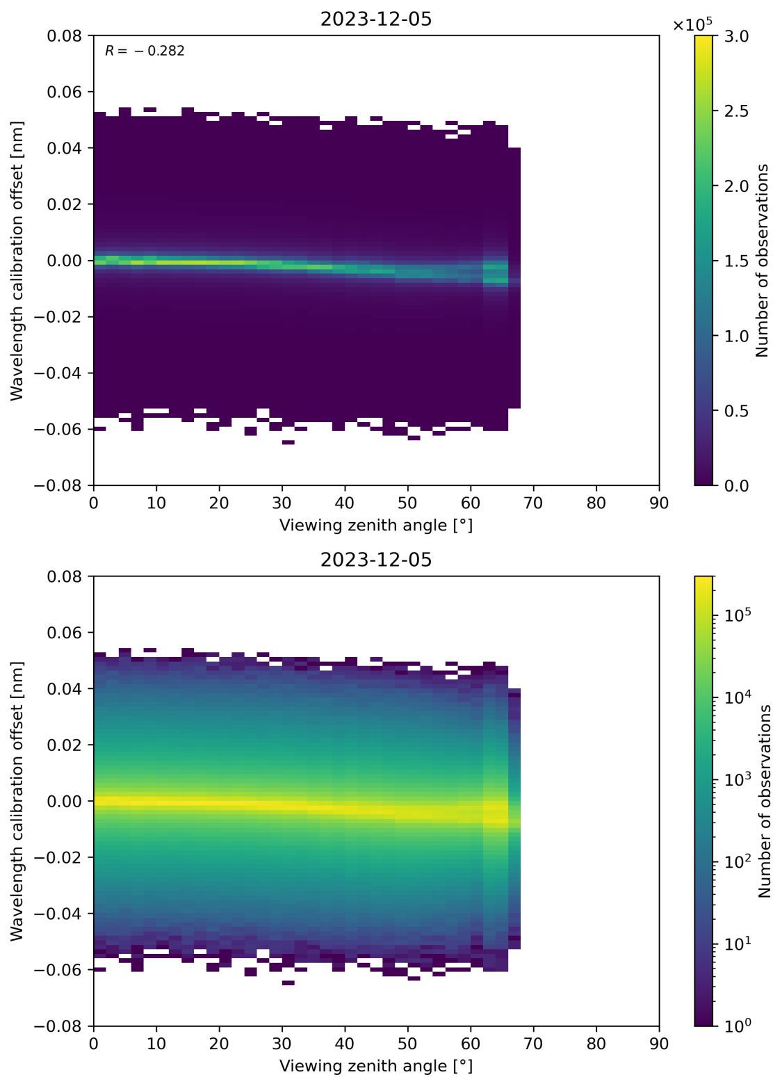
Figure 173: Scatter density plot of “Viewing zenith angle” against “Wavelength calibration offset” for 2023-12-04 to 2023-12-06.
