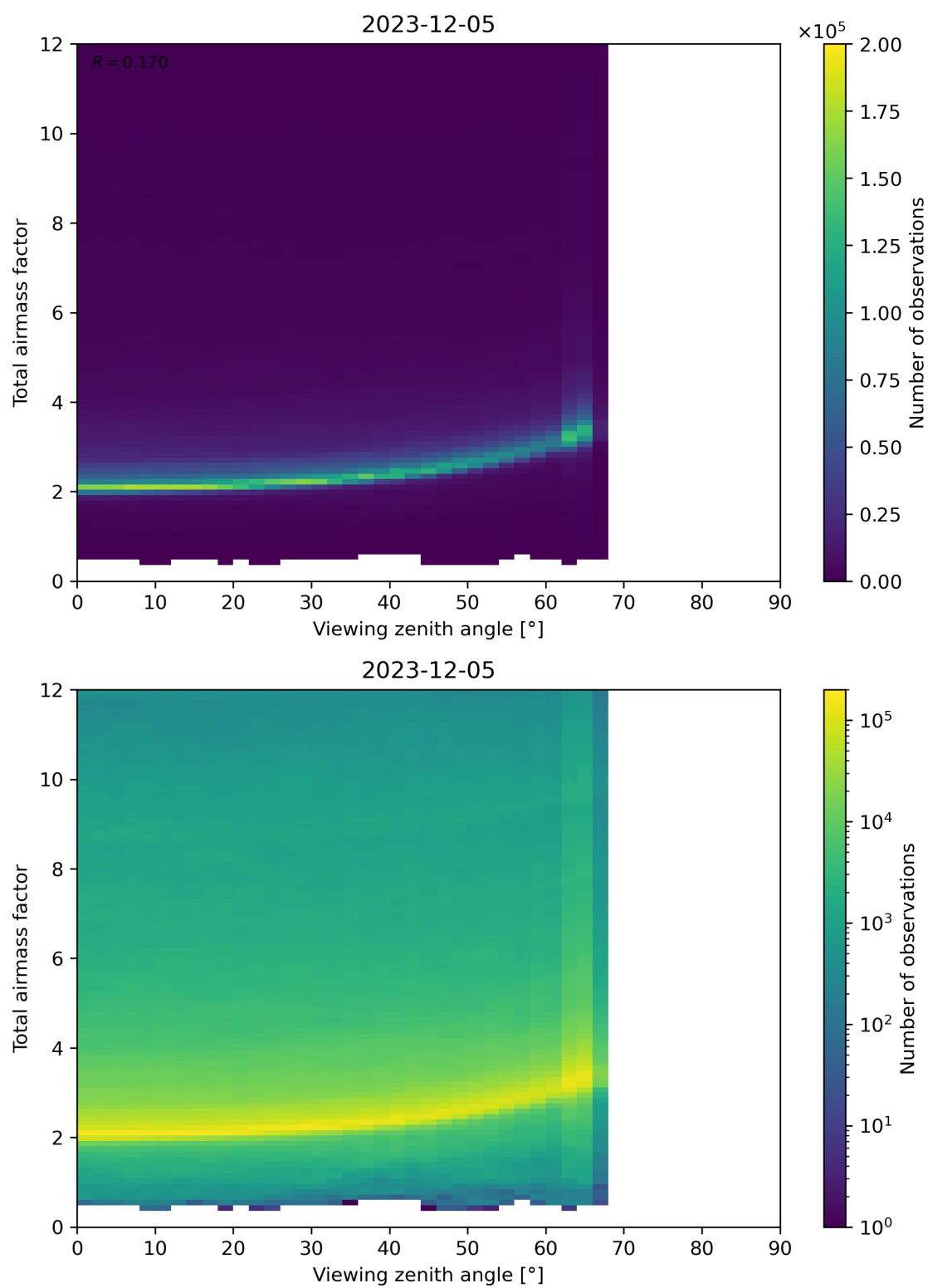
Figure 160: Scatter density plot of “Viewing zenith angle” against “Total airmass factor” for 2023-12-04 to 2023-12-06.
