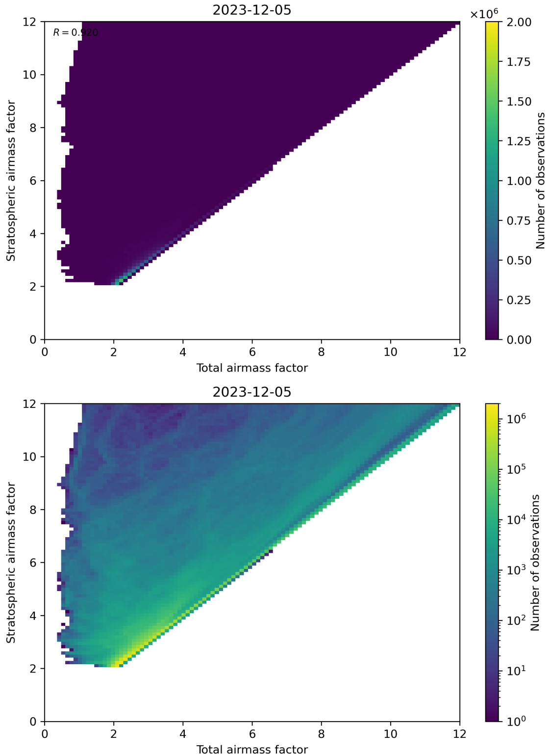
Figure 62: Scatter density plot of “Total airmass factor” against “Stratospheric airmass factor” for 2023-12-04 to 2023-12-06.
