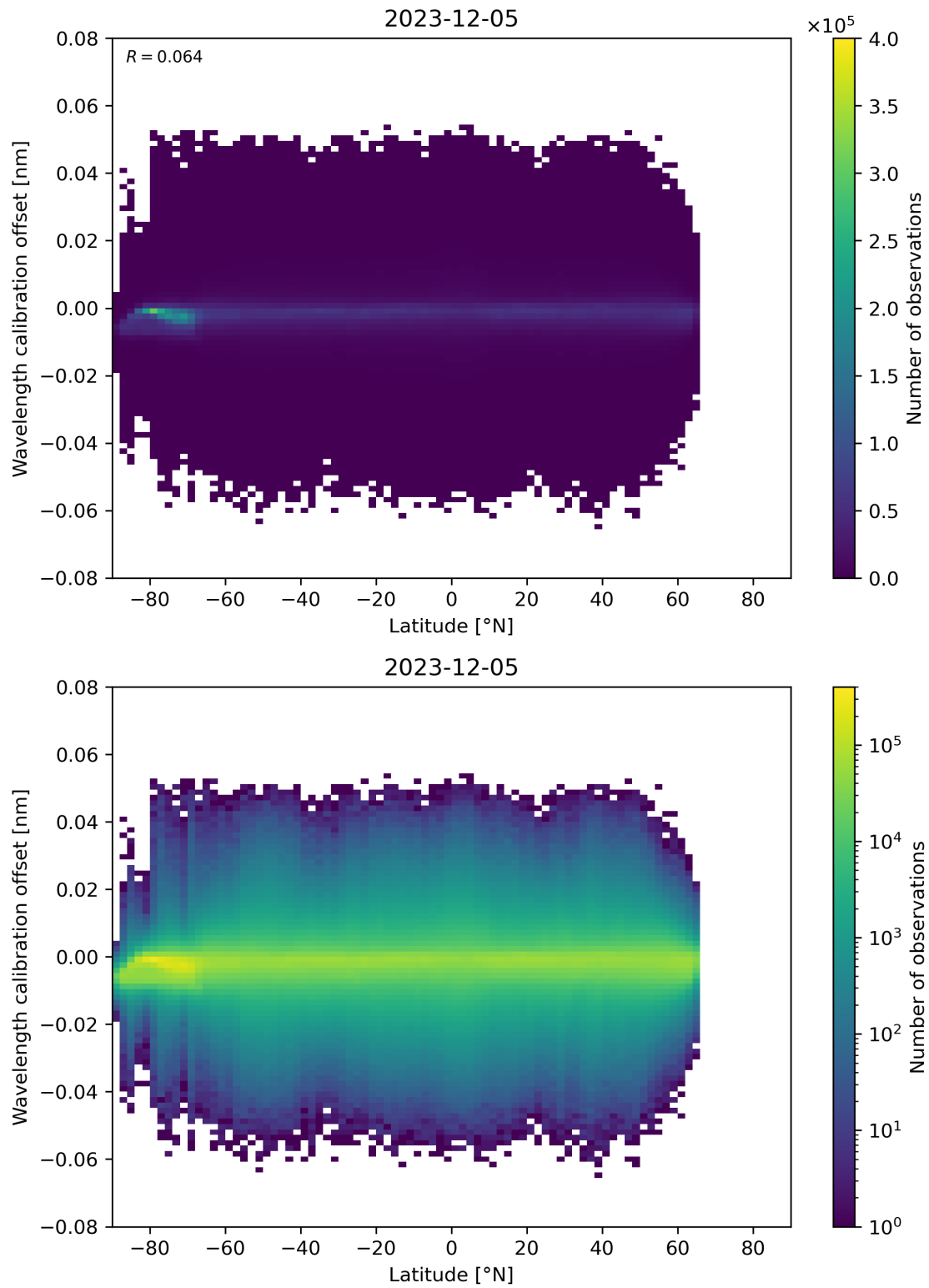
Figure 95: Scatter density plot of “Latitude” against “Wavelength calibration offset” for 2023-12-04 to 2023-12-06.
