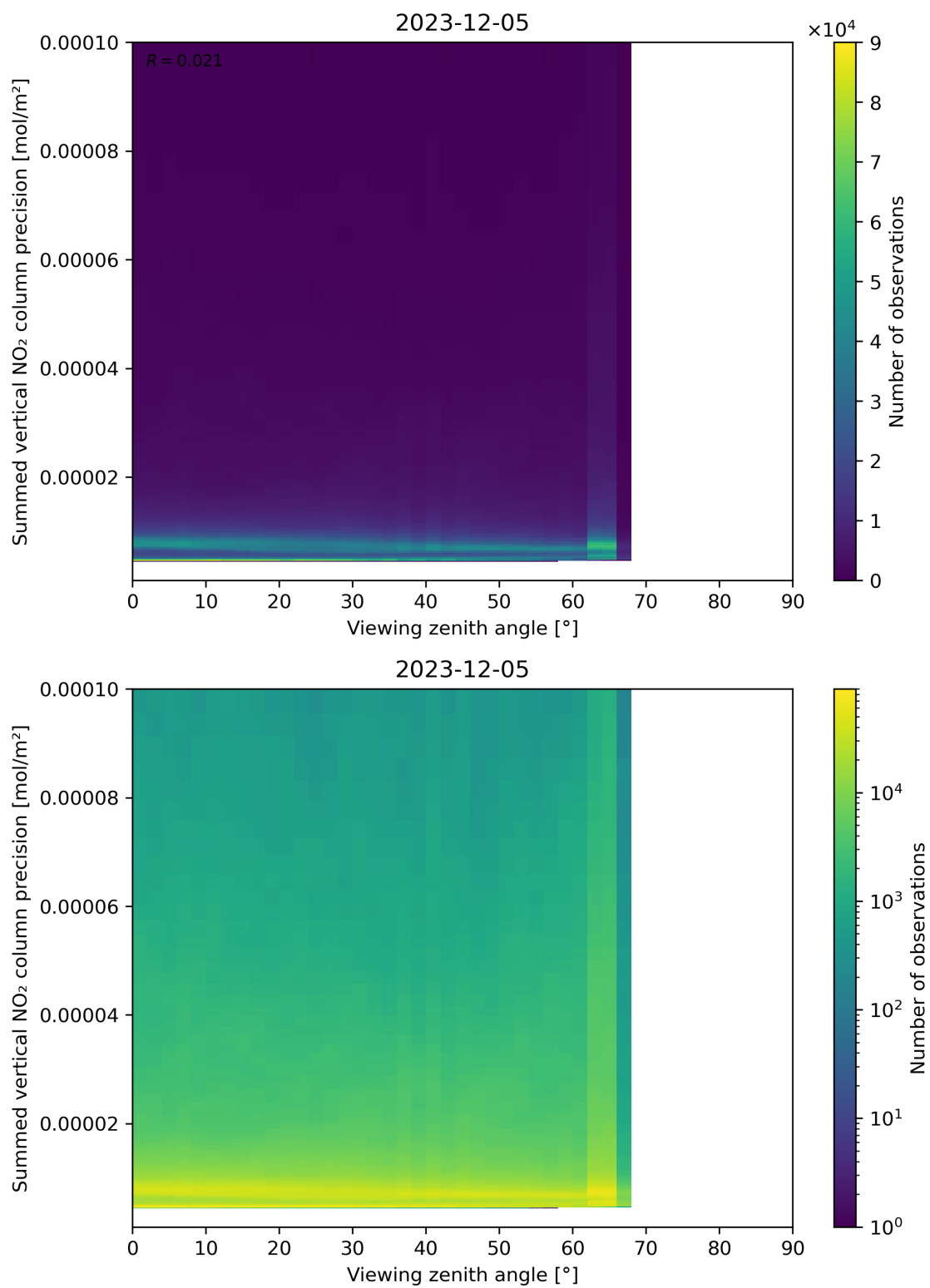
Figure 166: Scatter density plot of “Viewing zenith angle” against “Summed vertical NO 2 column precision” for 2023-12-04 to 2023-12-06.
