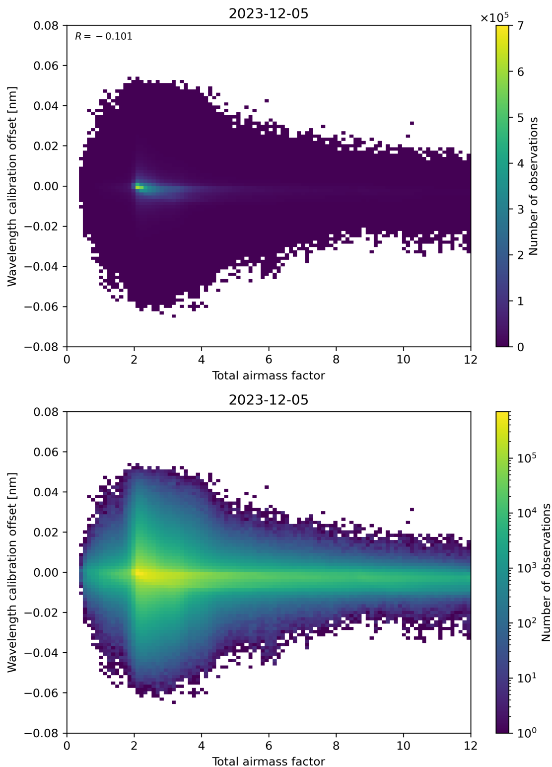
Figure 70: Scatter density plot of “Total airmass factor” against “Wavelength calibration offset” for 2023-12-04 to 2023-12-06.
