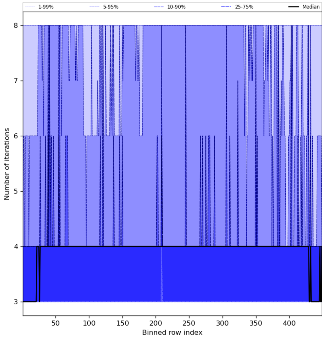
Figure 51: Along track statistics of “Number of iterations” for 2023-12-04 to 2023-12-06
