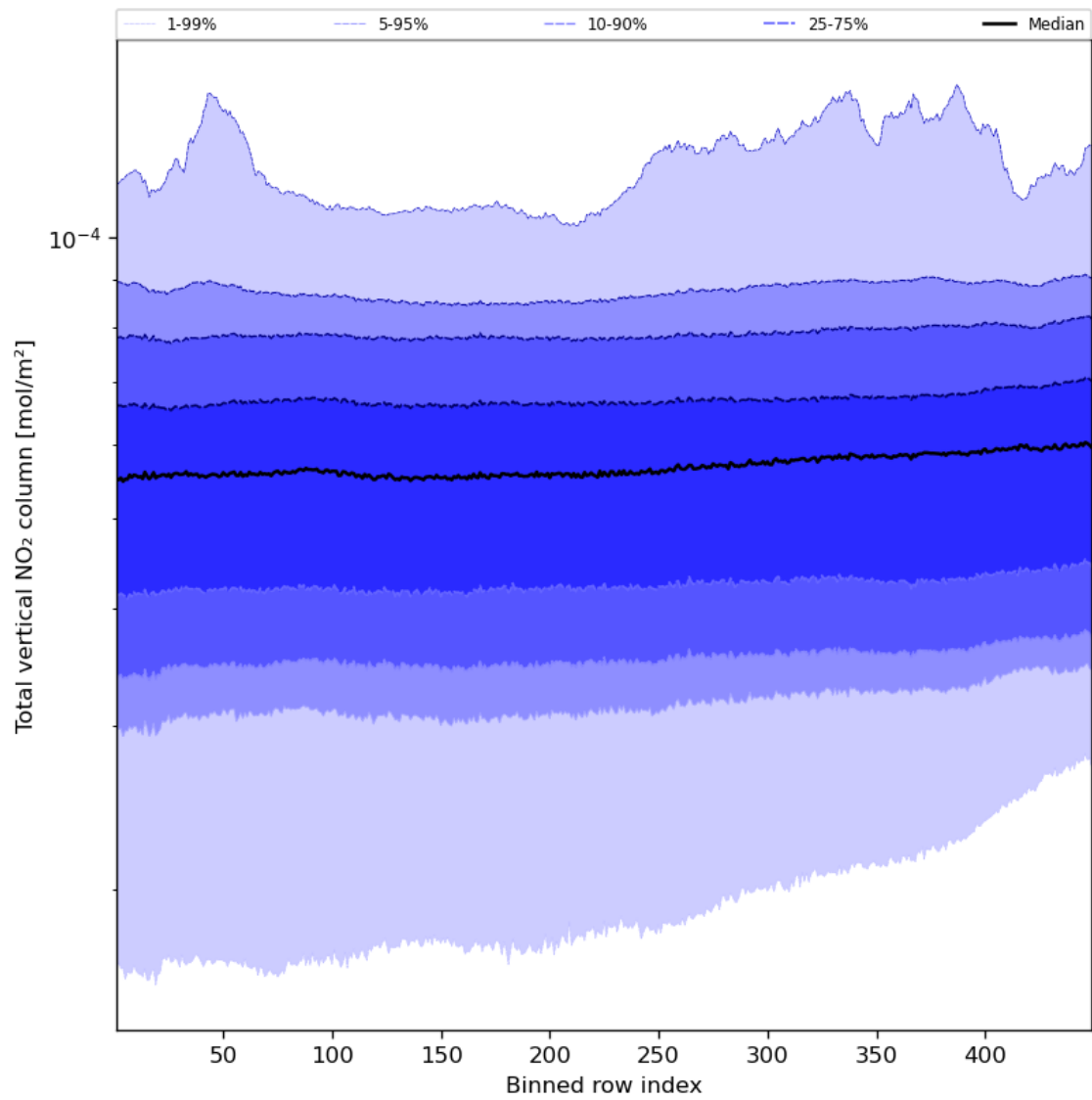
Figure 55: Along track statistics of “Total vertical NO 2 column” for 2023-12-04 to 2023-12-06
