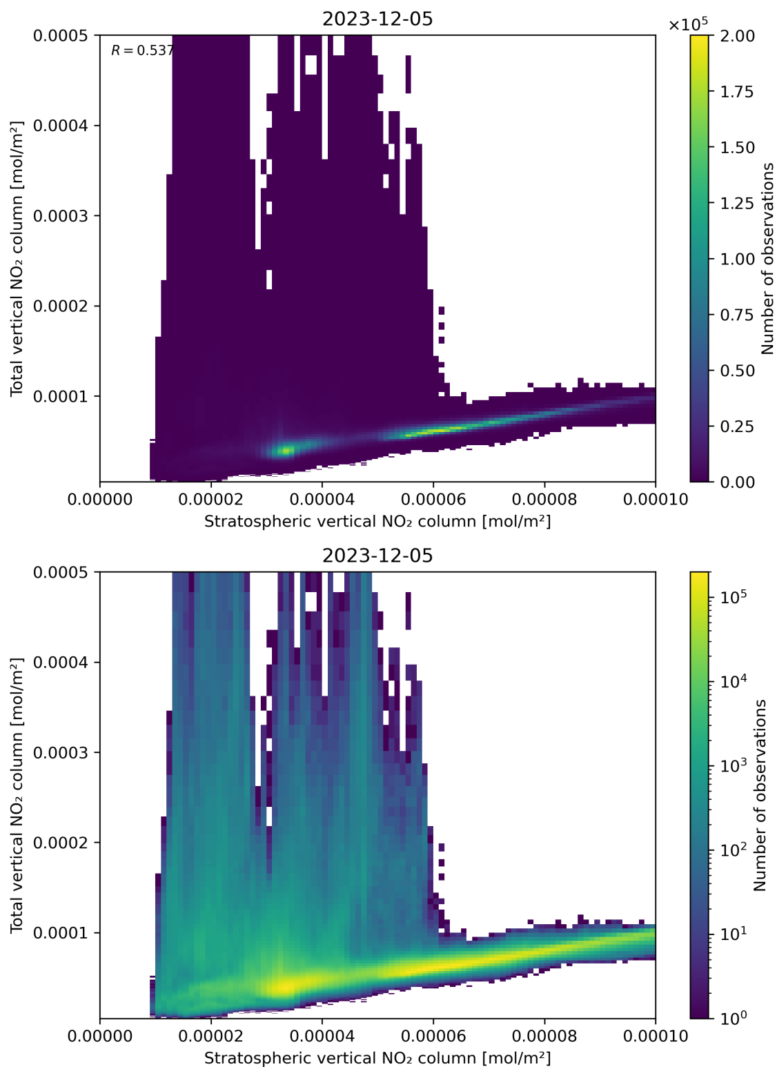
Figure 100: Scatter density plot of “Stratospheric vertical NO 2 column” against “Total vertical NO 2 column” for 2023-12-04 to 2023-12-06.
