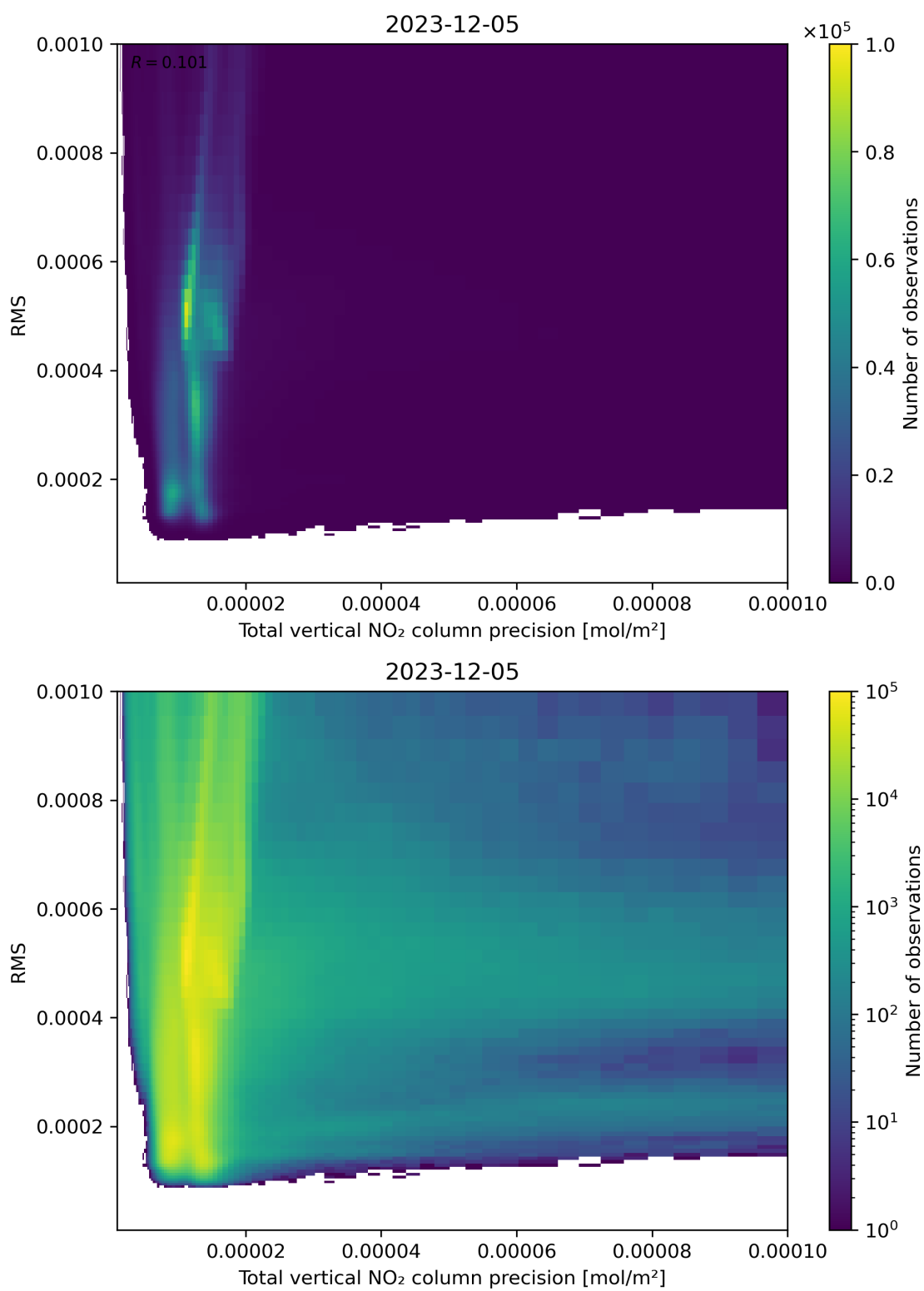
Figure 119: Scatter density plot of “Total vertical NO 2 column precision” against “RMS” for 2023-12-04 to 2023-12-06.
