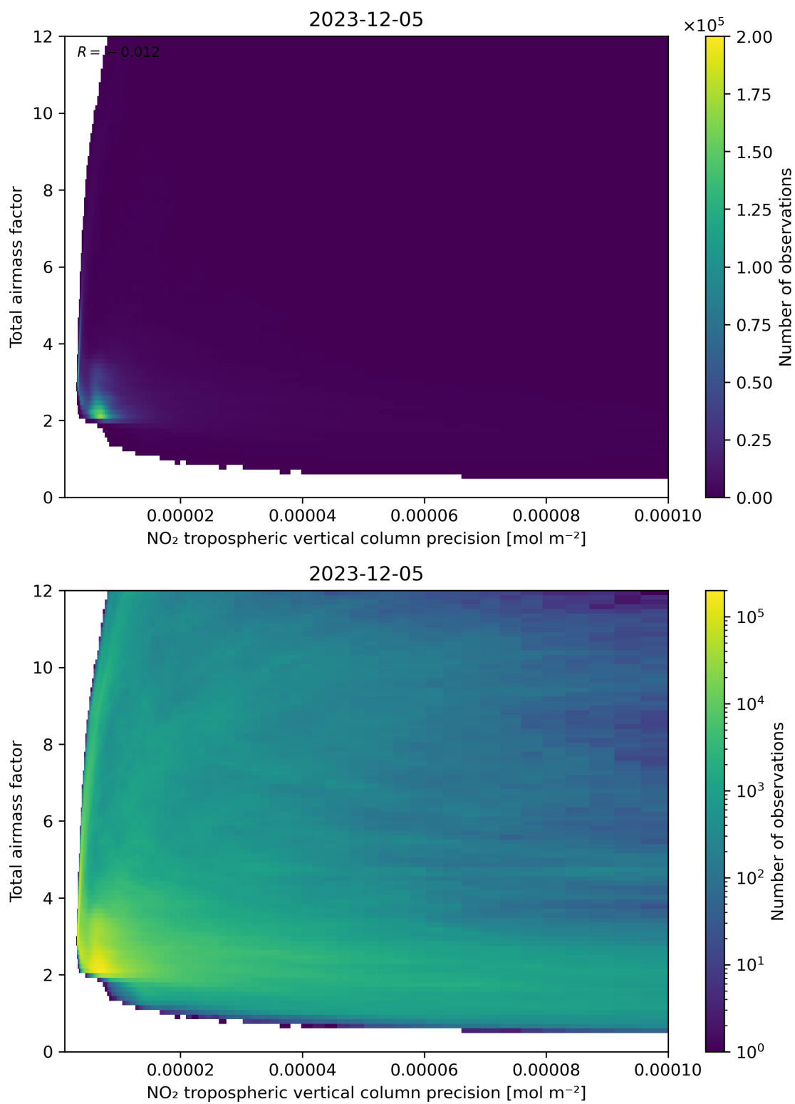
Figure 132: Scatter density plot of “NO 2 tropospheric vertical column precision” against “Total air mass factor” for 2023-12-04 to 2023-12-06.
