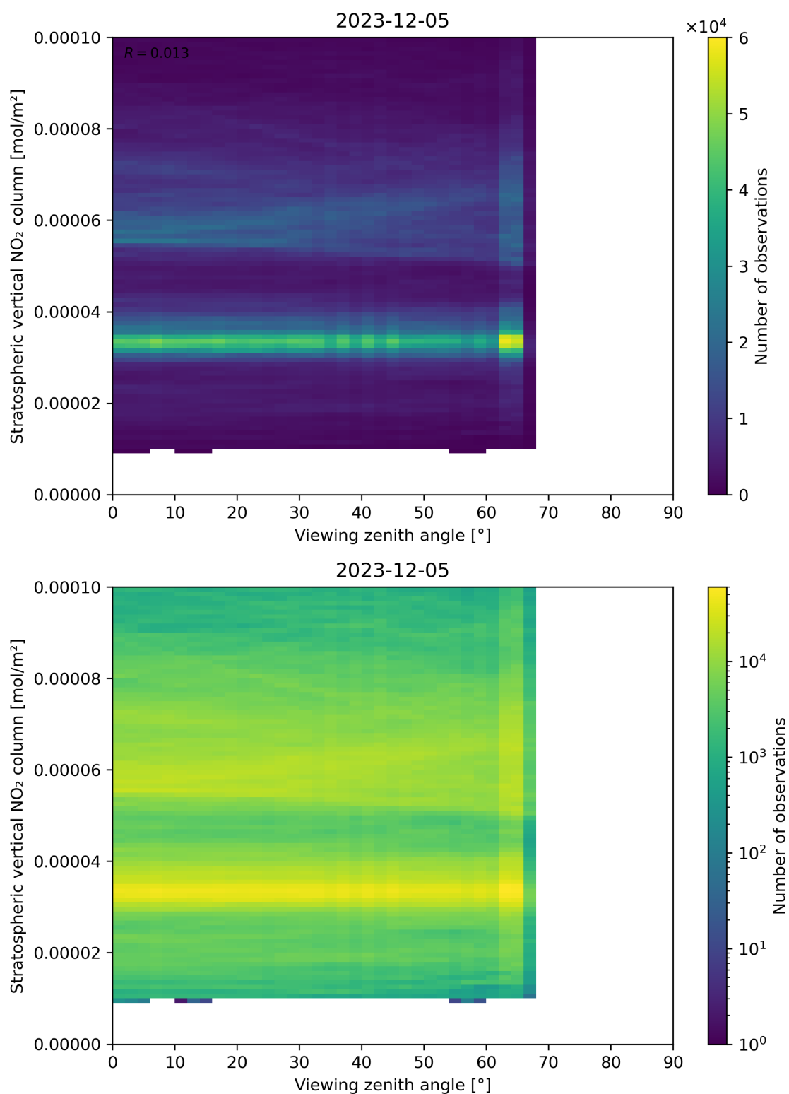
Figure 164: Scatter density plot of “Viewing zenith angle” against “Stratospheric vertical NO 2 column” for 2023-12-04 to 2023-12-06.
