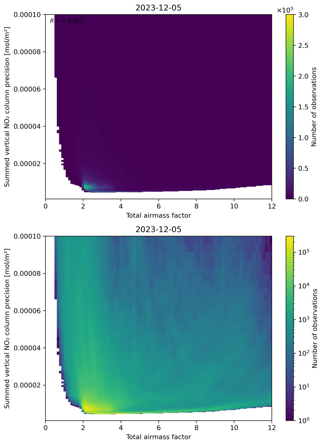
Figure 66: Scatter density plot of “Total airmass factor” against “Summed vertical NO 2 column precision” for 2023-12-04 to 2023-12-06.
