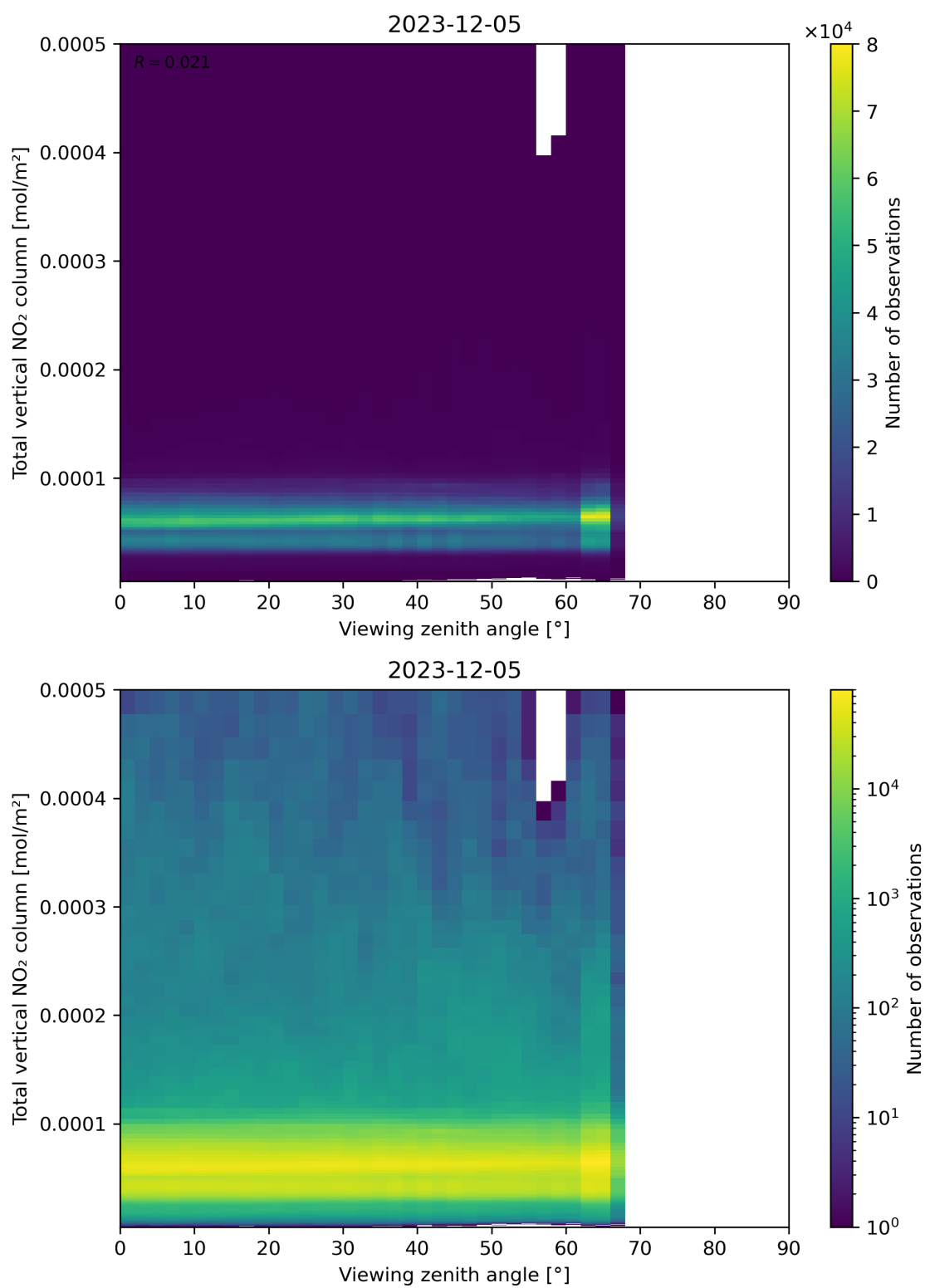
Figure 167: Scatter density plot of “Viewing zenith angle” against “Total vertical NO 2 column” for 2023-12-04 to 2023-12-06.
