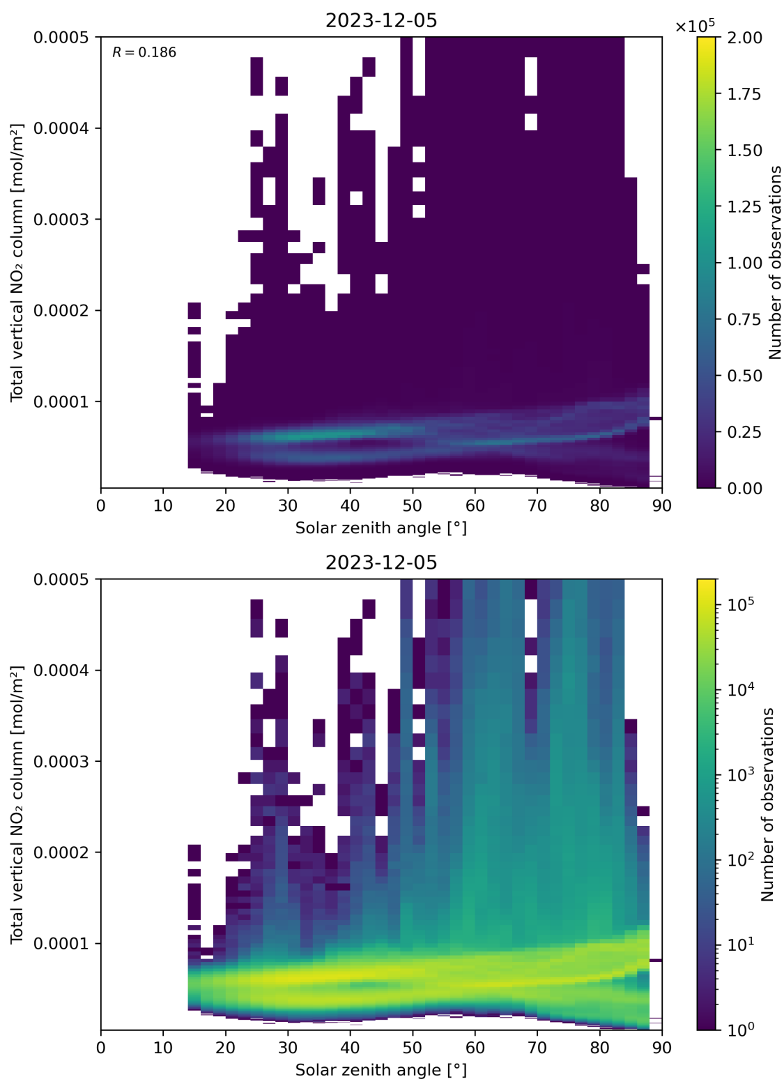
Figure 153: Scatter density plot of “Solar zenith angle” against “Total vertical NO 2 column” for 2023-12-04 to 2023-12-06.
