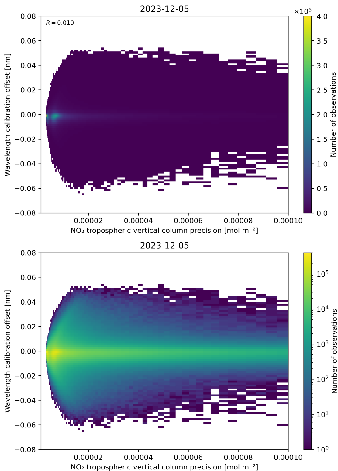
Figure 141: Scatter density plot of “NO 2 tropospheric vertical column precision” against “Wavelength calibration offset” for 2023-12-04 to 2023-12-06.
