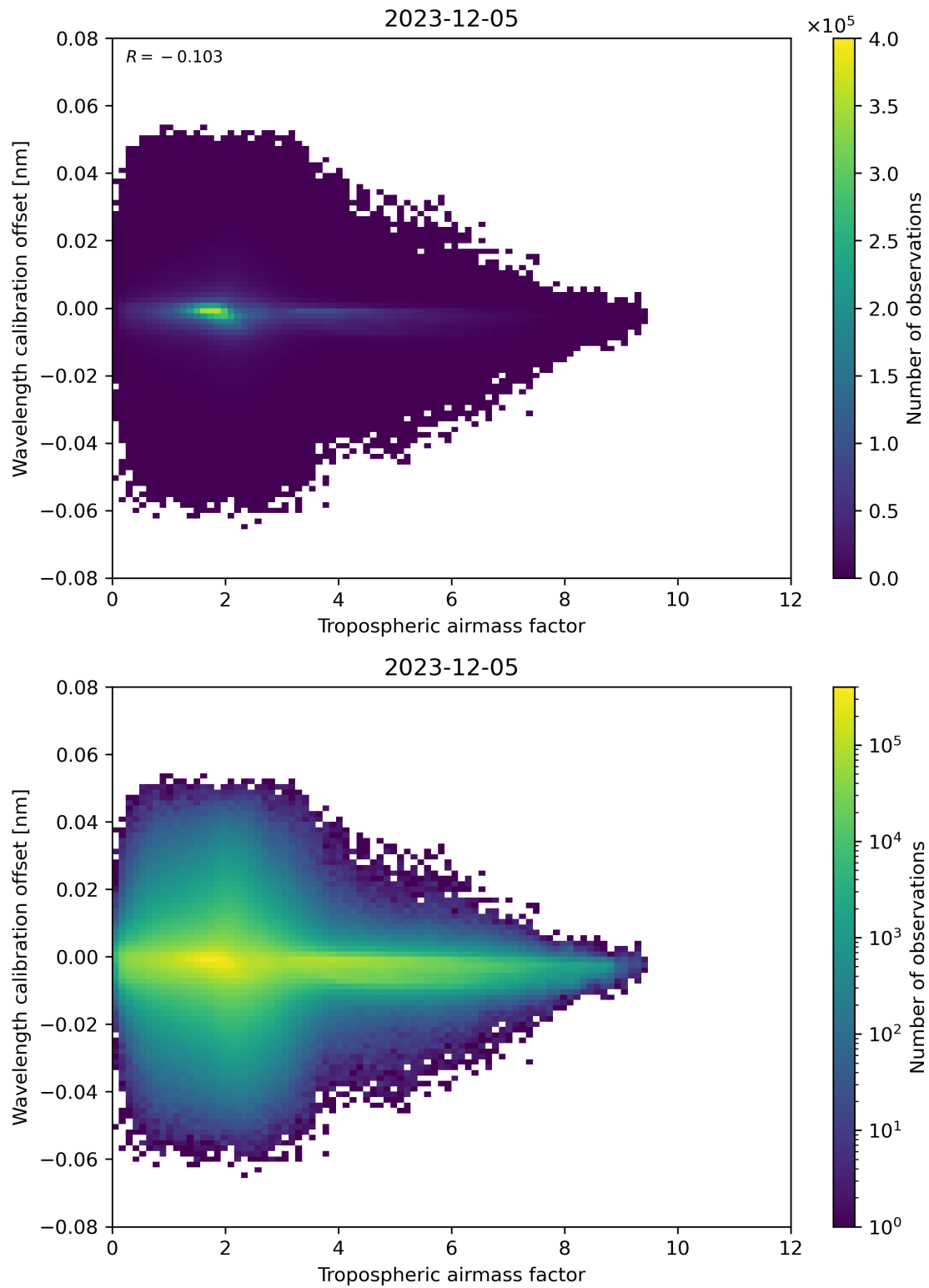
Figure 80: Scatter density plot of “Tropospheric airmass factor” against “Wavelength calibration offset” for 2023-12-04 to 2023-12-06.
