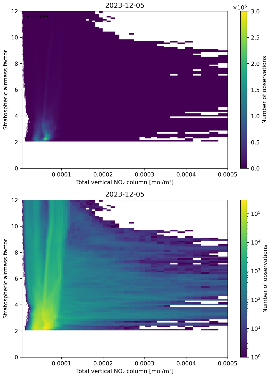
Figure 110: Scatter density plot of “Total vertical NO 2 column” against “Stratospheric air mass factor” for 2023-12-04 to 2023-12-06.
