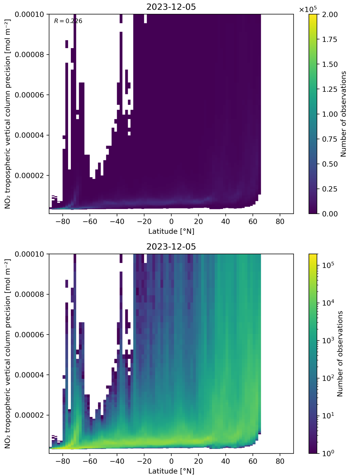
Figure 93: Scatter density plot of “Latitude” against “NO 2 tropospheric vertical column precision” for 2023-12-04 to 2023-12-06.
