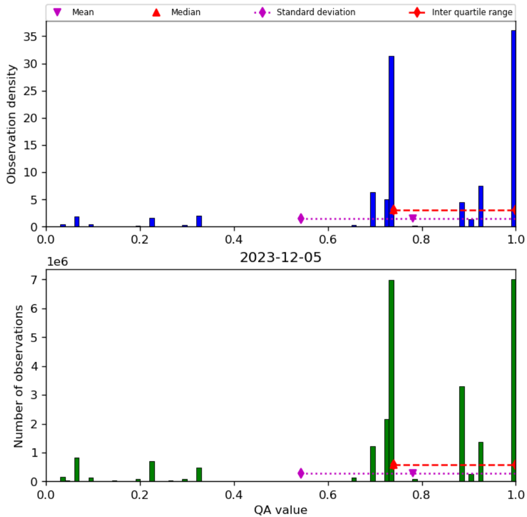
Figure 28: Histogram of “QA value” for 2023-12-04 to 2023-12-06
