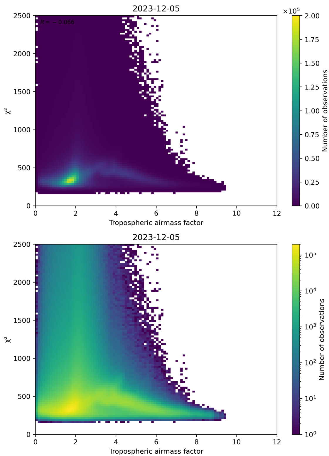
Figure 73: Scatter density plot of “Tropospheric airmass factor” against “ \chi^2 ” for 2023-12-04 to 2023-12-06.
