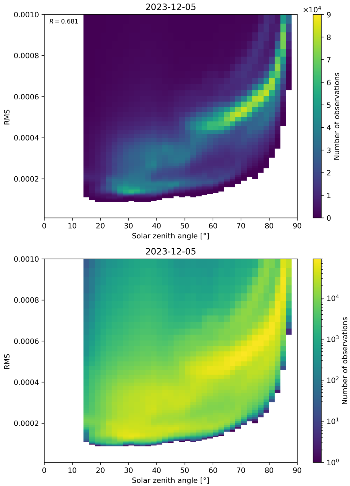
Figure 157: Scatter density plot of “Solar zenith angle” against “RMS” for 2023-12-04 to 2023-12-06.
