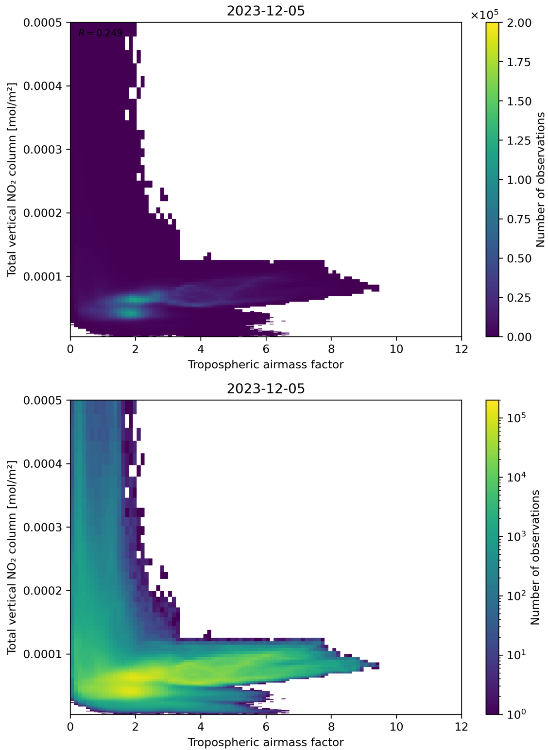
Figure 77: Scatter density plot of “Tropospheric airmass factor” against “Total vertical NO 2 column” for 2023-12-04 to 2023-12-06.
