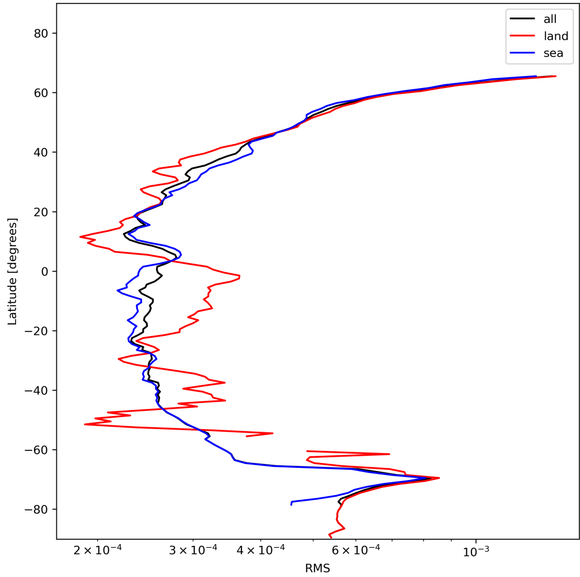
Figure 26: Zonal average of “RMS” for 2023-12-04 to 2023-12-06.
