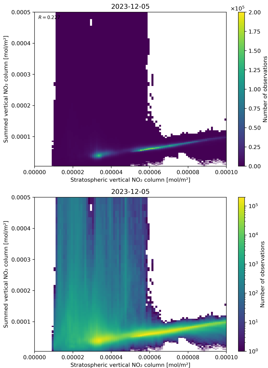
Figure 98: Scatter density plot of “Stratospheric vertical NO 2 column” against “Summed vertical NO 2 column” for 2023-12-04 to 2023-12-06.
