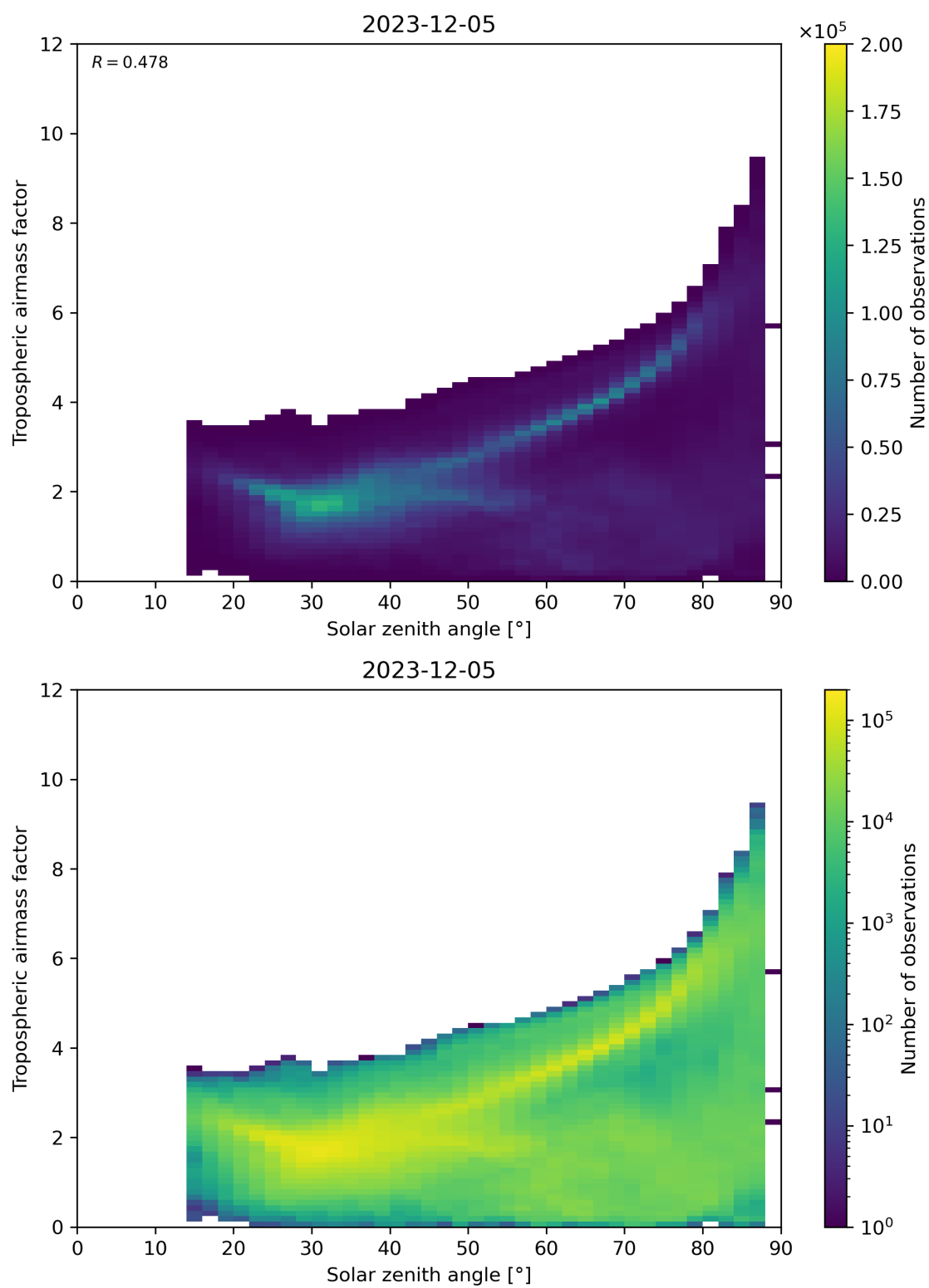
Figure 147: Scatter density plot of “Solar zenith angle” against “Tropospheric airmass factor” for 2023-12-04 to 2023-12-06.
