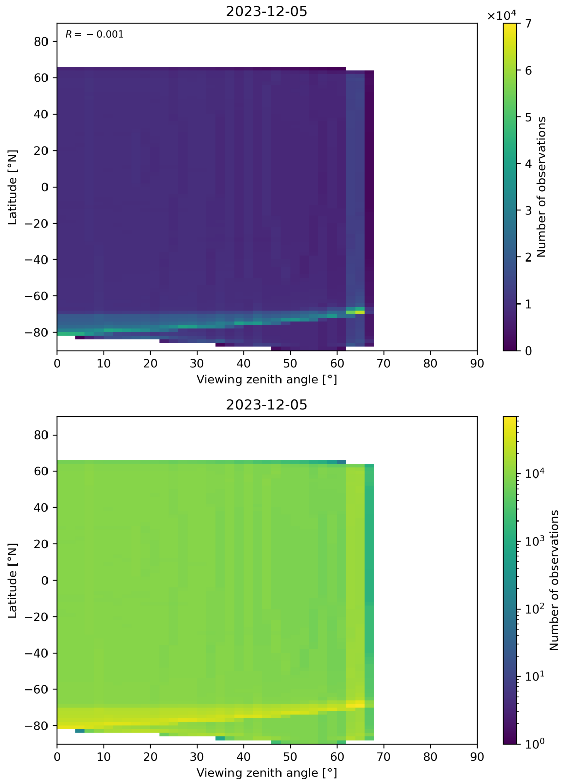
Figure 163: Scatter density plot of “Viewing zenith angle” against “Latitude” for 2023-12-04 to 2023-12-06.
