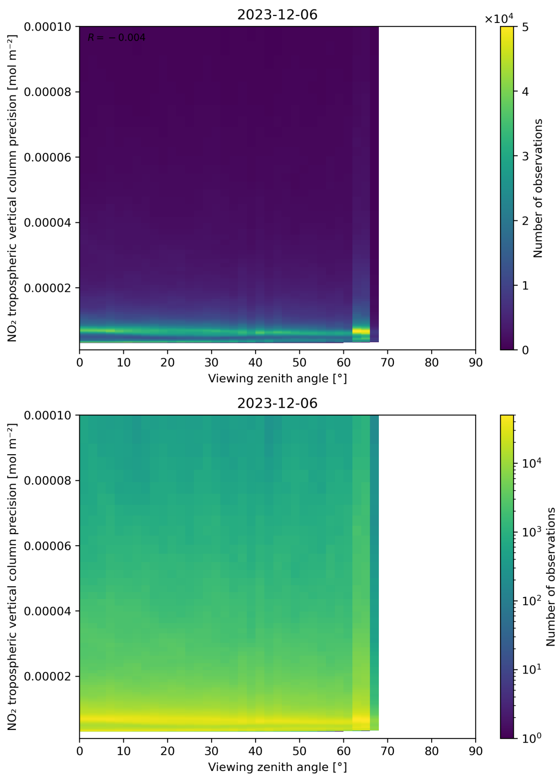
Figure 170: Scatter density plot of “Viewing zenith angle” against “NO 2 tropospheric vertical column precision” for 2023-12-05 to 2023-12-07.
