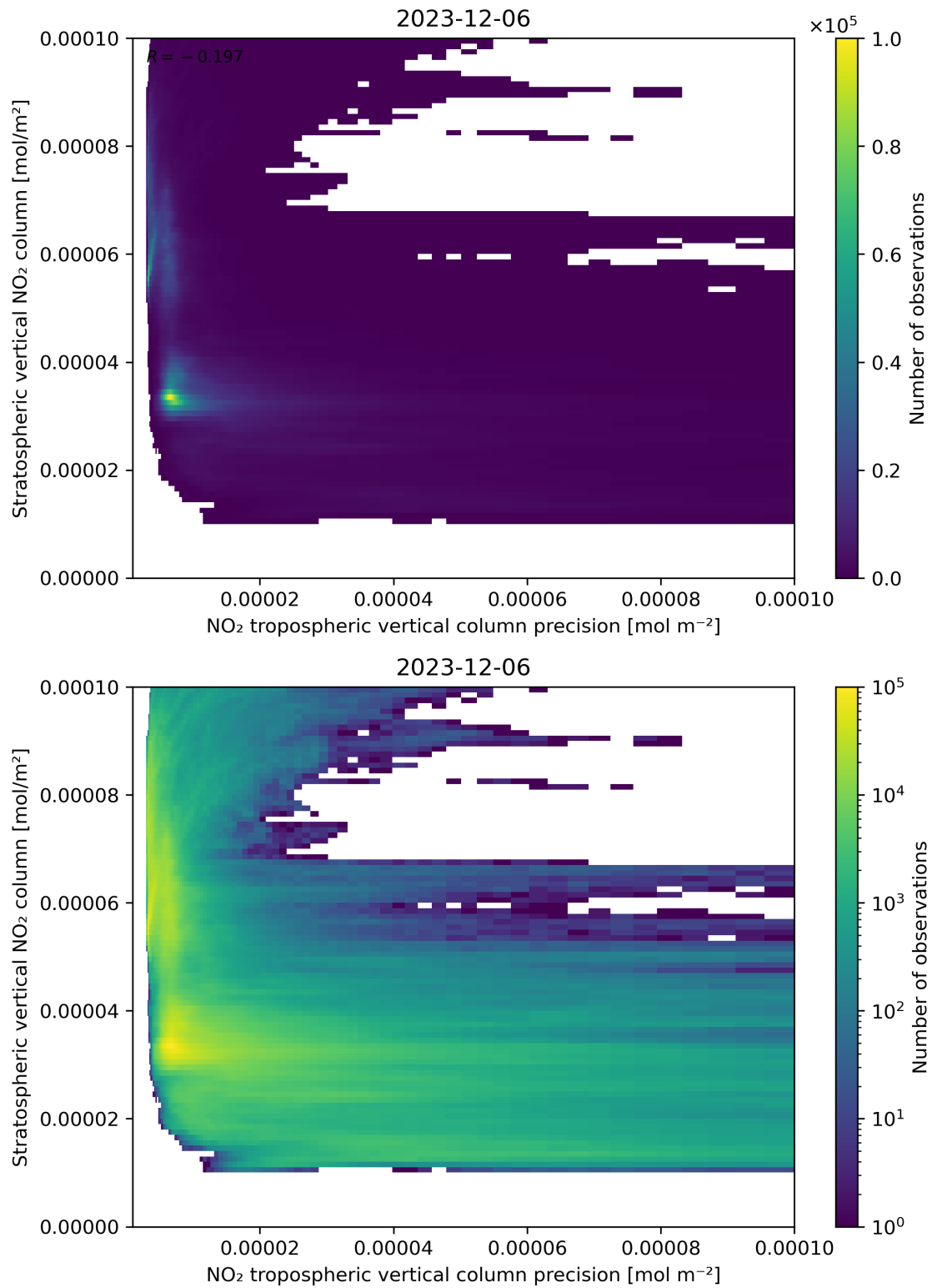
Figure 135: Scatter density plot of “NO 2 tropospheric vertical column precision” against “Stratospheric vertical NO 2 column” for 2023-12-05 to 2023-12-07.
