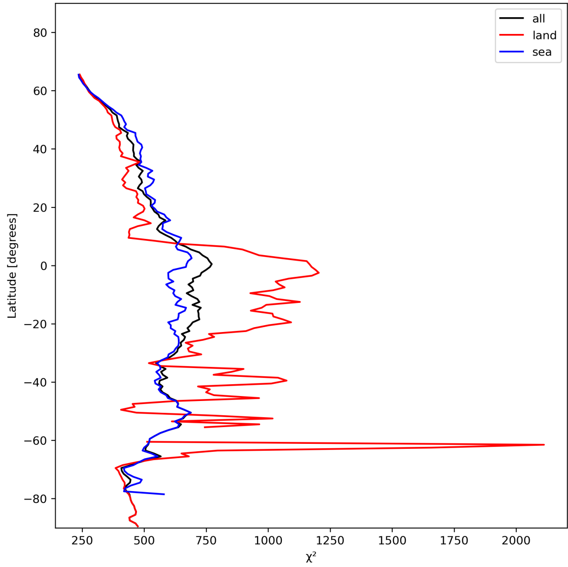
Figure 25: Zonal average of “ \chi^2 ” for 2023-12-05 to 2023-12-07.
