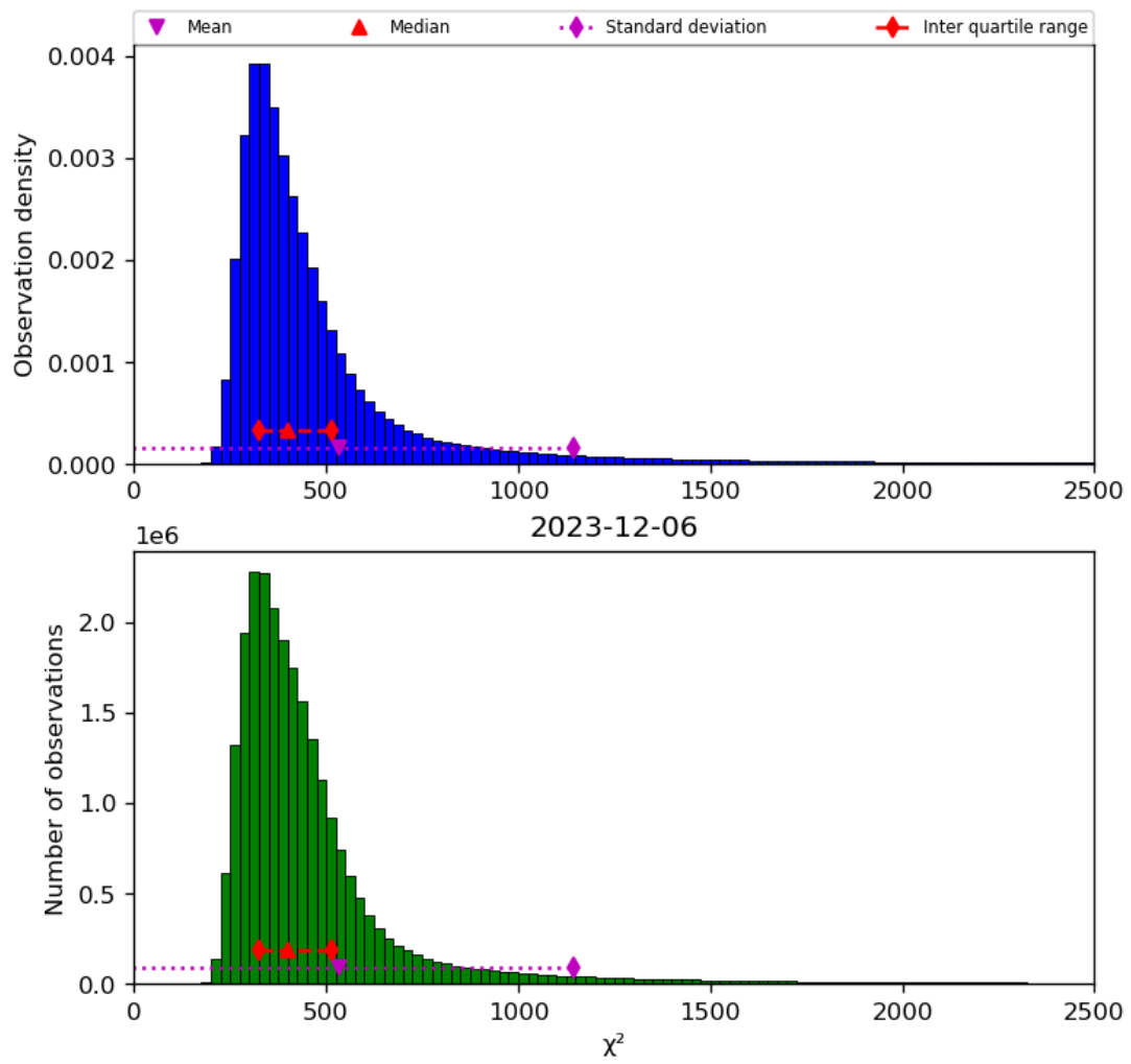
Figure 42: Histogram of “ \chi^2 ” for 2023-12-05 to 2023-12-07
