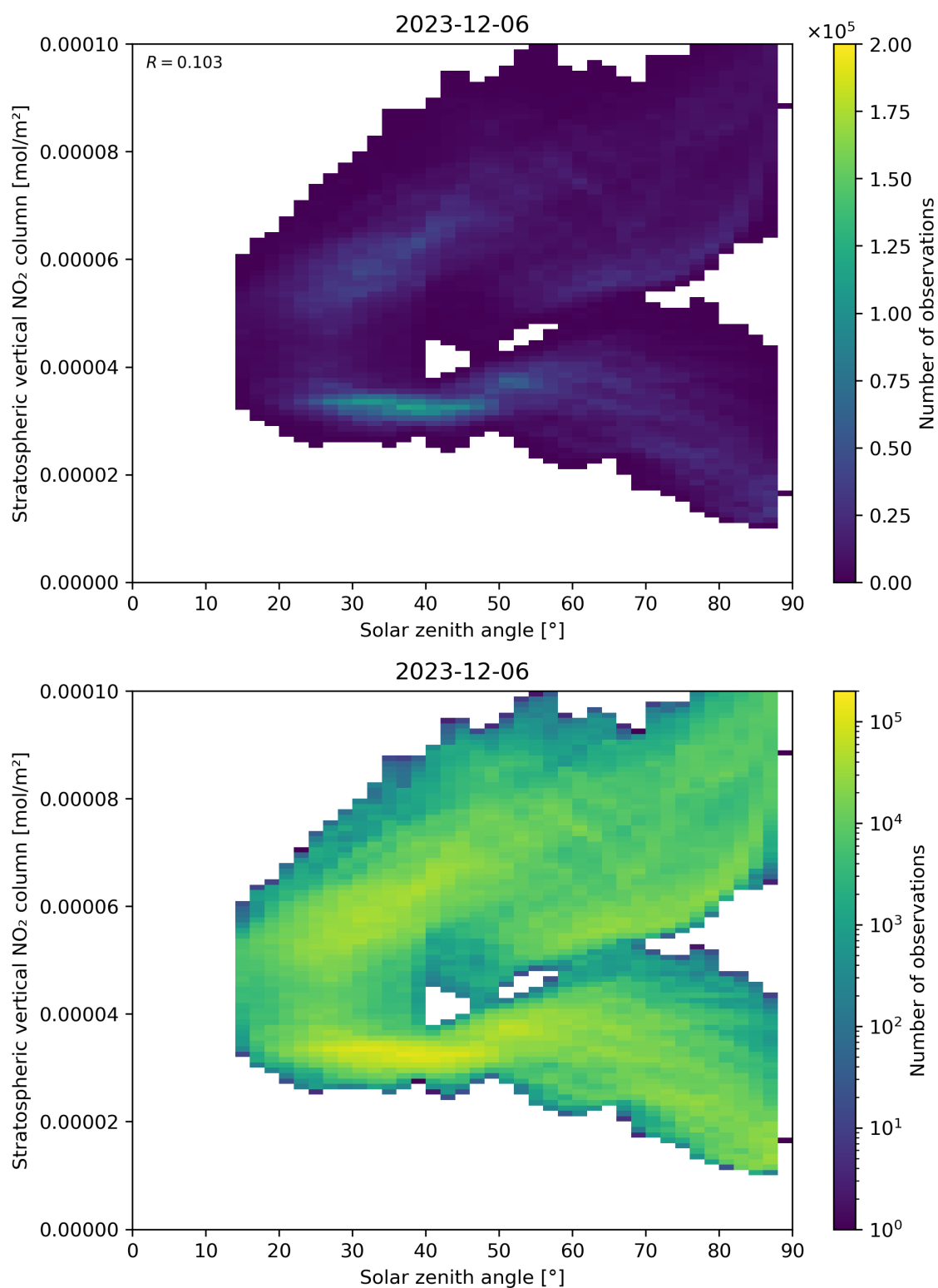
Figure 150: Scatter density plot of “Solar zenith angle” against “Stratospheric vertical NO 2 column” for 2023-12-05 to 2023-12-07.
