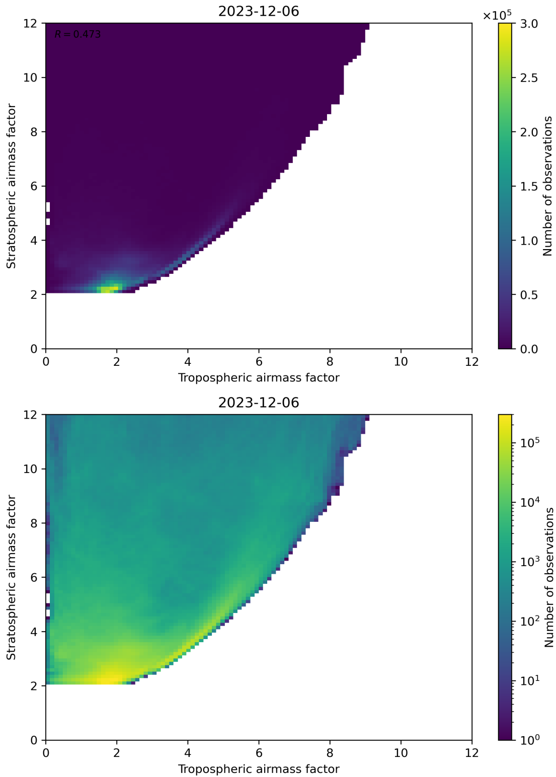
Figure 71: Scatter density plot of “Tropospheric airmass factor” against “Stratospheric airmass factor” for 2023-12-05 to 2023-12-07.
