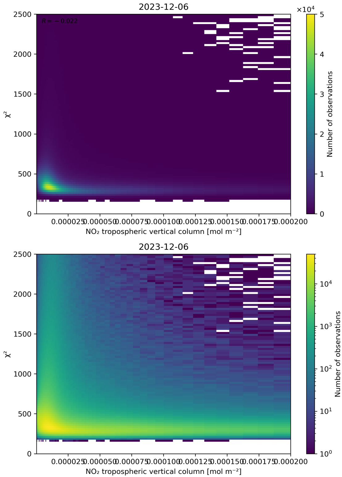
Figure 124: Scatter density plot of “NO 2 tropospheric vertical column” against “ \chi^2 ” for 2023-12-05 to 2023-12-07.
