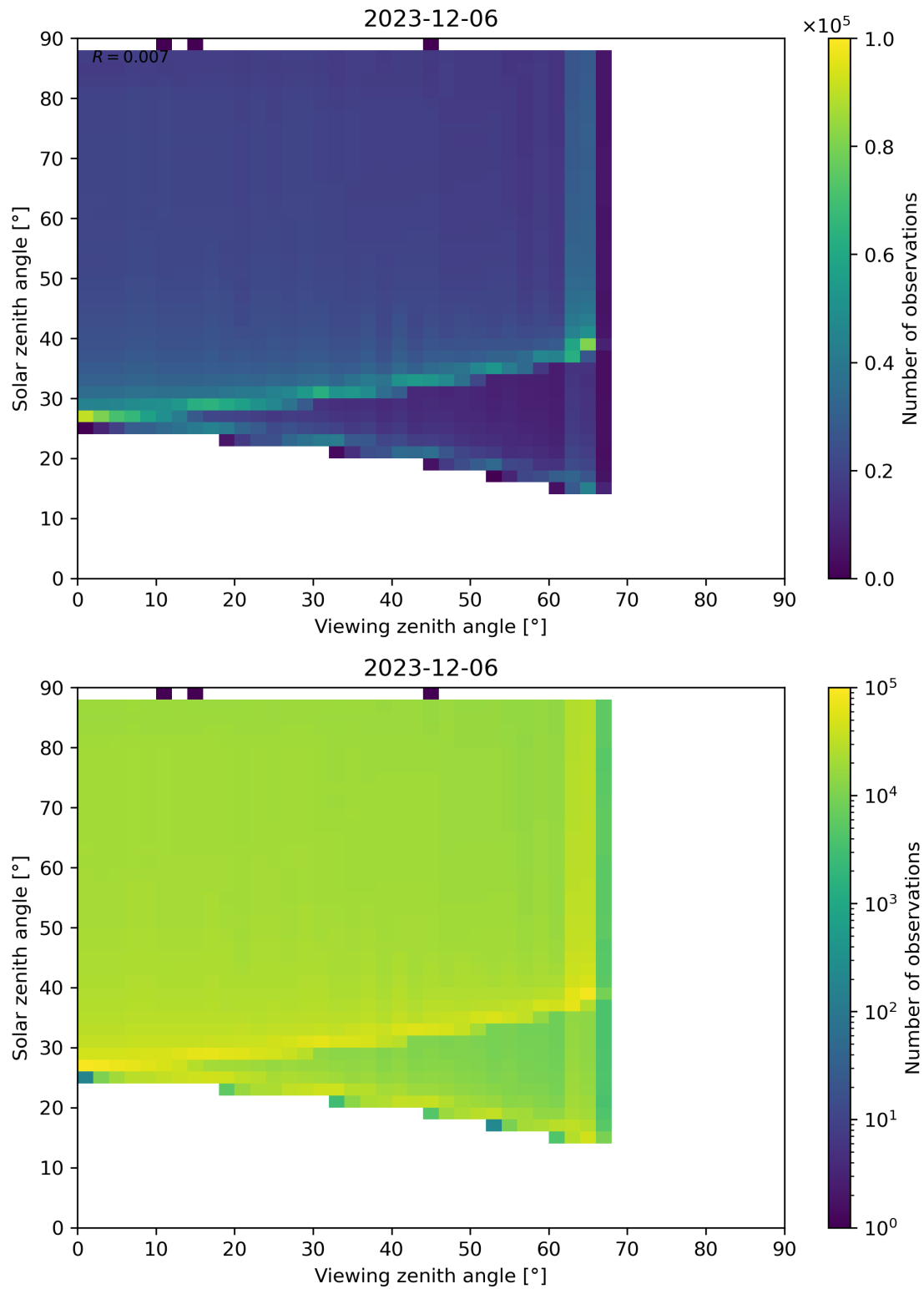
Figure 172: Scatter density plot of “Viewing zenith angle” against “Solar zenith angle” for 2023-12-05 to 2023-12-07.
