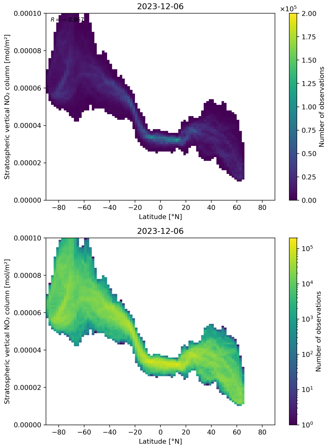
Figure 87: Scatter density plot of “Latitude” against “Stratospheric vertical NO 2 column” for 2023-12-05 to 2023-12-07.
