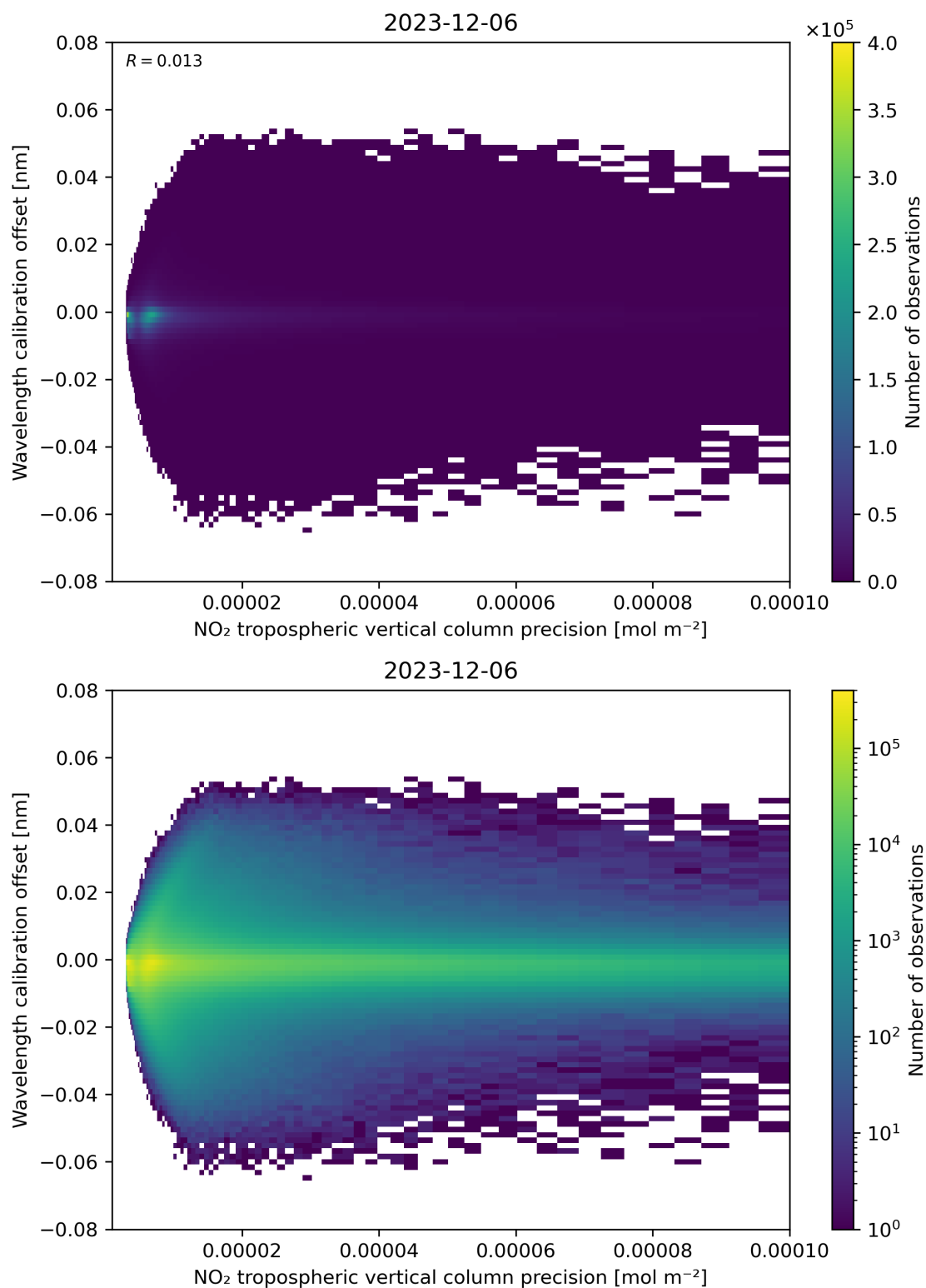
Figure 141: Scatter density plot of “NO 2 tropospheric vertical column precision” against “Wavelength calibration offset” for 2023-12-05 to 2023-12-07.
