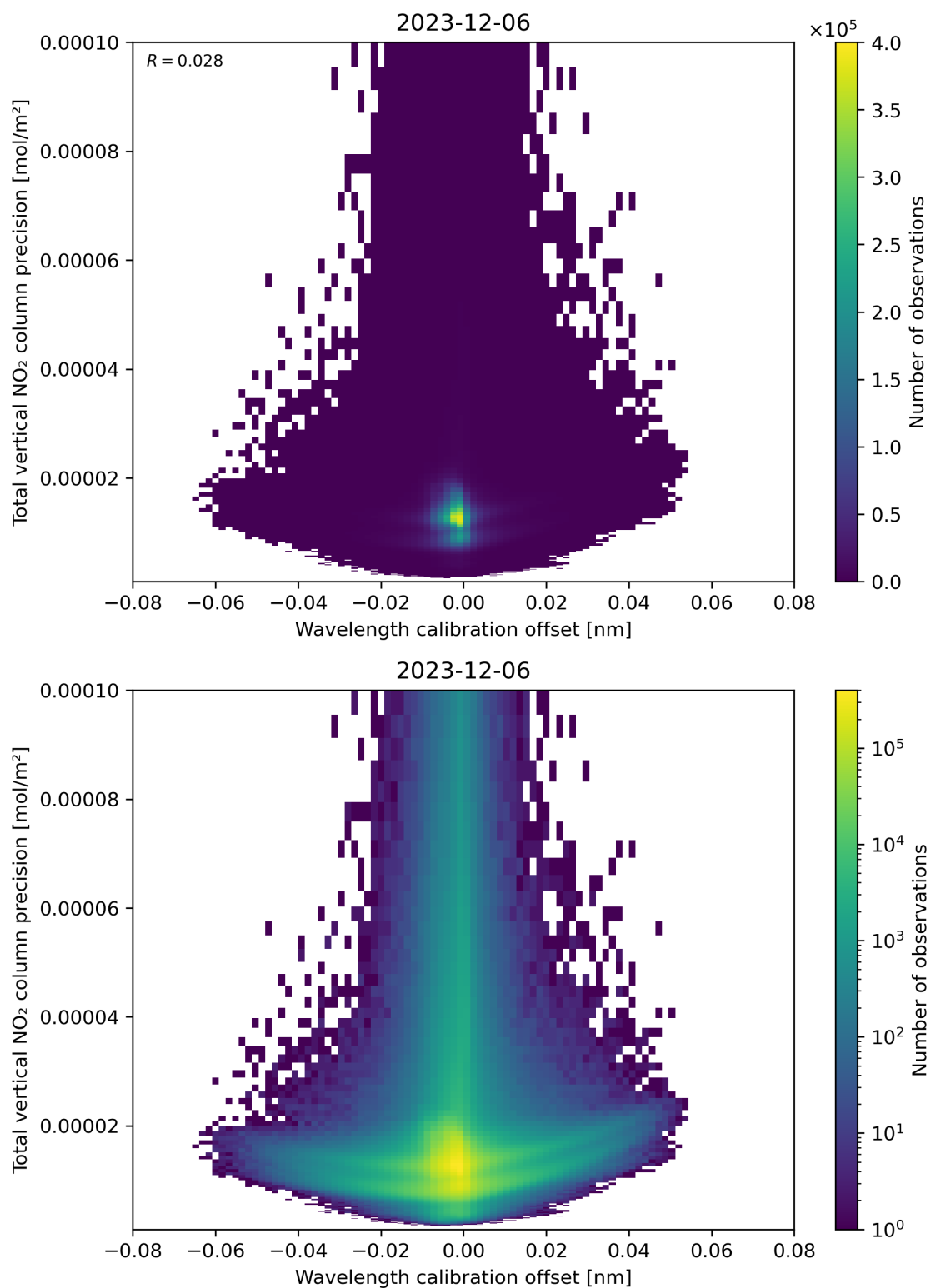
Figure 180: Scatter density plot of “Wavelength calibration offset” against “Total vertical NO 2 column precision” for 2023-12-05 to 2023-12-07.
