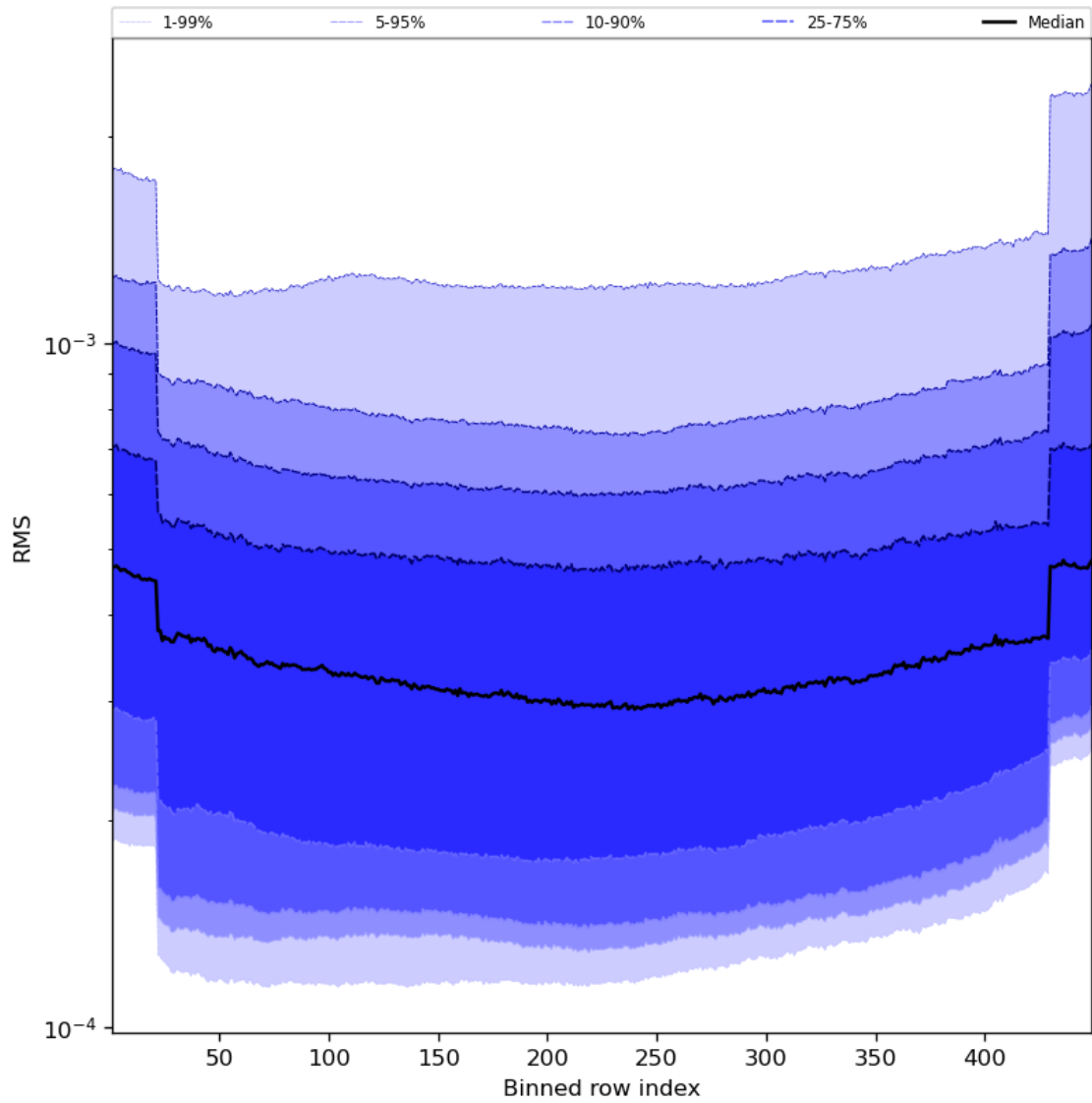
Figure 60: Along track statistics of “RMS” for 2023-12-05 to 2023-12-07
