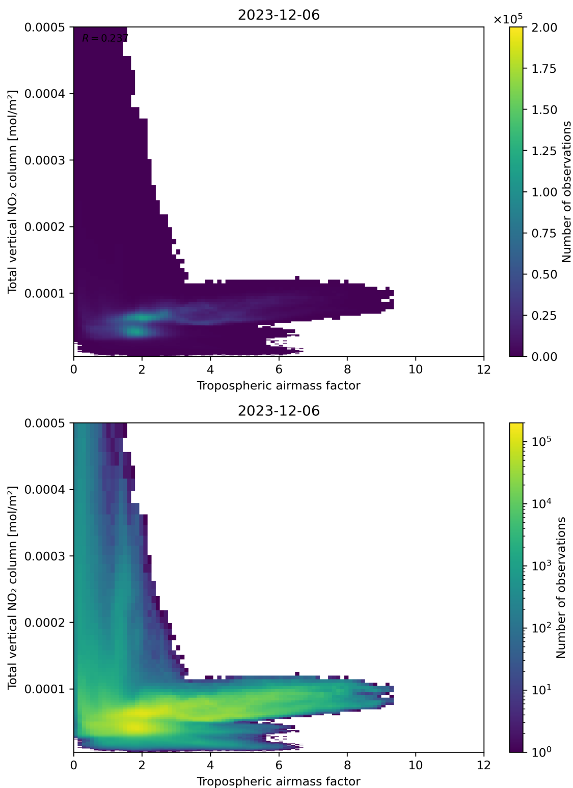
Figure 77: Scatter density plot of “Tropospheric airmass factor” against “Total vertical \text{NO}_2 column” for 2023-12-05 to 2023-12-07.
