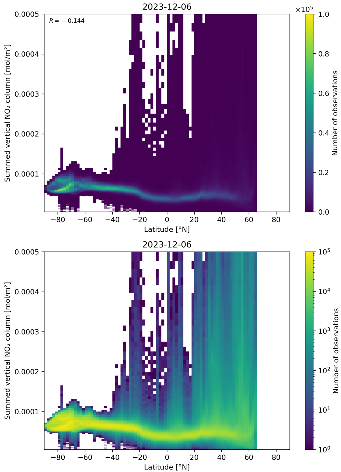
Figure 88: Scatter density plot of “Latitude” against “Summed vertical NO 2 column” for 2023-12-05 to 2023-12-07.
