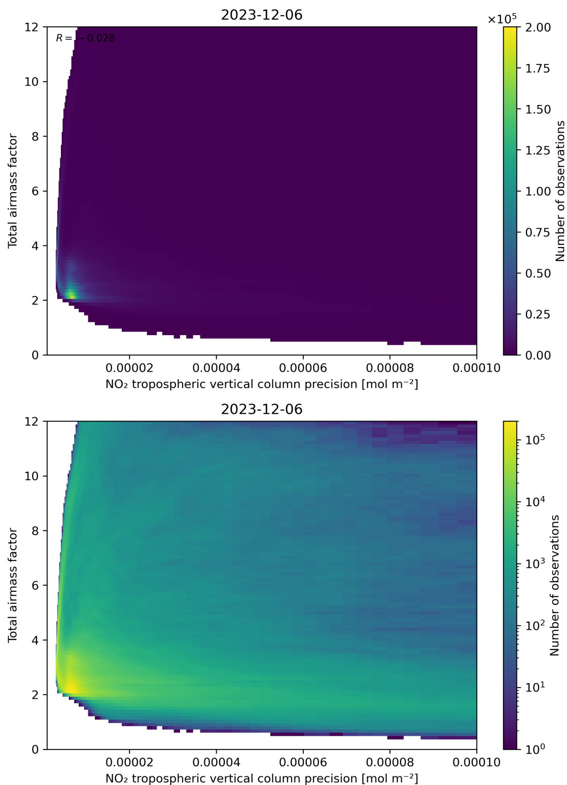
Figure 132: Scatter density plot of “NO 2 tropospheric vertical column precision” against “Total air mass factor” for 2023-12-05 to 2023-12-07.
