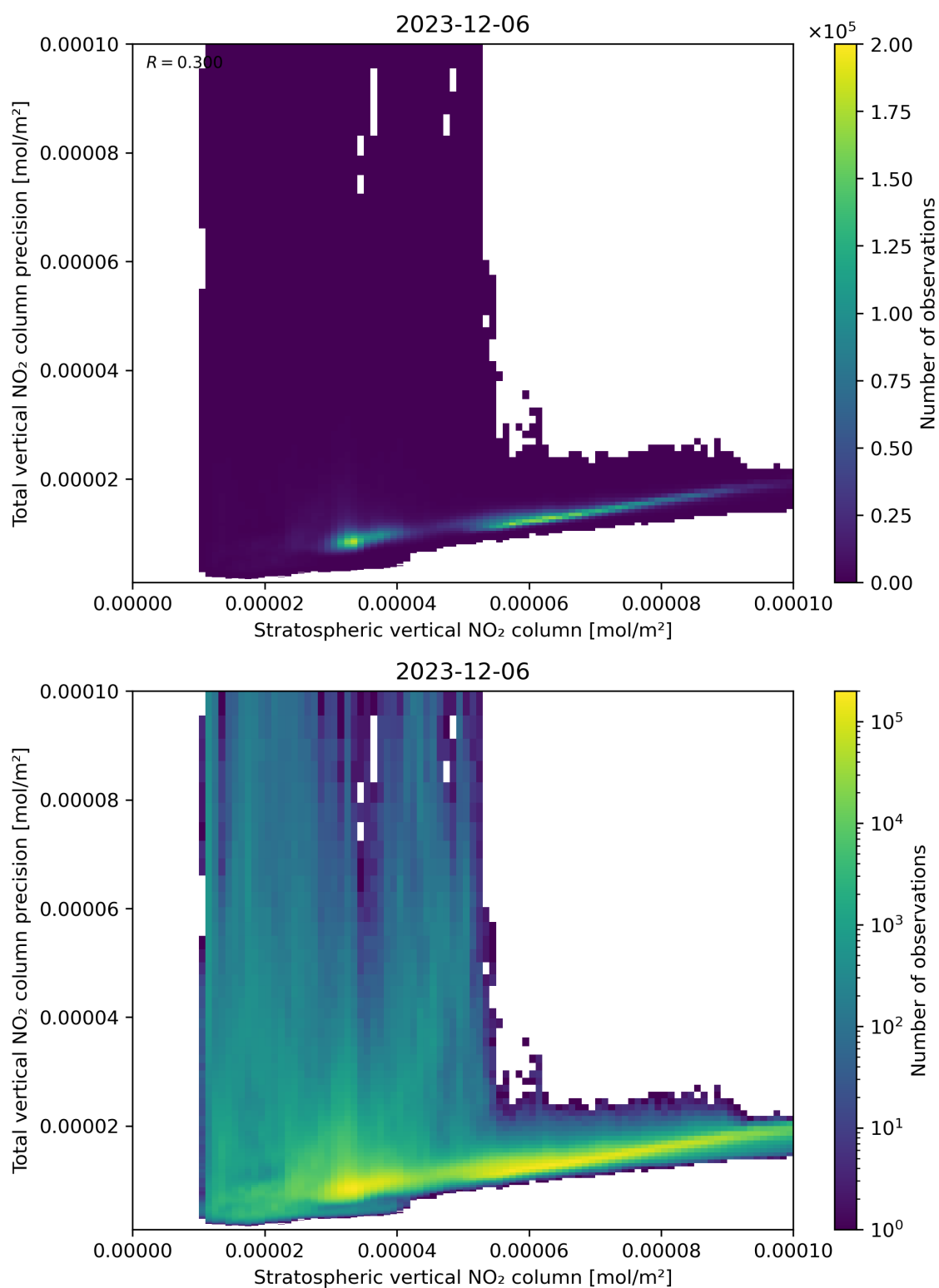
Figure 101: Scatter density plot of “Stratospheric vertical NO 2 column” against “Total vertical NO 2 column precision” for 2023-12-05 to 2023-12-07.
