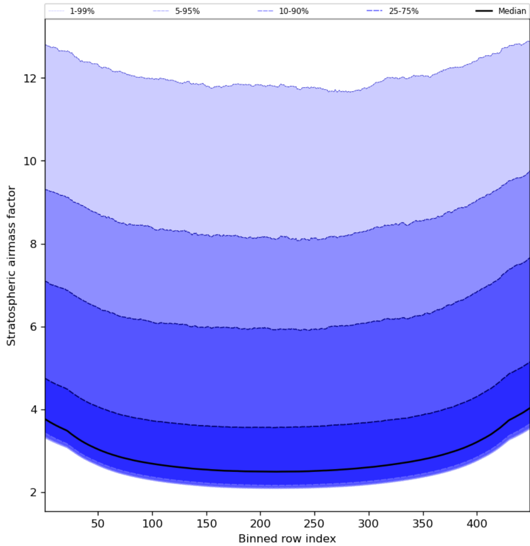
Figure 61: Along track statistics of “Stratospheric air mass factor” for 2023-12-05 to 2023-12-07
