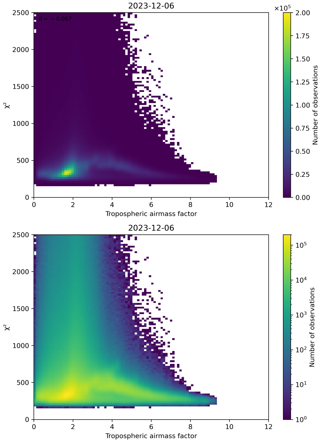
Figure 73: Scatter density plot of “Tropospheric airmass factor” against “ \chi^2 ” for 2023-12-05 to 2023-12-07.
