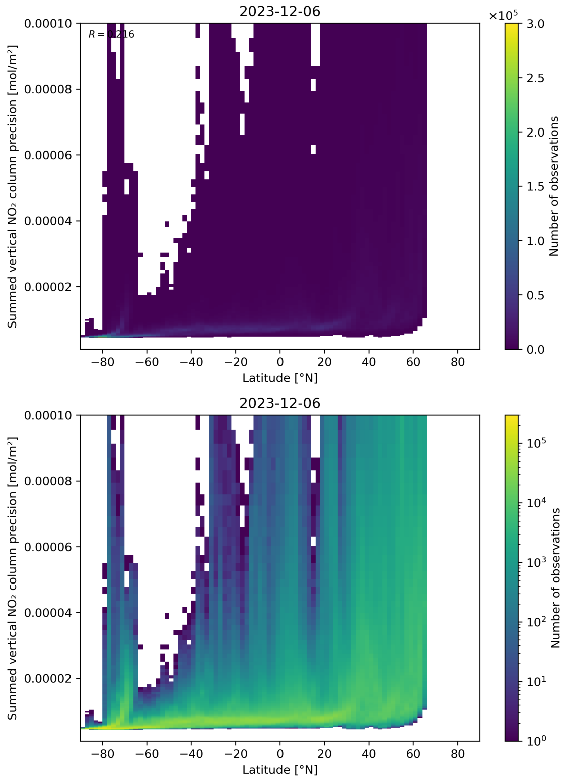
Figure 89: Scatter density plot of “Latitude” against “Summed vertical NO 2 column precision” for 2023-12-05 to 2023-12-07.
