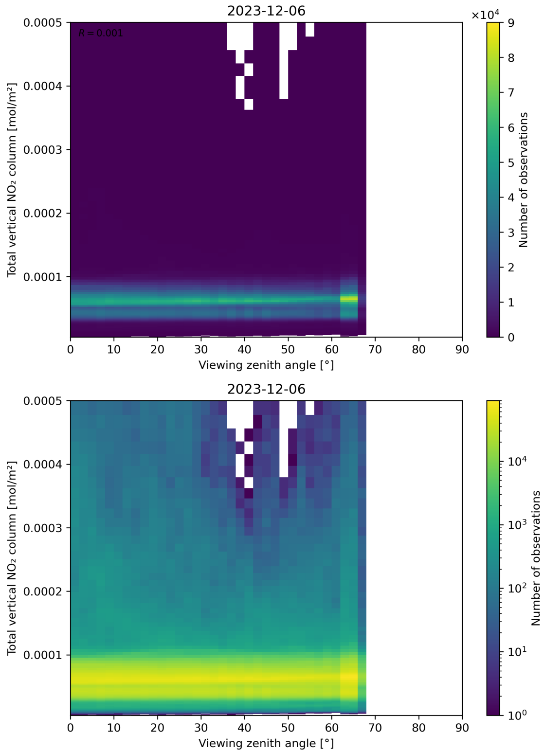
Figure 167: Scatter density plot of “Viewing zenith angle” against “Total vertical NO 2 column” for 2023-12-05 to 2023-12-07.
