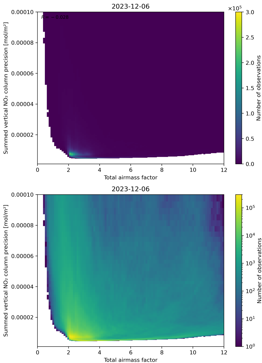
Figure 66: Scatter density plot of “Total airmass factor” against “Summed vertical NO 2 column precision” for 2023-12-05 to 2023-12-07.
