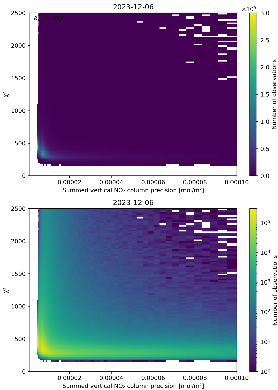
Figure 107: Scatter density plot of “Summed vertical NO 2 column precision” against “ \chi^2 ” for 2023-12-05 to 2023-12-07.
