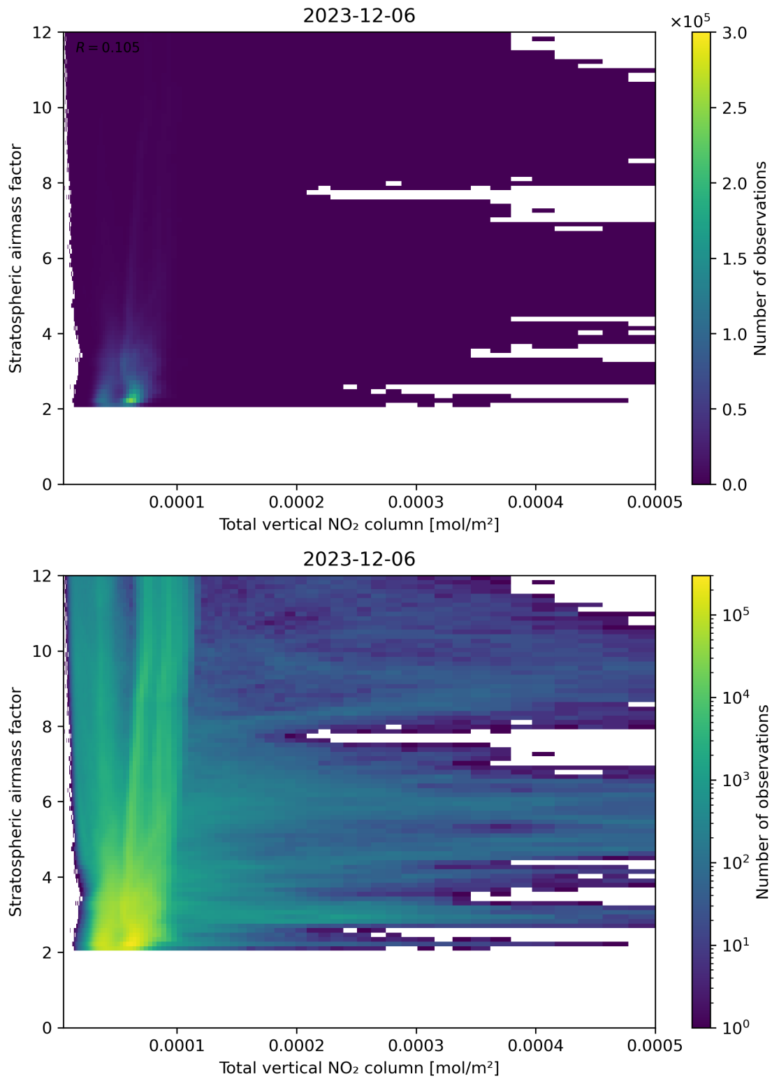
Figure 110: Scatter density plot of “Total vertical NO 2 column” against “Stratospheric airmass factor” for 2023-12-05 to 2023-12-07.
