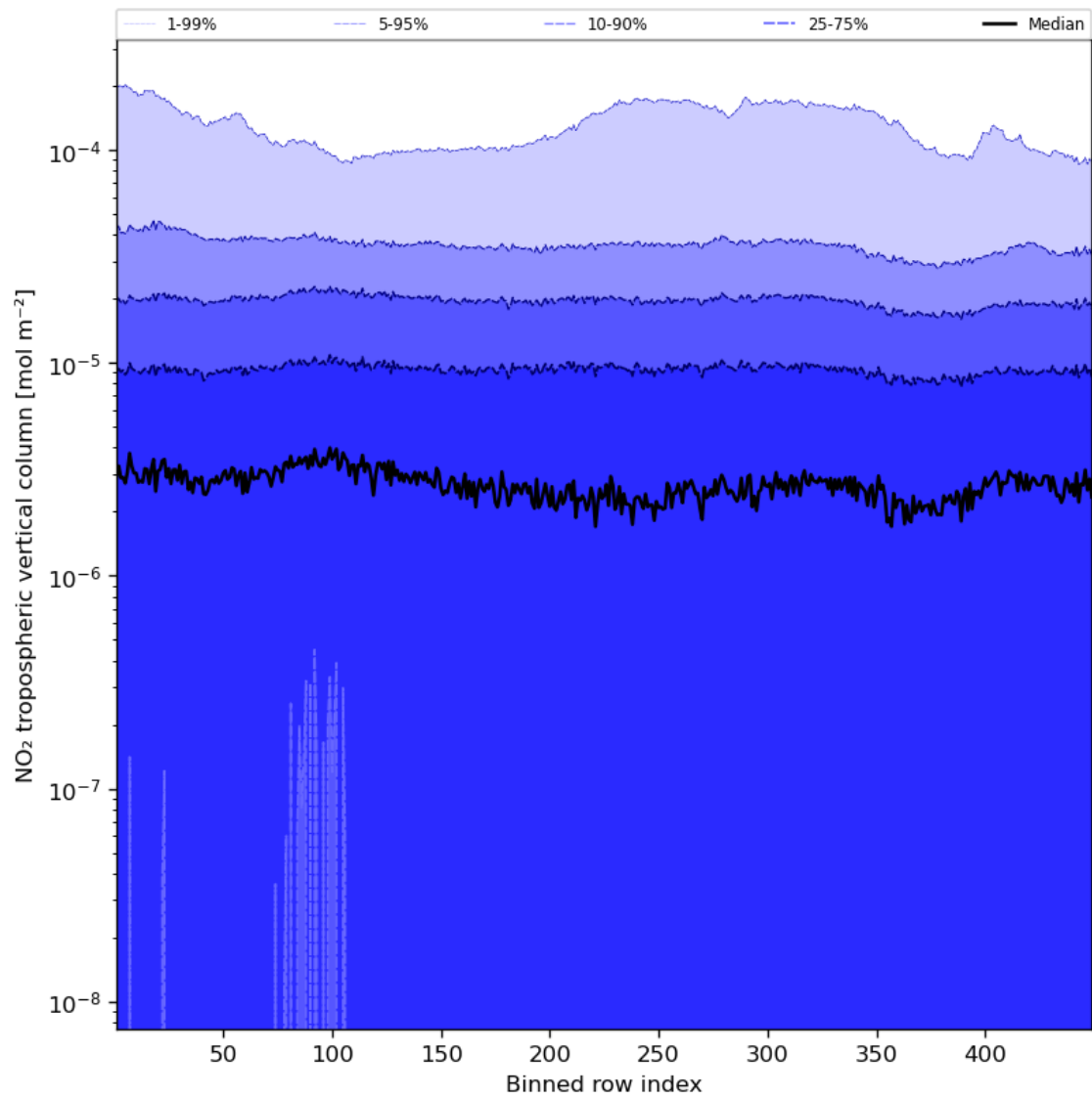
Figure 46: Along track statistics of “NO 2 tropospheric vertical column” for 2023-12-05 to 2023-12-07
