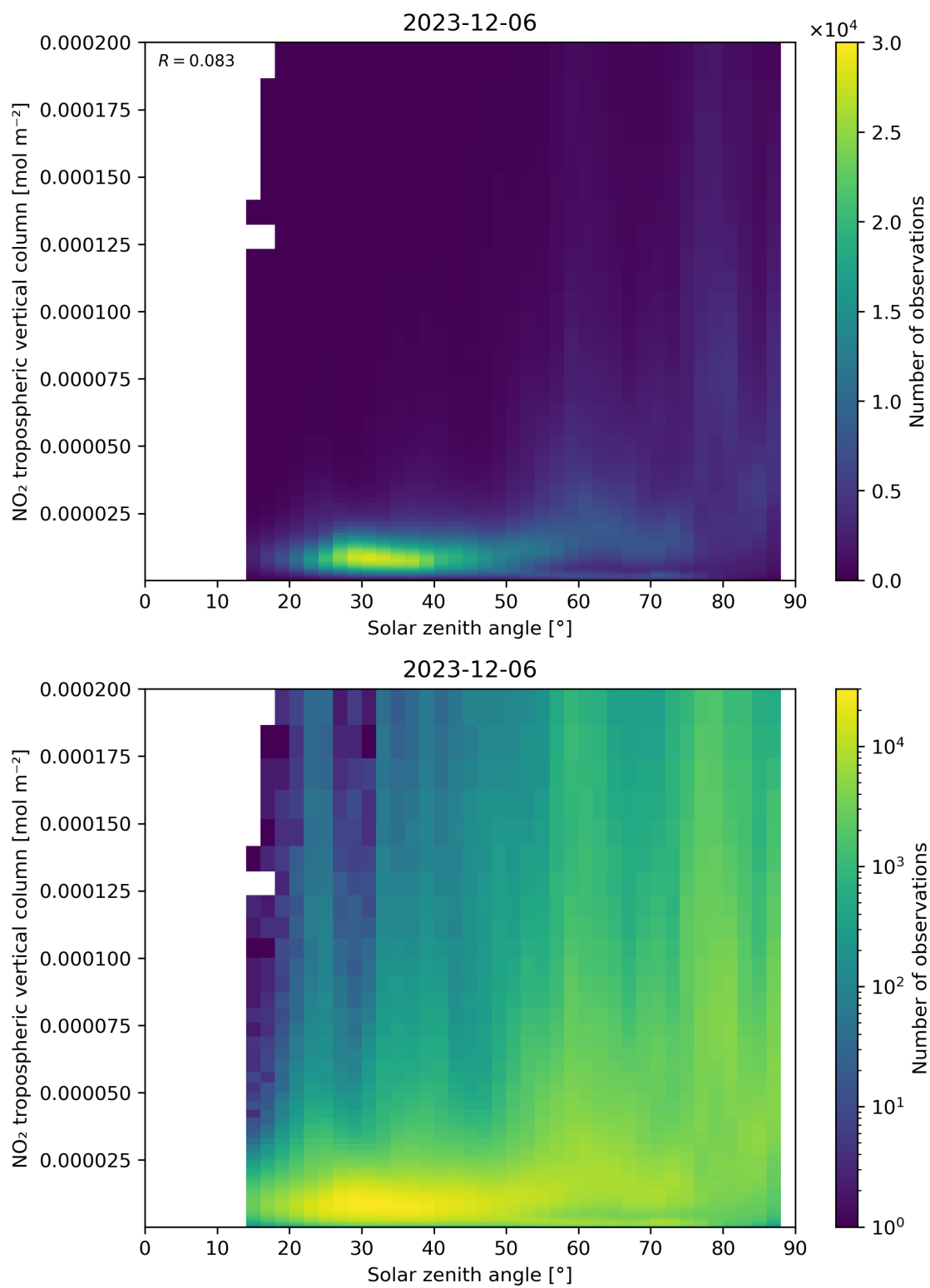
Figure 155: Scatter density plot of “Solar zenith angle” against “NO 2 tropospheric vertical column” for 2023-12-05 to 2023-12-07.
