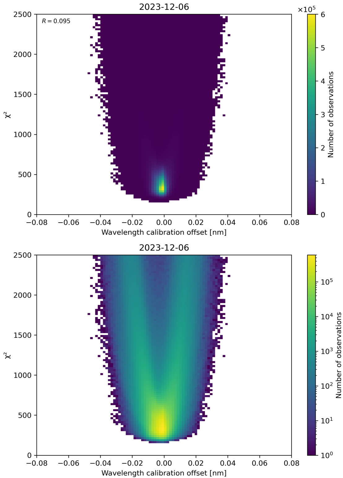
Figure 175: Scatter density plot of “Wavelength calibration offset” against “ \chi^2 ” for 2023-12-05 to 2023-12-07.
