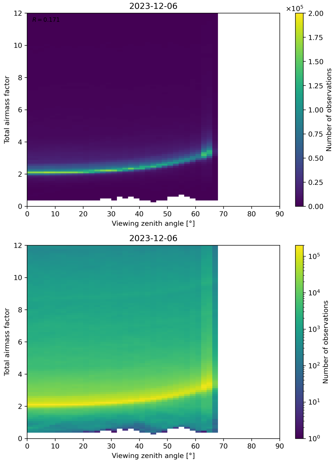
Figure 160: Scatter density plot of “Viewing zenith angle” against “Total airmass factor” for 2023-12-05 to 2023-12-07.
