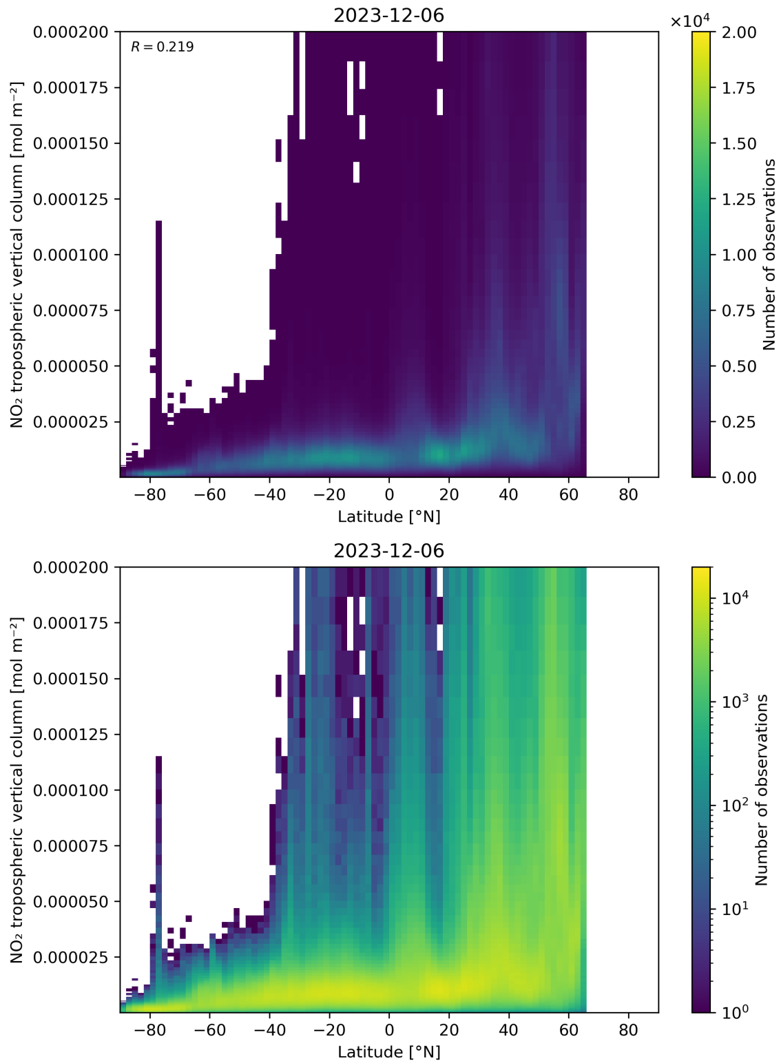
Figure 92: Scatter density plot of “Latitude” against “NO 2 tropospheric vertical column” for 2023-12-05 to 2023-12-07.
