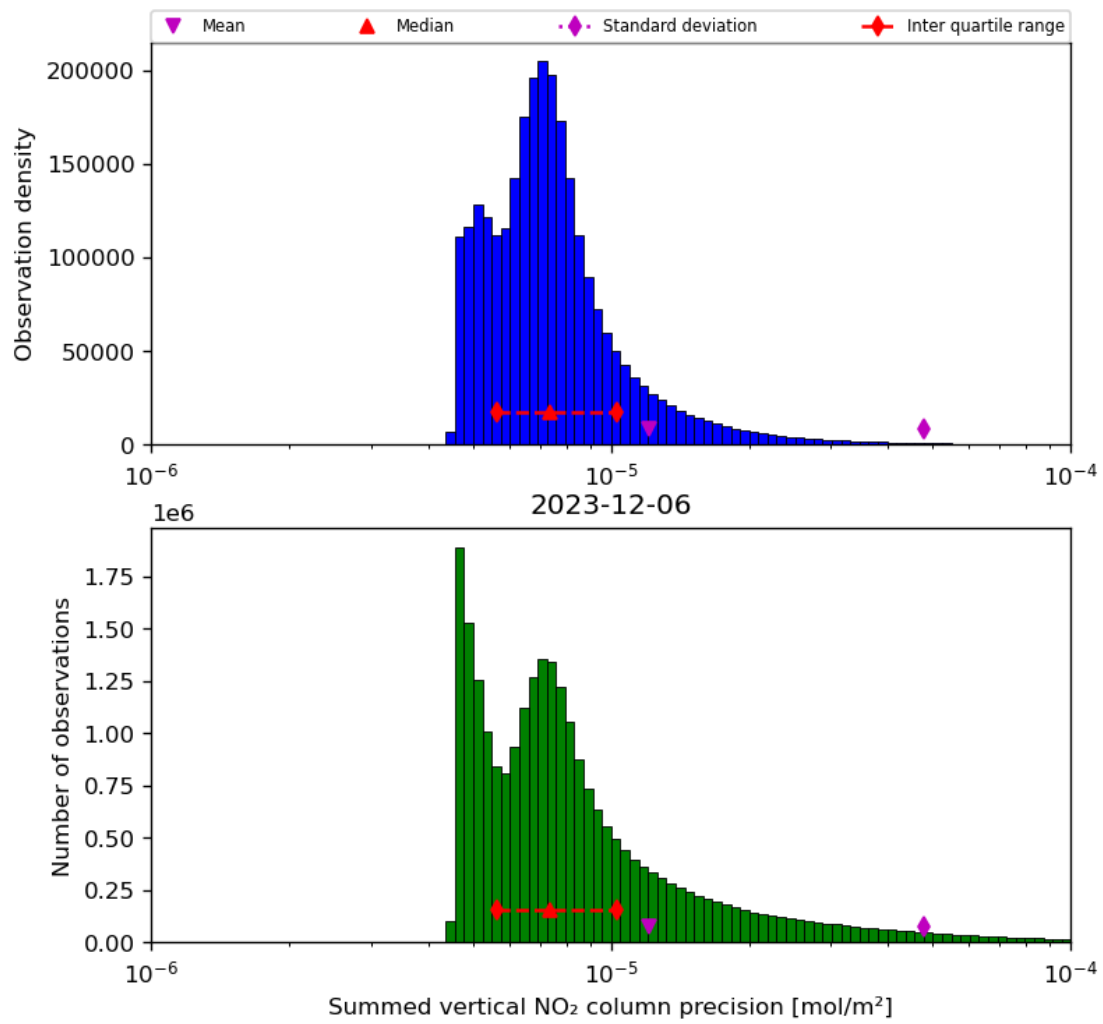
Figure 41: Histogram of "Summed vertical NO 2 column precision" for 2023-12-05 to 2023-12-07
