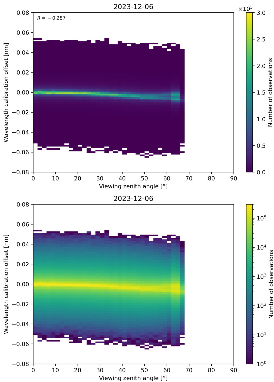
Figure 173: Scatter density plot of “Viewing zenith angle” against “Wavelength calibration offset” for 2023-12-05 to 2023-12-07.
