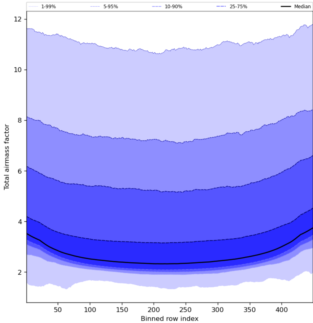
Figure 49: Along track statistics of “Total airmass factor” for 2023-12-05 to 2023-12-07
