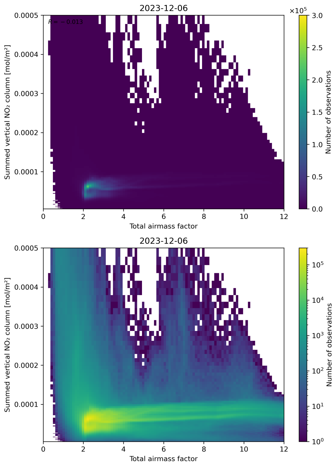
Figure 65: Scatter density plot of “Total airmass factor” against “Summed vertical NO 2 column” for 2023-12-05 to 2023-12-07.
