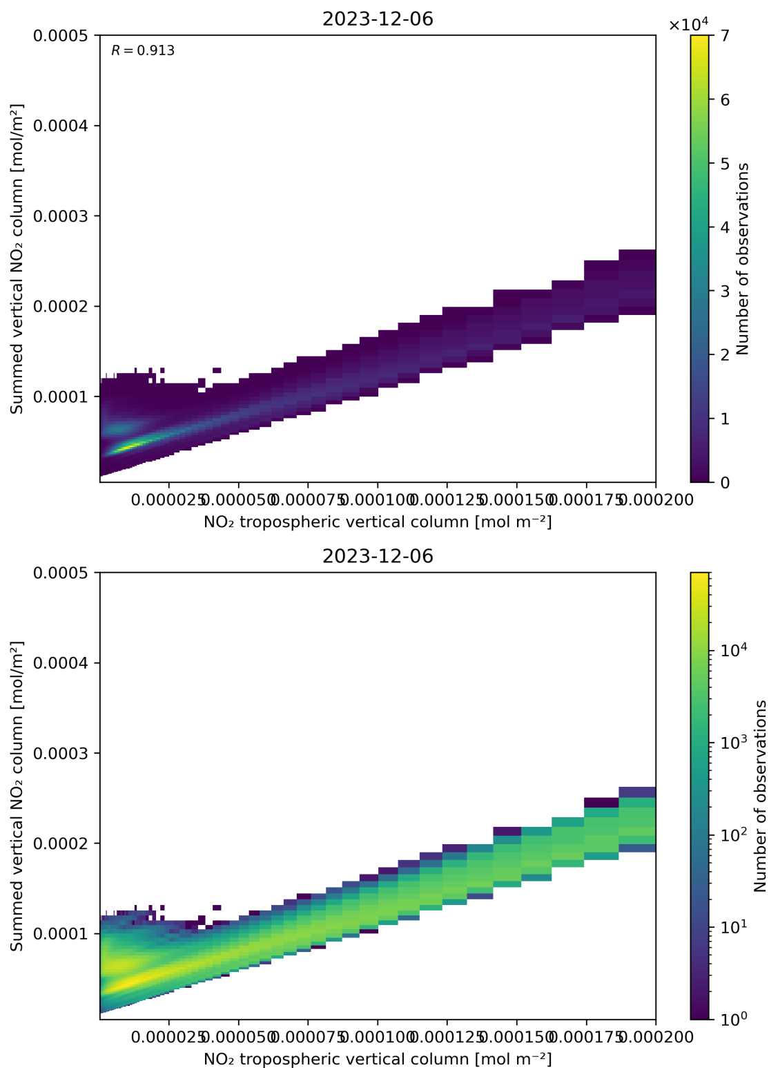
Figure 126: Scatter density plot of “NO 2 tropospheric vertical column” against “Summed vertical NO 2 column” for 2023-12-05 to 2023-12-07.
