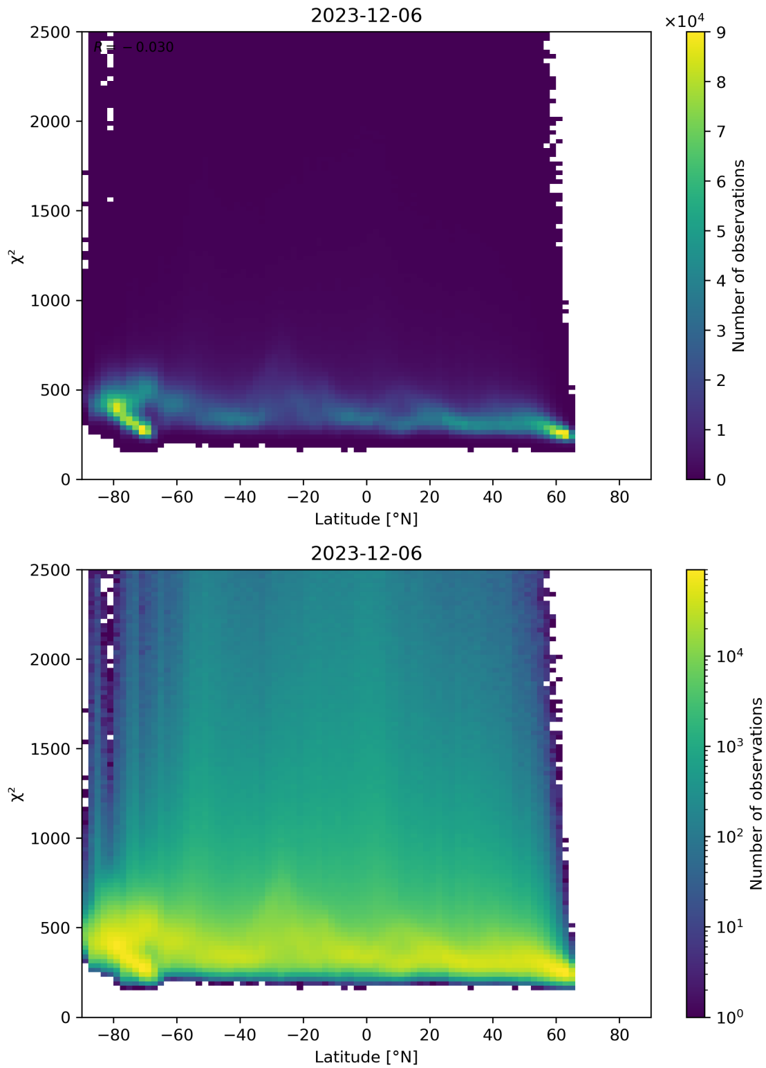
Figure 86: Scatter density plot of “Latitude” against “ \chi^2 ” for 2023-12-05 to 2023-12-07.
