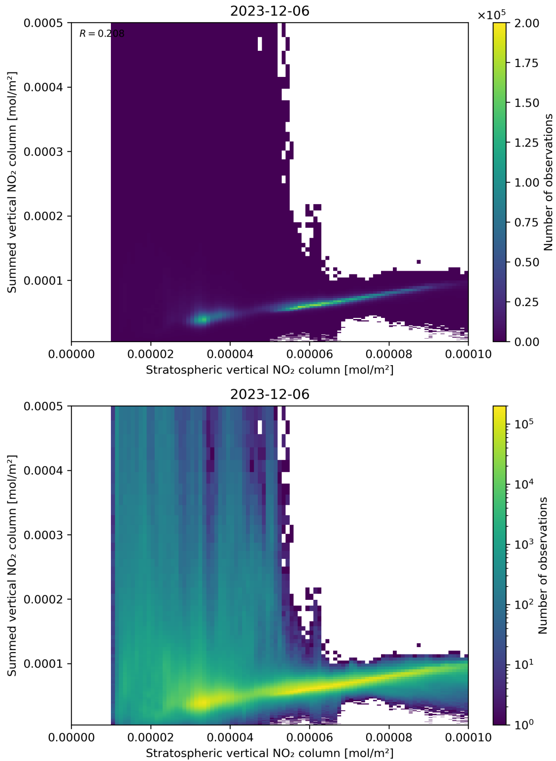
Figure 98: Scatter density plot of “Stratospheric vertical NO 2 column” against “Summed vertical NO 2 column” for 2023-12-05 to 2023-12-07.
