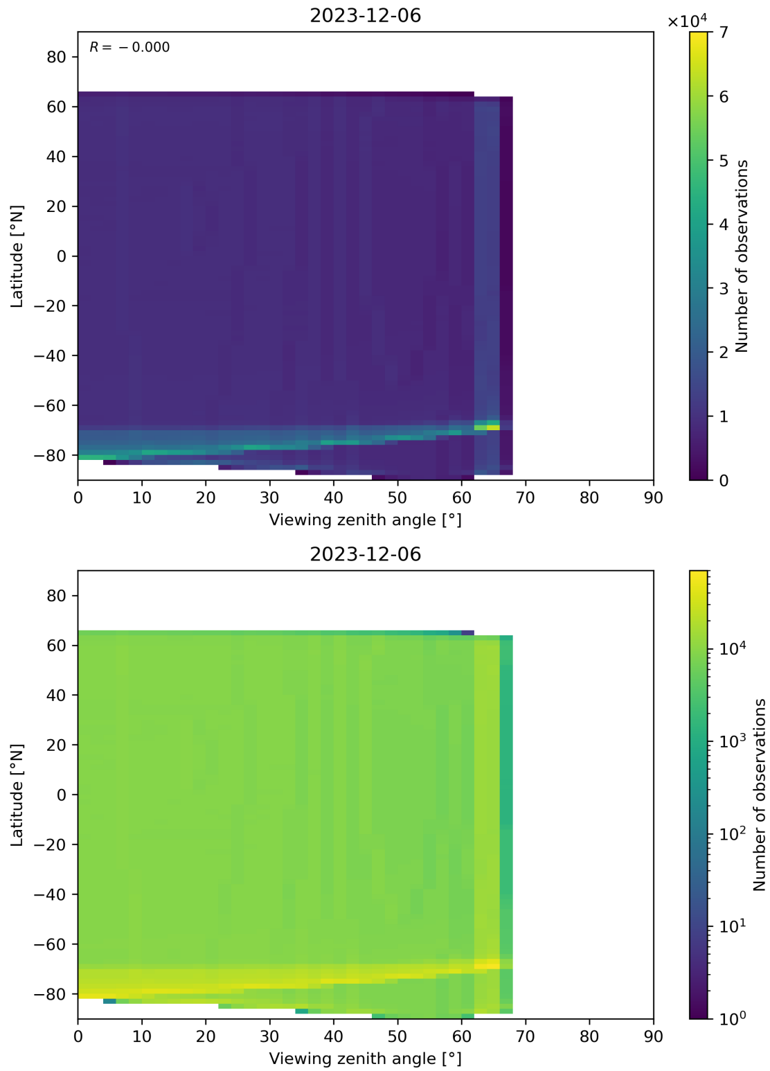
Figure 163: Scatter density plot of “Viewing zenith angle” against “Latitude” for 2023-12-05 to 2023-12-07.
