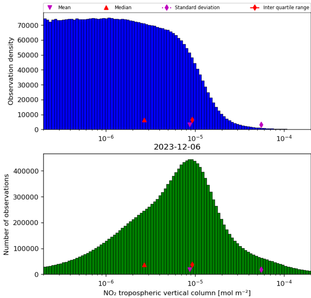
Figure 29: Histogram of “NO 2 tropospheric vertical column” for 2023-12-05 to 2023-12-07
