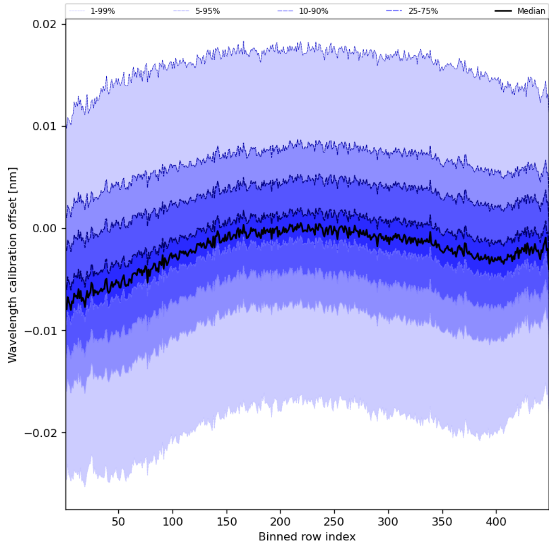
Figure 52: Along track statistics of “Wavelength calibration offset” for 2023-12-05 to 2023-12-07
