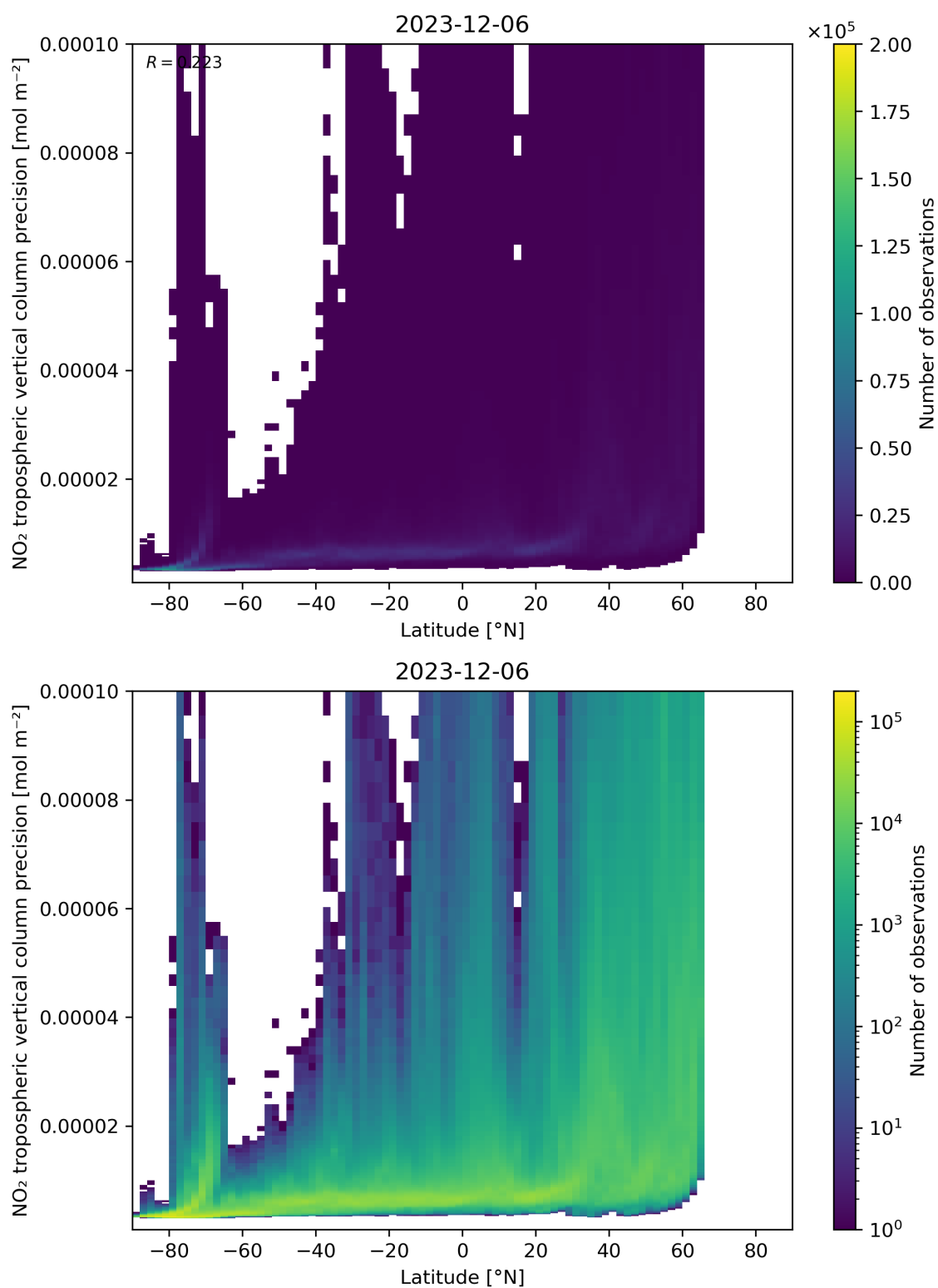
Figure 93: Scatter density plot of “Latitude” against “NO 2 tropospheric vertical column precision” for 2023-12-05 to 2023-12-07.
