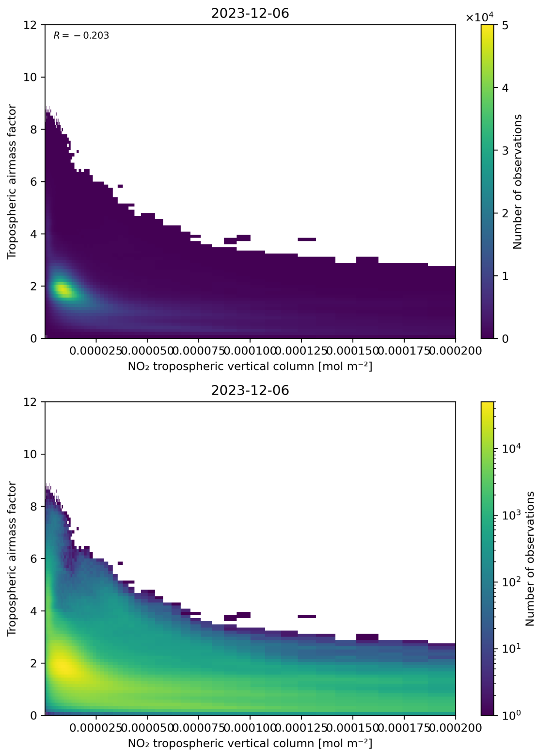
Figure 123: Scatter density plot of “NO 2 tropospheric vertical column” against “Tropospheric air mass factor” for 2023-12-05 to 2023-12-07.
