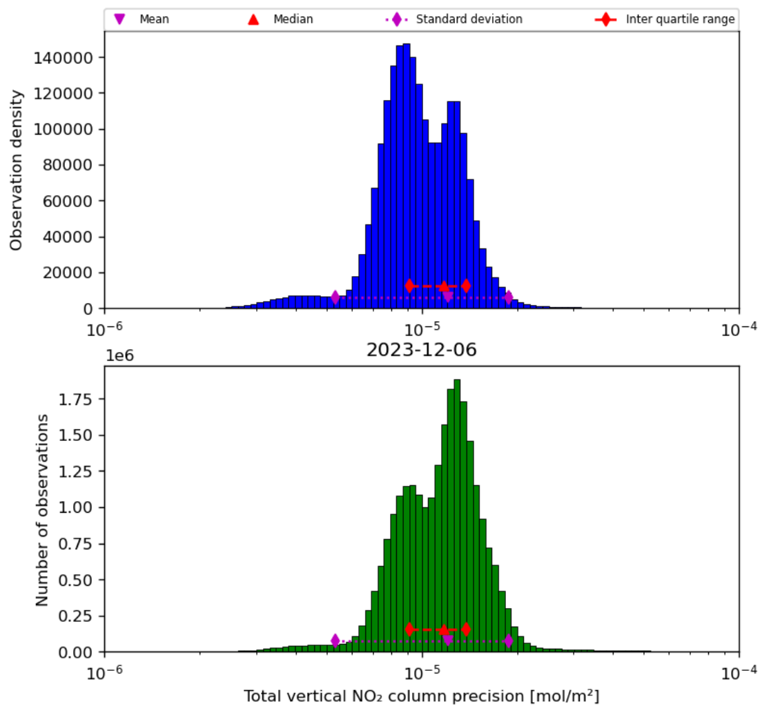
Figure 39: Histogram of “Total vertical NO 2 column precision” for 2023-12-05 to 2023-12-07
