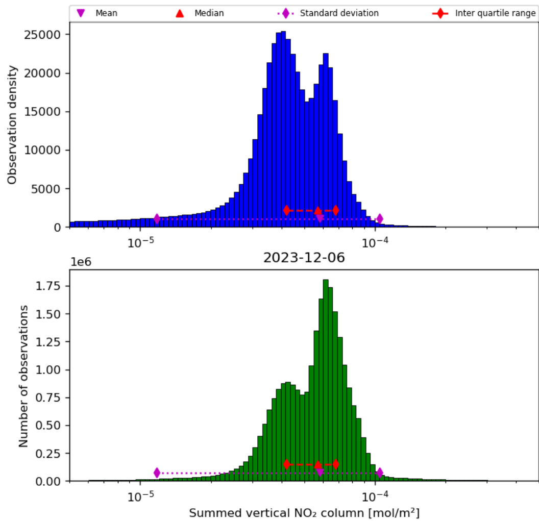
Figure 40: Histogram of “Summed vertical NO 2 column” for 2023-12-05 to 2023-12-07
