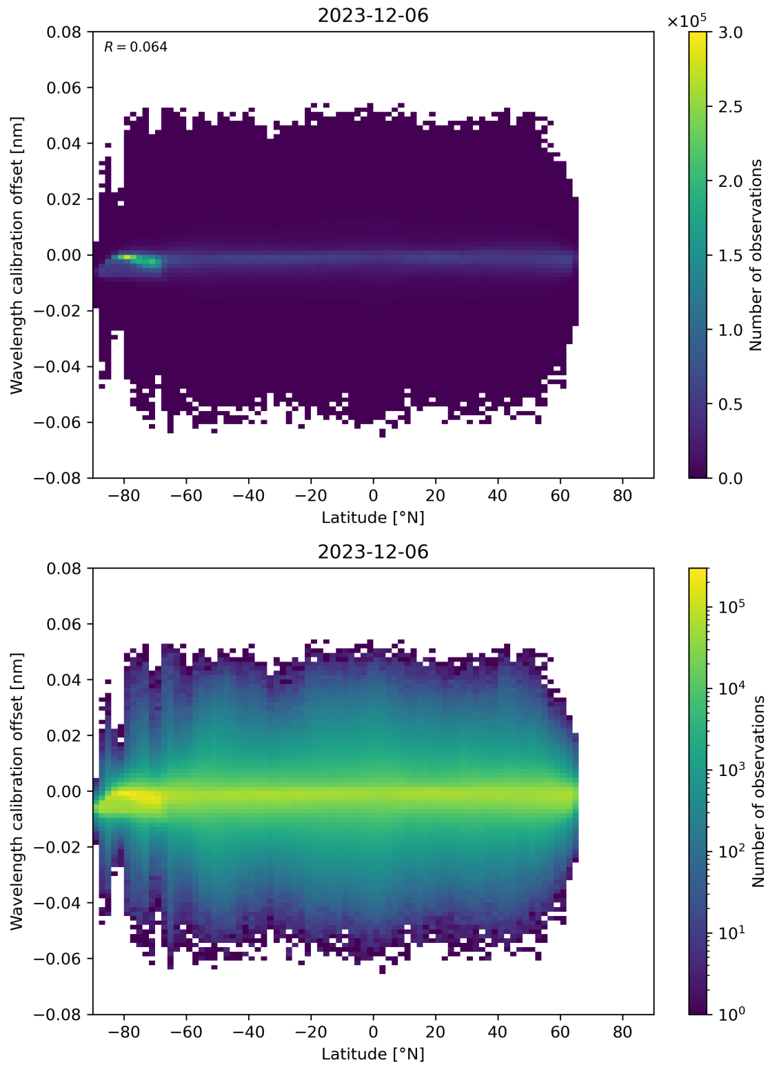
Figure 95: Scatter density plot of “Latitude” against “Wavelength calibration offset” for 2023-12-05 to 2023-12-07.
