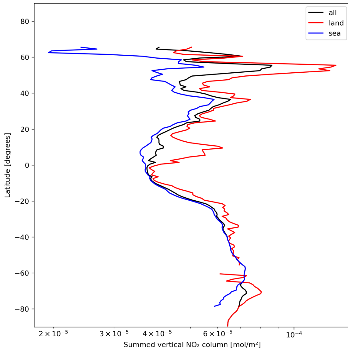
Figure 23: Zonal average of “Summed vertical NO 2 column” for 2023-12-05 to 2023-12-07.
