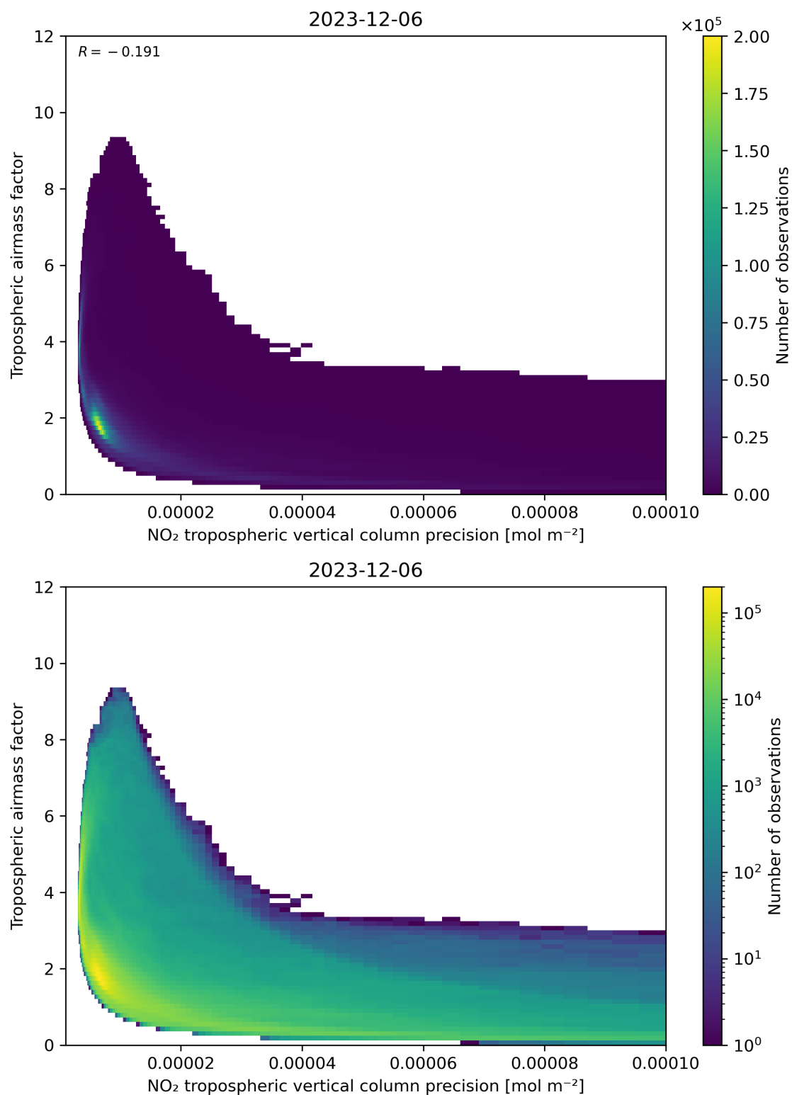
Figure 133: Scatter density plot of “NO 2 tropospheric vertical column precision” against “Tropospheric air mass factor” for 2023-12-05 to 2023-12-07.
