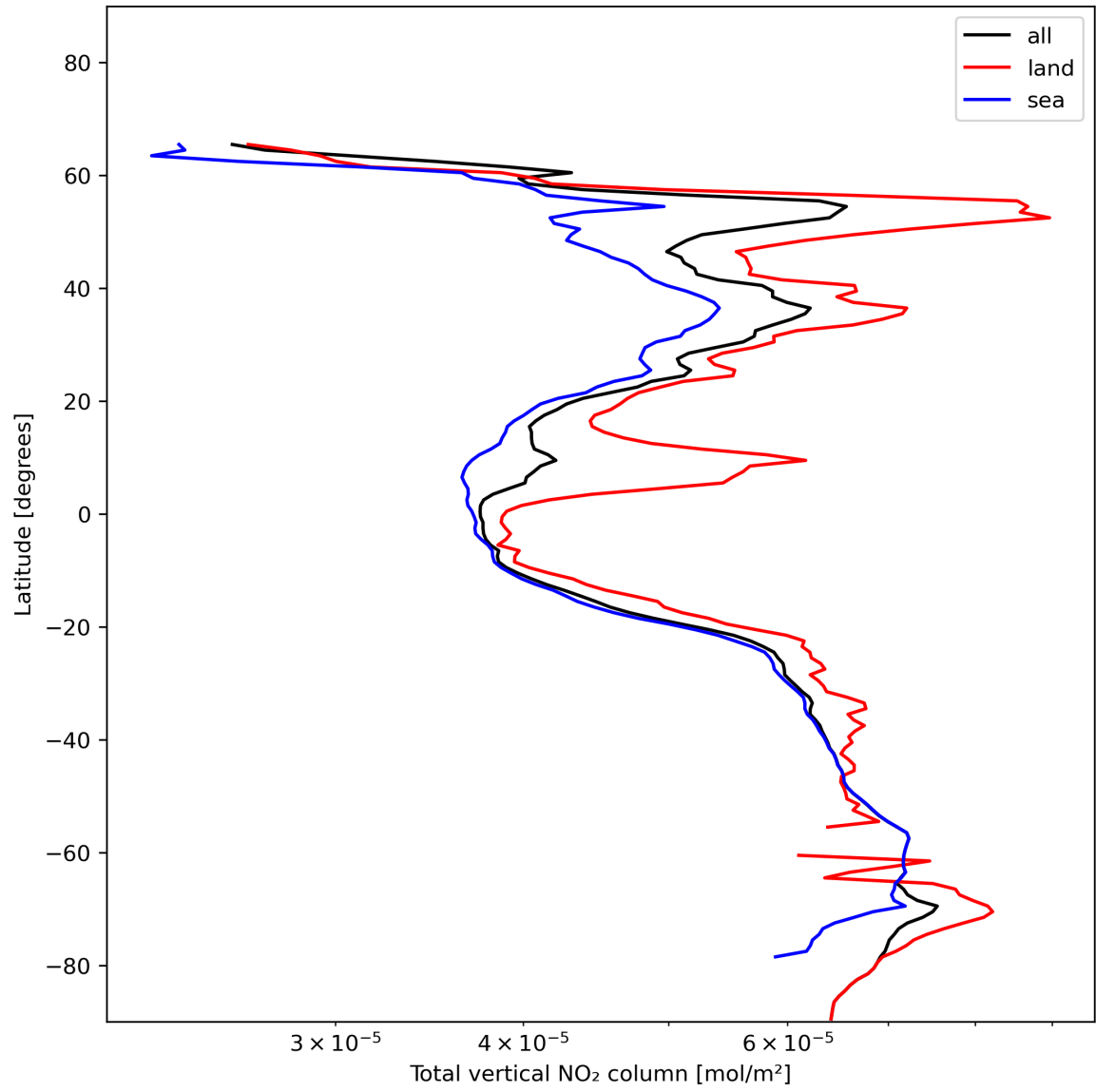
Figure 21: Zonal average of “Total vertical NO 2 column” for 2023-12-05 to 2023-12-07.
