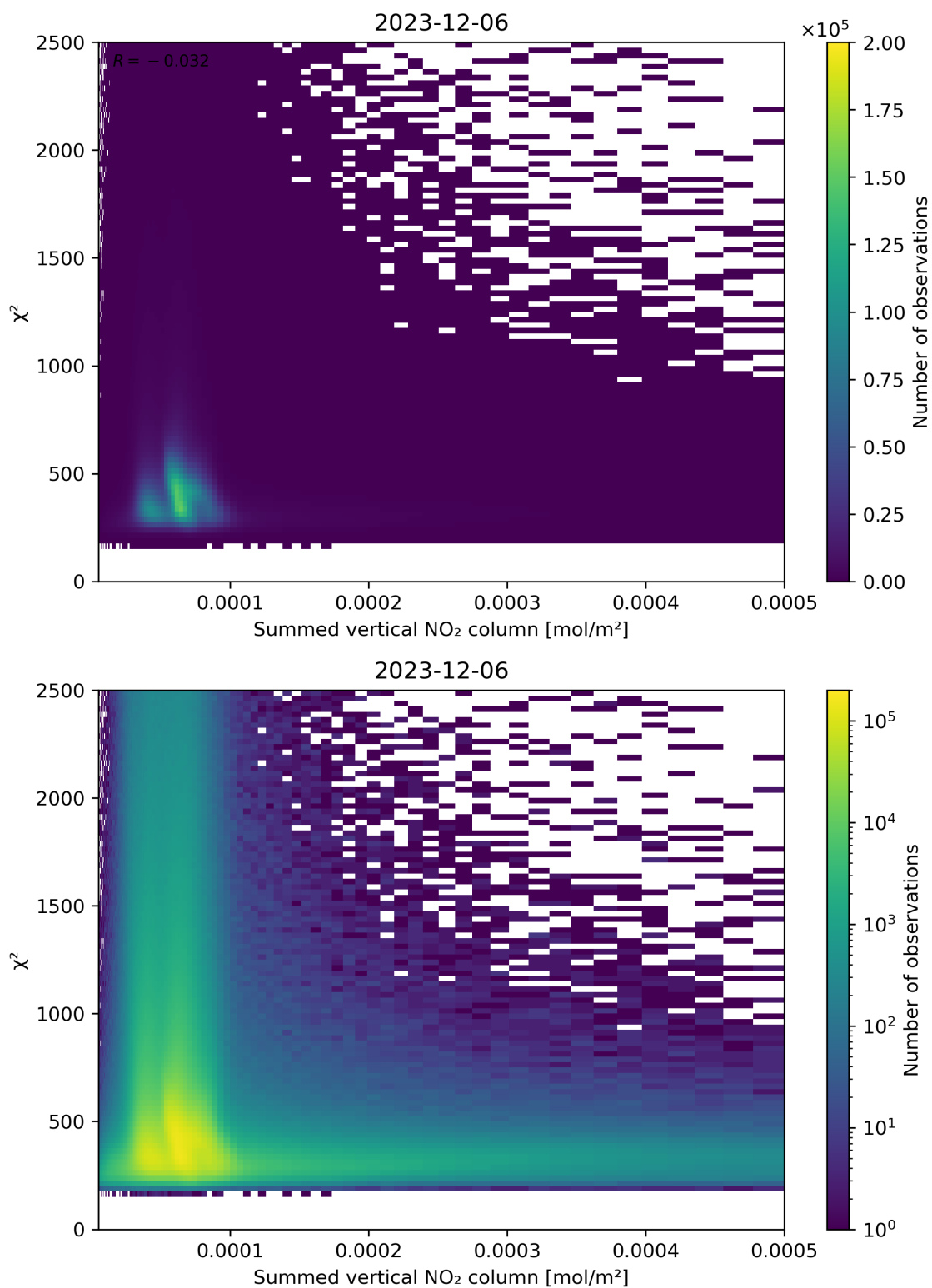
Figure 104: Scatter density plot of “Summed vertical NO 2 column” against “ \chi^2 ” for 2023-12-05 to 2023-12-07.
