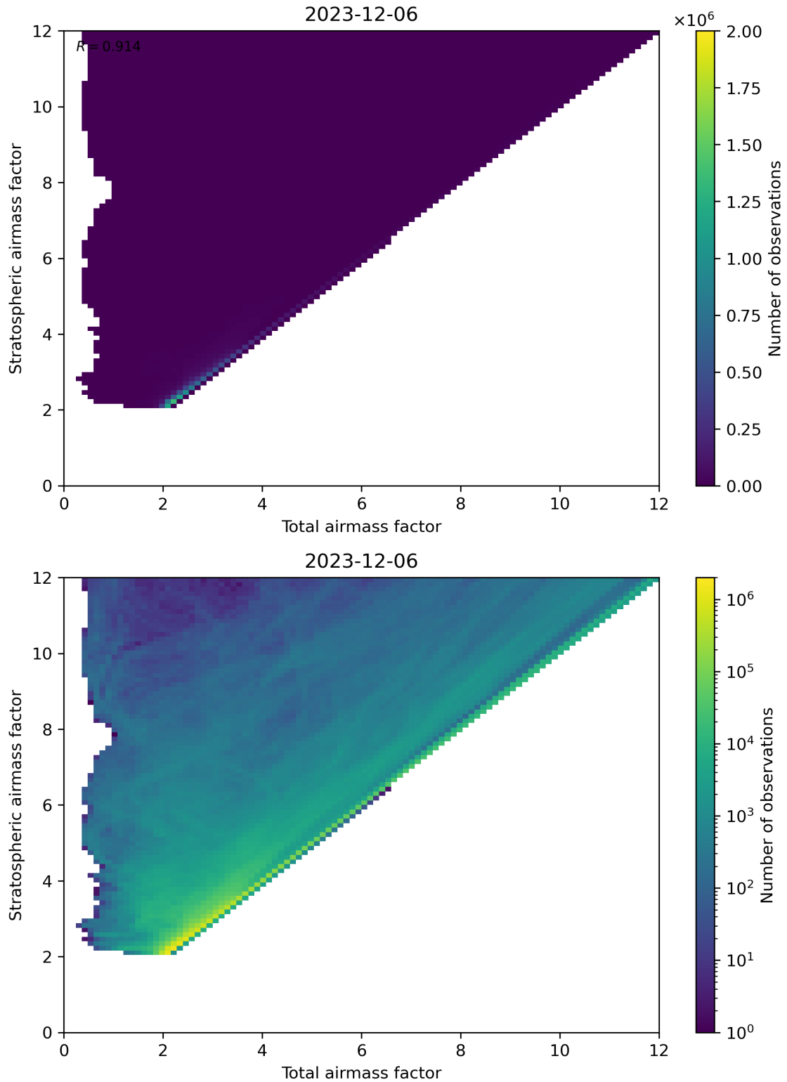
Figure 62: Scatter density plot of “Total airmass factor” against “Stratospheric airmass factor” for 2023-12-05 to 2023-12-07.
