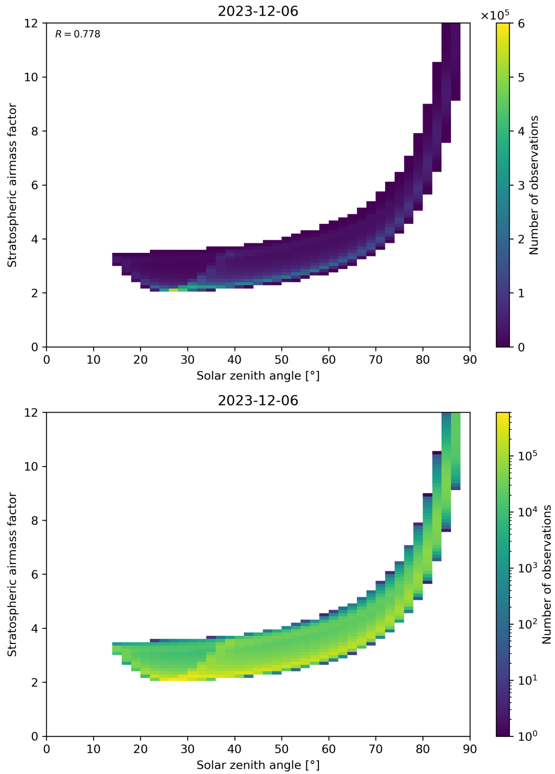
Figure 145: Scatter density plot of “Solar zenith angle” against “Stratospheric airmass factor” for 2023-12-05 to 2023-12-07.
