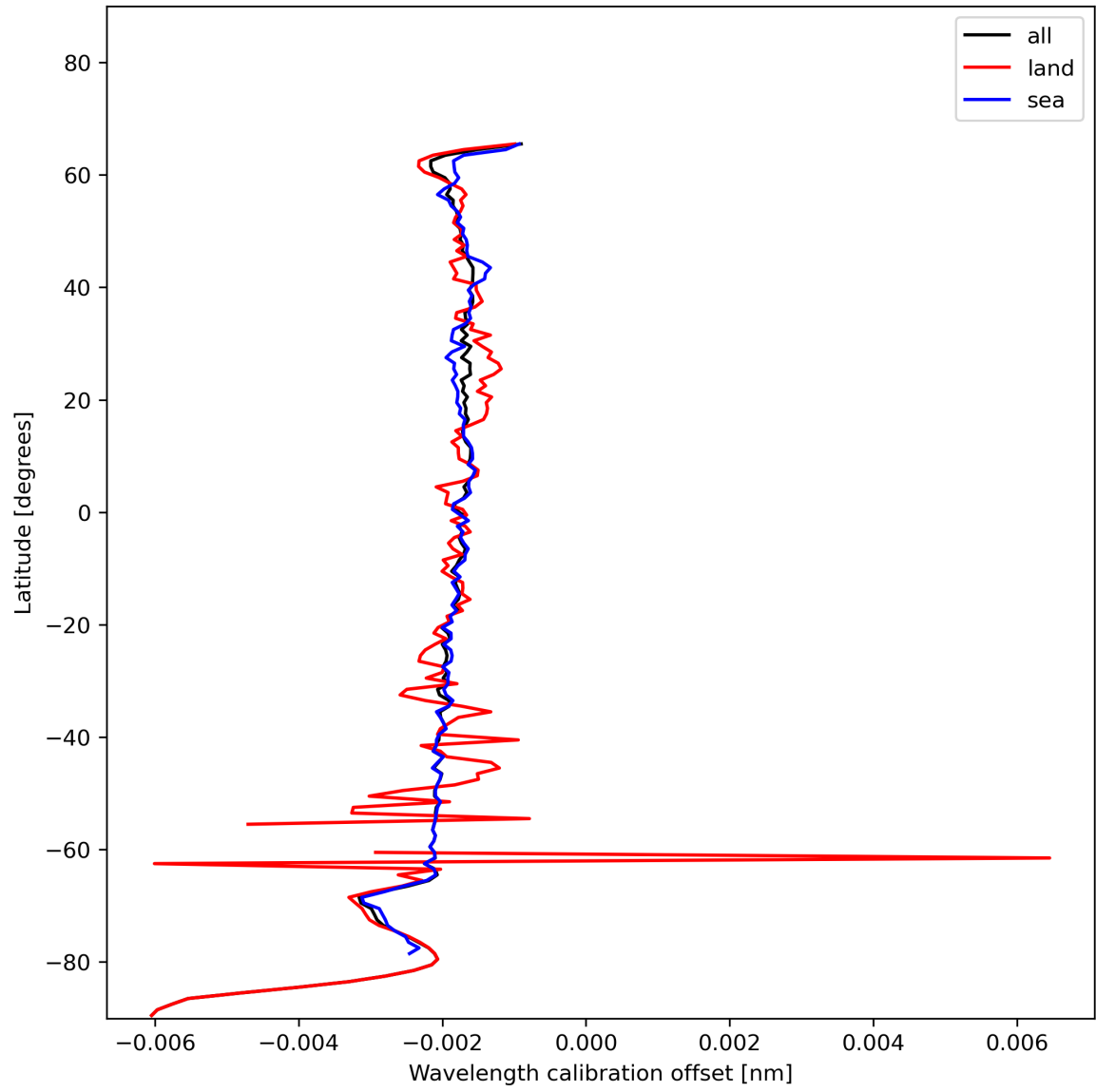
Figure 18: Zonal average of “Wavelength calibration offset” for 2023-12-05 to 2023-12-07.
