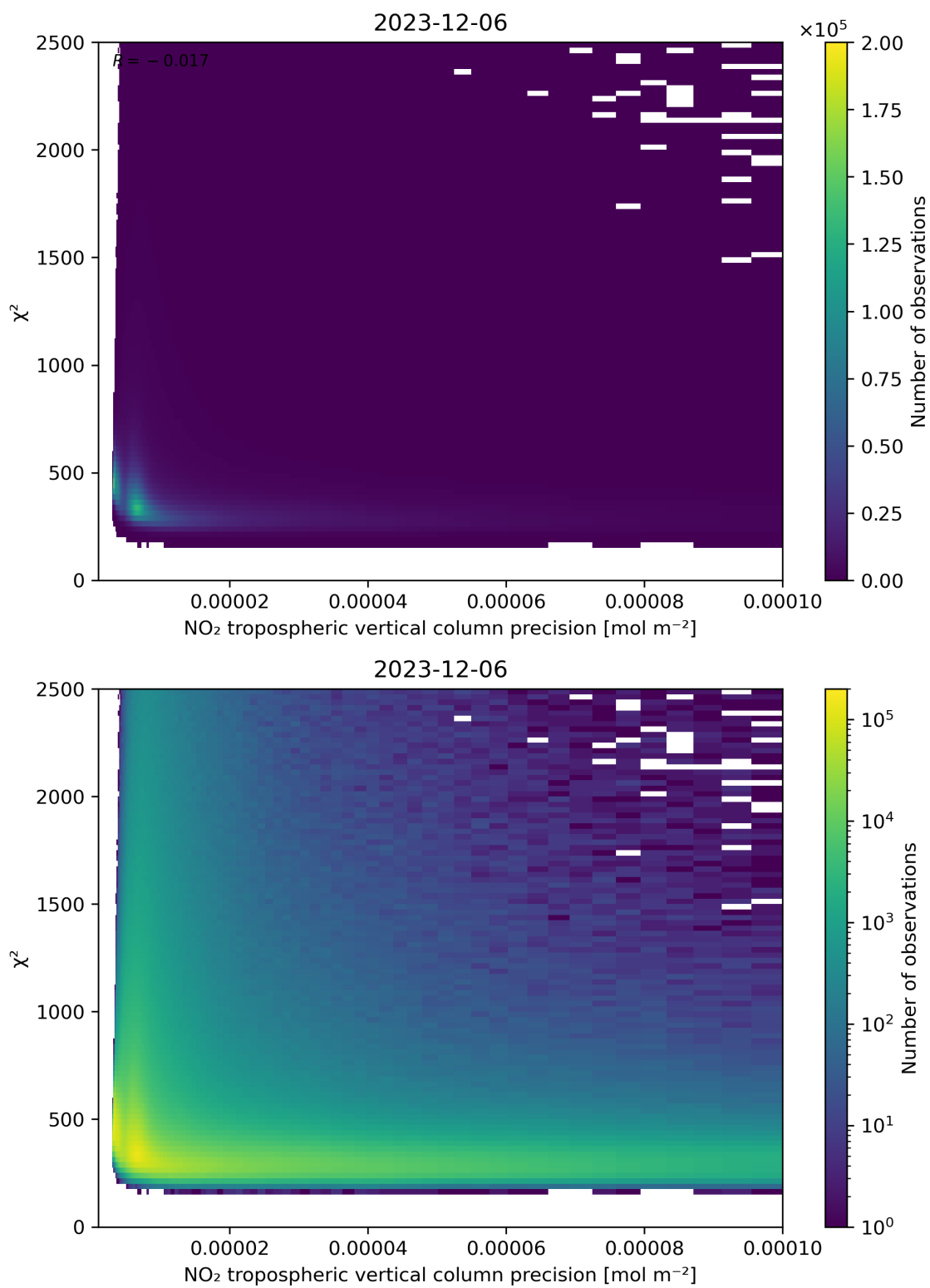
Figure 134: Scatter density plot of “NO 2 tropospheric vertical column precision” against “ \chi^2 ” for 2023-12-05 to 2023-12-07.
