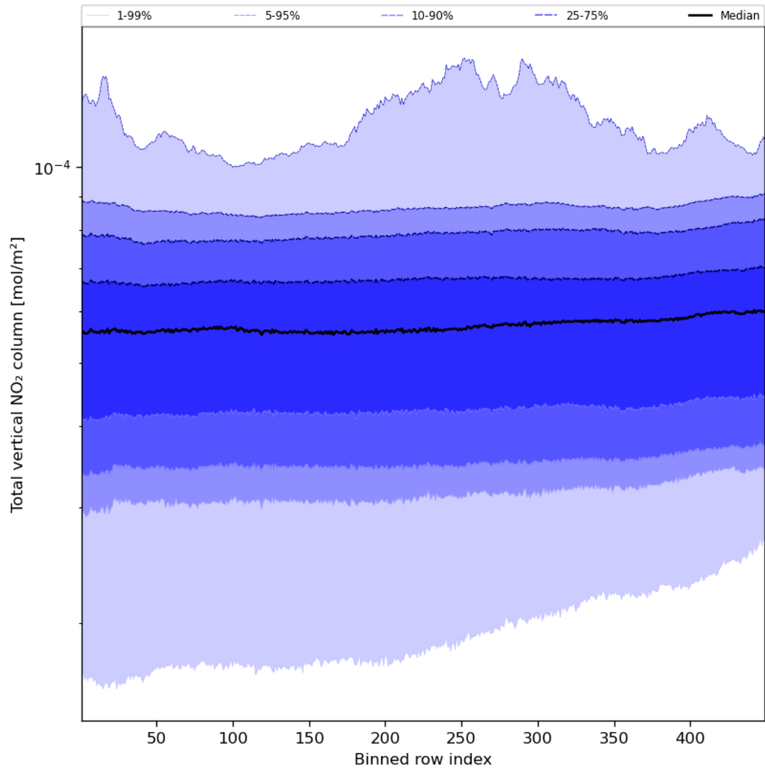
Figure 55: Along track statistics of “Total vertical NO 2 column” for 2023-12-05 to 2023-12-07
