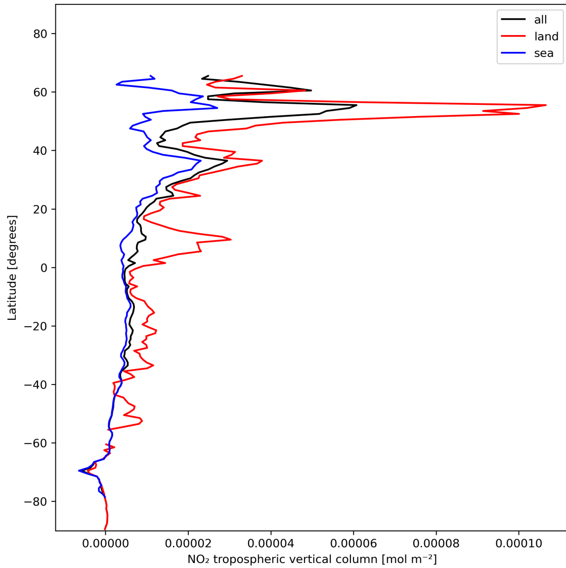
Figure 12: Zonal average of “NO 2 tropospheric vertical column” for 2023-12-05 to 2023-12-07.
