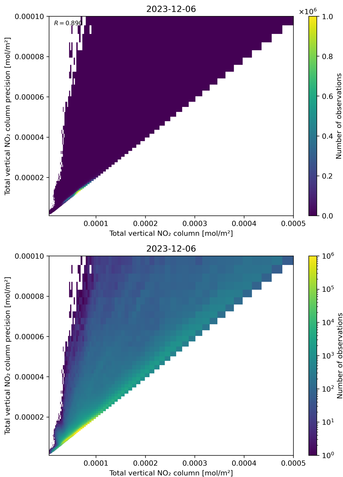
Figure 114: Scatter density plot of “Total vertical NO 2 column” against “Total vertical NO 2 column precision” for 2023-12-05 to 2023-12-07.
