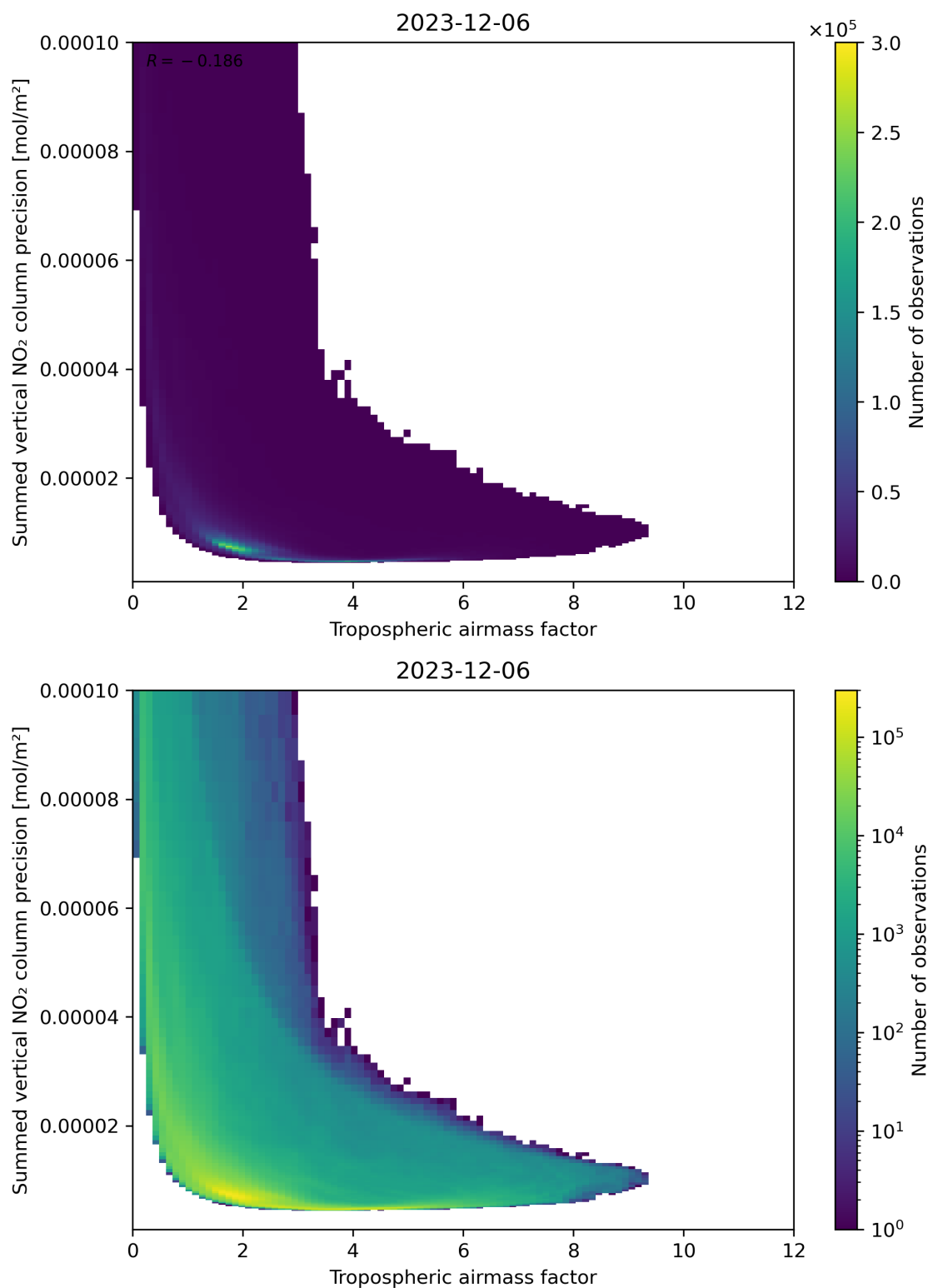
Figure 76: Scatter density plot of “Tropospheric air mass factor” against “Summed vertical NO 2 column precision” for 2023-12-05 to 2023-12-07.
