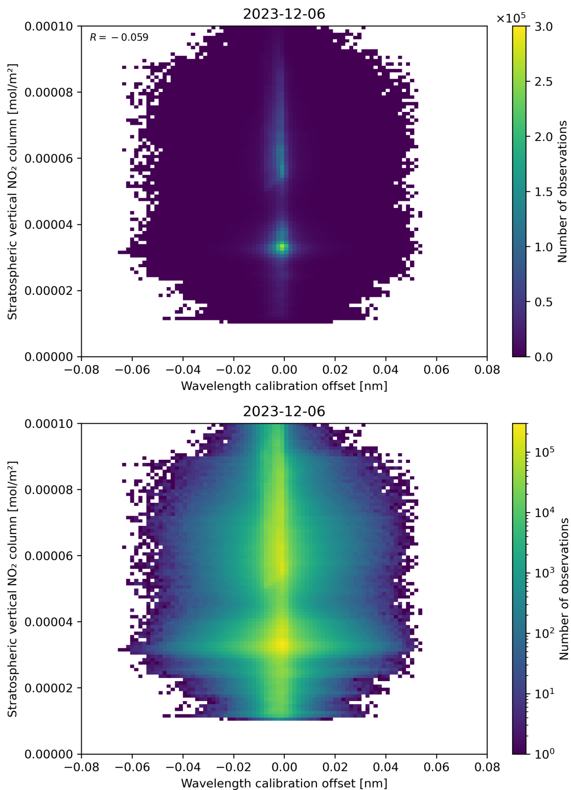
Figure 176: Scatter density plot of “Wavelength calibration offset” against “Stratospheric vertical NO 2 column” for 2023-12-05 to 2023-12-07.
