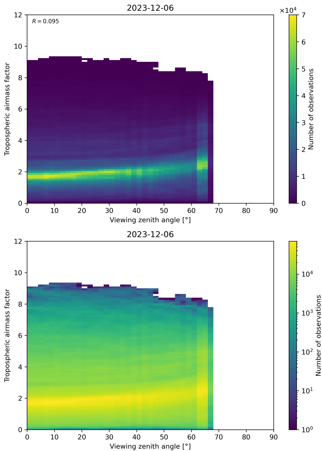
Figure 161: Scatter density plot of “Viewing zenith angle” against “Tropospheric airmass factor” for 2023-12-05 to 2023-12-07.
