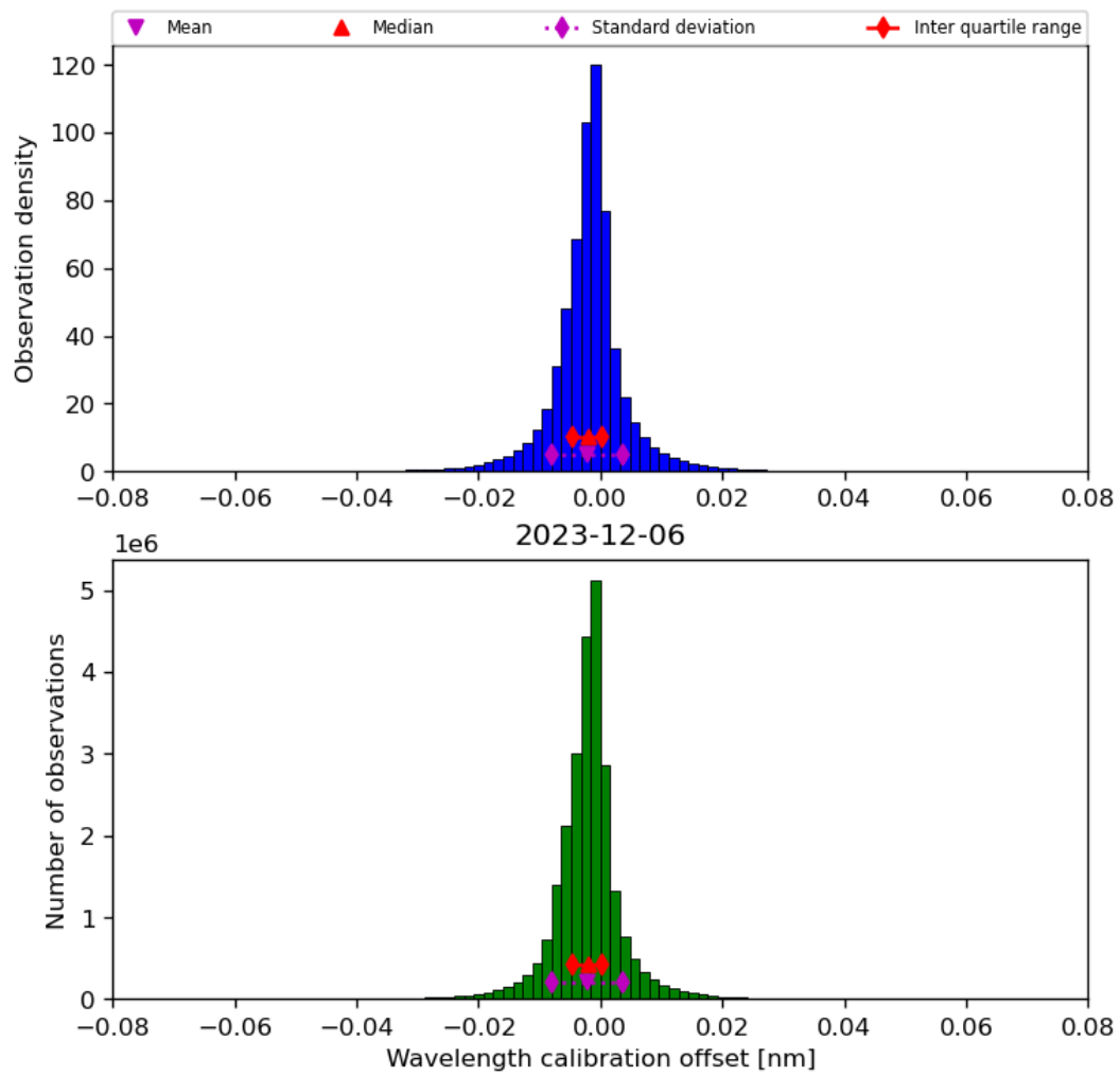
Figure 35: Histogram of “Wavelength calibration offset” for 2023-12-05 to 2023-12-07
