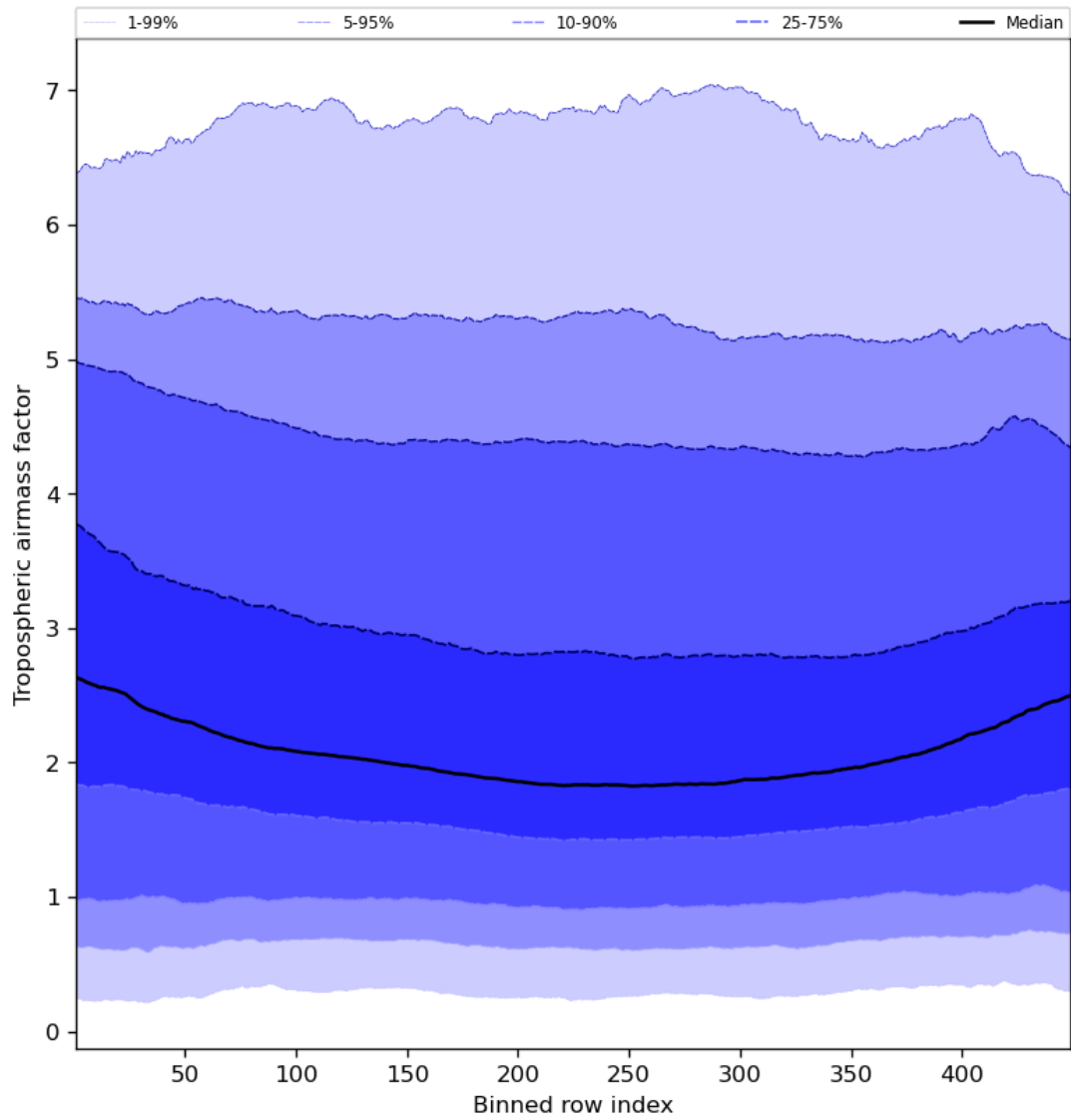
Figure 48: Along track statistics of “Tropospheric airmass factor” for 2023-12-05 to 2023-12-07
