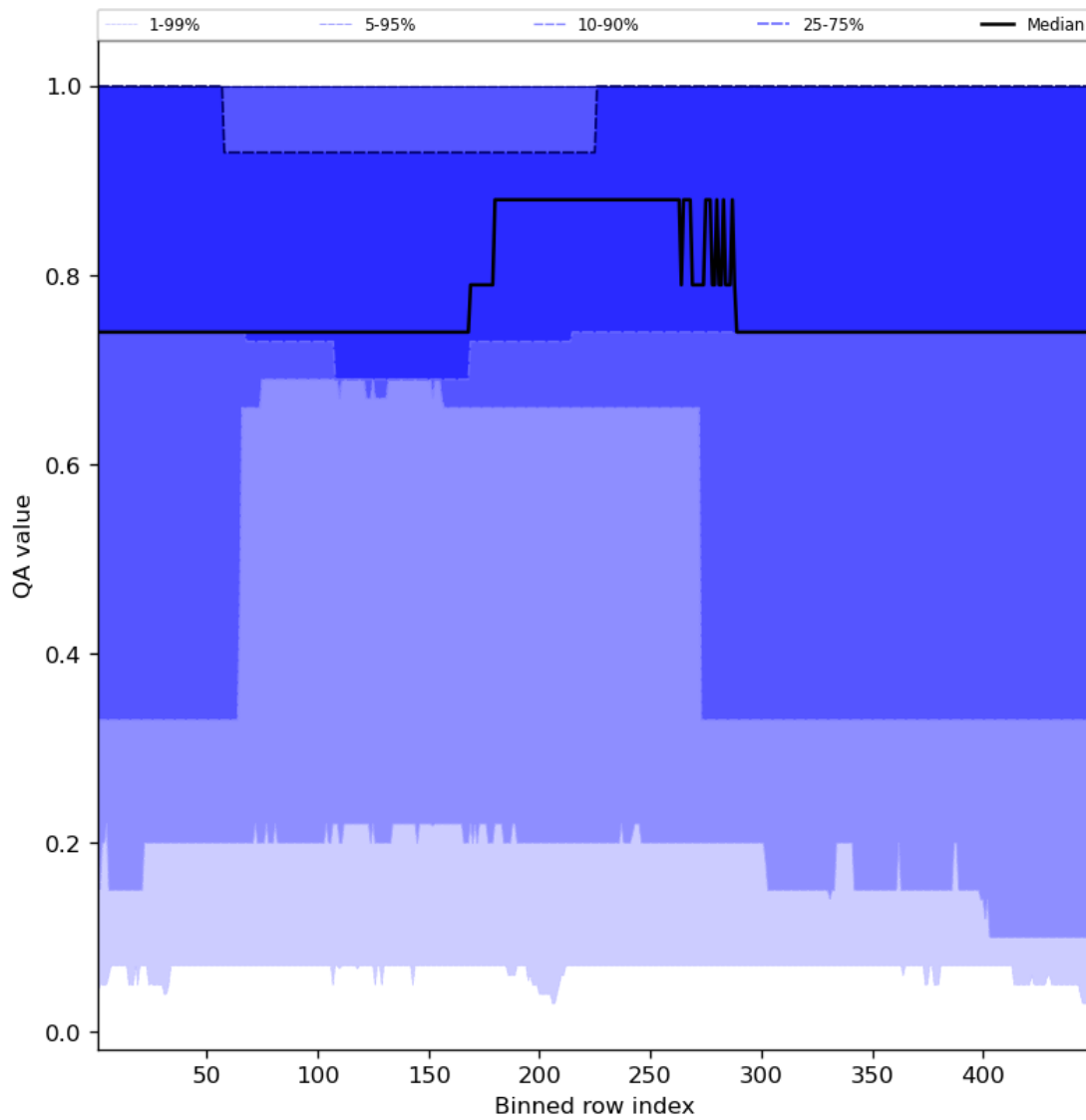
Figure 45: Along track statistics of “QA value” for 2023-12-05 to 2023-12-07
