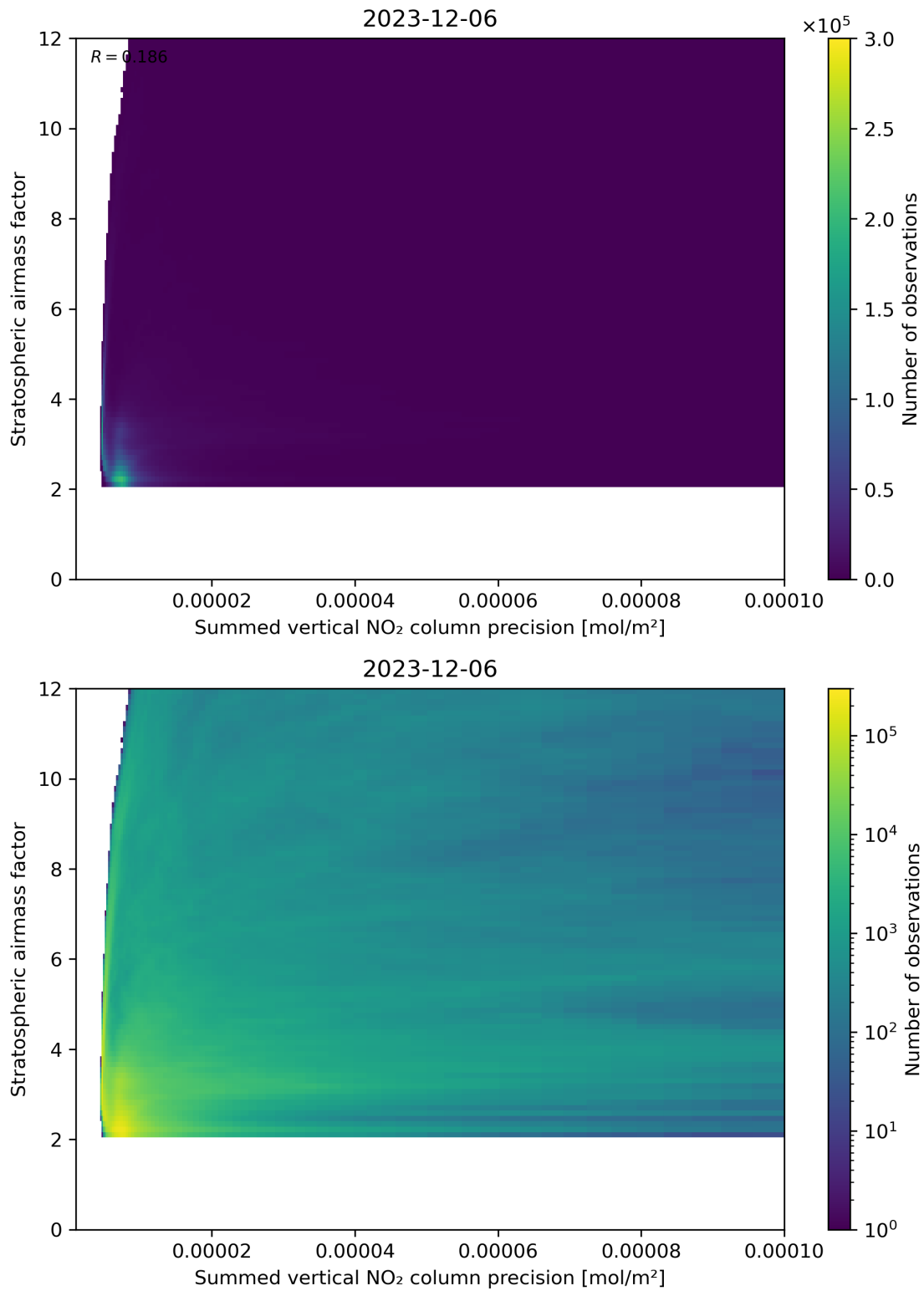
Figure 106: Scatter density plot of “Summed vertical NO 2 column precision” against “Stratospheric airmass factor” for 2023-12-05 to 2023-12-07.
