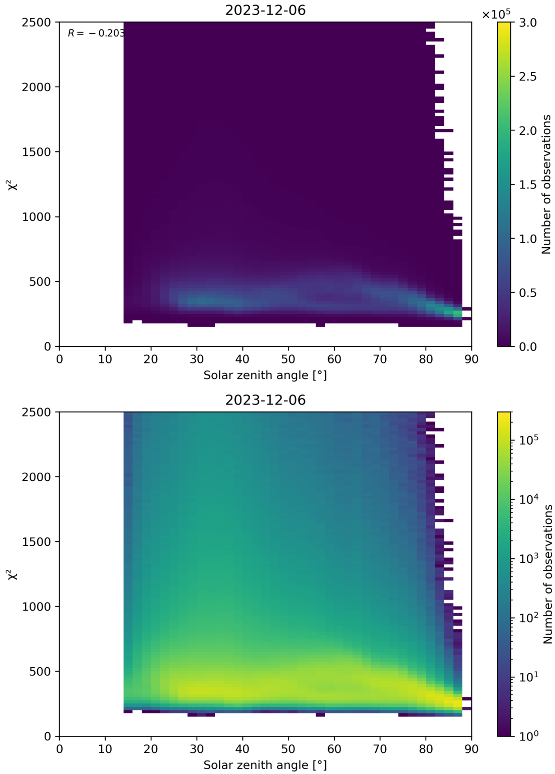
Figure 148: Scatter density plot of “Solar zenith angle” against “ \chi^2 ” for 2023-12-05 to 2023-12-07.
