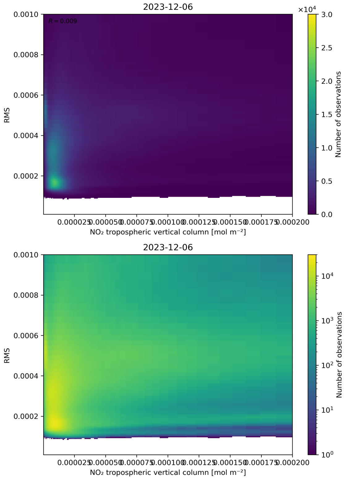
Figure 142: Scatter density plot of “NO 2 tropospheric vertical column” against “RMS” for 2023-12-05 to 2023-12-07.
