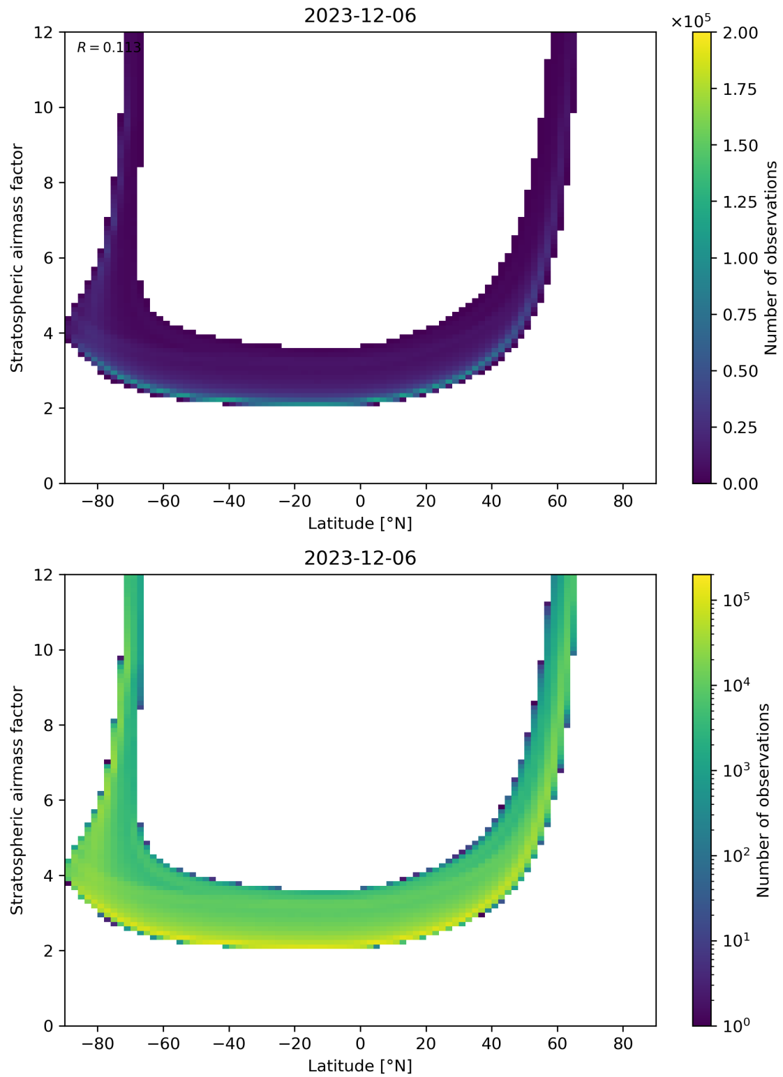
Figure 83: Scatter density plot of “Latitude” against “Stratospheric air mass factor” for 2023-12-05 to 2023-12-07.
