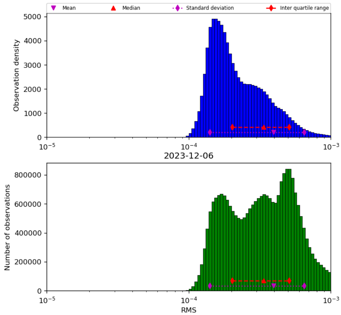
Figure 43: Histogram of “RMS” for 2023-12-05 to 2023-12-07
