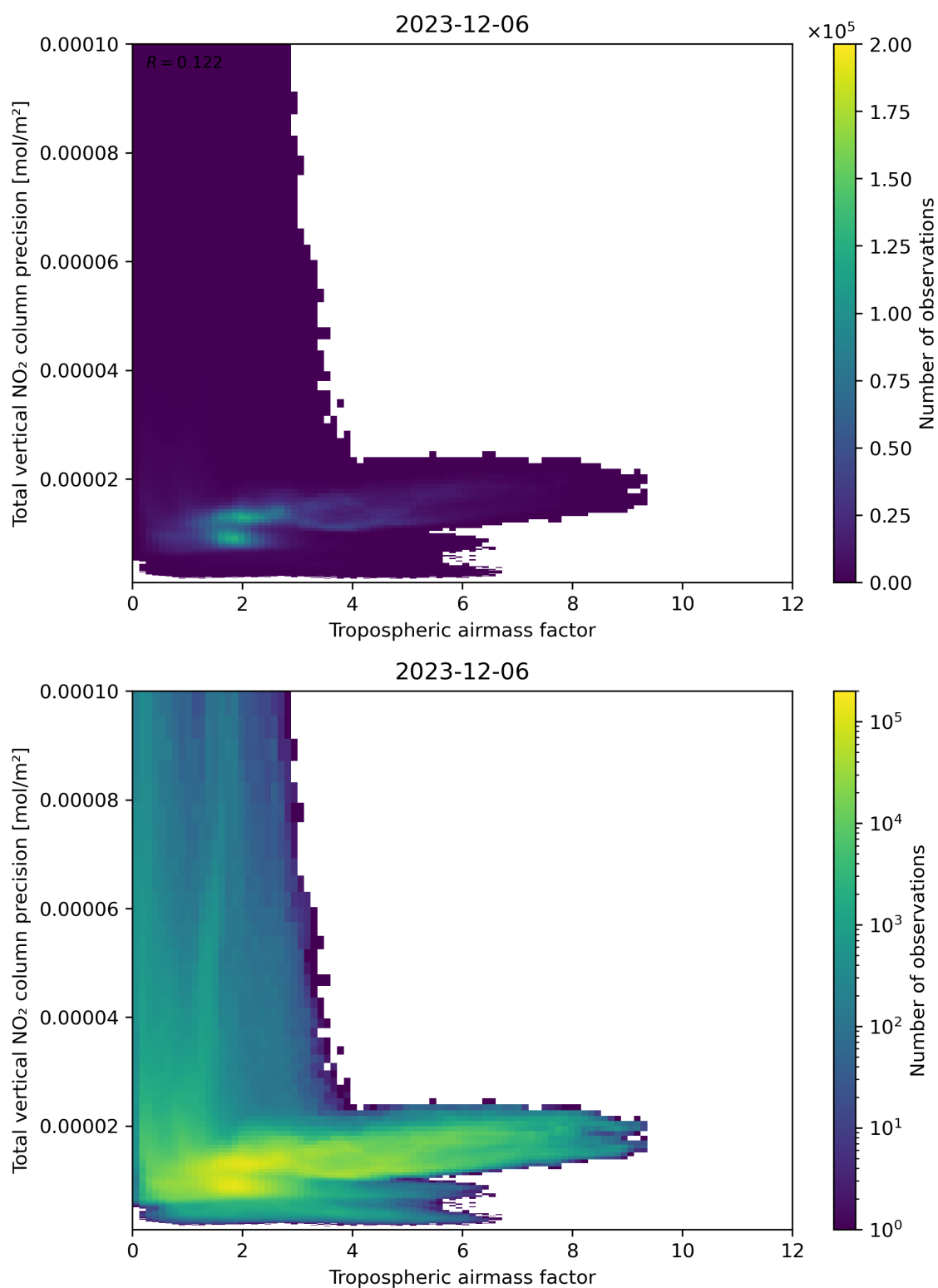
Figure 78: Scatter density plot of “Tropospheric air mass factor” against “Total vertical NO 2 column precision” for 2023-12-05 to 2023-12-07.
