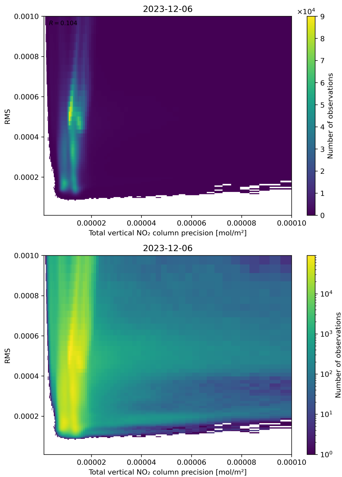
Figure 119: Scatter density plot of “Total vertical NO 2 column precision” against “RMS” for 2023-12-05 to 2023-12-07.
