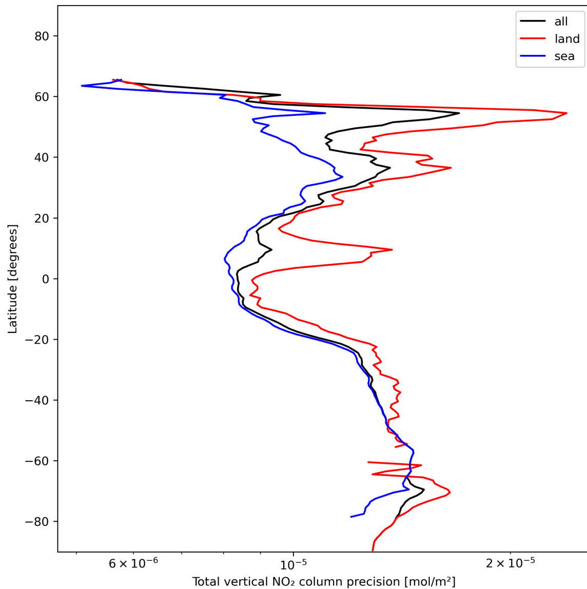
Figure 22: Zonal average of “Total vertical NO 2 column precision” for 2023-12-05 to 2023-12-07.
