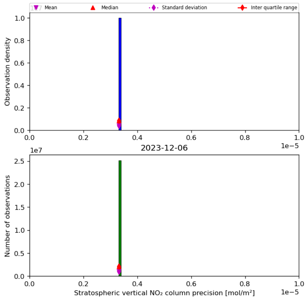
Figure 37: Histogram of “Stratospheric vertical NO 2 column precision” for 2023-12-05 to 2023-12-07
