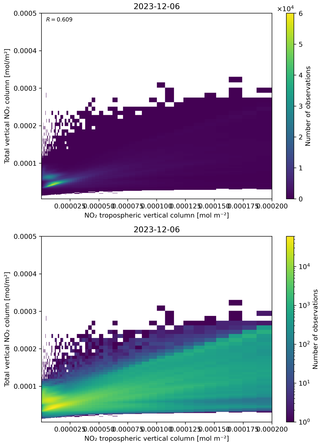
Figure 128: Scatter density plot of “NO 2 tropospheric vertical column” against “Total vertical NO 2 column” for 2023-12-05 to 2023-12-07.
