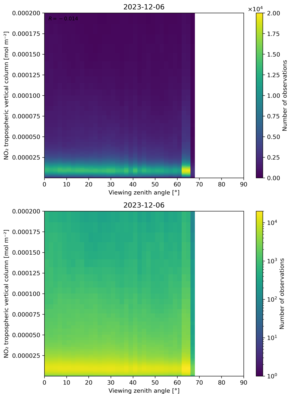
Figure 169: Scatter density plot of “Viewing zenith angle” against “NO 2 tropospheric vertical column” for 2023-12-05 to 2023-12-07.
