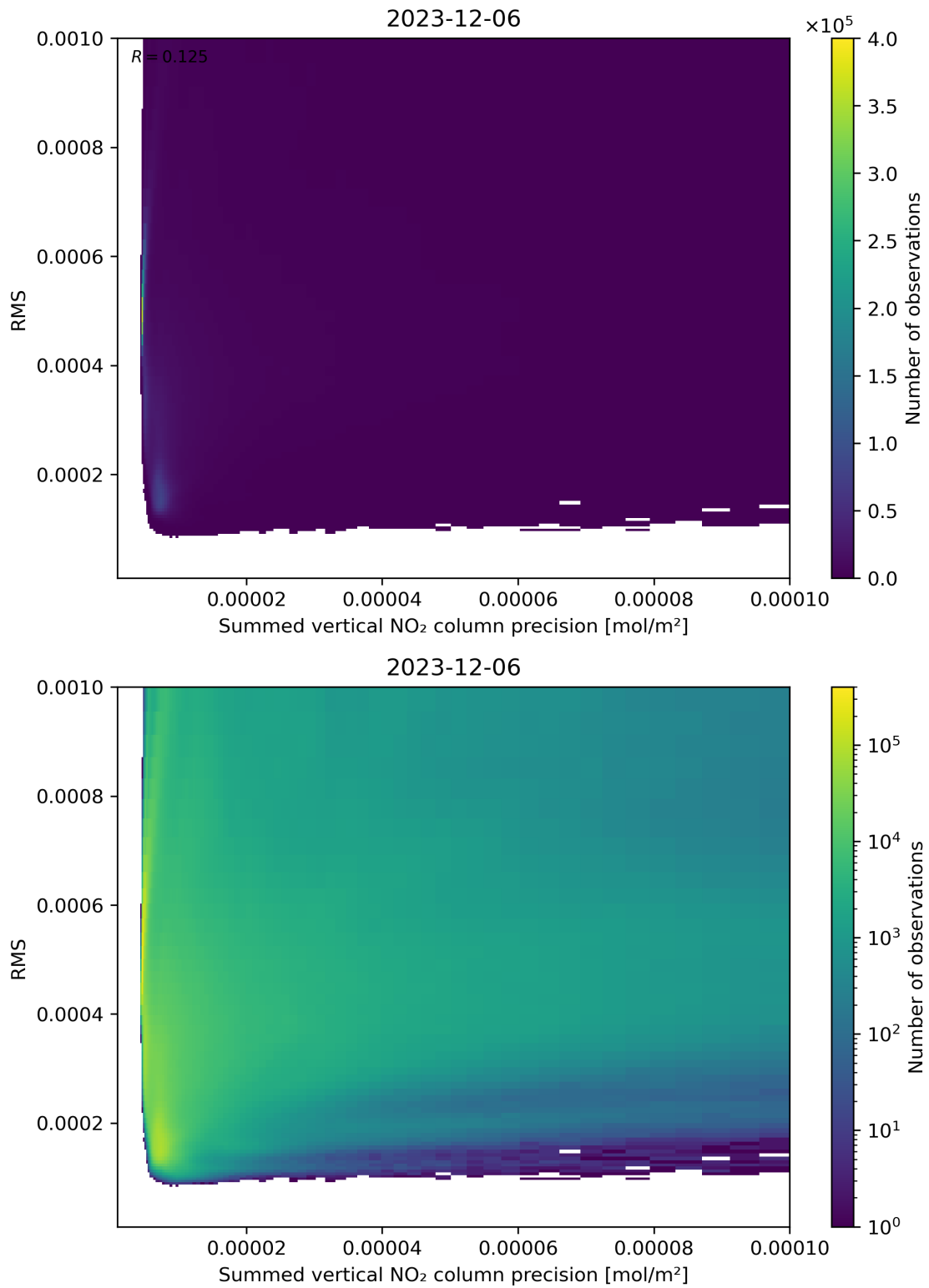
Figure 108: Scatter density plot of “Summed vertical NO 2 column precision” against “RMS” for 2023-12-05 to 2023-12-07.
