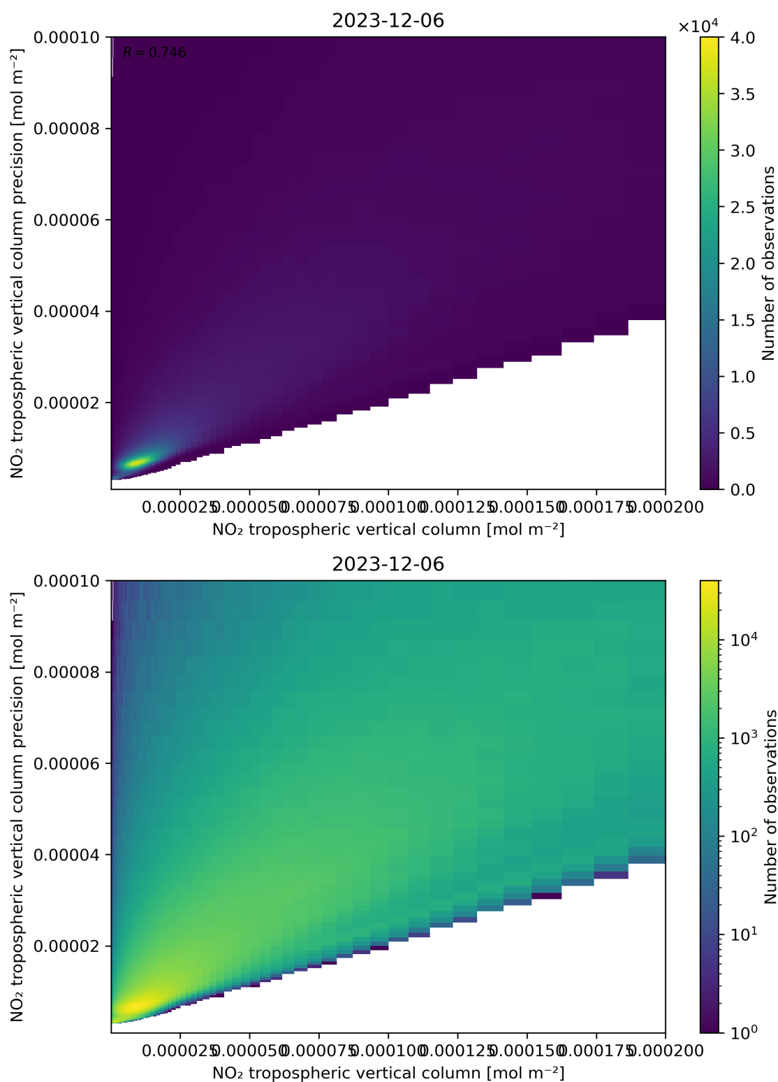
Figure 130: Scatter density plot of “NO 2 tropospheric vertical column” against “NO 2 tropospheric vertical column precision” for 2023-12-05 to 2023-12-07.
