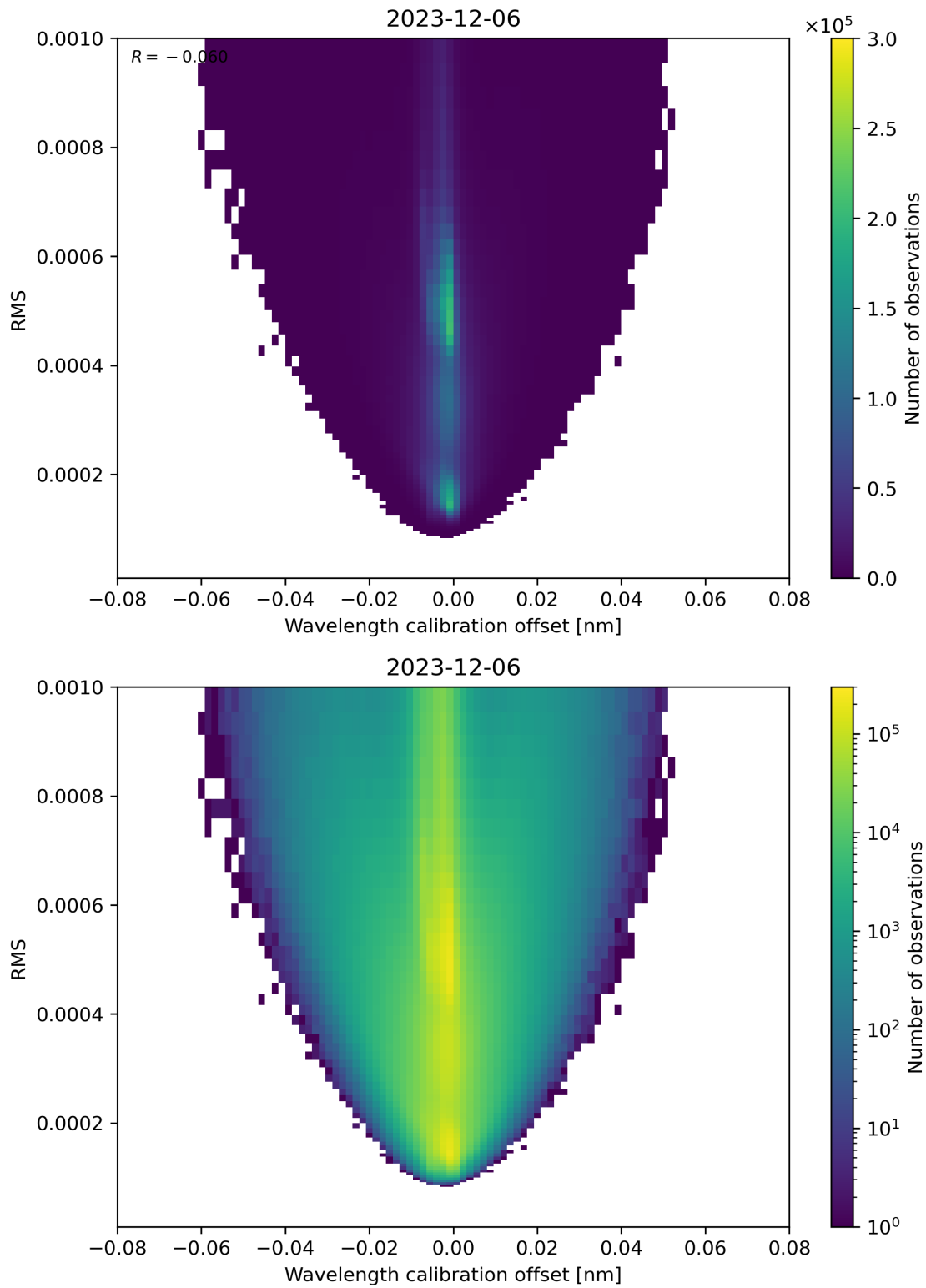
Figure 181: Scatter density plot of “Wavelength calibration offset” against “RMS” for 2023-12-05 to 2023-12-07.
