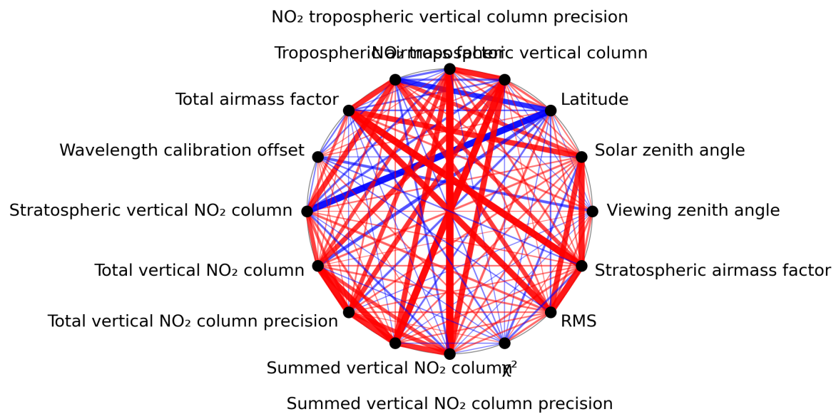
Figure 1: Map of correlation graph for 2023-12-05 to 2023-12-07.
