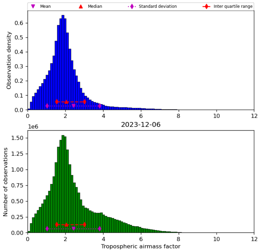
Figure 31: Histogram of “Tropospheric airmass factor” for 2023-12-05 to 2023-12-07
