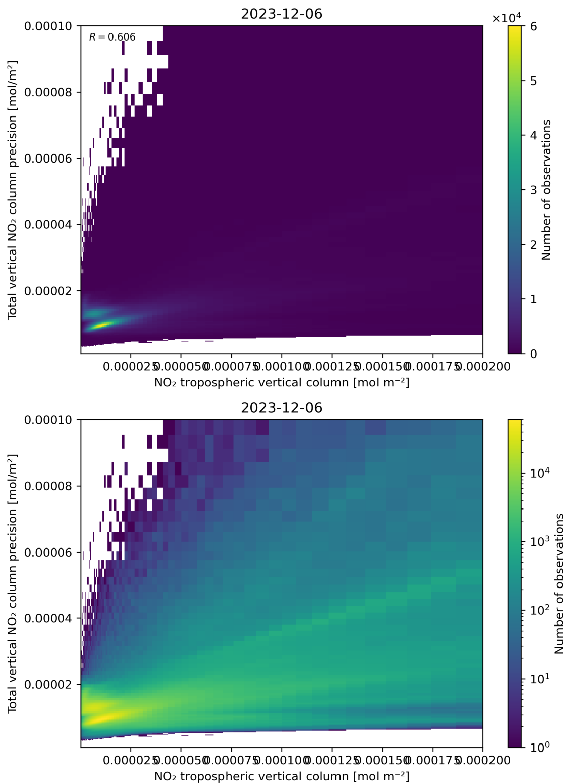
Figure 129: Scatter density plot of “NO 2 tropospheric vertical column” against “Total vertical NO 2 column precision” for 2023-12-05 to 2023-12-07.
