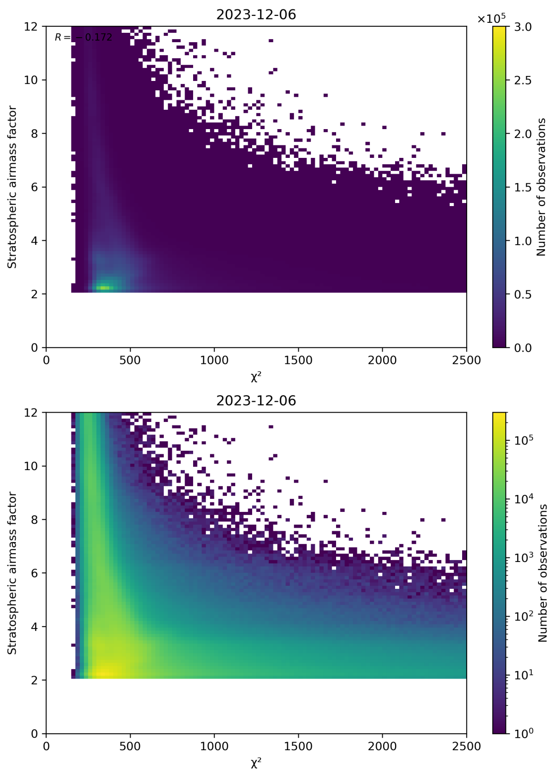
Figure 81: Scatter density plot of “ \chi^2 ” against “Stratospheric airmass factor” for 2023-12-05 to 2023-12-07.
