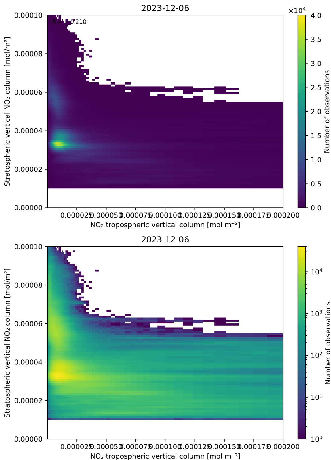
Figure 125: Scatter density plot of “NO 2 tropospheric vertical column” against “Stratospheric vertical NO 2 column” for 2023-12-05 to 2023-12-07.
