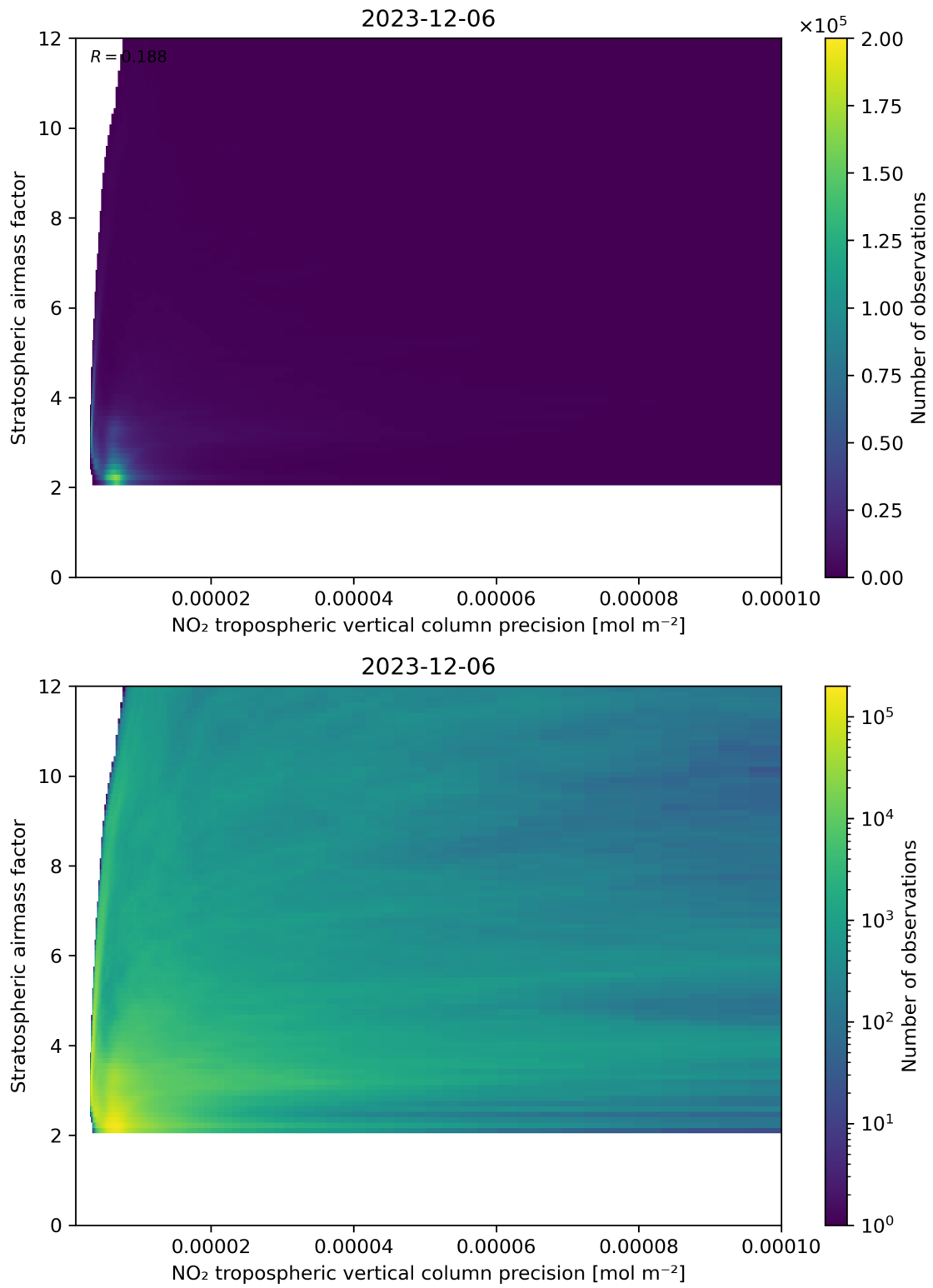
Figure 131: Scatter density plot of “NO 2 tropospheric vertical column precision” against “Stratospheric airmass factor” for 2023-12-05 to 2023-12-07.
