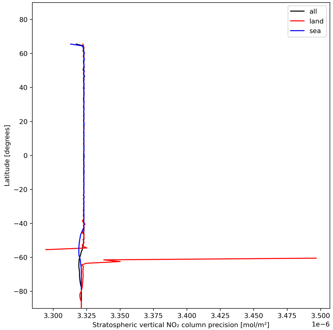
Figure 20: Zonal average of "Stratospheric vertical NO 2 column precision" for 2023-12-05 to 2023-12-07.
