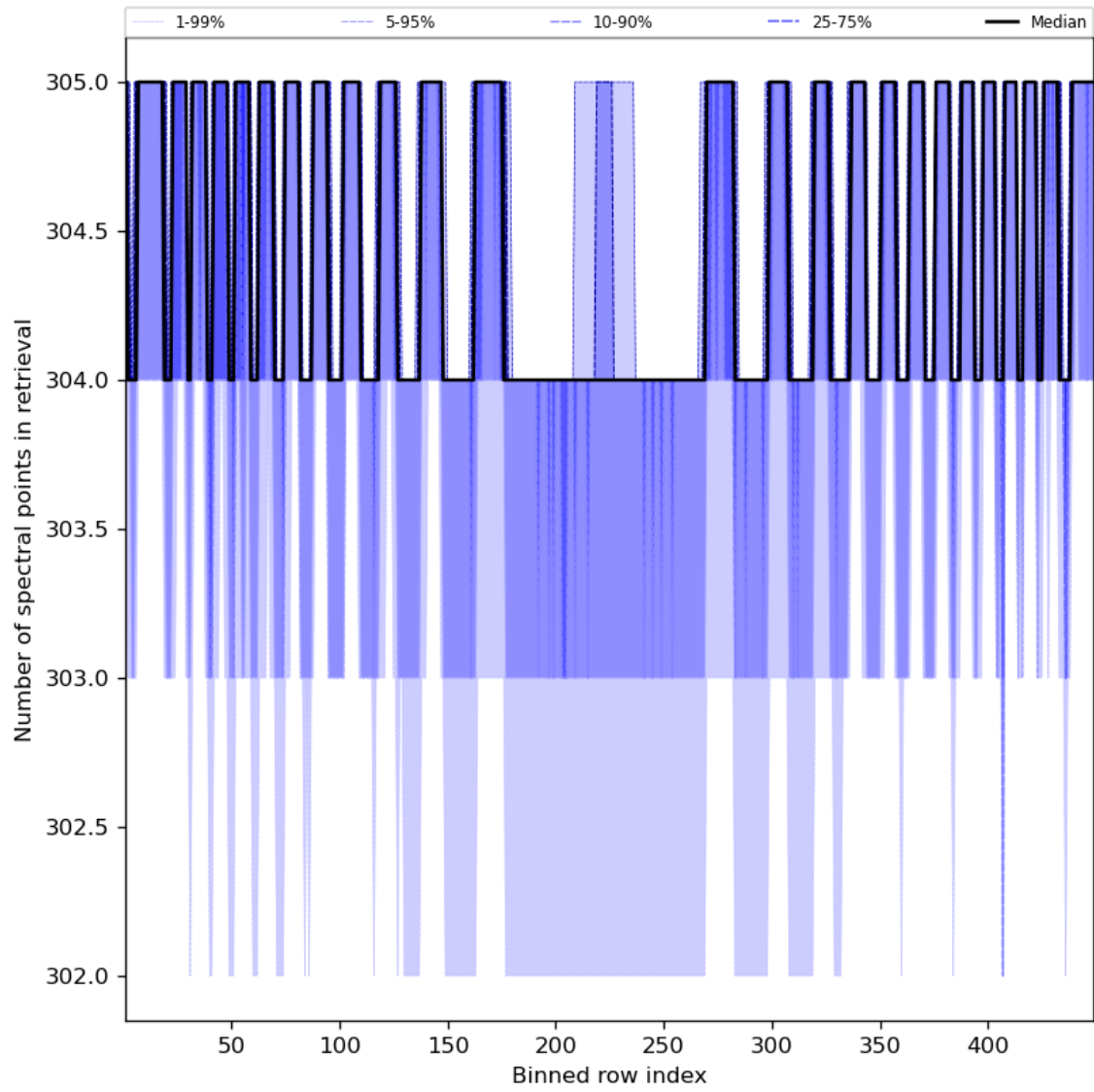
Figure 50: Along track statistics of “Number of spectral points in retrieval” for 2023-12-05 to 2023-12-07
