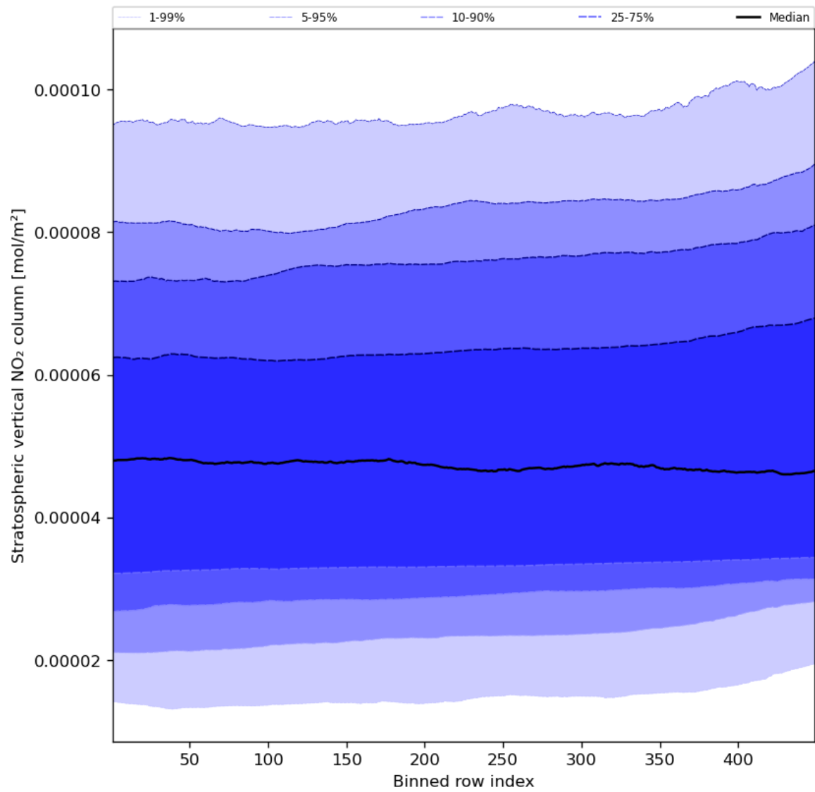
Figure 53: Along track statistics of “Stratospheric vertical NO 2 column” for 2023-12-05 to 2023-12-07
