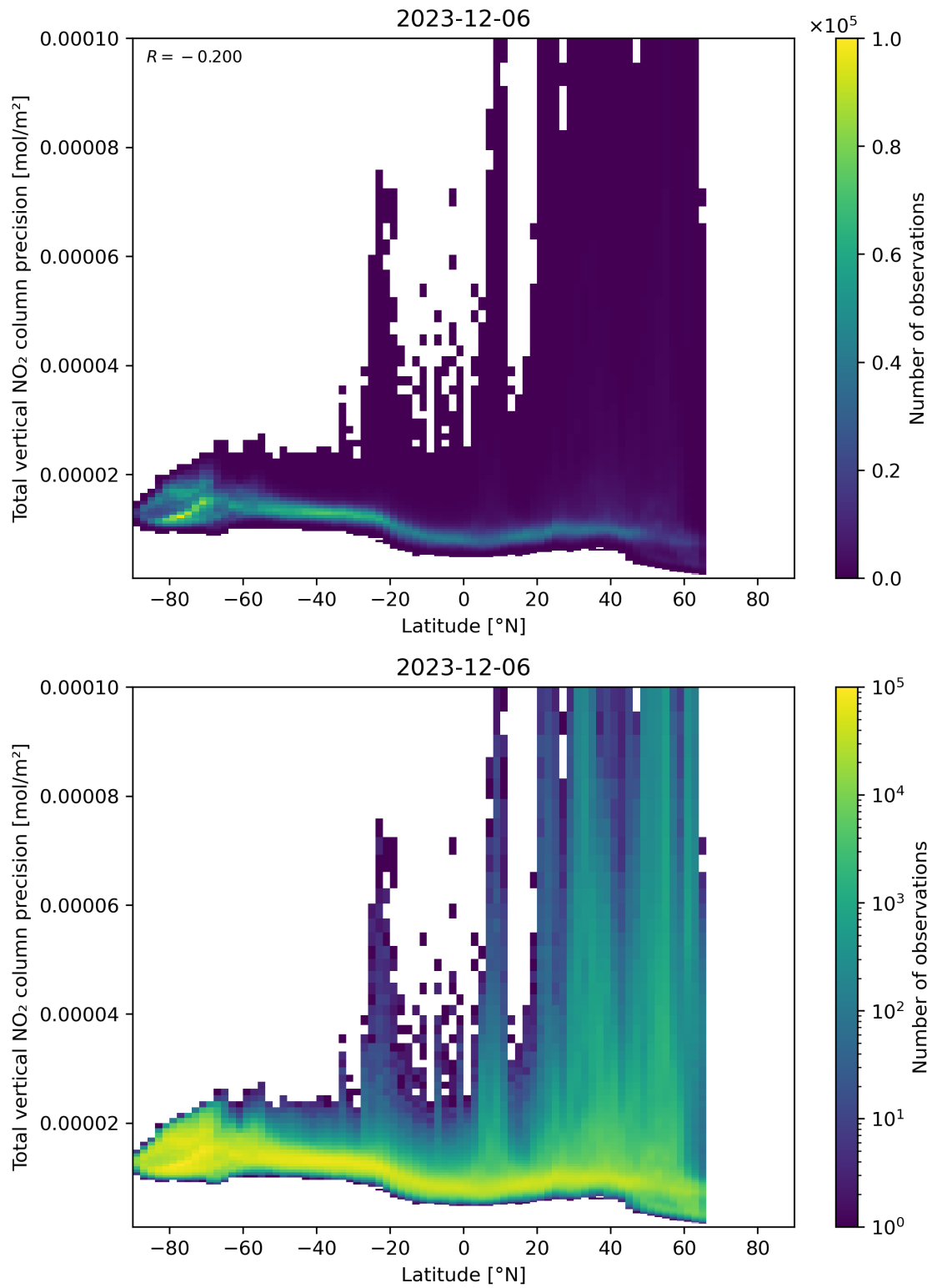
Figure 91: Scatter density plot of “Latitude” against “Total vertical NO 2 column precision” for 2023-12-05 to 2023-12-07.
