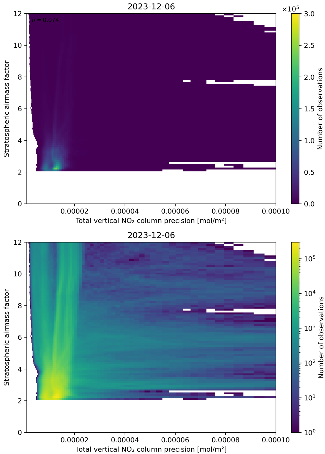
Figure 115: Scatter density plot of “Total vertical NO 2 column precision” against “Stratospheric air mass factor” for 2023-12-05 to 2023-12-07.
