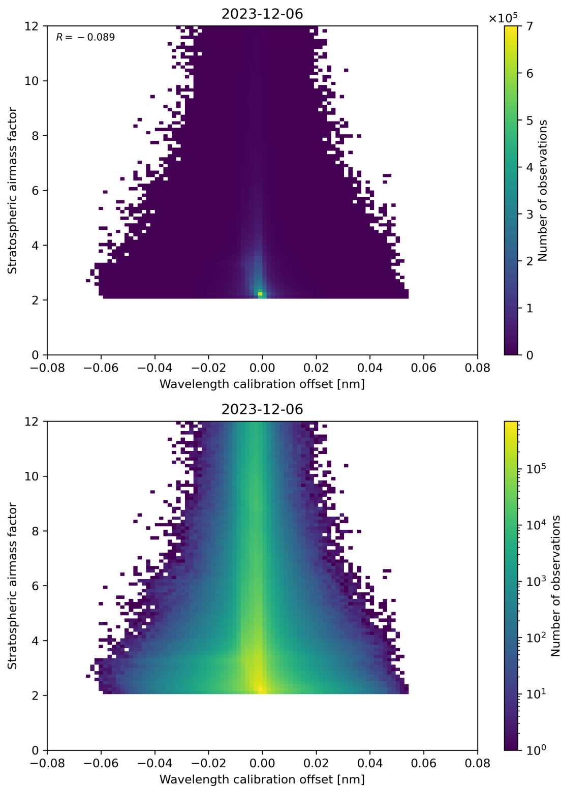
Figure 174: Scatter density plot of “Wavelength calibration offset” against “Stratospheric airmass factor” for 2023-12-05 to 2023-12-07.
