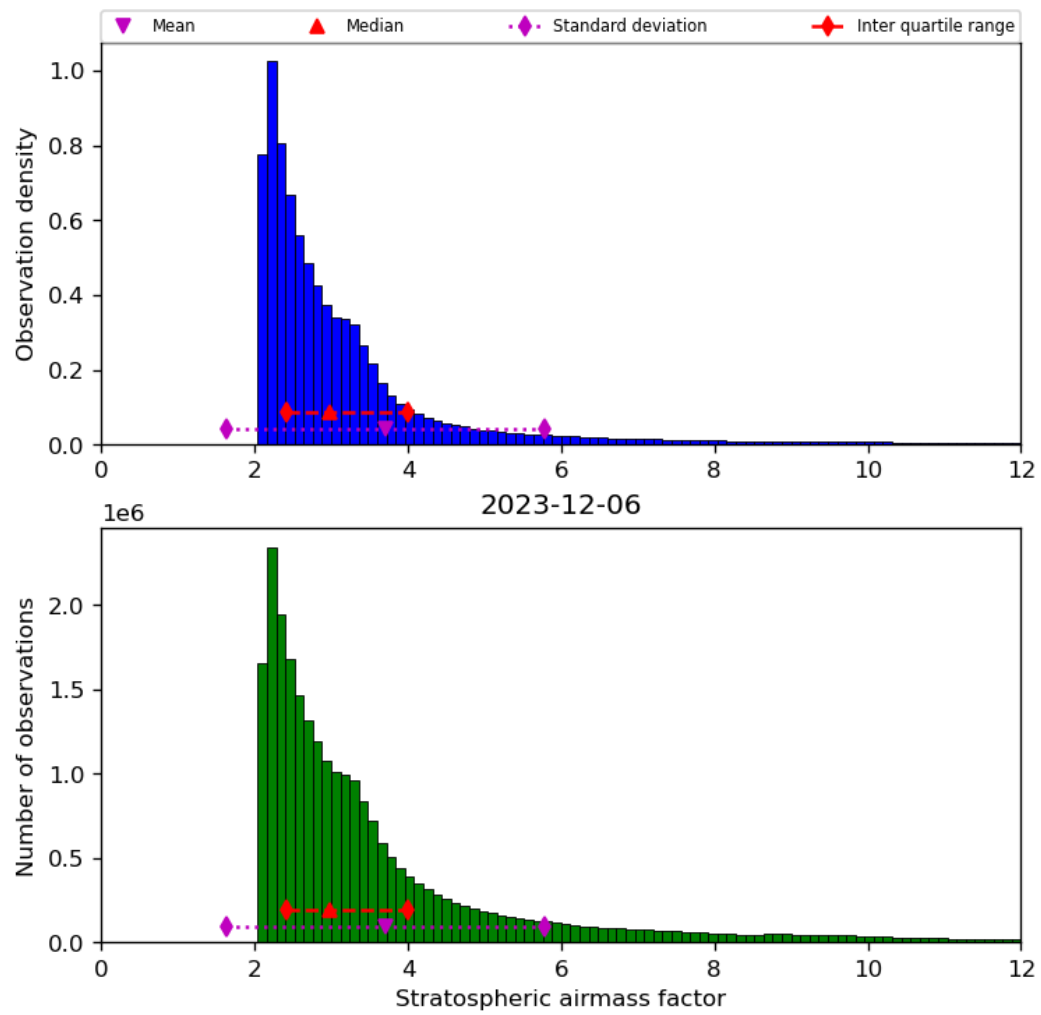
Figure 44: Histogram of “Stratospheric airmass factor” for 2023-12-05 to 2023-12-07
