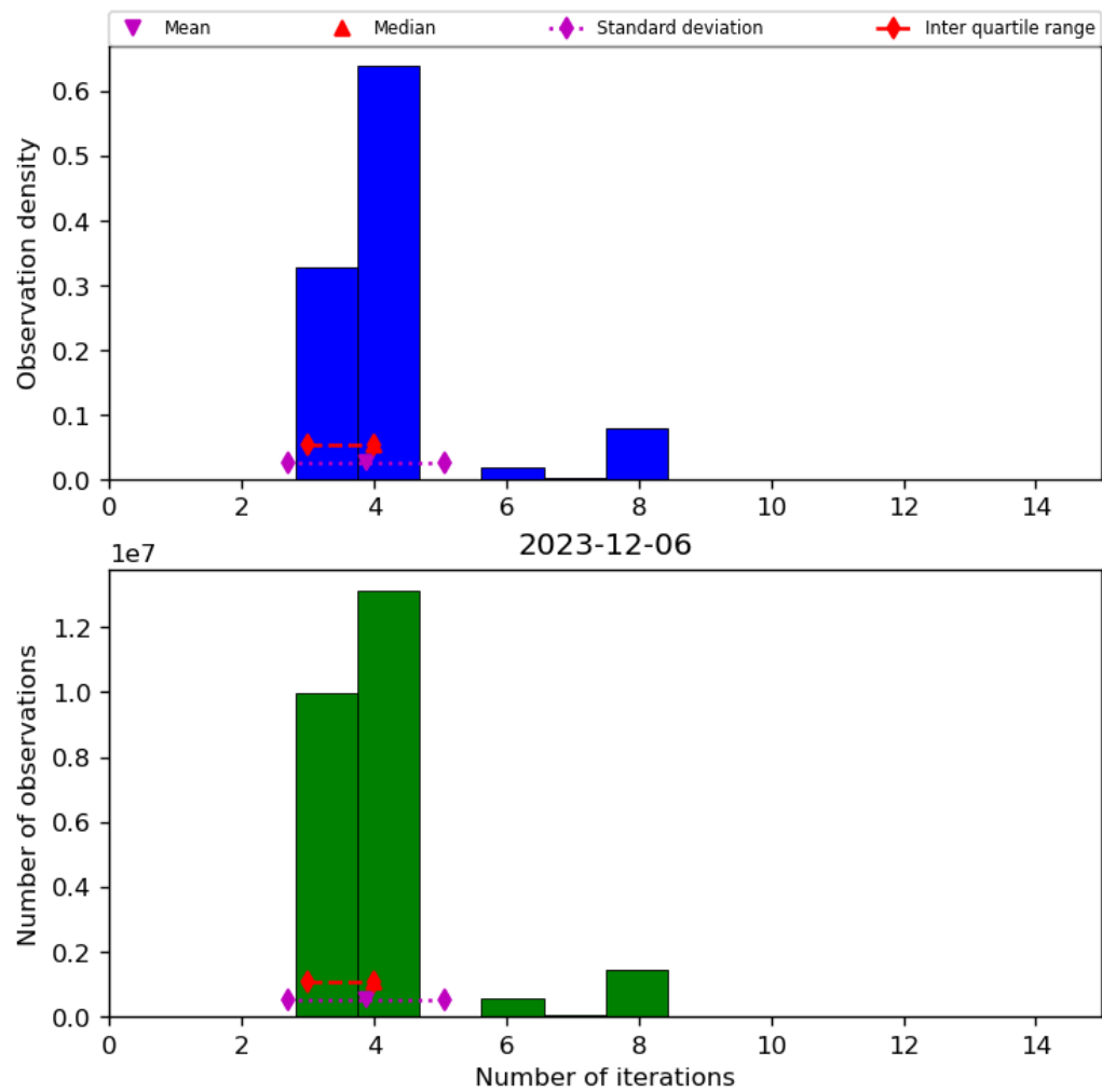
Figure 34: Histogram of “Number of iterations” for 2023-12-05 to 2023-12-07
