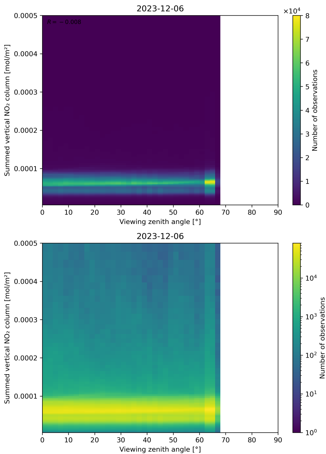
Figure 165: Scatter density plot of “Viewing zenith angle” against “Summed vertical NO 2 column” for 2023-12-05 to 2023-12-07.
