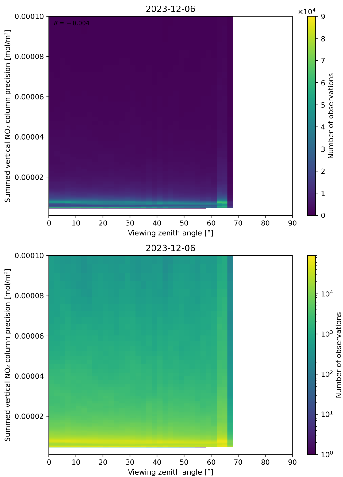
Figure 166: Scatter density plot of “Viewing zenith angle” against “Summed vertical NO 2 column precision” for 2023-12-05 to 2023-12-07.
