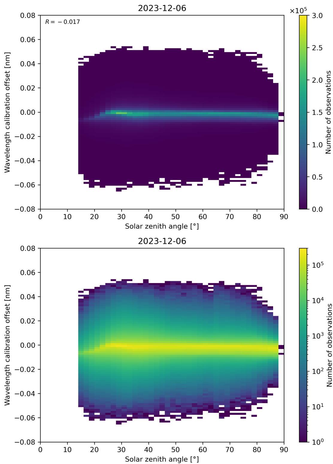
Figure 158: Scatter density plot of “Solar zenith angle” against “Wavelength calibration offset” for 2023-12-05 to 2023-12-07.
