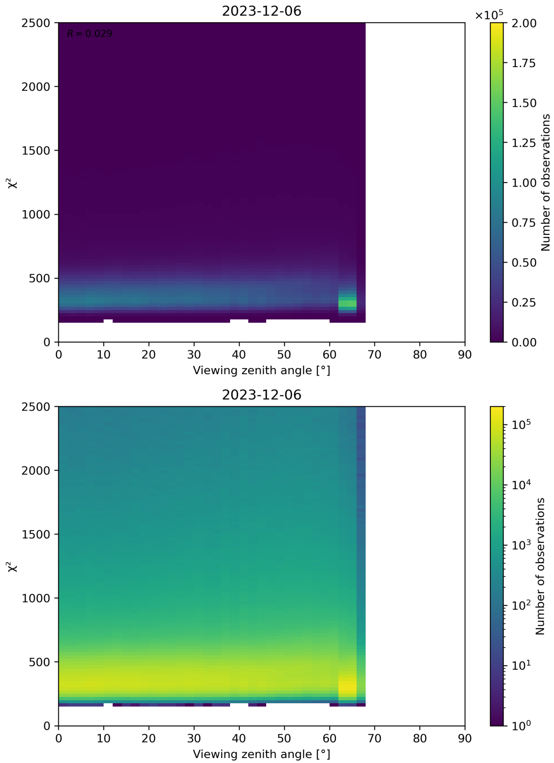
Figure 162: Scatter density plot of “Viewing zenith angle” against “ \chi^2 ” for 2023-12-05 to 2023-12-07.
