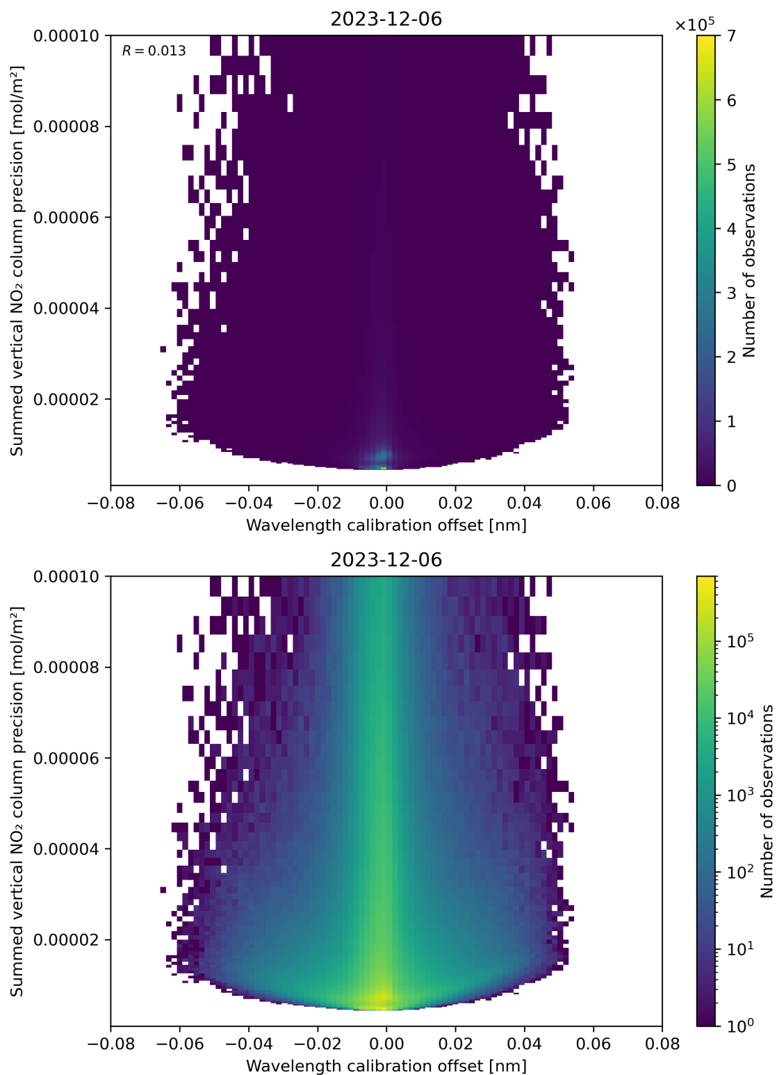
Figure 178: Scatter density plot of “Wavelength calibration offset” against “Summed vertical NO 2 column precision” for 2023-12-05 to 2023-12-07.
