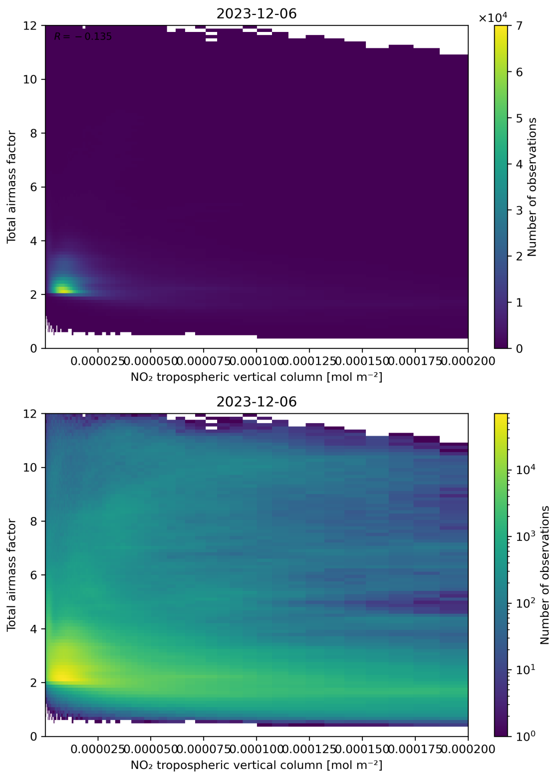
Figure 122: Scatter density plot of “NO 2 tropospheric vertical column” against “Total air mass factor” for 2023-12-05 to 2023-12-07.
