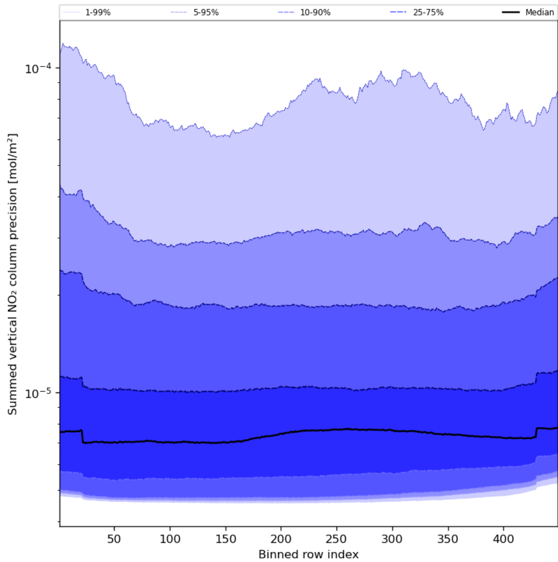
Figure 58: Along track statistics of “Summed vertical NO 2 column precision” for 2023-12-05 to 2023-12-07
