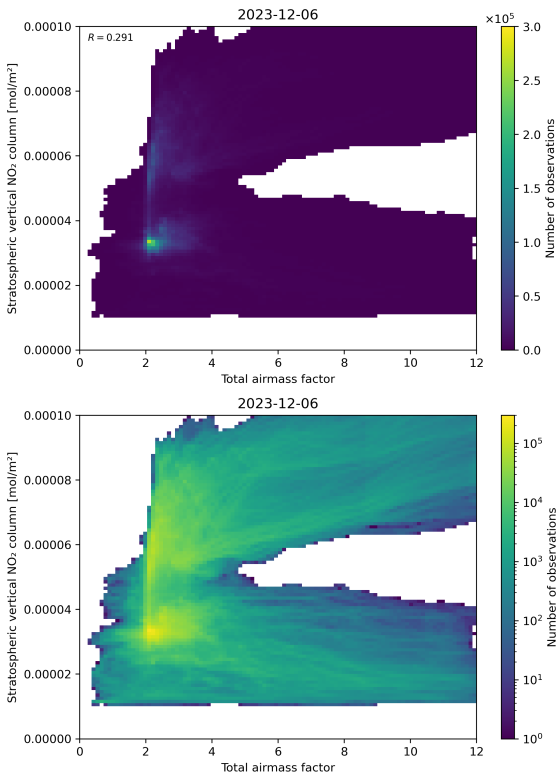
Figure 64: Scatter density plot of “Total airmass factor” against “Stratospheric vertical \text{NO}_2 column” for 2023-12-05 to 2023-12-07.
