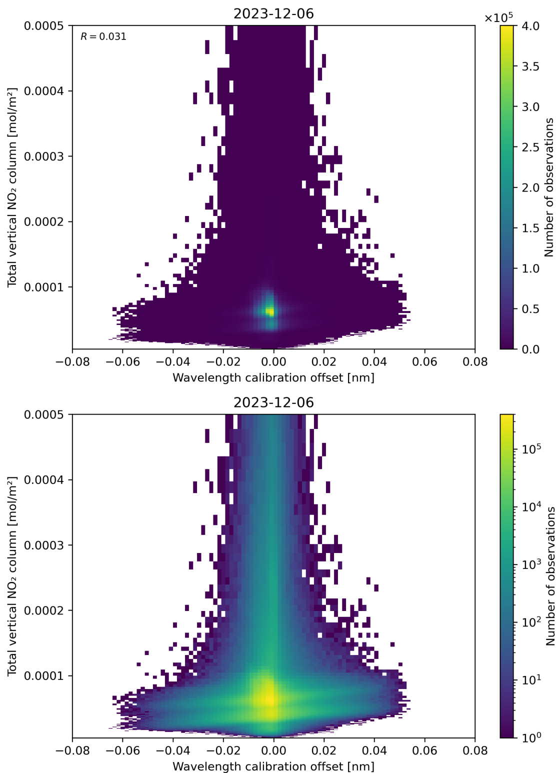
Figure 179: Scatter density plot of “Wavelength calibration offset” against “Total vertical NO 2 column” for 2023-12-05 to 2023-12-07.
