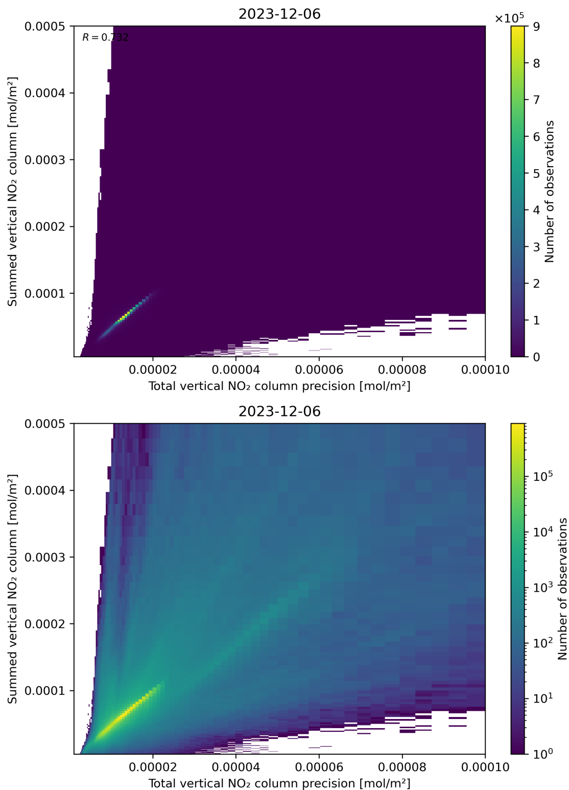
Figure 117: Scatter density plot of “Total vertical NO 2 column precision” against “Summed vertical NO 2 column” for 2023-12-05 to 2023-12-07.
