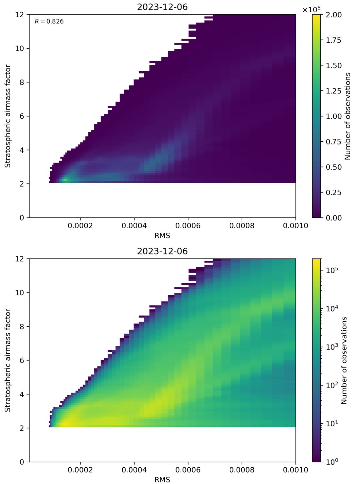
Figure 144: Scatter density plot of “RMS” against “Stratospheric airmass factor” for 2023-12-05 to 2023-12-07.
