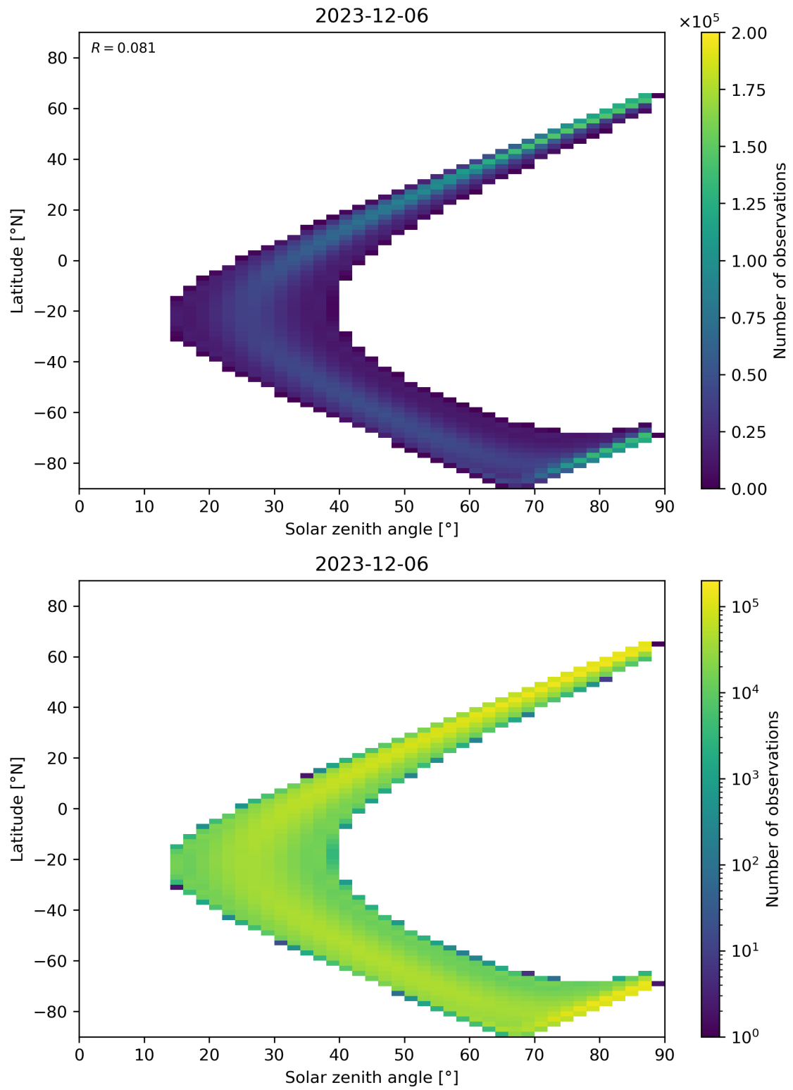
Figure 149: Scatter density plot of “Solar zenith angle” against “Latitude” for 2023-12-05 to 2023-12-07.
