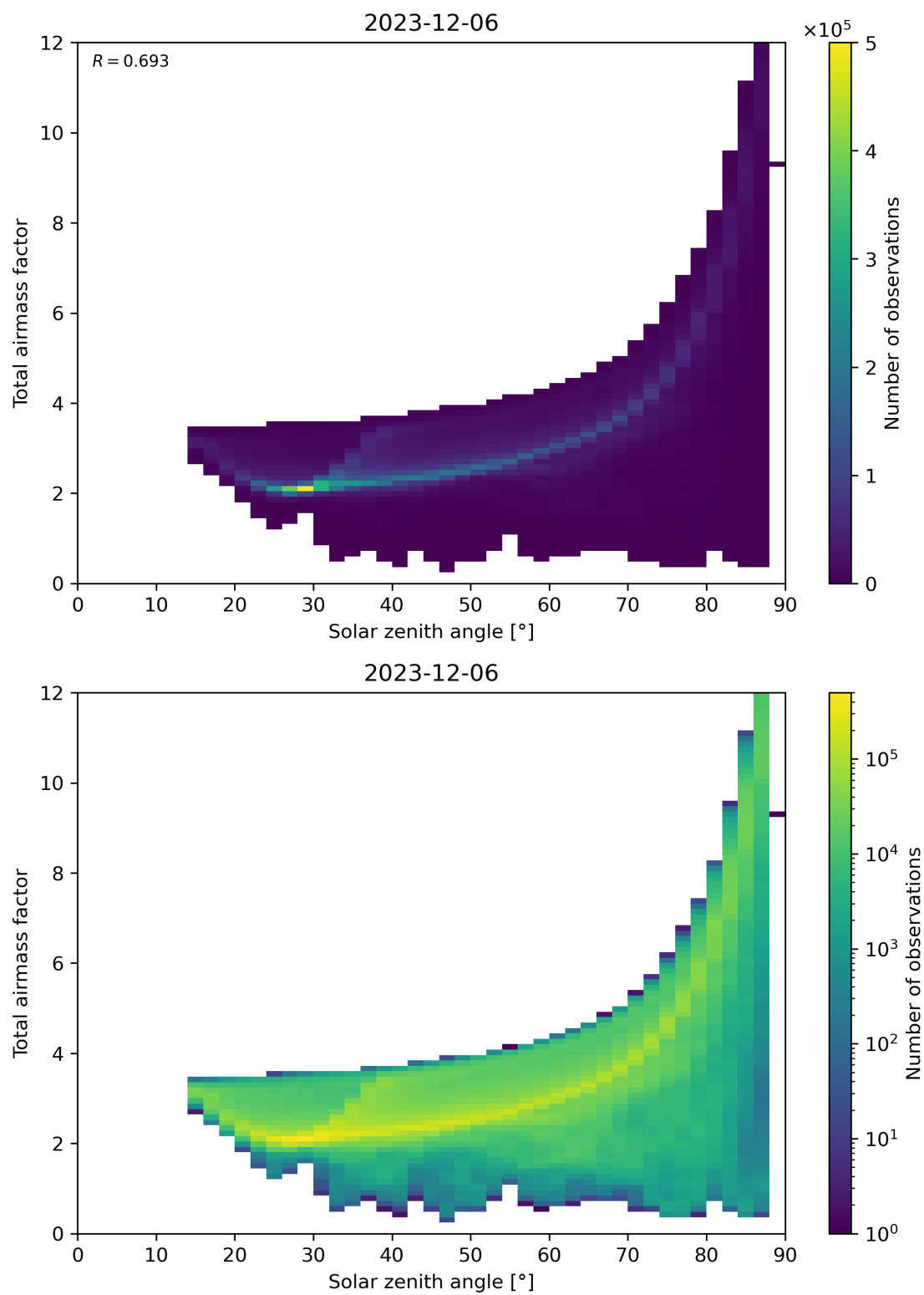
Figure 146: Scatter density plot of “Solar zenith angle” against “Total air mass factor” for 2023-12-05 to 2023-12-07.
