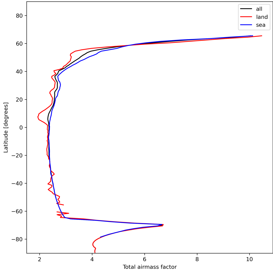
Figure 15: Zonal average of “Total airmass factor” for 2023-12-05 to 2023-12-07.
