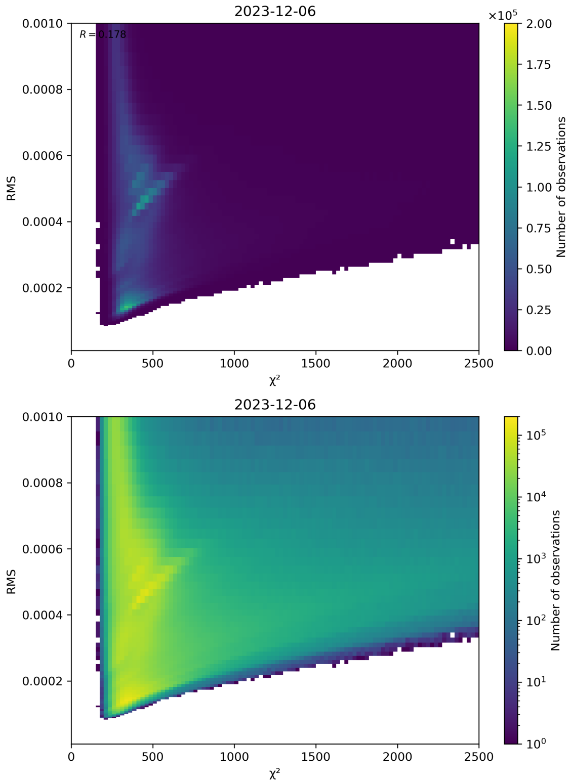
Figure 82: Scatter density plot of “ \chi^2 ” against “RMS” for 2023-12-05 to 2023-12-07.
