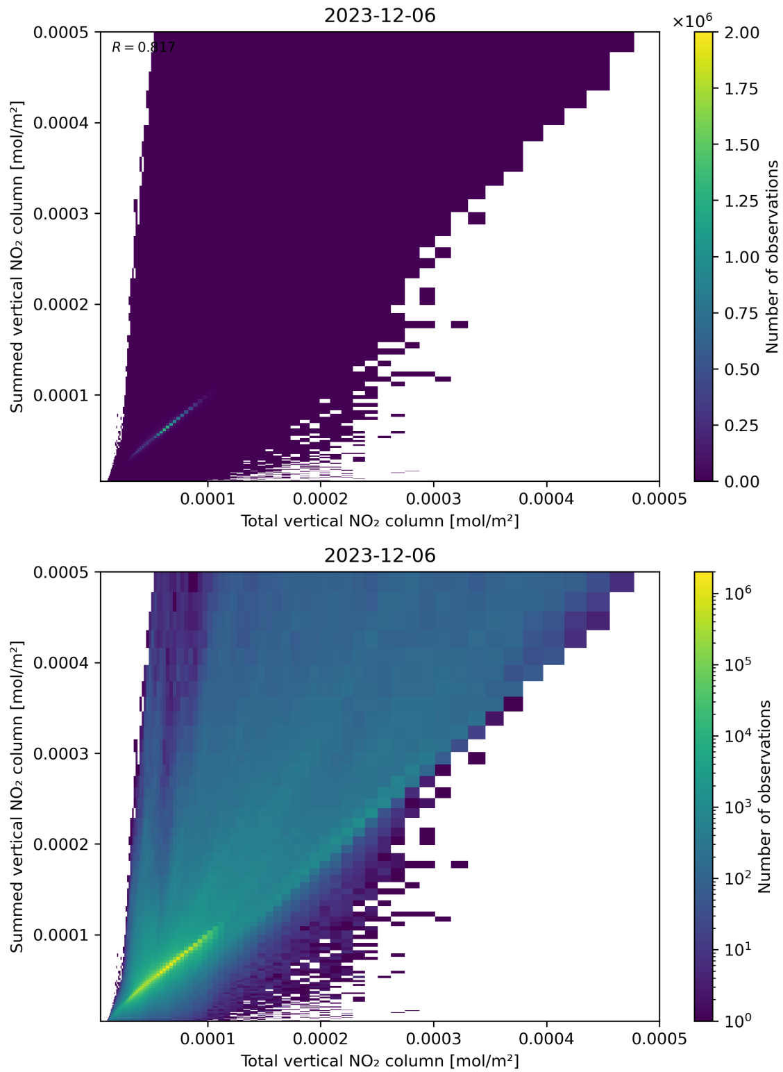
Figure 112: Scatter density plot of “Total vertical NO 2 column” against “Summed vertical NO 2 column” for 2023-12-05 to 2023-12-07.
