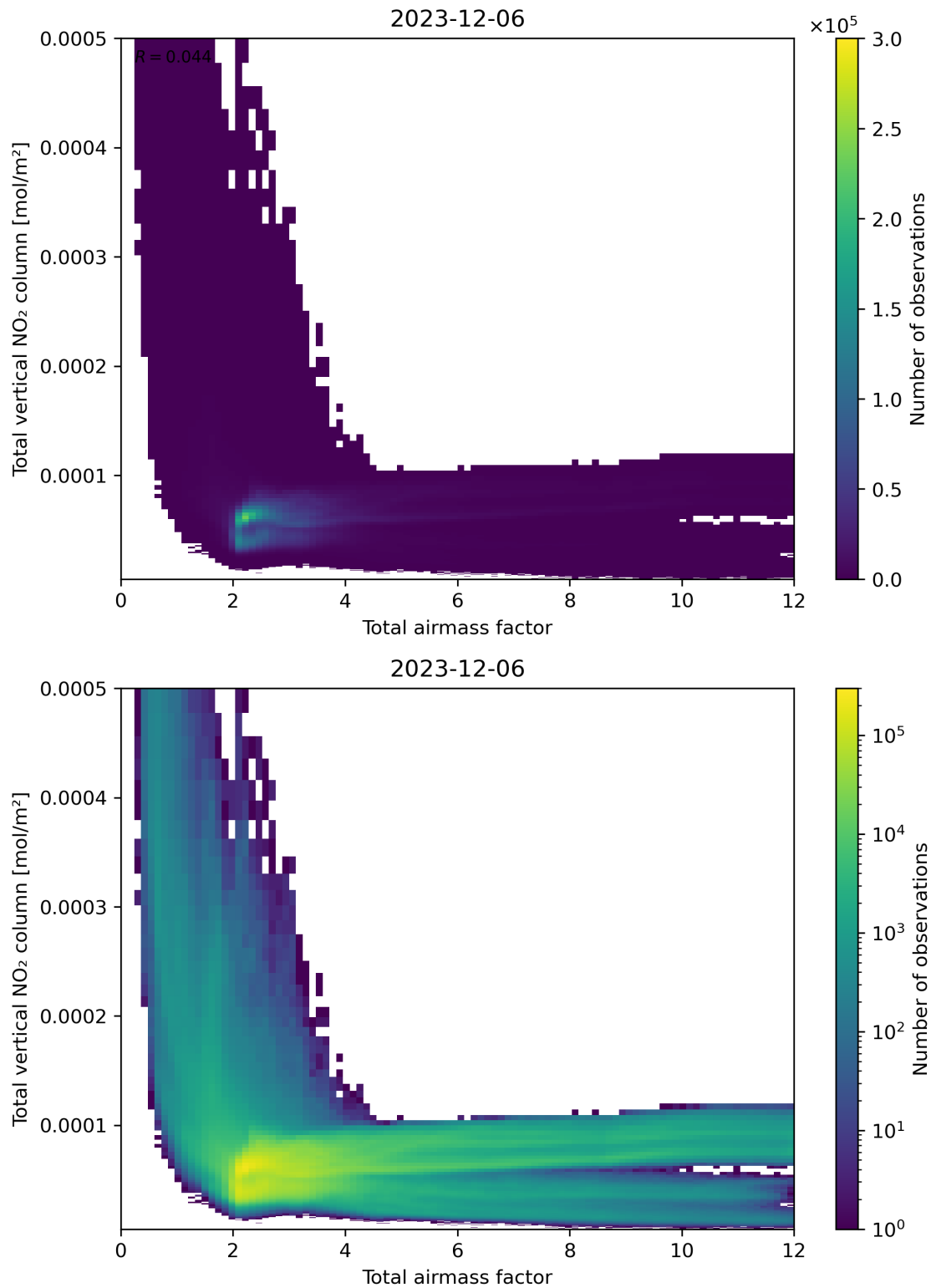
Figure 67: Scatter density plot of “Total airmass factor” against “Total vertical NO 2 column” for 2023-12-05 to 2023-12-07.
