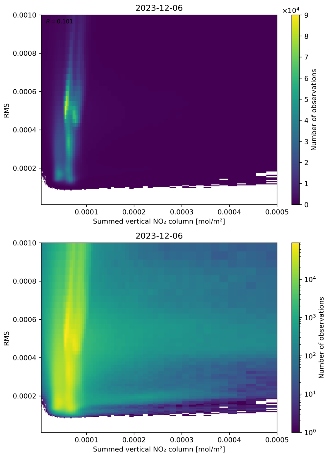
Figure 109: Scatter density plot of “Summed vertical NO 2 column” against “RMS” for 2023-12-05 to 2023-12-07.
