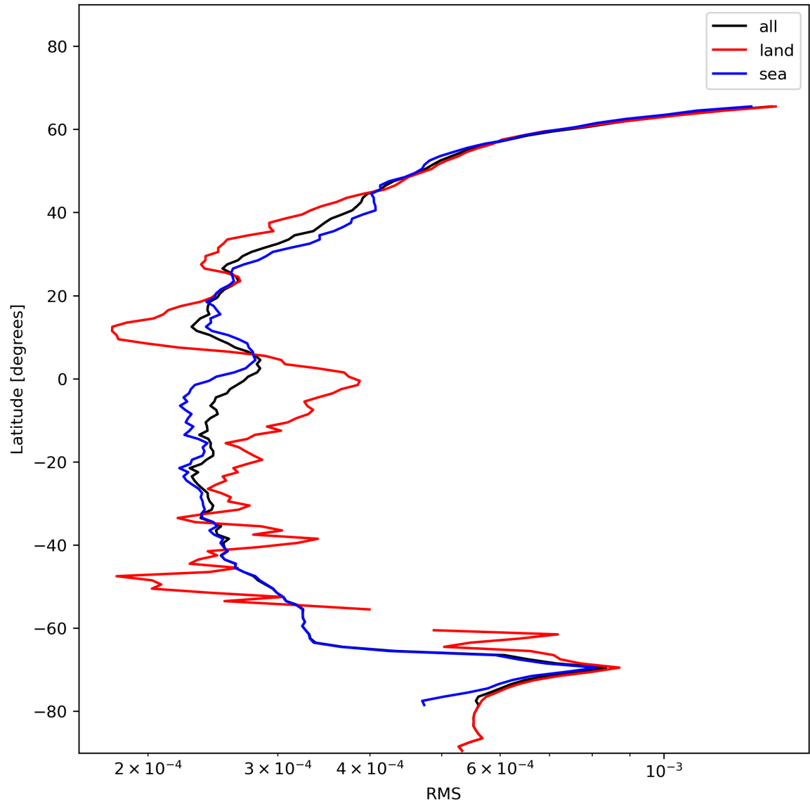
Figure 26: Zonal average of “RMS” for 2023-12-05 to 2023-12-07.
