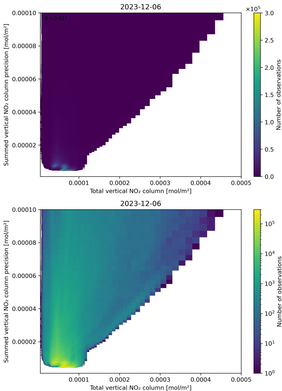
Figure 113: Scatter density plot of “Total vertical NO 2 column” against “Summed vertical NO 2 column precision” for 2023-12-05 to 2023-12-07.
