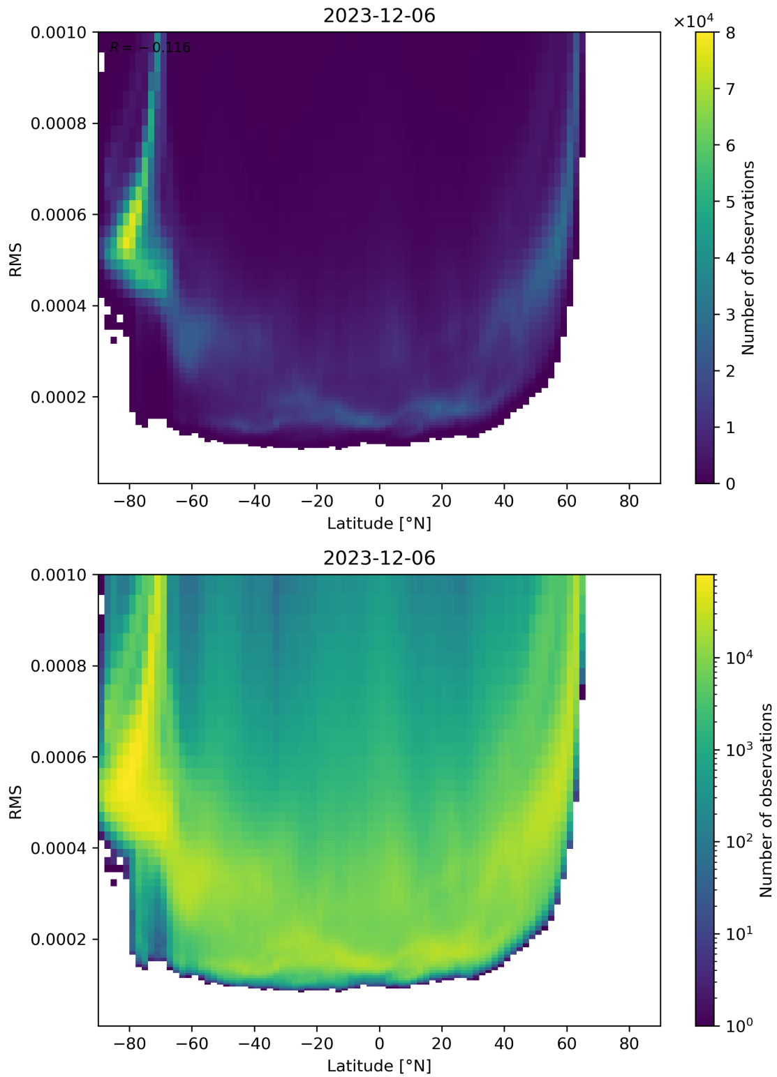
Figure 94: Scatter density plot of “Latitude” against “RMS” for 2023-12-05 to 2023-12-07.
