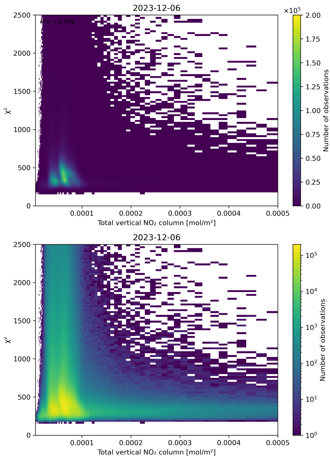
Figure 111: Scatter density plot of “Total vertical NO 2 column” against “ \chi^2 ” for 2023-12-05 to 2023-12-07.
