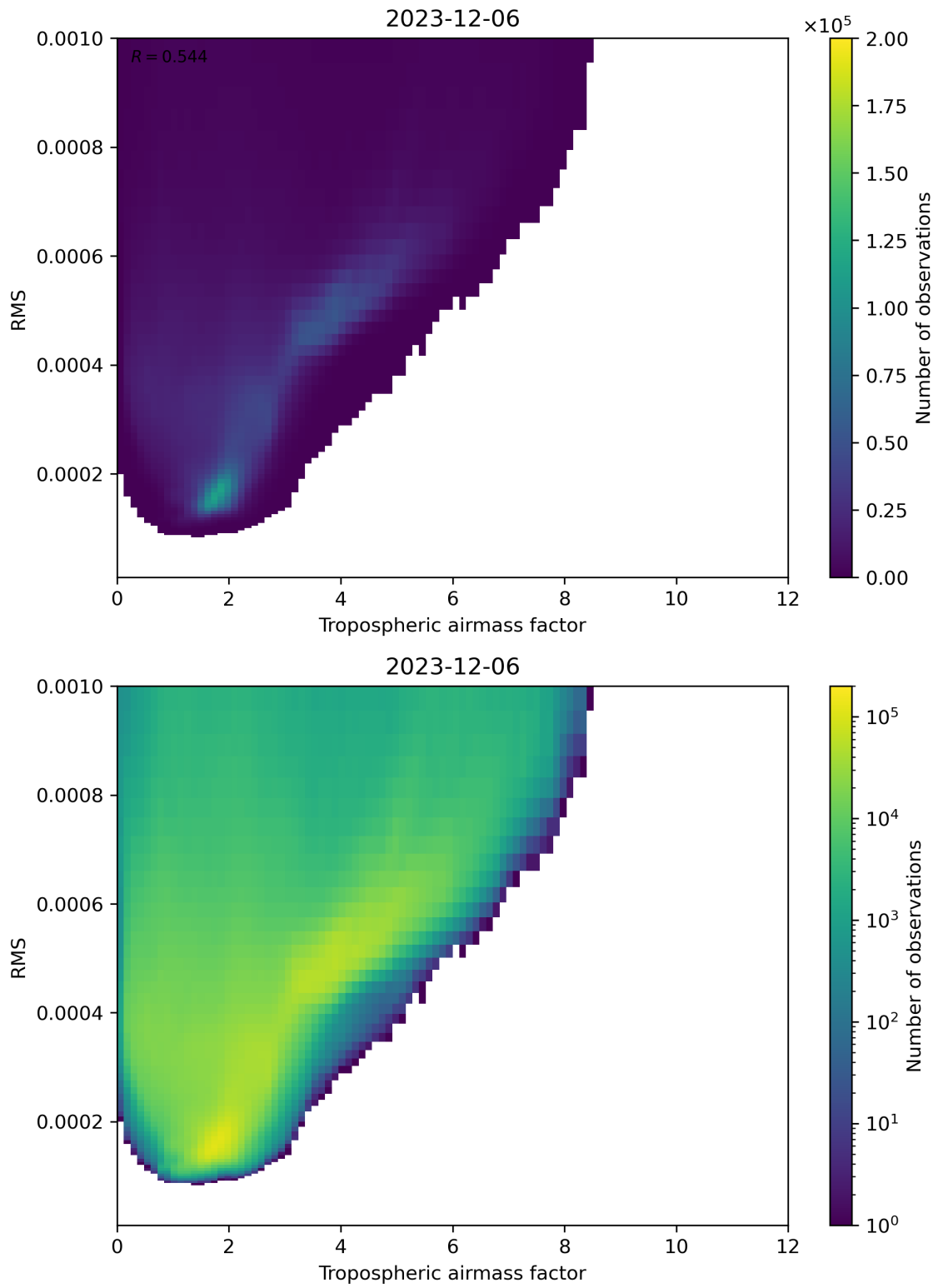
Figure 79: Scatter density plot of “Tropospheric airmass factor” against “RMS” for 2023-12-05 to 2023-12-07.
