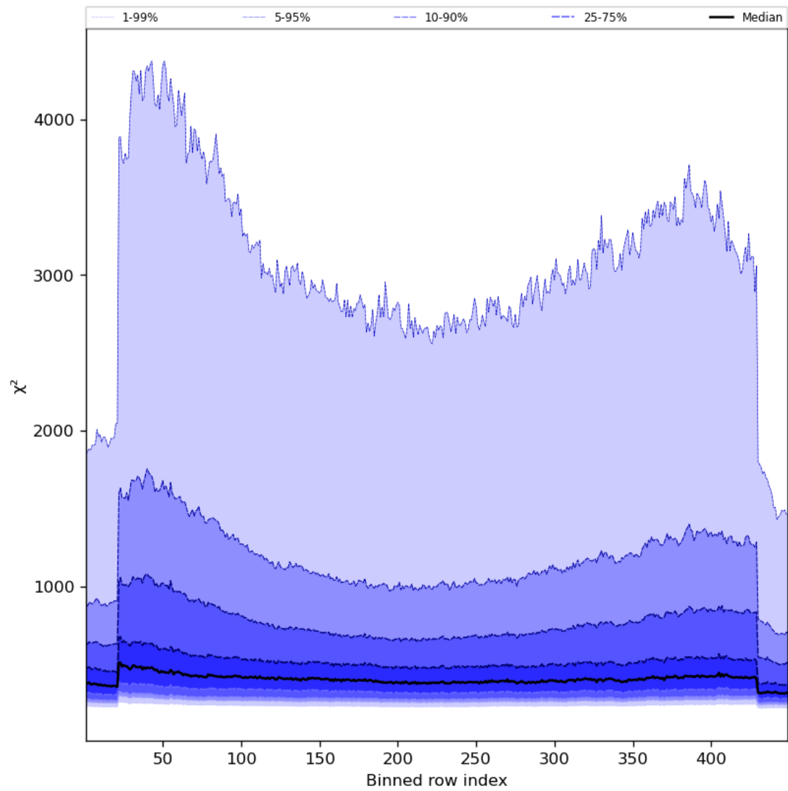
Figure 59: Along track statistics of “ \chi^2 ” for 2023-12-05 to 2023-12-07
