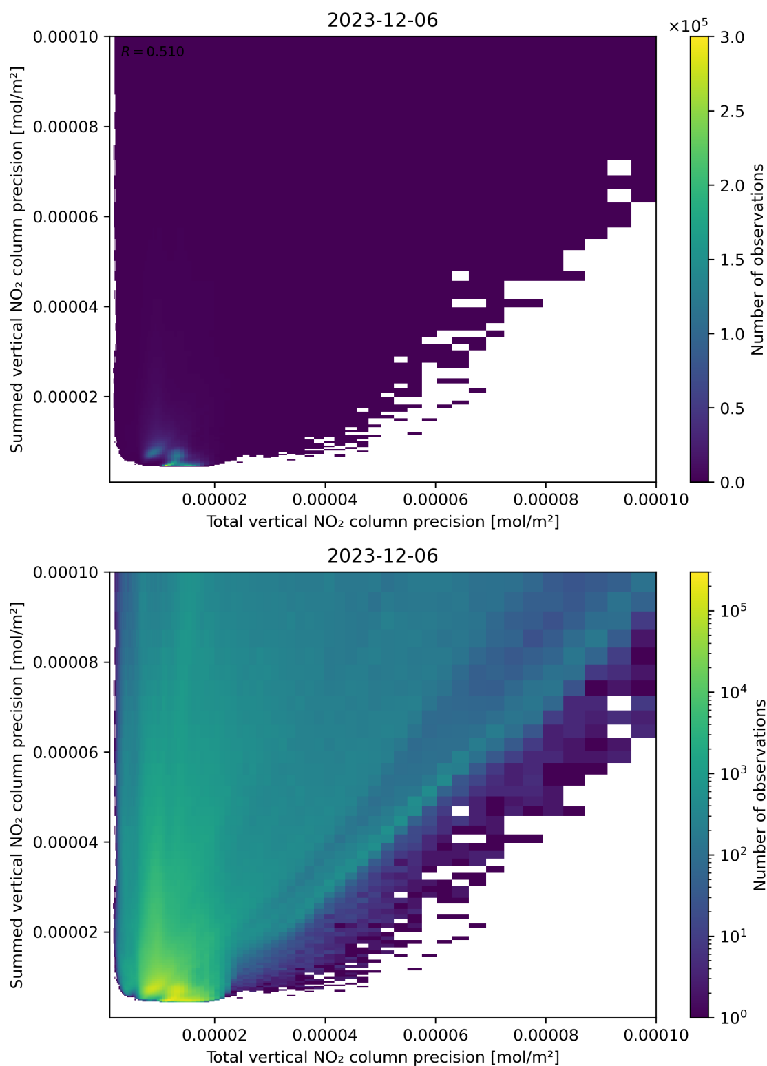
Figure 118: Scatter density plot of “Total vertical NO 2 column precision” against “Summed vertical NO 2 column precision” for 2023-12-05 to 2023-12-07.
