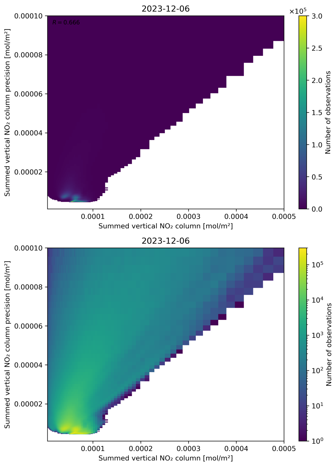
Figure 105: Scatter density plot of “Summed vertical NO 2 column” against “Summed vertical NO 2 column precision” for 2023-12-05 to 2023-12-07.
