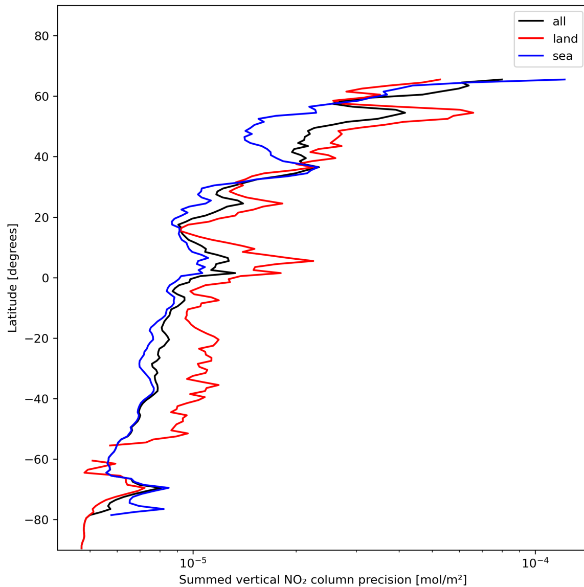
Figure 24: Zonal average of “Summed vertical NO 2 column precision” for 2023-12-05 to 2023-12-07.
