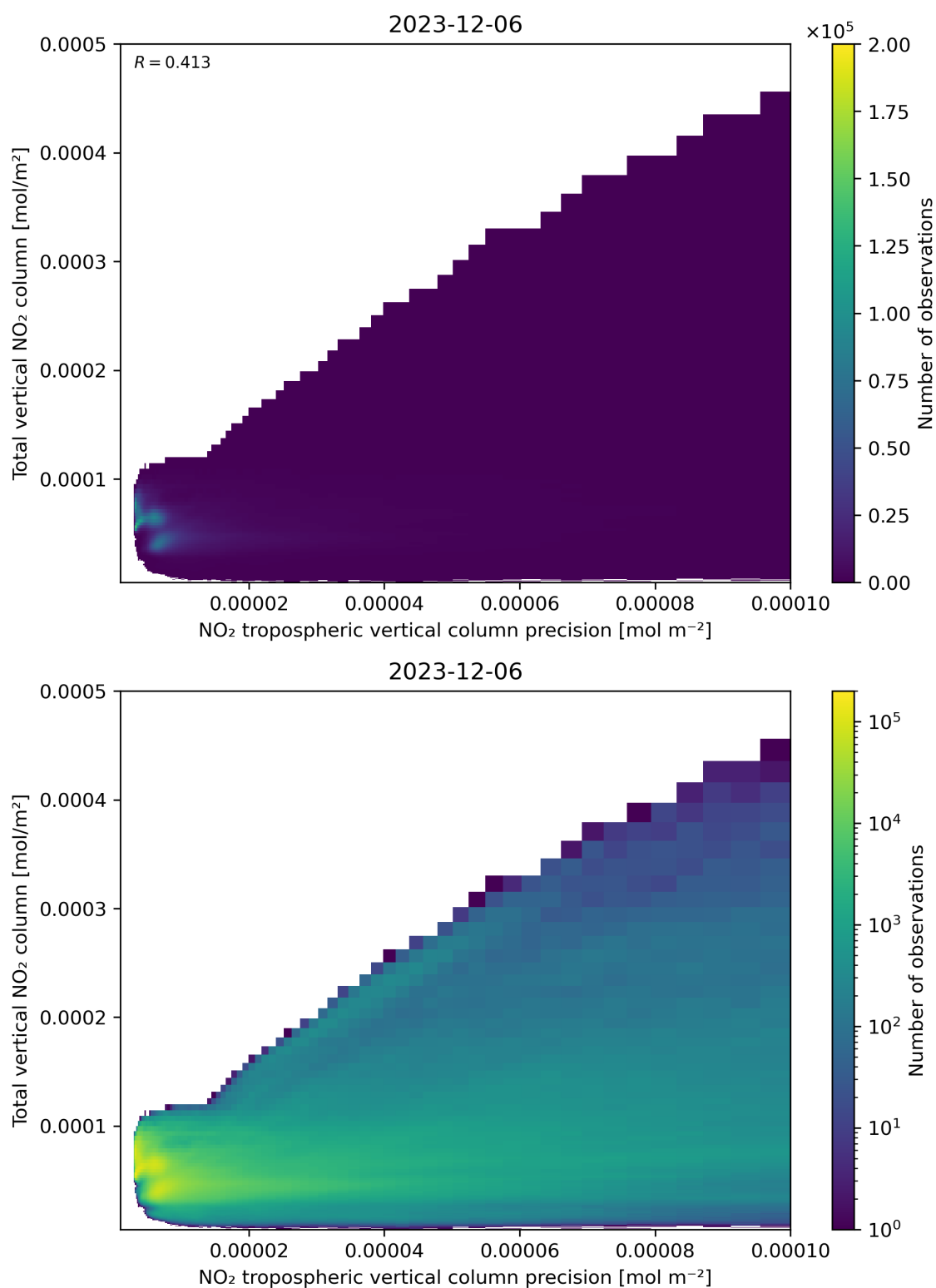
Figure 138: Scatter density plot of “NO 2 tropospheric vertical column precision” against “Total vertical NO 2 column” for 2023-12-05 to 2023-12-07.
