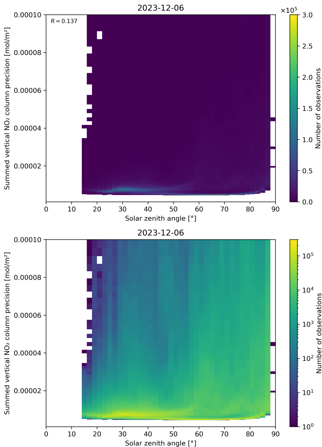
Figure 152: Scatter density plot of “Solar zenith angle” against “Summed vertical NO 2 column precision” for 2023-12-05 to 2023-12-07.
