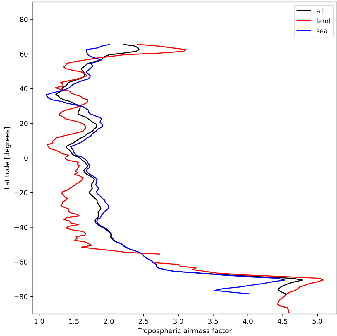
Figure 14: Zonal average of “Tropospheric airmass factor” for 2023-12-05 to 2023-12-07.
