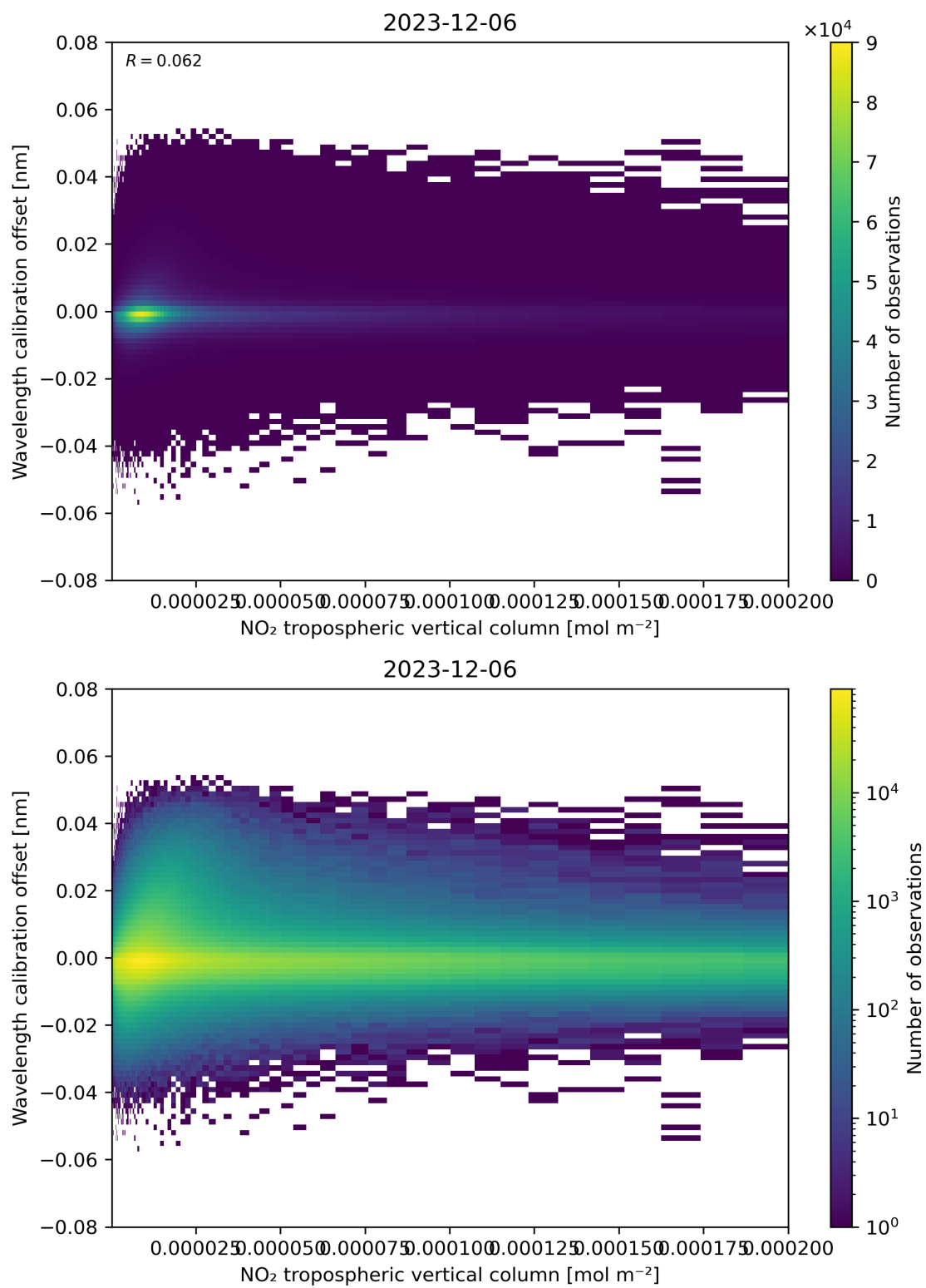
Figure 143: Scatter density plot of “NO 2 tropospheric vertical column” against “Wavelength calibration offset” for 2023-12-05 to 2023-12-07.
