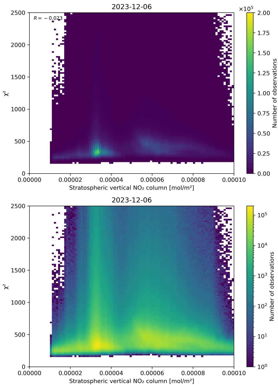
Figure 97: Scatter density plot of “Stratospheric vertical NO 2 column” against “ \chi^2 ” for 2023-12-05 to 2023-12-07.
