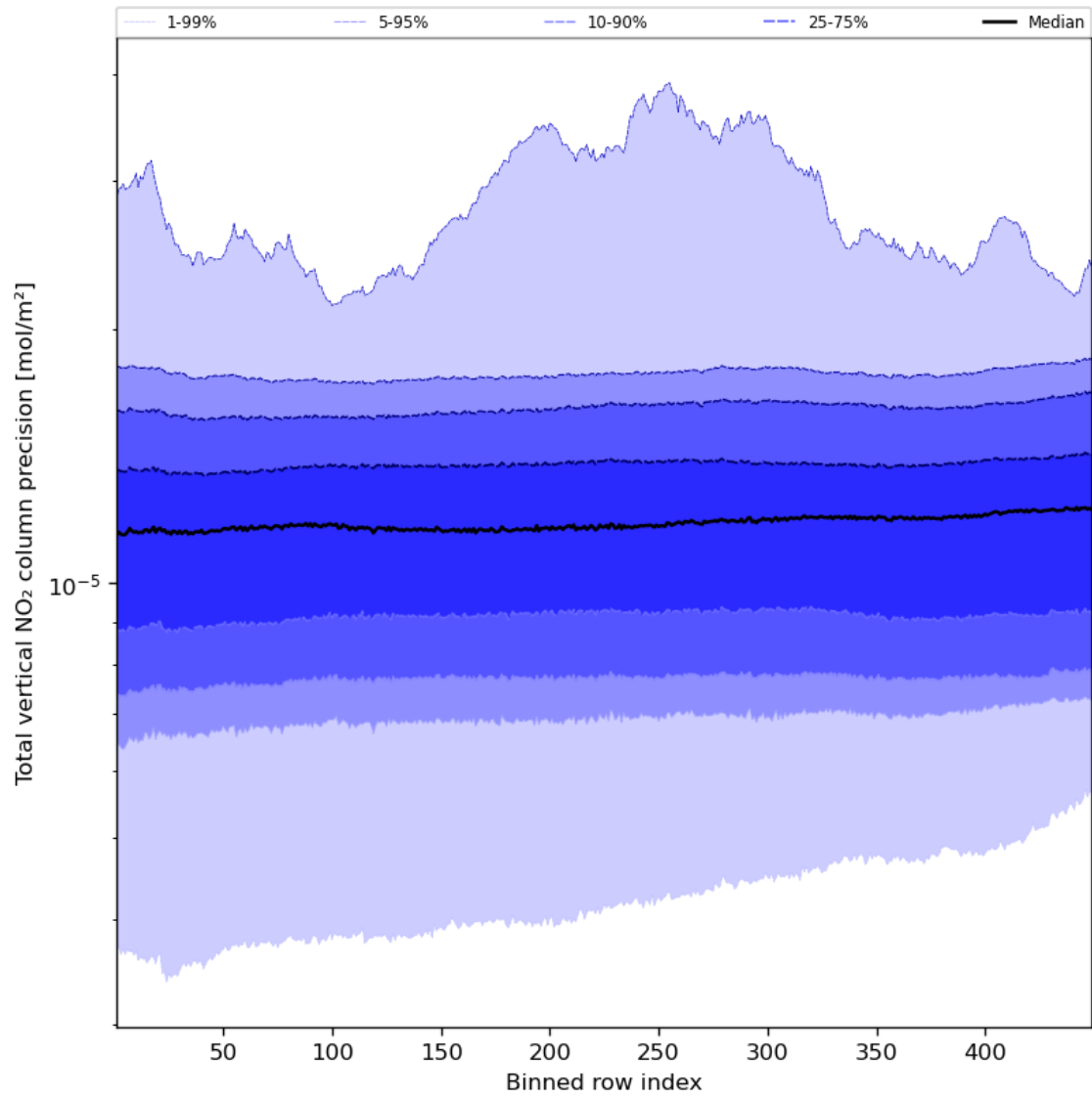
Figure 56: Along track statistics of “Total vertical NO 2 column precision” for 2023-12-05 to 2023-12-07
