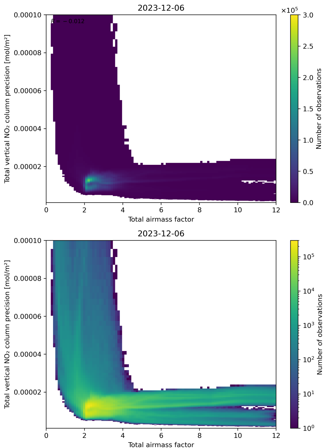
Figure 68: Scatter density plot of “Total airmass factor” against “Total vertical NO 2 column precision” for 2023-12-05 to 2023-12-07.
