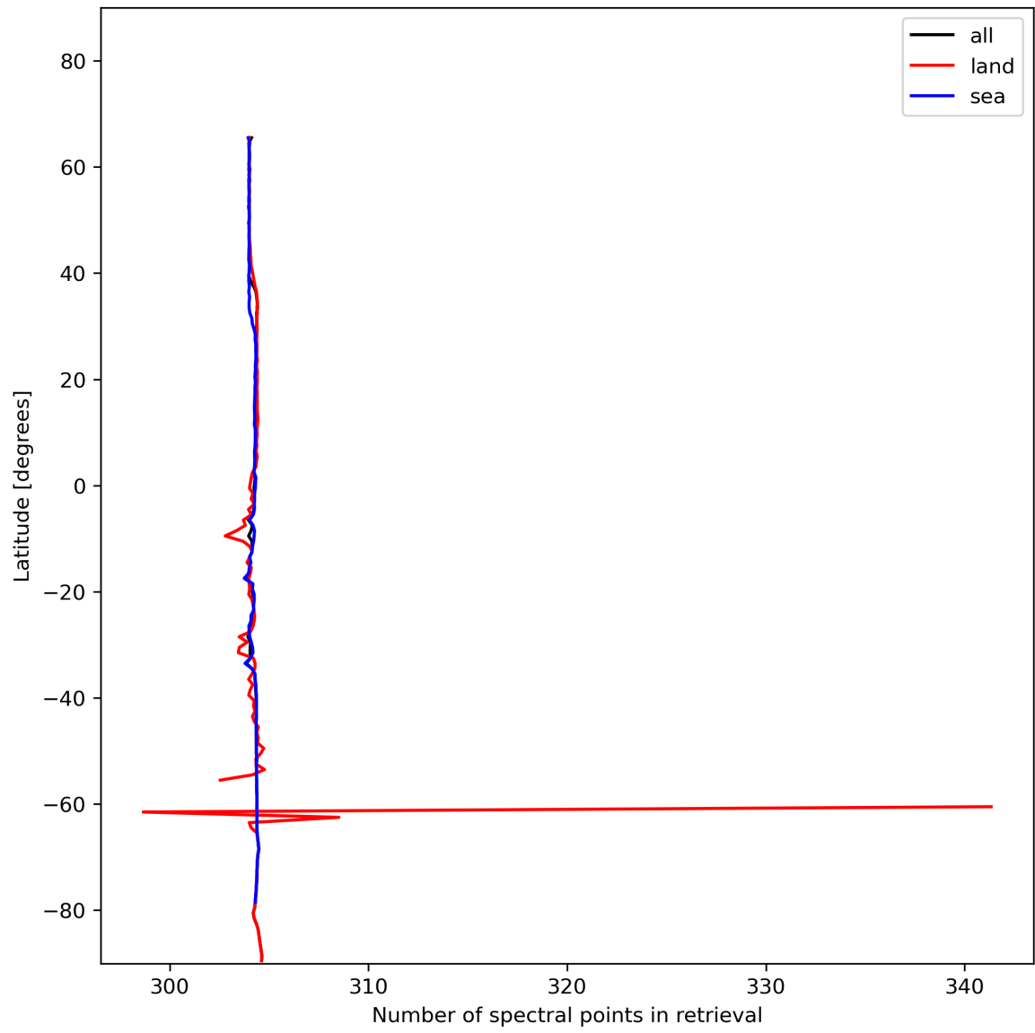
Figure 16: Zonal average of “Number of spectral points in retrieval” for 2023-12-05 to 2023-12-07.
