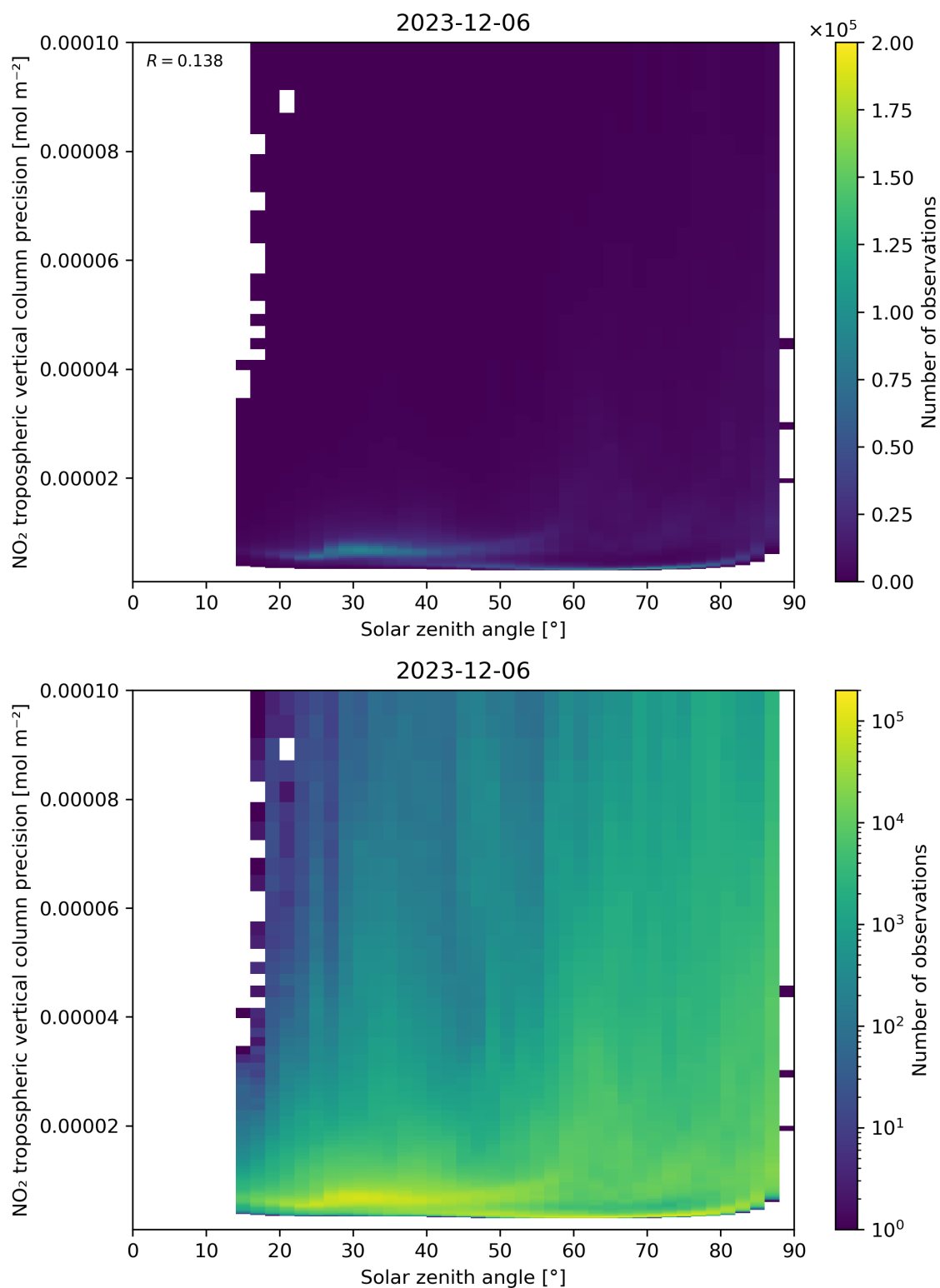
Figure 156: Scatter density plot of “Solar zenith angle” against “NO 2 tropospheric vertical column precision” for 2023-12-05 to 2023-12-07.
