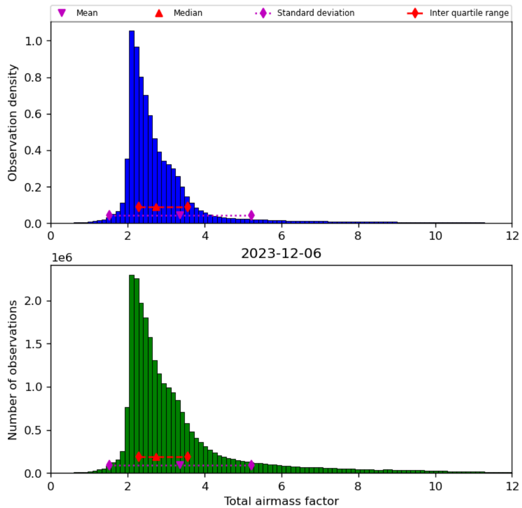
Figure 32: Histogram of “Total airmass factor” for 2023-12-05 to 2023-12-07
