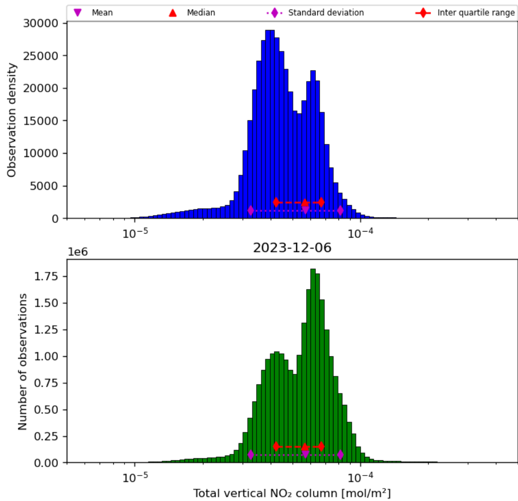
Figure 38: Histogram of “Total vertical NO 2 column” for 2023-12-05 to 2023-12-07
