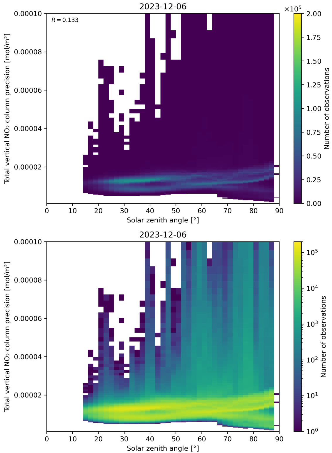
Figure 154: Scatter density plot of “Solar zenith angle” against “Total vertical NO 2 column precision” for 2023-12-05 to 2023-12-07.
