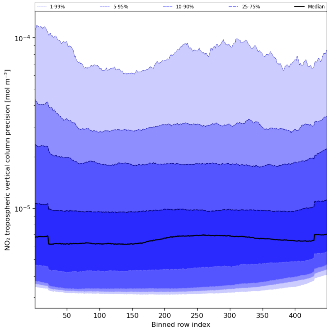
Figure 47: Along track statistics of “NO 2 tropospheric vertical column precision” for 2023-12-05 to 2023-12-07
