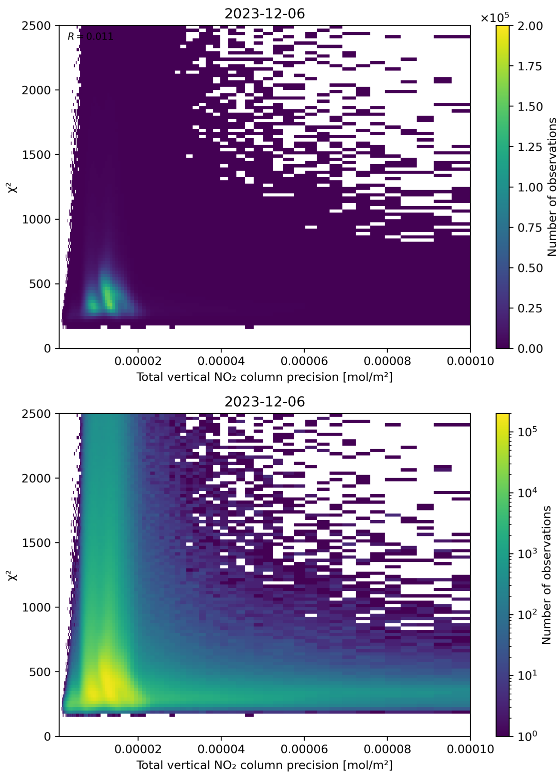
Figure 116: Scatter density plot of “Total vertical NO 2 column precision” against “ \chi^2 ” for 2023-12-05 to 2023-12-07.
