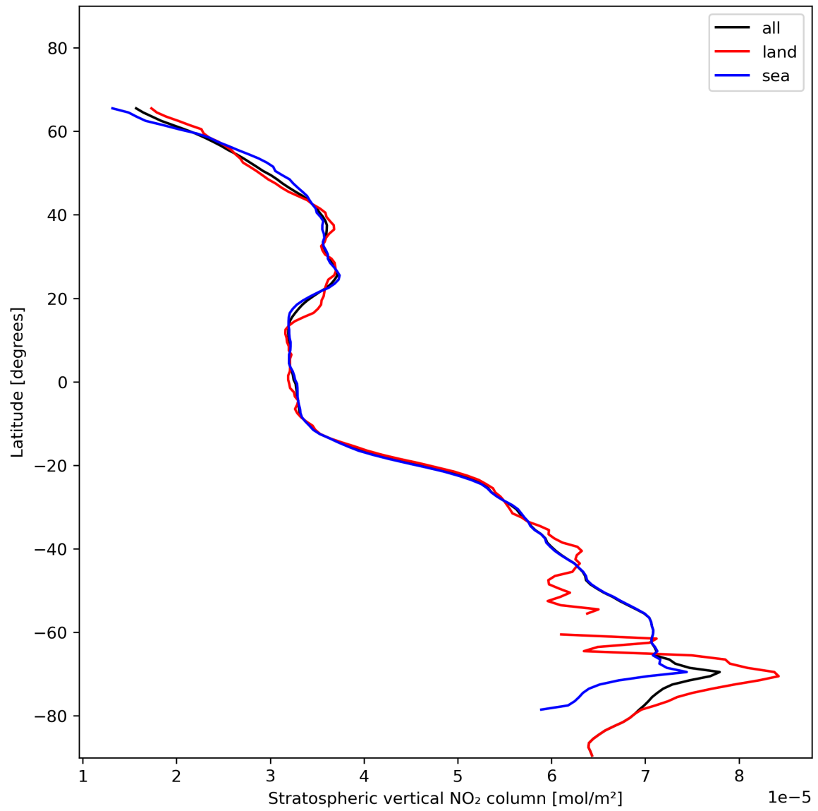
Figure 19: Zonal average of “Stratospheric vertical NO 2 column” for 2023-12-05 to 2023-12-07.
