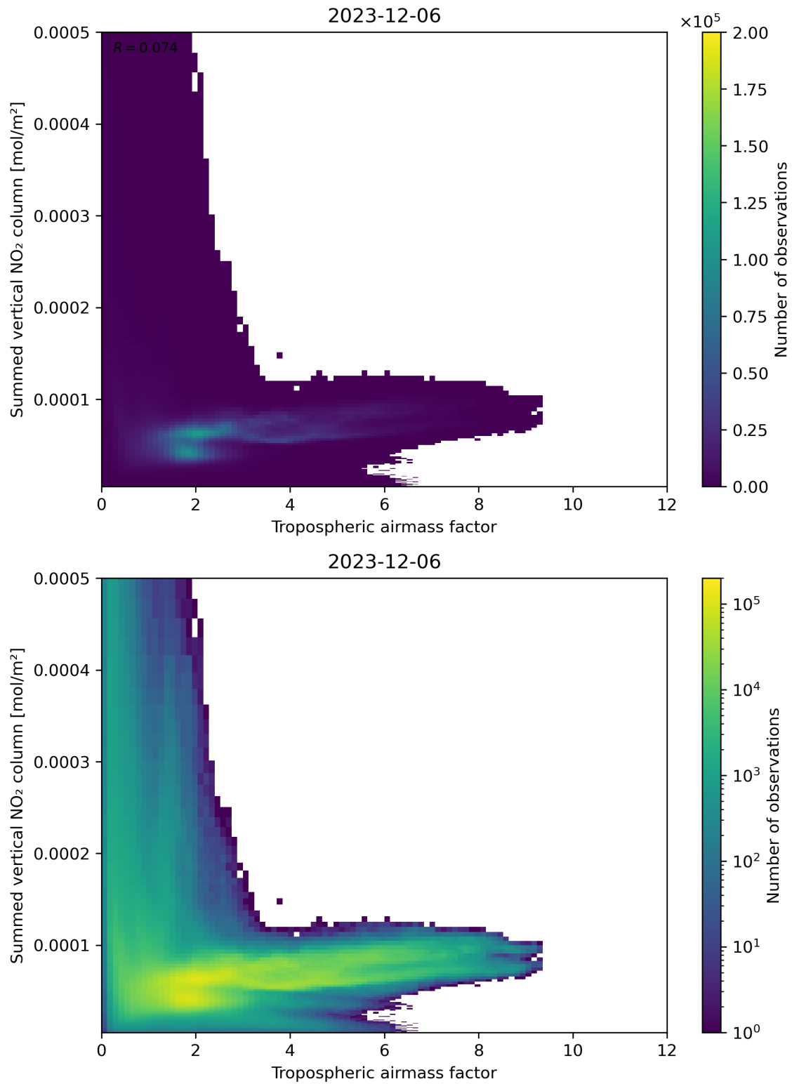
Figure 75: Scatter density plot of “Tropospheric airmass factor” against “Summed vertical NO 2 column” for 2023-12-05 to 2023-12-07.
