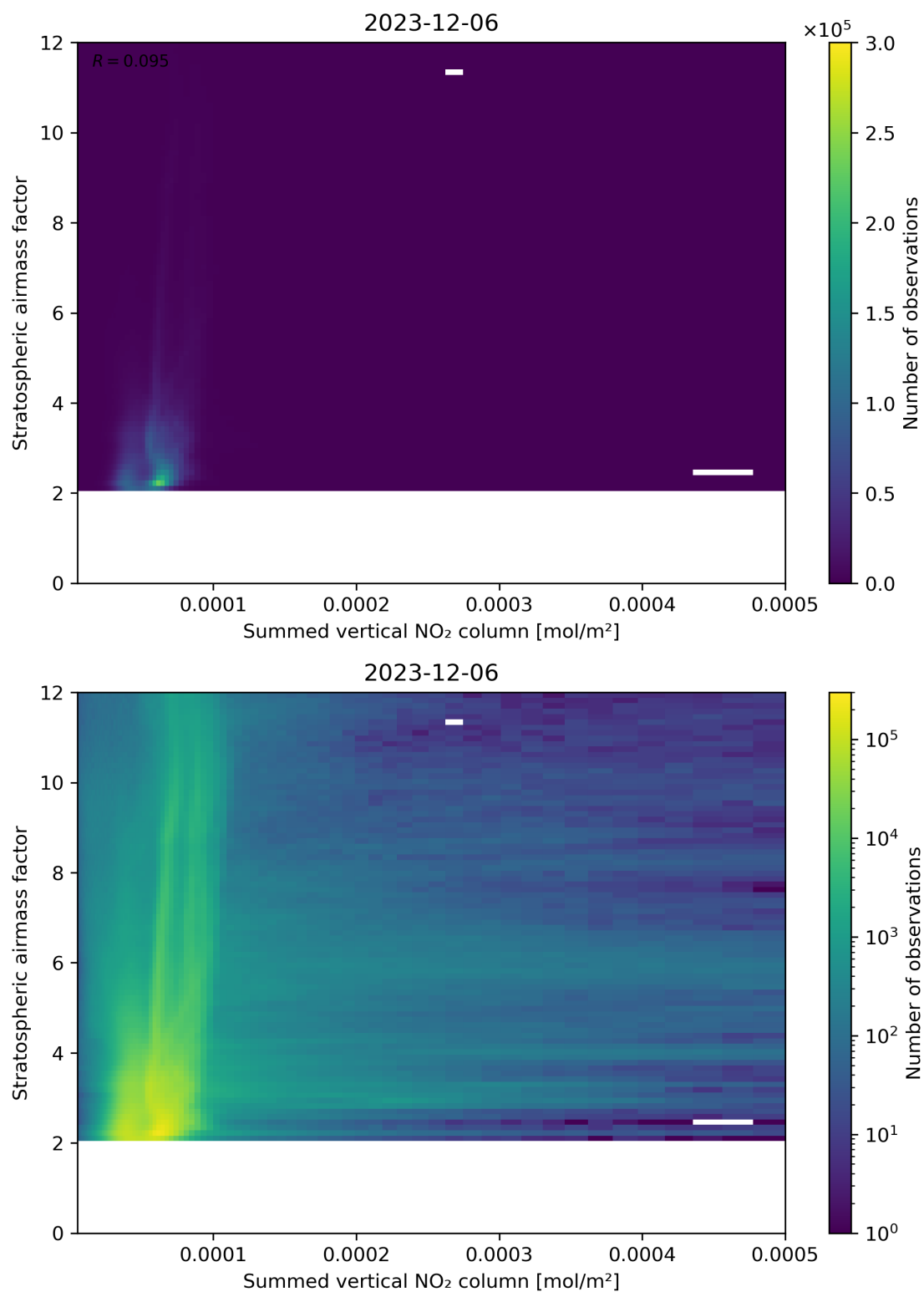
Figure 103: Scatter density plot of “Summed vertical NO 2 column” against “Stratospheric airmass factor” for 2023-12-05 to 2023-12-07.
