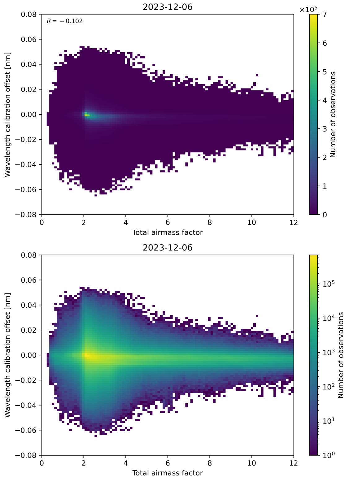
Figure 70: Scatter density plot of “Total airmass factor” against “Wavelength calibration offset” for 2023-12-05 to 2023-12-07.
