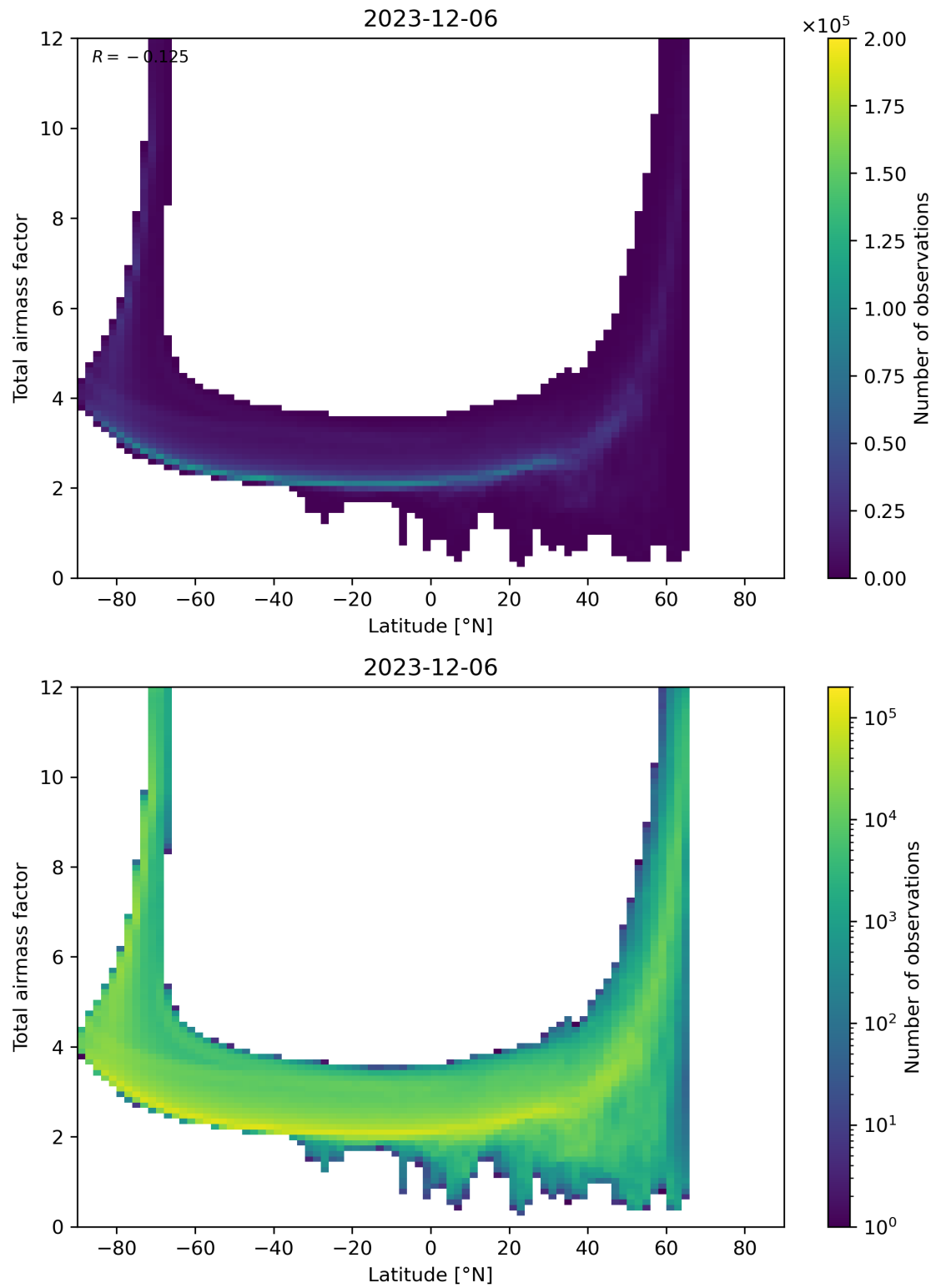
Figure 84: Scatter density plot of “Latitude” against “Total airmass factor” for 2023-12-05 to 2023-12-07.
