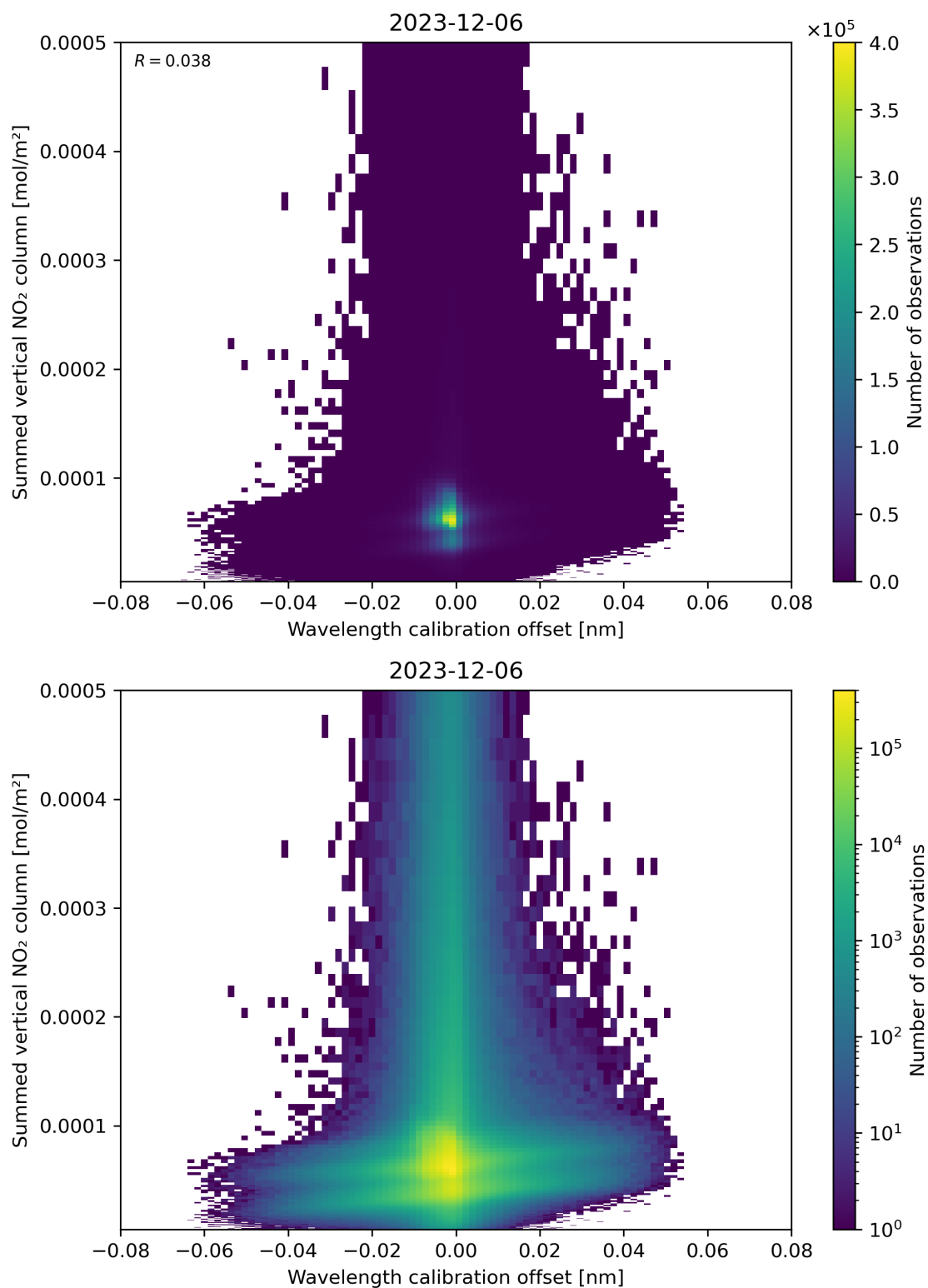
Figure 177: Scatter density plot of “Wavelength calibration offset” against “Summed vertical NO 2 column” for 2023-12-05 to 2023-12-07.
