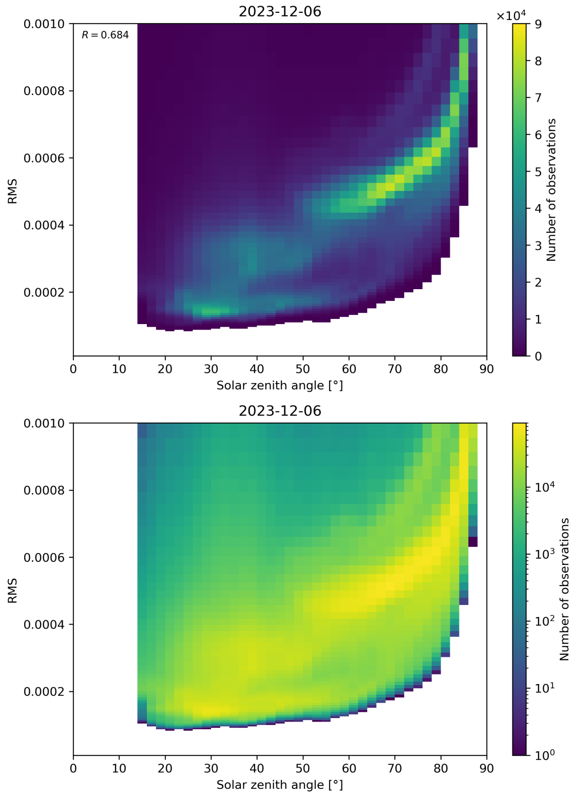
Figure 157: Scatter density plot of “Solar zenith angle” against “RMS” for 2023-12-05 to 2023-12-07.
