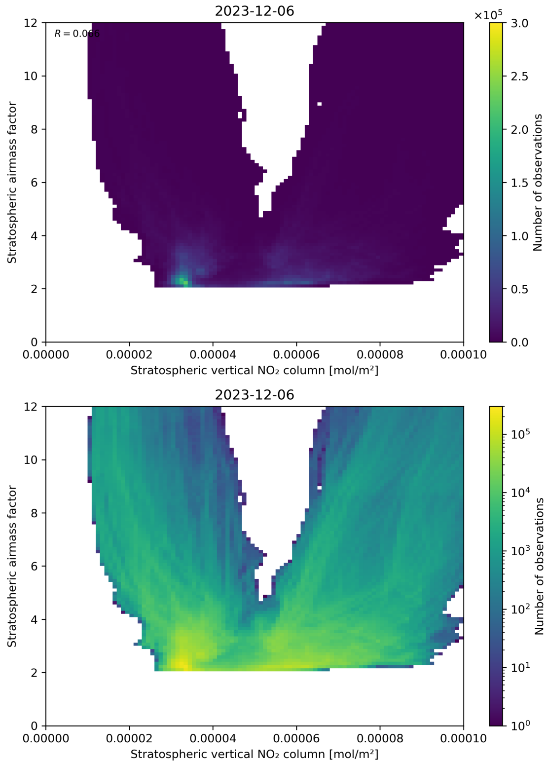
Figure 96: Scatter density plot of “Stratospheric vertical NO 2 column” against “Stratospheric airmass factor” for 2023-12-05 to 2023-12-07.
