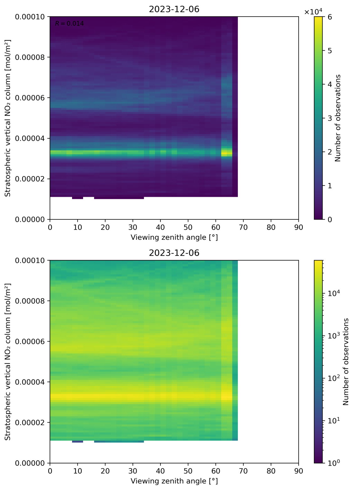
Figure 164: Scatter density plot of “Viewing zenith angle” against “Stratospheric vertical NO 2 column” for 2023-12-05 to 2023-12-07.
