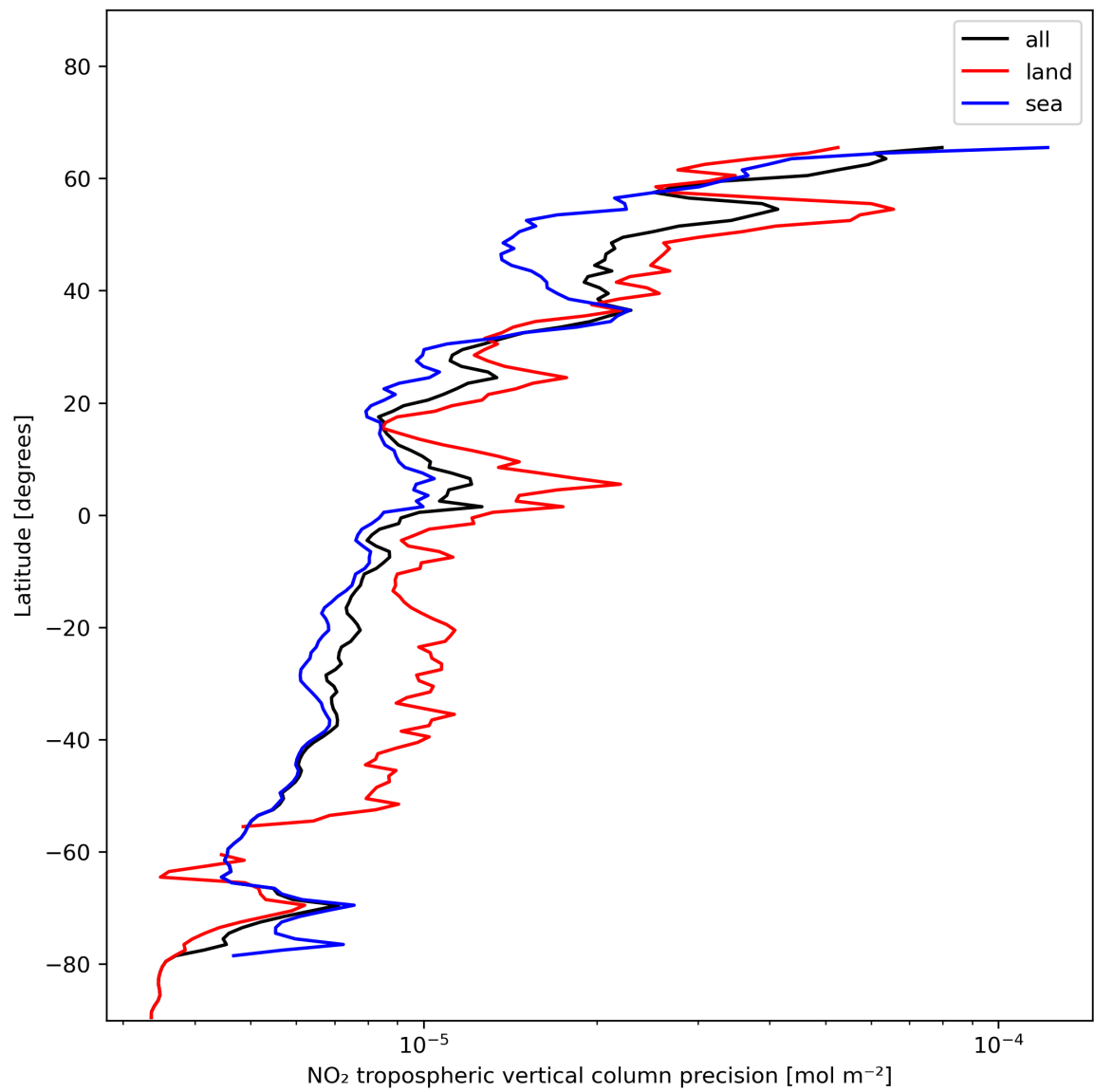
Figure 13: Zonal average of “NO 2 tropospheric vertical column precision” for 2023-12-05 to 2023-12-07.
