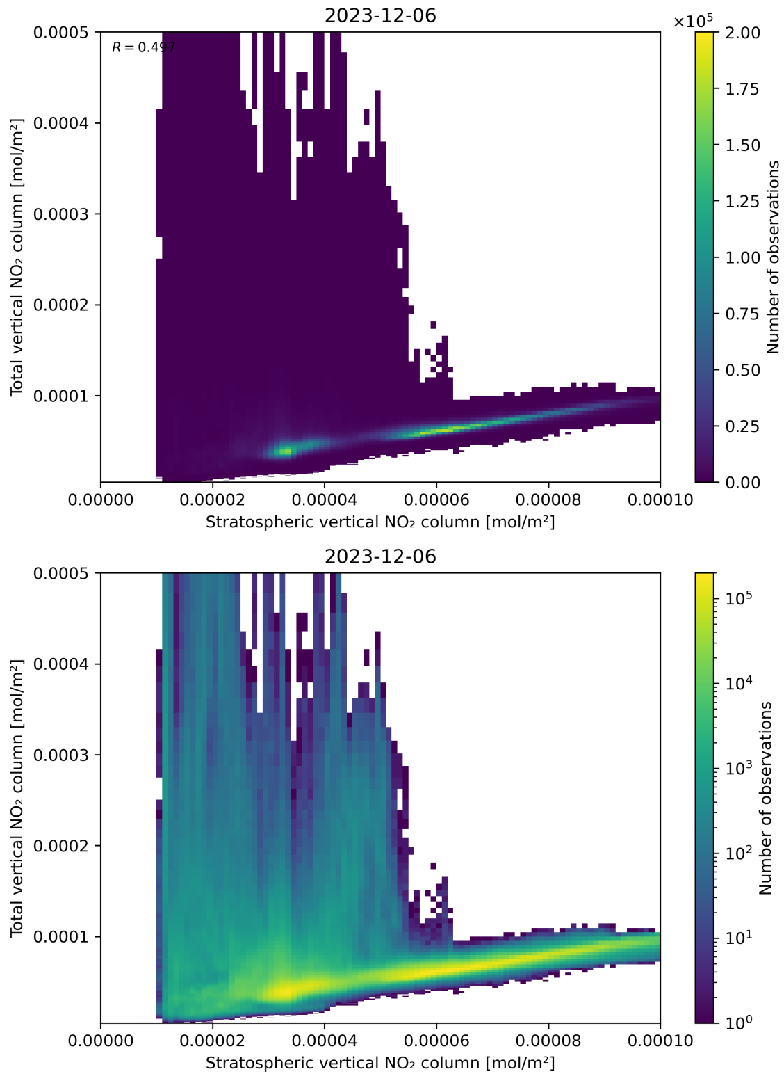
Figure 100: Scatter density plot of “Stratospheric vertical NO 2 column” against “Total vertical NO 2 column” for 2023-12-05 to 2023-12-07.
