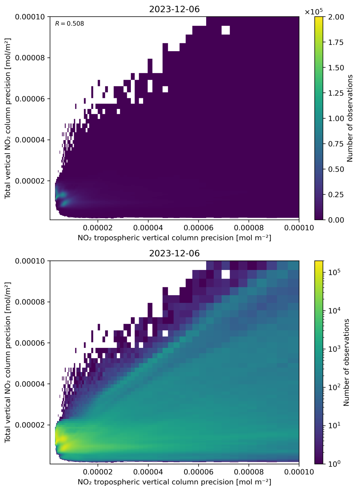
Figure 139: Scatter density plot of “NO 2 tropospheric vertical column precision” against “Total vertical NO 2 column precision” for 2023-12-05 to 2023-12-07.
