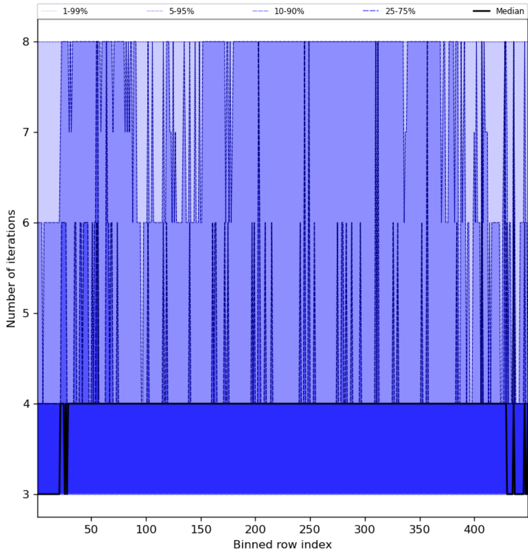
Figure 51: Along track statistics of “Number of iterations” for 2023-12-05 to 2023-12-07
