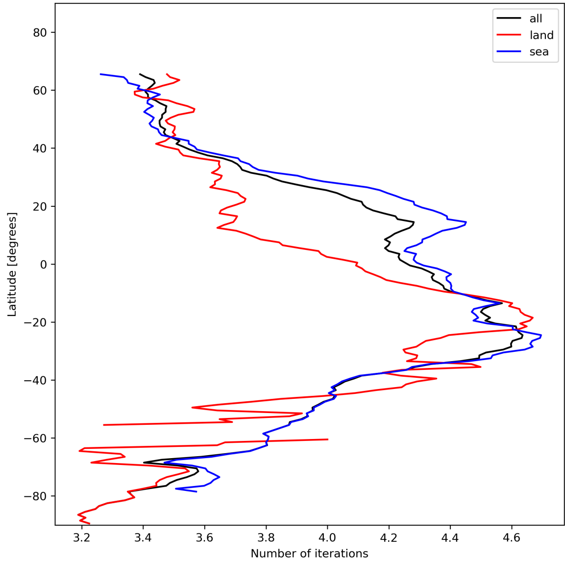
Figure 17: Zonal average of “Number of iterations” for 2023-12-05 to 2023-12-07.
