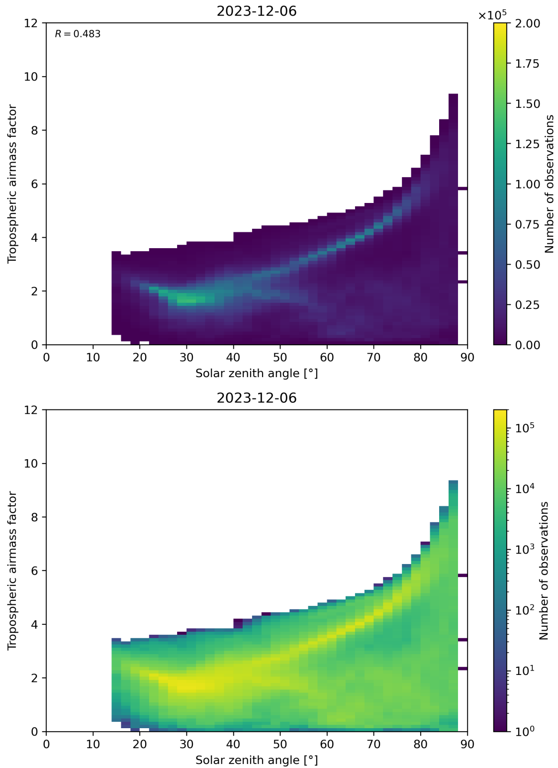
Figure 147: Scatter density plot of “Solar zenith angle” against “Tropospheric airmass factor” for 2023-12-05 to 2023-12-07.
