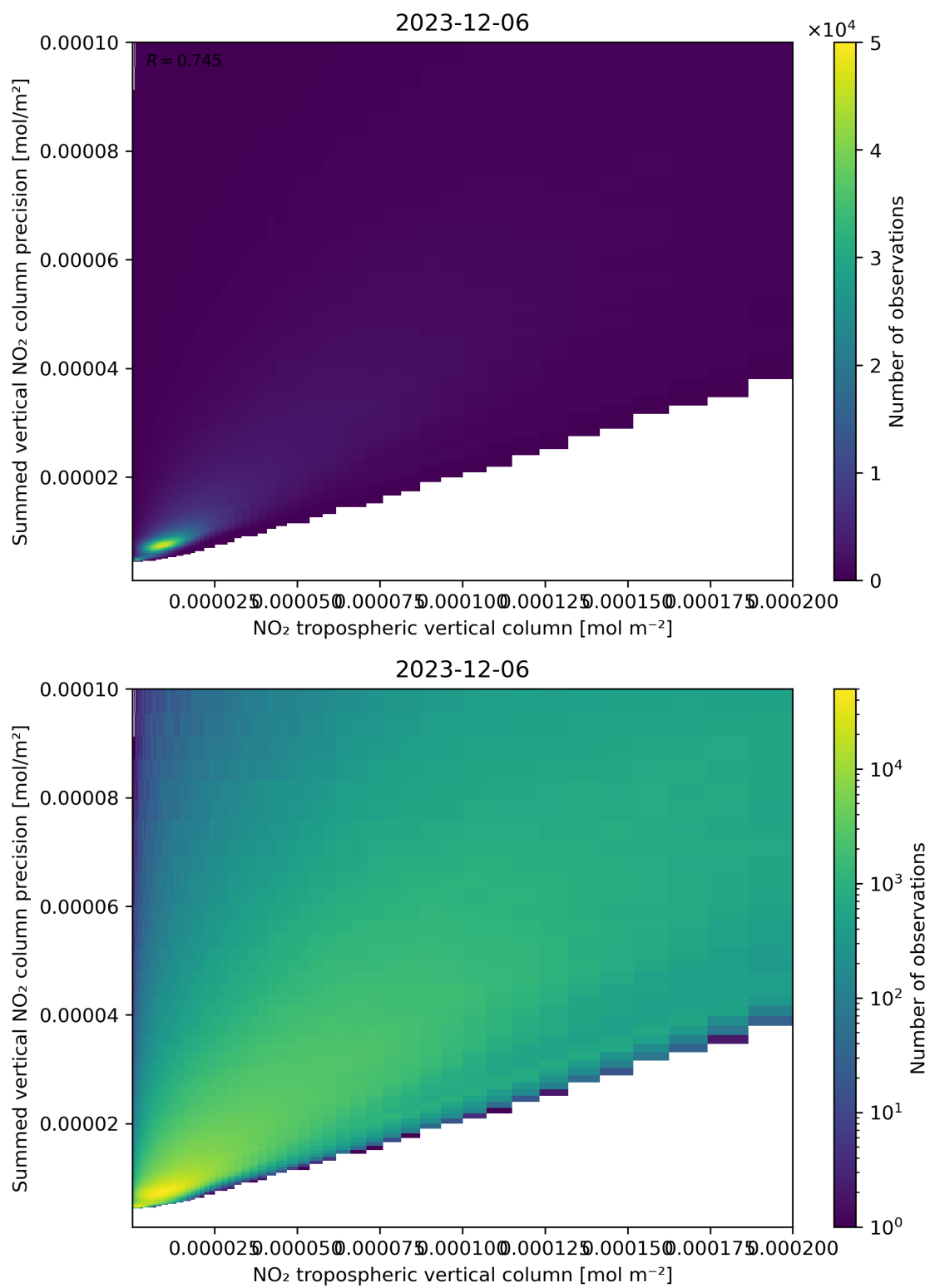
Figure 127: Scatter density plot of “NO 2 tropospheric vertical column” against “Summed vertical NO 2 column precision” for 2023-12-05 to 2023-12-07.
