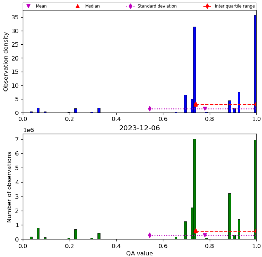
Figure 28: Histogram of “QA value” for 2023-12-05 to 2023-12-07
