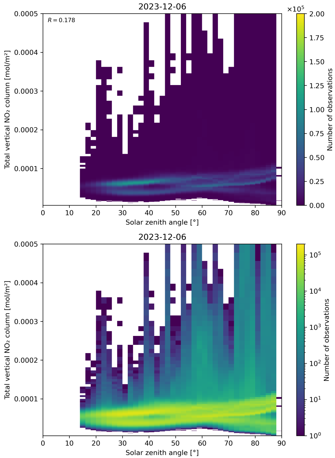
Figure 153: Scatter density plot of “Solar zenith angle” against “Total vertical NO 2 column” for 2023-12-05 to 2023-12-07.
