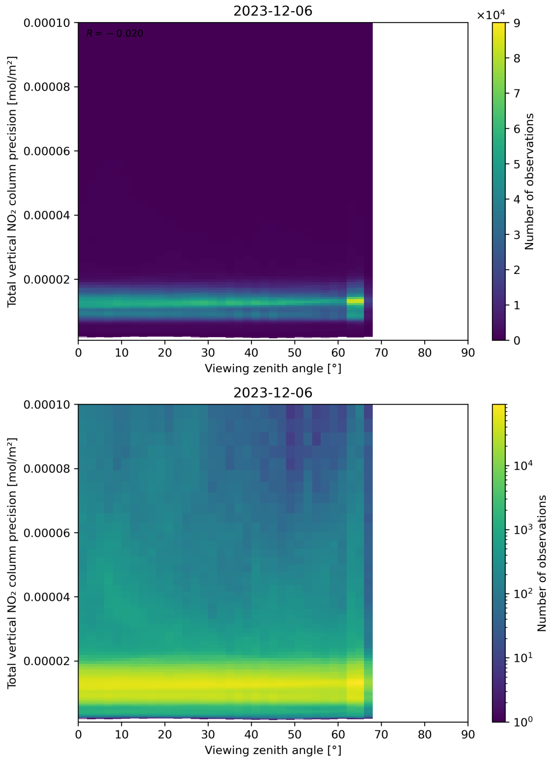
Figure 168: Scatter density plot of “Viewing zenith angle” against “Total vertical NO 2 column precision” for 2023-12-05 to 2023-12-07.
