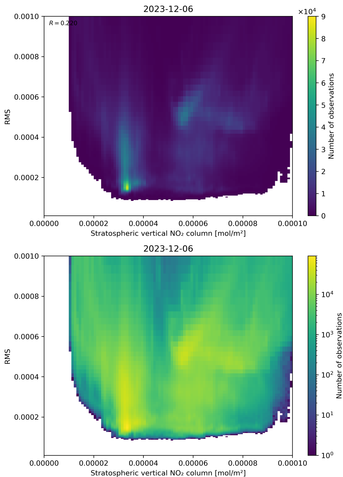
Figure 102: Scatter density plot of “Stratospheric vertical NO 2 column” against “RMS” for 2023-12-05 to 2023-12-07.
