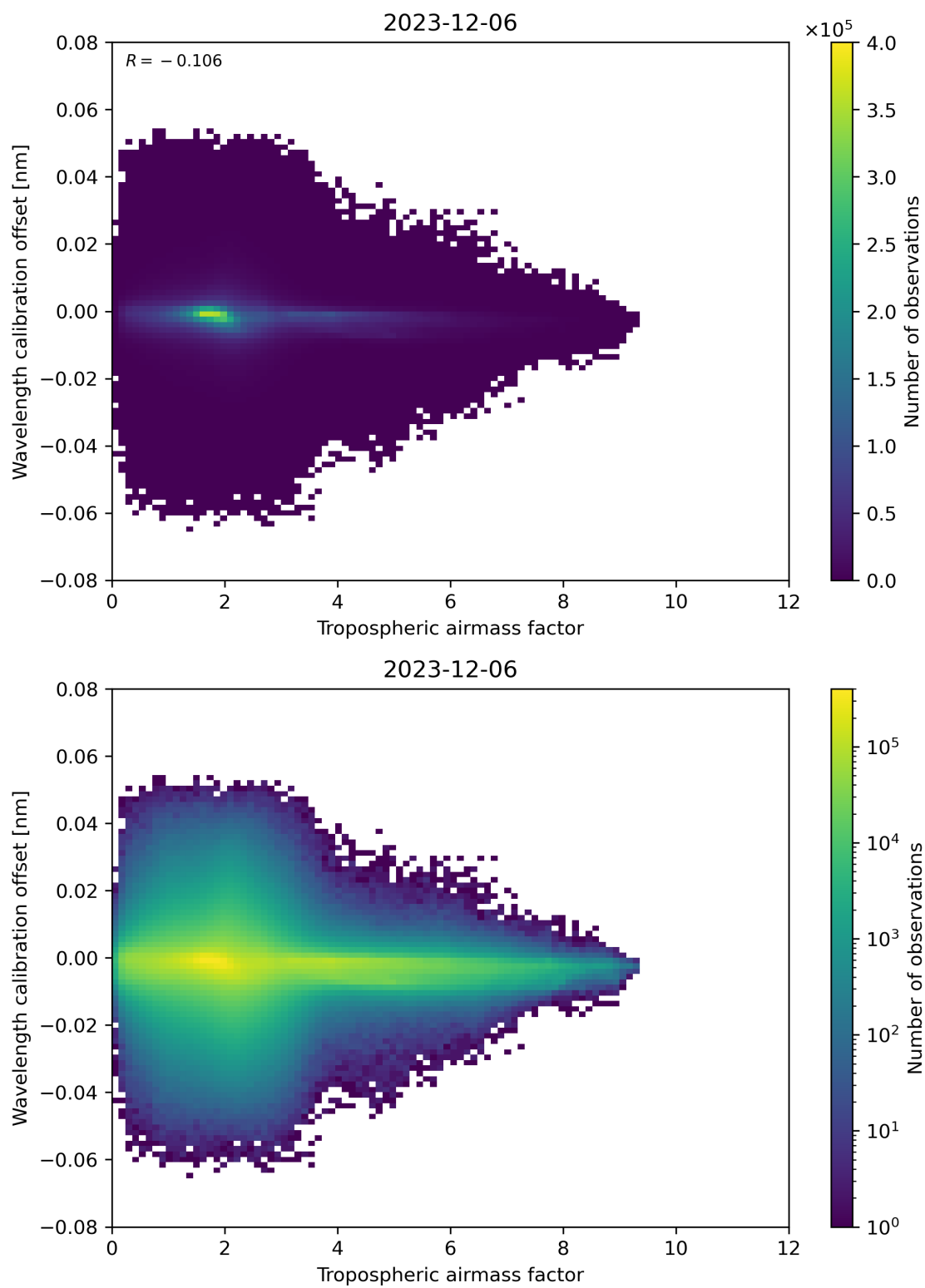
Figure 80: Scatter density plot of “Tropospheric air mass factor” against “Wavelength calibration offset” for 2023-12-05 to 2023-12-07.
