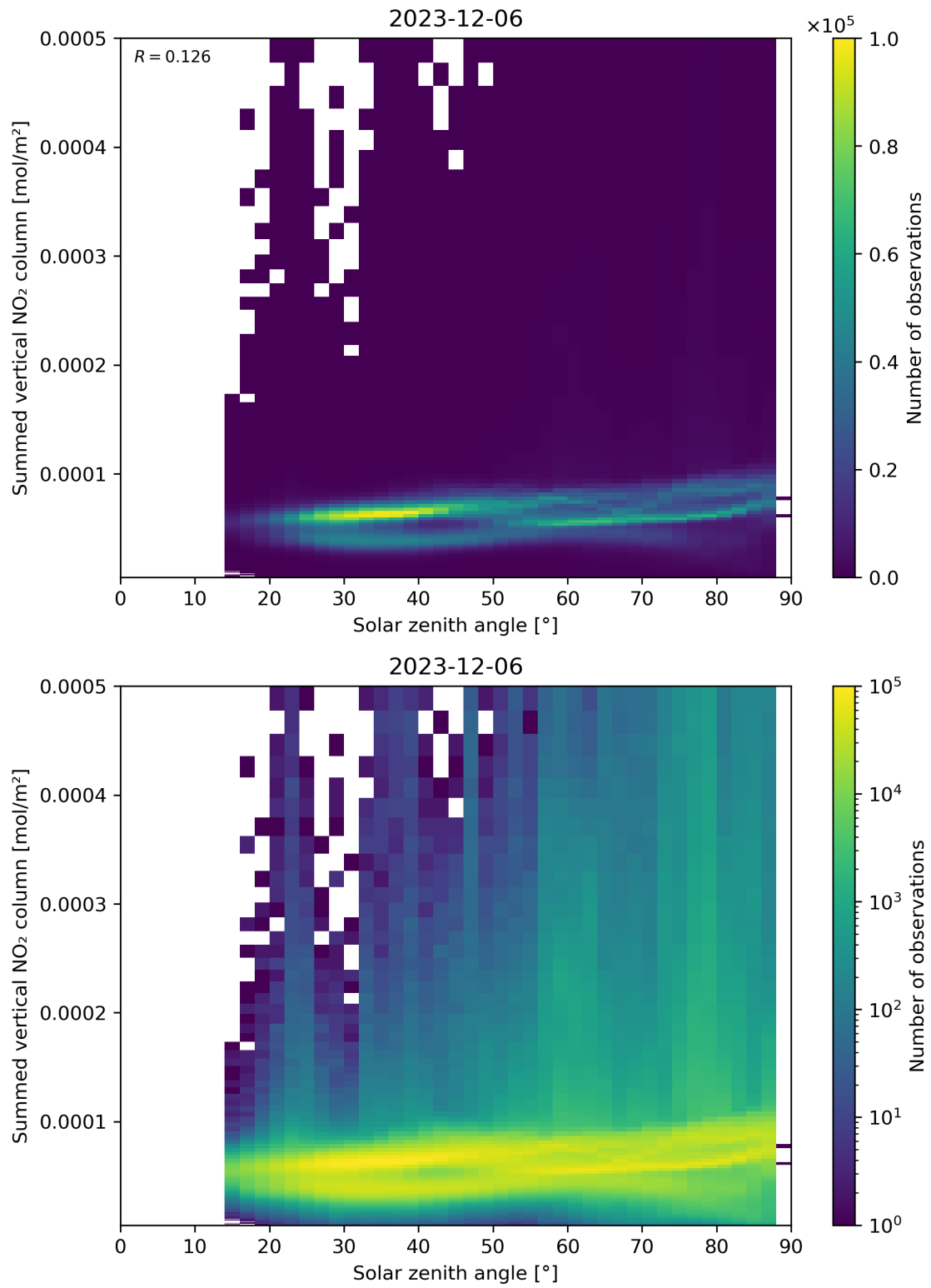
Figure 151: Scatter density plot of “Solar zenith angle” against “Summed vertical NO 2 column” for 2023-12-05 to 2023-12-07.
