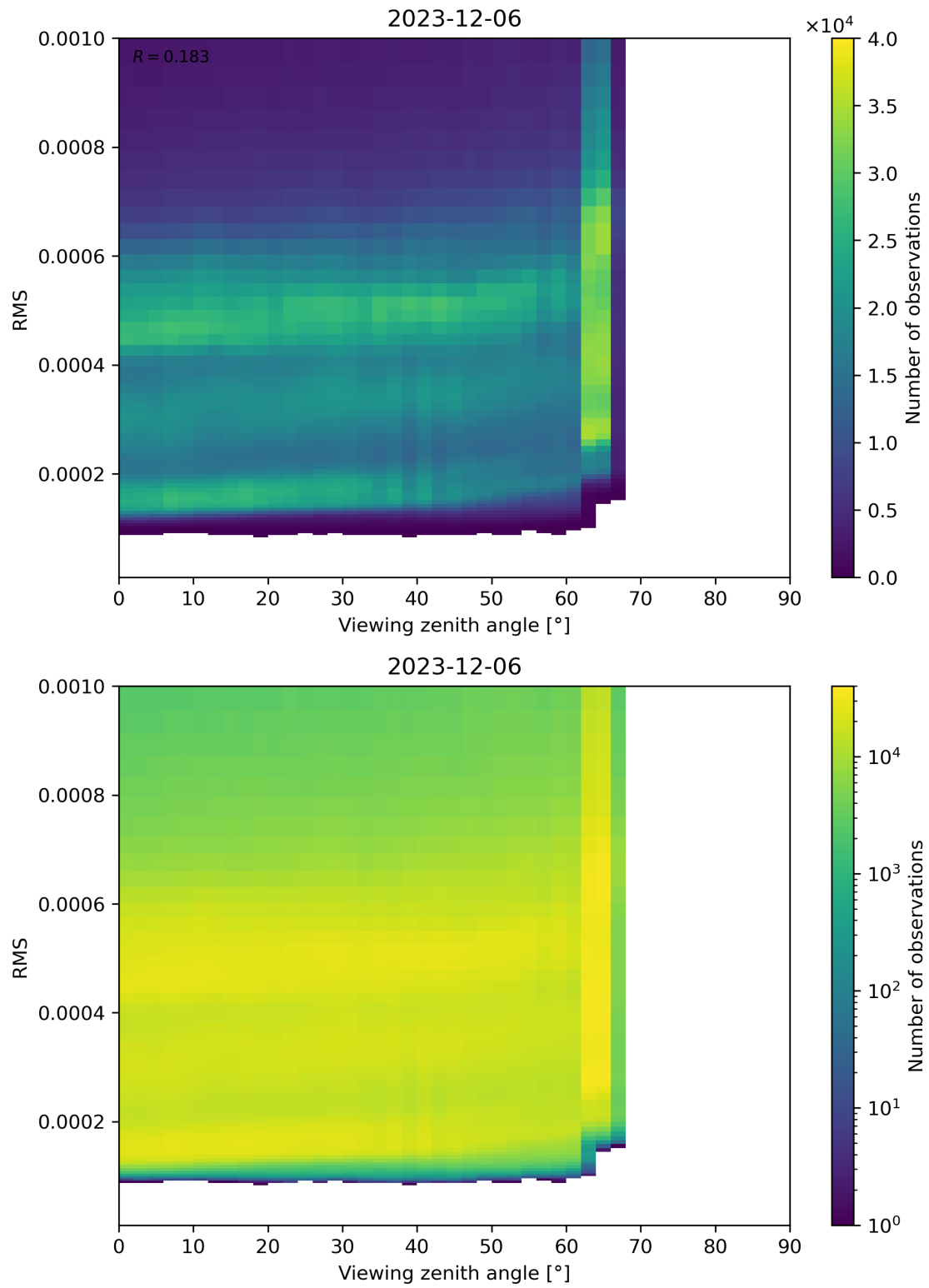
Figure 171: Scatter density plot of “Viewing zenith angle” against “RMS” for 2023-12-05 to 2023-12-07.
