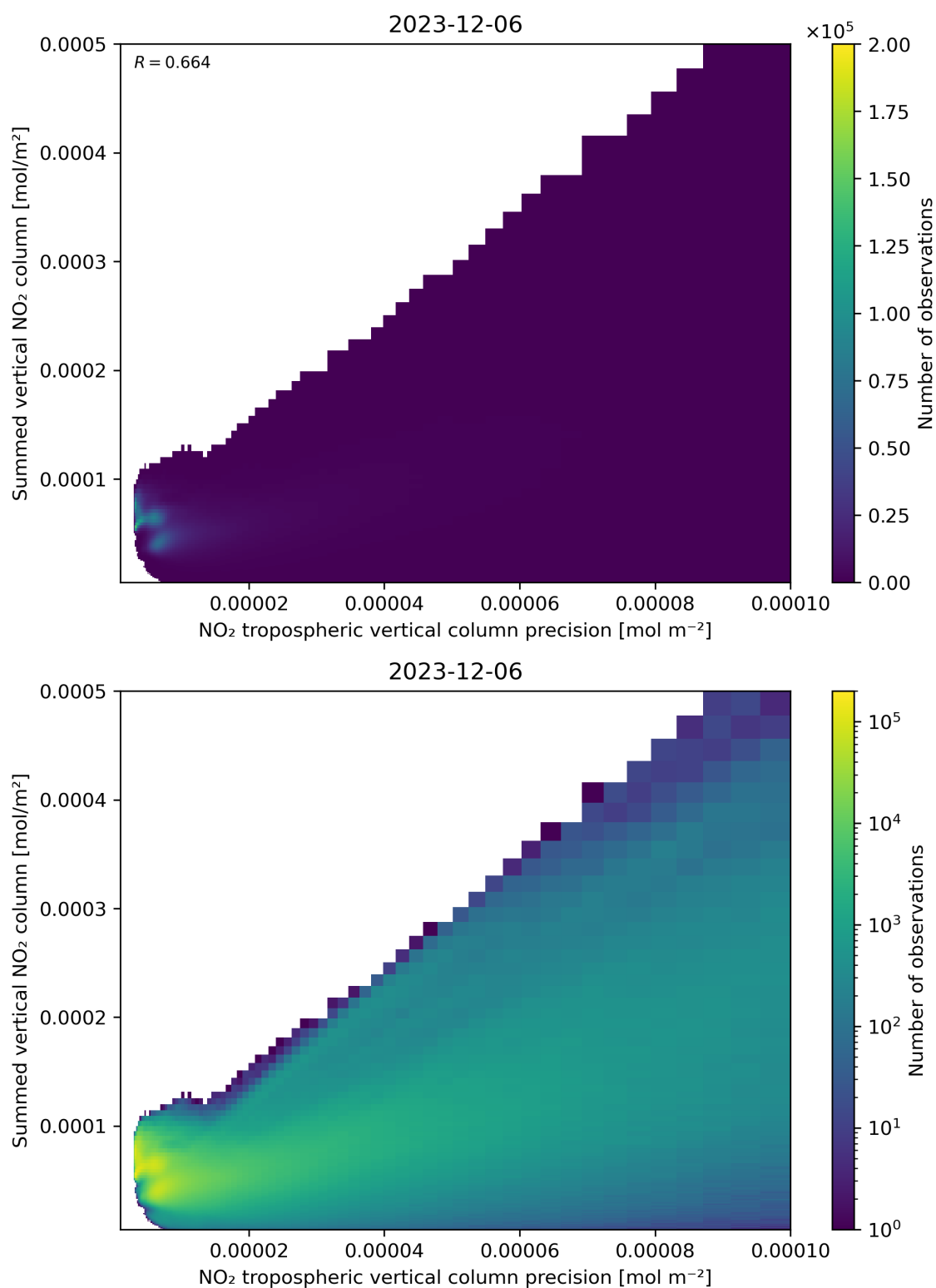
Figure 136: Scatter density plot of “NO 2 tropospheric vertical column precision” against “Summed vertical NO 2 column” for 2023-12-05 to 2023-12-07.
