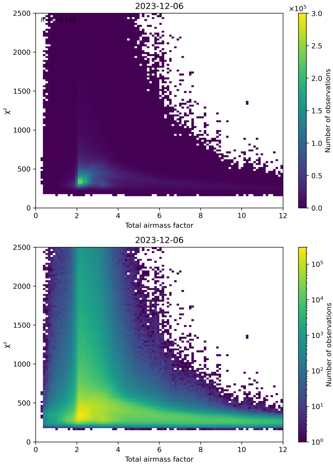
Figure 63: Scatter density plot of “Total airmass factor” against “ \chi^2 ” for 2023-12-05 to 2023-12-07.
