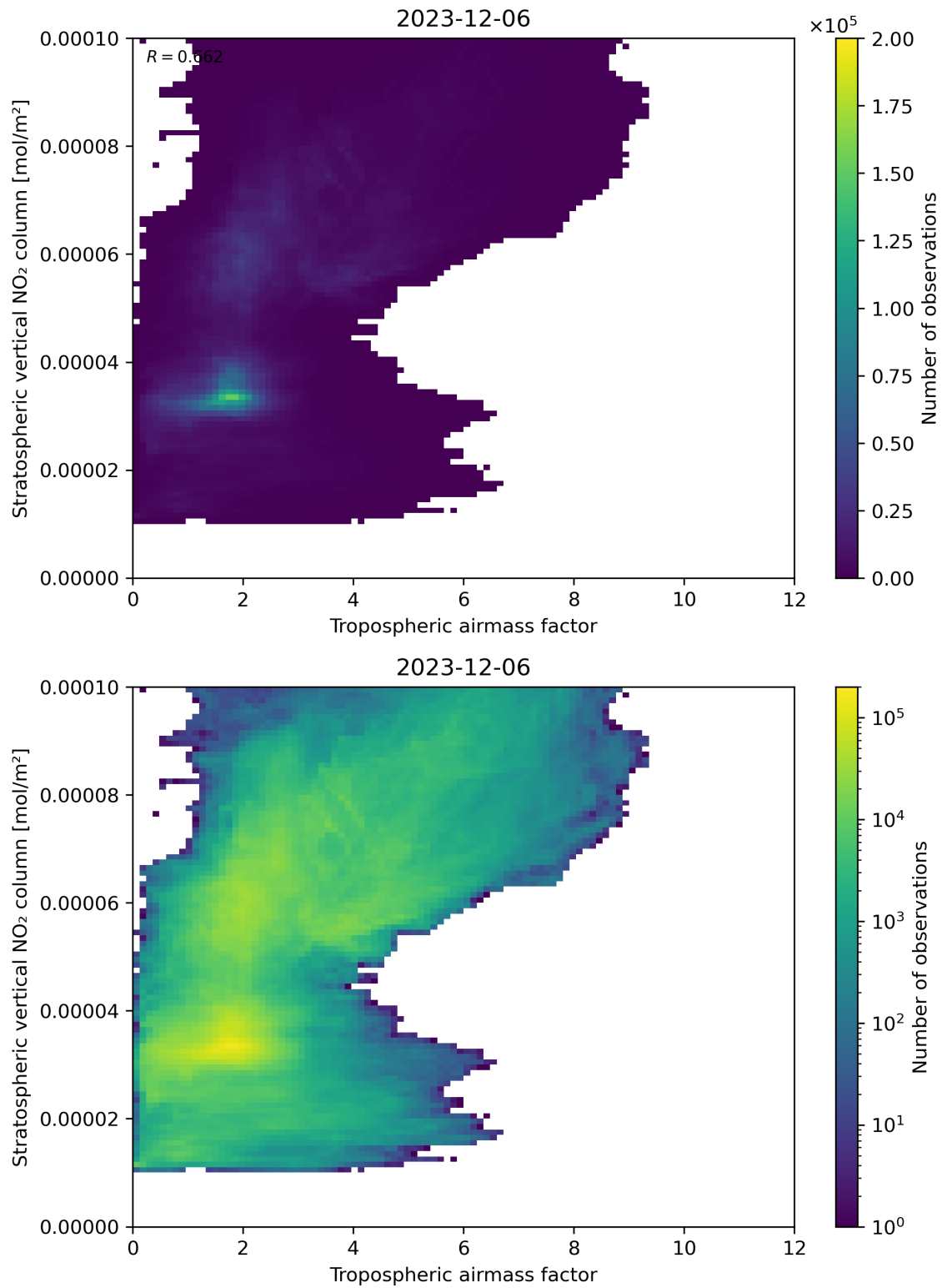
Figure 74: Scatter density plot of “Tropospheric air mass factor” against “Stratospheric vertical NO 2 column” for 2023-12-05 to 2023-12-07.
