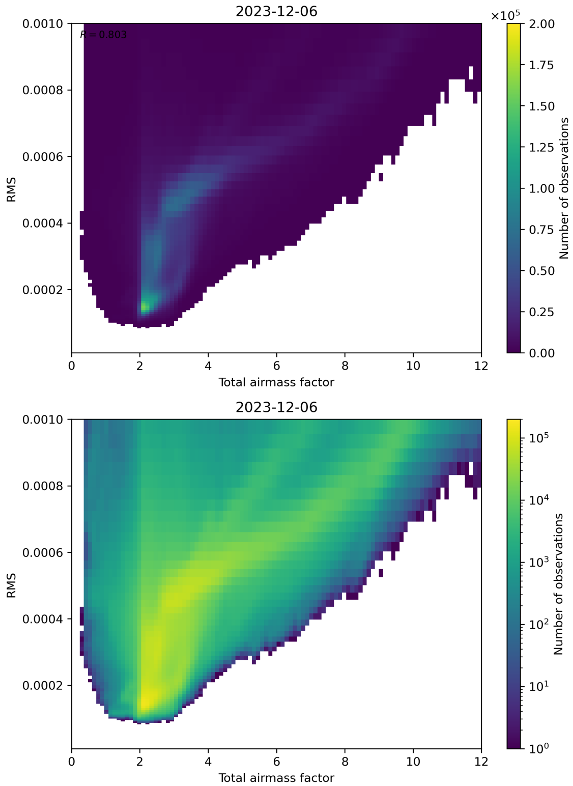
Figure 69: Scatter density plot of “Total airmass factor” against “RMS” for 2023-12-05 to 2023-12-07.
