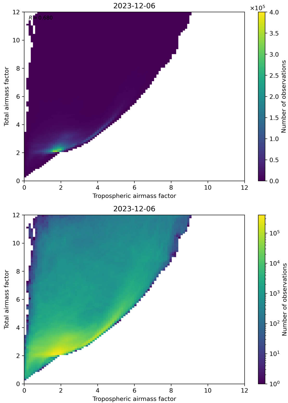
Figure 72: Scatter density plot of “Tropospheric airmass factor” against “Total airmass factor” for 2023-12-05 to 2023-12-07.
