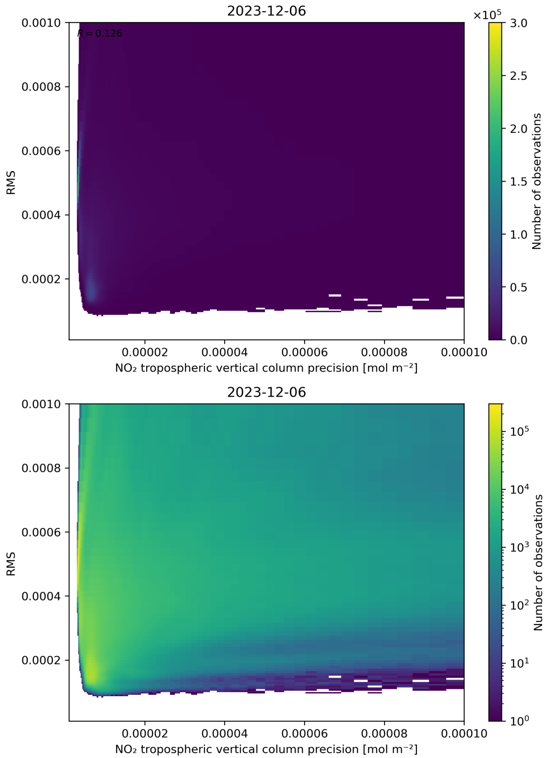
Figure 140: Scatter density plot of “NO 2 tropospheric vertical column precision” against “RMS” for 2023-12-05 to 2023-12-07.
