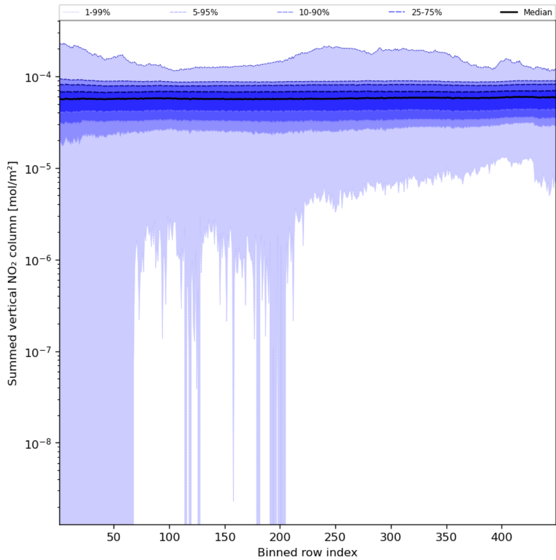
Figure 57: Along track statistics of “Summed vertical NO 2 column” for 2023-12-05 to 2023-12-07
