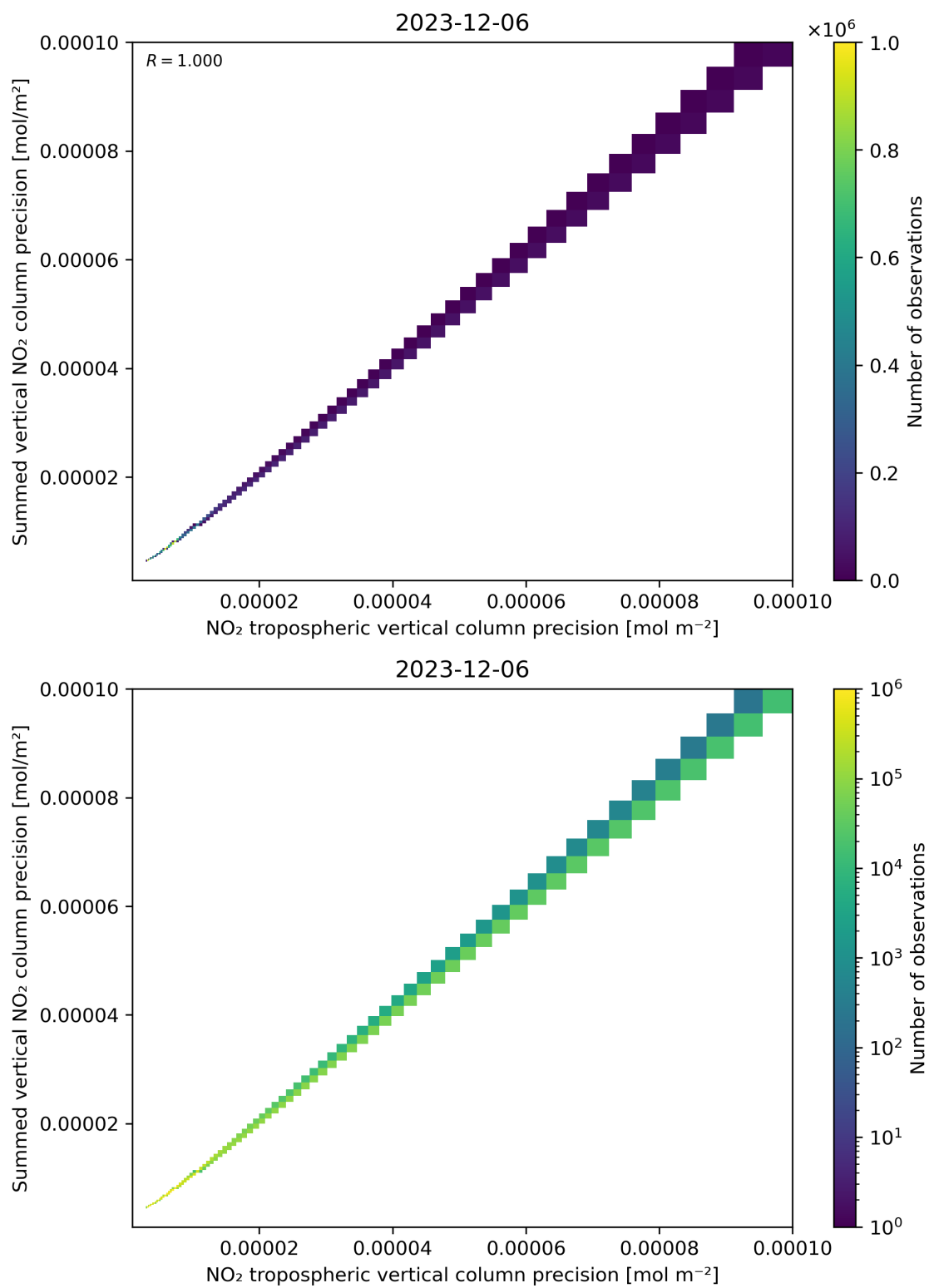
Figure 137: Scatter density plot of “NO 2 tropospheric vertical column precision” against “Summed vertical NO 2 column precision” for 2023-12-05 to 2023-12-07.
