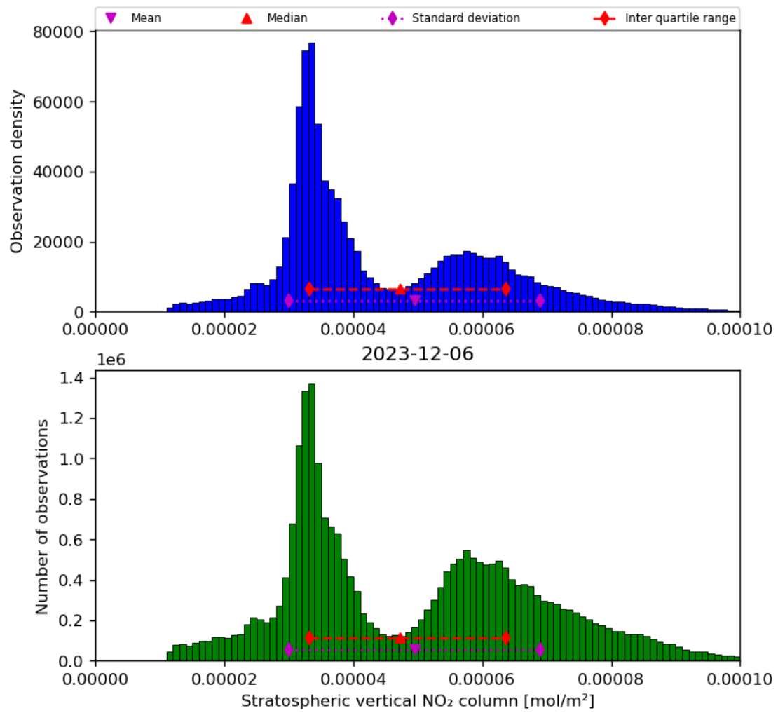
Figure 36: Histogram of “Stratospheric vertical NO 2 column” for 2023-12-05 to 2023-12-07
