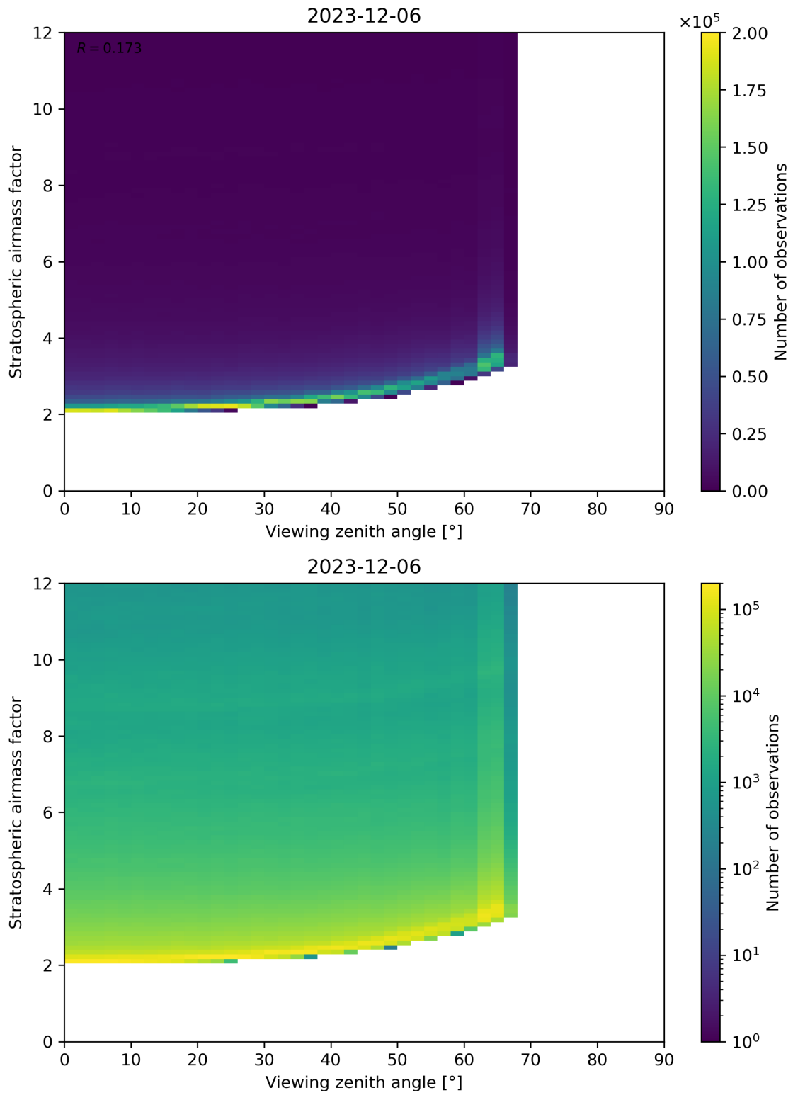
Figure 159: Scatter density plot of “Viewing zenith angle” against “Stratospheric airmass factor” for 2023-12-05 to 2023-12-07.
