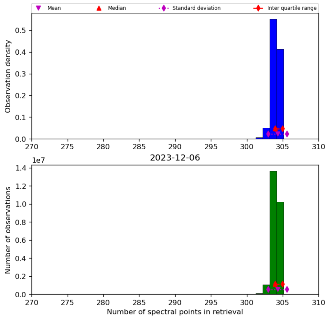
Figure 33: Histogram of “Number of spectral points in retrieval” for 2023-12-05 to 2023-12-07
