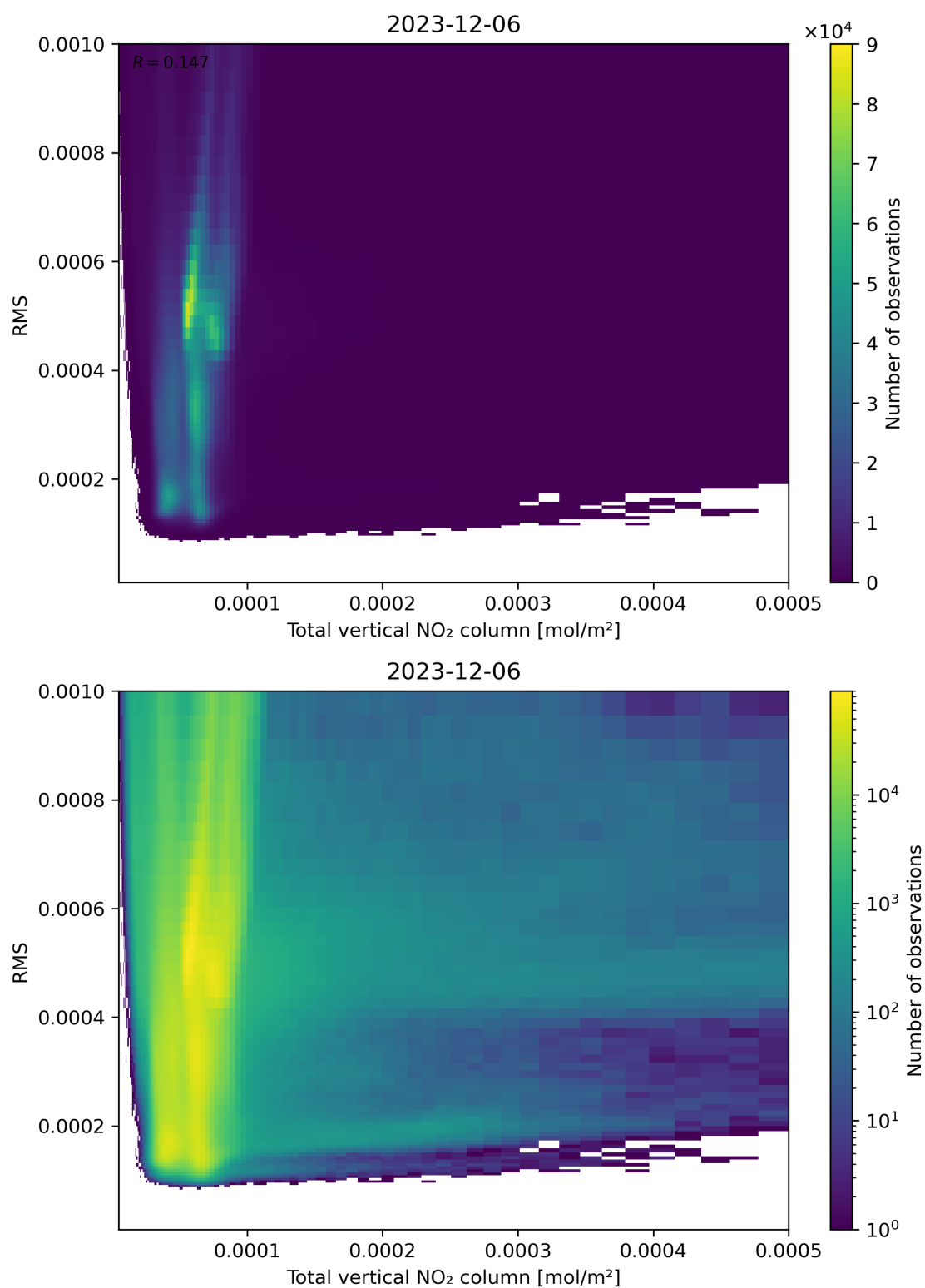
Figure 120: Scatter density plot of “Total vertical NO 2 column” against “RMS” for 2023-12-05 to 2023-12-07.
