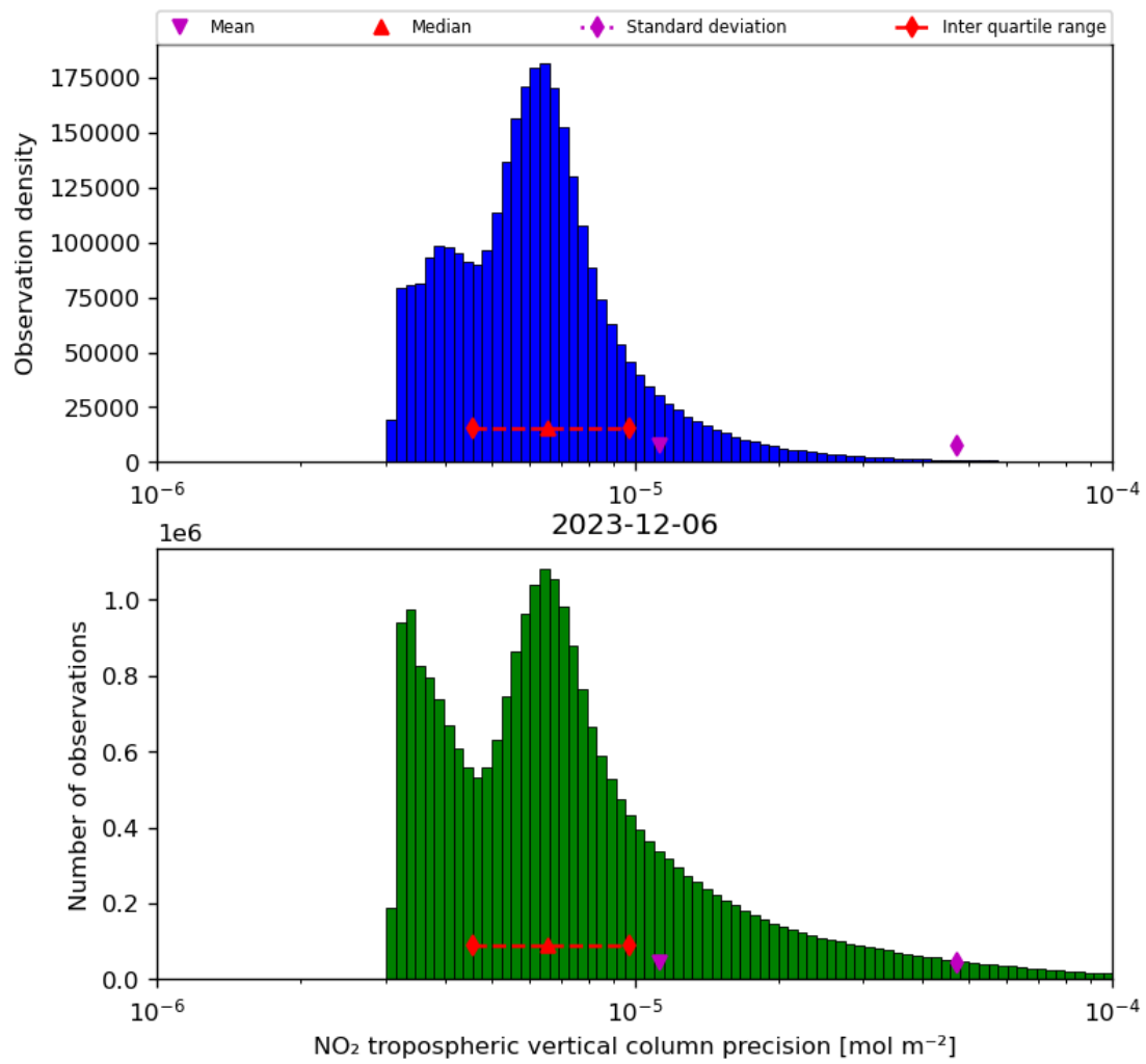
Figure 30: Histogram of “NO 2 tropospheric vertical column precision” for 2023-12-05 to 2023-12-07
