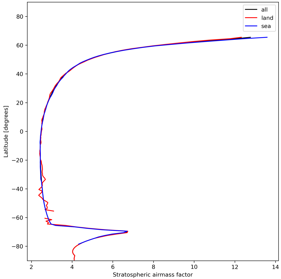
Figure 27: Zonal average of “Stratospheric air mass factor” for 2023-12-05 to 2023-12-07.
