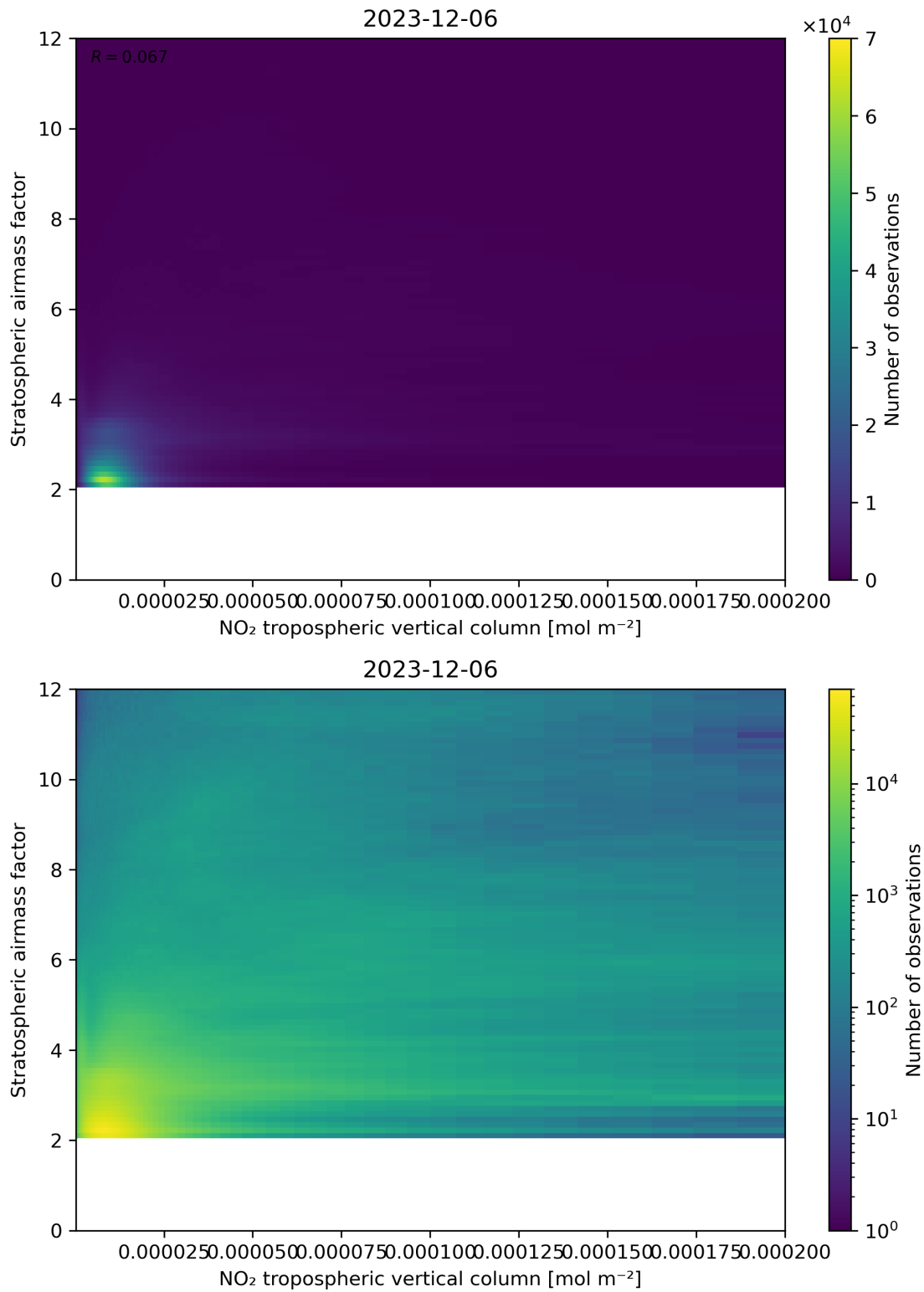
Figure 121: Scatter density plot of “NO 2 tropospheric vertical column” against “Stratospheric airmass factor” for 2023-12-05 to 2023-12-07.
