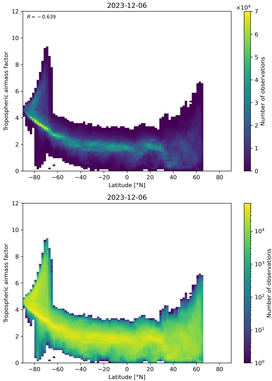
Figure 85: Scatter density plot of “Latitude” against “Tropospheric airmass factor” for 2023-12-05 to 2023-12-07.
