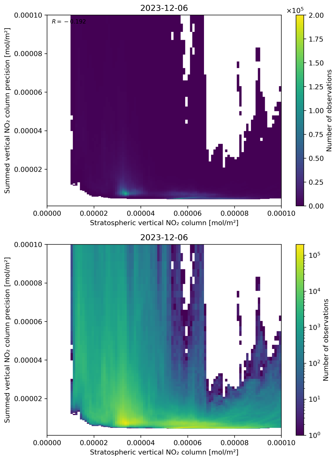
Figure 99: Scatter density plot of “Stratospheric vertical NO 2 column” against “Summed vertical NO 2 column precision” for 2023-12-05 to 2023-12-07.
