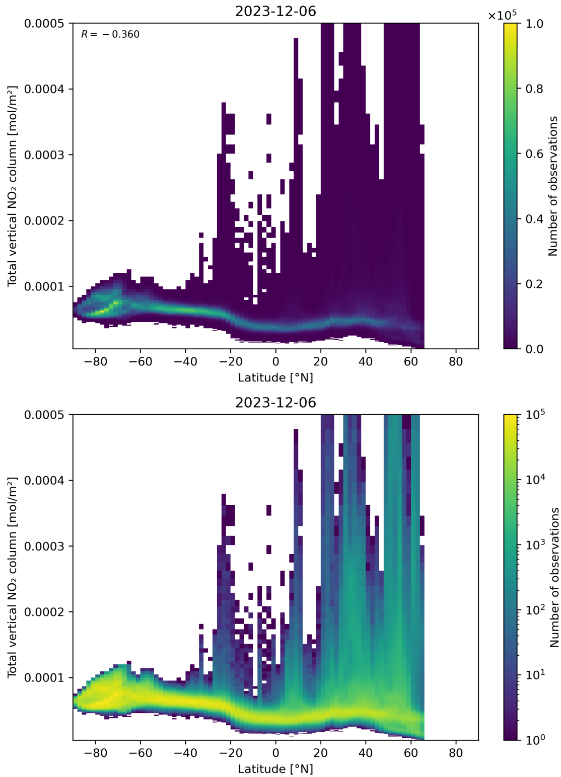
Figure 90: Scatter density plot of “Latitude” against “Total vertical NO 2 column” for 2023-12-05 to 2023-12-07.
