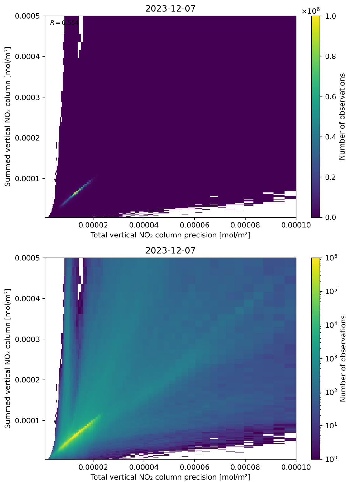
Figure 117: Scatter density plot of “Total vertical NO 2 column precision” against “Summed vertical NO 2 column” for 2023-12-06 to 2023-12-08.
