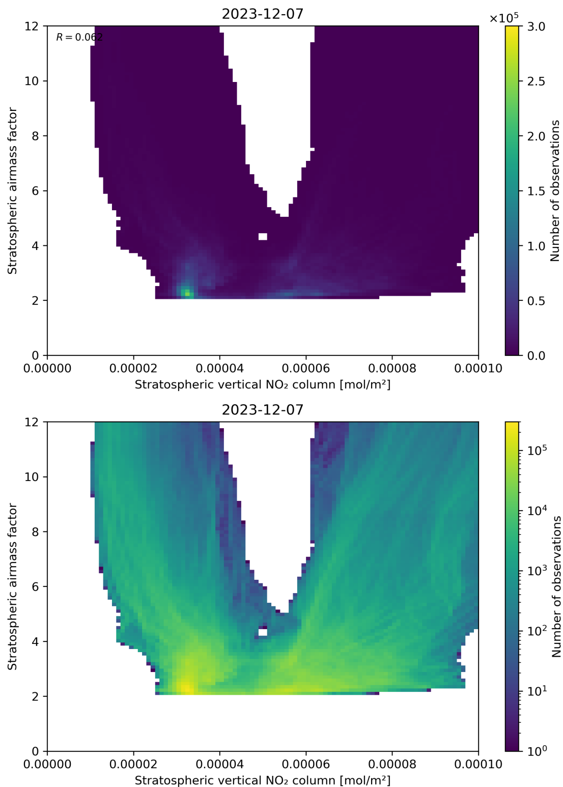
Figure 96: Scatter density plot of “Stratospheric vertical NO 2 column” against “Stratospheric airmass factor” for 2023-12-06 to 2023-12-08.
