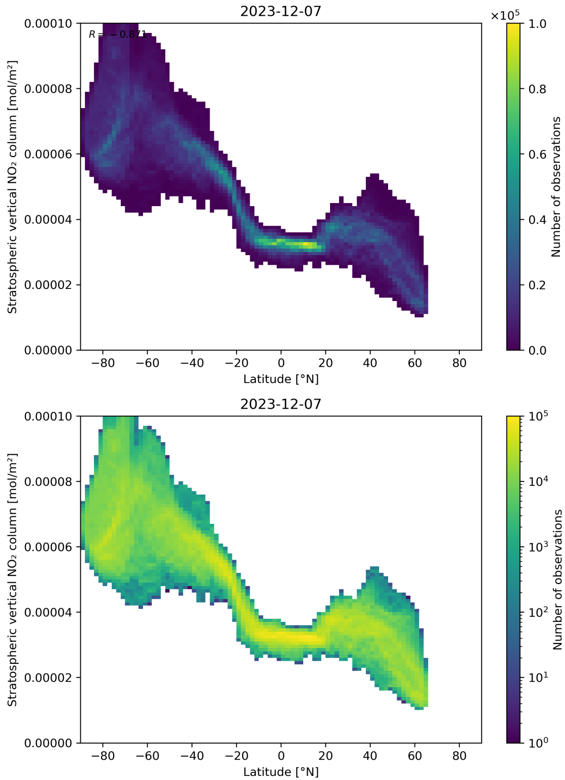
Figure 87: Scatter density plot of “Latitude” against “Stratospheric vertical NO 2 column” for 2023-12-06 to 2023-12-08.
