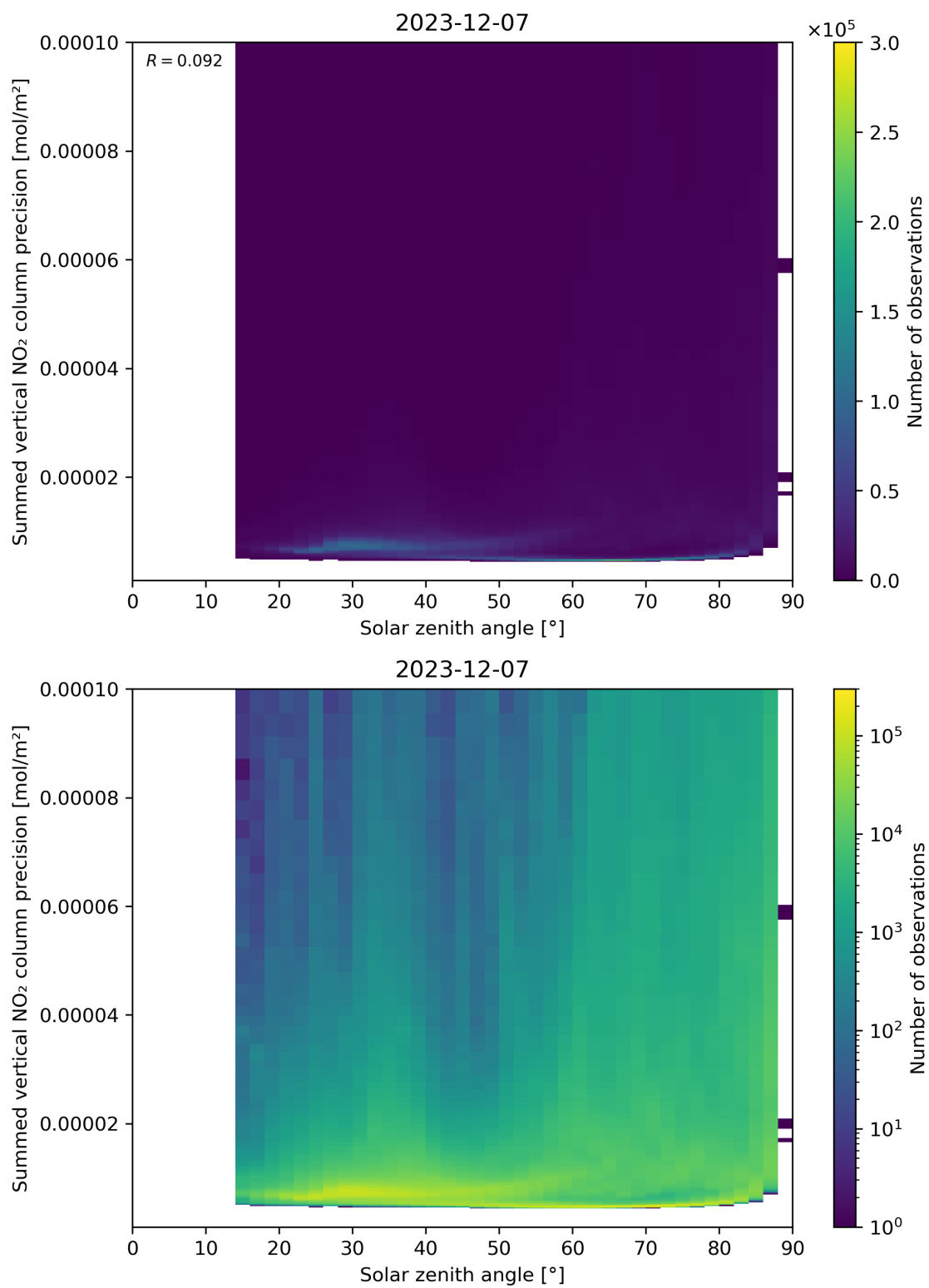
Figure 152: Scatter density plot of “Solar zenith angle” against “Summed vertical NO 2 column precision” for 2023-12-06 to 2023-12-08.
