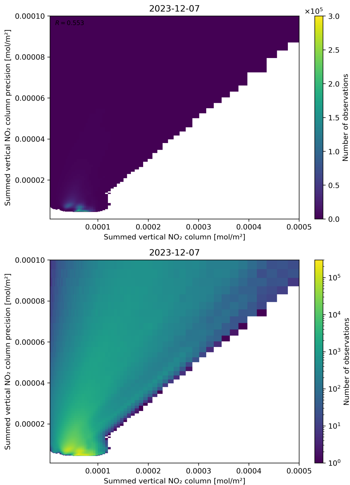
Figure 105: Scatter density plot of “Summed vertical NO 2 column” against “Summed vertical NO 2 column precision” for 2023-12-06 to 2023-12-08.
