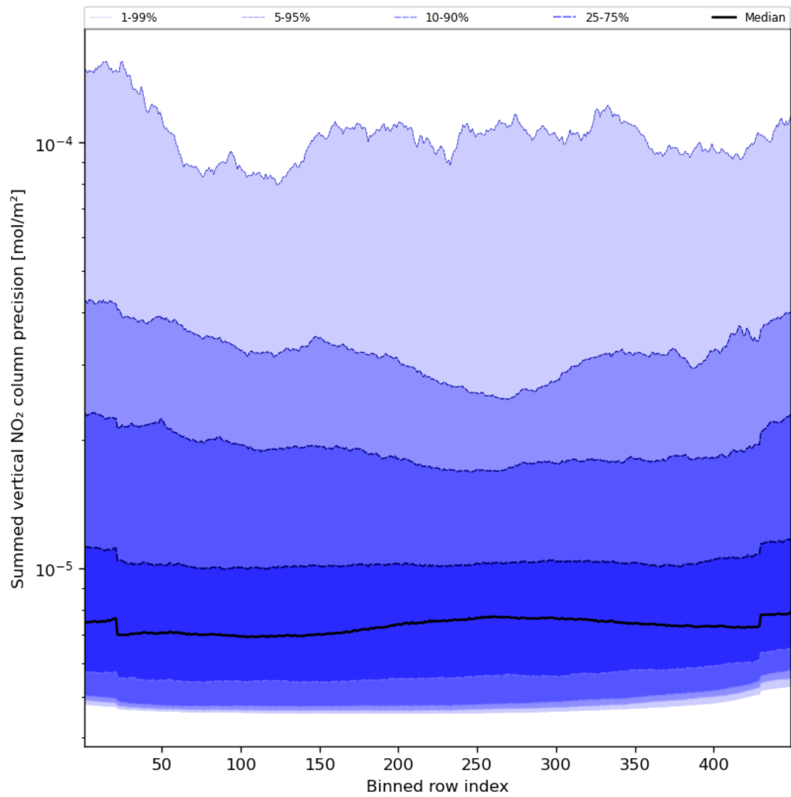
Figure 58: Along track statistics of “Summed vertical NO 2 column precision” for 2023-12-06 to 2023-12-08
