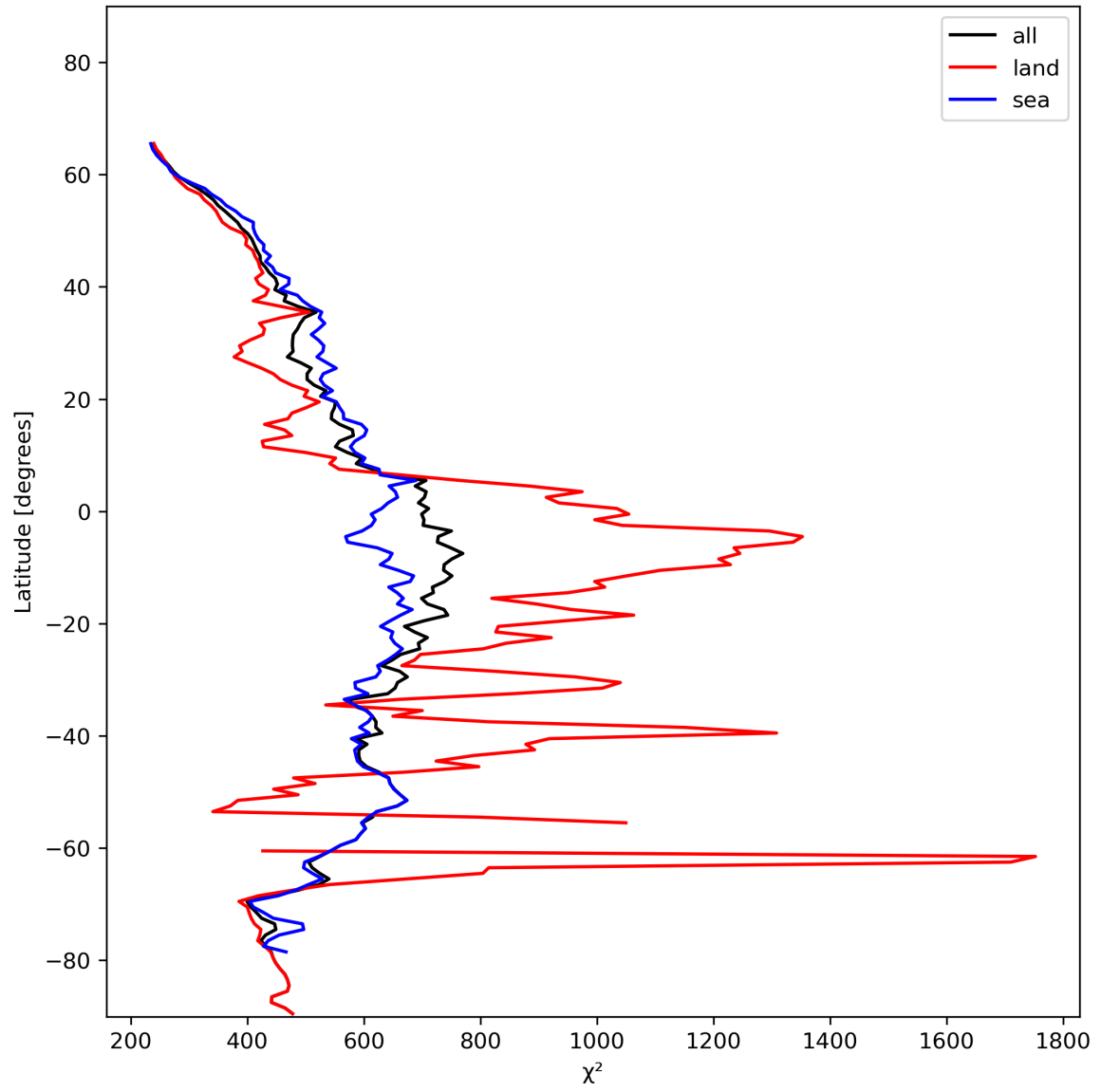
Figure 25: Zonal average of “ \chi^2 ” for 2023-12-06 to 2023-12-08.
