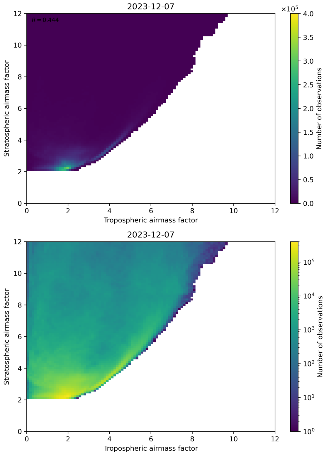
Figure 71: Scatter density plot of “Tropospheric airmass factor” against “Stratospheric airmass factor” for 2023-12-06 to 2023-12-08.
