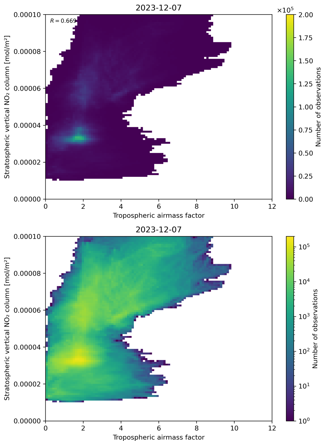
Figure 74: Scatter density plot of “Tropospheric airmass factor” against “Stratospheric vertical NO 2 column” for 2023-12-06 to 2023-12-08.
