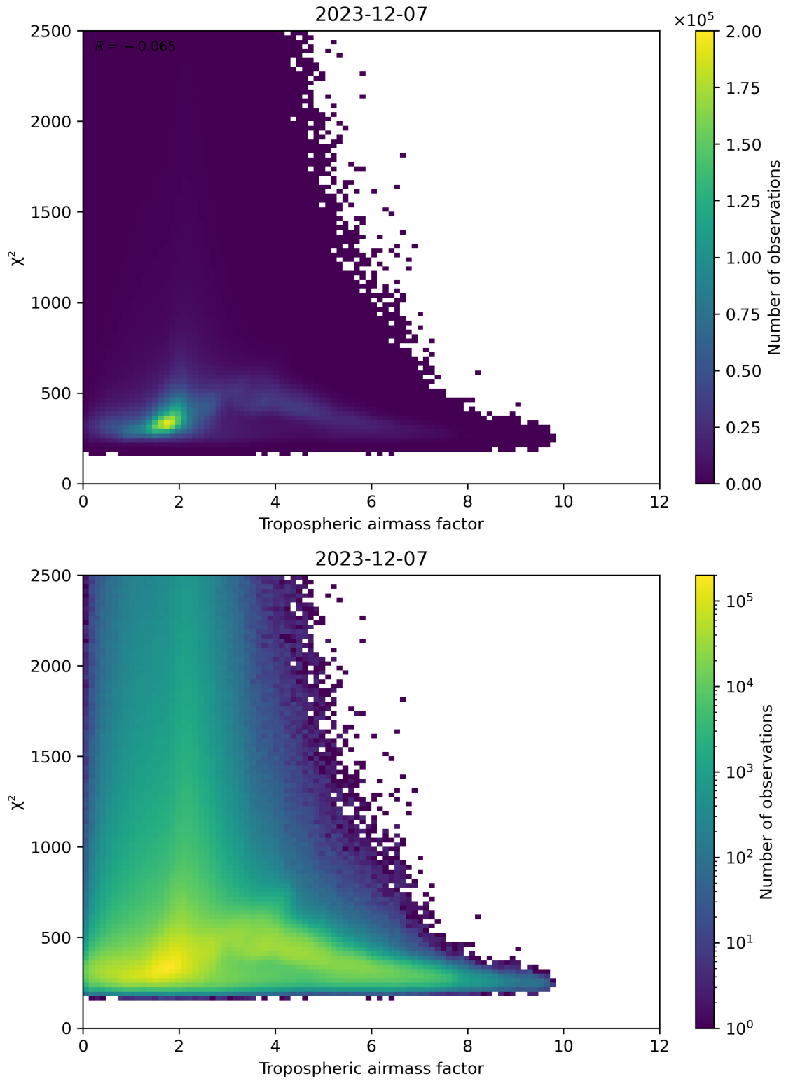
Figure 73: Scatter density plot of “Tropospheric airmass factor” against “ \chi^2 ” for 2023-12-06 to 2023-12-08.
