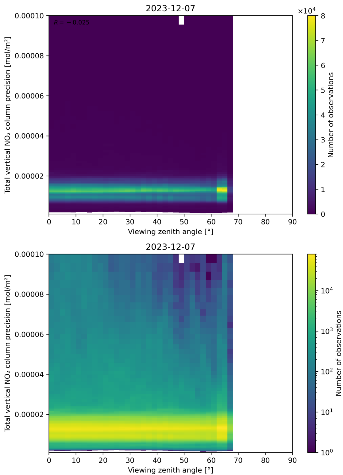
Figure 168: Scatter density plot of “Viewing zenith angle” against “Total vertical NO 2 column precision” for 2023-12-06 to 2023-12-08.
