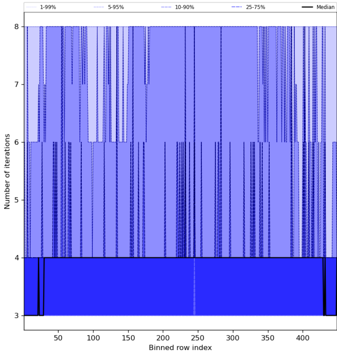
Figure 51: Along track statistics of “Number of iterations” for 2023-12-06 to 2023-12-08
