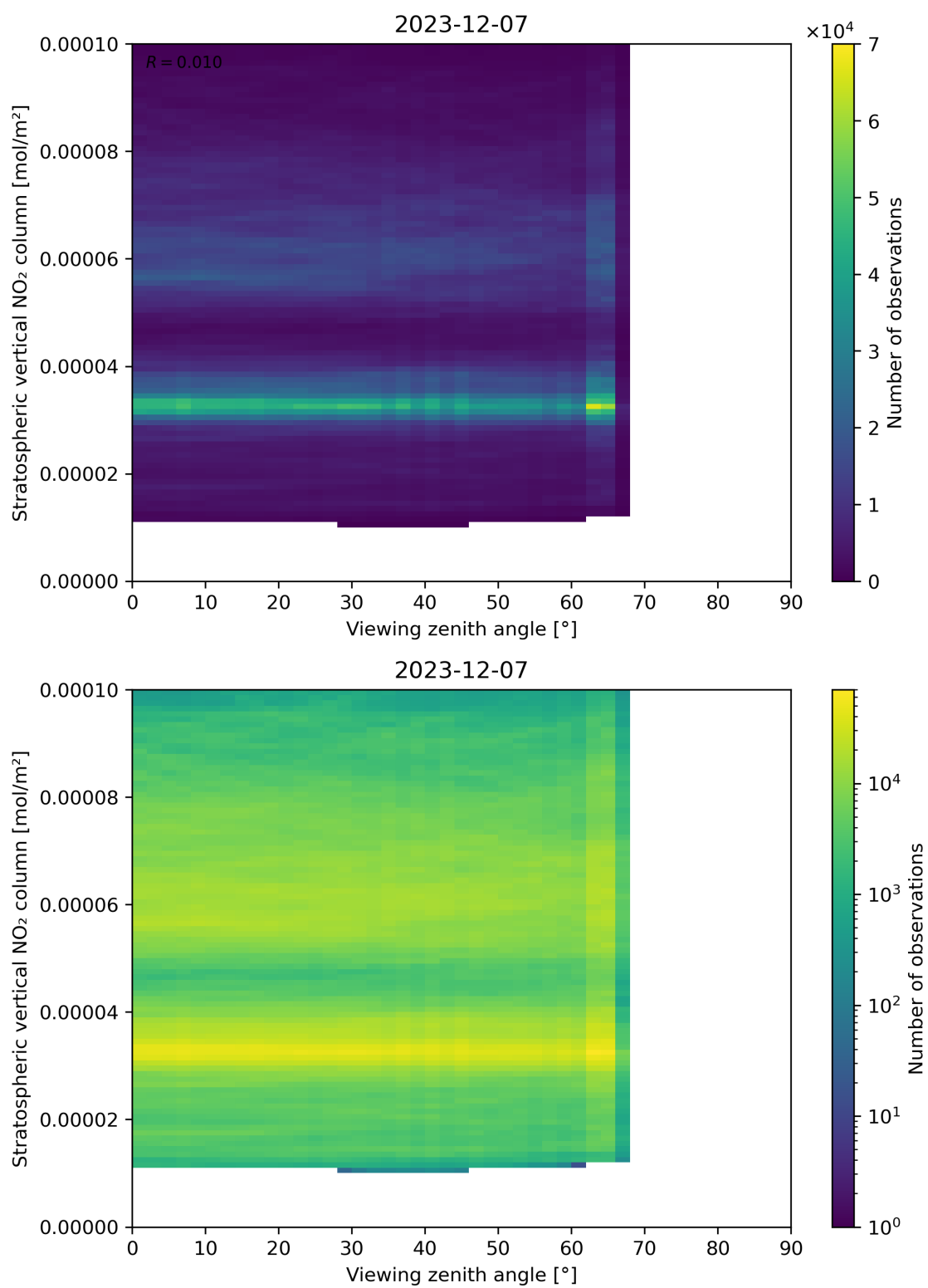
Figure 164: Scatter density plot of “Viewing zenith angle” against “Stratospheric vertical NO 2 column” for 2023-12-06 to 2023-12-08.
