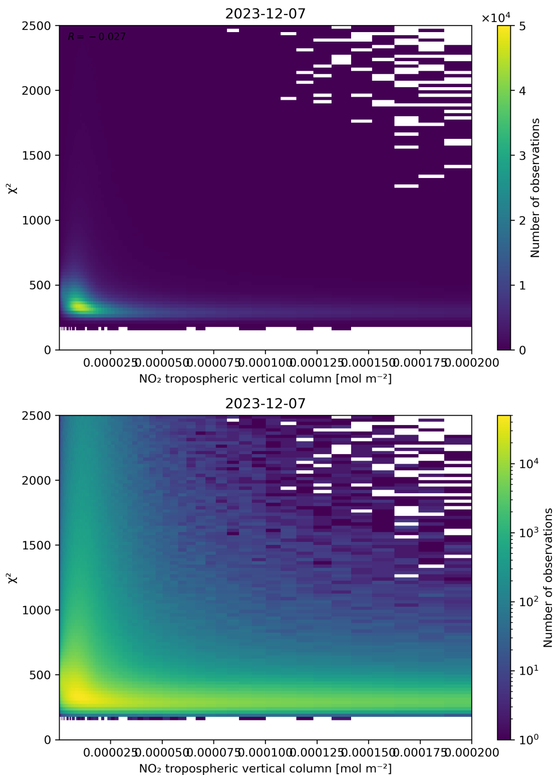
Figure 124: Scatter density plot of “NO 2 tropospheric vertical column” against “ \chi^2 ” for 2023-12-06 to 2023-12-08.
