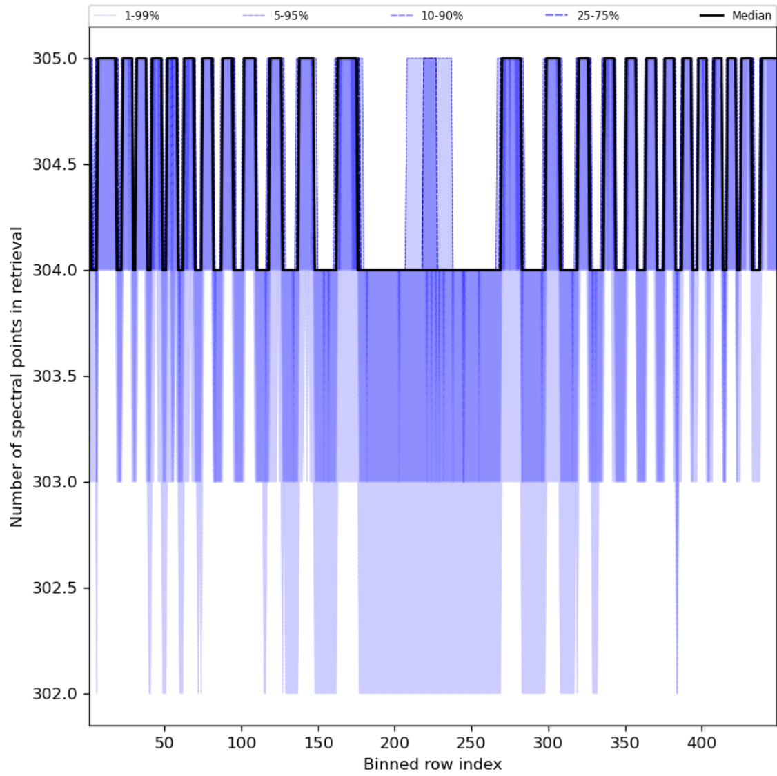
Figure 50: Along track statistics of “Number of spectral points in retrieval” for 2023-12-06 to 2023-12-08
