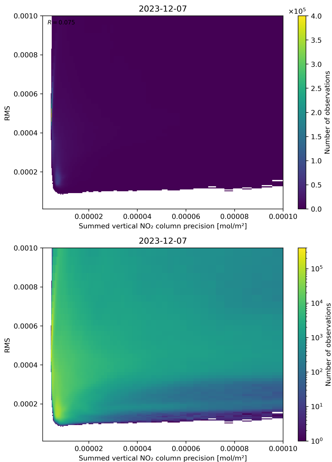
Figure 108: Scatter density plot of “Summed vertical NO 2 column precision” against “RMS” for 2023-12-06 to 2023-12-08.
