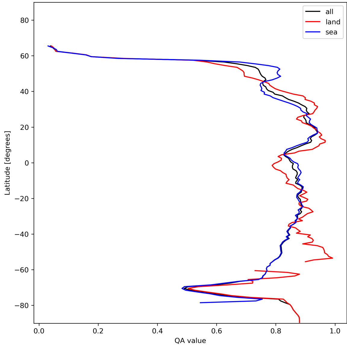
Figure 11: Zonal average of “QA value” for 2023-12-06 to 2023-12-08.
