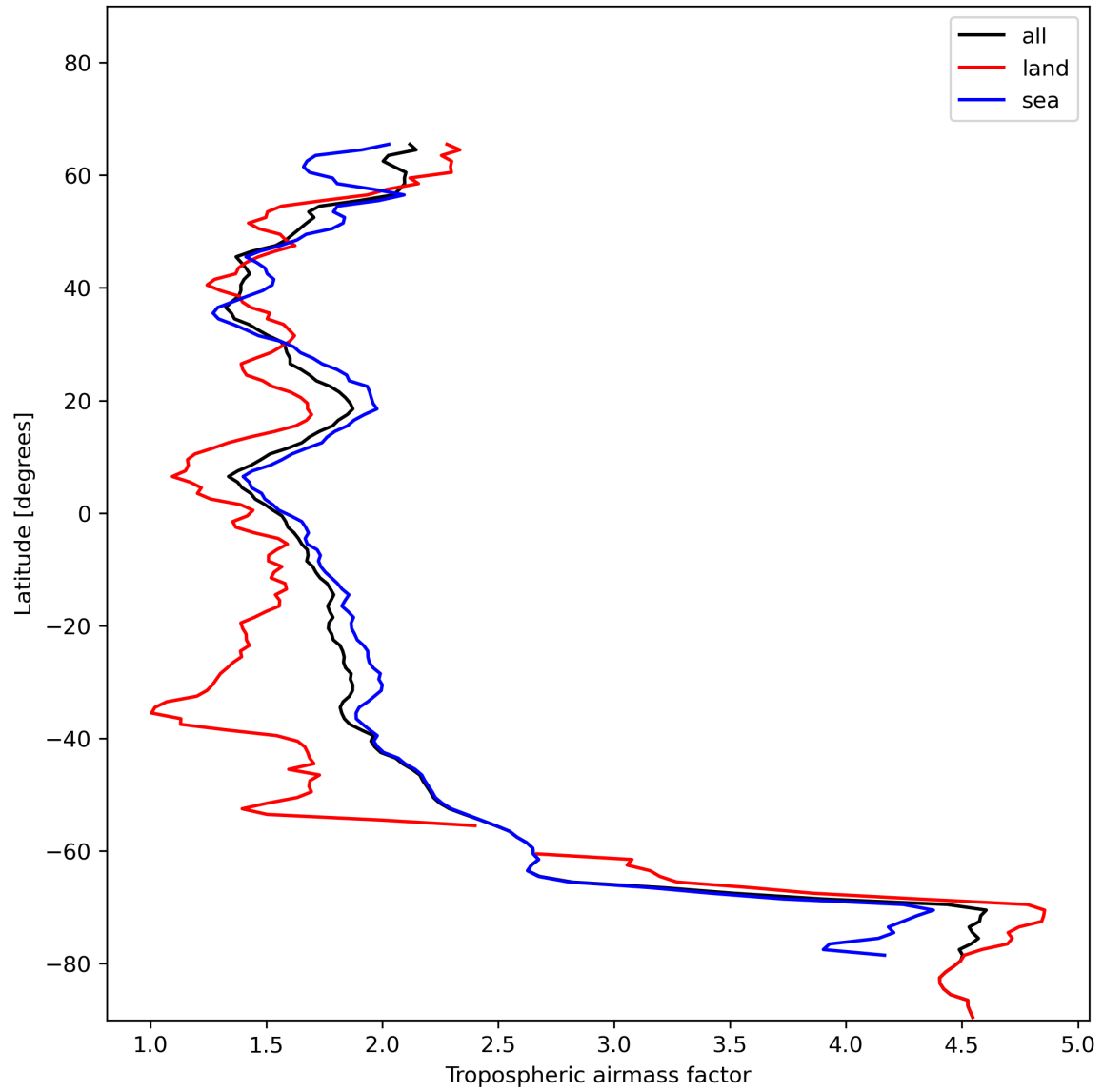
Figure 14: Zonal average of “Tropospheric airmass factor” for 2023-12-06 to 2023-12-08.
