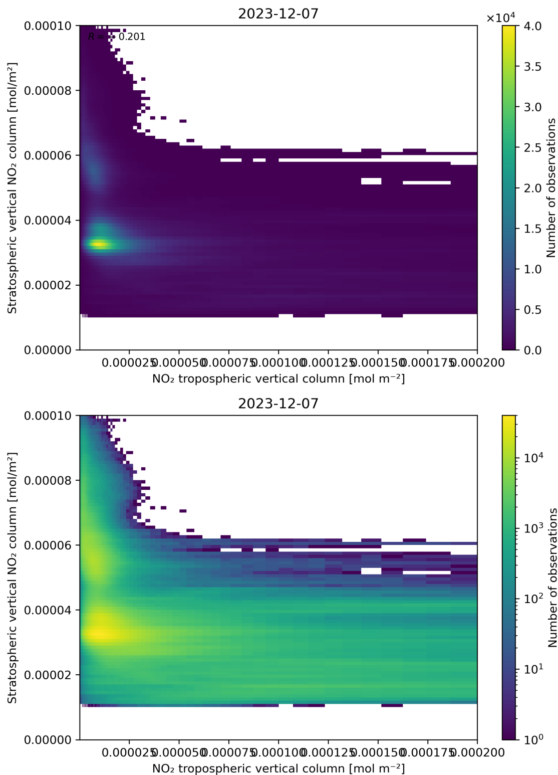
Figure 125: Scatter density plot of “NO 2 tropospheric vertical column” against “Stratospheric vertical NO 2 column” for 2023-12-06 to 2023-12-08.
