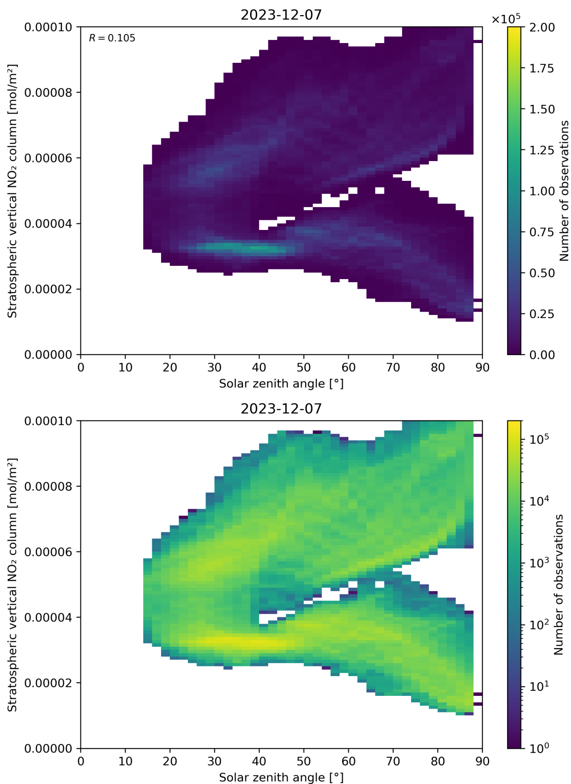
Figure 150: Scatter density plot of “Solar zenith angle” against “Stratospheric vertical NO 2 column” for 2023-12-06 to 2023-12-08.
