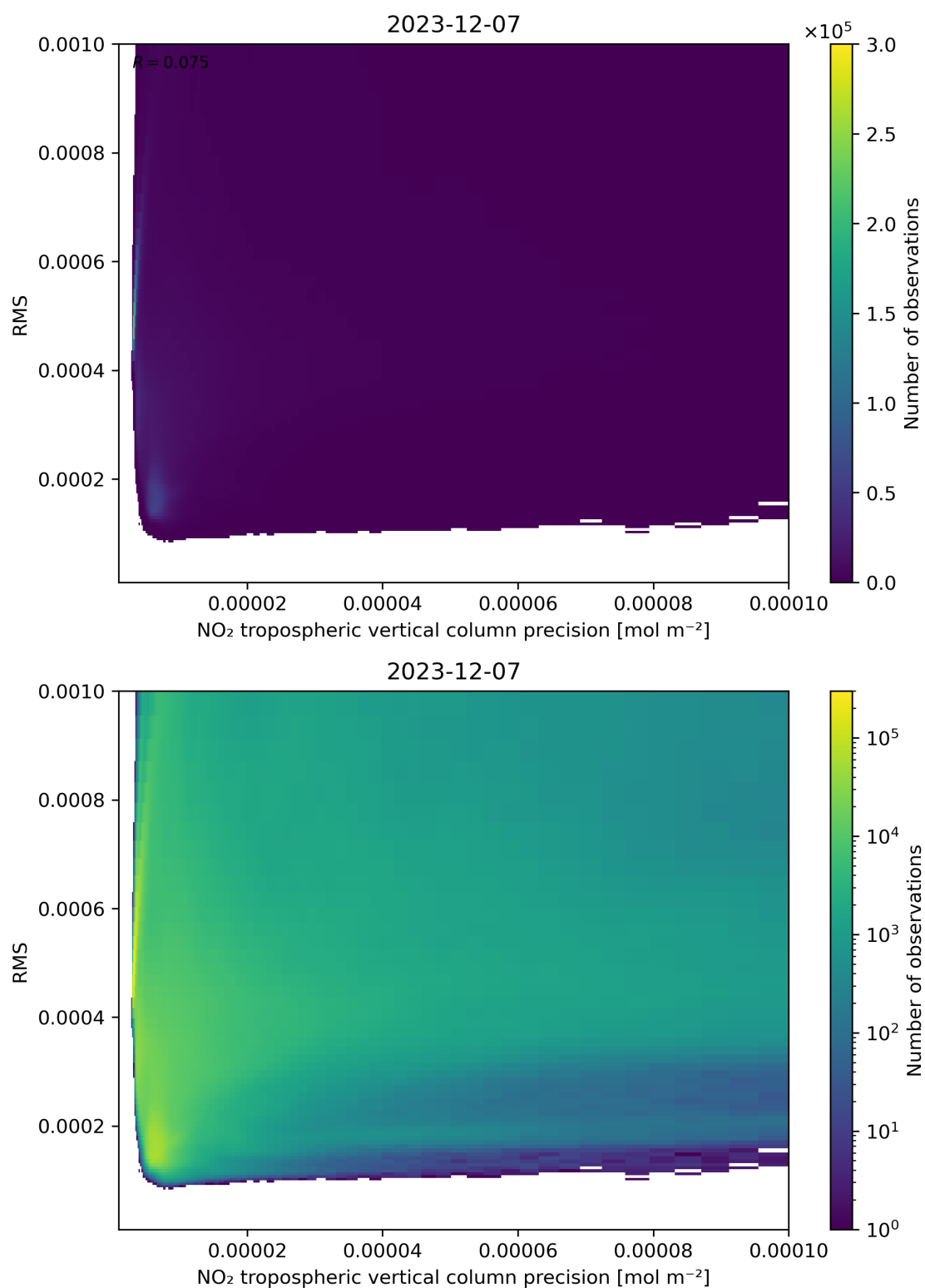
Figure 140: Scatter density plot of “NO 2 tropospheric vertical column precision” against “RMS” for 2023-12-06 to 2023-12-08.
