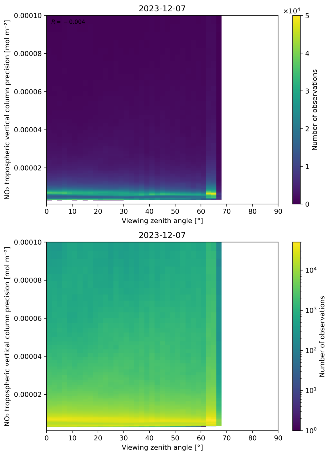
Figure 170: Scatter density plot of “Viewing zenith angle” against “NO 2 tropospheric vertical column precision” for 2023-12-06 to 2023-12-08.
