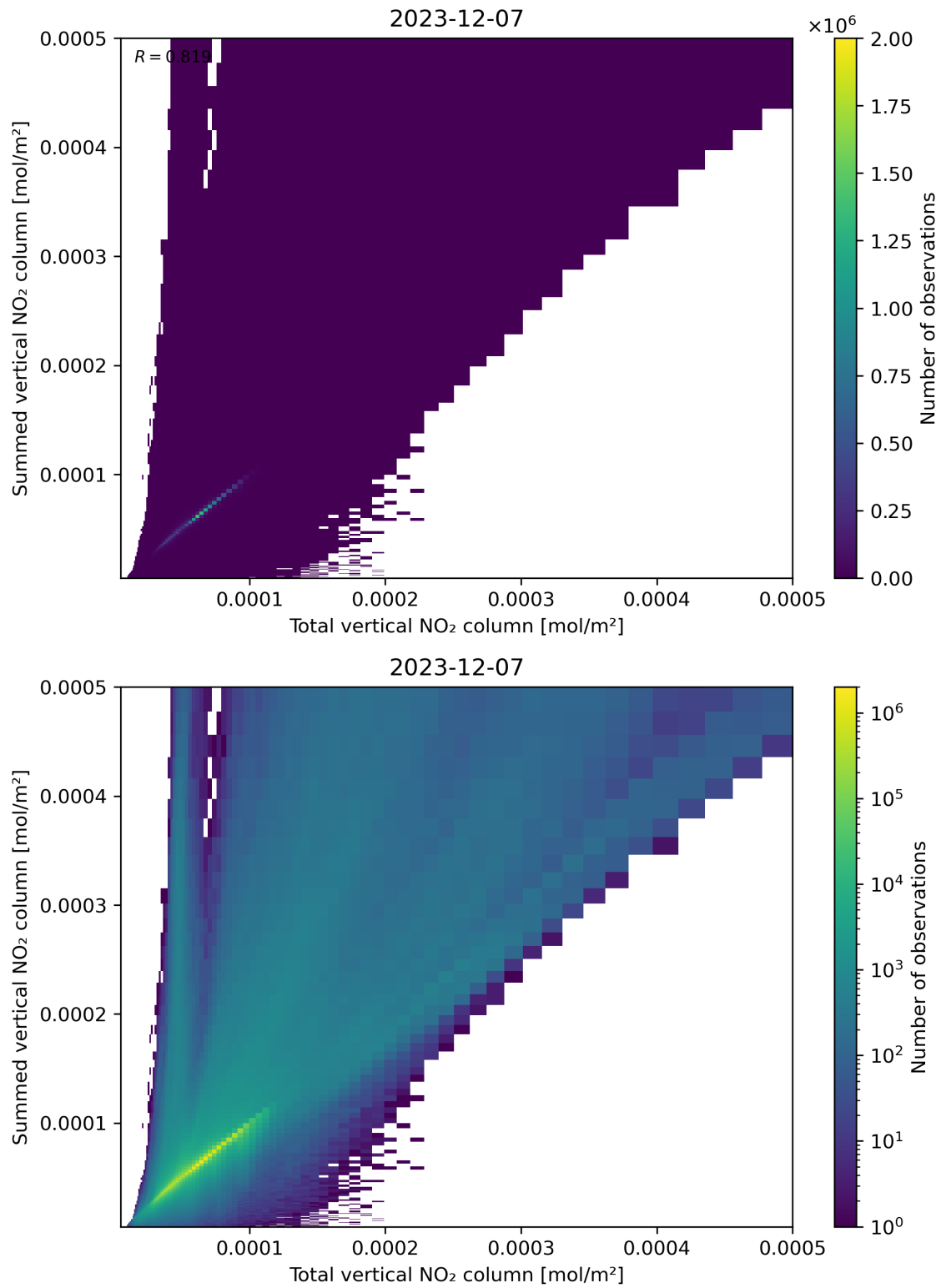
Figure 112: Scatter density plot of “Total vertical NO 2 column” against “Summed vertical NO 2 column” for 2023-12-06 to 2023-12-08.
