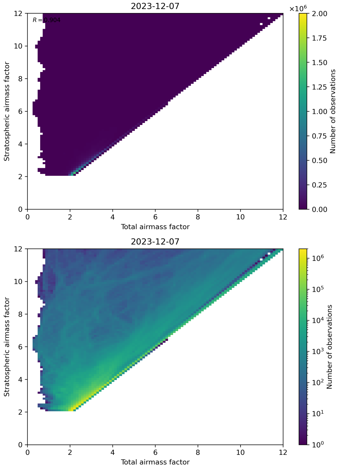
Figure 62: Scatter density plot of “Total airmass factor” against “Stratospheric airmass factor” for 2023-12-06 to 2023-12-08.
