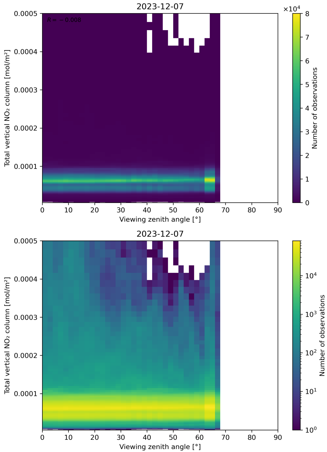
Figure 167: Scatter density plot of “Viewing zenith angle” against “Total vertical NO 2 column” for 2023-12-06 to 2023-12-08.
