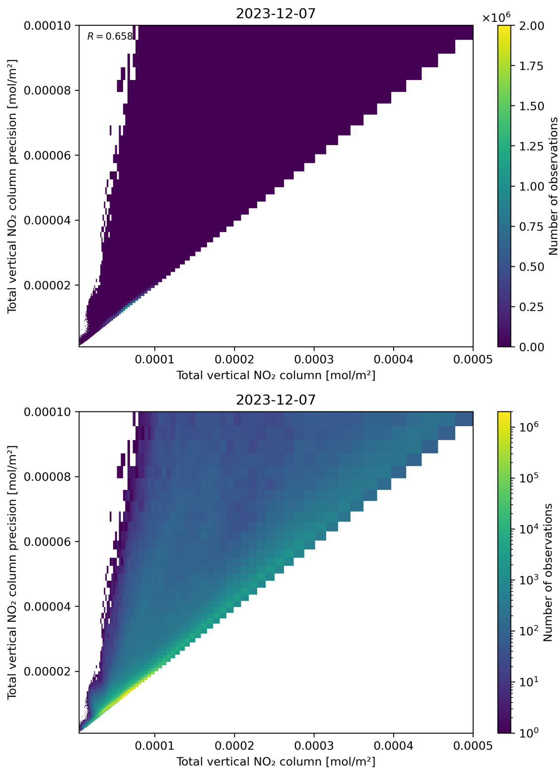
Figure 114: Scatter density plot of “Total vertical NO 2 column” against “Total vertical NO 2 column precision” for 2023-12-06 to 2023-12-08.
