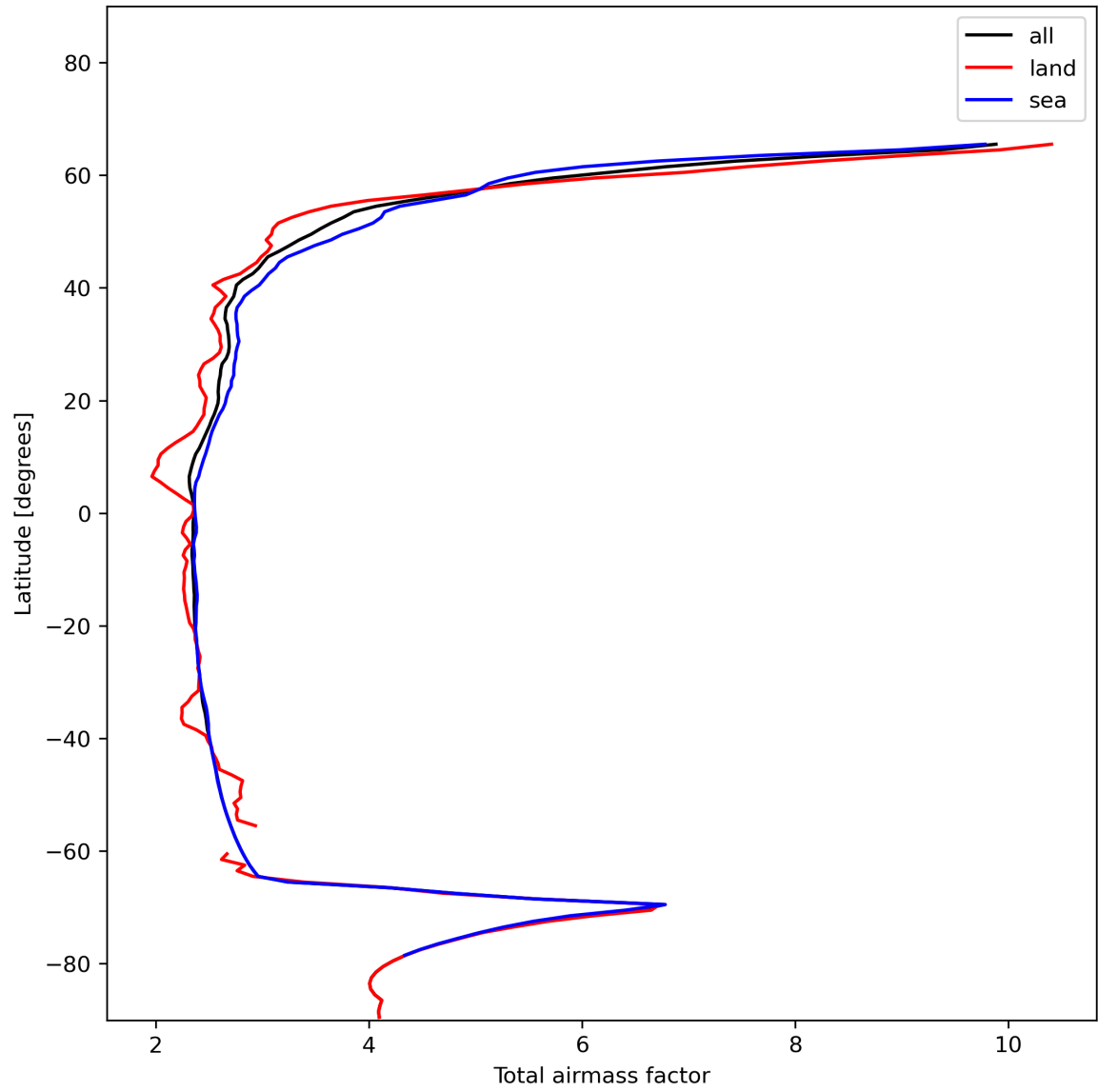
Figure 15: Zonal average of “Total airmass factor” for 2023-12-06 to 2023-12-08.
