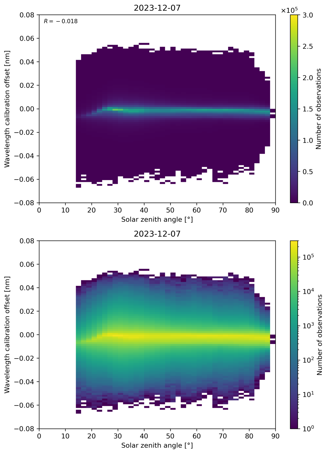
Figure 158: Scatter density plot of “Solar zenith angle” against “Wavelength calibration offset” for 2023-12-06 to 2023-12-08.
