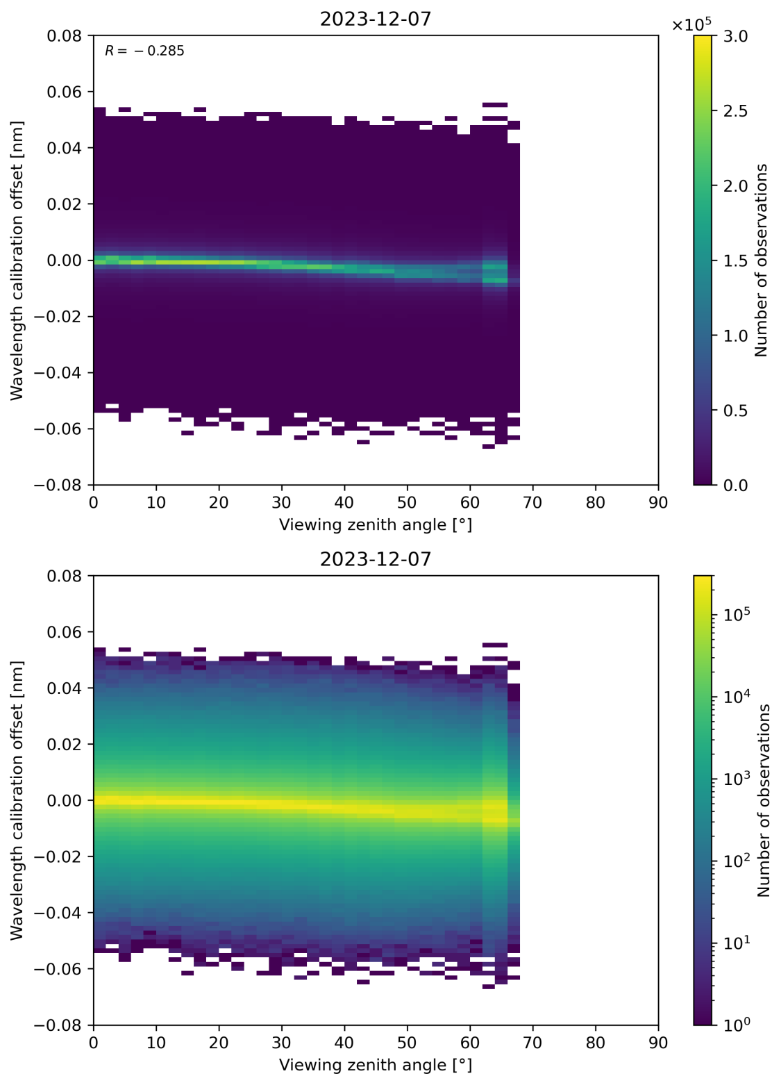
Figure 173: Scatter density plot of “Viewing zenith angle” against “Wavelength calibration offset” for 2023-12-06 to 2023-12-08.
