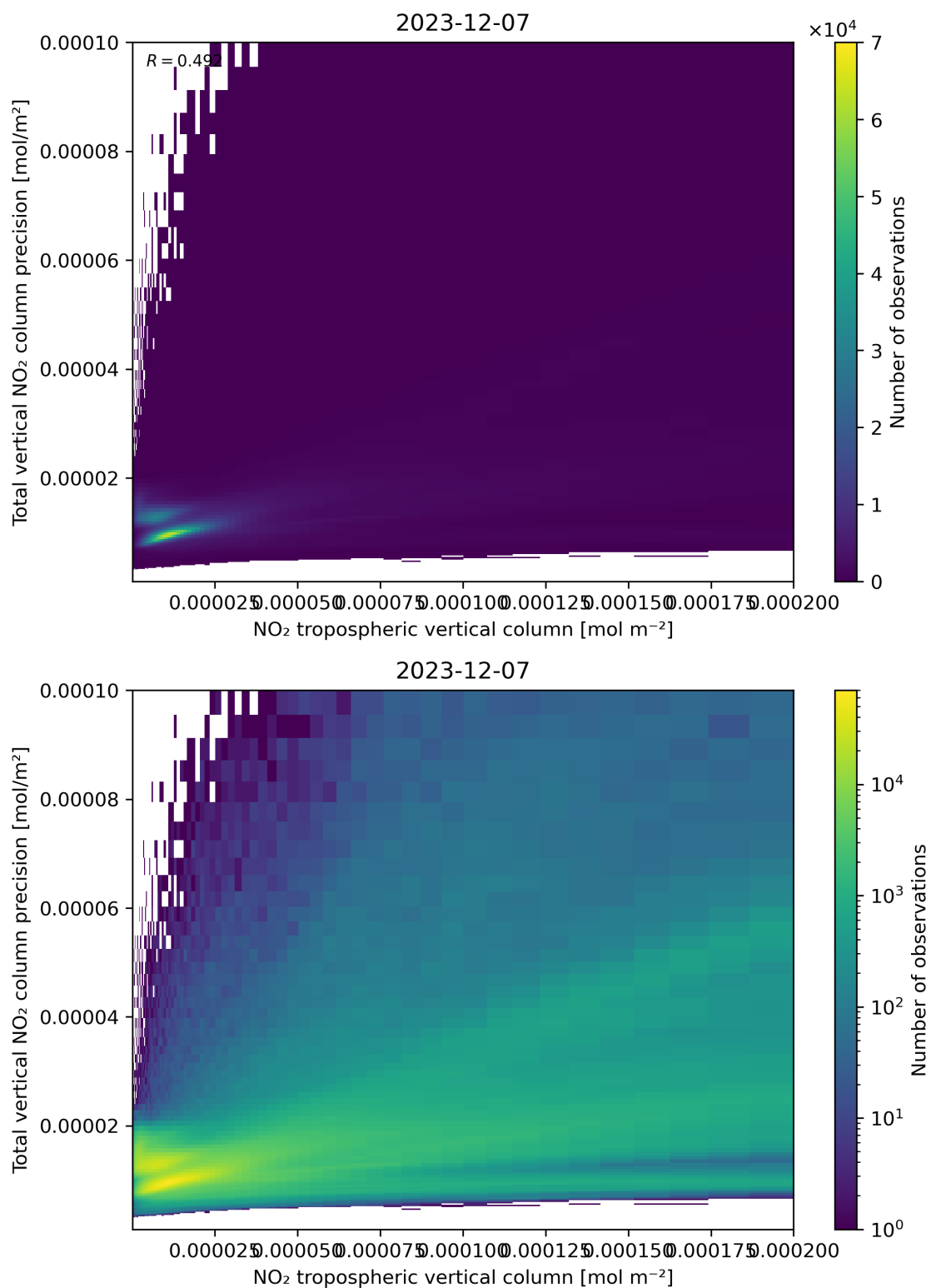
Figure 129: Scatter density plot of “NO 2 tropospheric vertical column” against “Total vertical NO 2 column precision” for 2023-12-06 to 2023-12-08.
