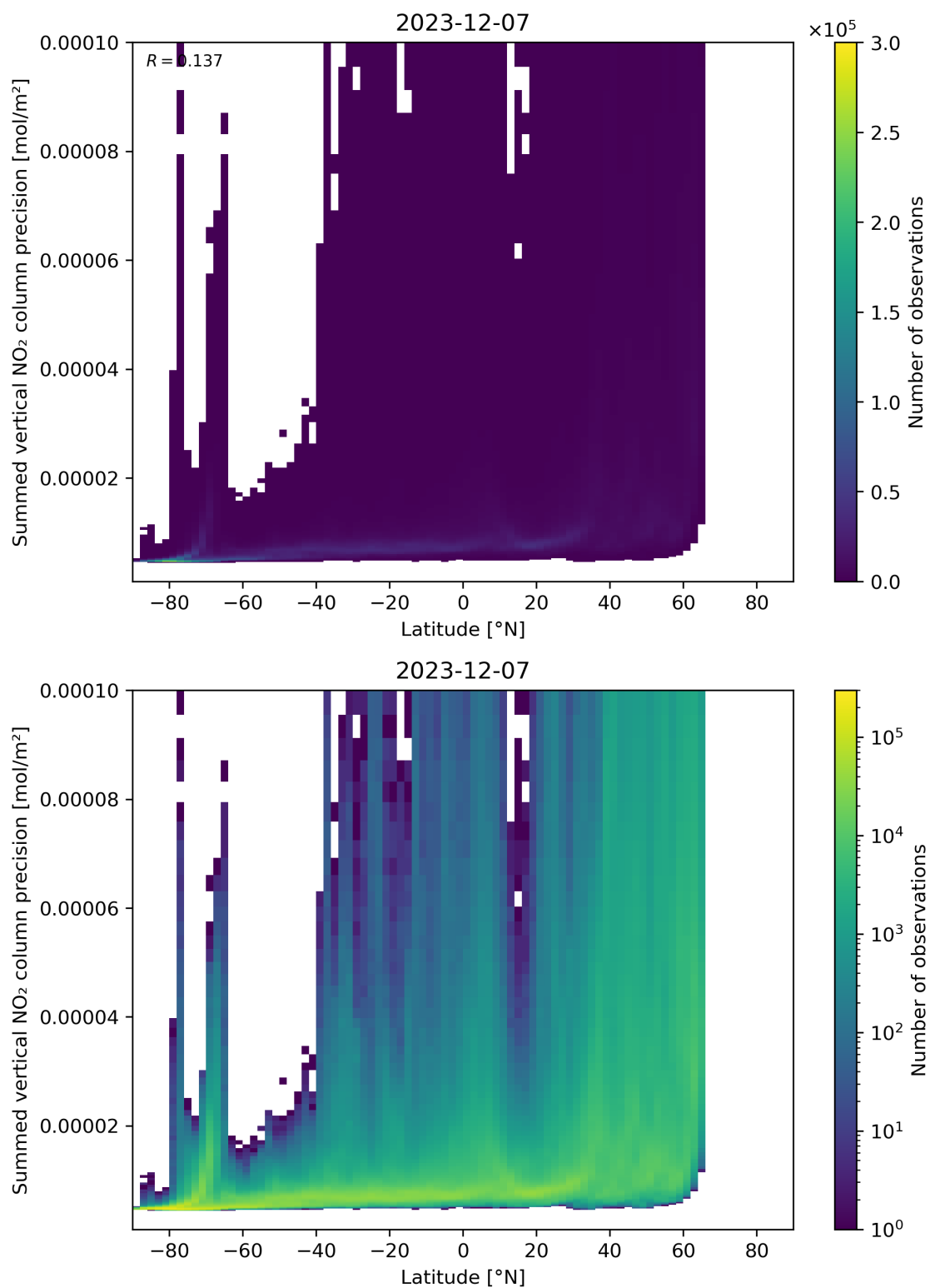
Figure 89: Scatter density plot of “Latitude” against “Summed vertical NO 2 column precision” for 2023-12-06 to 2023-12-08.
