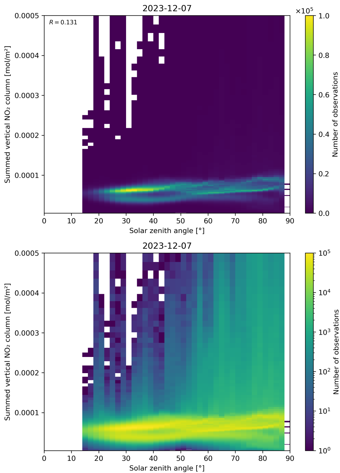
Figure 151: Scatter density plot of “Solar zenith angle” against “Summed vertical NO 2 column” for 2023-12-06 to 2023-12-08.
