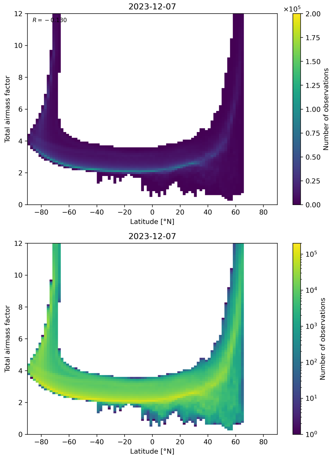
Figure 84: Scatter density plot of “Latitude” against “Total airmass factor” for 2023-12-06 to 2023-12-08.
