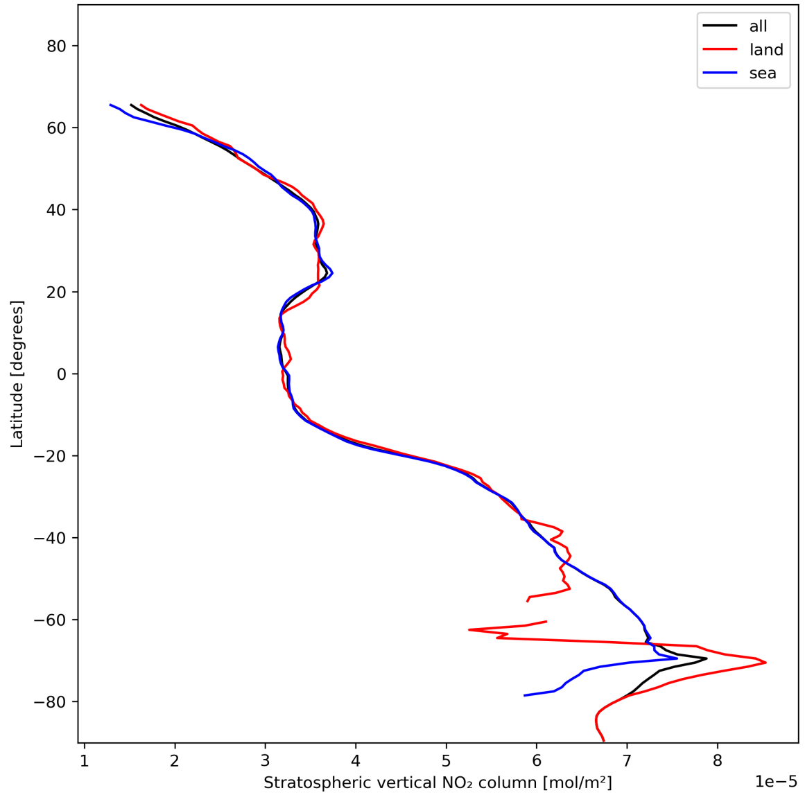
Figure 19: Zonal average of “Stratospheric vertical NO 2 column” for 2023-12-06 to 2023-12-08.
