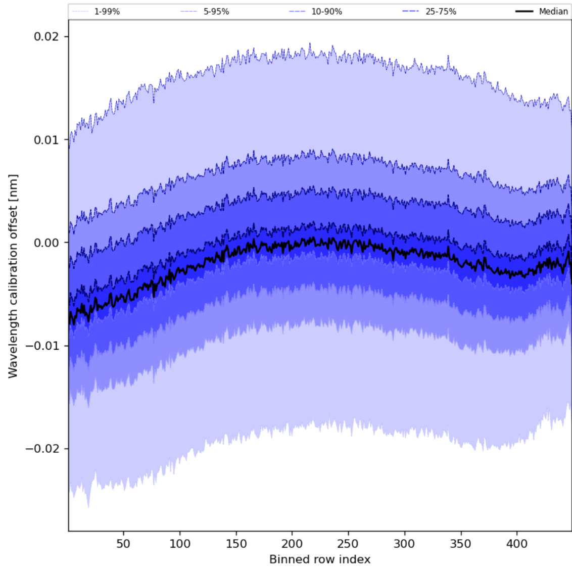
Figure 52: Along track statistics of “Wavelength calibration offset” for 2023-12-06 to 2023-12-08
