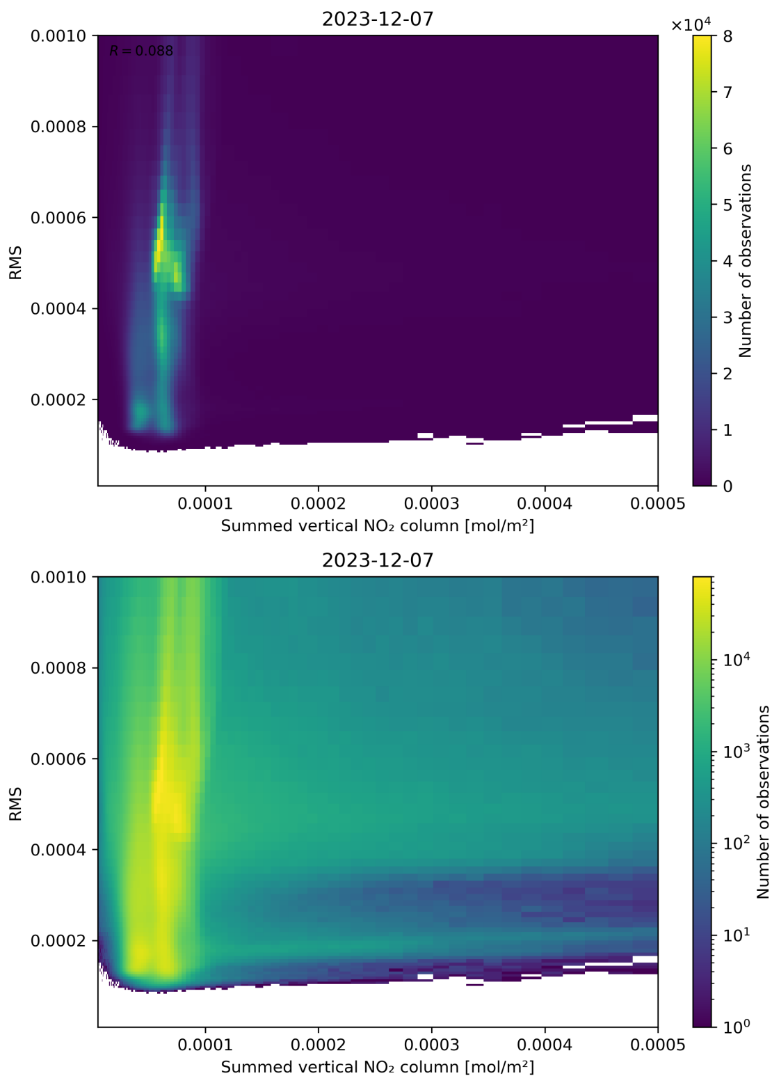
Figure 109: Scatter density plot of “Summed vertical NO 2 column” against “RMS” for 2023-12-06 to 2023-12-08.
