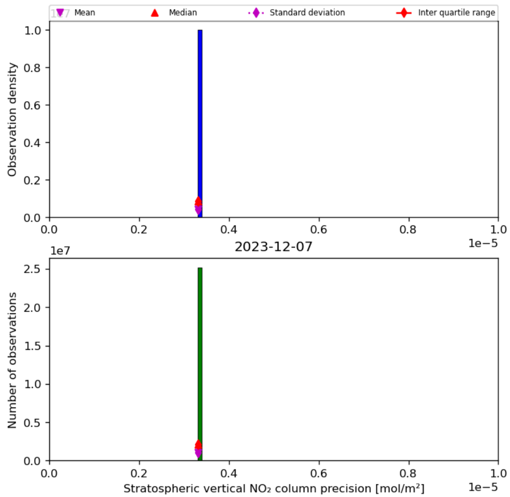
Figure 37: Histogram of “Stratospheric vertical NO 2 column precision” for 2023-12-06 to 2023-12-08
