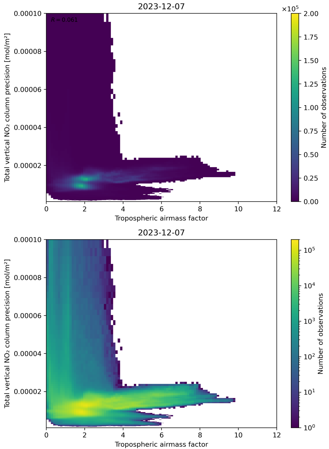
Figure 78: Scatter density plot of “Tropospheric air mass factor” against “Total vertical NO 2 column precision” for 2023-12-06 to 2023-12-08.
