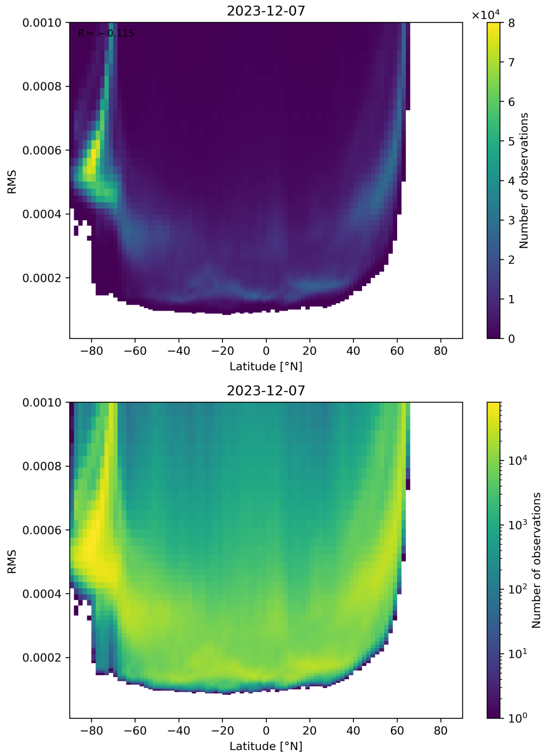
Figure 94: Scatter density plot of “Latitude” against “RMS” for 2023-12-06 to 2023-12-08.
