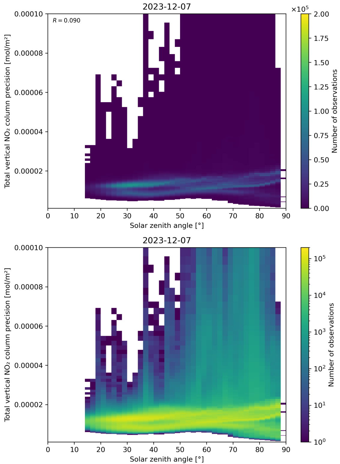
Figure 154: Scatter density plot of “Solar zenith angle” against “Total vertical NO 2 column precision” for 2023-12-06 to 2023-12-08.
