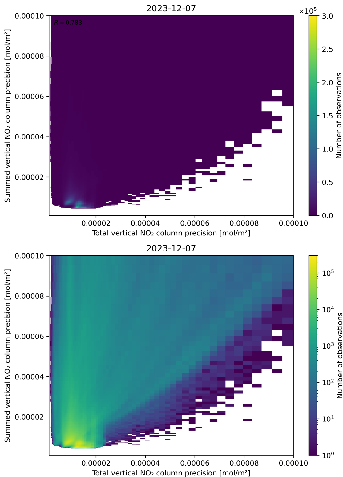
Figure 118: Scatter density plot of “Total vertical NO 2 column precision” against “Summed vertical NO 2 column precision” for 2023-12-06 to 2023-12-08.
