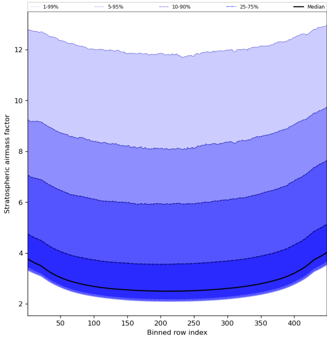
Figure 61: Along track statistics of “Stratospheric air mass factor” for 2023-12-06 to 2023-12-08
