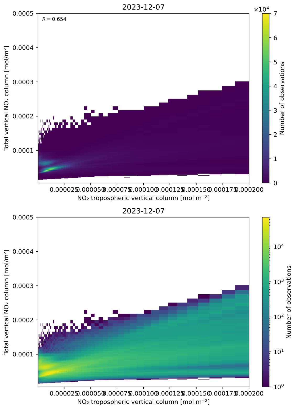
Figure 128: Scatter density plot of “NO 2 tropospheric vertical column” against “Total vertical NO 2 column” for 2023-12-06 to 2023-12-08.
