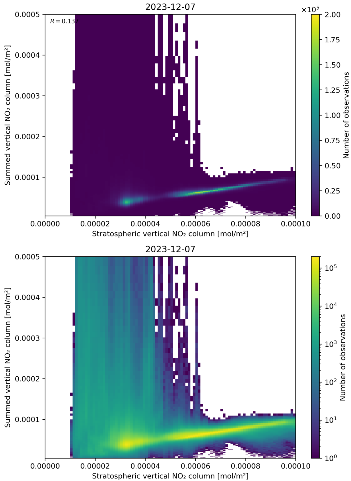
Figure 98: Scatter density plot of “Stratospheric vertical NO 2 column” against “Summed vertical NO 2 column” for 2023-12-06 to 2023-12-08.
