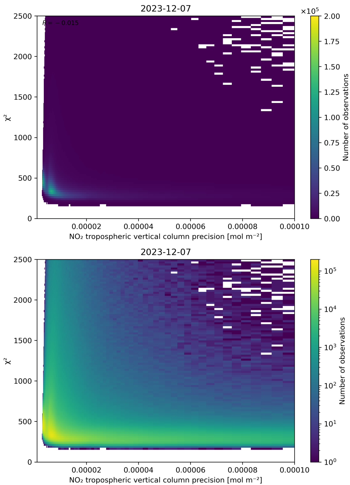
Figure 134: Scatter density plot of “NO 2 tropospheric vertical column precision” against “ \chi^2 ” for 2023-12-06 to 2023-12-08.
