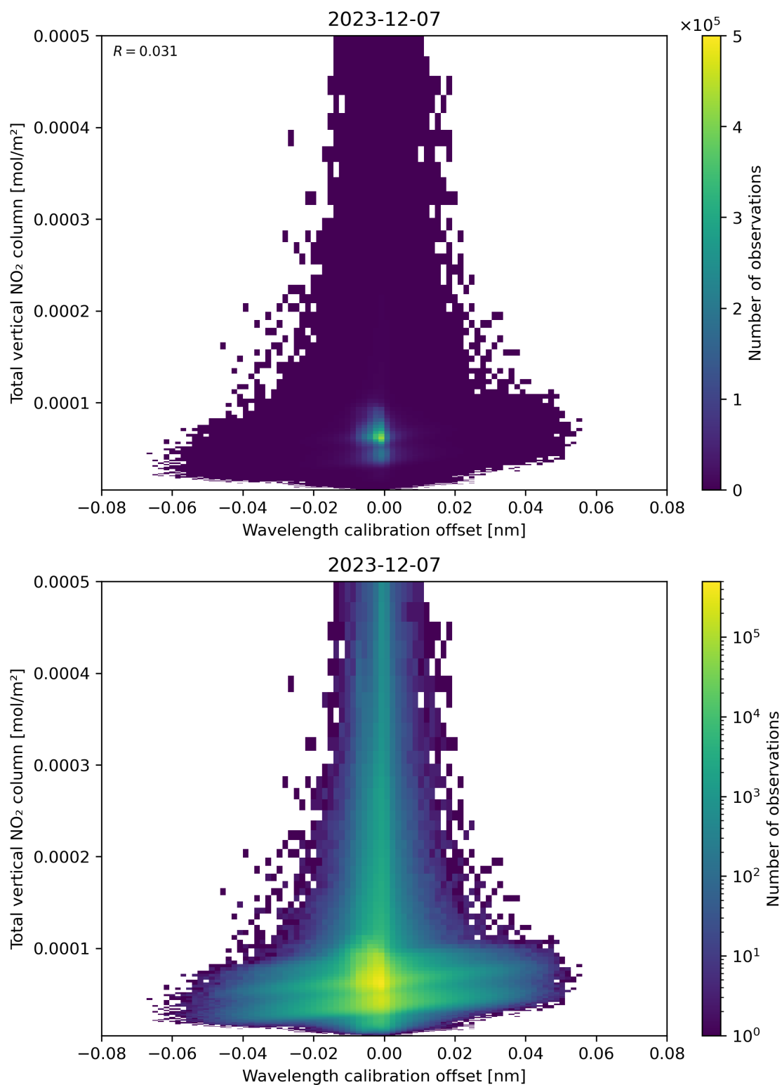
Figure 179: Scatter density plot of “Wavelength calibration offset” against “Total vertical NO 2 column” for 2023-12-06 to 2023-12-08.
