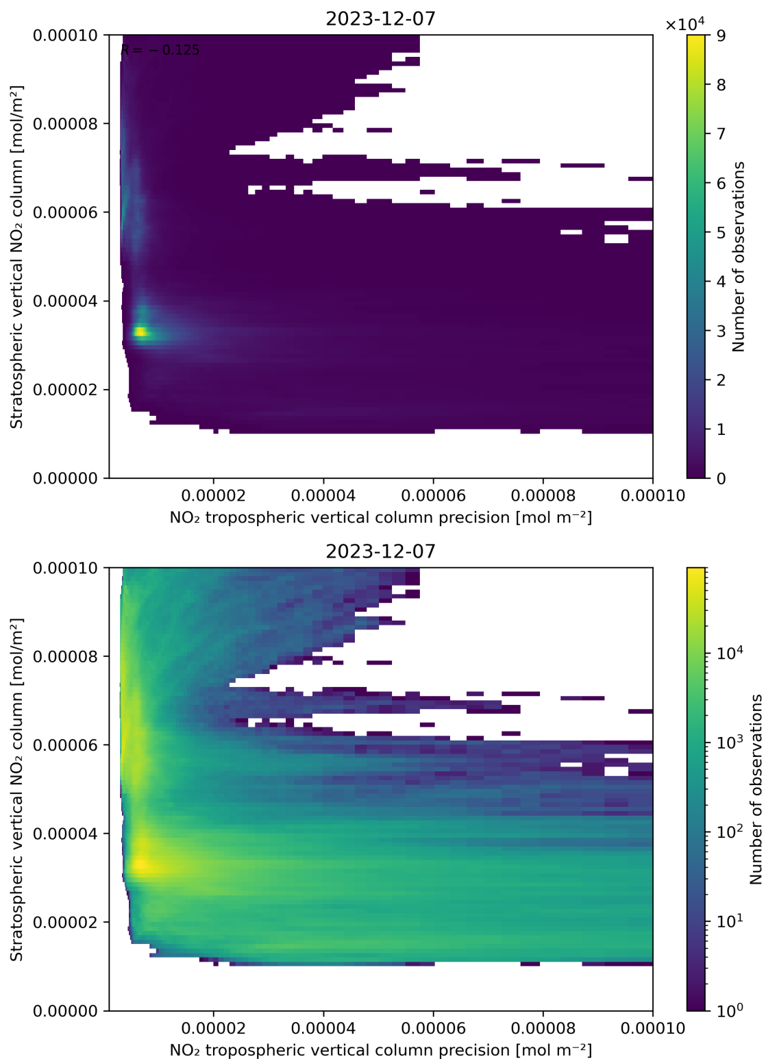
Figure 135: Scatter density plot of “NO 2 tropospheric vertical column precision” against “Stratospheric vertical NO 2 column” for 2023-12-06 to 2023-12-08.
