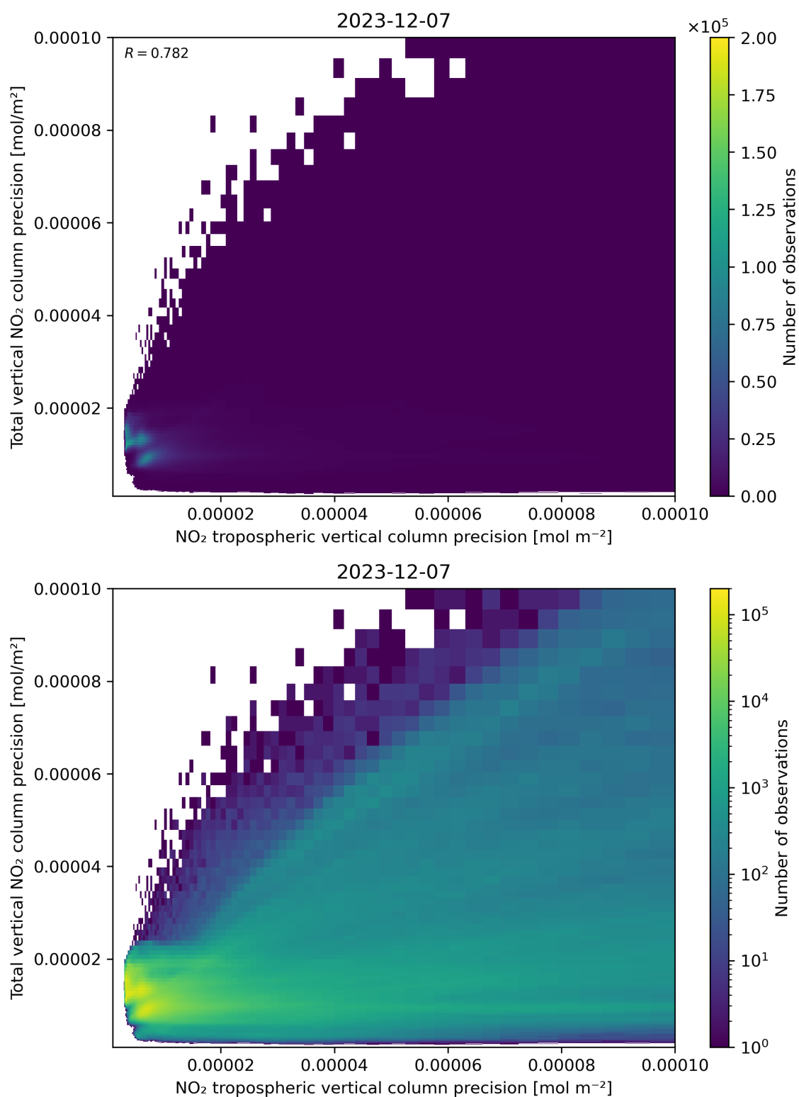
Figure 139: Scatter density plot of “NO 2 tropospheric vertical column precision” against “Total vertical NO 2 column precision” for 2023-12-06 to 2023-12-08.
