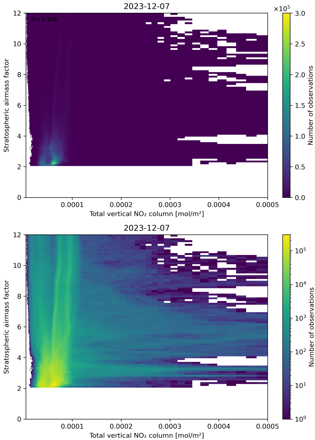
Figure 110: Scatter density plot of “Total vertical NO 2 column” against “Stratospheric air mass factor” for 2023-12-06 to 2023-12-08.
