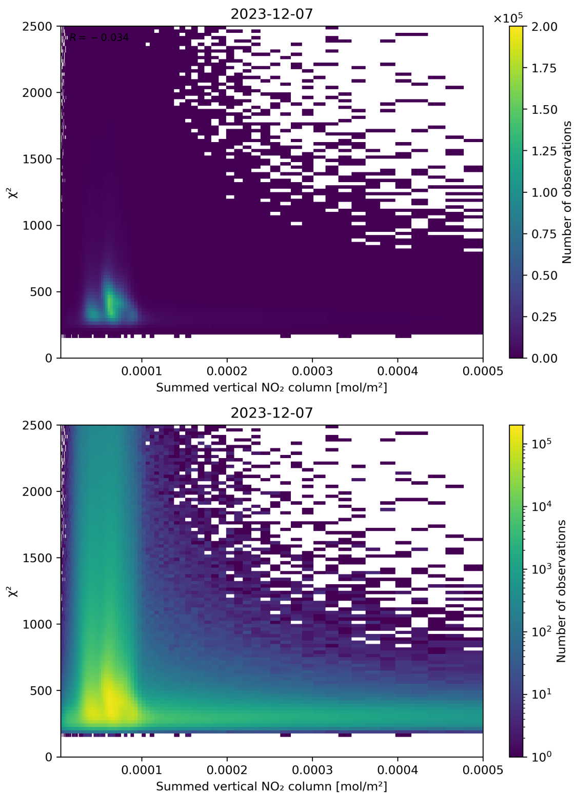
Figure 104: Scatter density plot of “Summed vertical NO 2 column” against “ \chi^2 ” for 2023-12-06 to 2023-12-08.
