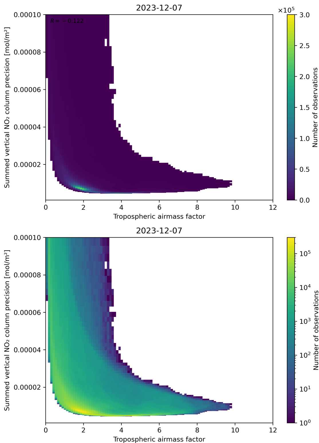
Figure 76: Scatter density plot of “Tropospheric air mass factor” against “Summed vertical NO 2 column precision” for 2023-12-06 to 2023-12-08.
