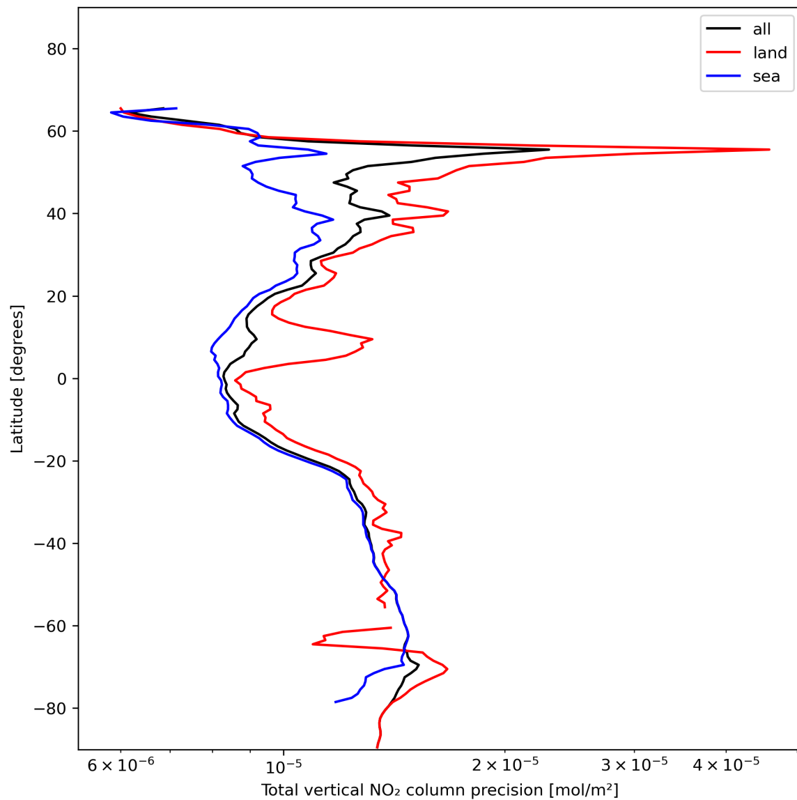
Figure 22: Zonal average of “Total vertical NO 2 column precision” for 2023-12-06 to 2023-12-08.
