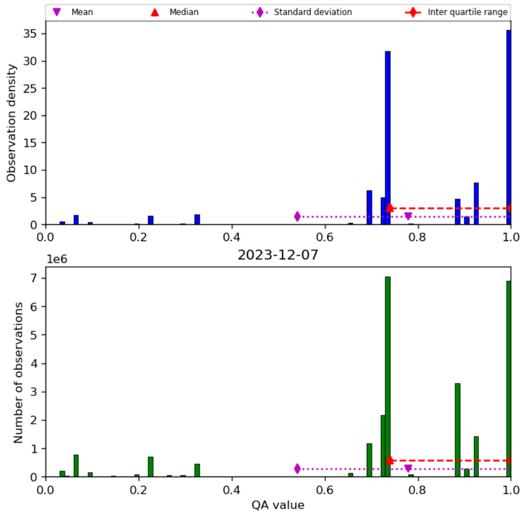
Figure 28: Histogram of “QA value” for 2023-12-06 to 2023-12-08
