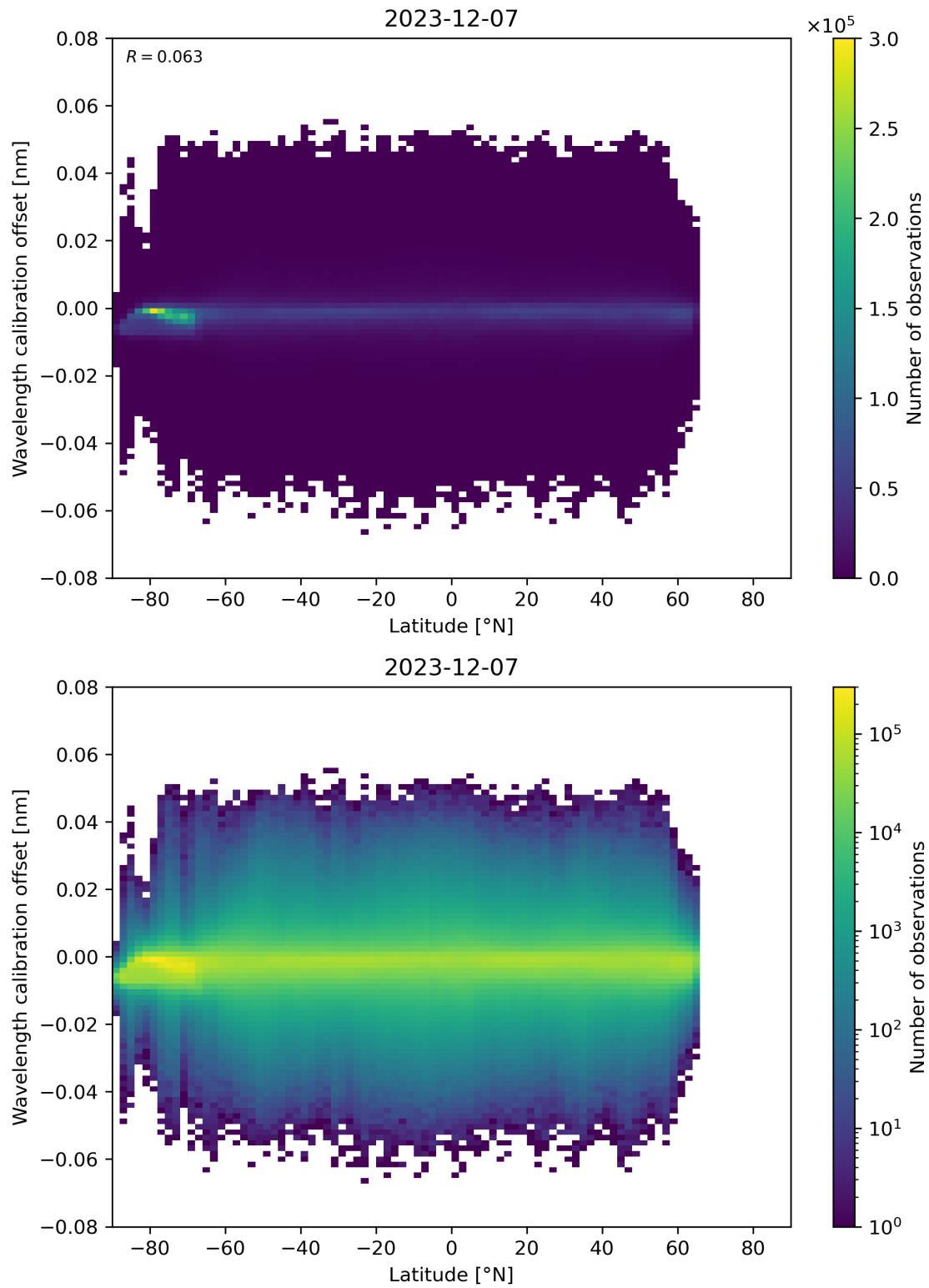
Figure 95: Scatter density plot of “Latitude” against “Wavelength calibration offset” for 2023-12-06 to 2023-12-08.
