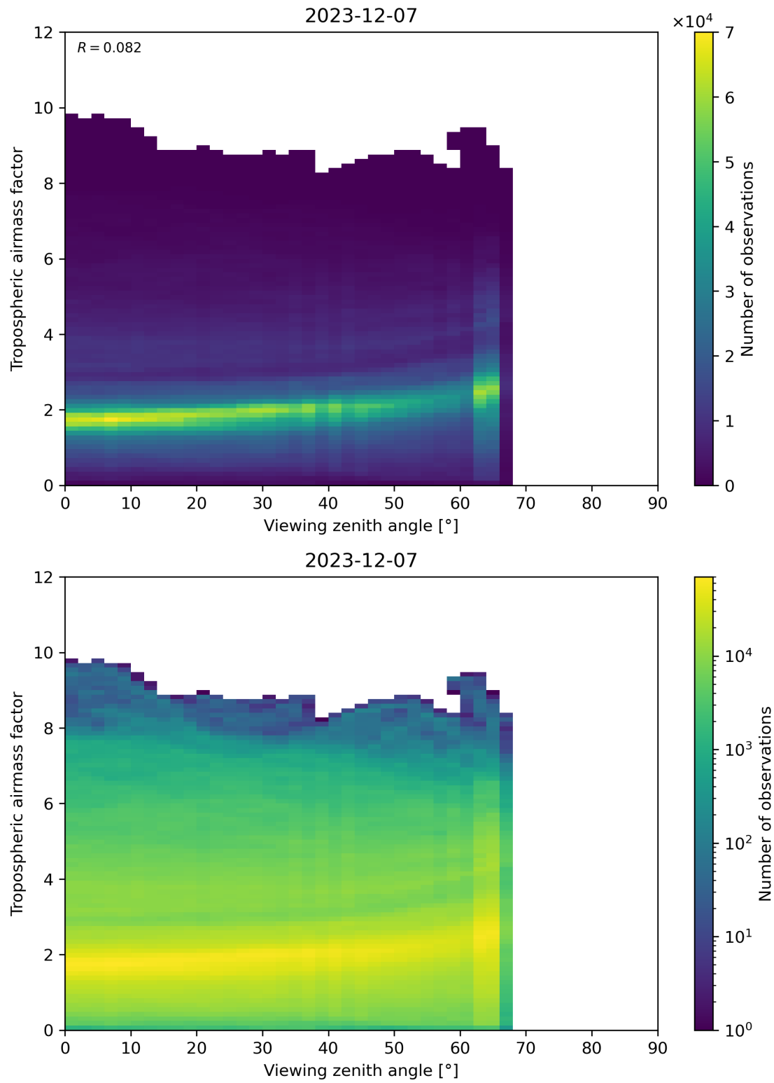
Figure 161: Scatter density plot of “Viewing zenith angle” against “Tropospheric airmass factor” for 2023-12-06 to 2023-12-08.
