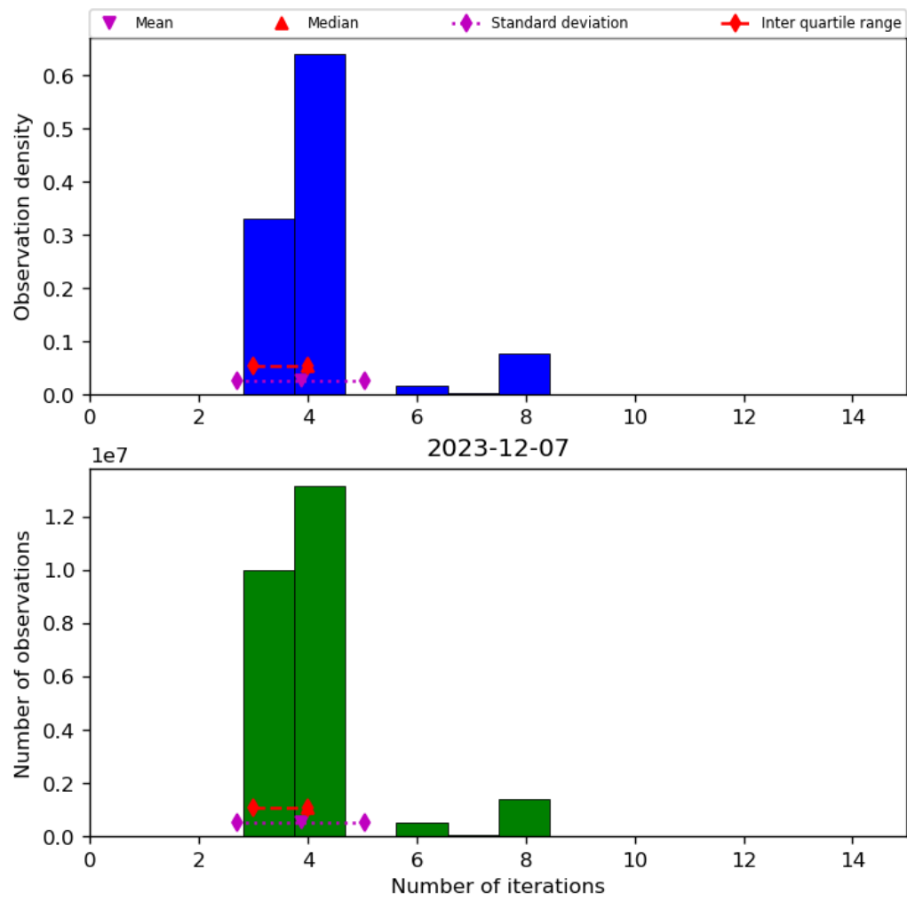
Figure 34: Histogram of “Number of iterations” for 2023-12-06 to 2023-12-08
