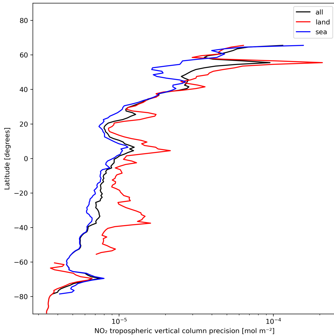
Figure 13: Zonal average of “NO 2 tropospheric vertical column precision” for 2023-12-06 to 2023-12-08.
