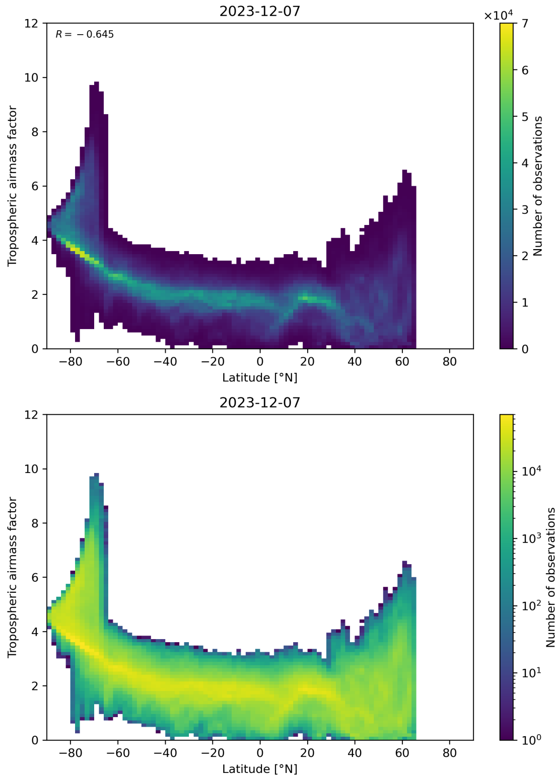
Figure 85: Scatter density plot of “Latitude” against “Tropospheric airmass factor” for 2023-12-06 to 2023-12-08.
