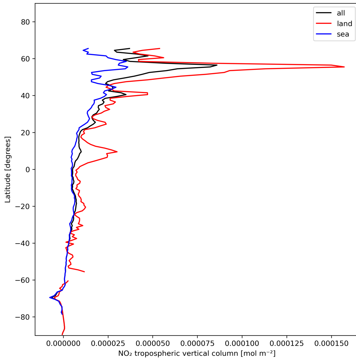
Figure 12: Zonal average of “NO 2 tropospheric vertical column” for 2023-12-06 to 2023-12-08.
