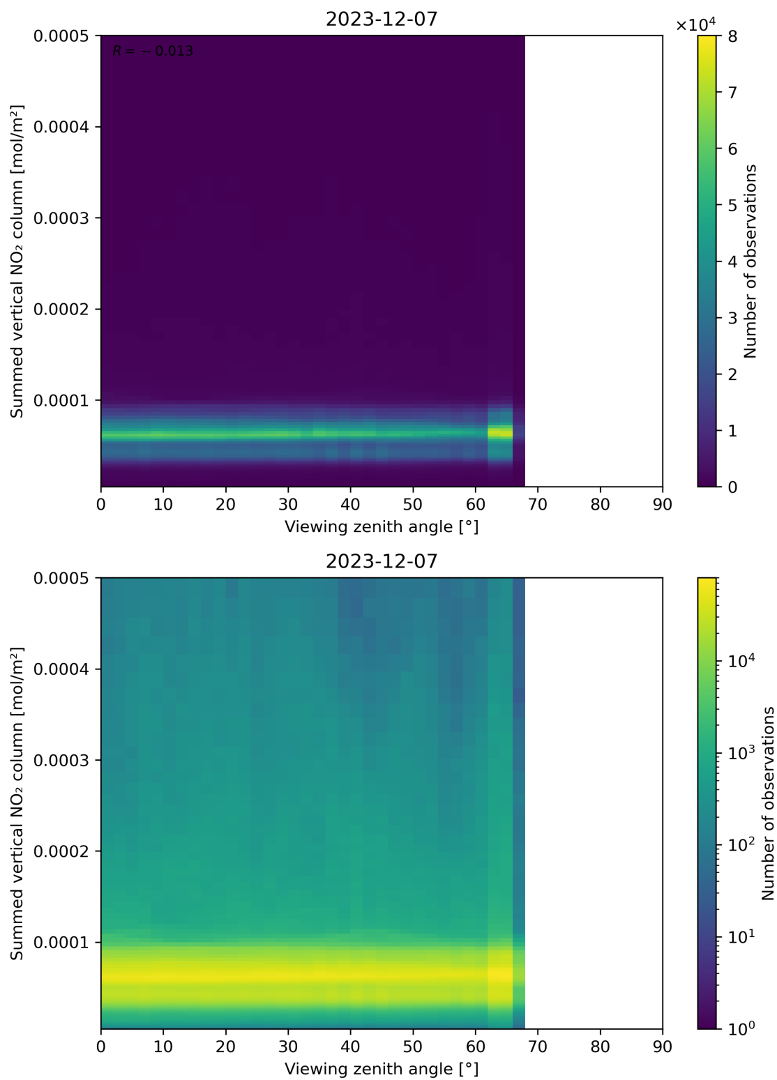
Figure 165: Scatter density plot of “Viewing zenith angle” against “Summed vertical NO 2 column” for 2023-12-06 to 2023-12-08.
