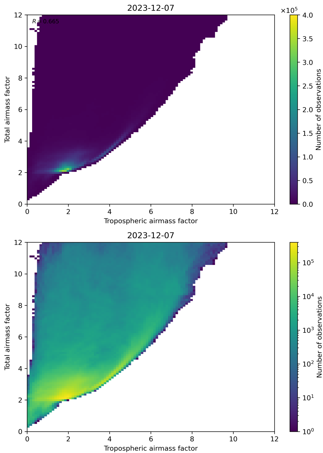
Figure 72: Scatter density plot of “Tropospheric airmass factor” against “Total airmass factor” for 2023-12-06 to 2023-12-08.
