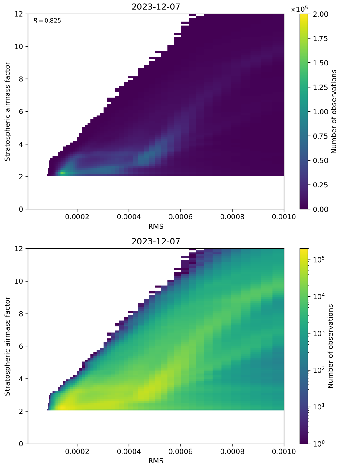
Figure 144: Scatter density plot of “RMS” against “Stratospheric airmass factor” for 2023-12-06 to 2023-12-08.
