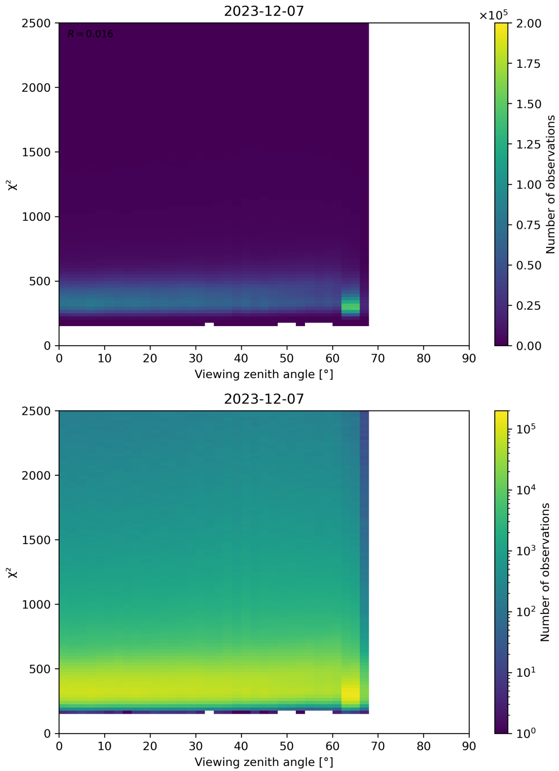
Figure 162: Scatter density plot of “Viewing zenith angle” against “ \chi^2 ” for 2023-12-06 to 2023-12-08.
