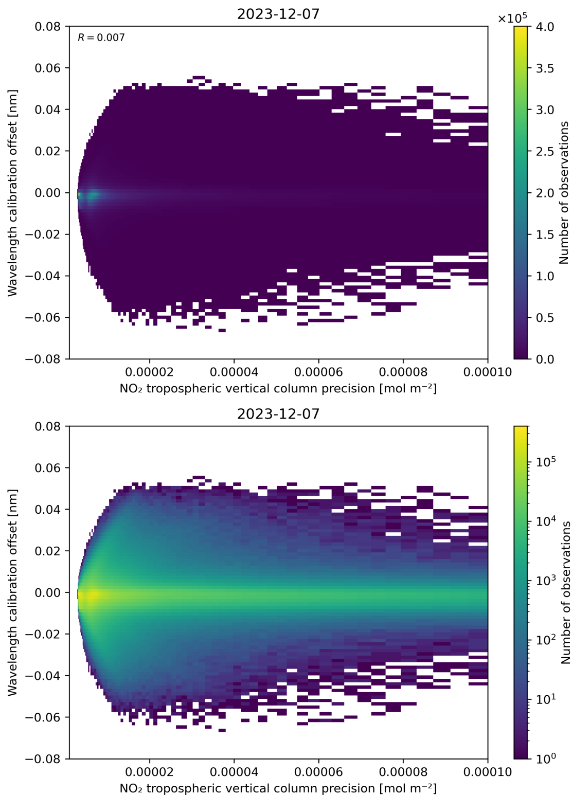
Figure 141: Scatter density plot of “NO 2 tropospheric vertical column precision” against “Wavelength calibration offset” for 2023-12-06 to 2023-12-08.
