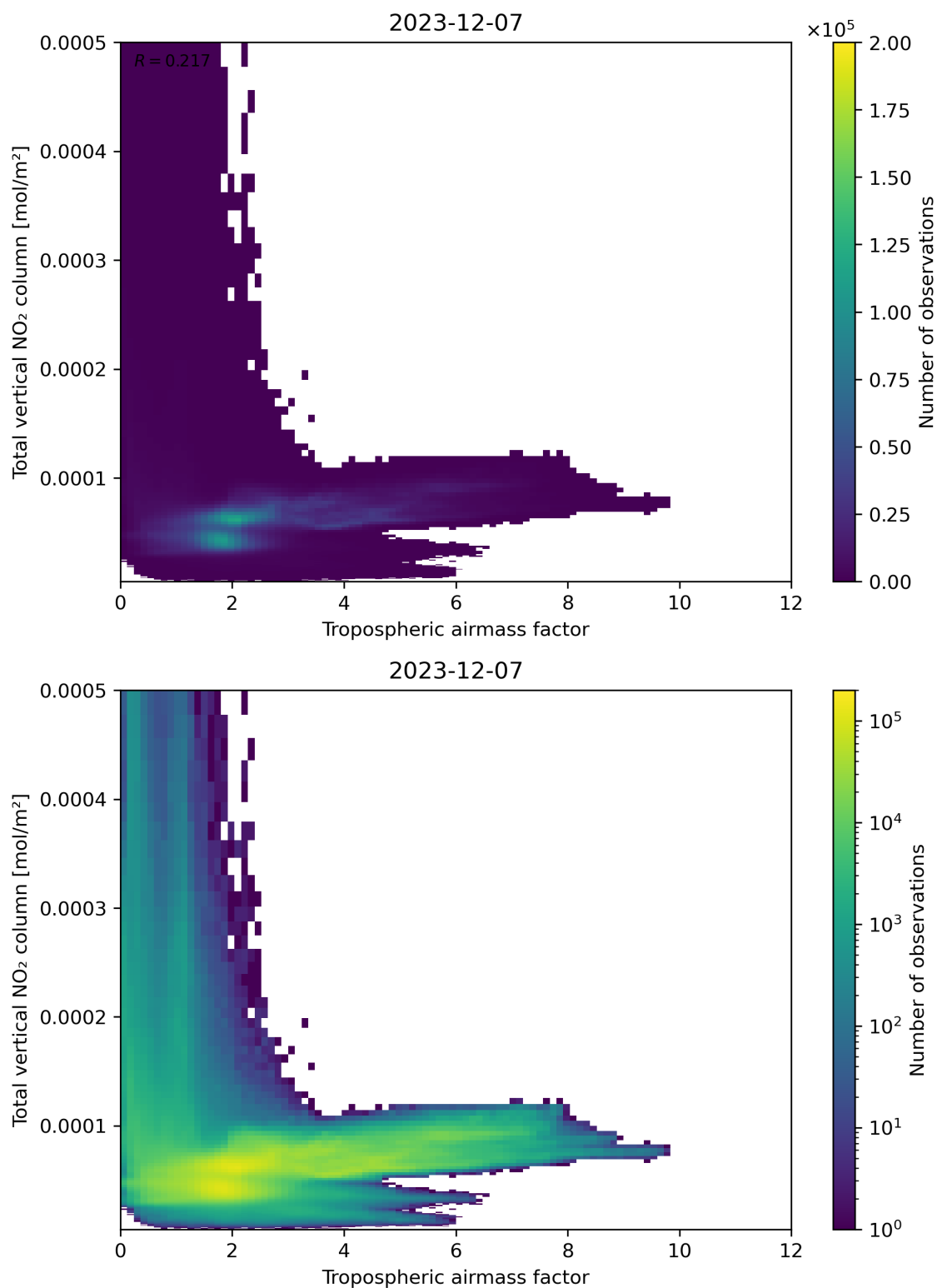
Figure 77: Scatter density plot of “Tropospheric airmass factor” against “Total vertical NO 2 column” for 2023-12-06 to 2023-12-08.
