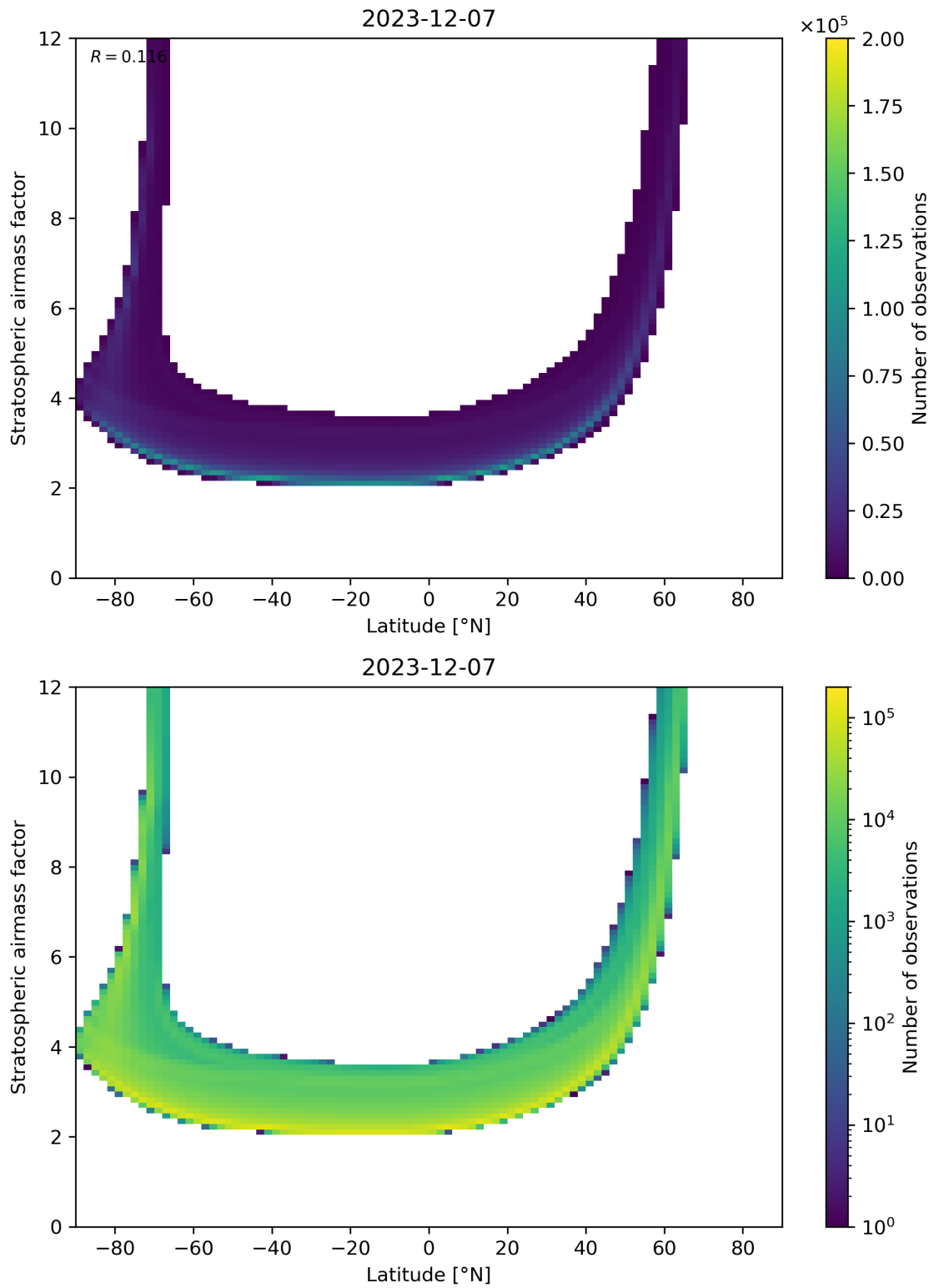
Figure 83: Scatter density plot of “Latitude” against “Stratospheric airmass factor” for 2023-12-06 to 2023-12-08.
