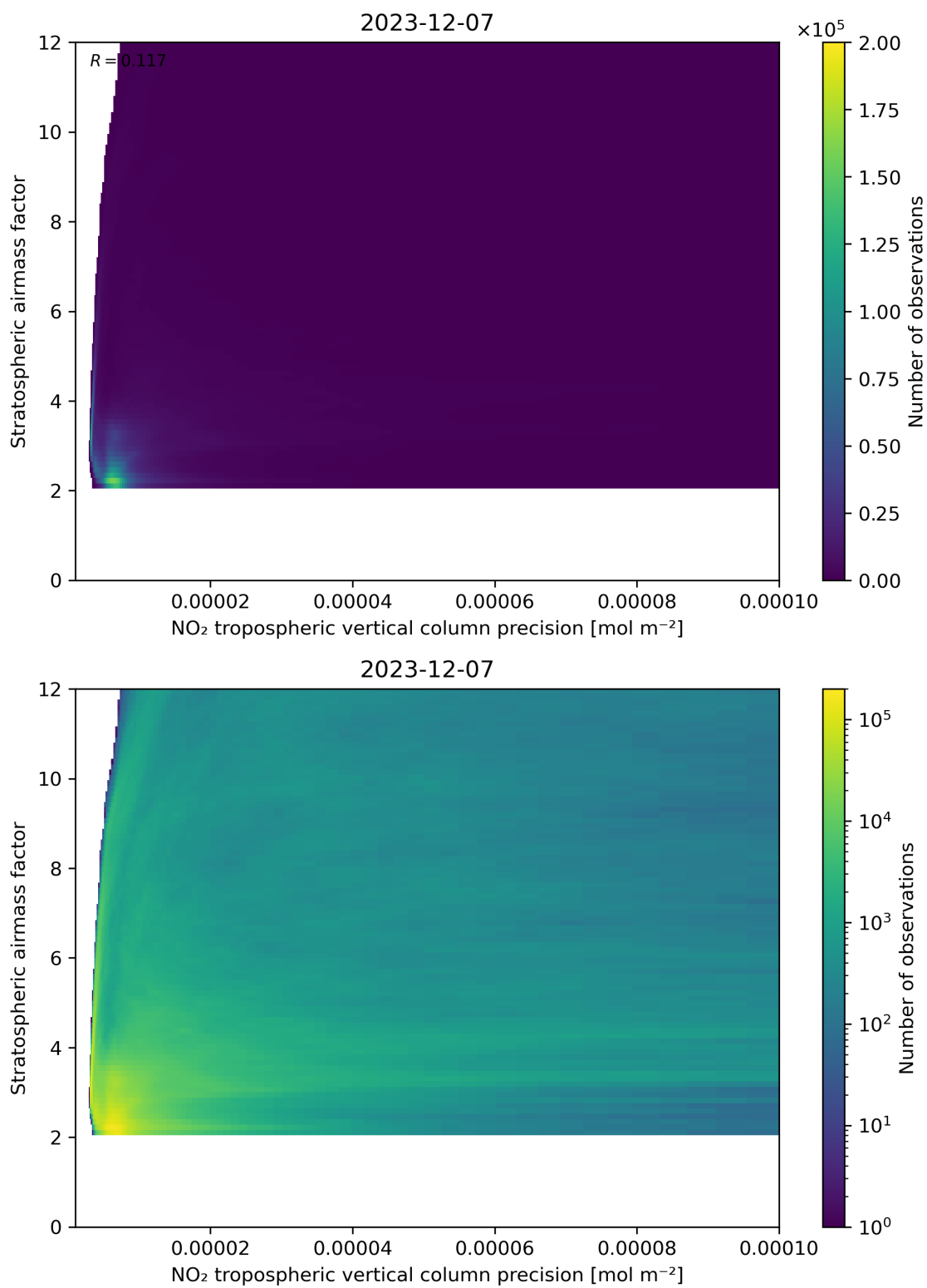
Figure 131: Scatter density plot of “NO 2 tropospheric vertical column precision” against “Stratospheric airmass factor” for 2023-12-06 to 2023-12-08.
