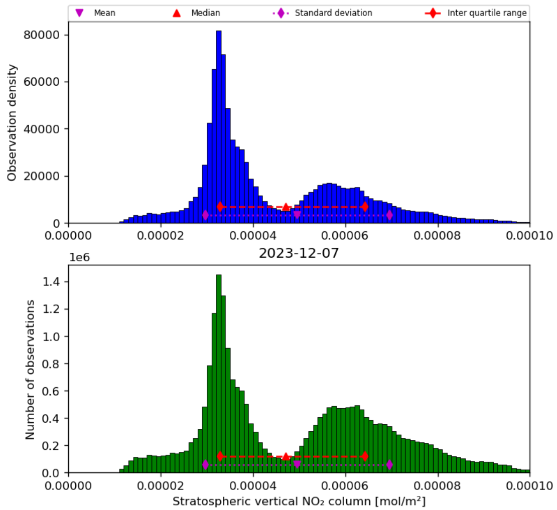
Figure 36: Histogram of “Stratospheric vertical NO 2 column” for 2023-12-06 to 2023-12-08
