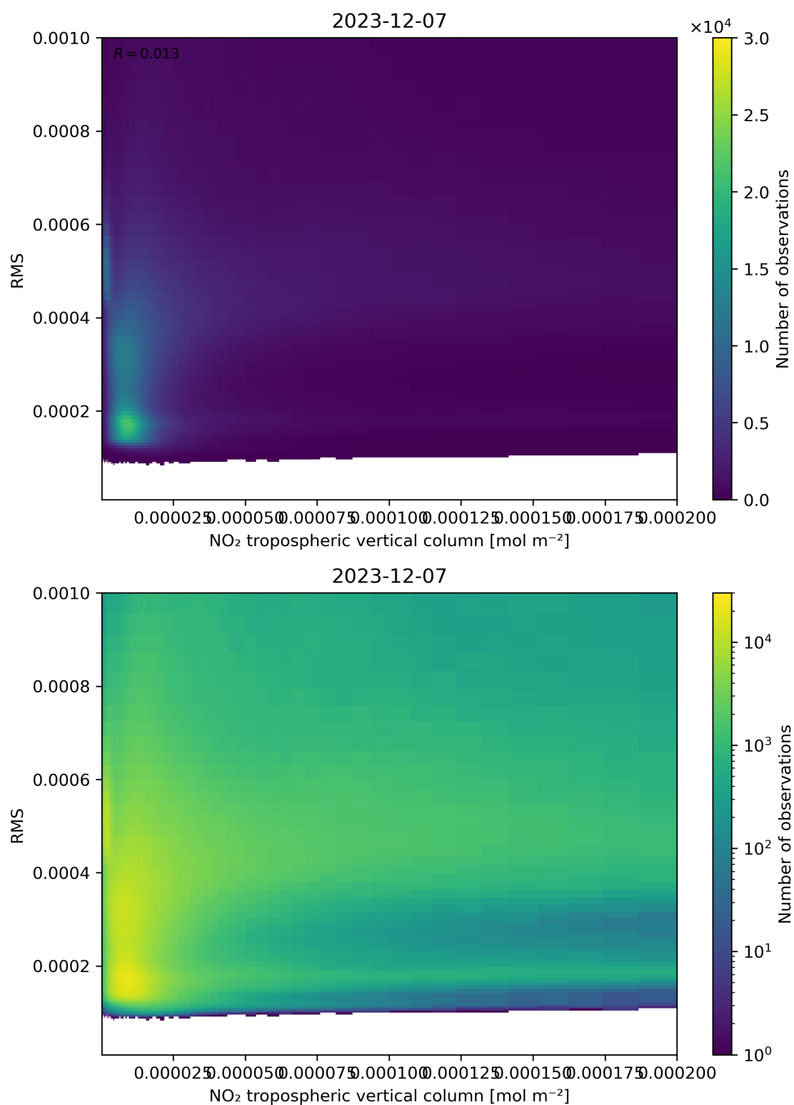
Figure 142: Scatter density plot of “NO 2 tropospheric vertical column” against “RMS” for 2023-12-06 to 2023-12-08.
