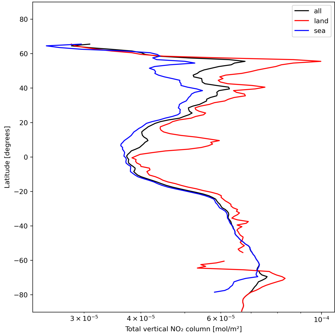
Figure 21: Zonal average of “Total vertical NO 2 column” for 2023-12-06 to 2023-12-08.
