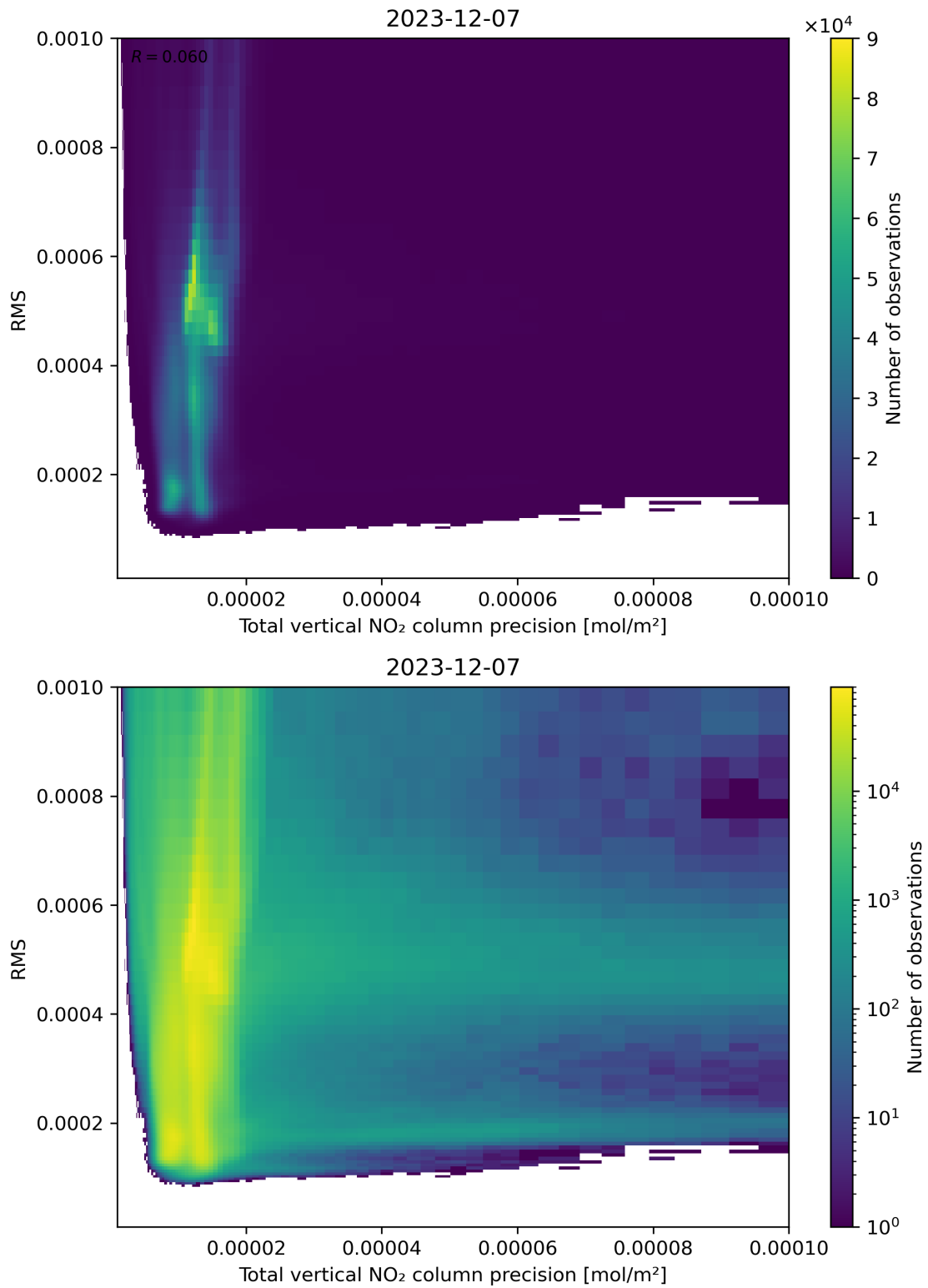
Figure 119: Scatter density plot of “Total vertical NO 2 column precision” against “RMS” for 2023-12-06 to 2023-12-08.
