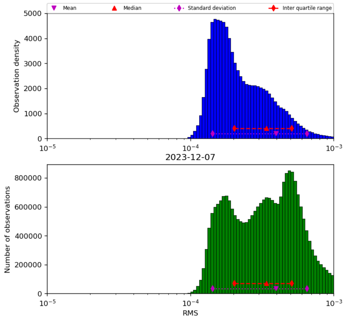
Figure 43: Histogram of “RMS” for 2023-12-06 to 2023-12-08
