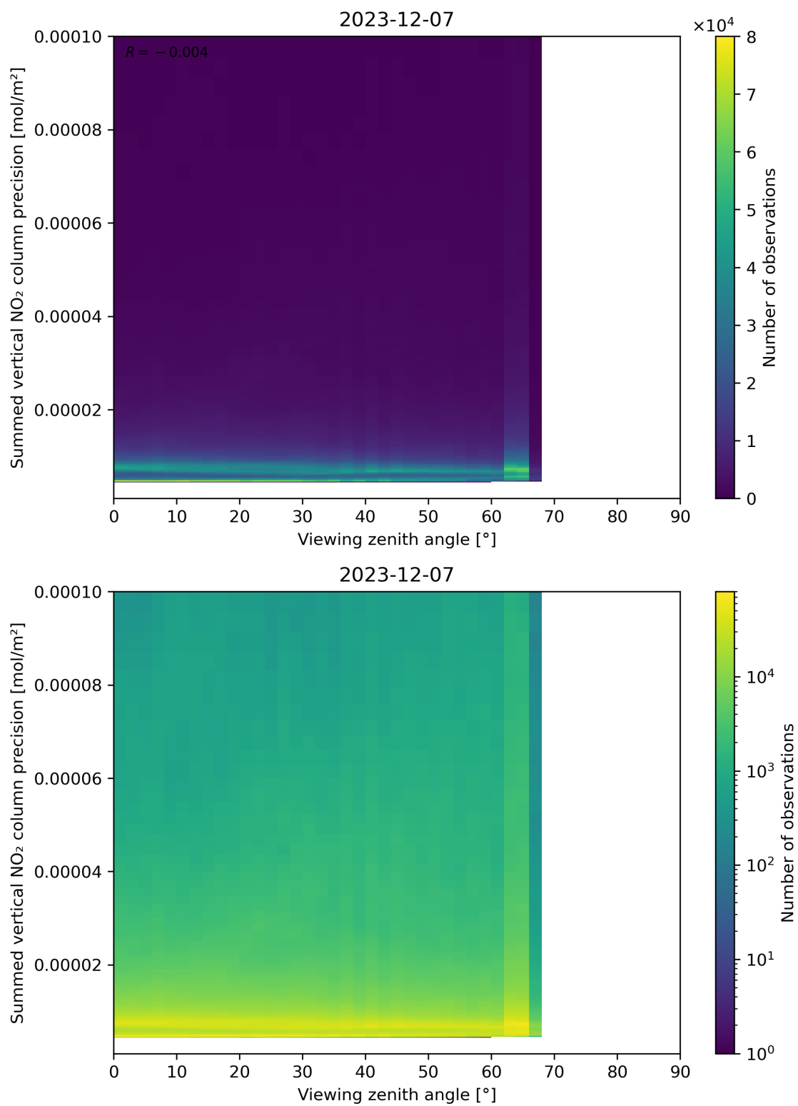
Figure 166: Scatter density plot of “Viewing zenith angle” against “Summed vertical NO 2 column precision” for 2023-12-06 to 2023-12-08.
