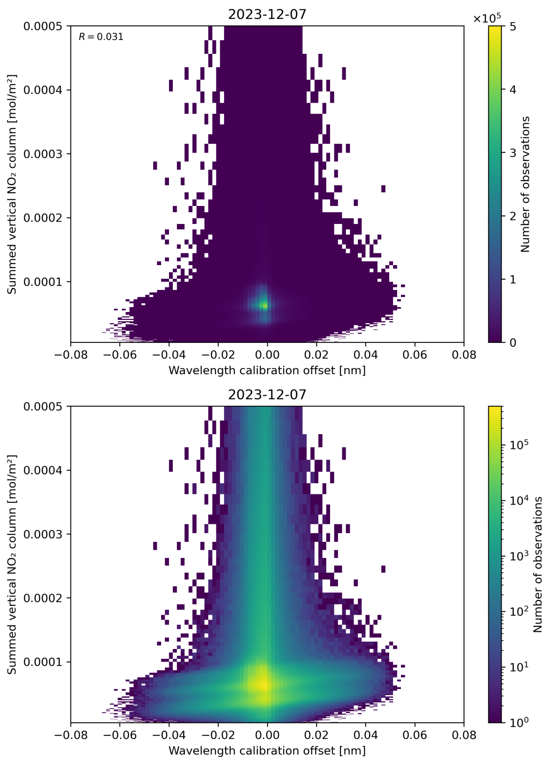
Figure 177: Scatter density plot of “Wavelength calibration offset” against “Summed vertical NO 2 column” for 2023-12-06 to 2023-12-08.
