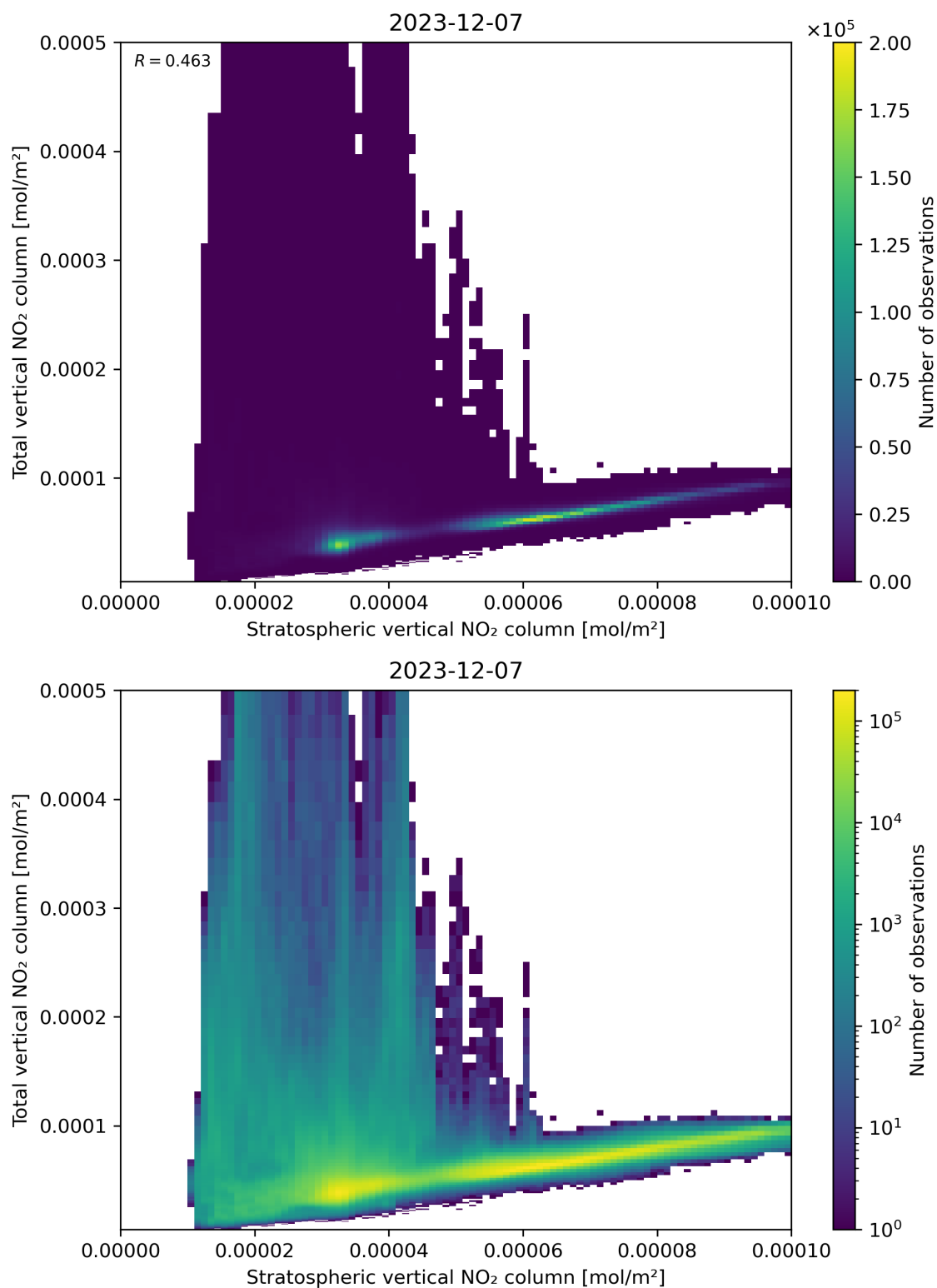
Figure 100: Scatter density plot of “Stratospheric vertical NO 2 column” against “Total vertical NO 2 column” for 2023-12-06 to 2023-12-08.
