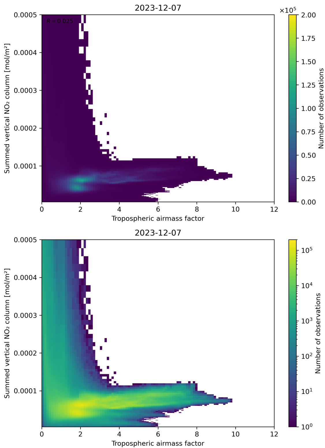
Figure 75: Scatter density plot of “Tropospheric airmass factor” against “Summed vertical NO 2 column” for 2023-12-06 to 2023-12-08.
