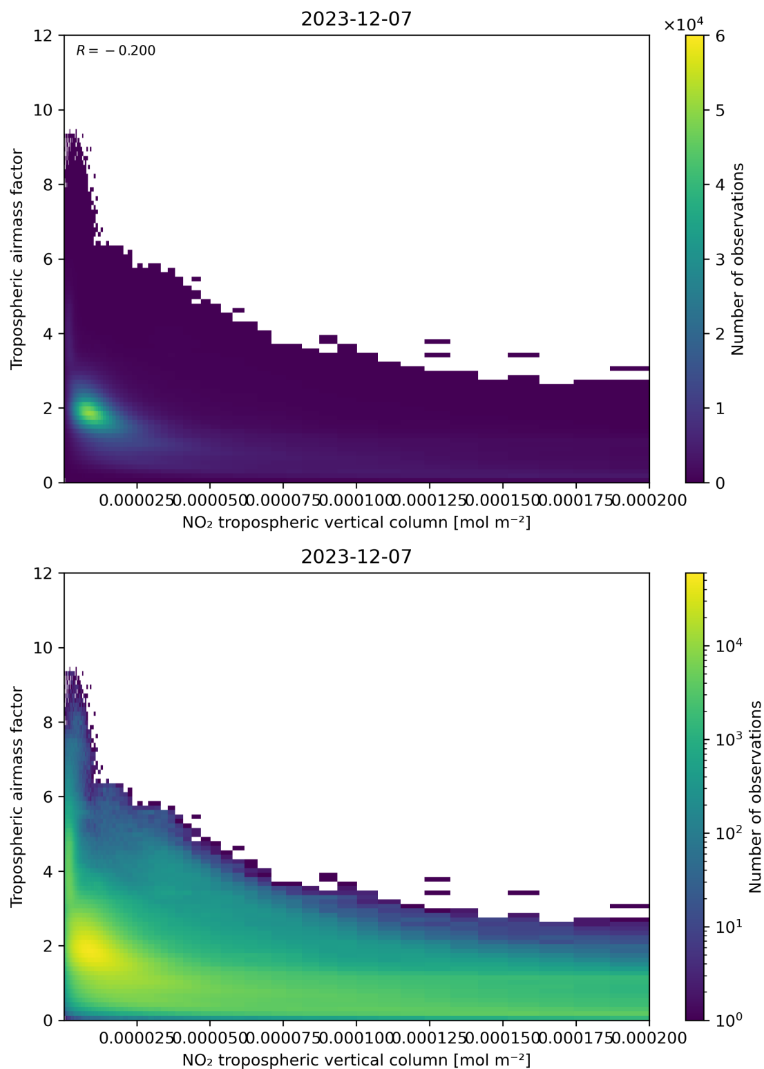
Figure 123: Scatter density plot of “NO 2 tropospheric vertical column” against “Tropospheric airmass factor” for 2023-12-06 to 2023-12-08.
