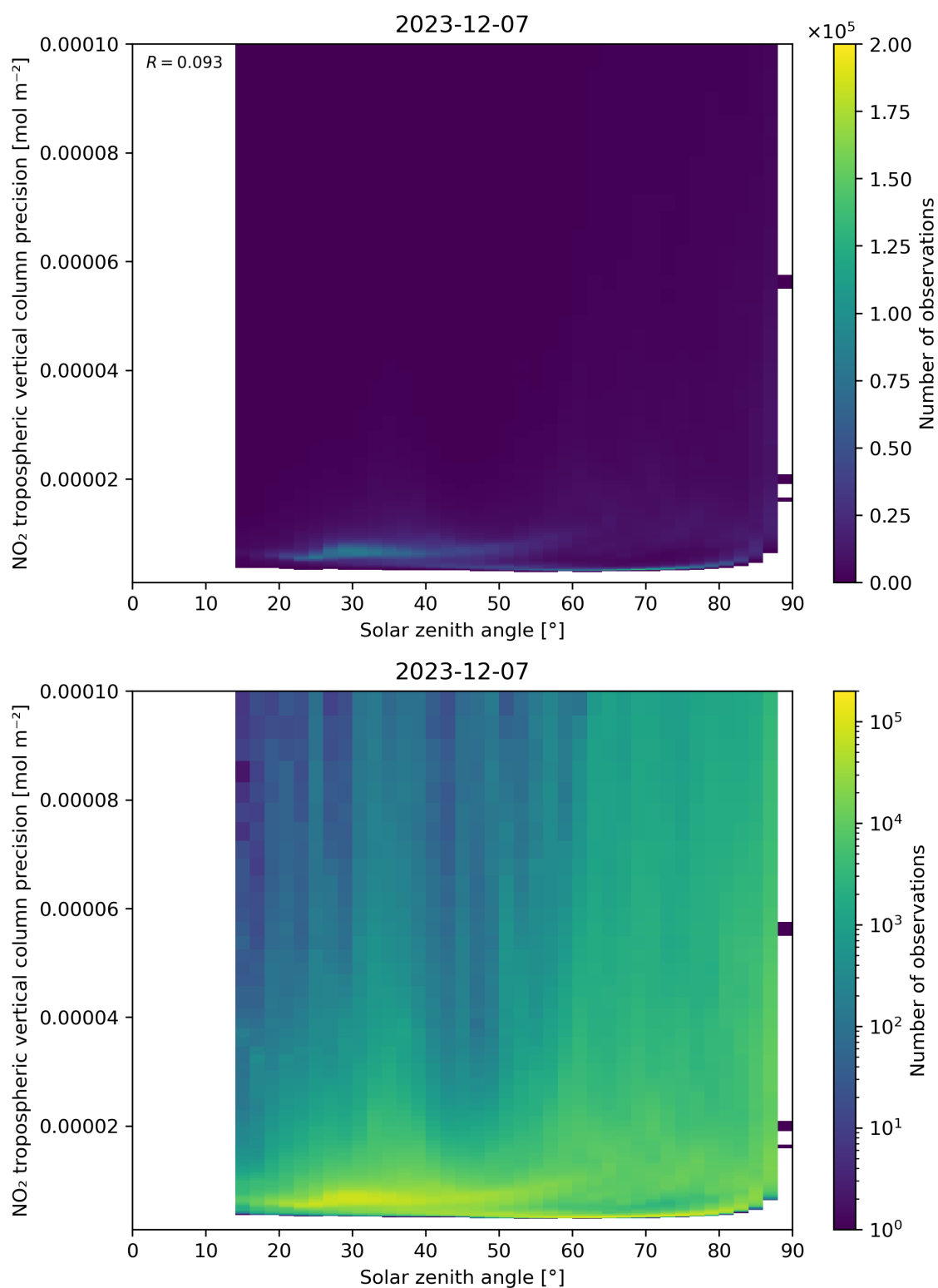
Figure 156: Scatter density plot of “Solar zenith angle” against “NO 2 tropospheric vertical column precision” for 2023-12-06 to 2023-12-08.
