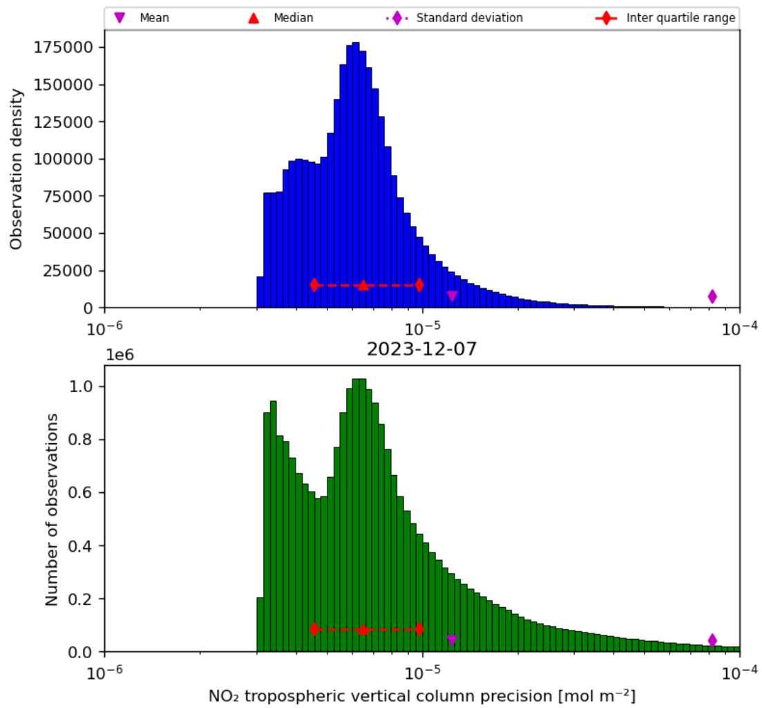
Figure 30: Histogram of “NO 2 tropospheric vertical column precision” for 2023-12-06 to 2023-12-08
