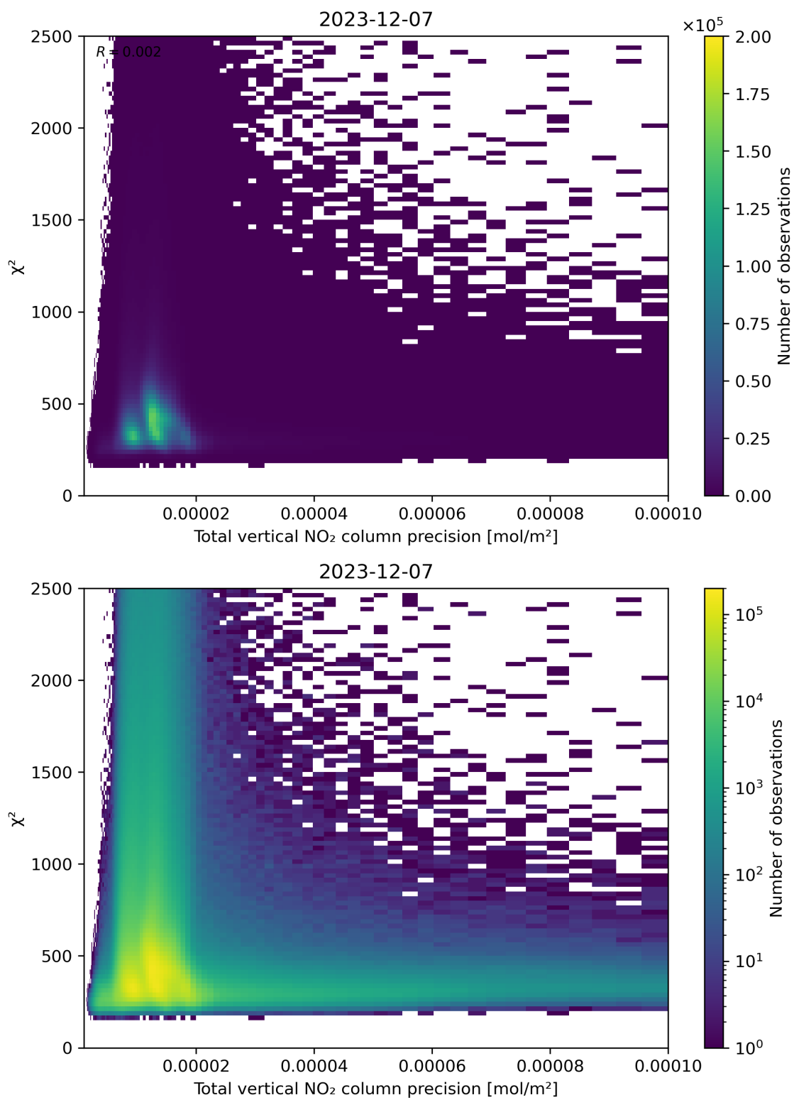
Figure 116: Scatter density plot of “Total vertical NO 2 column precision” against “ \chi^2 ” for 2023-12-06 to 2023-12-08.
