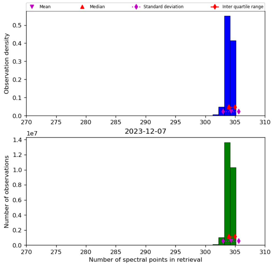
Figure 33: Histogram of “Number of spectral points in retrieval” for 2023-12-06 to 2023-12-08
