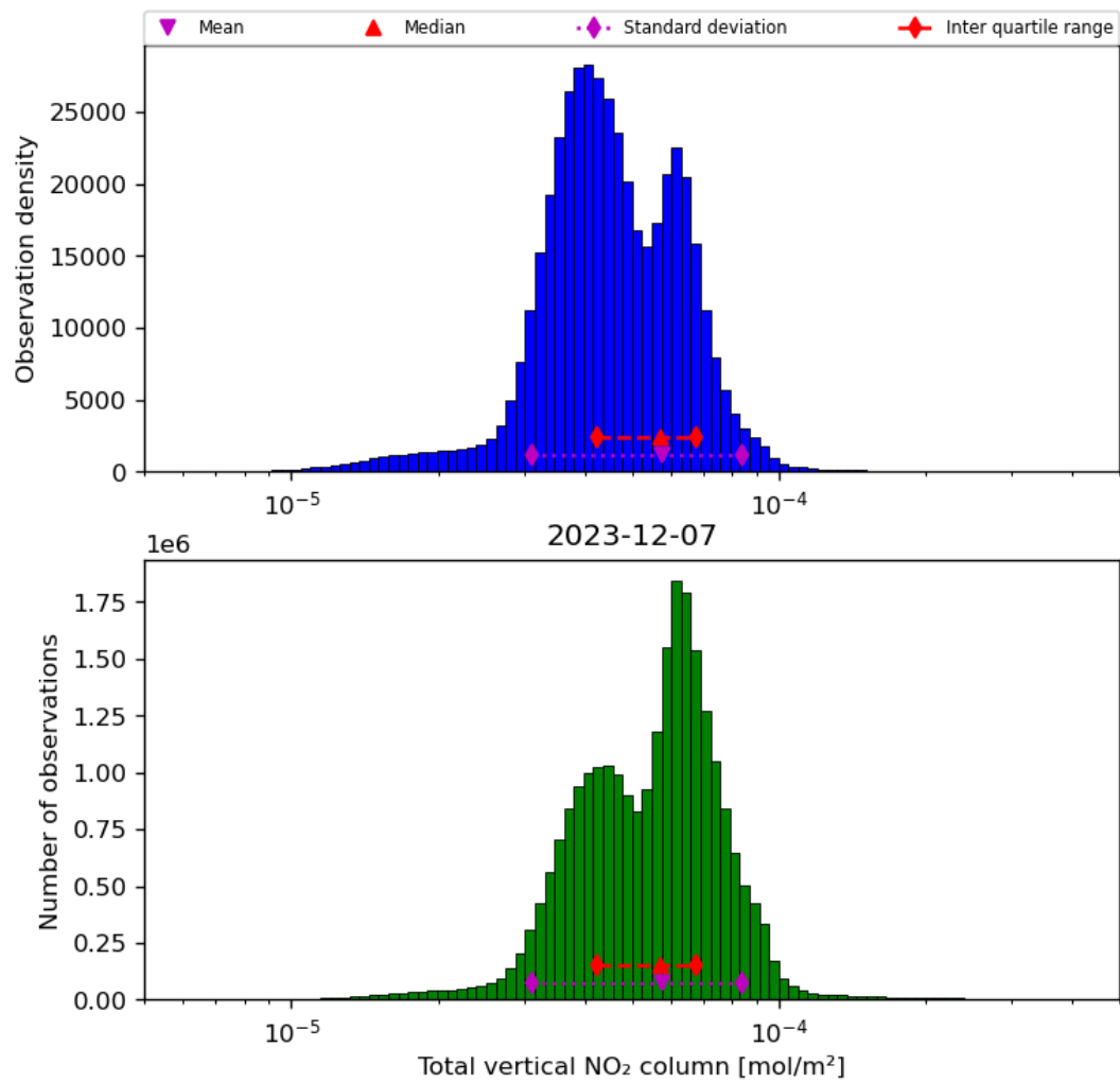
Figure 38: Histogram of “Total vertical NO 2 column” for 2023-12-06 to 2023-12-08
