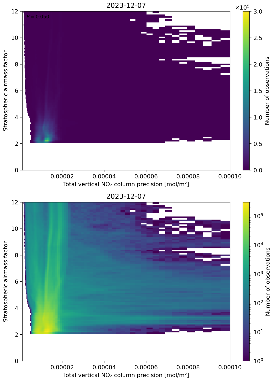
Figure 115: Scatter density plot of “Total vertical NO 2 column precision” against “Stratospheric airmass factor” for 2023-12-06 to 2023-12-08.
