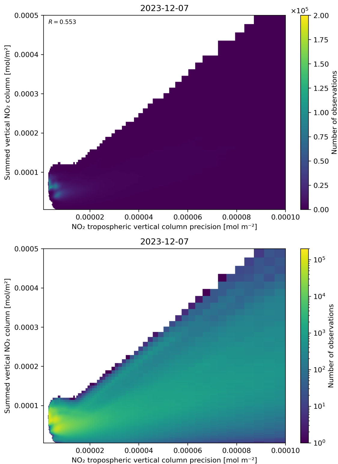
Figure 136: Scatter density plot of “NO 2 tropospheric vertical column precision” against “Summed vertical NO 2 column” for 2023-12-06 to 2023-12-08.
