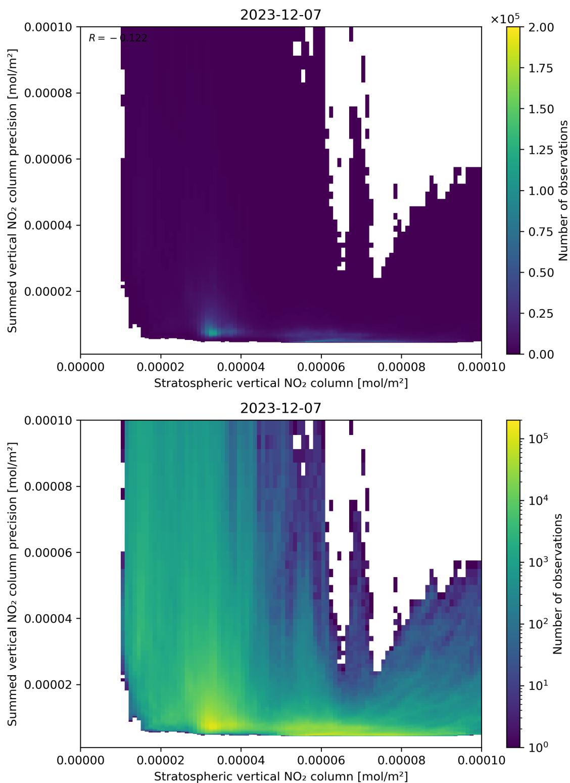
Figure 99: Scatter density plot of “Stratospheric vertical NO 2 column” against “Summed vertical NO 2 column precision” for 2023-12-06 to 2023-12-08.
