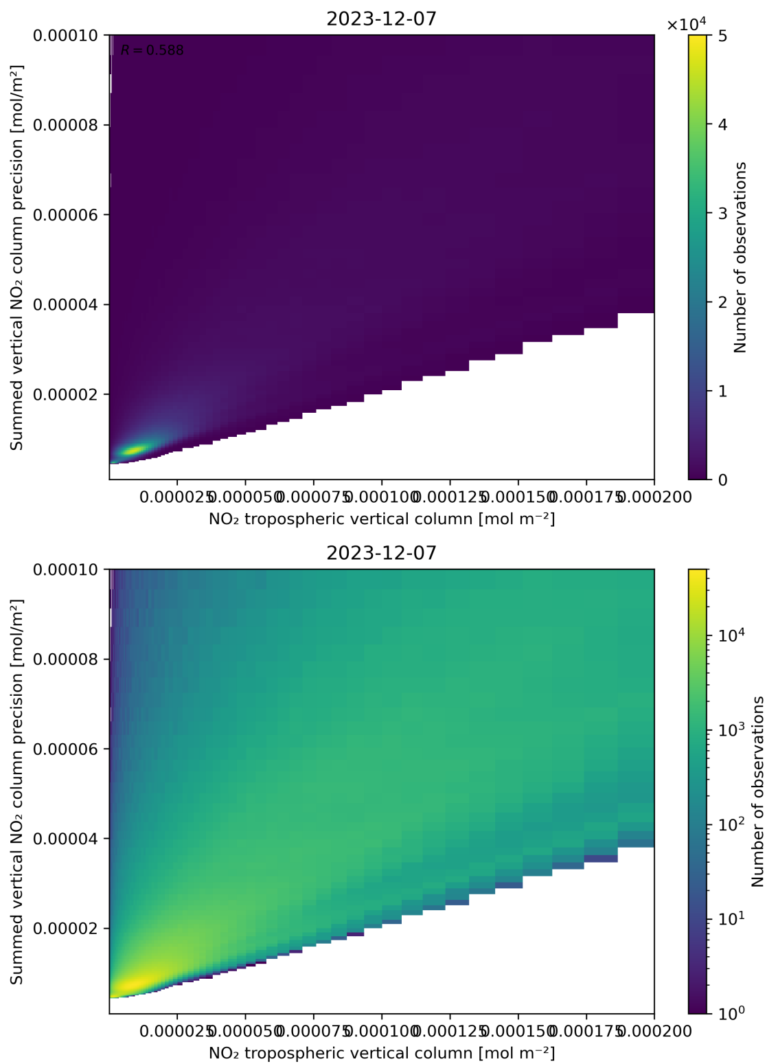
Figure 127: Scatter density plot of “NO 2 tropospheric vertical column” against “Summed vertical NO 2 column precision” for 2023-12-06 to 2023-12-08.
