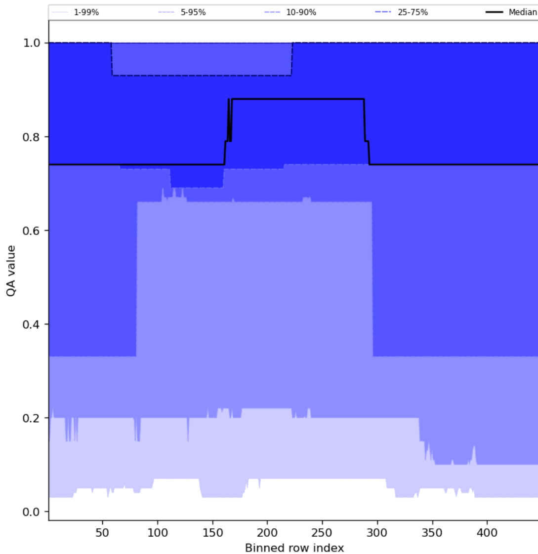
Figure 45: Along track statistics of “QA value” for 2023-12-06 to 2023-12-08
