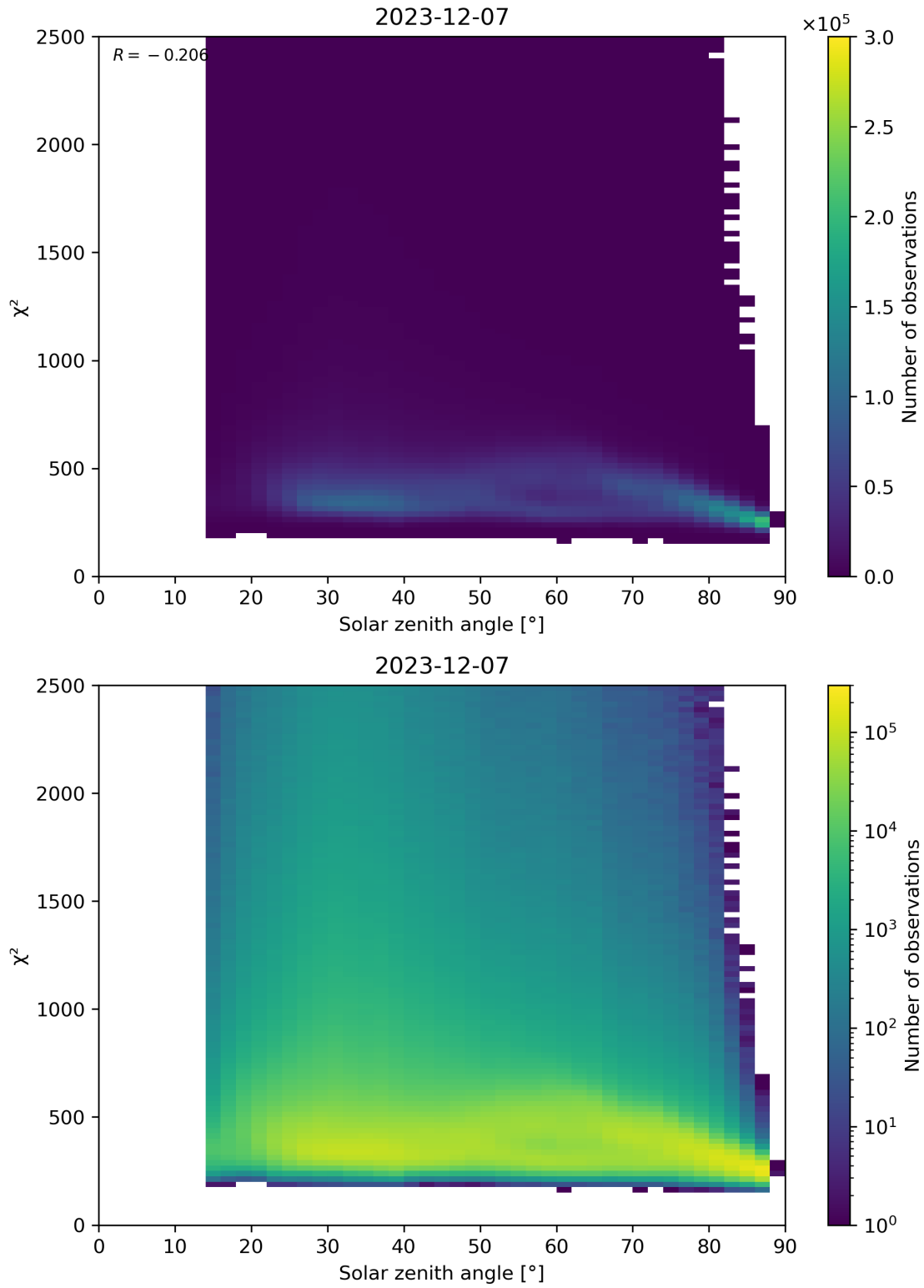
Figure 148: Scatter density plot of “Solar zenith angle” against “ \chi^2 ” for 2023-12-06 to 2023-12-08.
