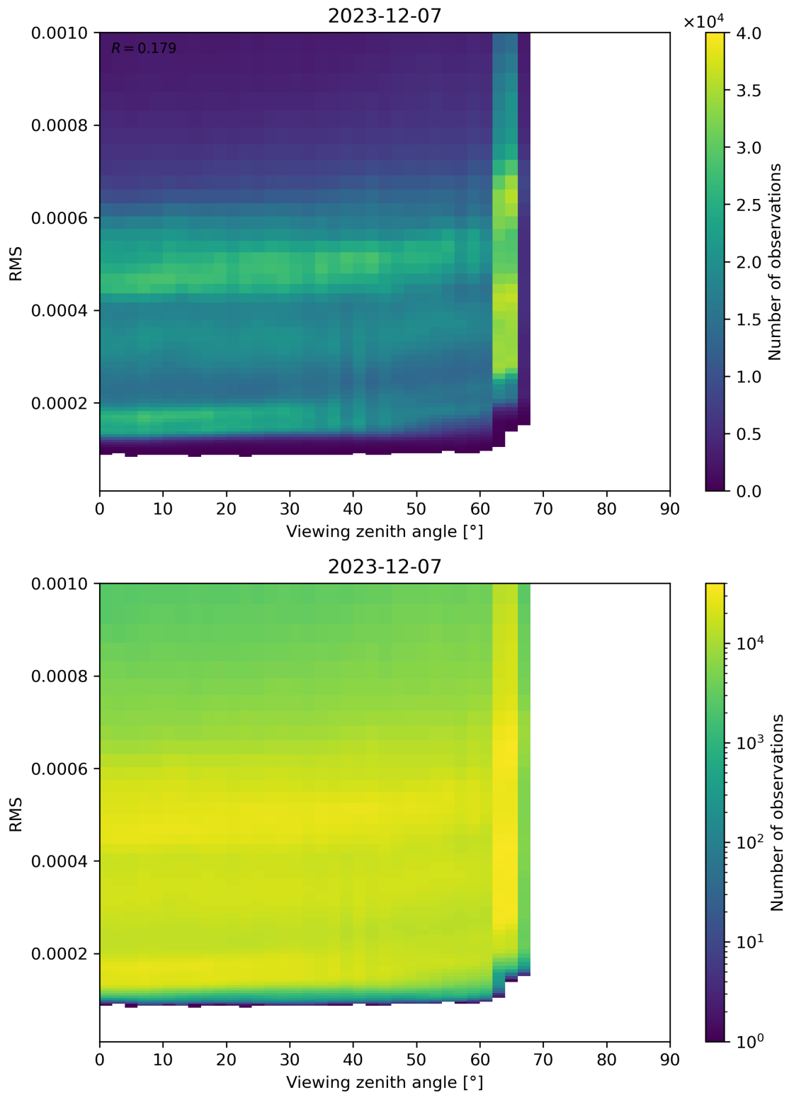
Figure 171: Scatter density plot of “Viewing zenith angle” against “RMS” for 2023-12-06 to 2023-12-08.
