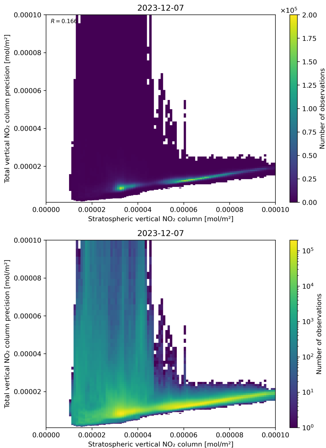
Figure 101: Scatter density plot of “Stratospheric vertical NO 2 column” against “Total vertical NO 2 column precision” for 2023-12-06 to 2023-12-08.
