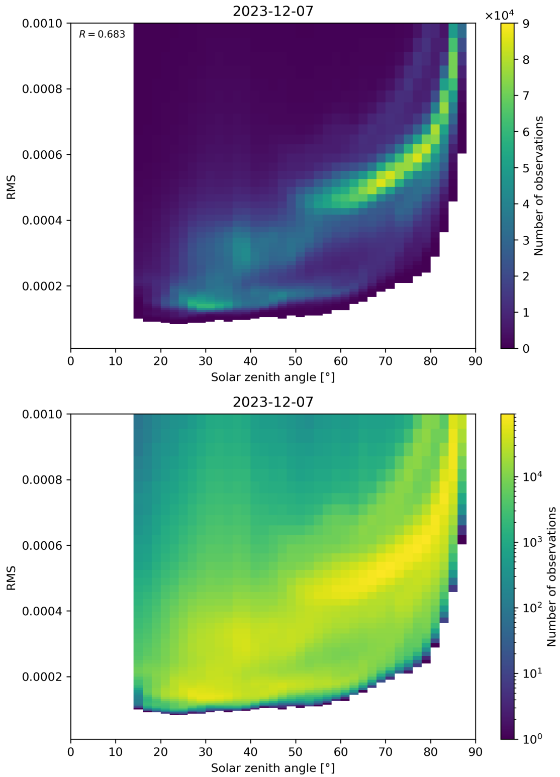
Figure 157: Scatter density plot of “Solar zenith angle” against “RMS” for 2023-12-06 to 2023-12-08.
