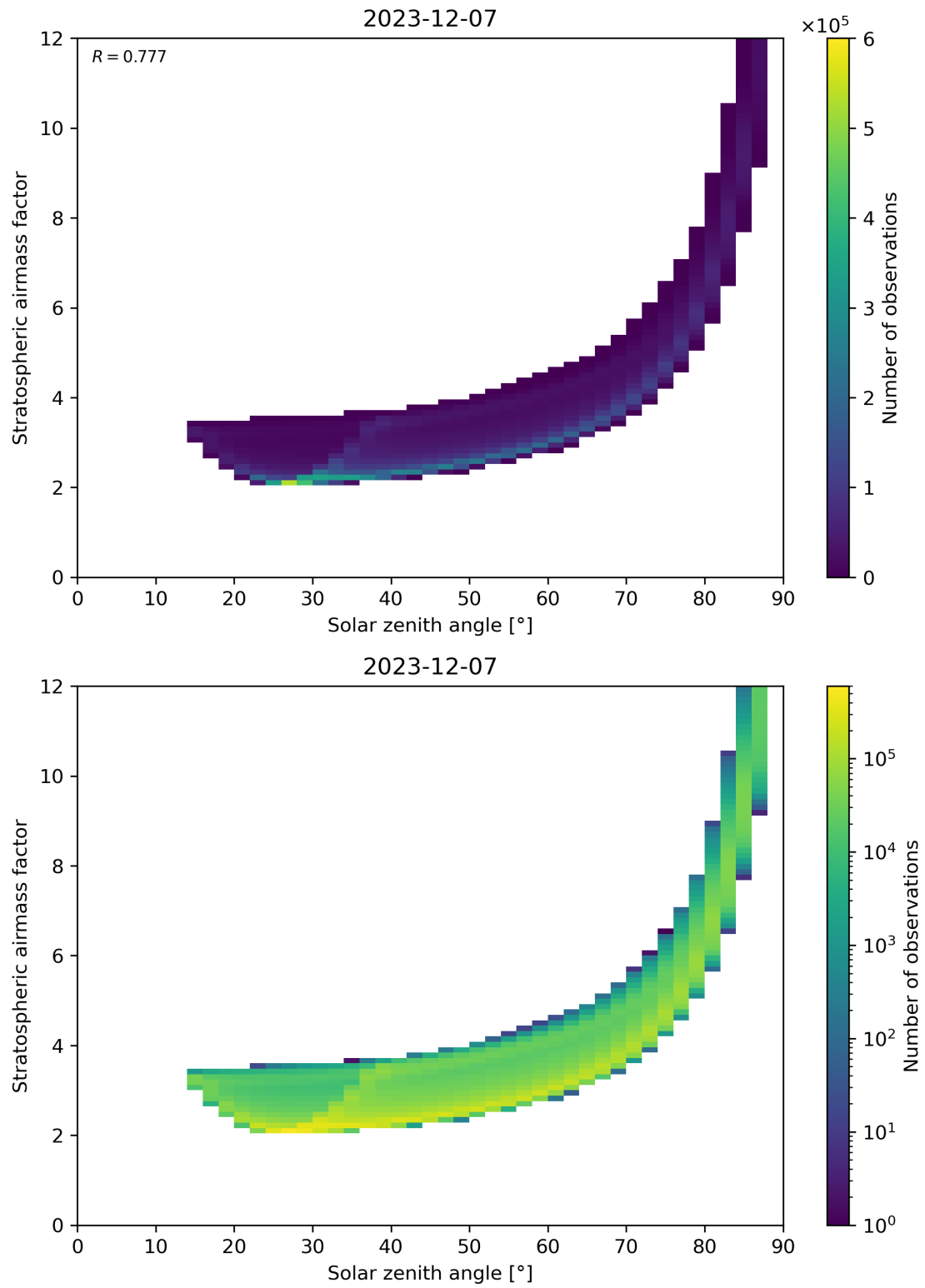
Figure 145: Scatter density plot of “Solar zenith angle” against “Stratospheric airmass factor” for 2023-12-06 to 2023-12-08.
