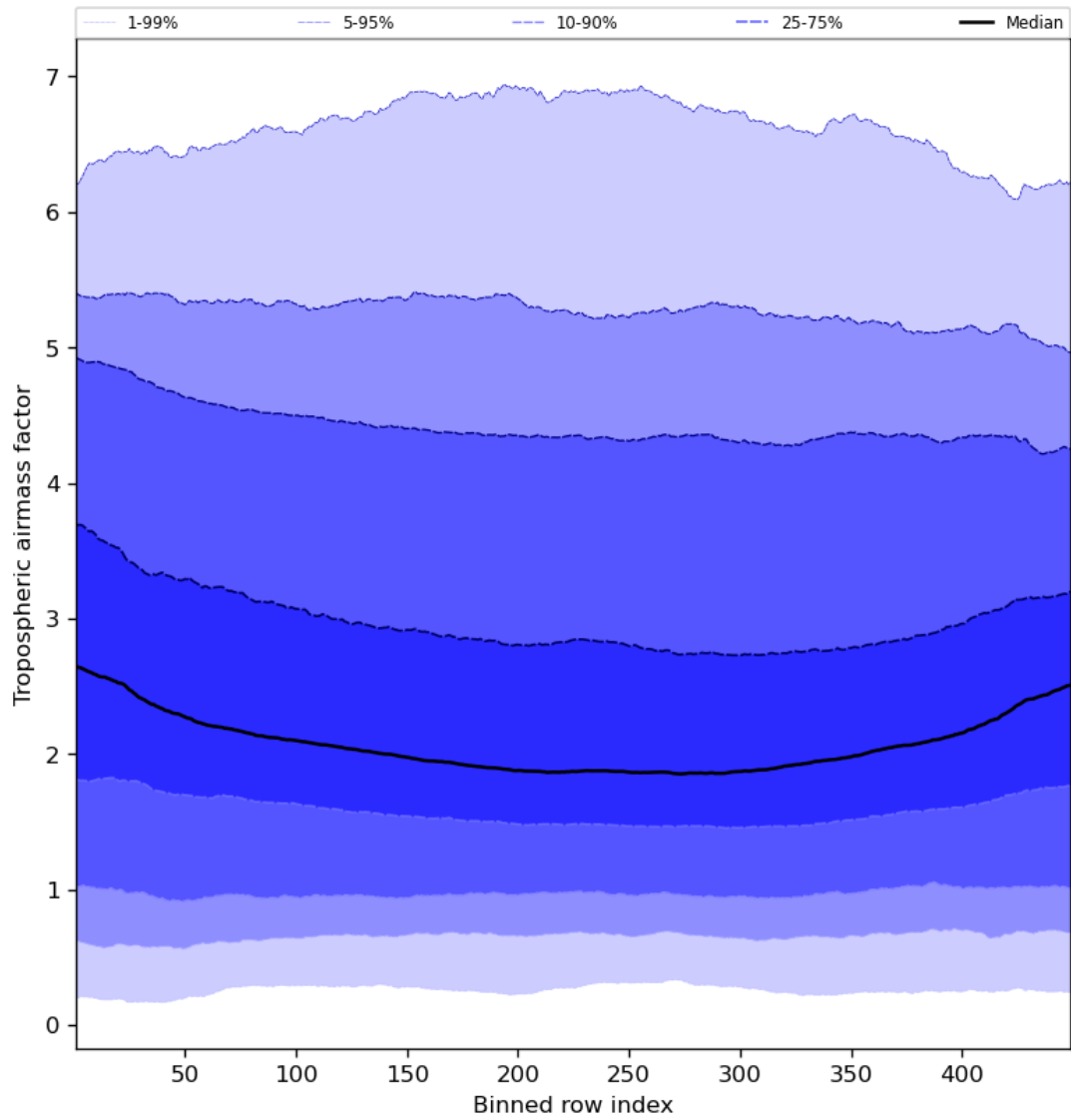
Figure 48: Along track statistics of “Tropospheric airmass factor” for 2023-12-06 to 2023-12-08
