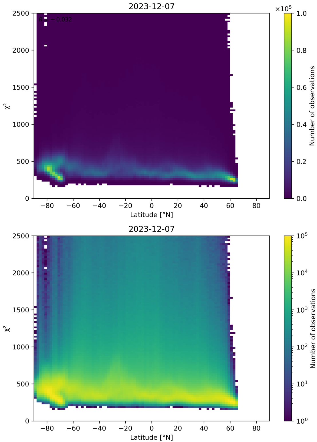
Figure 86: Scatter density plot of “Latitude” against “ \chi^2 ” for 2023-12-06 to 2023-12-08.
