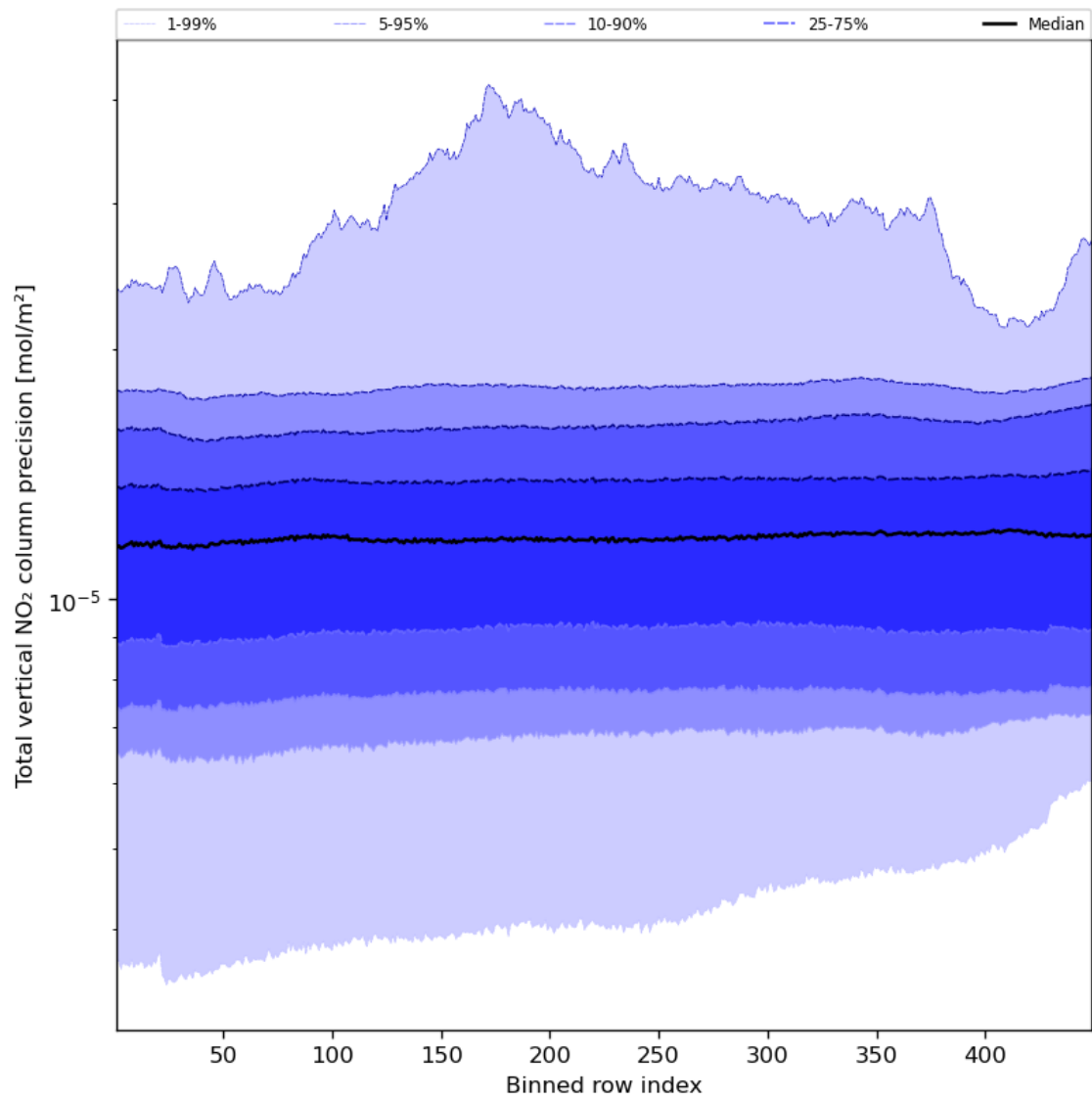
Figure 56: Along track statistics of “Total vertical NO 2 column precision” for 2023-12-06 to 2023-12-08
