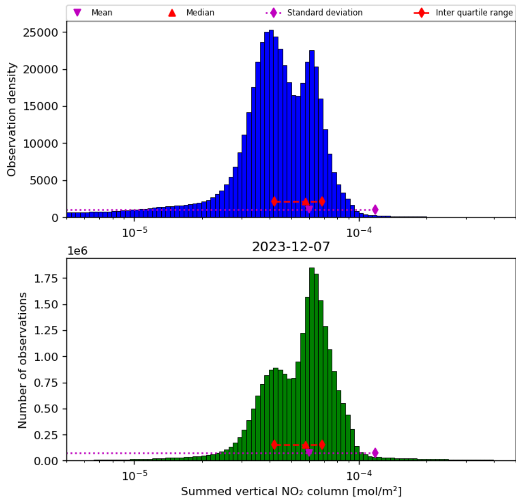
Figure 40: Histogram of “Summed vertical NO 2 column” for 2023-12-06 to 2023-12-08
