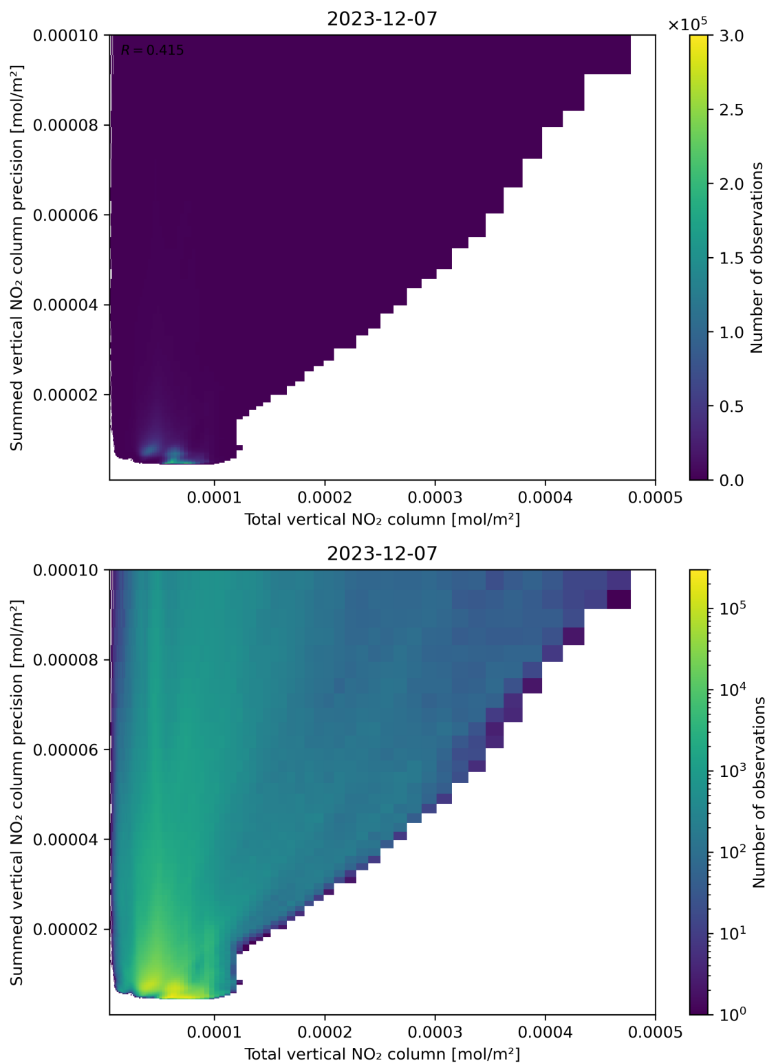
Figure 113: Scatter density plot of “Total vertical NO 2 column” against “Summed vertical NO 2 column precision” for 2023-12-06 to 2023-12-08.
