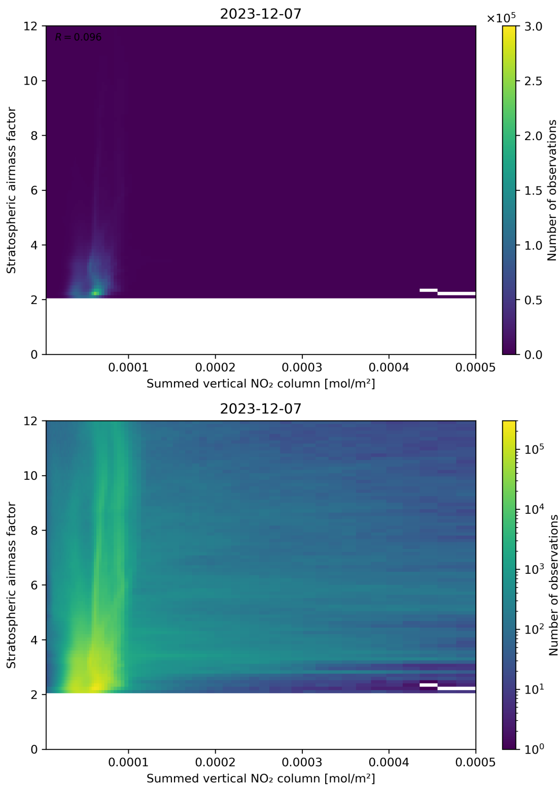
Figure 103: Scatter density plot of “Summed vertical NO 2 column” against “Stratospheric airmass factor” for 2023-12-06 to 2023-12-08.
