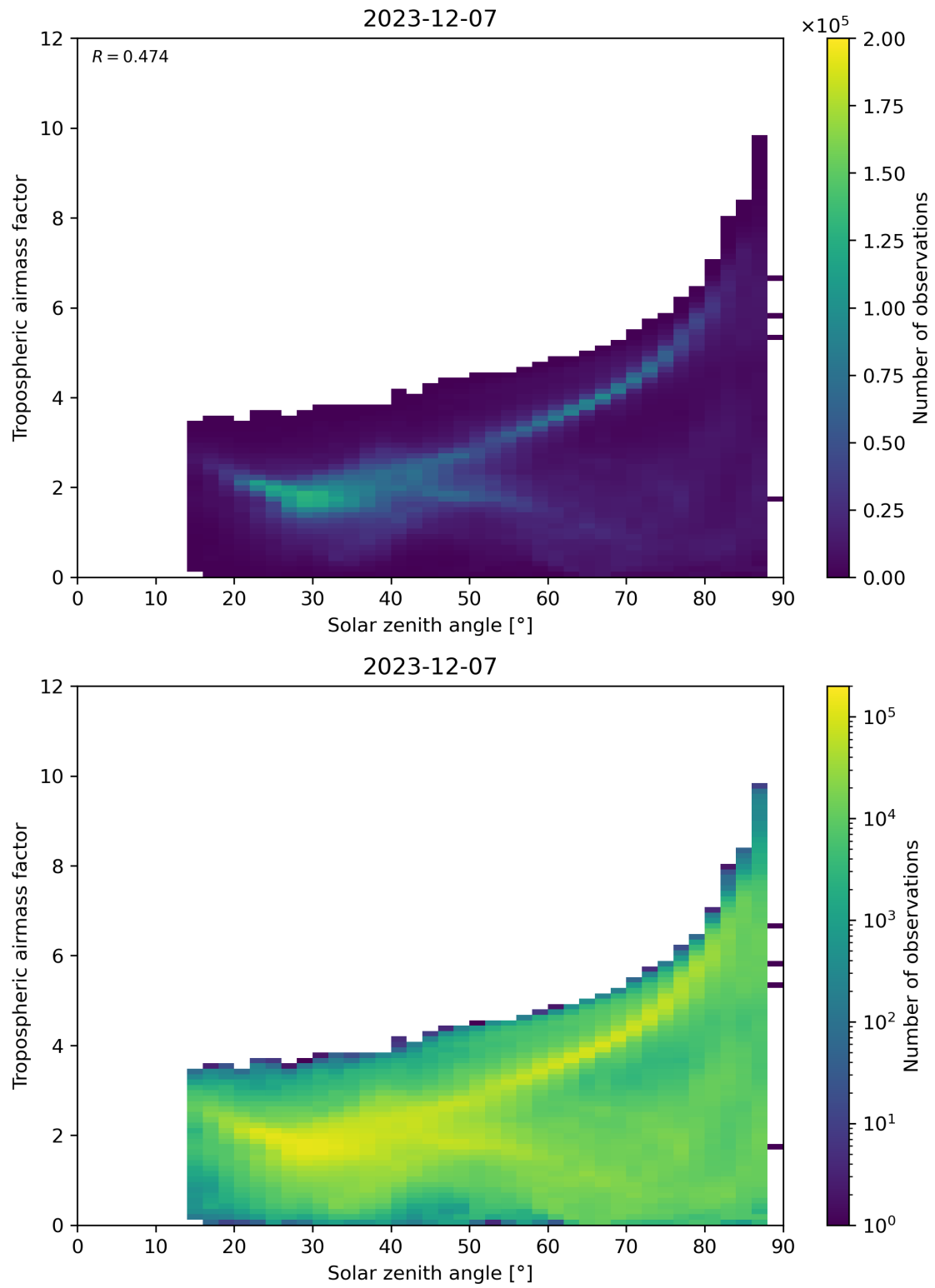
Figure 147: Scatter density plot of “Solar zenith angle” against “Tropospheric airmass factor” for 2023-12-06 to 2023-12-08.
