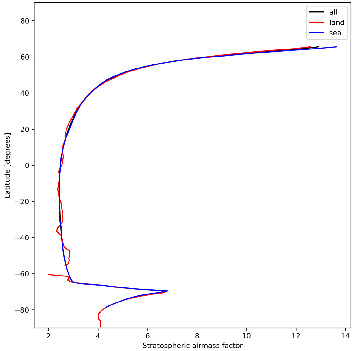
Figure 27: Zonal average of “Stratospheric airmass factor” for 2023-12-06 to 2023-12-08.
