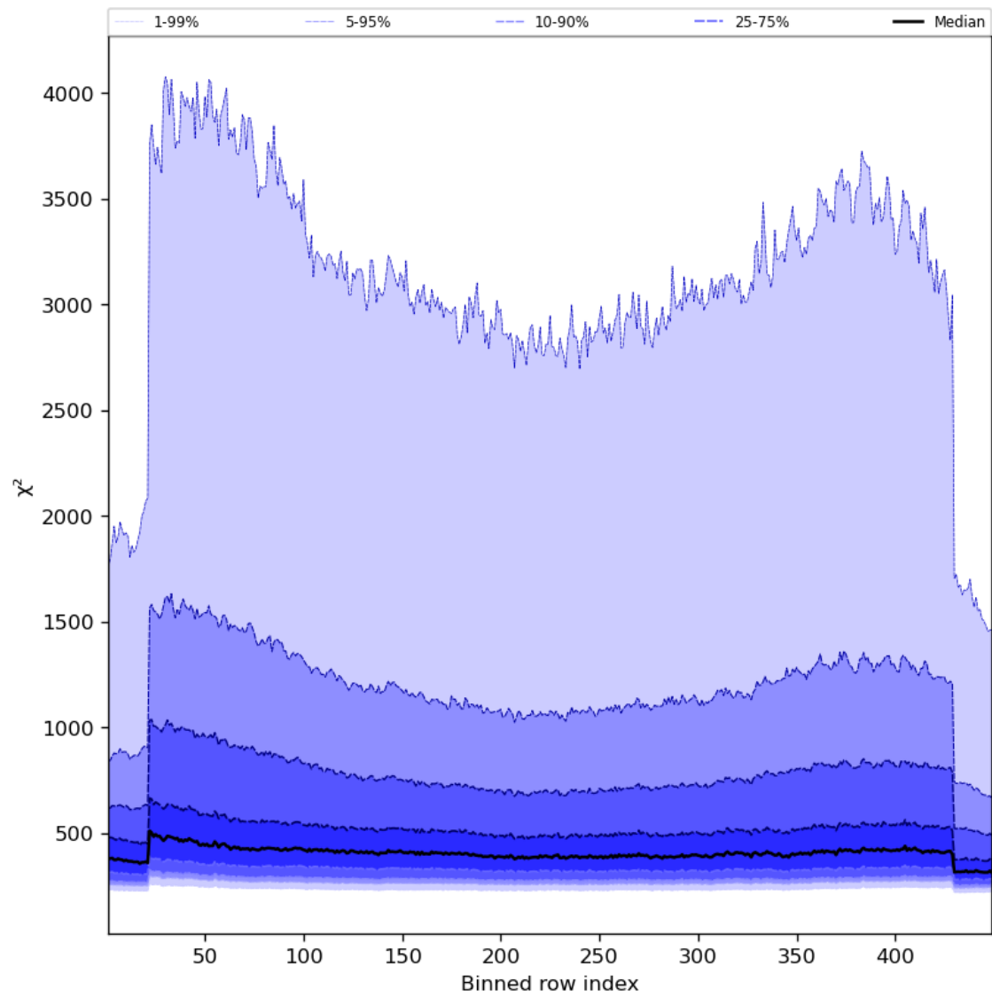
Figure 59: Along track statistics of “ \chi^2 ” for 2023-12-06 to 2023-12-08
