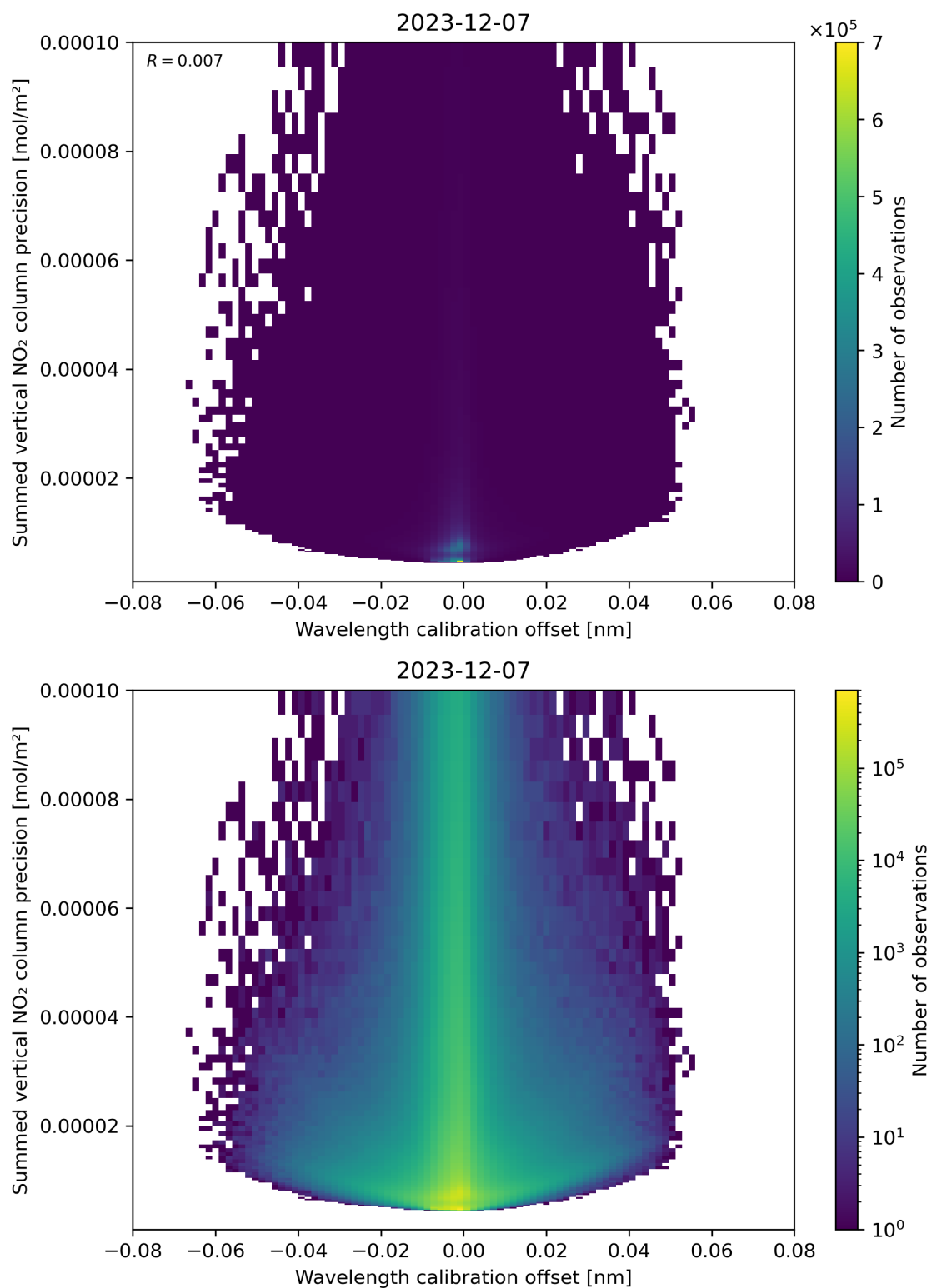
Figure 178: Scatter density plot of “Wavelength calibration offset” against “Summed vertical NO 2 column precision” for 2023-12-06 to 2023-12-08.
