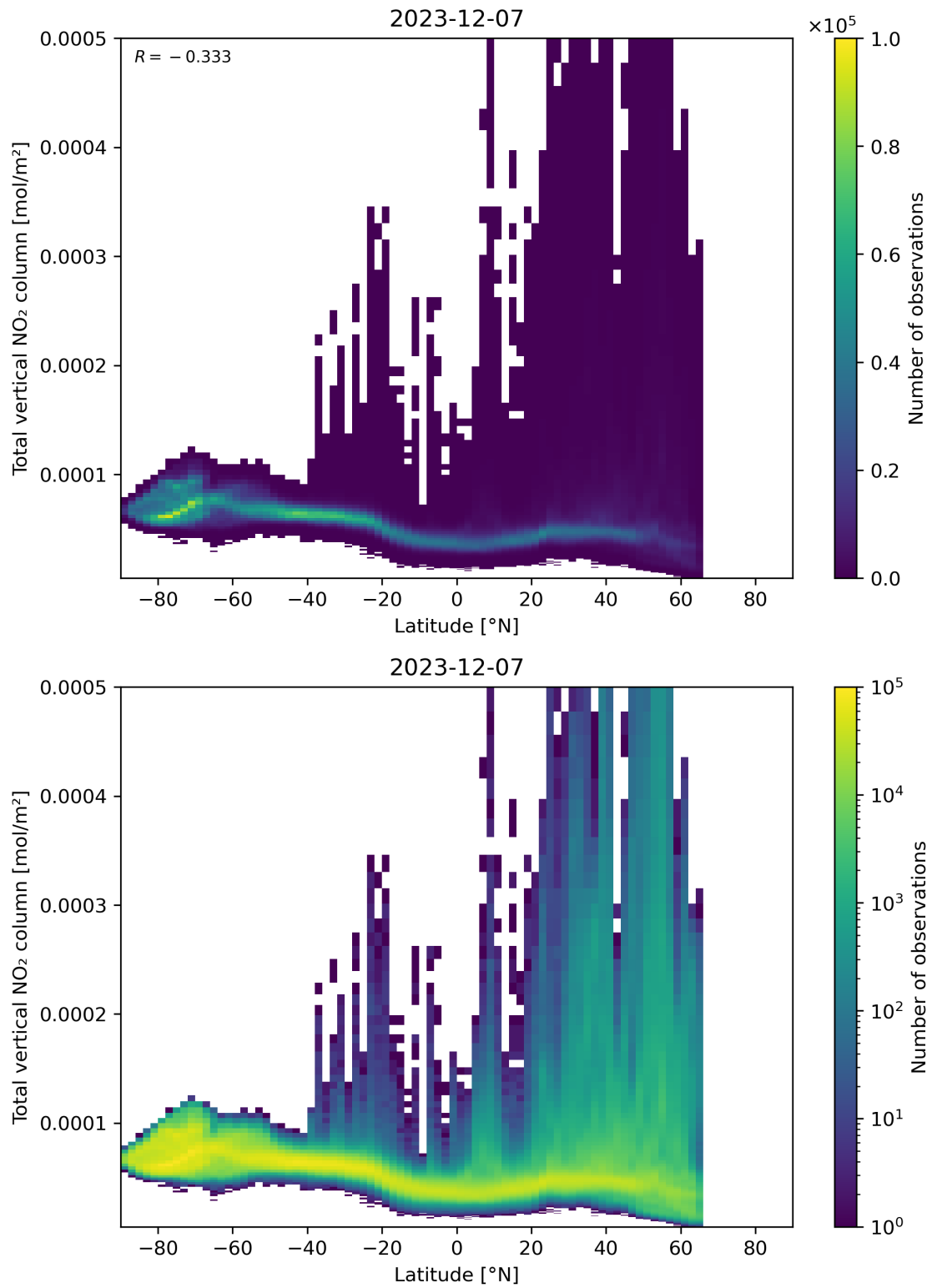
Figure 90: Scatter density plot of “Latitude” against “Total vertical NO 2 column” for 2023-12-06 to 2023-12-08.
