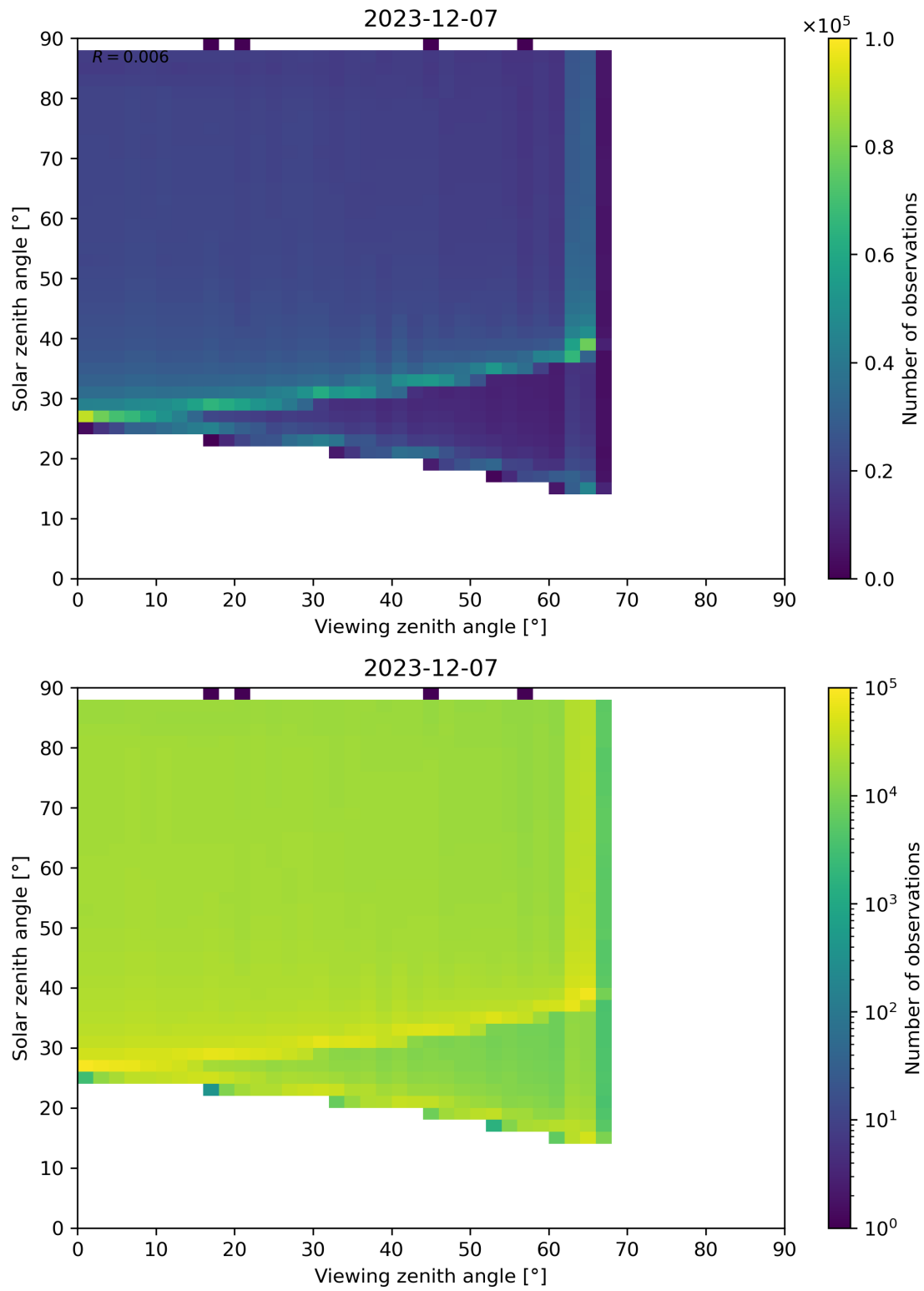
Figure 172: Scatter density plot of “Viewing zenith angle” against “Solar zenith angle” for 2023-12-06 to 2023-12-08.
