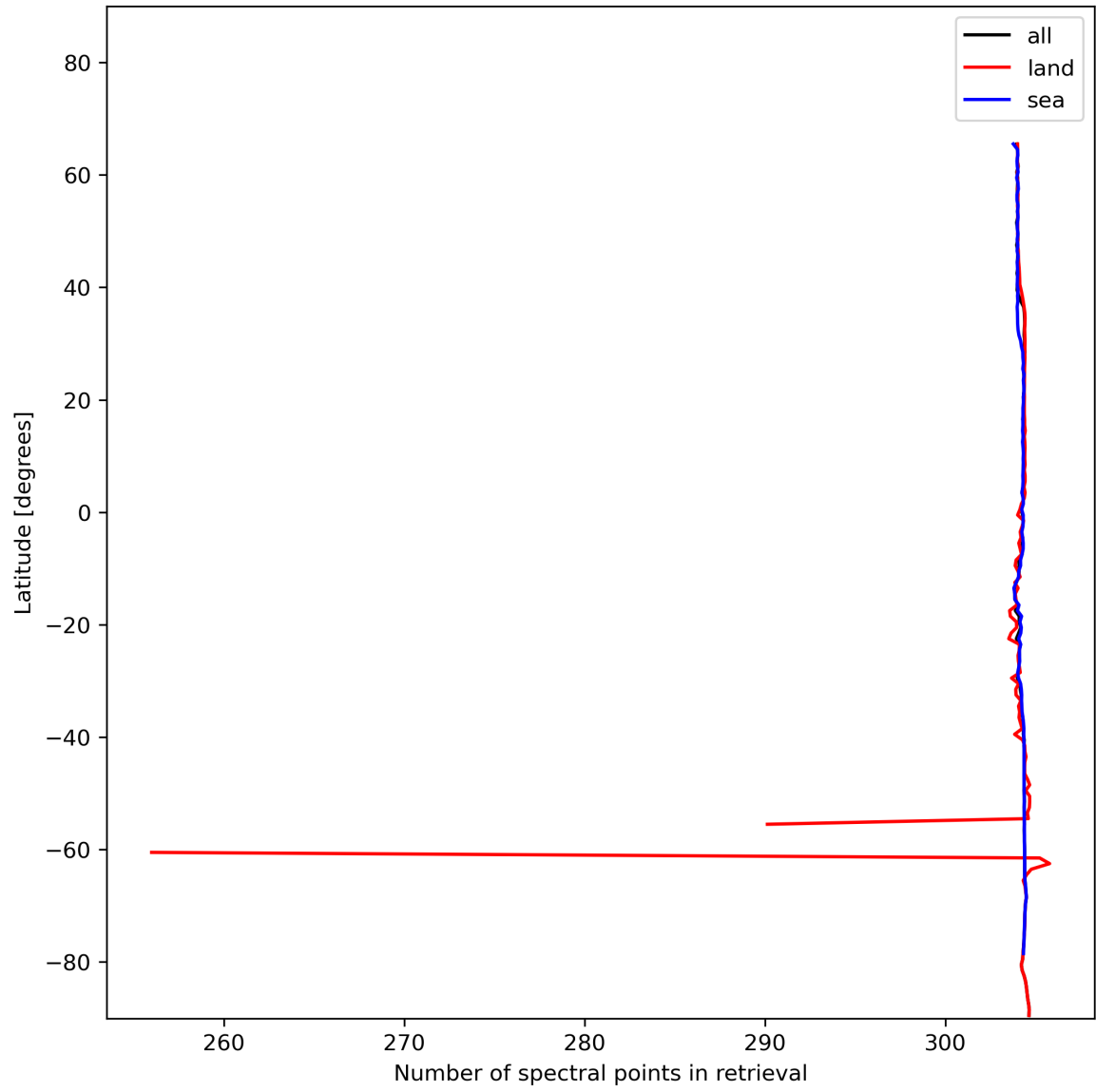
Figure 16: Zonal average of “Number of spectral points in retrieval” for 2023-12-06 to 2023-12-08.
