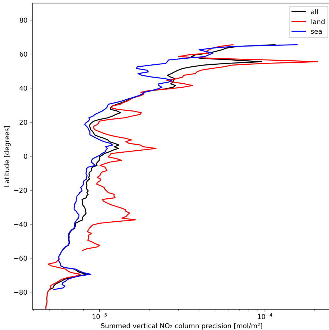
Figure 24: Zonal average of “Summed vertical NO 2 column precision” for 2023-12-06 to 2023-12-08.
