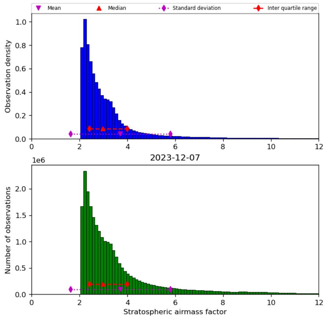
Figure 44: Histogram of “Stratospheric airmass factor” for 2023-12-06 to 2023-12-08
