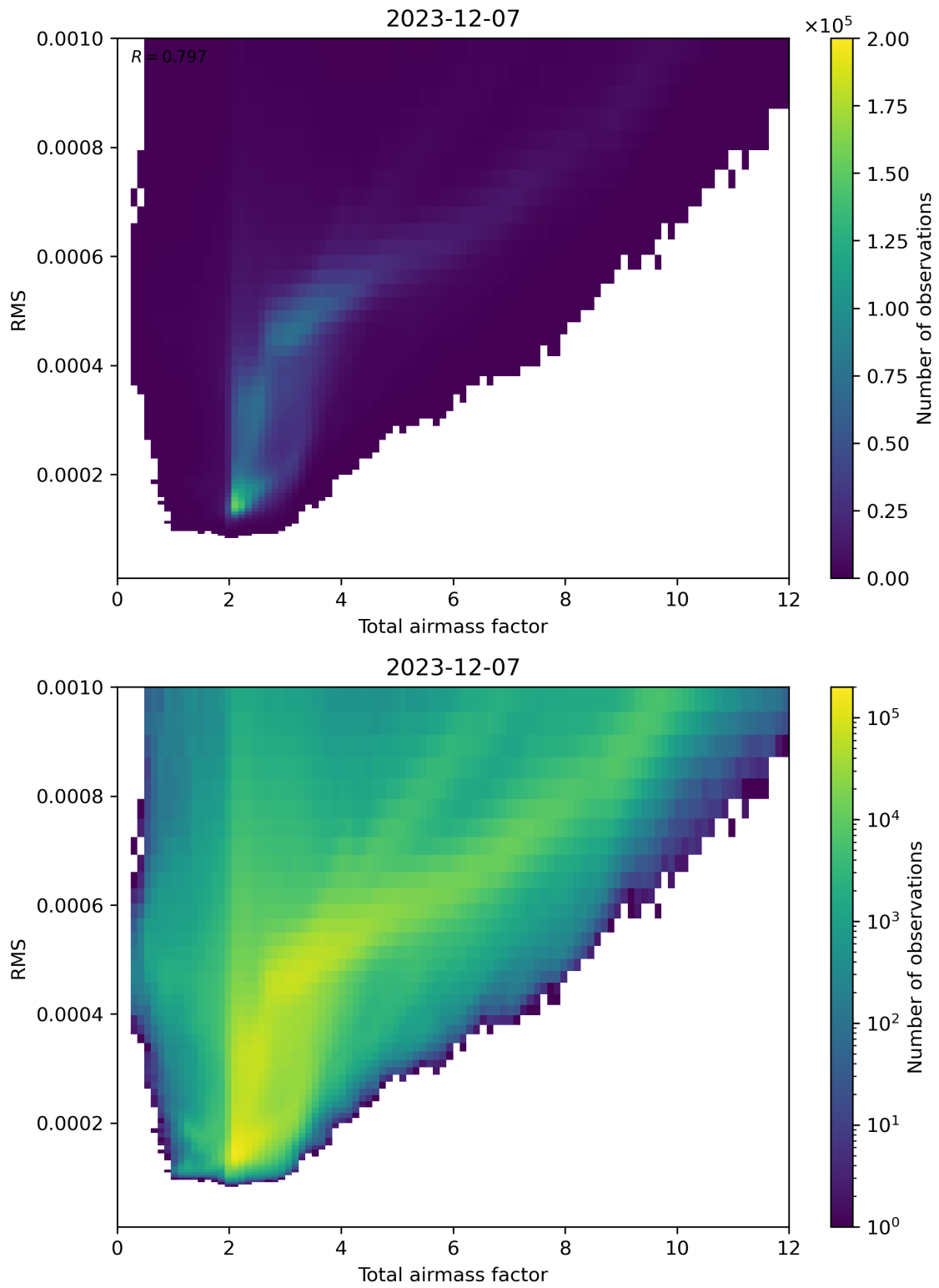
Figure 69: Scatter density plot of “Total airmass factor” against “RMS” for 2023-12-06 to 2023-12-08.
