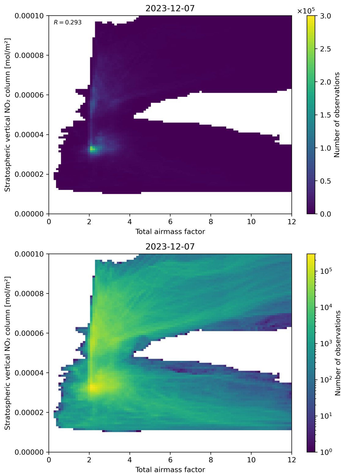
Figure 64: Scatter density plot of “Total airmass factor” against “Stratospheric vertical NO 2 column” for 2023-12-06 to 2023-12-08.
