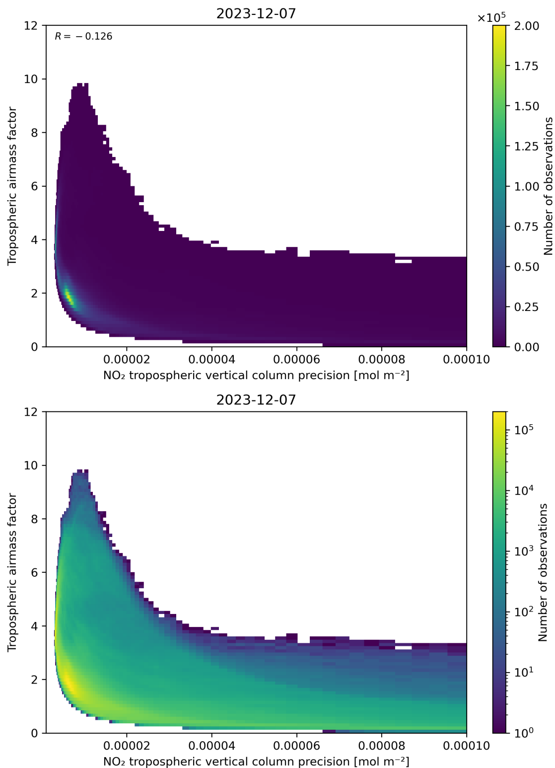
Figure 133: Scatter density plot of “NO 2 tropospheric vertical column precision” against “Tropospheric airmass factor” for 2023-12-06 to 2023-12-08.
