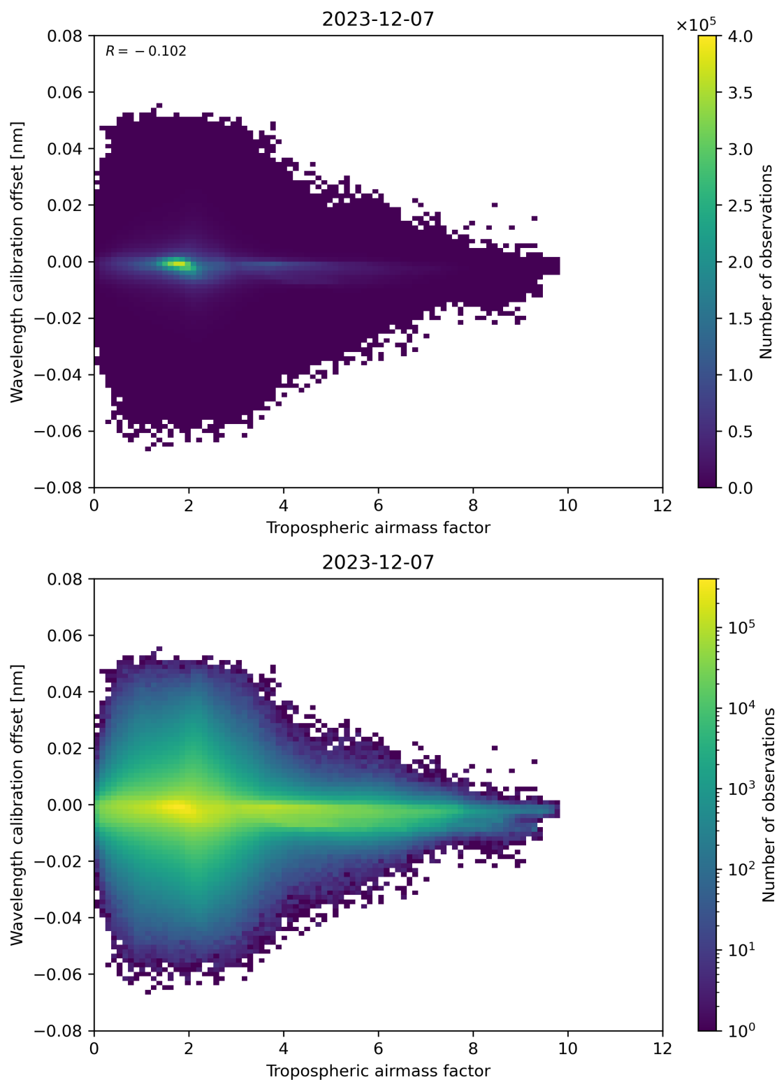
Figure 80: Scatter density plot of “Tropospheric airmass factor” against “Wavelength calibration offset” for 2023-12-06 to 2023-12-08.
