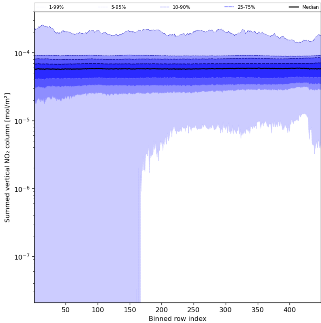
Figure 57: Along track statistics of “Summed vertical NO 2 column” for 2023-12-06 to 2023-12-08
