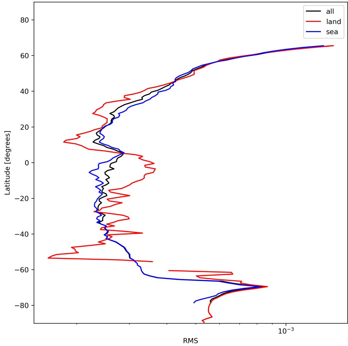
Figure 26: Zonal average of “RMS” for 2023-12-06 to 2023-12-08.
