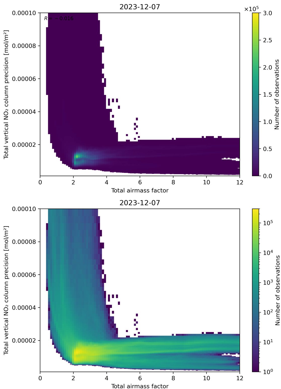
Figure 68: Scatter density plot of “Total airmass factor” against “Total vertical NO 2 column precision” for 2023-12-06 to 2023-12-08.
