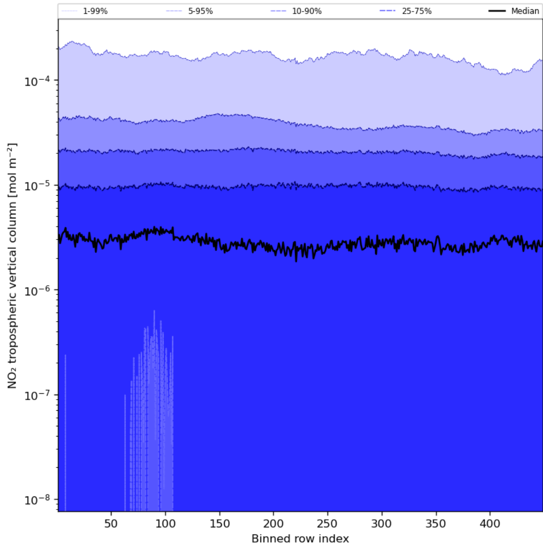
Figure 46: Along track statistics of “NO 2 tropospheric vertical column” for 2023-12-06 to 2023-12-08
