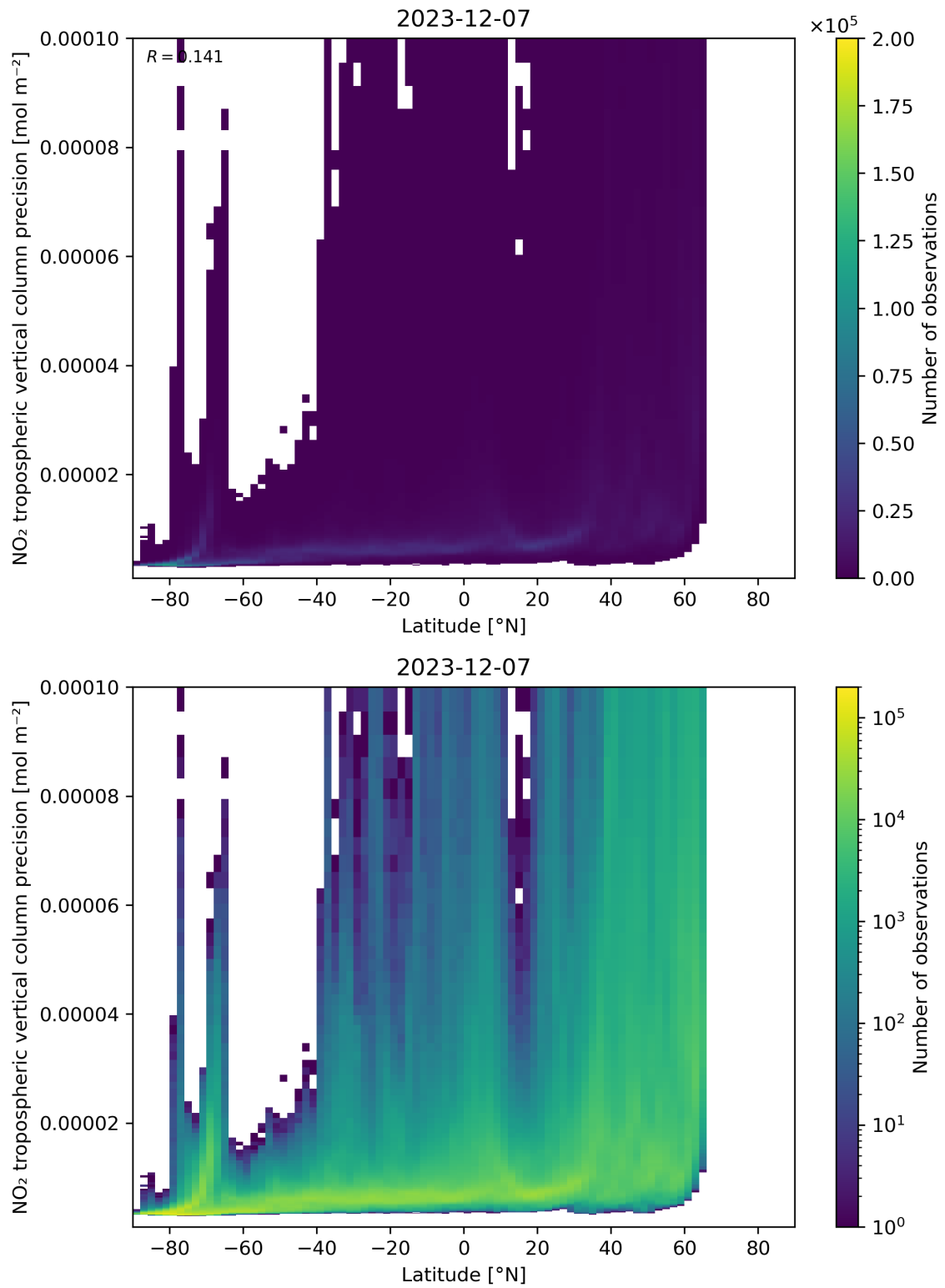
Figure 93: Scatter density plot of “Latitude” against “NO 2 tropospheric vertical column precision” for 2023-12-06 to 2023-12-08.
