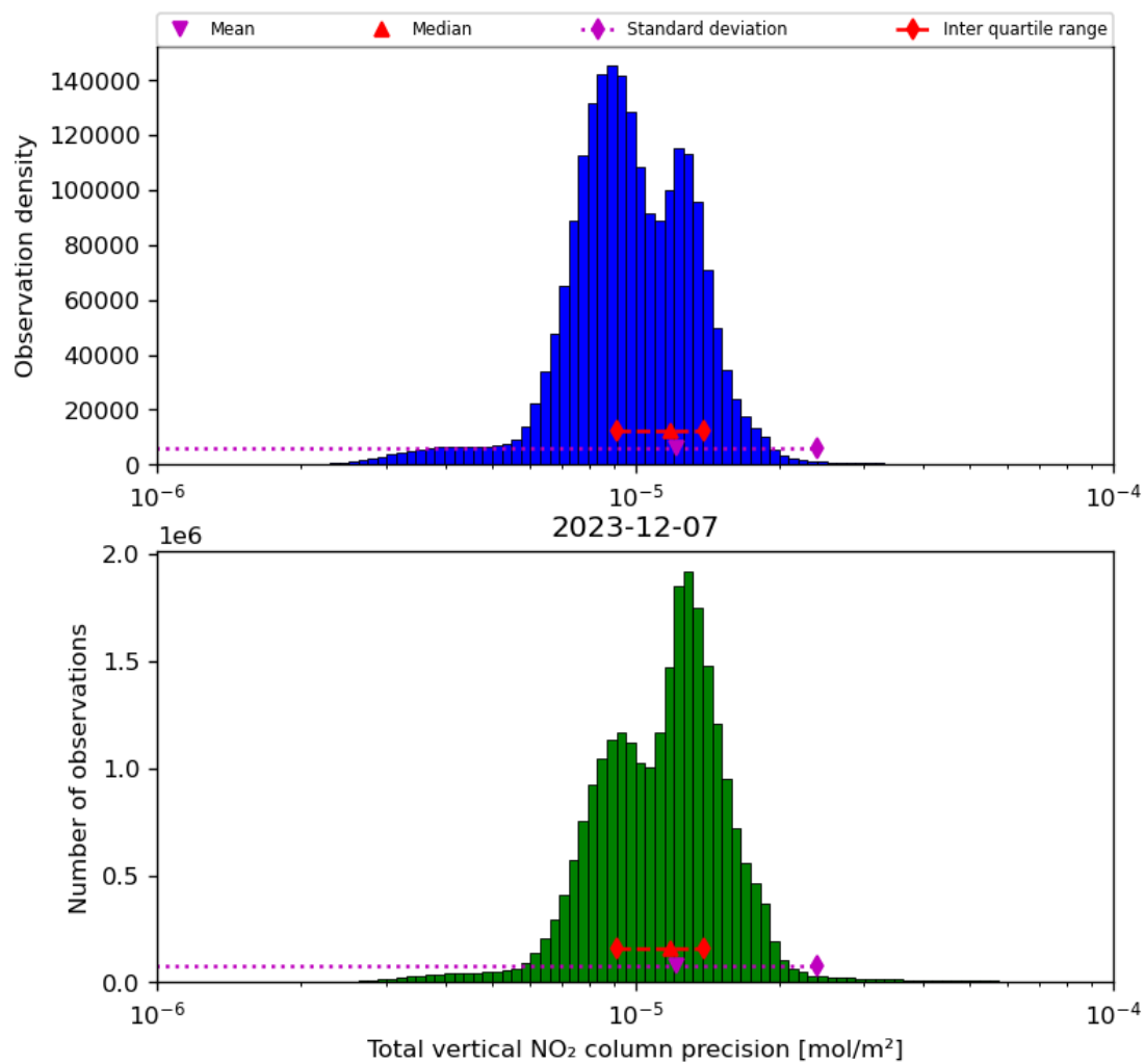
Figure 39: Histogram of “Total vertical NO 2 column precision” for 2023-12-06 to 2023-12-08
