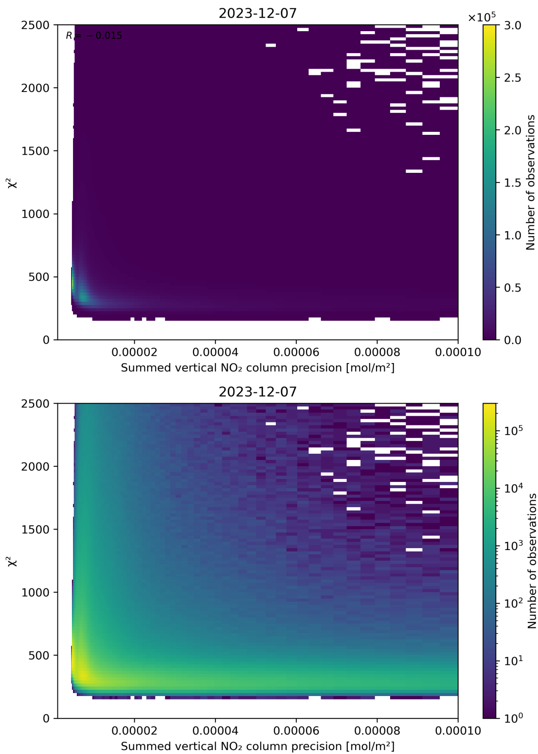
Figure 107: Scatter density plot of “Summed vertical NO 2 column precision” against “ \chi^2 ” for 2023-12-06 to 2023-12-08.
