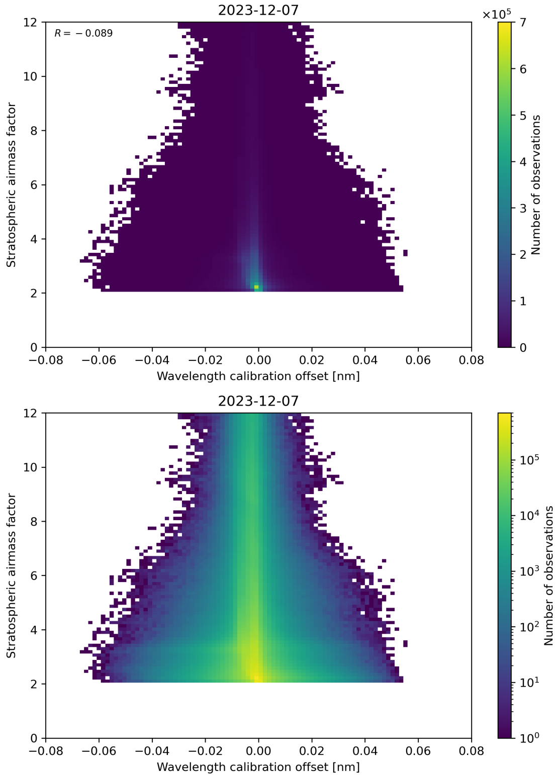
Figure 174: Scatter density plot of “Wavelength calibration offset” against “Stratospheric airmass factor” for 2023-12-06 to 2023-12-08.
