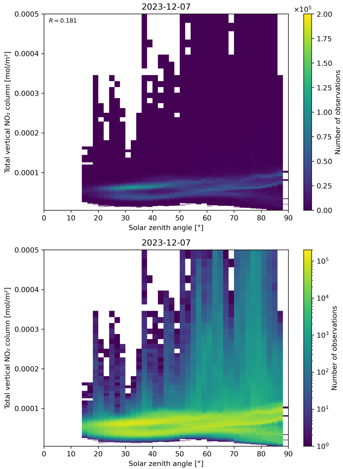
Figure 153: Scatter density plot of “Solar zenith angle” against “Total vertical NO 2 column” for 2023-12-06 to 2023-12-08.
