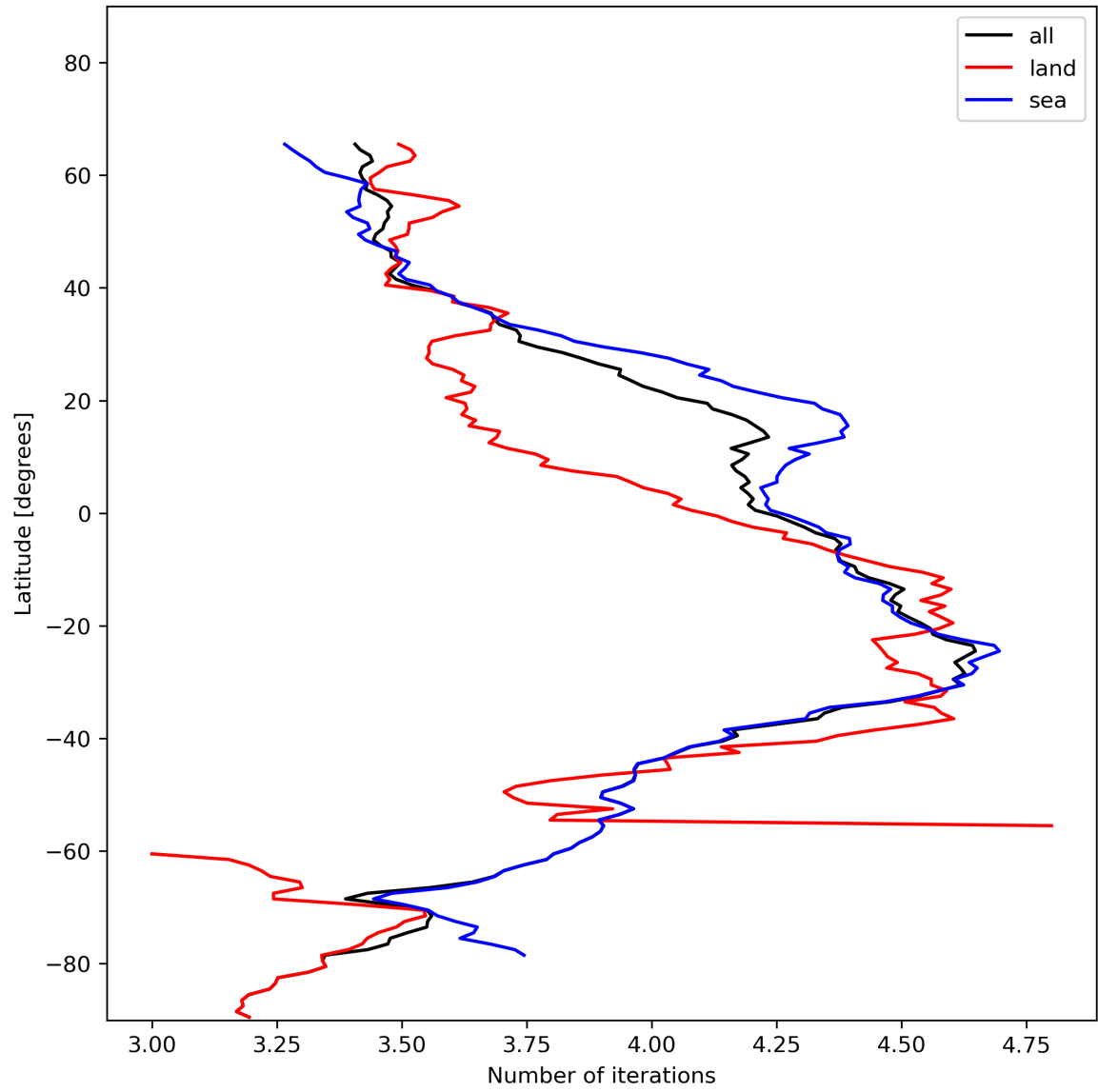
Figure 17: Zonal average of “Number of iterations” for 2023-12-06 to 2023-12-08.
