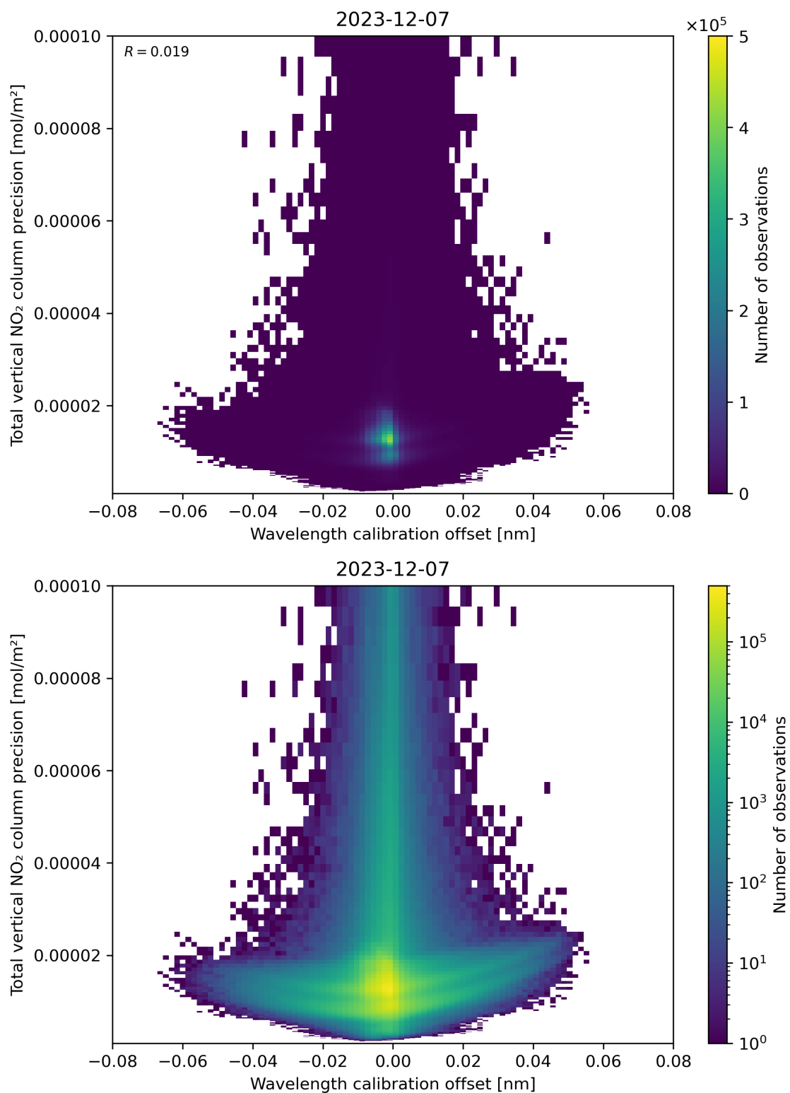
Figure 180: Scatter density plot of “Wavelength calibration offset” against “Total vertical NO 2 column precision” for 2023-12-06 to 2023-12-08.
