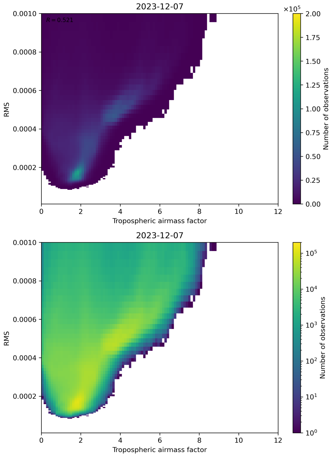
Figure 79: Scatter density plot of “Tropospheric airmass factor” against “RMS” for 2023-12-06 to 2023-12-08.
