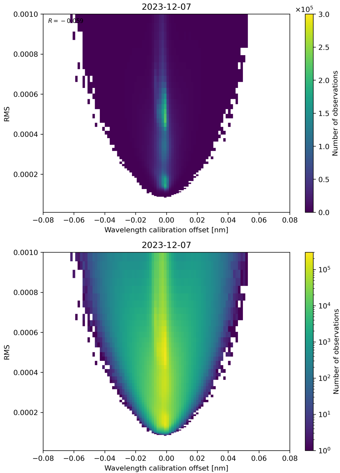
Figure 181: Scatter density plot of “Wavelength calibration offset” against “RMS” for 2023-12-06 to 2023-12-08.
