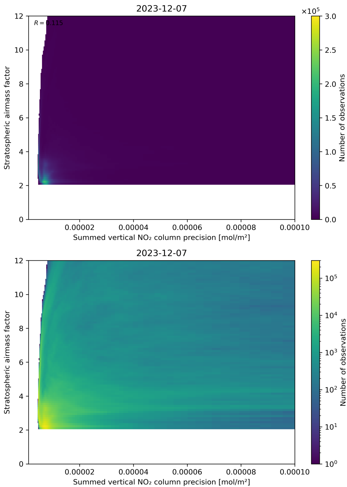
Figure 106: Scatter density plot of “Summed vertical NO 2 column precision” against “Stratospheric airmass factor” for 2023-12-06 to 2023-12-08.
