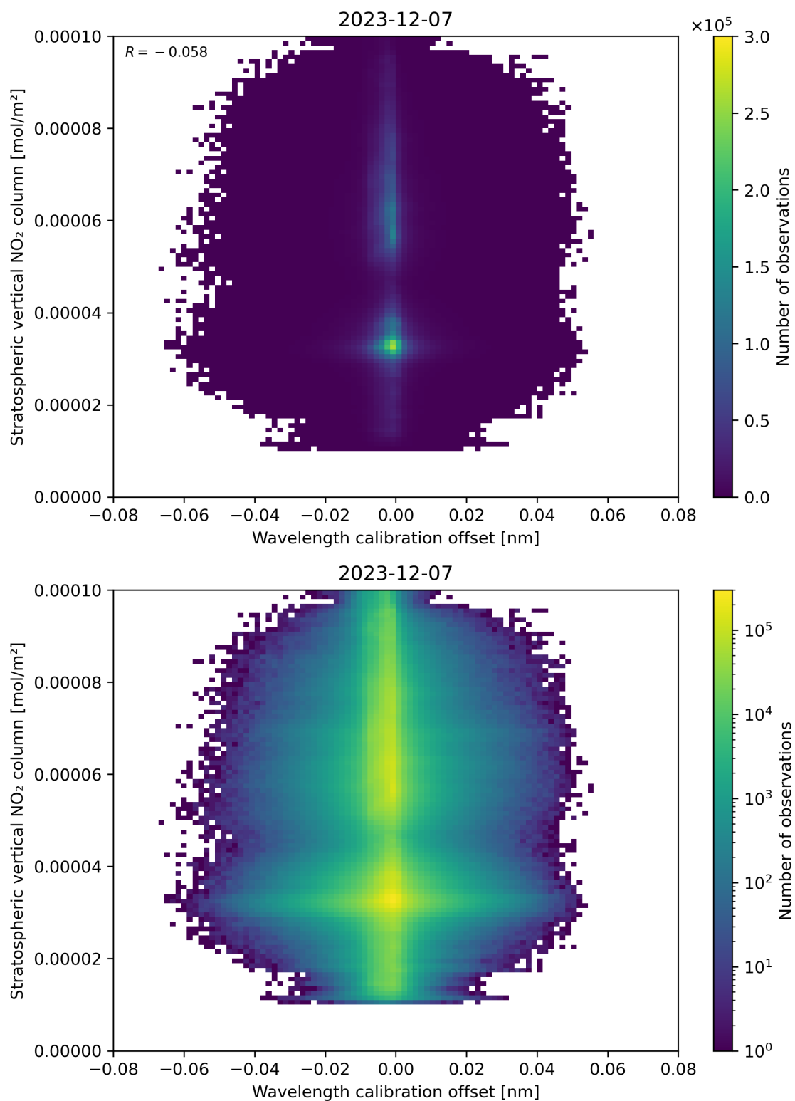
Figure 176: Scatter density plot of “Wavelength calibration offset” against “Stratospheric vertical NO 2 column” for 2023-12-06 to 2023-12-08.
