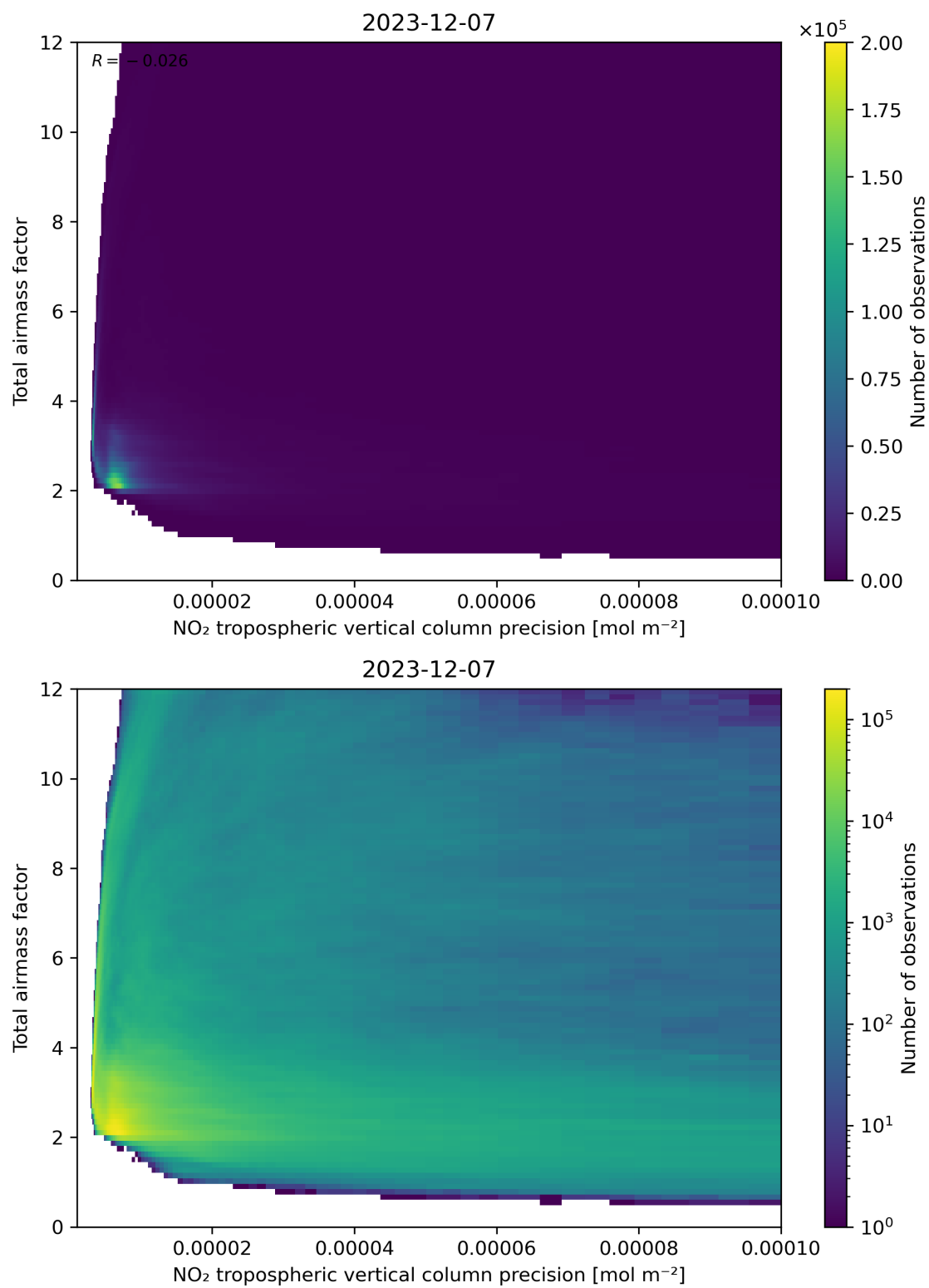
Figure 132: Scatter density plot of “NO 2 tropospheric vertical column precision” against “Total air mass factor” for 2023-12-06 to 2023-12-08.
