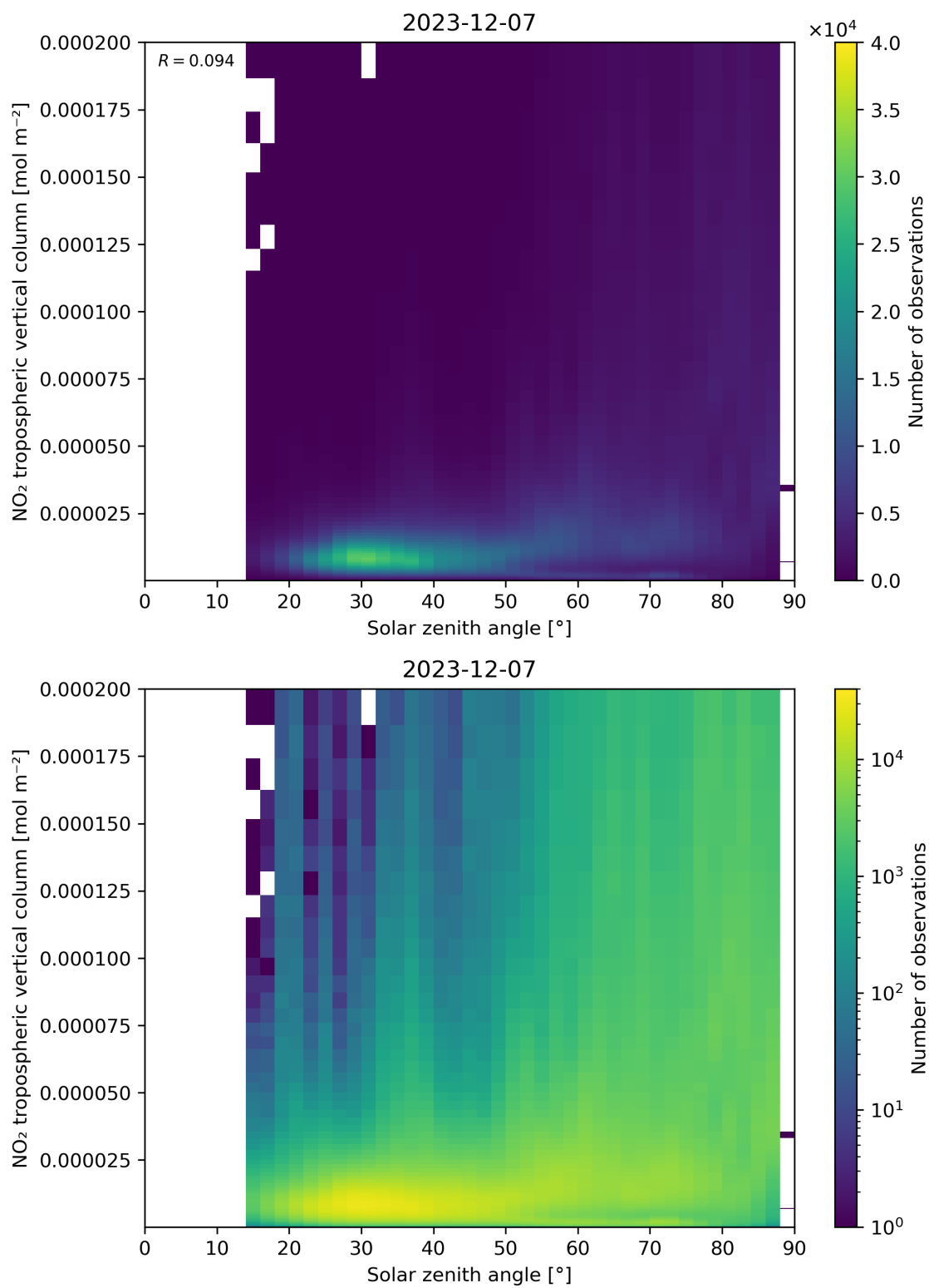
Figure 155: Scatter density plot of “Solar zenith angle” against “NO 2 tropospheric vertical column” for 2023-12-06 to 2023-12-08.
