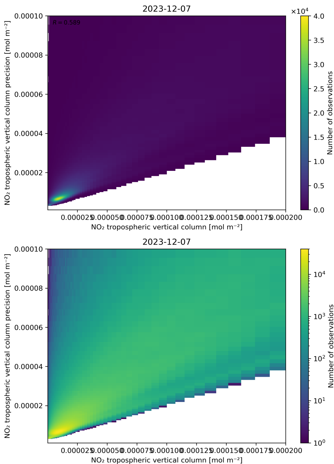
Figure 130: Scatter density plot of “NO 2 tropospheric vertical column” against “NO 2 tropospheric vertical column precision” for 2023-12-06 to 2023-12-08.
