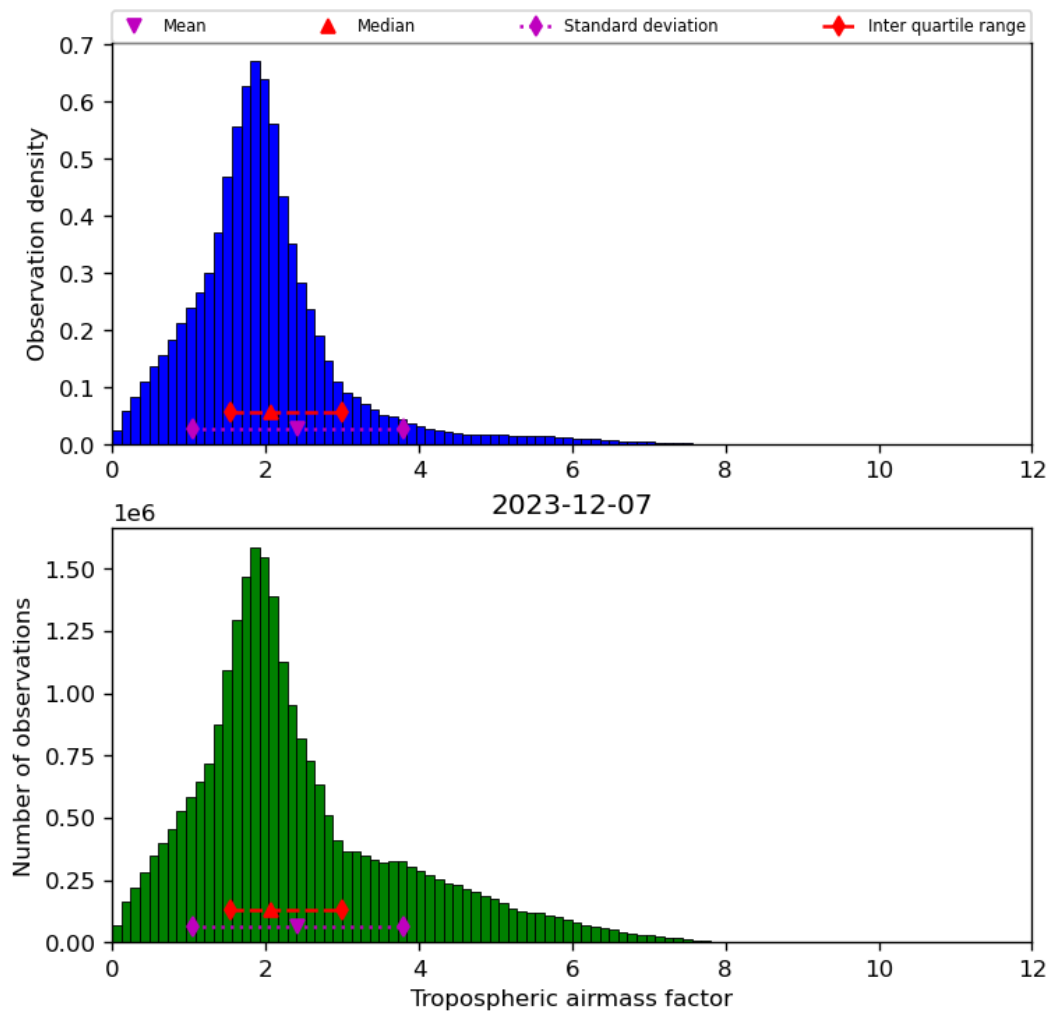
Figure 31: Histogram of “Tropospheric airmass factor” for 2023-12-06 to 2023-12-08
