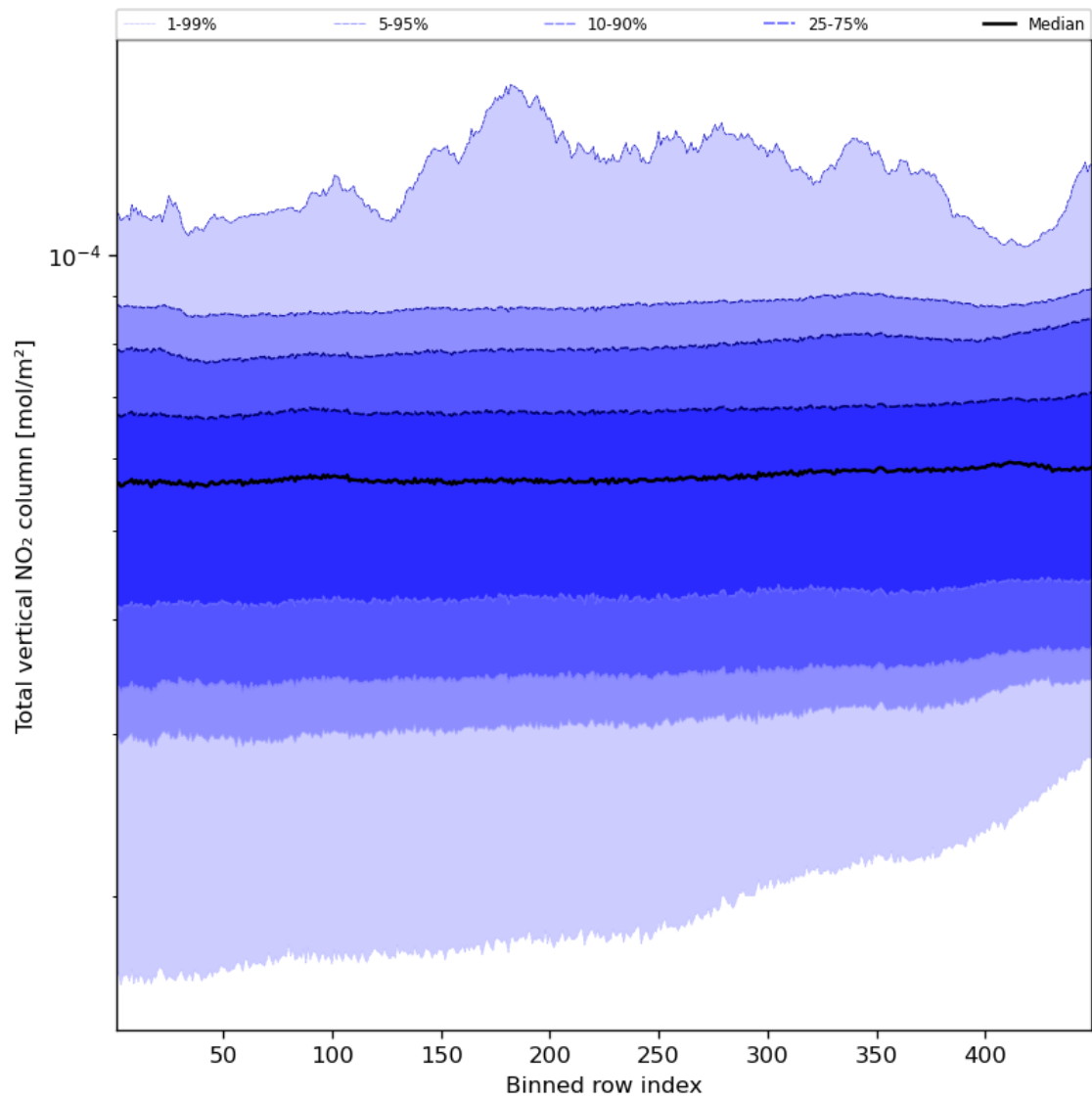
Figure 55: Along track statistics of “Total vertical NO 2 column” for 2023-12-06 to 2023-12-08
