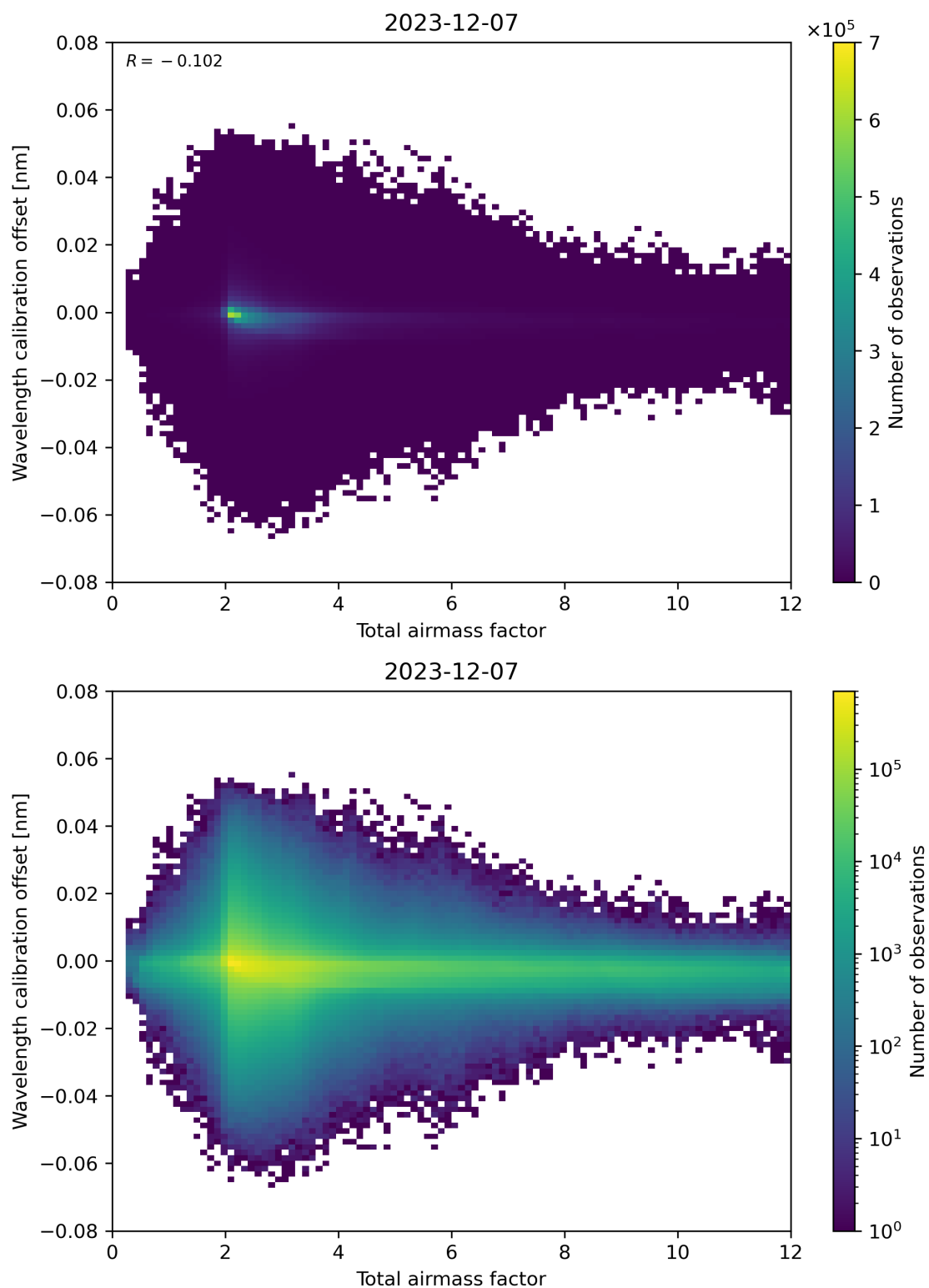
Figure 70: Scatter density plot of “Total airmass factor” against “Wavelength calibration offset” for 2023-12-06 to 2023-12-08.
