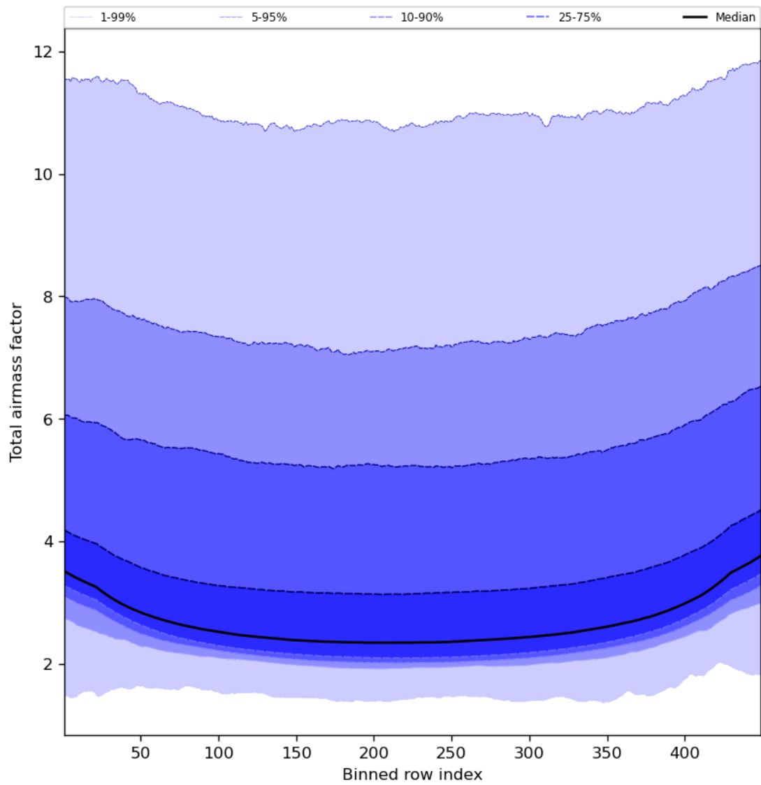
Figure 49: Along track statistics of “Total airmass factor” for 2023-12-06 to 2023-12-08
