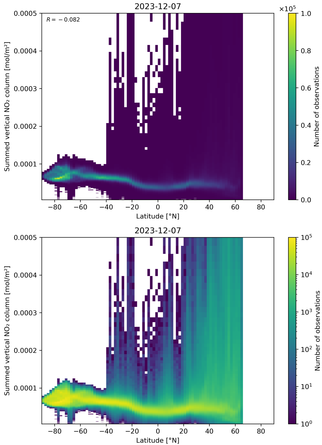
Figure 88: Scatter density plot of “Latitude” against “Summed vertical NO 2 column” for 2023-12-06 to 2023-12-08.
