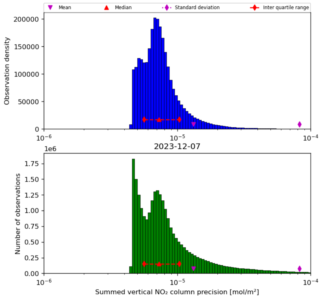
Figure 41: Histogram of “Summed vertical NO 2 column precision” for 2023-12-06 to 2023-12-08
