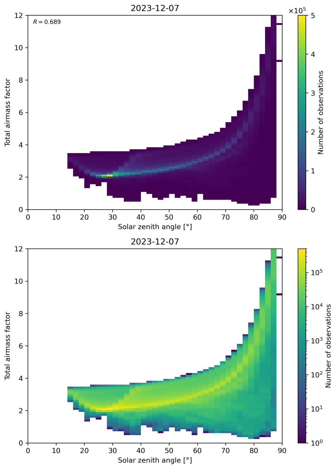
Figure 146: Scatter density plot of “Solar zenith angle” against “Total air mass factor” for 2023-12-06 to 2023-12-08.
