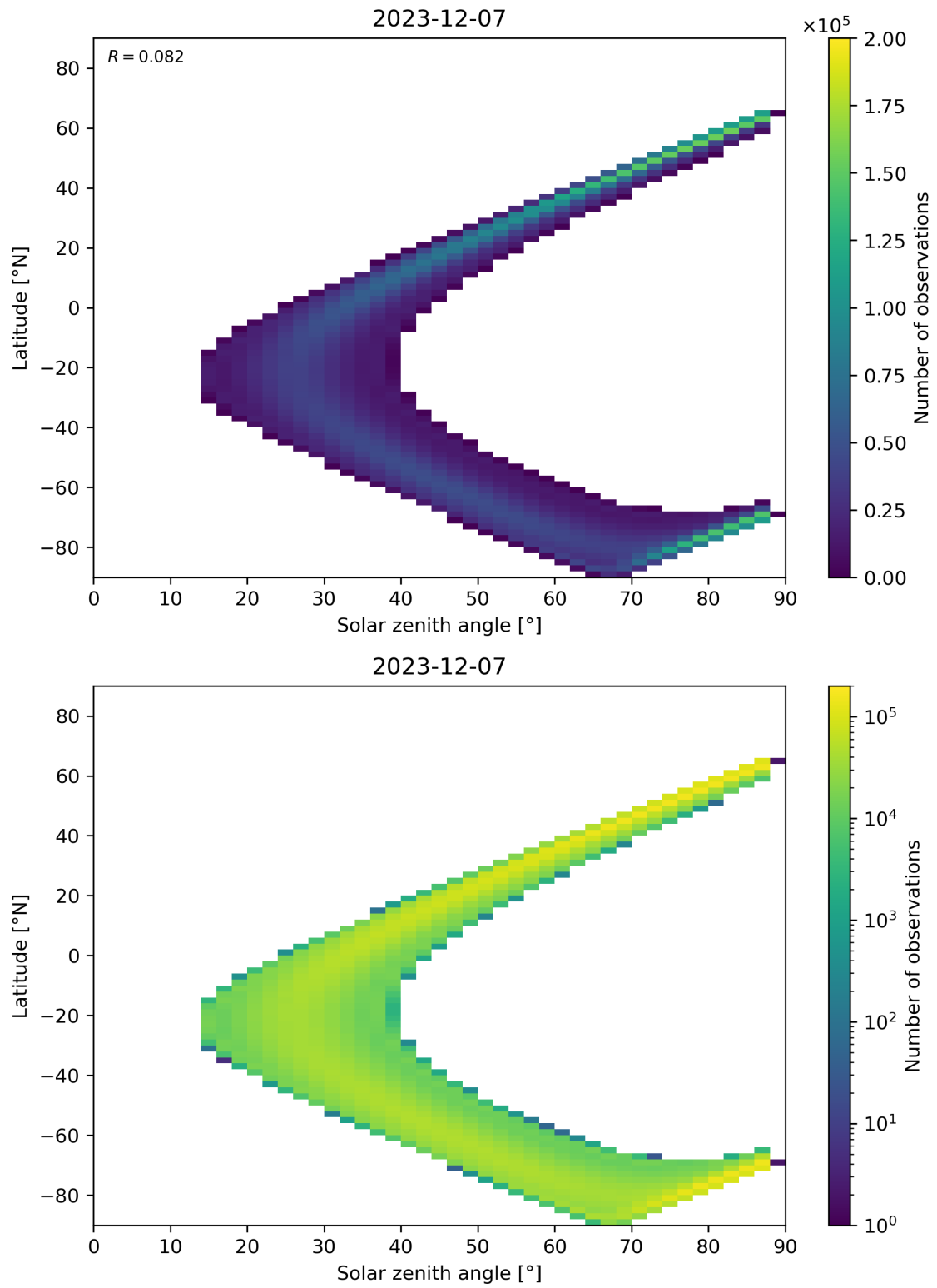
Figure 149: Scatter density plot of “Solar zenith angle” against “Latitude” for 2023-12-06 to 2023-12-08.
