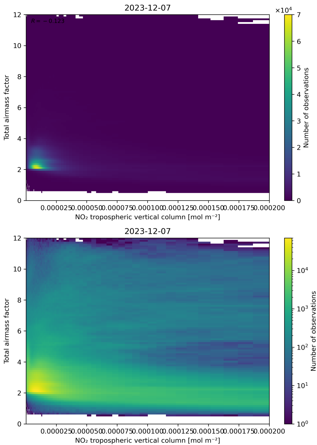
Figure 122: Scatter density plot of “NO 2 tropospheric vertical column” against “Total air mass factor” for 2023-12-06 to 2023-12-08.
