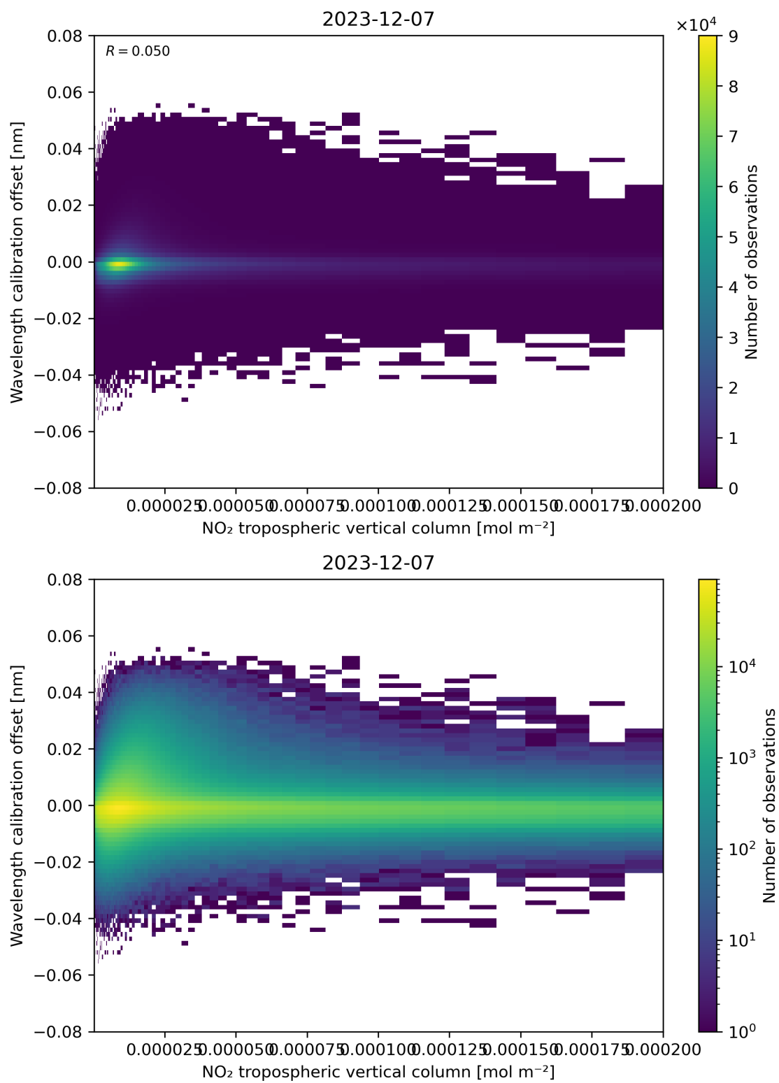
Figure 143: Scatter density plot of “NO 2 tropospheric vertical column” against “Wavelength calibration offset” for 2023-12-06 to 2023-12-08.
