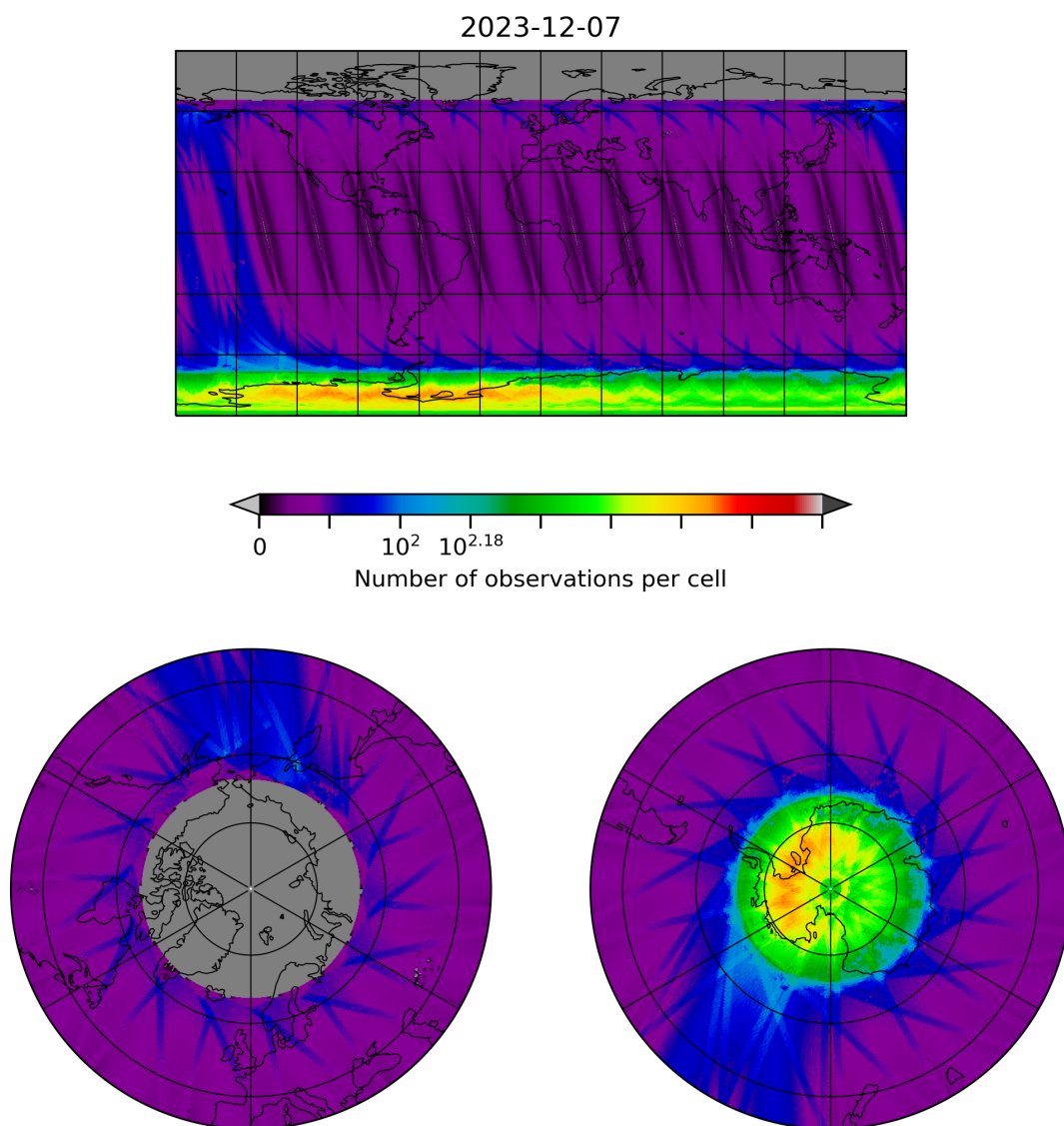
Figure 10: Map of the number of observations for 2023-12-06 to 2023-12-08
