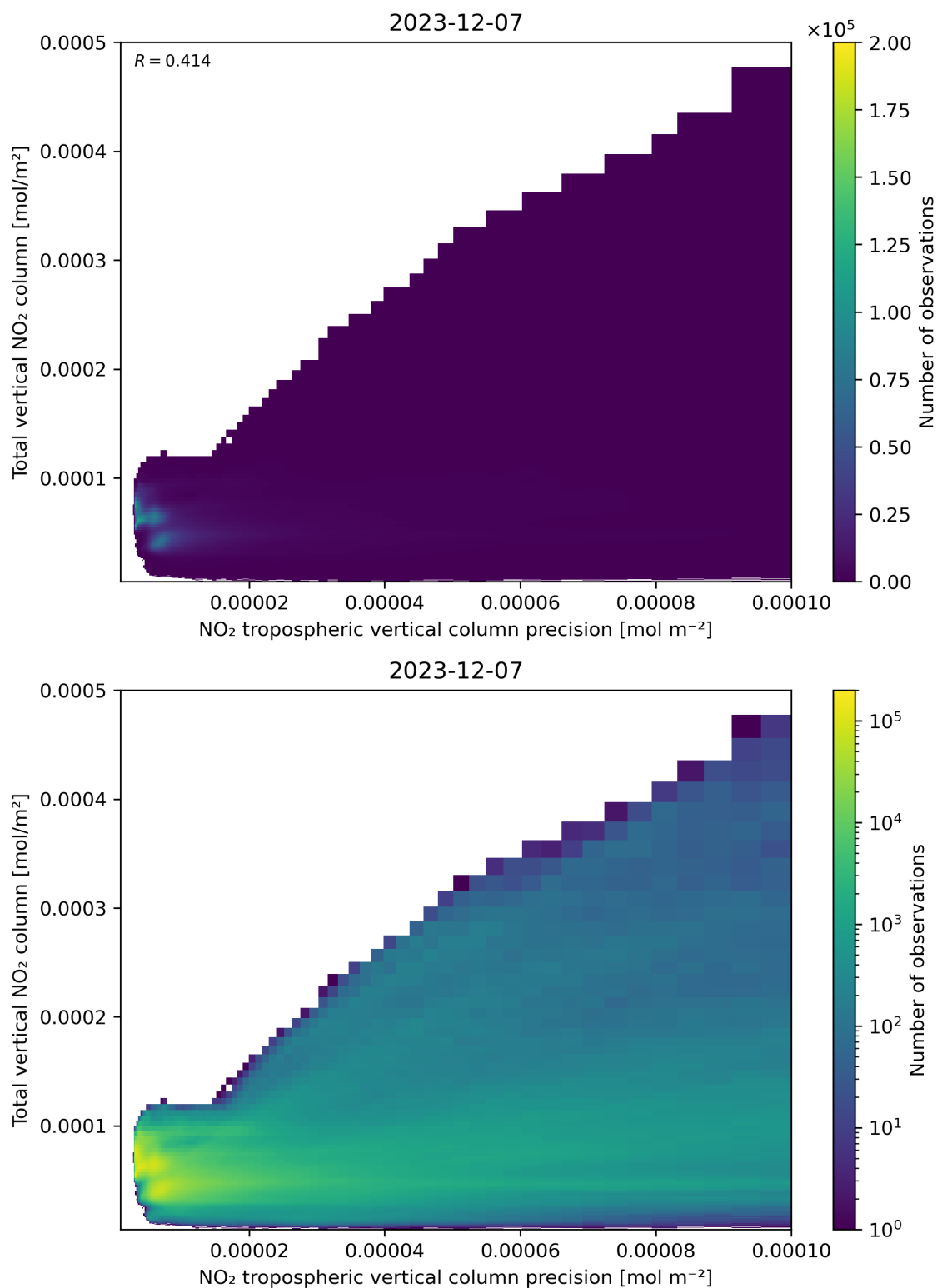
Figure 138: Scatter density plot of “NO 2 tropospheric vertical column precision” against “Total vertical NO 2 column” for 2023-12-06 to 2023-12-08.
