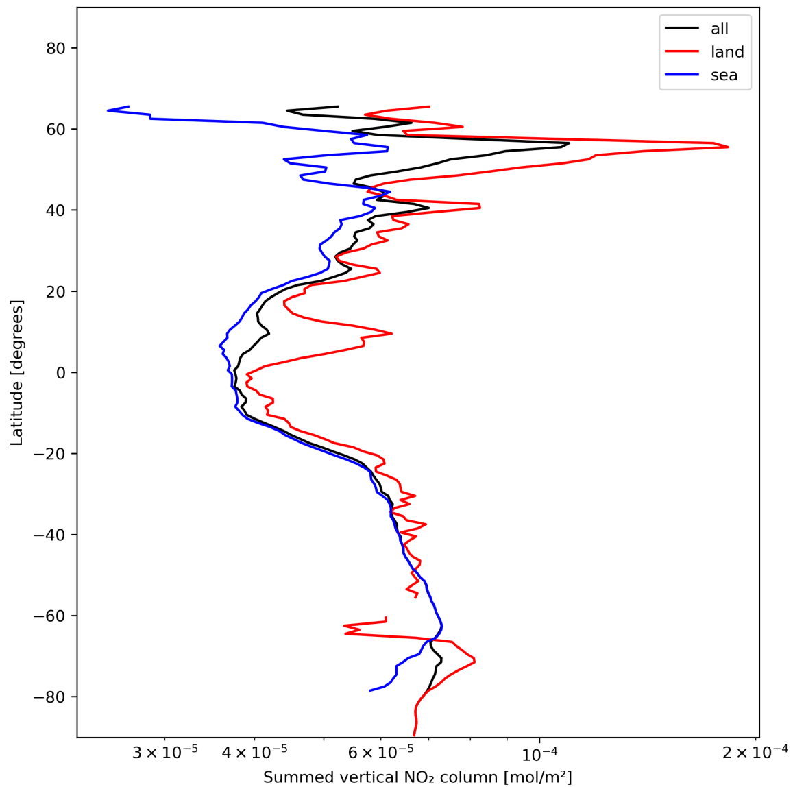
Figure 23: Zonal average of “Summed vertical NO 2 column” for 2023-12-06 to 2023-12-08.
