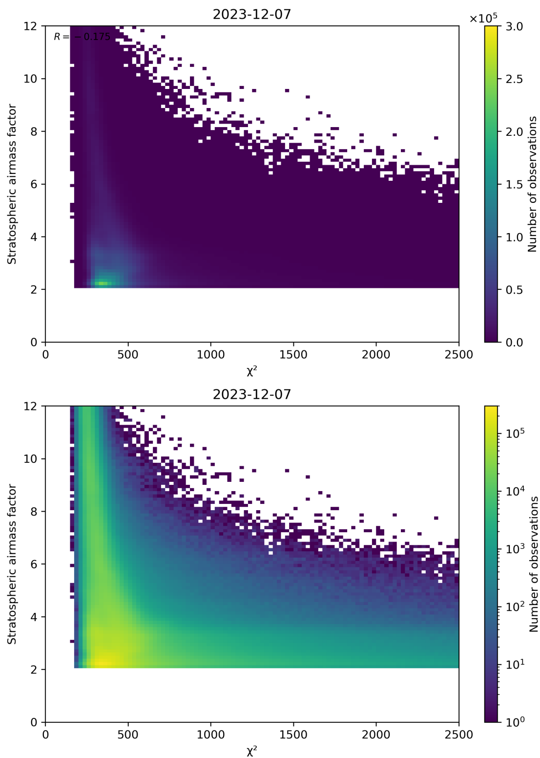
Figure 81: Scatter density plot of “ \chi^2 ” against “Stratospheric airmass factor” for 2023-12-06 to 2023-12-08.
