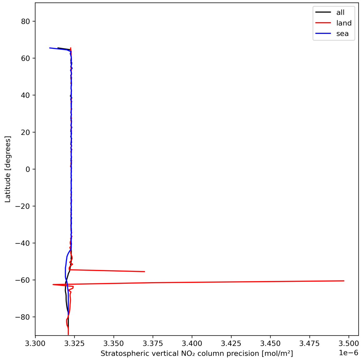
Figure 20: Zonal average of “Stratospheric vertical NO 2 column precision” for 2023-12-06 to 2023-12-08.
