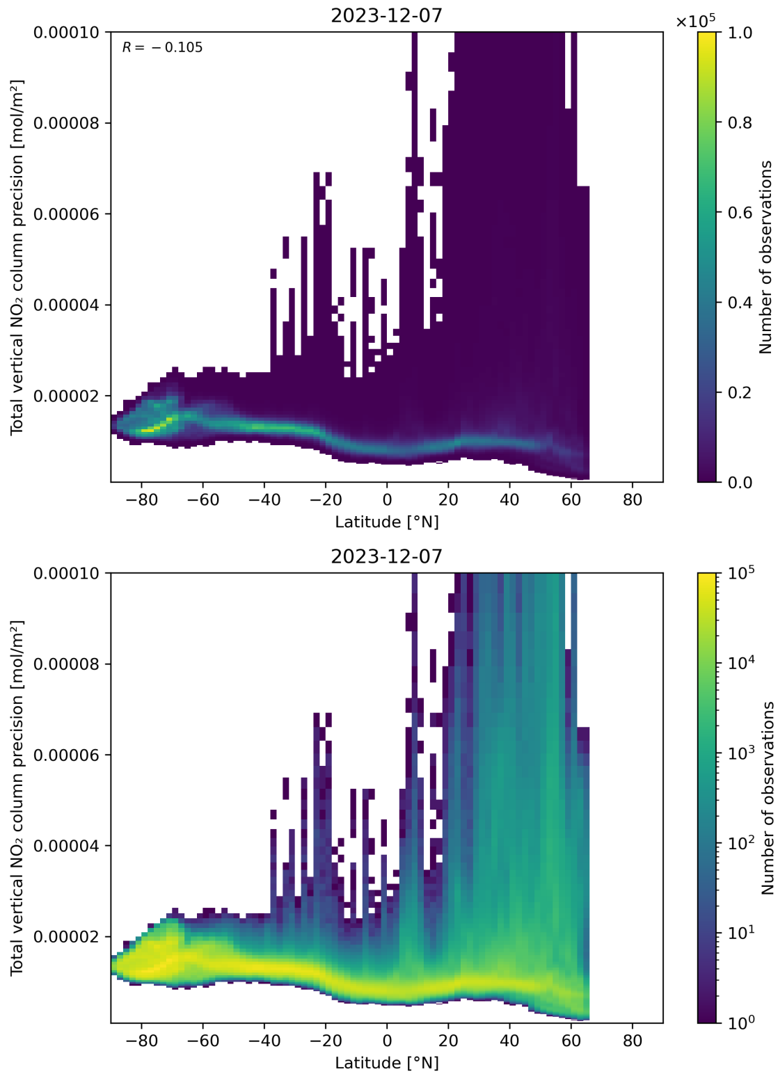
Figure 91: Scatter density plot of “Latitude” against “Total vertical NO 2 column precision” for 2023-12-06 to 2023-12-08.
