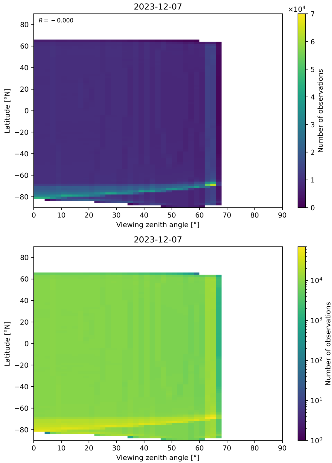
Figure 163: Scatter density plot of “Viewing zenith angle” against “Latitude” for 2023-12-06 to 2023-12-08.
