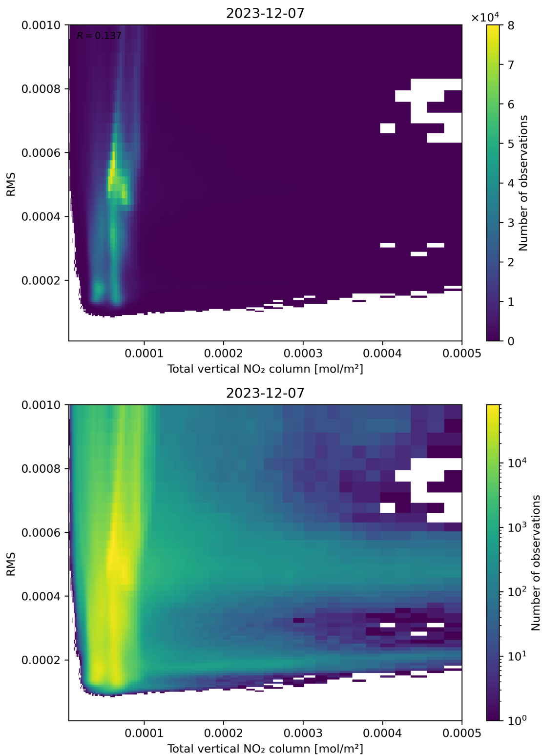
Figure 120: Scatter density plot of “Total vertical NO 2 column” against “RMS” for 2023-12-06 to 2023-12-08.
