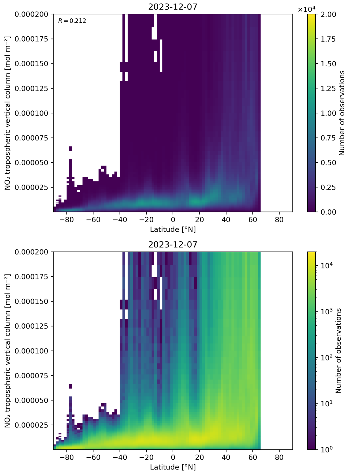
Figure 92: Scatter density plot of “Latitude” against “NO 2 tropospheric vertical column” for 2023-12-06 to 2023-12-08.
