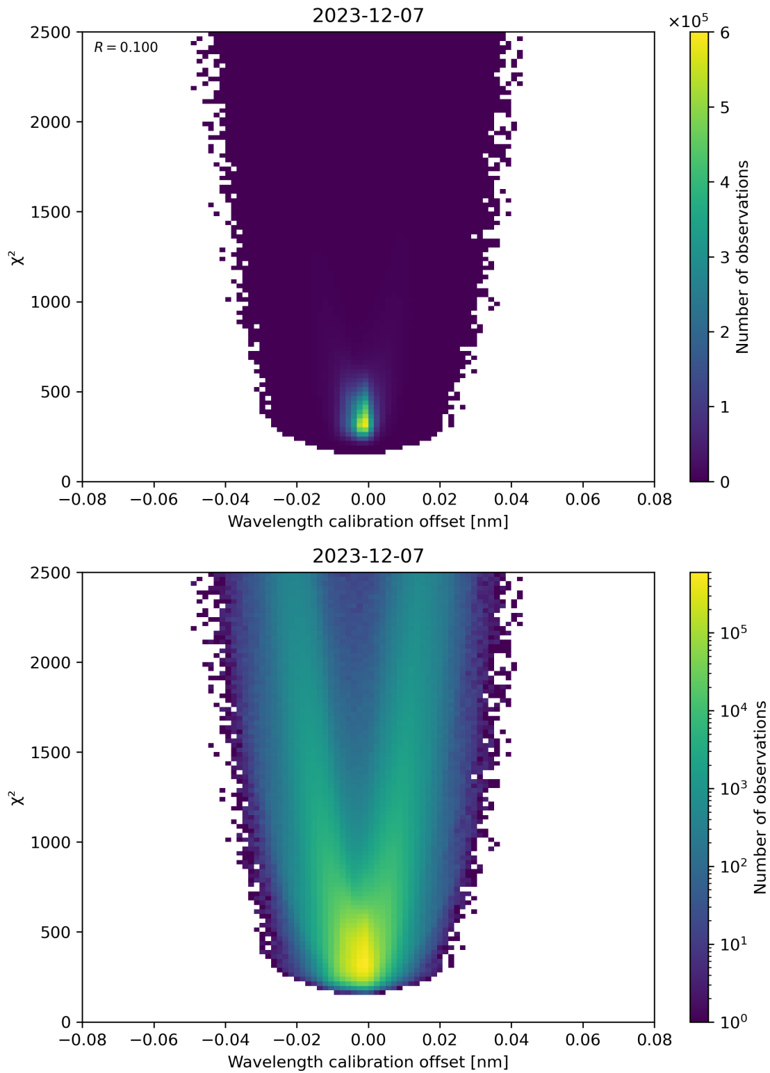
Figure 175: Scatter density plot of “Wavelength calibration offset” against “ \chi^2 ” for 2023-12-06 to 2023-12-08.
