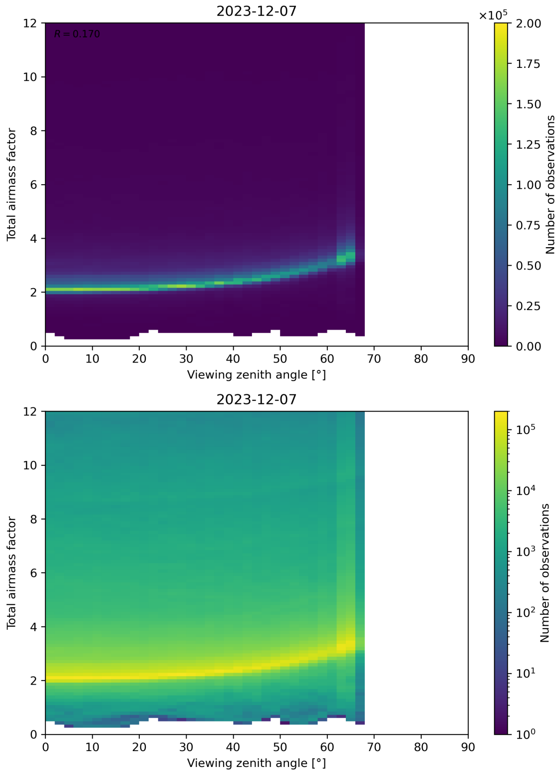
Figure 160: Scatter density plot of “Viewing zenith angle” against “Total airmass factor” for 2023-12-06 to 2023-12-08.
