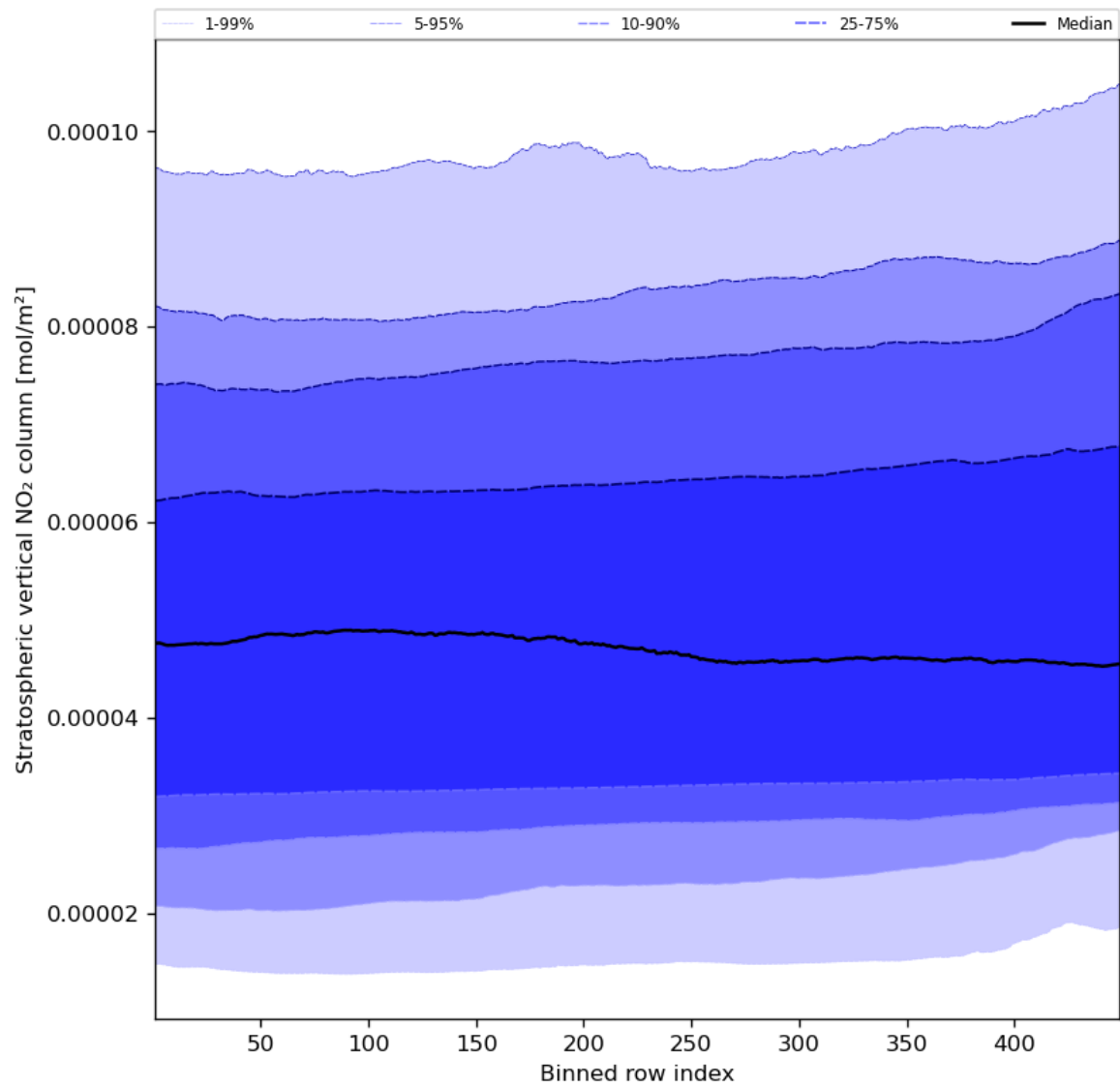
Figure 53: Along track statistics of “Stratospheric vertical NO 2 column” for 2023-12-06 to 2023-12-08
