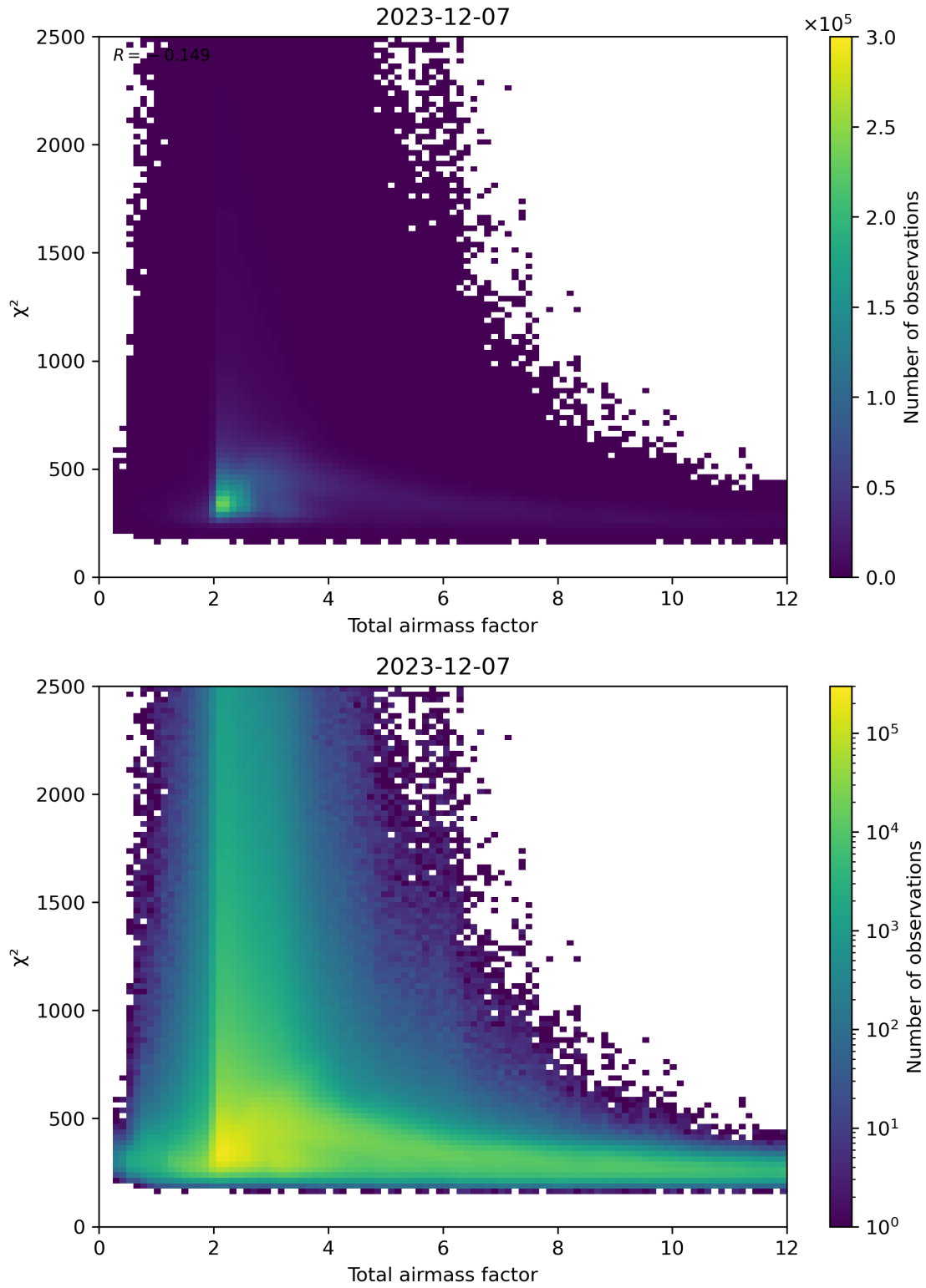
Figure 63: Scatter density plot of “Total airmass factor” against “ \chi^2 ” for 2023-12-06 to 2023-12-08.
