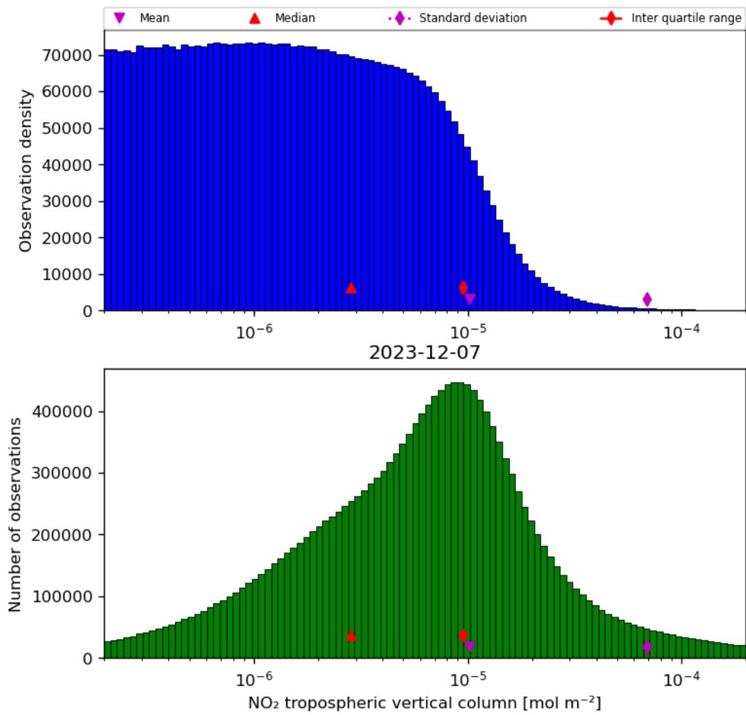
Figure 29: Histogram of “NO 2 tropospheric vertical column” for 2023-12-06 to 2023-12-08
