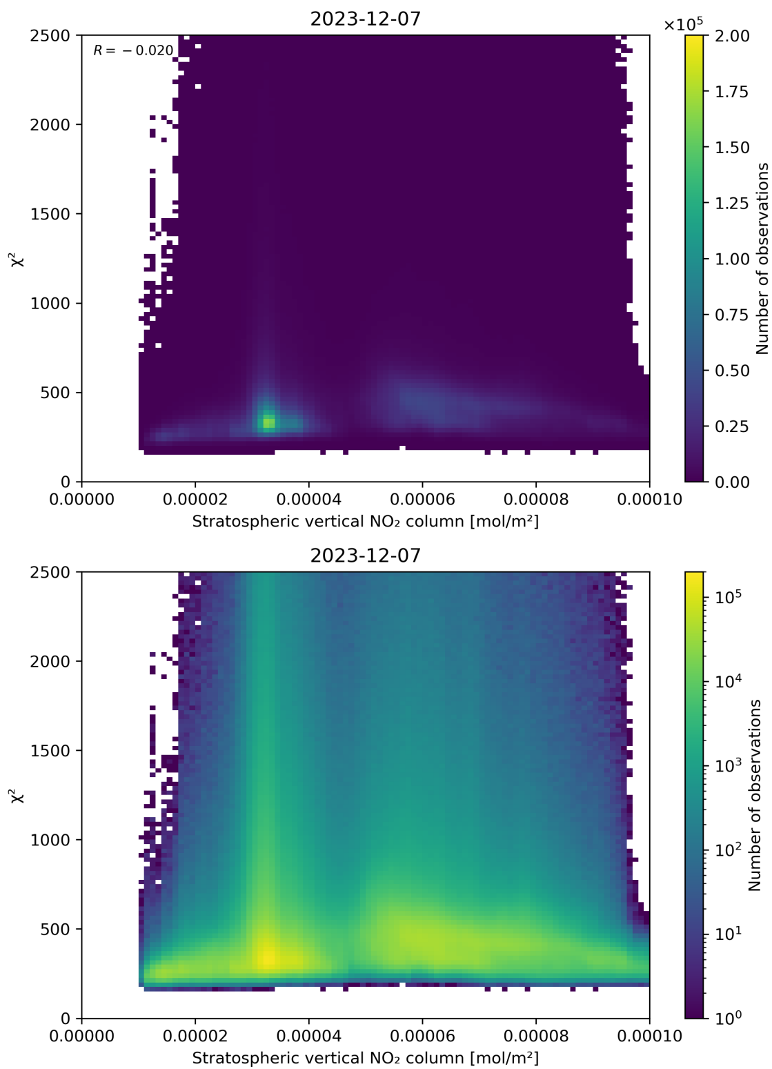
Figure 97: Scatter density plot of “Stratospheric vertical NO 2 column” against “ \chi^2 ” for 2023-12-06 to 2023-12-08.
