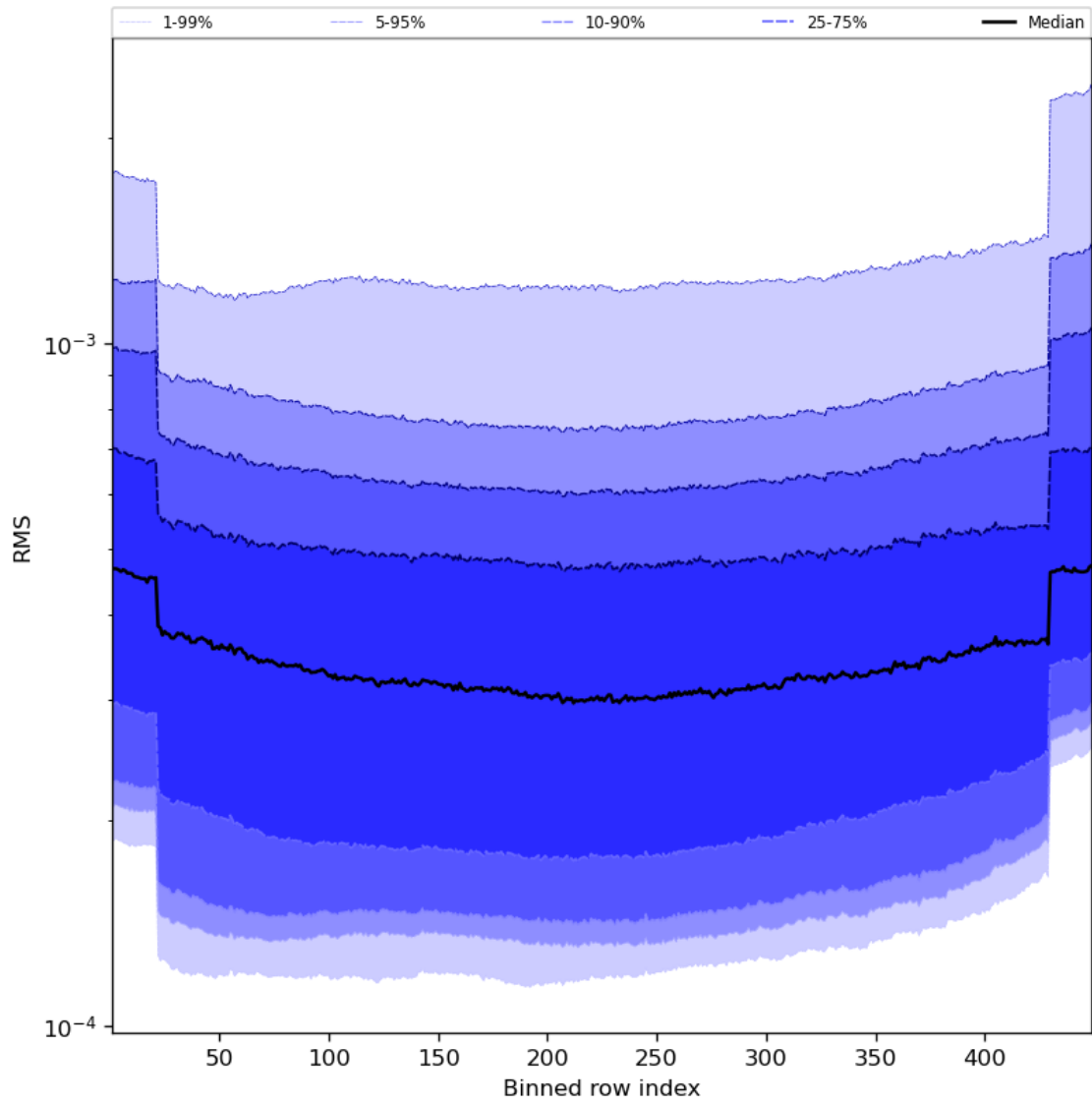
Figure 60: Along track statistics of “RMS” for 2023-12-06 to 2023-12-08
