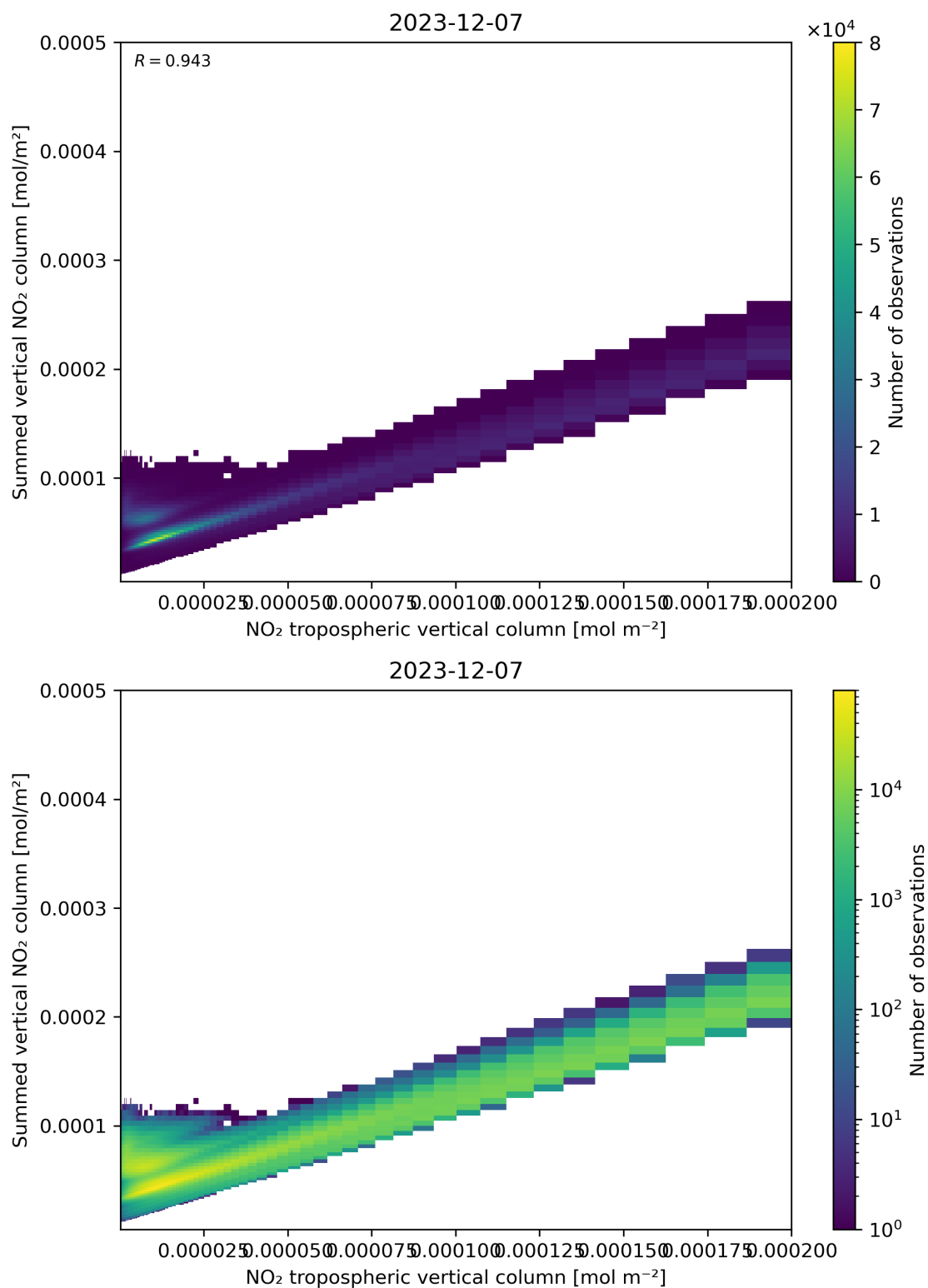
Figure 126: Scatter density plot of “NO 2 tropospheric vertical column” against “Summed vertical NO 2 column” for 2023-12-06 to 2023-12-08.
