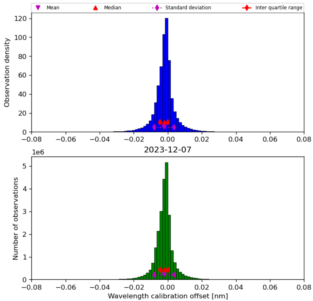
Figure 35: Histogram of “Wavelength calibration offset” for 2023-12-06 to 2023-12-08
