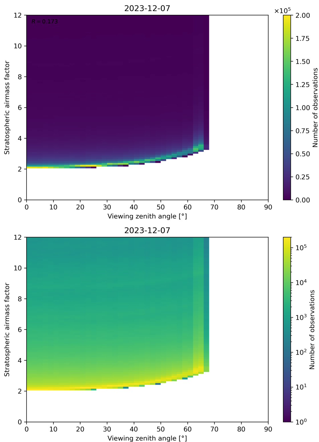
Figure 159: Scatter density plot of “Viewing zenith angle” against “Stratospheric airmass factor” for 2023-12-06 to 2023-12-08.
