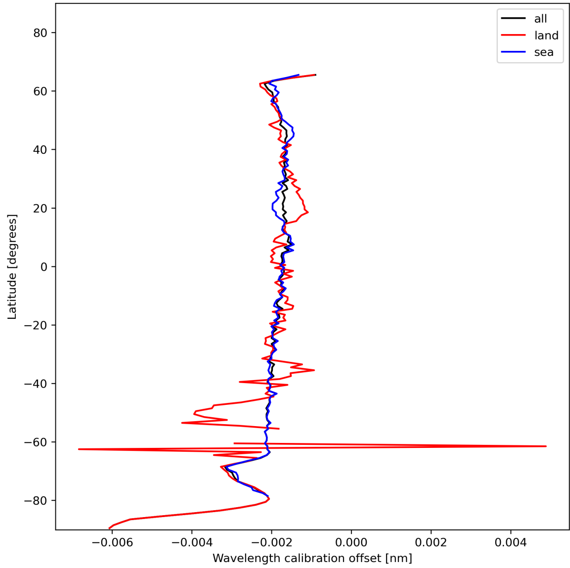
Figure 18: Zonal average of “Wavelength calibration offset” for 2023-12-06 to 2023-12-08.
