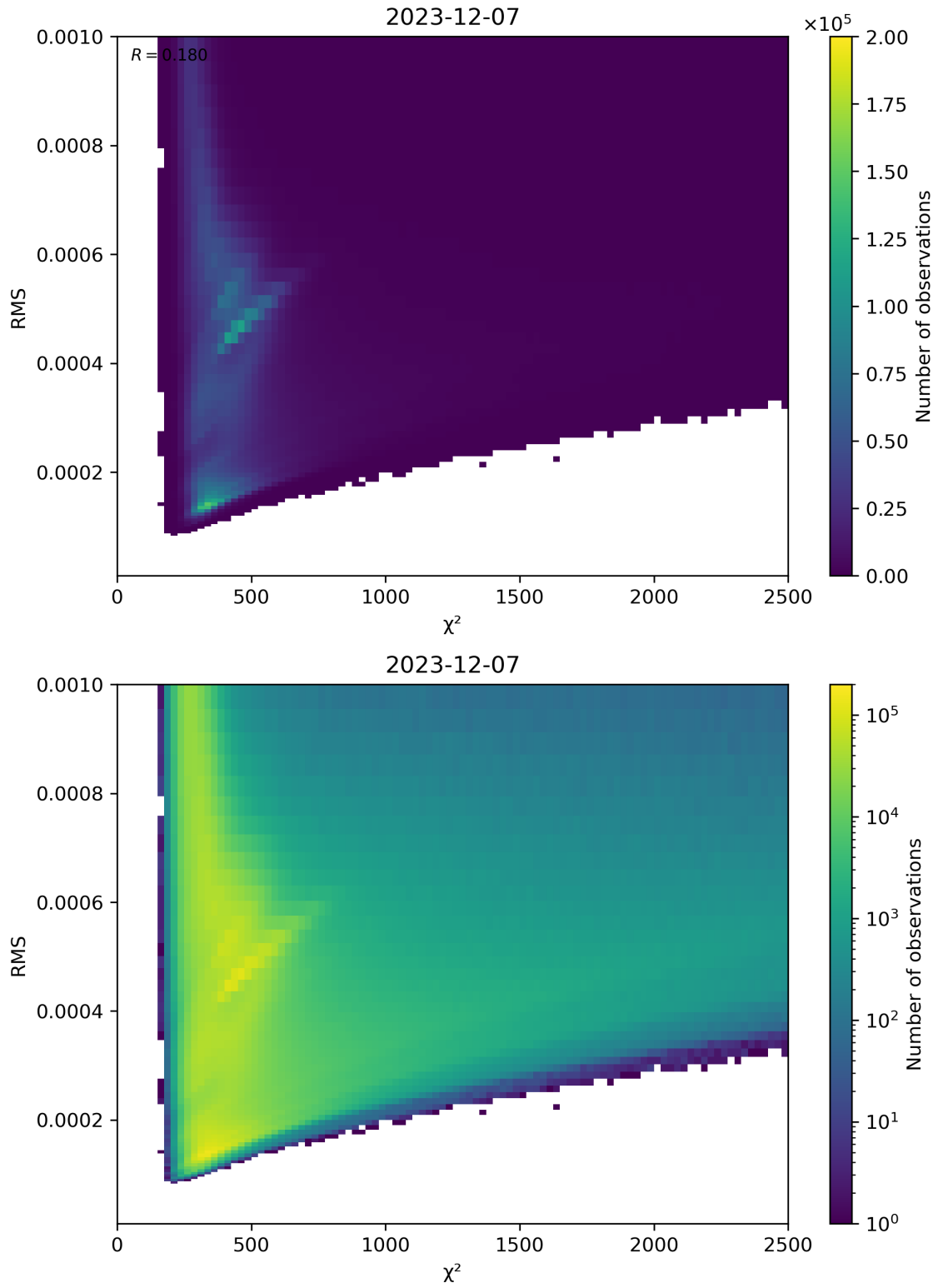
Figure 82: Scatter density plot of “ \chi^2 ” against “RMS” for 2023-12-06 to 2023-12-08.
