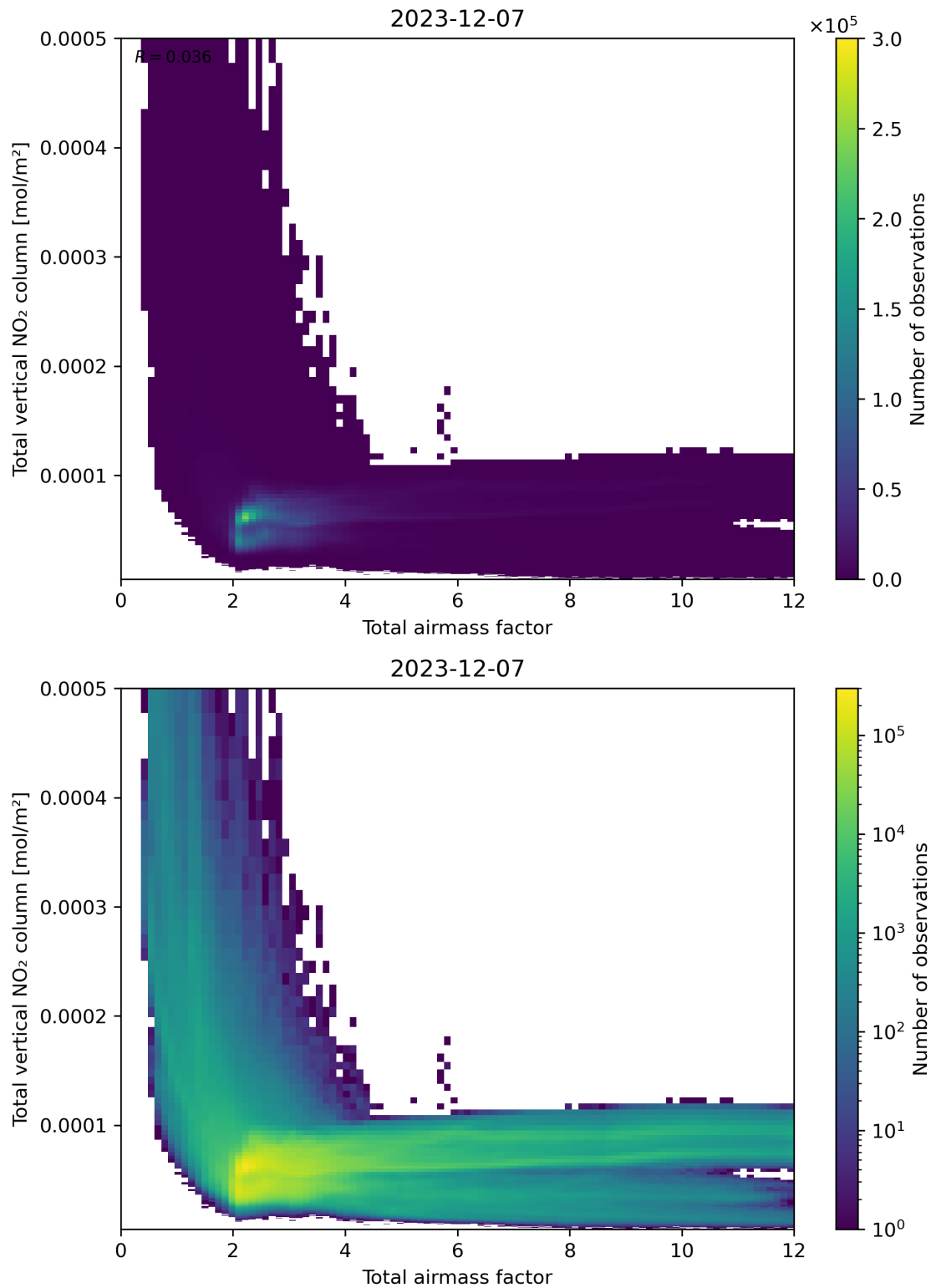
Figure 67: Scatter density plot of “Total airmass factor” against “Total vertical NO 2 column” for 2023-12-06 to 2023-12-08.
