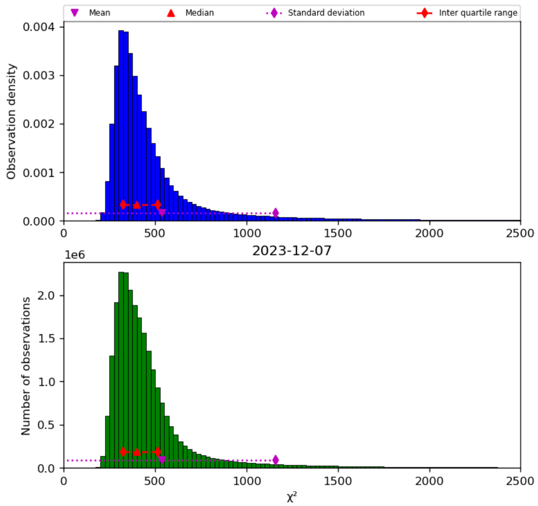
Figure 42: Histogram of “ \chi^2 ” for 2023-12-06 to 2023-12-08
