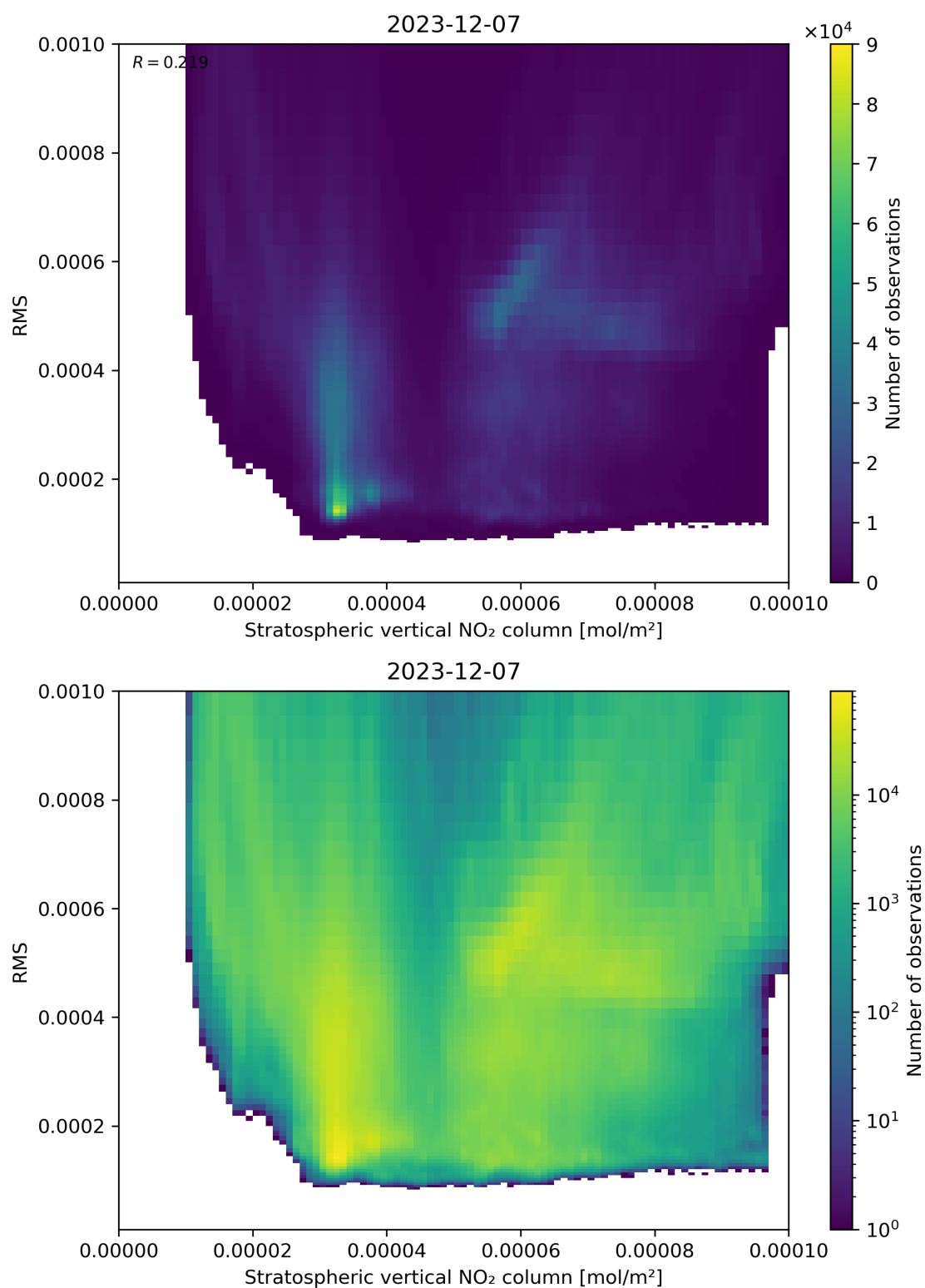
Figure 102: Scatter density plot of “Stratospheric vertical NO 2 column” against “RMS” for 2023-12-06 to 2023-12-08.
