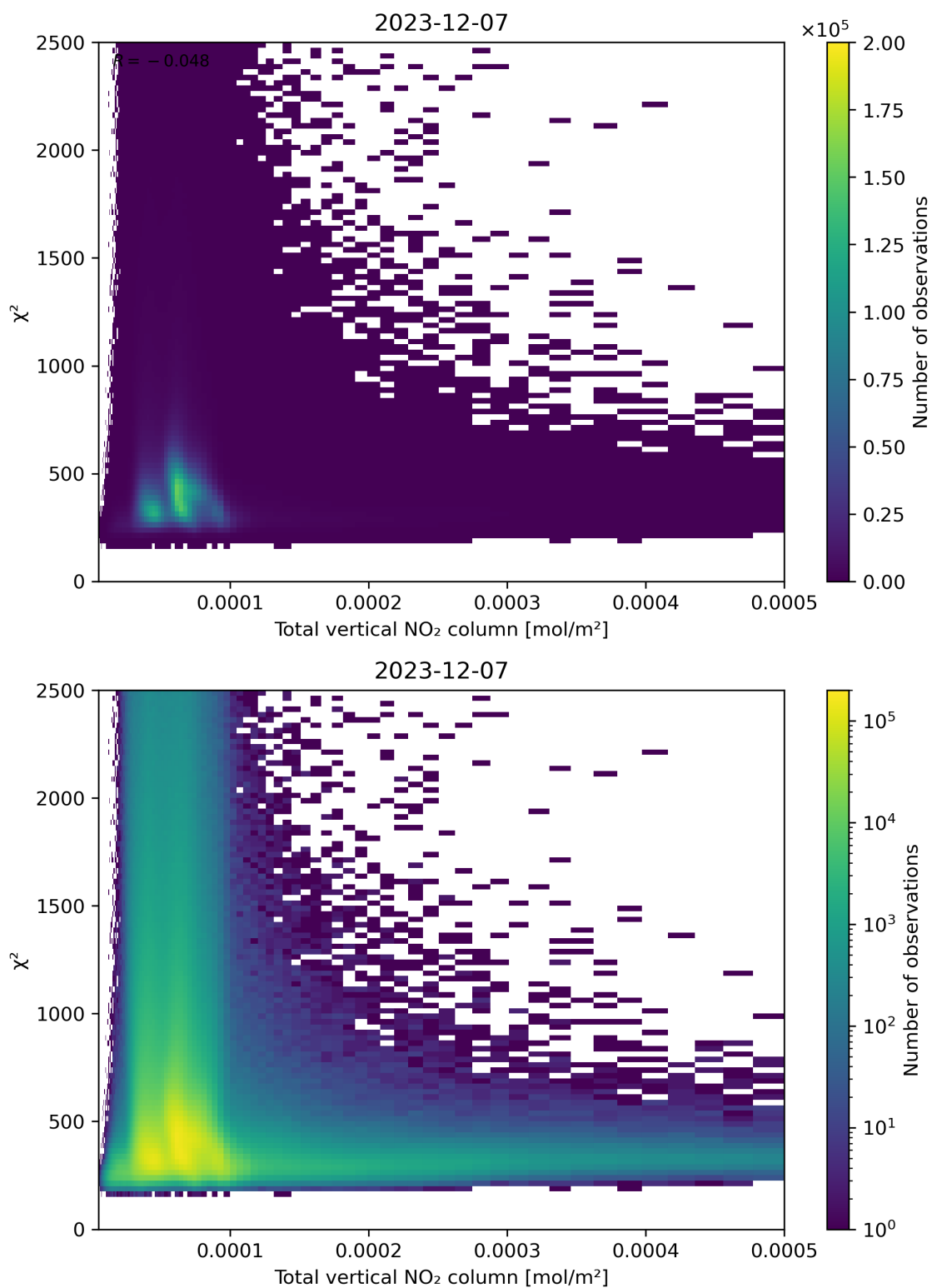
Figure 111: Scatter density plot of “Total vertical NO 2 column” against “ \chi^2 ” for 2023-12-06 to 2023-12-08.
