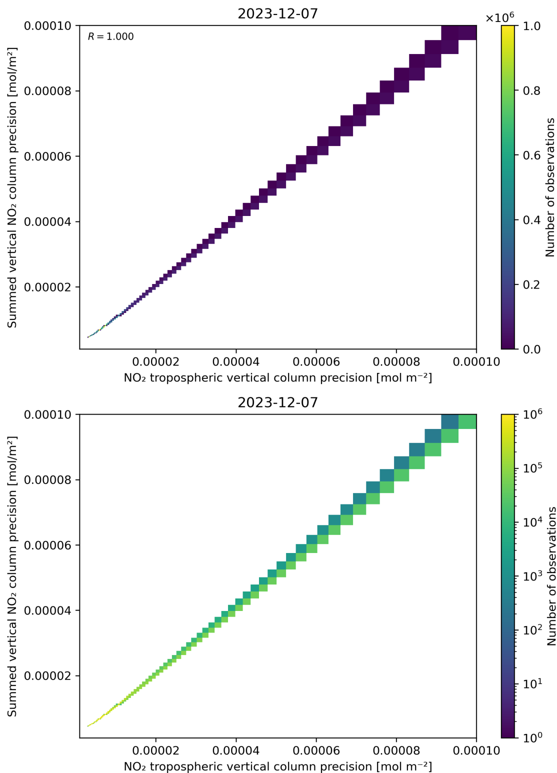
Figure 137: Scatter density plot of “NO 2 tropospheric vertical column precision” against “Summed vertical NO 2 column precision” for 2023-12-06 to 2023-12-08.
