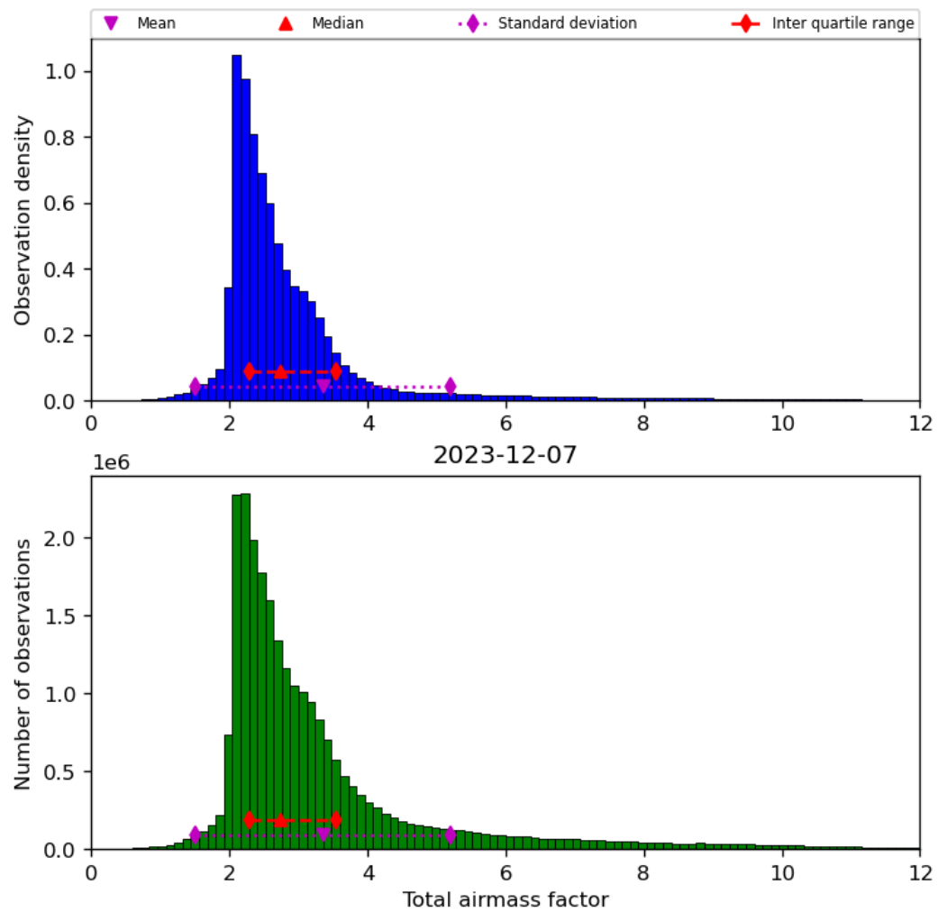
Figure 32: Histogram of “Total airmass factor” for 2023-12-06 to 2023-12-08
