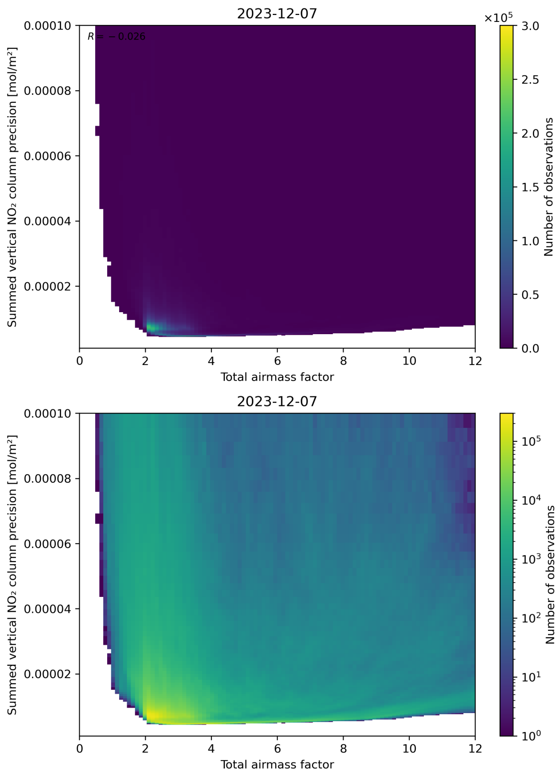
Figure 66: Scatter density plot of “Total airmass factor” against “Summed vertical NO 2 column precision” for 2023-12-06 to 2023-12-08.
