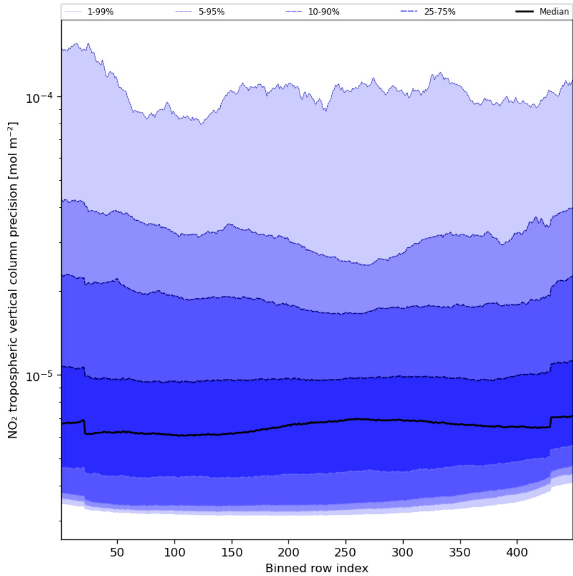
Figure 47: Along track statistics of “NO 2 tropospheric vertical column precision” for 2023-12-06 to 2023-12-08
