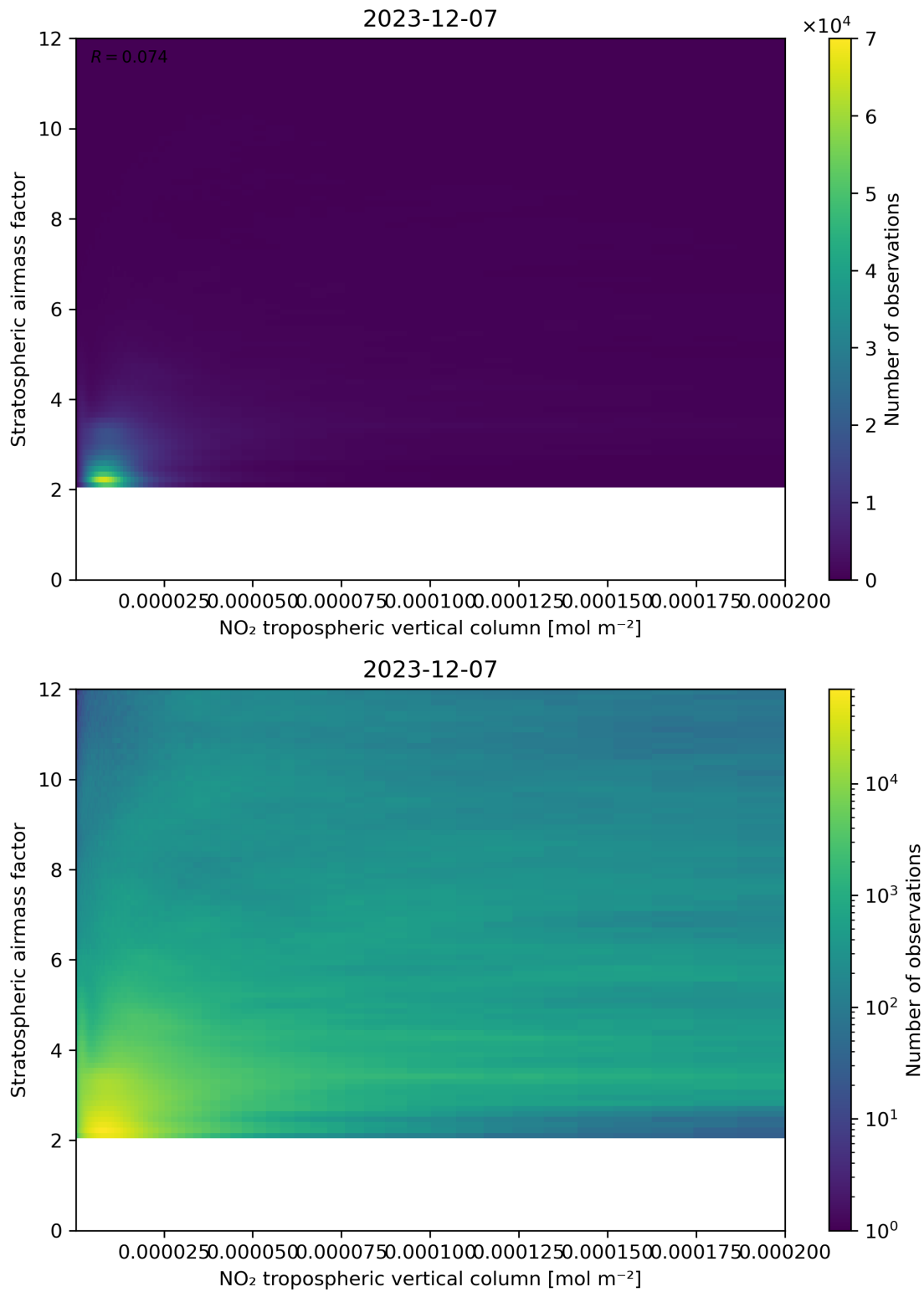
Figure 121: Scatter density plot of “NO 2 tropospheric vertical column” against “Stratospheric airmass factor” for 2023-12-06 to 2023-12-08.
