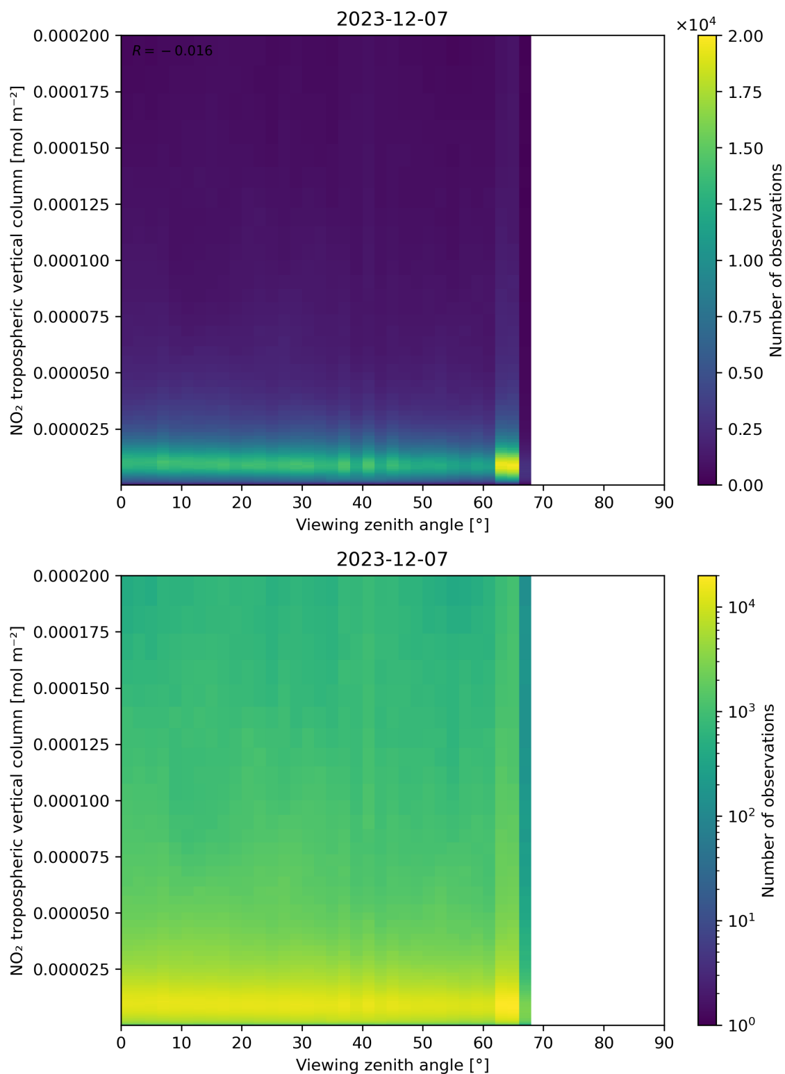
Figure 169: Scatter density plot of “Viewing zenith angle” against “NO 2 tropospheric vertical column” for 2023-12-06 to 2023-12-08.
