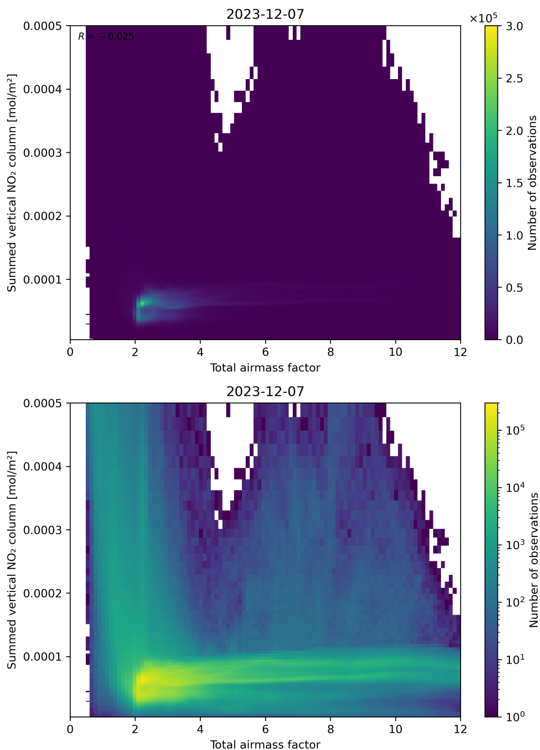
Figure 65: Scatter density plot of “Total airmass factor” against “Summed vertical NO 2 column” for 2023-12-06 to 2023-12-08.
