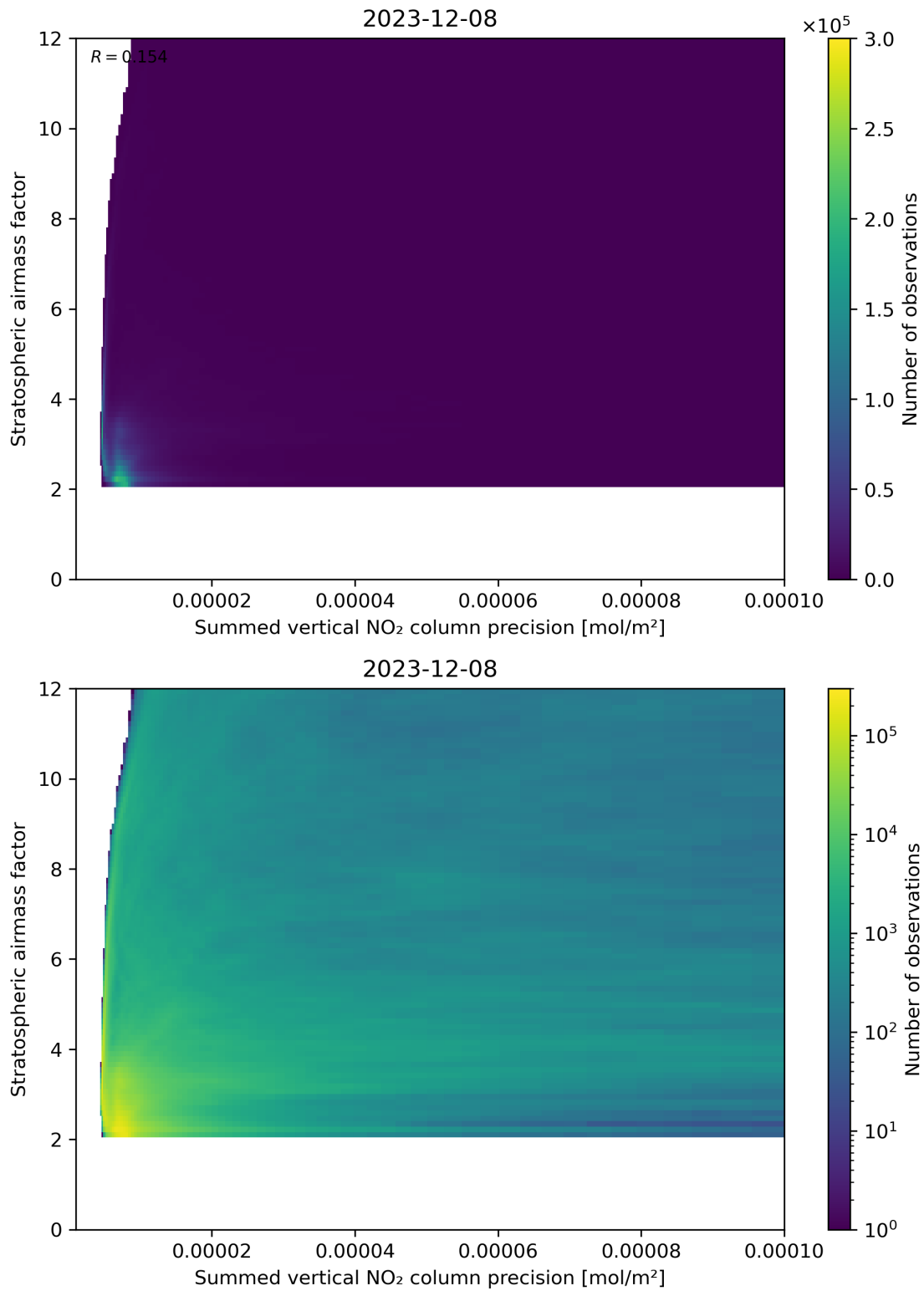
Figure 106: Scatter density plot of “Summed vertical NO 2 column precision” against “Stratospheric airmass factor” for 2023-12-07 to 2023-12-09.
