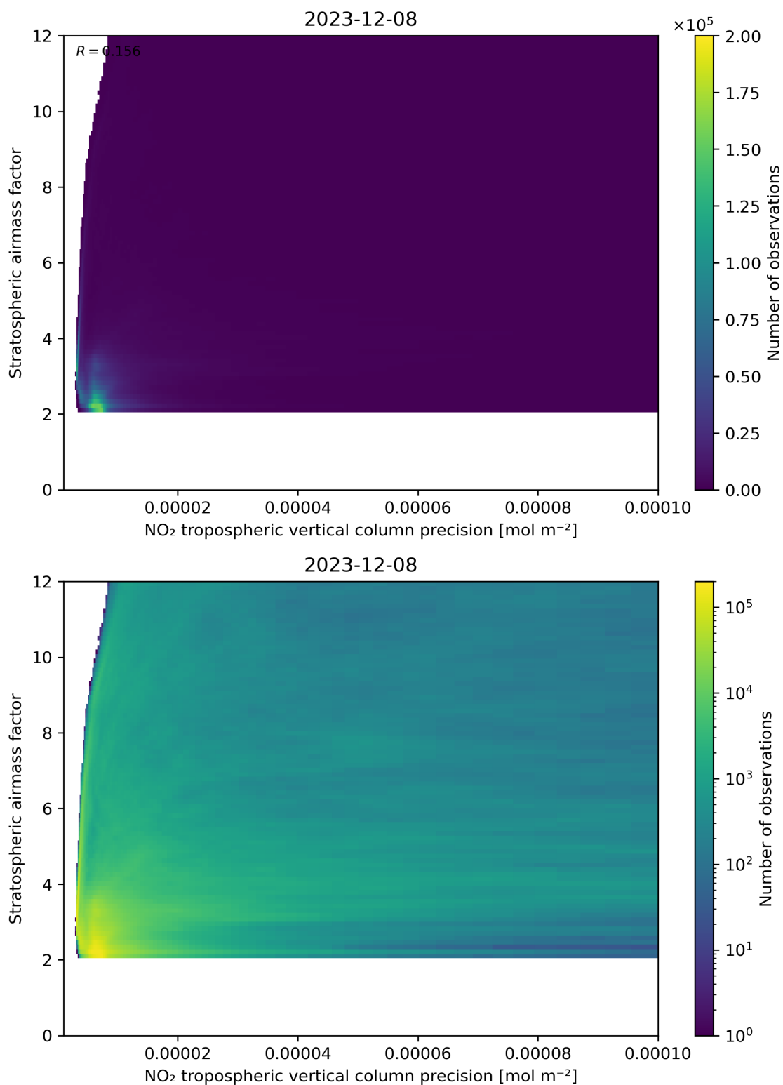
Figure 131: Scatter density plot of “NO 2 tropospheric vertical column precision” against “Stratospheric airmass factor” for 2023-12-07 to 2023-12-09.
