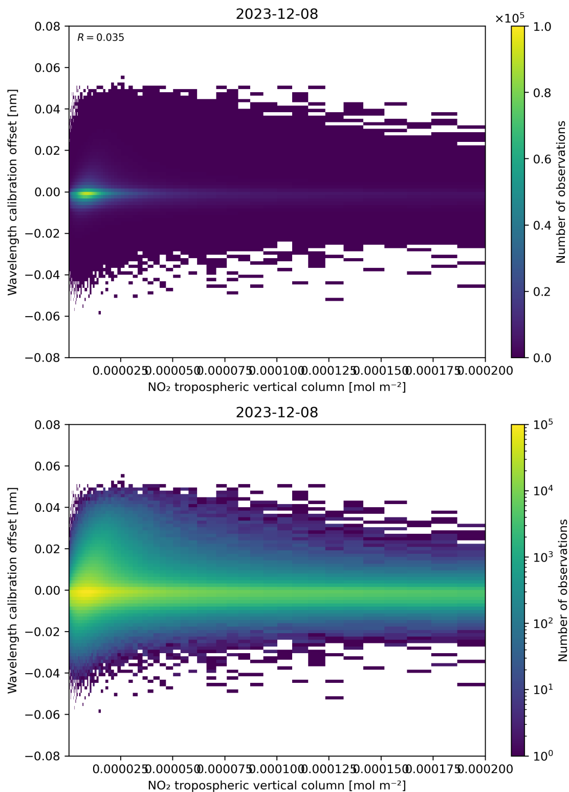
Figure 143: Scatter density plot of “NO 2 tropospheric vertical column” against “Wavelength calibration offset” for 2023-12-07 to 2023-12-09.
