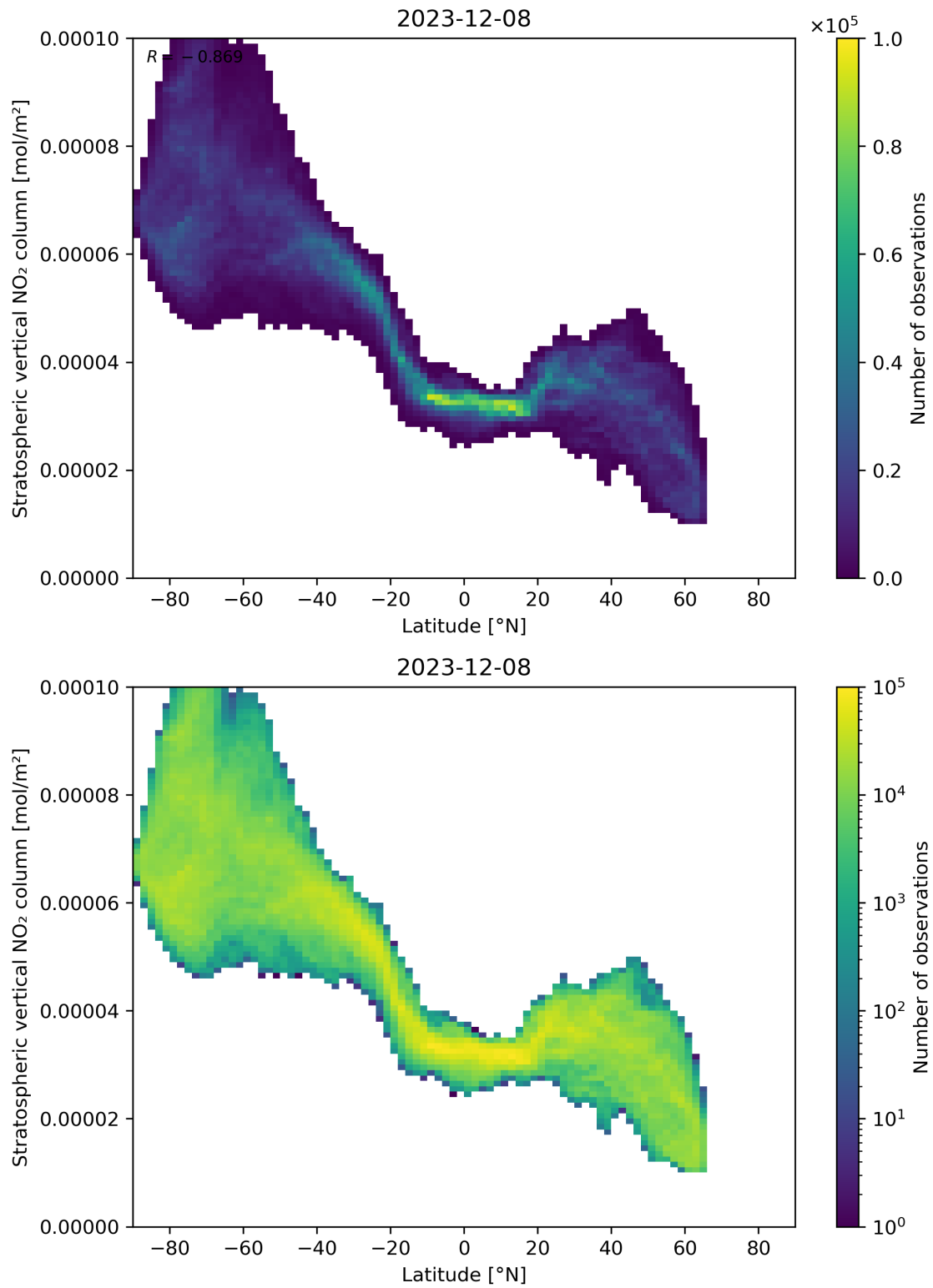
Figure 87: Scatter density plot of “Latitude” against “Stratospheric vertical NO 2 column” for 2023-12-07 to 2023-12-09.
