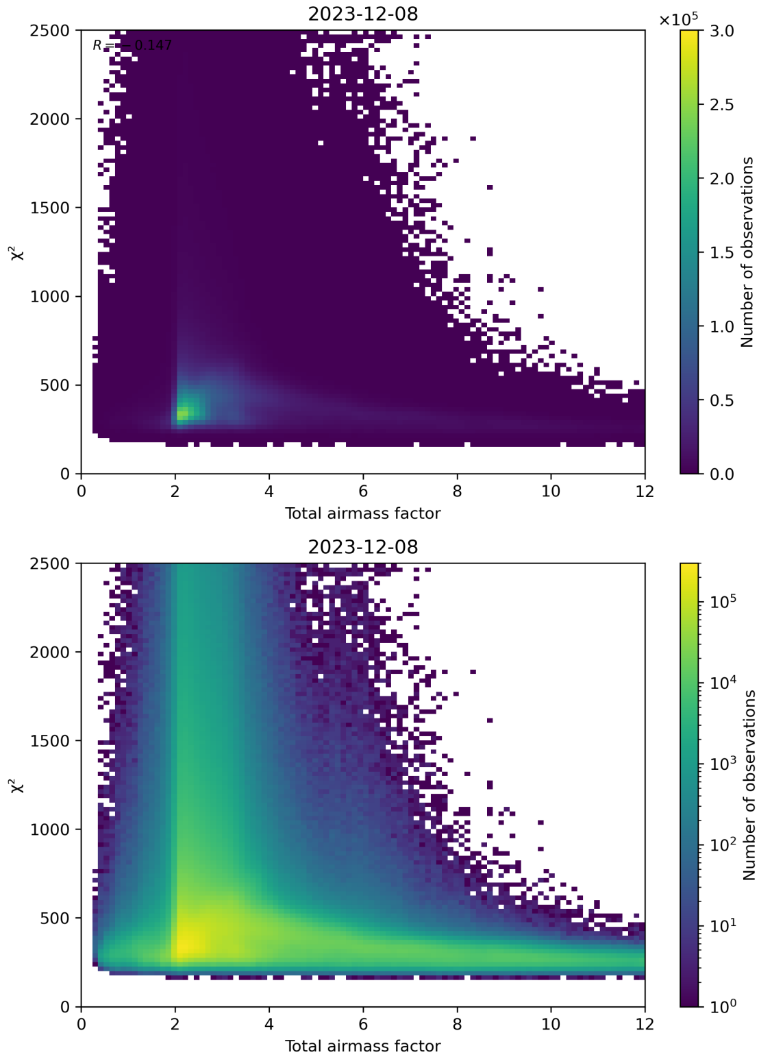
Figure 63: Scatter density plot of “Total airmass factor” against “ \chi^2 ” for 2023-12-07 to 2023-12-09.
