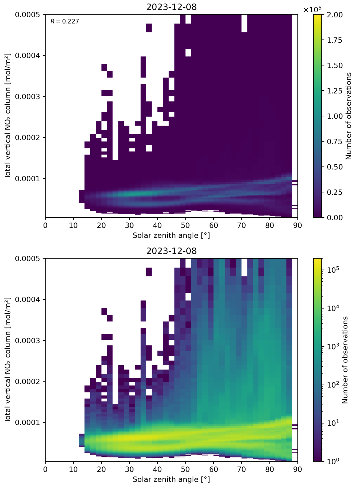
Figure 153: Scatter density plot of “Solar zenith angle” against “Total vertical NO 2 column” for 2023-12-07 to 2023-12-09.
