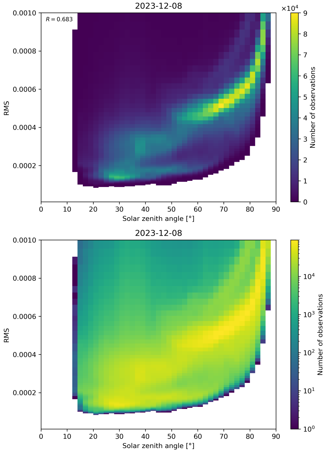
Figure 157: Scatter density plot of “Solar zenith angle” against “RMS” for 2023-12-07 to 2023-12-09.
