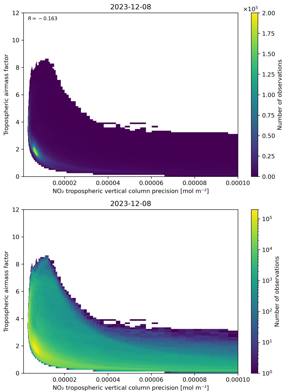
Figure 133: Scatter density plot of “NO 2 tropospheric vertical column precision” against “Tropospheric air mass factor” for 2023-12-07 to 2023-12-09.
