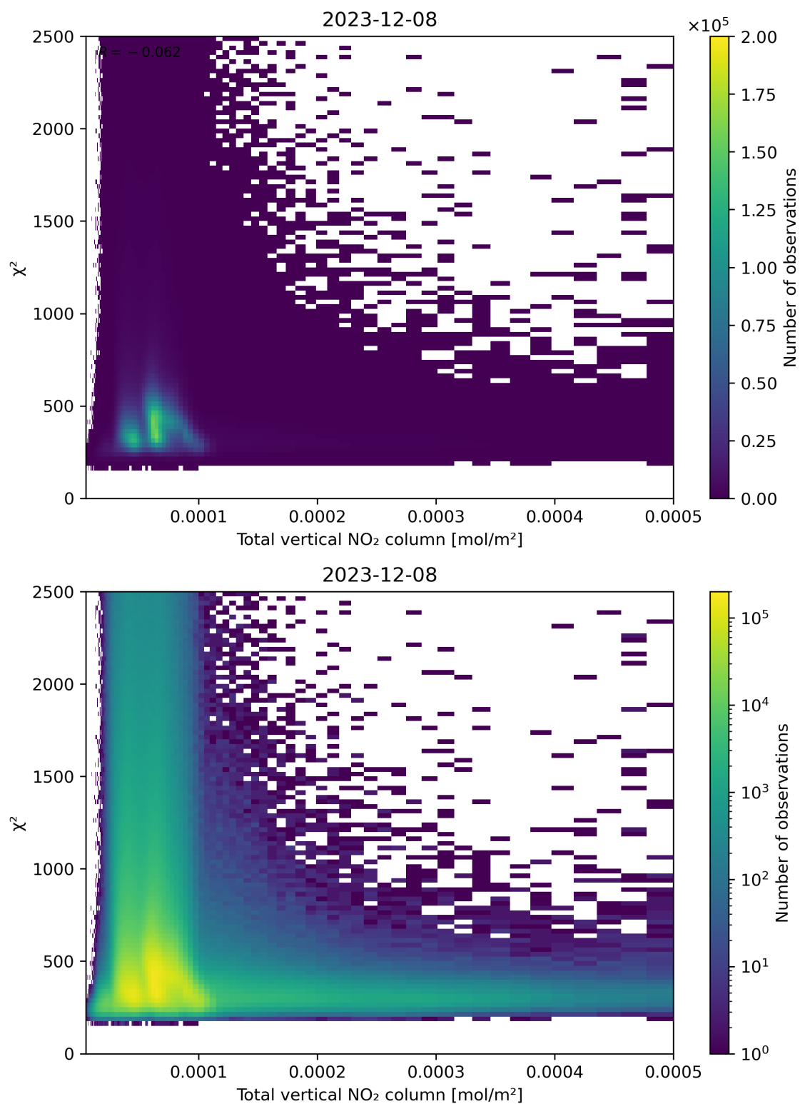
Figure 111: Scatter density plot of “Total vertical NO 2 column” against “ \chi^2 ” for 2023-12-07 to 2023-12-09.
