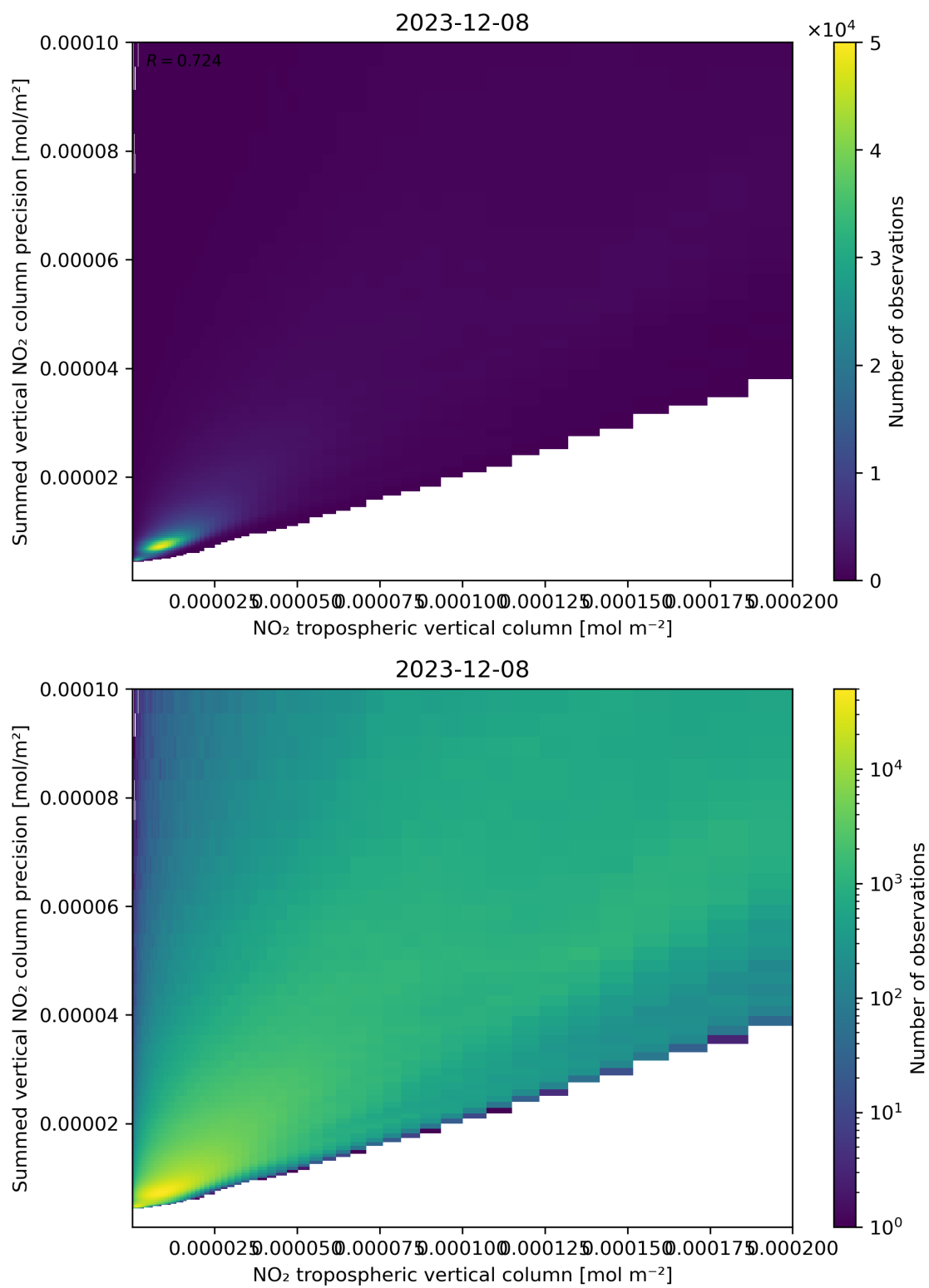
Figure 127: Scatter density plot of “NO 2 tropospheric vertical column” against “Summed vertical NO 2 column precision” for 2023-12-07 to 2023-12-09.
