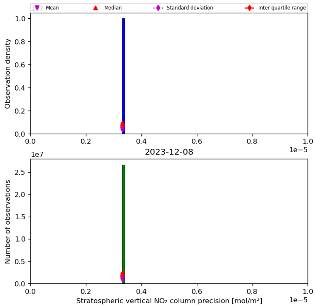
Figure 37: Histogram of “Stratospheric vertical NO 2 column precision” for 2023-12-07 to 2023-12-09
