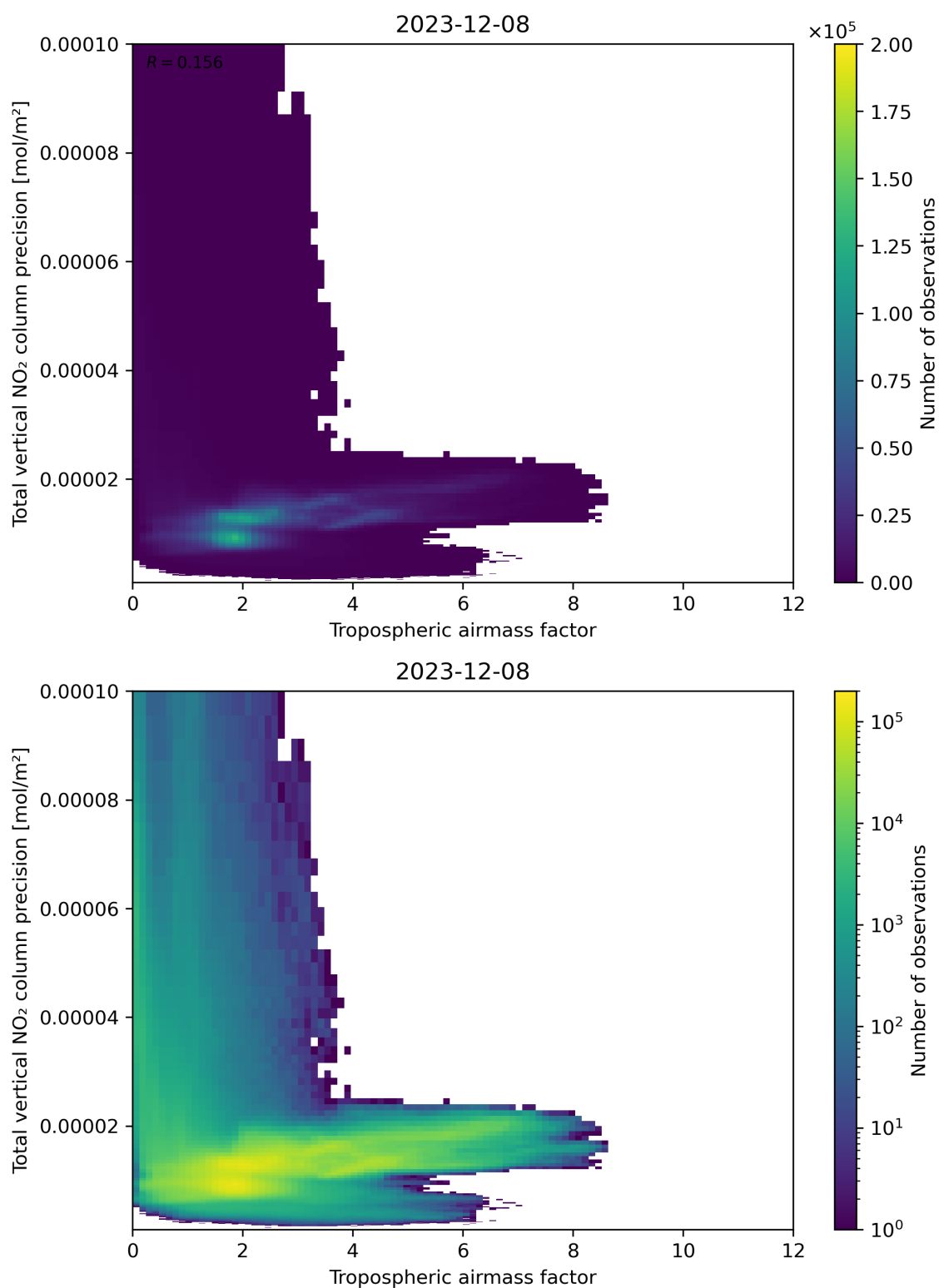
Figure 78: Scatter density plot of “Tropospheric airmass factor” against “Total vertical NO 2 column precision” for 2023-12-07 to 2023-12-09.
