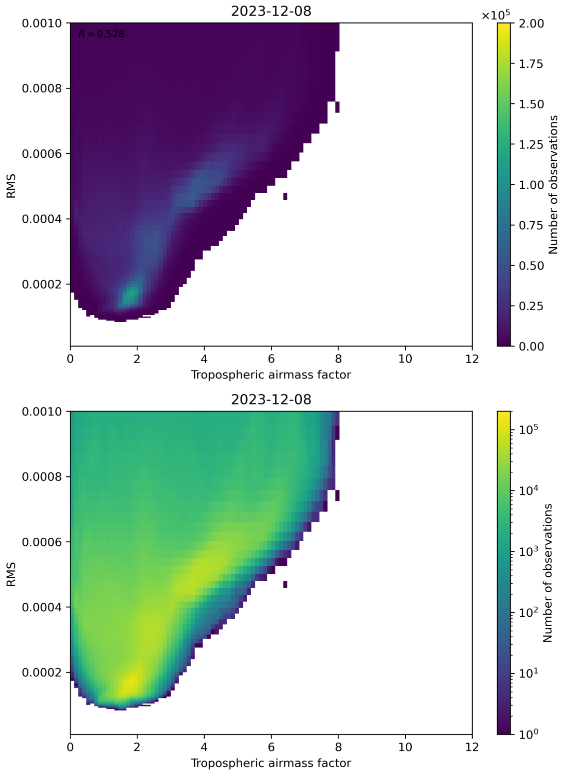
Figure 79: Scatter density plot of “Tropospheric airmass factor” against “RMS” for 2023-12-07 to 2023-12-09.
