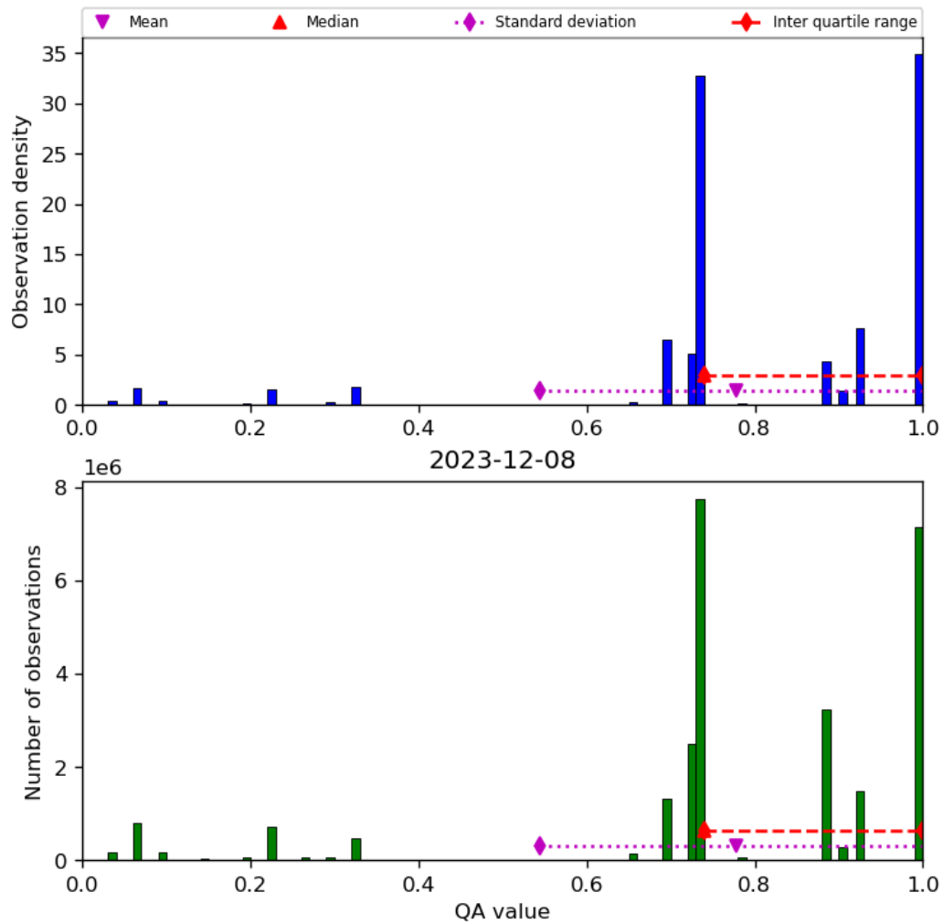
Figure 28: Histogram of “QA value” for 2023-12-07 to 2023-12-09
