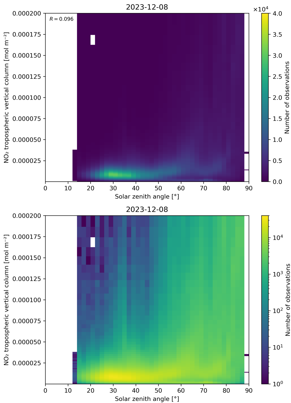
Figure 155: Scatter density plot of “Solar zenith angle” against “NO 2 tropospheric vertical column” for 2023-12-07 to 2023-12-09.
