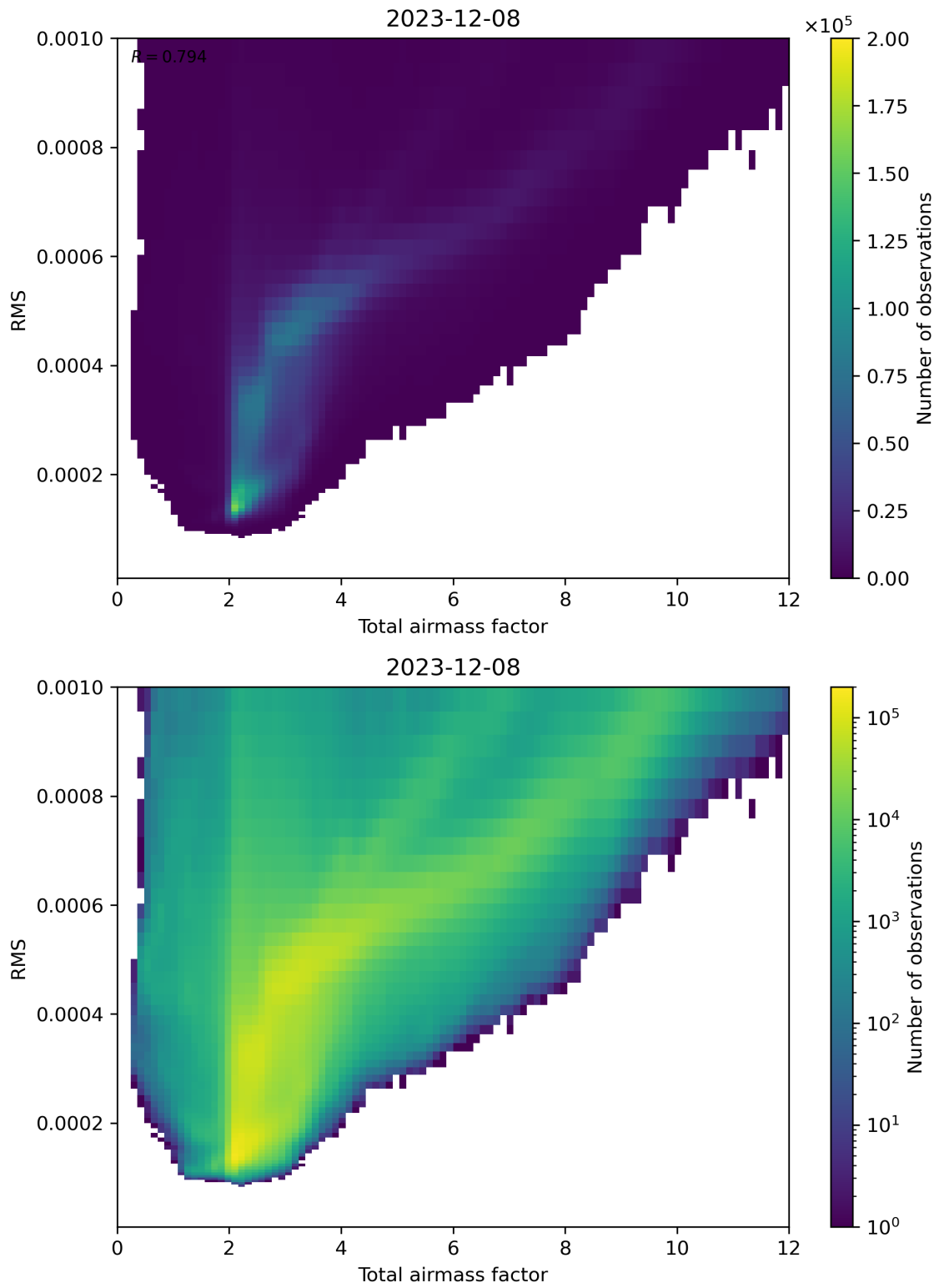
Figure 69: Scatter density plot of “Total airmass factor” against “RMS” for 2023-12-07 to 2023-12-09.
