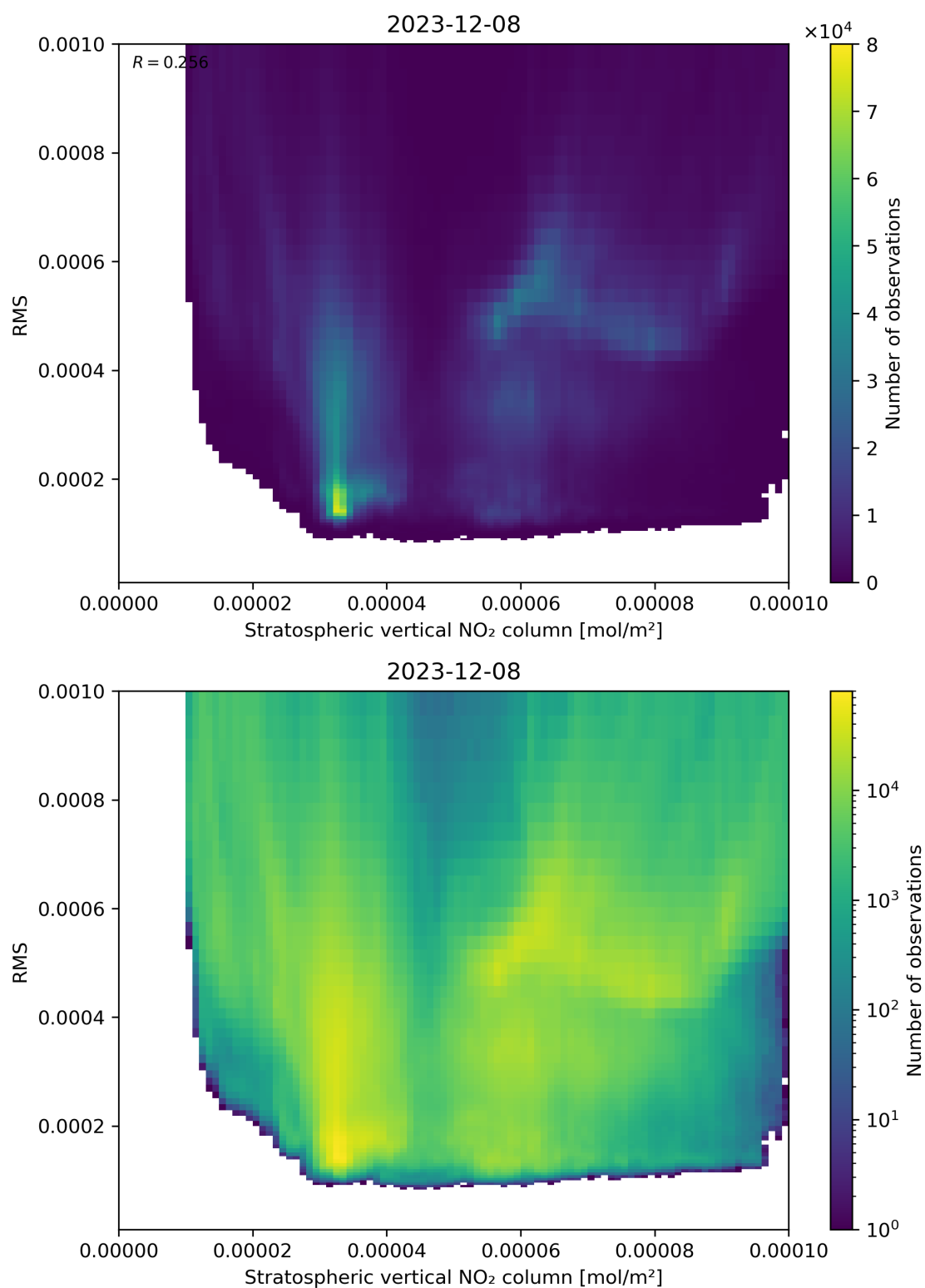
Figure 102: Scatter density plot of “Stratospheric vertical NO 2 column” against “RMS” for 2023-12-07 to 2023-12-09.
