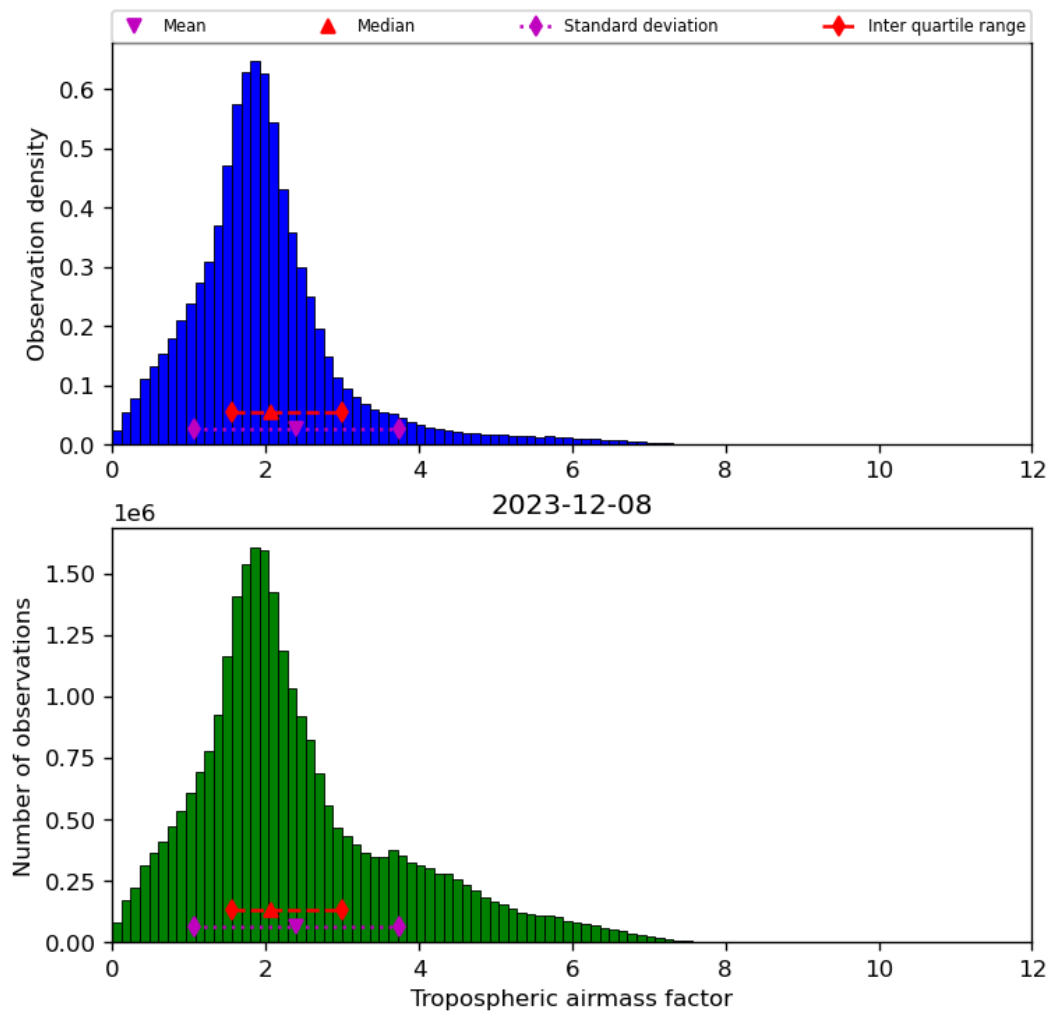
Figure 31: Histogram of “Tropospheric airmass factor” for 2023-12-07 to 2023-12-09
