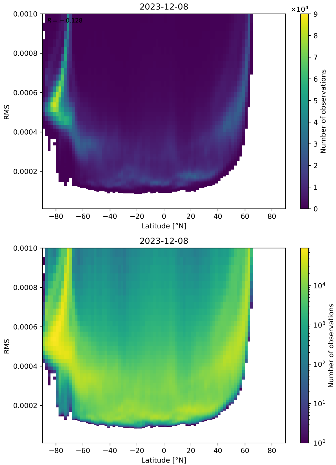
Figure 94: Scatter density plot of “Latitude” against “RMS” for 2023-12-07 to 2023-12-09.
