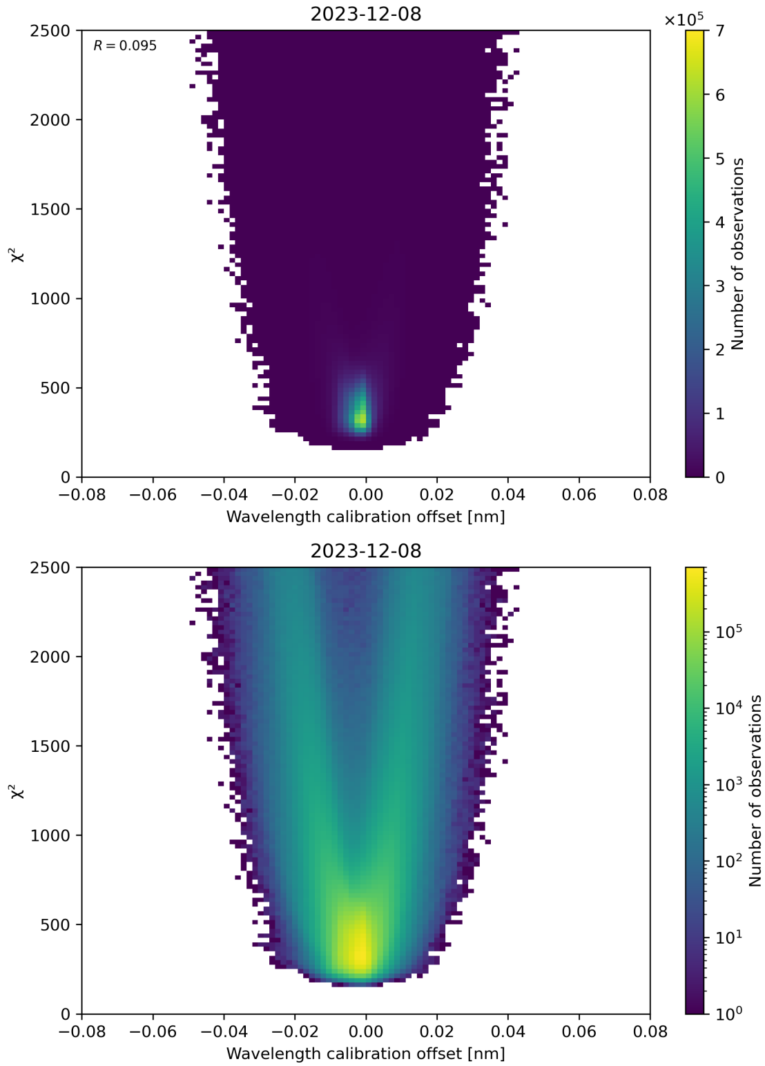
Figure 175: Scatter density plot of “Wavelength calibration offset” against “ \chi^2 ” for 2023-12-07 to 2023-12-09.
