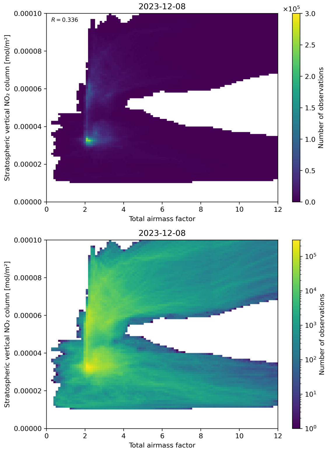
Figure 64: Scatter density plot of “Total airmass factor” against “Stratospheric vertical \text{NO}_2 column” for 2023-12-07 to 2023-12-09.
