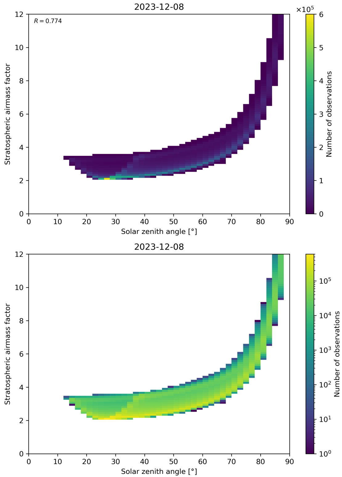
Figure 145: Scatter density plot of “Solar zenith angle” against “Stratospheric airmass factor” for 2023-12-07 to 2023-12-09.
