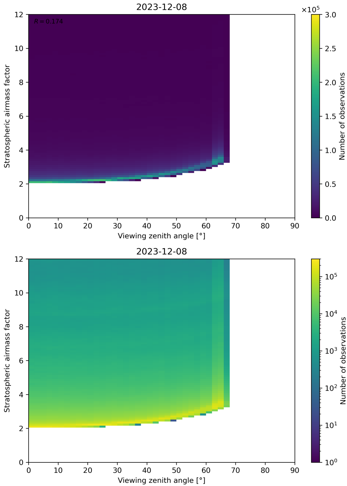
Figure 159: Scatter density plot of “Viewing zenith angle” against “Stratospheric airmass factor” for 2023-12-07 to 2023-12-09.
