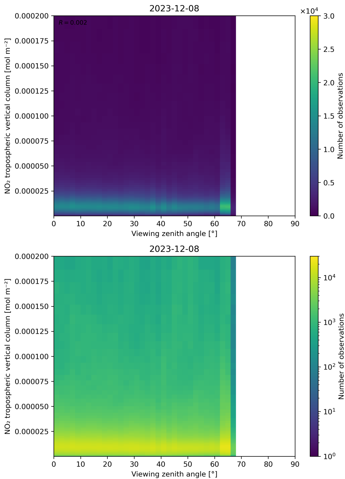
Figure 169: Scatter density plot of “Viewing zenith angle” against “NO 2 tropospheric vertical column” for 2023-12-07 to 2023-12-09.
