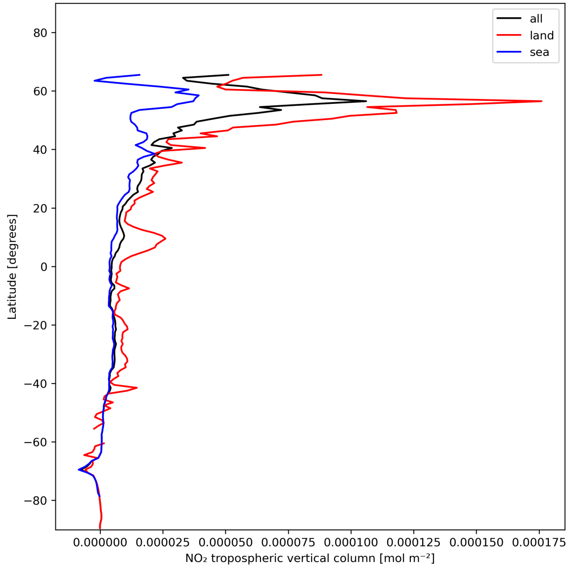
Figure 12: Zonal average of “NO 2 tropospheric vertical column” for 2023-12-07 to 2023-12-09.
