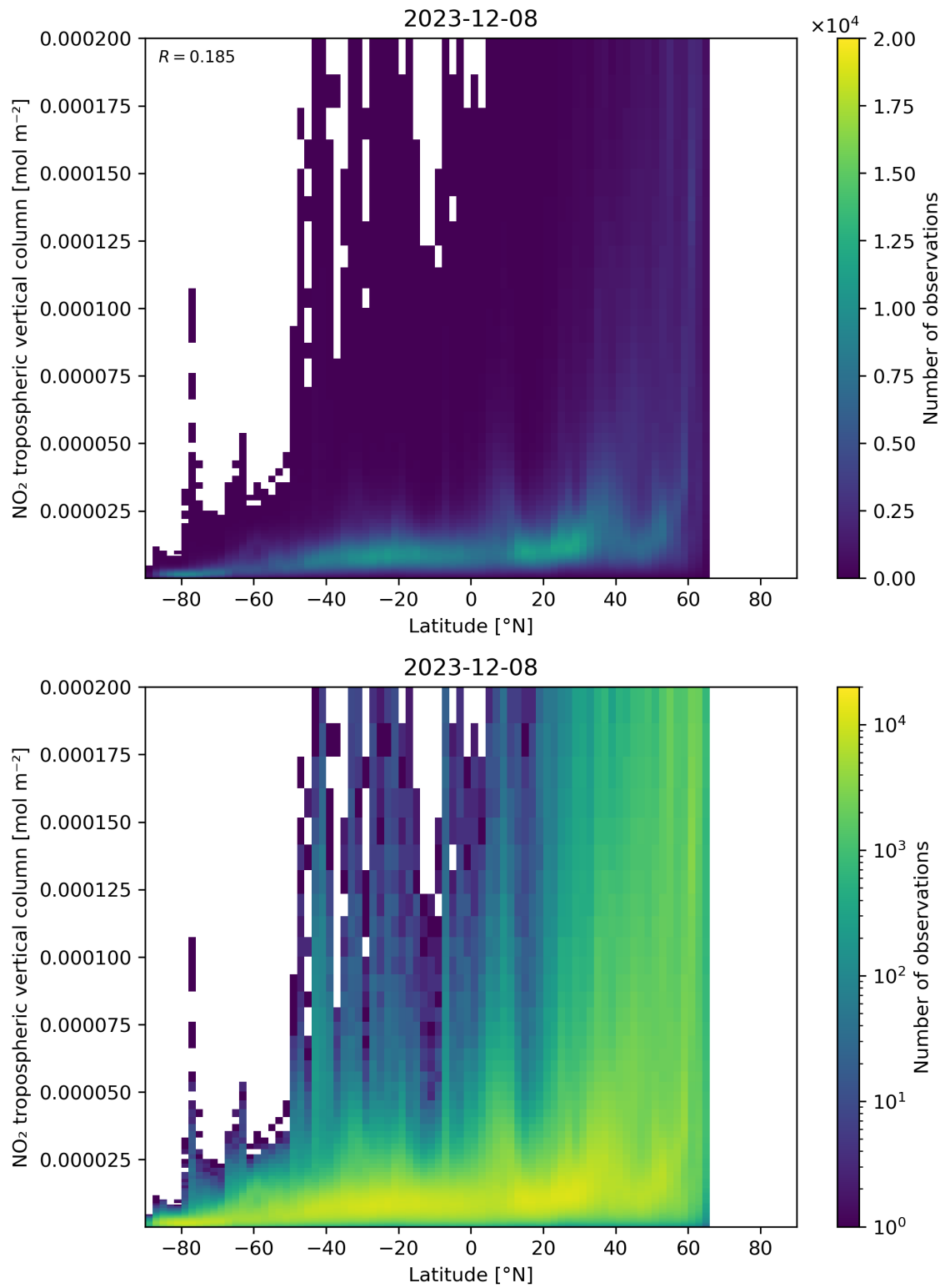
Figure 92: Scatter density plot of “Latitude” against “NO 2 tropospheric vertical column” for 2023-12-07 to 2023-12-09.
