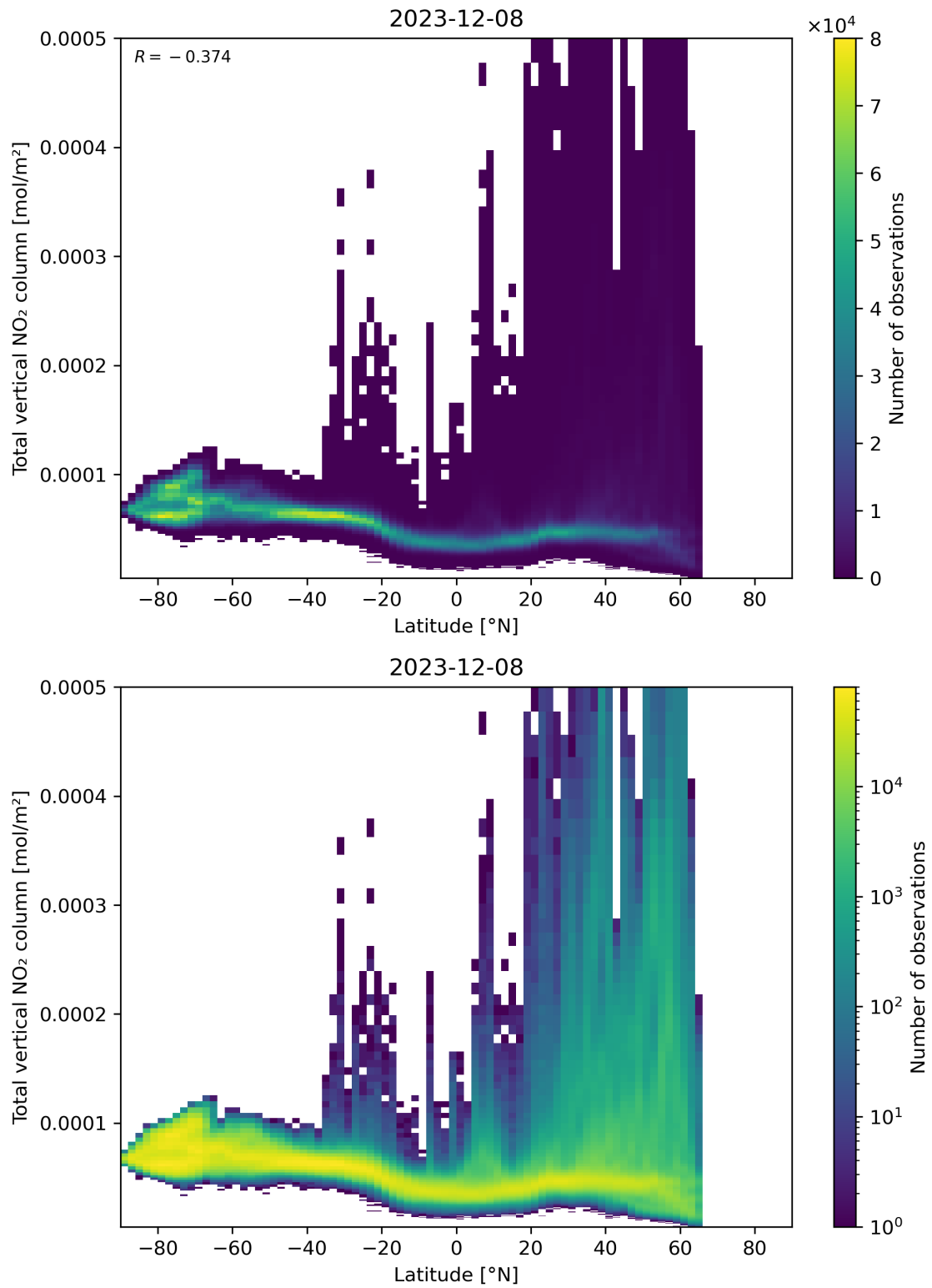
Figure 90: Scatter density plot of “Latitude” against “Total vertical NO 2 column” for 2023-12-07 to 2023-12-09.
