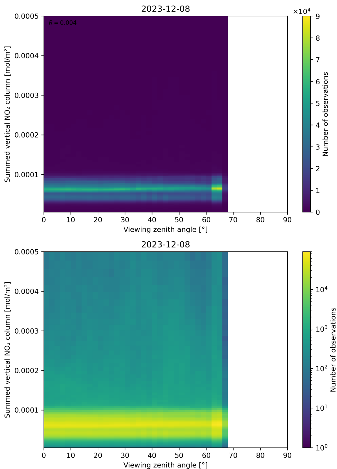
Figure 165: Scatter density plot of “Viewing zenith angle” against “Summed vertical NO 2 column” for 2023-12-07 to 2023-12-09.
