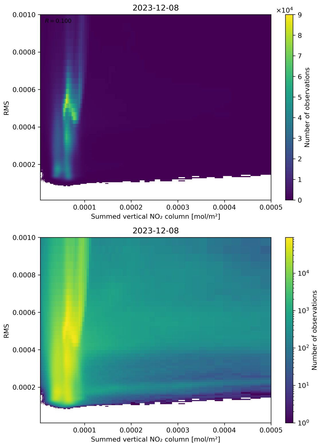
Figure 109: Scatter density plot of “Summed vertical NO 2 column” against “RMS” for 2023-12-07 to 2023-12-09.
