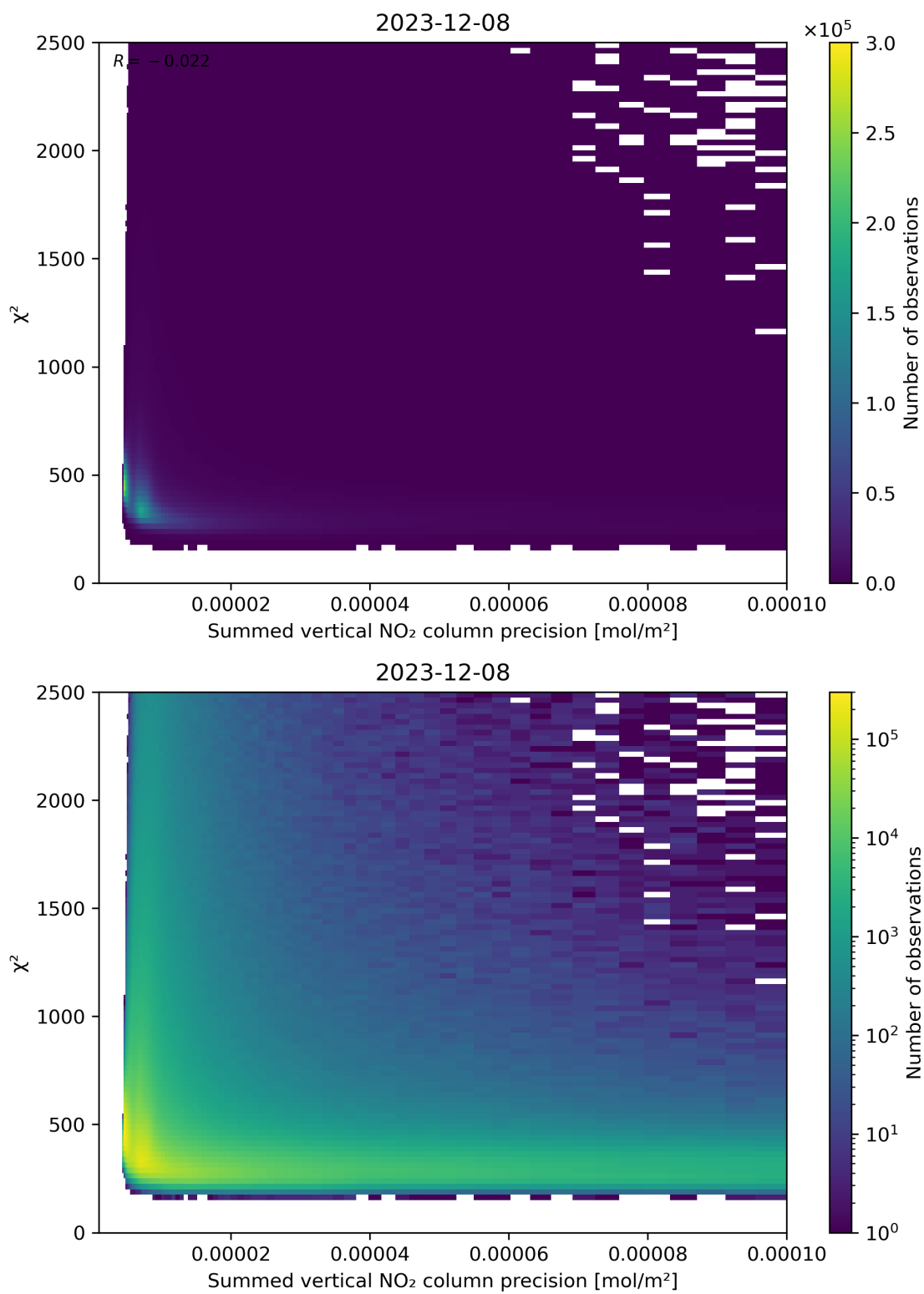
Figure 107: Scatter density plot of “Summed vertical NO 2 column precision” against “ \chi^2 ” for 2023-12-07 to 2023-12-09.
