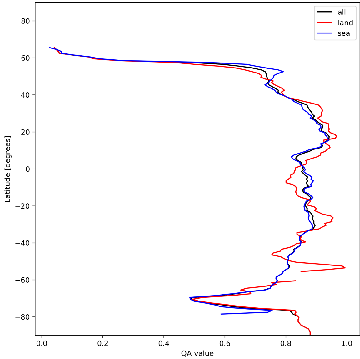
Figure 11: Zonal average of “QA value” for 2023-12-07 to 2023-12-09.
