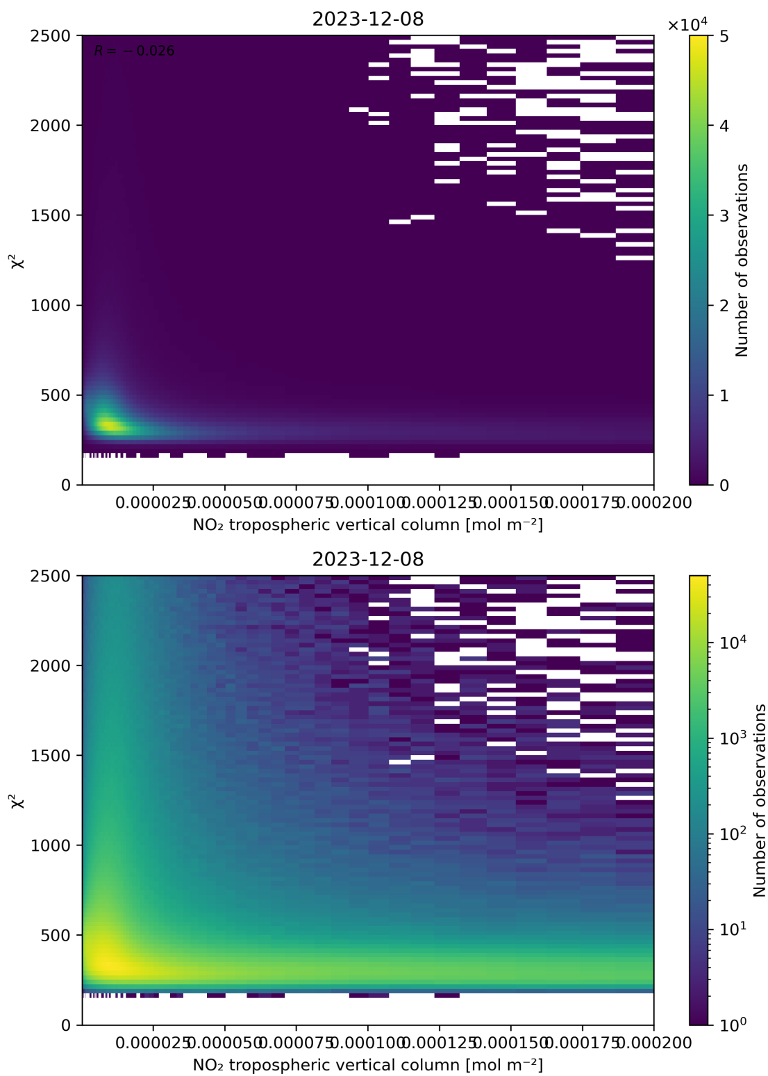
Figure 124: Scatter density plot of “NO 2 tropospheric vertical column” against “ \chi^2 ” for 2023-12-07 to 2023-12-09.
