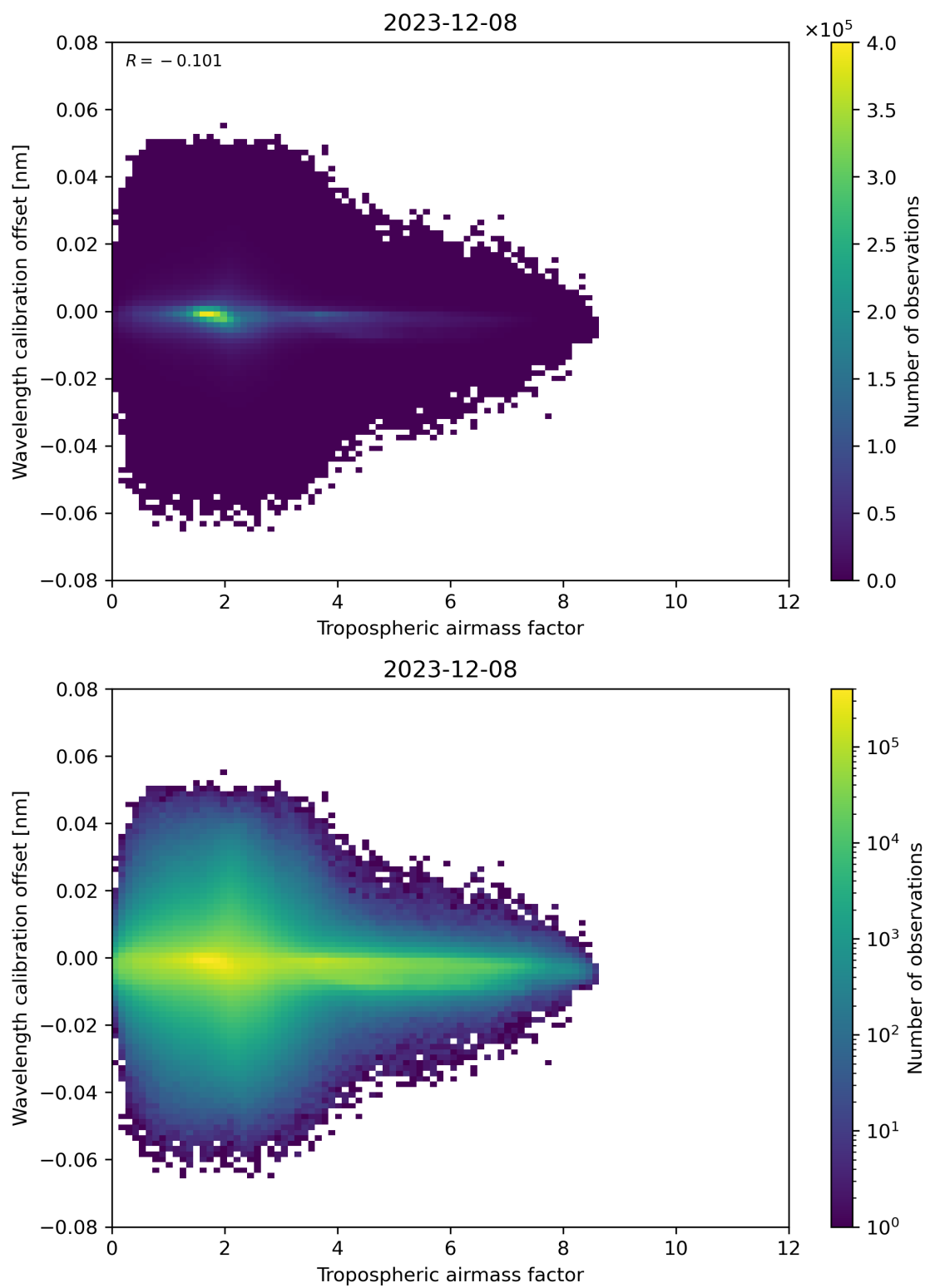
Figure 80: Scatter density plot of “Tropospheric airmass factor” against “Wavelength calibration offset” for 2023-12-07 to 2023-12-09.
