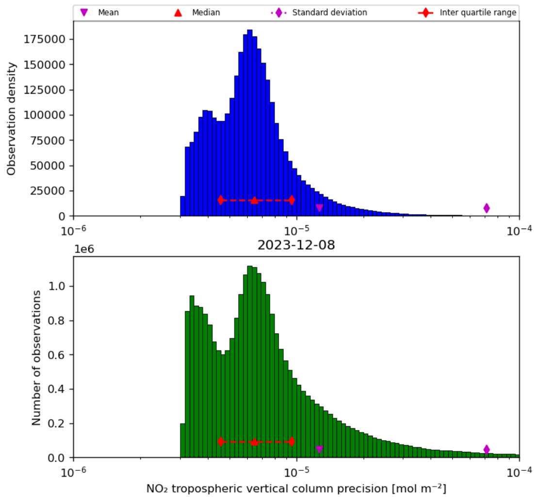
Figure 30: Histogram of “NO 2 tropospheric vertical column precision” for 2023-12-07 to 2023-12-09
