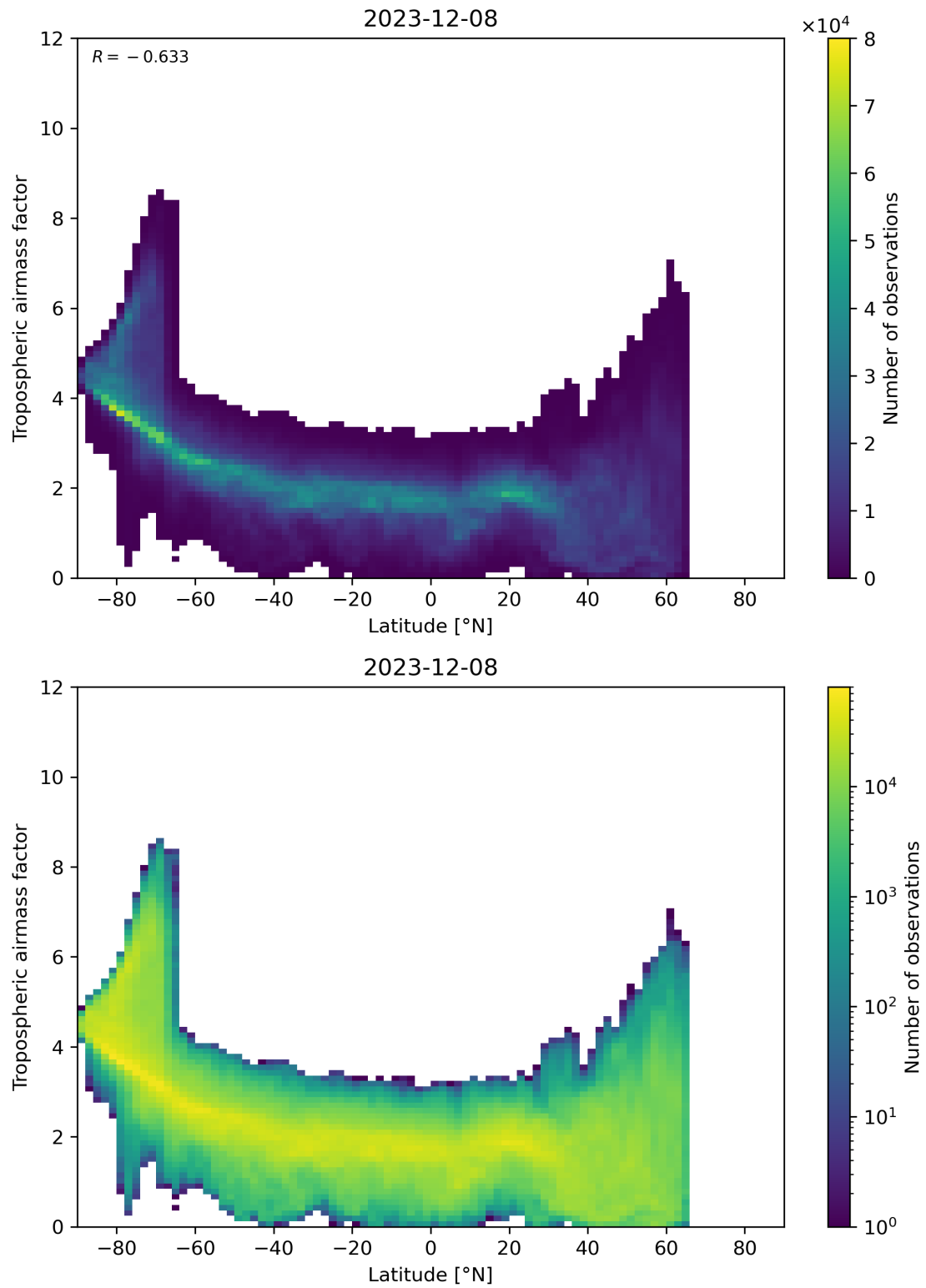
Figure 85: Scatter density plot of “Latitude” against “Tropospheric air mass factor” for 2023-12-07 to 2023-12-09.
