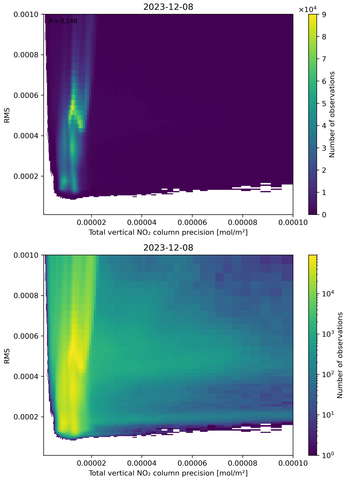
Figure 119: Scatter density plot of “Total vertical NO 2 column precision” against “RMS” for 2023-12-07 to 2023-12-09.
