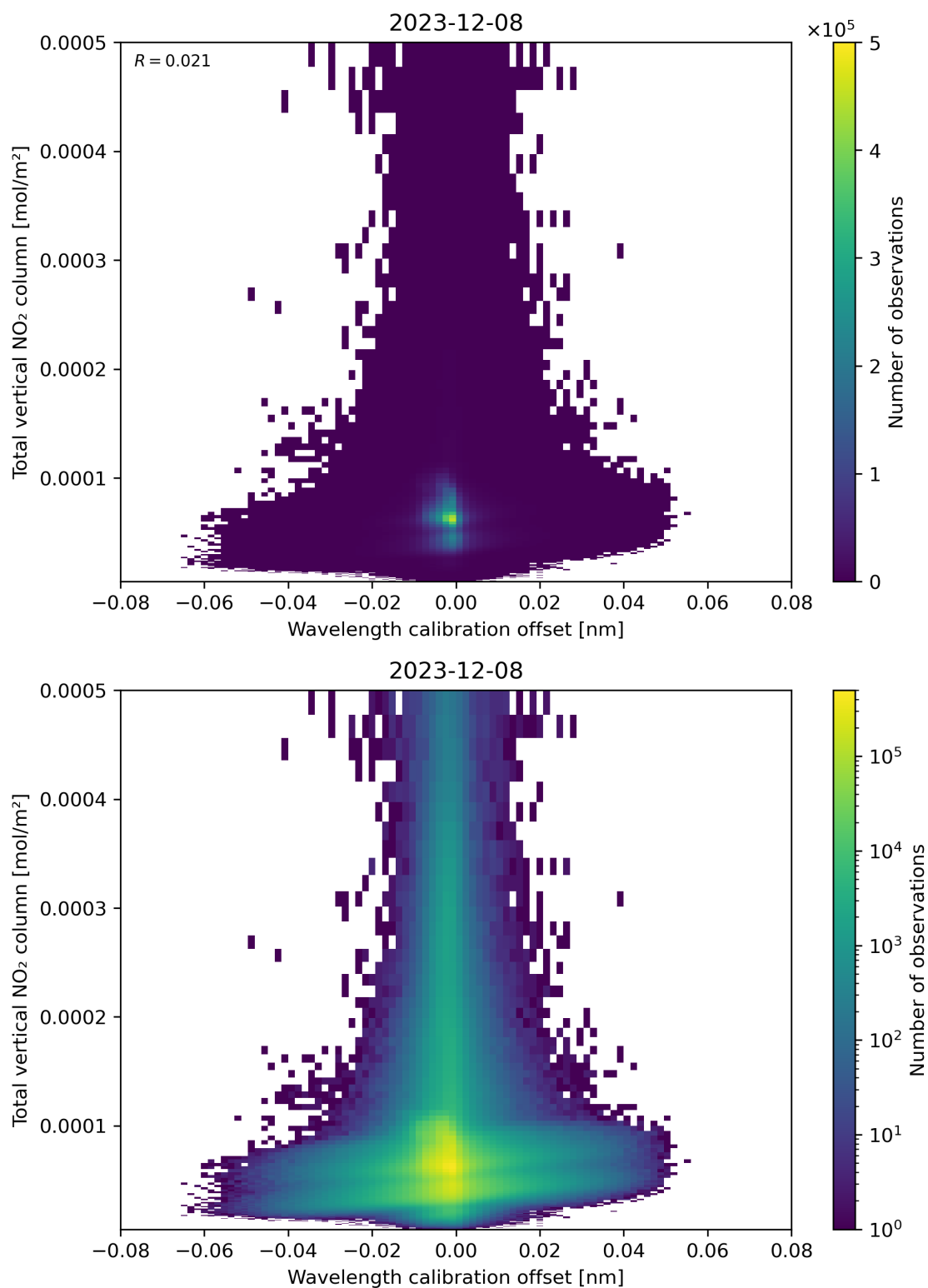
Figure 179: Scatter density plot of “Wavelength calibration offset” against “Total vertical NO 2 column” for 2023-12-07 to 2023-12-09.
