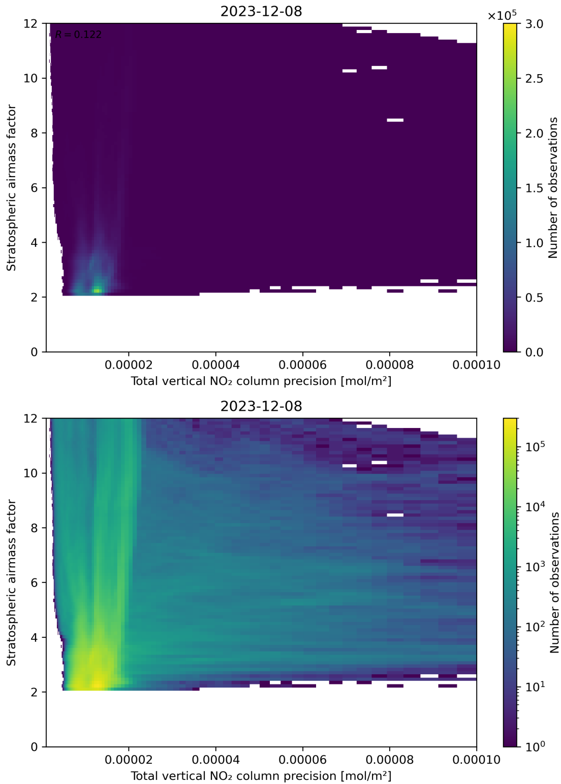
Figure 115: Scatter density plot of “Total vertical NO 2 column precision” against “Stratospheric airmass factor” for 2023-12-07 to 2023-12-09.
