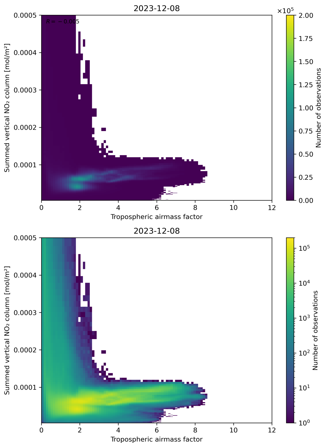
Figure 75: Scatter density plot of “Tropospheric airmass factor” against “Summed vertical NO 2 column” for 2023-12-07 to 2023-12-09.
