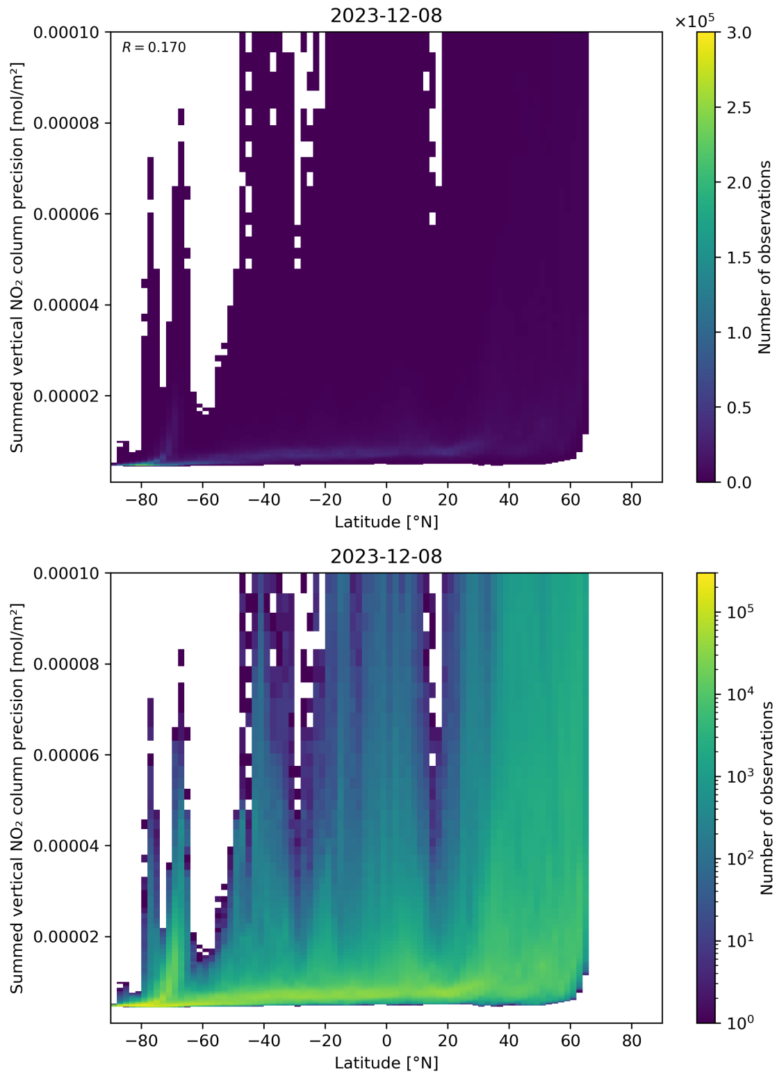
Figure 89: Scatter density plot of “Latitude” against “Summed vertical NO 2 column precision” for 2023-12-07 to 2023-12-09.
