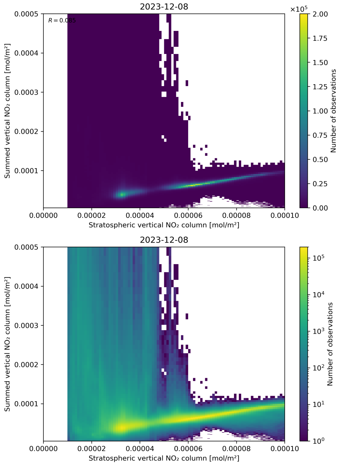
Figure 98: Scatter density plot of “Stratospheric vertical NO 2 column” against “Summed vertical NO 2 column” for 2023-12-07 to 2023-12-09.
