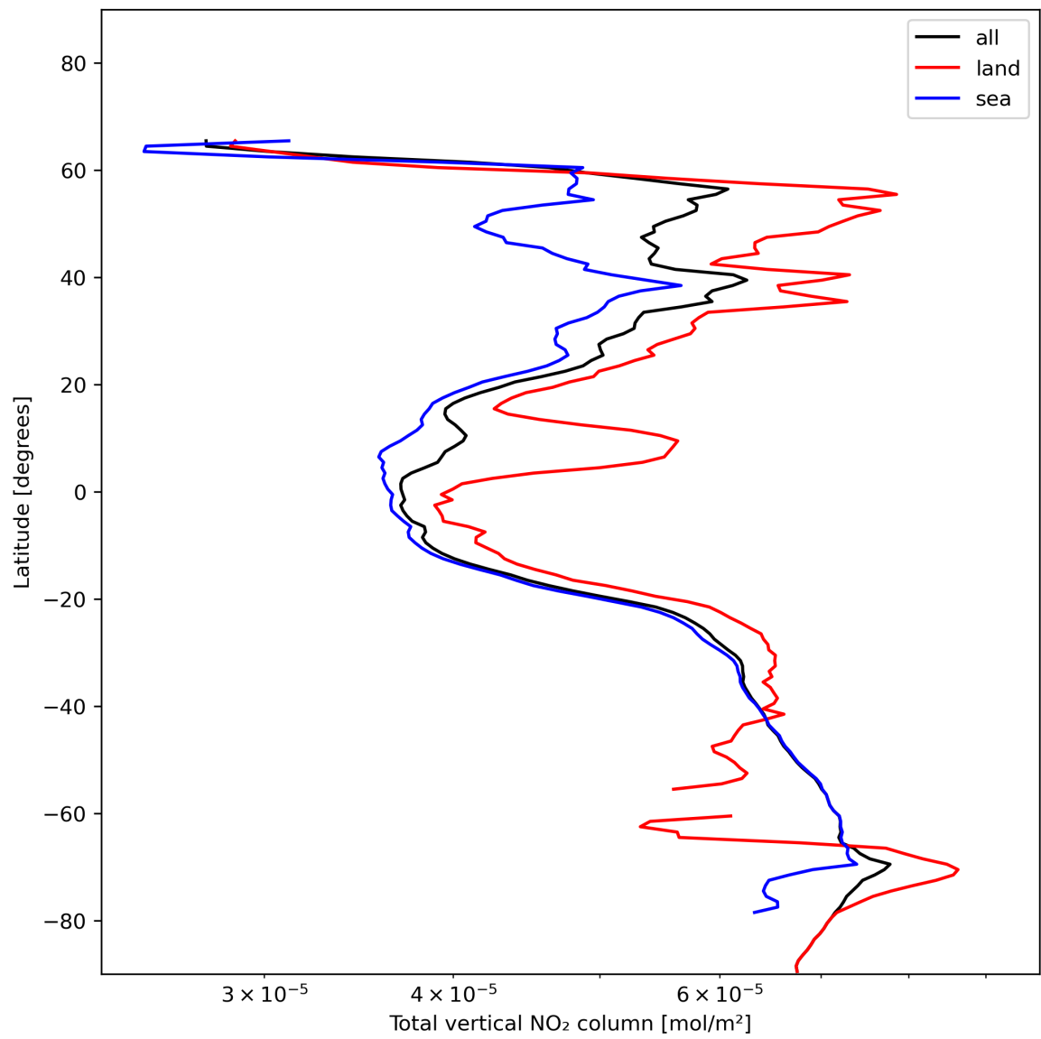
Figure 21: Zonal average of “Total vertical NO 2 column” for 2023-12-07 to 2023-12-09.
