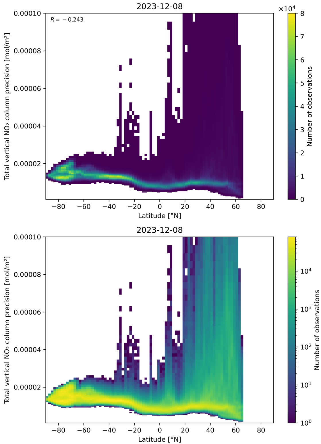
Figure 91: Scatter density plot of “Latitude” against “Total vertical NO 2 column precision” for 2023-12-07 to 2023-12-09.
