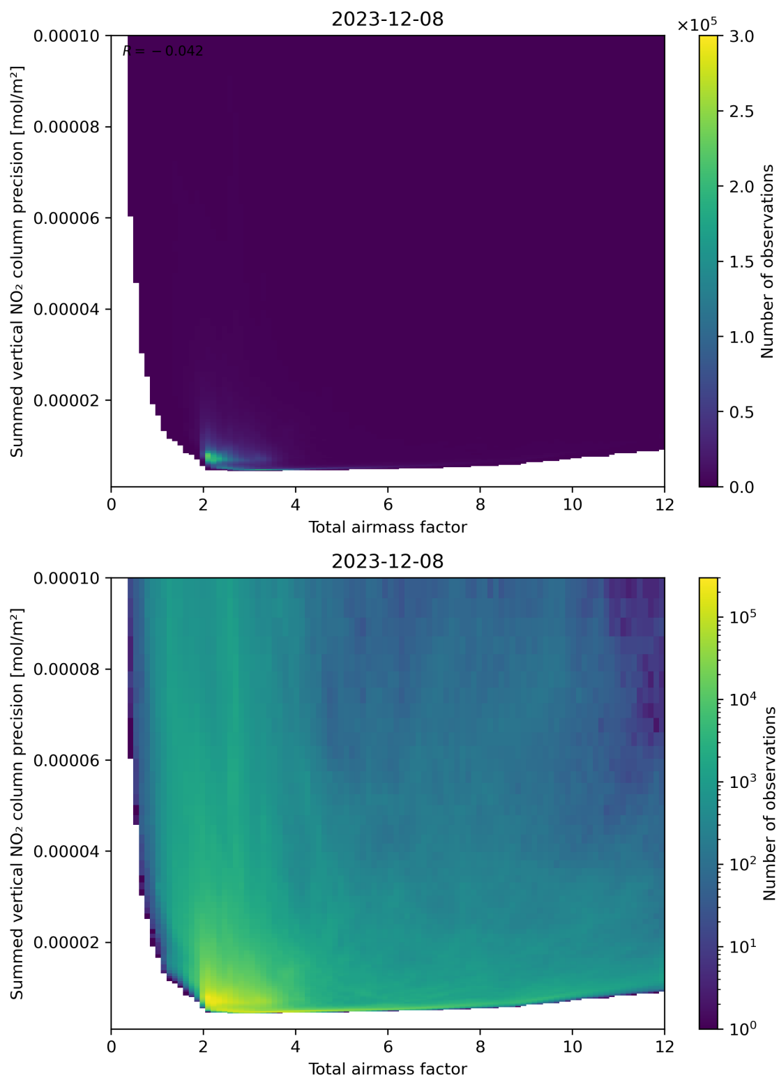
Figure 66: Scatter density plot of “Total airmass factor” against “Summed vertical NO 2 column precision” for 2023-12-07 to 2023-12-09.
