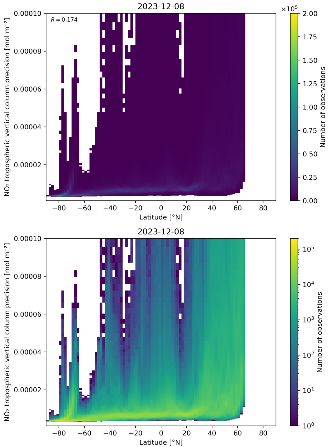
Figure 93: Scatter density plot of “Latitude” against “NO 2 tropospheric vertical column precision” for 2023-12-07 to 2023-12-09.
