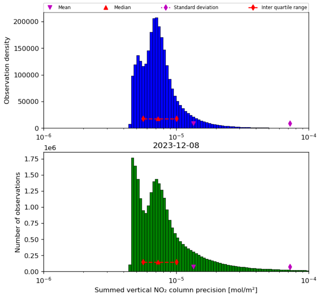
Figure 41: Histogram of “Summed vertical NO 2 column precision” for 2023-12-07 to 2023-12-09
