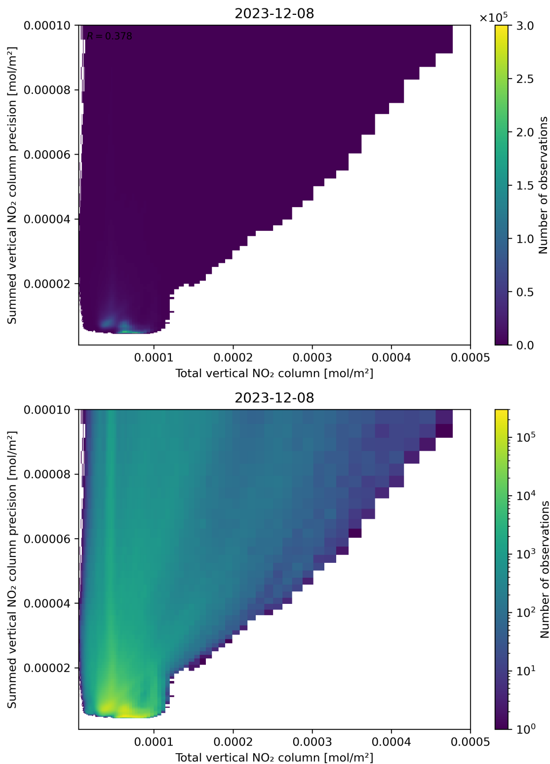
Figure 113: Scatter density plot of “Total vertical NO 2 column” against “Summed vertical NO 2 column precision” for 2023-12-07 to 2023-12-09.
