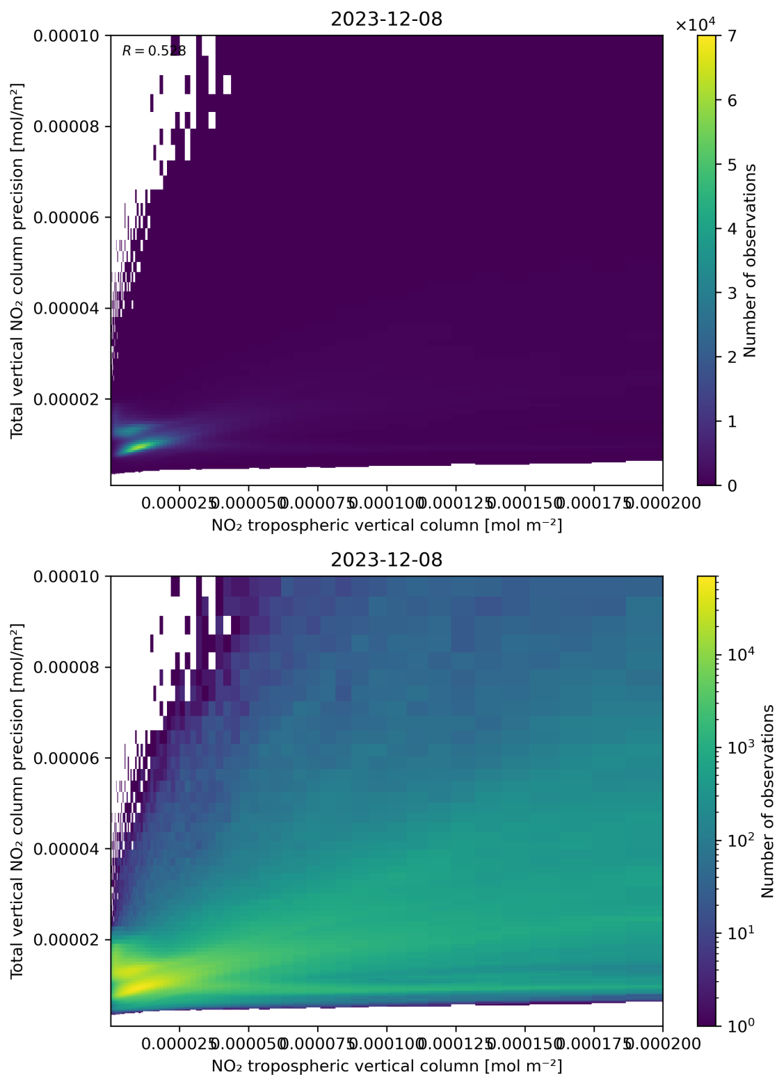
Figure 129: Scatter density plot of “NO 2 tropospheric vertical column” against “Total vertical NO 2 column precision” for 2023-12-07 to 2023-12-09.
