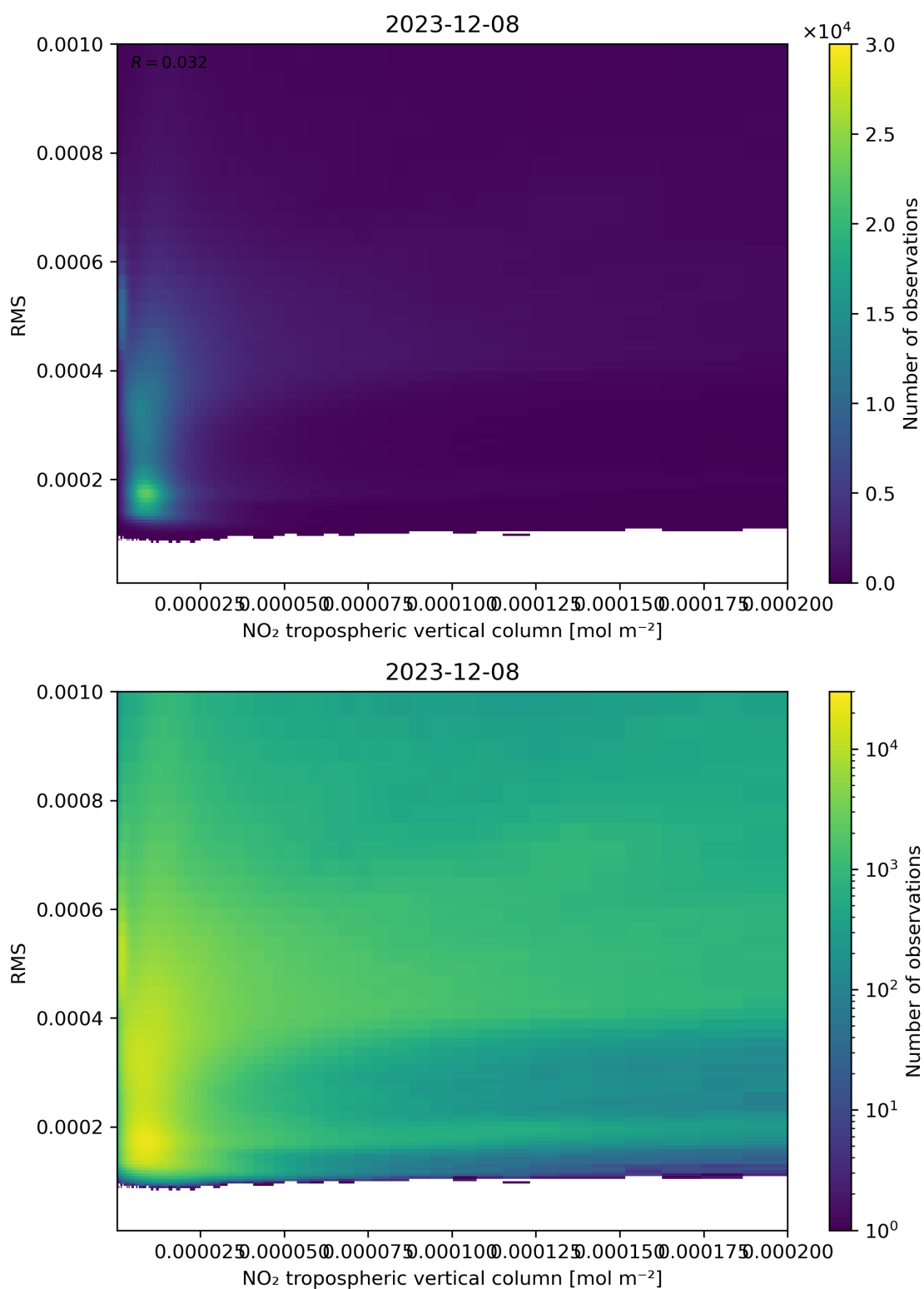
Figure 142: Scatter density plot of “NO 2 tropospheric vertical column” against “RMS” for 2023-12-07 to 2023-12-09.
