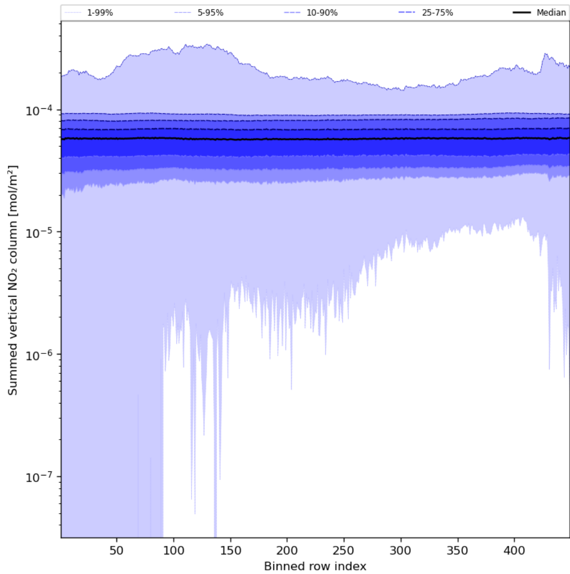
Figure 57: Along track statistics of “Summed vertical NO 2 column” for 2023-12-07 to 2023-12-09
