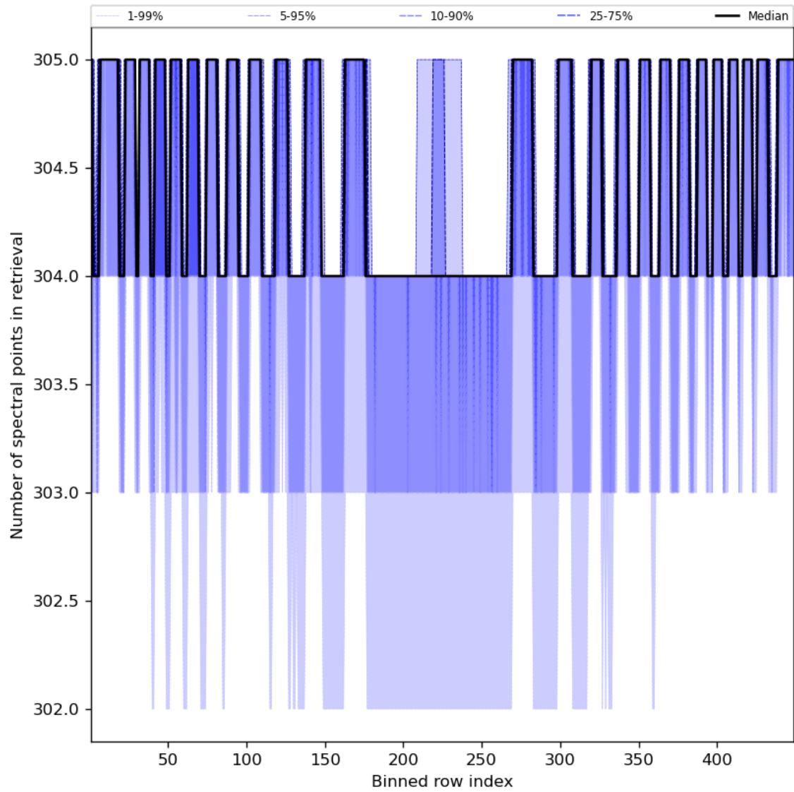
Figure 50: Along track statistics of “Number of spectral points in retrieval” for 2023-12-07 to 2023-12-09
