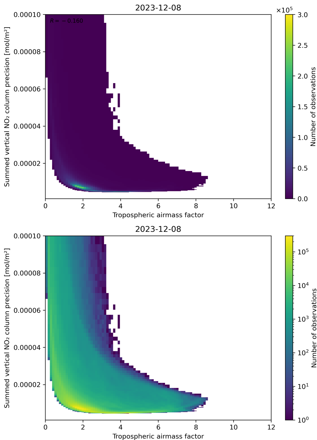
Figure 76: Scatter density plot of “Tropospheric air mass factor” against “Summed vertical NO 2 column precision” for 2023-12-07 to 2023-12-09.
