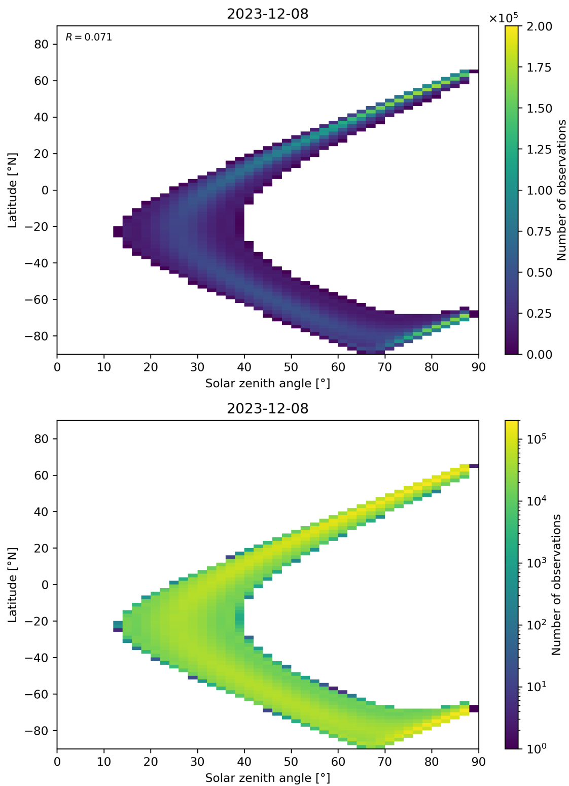
Figure 149: Scatter density plot of “Solar zenith angle” against “Latitude” for 2023-12-07 to 2023-12-09.
