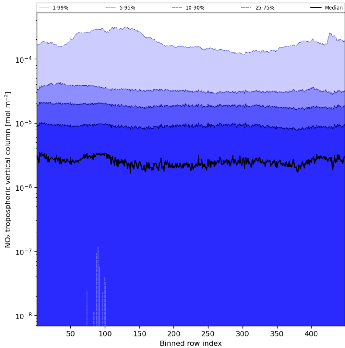
Figure 46: Along track statistics of “NO 2 tropospheric vertical column” for 2023-12-07 to 2023-12-09
