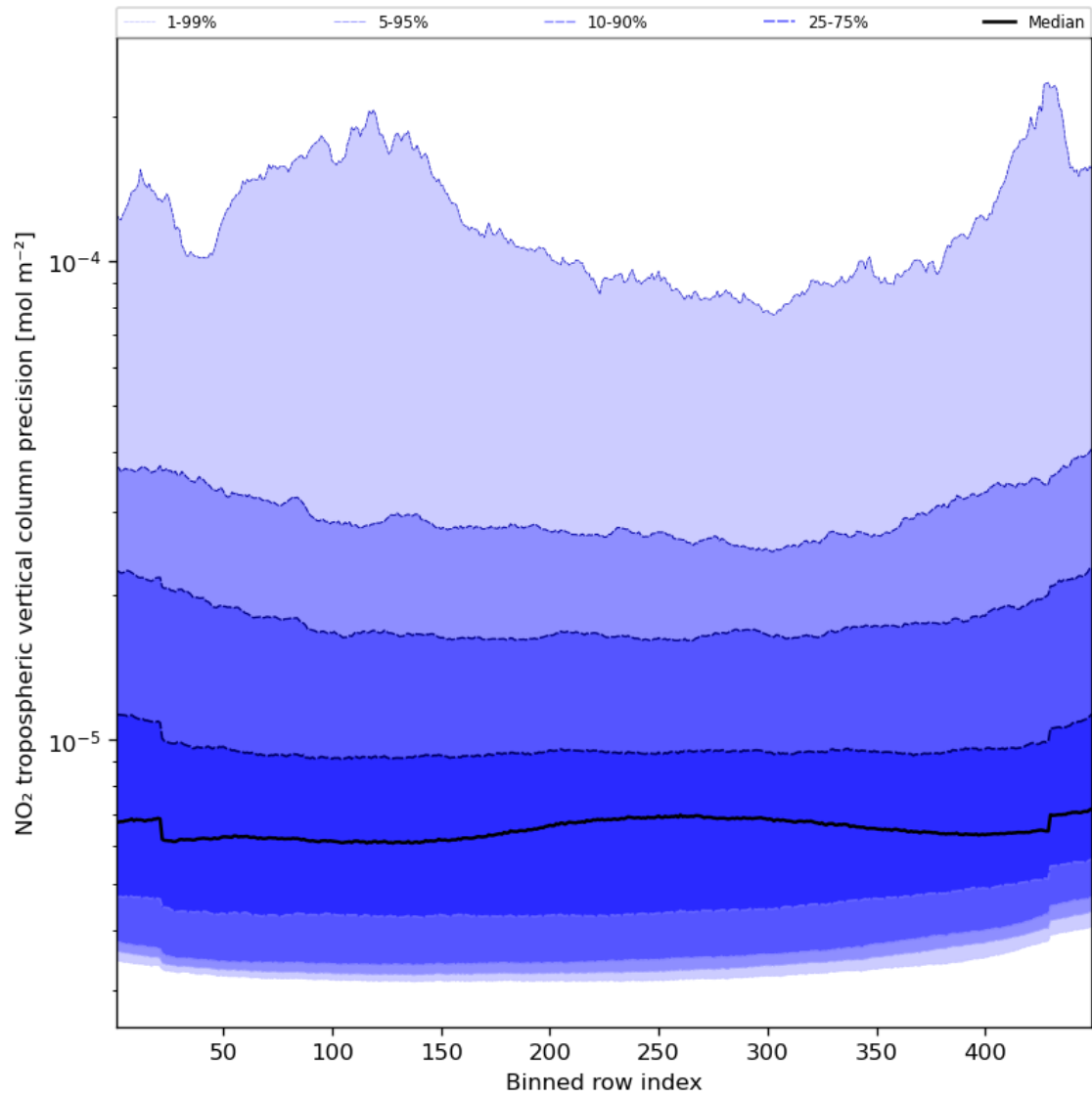
Figure 47: Along track statistics of “NO 2 tropospheric vertical column precision” for 2023-12-07 to 2023-12-09
