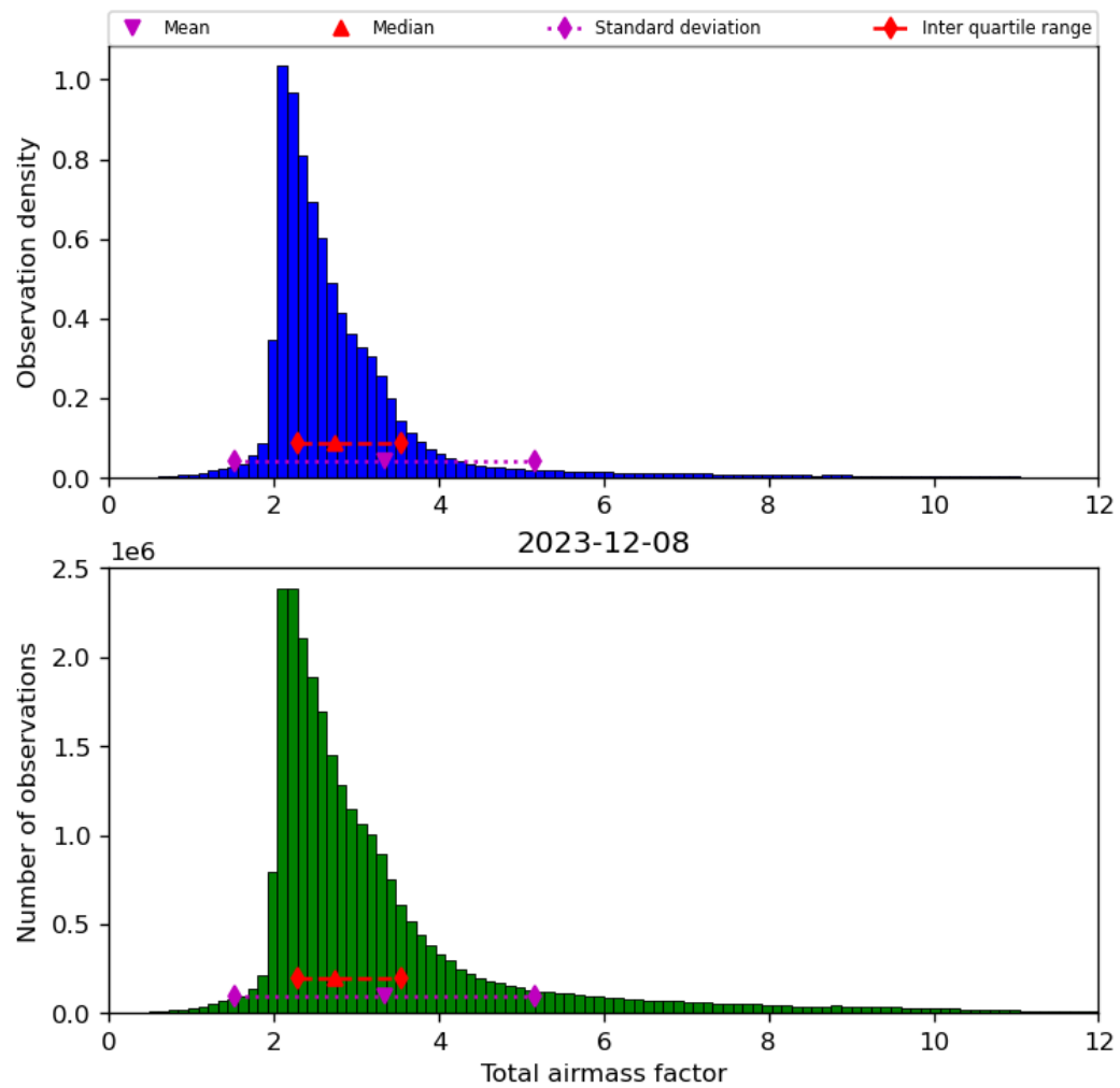
Figure 32: Histogram of “Total airmass factor” for 2023-12-07 to 2023-12-09
