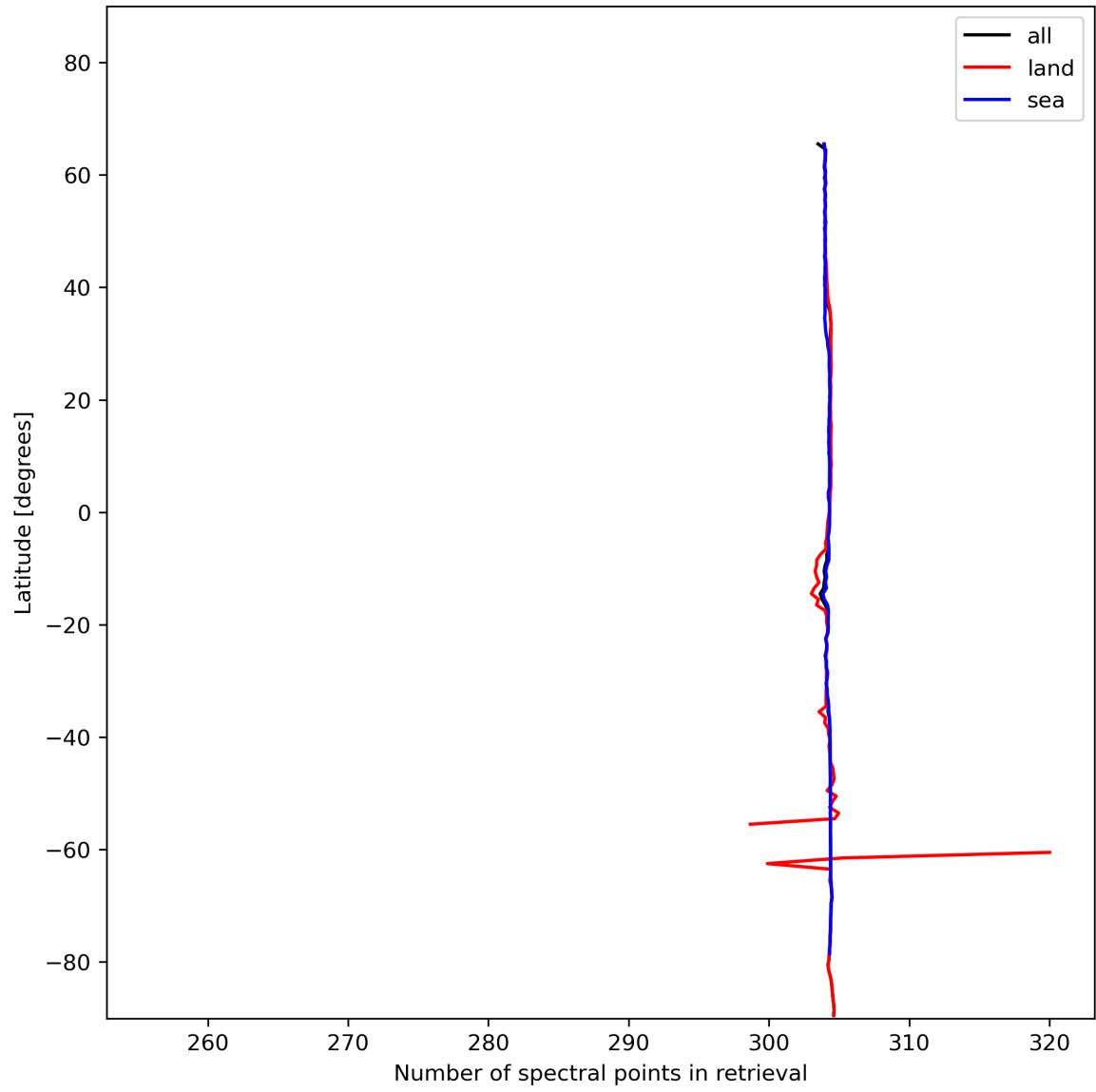
Figure 16: Zonal average of “Number of spectral points in retrieval” for 2023-12-07 to 2023-12-09.
