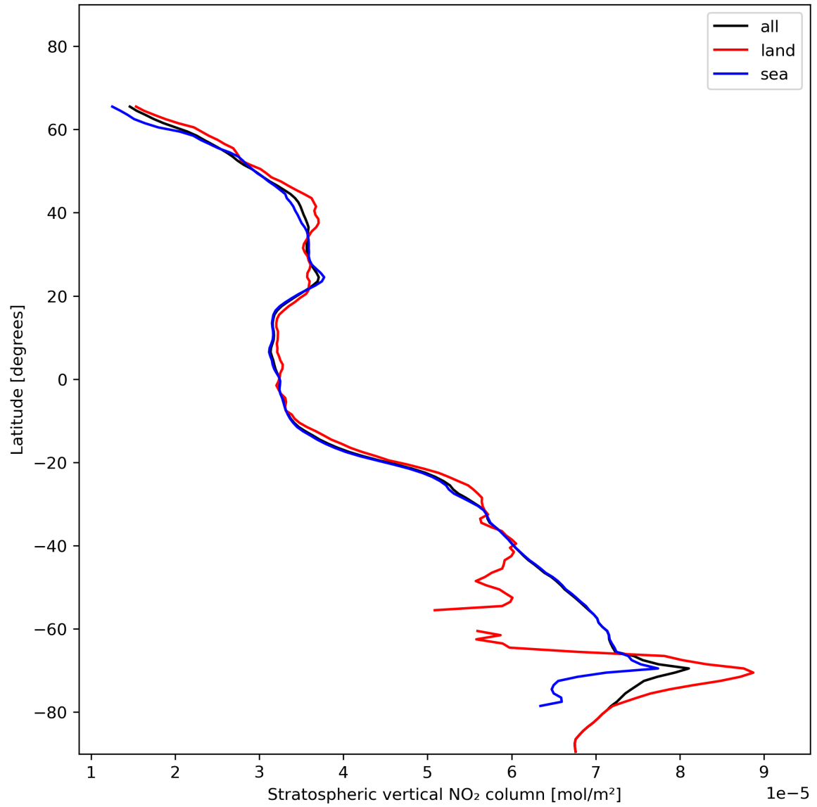
Figure 19: Zonal average of “Stratospheric vertical NO 2 column” for 2023-12-07 to 2023-12-09.
