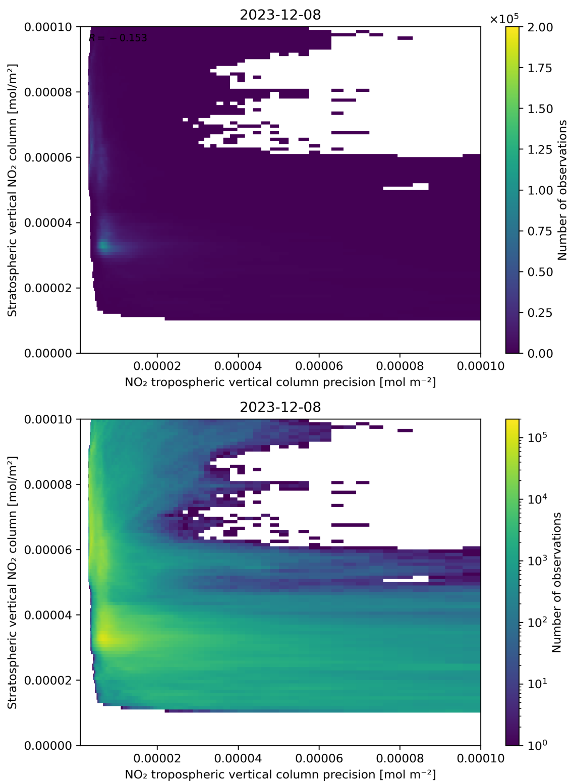
Figure 135: Scatter density plot of “NO 2 tropospheric vertical column precision” against “Stratospheric vertical NO 2 column” for 2023-12-07 to 2023-12-09.
