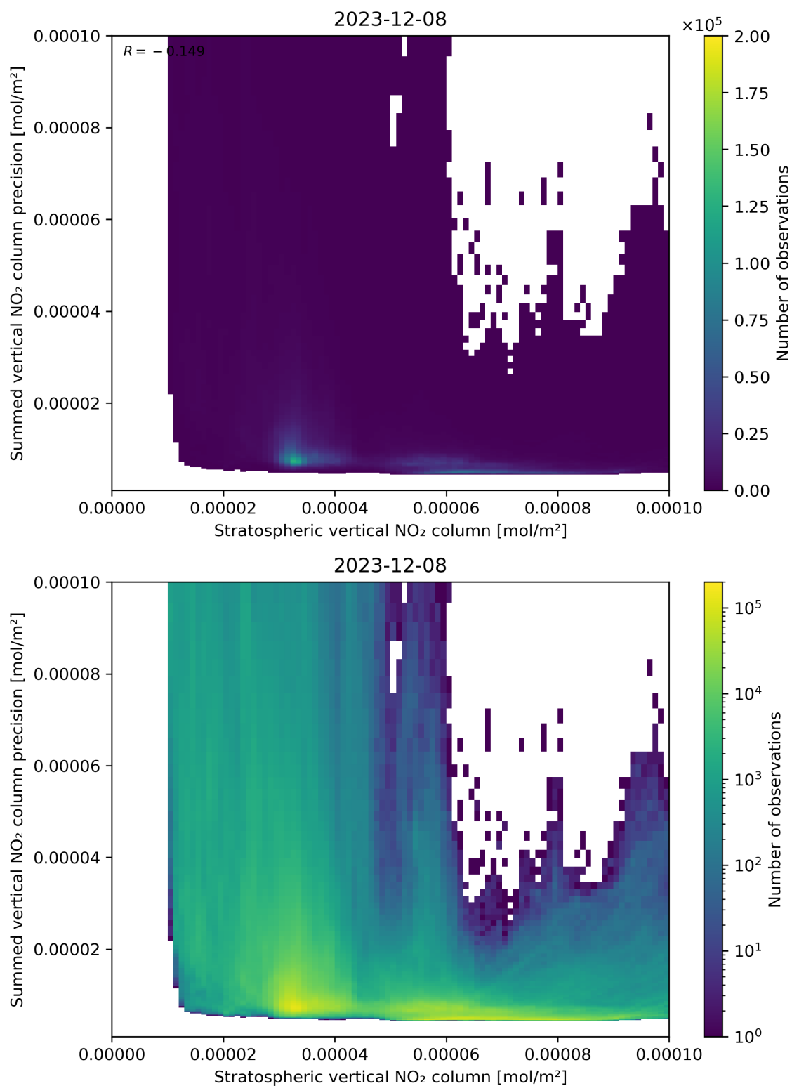
Figure 99: Scatter density plot of “Stratospheric vertical NO 2 column” against “Summed vertical NO 2 column precision” for 2023-12-07 to 2023-12-09.
