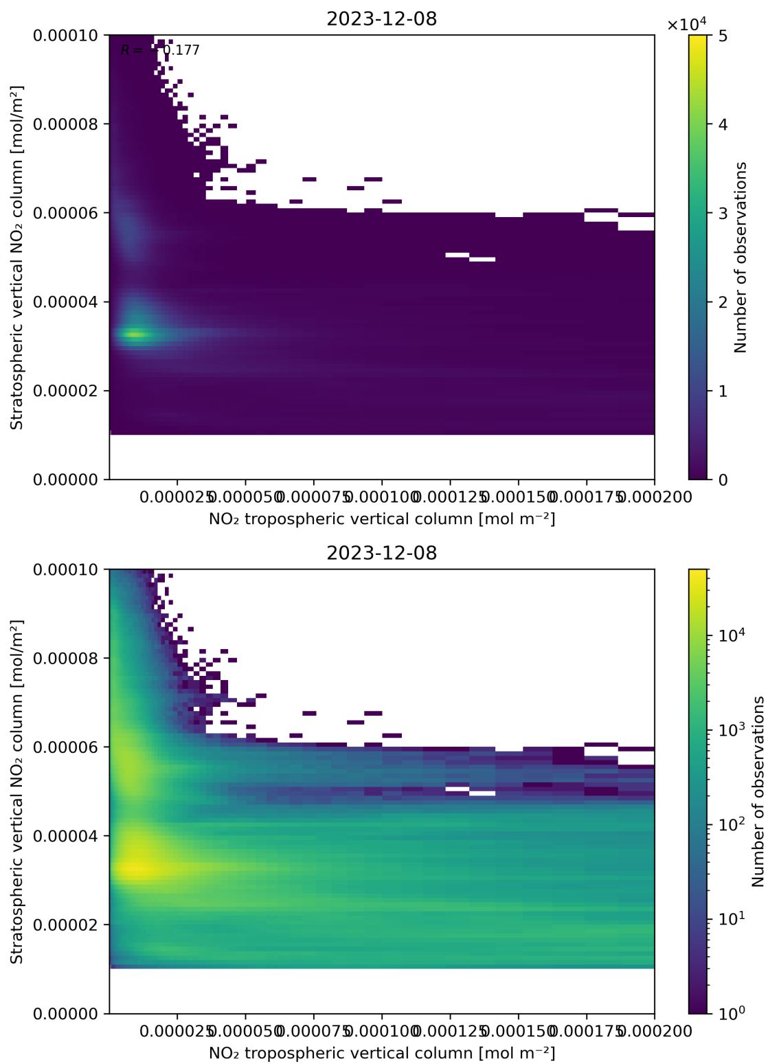
Figure 125: Scatter density plot of “NO 2 tropospheric vertical column” against “Stratospheric vertical NO 2 column” for 2023-12-07 to 2023-12-09.
