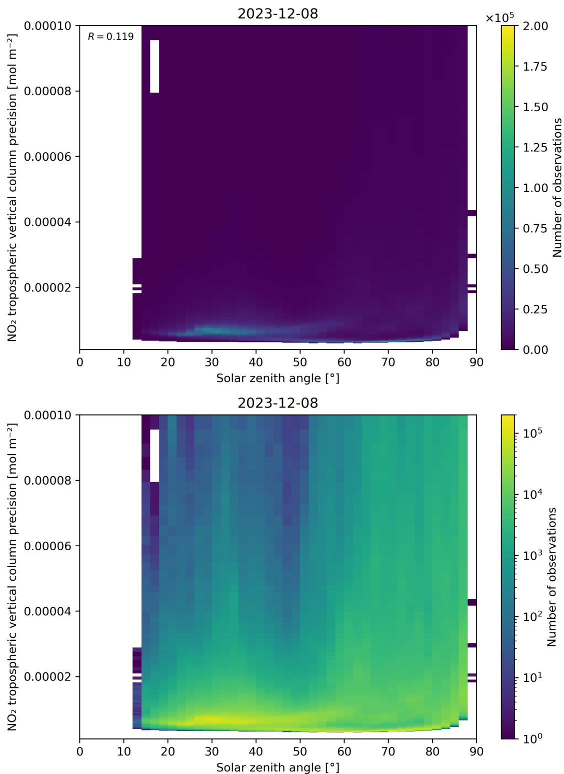
Figure 156: Scatter density plot of “Solar zenith angle” against “NO 2 tropospheric vertical column precision” for 2023-12-07 to 2023-12-09.
