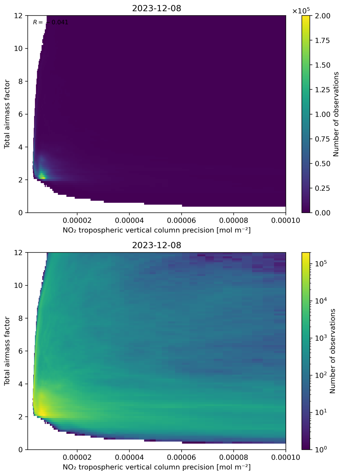
Figure 132: Scatter density plot of “NO 2 tropospheric vertical column precision” against “Total air mass factor” for 2023-12-07 to 2023-12-09.
