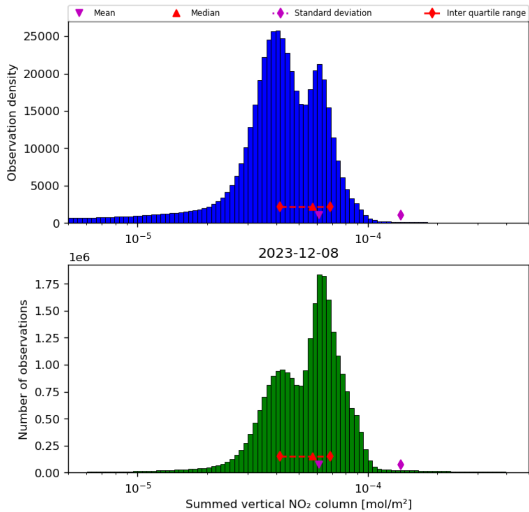
Figure 40: Histogram of “Summed vertical NO 2 column” for 2023-12-07 to 2023-12-09
