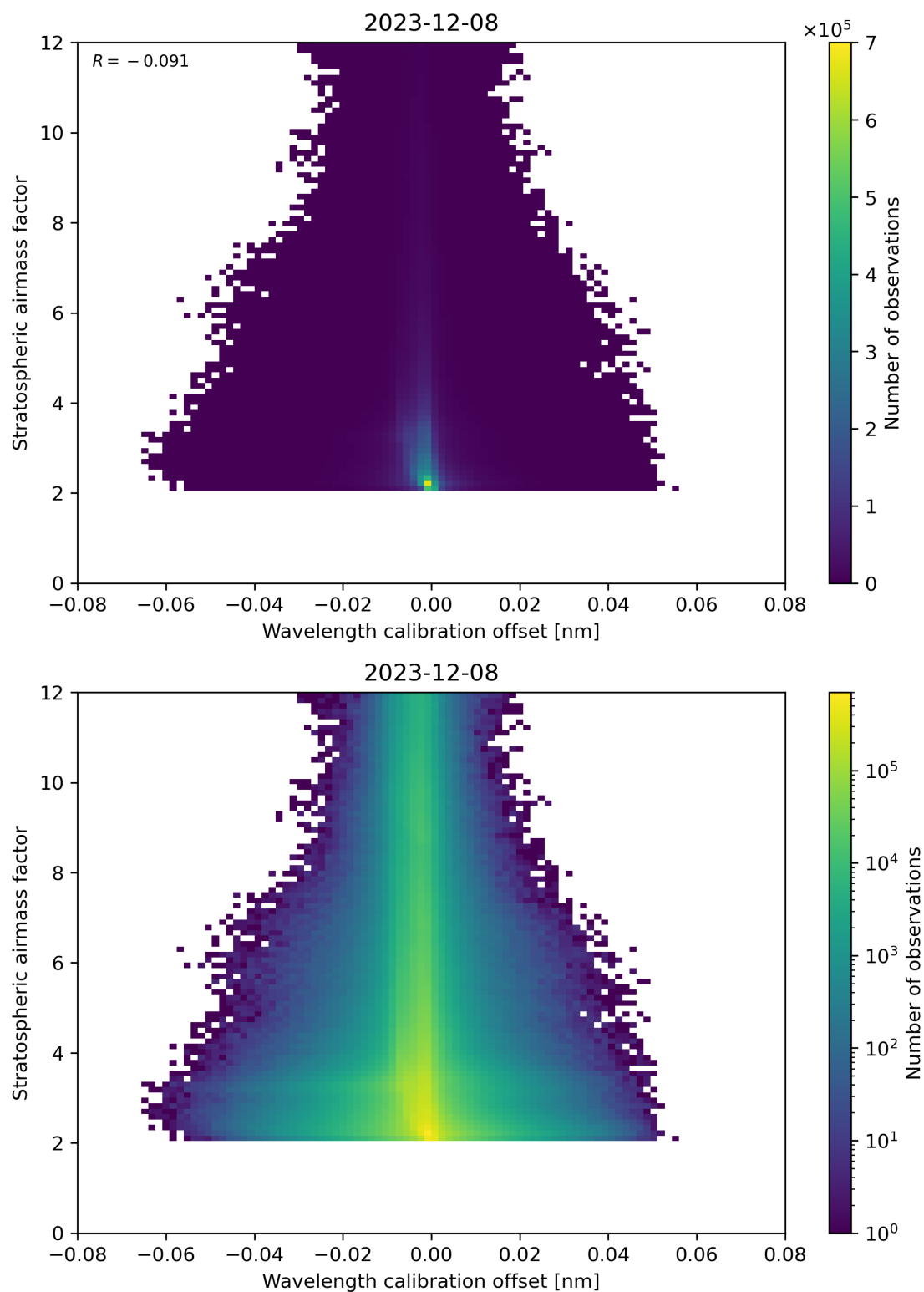
Figure 174: Scatter density plot of “Wavelength calibration offset” against “Stratospheric airmass factor” for 2023-12-07 to 2023-12-09.
