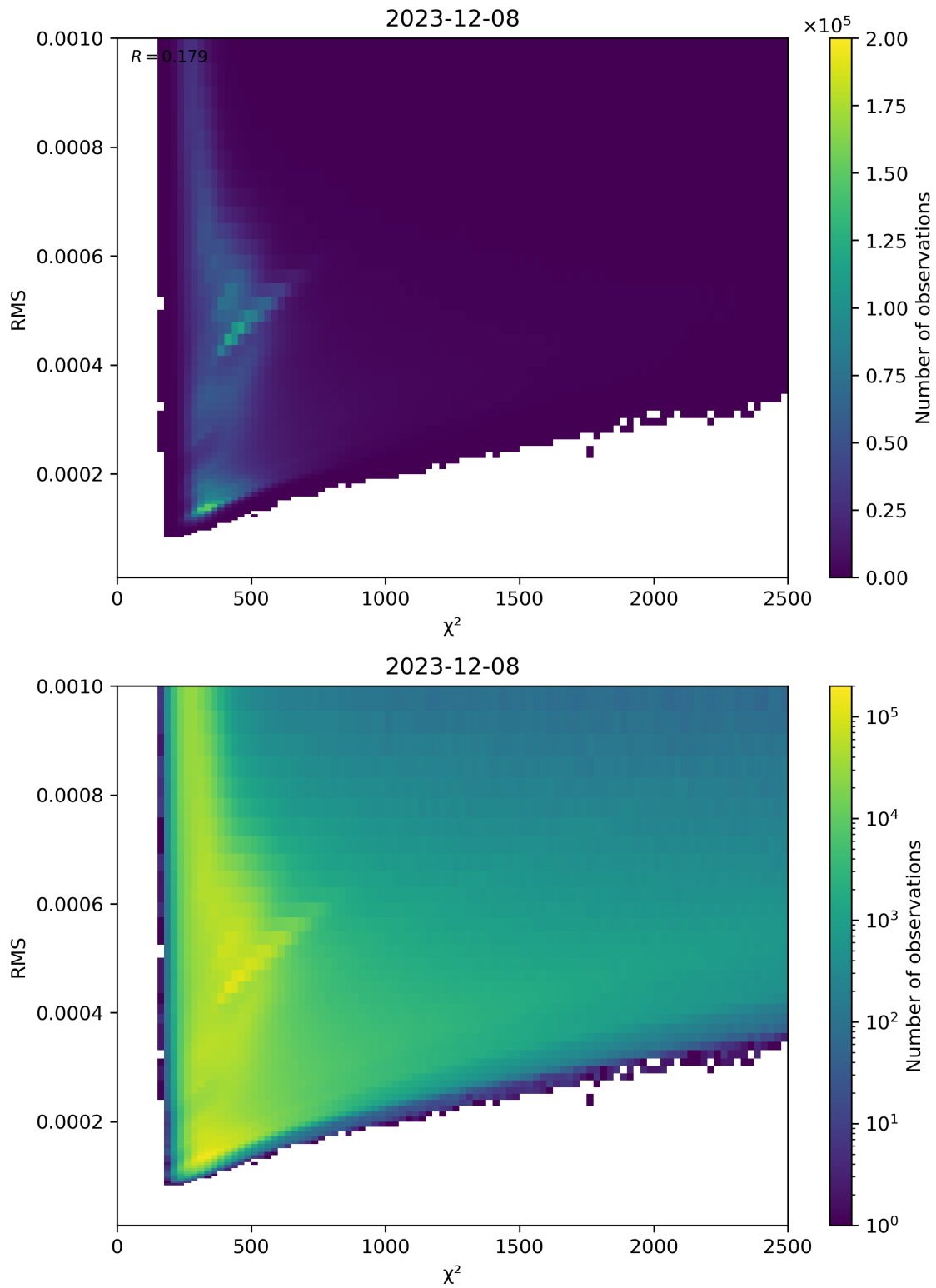
Figure 82: Scatter density plot of “ \chi^2 ” against “RMS” for 2023-12-07 to 2023-12-09.
