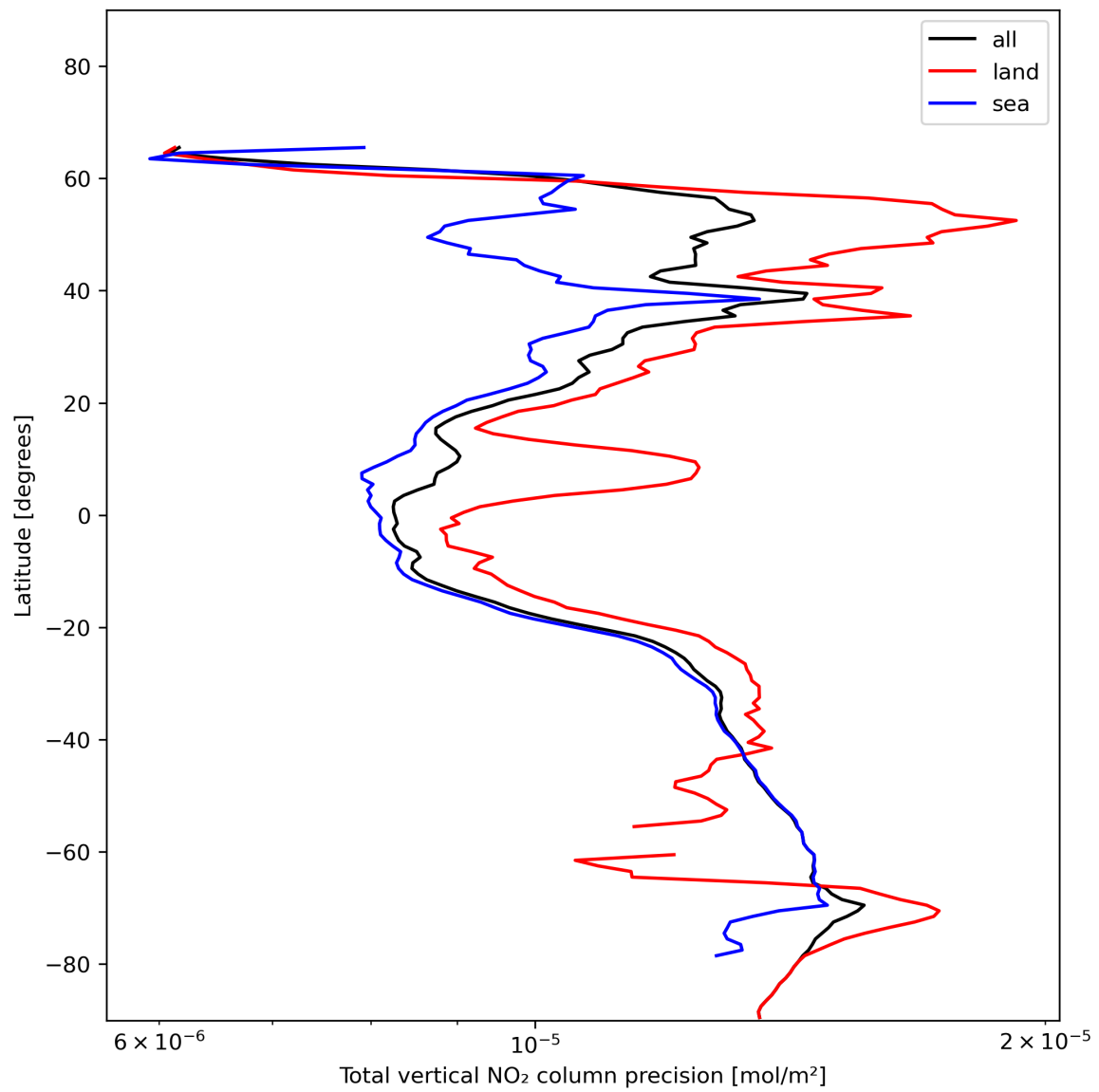
Figure 22: Zonal average of “Total vertical NO 2 column precision” for 2023-12-07 to 2023-12-09.
