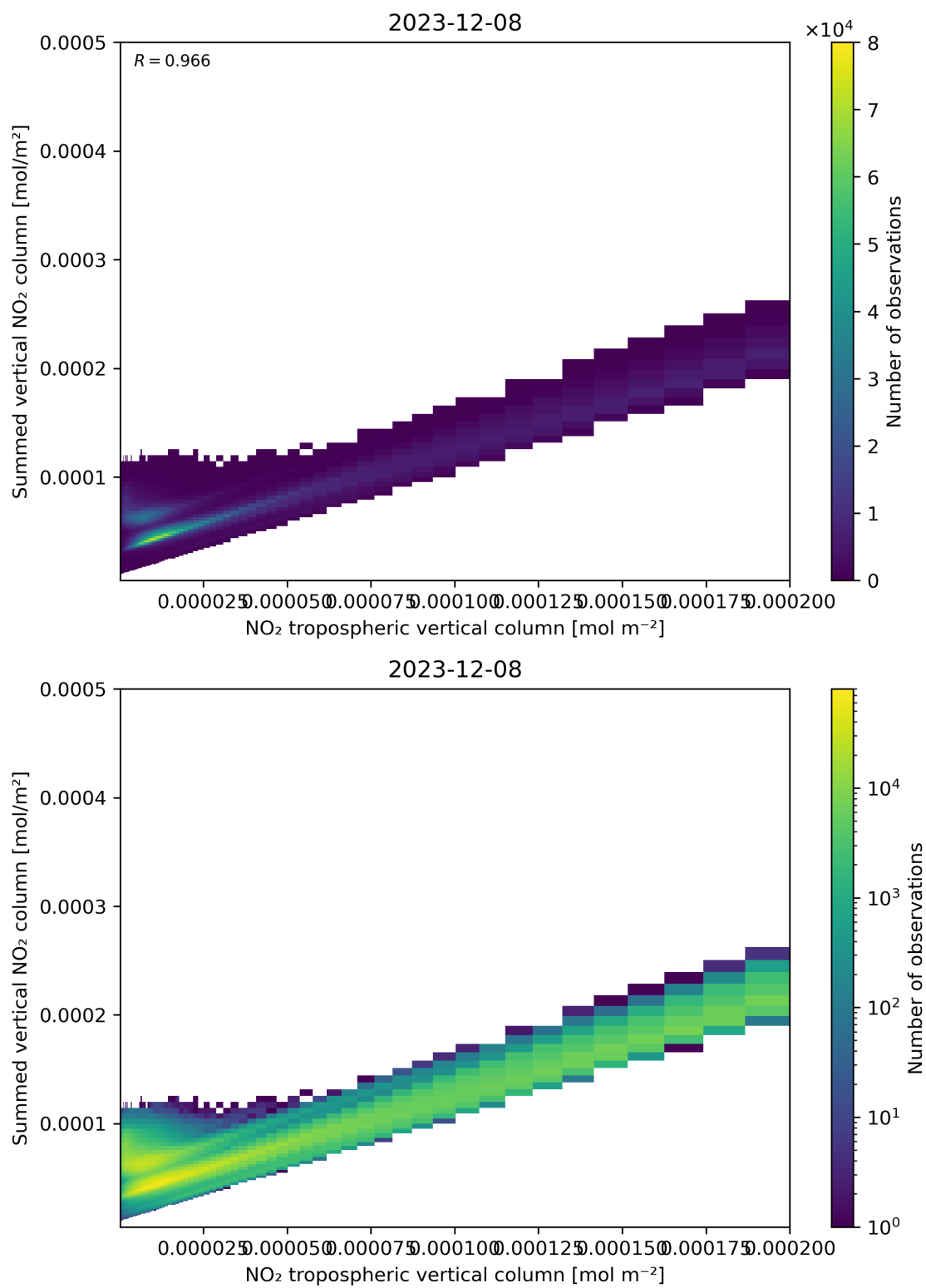
Figure 126: Scatter density plot of “NO 2 tropospheric vertical column” against “Summed vertical NO 2 column” for 2023-12-07 to 2023-12-09.
