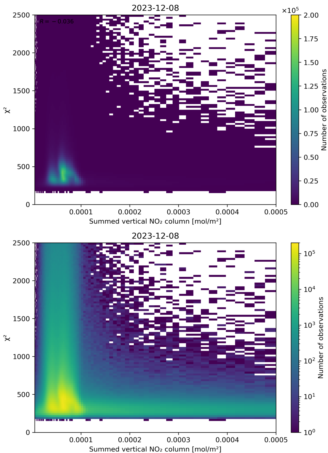
Figure 104: Scatter density plot of “Summed vertical NO 2 column” against “ \chi^2 ” for 2023-12-07 to 2023-12-09.
