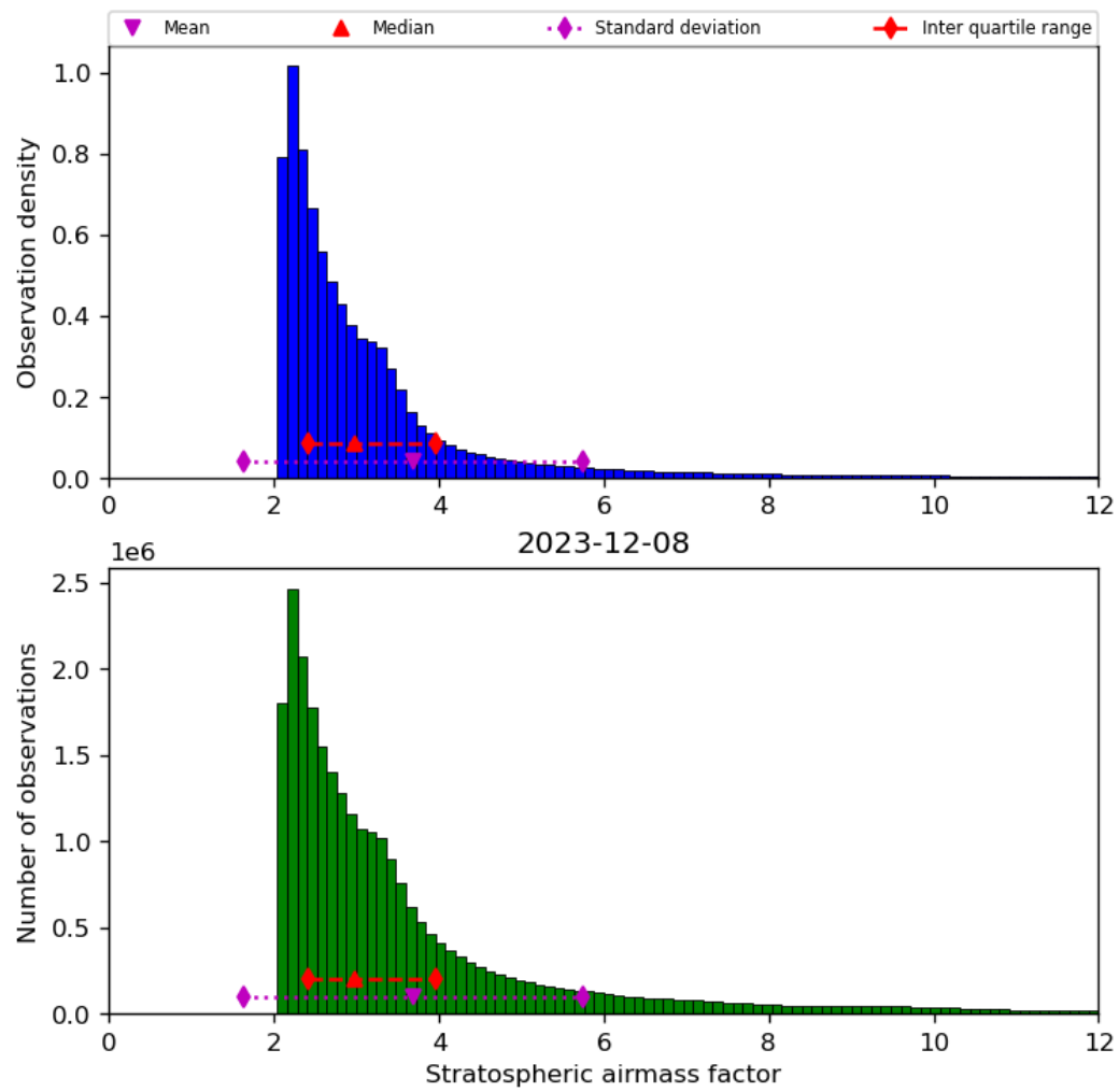
Figure 44: Histogram of “Stratospheric airmass factor” for 2023-12-07 to 2023-12-09
