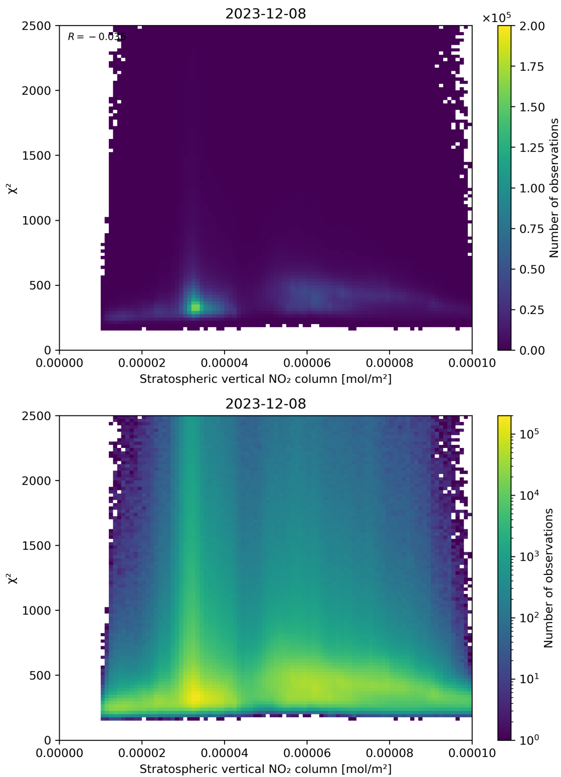
Figure 97: Scatter density plot of “Stratospheric vertical NO 2 column” against “ \chi^2 ” for 2023-12-07 to 2023-12-09.
