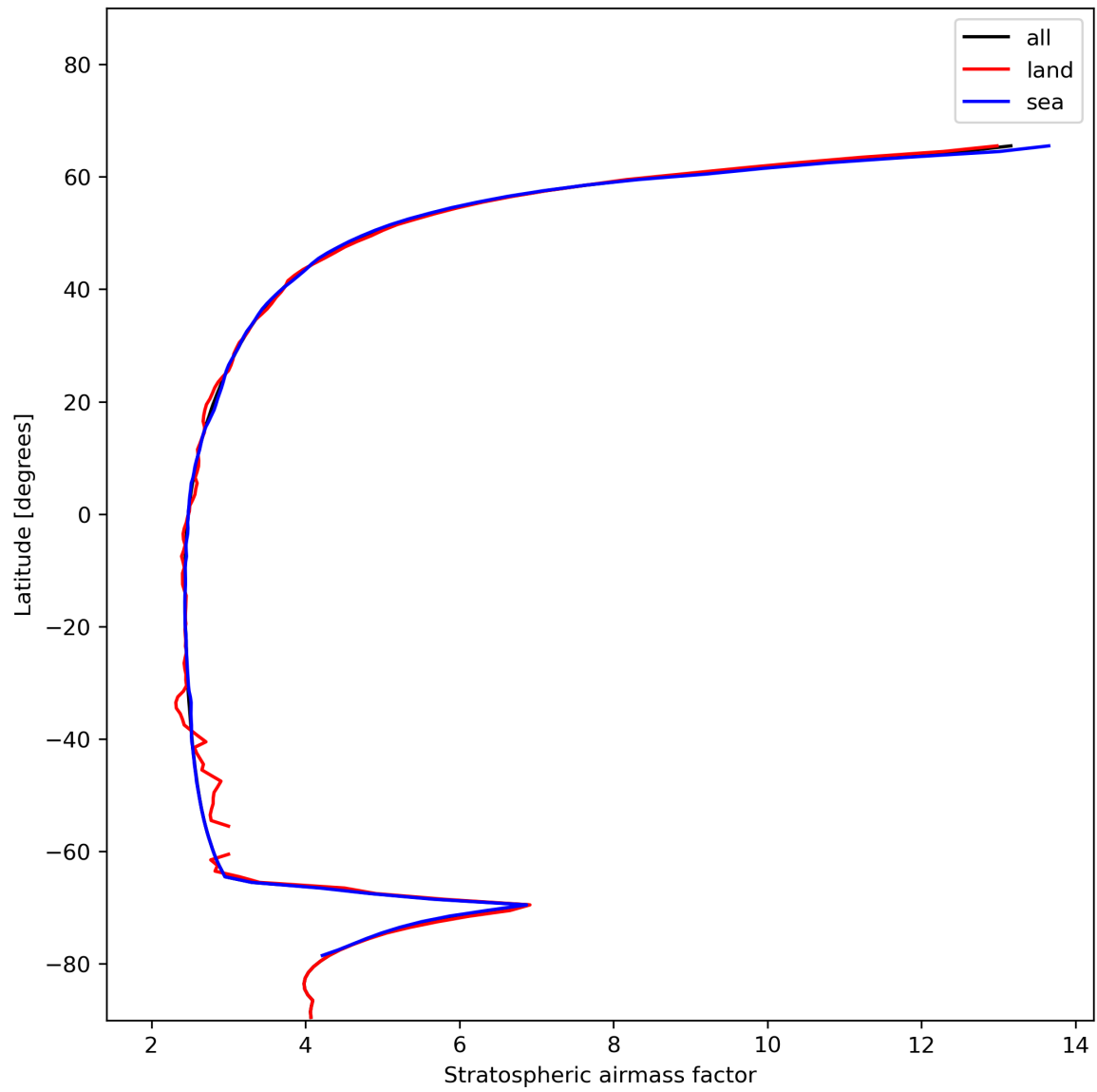
Figure 27: Zonal average of “Stratospheric air mass factor” for 2023-12-07 to 2023-12-09.
