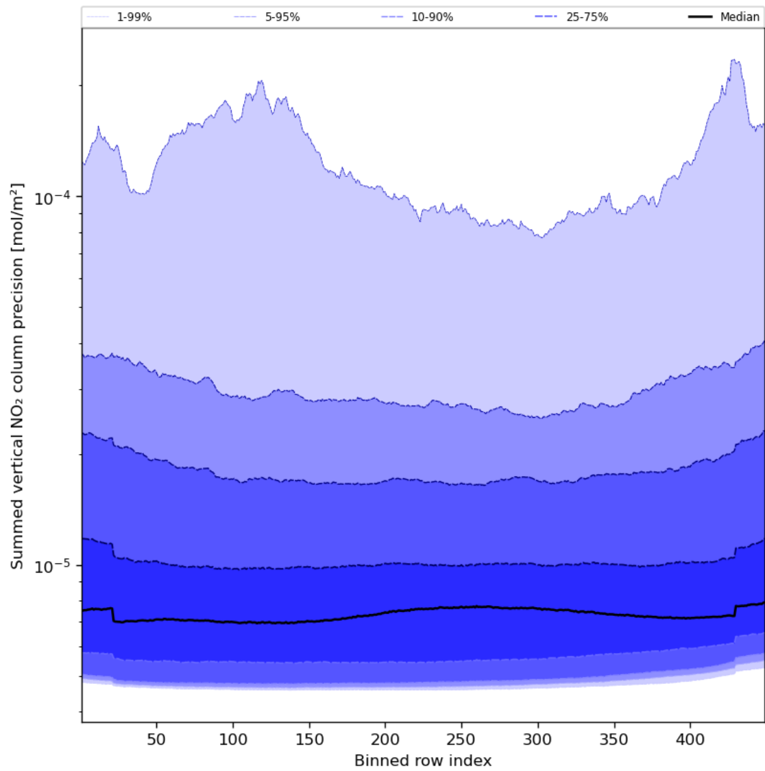
Figure 58: Along track statistics of “Summed vertical NO 2 column precision” for 2023-12-07 to 2023-12-09
