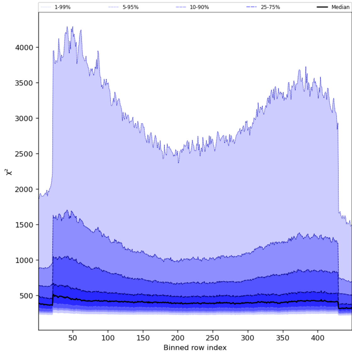
Figure 59: Along track statistics of “ \chi^2 ” for 2023-12-07 to 2023-12-09
