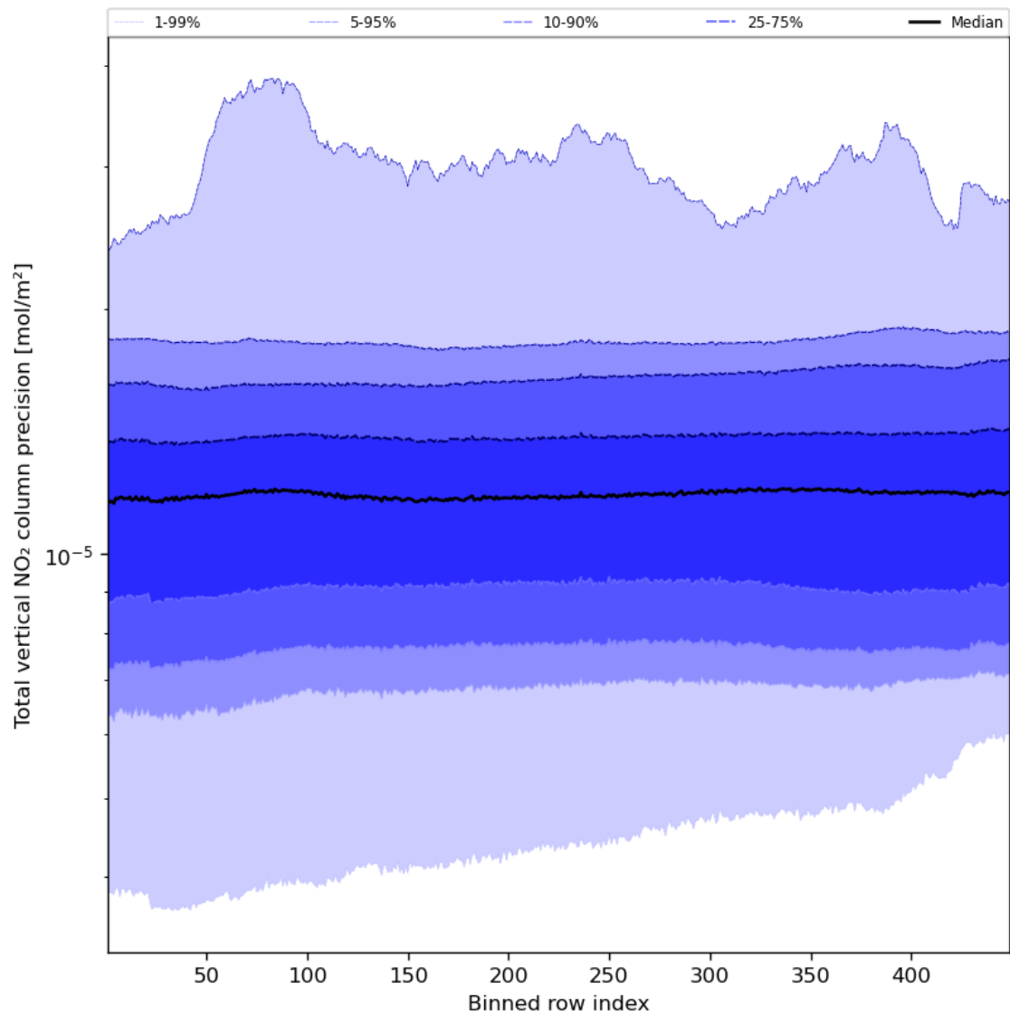
Figure 56: Along track statistics of “Total vertical NO 2 column precision” for 2023-12-07 to 2023-12-09
