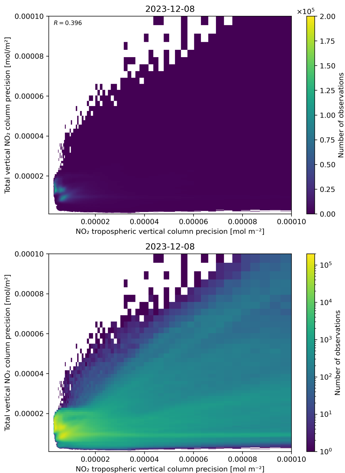
Figure 139: Scatter density plot of “NO 2 tropospheric vertical column precision” against “Total vertical NO 2 column precision” for 2023-12-07 to 2023-12-09.
