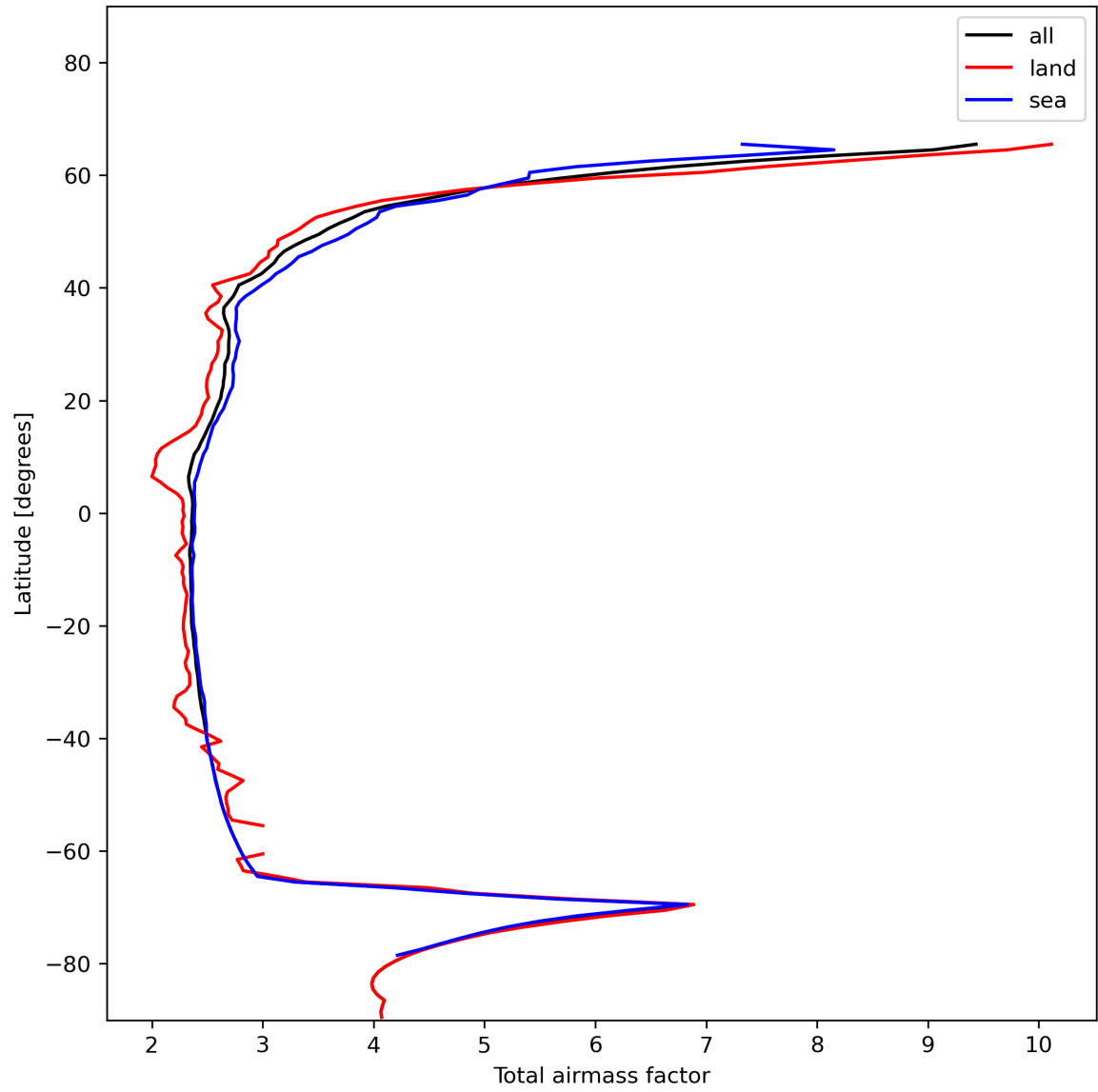
Figure 15: Zonal average of “Total airmass factor” for 2023-12-07 to 2023-12-09.
