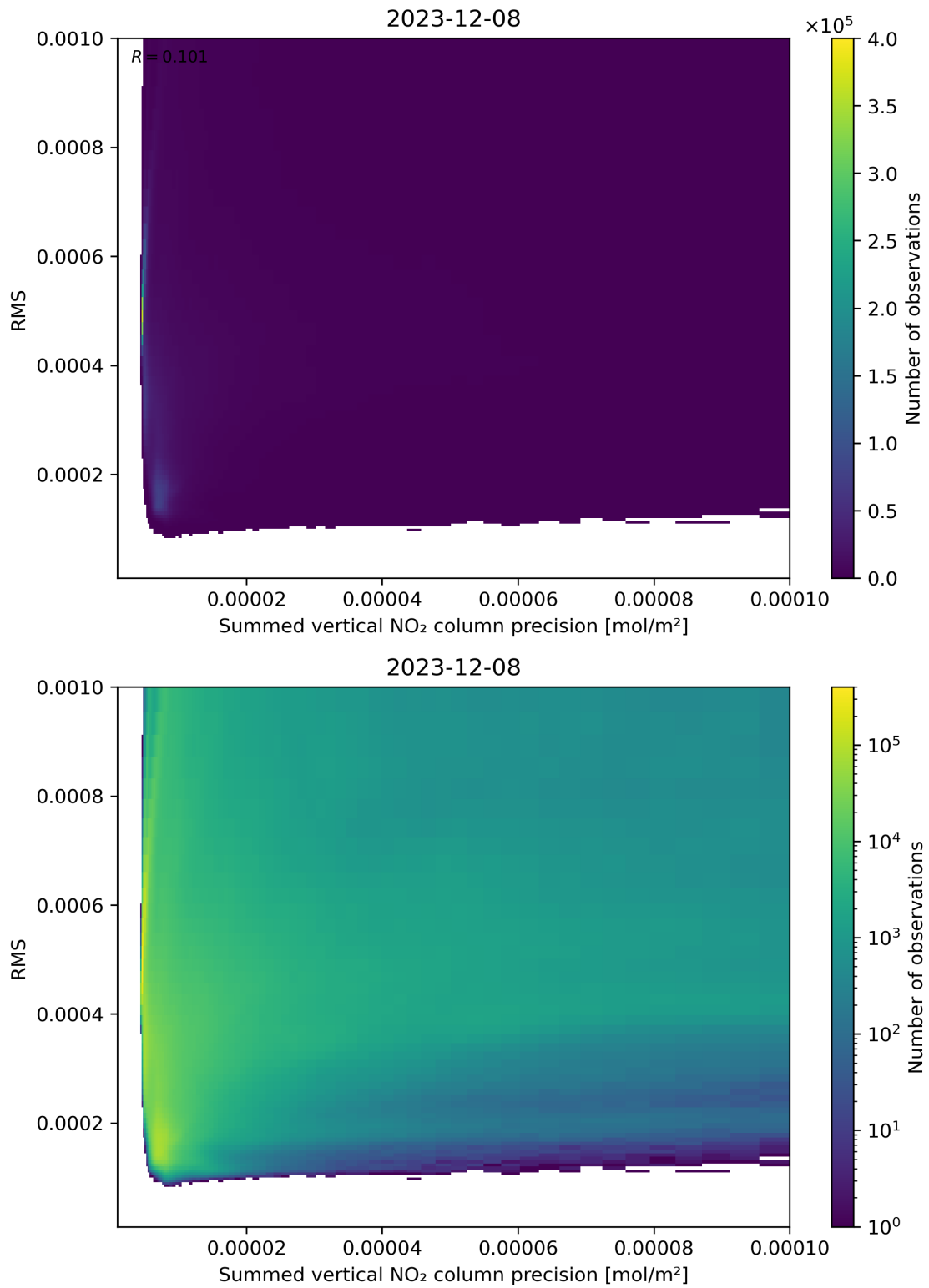
Figure 108: Scatter density plot of “Summed vertical NO 2 column precision” against “RMS” for 2023-12-07 to 2023-12-09.
