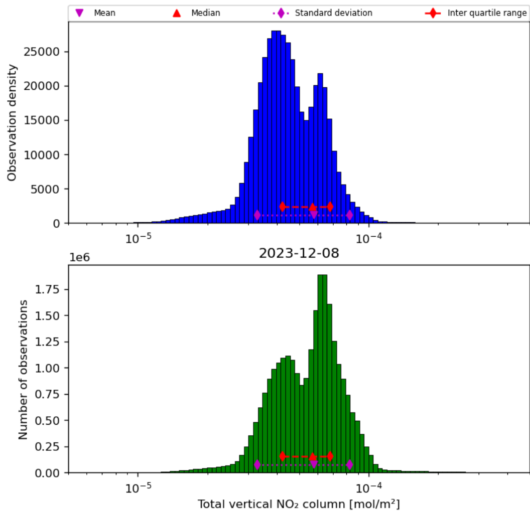
Figure 38: Histogram of “Total vertical NO 2 column” for 2023-12-07 to 2023-12-09
