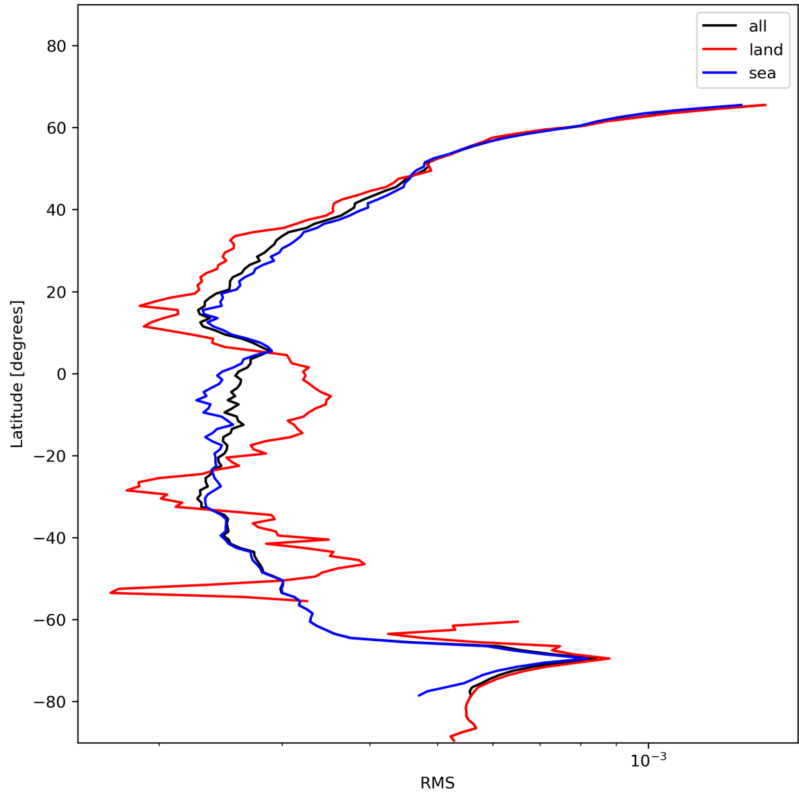
Figure 26: Zonal average of “RMS” for 2023-12-07 to 2023-12-09.
