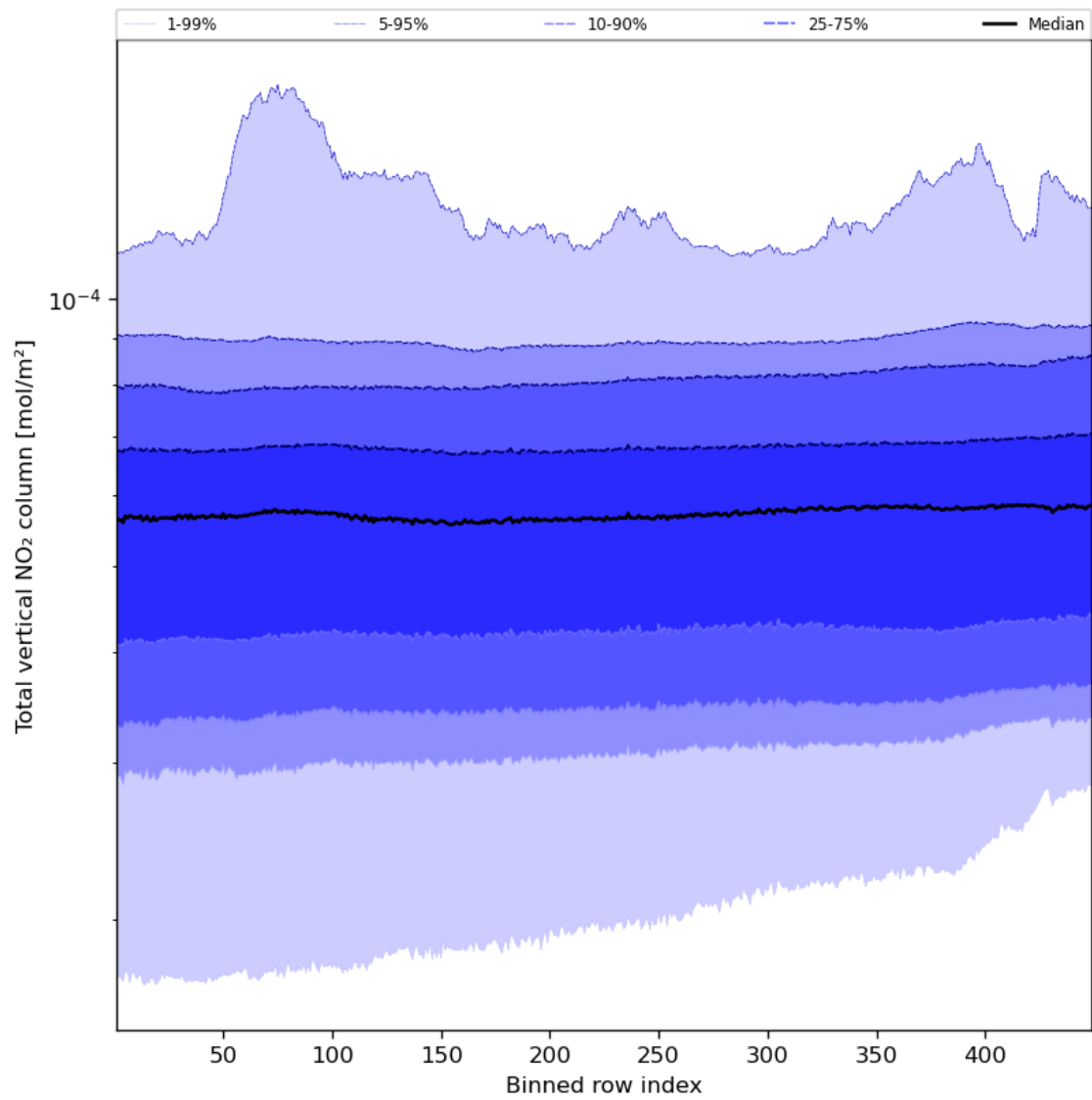
Figure 55: Along track statistics of “Total vertical NO 2 column” for 2023-12-07 to 2023-12-09
