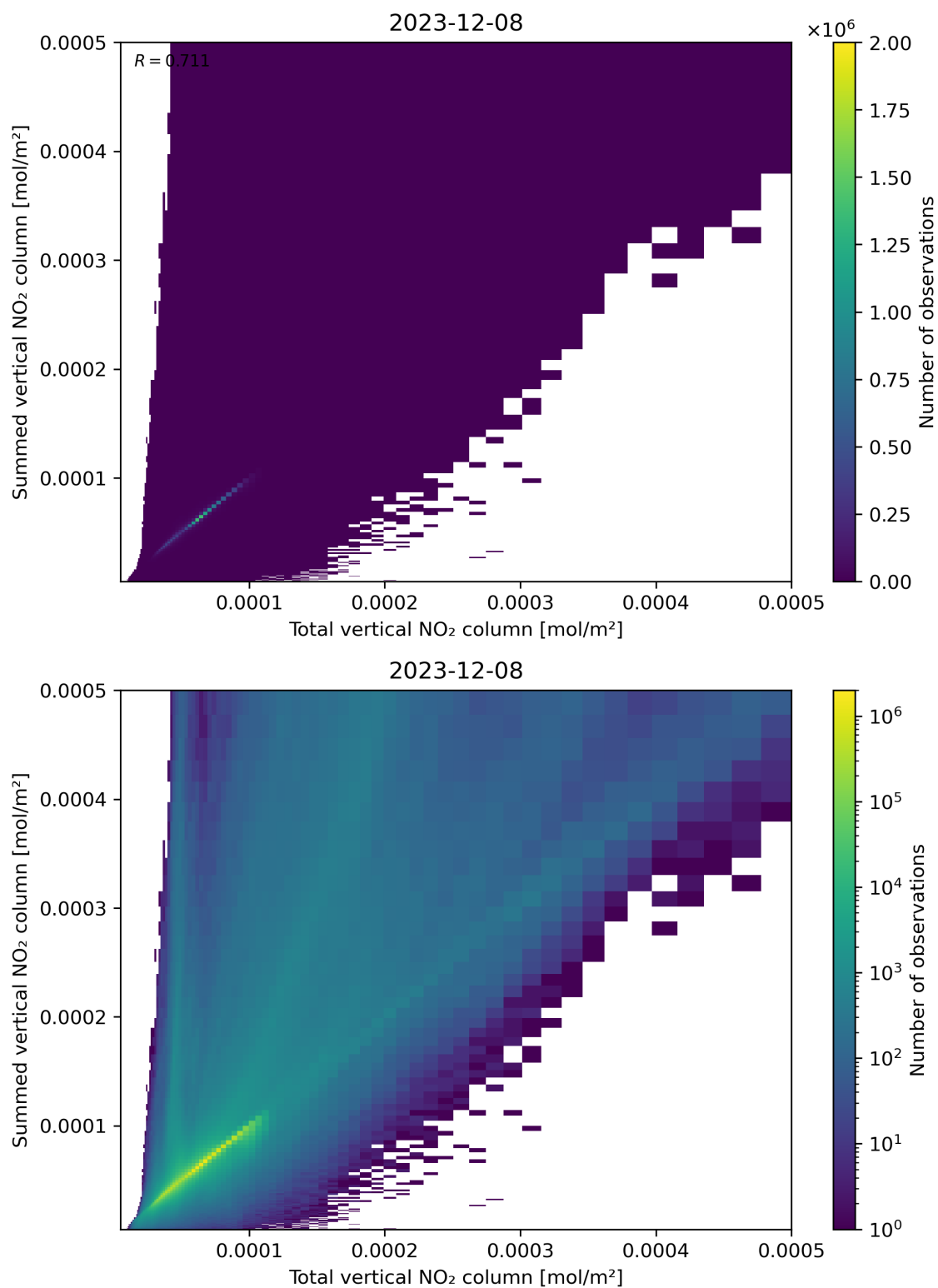
Figure 112: Scatter density plot of “Total vertical NO 2 column” against “Summed vertical NO 2 column” for 2023-12-07 to 2023-12-09.
