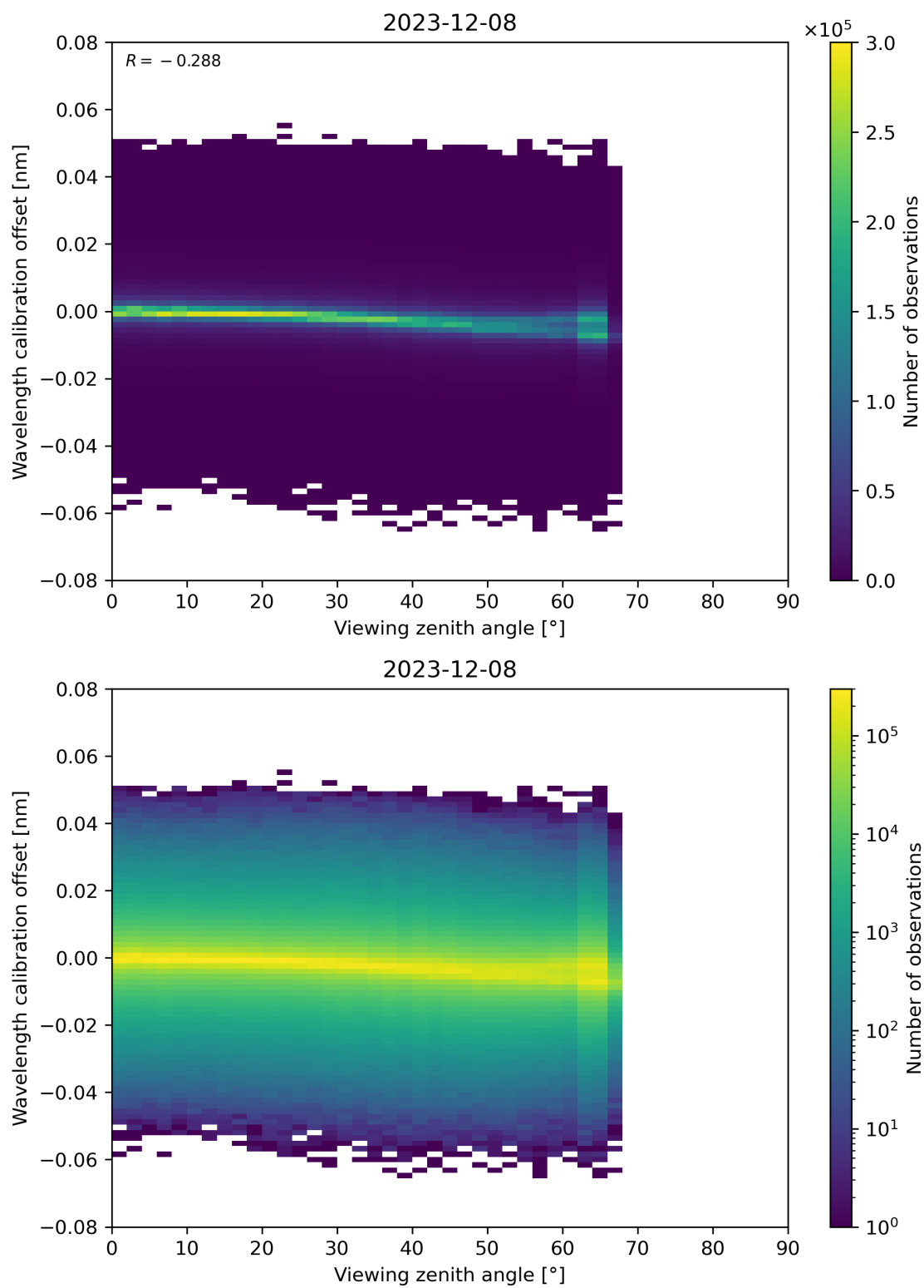
Figure 173: Scatter density plot of “Viewing zenith angle” against “Wavelength calibration offset” for 2023-12-07 to 2023-12-09.
