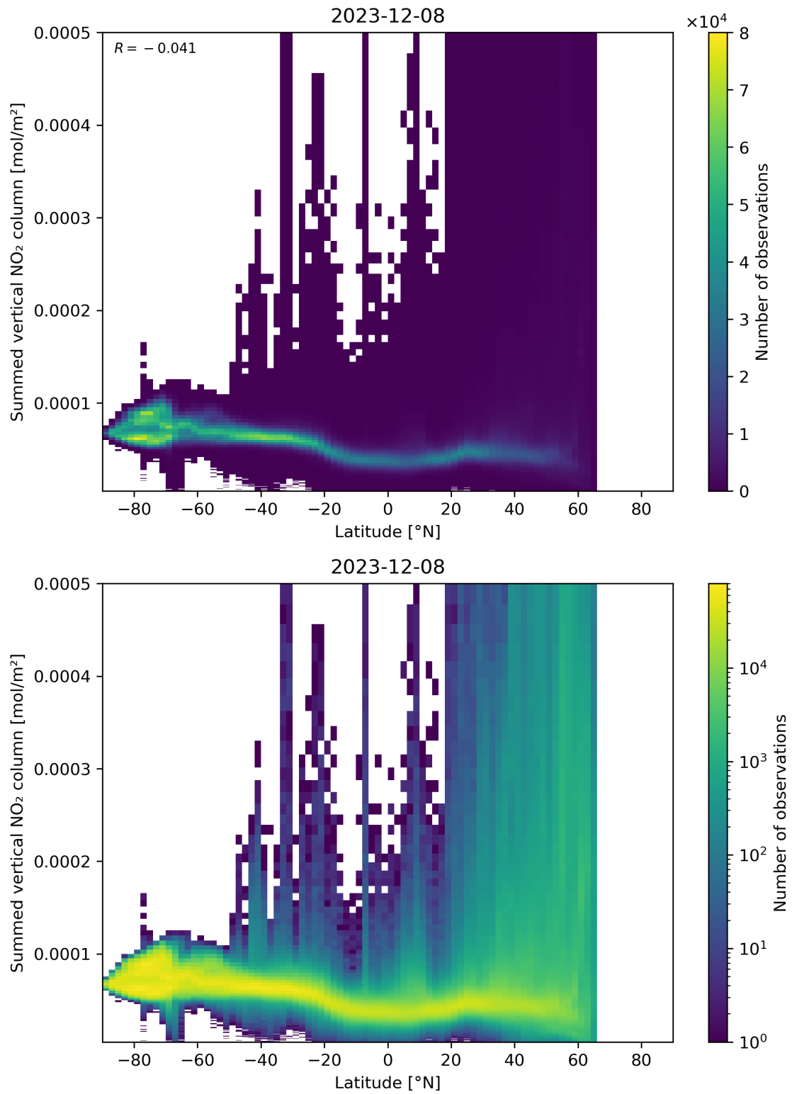
Figure 88: Scatter density plot of “Latitude” against “Summed vertical NO 2 column” for 2023-12-07 to 2023-12-09.
