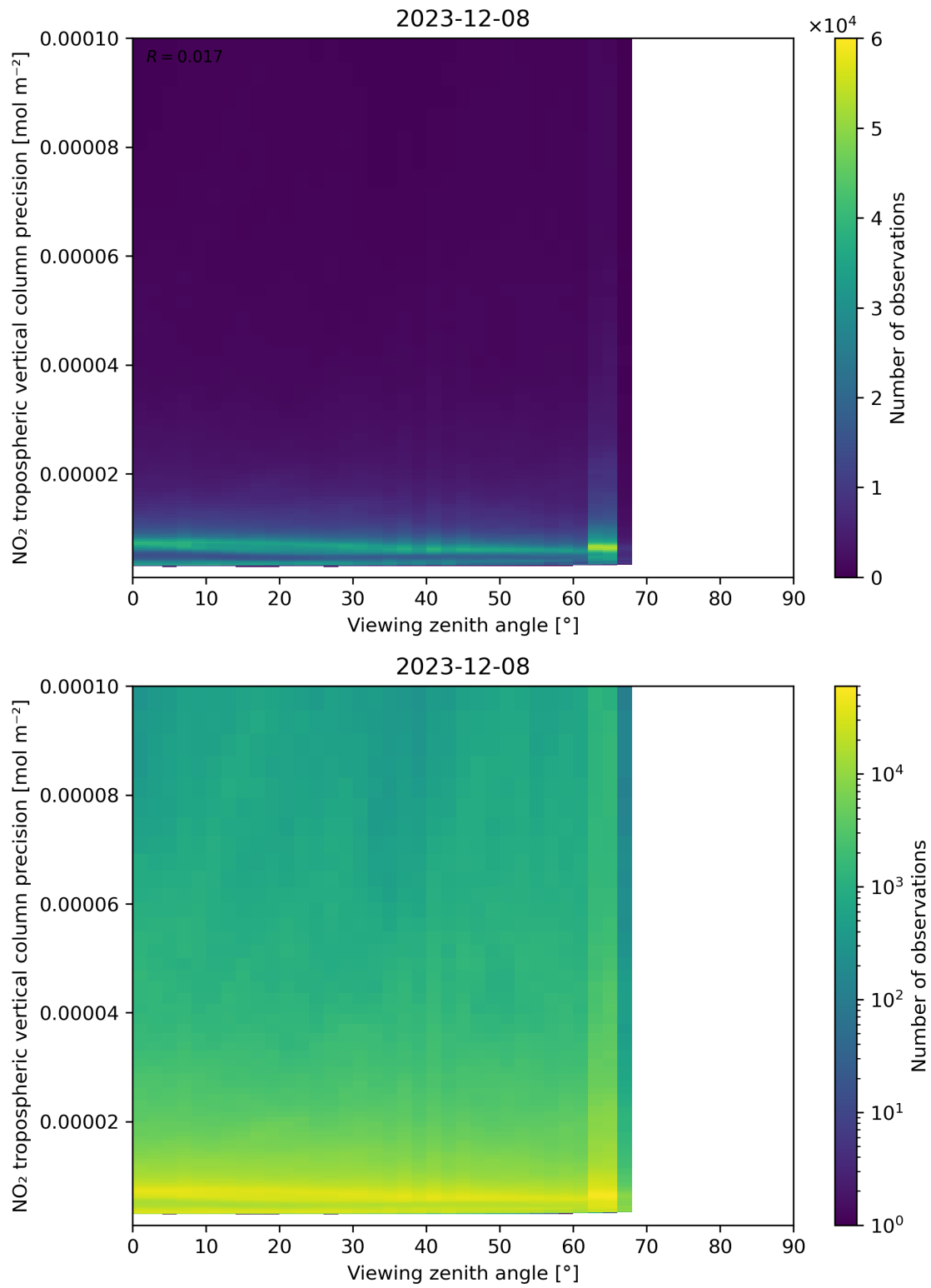
Figure 170: Scatter density plot of “Viewing zenith angle” against “NO 2 tropospheric vertical column precision” for 2023-12-07 to 2023-12-09.
