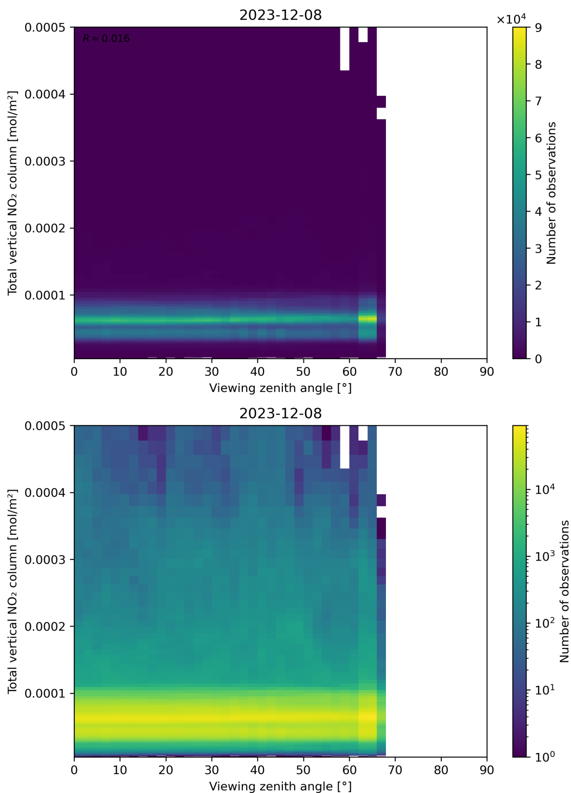
Figure 167: Scatter density plot of “Viewing zenith angle” against “Total vertical NO 2 column” for 2023-12-07 to 2023-12-09.
