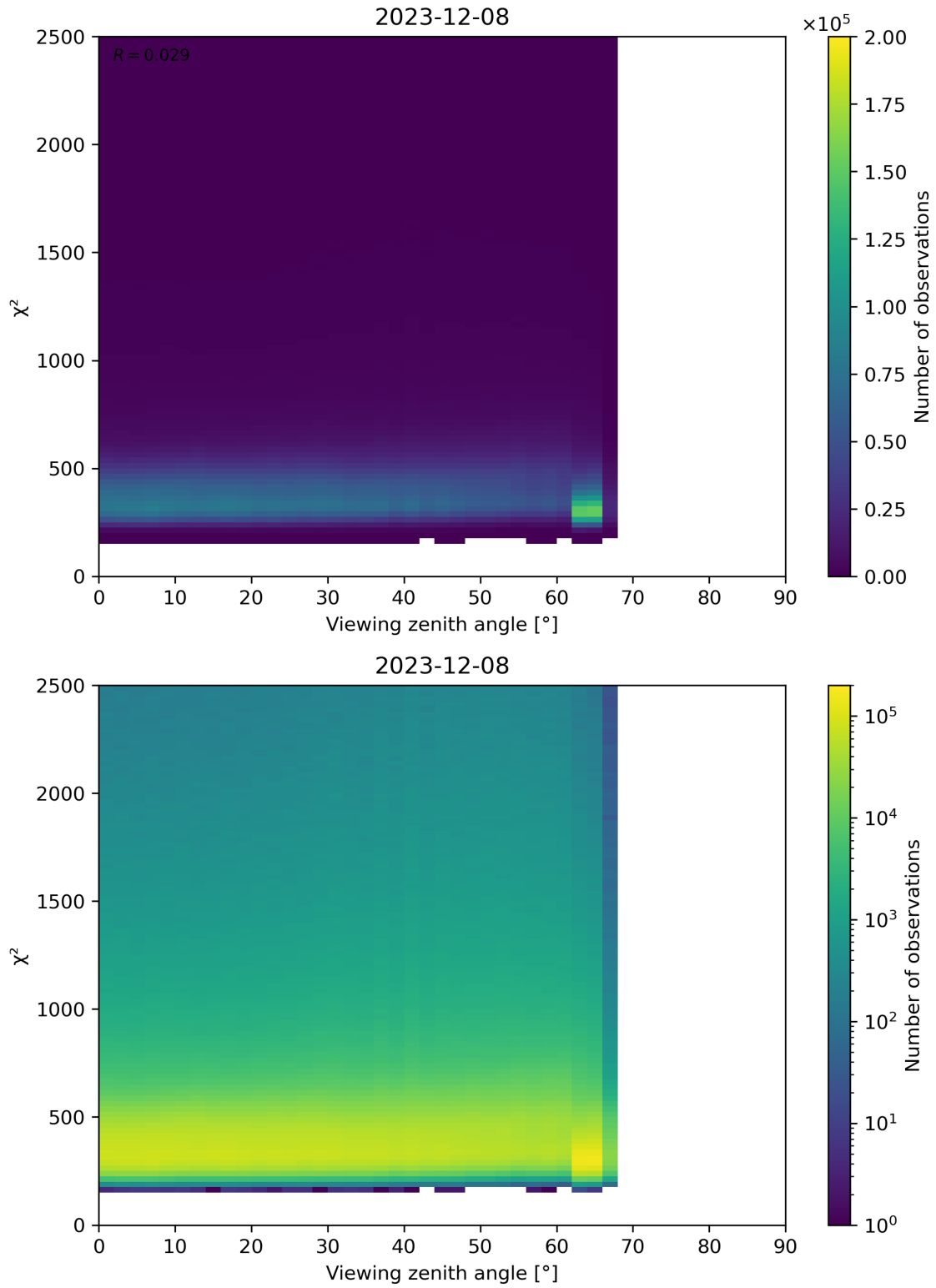
Figure 162: Scatter density plot of “Viewing zenith angle” against “ \chi^2 ” for 2023-12-07 to 2023-12-09.
