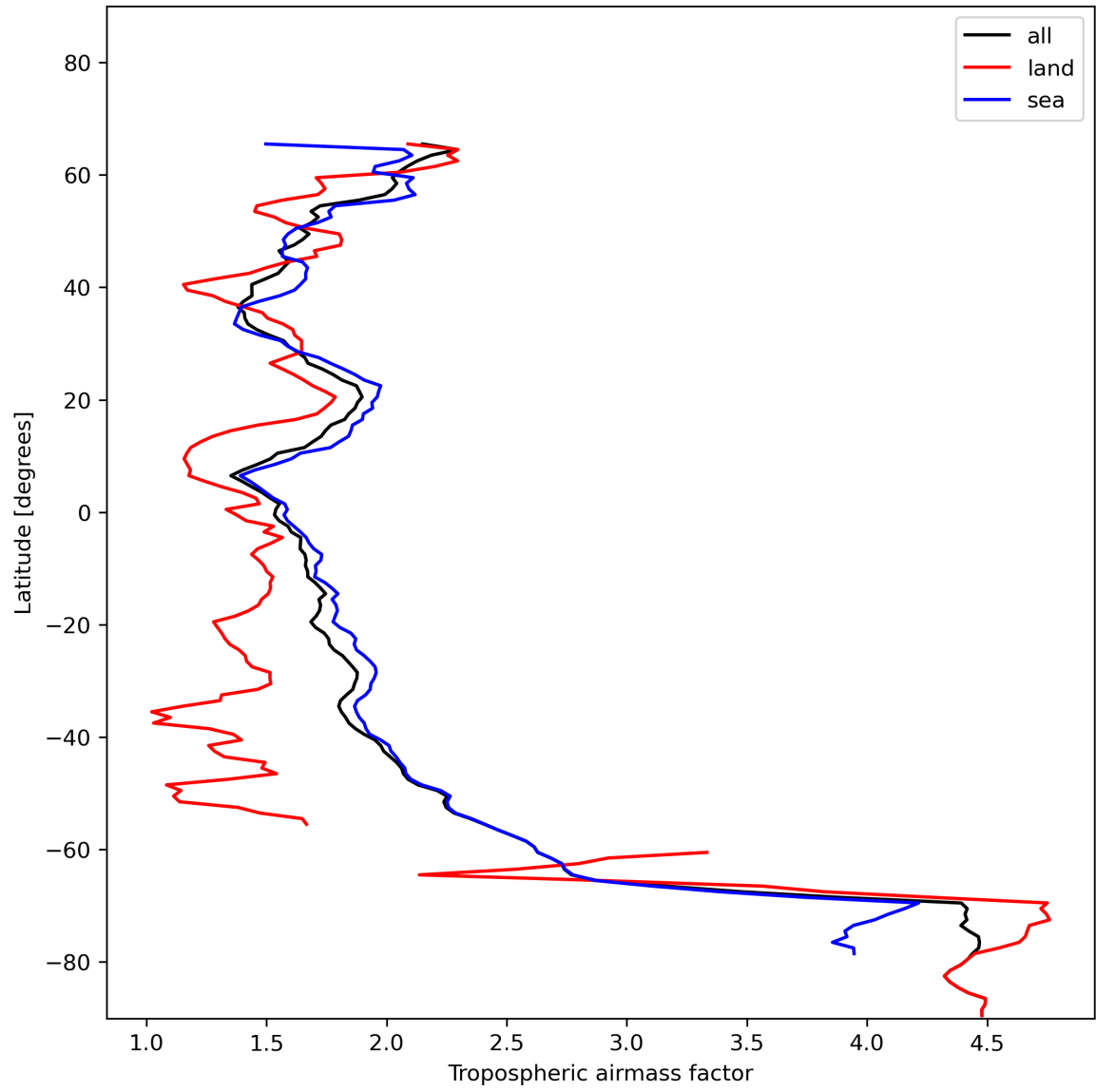
Figure 14: Zonal average of “Tropospheric airmass factor” for 2023-12-07 to 2023-12-09.
