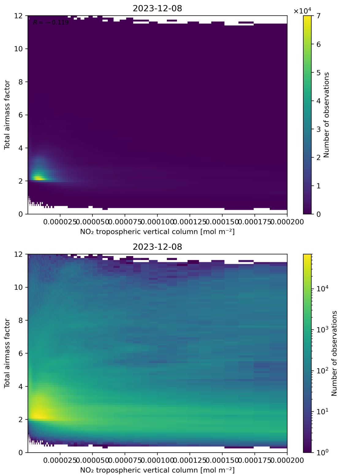
Figure 122: Scatter density plot of “NO 2 tropospheric vertical column” against “Total air mass factor” for 2023-12-07 to 2023-12-09.
