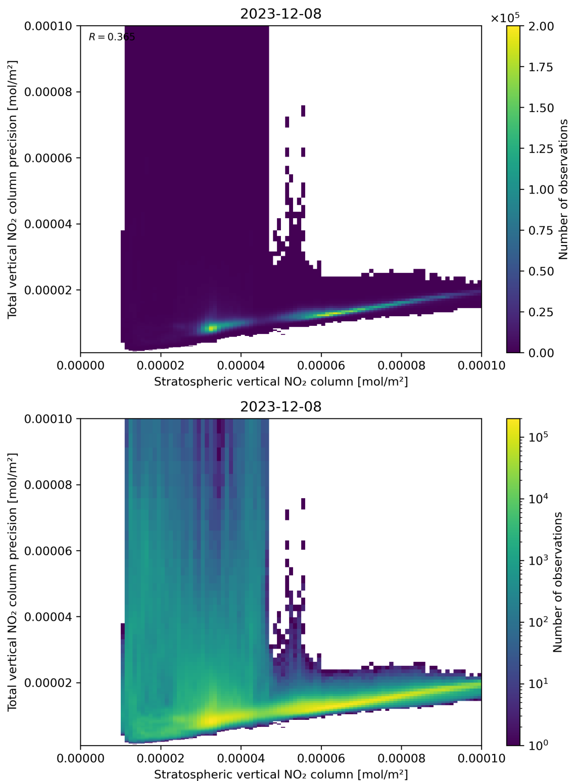
Figure 101: Scatter density plot of “Stratospheric vertical NO 2 column” against “Total vertical NO 2 column precision” for 2023-12-07 to 2023-12-09.
