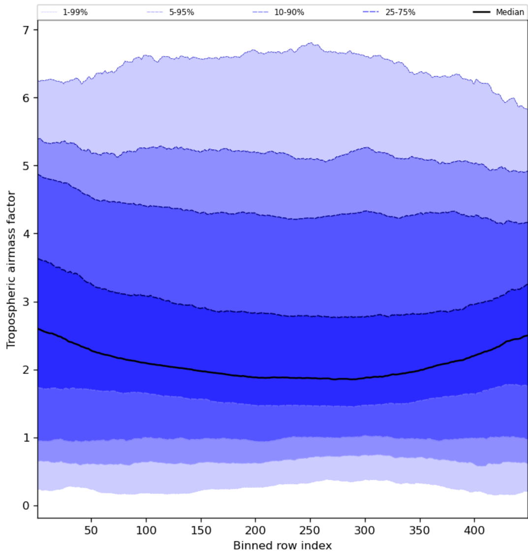
Figure 48: Along track statistics of “Tropospheric airmass factor” for 2023-12-07 to 2023-12-09
