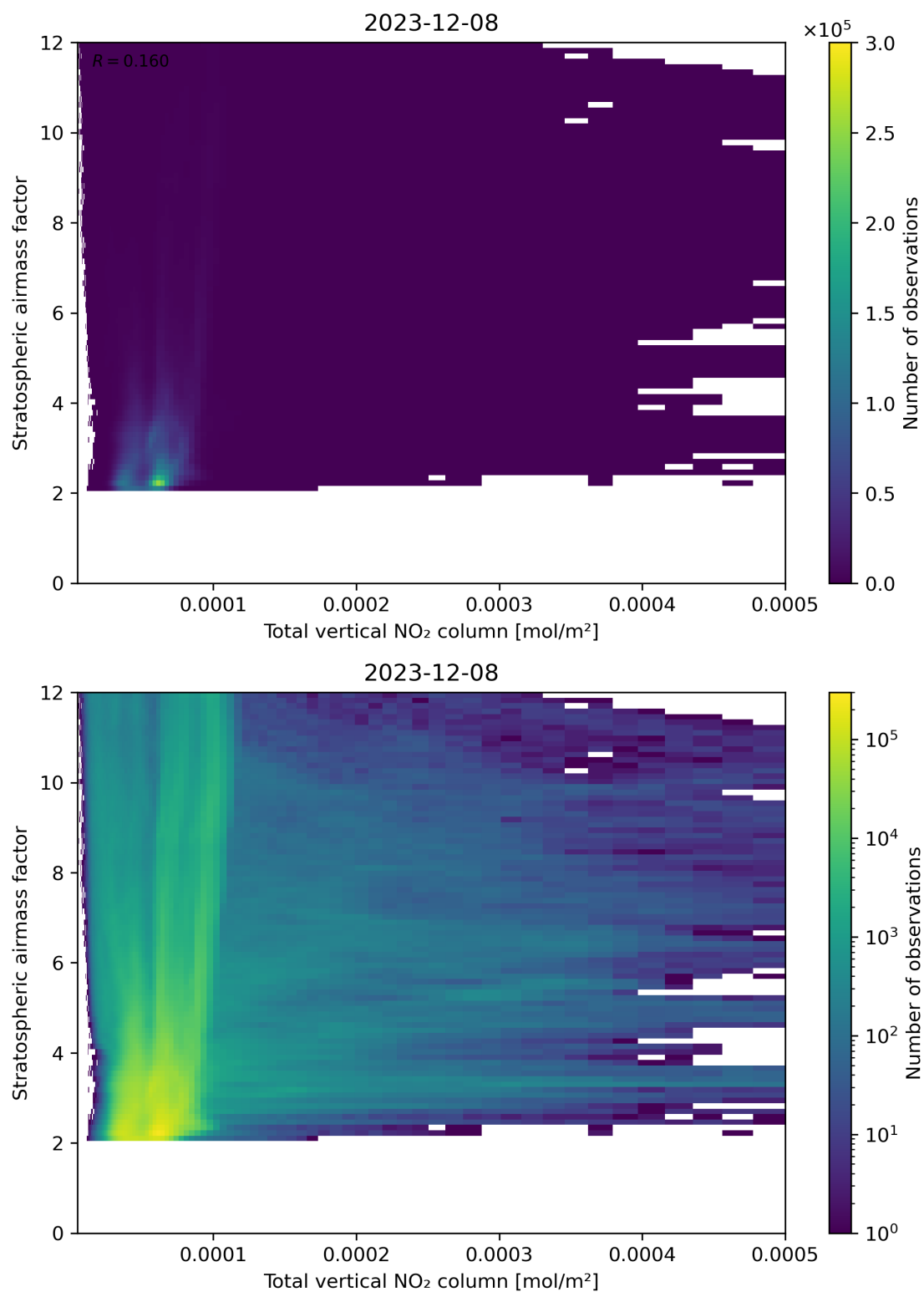
Figure 110: Scatter density plot of “Total vertical NO 2 column” against “Stratospheric airmass factor” for 2023-12-07 to 2023-12-09.
