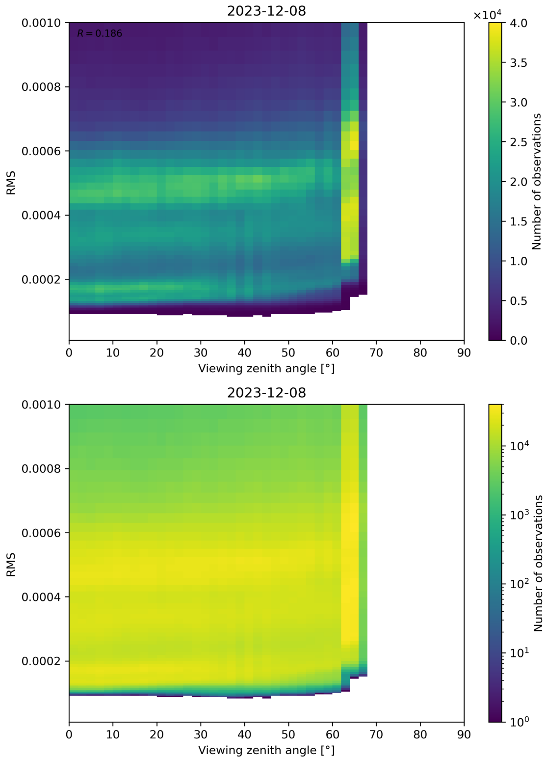
Figure 171: Scatter density plot of “Viewing zenith angle” against “RMS” for 2023-12-07 to 2023-12-09.
