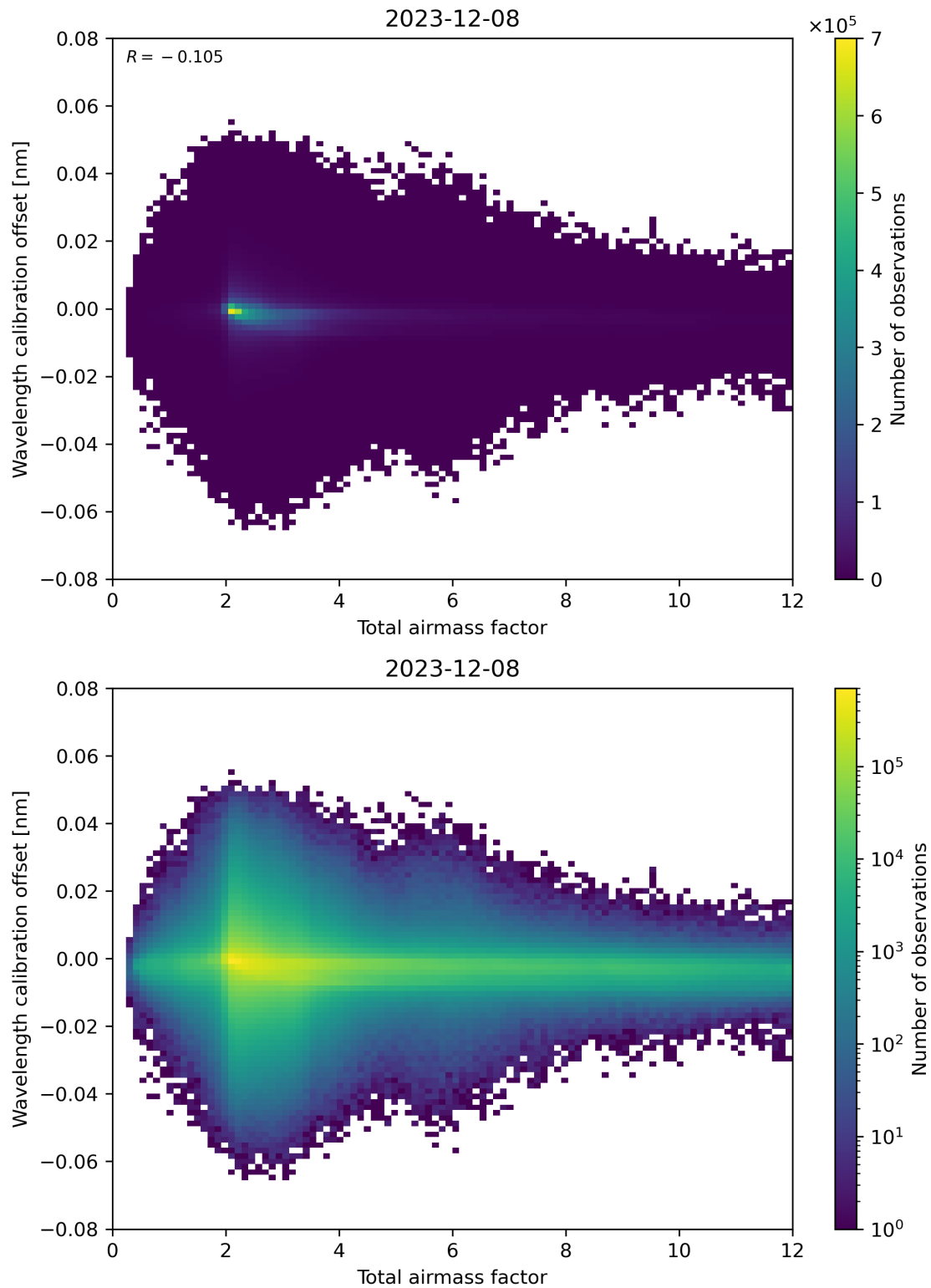
Figure 70: Scatter density plot of “Total airmass factor” against “Wavelength calibration offset” for 2023-12-07 to 2023-12-09.
