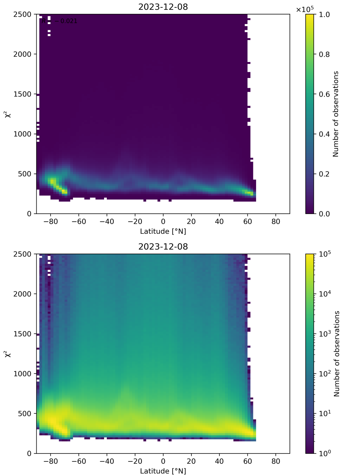
Figure 86: Scatter density plot of “Latitude” against “ \chi^2 ” for 2023-12-07 to 2023-12-09.
