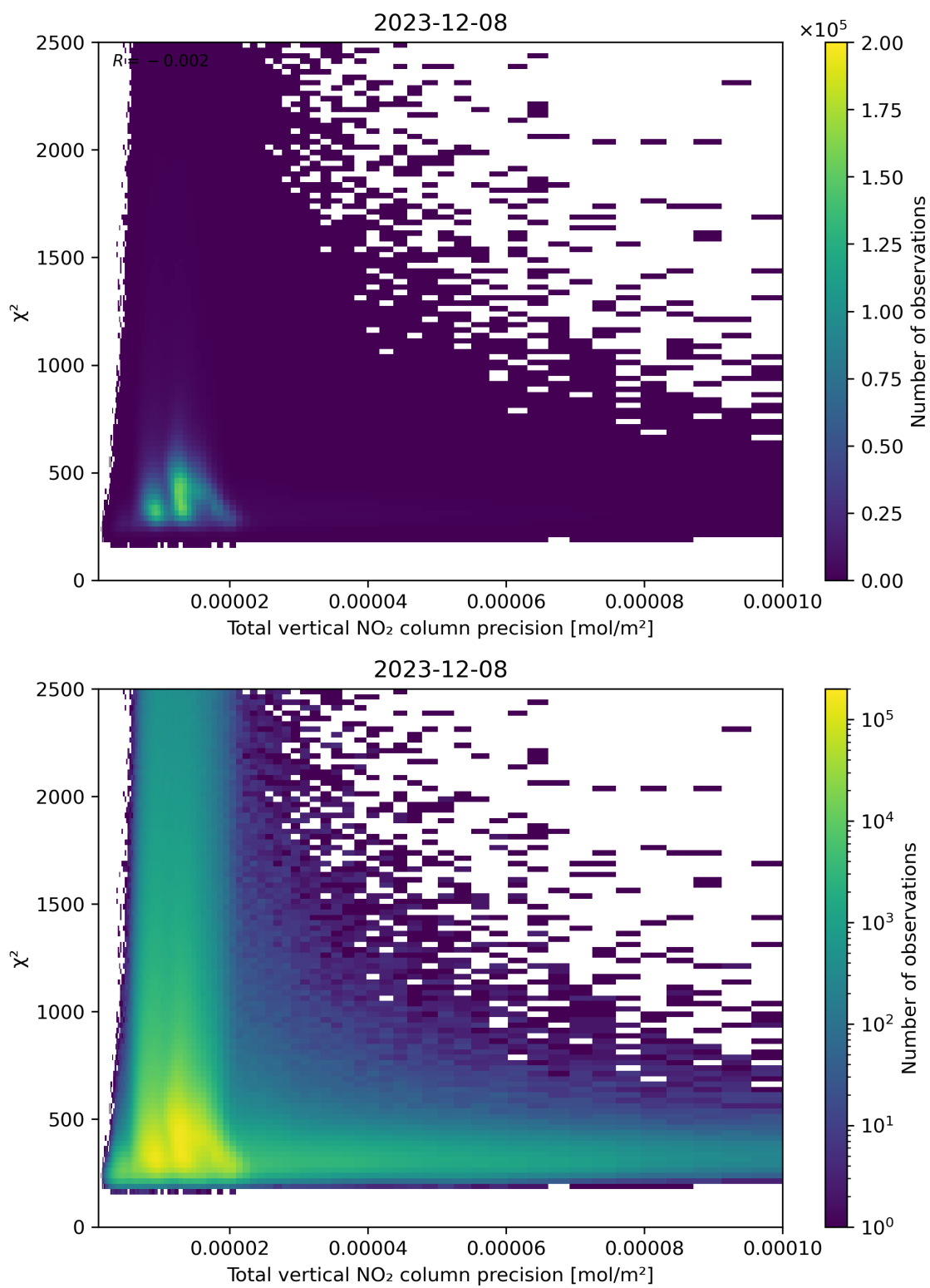
Figure 116: Scatter density plot of “Total vertical NO 2 column precision” against “ \chi^2 ” for 2023-12-07 to 2023-12-09.
