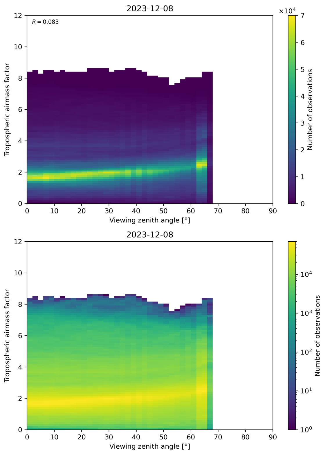
Figure 161: Scatter density plot of “Viewing zenith angle” against “Tropospheric airmass factor” for 2023-12-07 to 2023-12-09.
