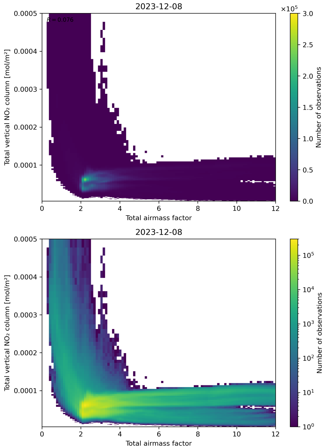
Figure 67: Scatter density plot of “Total airmass factor” against “Total vertical NO 2 column” for 2023-12-07 to 2023-12-09.
