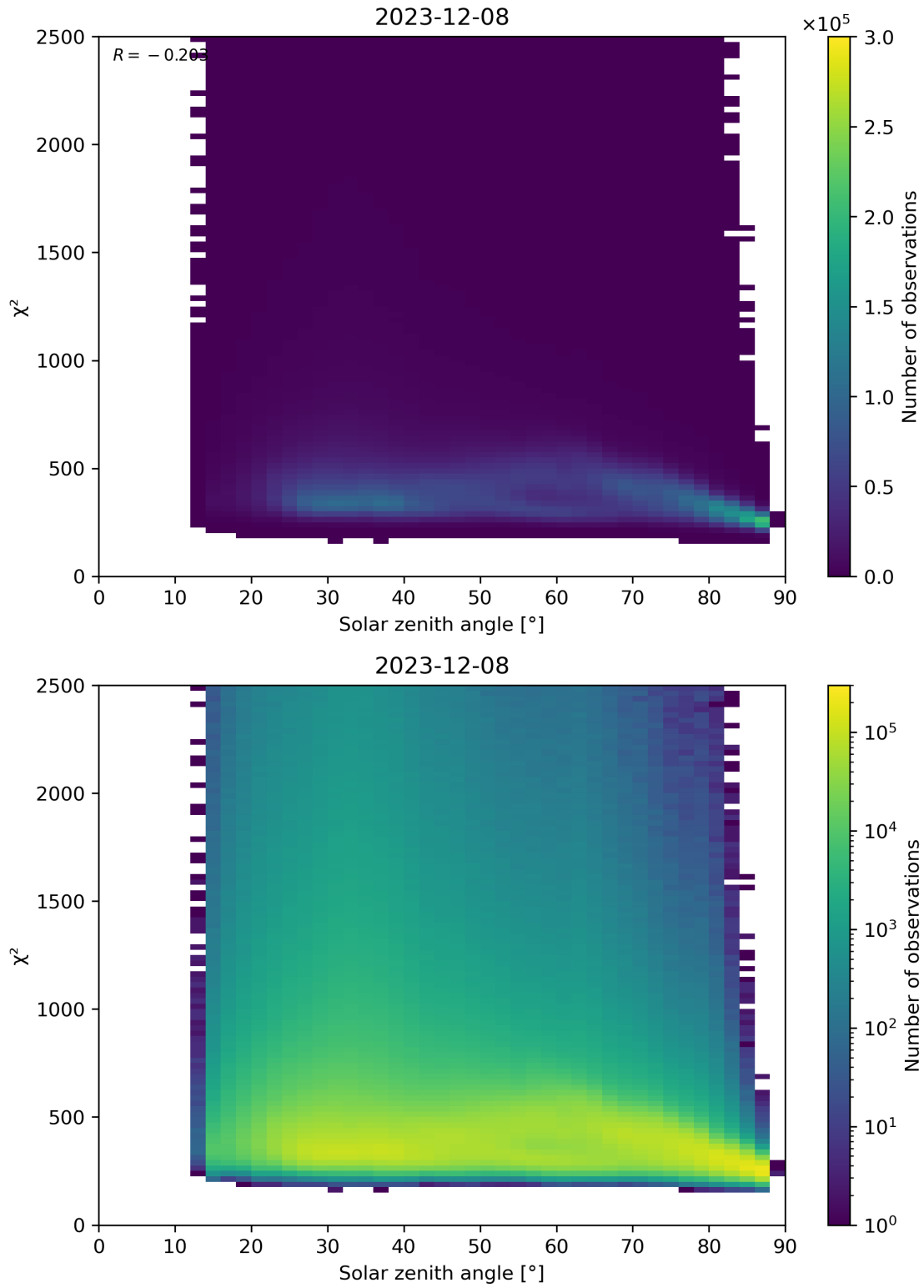
Figure 148: Scatter density plot of “Solar zenith angle” against “ \chi^2 ” for 2023-12-07 to 2023-12-09.
