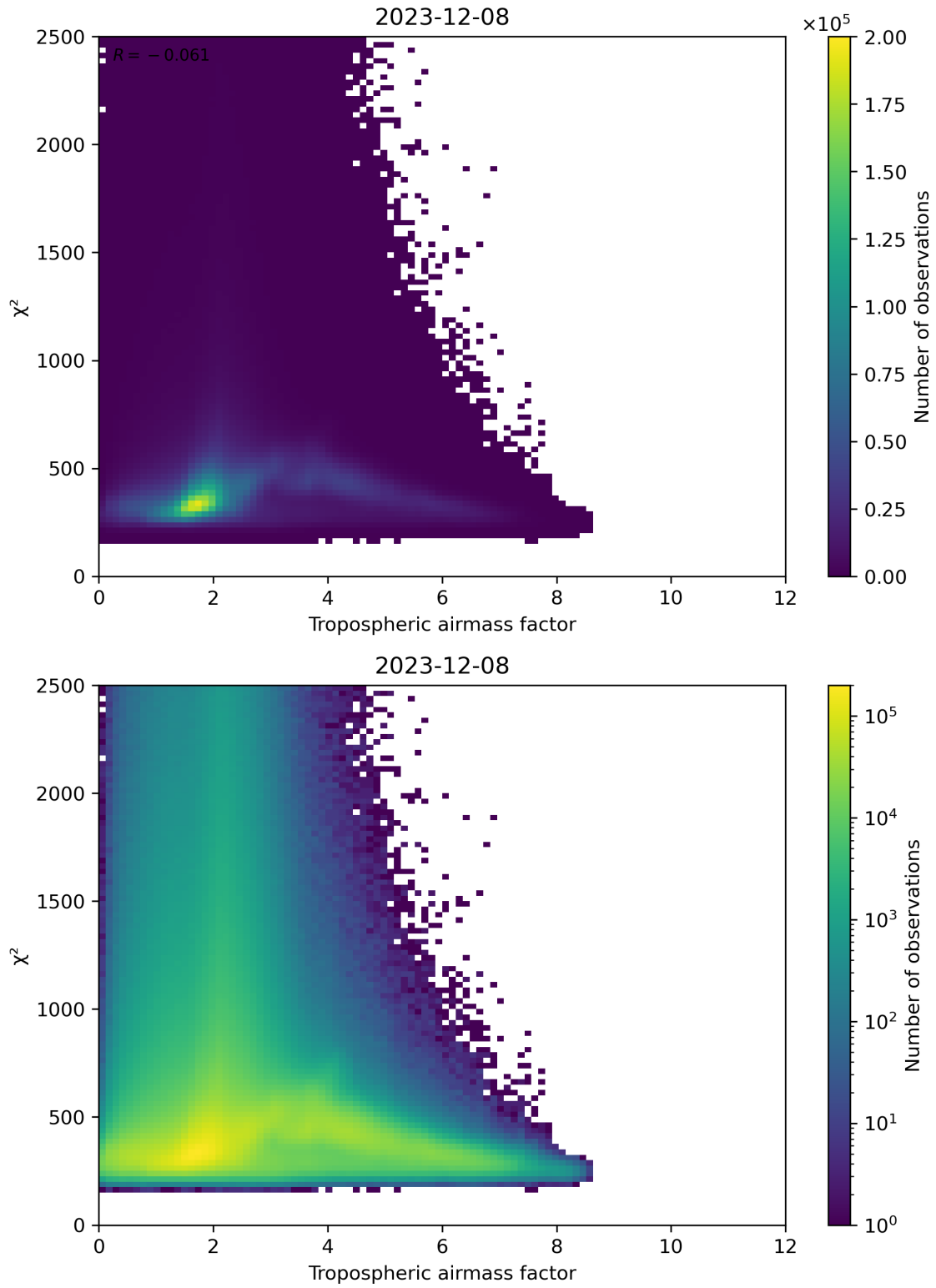
Figure 73: Scatter density plot of “Tropospheric airmass factor” against “ \chi^2 ” for 2023-12-07 to 2023-12-09.
