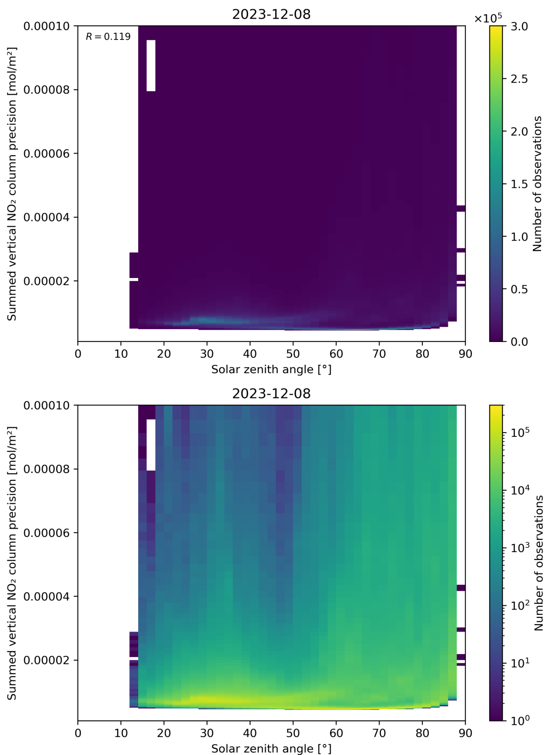
Figure 152: Scatter density plot of “Solar zenith angle” against “Summed vertical NO 2 column precision” for 2023-12-07 to 2023-12-09.
