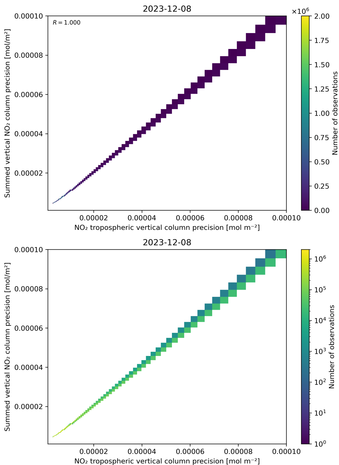
Figure 137: Scatter density plot of “NO 2 tropospheric vertical column precision” against “Summed vertical NO 2 column precision” for 2023-12-07 to 2023-12-09.
