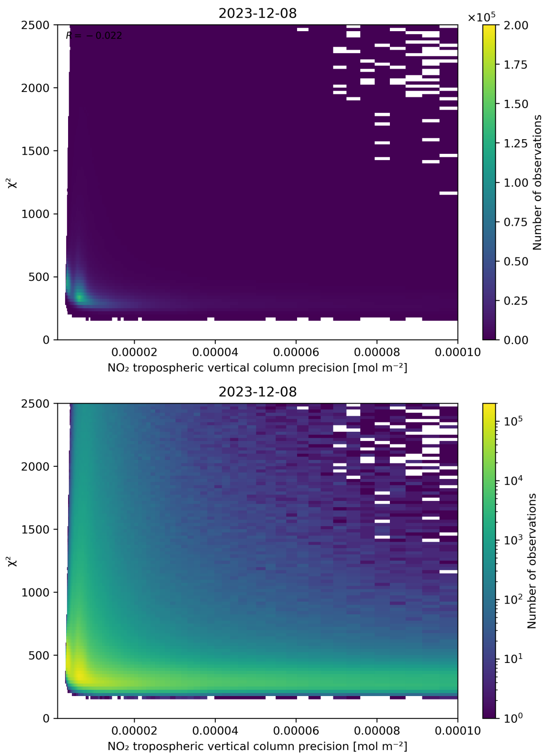
Figure 134: Scatter density plot of “NO 2 tropospheric vertical column precision” against “ \chi^2 ” for 2023-12-07 to 2023-12-09.
