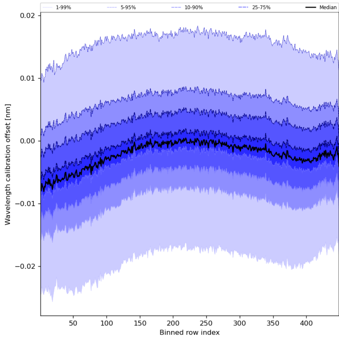
Figure 52: Along track statistics of “Wavelength calibration offset” for 2023-12-07 to 2023-12-09
