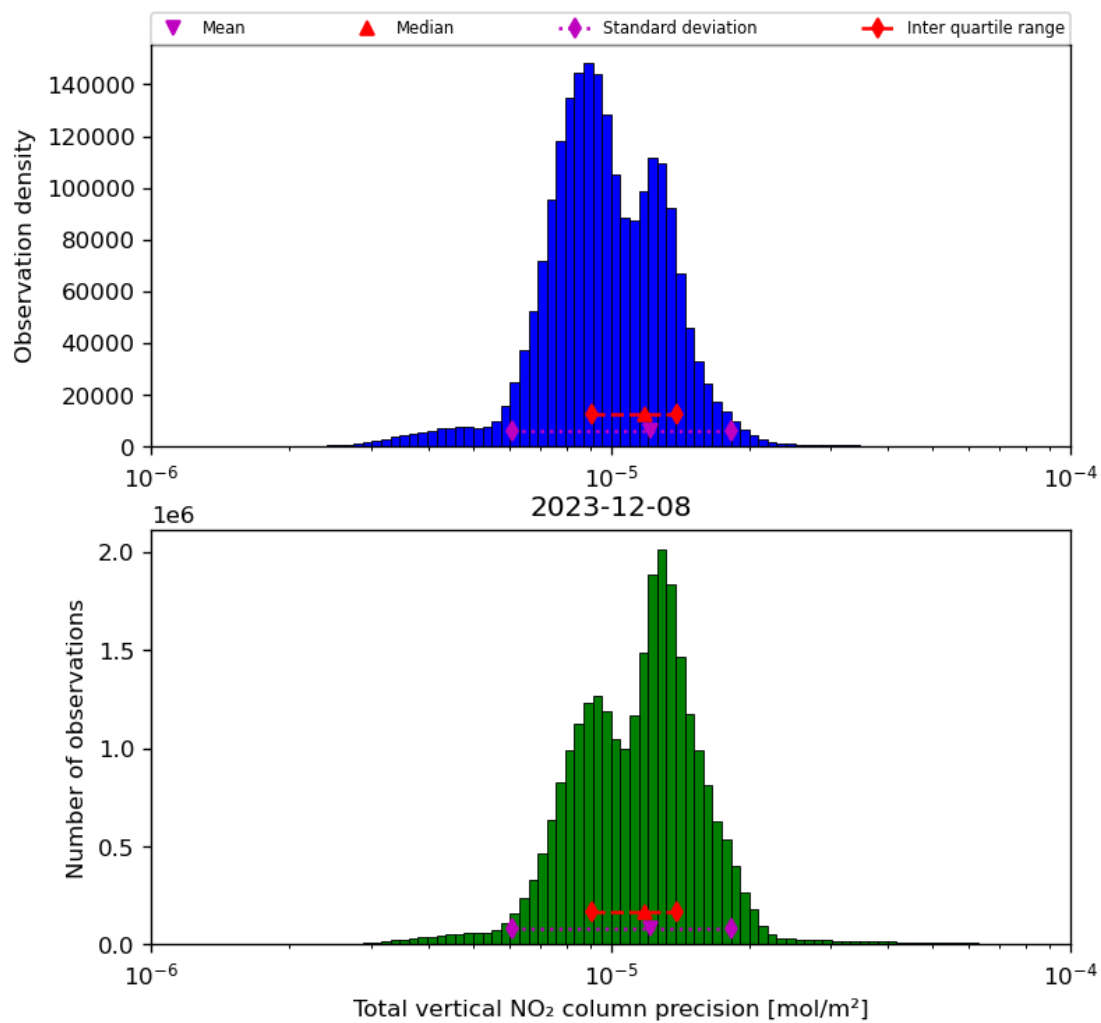
Figure 39: Histogram of "Total vertical NO 2 column precision" for 2023-12-07 to 2023-12-09
