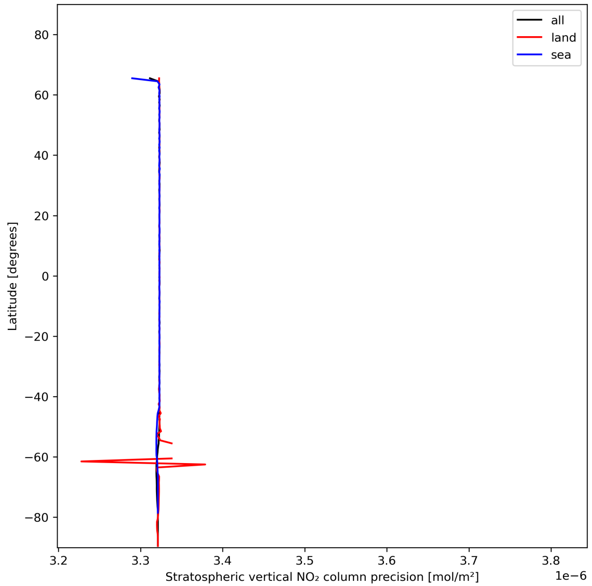
Figure 20: Zonal average of "Stratospheric vertical NO 2 column precision" for 2023-12-07 to 2023-12-09.
