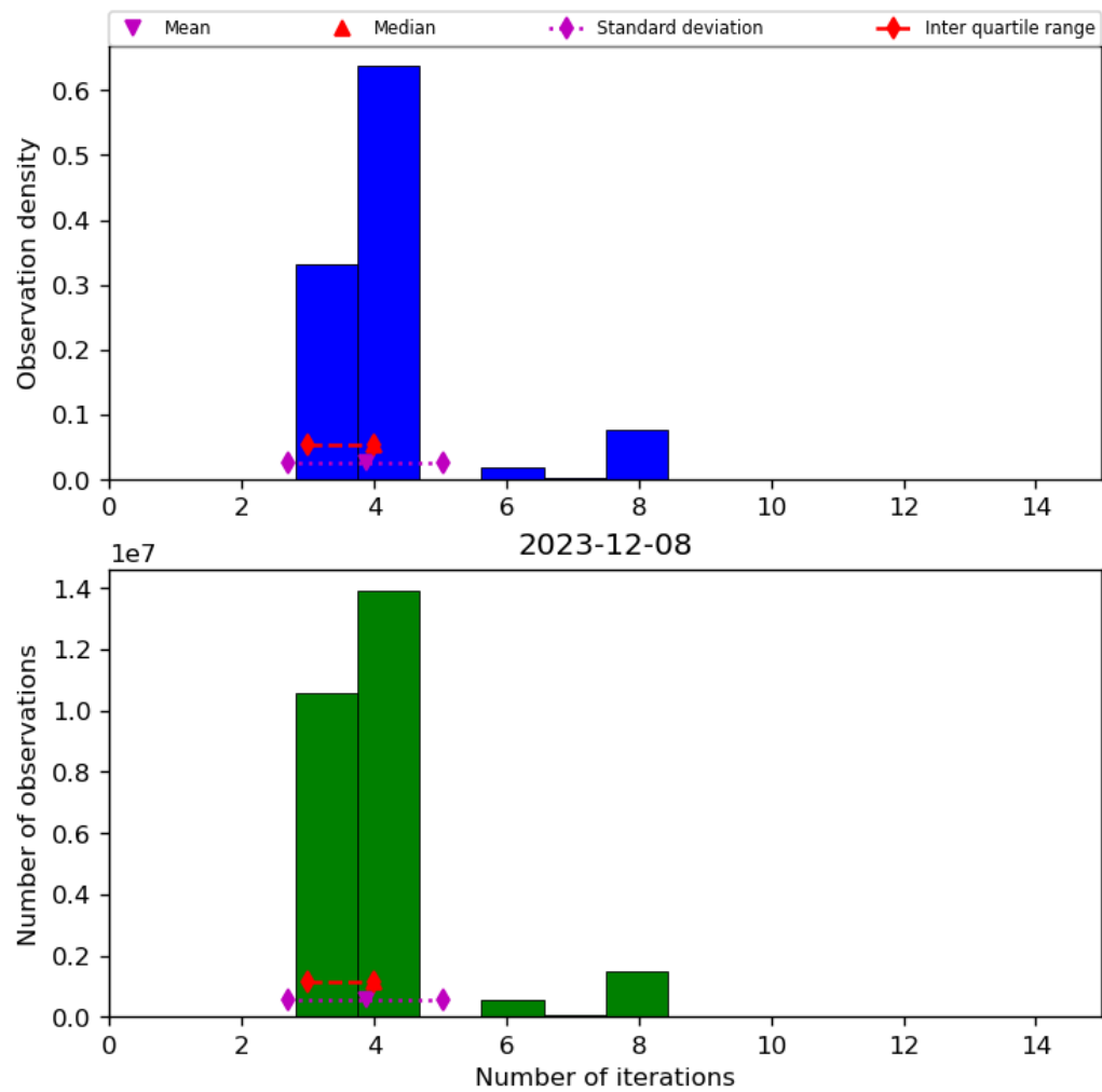
Figure 34: Histogram of “Number of iterations” for 2023-12-07 to 2023-12-09
