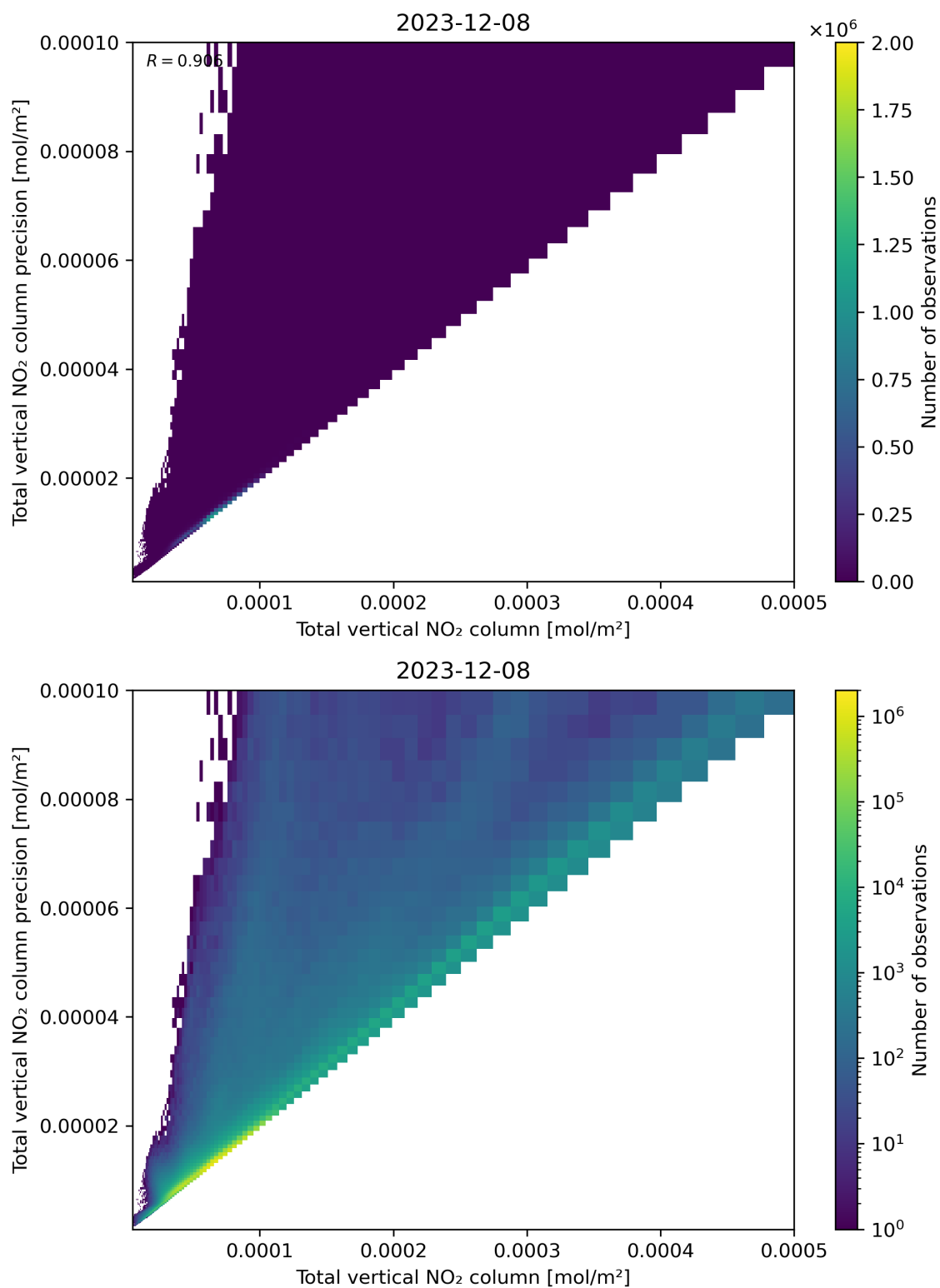
Figure 114: Scatter density plot of “Total vertical NO 2 column” against “Total vertical NO 2 column precision” for 2023-12-07 to 2023-12-09.
