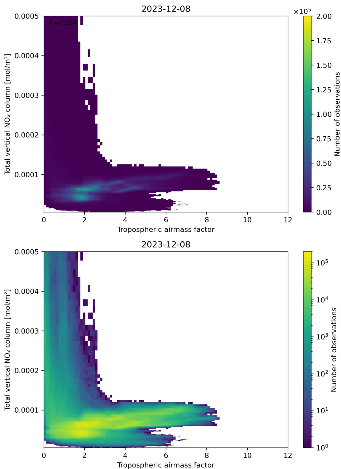
Figure 77: Scatter density plot of “Tropospheric airmass factor” against “Total vertical NO 2 column” for 2023-12-07 to 2023-12-09.
