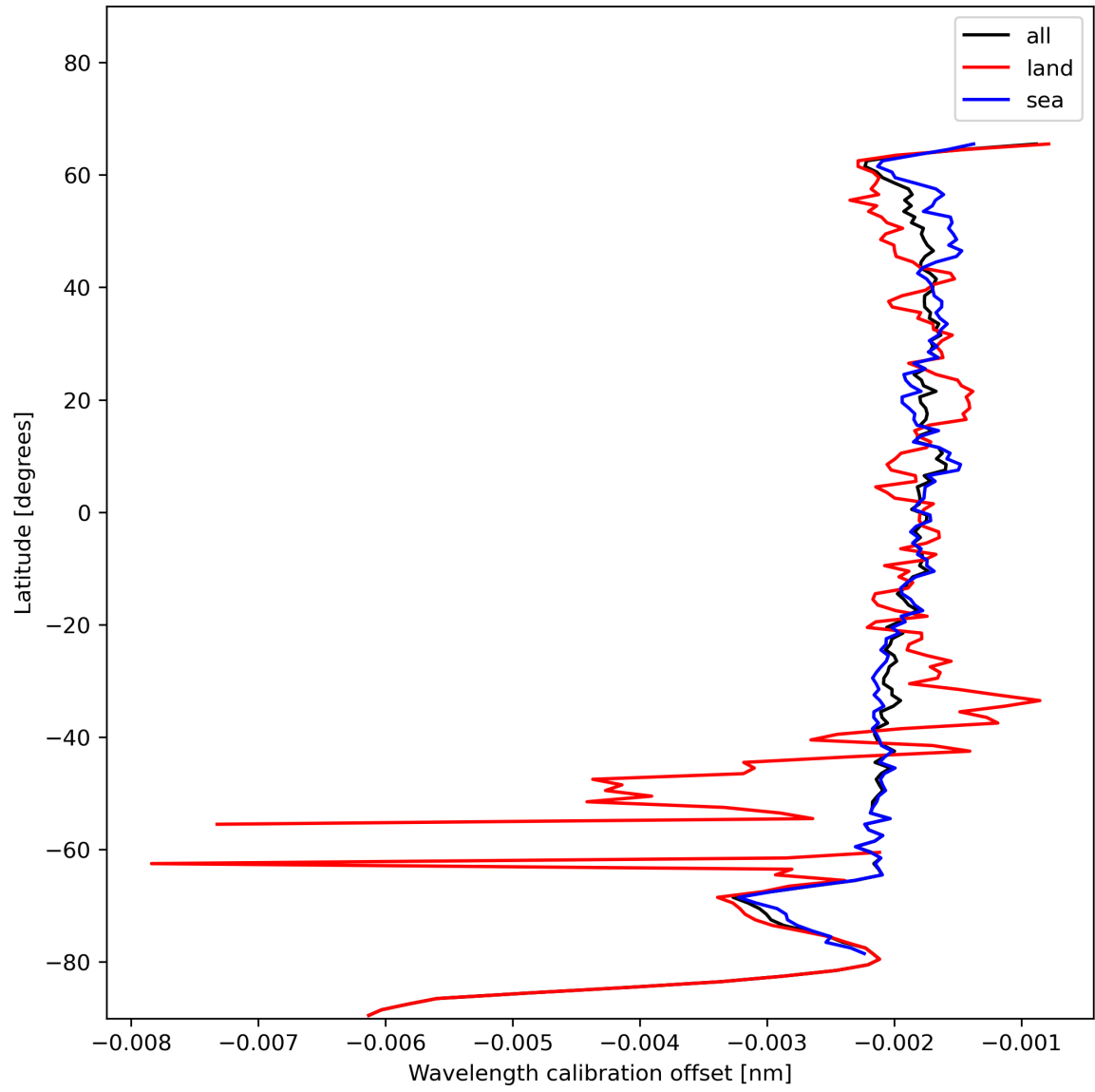
Figure 18: Zonal average of “Wavelength calibration offset” for 2023-12-07 to 2023-12-09.
