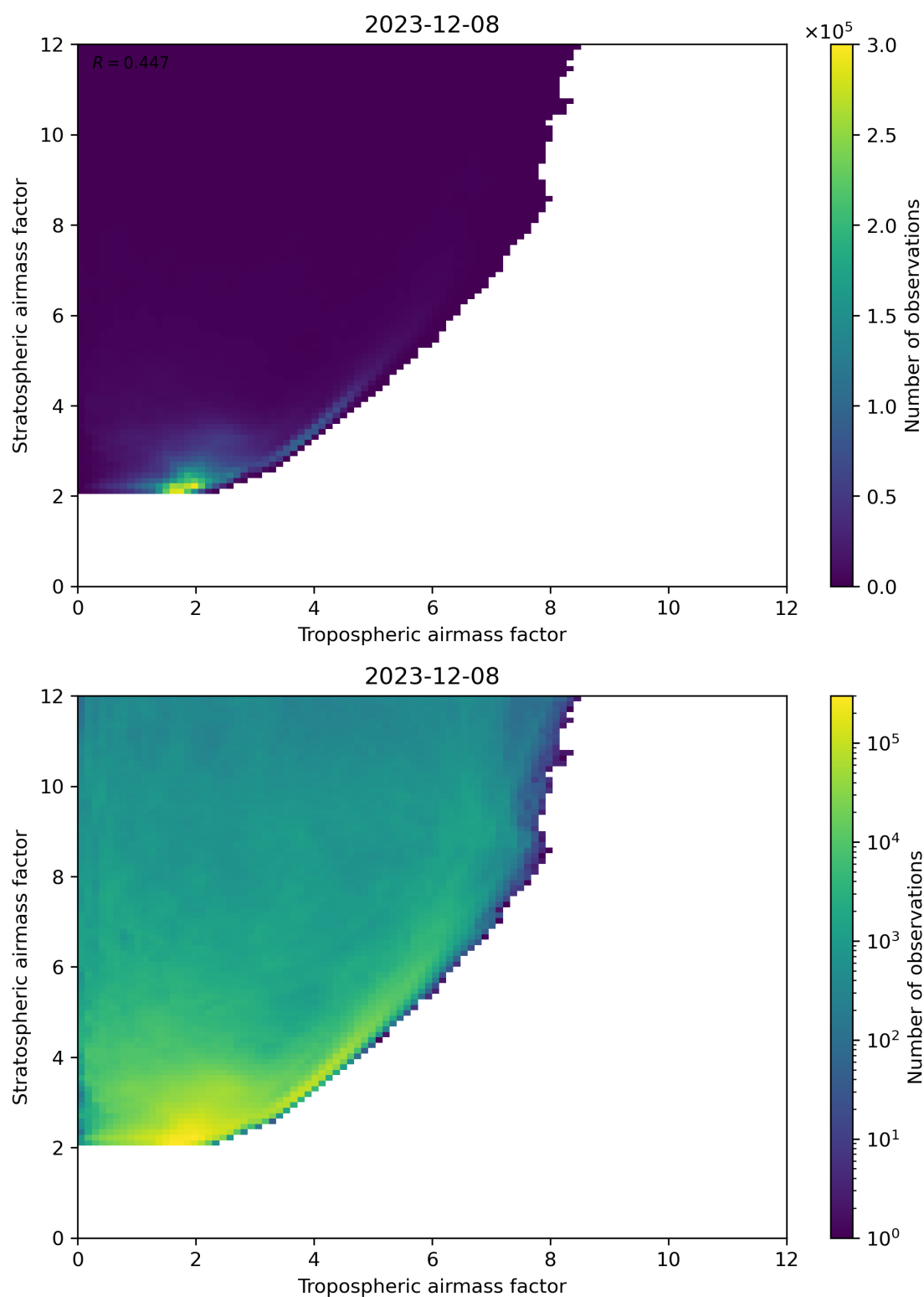
Figure 71: Scatter density plot of “Tropospheric airmass factor” against “Stratospheric airmass factor” for 2023-12-07 to 2023-12-09.
