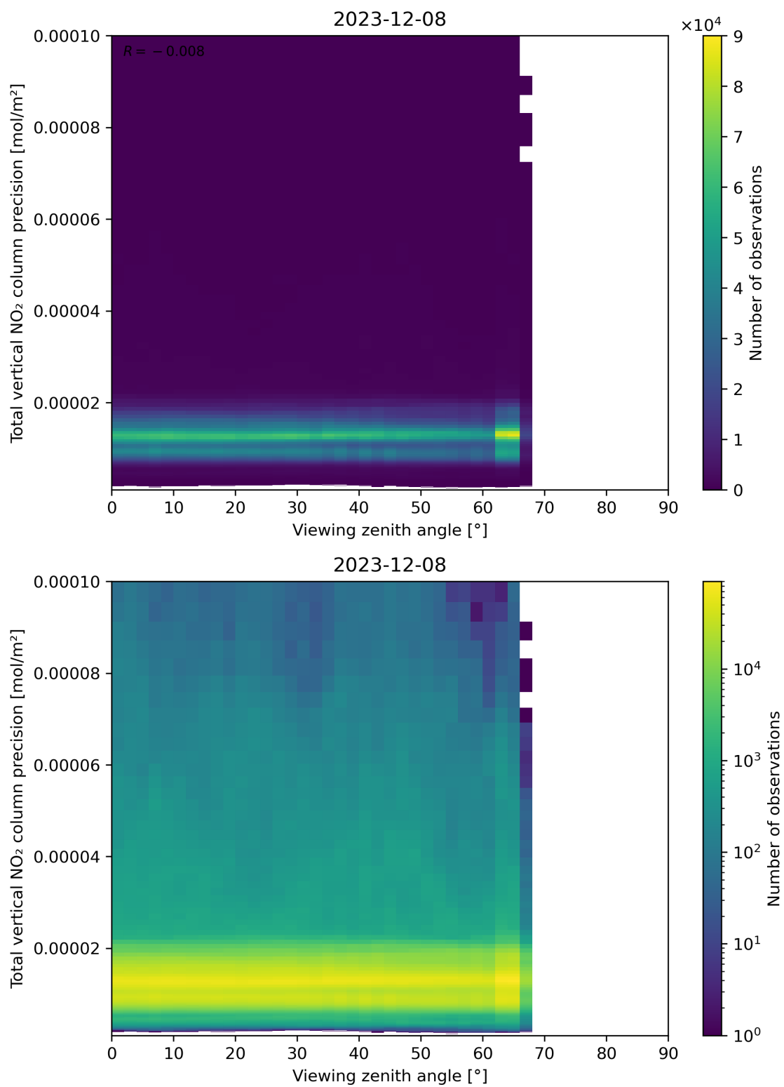
Figure 168: Scatter density plot of “Viewing zenith angle” against “Total vertical NO 2 column precision” for 2023-12-07 to 2023-12-09.
