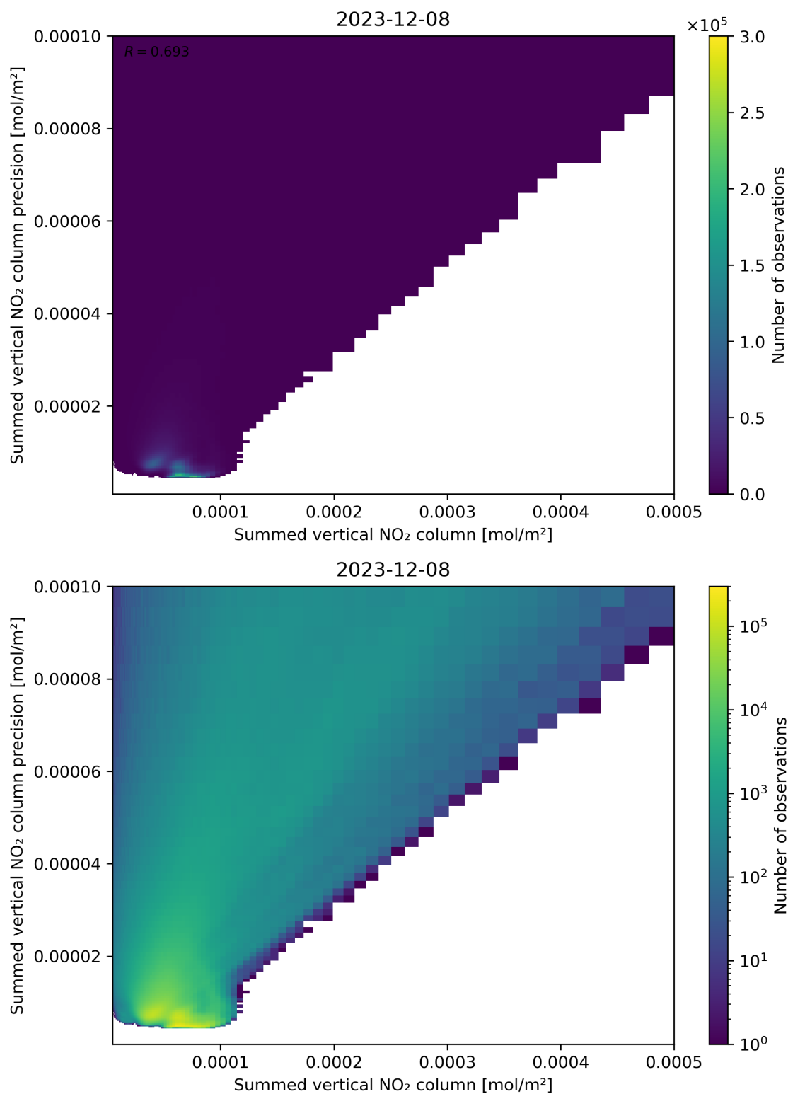
Figure 105: Scatter density plot of “Summed vertical NO 2 column” against “Summed vertical NO 2 column precision” for 2023-12-07 to 2023-12-09.
