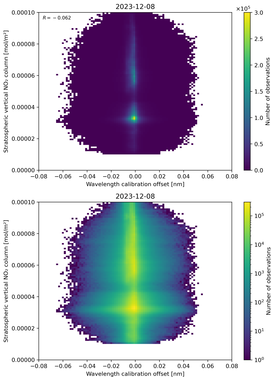
Figure 176: Scatter density plot of “Wavelength calibration offset” against “Stratospheric vertical NO 2 column” for 2023-12-07 to 2023-12-09.
