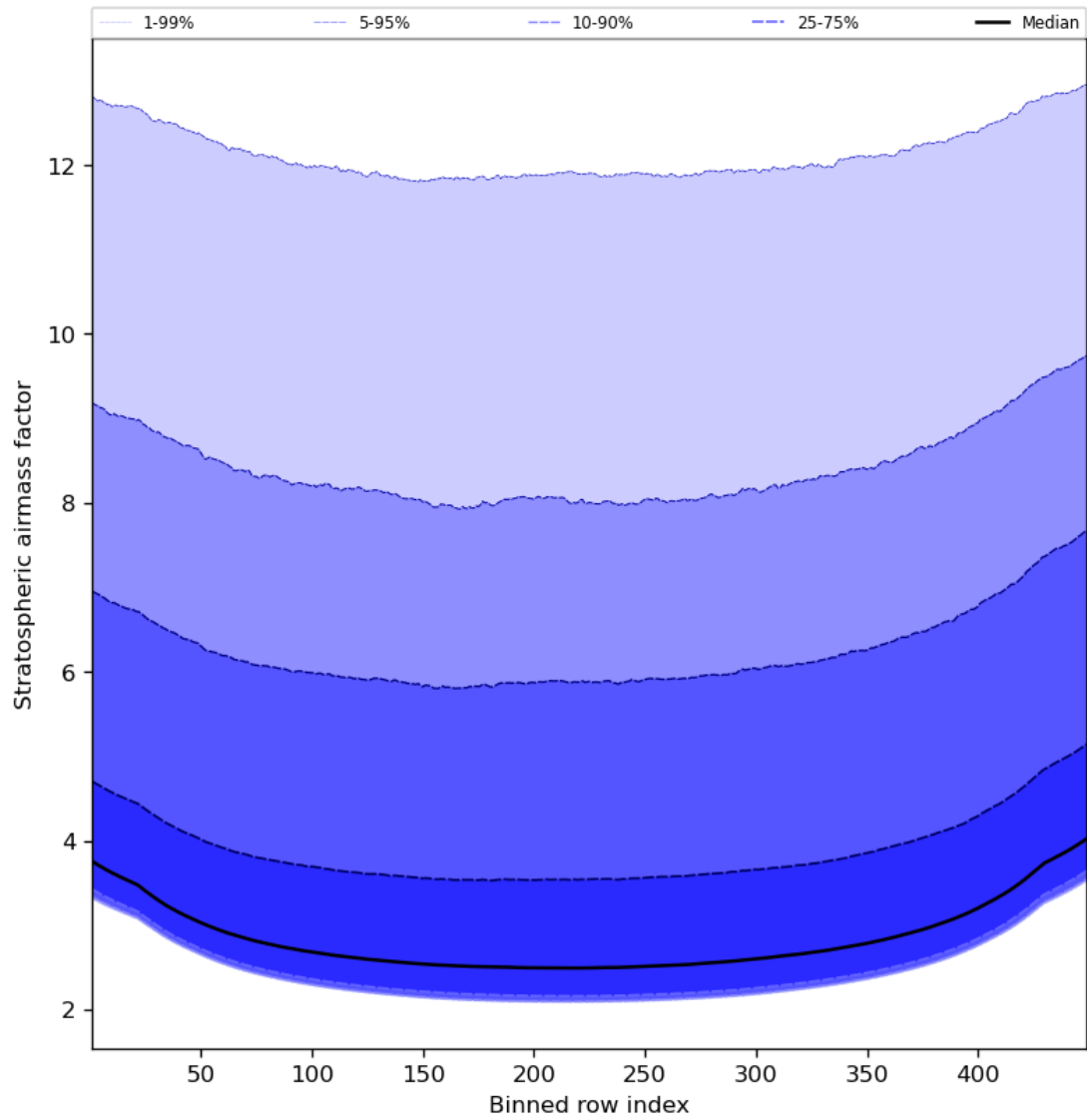
Figure 61: Along track statistics of “Stratospheric airmass factor” for 2023-12-07 to 2023-12-09
