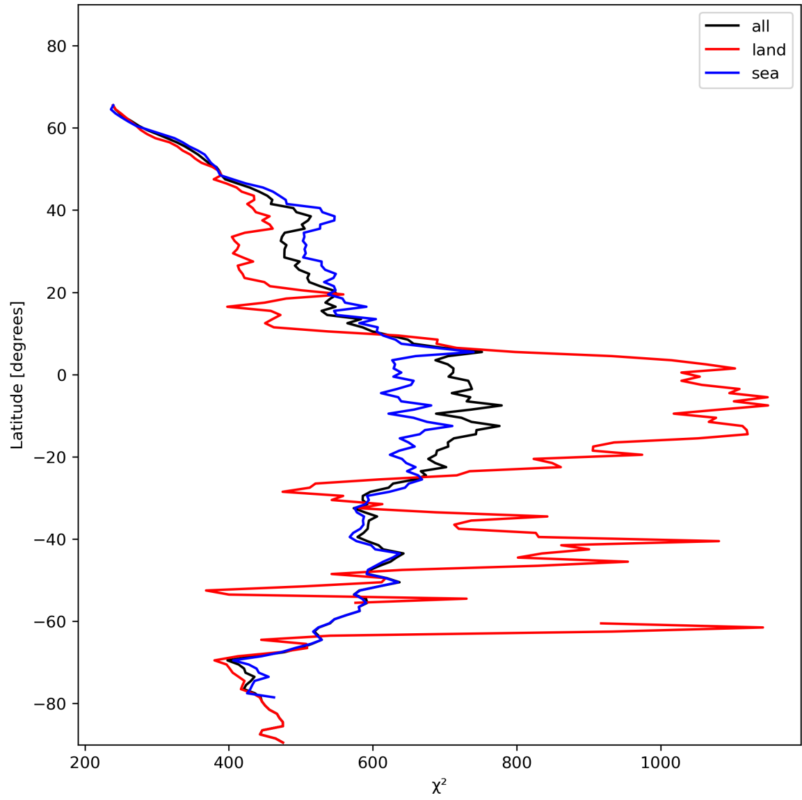
Figure 25: Zonal average of “ \chi^2 ” for 2023-12-07 to 2023-12-09.
