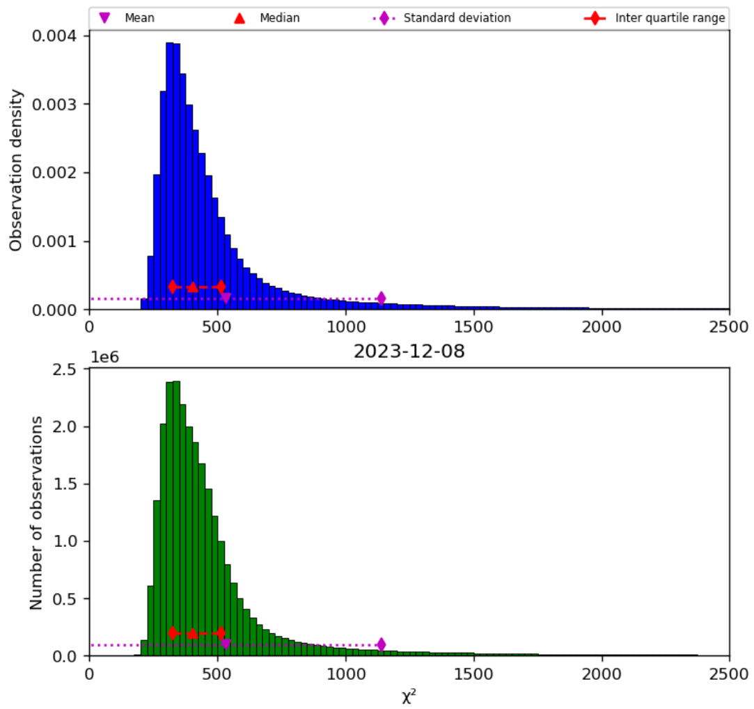
Figure 42: Histogram of “ \chi^2 ” for 2023-12-07 to 2023-12-09
