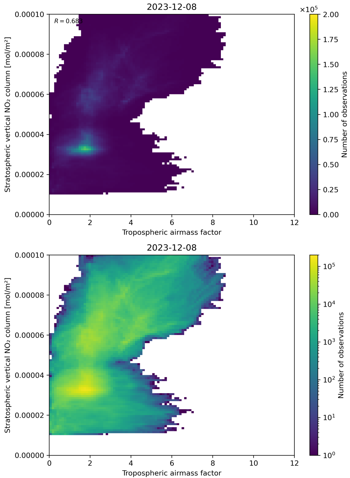
Figure 74: Scatter density plot of “Tropospheric air mass factor” against “Stratospheric vertical NO 2 column” for 2023-12-07 to 2023-12-09.
