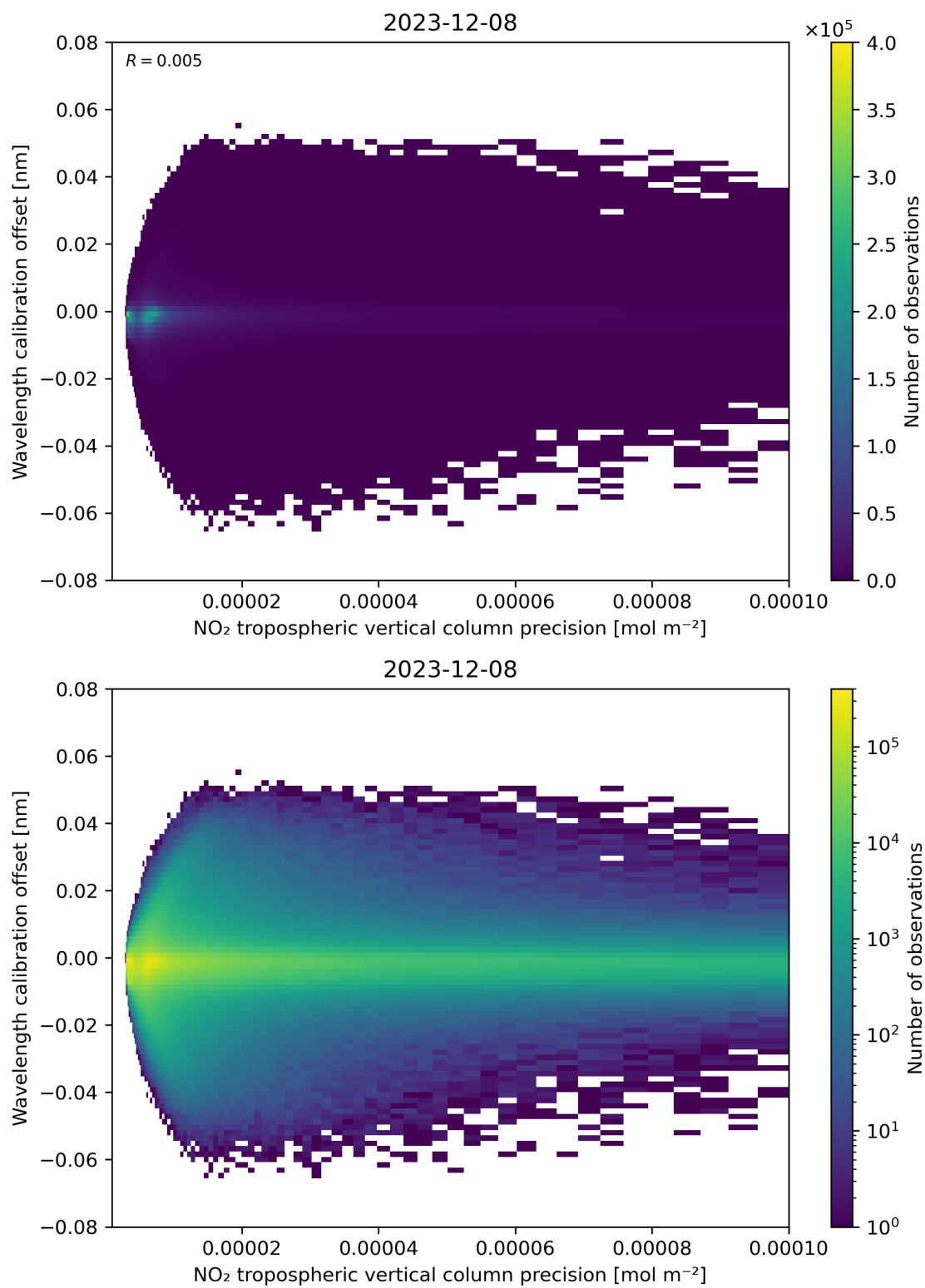
Figure 141: Scatter density plot of “NO 2 tropospheric vertical column precision” against “Wavelength calibration offset” for 2023-12-07 to 2023-12-09.
