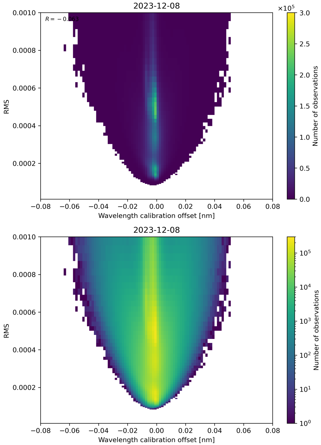
Figure 181: Scatter density plot of “Wavelength calibration offset” against “RMS” for 2023-12-07 to 2023-12-09.
