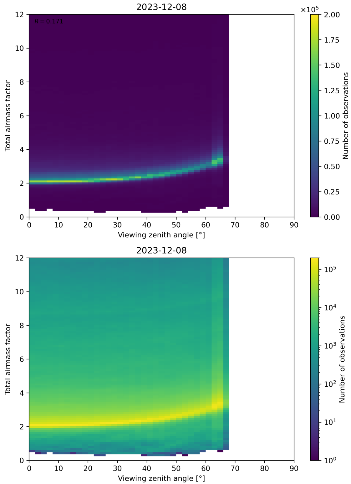
Figure 160: Scatter density plot of “Viewing zenith angle” against “Total airmass factor” for 2023-12-07 to 2023-12-09.
