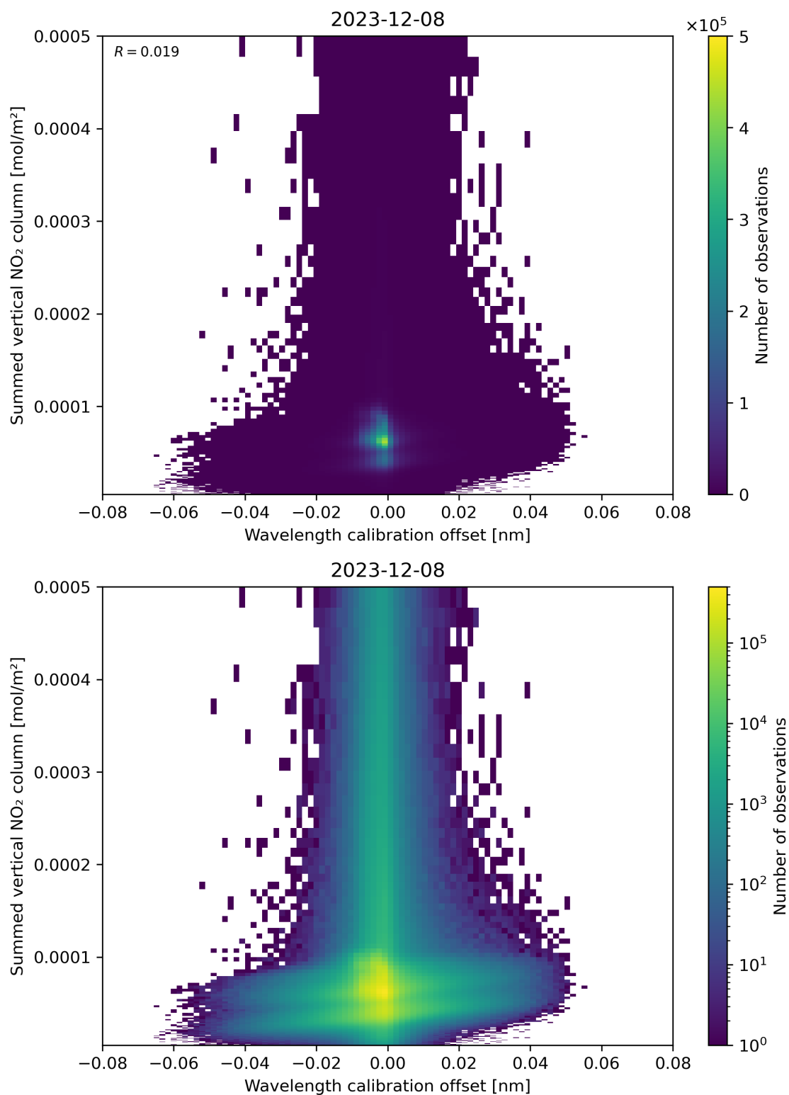
Figure 177: Scatter density plot of “Wavelength calibration offset” against “Summed vertical NO 2 column” for 2023-12-07 to 2023-12-09.
