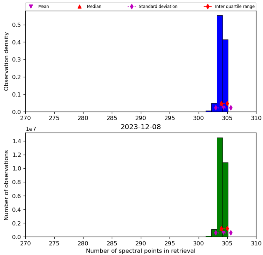
Figure 33: Histogram of “Number of spectral points in retrieval” for 2023-12-07 to 2023-12-09
