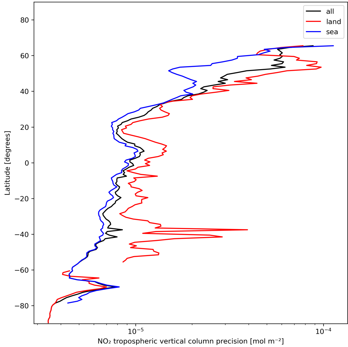
Figure 13: Zonal average of “NO 2 tropospheric vertical column precision” for 2023-12-07 to 2023-12-09.
