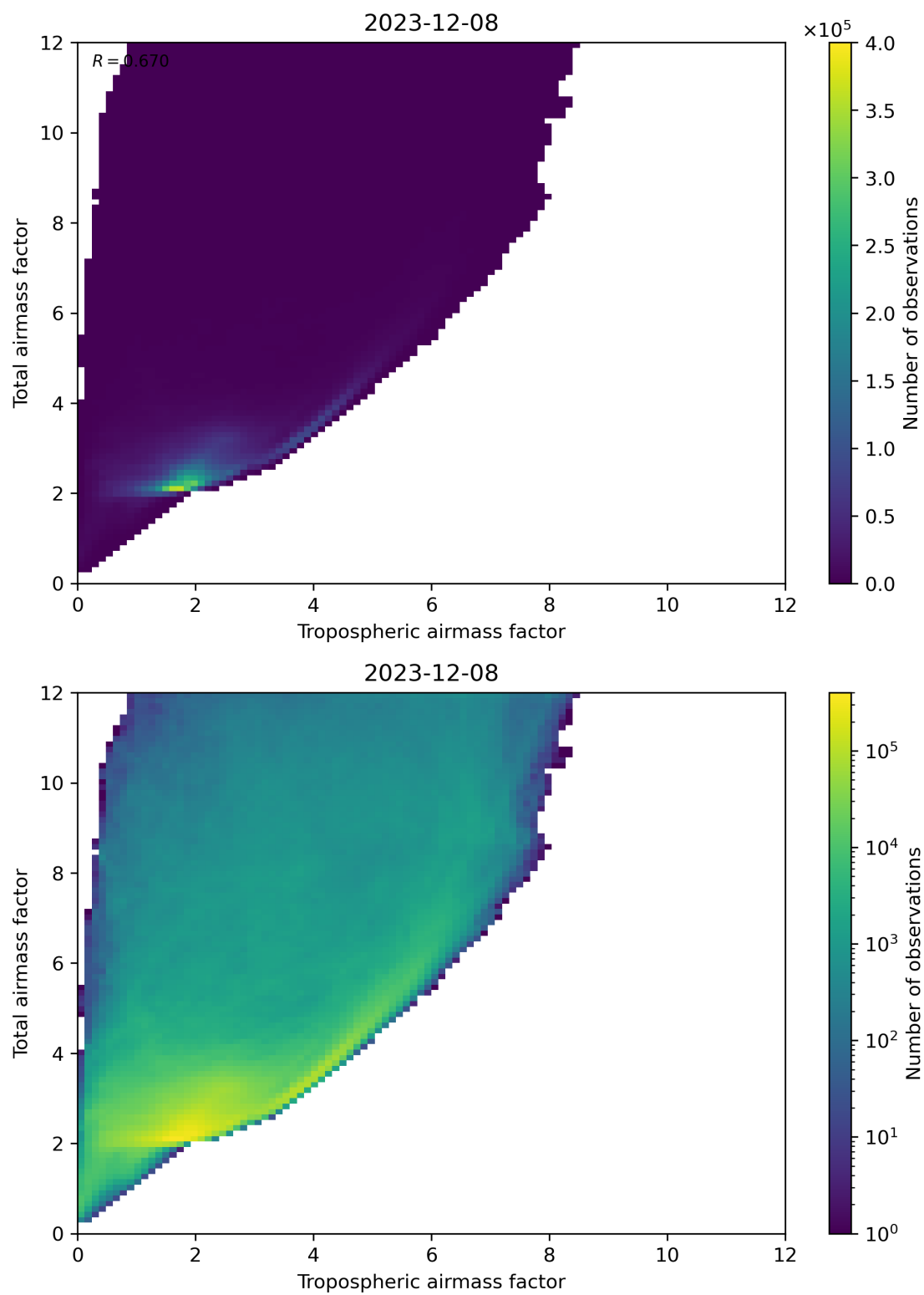
Figure 72: Scatter density plot of “Tropospheric airmass factor” against “Total airmass factor” for 2023-12-07 to 2023-12-09.
