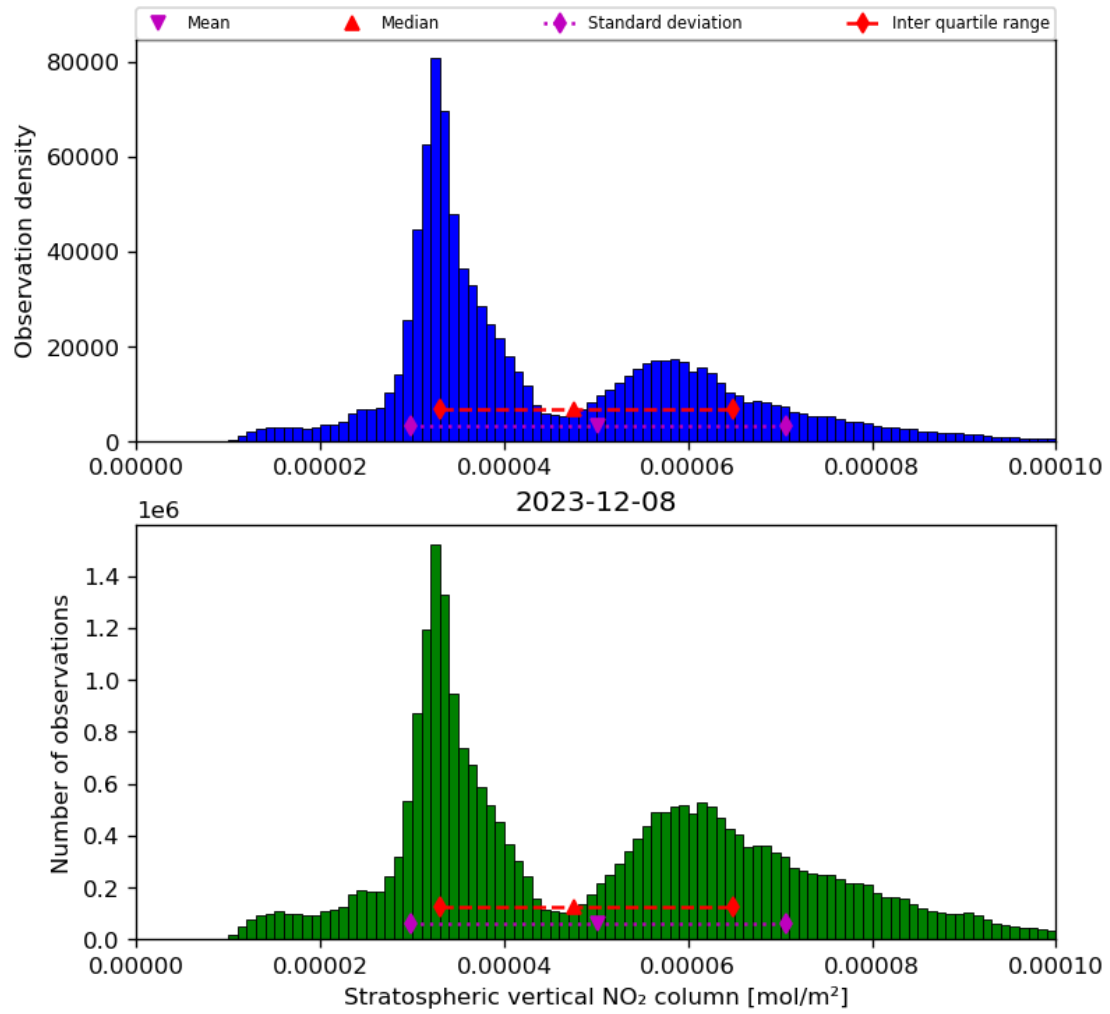
Figure 36: Histogram of “Stratospheric vertical NO 2 column” for 2023-12-07 to 2023-12-09
