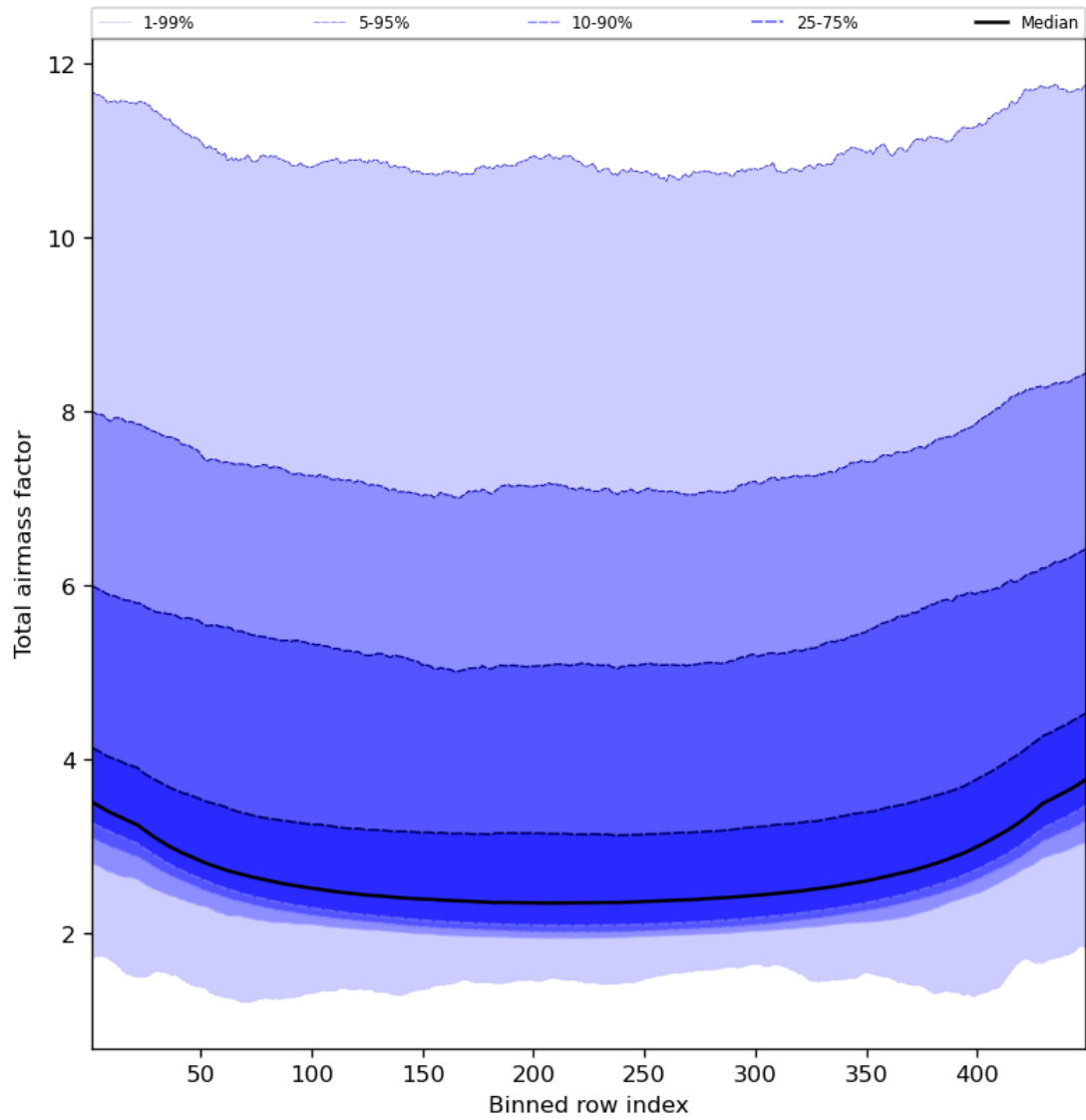
Figure 49: Along track statistics of “Total airmass factor” for 2023-12-07 to 2023-12-09
