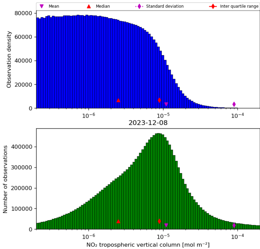
Figure 29: Histogram of “NO 2 tropospheric vertical column” for 2023-12-07 to 2023-12-09
