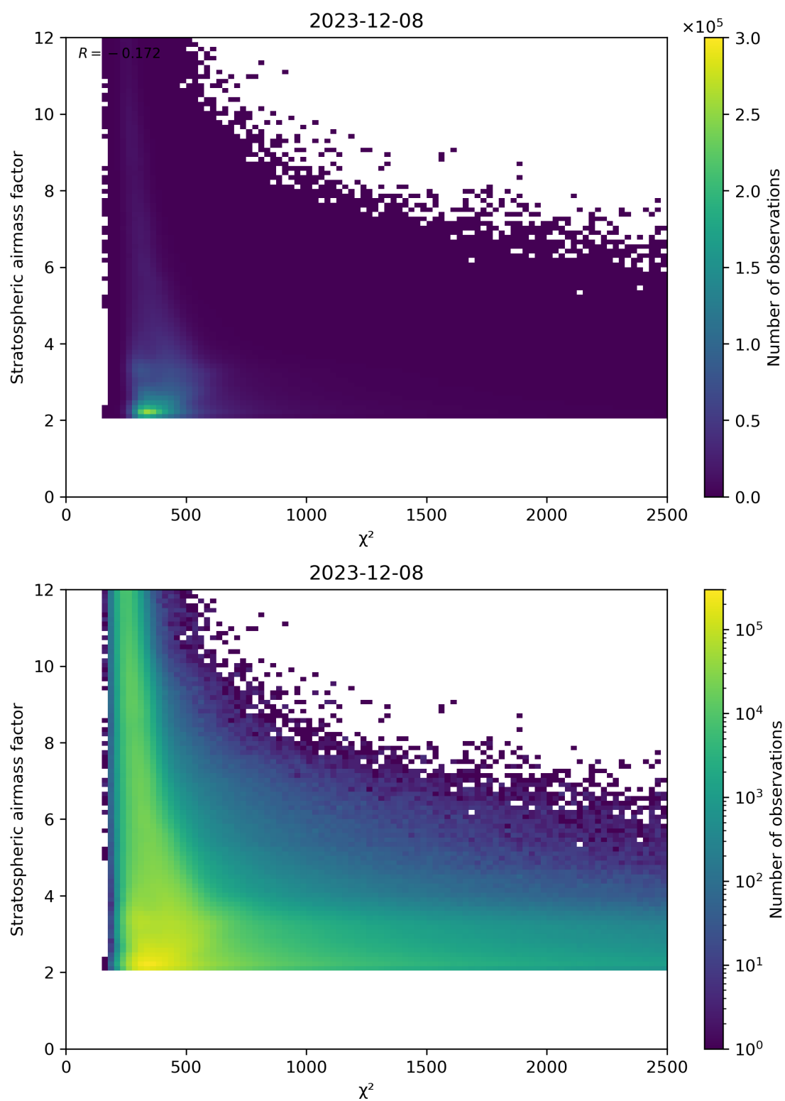
Figure 81: Scatter density plot of “ \chi^2 ” against “Stratospheric airmass factor” for 2023-12-07 to 2023-12-09.
