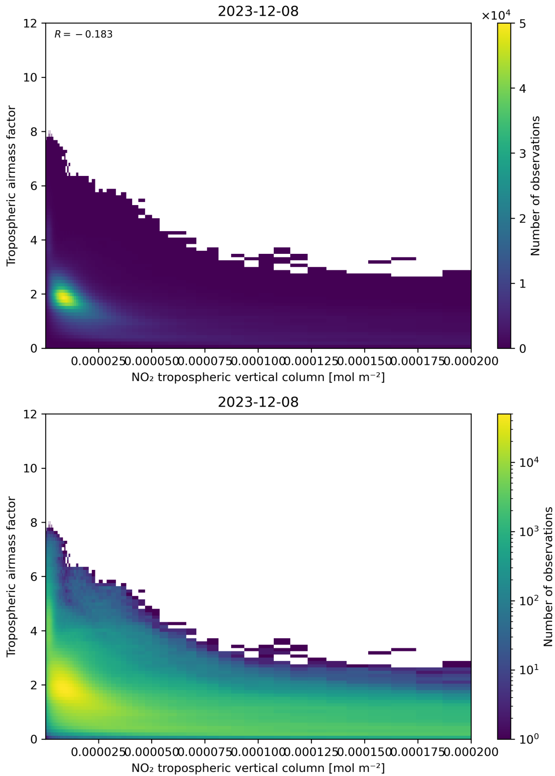
Figure 123: Scatter density plot of “NO 2 tropospheric vertical column” against “Tropospheric airmass factor” for 2023-12-07 to 2023-12-09.
