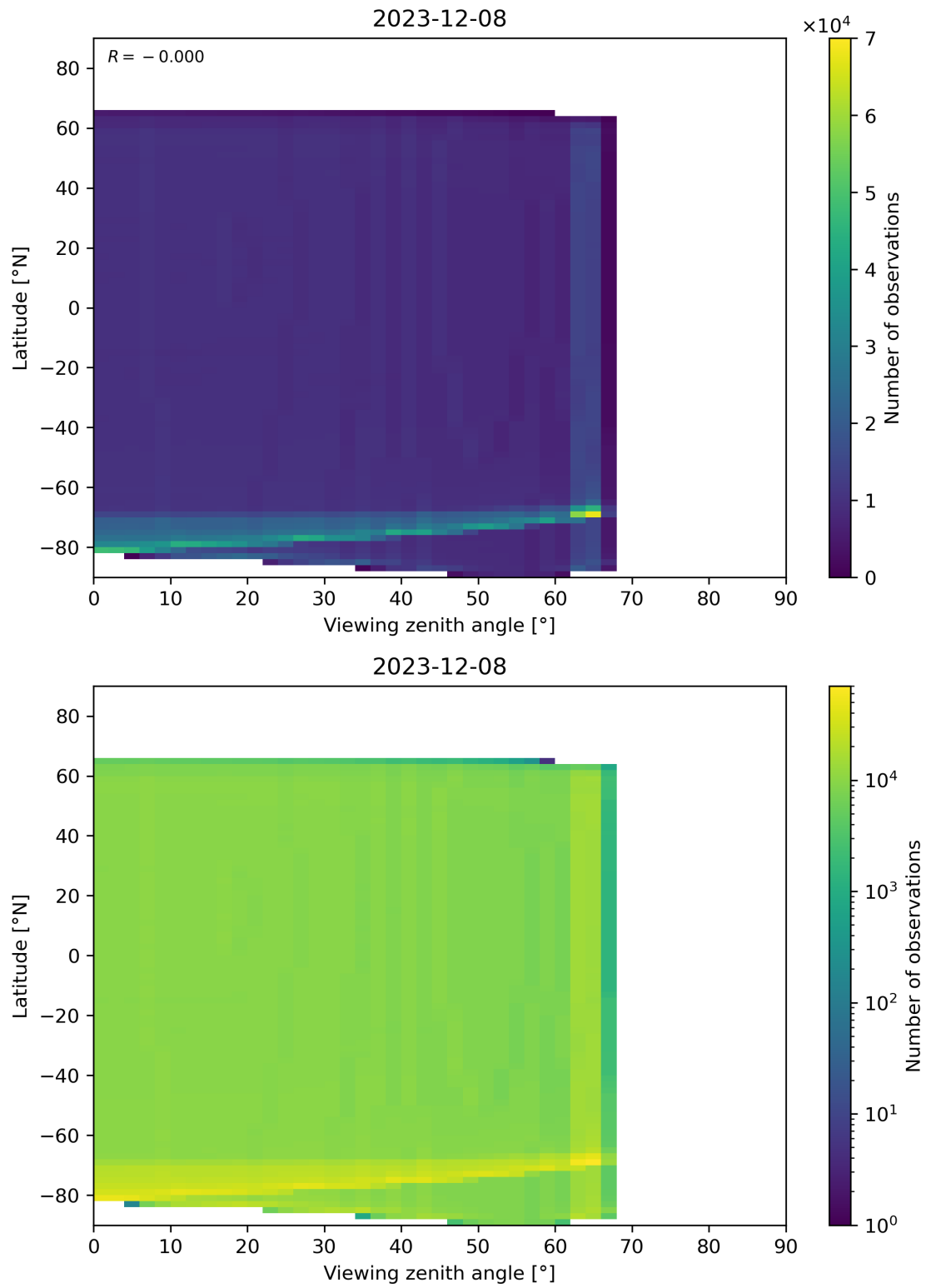
Figure 163: Scatter density plot of “Viewing zenith angle” against “Latitude” for 2023-12-07 to 2023-12-09.
