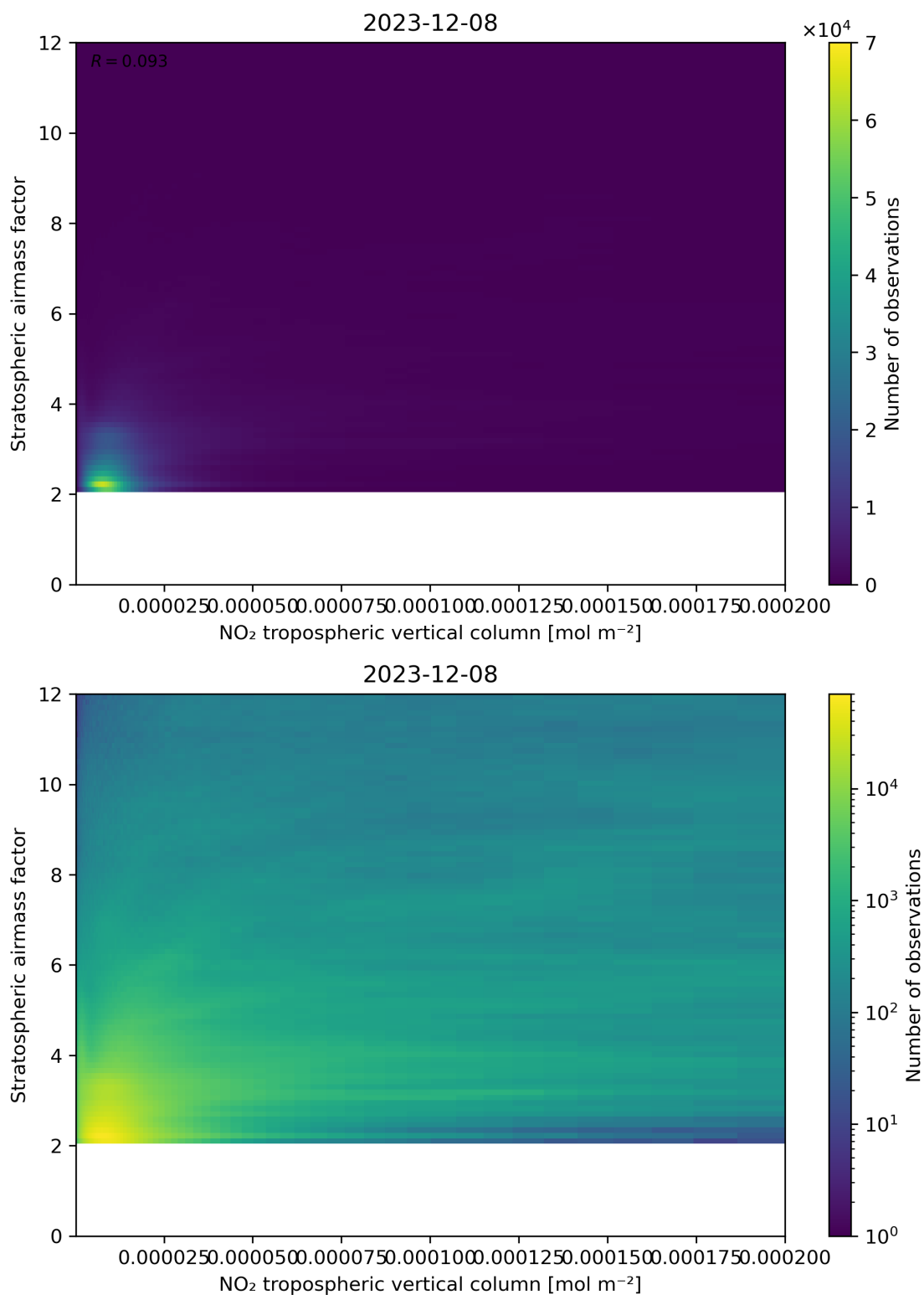
Figure 121: Scatter density plot of “NO 2 tropospheric vertical column” against “Stratospheric airmass factor” for 2023-12-07 to 2023-12-09.
