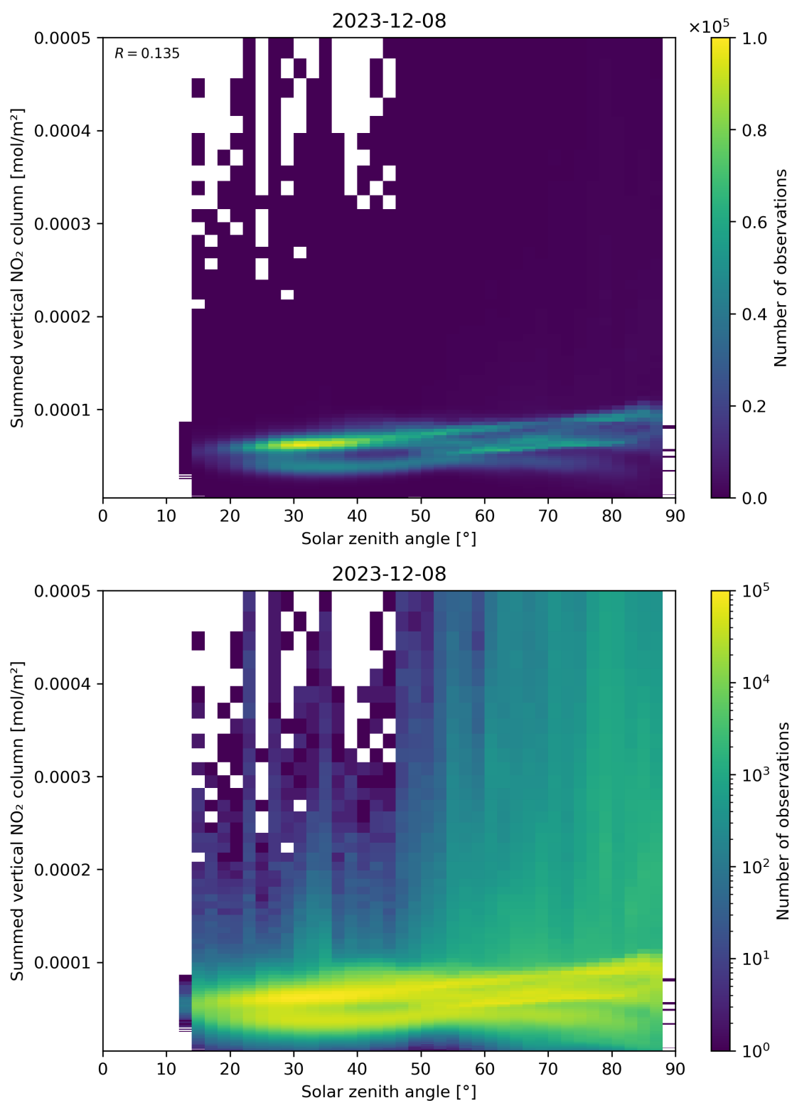
Figure 151: Scatter density plot of “Solar zenith angle” against “Summed vertical NO 2 column” for 2023-12-07 to 2023-12-09.
