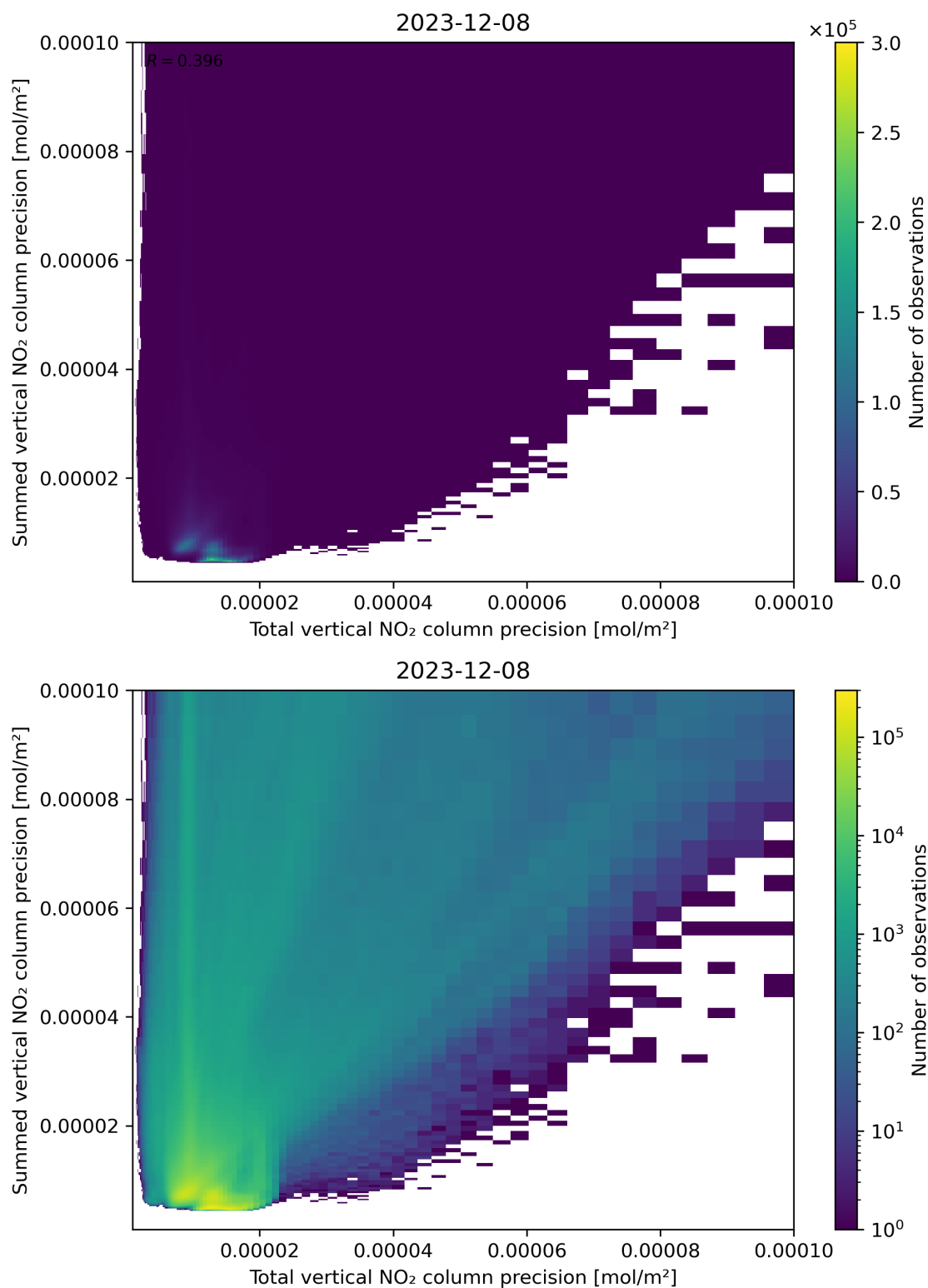
Figure 118: Scatter density plot of “Total vertical NO 2 column precision” against “Summed vertical NO 2 column precision” for 2023-12-07 to 2023-12-09.
