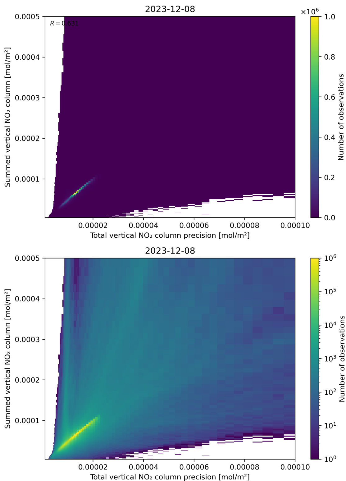
Figure 117: Scatter density plot of “Total vertical NO 2 column precision” against “Summed vertical NO 2 column” for 2023-12-07 to 2023-12-09.
