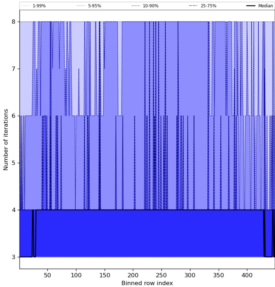
Figure 51: Along track statistics of “Number of iterations” for 2023-12-07 to 2023-12-09
