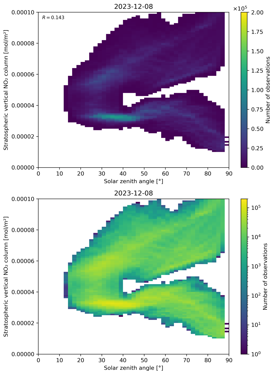
Figure 150: Scatter density plot of “Solar zenith angle” against “Stratospheric vertical NO 2 column” for 2023-12-07 to 2023-12-09.
