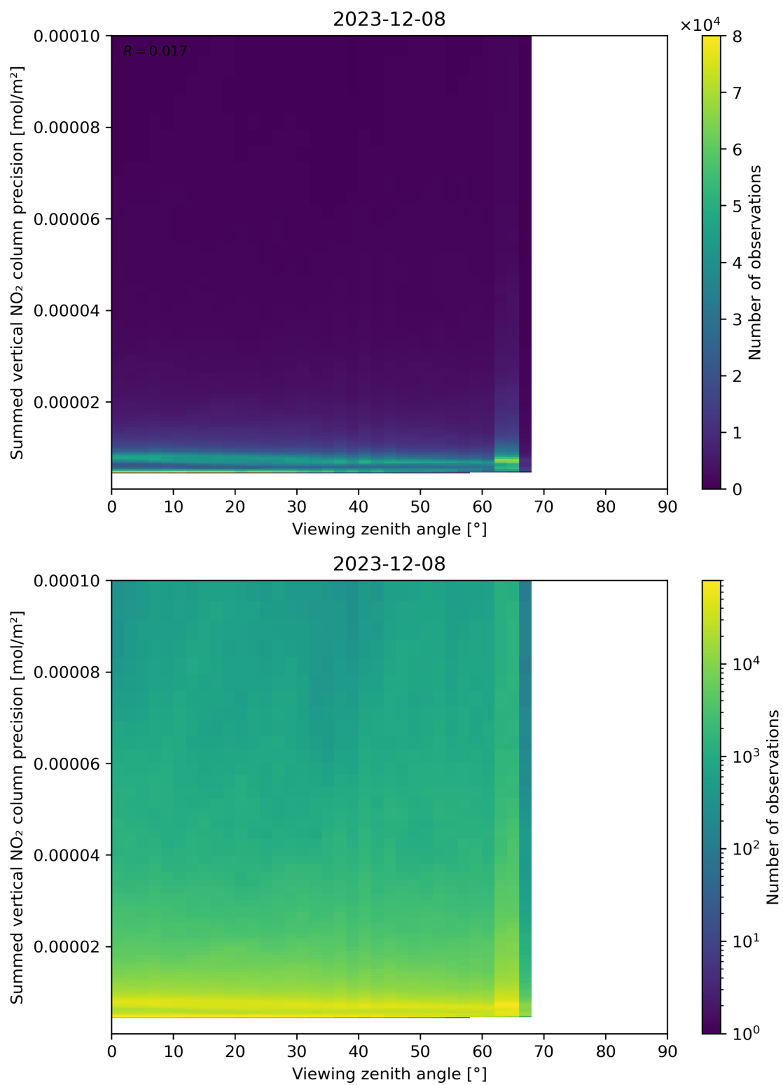
Figure 166: Scatter density plot of “Viewing zenith angle” against “Summed vertical NO 2 column precision” for 2023-12-07 to 2023-12-09.
