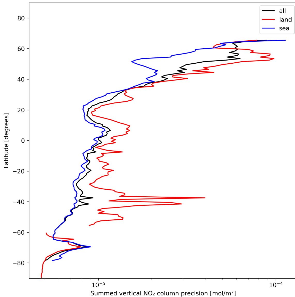
Figure 24: Zonal average of “Summed vertical NO 2 column precision” for 2023-12-07 to 2023-12-09.
