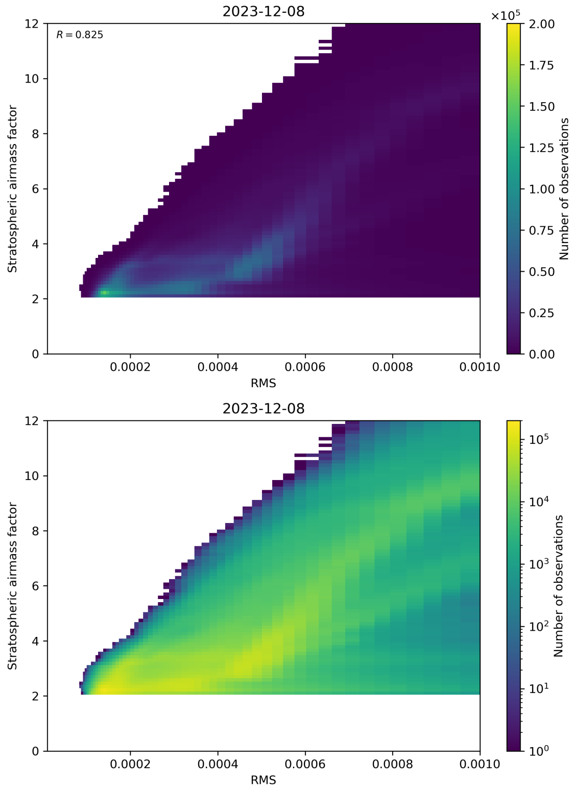
Figure 144: Scatter density plot of “RMS” against “Stratospheric airmass factor” for 2023-12-07 to 2023-12-09.
