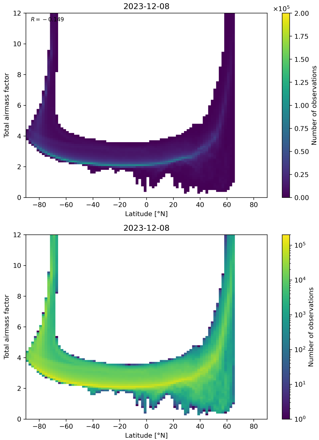
Figure 84: Scatter density plot of “Latitude” against “Total airmass factor” for 2023-12-07 to 2023-12-09.
