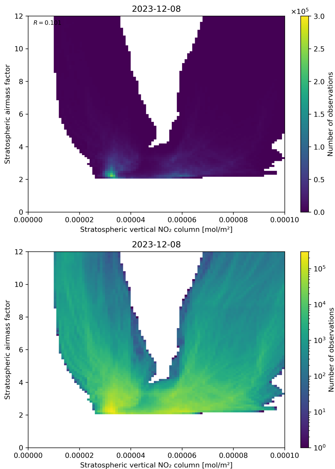
Figure 96: Scatter density plot of “Stratospheric vertical NO 2 column” against “Stratospheric airmass factor” for 2023-12-07 to 2023-12-09.
