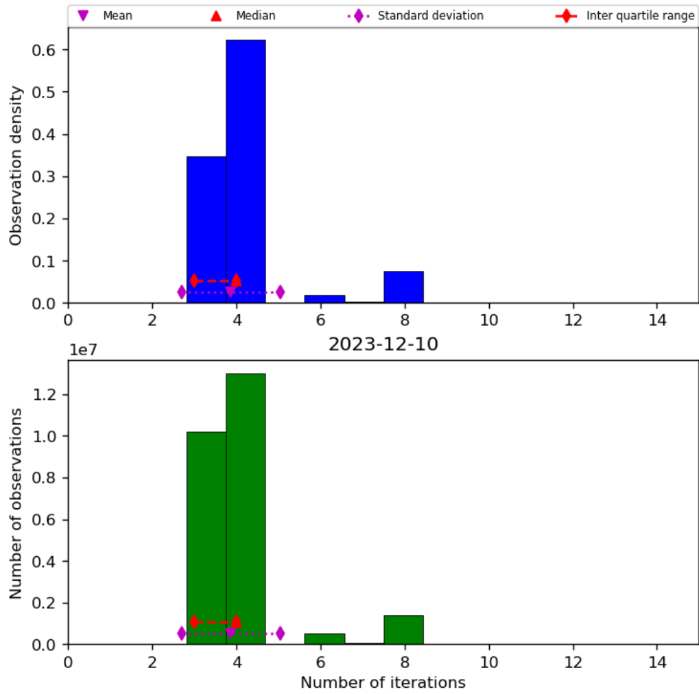
Figure 34: Histogram of “Number of iterations” for 2023-12-09 to 2023-12-11
