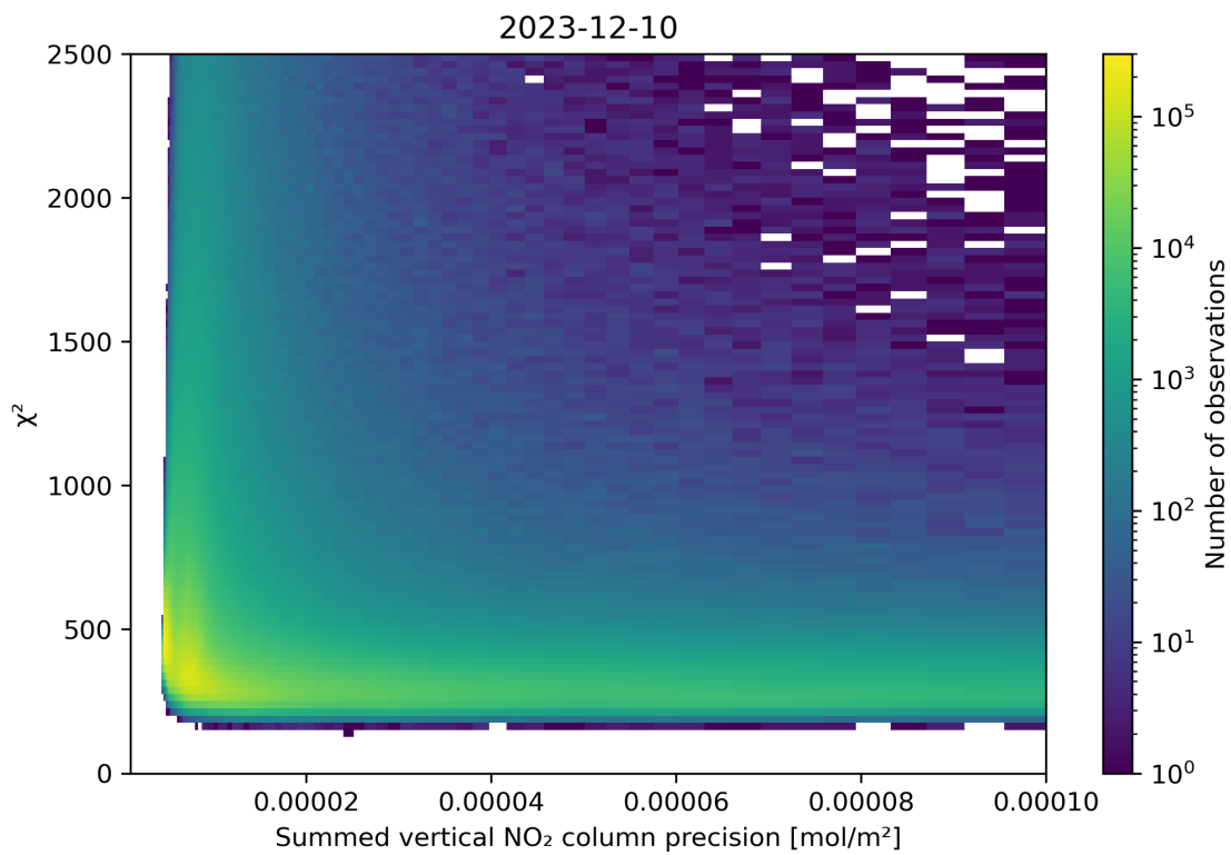
Figure 107: Scatter density plot of “Summed vertical NO 2 column precision” against “ \chi^2 ” for 2023-12-09 to 2023-12-11.
