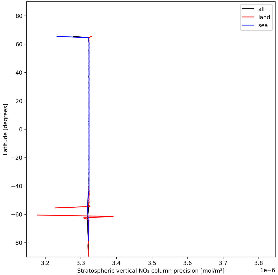
Figure 20: Zonal average of “Stratospheric vertical NO 2 column precision” for 2023-12-09 to 2023-12-11.
