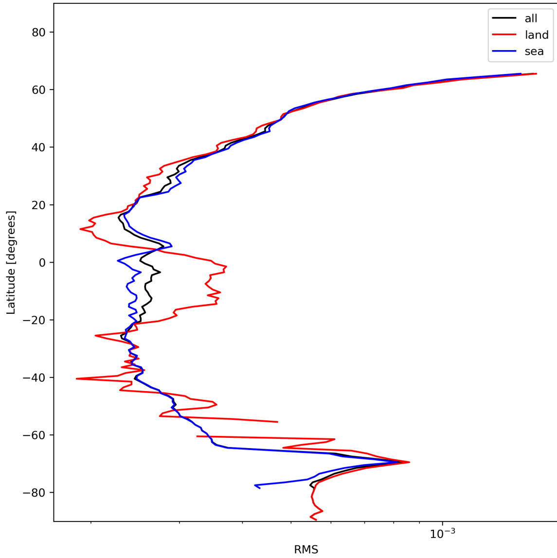
Figure 26: Zonal average of “RMS” for 2023-12-09 to 2023-12-11.
