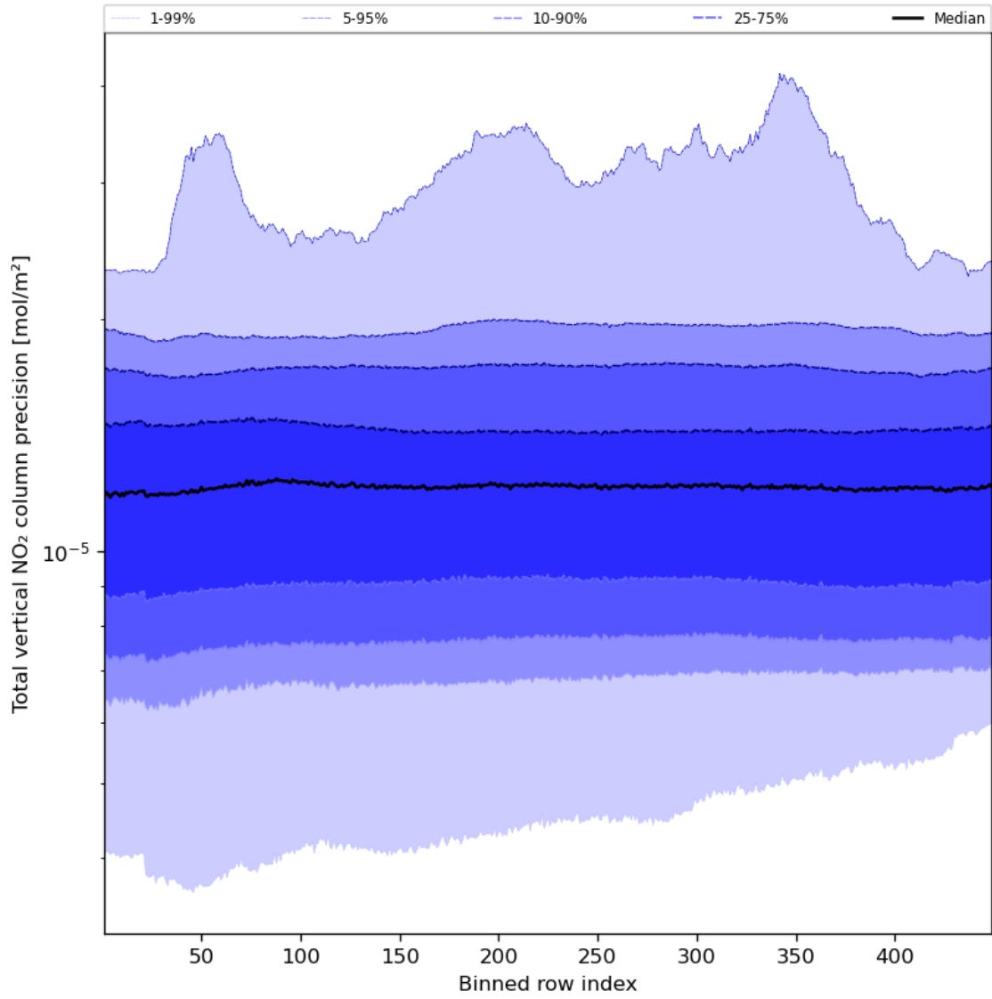
Figure 56: Along track statistics of “Total vertical NO 2 column precision” for 2023-12-09 to 2023-12-11
