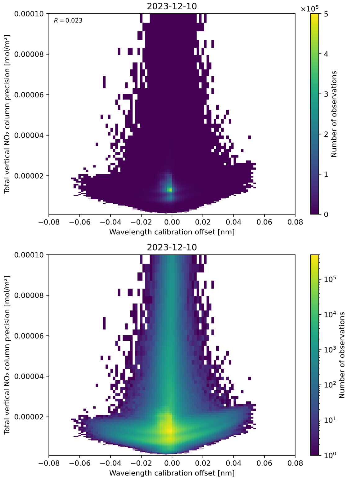
Figure 180: Scatter density plot of “Wavelength calibration offset” against “Total vertical NO 2 column precision” for 2023-12-09 to 2023-12-11.
