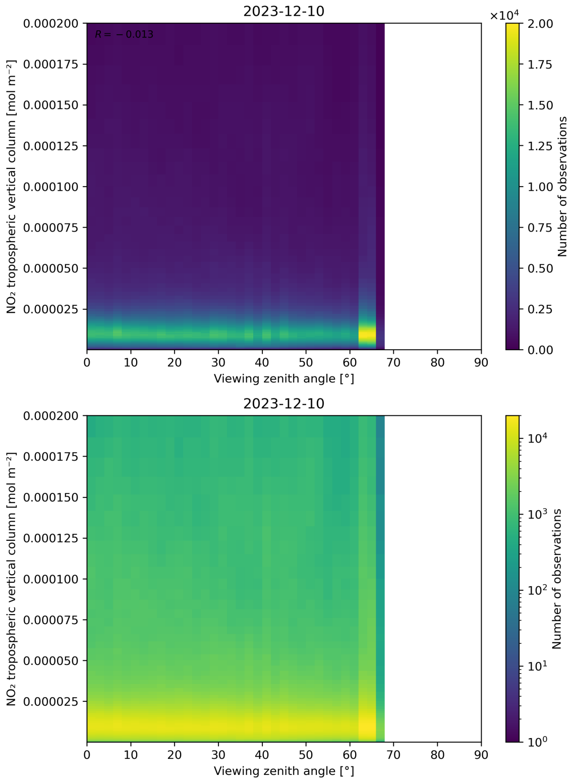
Figure 169: Scatter density plot of “Viewing zenith angle” against “NO 2 tropospheric vertical column” for 2023-12-09 to 2023-12-11.
