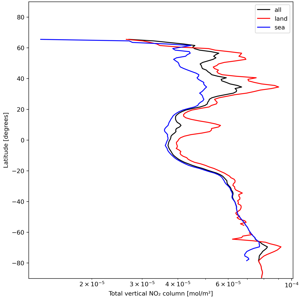
Figure 21: Zonal average of “Total vertical NO 2 column” for 2023-12-09 to 2023-12-11.
