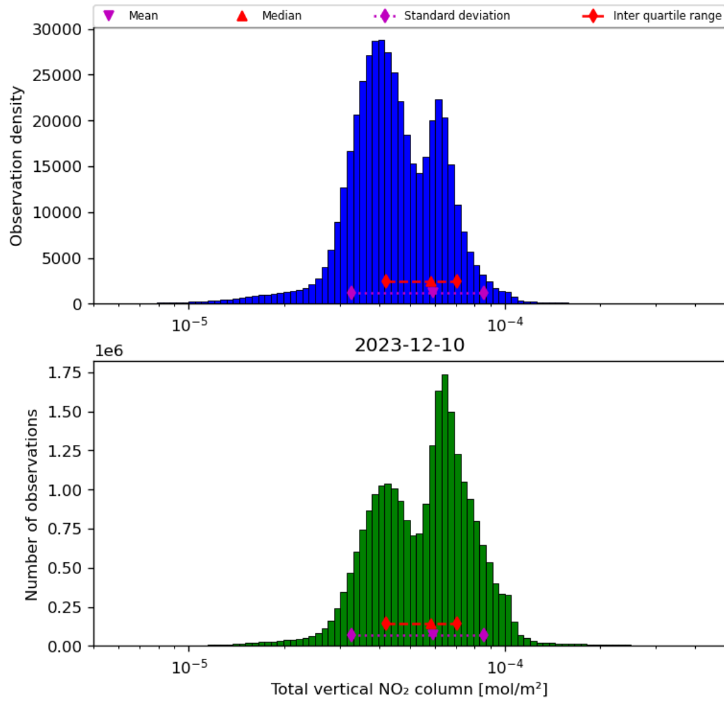
Figure 38: Histogram of “Total vertical NO 2 column” for 2023-12-09 to 2023-12-11
