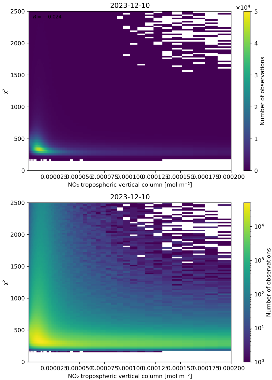
Figure 124: Scatter density plot of “NO 2 tropospheric vertical column” against “ \chi^2 ” for 2023-12-09 to 2023-12-11.
