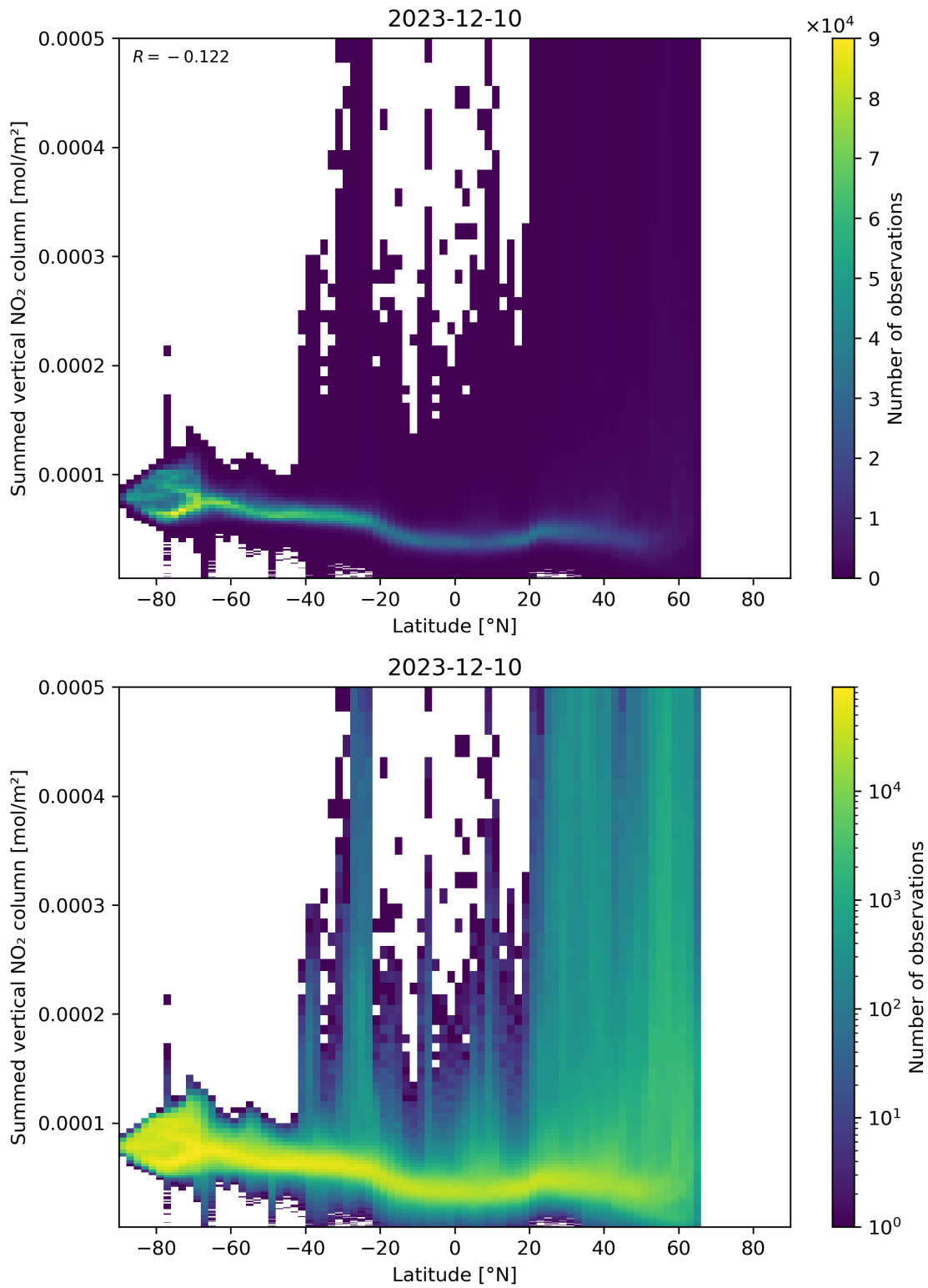
Figure 88: Scatter density plot of “Latitude” against “Summed vertical NO 2 column” for 2023-12-09 to 2023-12-11.
