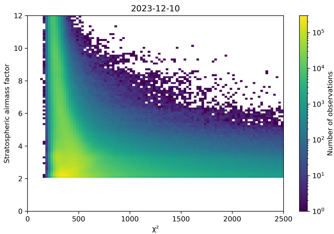
Figure 81: Scatter density plot of “ \chi^2 ” against “Stratospheric airmass factor” for 2023-12-09 to 2023-12-11.
