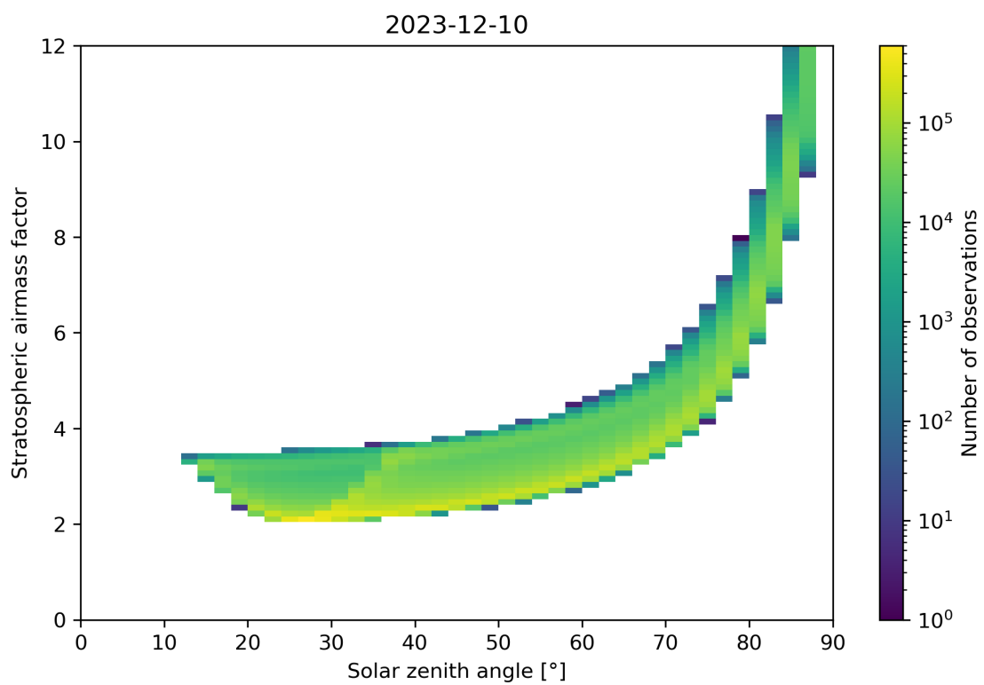
Figure 145: Scatter density plot of “Solar zenith angle” against “Stratospheric airmass factor” for 2023-12-09 to 2023-12-11.
