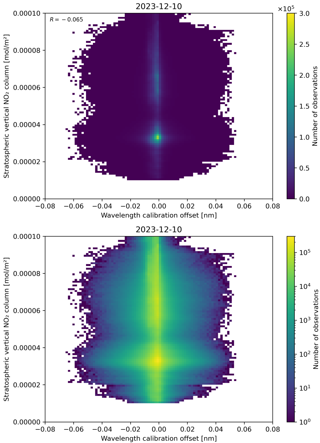
Figure 176: Scatter density plot of “Wavelength calibration offset” against “Stratospheric vertical NO 2 column” for 2023-12-09 to 2023-12-11.
