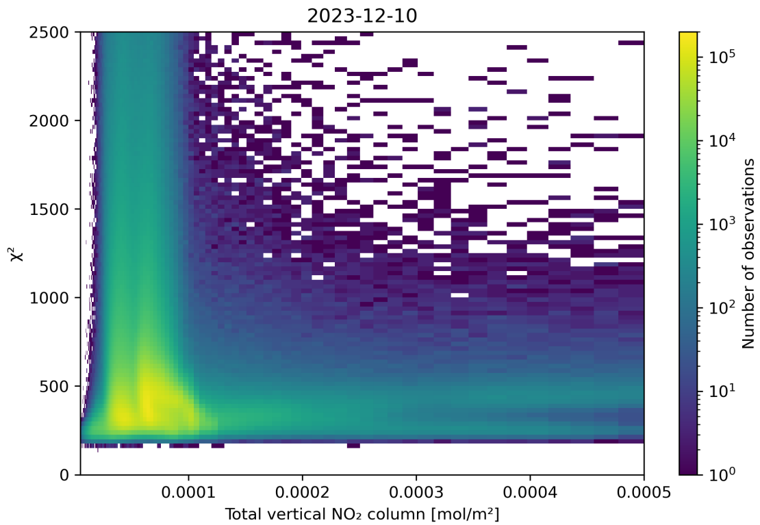
Figure 111: Scatter density plot of “Total vertical NO 2 column” against “ \chi^2 ” for 2023-12-09 to 2023-12-11.
