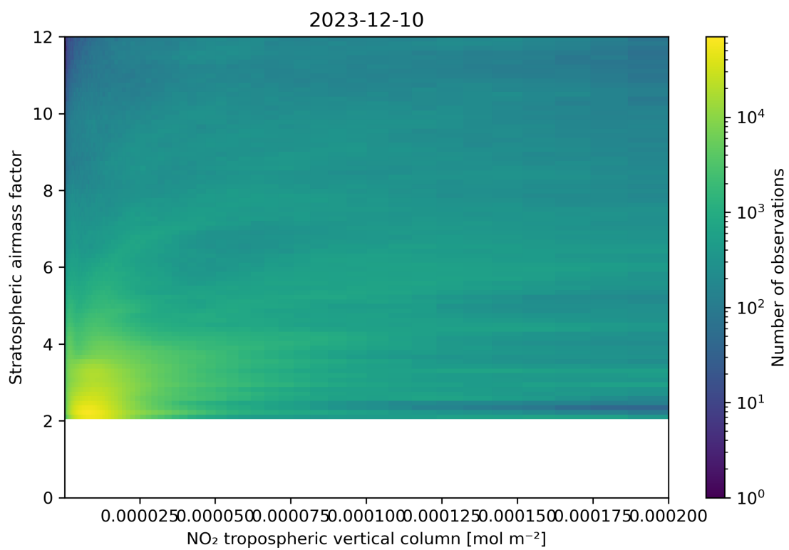
Figure 121: Scatter density plot of “NO 2 tropospheric vertical column” against “Stratospheric airmass factor” for 2023-12-09 to 2023-12-11.
