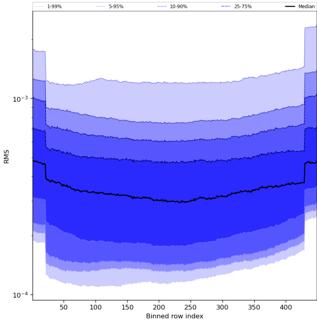
Figure 60: Along track statistics of “RMS” for 2023-12-09 to 2023-12-11
