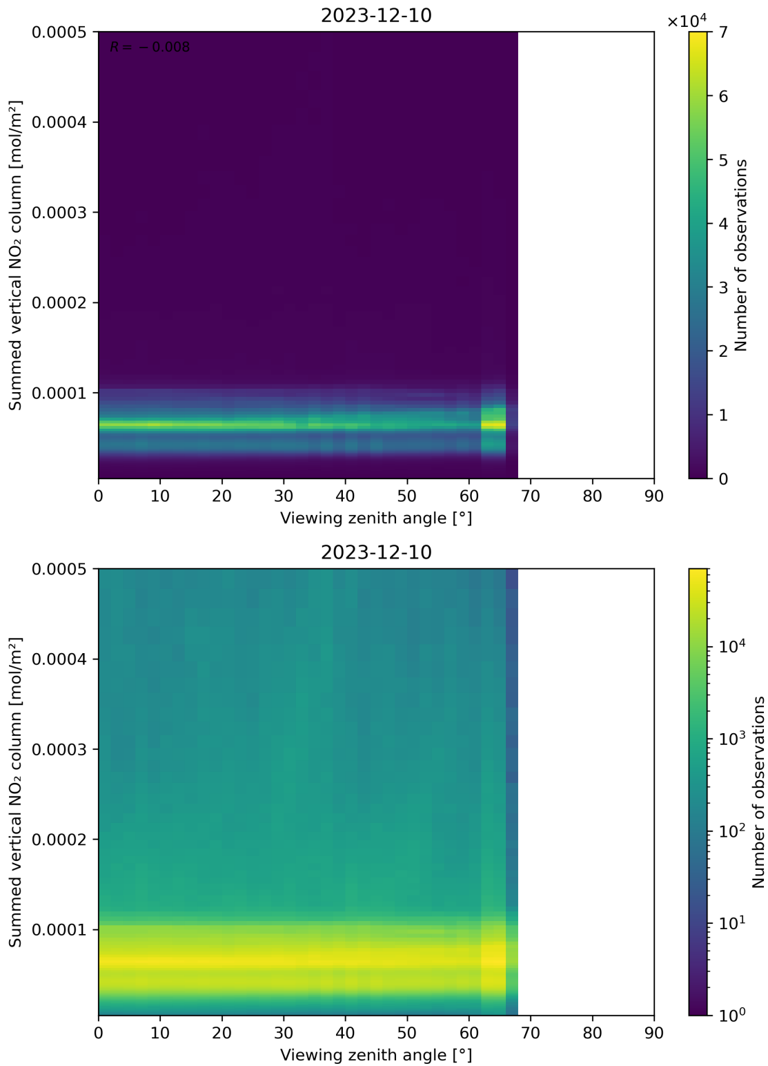
Figure 165: Scatter density plot of “Viewing zenith angle” against “Summed vertical NO 2 column” for 2023-12-09 to 2023-12-11.
