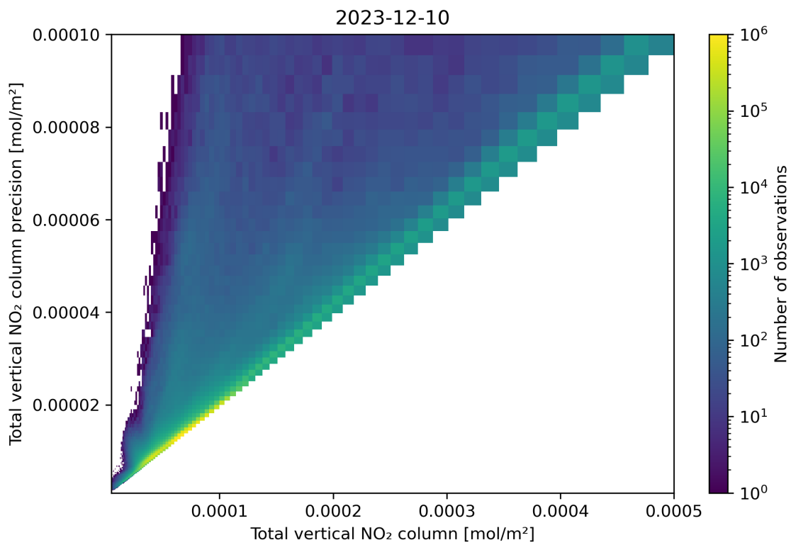
Figure 114: Scatter density plot of “Total vertical NO 2 column” against “Total vertical NO 2 column precision” for 2023-12-09 to 2023-12-11.
