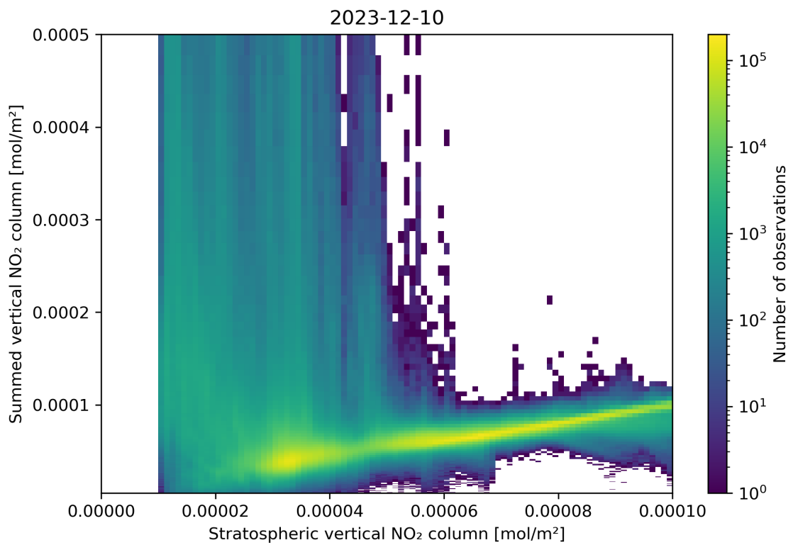
Figure 98: Scatter density plot of “Stratospheric vertical NO 2 column” against “Summed vertical NO 2 column” for 2023-12-09 to 2023-12-11.
