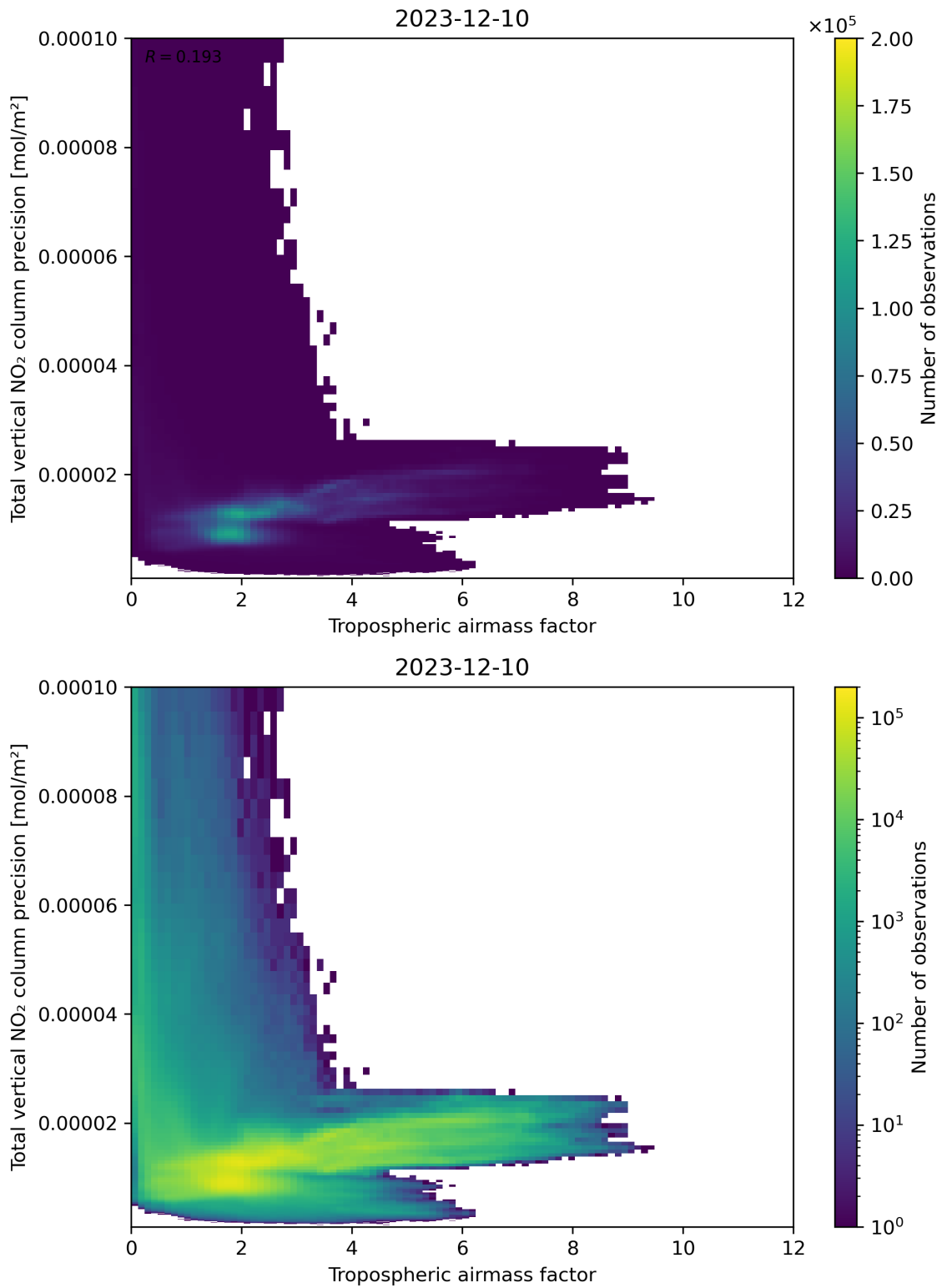
Figure 78: Scatter density plot of “Tropospheric airmass factor” against “Total vertical NO 2 column precision” for 2023-12-09 to 2023-12-11.
