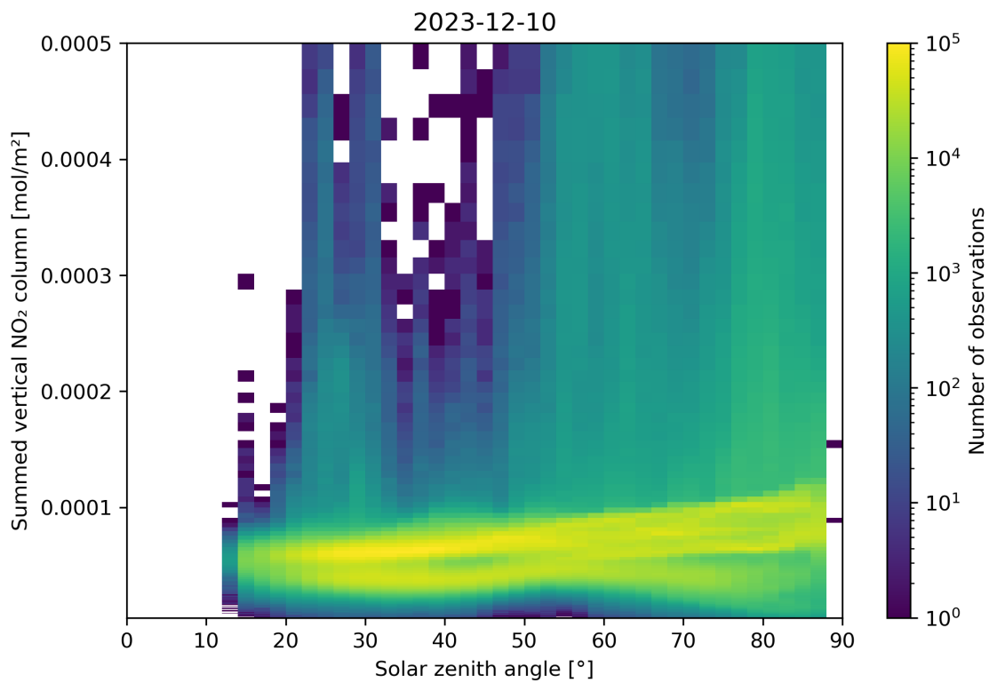
Figure 151: Scatter density plot of “Solar zenith angle” against “Summed vertical NO 2 column” for 2023-12-09 to 2023-12-11.
