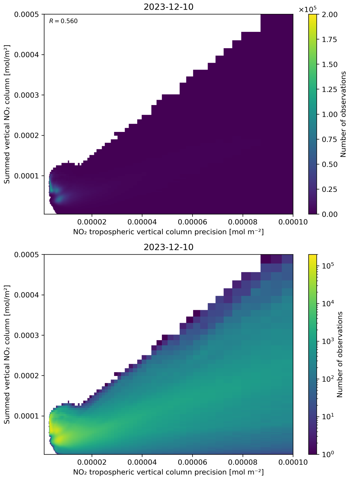
Figure 136: Scatter density plot of “NO 2 tropospheric vertical column precision” against “Summed vertical NO 2 column” for 2023-12-09 to 2023-12-11.
