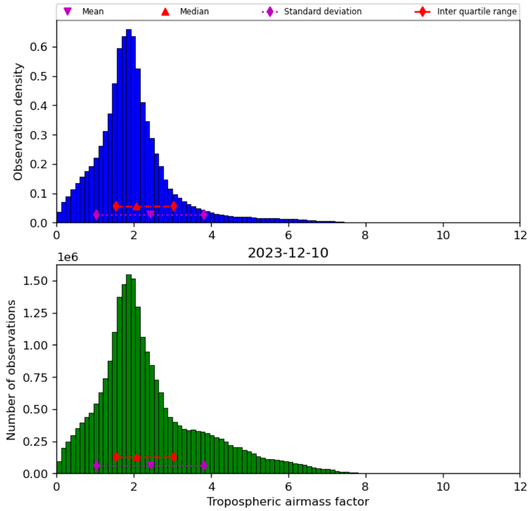
Figure 31: Histogram of “Tropospheric airmass factor” for 2023-12-09 to 2023-12-11
