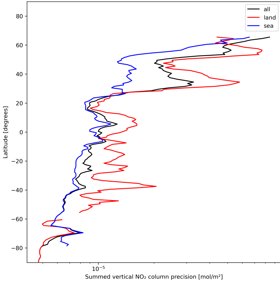
Figure 24: Zonal average of “Summed vertical NO 2 column precision” for 2023-12-09 to 2023-12-11.
