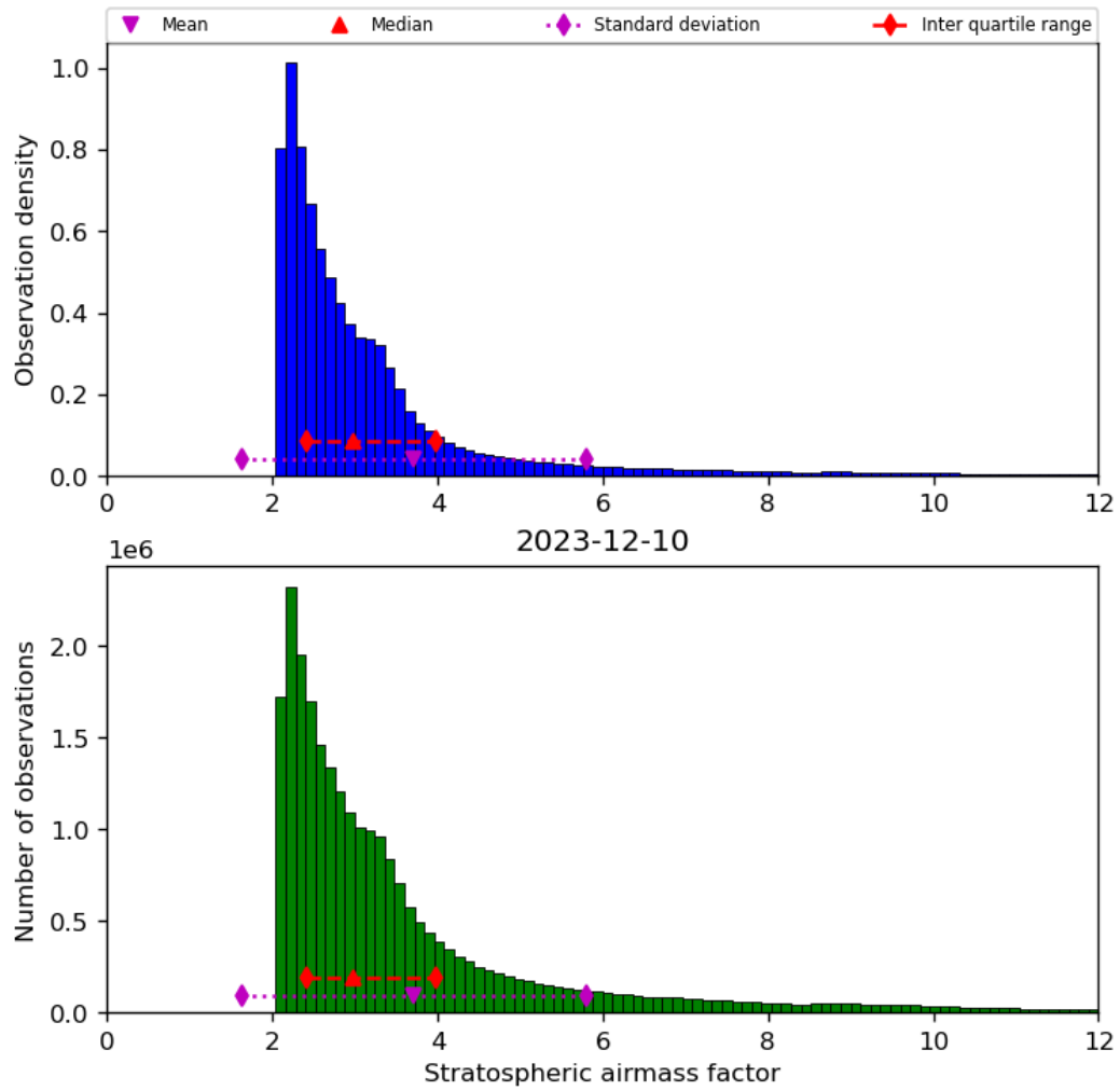
Figure 44: Histogram of “Stratospheric airmass factor” for 2023-12-09 to 2023-12-11
