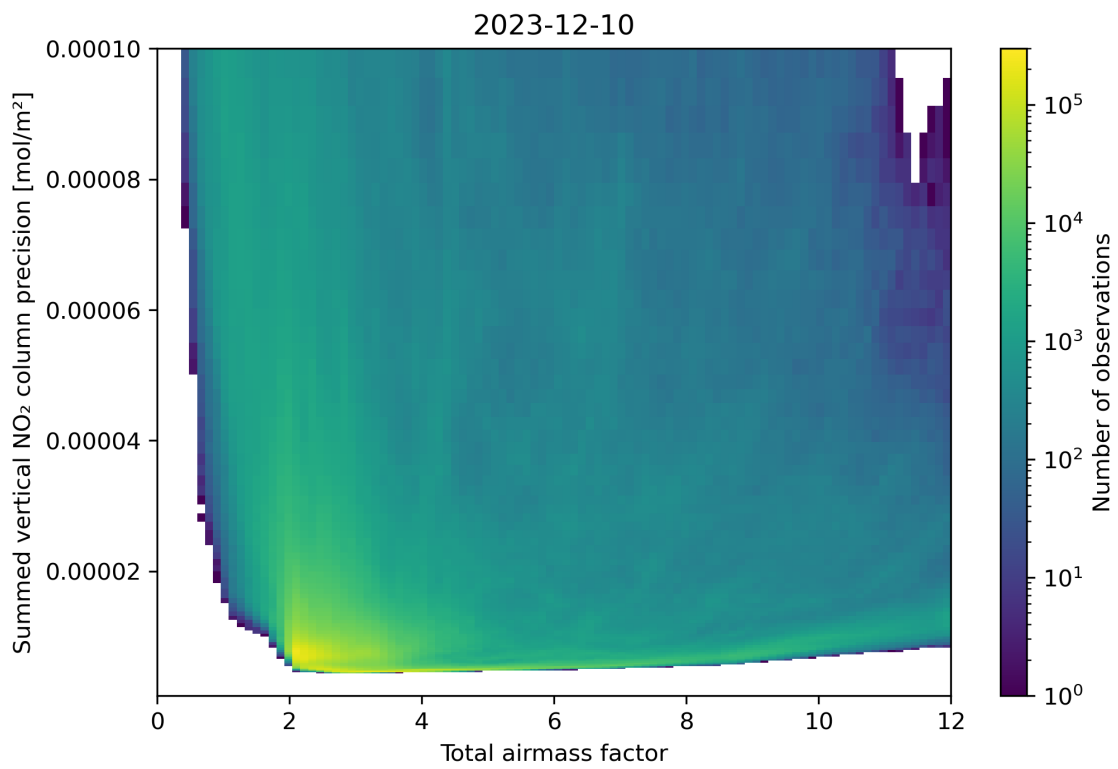
Figure 66: Scatter density plot of “Total airmass factor” against “Summed vertical NO 2 column precision” for 2023-12-09 to 2023-12-11.
