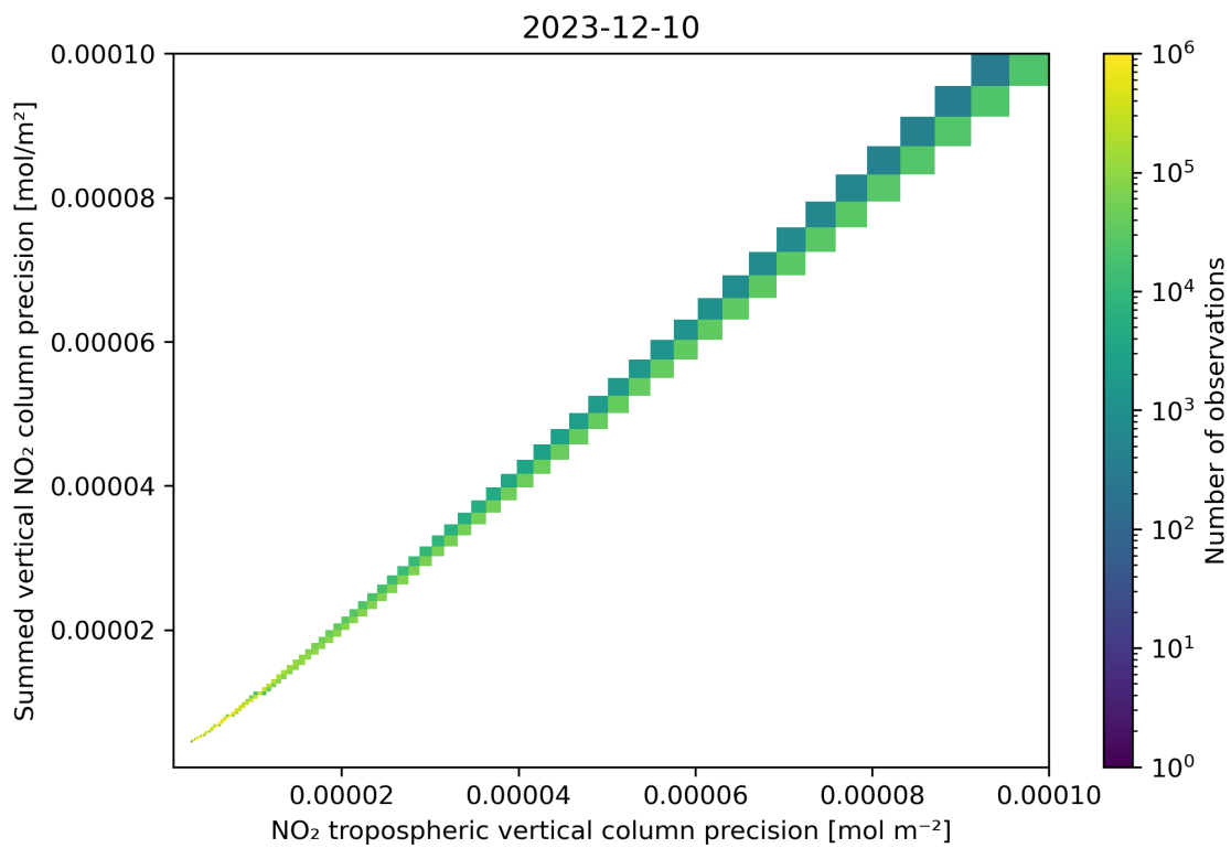
Figure 137: Scatter density plot of “NO 2 tropospheric vertical column precision” against “Summed vertical NO 2 column precision” for 2023-12-09 to 2023-12-11.
