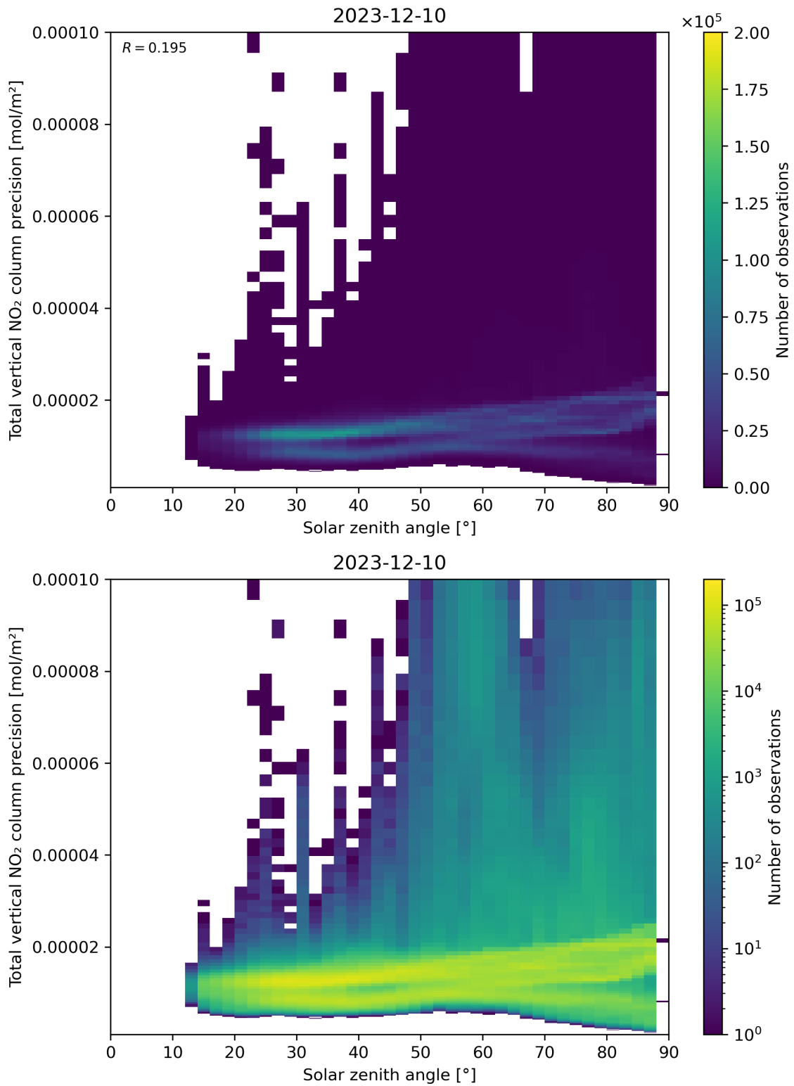
Figure 154: Scatter density plot of “Solar zenith angle” against “Total vertical NO 2 column precision” for 2023-12-09 to 2023-12-11.
