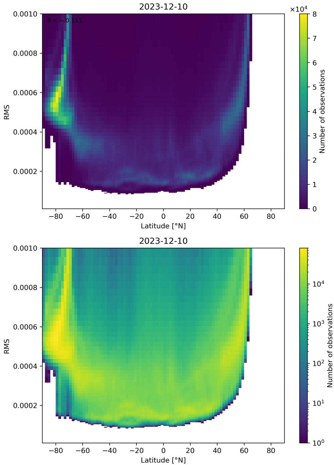
Figure 94: Scatter density plot of “Latitude” against “RMS” for 2023-12-09 to 2023-12-11.
