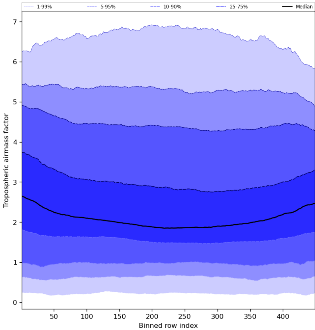
Figure 48: Along track statistics of “Tropospheric airmass factor” for 2023-12-09 to 2023-12-11
