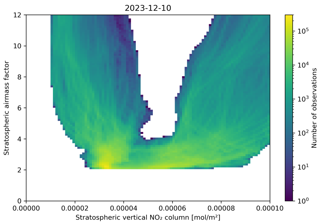
Figure 96: Scatter density plot of “Stratospheric vertical NO 2 column” against “Stratospheric airmass factor” for 2023-12-09 to 2023-12-11.
