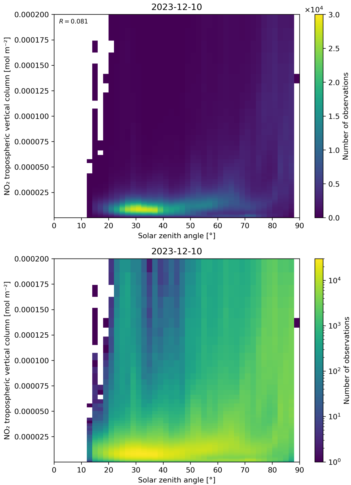
Figure 155: Scatter density plot of “Solar zenith angle” against “NO 2 tropospheric vertical column” for 2023-12-09 to 2023-12-11.
