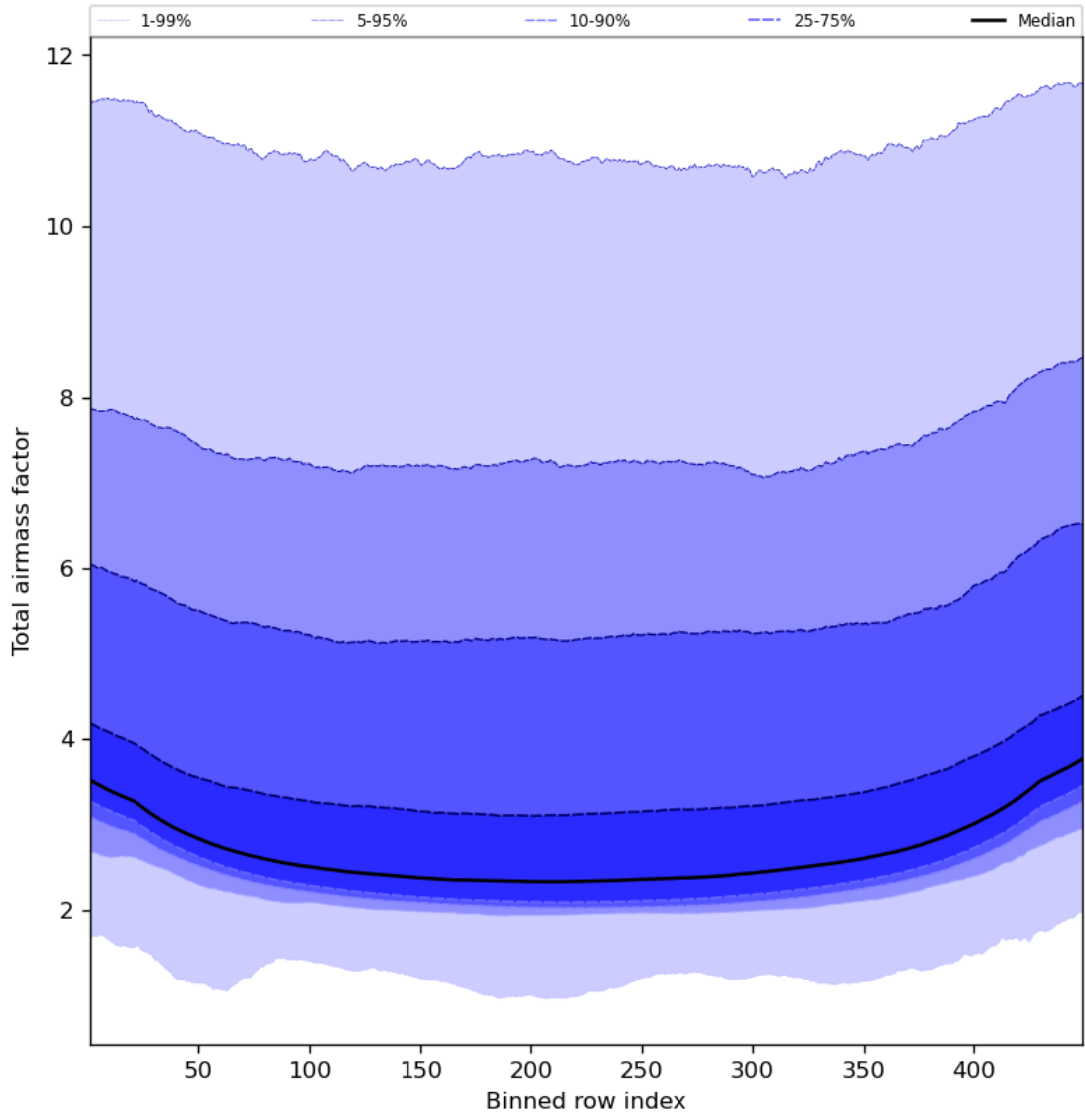
Figure 49: Along track statistics of “Total airmass factor” for 2023-12-09 to 2023-12-11
