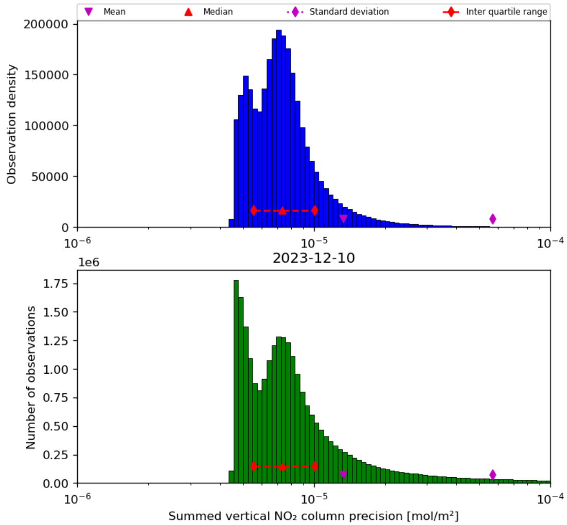
Figure 41: Histogram of “Summed vertical NO 2 column precision” for 2023-12-09 to 2023-12-11
