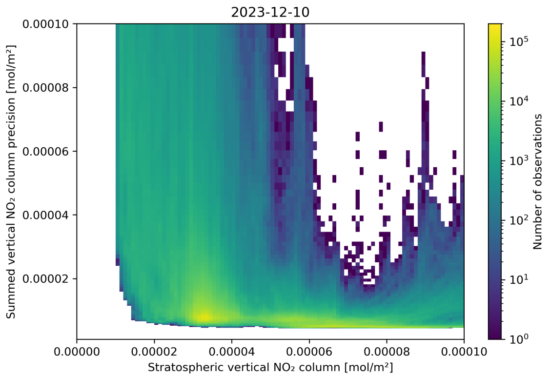
Figure 99: Scatter density plot of “Stratospheric vertical NO 2 column” against “Summed vertical NO 2 column precision” for 2023-12-09 to 2023-12-11.
