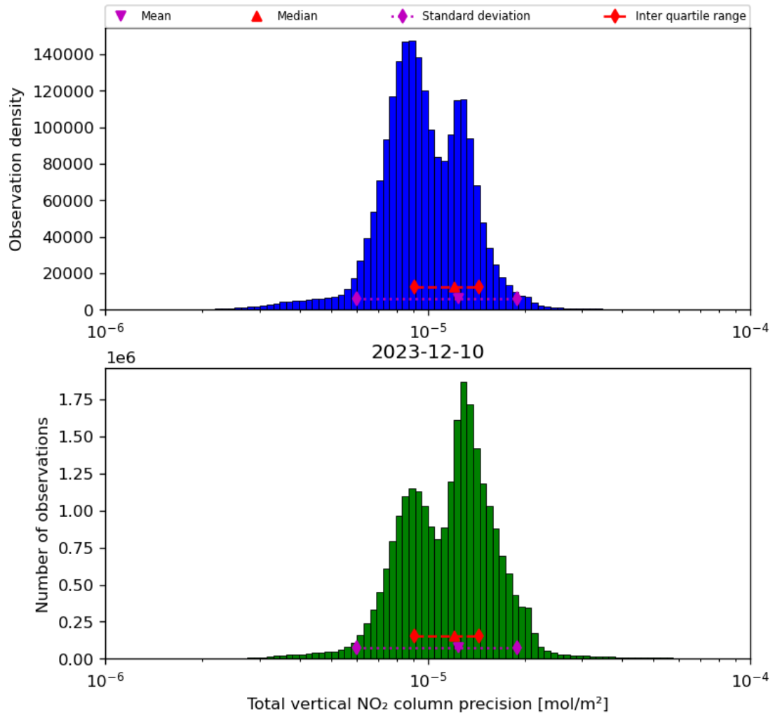
Figure 39: Histogram of “Total vertical NO 2 column precision” for 2023-12-09 to 2023-12-11
