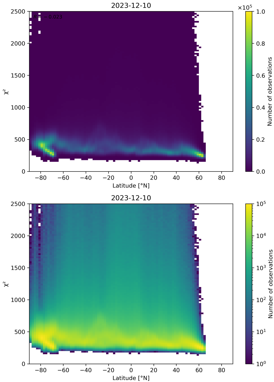
Figure 86: Scatter density plot of “Latitude” against “ \chi^2 ” for 2023-12-09 to 2023-12-11.
