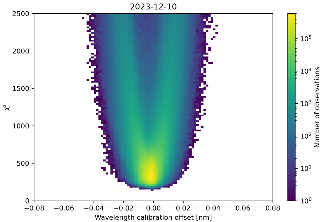
Figure 175: Scatter density plot of “Wavelength calibration offset” against “ \chi^2 ” for 2023-12-09 to 2023-12-11.
