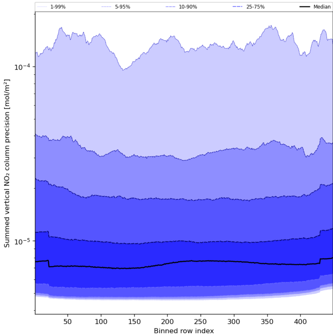
Figure 58: Along track statistics of “Summed vertical NO 2 column precision” for 2023-12-09 to 2023-12-11
