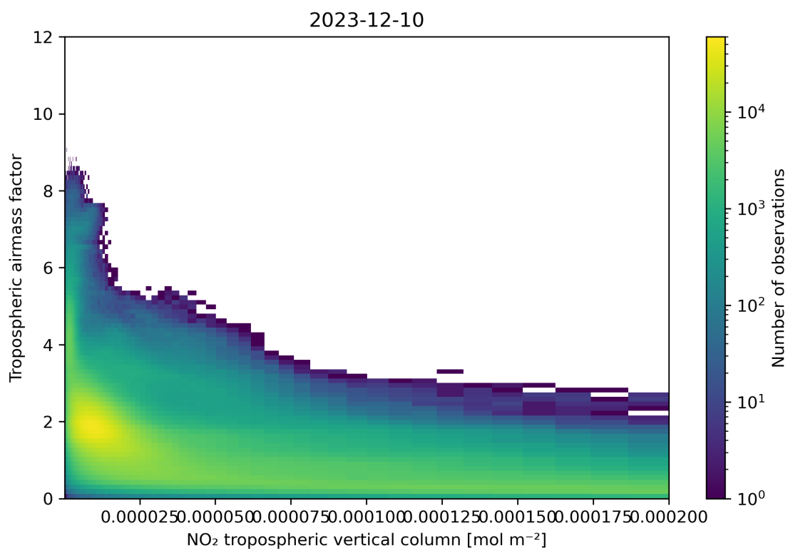
Figure 123: Scatter density plot of “NO 2 tropospheric vertical column” against “Tropospheric airmass factor” for 2023-12-09 to 2023-12-11.
