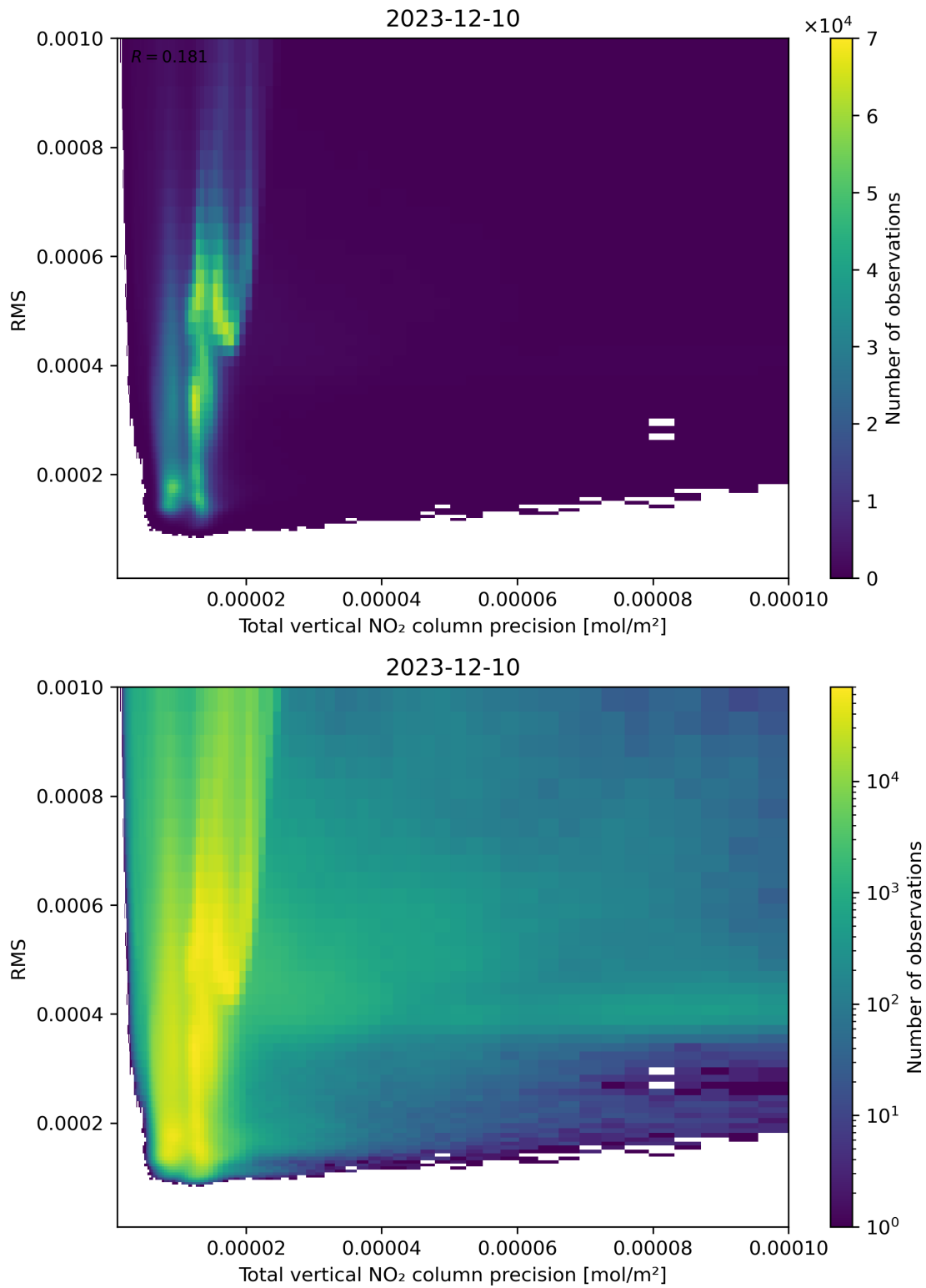
Figure 119: Scatter density plot of “Total vertical NO 2 column precision” against “RMS” for 2023-12-09 to 2023-12-11.
