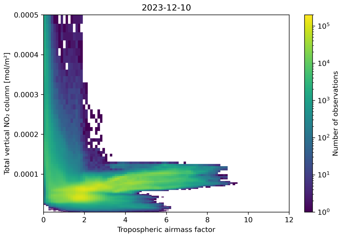
Figure 77: Scatter density plot of “Tropospheric airmass factor” against “Total vertical NO 2 column” for 2023-12-09 to 2023-12-11.
