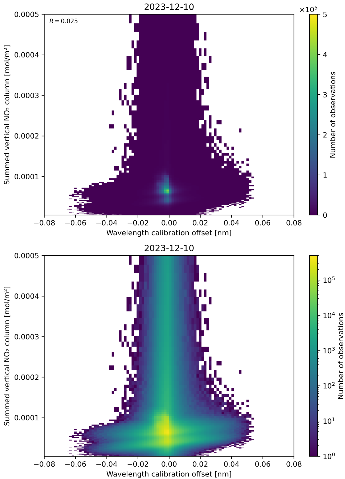
Figure 177: Scatter density plot of “Wavelength calibration offset” against “Summed vertical NO 2 column” for 2023-12-09 to 2023-12-11.
