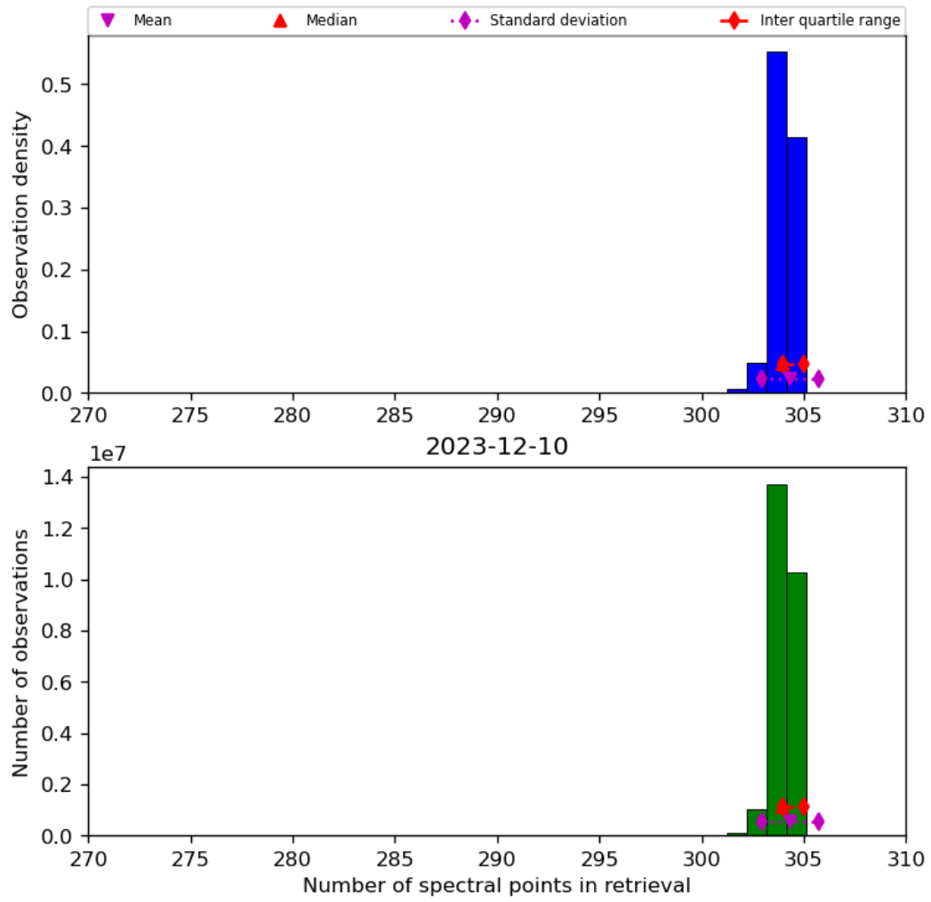
Figure 33: Histogram of “Number of spectral points in retrieval” for 2023-12-09 to 2023-12-11
