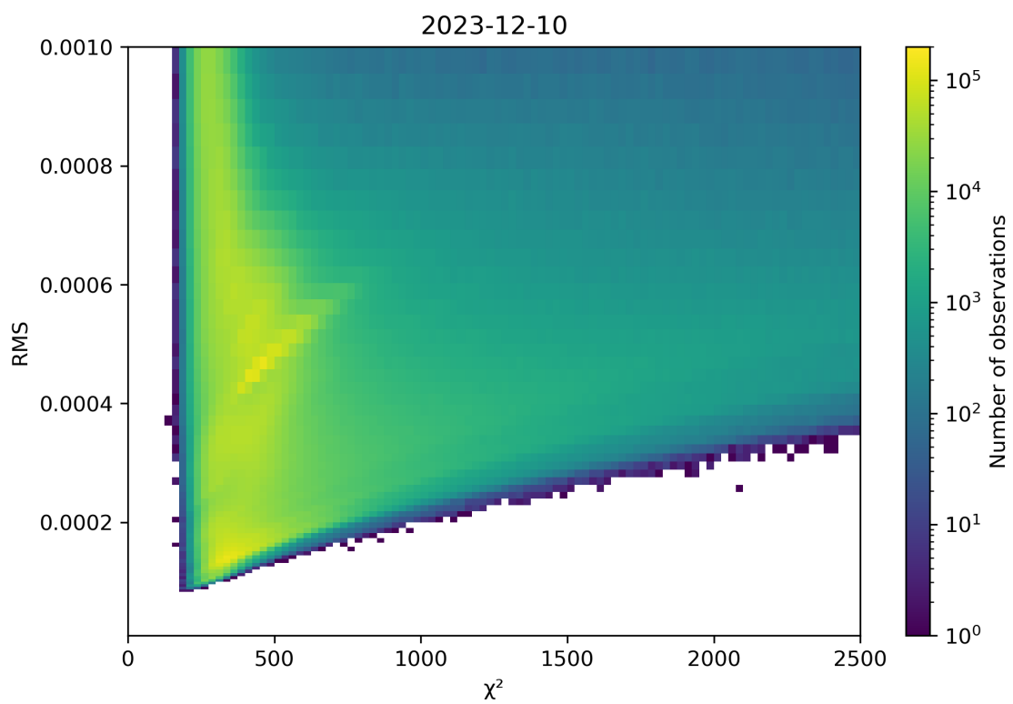
Figure 82: Scatter density plot of " \chi^2 " against "RMS" for 2023-12-09 to 2023-12-11.
