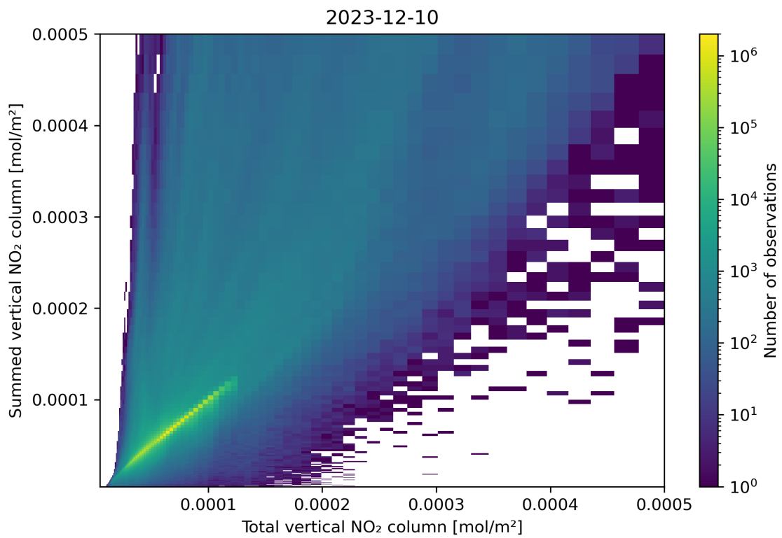
Figure 112: Scatter density plot of “Total vertical NO 2 column” against “Summed vertical NO 2 column” for 2023-12-09 to 2023-12-11.
