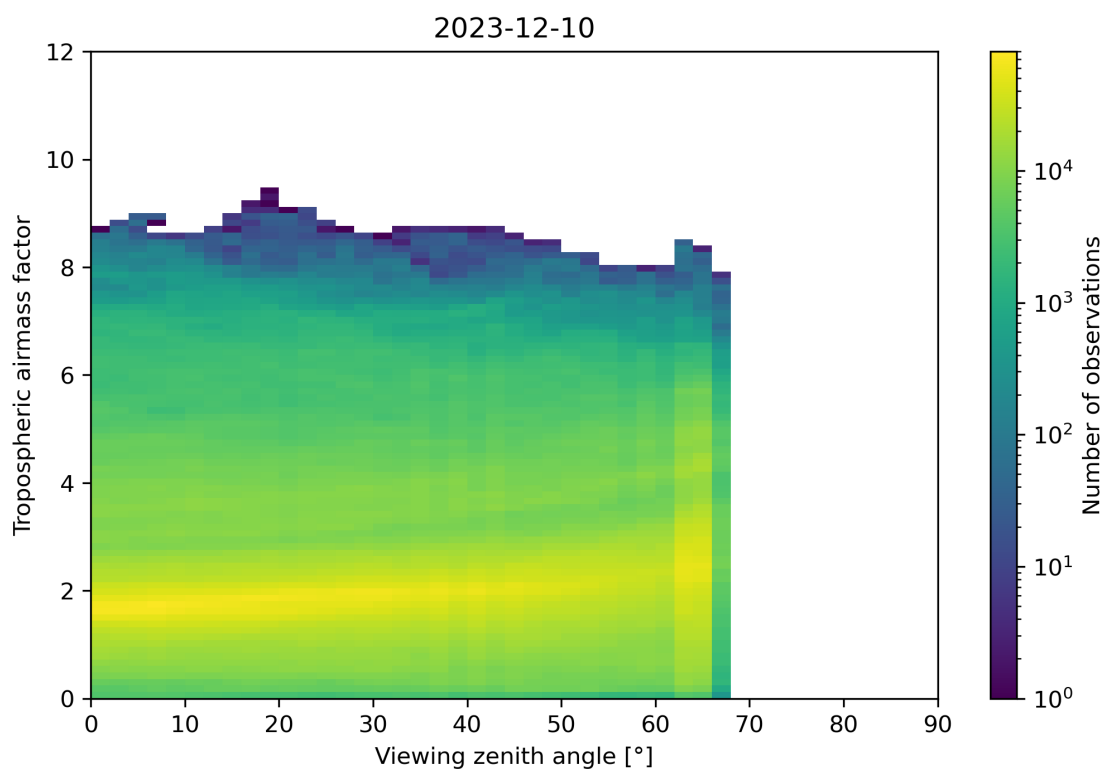
Figure 161: Scatter density plot of “Viewing zenith angle” against “Tropospheric airmass factor” for 2023-12-09 to 2023-12-11.
