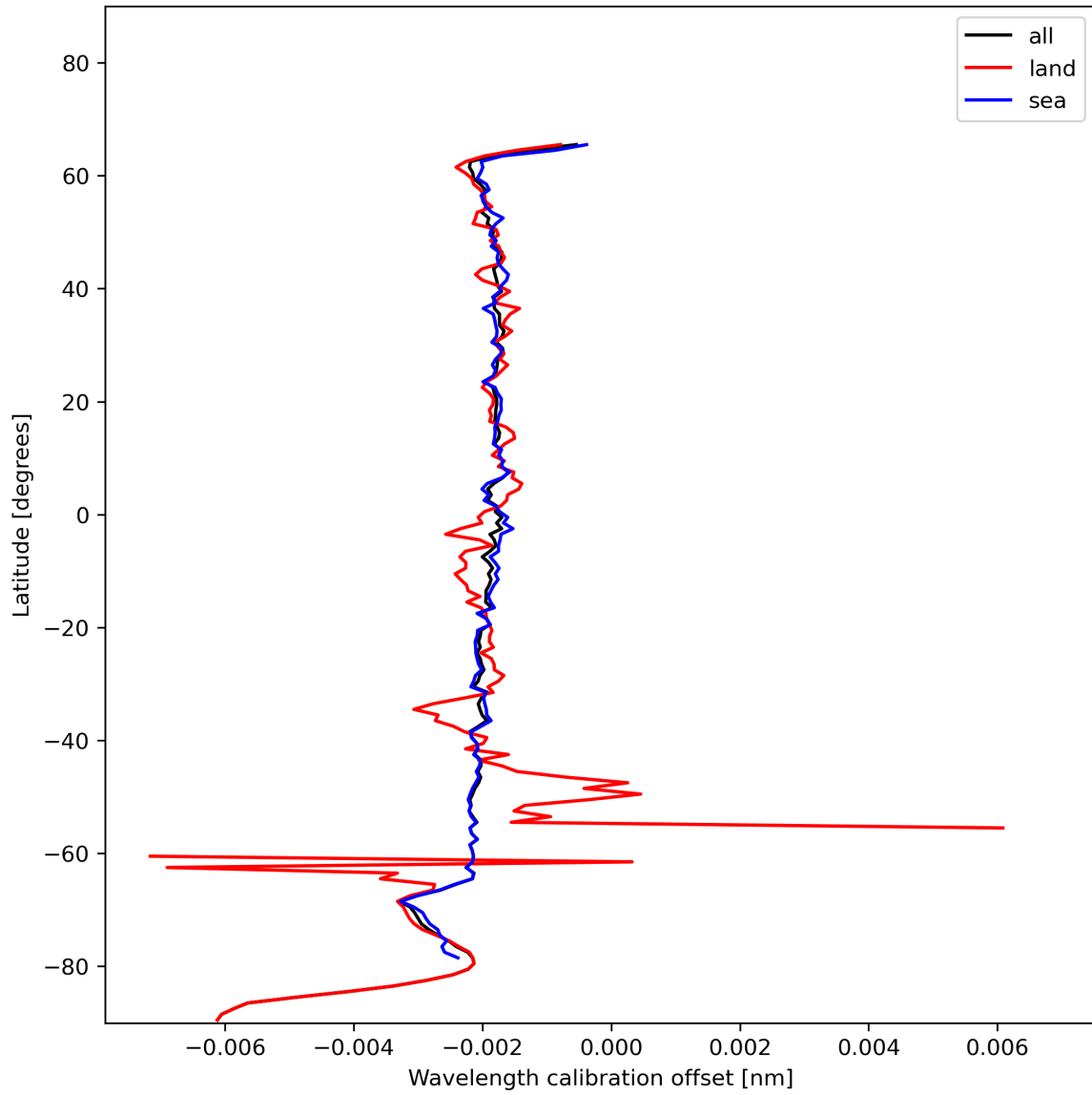
Figure 18: Zonal average of “Wavelength calibration offset” for 2023-12-09 to 2023-12-11.
