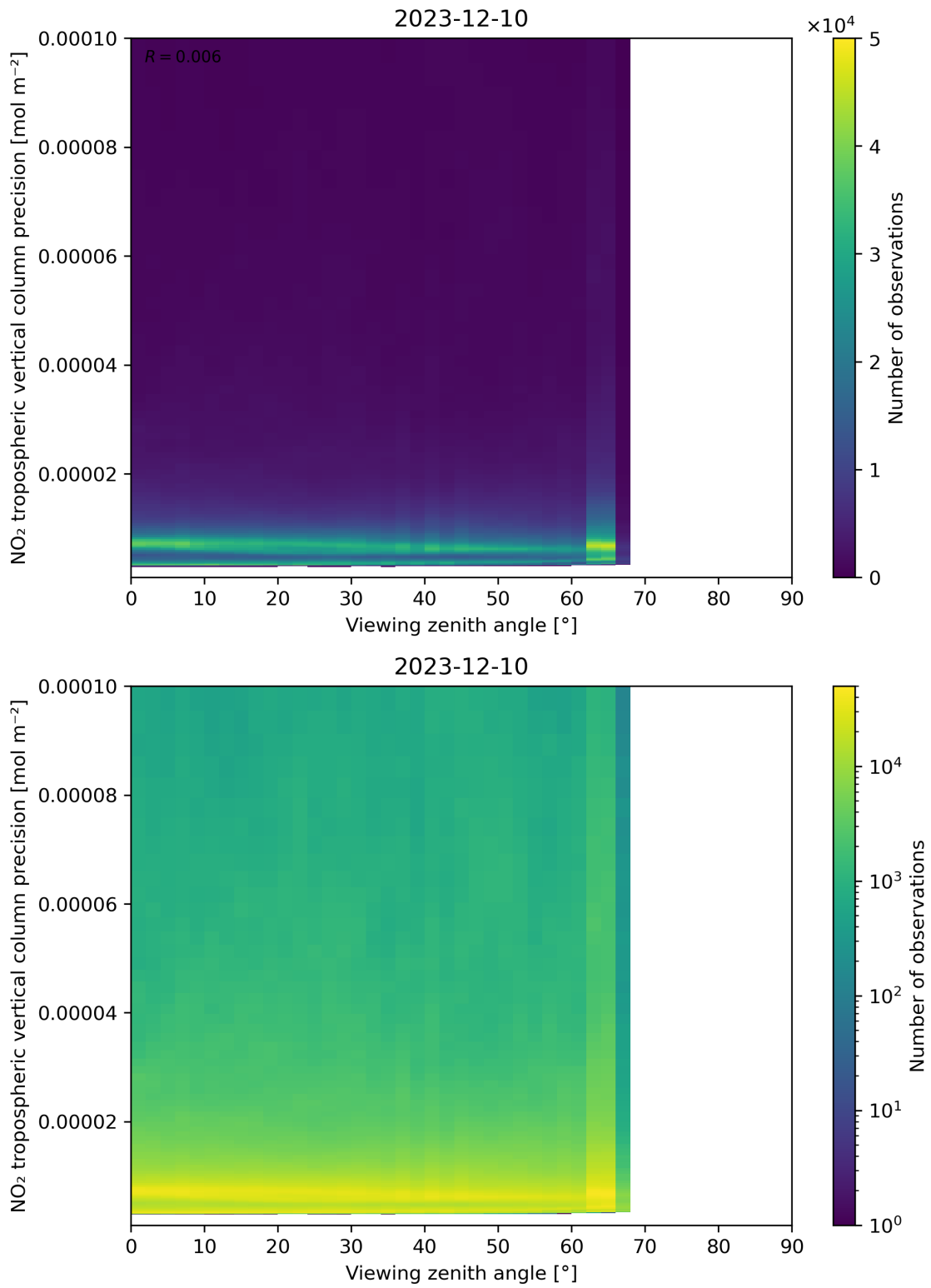
Figure 170: Scatter density plot of “Viewing zenith angle” against “NO 2 tropospheric vertical column precision” for 2023-12-09 to 2023-12-11.
