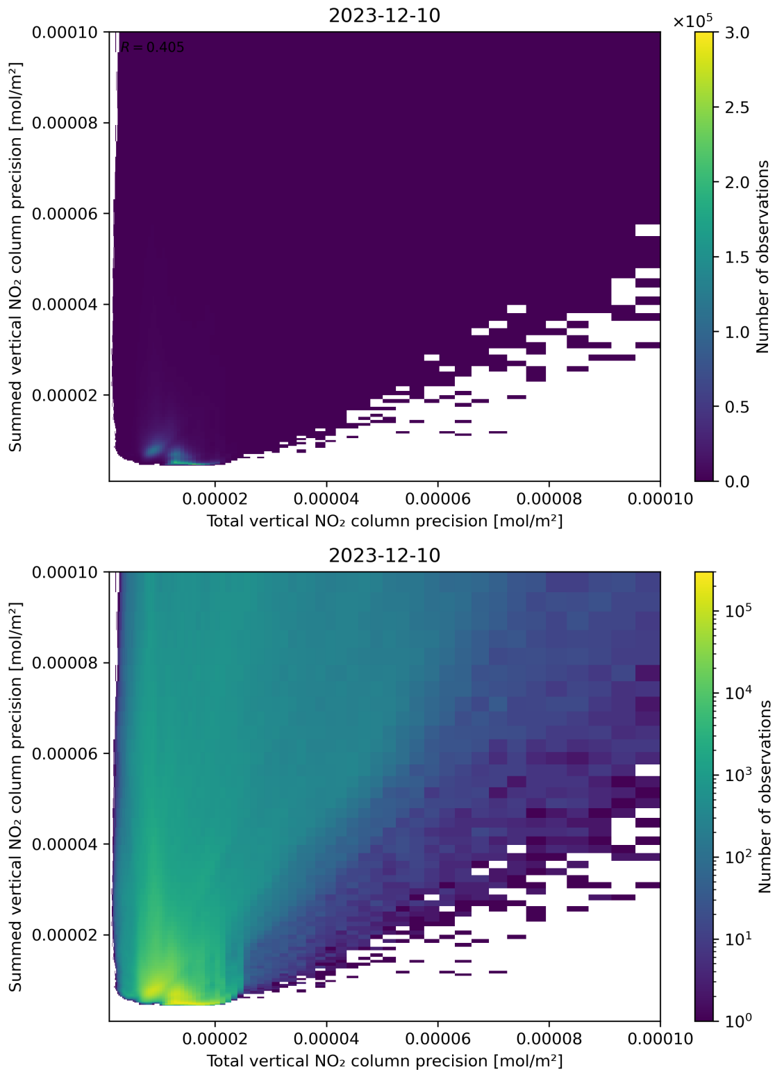
Figure 118: Scatter density plot of “Total vertical NO 2 column precision” against “Summed vertical NO 2 column precision” for 2023-12-09 to 2023-12-11.
