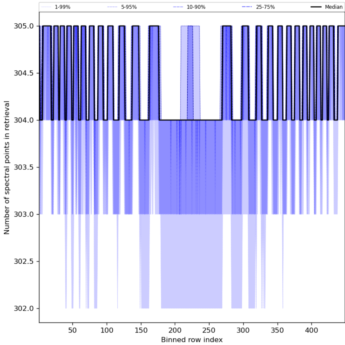
Figure 50: Along track statistics of “Number of spectral points in retrieval” for 2023-12-09 to 2023-12-11
