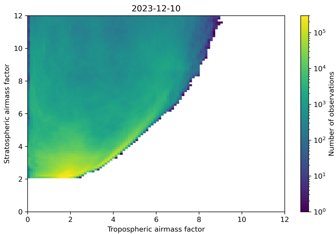
Figure 71: Scatter density plot of “Tropospheric airmass factor” against “Stratospheric airmass factor” for 2023-12-09 to 2023-12-11.
