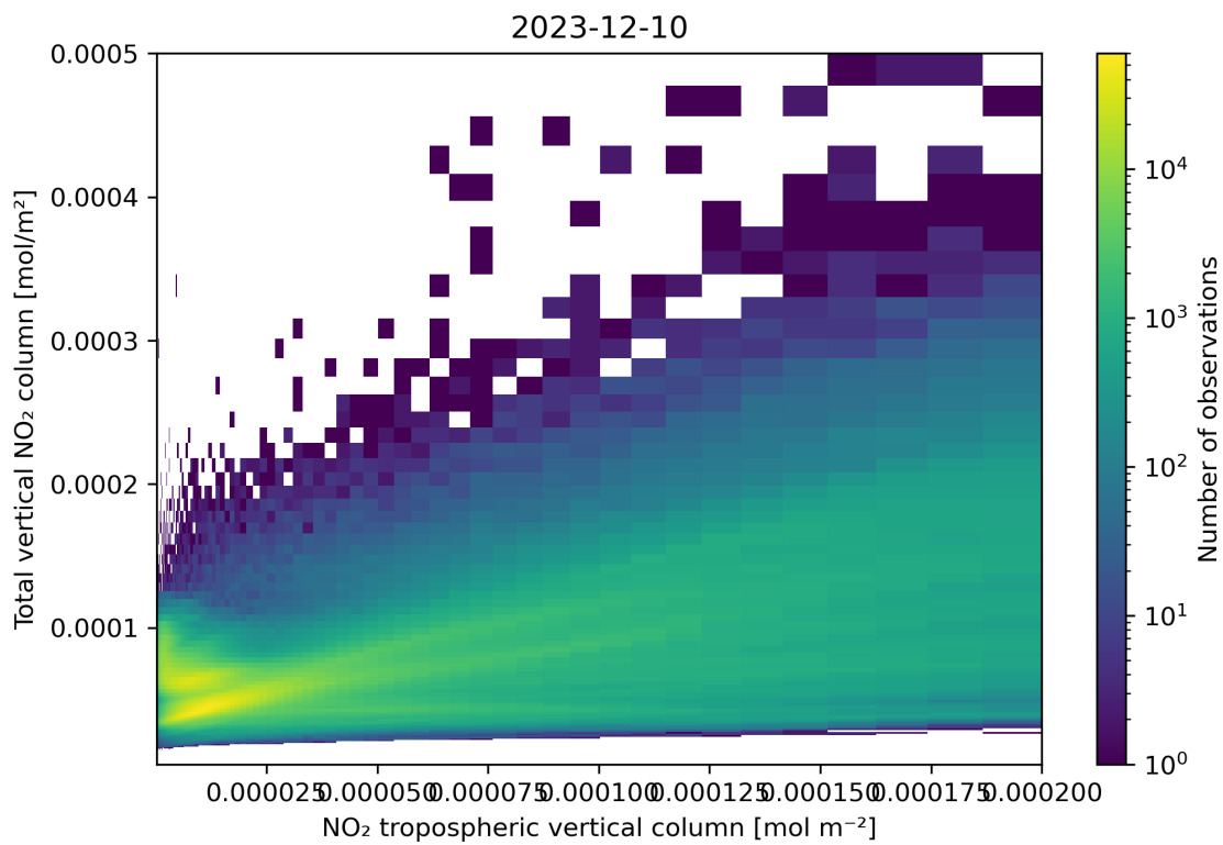
Figure 128: Scatter density plot of “NO 2 tropospheric vertical column” against “Total vertical NO 2 column” for 2023-12-09 to 2023-12-11.
