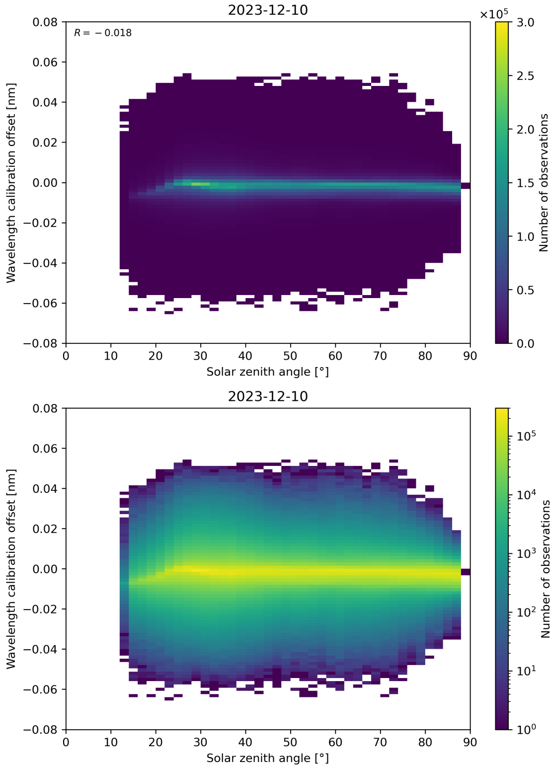
Figure 158: Scatter density plot of “Solar zenith angle” against “Wavelength calibration offset” for 2023-12-09 to 2023-12-11.
