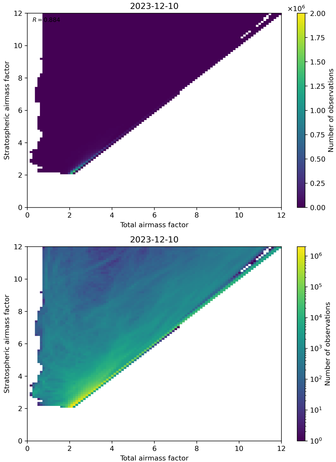
Figure 62: Scatter density plot of “Total airmass factor” against “Stratospheric airmass factor” for 2023-12-09 to 2023-12-11.
