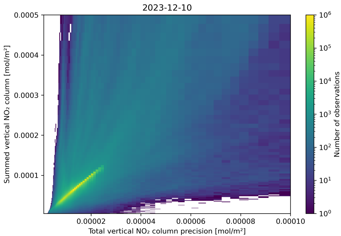
Figure 117: Scatter density plot of “Total vertical NO 2 column precision” against “Summed vertical NO 2 column” for 2023-12-09 to 2023-12-11.
