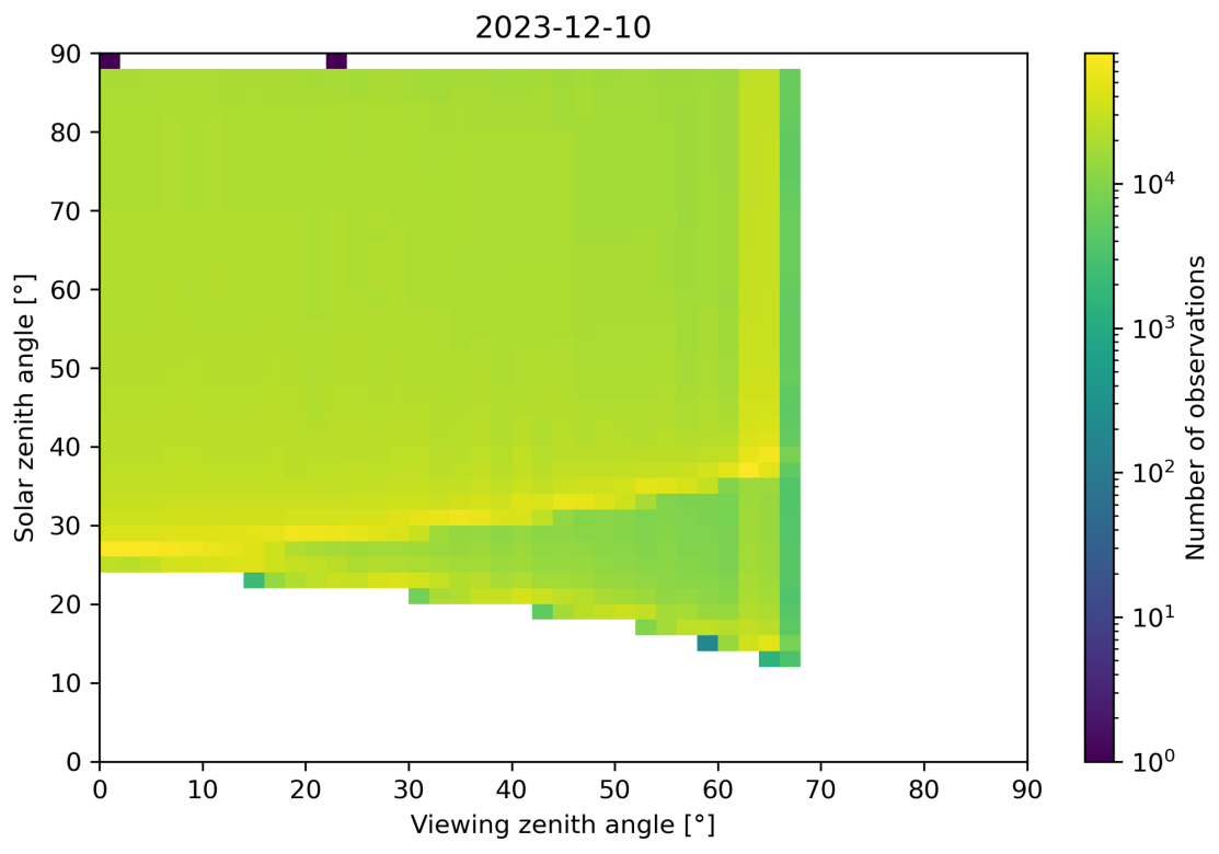
Figure 172: Scatter density plot of “Viewing zenith angle” against “Solar zenith angle” for 2023-12-09 to 2023-12-11.
