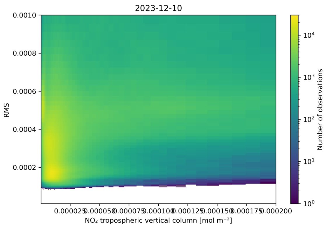
Figure 142: Scatter density plot of “NO 2 tropospheric vertical column” against “RMS” for 2023-12-09 to 2023-12-11.
