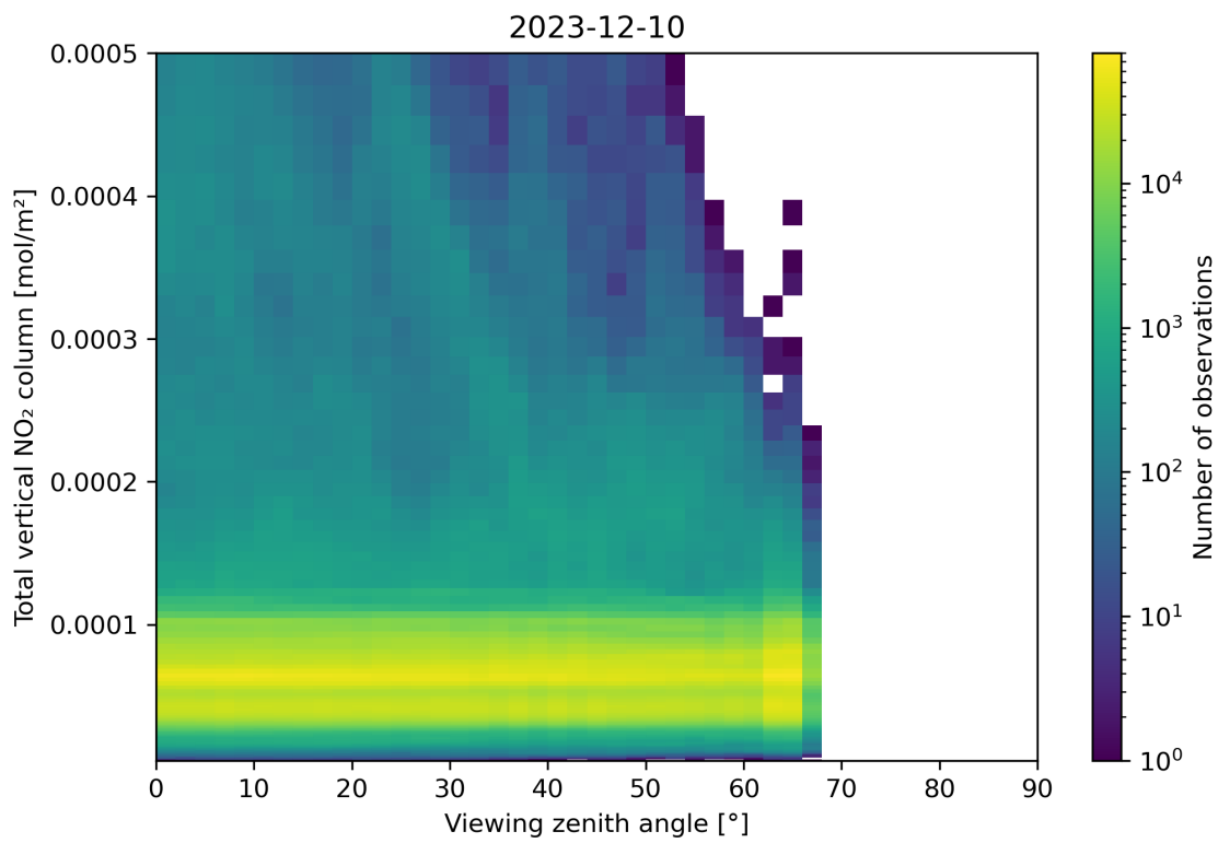
Figure 167: Scatter density plot of “Viewing zenith angle” against “Total vertical NO 2 column” for 2023-12-09 to 2023-12-11.
