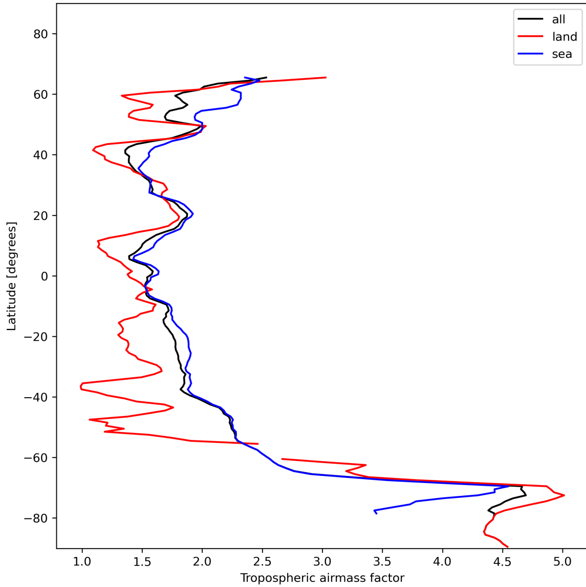
Figure 14: Zonal average of “Tropospheric airmass factor” for 2023-12-09 to 2023-12-11.
