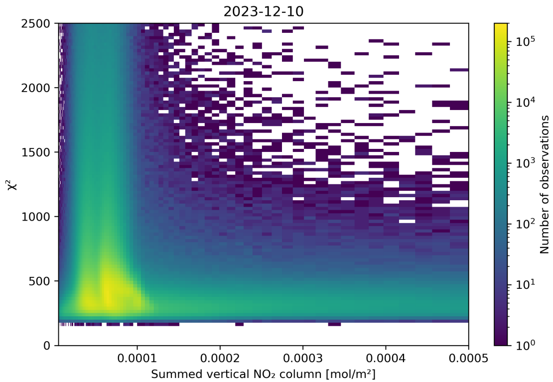
Figure 104: Scatter density plot of “Summed vertical NO 2 column” against “ \chi^2 ” for 2023-12-09 to 2023-12-11.
