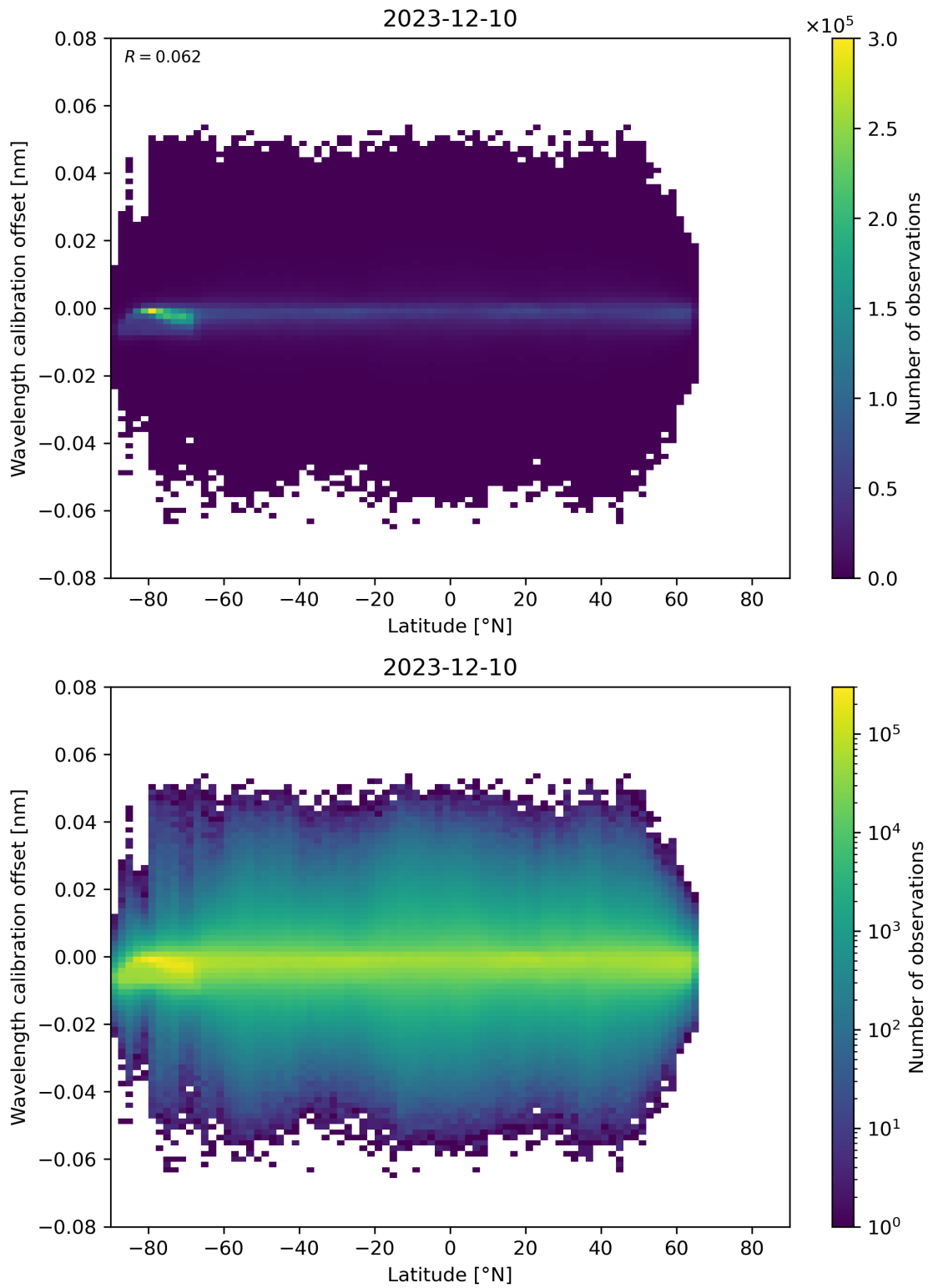
Figure 95: Scatter density plot of “Latitude” against “Wavelength calibration offset” for 2023-12-09 to 2023-12-11.
