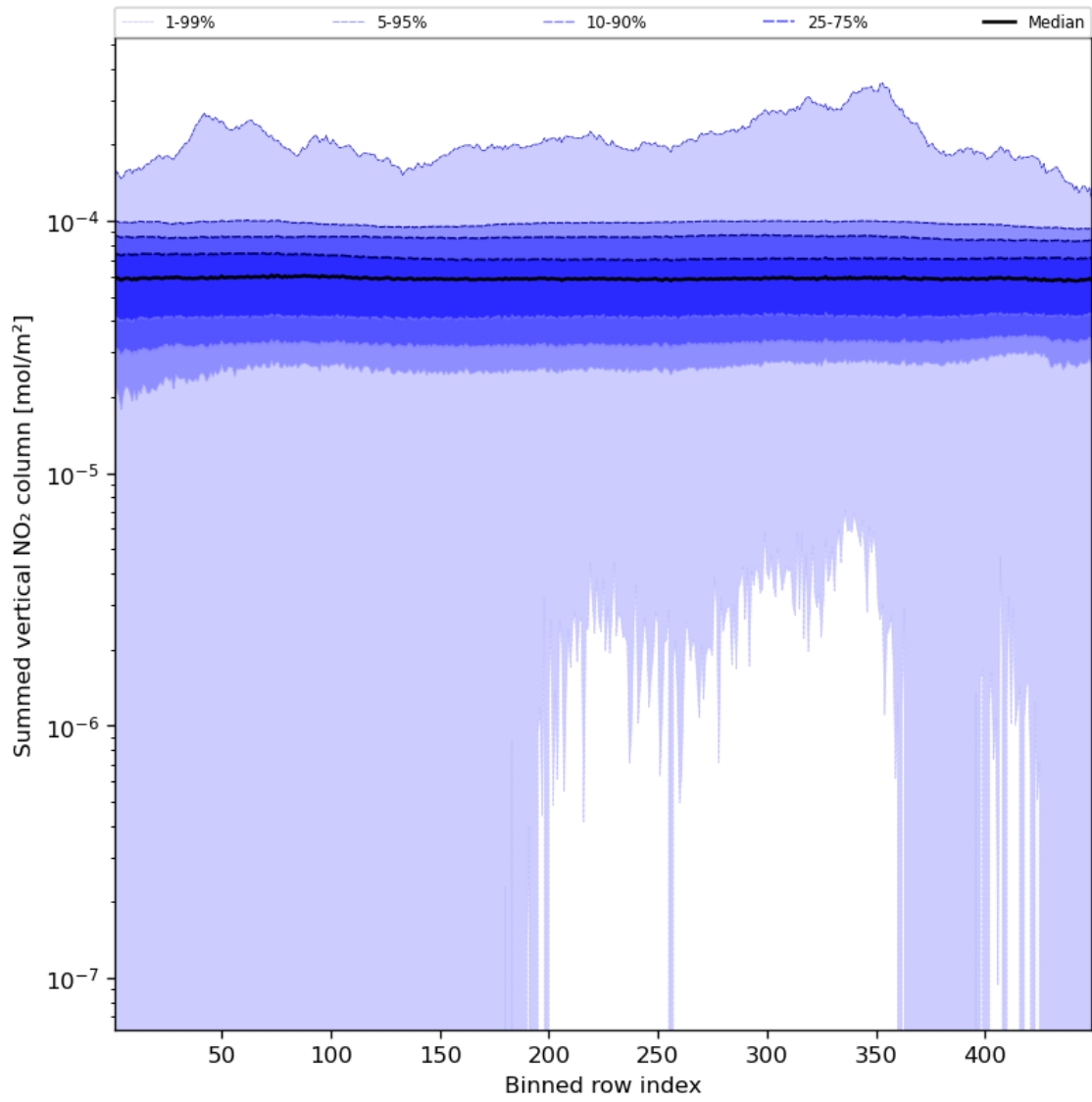
Figure 57: Along track statistics of “Summed vertical NO 2 column” for 2023-12-09 to 2023-12-11
