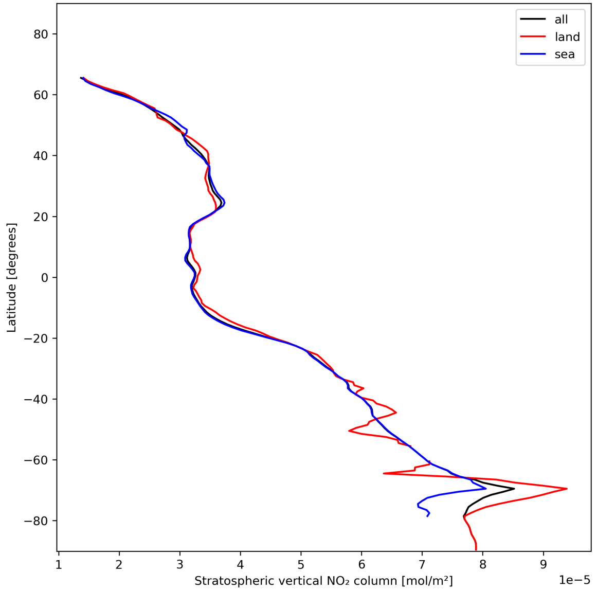
Figure 19: Zonal average of “Stratospheric vertical NO 2 column” for 2023-12-09 to 2023-12-11.
