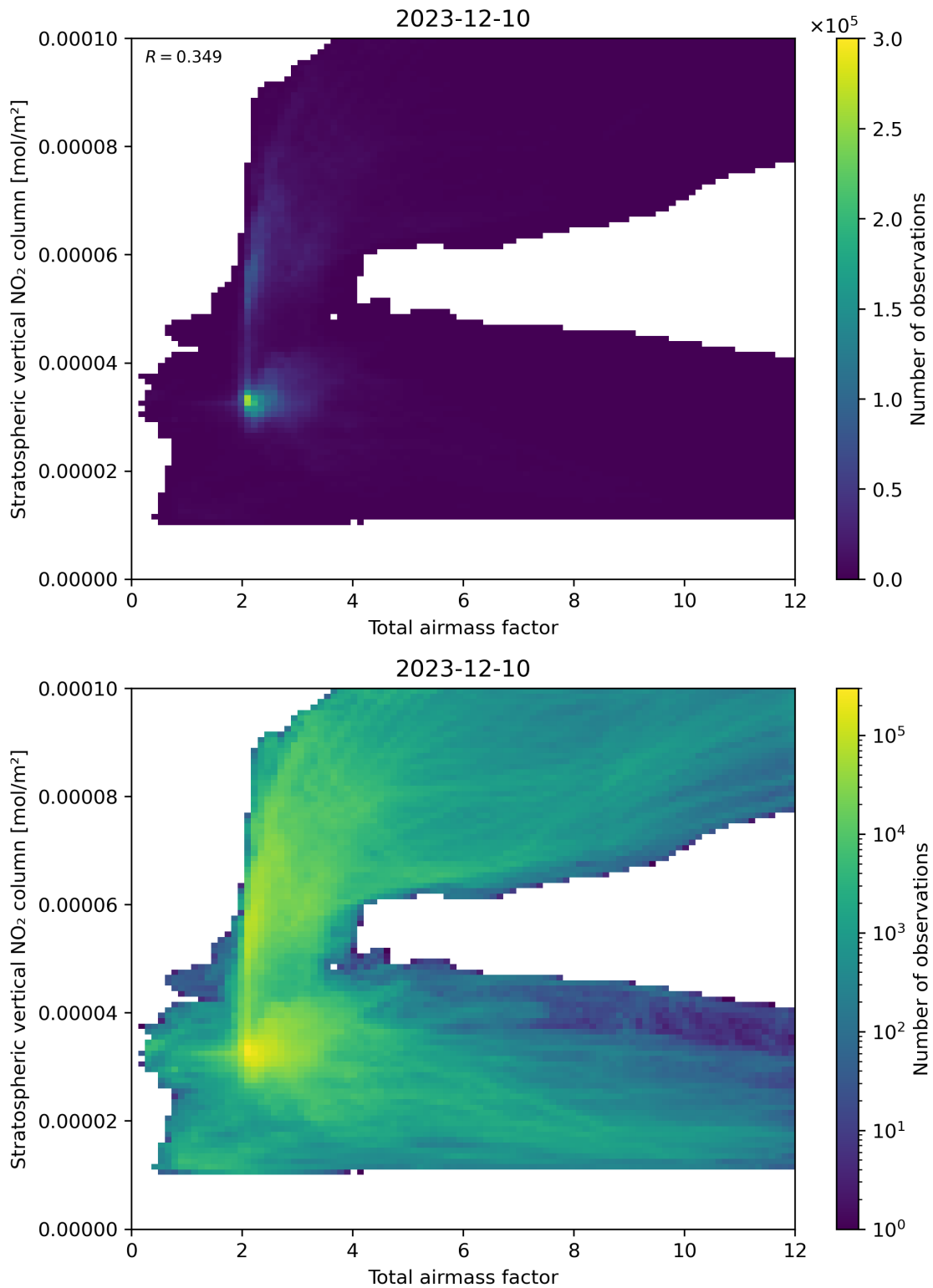
Figure 64: Scatter density plot of “Total airmass factor” against “Stratospheric vertical NO 2 column” for 2023-12-09 to 2023-12-11.
