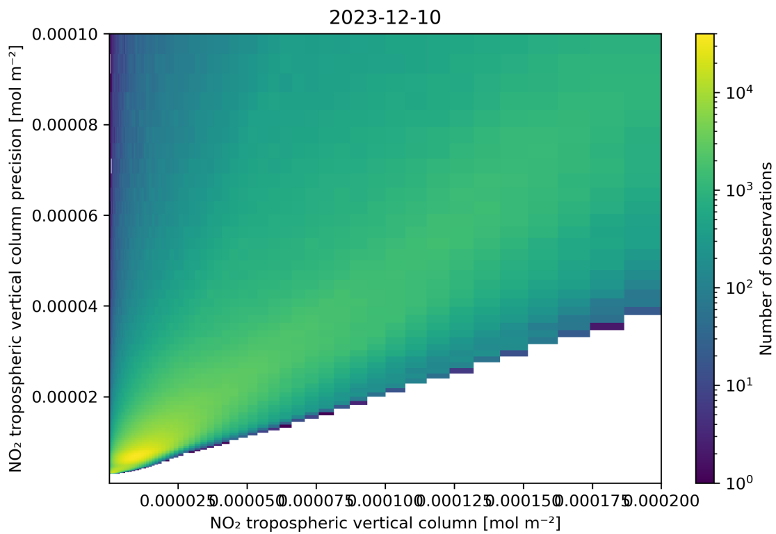
Figure 130: Scatter density plot of “NO 2 tropospheric vertical column” against “NO 2 tropospheric vertical column precision” for 2023-12-09 to 2023-12-11.
