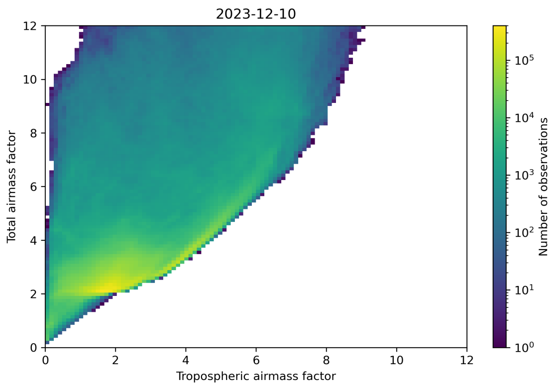
Figure 72: Scatter density plot of “Tropospheric airmass factor” against “Total airmass factor” for 2023-12-09 to 2023-12-11.
