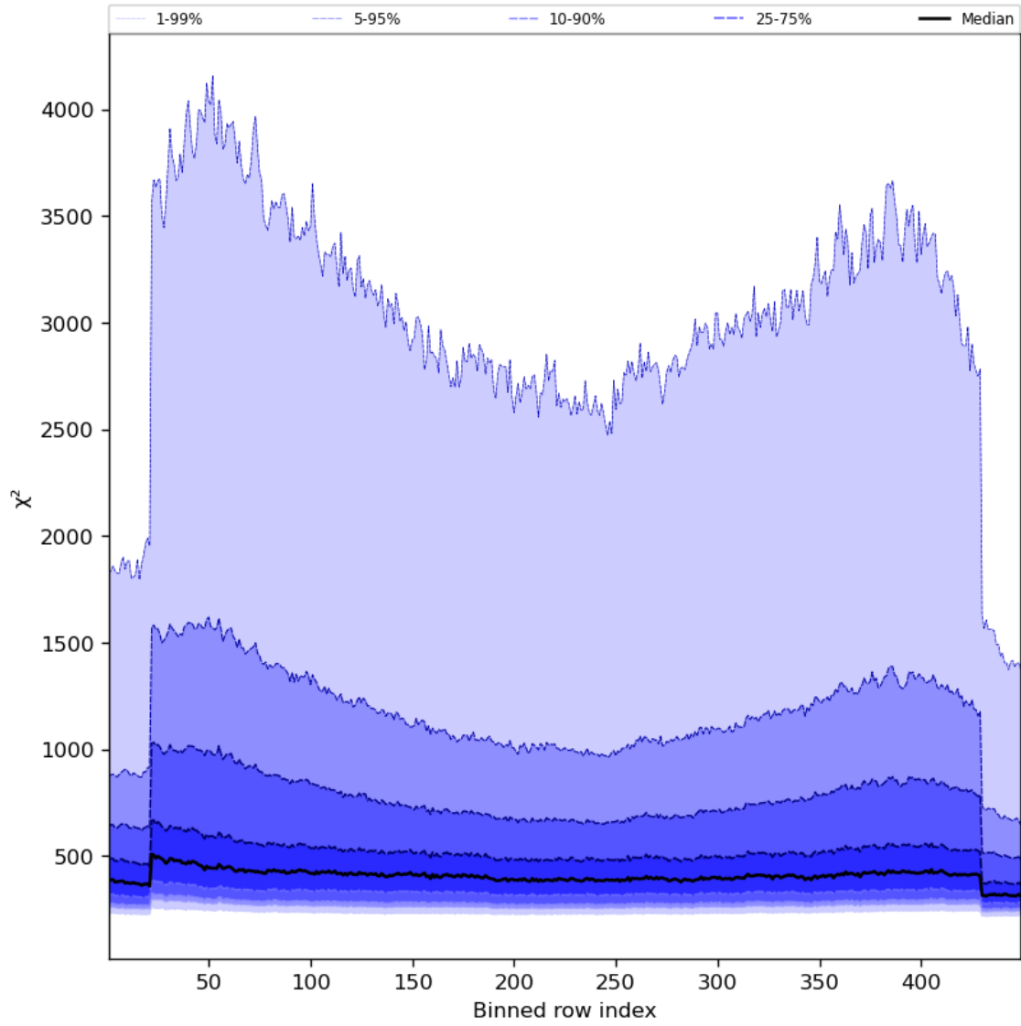
Figure 59: Along track statistics of “ \chi^2 ” for 2023-12-09 to 2023-12-11
