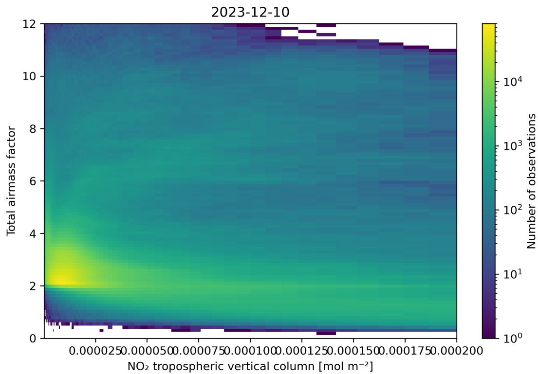
Figure 122: Scatter density plot of “NO 2 tropospheric vertical column” against “Total airmass factor” for 2023-12-09 to 2023-12-11.
