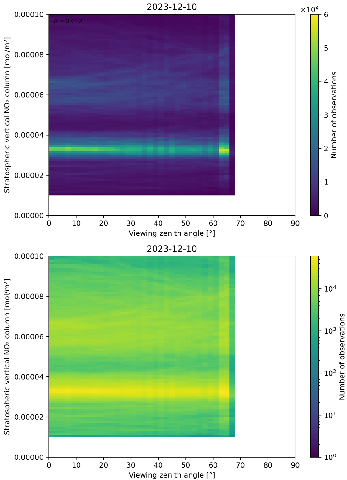
Figure 164: Scatter density plot of “Viewing zenith angle” against “Stratospheric vertical NO 2 column” for 2023-12-09 to 2023-12-11.
