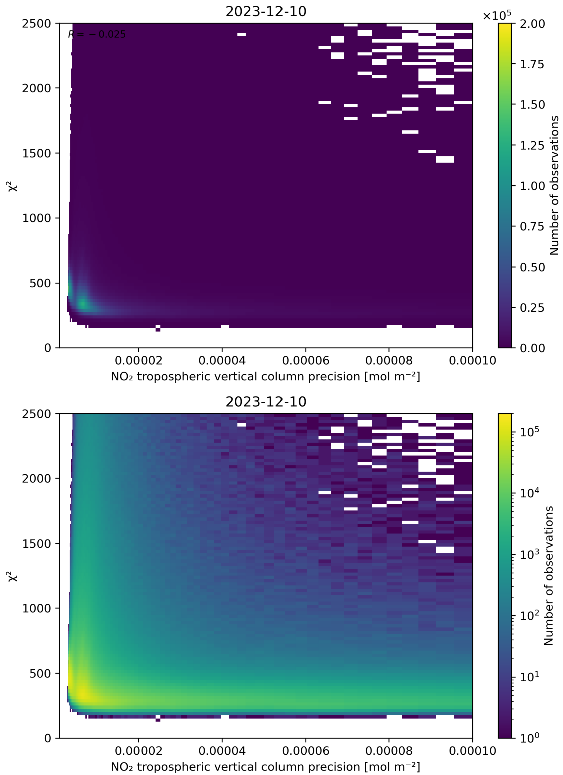
Figure 134: Scatter density plot of “NO 2 tropospheric vertical column precision” against “χ 2 ” for 2023-12-09 to 2023-12-11.
