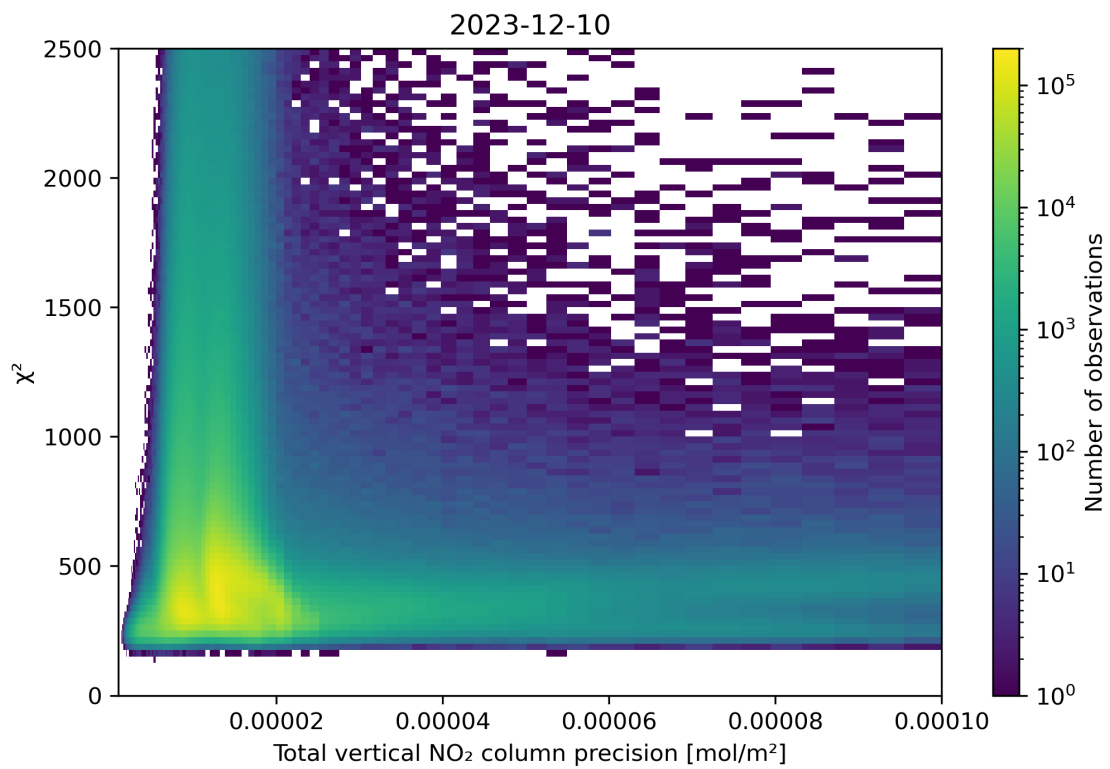
Figure 116: Scatter density plot of “Total vertical NO 2 column precision” against “ \chi^2 ” for 2023-12-09 to 2023-12-11.
