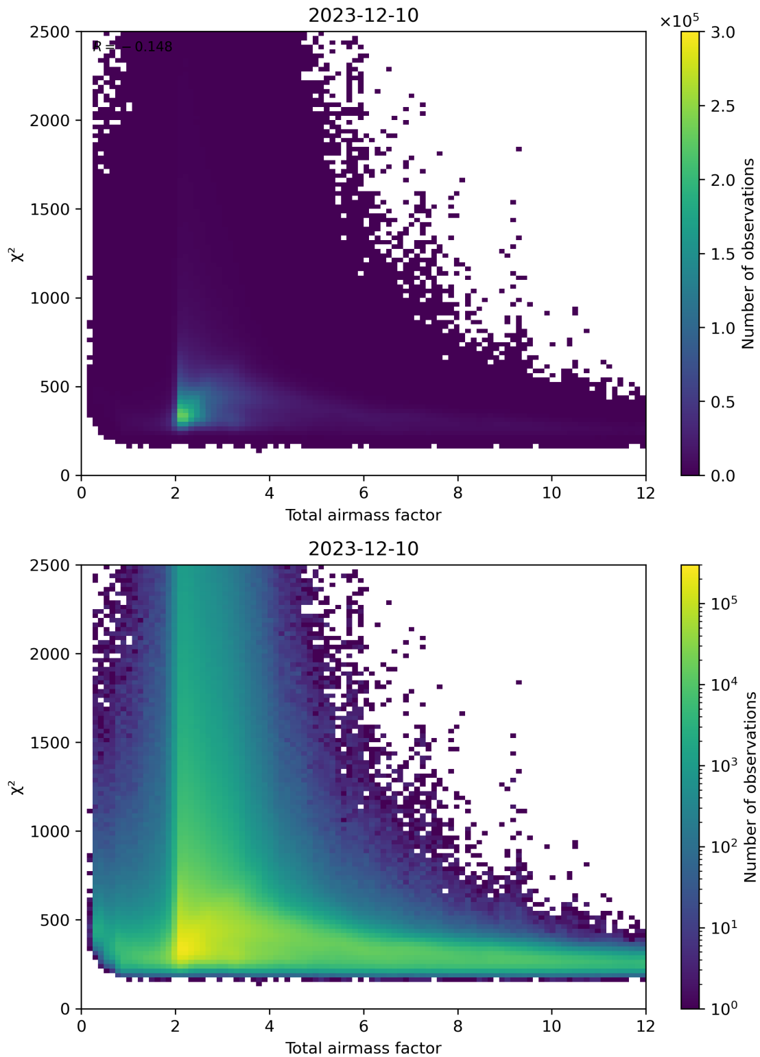
Figure 63: Scatter density plot of “Total airmass factor” against “ \chi^2 ” for 2023-12-09 to 2023-12-11.
