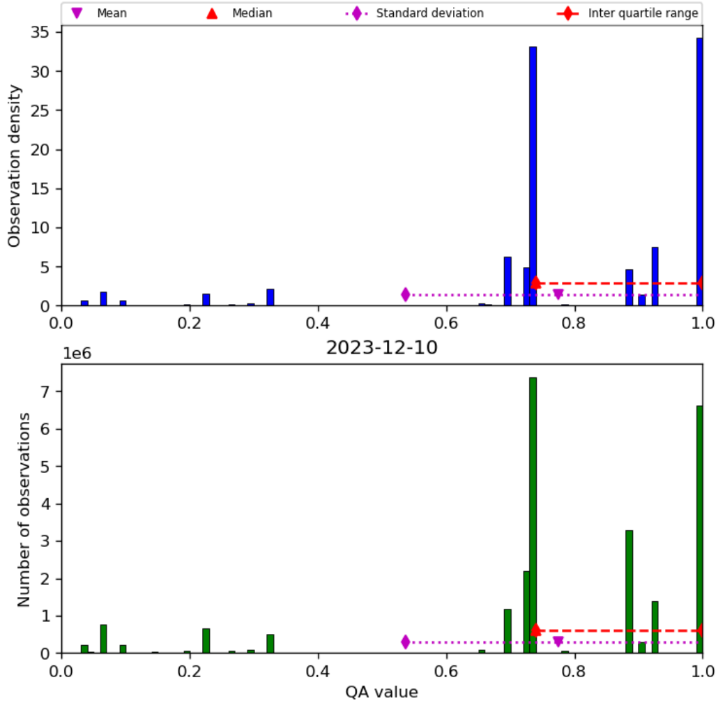
Figure 28: Histogram of “QA value” for 2023-12-09 to 2023-12-11
