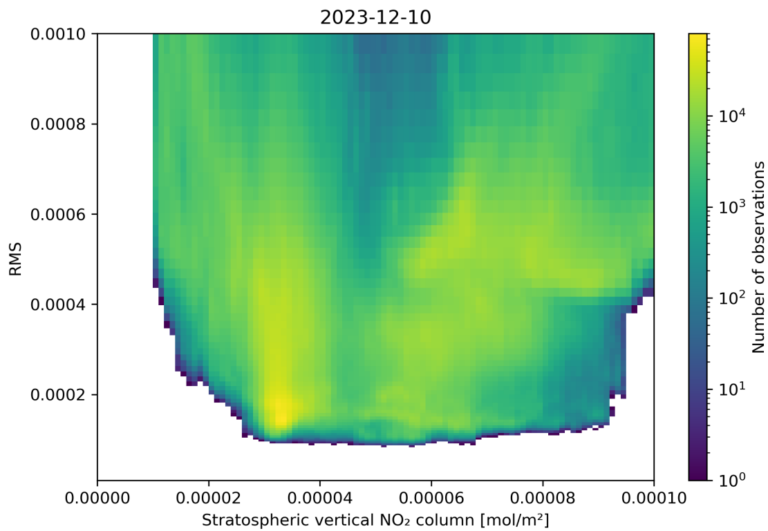
Figure 102: Scatter density plot of “Stratospheric vertical NO 2 column” against “RMS” for 2023-12-09 to 2023-12-11.
