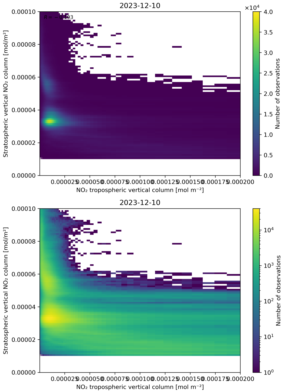
Figure 125: Scatter density plot of “NO 2 tropospheric vertical column” against “Stratospheric vertical NO 2 column” for 2023-12-09 to 2023-12-11.
