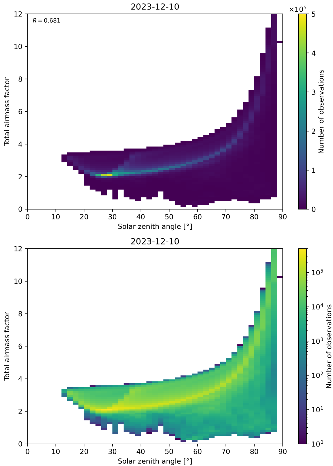
Figure 146: Scatter density plot of “Solar zenith angle” against “Total airmass factor” for 2023-12-09 to 2023-12-11.
