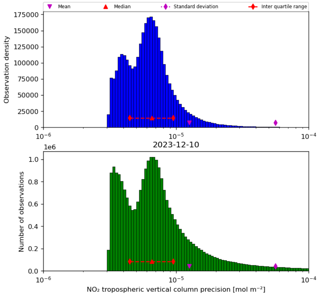
Figure 30: Histogram of “NO 2 tropospheric vertical column precision” for 2023-12-09 to 2023-12-11
