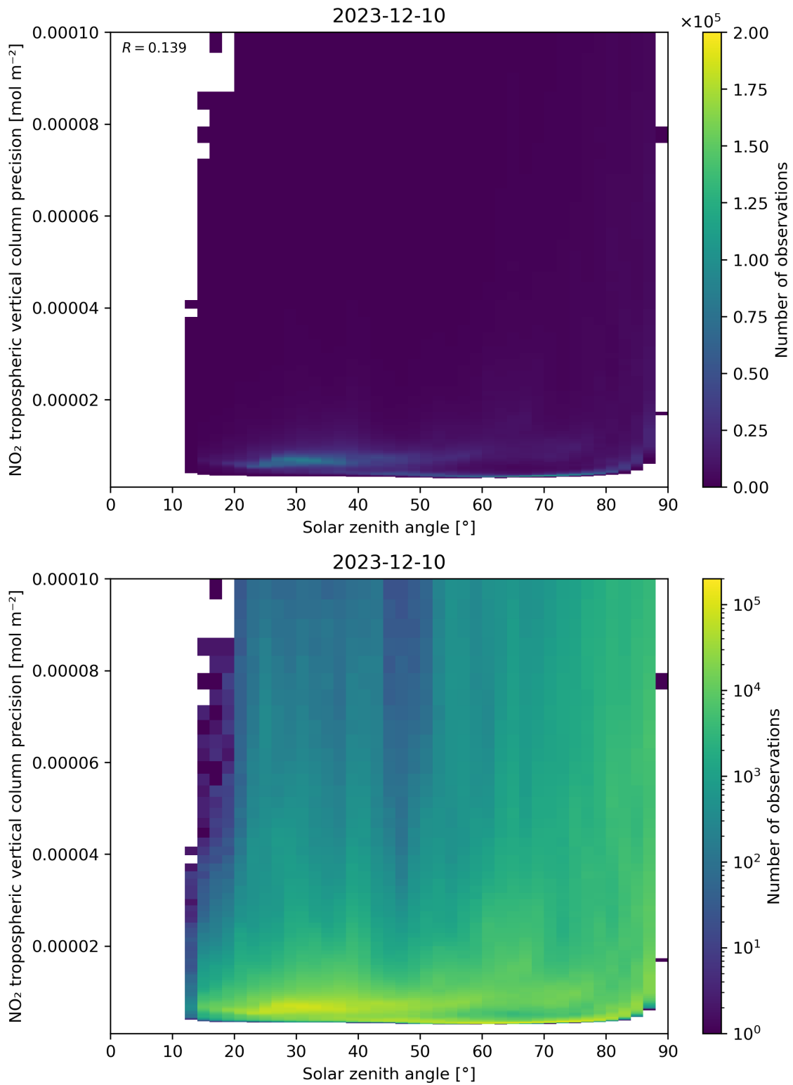
Figure 156: Scatter density plot of “Solar zenith angle” against “NO 2 tropospheric vertical column precision” for 2023-12-09 to 2023-12-11.
