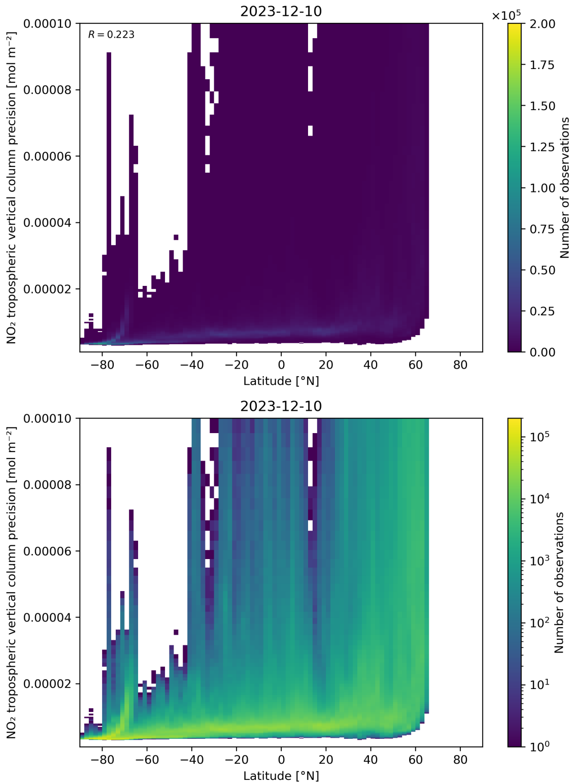
Figure 93: Scatter density plot of “Latitude” against “NO 2 tropospheric vertical column precision” for 2023-12-09 to 2023-12-11.
