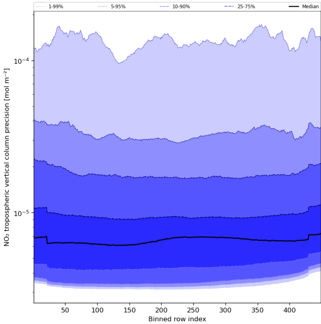
Figure 47: Along track statistics of “NO 2 tropospheric vertical column precision” for 2023-12-09 to 2023-12-11
