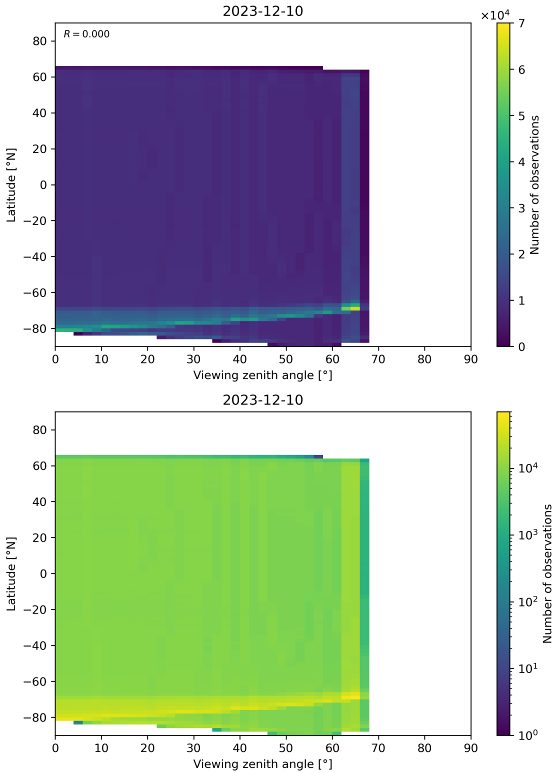
Figure 163: Scatter density plot of “Viewing zenith angle” against “Latitude” for 2023-12-09 to 2023-12-11.
