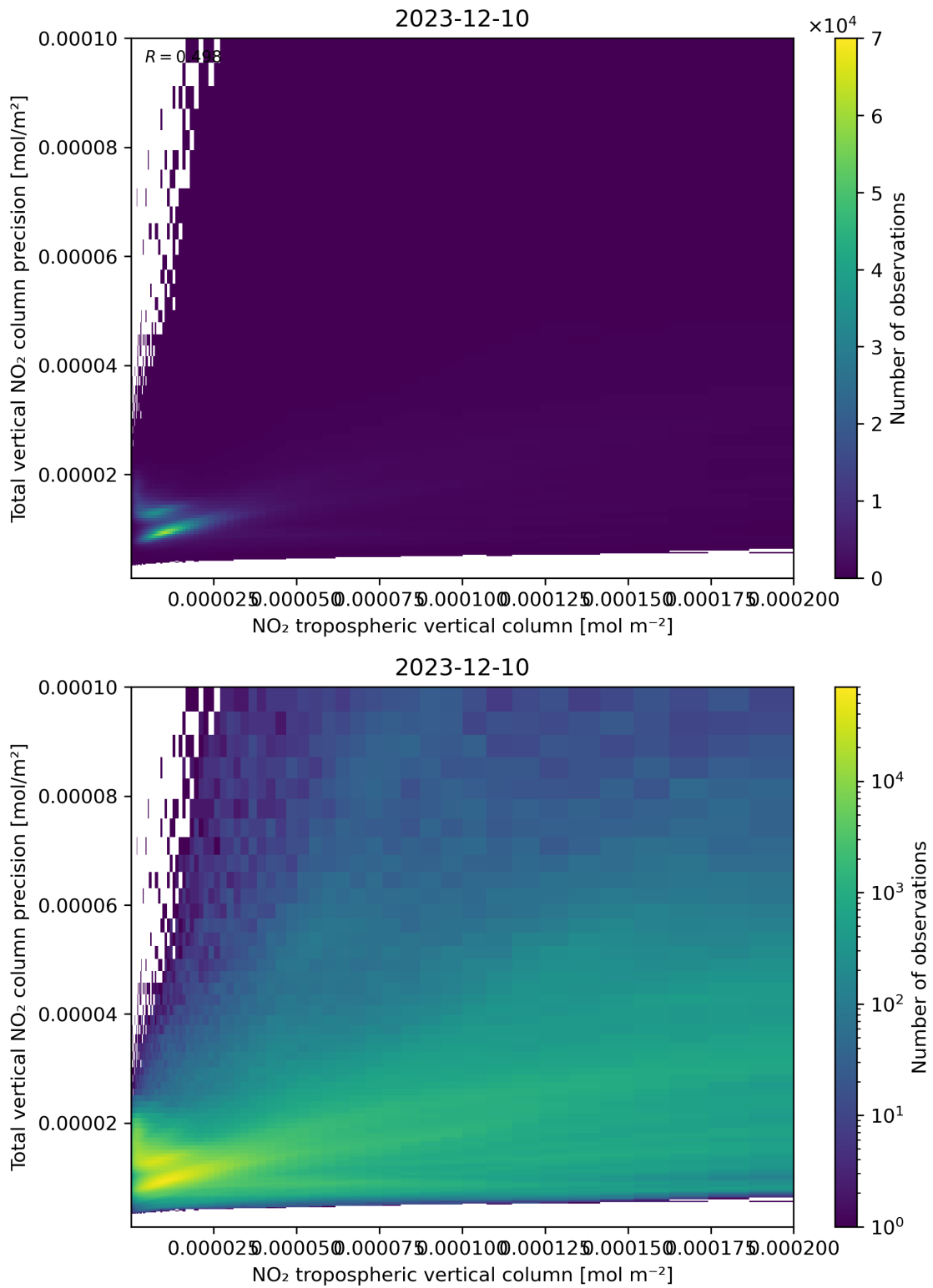
Figure 129: Scatter density plot of “NO 2 tropospheric vertical column” against “Total vertical NO 2 column precision” for 2023-12-09 to 2023-12-11.
