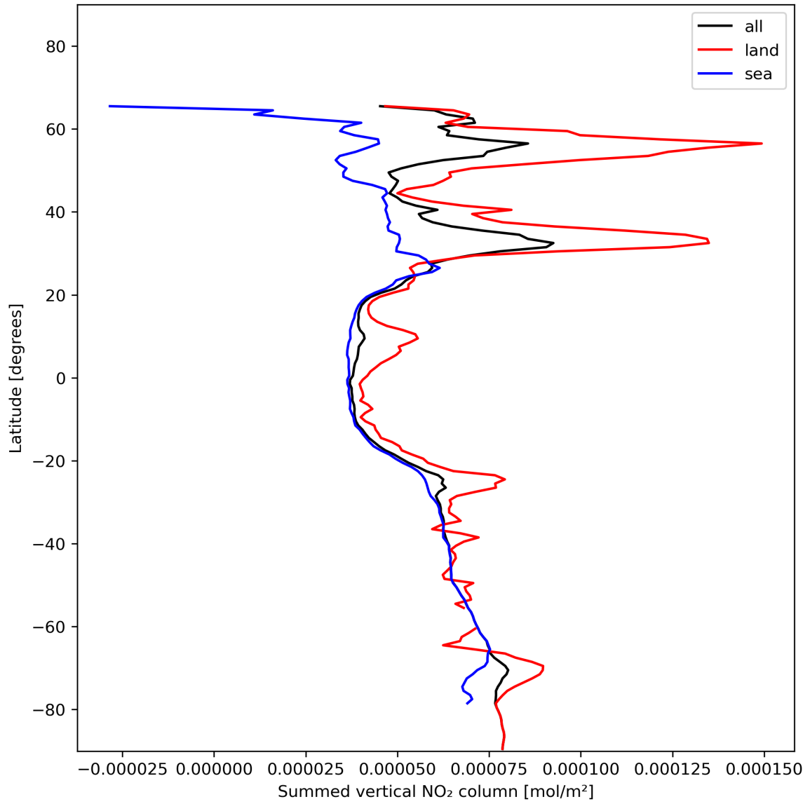
Figure 23: Zonal average of “Summed vertical NO 2 column” for 2023-12-09 to 2023-12-11.
