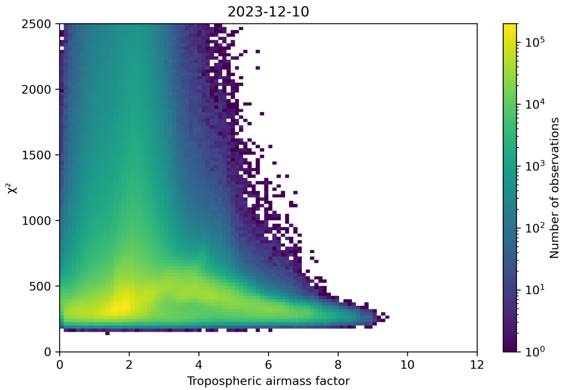
Figure 73: Scatter density plot of “Tropospheric airmass factor” against “ \chi^2 ” for 2023-12-09 to 2023-12-11.
