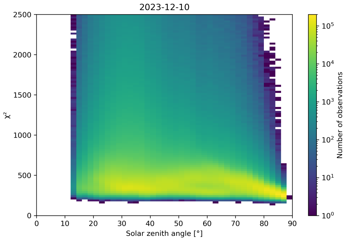
Figure 148: Scatter density plot of “Solar zenith angle” against “ \chi^2 ” for 2023-12-09 to 2023-12-11.
