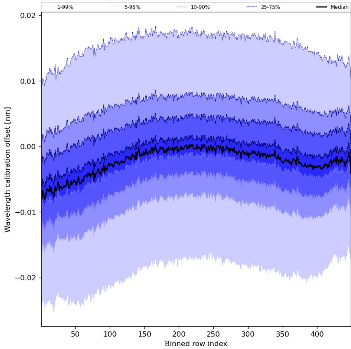
Figure 52: Along track statistics of “Wavelength calibration offset” for 2023-12-09 to 2023-12-11
