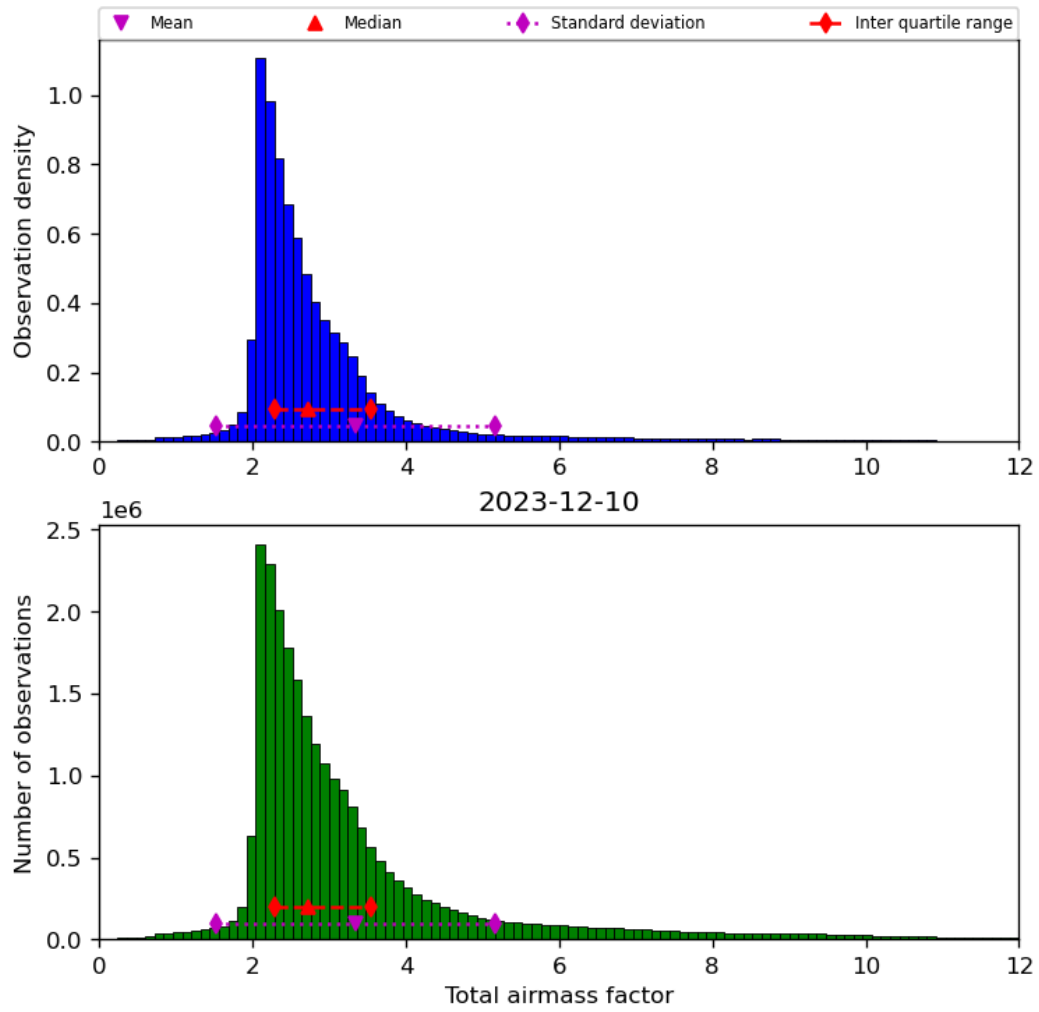
Figure 32: Histogram of “Total airmass factor” for 2023-12-09 to 2023-12-11
