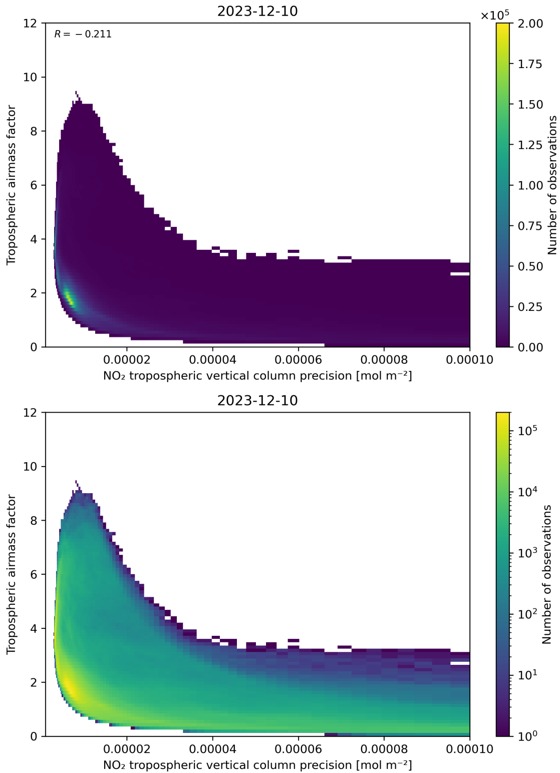
Figure 133: Scatter density plot of “NO 2 tropospheric vertical column precision” against “Tropospheric air mass factor” for 2023-12-09 to 2023-12-11.
