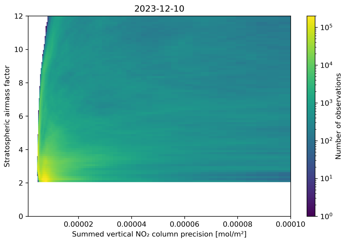
Figure 106: Scatter density plot of “Summed vertical NO 2 column precision” against “Stratospheric airmass factor” for 2023-12-09 to 2023-12-11.
