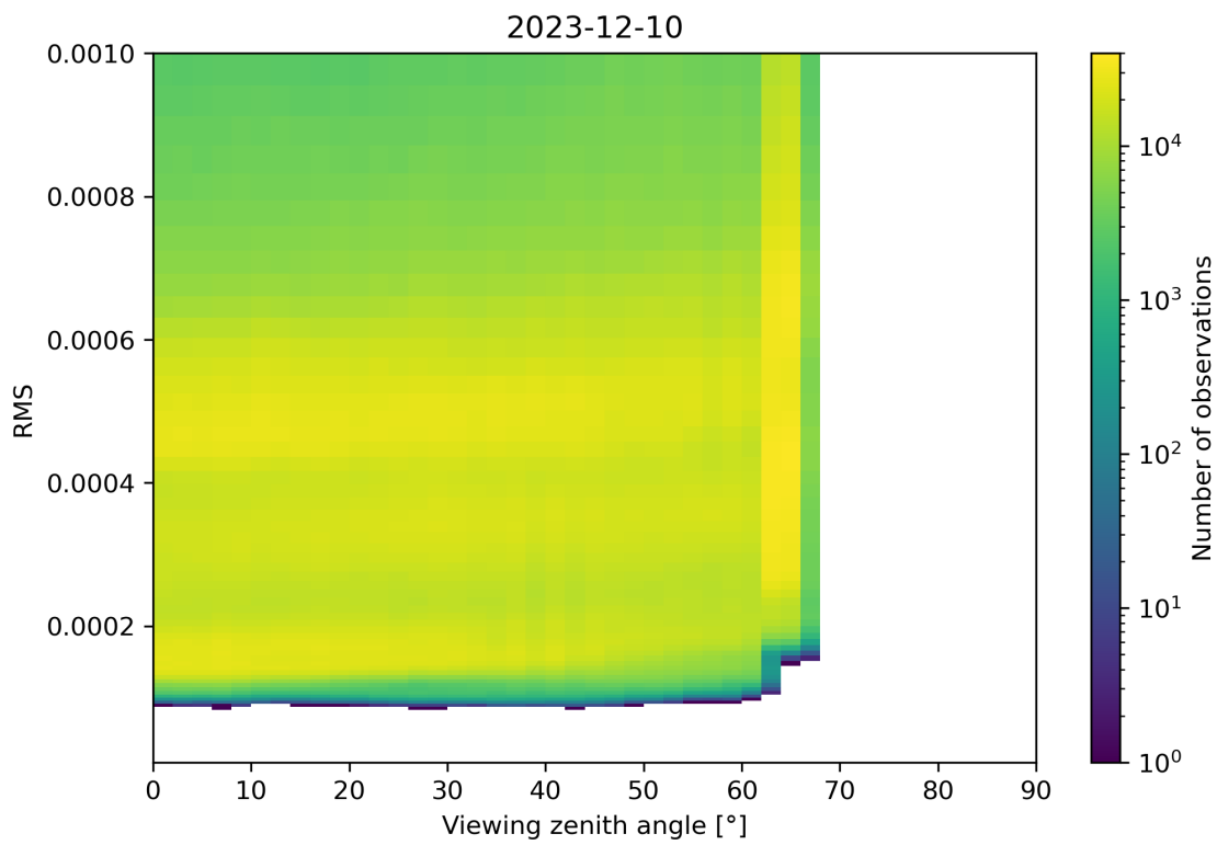
Figure 171: Scatter density plot of “Viewing zenith angle” against “RMS” for 2023-12-09 to 2023-12-11.
