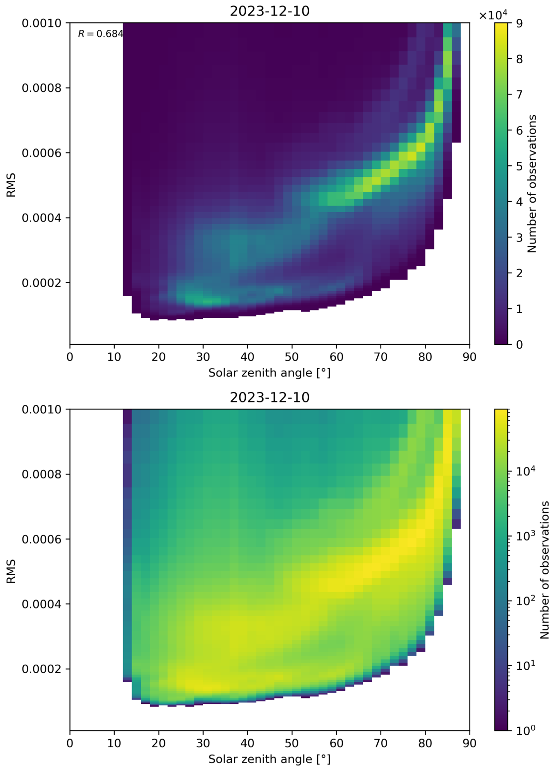
Figure 157: Scatter density plot of “Solar zenith angle” against “RMS” for 2023-12-09 to 2023-12-11.
