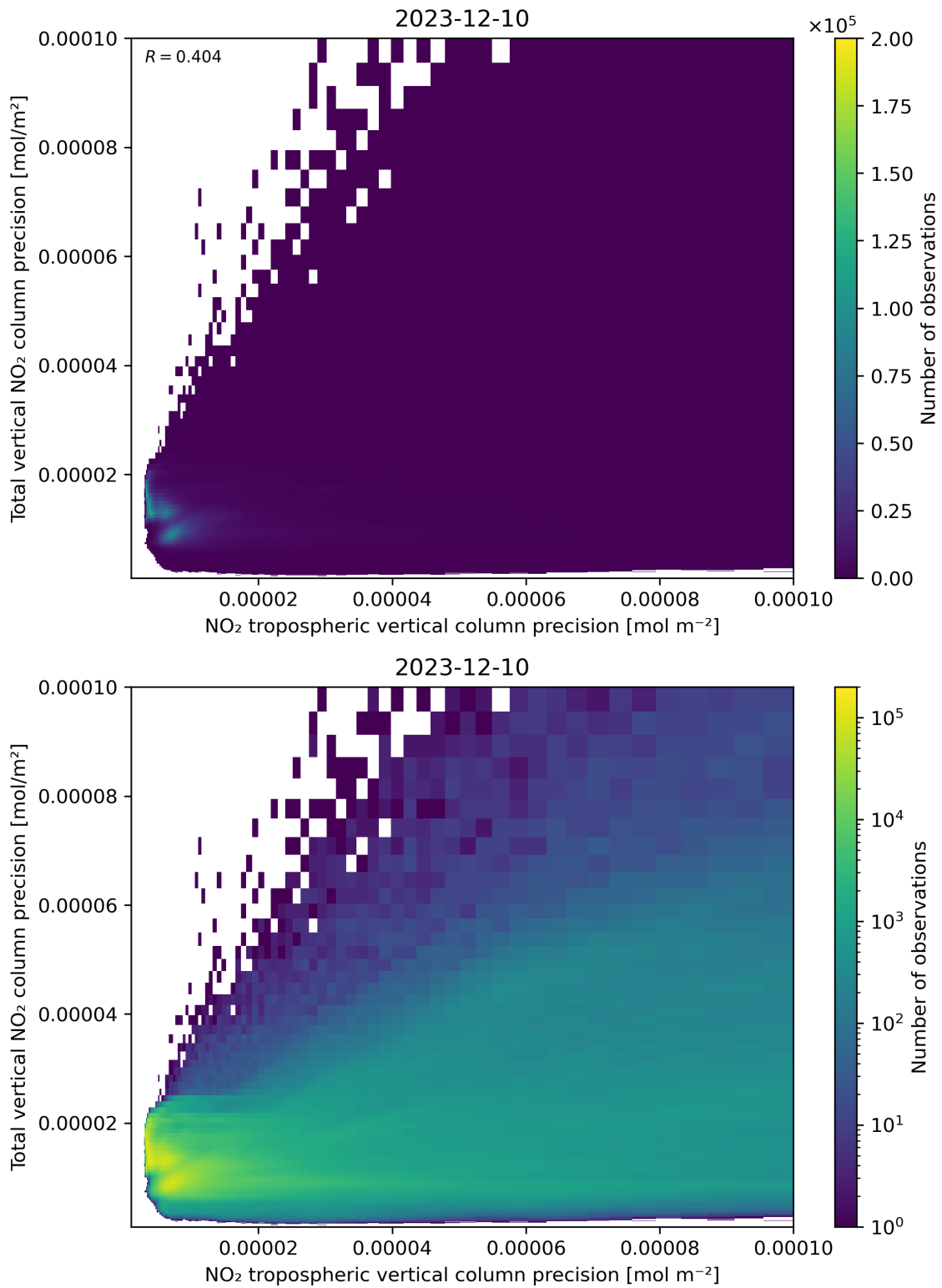
Figure 139: Scatter density plot of “NO 2 tropospheric vertical column precision” against “Total vertical NO 2 column precision” for 2023-12-09 to 2023-12-11.
