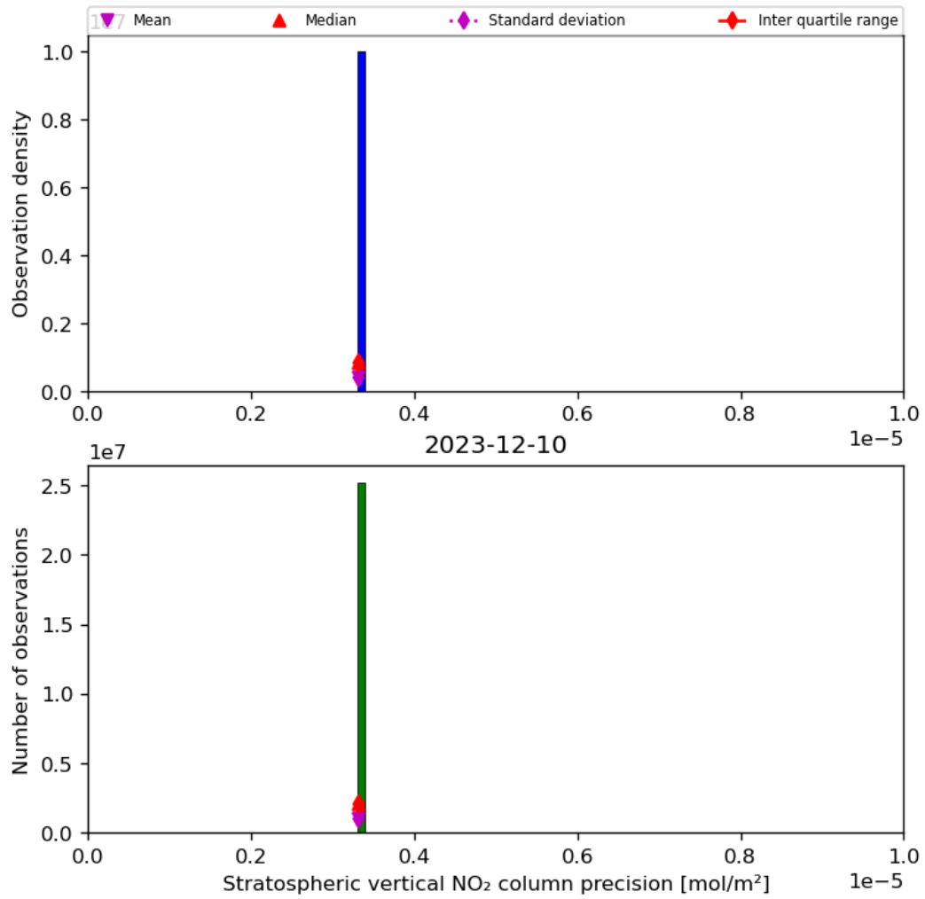
Figure 37: Histogram of “Stratospheric vertical NO 2 column precision” for 2023-12-09 to 2023-12-11
