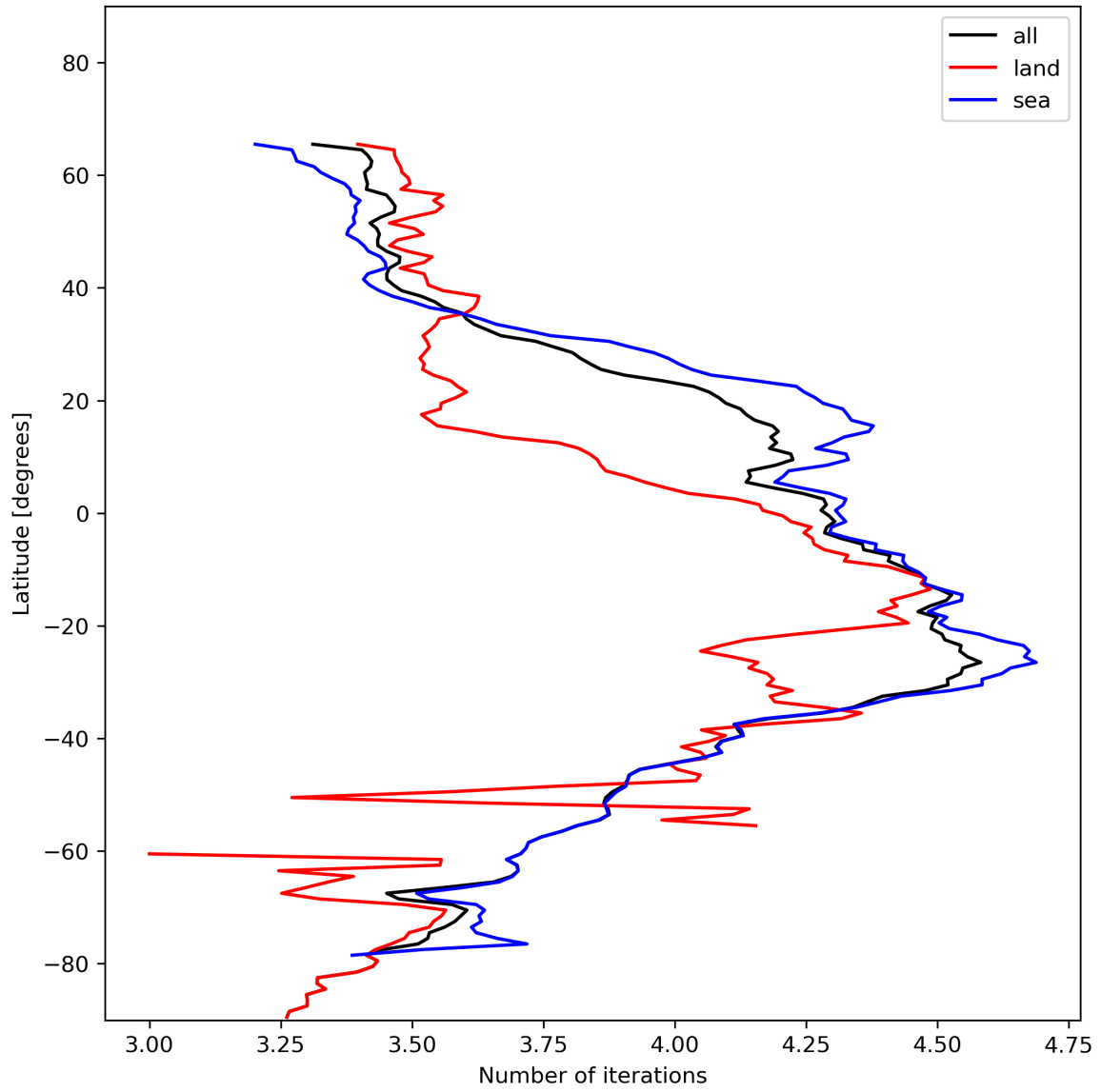
Figure 17: Zonal average of “Number of iterations” for 2023-12-09 to 2023-12-11.
