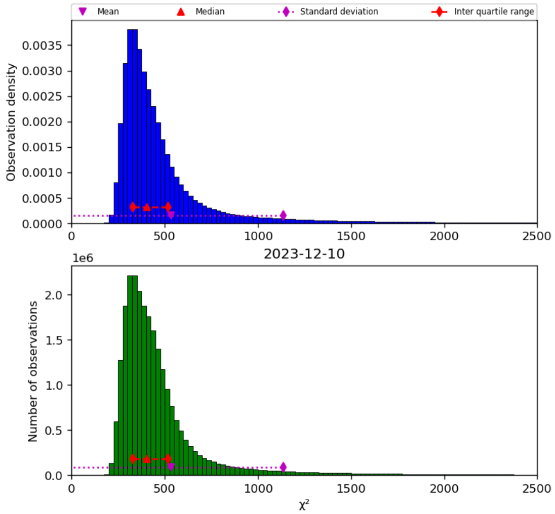
Figure 42: Histogram of “ \chi^2 ” for 2023-12-09 to 2023-12-11
