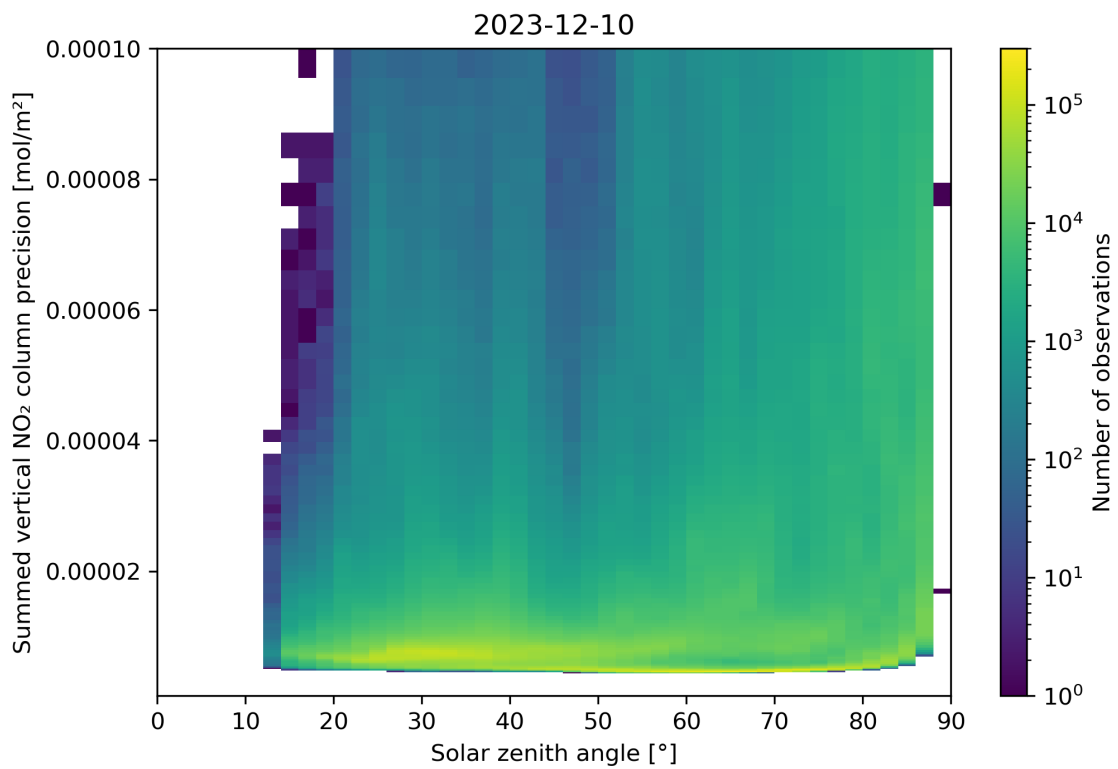
Figure 152: Scatter density plot of “Solar zenith angle” against “Summed vertical NO 2 column precision” for 2023-12-09 to 2023-12-11.
