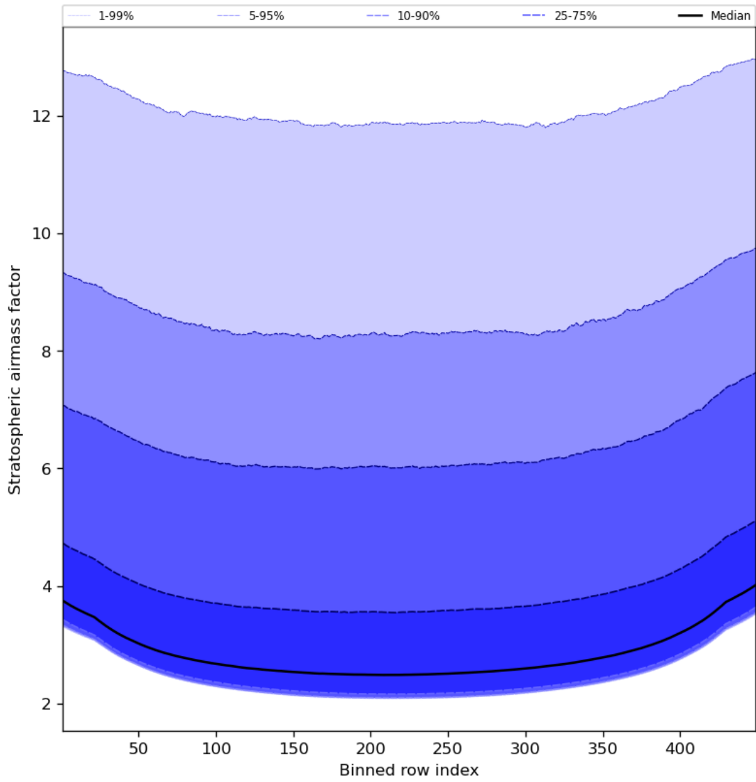
Figure 61: Along track statistics of “Stratospheric airmass factor” for 2023-12-09 to 2023-12-11
