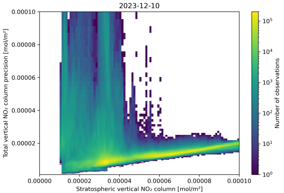
Figure 101: Scatter density plot of “Stratospheric vertical NO 2 column” against “Total vertical NO 2 column precision” for 2023-12-09 to 2023-12-11.
