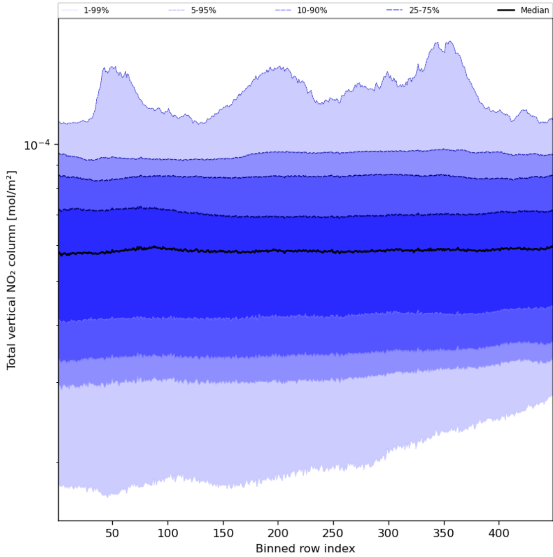
Figure 55: Along track statistics of “Total vertical NO 2 column” for 2023-12-09 to 2023-12-11
