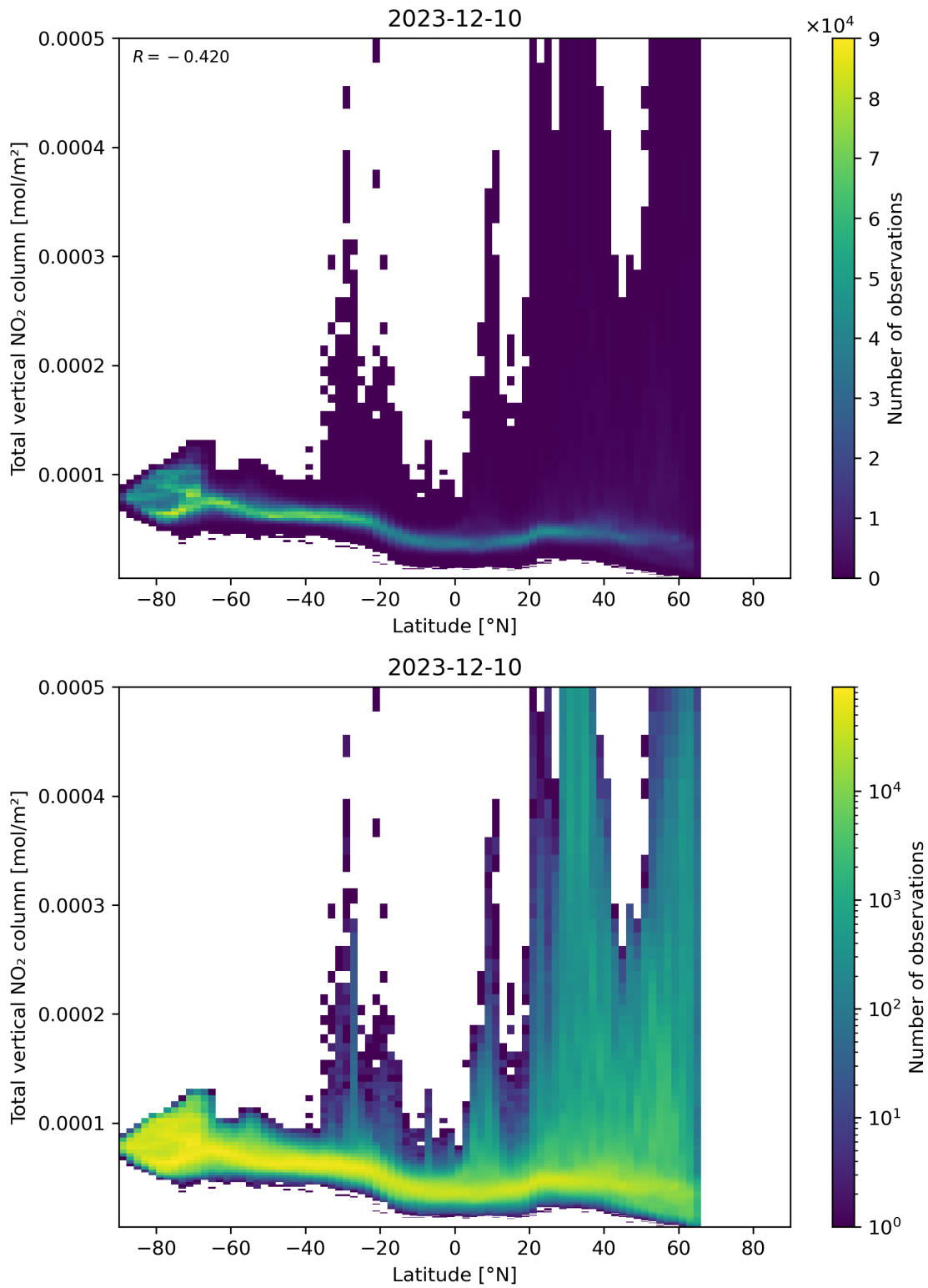
Figure 90: Scatter density plot of “Latitude” against “Total vertical NO 2 column” for 2023-12-09 to 2023-12-11.
