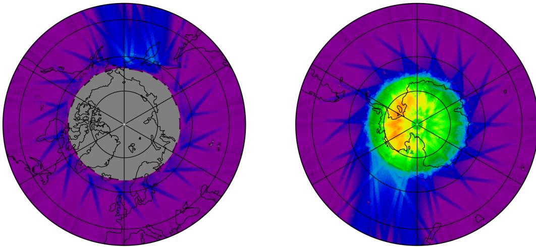
Figure 10: Map of the number of observations for 2023-12-09 to 2023-12-11
