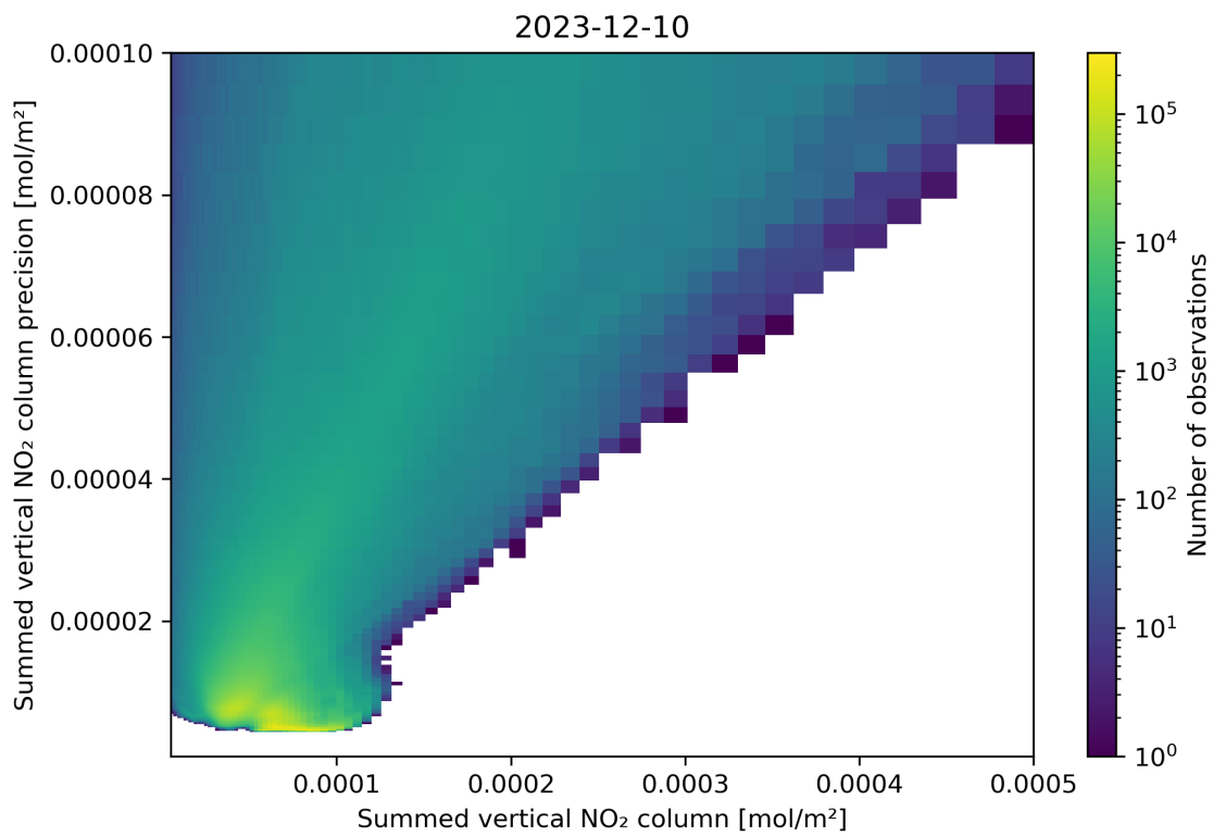
Figure 105: Scatter density plot of “Summed vertical NO 2 column” against “Summed vertical NO 2 column precision” for 2023-12-09 to 2023-12-11.
