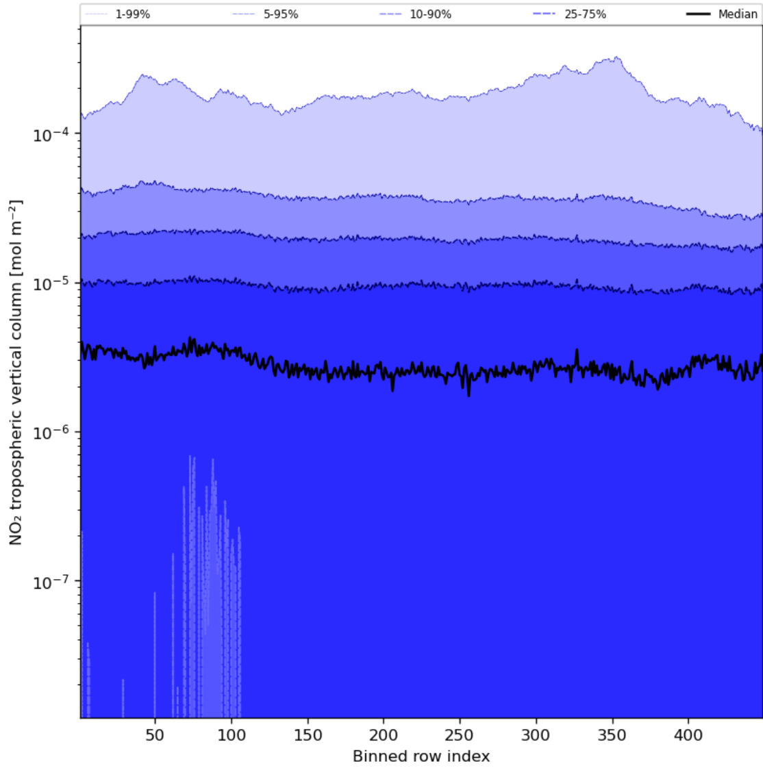
Figure 46: Along track statistics of “NO 2 tropospheric vertical column” for 2023-12-09 to 2023-12-11
