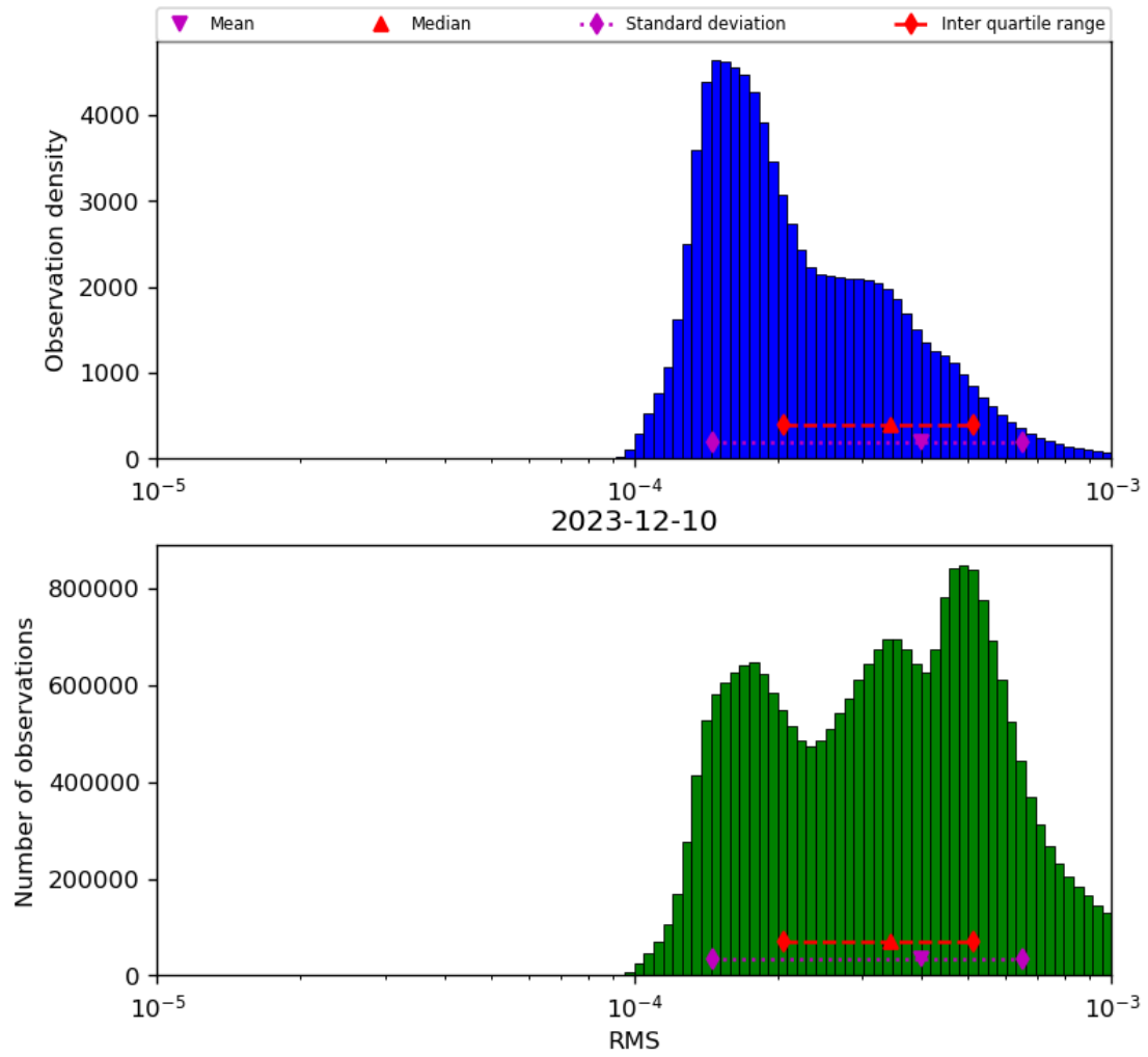
Figure 43: Histogram of “RMS” for 2023-12-09 to 2023-12-11
