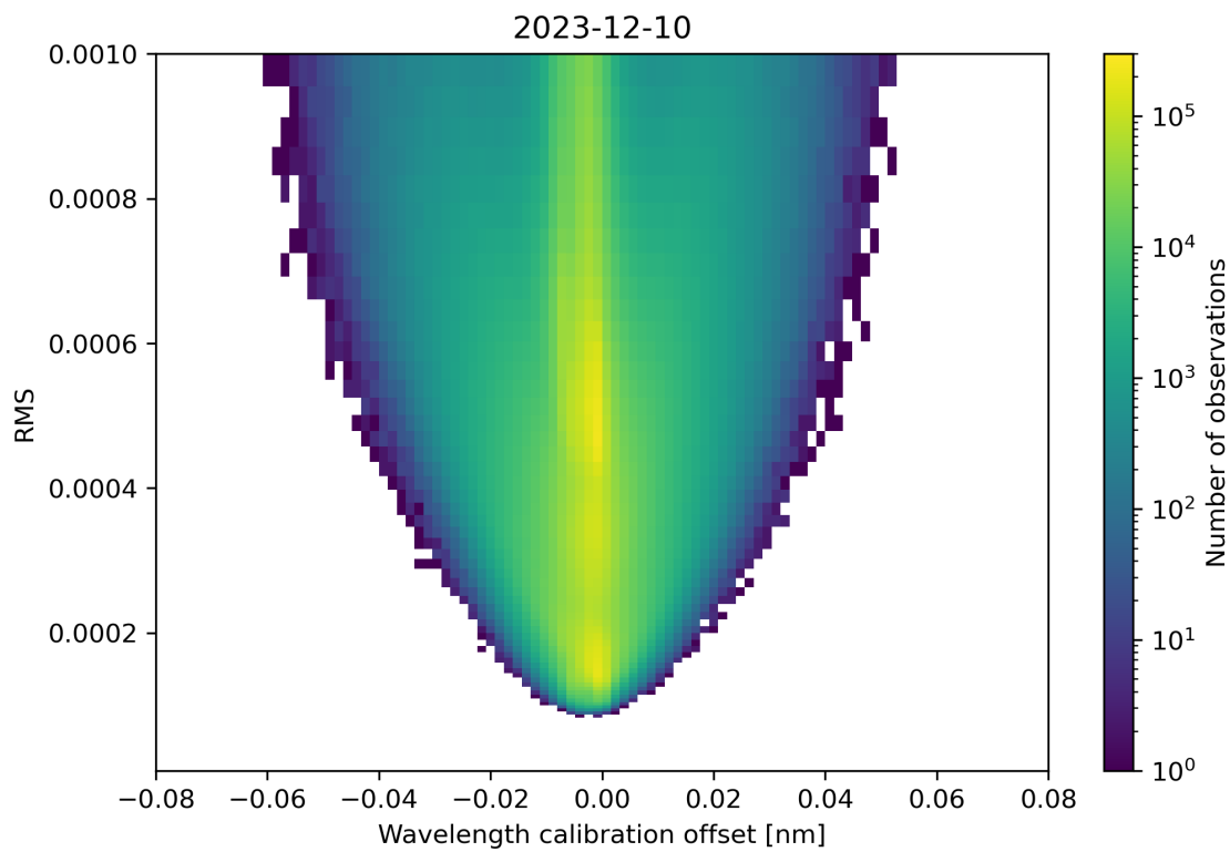
Figure 181: Scatter density plot of “Wavelength calibration offset” against “RMS” for 2023-12-09 to 2023-12-11.
