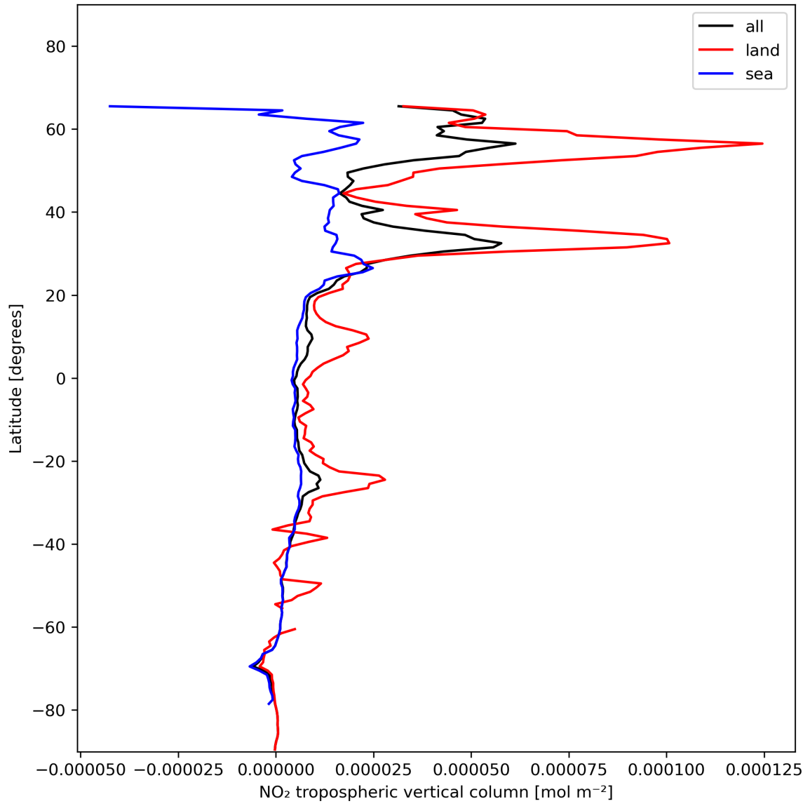
Figure 12: Zonal average of “NO 2 tropospheric vertical column” for 2023-12-09 to 2023-12-11.
