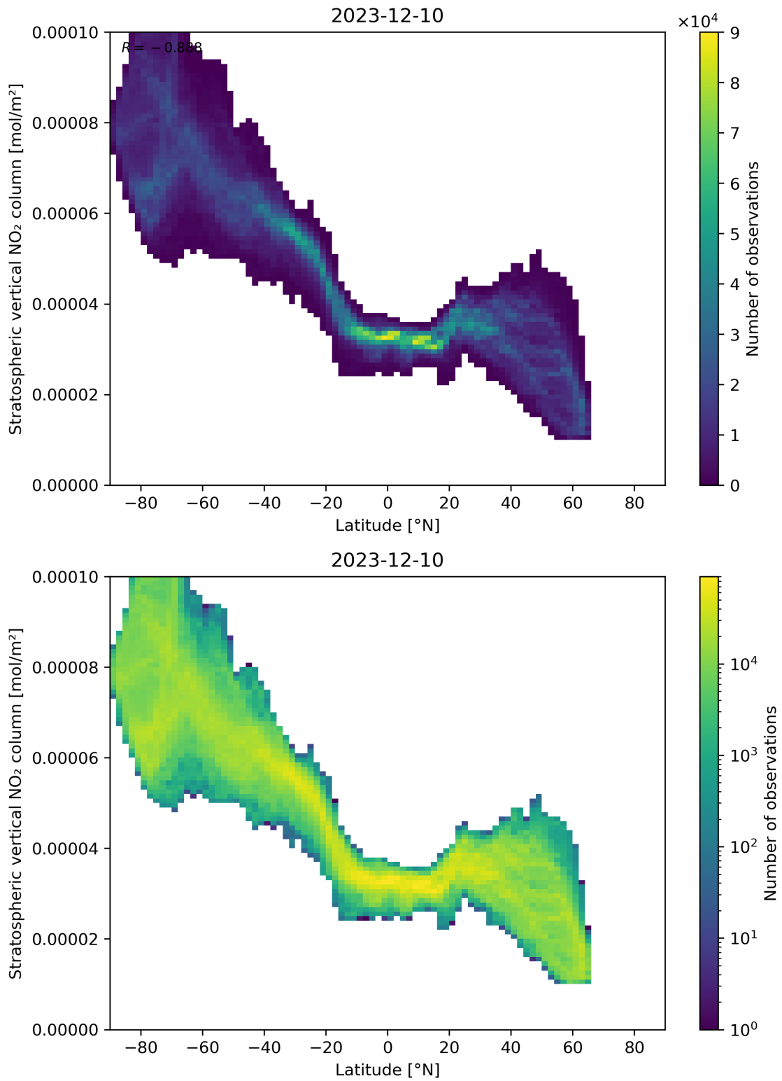
Figure 87: Scatter density plot of “Latitude” against “Stratospheric vertical NO 2 column” for 2023-12-09 to 2023-12-11.
