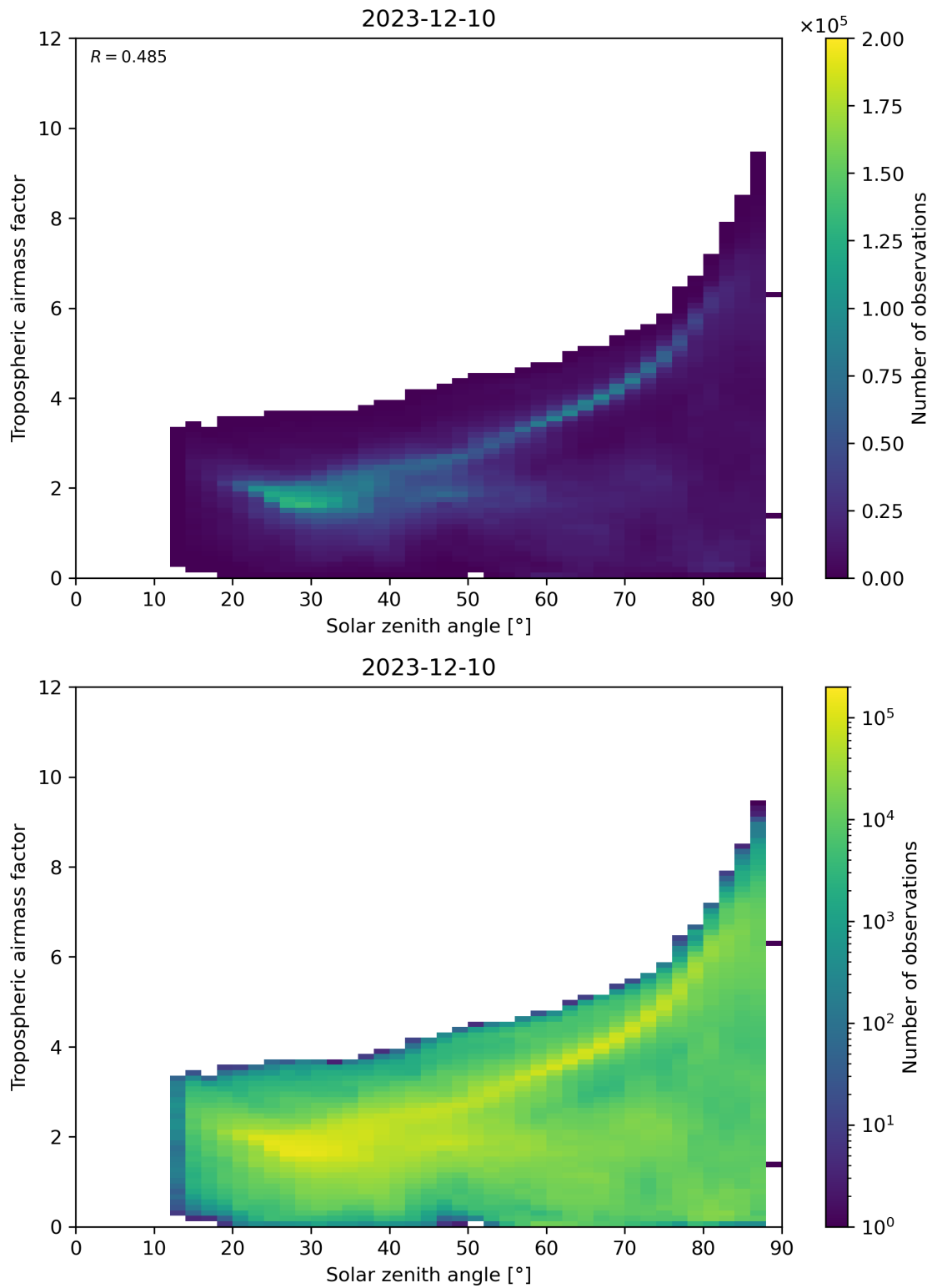
Figure 147: Scatter density plot of “Solar zenith angle” against “Tropospheric airmass factor” for 2023-12-09 to 2023-12-11.
