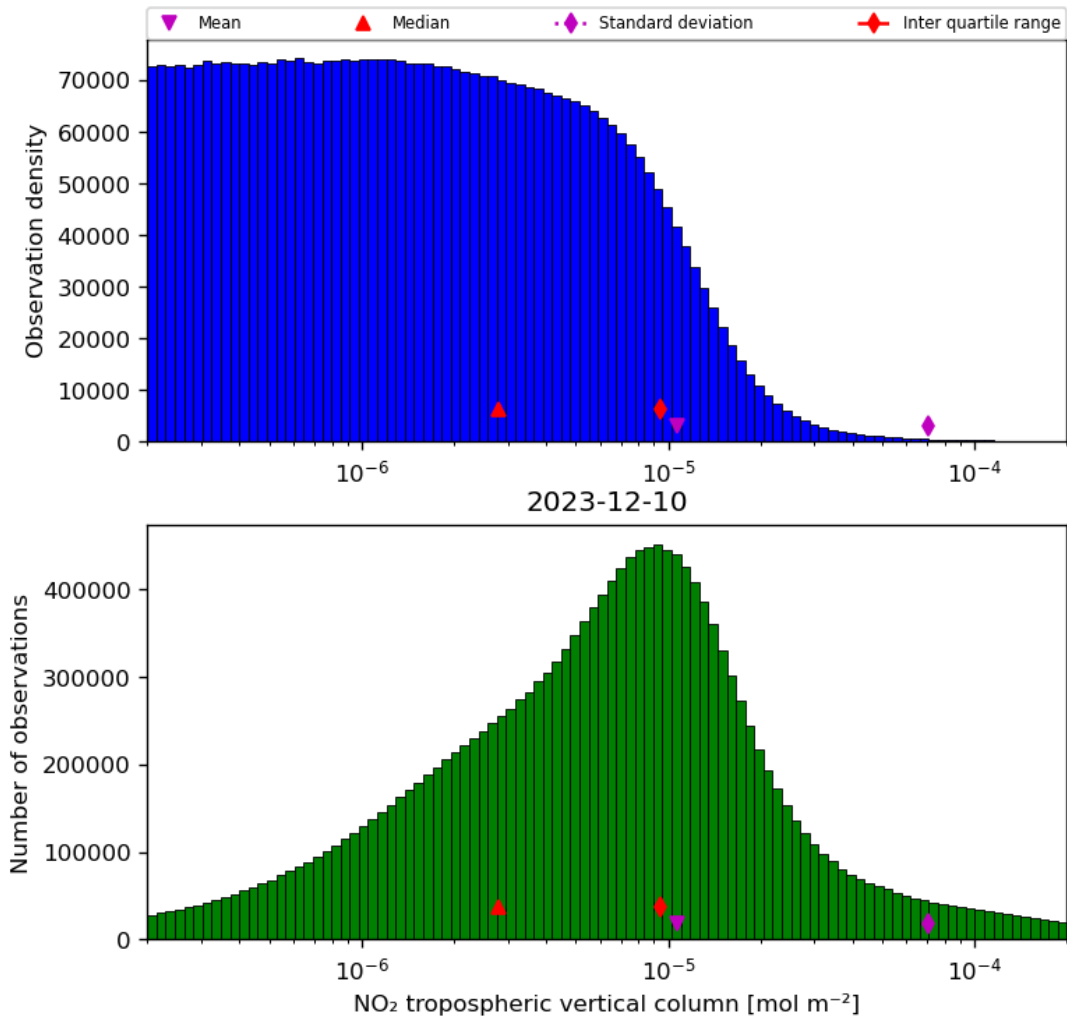
Figure 29: Histogram of “NO 2 tropospheric vertical column” for 2023-12-09 to 2023-12-11
