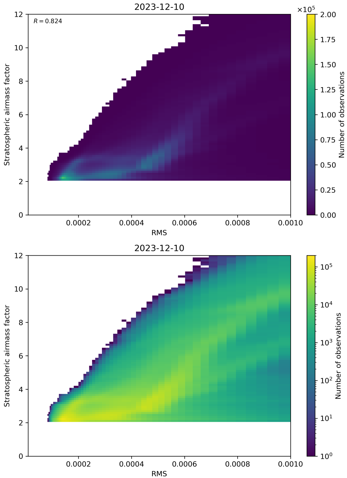
Figure 144: Scatter density plot of “RMS” against “Stratospheric airmass factor” for 2023-12-09 to 2023-12-11.
