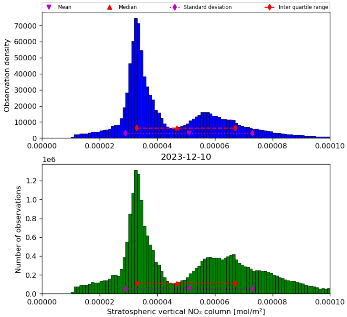
Figure 36: Histogram of “Stratospheric vertical NO 2 column” for 2023-12-09 to 2023-12-11
