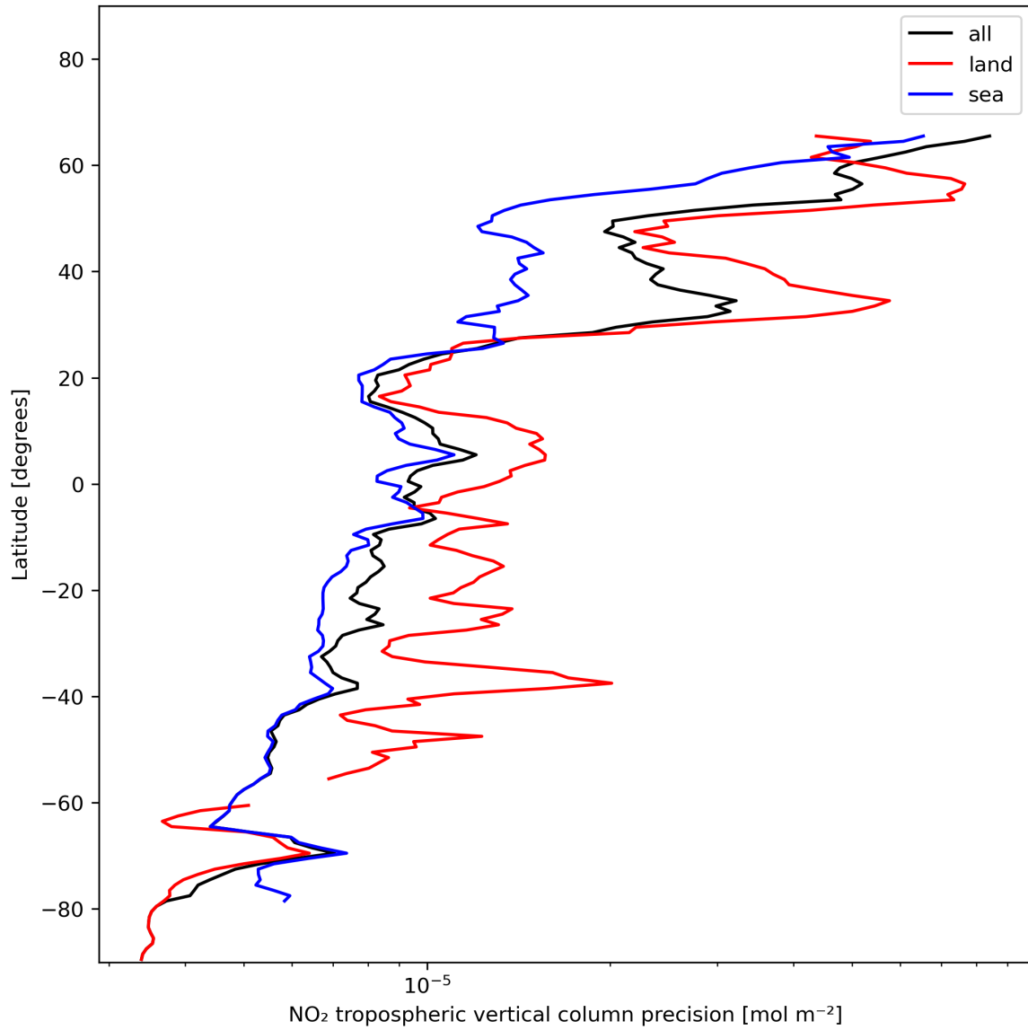
Figure 13: Zonal average of “NO 2 tropospheric vertical column precision” for 2023-12-09 to 2023-12-11.
