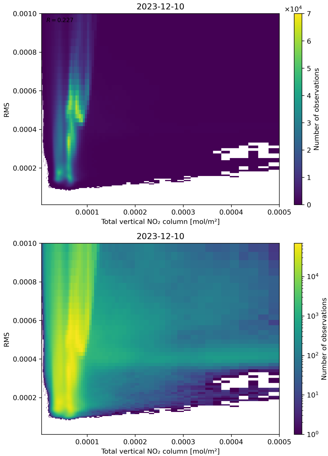
Figure 120: Scatter density plot of “Total vertical NO 2 column” against “RMS” for 2023-12-09 to 2023-12-11.
