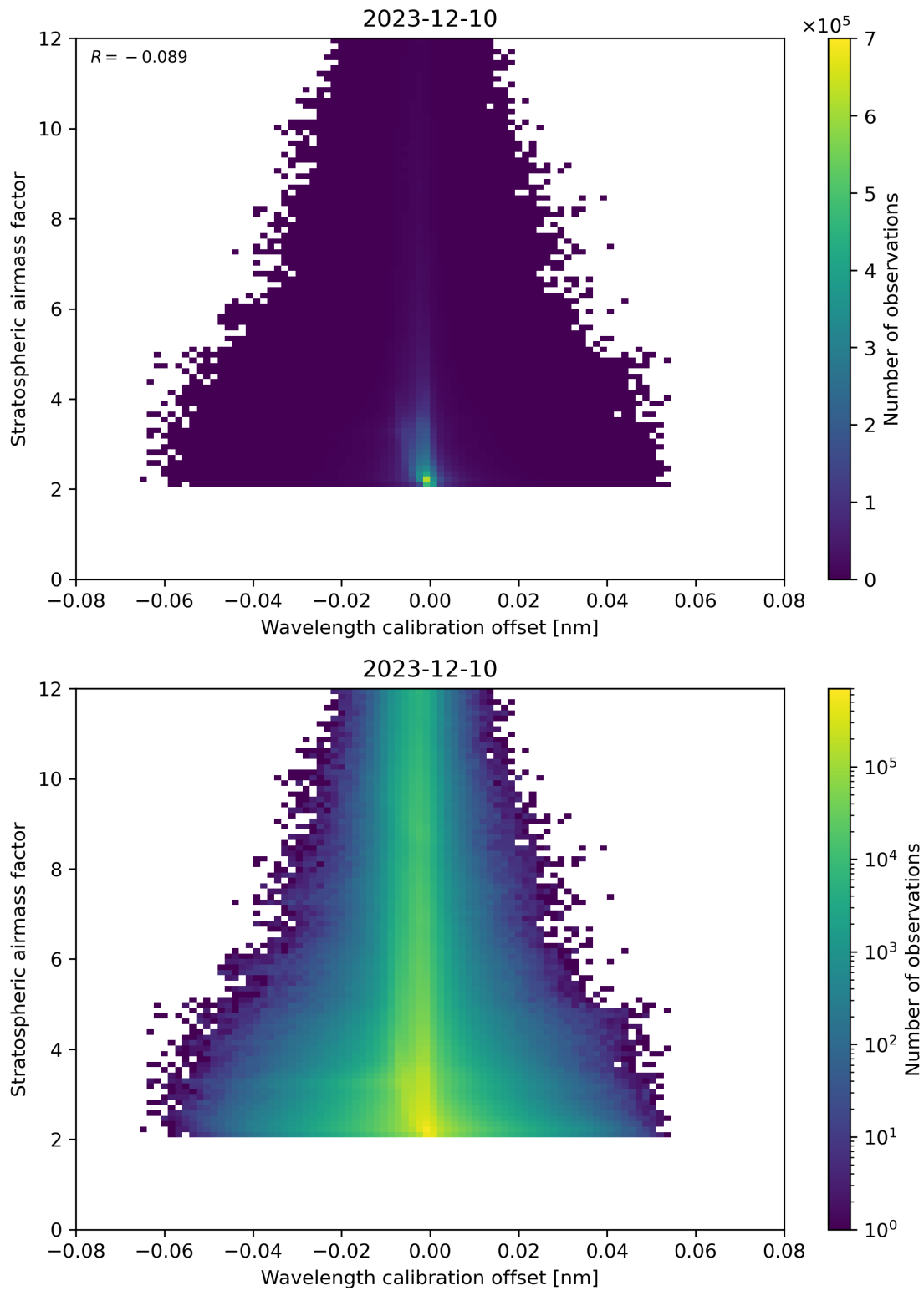
Figure 174: Scatter density plot of “Wavelength calibration offset” against “Stratospheric airmass factor” for 2023-12-09 to 2023-12-11.
