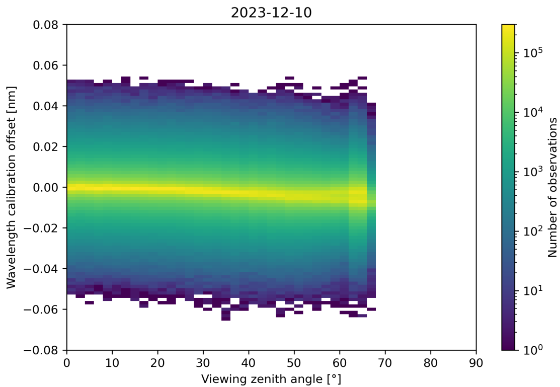
Figure 173: Scatter density plot of “Viewing zenith angle” against “Wavelength calibration offset” for 2023-12-09 to 2023-12-11.
