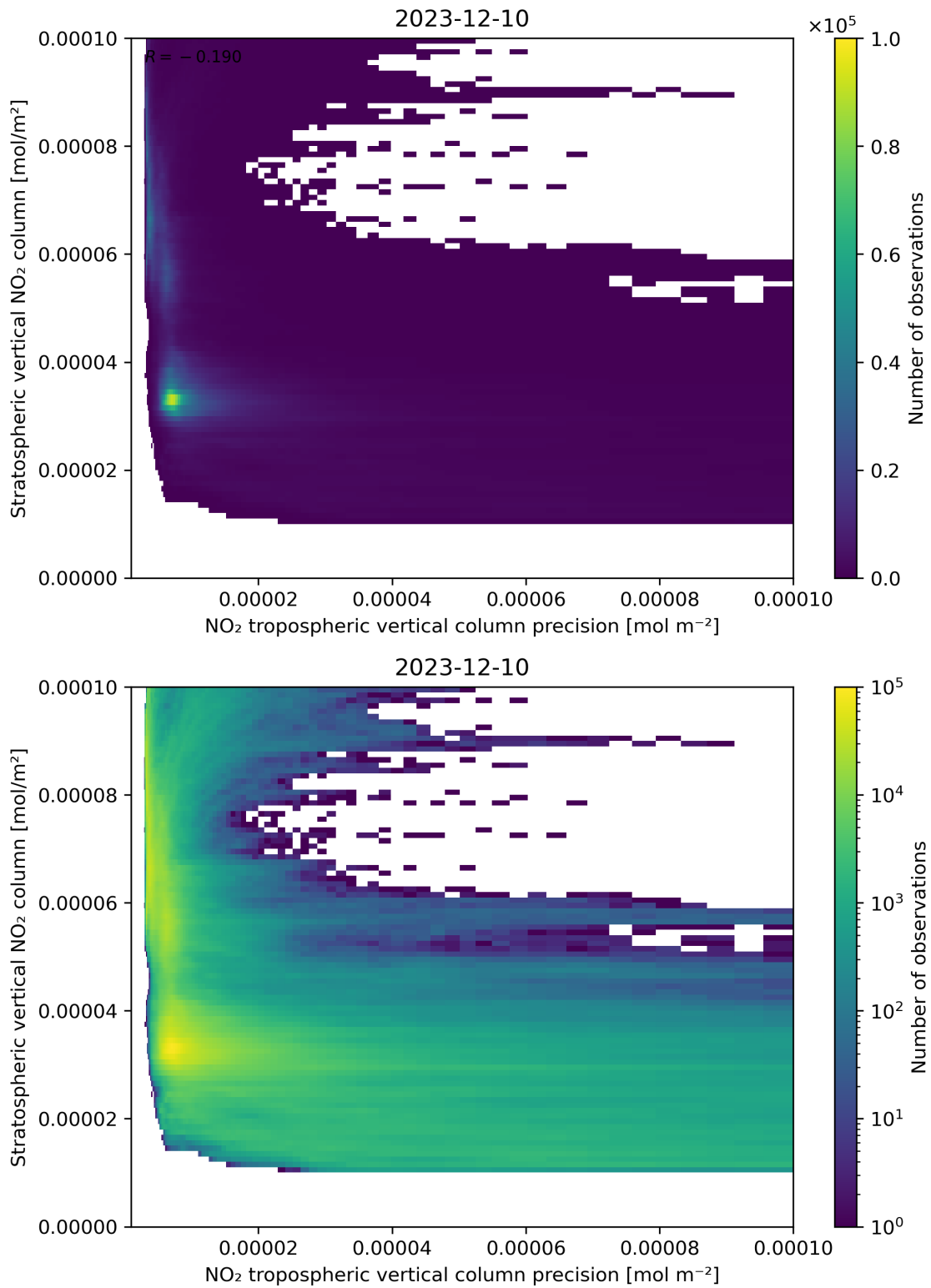
Figure 135: Scatter density plot of “NO 2 tropospheric vertical column precision” against “Stratospheric vertical NO 2 column” for 2023-12-09 to 2023-12-11.
