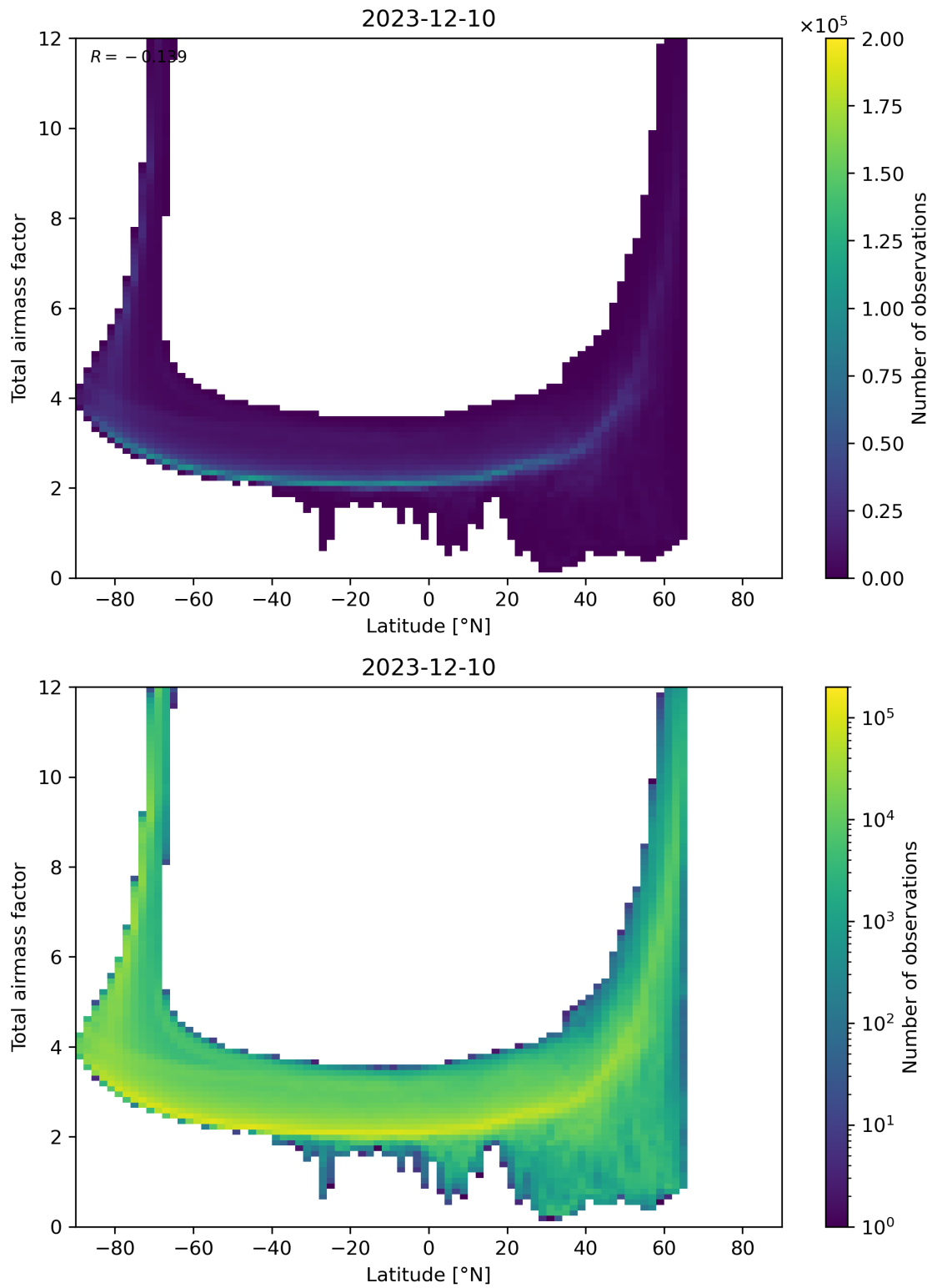
Figure 84: Scatter density plot of “Latitude” against “Total airmass factor” for 2023-12-09 to 2023-12-11.
