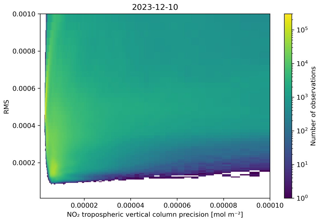
Figure 140: Scatter density plot of “NO 2 tropospheric vertical column precision” against “RMS” for 2023-12-09 to 2023-12-11.
