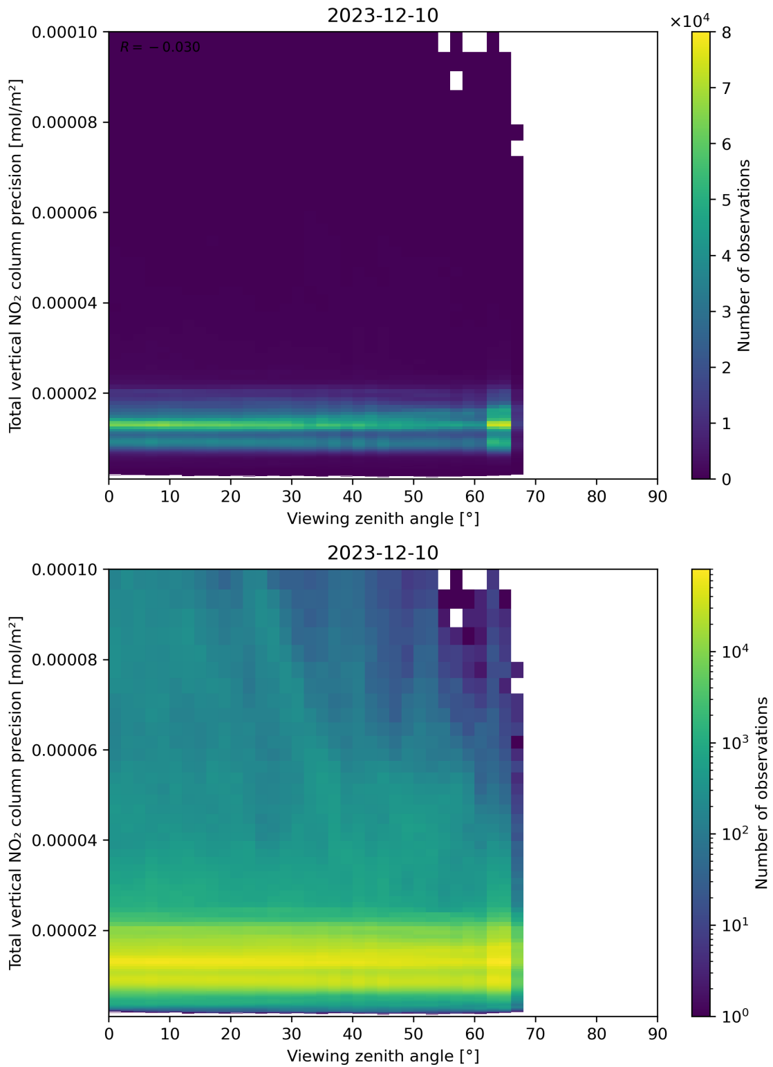
Figure 168: Scatter density plot of “Viewing zenith angle” against “Total vertical NO 2 column precision” for 2023-12-09 to 2023-12-11.
