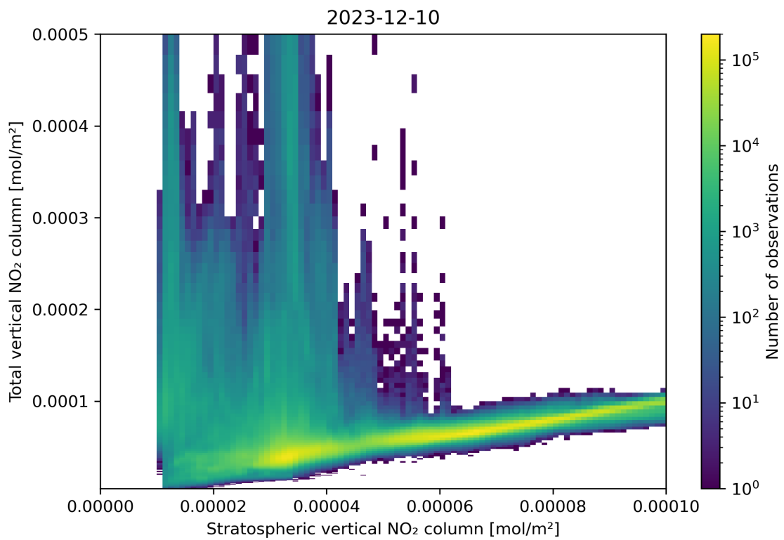
Figure 100: Scatter density plot of “Stratospheric vertical NO 2 column” against “Total vertical NO 2 column” for 2023-12-09 to 2023-12-11.
