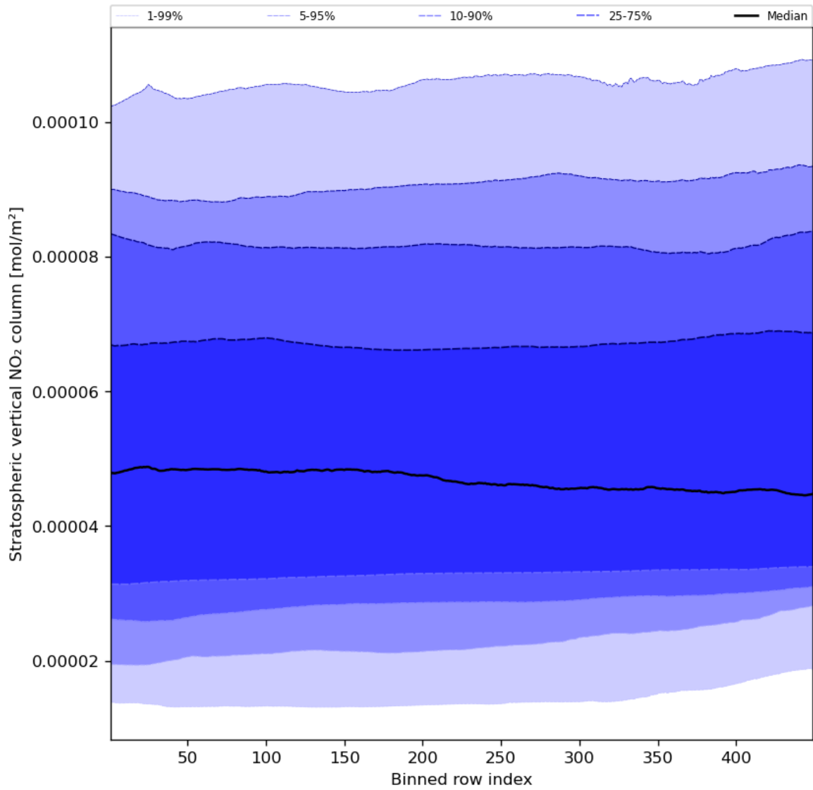
Figure 53: Along track statistics of “Stratospheric vertical NO 2 column” for 2023-12-09 to 2023-12-11
