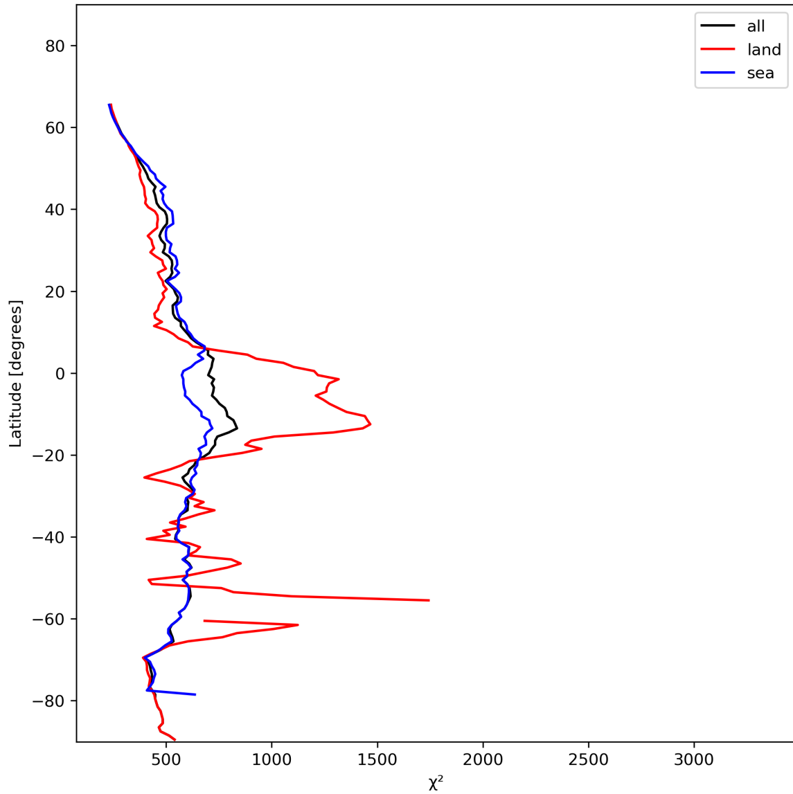
Figure 25: Zonal average of " \chi^2 " for 2023-12-09 to 2023-12-11.
