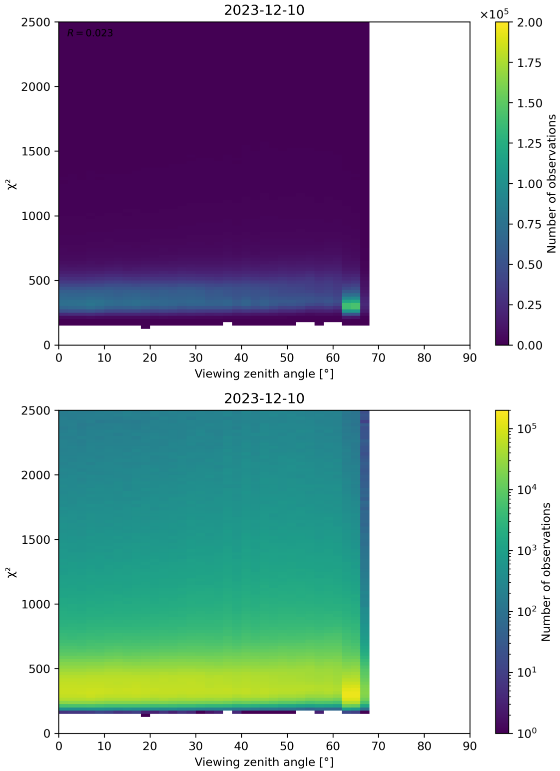
Figure 162: Scatter density plot of “Viewing zenith angle” against “ \chi^2 ” for 2023-12-09 to 2023-12-11.
