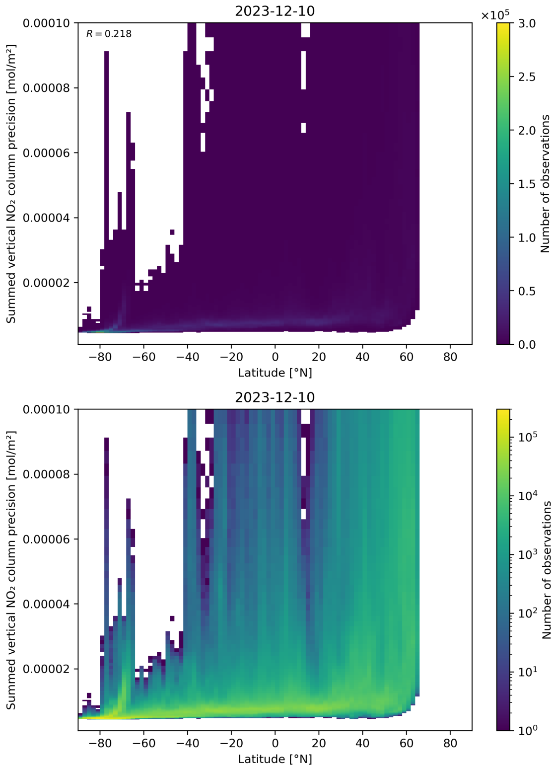
Figure 89: Scatter density plot of “Latitude” against “Summed vertical NO 2 column precision” for 2023-12-09 to 2023-12-11.
