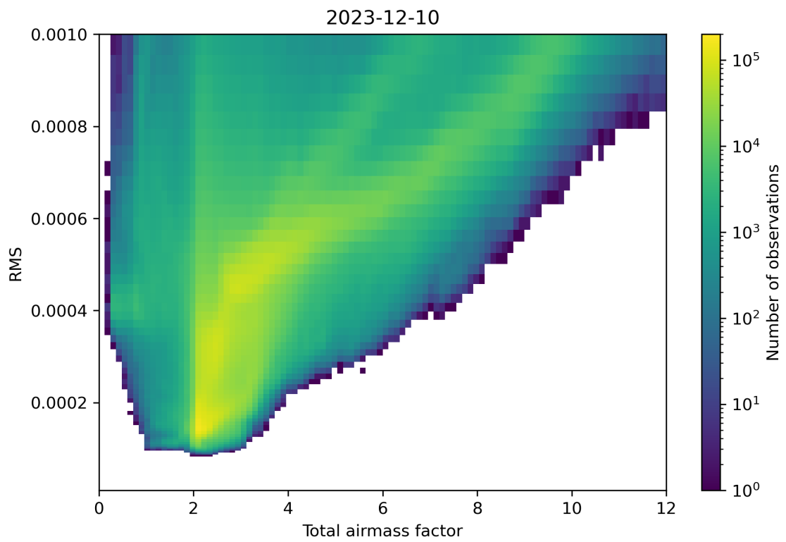
Figure 69: Scatter density plot of “Total airmass factor” against “RMS” for 2023-12-09 to 2023-12-11.
