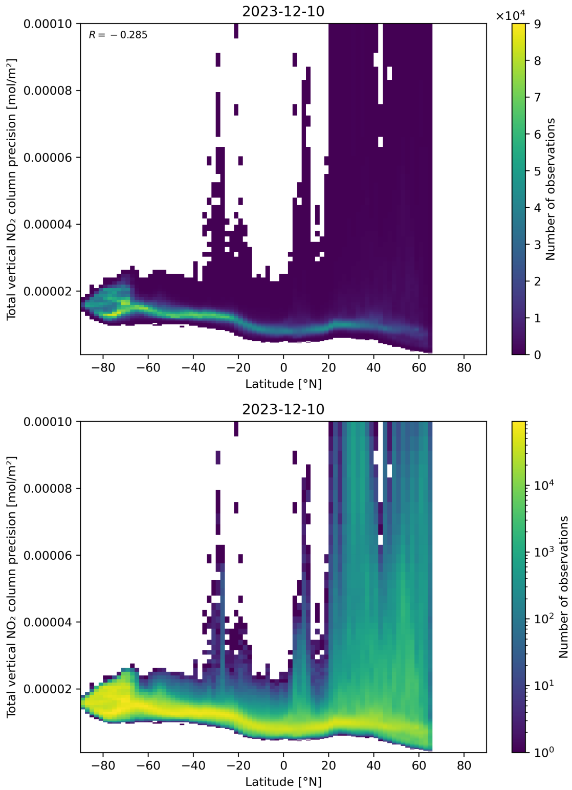
Figure 91: Scatter density plot of “Latitude” against “Total vertical NO 2 column precision” for 2023-12-09 to 2023-12-11.
