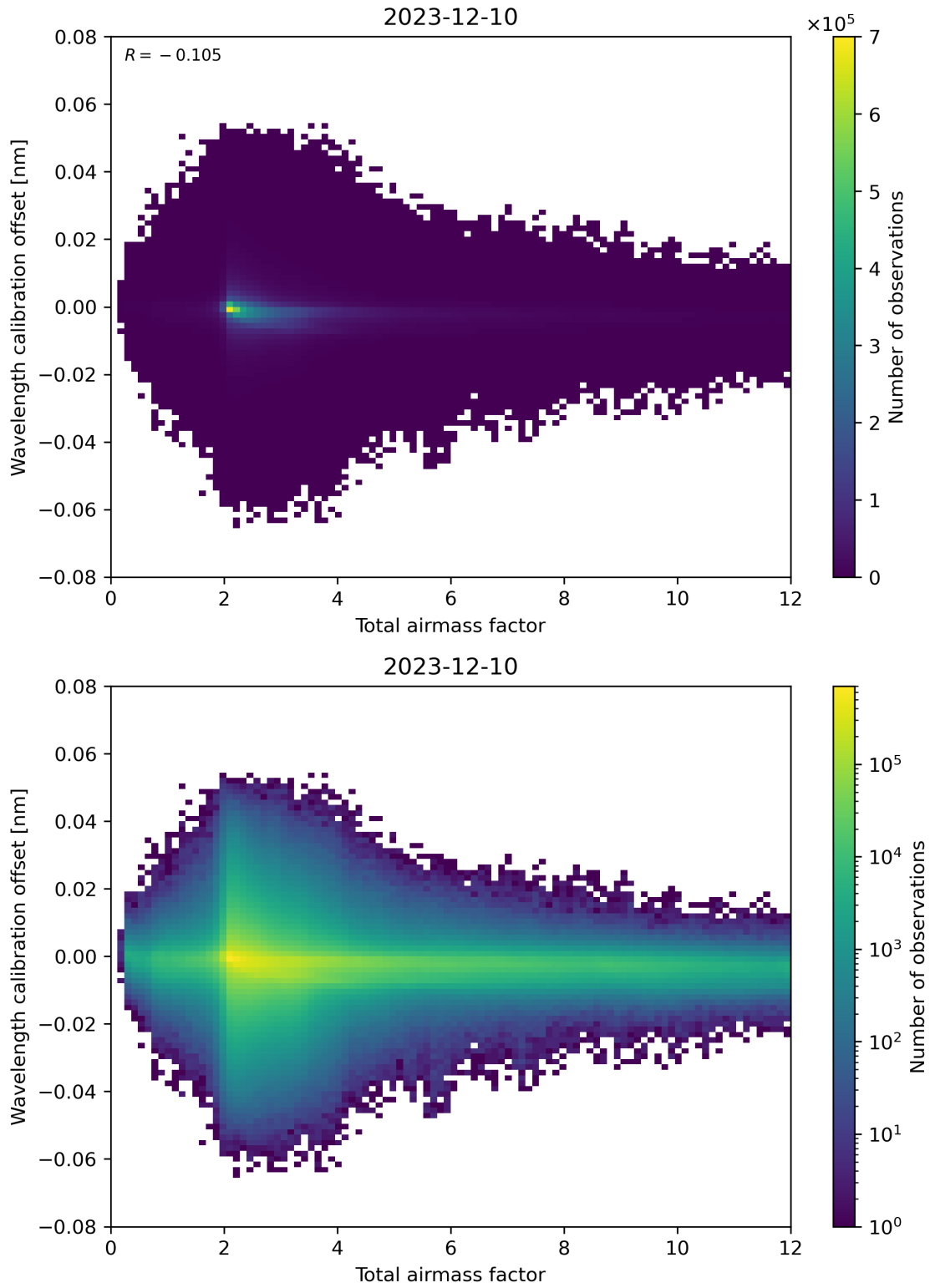
Figure 70: Scatter density plot of “Total airmass factor” against “Wavelength calibration offset” for 2023-12-09 to 2023-12-11.
