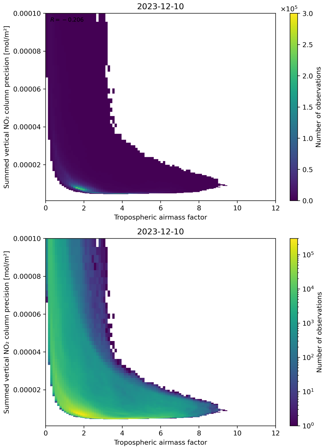
Figure 76: Scatter density plot of “Tropospheric airmass factor” against “Summed vertical NO 2 column precision” for 2023-12-09 to 2023-12-11.
