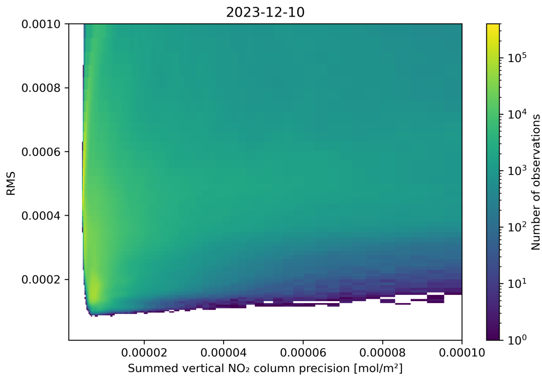
Figure 108: Scatter density plot of “Summed vertical NO 2 column precision” against “RMS” for 2023-12-09 to 2023-12-11.
