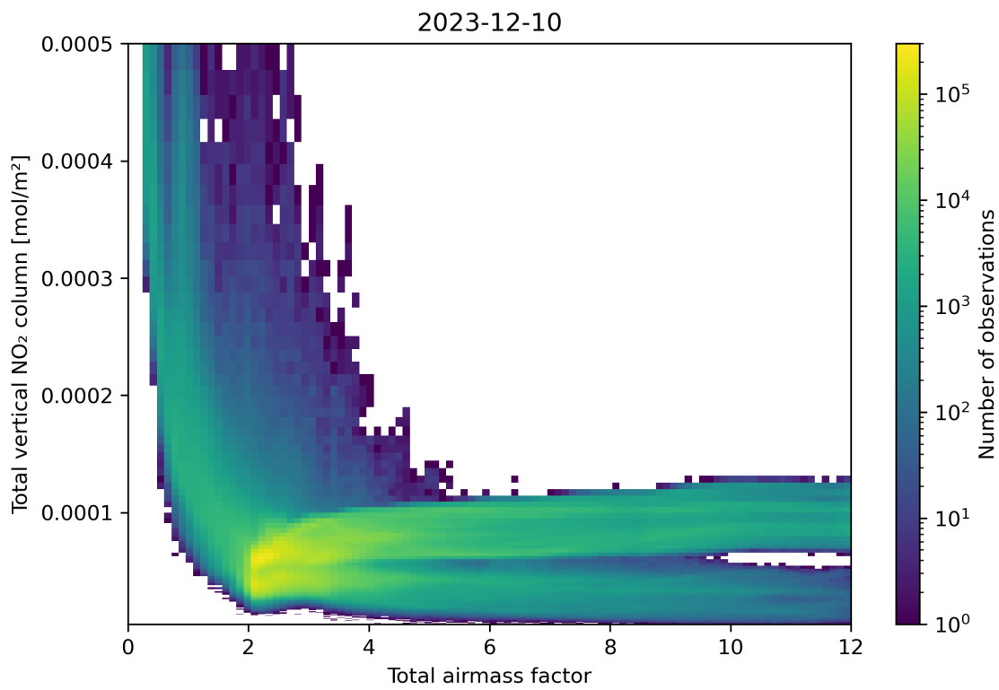
Figure 67: Scatter density plot of “Total airmass factor” against “Total vertical NO 2 column” for 2023-12-09 to 2023-12-11.
