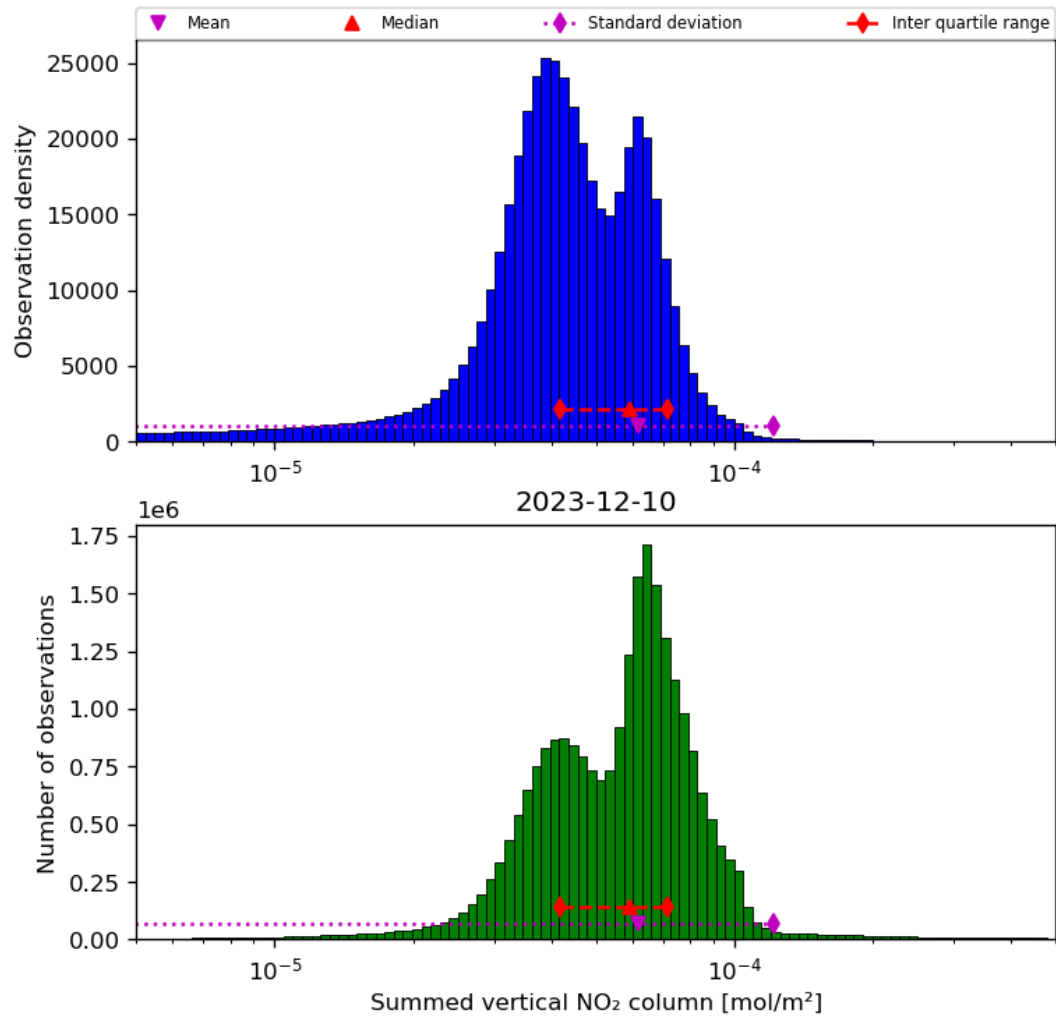
Figure 40: Histogram of “Summed vertical NO 2 column” for 2023-12-09 to 2023-12-11
