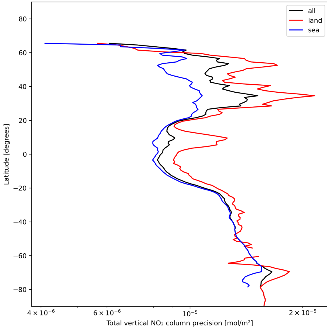
Figure 22: Zonal average of “Total vertical NO 2 column precision” for 2023-12-09 to 2023-12-11.
