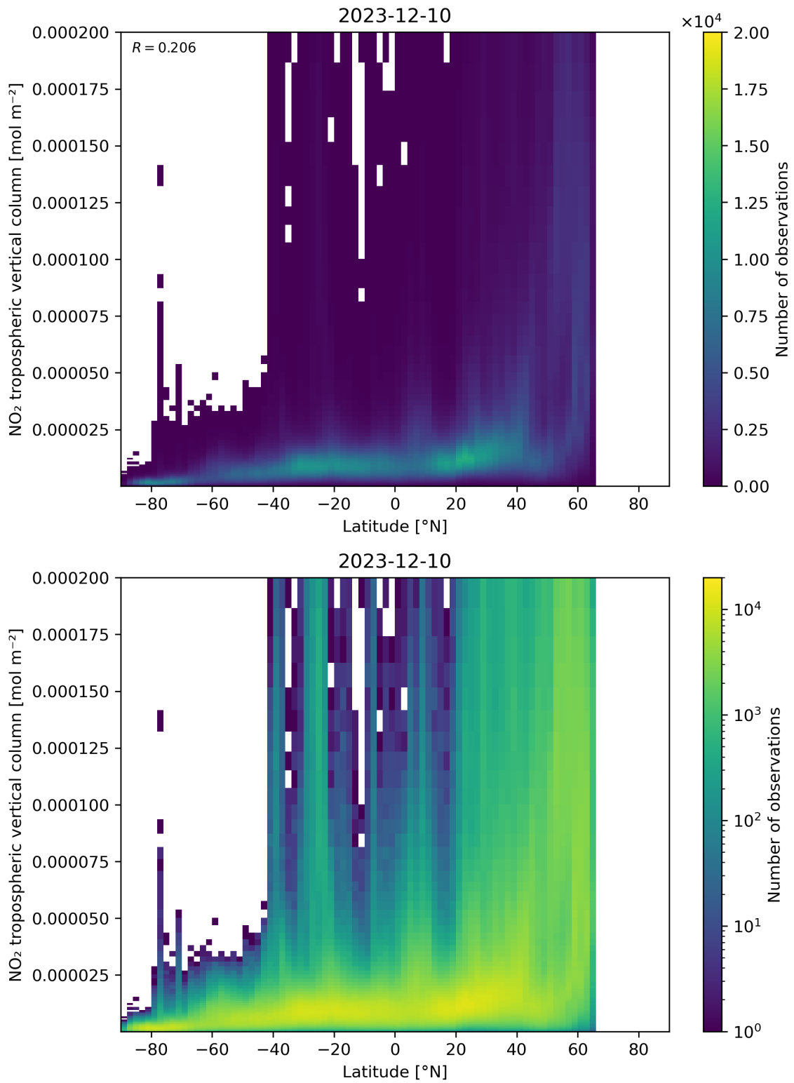
Figure 92: Scatter density plot of “Latitude” against “NO 2 tropospheric vertical column” for 2023-12-09 to 2023-12-11.
