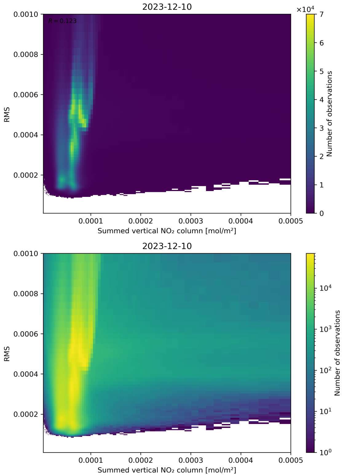
Figure 109: Scatter density plot of “Summed vertical NO 2 column” against “RMS” for 2023-12-09 to 2023-12-11.
