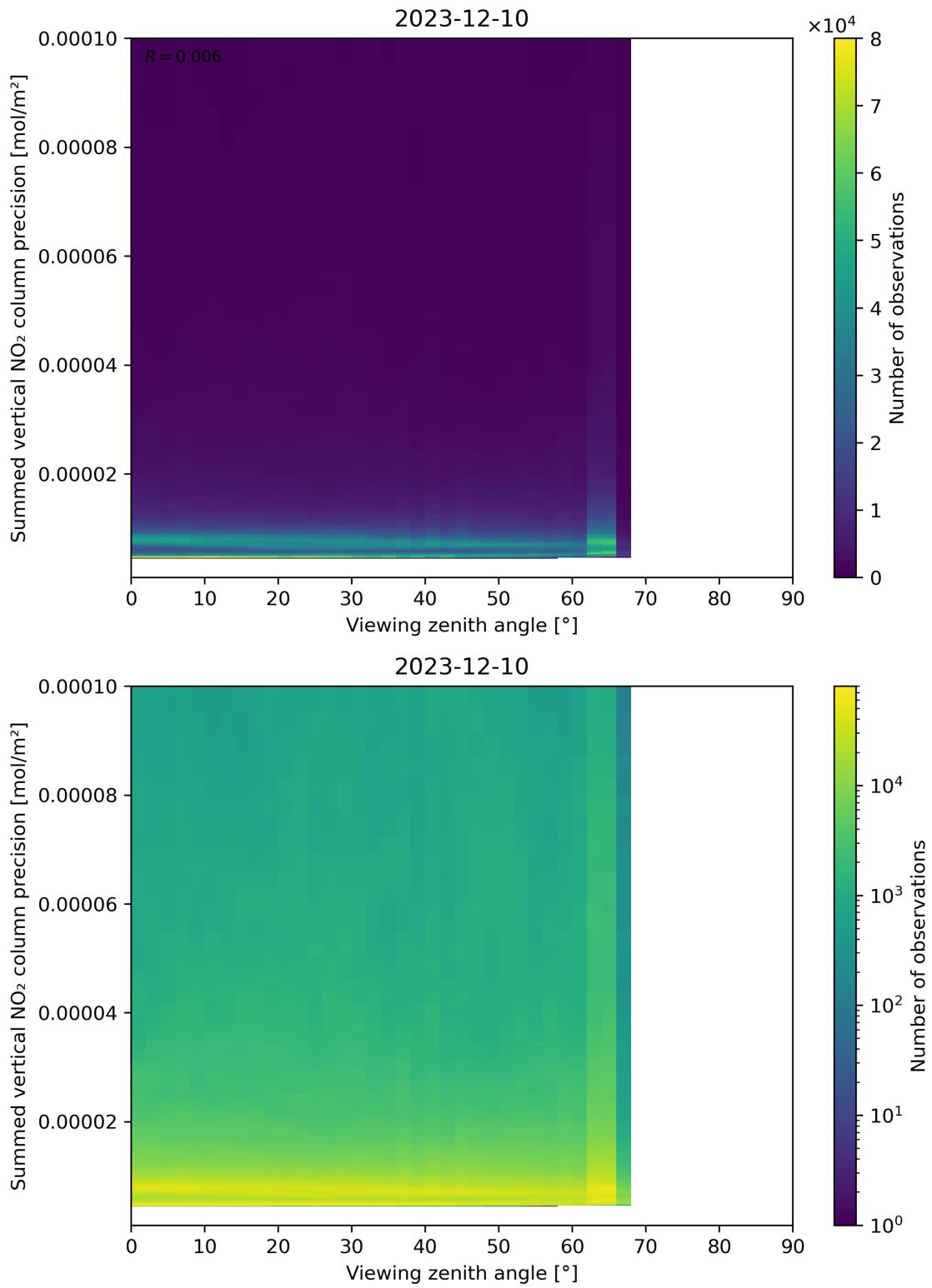
Figure 166: Scatter density plot of “Viewing zenith angle” against “Summed vertical NO 2 column precision” for 2023-12-09 to 2023-12-11.
