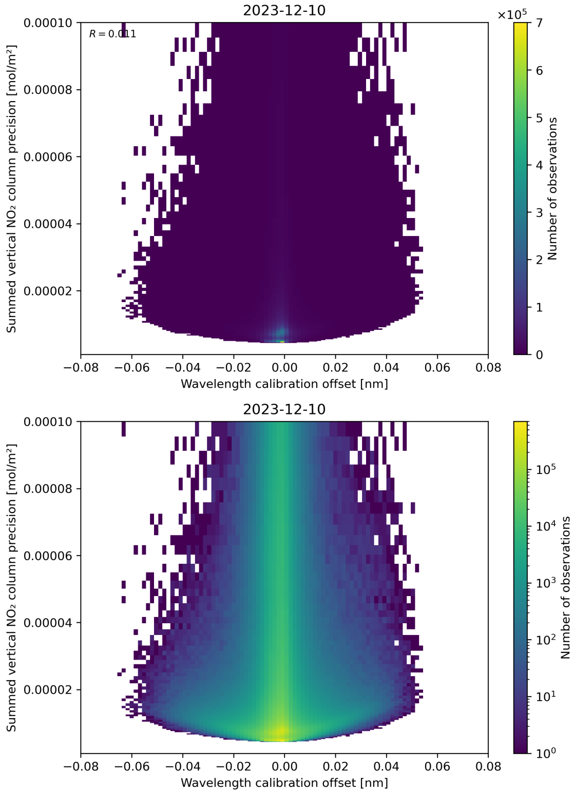
Figure 178: Scatter density plot of “Wavelength calibration offset” against “Summed vertical NO 2 column precision” for 2023-12-09 to 2023-12-11.
