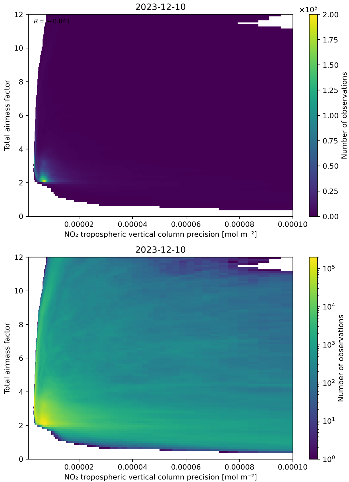
Figure 132: Scatter density plot of “NO 2 tropospheric vertical column precision” against “Total airmass factor” for 2023-12-09 to 2023-12-11.
