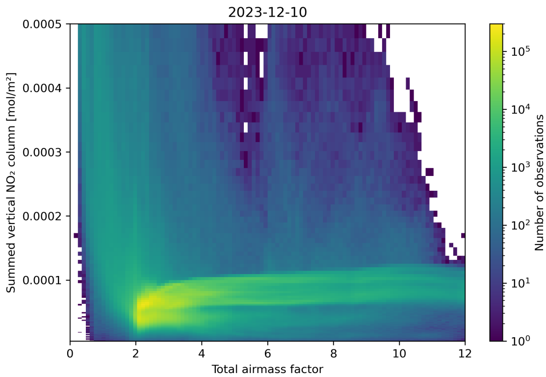
Figure 65: Scatter density plot of “Total airmass factor” against “Summed vertical NO 2 column” for 2023-12-09 to 2023-12-11.
