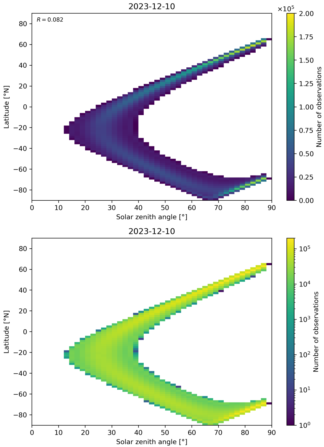
Figure 149: Scatter density plot of “Solar zenith angle” against “Latitude” for 2023-12-09 to 2023-12-11.
