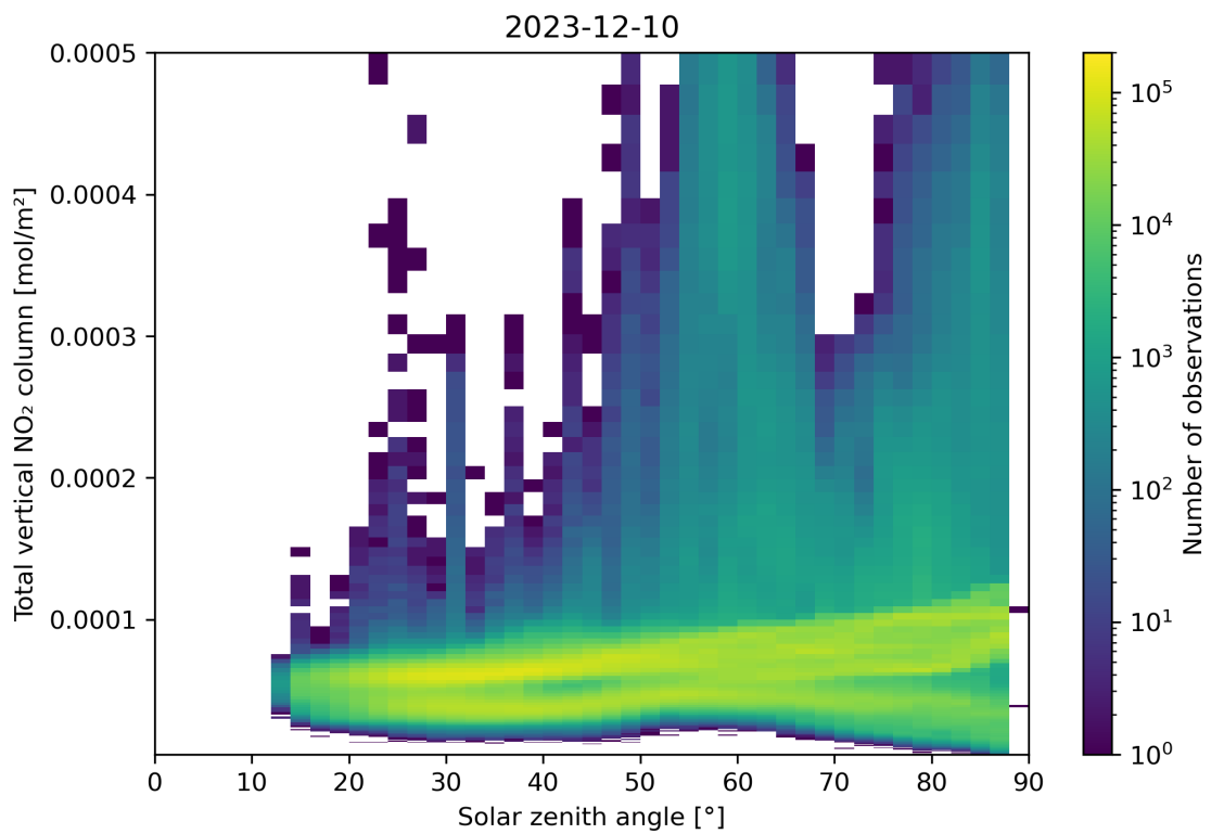
Figure 153: Scatter density plot of “Solar zenith angle” against “Total vertical NO 2 column” for 2023-12-09 to 2023-12-11.
