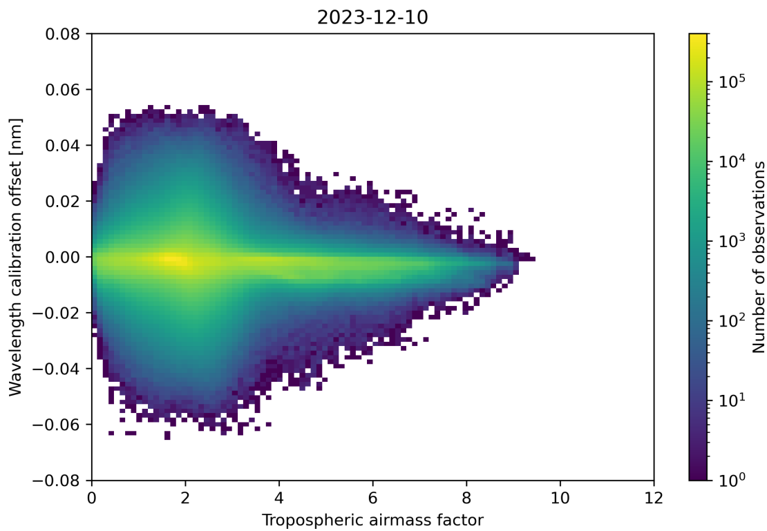
Figure 80: Scatter density plot of “Tropospheric airmass factor” against “Wavelength calibration offset” for 2023-12-09 to 2023-12-11.
