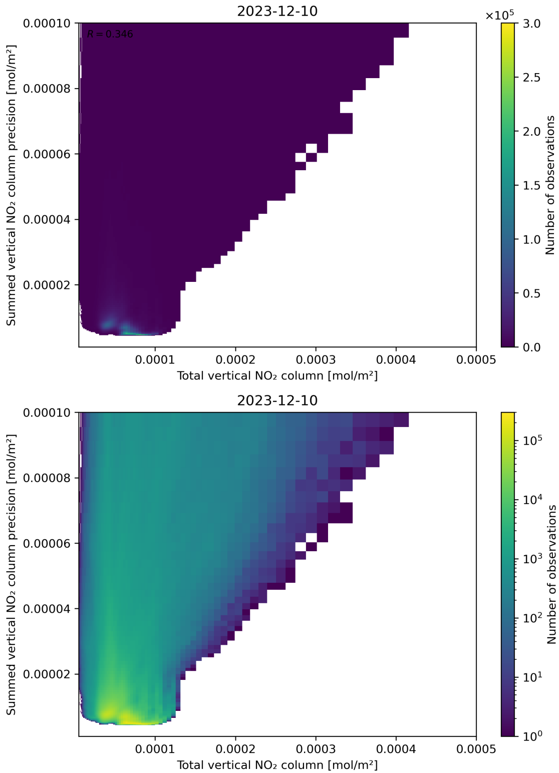
Figure 113: Scatter density plot of “Total vertical NO 2 column” against “Summed vertical NO 2 column precision” for 2023-12-09 to 2023-12-11.
