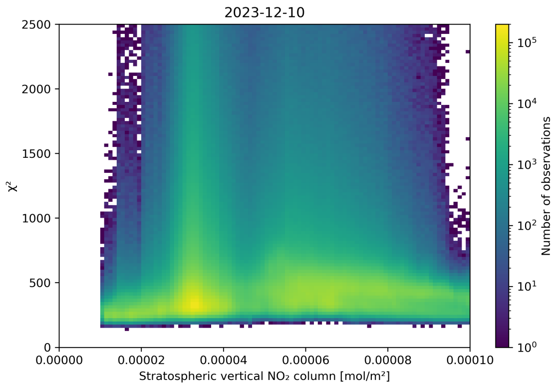
Figure 97: Scatter density plot of “Stratospheric vertical NO 2 column” against “ \chi^2 ” for 2023-12-09 to 2023-12-11.
