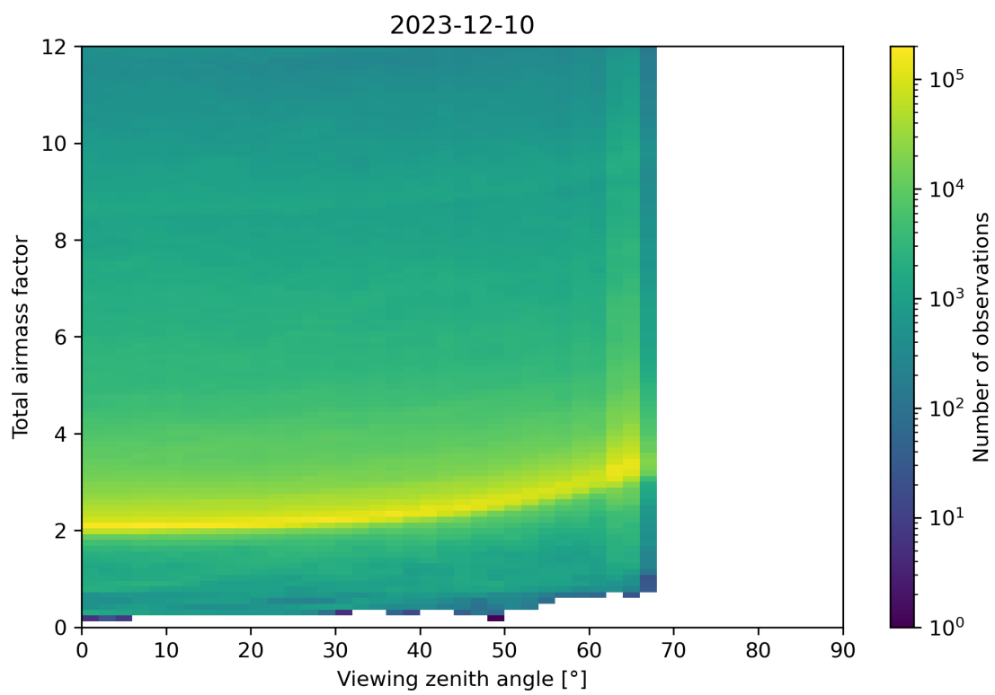
Figure 160: Scatter density plot of “Viewing zenith angle” against “Total airmass factor” for 2023-12-09 to 2023-12-11.
