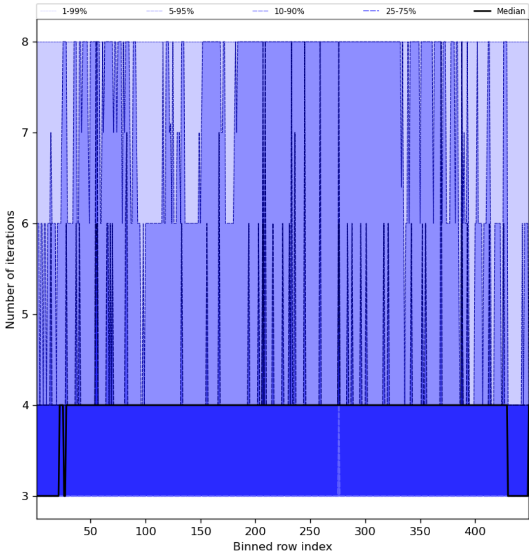
Figure 51: Along track statistics of “Number of iterations” for 2023-12-09 to 2023-12-11
