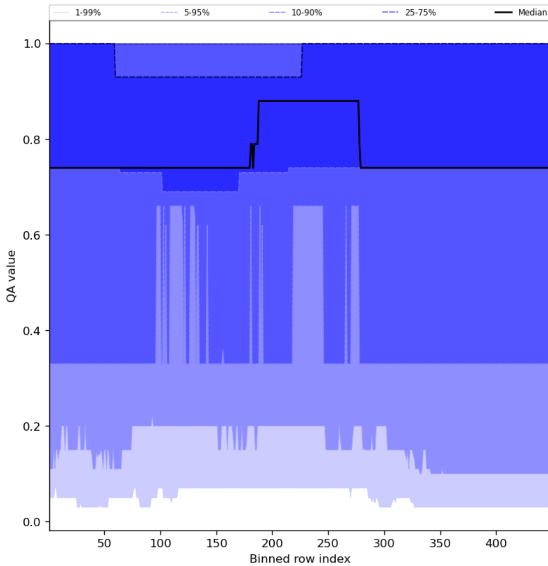
Figure 45: Along track statistics of “QA value” for 2023-12-09 to 2023-12-11
