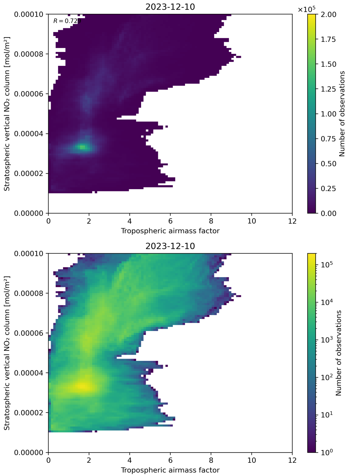
Figure 74: Scatter density plot of “Tropospheric airmass factor” against “Stratospheric vertical NO 2 column” for 2023-12-09 to 2023-12-11.
