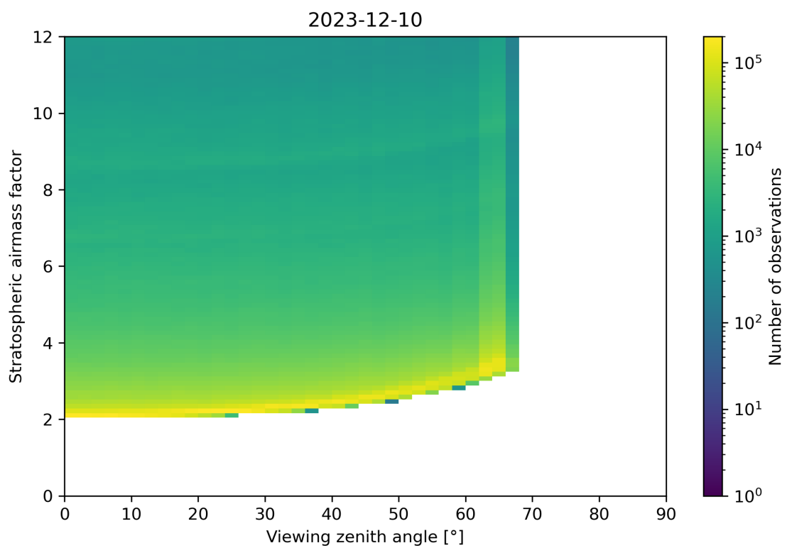
Figure 159: Scatter density plot of “Viewing zenith angle” against “Stratospheric airmass factor” for 2023-12-09 to 2023-12-11.
