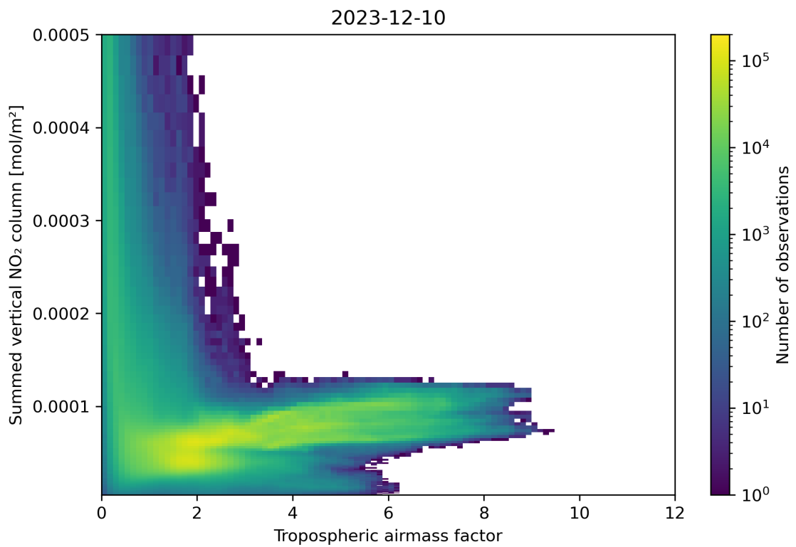
Figure 75: Scatter density plot of “Tropospheric airmass factor” against “Summed vertical NO 2 column” for 2023-12-09 to 2023-12-11.
