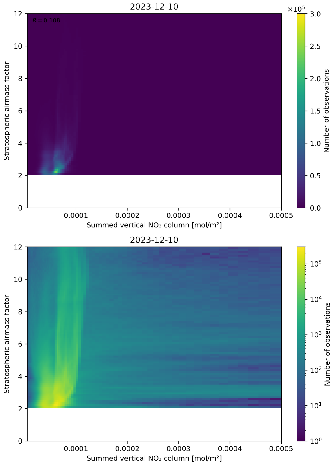
Figure 103: Scatter density plot of “Summed vertical NO 2 column” against “Stratospheric airmass factor” for 2023-12-09 to 2023-12-11.
