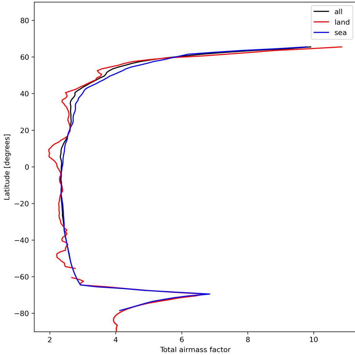
Figure 15: Zonal average of “Total air mass factor” for 2023-12-09 to 2023-12-11.
