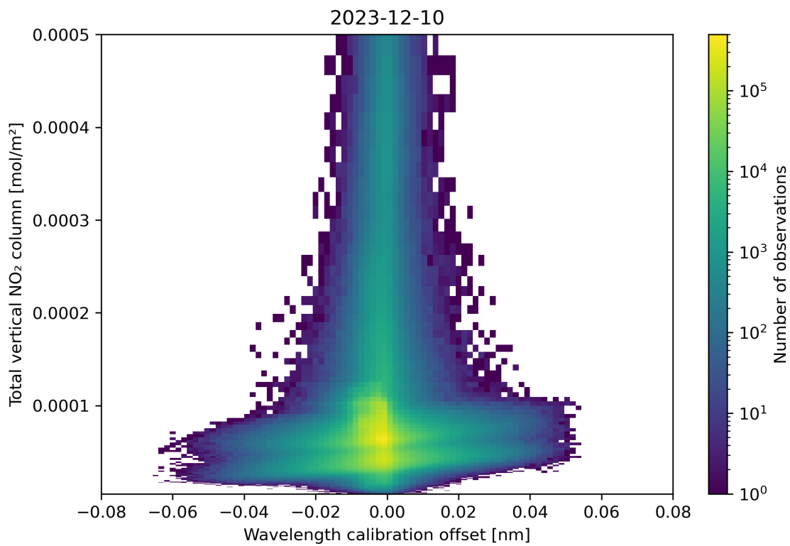
Figure 179: Scatter density plot of “Wavelength calibration offset” against “Total vertical NO 2 column” for 2023-12-09 to 2023-12-11.
