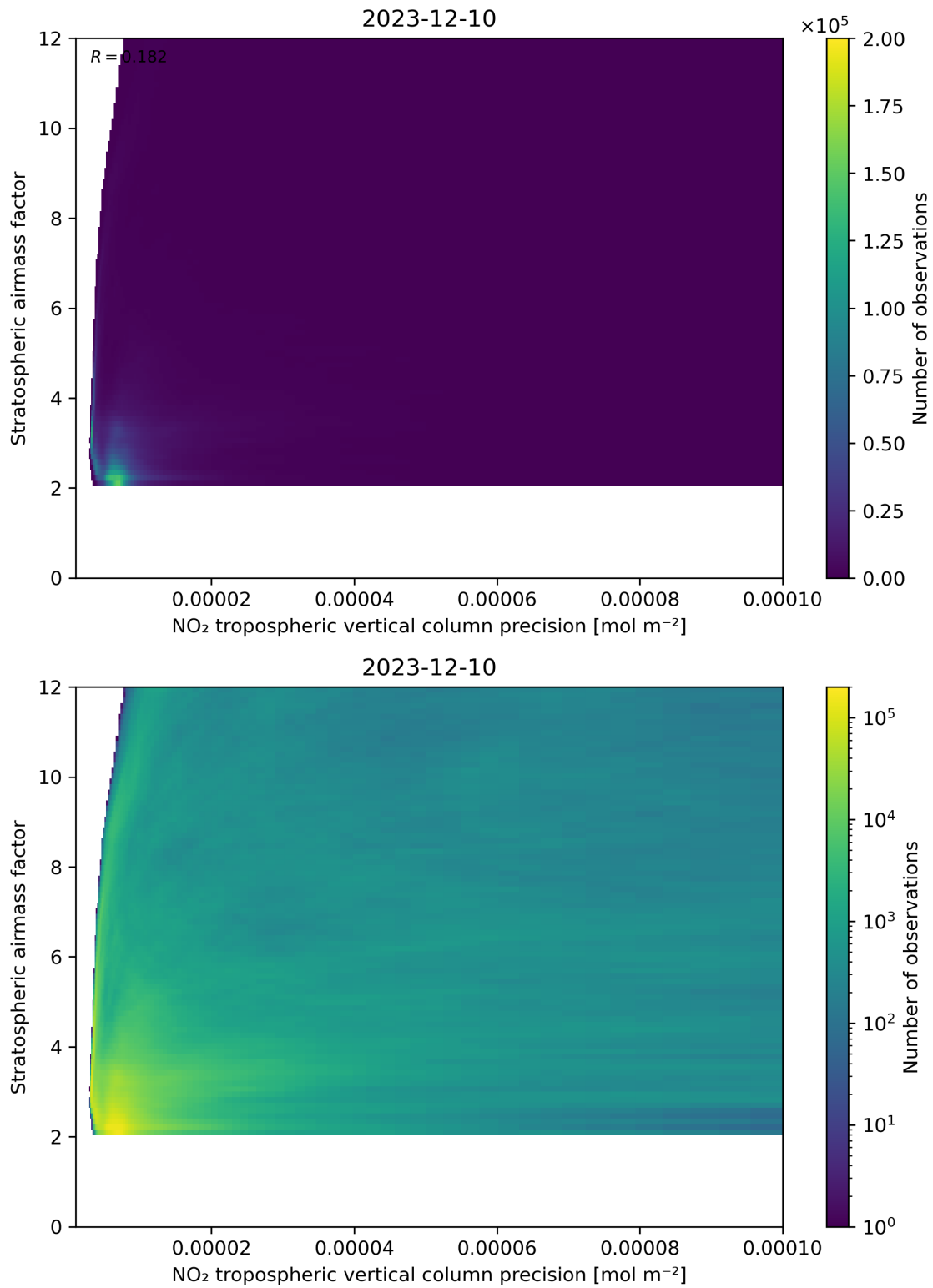
Figure 131: Scatter density plot of “NO 2 tropospheric vertical column precision” against “Stratospheric airmass factor” for 2023-12-09 to 2023-12-11.
