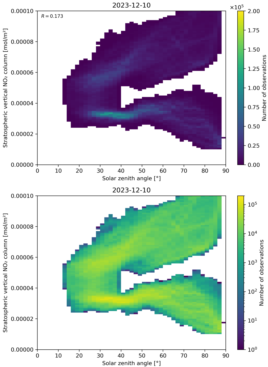
Figure 150: Scatter density plot of “Solar zenith angle” against “Stratospheric vertical NO 2 column” for 2023-12-09 to 2023-12-11.
