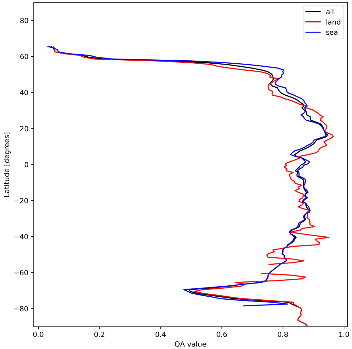
Figure 11: Zonal average of “QA value” for 2023-12-09 to 2023-12-11.
