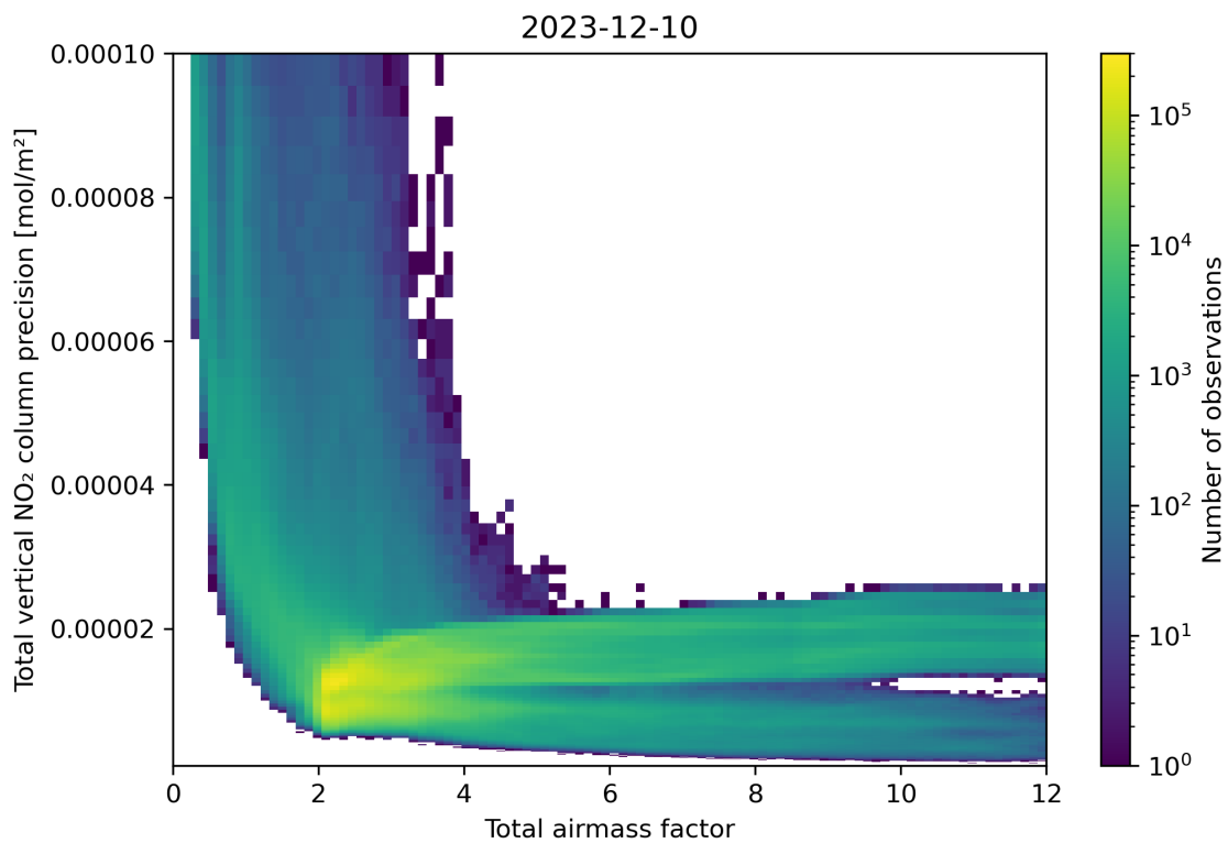
Figure 68: Scatter density plot of “Total airmass factor” against “Total vertical NO 2 column precision” for 2023-12-09 to 2023-12-11.
