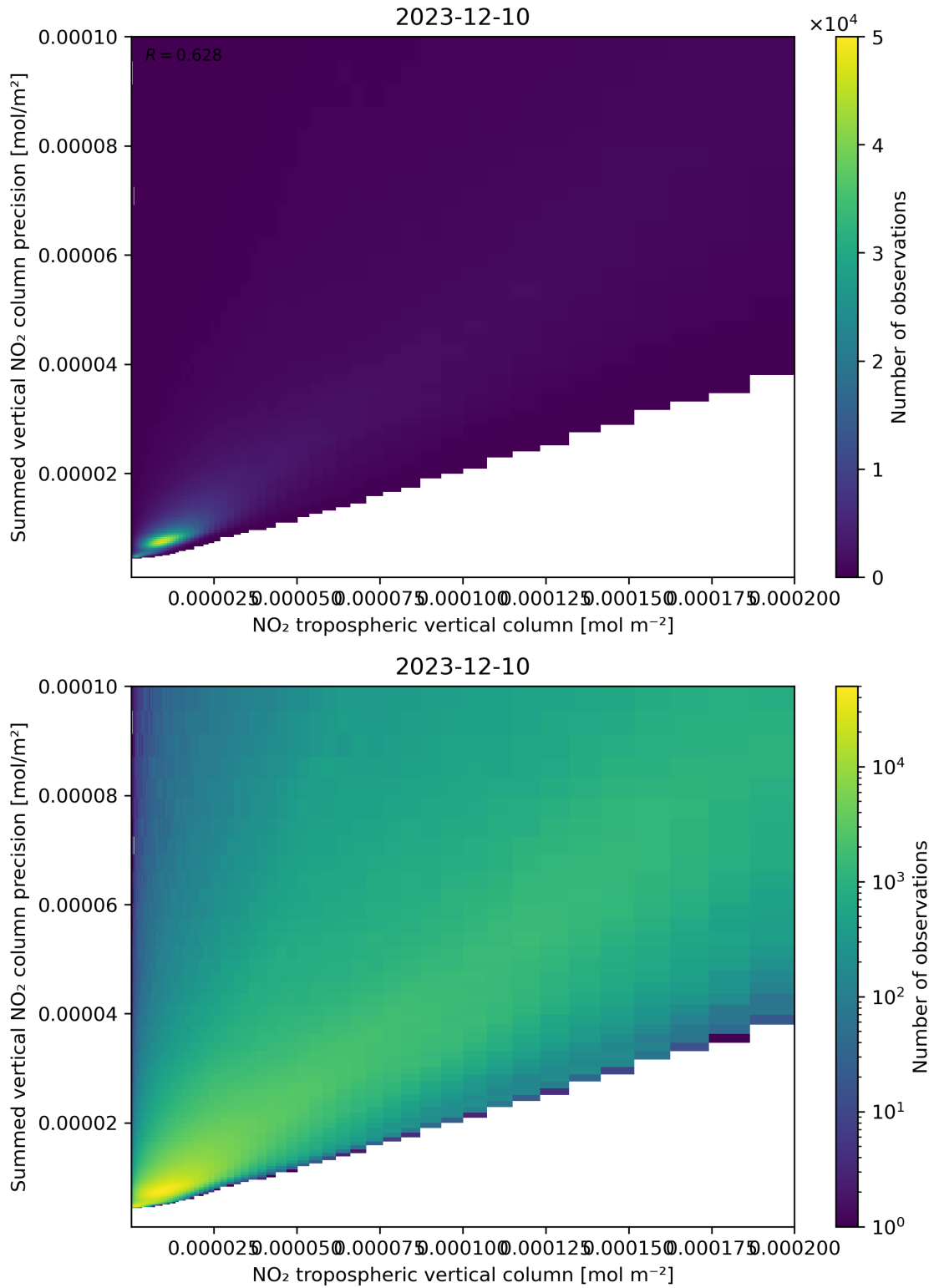
Figure 127: Scatter density plot of “NO 2 tropospheric vertical column” against “Summed vertical NO 2 column precision” for 2023-12-09 to 2023-12-11.
