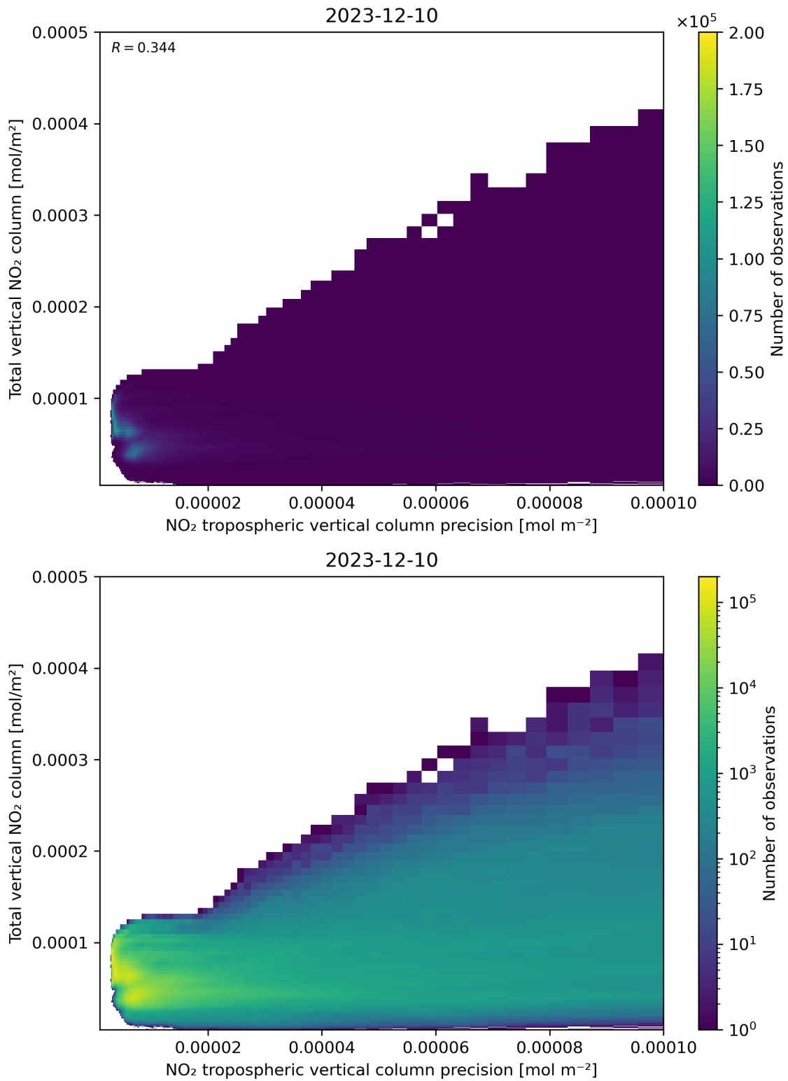
Figure 138: Scatter density plot of “NO 2 tropospheric vertical column precision” against “Total vertical NO 2 column” for 2023-12-09 to 2023-12-11.
