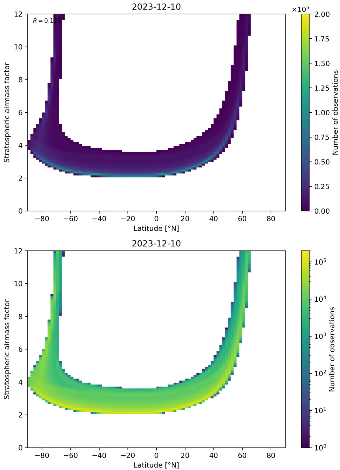
Figure 83: Scatter density plot of “Latitude” against “Stratospheric airmass factor” for 2023-12-09 to 2023-12-11.
