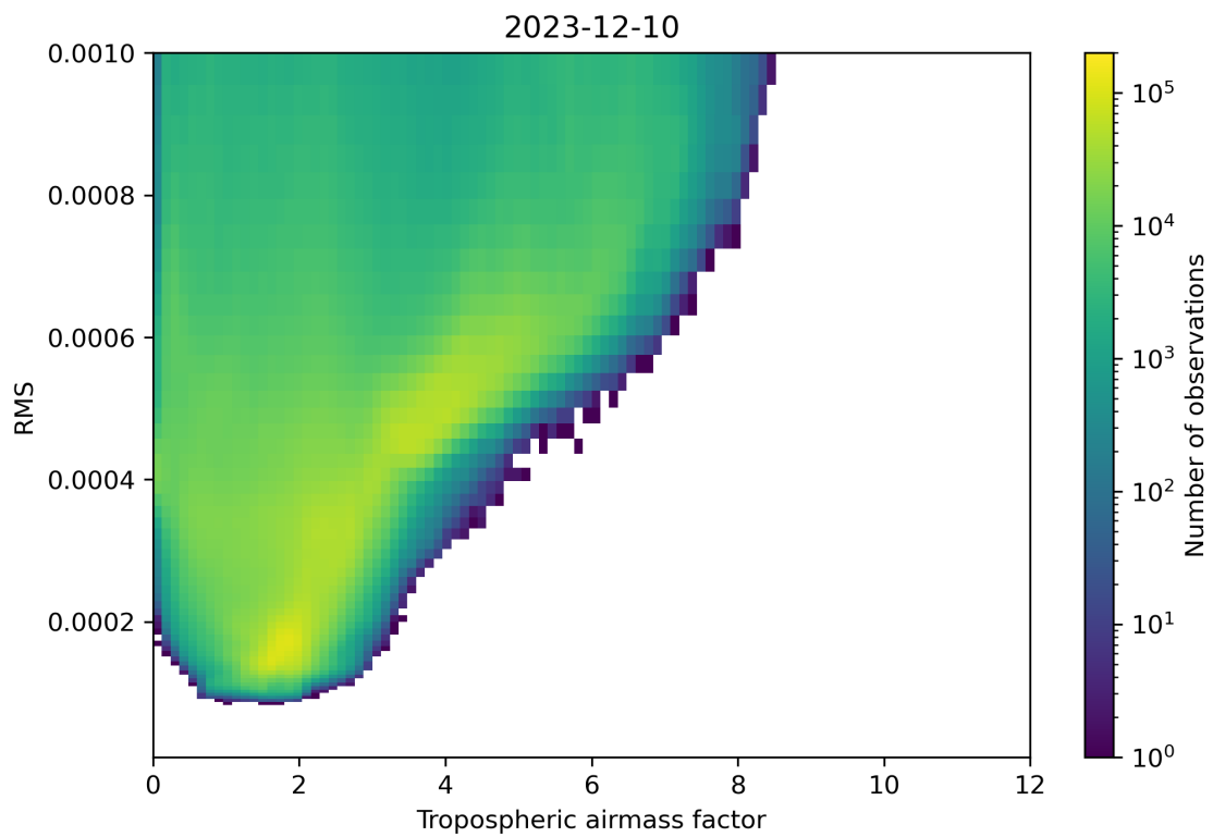
Figure 79: Scatter density plot of “Tropospheric airmass factor” against “RMS” for 2023-12-09 to 2023-12-11.
