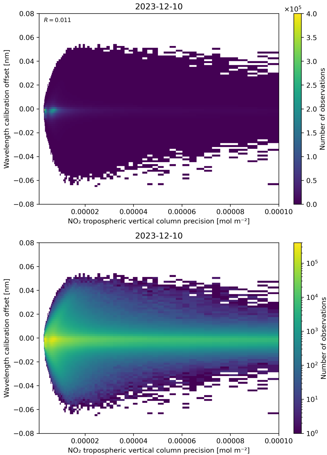
Figure 141: Scatter density plot of “NO 2 tropospheric vertical column precision” against “Wavelength calibration offset” for 2023-12-09 to 2023-12-11.
