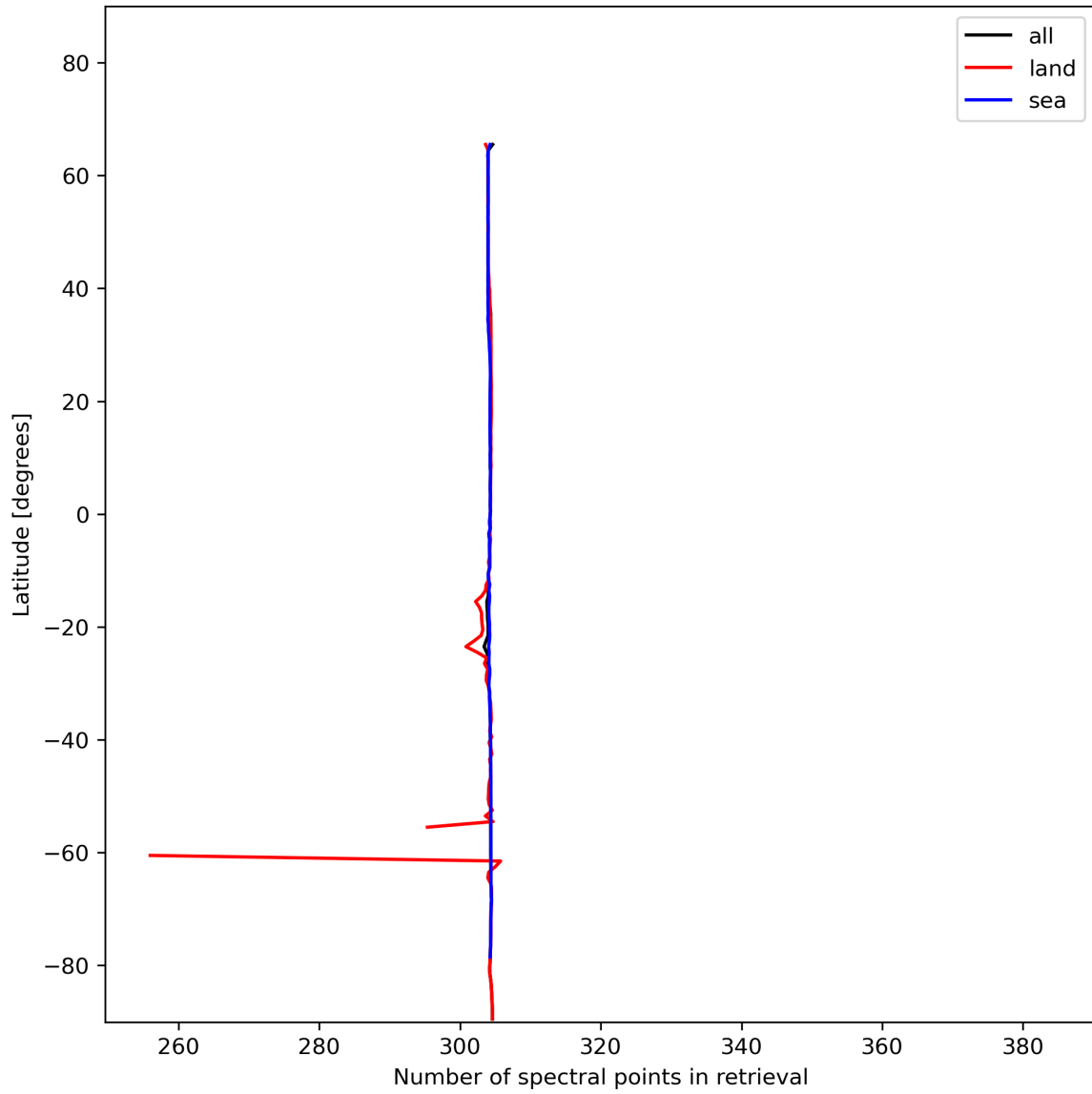
Figure 16: Zonal average of “Number of spectral points in retrieval” for 2023-12-09 to 2023-12-11.
