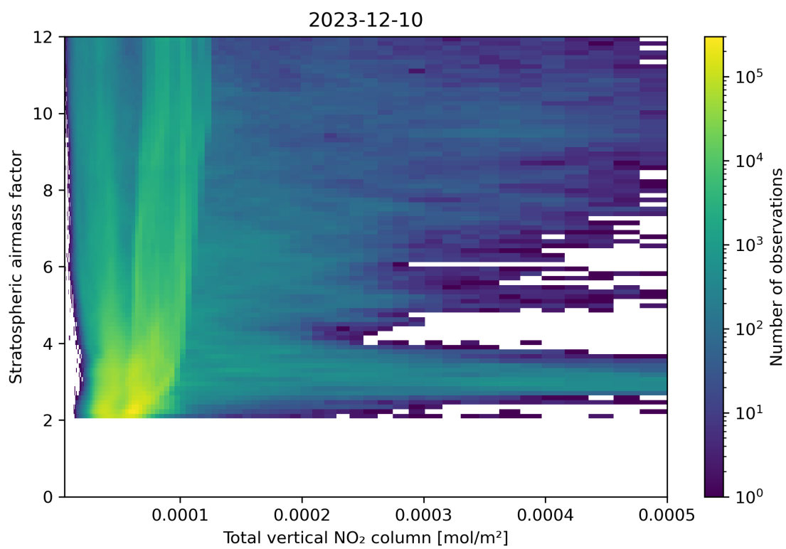
Figure 110: Scatter density plot of “Total vertical NO 2 column” against “Stratospheric airmass factor” for 2023-12-09 to 2023-12-11.
