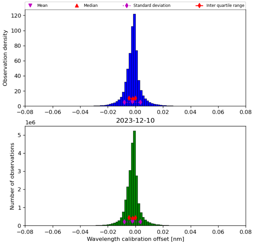
Figure 35: Histogram of “Wavelength calibration offset” for 2023-12-09 to 2023-12-11
