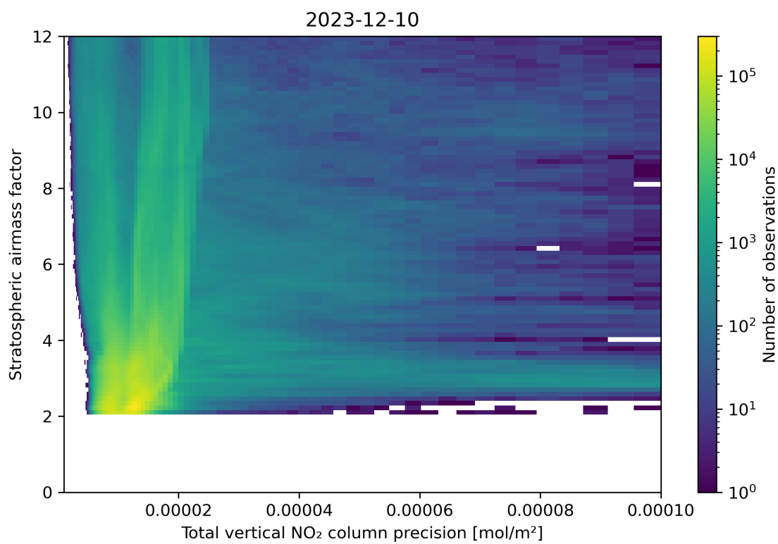
Figure 115: Scatter density plot of “Total vertical NO 2 column precision” against “Stratospheric airmass factor” for 2023-12-09 to 2023-12-11.
