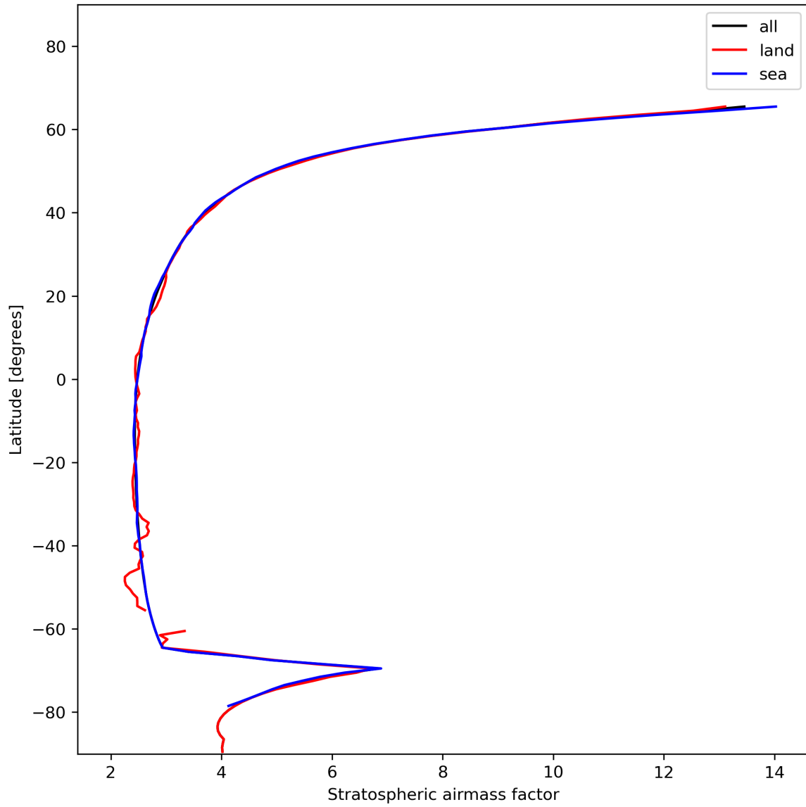
Figure 27: Zonal average of “Stratospheric air mass factor” for 2023-12-09 to 2023-12-11.
