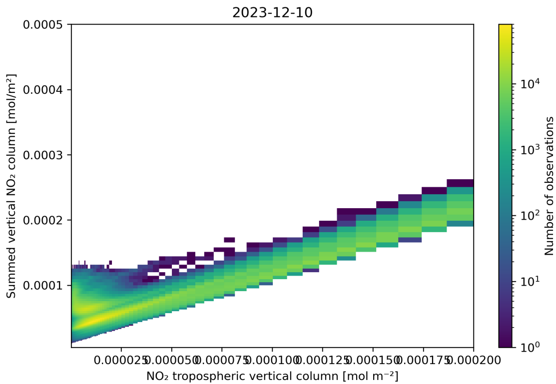
Figure 126: Scatter density plot of “NO 2 tropospheric vertical column” against “Summed vertical NO 2 column” for 2023-12-09 to 2023-12-11.
