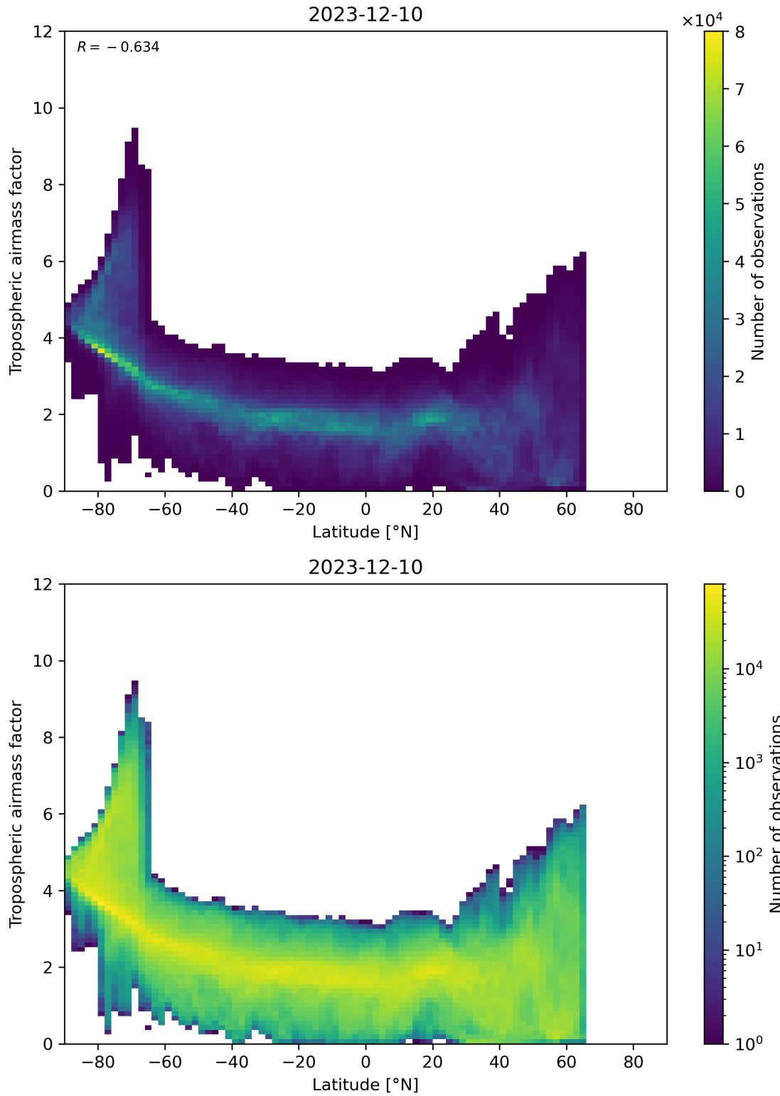
Figure 85: Scatter density plot of “Latitude” against “Tropospheric airmass factor” for 2023-12-09 to 2023-12-11.
