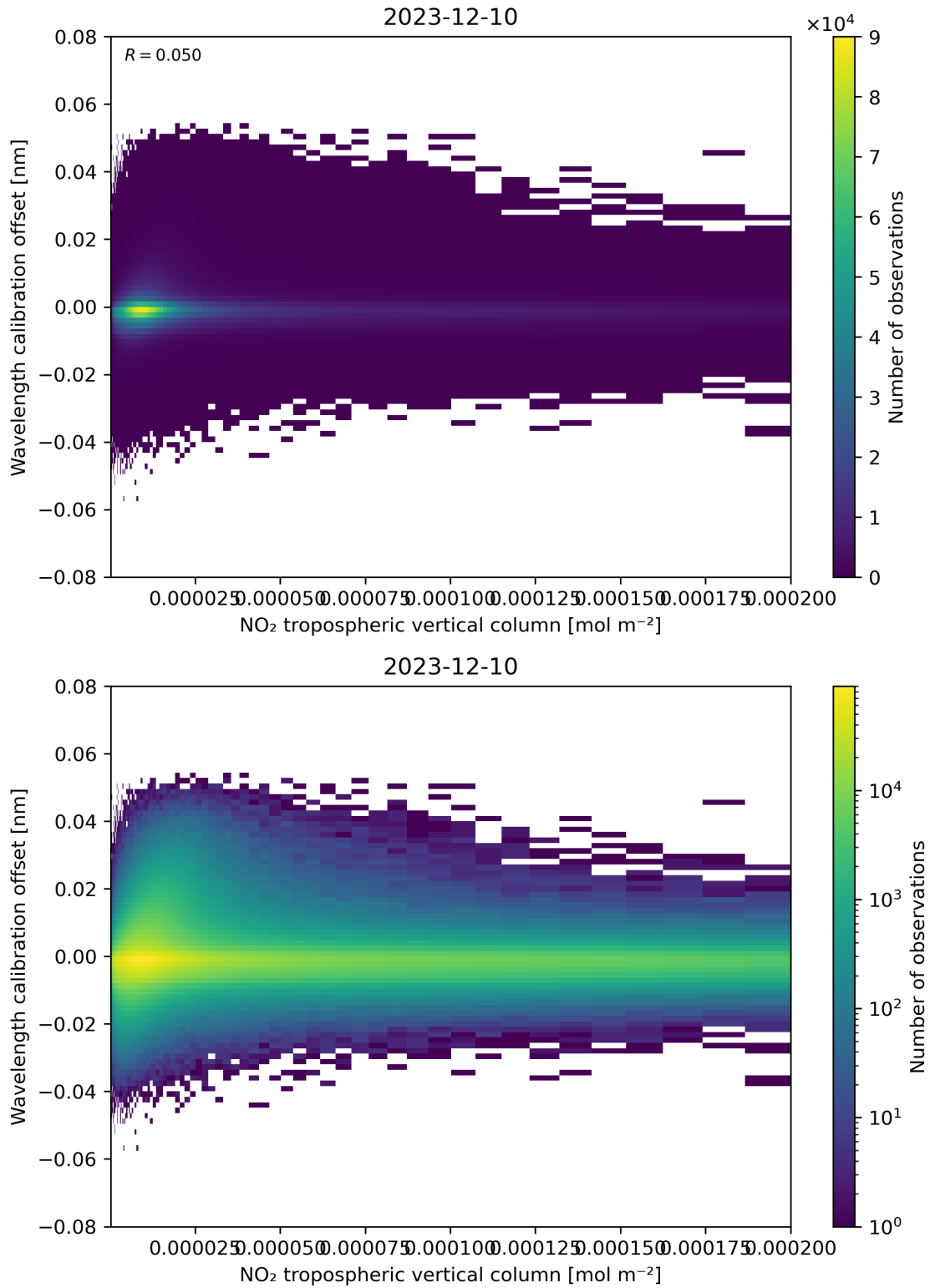
Figure 143: Scatter density plot of “NO 2 tropospheric vertical column” against “Wavelength calibration offset” for 2023-12-09 to 2023-12-11.
