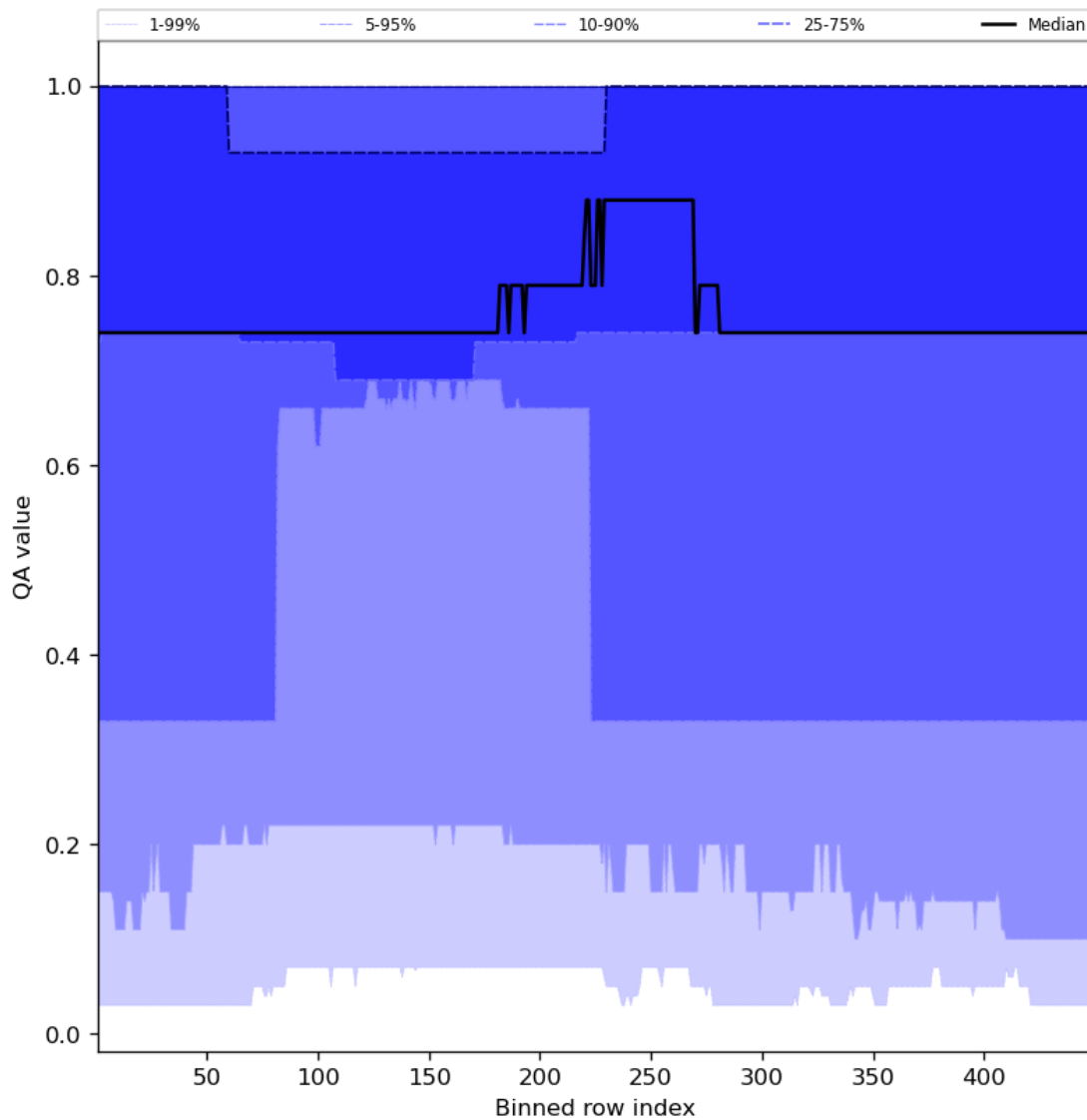
Figure 45: Along track statistics of “QA value” for 2023-12-10 to 2023-12-12
