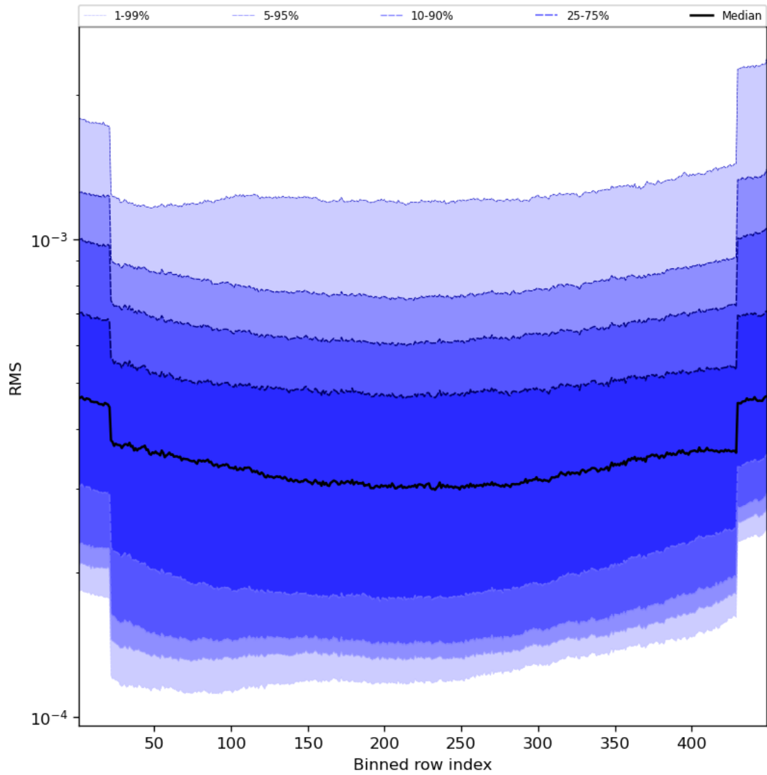
Figure 60: Along track statistics of “RMS” for 2023-12-10 to 2023-12-12
