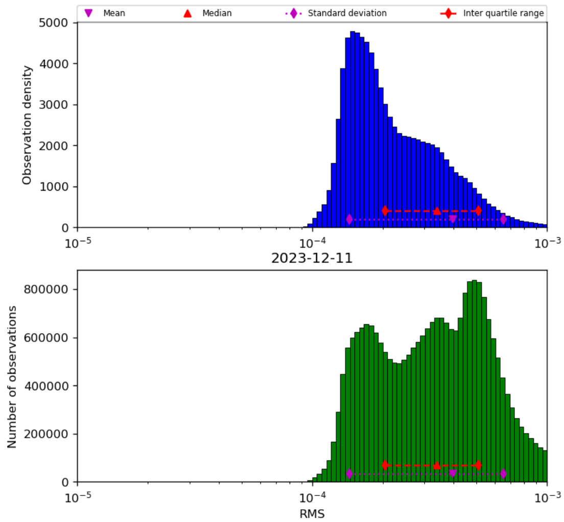
Figure 43: Histogram of “RMS” for 2023-12-10 to 2023-12-12
