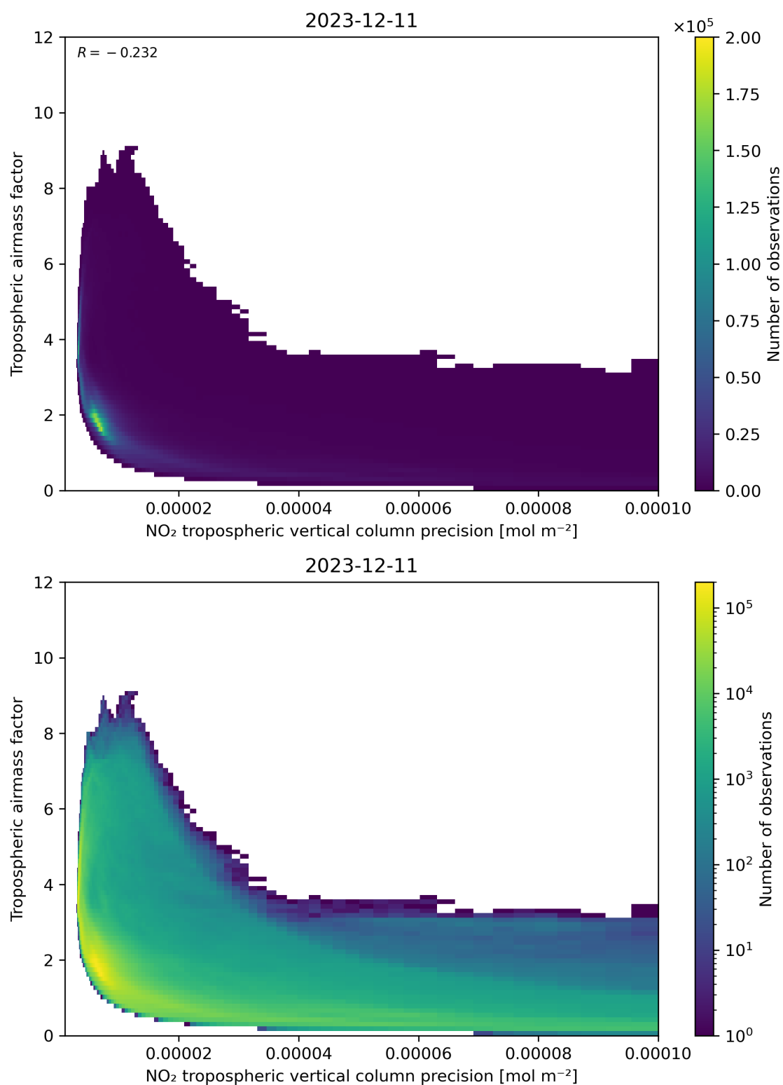
Figure 133: Scatter density plot of “NO 2 tropospheric vertical column precision” against “Tropospheric air mass factor” for 2023-12-10 to 2023-12-12.
