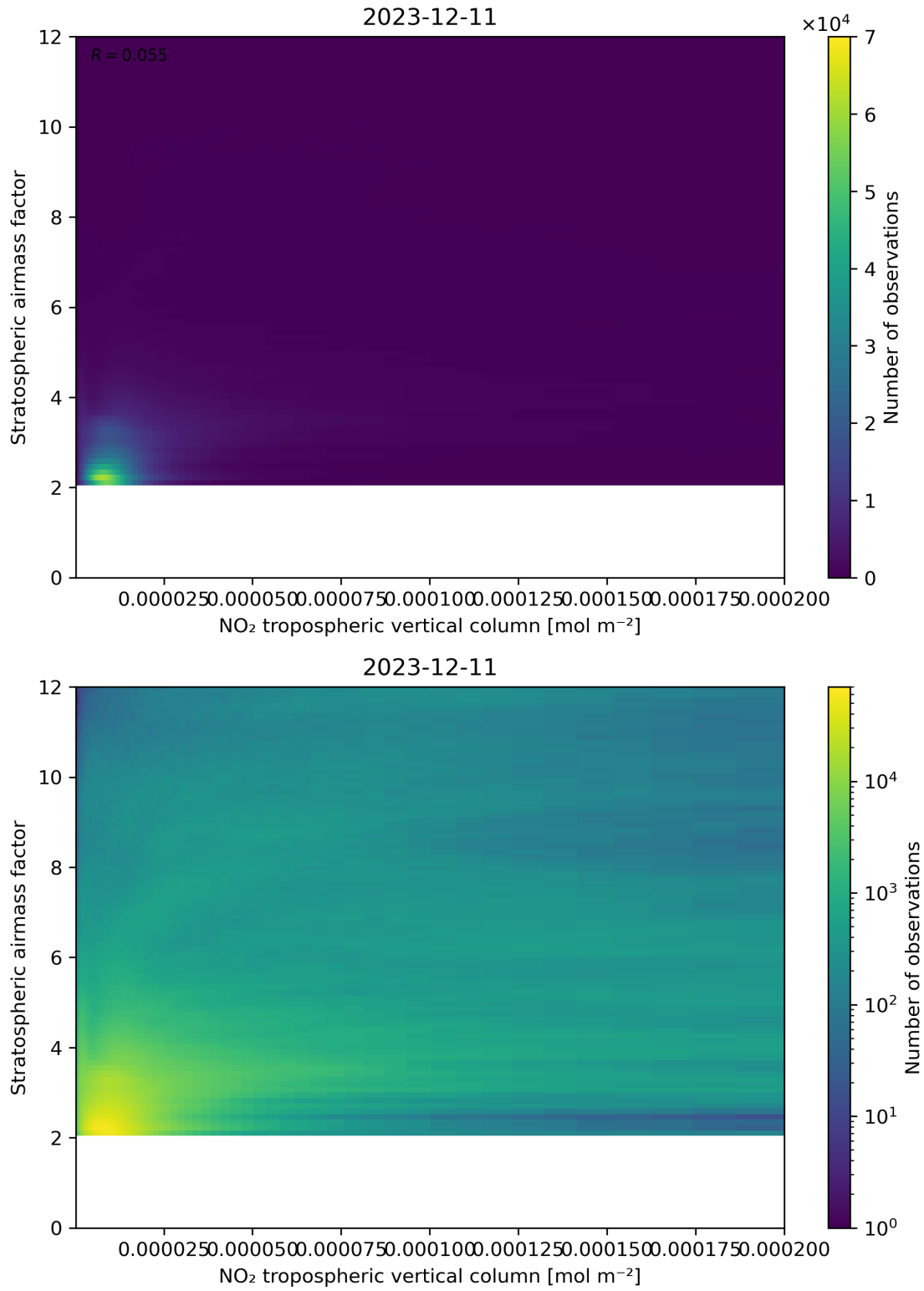
Figure 121: Scatter density plot of “NO 2 tropospheric vertical column” against “Stratospheric airmass factor” for 2023-12-10 to 2023-12-12.
