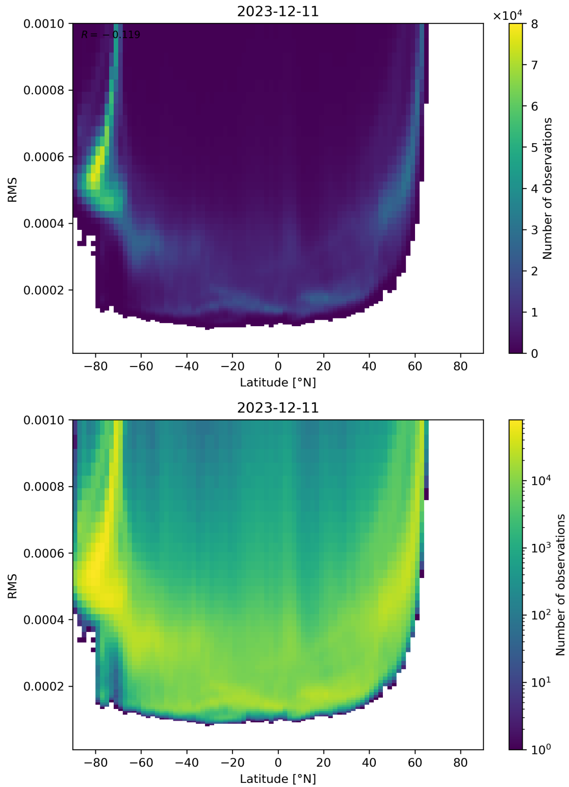
Figure 94: Scatter density plot of “Latitude” against “RMS” for 2023-12-10 to 2023-12-12.
