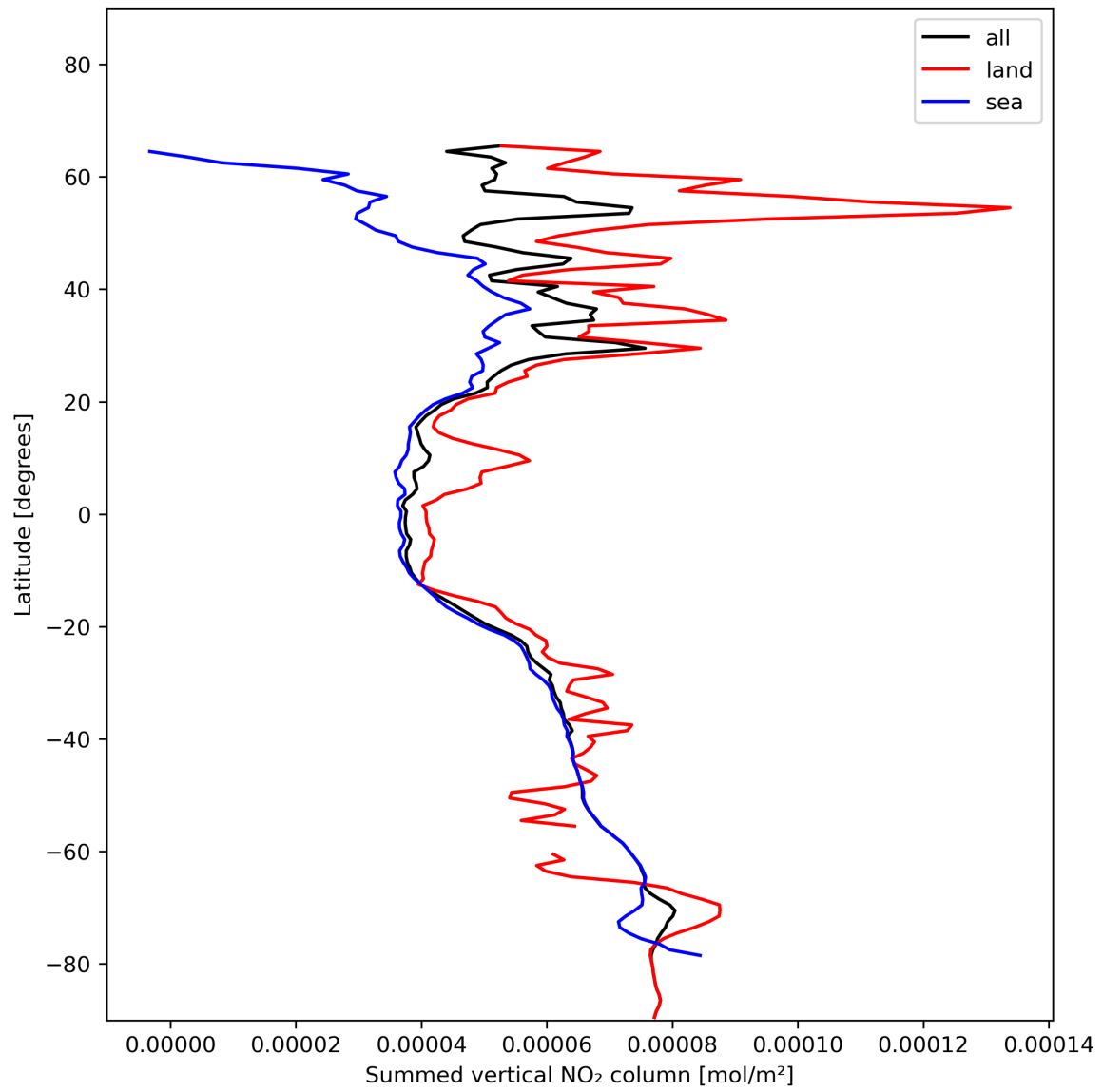
Figure 23: Zonal average of “Summed vertical NO 2 column” for 2023-12-10 to 2023-12-12.
