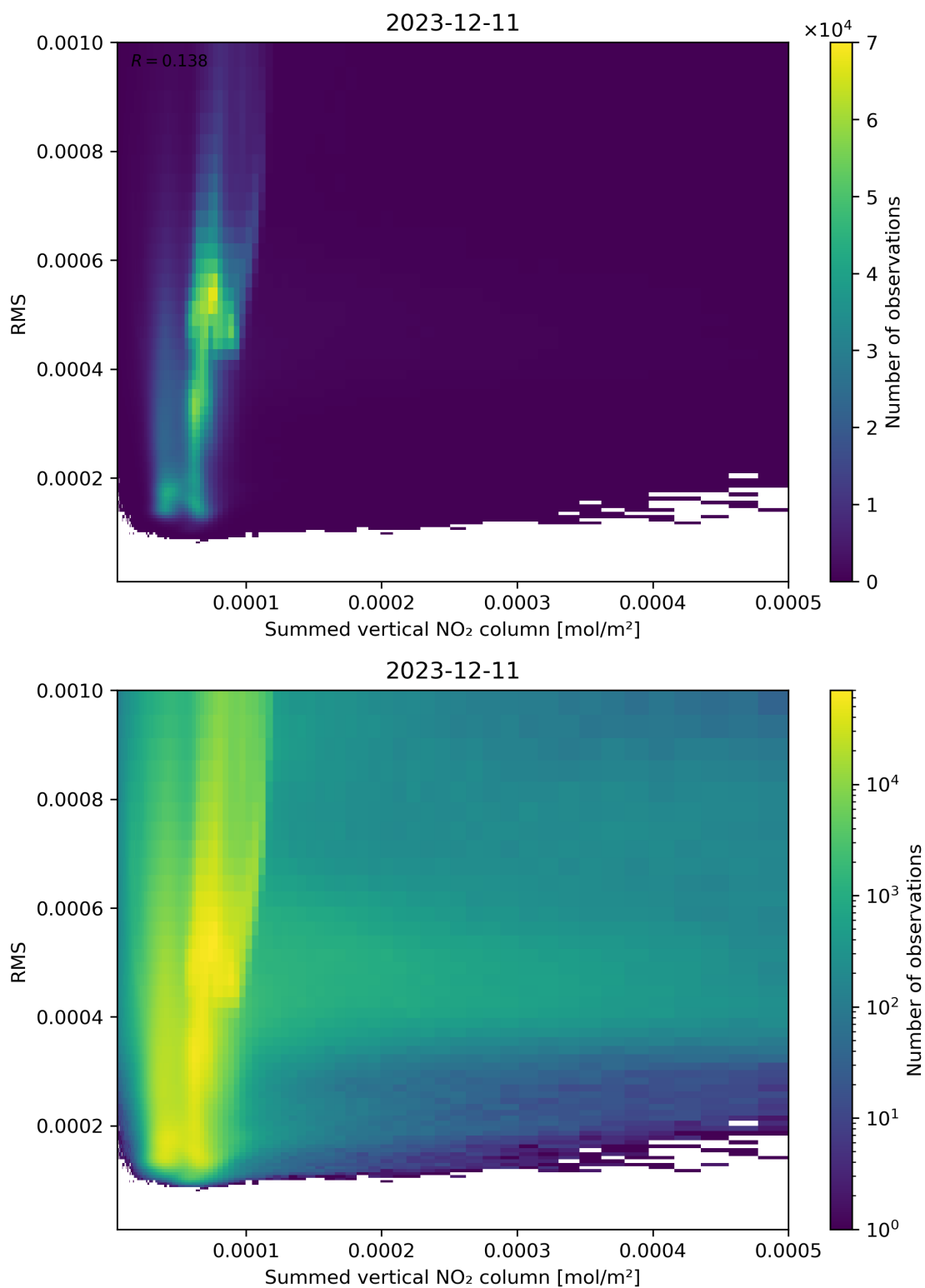
Figure 109: Scatter density plot of “Summed vertical NO 2 column” against “RMS” for 2023-12-10 to 2023-12-12.
