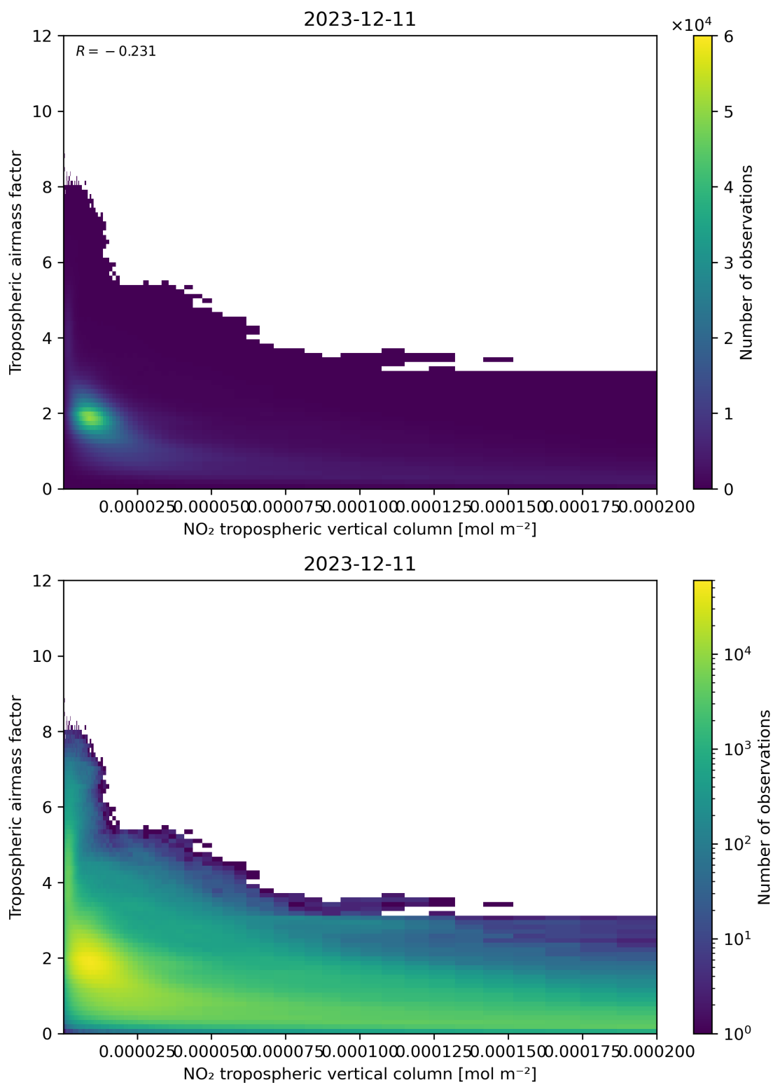
Figure 123: Scatter density plot of “NO 2 tropospheric vertical column” against “Tropospheric air mass factor” for 2023-12-10 to 2023-12-12.
