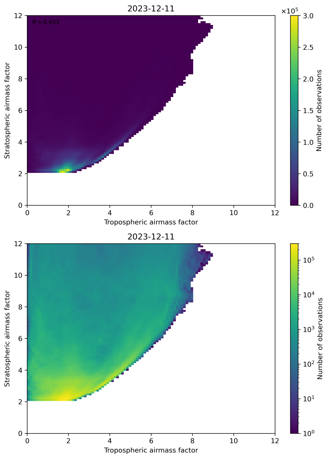
Figure 71: Scatter density plot of “Tropospheric airmass factor” against “Stratospheric airmass factor” for 2023-12-10 to 2023-12-12.
