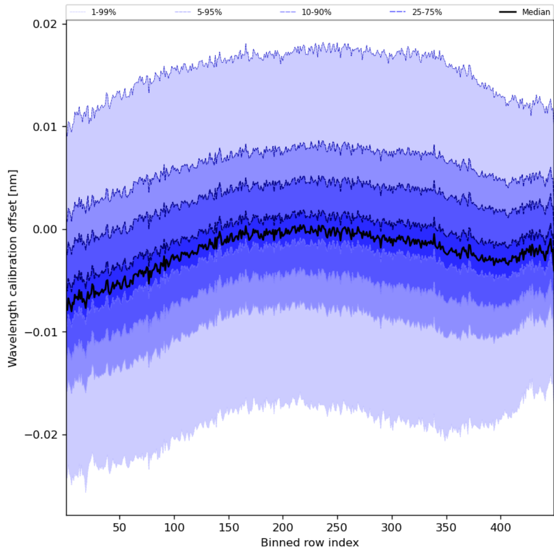
Figure 52: Along track statistics of “Wavelength calibration offset” for 2023-12-10 to 2023-12-12
