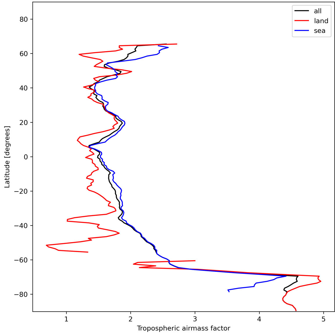
Figure 14: Zonal average of “Tropospheric airmass factor” for 2023-12-10 to 2023-12-12.
