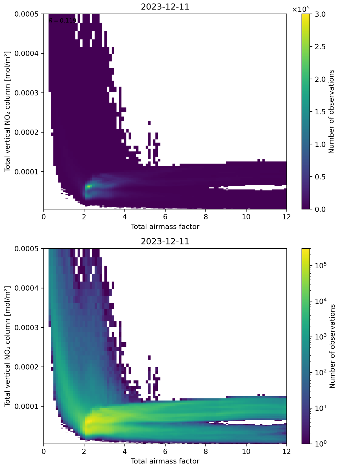
Figure 67: Scatter density plot of “Total airmass factor” against “Total vertical NO 2 column” for 2023-12-10 to 2023-12-12.
