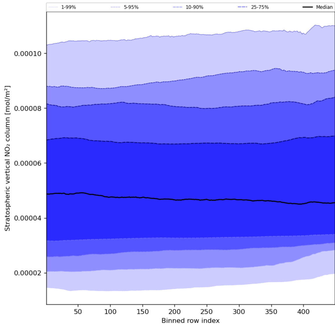
Figure 53: Along track statistics of “Stratospheric vertical NO 2 column” for 2023-12-10 to 2023-12-12
