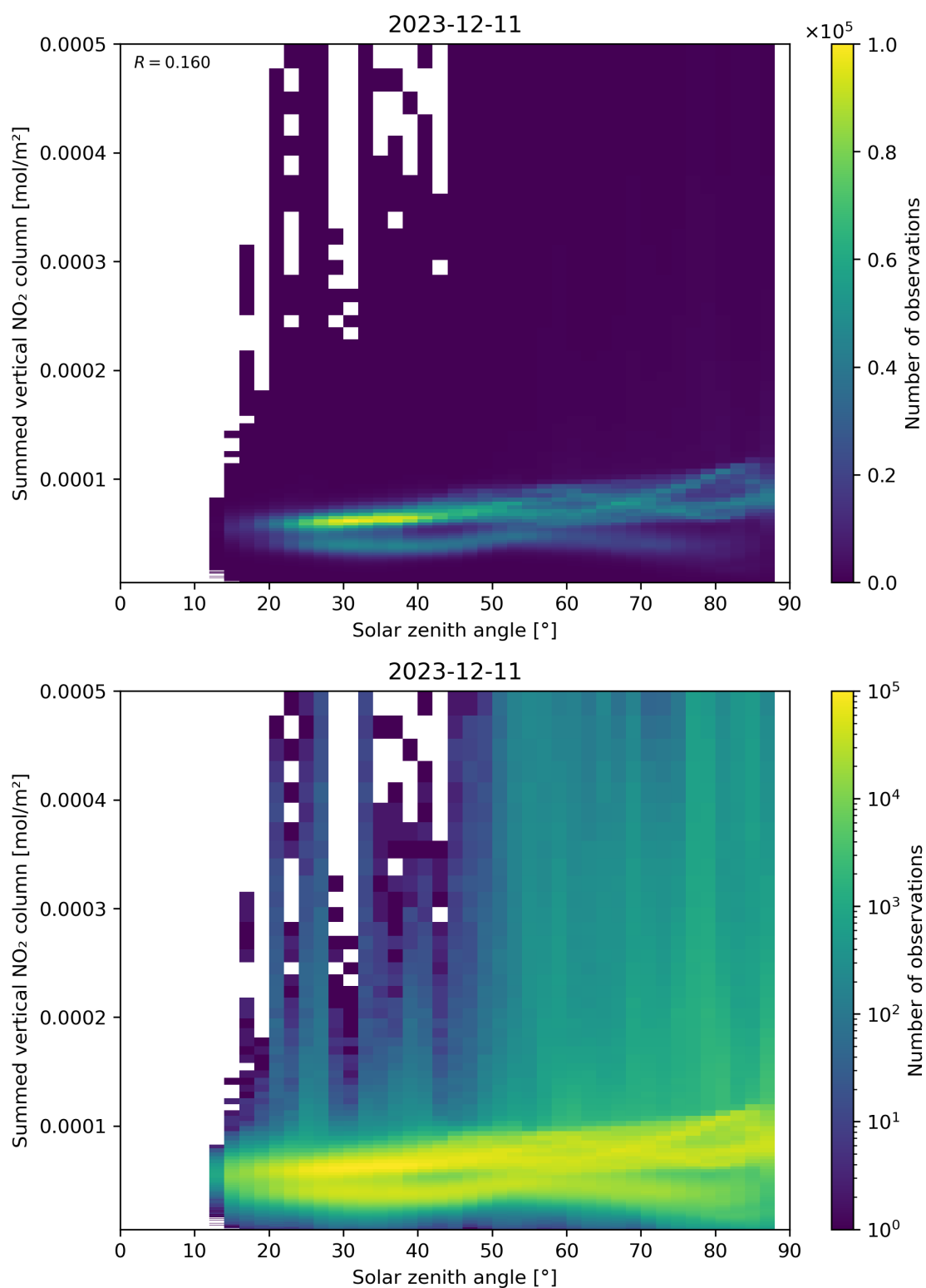
Figure 151: Scatter density plot of “Solar zenith angle” against “Summed vertical NO 2 column” for 2023-12-10 to 2023-12-12.
