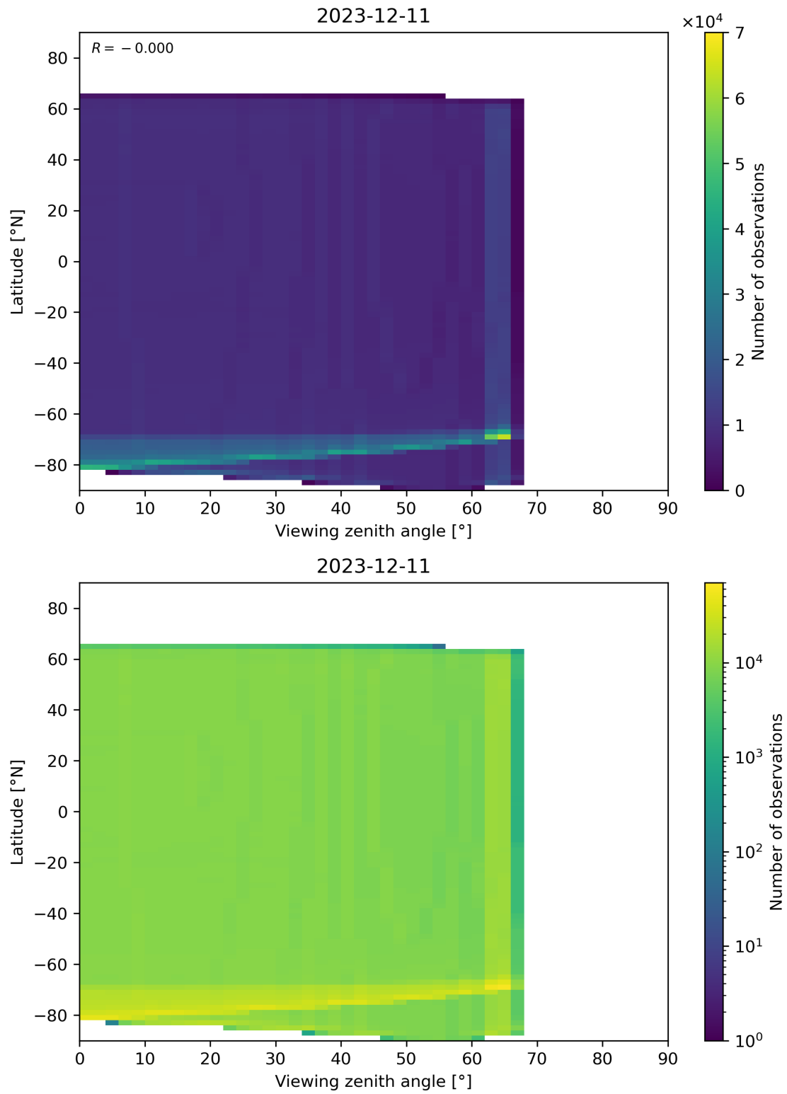
Figure 163: Scatter density plot of “Viewing zenith angle” against “Latitude” for 2023-12-10 to 2023-12-12.
