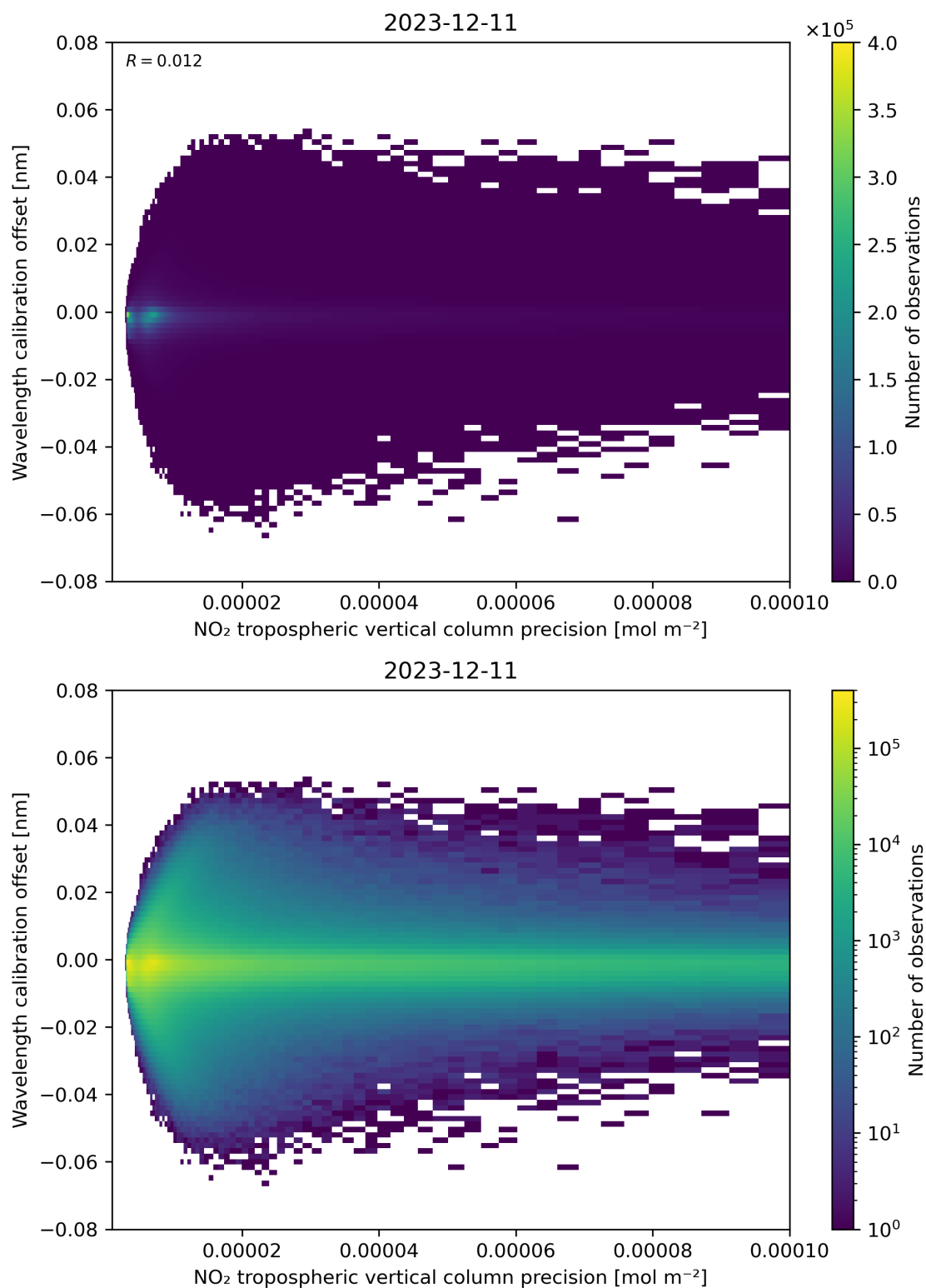
Figure 141: Scatter density plot of “NO 2 tropospheric vertical column precision” against “Wavelength calibration offset” for 2023-12-10 to 2023-12-12.
