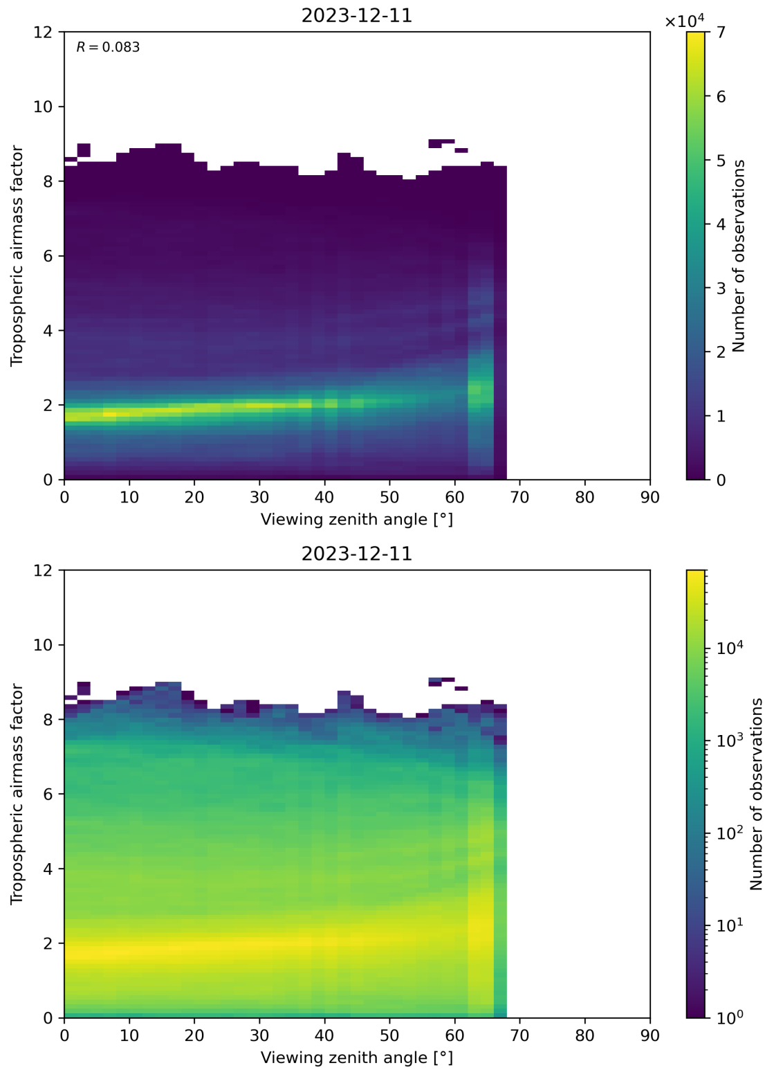
Figure 161: Scatter density plot of “Viewing zenith angle” against “Tropospheric airmass factor” for 2023-12-10 to 2023-12-12.
