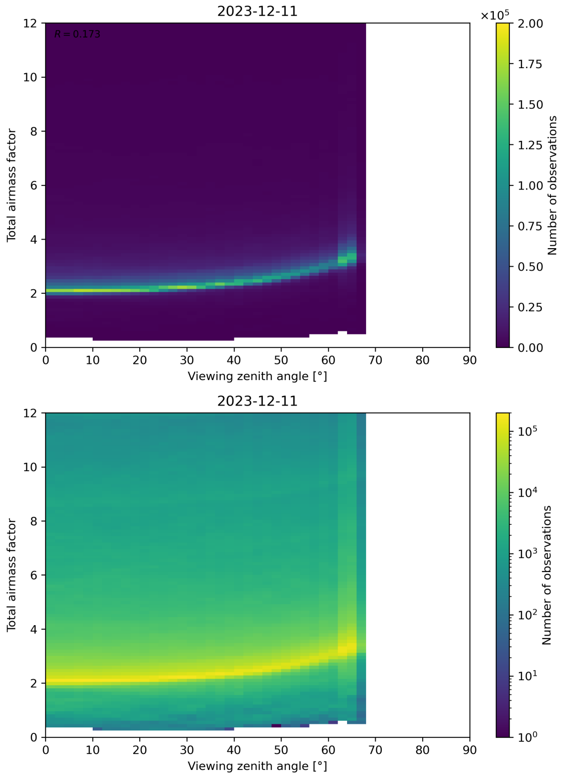
Figure 160: Scatter density plot of “Viewing zenith angle” against “Total airmass factor” for 2023-12-10 to 2023-12-12.
