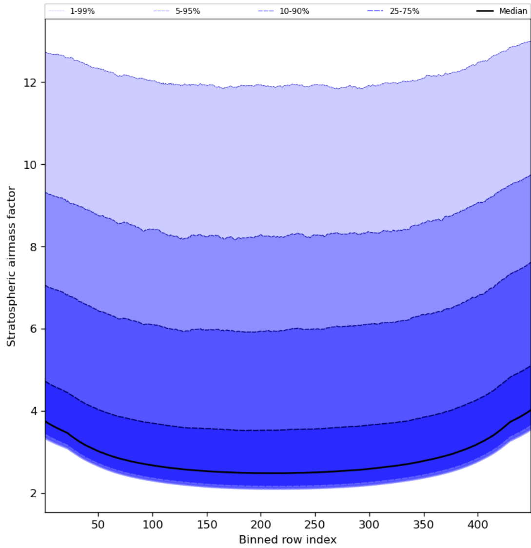
Figure 61: Along track statistics of “Stratospheric airmass factor” for 2023-12-10 to 2023-12-12
