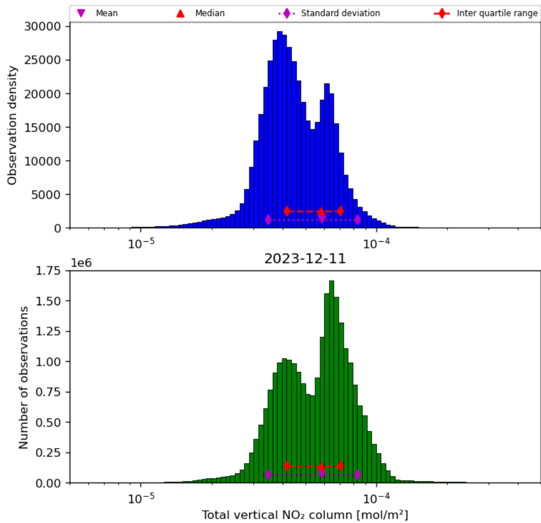
Figure 38: Histogram of “Total vertical NO 2 column” for 2023-12-10 to 2023-12-12
