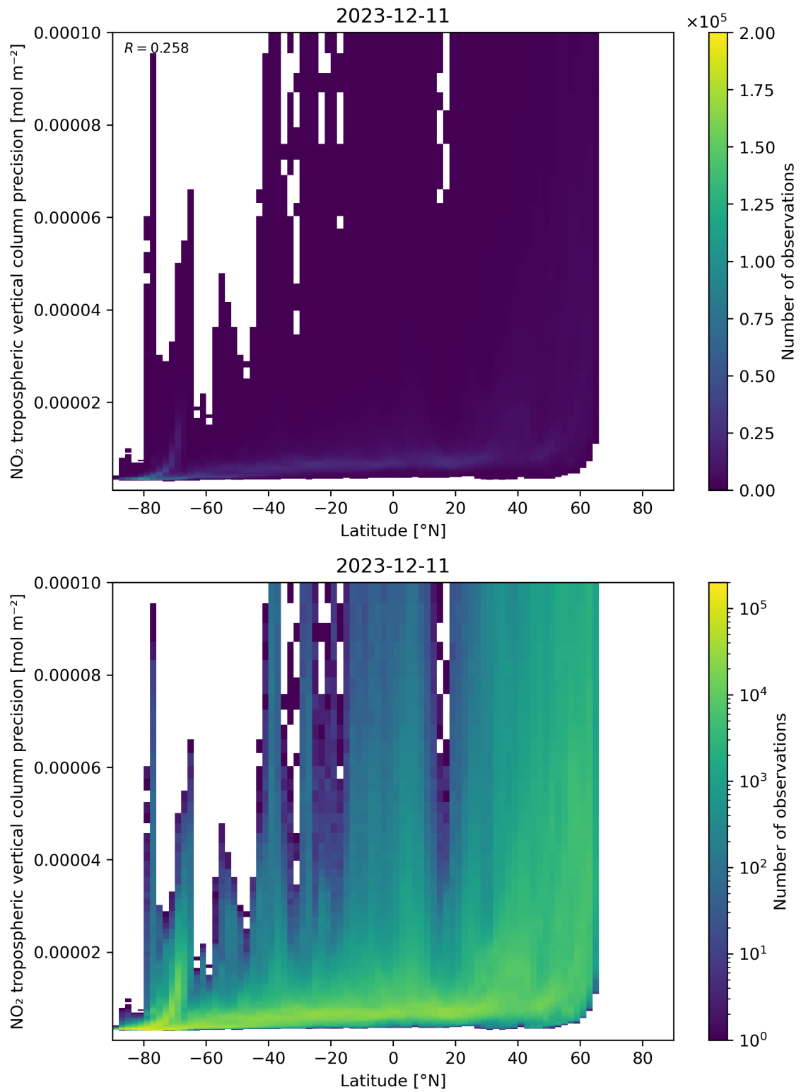
Figure 93: Scatter density plot of “Latitude” against “NO 2 tropospheric vertical column precision” for 2023-12-10 to 2023-12-12.
