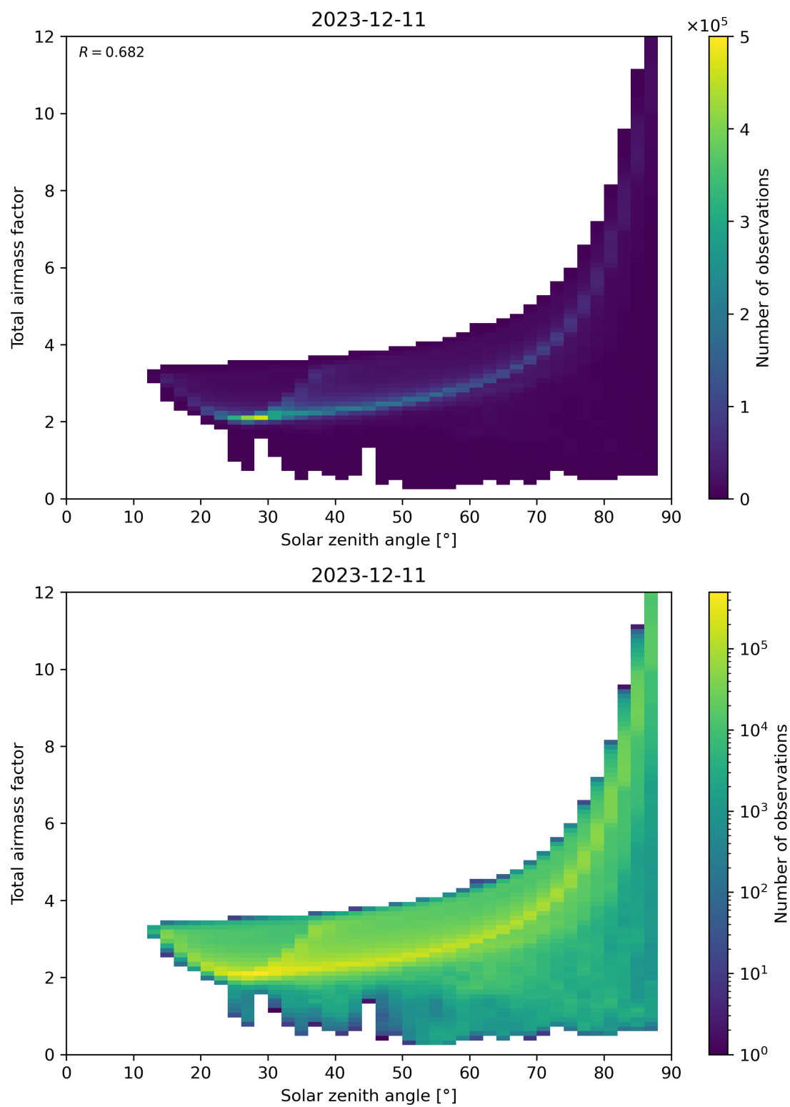
Figure 146: Scatter density plot of “Solar zenith angle” against “Total air mass factor” for 2023-12-10 to 2023-12-12.
