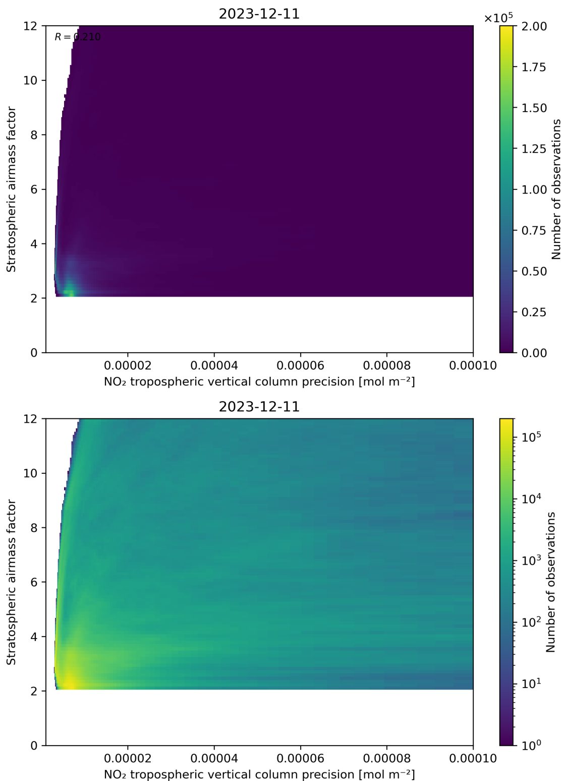
Figure 131: Scatter density plot of “NO 2 tropospheric vertical column precision” against “Stratospheric airmass factor” for 2023-12-10 to 2023-12-12.
