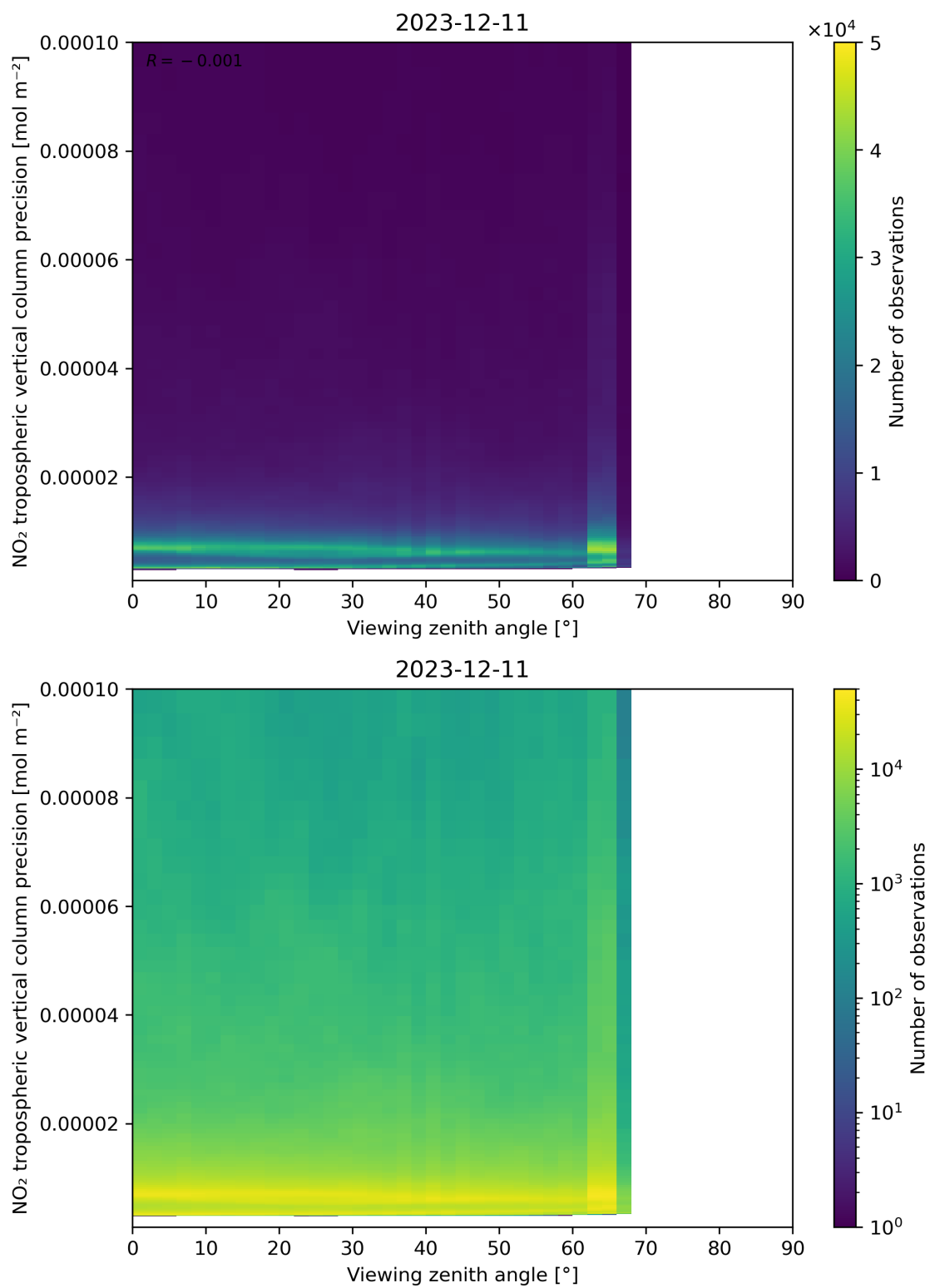
Figure 170: Scatter density plot of “Viewing zenith angle” against “NO 2 tropospheric vertical column precision” for 2023-12-10 to 2023-12-12.
