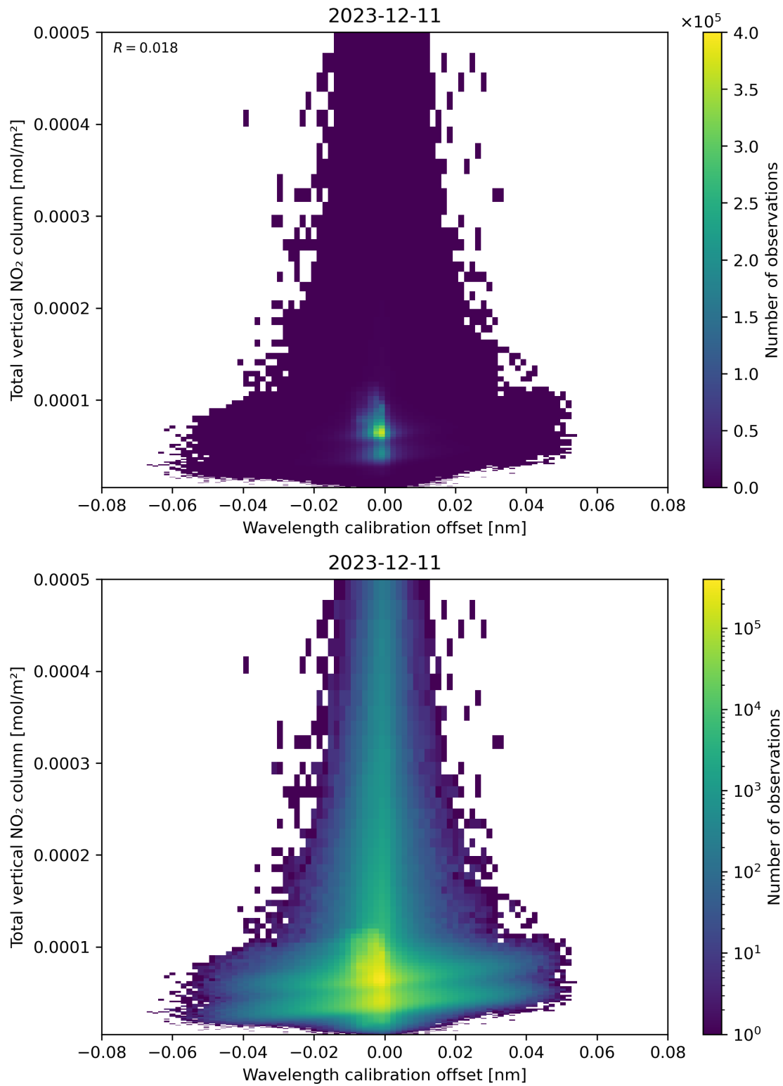
Figure 179: Scatter density plot of “Wavelength calibration offset” against “Total vertical NO 2 column” for 2023-12-10 to 2023-12-12.
