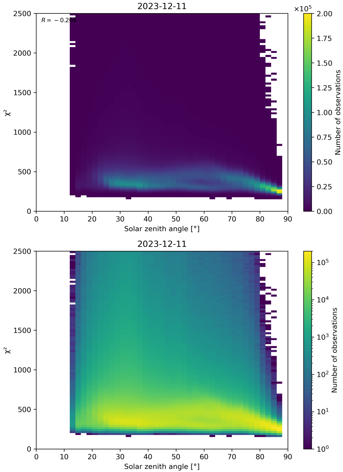
Figure 148: Scatter density plot of “Solar zenith angle” against “ \chi^2 ” for 2023-12-10 to 2023-12-12.
