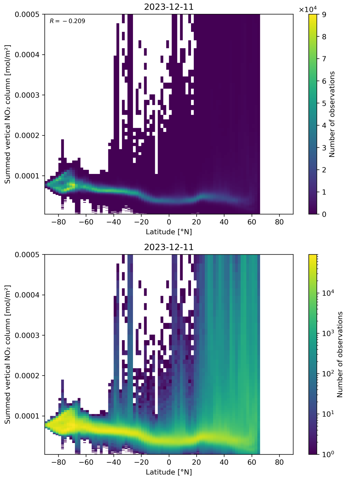
Figure 88: Scatter density plot of “Latitude” against “Summed vertical NO 2 column” for 2023-12-10 to 2023-12-12.
