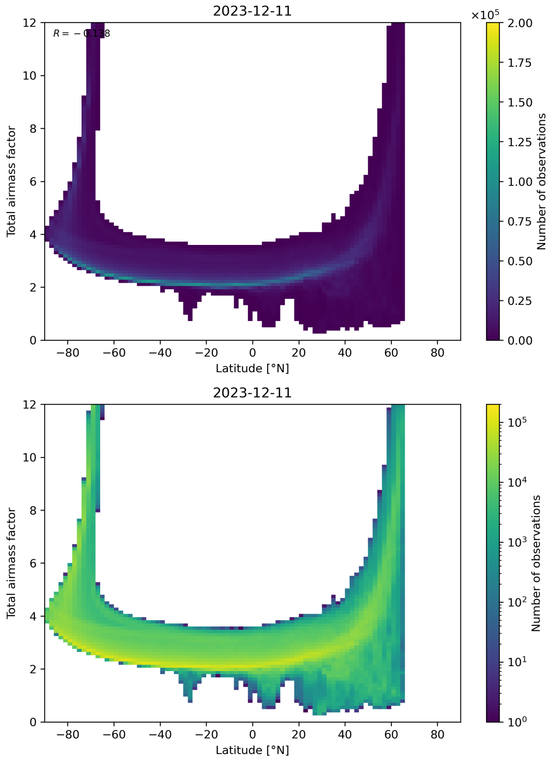
Figure 84: Scatter density plot of “Latitude” against “Total airmass factor” for 2023-12-10 to 2023-12-12.
