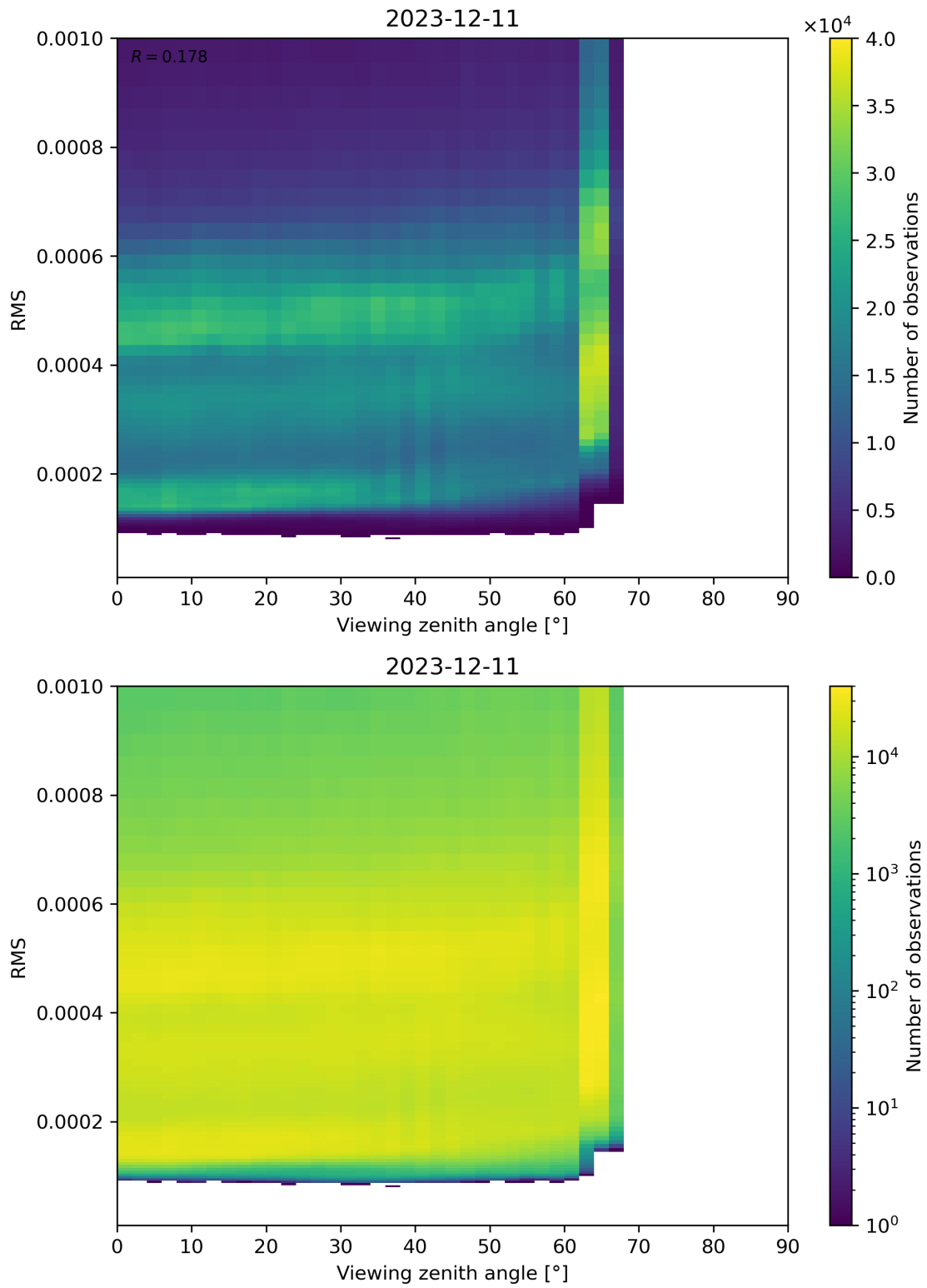
Figure 171: Scatter density plot of “Viewing zenith angle” against “RMS” for 2023-12-10 to 2023-12-12.
