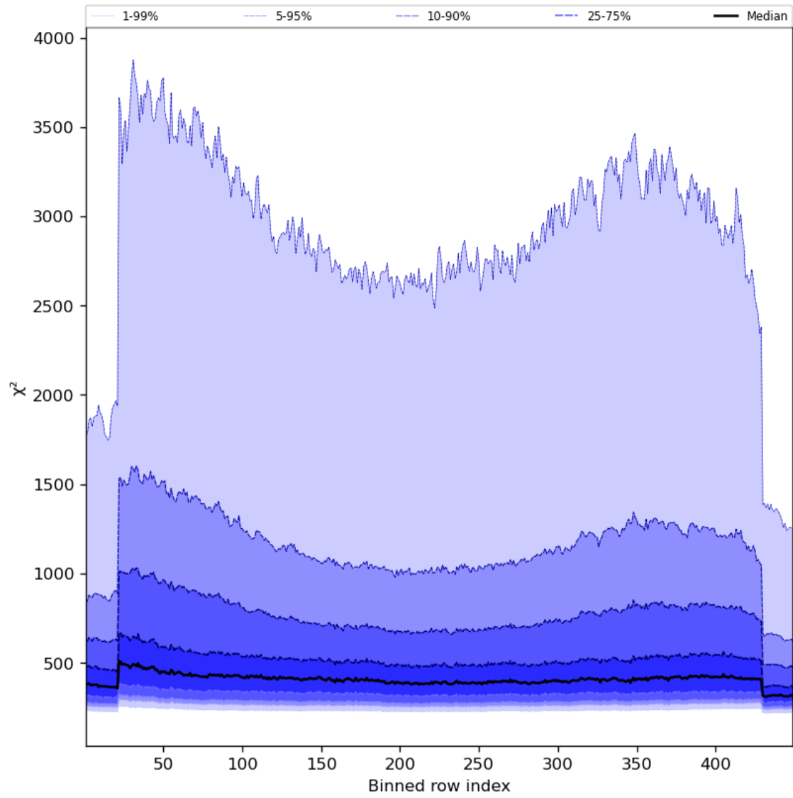
Figure 59: Along track statistics of “ \chi^2 ” for 2023-12-10 to 2023-12-12
