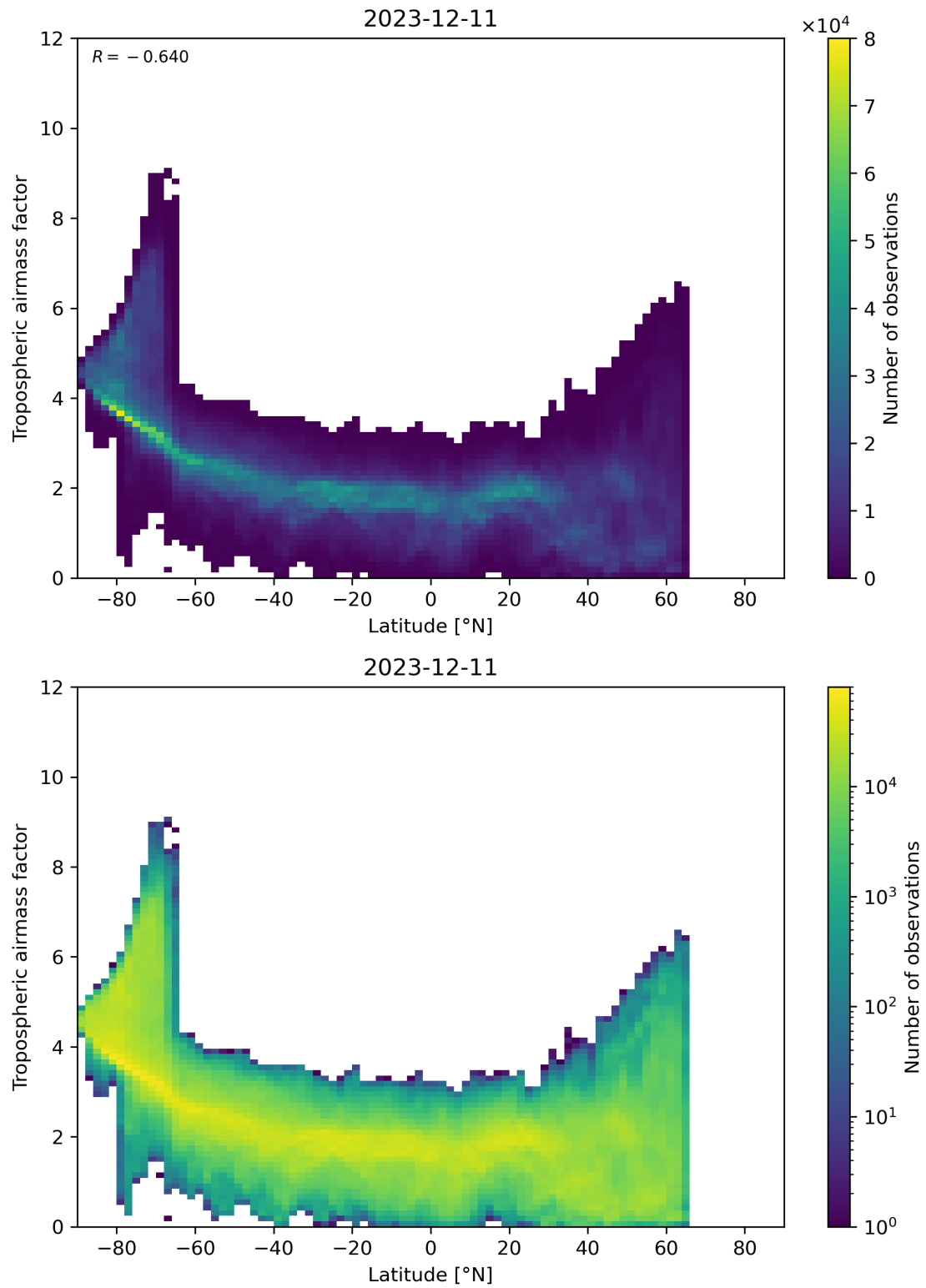
Figure 85: Scatter density plot of “Latitude” against “Tropospheric airmass factor” for 2023-12-10 to 2023-12-12.
