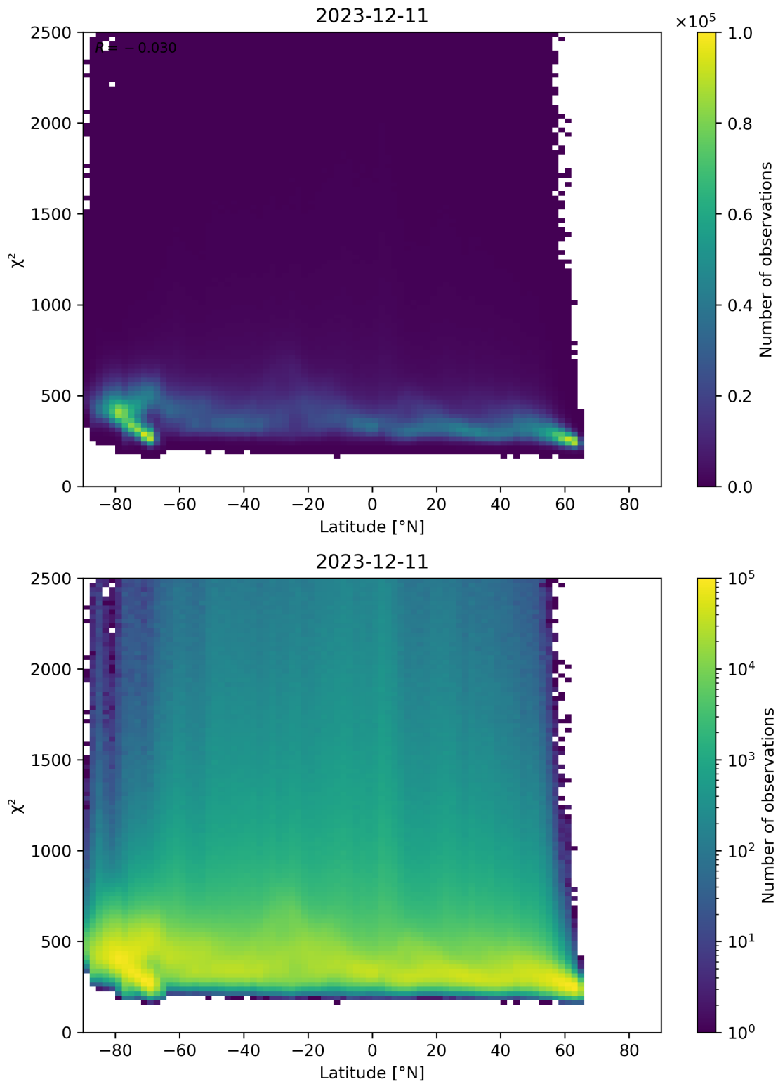
Figure 86: Scatter density plot of “Latitude” against “ \chi^2 ” for 2023-12-10 to 2023-12-12.
