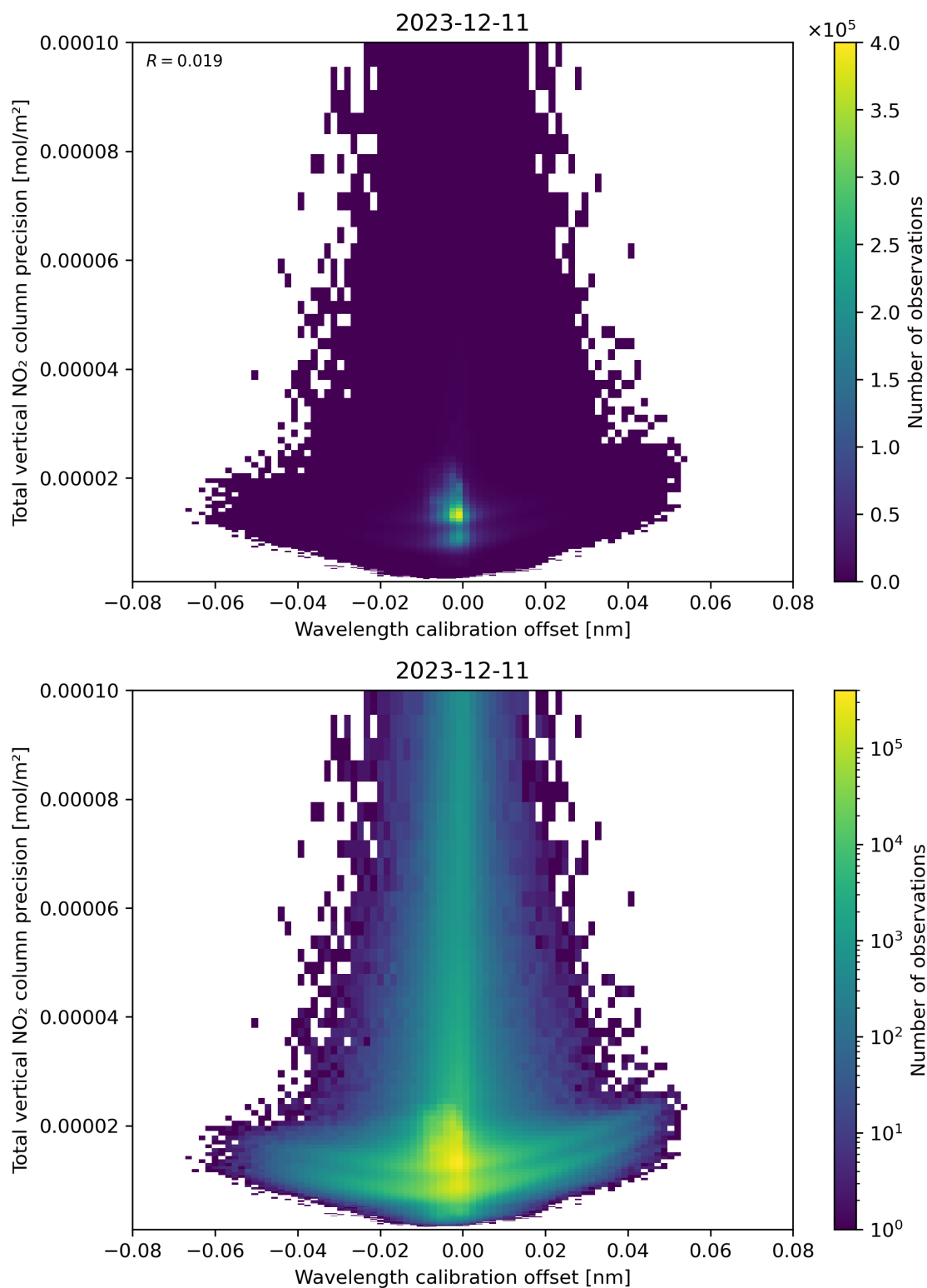
Figure 180: Scatter density plot of “Wavelength calibration offset” against “Total vertical NO 2 column precision” for 2023-12-10 to 2023-12-12.
