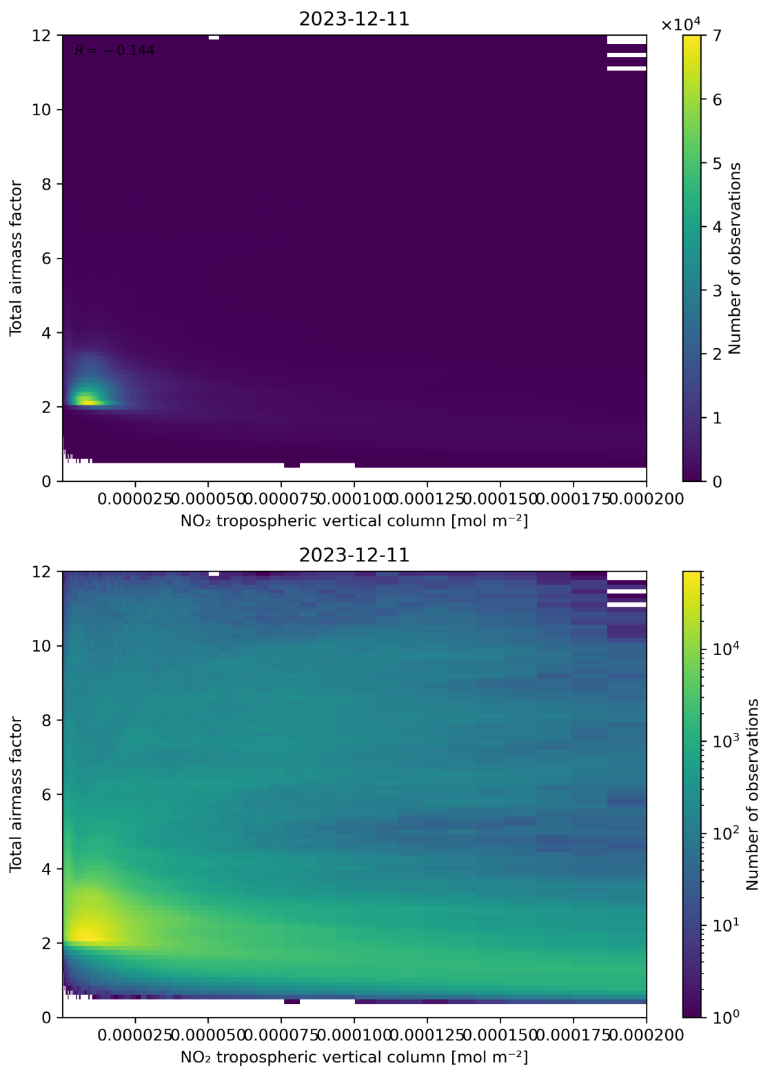
Figure 122: Scatter density plot of “NO 2 tropospheric vertical column” against “Total air mass factor” for 2023-12-10 to 2023-12-12.
