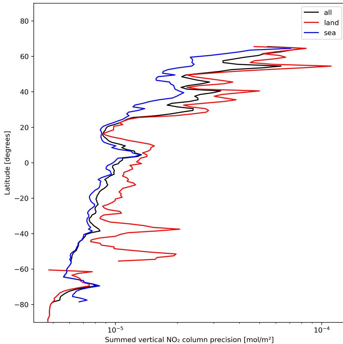
Figure 24: Zonal average of “Summed vertical NO 2 column precision” for 2023-12-10 to 2023-12-12.
