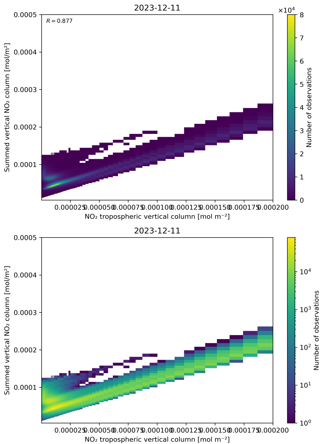
Figure 126: Scatter density plot of “NO 2 tropospheric vertical column” against “Summed vertical NO 2 column” for 2023-12-10 to 2023-12-12.
