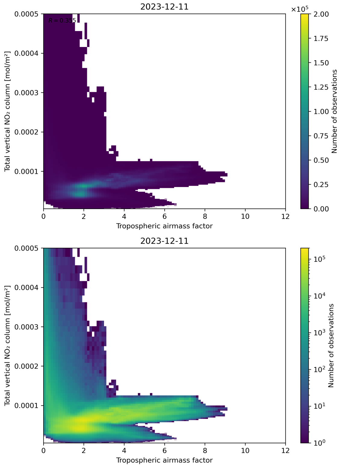
Figure 77: Scatter density plot of “Tropospheric airmass factor” against “Total vertical NO 2 column” for 2023-12-10 to 2023-12-12.
