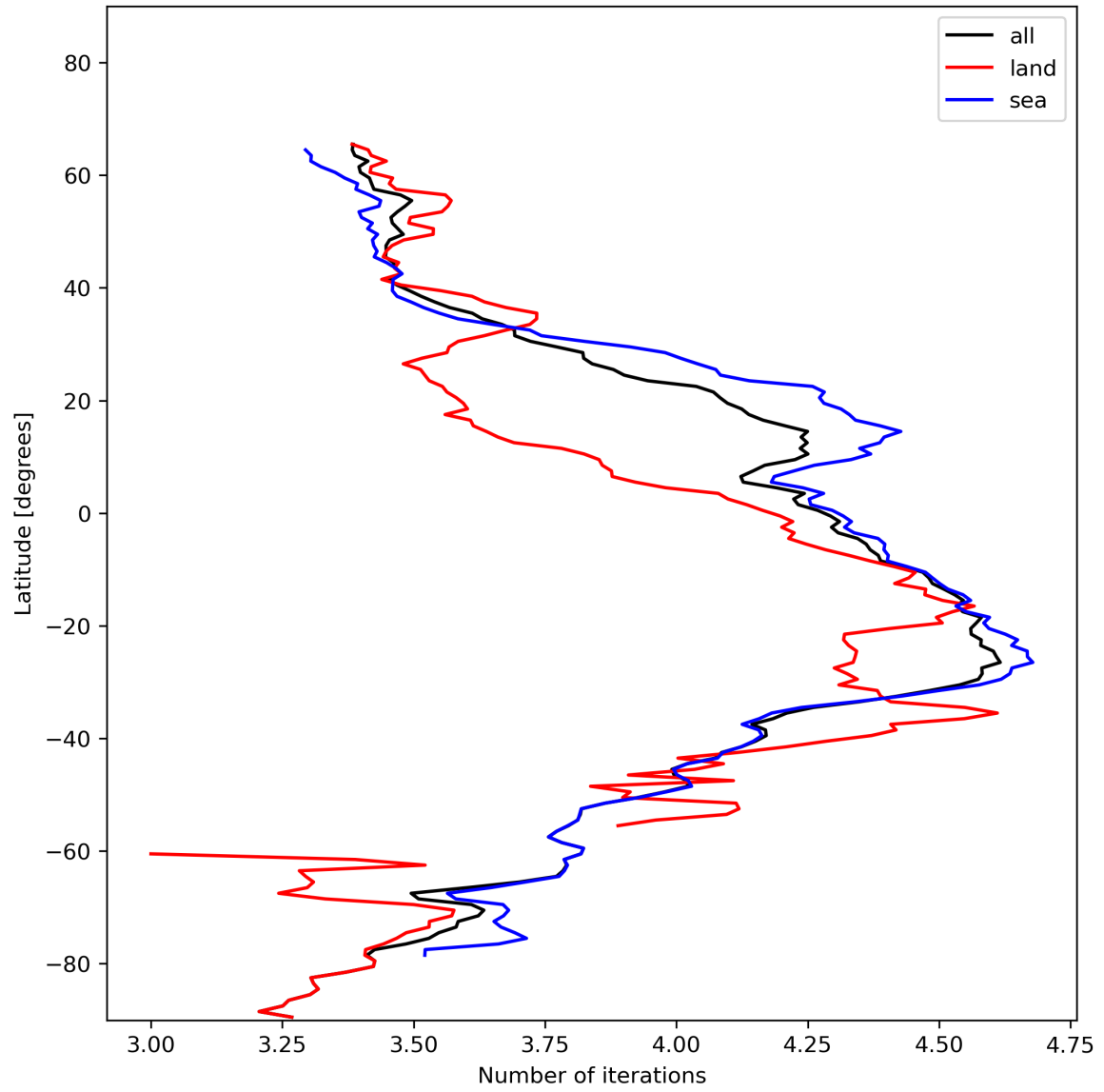
Figure 17: Zonal average of “Number of iterations” for 2023-12-10 to 2023-12-12.
