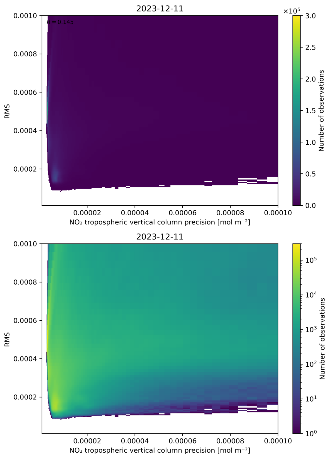
Figure 140: Scatter density plot of “NO 2 tropospheric vertical column precision” against “RMS” for 2023-12-10 to 2023-12-12.
