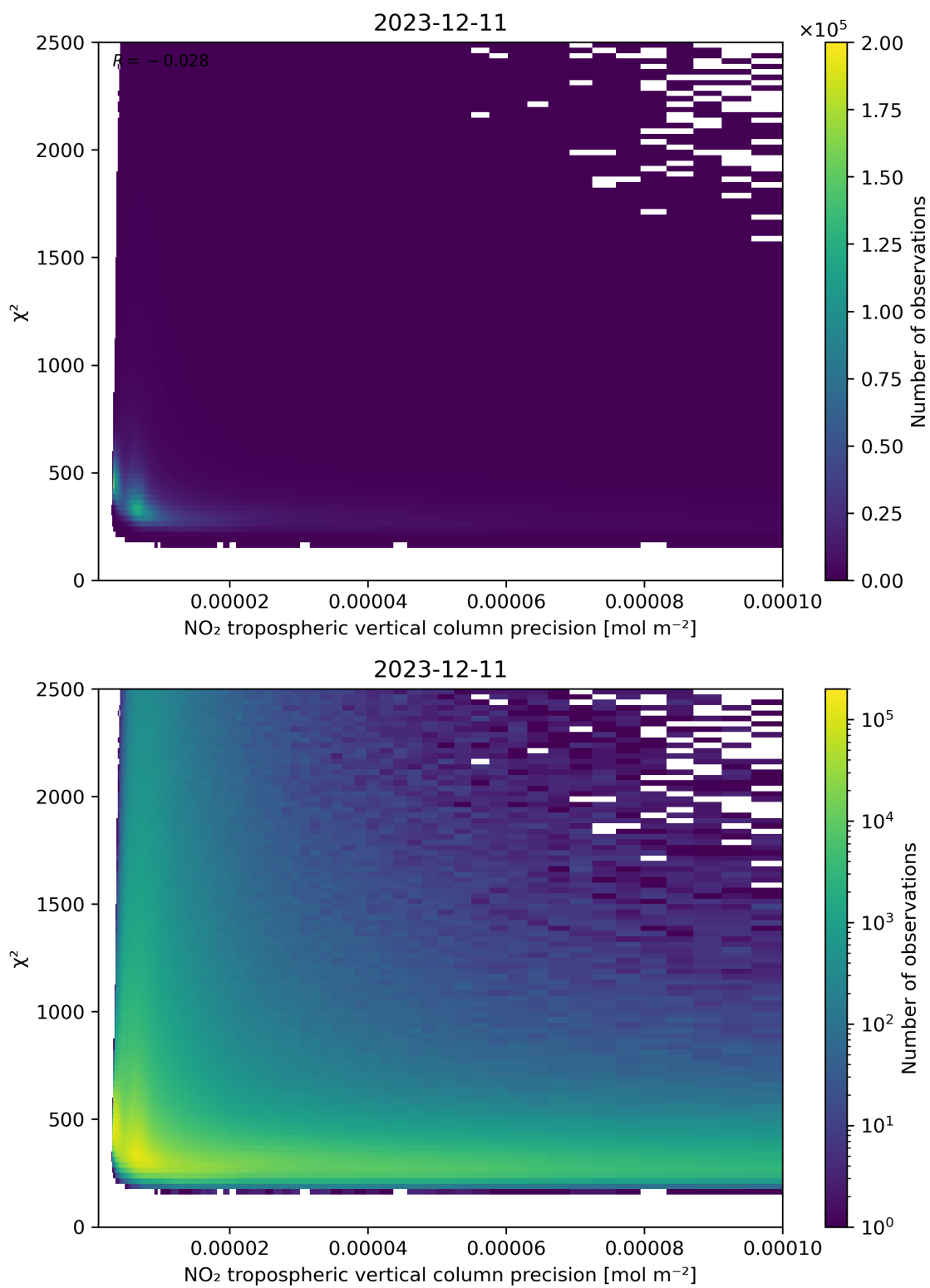
Figure 134: Scatter density plot of “NO 2 tropospheric vertical column precision” against “ \chi^2 ” for 2023-12-10 to 2023-12-12.
