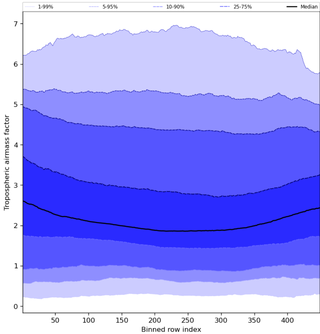
Figure 48: Along track statistics of “Tropospheric airmass factor” for 2023-12-10 to 2023-12-12
