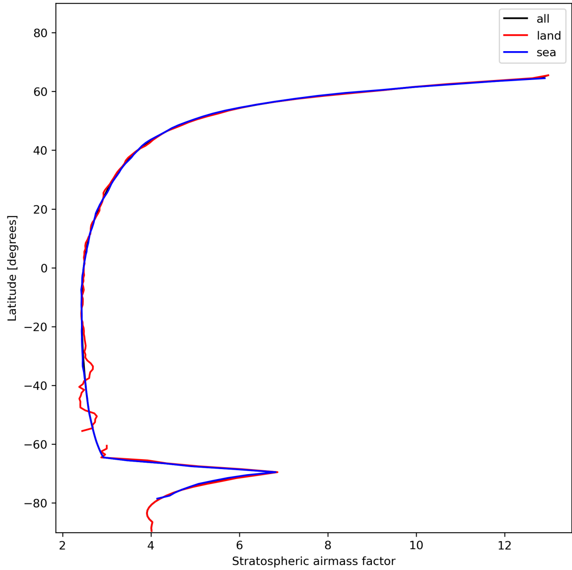
Figure 27: Zonal average of “Stratospheric air mass factor” for 2023-12-10 to 2023-12-12.
