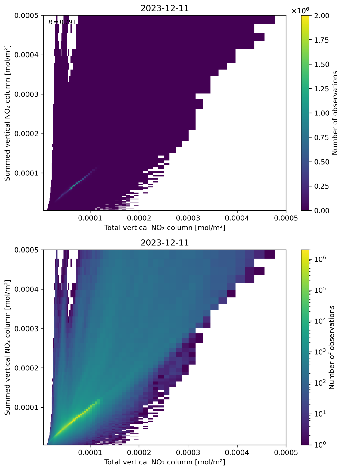
Figure 112: Scatter density plot of “Total vertical NO 2 column” against “Summed vertical NO 2 column” for 2023-12-10 to 2023-12-12.
