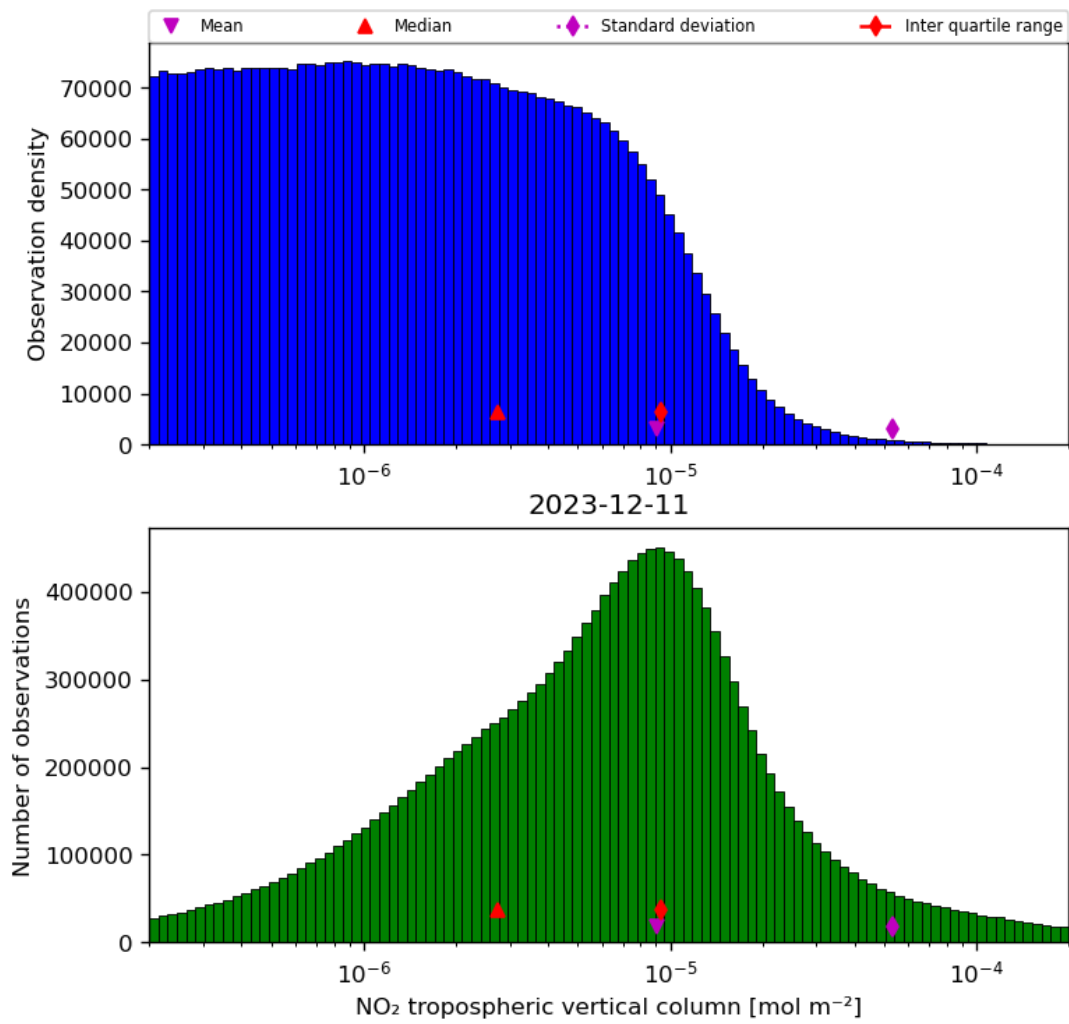
Figure 29: Histogram of “NO 2 tropospheric vertical column” for 2023-12-10 to 2023-12-12
