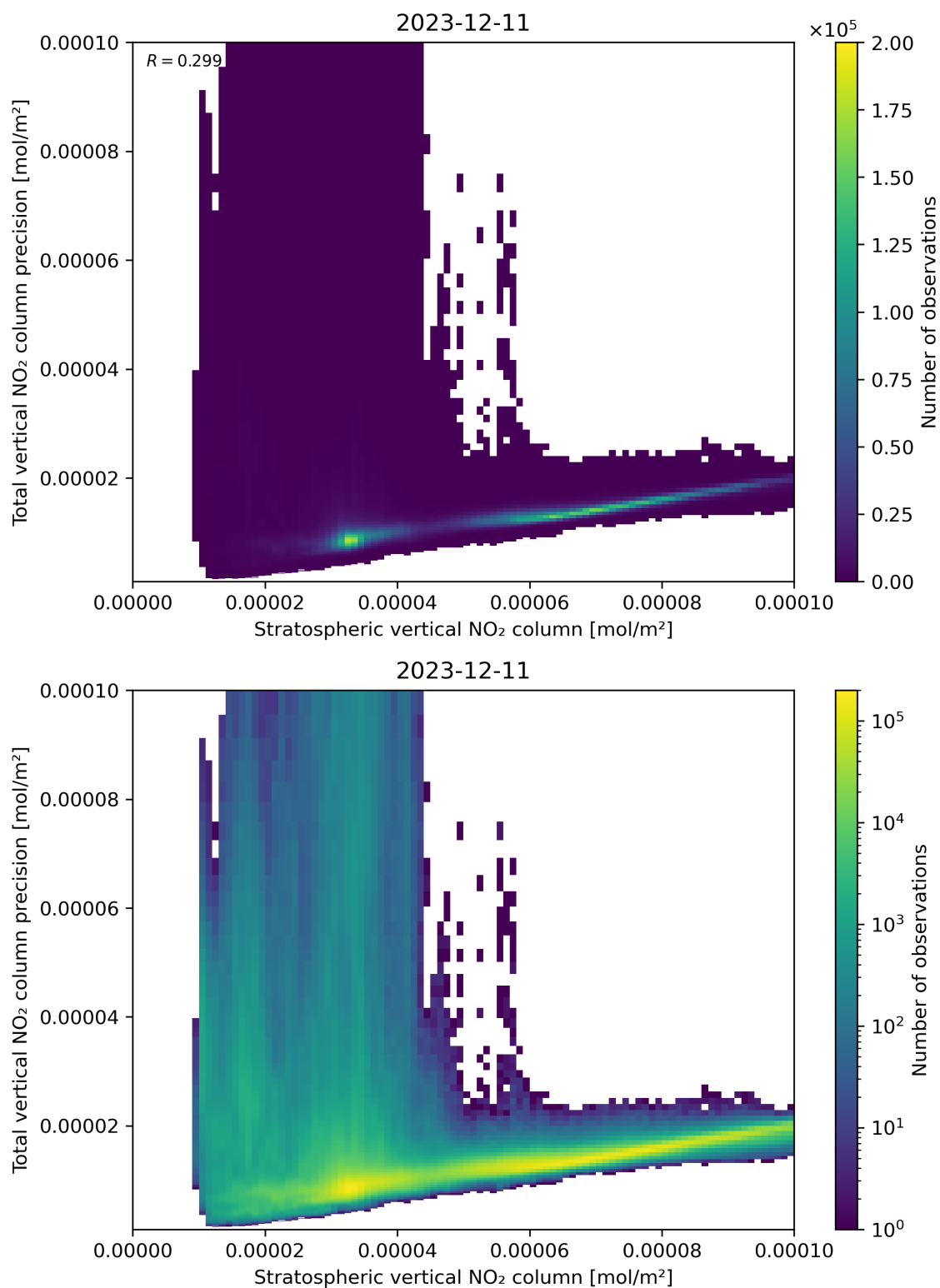
Figure 101: Scatter density plot of “Stratospheric vertical NO 2 column” against “Total vertical NO 2 column precision” for 2023-12-10 to 2023-12-12.
