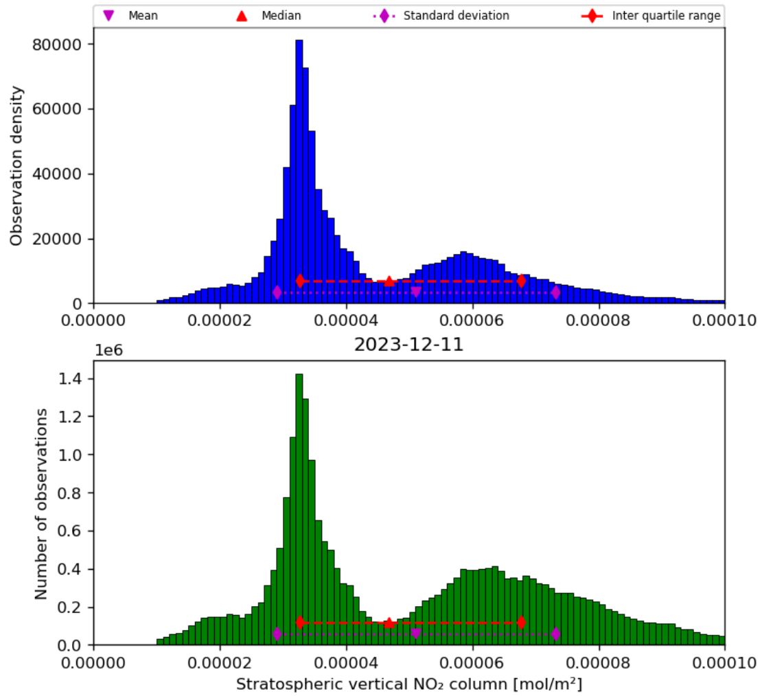
Figure 36: Histogram of “Stratospheric vertical NO 2 column” for 2023-12-10 to 2023-12-12
