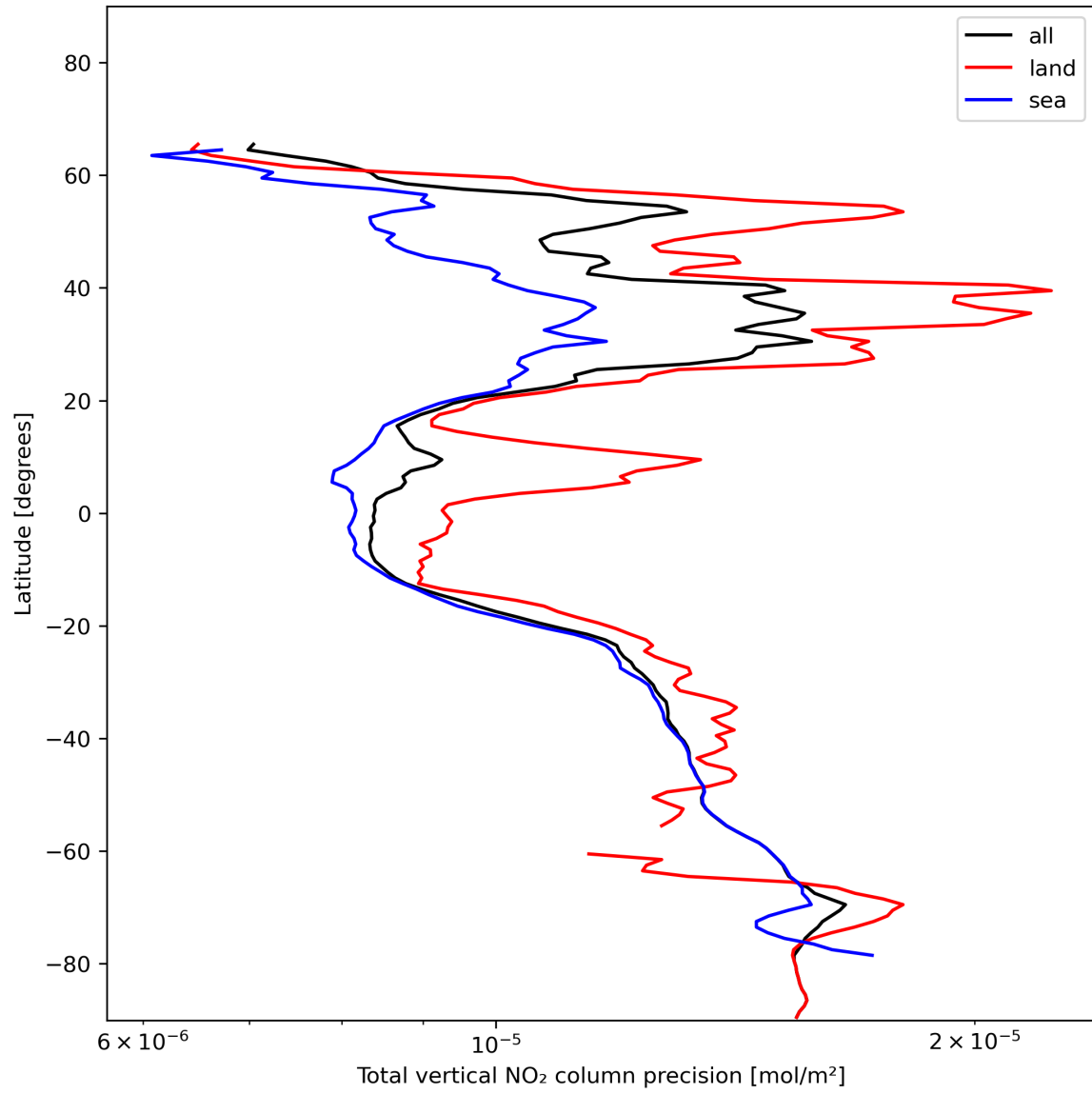
Figure 22: Zonal average of “Total vertical NO 2 column precision” for 2023-12-10 to 2023-12-12.
