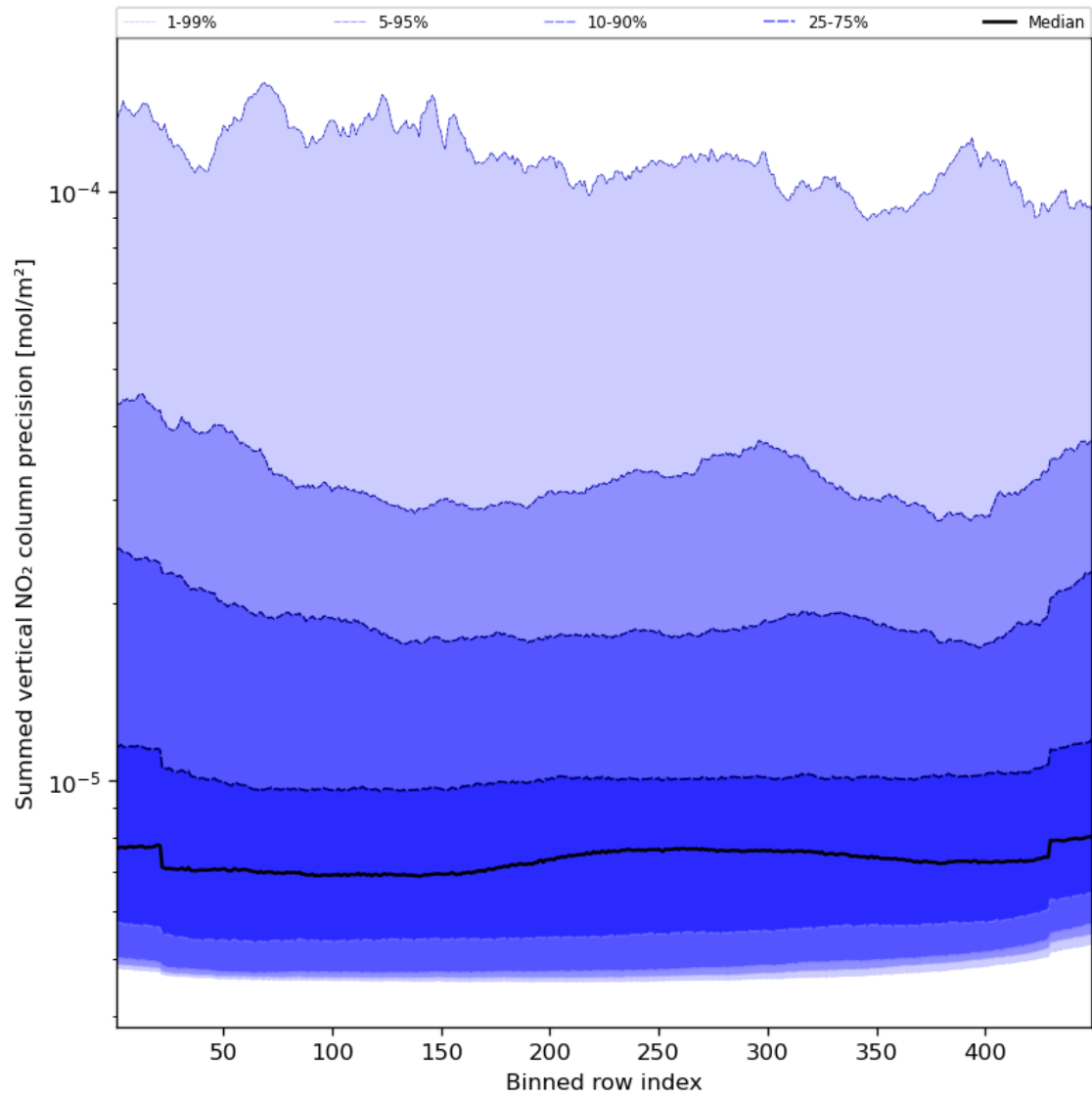
Figure 58: Along track statistics of “Summed vertical NO 2 column precision” for 2023-12-10 to 2023-12-12
