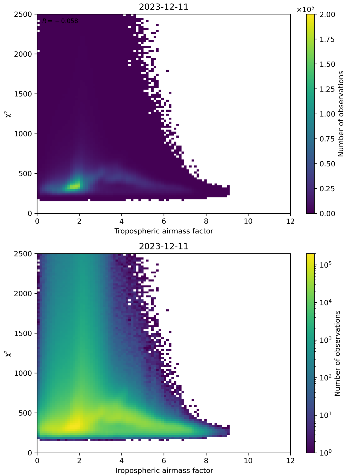
Figure 73: Scatter density plot of “Tropospheric airmass factor” against “ \chi^2 ” for 2023-12-10 to 2023-12-12.
