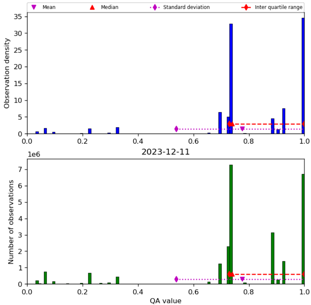
Figure 28: Histogram of “QA value” for 2023-12-10 to 2023-12-12
