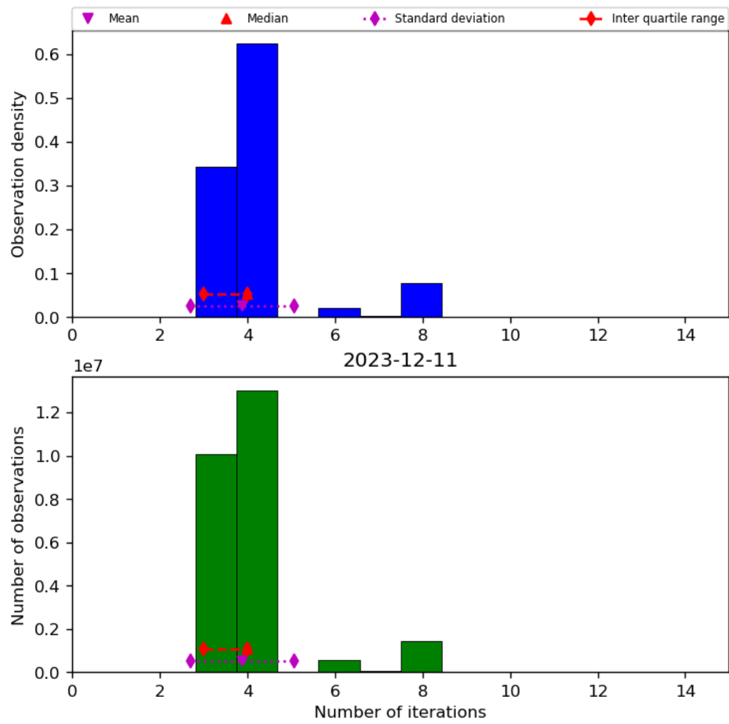
Figure 34: Histogram of “Number of iterations” for 2023-12-10 to 2023-12-12
