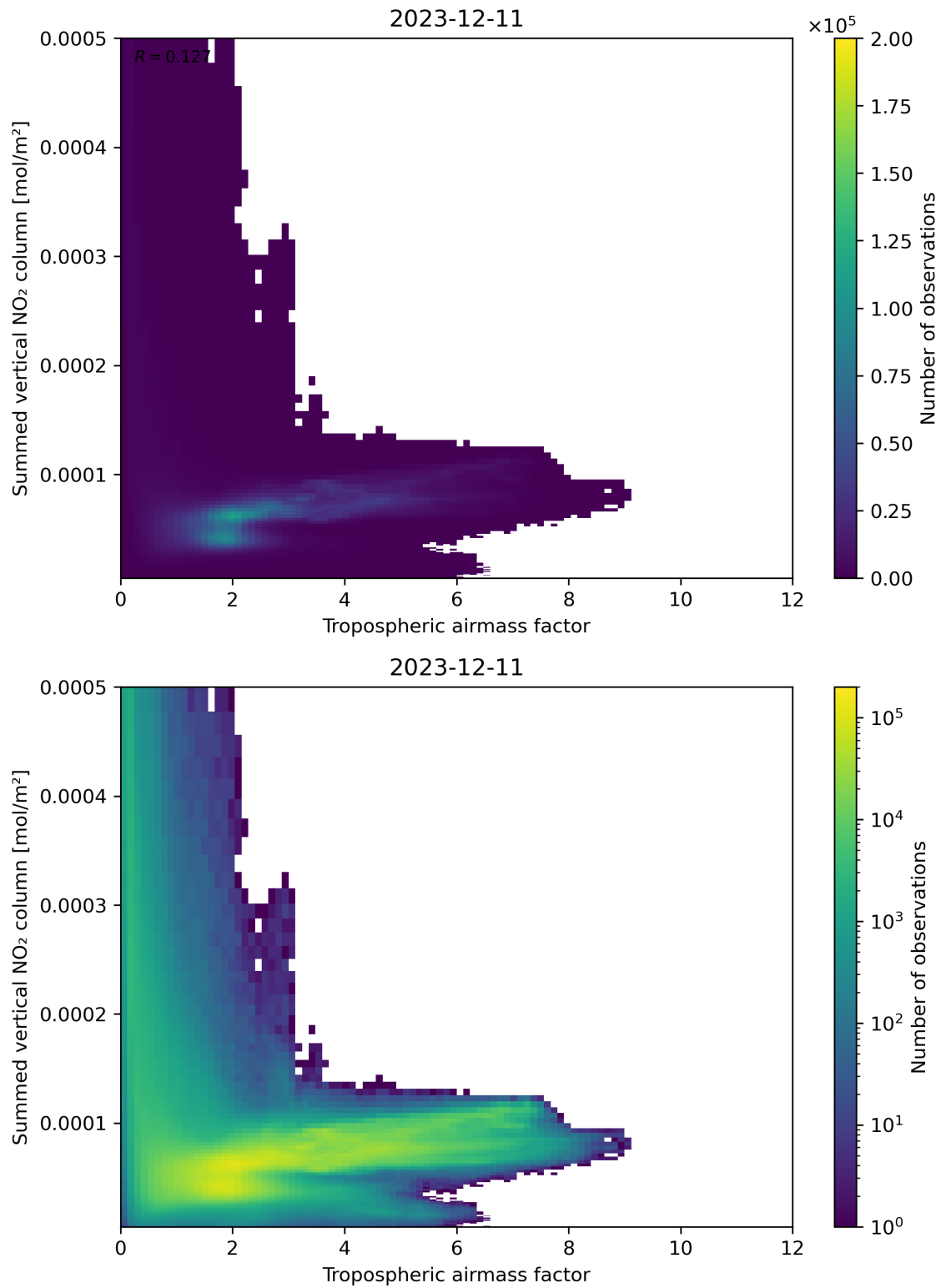
Figure 75: Scatter density plot of “Tropospheric air mass factor” against “Summed vertical NO 2 column” for 2023-12-10 to 2023-12-12.
