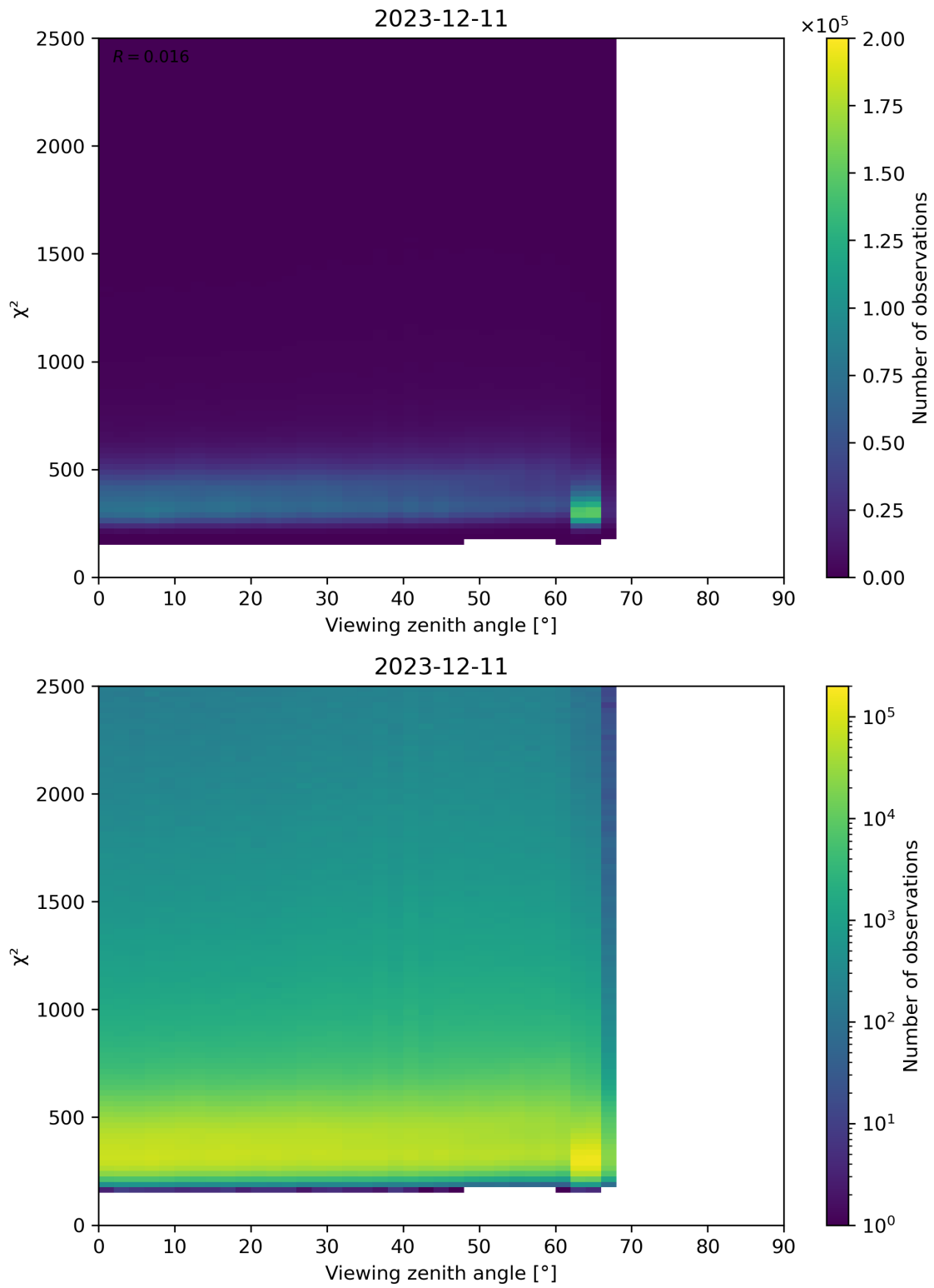
Figure 162: Scatter density plot of “Viewing zenith angle” against “ \chi^2 ” for 2023-12-10 to 2023-12-12.
