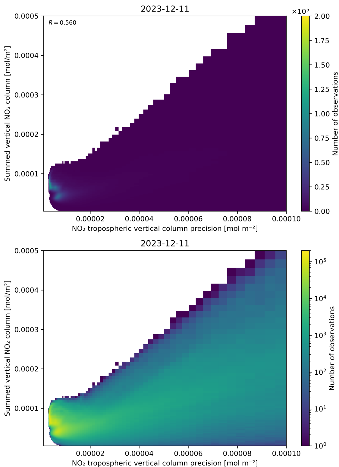
Figure 136: Scatter density plot of “NO 2 tropospheric vertical column precision” against “Summed vertical NO 2 column” for 2023-12-10 to 2023-12-12.
