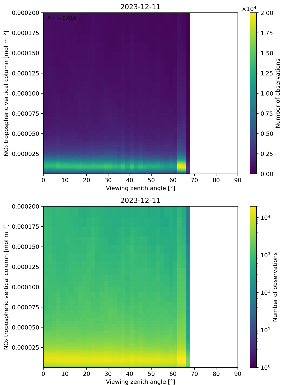
Figure 169: Scatter density plot of “Viewing zenith angle” against “NO 2 tropospheric vertical column” for 2023-12-10 to 2023-12-12.
