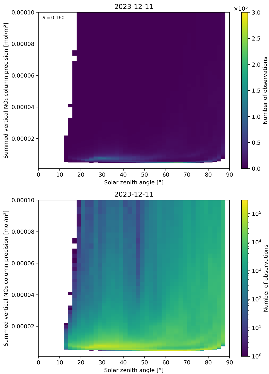
Figure 152: Scatter density plot of “Solar zenith angle” against “Summed vertical NO 2 column precision” for 2023-12-10 to 2023-12-12.
