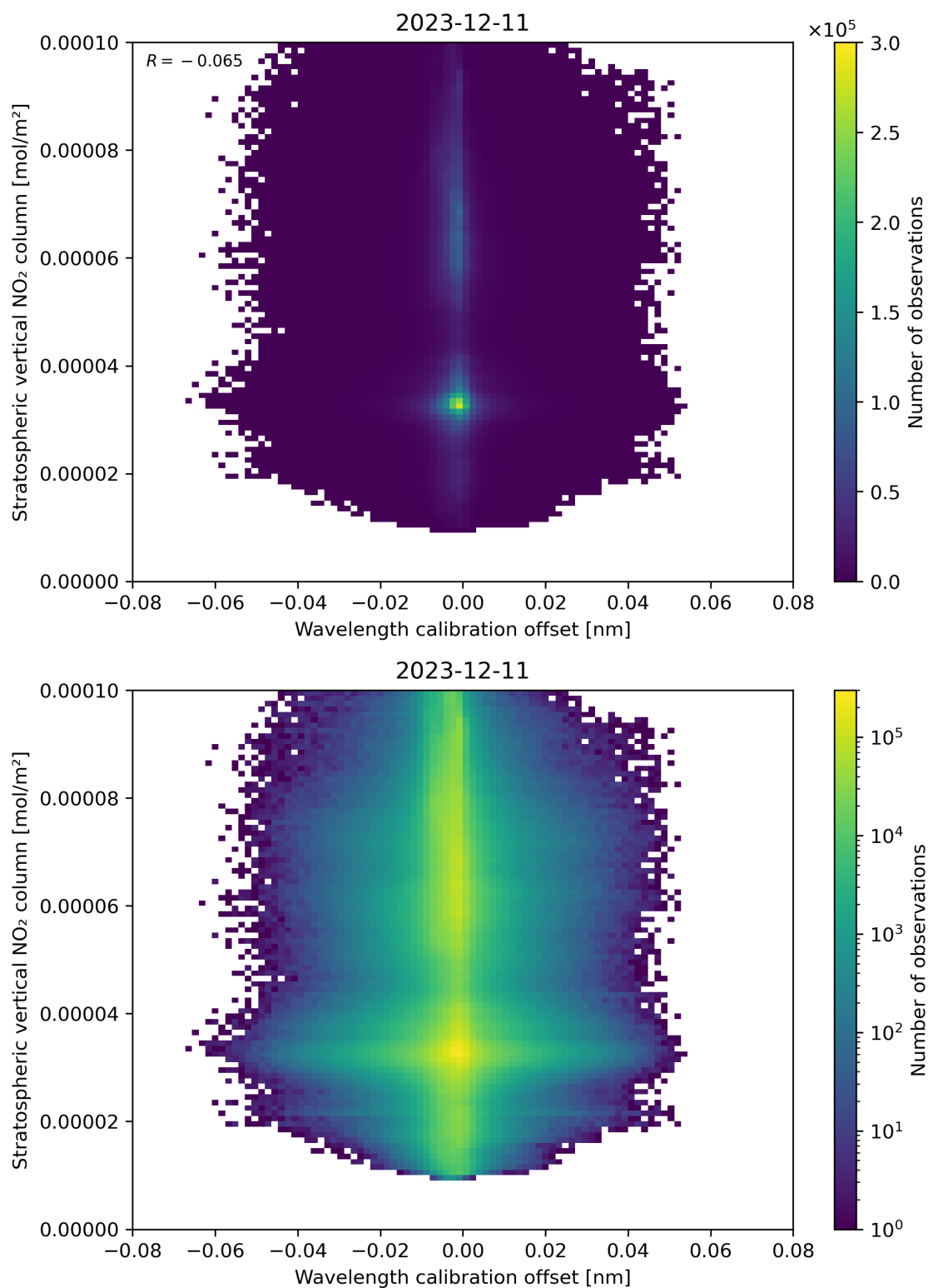
Figure 176: Scatter density plot of “Wavelength calibration offset” against “Stratospheric vertical NO 2 column” for 2023-12-10 to 2023-12-12.
