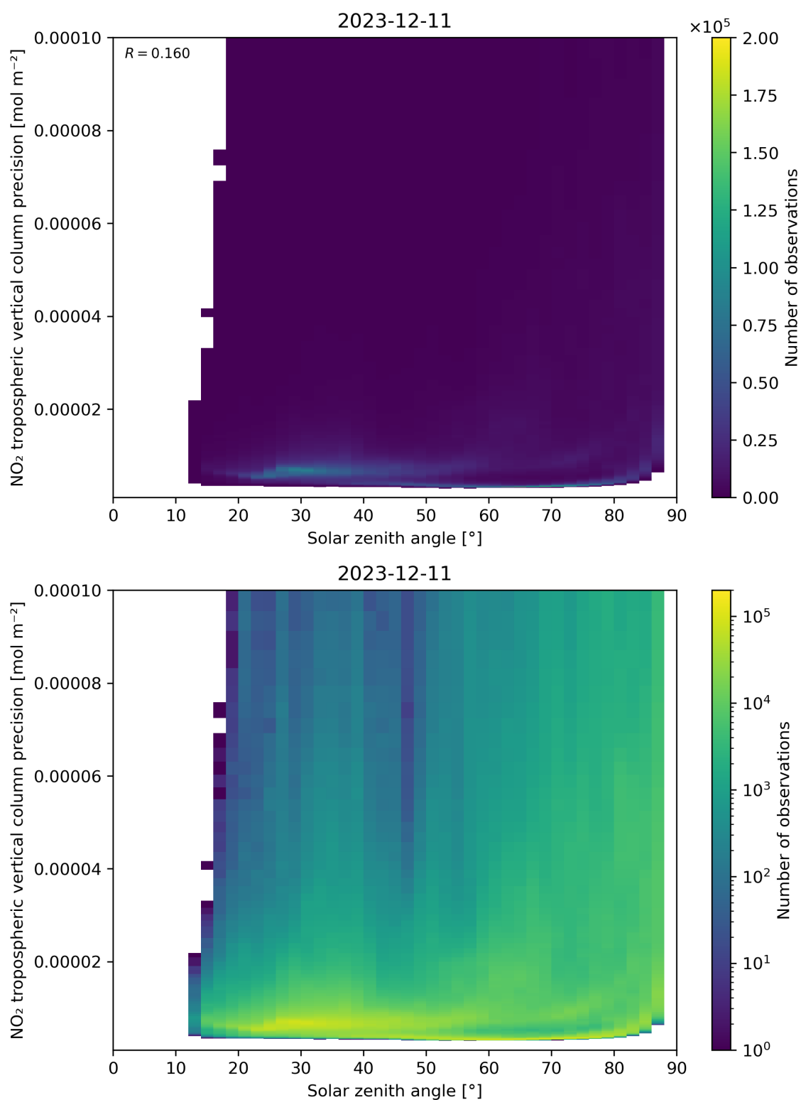
Figure 156: Scatter density plot of “Solar zenith angle” against “NO 2 tropospheric vertical column precision” for 2023-12-10 to 2023-12-12.
