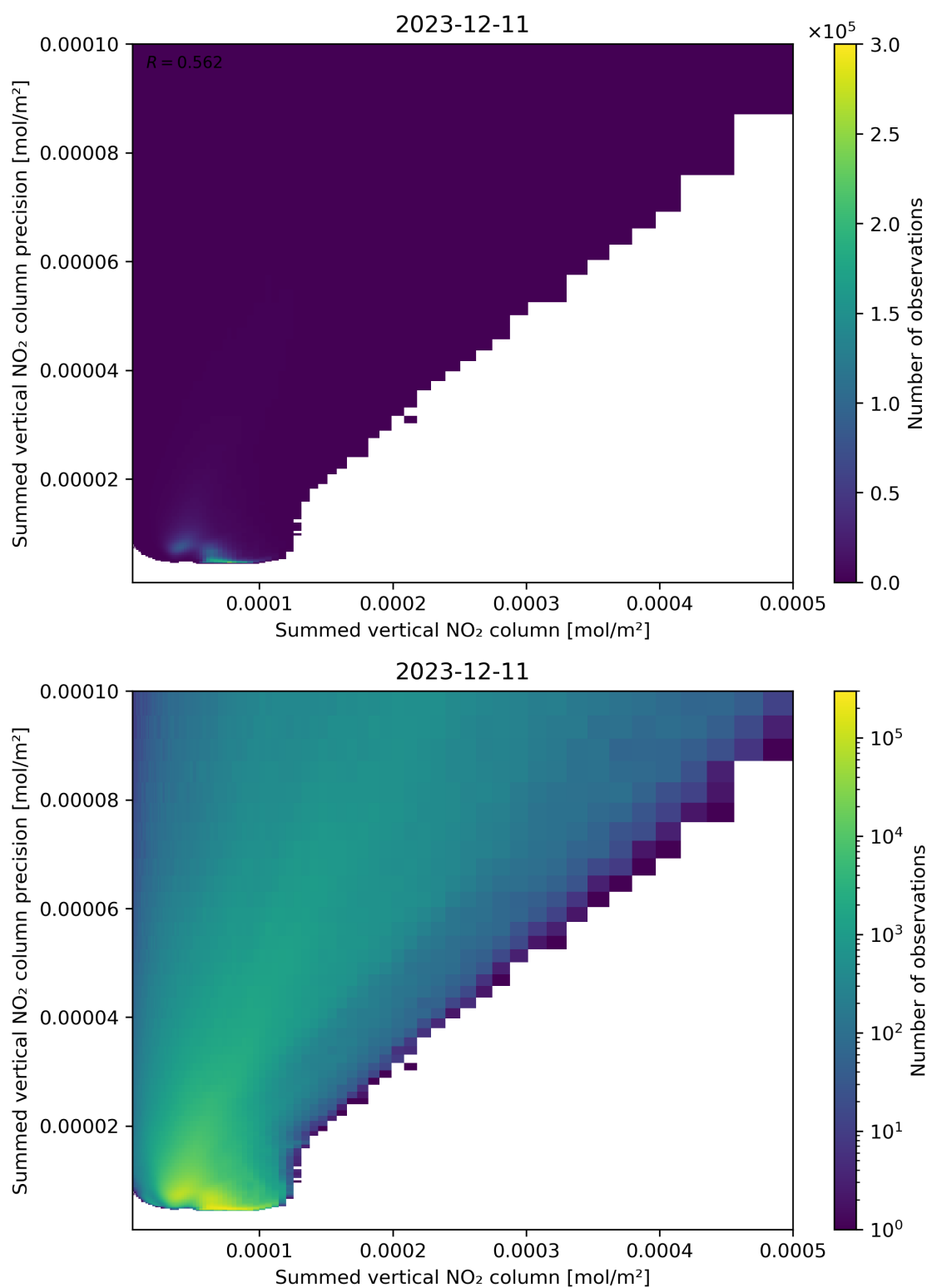
Figure 105: Scatter density plot of “Summed vertical NO 2 column” against “Summed vertical NO 2 column precision” for 2023-12-10 to 2023-12-12.
