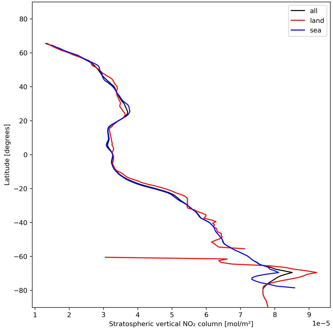
Figure 19: Zonal average of “Stratospheric vertical NO 2 column” for 2023-12-10 to 2023-12-12.
