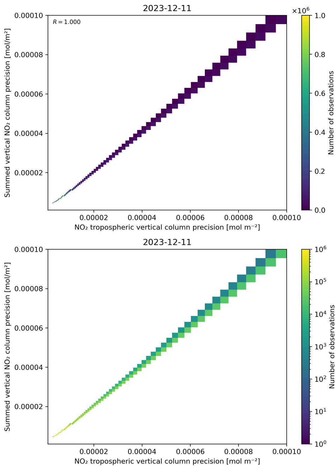
Figure 137: Scatter density plot of “NO 2 tropospheric vertical column precision” against “Summed vertical NO 2 column precision” for 2023-12-10 to 2023-12-12.
