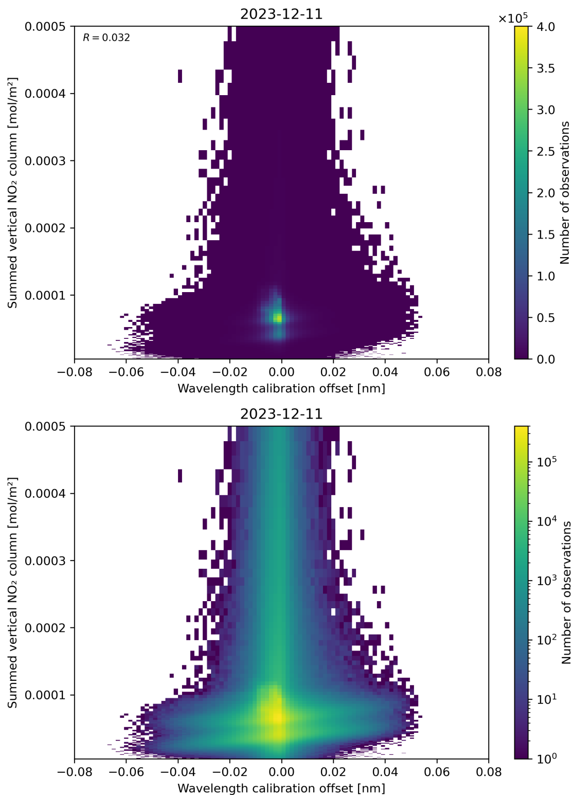
Figure 177: Scatter density plot of “Wavelength calibration offset” against “Summed vertical NO 2 column” for 2023-12-10 to 2023-12-12.
