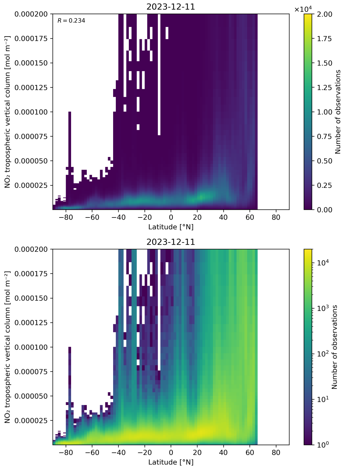
Figure 92: Scatter density plot of “Latitude” against “NO 2 tropospheric vertical column” for 2023-12-10 to 2023-12-12.
