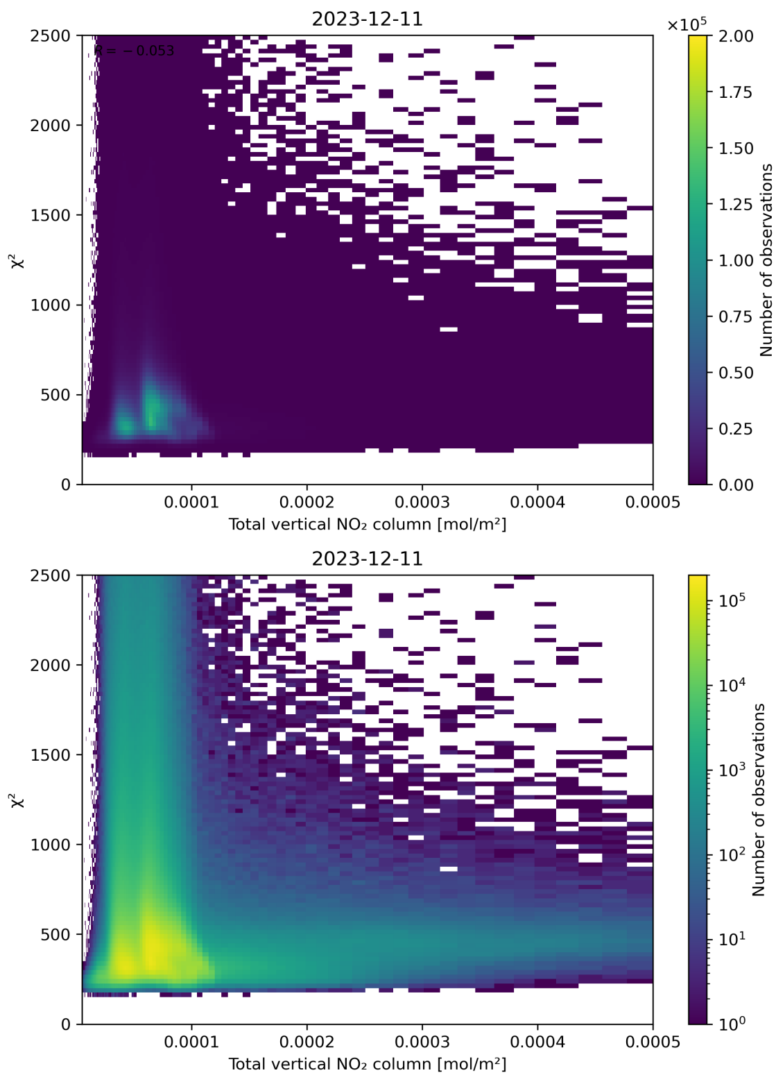
Figure 111: Scatter density plot of “Total vertical NO 2 column” against “ \chi^2 ” for 2023-12-10 to 2023-12-12.
