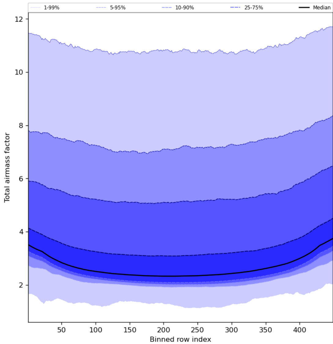
Figure 49: Along track statistics of “Total airmass factor” for 2023-12-10 to 2023-12-12
