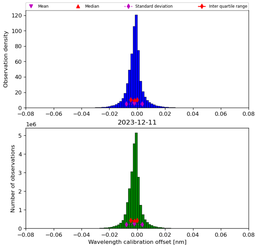
Figure 35: Histogram of “Wavelength calibration offset” for 2023-12-10 to 2023-12-12
