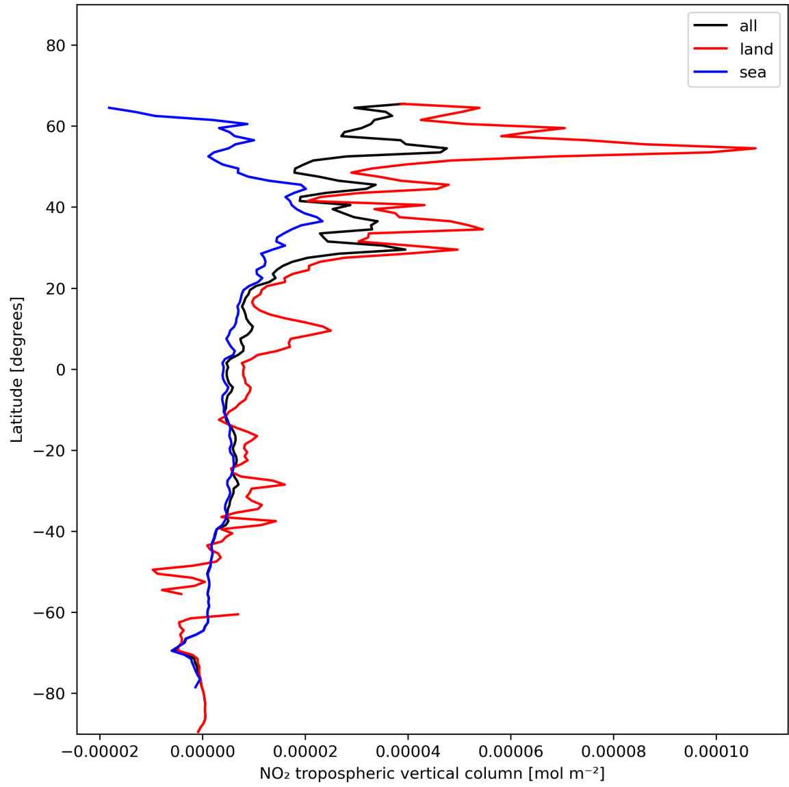
Figure 12: Zonal average of “NO 2 tropospheric vertical column” for 2023-12-10 to 2023-12-12.
