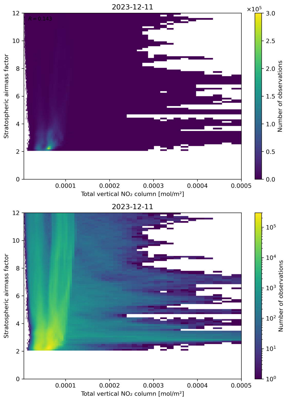
Figure 110: Scatter density plot of “Total vertical NO 2 column” against “Stratospheric airmass factor” for 2023-12-10 to 2023-12-12.
