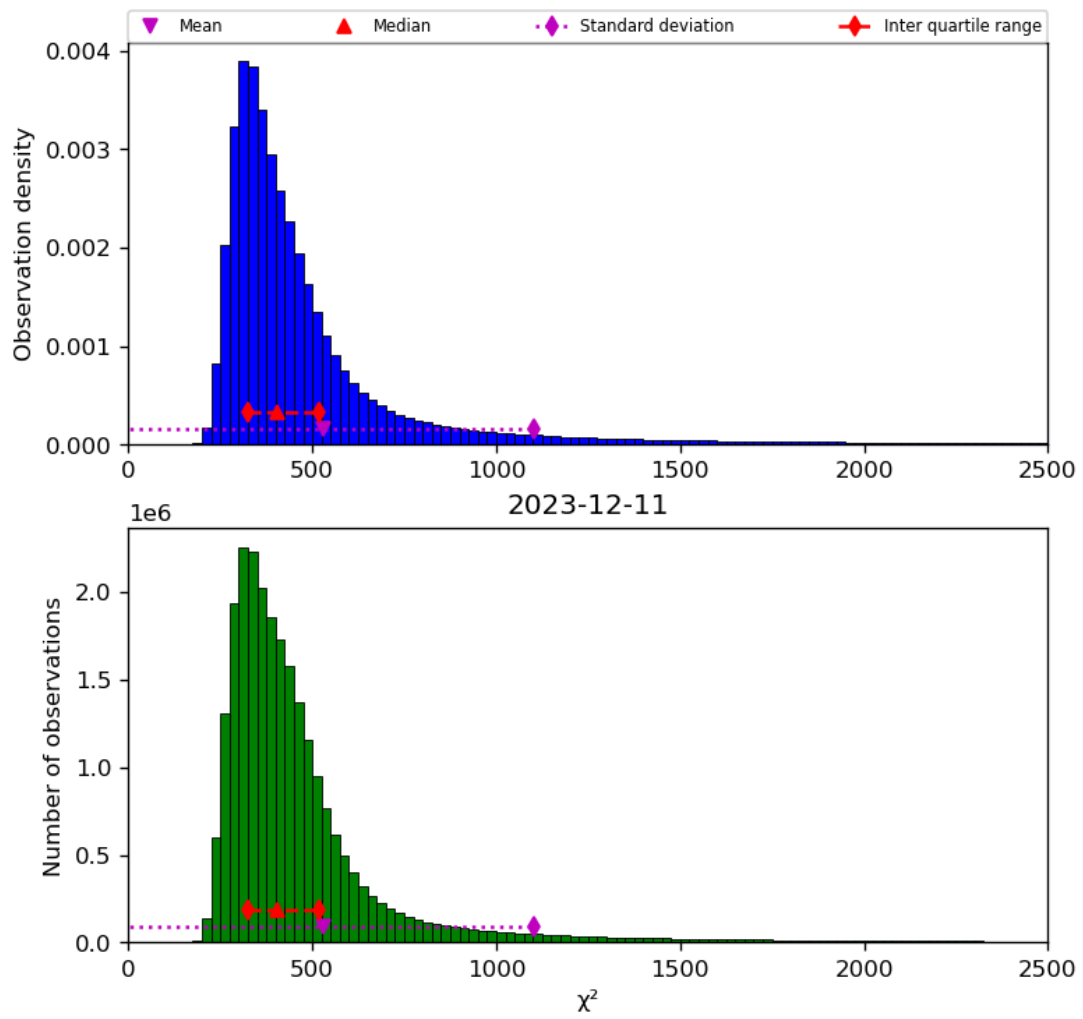
Figure 42: Histogram of “ \chi^2 ” for 2023-12-10 to 2023-12-12
