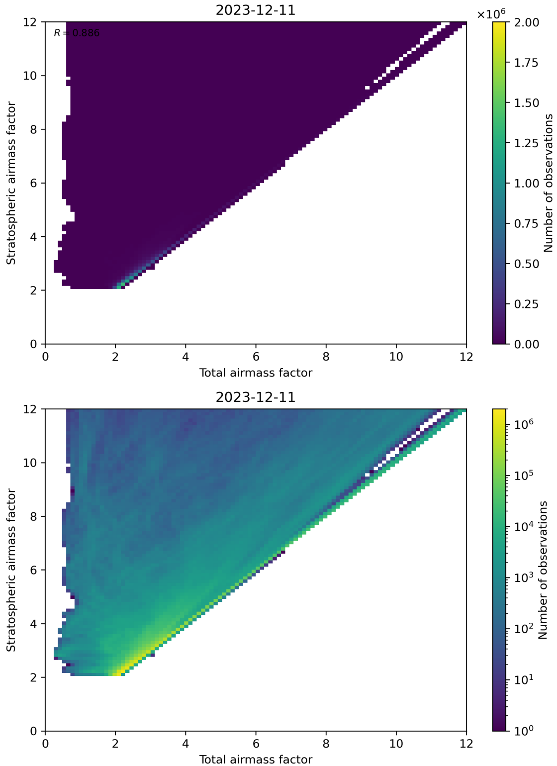
Figure 62: Scatter density plot of “Total airmass factor” against “Stratospheric airmass factor” for 2023-12-10 to 2023-12-12.
