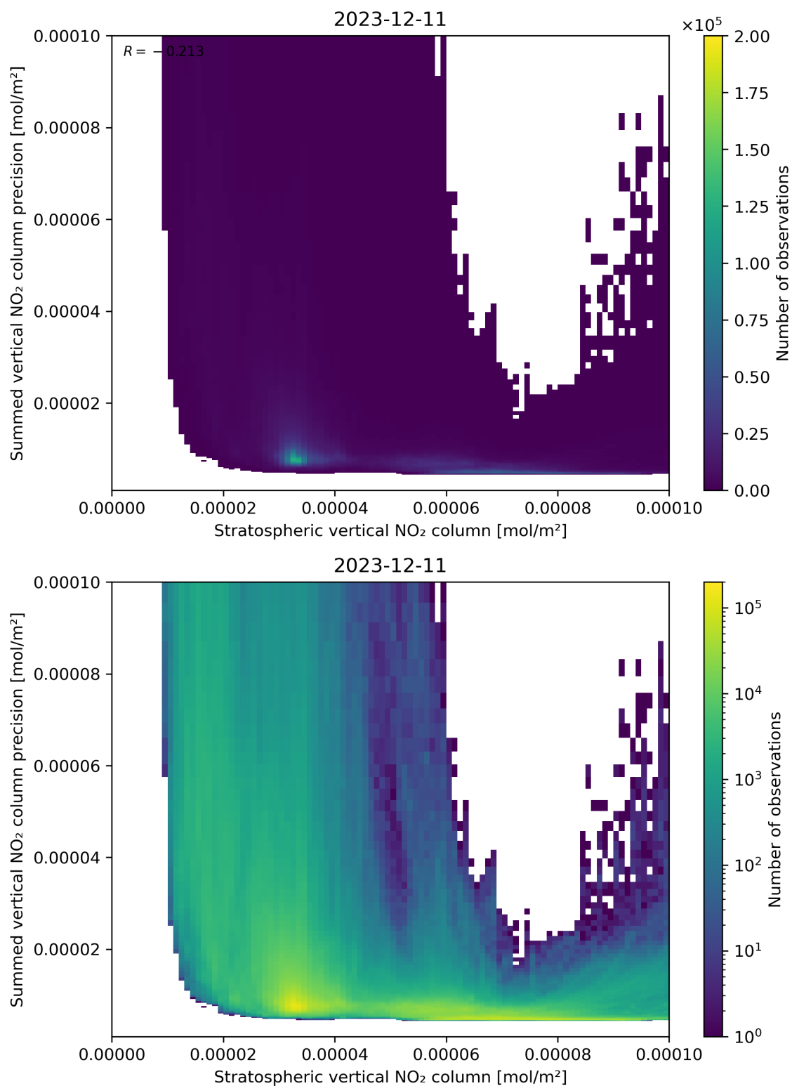
Figure 99: Scatter density plot of “Stratospheric vertical NO 2 column” against “Summed vertical NO 2 column precision” for 2023-12-10 to 2023-12-12.
