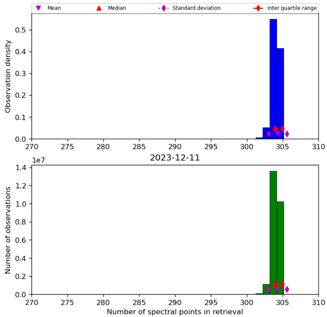
Figure 33: Histogram of “Number of spectral points in retrieval” for 2023-12-10 to 2023-12-12
