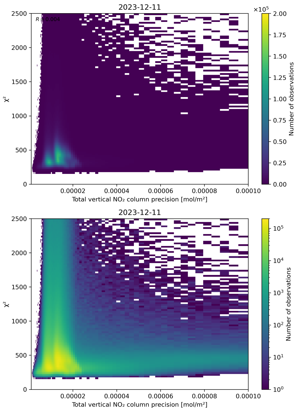
Figure 116: Scatter density plot of “Total vertical NO 2 column precision” against “ \chi^2 ” for 2023-12-10 to 2023-12-12.
