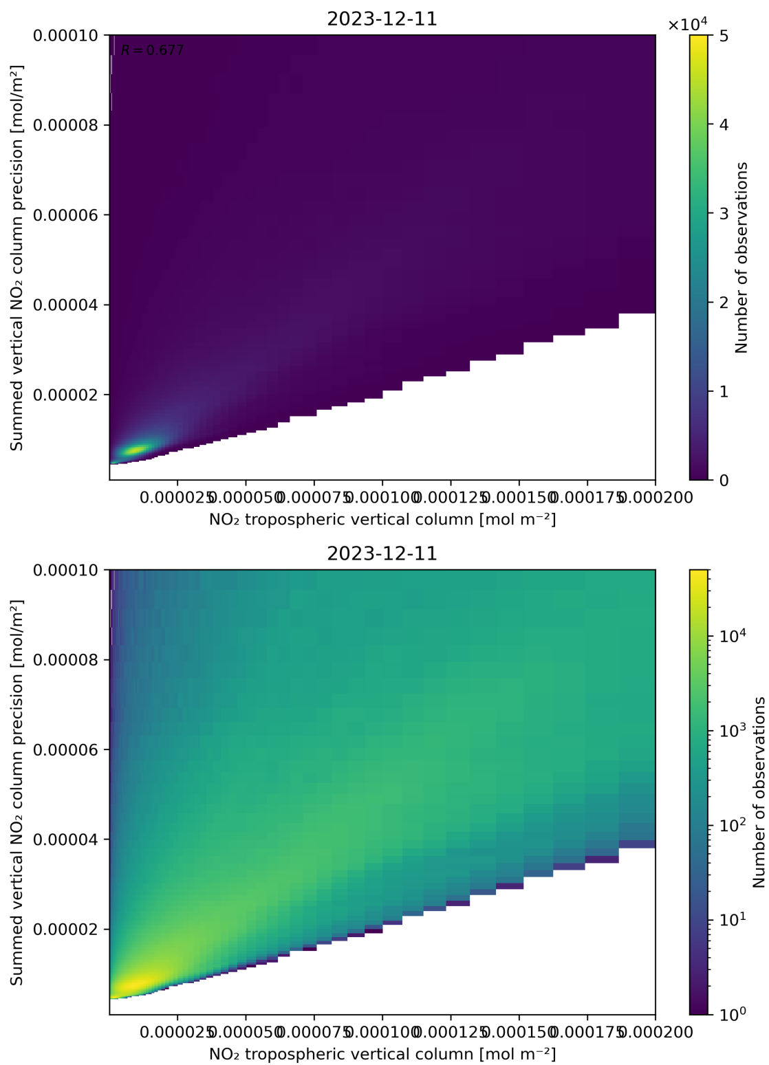
Figure 127: Scatter density plot of “NO 2 tropospheric vertical column” against “Summed vertical NO 2 column precision” for 2023-12-10 to 2023-12-12.
