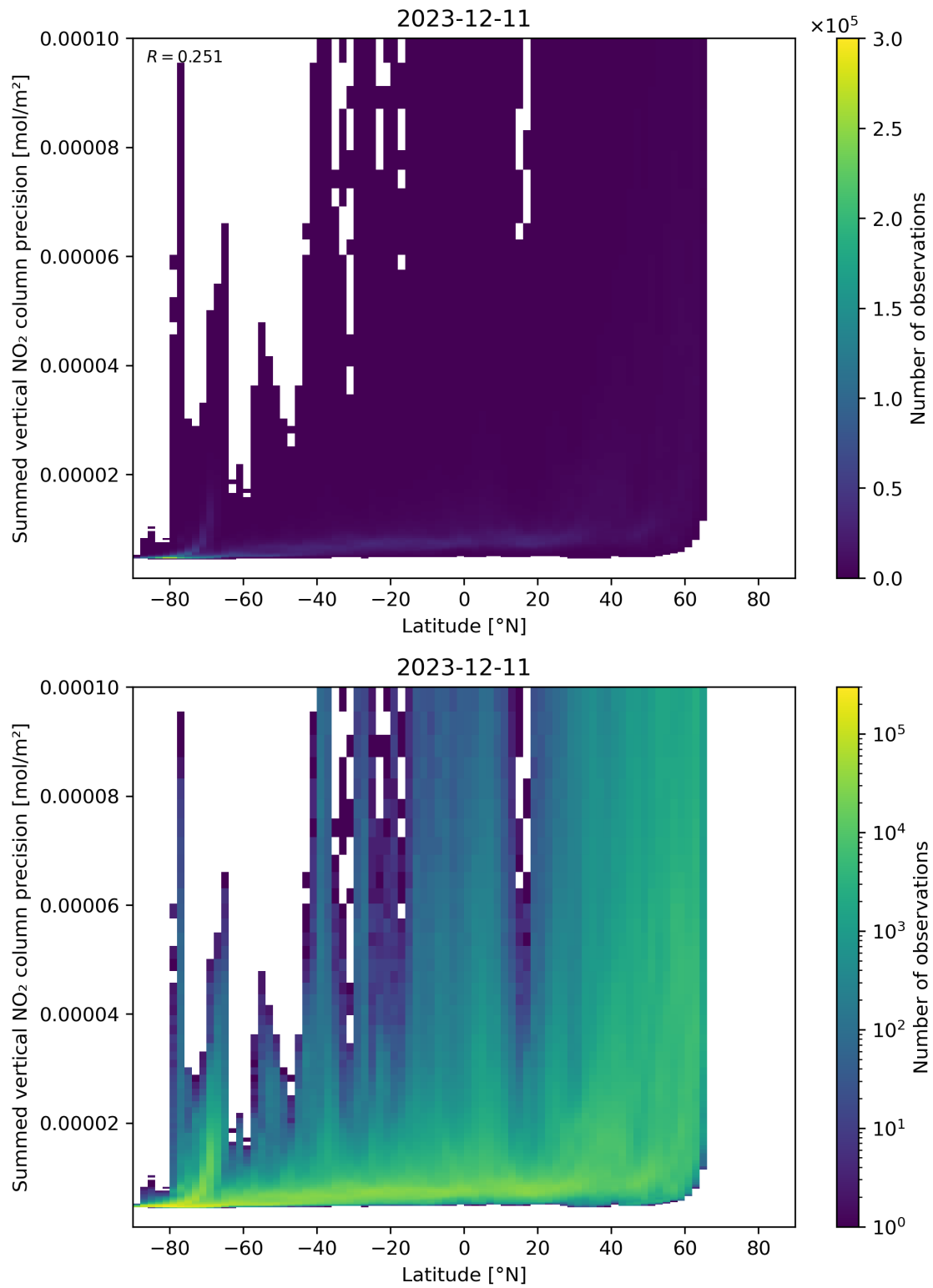
Figure 89: Scatter density plot of “Latitude” against “Summed vertical NO 2 column precision” for 2023-12-10 to 2023-12-12.
