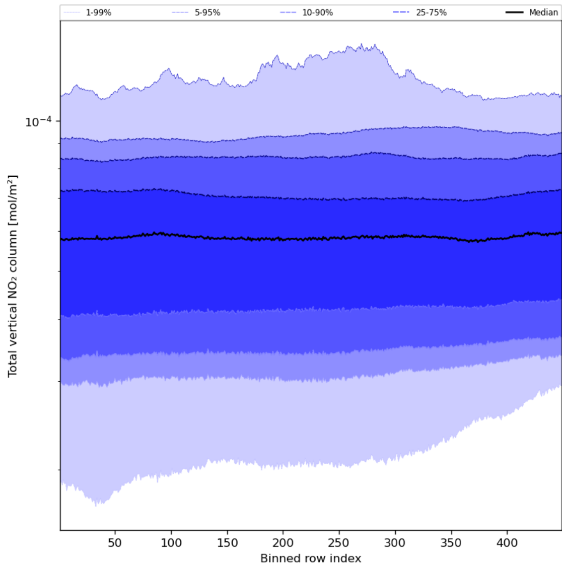
Figure 55: Along track statistics of “Total vertical NO 2 column” for 2023-12-10 to 2023-12-12
