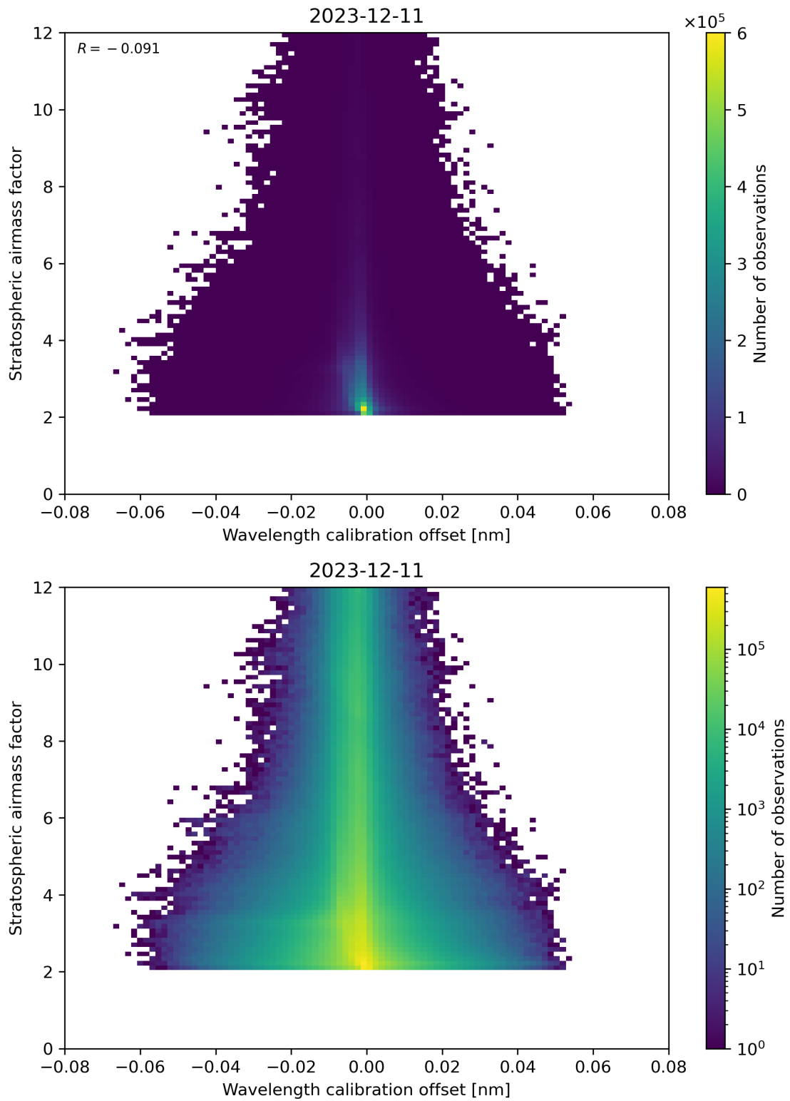
Figure 174: Scatter density plot of “Wavelength calibration offset” against “Stratospheric airmass factor” for 2023-12-10 to 2023-12-12.
