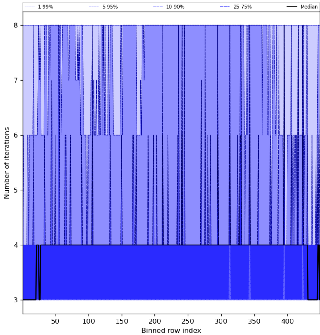
Figure 51: Along track statistics of “Number of iterations” for 2023-12-10 to 2023-12-12
