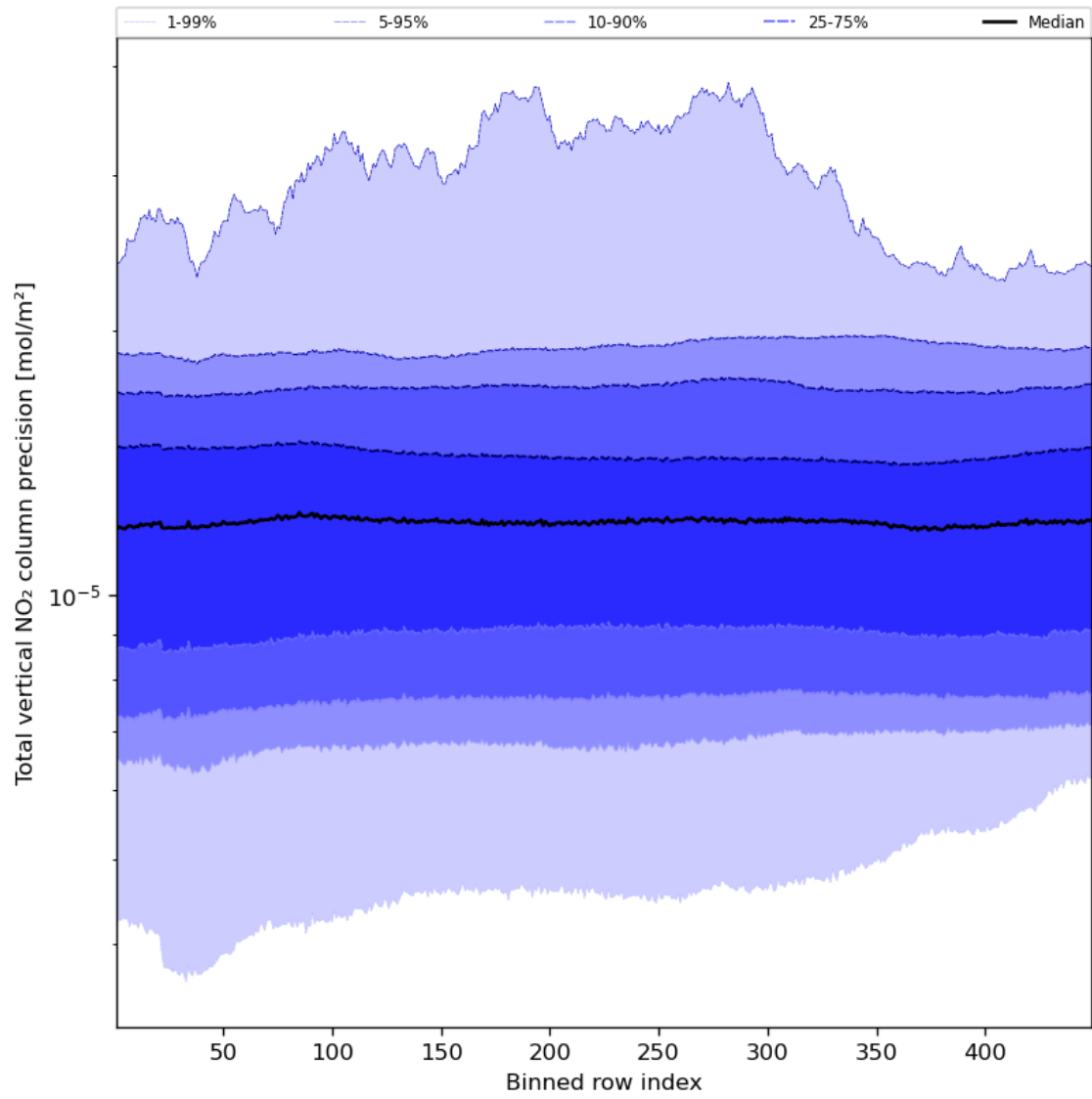
Figure 56: Along track statistics of “Total vertical NO 2 column precision” for 2023-12-10 to 2023-12-12
