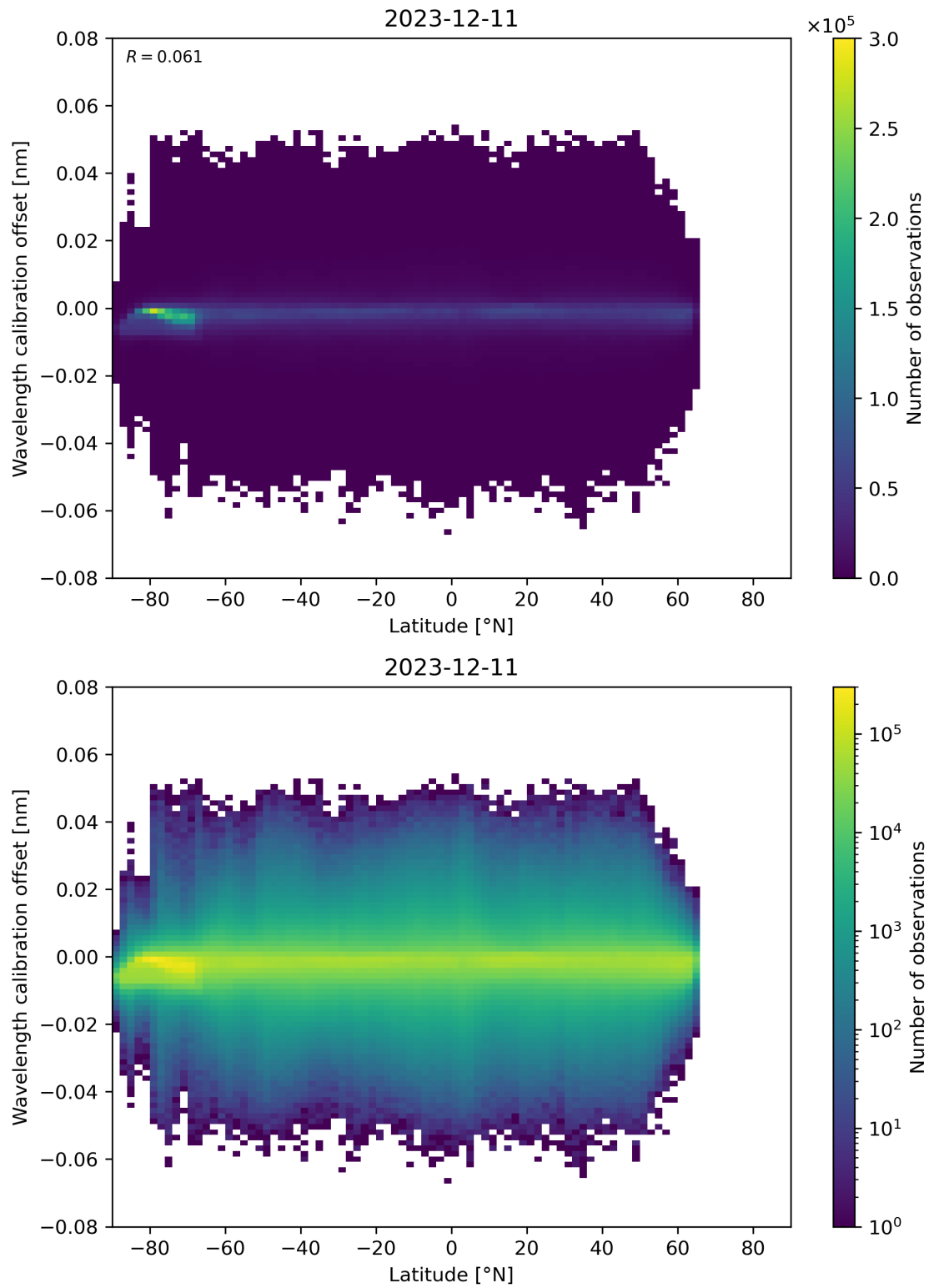
Figure 95: Scatter density plot of “Latitude” against “Wavelength calibration offset” for 2023-12-10 to 2023-12-12.
