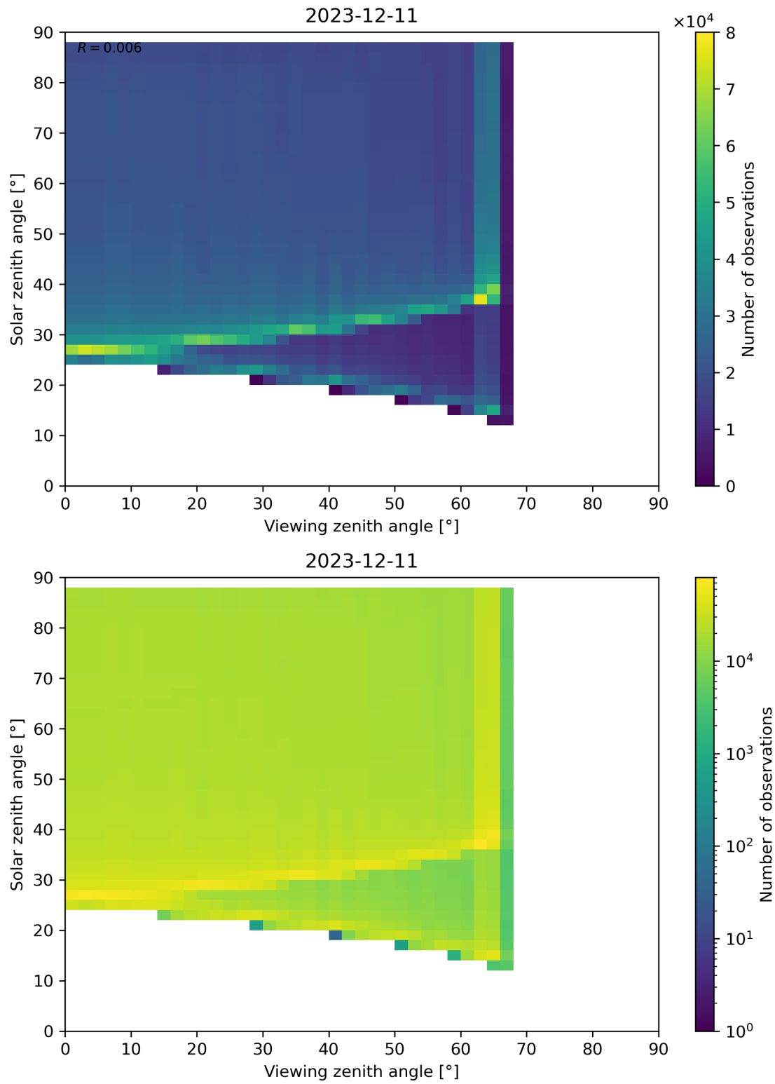
Figure 172: Scatter density plot of “Viewing zenith angle” against “Solar zenith angle” for 2023-12-10 to 2023-12-12.
