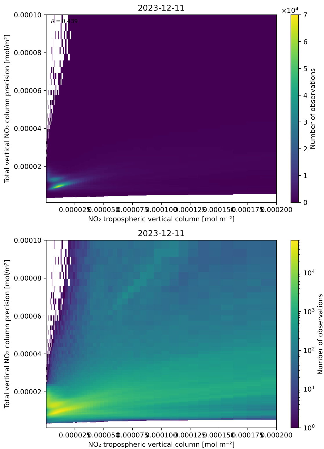
Figure 129: Scatter density plot of “NO 2 tropospheric vertical column” against “Total vertical NO 2 column precision” for 2023-12-10 to 2023-12-12.
