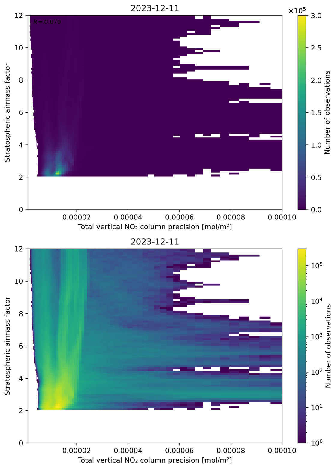
Figure 115: Scatter density plot of “Total vertical NO 2 column precision” against “Stratospheric airmass factor” for 2023-12-10 to 2023-12-12.
