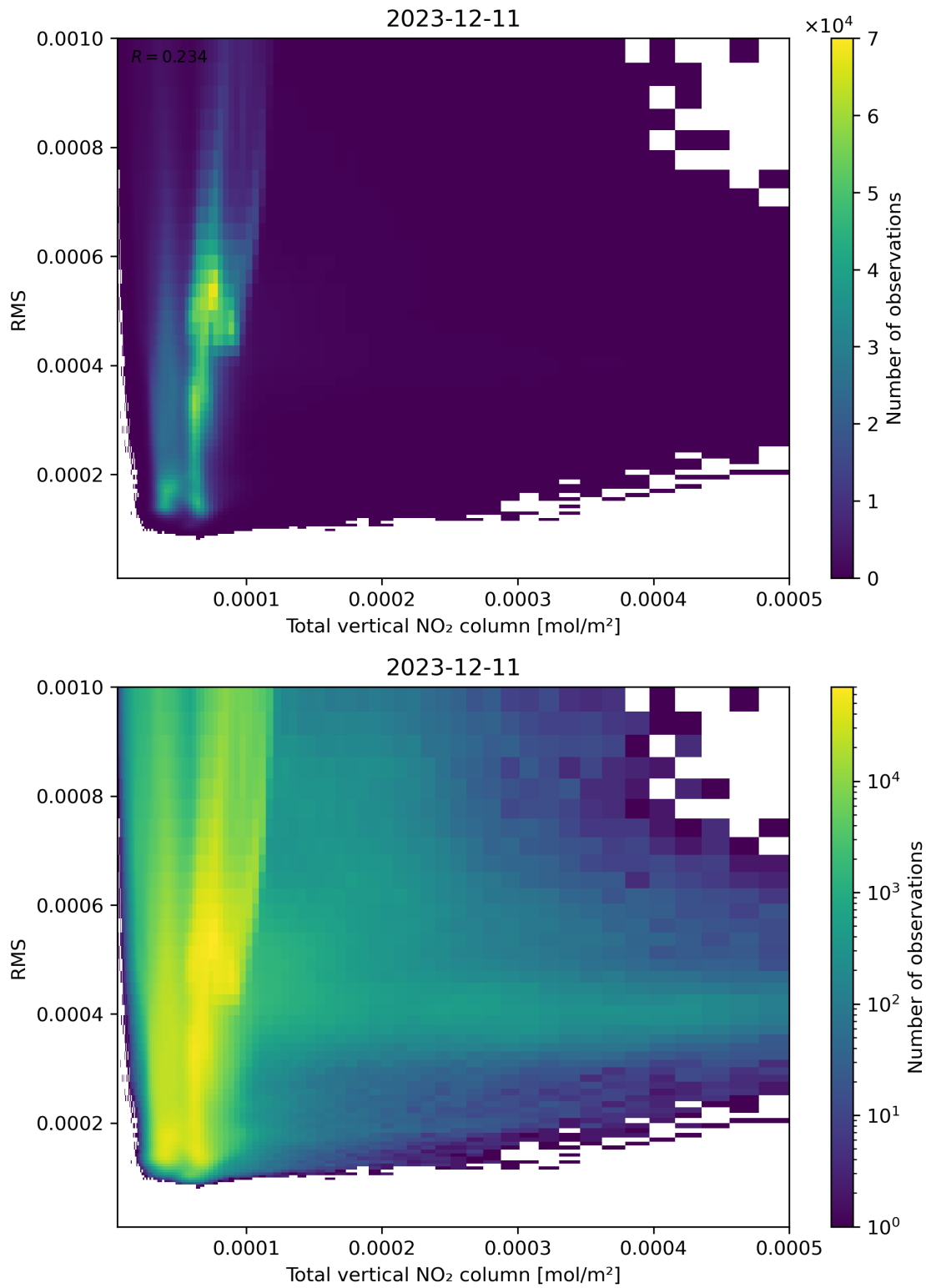
Figure 120: Scatter density plot of “Total vertical NO 2 column” against “RMS” for 2023-12-10 to 2023-12-12.
