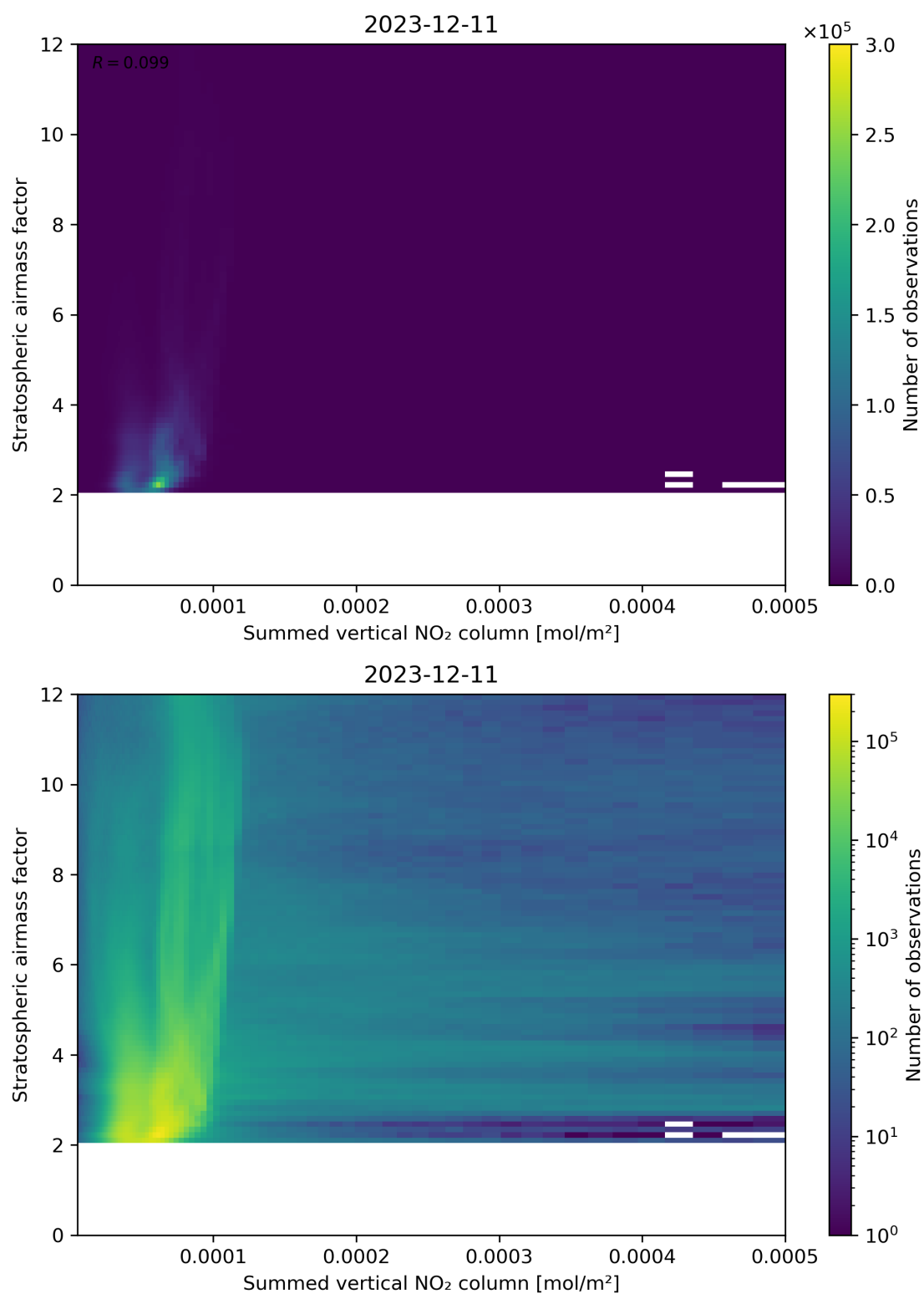
Figure 103: Scatter density plot of “Summed vertical NO 2 column” against “Stratospheric airmass factor” for 2023-12-10 to 2023-12-12.
