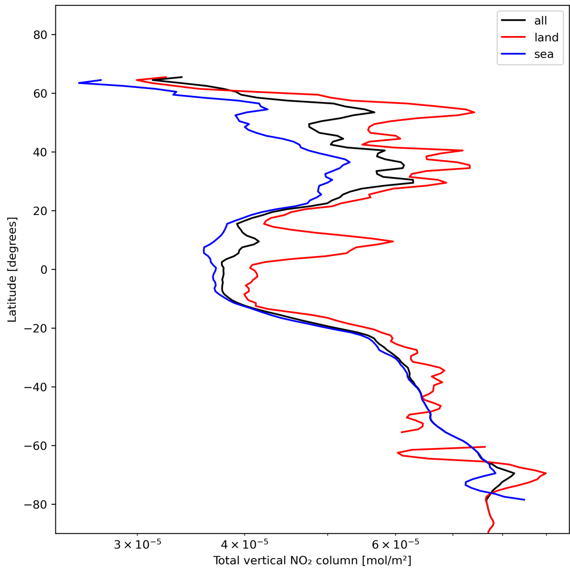
Figure 21: Zonal average of “Total vertical NO 2 column” for 2023-12-10 to 2023-12-12.
