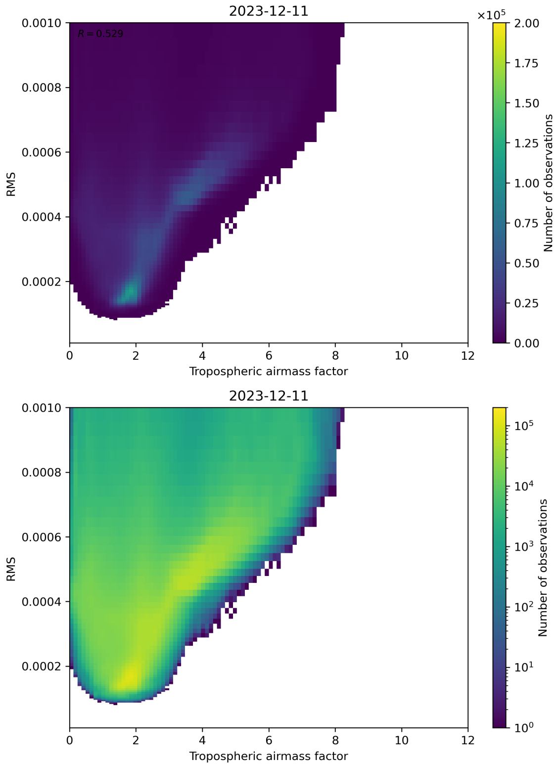
Figure 79: Scatter density plot of “Tropospheric airmass factor” against “RMS” for 2023-12-10 to 2023-12-12.
