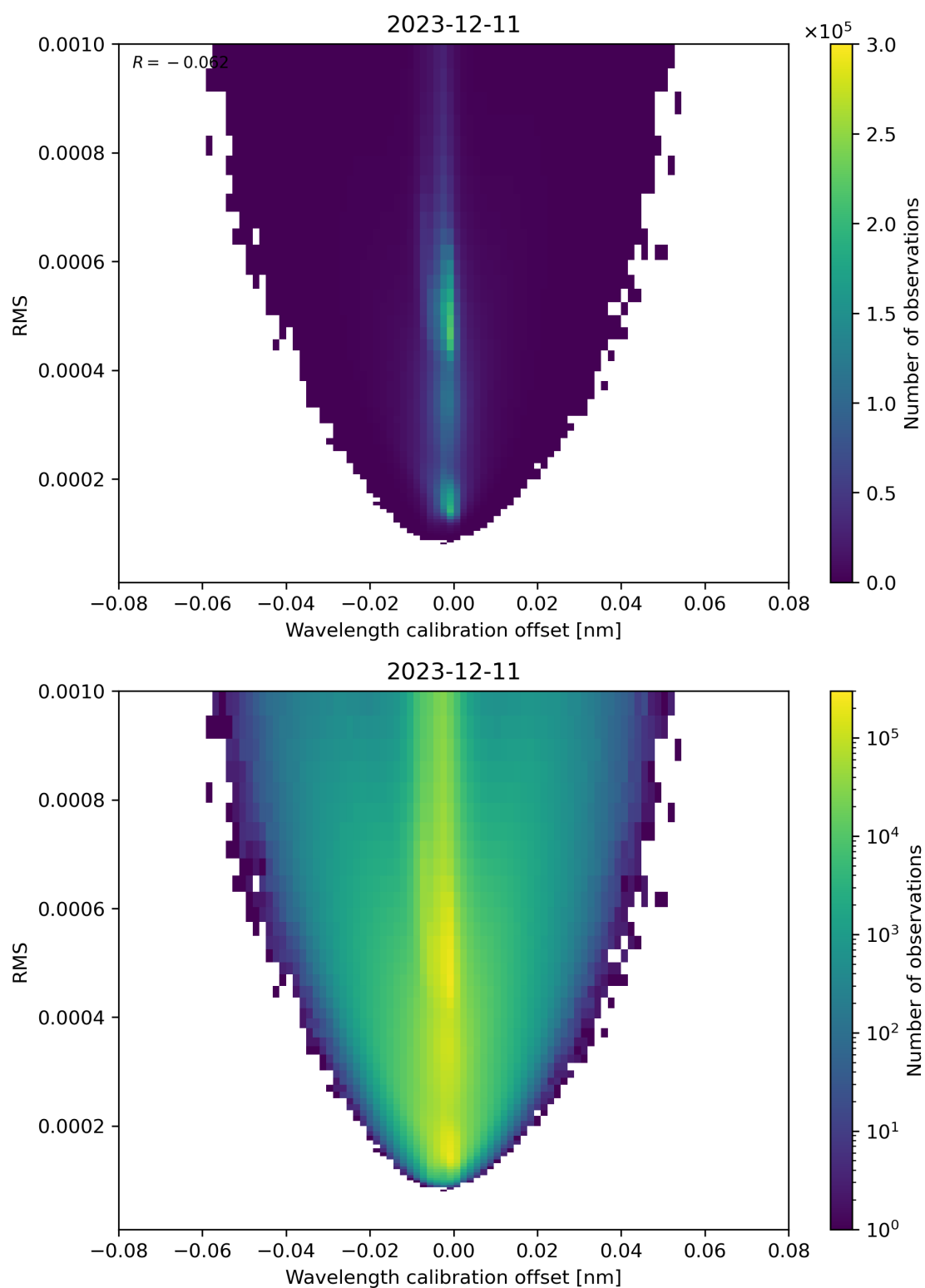
Figure 181: Scatter density plot of “Wavelength calibration offset” against “RMS” for 2023-12-10 to 2023-12-12.
