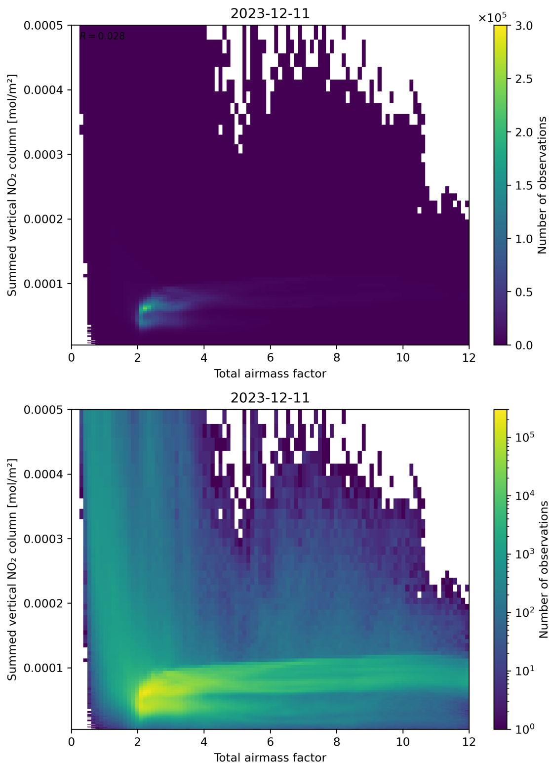
Figure 65: Scatter density plot of “Total airmass factor” against “Summed vertical NO 2 column” for 2023-12-10 to 2023-12-12.
