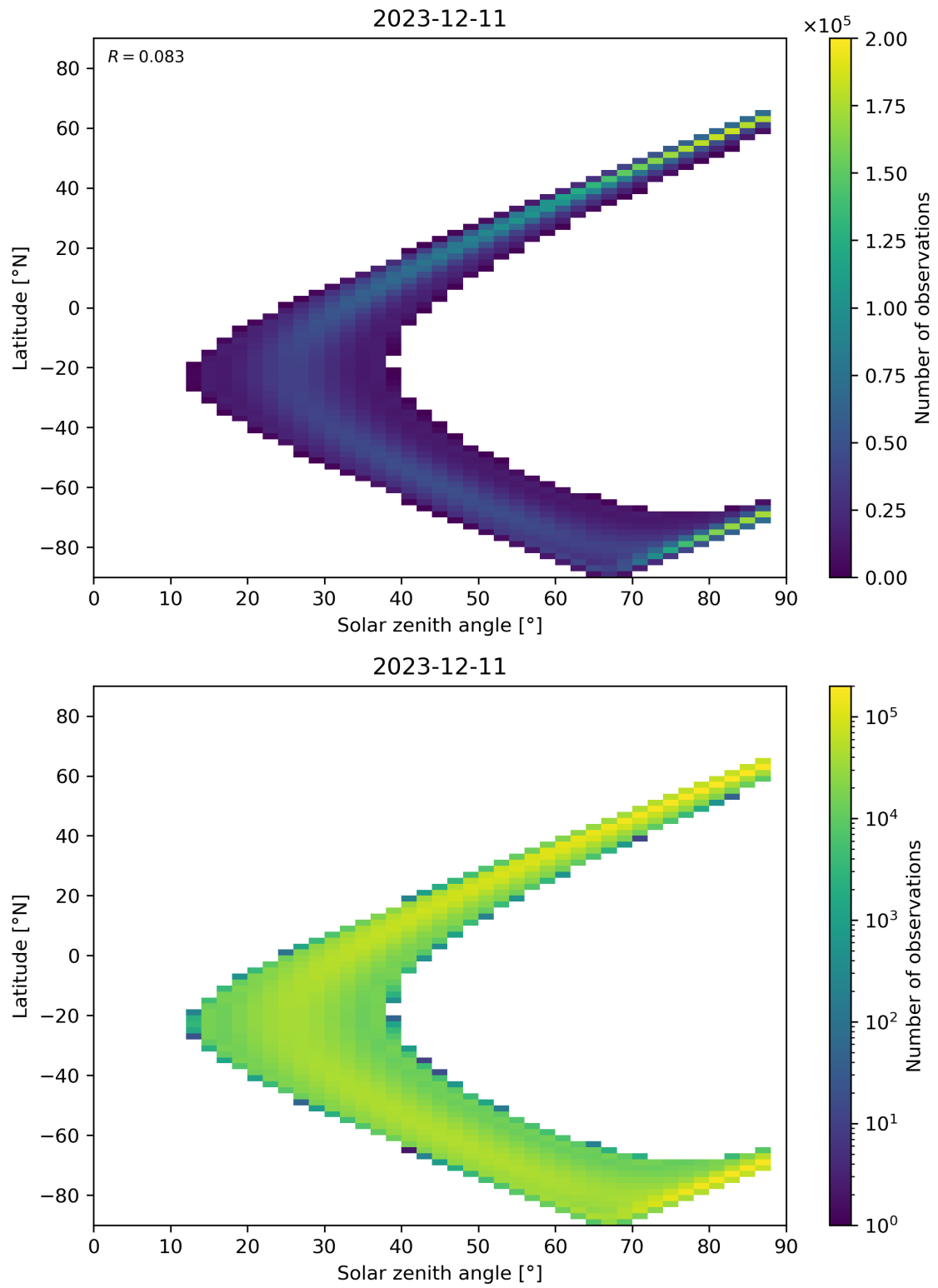
Figure 149: Scatter density plot of “Solar zenith angle” against “Latitude” for 2023-12-10 to 2023-12-12.
