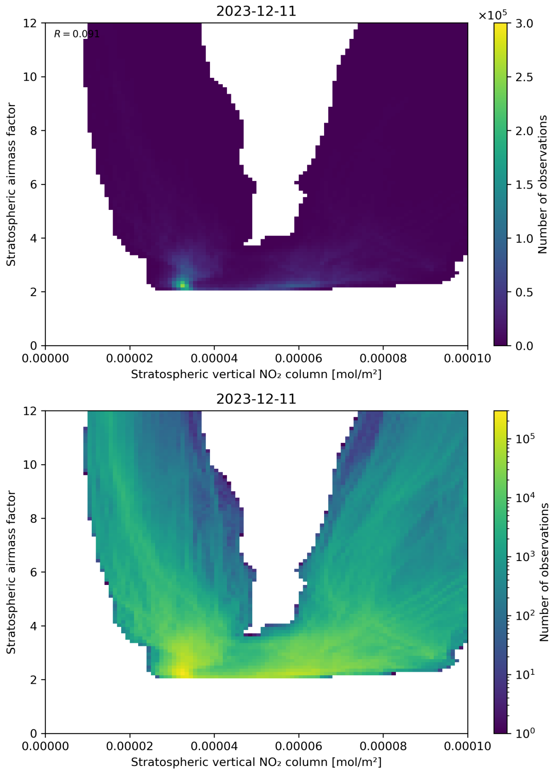
Figure 96: Scatter density plot of “Stratospheric vertical NO 2 column” against “Stratospheric airmass factor” for 2023-12-10 to 2023-12-12.
