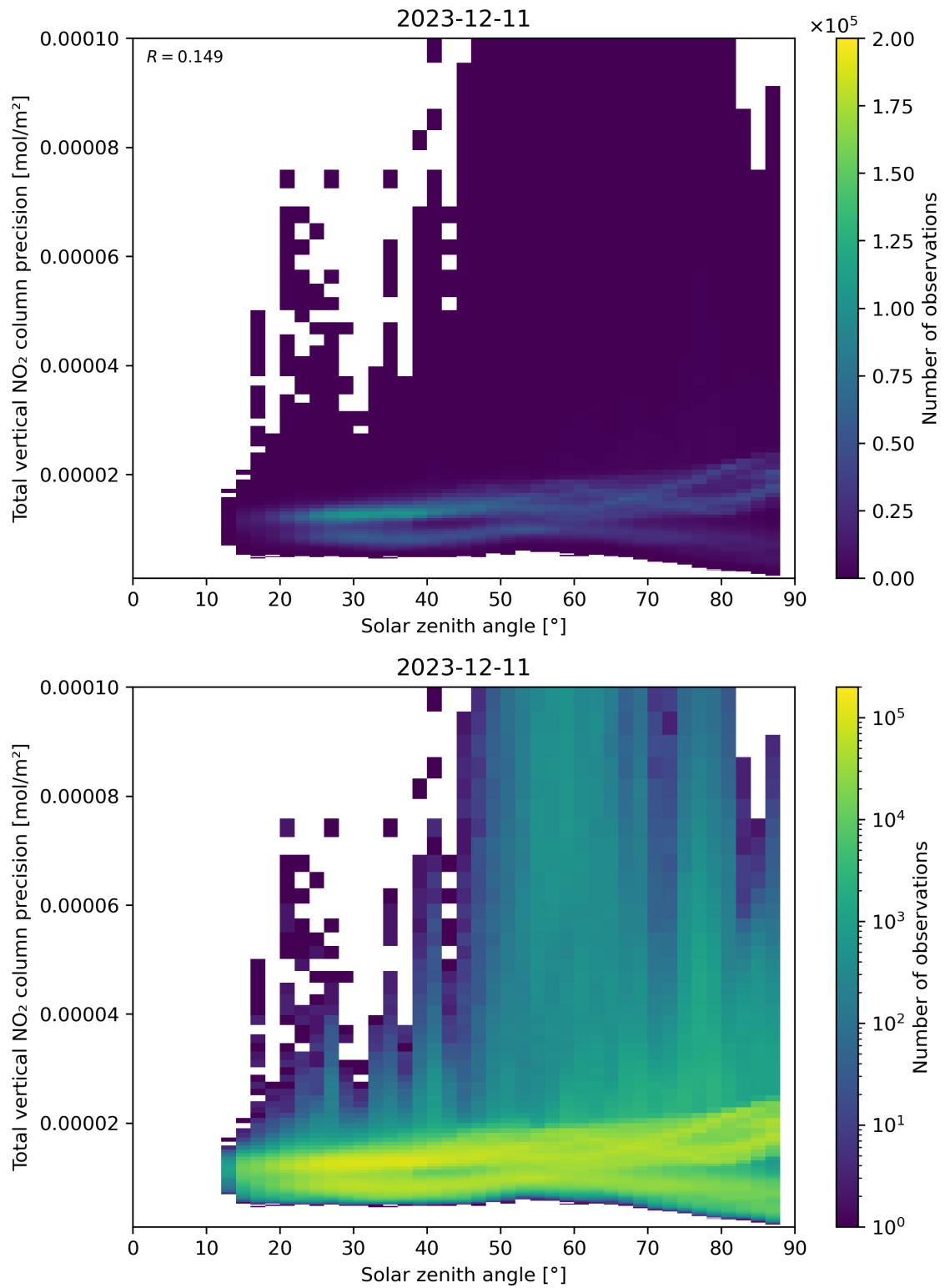
Figure 154: Scatter density plot of “Solar zenith angle” against “Total vertical NO 2 column precision” for 2023-12-10 to 2023-12-12.
