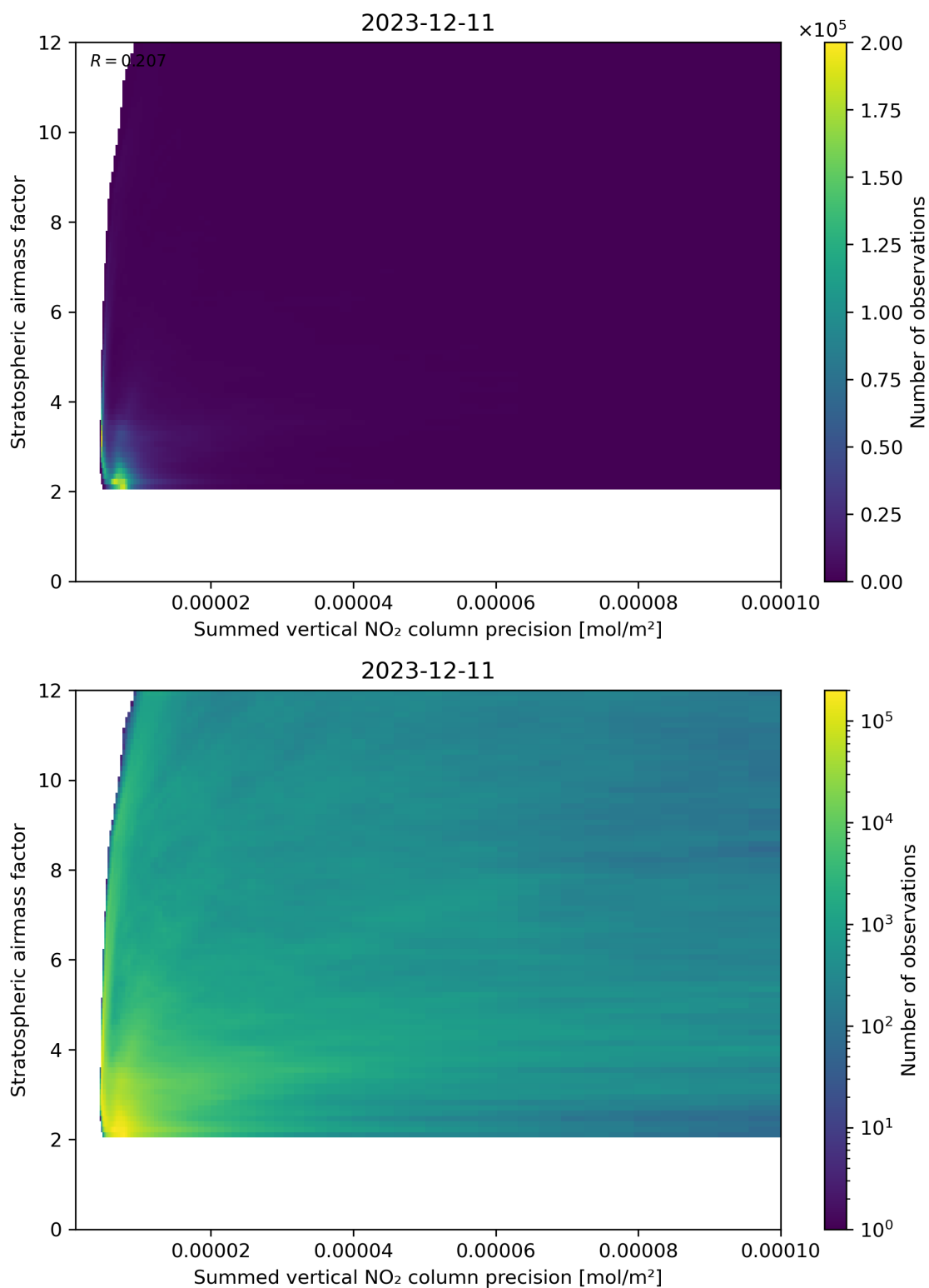
Figure 106: Scatter density plot of “Summed vertical NO 2 column precision” against “Stratospheric airmass factor” for 2023-12-10 to 2023-12-12.
