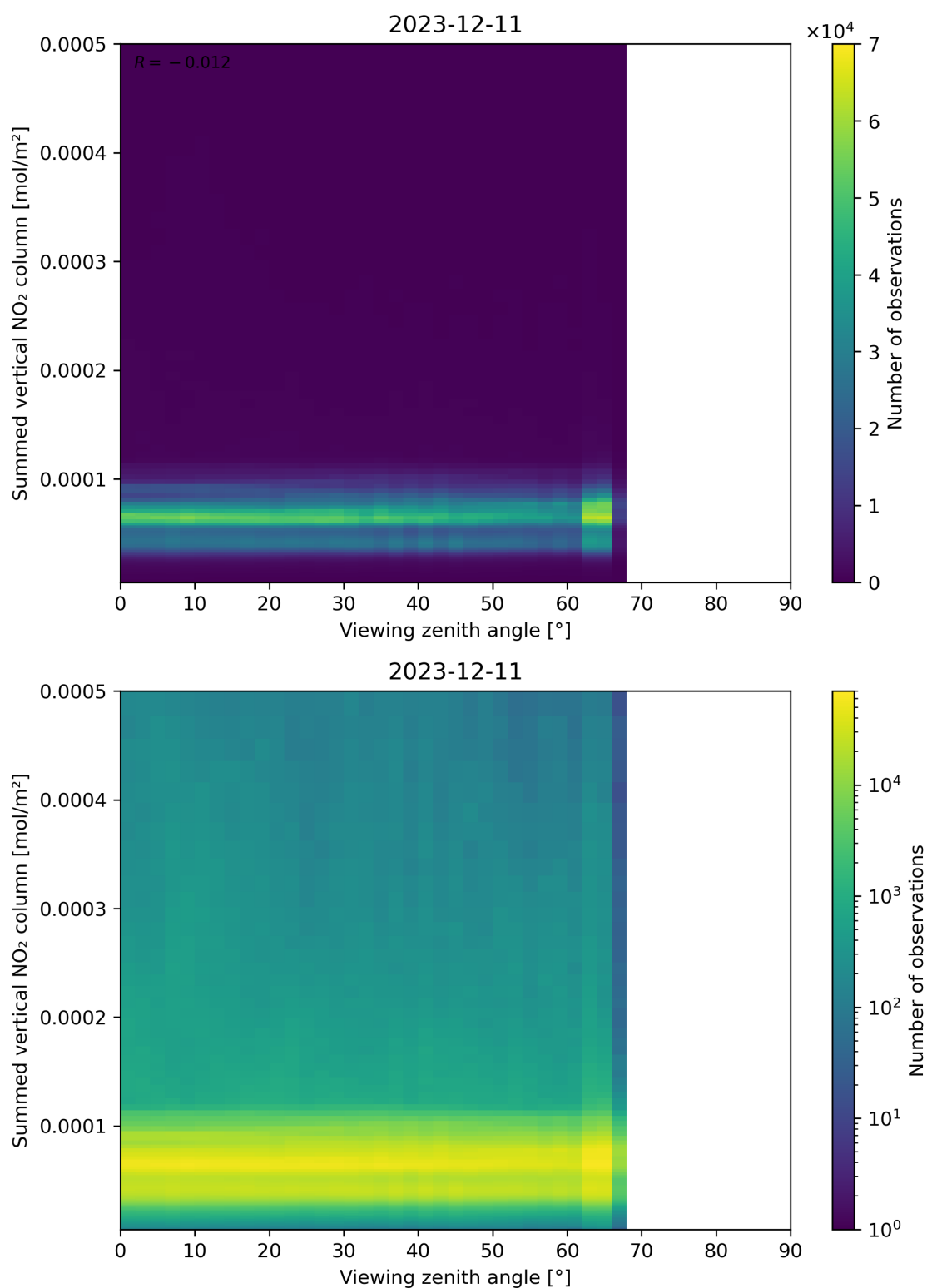
Figure 165: Scatter density plot of “Viewing zenith angle” against “Summed vertical NO 2 column” for 2023-12-10 to 2023-12-12.
