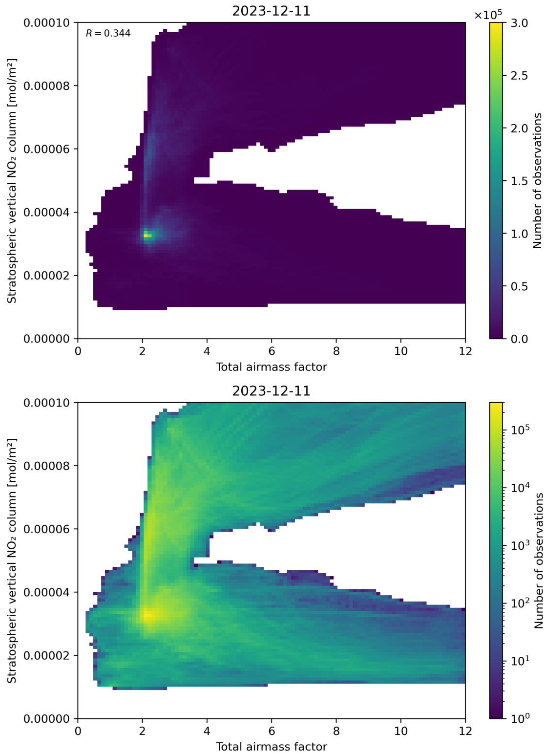
Figure 64: Scatter density plot of “Total airmass factor” against “Stratospheric vertical \text{NO}_2 column” for 2023-12-10 to 2023-12-12.
