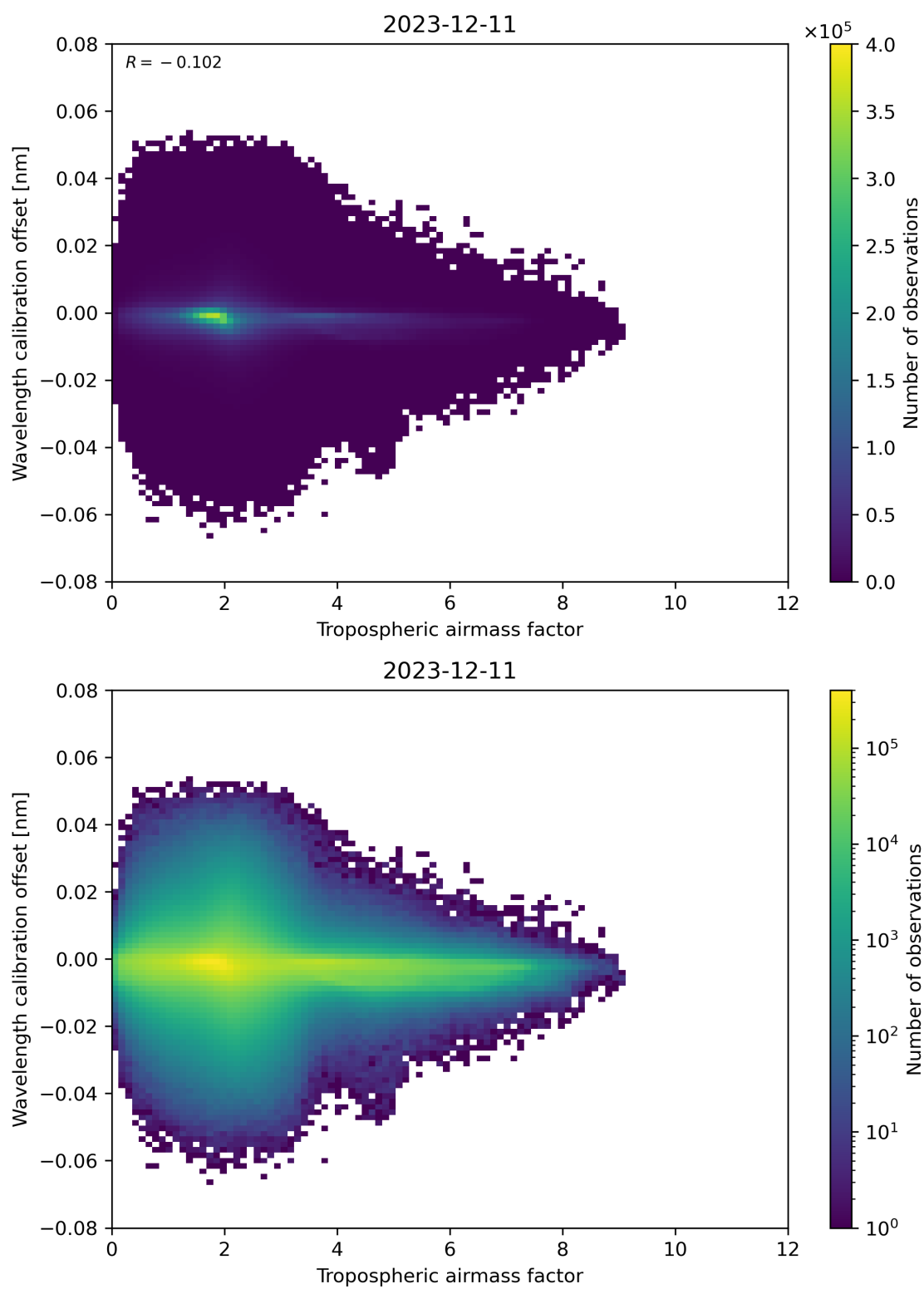
Figure 80: Scatter density plot of “Tropospheric airmass factor” against “Wavelength calibration offset” for 2023-12-10 to 2023-12-12.
