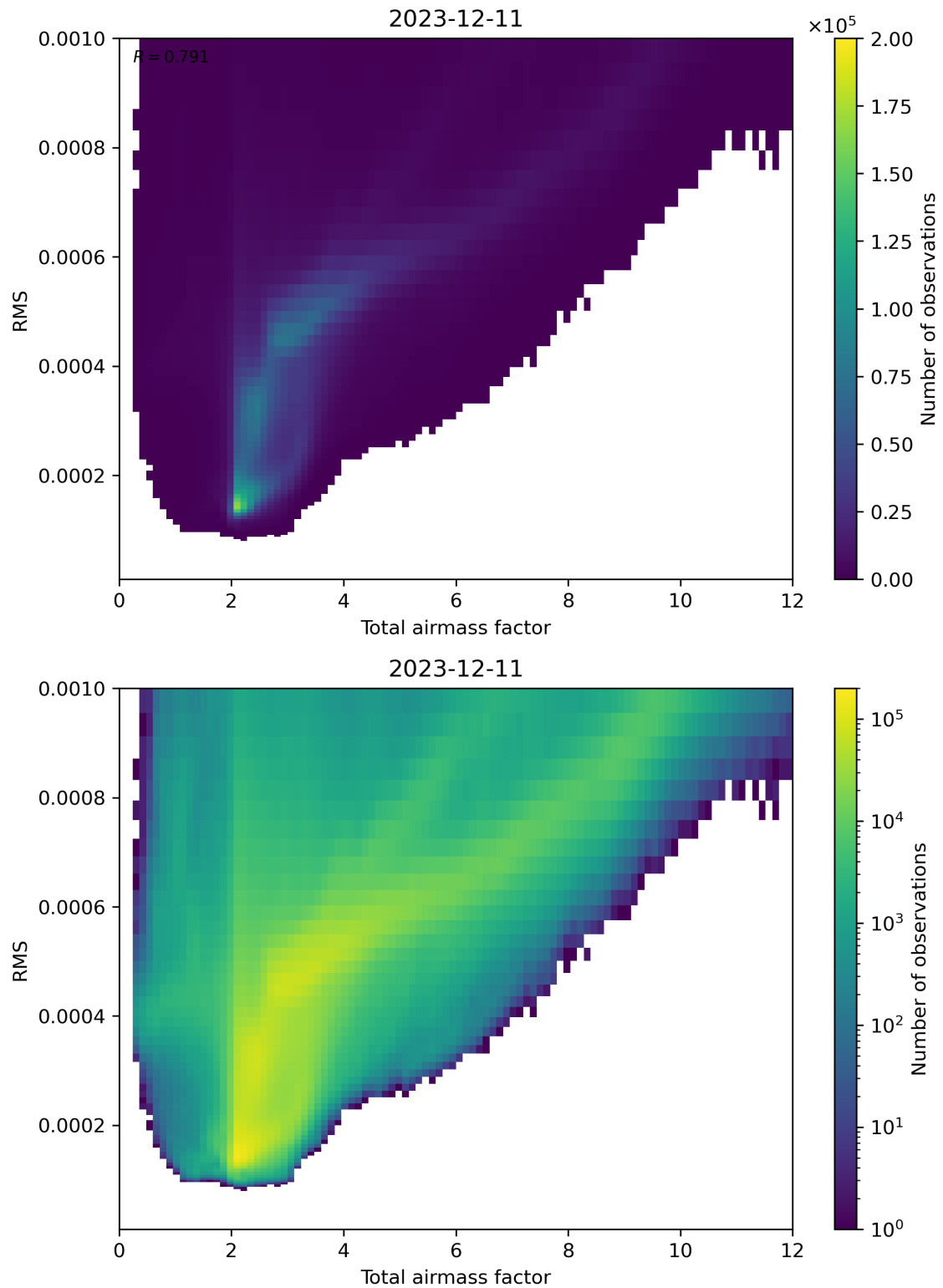
Figure 69: Scatter density plot of “Total airmass factor” against “RMS” for 2023-12-10 to 2023-12-12.
