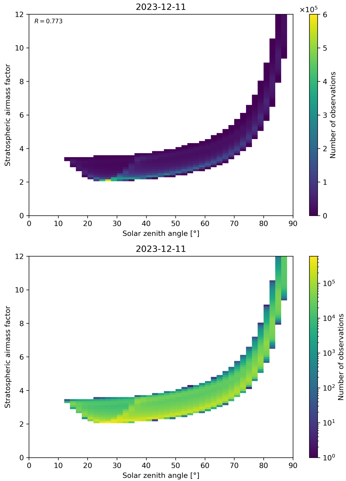
Figure 145: Scatter density plot of “Solar zenith angle” against “Stratospheric airmass factor” for 2023-12-10 to 2023-12-12.
