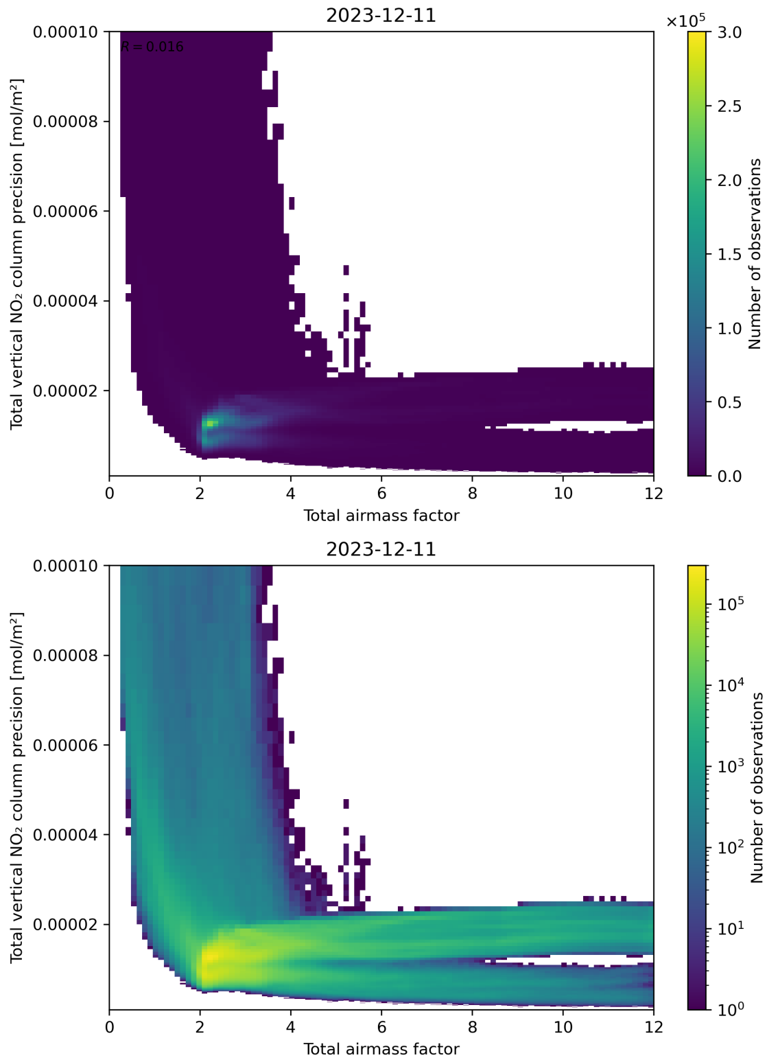
Figure 68: Scatter density plot of “Total airmass factor” against “Total vertical NO 2 column precision” for 2023-12-10 to 2023-12-12.
