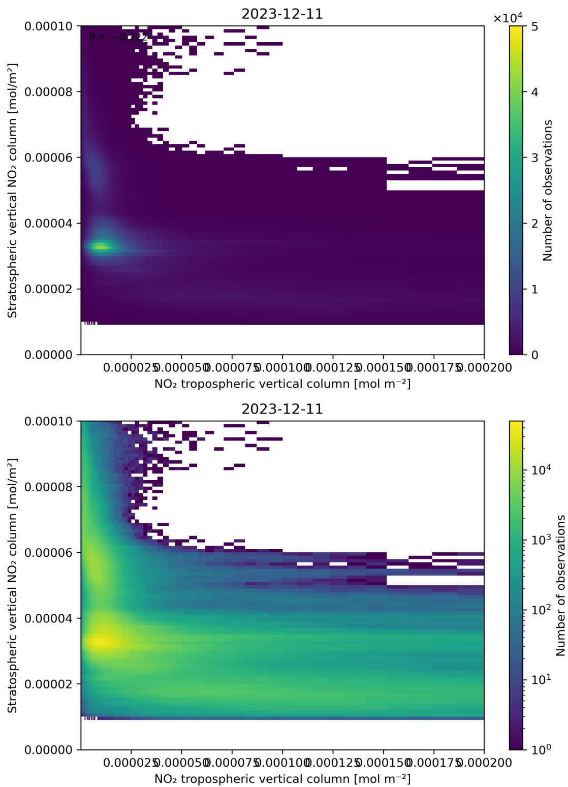
Figure 125: Scatter density plot of “NO 2 tropospheric vertical column” against “Stratospheric vertical NO 2 column” for 2023-12-10 to 2023-12-12.
