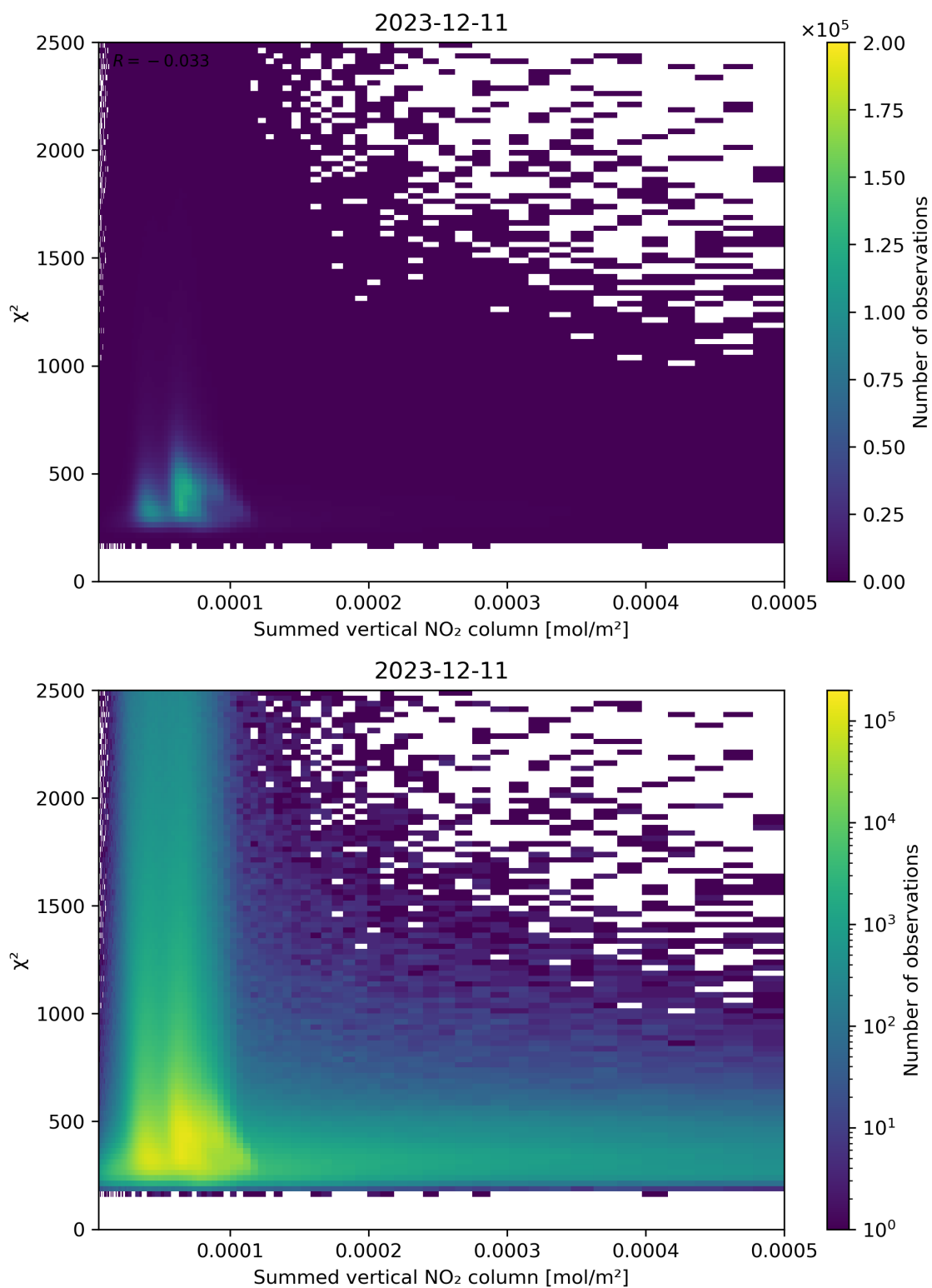
Figure 104: Scatter density plot of “Summed vertical NO 2 column” against “ \chi^2 ” for 2023-12-10 to 2023-12-12.
