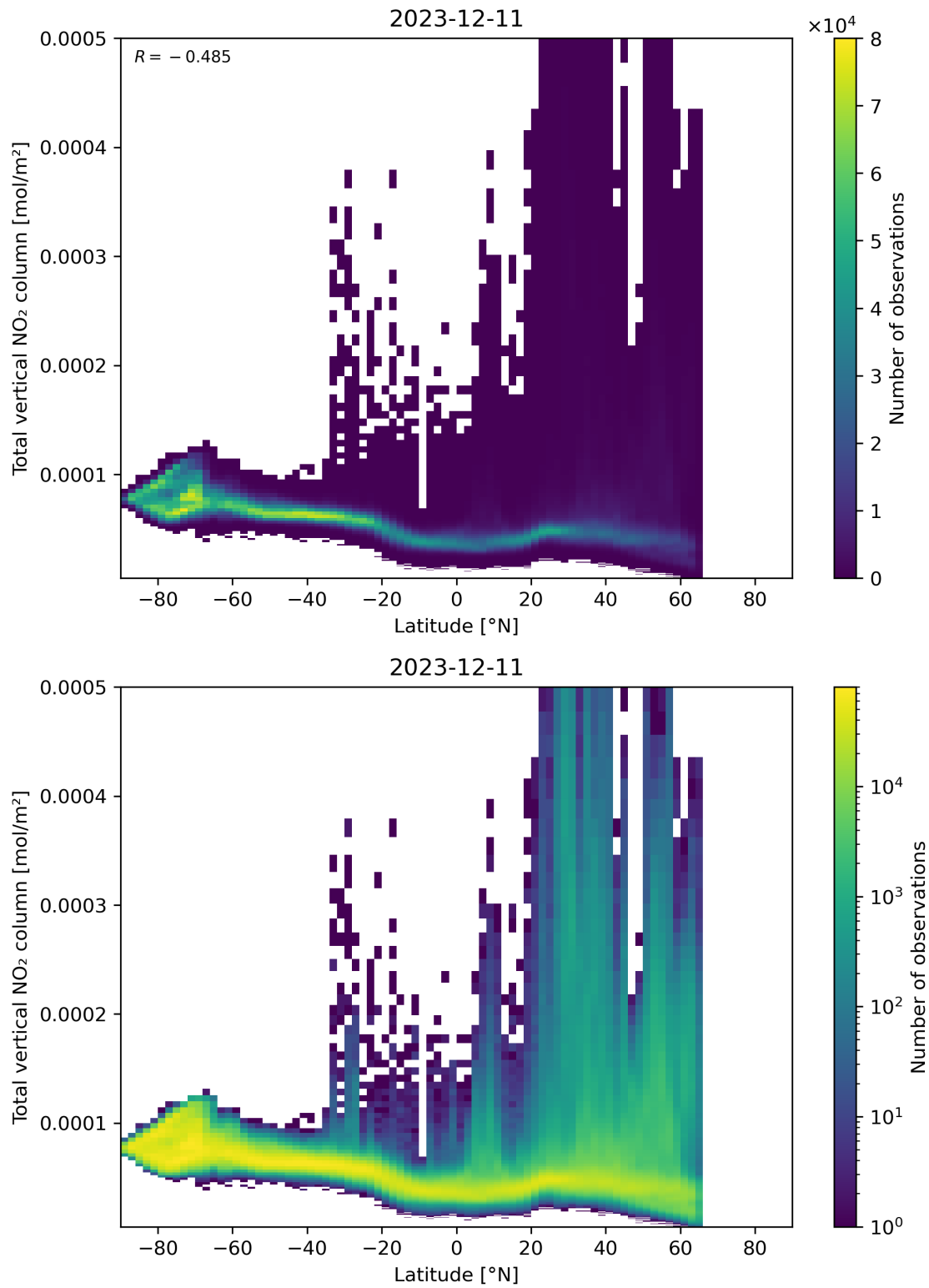
Figure 90: Scatter density plot of “Latitude” against “Total vertical NO 2 column” for 2023-12-10 to 2023-12-12.
