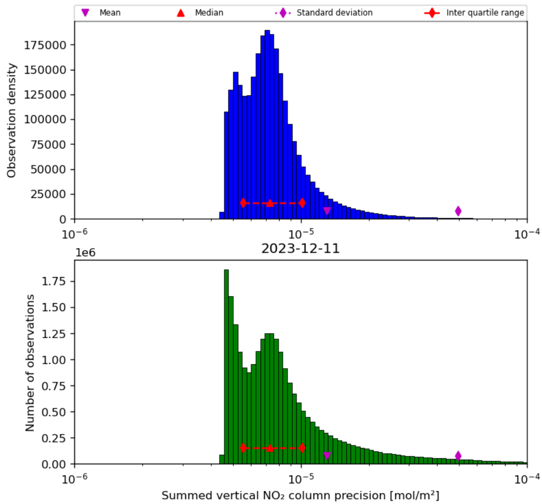
Figure 41: Histogram of “Summed vertical NO 2 column precision” for 2023-12-10 to 2023-12-12
