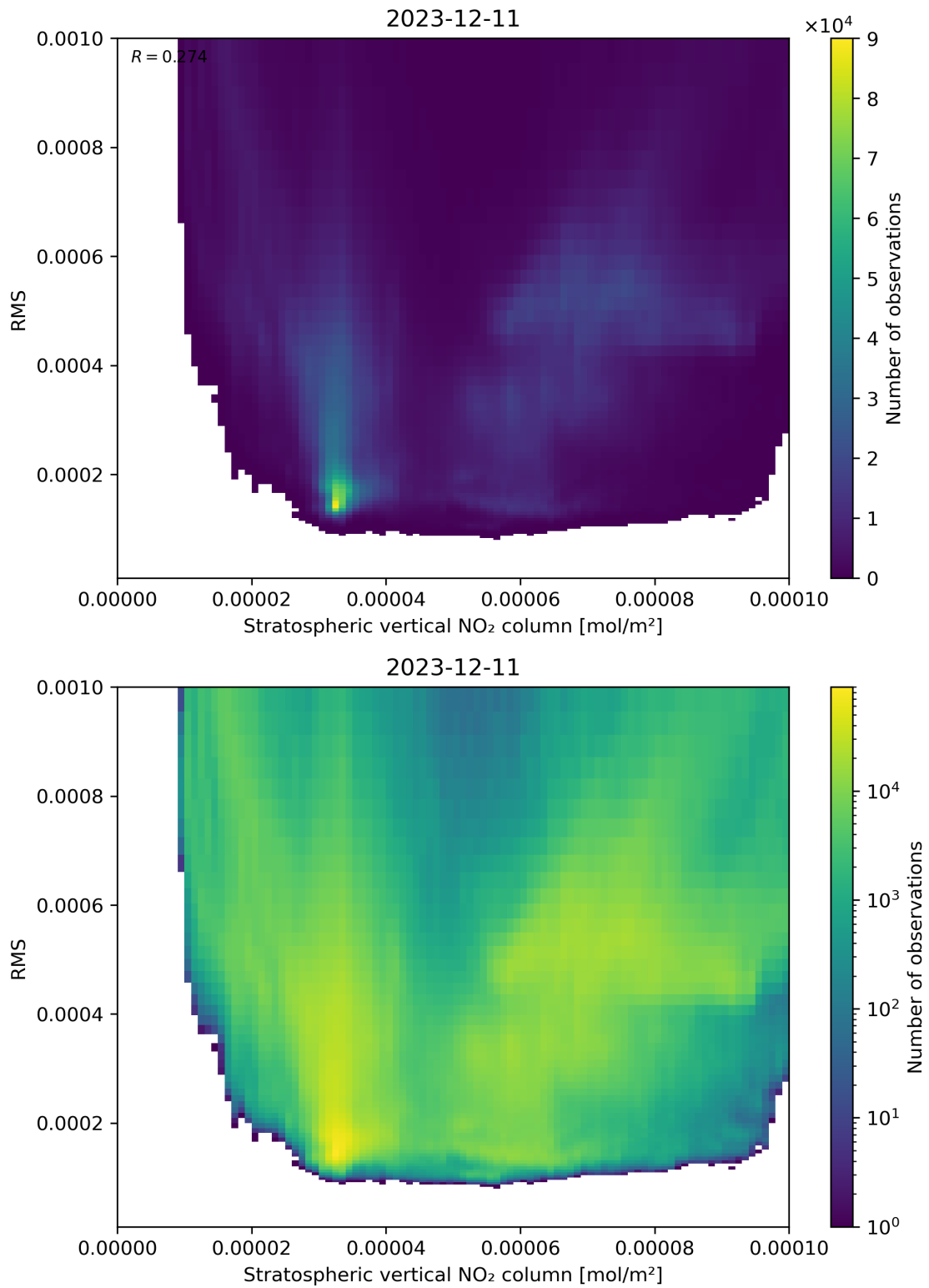
Figure 102: Scatter density plot of “Stratospheric vertical NO 2 column” against “RMS” for 2023-12-10 to 2023-12-12.
