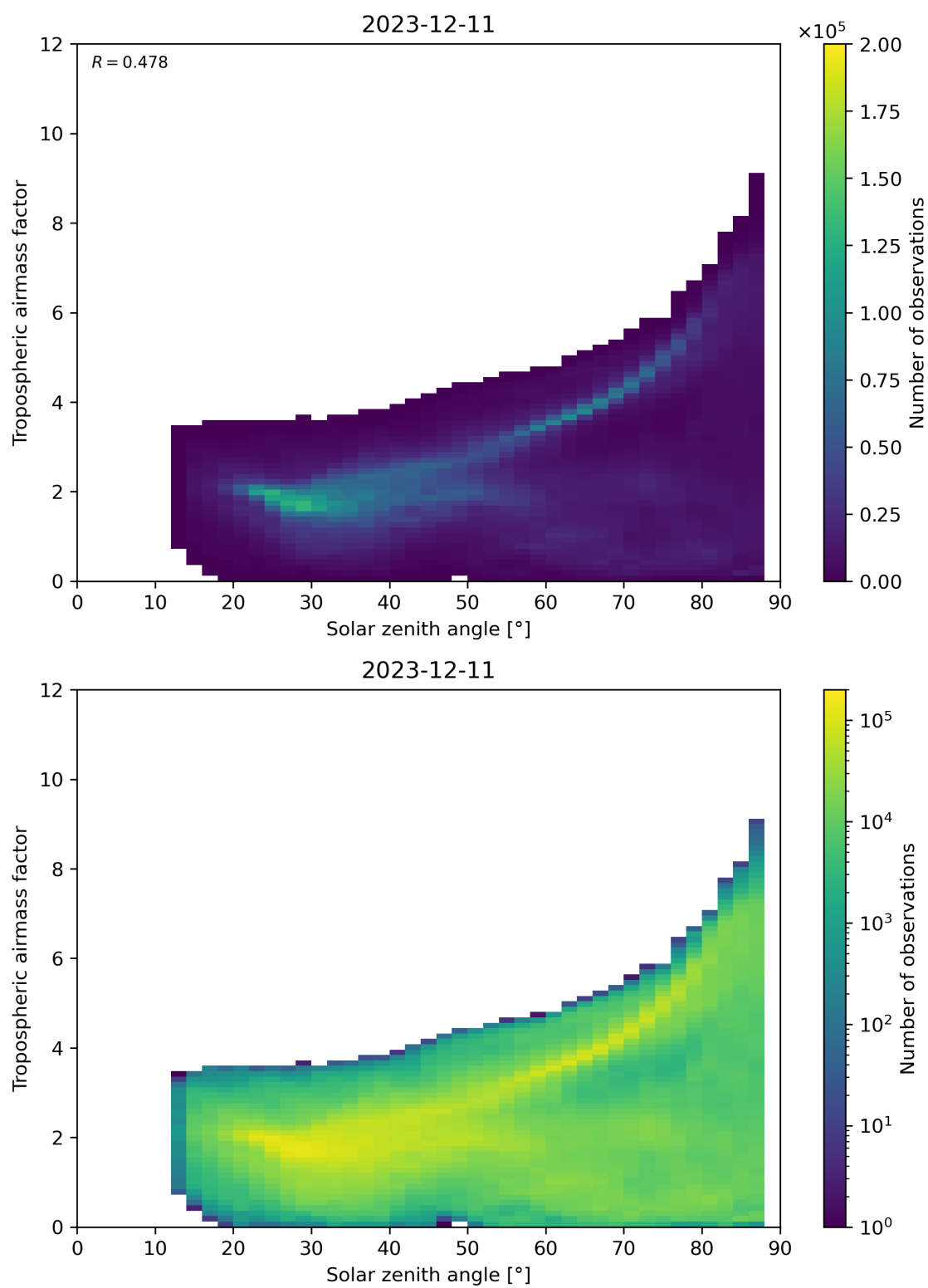
Figure 147: Scatter density plot of “Solar zenith angle” against “Tropospheric airmass factor” for 2023-12-10 to 2023-12-12.
