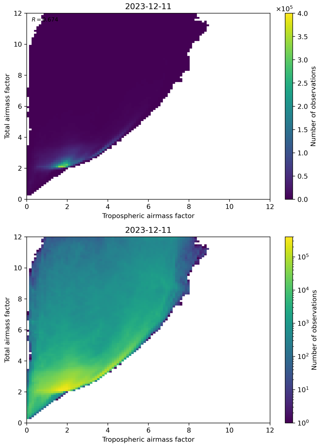
Figure 72: Scatter density plot of “Tropospheric airmass factor” against “Total airmass factor” for 2023-12-10 to 2023-12-12.
