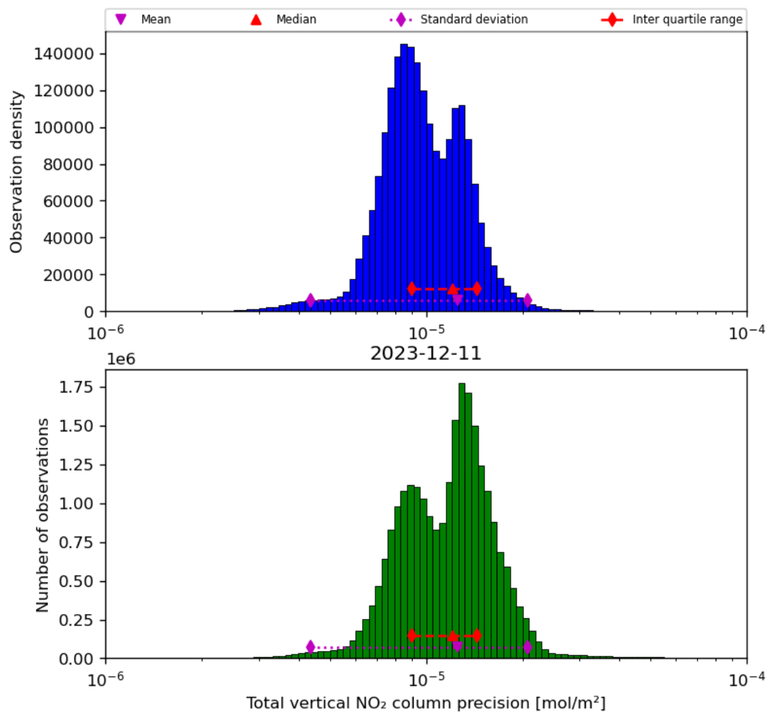
Figure 39: Histogram of “Total vertical NO 2 column precision” for 2023-12-10 to 2023-12-12
