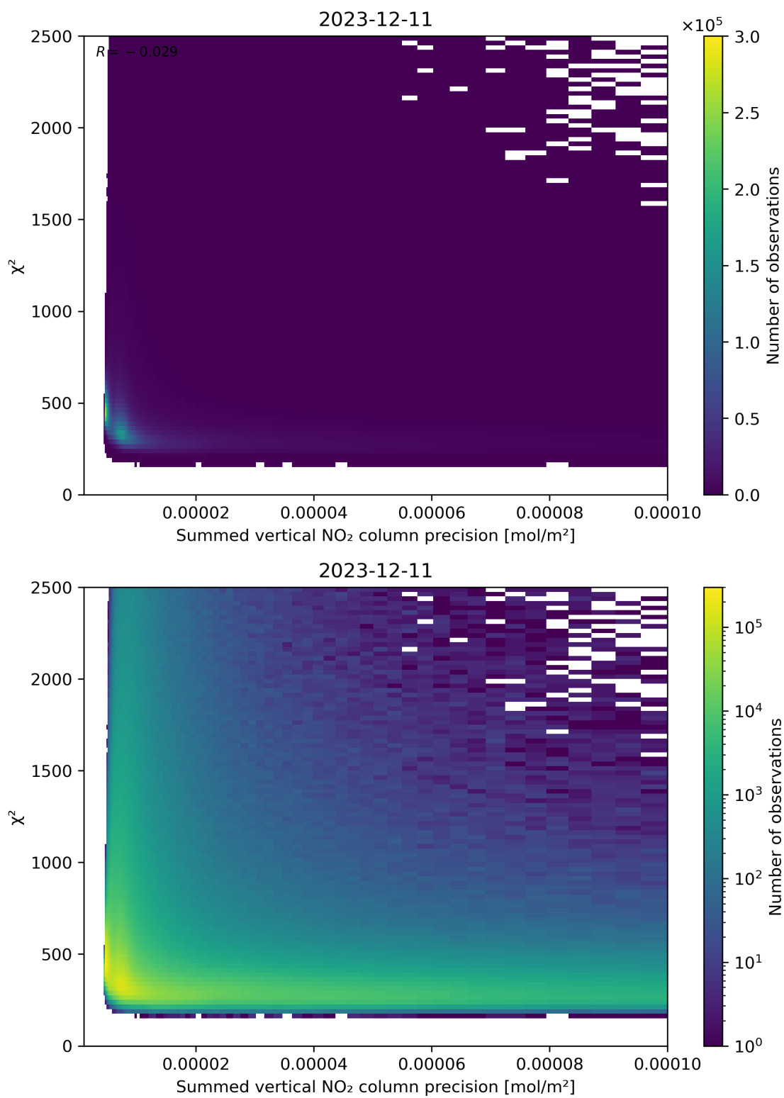
Figure 107: Scatter density plot of “Summed vertical NO 2 column precision” against “ \chi^2 ” for 2023-12-10 to 2023-12-12.
