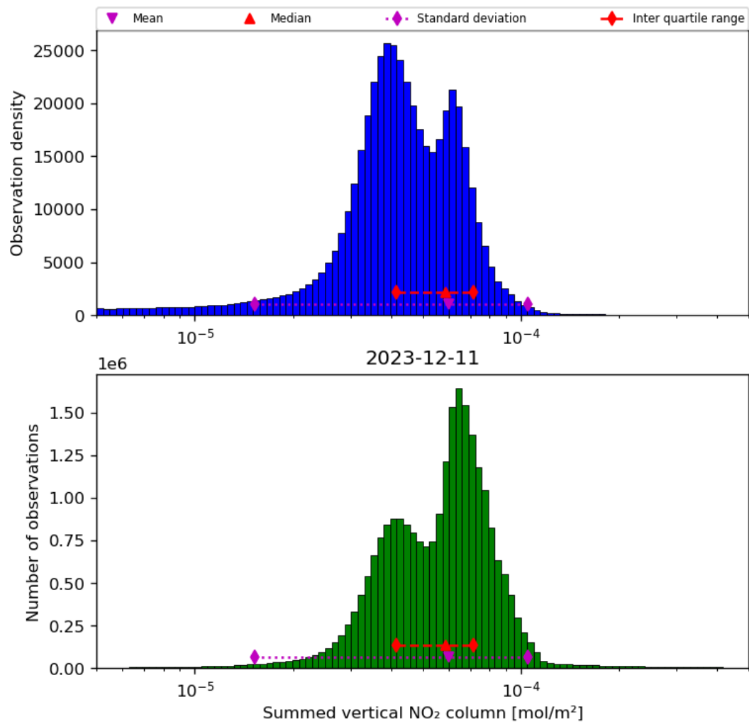
Figure 40: Histogram of “Summed vertical NO 2 column” for 2023-12-10 to 2023-12-12
