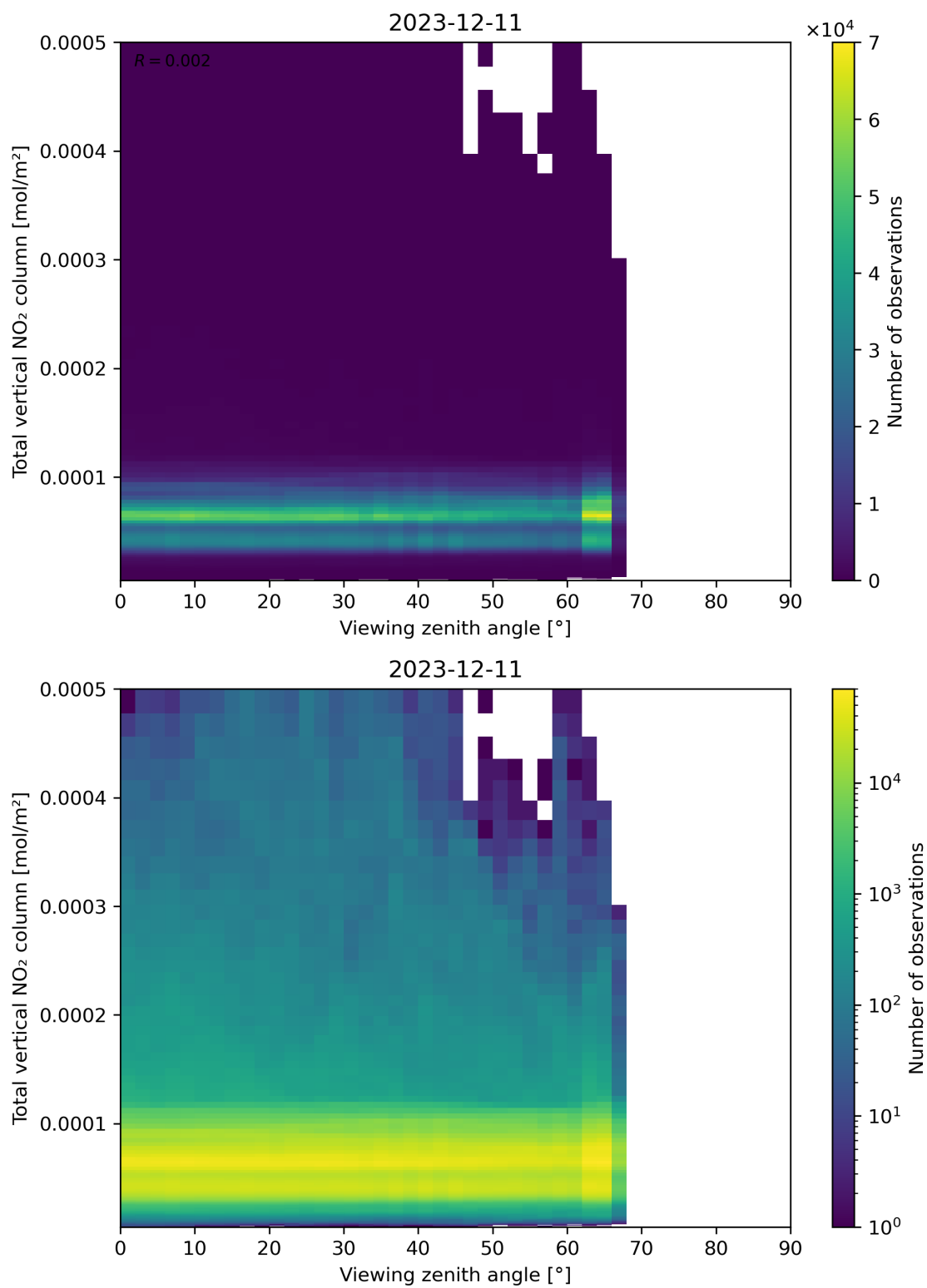
Figure 167: Scatter density plot of “Viewing zenith angle” against “Total vertical NO 2 column” for 2023-12-10 to 2023-12-12.
