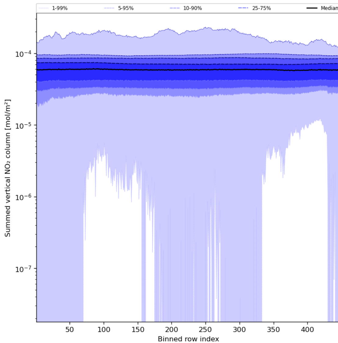
Figure 57: Along track statistics of “Summed vertical NO 2 column” for 2023-12-10 to 2023-12-12
