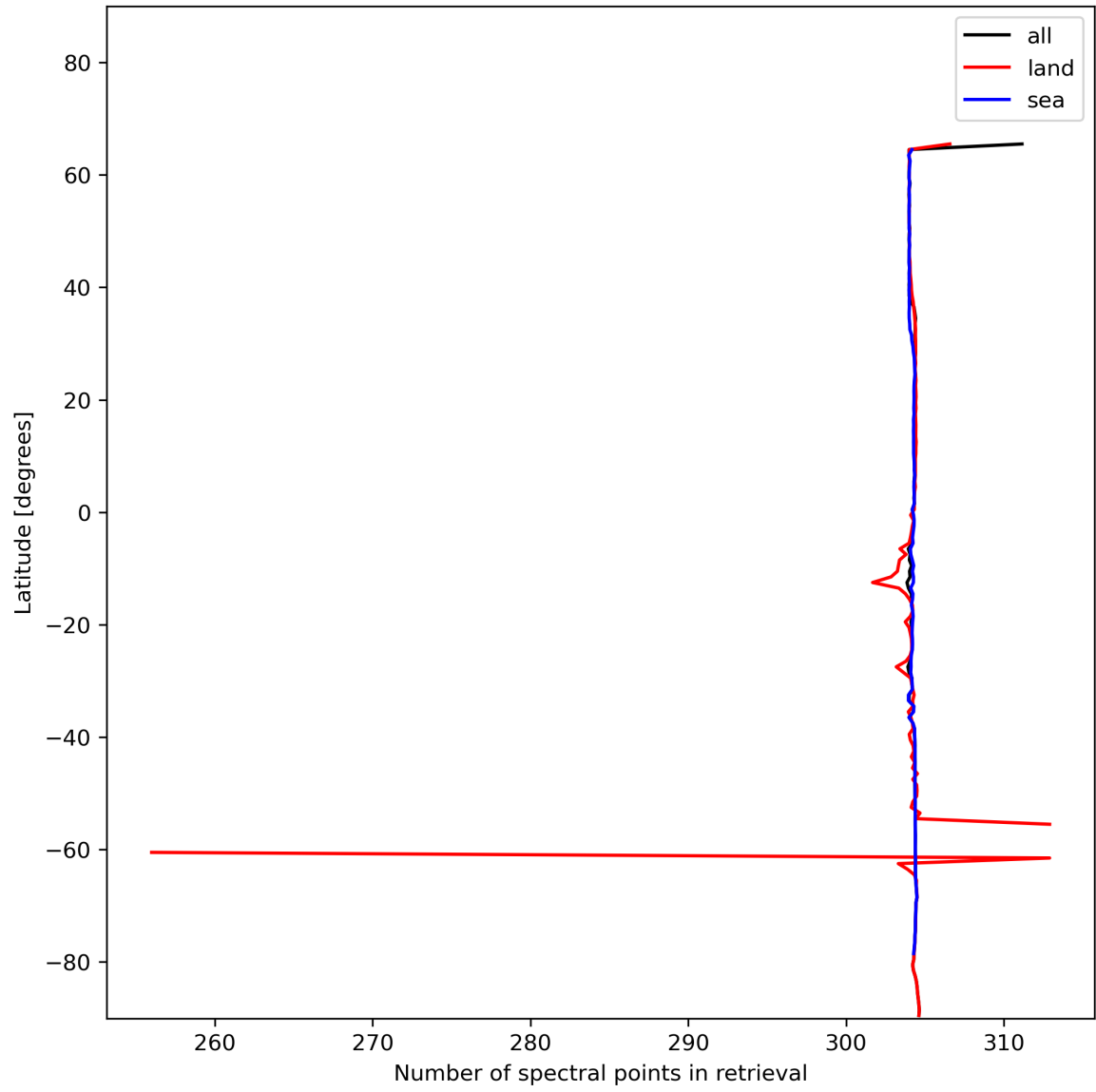
Figure 16: Zonal average of “Number of spectral points in retrieval” for 2023-12-10 to 2023-12-12.
