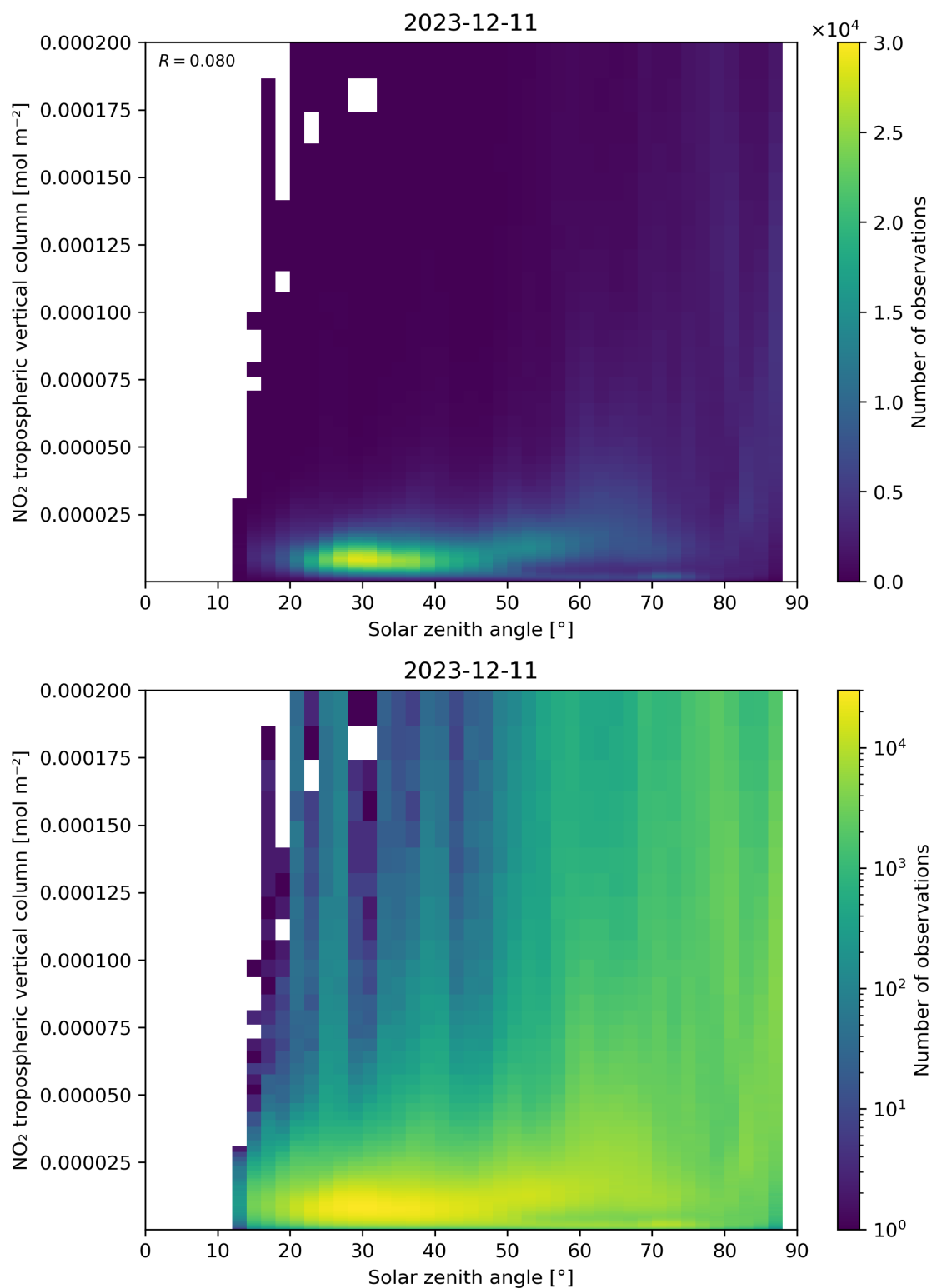
Figure 155: Scatter density plot of “Solar zenith angle” against “NO 2 tropospheric vertical column” for 2023-12-10 to 2023-12-12.
