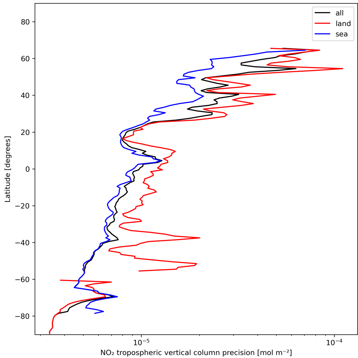
Figure 13: Zonal average of “NO 2 tropospheric vertical column precision” for 2023-12-10 to 2023-12-12.
