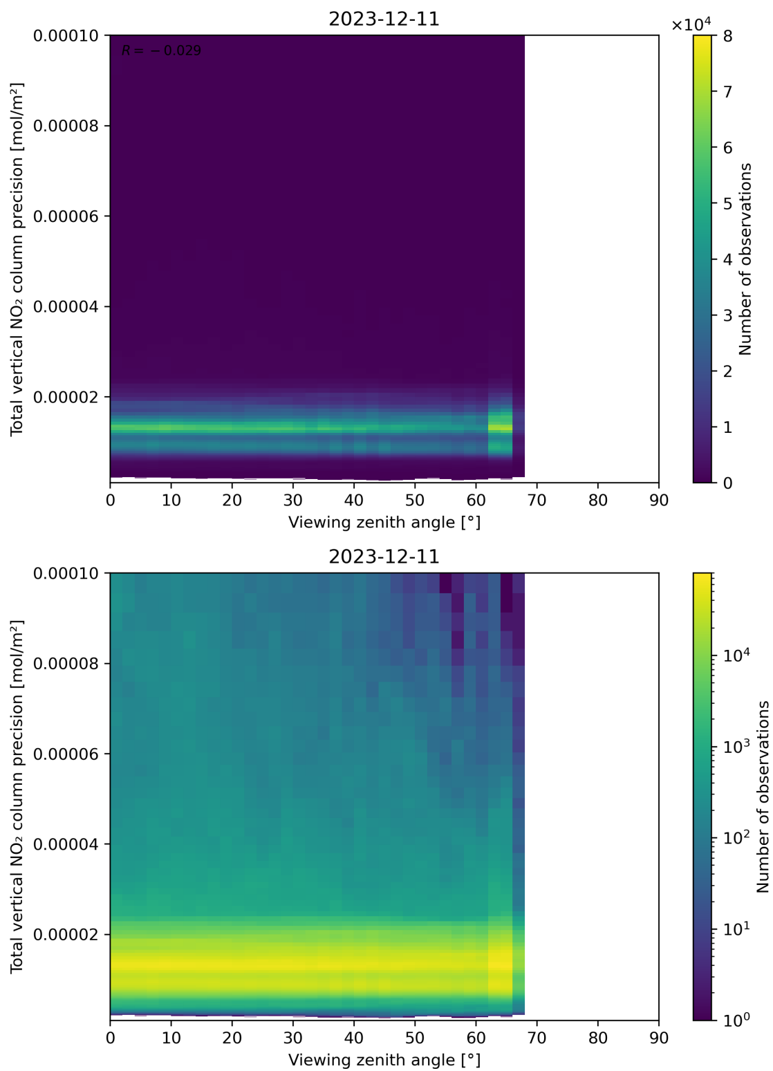
Figure 168: Scatter density plot of “Viewing zenith angle” against “Total vertical NO 2 column precision” for 2023-12-10 to 2023-12-12.
