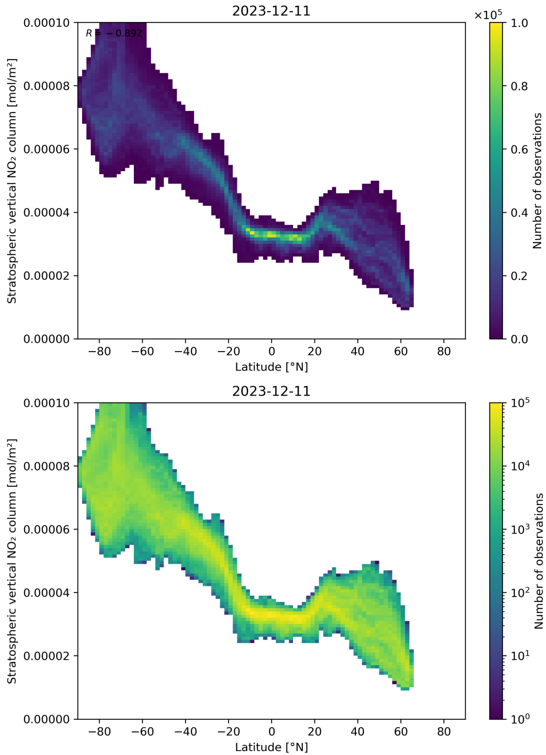
Figure 87: Scatter density plot of “Latitude” against “Stratospheric vertical NO 2 column” for 2023-12-10 to 2023-12-12.
