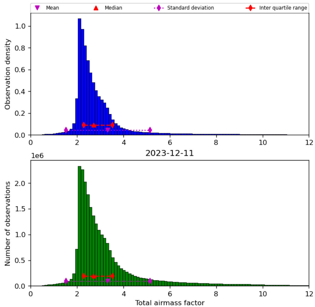
Figure 32: Histogram of “Total airmass factor” for 2023-12-10 to 2023-12-12
