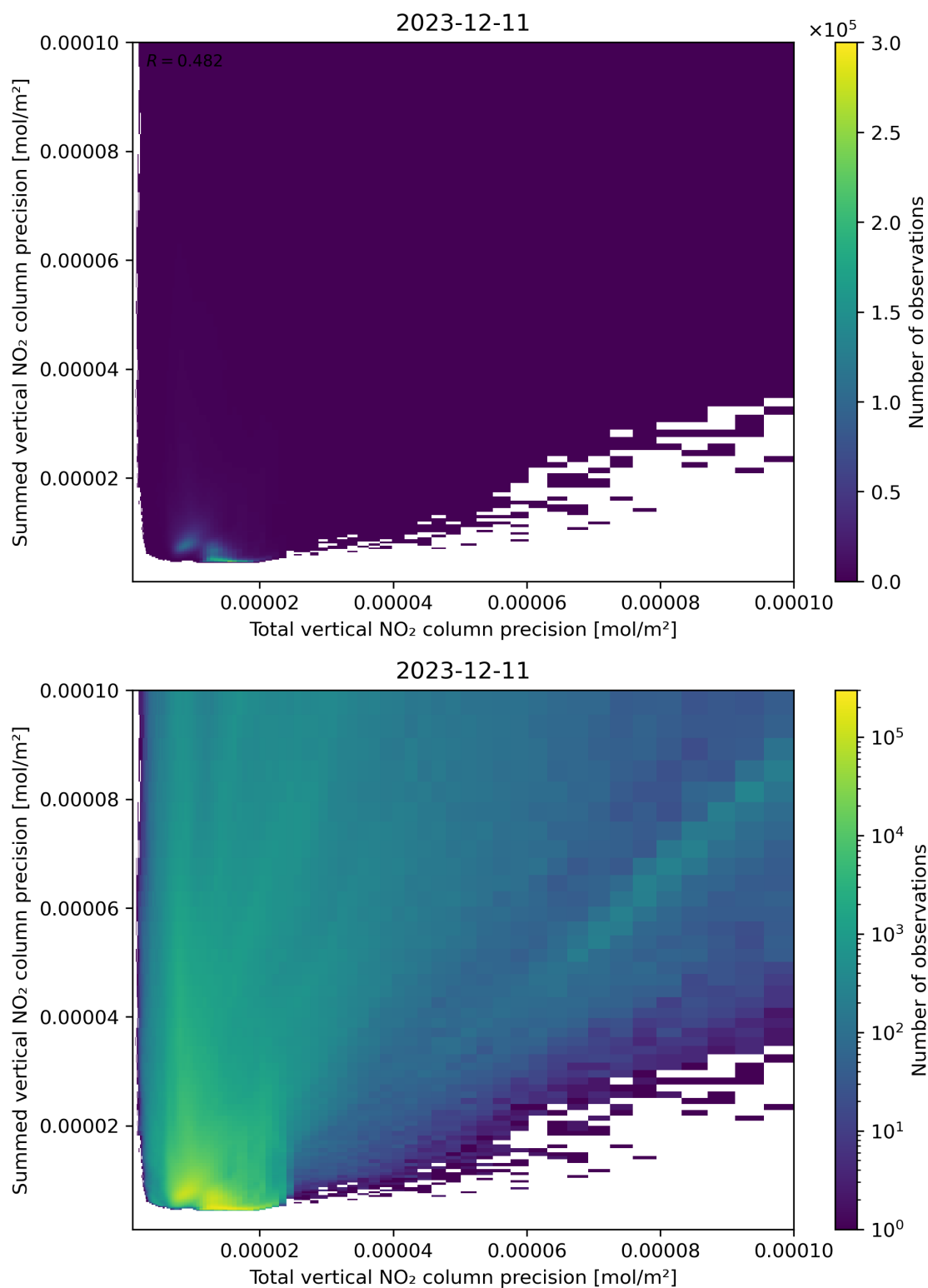
Figure 118: Scatter density plot of “Total vertical NO 2 column precision” against “Summed vertical NO 2 column precision” for 2023-12-10 to 2023-12-12.
