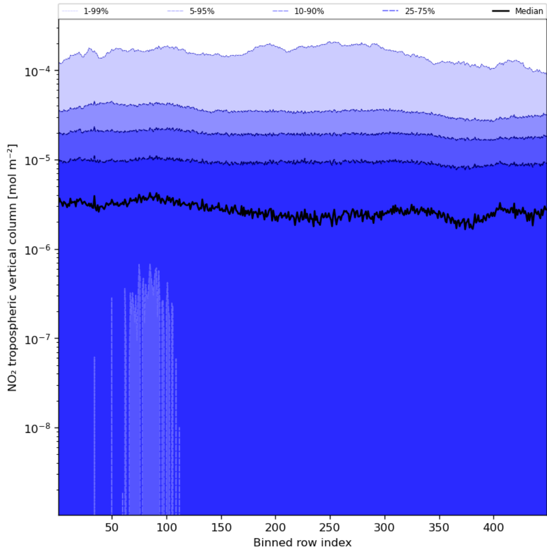
Figure 46: Along track statistics of “NO 2 tropospheric vertical column” for 2023-12-10 to 2023-12-12
