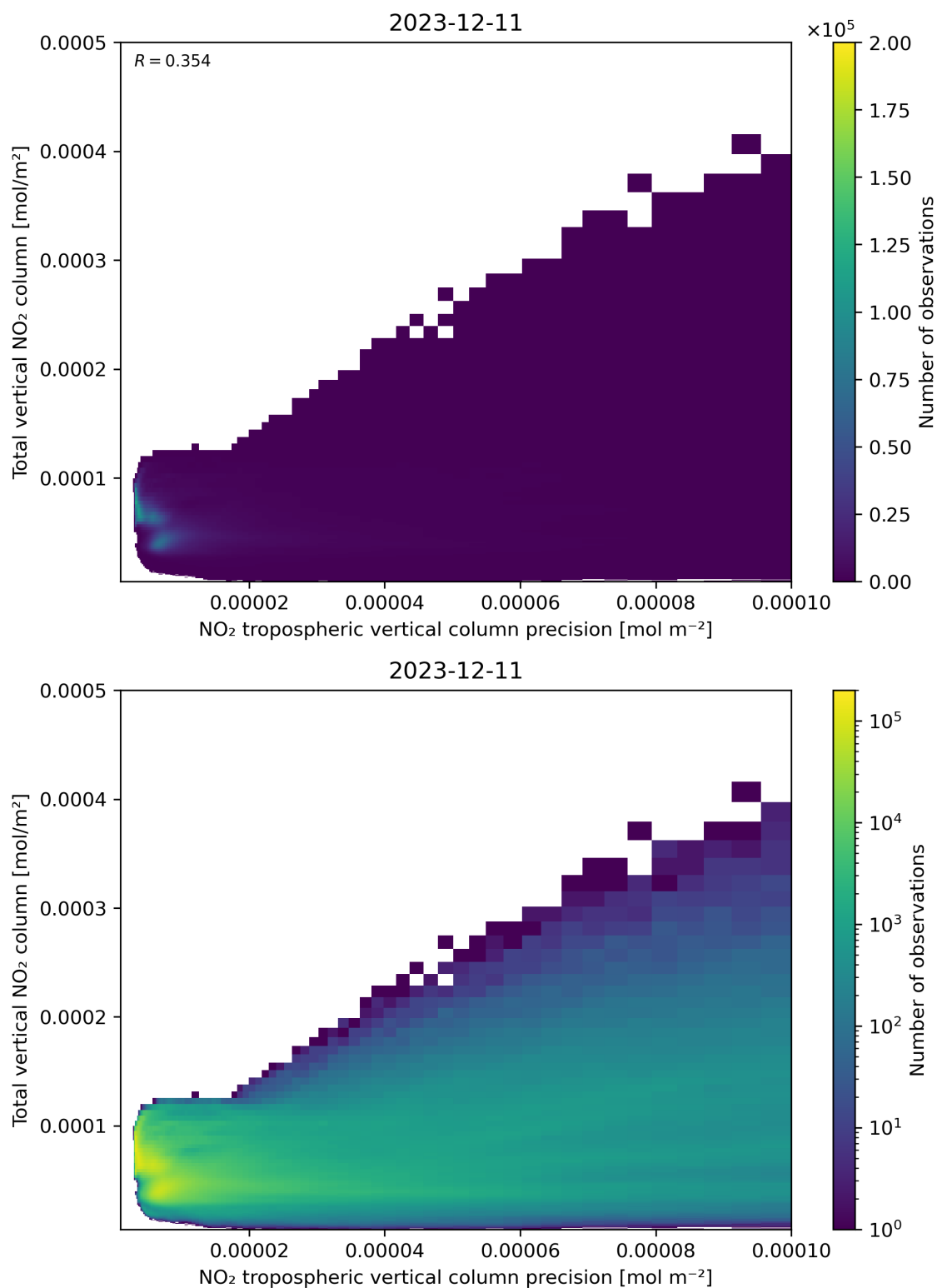
Figure 138: Scatter density plot of “NO 2 tropospheric vertical column precision” against “Total vertical NO 2 column” for 2023-12-10 to 2023-12-12.
