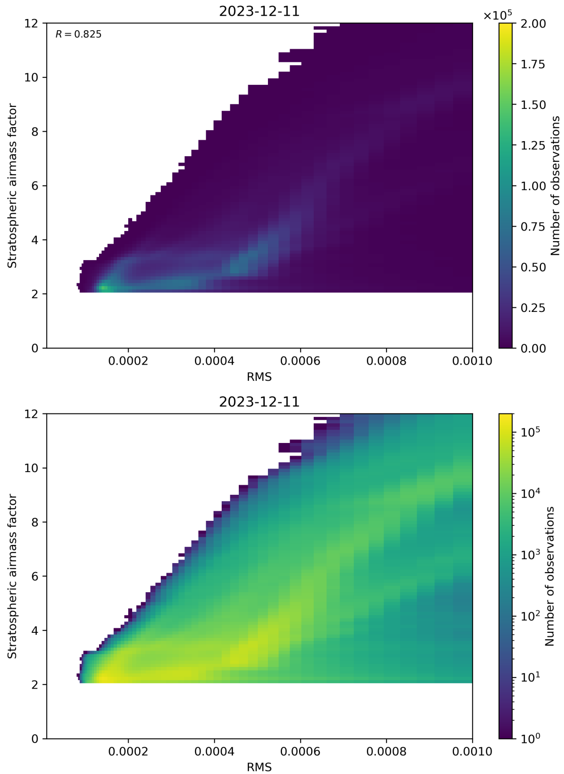
Figure 144: Scatter density plot of “RMS” against “Stratospheric airmass factor” for 2023-12-10 to 2023-12-12.
