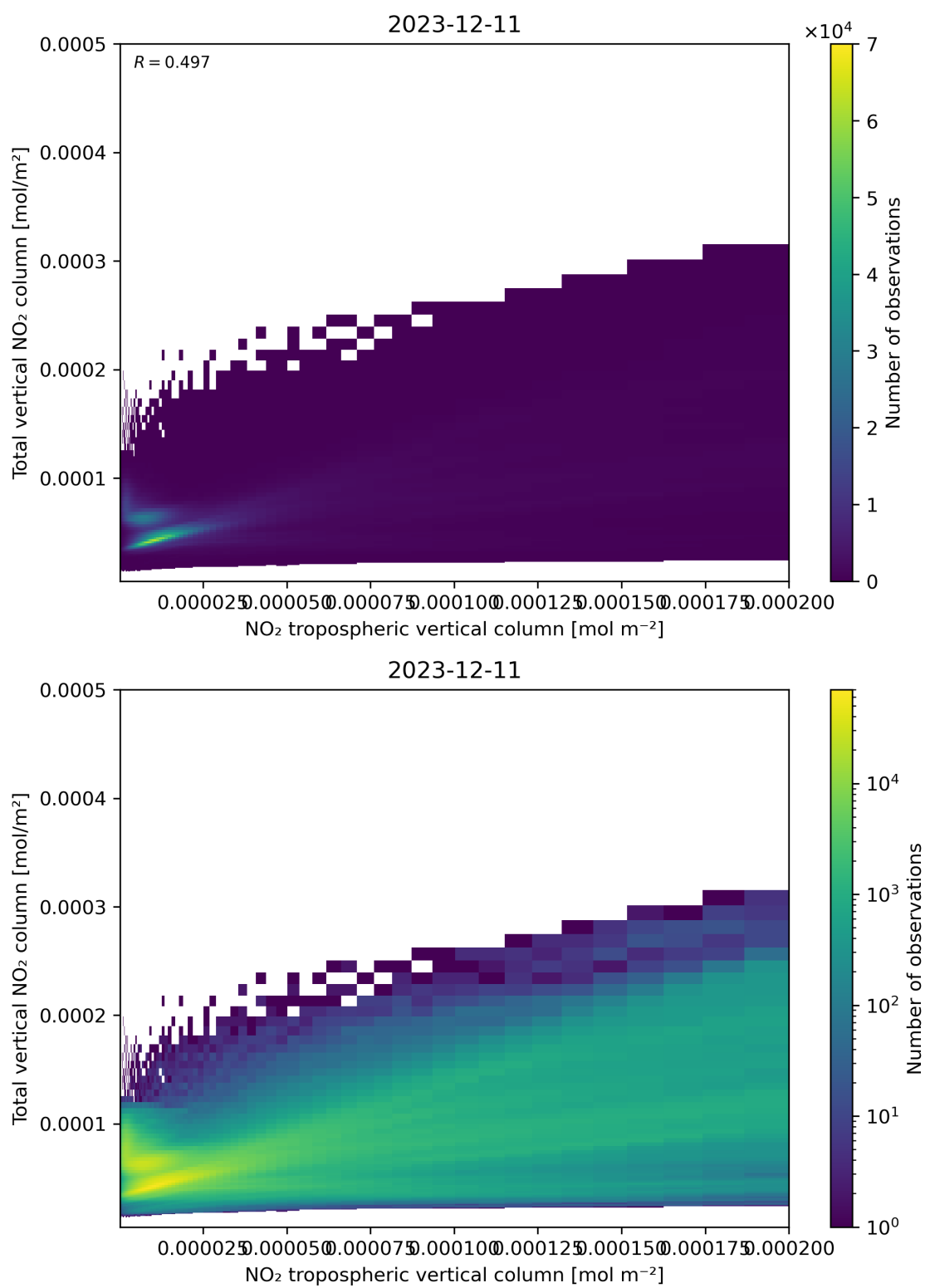
Figure 128: Scatter density plot of “NO 2 tropospheric vertical column” against “Total vertical NO 2 column” for 2023-12-10 to 2023-12-12.
