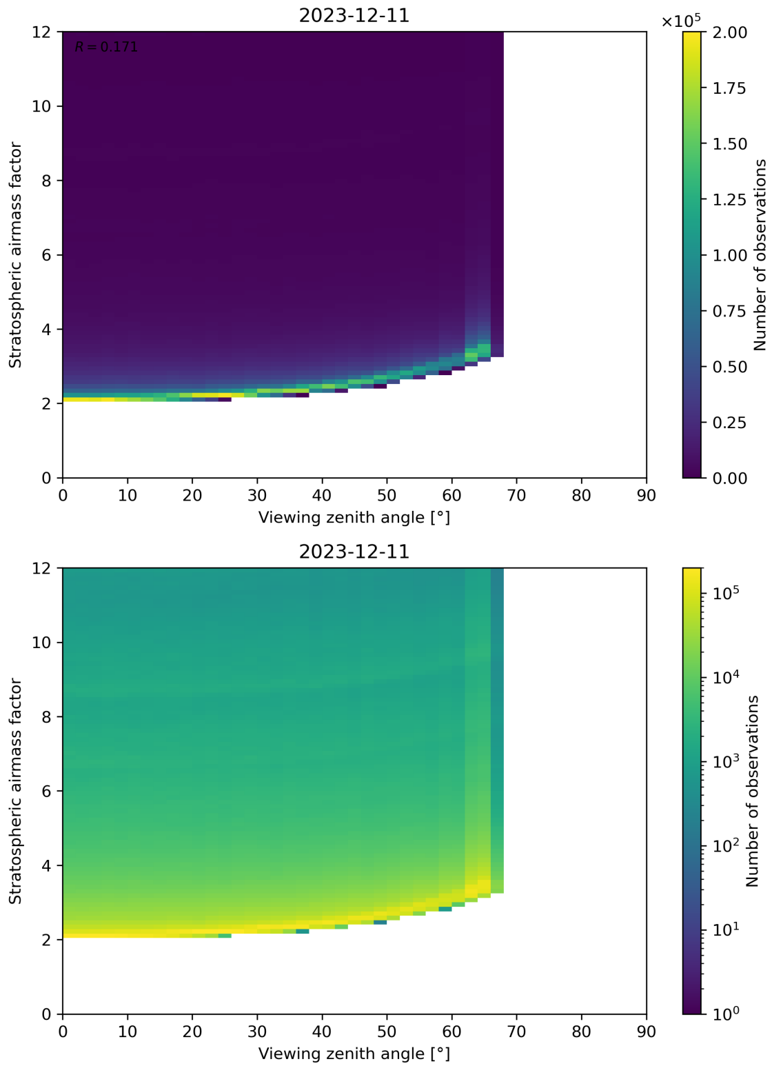
Figure 159: Scatter density plot of “Viewing zenith angle” against “Stratospheric airmass factor” for 2023-12-10 to 2023-12-12.
