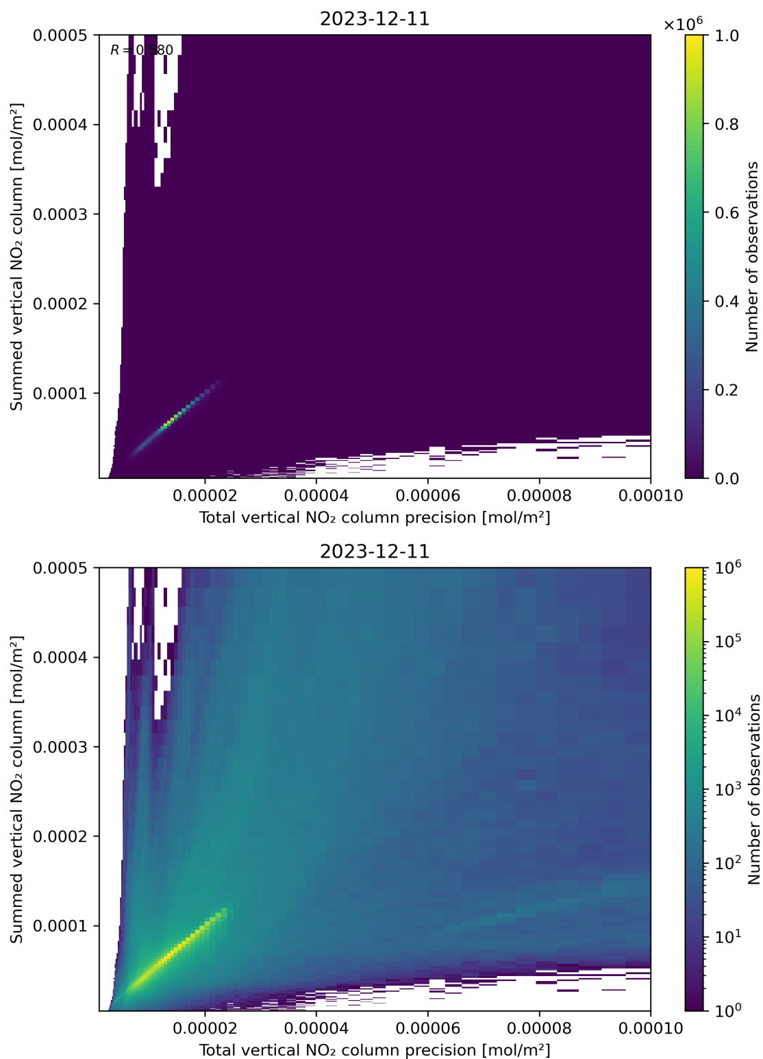
Figure 117: Scatter density plot of “Total vertical NO 2 column precision” against “Summed vertical NO 2 column” for 2023-12-10 to 2023-12-12.
