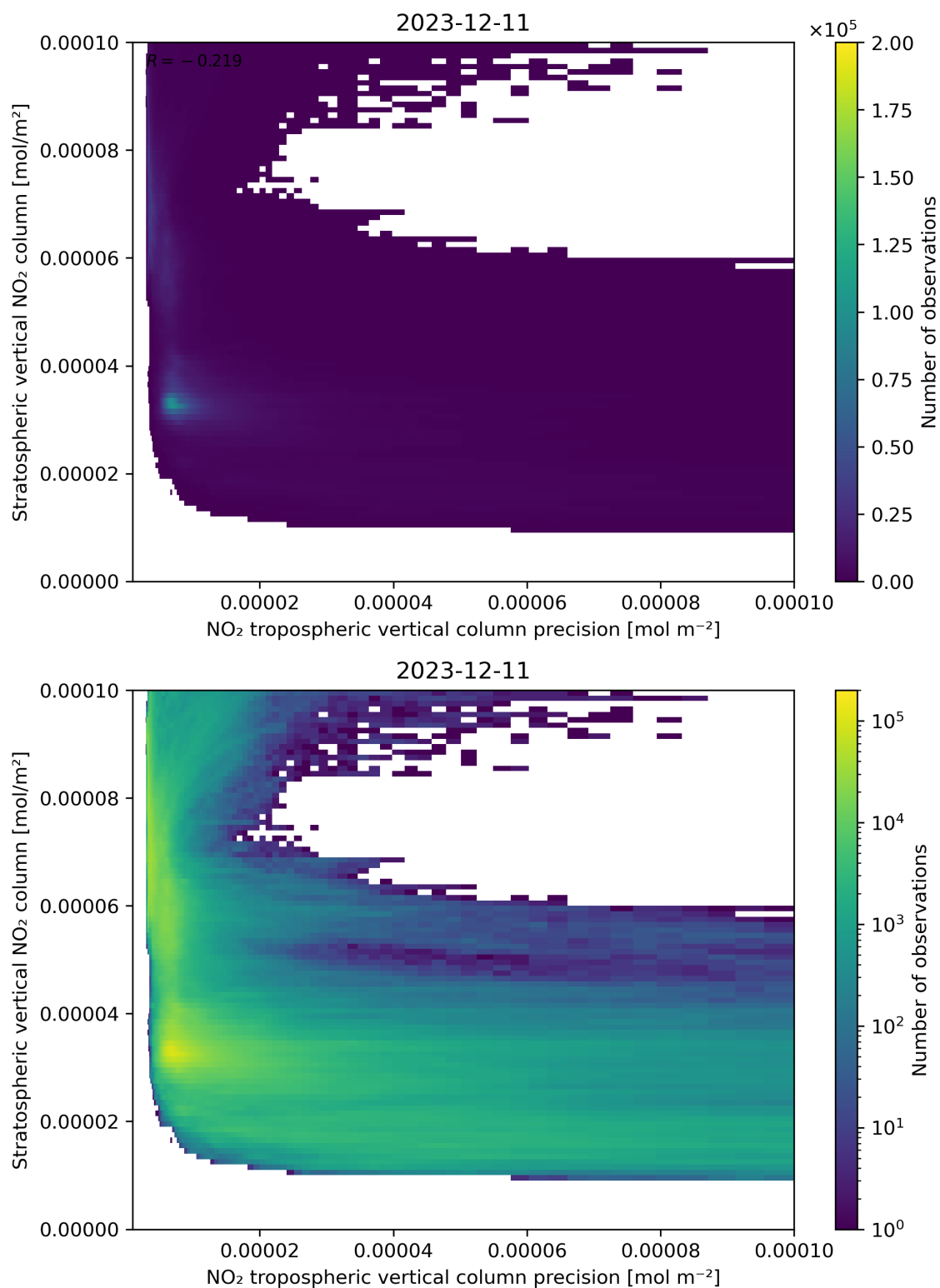
Figure 135: Scatter density plot of “NO 2 tropospheric vertical column precision” against “Stratospheric vertical NO 2 column” for 2023-12-10 to 2023-12-12.
