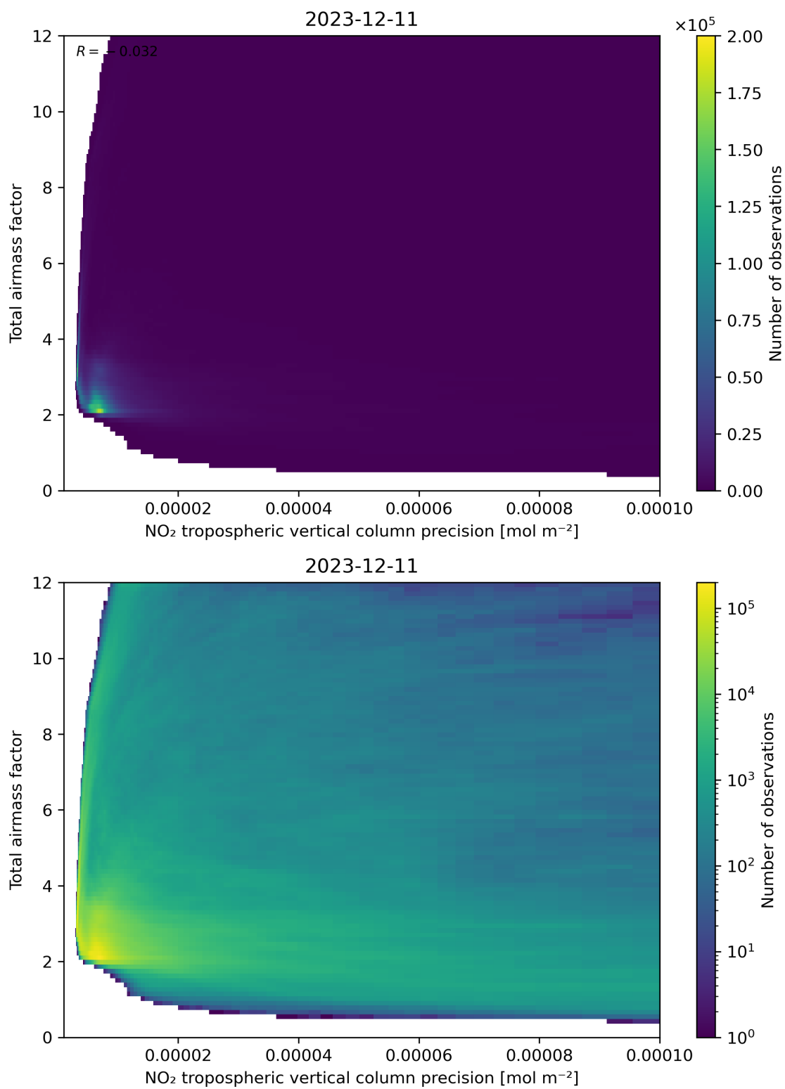
Figure 132: Scatter density plot of “NO 2 tropospheric vertical column precision” against “Total air mass factor” for 2023-12-10 to 2023-12-12.
