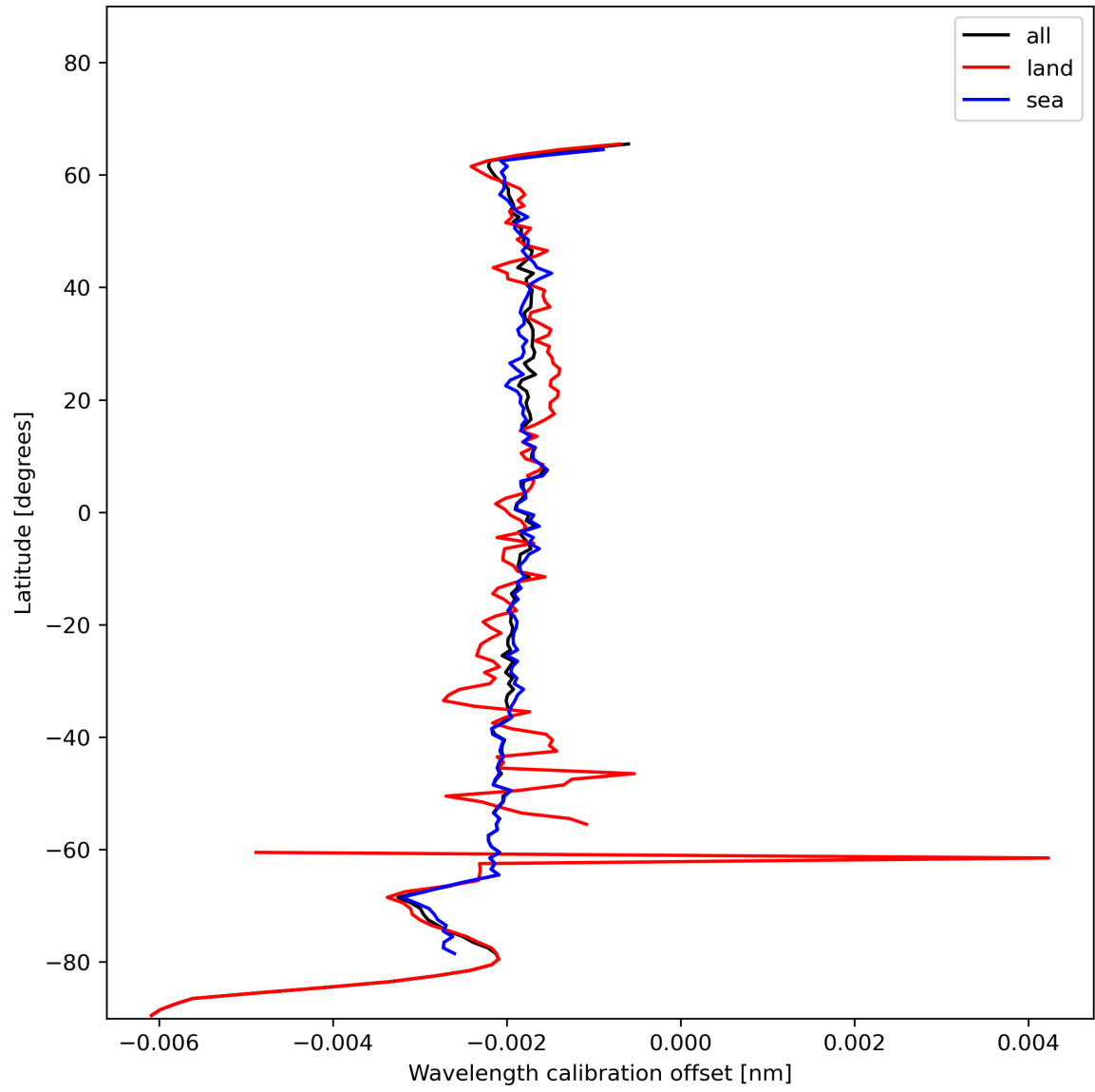
Figure 18: Zonal average of “Wavelength calibration offset” for 2023-12-10 to 2023-12-12.
