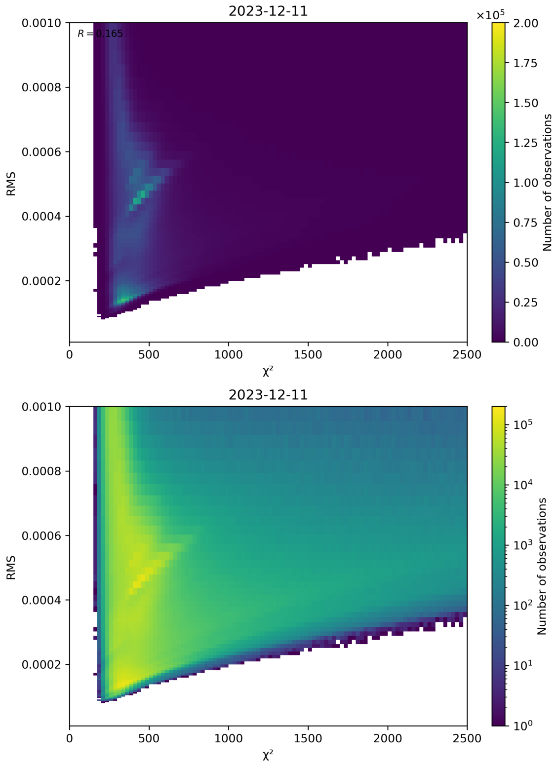
Figure 82: Scatter density plot of “ \chi^2 ” against “RMS” for 2023-12-10 to 2023-12-12.
