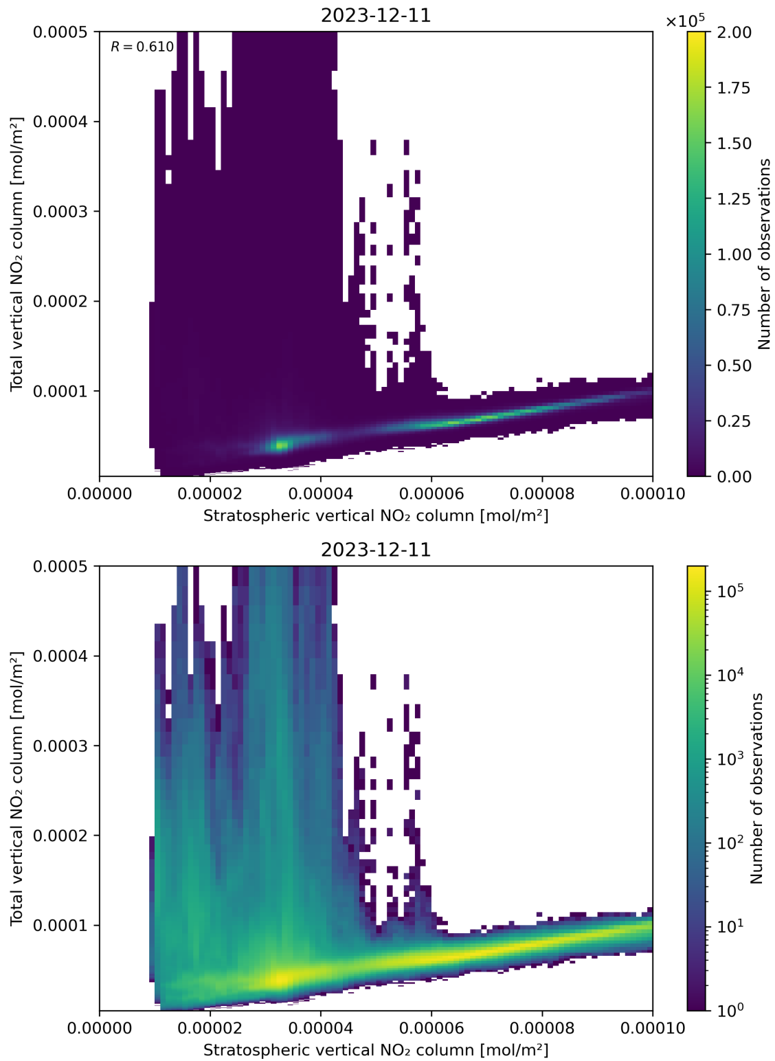
Figure 100: Scatter density plot of “Stratospheric vertical NO 2 column” against “Total vertical NO 2 column” for 2023-12-10 to 2023-12-12.
