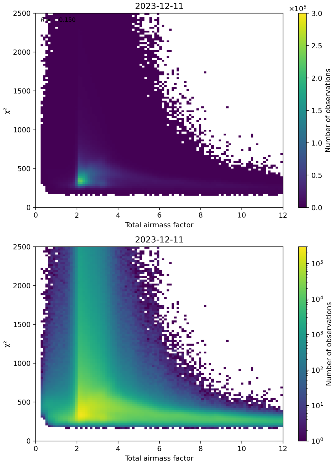
Figure 63: Scatter density plot of “Total airmass factor” against “ \chi^2 ” for 2023-12-10 to 2023-12-12.
