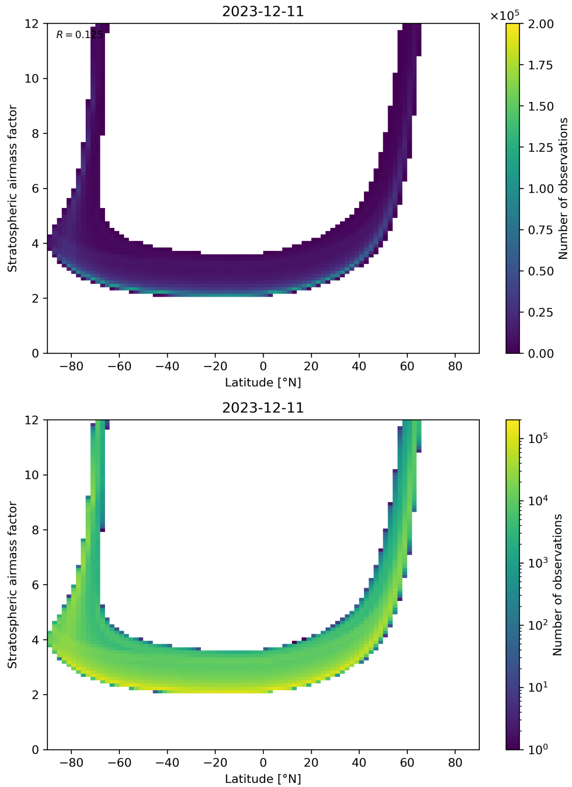
Figure 83: Scatter density plot of “Latitude” against “Stratospheric air mass factor” for 2023-12-10 to 2023-12-12.
