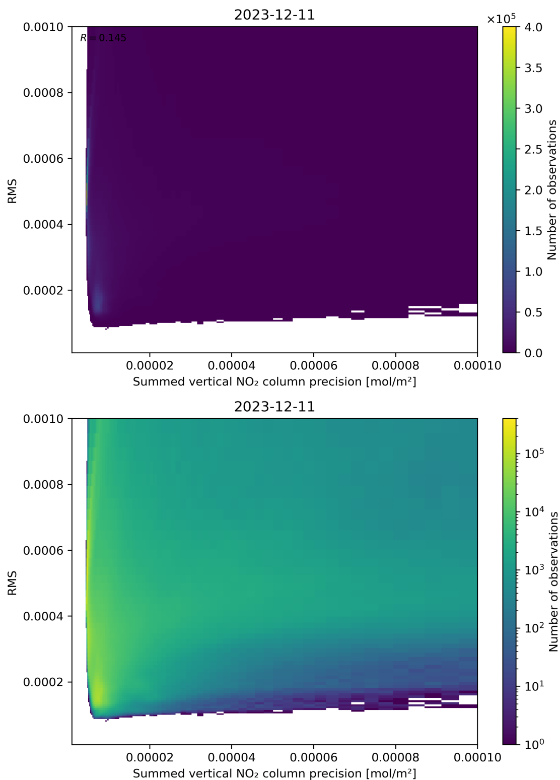
Figure 108: Scatter density plot of “Summed vertical NO 2 column precision” against “RMS” for 2023-12-10 to 2023-12-12.
