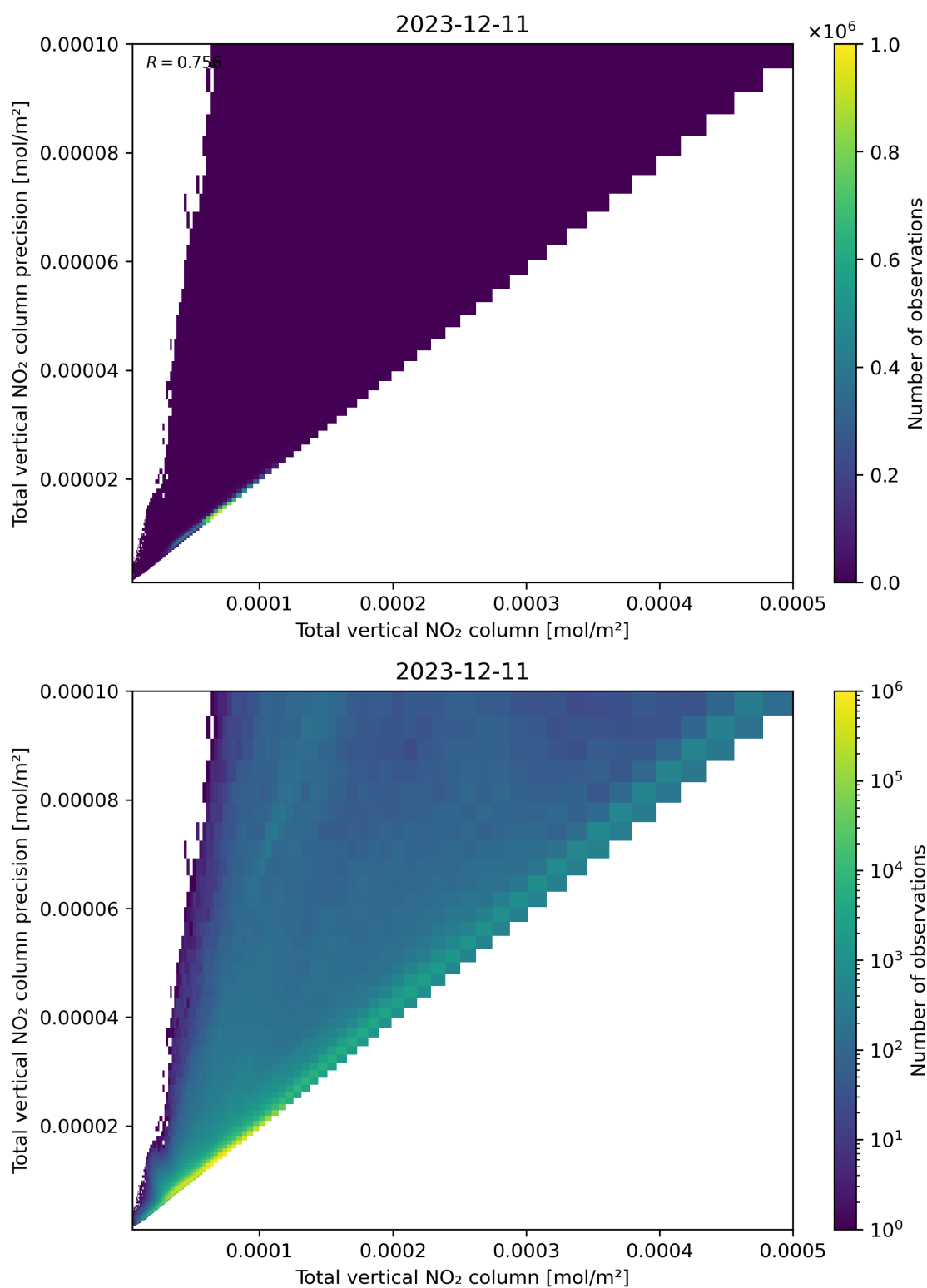
Figure 114: Scatter density plot of “Total vertical NO 2 column” against “Total vertical NO 2 column precision” for 2023-12-10 to 2023-12-12.
