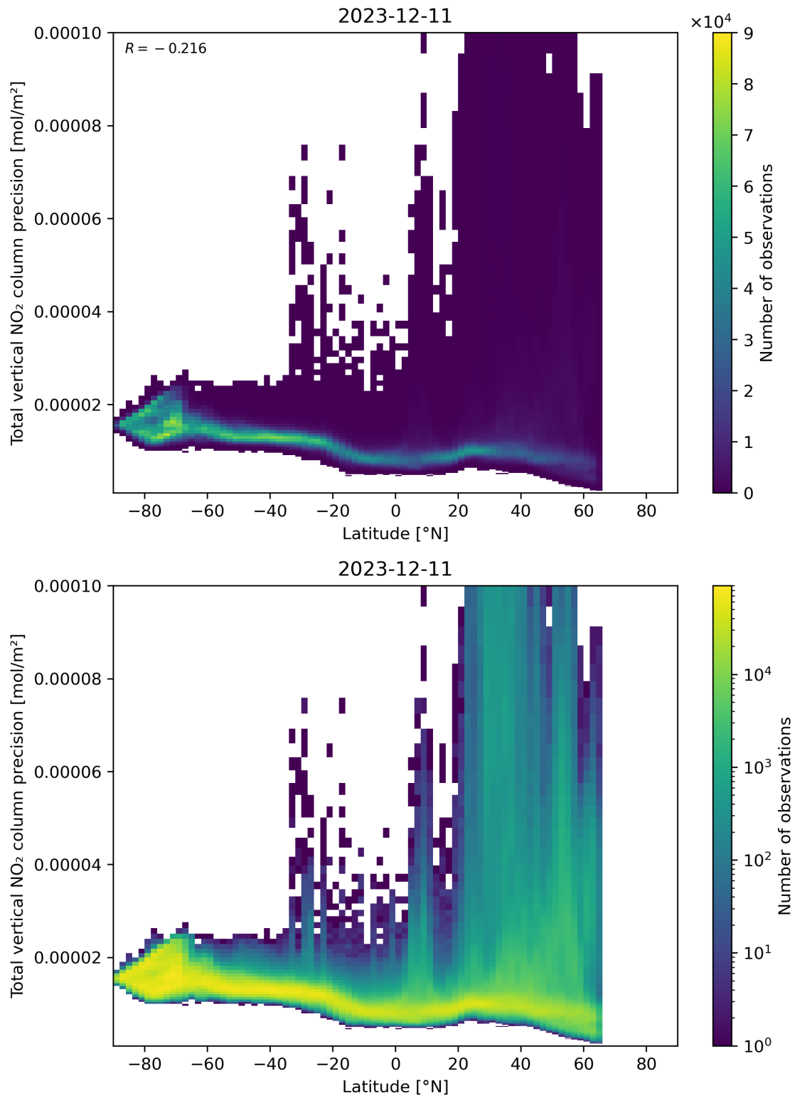
Figure 91: Scatter density plot of “Latitude” against “Total vertical NO 2 column precision” for 2023-12-10 to 2023-12-12.
