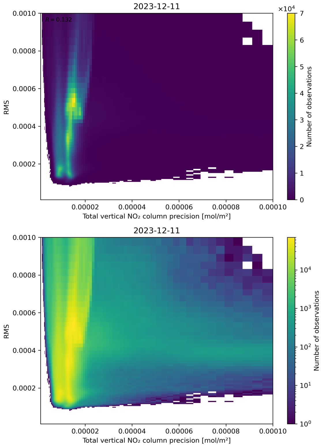
Figure 119: Scatter density plot of “Total vertical NO 2 column precision” against “RMS” for 2023-12-10 to 2023-12-12.
