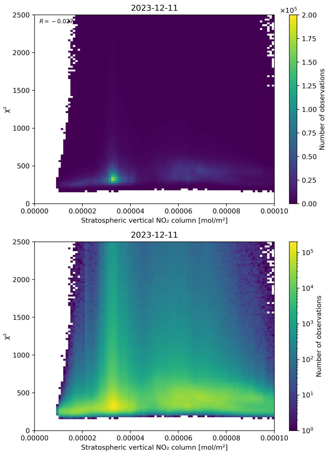
Figure 97: Scatter density plot of “Stratospheric vertical NO 2 column” against “ \chi^2 ” for 2023-12-10 to 2023-12-12.
