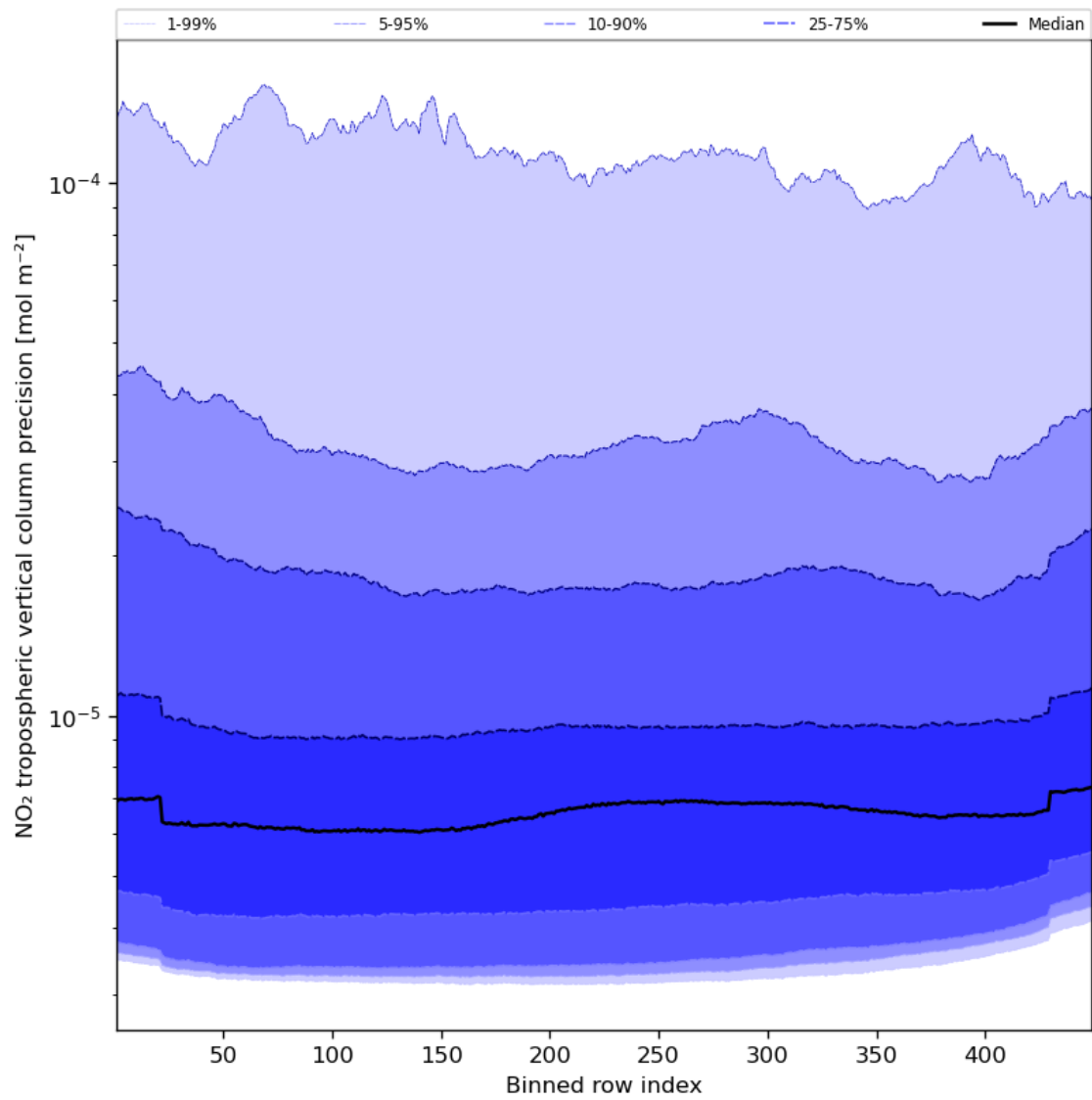
Figure 47: Along track statistics of “NO 2 tropospheric vertical column precision” for 2023-12-10 to 2023-12-12
