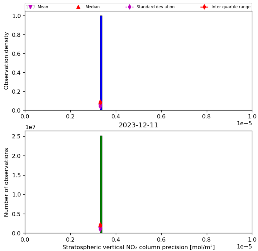
Figure 37: Histogram of “Stratospheric vertical NO 2 column precision” for 2023-12-10 to 2023-12-12
