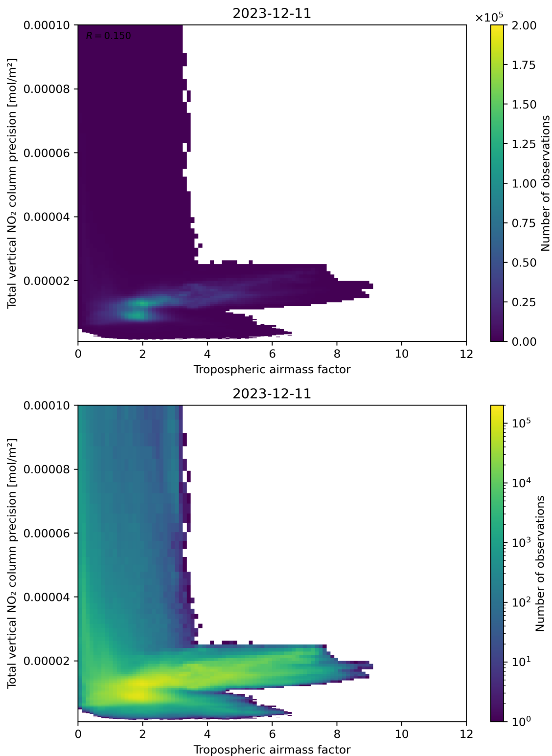
Figure 78: Scatter density plot of “Tropospheric air mass factor” against “Total vertical NO 2 column precision” for 2023-12-10 to 2023-12-12.
