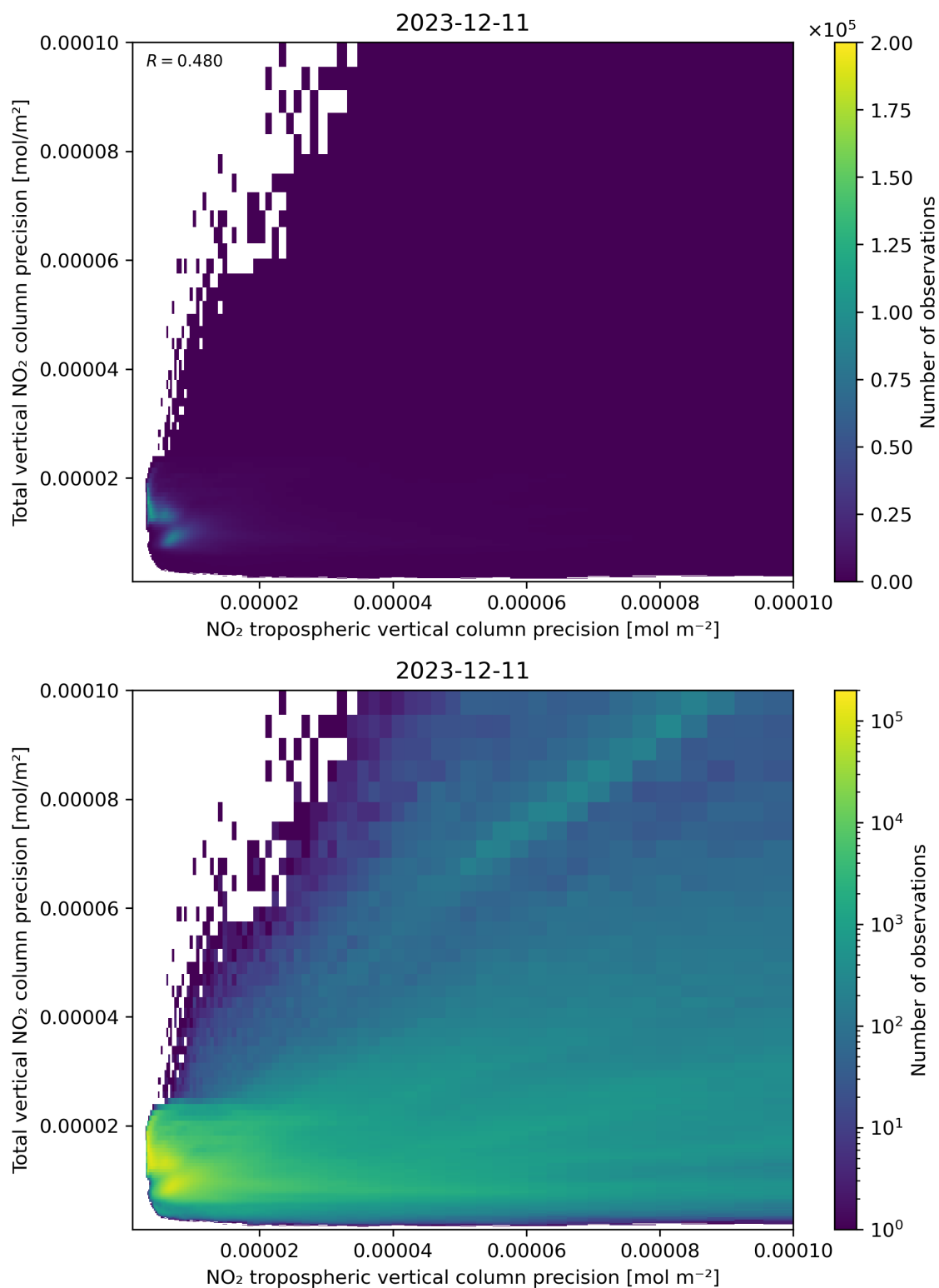
Figure 139: Scatter density plot of “NO 2 tropospheric vertical column precision” against “Total vertical NO 2 column precision” for 2023-12-10 to 2023-12-12.
