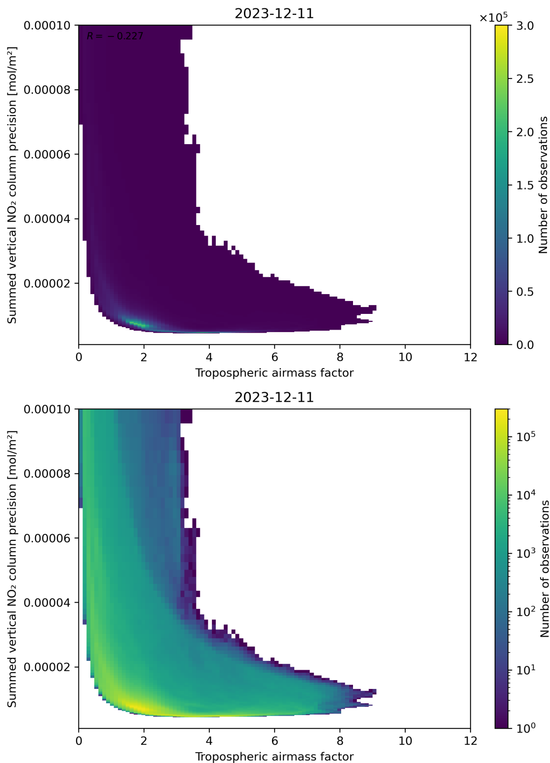
Figure 76: Scatter density plot of “Tropospheric air mass factor” against “Summed vertical NO 2 column precision” for 2023-12-10 to 2023-12-12.
