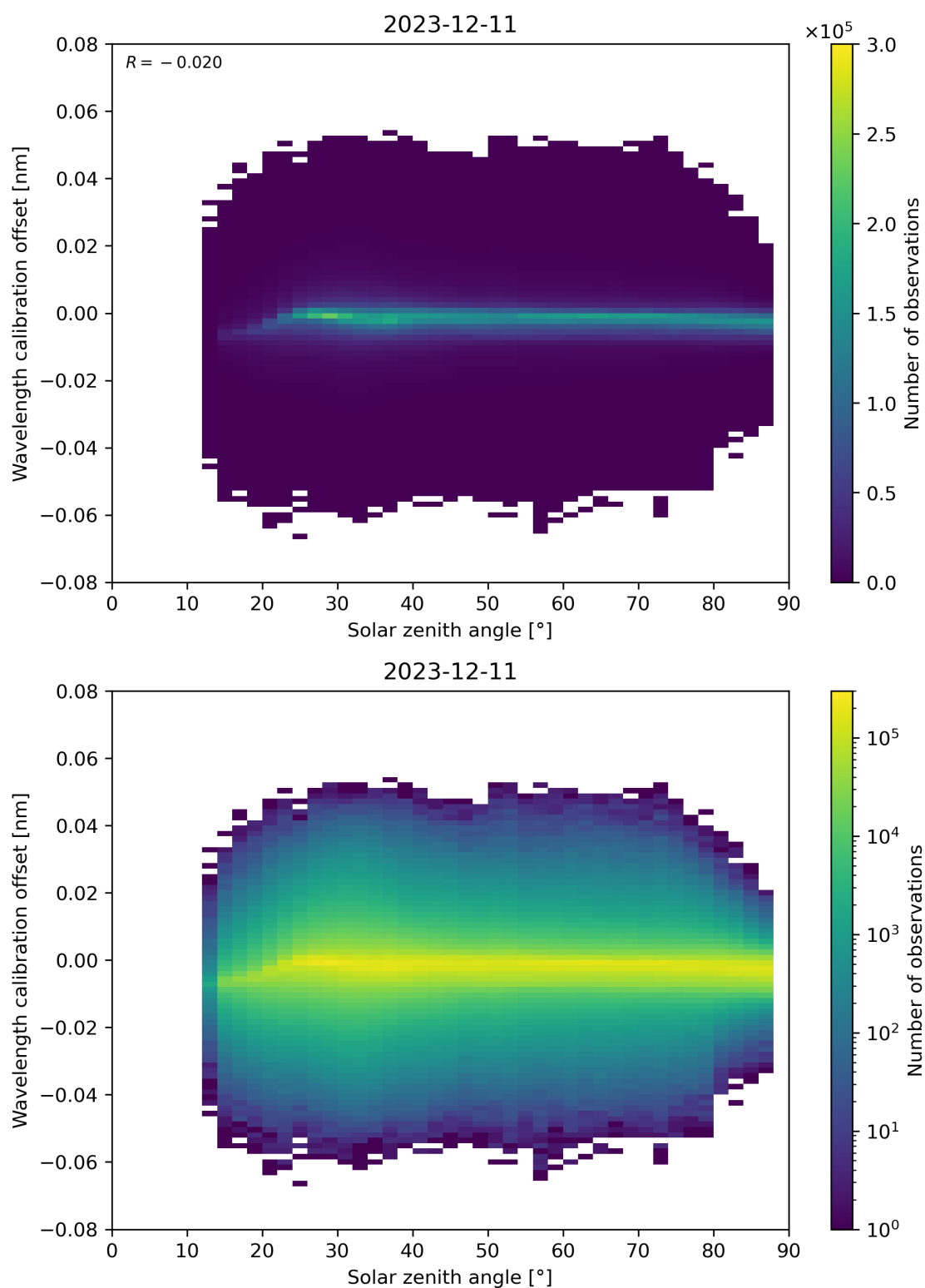
Figure 158: Scatter density plot of “Solar zenith angle” against “Wavelength calibration offset” for 2023-12-10 to 2023-12-12.
