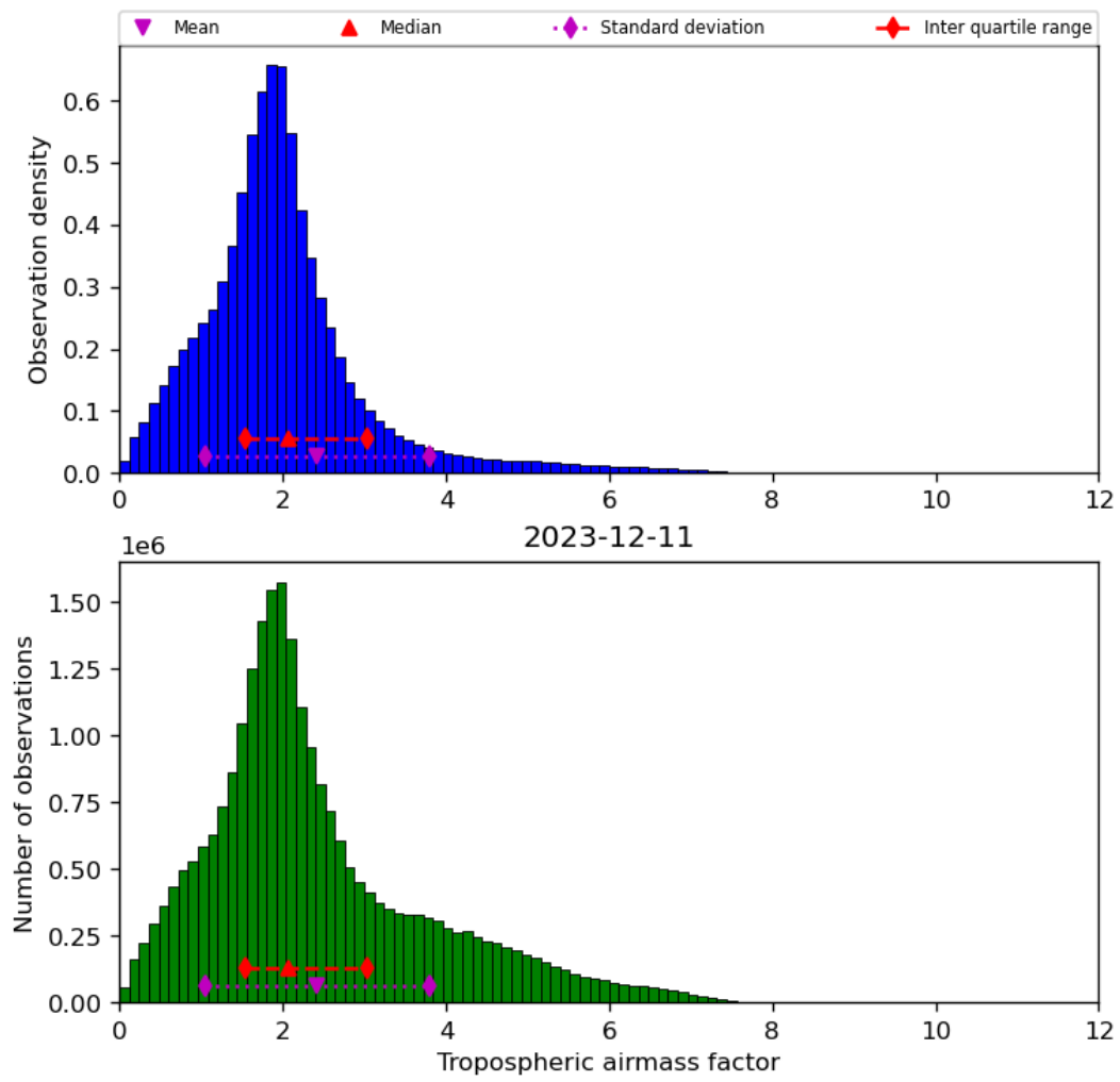
Figure 31: Histogram of “Tropospheric airmass factor” for 2023-12-10 to 2023-12-12
