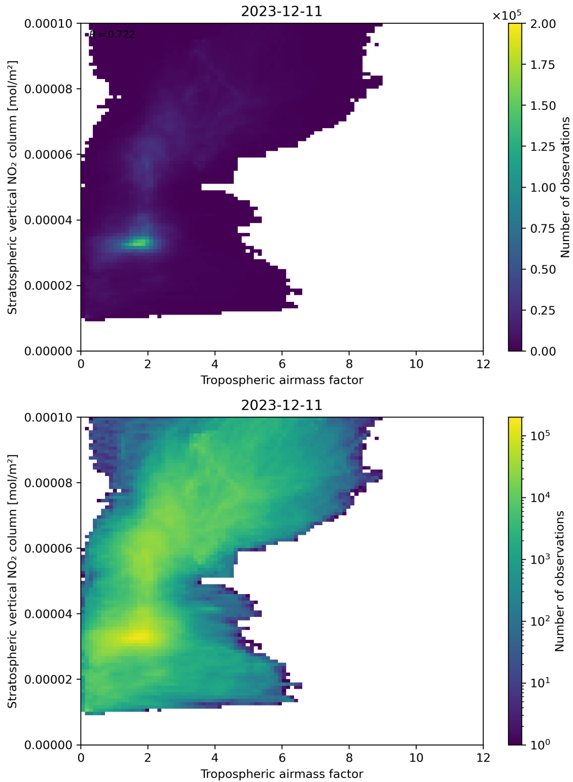
Figure 74: Scatter density plot of “Tropospheric air mass factor” against “Stratospheric vertical NO 2 column” for 2023-12-10 to 2023-12-12.
