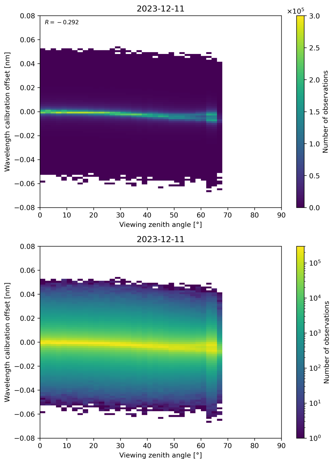
Figure 173: Scatter density plot of “Viewing zenith angle” against “Wavelength calibration offset” for 2023-12-10 to 2023-12-12.
