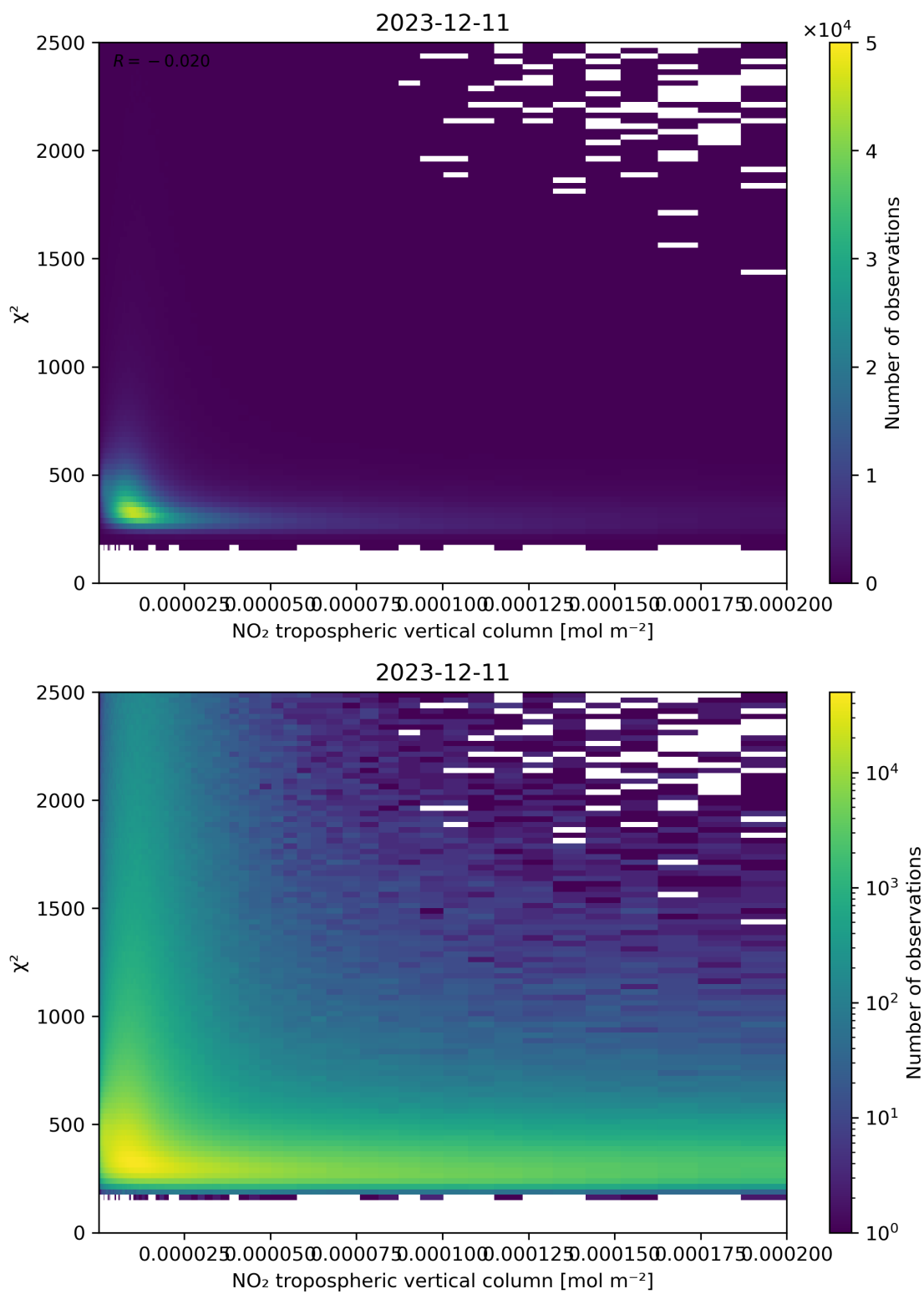
Figure 124: Scatter density plot of “NO 2 tropospheric vertical column” against “ \chi^2 ” for 2023-12-10 to 2023-12-12.
