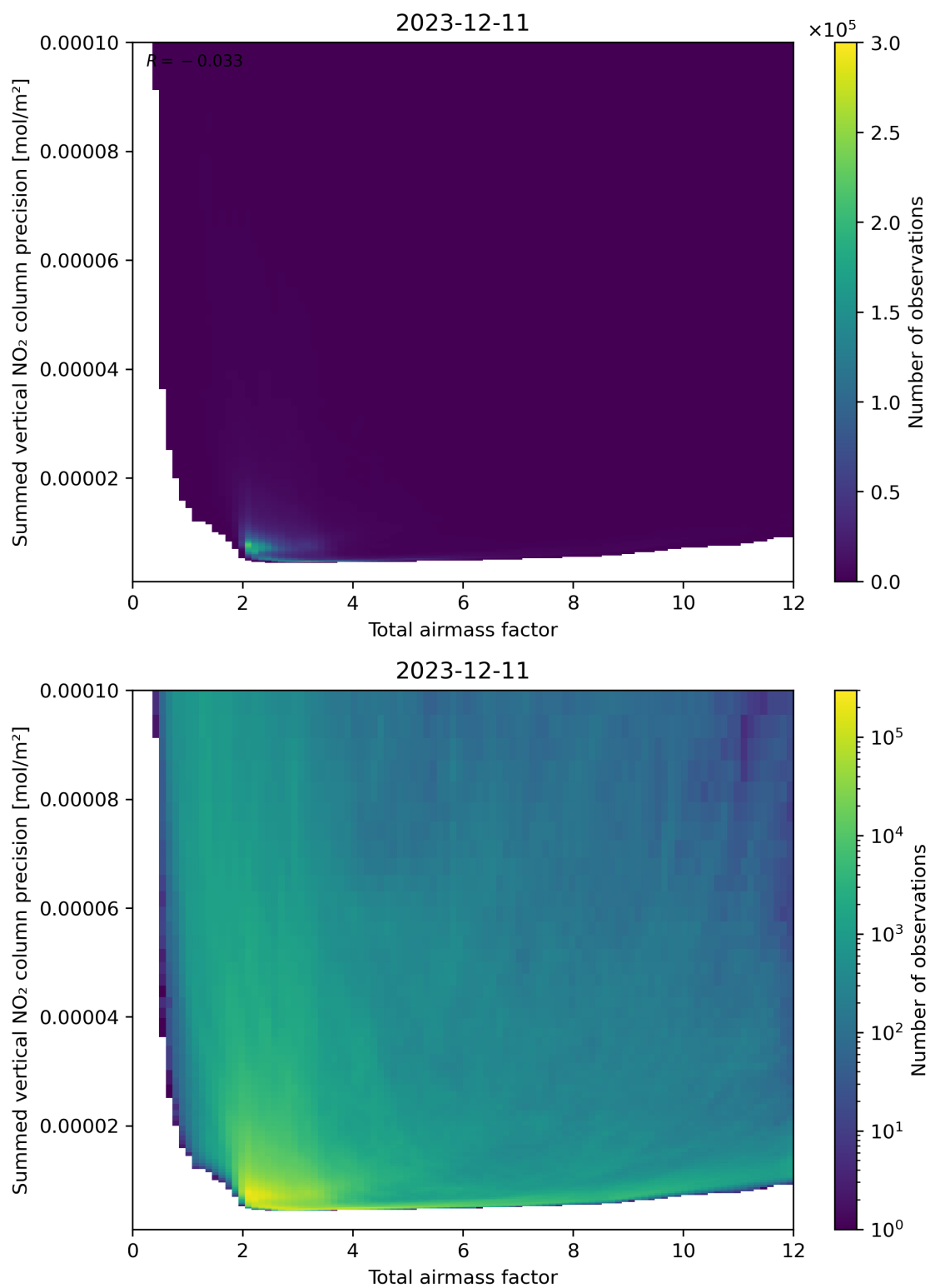
Figure 66: Scatter density plot of “Total airmass factor” against “Summed vertical NO 2 column precision” for 2023-12-10 to 2023-12-12.
