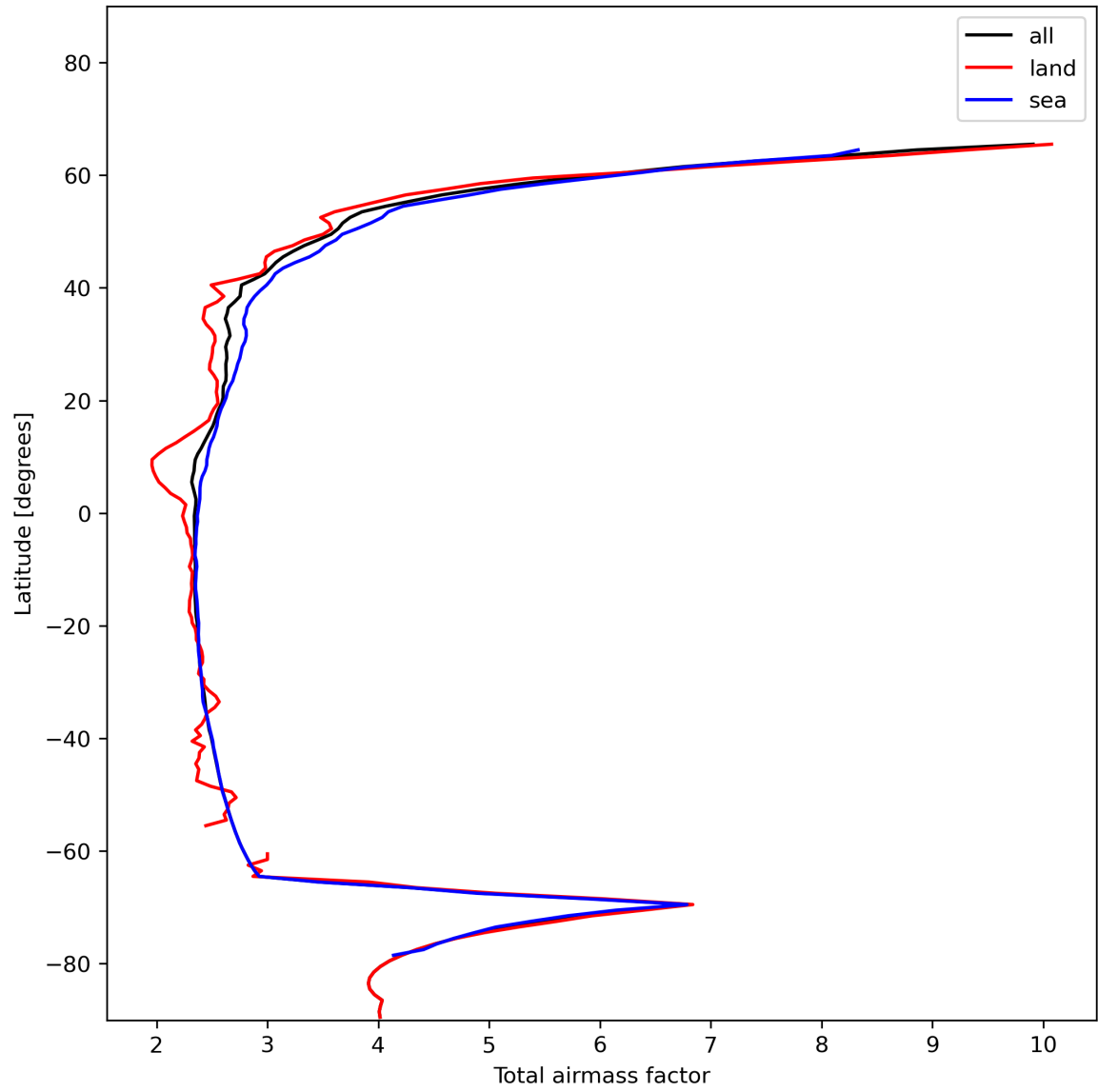
Figure 15: Zonal average of “Total airmass factor” for 2023-12-10 to 2023-12-12.
