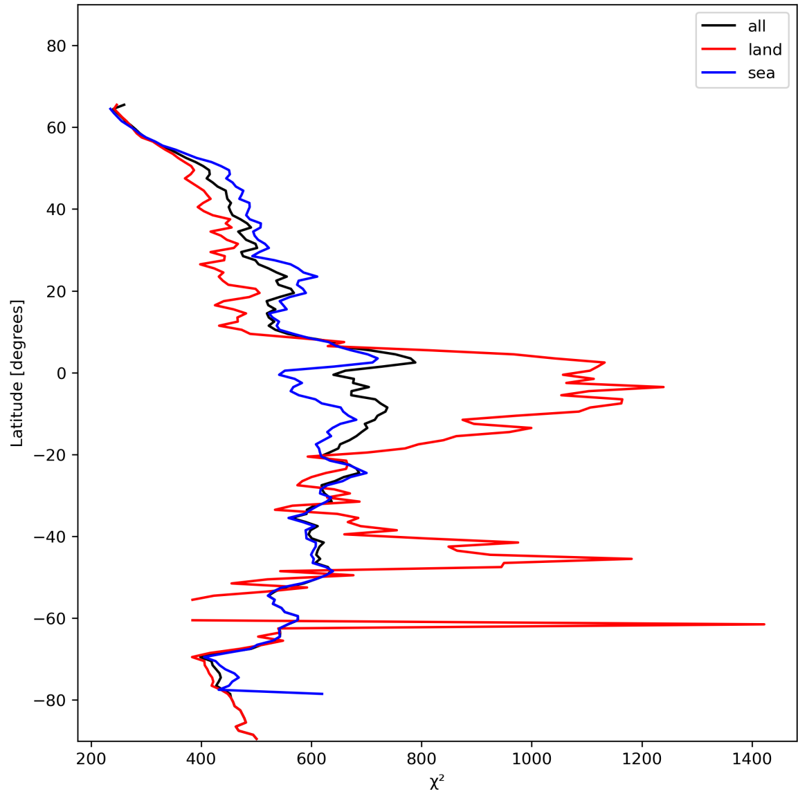
Figure 25: Zonal average of “ \chi^2 ” for 2023-12-10 to 2023-12-12.
