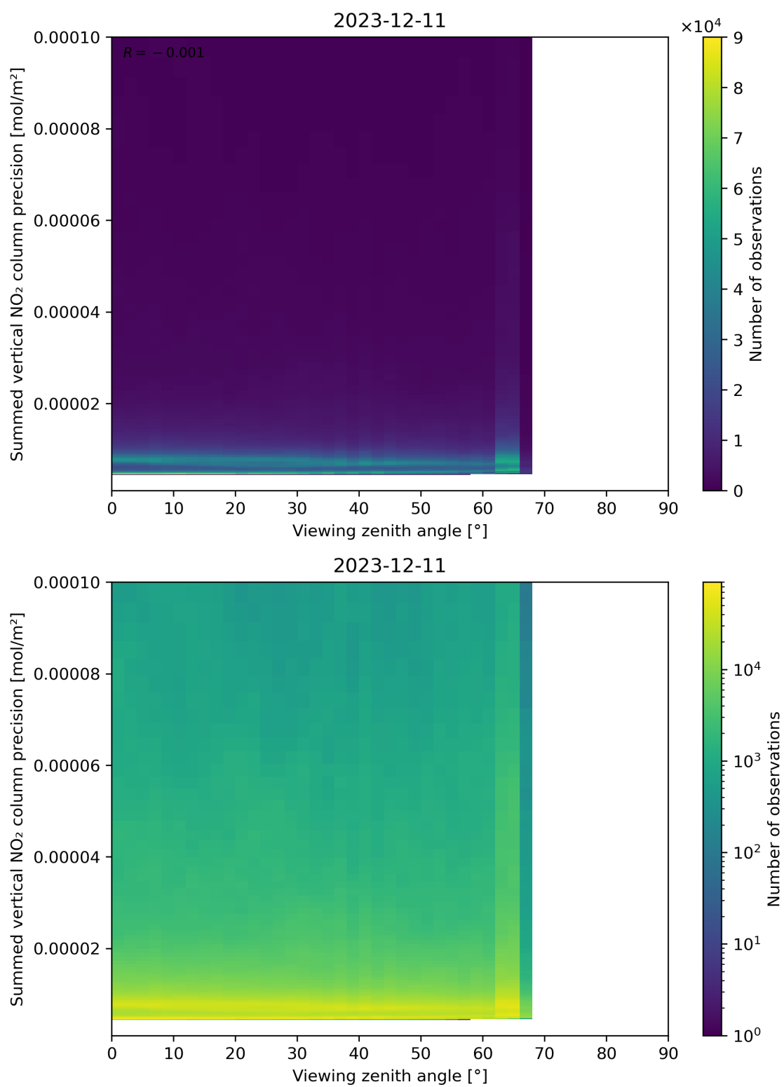
Figure 166: Scatter density plot of “Viewing zenith angle” against “Summed vertical NO 2 column precision” for 2023-12-10 to 2023-12-12.
