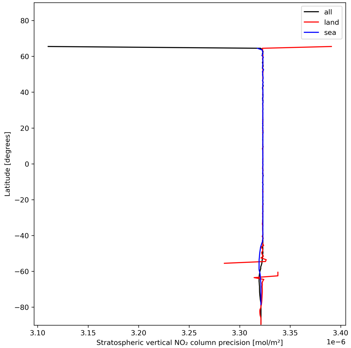
Figure 20: Zonal average of “Stratospheric vertical NO 2 column precision” for 2023-12-10 to 2023-12-12.
