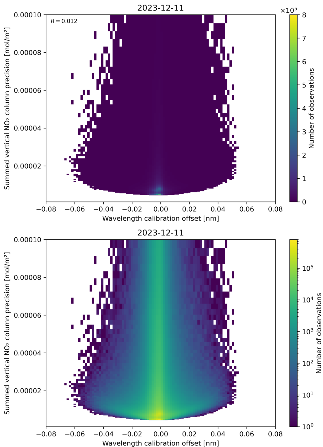
Figure 178: Scatter density plot of “Wavelength calibration offset” against “Summed vertical NO 2 column precision” for 2023-12-10 to 2023-12-12.
