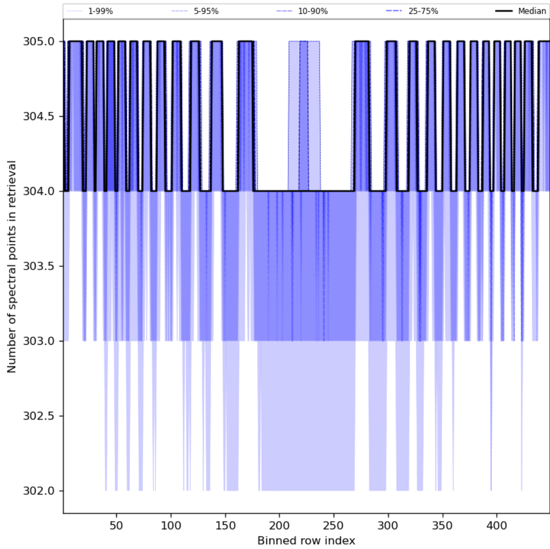
Figure 50: Along track statistics of “Number of spectral points in retrieval” for 2023-12-10 to 2023-12-12
