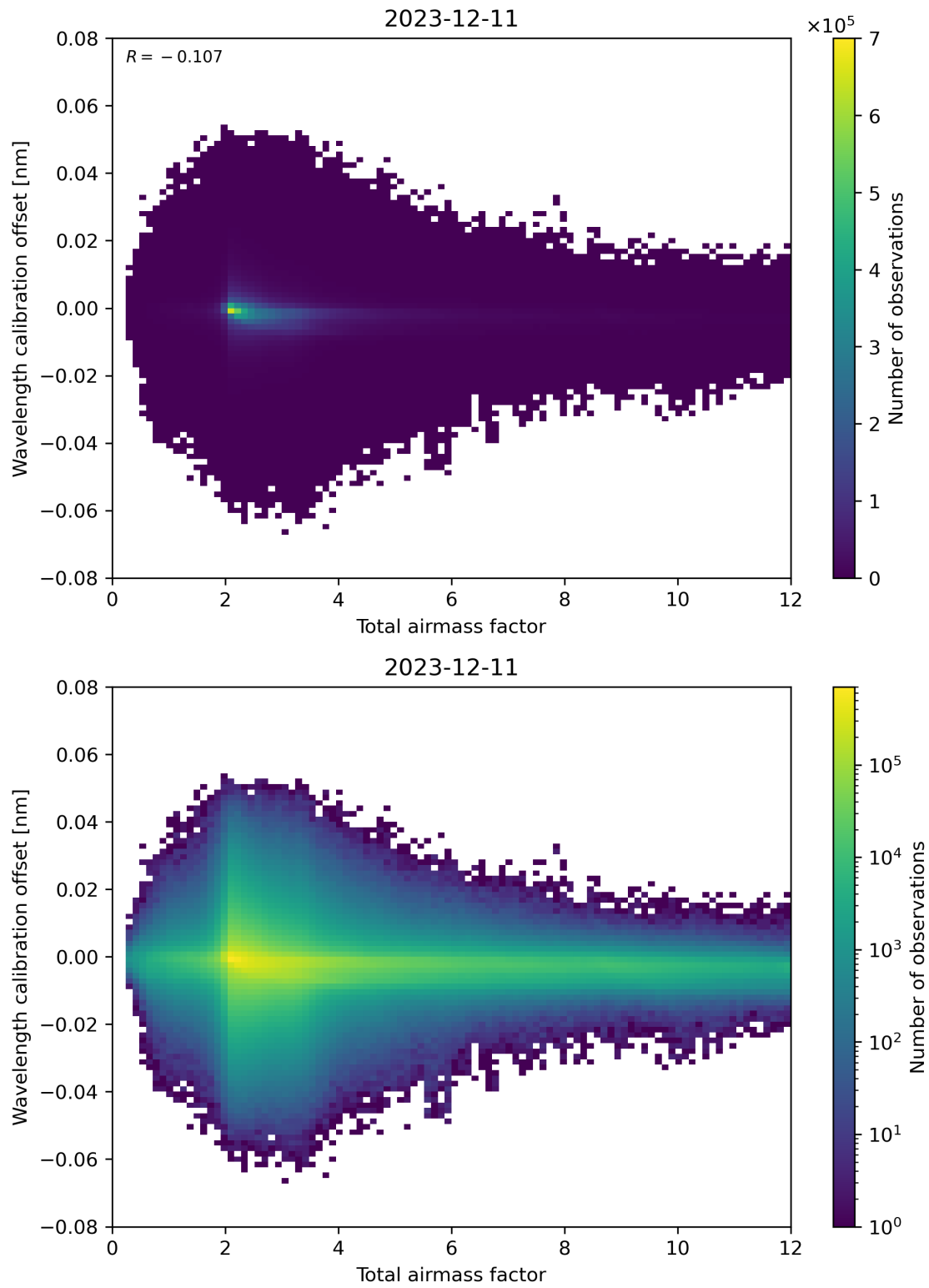
Figure 70: Scatter density plot of “Total airmass factor” against “Wavelength calibration offset” for 2023-12-10 to 2023-12-12.
