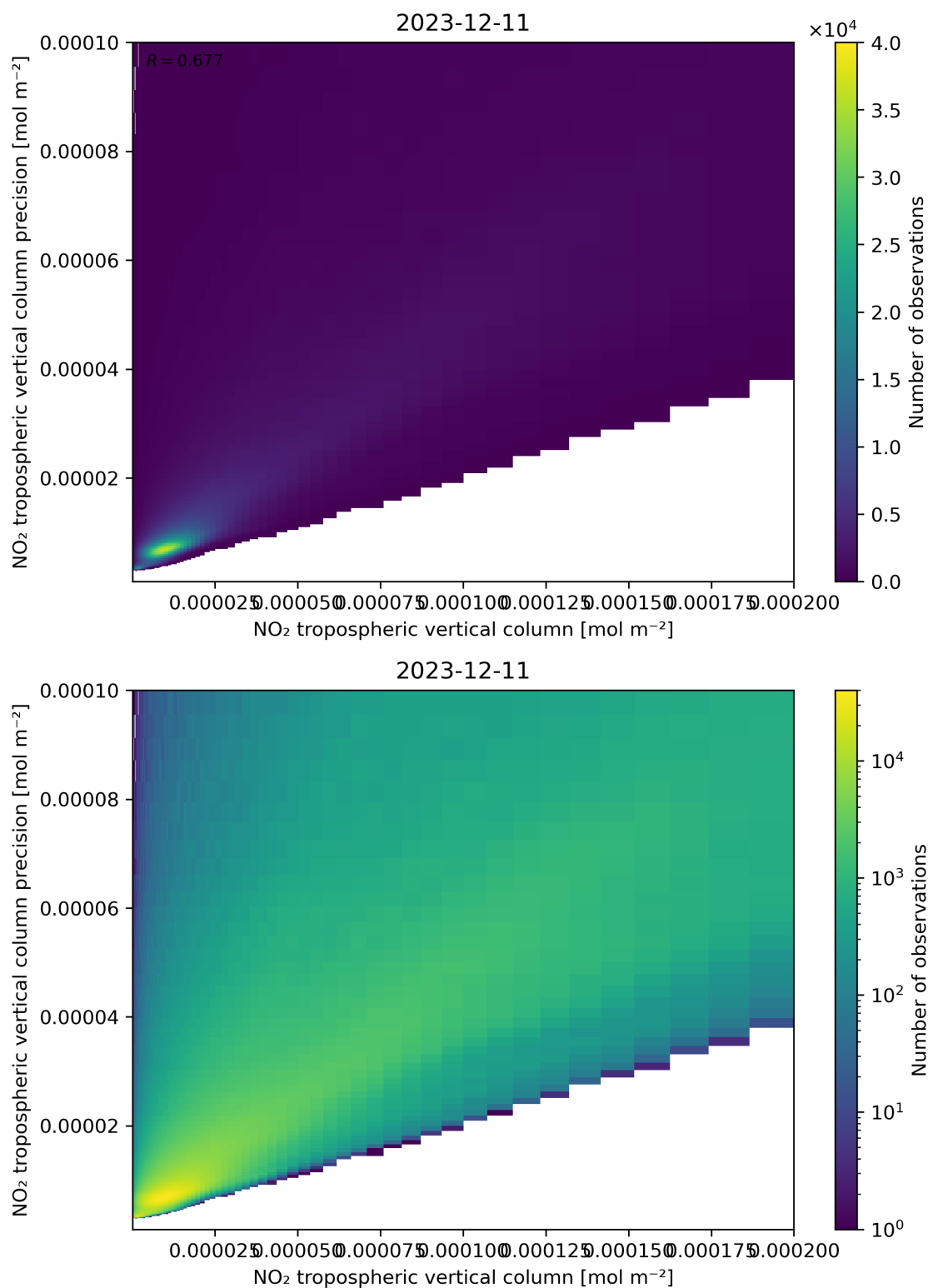
Figure 130: Scatter density plot of “NO 2 tropospheric vertical column” against “NO 2 tropospheric vertical column precision” for 2023-12-10 to 2023-12-12.
