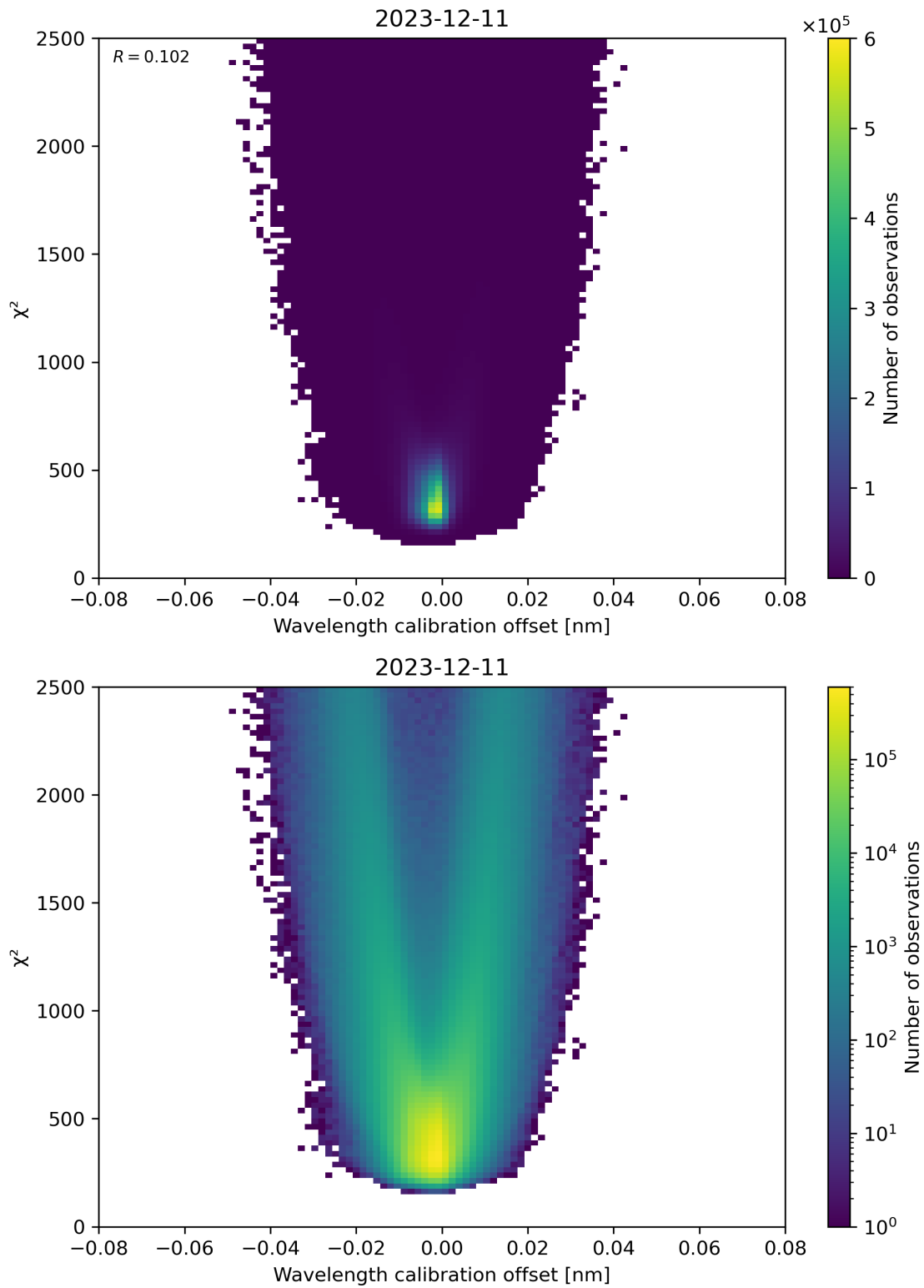
Figure 175: Scatter density plot of “Wavelength calibration offset” against “ \chi^2 ” for 2023-12-10 to 2023-12-12.
