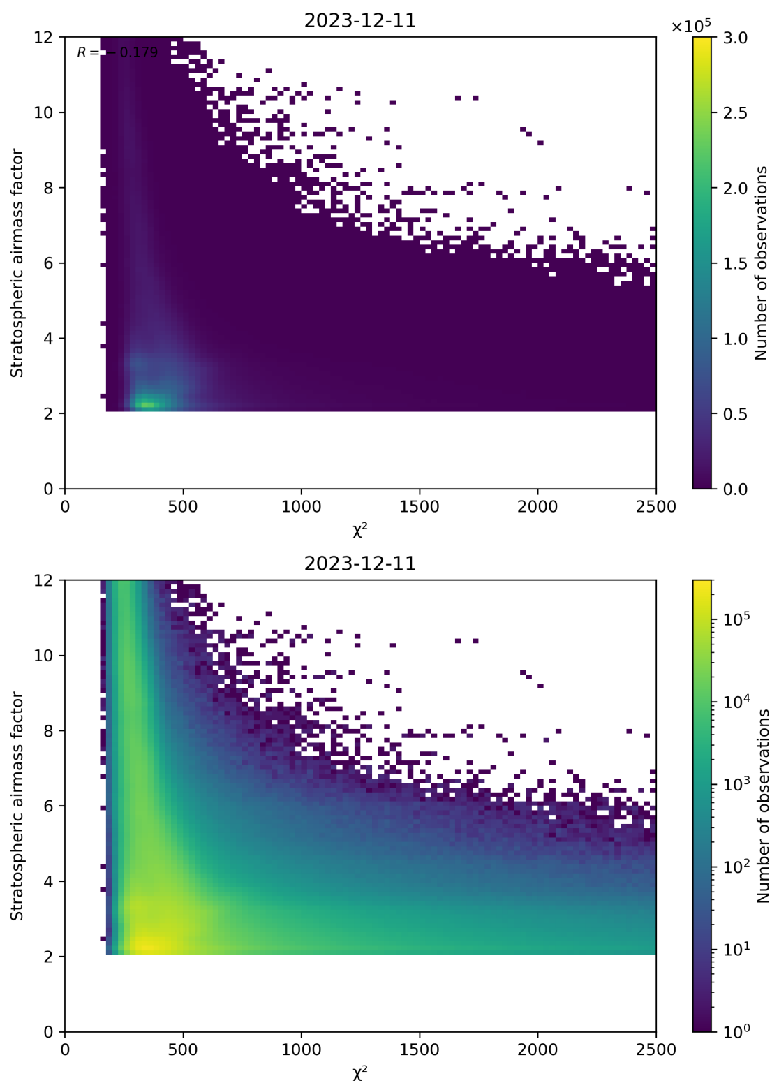
Figure 81: Scatter density plot of “ \chi^2 ” against “Stratospheric airmass factor” for 2023-12-10 to 2023-12-12.
