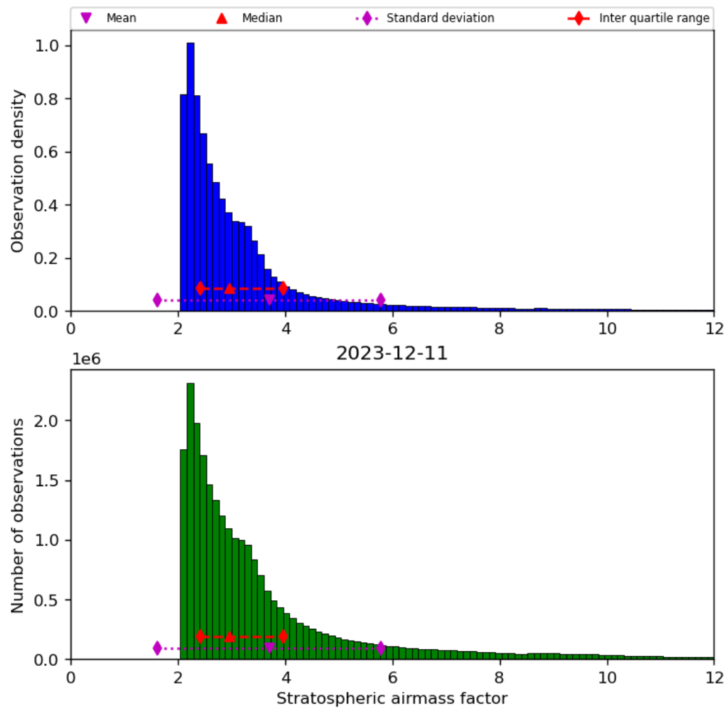
Figure 44: Histogram of “Stratospheric airmass factor” for 2023-12-10 to 2023-12-12
