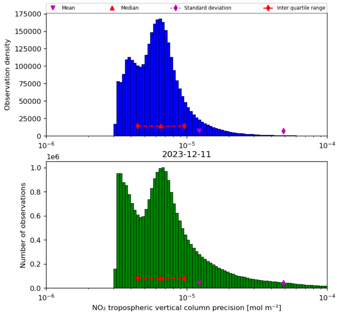
Figure 30: Histogram of “NO 2 tropospheric vertical column precision” for 2023-12-10 to 2023-12-12
