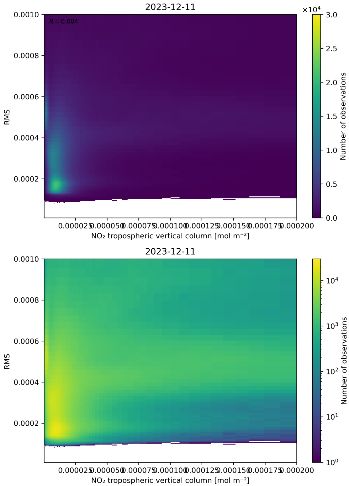
Figure 142: Scatter density plot of “NO 2 tropospheric vertical column” against “RMS” for 2023-12-10 to 2023-12-12.
