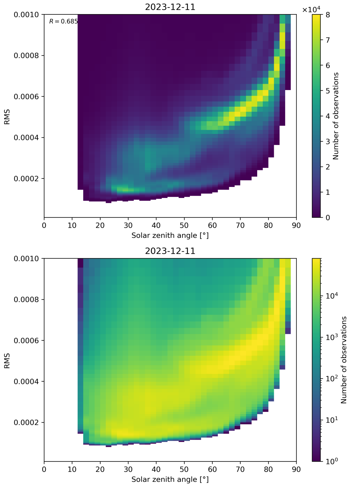
Figure 157: Scatter density plot of “Solar zenith angle” against “RMS” for 2023-12-10 to 2023-12-12.
