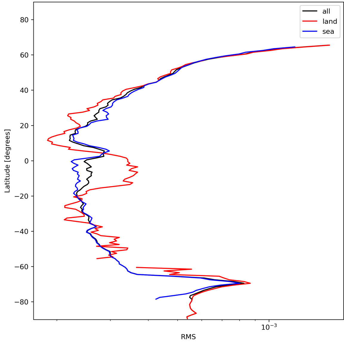
Figure 26: Zonal average of “RMS” for 2023-12-10 to 2023-12-12.
