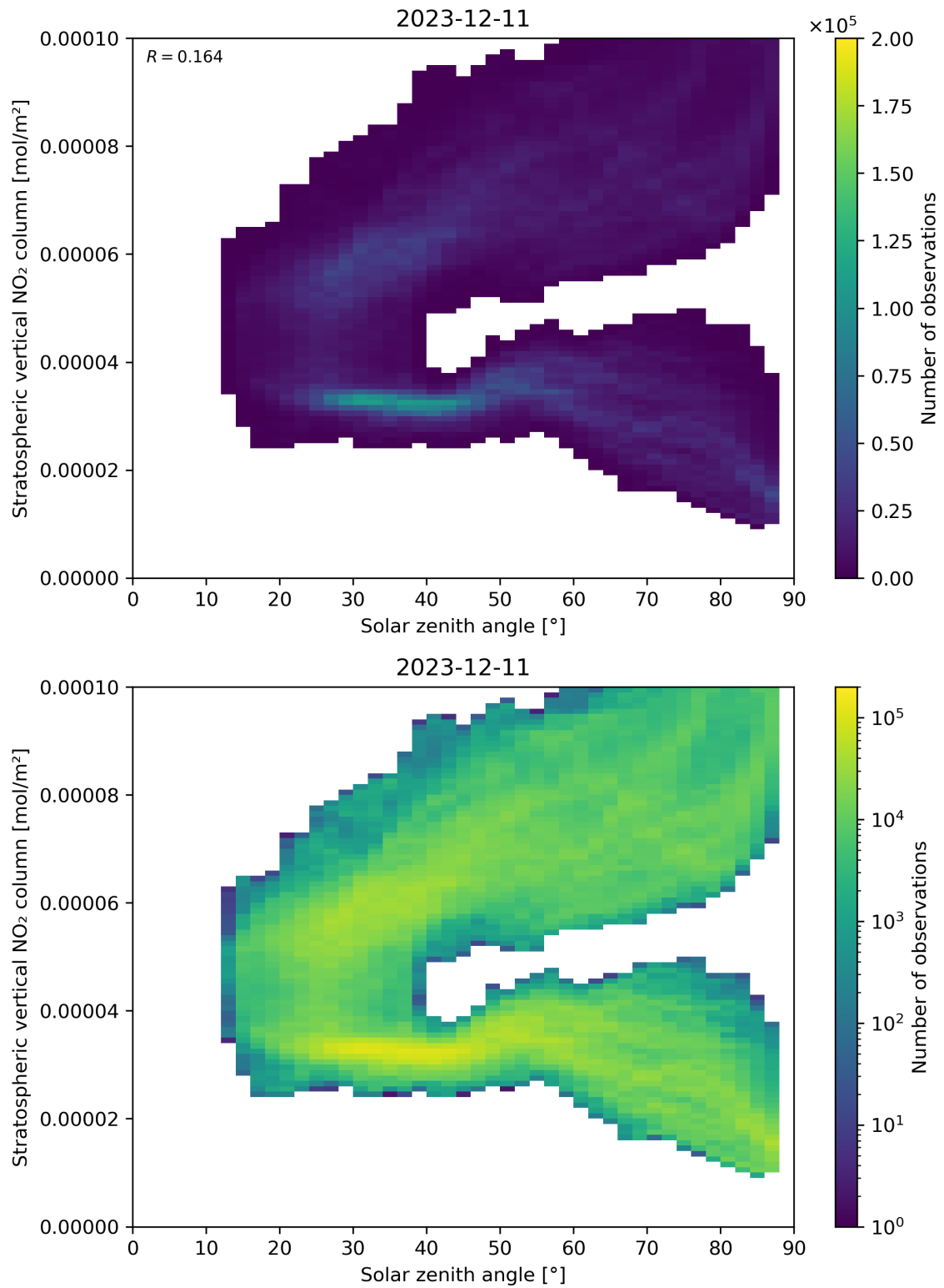
Figure 150: Scatter density plot of “Solar zenith angle” against “Stratospheric vertical NO 2 column” for 2023-12-10 to 2023-12-12.
