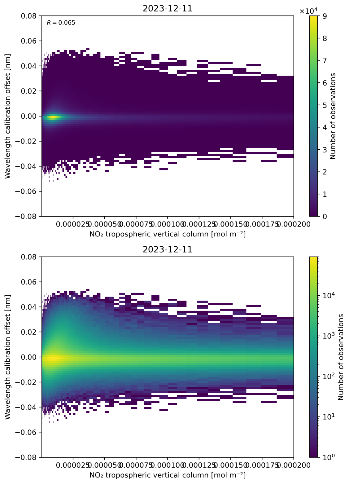
Figure 143: Scatter density plot of “NO 2 tropospheric vertical column” against “Wavelength calibration offset” for 2023-12-10 to 2023-12-12.
