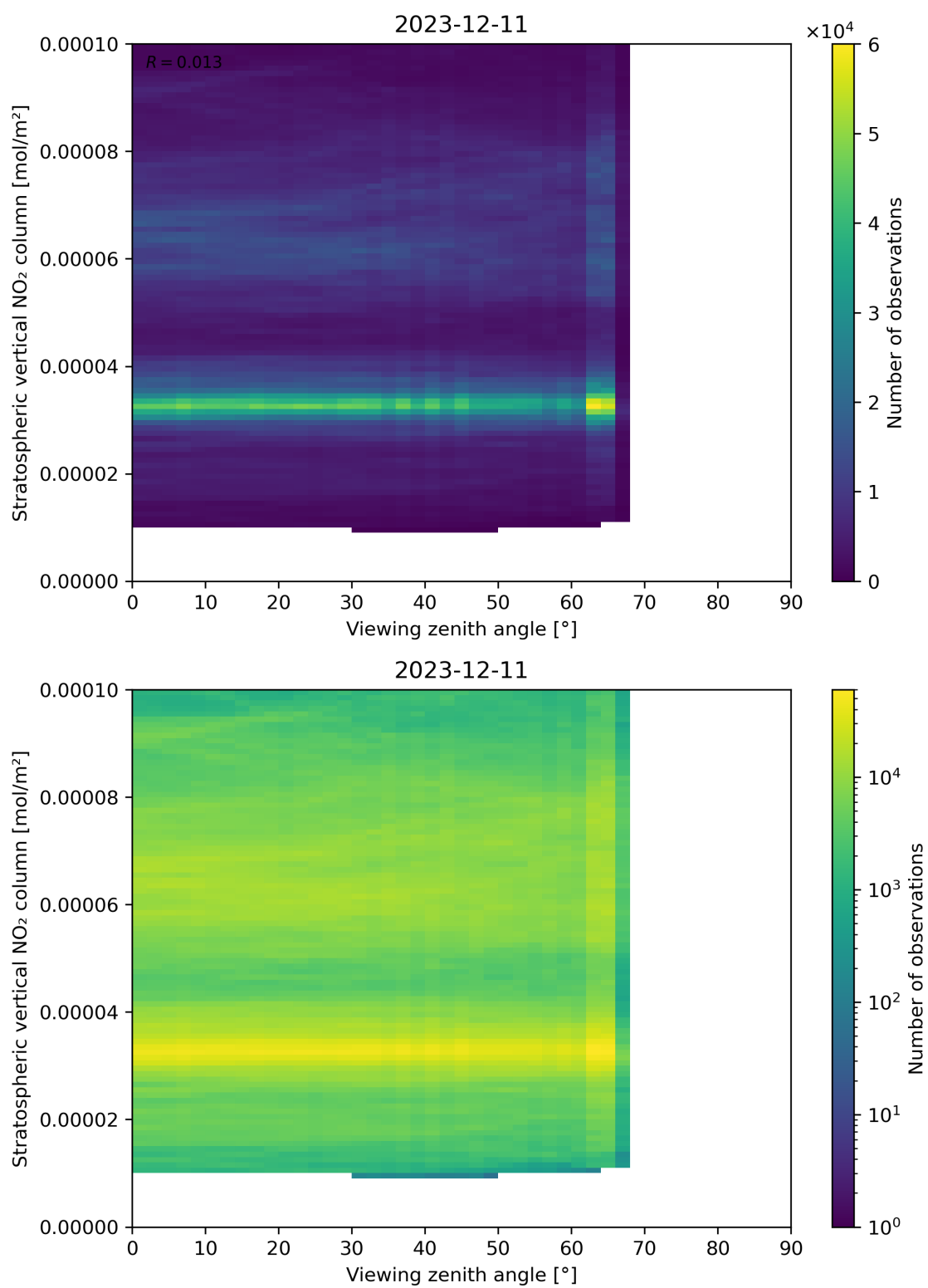
Figure 164: Scatter density plot of “Viewing zenith angle” against “Stratospheric vertical NO 2 column” for 2023-12-10 to 2023-12-12.
