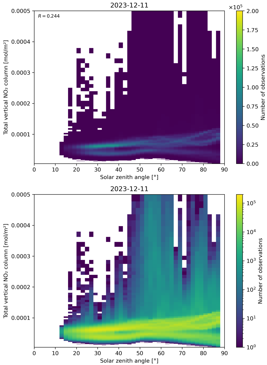
Figure 153: Scatter density plot of “Solar zenith angle” against “Total vertical NO 2 column” for 2023-12-10 to 2023-12-12.
