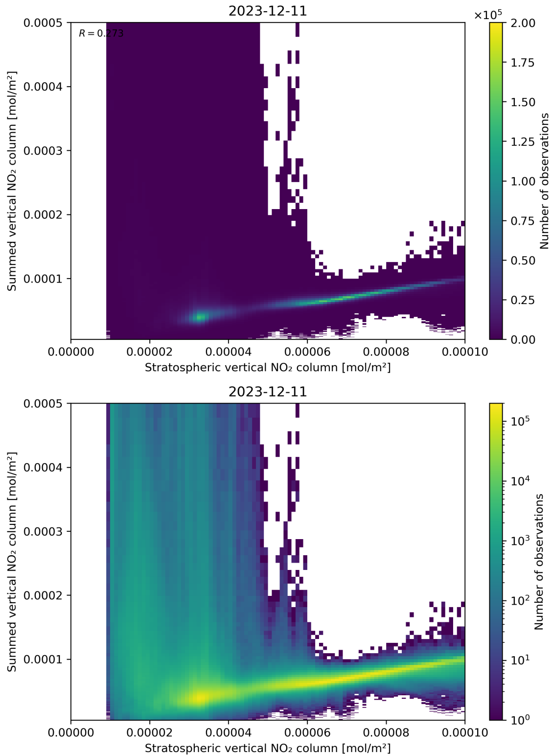
Figure 98: Scatter density plot of “Stratospheric vertical NO 2 column” against “Summed vertical NO 2 column” for 2023-12-10 to 2023-12-12.
