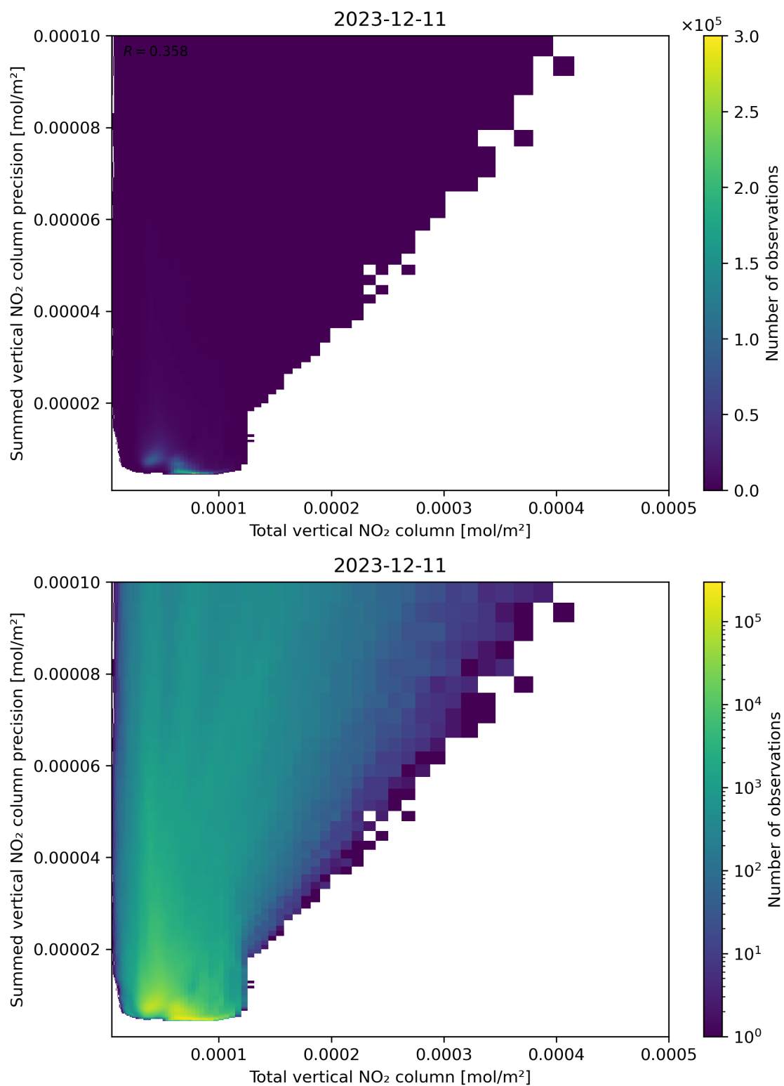
Figure 113: Scatter density plot of “Total vertical NO 2 column” against “Summed vertical NO 2 column precision” for 2023-12-10 to 2023-12-12.
