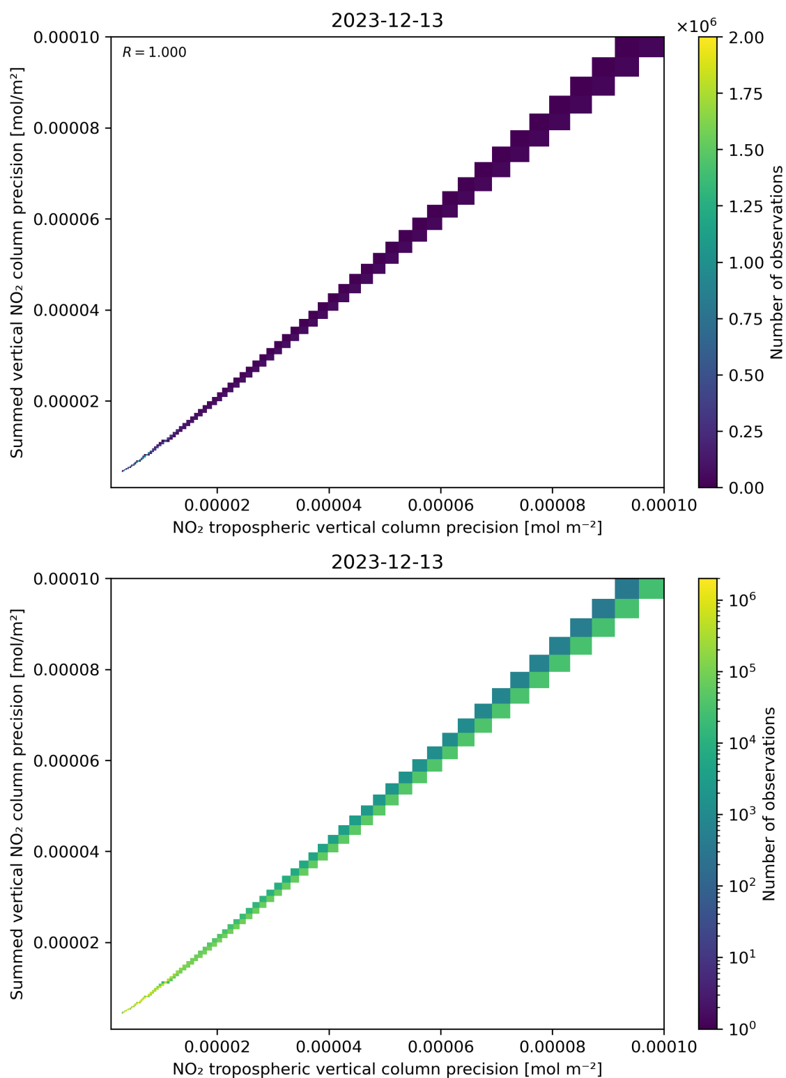
Figure 137: Scatter density plot of “NO 2 tropospheric vertical column precision” against “Summed vertical NO 2 column precision” for 2023-12-12 to 2023-12-14.
