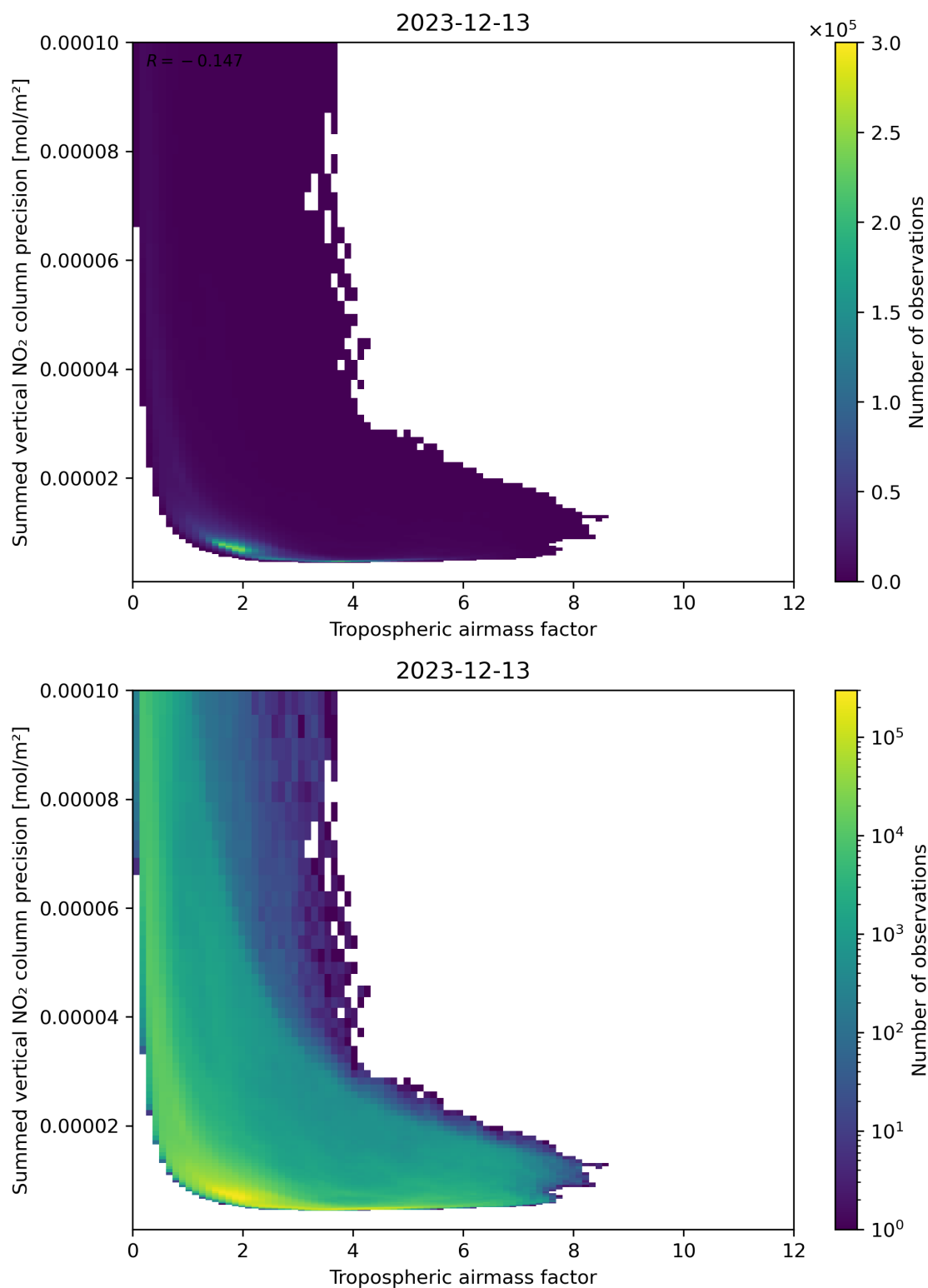
Figure 76: Scatter density plot of “Tropospheric air mass factor” against “Summed vertical NO 2 column precision” for 2023-12-12 to 2023-12-14.
