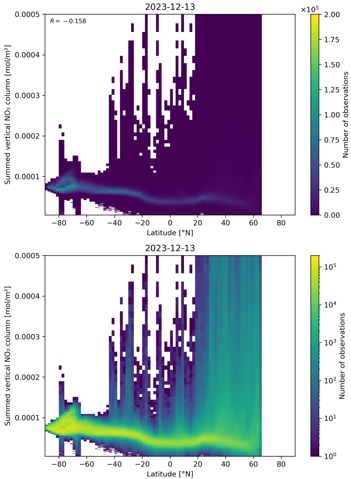
Figure 88: Scatter density plot of “Latitude” against “Summed vertical NO 2 column” for 2023-12-12 to 2023-12-14.
