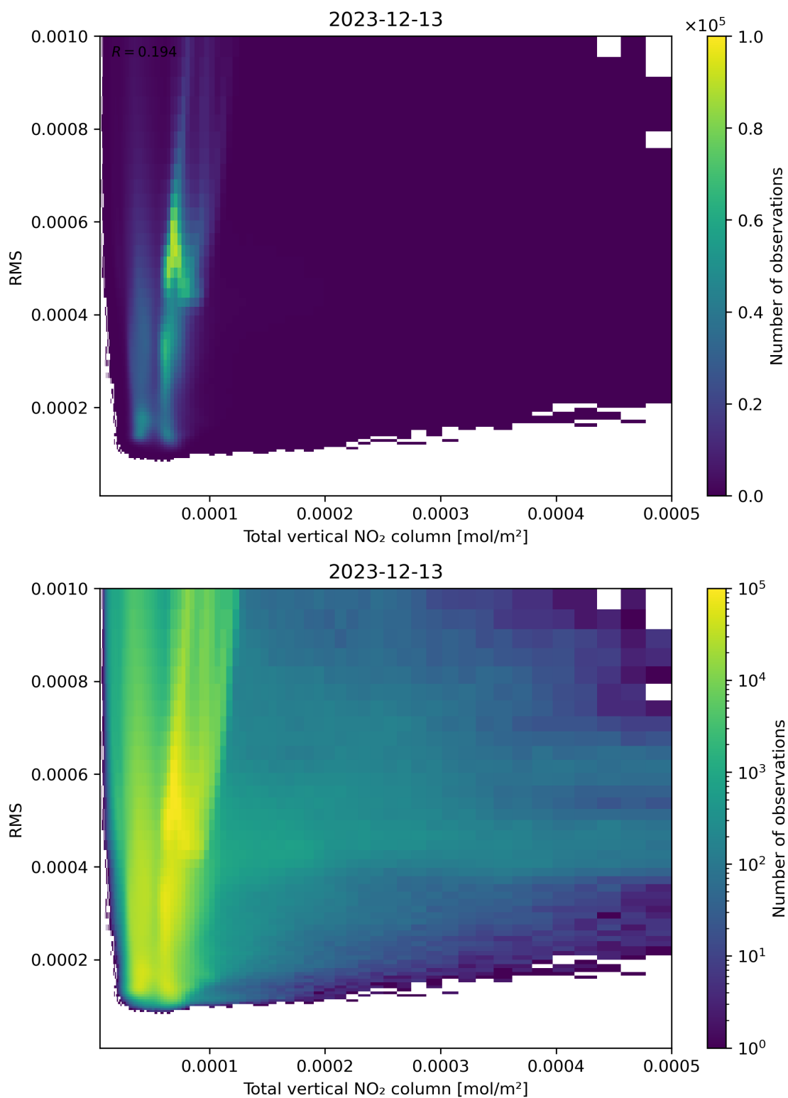
Figure 120: Scatter density plot of “Total vertical NO 2 column” against “RMS” for 2023-12-12 to 2023-12-14.
