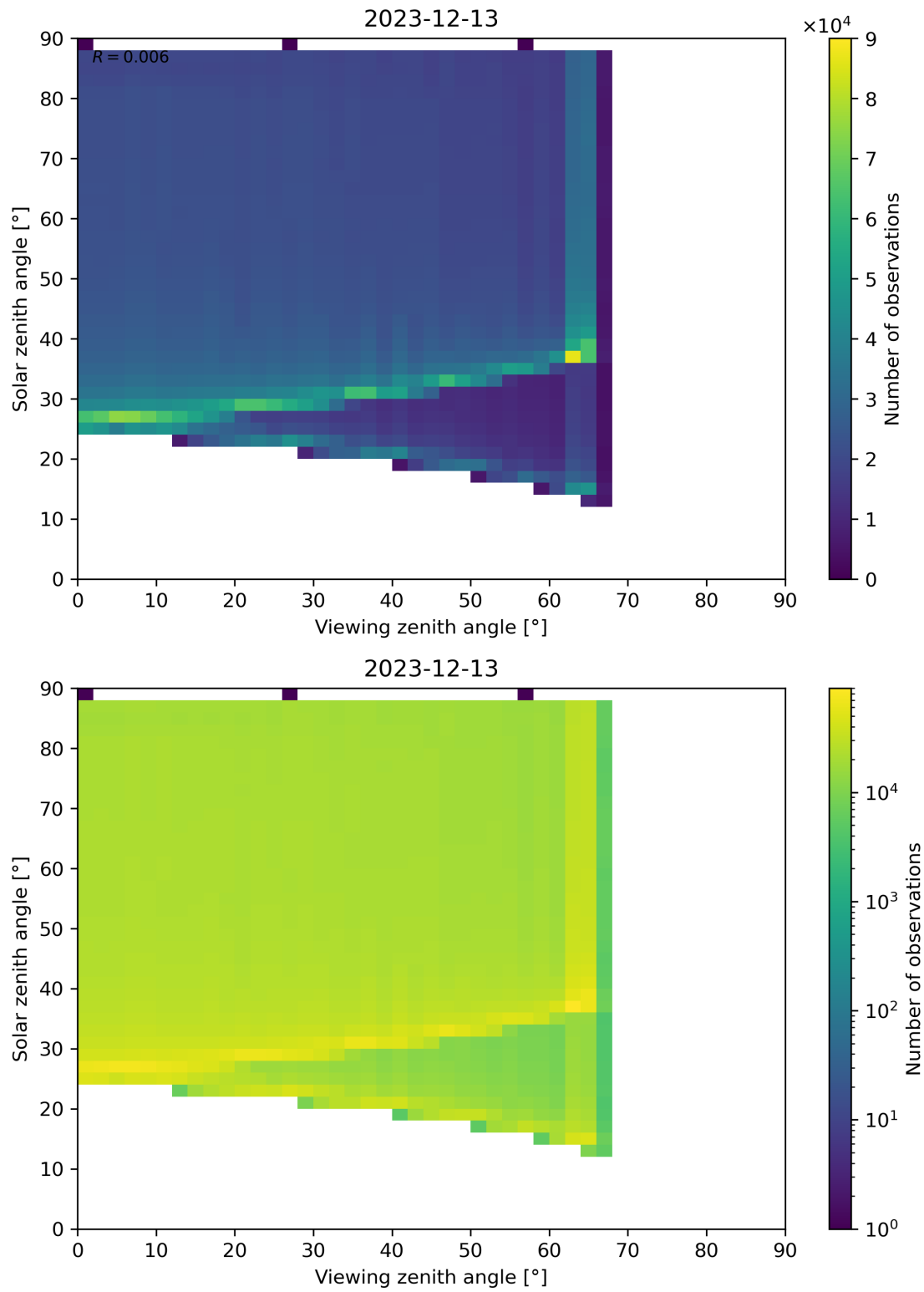
Figure 172: Scatter density plot of “Viewing zenith angle” against “Solar zenith angle” for 2023-12-12 to 2023-12-14.
