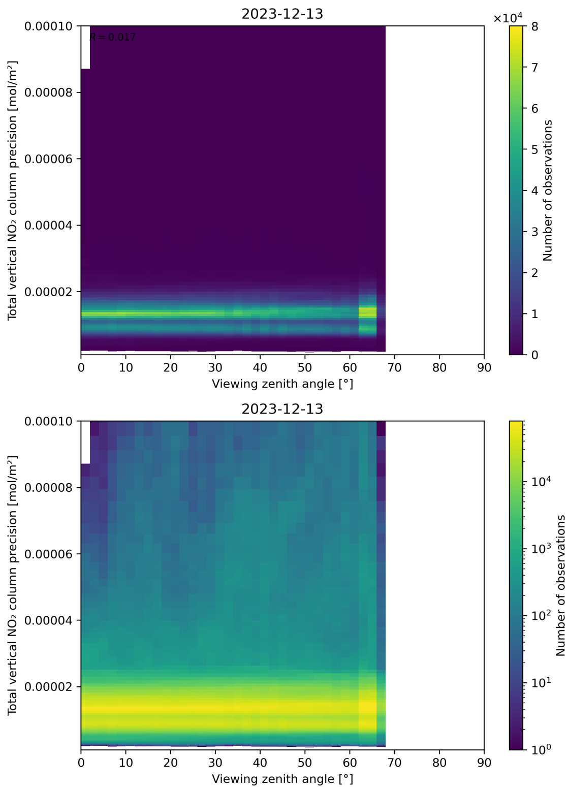
Figure 168: Scatter density plot of “Viewing zenith angle” against “Total vertical NO 2 column precision” for 2023-12-12 to 2023-12-14.
