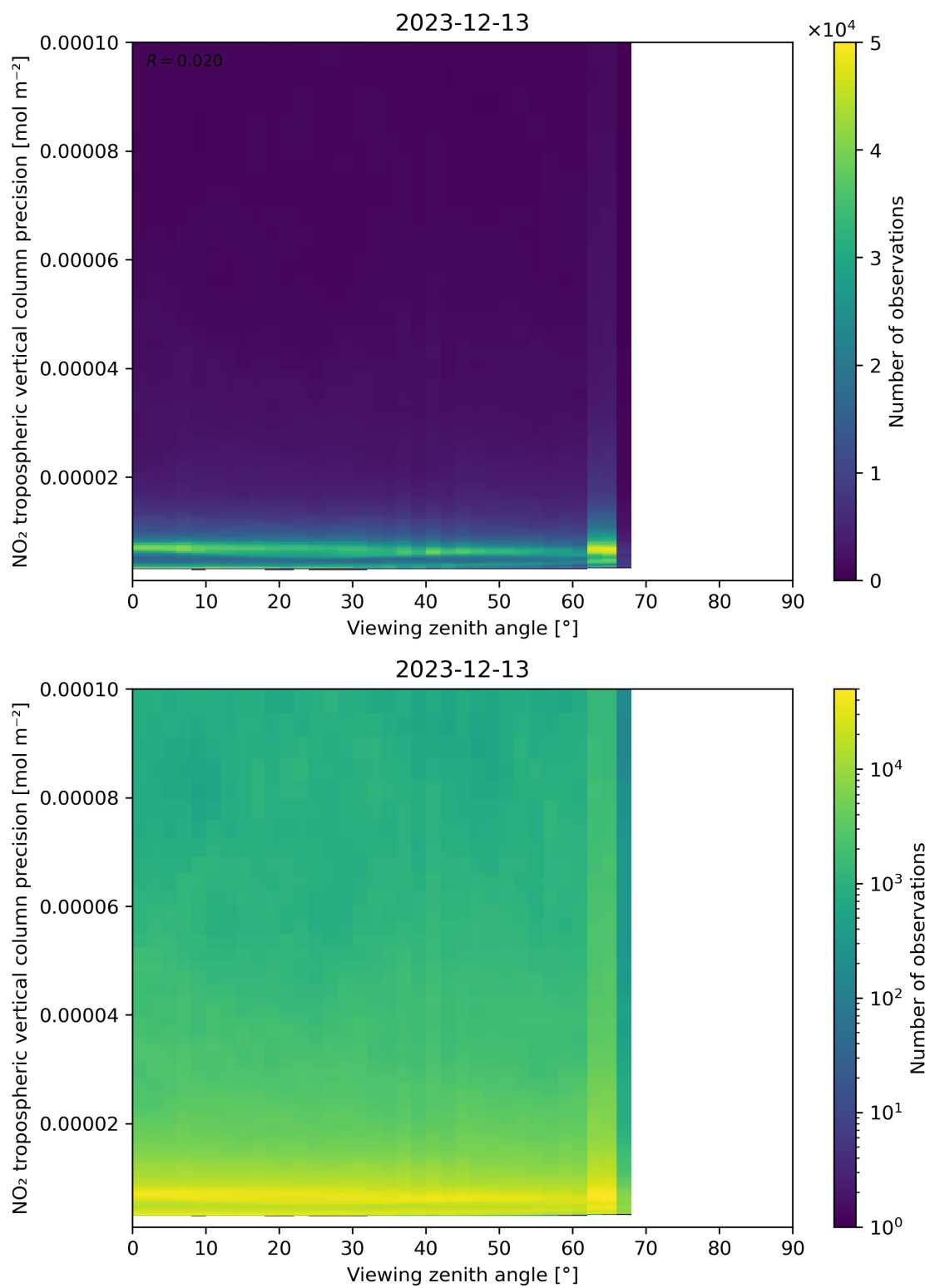
Figure 170: Scatter density plot of “Viewing zenith angle” against “NO 2 tropospheric vertical column precision” for 2023-12-12 to 2023-12-14.
