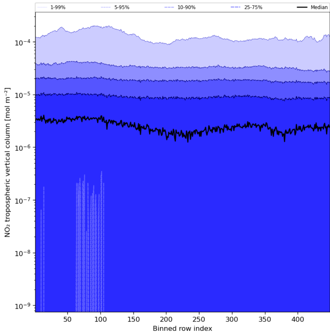
Figure 46: Along track statistics of “NO 2 tropospheric vertical column” for 2023-12-12 to 2023-12-14
