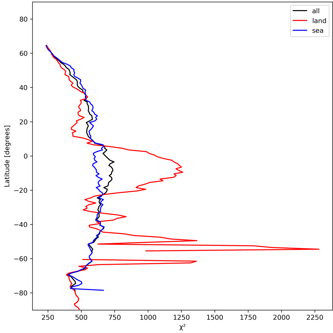
Figure 25: Zonal average of “ \chi^2 ” for 2023-12-12 to 2023-12-14.
