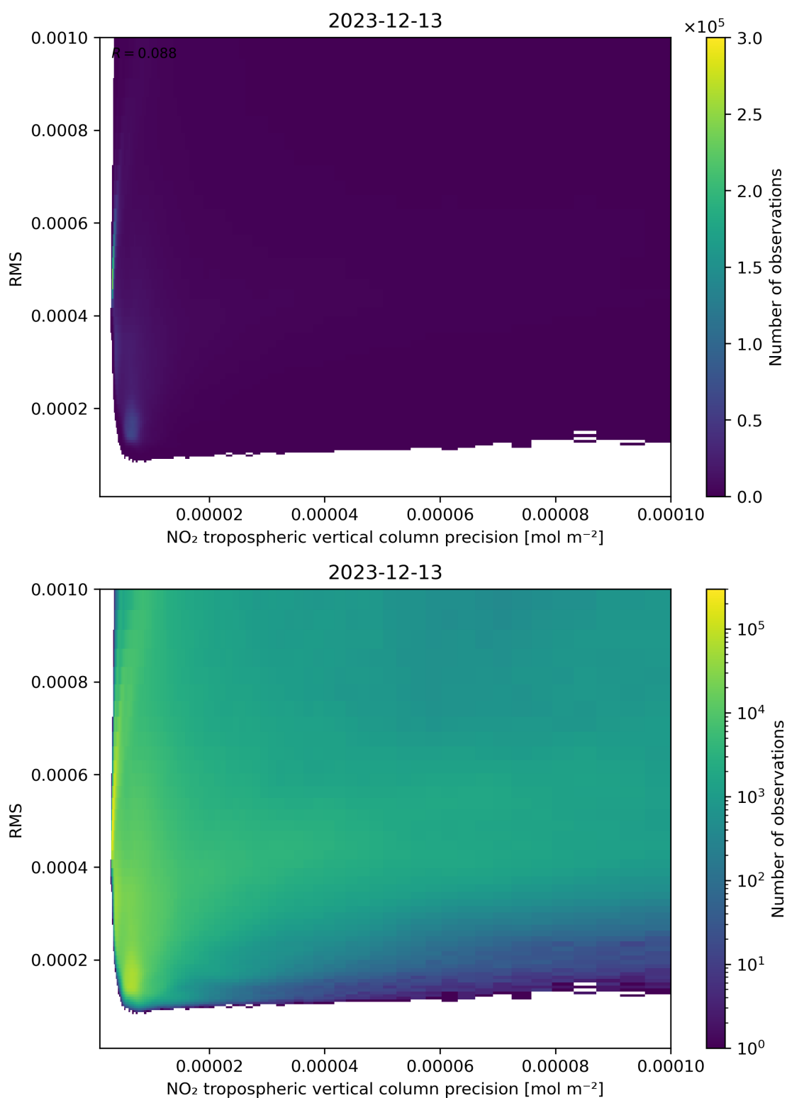
Figure 140: Scatter density plot of “NO 2 tropospheric vertical column precision” against “RMS” for 2023-12-12 to 2023-12-14.
