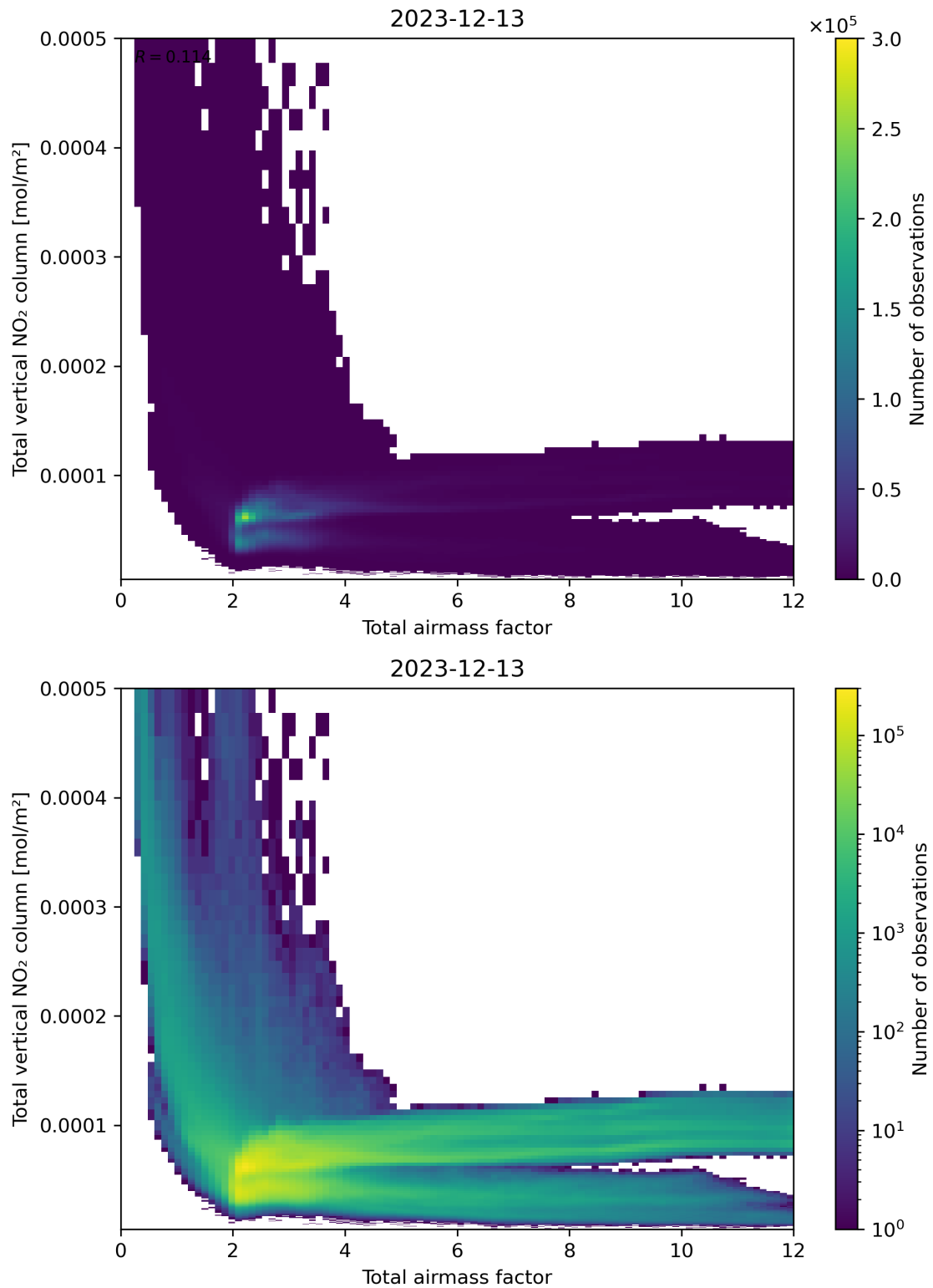
Figure 67: Scatter density plot of “Total air mass factor” against “Total vertical NO 2 column” for 2023-12-12 to 2023-12-14.
