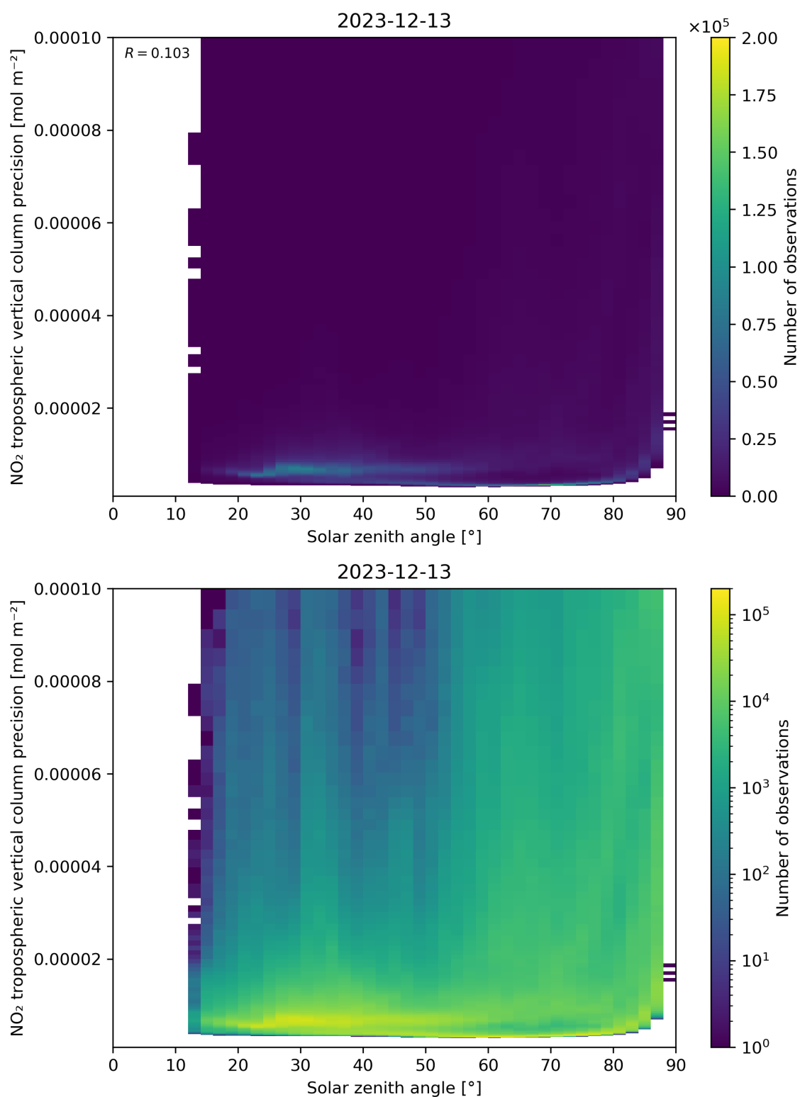
Figure 156: Scatter density plot of “Solar zenith angle” against “NO 2 tropospheric vertical column precision” for 2023-12-12 to 2023-12-14.
