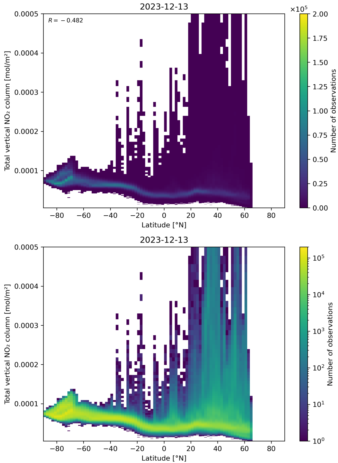
Figure 90: Scatter density plot of “Latitude” against “Total vertical NO 2 column” for 2023-12-12 to 2023-12-14.
