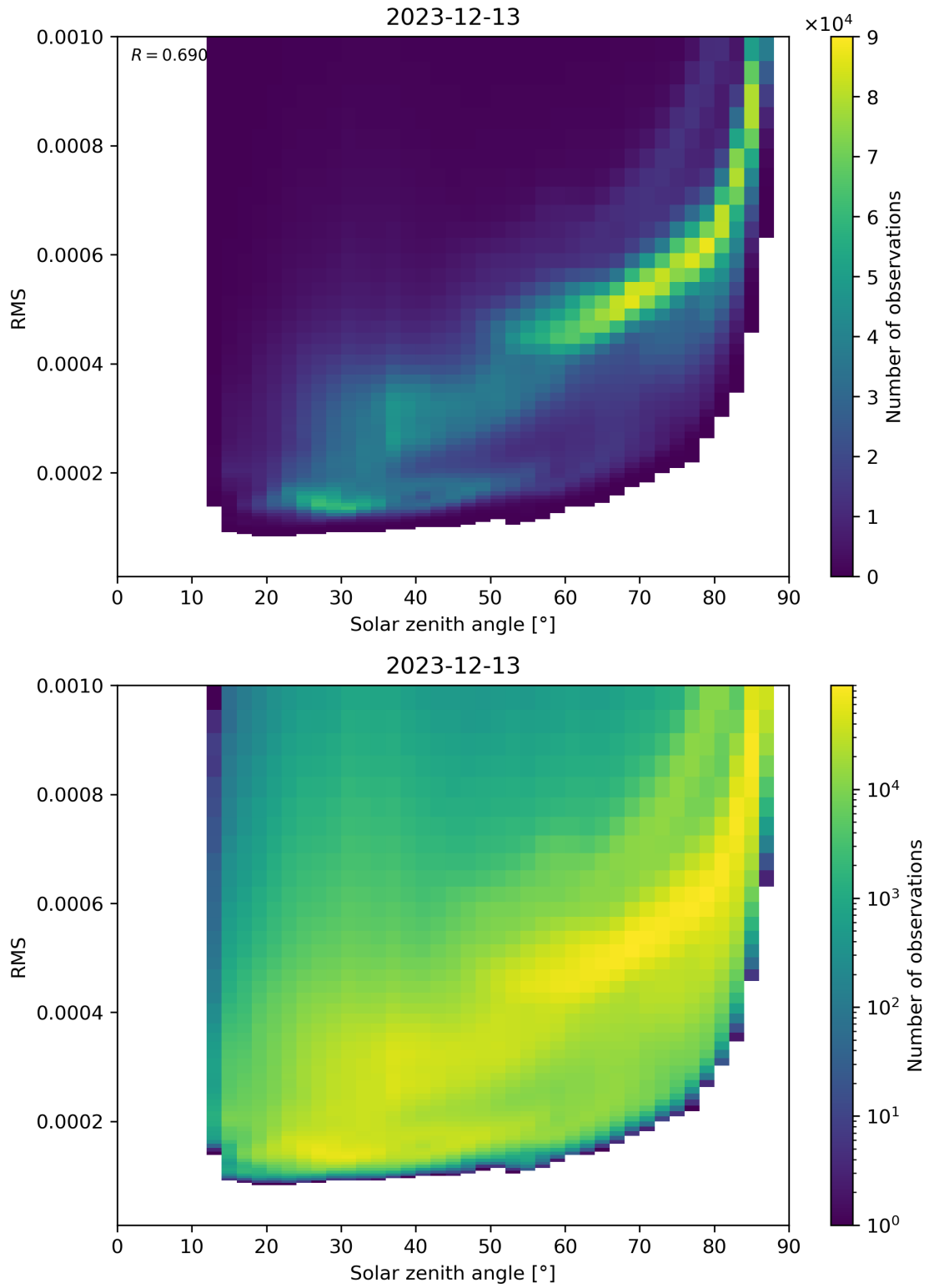
Figure 157: Scatter density plot of “Solar zenith angle” against “RMS” for 2023-12-12 to 2023-12-14.
