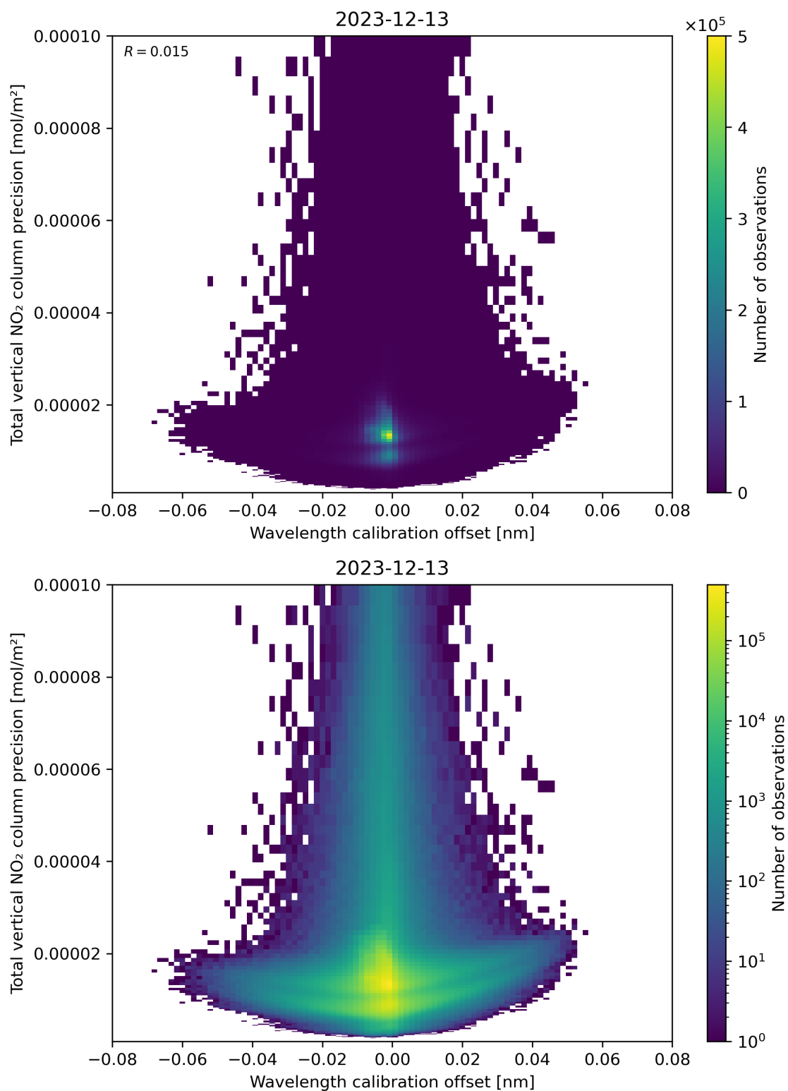
Figure 180: Scatter density plot of “Wavelength calibration offset” against “Total vertical NO 2 column precision” for 2023-12-12 to 2023-12-14.
