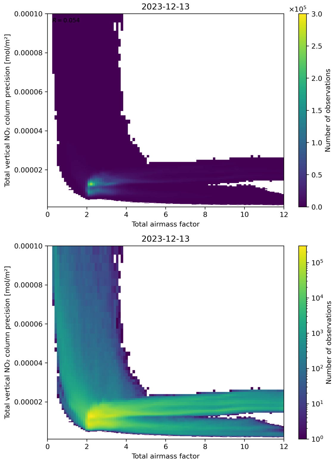
Figure 68: Scatter density plot of “Total airmass factor” against “Total vertical NO 2 column precision” for 2023-12-12 to 2023-12-14.
