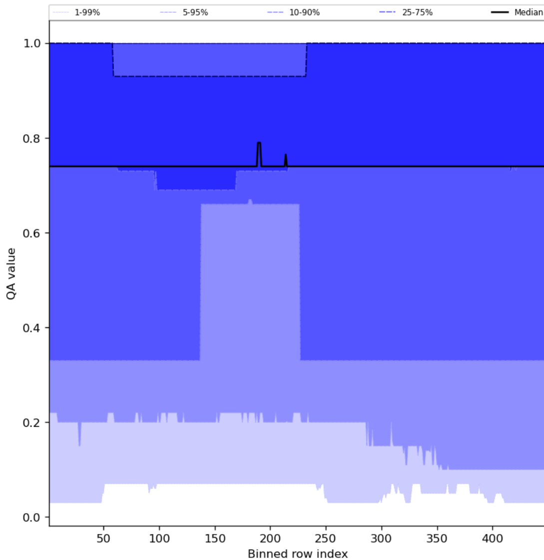
Figure 45: Along track statistics of “QA value” for 2023-12-12 to 2023-12-14
