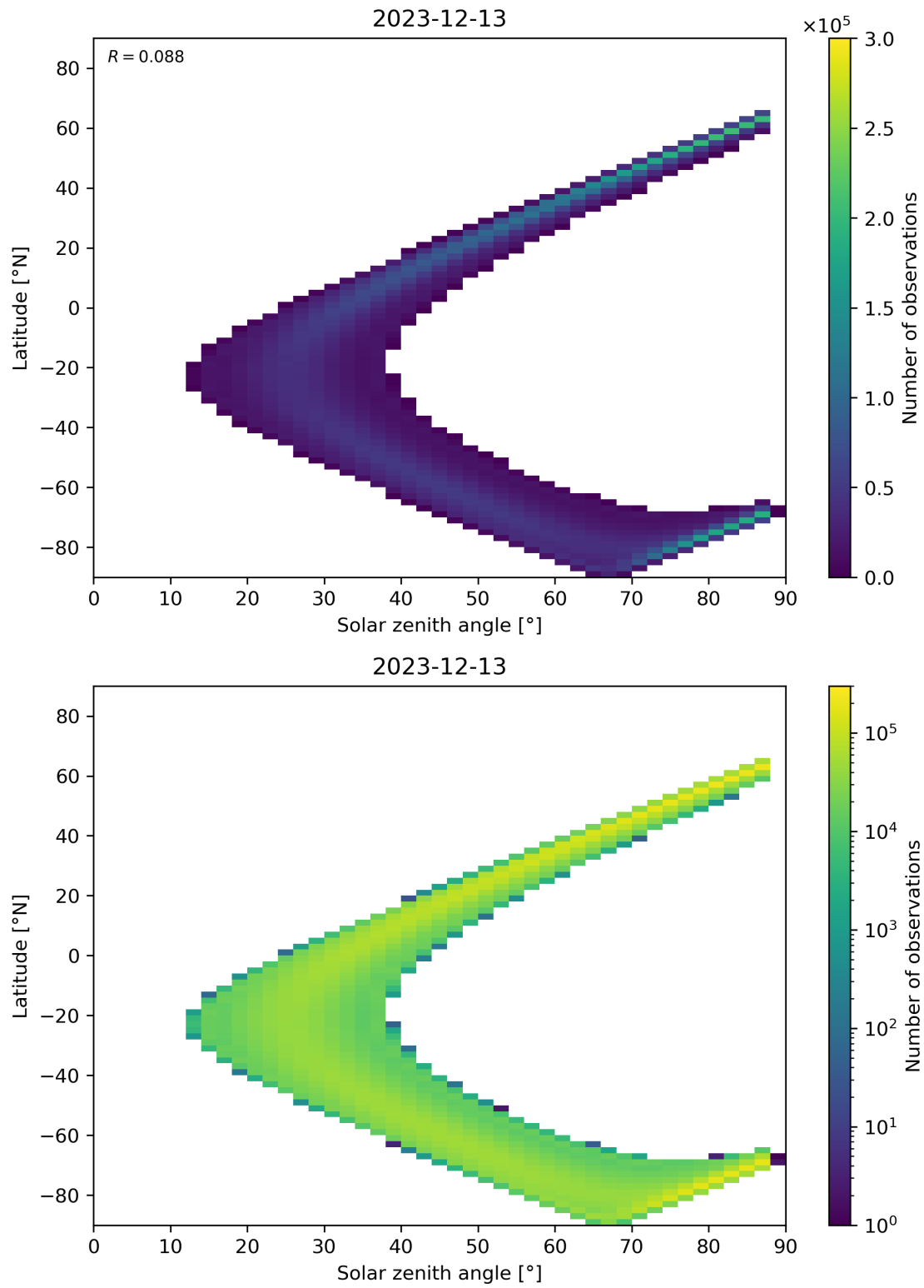
Figure 149: Scatter density plot of “Solar zenith angle” against “Latitude” for 2023-12-12 to 2023-12-14.
