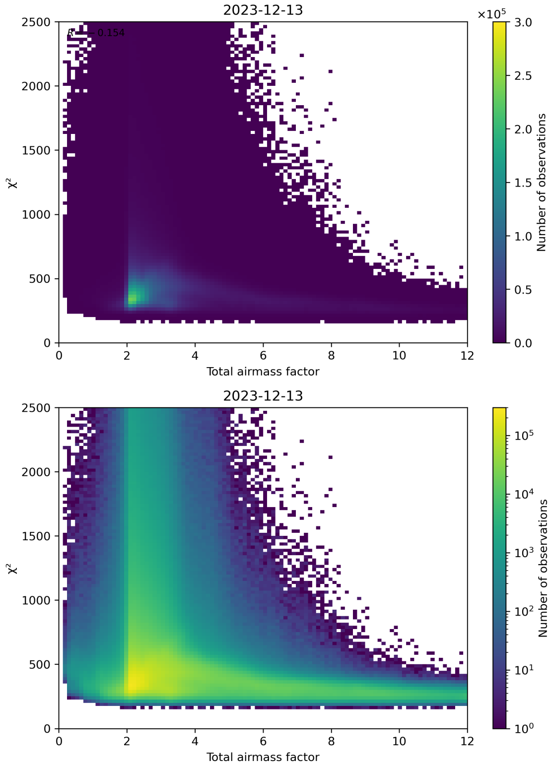
Figure 63: Scatter density plot of “Total airmass factor” against “ \chi^2 ” for 2023-12-12 to 2023-12-14.
