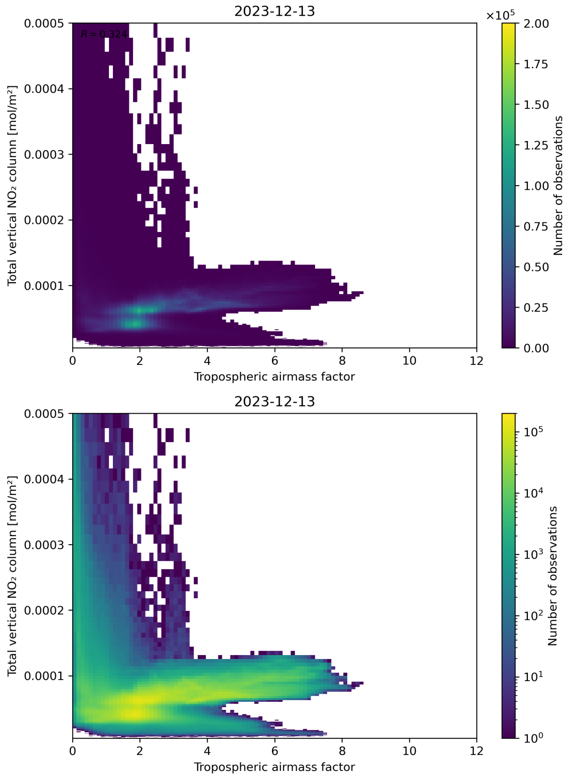
Figure 77: Scatter density plot of “Tropospheric airmass factor” against “Total vertical NO 2 column” for 2023-12-12 to 2023-12-14.
