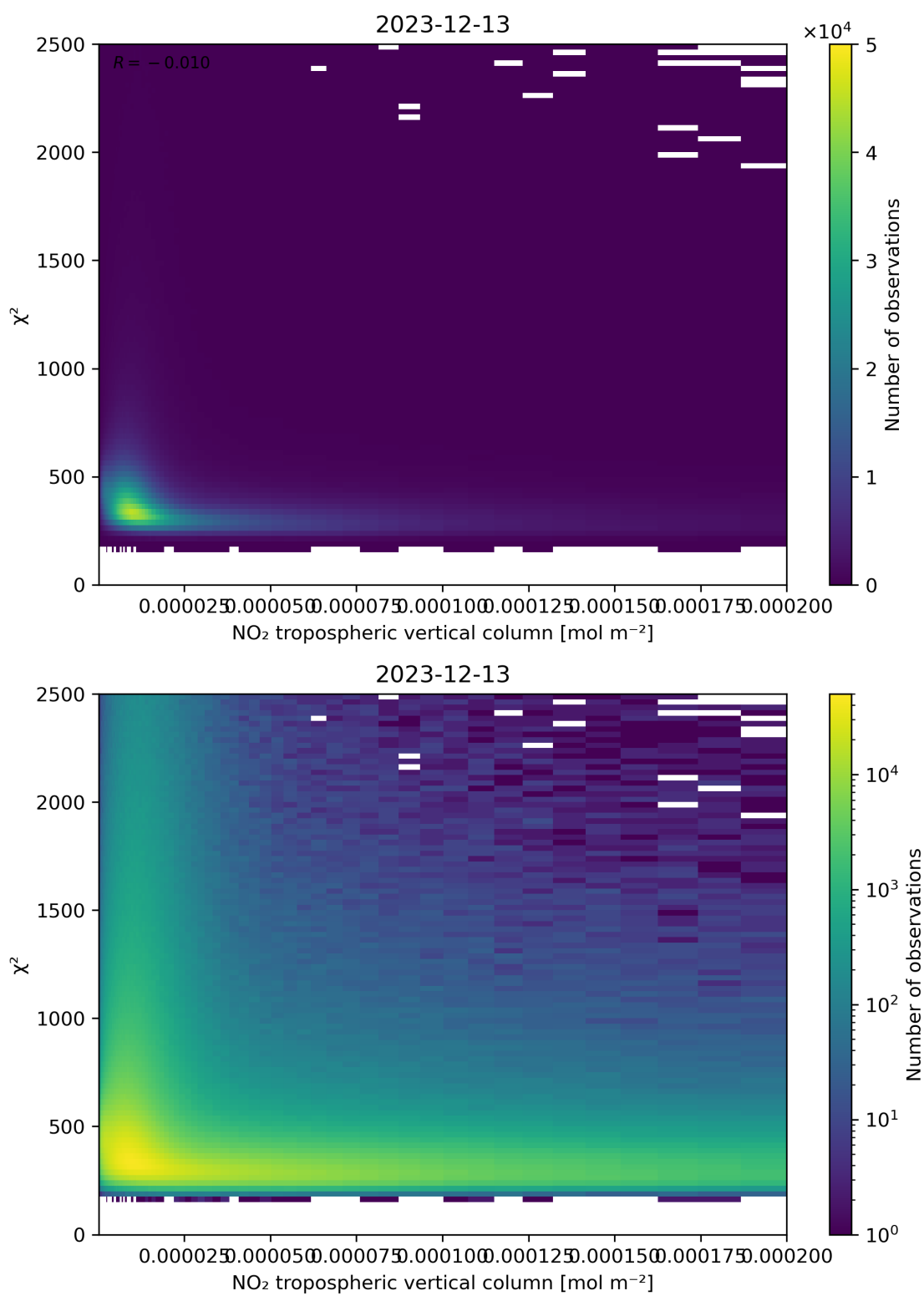
Figure 124: Scatter density plot of “NO 2 tropospheric vertical column” against “ \chi^2 ” for 2023-12-12 to 2023-12-14.
