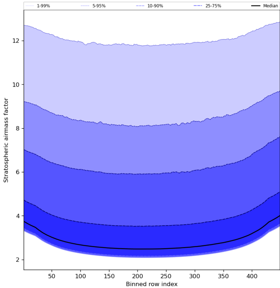
Figure 61: Along track statistics of “Stratospheric airmass factor” for 2023-12-12 to 2023-12-14
