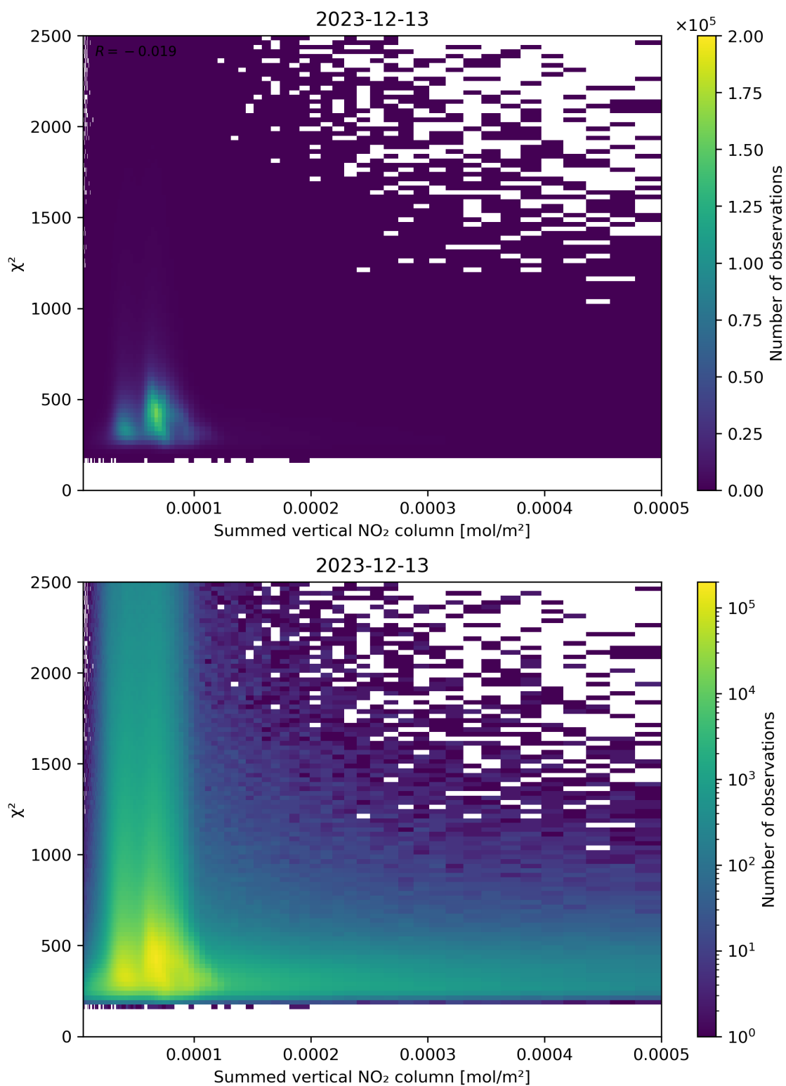
Figure 104: Scatter density plot of “Summed vertical NO 2 column” against “ \chi^2 ” for 2023-12-12 to 2023-12-14.
