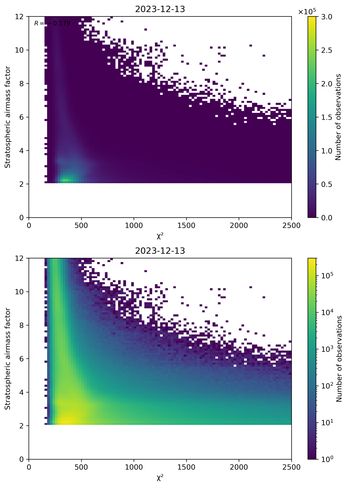
Figure 81: Scatter density plot of “ \chi^2 ” against “Stratospheric air mass factor” for 2023-12-12 to 2023-12-14.
