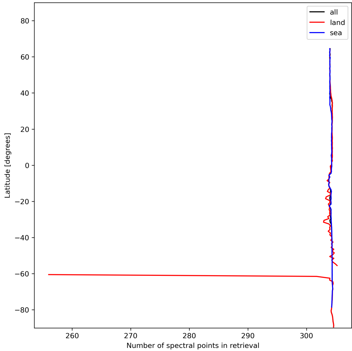
Figure 16: Zonal average of “Number of spectral points in retrieval” for 2023-12-12 to 2023-12-14.
