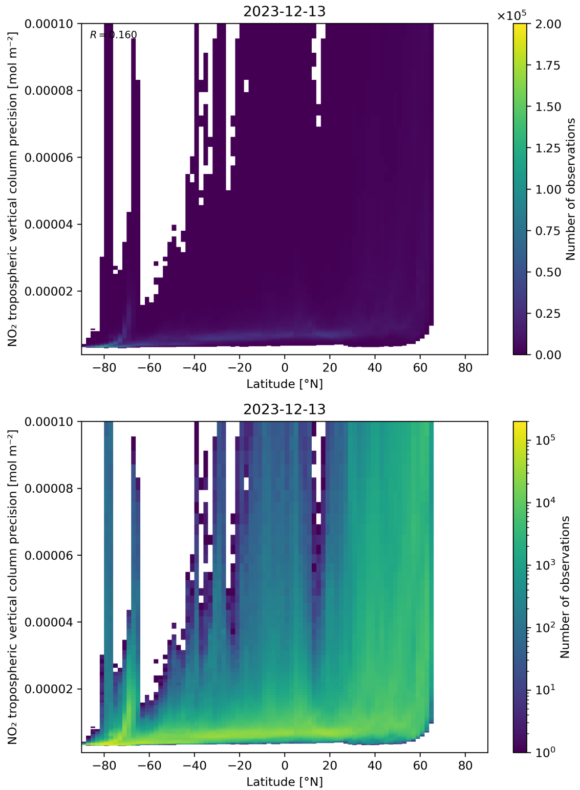
Figure 93: Scatter density plot of “Latitude” against “NO 2 tropospheric vertical column precision” for 2023-12-12 to 2023-12-14.
