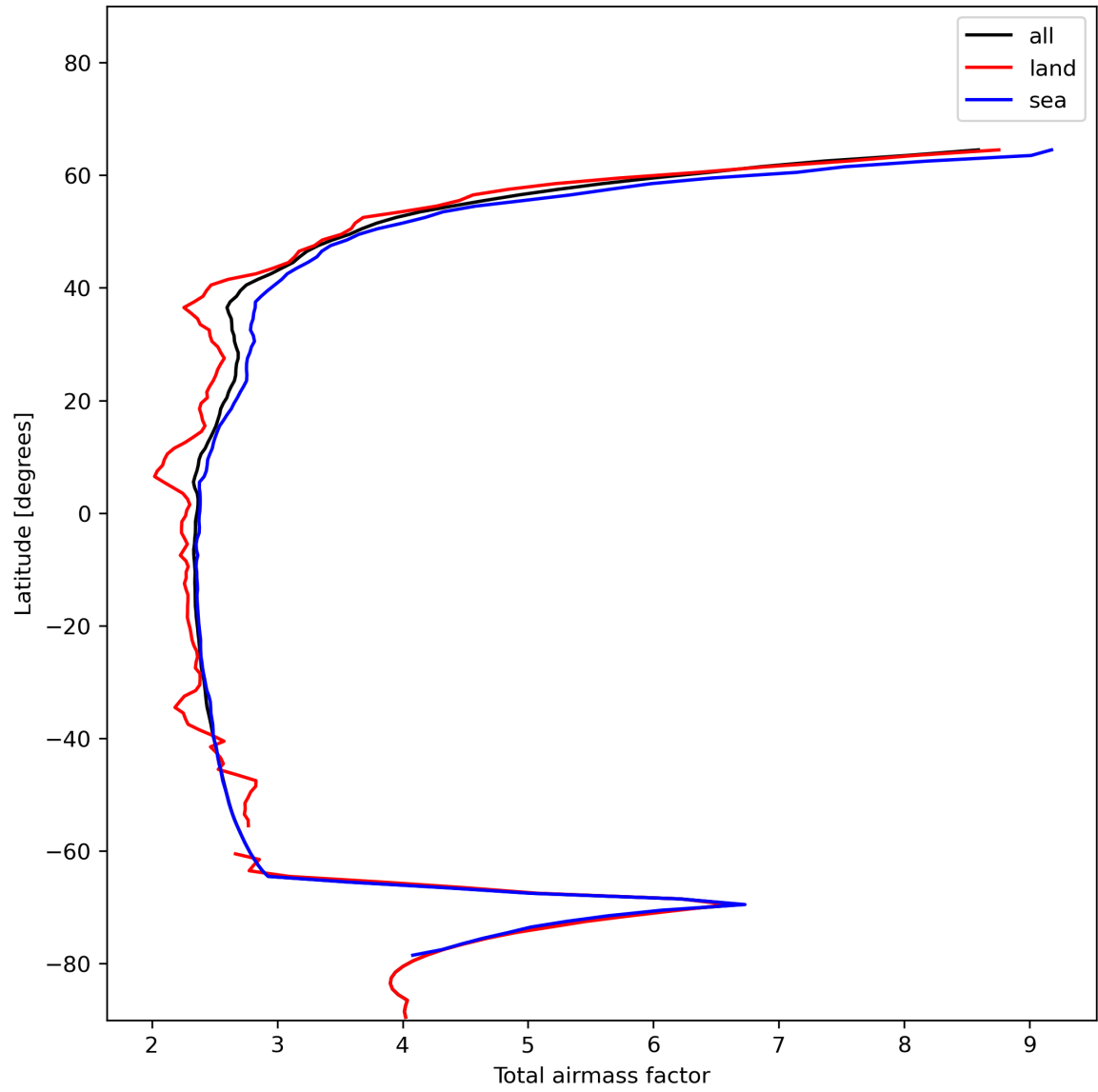
Figure 15: Zonal average of “Total airmass factor” for 2023-12-12 to 2023-12-14.
