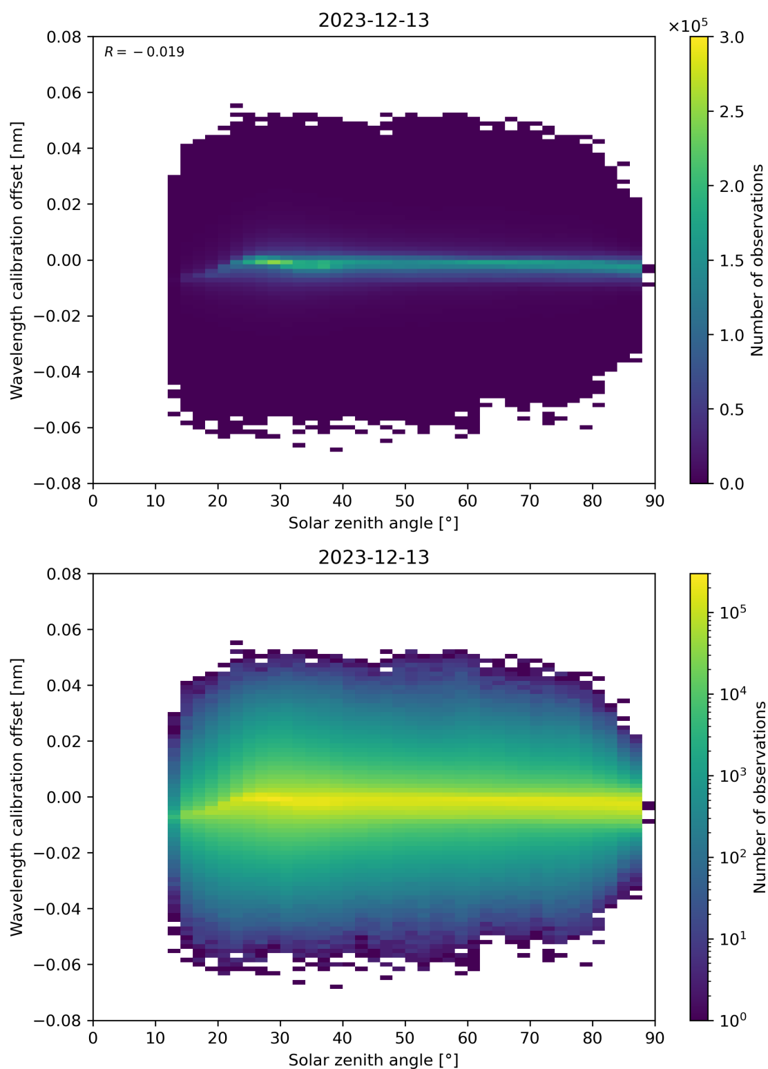
Figure 158: Scatter density plot of “Solar zenith angle” against “Wavelength calibration offset” for 2023-12-12 to 2023-12-14.
