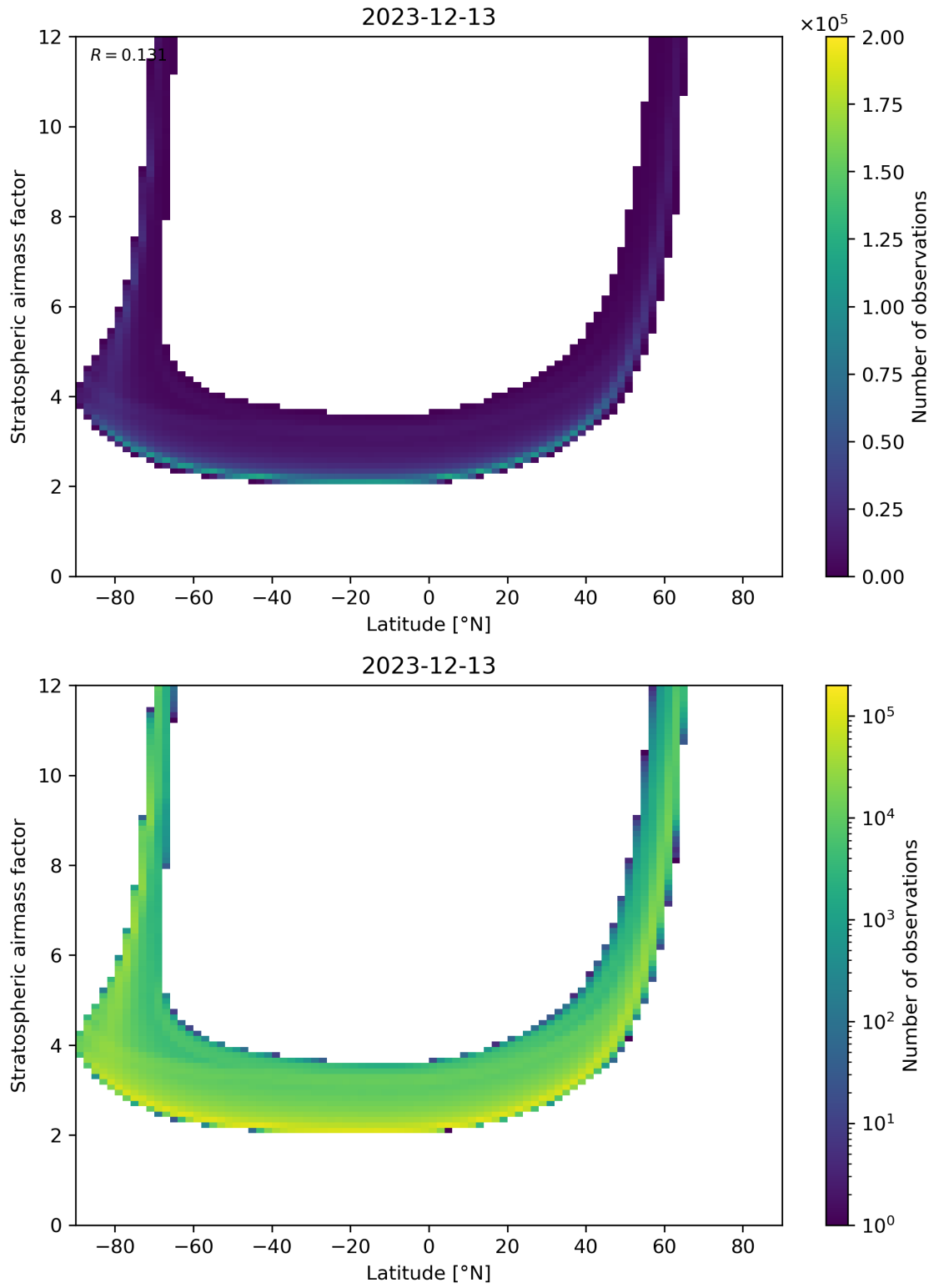
Figure 83: Scatter density plot of “Latitude” against “Stratospheric air mass factor” for 2023-12-12 to 2023-12-14.
