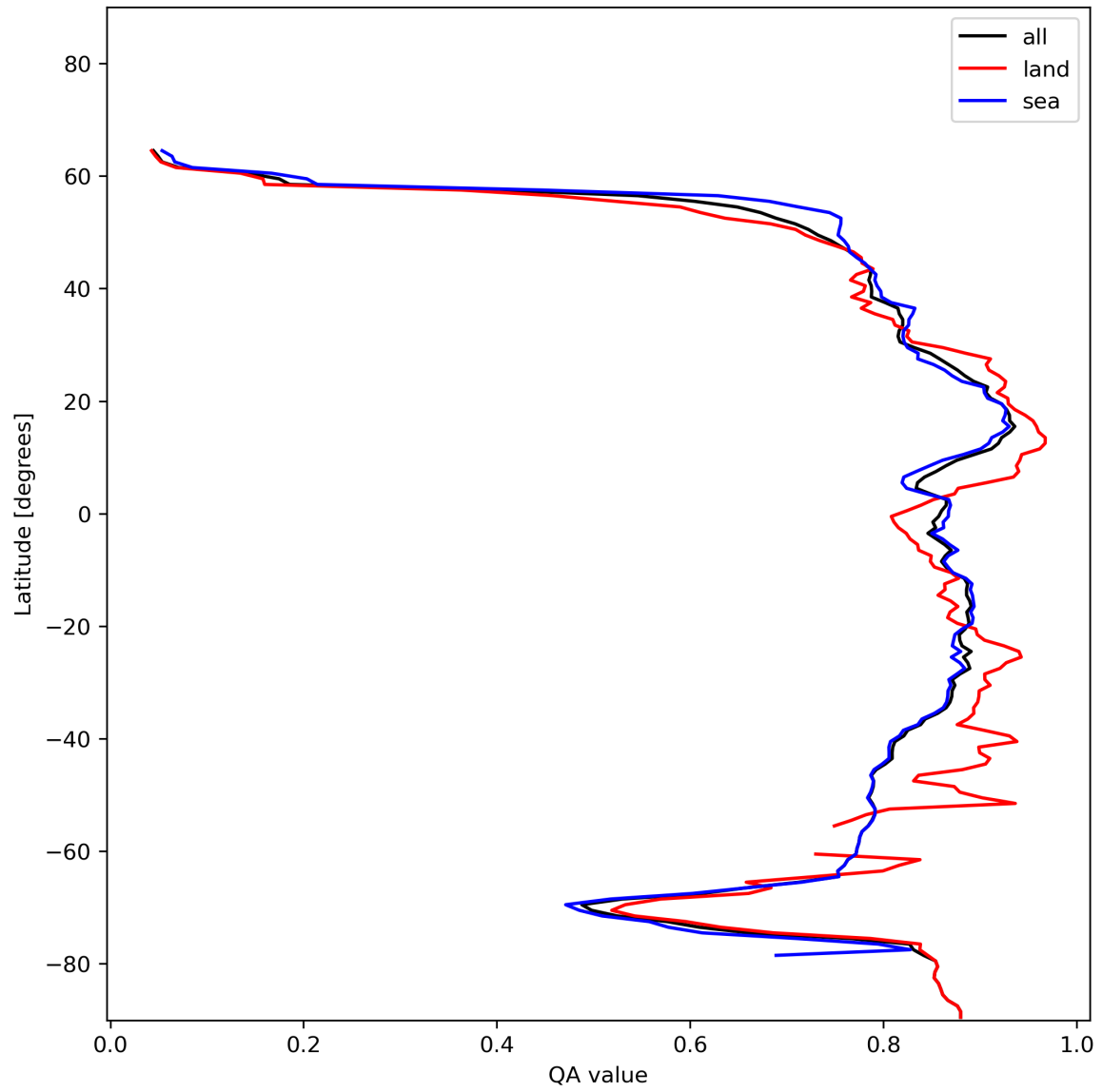
Figure 11: Zonal average of “QA value” for 2023-12-12 to 2023-12-14.
