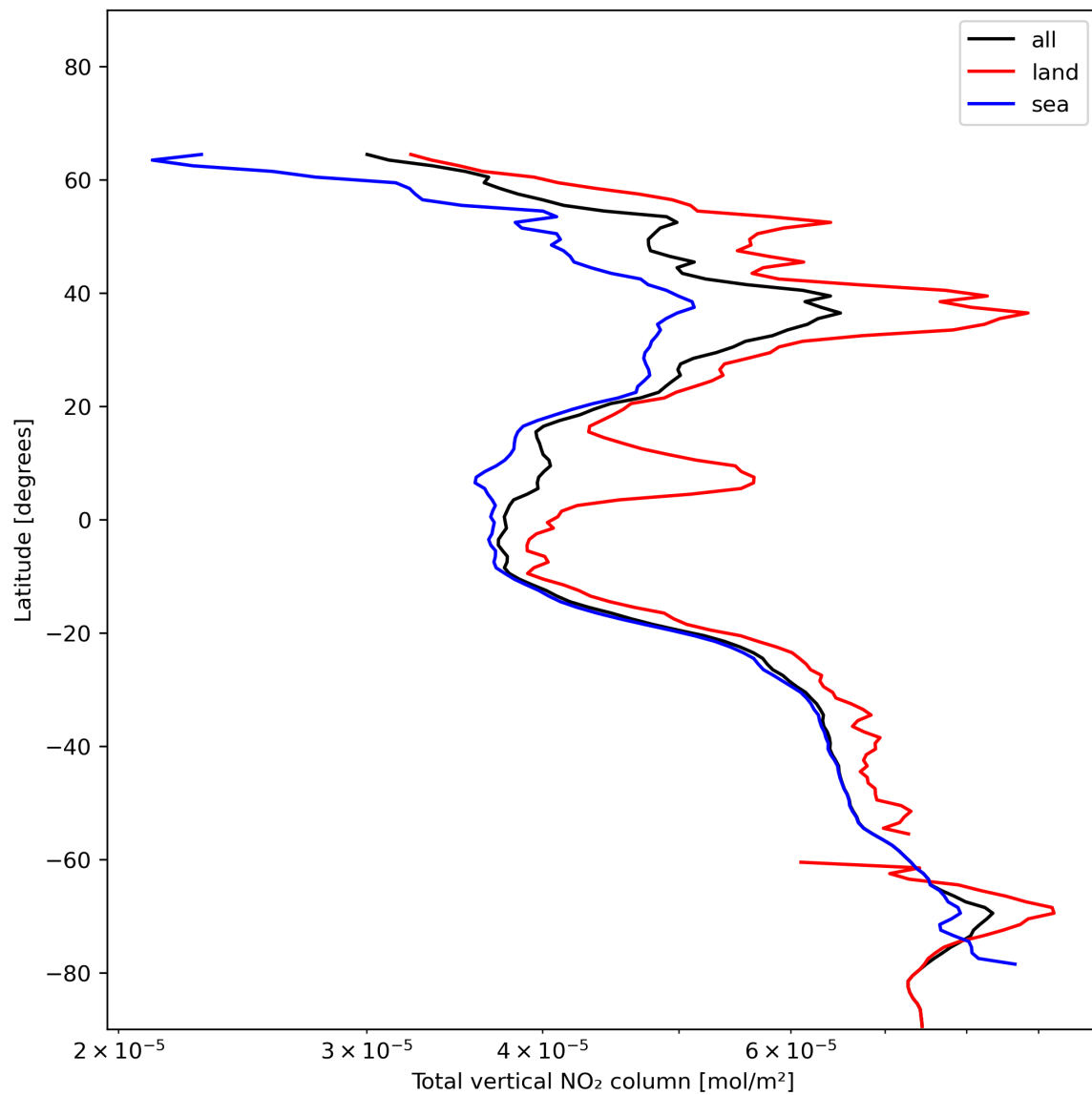
Figure 21: Zonal average of “Total vertical NO 2 column” for 2023-12-12 to 2023-12-14.
