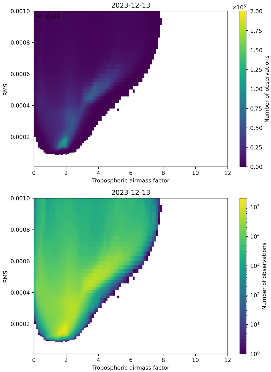
Figure 79: Scatter density plot of “Tropospheric airmass factor” against “RMS” for 2023-12-12 to 2023-12-14.
