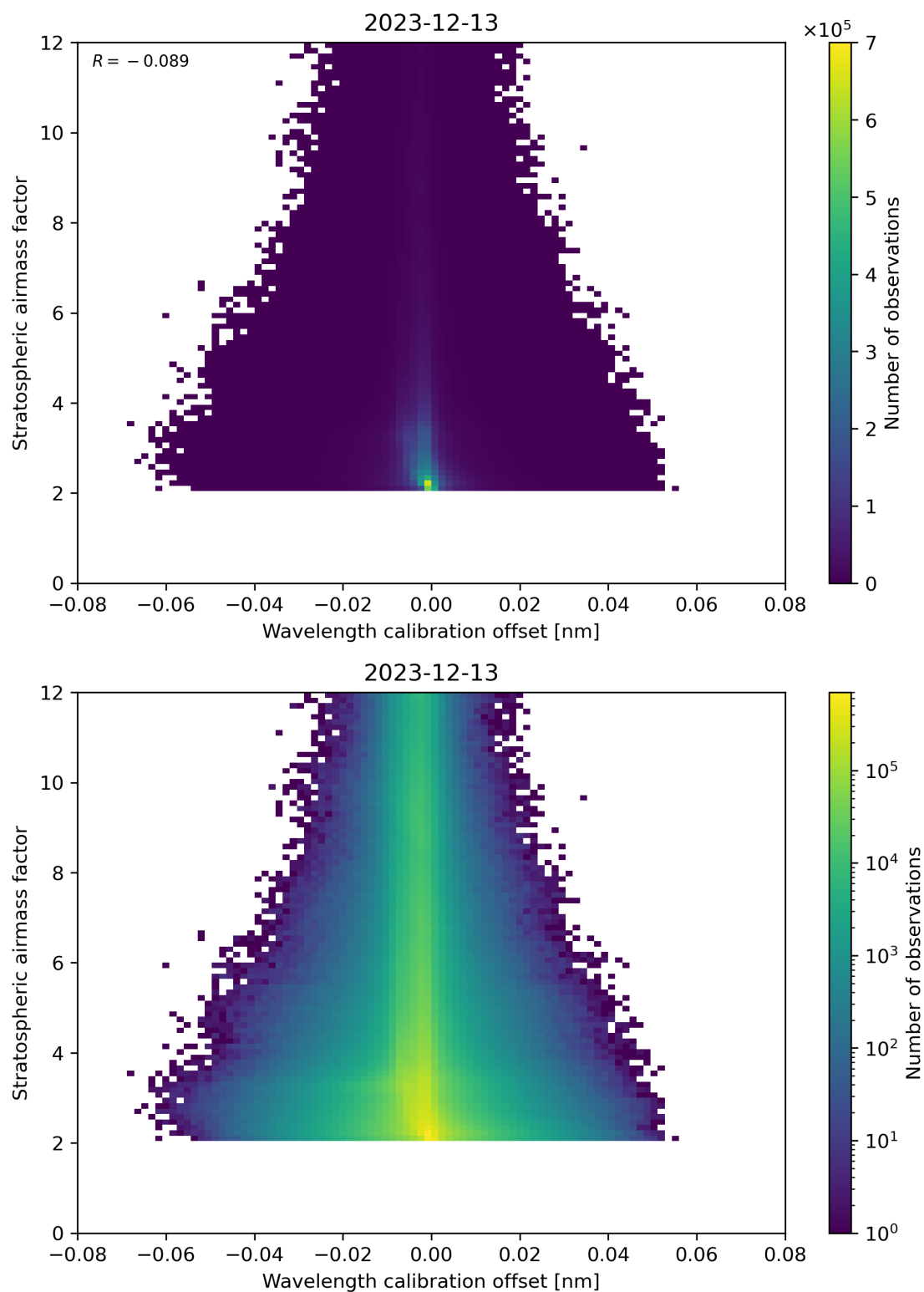
Figure 174: Scatter density plot of “Wavelength calibration offset” against “Stratospheric air mass factor” for 2023-12-12 to 2023-12-14.
