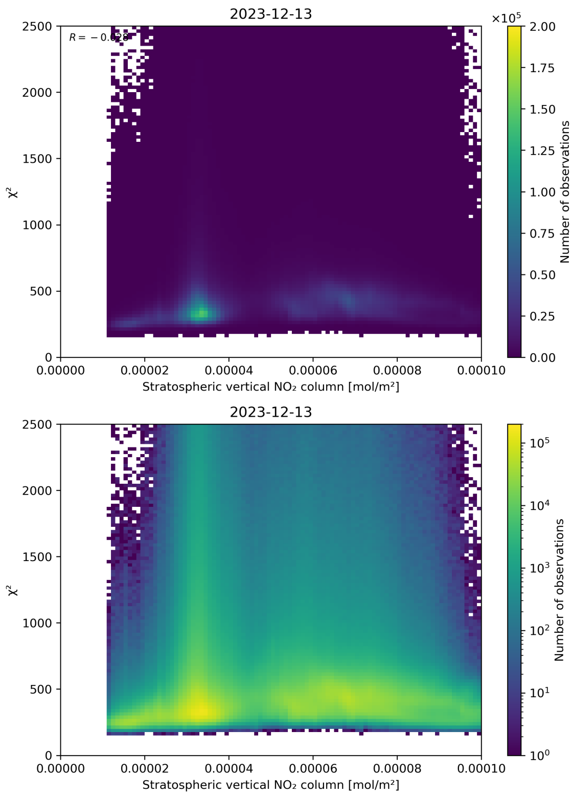
Figure 97: Scatter density plot of “Stratospheric vertical NO 2 column” against “ \chi^2 ” for 2023-12-12 to 2023-12-14.
