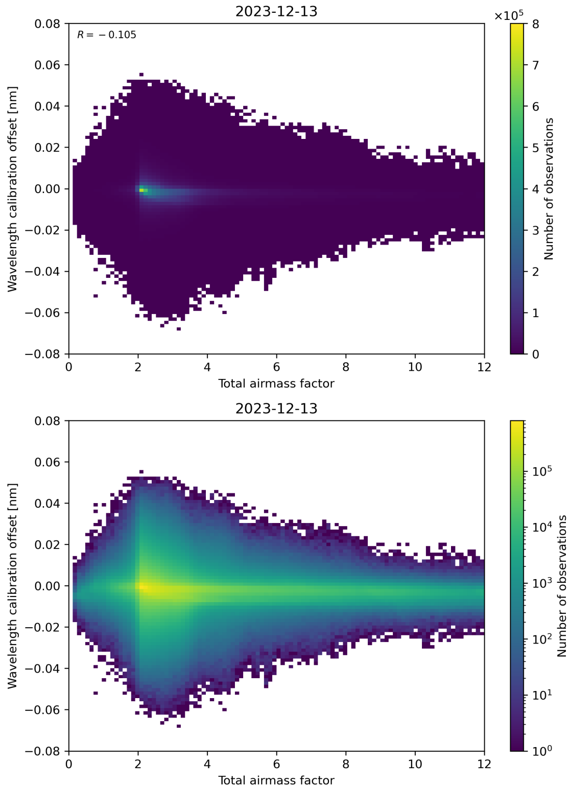
Figure 70: Scatter density plot of “Total airmass factor” against “Wavelength calibration offset” for 2023-12-12 to 2023-12-14.
