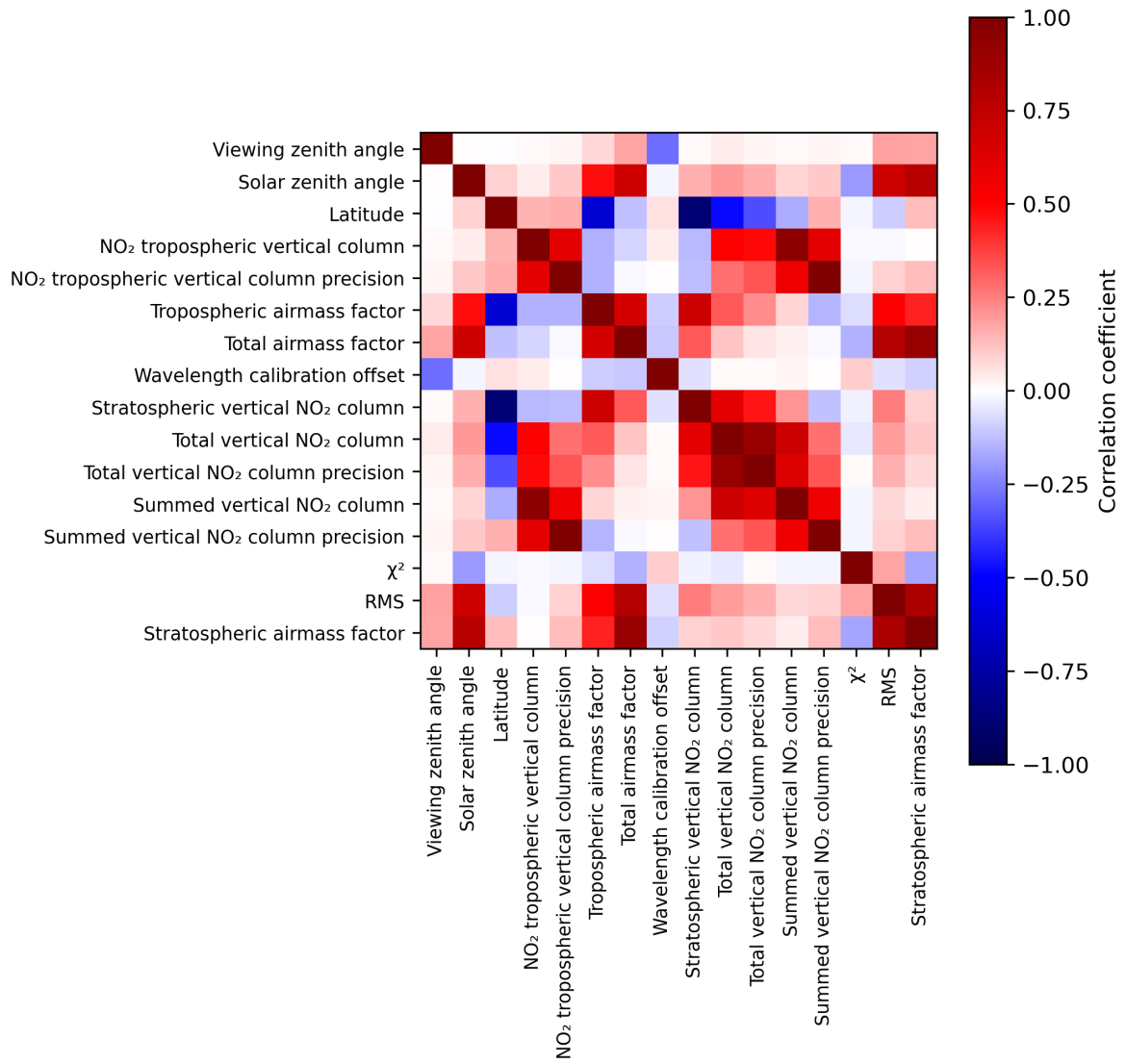
Figure 2: Map of correlation matrix for 2023-12-12 to 2023-12-14.
