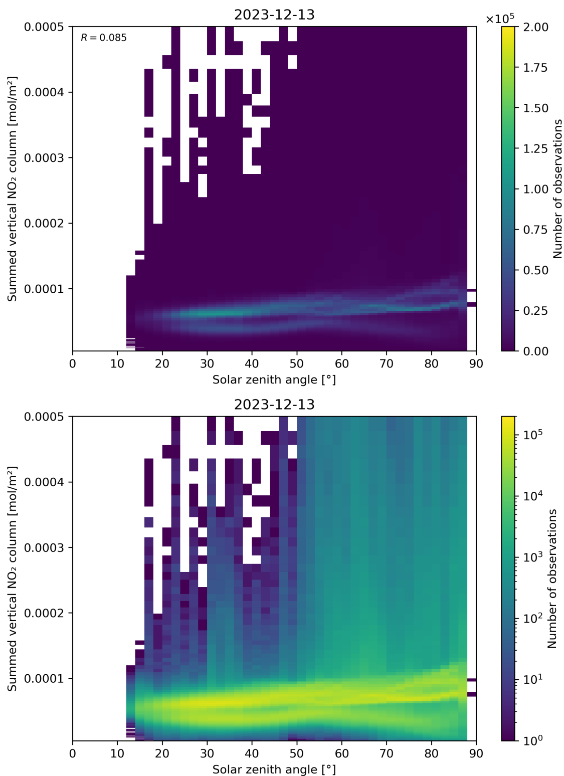
Figure 151: Scatter density plot of “Solar zenith angle” against “Summed vertical NO 2 column” for 2023-12-12 to 2023-12-14.
