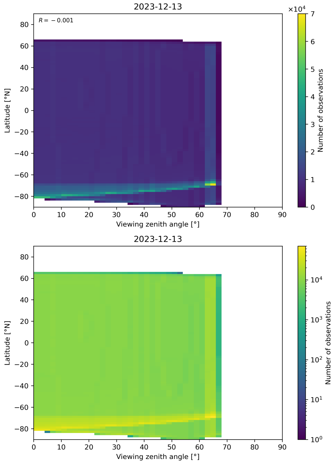
Figure 163: Scatter density plot of “Viewing zenith angle” against “Latitude” for 2023-12-12 to 2023-12-14.
