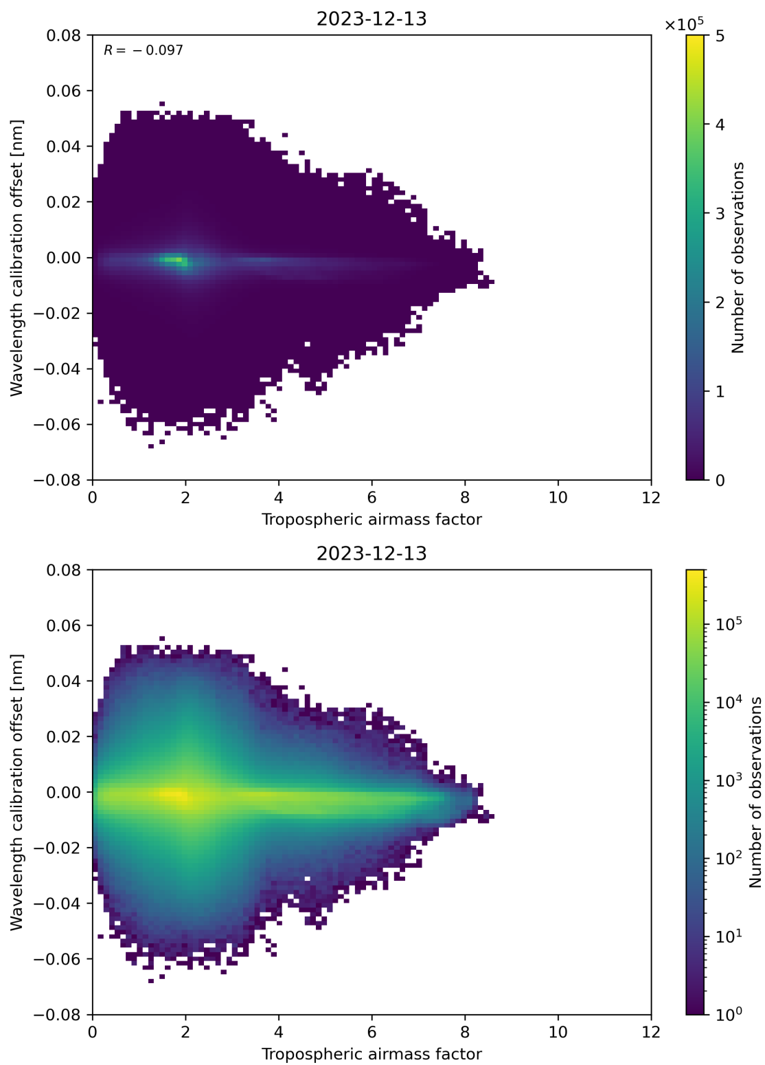
Figure 80: Scatter density plot of “Tropospheric airmass factor” against “Wavelength calibration offset” for 2023-12-12 to 2023-12-14.
