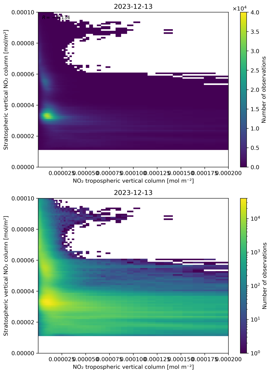
Figure 125: Scatter density plot of “NO 2 tropospheric vertical column” against “Stratospheric vertical NO 2 column” for 2023-12-12 to 2023-12-14.
