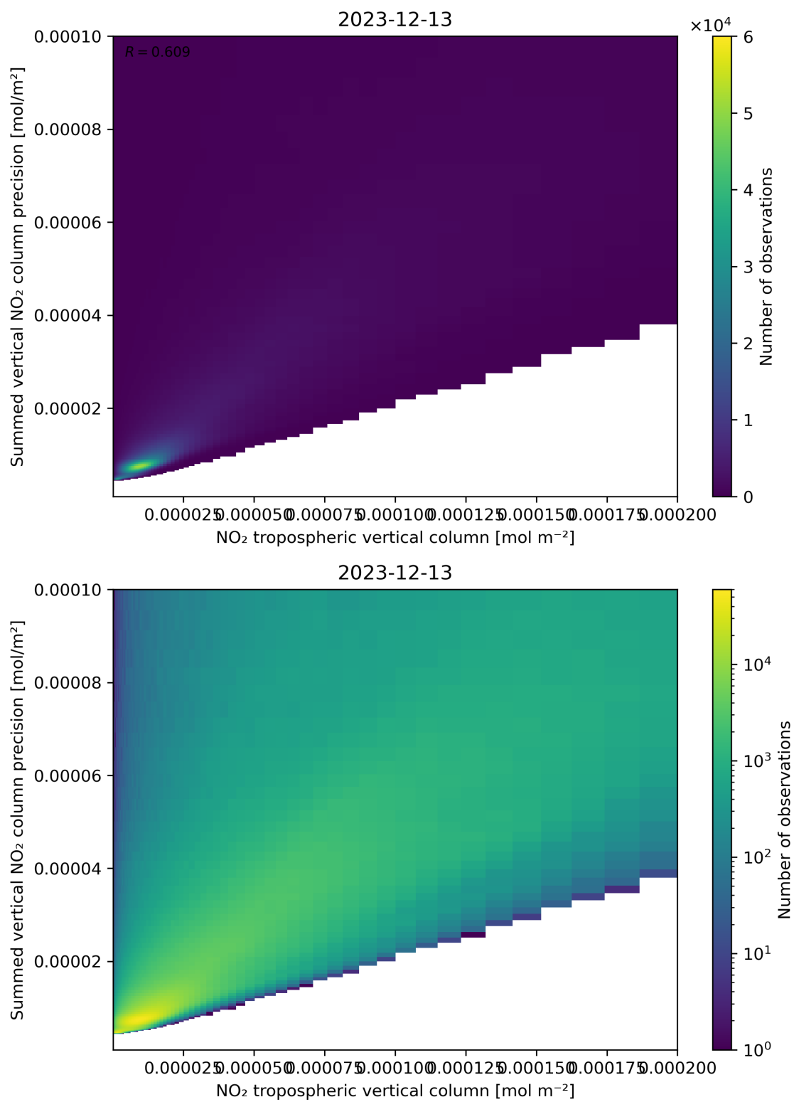
Figure 127: Scatter density plot of “NO 2 tropospheric vertical column” against “Summed vertical NO 2 column precision” for 2023-12-12 to 2023-12-14.
