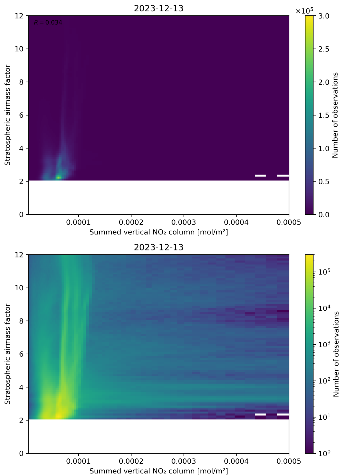
Figure 103: Scatter density plot of “Summed vertical NO 2 column” against “Stratospheric airmass factor” for 2023-12-12 to 2023-12-14.
