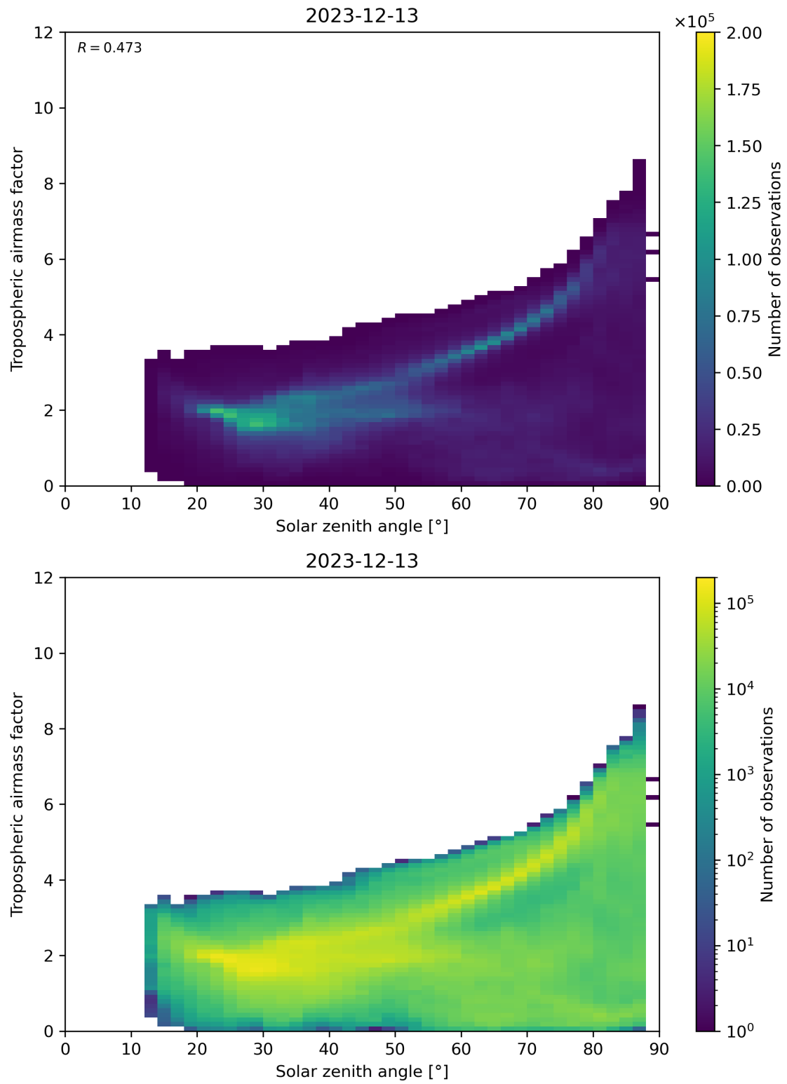
Figure 147: Scatter density plot of “Solar zenith angle” against “Tropospheric airmass factor” for 2023-12-12 to 2023-12-14.
