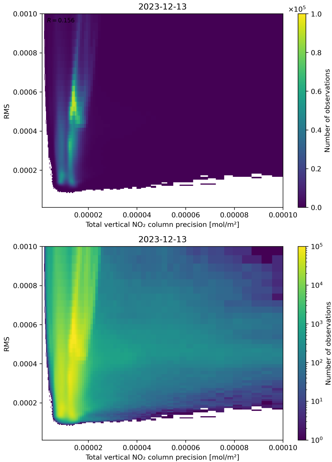
Figure 119: Scatter density plot of “Total vertical NO 2 column precision” against “RMS” for 2023-12-12 to 2023-12-14.
