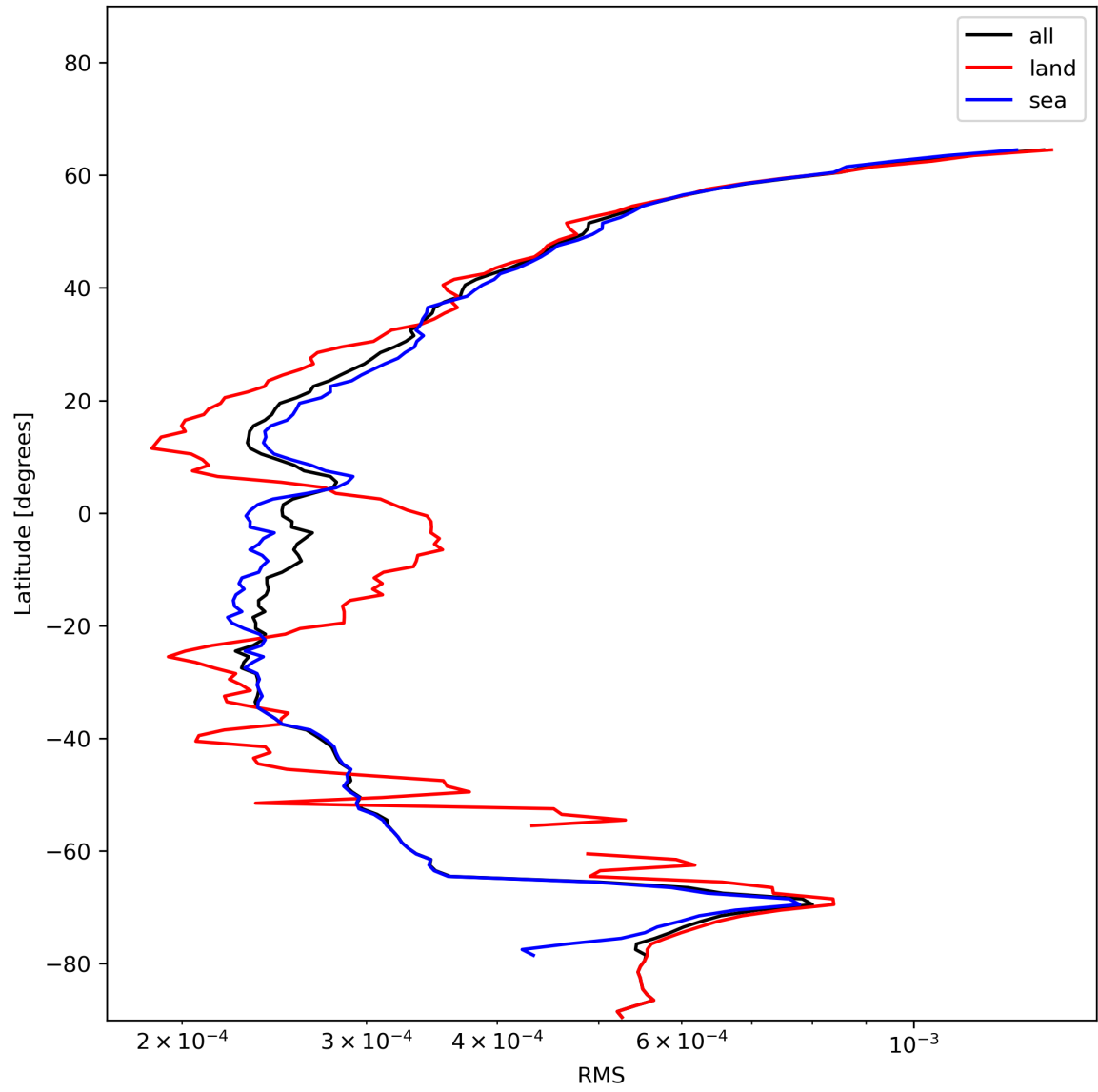
Figure 26: Zonal average of “RMS” for 2023-12-12 to 2023-12-14.
