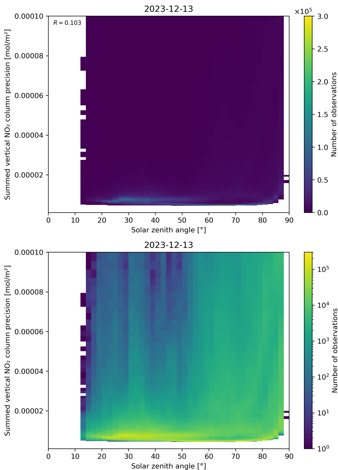
Figure 152: Scatter density plot of “Solar zenith angle” against “Summed vertical NO 2 column precision” for 2023-12-12 to 2023-12-14.
