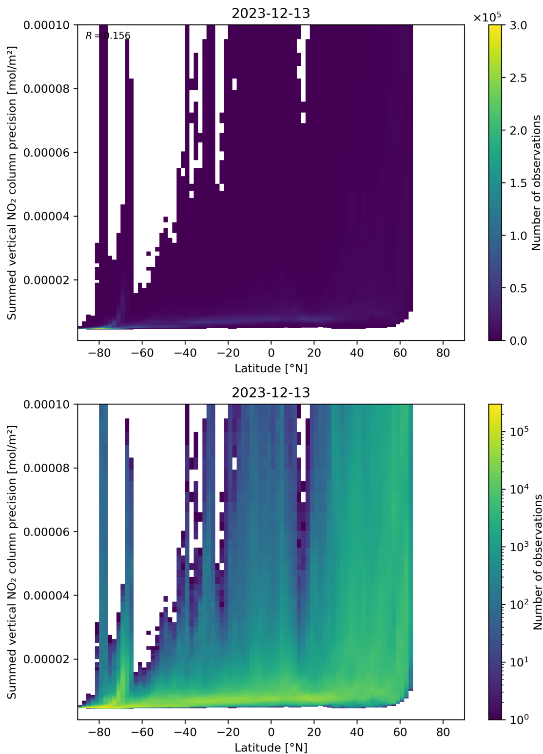
Figure 89: Scatter density plot of “Latitude” against “Summed vertical NO 2 column precision” for 2023-12-12 to 2023-12-14.
