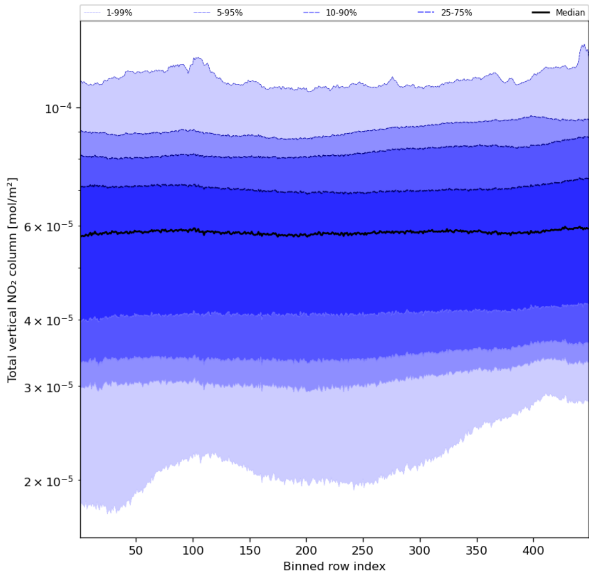
Figure 55: Along track statistics of “Total vertical NO 2 column” for 2023-12-12 to 2023-12-14
