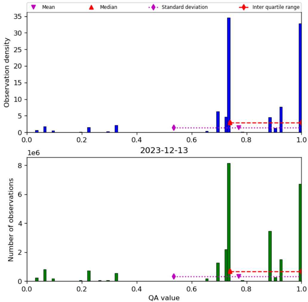
Figure 28: Histogram of “QA value” for 2023-12-12 to 2023-12-14
