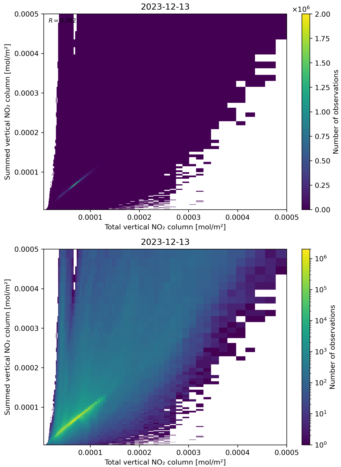
Figure 112: Scatter density plot of “Total vertical NO 2 column” against “Summed vertical NO 2 column” for 2023-12-12 to 2023-12-14.
