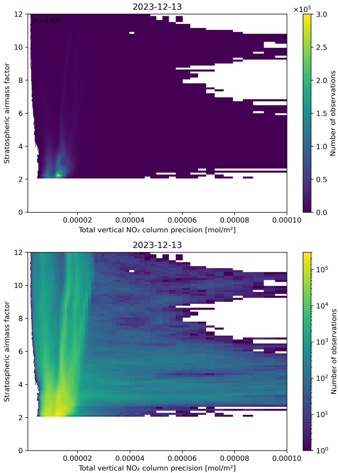
Figure 115: Scatter density plot of “Total vertical NO 2 column precision” against “Stratospheric air mass factor” for 2023-12-12 to 2023-12-14.
