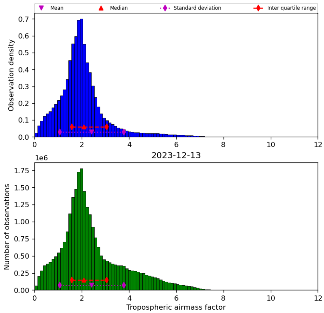
Figure 31: Histogram of “Tropospheric airmass factor” for 2023-12-12 to 2023-12-14
