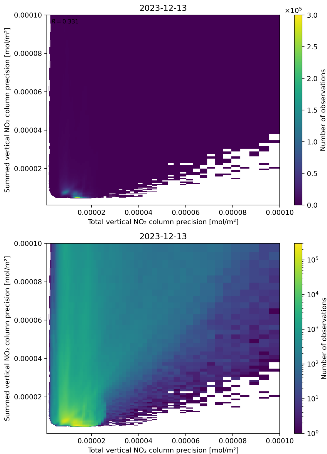
Figure 118: Scatter density plot of “Total vertical NO 2 column precision” against “Summed vertical NO 2 column precision” for 2023-12-12 to 2023-12-14.
