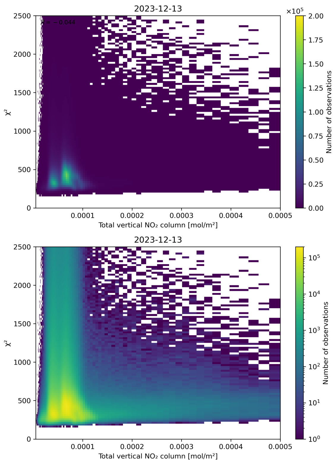
Figure 111: Scatter density plot of “Total vertical NO 2 column” against “ \chi^2 ” for 2023-12-12 to 2023-12-14.
