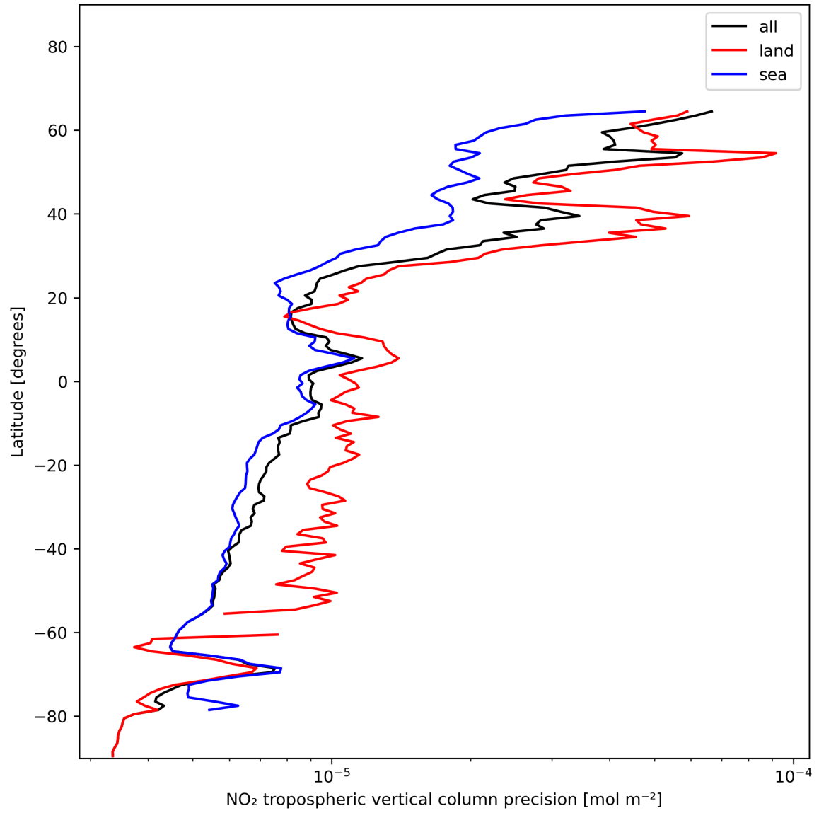
Figure 13: Zonal average of “NO 2 tropospheric vertical column precision” for 2023-12-12 to 2023-12-14.
