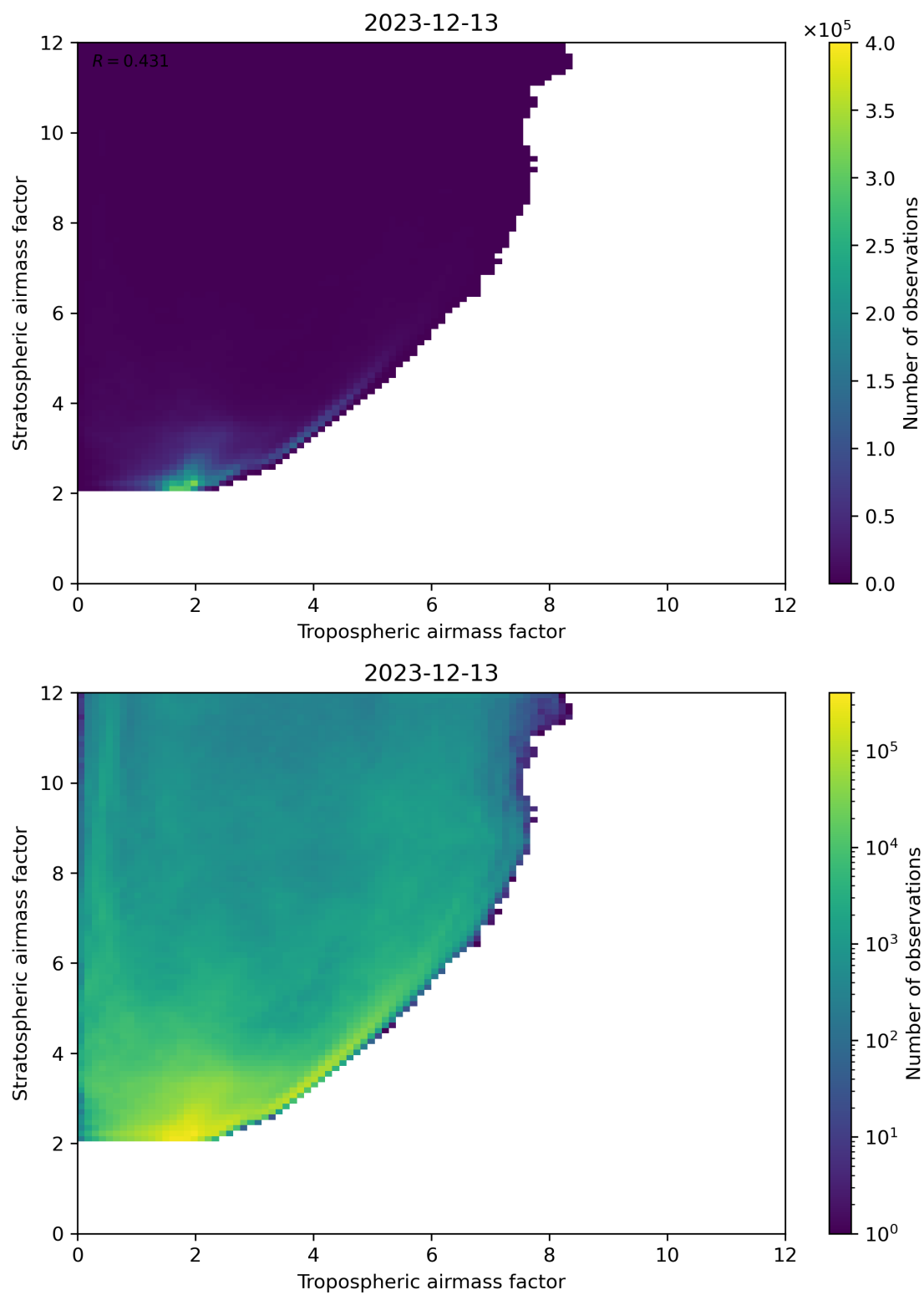
Figure 71: Scatter density plot of “Tropospheric airmass factor” against “Stratospheric airmass factor” for 2023-12-12 to 2023-12-14.
