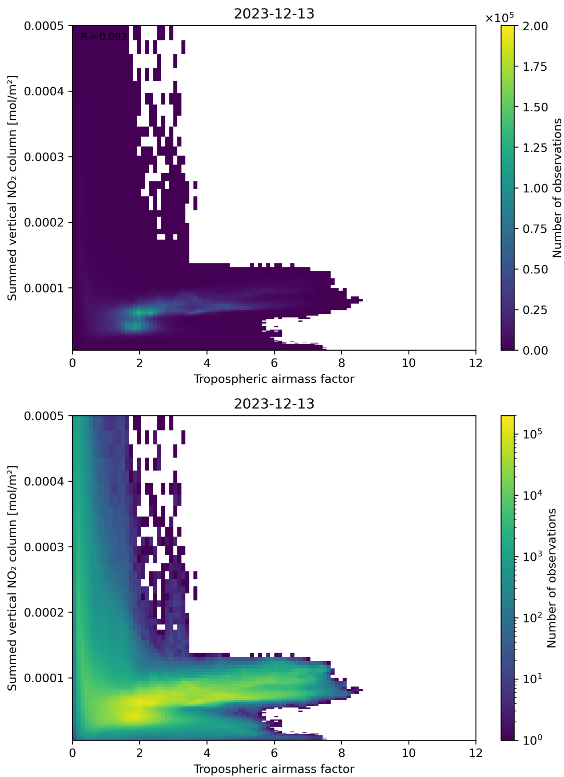
Figure 75: Scatter density plot of “Tropospheric air mass factor” against “Summed vertical NO 2 column” for 2023-12-12 to 2023-12-14.
