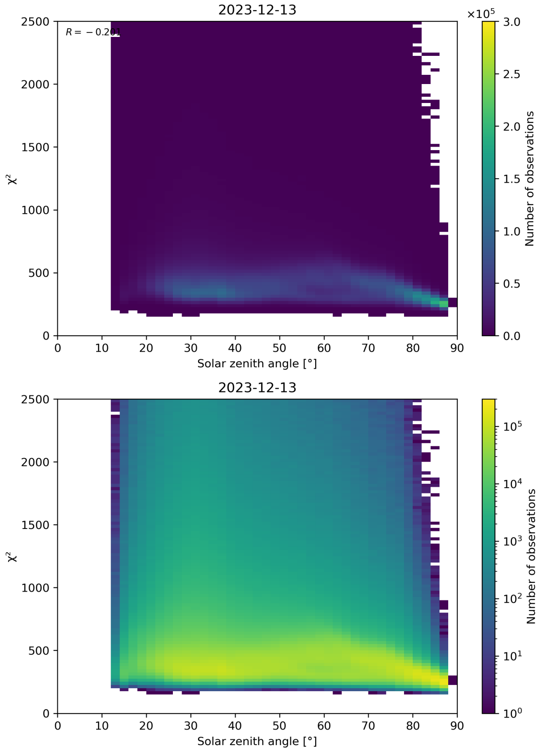
Figure 148: Scatter density plot of “Solar zenith angle” against “ \chi^2 ” for 2023-12-12 to 2023-12-14.
