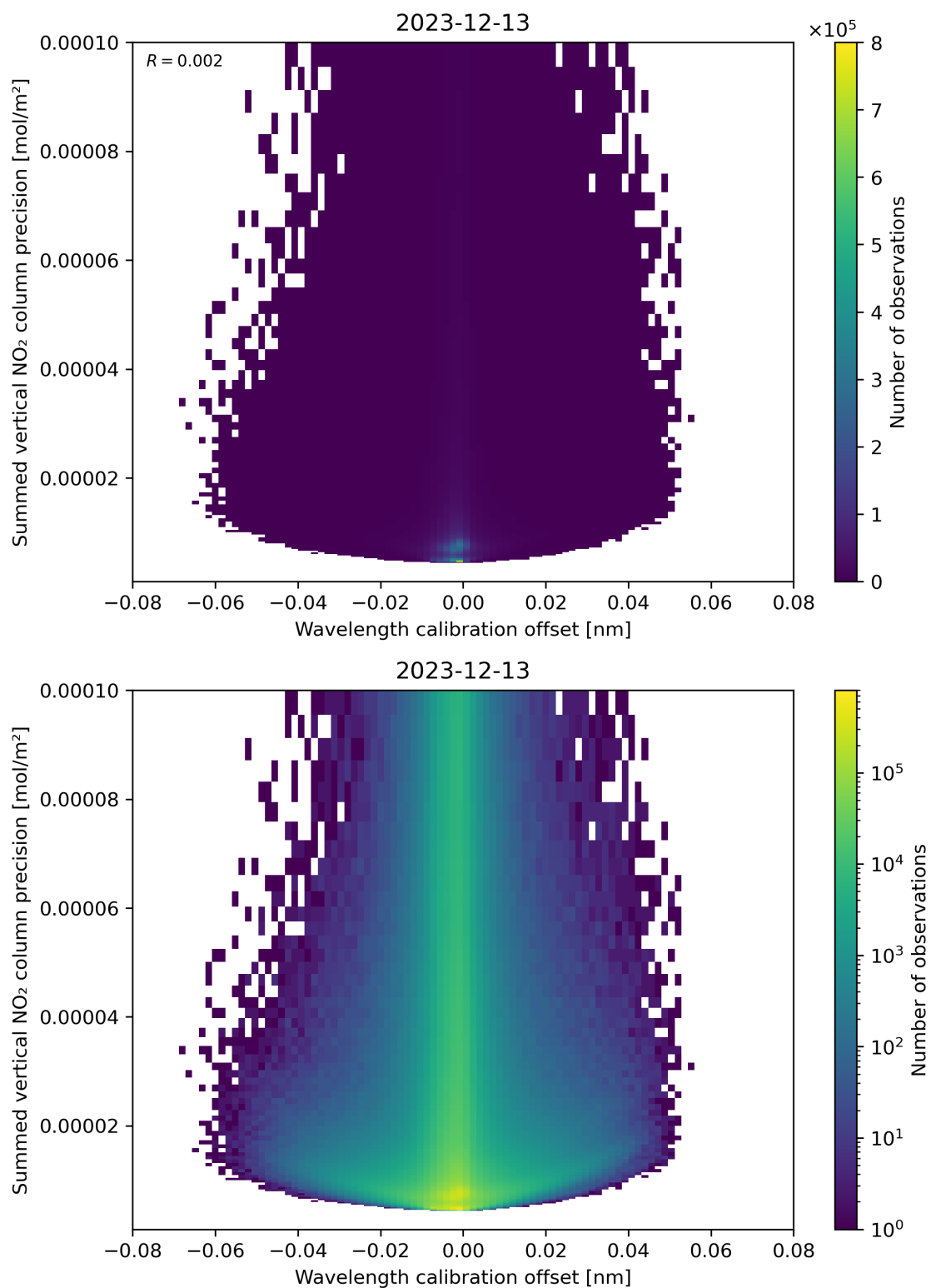
Figure 178: Scatter density plot of “Wavelength calibration offset” against “Summed vertical NO 2 column precision” for 2023-12-12 to 2023-12-14.
