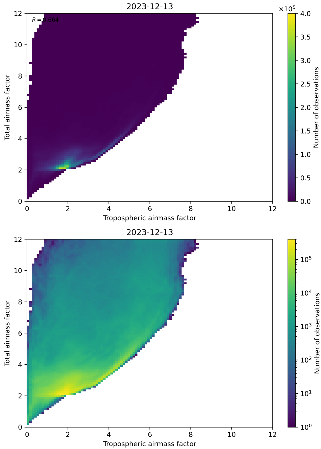
Figure 72: Scatter density plot of “Tropospheric airmass factor” against “Total airmass factor” for 2023-12-12 to 2023-12-14.
