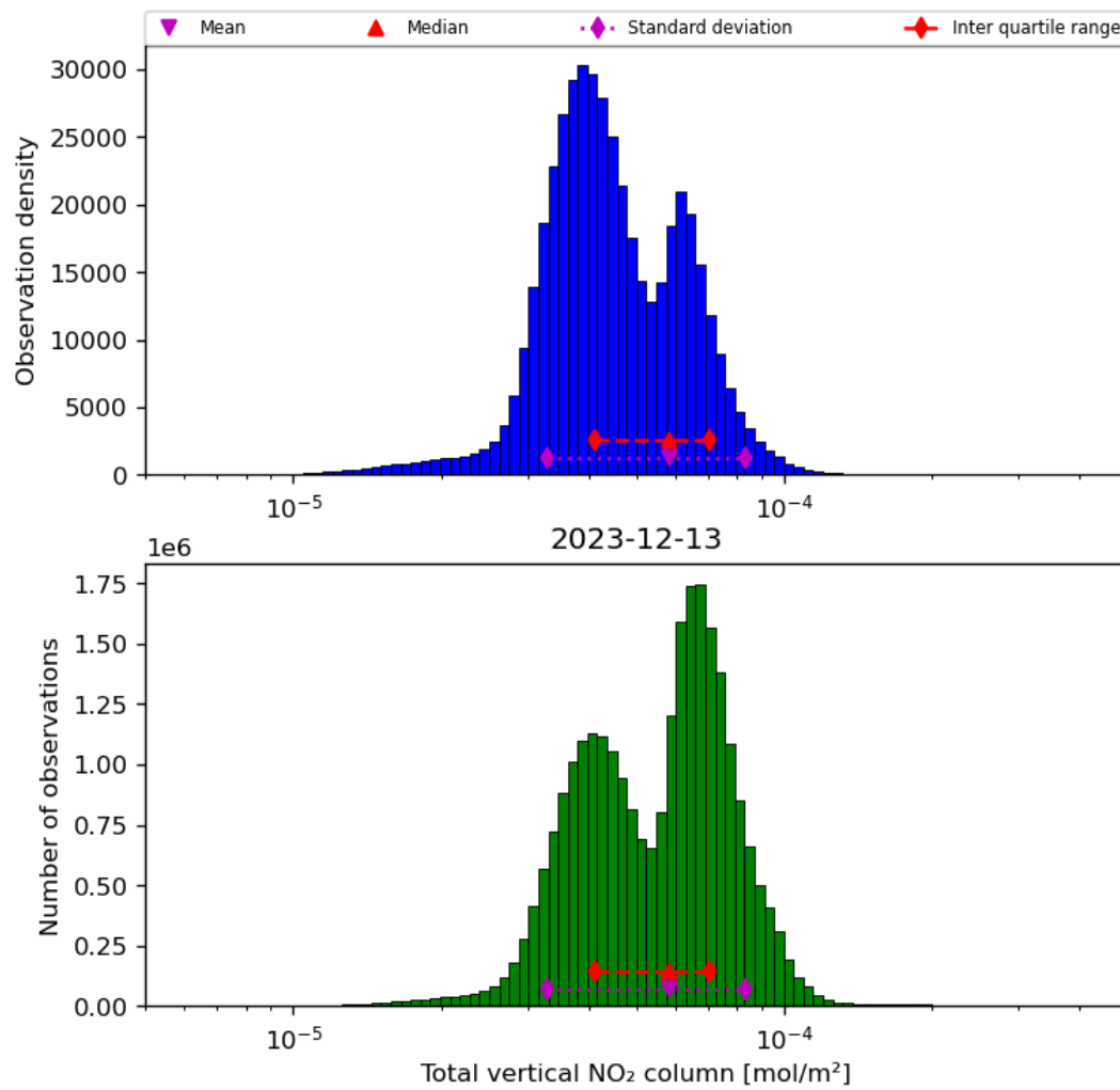
Figure 38: Histogram of “Total vertical NO 2 column” for 2023-12-12 to 2023-12-14
