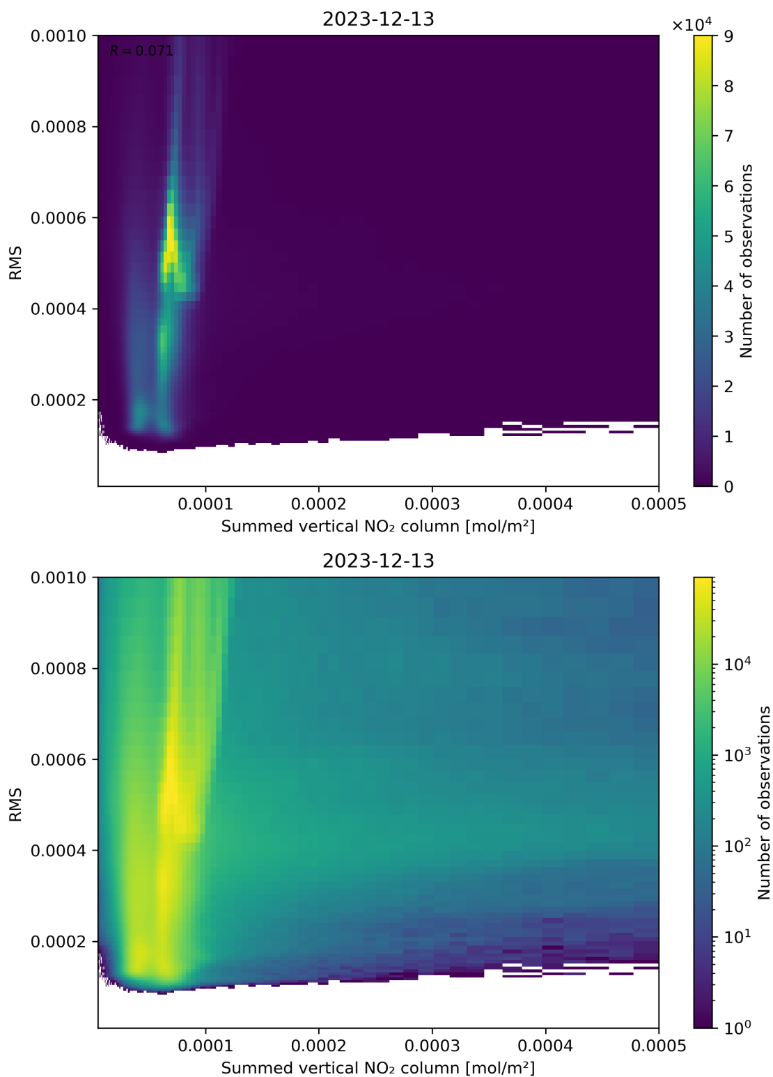
Figure 109: Scatter density plot of “Summed vertical NO 2 column” against “RMS” for 2023-12-12 to 2023-12-14.
