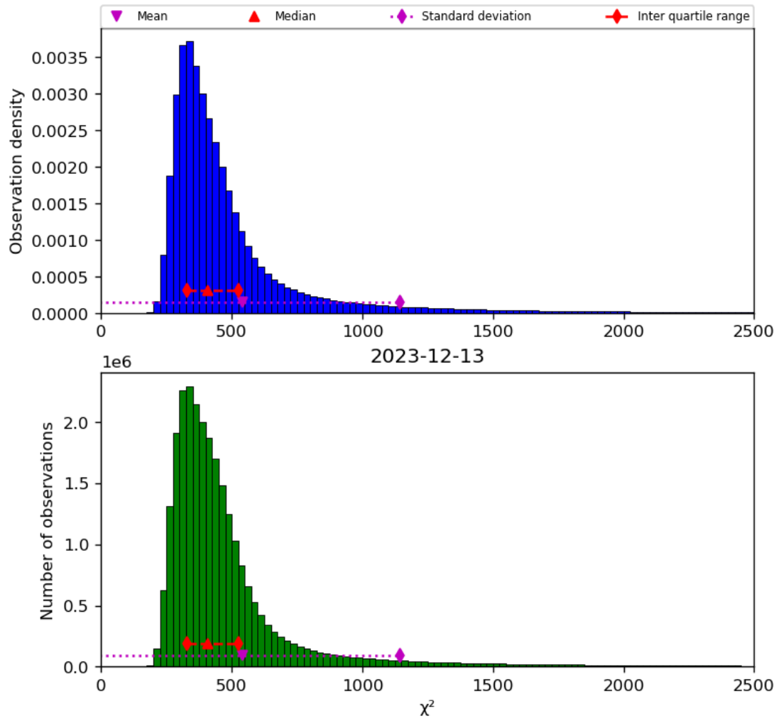
Figure 42: Histogram of “ \chi^2 ” for 2023-12-12 to 2023-12-14
