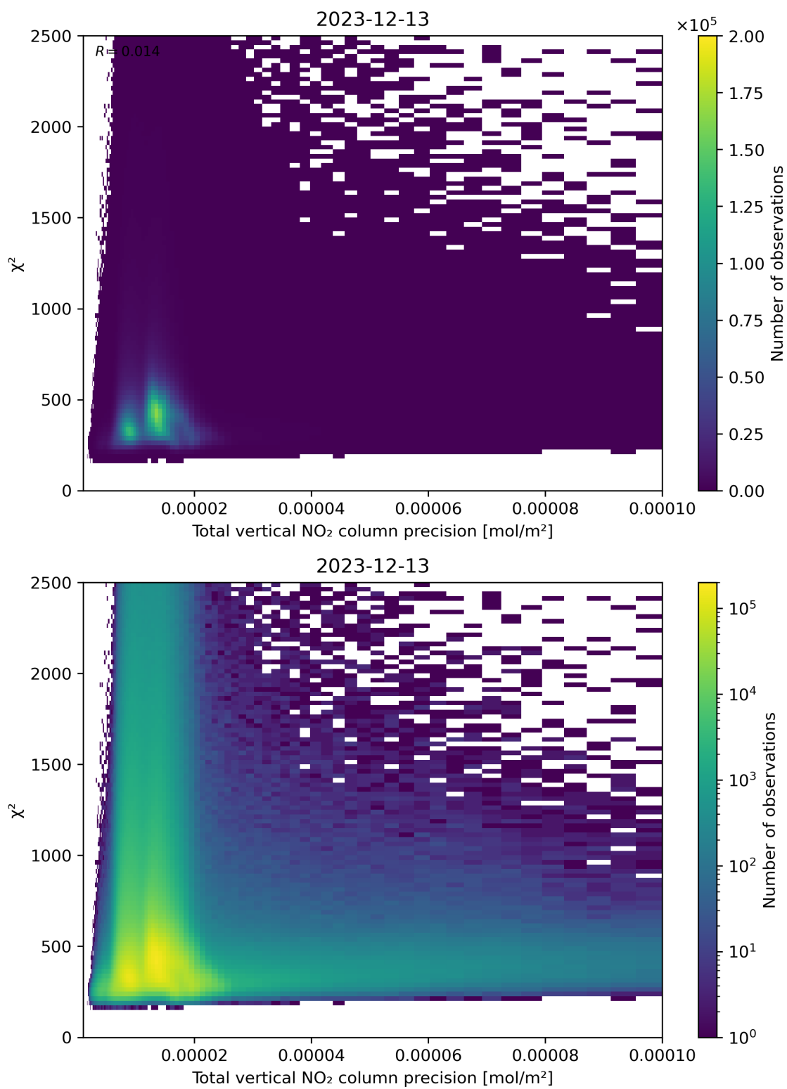
Figure 116: Scatter density plot of “Total vertical NO 2 column precision” against “ \chi^2 ” for 2023-12-12 to 2023-12-14.
