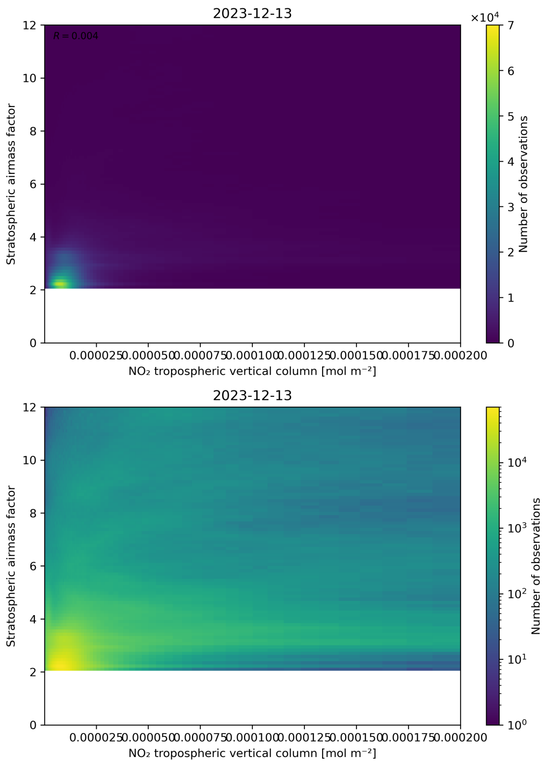
Figure 121: Scatter density plot of “NO 2 tropospheric vertical column” against “Stratospheric air mass factor” for 2023-12-12 to 2023-12-14.
