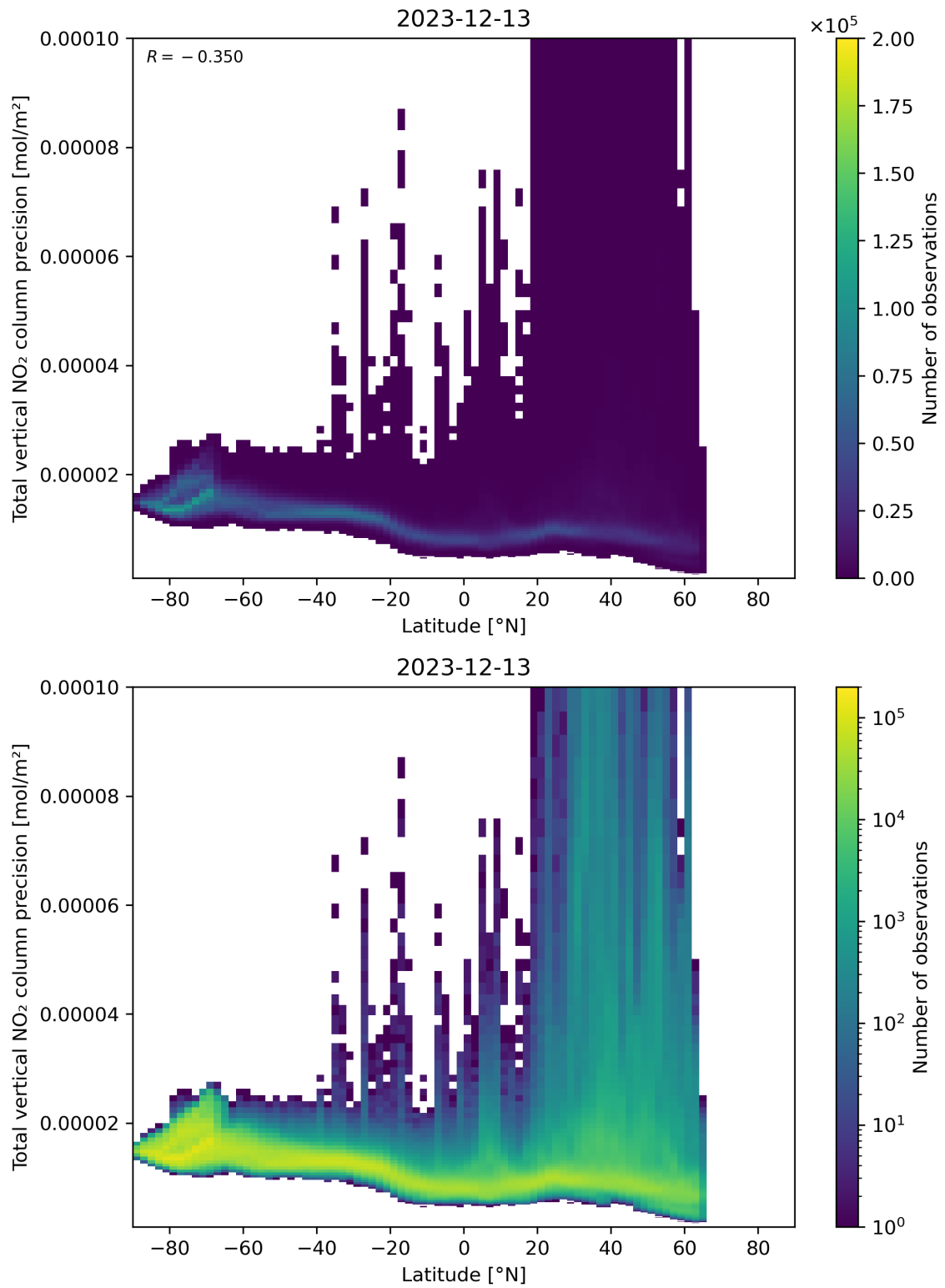
Figure 91: Scatter density plot of “Latitude” against “Total vertical NO 2 column precision” for 2023-12-12 to 2023-12-14.
