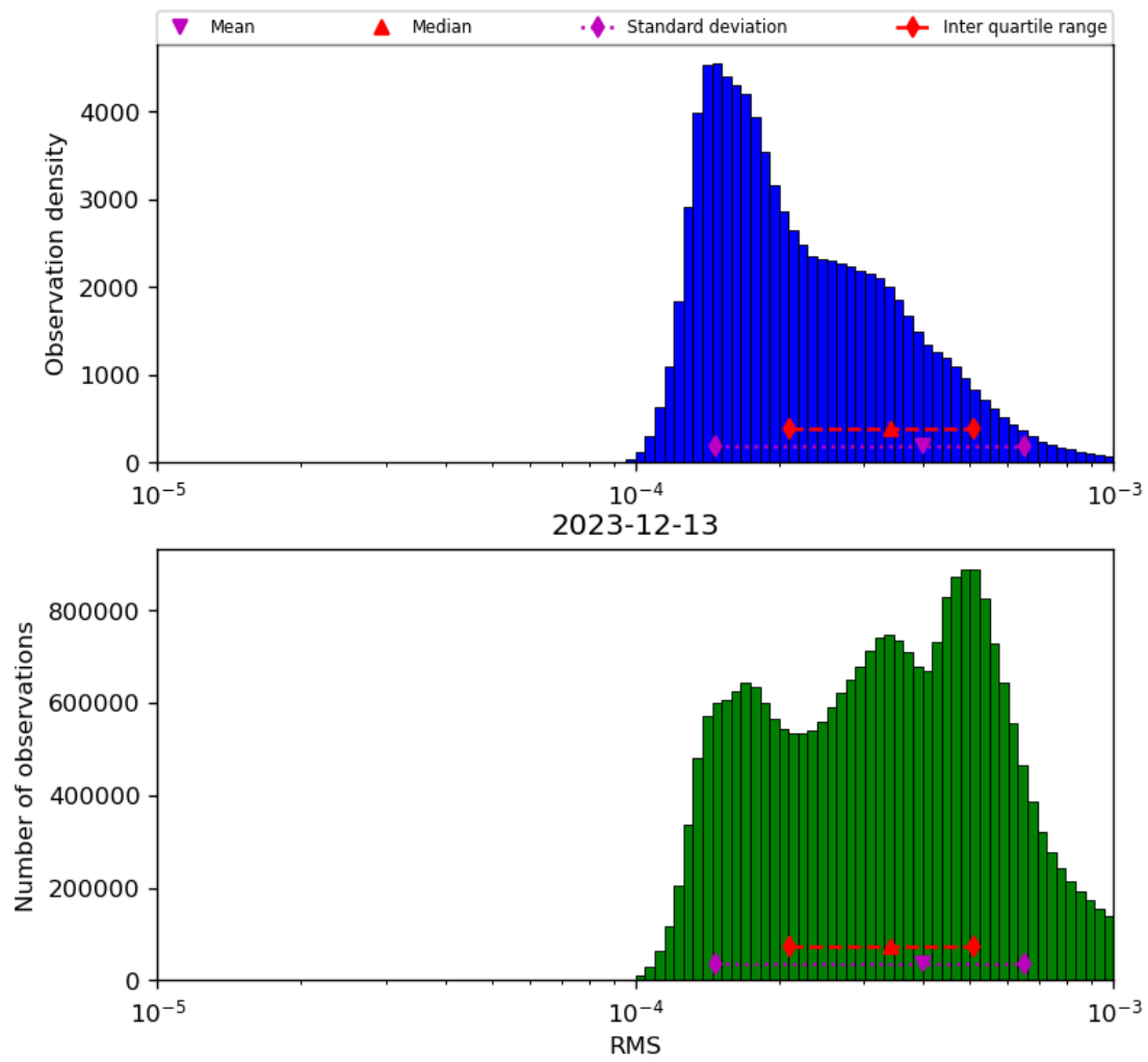
Figure 43: Histogram of “RMS” for 2023-12-12 to 2023-12-14
