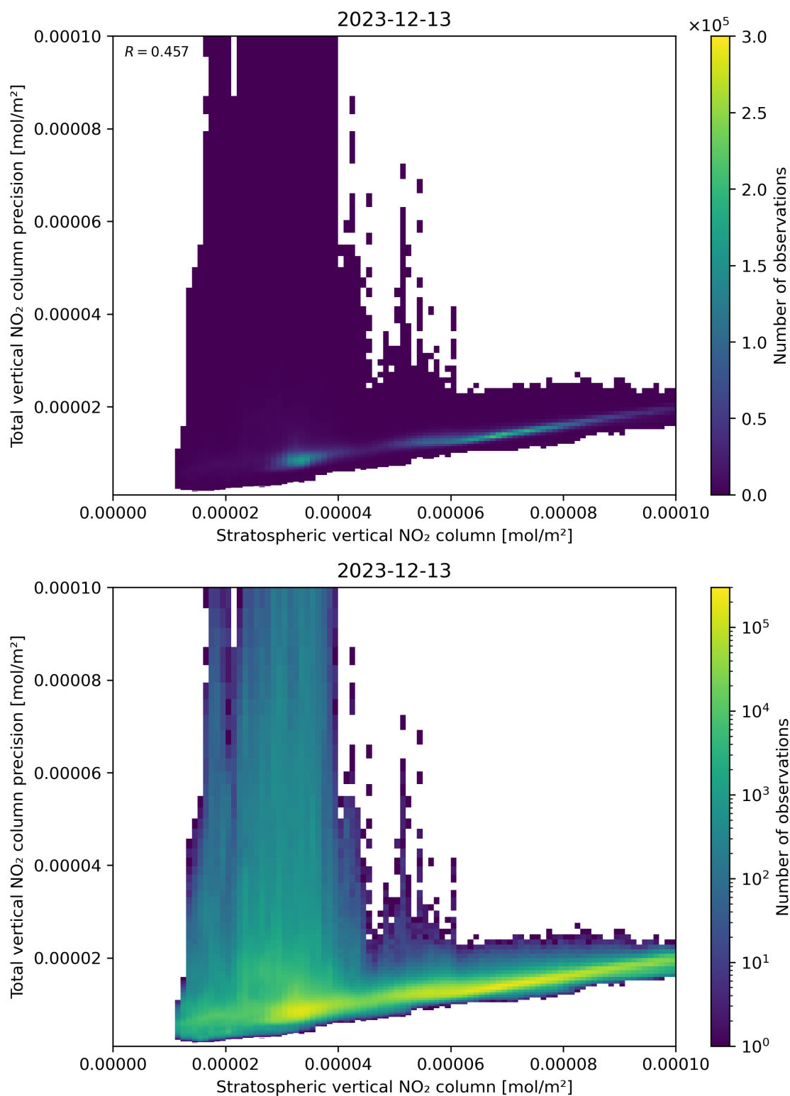
Figure 101: Scatter density plot of “Stratospheric vertical NO 2 column” against “Total vertical NO 2 column precision” for 2023-12-12 to 2023-12-14.
