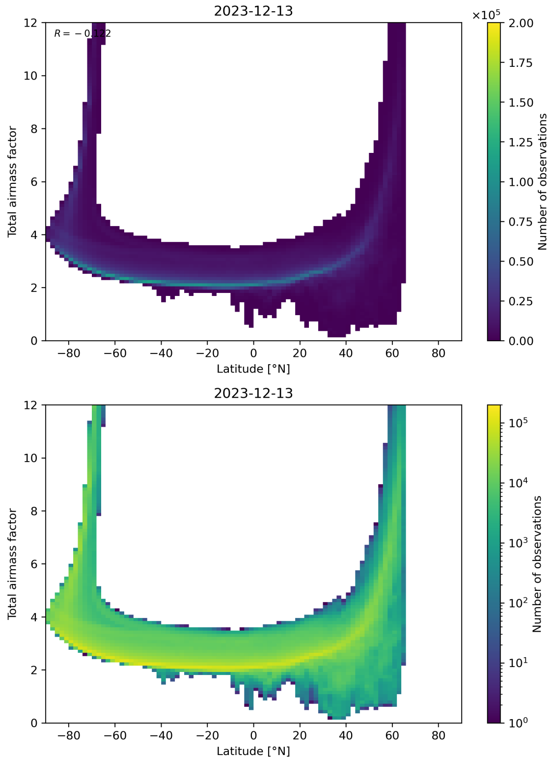
Figure 84: Scatter density plot of “Latitude” against “Total airmass factor” for 2023-12-12 to 2023-12-14.
