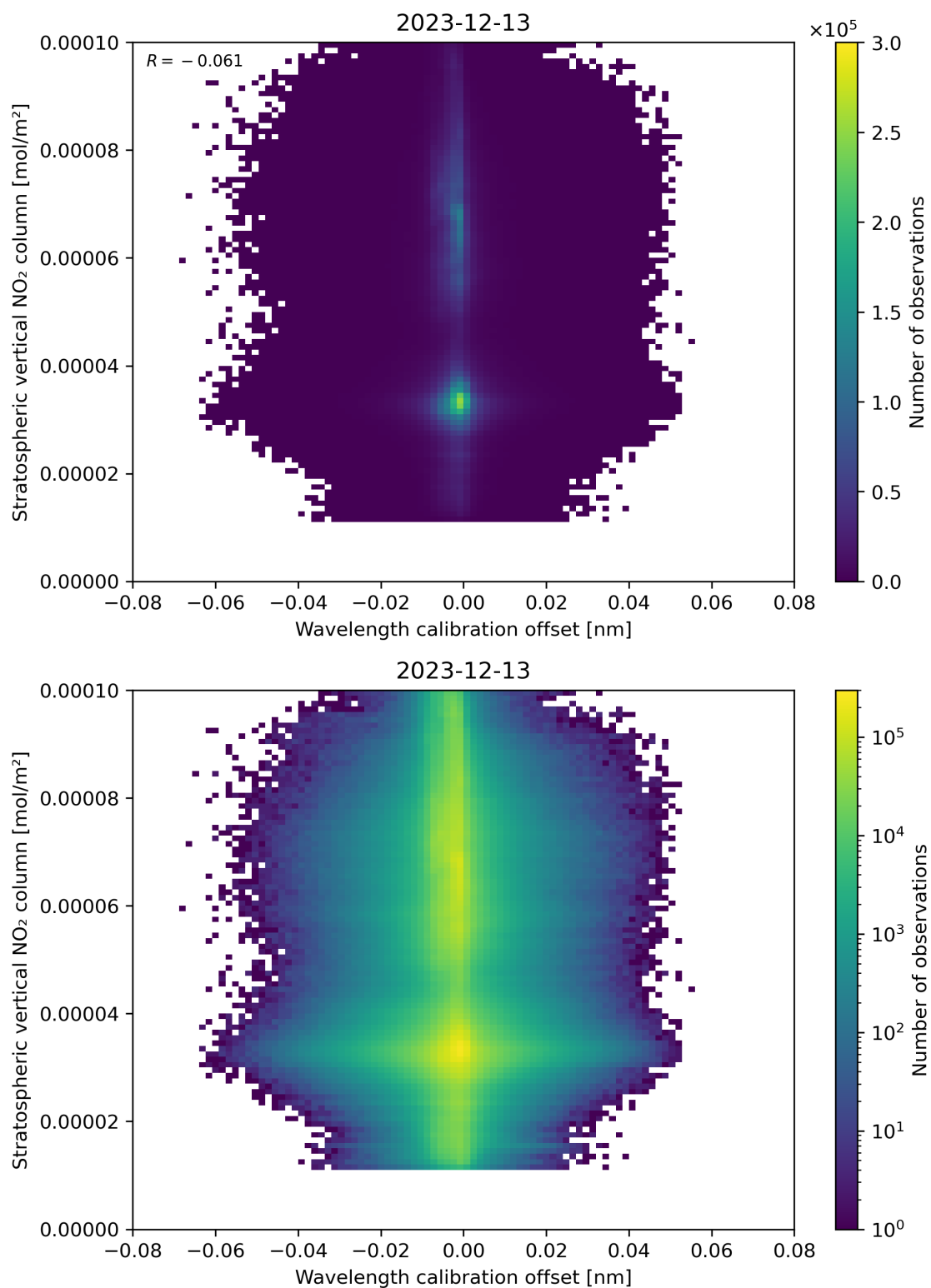
Figure 176: Scatter density plot of “Wavelength calibration offset” against “Stratospheric vertical NO 2 column” for 2023-12-12 to 2023-12-14.
