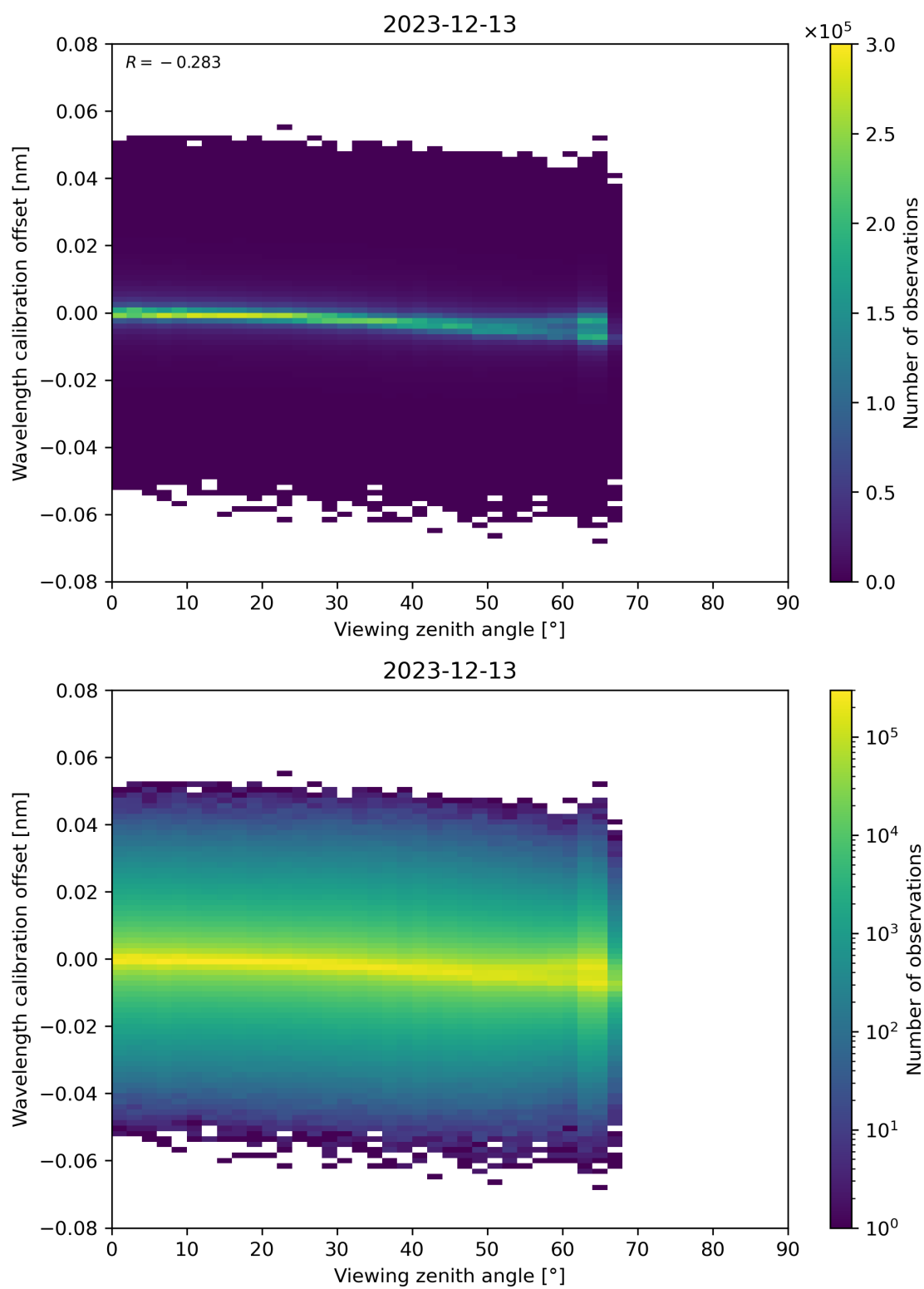
Figure 173: Scatter density plot of “Viewing zenith angle” against “Wavelength calibration offset” for 2023-12-12 to 2023-12-14.
