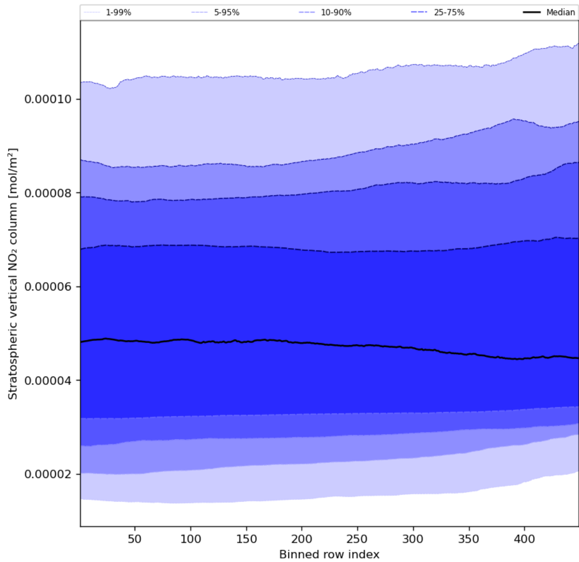
Figure 53: Along track statistics of “Stratospheric vertical NO 2 column” for 2023-12-12 to 2023-12-14
