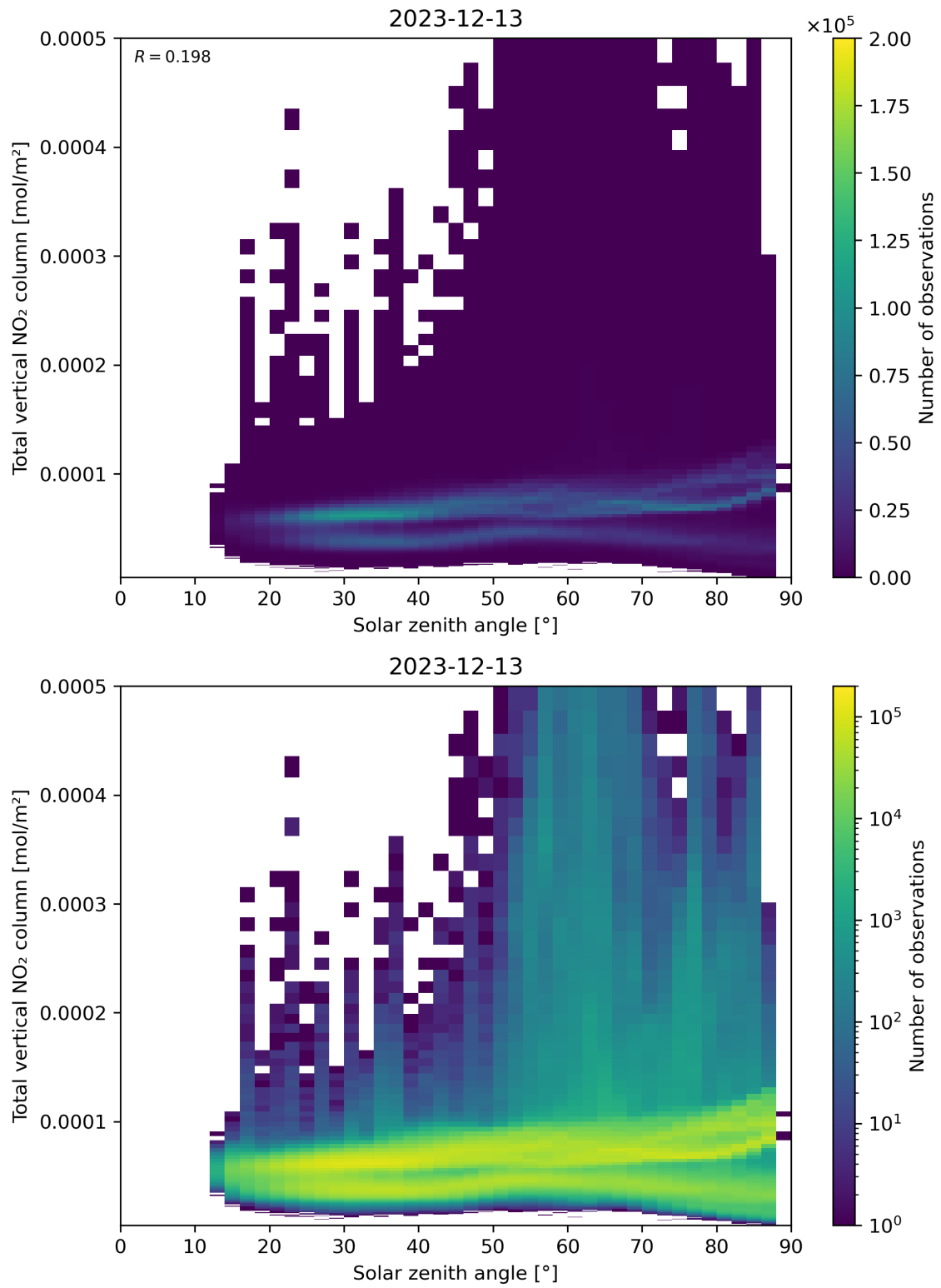
Figure 153: Scatter density plot of “Solar zenith angle” against “Total vertical NO 2 column” for 2023-12-12 to 2023-12-14.
