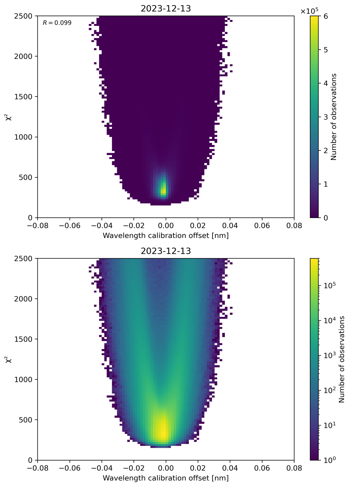
Figure 175: Scatter density plot of “Wavelength calibration offset” against “ \chi^2 ” for 2023-12-12 to 2023-12-14.
