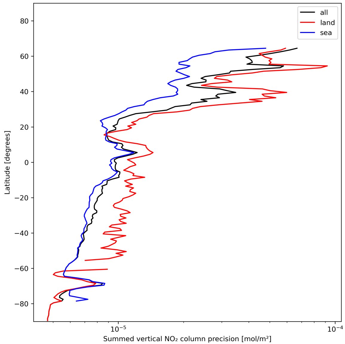
Figure 24: Zonal average of “Summed vertical NO 2 column precision” for 2023-12-12 to 2023-12-14.
