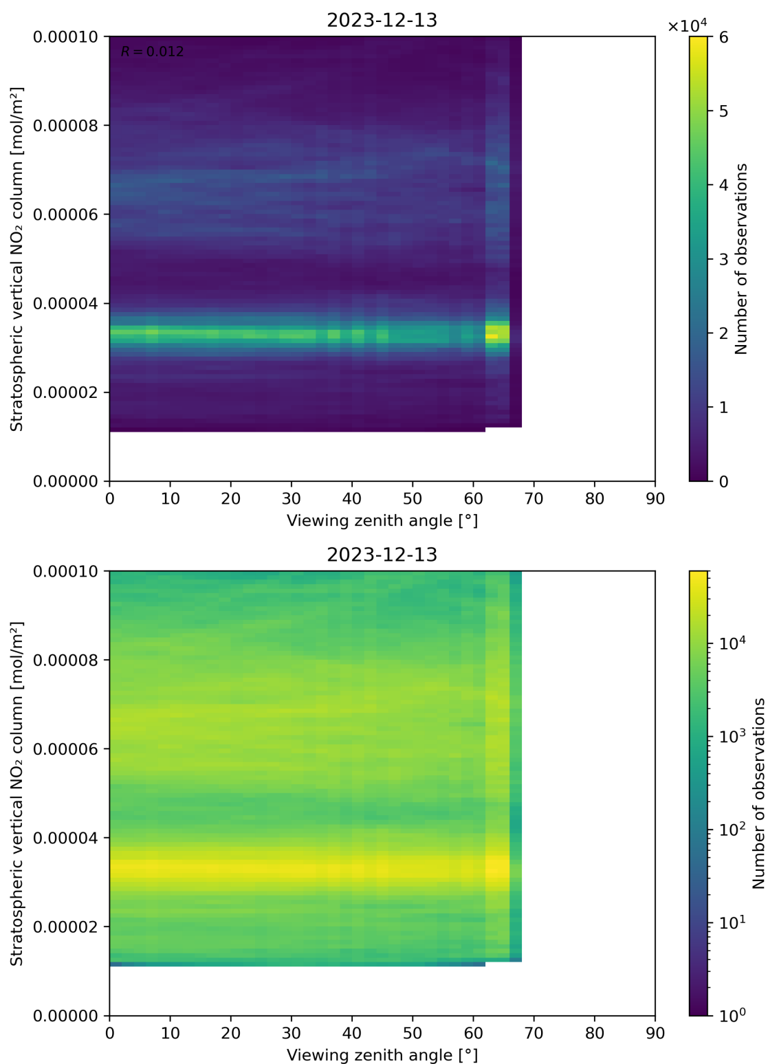
Figure 164: Scatter density plot of “Viewing zenith angle” against “Stratospheric vertical NO 2 column” for 2023-12-12 to 2023-12-14.
