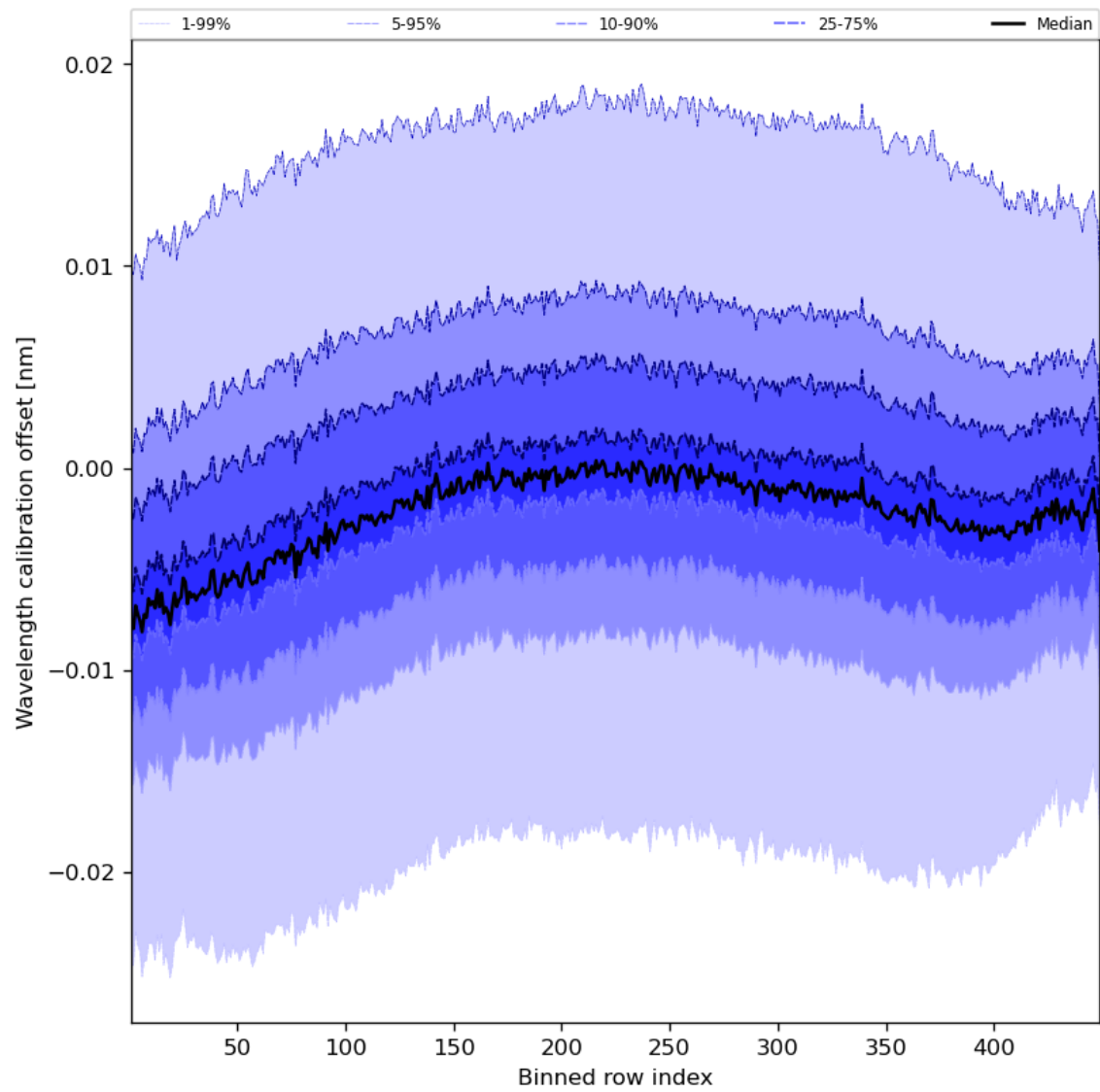
Figure 52: Along track statistics of “Wavelength calibration offset” for 2023-12-12 to 2023-12-14
