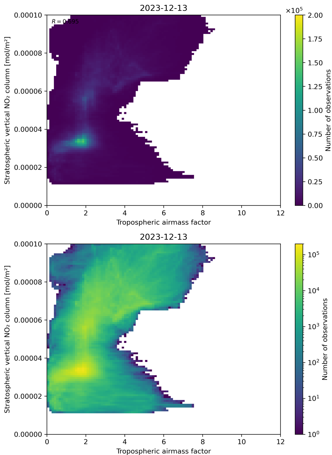
Figure 74: Scatter density plot of “Tropospheric airmass factor” against “Stratospheric vertical NO 2 column” for 2023-12-12 to 2023-12-14.
