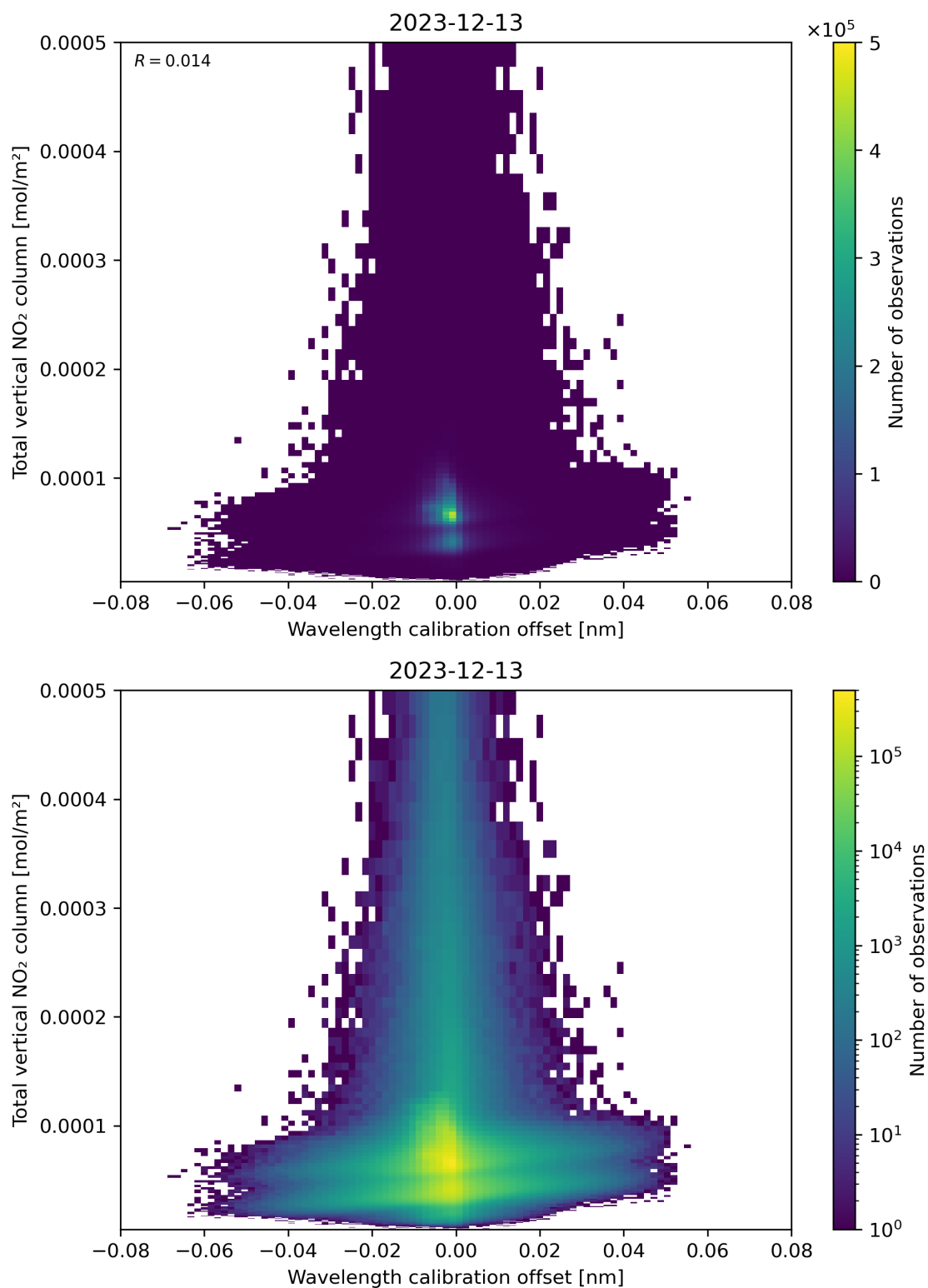
Figure 179: Scatter density plot of “Wavelength calibration offset” against “Total vertical NO 2 column” for 2023-12-12 to 2023-12-14.
