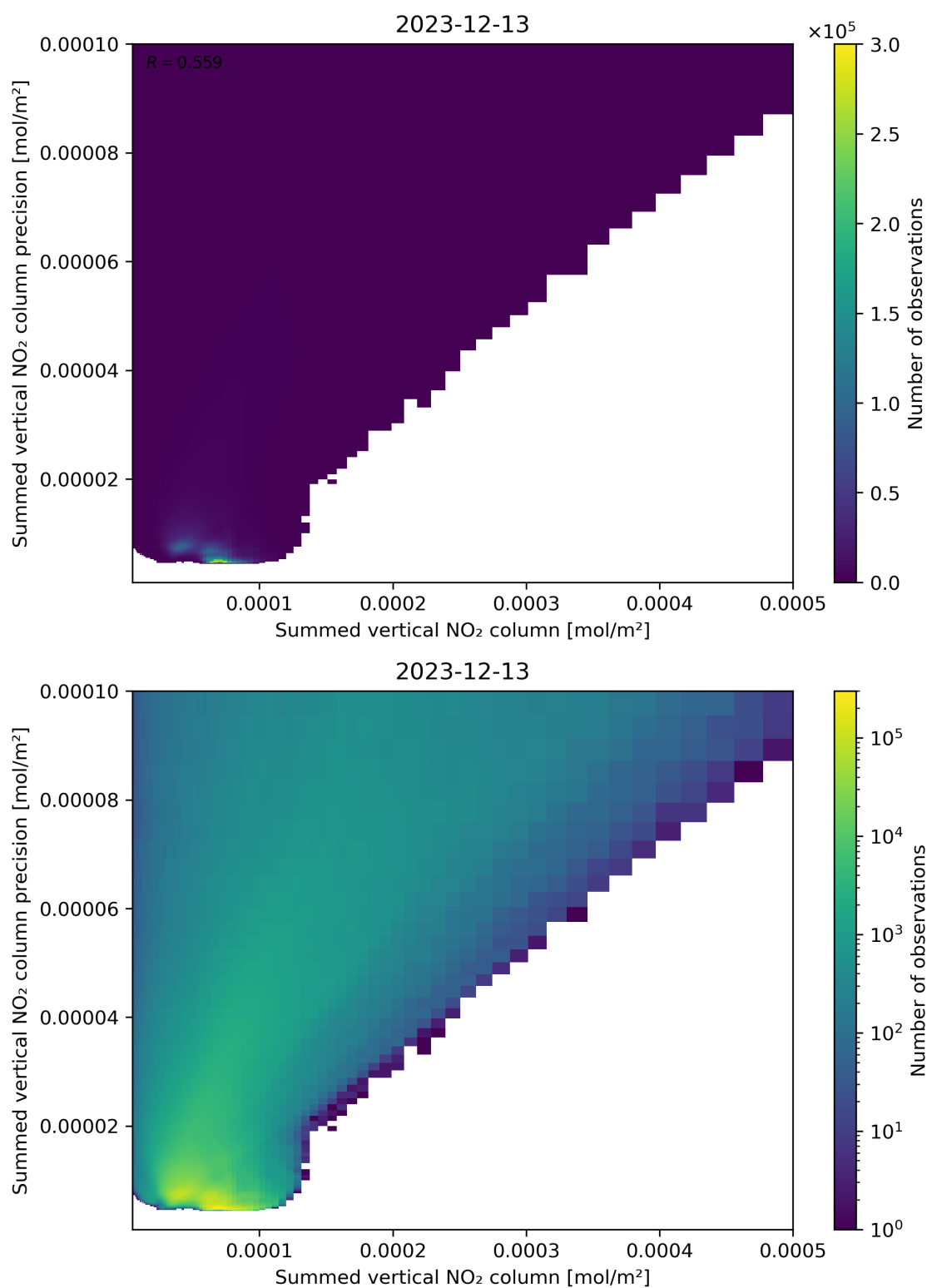
Figure 105: Scatter density plot of “Summed vertical NO 2 column” against “Summed vertical NO 2 column precision” for 2023-12-12 to 2023-12-14.
