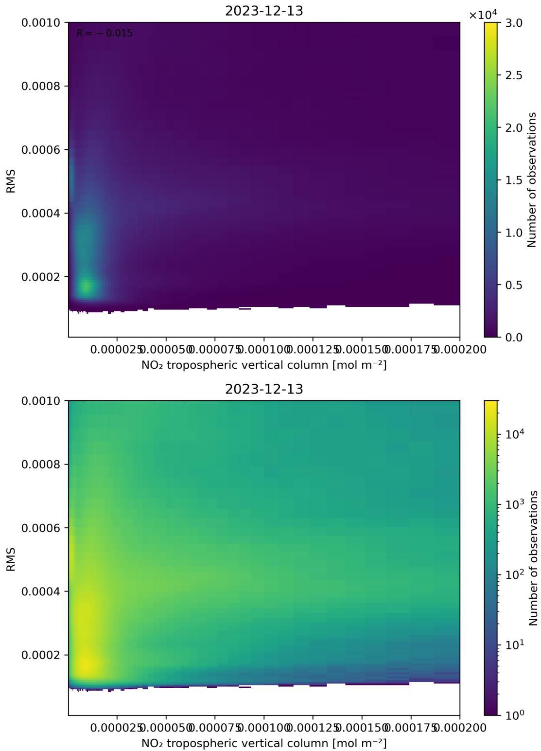
Figure 142: Scatter density plot of “NO 2 tropospheric vertical column” against “RMS” for 2023-12-12 to 2023-12-14.
