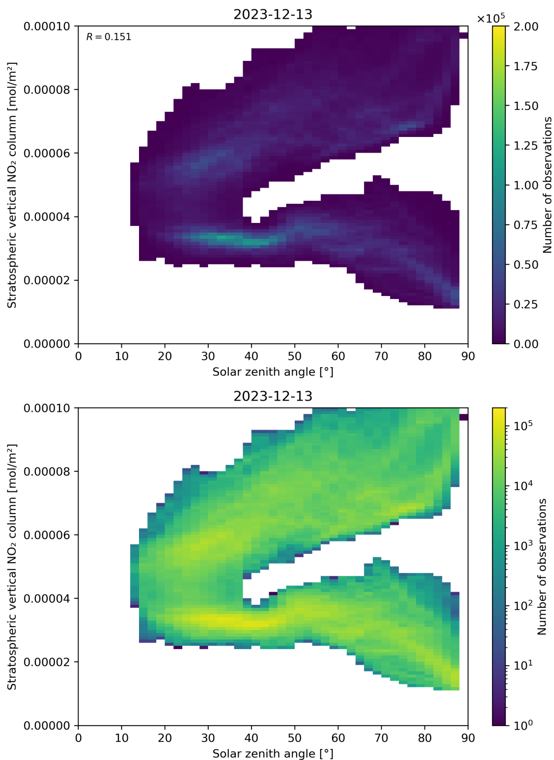
Figure 150: Scatter density plot of “Solar zenith angle” against “Stratospheric vertical NO 2 column” for 2023-12-12 to 2023-12-14.
