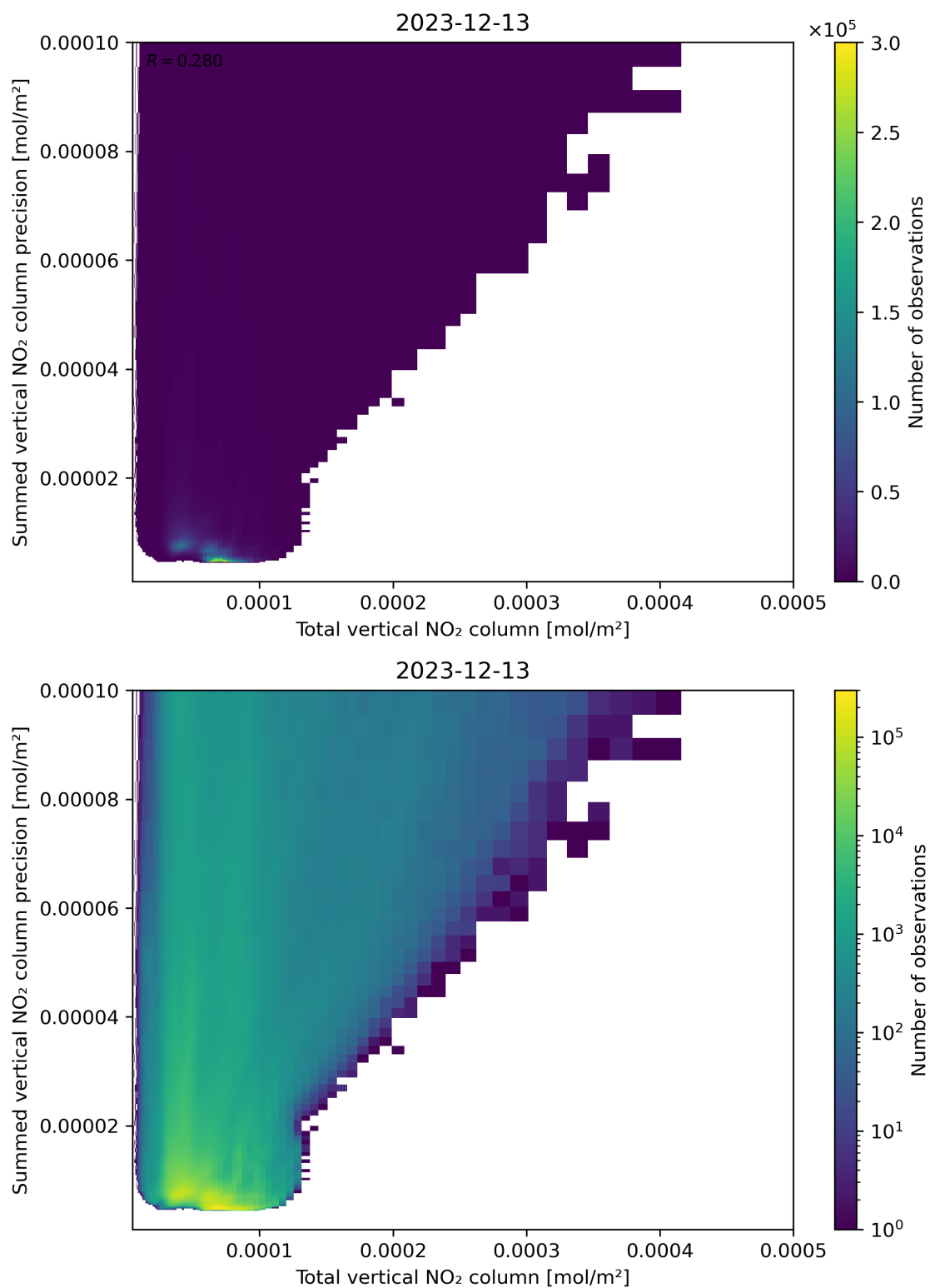
Figure 113: Scatter density plot of “Total vertical NO 2 column” against “Summed vertical NO 2 column precision” for 2023-12-12 to 2023-12-14.
