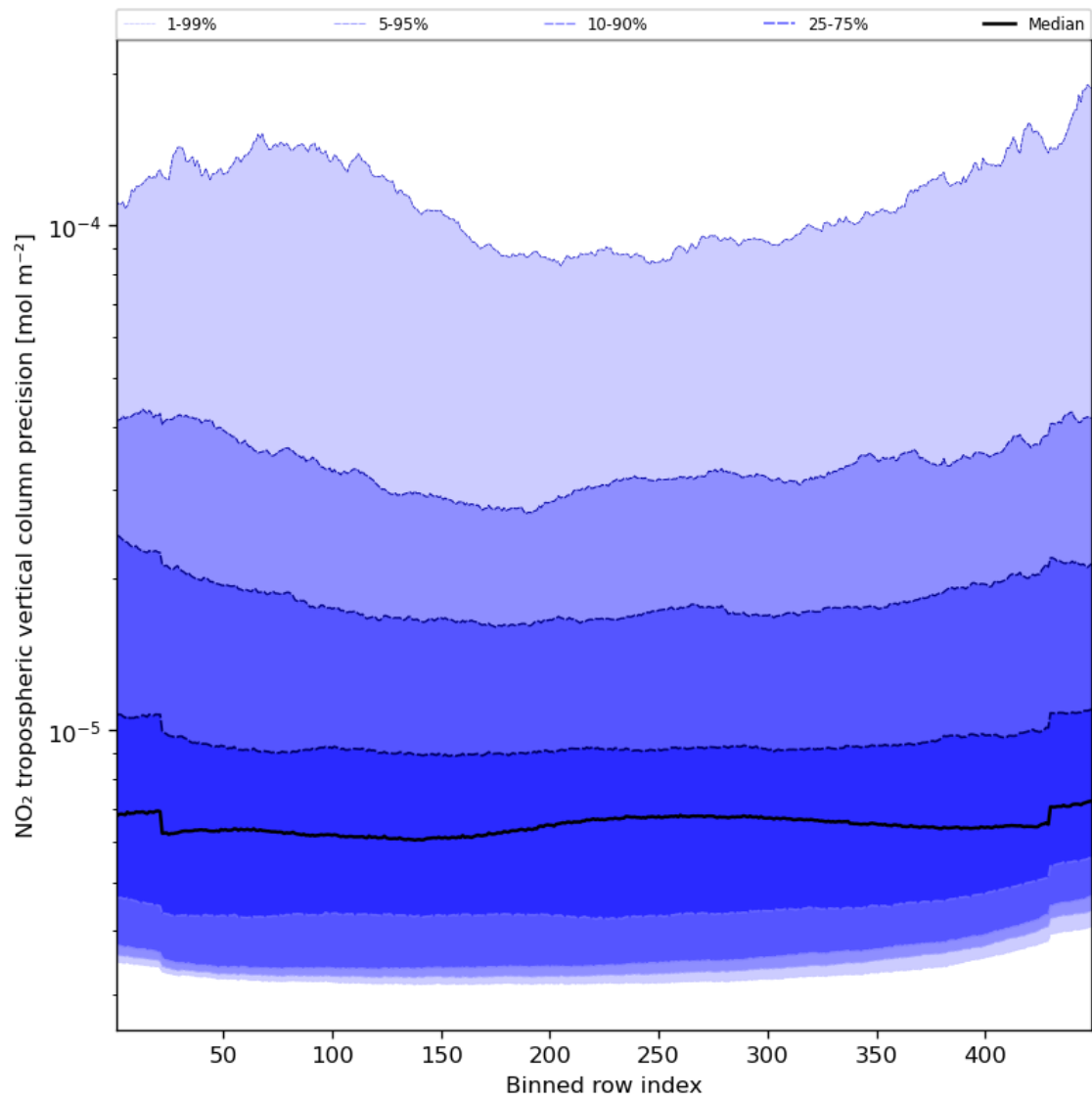
Figure 47: Along track statistics of “NO 2 tropospheric vertical column precision” for 2023-12-12 to 2023-12-14
