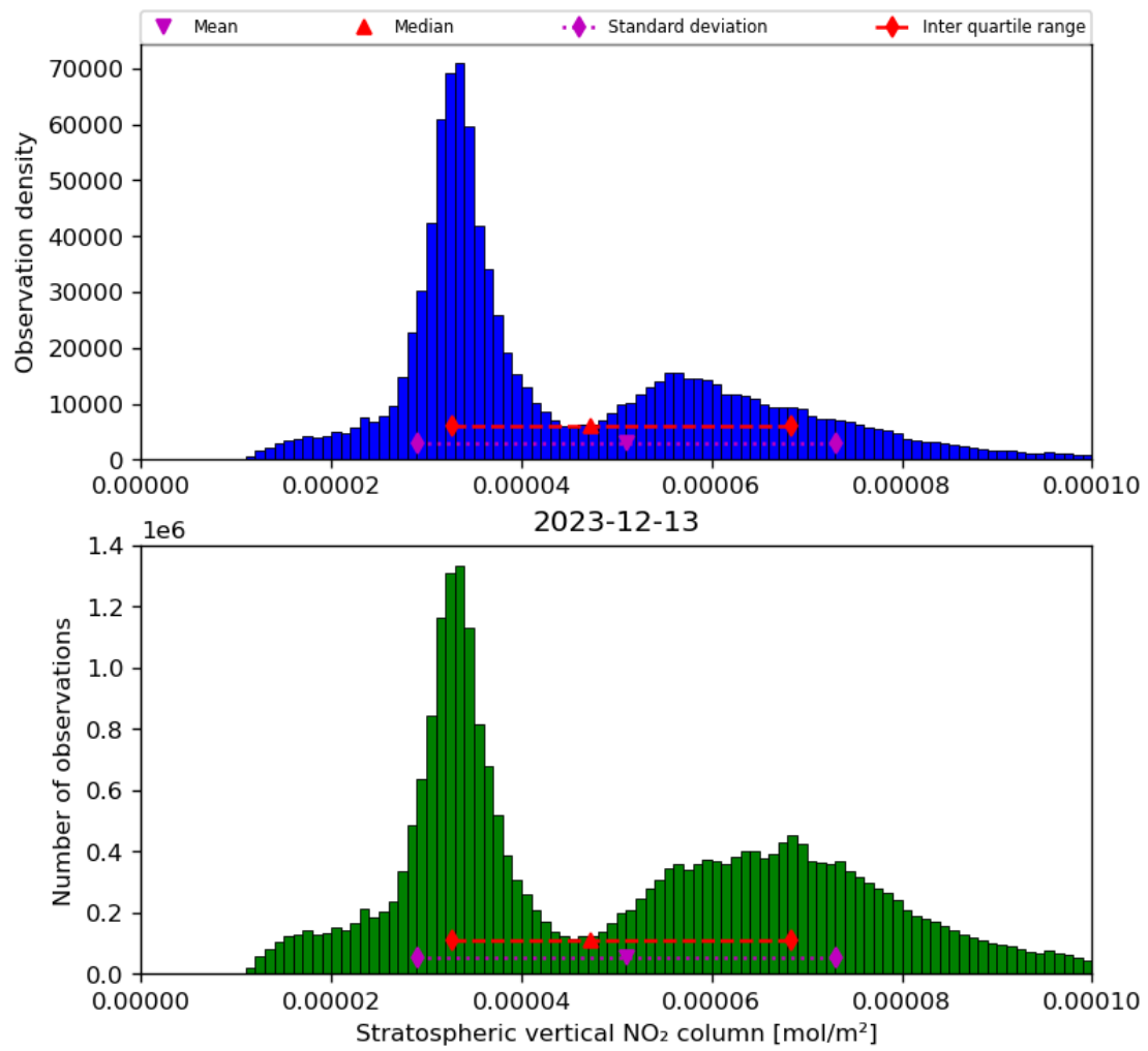
Figure 36: Histogram of “Stratospheric vertical NO 2 column” for 2023-12-12 to 2023-12-14
