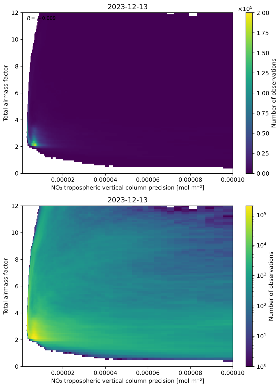
Figure 132: Scatter density plot of “NO 2 tropospheric vertical column precision” against “Total air mass factor” for 2023-12-12 to 2023-12-14.
