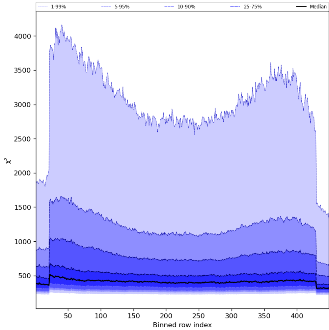
Figure 59: Along track statistics of “ \chi^2 ” for 2023-12-12 to 2023-12-14
