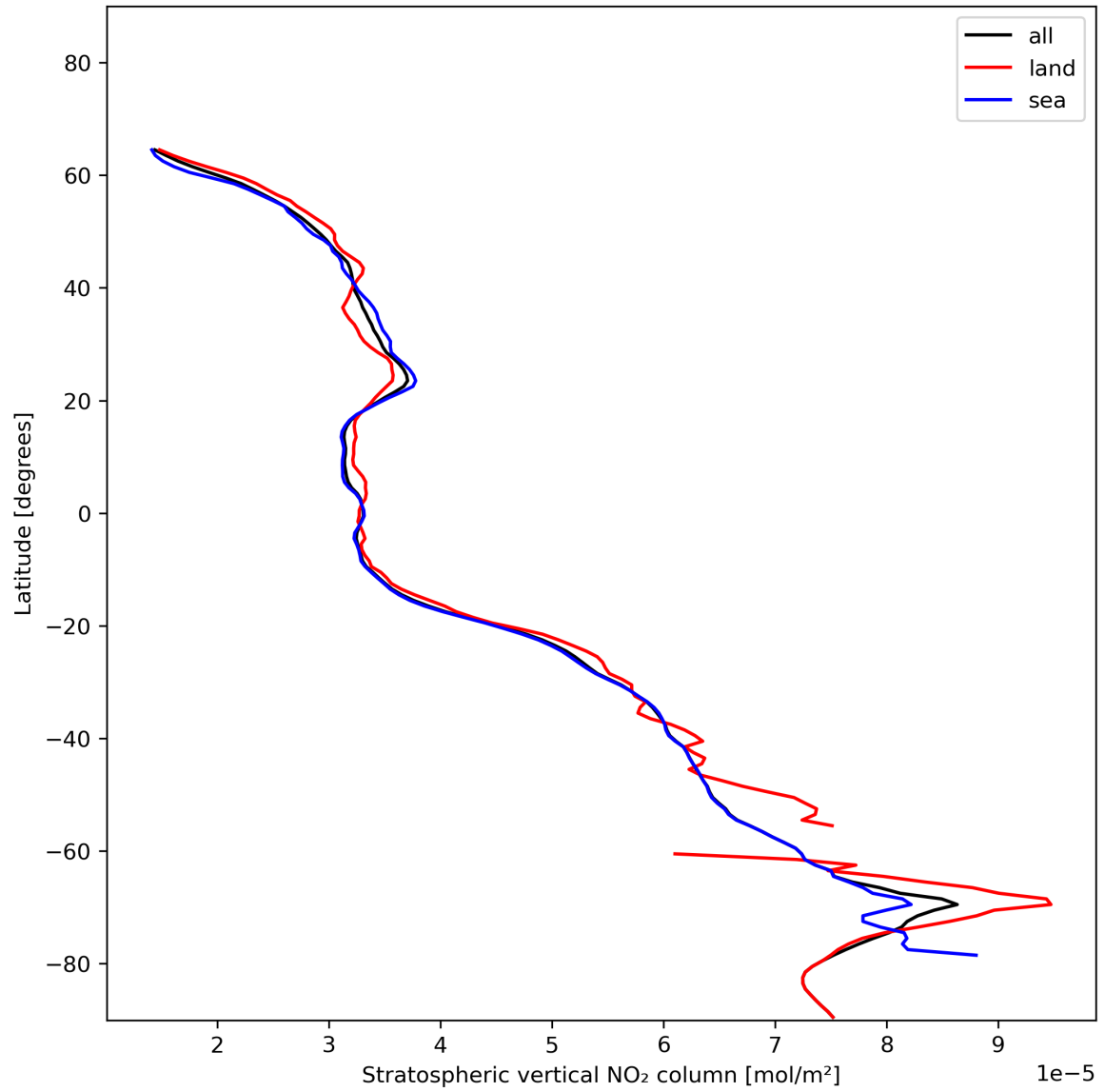
Figure 19: Zonal average of “Stratospheric vertical NO 2 column” for 2023-12-12 to 2023-12-14.
