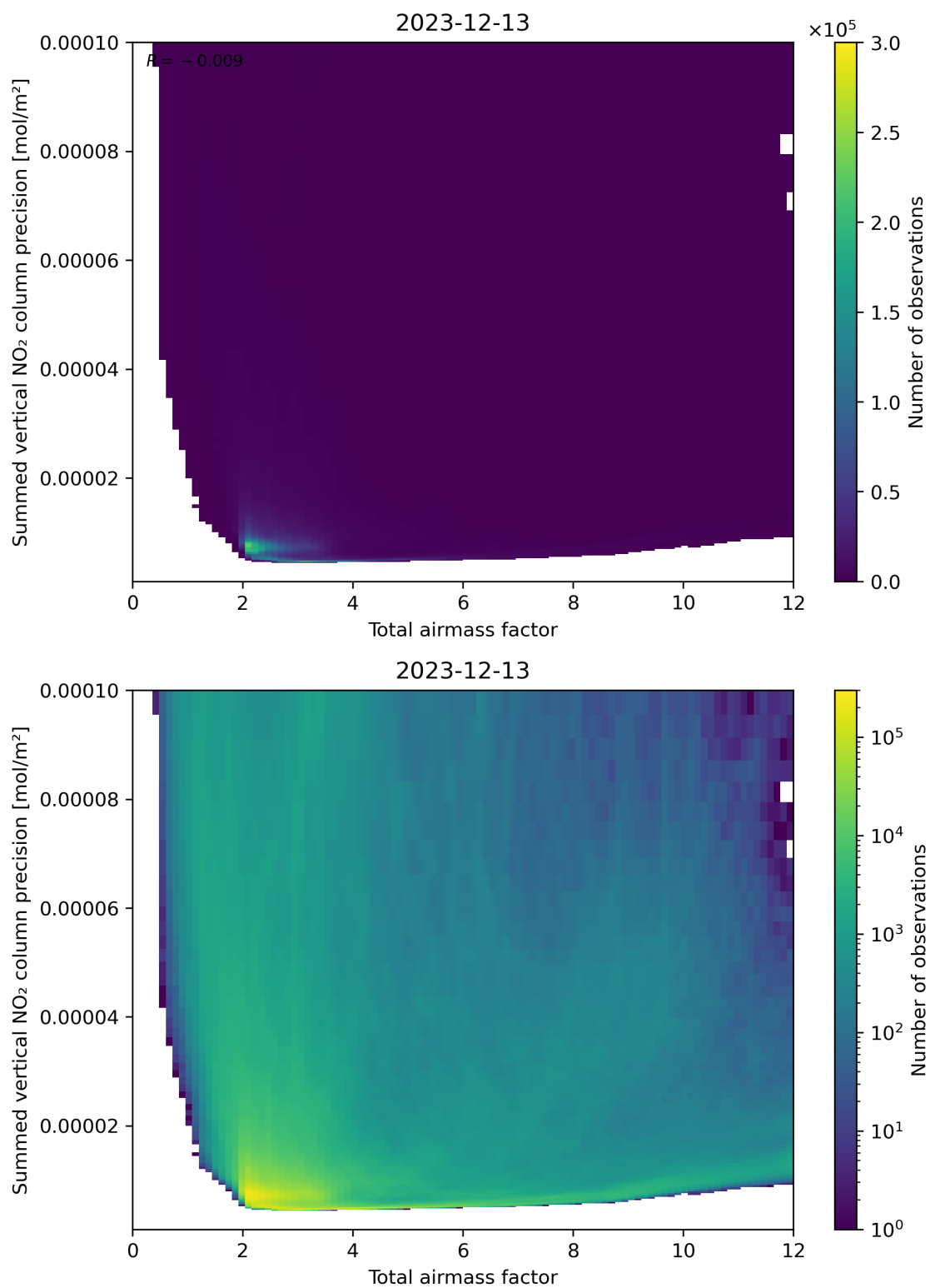
Figure 66: Scatter density plot of “Total airmass factor” against “Summed vertical NO 2 column precision” for 2023-12-12 to 2023-12-14.
