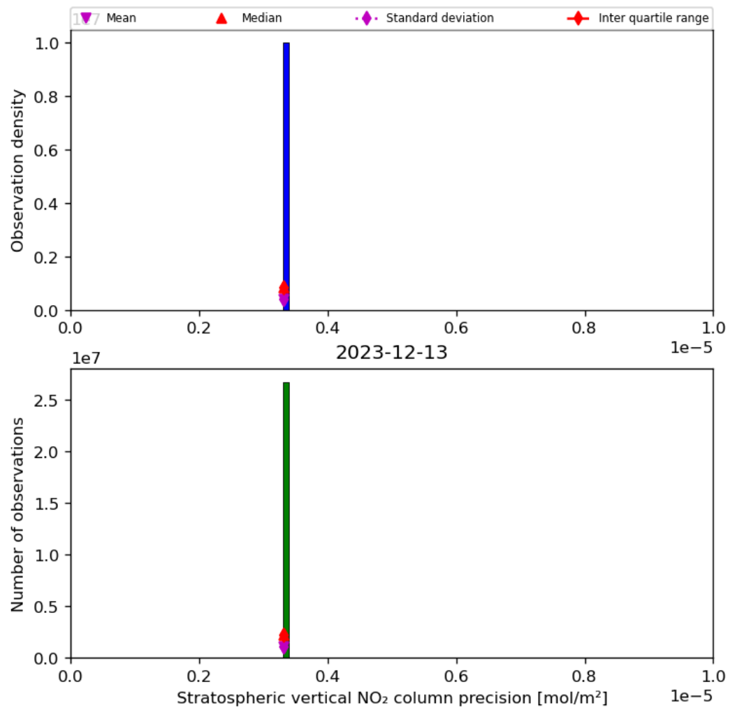
Figure 37: Histogram of “Stratospheric vertical NO 2 column precision” for 2023-12-12 to 2023-12-14
