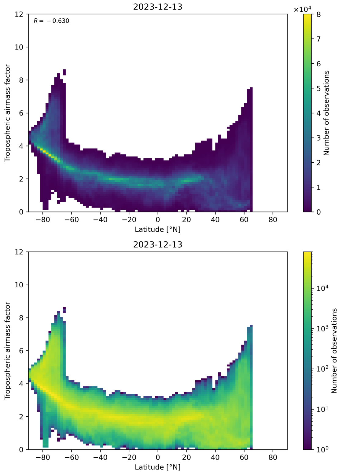
Figure 85: Scatter density plot of “Latitude” against “Tropospheric airmass factor” for 2023-12-12 to 2023-12-14.
