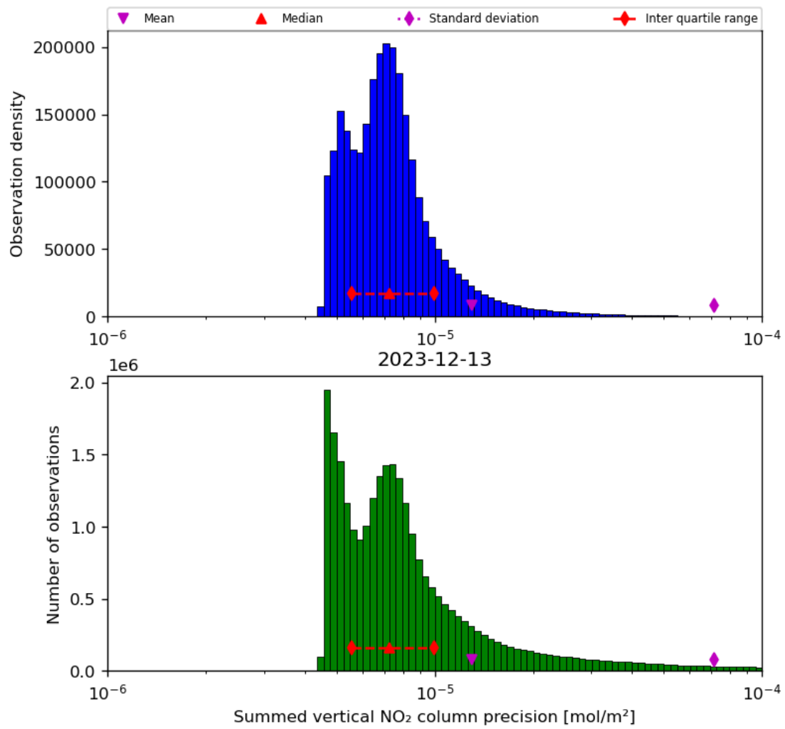
Figure 41: Histogram of “Summed vertical NO 2 column precision” for 2023-12-12 to 2023-12-14
