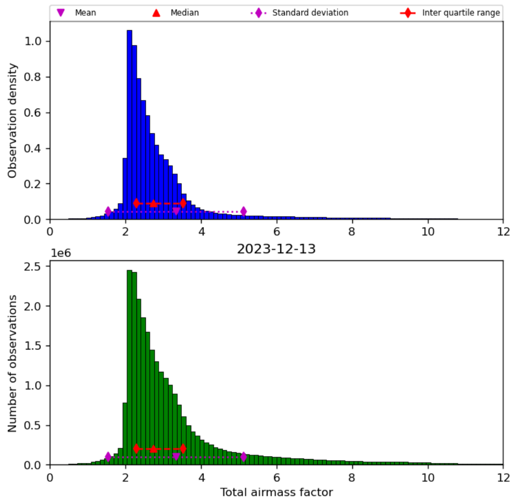
Figure 32: Histogram of “Total airmass factor” for 2023-12-12 to 2023-12-14
