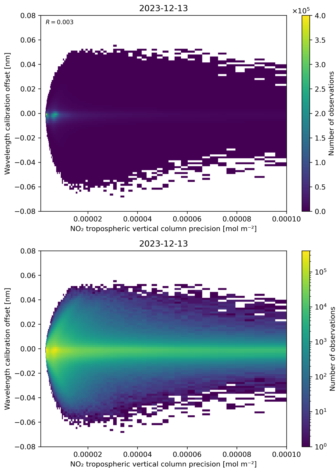
Figure 141: Scatter density plot of “NO 2 tropospheric vertical column precision” against “Wavelength calibration offset” for 2023-12-12 to 2023-12-14.
