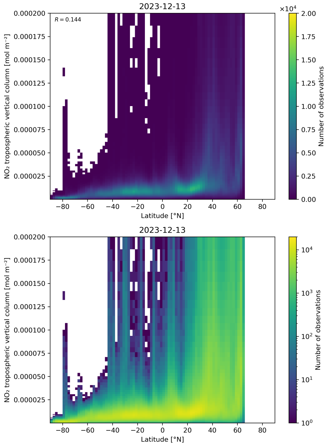
Figure 92: Scatter density plot of “Latitude” against “NO 2 tropospheric vertical column” for 2023-12-12 to 2023-12-14.
