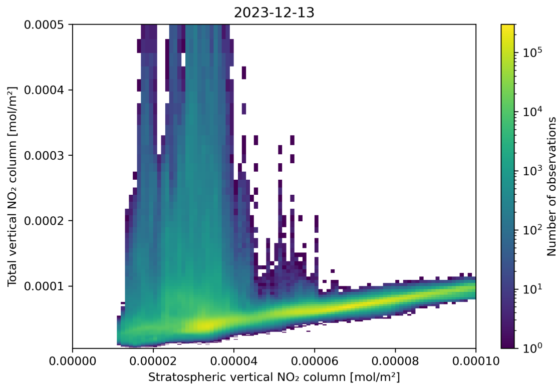
Figure 100: Scatter density plot of “Stratospheric vertical NO 2 column” against “Total vertical NO 2 column” for 2023-12-12 to 2023-12-14.
