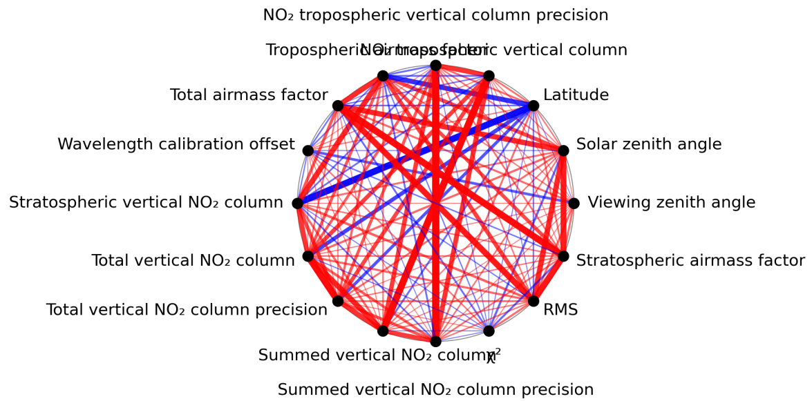
Figure 1: Map of correlation graph for 2023-12-12 to 2023-12-14.
