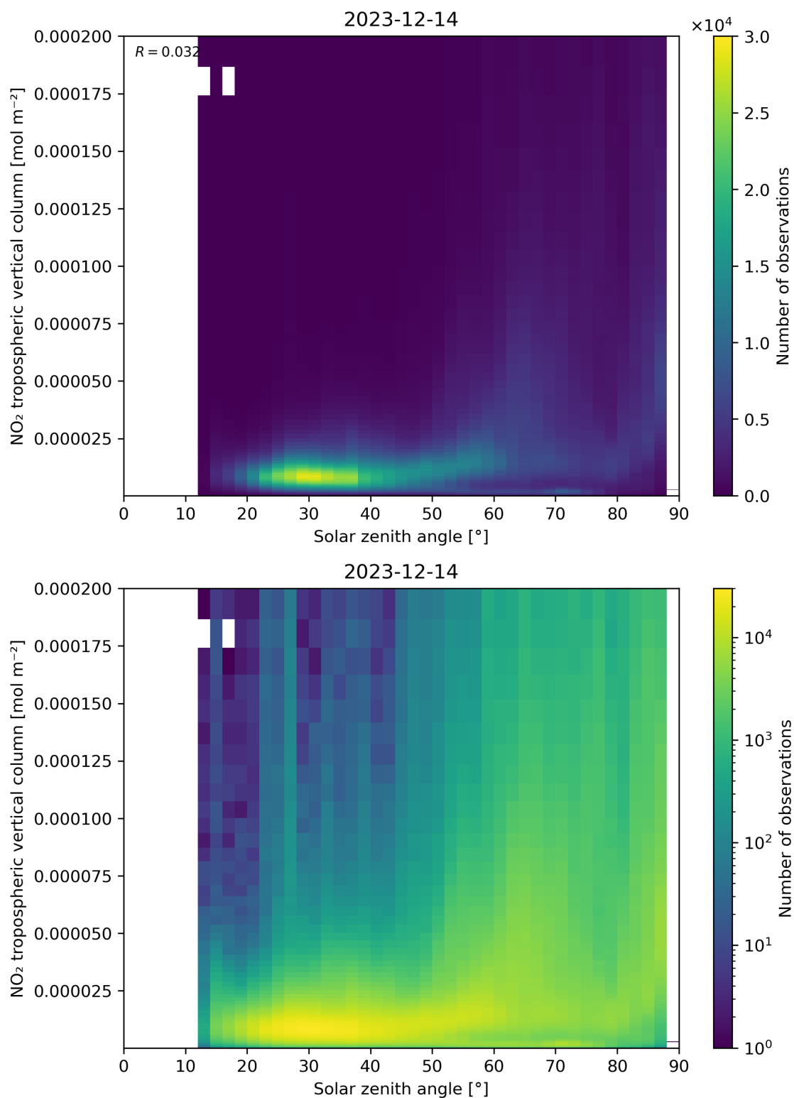
Figure 155: Scatter density plot of “Solar zenith angle” against “NO 2 tropospheric vertical column” for 2023-12-14 to 2023-12-15.
