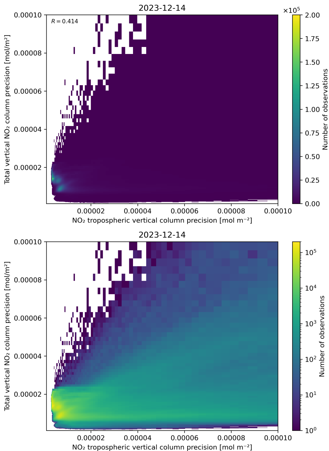
Figure 139: Scatter density plot of “NO 2 tropospheric vertical column precision” against “Total vertical NO 2 column precision” for 2023-12-14 to 2023-12-15.
