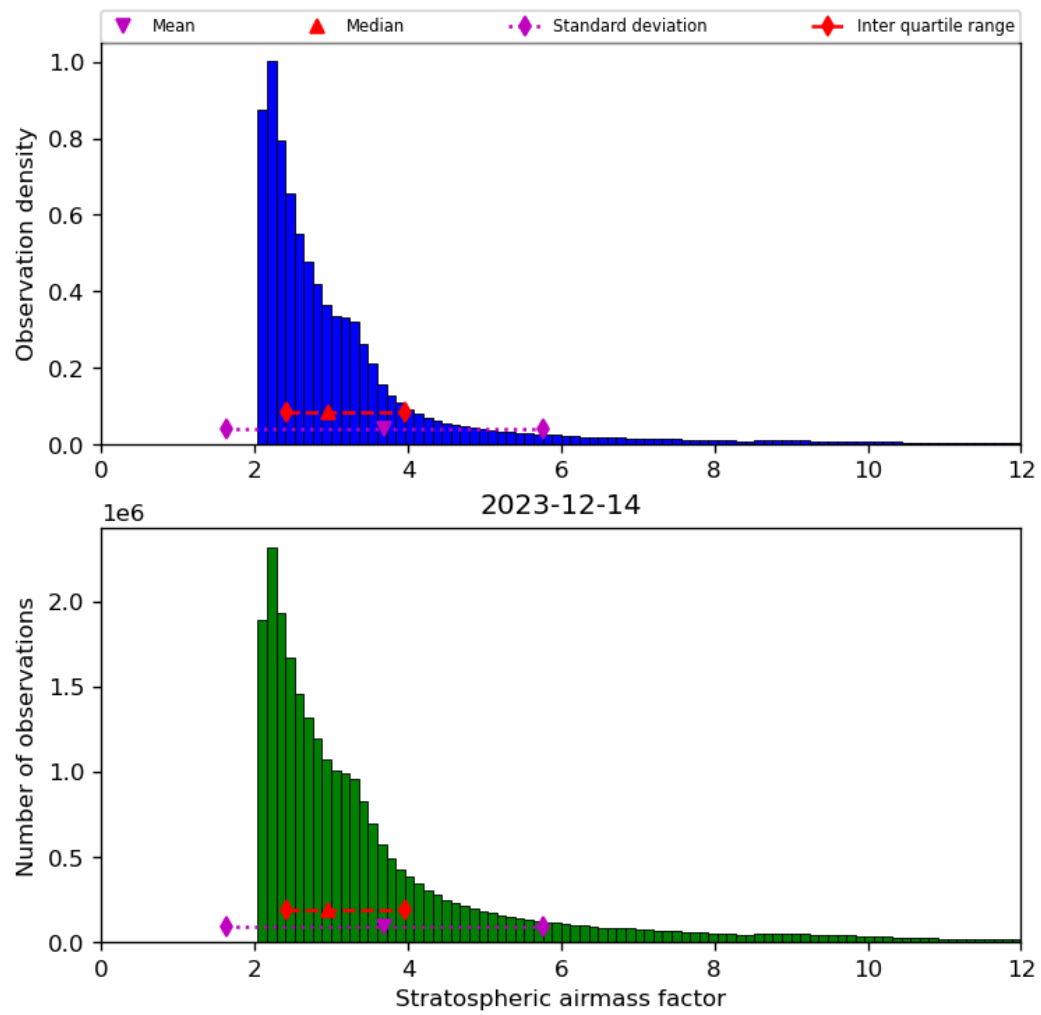
Figure 44: Histogram of “Stratospheric airmass factor” for 2023-12-14 to 2023-12-15
