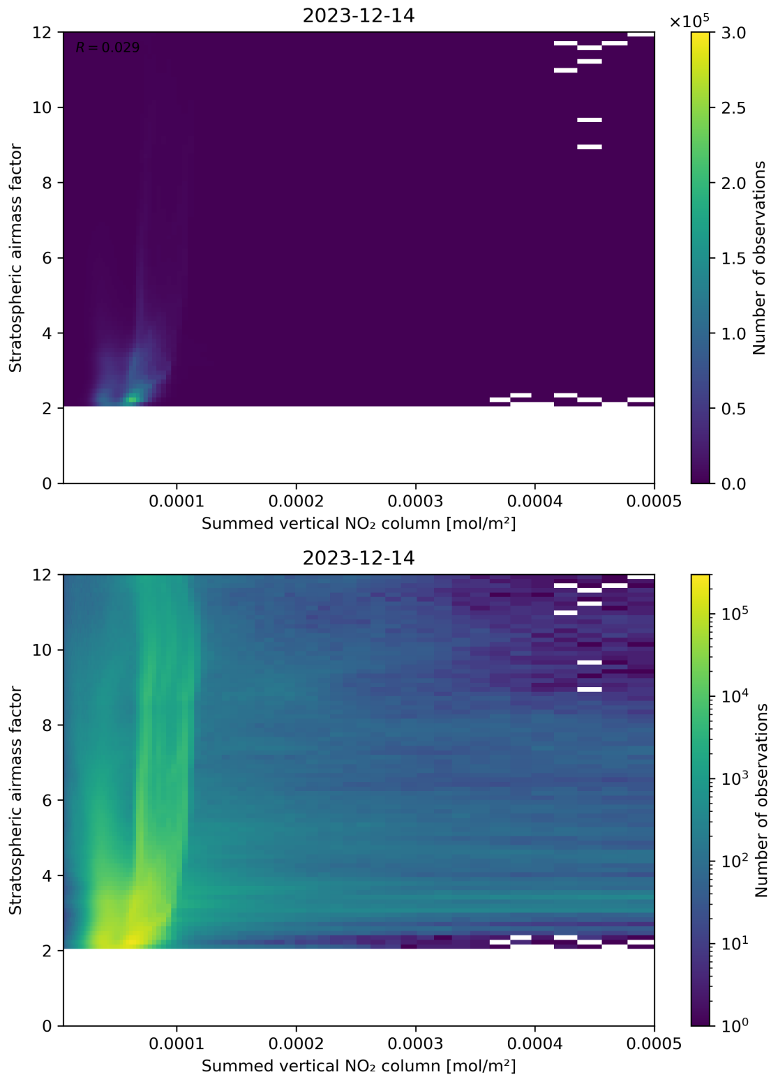
Figure 103: Scatter density plot of “Summed vertical NO 2 column” against “Stratospheric airmass factor” for 2023-12-14 to 2023-12-15.
