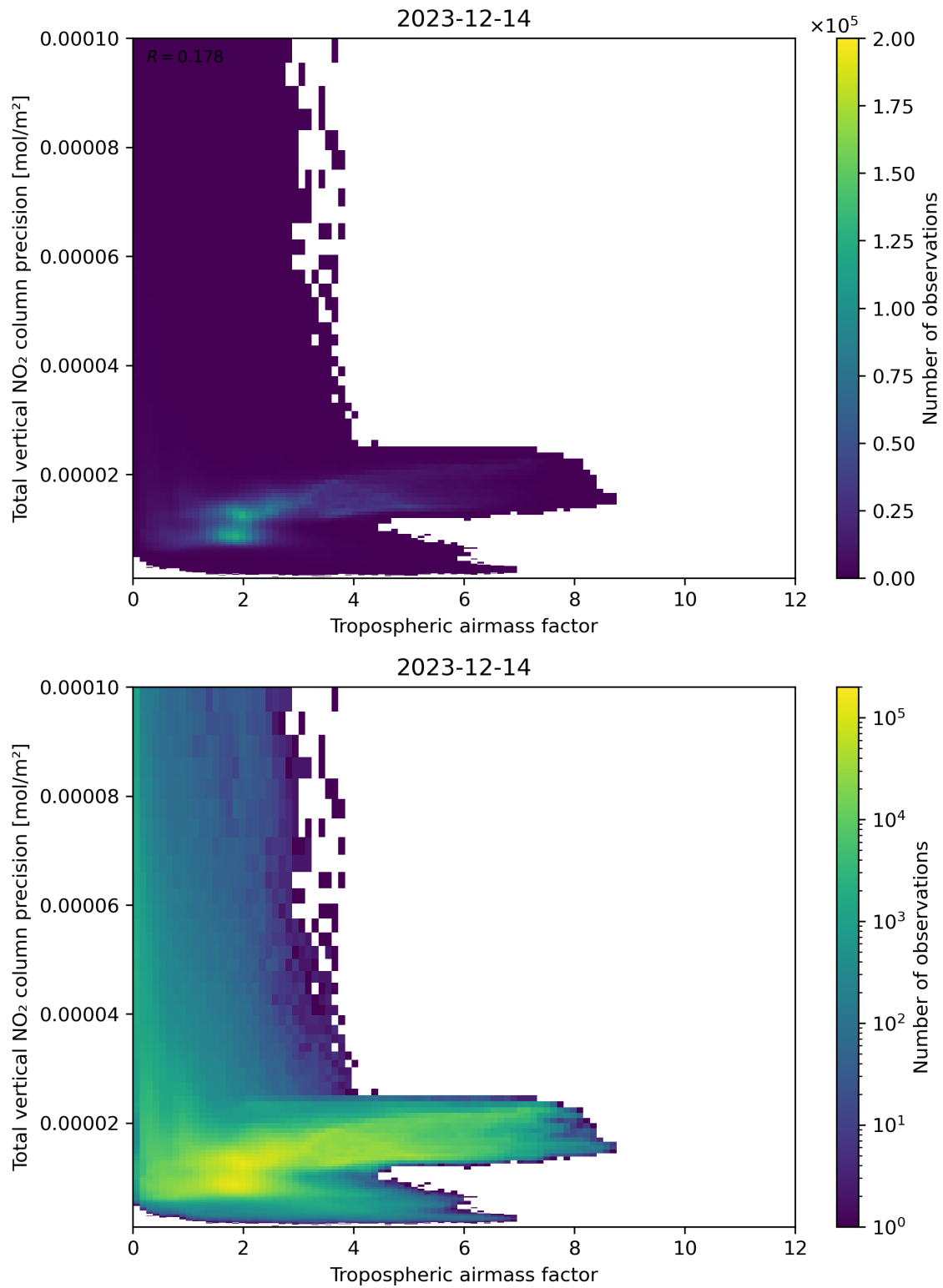
Figure 78: Scatter density plot of “Tropospheric air mass factor” against “Total vertical NO 2 column precision” for 2023-12-14 to 2023-12-15.
