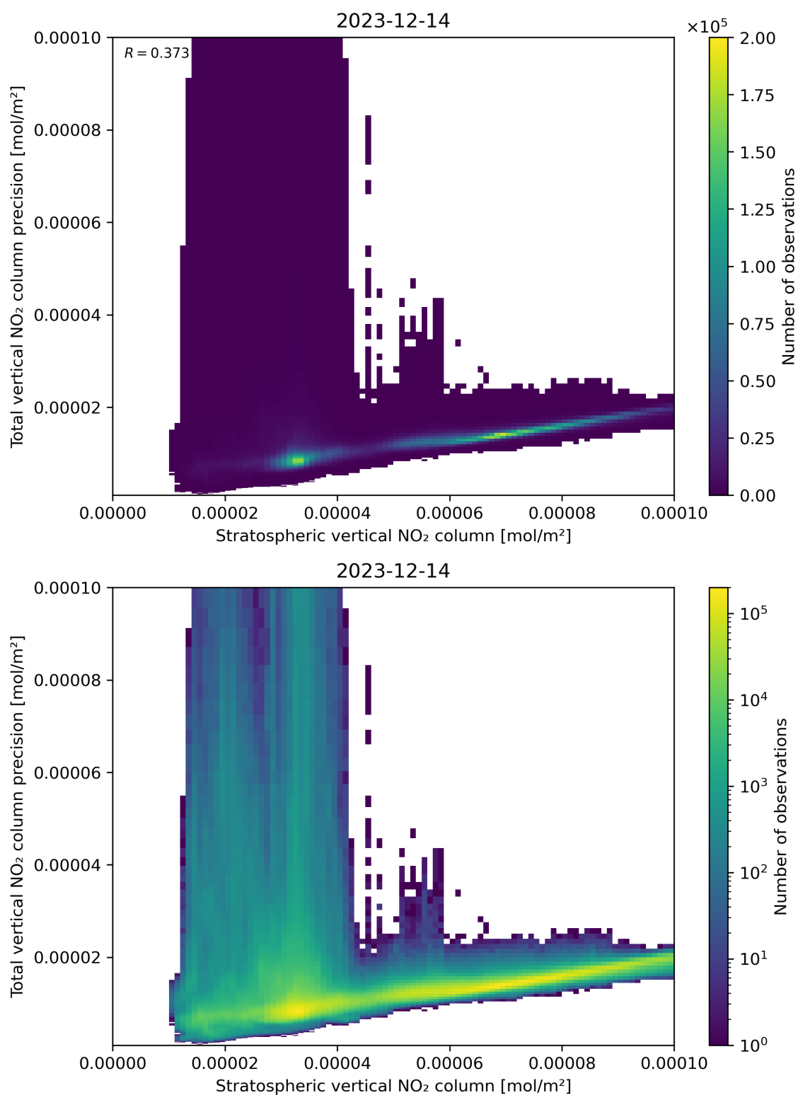
Figure 101: Scatter density plot of “Stratospheric vertical NO 2 column” against “Total vertical NO 2 column precision” for 2023-12-14 to 2023-12-15.
