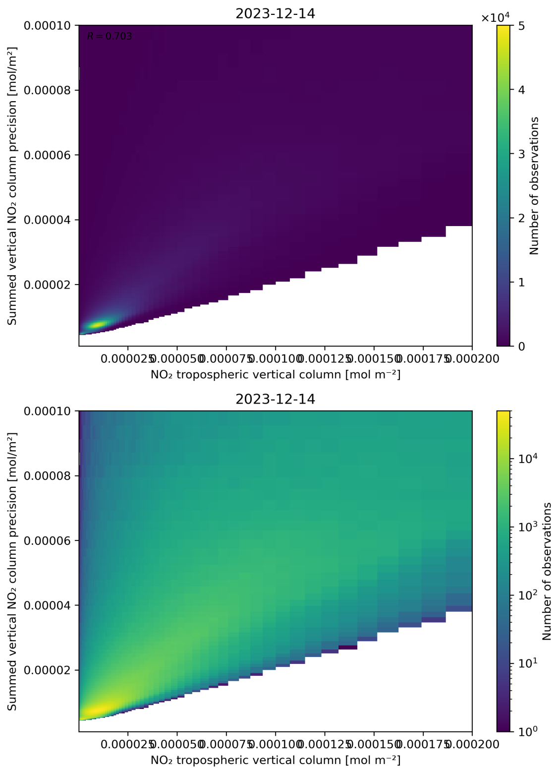
Figure 127: Scatter density plot of “NO 2 tropospheric vertical column” against “Summed vertical NO 2 column precision” for 2023-12-14 to 2023-12-15.
