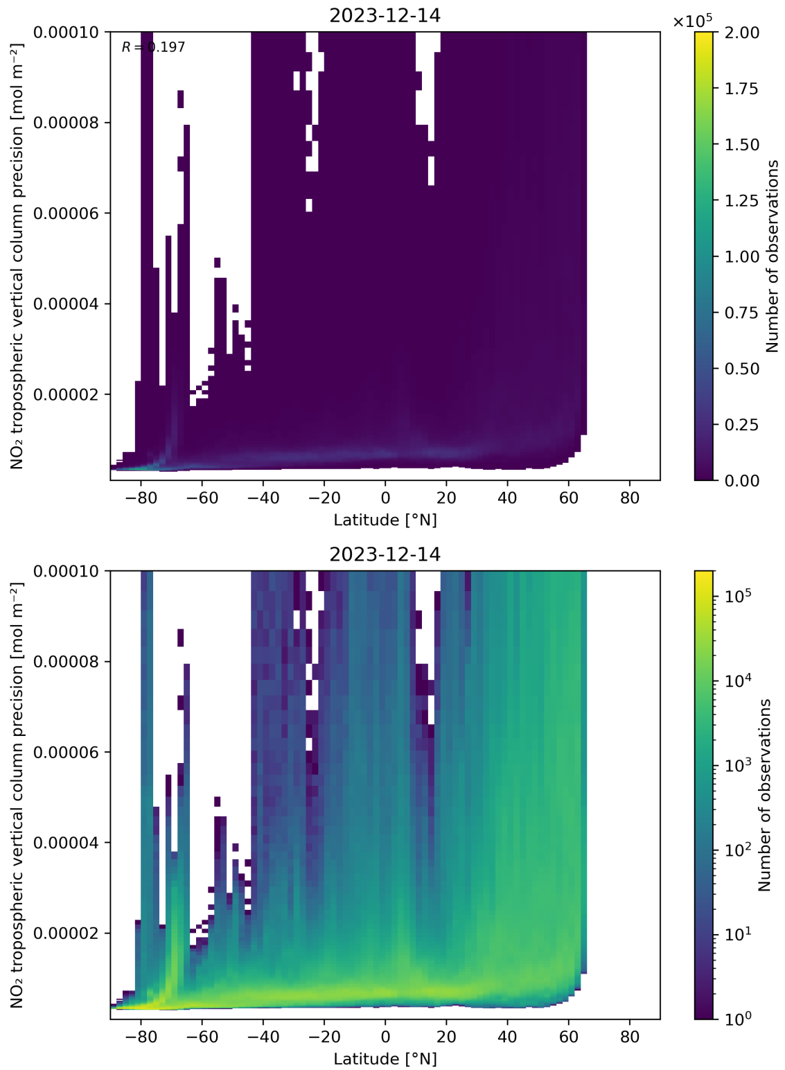
Figure 93: Scatter density plot of “Latitude” against “NO 2 tropospheric vertical column precision” for 2023-12-14 to 2023-12-15.
