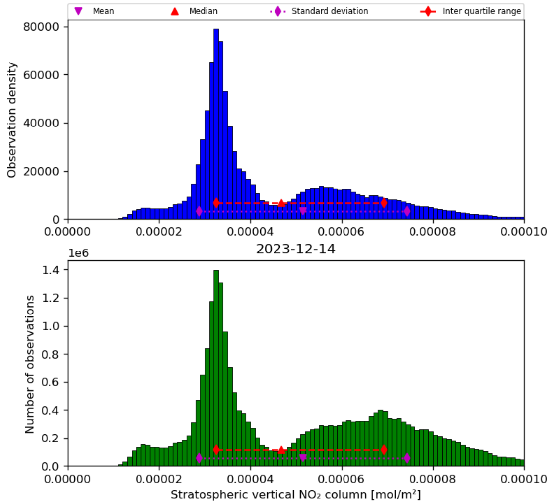
Figure 36: Histogram of “Stratospheric vertical NO 2 column” for 2023-12-14 to 2023-12-15
