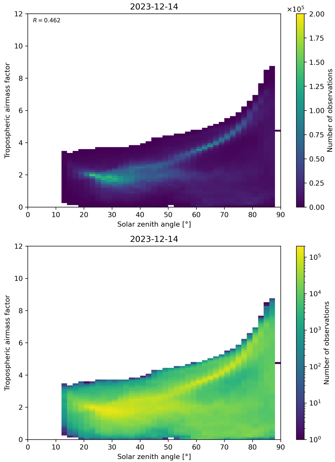
Figure 147: Scatter density plot of “Solar zenith angle” against “Tropospheric airmass factor” for 2023-12-14 to 2023-12-15.
