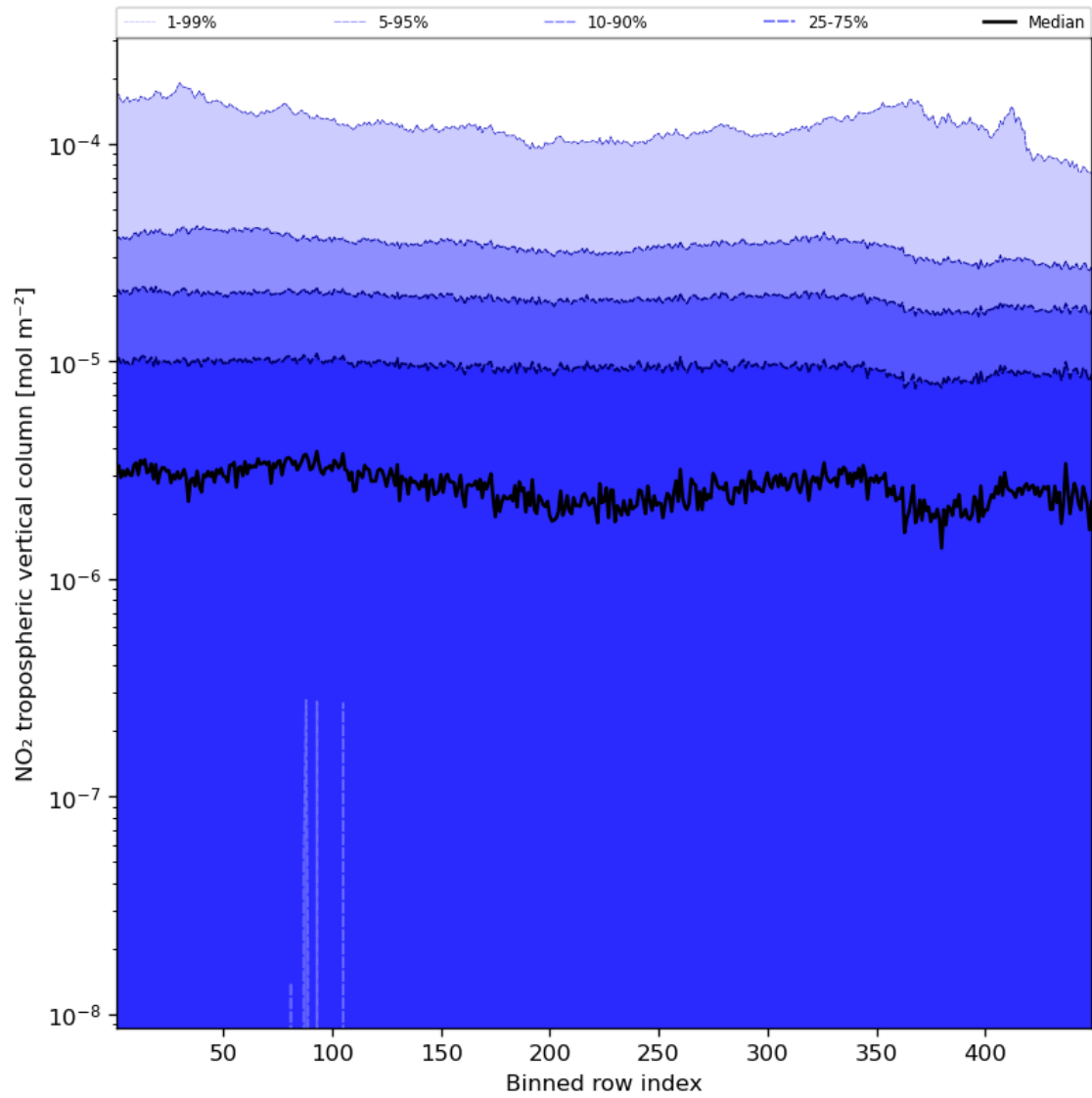
Figure 46: Along track statistics of “NO 2 tropospheric vertical column” for 2023-12-14 to 2023-12-15
