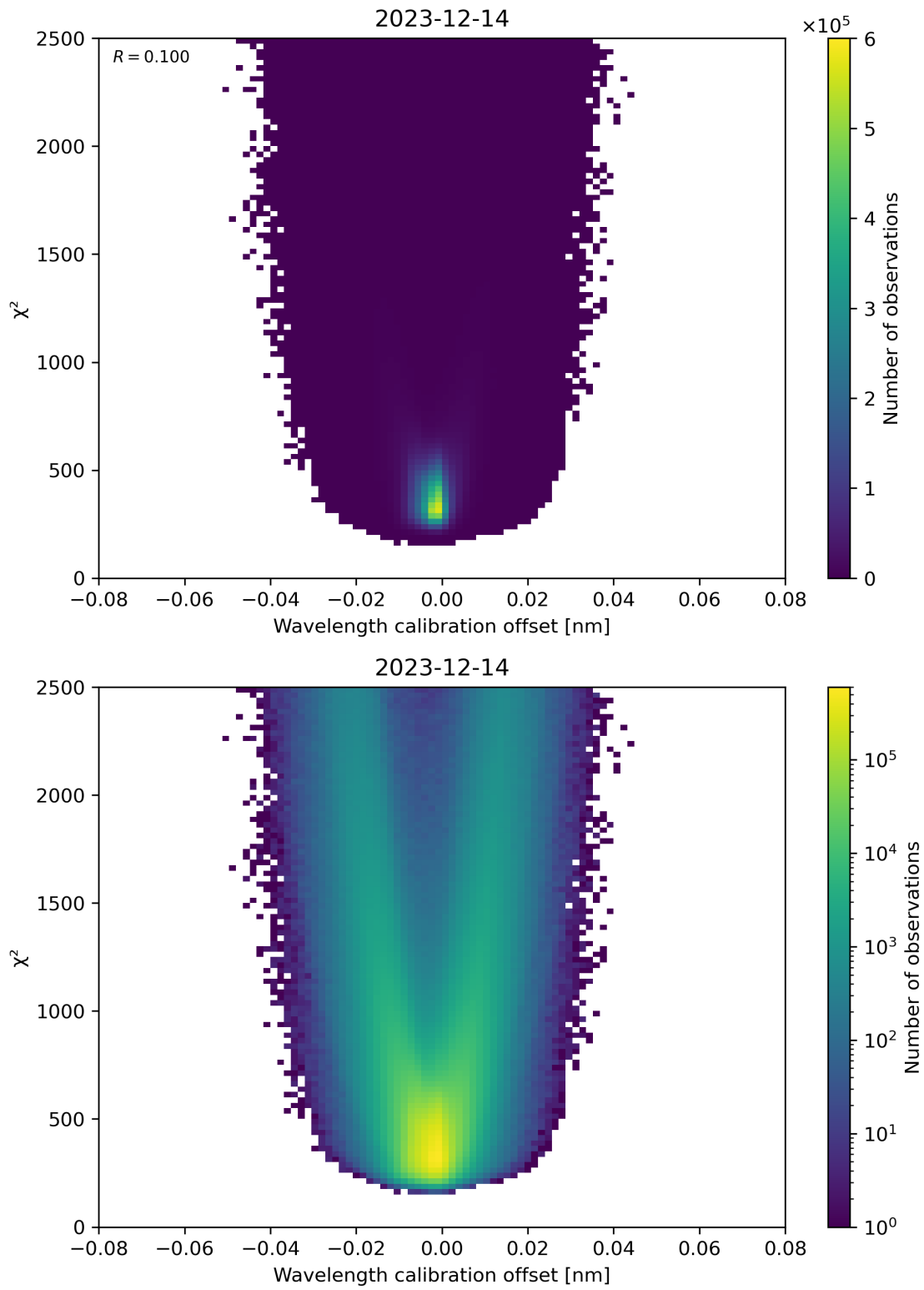
Figure 175: Scatter density plot of “Wavelength calibration offset” against “ \chi^2 ” for 2023-12-14 to 2023-12-15.
