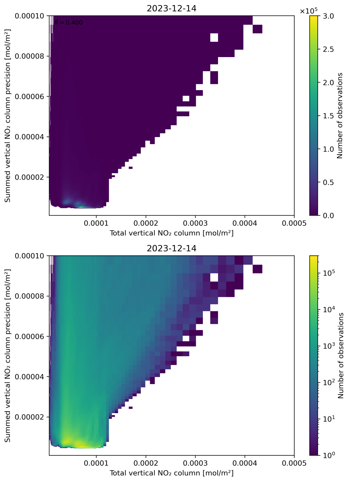
Figure 113: Scatter density plot of “Total vertical NO 2 column” against “Summed vertical NO 2 column precision” for 2023-12-14 to 2023-12-15.
