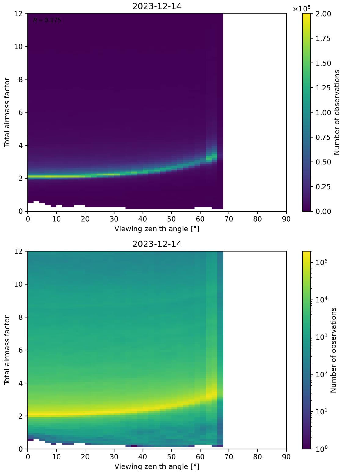
Figure 160: Scatter density plot of “Viewing zenith angle” against “Total airmass factor” for 2023-12-14 to 2023-12-15.
