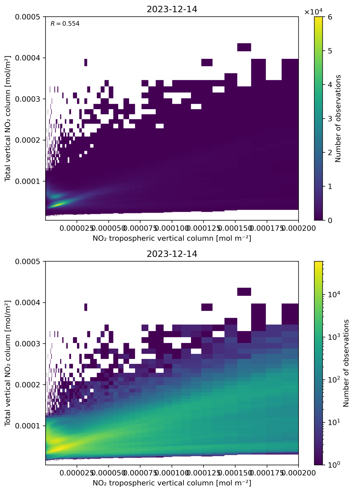
Figure 128: Scatter density plot of “NO 2 tropospheric vertical column” against “Total vertical NO 2 column” for 2023-12-14 to 2023-12-15.
