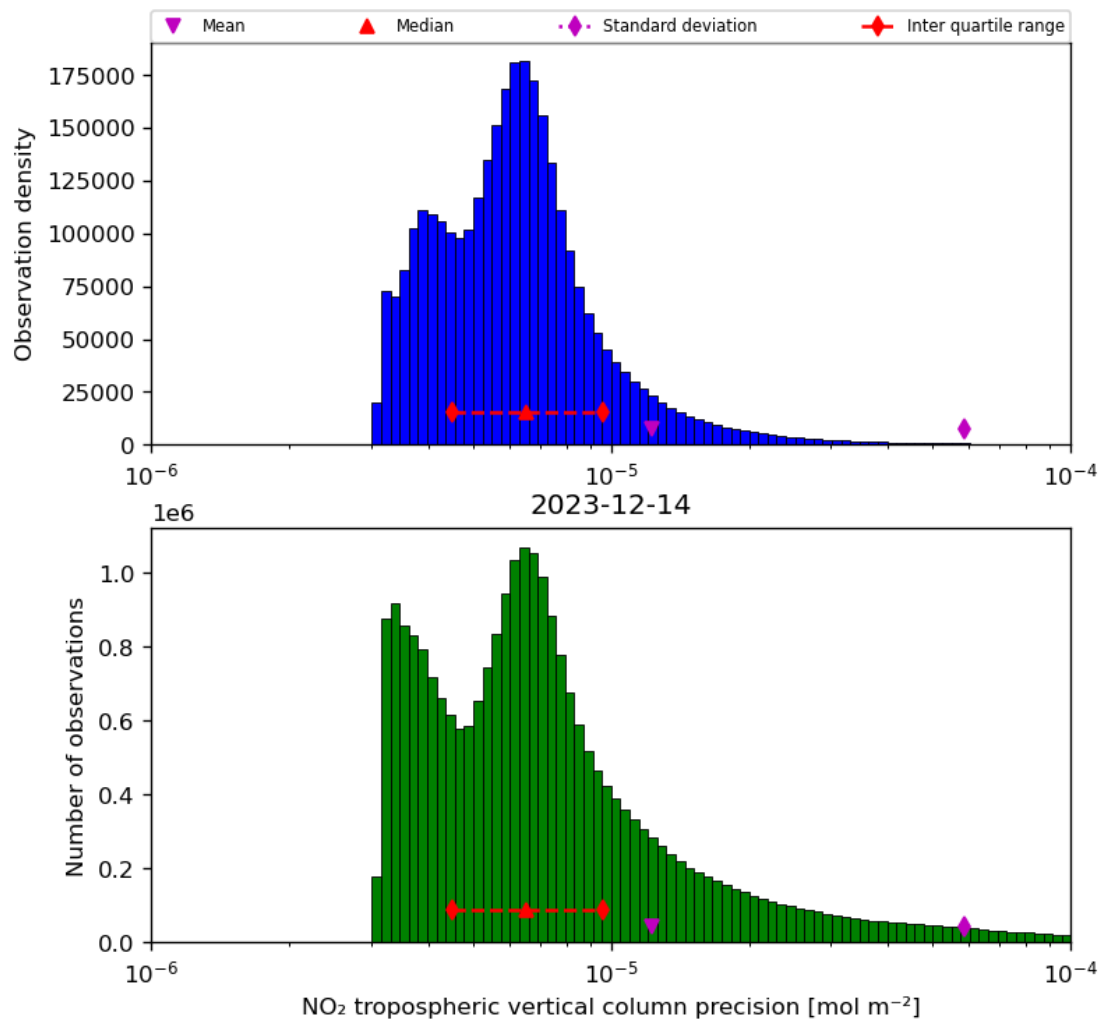
Figure 30: Histogram of “NO 2 tropospheric vertical column precision” for 2023-12-14 to 2023-12-15
