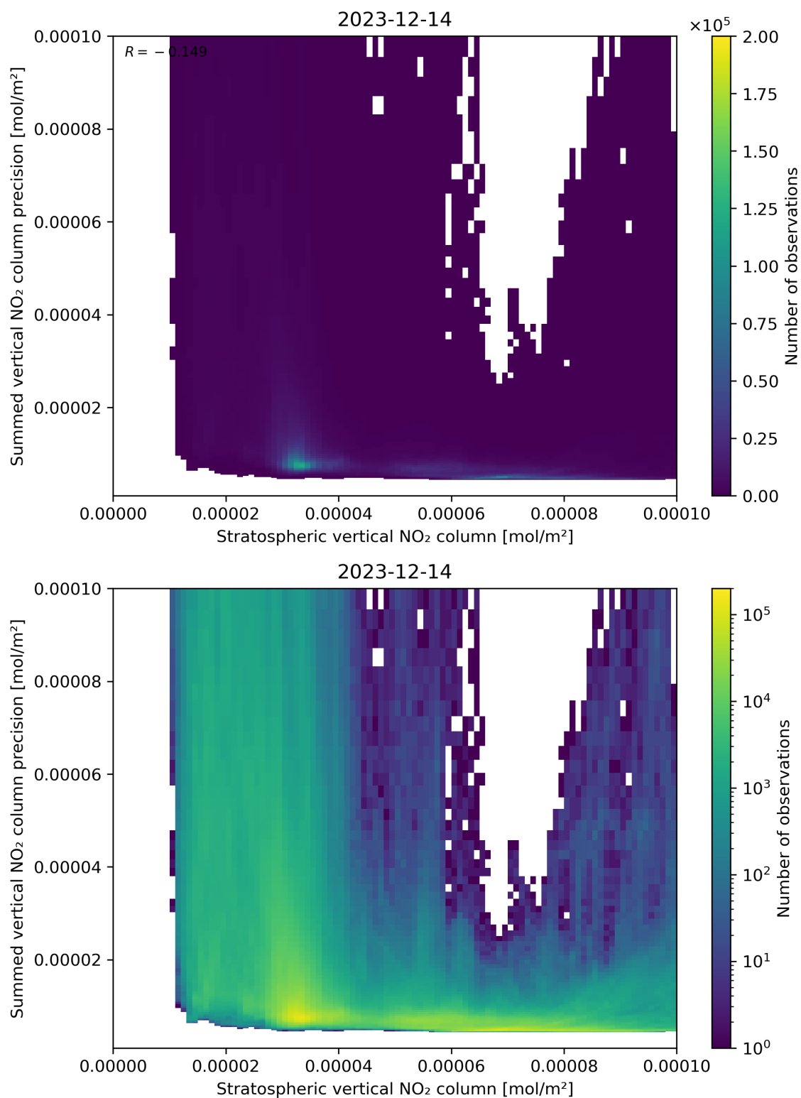
Figure 99: Scatter density plot of “Stratospheric vertical NO 2 column” against “Summed vertical NO 2 column precision” for 2023-12-14 to 2023-12-15.
