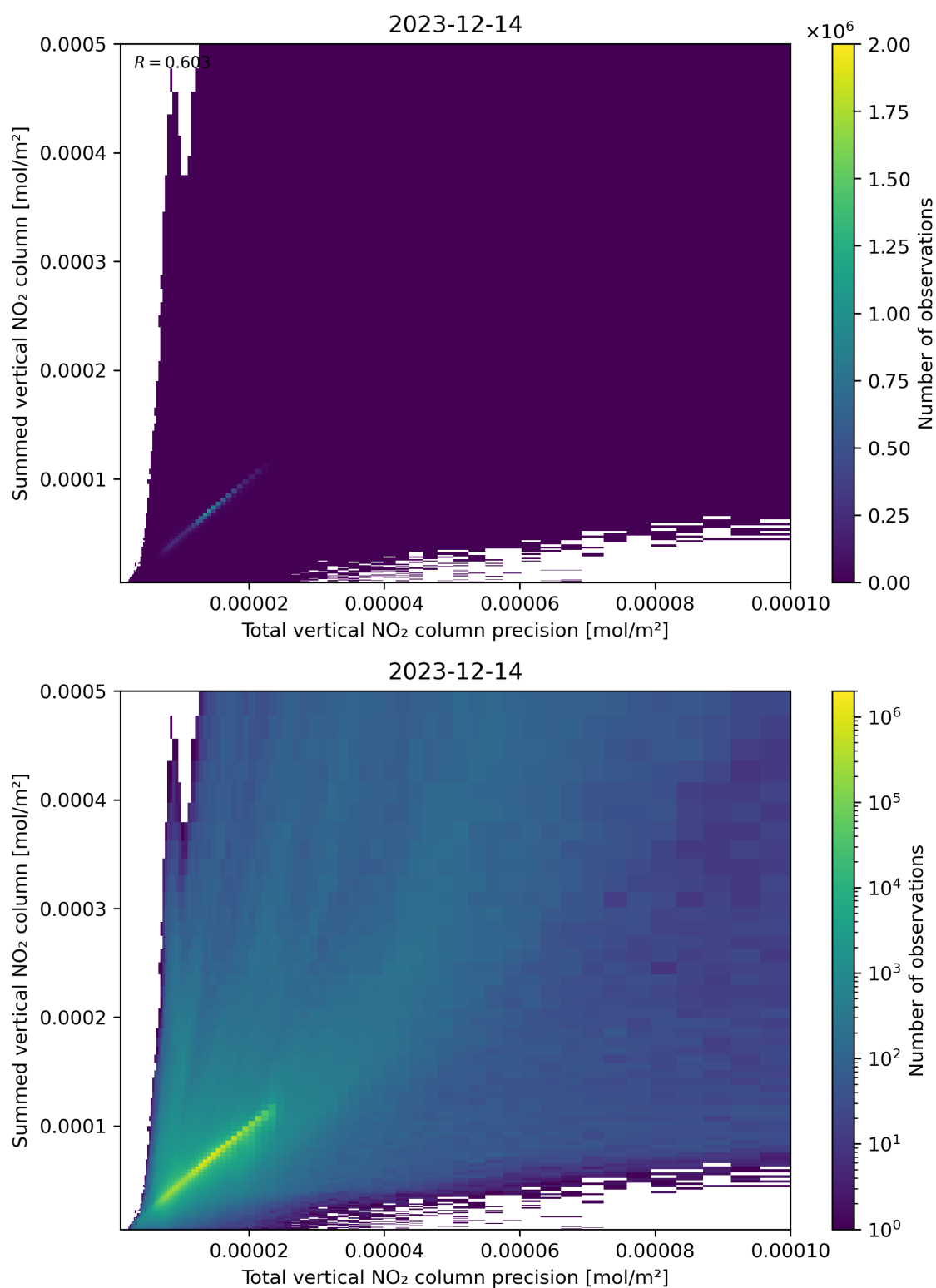
Figure 117: Scatter density plot of “Total vertical NO 2 column precision” against “Summed vertical NO 2 column” for 2023-12-14 to 2023-12-15.
