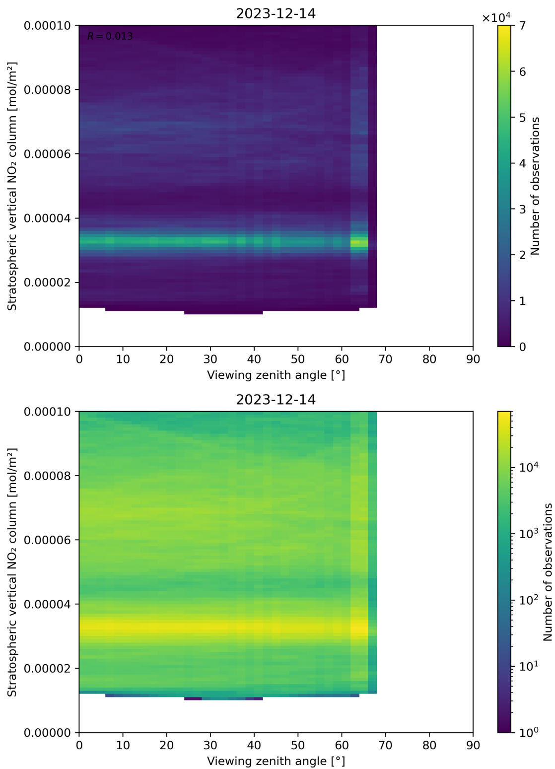
Figure 164: Scatter density plot of “Viewing zenith angle” against “Stratospheric vertical NO 2 column” for 2023-12-14 to 2023-12-15.
