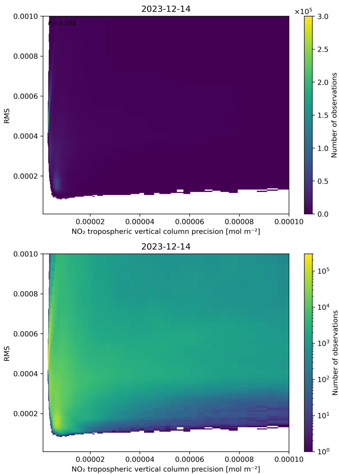
Figure 140: Scatter density plot of “NO 2 tropospheric vertical column precision” against “RMS” for 2023-12-14 to 2023-12-15.
