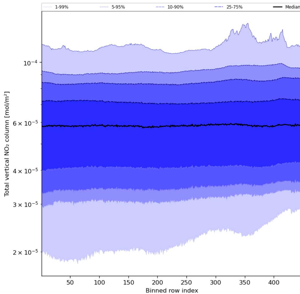
Figure 55: Along track statistics of “Total vertical NO 2 column” for 2023-12-14 to 2023-12-15
