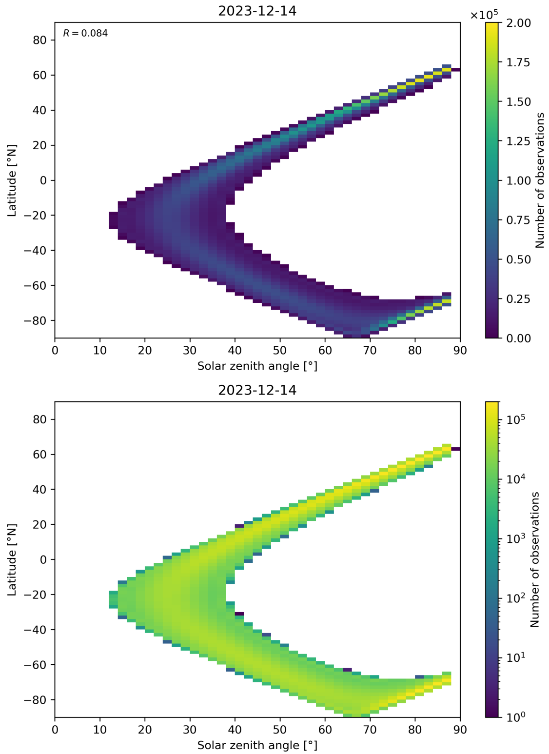
Figure 149: Scatter density plot of “Solar zenith angle” against “Latitude” for 2023-12-14 to 2023-12-15.
