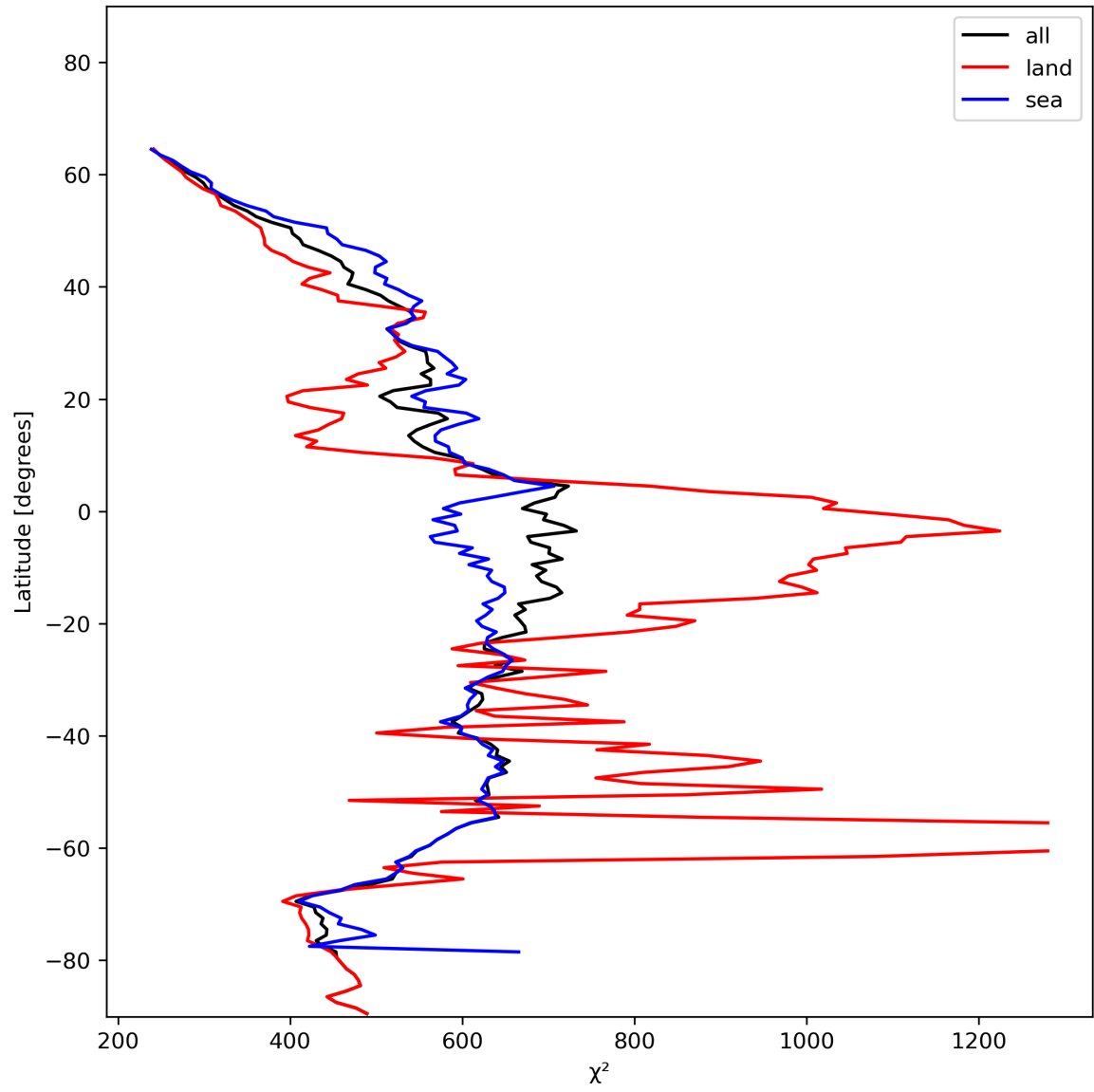
Figure 25: Zonal average of “ \chi^2 ” for 2023-12-14 to 2023-12-15.
