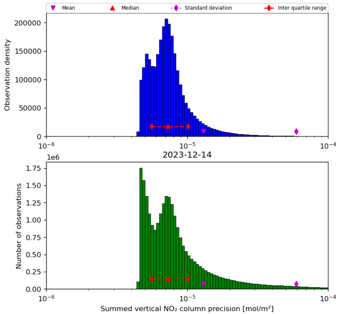
Figure 41: Histogram of “Summed vertical NO 2 column precision” for 2023-12-14 to 2023-12-15
