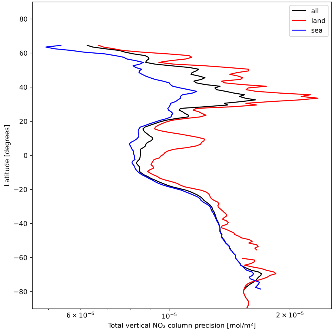
Figure 22: Zonal average of “Total vertical NO 2 column precision” for 2023-12-14 to 2023-12-15.
