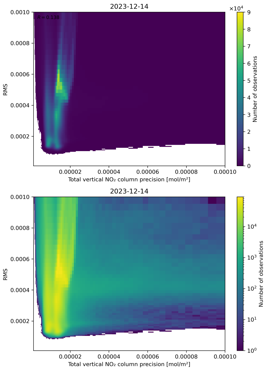
Figure 119: Scatter density plot of “Total vertical NO 2 column precision” against “RMS” for 2023-12-14 to 2023-12-15.
