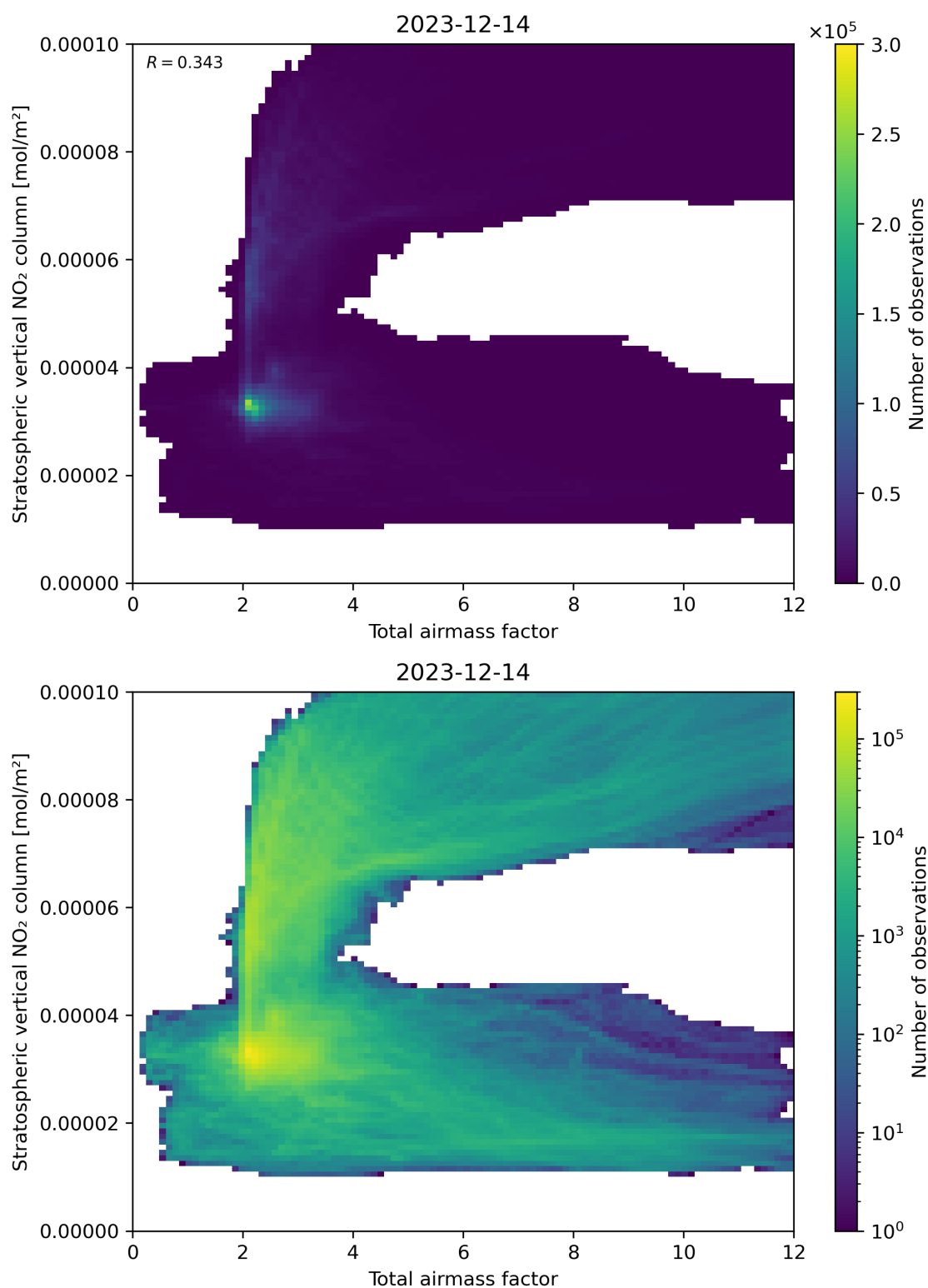
Figure 64: Scatter density plot of “Total airmass factor” against “Stratospheric vertical NO 2 column” for 2023-12-14 to 2023-12-15.
