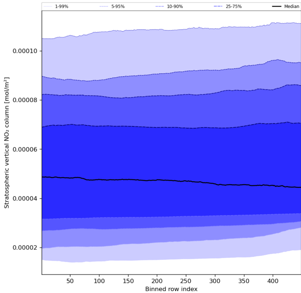
Figure 53: Along track statistics of “Stratospheric vertical NO 2 column” for 2023-12-14 to 2023-12-15
