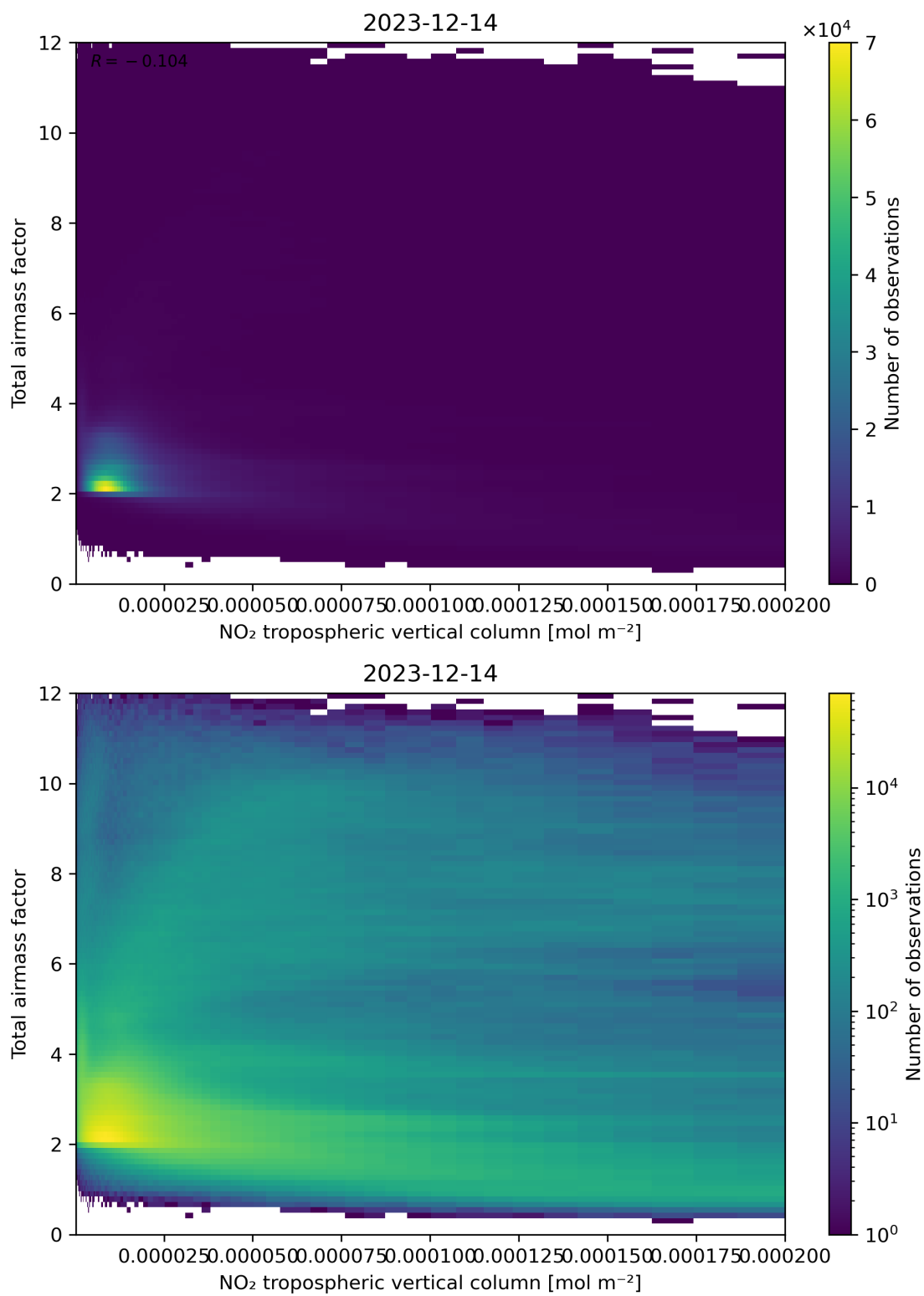
Figure 122: Scatter density plot of “NO 2 tropospheric vertical column” against “Total air mass factor” for 2023-12-14 to 2023-12-15.
