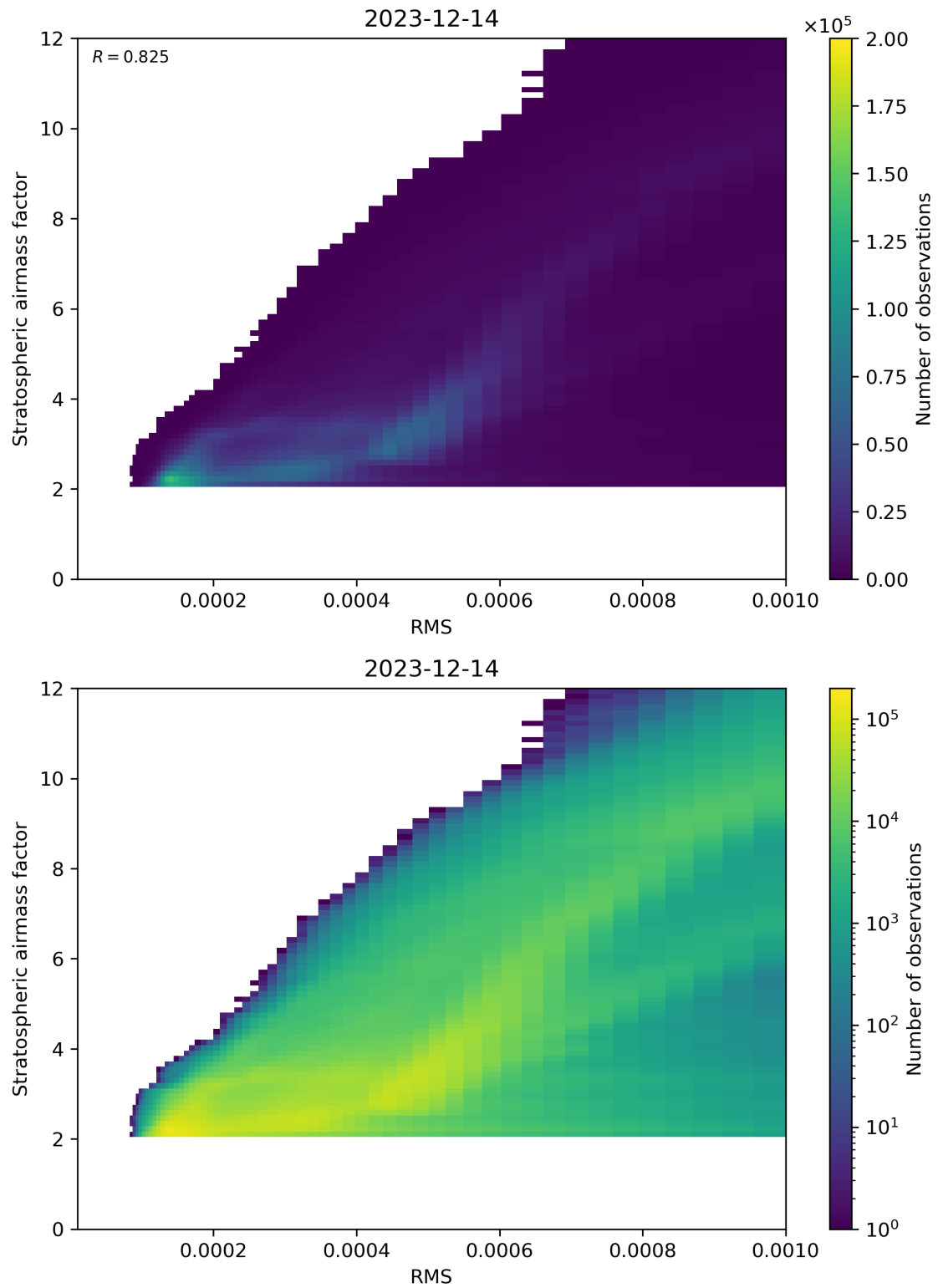
Figure 144: Scatter density plot of “RMS” against “Stratospheric airmass factor” for 2023-12-14 to 2023-12-15.
