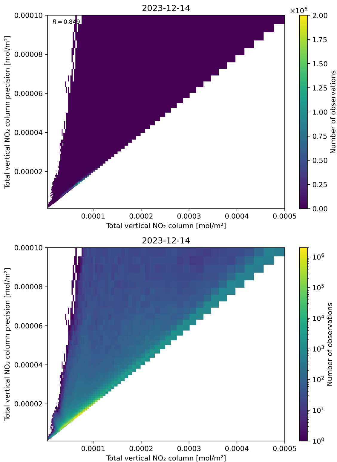
Figure 114: Scatter density plot of “Total vertical NO 2 column” against “Total vertical NO 2 column precision” for 2023-12-14 to 2023-12-15.
