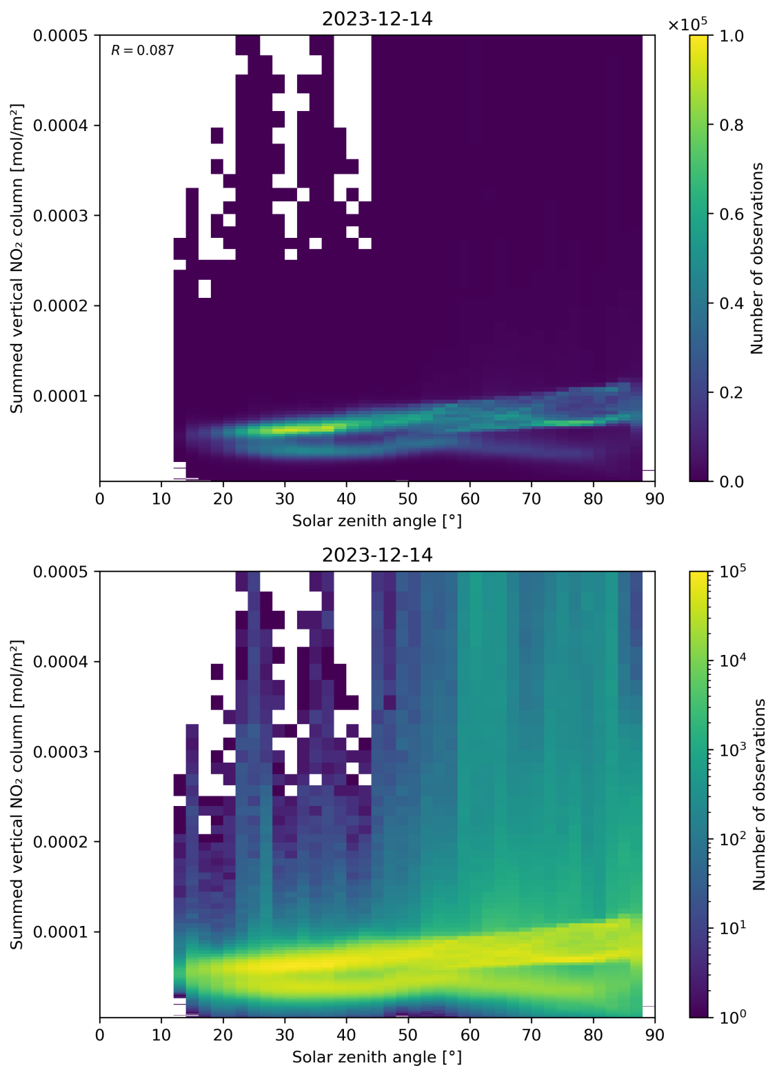
Figure 151: Scatter density plot of “Solar zenith angle” against “Summed vertical NO 2 column” for 2023-12-14 to 2023-12-15.
