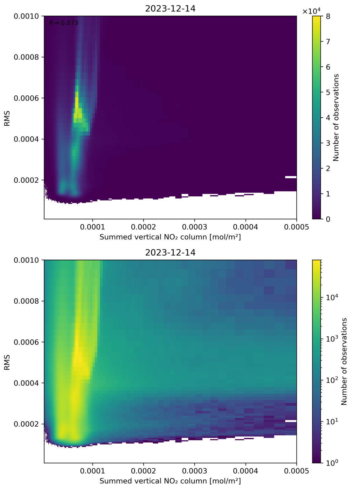
Figure 109: Scatter density plot of “Summed vertical NO 2 column” against “RMS” for 2023-12-14 to 2023-12-15.
