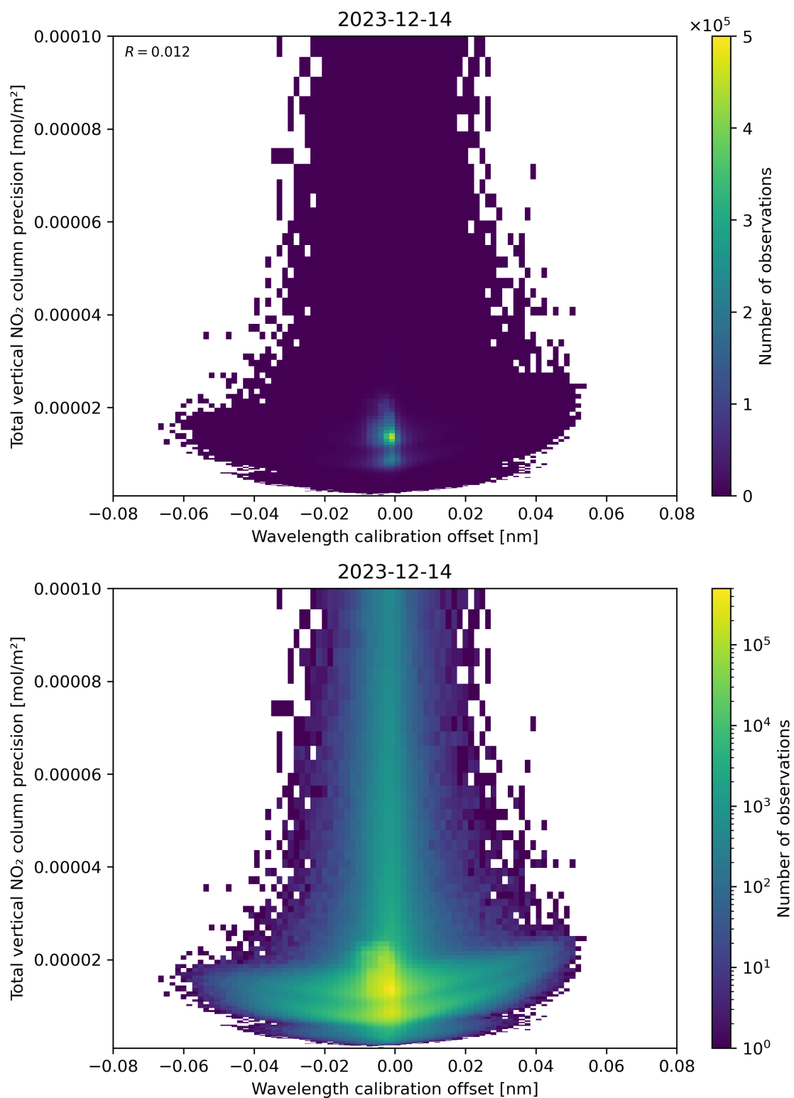
Figure 180: Scatter density plot of “Wavelength calibration offset” against “Total vertical NO 2 column precision” for 2023-12-14 to 2023-12-15.
