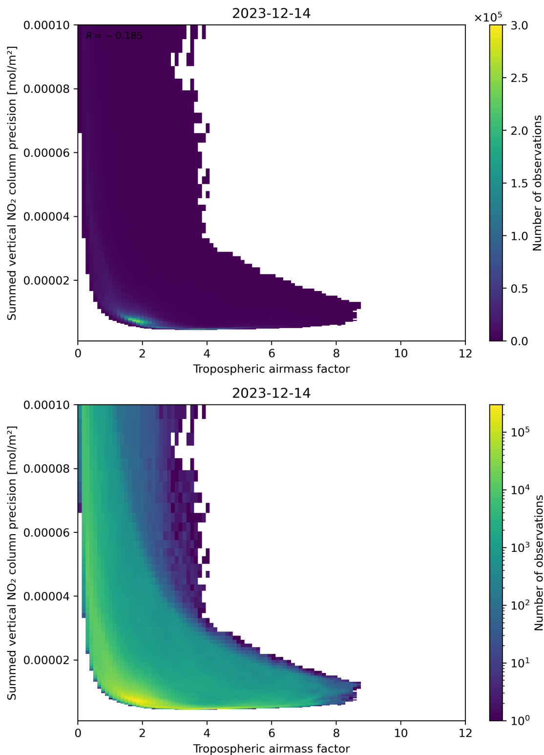
Figure 76: Scatter density plot of “Tropospheric air mass factor” against “Summed vertical NO 2 column precision” for 2023-12-14 to 2023-12-15.
