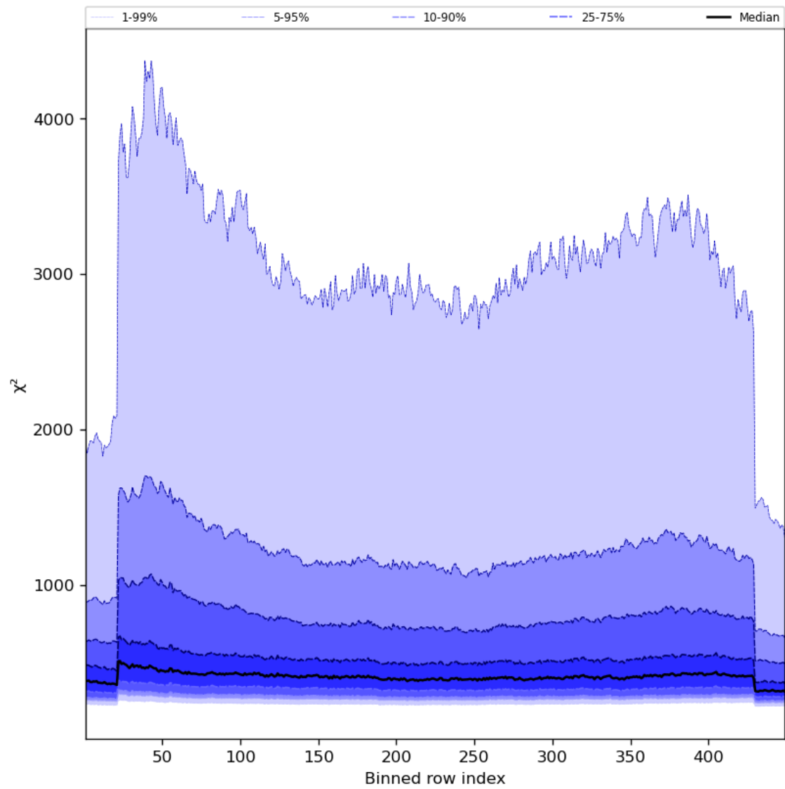
Figure 59: Along track statistics of “ \chi^2 ” for 2023-12-14 to 2023-12-15
