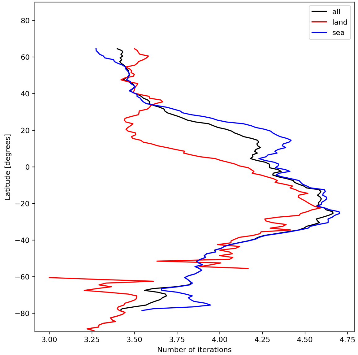
Figure 17: Zonal average of “Number of iterations” for 2023-12-14 to 2023-12-15.
