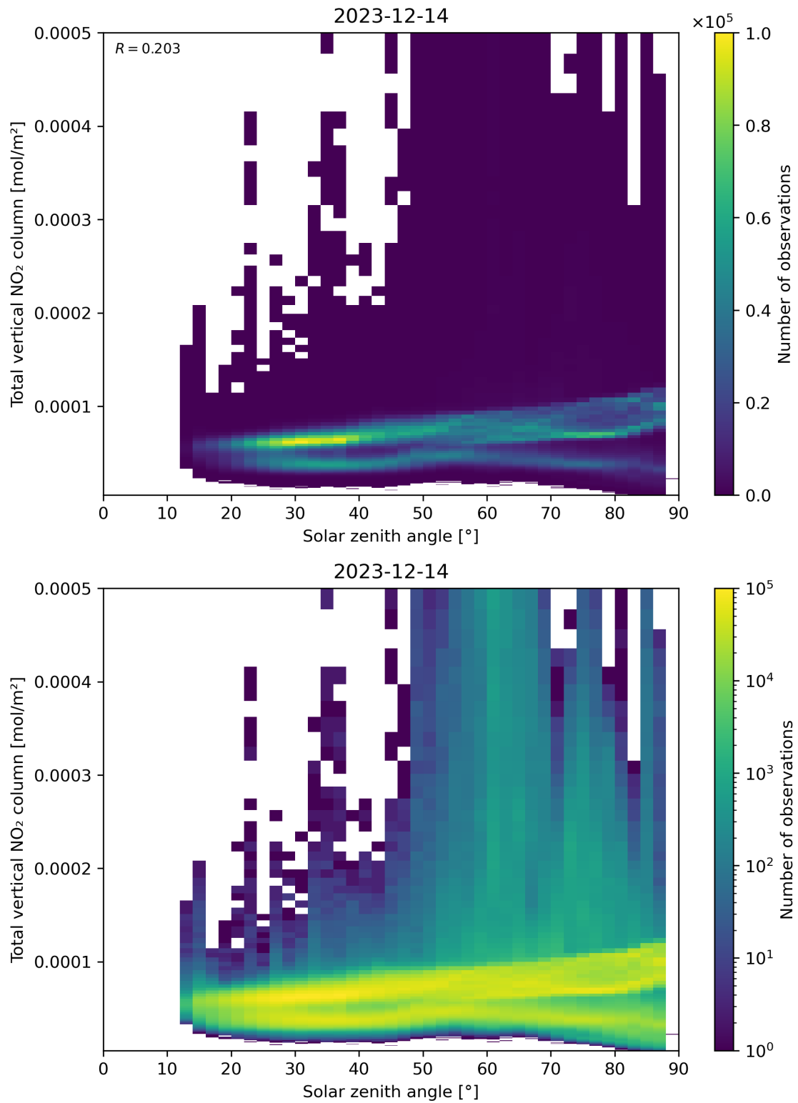
Figure 153: Scatter density plot of “Solar zenith angle” against “Total vertical NO 2 column” for 2023-12-14 to 2023-12-15.
