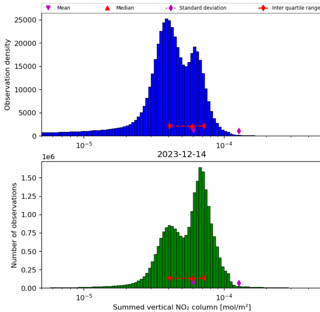
Figure 40: Histogram of “Summed vertical NO 2 column” for 2023-12-14 to 2023-12-15
