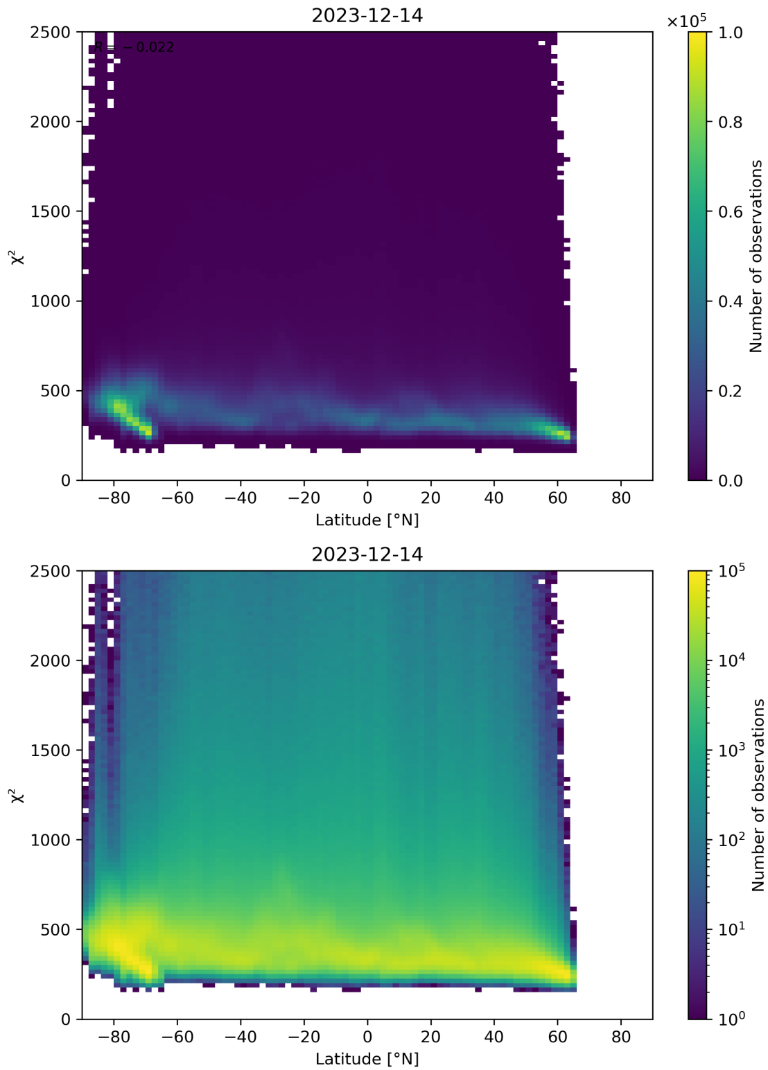
Figure 86: Scatter density plot of “Latitude” against “ \chi^2 ” for 2023-12-14 to 2023-12-15.
