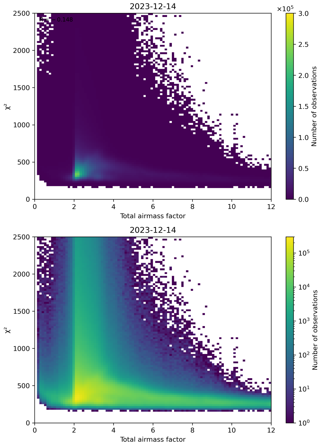
Figure 63: Scatter density plot of “Total airmass factor” against “ \chi^2 ” for 2023-12-14 to 2023-12-15.
