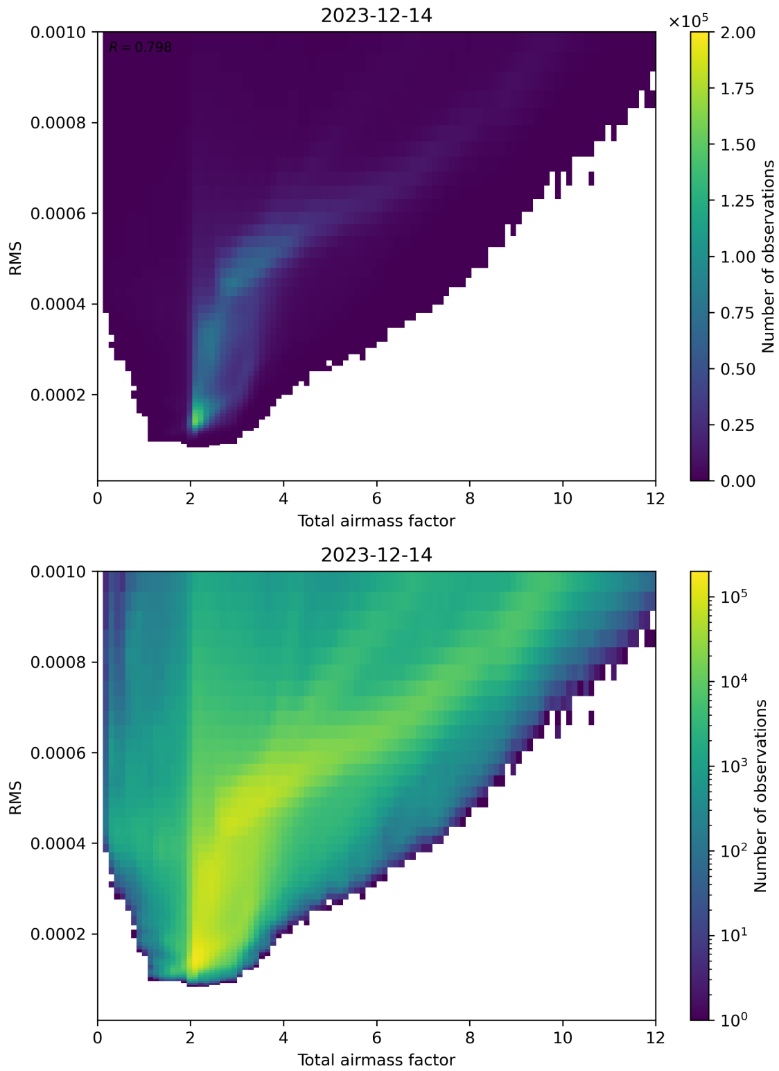
Figure 69: Scatter density plot of “Total airmass factor” against “RMS” for 2023-12-14 to 2023-12-15.
