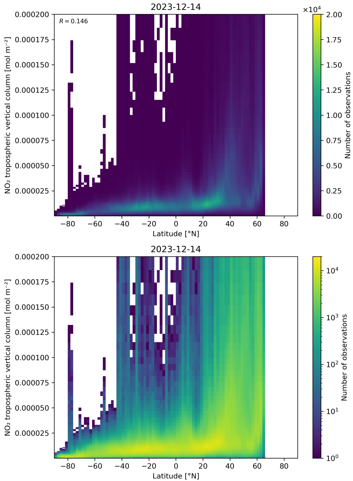
Figure 92: Scatter density plot of “Latitude” against “NO 2 tropospheric vertical column” for 2023-12-14 to 2023-12-15.
