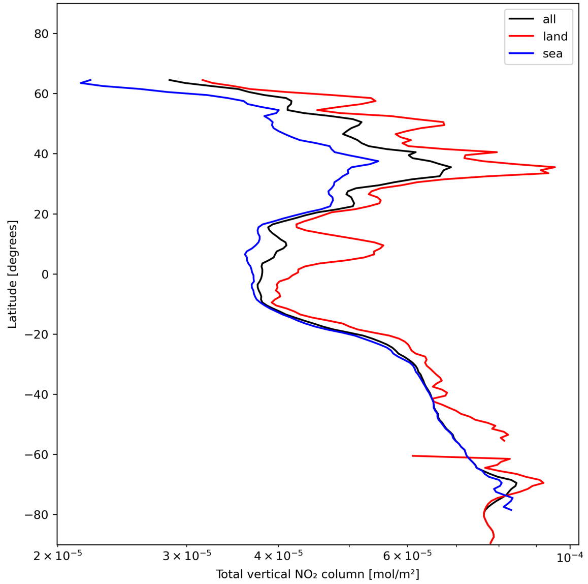
Figure 21: Zonal average of “Total vertical NO 2 column” for 2023-12-14 to 2023-12-15.
