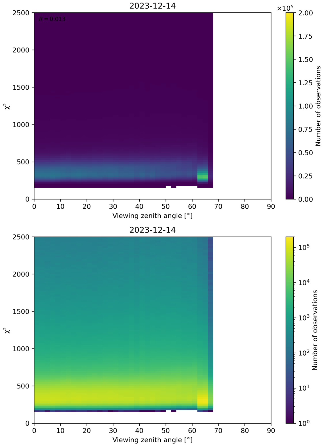
Figure 162: Scatter density plot of “Viewing zenith angle” against “ \chi^2 ” for 2023-12-14 to 2023-12-15.
