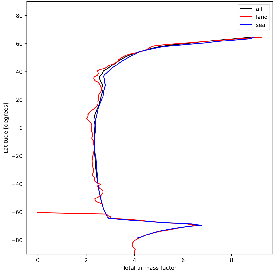
Figure 15: Zonal average of “Total airmass factor” for 2023-12-14 to 2023-12-15.
