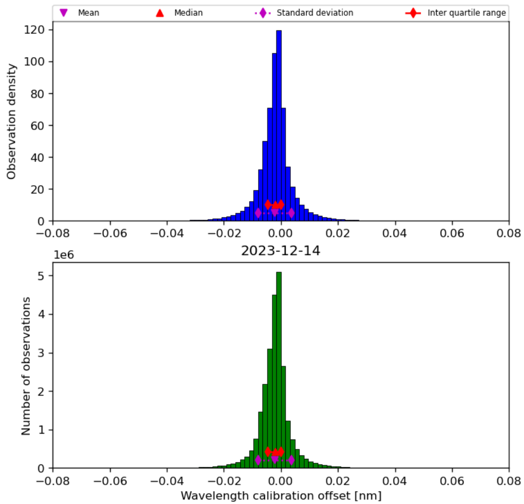
Figure 35: Histogram of “Wavelength calibration offset” for 2023-12-14 to 2023-12-15
