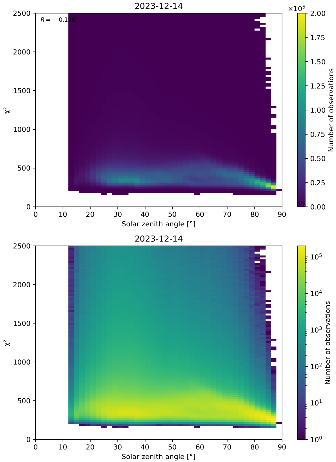
Figure 148: Scatter density plot of “Solar zenith angle” against “ \chi^2 ” for 2023-12-14 to 2023-12-15.
