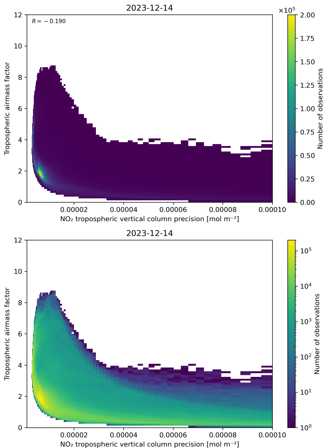
Figure 133: Scatter density plot of “NO 2 tropospheric vertical column precision” against “Tropospheric airmass factor” for 2023-12-14 to 2023-12-15.
