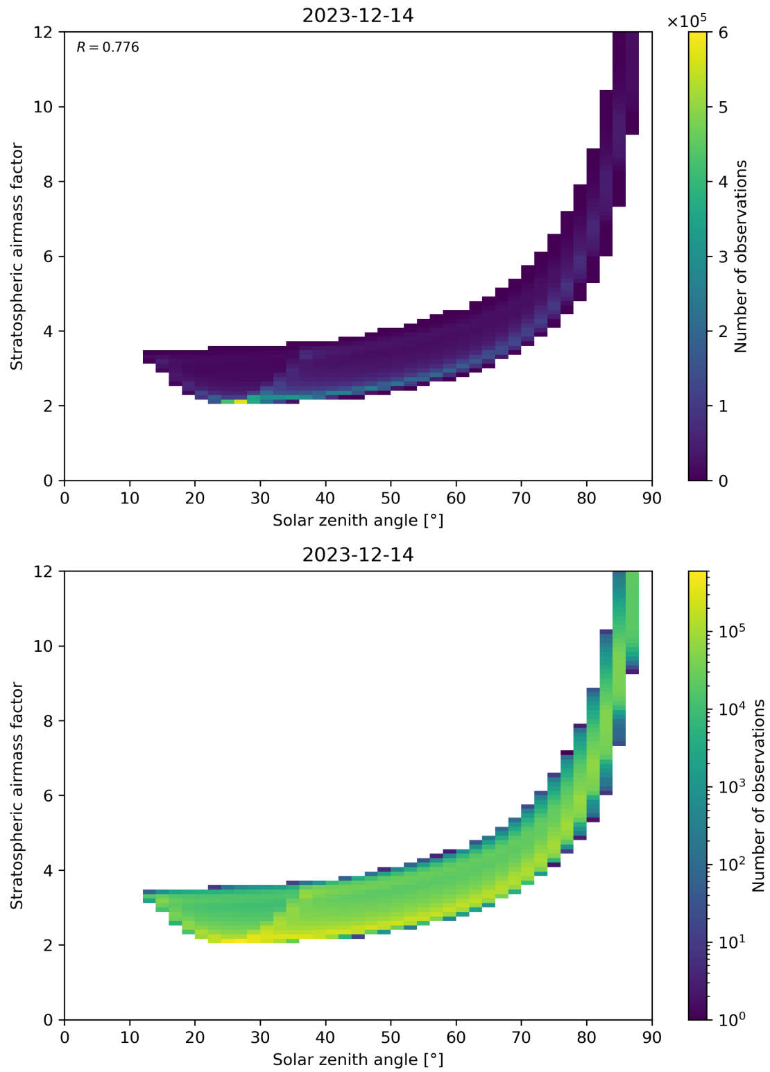
Figure 145: Scatter density plot of “Solar zenith angle” against “Stratospheric airmass factor” for 2023-12-14 to 2023-12-15.
