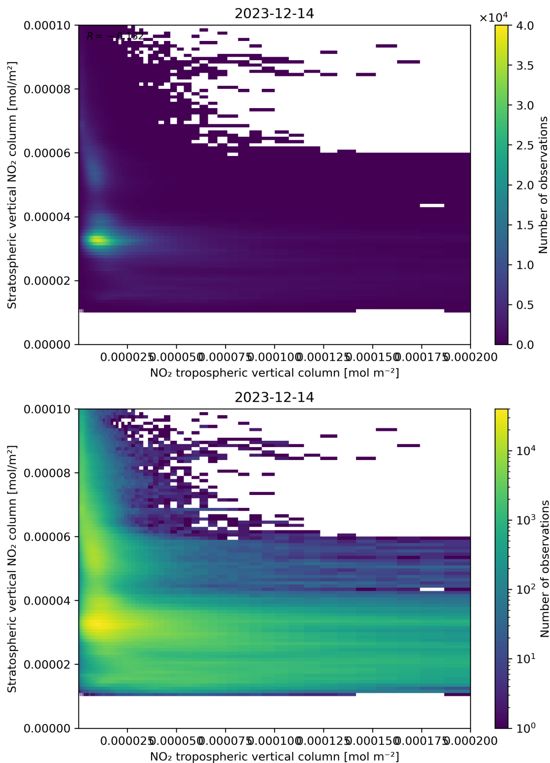
Figure 125: Scatter density plot of “NO 2 tropospheric vertical column” against “Stratospheric vertical NO 2 column” for 2023-12-14 to 2023-12-15.
