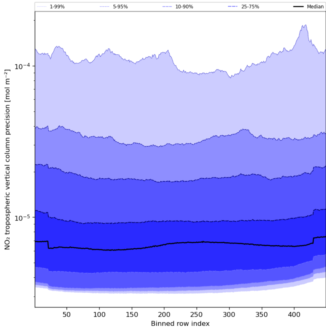
Figure 47: Along track statistics of “NO 2 tropospheric vertical column precision” for 2023-12-14 to 2023-12-15
