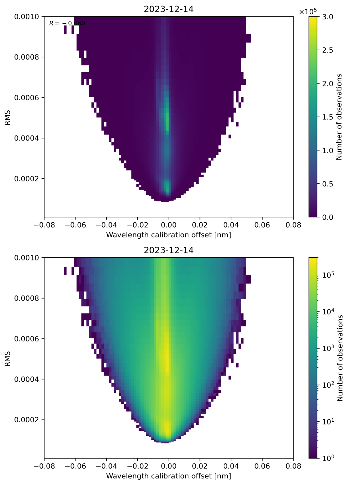
Figure 181: Scatter density plot of “Wavelength calibration offset” against “RMS” for 2023-12-14 to 2023-12-15.
