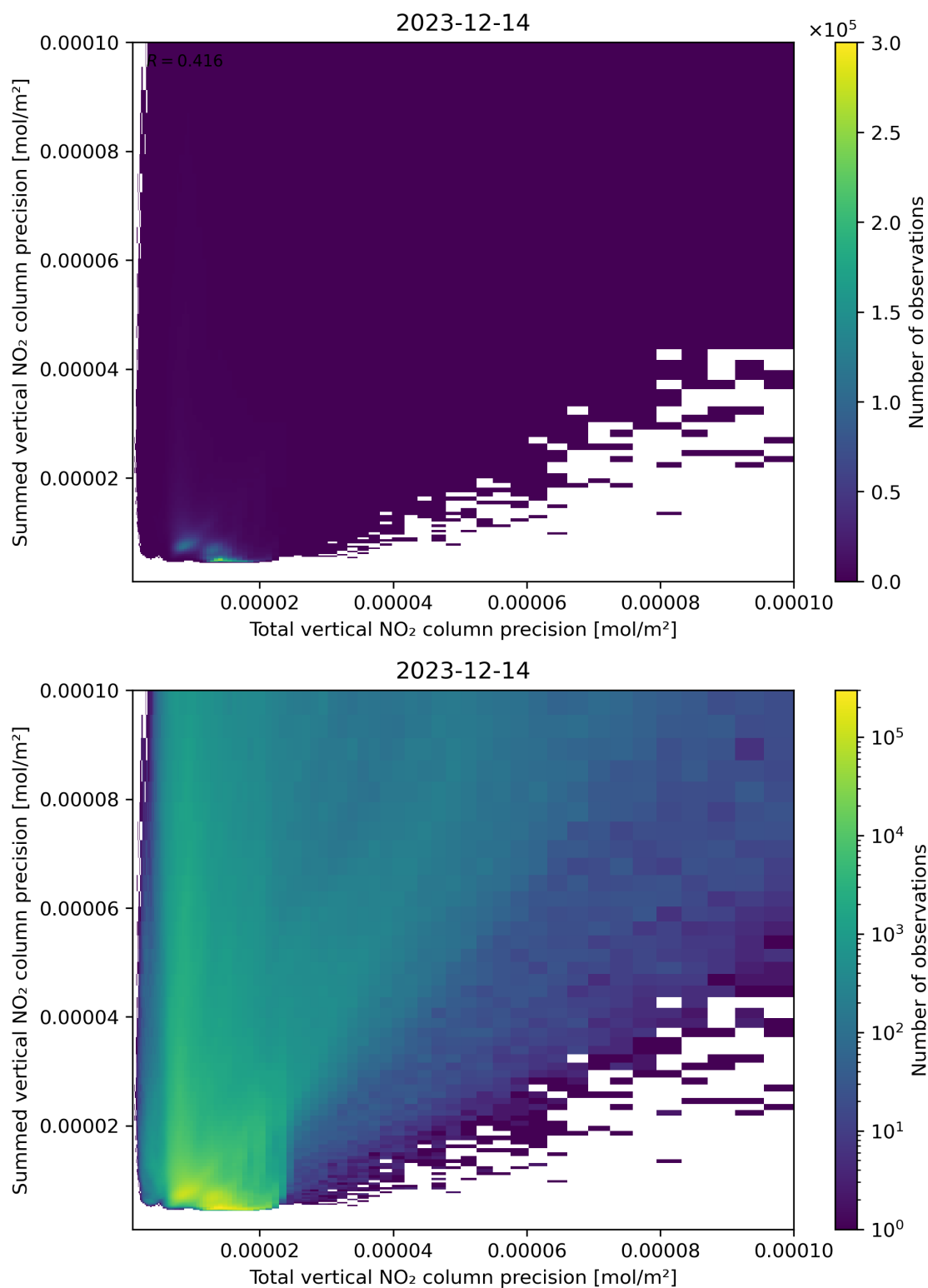
Figure 118: Scatter density plot of “Total vertical NO 2 column precision” against “Summed vertical NO 2 column precision” for 2023-12-14 to 2023-12-15.
