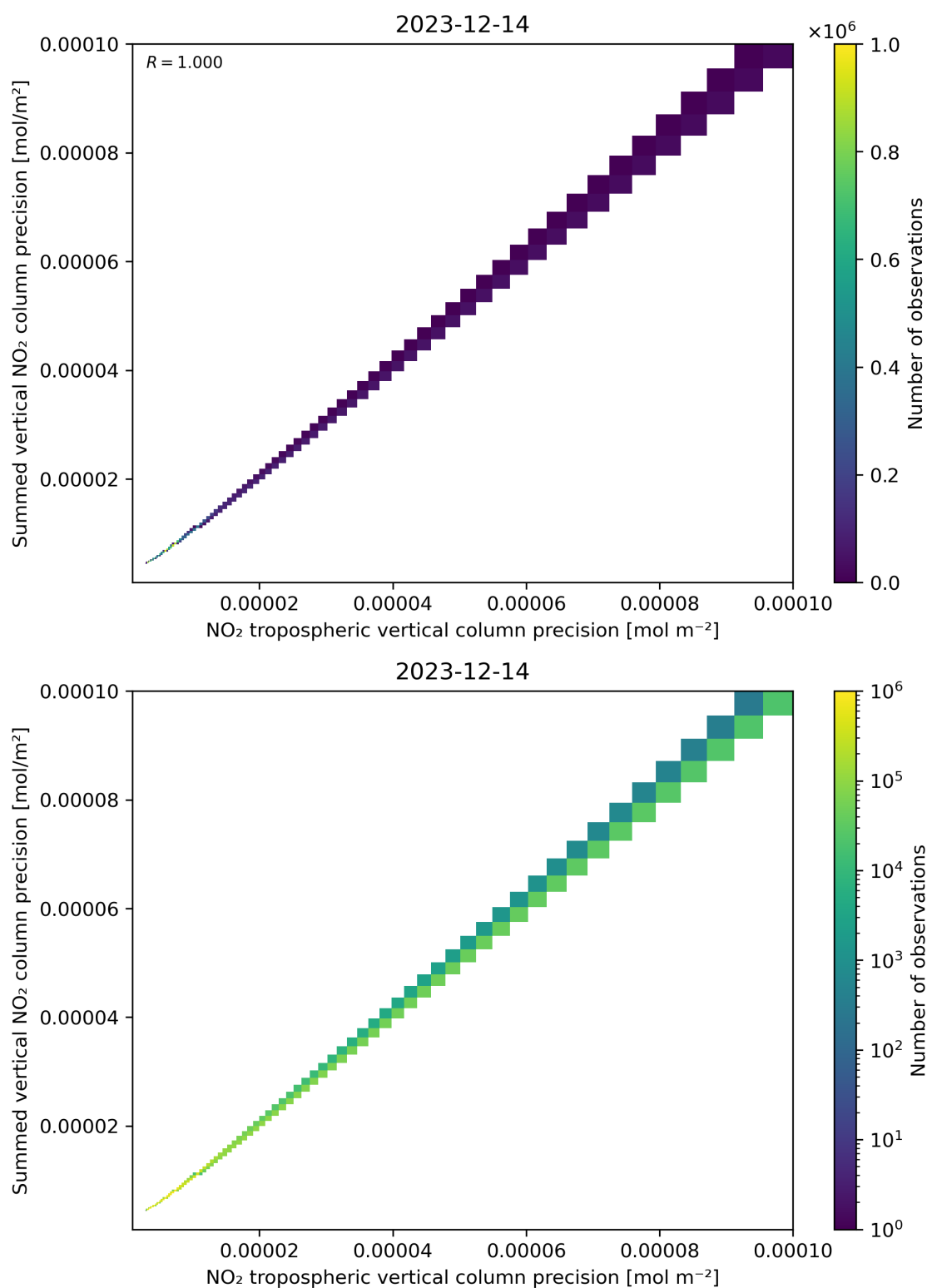
Figure 137: Scatter density plot of “NO 2 tropospheric vertical column precision” against “Summed vertical NO 2 column precision” for 2023-12-14 to 2023-12-15.
