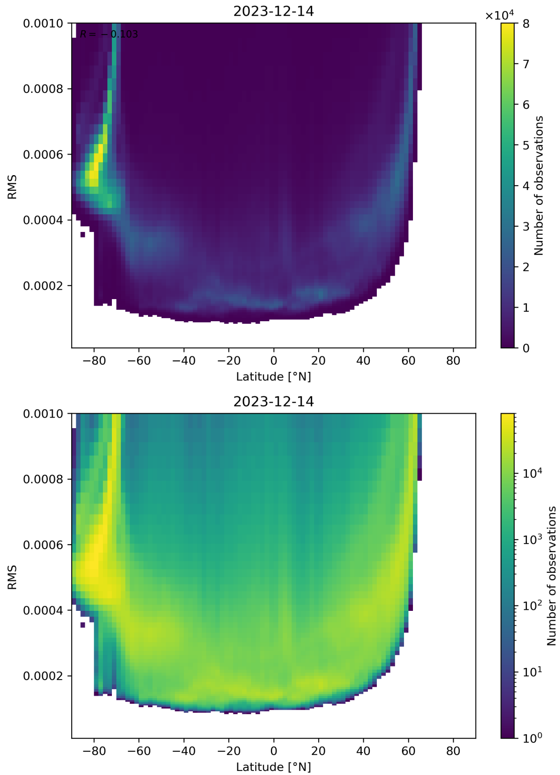
Figure 94: Scatter density plot of “Latitude” against “RMS” for 2023-12-14 to 2023-12-15.
