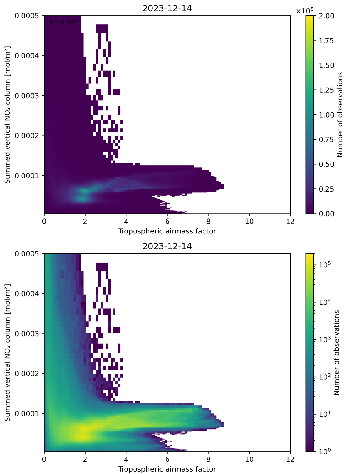
Figure 75: Scatter density plot of “Tropospheric airmass factor” against “Summed vertical NO 2 column” for 2023-12-14 to 2023-12-15.
