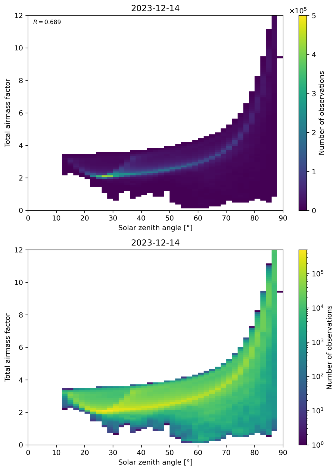
Figure 146: Scatter density plot of “Solar zenith angle” against “Total airmass factor” for 2023-12-14 to 2023-12-15.
