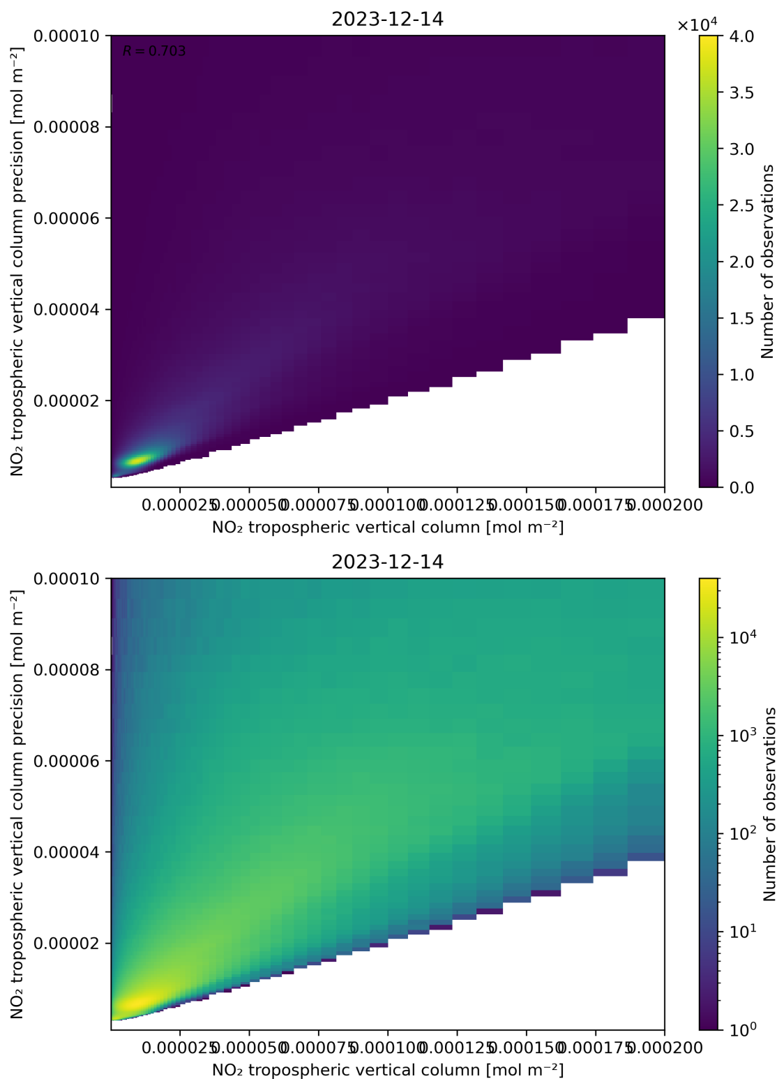
Figure 130: Scatter density plot of “NO 2 tropospheric vertical column” against “NO 2 tropospheric vertical column precision” for 2023-12-14 to 2023-12-15.
