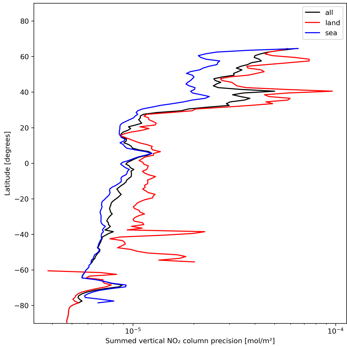
Figure 24: Zonal average of “Summed vertical NO 2 column precision” for 2023-12-14 to 2023-12-15.
