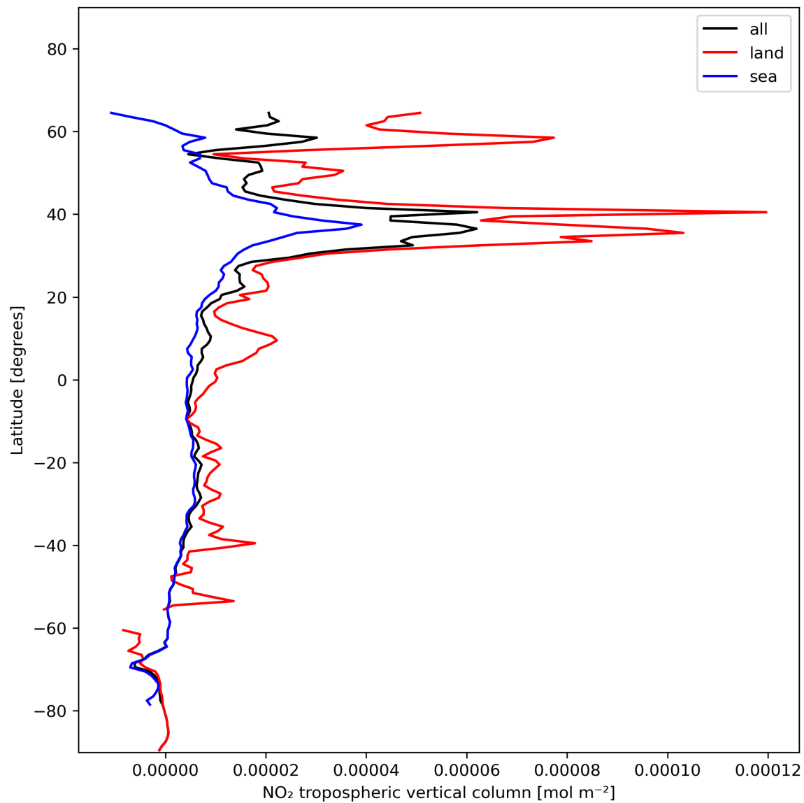
Figure 12: Zonal average of “NO 2 tropospheric vertical column” for 2023-12-14 to 2023-12-15.
