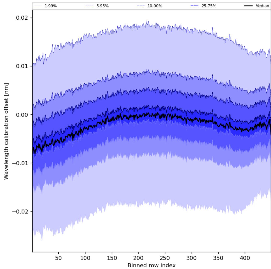
Figure 52: Along track statistics of “Wavelength calibration offset” for 2023-12-14 to 2023-12-15
