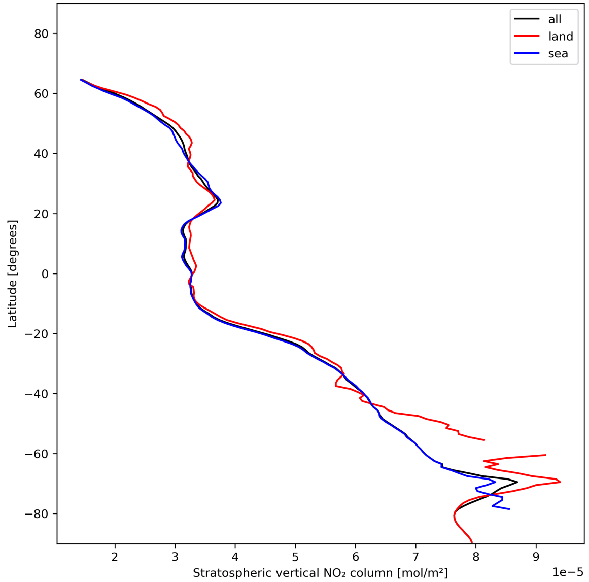
Figure 19: Zonal average of “Stratospheric vertical NO 2 column” for 2023-12-14 to 2023-12-15.
