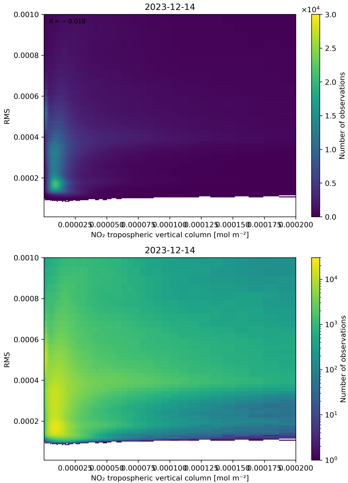
Figure 142: Scatter density plot of “NO 2 tropospheric vertical column” against “RMS” for 2023-12-14 to 2023-12-15.
