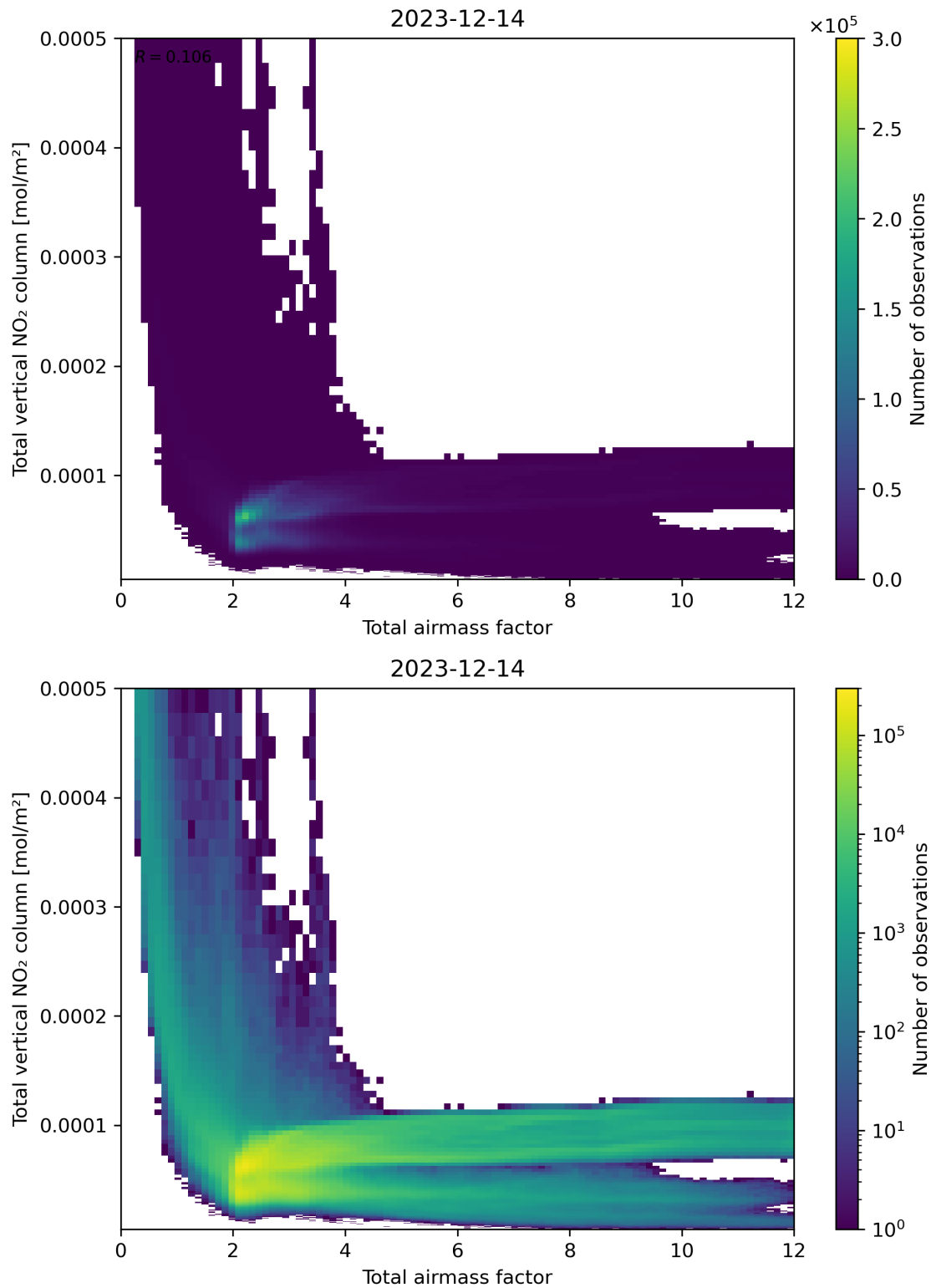
Figure 67: Scatter density plot of “Total airmass factor” against “Total vertical NO 2 column” for 2023-12-14 to 2023-12-15.
