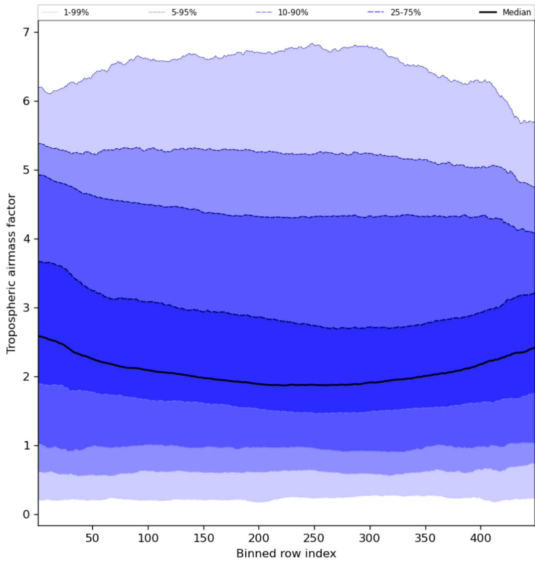
Figure 48: Along track statistics of “Tropospheric air mass factor” for 2023-12-14 to 2023-12-15
