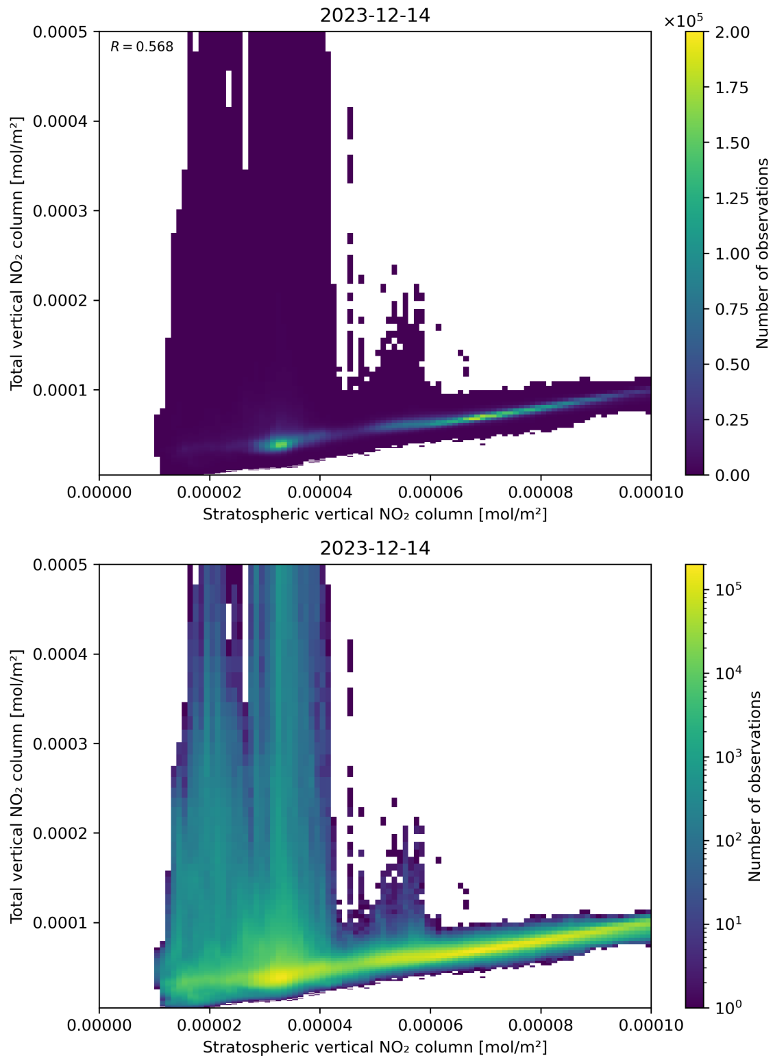
Figure 100: Scatter density plot of “Stratospheric vertical NO 2 column” against “Total vertical NO 2 column” for 2023-12-14 to 2023-12-15.
