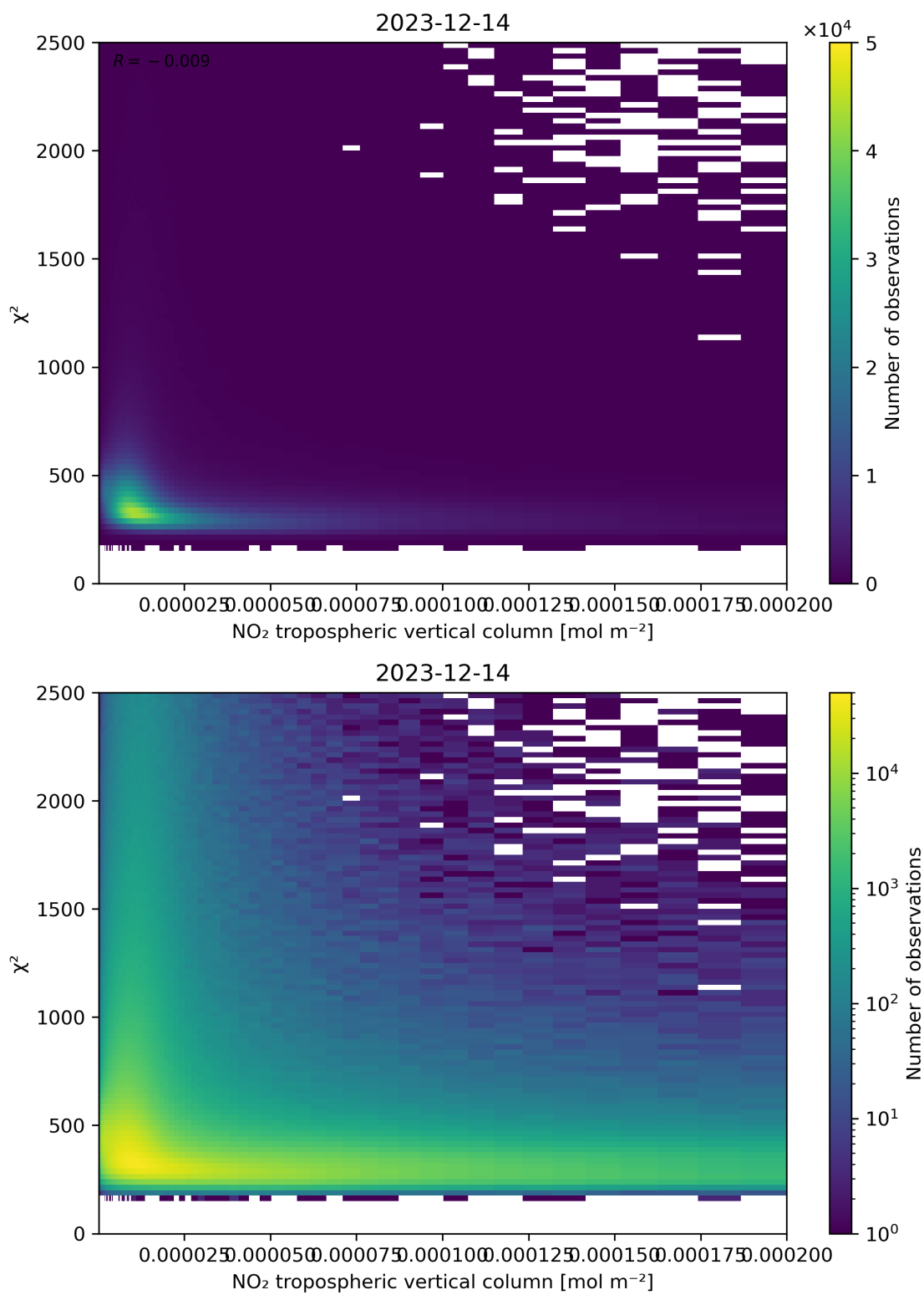
Figure 124: Scatter density plot of “NO 2 tropospheric vertical column” against “ \chi^2 ” for 2023-12-14 to 2023-12-15.
