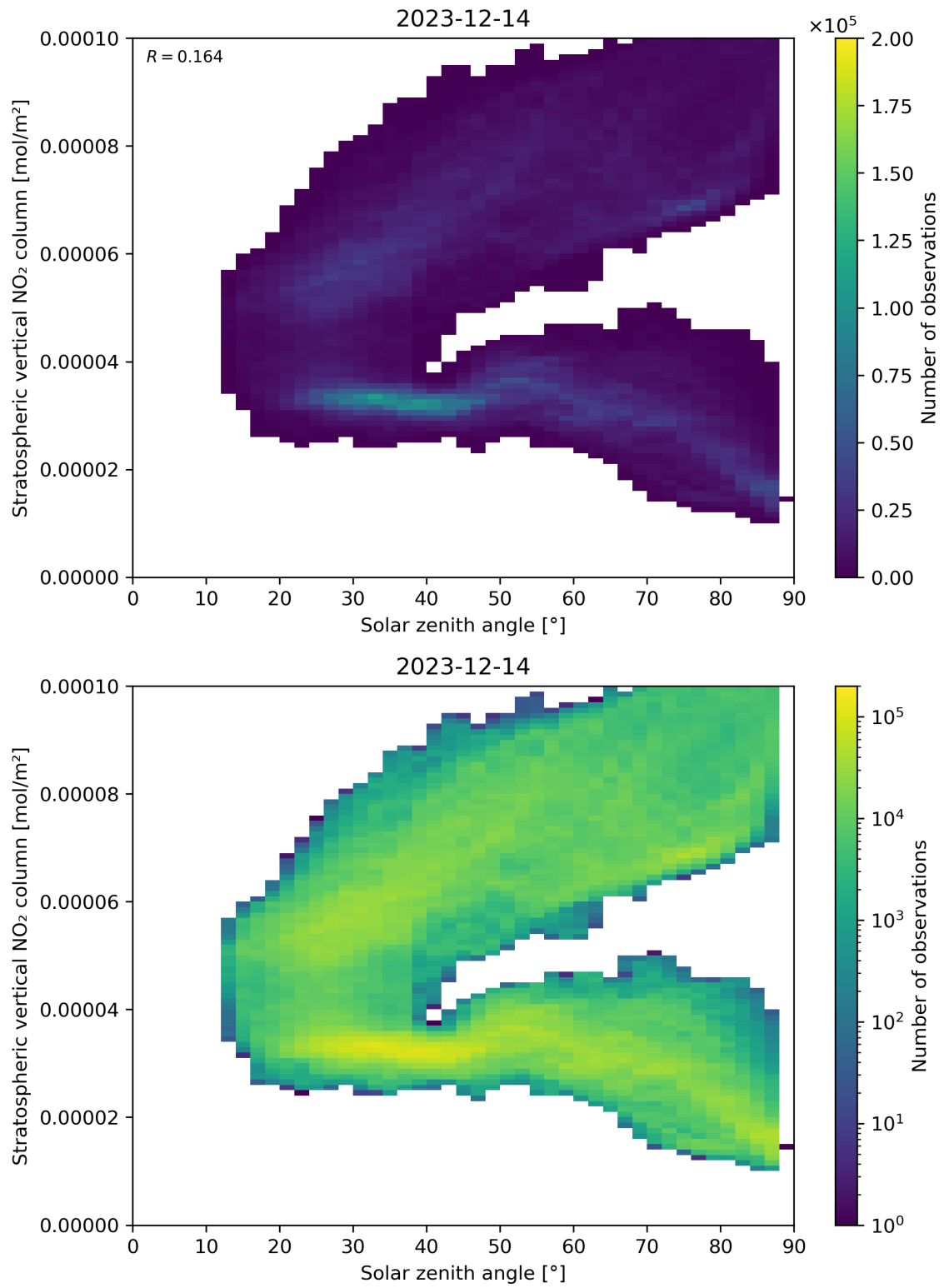
Figure 150: Scatter density plot of “Solar zenith angle” against “Stratospheric vertical NO 2 column” for 2023-12-14 to 2023-12-15.
