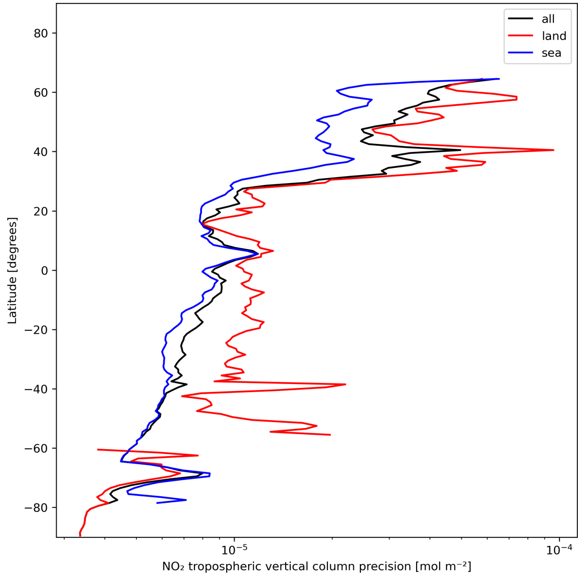
Figure 13: Zonal average of “NO 2 tropospheric vertical column precision” for 2023-12-14 to 2023-12-15.
