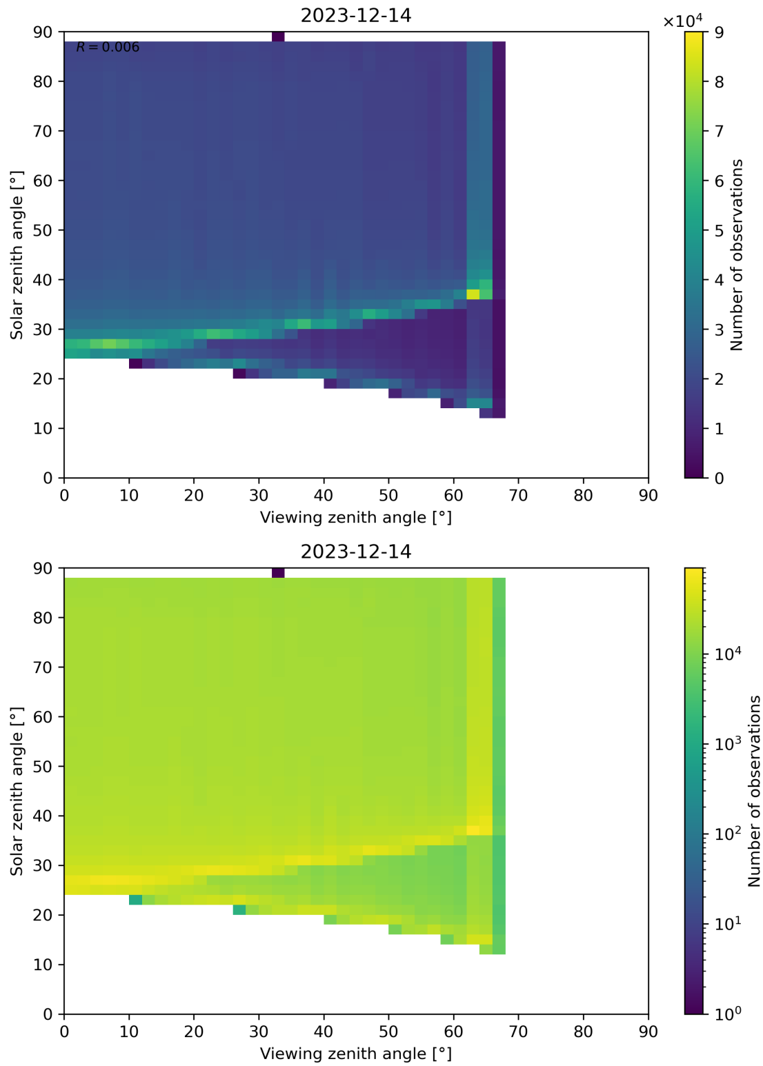
Figure 172: Scatter density plot of “Viewing zenith angle” against “Solar zenith angle” for 2023-12-14 to 2023-12-15.
