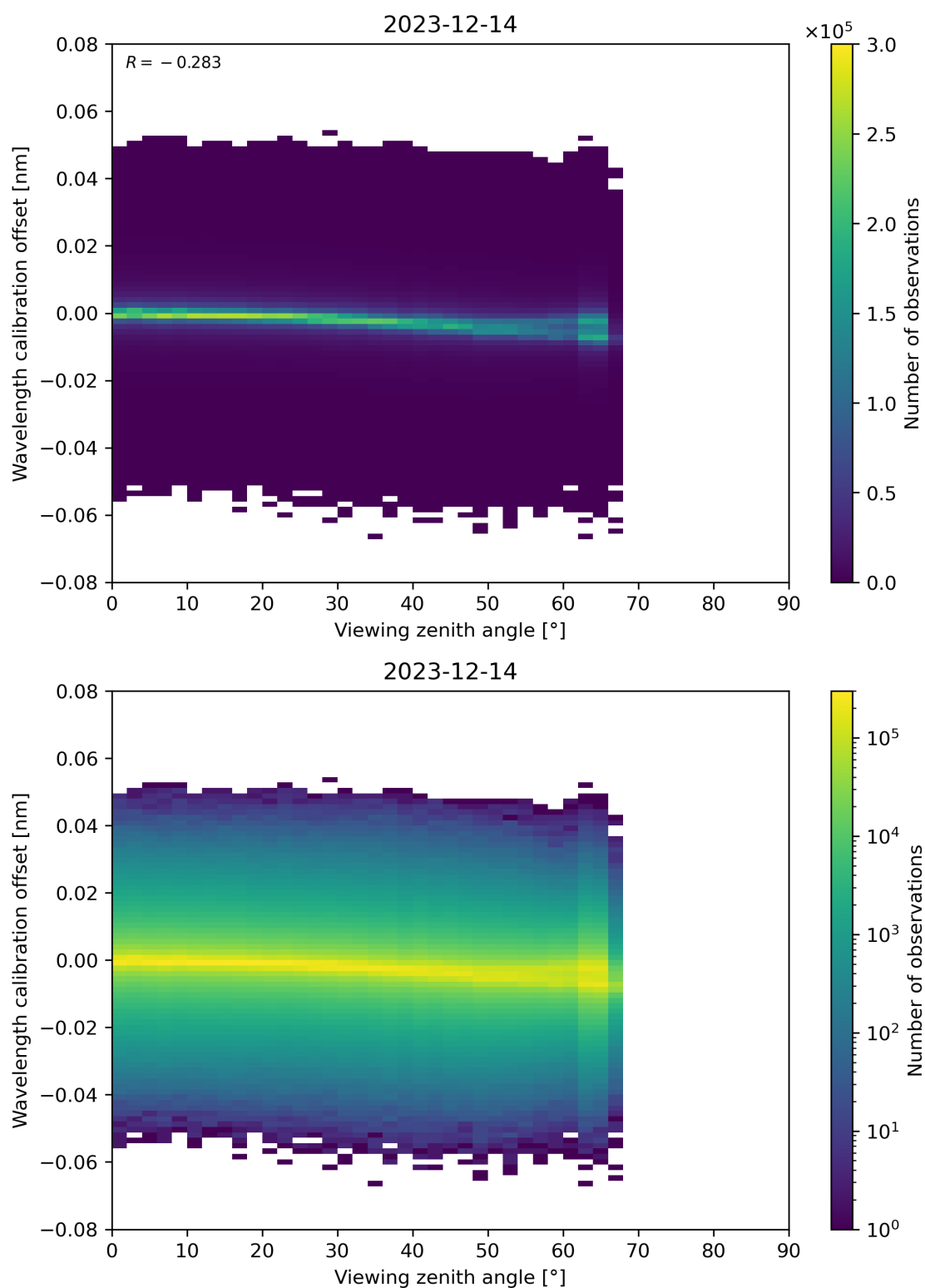
Figure 173: Scatter density plot of “Viewing zenith angle” against “Wavelength calibration offset” for 2023-12-14 to 2023-12-15.
