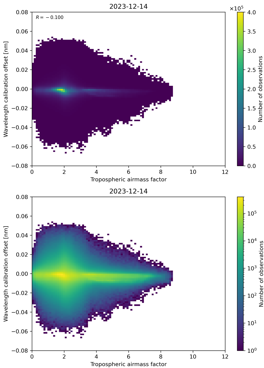
Figure 80: Scatter density plot of “Tropospheric airmass factor” against “Wavelength calibration offset” for 2023-12-14 to 2023-12-15.
