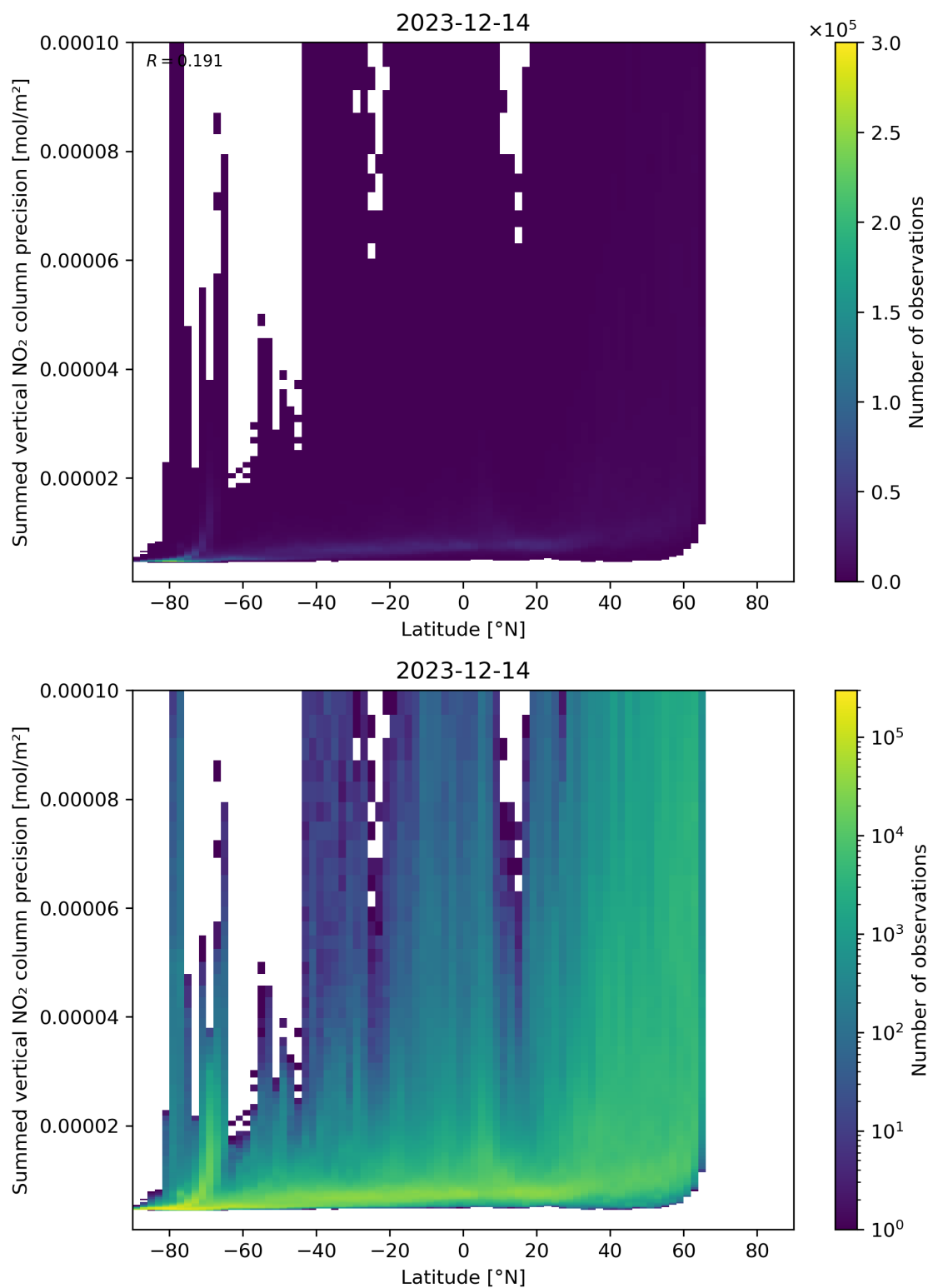
Figure 89: Scatter density plot of “Latitude” against “Summed vertical NO 2 column precision” for 2023-12-14 to 2023-12-15.
