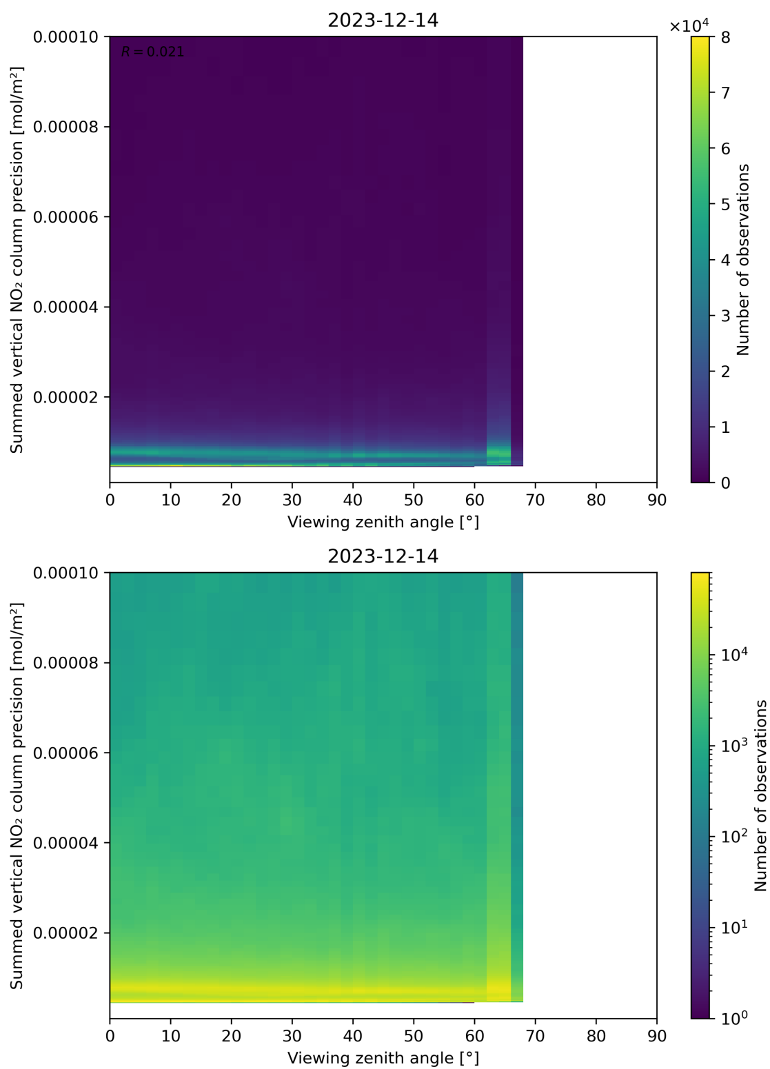
Figure 166: Scatter density plot of “Viewing zenith angle” against “Summed vertical NO 2 column precision” for 2023-12-14 to 2023-12-15.
