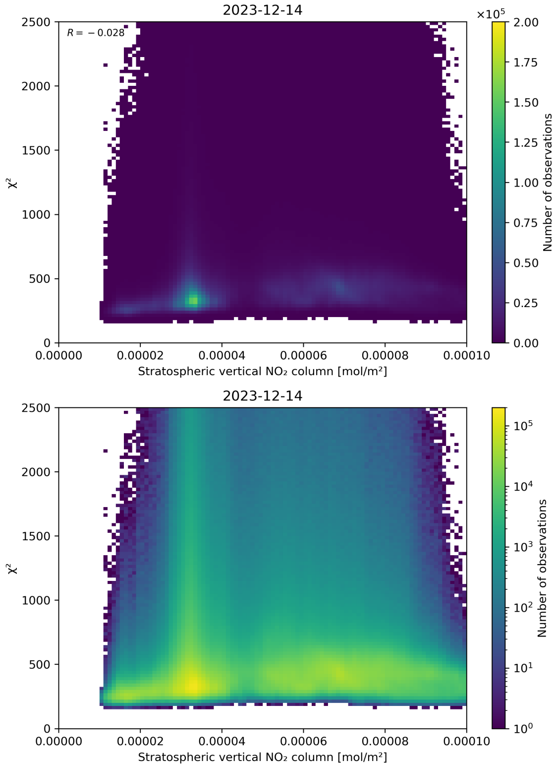
Figure 97: Scatter density plot of “Stratospheric vertical NO 2 column” against “ \chi^2 ” for 2023-12-14 to 2023-12-15.
