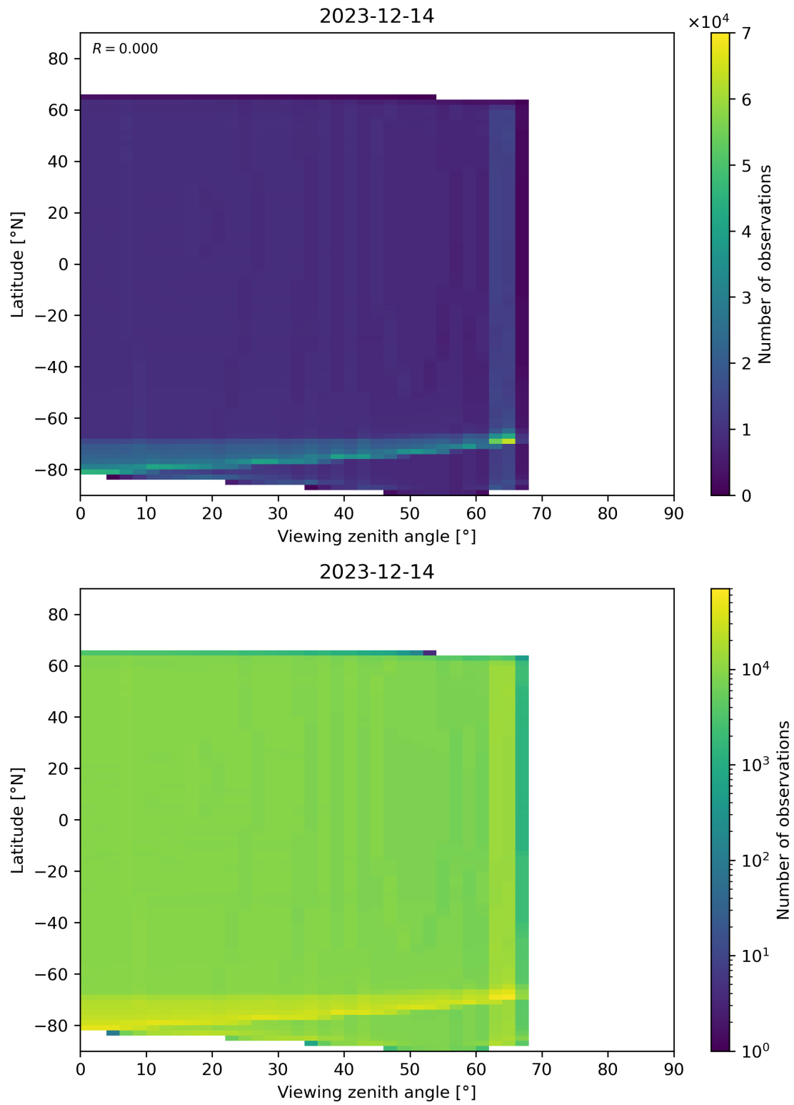
Figure 163: Scatter density plot of “Viewing zenith angle” against “Latitude” for 2023-12-14 to 2023-12-15.
