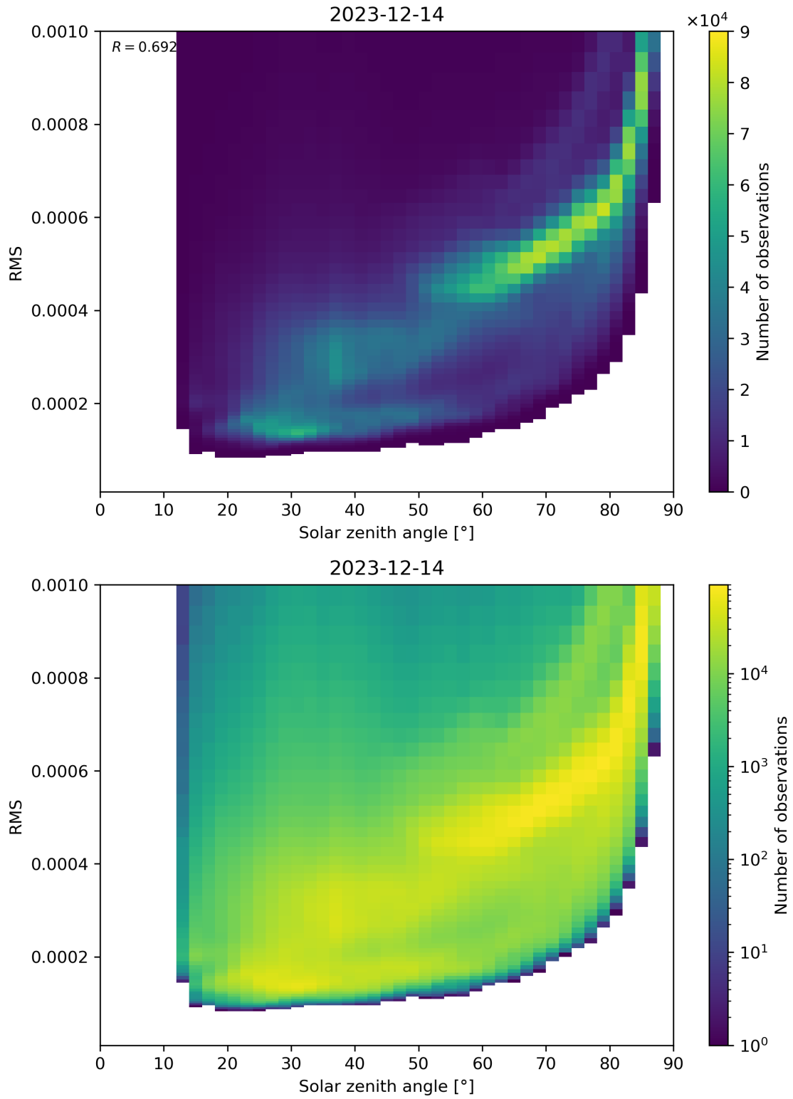
Figure 157: Scatter density plot of “Solar zenith angle” against “RMS” for 2023-12-14 to 2023-12-15.
