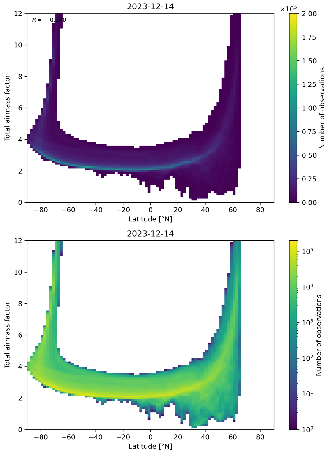
Figure 84: Scatter density plot of “Latitude” against “Total airmass factor” for 2023-12-14 to 2023-12-15.
