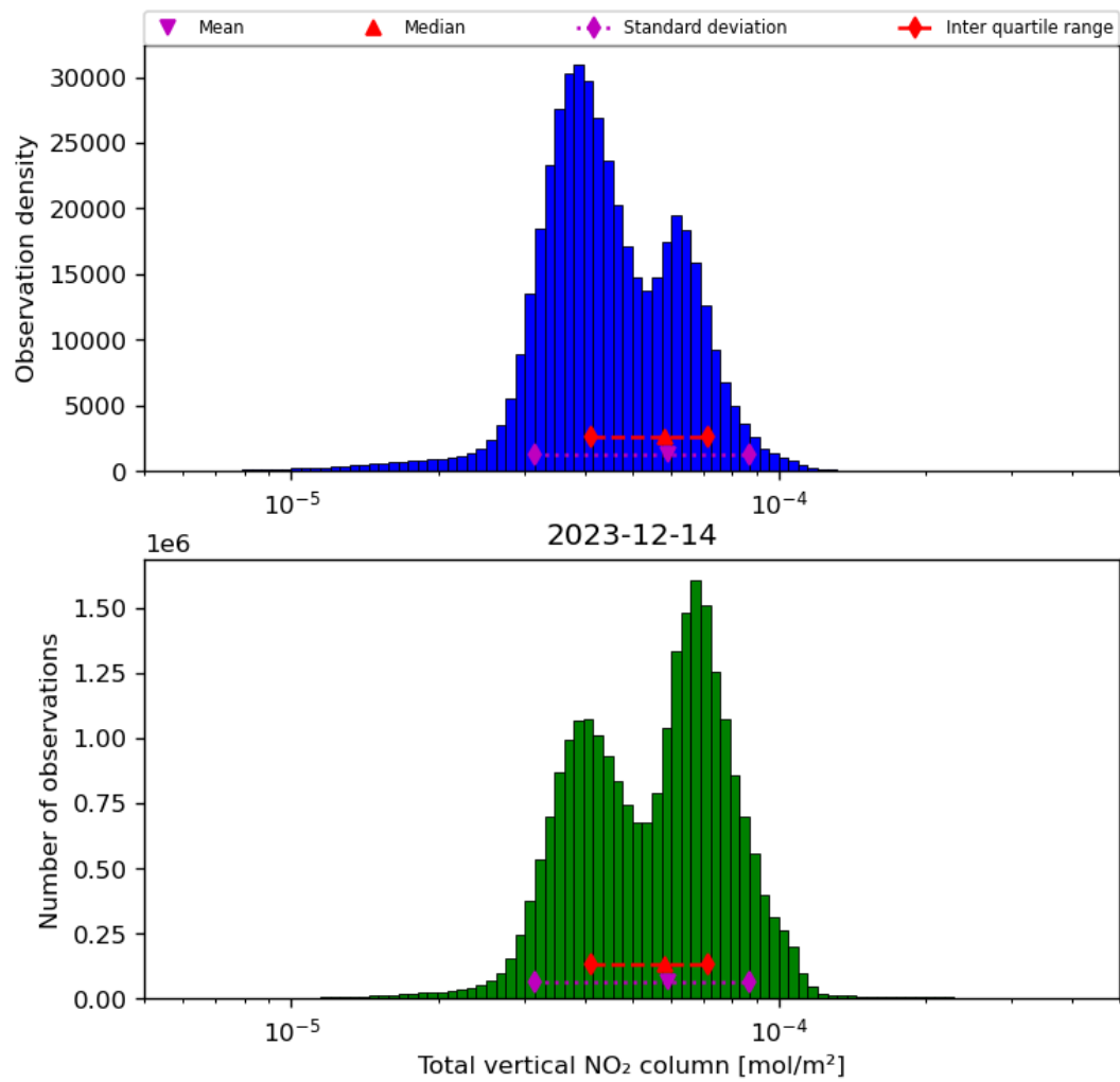
Figure 38: Histogram of “Total vertical NO 2 column” for 2023-12-14 to 2023-12-15
