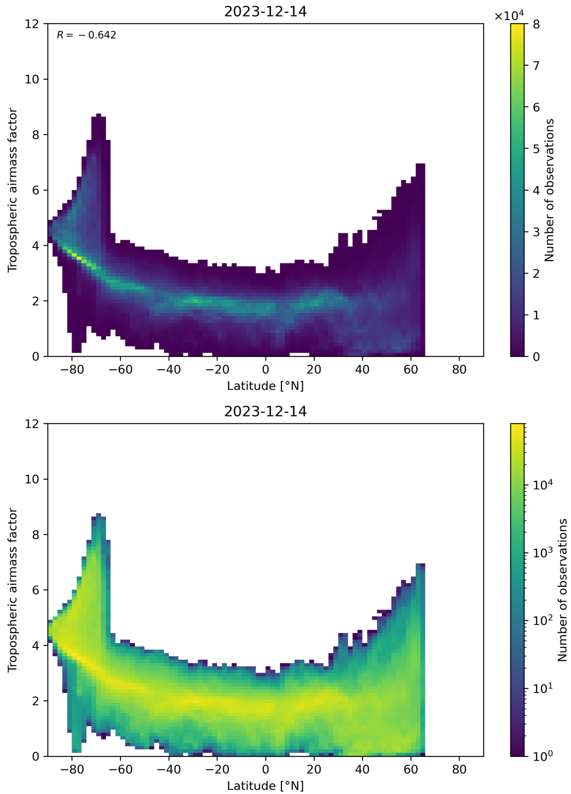
Figure 85: Scatter density plot of “Latitude” against “Tropospheric airmass factor” for 2023-12-14 to 2023-12-15.
