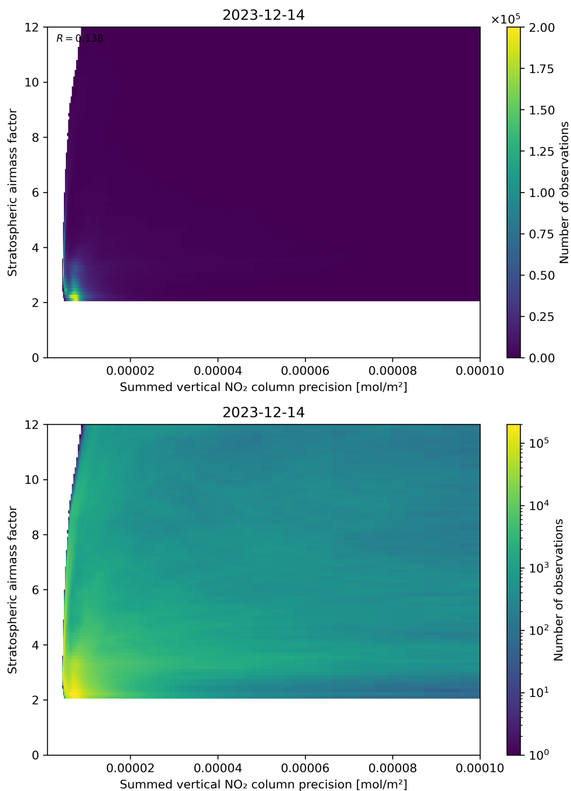
Figure 106: Scatter density plot of “Summed vertical NO 2 column precision” against “Stratospheric airmass factor” for 2023-12-14 to 2023-12-15.
