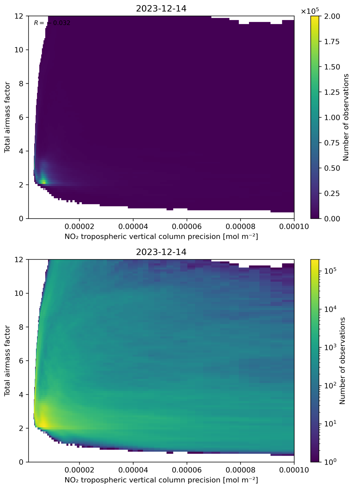
Figure 132: Scatter density plot of “NO 2 tropospheric vertical column precision” against “Total air mass factor” for 2023-12-14 to 2023-12-15.
