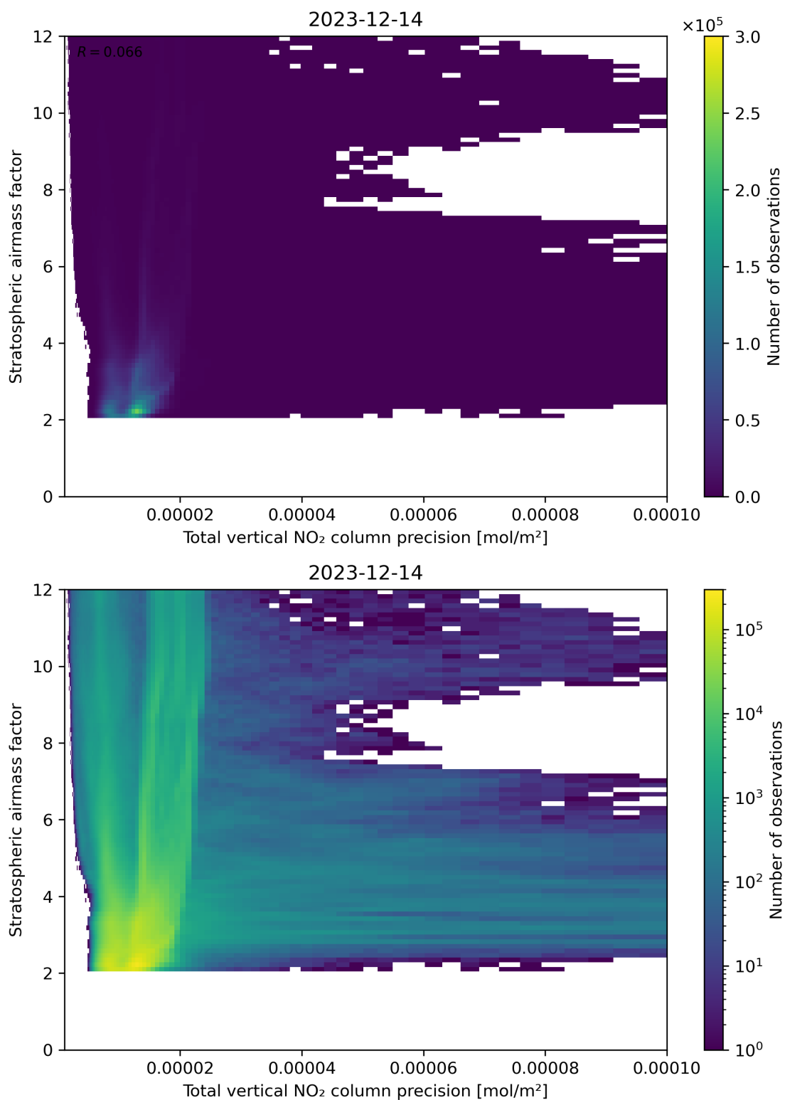
Figure 115: Scatter density plot of “Total vertical NO 2 column precision” against “Stratospheric air mass factor” for 2023-12-14 to 2023-12-15.
