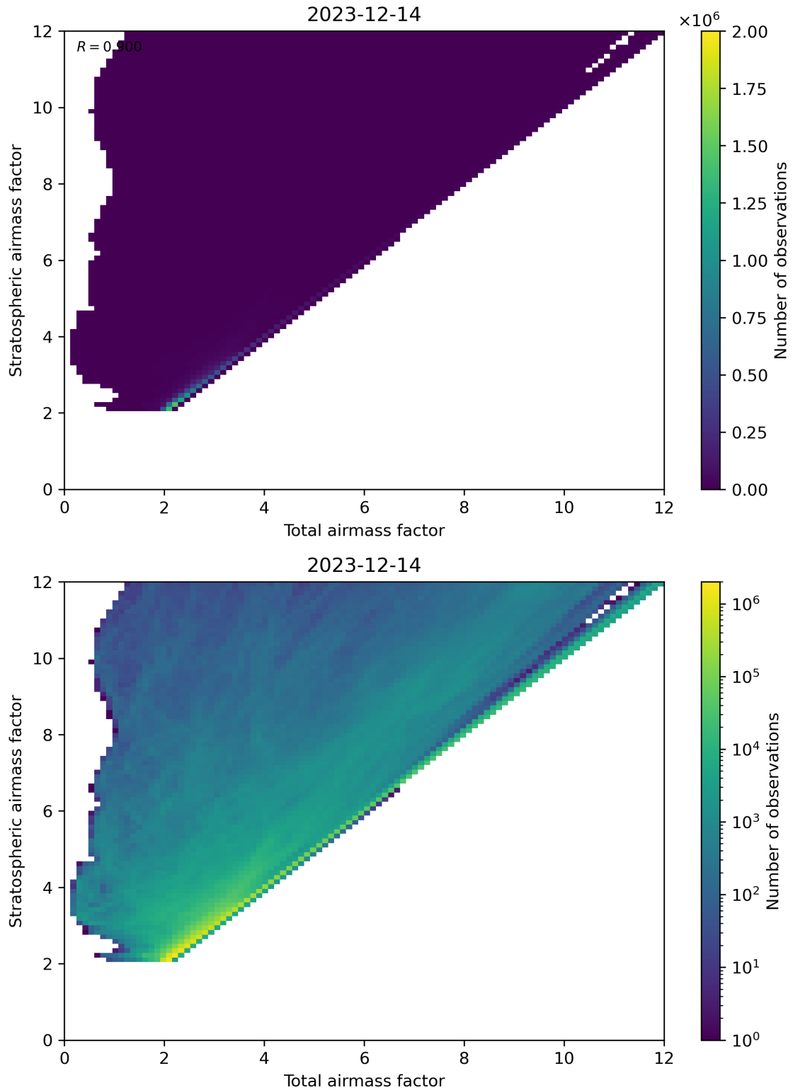
Figure 62: Scatter density plot of “Total air mass factor” against “Stratospheric air mass factor” for 2023-12-14 to 2023-12-15.
