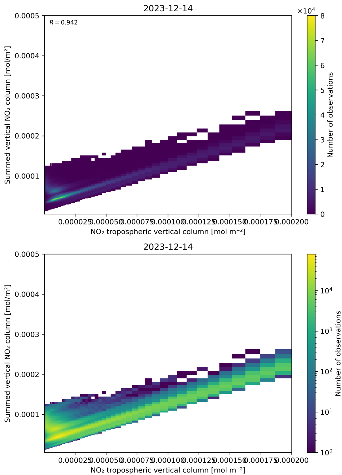
Figure 126: Scatter density plot of “NO 2 tropospheric vertical column” against “Summed vertical NO 2 column” for 2023-12-14 to 2023-12-15.
