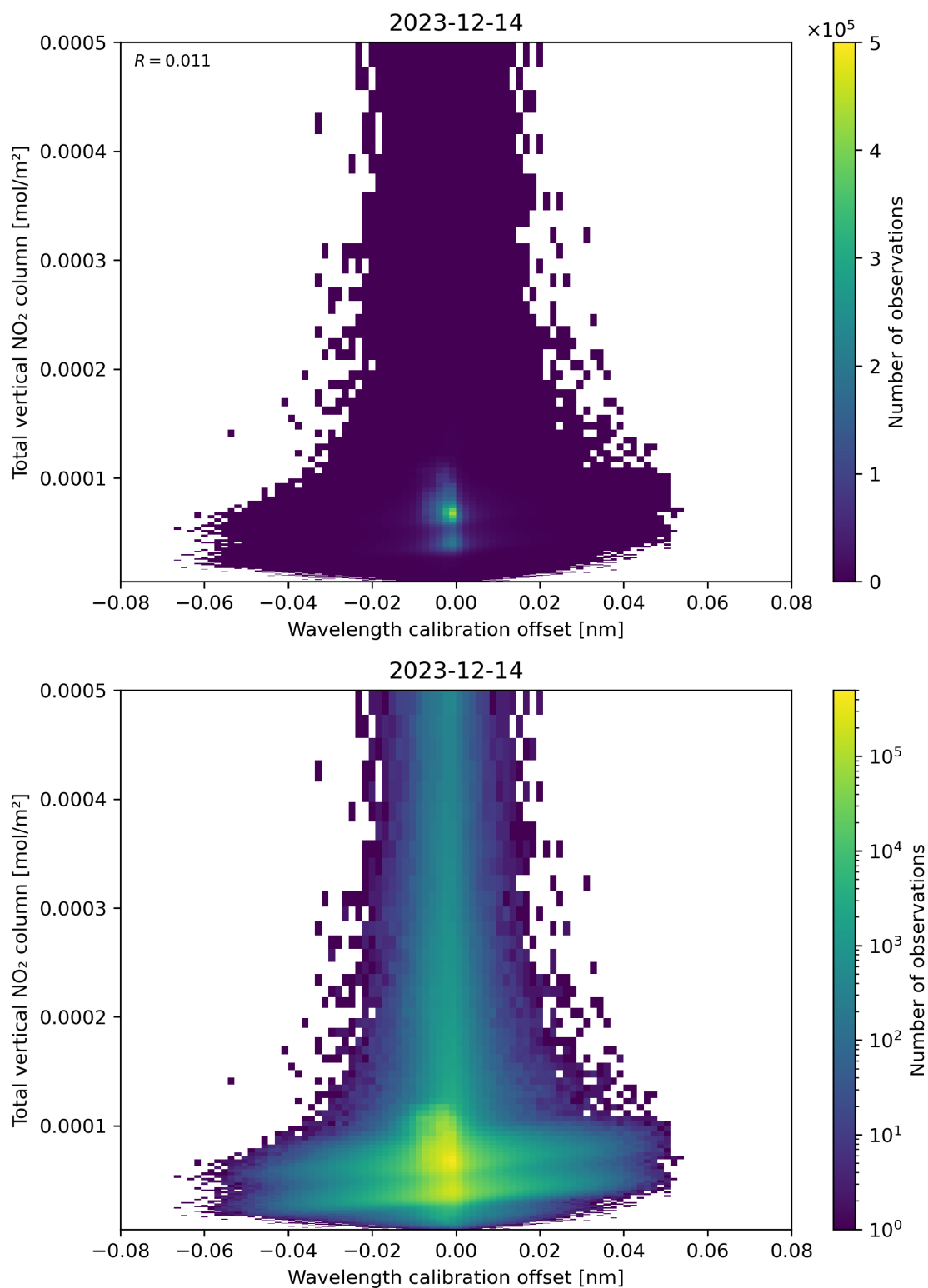
Figure 179: Scatter density plot of “Wavelength calibration offset” against “Total vertical NO 2 column” for 2023-12-14 to 2023-12-15.
