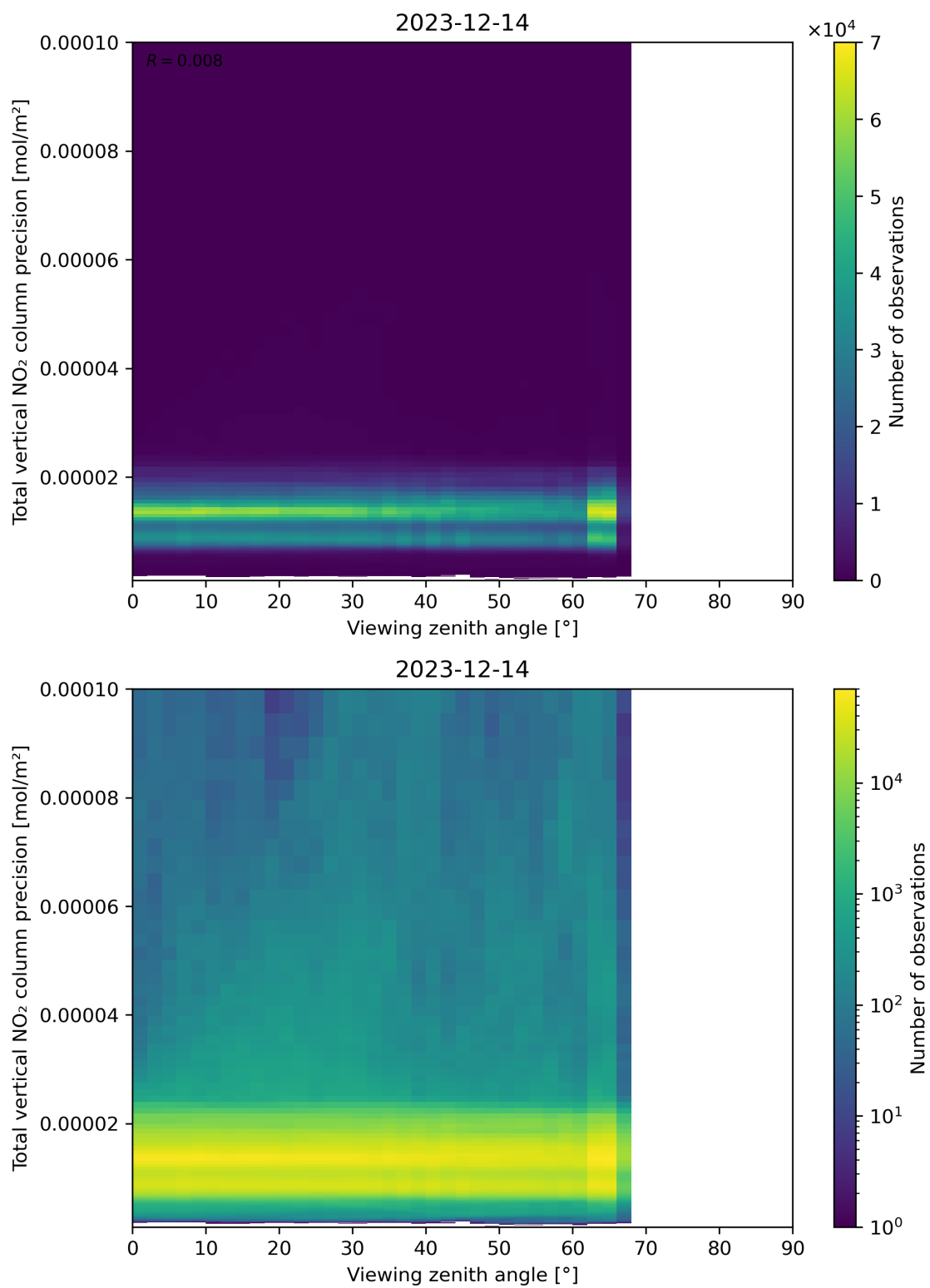
Figure 168: Scatter density plot of “Viewing zenith angle” against “Total vertical NO 2 column precision” for 2023-12-14 to 2023-12-15.
