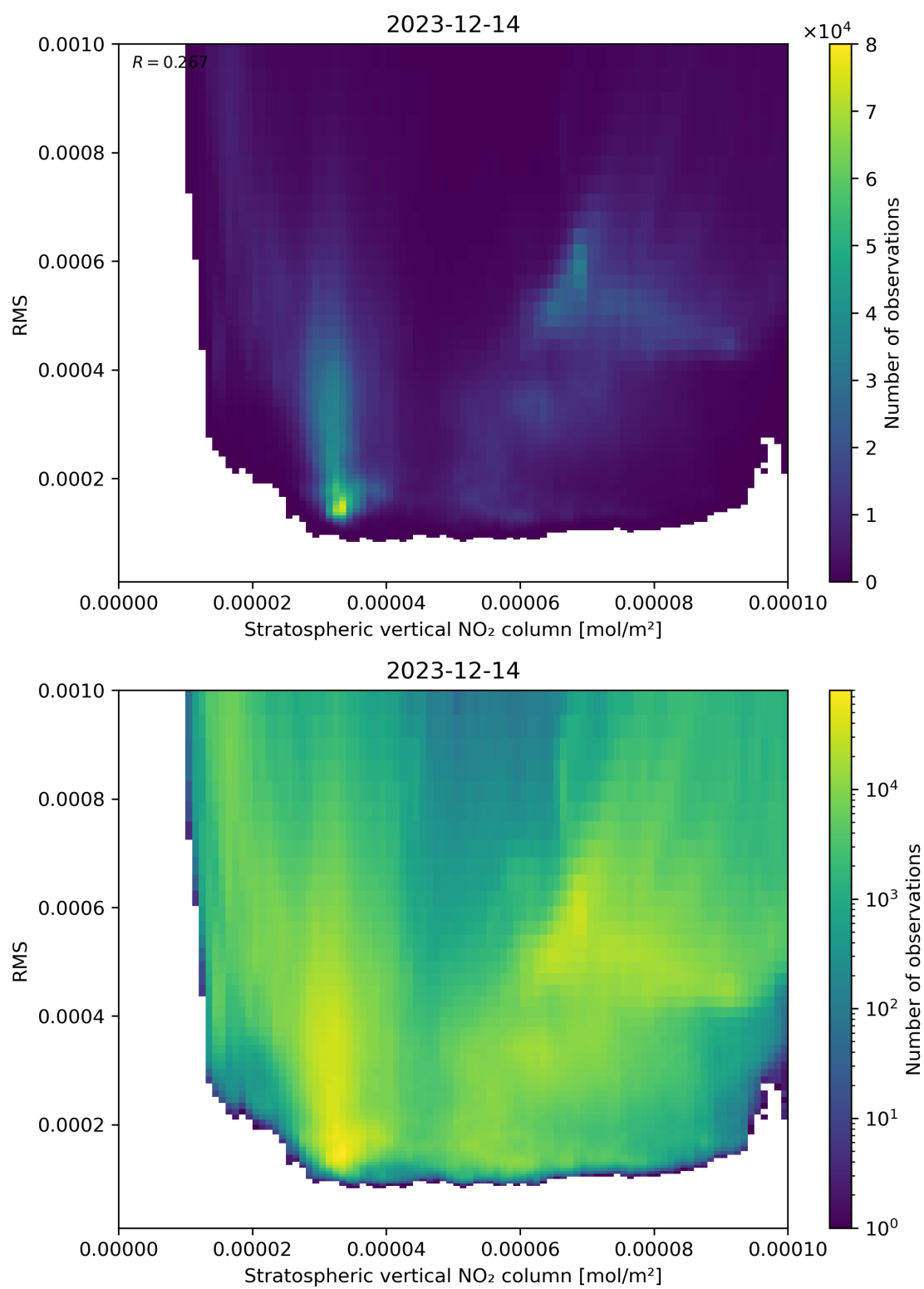
Figure 102: Scatter density plot of “Stratospheric vertical NO 2 column” against “RMS” for 2023-12-14 to 2023-12-15.
