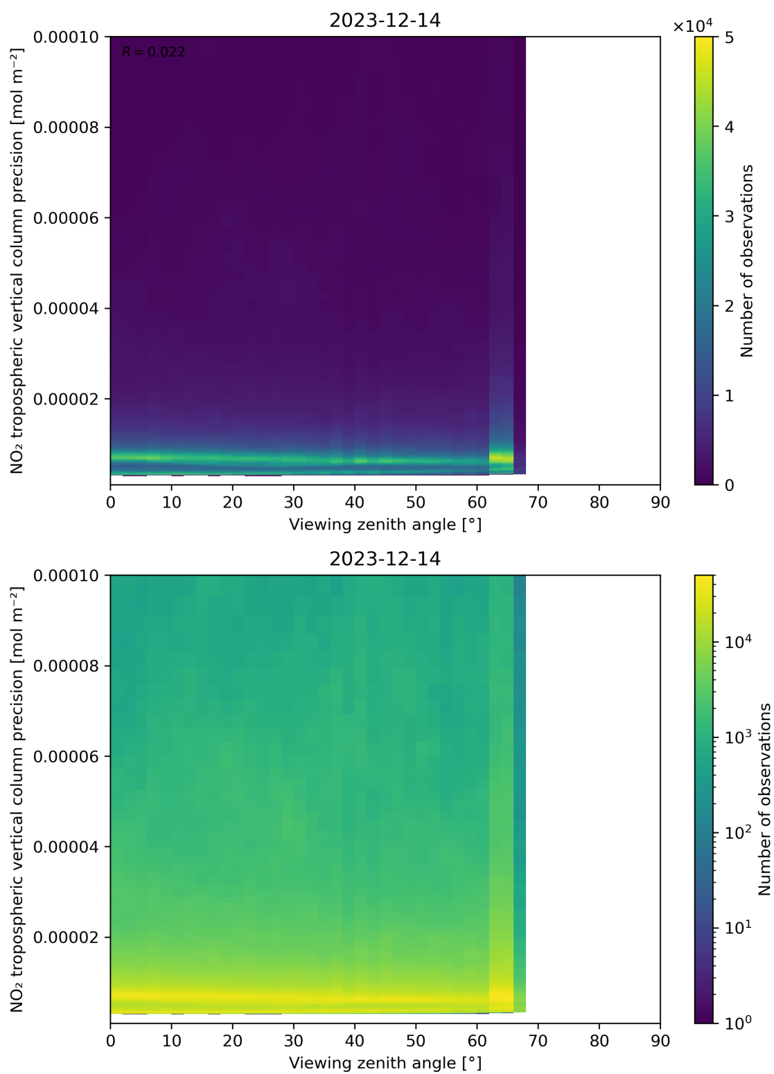
Figure 170: Scatter density plot of “Viewing zenith angle” against “NO 2 tropospheric vertical column precision” for 2023-12-14 to 2023-12-15.
