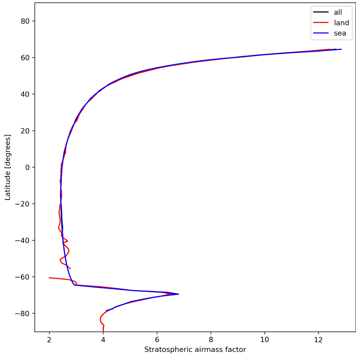
Figure 27: Zonal average of “Stratospheric airmass factor” for 2023-12-14 to 2023-12-15.
