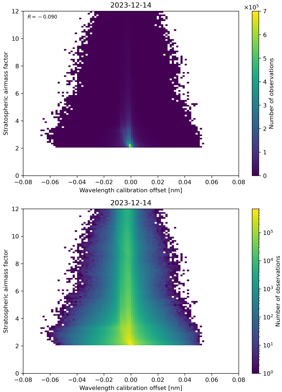
Figure 174: Scatter density plot of “Wavelength calibration offset” against “Stratospheric airmass factor” for 2023-12-14 to 2023-12-15.
