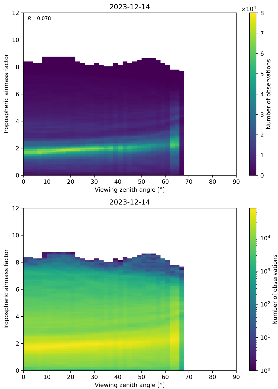
Figure 161: Scatter density plot of “Viewing zenith angle” against “Tropospheric airmass factor” for 2023-12-14 to 2023-12-15.
