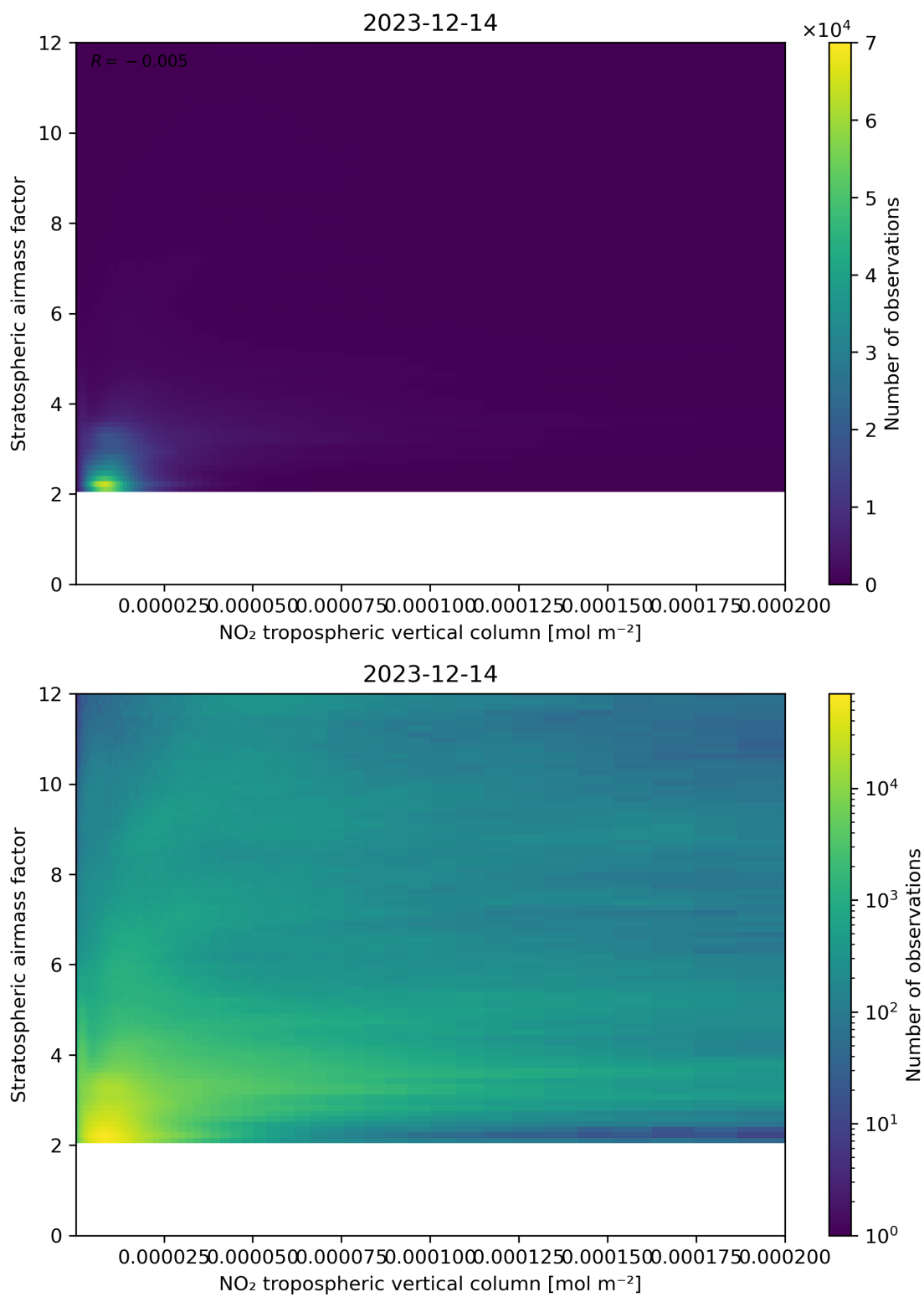
Figure 121: Scatter density plot of “NO 2 tropospheric vertical column” against “Stratospheric airmass factor” for 2023-12-14 to 2023-12-15.
