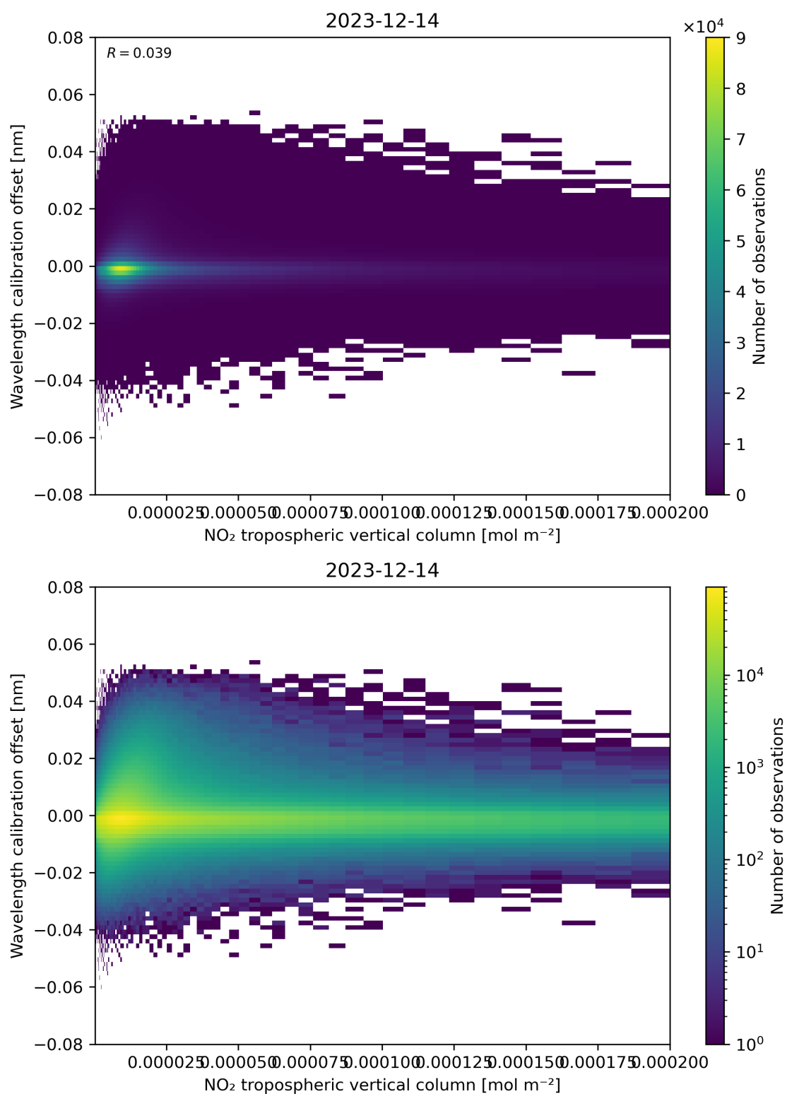
Figure 143: Scatter density plot of “NO 2 tropospheric vertical column” against “Wavelength calibration offset” for 2023-12-14 to 2023-12-15.
