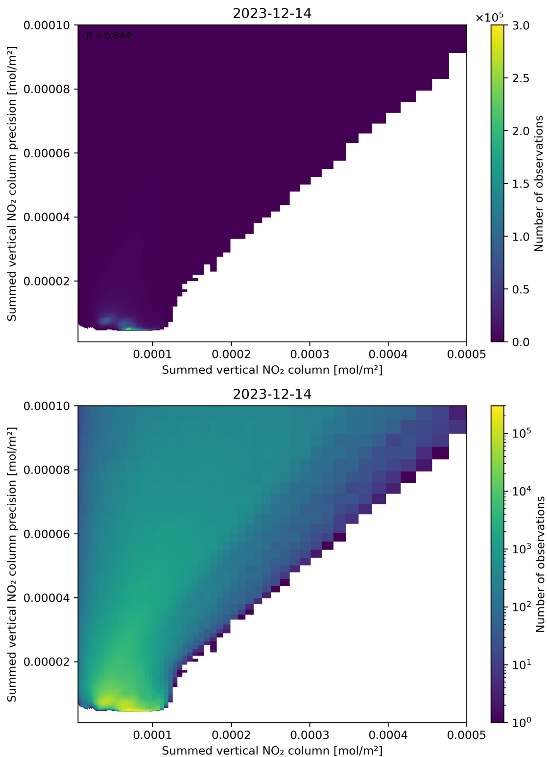
Figure 105: Scatter density plot of “Summed vertical NO 2 column” against “Summed vertical NO 2 column precision” for 2023-12-14 to 2023-12-15.
