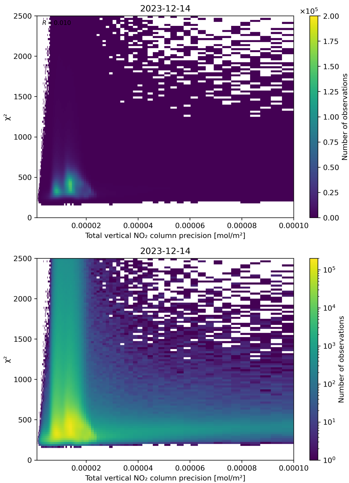
Figure 116: Scatter density plot of “Total vertical NO 2 column precision” against “ \chi^2 ” for 2023-12-14 to 2023-12-15.
