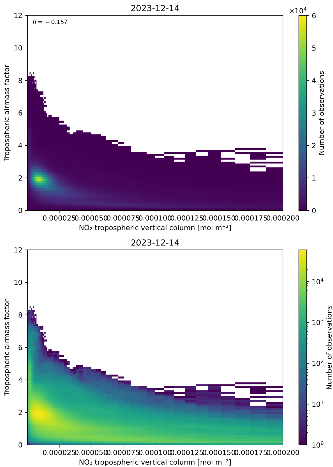
Figure 123: Scatter density plot of “NO 2 tropospheric vertical column” against “Tropospheric airmass factor” for 2023-12-14 to 2023-12-15.
