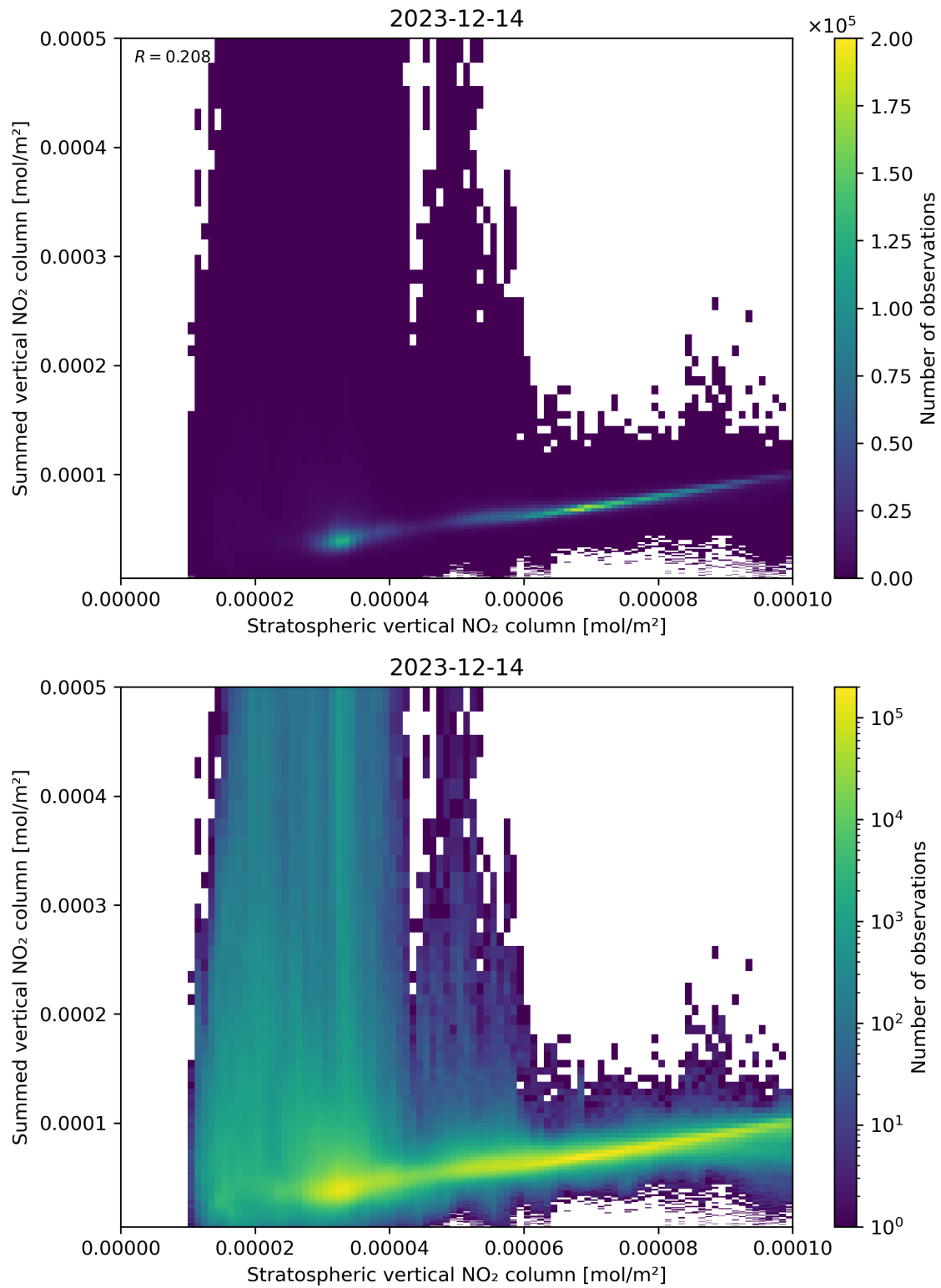
Figure 98: Scatter density plot of “Stratospheric vertical NO 2 column” against “Summed vertical NO 2 column” for 2023-12-14 to 2023-12-15.
