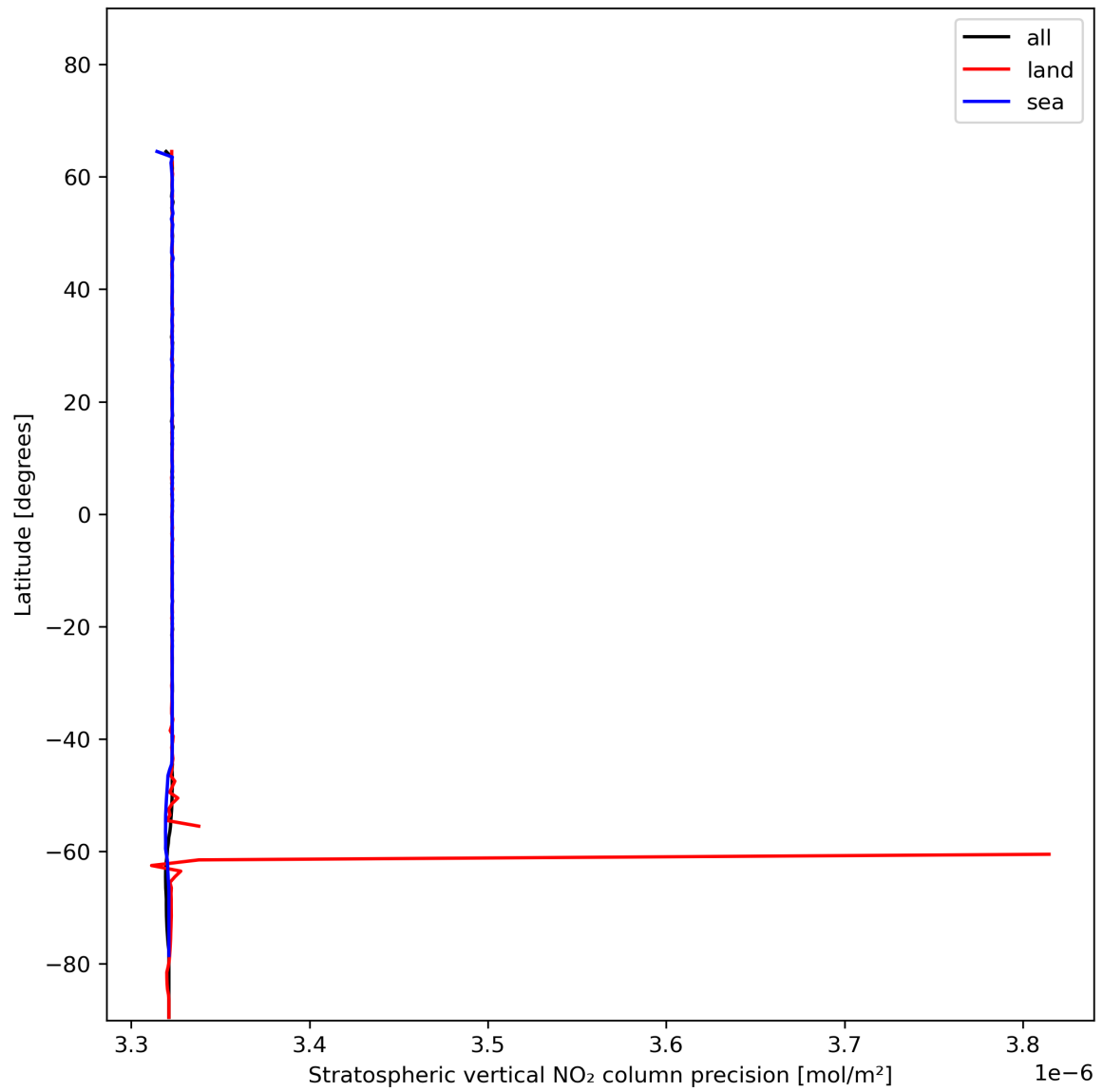
Figure 20: Zonal average of “Stratospheric vertical NO 2 column precision” for 2023-12-14 to 2023-12-15.
