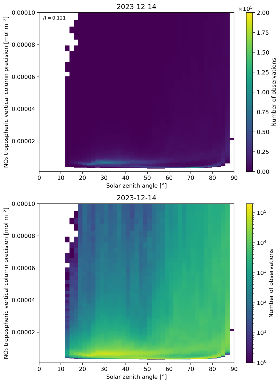
Figure 156: Scatter density plot of “Solar zenith angle” against “NO 2 tropospheric vertical column precision” for 2023-12-14 to 2023-12-15.
