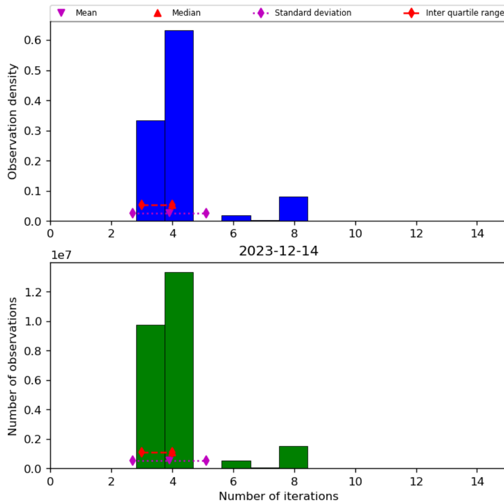
Figure 34: Histogram of “Number of iterations” for 2023-12-14 to 2023-12-15
