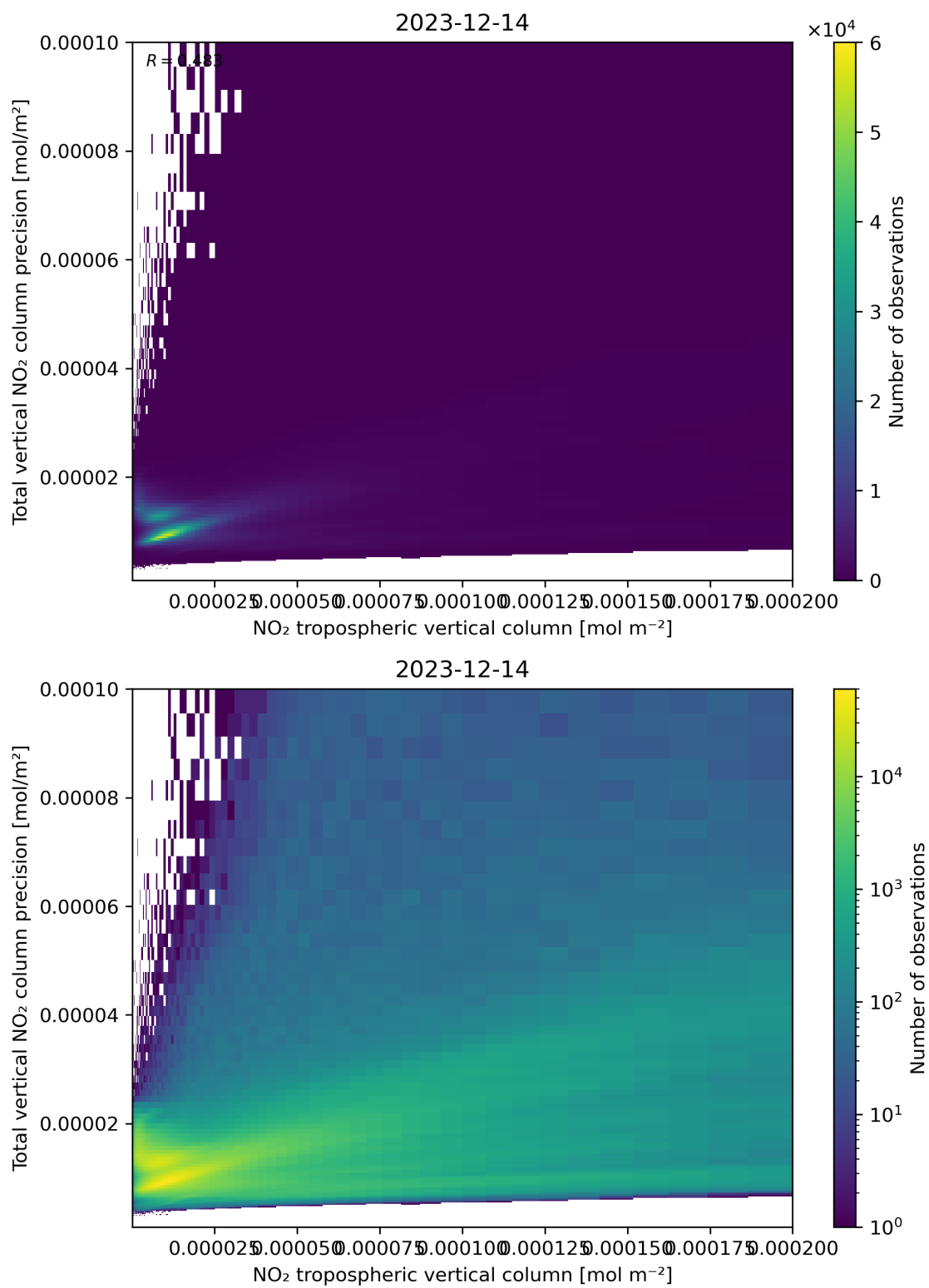
Figure 129: Scatter density plot of “NO 2 tropospheric vertical column” against “Total vertical NO 2 column precision” for 2023-12-14 to 2023-12-15.
