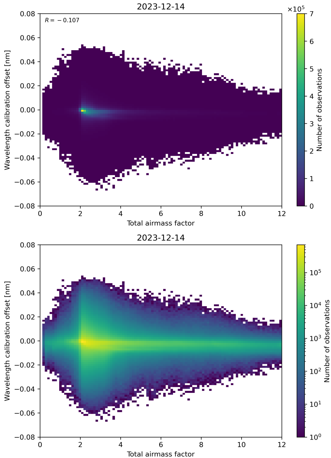
Figure 70: Scatter density plot of “Total airmass factor” against “Wavelength calibration offset” for 2023-12-14 to 2023-12-15.
