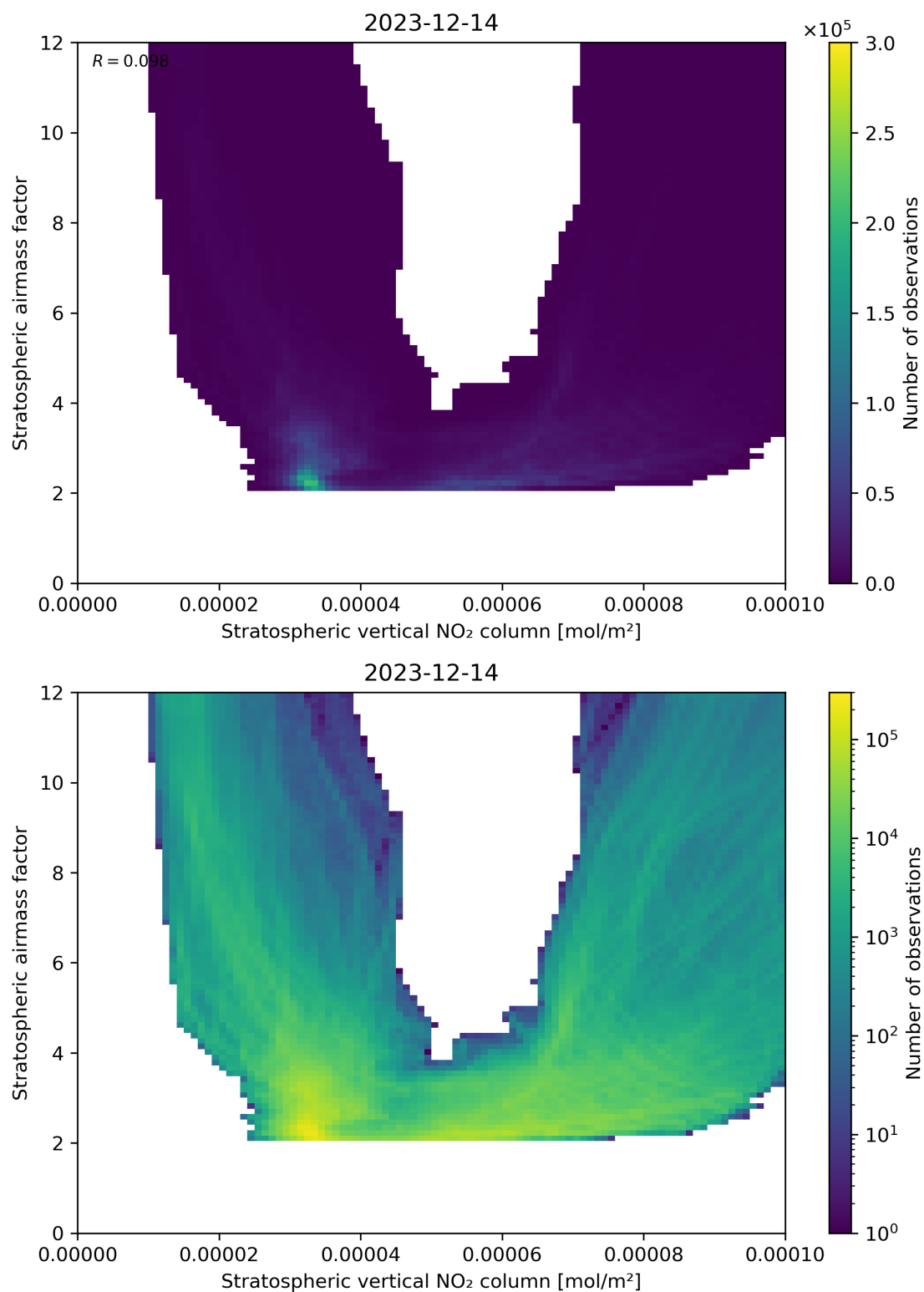
Figure 96: Scatter density plot of “Stratospheric vertical NO 2 column” against “Stratospheric airmass factor” for 2023-12-14 to 2023-12-15.
