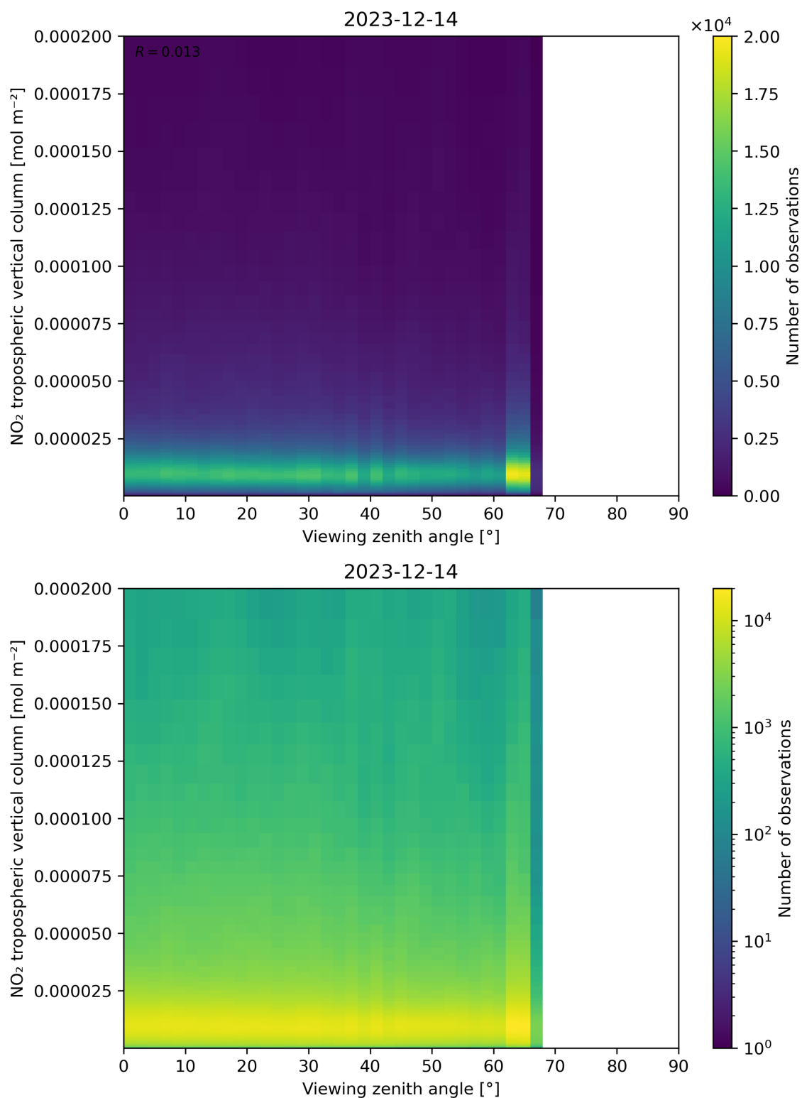
Figure 169: Scatter density plot of “Viewing zenith angle” against “NO 2 tropospheric vertical column” for 2023-12-14 to 2023-12-15.
