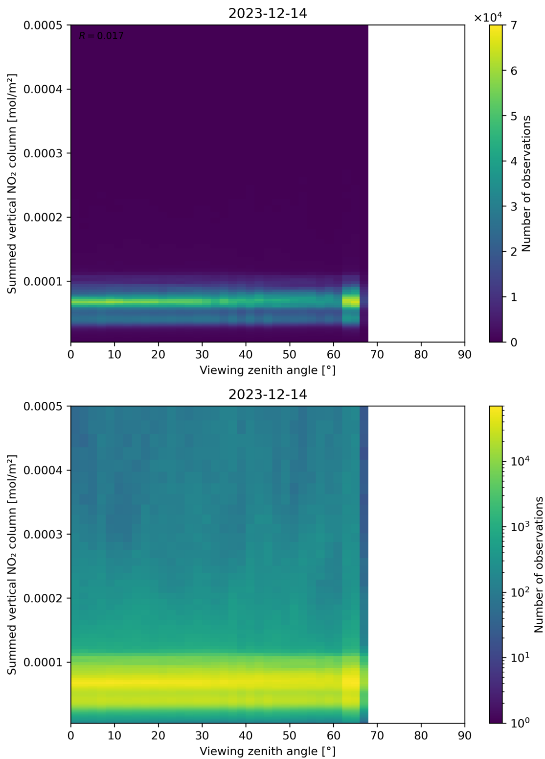
Figure 165: Scatter density plot of “Viewing zenith angle” against “Summed vertical NO 2 column” for 2023-12-14 to 2023-12-15.
