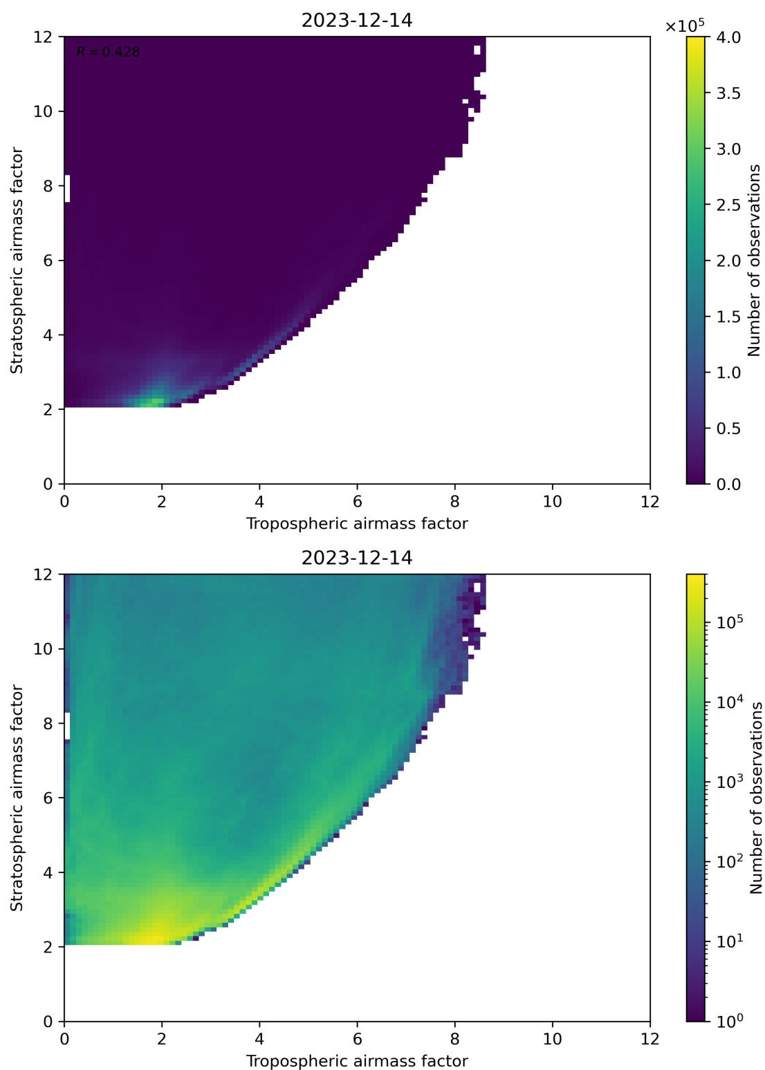
Figure 71: Scatter density plot of “Tropospheric airmass factor” against “Stratospheric airmass factor” for 2023-12-14 to 2023-12-15.
