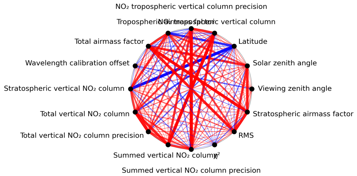
Figure 1: Map of correlation graph for 2023-12-14 to 2023-12-15.
