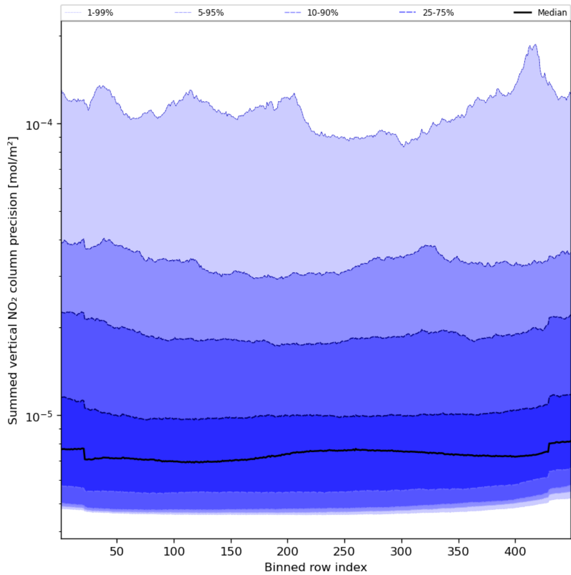
Figure 58: Along track statistics of “Summed vertical NO 2 column precision” for 2023-12-14 to 2023-12-15
