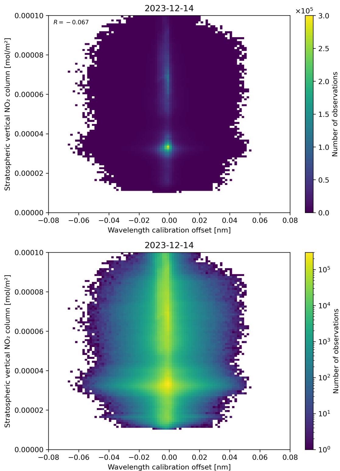
Figure 176: Scatter density plot of “Wavelength calibration offset” against “Stratospheric vertical NO 2 column” for 2023-12-14 to 2023-12-15.
