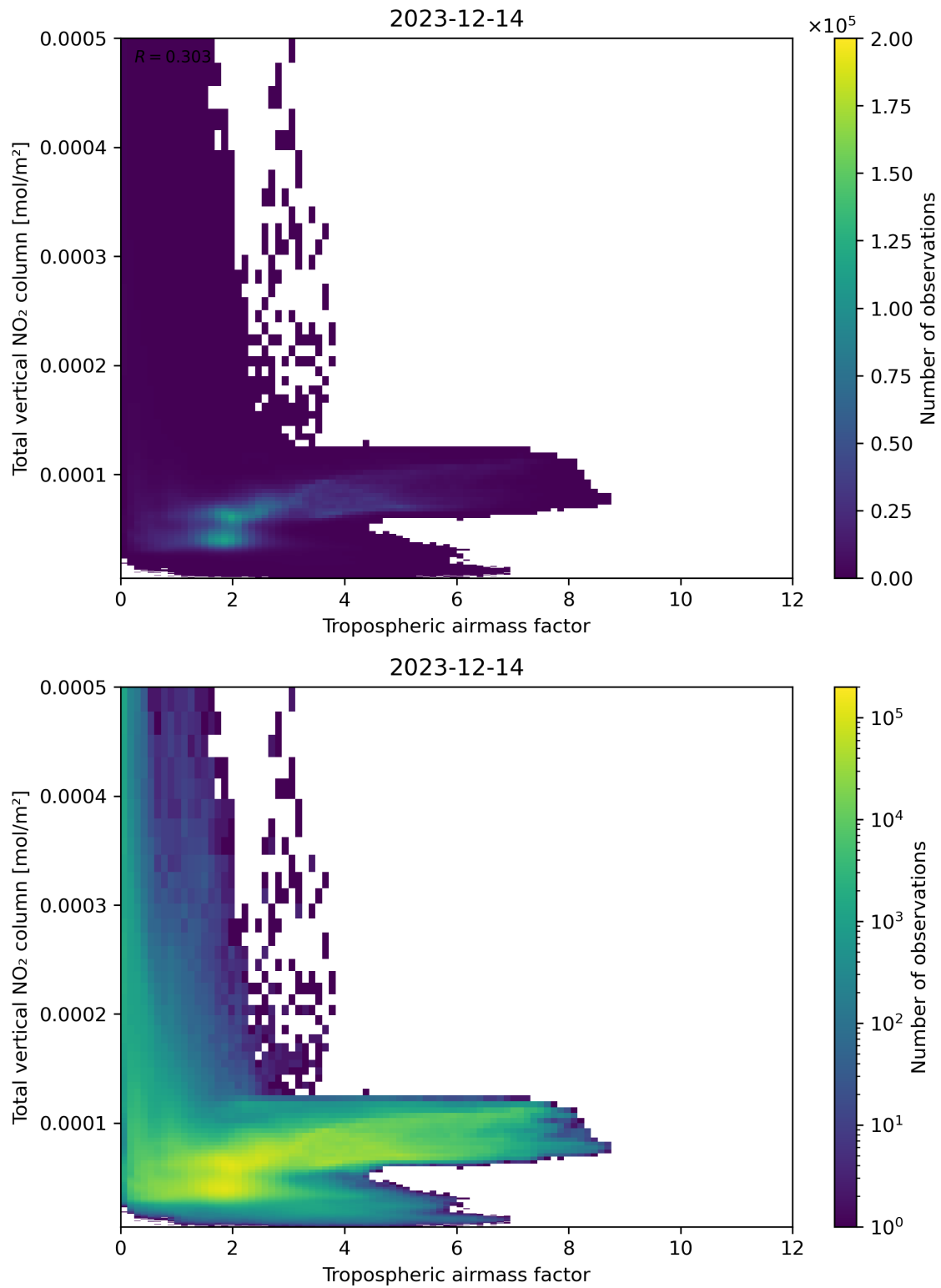
Figure 77: Scatter density plot of “Tropospheric airmass factor” against “Total vertical NO 2 column” for 2023-12-14 to 2023-12-15.
