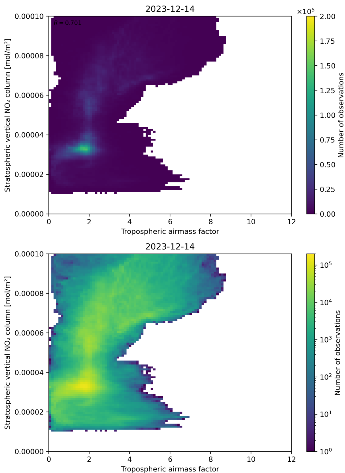
Figure 74: Scatter density plot of “Tropospheric air mass factor” against “Stratospheric vertical NO 2 column” for 2023-12-14 to 2023-12-15.
