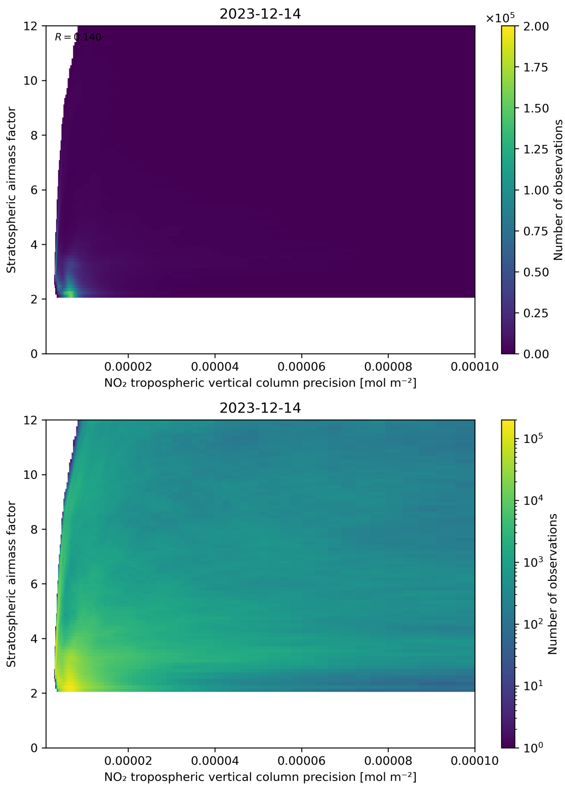
Figure 131: Scatter density plot of “NO 2 tropospheric vertical column precision” against “Stratospheric airmass factor” for 2023-12-14 to 2023-12-15.
