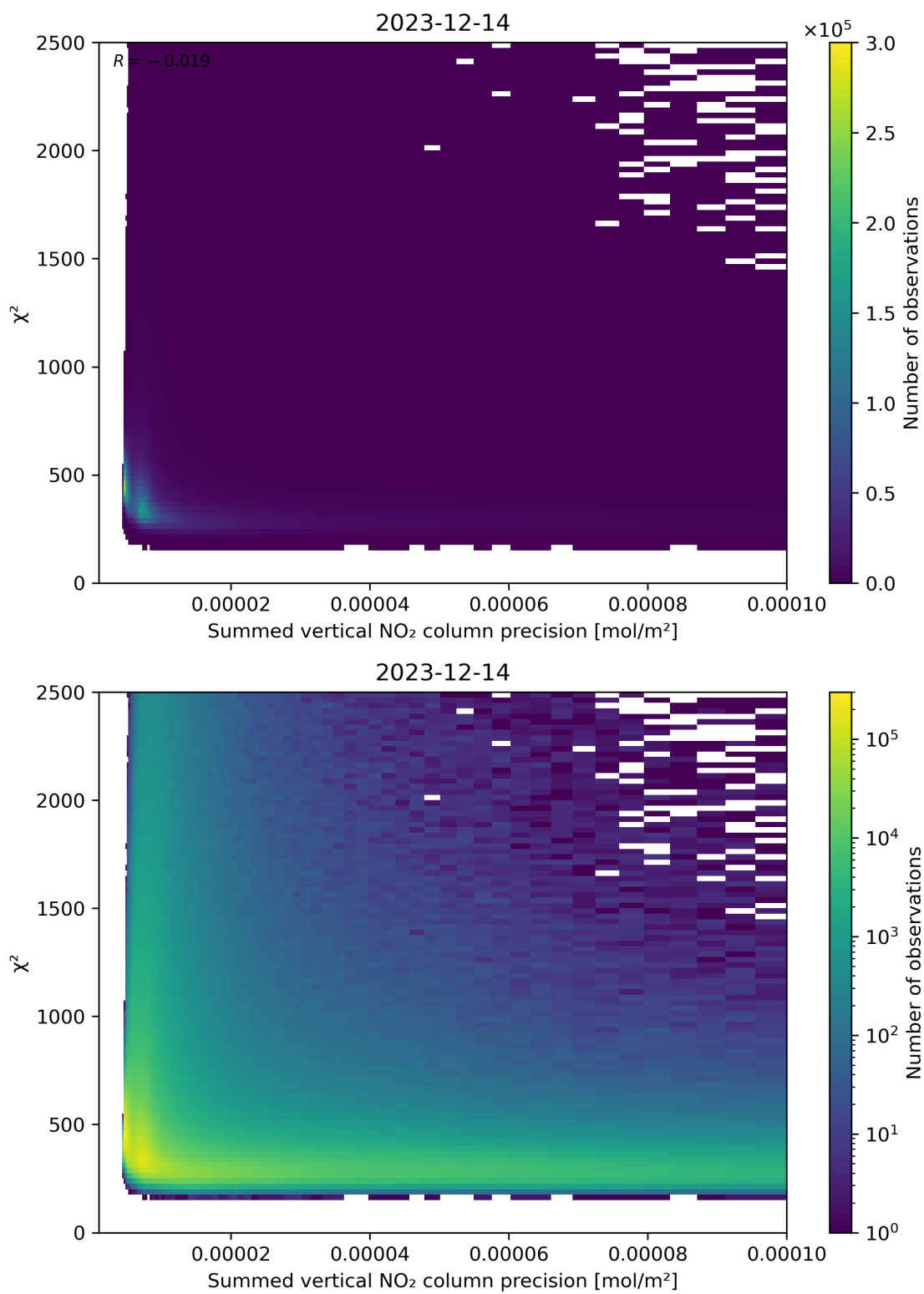
Figure 107: Scatter density plot of “Summed vertical NO 2 column precision” against “ \chi^2 ” for 2023-12-14 to 2023-12-15.
