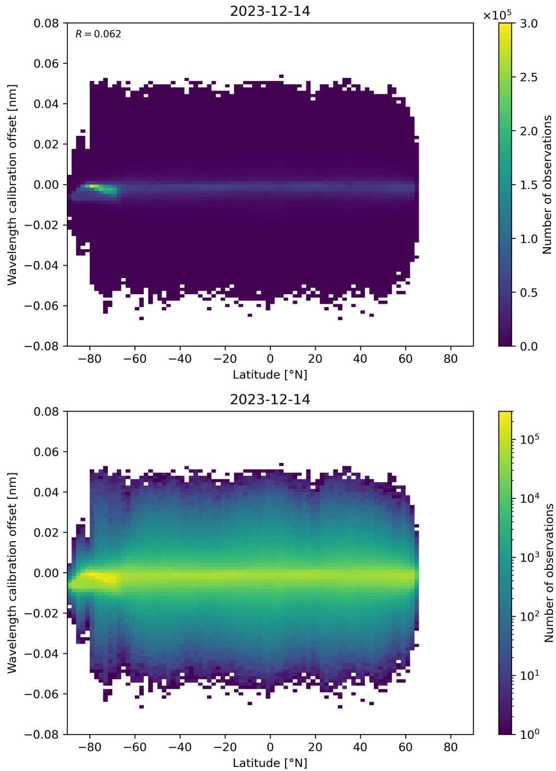
Figure 95: Scatter density plot of “Latitude” against “Wavelength calibration offset” for 2023-12-14 to 2023-12-15.
