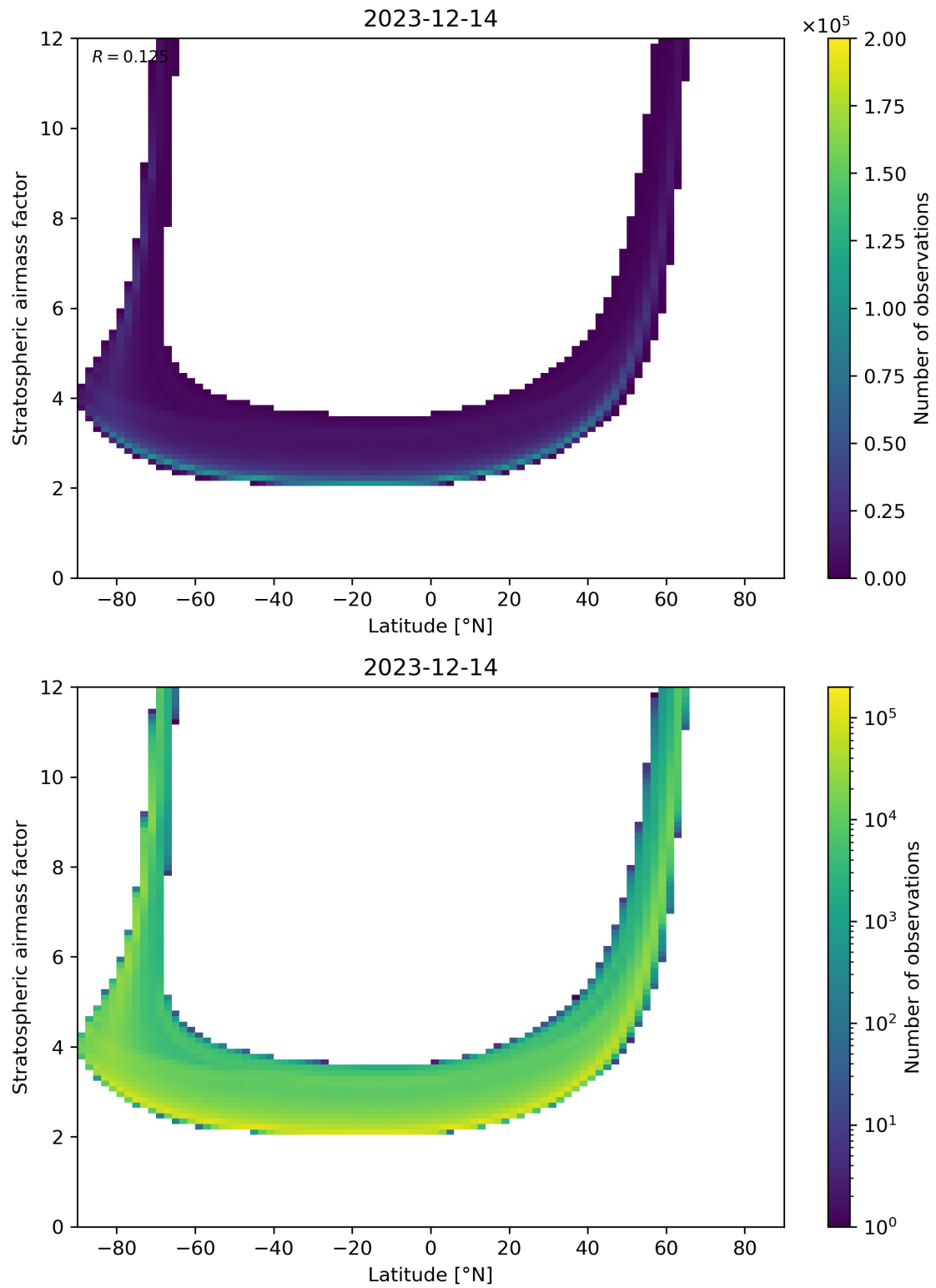
Figure 83: Scatter density plot of “Latitude” against “Stratospheric air mass factor” for 2023-12-14 to 2023-12-15.
