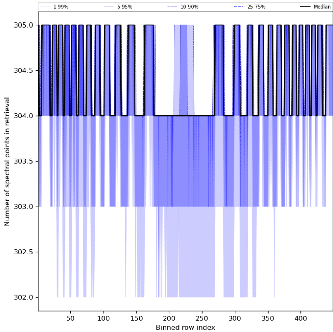
Figure 50: Along track statistics of “Number of spectral points in retrieval” for 2023-12-14 to 2023-12-15
