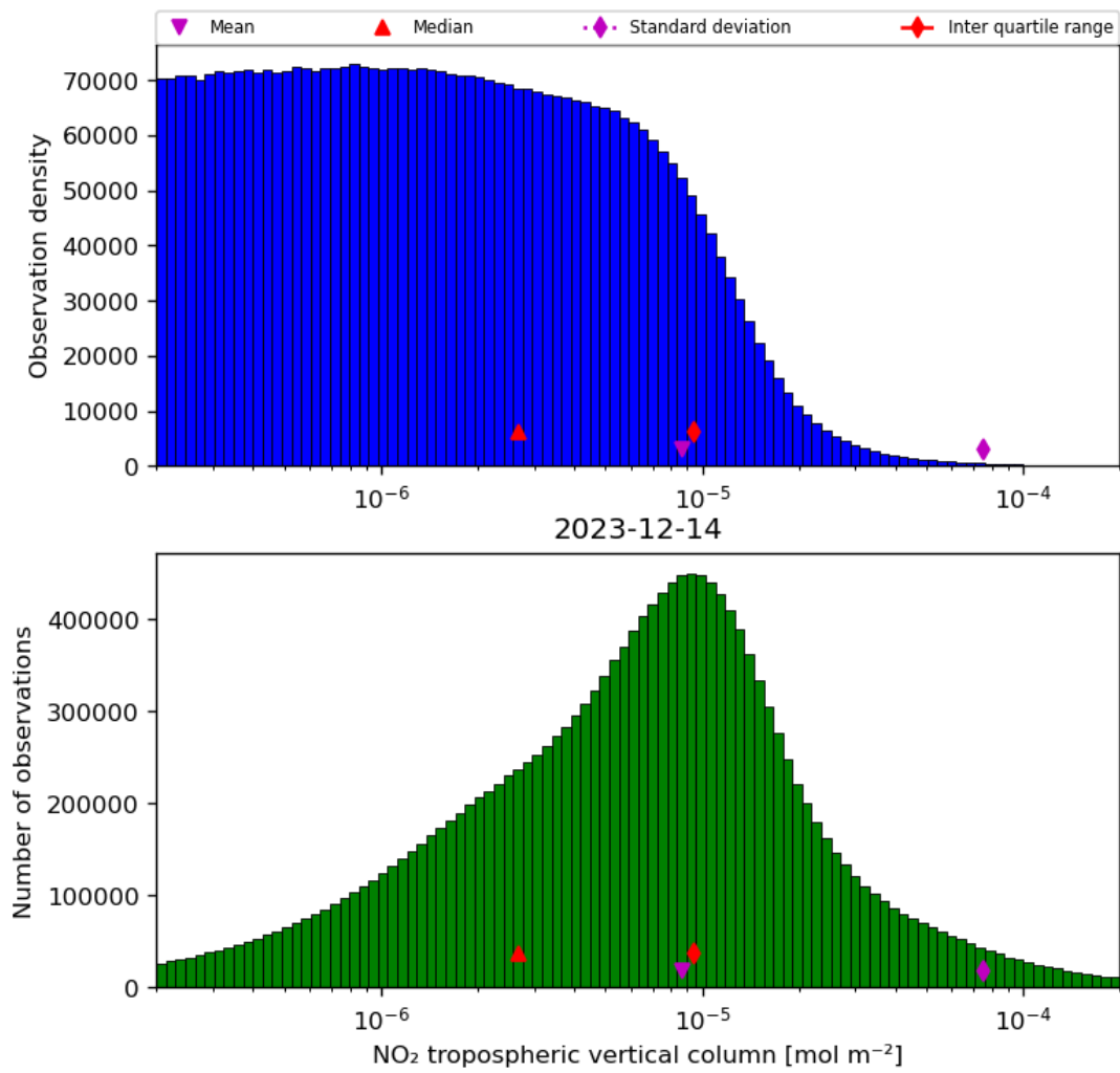
Figure 29: Histogram of “NO 2 tropospheric vertical column” for 2023-12-14 to 2023-12-15
