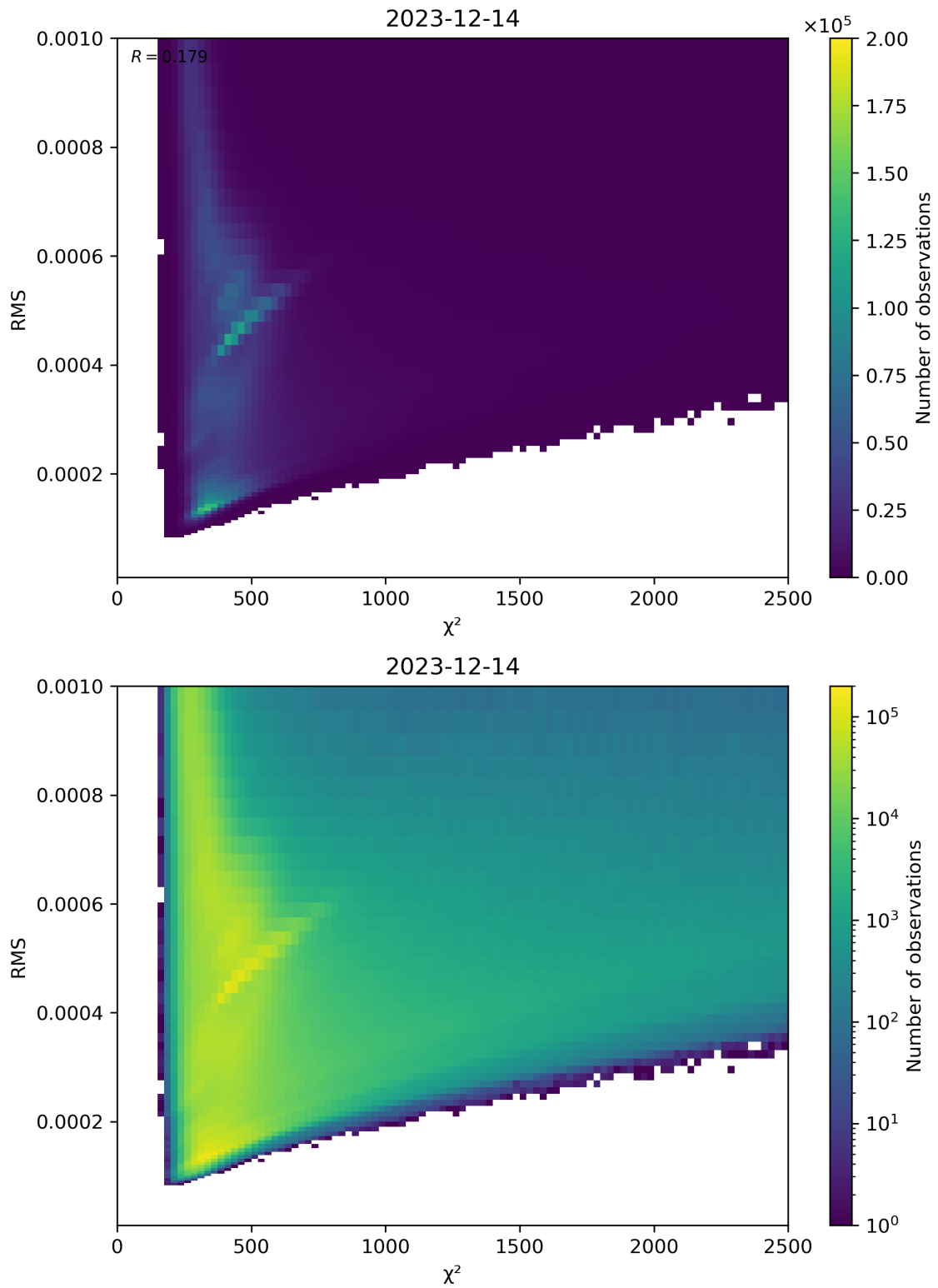
Figure 82: Scatter density plot of “ \chi^2 ” against “RMS” for 2023-12-14 to 2023-12-15.
