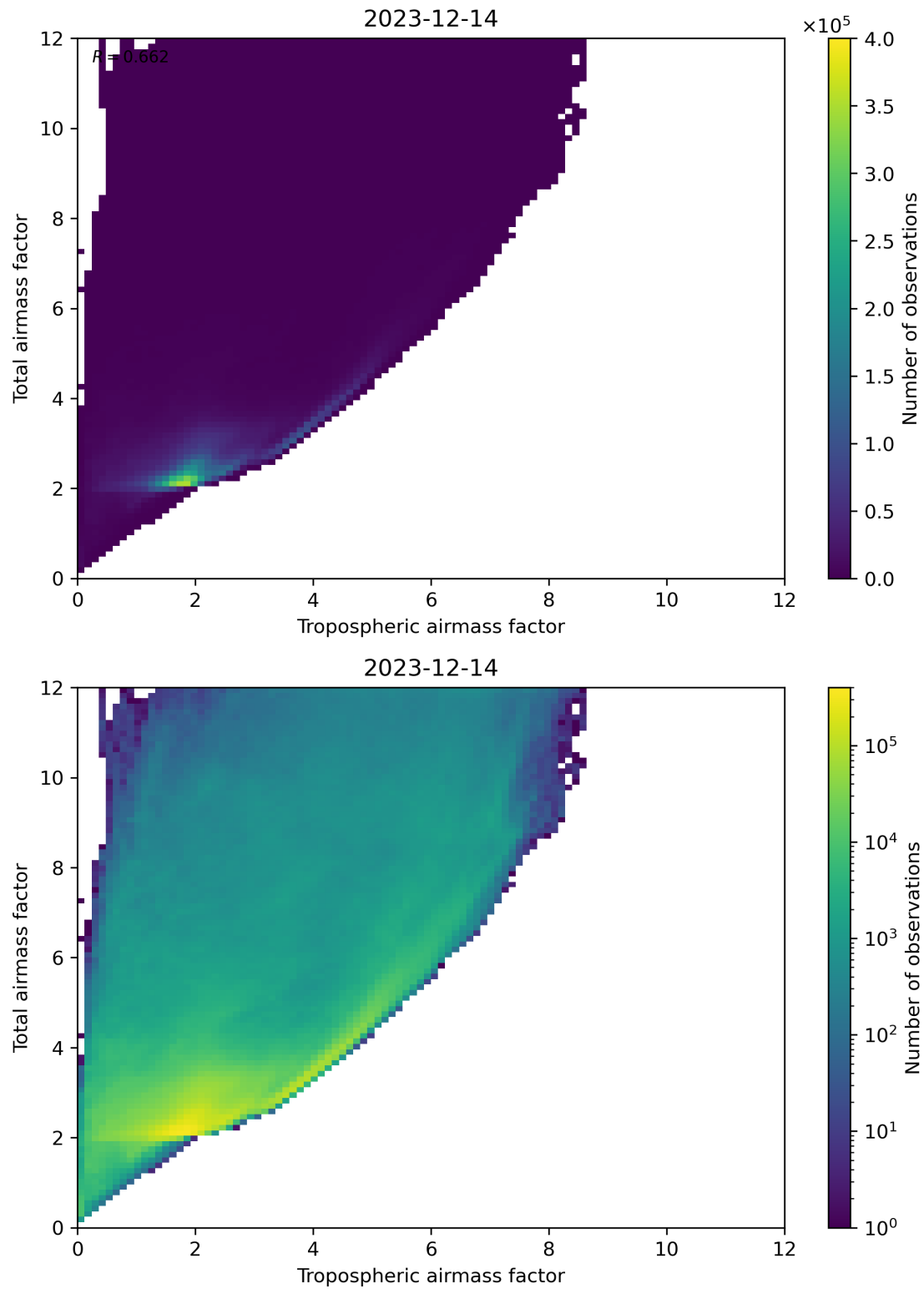
Figure 72: Scatter density plot of “Tropospheric airmass factor” against “Total airmass factor” for 2023-12-14 to 2023-12-15.
