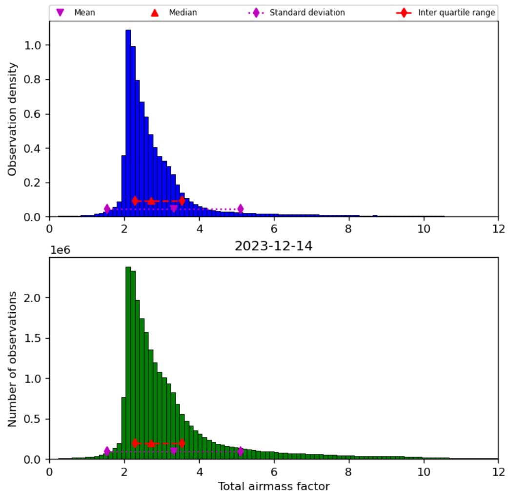
Figure 32: Histogram of “Total airmass factor” for 2023-12-14 to 2023-12-15
