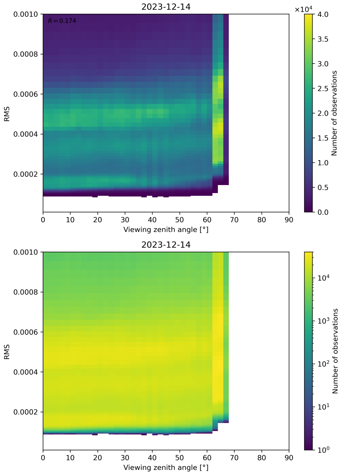
Figure 171: Scatter density plot of “Viewing zenith angle” against “RMS” for 2023-12-14 to 2023-12-15.
