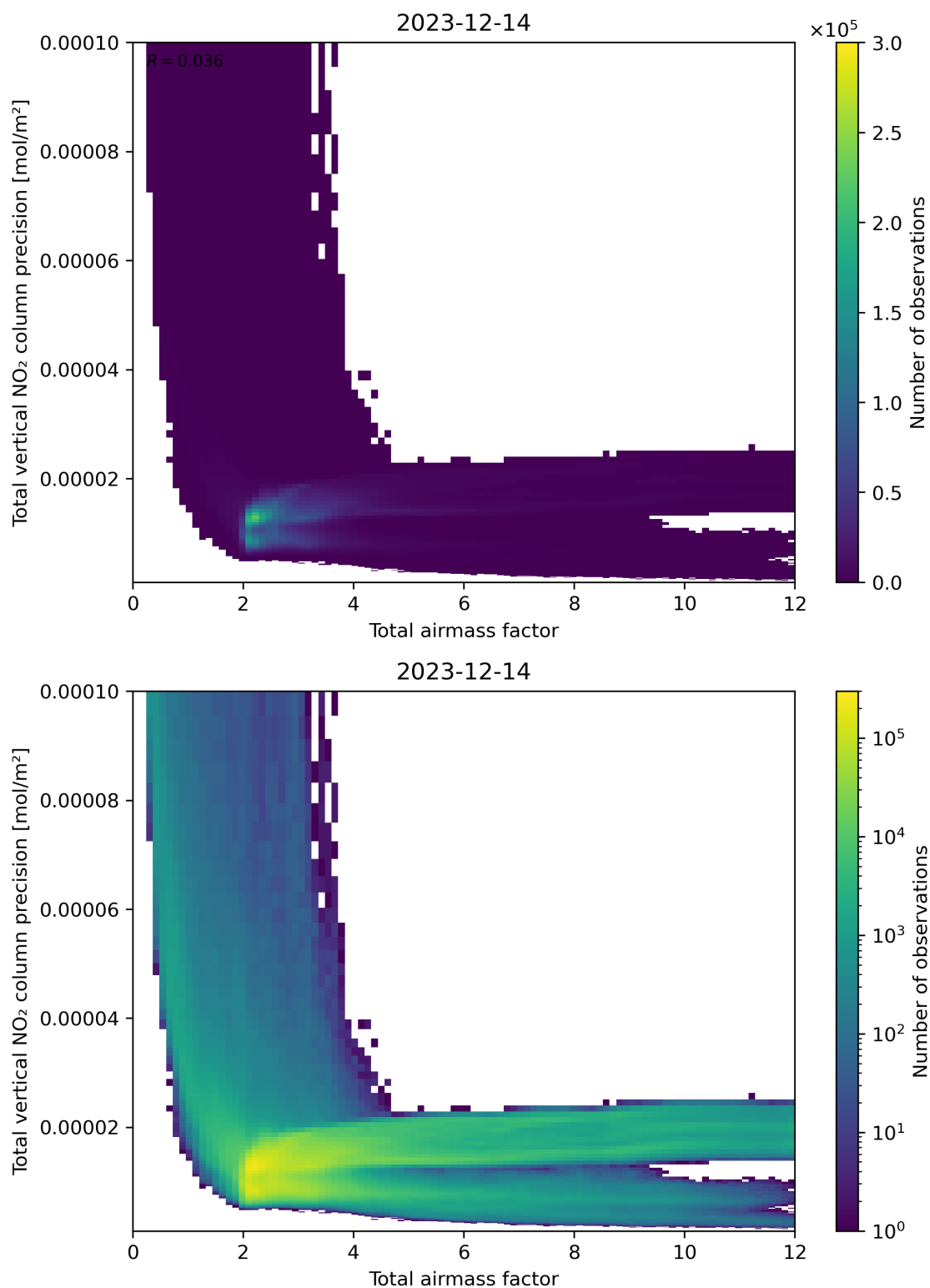
Figure 68: Scatter density plot of “Total airmass factor” against “Total vertical NO 2 column precision” for 2023-12-14 to 2023-12-15.
