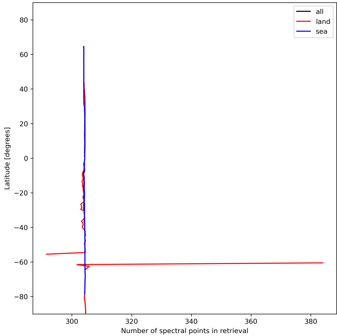
Figure 16: Zonal average of “Number of spectral points in retrieval” for 2023-12-14 to 2023-12-15.
