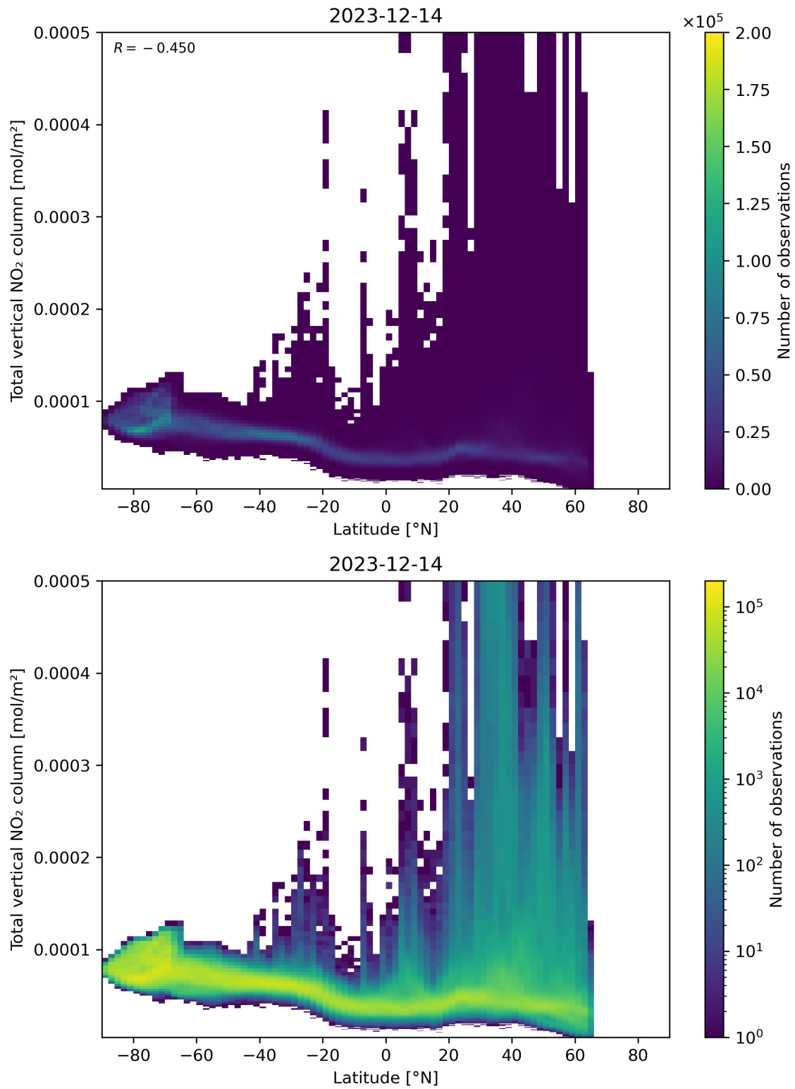
Figure 90: Scatter density plot of “Latitude” against “Total vertical NO 2 column” for 2023-12-14 to 2023-12-15.
