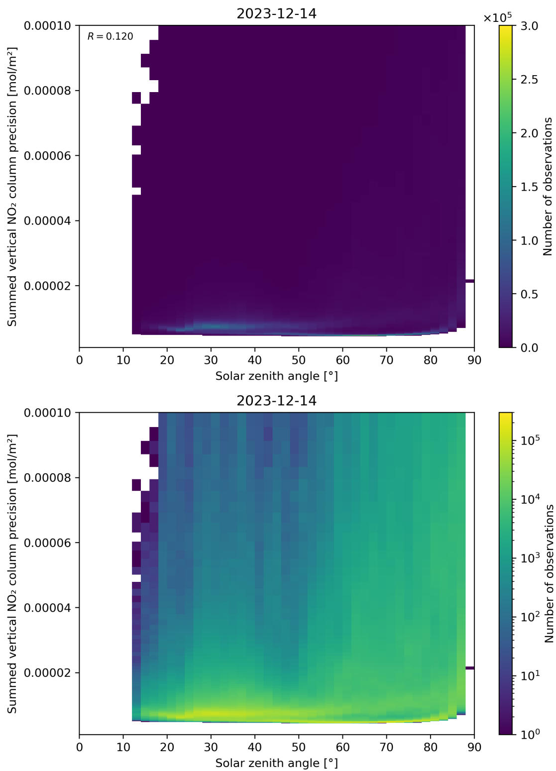
Figure 152: Scatter density plot of “Solar zenith angle” against “Summed vertical NO 2 column precision” for 2023-12-14 to 2023-12-15.
