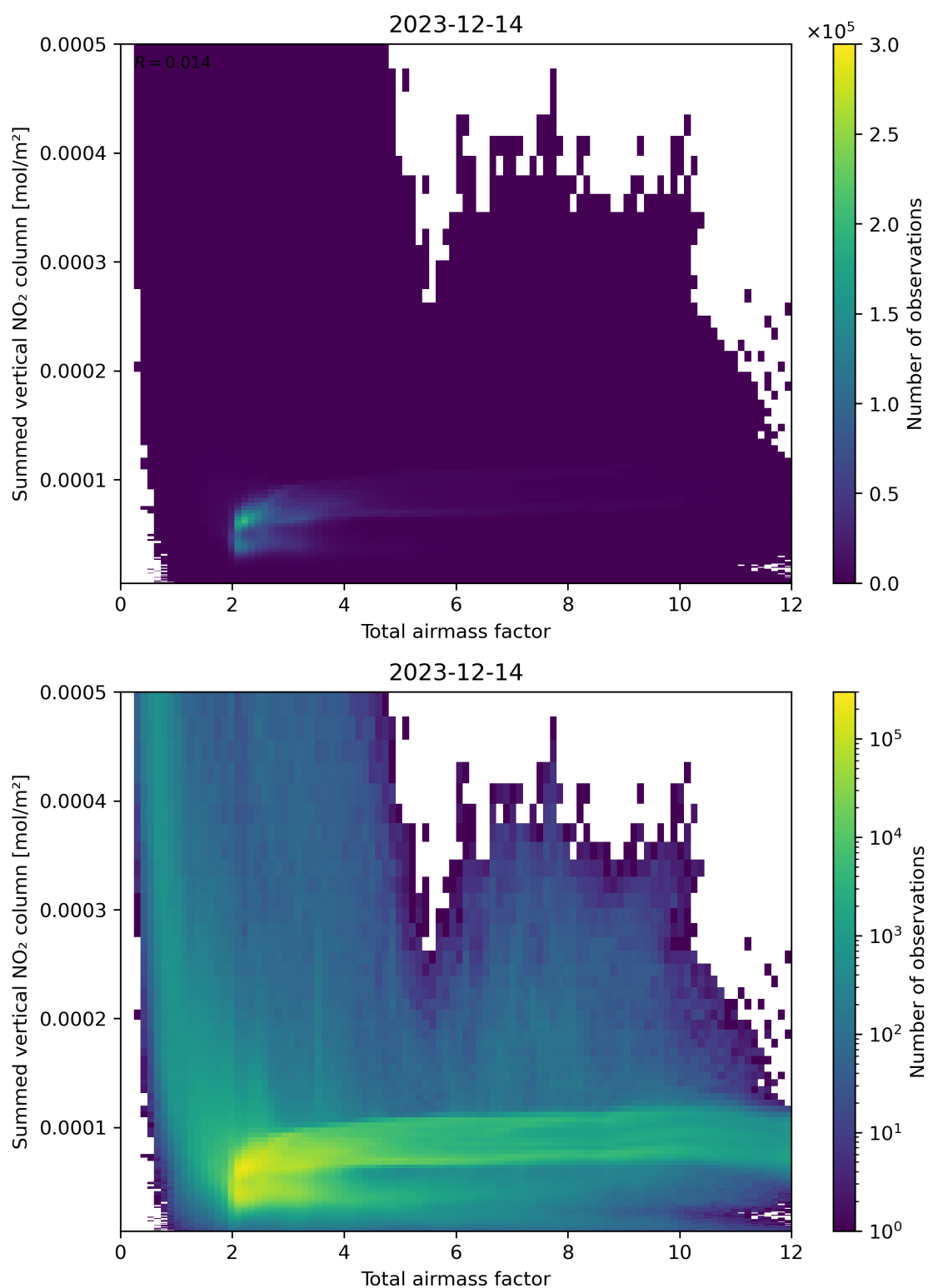
Figure 65: Scatter density plot of “Total airmass factor” against “Summed vertical NO 2 column” for 2023-12-14 to 2023-12-15.
