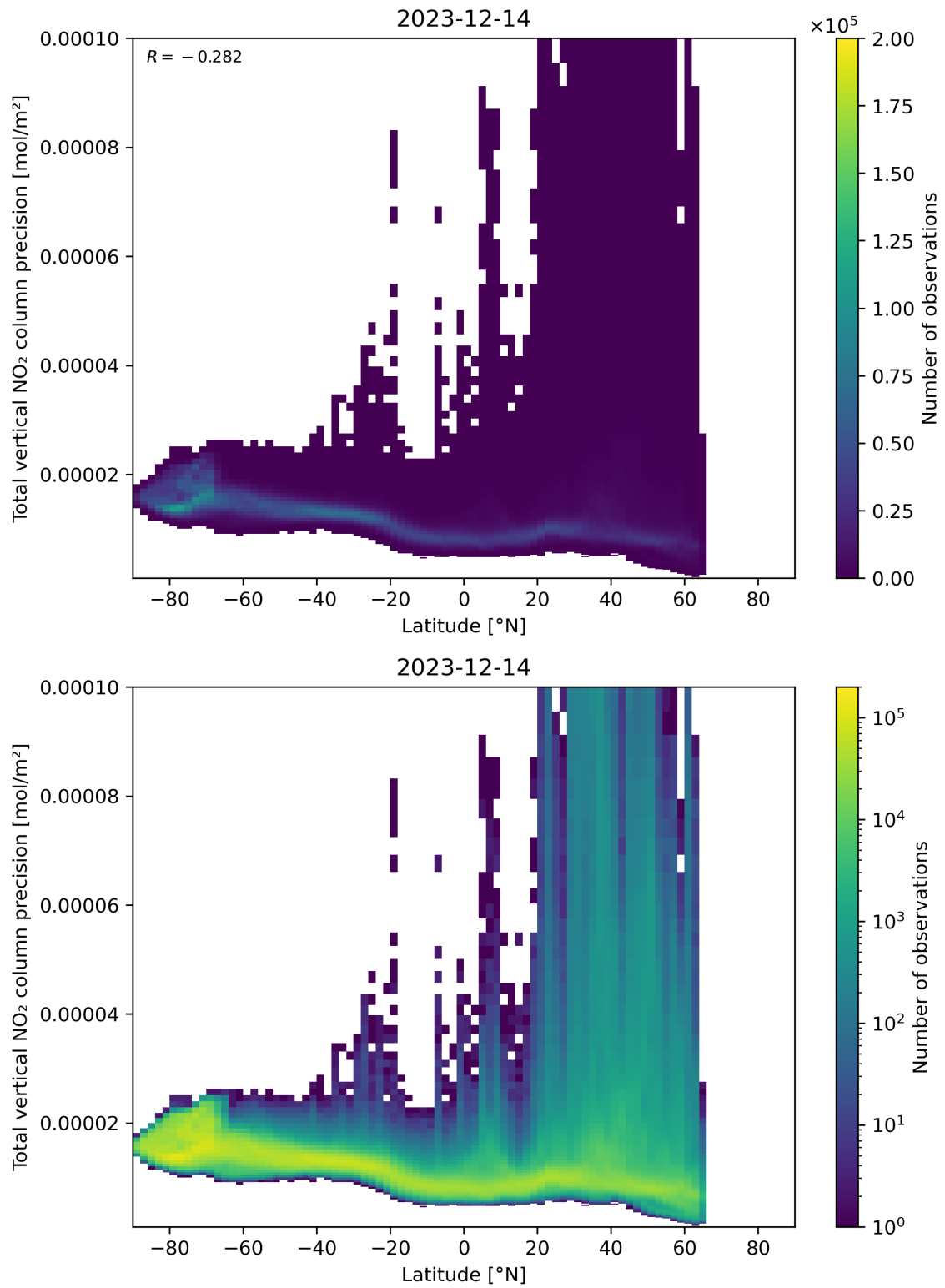
Figure 91: Scatter density plot of “Latitude” against “Total vertical NO 2 column precision” for 2023-12-14 to 2023-12-15.
