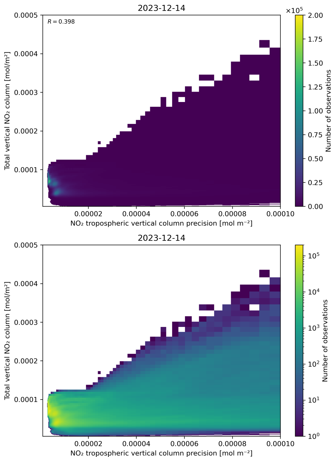
Figure 138: Scatter density plot of “NO 2 tropospheric vertical column precision” against “Total vertical NO 2 column” for 2023-12-14 to 2023-12-15.
