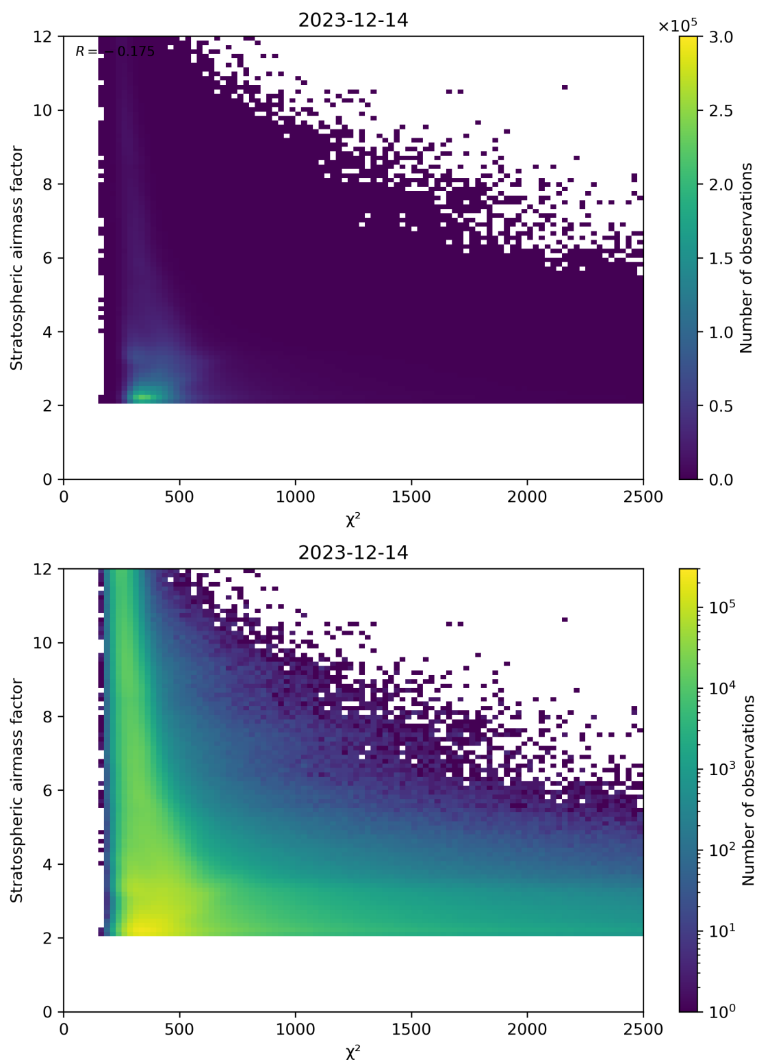
Figure 81: Scatter density plot of " \chi^2 " against "Stratospheric airmass factor" for 2023-12-14 to 2023-12-15.
