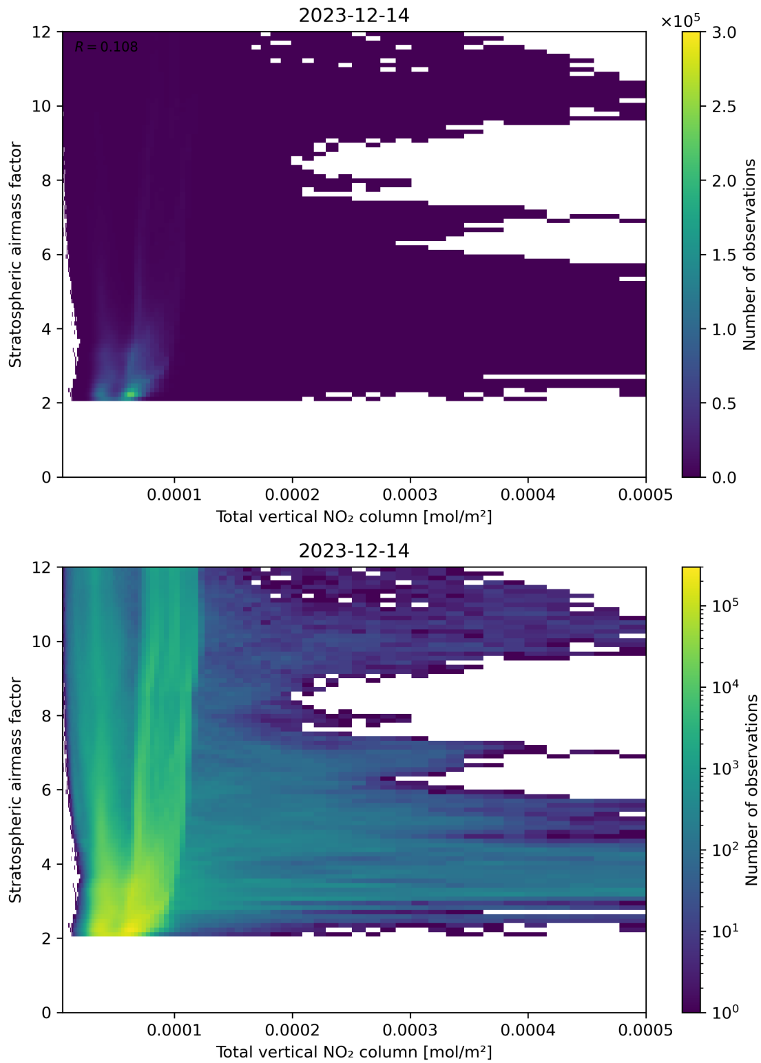
Figure 110: Scatter density plot of “Total vertical NO 2 column” against “Stratospheric air mass factor” for 2023-12-14 to 2023-12-15.
