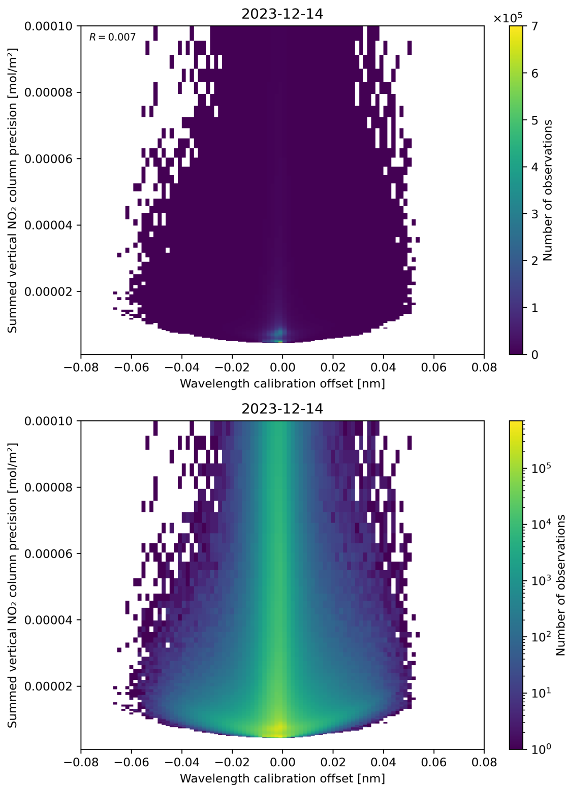
Figure 178: Scatter density plot of “Wavelength calibration offset” against “Summed vertical NO 2 column precision” for 2023-12-14 to 2023-12-15.
