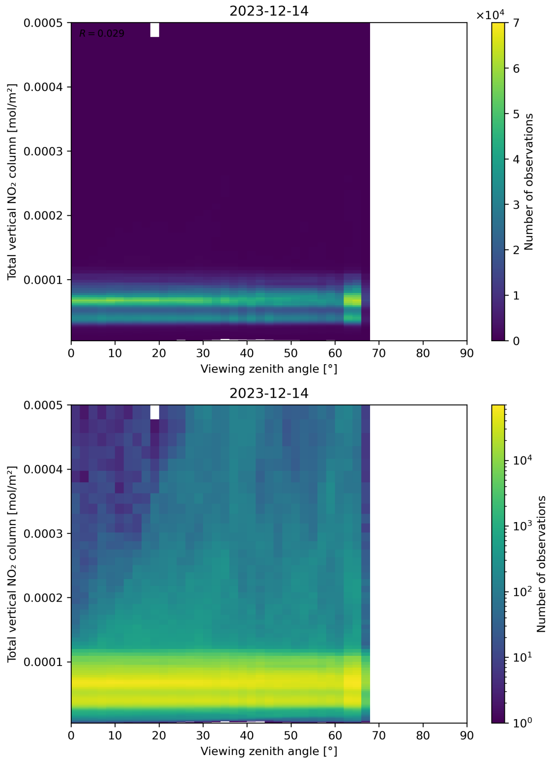
Figure 167: Scatter density plot of “Viewing zenith angle” against “Total vertical NO 2 column” for 2023-12-14 to 2023-12-15.
