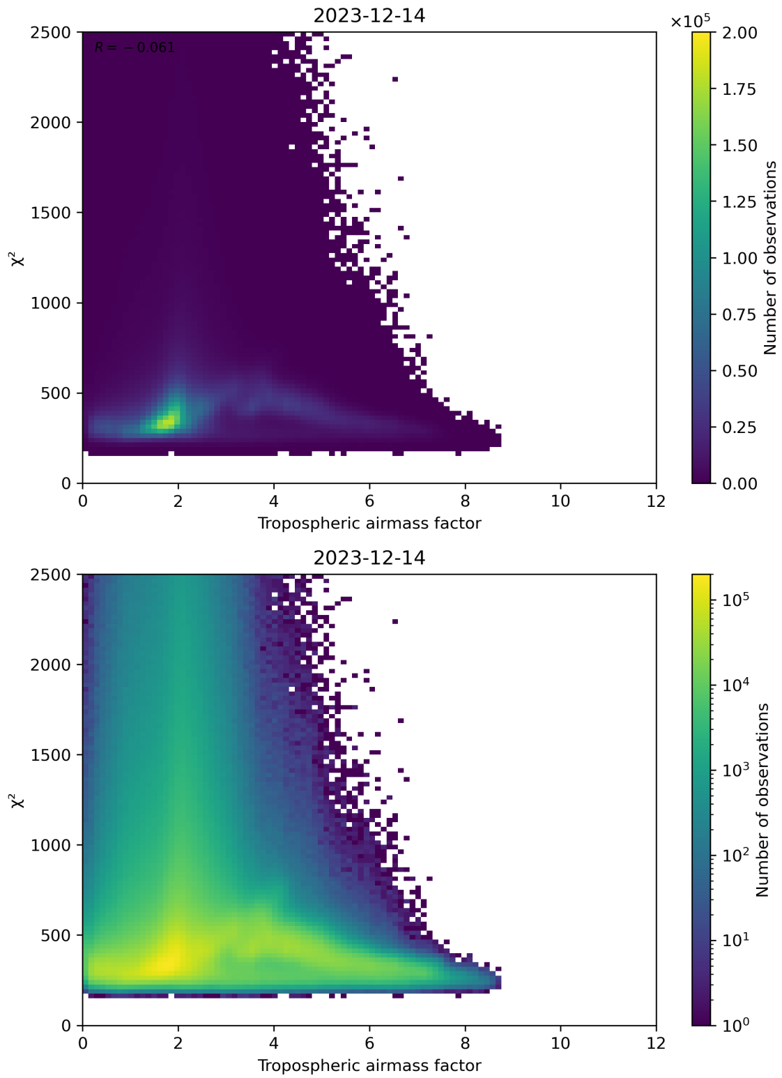
Figure 73: Scatter density plot of “Tropospheric airmass factor” against “ \chi^2 ” for 2023-12-14 to 2023-12-15.
