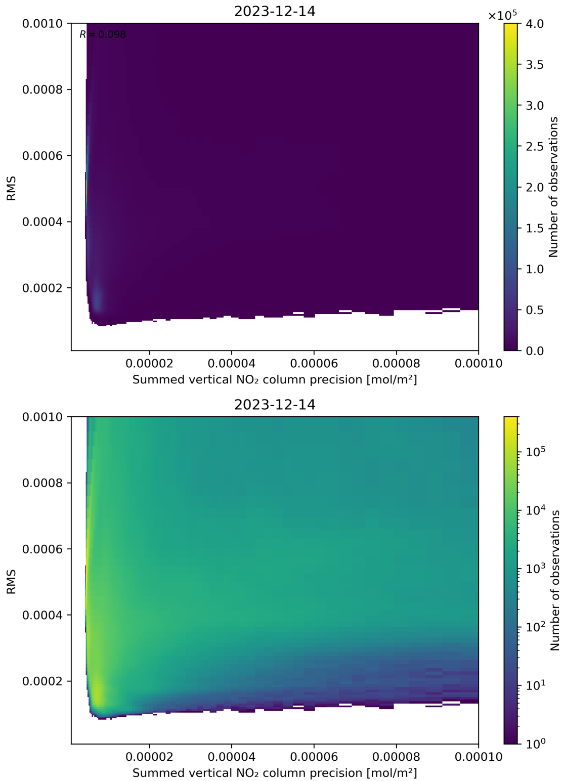
Figure 108: Scatter density plot of “Summed vertical NO 2 column precision” against “RMS” for 2023-12-14 to 2023-12-15.
