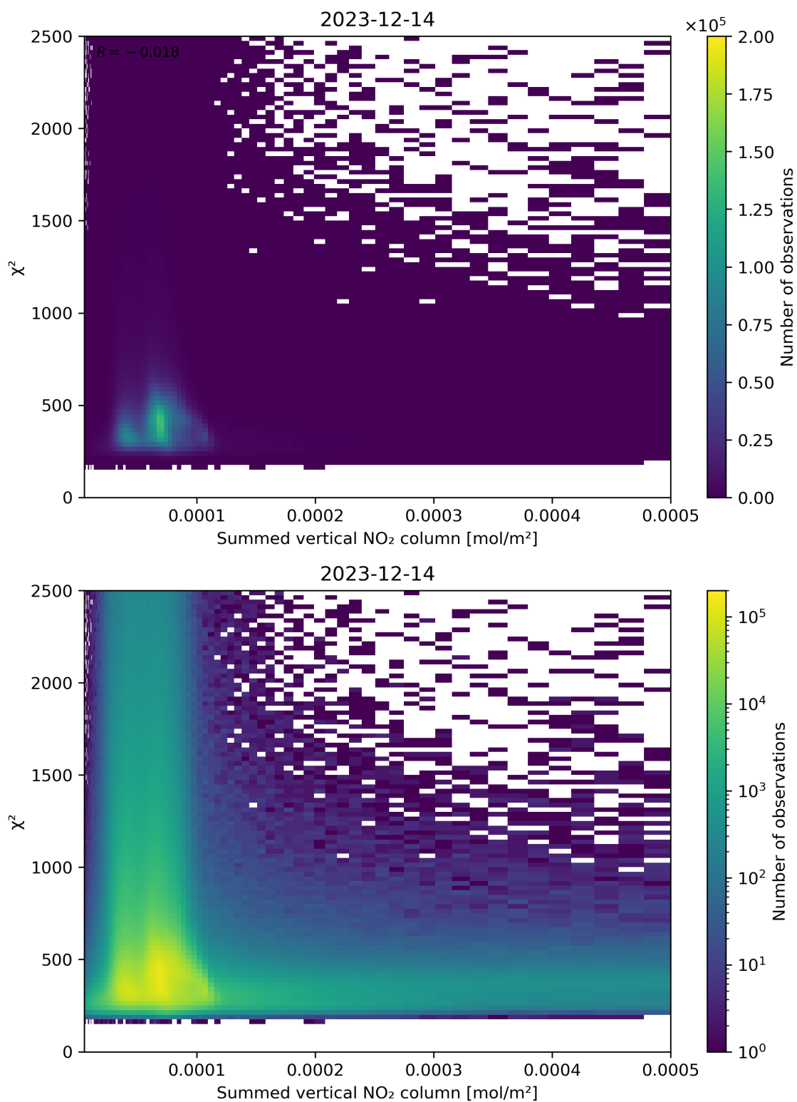
Figure 104: Scatter density plot of “Summed vertical NO 2 column” against “ \chi^2 ” for 2023-12-14 to 2023-12-15.
