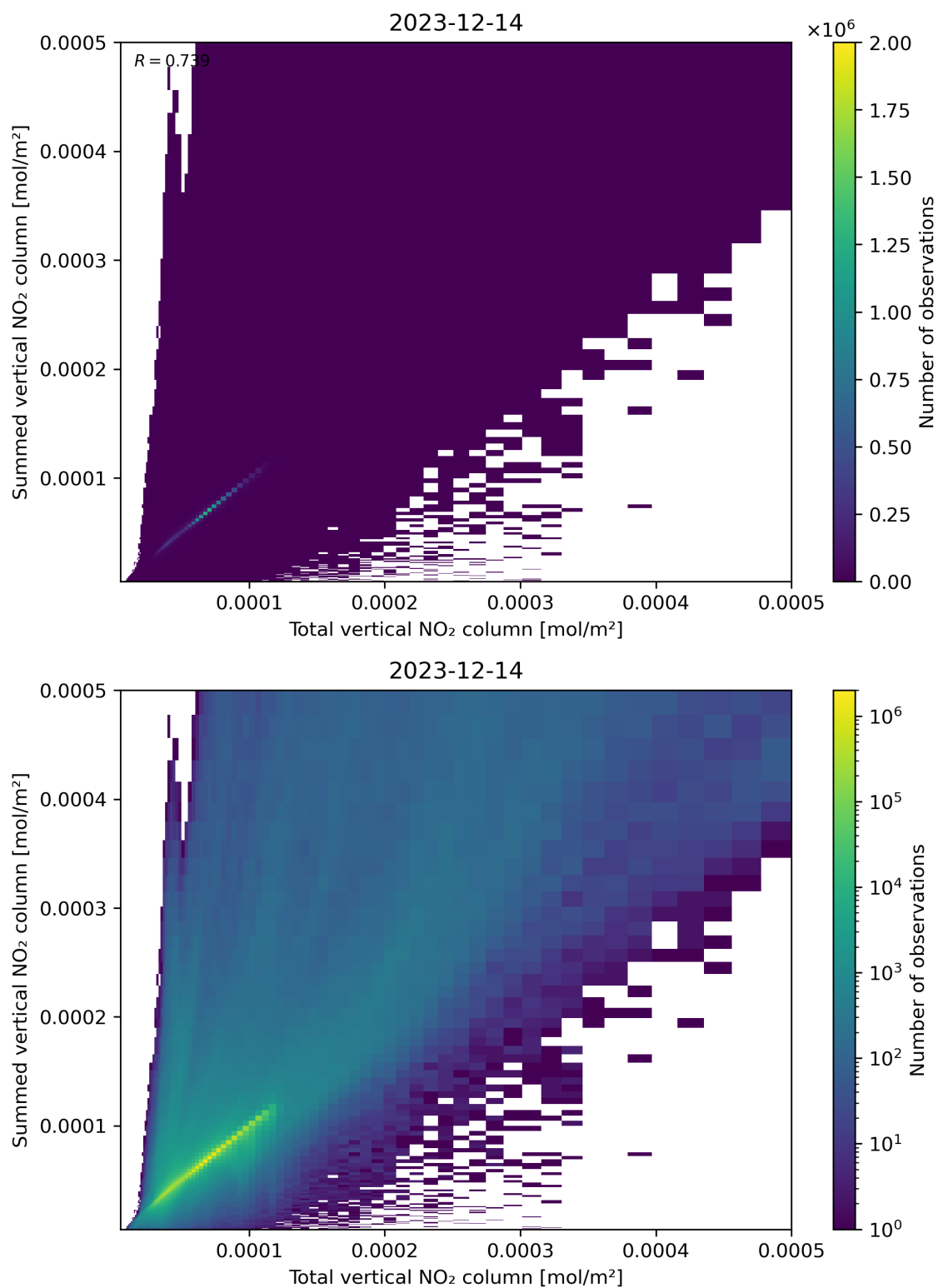
Figure 112: Scatter density plot of “Total vertical NO 2 column” against “Summed vertical NO 2 column” for 2023-12-14 to 2023-12-15.
