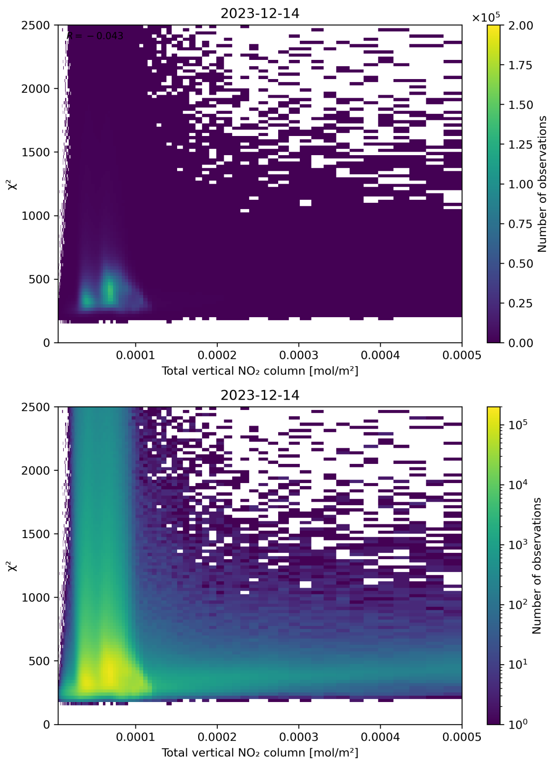
Figure 111: Scatter density plot of “Total vertical NO 2 column” against “ \chi^2 ” for 2023-12-14 to 2023-12-15.
