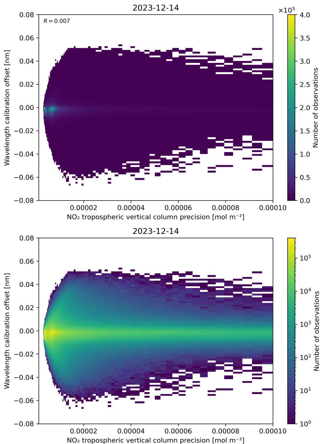
Figure 141: Scatter density plot of “NO 2 tropospheric vertical column precision” against “Wavelength calibration offset” for 2023-12-14 to 2023-12-15.
