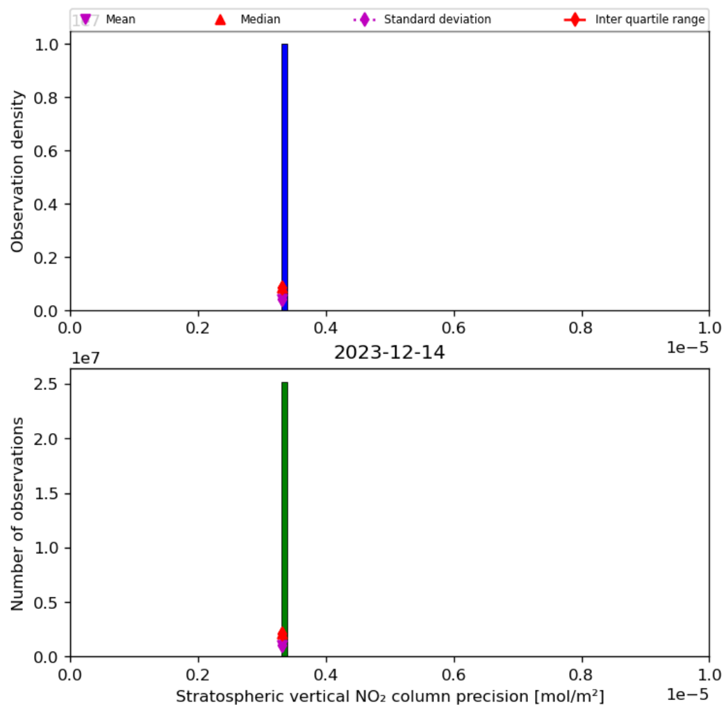
Figure 37: Histogram of “Stratospheric vertical NO 2 column precision” for 2023-12-14 to 2023-12-15
