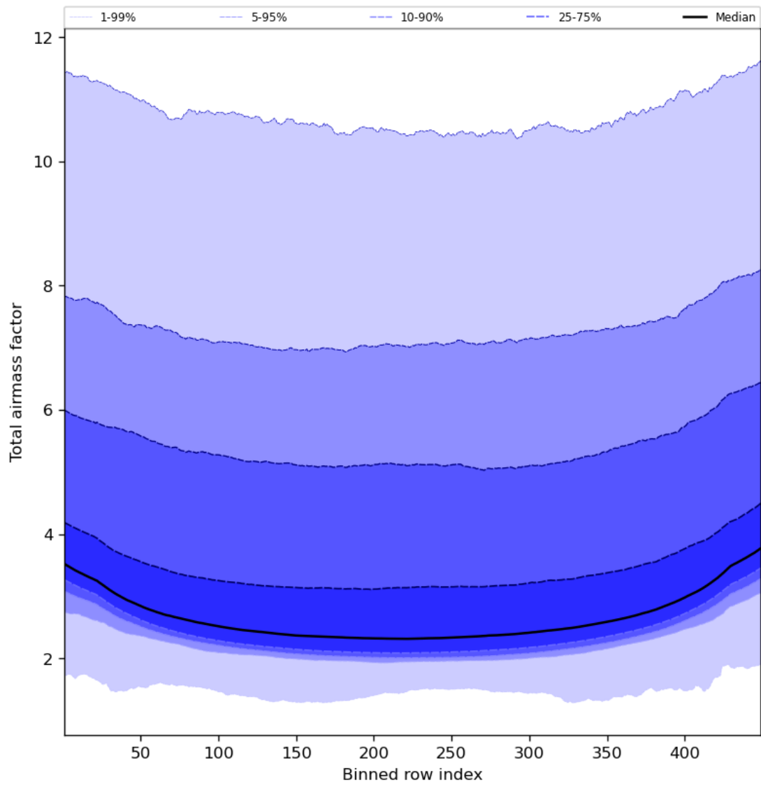
Figure 49: Along track statistics of “Total airmass factor” for 2023-12-14 to 2023-12-15
