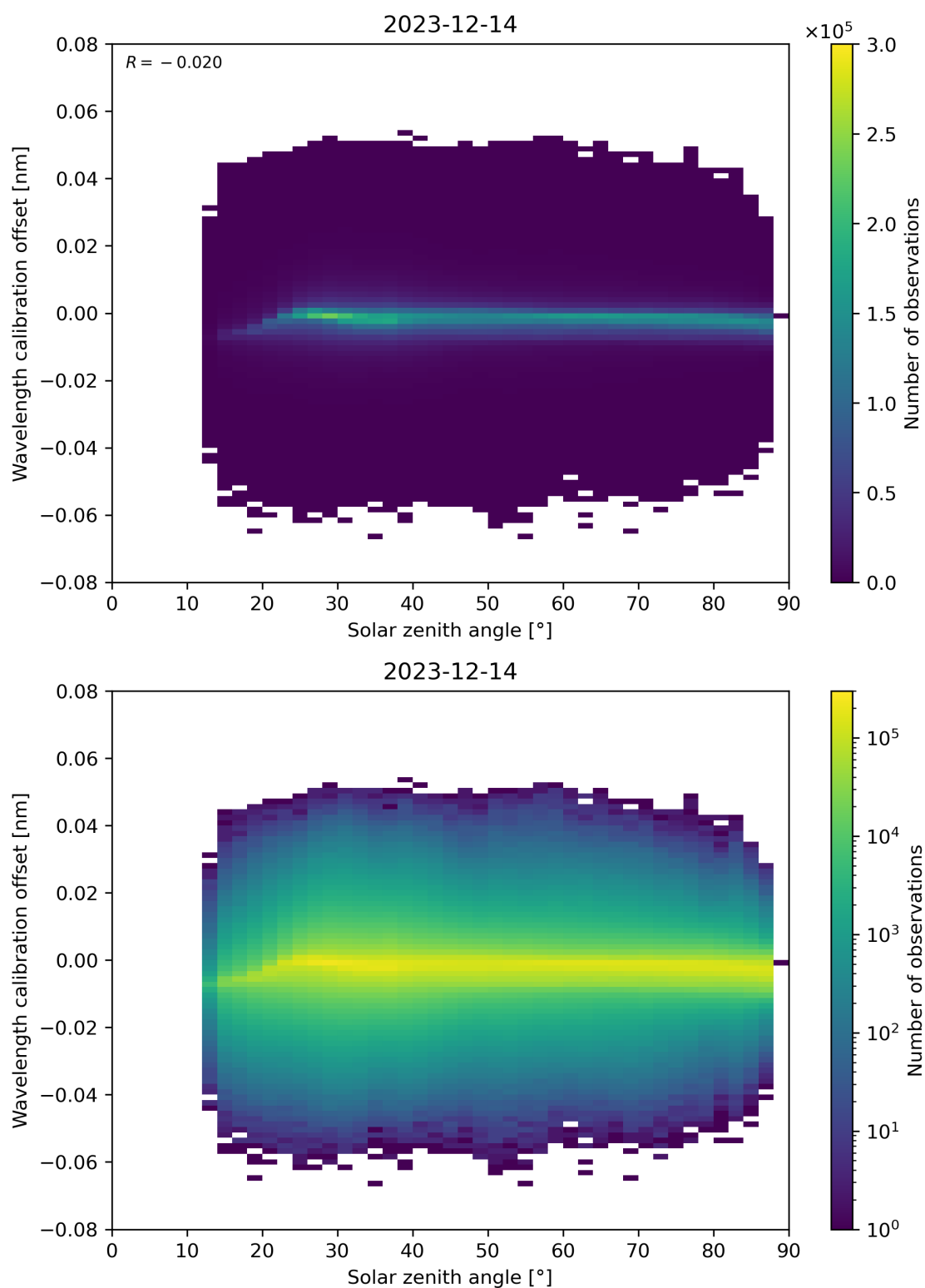
Figure 158: Scatter density plot of “Solar zenith angle” against “Wavelength calibration offset” for 2023-12-14 to 2023-12-15.
