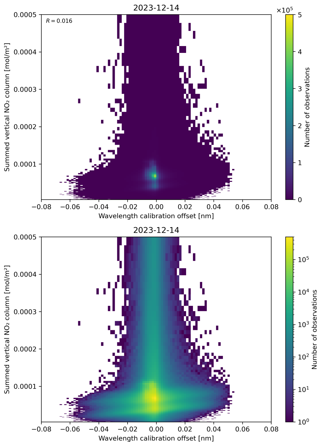
Figure 177: Scatter density plot of “Wavelength calibration offset” against “Summed vertical NO 2 column” for 2023-12-14 to 2023-12-15.
