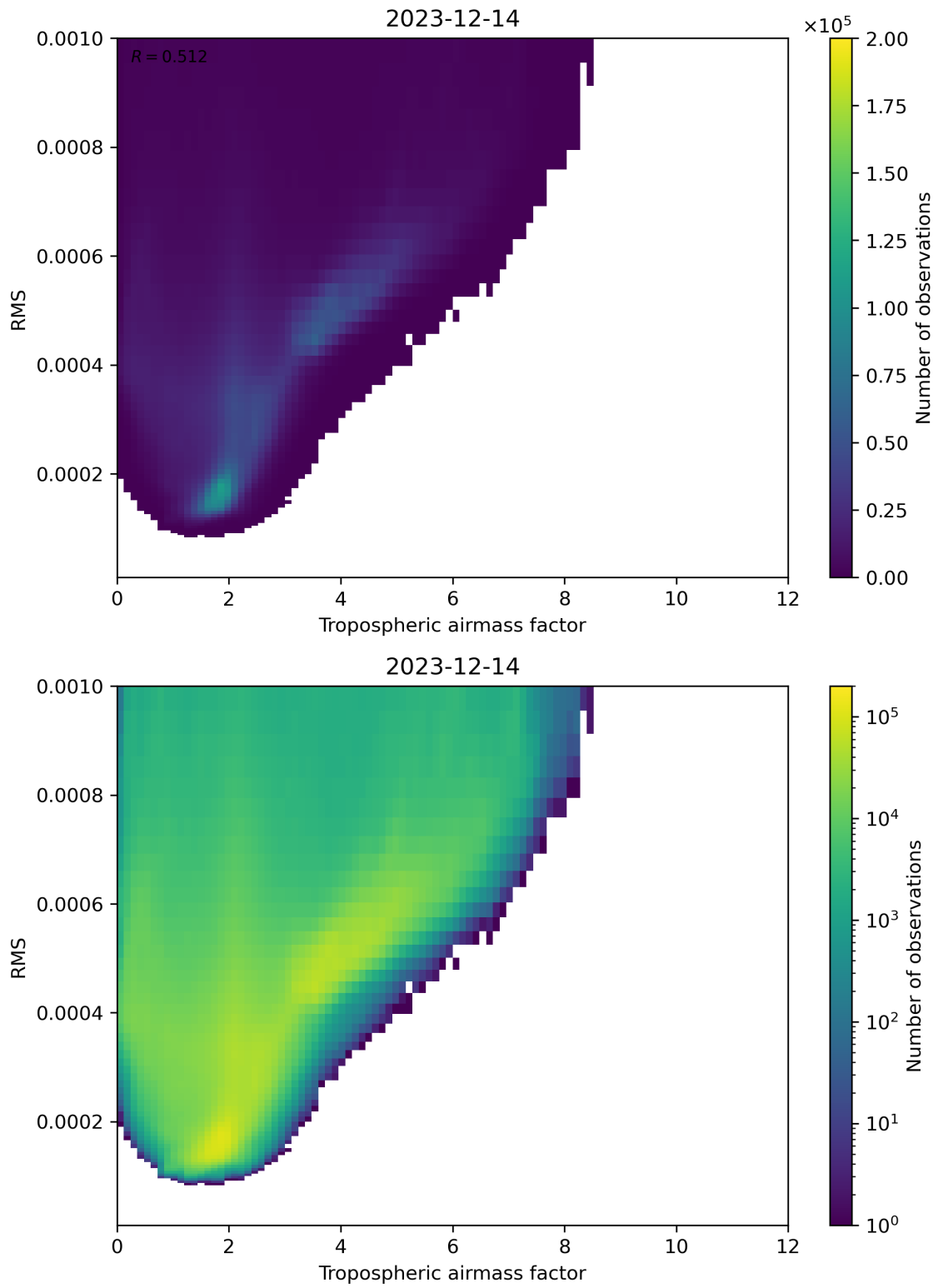
Figure 79: Scatter density plot of “Tropospheric airmass factor” against “RMS” for 2023-12-14 to 2023-12-15.
