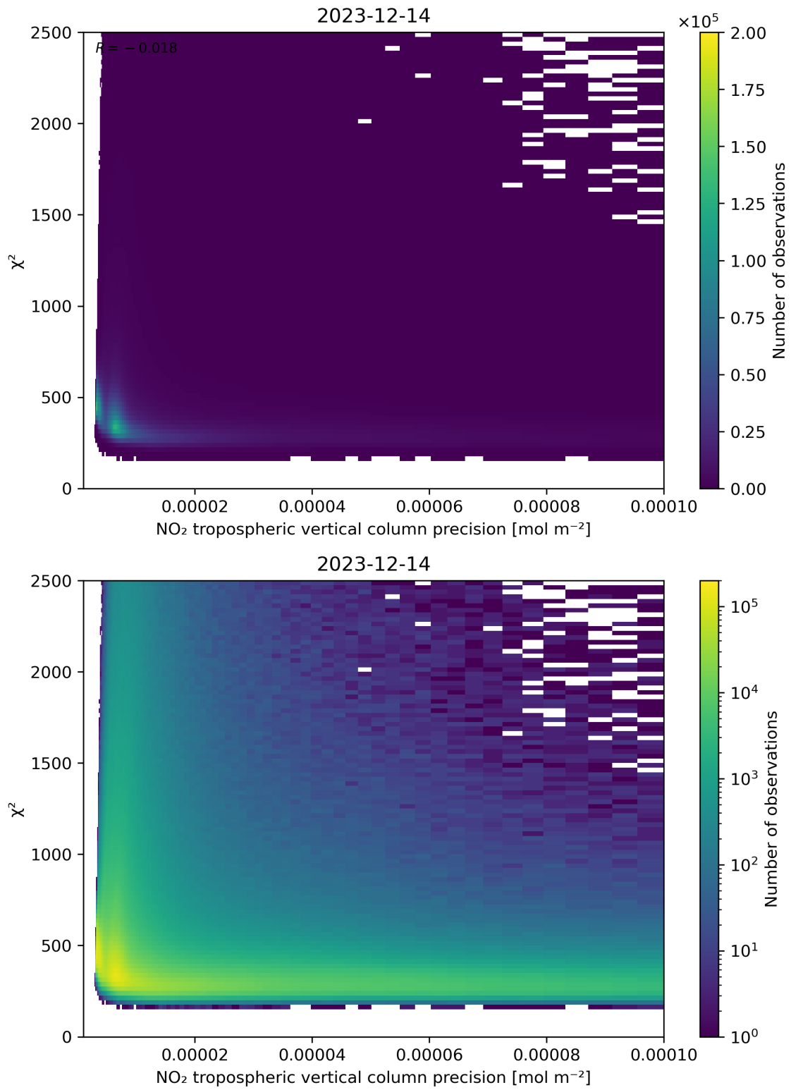
Figure 134: Scatter density plot of “NO 2 tropospheric vertical column precision” against “ \chi^2 ” for 2023-12-14 to 2023-12-15.
