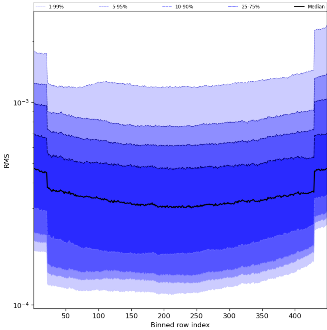
Figure 60: Along track statistics of “RMS” for 2023-12-14 to 2023-12-15
