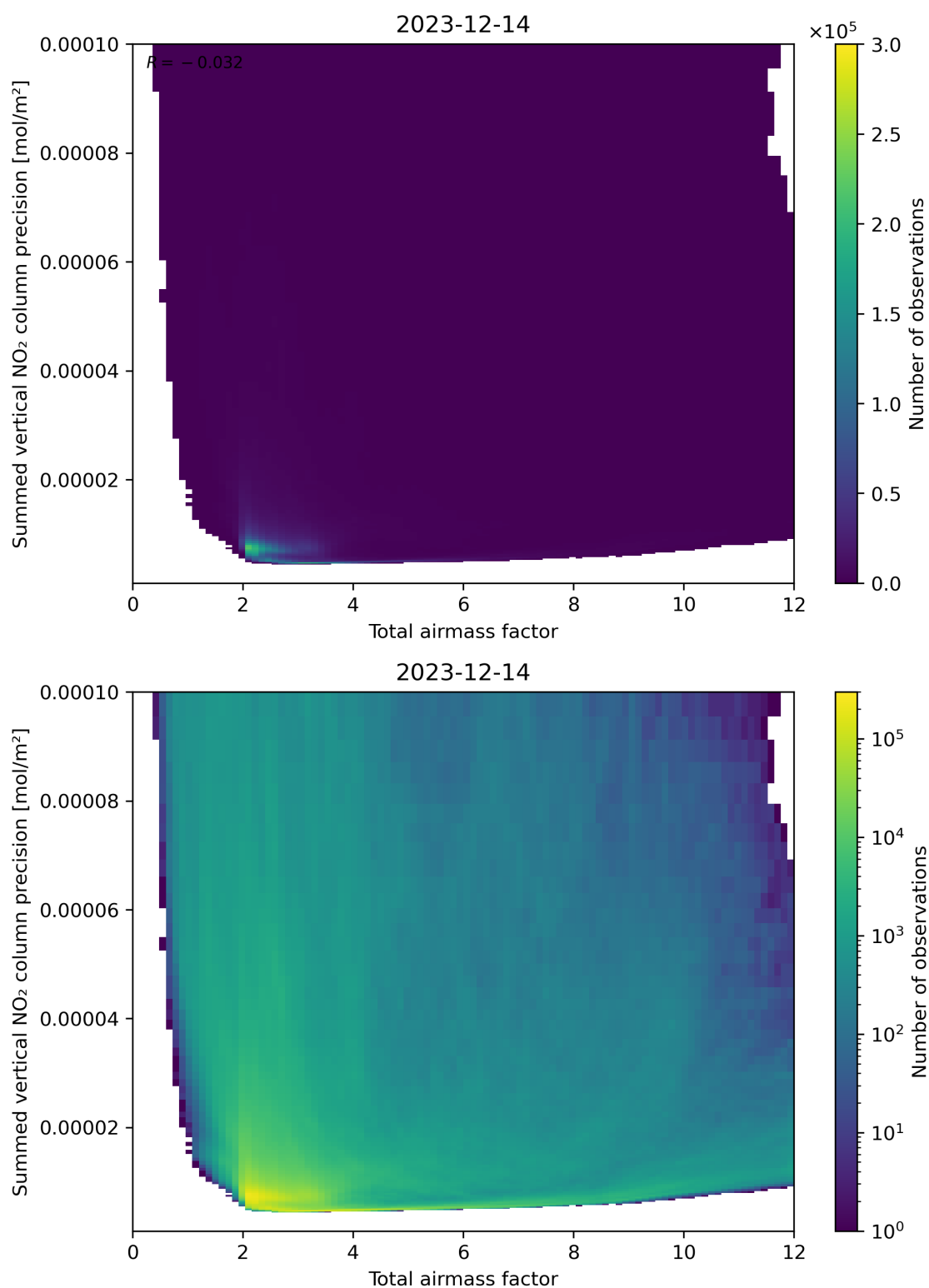
Figure 66: Scatter density plot of “Total airmass factor” against “Summed vertical NO 2 column precision” for 2023-12-14 to 2023-12-15.
