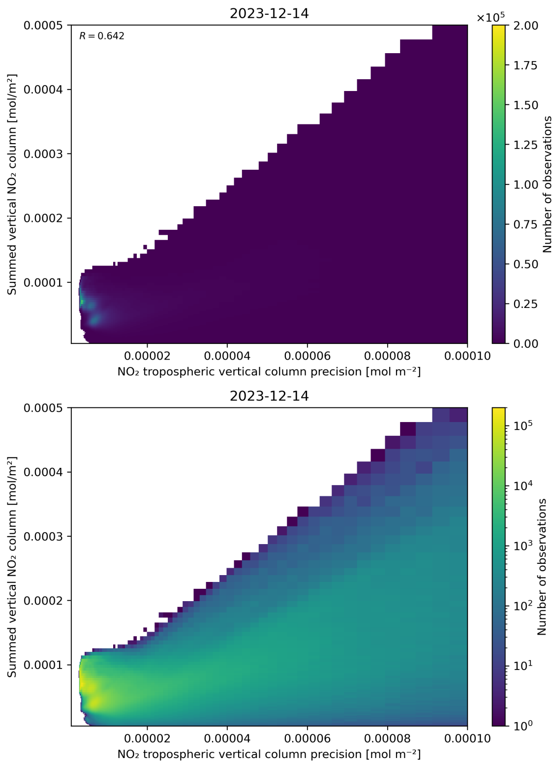
Figure 136: Scatter density plot of “NO 2 tropospheric vertical column precision” against “Summed vertical NO 2 column” for 2023-12-14 to 2023-12-15.
