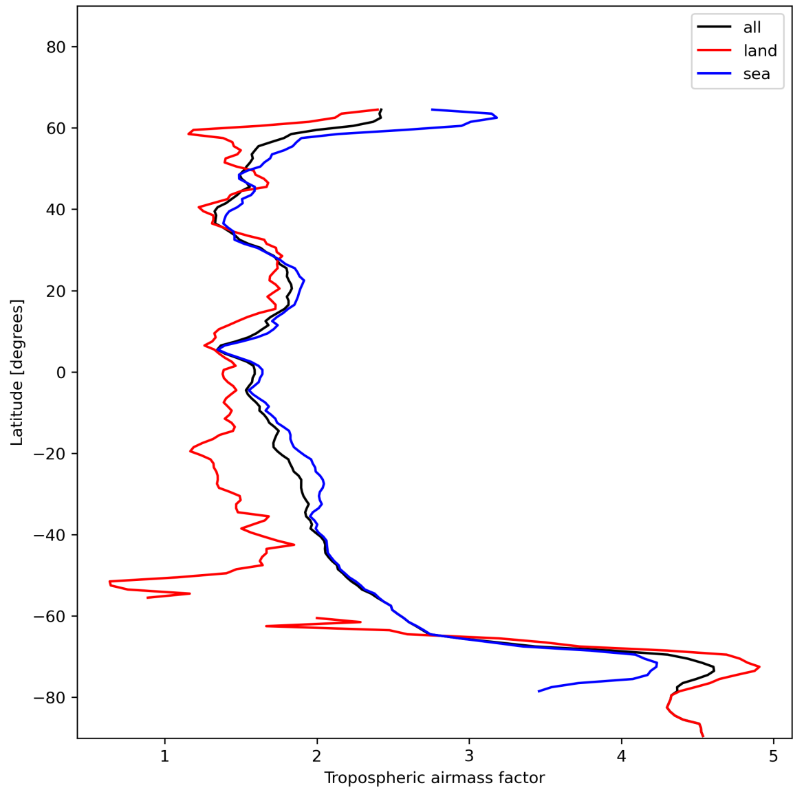
Figure 14: Zonal average of “Tropospheric airmass factor” for 2023-12-14 to 2023-12-15.
