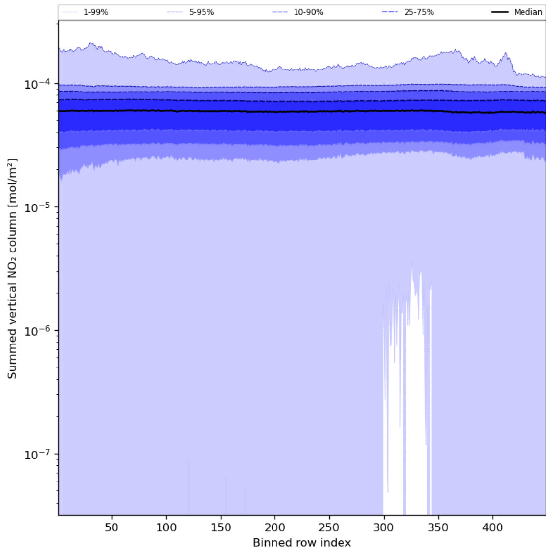
Figure 57: Along track statistics of “Summed vertical NO 2 column” for 2023-12-14 to 2023-12-15
