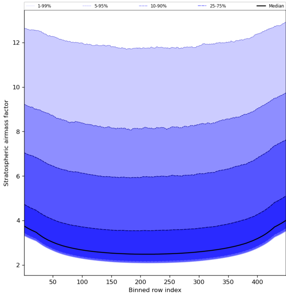
Figure 61: Along track statistics of “Stratospheric air mass factor” for 2023-12-14 to 2023-12-15
