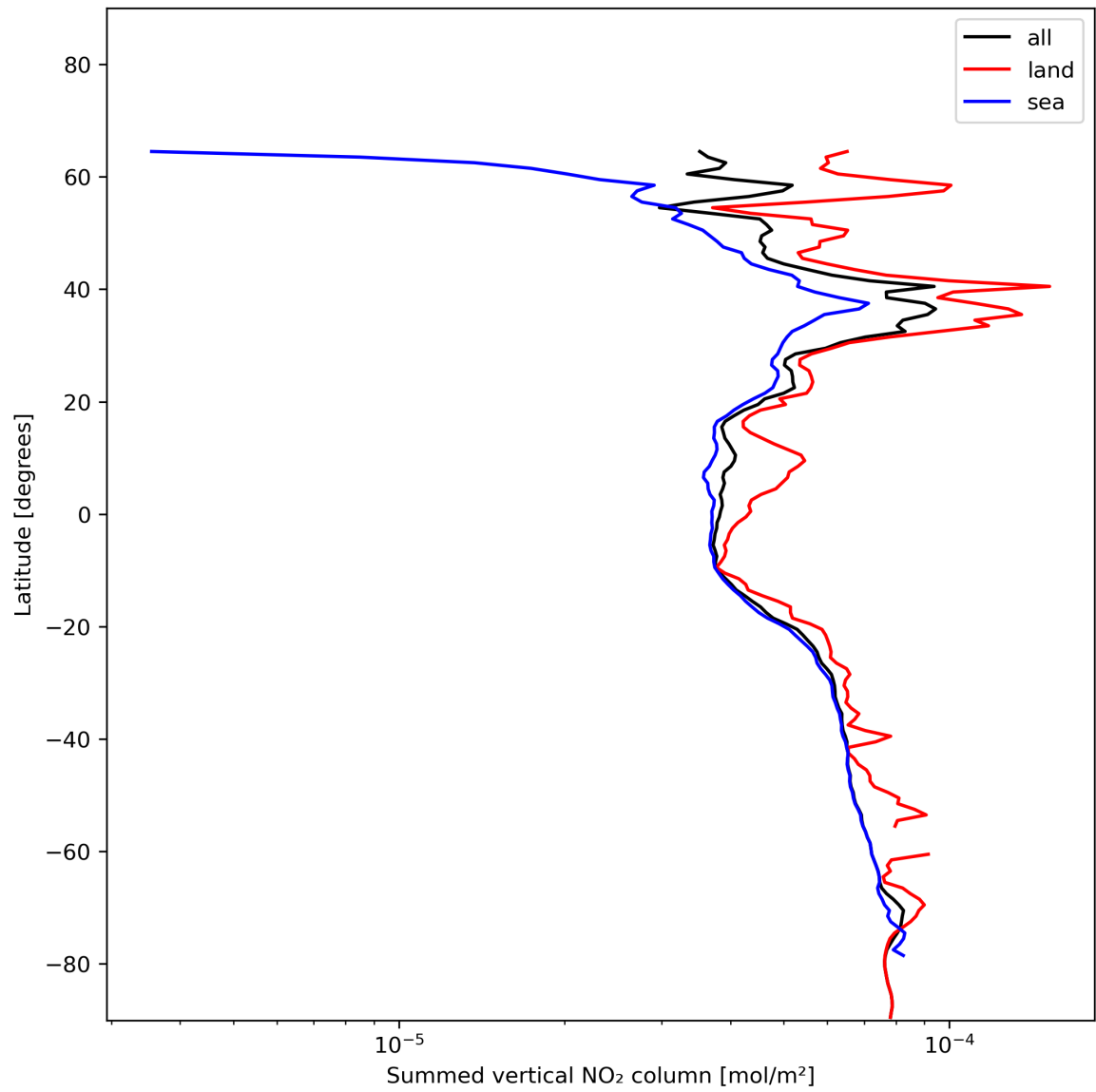
Figure 23: Zonal average of “Summed vertical NO 2 column” for 2023-12-14 to 2023-12-15.
