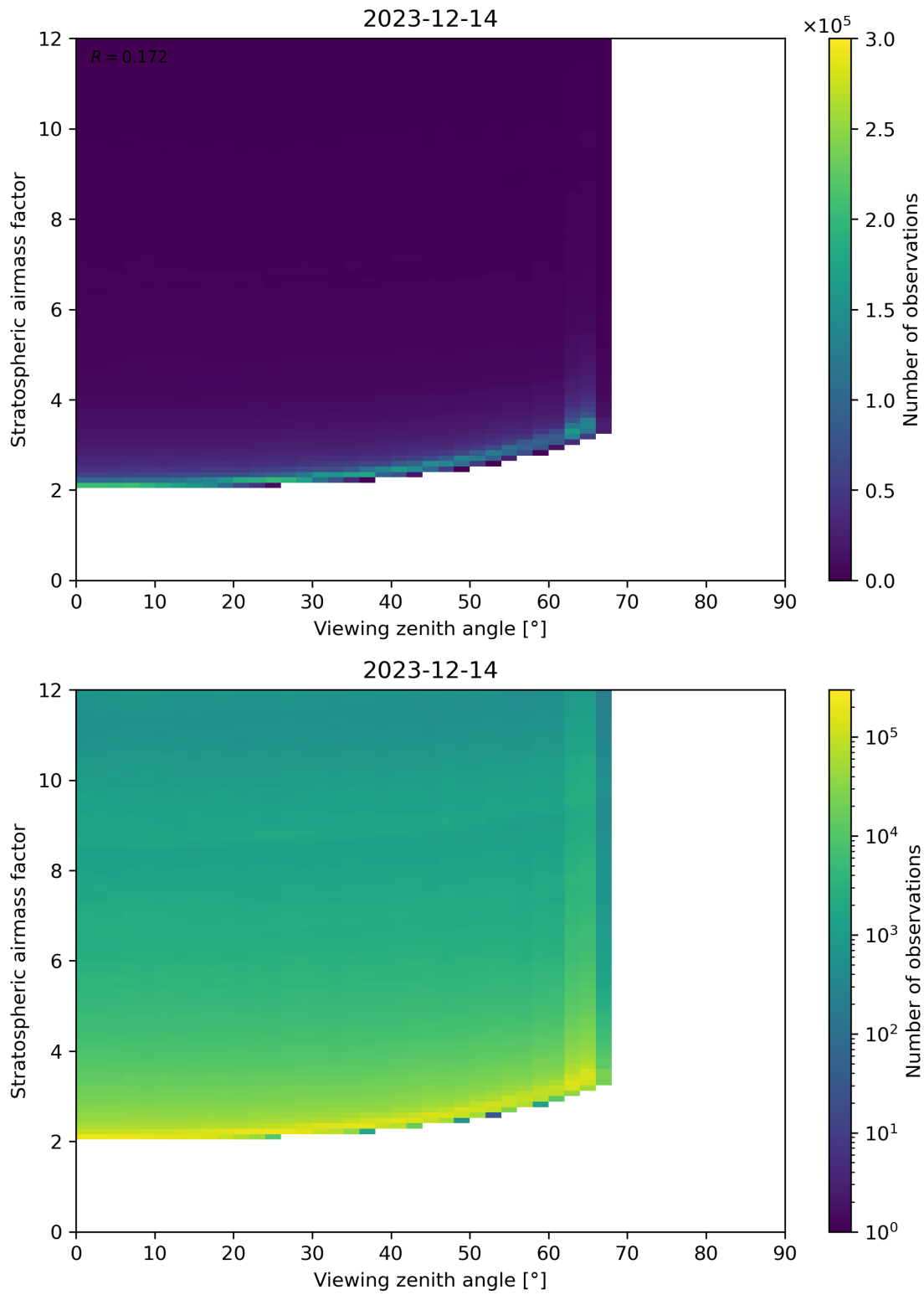
Figure 159: Scatter density plot of “Viewing zenith angle” against “Stratospheric airmass factor” for 2023-12-14 to 2023-12-15.
