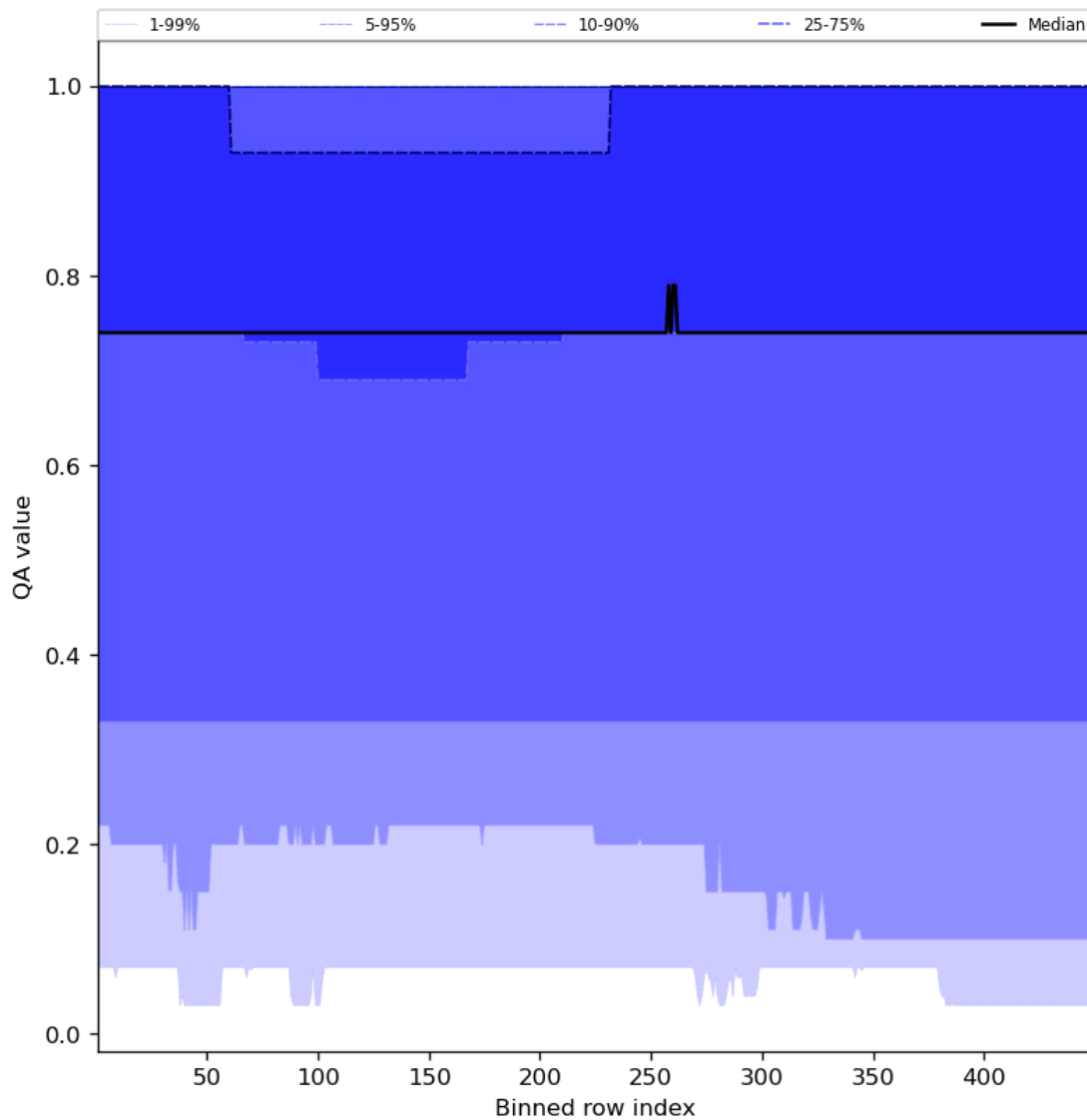
Figure 45: Along track statistics of “QA value” for 2023-12-14 to 2023-12-15
