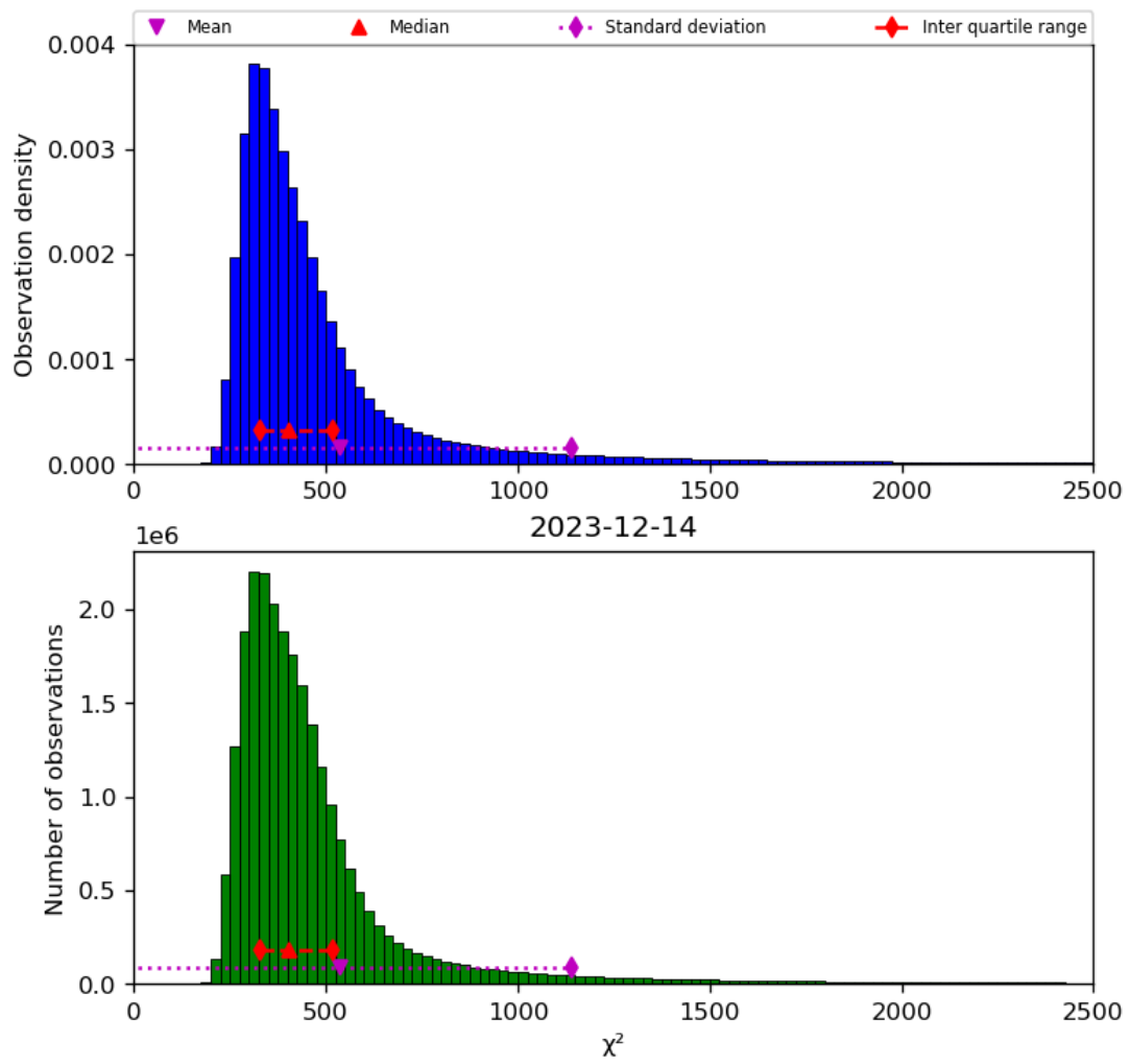
Figure 42: Histogram of “ \chi^2 ” for 2023-12-14 to 2023-12-15
