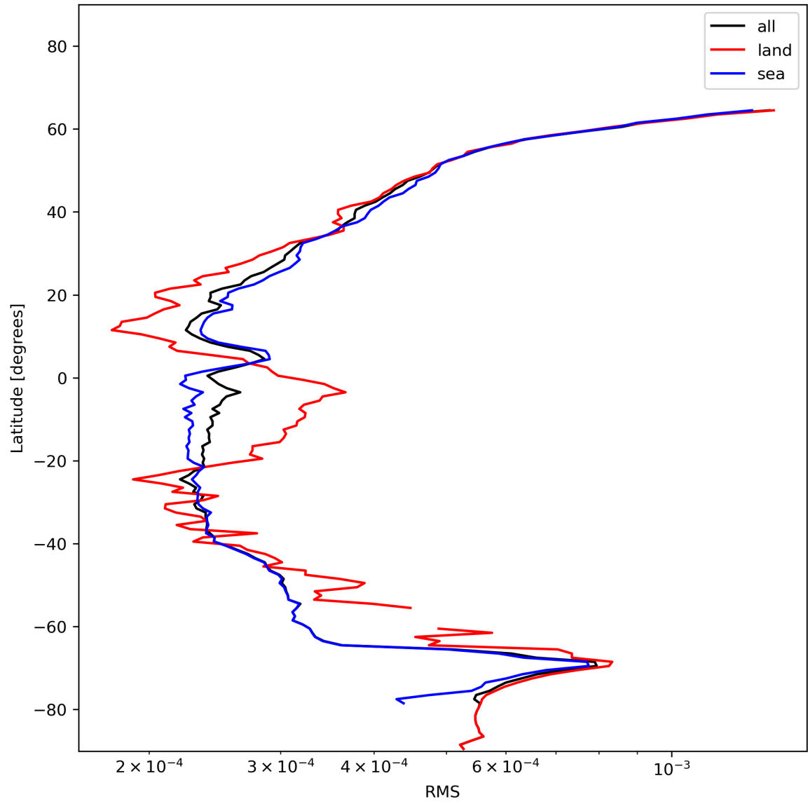
Figure 26: Zonal average of “RMS” for 2023-12-14 to 2023-12-15.
