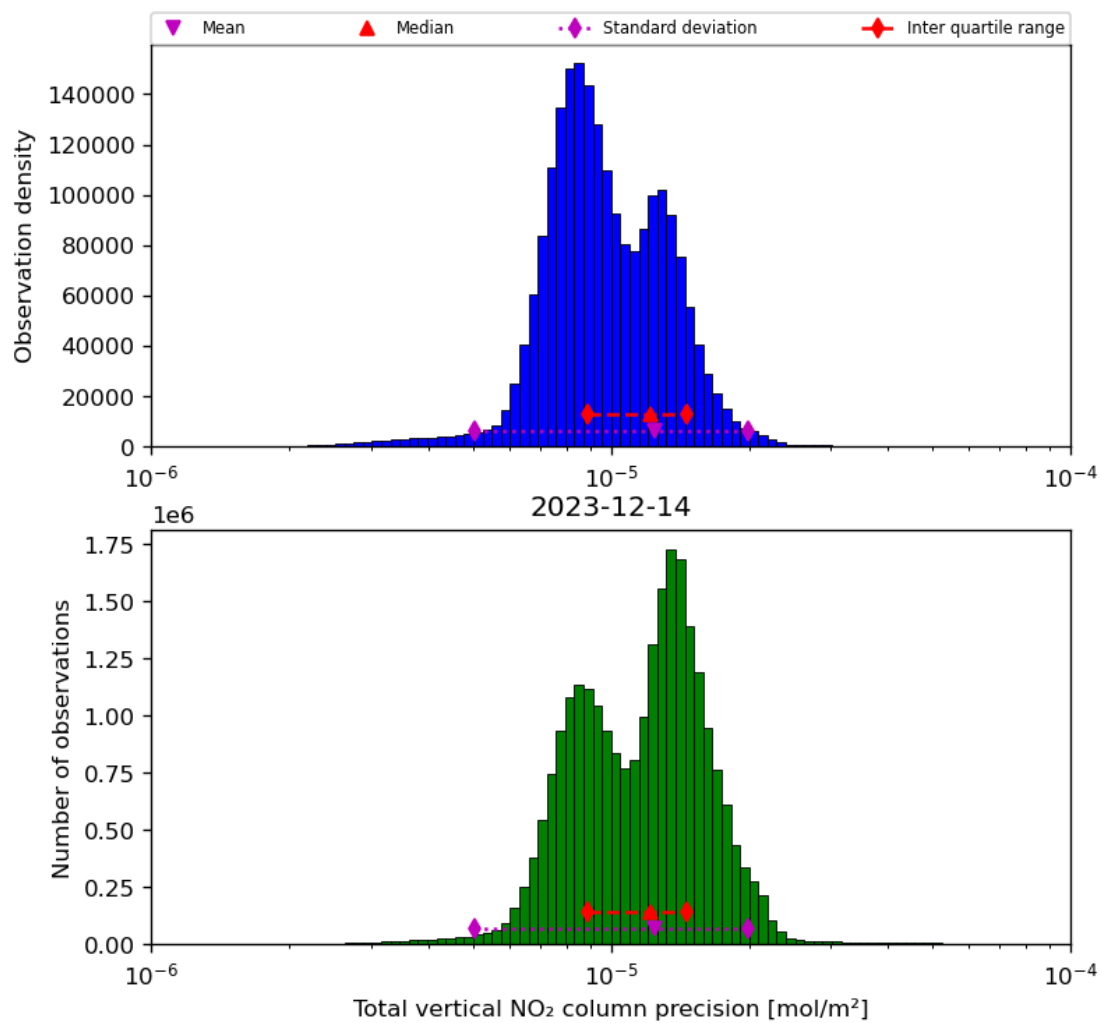
Figure 39: Histogram of “Total vertical NO 2 column precision” for 2023-12-14 to 2023-12-15
