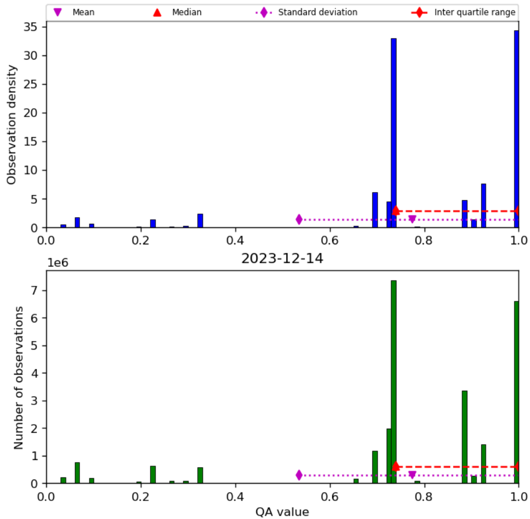
Figure 28: Histogram of “QA value” for 2023-12-14 to 2023-12-15
