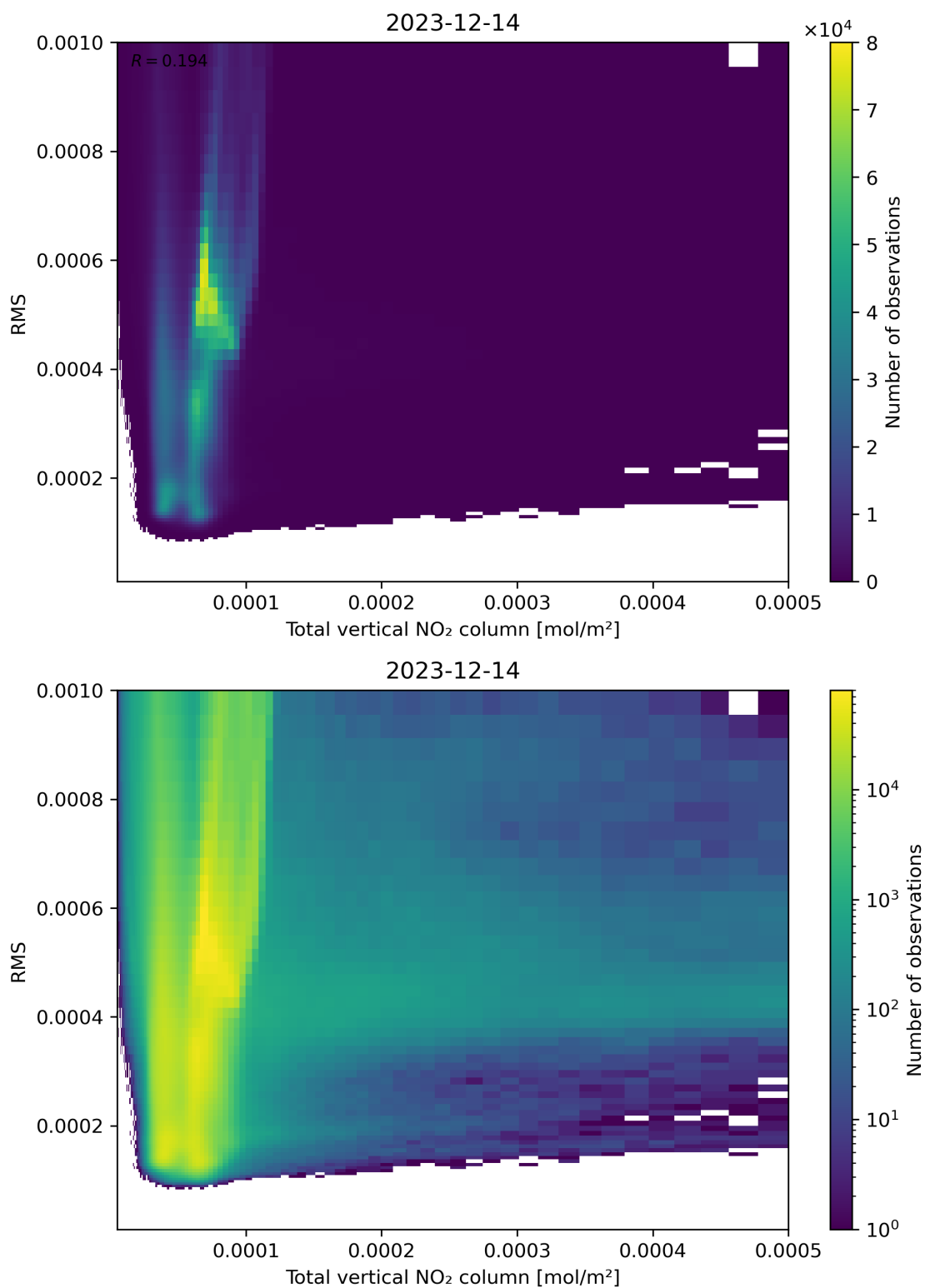
Figure 120: Scatter density plot of “Total vertical NO 2 column” against “RMS” for 2023-12-14 to 2023-12-15.
