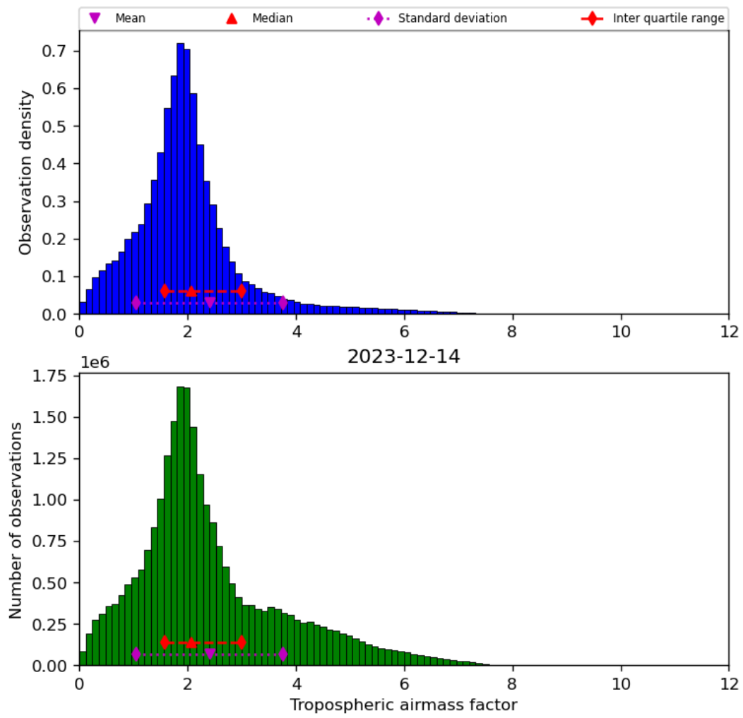
Figure 31: Histogram of “Tropospheric airmass factor” for 2023-12-14 to 2023-12-15
