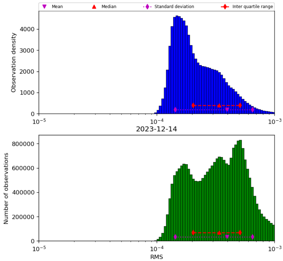
Figure 43: Histogram of “RMS” for 2023-12-14 to 2023-12-15
