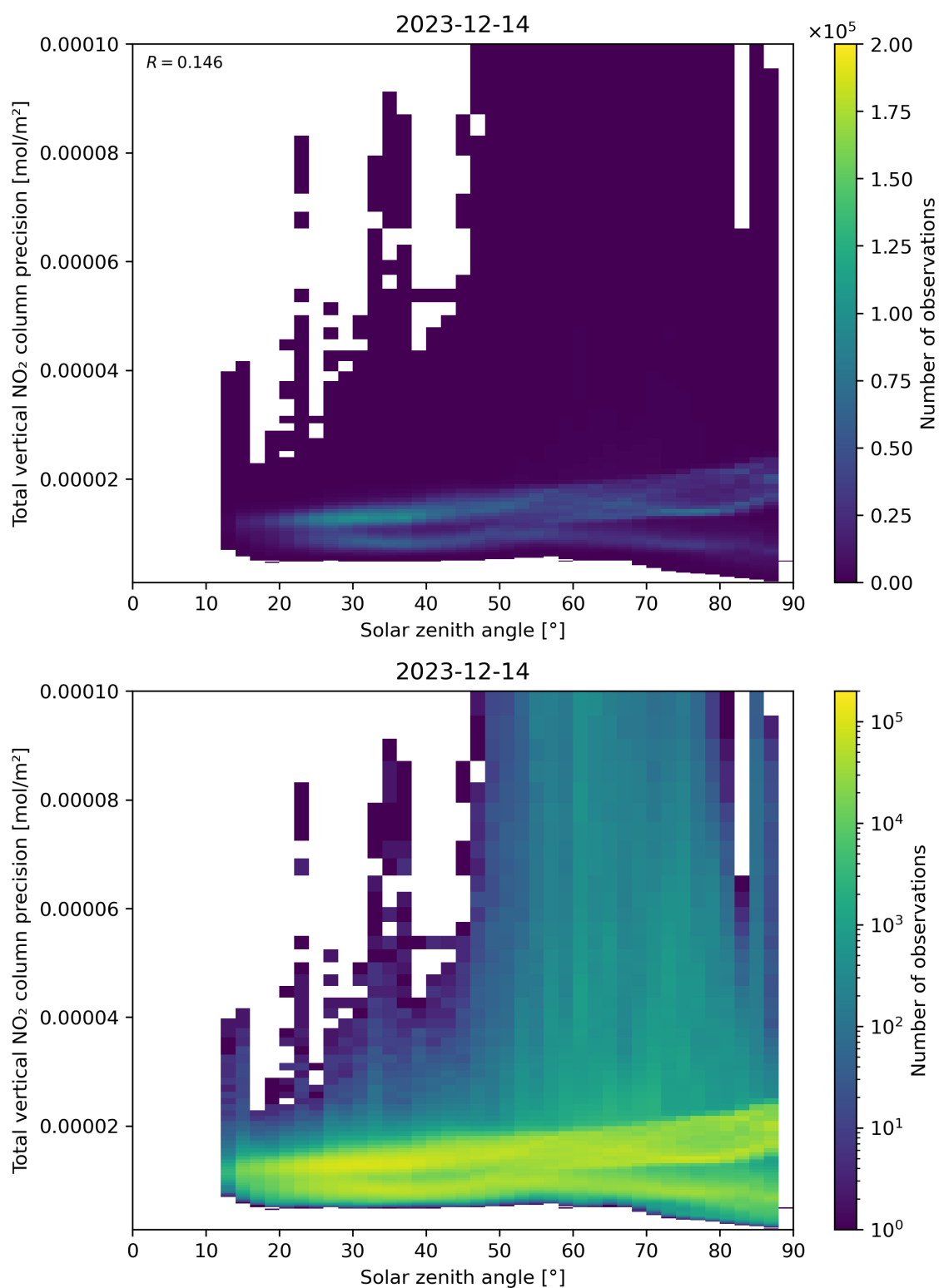
Figure 154: Scatter density plot of “Solar zenith angle” against “Total vertical NO 2 column precision” for 2023-12-14 to 2023-12-15.
