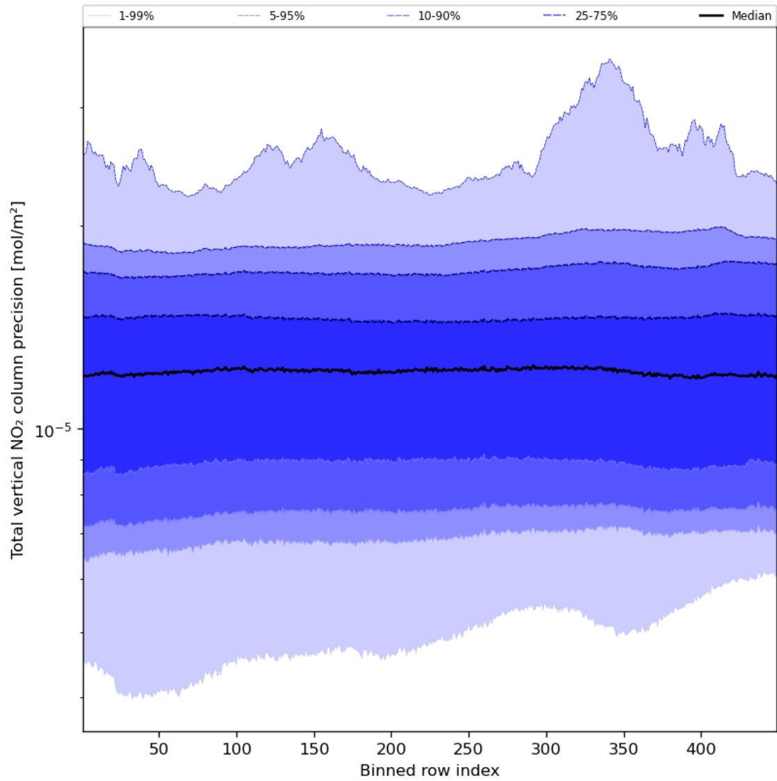
Figure 56: Along track statistics of “Total vertical NO 2 column precision” for 2023-12-14 to 2023-12-15
