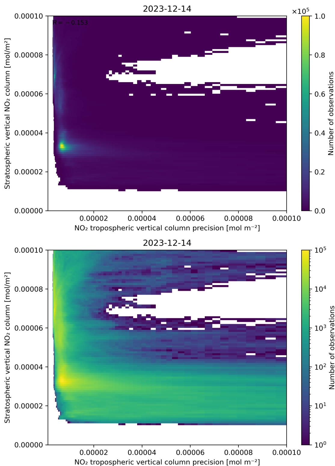
Figure 135: Scatter density plot of “NO 2 tropospheric vertical column precision” against “Stratospheric vertical NO 2 column” for 2023-12-14 to 2023-12-15.
