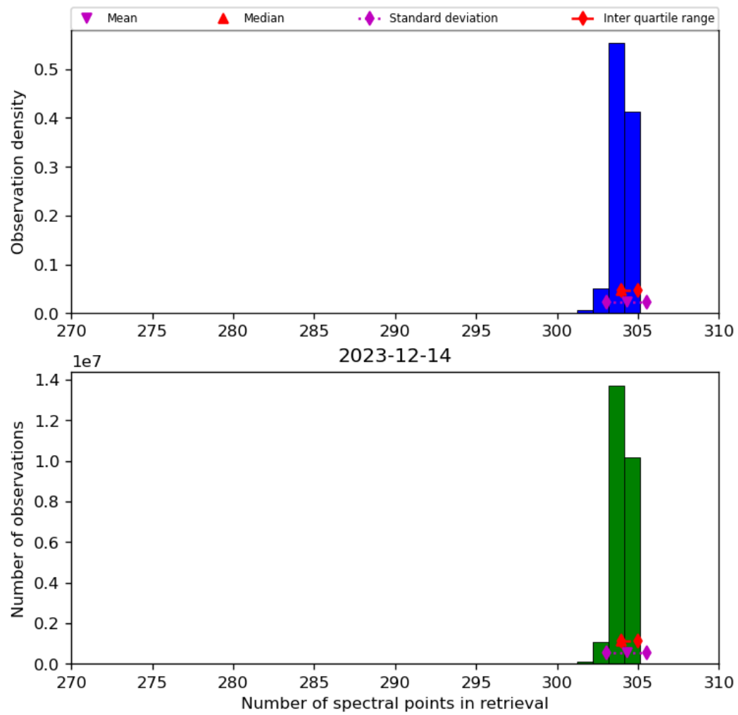
Figure 33: Histogram of “Number of spectral points in retrieval” for 2023-12-14 to 2023-12-15
