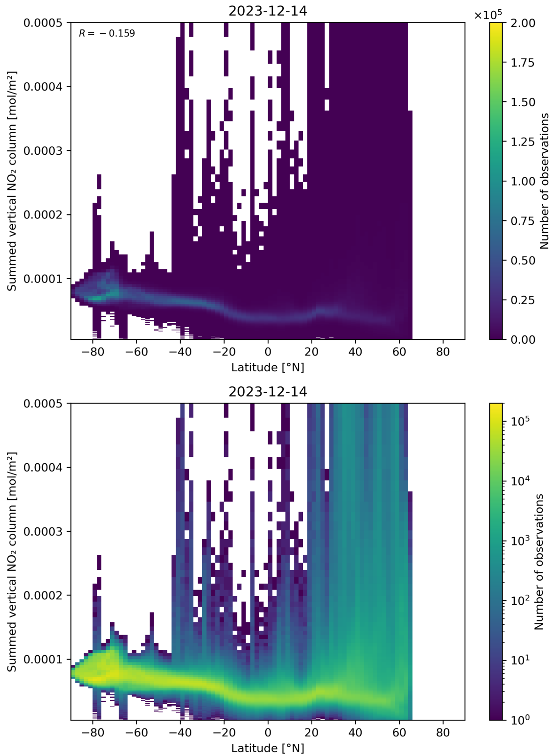
Figure 88: Scatter density plot of “Latitude” against “Summed vertical NO 2 column” for 2023-12-14 to 2023-12-15.
