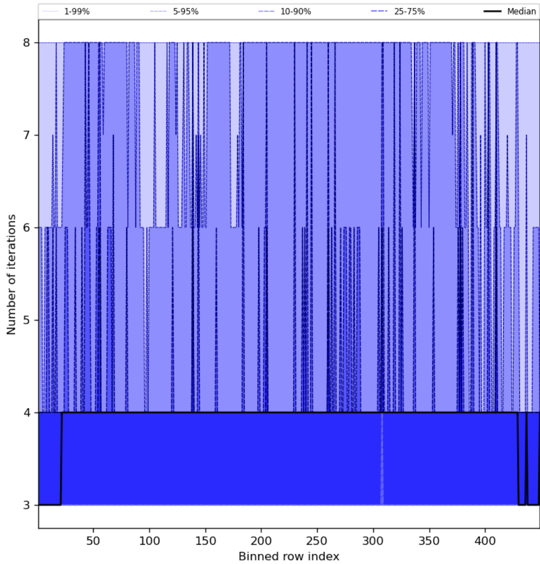
Figure 51: Along track statistics of “Number of iterations” for 2023-12-14 to 2023-12-15
