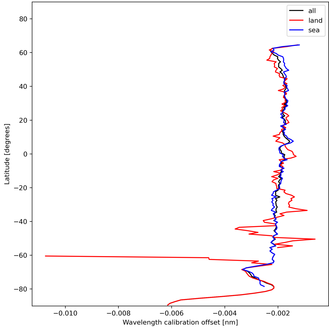
Figure 18: Zonal average of “Wavelength calibration offset” for 2023-12-14 to 2023-12-15.
