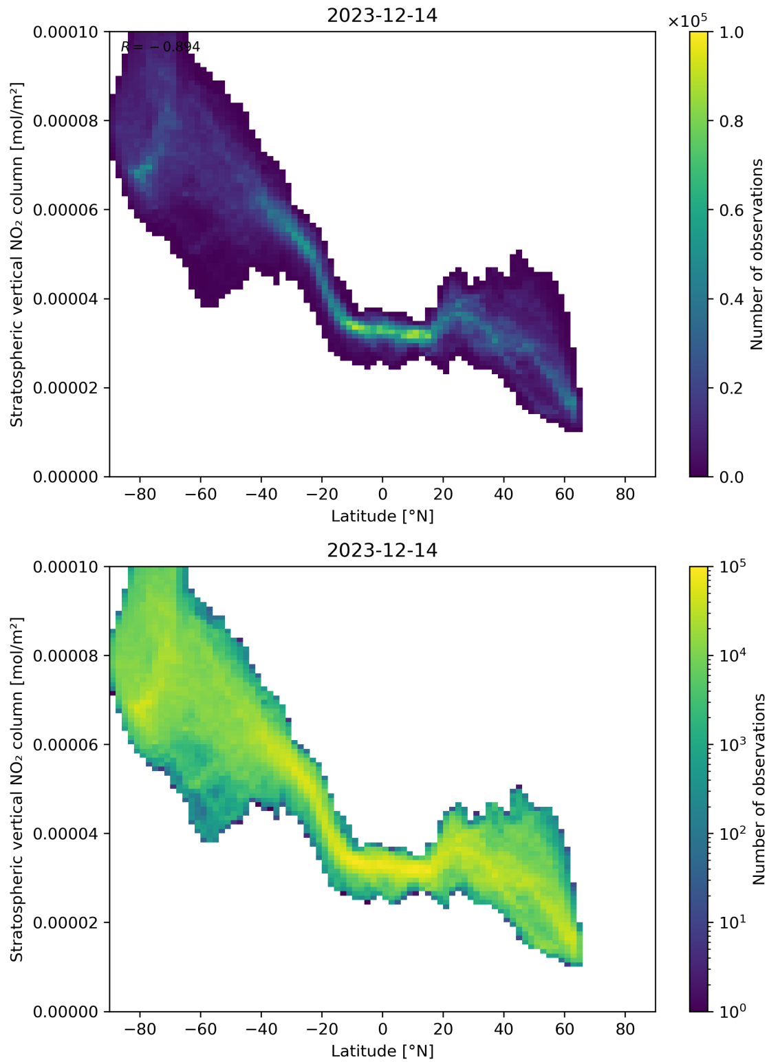
Figure 87: Scatter density plot of “Latitude” against “Stratospheric vertical NO 2 column” for 2023-12-14 to 2023-12-15.
