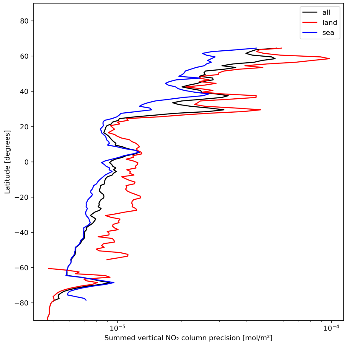
Figure 24: Zonal average of “Summed vertical NO 2 column precision” for 2023-12-14 to 2023-12-16.
