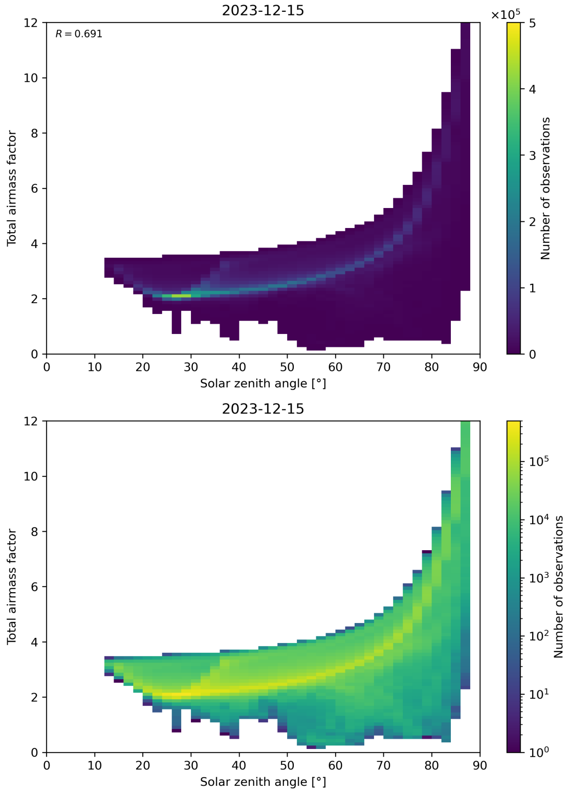
Figure 146: Scatter density plot of “Solar zenith angle” against “Total airmass factor” for 2023-12-14 to 2023-12-16.
