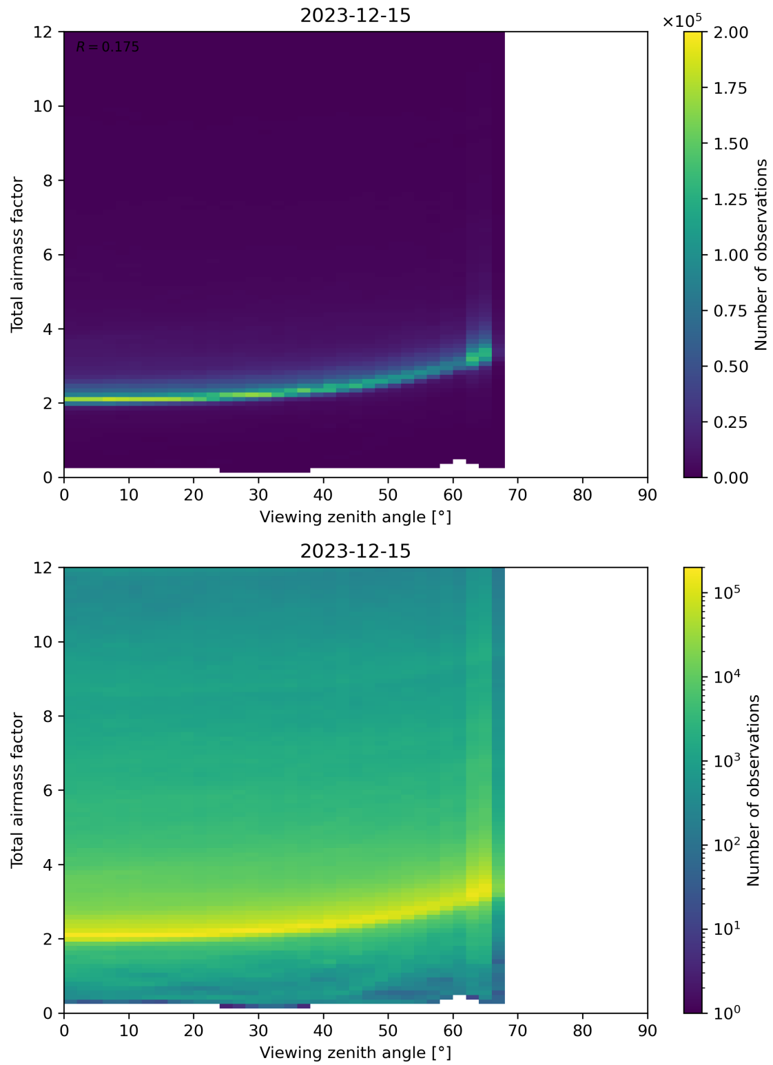
Figure 160: Scatter density plot of “Viewing zenith angle” against “Total airmass factor” for 2023-12-14 to 2023-12-16.
