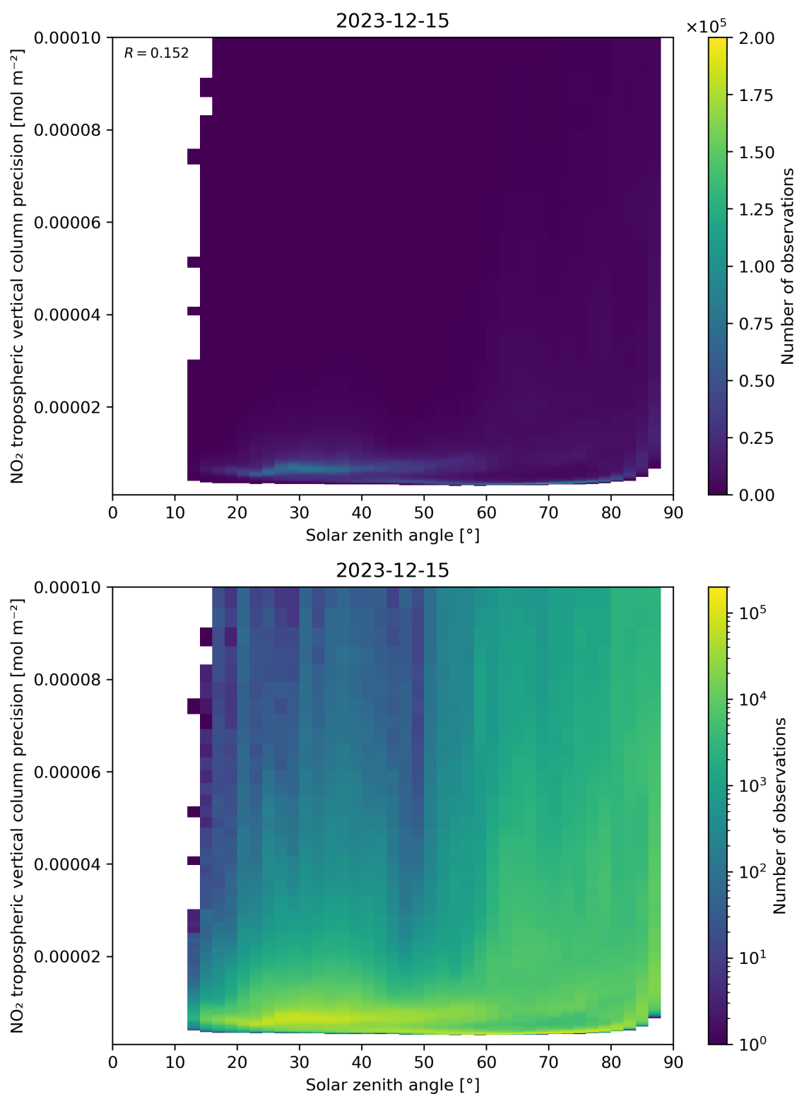
Figure 156: Scatter density plot of “Solar zenith angle” against “NO 2 tropospheric vertical column precision” for 2023-12-14 to 2023-12-16.
