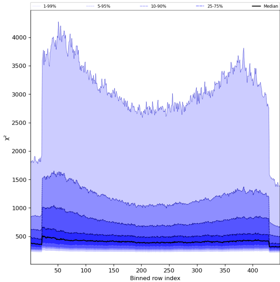
Figure 59: Along track statistics of “ \chi^2 ” for 2023-12-14 to 2023-12-16
