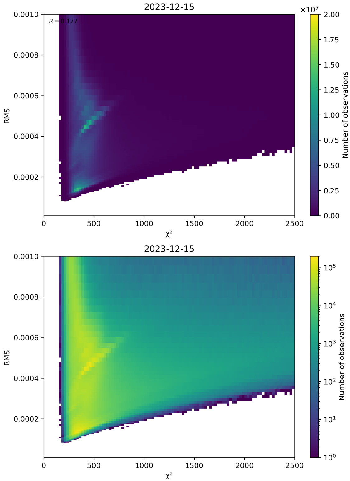
Figure 82: Scatter density plot of “ \chi^2 ” against “RMS” for 2023-12-14 to 2023-12-16.
