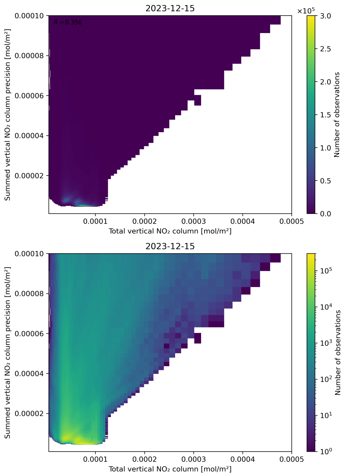
Figure 113: Scatter density plot of “Total vertical NO 2 column” against “Summed vertical NO 2 column precision” for 2023-12-14 to 2023-12-16.
