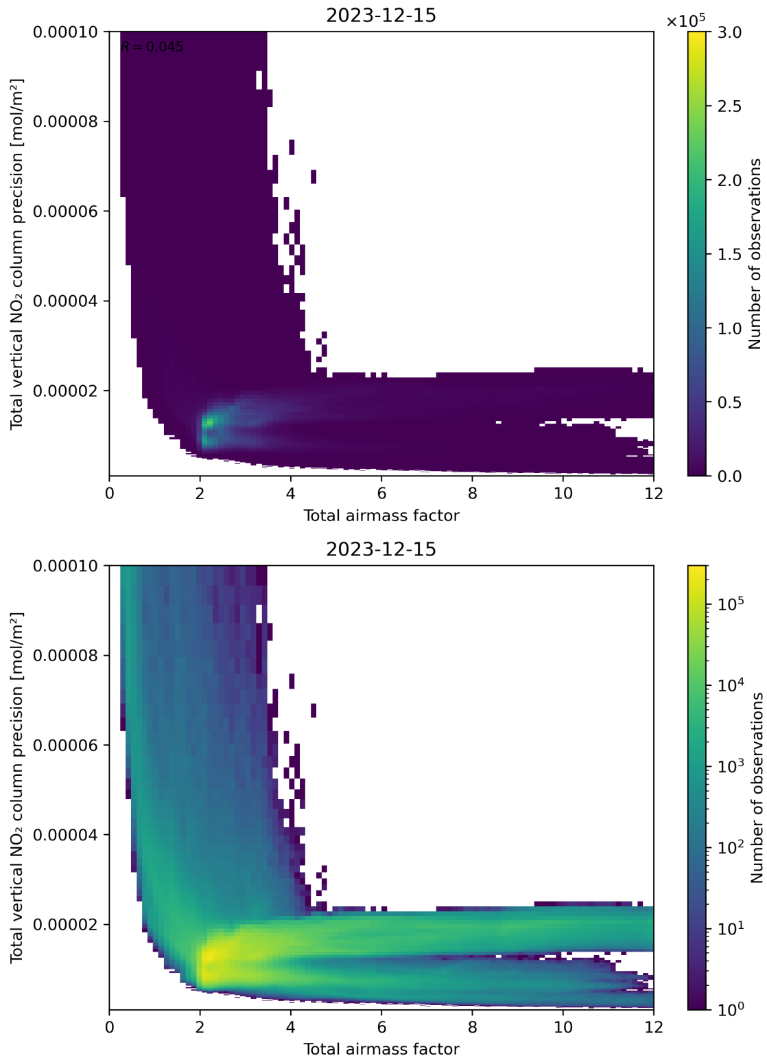
Figure 68: Scatter density plot of “Total airmass factor” against “Total vertical NO 2 column precision” for 2023-12-14 to 2023-12-16.
