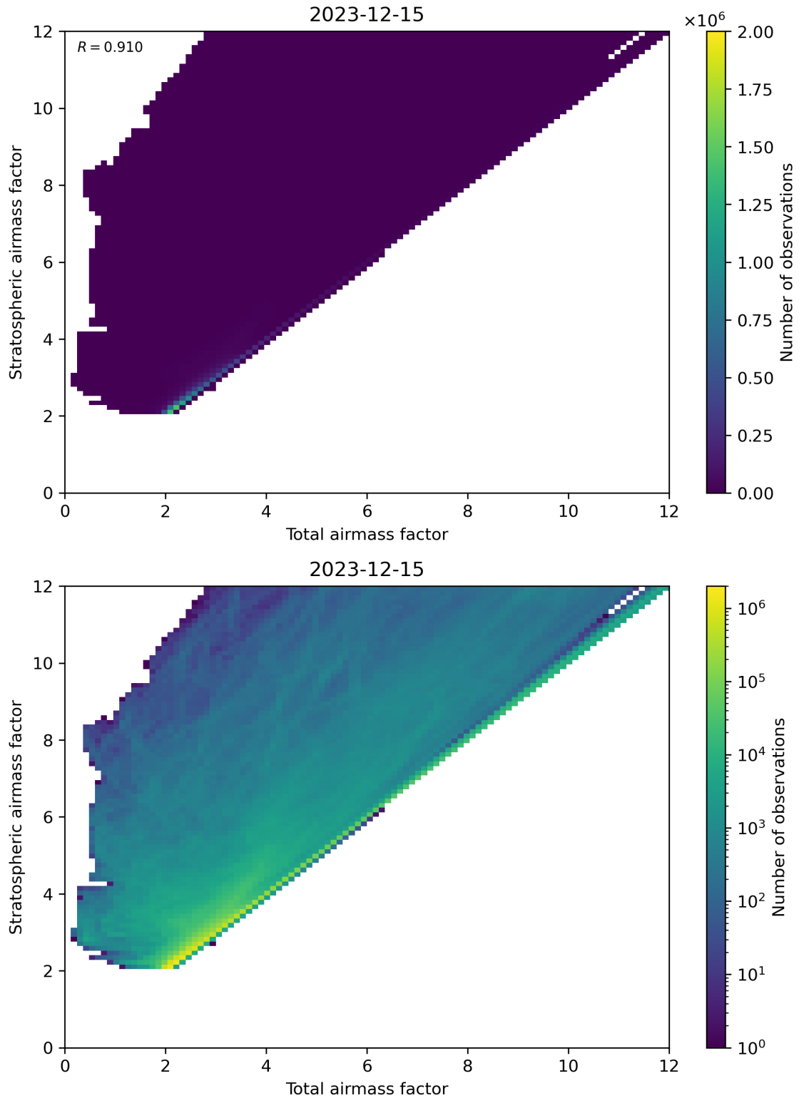
Figure 62: Scatter density plot of “Total airmass factor” against “Stratospheric airmass factor” for 2023-12-14 to 2023-12-16.
