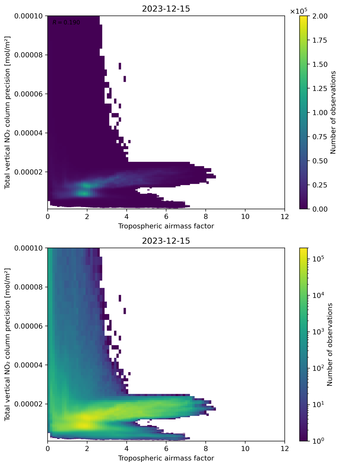
Figure 78: Scatter density plot of “Tropospheric air mass factor” against “Total vertical NO 2 column precision” for 2023-12-14 to 2023-12-16.
