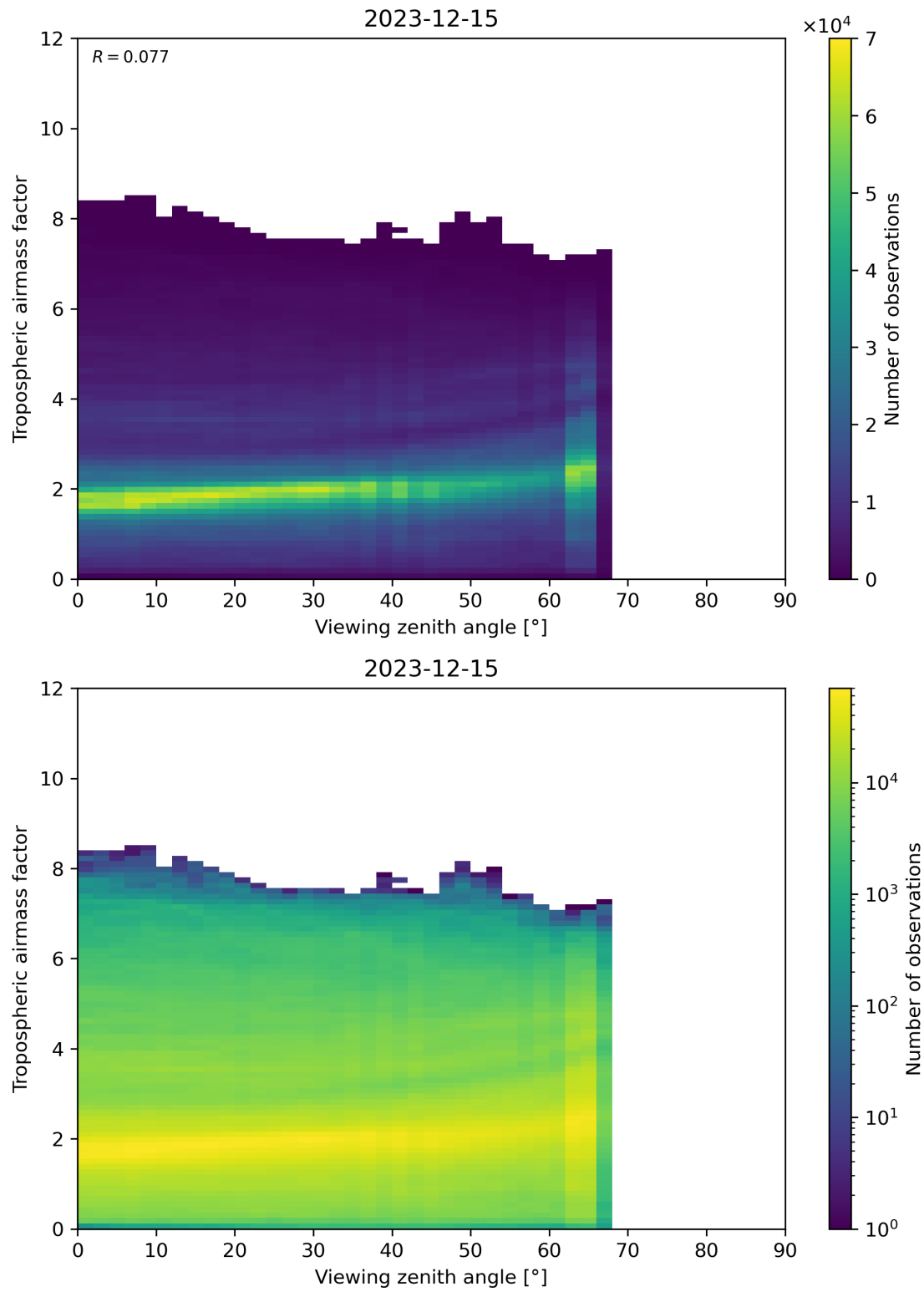
Figure 161: Scatter density plot of “Viewing zenith angle” against “Tropospheric airmass factor” for 2023-12-14 to 2023-12-16.
