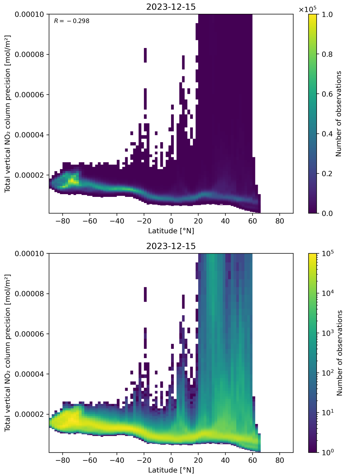
Figure 91: Scatter density plot of “Latitude” against “Total vertical NO 2 column precision” for 2023-12-14 to 2023-12-16.
