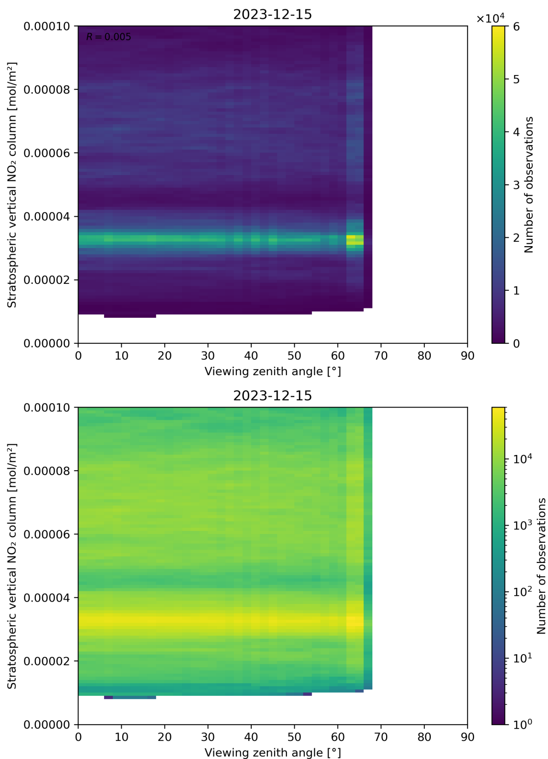
Figure 164: Scatter density plot of “Viewing zenith angle” against “Stratospheric vertical NO 2 column” for 2023-12-14 to 2023-12-16.
