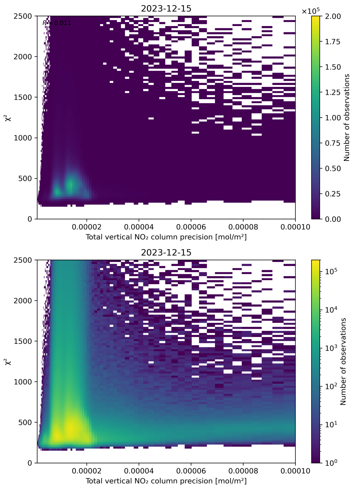
Figure 116: Scatter density plot of "Total vertical NO 2 column precision" against " \chi^2 " for 2023-12-14 to 2023-12-16.
