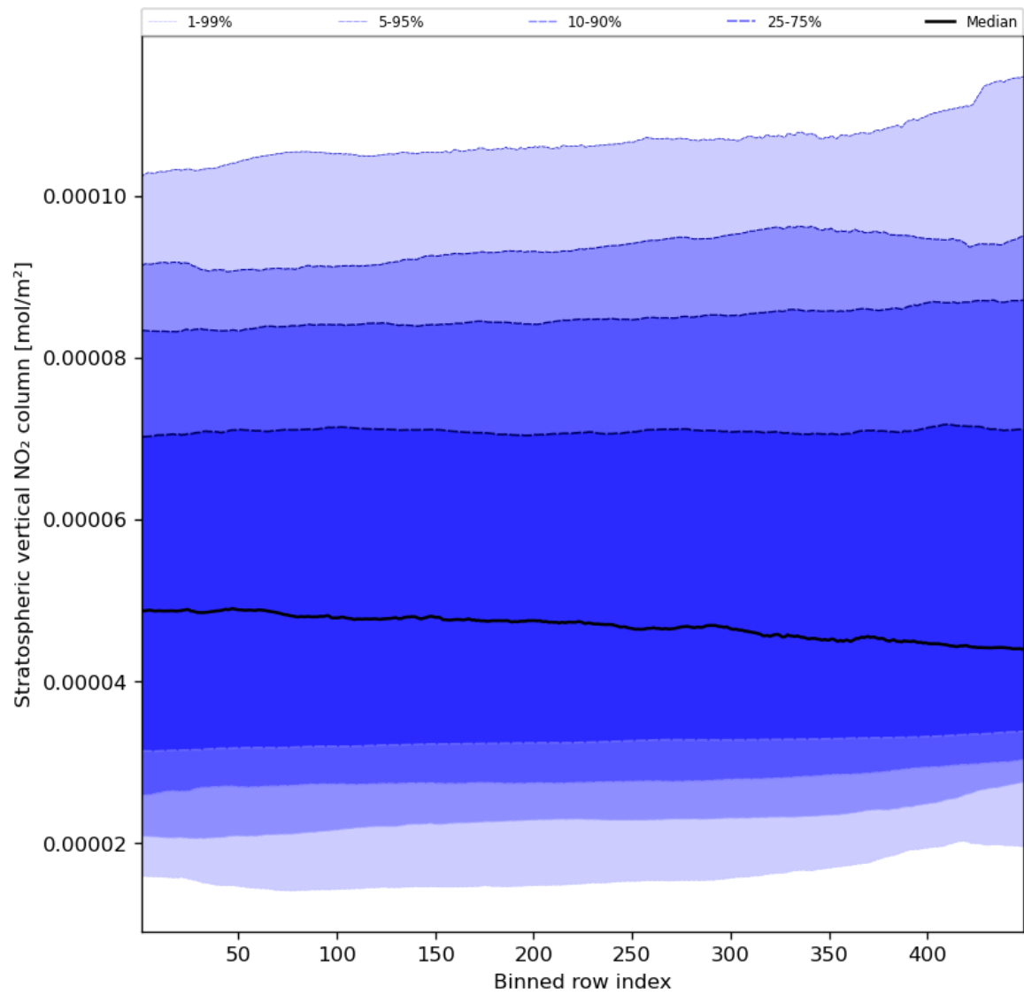
Figure 53: Along track statistics of “Stratospheric vertical NO 2 column” for 2023-12-14 to 2023-12-16
