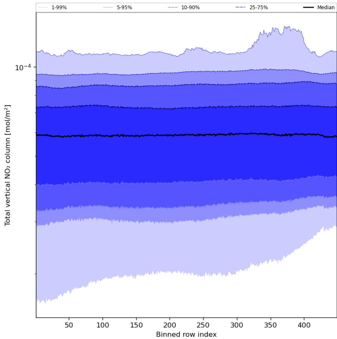
Figure 55: Along track statistics of “Total vertical NO 2 column” for 2023-12-14 to 2023-12-16
