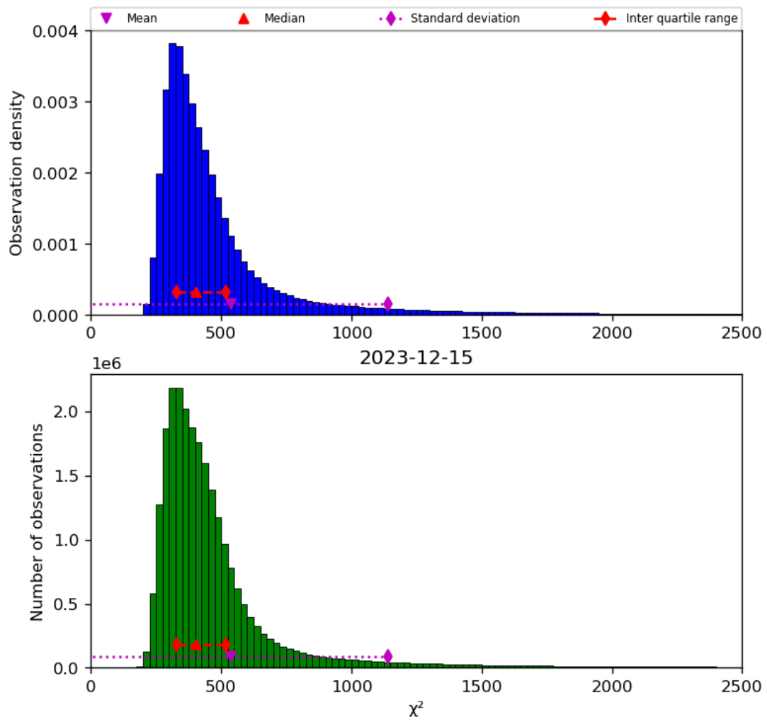
Figure 42: Histogram of “ \chi^2 ” for 2023-12-14 to 2023-12-16
