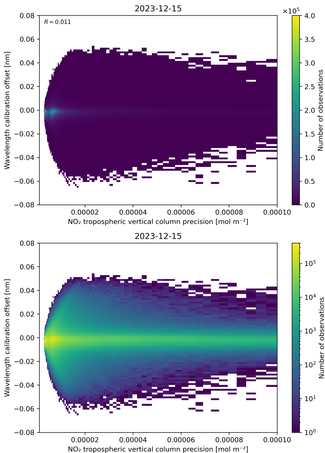
Figure 141: Scatter density plot of “NO 2 tropospheric vertical column precision” against “Wavelength calibration offset” for 2023-12-14 to 2023-12-16.
