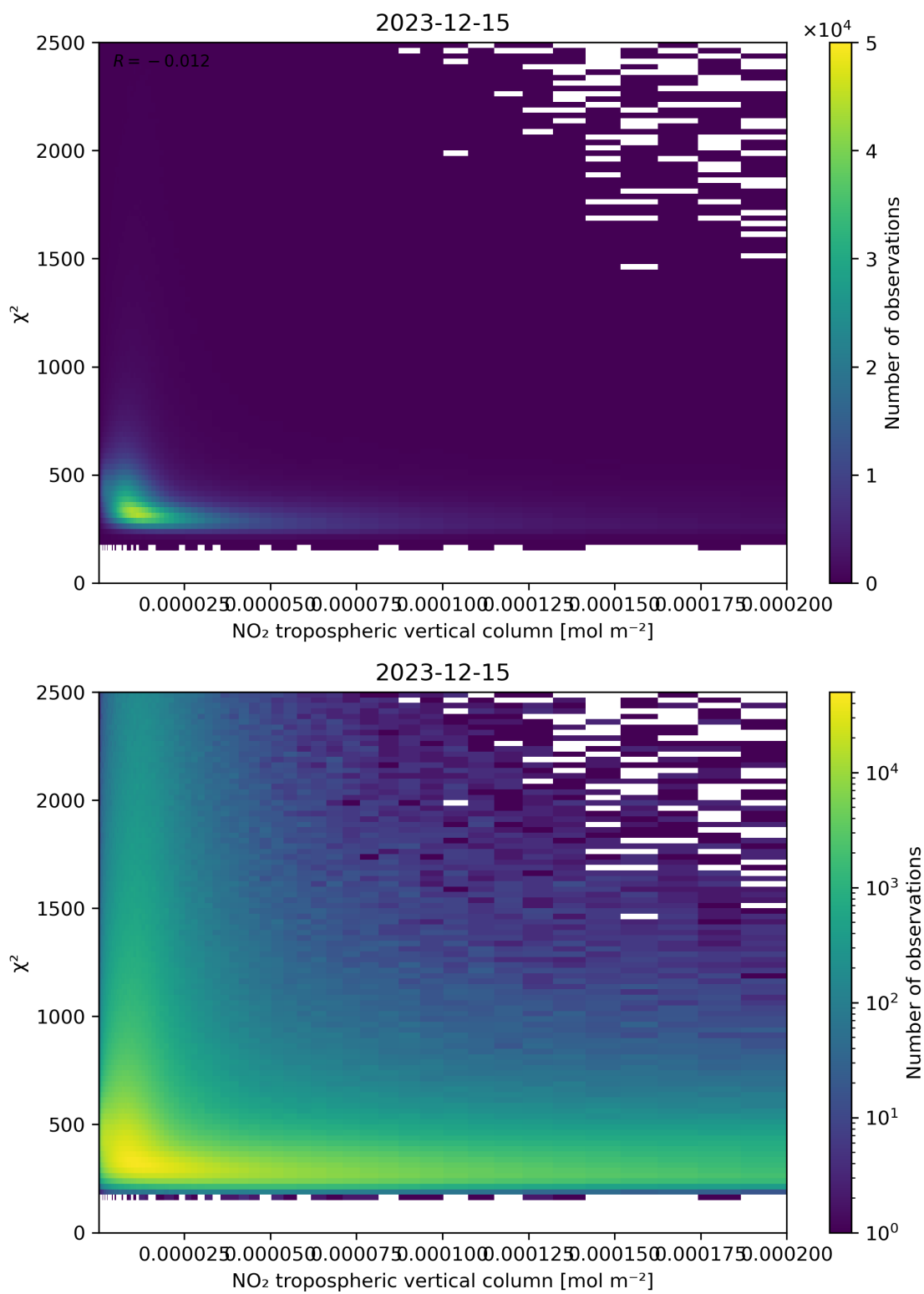
Figure 124: Scatter density plot of “NO 2 tropospheric vertical column” against “ \chi^2 ” for 2023-12-14 to 2023-12-16.
