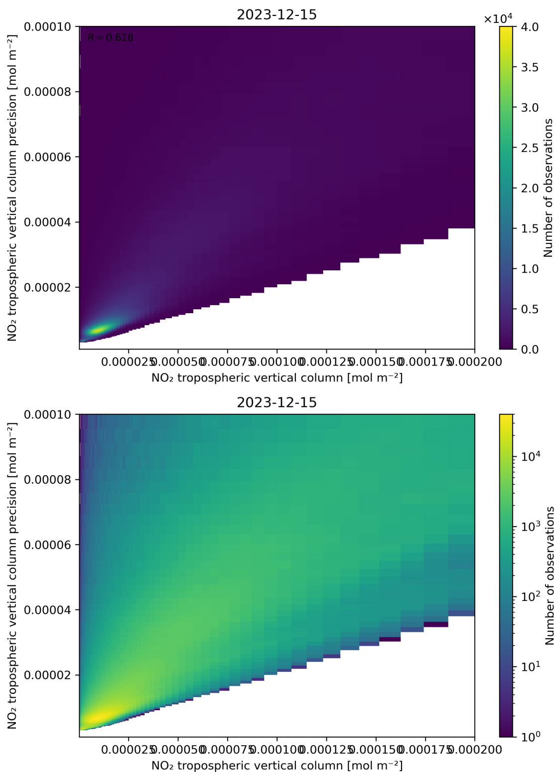
Figure 130: Scatter density plot of “NO 2 tropospheric vertical column” against “NO 2 tropospheric vertical column precision” for 2023-12-14 to 2023-12-16.
