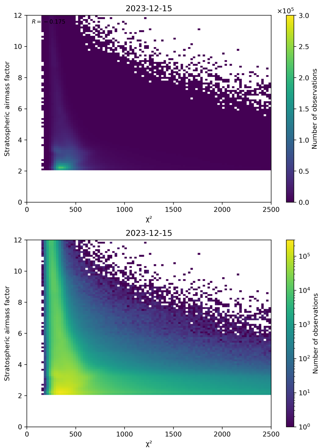
Figure 81: Scatter density plot of “ \chi^2 ” against “Stratospheric airmass factor” for 2023-12-14 to 2023-12-16.
