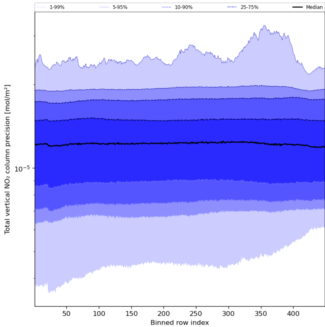
Figure 56: Along track statistics of “Total vertical NO 2 column precision” for 2023-12-14 to 2023-12-16
