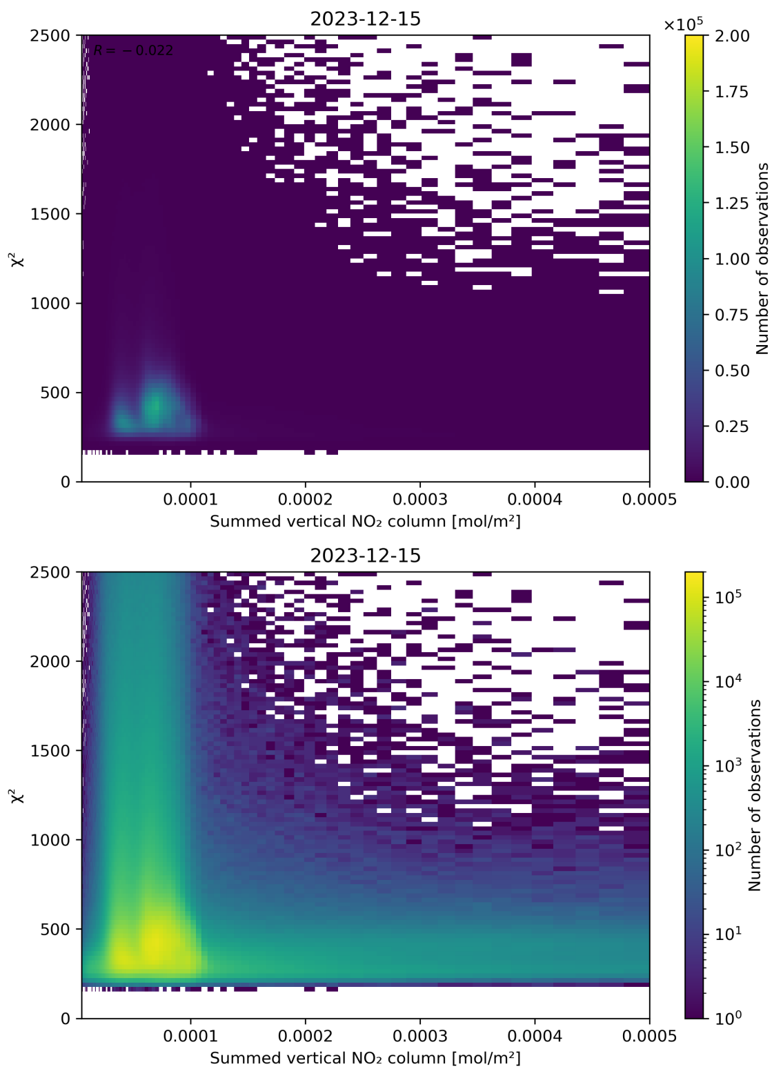
Figure 104: Scatter density plot of “Summed vertical NO 2 column” against “ \chi^2 ” for 2023-12-14 to 2023-12-16.
