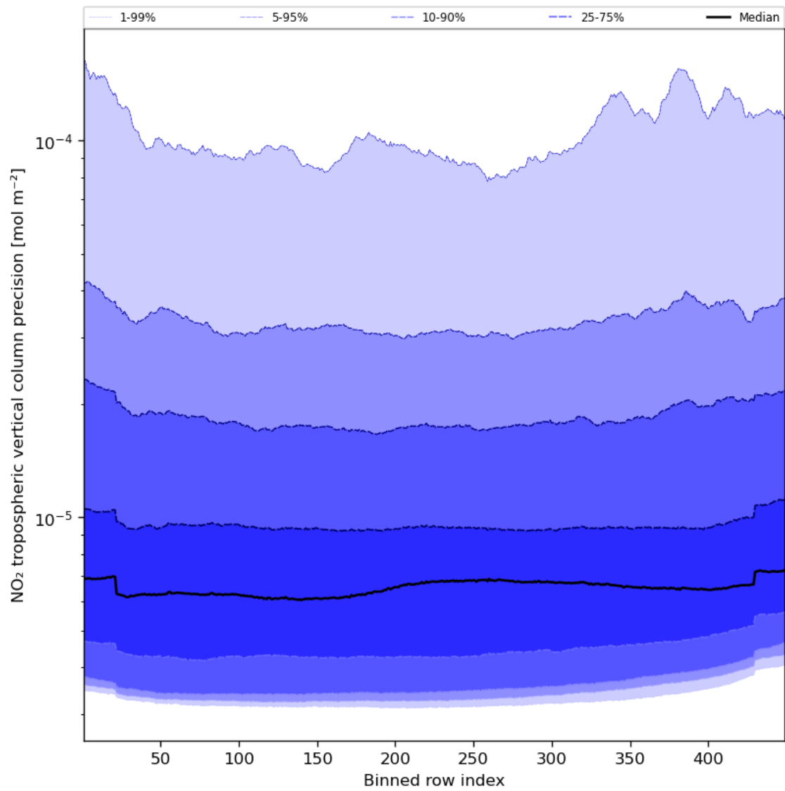
Figure 47: Along track statistics of “NO 2 tropospheric vertical column precision” for 2023-12-14 to 2023-12-16
