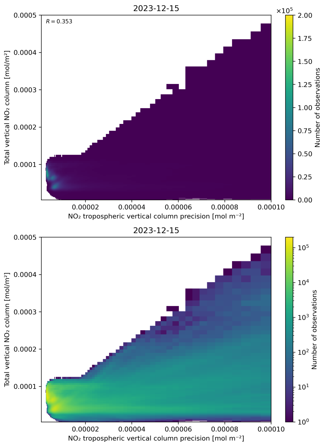
Figure 138: Scatter density plot of “NO 2 tropospheric vertical column precision” against “Total vertical NO 2 column” for 2023-12-14 to 2023-12-16.
