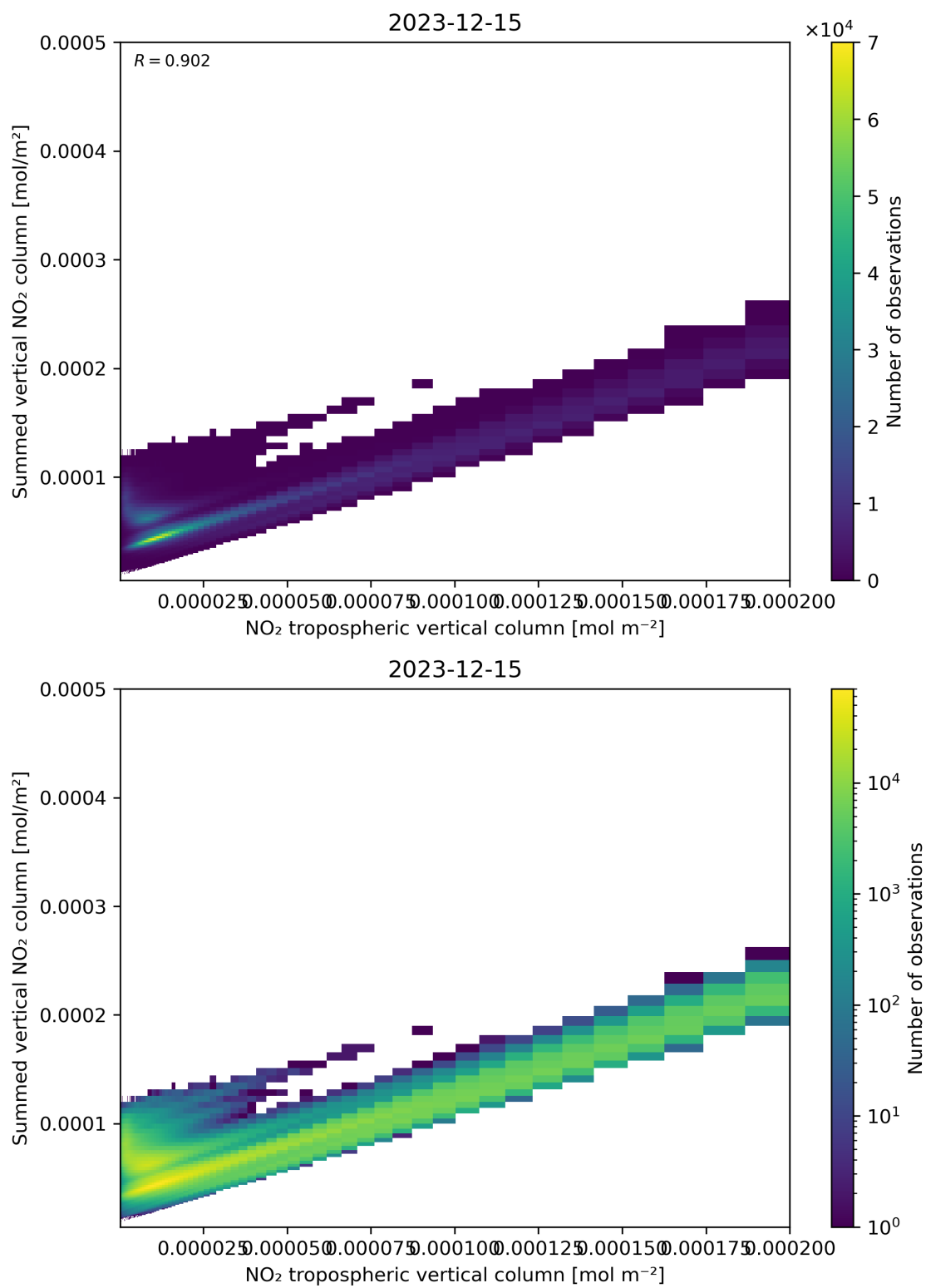
Figure 126: Scatter density plot of “NO 2 tropospheric vertical column” against “Summed vertical NO 2 column” for 2023-12-14 to 2023-12-16.
