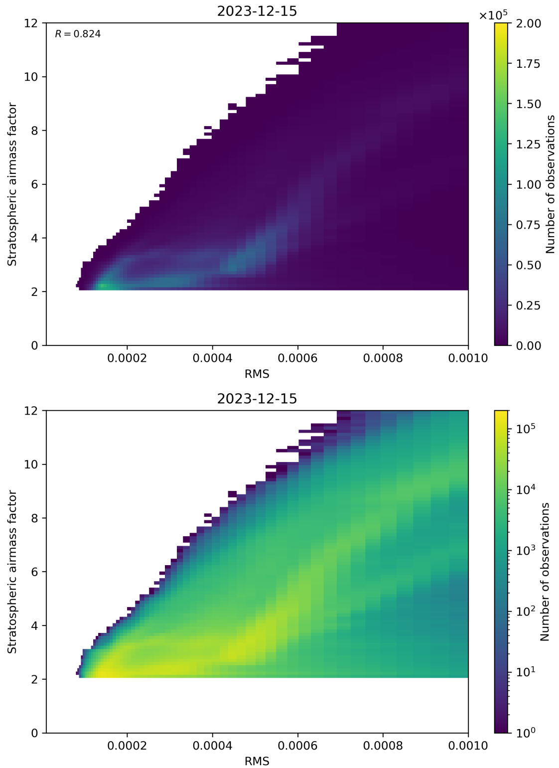
Figure 144: Scatter density plot of “RMS” against “Stratospheric airmass factor” for 2023-12-14 to 2023-12-16.
