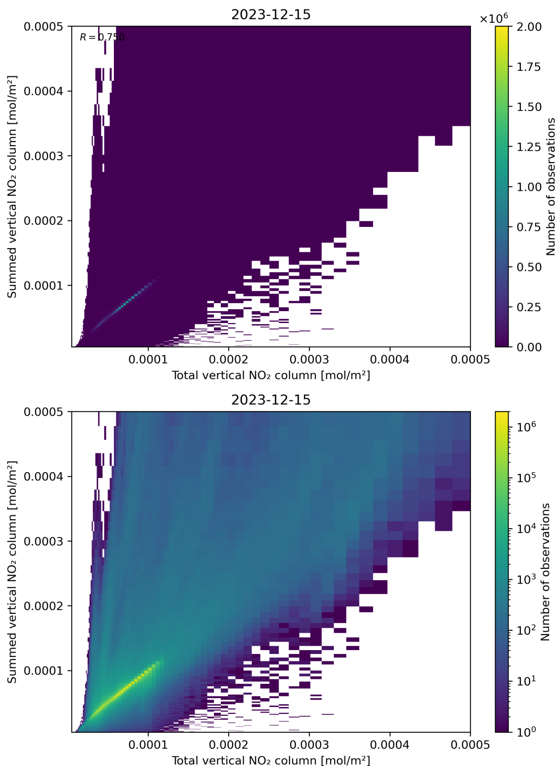
Figure 112: Scatter density plot of “Total vertical NO 2 column” against “Summed vertical NO 2 column” for 2023-12-14 to 2023-12-16.
