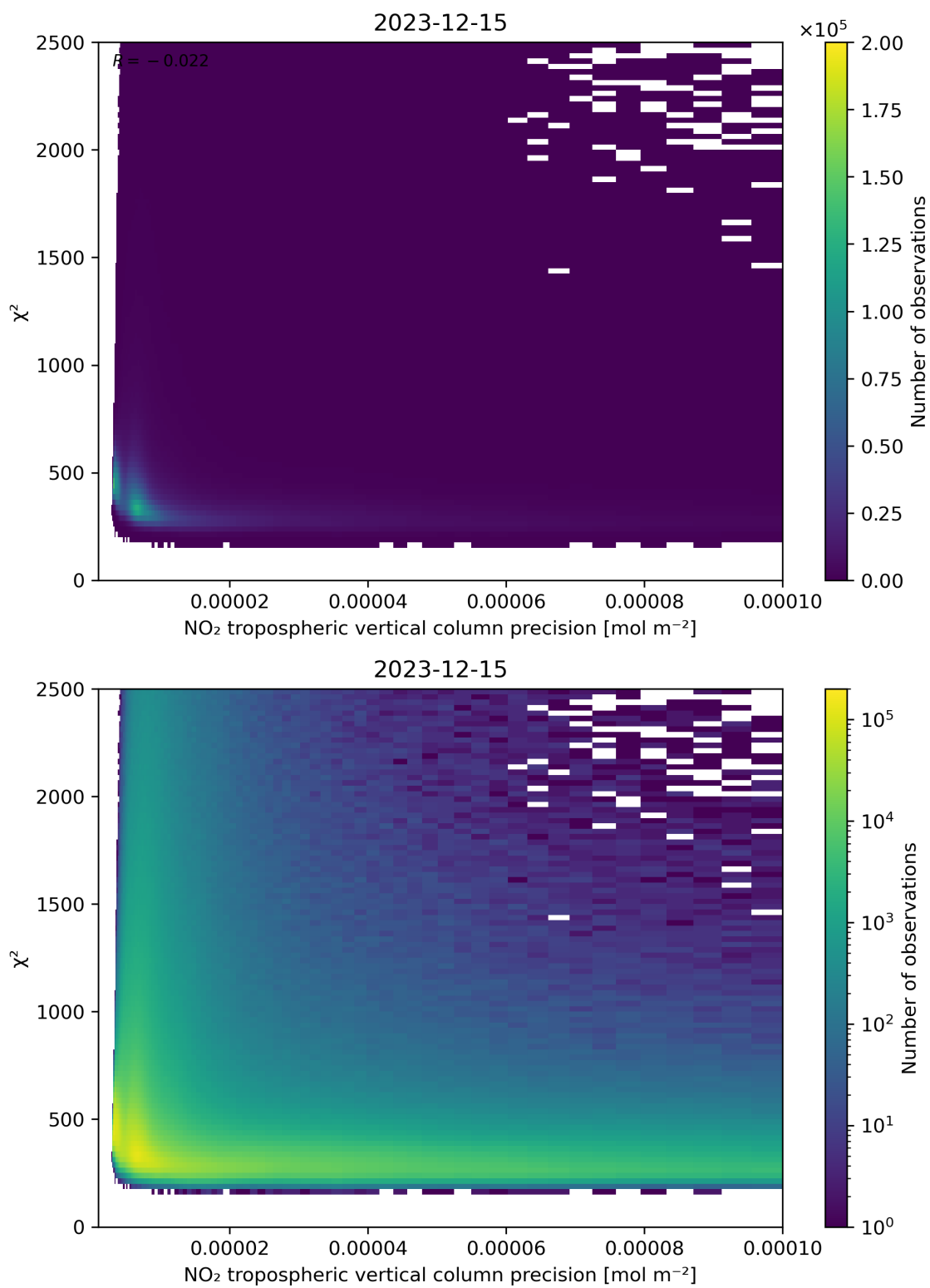
Figure 134: Scatter density plot of “NO 2 tropospheric vertical column precision” against “ \chi^2 ” for 2023-12-14 to 2023-12-16.
