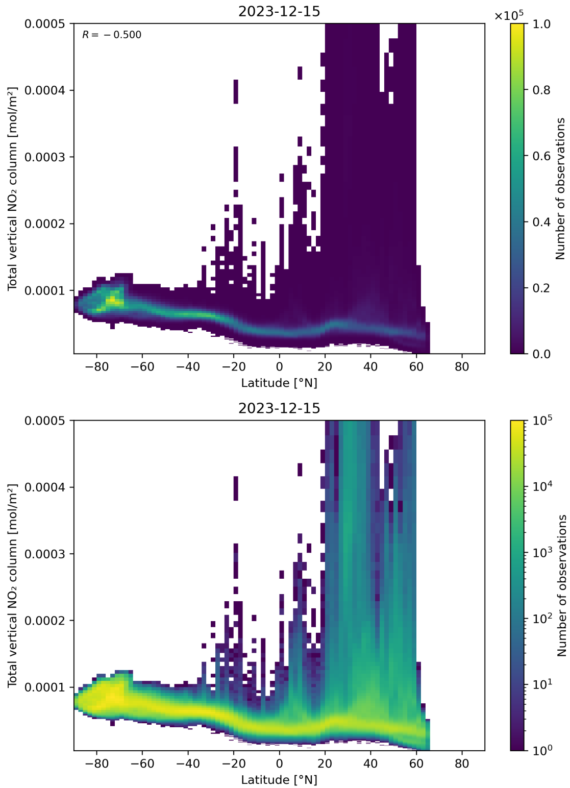
Figure 90: Scatter density plot of “Latitude” against “Total vertical NO 2 column” for 2023-12-14 to 2023-12-16.
