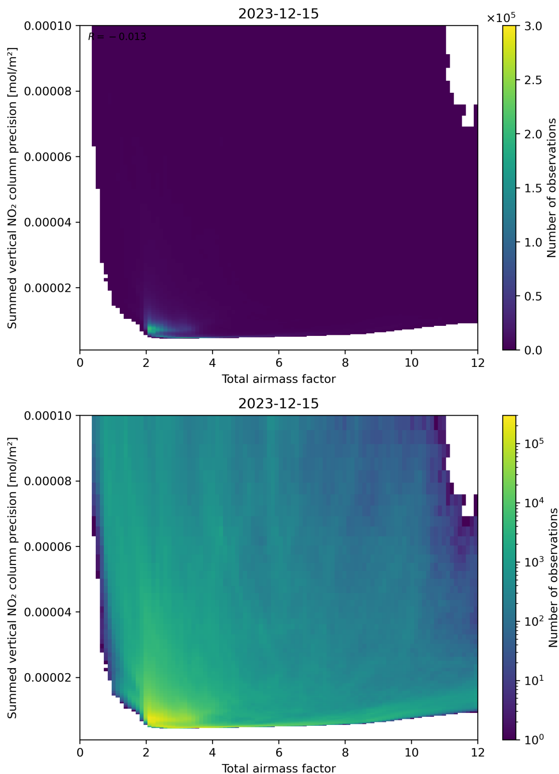
Figure 66: Scatter density plot of “Total airmass factor” against “Summed vertical NO 2 column precision” for 2023-12-14 to 2023-12-16.
