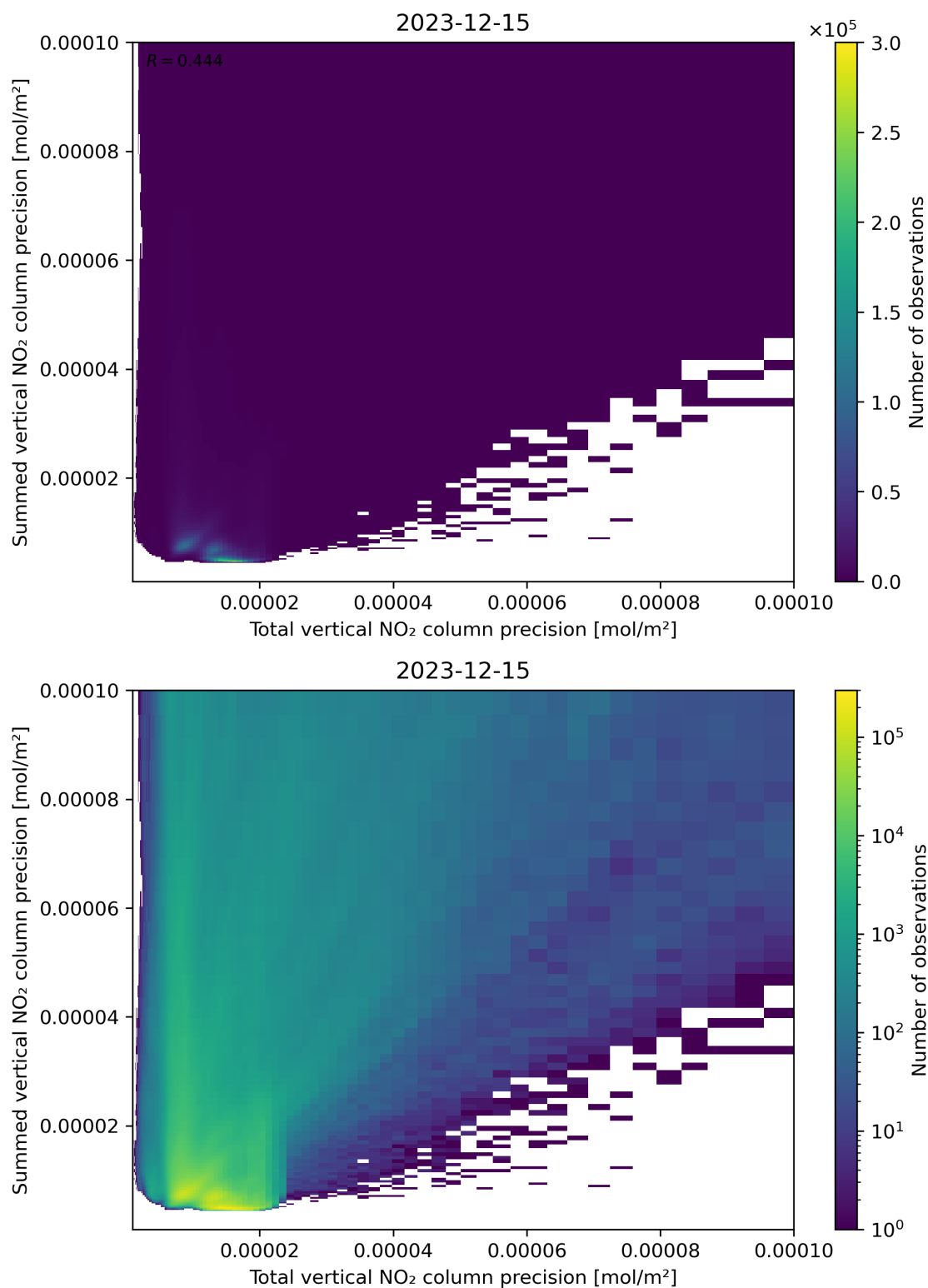
Figure 118: Scatter density plot of “Total vertical NO 2 column precision” against “Summed vertical NO 2 column precision” for 2023-12-14 to 2023-12-16.
