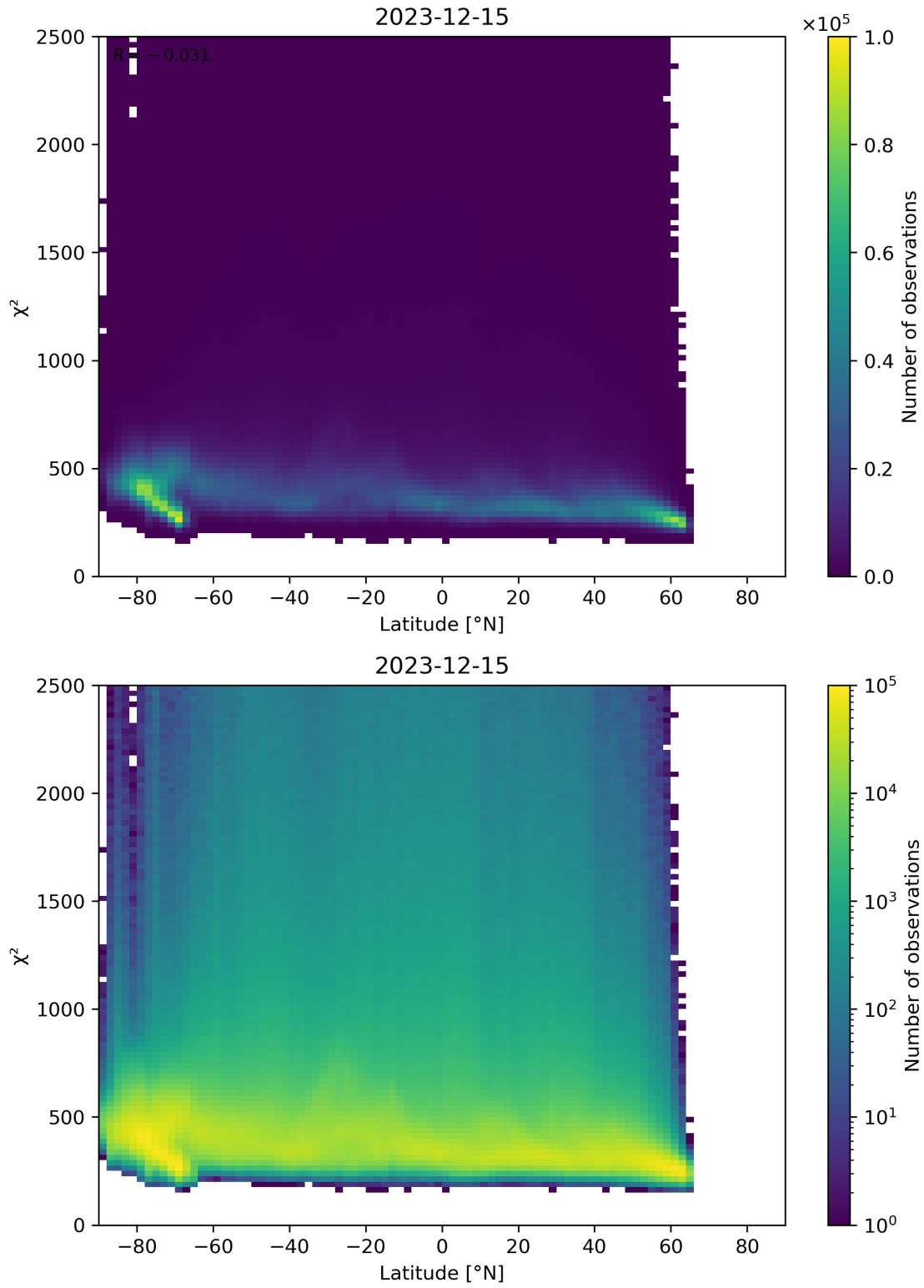
Figure 86: Scatter density plot of “Latitude” against “ \chi^2 ” for 2023-12-14 to 2023-12-16.
