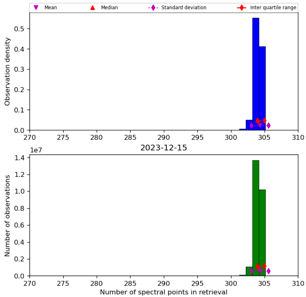
Figure 33: Histogram of “Number of spectral points in retrieval” for 2023-12-14 to 2023-12-16
