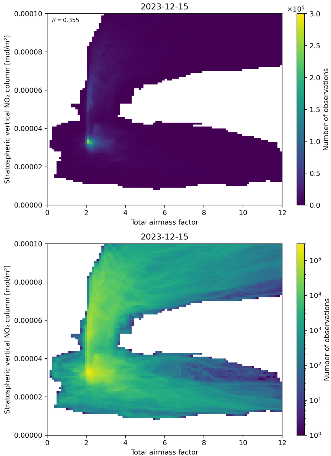
Figure 64: Scatter density plot of “Total airmass factor” against “Stratospheric vertical NO 2 column” for 2023-12-14 to 2023-12-16.
