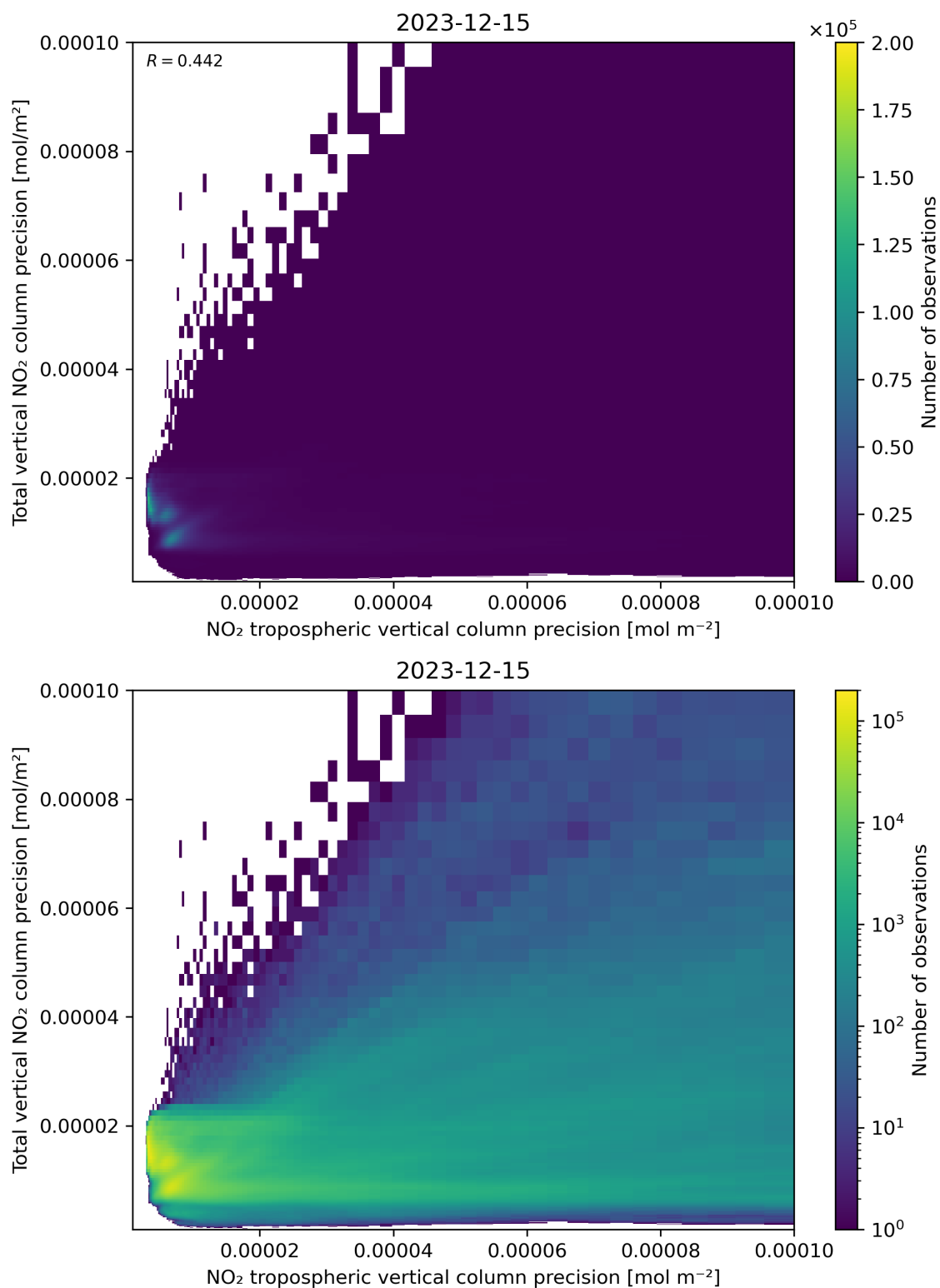
Figure 139: Scatter density plot of “NO 2 tropospheric vertical column precision” against “Total vertical NO 2 column precision” for 2023-12-14 to 2023-12-16.
