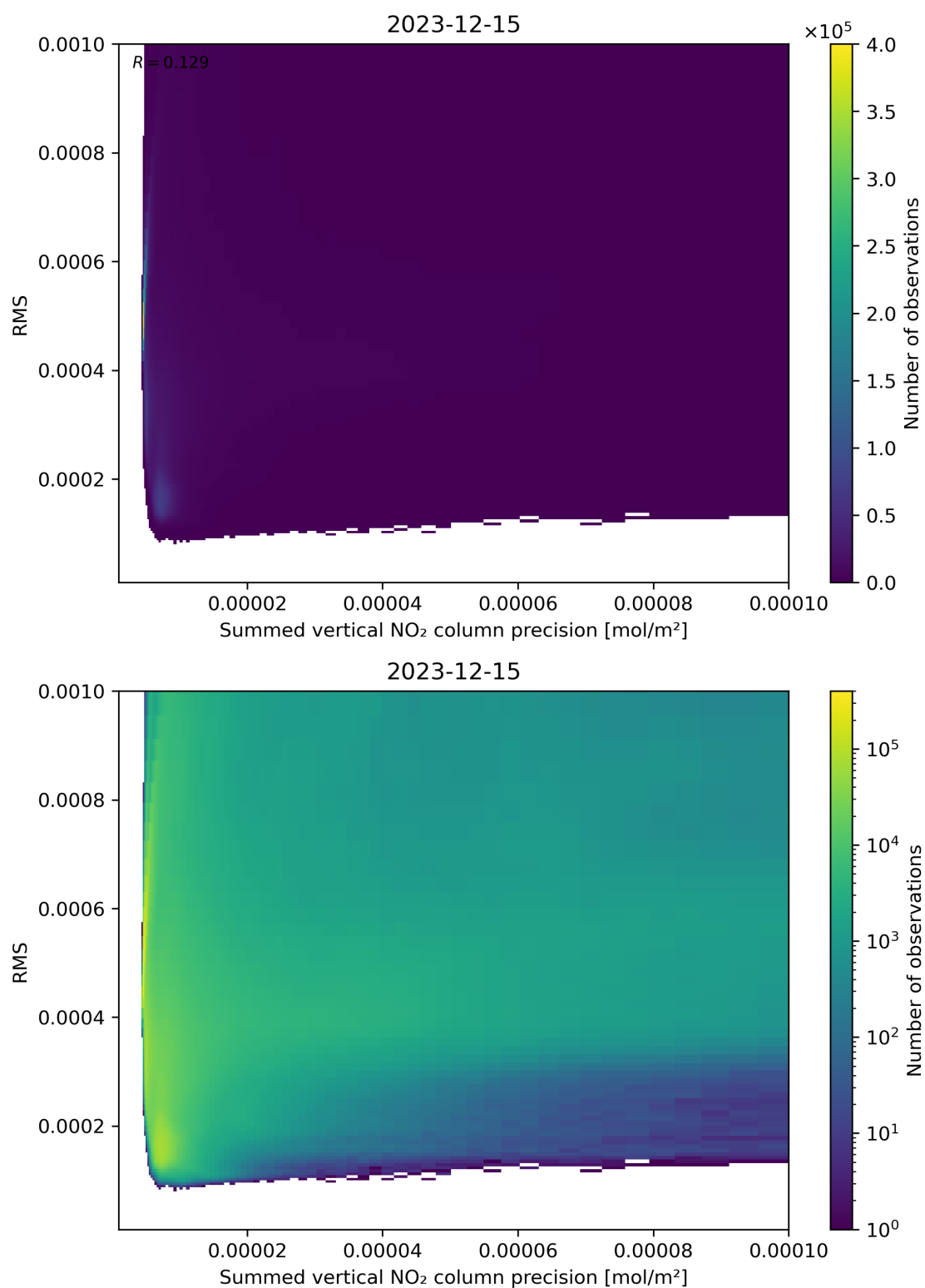
Figure 108: Scatter density plot of “Summed vertical NO 2 column precision” against “RMS” for 2023-12-14 to 2023-12-16.
