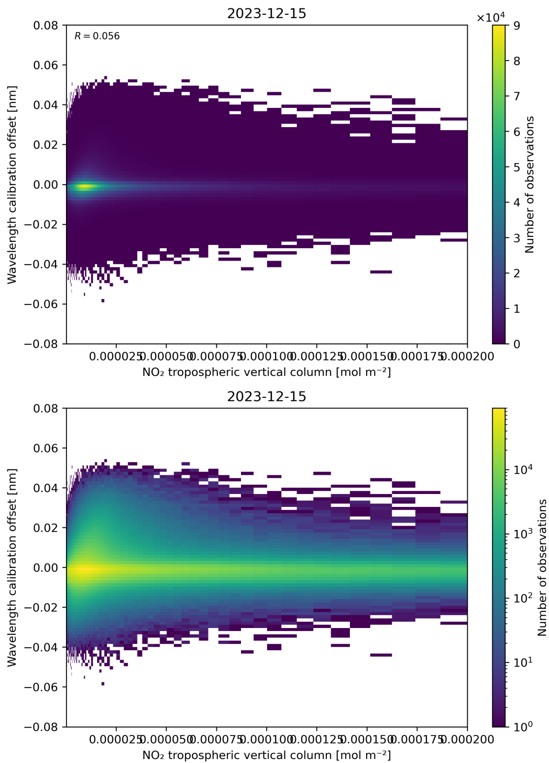
Figure 143: Scatter density plot of “NO 2 tropospheric vertical column” against “Wavelength calibration offset” for 2023-12-14 to 2023-12-16.
