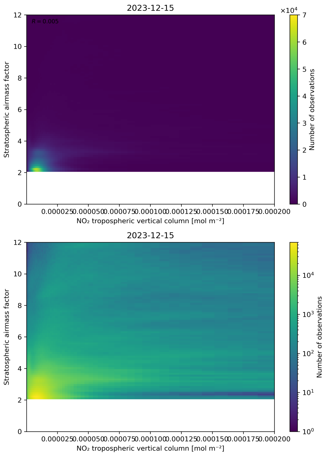
Figure 121: Scatter density plot of “NO 2 tropospheric vertical column” against “Stratospheric airmass factor” for 2023-12-14 to 2023-12-16.
