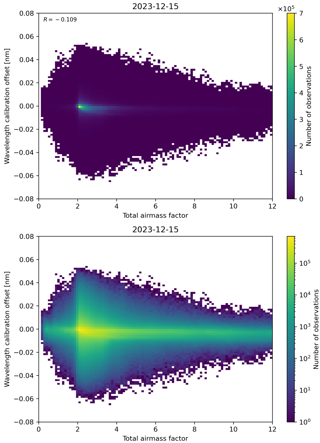
Figure 70: Scatter density plot of “Total airmass factor” against “Wavelength calibration offset” for 2023-12-14 to 2023-12-16.
