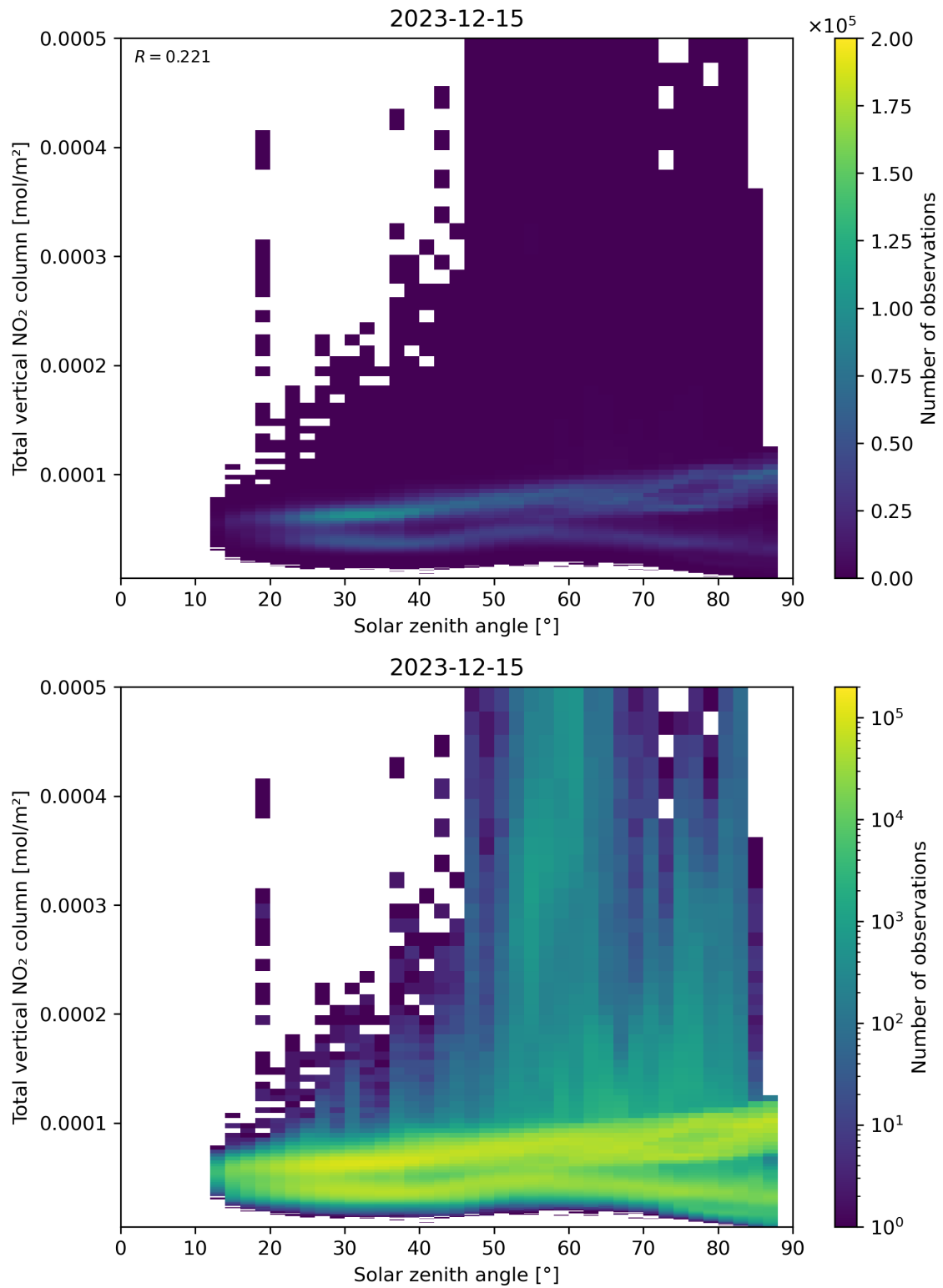
Figure 153: Scatter density plot of “Solar zenith angle” against “Total vertical NO 2 column” for 2023-12-14 to 2023-12-16.
