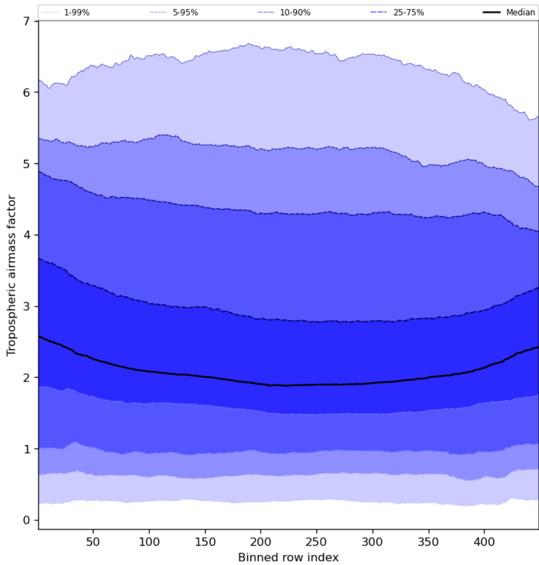
Figure 48: Along track statistics of “Tropospheric airmass factor” for 2023-12-14 to 2023-12-16
