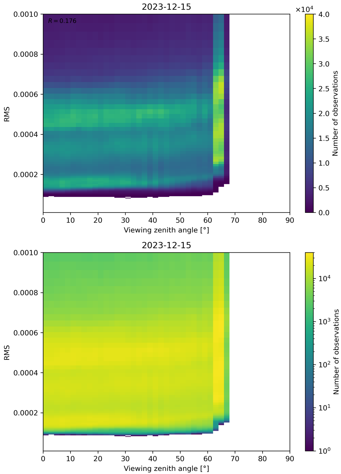
Figure 171: Scatter density plot of “Viewing zenith angle” against “RMS” for 2023-12-14 to 2023-12-16.
