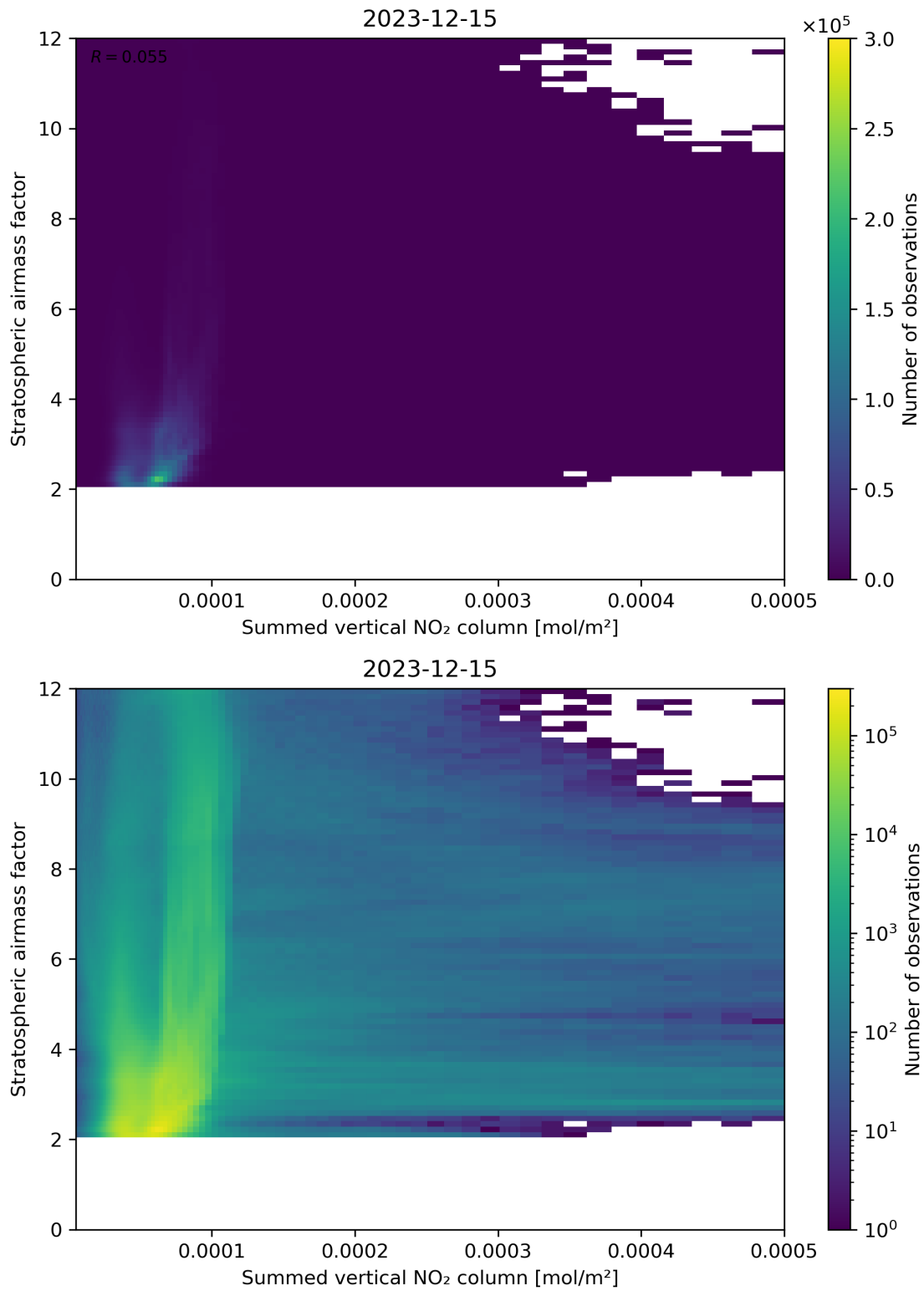
Figure 103: Scatter density plot of “Summed vertical NO 2 column” against “Stratospheric air mass factor” for 2023-12-14 to 2023-12-16.
