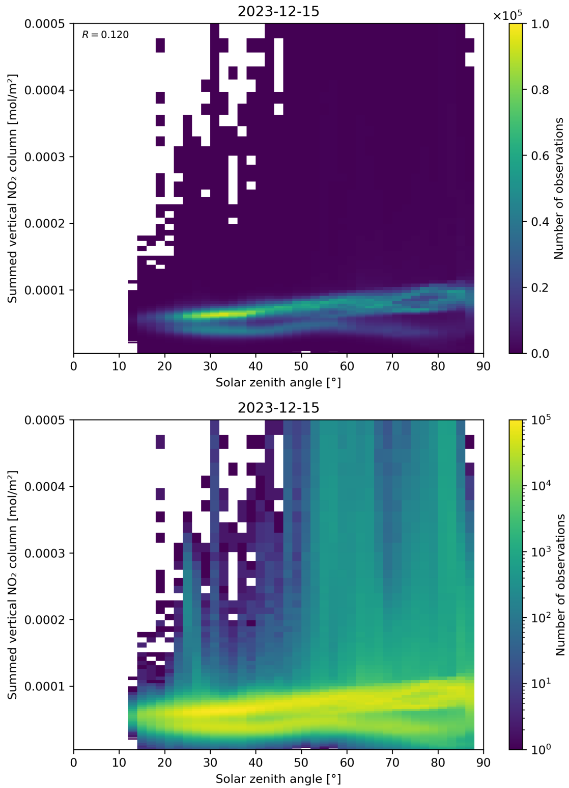
Figure 151: Scatter density plot of “Solar zenith angle” against “Summed vertical NO 2 column” for 2023-12-14 to 2023-12-16.
