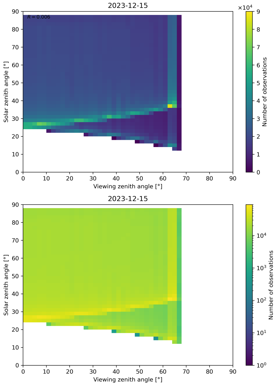
Figure 172: Scatter density plot of “Viewing zenith angle” against “Solar zenith angle” for 2023-12-14 to 2023-12-16.
