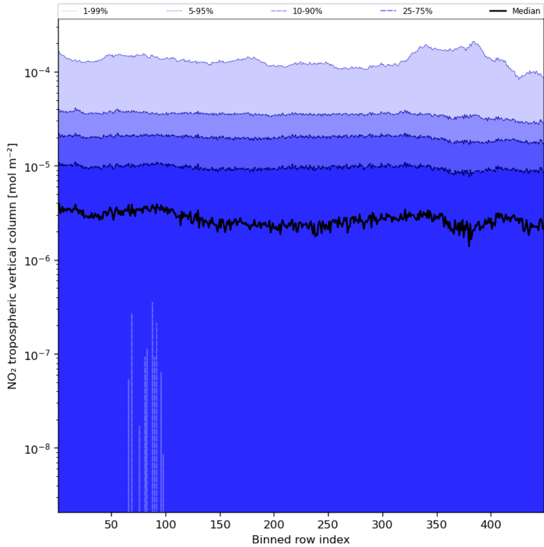
Figure 46: Along track statistics of “NO 2 tropospheric vertical column” for 2023-12-14 to 2023-12-16
