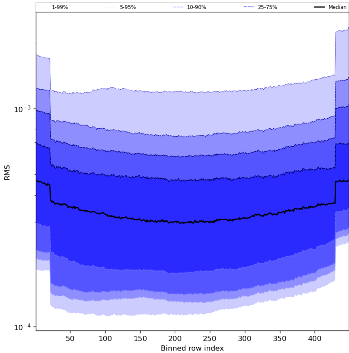
Figure 60: Along track statistics of “RMS” for 2023-12-14 to 2023-12-16
