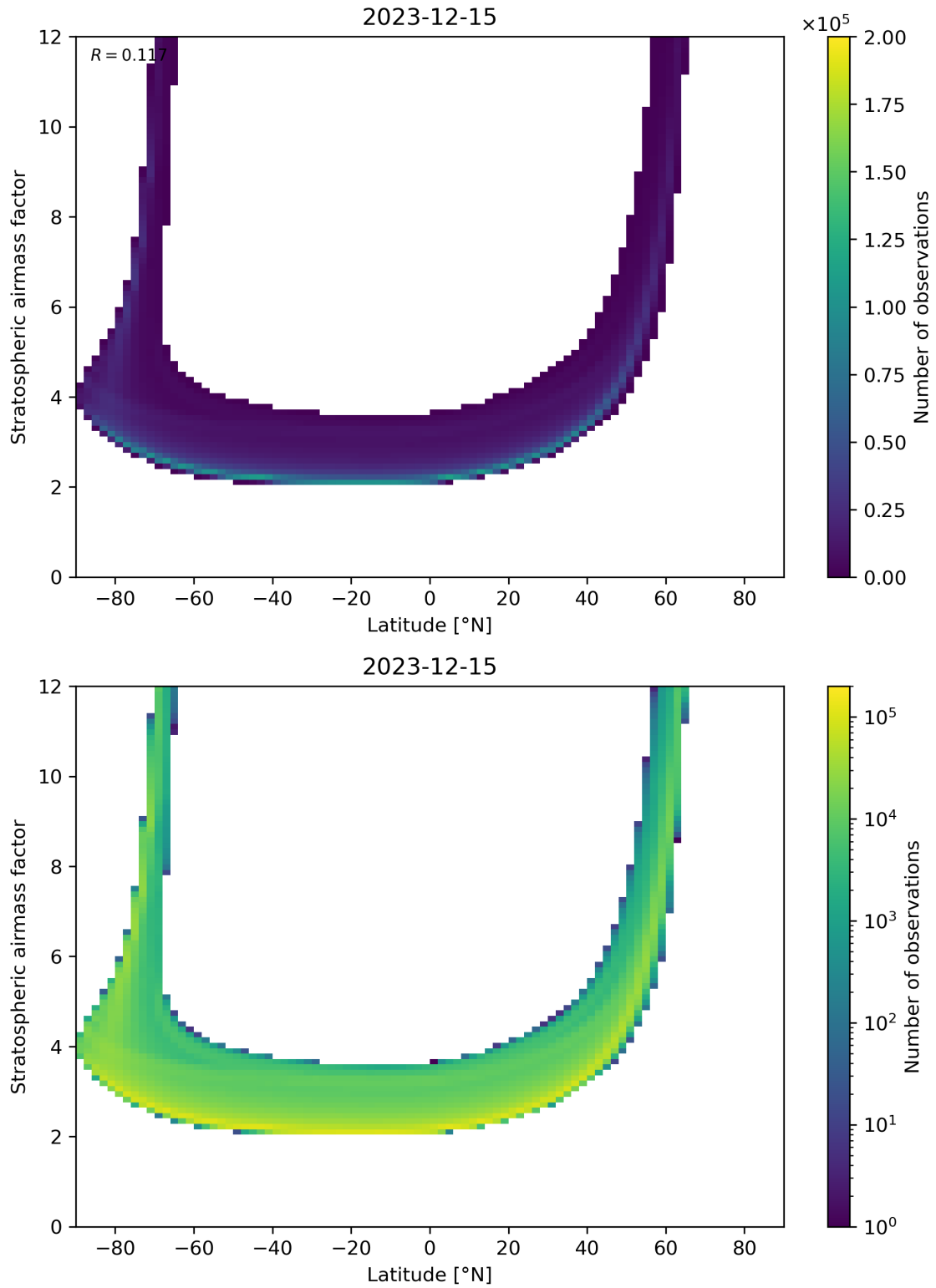
Figure 83: Scatter density plot of “Latitude” against “Stratospheric airmass factor” for 2023-12-14 to 2023-12-16.
