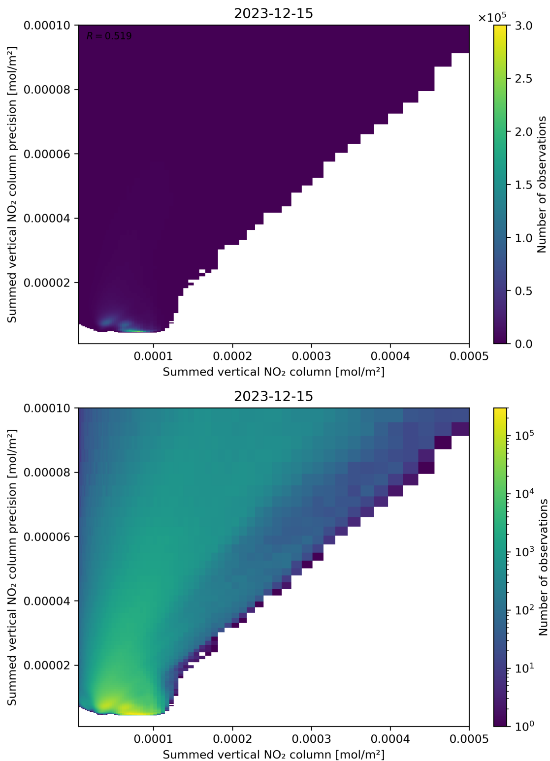
Figure 105: Scatter density plot of “Summed vertical NO 2 column” against “Summed vertical NO 2 column precision” for 2023-12-14 to 2023-12-16.
