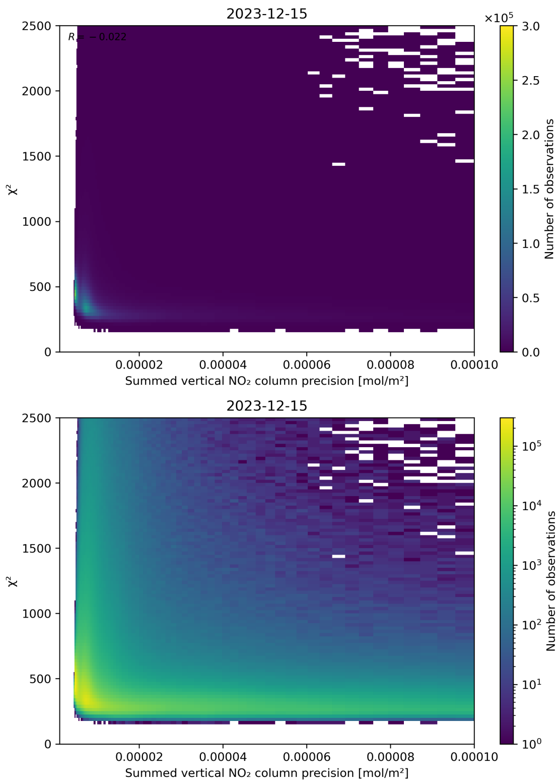
Figure 107: Scatter density plot of “Summed vertical NO 2 column precision” against “ \chi^2 ” for 2023-12-14 to 2023-12-16.
