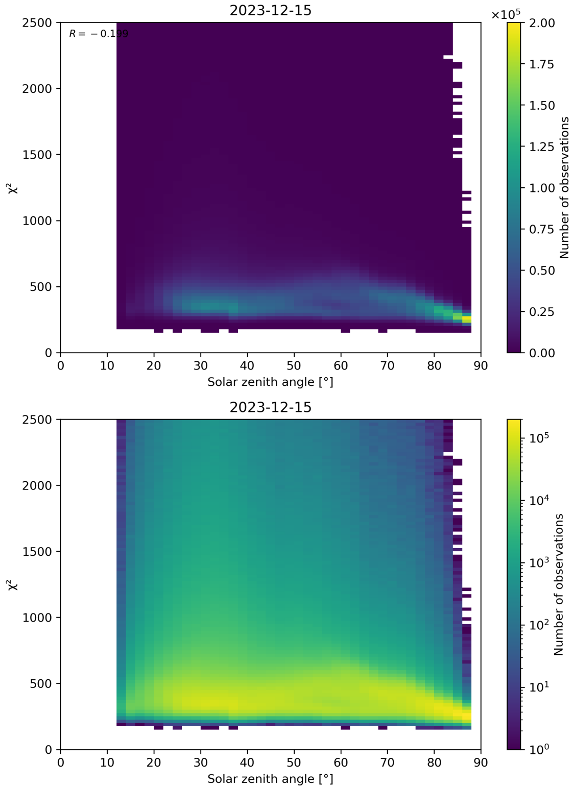
Figure 148: Scatter density plot of “Solar zenith angle” against “ \chi^2 ” for 2023-12-14 to 2023-12-16.
