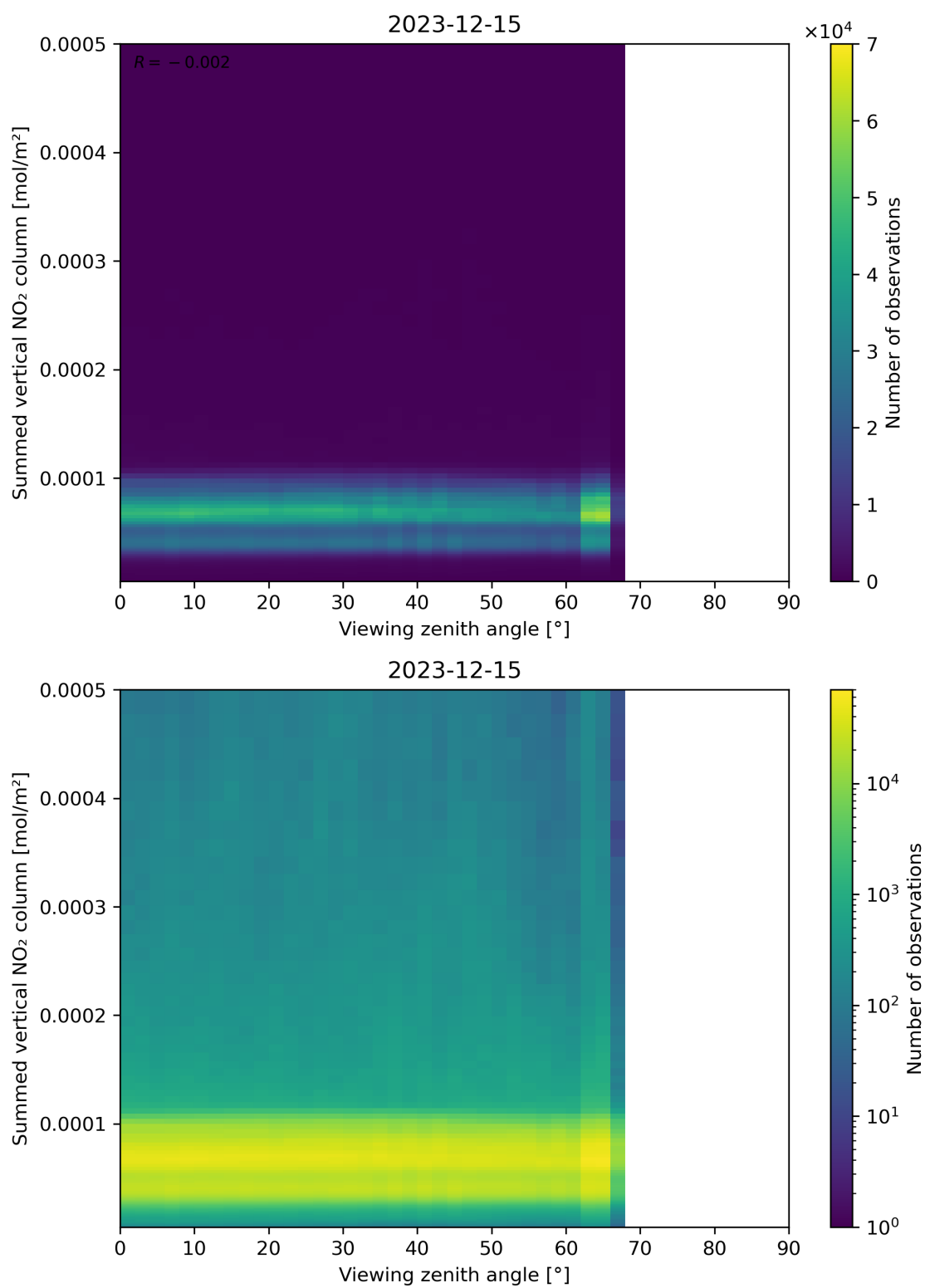
Figure 165: Scatter density plot of “Viewing zenith angle” against “Summed vertical NO 2 column” for 2023-12-14 to 2023-12-16.
