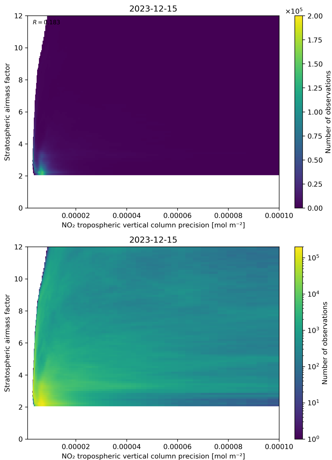
Figure 131: Scatter density plot of “NO 2 tropospheric vertical column precision” against “Stratospheric airmass factor” for 2023-12-14 to 2023-12-16.
