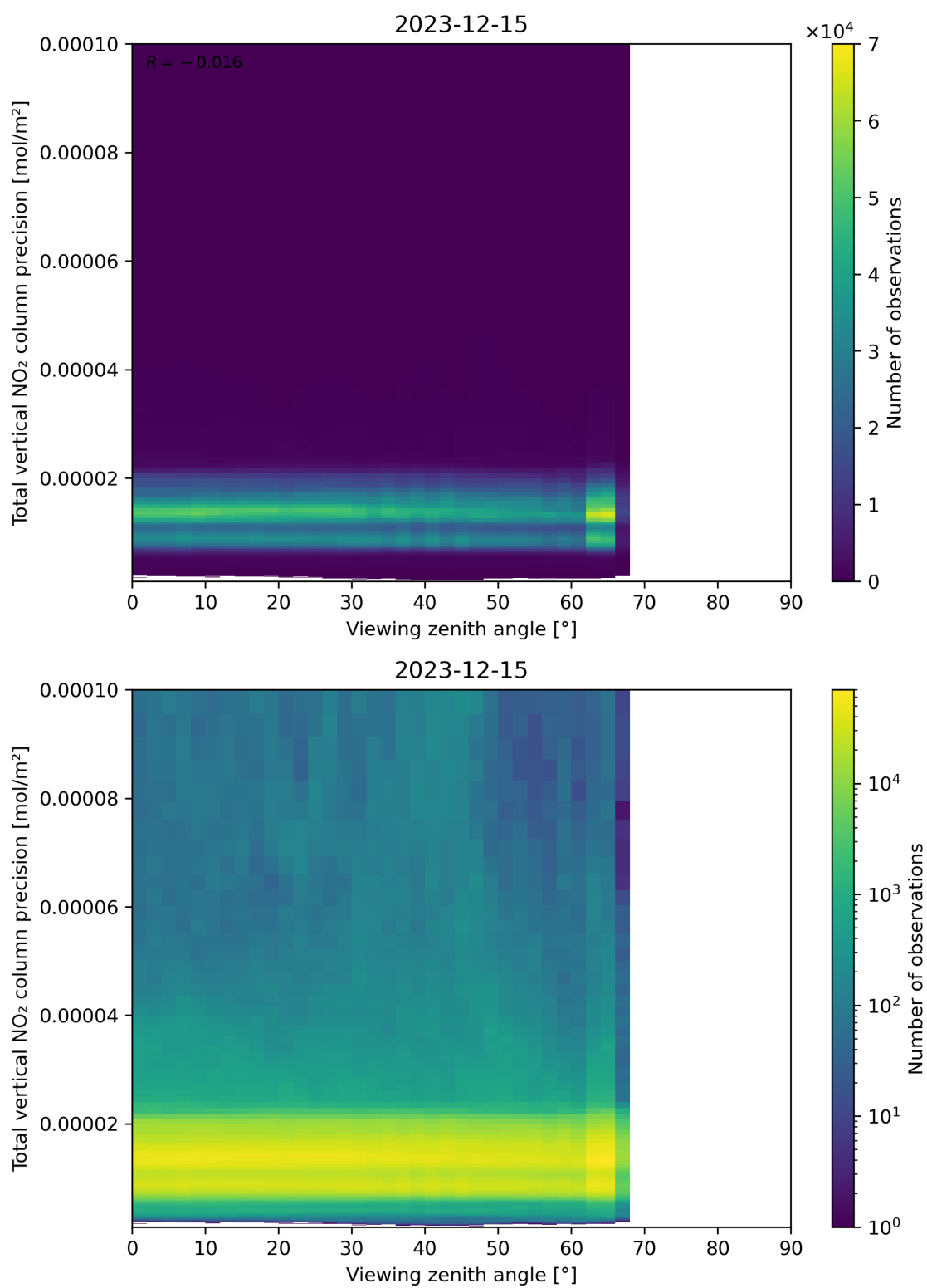
Figure 168: Scatter density plot of “Viewing zenith angle” against “Total vertical NO 2 column precision” for 2023-12-14 to 2023-12-16.
