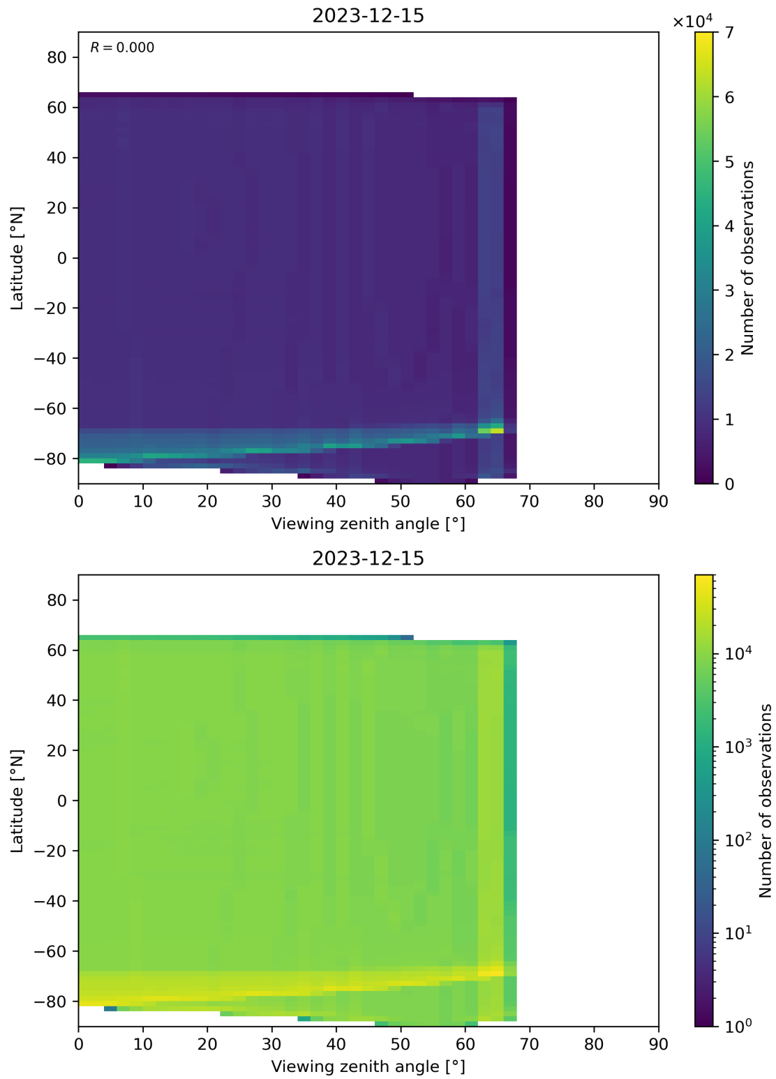
Figure 163: Scatter density plot of “Viewing zenith angle” against “Latitude” for 2023-12-14 to 2023-12-16.
