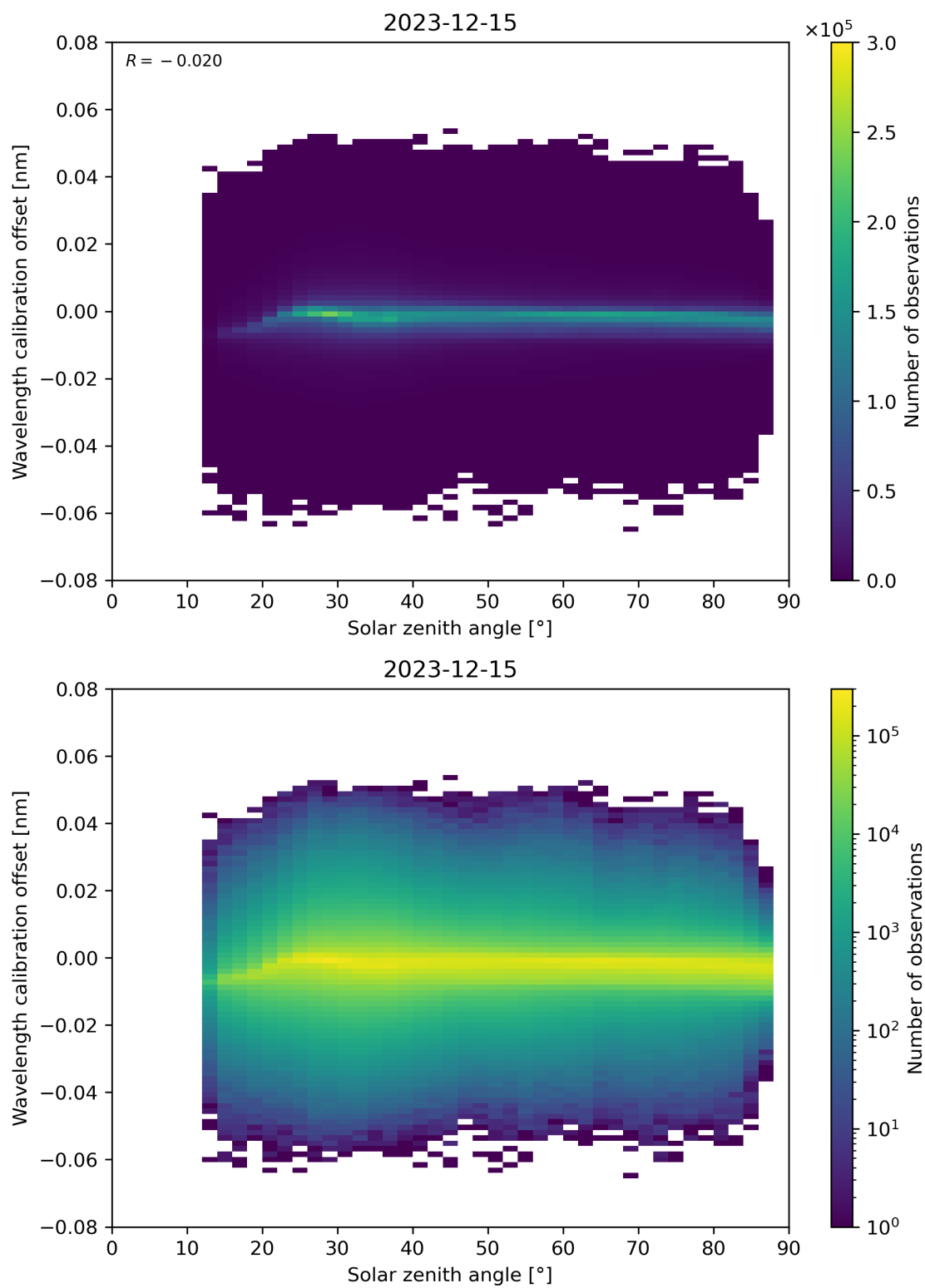
Figure 158: Scatter density plot of “Solar zenith angle” against “Wavelength calibration offset” for 2023-12-14 to 2023-12-16.
