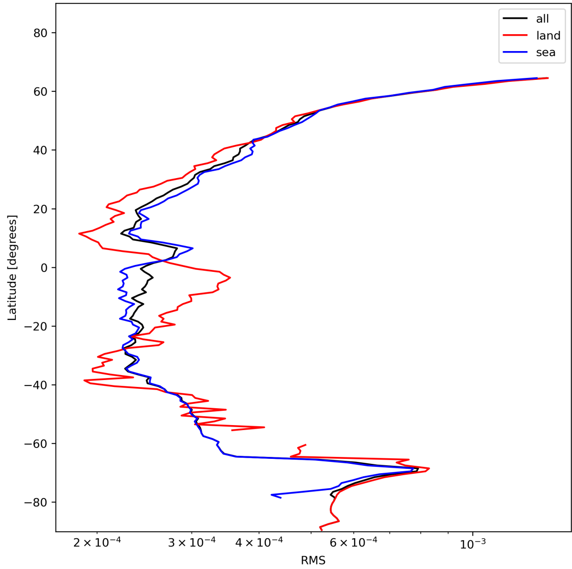
Figure 26: Zonal average of “RMS” for 2023-12-14 to 2023-12-16.
