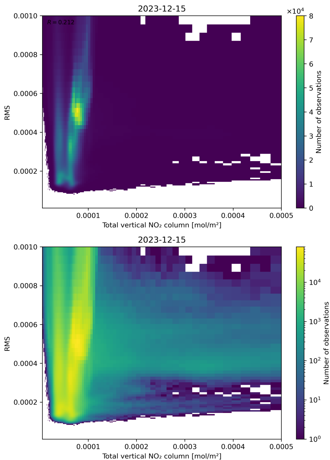
Figure 120: Scatter density plot of “Total vertical NO 2 column” against “RMS” for 2023-12-14 to 2023-12-16.
