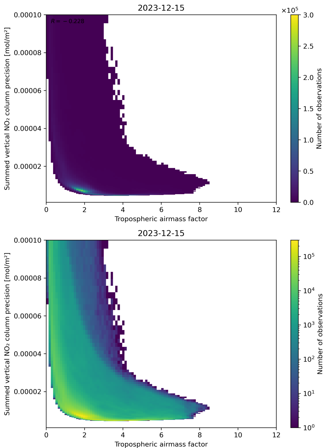
Figure 76: Scatter density plot of “Tropospheric air mass factor” against “Summed vertical NO 2 column precision” for 2023-12-14 to 2023-12-16.
