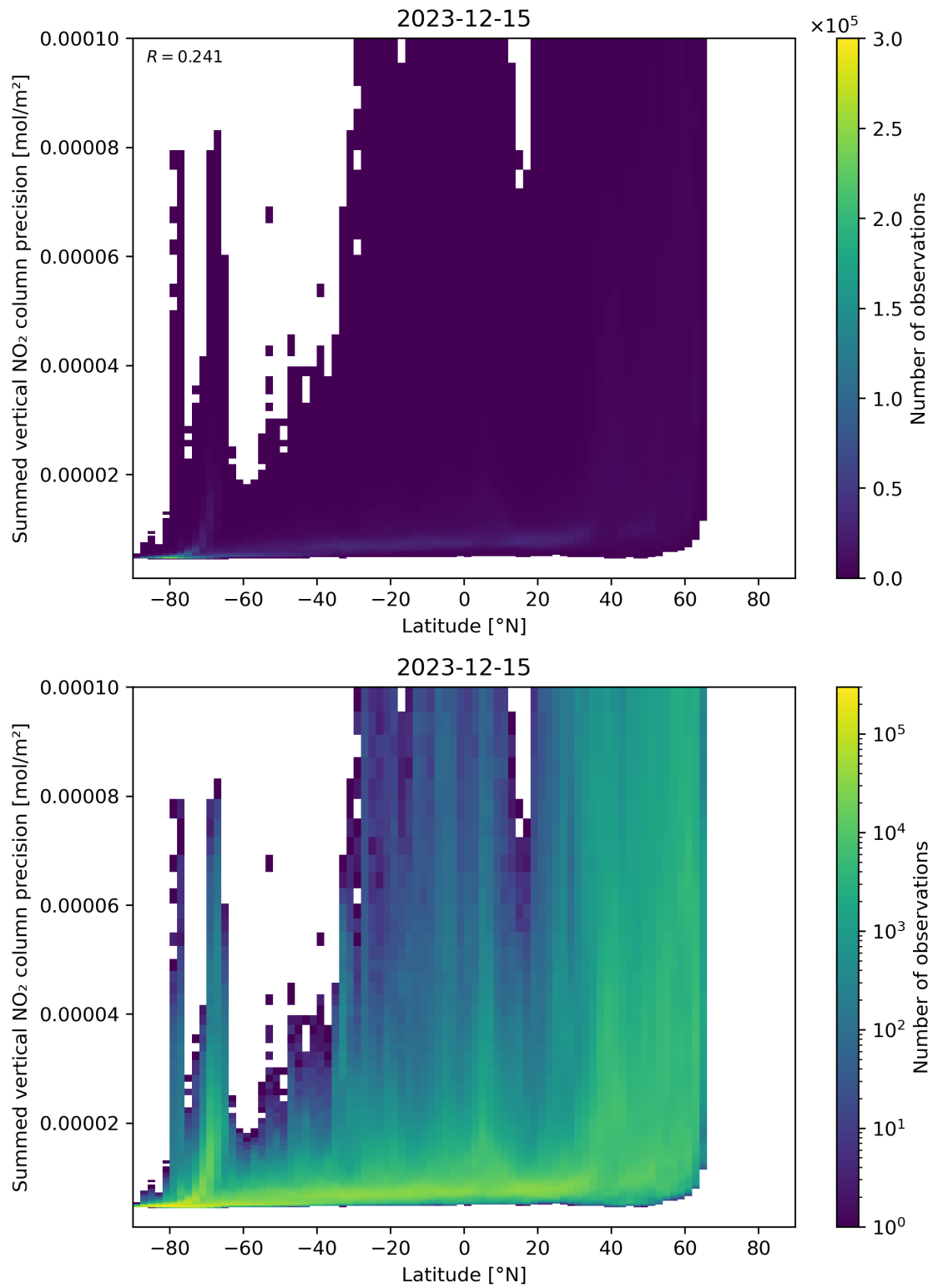
Figure 89: Scatter density plot of “Latitude” against “Summed vertical NO 2 column precision” for 2023-12-14 to 2023-12-16.
