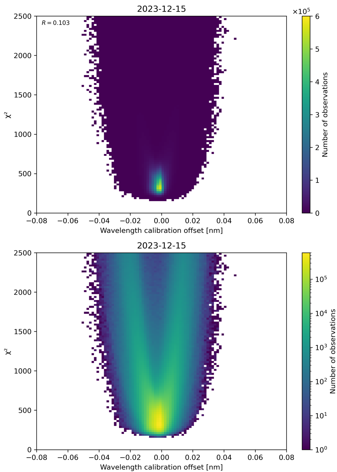
Figure 175: Scatter density plot of “Wavelength calibration offset” against “ \chi^2 ” for 2023-12-14 to 2023-12-16.
