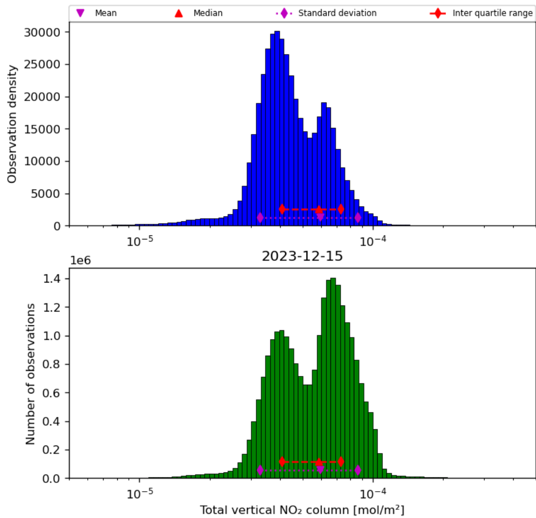
Figure 38: Histogram of “Total vertical NO 2 column” for 2023-12-14 to 2023-12-16
