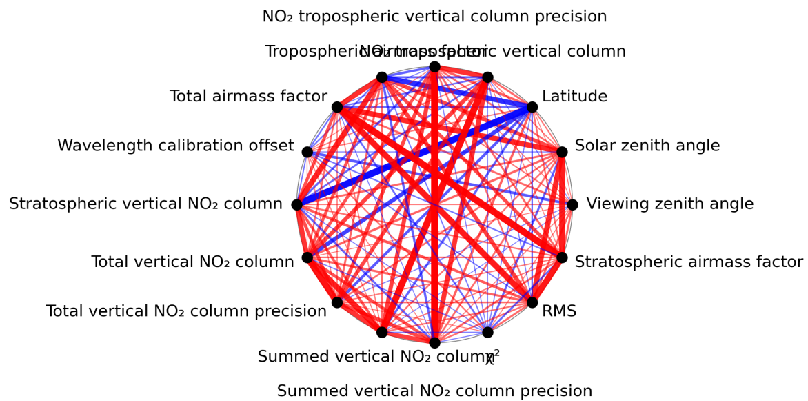
Figure 1: Map of correlation graph for 2023-12-14 to 2023-12-16.
