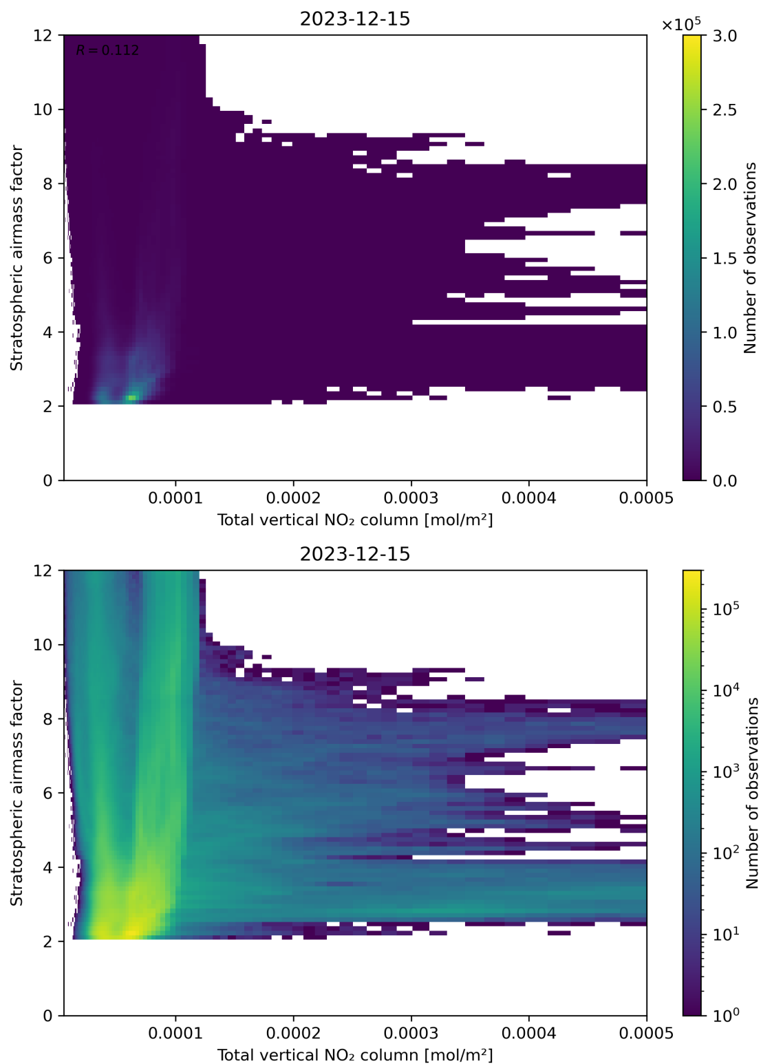
Figure 110: Scatter density plot of “Total vertical NO 2 column” against “Stratospheric airmass factor” for 2023-12-14 to 2023-12-16.
