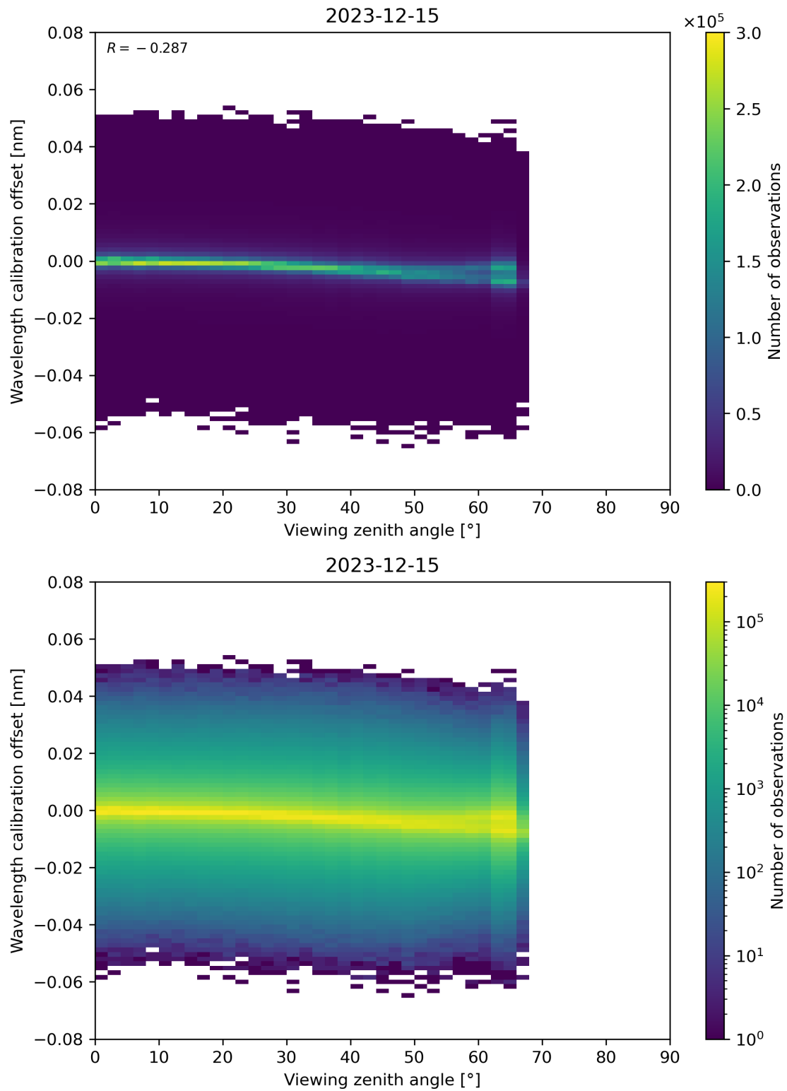
Figure 173: Scatter density plot of “Viewing zenith angle” against “Wavelength calibration offset” for 2023-12-14 to 2023-12-16.
