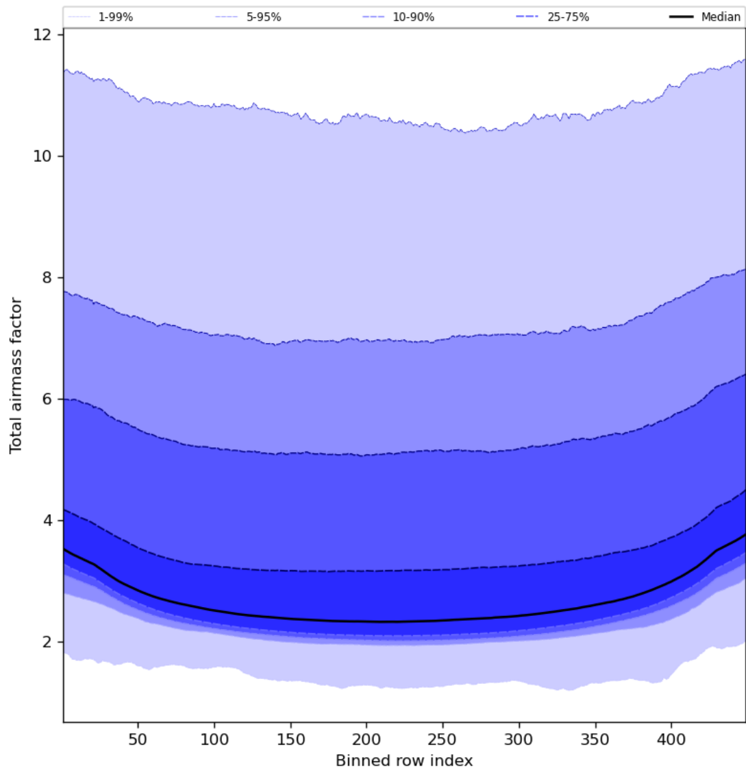
Figure 49: Along track statistics of “Total airmass factor” for 2023-12-14 to 2023-12-16
