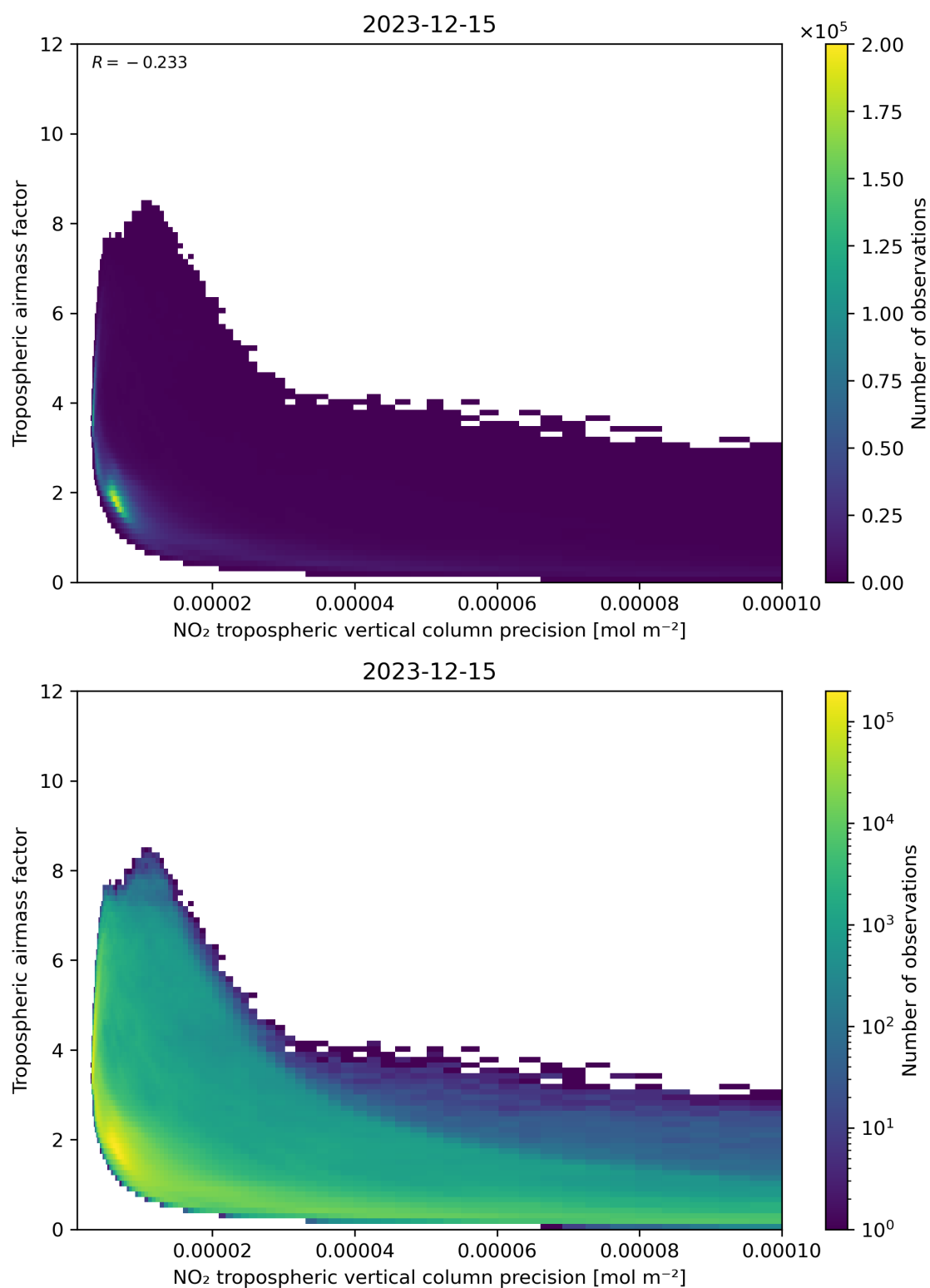
Figure 133: Scatter density plot of “NO 2 tropospheric vertical column precision” against “Tropospheric airmass factor” for 2023-12-14 to 2023-12-16.
