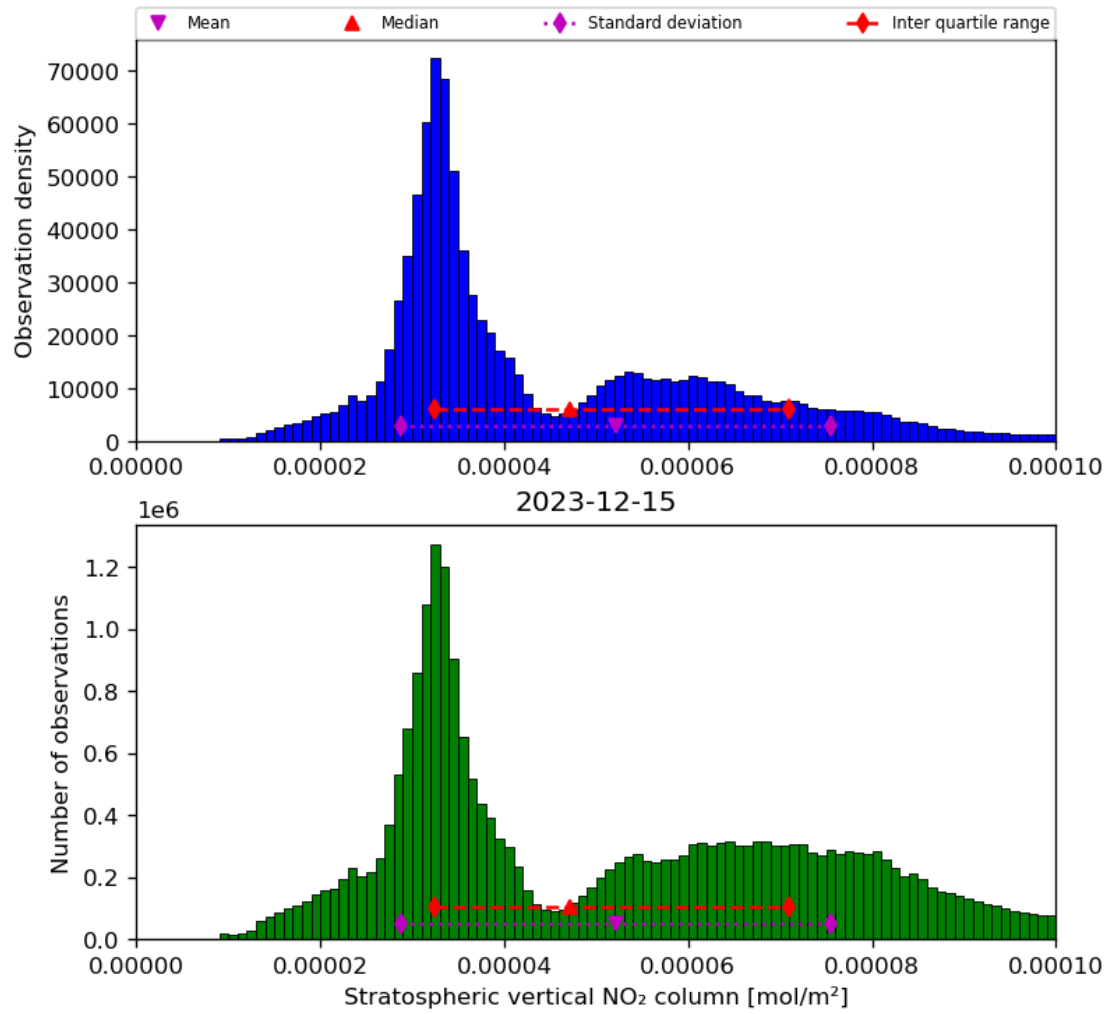
Figure 36: Histogram of “Stratospheric vertical NO 2 column” for 2023-12-14 to 2023-12-16
