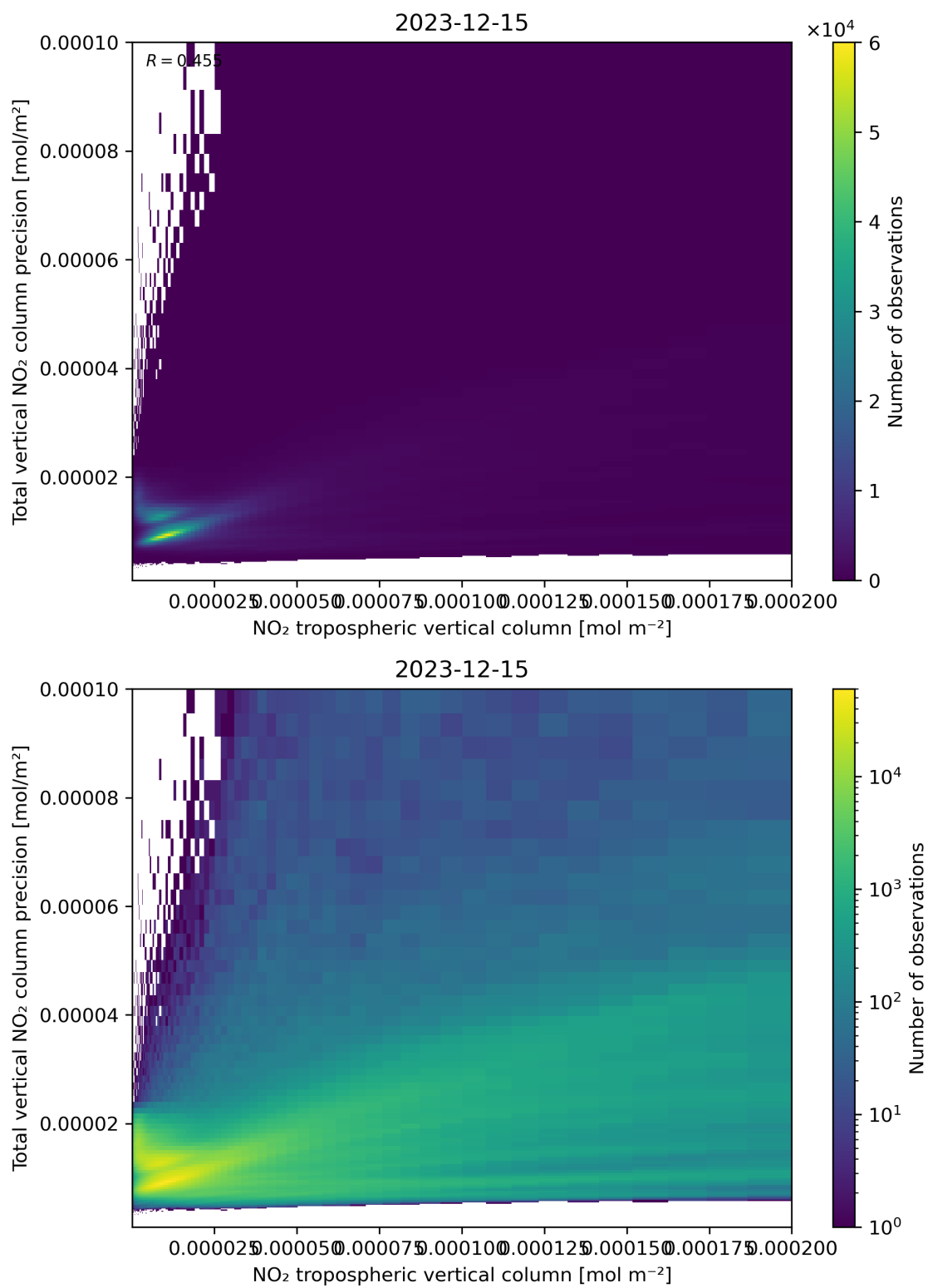
Figure 129: Scatter density plot of “NO 2 tropospheric vertical column” against “Total vertical NO 2 column precision” for 2023-12-14 to 2023-12-16.
