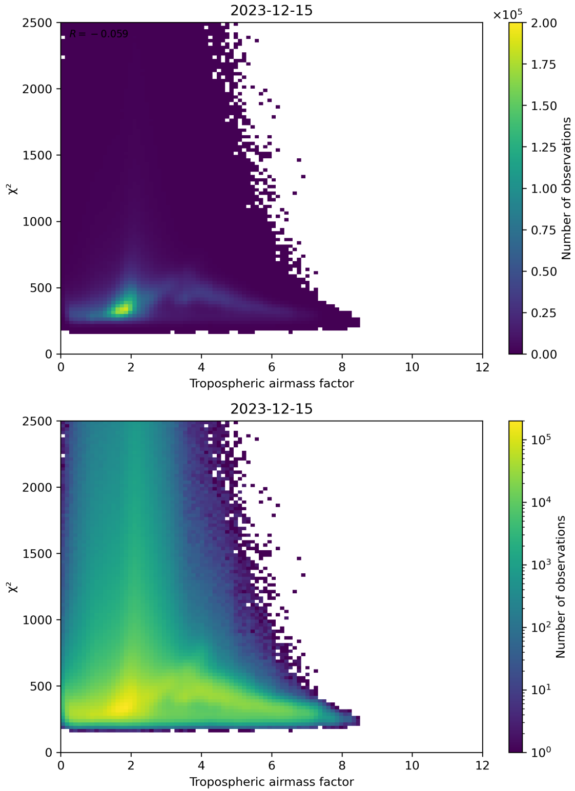
Figure 73: Scatter density plot of “Tropospheric airmass factor” against “ \chi^2 ” for 2023-12-14 to 2023-12-16.
