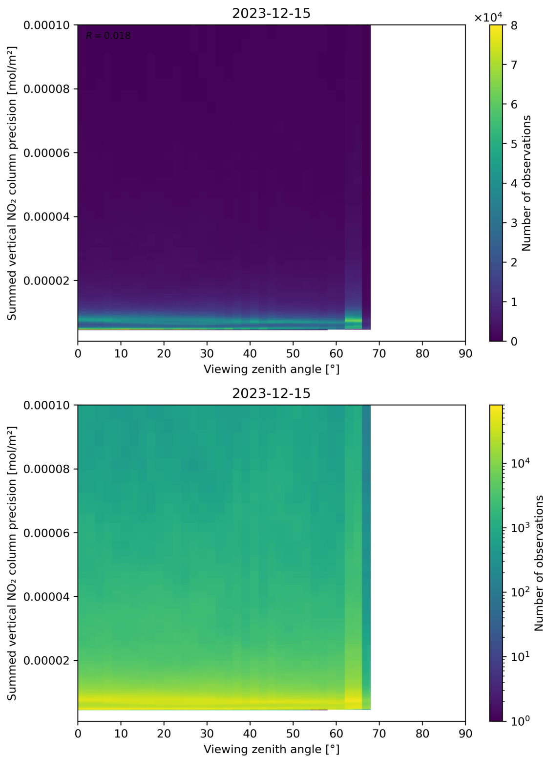
Figure 166: Scatter density plot of “Viewing zenith angle” against “Summed vertical NO 2 column precision” for 2023-12-14 to 2023-12-16.
