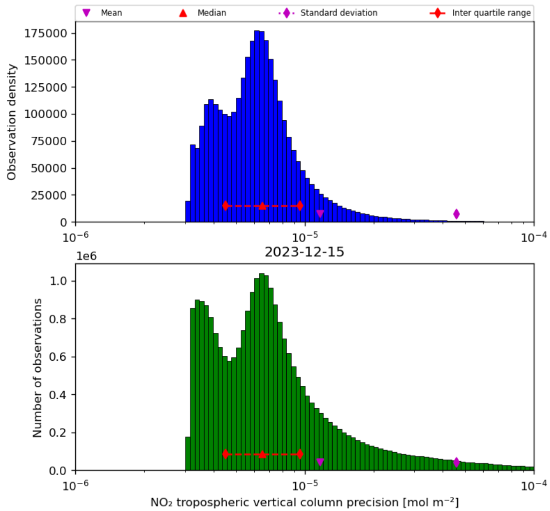
Figure 30: Histogram of “NO 2 tropospheric vertical column precision” for 2023-12-14 to 2023-12-16
