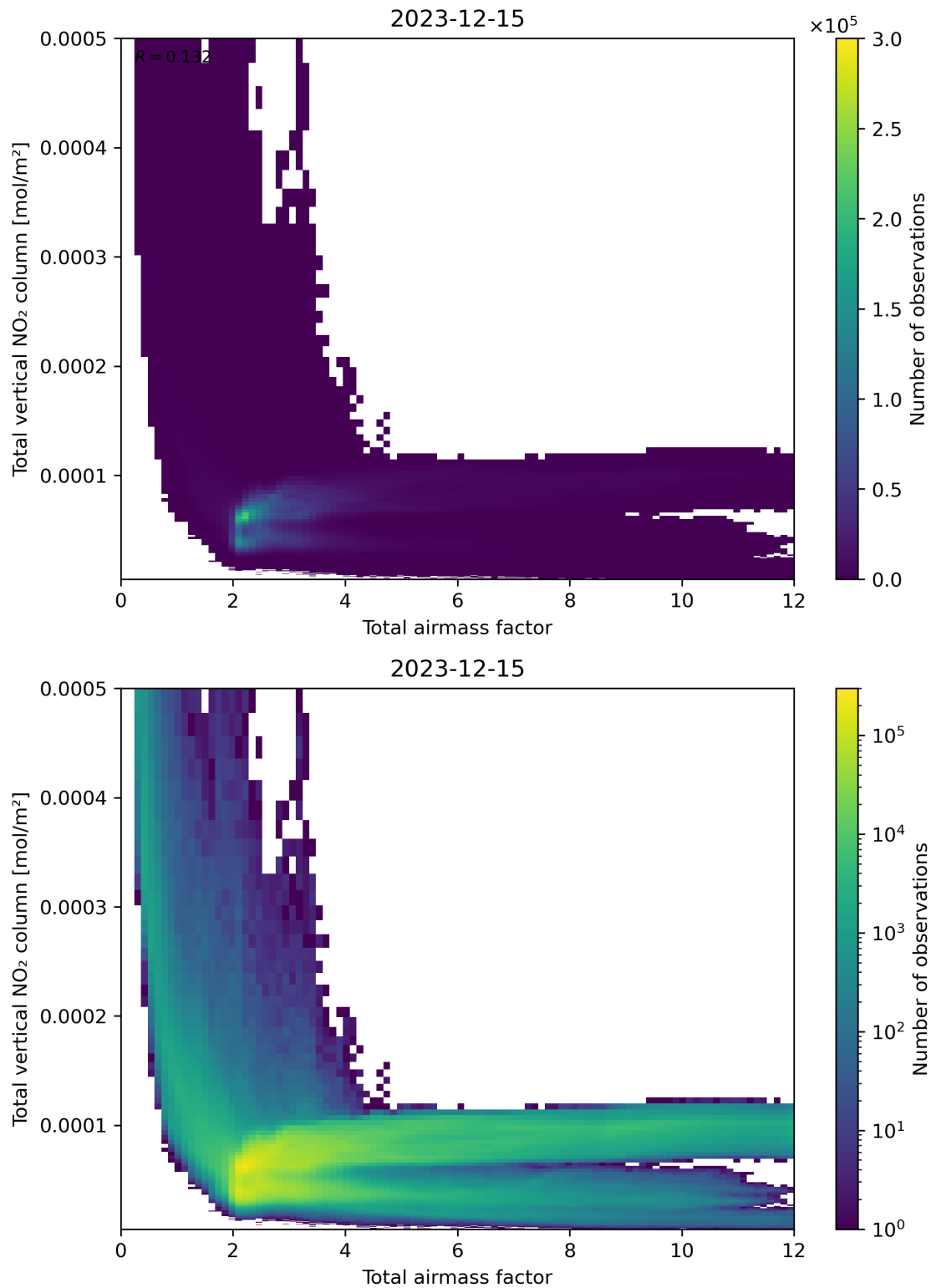
Figure 67: Scatter density plot of “Total airmass factor” against “Total vertical NO 2 column” for 2023-12-14 to 2023-12-16.
