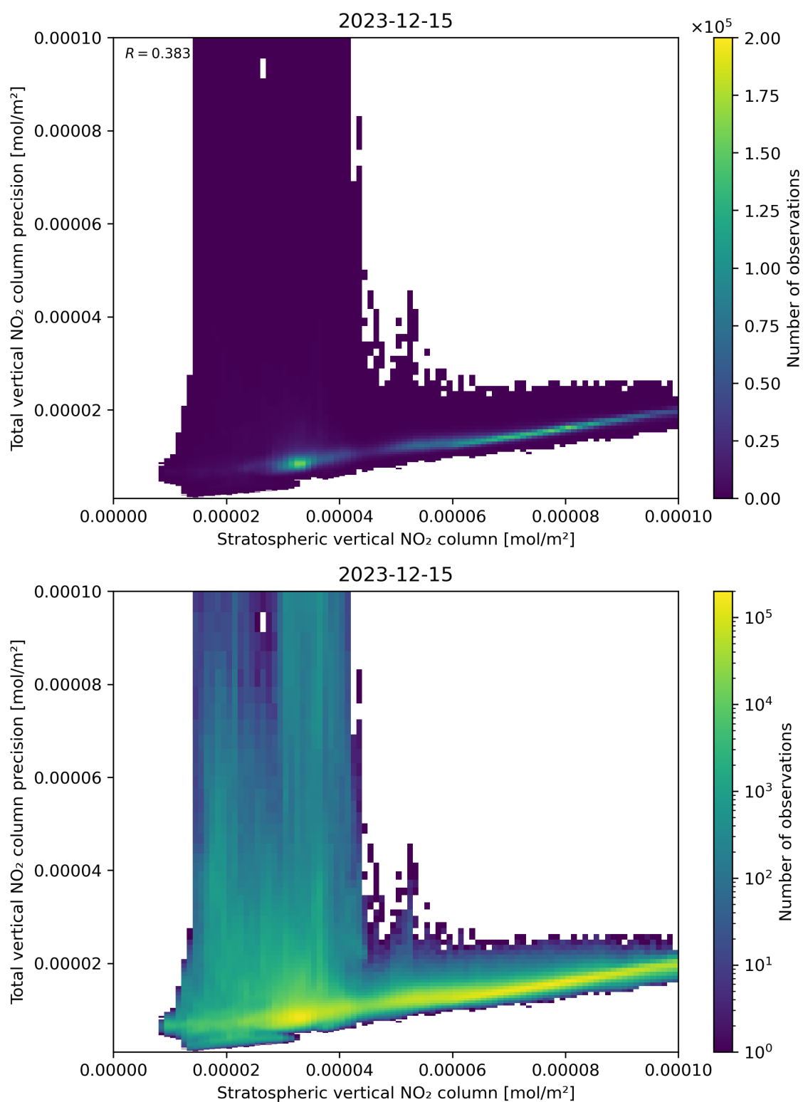
Figure 101: Scatter density plot of “Stratospheric vertical NO 2 column” against “Total vertical NO 2 column precision” for 2023-12-14 to 2023-12-16.
