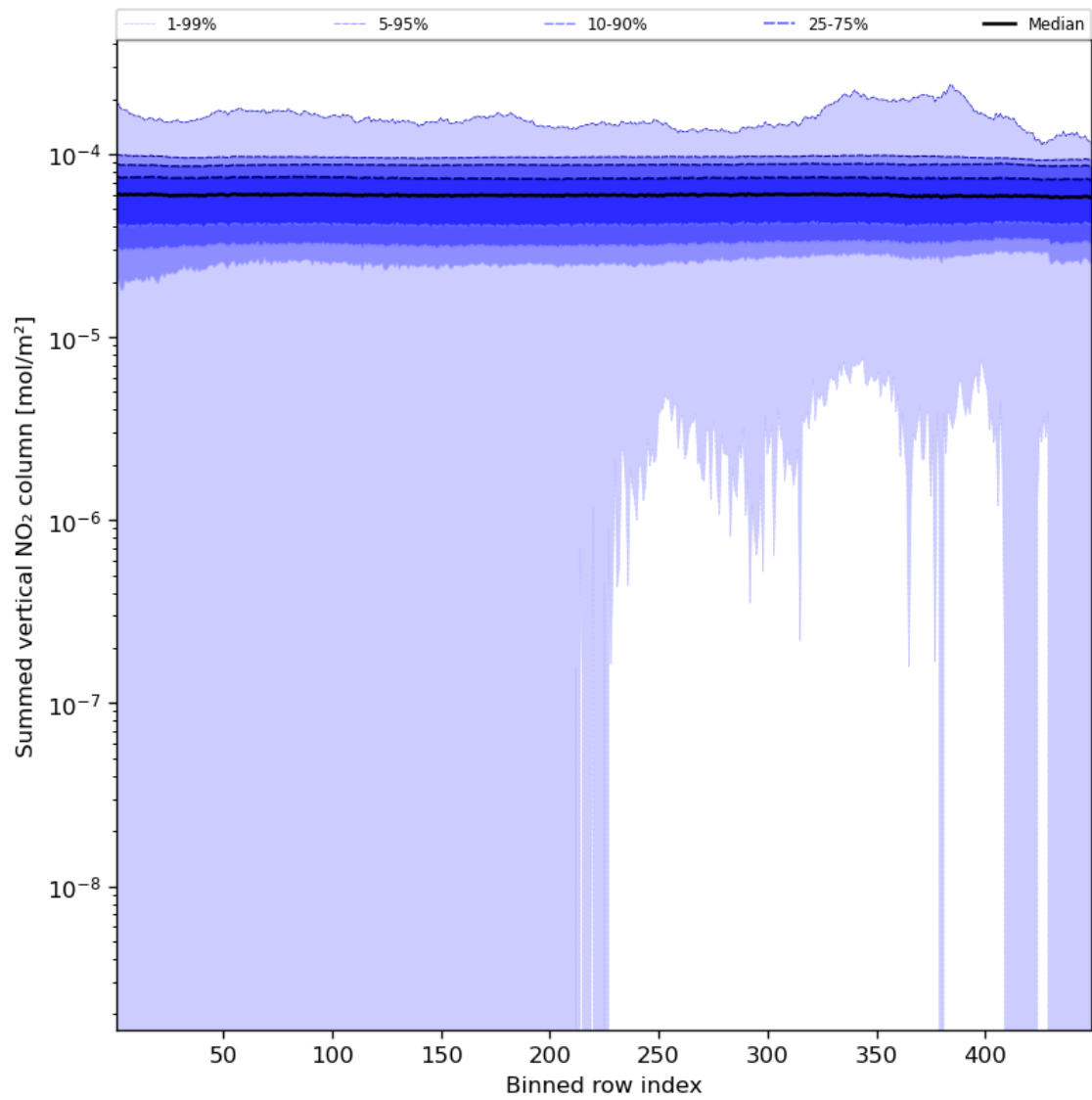
Figure 57: Along track statistics of “Summed vertical NO 2 column” for 2023-12-14 to 2023-12-16
