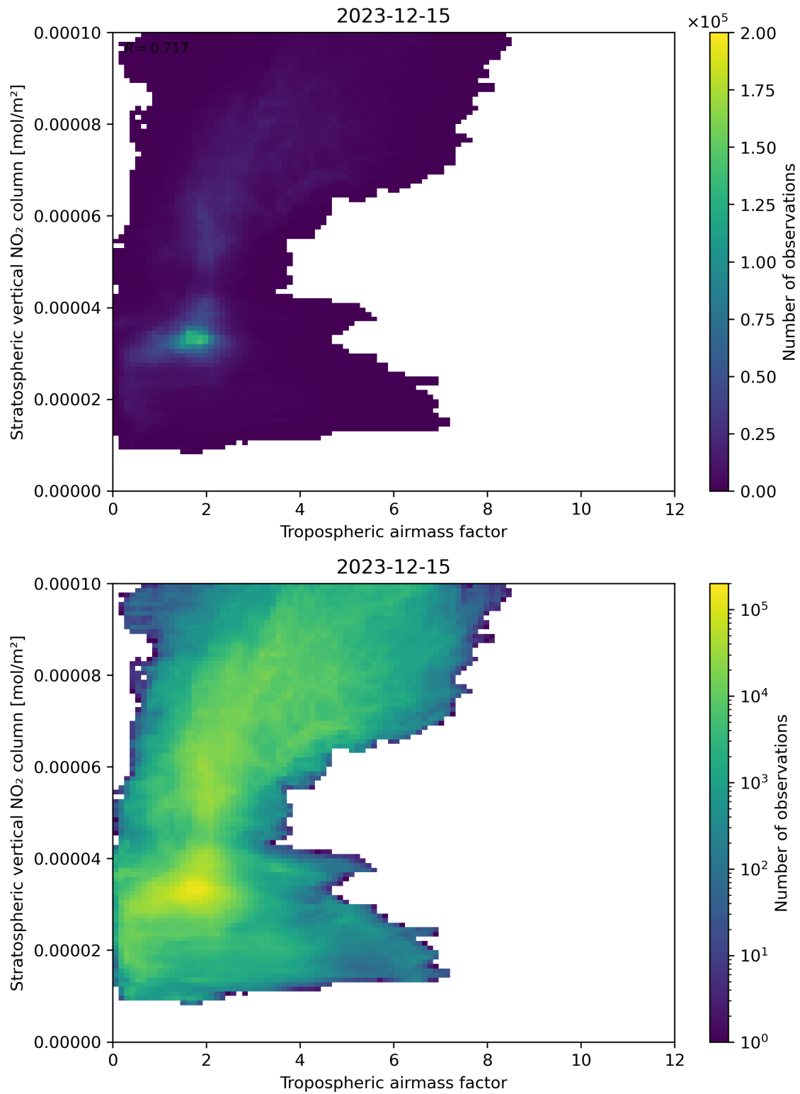
Figure 74: Scatter density plot of “Tropospheric air mass factor” against “Stratospheric vertical NO 2 column” for 2023-12-14 to 2023-12-16.
