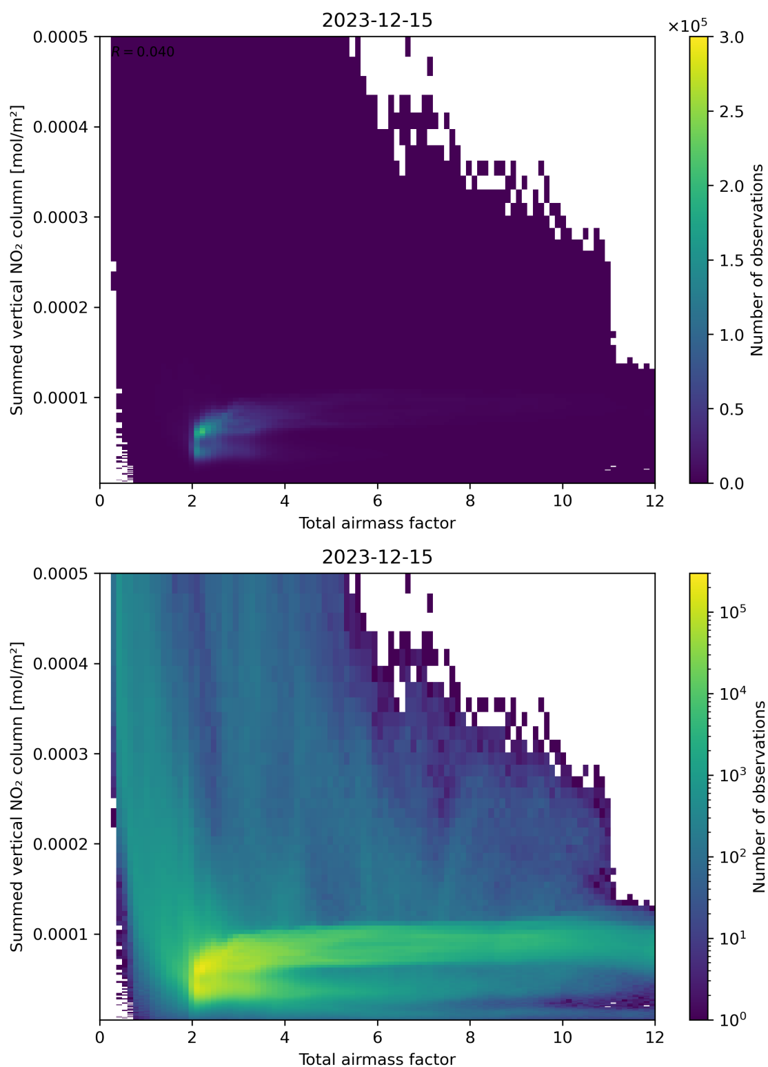
Figure 65: Scatter density plot of “Total airmass factor” against “Summed vertical NO 2 column” for 2023-12-14 to 2023-12-16.
