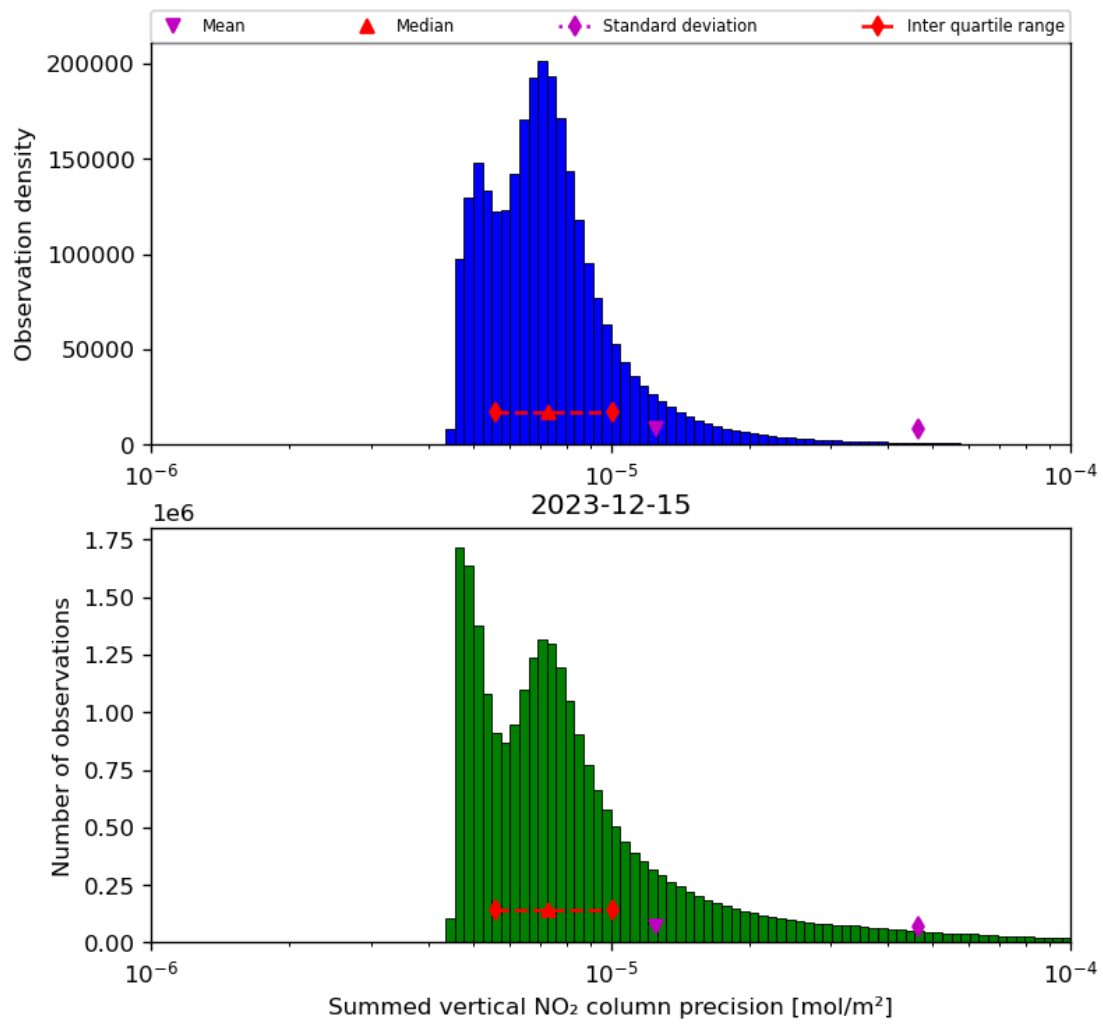
Figure 41: Histogram of “Summed vertical NO 2 column precision” for 2023-12-14 to 2023-12-16
