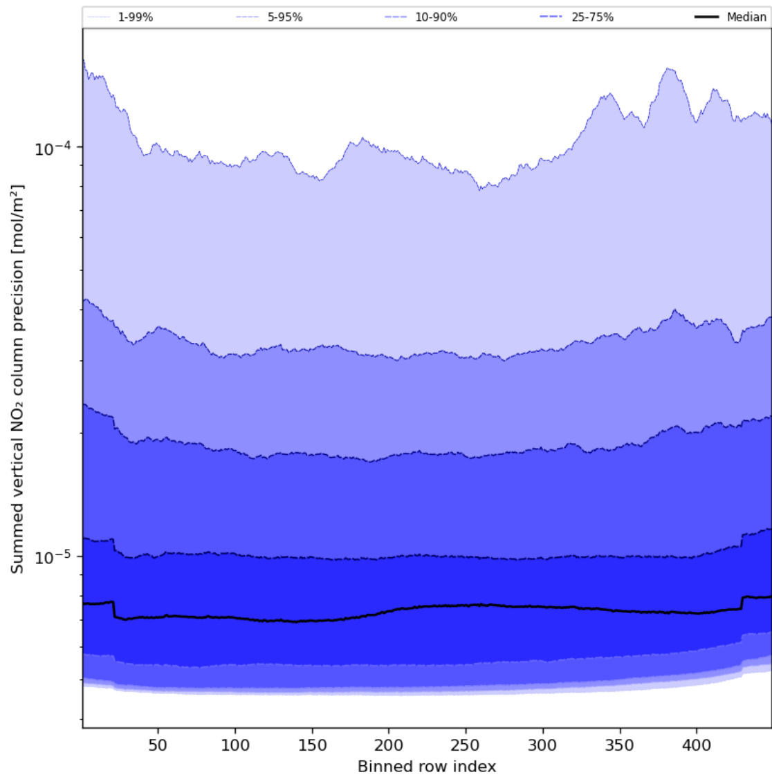
Figure 58: Along track statistics of “Summed vertical NO 2 column precision” for 2023-12-14 to 2023-12-16
