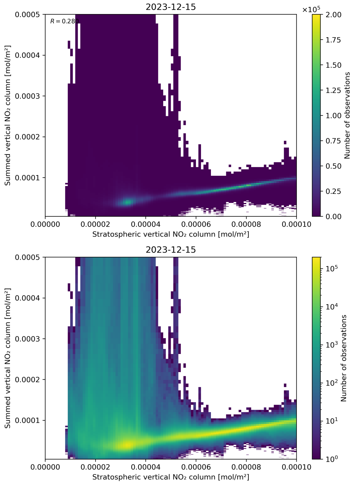
Figure 98: Scatter density plot of “Stratospheric vertical NO 2 column” against “Summed vertical NO 2 column” for 2023-12-14 to 2023-12-16.
