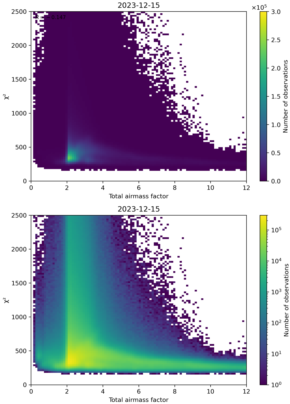
Figure 63: Scatter density plot of “Total airmass factor” against “ \chi^2 ” for 2023-12-14 to 2023-12-16.
