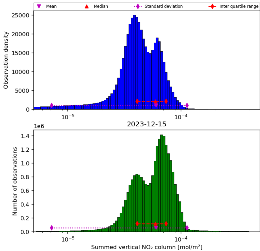
Figure 40: Histogram of "Summed vertical NO 2 column" for 2023-12-14 to 2023-12-16
