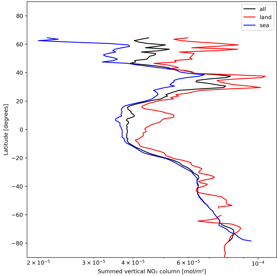
Figure 23: Zonal average of “Summed vertical NO 2 column” for 2023-12-14 to 2023-12-16.
