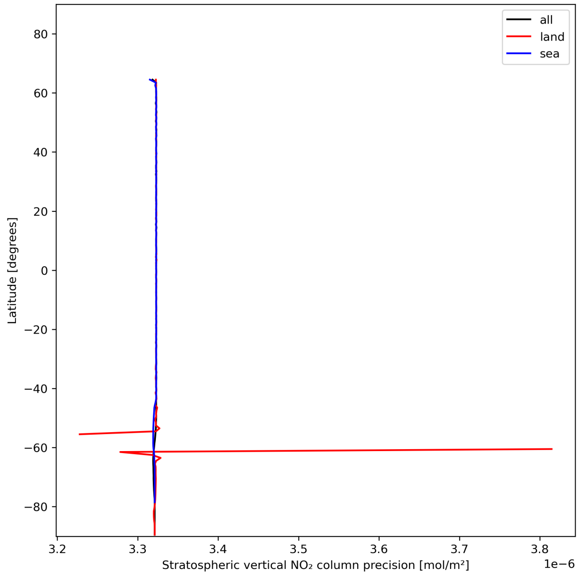
Figure 20: Zonal average of “Stratospheric vertical NO 2 column precision” for 2023-12-14 to 2023-12-16.
