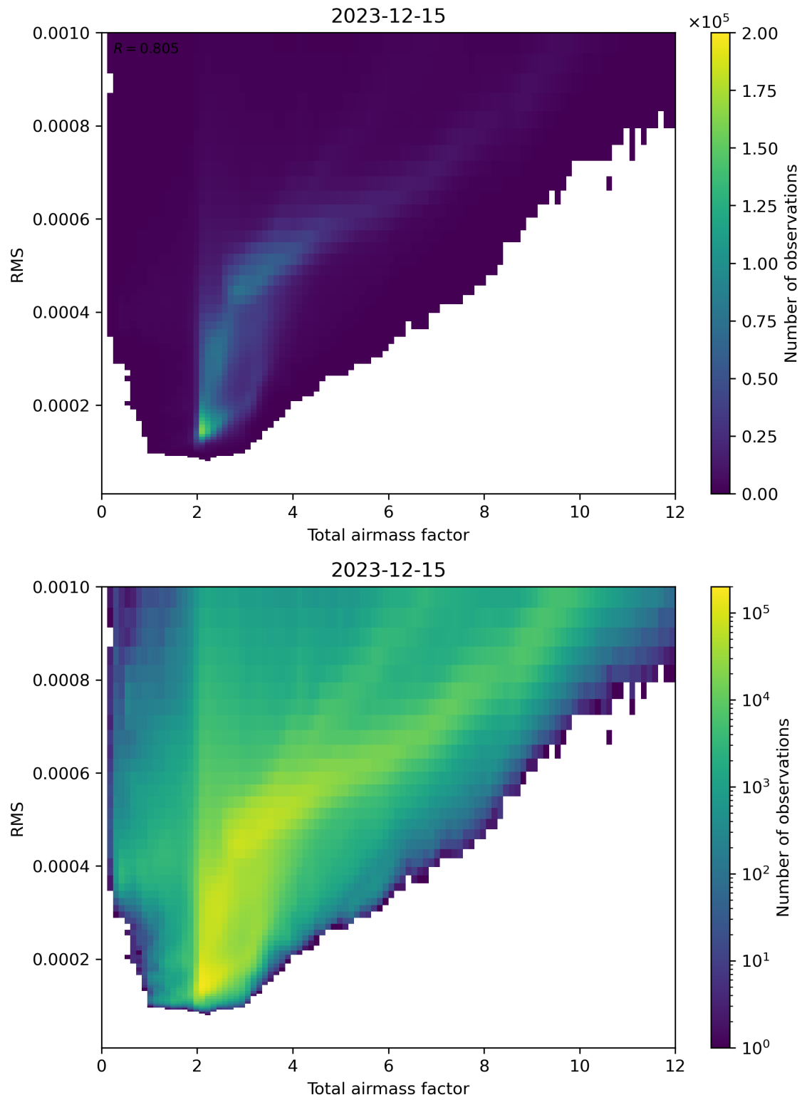
Figure 69: Scatter density plot of “Total airmass factor” against “RMS” for 2023-12-14 to 2023-12-16.
