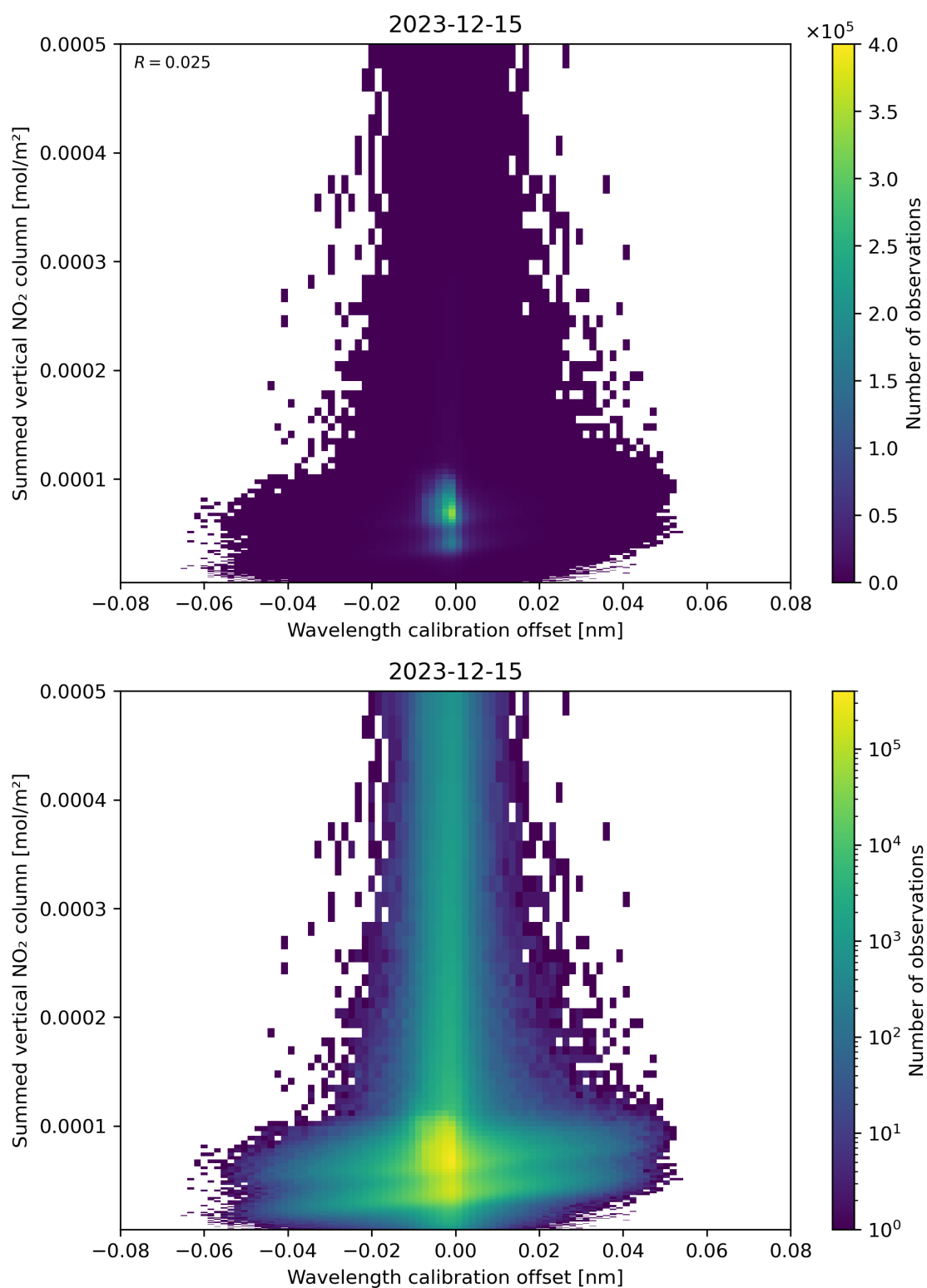
Figure 177: Scatter density plot of “Wavelength calibration offset” against “Summed vertical NO 2 column” for 2023-12-14 to 2023-12-16.
