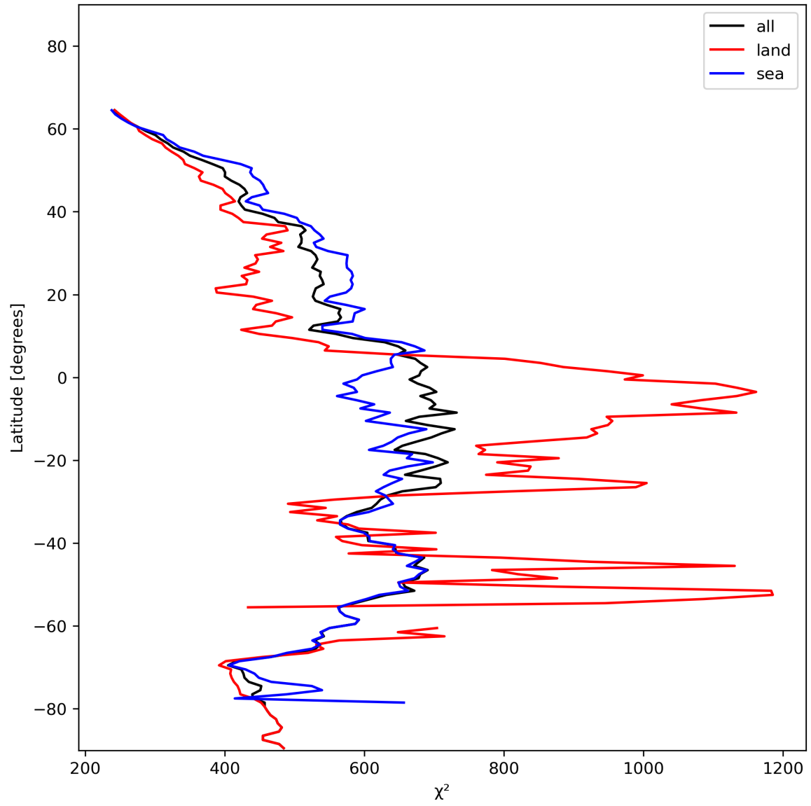
Figure 25: Zonal average of “ \chi^2 ” for 2023-12-14 to 2023-12-16.
