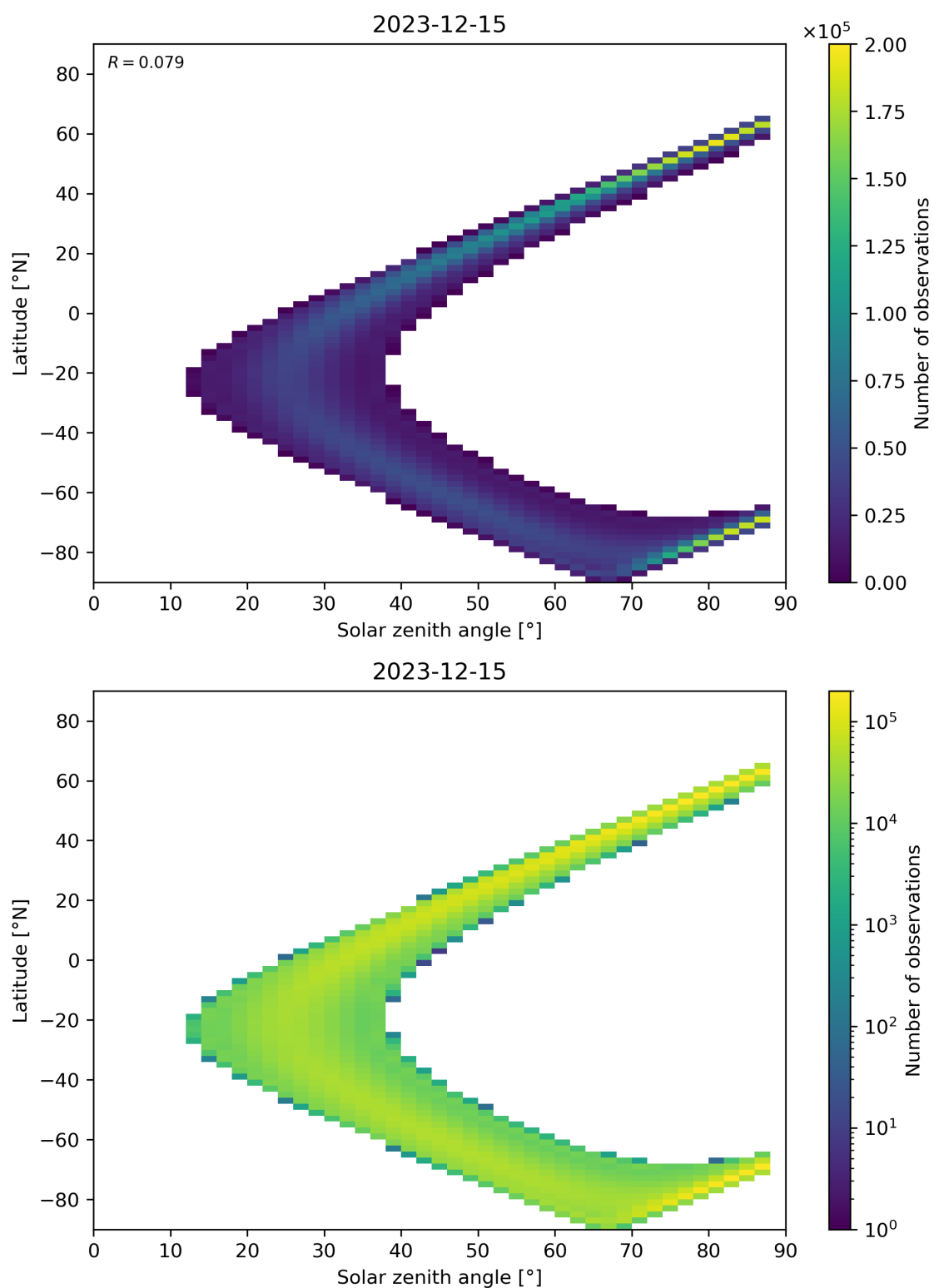
Figure 149: Scatter density plot of “Solar zenith angle” against “Latitude” for 2023-12-14 to 2023-12-16.
