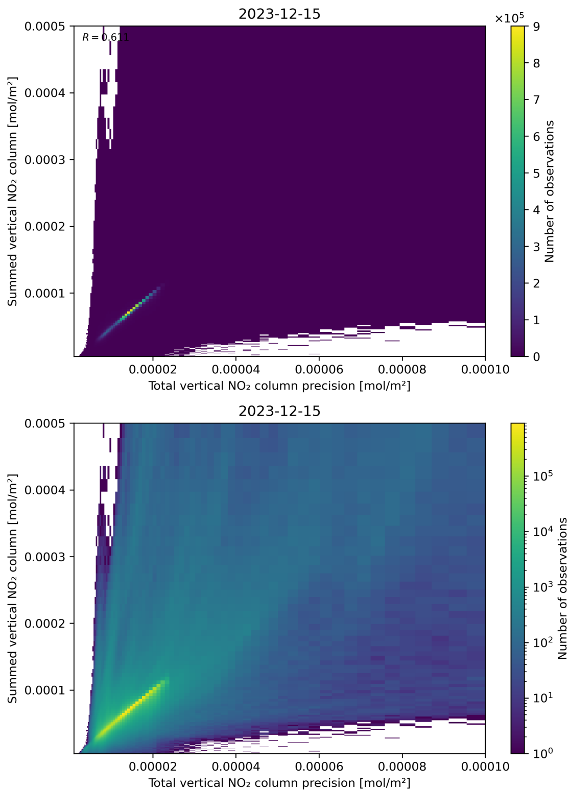
Figure 117: Scatter density plot of “Total vertical NO 2 column precision” against “Summed vertical NO 2 column” for 2023-12-14 to 2023-12-16.
