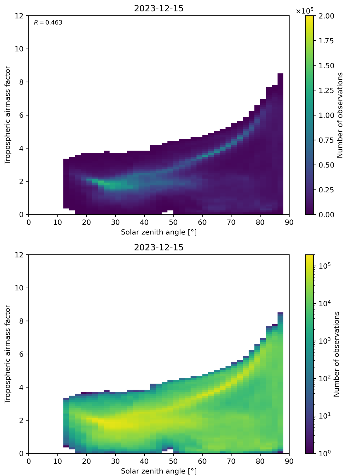
Figure 147: Scatter density plot of “Solar zenith angle” against “Tropospheric airmass factor” for 2023-12-14 to 2023-12-16.
