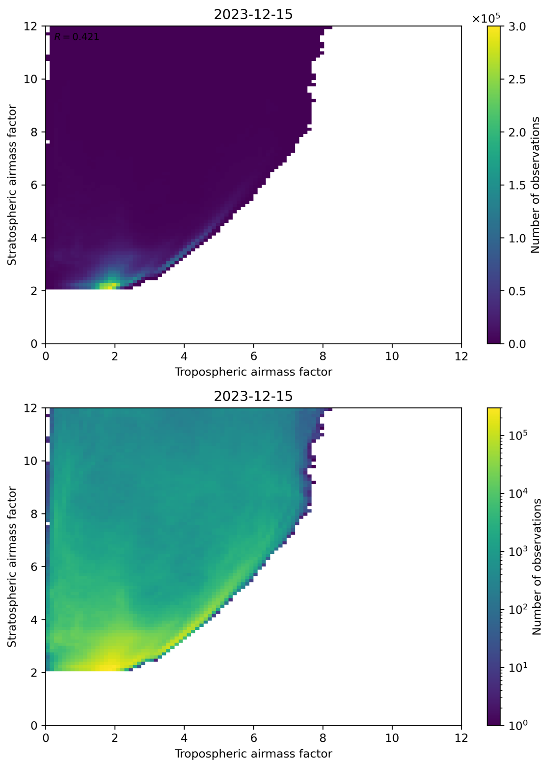
Figure 71: Scatter density plot of “Tropospheric airmass factor” against “Stratospheric airmass factor” for 2023-12-14 to 2023-12-16.
