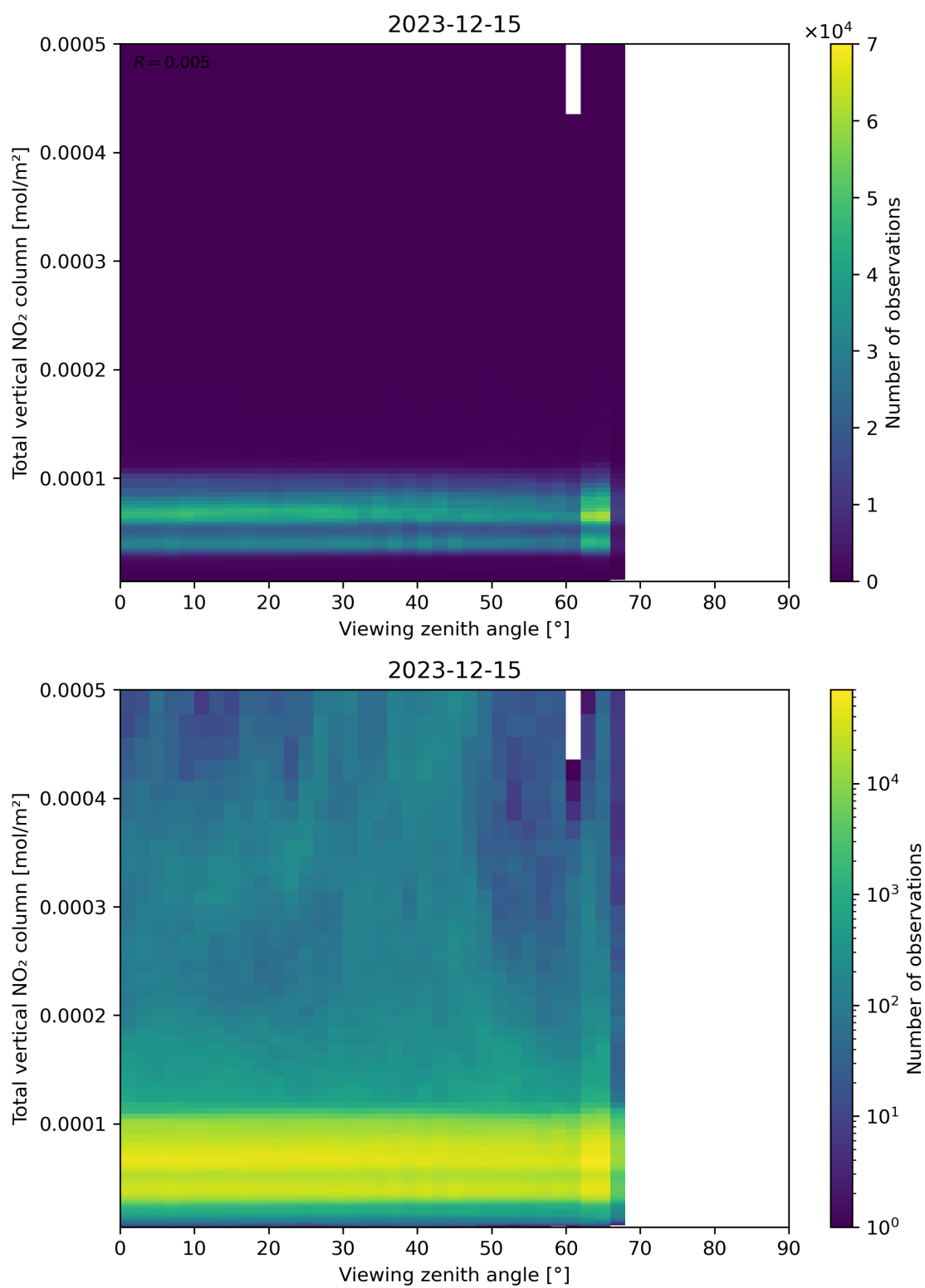
Figure 167: Scatter density plot of “Viewing zenith angle” against “Total vertical NO 2 column” for 2023-12-14 to 2023-12-16.
