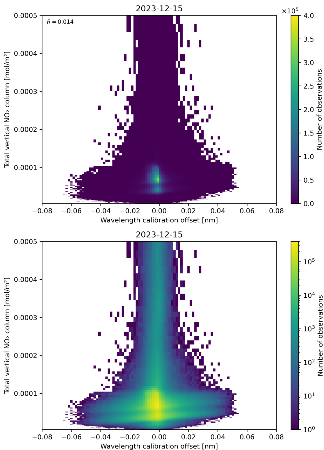
Figure 179: Scatter density plot of “Wavelength calibration offset” against “Total vertical NO 2 column” for 2023-12-14 to 2023-12-16.
