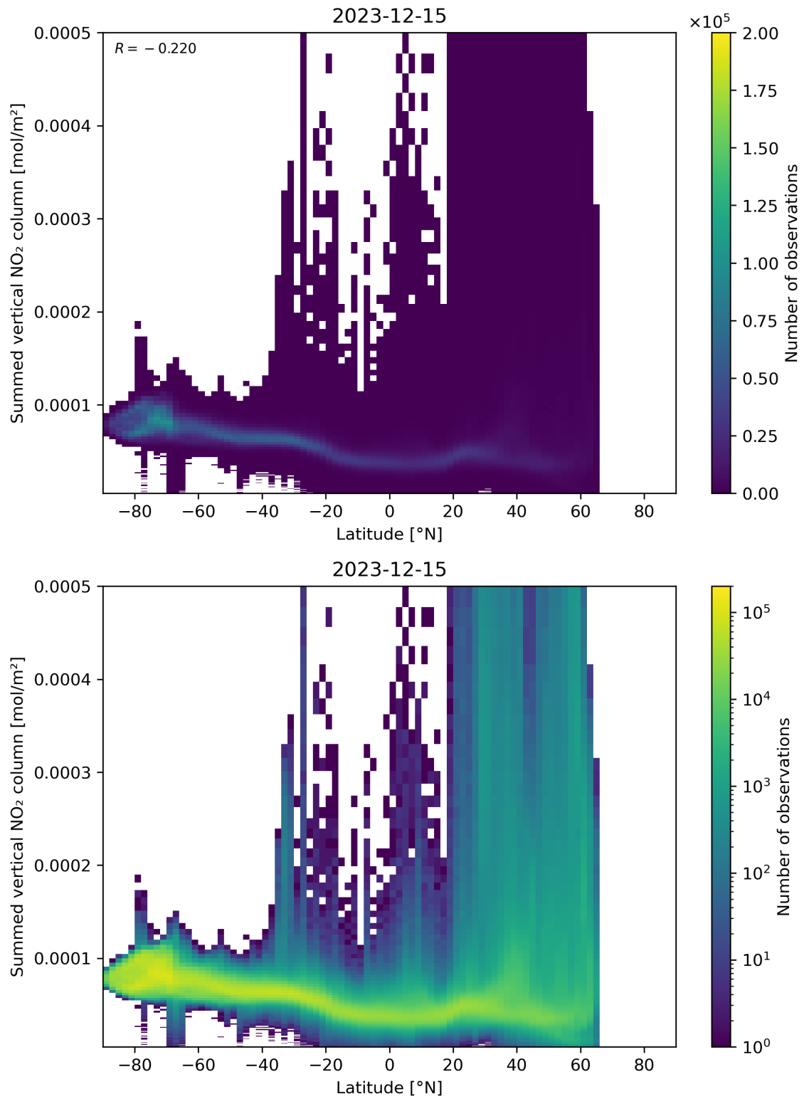
Figure 88: Scatter density plot of “Latitude” against “Summed vertical NO 2 column” for 2023-12-14 to 2023-12-16.
