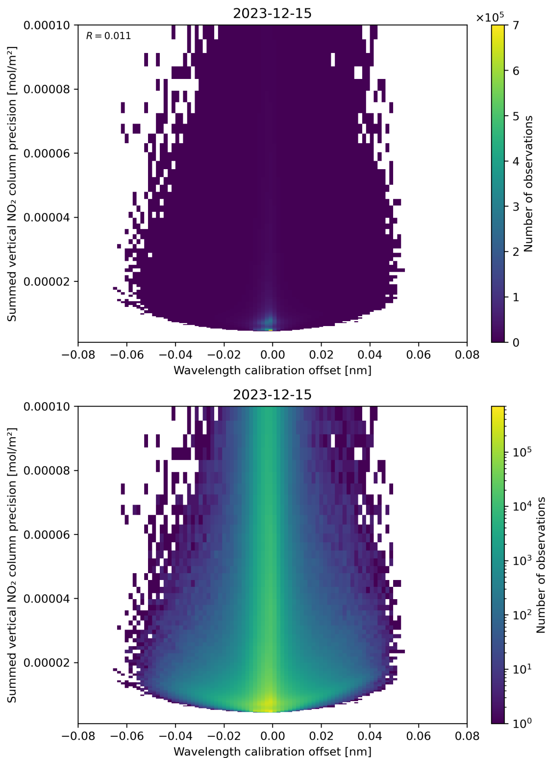
Figure 178: Scatter density plot of “Wavelength calibration offset” against “Summed vertical NO 2 column precision” for 2023-12-14 to 2023-12-16.
