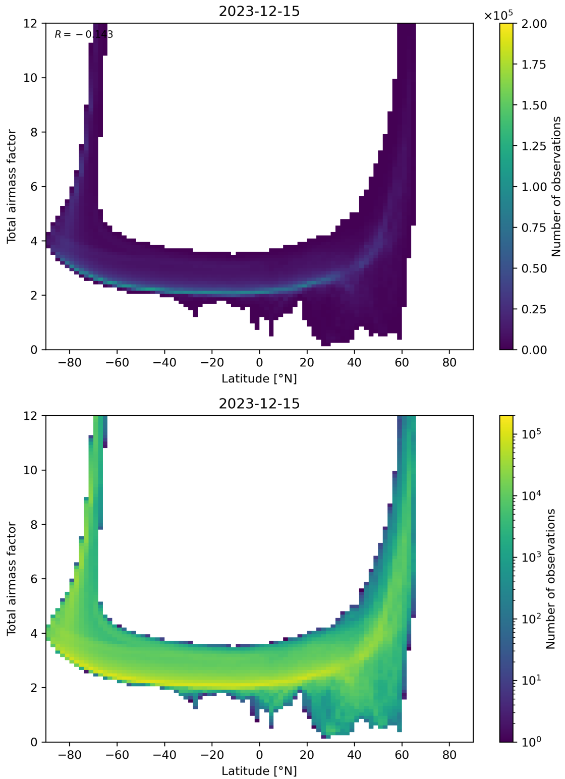
Figure 84: Scatter density plot of “Latitude” against “Total airmass factor” for 2023-12-14 to 2023-12-16.
