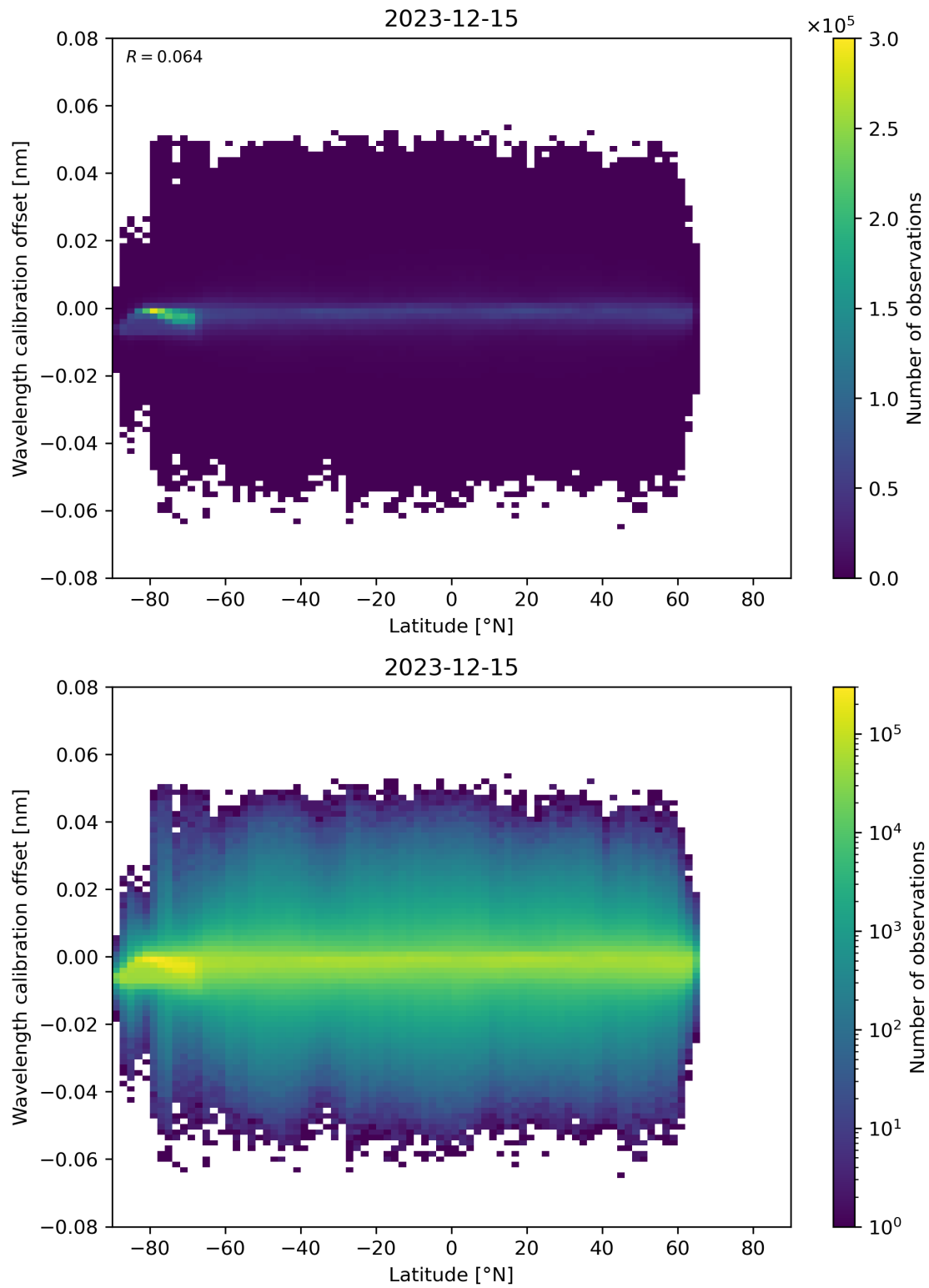
Figure 95: Scatter density plot of “Latitude” against “Wavelength calibration offset” for 2023-12-14 to 2023-12-16.
