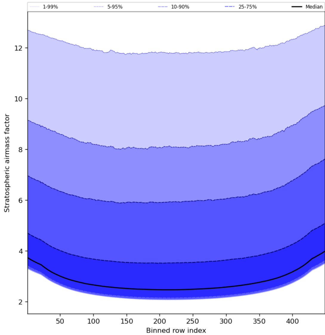
Figure 61: Along track statistics of “Stratospheric airmass factor” for 2023-12-14 to 2023-12-16
