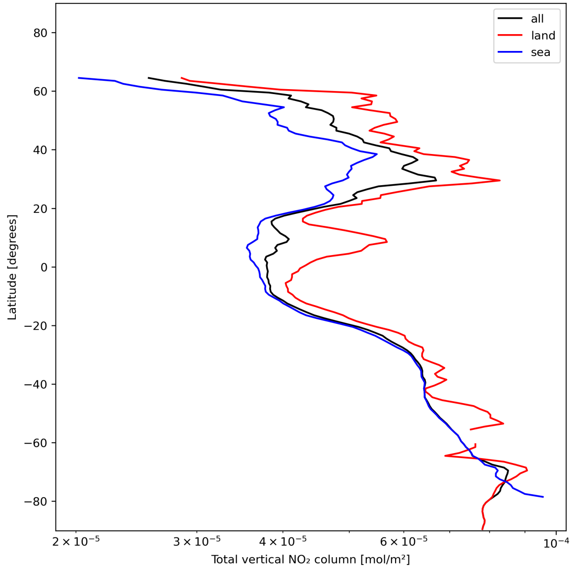
Figure 21: Zonal average of “Total vertical NO 2 column” for 2023-12-14 to 2023-12-16.
