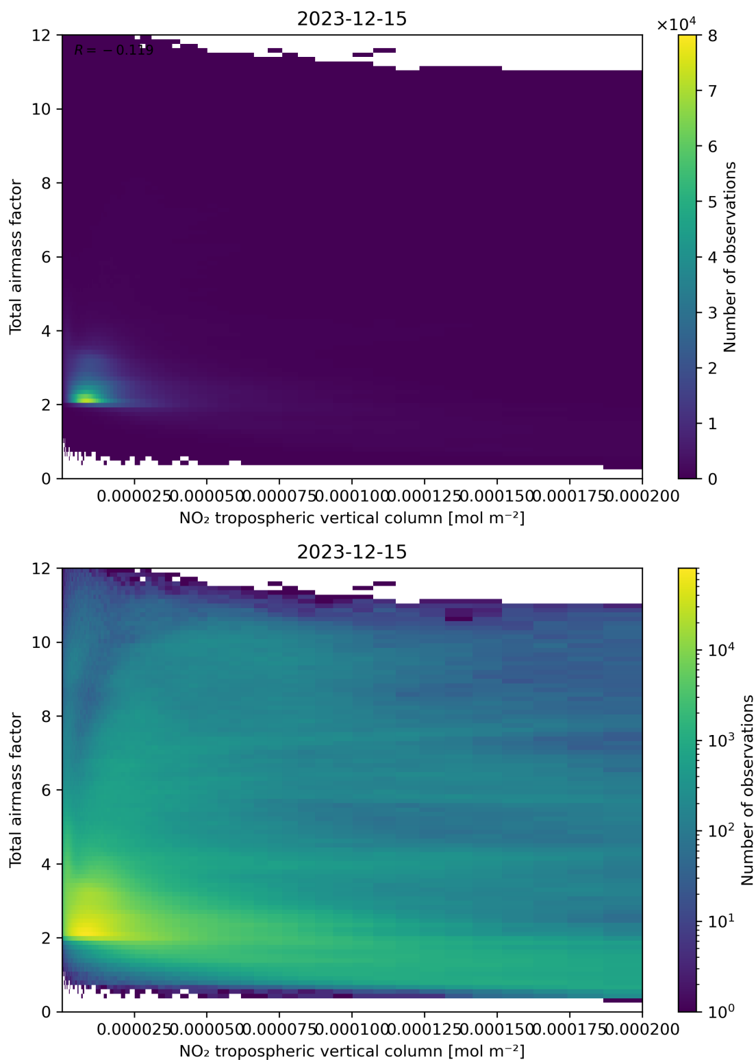
Figure 122: Scatter density plot of “NO 2 tropospheric vertical column” against “Total airmass factor” for 2023-12-14 to 2023-12-16.
