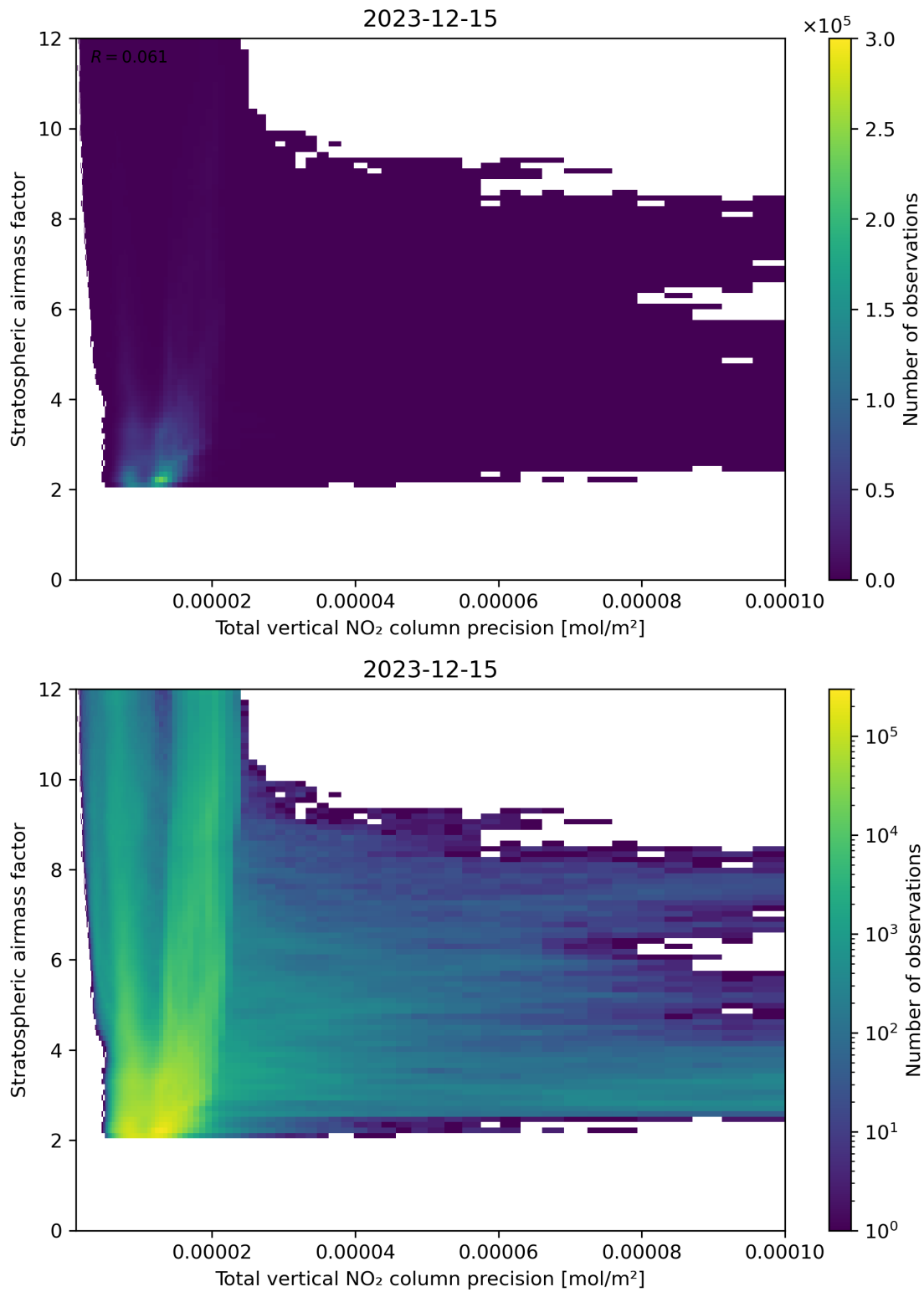
Figure 115: Scatter density plot of “Total vertical NO 2 column precision” against “Stratospheric airmass factor” for 2023-12-14 to 2023-12-16.
