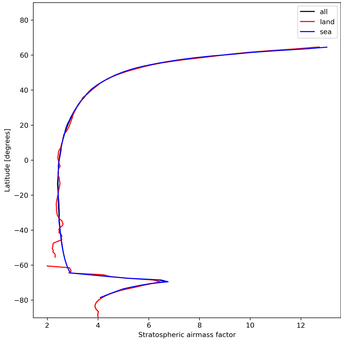
Figure 27: Zonal average of “Stratospheric airmass factor” for 2023-12-14 to 2023-12-16.
