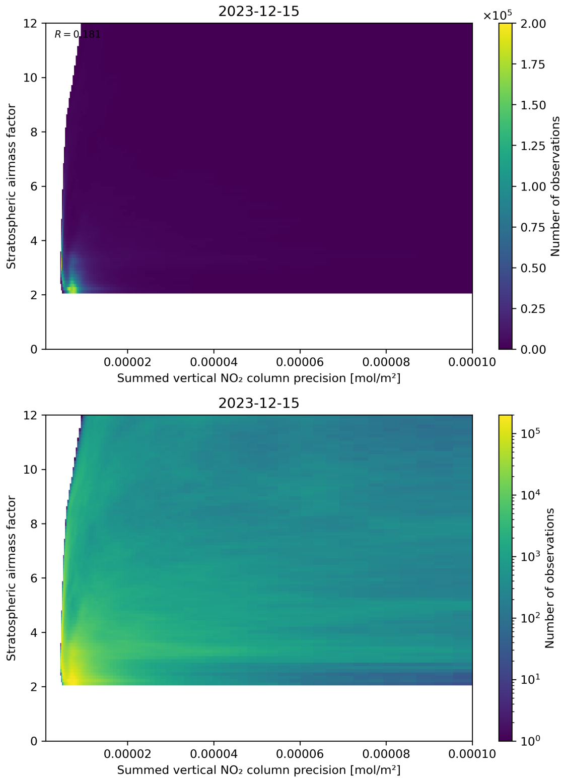
Figure 106: Scatter density plot of “Summed vertical NO 2 column precision” against “Stratospheric airmass factor” for 2023-12-14 to 2023-12-16.
