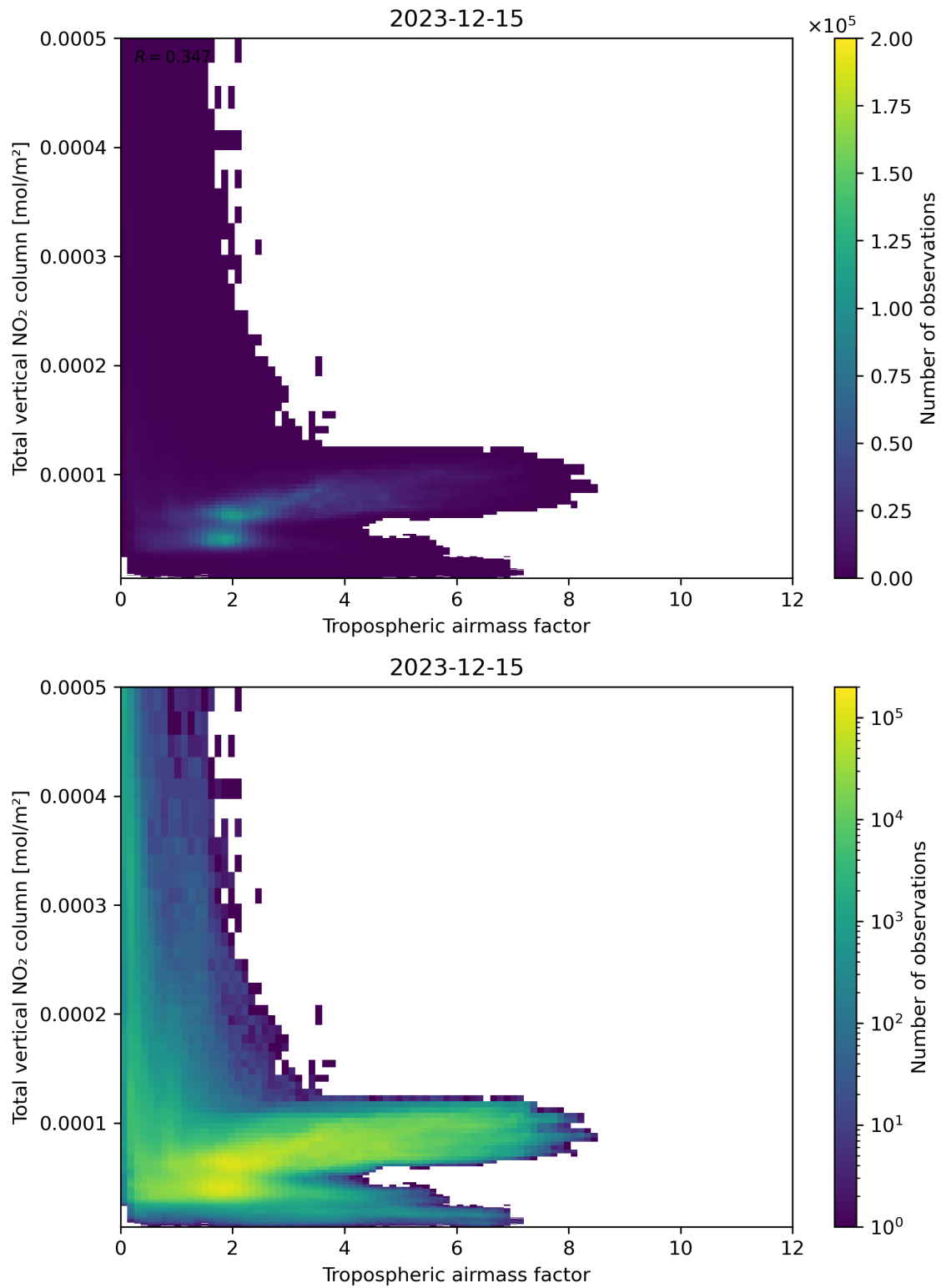
Figure 77: Scatter density plot of “Tropospheric airmass factor” against “Total vertical NO 2 column” for 2023-12-14 to 2023-12-16.
