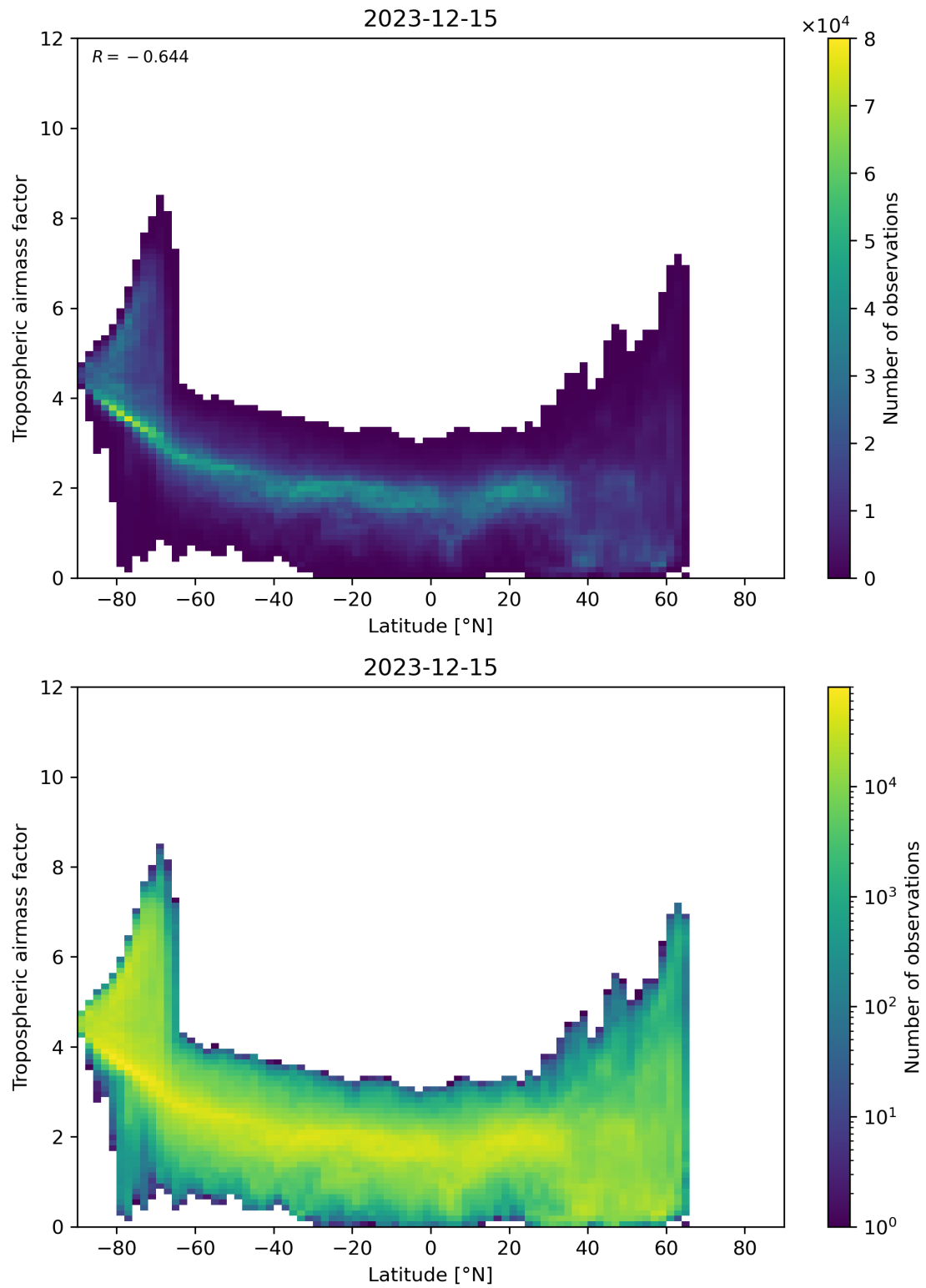
Figure 85: Scatter density plot of “Latitude” against “Tropospheric airmass factor” for 2023-12-14 to 2023-12-16.
