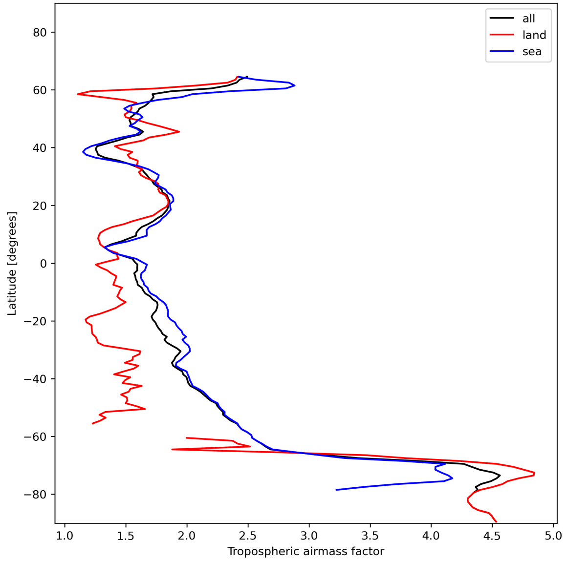
Figure 14: Zonal average of “Tropospheric airmass factor” for 2023-12-14 to 2023-12-16.
