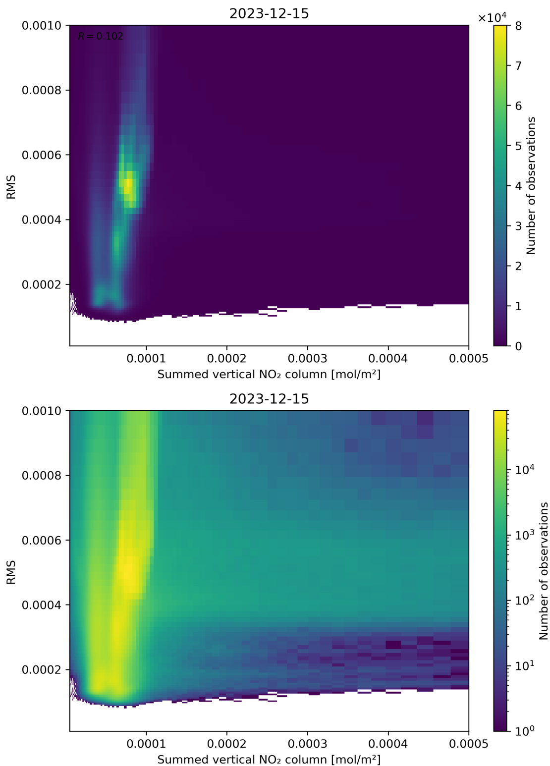
Figure 109: Scatter density plot of “Summed vertical NO 2 column” against “RMS” for 2023-12-14 to 2023-12-16.
