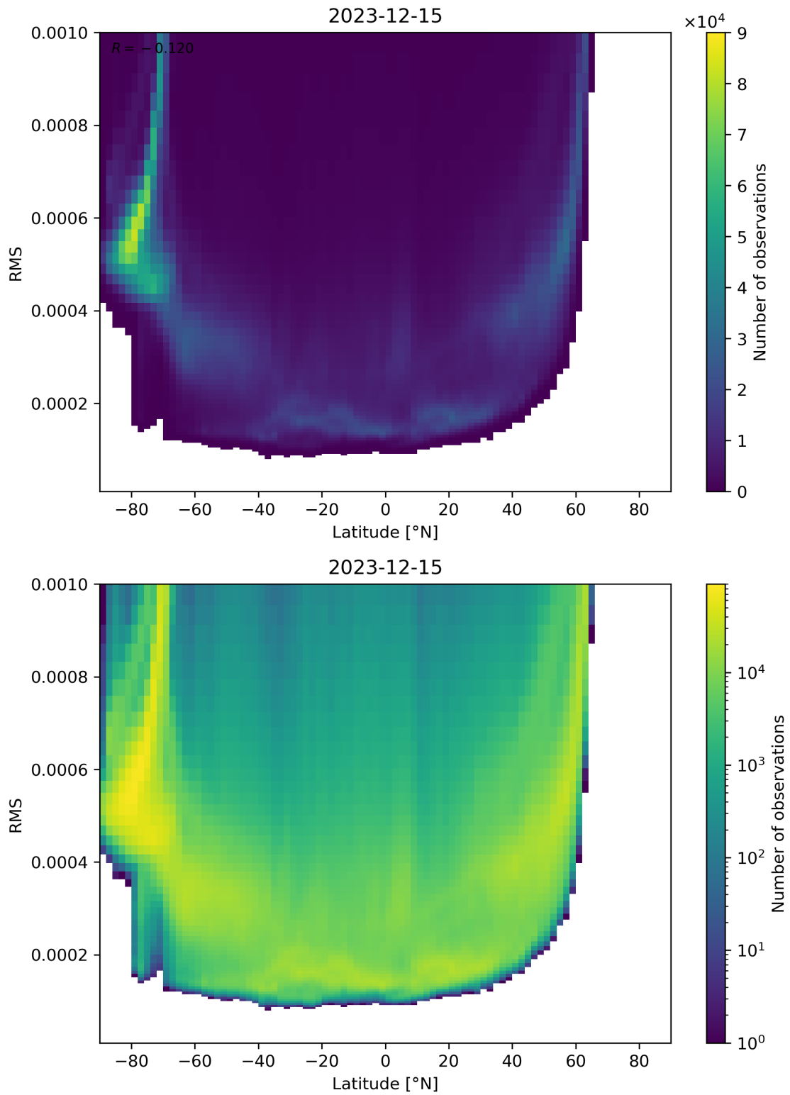
Figure 94: Scatter density plot of “Latitude” against “RMS” for 2023-12-14 to 2023-12-16.
