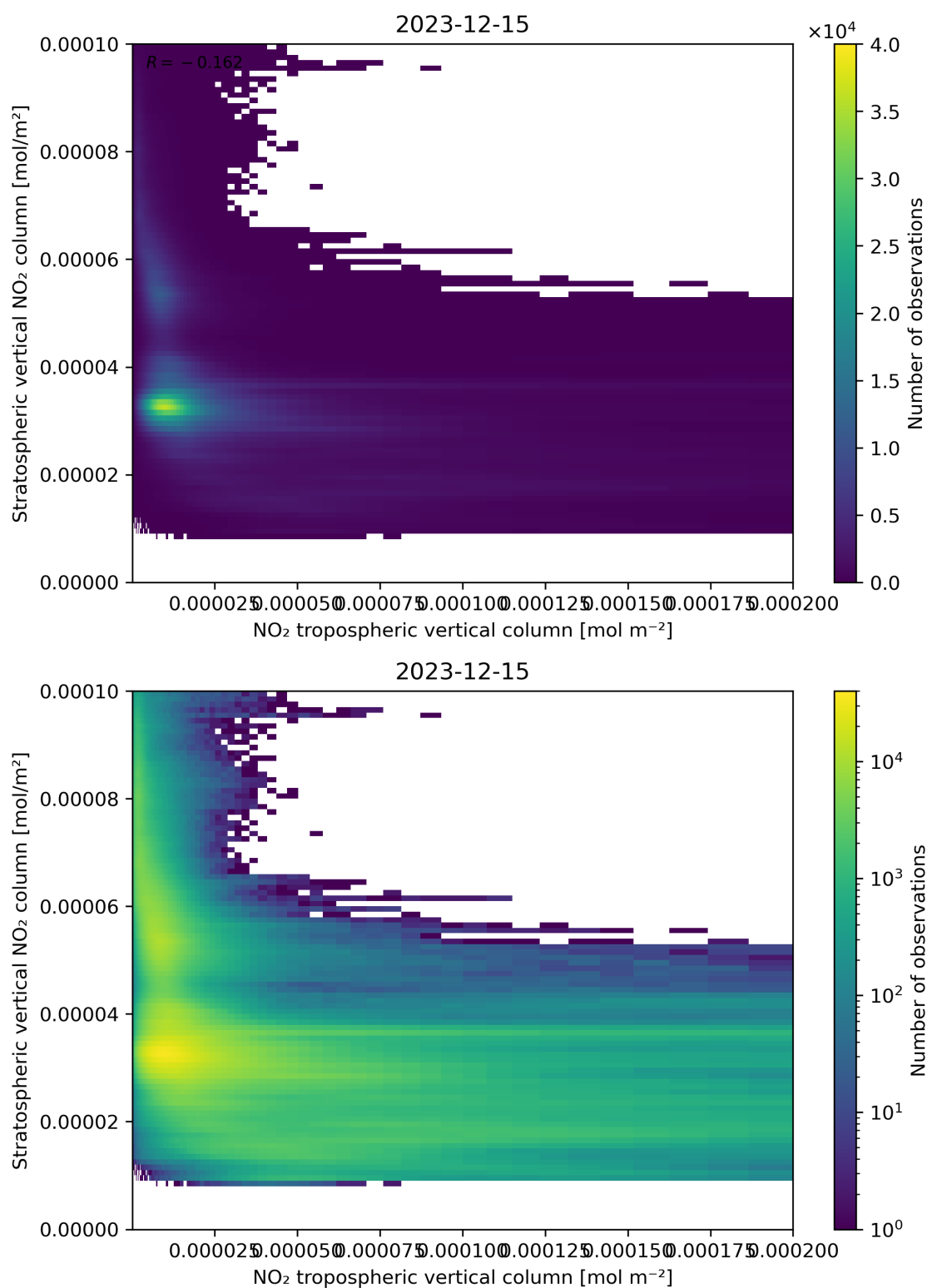
Figure 125: Scatter density plot of “NO 2 tropospheric vertical column” against “Stratospheric vertical NO 2 column” for 2023-12-14 to 2023-12-16.
