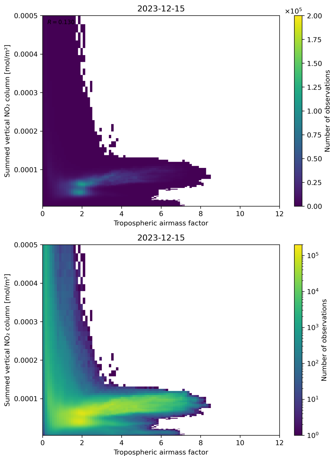
Figure 75: Scatter density plot of “Tropospheric air mass factor” against “Summed vertical NO 2 column” for 2023-12-14 to 2023-12-16.
