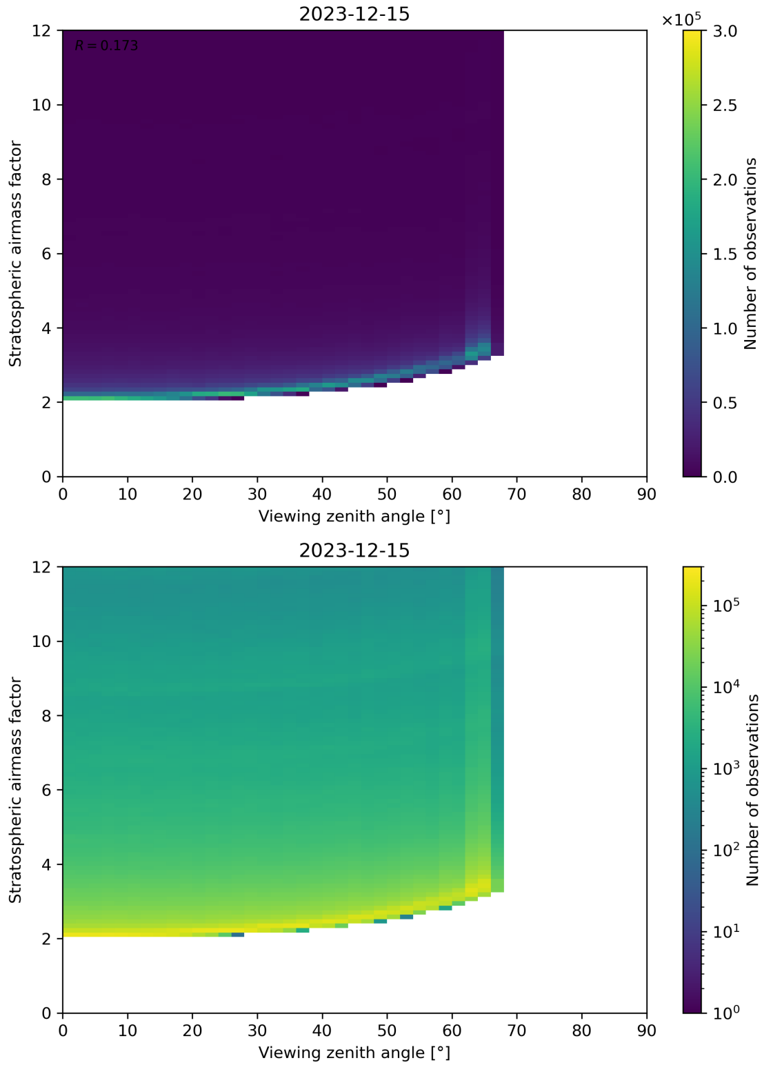
Figure 159: Scatter density plot of “Viewing zenith angle” against “Stratospheric airmass factor” for 2023-12-14 to 2023-12-16.
