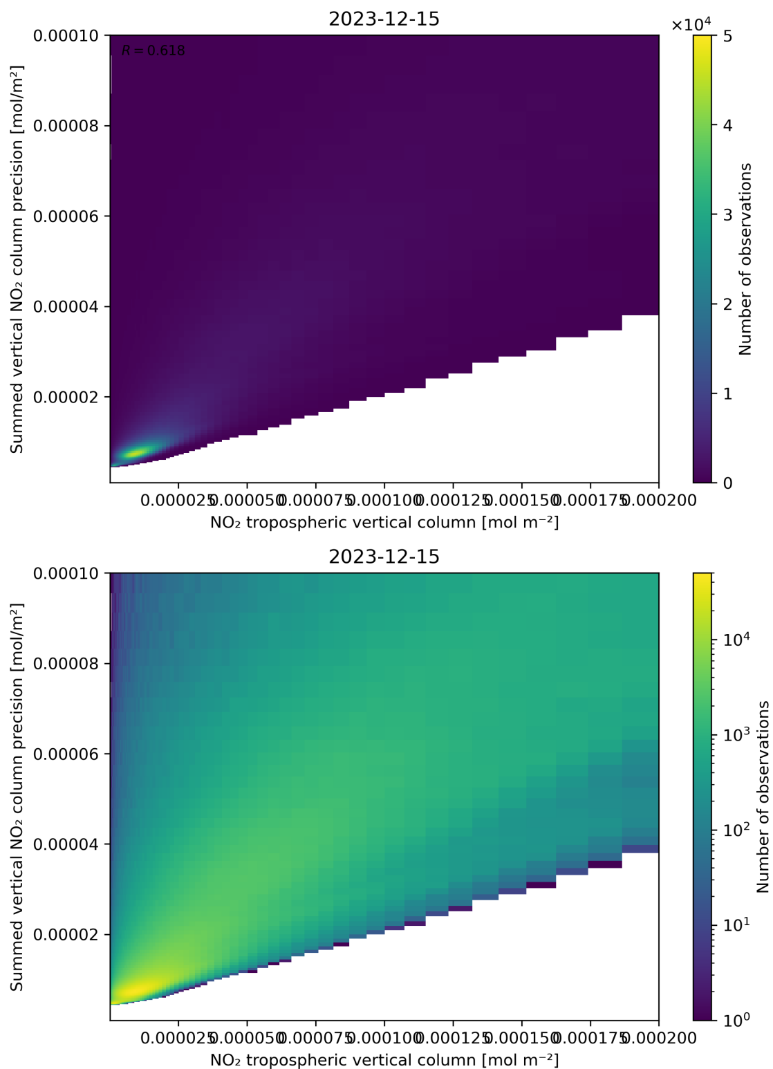
Figure 127: Scatter density plot of “NO 2 tropospheric vertical column” against “Summed vertical NO 2 column precision” for 2023-12-14 to 2023-12-16.
