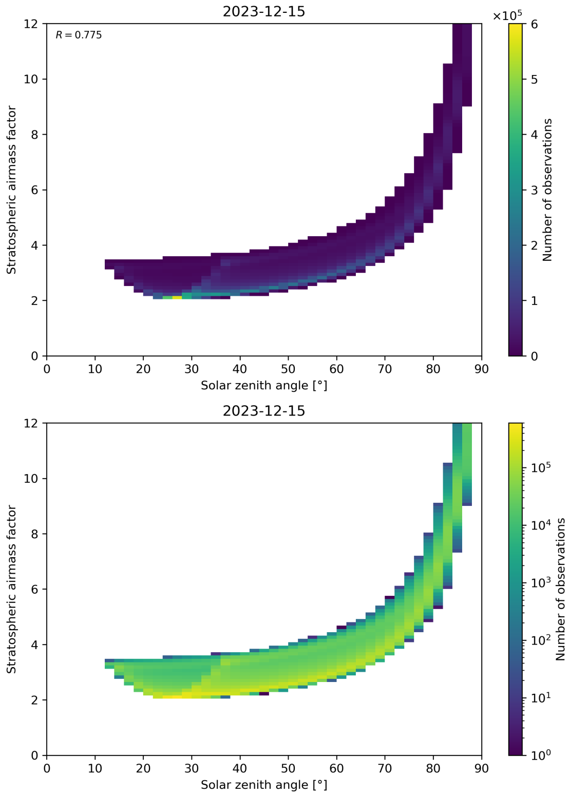
Figure 145: Scatter density plot of “Solar zenith angle” against “Stratospheric airmass factor” for 2023-12-14 to 2023-12-16.
