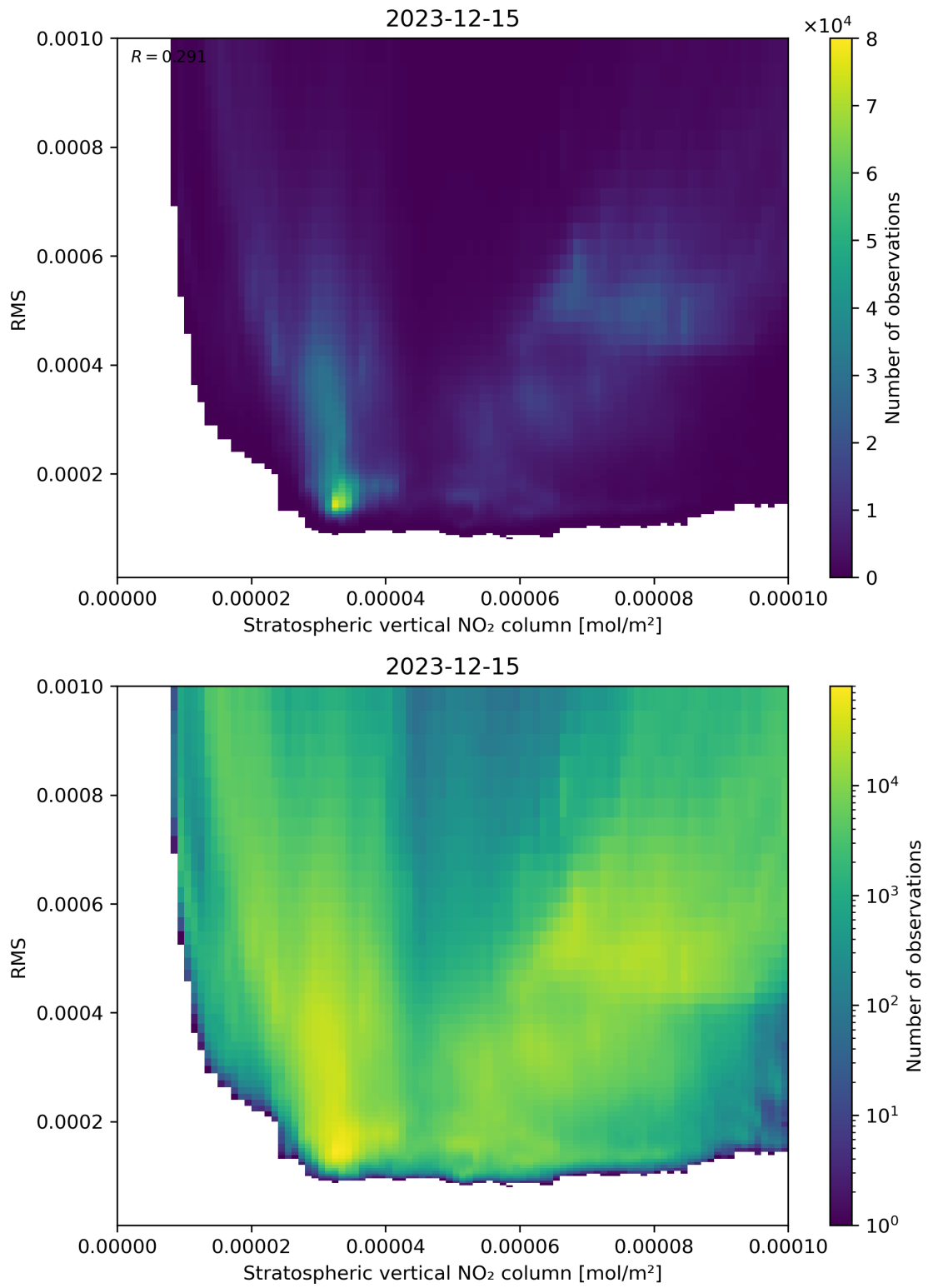
Figure 102: Scatter density plot of “Stratospheric vertical NO 2 column” against “RMS” for 2023-12-14 to 2023-12-16.
