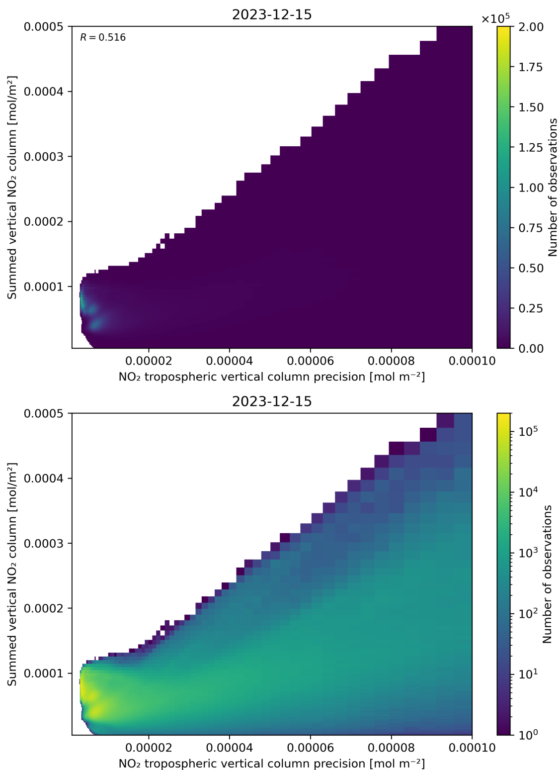
Figure 136: Scatter density plot of “NO 2 tropospheric vertical column precision” against “Summed vertical NO 2 column” for 2023-12-14 to 2023-12-16.
