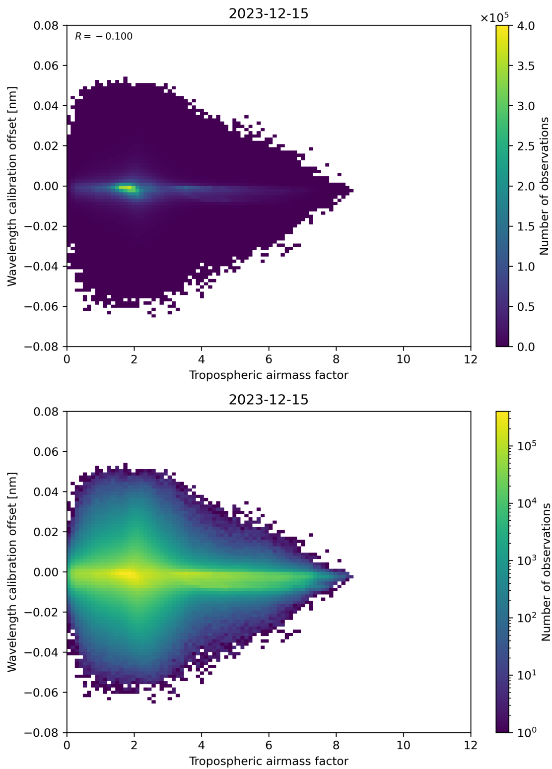
Figure 80: Scatter density plot of “Tropospheric airmass factor” against “Wavelength calibration offset” for 2023-12-14 to 2023-12-16.
