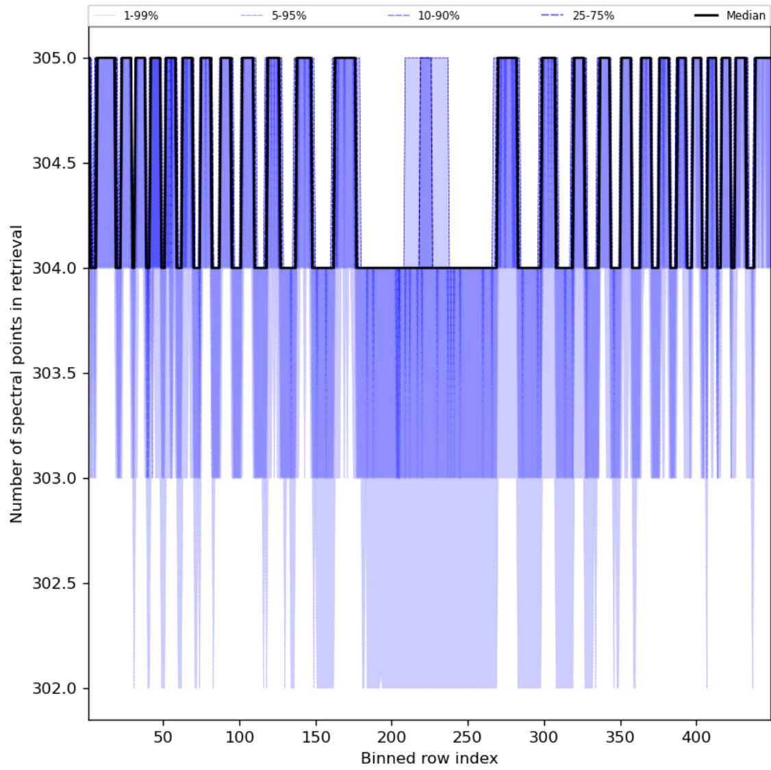
Figure 50: Along track statistics of “Number of spectral points in retrieval” for 2023-12-14 to 2023-12-16
