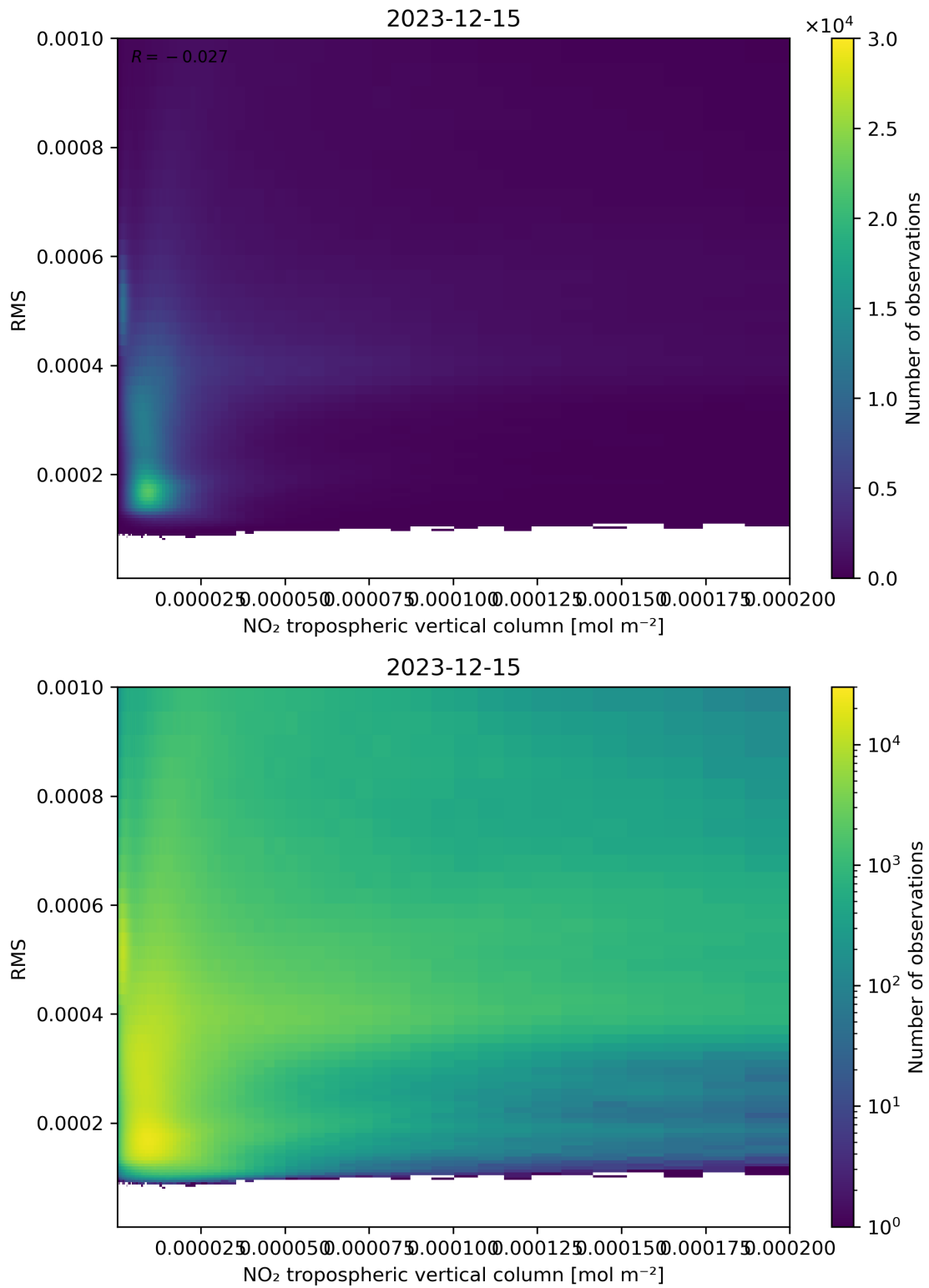
Figure 142: Scatter density plot of “NO 2 tropospheric vertical column” against “RMS” for 2023-12-14 to 2023-12-16.
