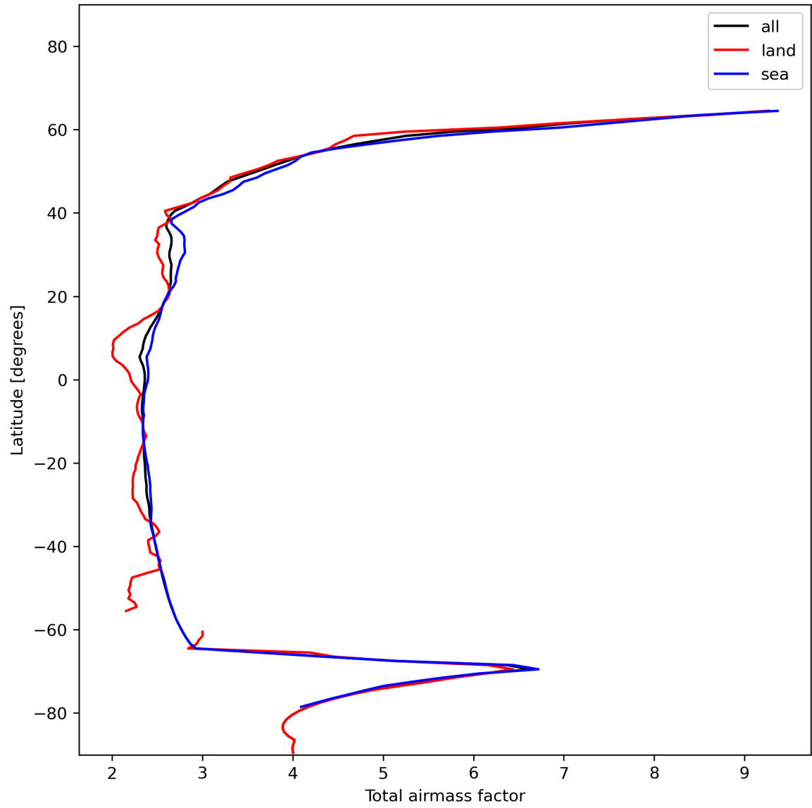
Figure 15: Zonal average of “Total airmass factor” for 2023-12-14 to 2023-12-16.
