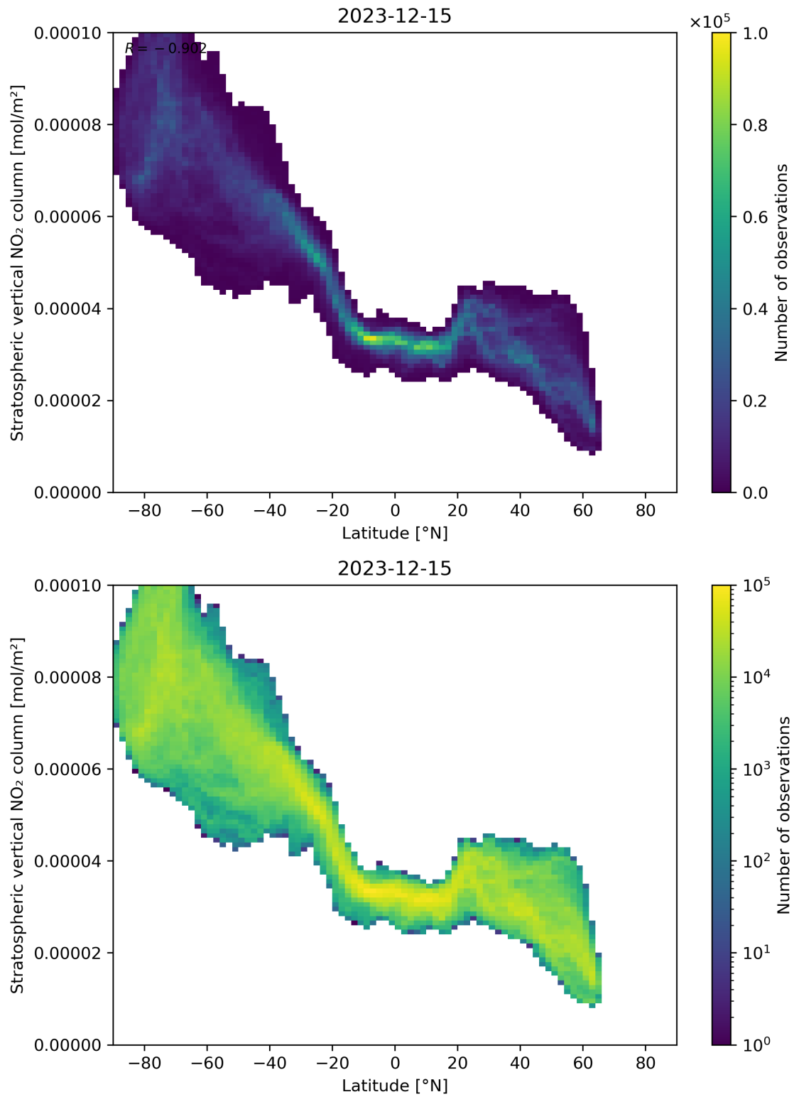
Figure 87: Scatter density plot of “Latitude” against “Stratospheric vertical NO 2 column” for 2023-12-14 to 2023-12-16.
