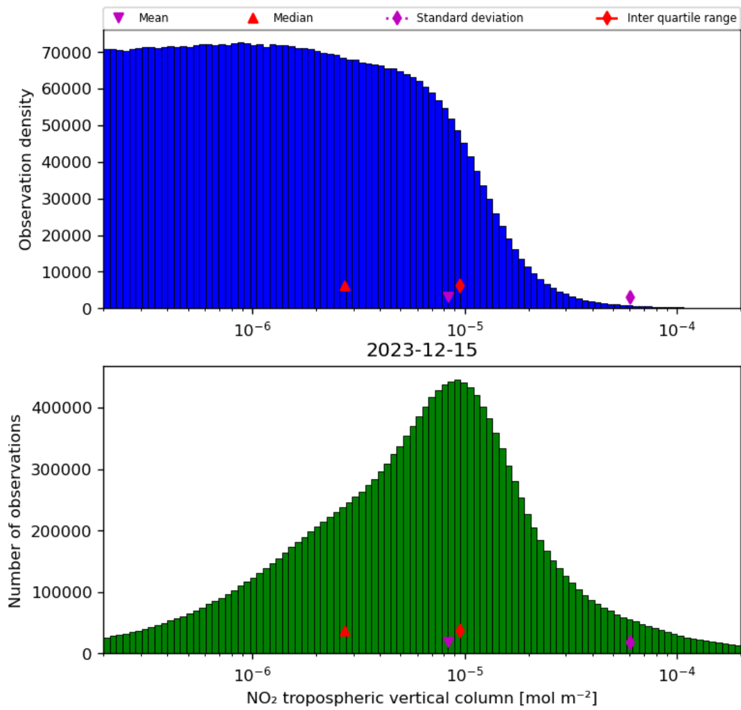
Figure 29: Histogram of “NO 2 tropospheric vertical column” for 2023-12-14 to 2023-12-16
