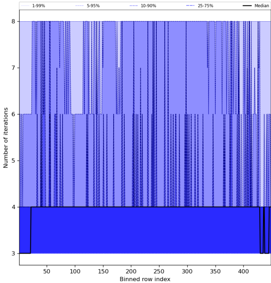
Figure 51: Along track statistics of “Number of iterations” for 2023-12-14 to 2023-12-16
