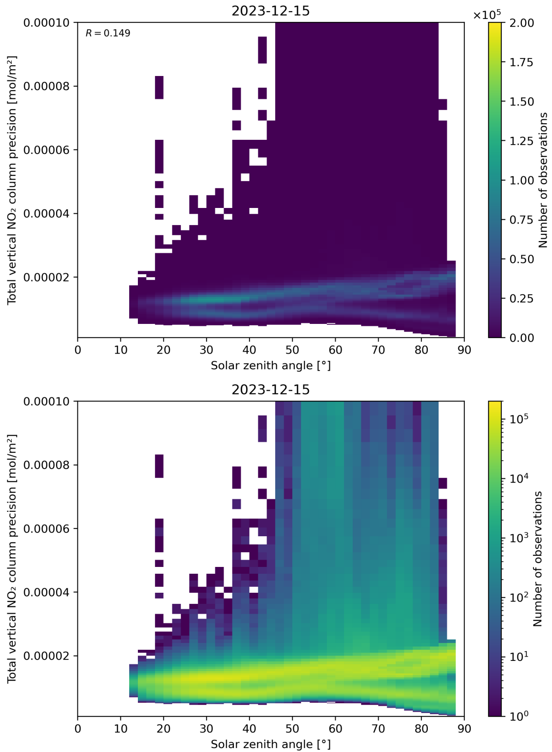
Figure 154: Scatter density plot of “Solar zenith angle” against “Total vertical NO 2 column precision” for 2023-12-14 to 2023-12-16.
