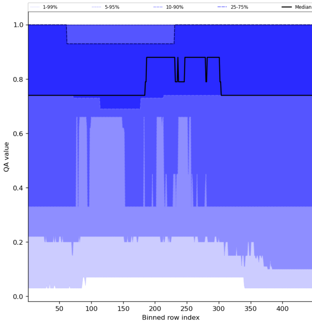
Figure 45: Along track statistics of “QA value” for 2023-12-14 to 2023-12-16
