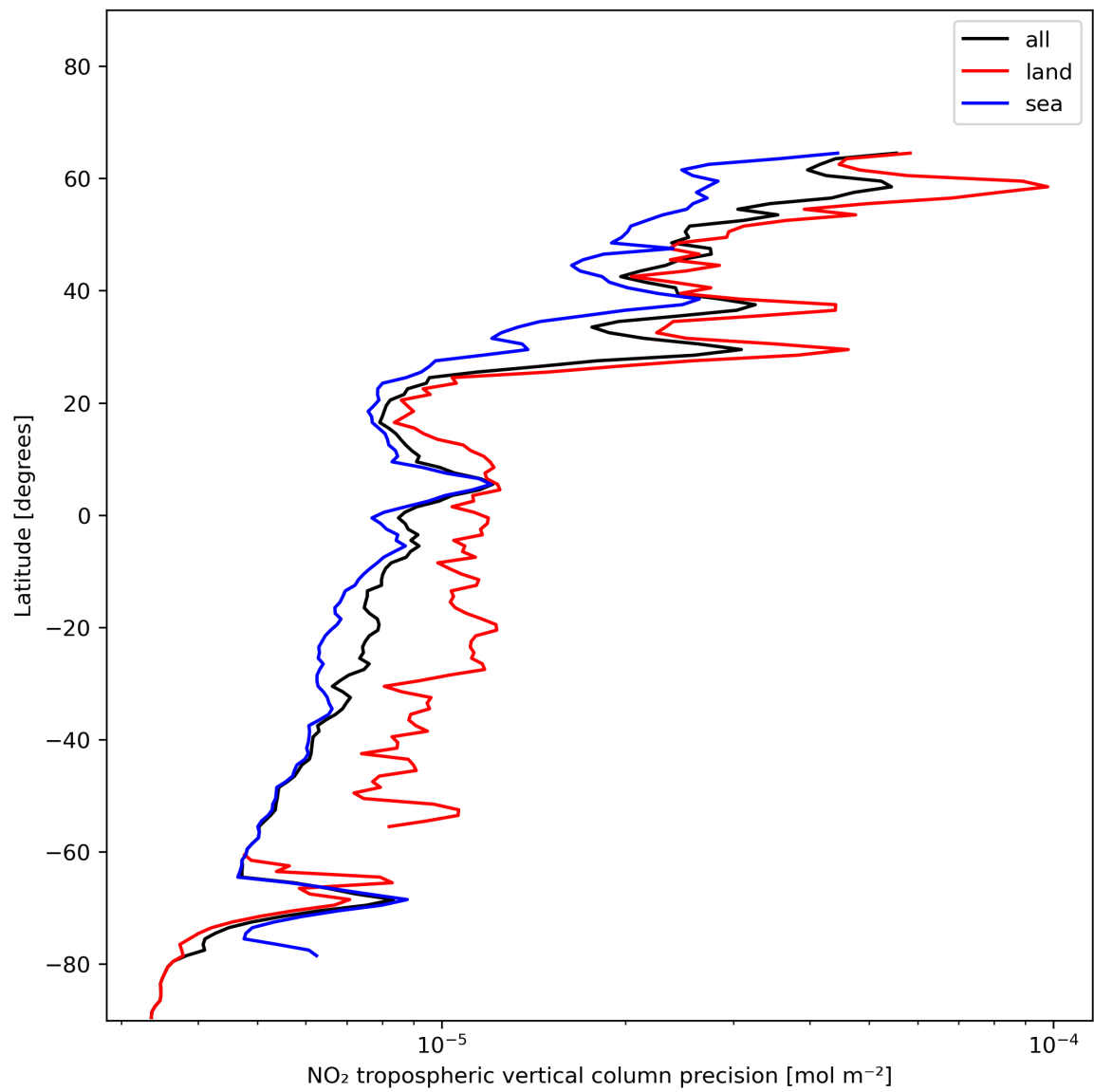
Figure 13: Zonal average of “NO 2 tropospheric vertical column precision” for 2023-12-14 to 2023-12-16.
