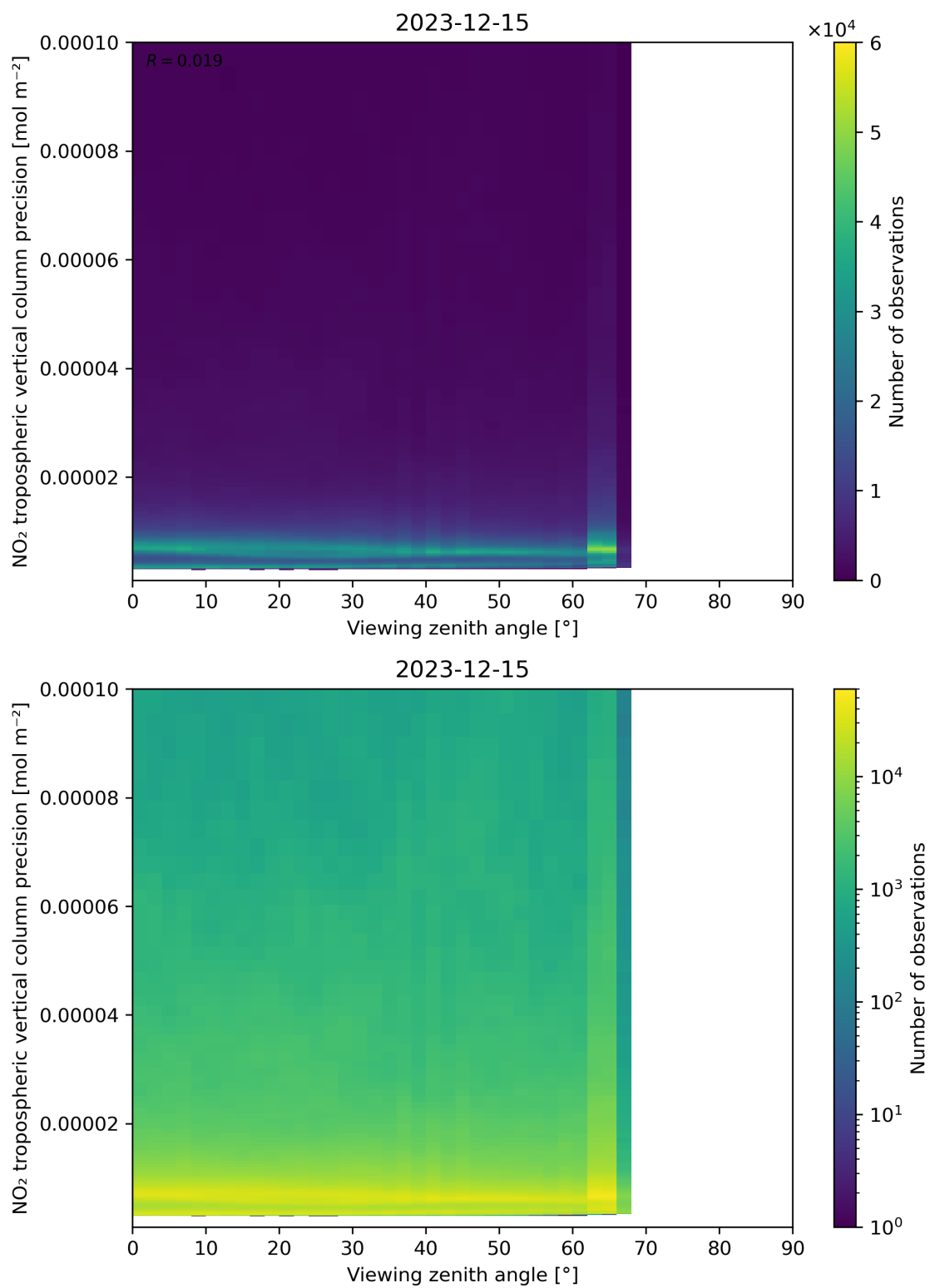
Figure 170: Scatter density plot of “Viewing zenith angle” against “NO 2 tropospheric vertical column precision” for 2023-12-14 to 2023-12-16.
