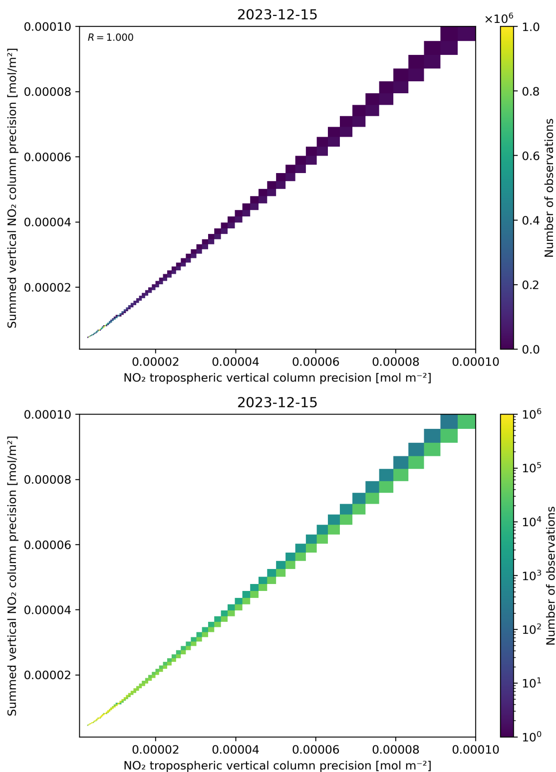
Figure 137: Scatter density plot of “NO 2 tropospheric vertical column precision” against “Summed vertical NO 2 column precision” for 2023-12-14 to 2023-12-16.
