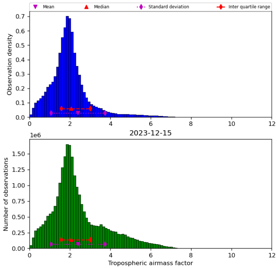
Figure 31: Histogram of “Tropospheric airmass factor” for 2023-12-14 to 2023-12-16
