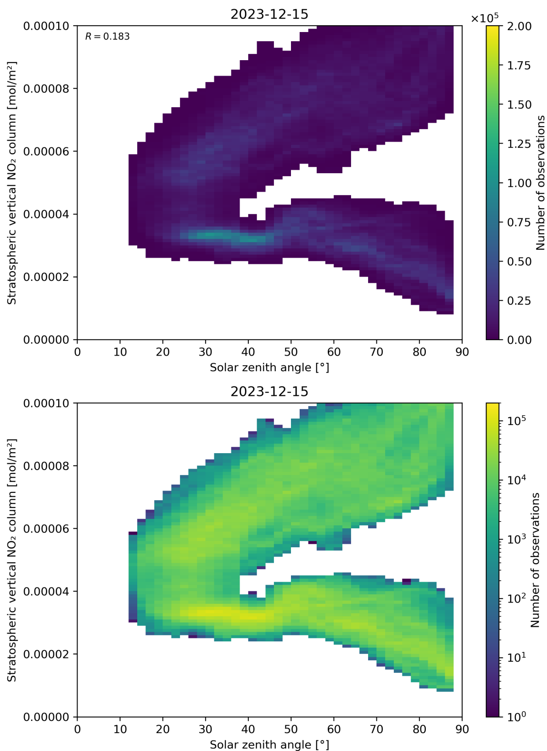
Figure 150: Scatter density plot of “Solar zenith angle” against “Stratospheric vertical NO 2 column” for 2023-12-14 to 2023-12-16.
