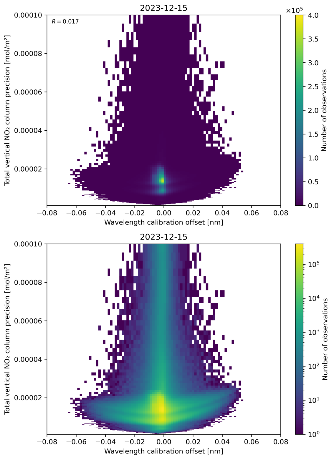
Figure 180: Scatter density plot of “Wavelength calibration offset” against “Total vertical NO 2 column precision” for 2023-12-14 to 2023-12-16.
