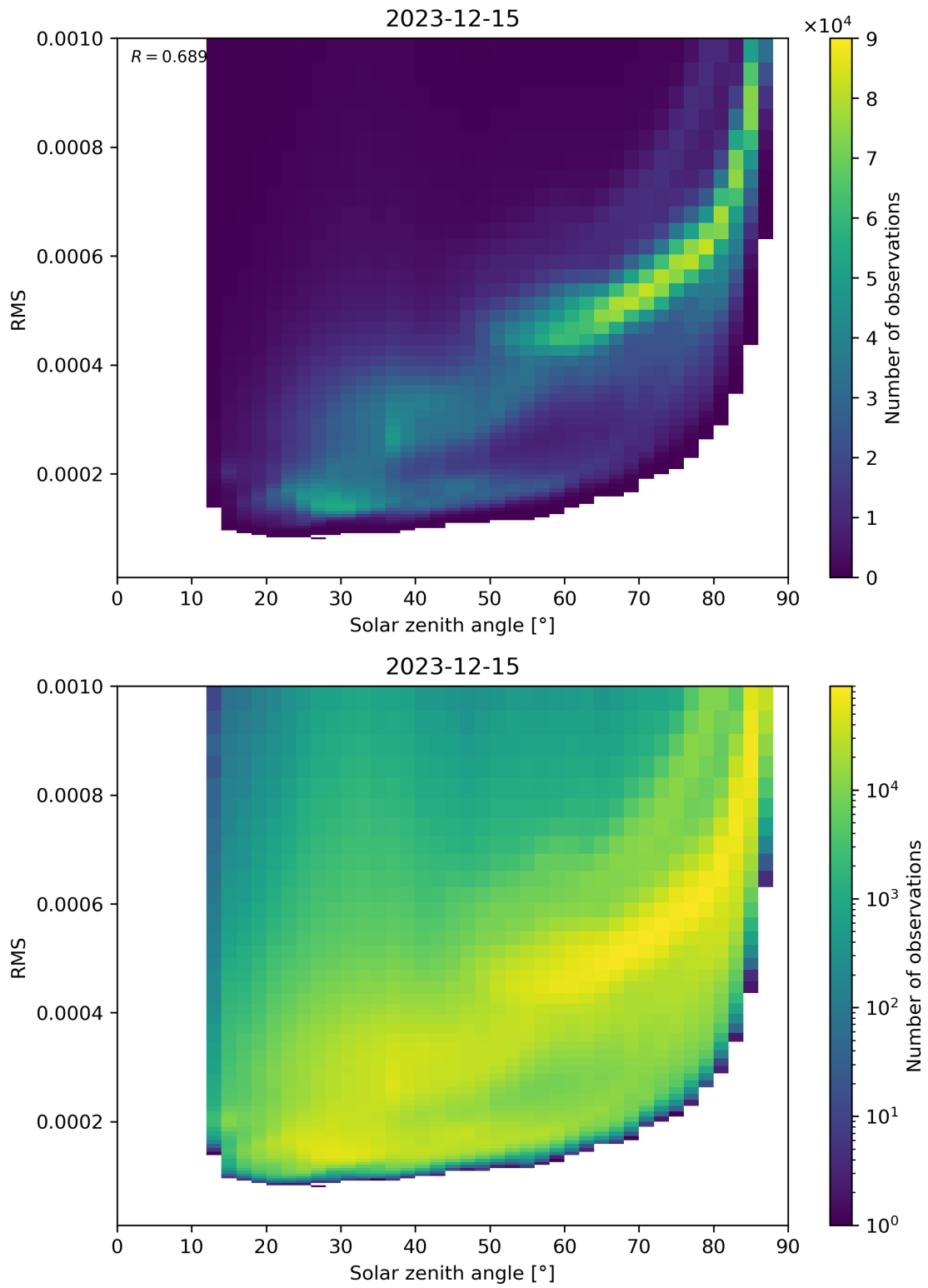
Figure 157: Scatter density plot of “Solar zenith angle” against “RMS” for 2023-12-14 to 2023-12-16.
