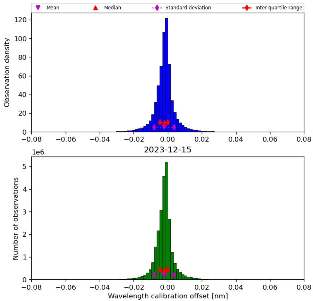
Figure 35: Histogram of “Wavelength calibration offset” for 2023-12-14 to 2023-12-16
