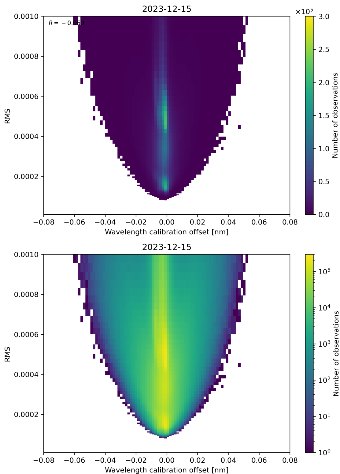
Figure 181: Scatter density plot of “Wavelength calibration offset” against “RMS” for 2023-12-14 to 2023-12-16.
