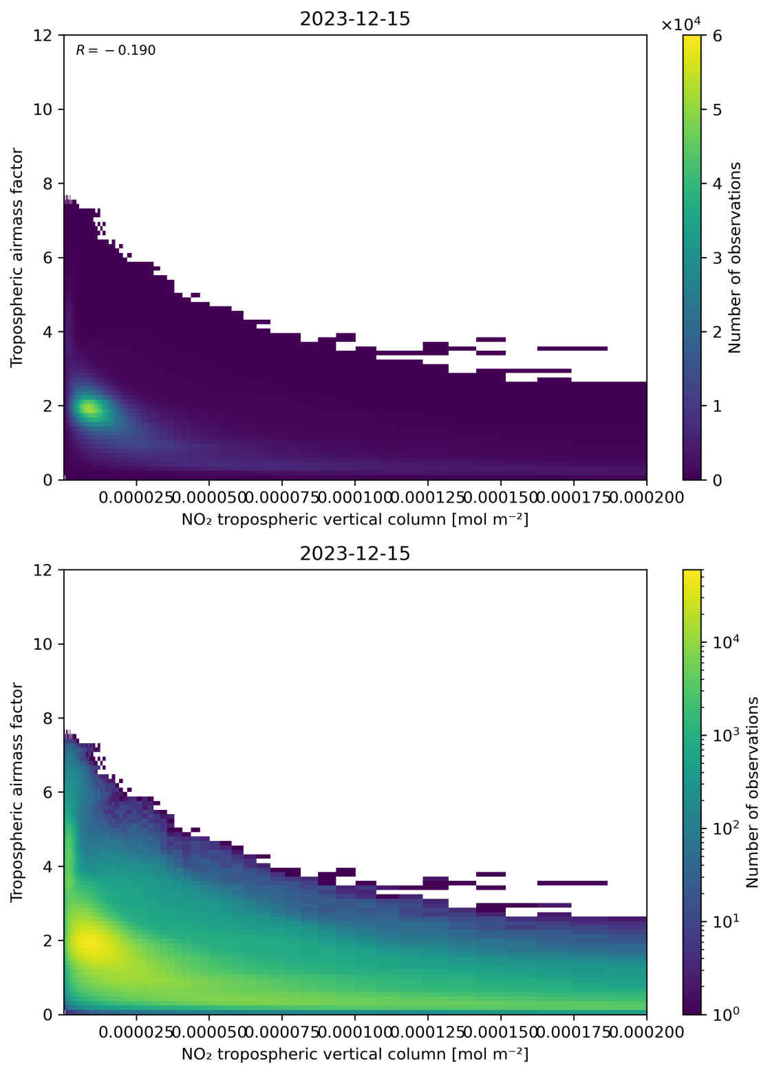
Figure 123: Scatter density plot of “NO 2 tropospheric vertical column” against “Tropospheric air mass factor” for 2023-12-14 to 2023-12-16.
