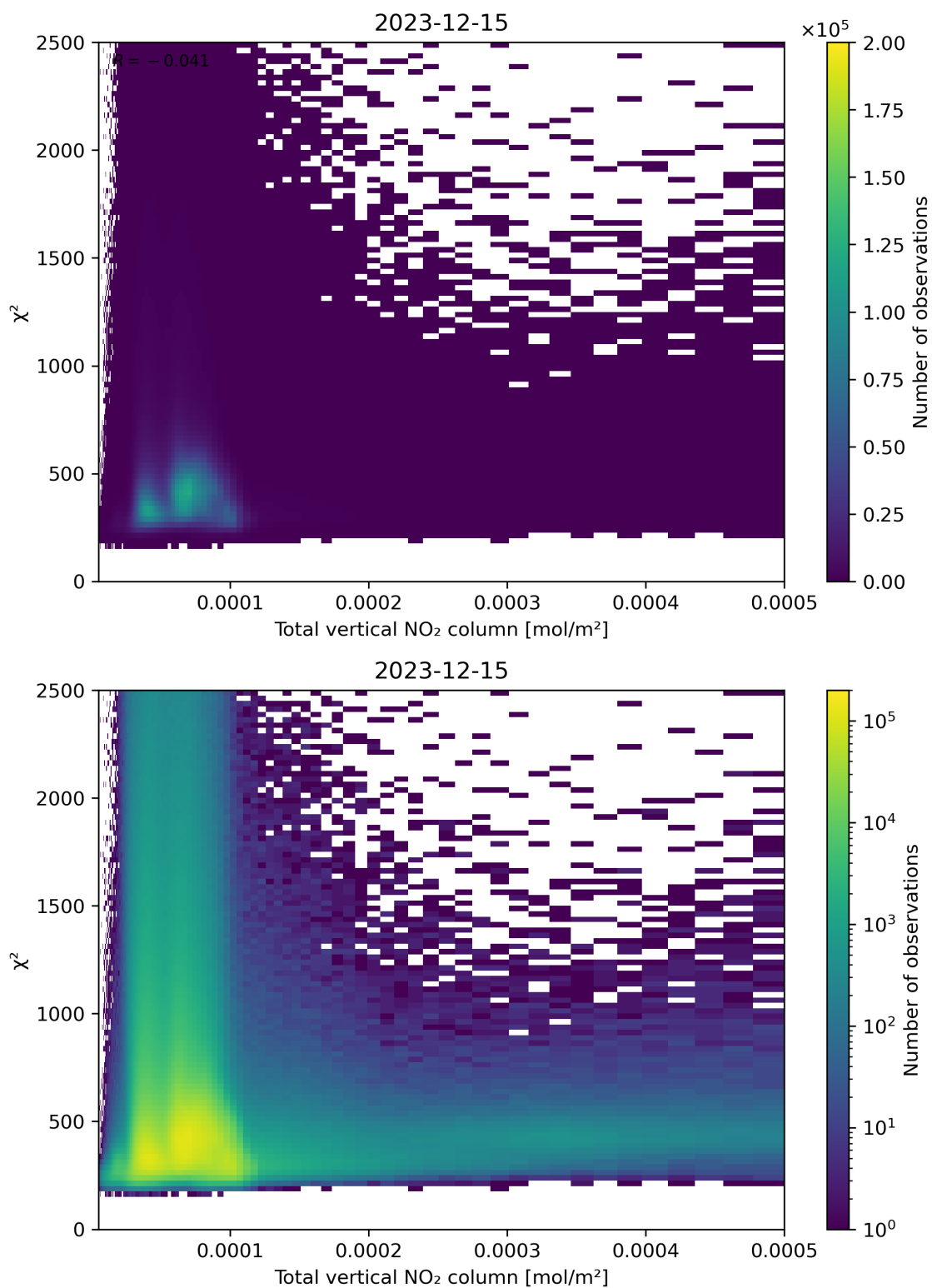
Figure 111: Scatter density plot of “Total vertical NO 2 column” against “ \chi^2 ” for 2023-12-14 to 2023-12-16.
