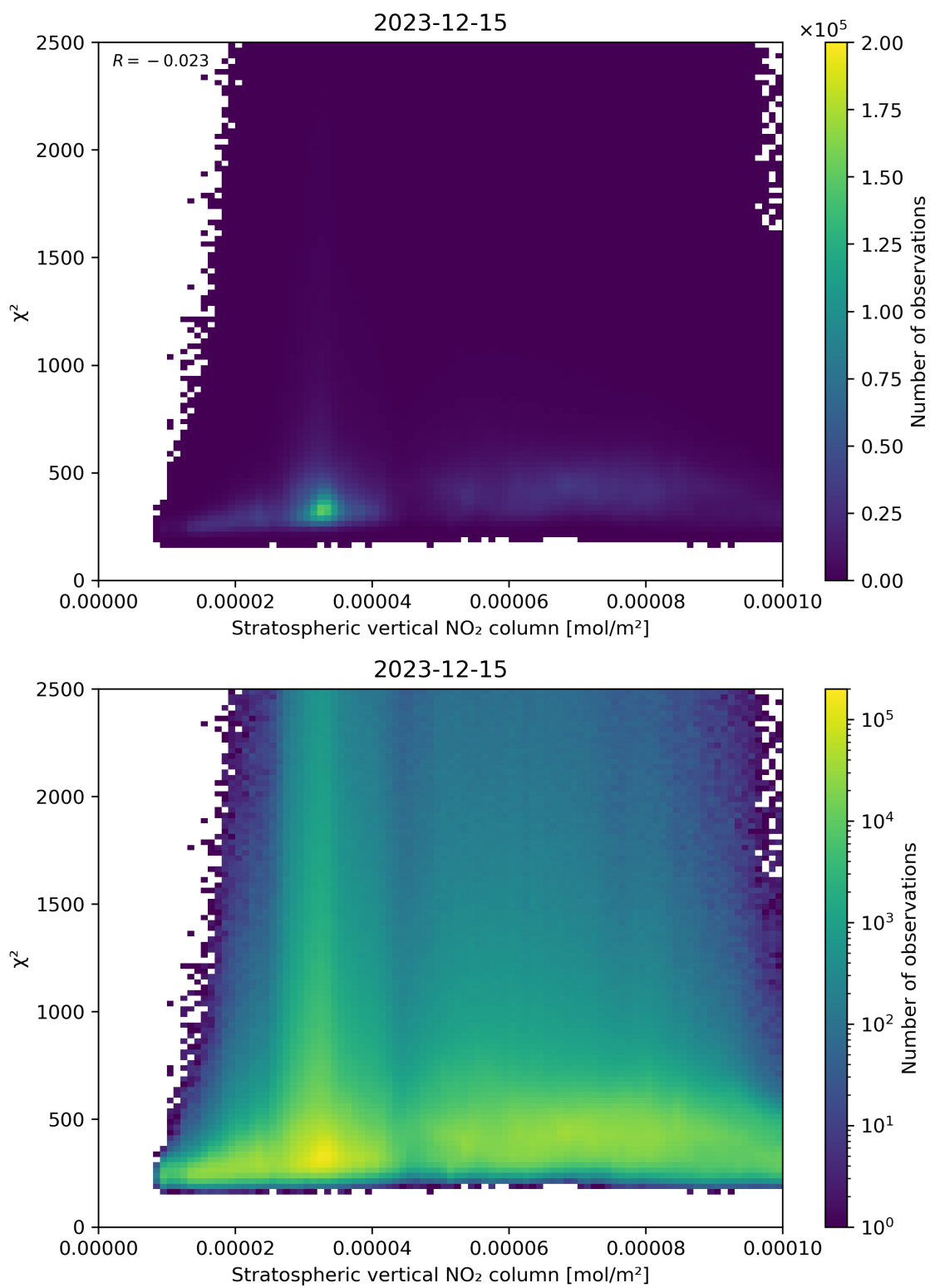
Figure 97: Scatter density plot of “Stratospheric vertical NO 2 column” against “ \chi^2 ” for 2023-12-14 to 2023-12-16.
