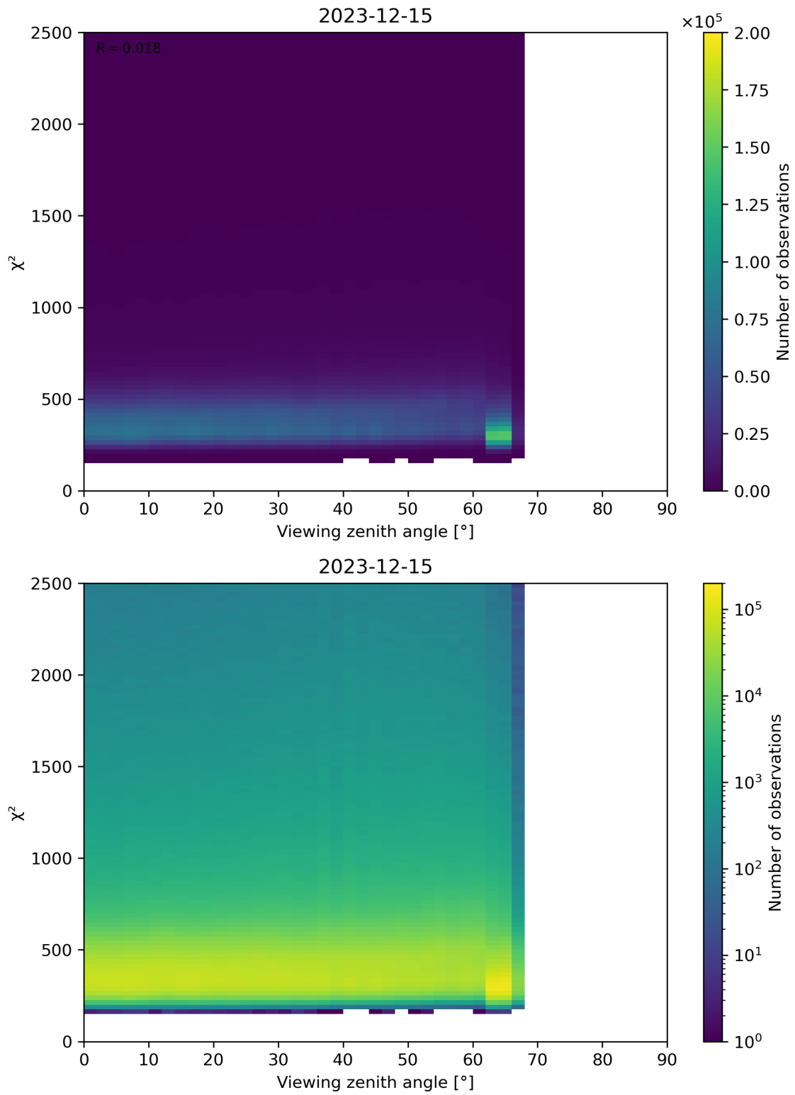
Figure 162: Scatter density plot of “Viewing zenith angle” against “ \chi^2 ” for 2023-12-14 to 2023-12-16.
