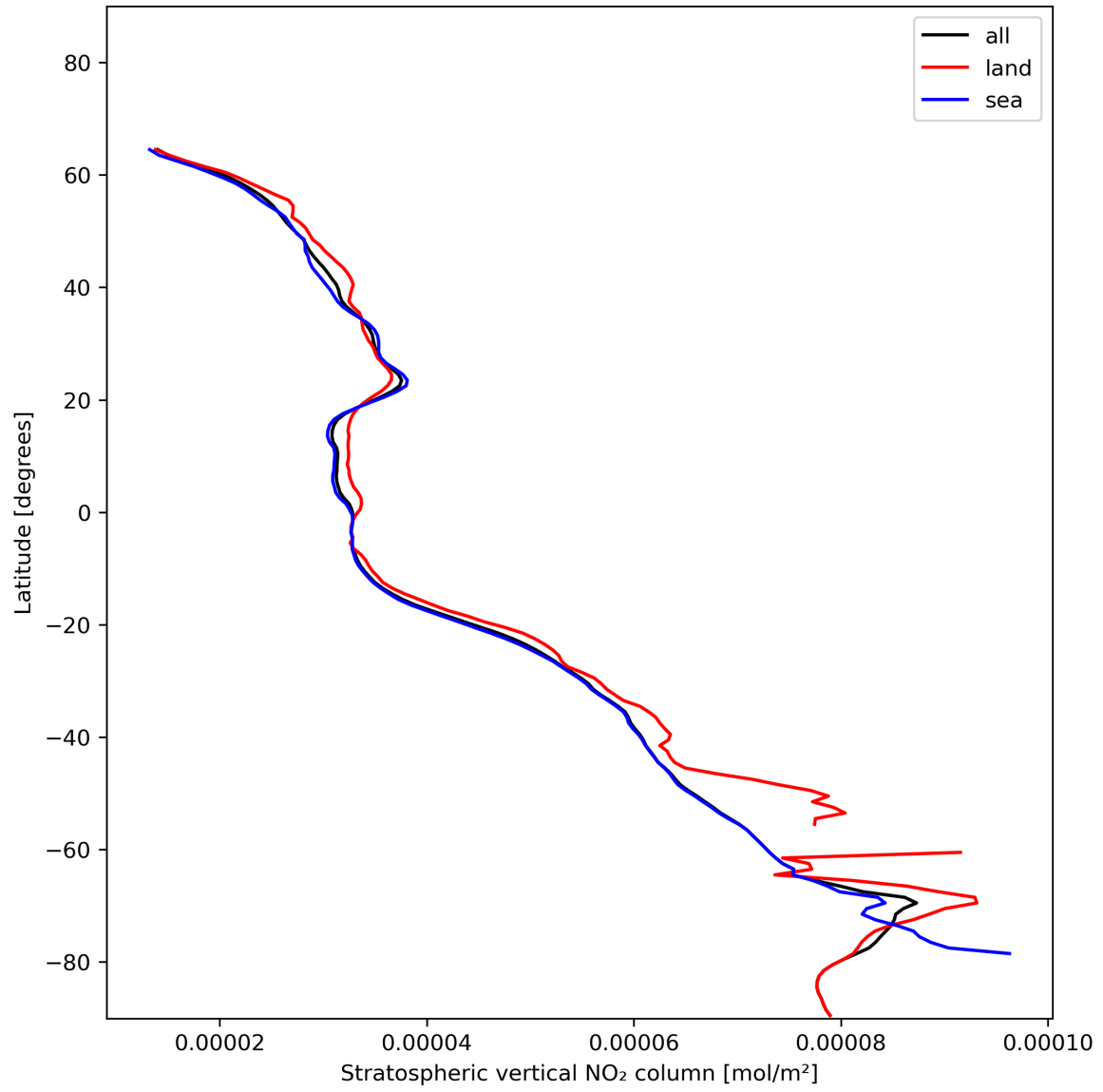
Figure 19: Zonal average of “Stratospheric vertical NO 2 column” for 2023-12-14 to 2023-12-16.
