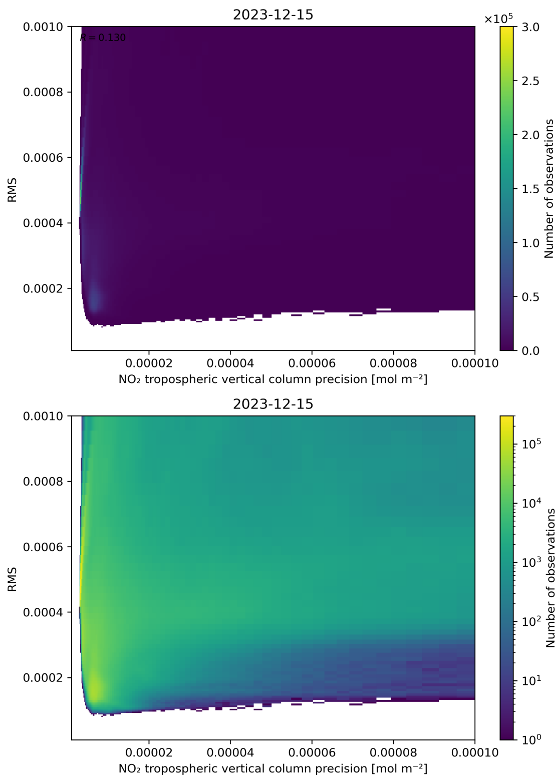
Figure 140: Scatter density plot of “NO 2 tropospheric vertical column precision” against “RMS” for 2023-12-14 to 2023-12-16.
