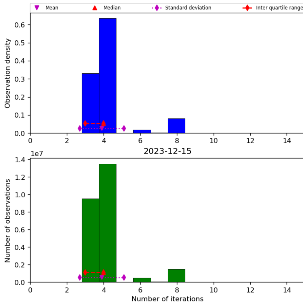
Figure 34: Histogram of “Number of iterations” for 2023-12-14 to 2023-12-16
