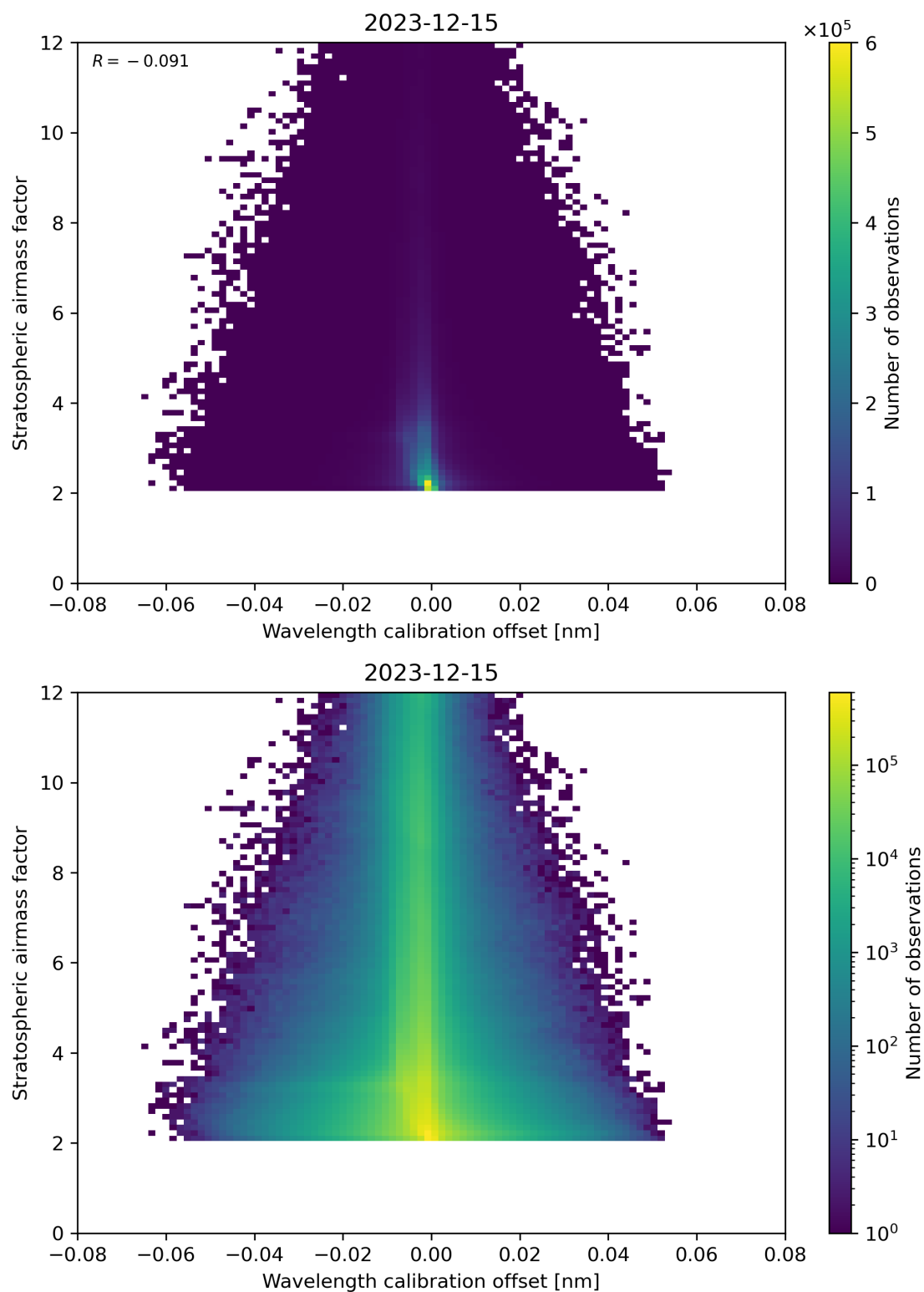
Figure 174: Scatter density plot of “Wavelength calibration offset” against “Stratospheric airmass factor” for 2023-12-14 to 2023-12-16.
