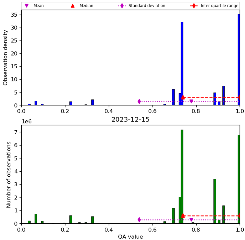
Figure 28: Histogram of “QA value” for 2023-12-14 to 2023-12-16
