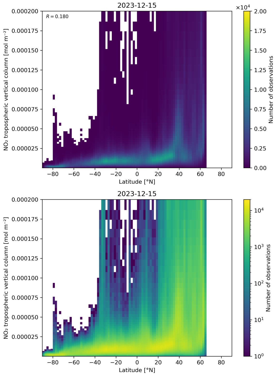
Figure 92: Scatter density plot of “Latitude” against “NO 2 tropospheric vertical column” for 2023-12-14 to 2023-12-16.
