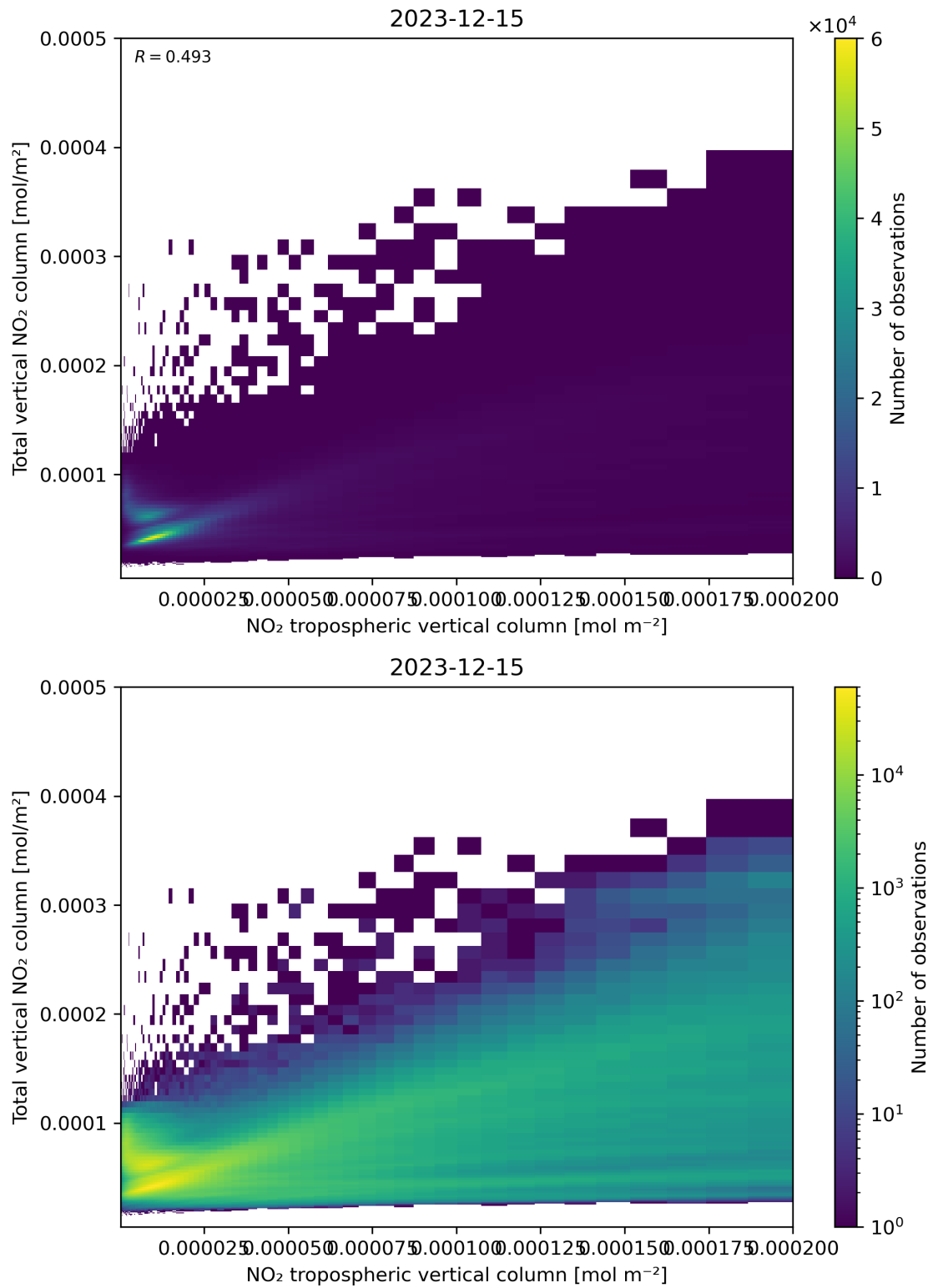
Figure 128: Scatter density plot of “NO 2 tropospheric vertical column” against “Total vertical NO 2 column” for 2023-12-14 to 2023-12-16.
