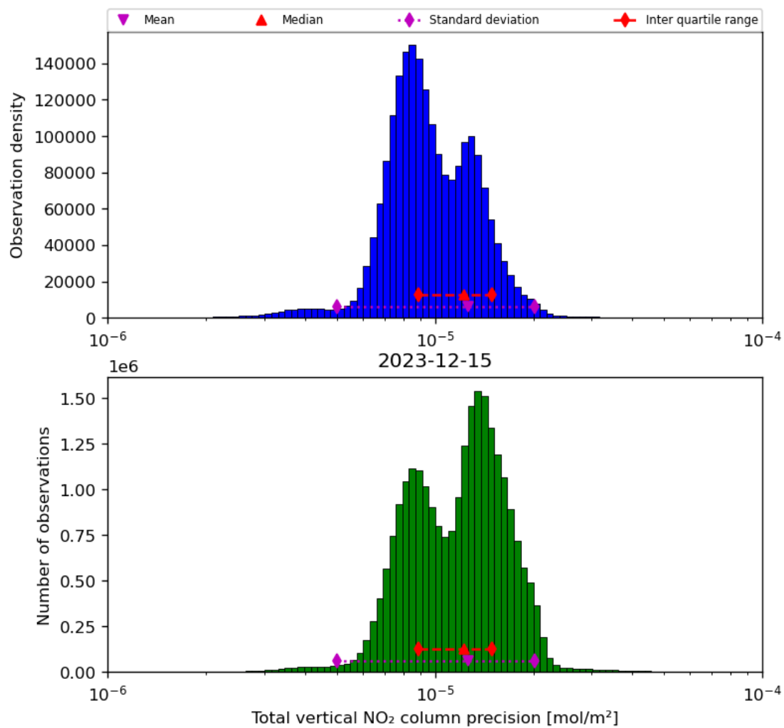
Figure 39: Histogram of “Total vertical NO 2 column precision” for 2023-12-14 to 2023-12-16
