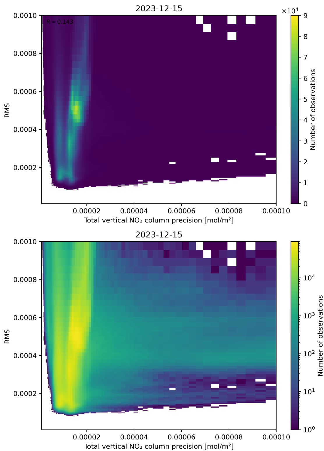
Figure 119: Scatter density plot of “Total vertical NO 2 column precision” against “RMS” for 2023-12-14 to 2023-12-16.
