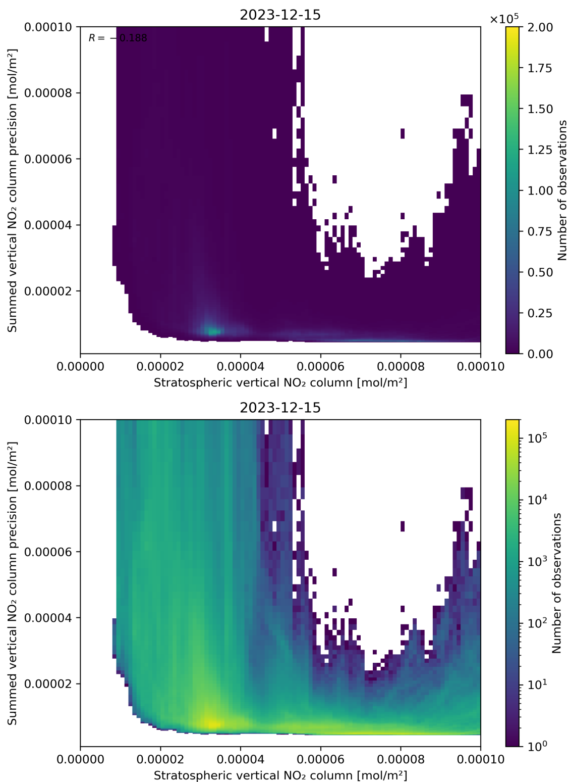
Figure 99: Scatter density plot of “Stratospheric vertical NO 2 column” against “Summed vertical NO 2 column precision” for 2023-12-14 to 2023-12-16.
