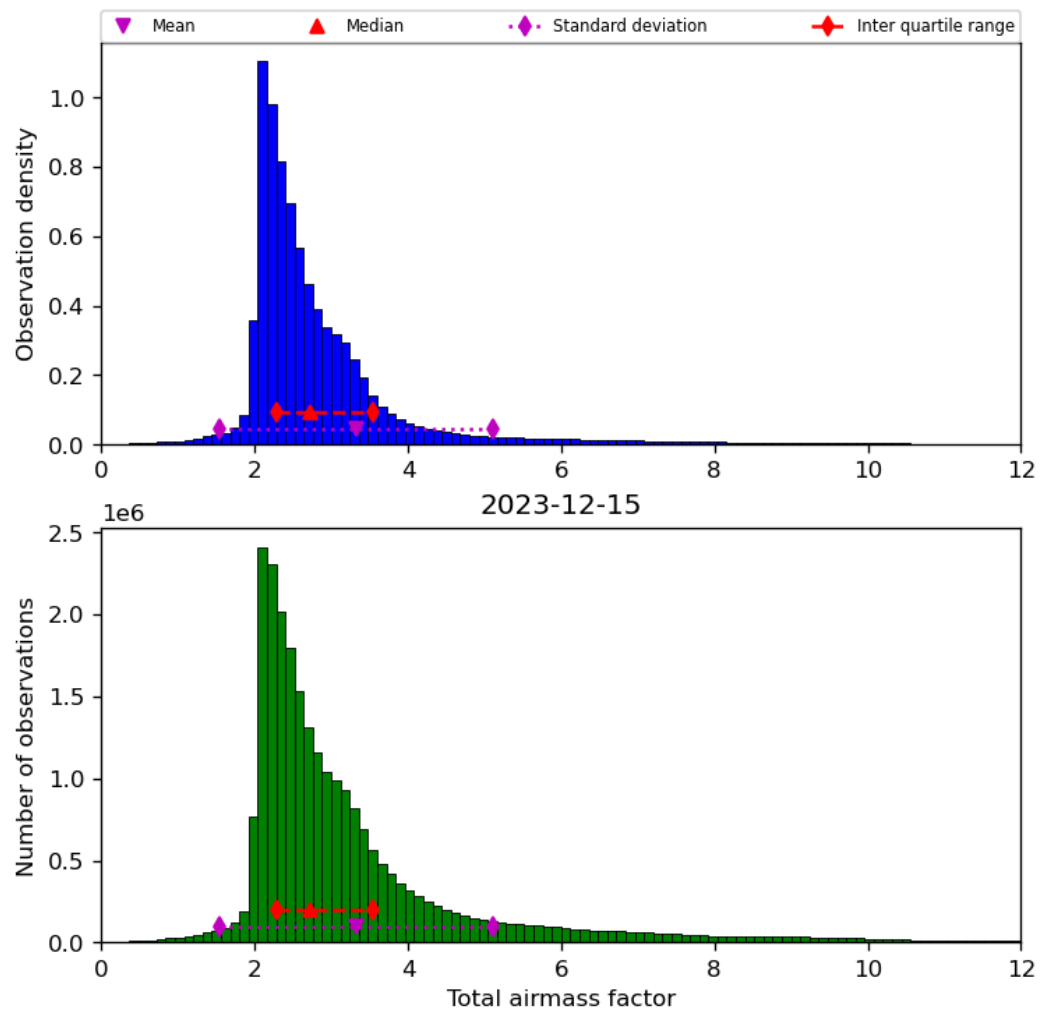
Figure 32: Histogram of “Total airmass factor” for 2023-12-14 to 2023-12-16
