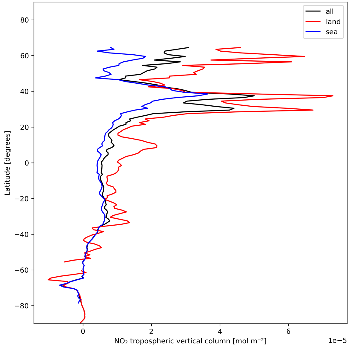
Figure 12: Zonal average of “NO 2 tropospheric vertical column” for 2023-12-14 to 2023-12-16.
