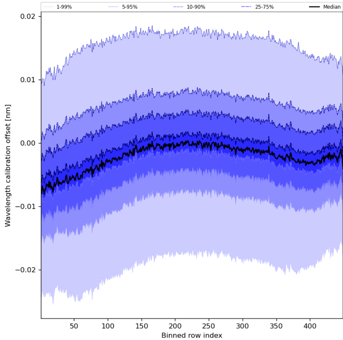
Figure 52: Along track statistics of “Wavelength calibration offset” for 2023-12-14 to 2023-12-16
