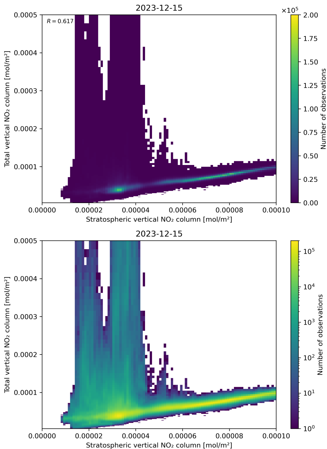
Figure 100: Scatter density plot of “Stratospheric vertical NO 2 column” against “Total vertical NO 2 column” for 2023-12-14 to 2023-12-16.
