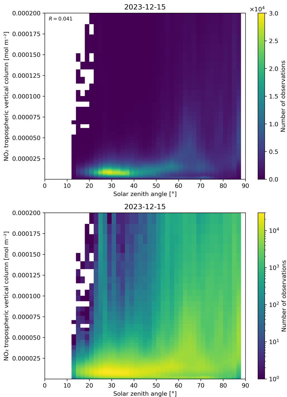
Figure 155: Scatter density plot of “Solar zenith angle” against “NO 2 tropospheric vertical column” for 2023-12-14 to 2023-12-16.
