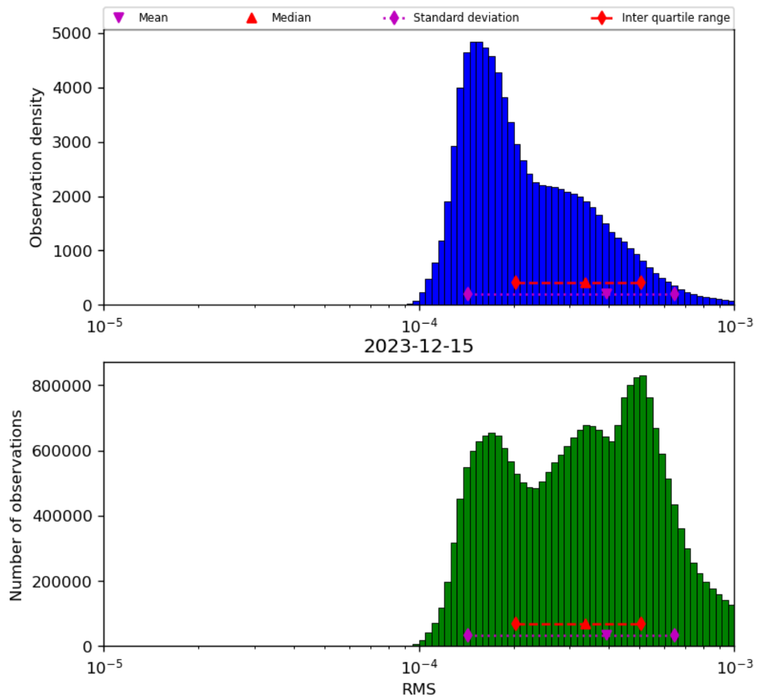
Figure 43: Histogram of “RMS” for 2023-12-14 to 2023-12-16
