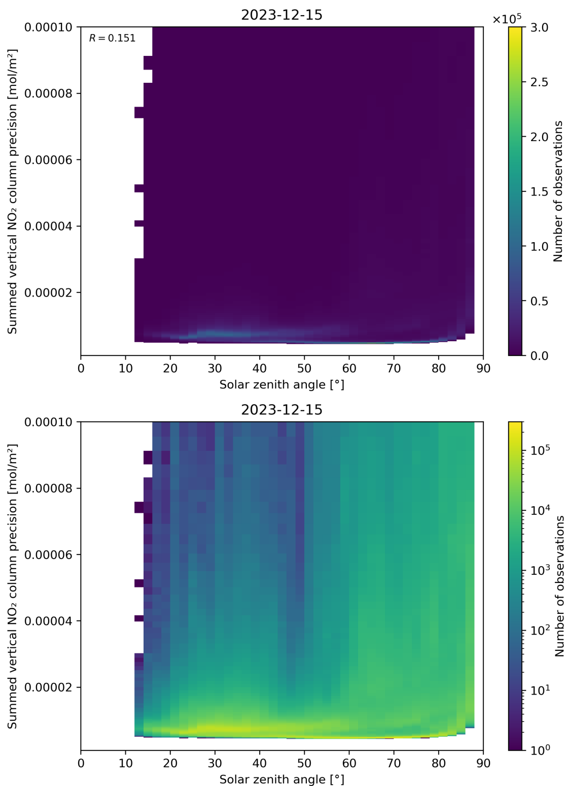
Figure 152: Scatter density plot of “Solar zenith angle” against “Summed vertical NO 2 column precision” for 2023-12-14 to 2023-12-16.
