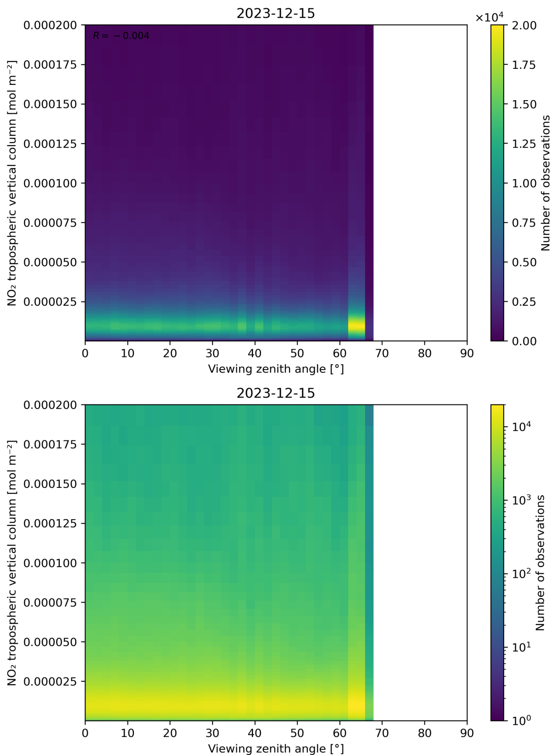
Figure 169: Scatter density plot of “Viewing zenith angle” against “NO 2 tropospheric vertical column” for 2023-12-14 to 2023-12-16.
