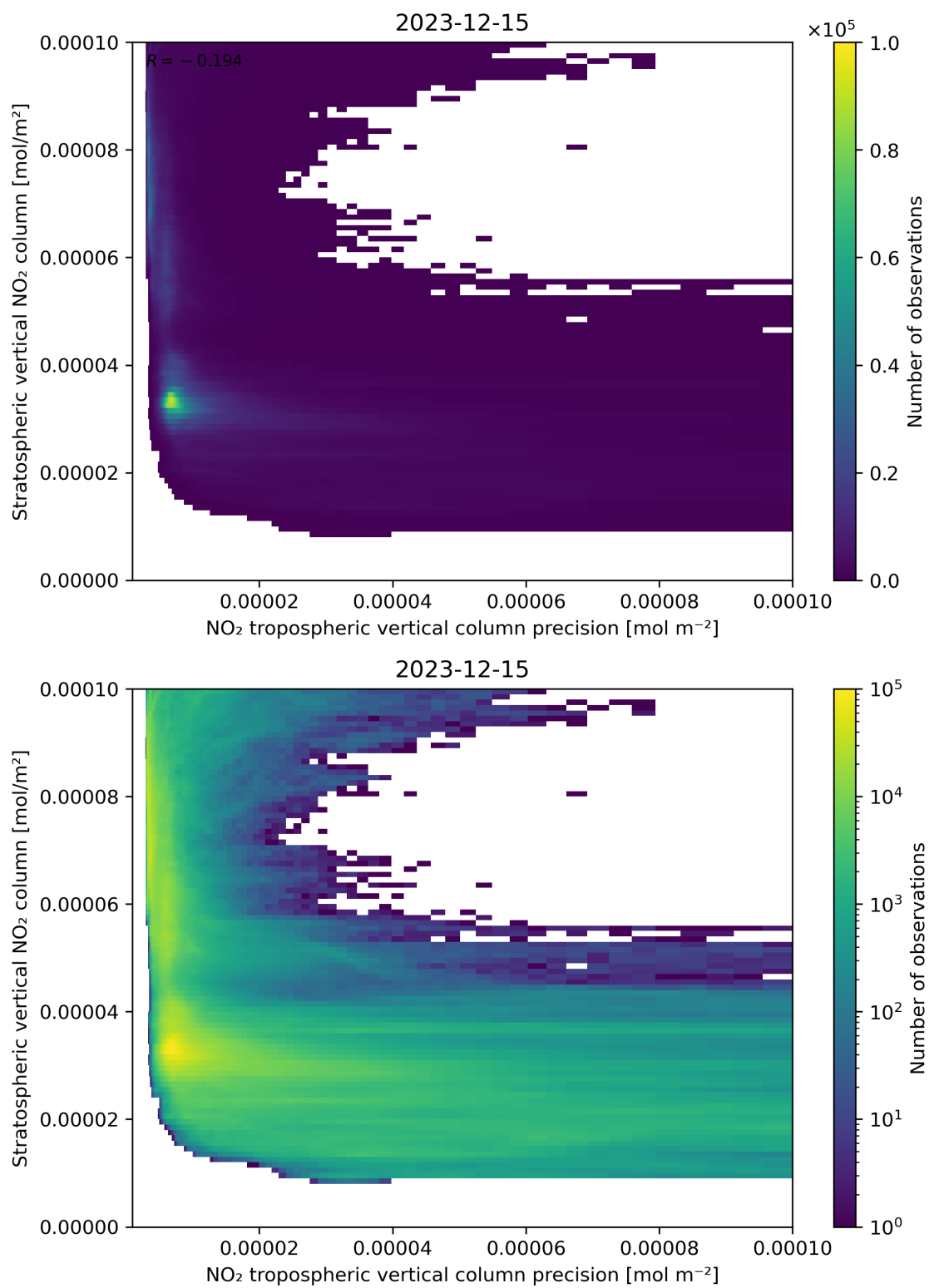
Figure 135: Scatter density plot of “NO 2 tropospheric vertical column precision” against “Stratospheric vertical NO 2 column” for 2023-12-14 to 2023-12-16.
