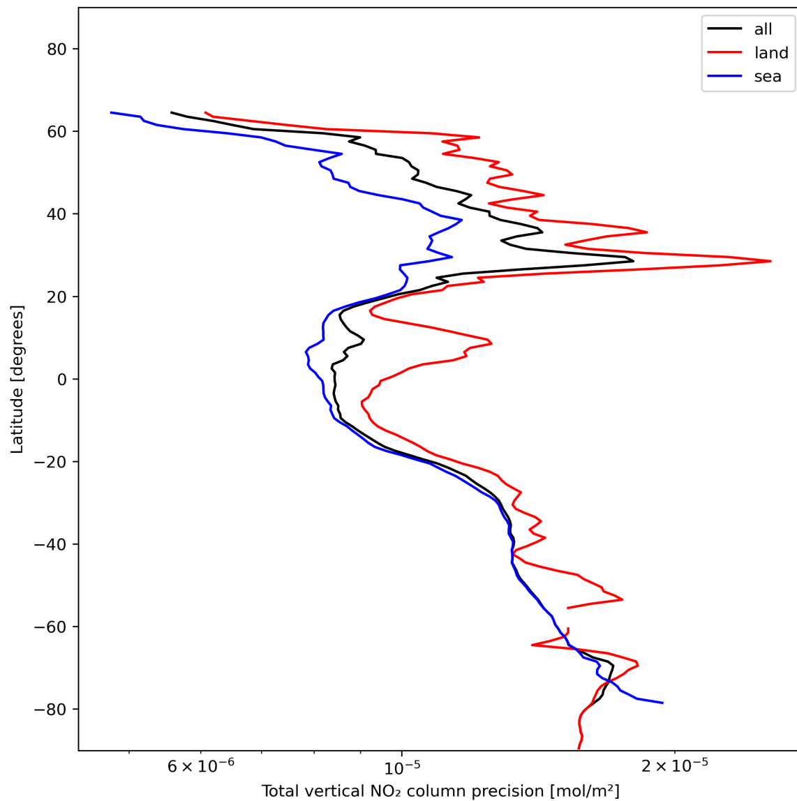
Figure 22: Zonal average of “Total vertical NO 2 column precision” for 2023-12-14 to 2023-12-16.
