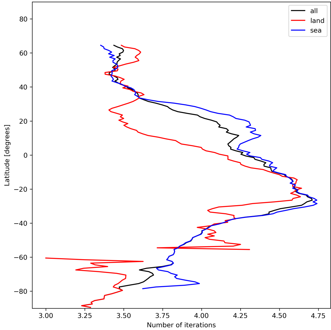
Figure 17: Zonal average of “Number of iterations” for 2023-12-14 to 2023-12-16.
