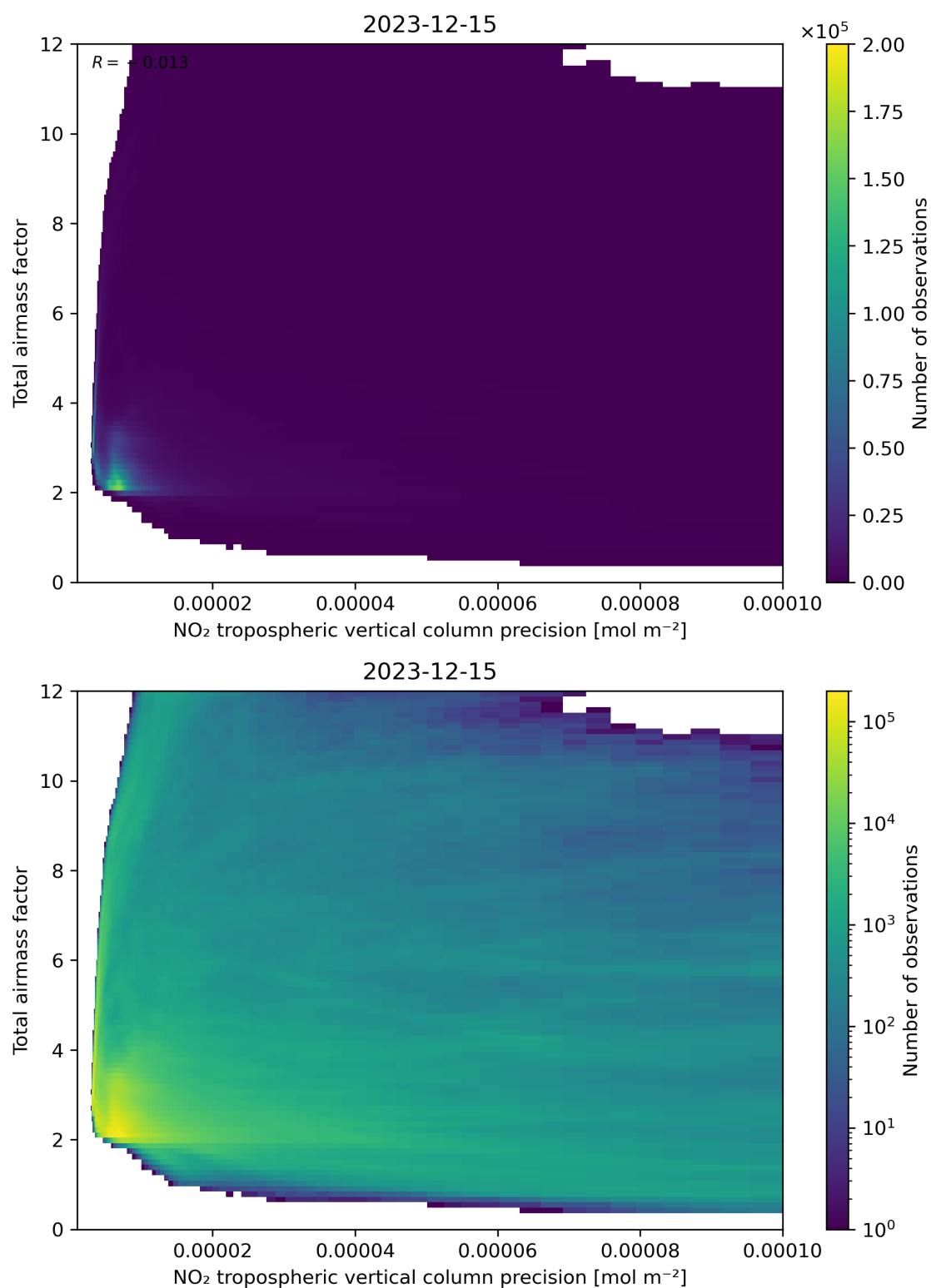
Figure 132: Scatter density plot of “NO 2 tropospheric vertical column precision” against “Total air mass factor” for 2023-12-14 to 2023-12-16.
