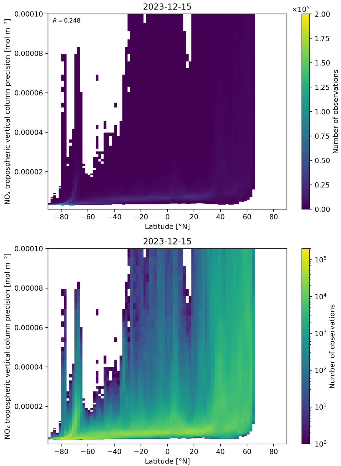
Figure 93: Scatter density plot of “Latitude” against “NO 2 tropospheric vertical column precision” for 2023-12-14 to 2023-12-16.
