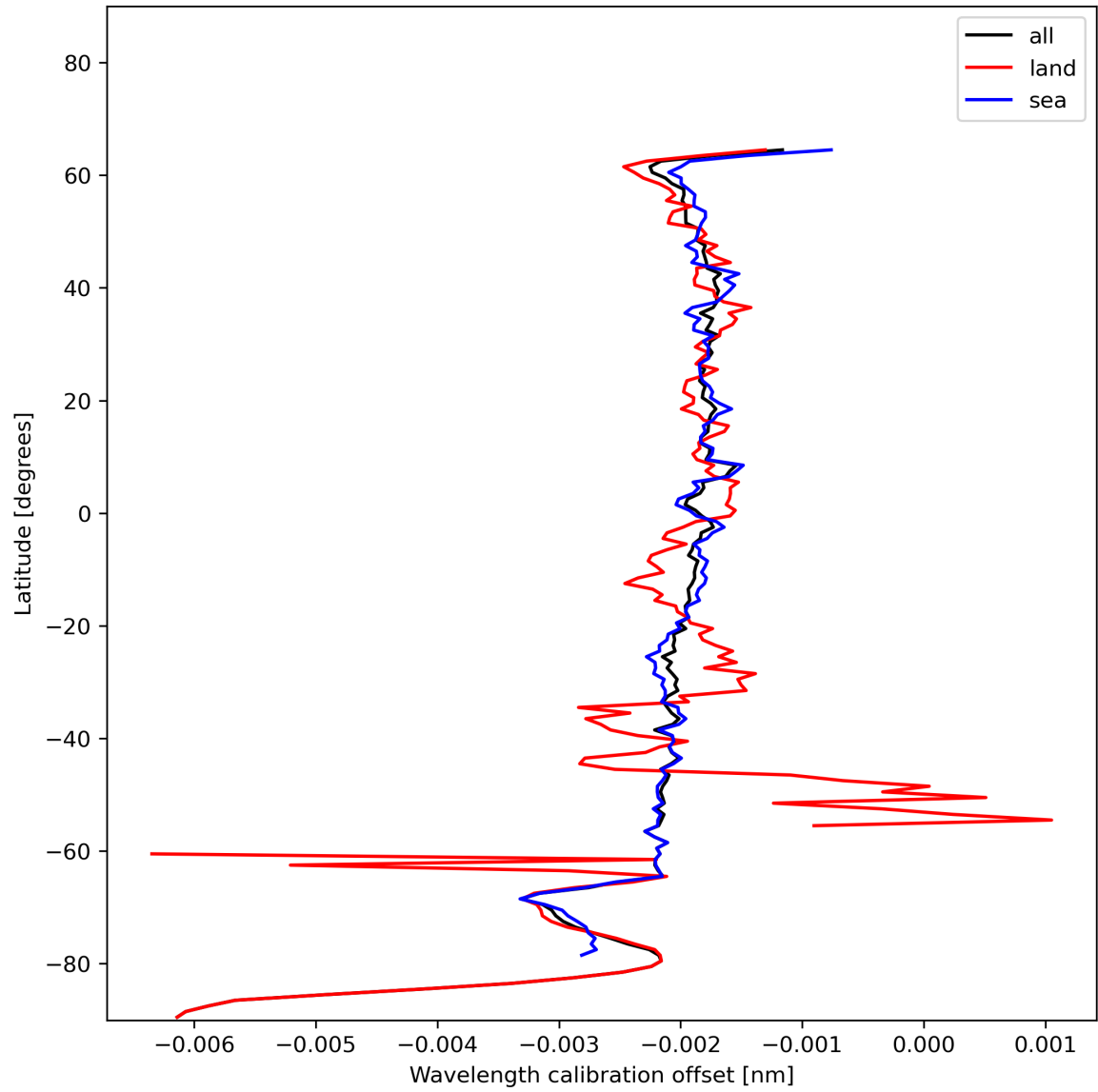
Figure 18: Zonal average of “Wavelength calibration offset” for 2023-12-14 to 2023-12-16.
