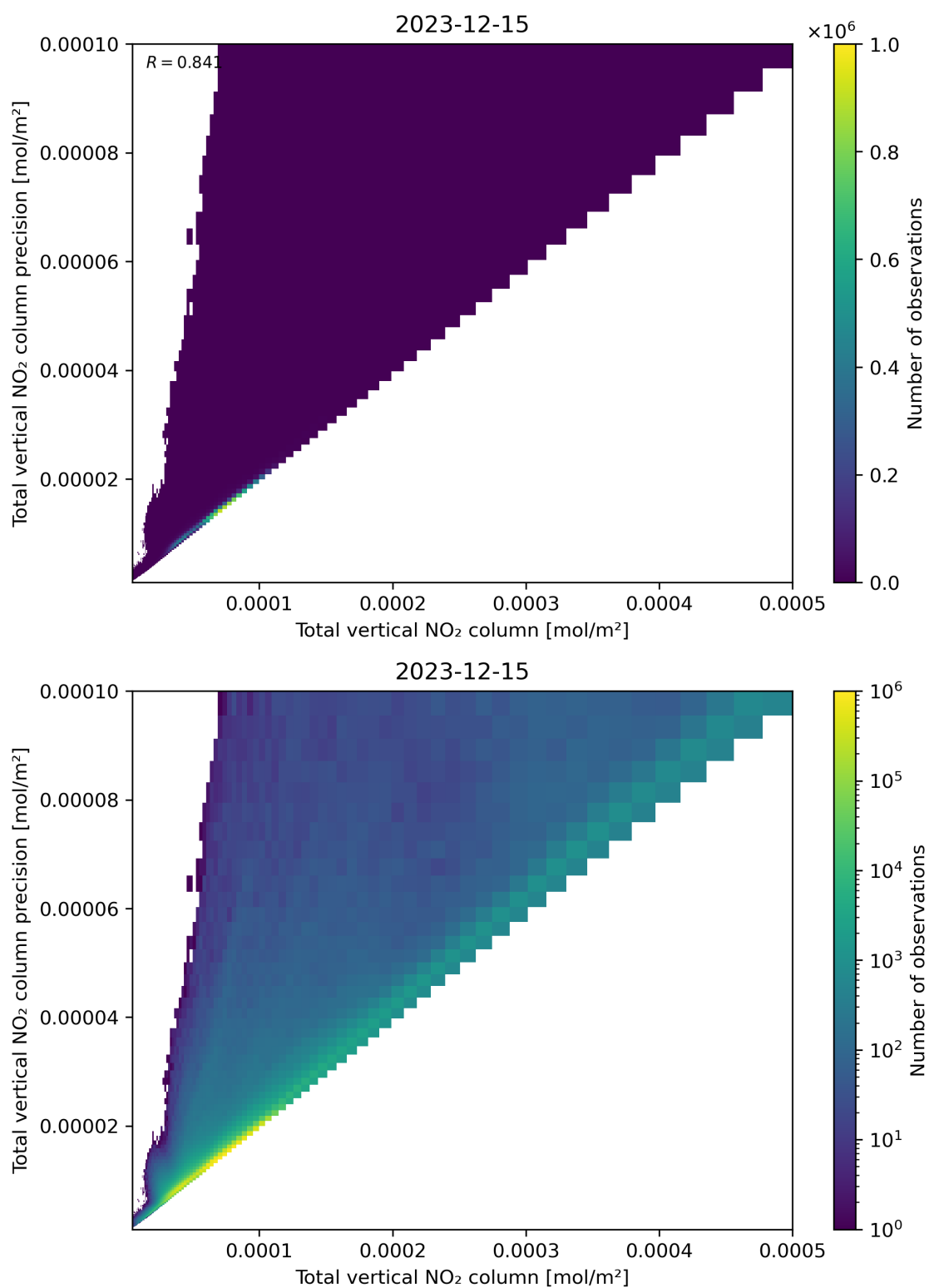
Figure 114: Scatter density plot of “Total vertical NO 2 column” against “Total vertical NO 2 column precision” for 2023-12-14 to 2023-12-16.
