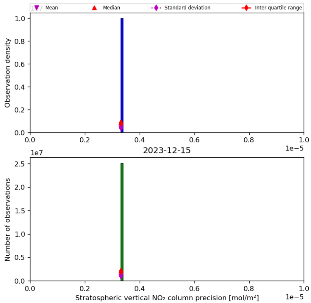
Figure 37: Histogram of “Stratospheric vertical NO 2 column precision” for 2023-12-14 to 2023-12-16
