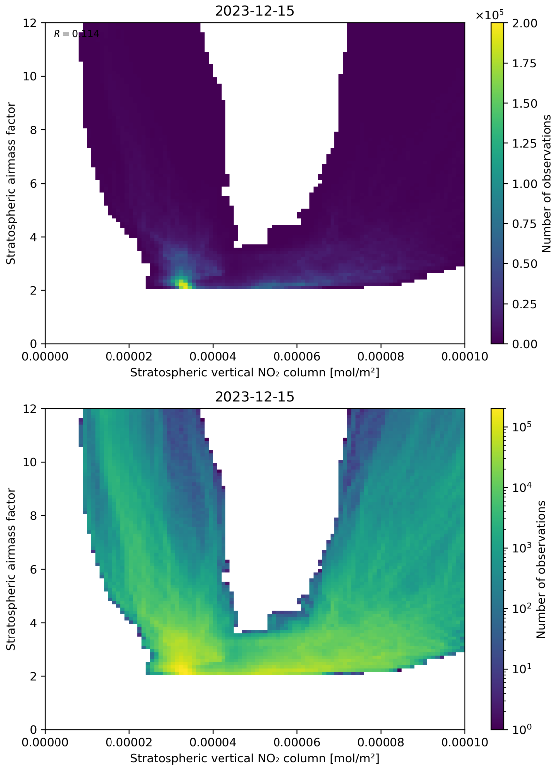
Figure 96: Scatter density plot of “Stratospheric vertical NO 2 column” against “Stratospheric airmass factor” for 2023-12-14 to 2023-12-16.
