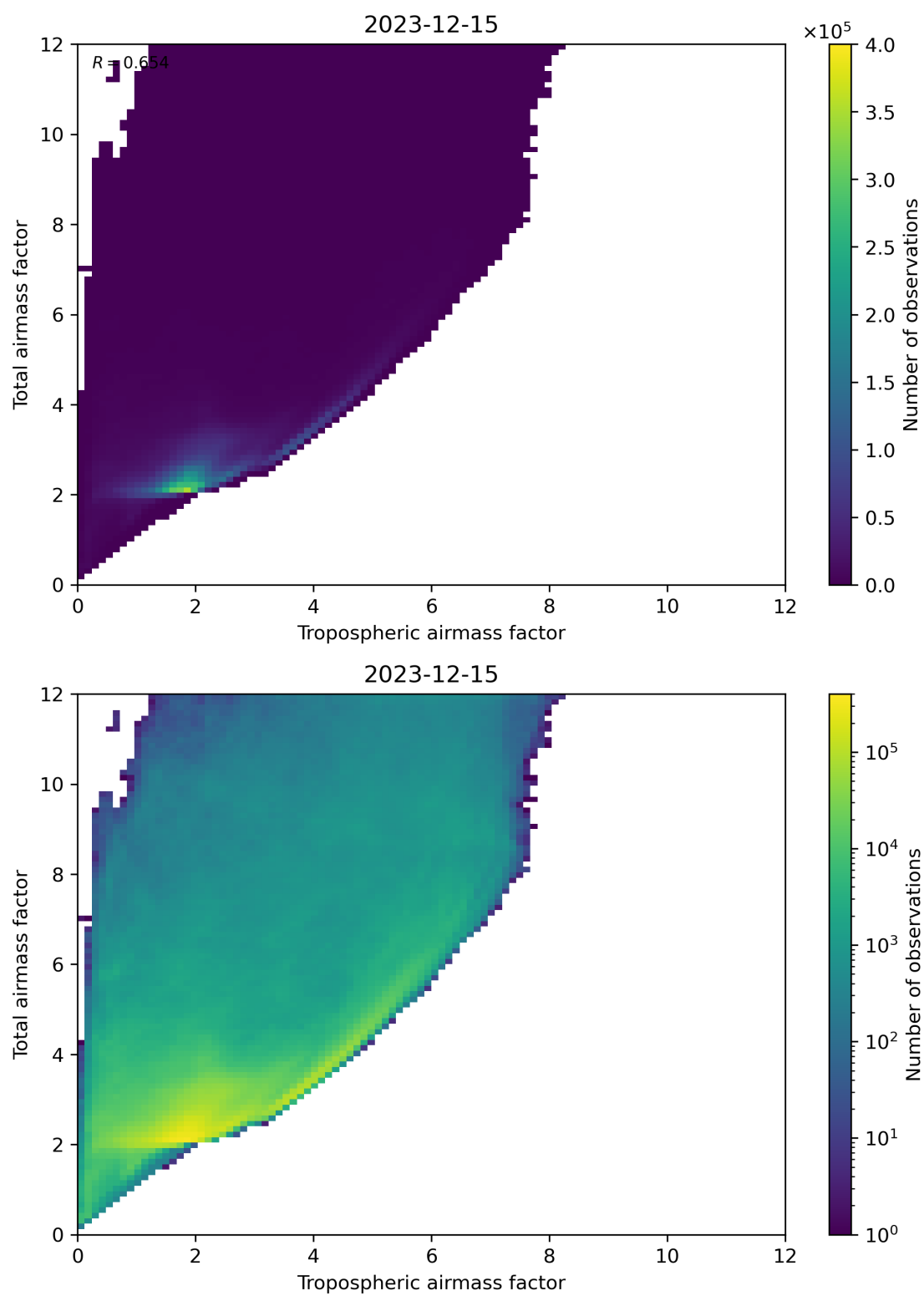
Figure 72: Scatter density plot of “Tropospheric airmass factor” against “Total airmass factor” for 2023-12-14 to 2023-12-16.
