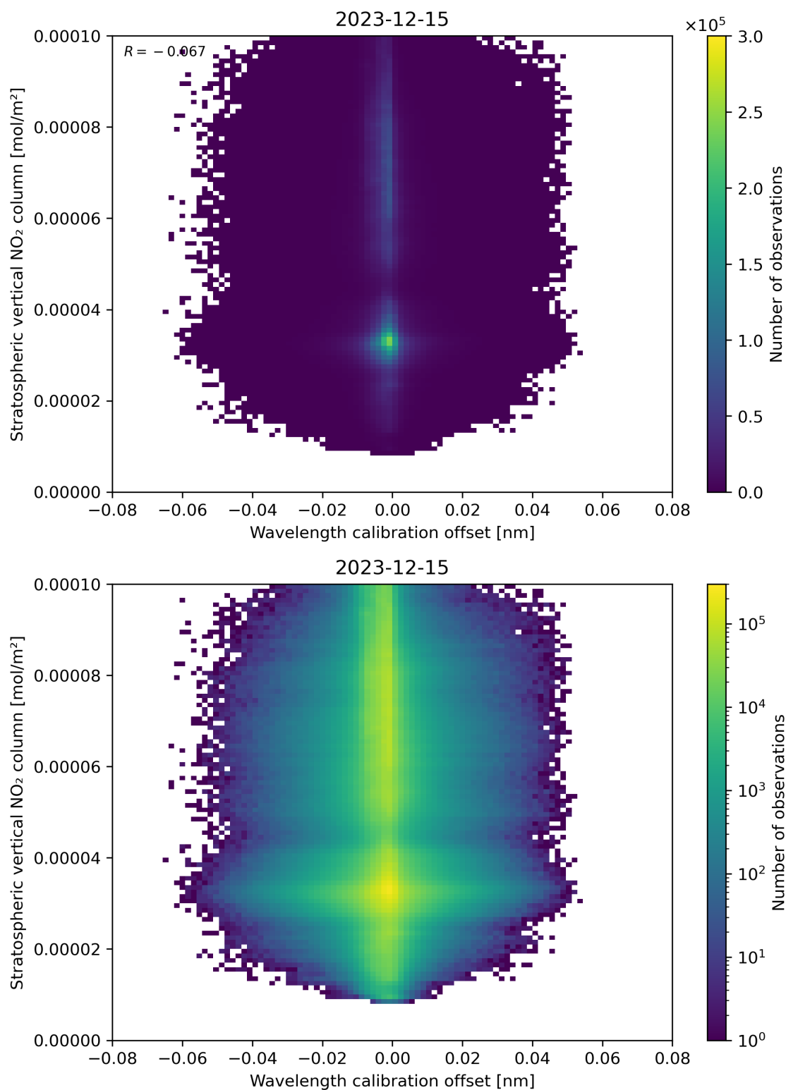
Figure 176: Scatter density plot of “Wavelength calibration offset” against “Stratospheric vertical NO 2 column” for 2023-12-14 to 2023-12-16.
