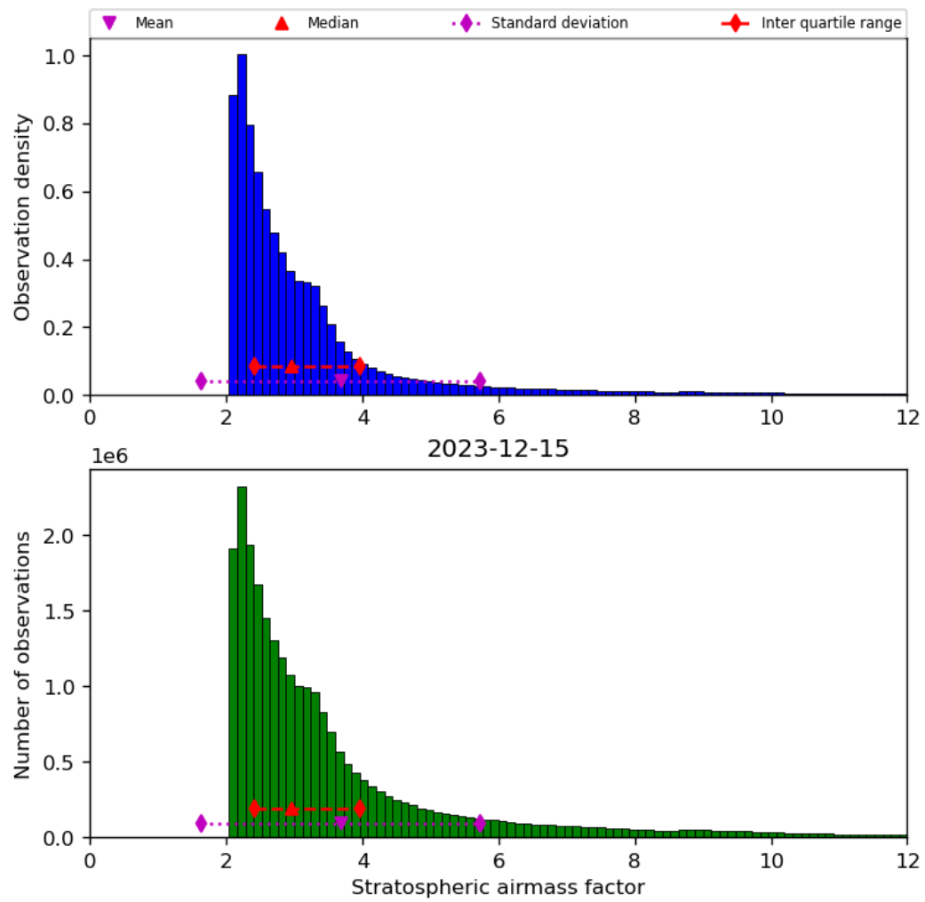
Figure 44: Histogram of “Stratospheric airmass factor” for 2023-12-14 to 2023-12-16
