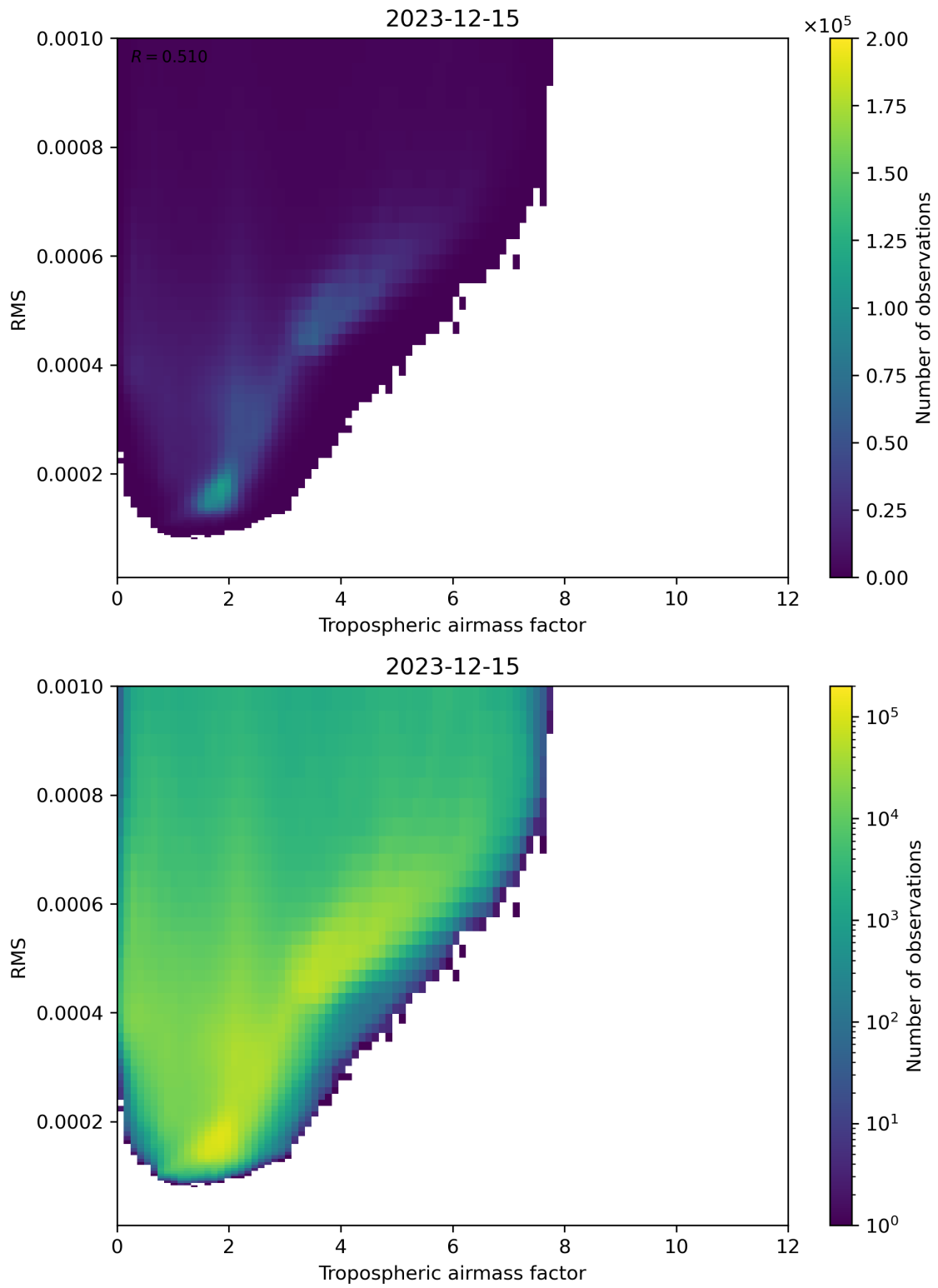
Figure 79: Scatter density plot of “Tropospheric airmass factor” against “RMS” for 2023-12-14 to 2023-12-16.
