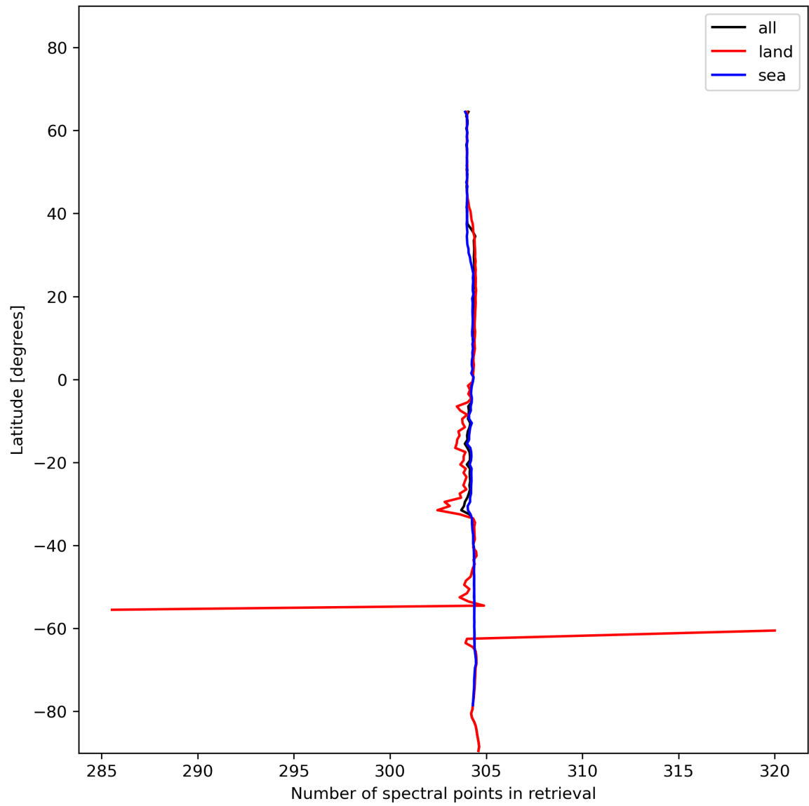
Figure 16: Zonal average of “Number of spectral points in retrieval” for 2023-12-14 to 2023-12-16.
