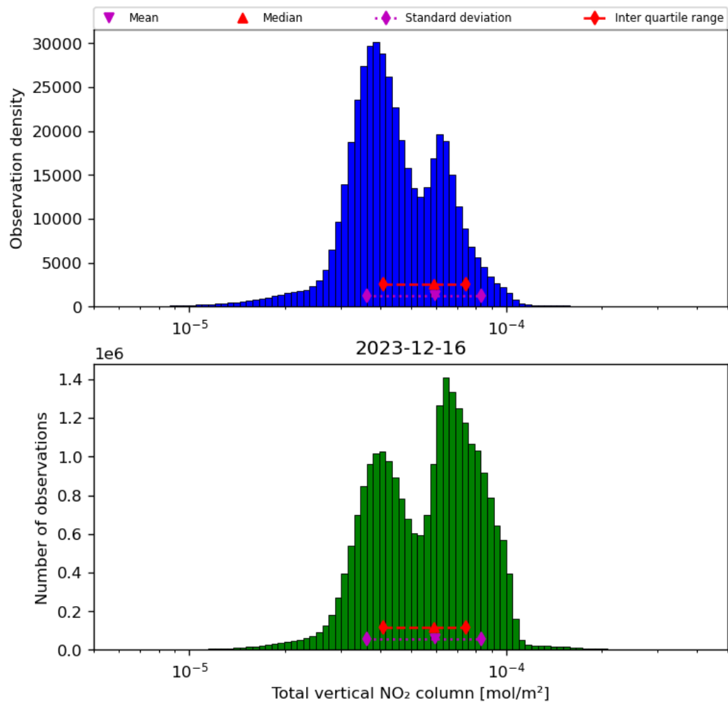
Figure 38: Histogram of "Total vertical NO 2 column" for 2023-12-15 to 2023-12-17
