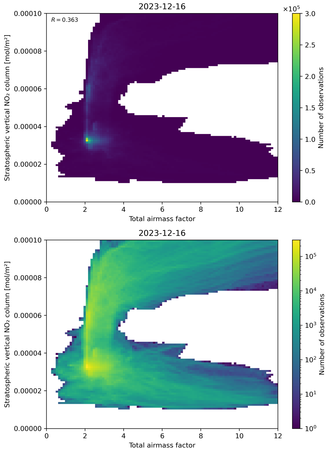
Figure 64: Scatter density plot of “Total airmass factor” against “Stratospheric vertical NO 2 column” for 2023-12-15 to 2023-12-17.
