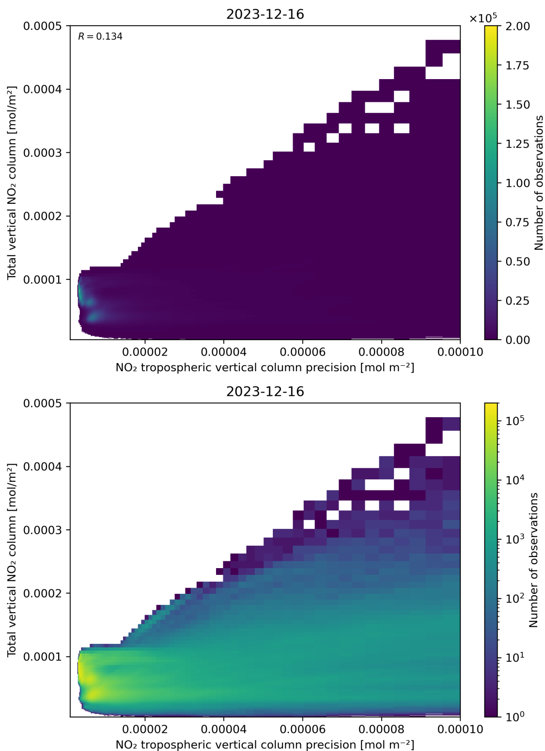
Figure 138: Scatter density plot of “NO 2 tropospheric vertical column precision” against “Total vertical NO 2 column” for 2023-12-15 to 2023-12-17.
