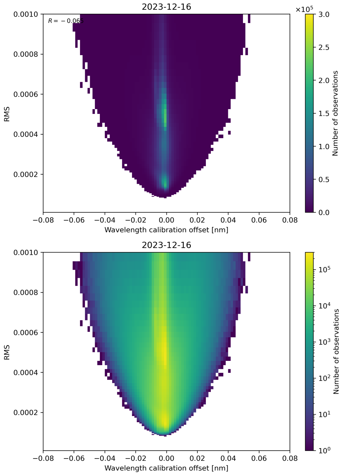
Figure 181: Scatter density plot of “Wavelength calibration offset” against “RMS” for 2023-12-15 to 2023-12-17.
