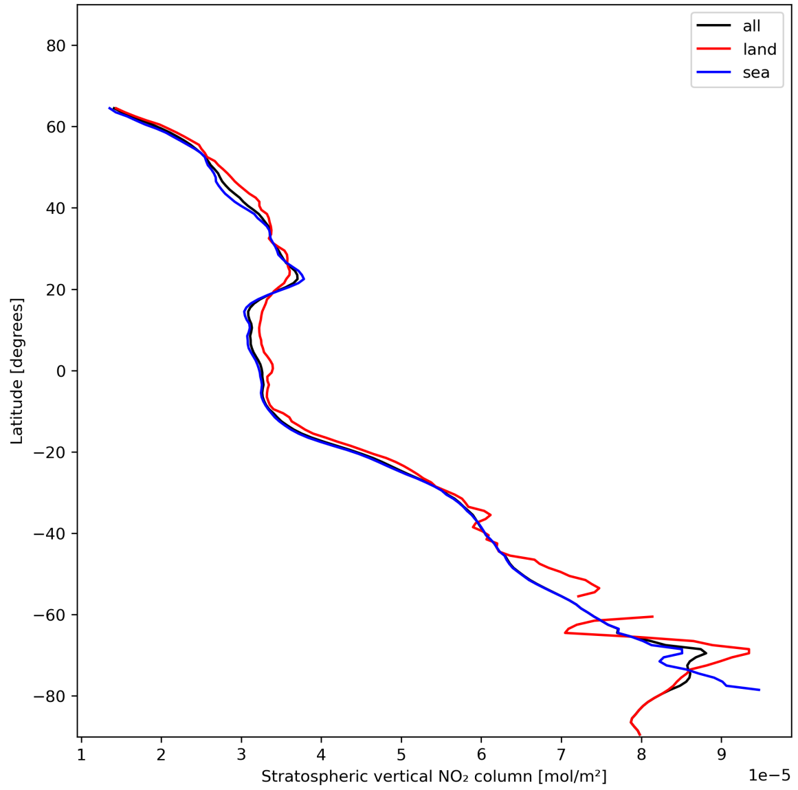
Figure 19: Zonal average of “Stratospheric vertical NO 2 column” for 2023-12-15 to 2023-12-17.
