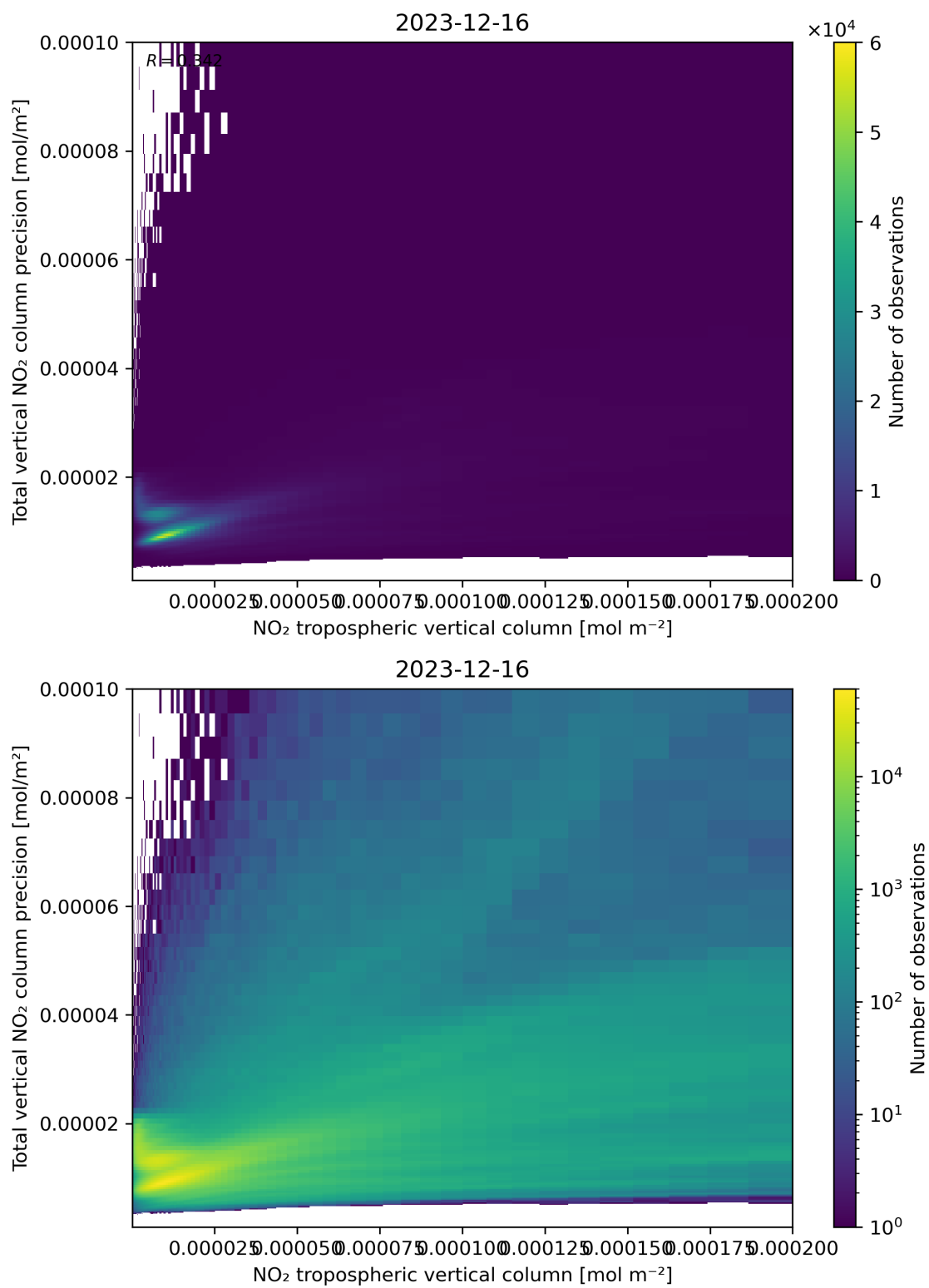
Figure 129: Scatter density plot of “NO 2 tropospheric vertical column” against “Total vertical NO 2 column precision” for 2023-12-15 to 2023-12-17.
