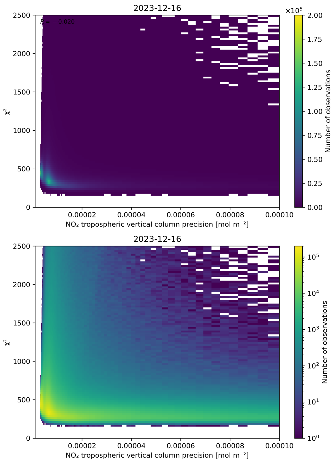
Figure 134: Scatter density plot of “NO 2 tropospheric vertical column precision” against “ \chi^2 ” for 2023-12-15 to 2023-12-17.
