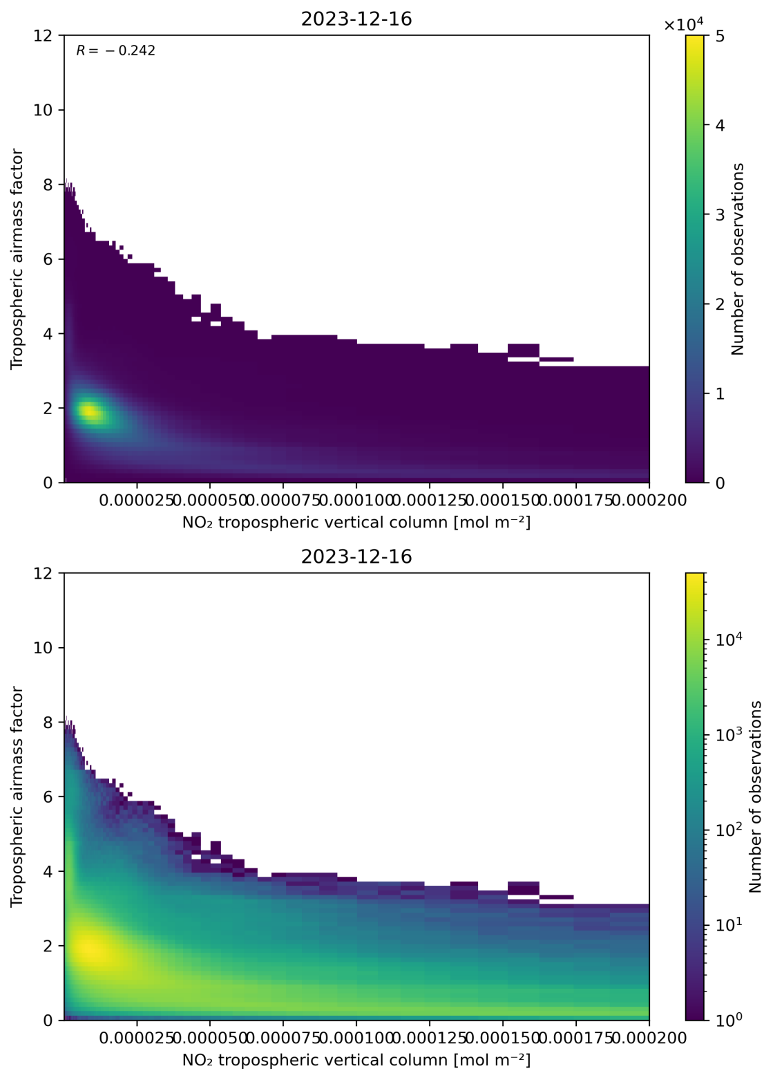
Figure 123: Scatter density plot of “NO 2 tropospheric vertical column” against “Tropospheric air mass factor” for 2023-12-15 to 2023-12-17.
