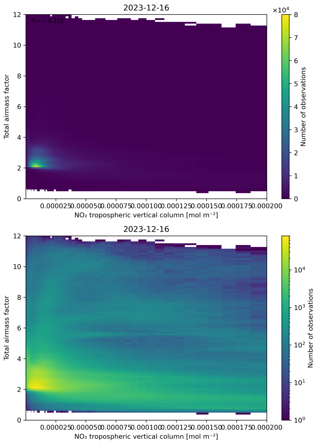
Figure 122: Scatter density plot of “NO 2 tropospheric vertical column” against “Total air mass factor” for 2023-12-15 to 2023-12-17.
