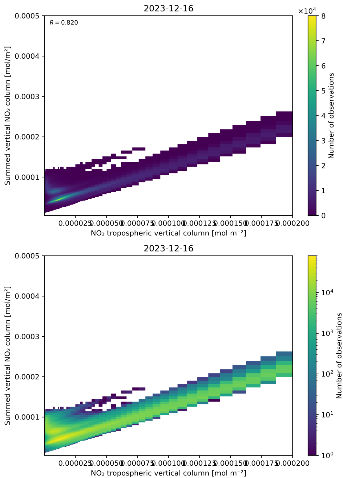
Figure 126: Scatter density plot of “NO 2 tropospheric vertical column” against “Summed vertical NO 2 column” for 2023-12-15 to 2023-12-17.
