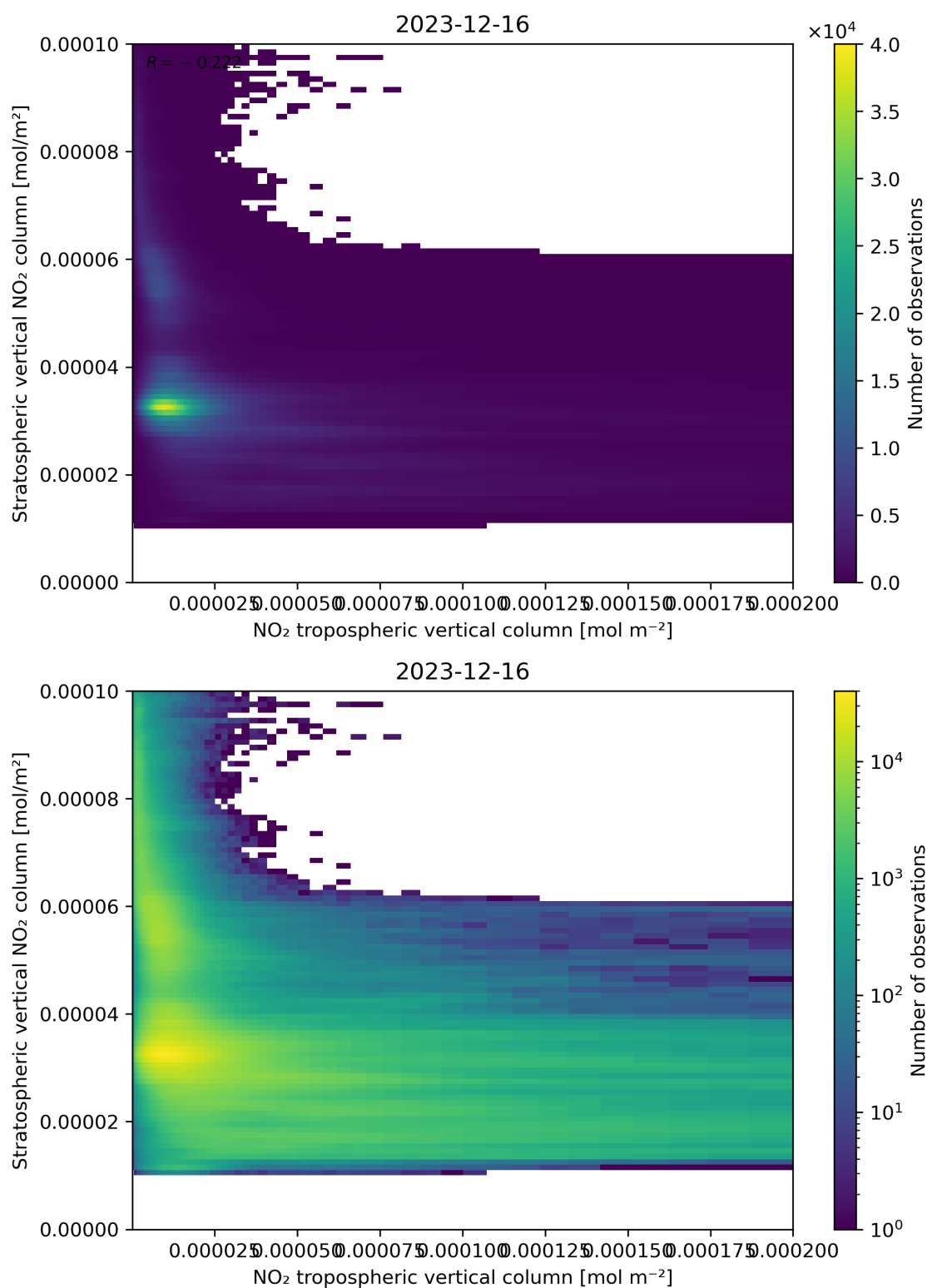
Figure 125: Scatter density plot of “NO 2 tropospheric vertical column” against “Stratospheric vertical NO 2 column” for 2023-12-15 to 2023-12-17.
