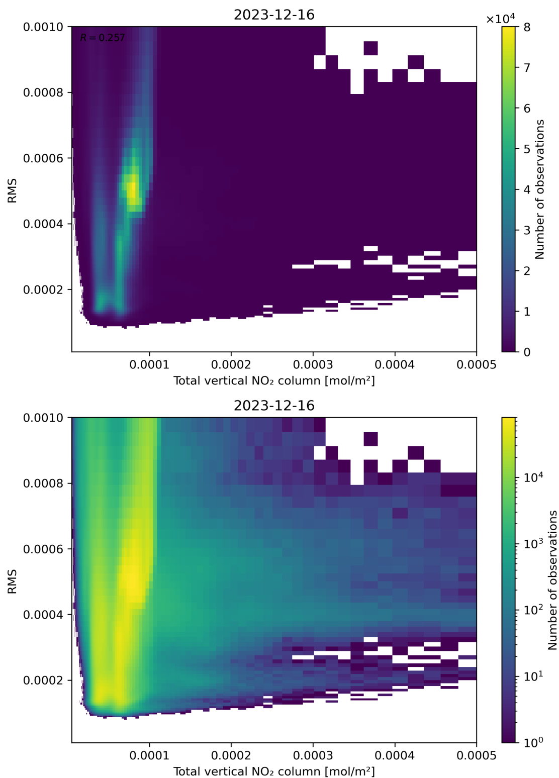
Figure 120: Scatter density plot of “Total vertical NO 2 column” against “RMS” for 2023-12-15 to 2023-12-17.
