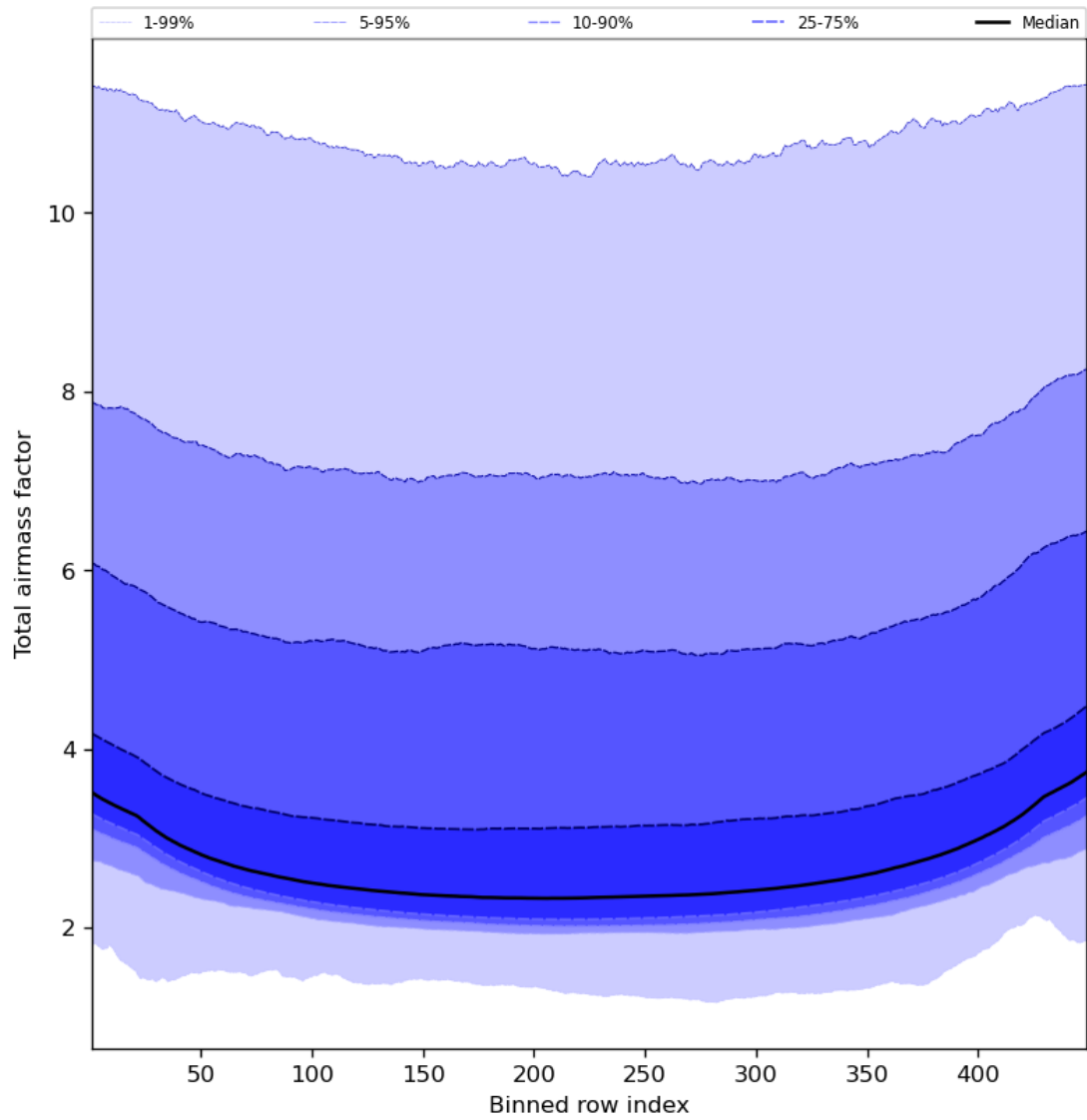
Figure 49: Along track statistics of “Total airmass factor” for 2023-12-15 to 2023-12-17
