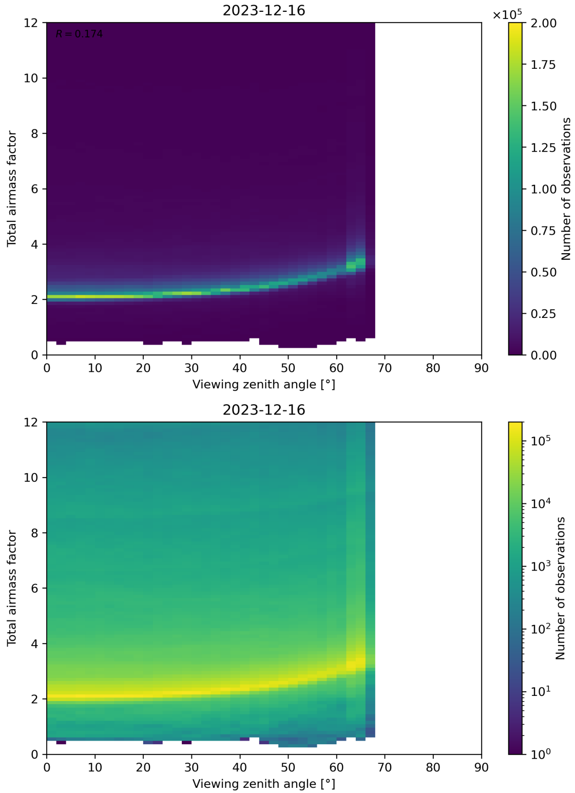
Figure 160: Scatter density plot of “Viewing zenith angle” against “Total airmass factor” for 2023-12-15 to 2023-12-17.
