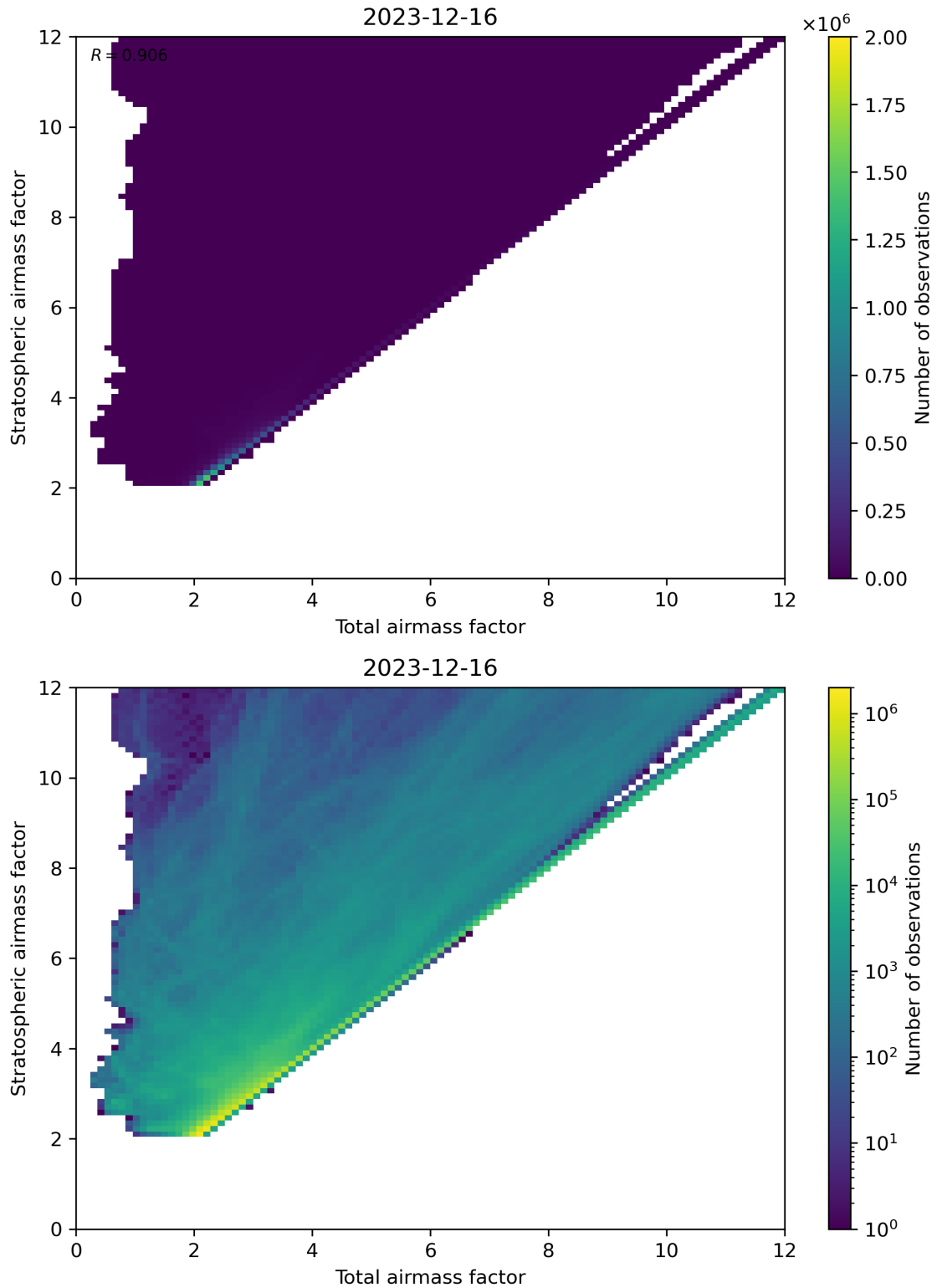
Figure 62: Scatter density plot of “Total airmass factor” against “Stratospheric airmass factor” for 2023-12-15 to 2023-12-17.
