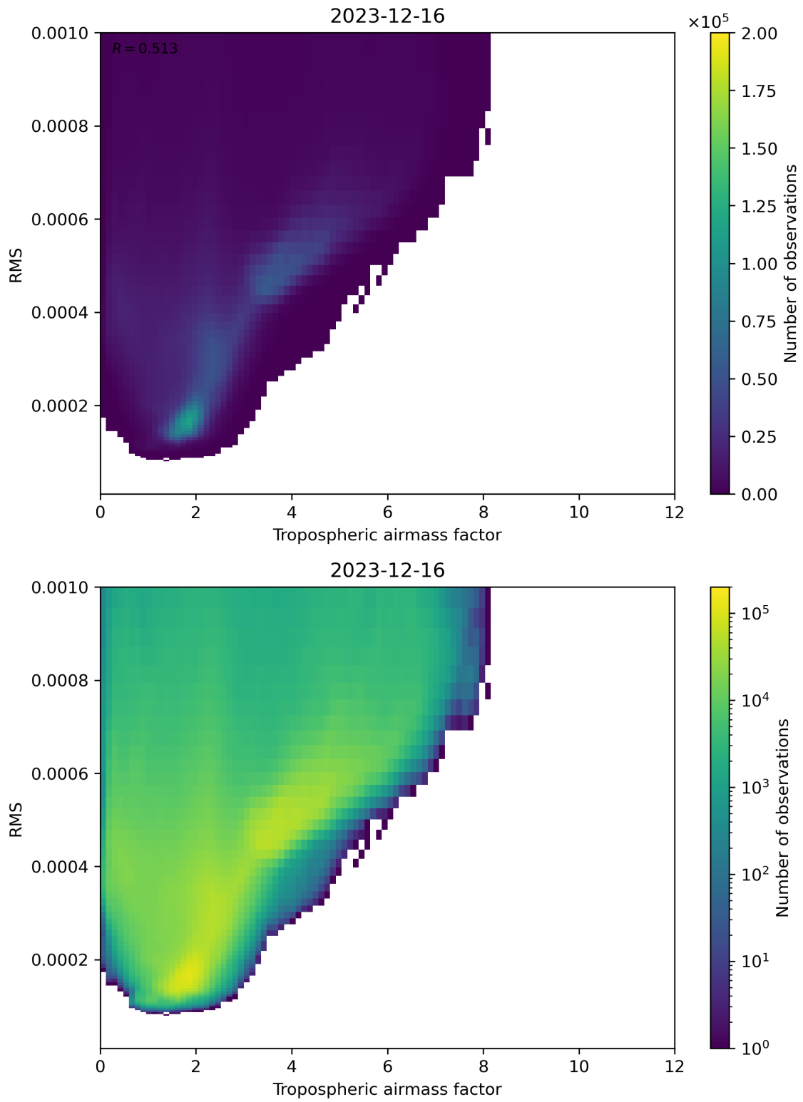
Figure 79: Scatter density plot of “Tropospheric airmass factor” against “RMS” for 2023-12-15 to 2023-12-17.
