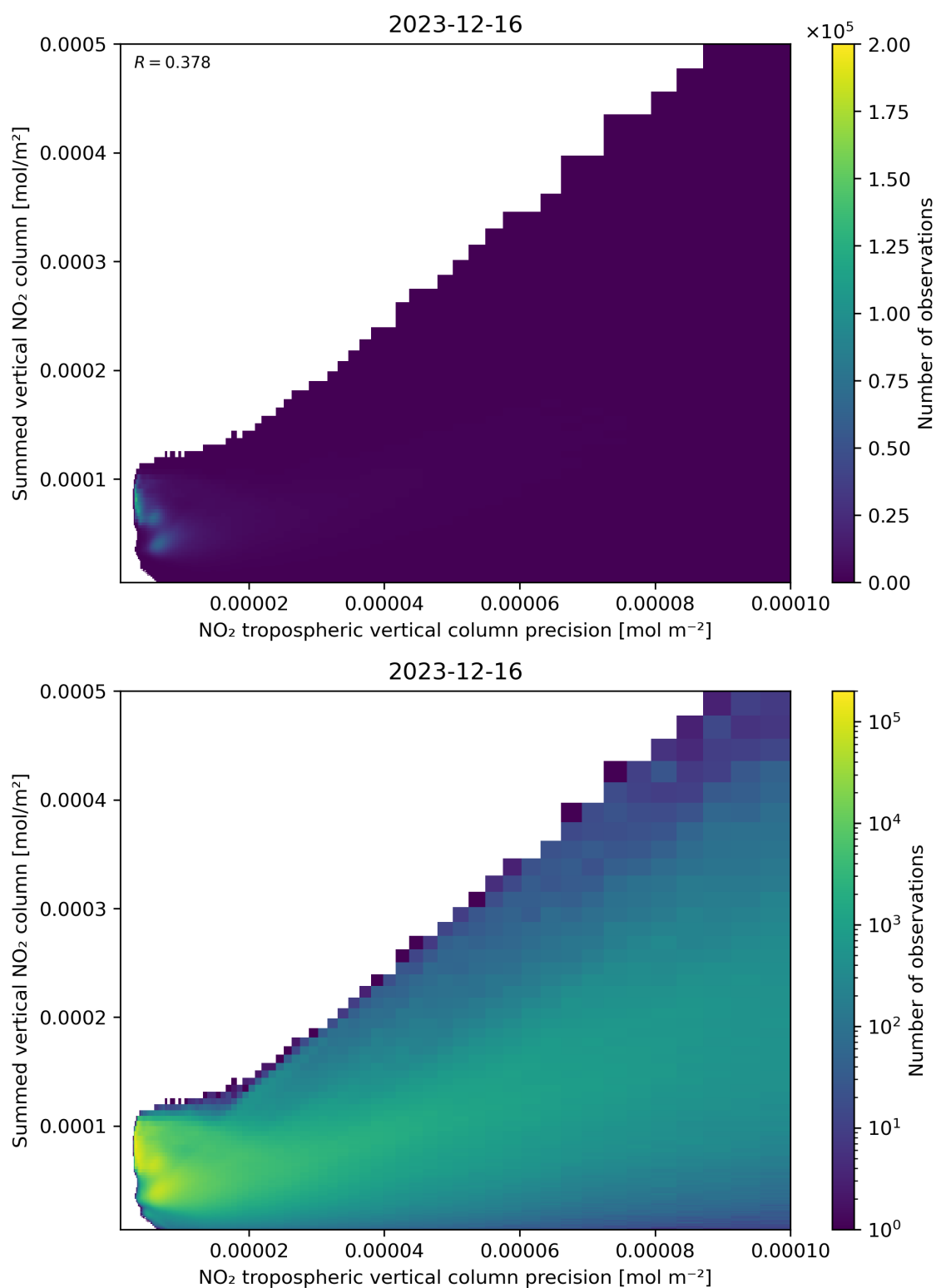
Figure 136: Scatter density plot of “NO 2 tropospheric vertical column precision” against “Summed vertical NO 2 column” for 2023-12-15 to 2023-12-17.
