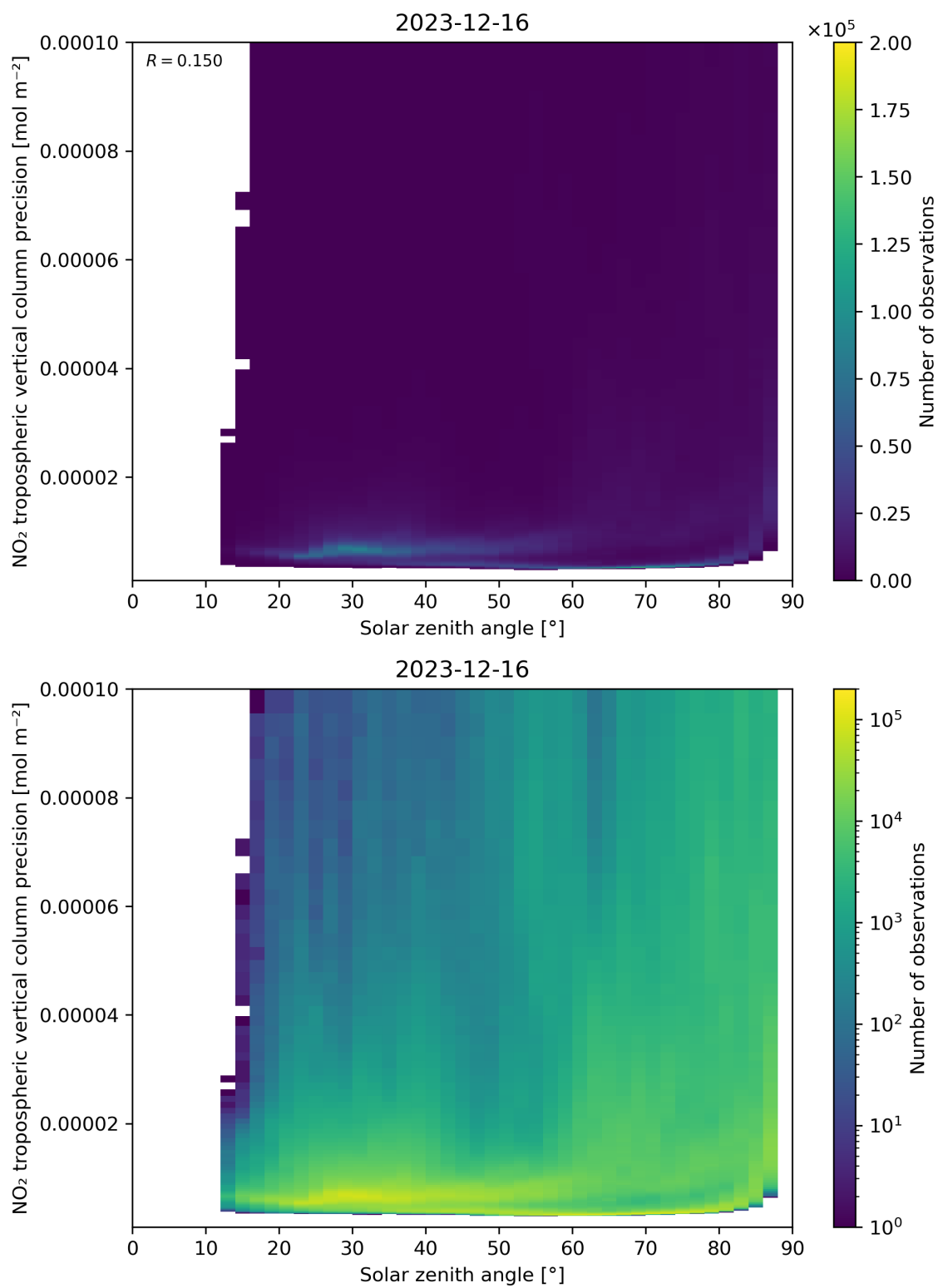
Figure 156: Scatter density plot of “Solar zenith angle” against “NO 2 tropospheric vertical column precision” for 2023-12-15 to 2023-12-17.
