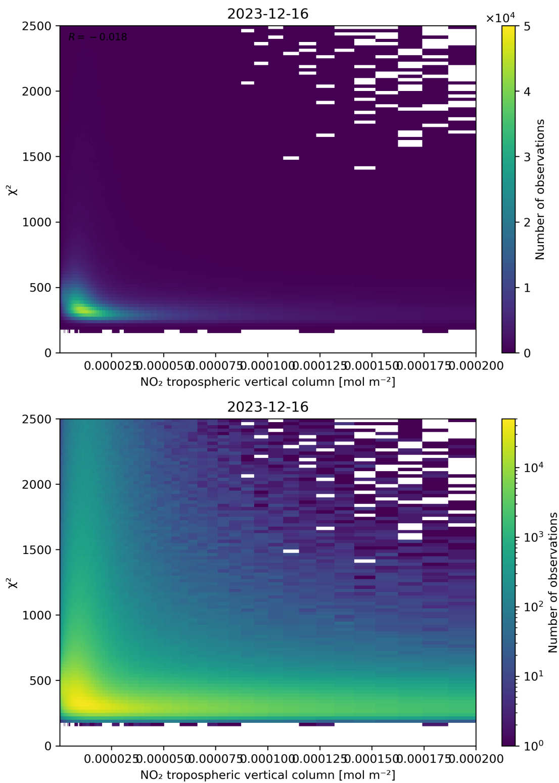
Figure 124: Scatter density plot of “NO 2 tropospheric vertical column” against “ \chi^2 ” for 2023-12-15 to 2023-12-17.
