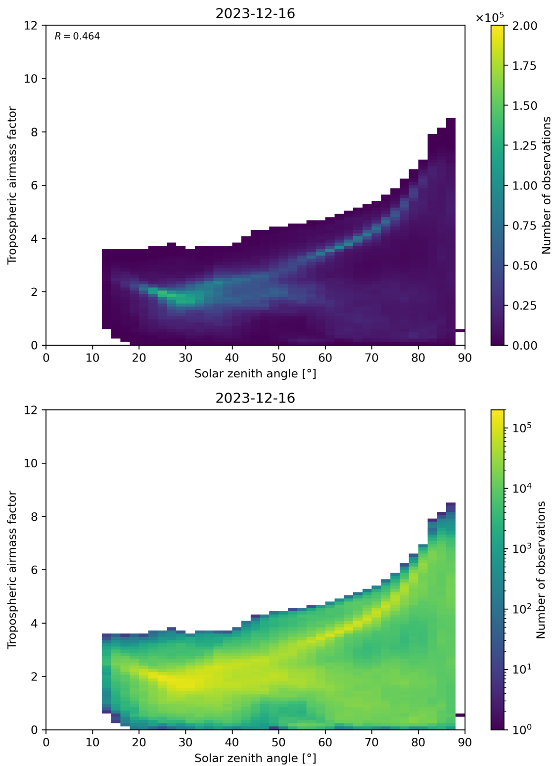
Figure 147: Scatter density plot of “Solar zenith angle” against “Tropospheric airmass factor” for 2023-12-15 to 2023-12-17.
