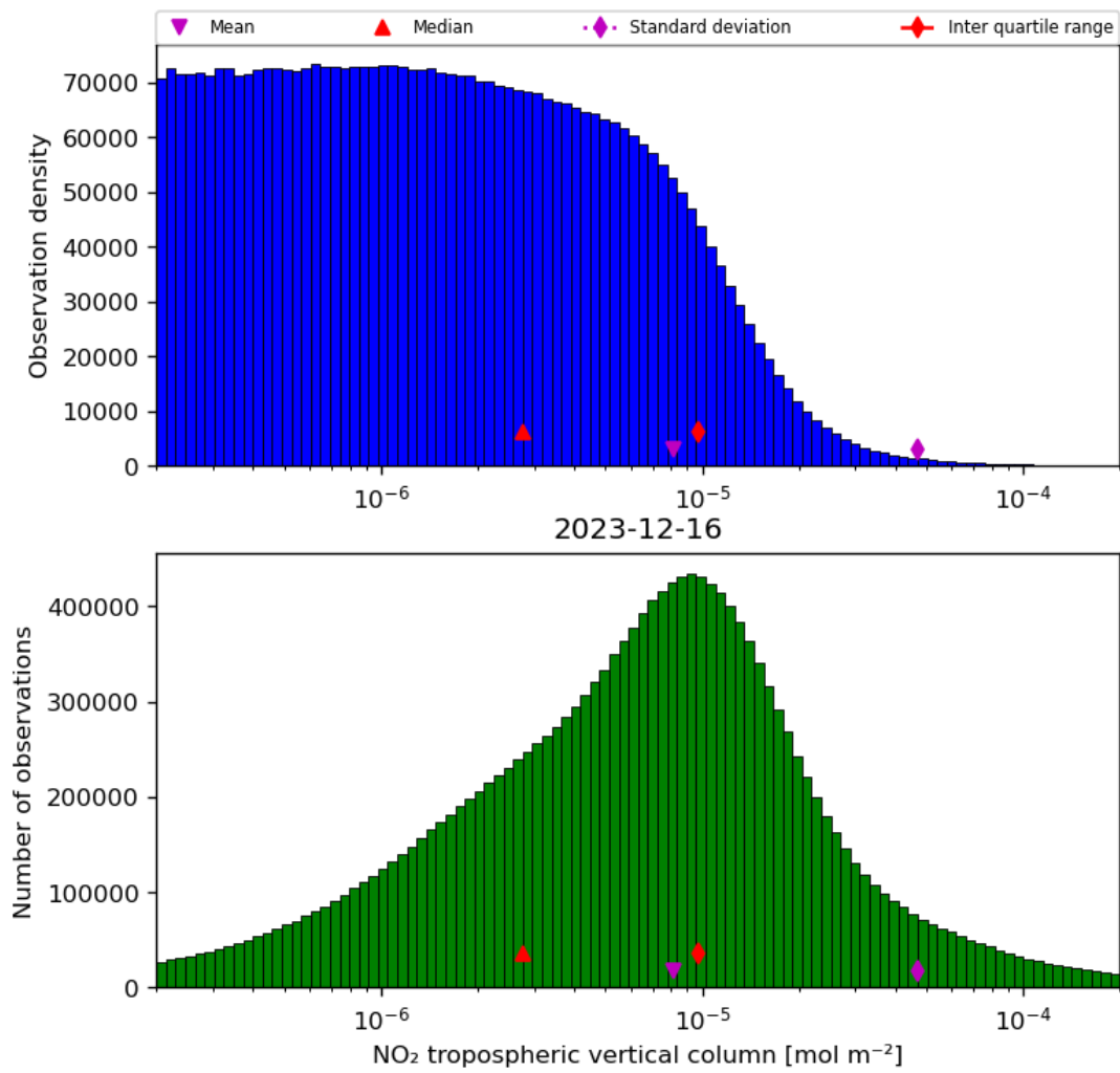
Figure 29: Histogram of “NO 2 tropospheric vertical column” for 2023-12-15 to 2023-12-17
