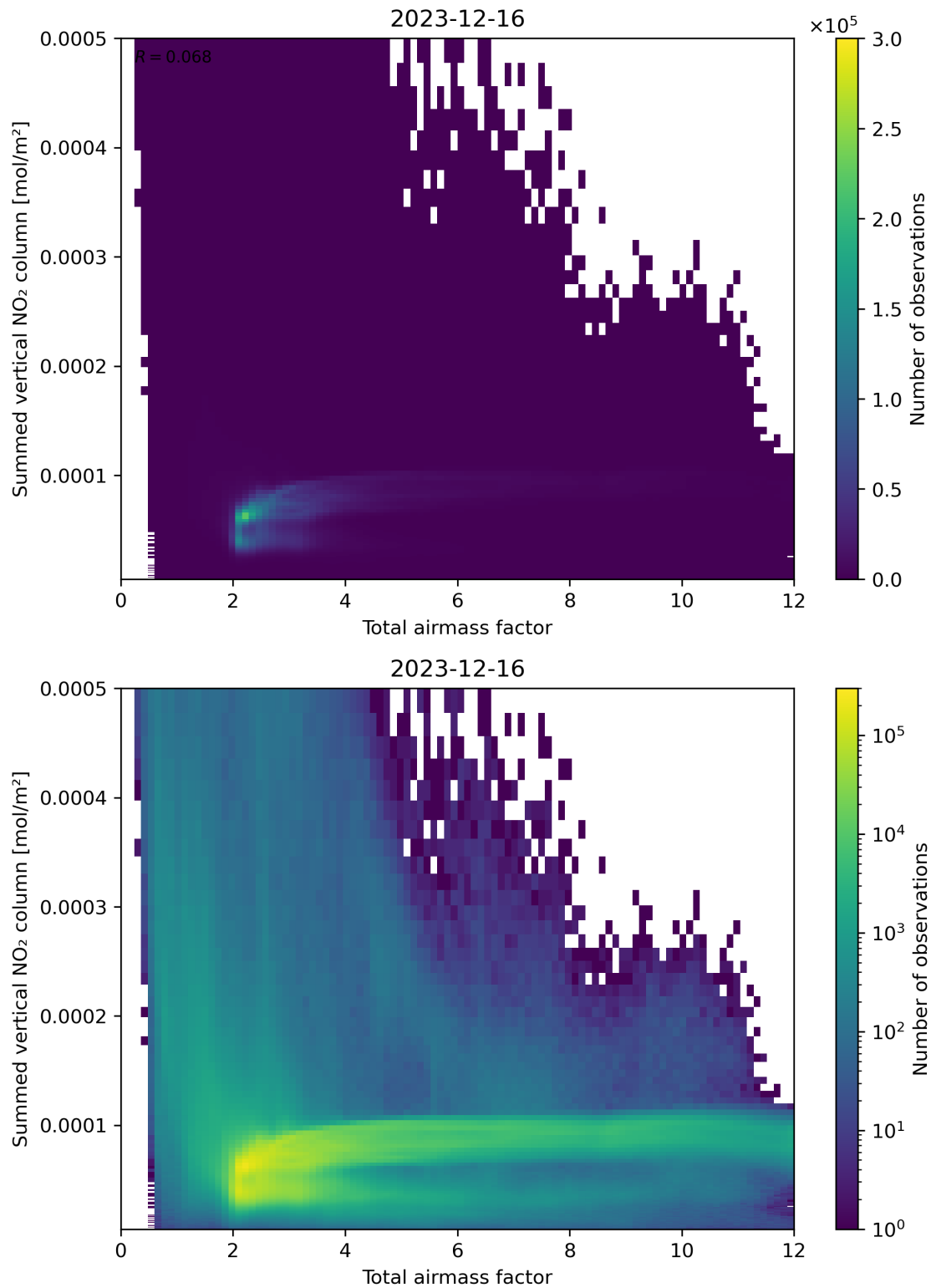
Figure 65: Scatter density plot of “Total airmass factor” against “Summed vertical NO 2 column” for 2023-12-15 to 2023-12-17.
