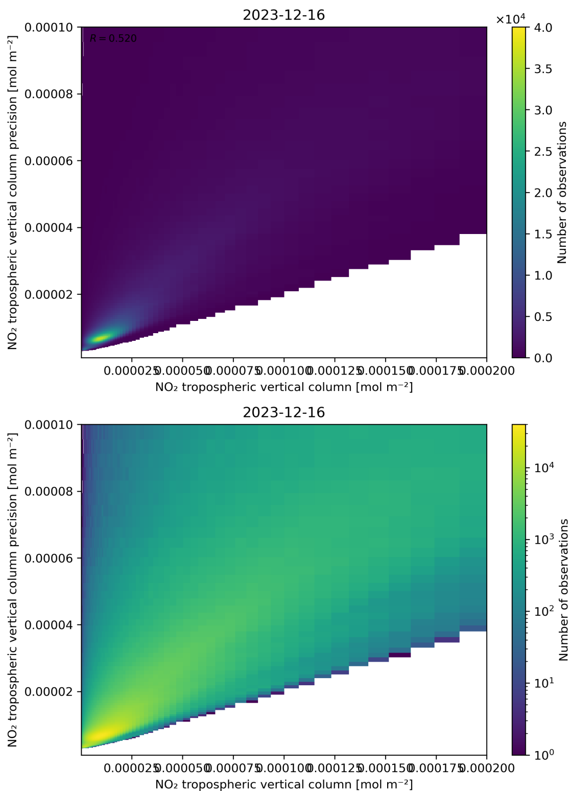
Figure 130: Scatter density plot of “NO 2 tropospheric vertical column” against “NO 2 tropospheric vertical column precision” for 2023-12-15 to 2023-12-17.
