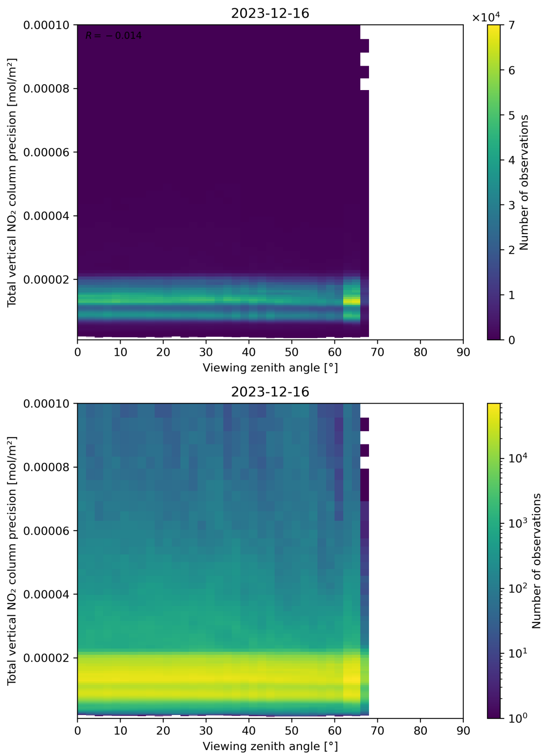
Figure 168: Scatter density plot of “Viewing zenith angle” against “Total vertical NO 2 column precision” for 2023-12-15 to 2023-12-17.
