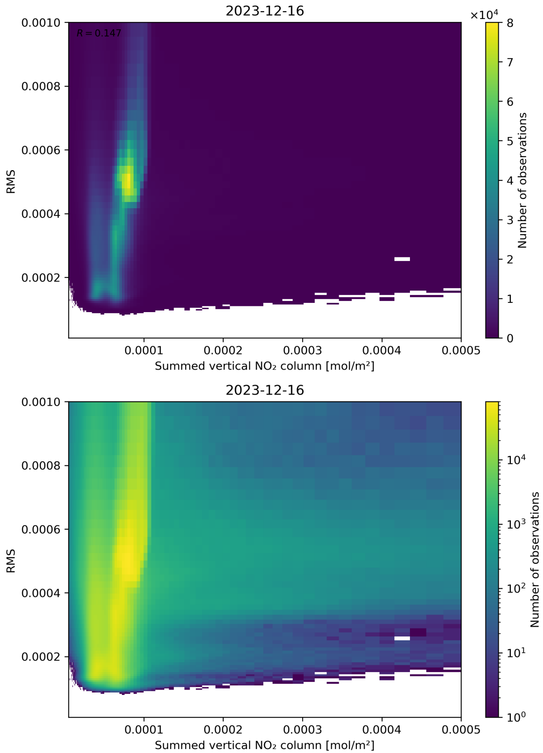
Figure 109: Scatter density plot of “Summed vertical NO 2 column” against “RMS” for 2023-12-15 to 2023-12-17.
