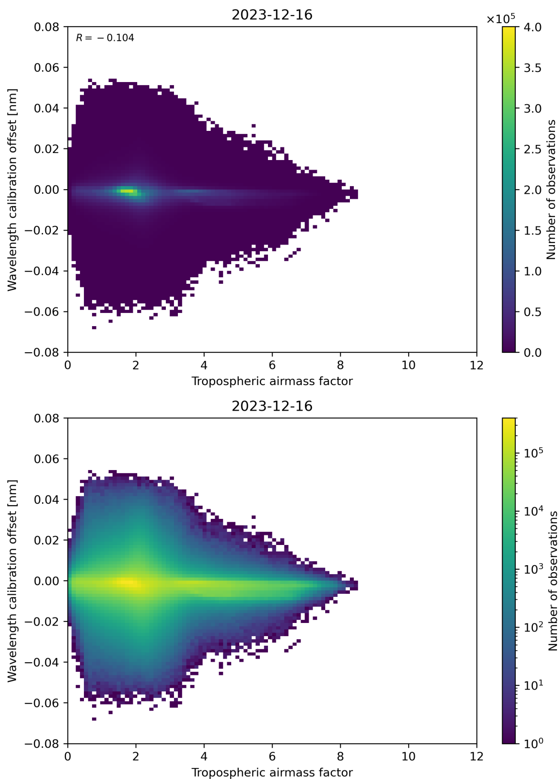
Figure 80: Scatter density plot of “Tropospheric airmass factor” against “Wavelength calibration offset” for 2023-12-15 to 2023-12-17.
