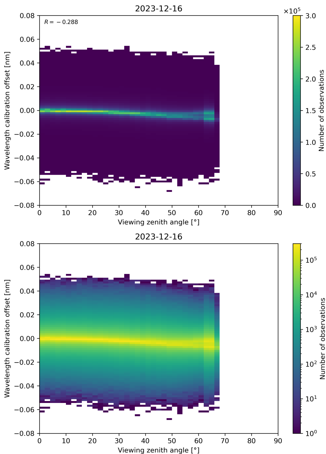
Figure 173: Scatter density plot of “Viewing zenith angle” against “Wavelength calibration offset” for 2023-12-15 to 2023-12-17.
