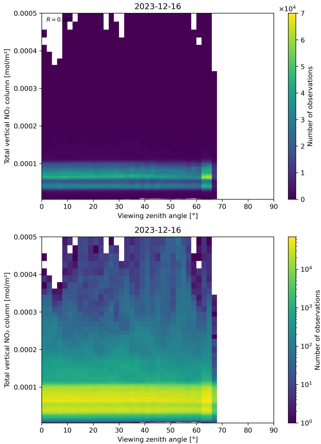
Figure 167: Scatter density plot of “Viewing zenith angle” against “Total vertical NO 2 column” for 2023-12-15 to 2023-12-17.
