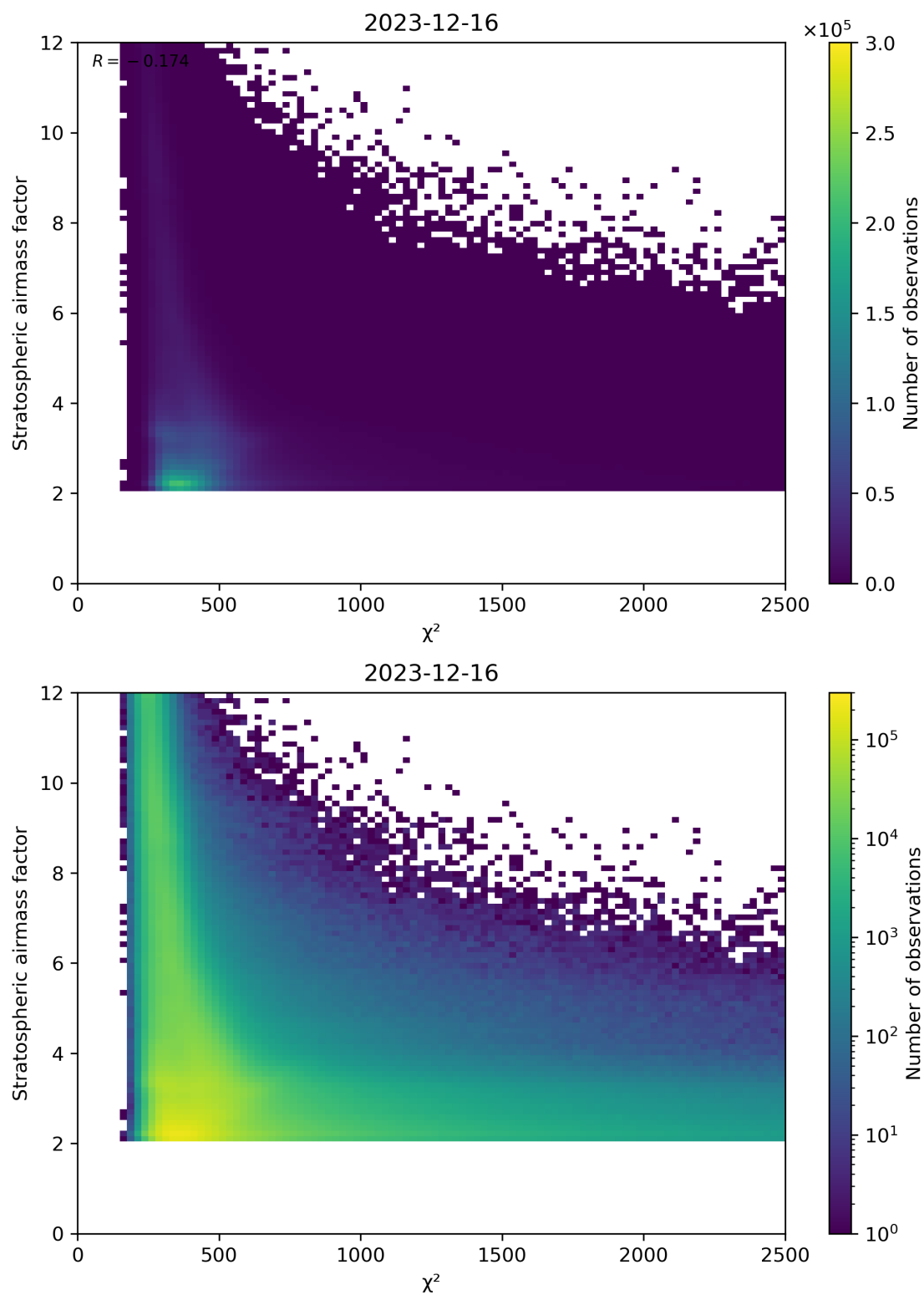
Figure 81: Scatter density plot of “ \chi^2 ” against “Stratospheric airmass factor” for 2023-12-15 to 2023-12-17.
