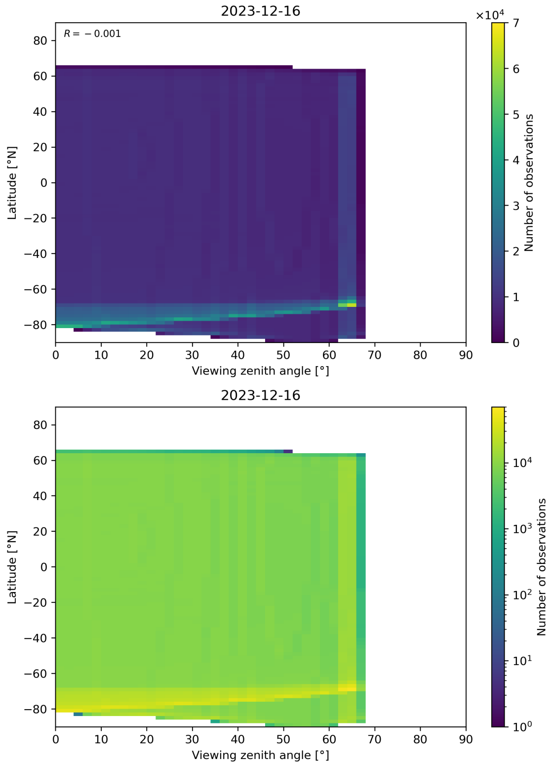
Figure 163: Scatter density plot of “Viewing zenith angle” against “Latitude” for 2023-12-15 to 2023-12-17.
