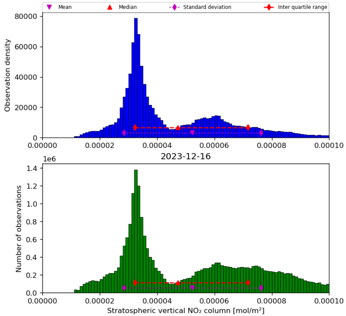
Figure 36: Histogram of “Stratospheric vertical NO 2 column” for 2023-12-15 to 2023-12-17
