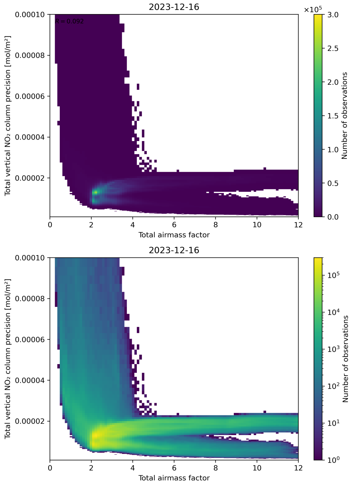
Figure 68: Scatter density plot of “Total airmass factor” against “Total vertical NO 2 column precision” for 2023-12-15 to 2023-12-17.
