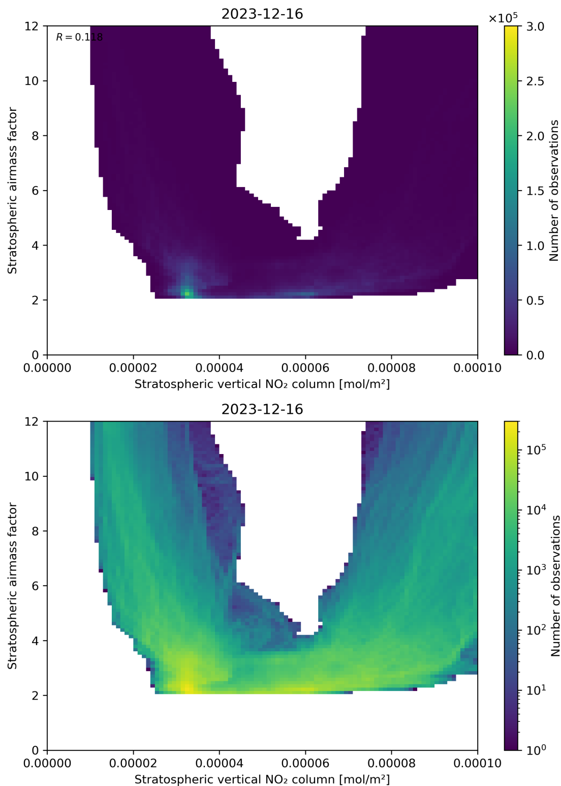
Figure 96: Scatter density plot of “Stratospheric vertical NO 2 column” against “Stratospheric airmass factor” for 2023-12-15 to 2023-12-17.
