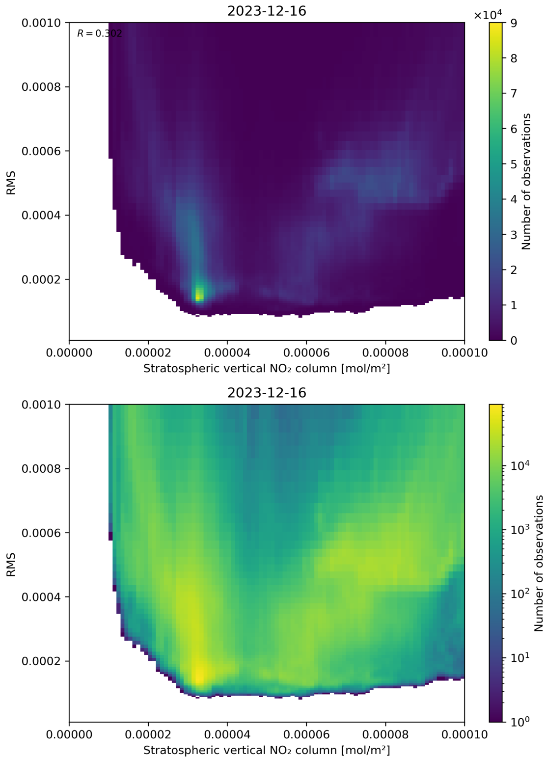
Figure 102: Scatter density plot of “Stratospheric vertical NO 2 column” against “RMS” for 2023-12-15 to 2023-12-17.
