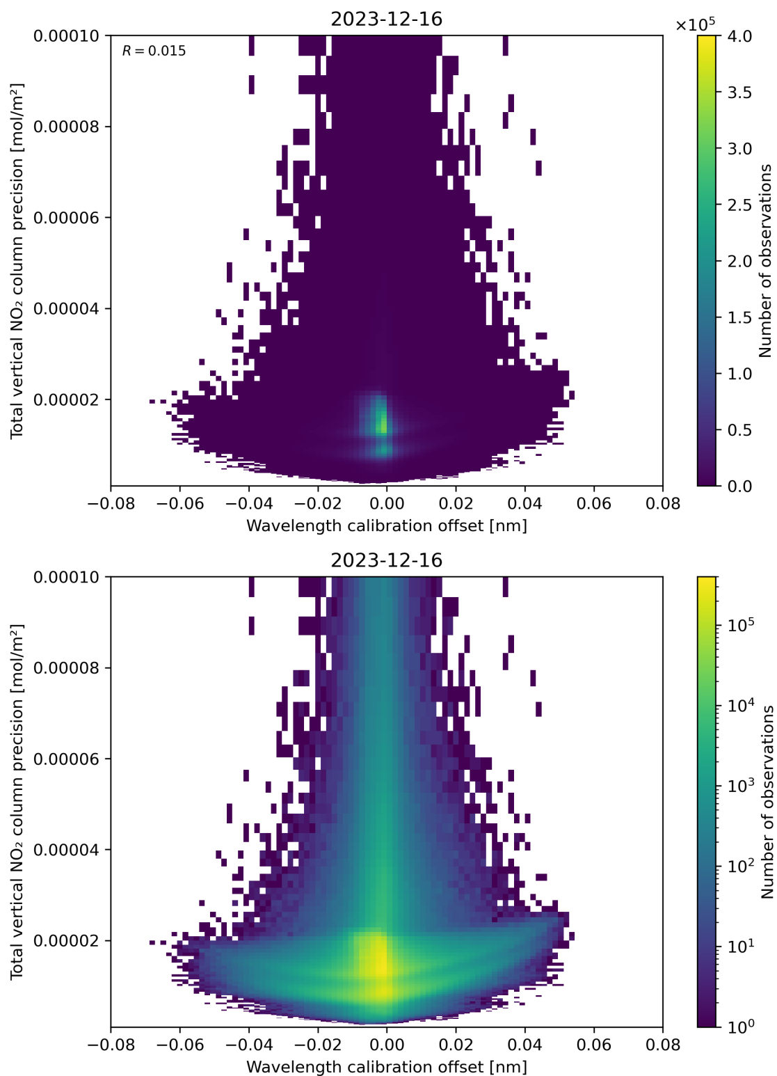
Figure 180: Scatter density plot of “Wavelength calibration offset” against “Total vertical NO 2 column precision” for 2023-12-15 to 2023-12-17.
