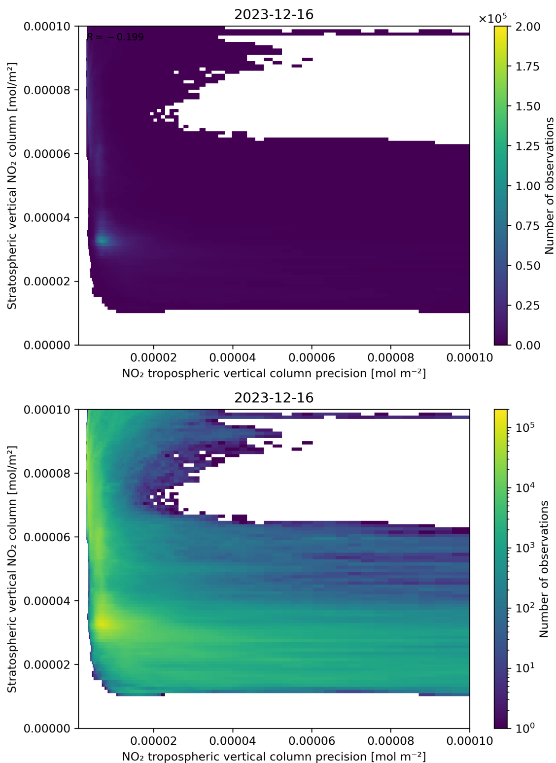
Figure 135: Scatter density plot of “NO 2 tropospheric vertical column precision” against “Stratospheric vertical NO 2 column” for 2023-12-15 to 2023-12-17.
