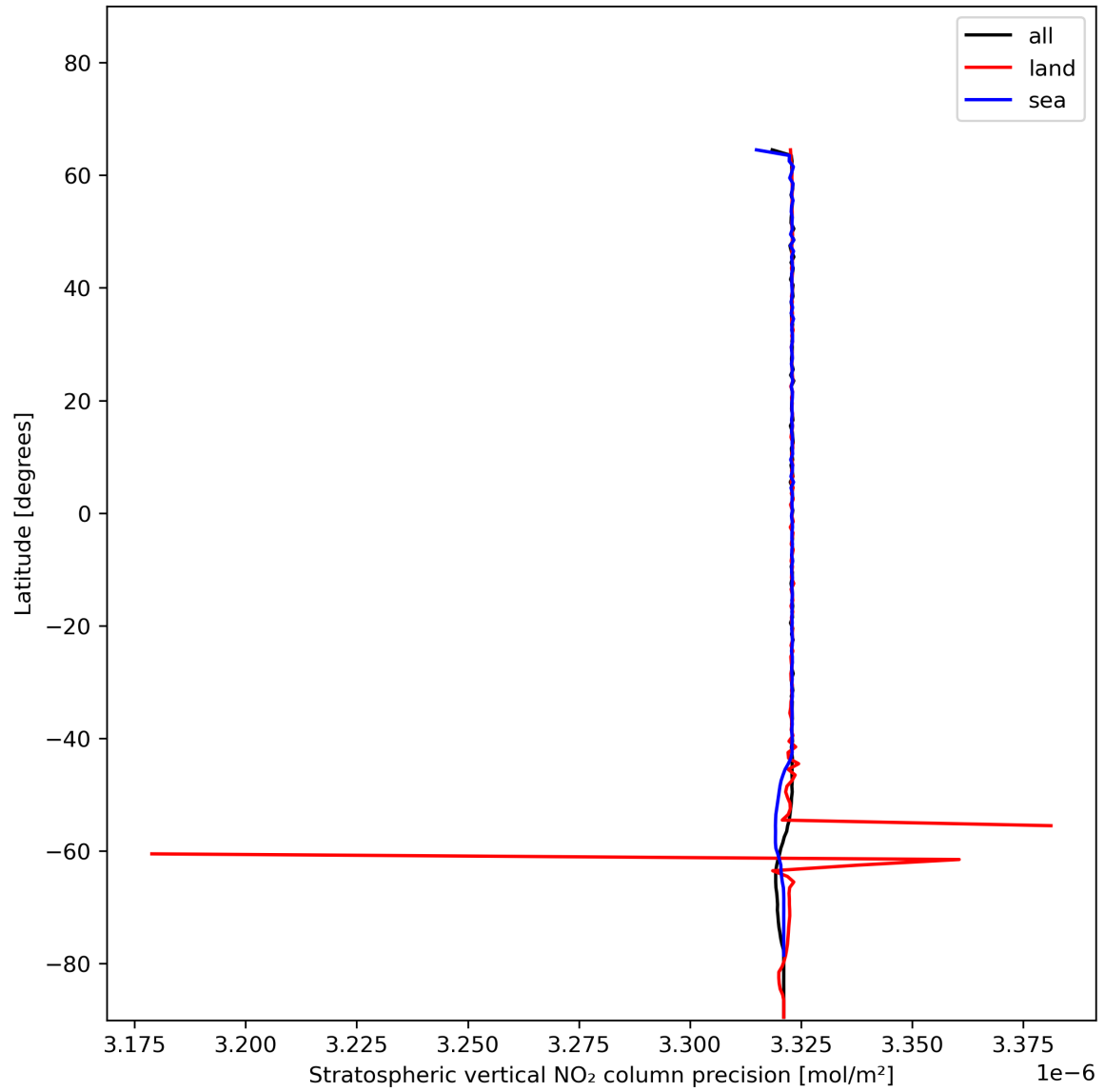
Figure 20: Zonal average of "Stratospheric vertical NO 2 column precision" for 2023-12-15 to 2023-12-17.
