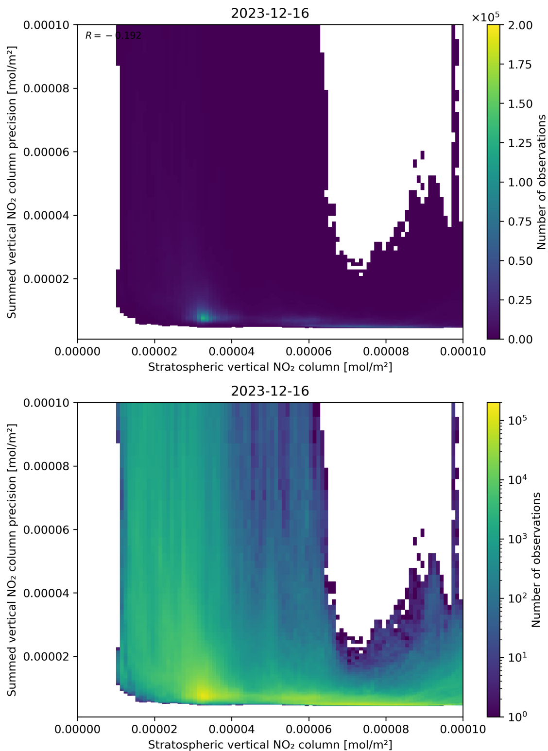
Figure 99: Scatter density plot of “Stratospheric vertical NO 2 column” against “Summed vertical NO 2 column precision” for 2023-12-15 to 2023-12-17.
