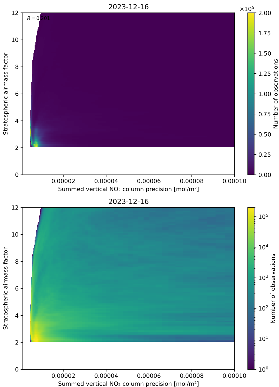
Figure 106: Scatter density plot of “Summed vertical NO 2 column precision” against “Stratospheric airmass factor” for 2023-12-15 to 2023-12-17.
