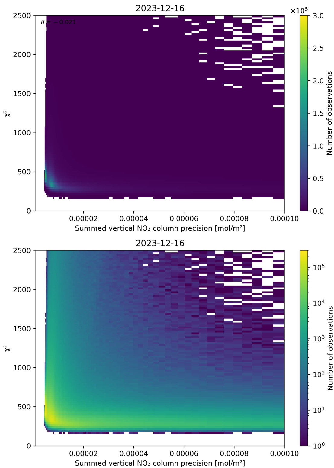
Figure 107: Scatter density plot of “Summed vertical NO 2 column precision” against “ \chi^2 ” for 2023-12-15 to 2023-12-17.
