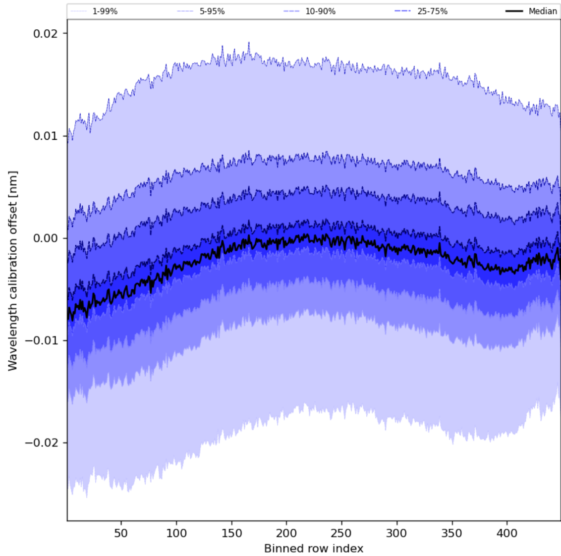
Figure 52: Along track statistics of “Wavelength calibration offset” for 2023-12-15 to 2023-12-17
