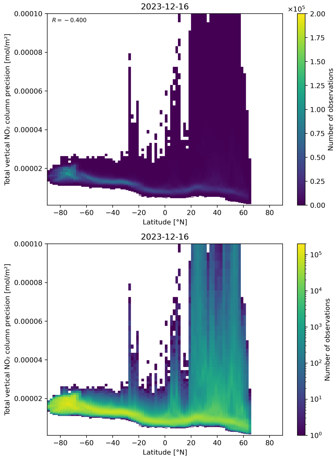
Figure 91: Scatter density plot of “Latitude” against “Total vertical NO 2 column precision” for 2023-12-15 to 2023-12-17.
