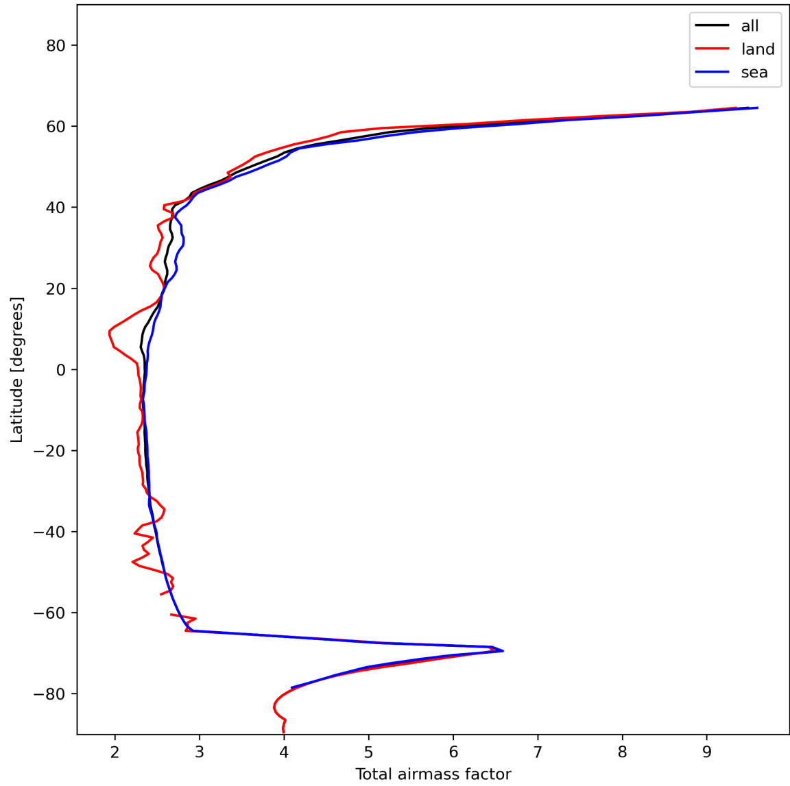
Figure 15: Zonal average of “Total airmass factor” for 2023-12-15 to 2023-12-17.
