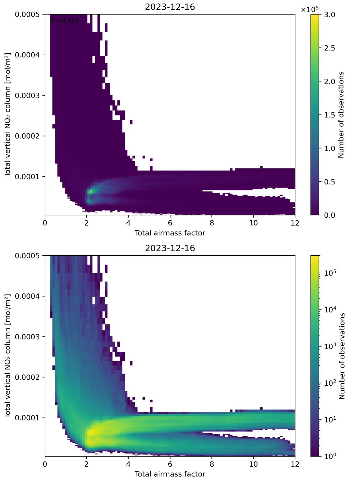
Figure 67: Scatter density plot of “Total airmass factor” against “Total vertical NO 2 column” for 2023-12-15 to 2023-12-17.
