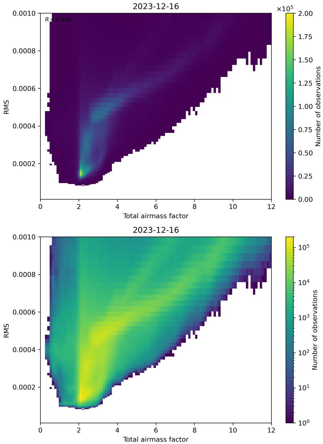
Figure 69: Scatter density plot of “Total airmass factor” against “RMS” for 2023-12-15 to 2023-12-17.
