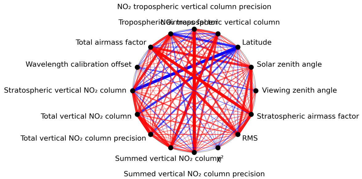
Figure 1: Map of correlation graph for 2023-12-15 to 2023-12-17.
