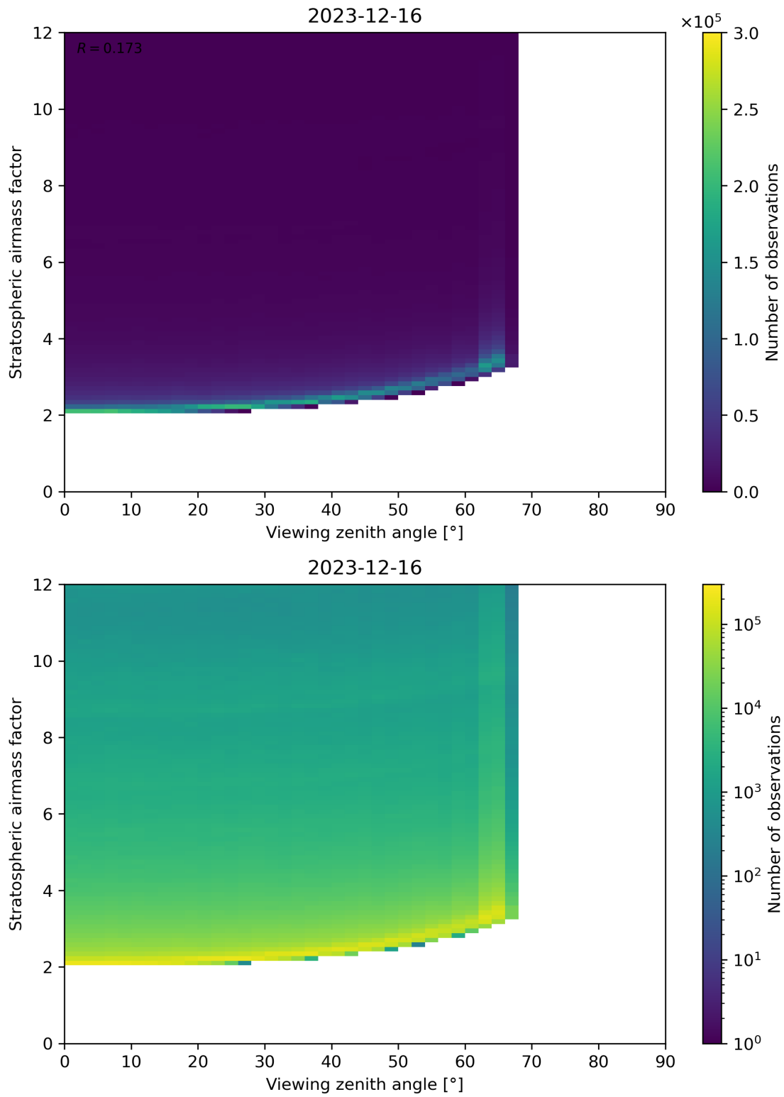
Figure 159: Scatter density plot of “Viewing zenith angle” against “Stratospheric airmass factor” for 2023-12-15 to 2023-12-17.
