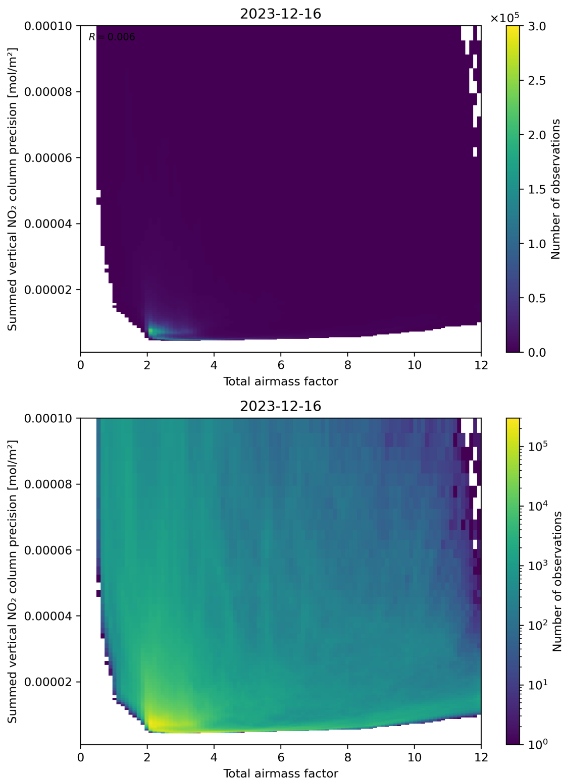
Figure 66: Scatter density plot of “Total airmass factor” against “Summed vertical NO 2 column precision” for 2023-12-15 to 2023-12-17.
