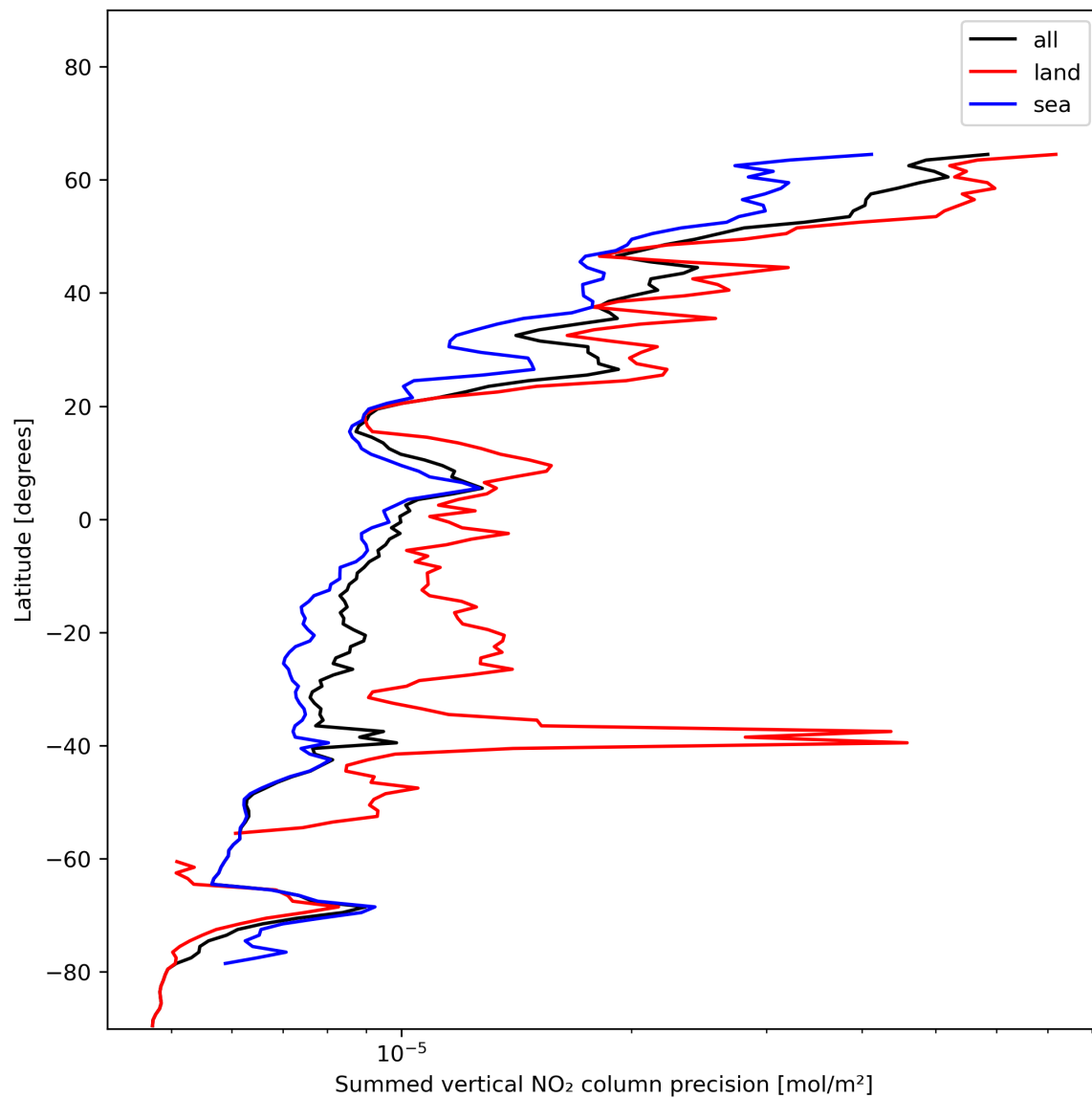
Figure 24: Zonal average of “Summed vertical NO 2 column precision” for 2023-12-15 to 2023-12-17.
