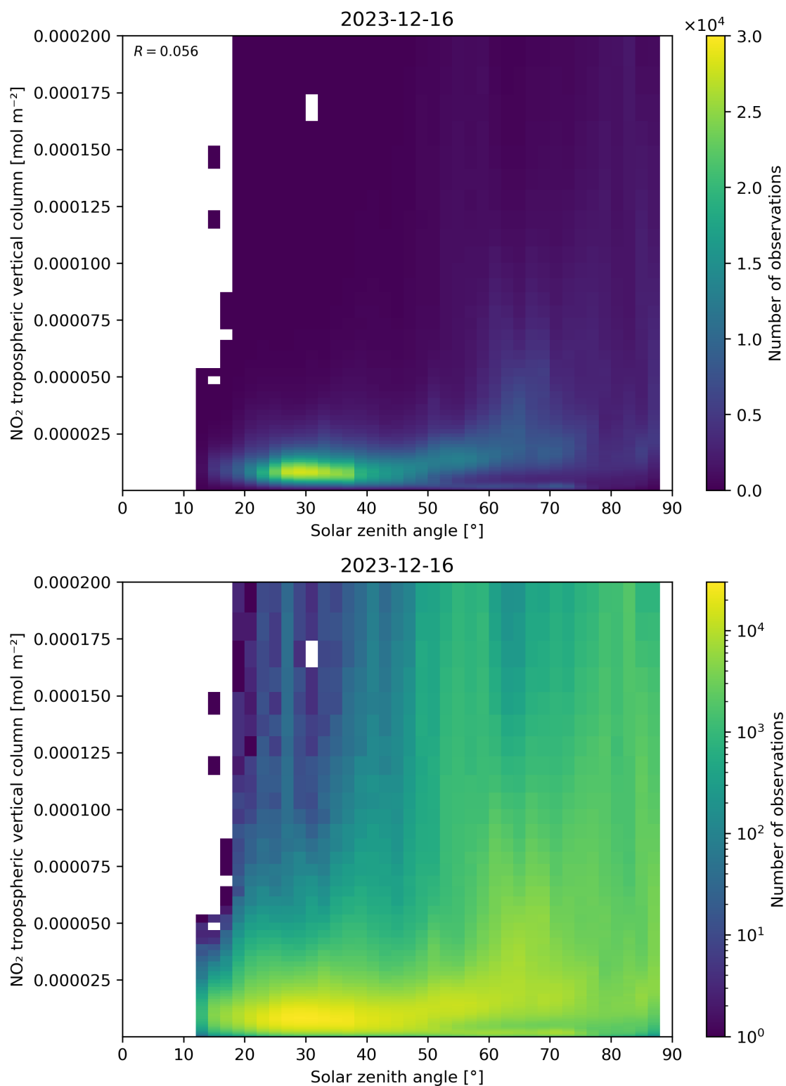
Figure 155: Scatter density plot of “Solar zenith angle” against “NO 2 tropospheric vertical column” for 2023-12-15 to 2023-12-17.
