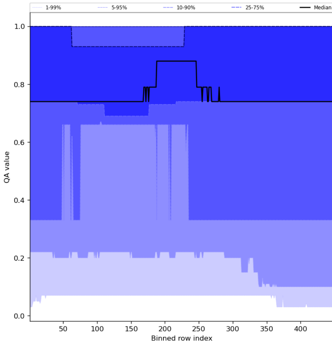
Figure 45: Along track statistics of “QA value” for 2023-12-15 to 2023-12-17
