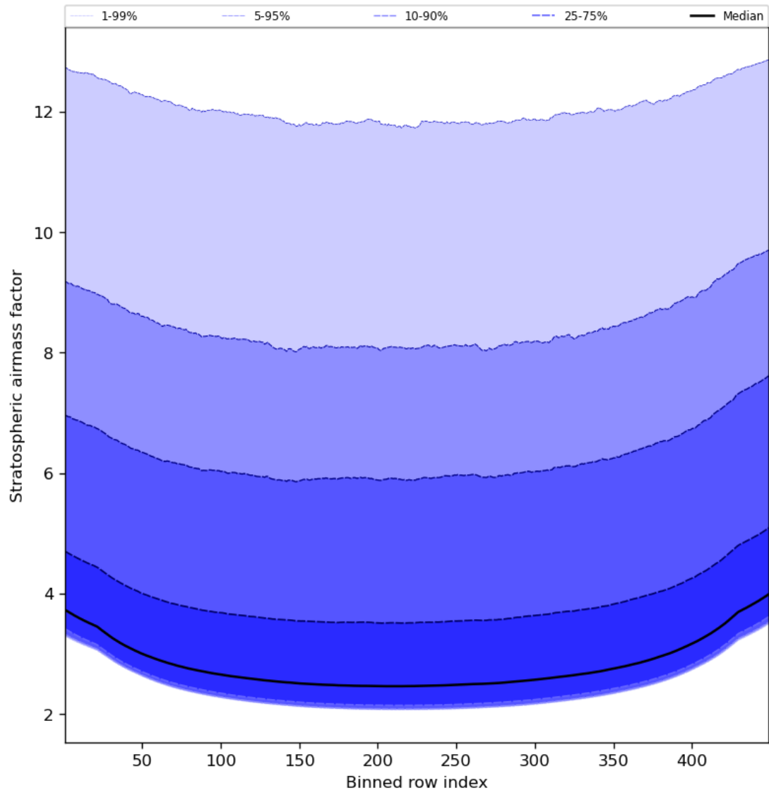
Figure 61: Along track statistics of “Stratospheric airmass factor” for 2023-12-15 to 2023-12-17
