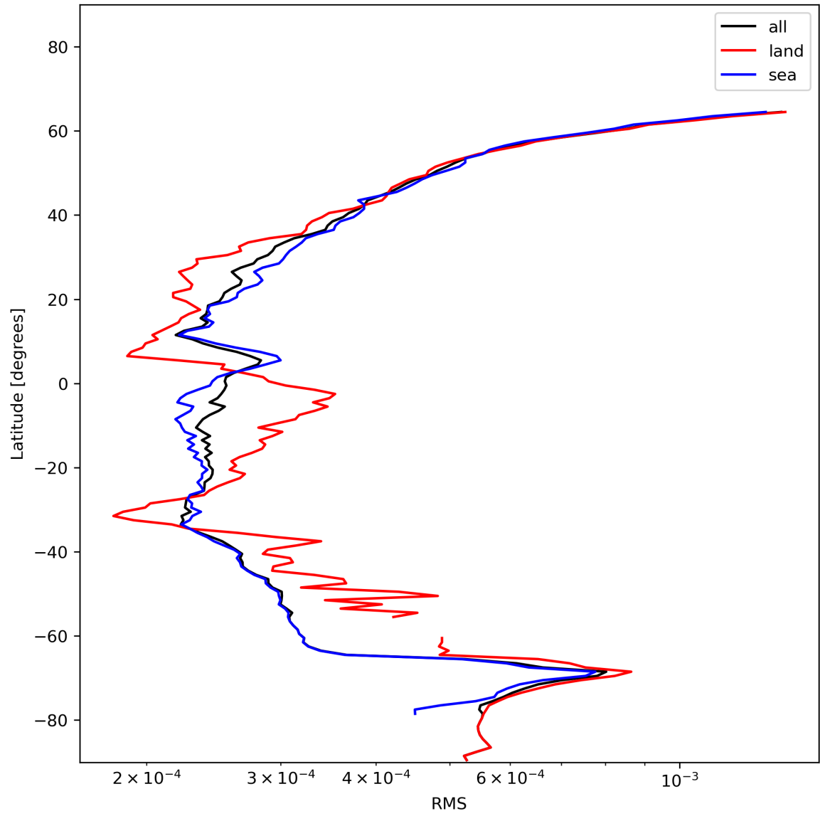
Figure 26: Zonal average of “RMS” for 2023-12-15 to 2023-12-17.
