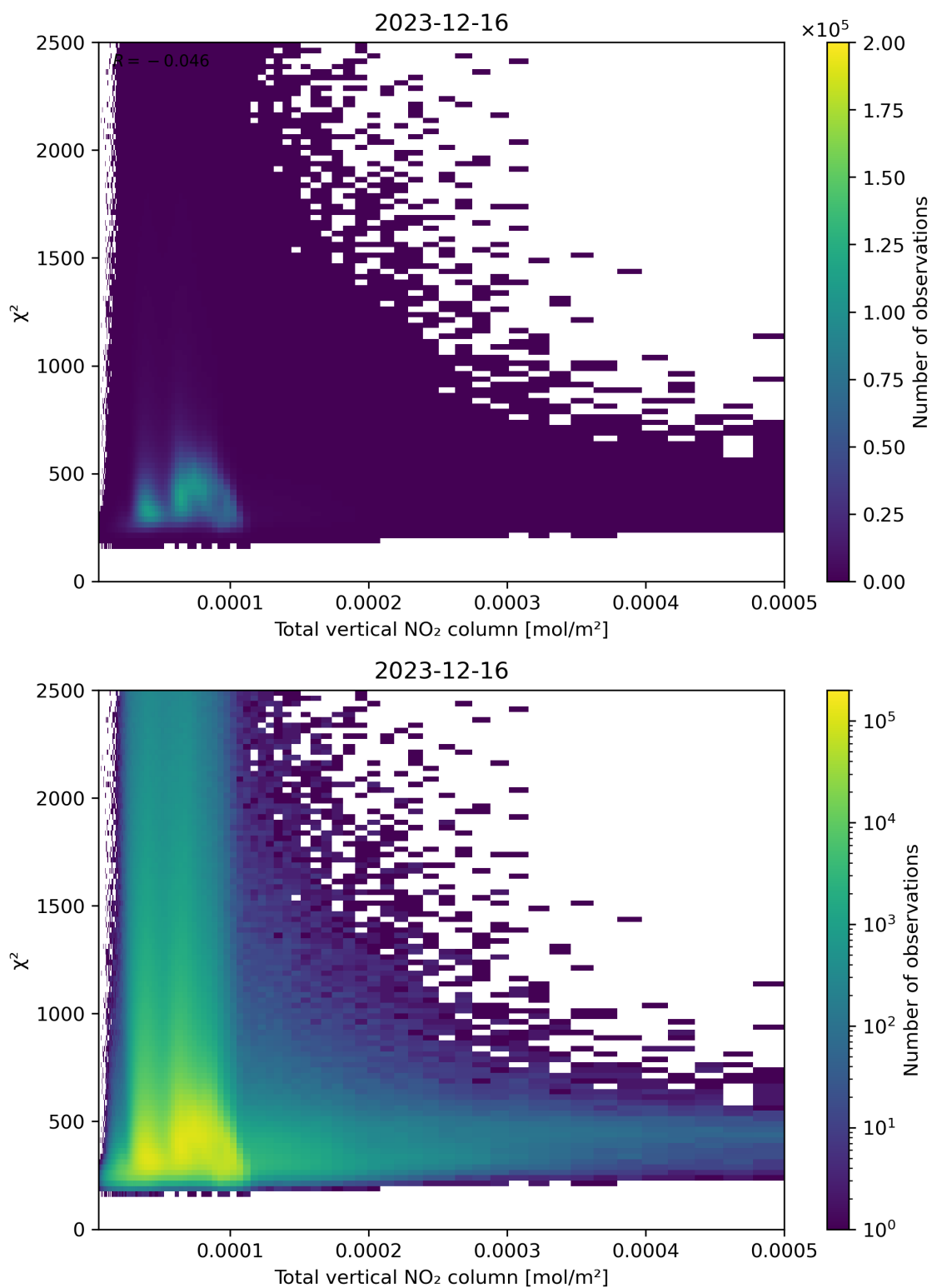
Figure 111: Scatter density plot of “Total vertical NO 2 column” against “ \chi^2 ” for 2023-12-15 to 2023-12-17.
