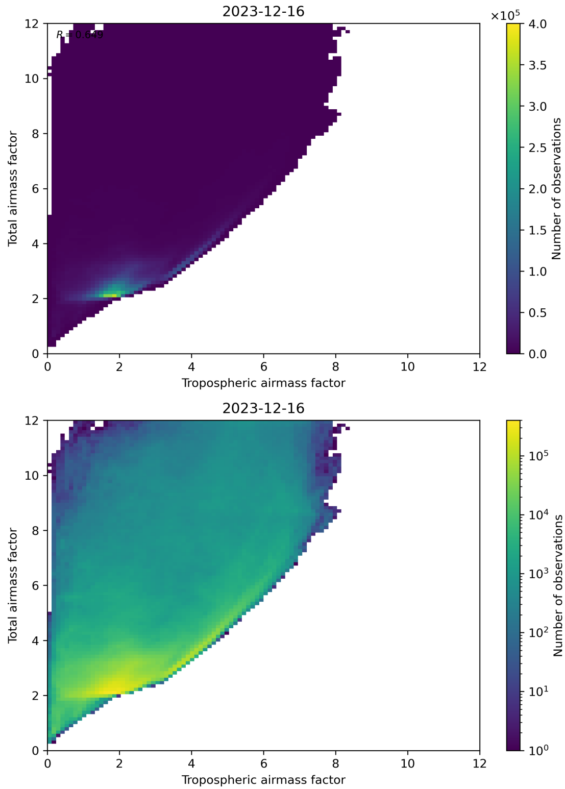
Figure 72: Scatter density plot of “Tropospheric airmass factor” against “Total airmass factor” for 2023-12-15 to 2023-12-17.
