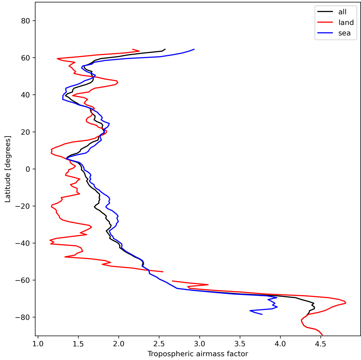
Figure 14: Zonal average of “Tropospheric airmass factor” for 2023-12-15 to 2023-12-17.
