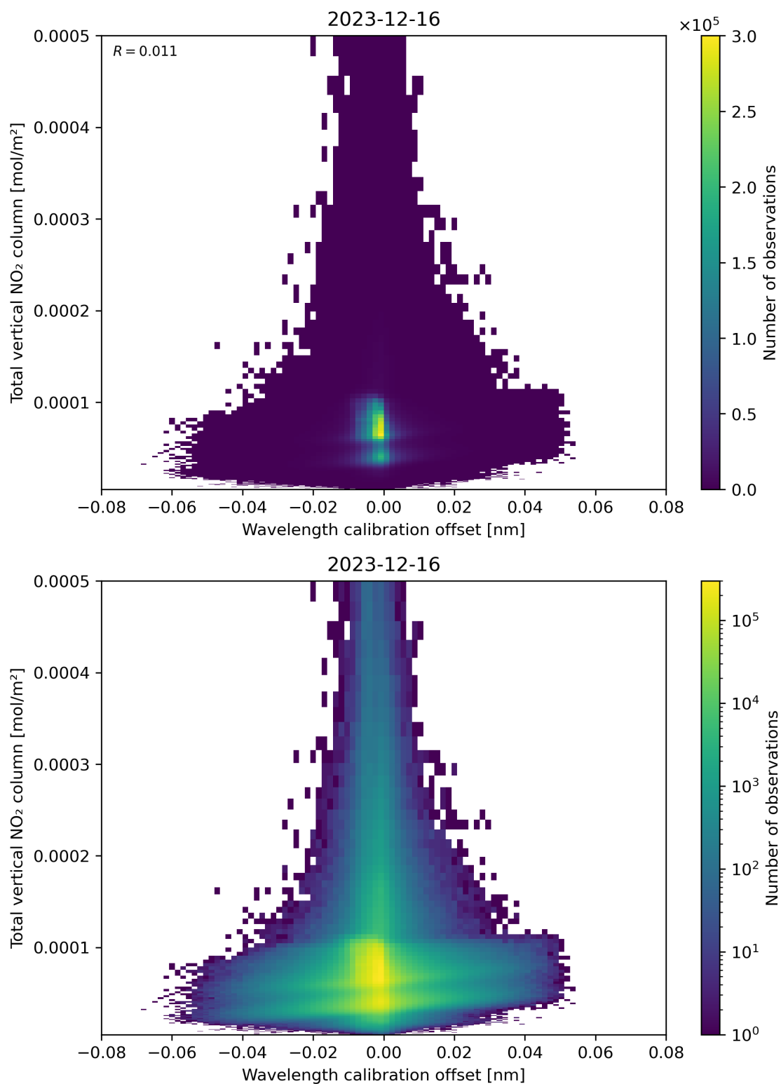
Figure 179: Scatter density plot of “Wavelength calibration offset” against “Total vertical NO 2 column” for 2023-12-15 to 2023-12-17.
