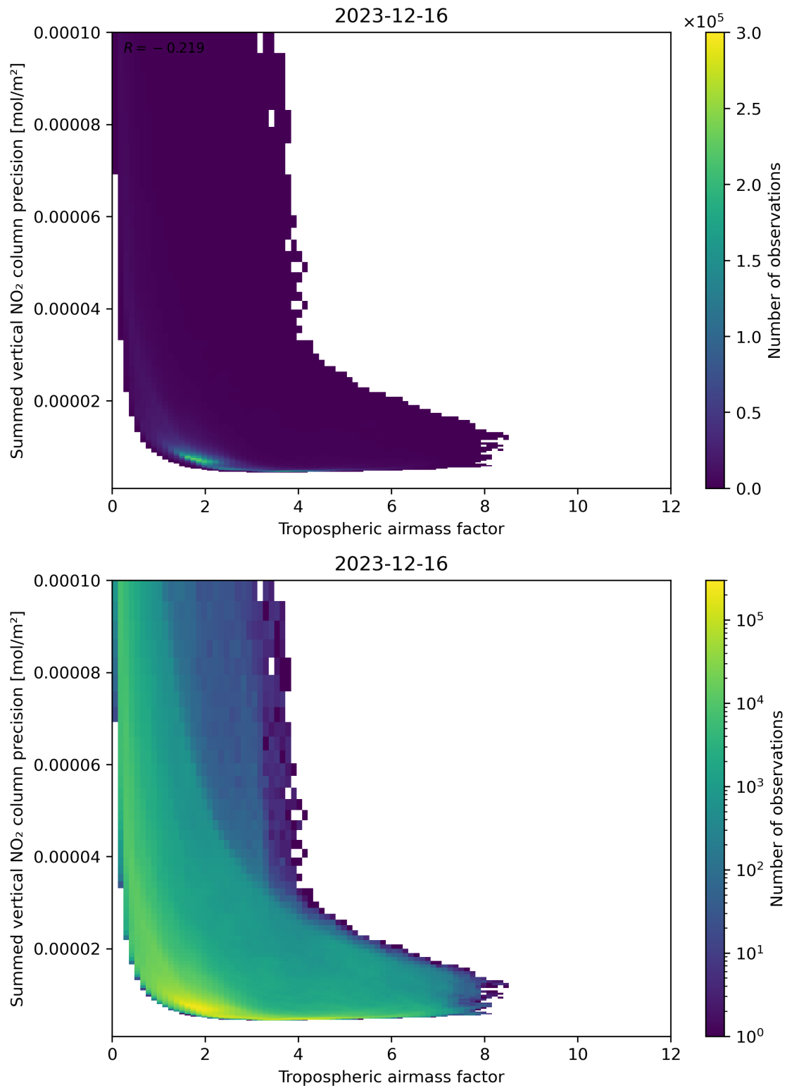
Figure 76: Scatter density plot of “Tropospheric air mass factor” against “Summed vertical NO 2 column precision” for 2023-12-15 to 2023-12-17.
