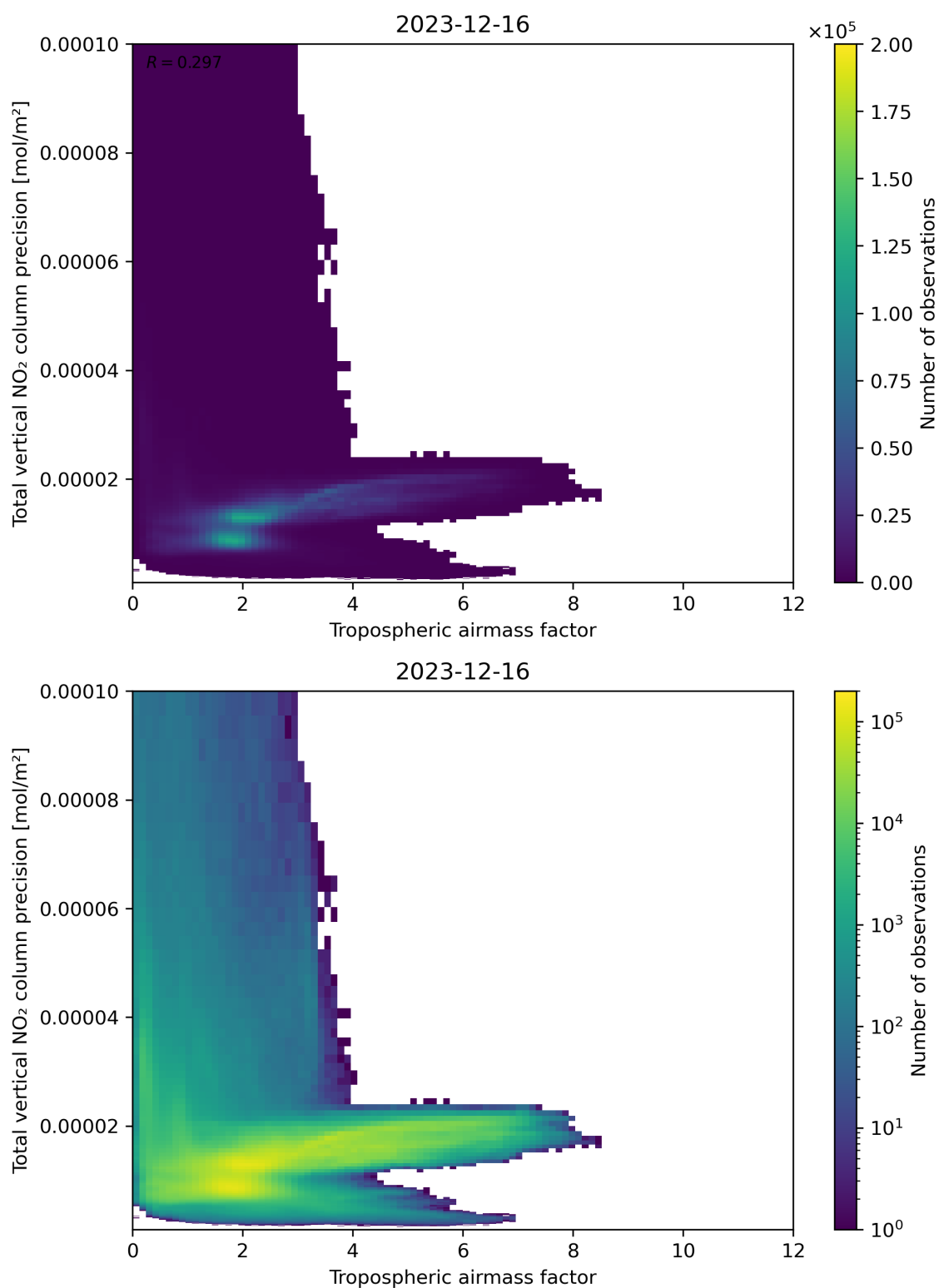
Figure 78: Scatter density plot of “Tropospheric air mass factor” against “Total vertical NO 2 column precision” for 2023-12-15 to 2023-12-17.
