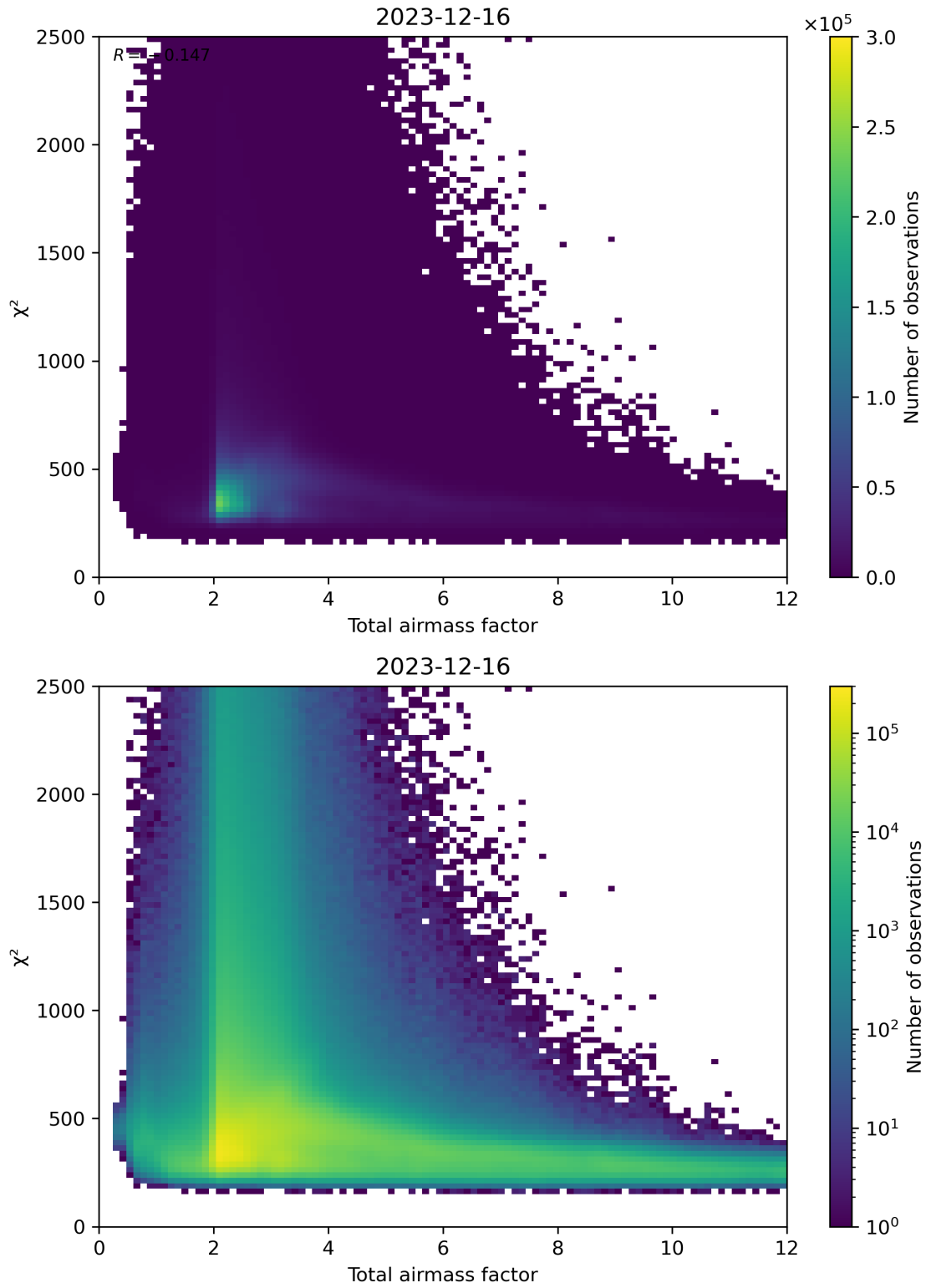
Figure 63: Scatter density plot of “Total airmass factor” against “ \chi^2 ” for 2023-12-15 to 2023-12-17.
