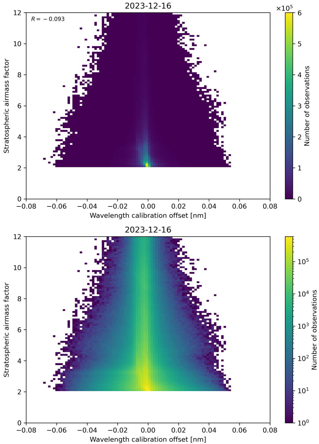
Figure 174: Scatter density plot of “Wavelength calibration offset” against “Stratospheric airmass factor” for 2023-12-15 to 2023-12-17.
