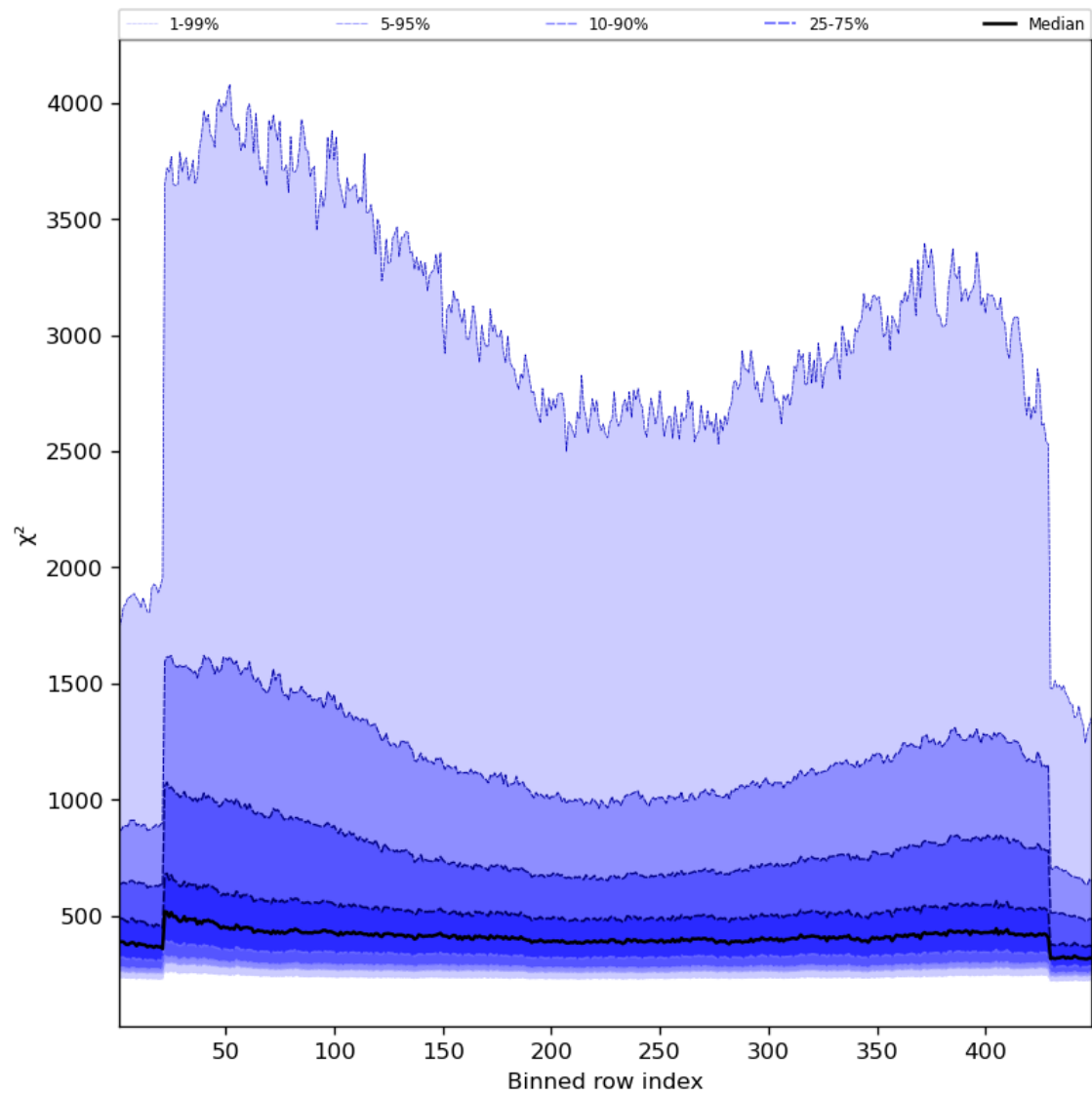
Figure 59: Along track statistics of “ \chi^2 ” for 2023-12-15 to 2023-12-17
