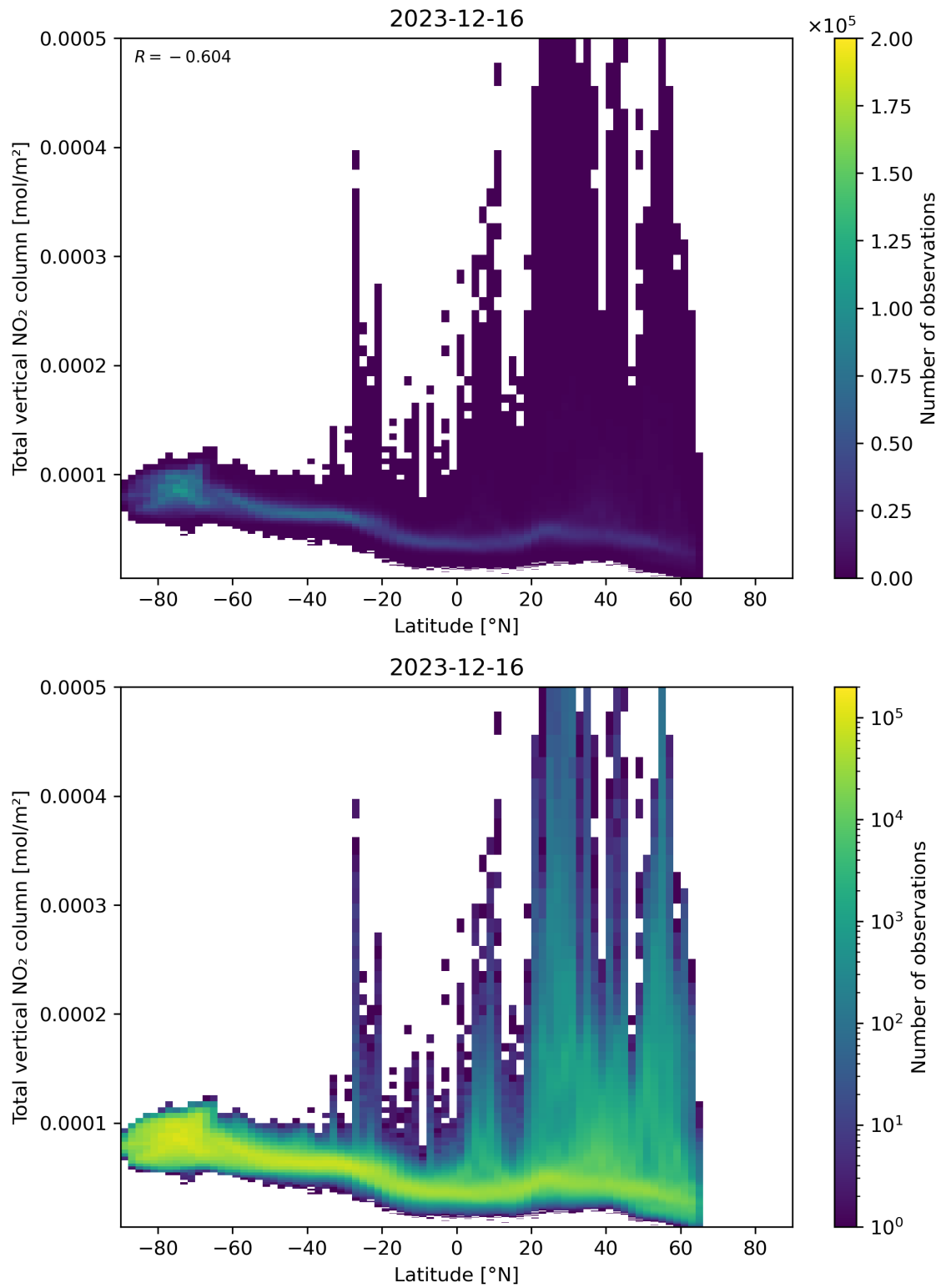
Figure 90: Scatter density plot of “Latitude” against “Total vertical NO 2 column” for 2023-12-15 to 2023-12-17.
