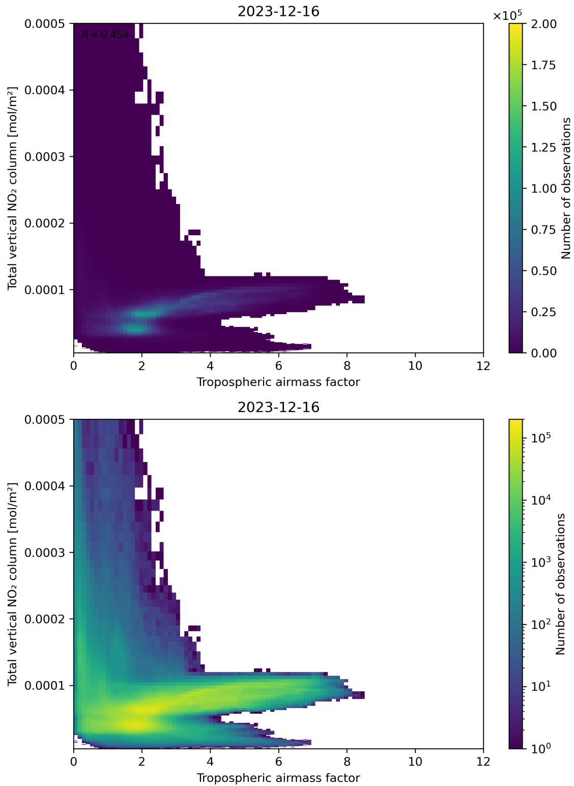
Figure 77: Scatter density plot of “Tropospheric airmass factor” against “Total vertical NO 2 column” for 2023-12-15 to 2023-12-17.
