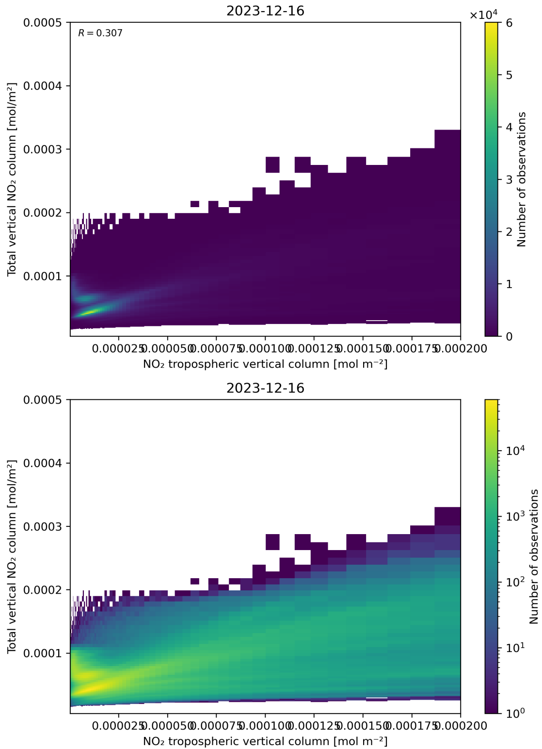
Figure 128: Scatter density plot of “NO 2 tropospheric vertical column” against “Total vertical NO 2 column” for 2023-12-15 to 2023-12-17.
