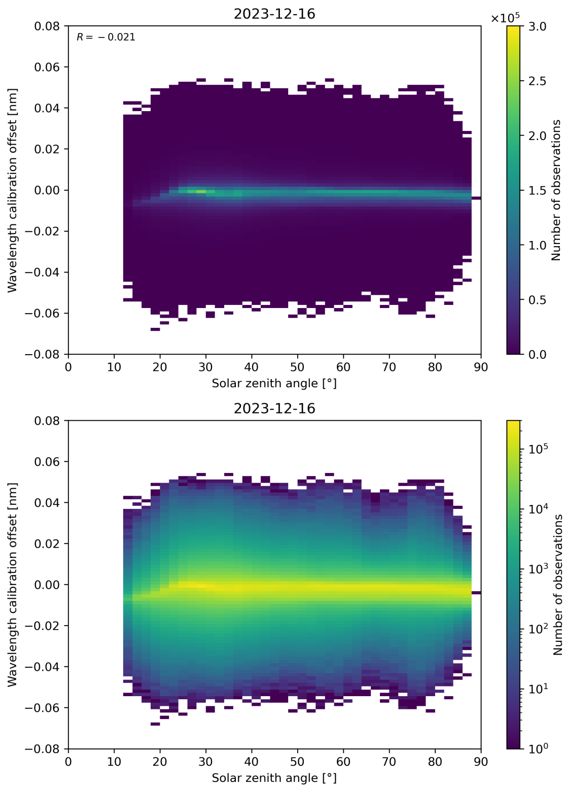
Figure 158: Scatter density plot of “Solar zenith angle” against “Wavelength calibration offset” for 2023-12-15 to 2023-12-17.
