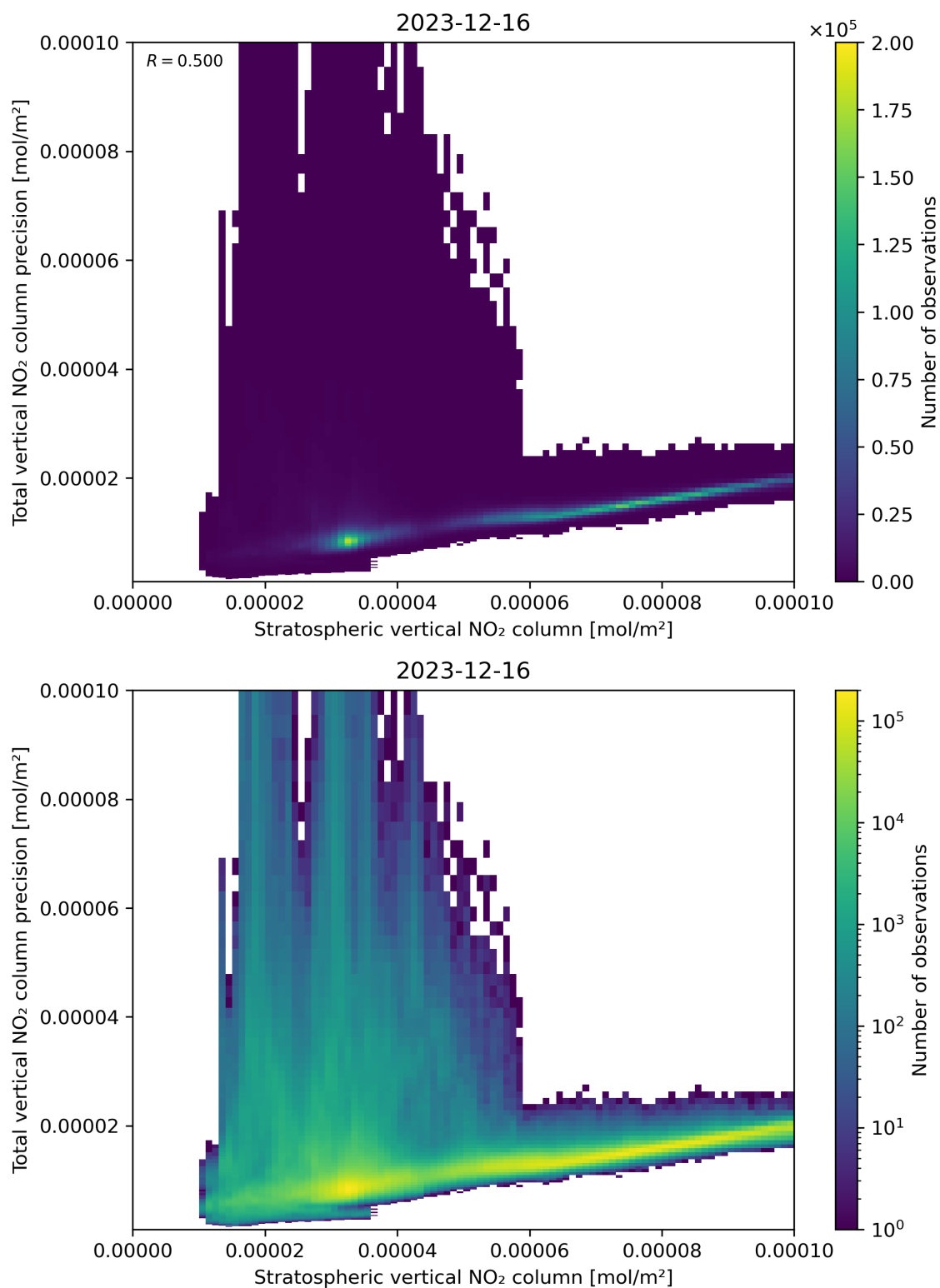
Figure 101: Scatter density plot of “Stratospheric vertical NO 2 column” against “Total vertical NO 2 column precision” for 2023-12-15 to 2023-12-17.
