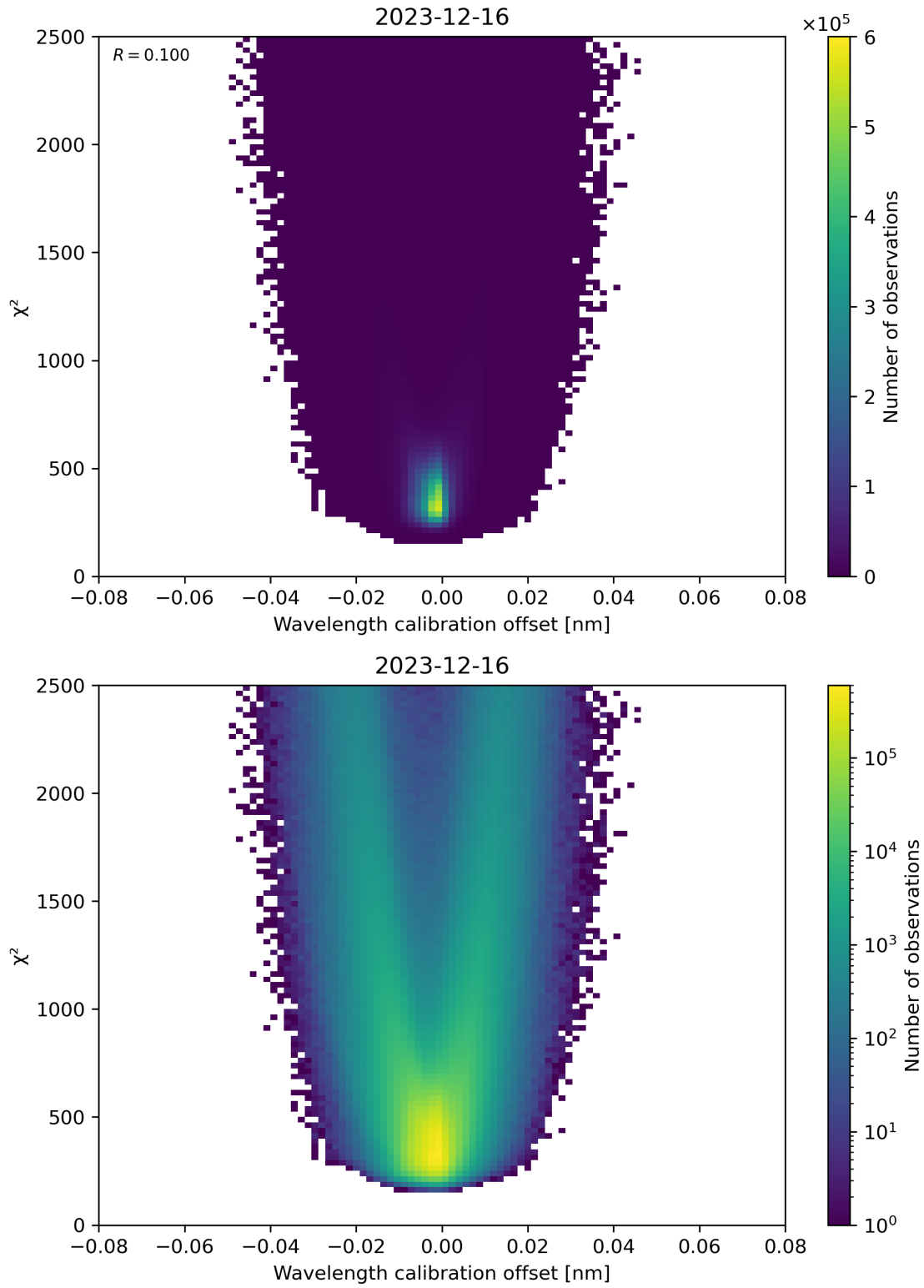
Figure 175: Scatter density plot of “Wavelength calibration offset” against “ \chi^2 ” for 2023-12-15 to 2023-12-17.
