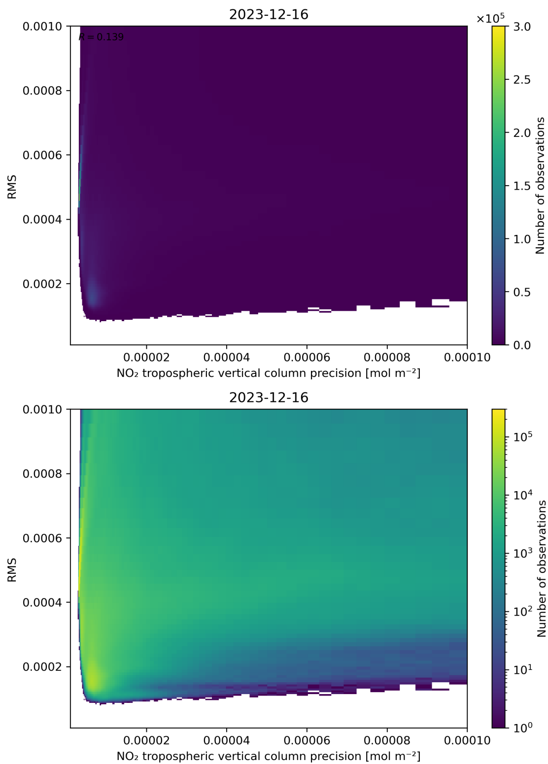
Figure 140: Scatter density plot of “NO 2 tropospheric vertical column precision” against “RMS” for 2023-12-15 to 2023-12-17.
