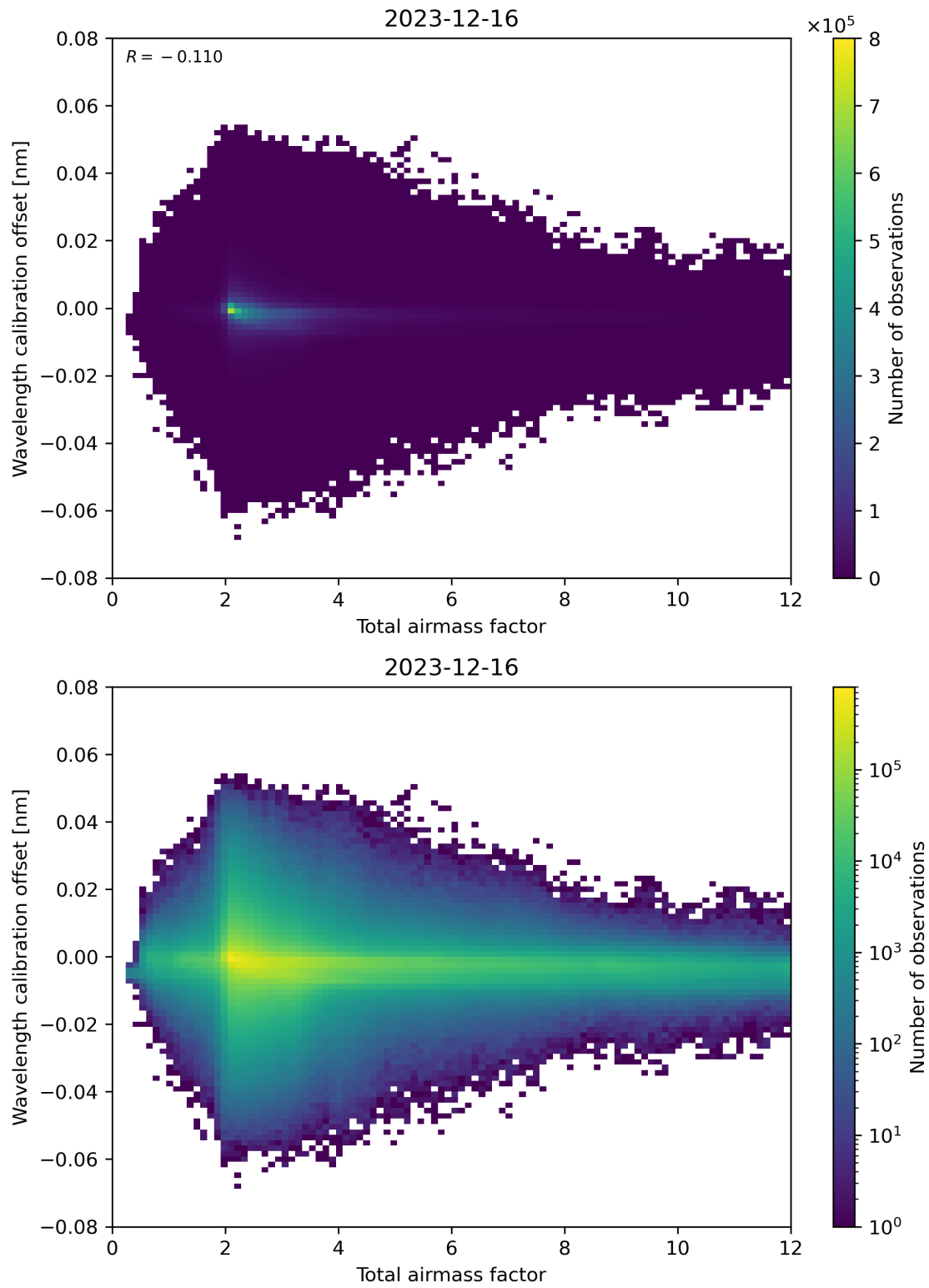
Figure 70: Scatter density plot of “Total airmass factor” against “Wavelength calibration offset” for 2023-12-15 to 2023-12-17.
