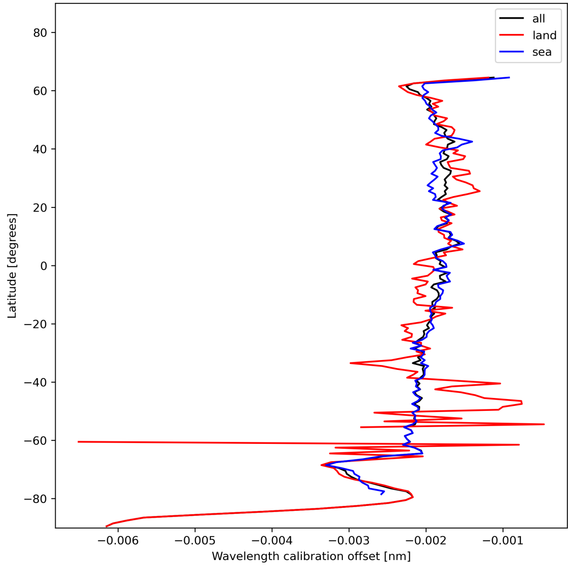
Figure 18: Zonal average of “Wavelength calibration offset” for 2023-12-15 to 2023-12-17.
