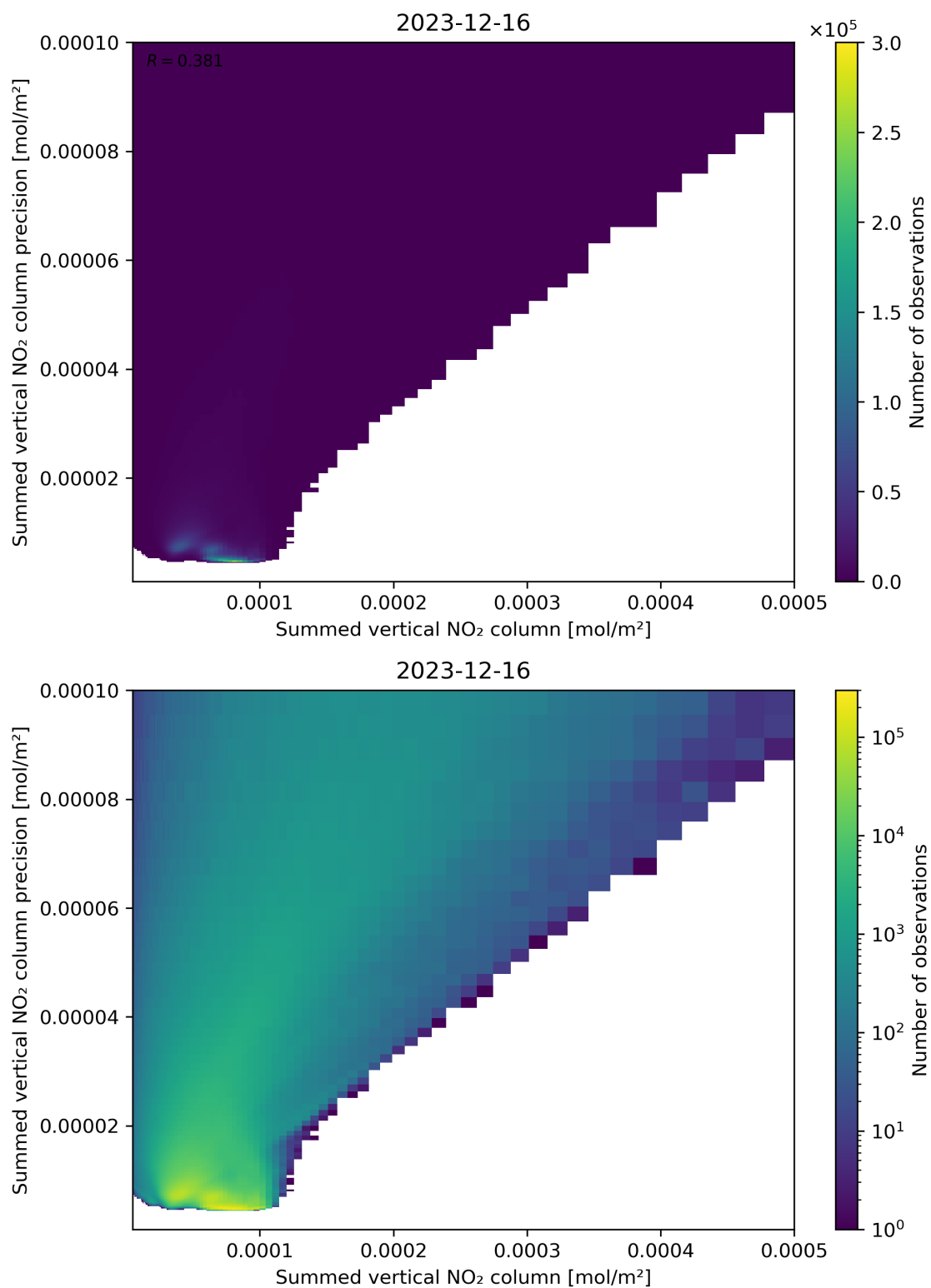
Figure 105: Scatter density plot of “Summed vertical NO 2 column” against “Summed vertical NO 2 column precision” for 2023-12-15 to 2023-12-17.
