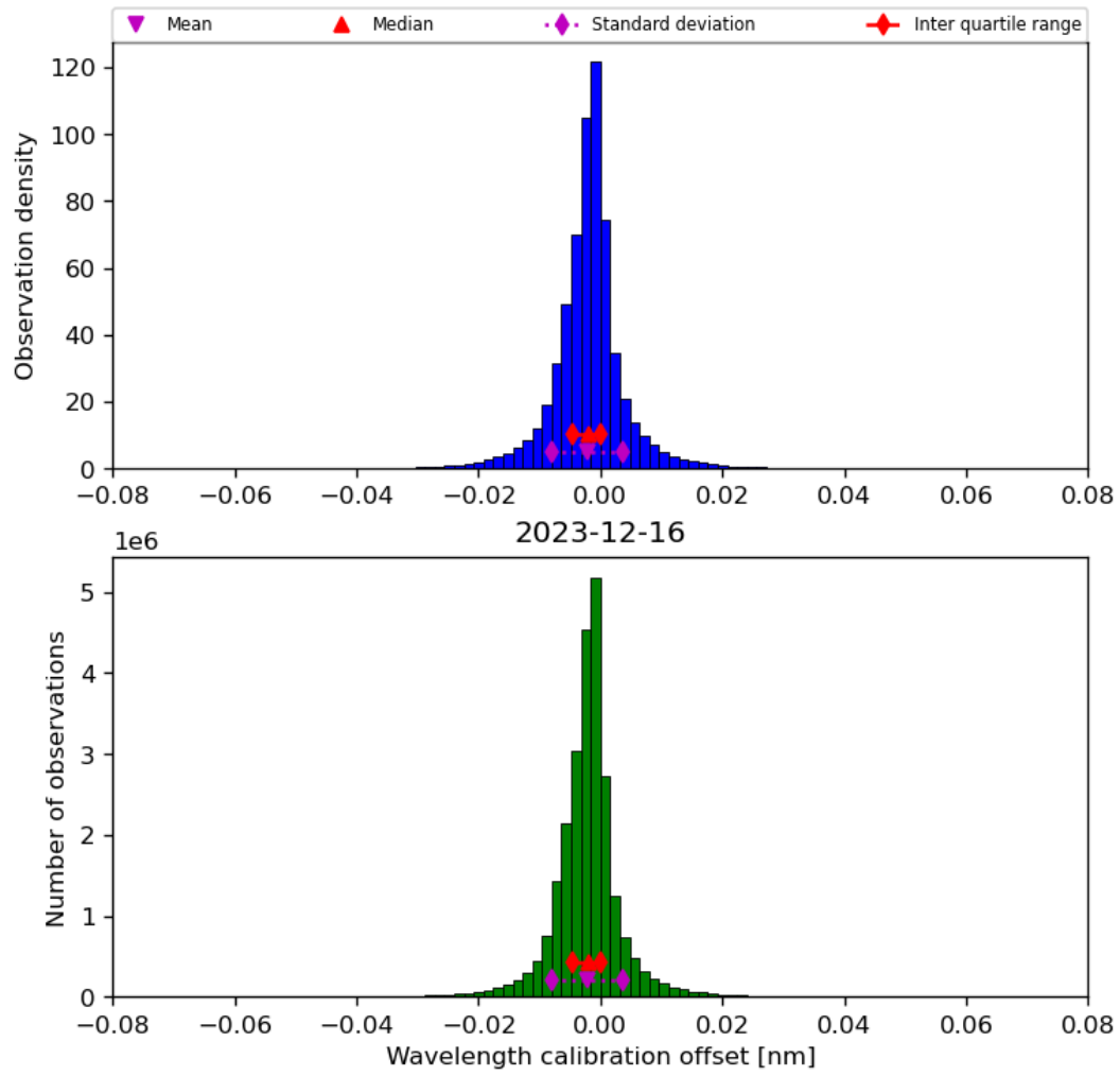
Figure 35: Histogram of “Wavelength calibration offset” for 2023-12-15 to 2023-12-17
