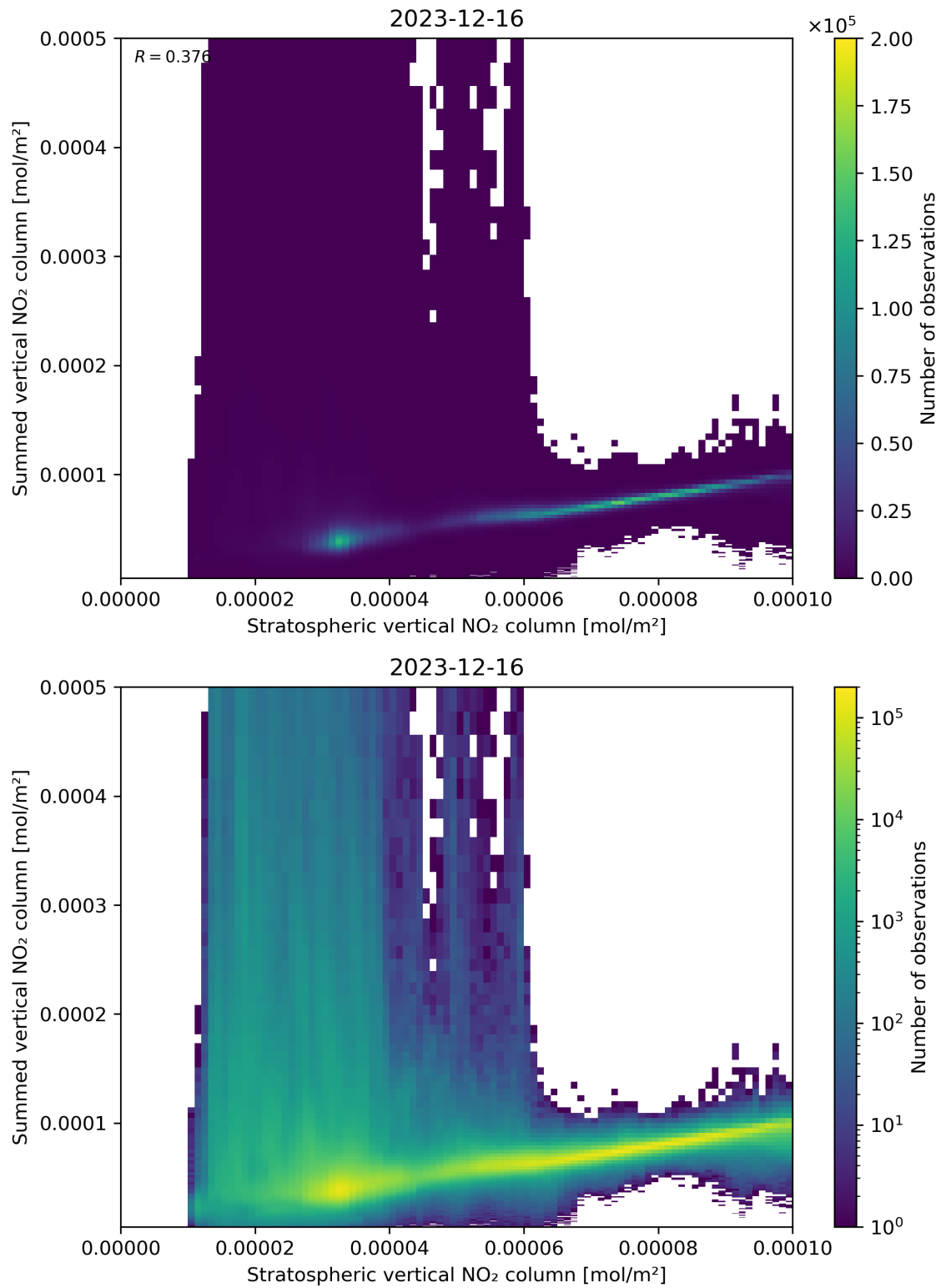
Figure 98: Scatter density plot of “Stratospheric vertical NO 2 column” against “Summed vertical NO 2 column” for 2023-12-15 to 2023-12-17.
