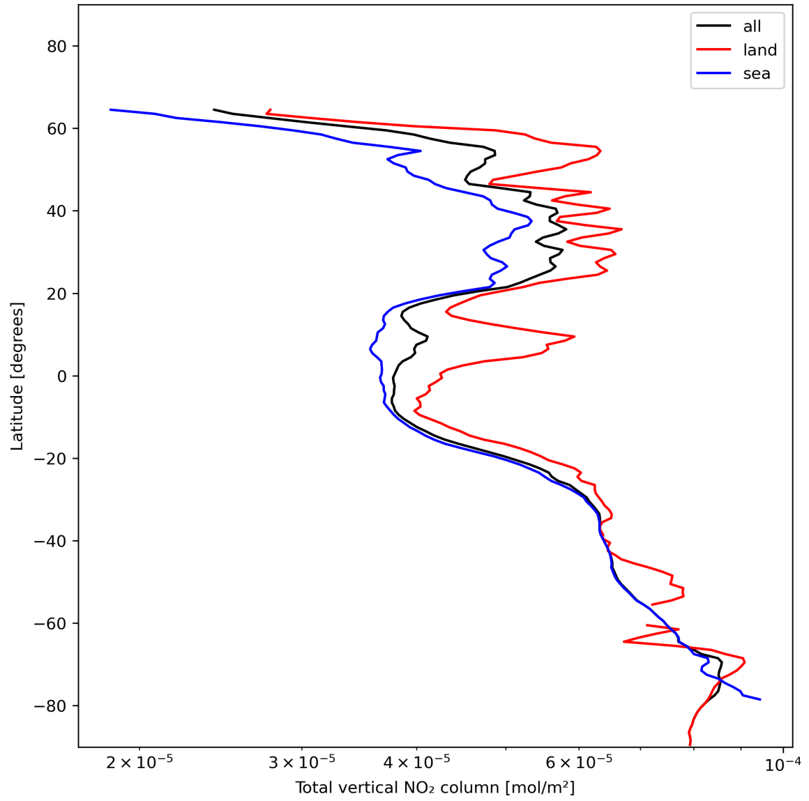
Figure 21: Zonal average of “Total vertical NO 2 column” for 2023-12-15 to 2023-12-17.
