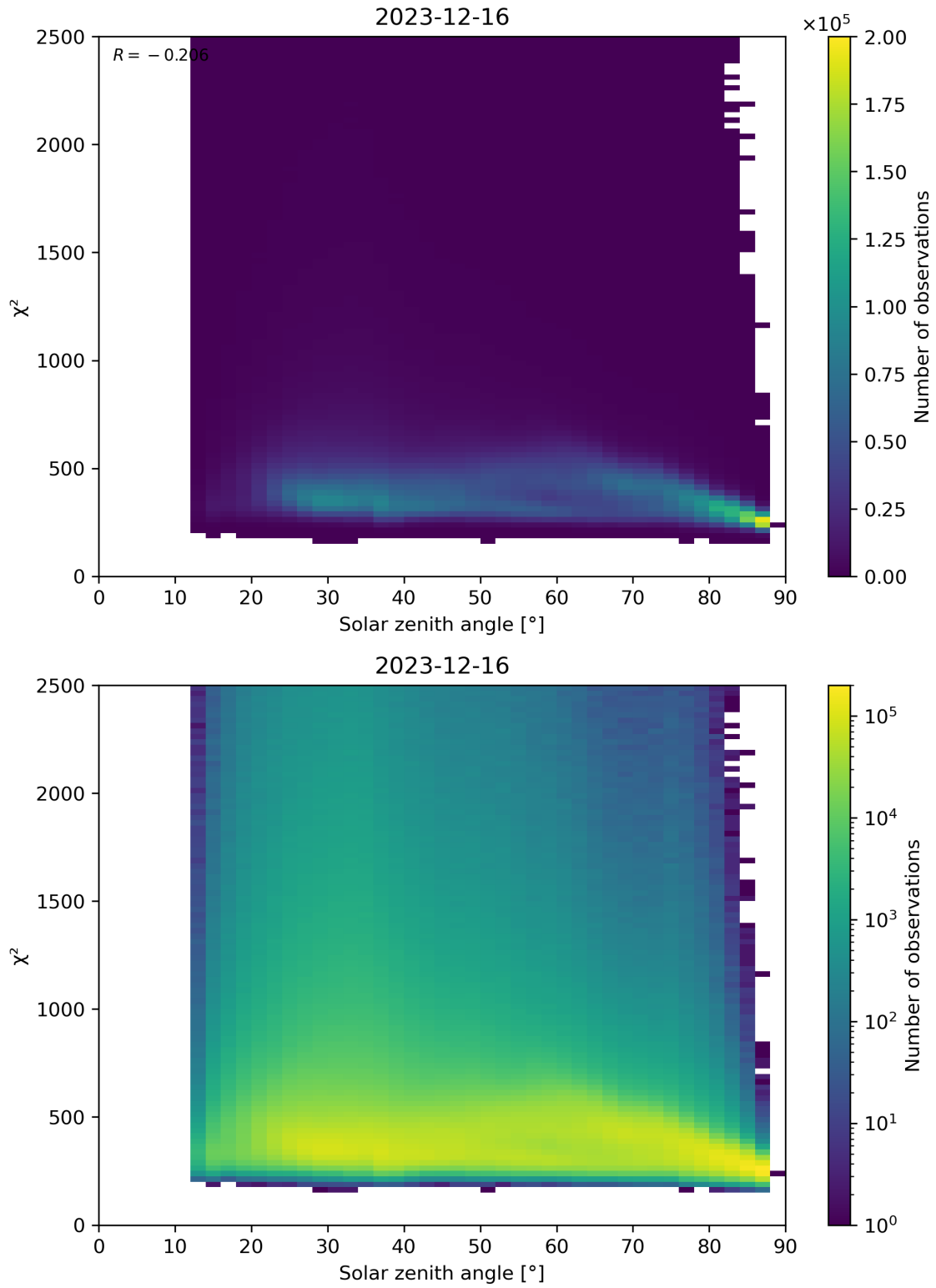
Figure 148: Scatter density plot of “Solar zenith angle” against “ \chi^2 ” for 2023-12-15 to 2023-12-17.
