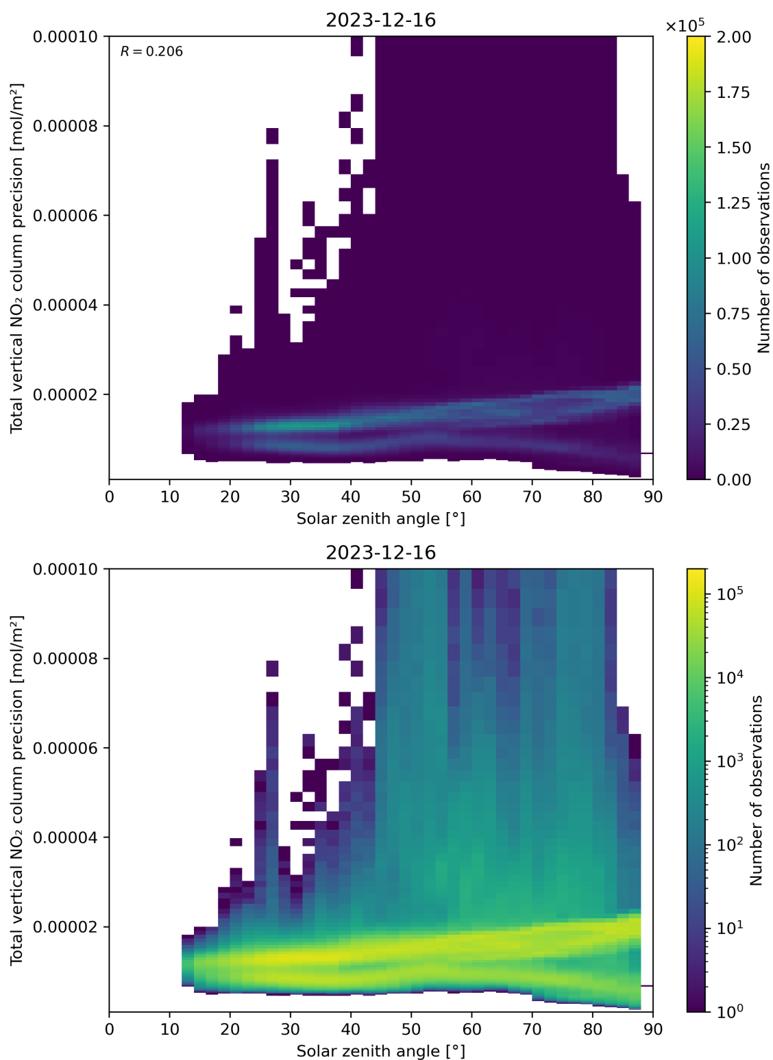
Figure 154: Scatter density plot of “Solar zenith angle” against “Total vertical NO 2 column precision” for 2023-12-15 to 2023-12-17.
