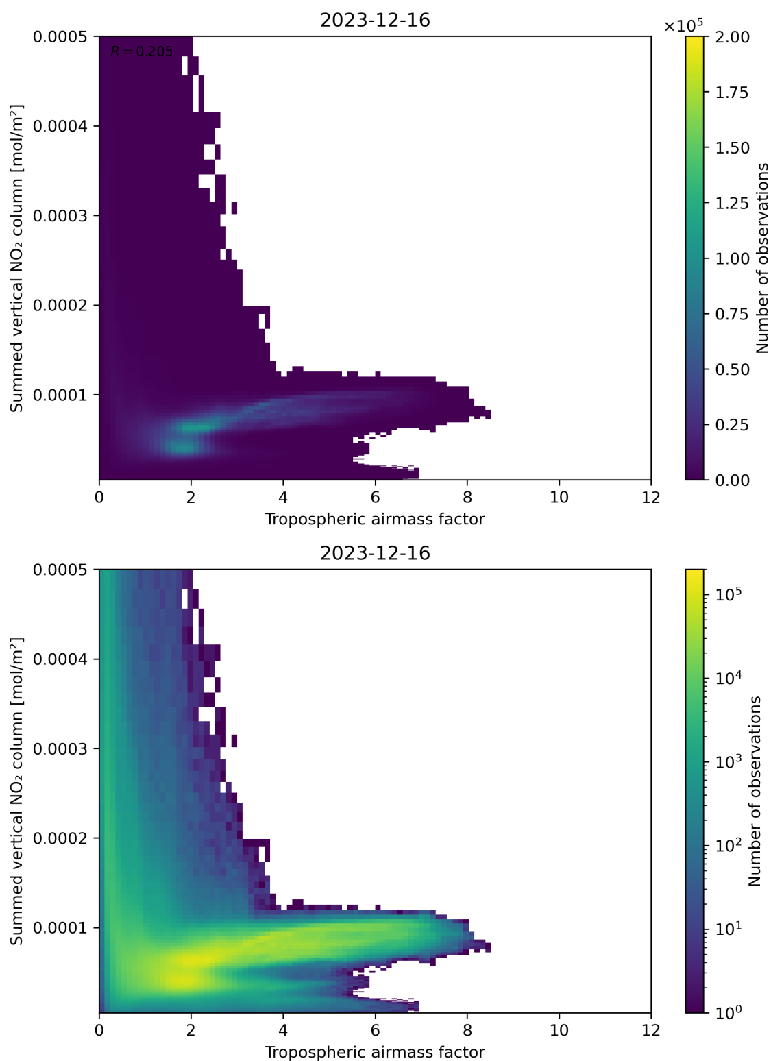
Figure 75: Scatter density plot of “Tropospheric airmass factor” against “Summed vertical NO 2 column” for 2023-12-15 to 2023-12-17.
