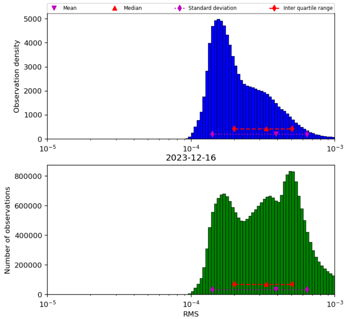
Figure 43: Histogram of “RMS” for 2023-12-15 to 2023-12-17
