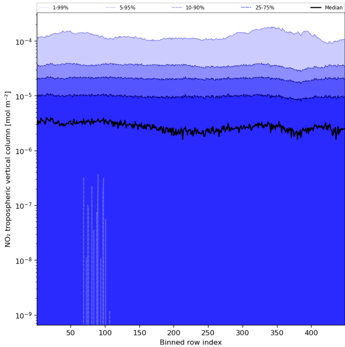
Figure 46: Along track statistics of “NO 2 tropospheric vertical column” for 2023-12-15 to 2023-12-17
