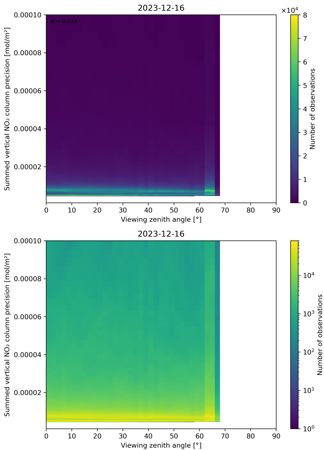
Figure 166: Scatter density plot of “Viewing zenith angle” against “Summed vertical NO 2 column precision” for 2023-12-15 to 2023-12-17.
