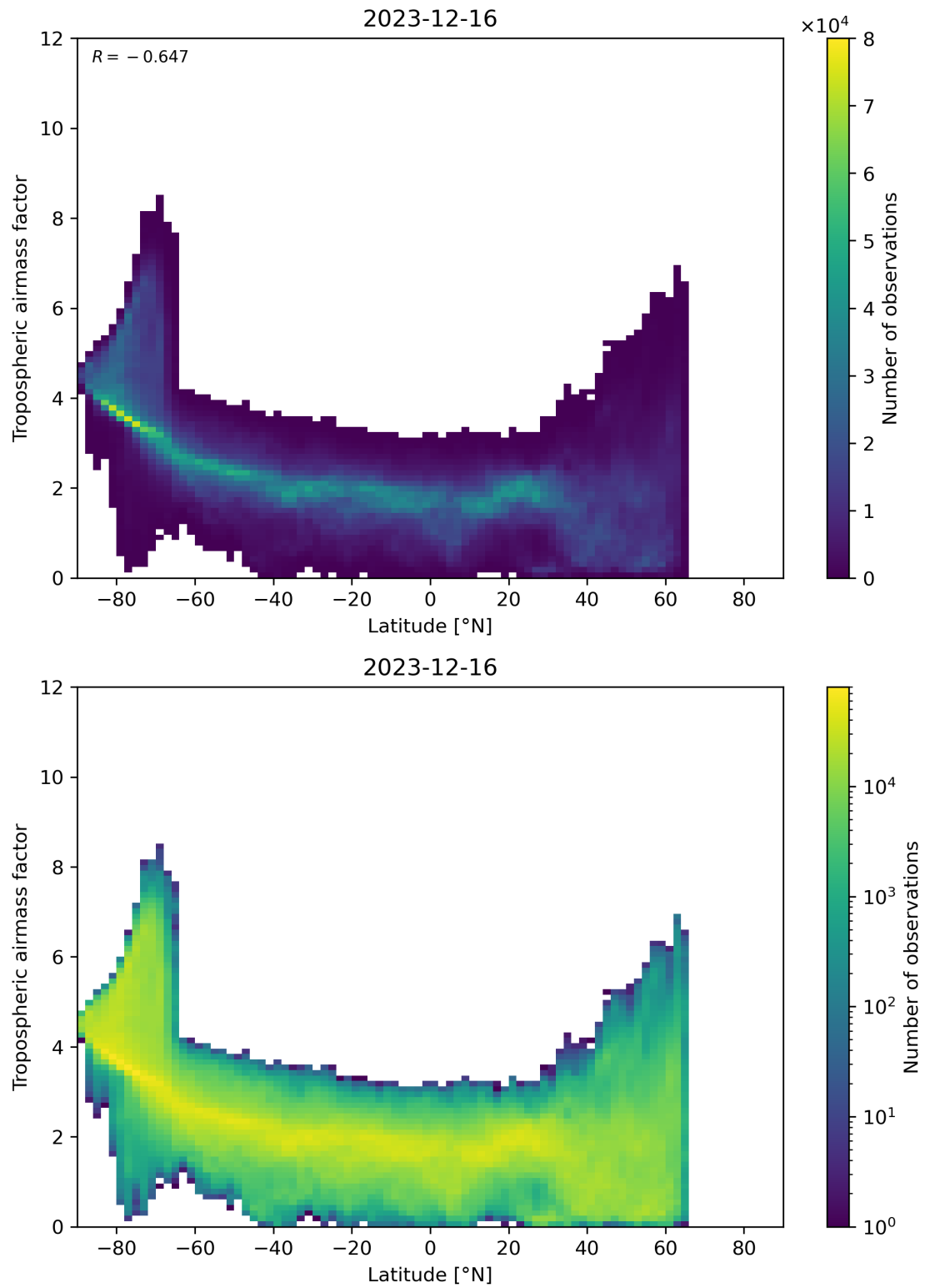
Figure 85: Scatter density plot of “Latitude” against “Tropospheric airmass factor” for 2023-12-15 to 2023-12-17.
