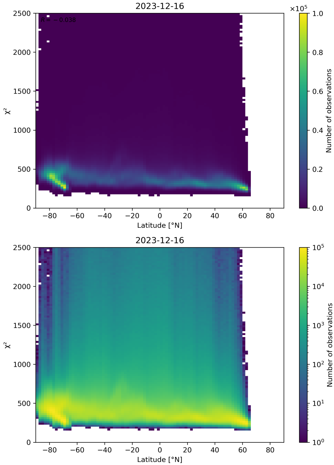
Figure 86: Scatter density plot of “Latitude” against “ \chi^2 ” for 2023-12-15 to 2023-12-17.
