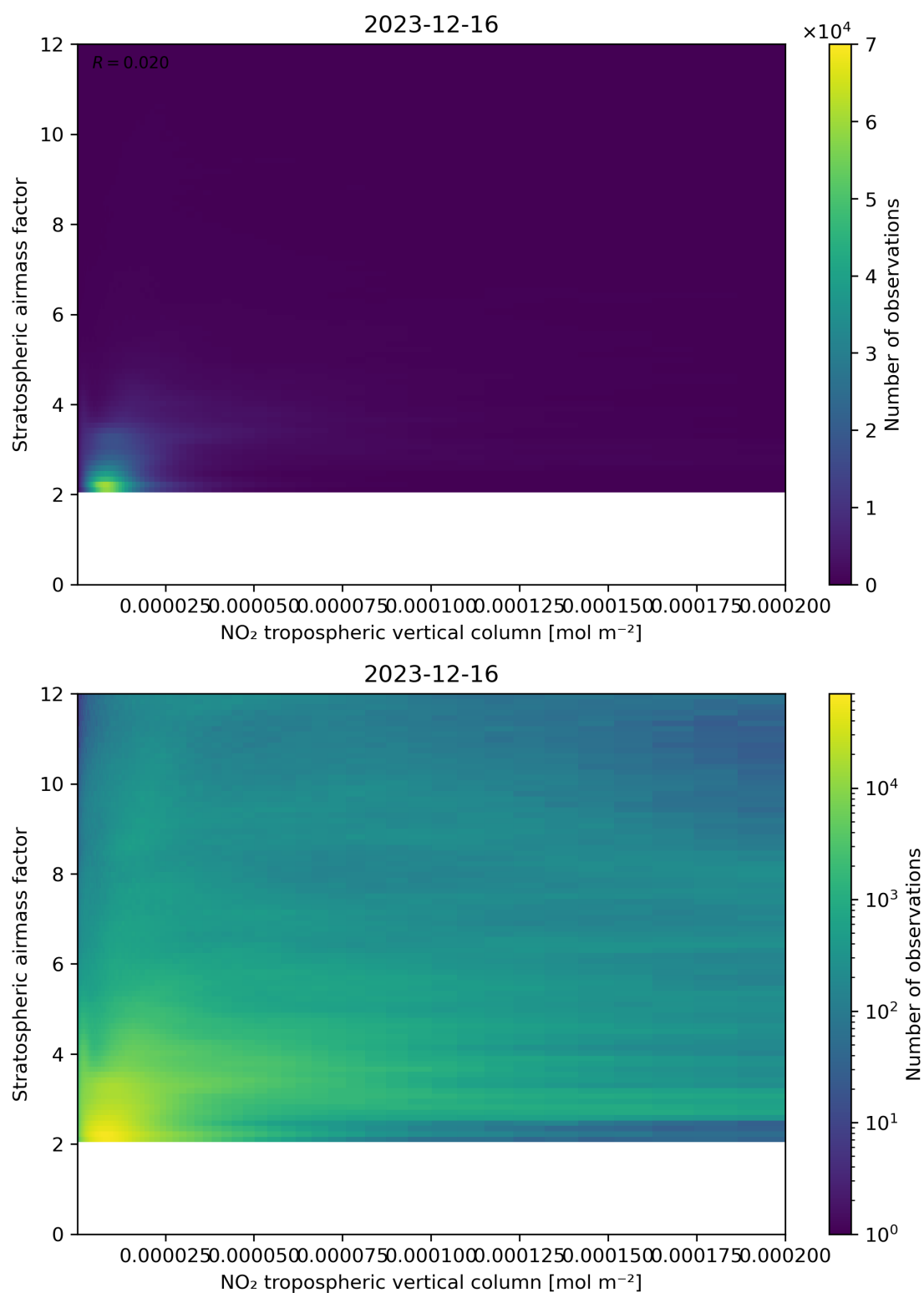
Figure 121: Scatter density plot of “NO 2 tropospheric vertical column” against “Stratospheric airmass factor” for 2023-12-15 to 2023-12-17.
