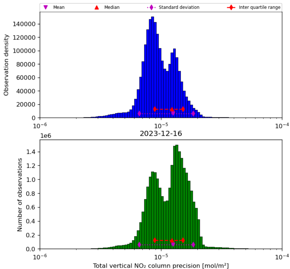
Figure 39: Histogram of "Total vertical NO 2 column precision" for 2023-12-15 to 2023-12-17
