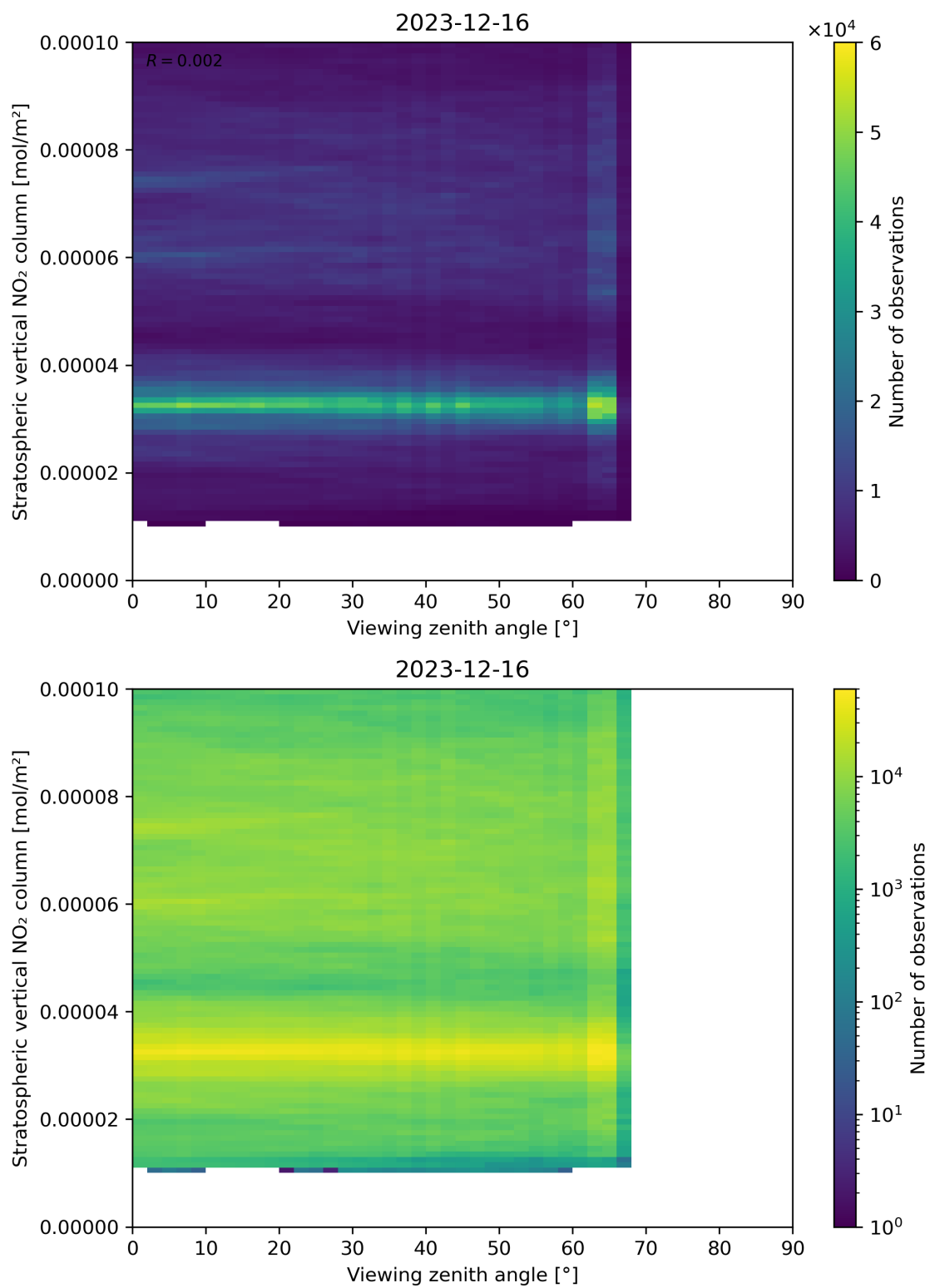
Figure 164: Scatter density plot of “Viewing zenith angle” against “Stratospheric vertical NO 2 column” for 2023-12-15 to 2023-12-17.
