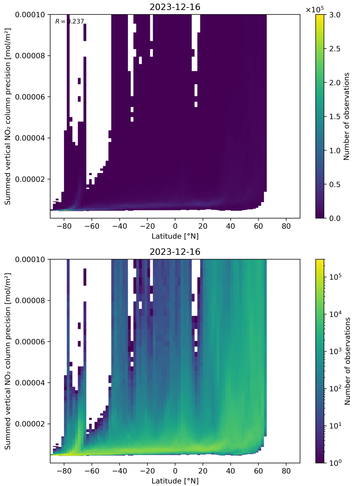
Figure 89: Scatter density plot of “Latitude” against “Summed vertical NO 2 column precision” for 2023-12-15 to 2023-12-17.
