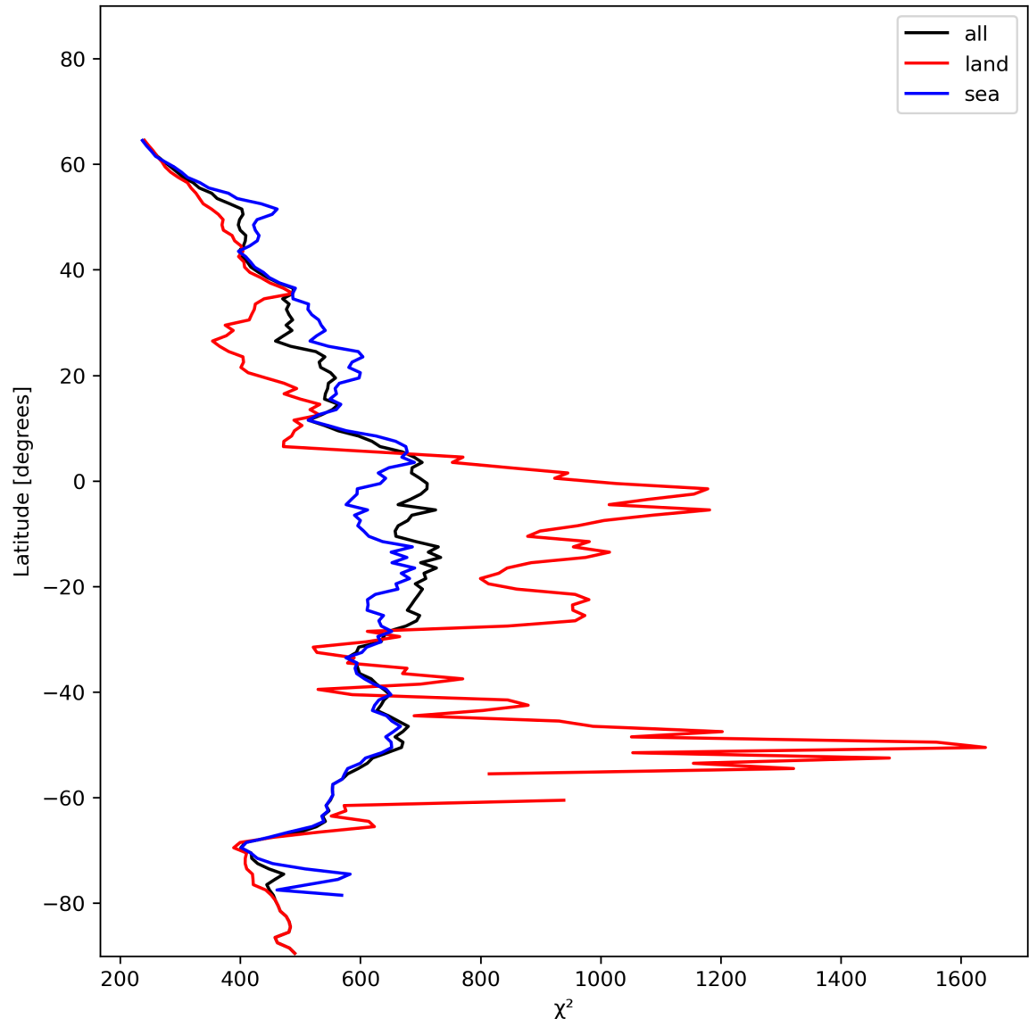
Figure 25: Zonal average of “ \chi^2 ” for 2023-12-15 to 2023-12-17.
