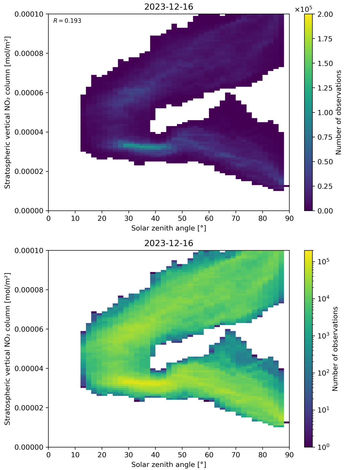
Figure 150: Scatter density plot of “Solar zenith angle” against “Stratospheric vertical NO 2 column” for 2023-12-15 to 2023-12-17.
