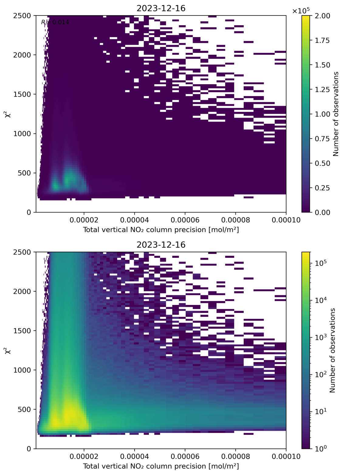
Figure 116: Scatter density plot of “Total vertical NO 2 column precision” against “ \chi^2 ” for 2023-12-15 to 2023-12-17.
