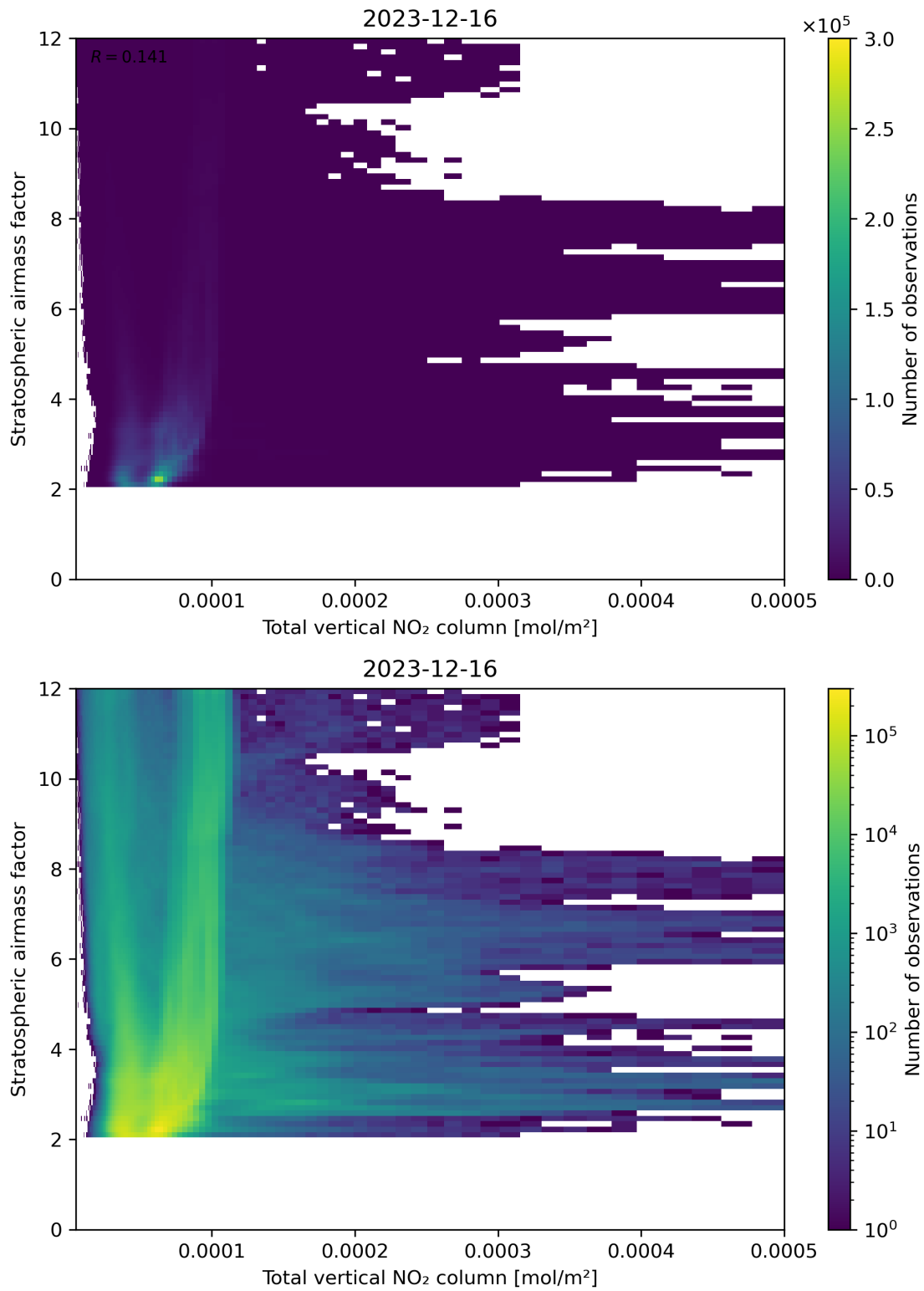
Figure 110: Scatter density plot of “Total vertical NO 2 column” against “Stratospheric airmass factor” for 2023-12-15 to 2023-12-17.
