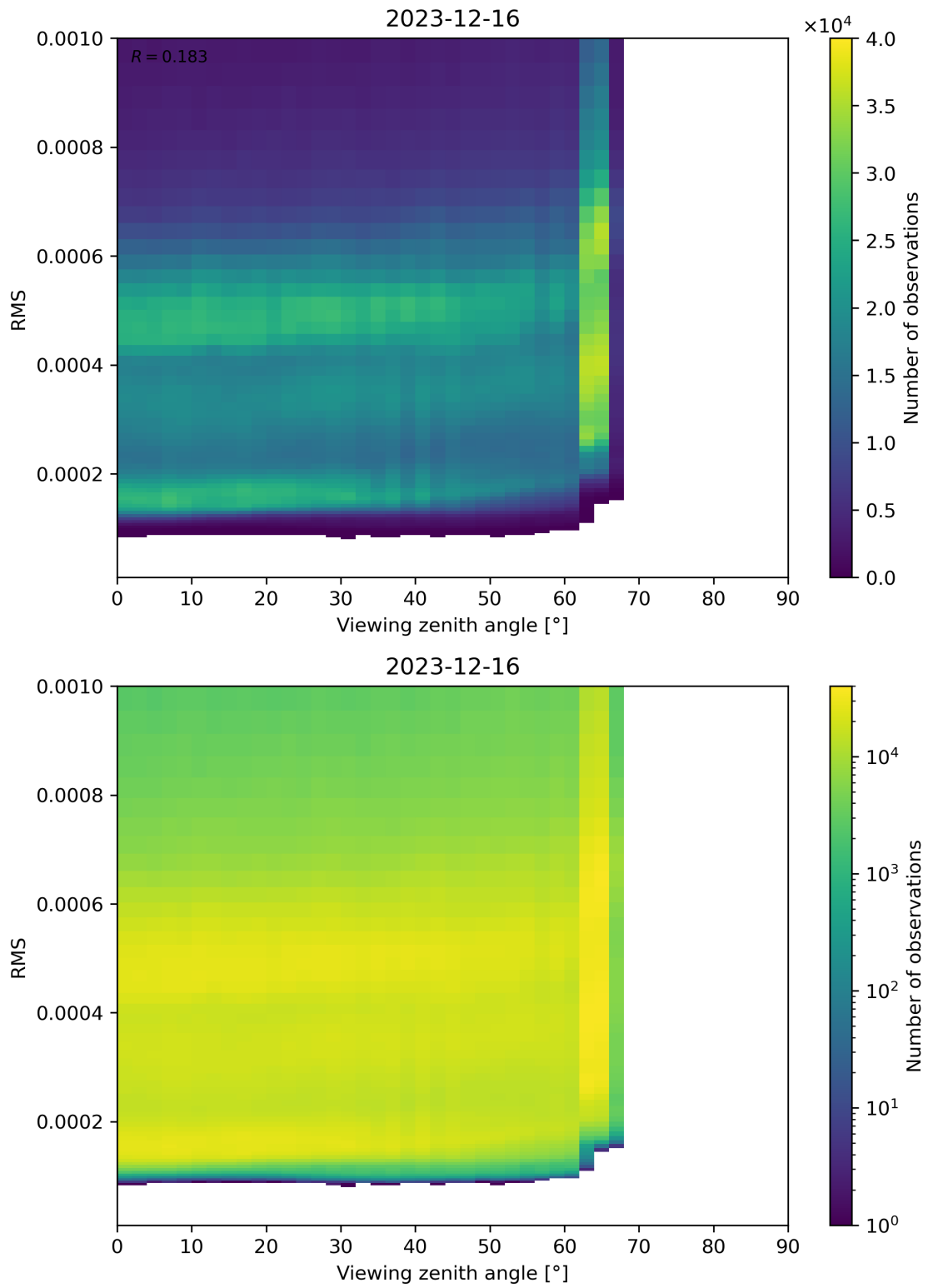
Figure 171: Scatter density plot of “Viewing zenith angle” against “RMS” for 2023-12-15 to 2023-12-17.
