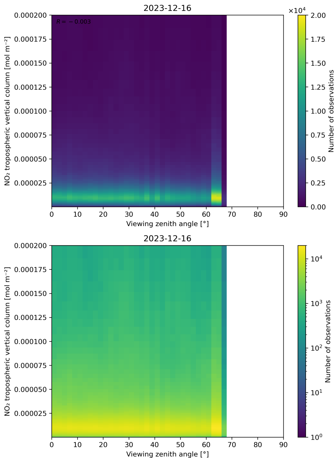
Figure 169: Scatter density plot of “Viewing zenith angle” against “NO 2 tropospheric vertical column” for 2023-12-15 to 2023-12-17.
