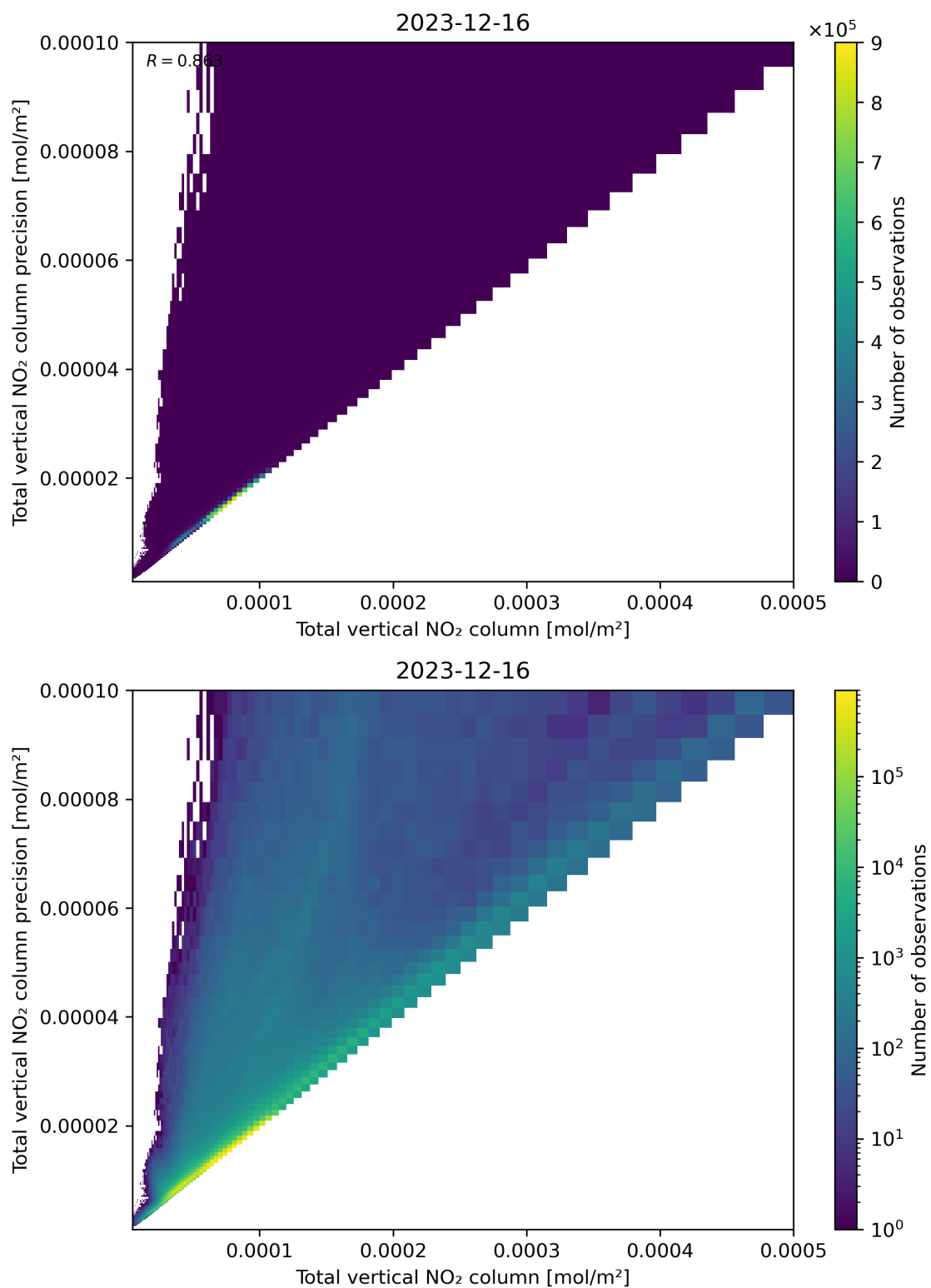
Figure 114: Scatter density plot of “Total vertical NO 2 column” against “Total vertical NO 2 column precision” for 2023-12-15 to 2023-12-17.
