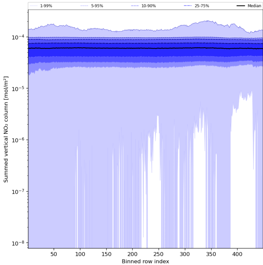
Figure 57: Along track statistics of “Summed vertical NO 2 column” for 2023-12-15 to 2023-12-17
