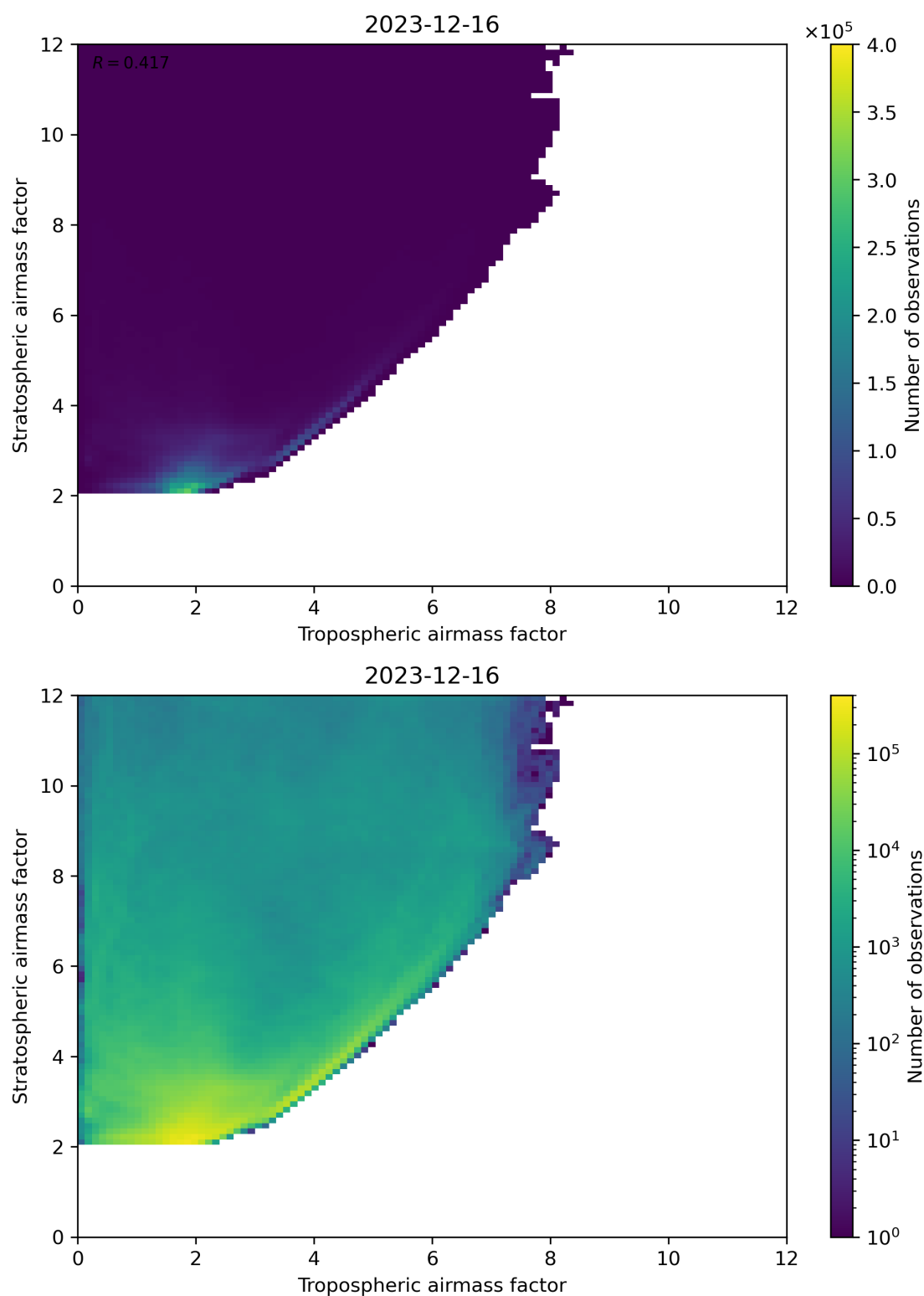
Figure 71: Scatter density plot of “Tropospheric airmass factor” against “Stratospheric airmass factor” for 2023-12-15 to 2023-12-17.
