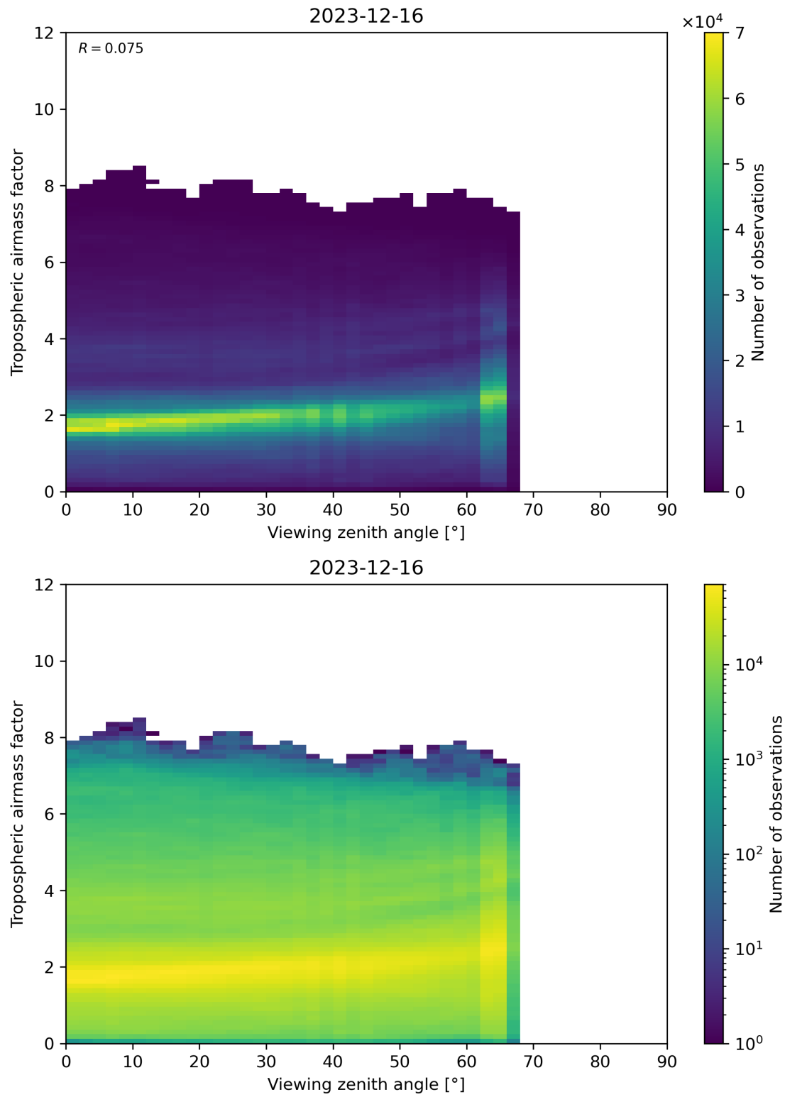
Figure 161: Scatter density plot of “Viewing zenith angle” against “Tropospheric airmass factor” for 2023-12-15 to 2023-12-17.
