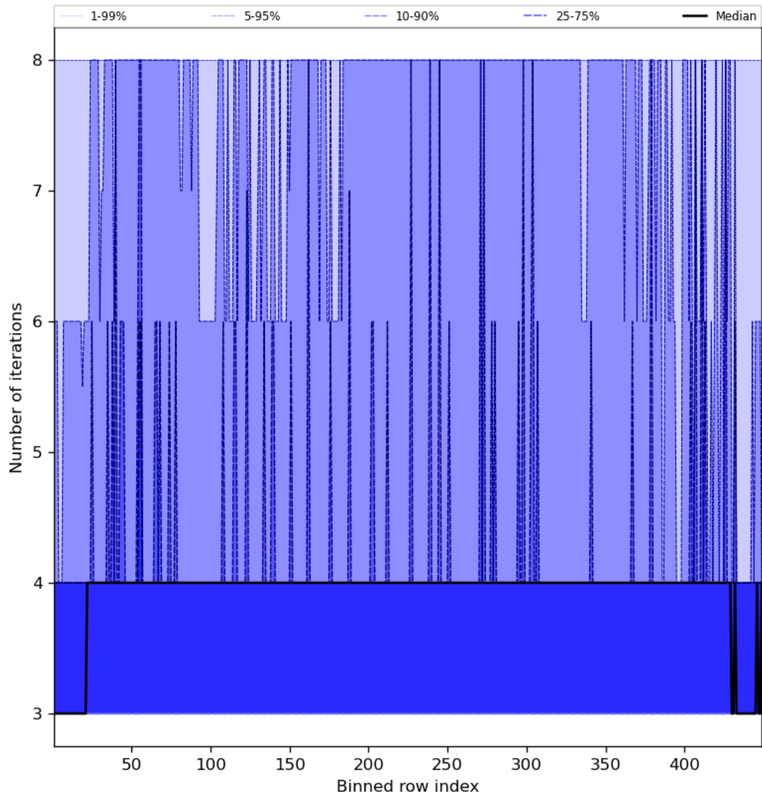
Figure 51: Along track statistics of “Number of iterations” for 2023-12-15 to 2023-12-17
