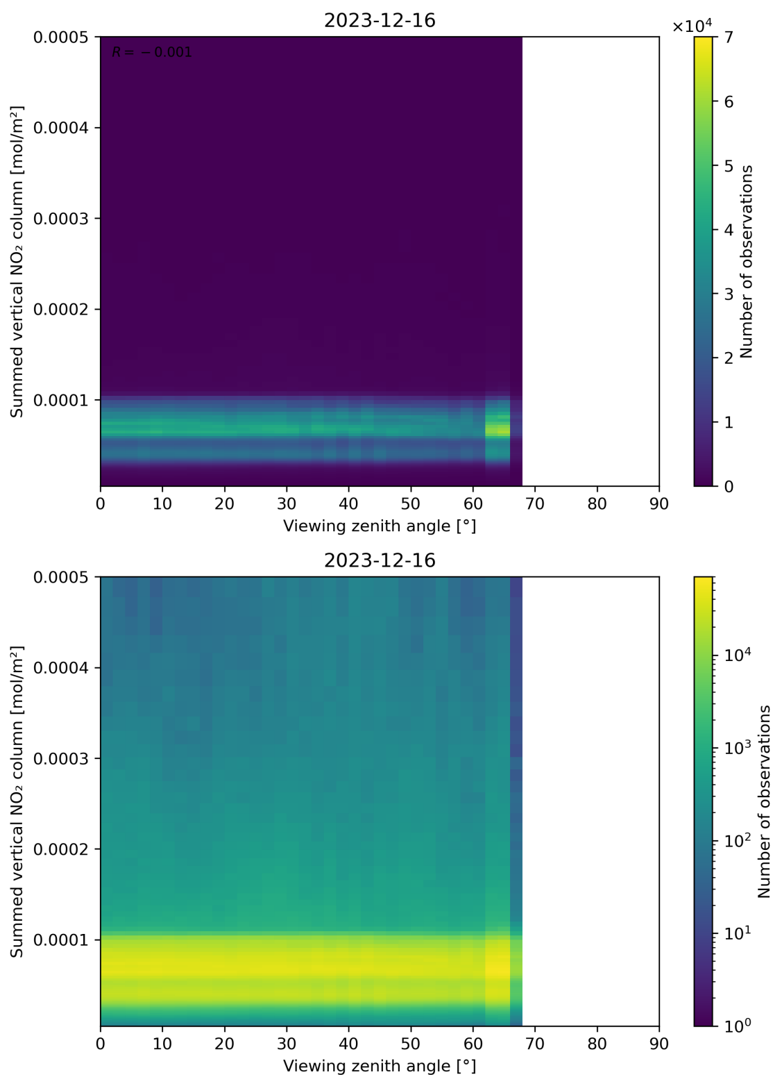
Figure 165: Scatter density plot of “Viewing zenith angle” against “Summed vertical NO 2 column” for 2023-12-15 to 2023-12-17.
