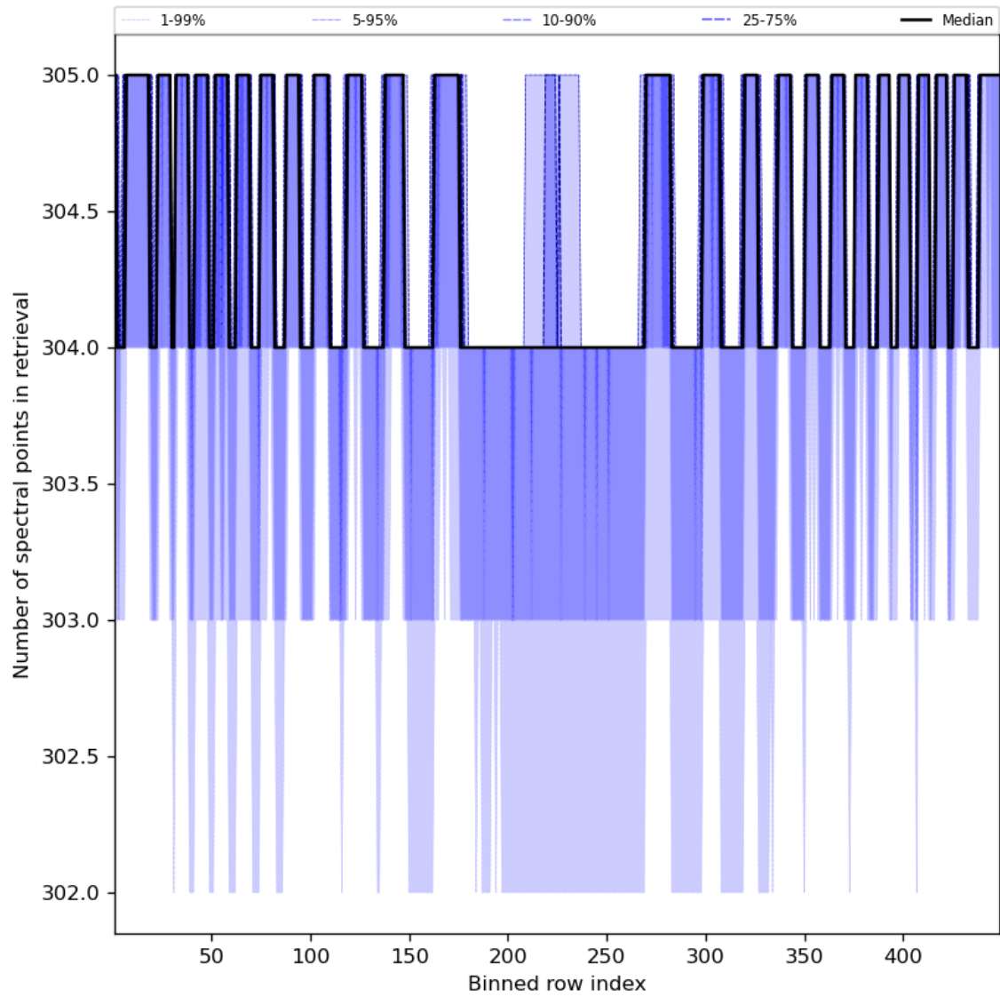
Figure 50: Along track statistics of “Number of spectral points in retrieval” for 2023-12-15 to 2023-12-17
