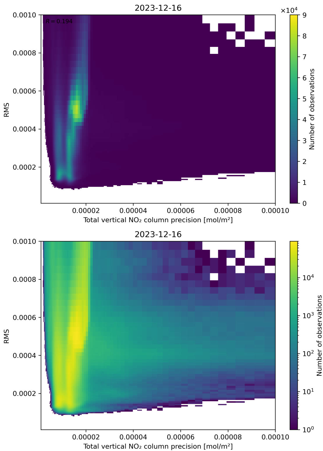
Figure 119: Scatter density plot of “Total vertical NO 2 column precision” against “RMS” for 2023-12-15 to 2023-12-17.
