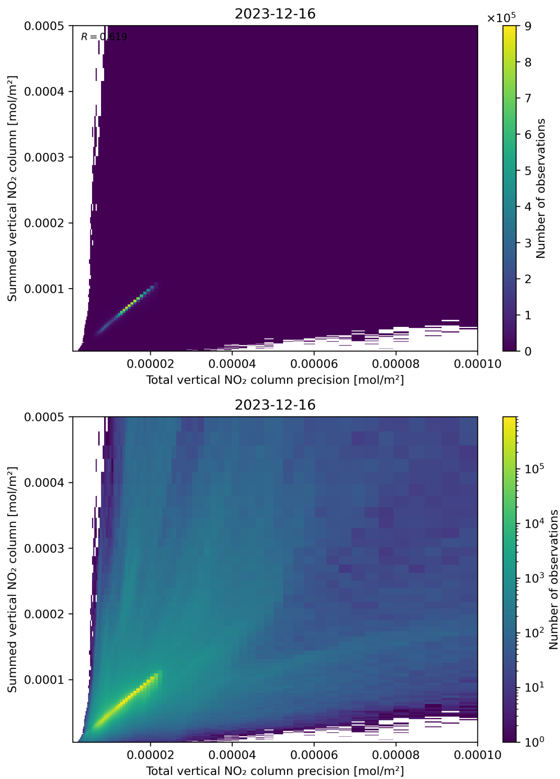
Figure 117: Scatter density plot of “Total vertical NO 2 column precision” against “Summed vertical NO 2 column” for 2023-12-15 to 2023-12-17.
