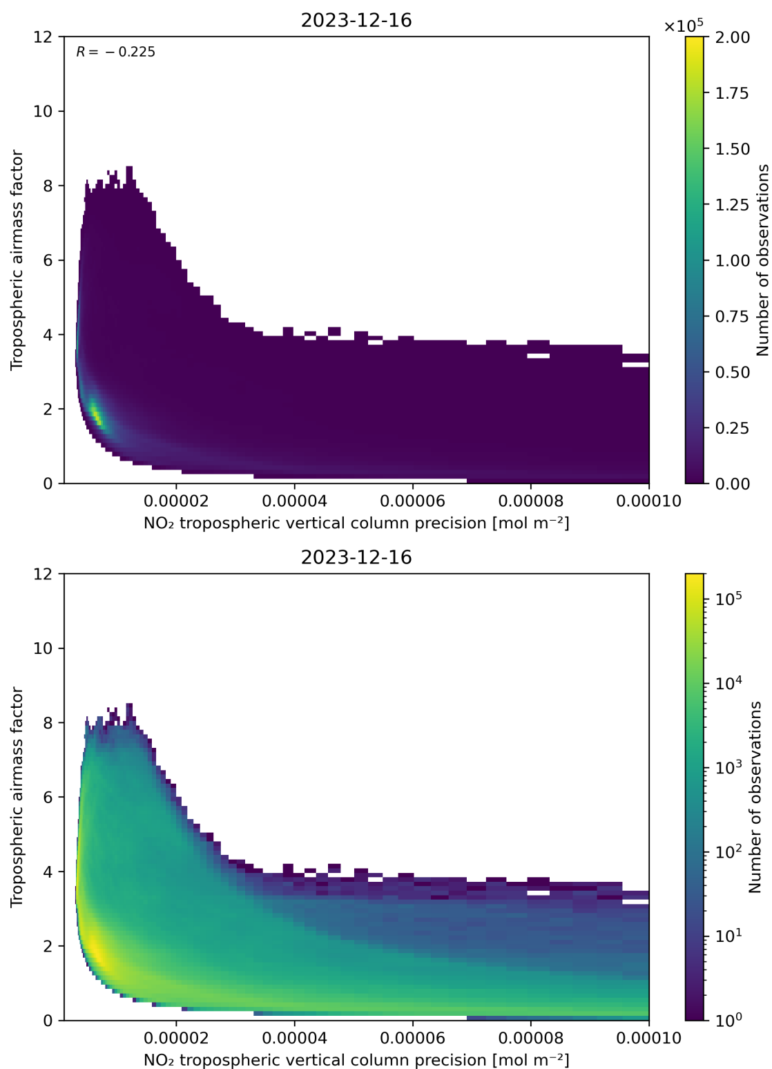
Figure 133: Scatter density plot of “NO 2 tropospheric vertical column precision” against “Tropospheric airmass factor” for 2023-12-15 to 2023-12-17.
