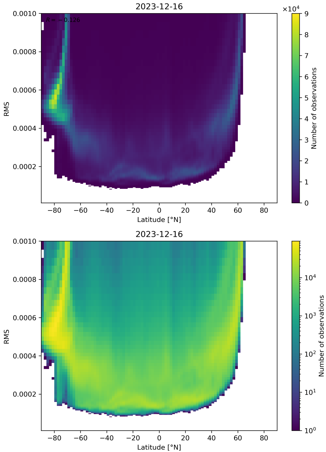
Figure 94: Scatter density plot of “Latitude” against “RMS” for 2023-12-15 to 2023-12-17.
