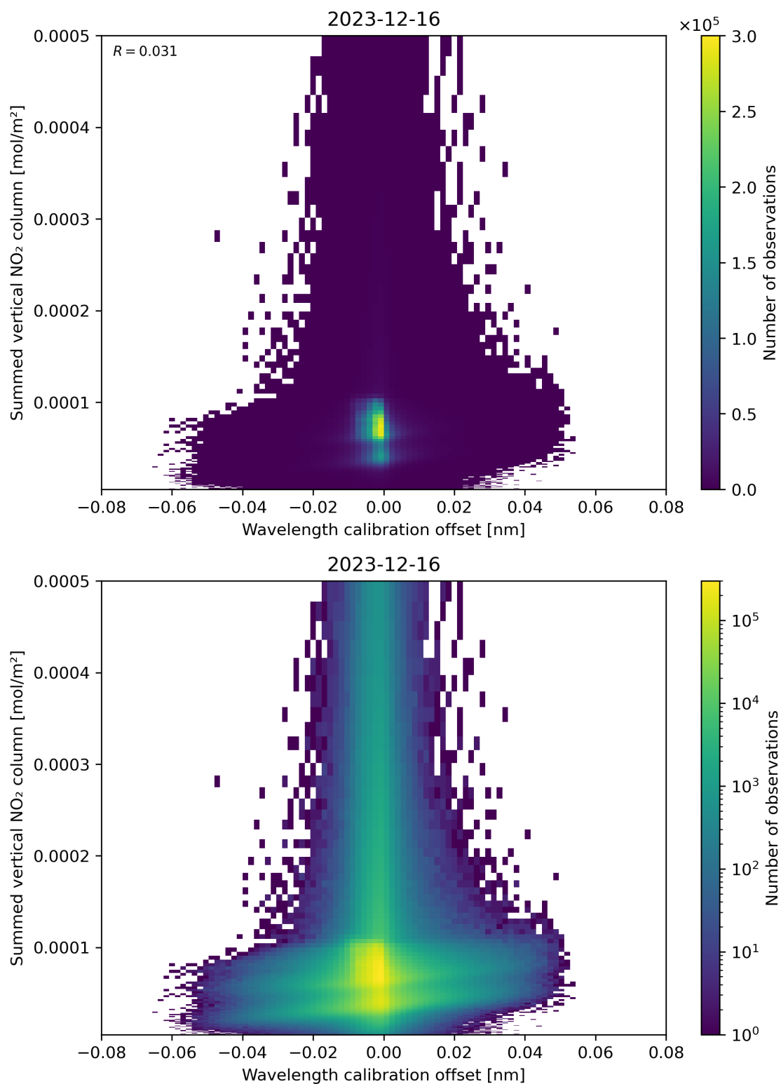
Figure 177: Scatter density plot of “Wavelength calibration offset” against “Summed vertical NO 2 column” for 2023-12-15 to 2023-12-17.
