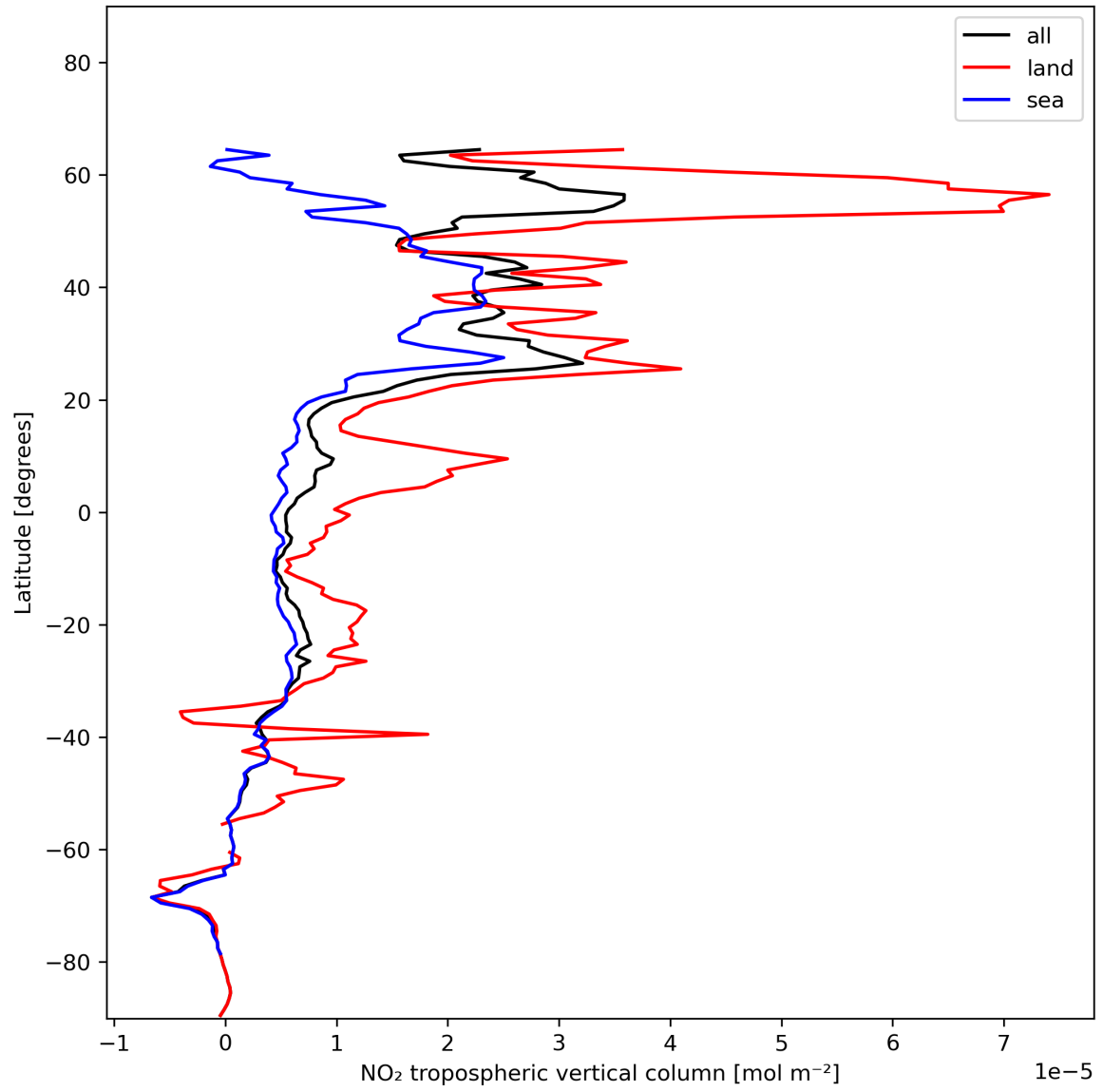
Figure 12: Zonal average of “NO 2 tropospheric vertical column” for 2023-12-15 to 2023-12-17.
