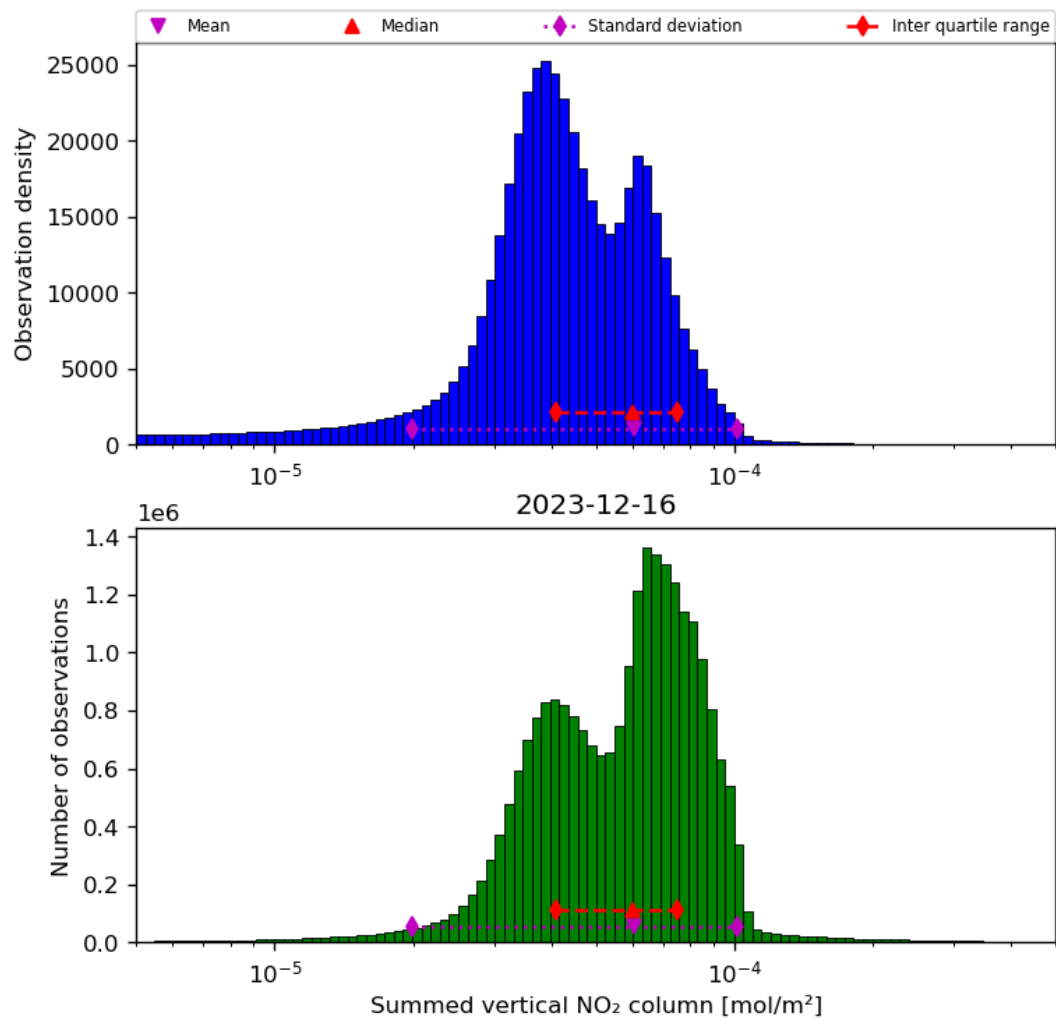
Figure 40: Histogram of “Summed vertical NO 2 column” for 2023-12-15 to 2023-12-17
