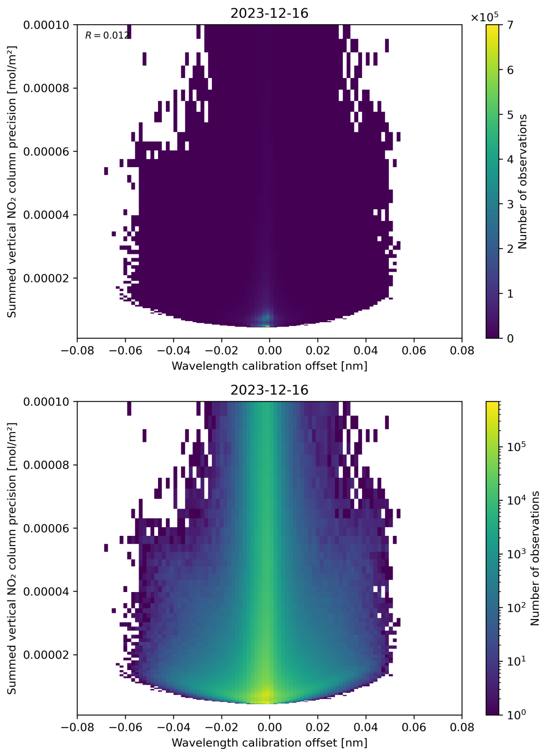
Figure 178: Scatter density plot of “Wavelength calibration offset” against “Summed vertical NO 2 column precision” for 2023-12-15 to 2023-12-17.
