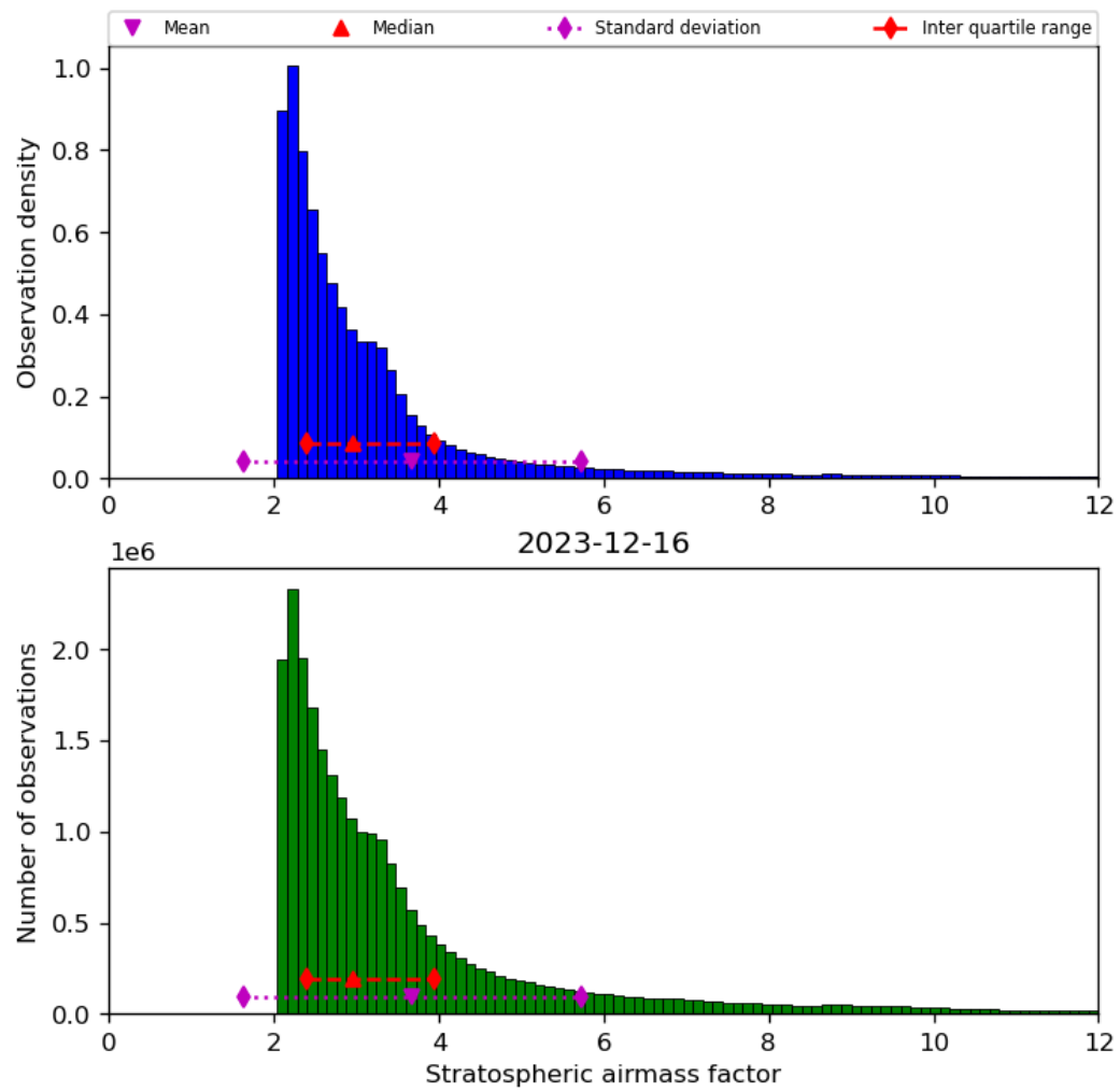
Figure 44: Histogram of “Stratospheric airmass factor” for 2023-12-15 to 2023-12-17
