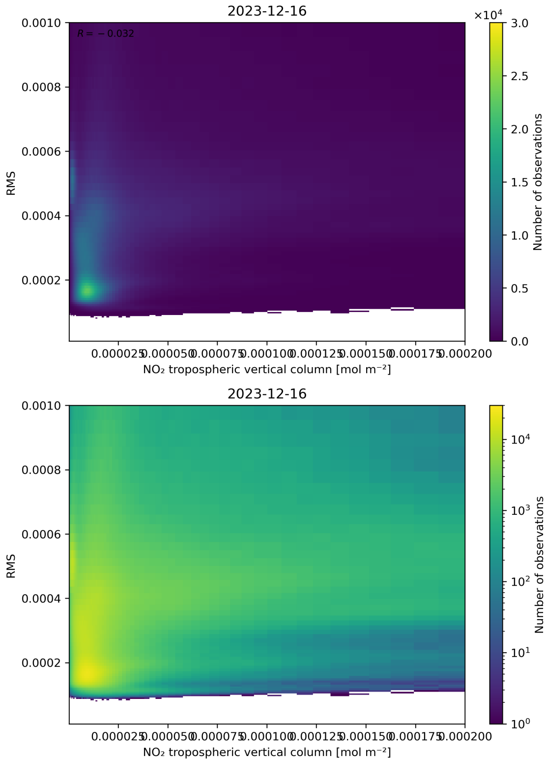
Figure 142: Scatter density plot of “NO 2 tropospheric vertical column” against “RMS” for 2023-12-15 to 2023-12-17.
