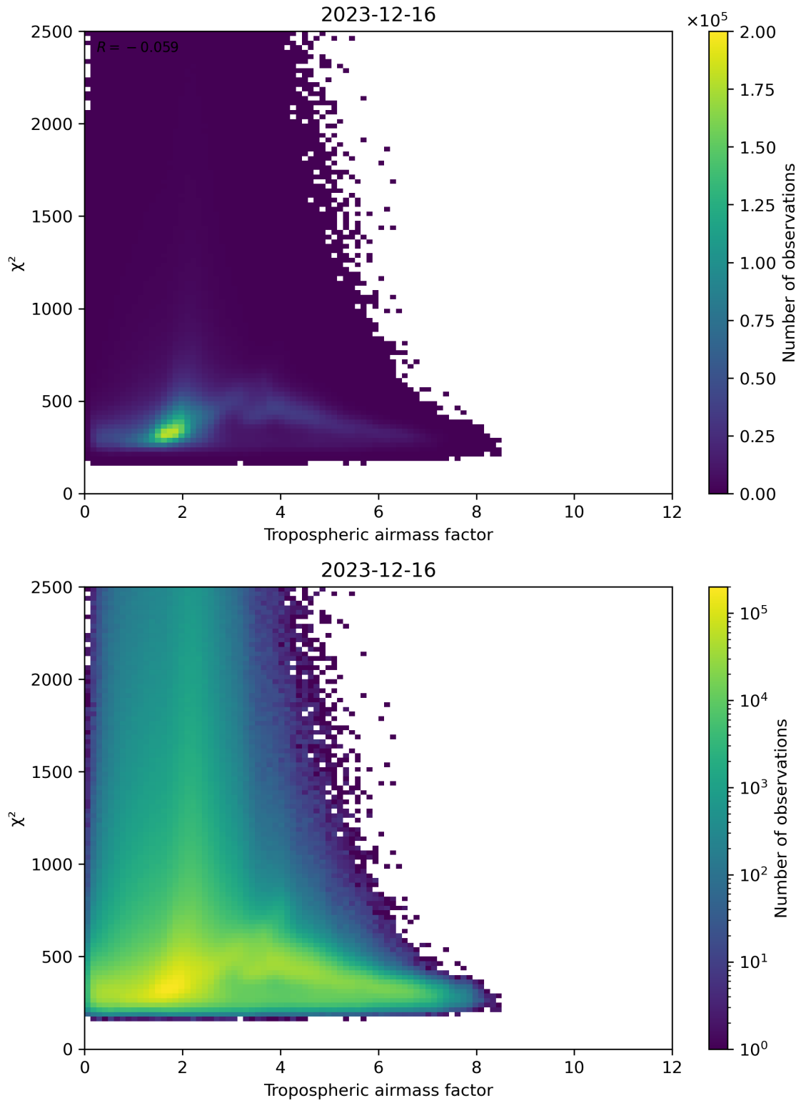
Figure 73: Scatter density plot of “Tropospheric airmass factor” against “ \chi^2 ” for 2023-12-15 to 2023-12-17.
