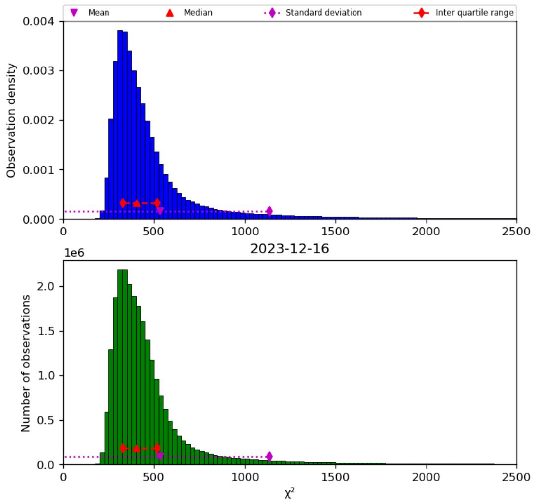
Figure 42: Histogram of “ \chi^2 ” for 2023-12-15 to 2023-12-17
