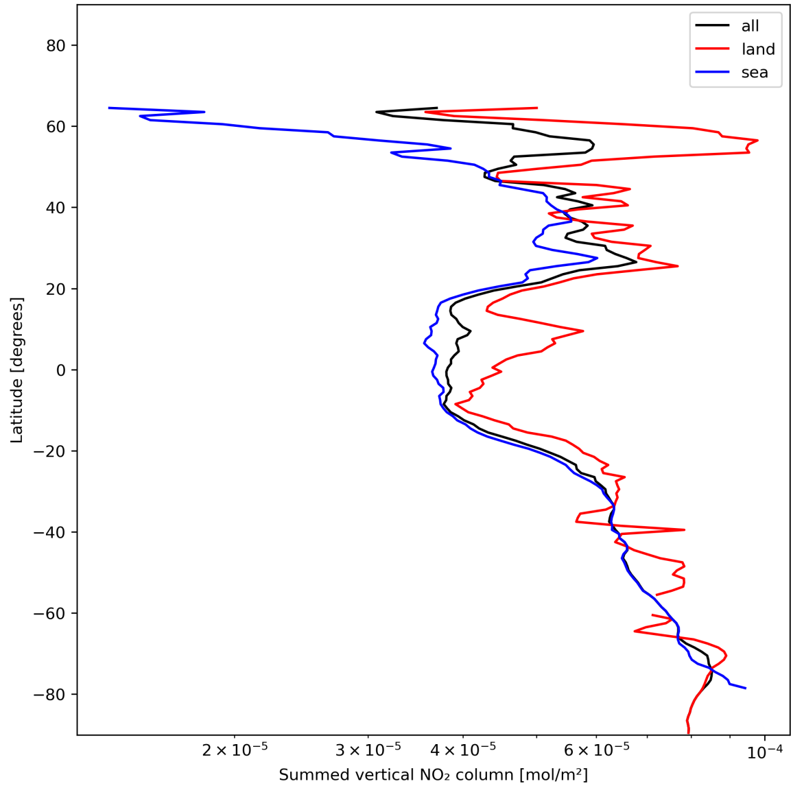
Figure 23: Zonal average of “Summed vertical NO 2 column” for 2023-12-15 to 2023-12-17.
