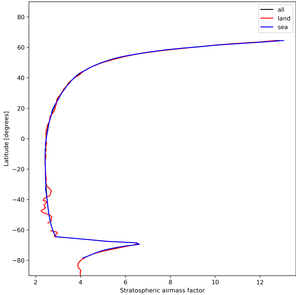
Figure 27: Zonal average of “Stratospheric airmass factor” for 2023-12-15 to 2023-12-17.
