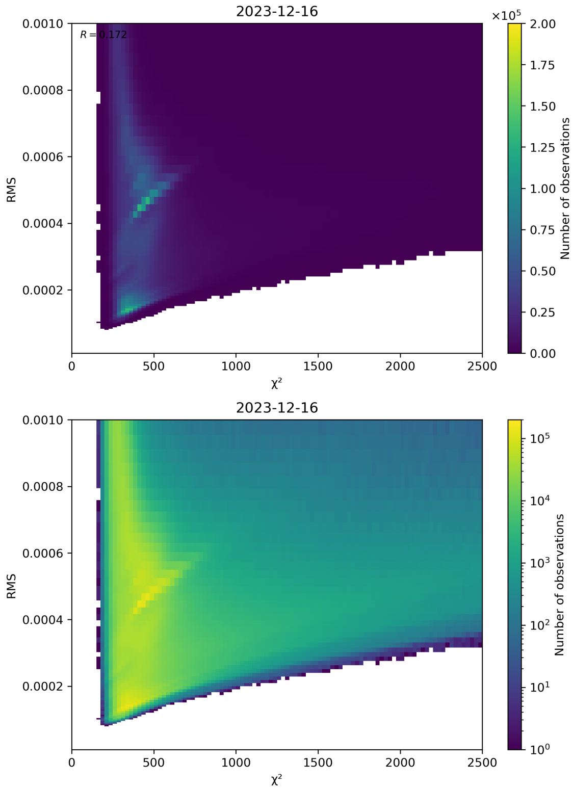
Figure 82: Scatter density plot of “ \chi^2 ” against “RMS” for 2023-12-15 to 2023-12-17.
