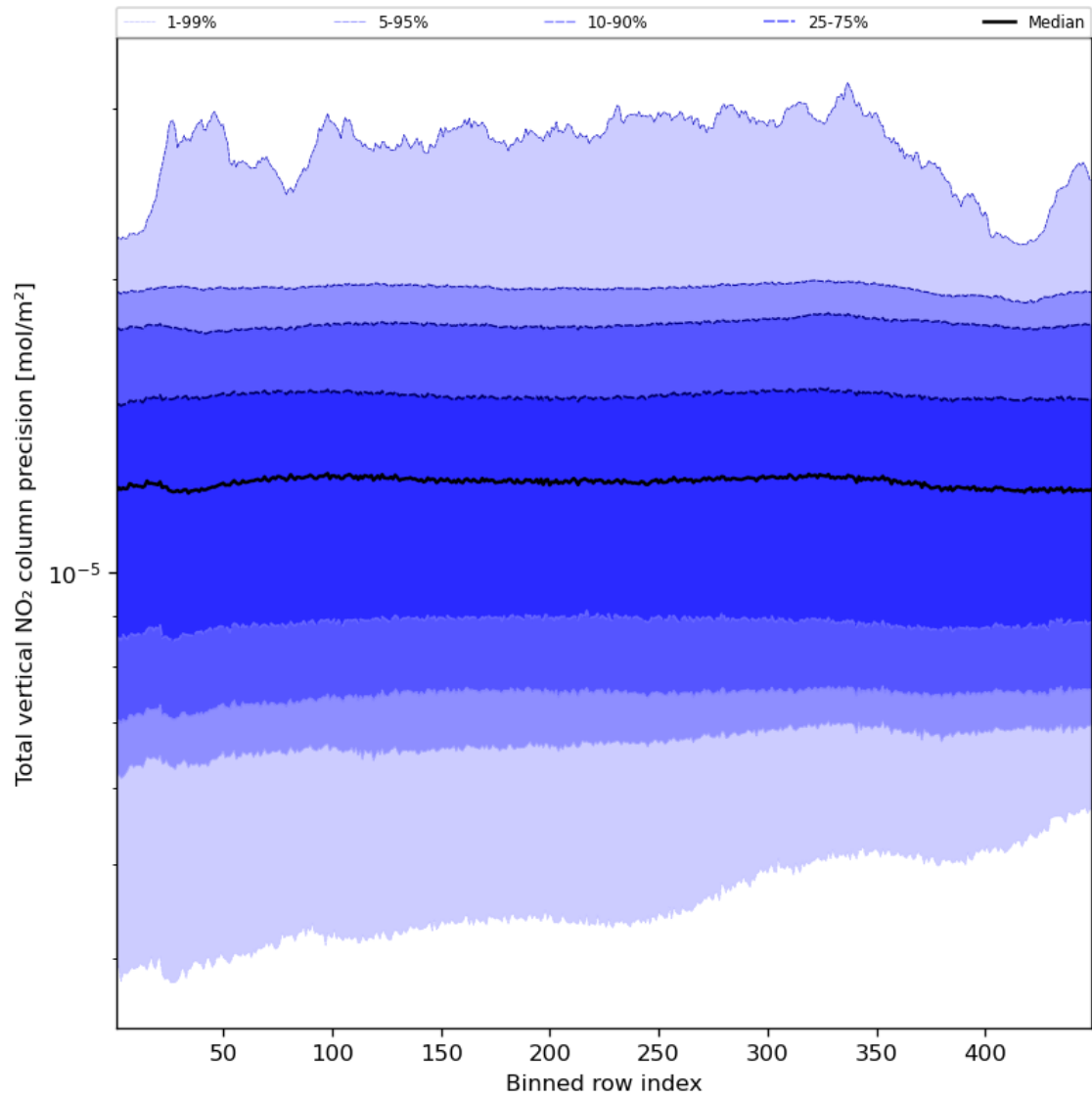
Figure 56: Along track statistics of “Total vertical NO 2 column precision” for 2023-12-15 to 2023-12-17
