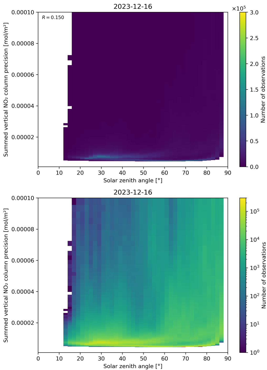
Figure 152: Scatter density plot of “Solar zenith angle” against “Summed vertical NO 2 column precision” for 2023-12-15 to 2023-12-17.
