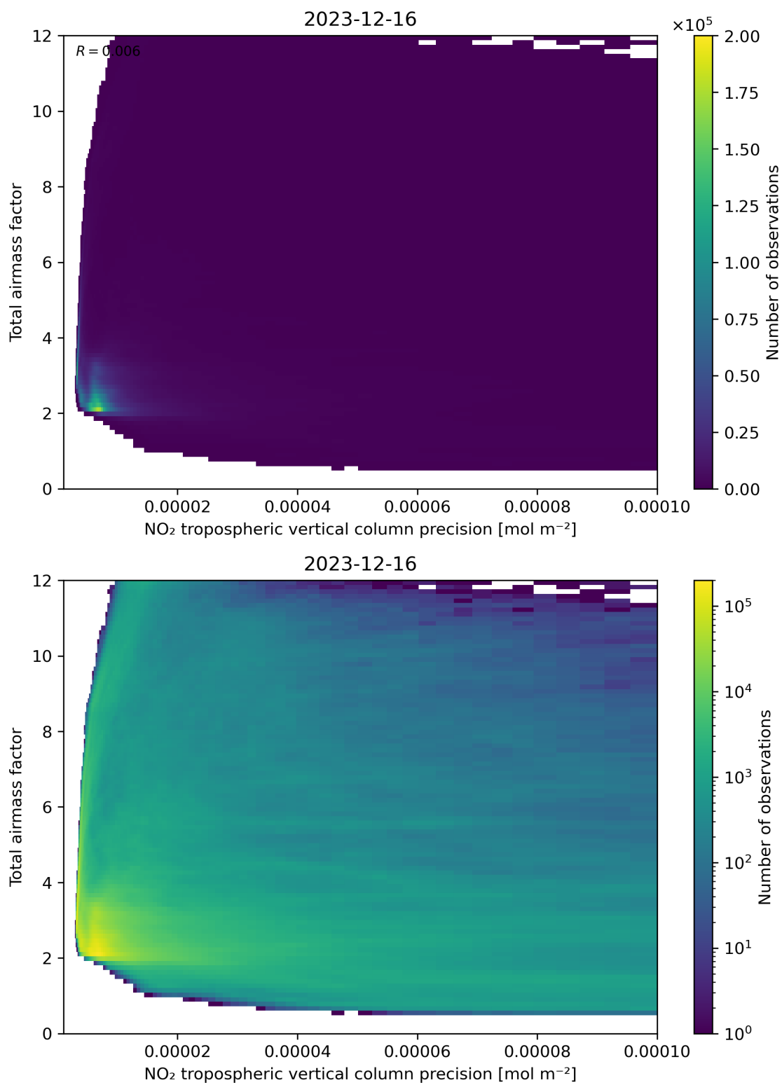
Figure 132: Scatter density plot of “NO 2 tropospheric vertical column precision” against “Total air mass factor” for 2023-12-15 to 2023-12-17.
