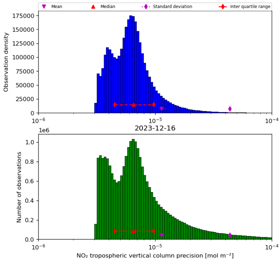
Figure 30: Histogram of “NO 2 tropospheric vertical column precision” for 2023-12-15 to 2023-12-17
