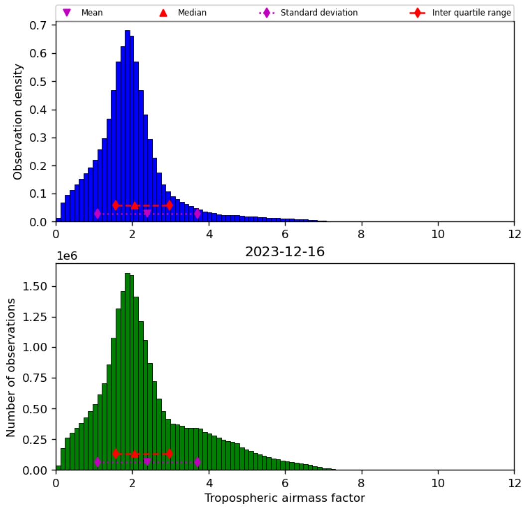
Figure 31: Histogram of “Tropospheric airmass factor” for 2023-12-15 to 2023-12-17
