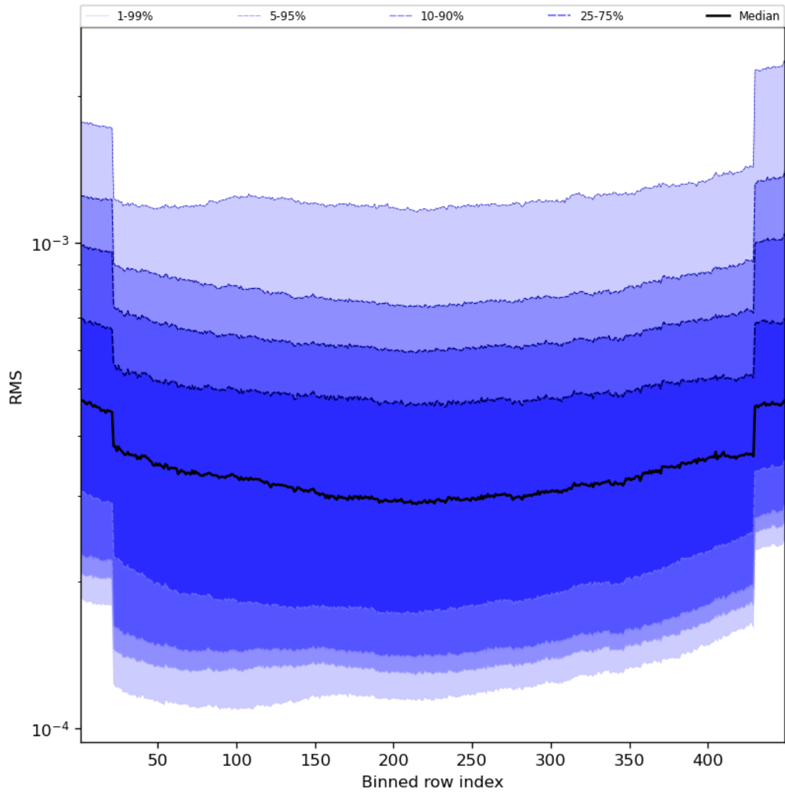
Figure 60: Along track statistics of “RMS” for 2023-12-15 to 2023-12-17
