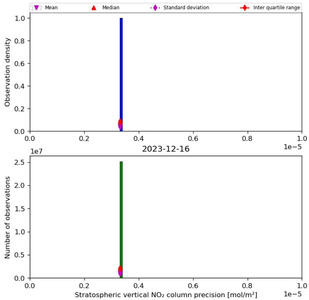
Figure 37: Histogram of “Stratospheric vertical NO 2 column precision” for 2023-12-15 to 2023-12-17
