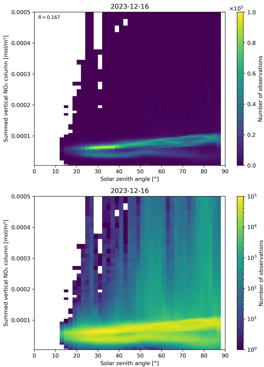
Figure 151: Scatter density plot of “Solar zenith angle” against “Summed vertical NO 2 column” for 2023-12-15 to 2023-12-17.
