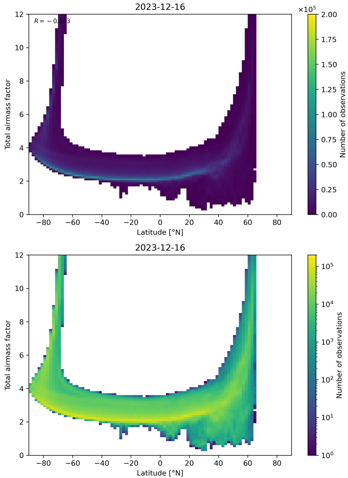
Figure 84: Scatter density plot of “Latitude” against “Total airmass factor” for 2023-12-15 to 2023-12-17.
