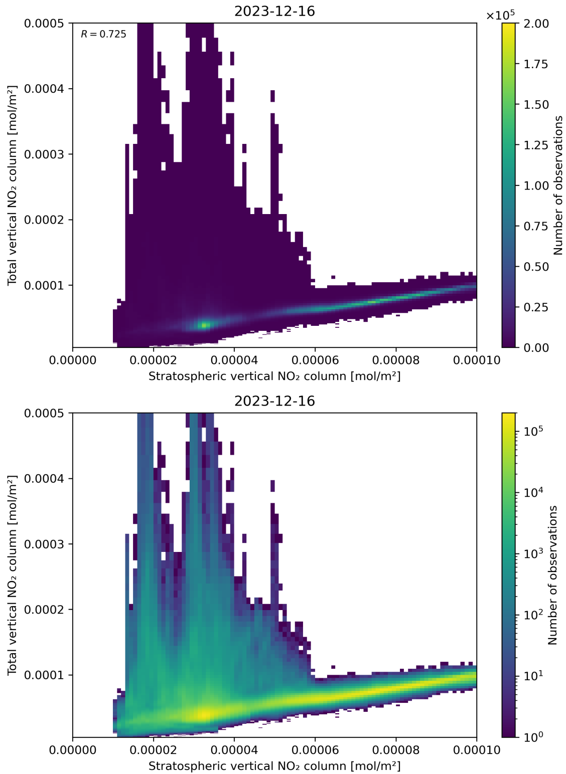
Figure 100: Scatter density plot of “Stratospheric vertical NO 2 column” against “Total vertical NO 2 column” for 2023-12-15 to 2023-12-17.
