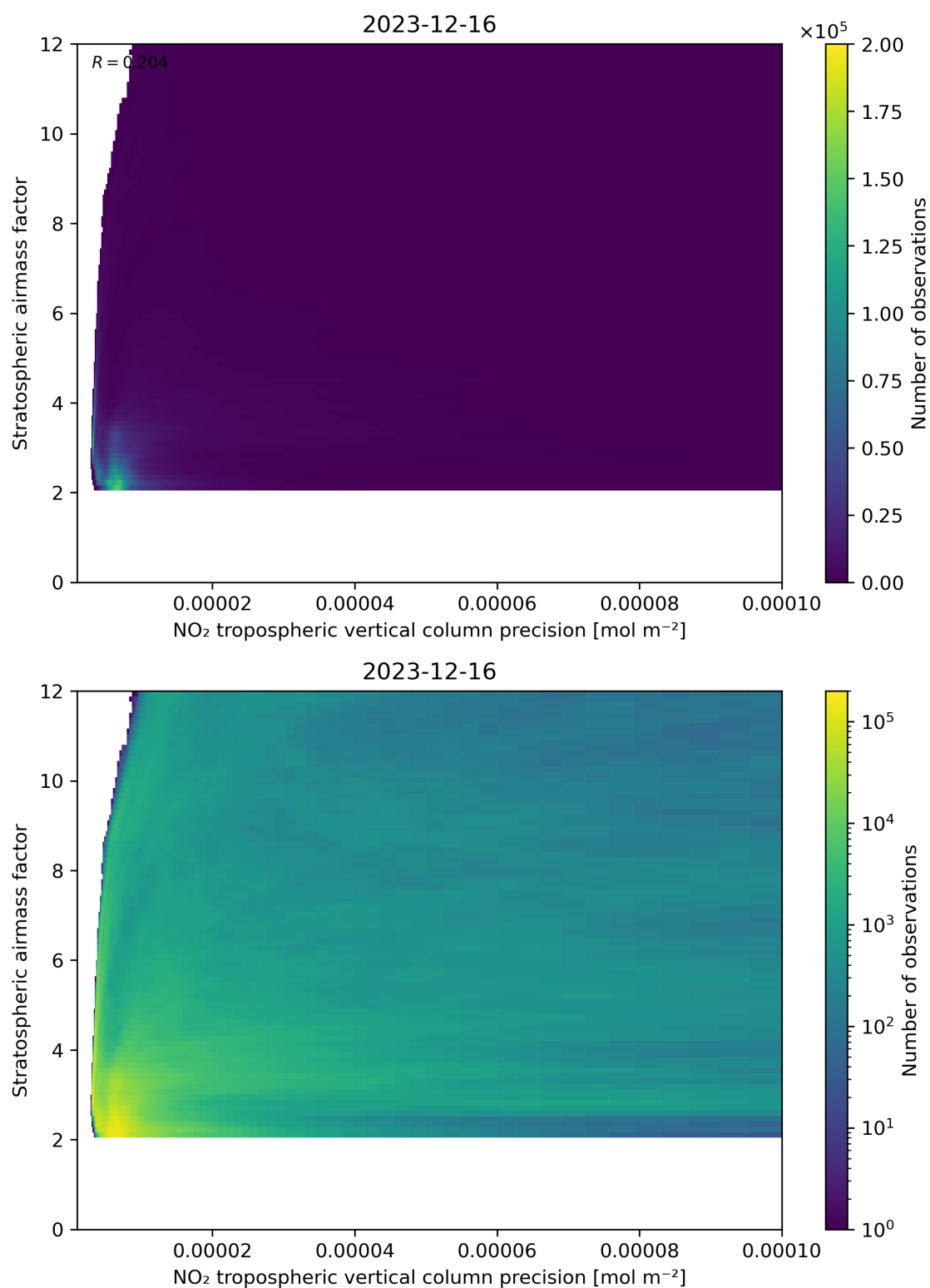
Figure 131: Scatter density plot of “NO 2 tropospheric vertical column precision” against “Stratospheric airmass factor” for 2023-12-15 to 2023-12-17.
