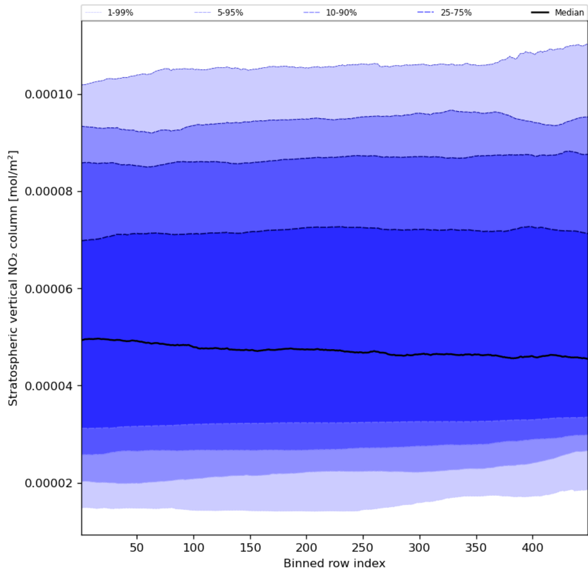
Figure 53: Along track statistics of “Stratospheric vertical NO 2 column” for 2023-12-15 to 2023-12-17
