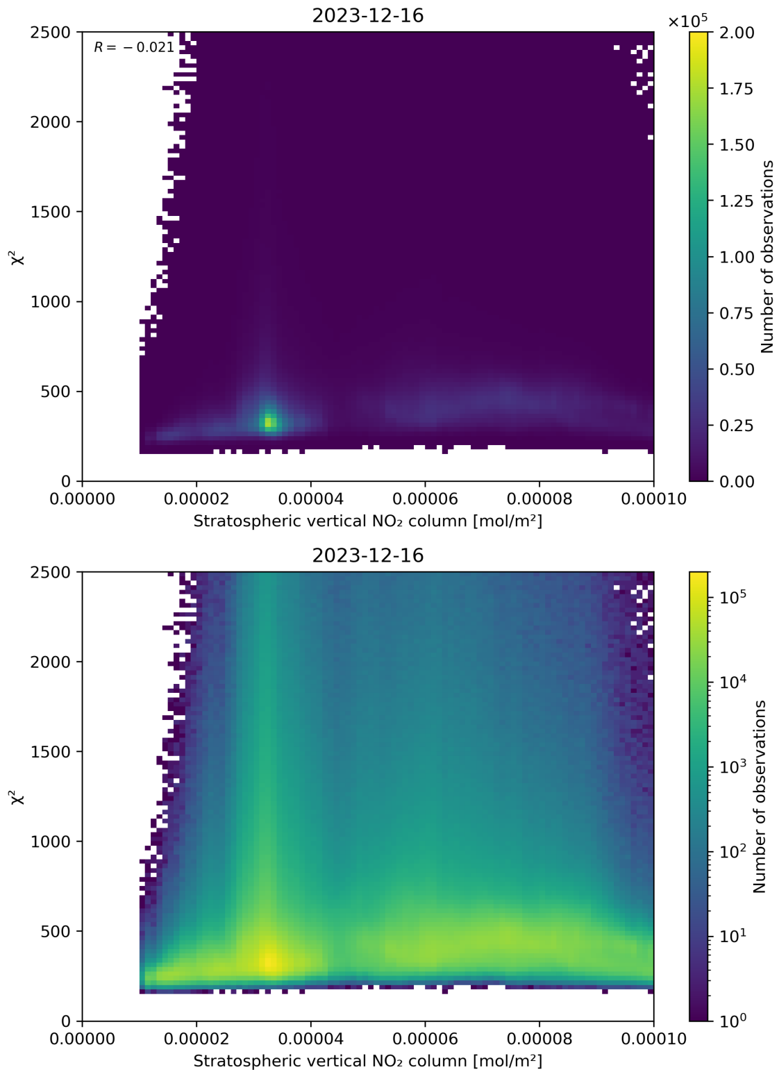
Figure 97: Scatter density plot of “Stratospheric vertical NO 2 column” against “ \chi^2 ” for 2023-12-15 to 2023-12-17.
