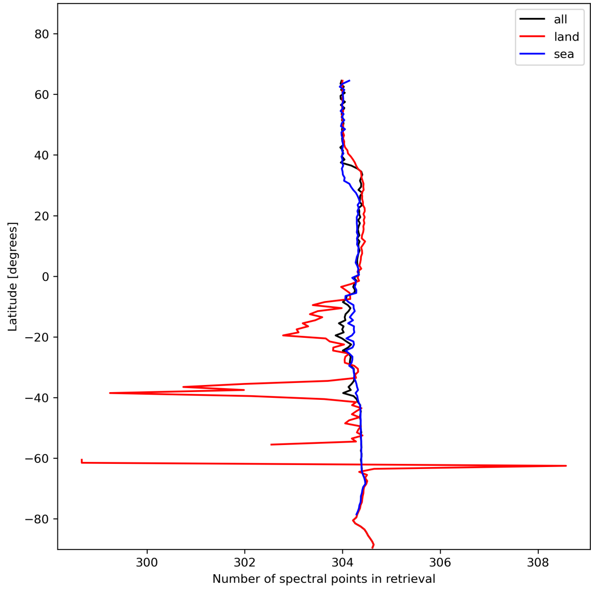
Figure 16: Zonal average of “Number of spectral points in retrieval” for 2023-12-15 to 2023-12-17.
