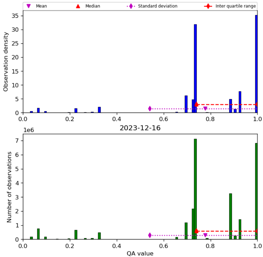
Figure 28: Histogram of “QA value” for 2023-12-15 to 2023-12-17
