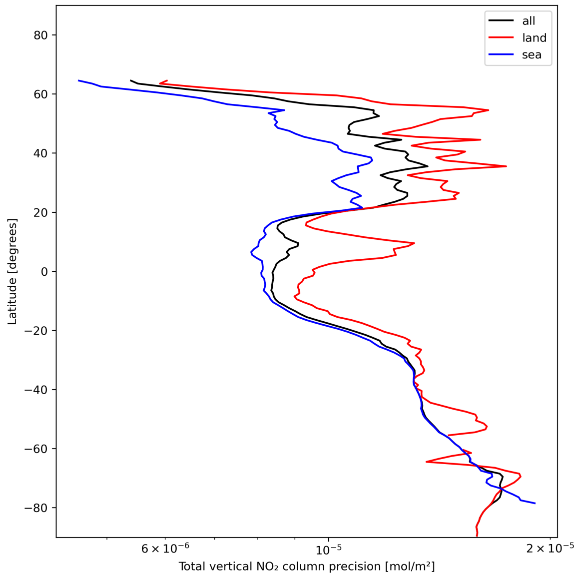
Figure 22: Zonal average of “Total vertical NO 2 column precision” for 2023-12-15 to 2023-12-17.
