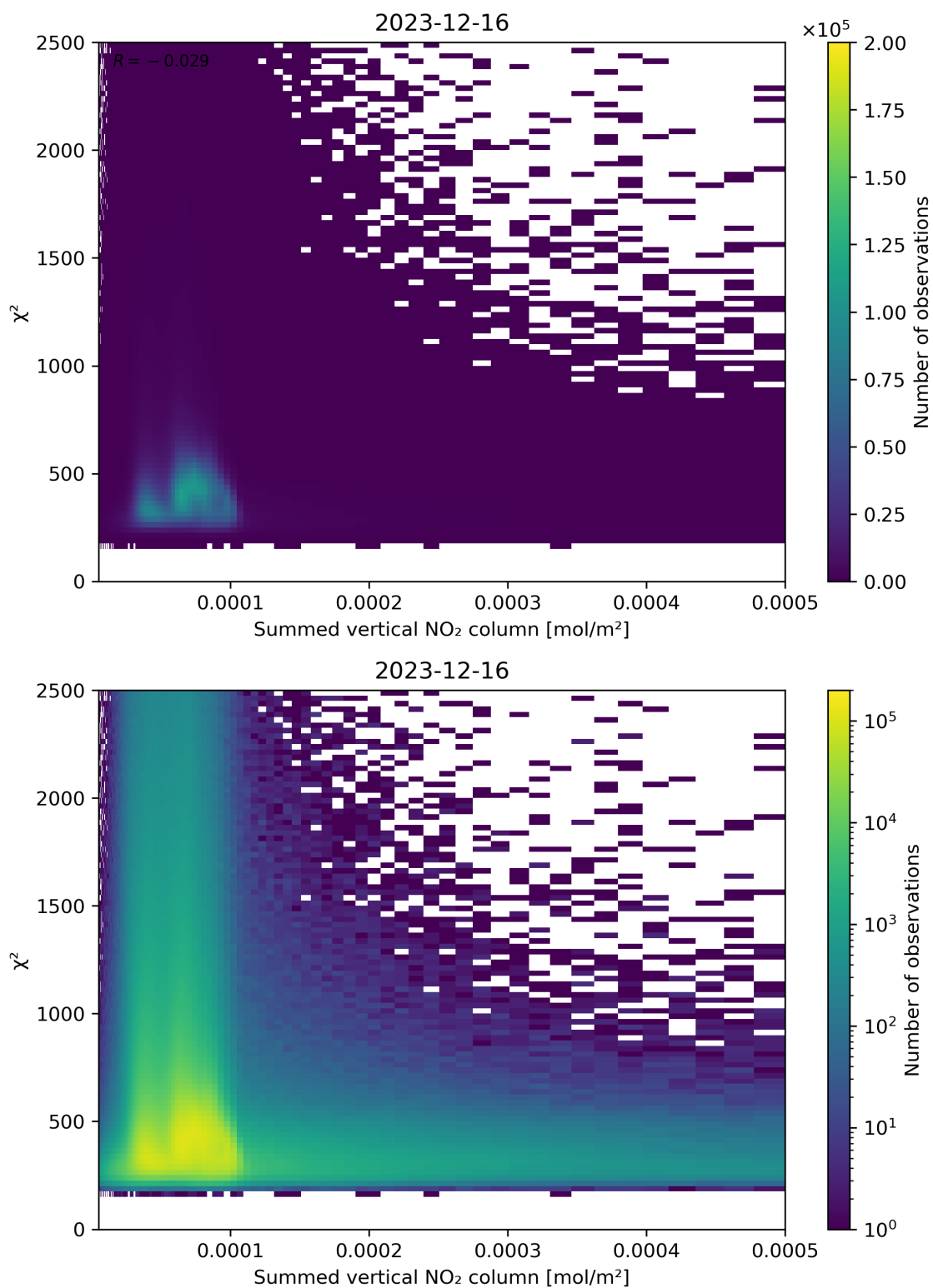
Figure 104: Scatter density plot of “Summed vertical NO 2 column” against “ \chi^2 ” for 2023-12-15 to 2023-12-17.
