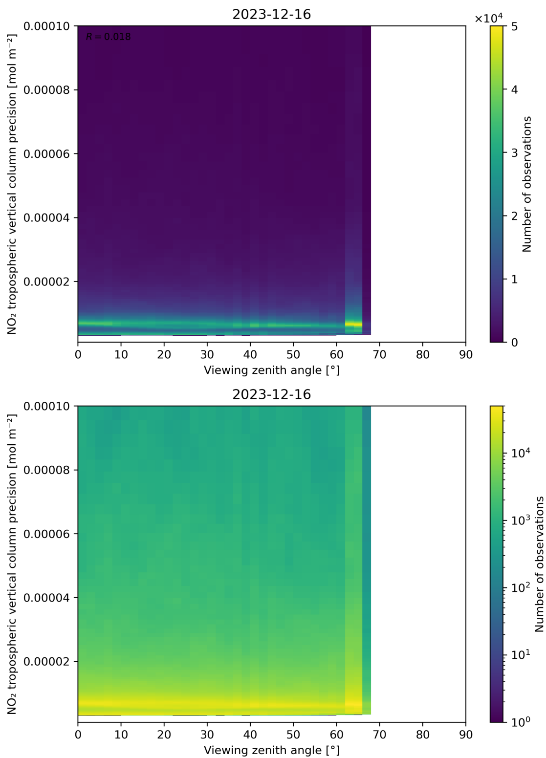
Figure 170: Scatter density plot of “Viewing zenith angle” against “NO 2 tropospheric vertical column precision” for 2023-12-15 to 2023-12-17.
