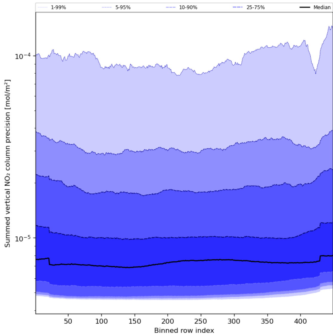
Figure 58: Along track statistics of “Summed vertical NO 2 column precision” for 2023-12-15 to 2023-12-17
