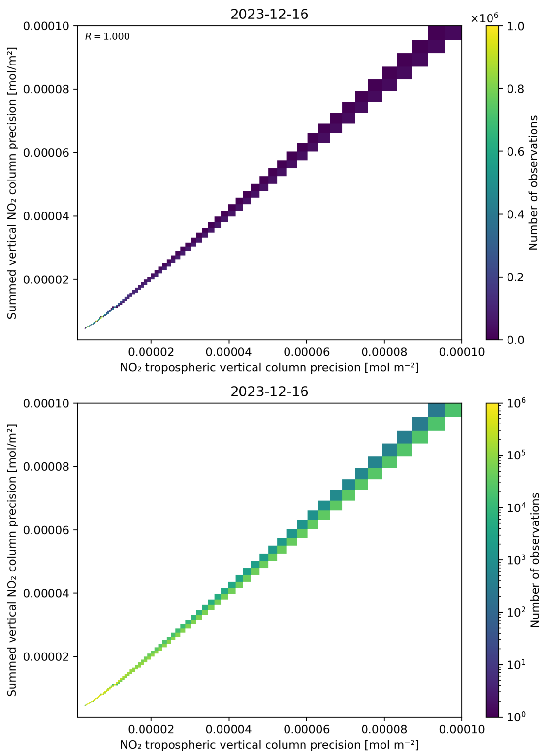
Figure 137: Scatter density plot of “NO 2 tropospheric vertical column precision” against “Summed vertical NO 2 column precision” for 2023-12-15 to 2023-12-17.
