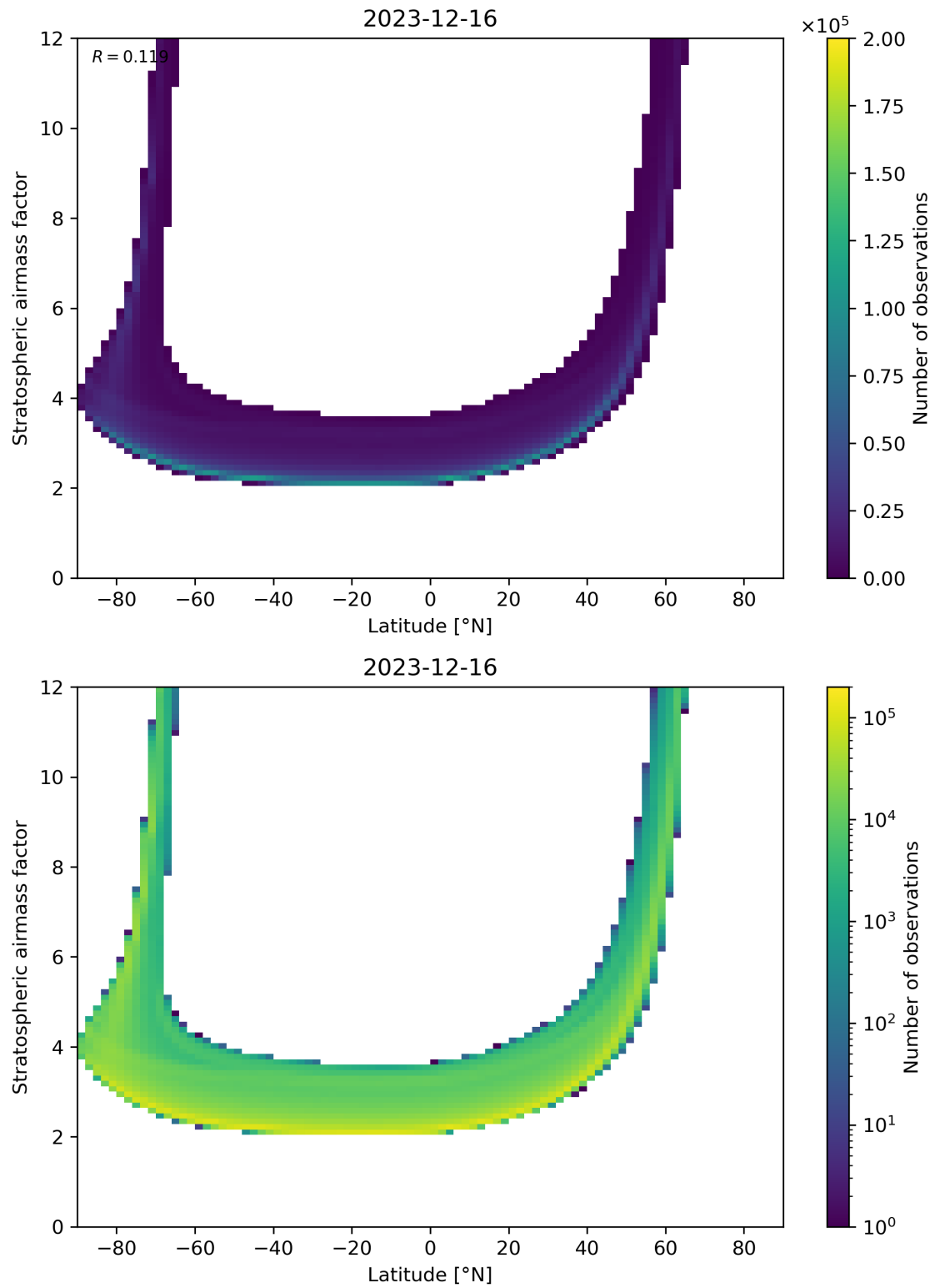
Figure 83: Scatter density plot of “Latitude” against “Stratospheric air mass factor” for 2023-12-15 to 2023-12-17.
