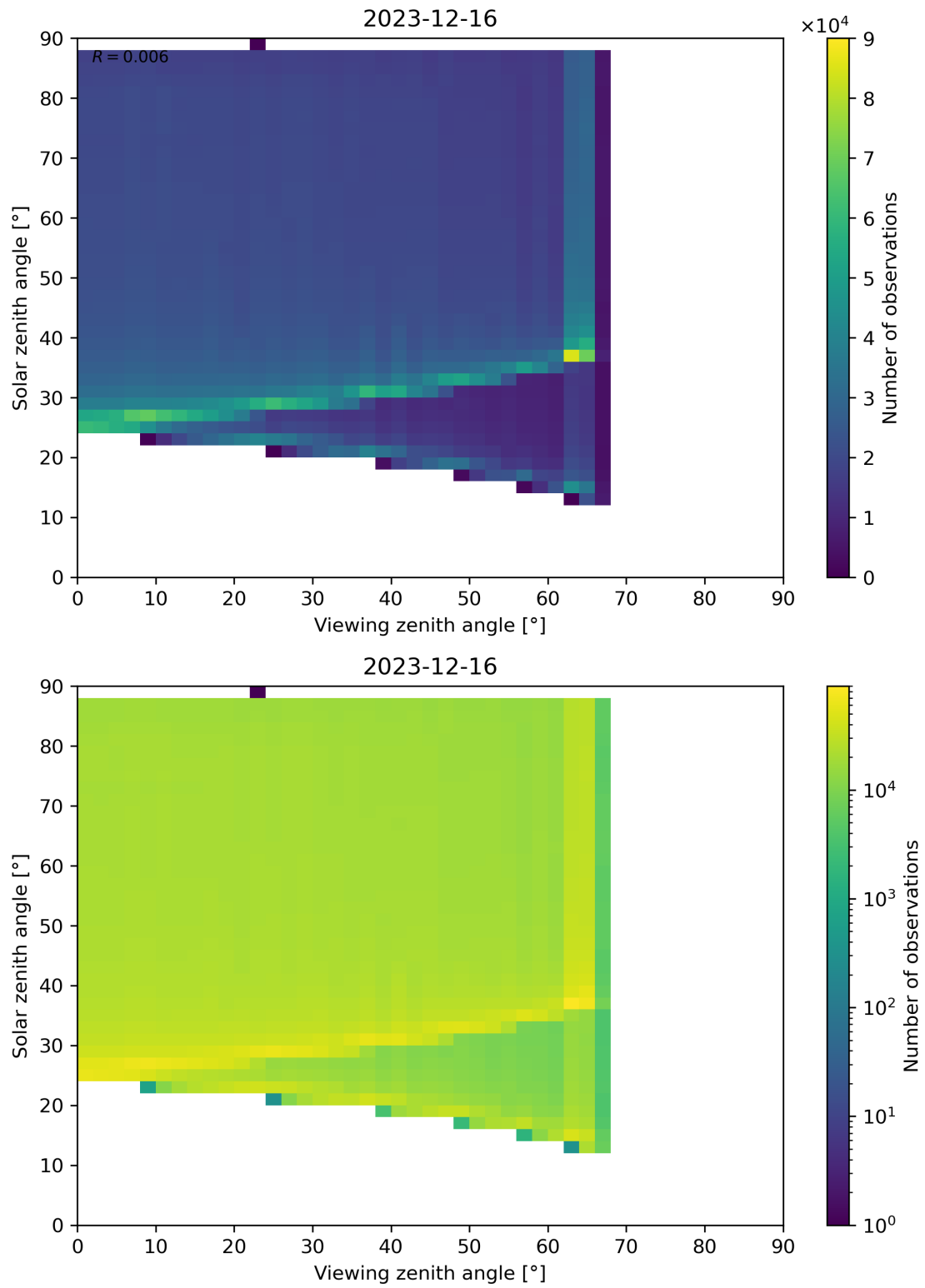
Figure 172: Scatter density plot of “Viewing zenith angle” against “Solar zenith angle” for 2023-12-15 to 2023-12-17.
