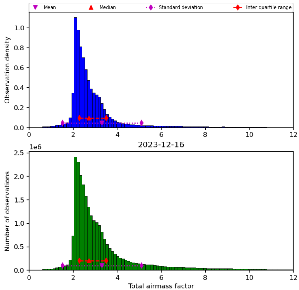
Figure 32: Histogram of “Total airmass factor” for 2023-12-15 to 2023-12-17
