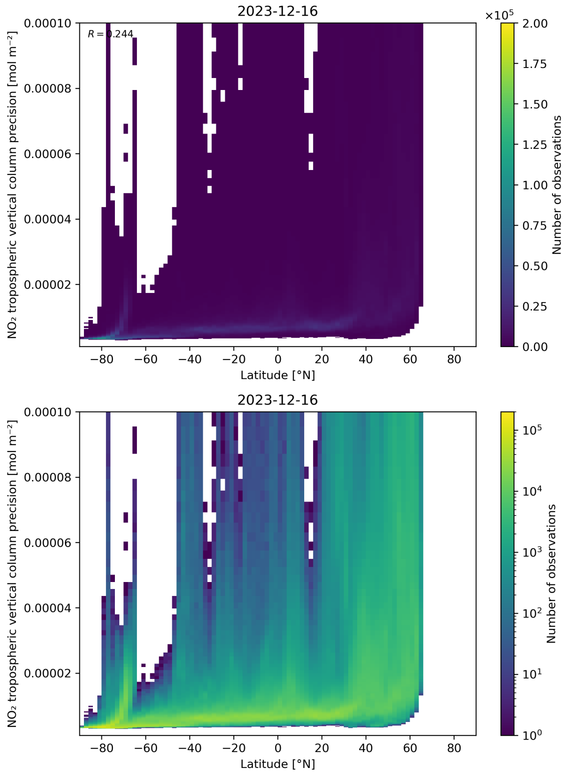
Figure 93: Scatter density plot of “Latitude” against “NO 2 tropospheric vertical column precision” for 2023-12-15 to 2023-12-17.
