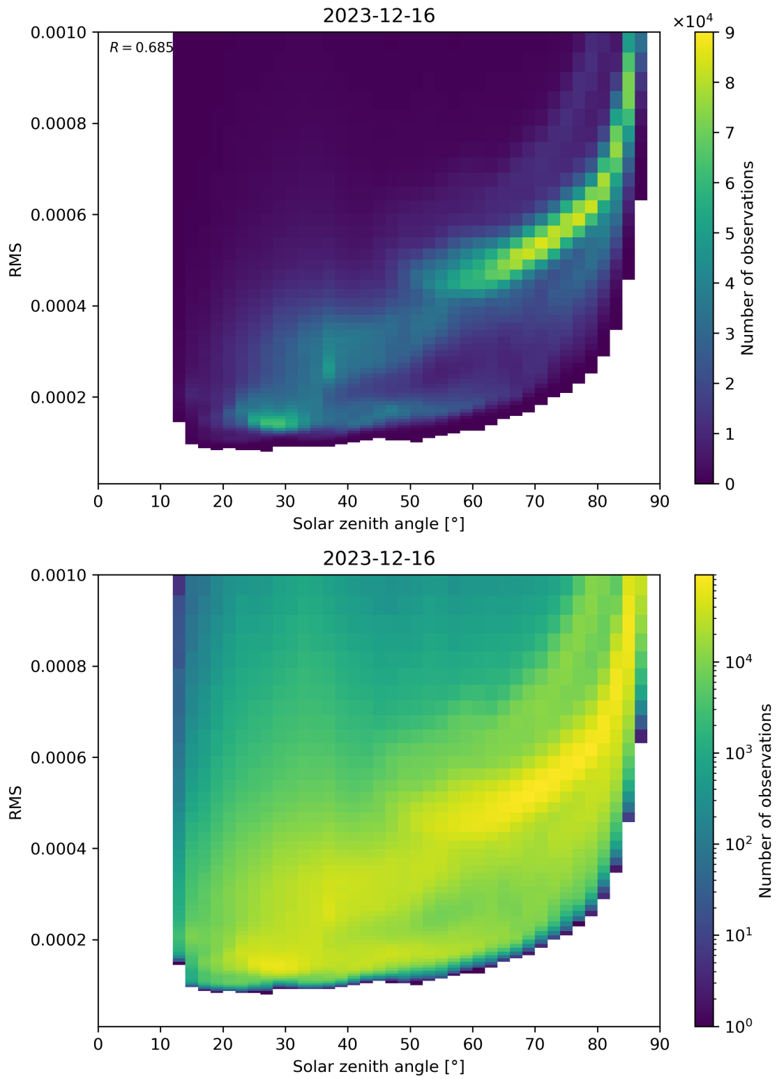
Figure 157: Scatter density plot of “Solar zenith angle” against “RMS” for 2023-12-15 to 2023-12-17.
