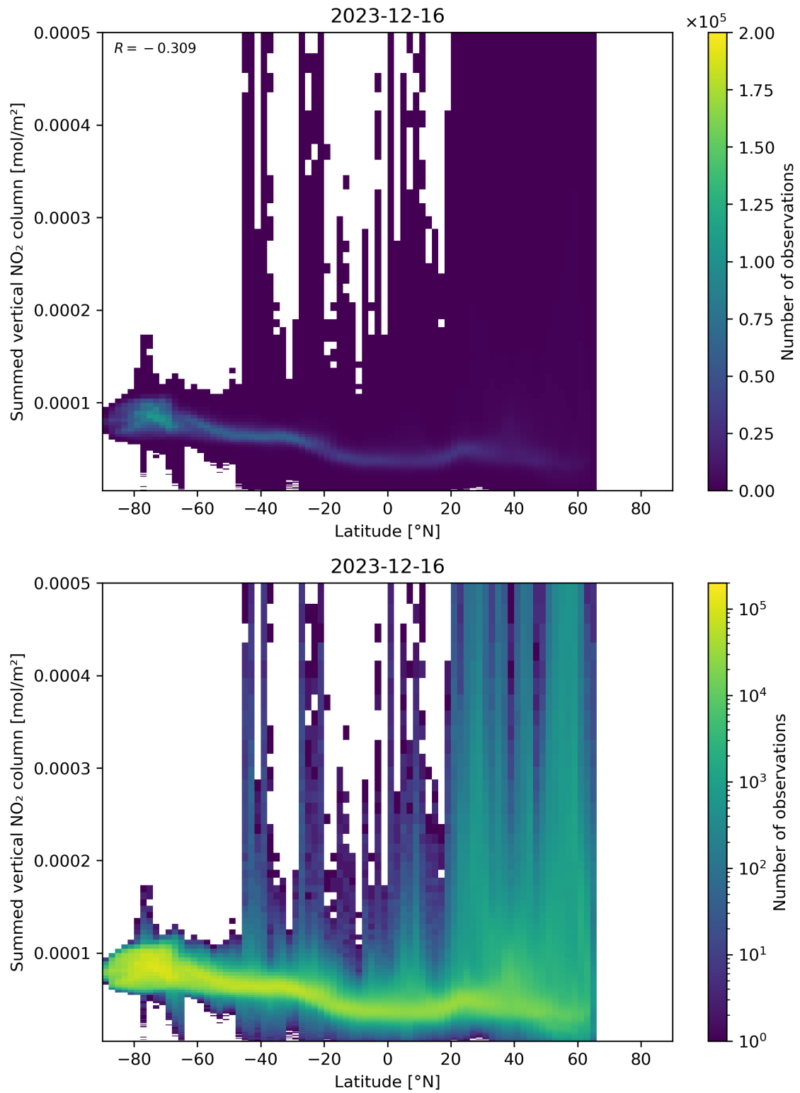
Figure 88: Scatter density plot of “Latitude” against “Summed vertical NO 2 column” for 2023-12-15 to 2023-12-17.
