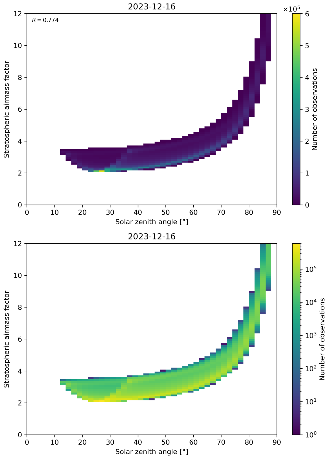
Figure 145: Scatter density plot of “Solar zenith angle” against “Stratospheric airmass factor” for 2023-12-15 to 2023-12-17.
