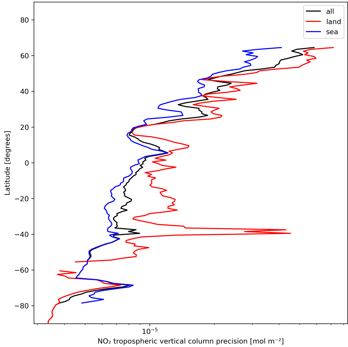
Figure 13: Zonal average of “NO 2 tropospheric vertical column precision” for 2023-12-15 to 2023-12-17.
