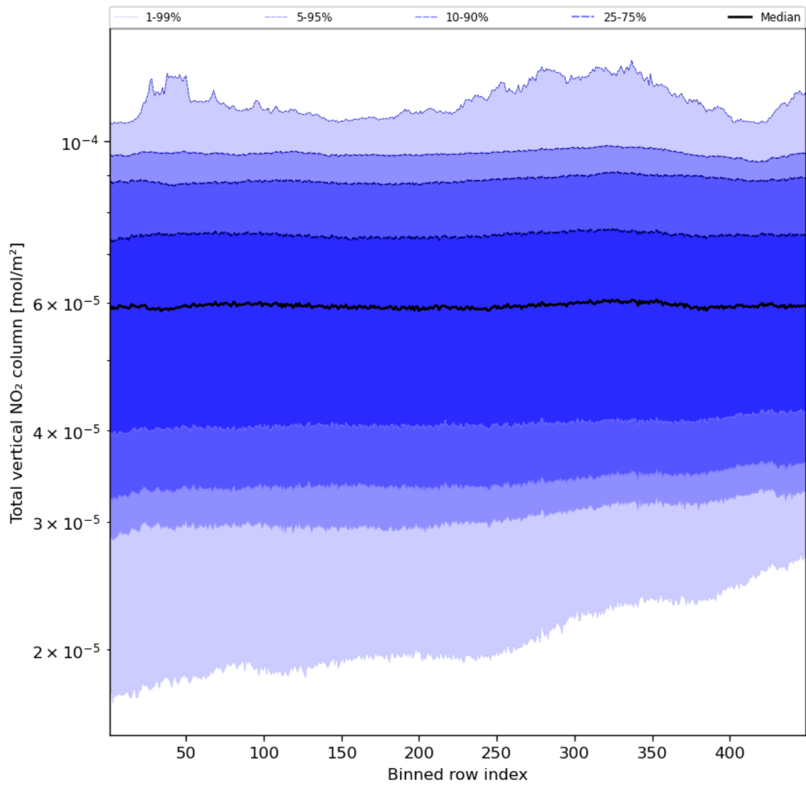
Figure 55: Along track statistics of “Total vertical NO 2 column” for 2023-12-15 to 2023-12-17
