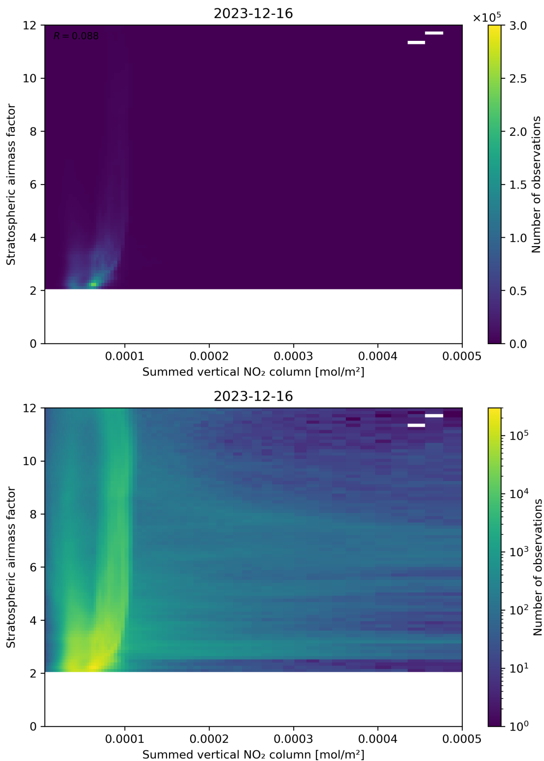
Figure 103: Scatter density plot of “Summed vertical NO 2 column” against “Stratospheric airmass factor” for 2023-12-15 to 2023-12-17.
