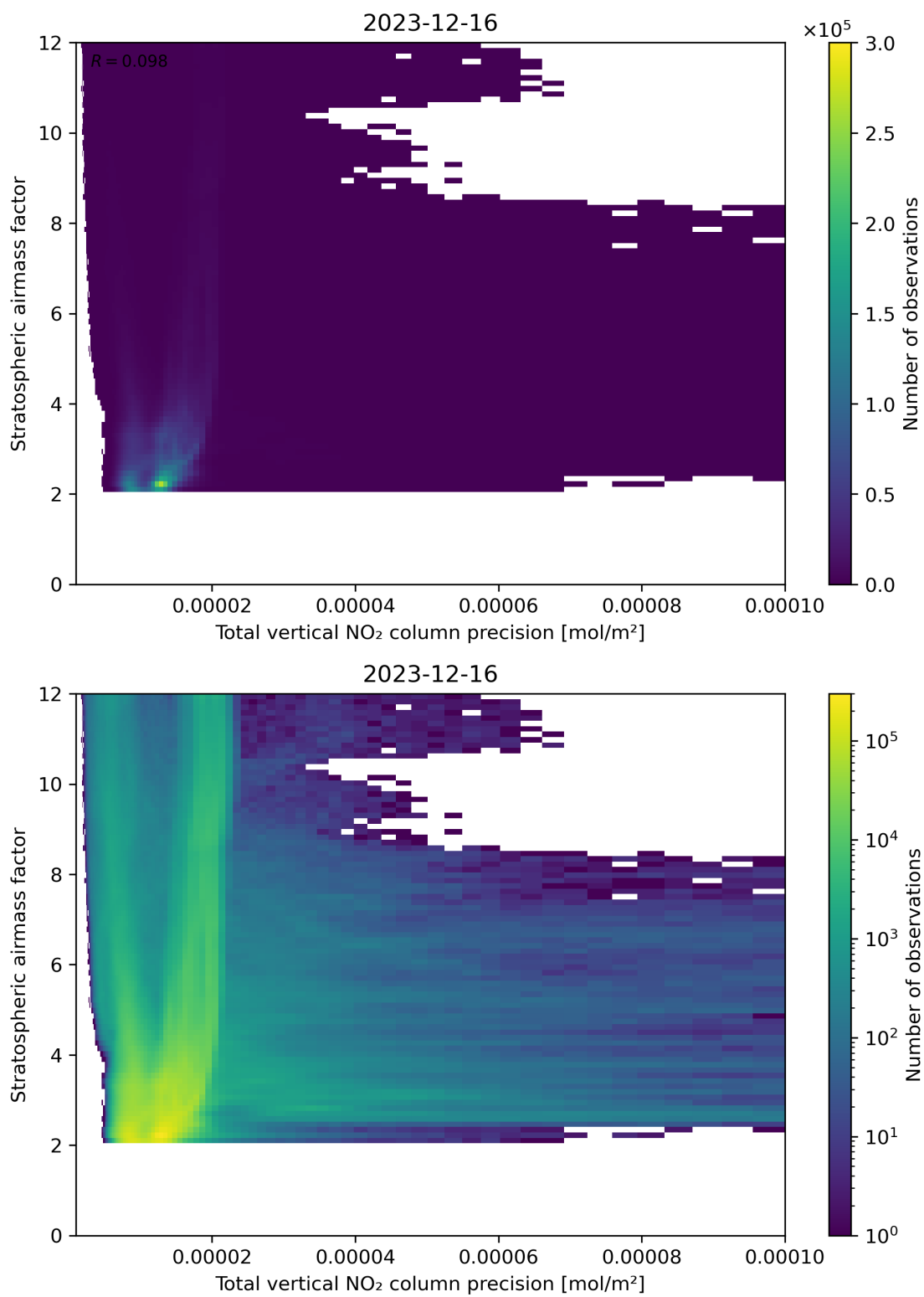
Figure 115: Scatter density plot of “Total vertical NO 2 column precision” against “Stratospheric air mass factor” for 2023-12-15 to 2023-12-17.
