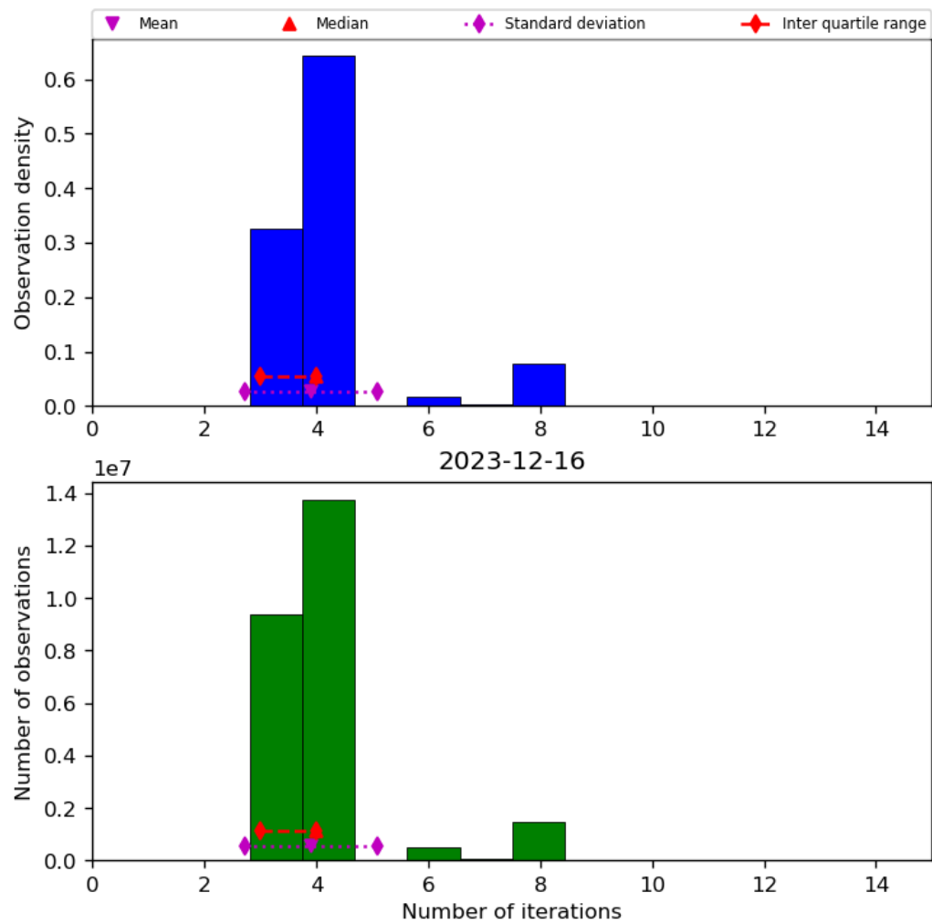
Figure 34: Histogram of “Number of iterations” for 2023-12-15 to 2023-12-17
