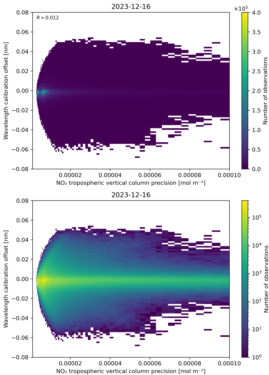
Figure 141: Scatter density plot of “NO 2 tropospheric vertical column precision” against “Wavelength calibration offset” for 2023-12-15 to 2023-12-17.
