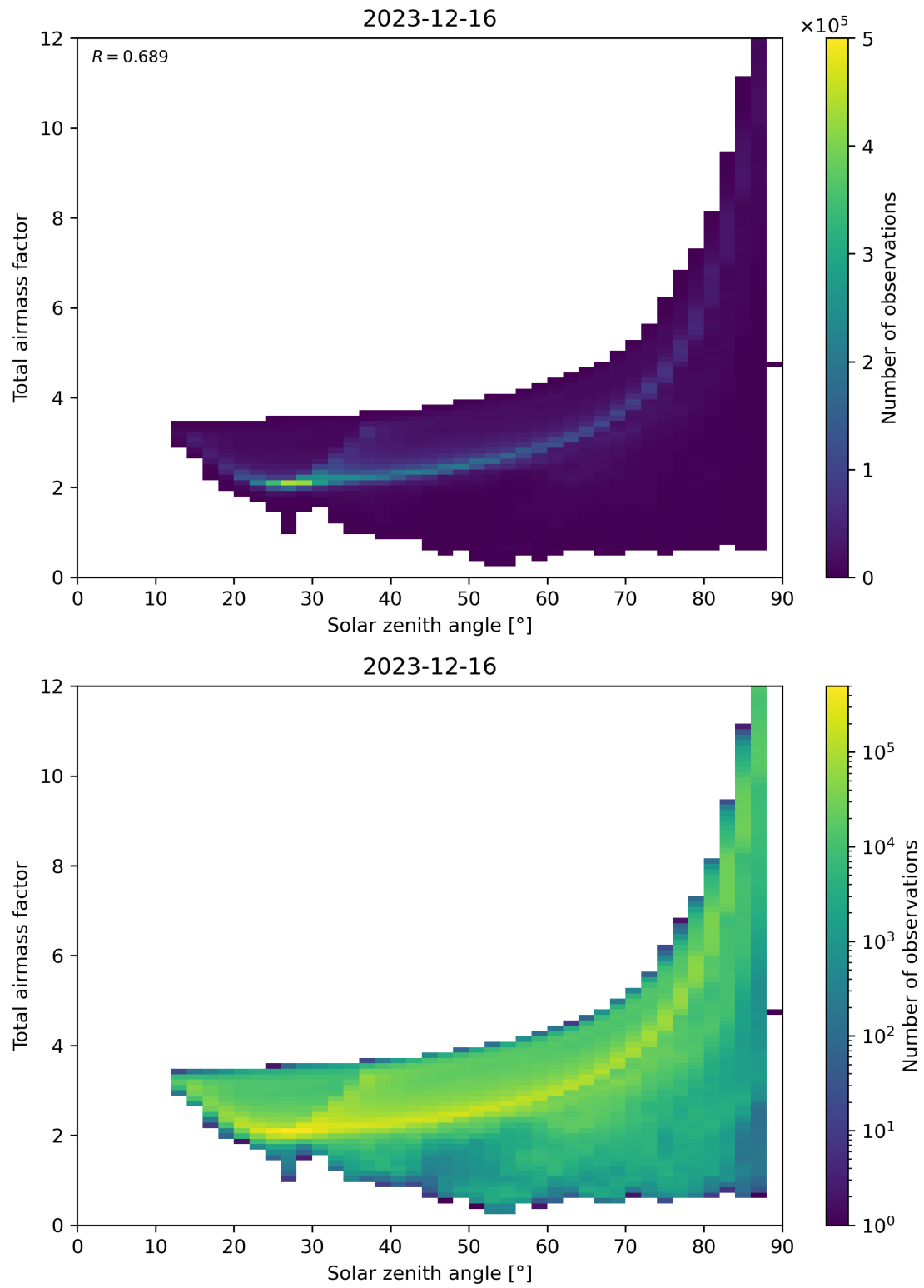
Figure 146: Scatter density plot of “Solar zenith angle” against “Total air mass factor” for 2023-12-15 to 2023-12-17.
