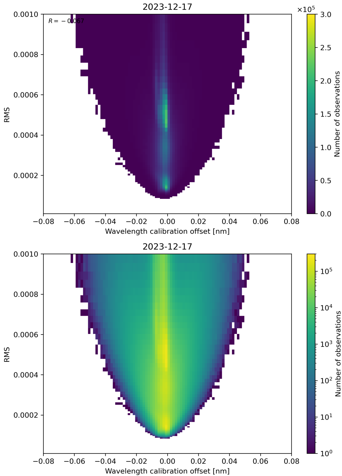
Figure 181: Scatter density plot of “Wavelength calibration offset” against “RMS” for 2023-12-16 to 2023-12-18.
