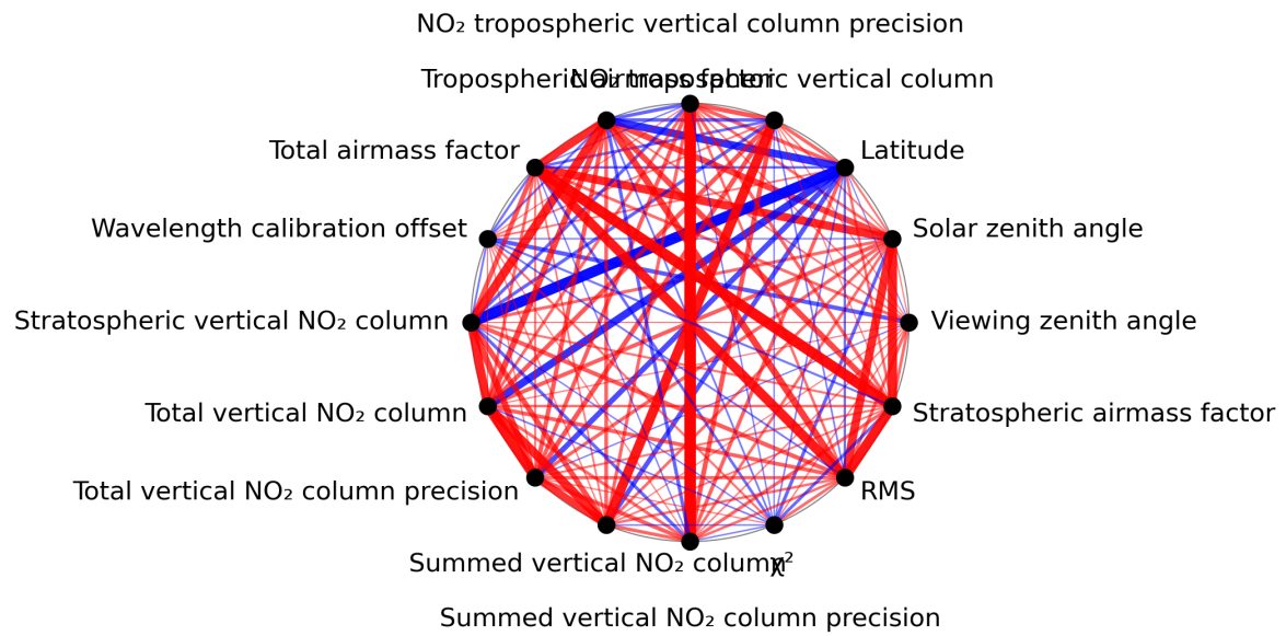
Figure 1: Map of correlation graph for 2023-12-16 to 2023-12-18.
