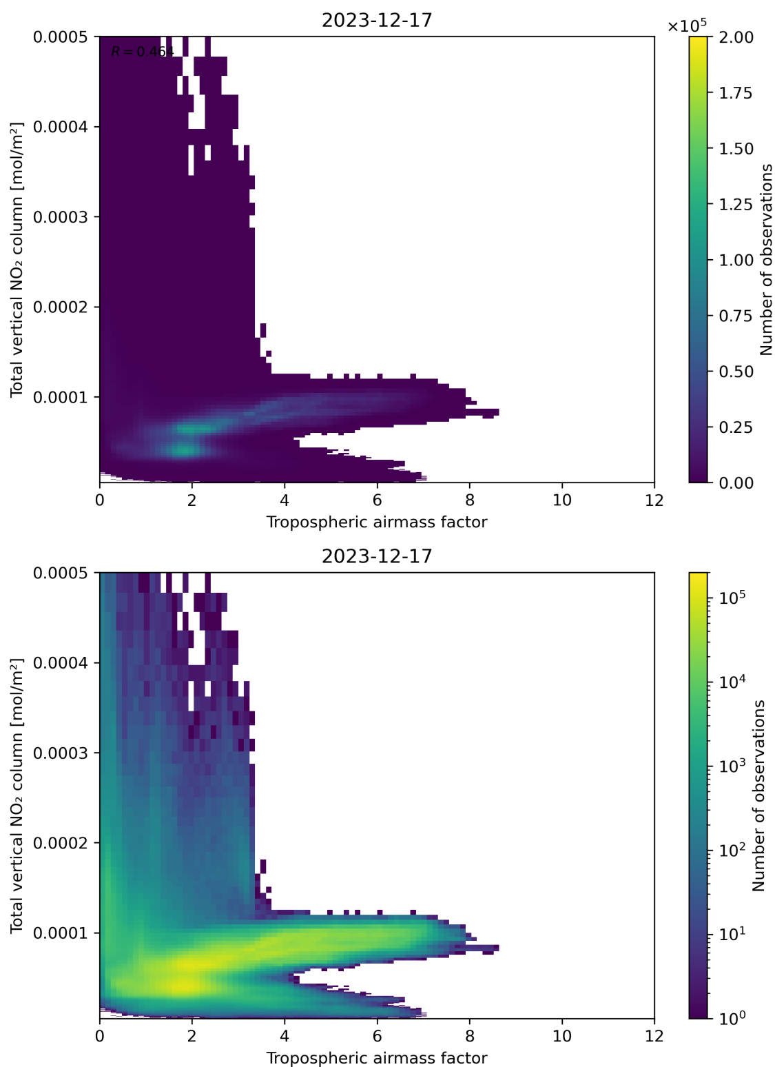
Figure 77: Scatter density plot of “Tropospheric airmass factor” against “Total vertical NO 2 column” for 2023-12-16 to 2023-12-18.
