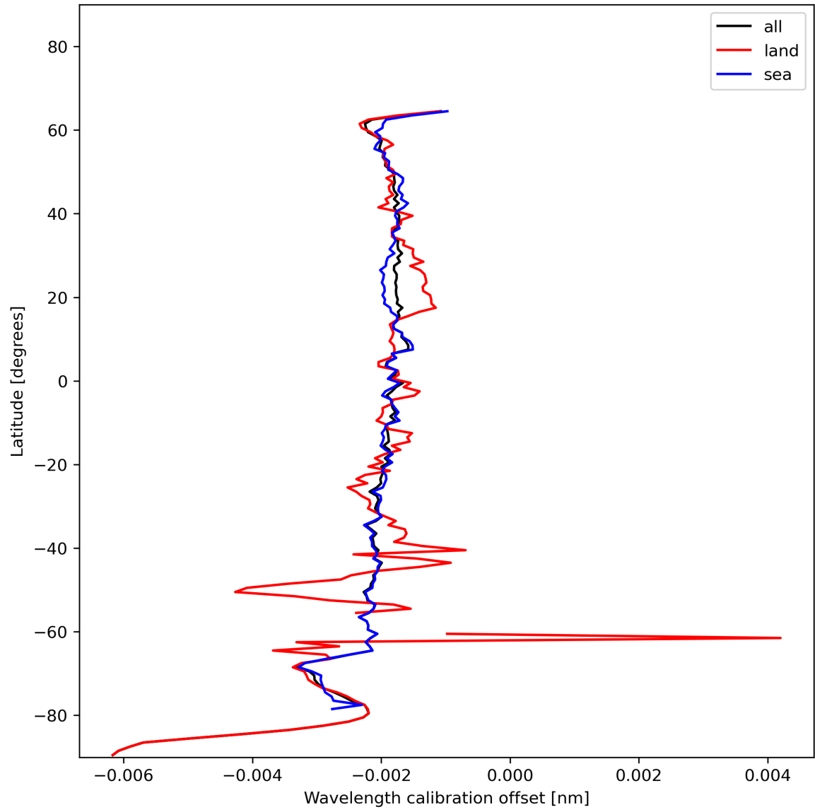
Figure 18: Zonal average of “Wavelength calibration offset” for 2023-12-16 to 2023-12-18.
