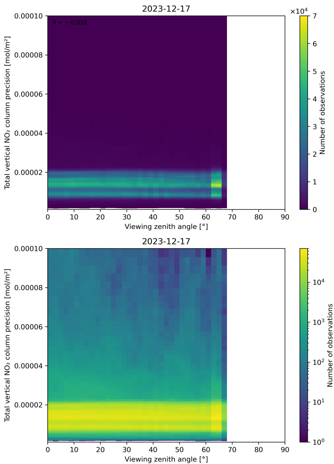
Figure 168: Scatter density plot of “Viewing zenith angle” against “Total vertical NO 2 column precision” for 2023-12-16 to 2023-12-18.
