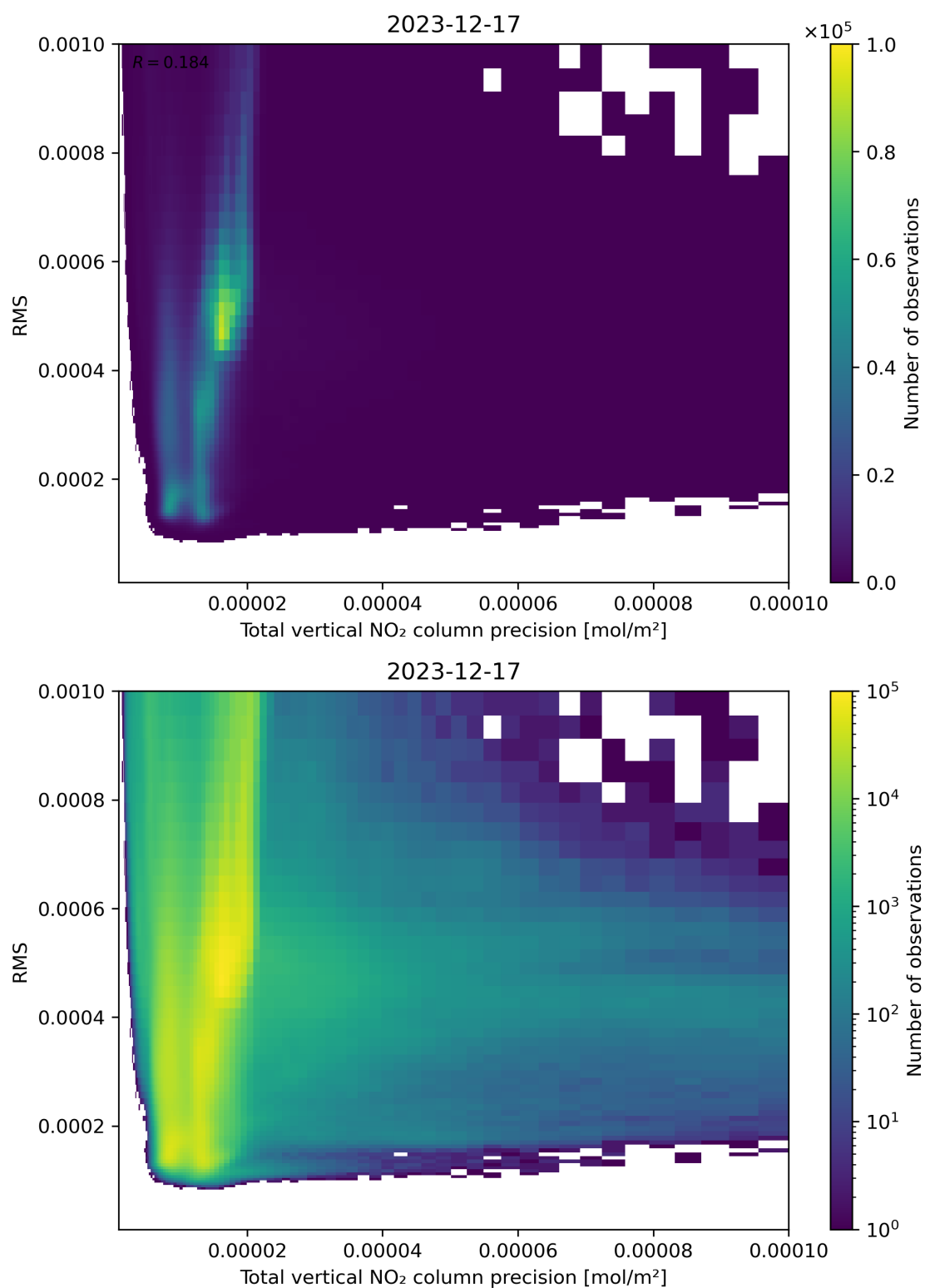
Figure 119: Scatter density plot of “Total vertical NO 2 column precision” against “RMS” for 2023-12-16 to 2023-12-18.
