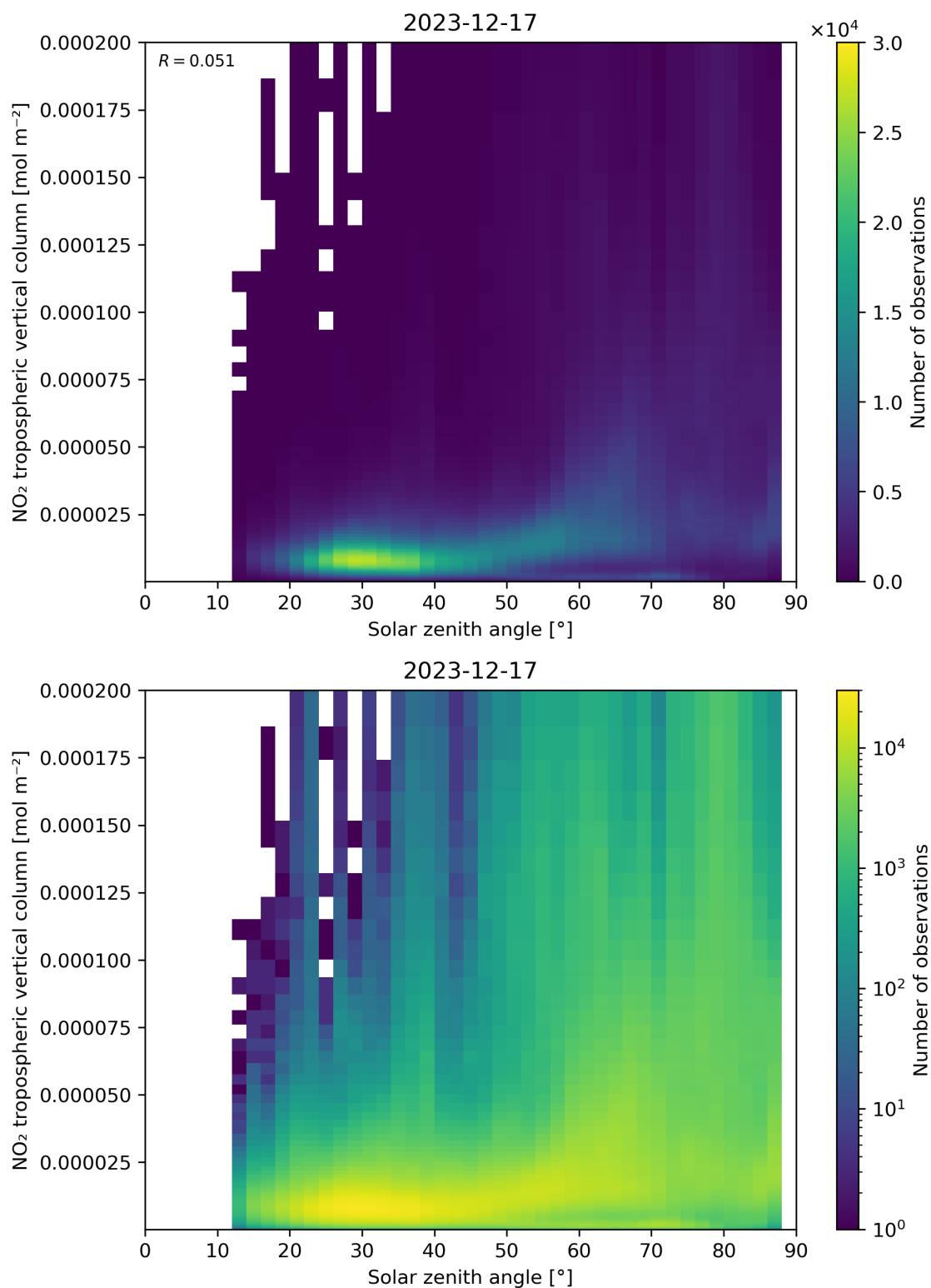
Figure 155: Scatter density plot of “Solar zenith angle” against “NO 2 tropospheric vertical column” for 2023-12-16 to 2023-12-18.
