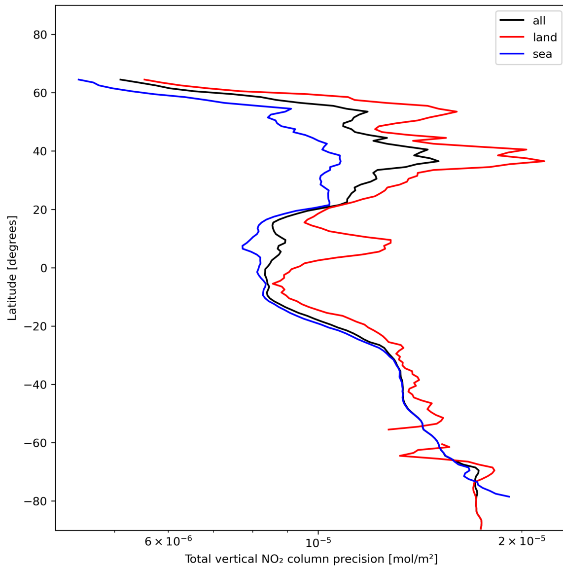
Figure 22: Zonal average of “Total vertical NO 2 column precision” for 2023-12-16 to 2023-12-18.
