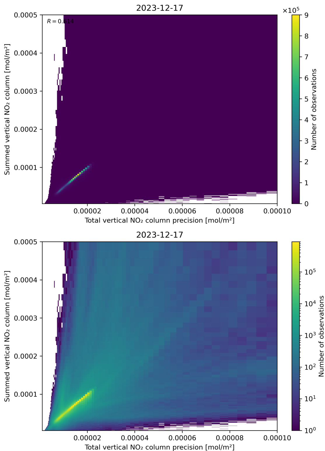
Figure 117: Scatter density plot of “Total vertical NO 2 column precision” against “Summed vertical NO 2 column” for 2023-12-16 to 2023-12-18.
