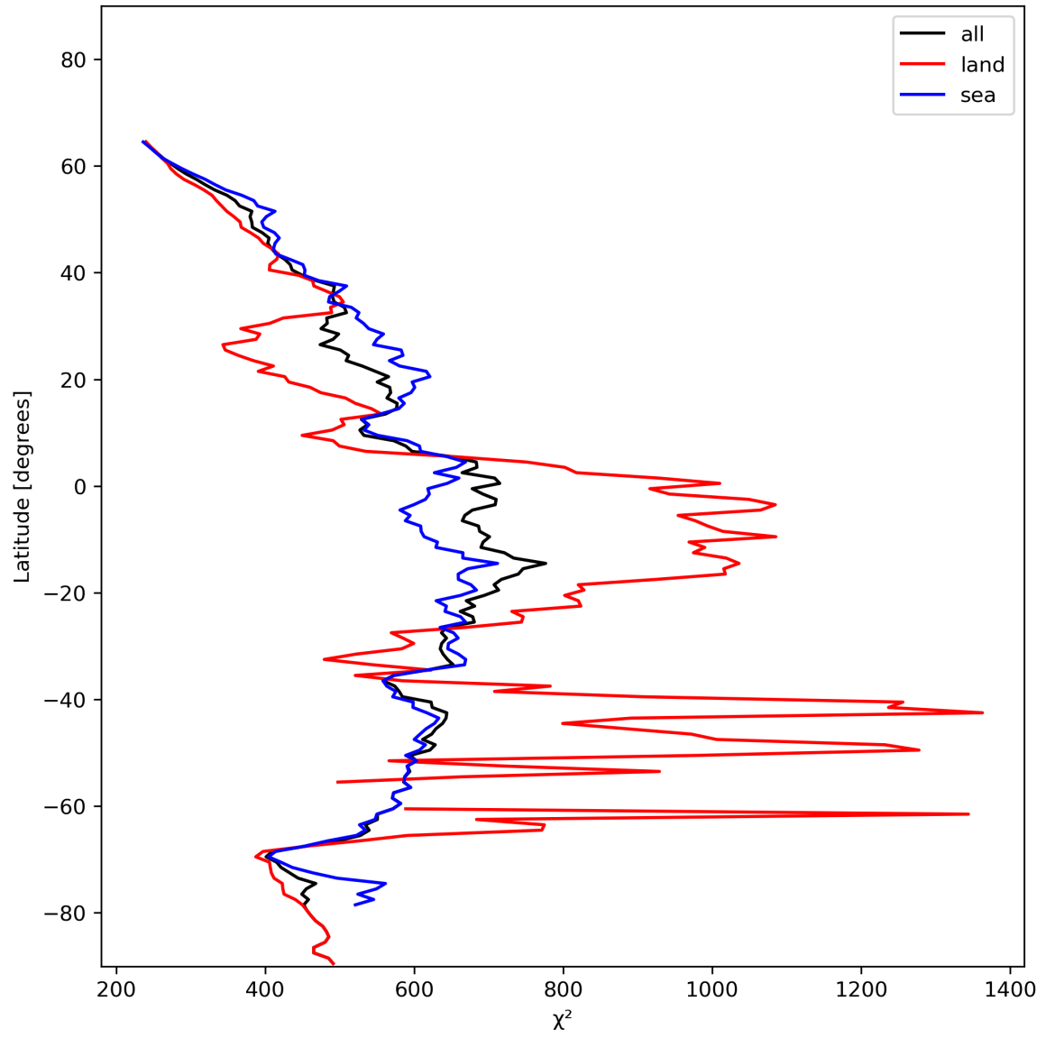
Figure 25: Zonal average of “ \chi^2 ” for 2023-12-16 to 2023-12-18.
