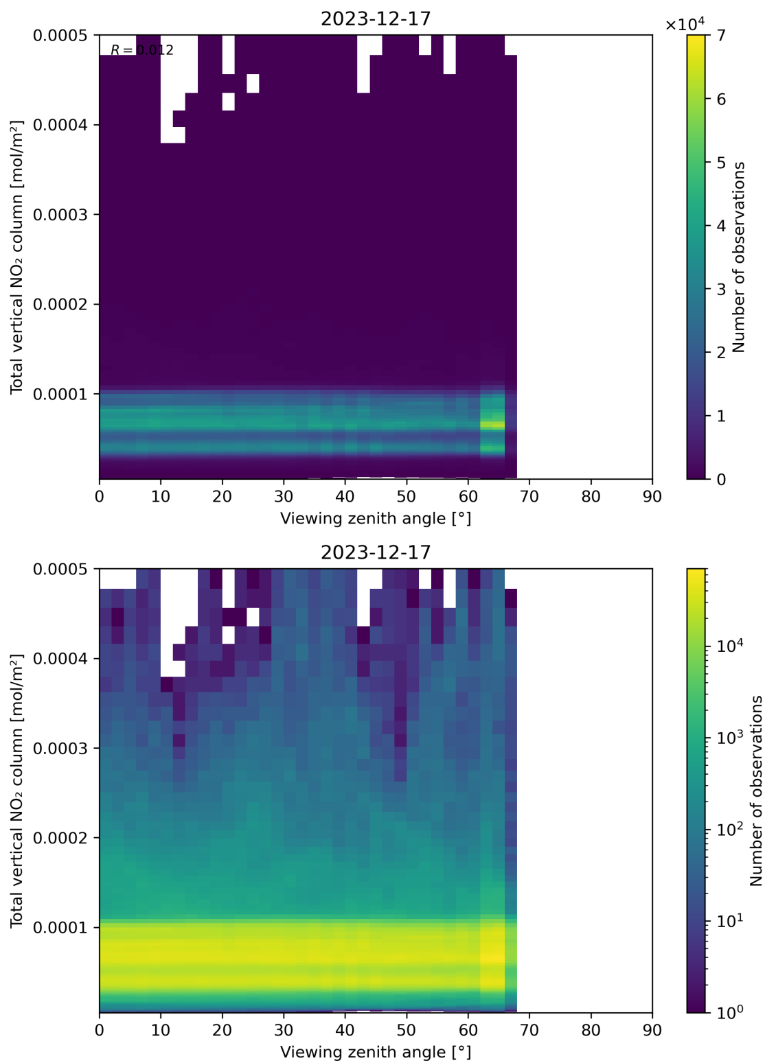
Figure 167: Scatter density plot of “Viewing zenith angle” against “Total vertical NO 2 column” for 2023-12-16 to 2023-12-18.
