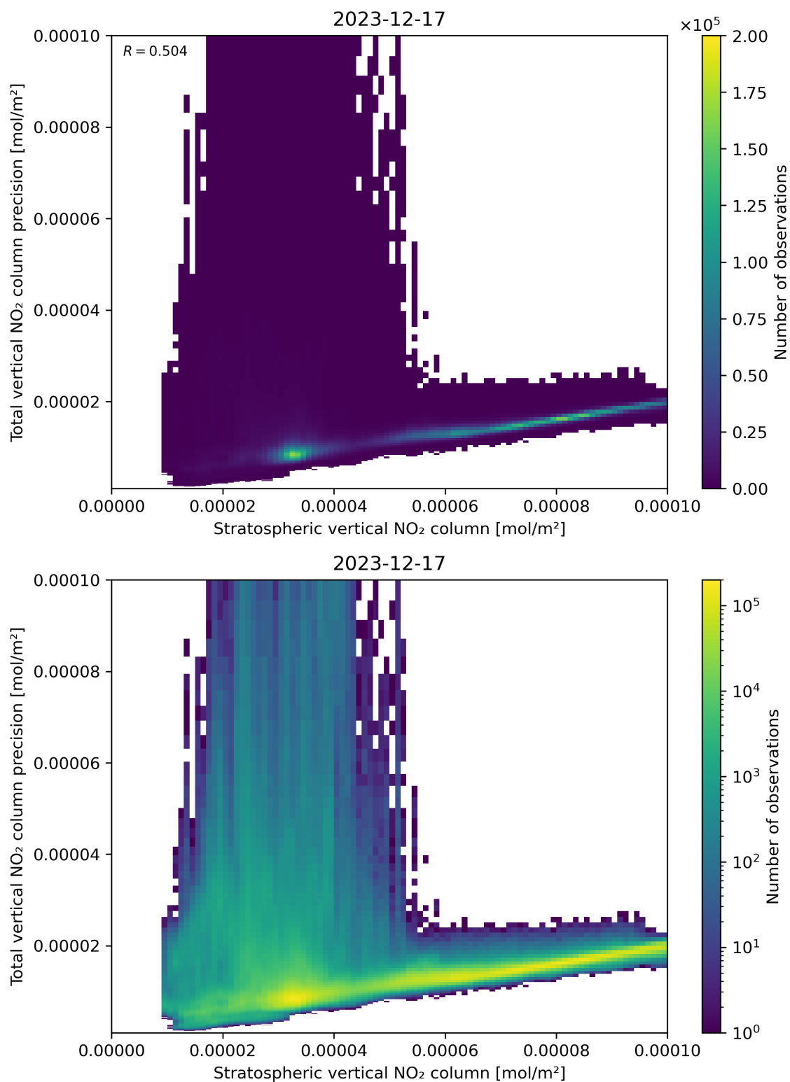
Figure 101: Scatter density plot of “Stratospheric vertical NO 2 column” against “Total vertical NO 2 column precision” for 2023-12-16 to 2023-12-18.
