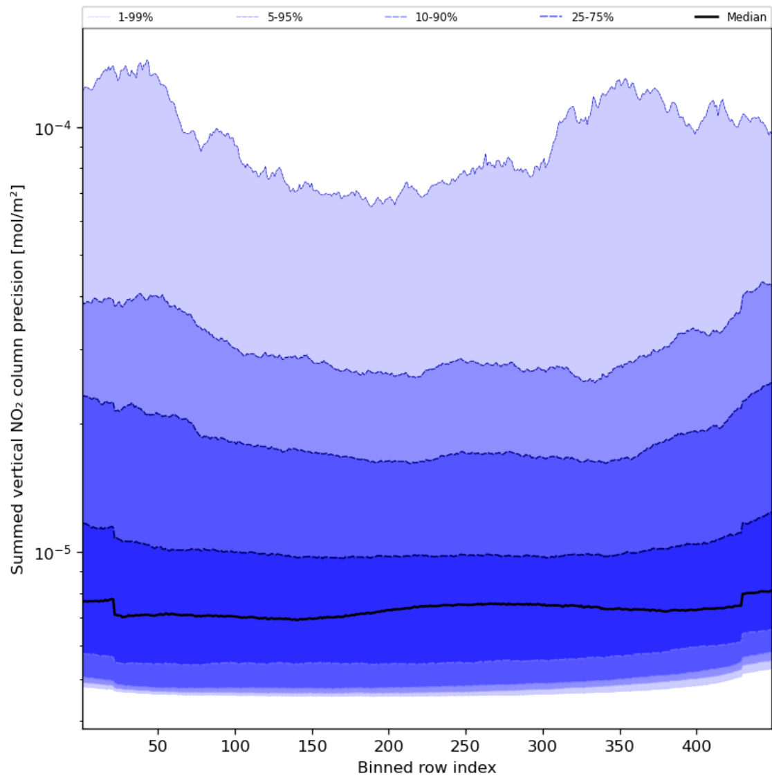
Figure 58: Along track statistics of “Summed vertical NO 2 column precision” for 2023-12-16 to 2023-12-18
