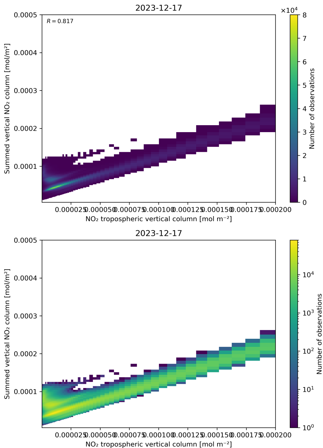
Figure 126: Scatter density plot of “NO 2 tropospheric vertical column” against “Summed vertical NO 2 column” for 2023-12-16 to 2023-12-18.
