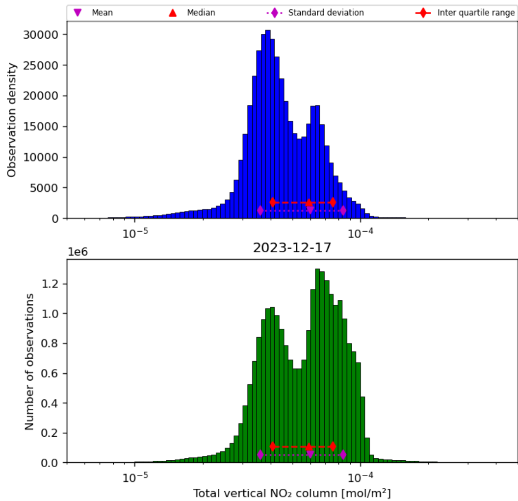
Figure 38: Histogram of “Total vertical NO 2 column” for 2023-12-16 to 2023-12-18
