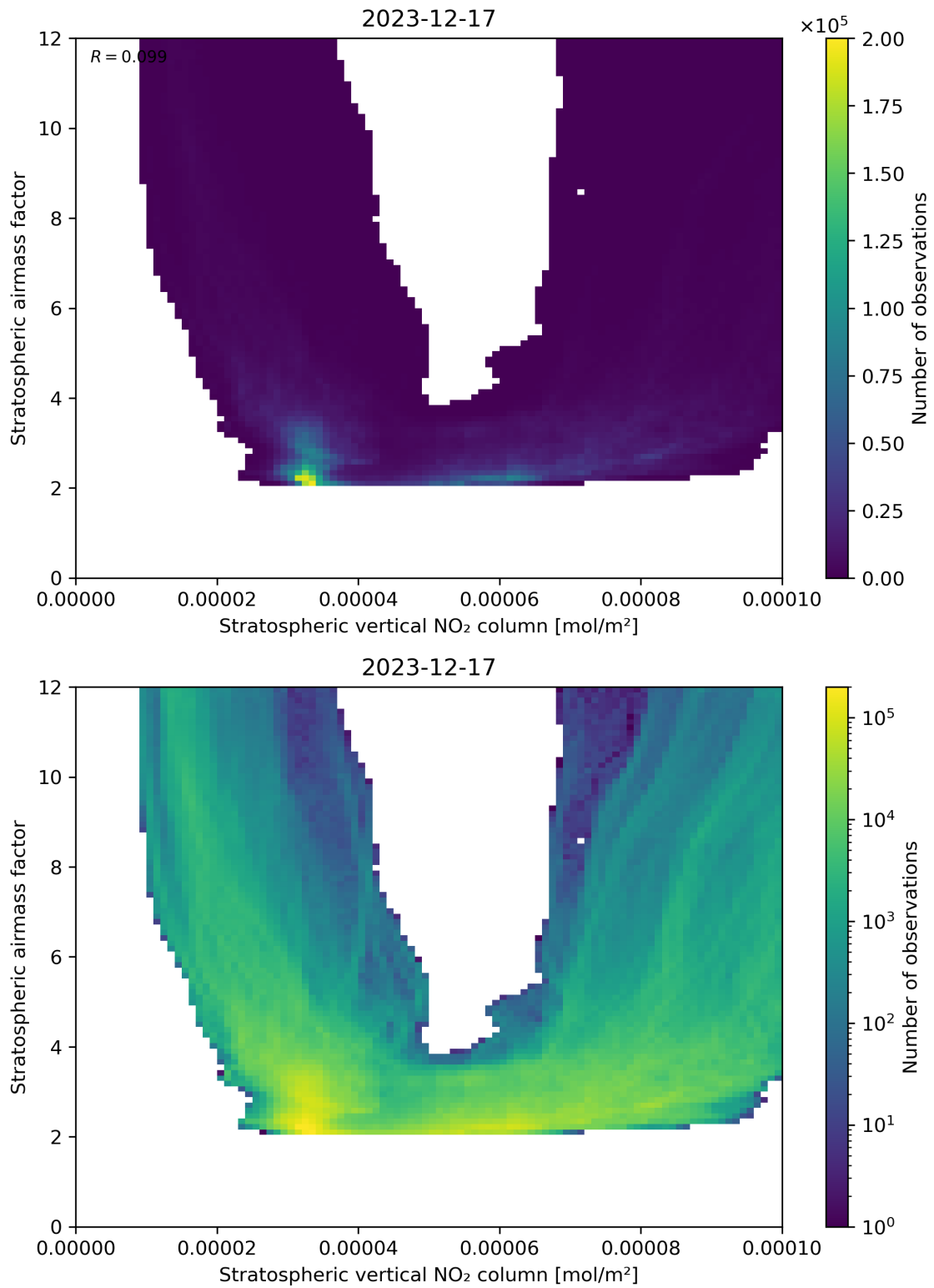
Figure 96: Scatter density plot of “Stratospheric vertical NO 2 column” against “Stratospheric airmass factor” for 2023-12-16 to 2023-12-18.
