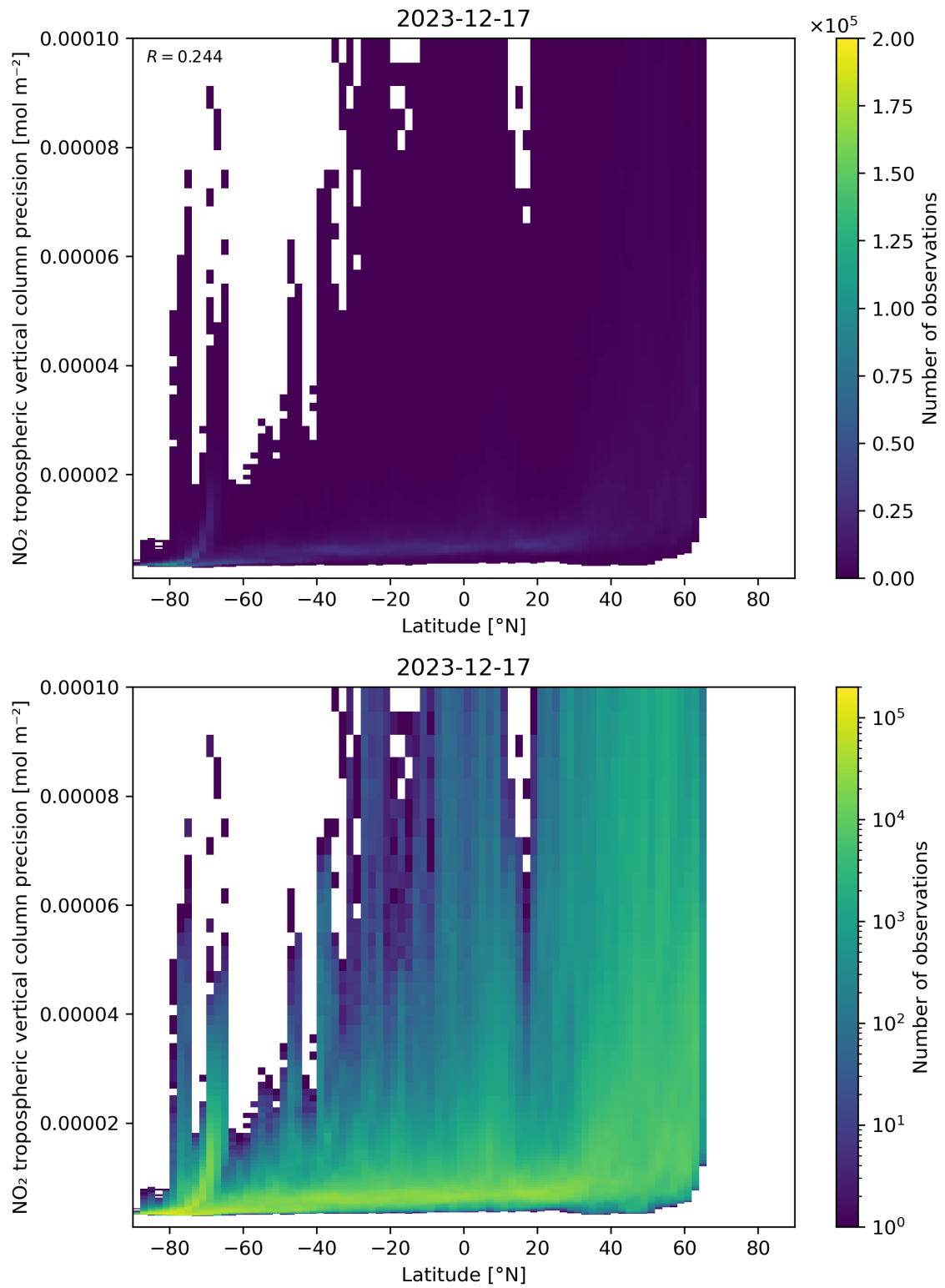
Figure 93: Scatter density plot of “Latitude” against “NO 2 tropospheric vertical column precision” for 2023-12-16 to 2023-12-18.
