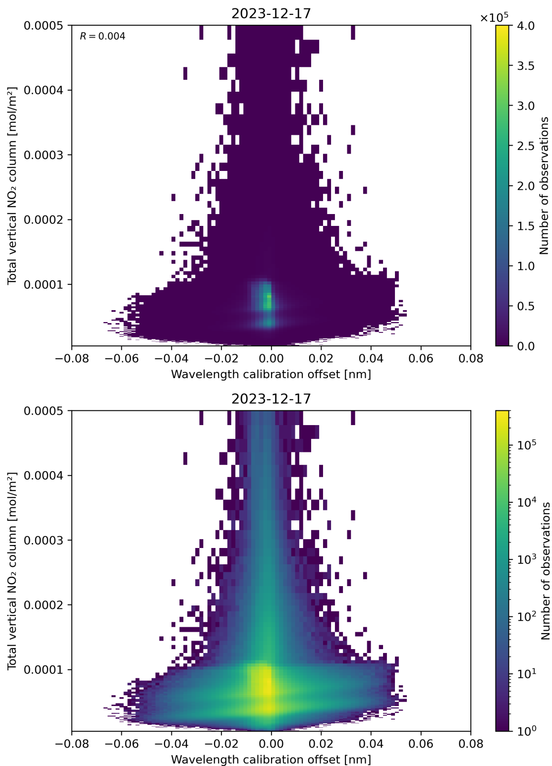
Figure 179: Scatter density plot of “Wavelength calibration offset” against “Total vertical NO 2 column” for 2023-12-16 to 2023-12-18.
