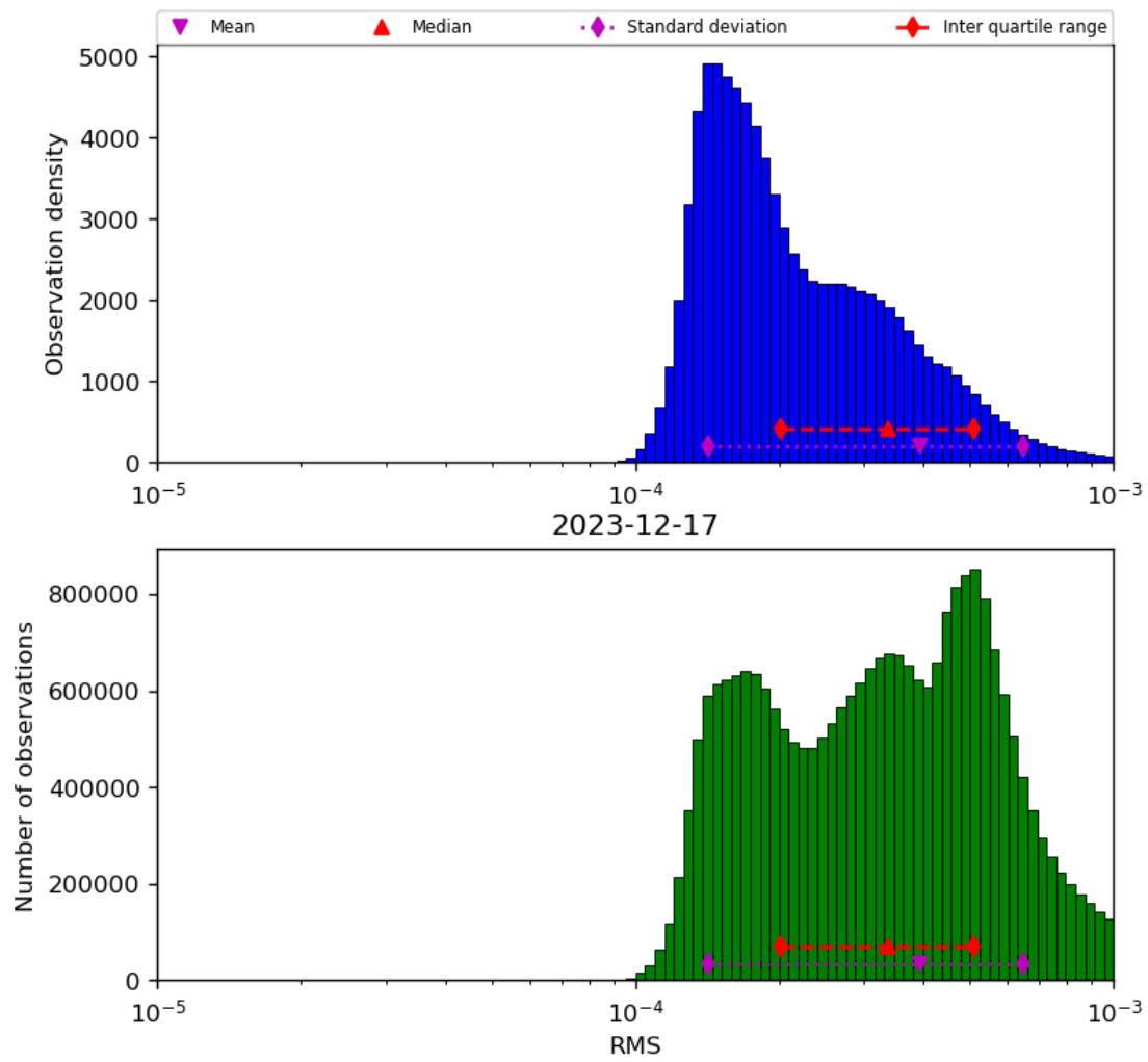
Figure 43: Histogram of “RMS” for 2023-12-16 to 2023-12-18
