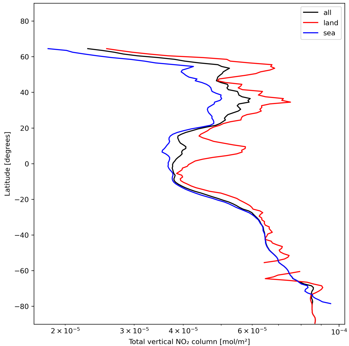
Figure 21: Zonal average of “Total vertical NO 2 column” for 2023-12-16 to 2023-12-18.
