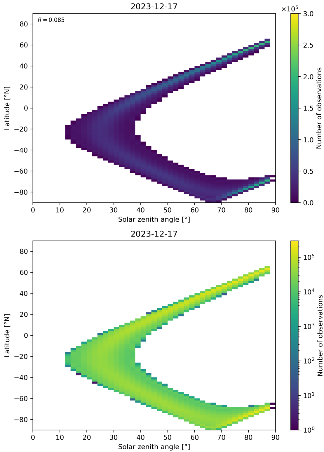
Figure 149: Scatter density plot of “Solar zenith angle” against “Latitude” for 2023-12-16 to 2023-12-18.
