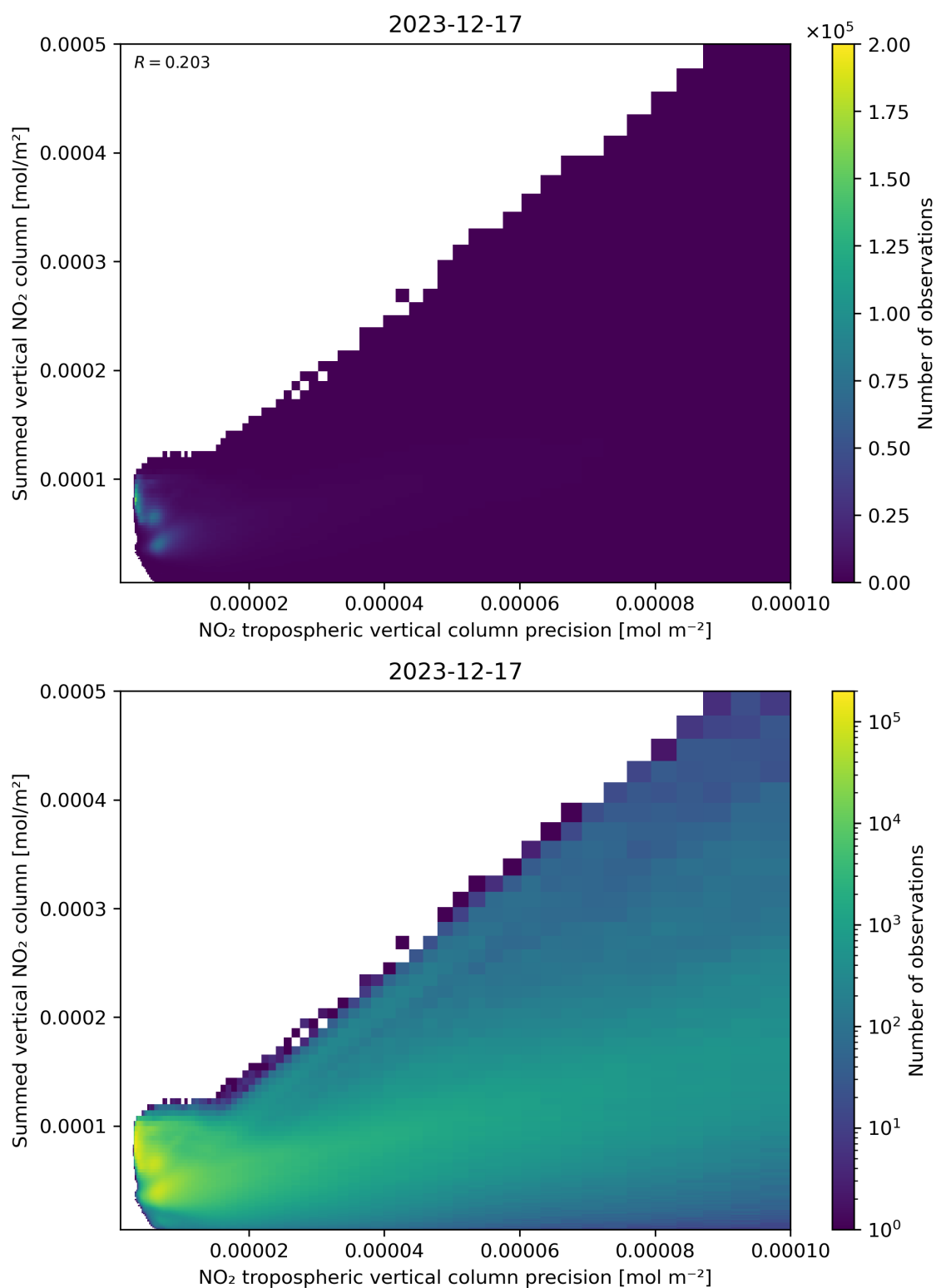
Figure 136: Scatter density plot of “NO 2 tropospheric vertical column precision” against “Summed vertical NO 2 column” for 2023-12-16 to 2023-12-18.
