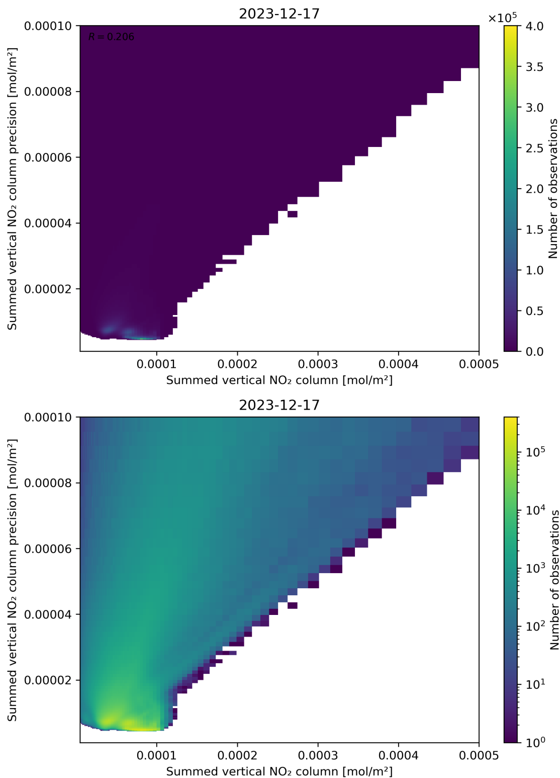
Figure 105: Scatter density plot of “Summed vertical NO 2 column” against “Summed vertical NO 2 column precision” for 2023-12-16 to 2023-12-18.
