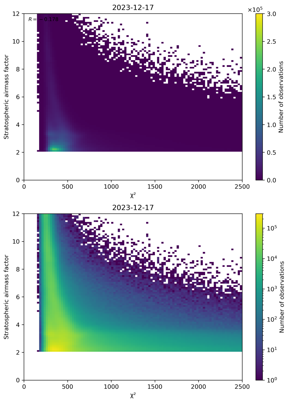
Figure 81: Scatter density plot of “ \chi^2 ” against “Stratospheric airmass factor” for 2023-12-16 to 2023-12-18.
