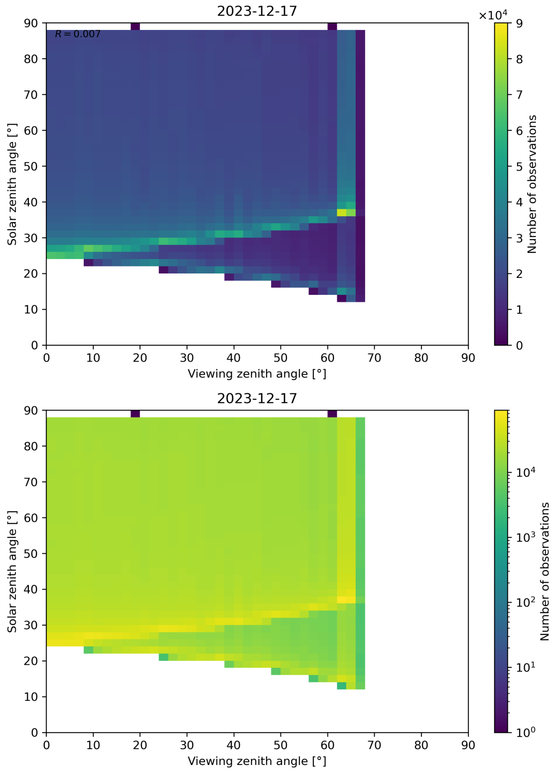
Figure 172: Scatter density plot of “Viewing zenith angle” against “Solar zenith angle” for 2023-12-16 to 2023-12-18.
