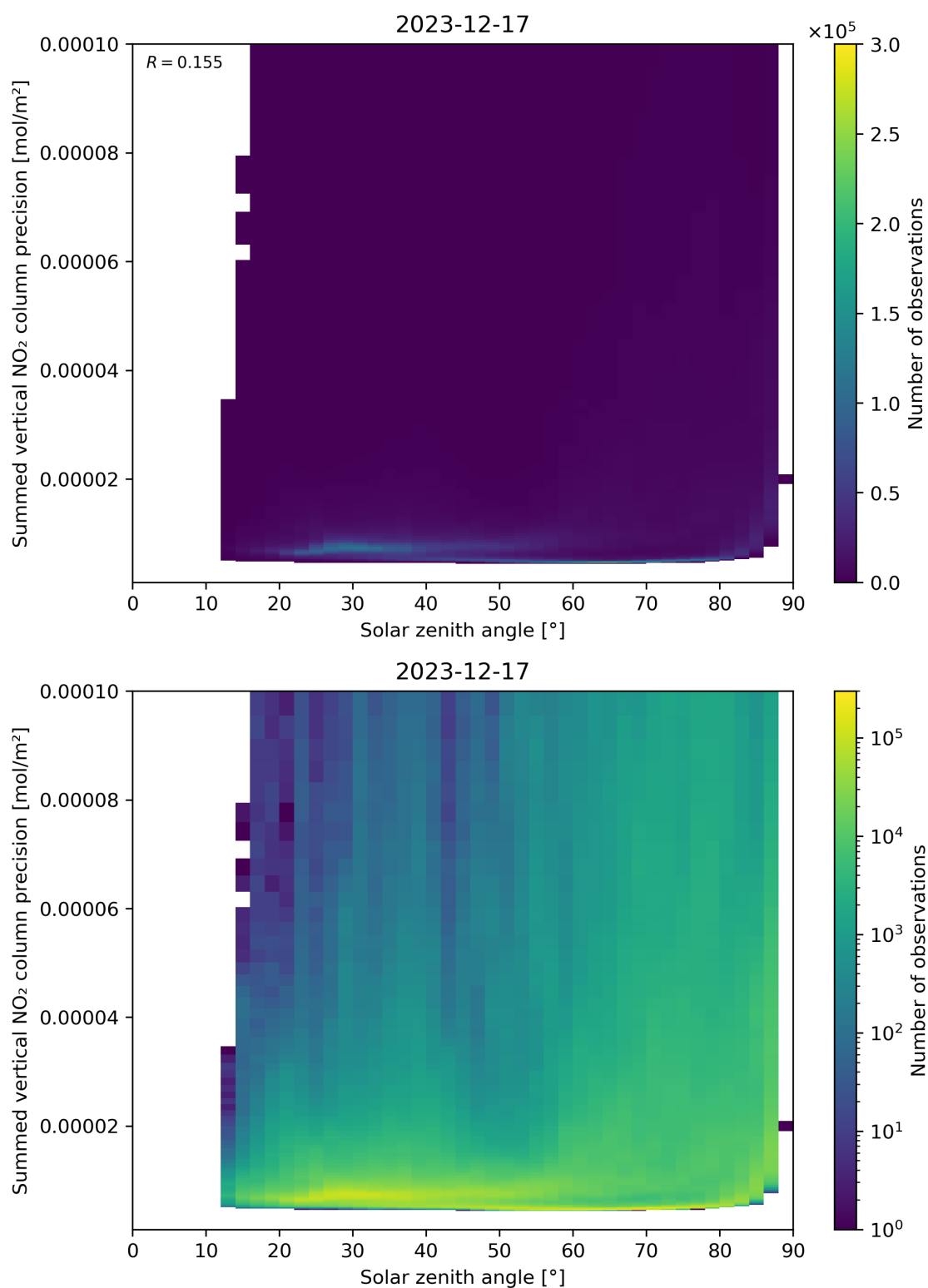
Figure 152: Scatter density plot of “Solar zenith angle” against “Summed vertical NO 2 column precision” for 2023-12-16 to 2023-12-18.
