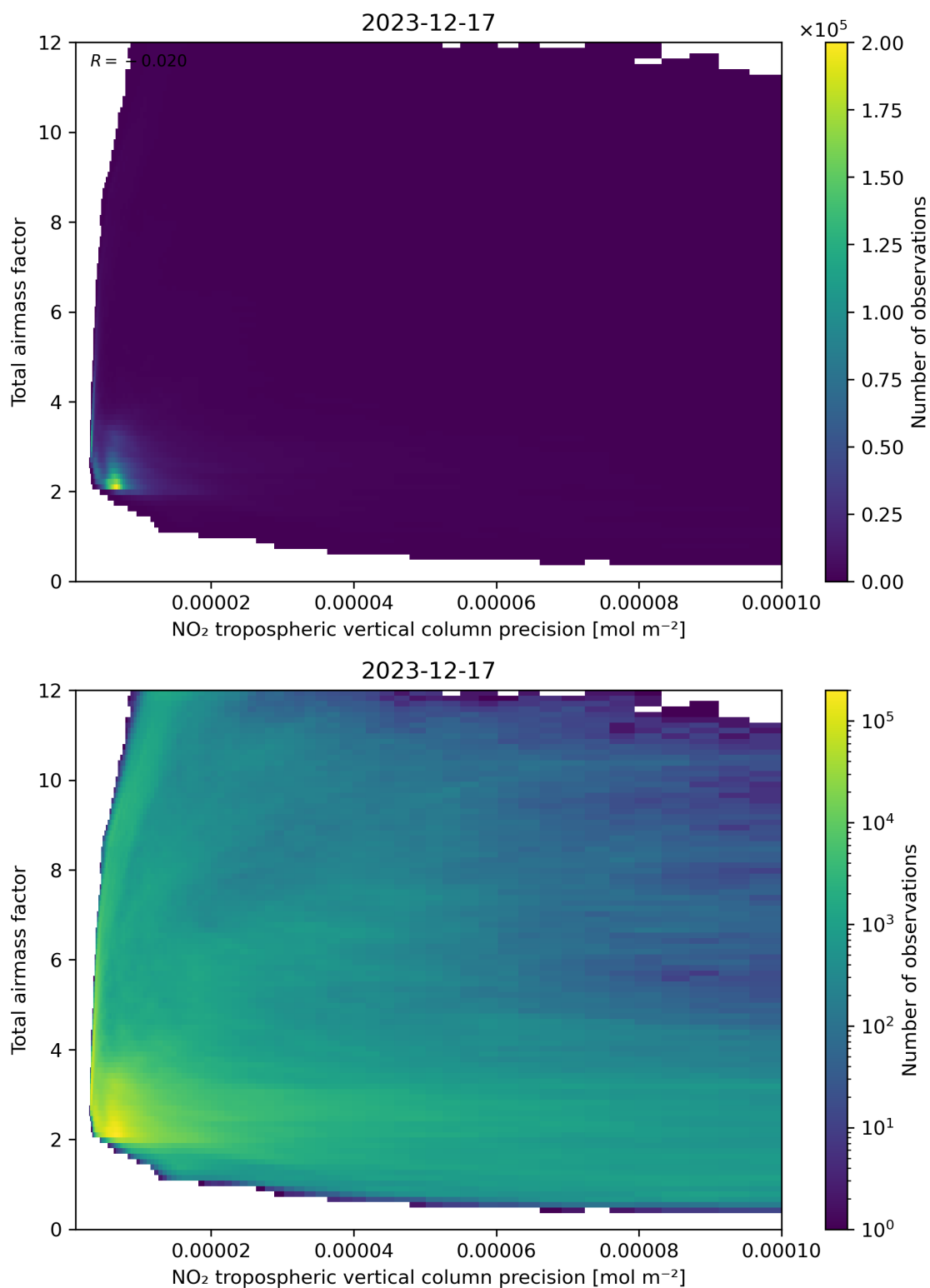
Figure 132: Scatter density plot of “NO 2 tropospheric vertical column precision” against “Total air mass factor” for 2023-12-16 to 2023-12-18.
