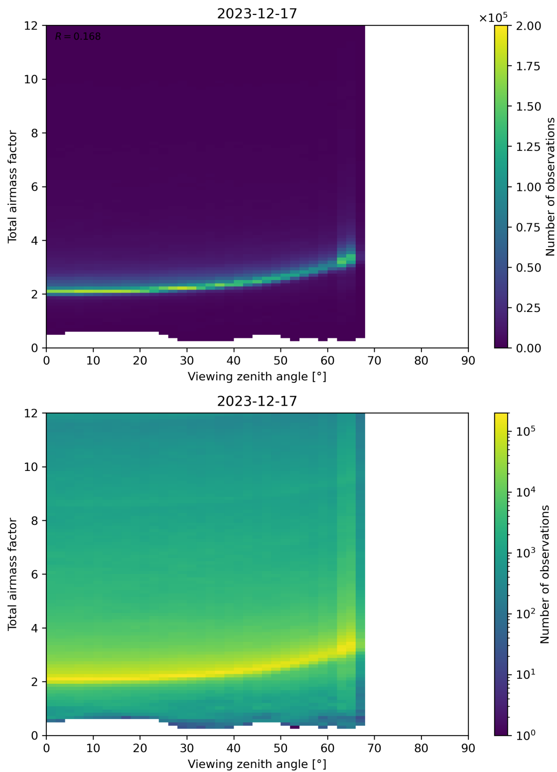
Figure 160: Scatter density plot of “Viewing zenith angle” against “Total airmass factor” for 2023-12-16 to 2023-12-18.
