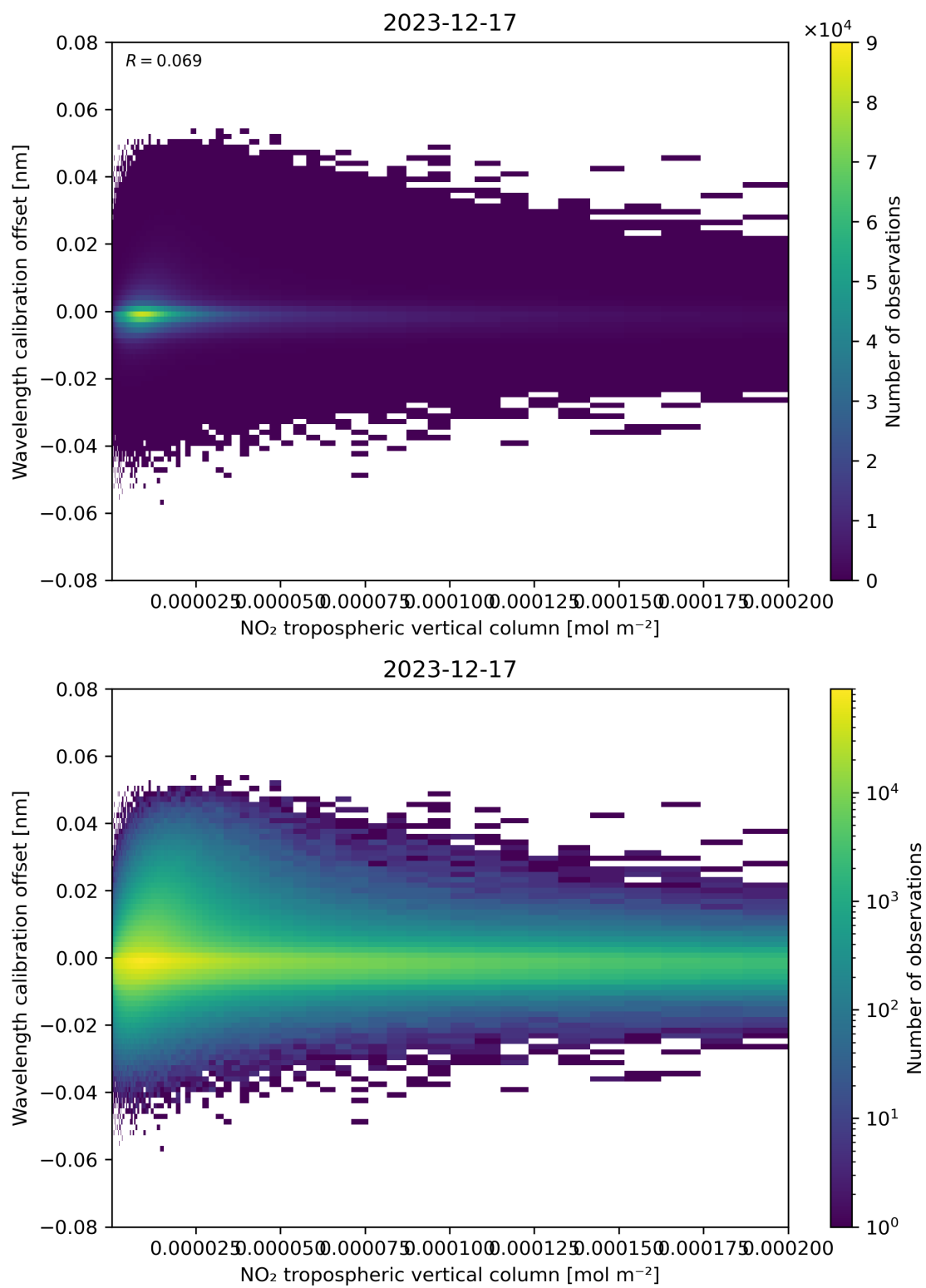
Figure 143: Scatter density plot of “NO 2 tropospheric vertical column” against “Wavelength calibration offset” for 2023-12-16 to 2023-12-18.
