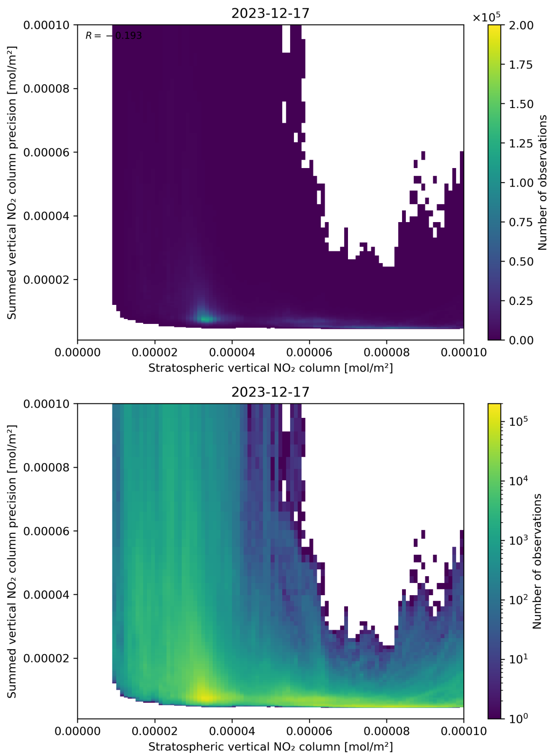
Figure 99: Scatter density plot of “Stratospheric vertical NO 2 column” against “Summed vertical NO 2 column precision” for 2023-12-16 to 2023-12-18.
