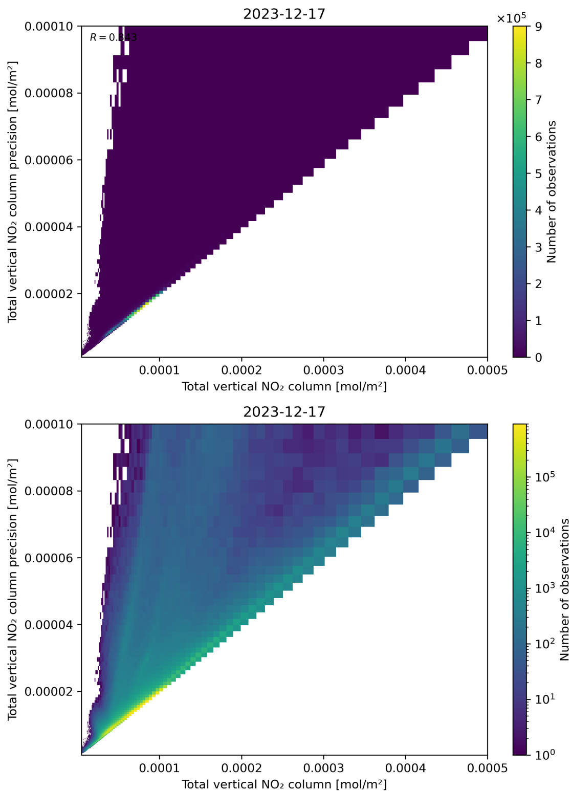
Figure 114: Scatter density plot of “Total vertical NO 2 column” against “Total vertical NO 2 column precision” for 2023-12-16 to 2023-12-18.
