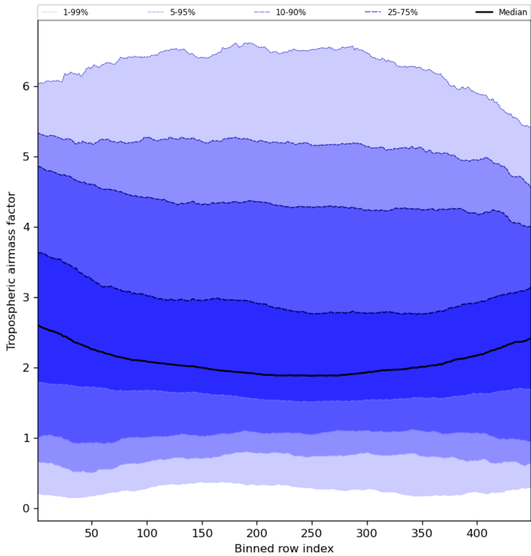
Figure 48: Along track statistics of “Tropospheric airmass factor” for 2023-12-16 to 2023-12-18
