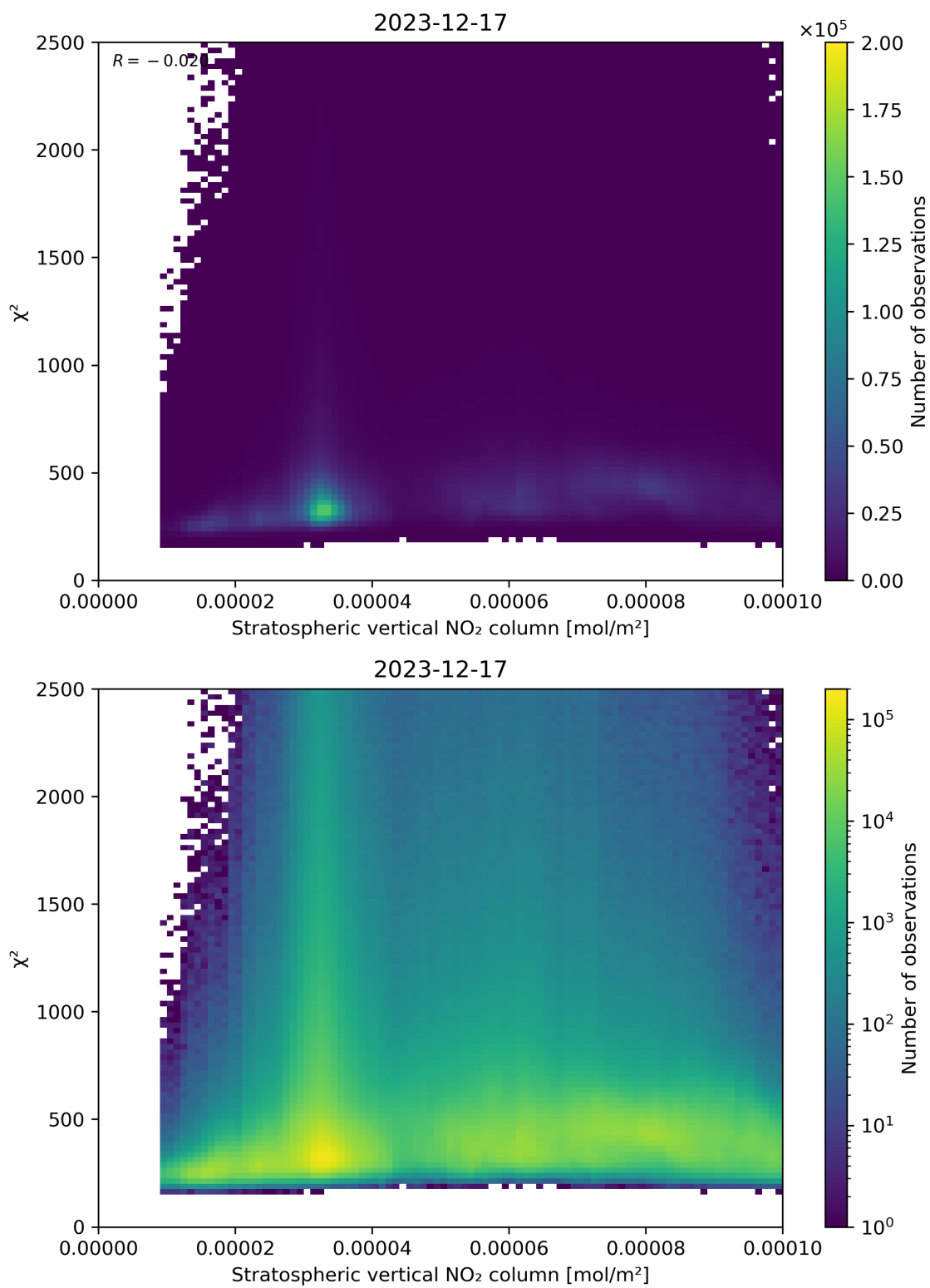
Figure 97: Scatter density plot of “Stratospheric vertical NO 2 column” against “ \chi^2 ” for 2023-12-16 to 2023-12-18.
