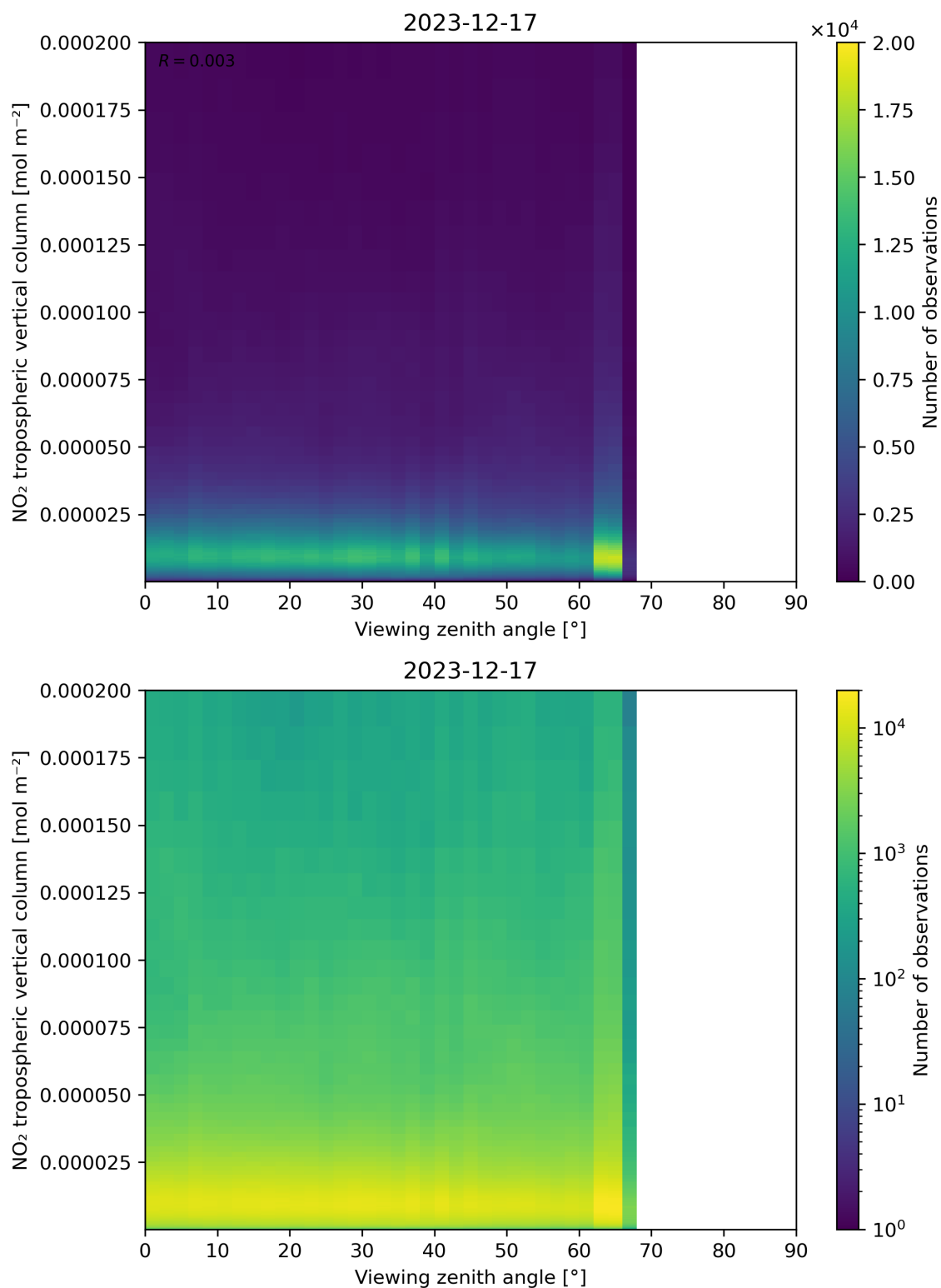
Figure 169: Scatter density plot of “Viewing zenith angle” against “NO 2 tropospheric vertical column” for 2023-12-16 to 2023-12-18.
