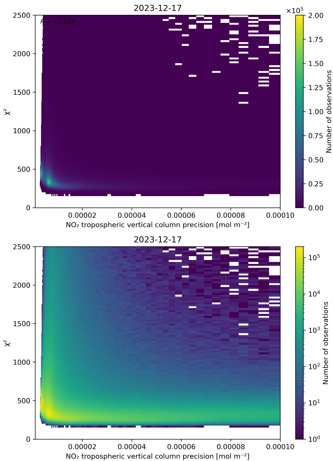
Figure 134: Scatter density plot of “NO 2 tropospheric vertical column precision” against “ \chi^2 ” for 2023-12-16 to 2023-12-18.
