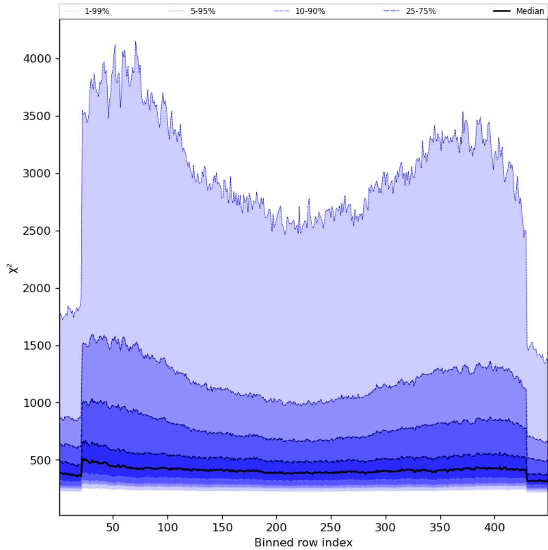
Figure 59: Along track statistics of “ \chi^2 ” for 2023-12-16 to 2023-12-18
