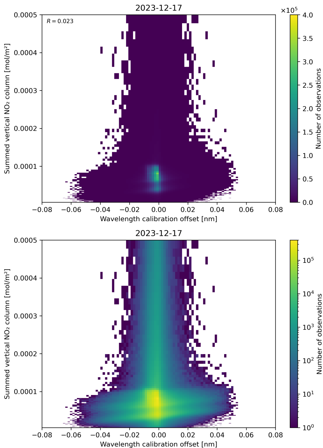
Figure 177: Scatter density plot of “Wavelength calibration offset” against “Summed vertical NO 2 column” for 2023-12-16 to 2023-12-18.
