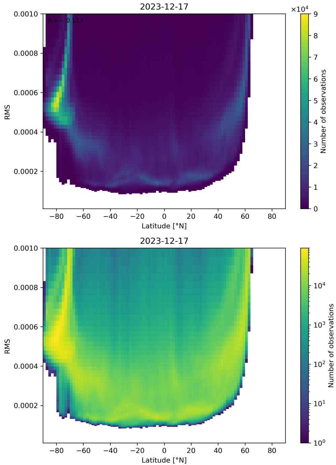
Figure 94: Scatter density plot of “Latitude” against “RMS” for 2023-12-16 to 2023-12-18.
