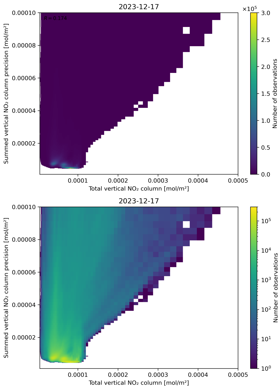
Figure 113: Scatter density plot of “Total vertical NO 2 column” against “Summed vertical NO 2 column precision” for 2023-12-16 to 2023-12-18.
