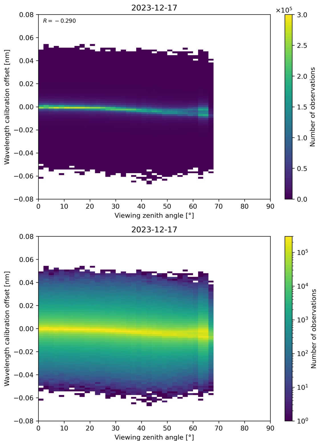
Figure 173: Scatter density plot of “Viewing zenith angle” against “Wavelength calibration offset” for 2023-12-16 to 2023-12-18.
