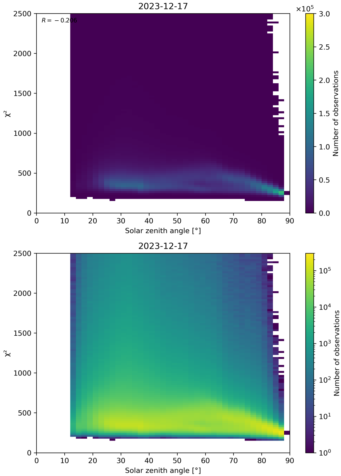
Figure 148: Scatter density plot of “Solar zenith angle” against “ \chi^2 ” for 2023-12-16 to 2023-12-18.
