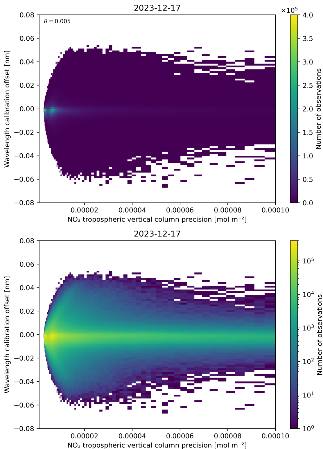
Figure 141: Scatter density plot of “NO 2 tropospheric vertical column precision” against “Wavelength calibration offset” for 2023-12-16 to 2023-12-18.
