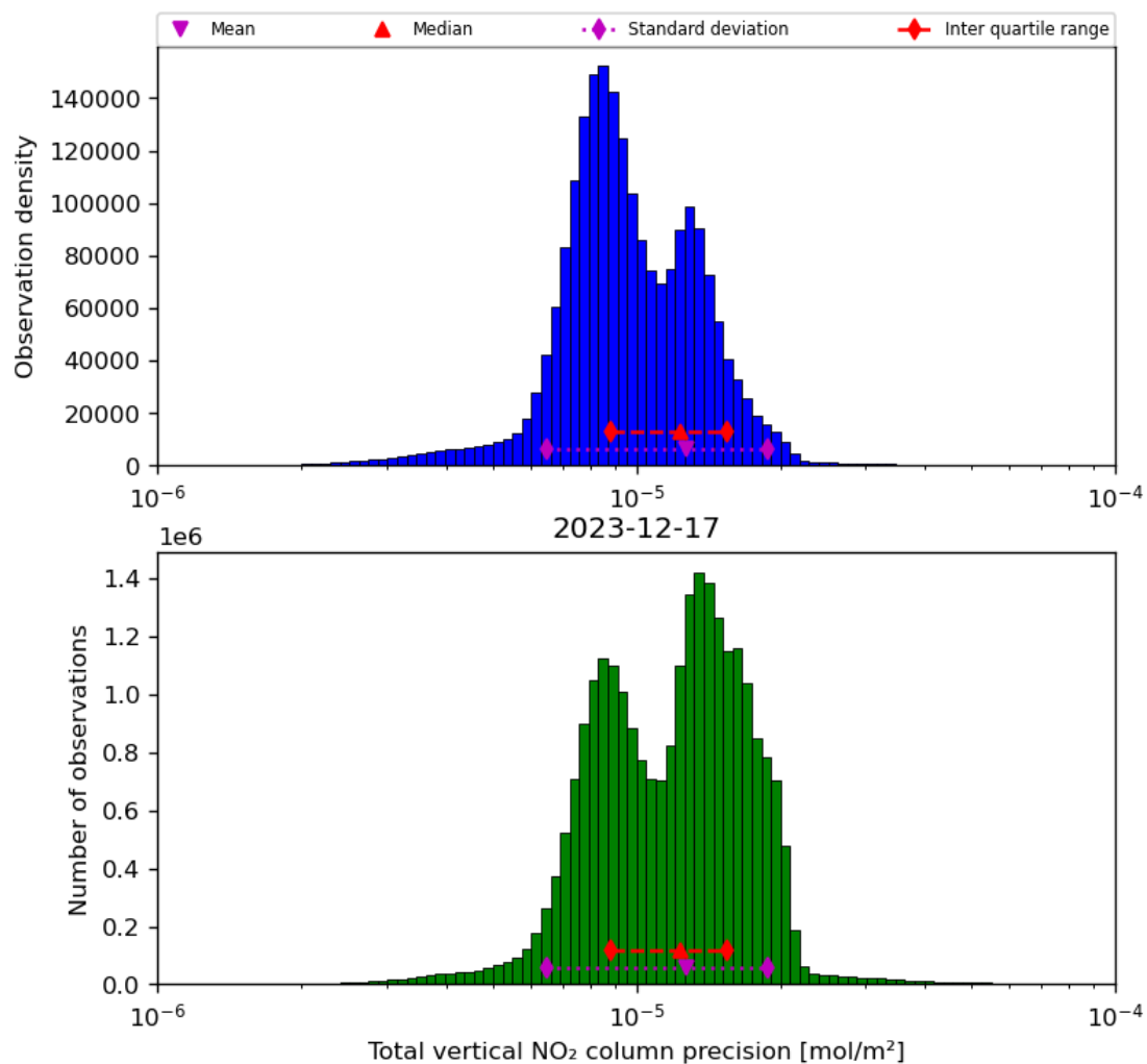
Figure 39: Histogram of “Total vertical NO 2 column precision” for 2023-12-16 to 2023-12-18
