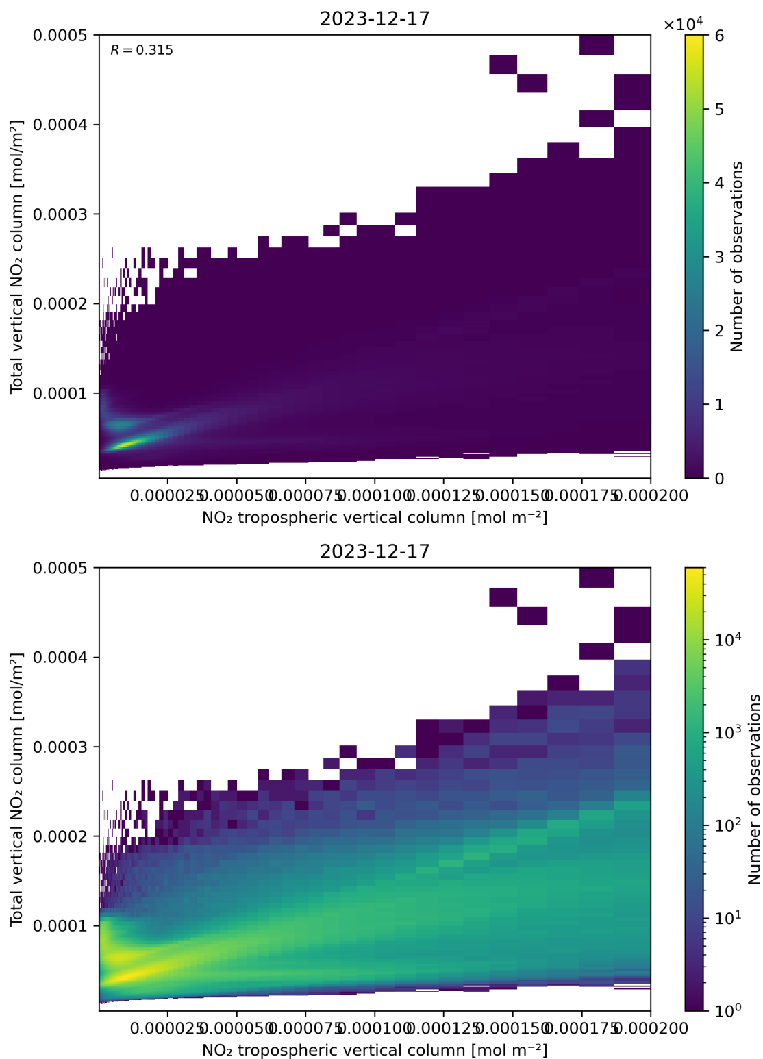
Figure 128: Scatter density plot of “NO 2 tropospheric vertical column” against “Total vertical NO 2 column” for 2023-12-16 to 2023-12-18.
