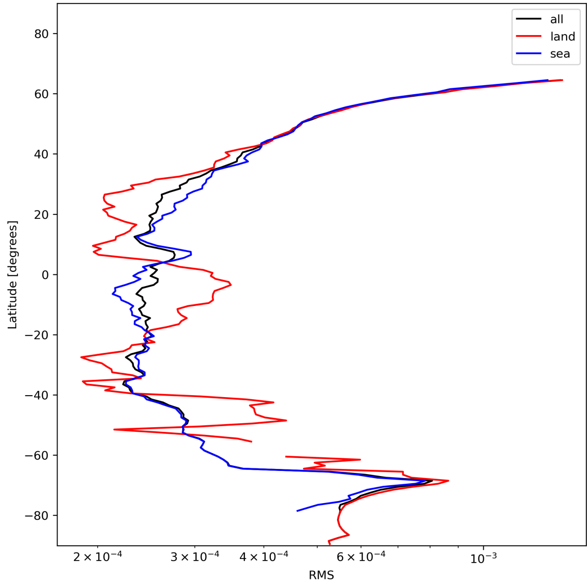
Figure 26: Zonal average of “RMS” for 2023-12-16 to 2023-12-18.
