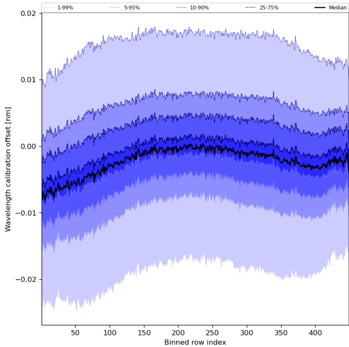
Figure 52: Along track statistics of “Wavelength calibration offset” for 2023-12-16 to 2023-12-18
