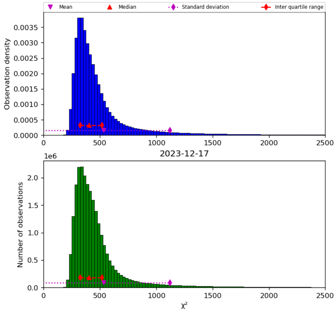
Figure 42: Histogram of “ \chi^2 ” for 2023-12-16 to 2023-12-18
