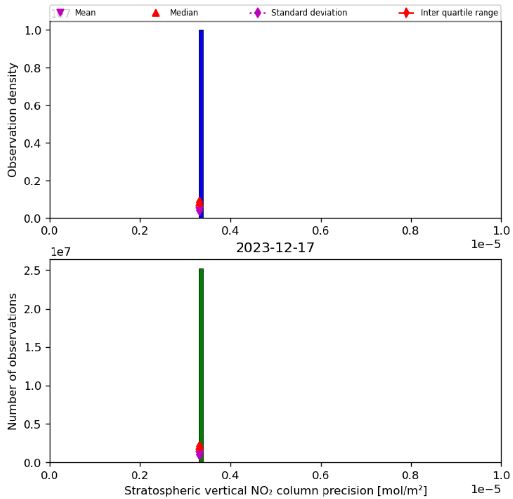
Figure 37: Histogram of “Stratospheric vertical NO 2 column precision” for 2023-12-16 to 2023-12-18
