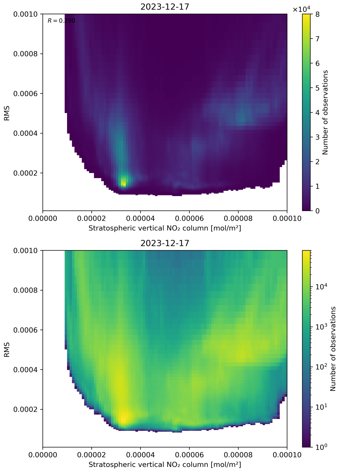
Figure 102: Scatter density plot of “Stratospheric vertical NO 2 column” against “RMS” for 2023-12-16 to 2023-12-18.
