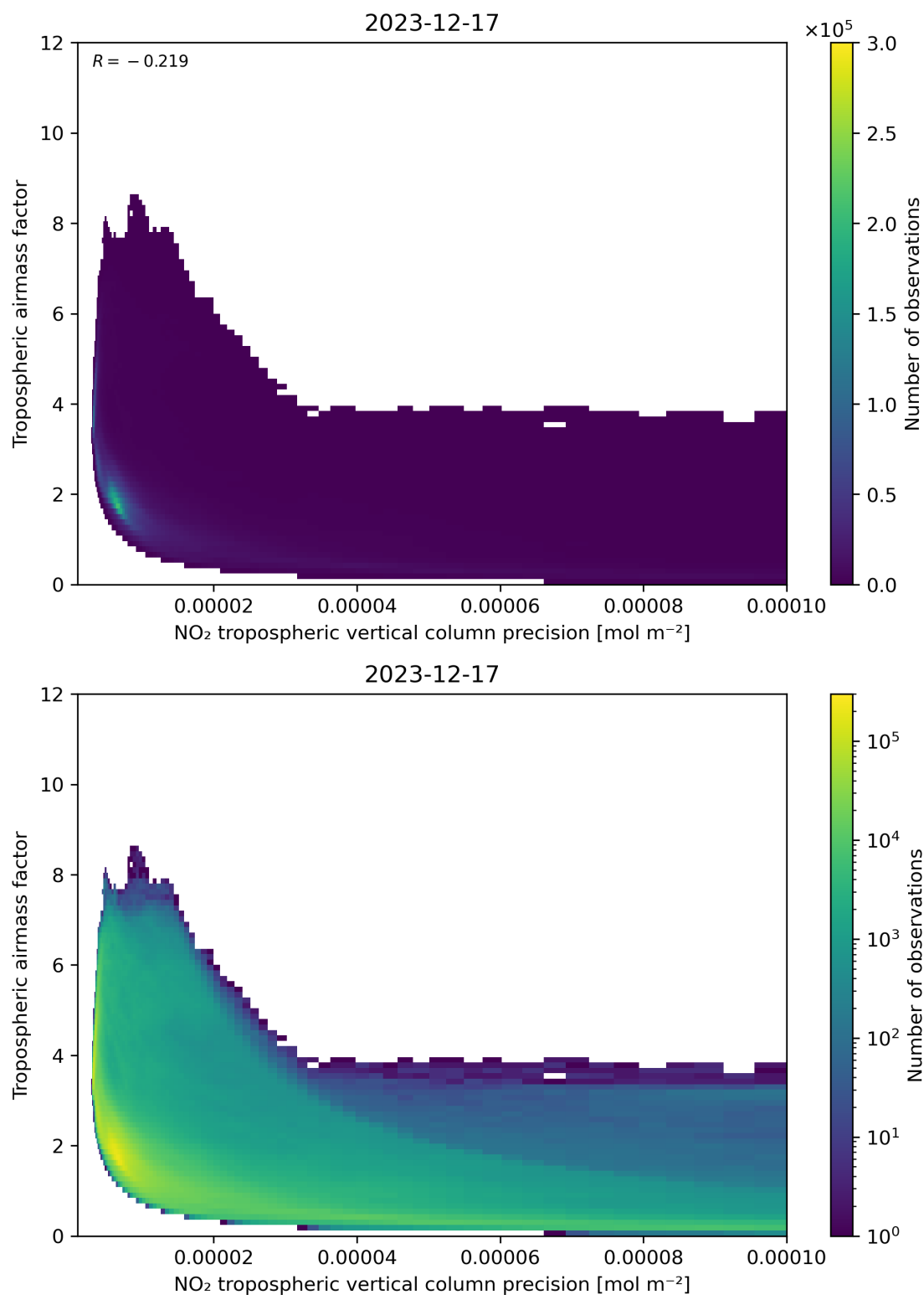
Figure 133: Scatter density plot of “NO 2 tropospheric vertical column precision” against “Tropospheric airmass factor” for 2023-12-16 to 2023-12-18.
