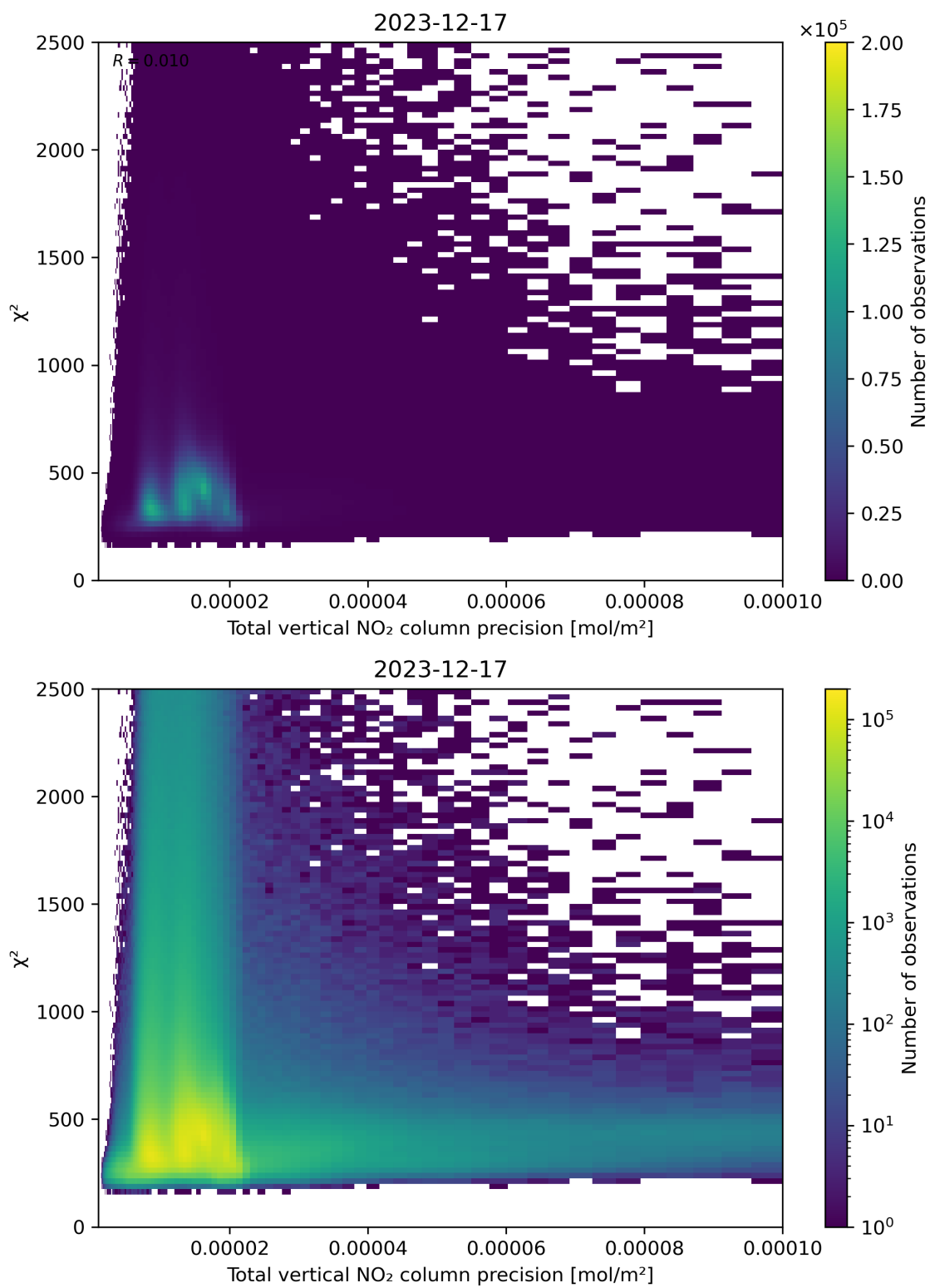
Figure 116: Scatter density plot of “Total vertical NO 2 column precision” against “ \chi^2 ” for 2023-12-16 to 2023-12-18.
