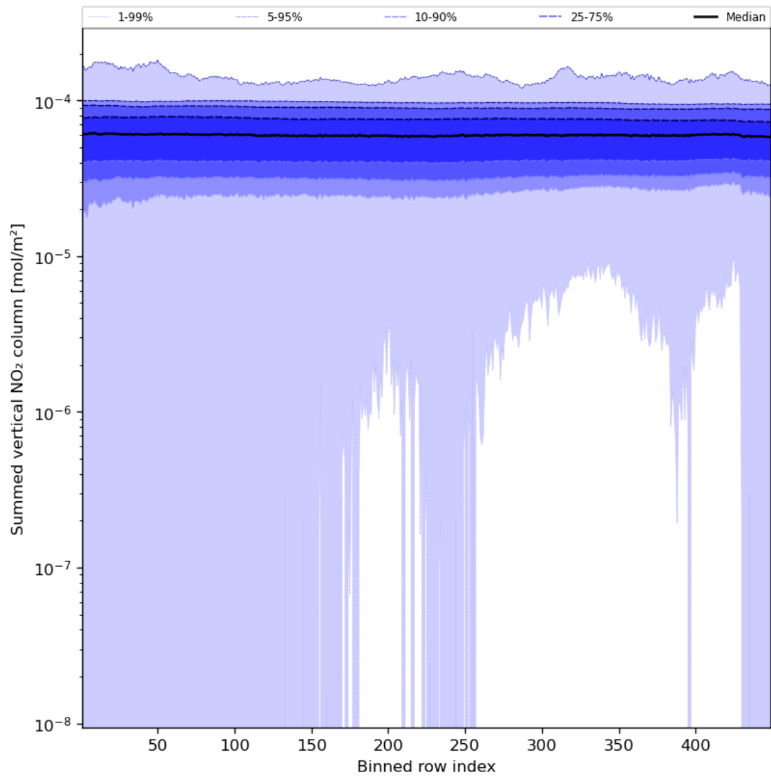
Figure 57: Along track statistics of “Summed vertical NO 2 column” for 2023-12-16 to 2023-12-18
