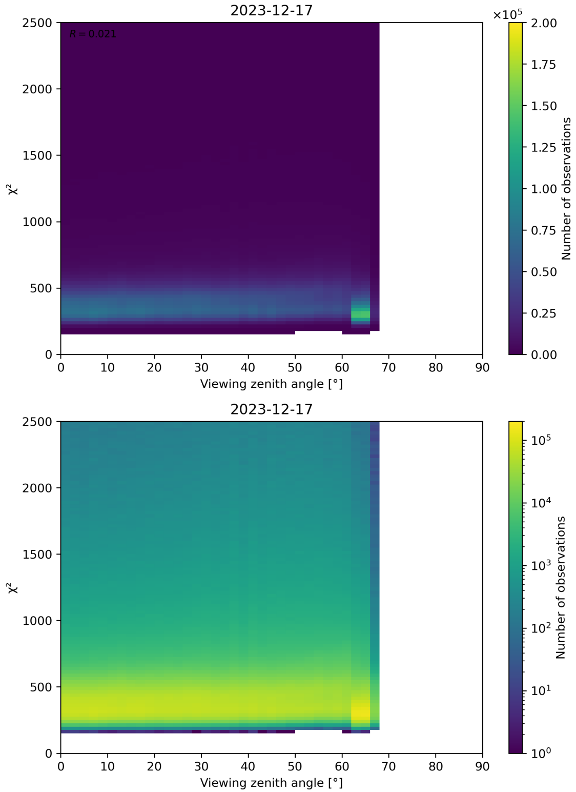
Figure 162: Scatter density plot of “Viewing zenith angle” against “ \chi^2 ” for 2023-12-16 to 2023-12-18.
