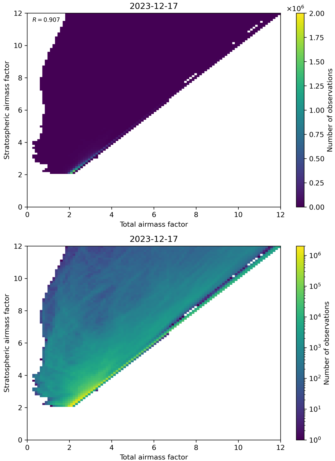
Figure 62: Scatter density plot of “Total airmass factor” against “Stratospheric airmass factor” for 2023-12-16 to 2023-12-18.
