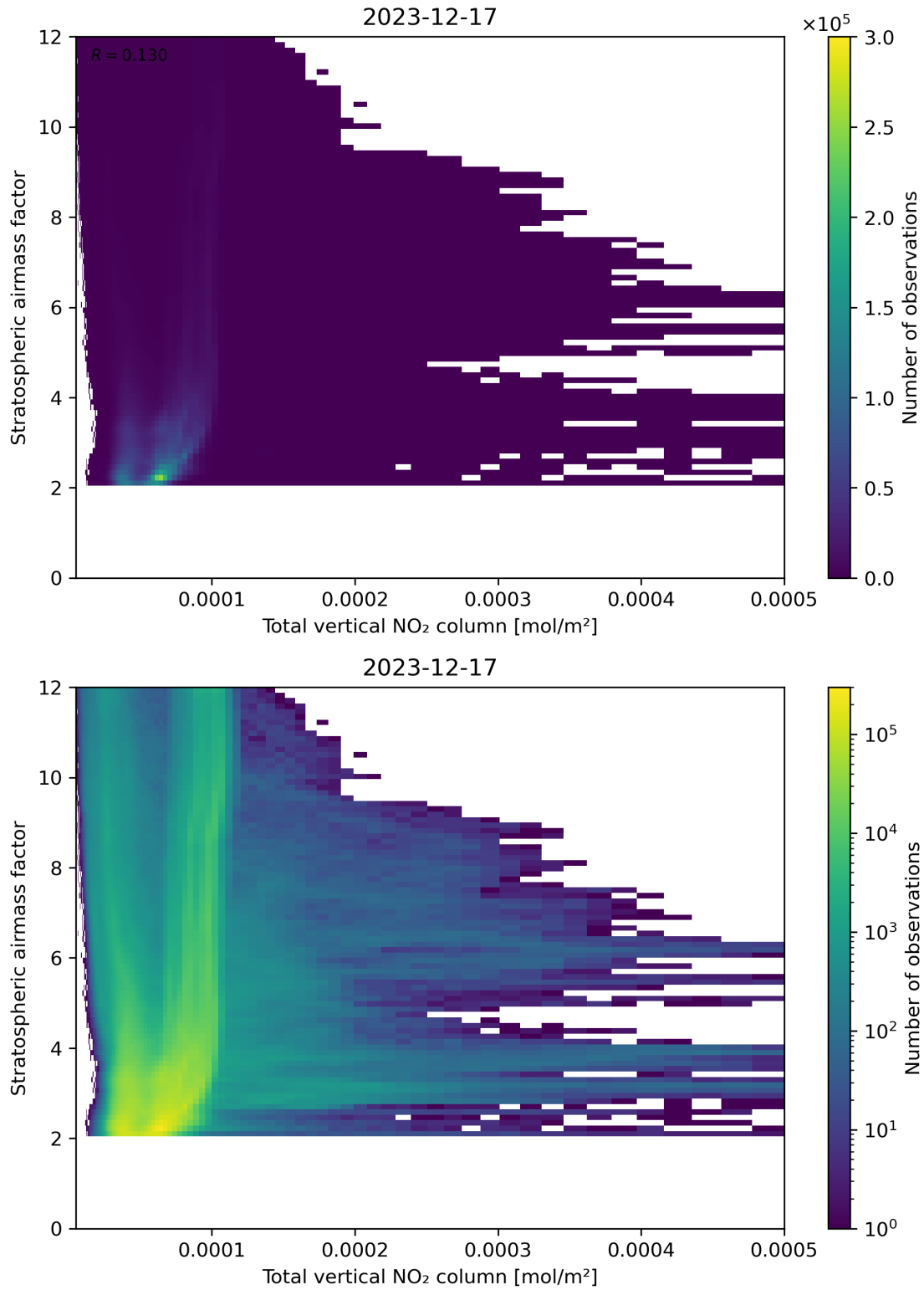
Figure 110: Scatter density plot of “Total vertical NO 2 column” against “Stratospheric air mass factor” for 2023-12-16 to 2023-12-18.
