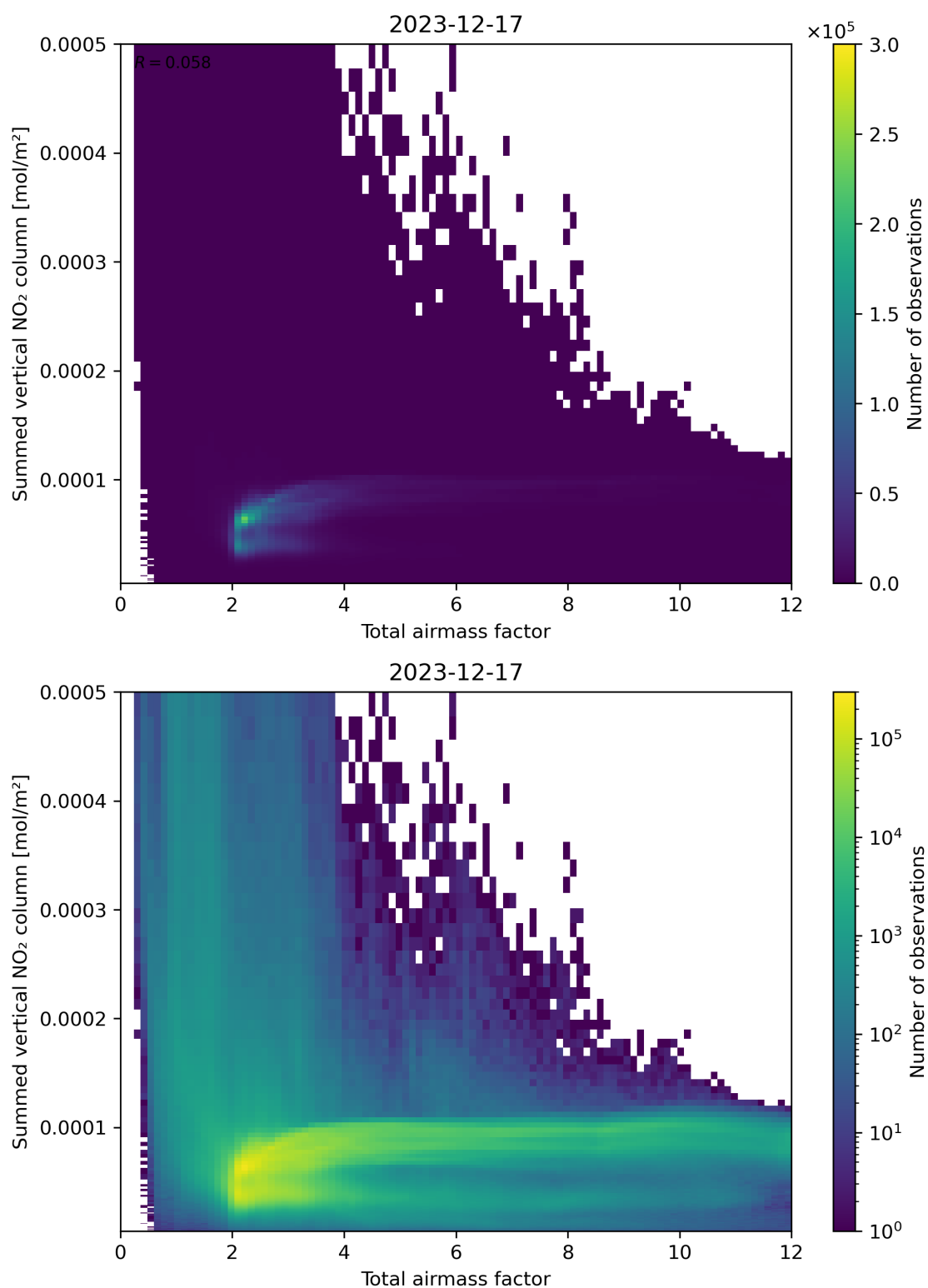
Figure 65: Scatter density plot of “Total airmass factor” against “Summed vertical NO 2 column” for 2023-12-16 to 2023-12-18.
