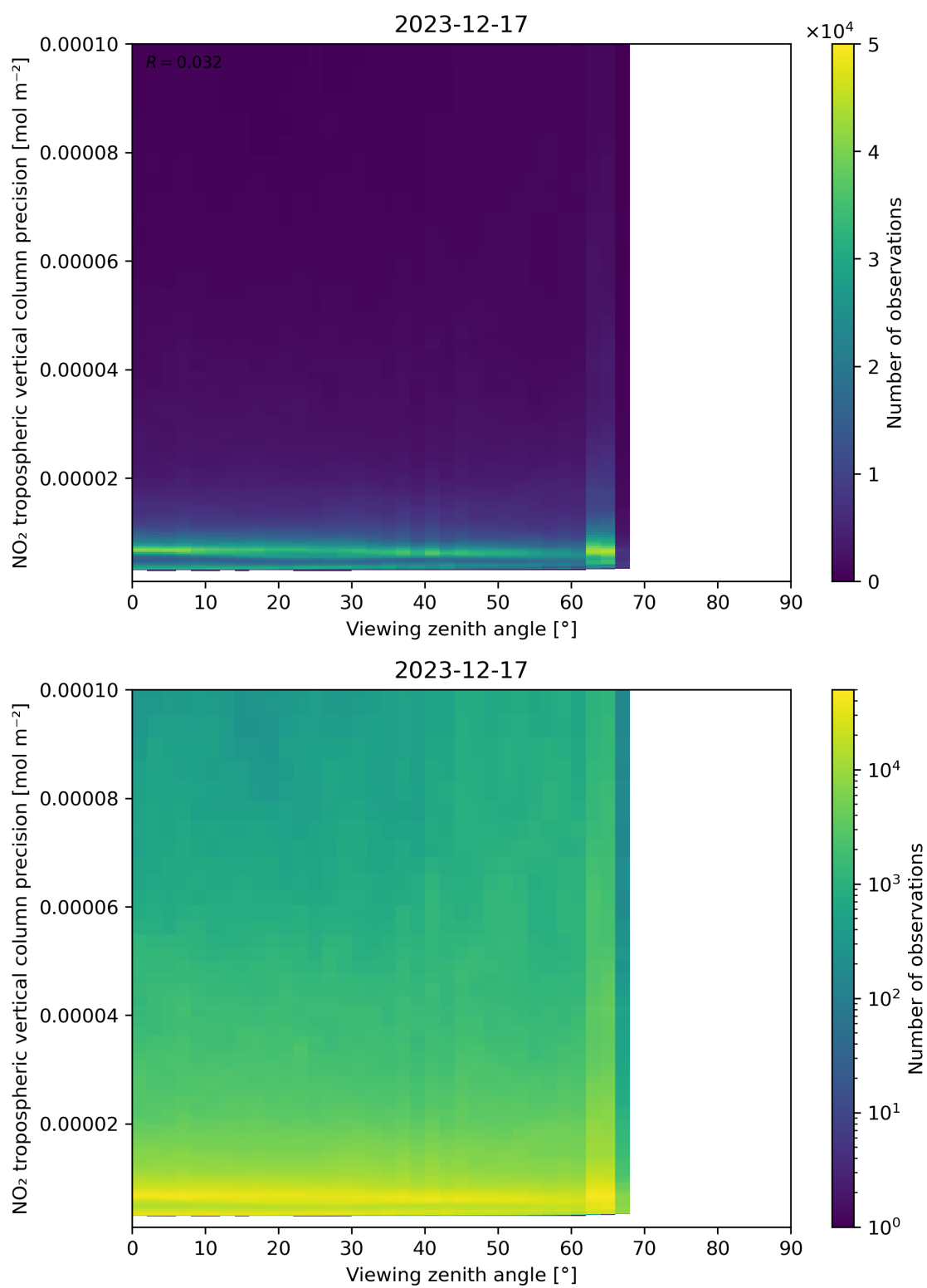
Figure 170: Scatter density plot of “Viewing zenith angle” against “NO 2 tropospheric vertical column precision” for 2023-12-16 to 2023-12-18.
