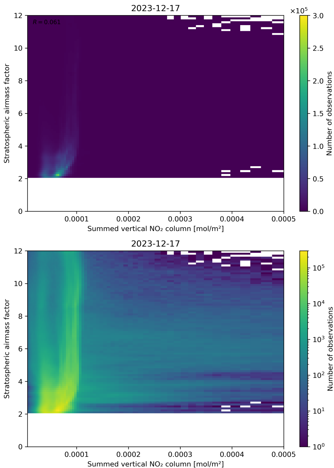
Figure 103: Scatter density plot of “Summed vertical NO 2 column” against “Stratospheric airmass factor” for 2023-12-16 to 2023-12-18.
