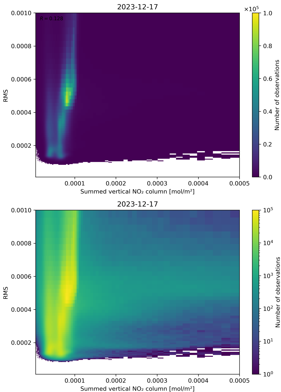
Figure 109: Scatter density plot of “Summed vertical NO 2 column” against “RMS” for 2023-12-16 to 2023-12-18.
