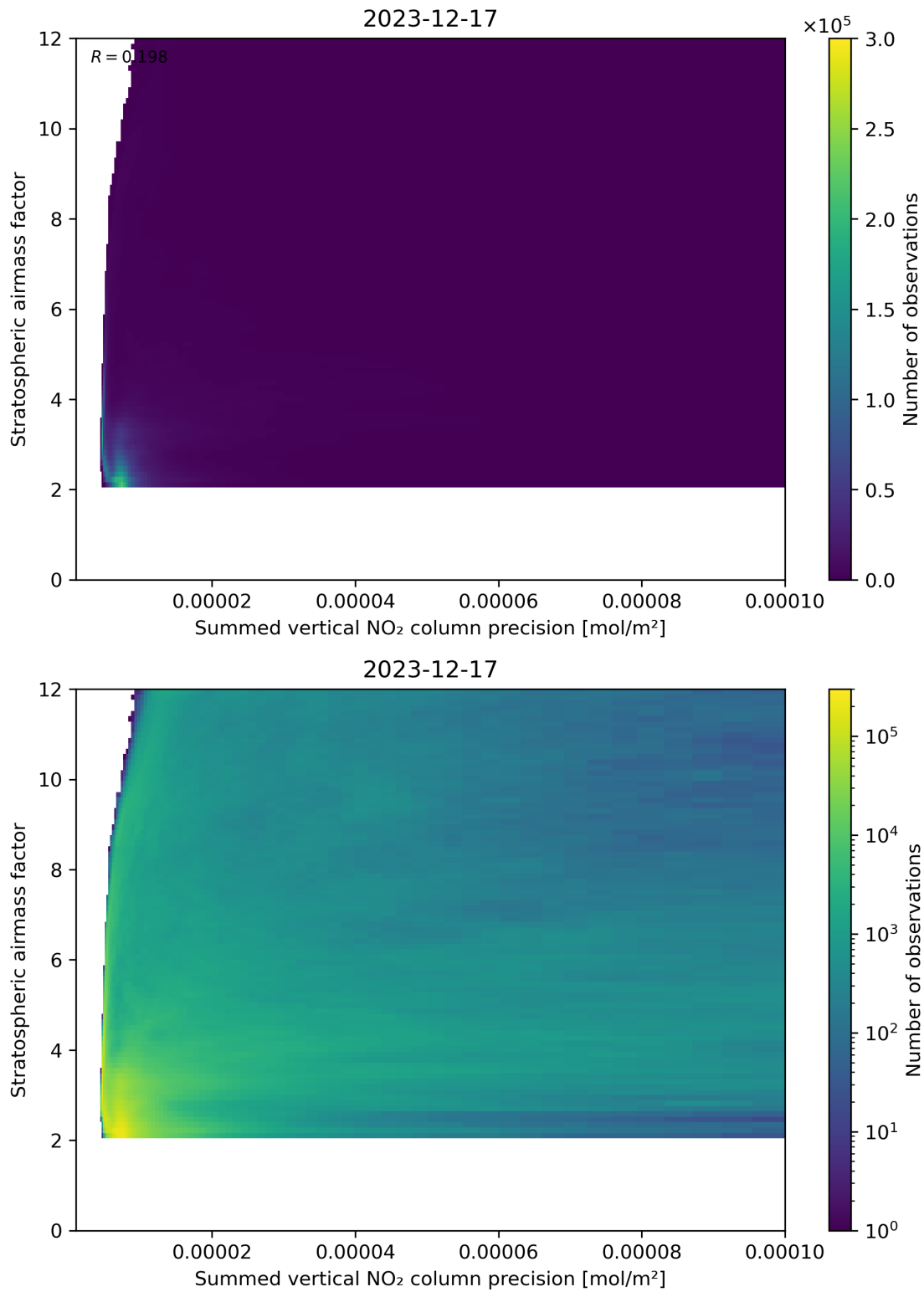
Figure 106: Scatter density plot of “Summed vertical NO 2 column precision” against “Stratospheric airmass factor” for 2023-12-16 to 2023-12-18.
