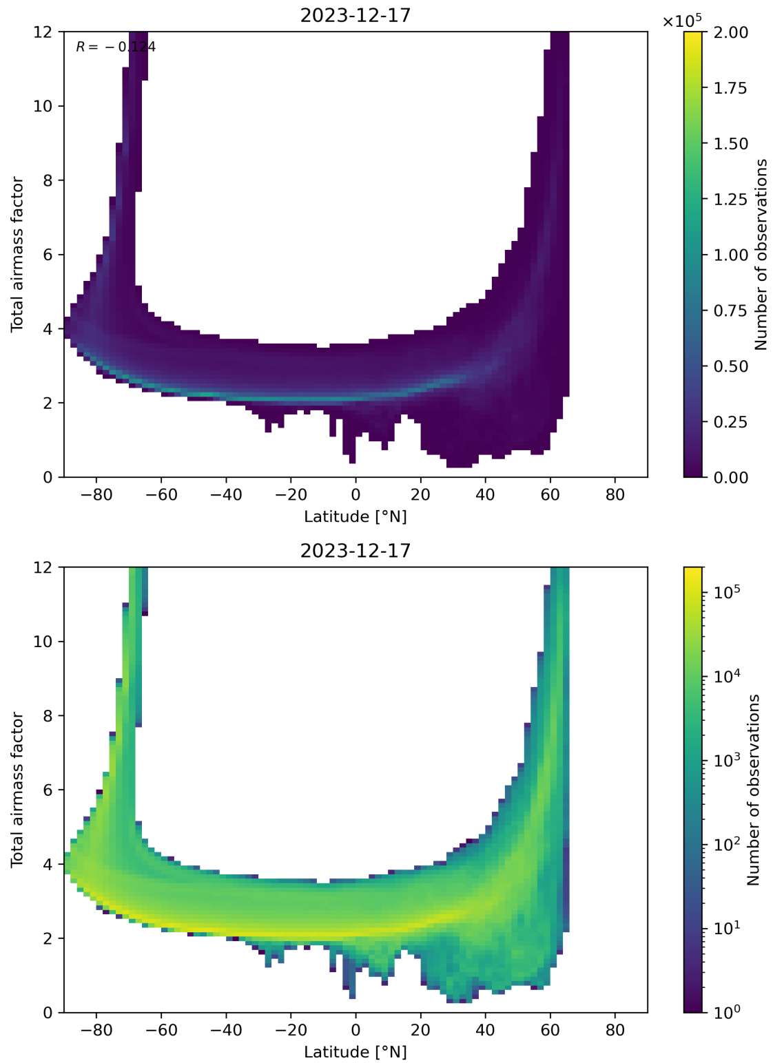
Figure 84: Scatter density plot of “Latitude” against “Total airmass factor” for 2023-12-16 to 2023-12-18.
