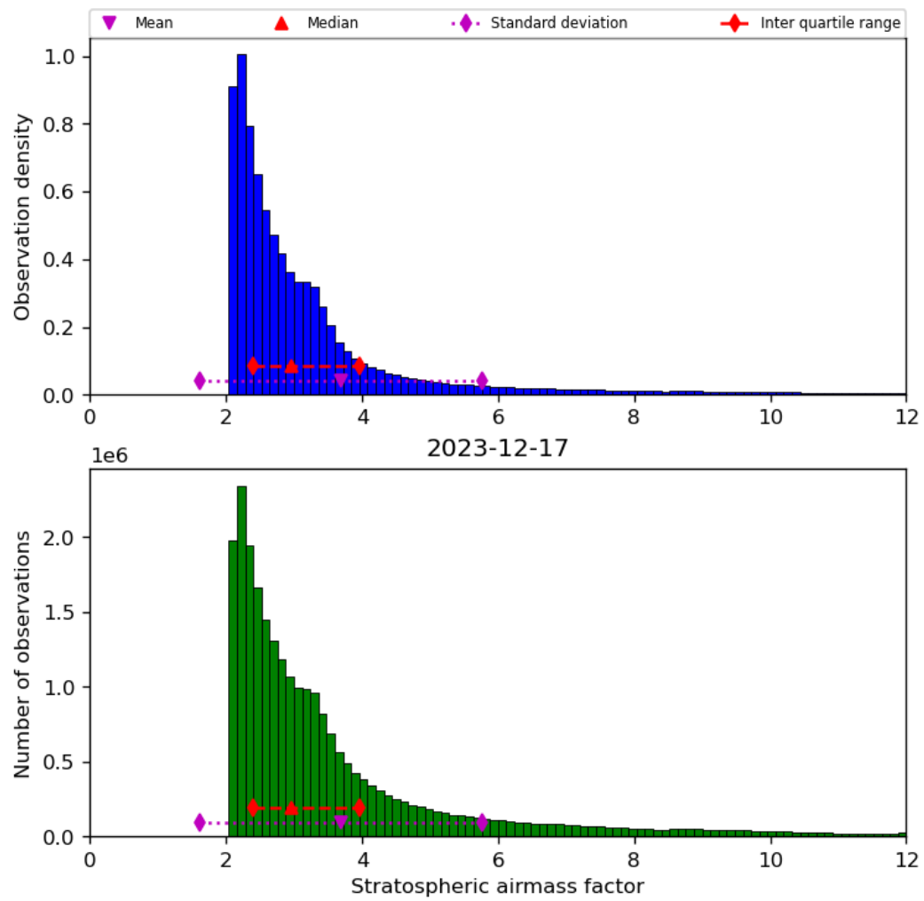
Figure 44: Histogram of “Stratospheric airmass factor” for 2023-12-16 to 2023-12-18
