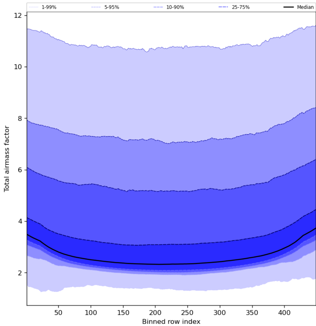
Figure 49: Along track statistics of “Total airmass factor” for 2023-12-16 to 2023-12-18
