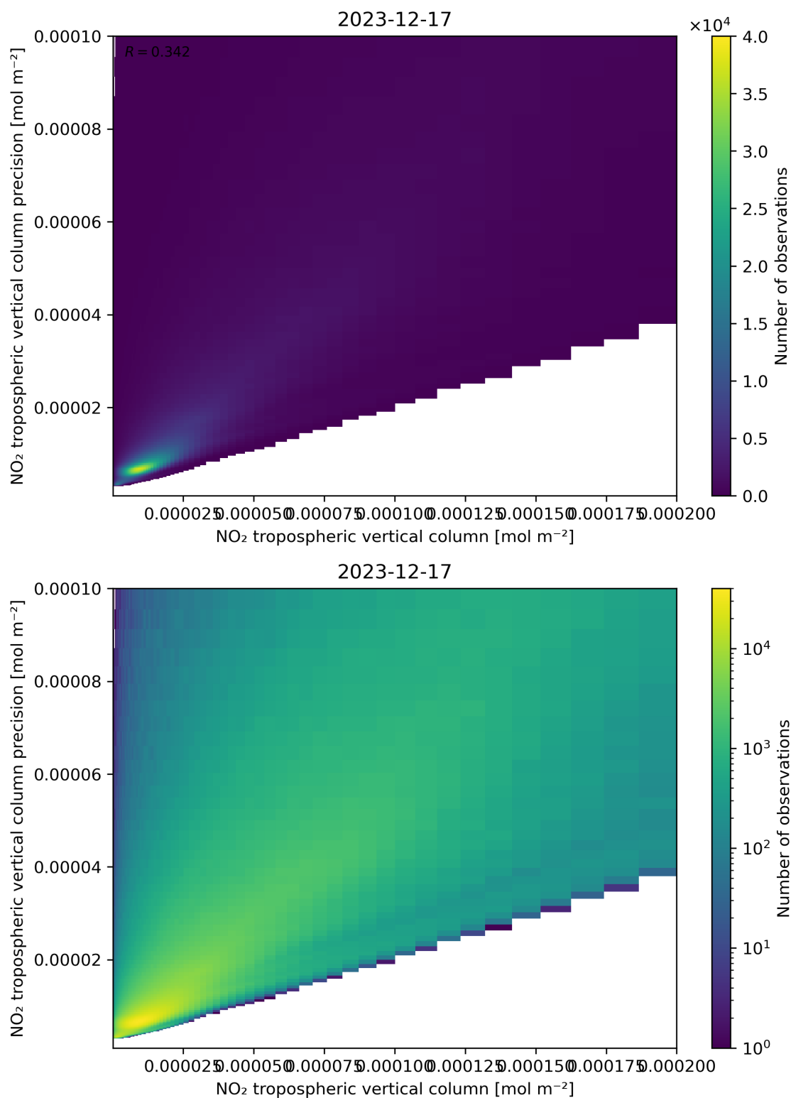
Figure 130: Scatter density plot of “NO 2 tropospheric vertical column” against “NO 2 tropospheric vertical column precision” for 2023-12-16 to 2023-12-18.
