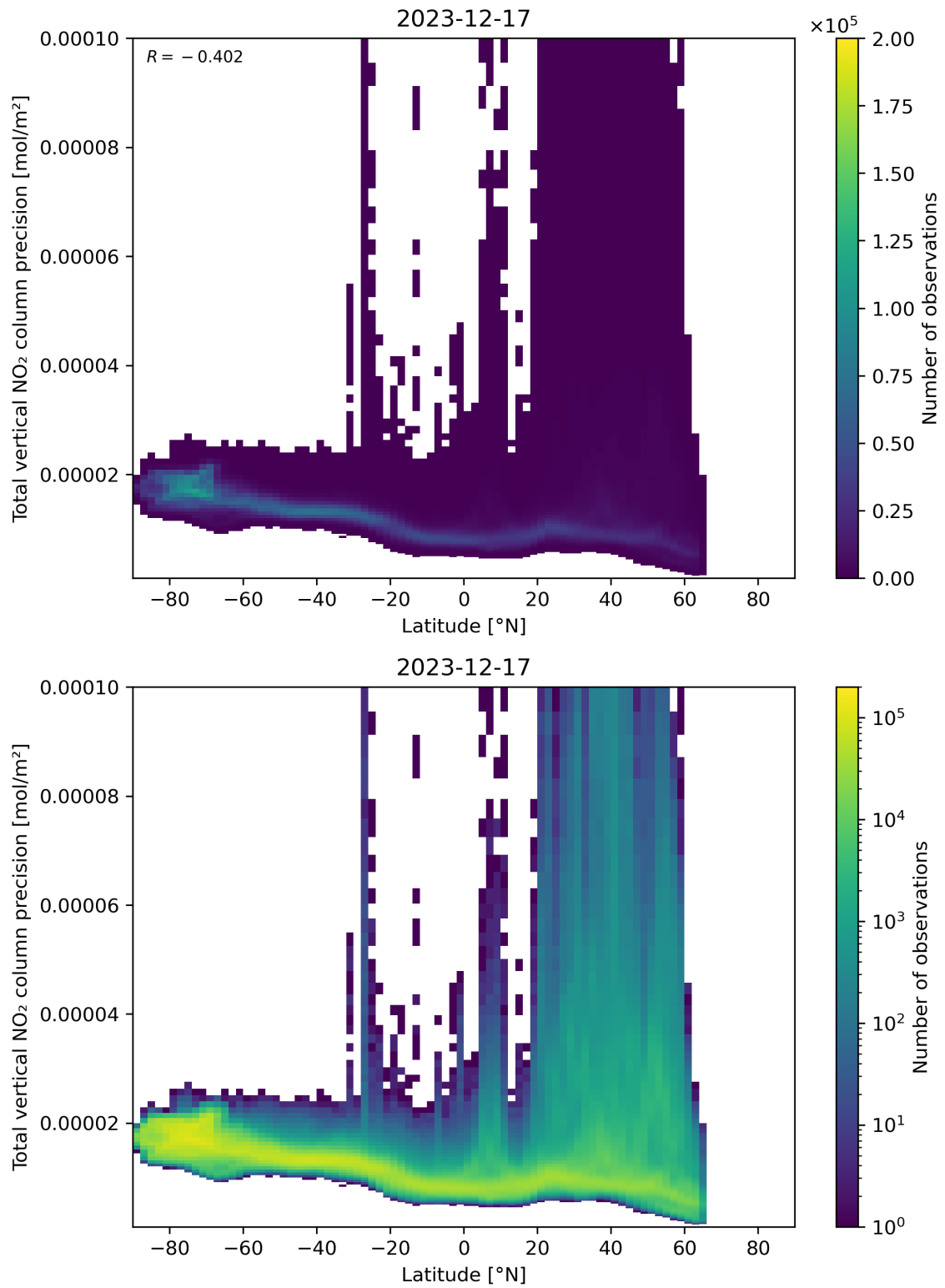
Figure 91: Scatter density plot of “Latitude” against “Total vertical NO 2 column precision” for 2023-12-16 to 2023-12-18.
