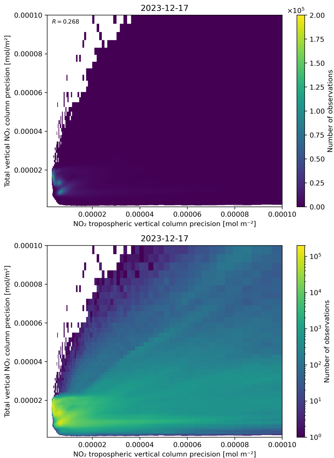
Figure 139: Scatter density plot of “NO 2 tropospheric vertical column precision” against “Total vertical NO 2 column precision” for 2023-12-16 to 2023-12-18.
