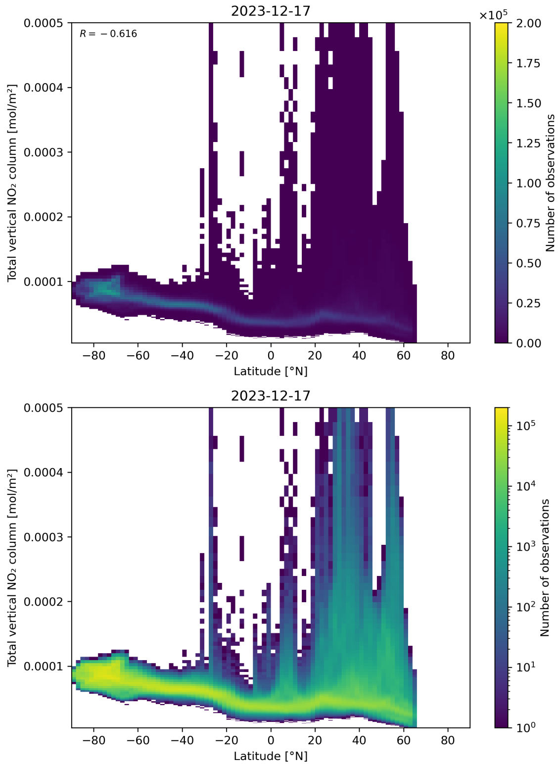
Figure 90: Scatter density plot of “Latitude” against “Total vertical NO 2 column” for 2023-12-16 to 2023-12-18.
