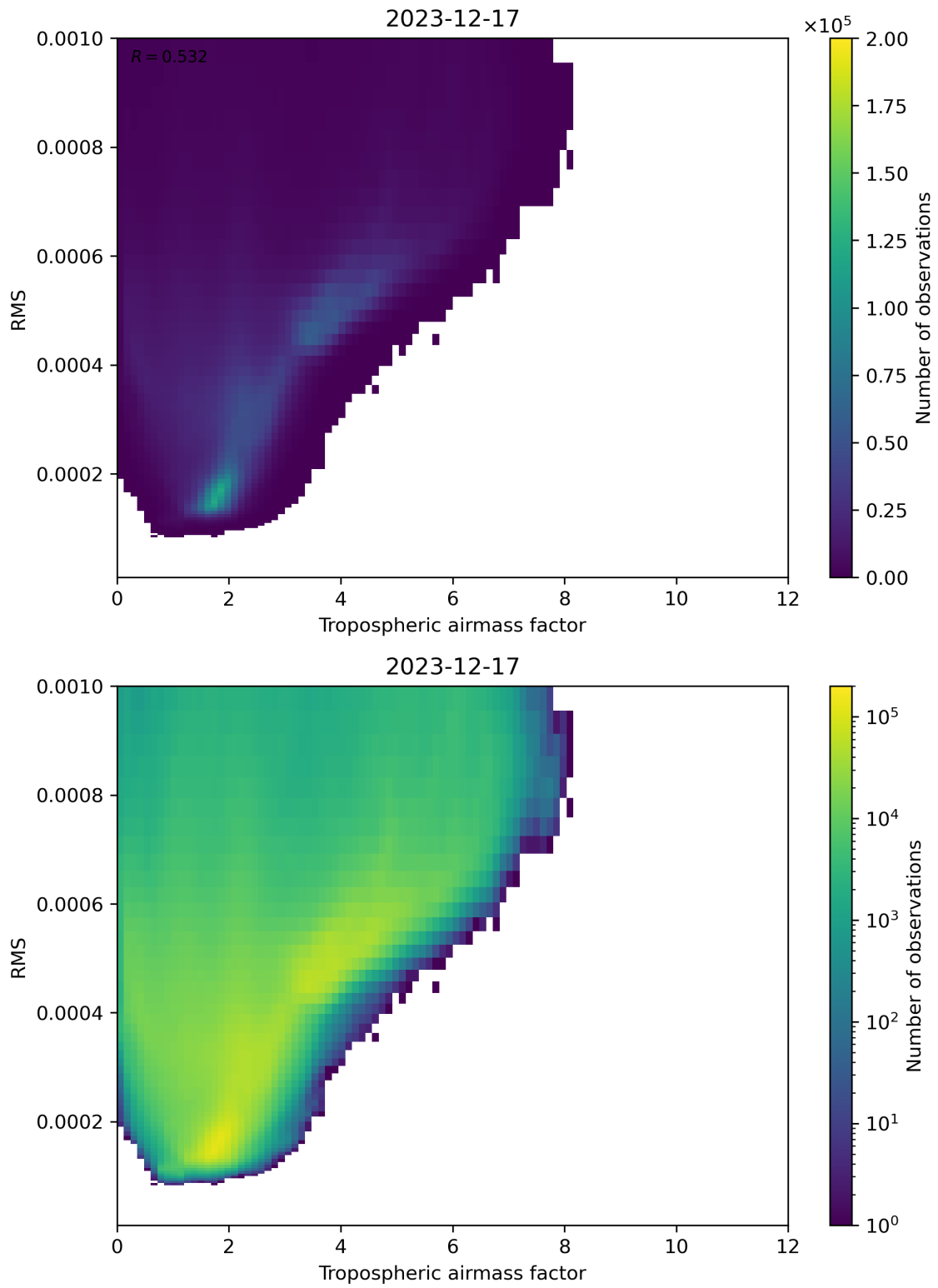
Figure 79: Scatter density plot of “Tropospheric airmass factor” against “RMS” for 2023-12-16 to 2023-12-18.
