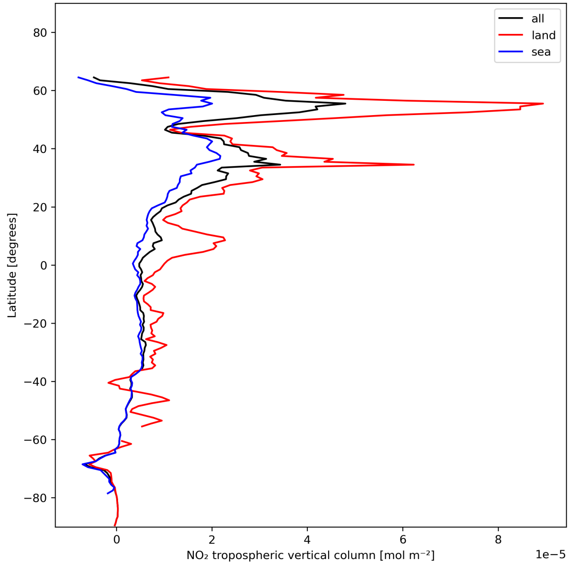
Figure 12: Zonal average of “NO 2 tropospheric vertical column” for 2023-12-16 to 2023-12-18.
