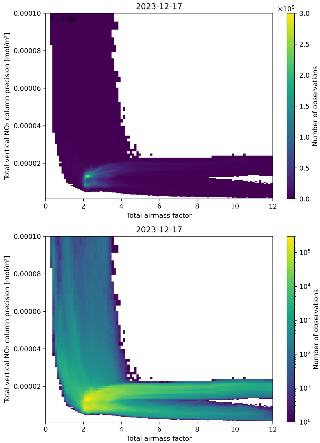
Figure 68: Scatter density plot of “Total airmass factor” against “Total vertical NO 2 column precision” for 2023-12-16 to 2023-12-18.
