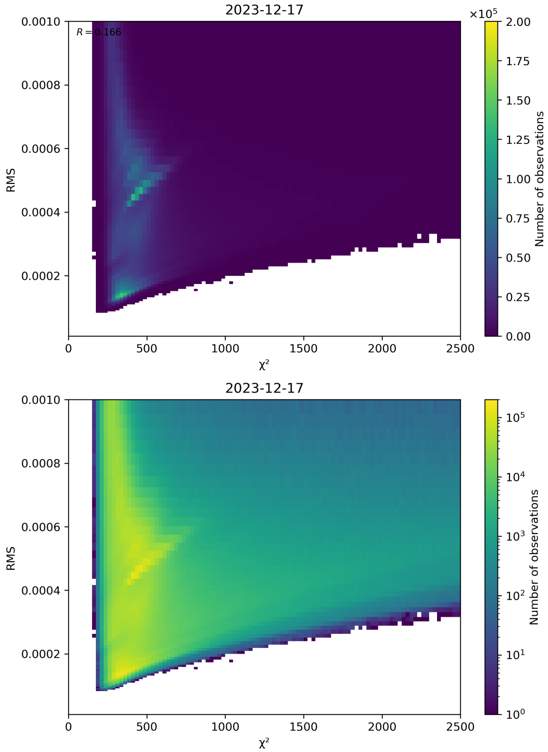
Figure 82: Scatter density plot of “ \chi^2 ” against “RMS” for 2023-12-16 to 2023-12-18.
