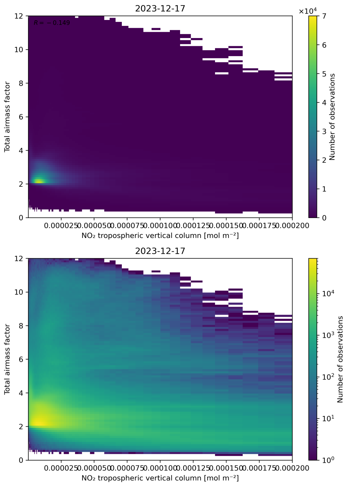
Figure 122: Scatter density plot of “NO 2 tropospheric vertical column” against “Total air mass factor” for 2023-12-16 to 2023-12-18.
