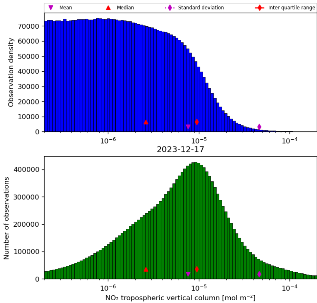
Figure 29: Histogram of “NO 2 tropospheric vertical column” for 2023-12-16 to 2023-12-18
