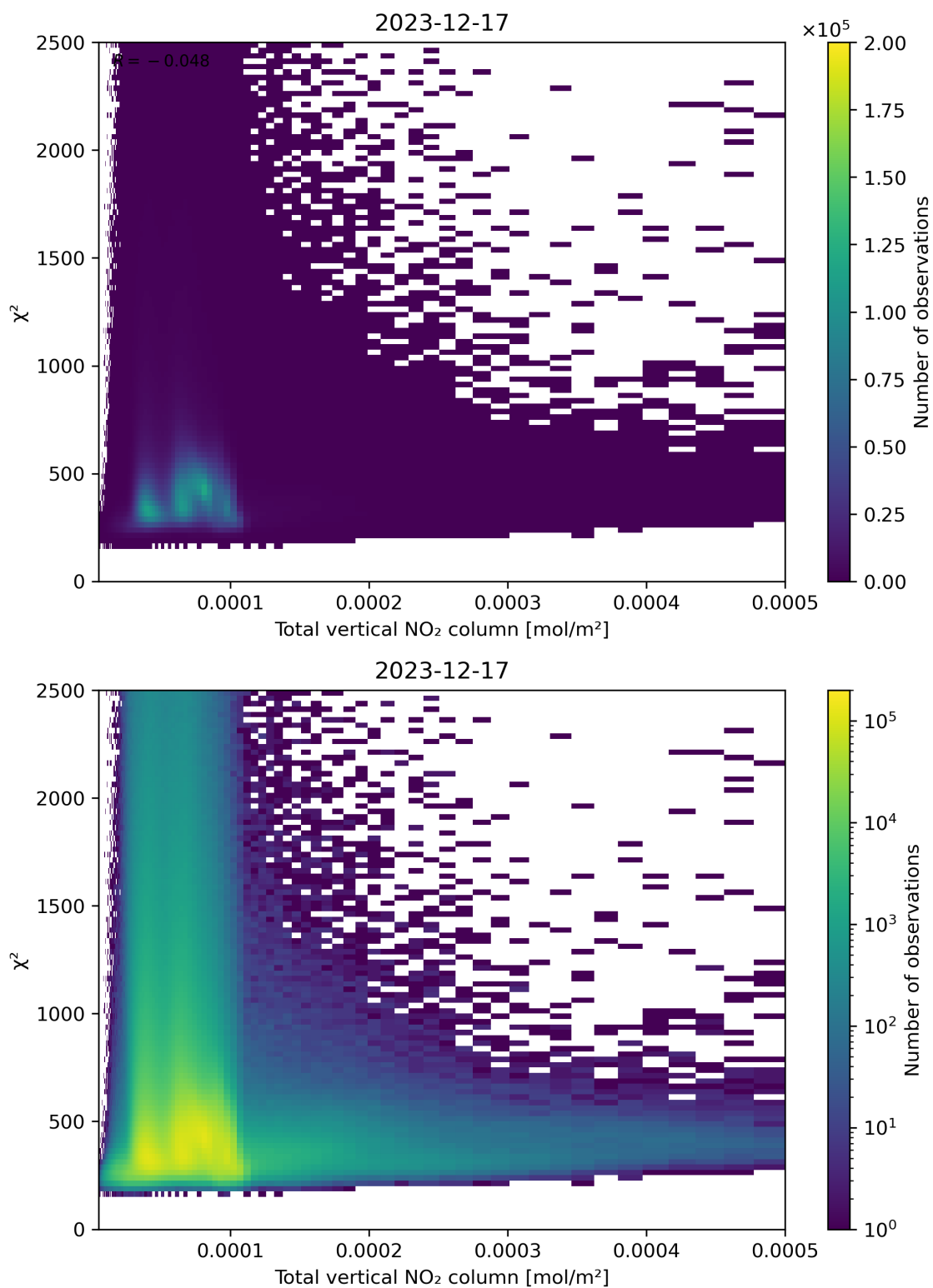
Figure 111: Scatter density plot of “Total vertical NO 2 column” against “ \chi^2 ” for 2023-12-16 to 2023-12-18.
