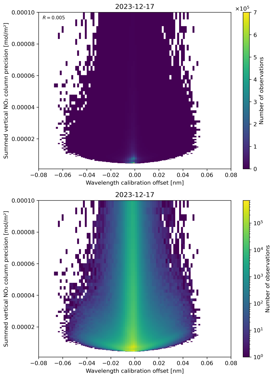
Figure 178: Scatter density plot of “Wavelength calibration offset” against “Summed vertical NO 2 column precision” for 2023-12-16 to 2023-12-18.
