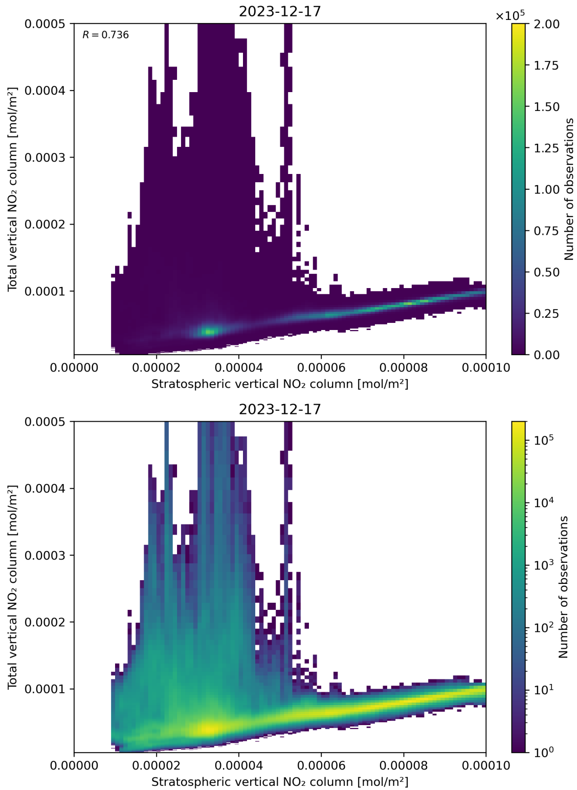
Figure 100: Scatter density plot of “Stratospheric vertical NO 2 column” against “Total vertical NO 2 column” for 2023-12-16 to 2023-12-18.
