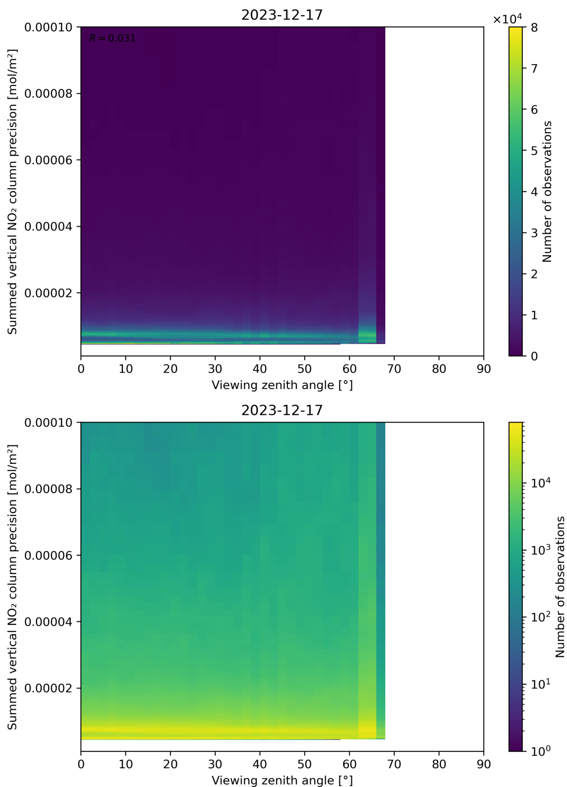
Figure 166: Scatter density plot of “Viewing zenith angle” against “Summed vertical NO 2 column precision” for 2023-12-16 to 2023-12-18.
