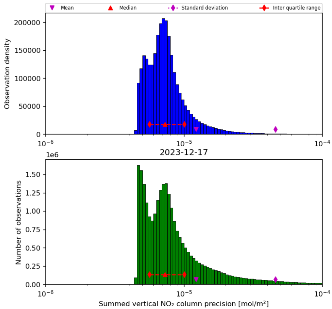
Figure 41: Histogram of “Summed vertical NO 2 column precision” for 2023-12-16 to 2023-12-18
