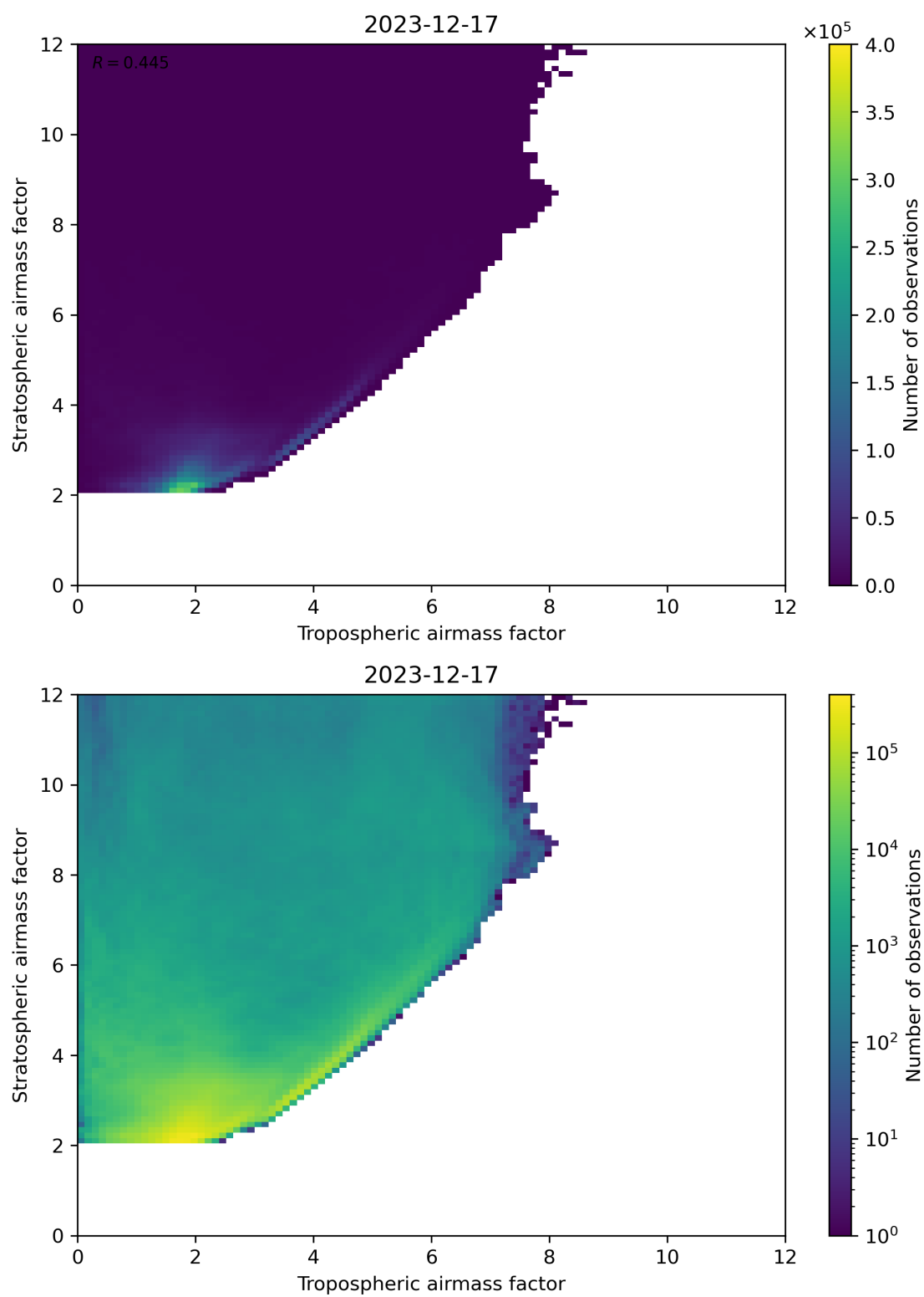
Figure 71: Scatter density plot of “Tropospheric airmass factor” against “Stratospheric airmass factor” for 2023-12-16 to 2023-12-18.
