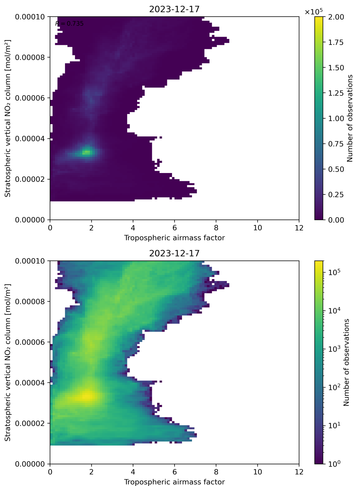
Figure 74: Scatter density plot of “Tropospheric air mass factor” against “Stratospheric vertical NO 2 column” for 2023-12-16 to 2023-12-18.
