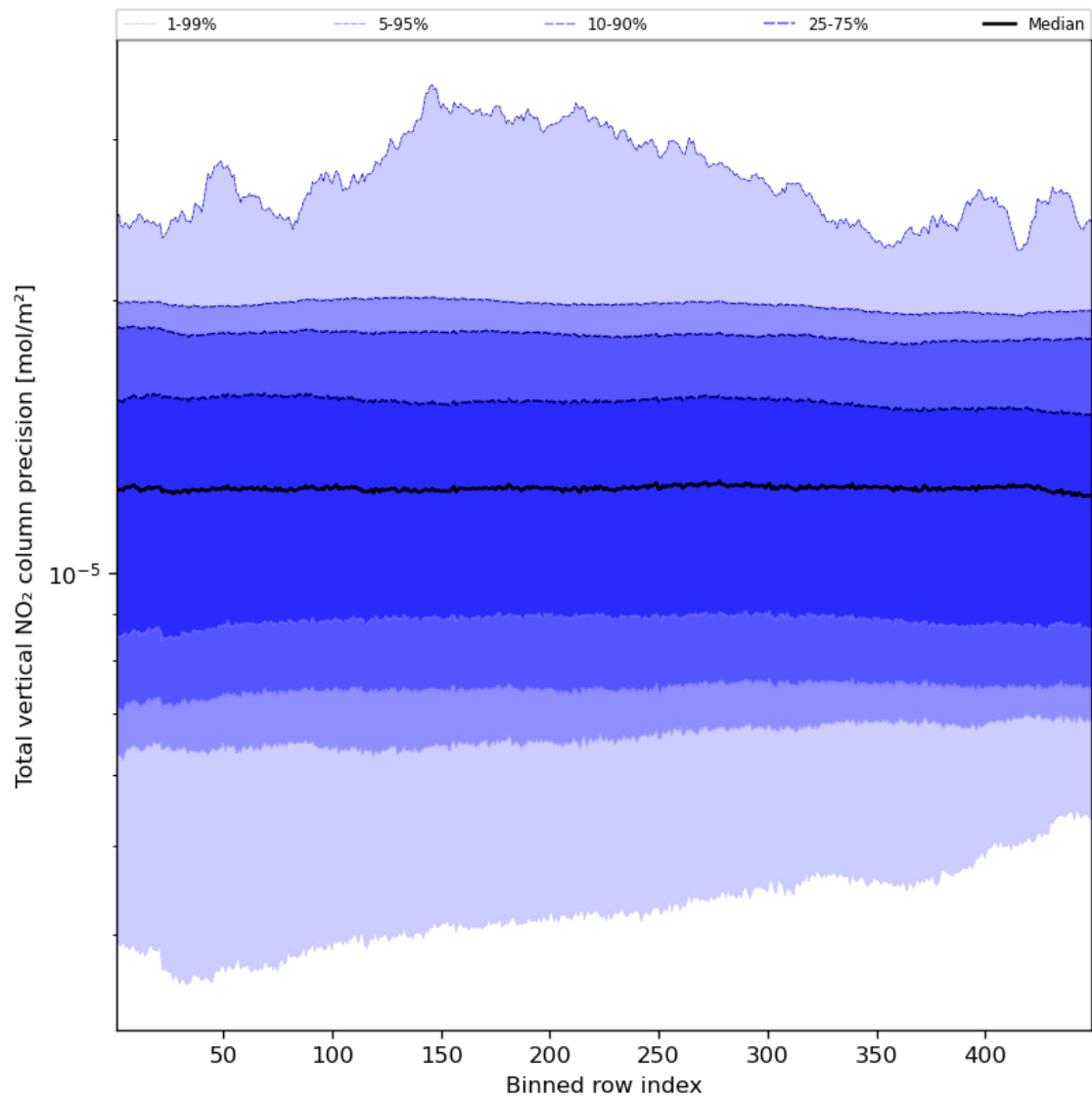
Figure 56: Along track statistics of “Total vertical NO 2 column precision” for 2023-12-16 to 2023-12-18
