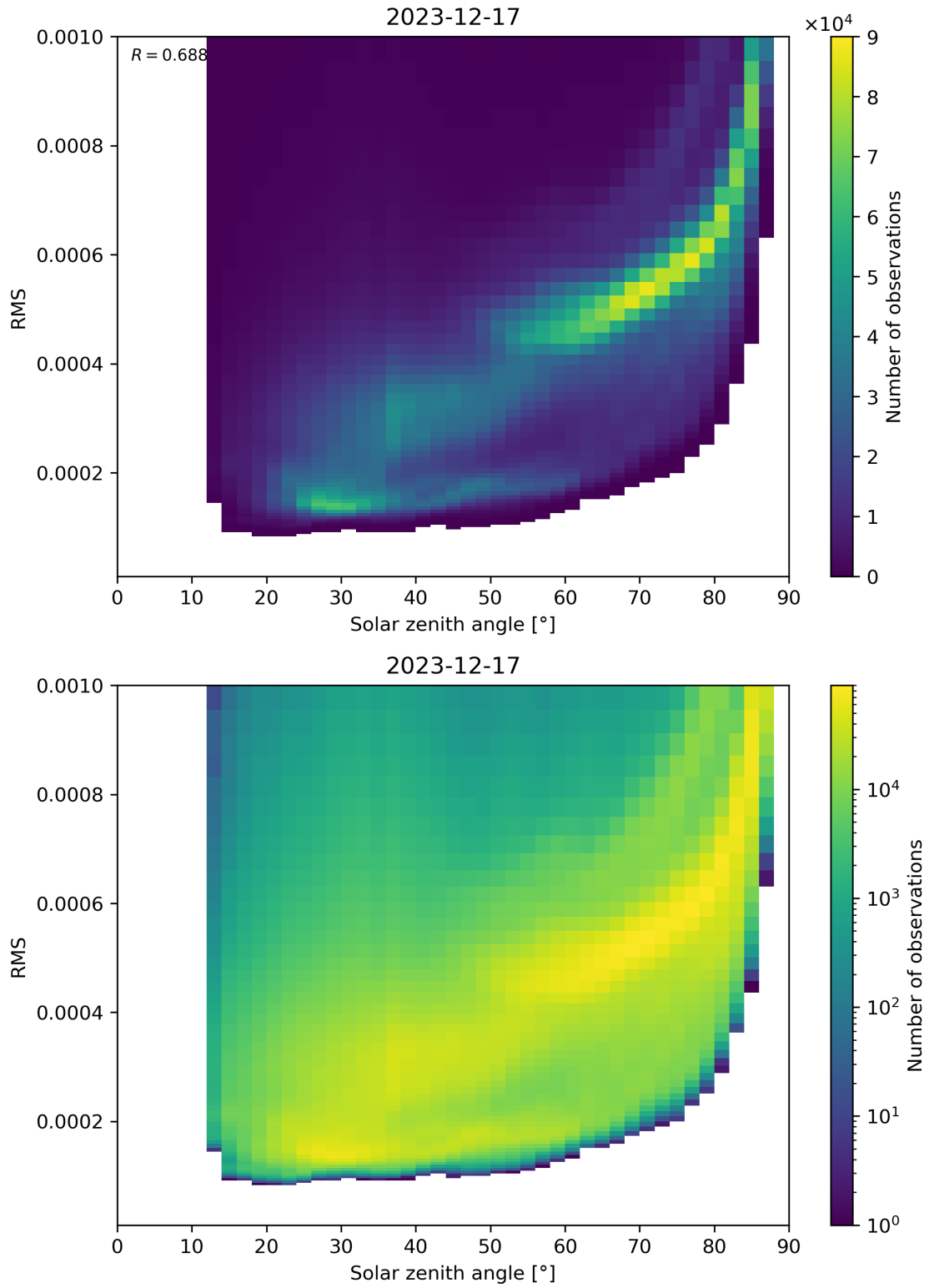
Figure 157: Scatter density plot of “Solar zenith angle” against “RMS” for 2023-12-16 to 2023-12-18.
