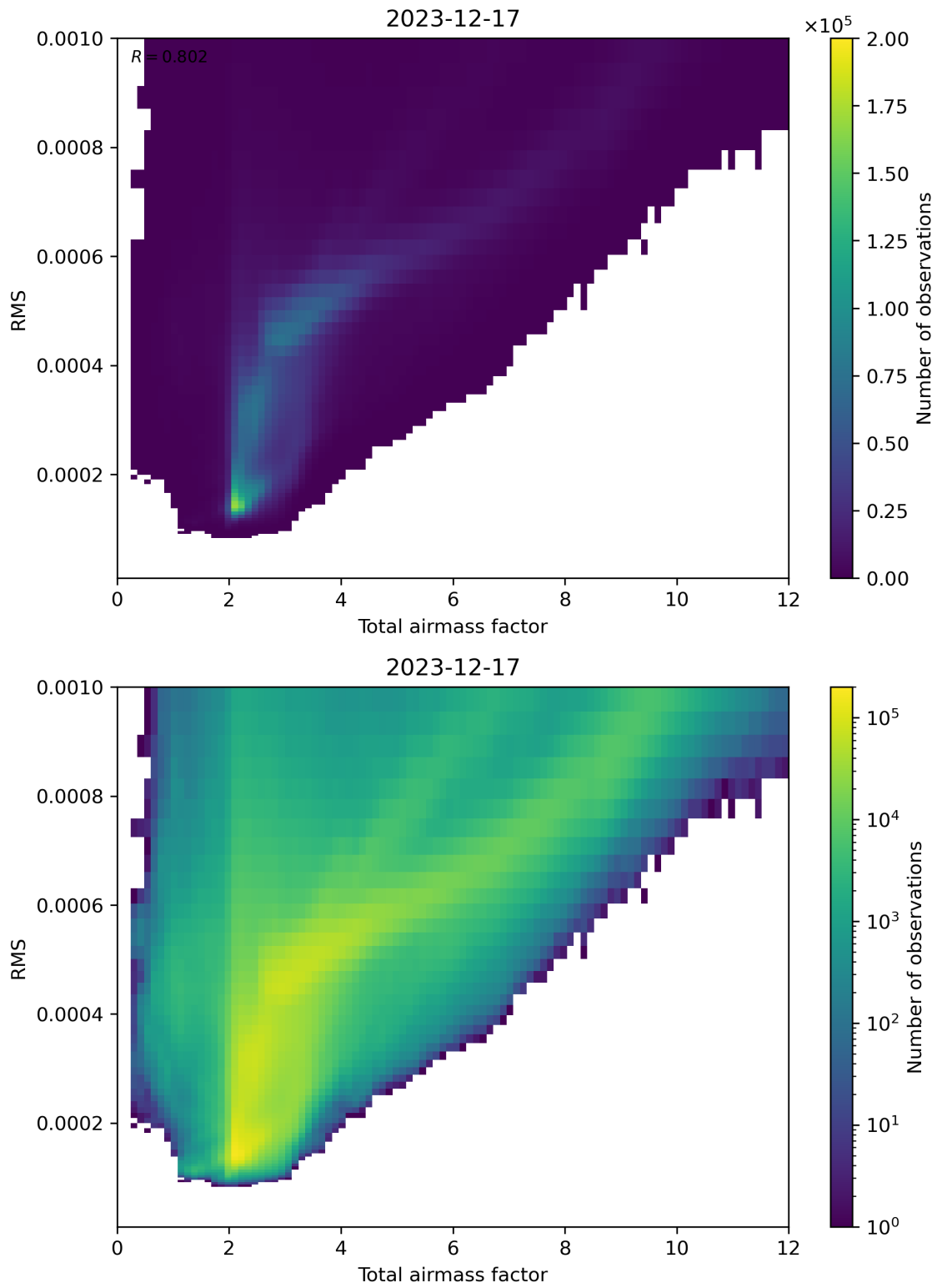
Figure 69: Scatter density plot of “Total airmass factor” against “RMS” for 2023-12-16 to 2023-12-18.
