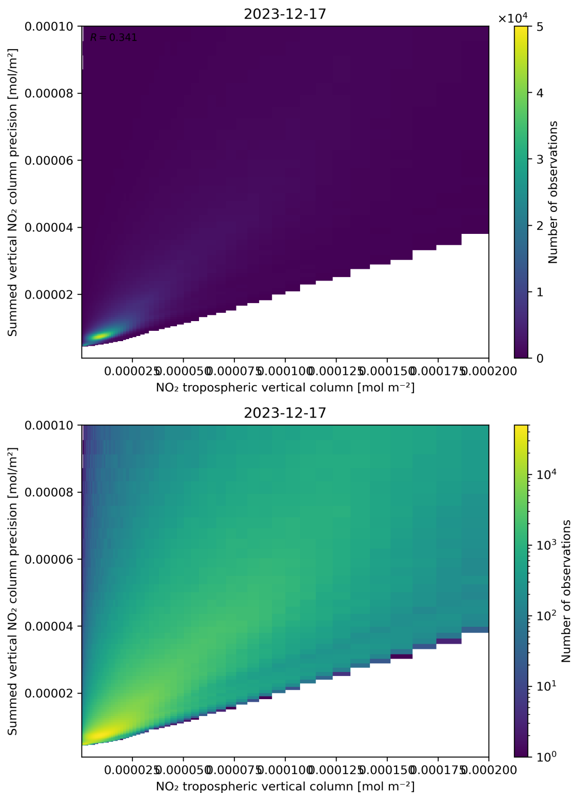
Figure 127: Scatter density plot of “NO 2 tropospheric vertical column” against “Summed vertical NO 2 column precision” for 2023-12-16 to 2023-12-18.
