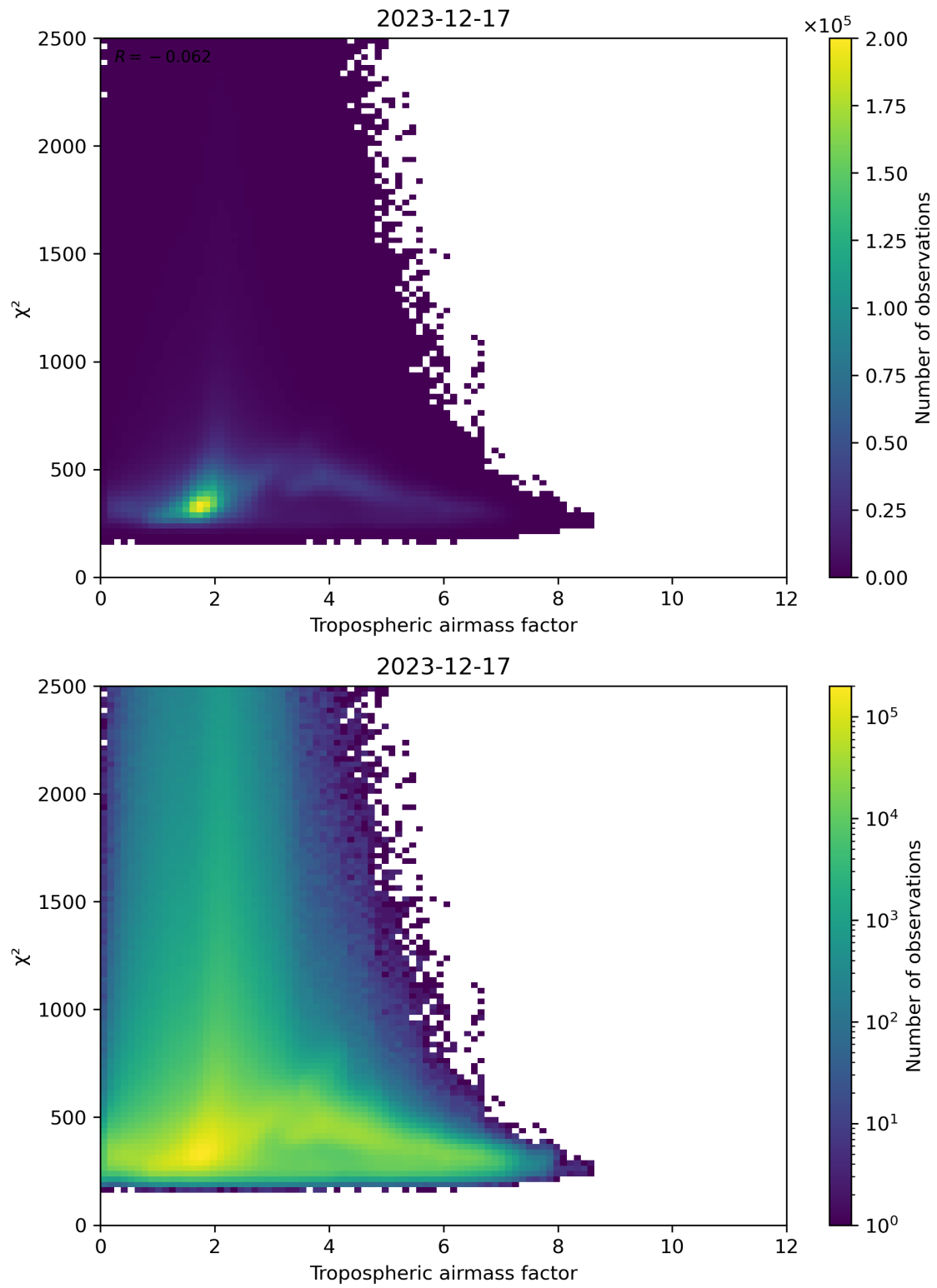
Figure 73: Scatter density plot of “Tropospheric airmass factor” against “ \chi^2 ” for 2023-12-16 to 2023-12-18.
