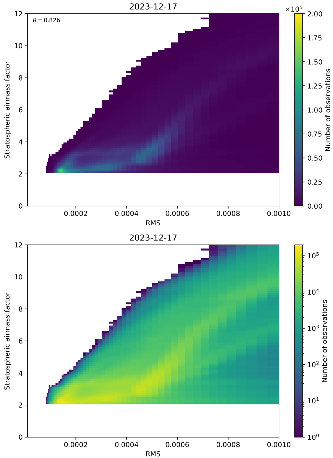
Figure 144: Scatter density plot of “RMS” against “Stratospheric airmass factor” for 2023-12-16 to 2023-12-18.
