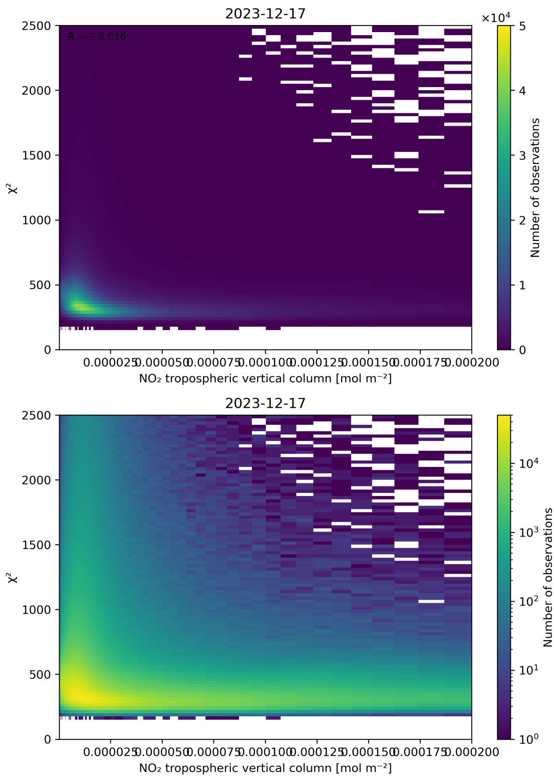
Figure 124: Scatter density plot of “NO 2 tropospheric vertical column” against “ \chi^2 ” for 2023-12-16 to 2023-12-18.
