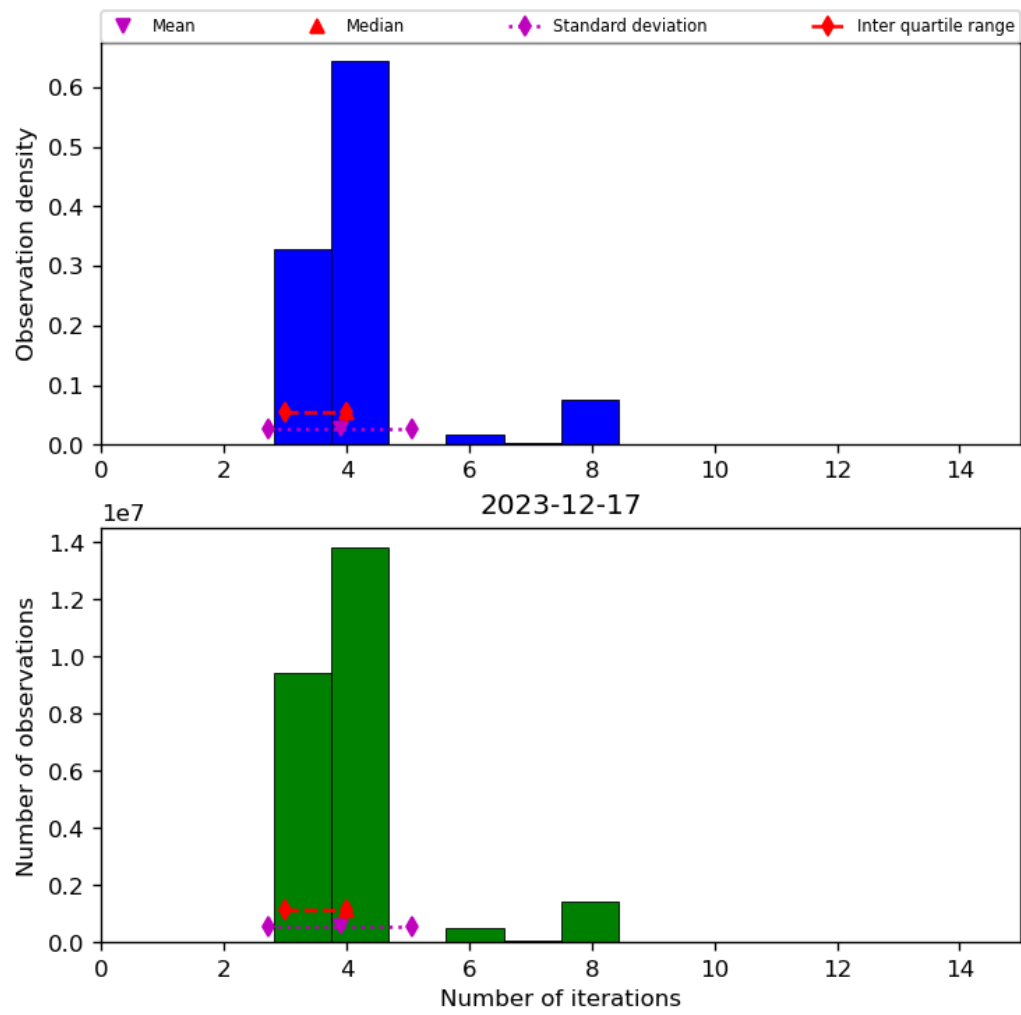
Figure 34: Histogram of “Number of iterations” for 2023-12-16 to 2023-12-18
