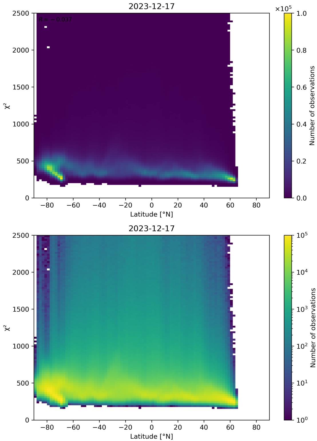
Figure 86: Scatter density plot of “Latitude” against “ \chi^2 ” for 2023-12-16 to 2023-12-18.
