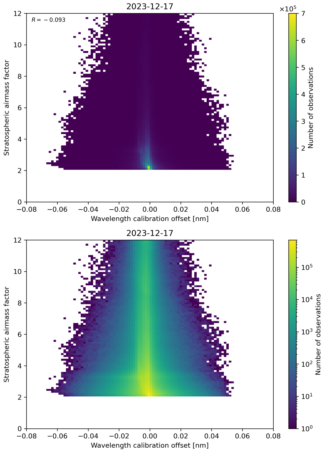
Figure 174: Scatter density plot of “Wavelength calibration offset” against “Stratospheric air mass factor” for 2023-12-16 to 2023-12-18.
