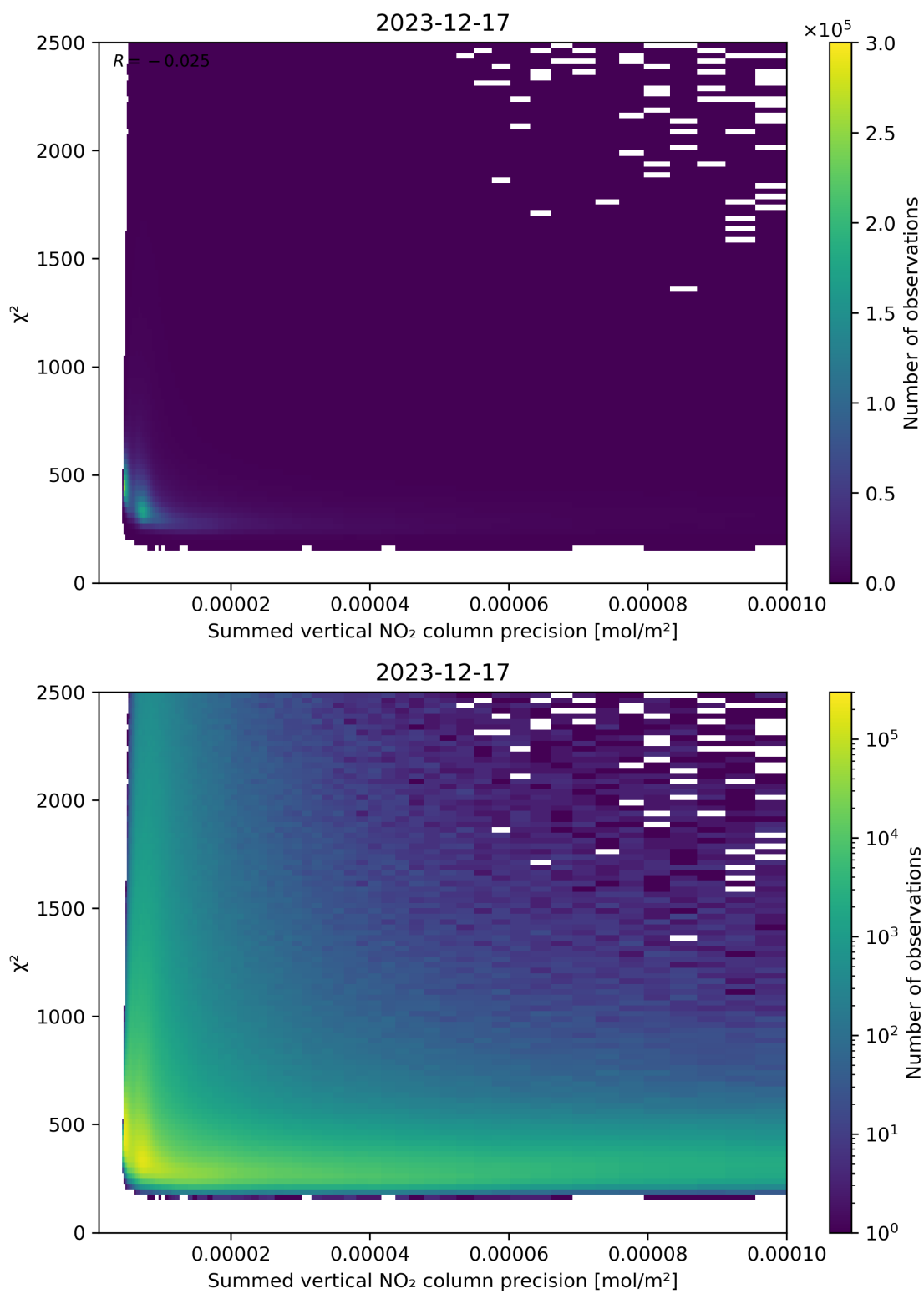
Figure 107: Scatter density plot of “Summed vertical NO 2 column precision” against “ \chi^2 ” for 2023-12-16 to 2023-12-18.
