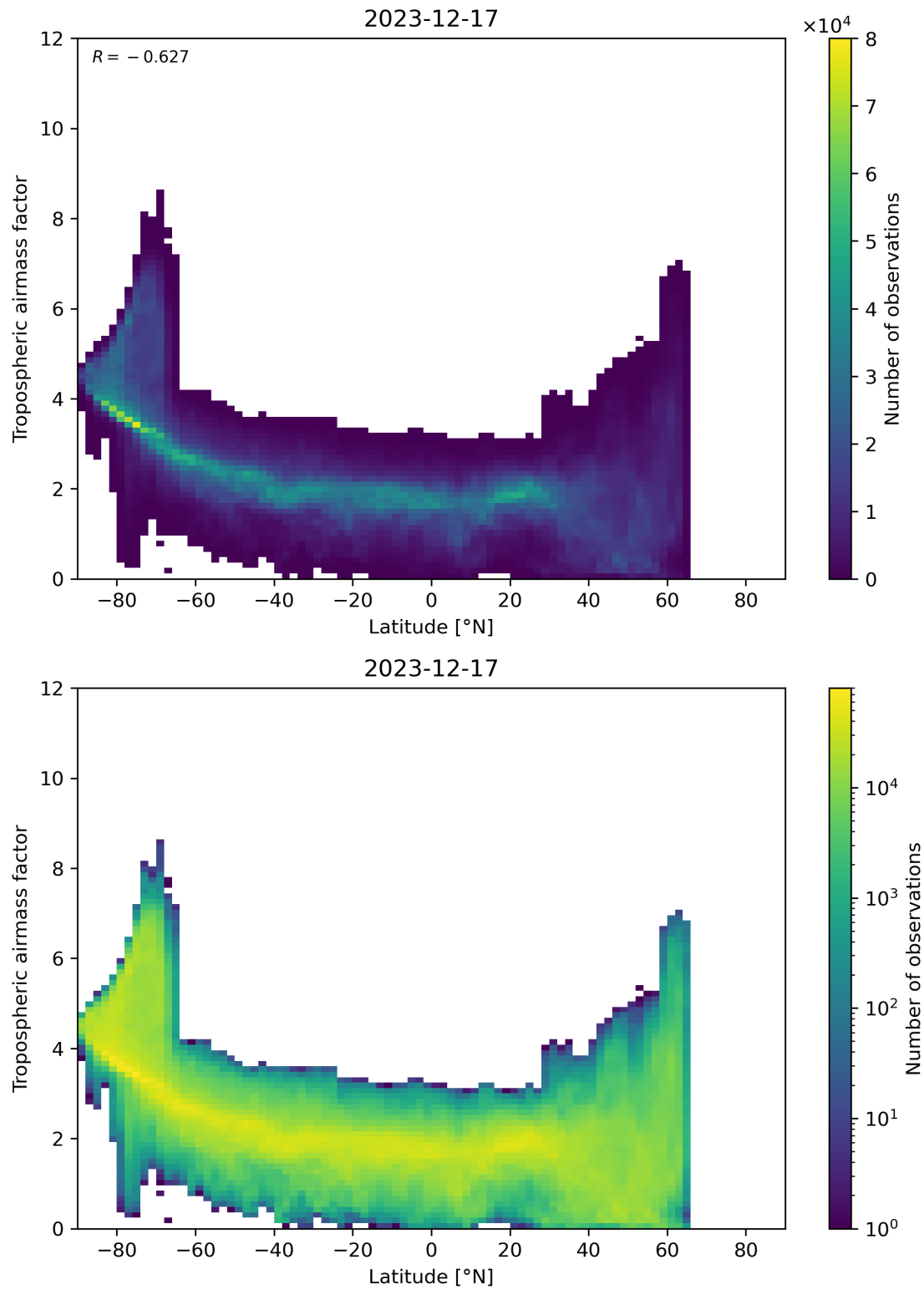
Figure 85: Scatter density plot of “Latitude” against “Tropospheric air mass factor” for 2023-12-16 to 2023-12-18.
