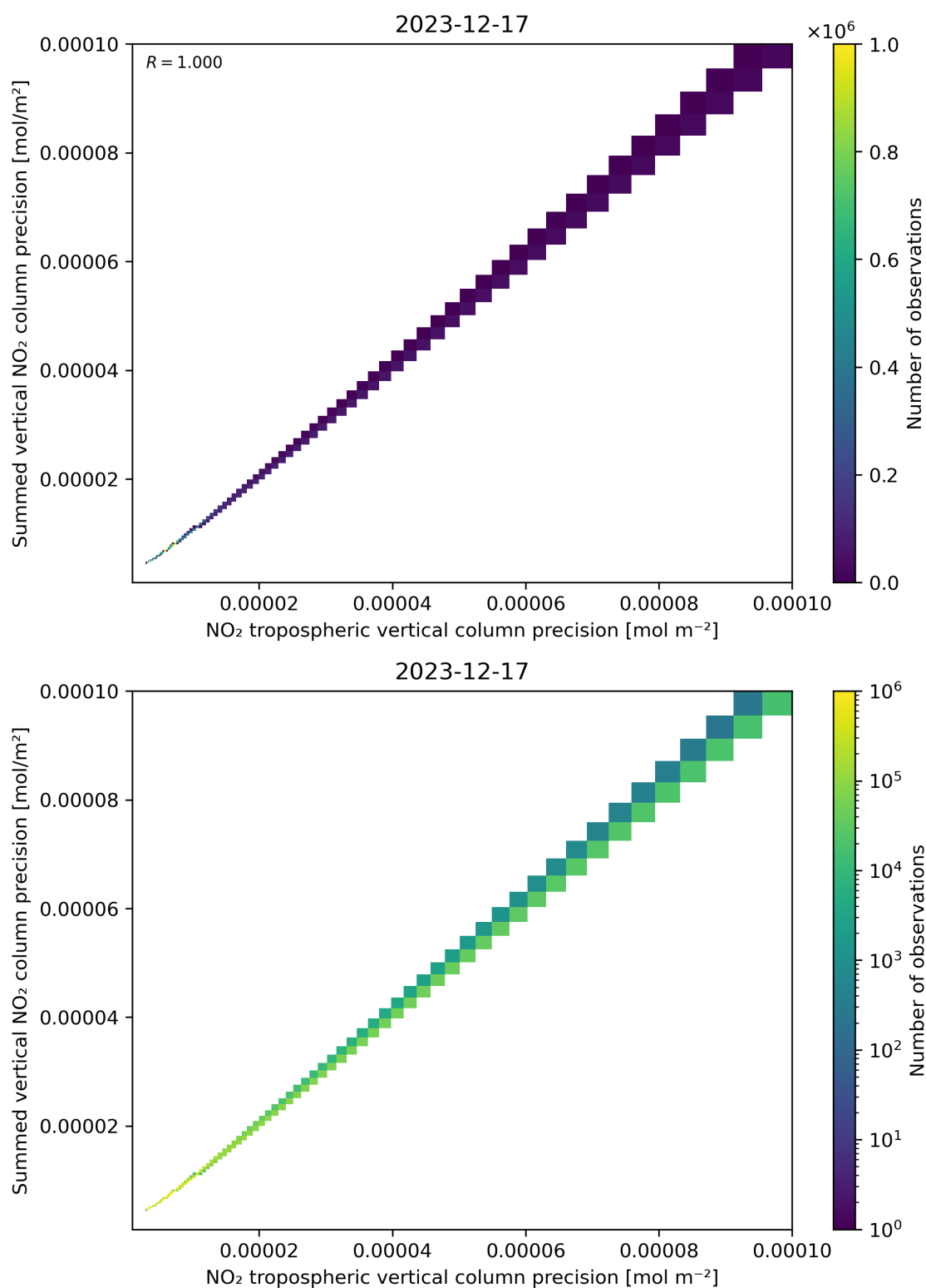
Figure 137: Scatter density plot of “NO 2 tropospheric vertical column precision” against “Summed vertical NO 2 column precision” for 2023-12-16 to 2023-12-18.
