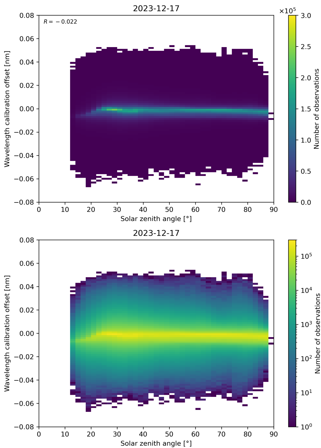
Figure 158: Scatter density plot of “Solar zenith angle” against “Wavelength calibration offset” for 2023-12-16 to 2023-12-18.
