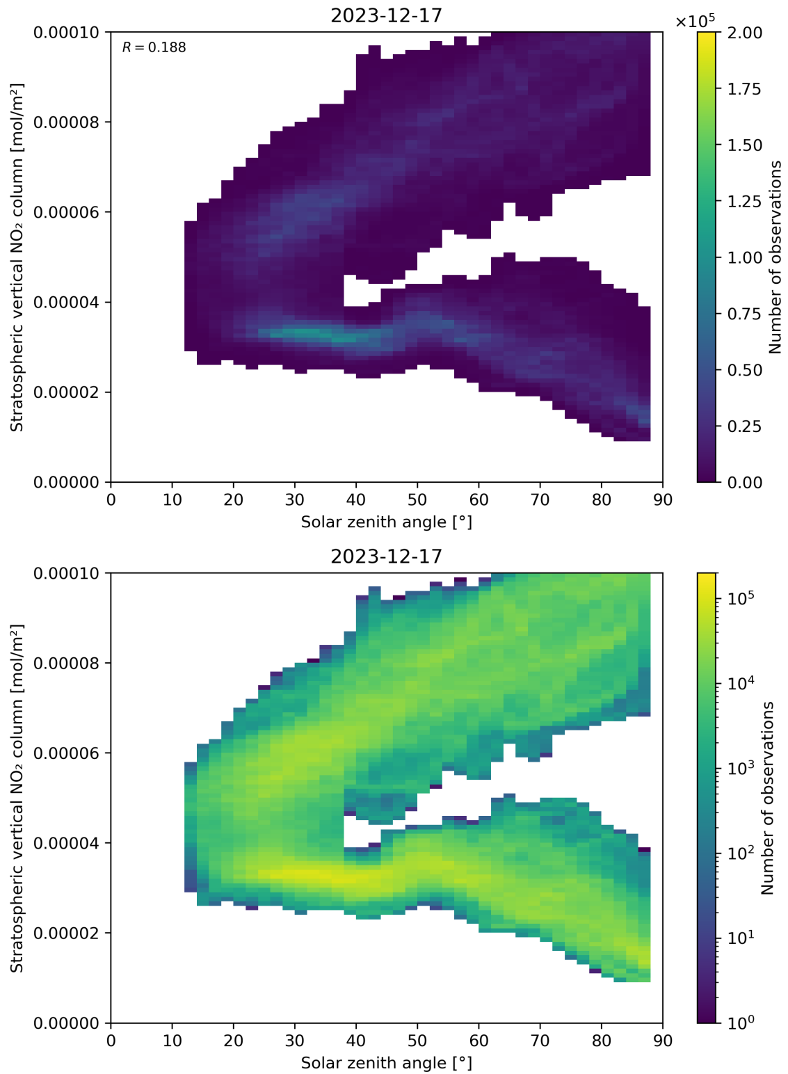
Figure 150: Scatter density plot of “Solar zenith angle” against “Stratospheric vertical NO 2 column” for 2023-12-16 to 2023-12-18.
