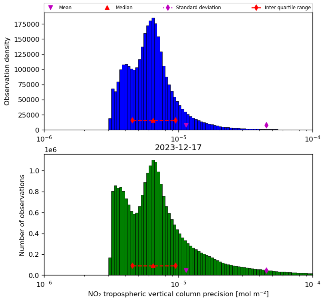
Figure 30: Histogram of “NO 2 tropospheric vertical column precision” for 2023-12-16 to 2023-12-18
