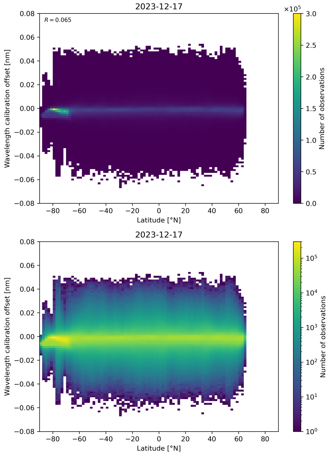
Figure 95: Scatter density plot of “Latitude” against “Wavelength calibration offset” for 2023-12-16 to 2023-12-18.
