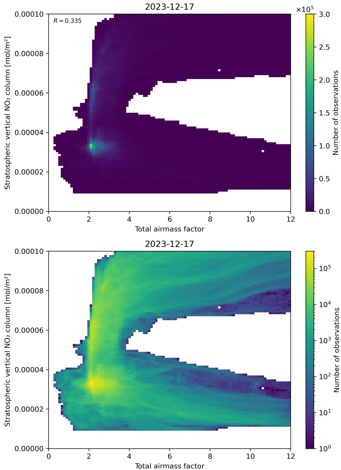
Figure 64: Scatter density plot of “Total airmass factor” against “Stratospheric vertical NO 2 column” for 2023-12-16 to 2023-12-18.
