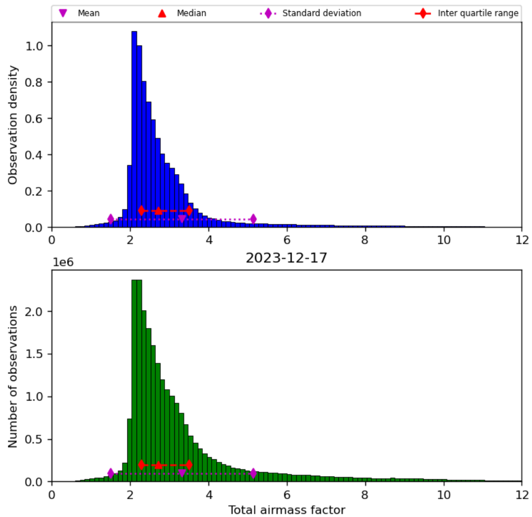
Figure 32: Histogram of “Total airmass factor” for 2023-12-16 to 2023-12-18
