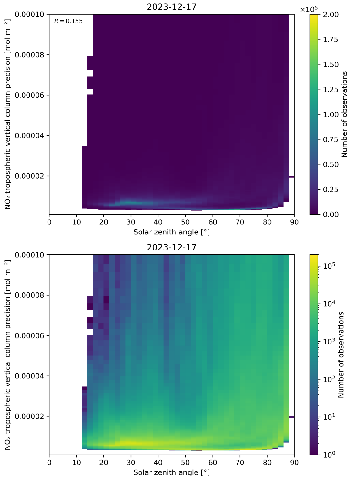
Figure 156: Scatter density plot of “Solar zenith angle” against “NO 2 tropospheric vertical column precision” for 2023-12-16 to 2023-12-18.
