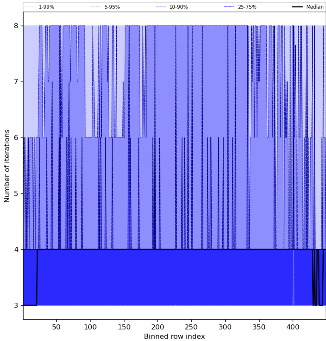
Figure 51: Along track statistics of “Number of iterations” for 2023-12-16 to 2023-12-18
