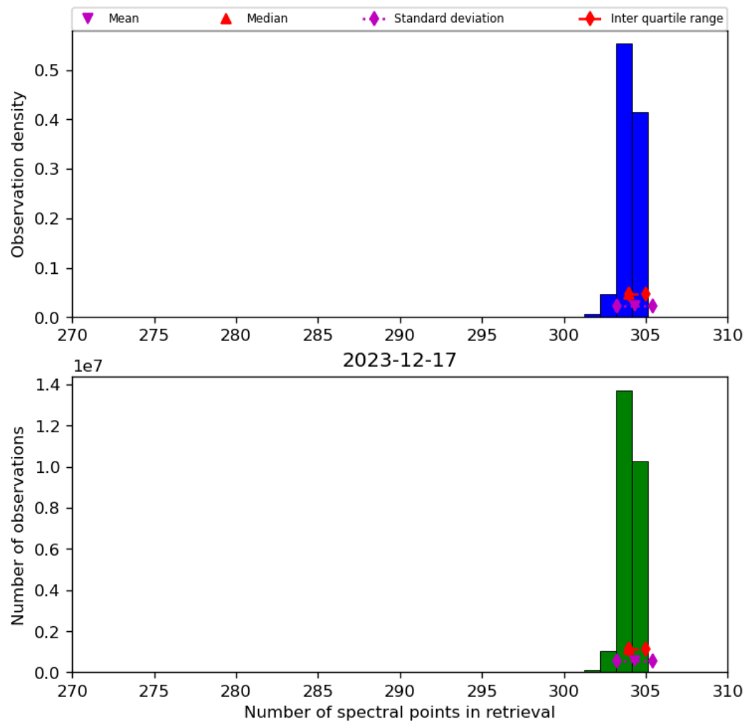
Figure 33: Histogram of “Number of spectral points in retrieval” for 2023-12-16 to 2023-12-18
