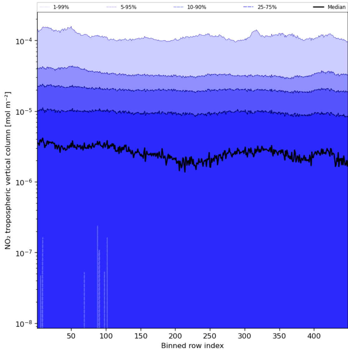
Figure 46: Along track statistics of “NO 2 tropospheric vertical column” for 2023-12-16 to 2023-12-18
