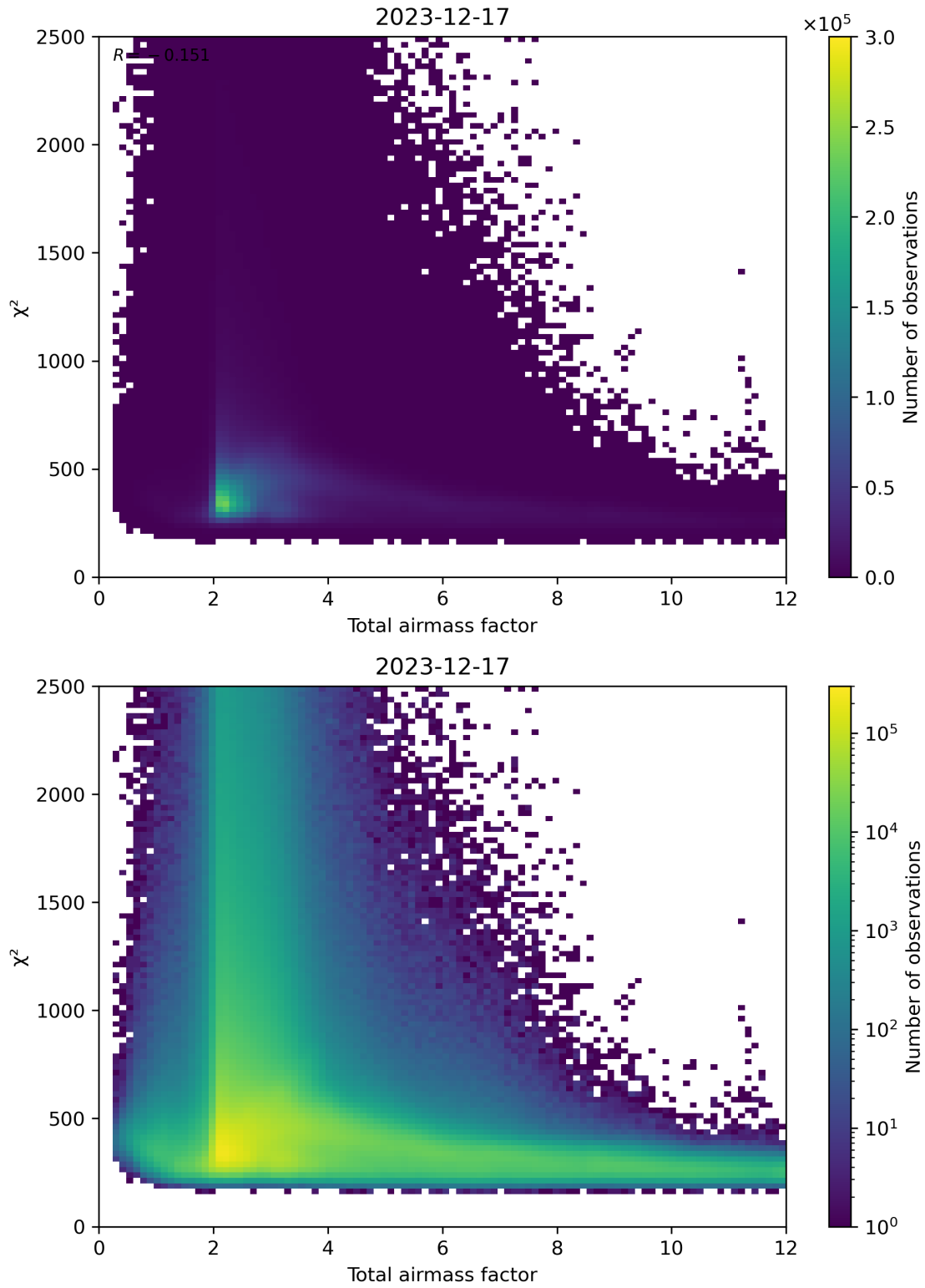
Figure 63: Scatter density plot of “Total airmass factor” against “ \chi^2 ” for 2023-12-16 to 2023-12-18.
