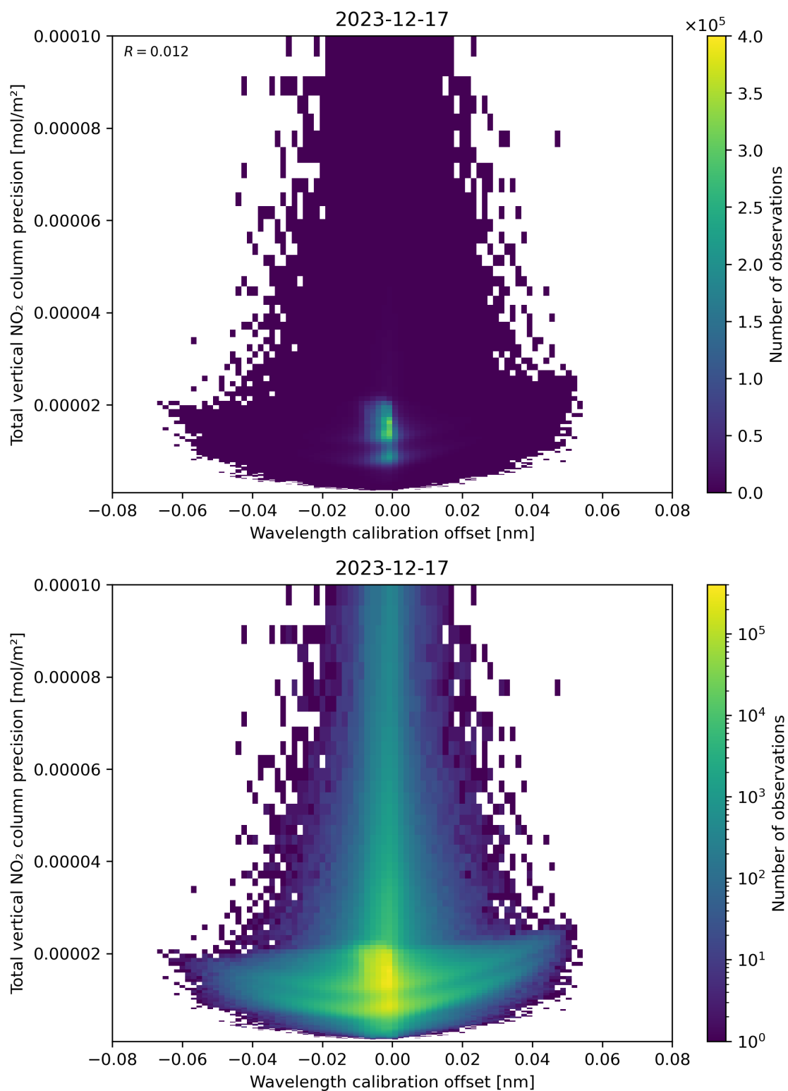
Figure 180: Scatter density plot of “Wavelength calibration offset” against “Total vertical NO 2 column precision” for 2023-12-16 to 2023-12-18.
