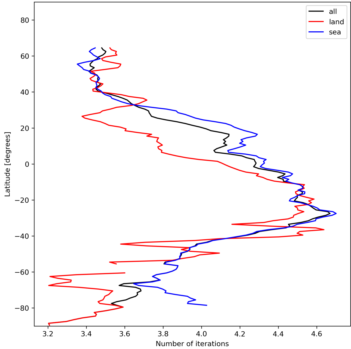
Figure 17: Zonal average of “Number of iterations” for 2023-12-16 to 2023-12-18.
