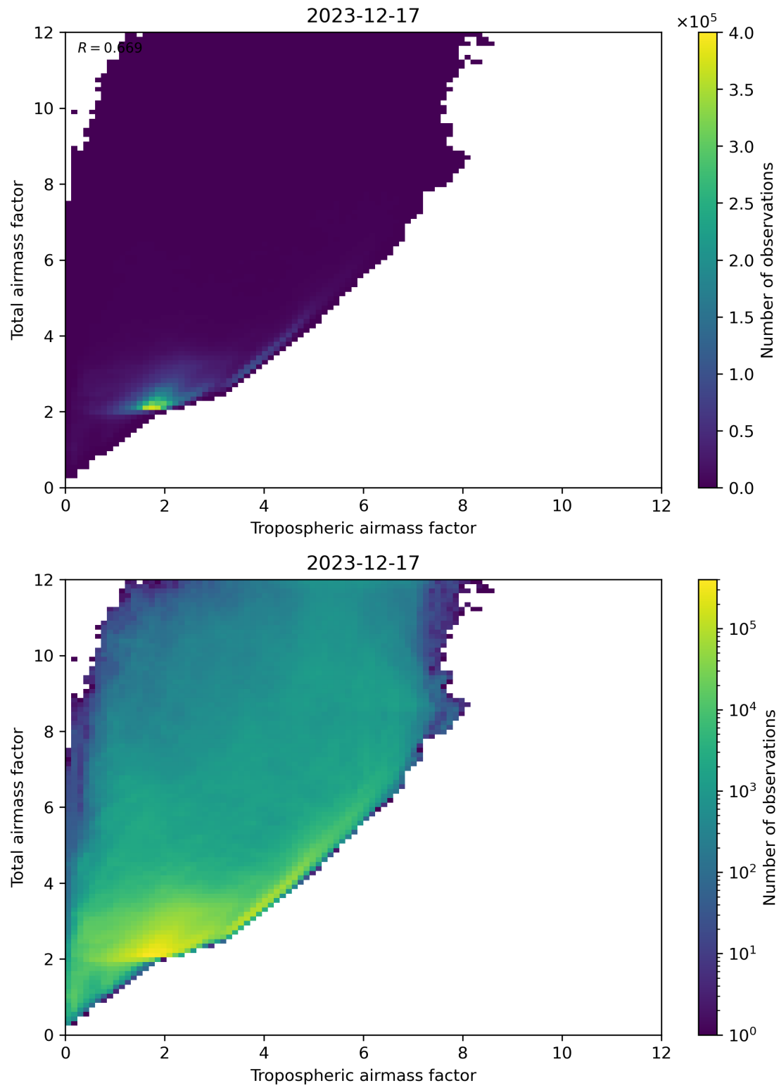
Figure 72: Scatter density plot of “Tropospheric airmass factor” against “Total airmass factor” for 2023-12-16 to 2023-12-18.
