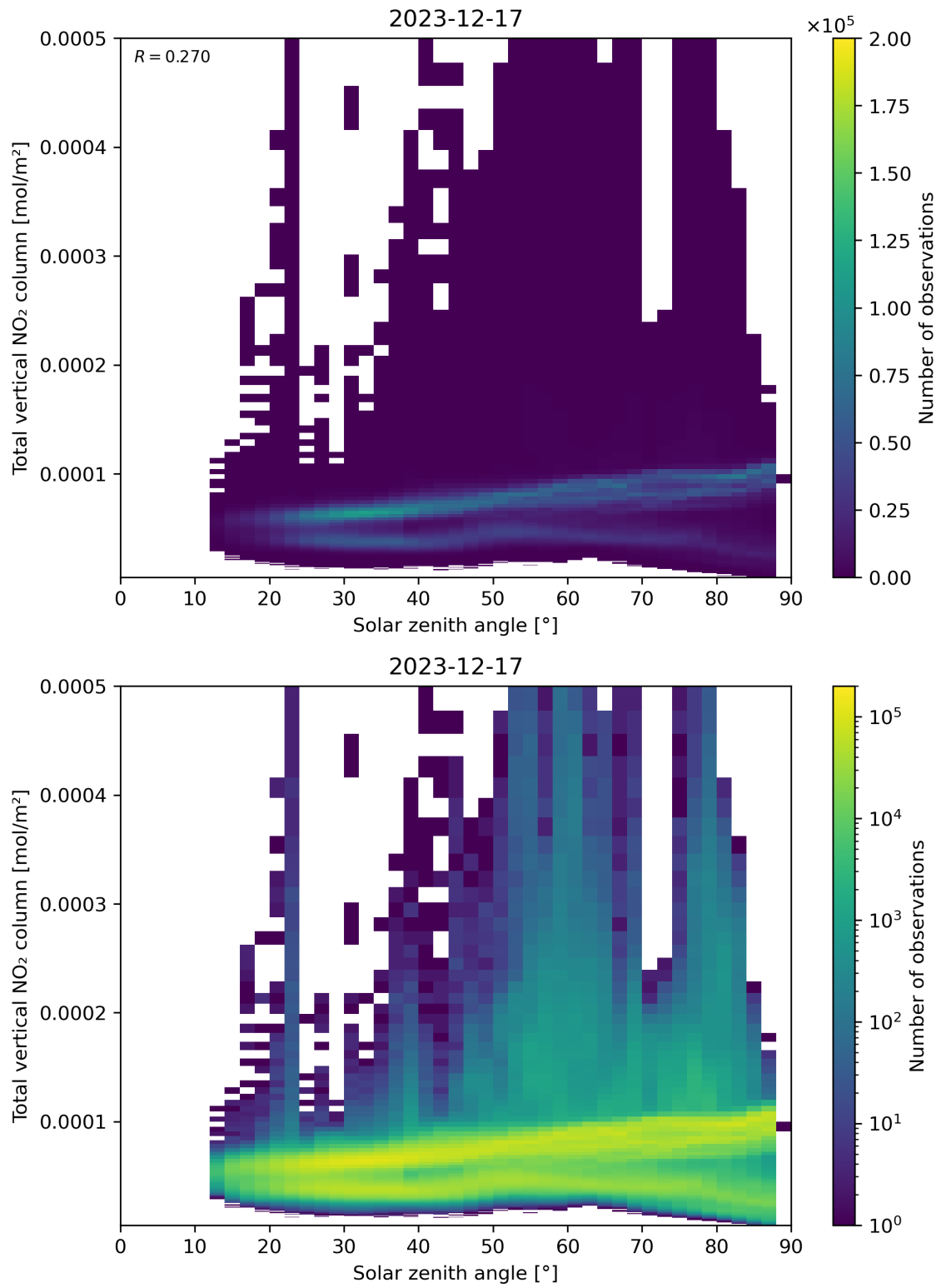
Figure 153: Scatter density plot of “Solar zenith angle” against “Total vertical NO 2 column” for 2023-12-16 to 2023-12-18.
