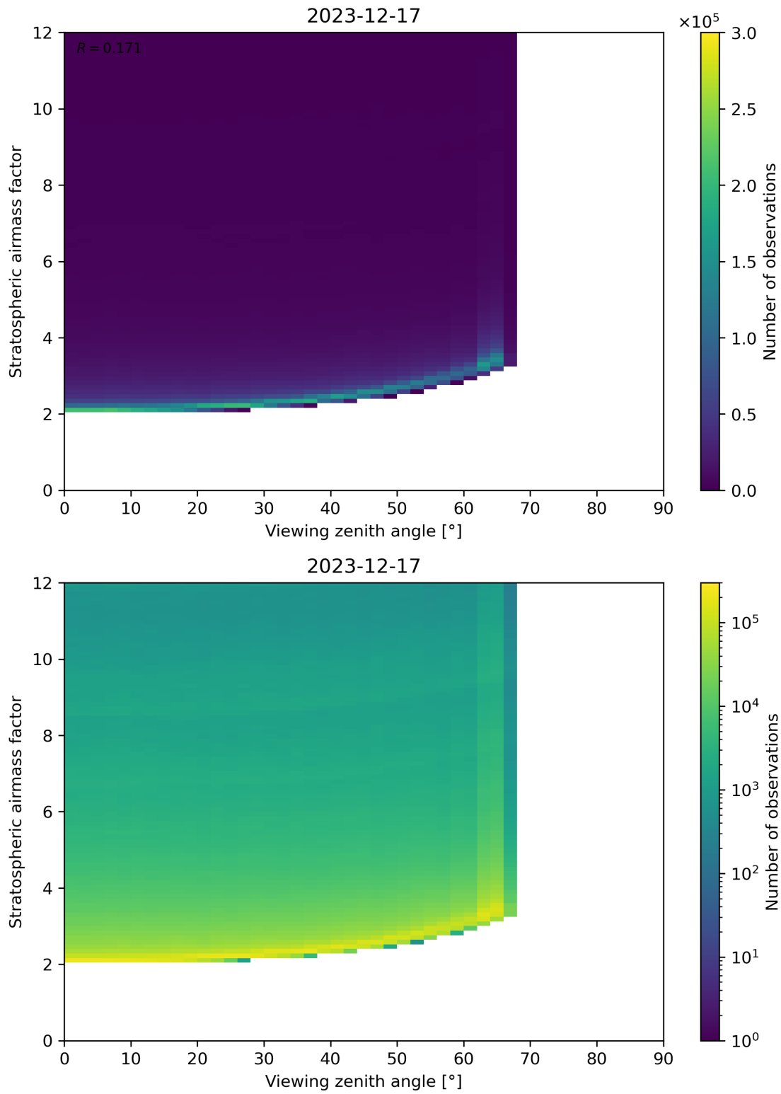
Figure 159: Scatter density plot of “Viewing zenith angle” against “Stratospheric airmass factor” for 2023-12-16 to 2023-12-18.
