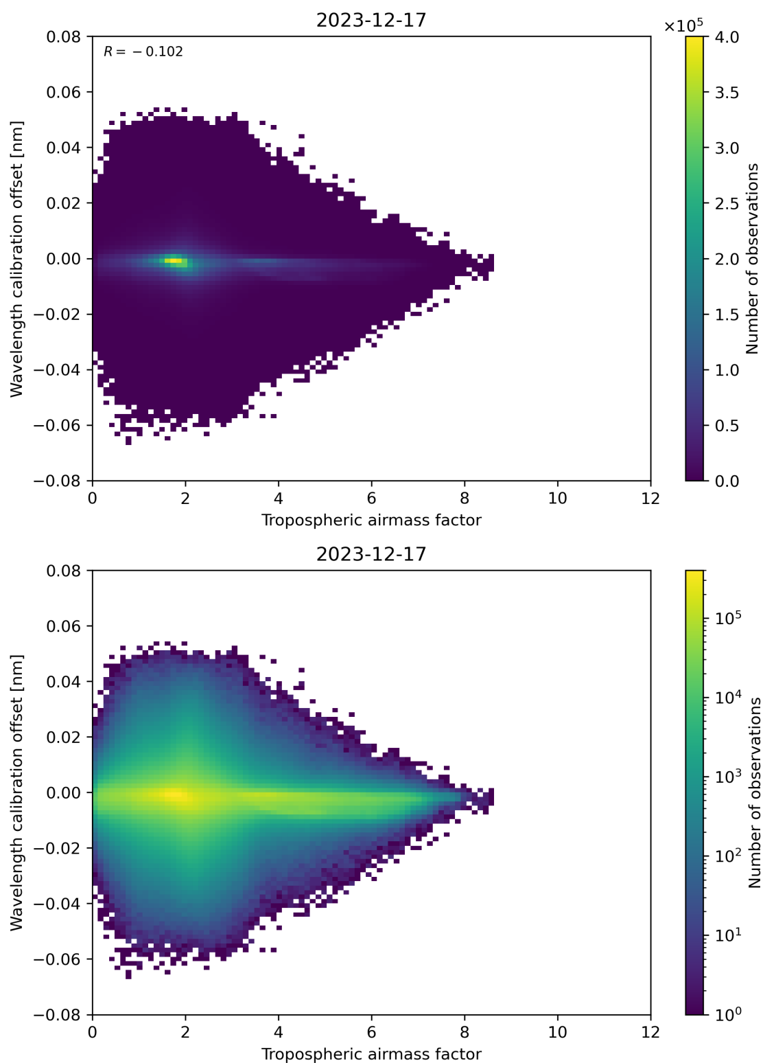
Figure 80: Scatter density plot of “Tropospheric airmass factor” against “Wavelength calibration offset” for 2023-12-16 to 2023-12-18.
