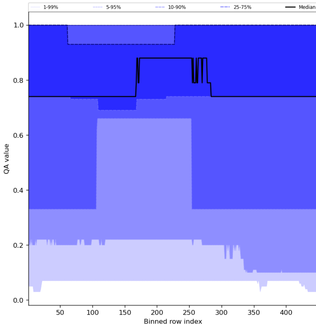
Figure 45: Along track statistics of “QA value” for 2023-12-16 to 2023-12-18
