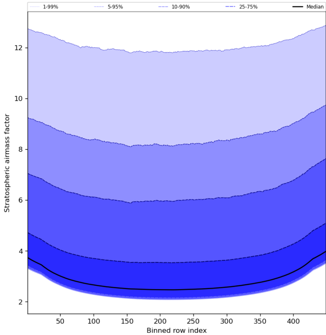
Figure 61: Along track statistics of “Stratospheric airmass factor” for 2023-12-16 to 2023-12-18
