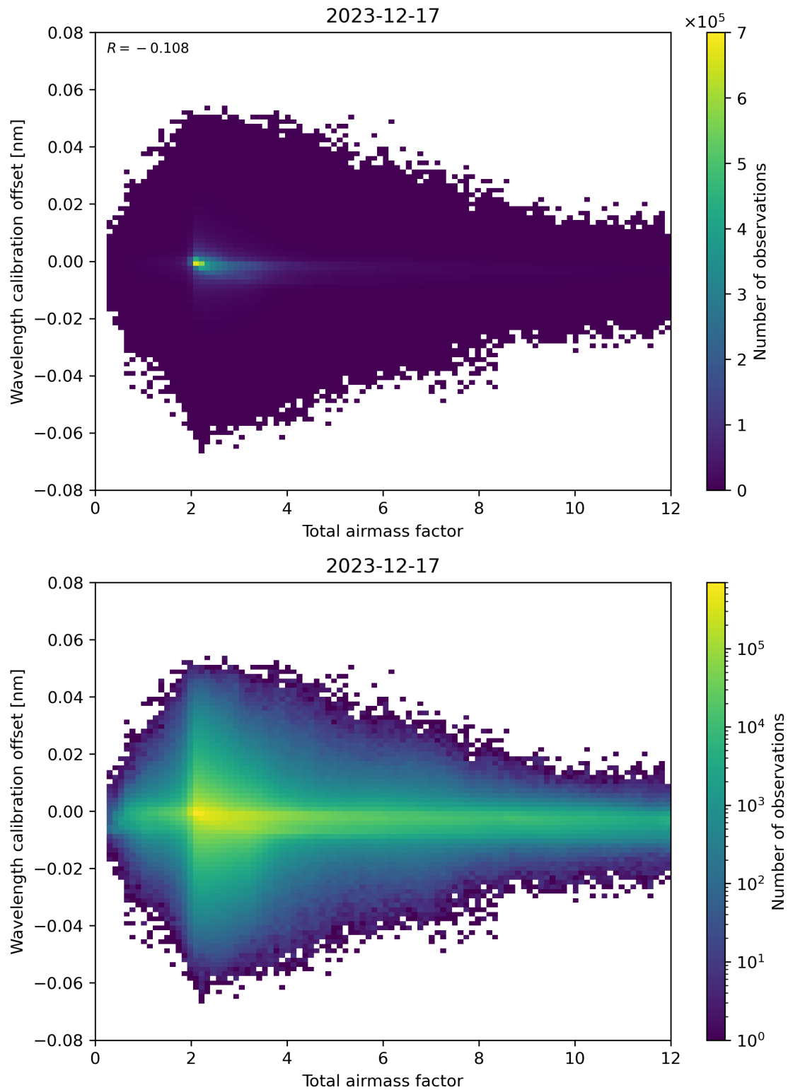
Figure 70: Scatter density plot of “Total airmass factor” against “Wavelength calibration offset” for 2023-12-16 to 2023-12-18.
