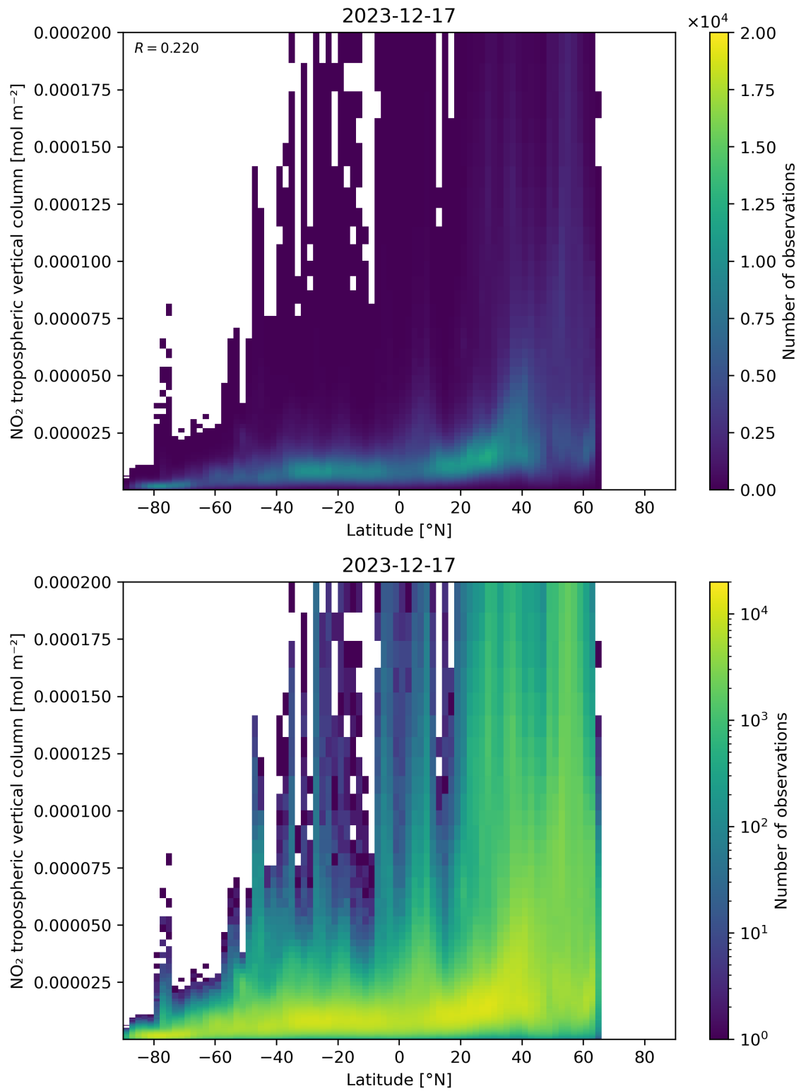
Figure 92: Scatter density plot of “Latitude” against “NO 2 tropospheric vertical column” for 2023-12-16 to 2023-12-18.
