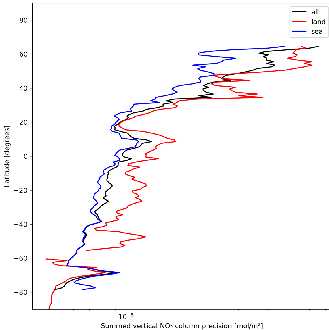
Figure 24: Zonal average of “Summed vertical NO 2 column precision” for 2023-12-16 to 2023-12-18.
