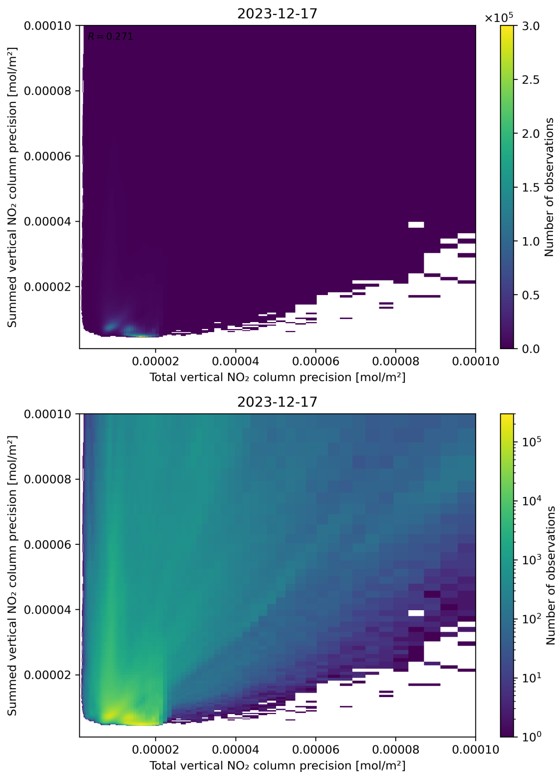
Figure 118: Scatter density plot of “Total vertical NO 2 column precision” against “Summed vertical NO 2 column precision” for 2023-12-16 to 2023-12-18.
