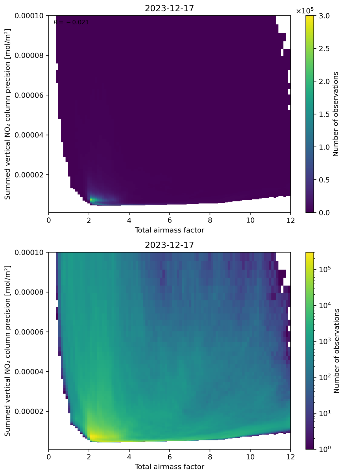
Figure 66: Scatter density plot of “Total airmass factor” against “Summed vertical NO 2 column precision” for 2023-12-16 to 2023-12-18.
