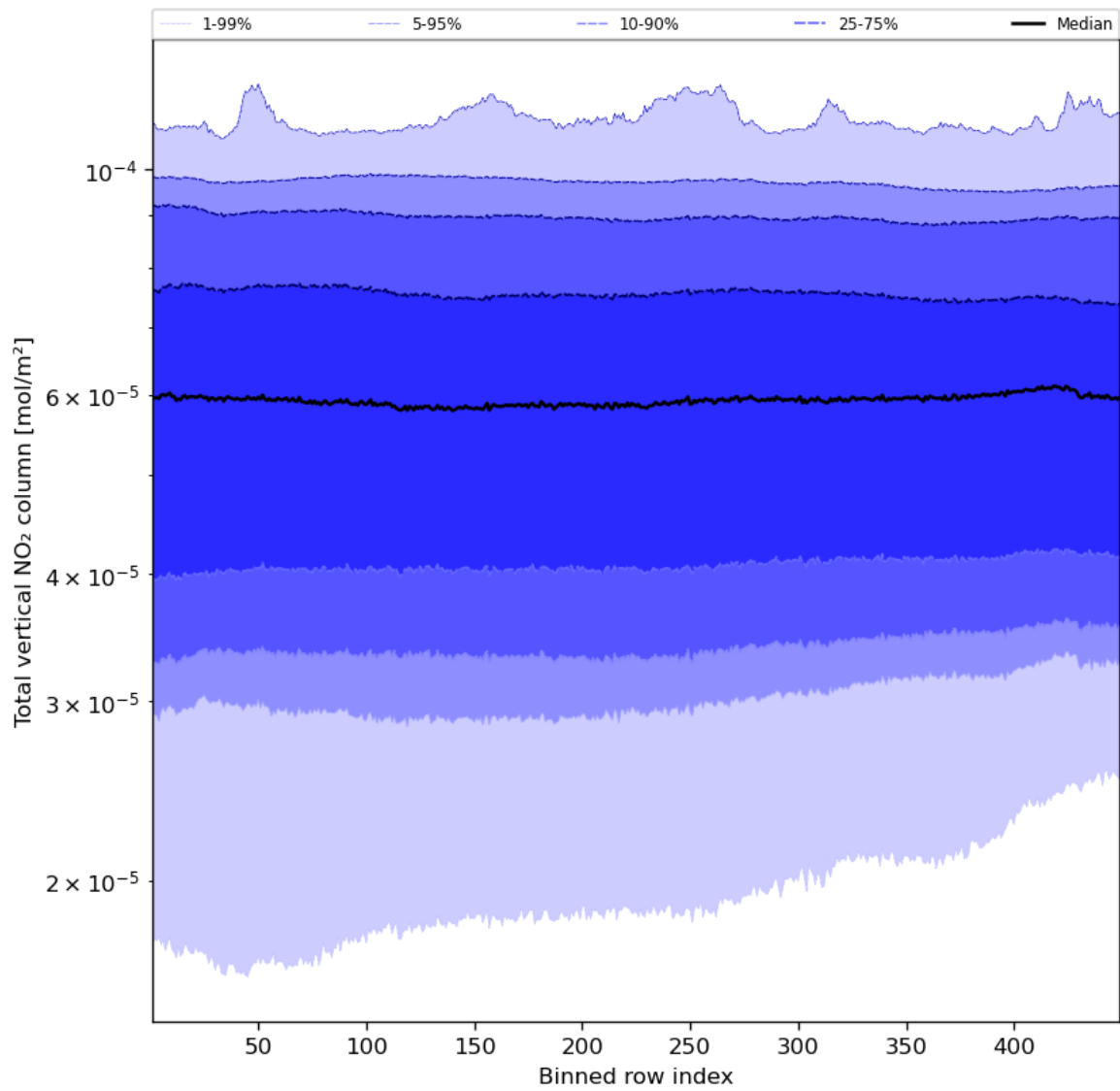
Figure 55: Along track statistics of “Total vertical NO 2 column” for 2023-12-16 to 2023-12-18
