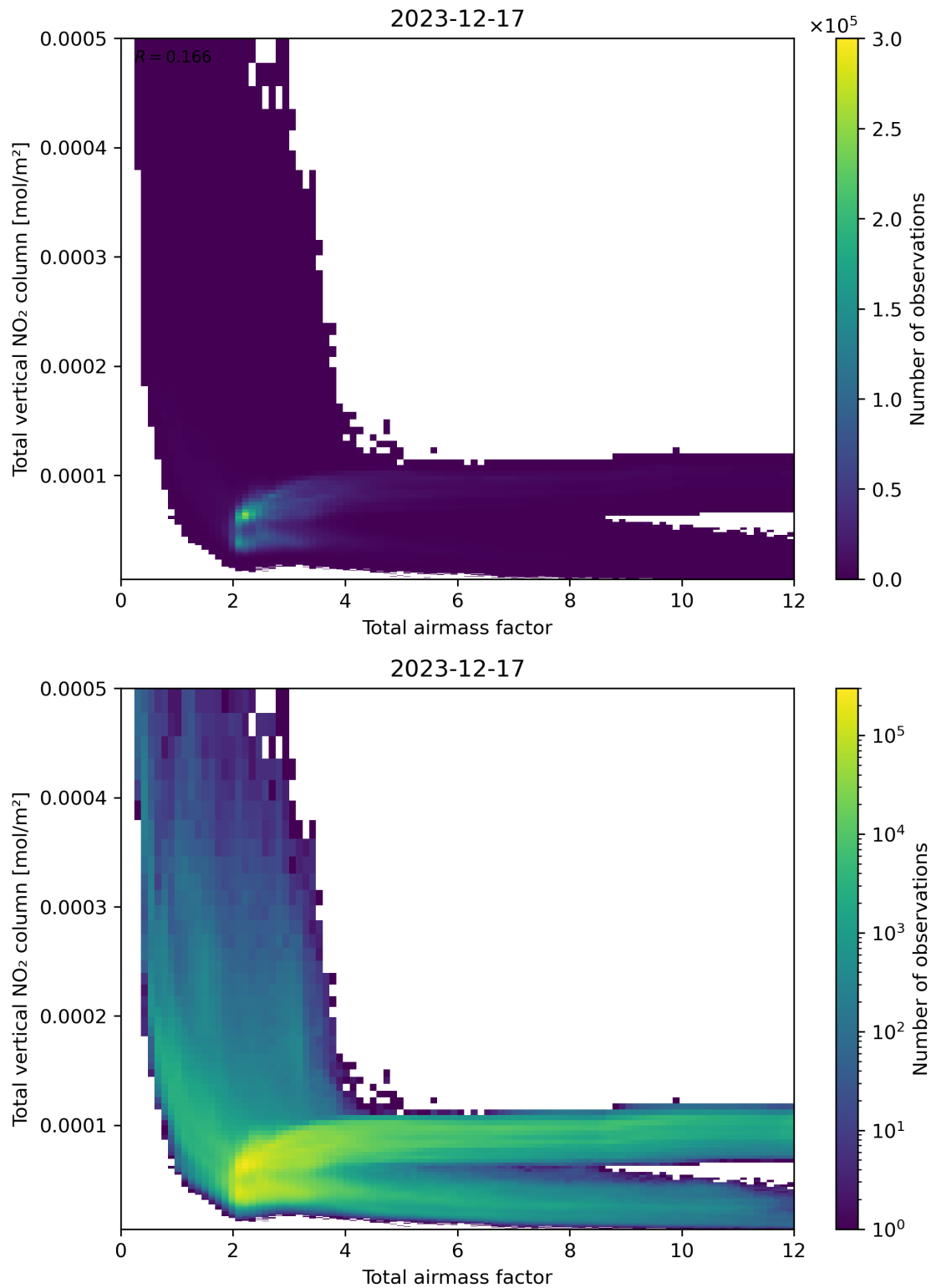
Figure 67: Scatter density plot of “Total airmass factor” against “Total vertical NO 2 column” for 2023-12-16 to 2023-12-18.
