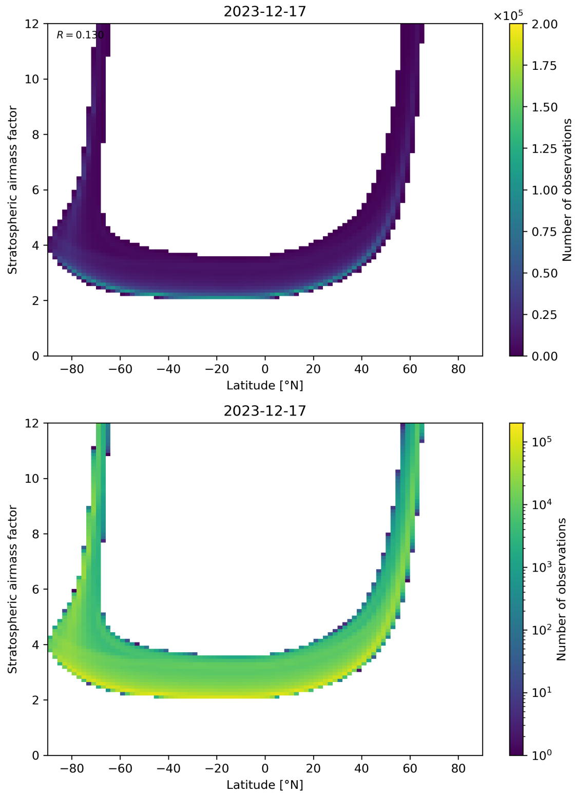
Figure 83: Scatter density plot of “Latitude” against “Stratospheric air mass factor” for 2023-12-16 to 2023-12-18.
