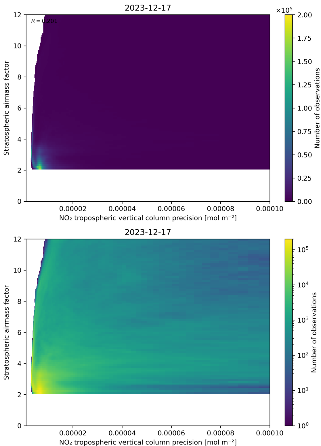
Figure 131: Scatter density plot of “NO 2 tropospheric vertical column precision” against “Stratospheric airmass factor” for 2023-12-16 to 2023-12-18.
