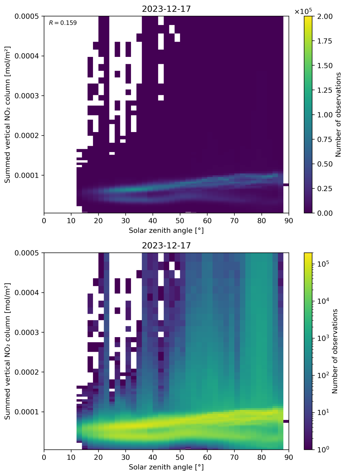
Figure 151: Scatter density plot of “Solar zenith angle” against “Summed vertical NO 2 column” for 2023-12-16 to 2023-12-18.
