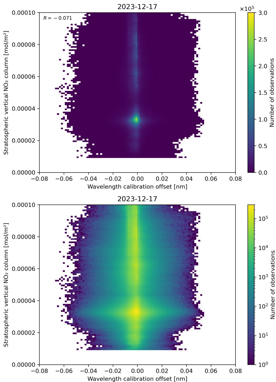
Figure 176: Scatter density plot of “Wavelength calibration offset” against “Stratospheric vertical NO 2 column” for 2023-12-16 to 2023-12-18.
