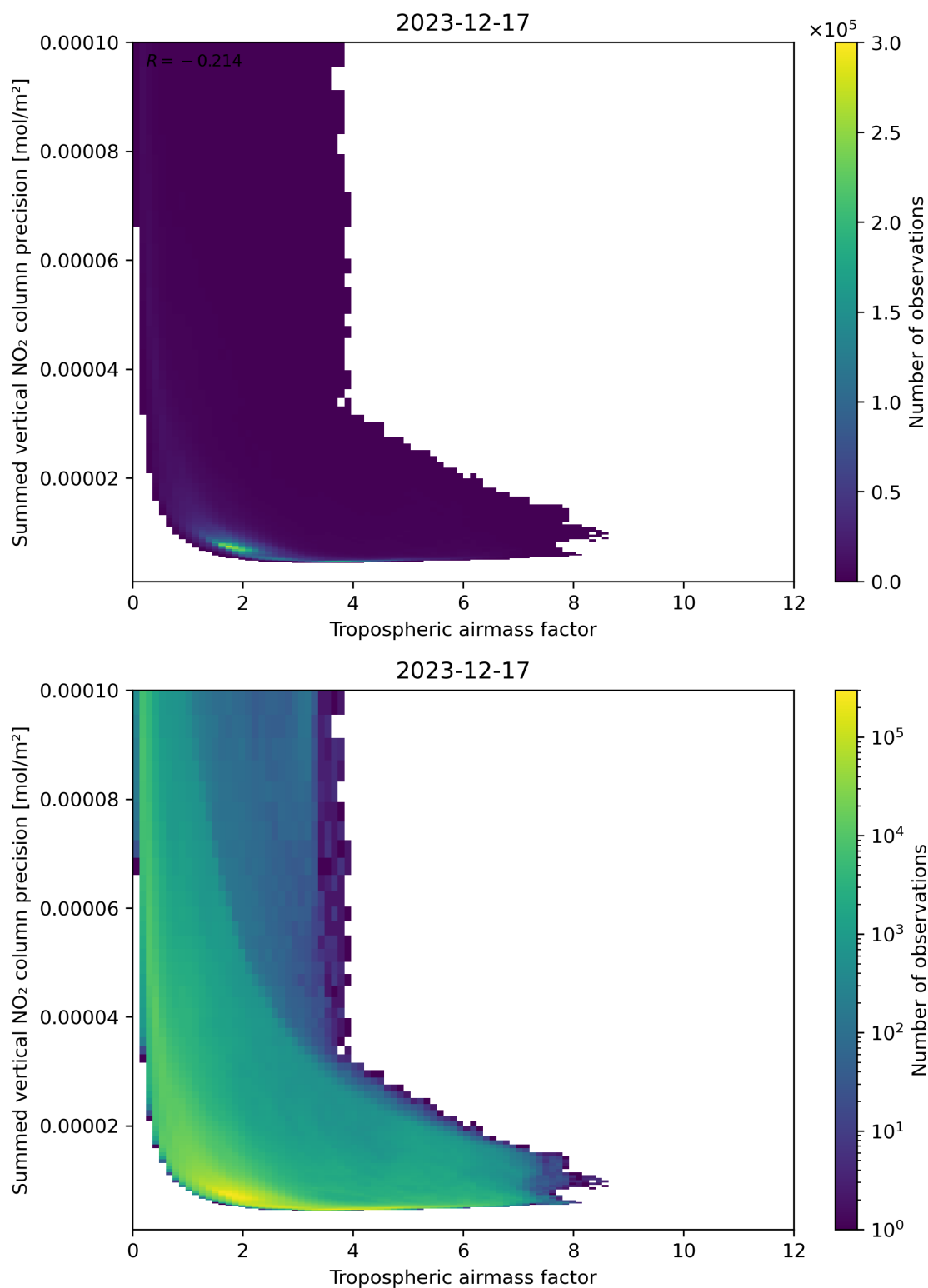
Figure 76: Scatter density plot of “Tropospheric air mass factor” against “Summed vertical NO 2 column precision” for 2023-12-16 to 2023-12-18.
