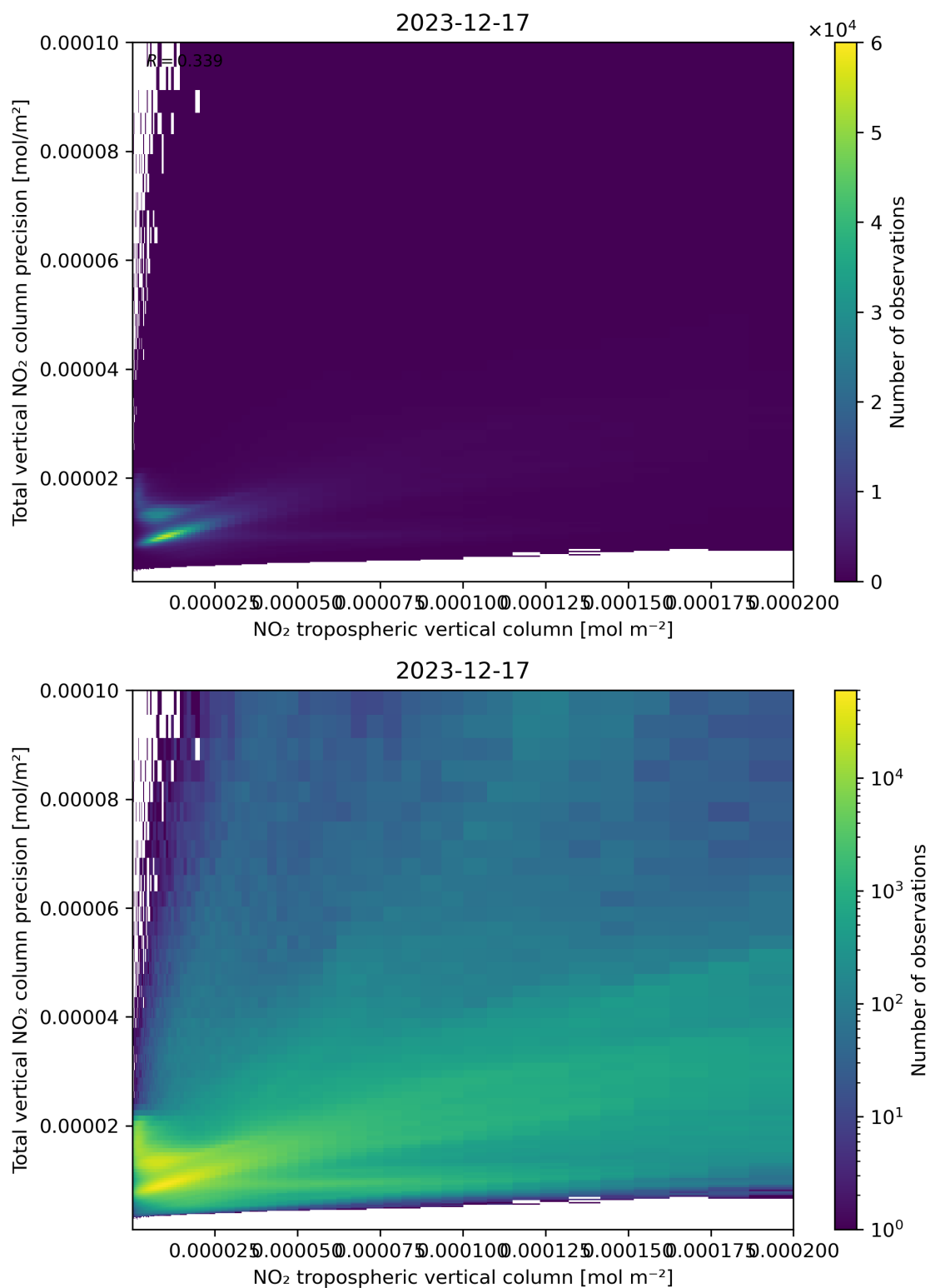
Figure 129: Scatter density plot of “NO 2 tropospheric vertical column” against “Total vertical NO 2 column precision” for 2023-12-16 to 2023-12-18.
