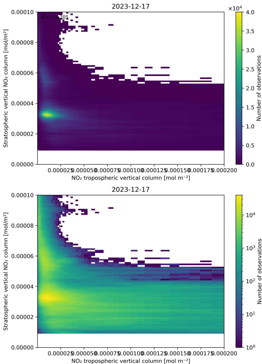
Figure 125: Scatter density plot of “NO 2 tropospheric vertical column” against “Stratospheric vertical NO 2 column” for 2023-12-16 to 2023-12-18.
