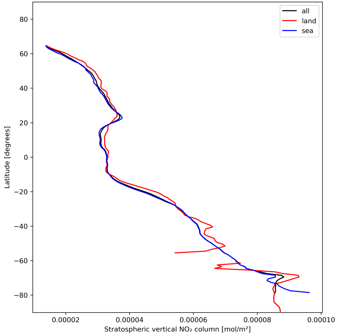
Figure 19: Zonal average of “Stratospheric vertical NO 2 column” for 2023-12-16 to 2023-12-18.
