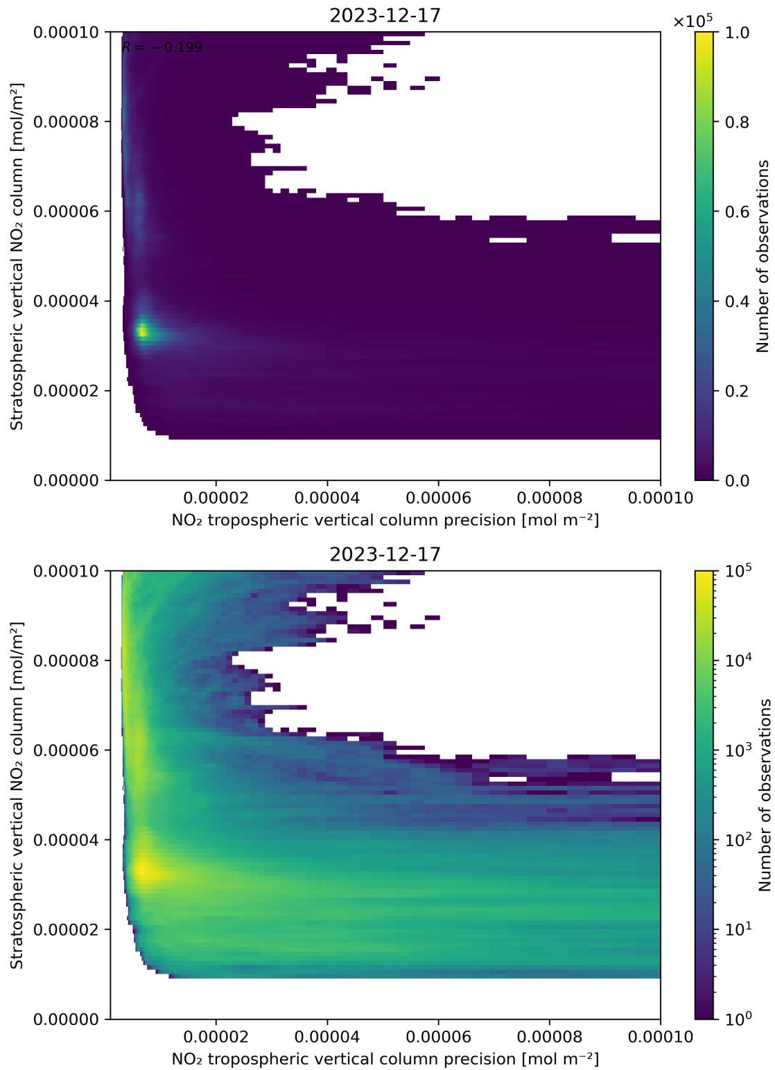
Figure 135: Scatter density plot of “NO 2 tropospheric vertical column precision” against “Stratospheric vertical NO 2 column” for 2023-12-16 to 2023-12-18.
