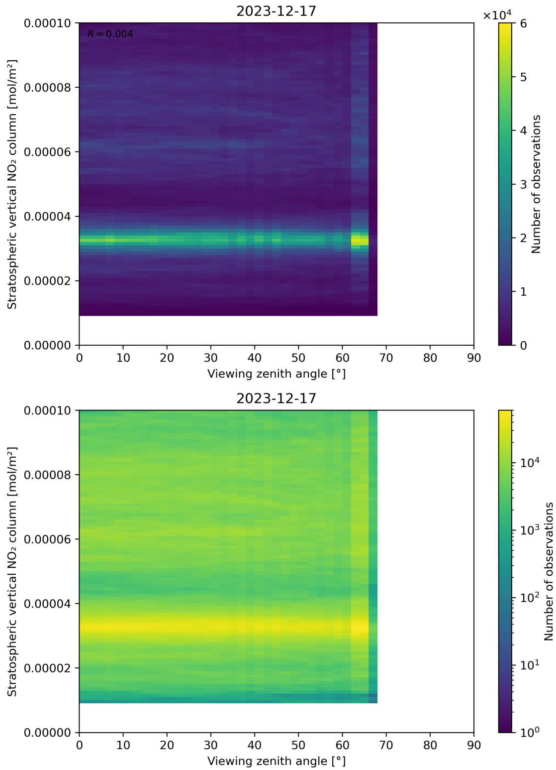
Figure 164: Scatter density plot of “Viewing zenith angle” against “Stratospheric vertical NO 2 column” for 2023-12-16 to 2023-12-18.
