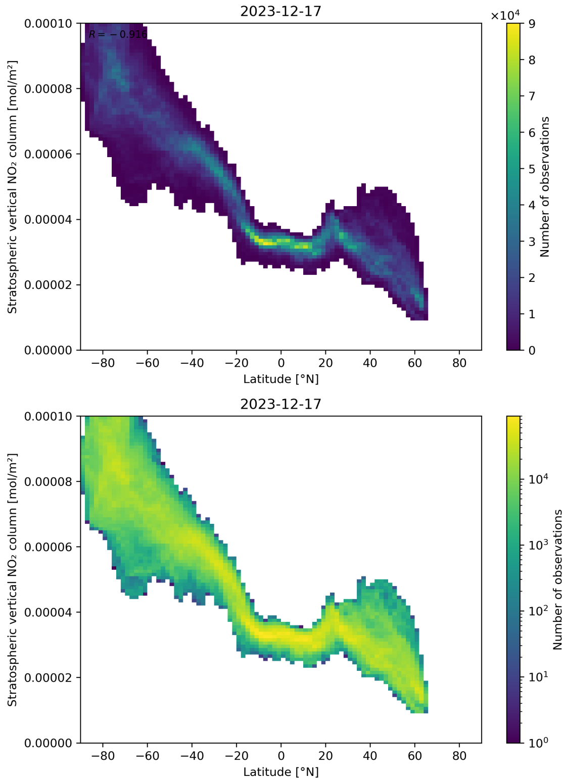
Figure 87: Scatter density plot of “Latitude” against “Stratospheric vertical NO 2 column” for 2023-12-16 to 2023-12-18.
