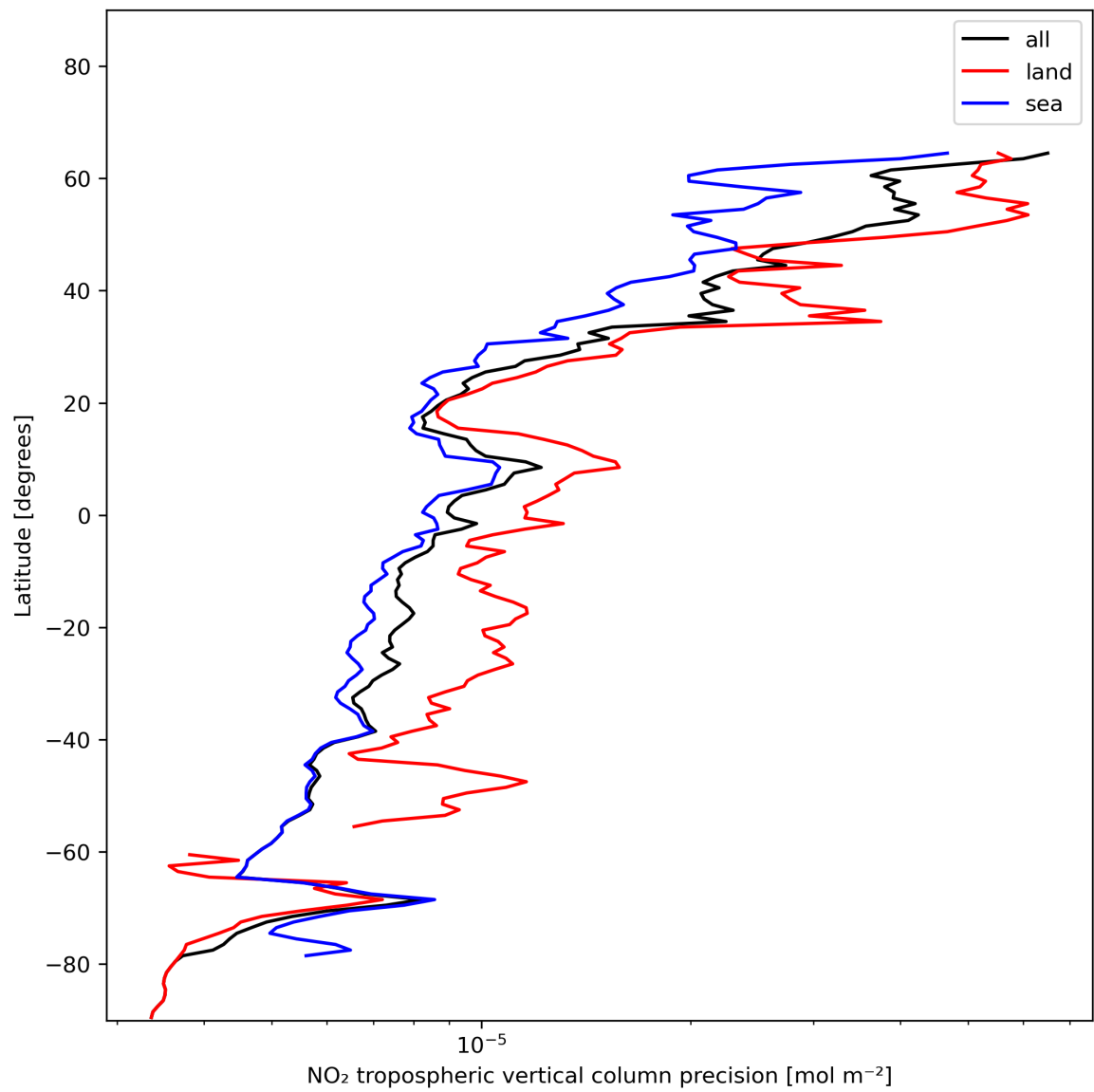
Figure 13: Zonal average of “NO 2 tropospheric vertical column precision” for 2023-12-16 to 2023-12-18.
