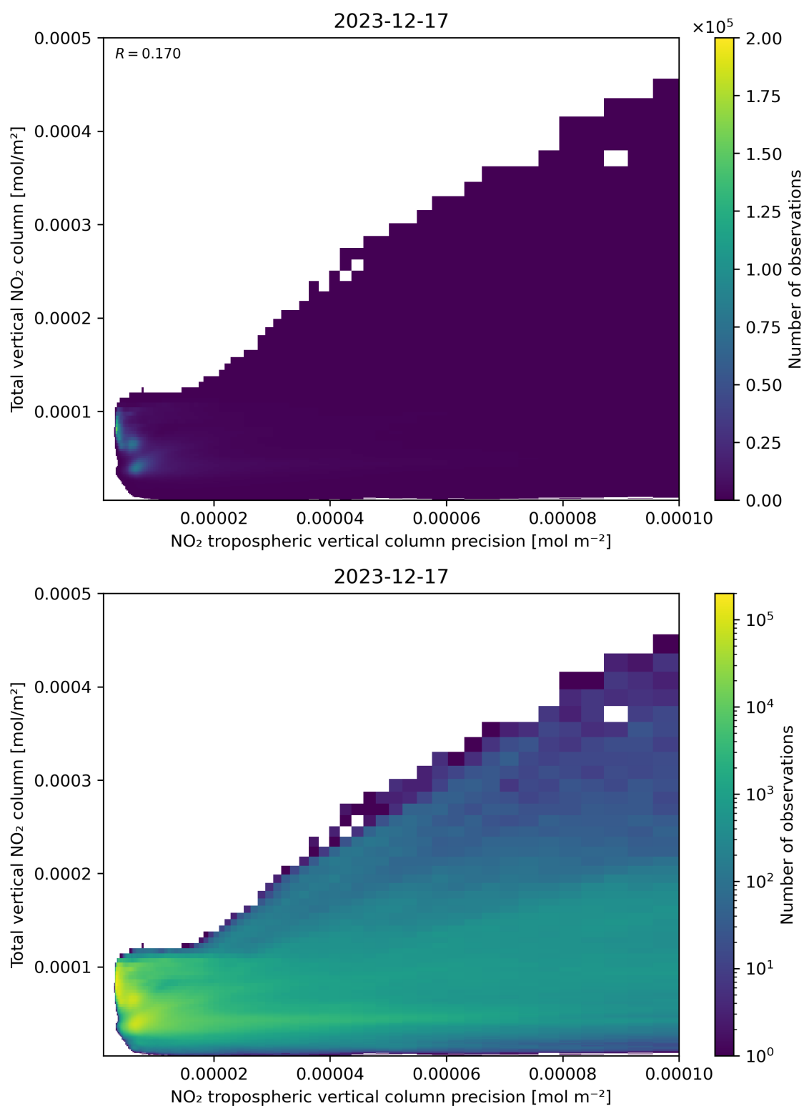
Figure 138: Scatter density plot of “NO 2 tropospheric vertical column precision” against “Total vertical NO 2 column” for 2023-12-16 to 2023-12-18.
