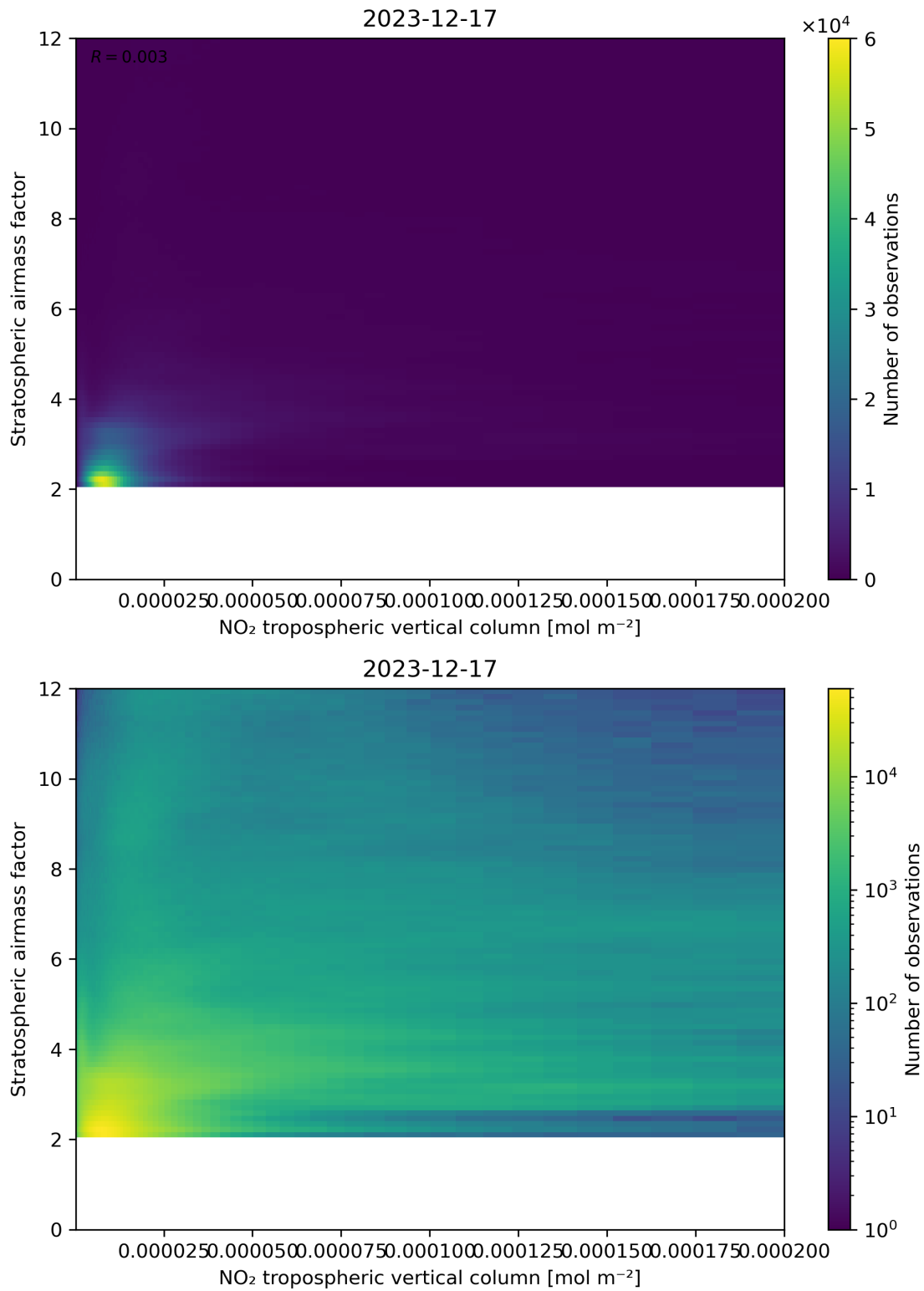
Figure 121: Scatter density plot of “NO 2 tropospheric vertical column” against “Stratospheric airmass factor” for 2023-12-16 to 2023-12-18.
