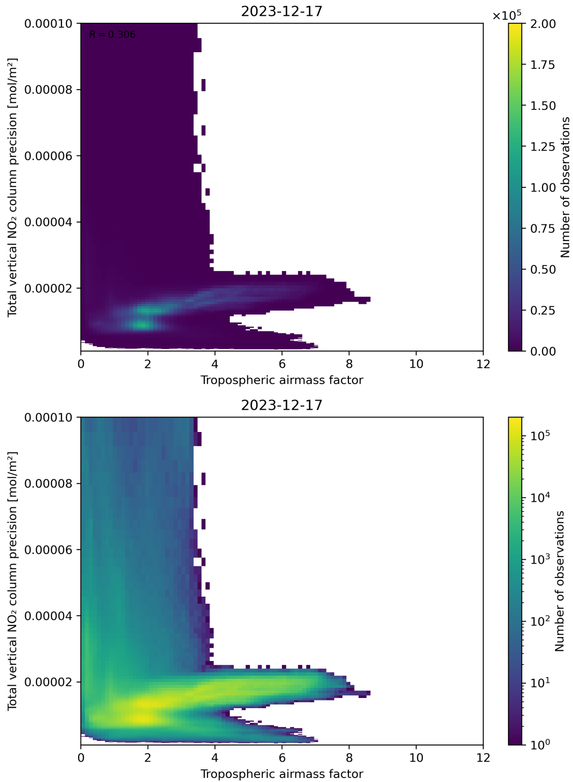
Figure 78: Scatter density plot of “Tropospheric air mass factor” against “Total vertical NO 2 column precision” for 2023-12-16 to 2023-12-18.
