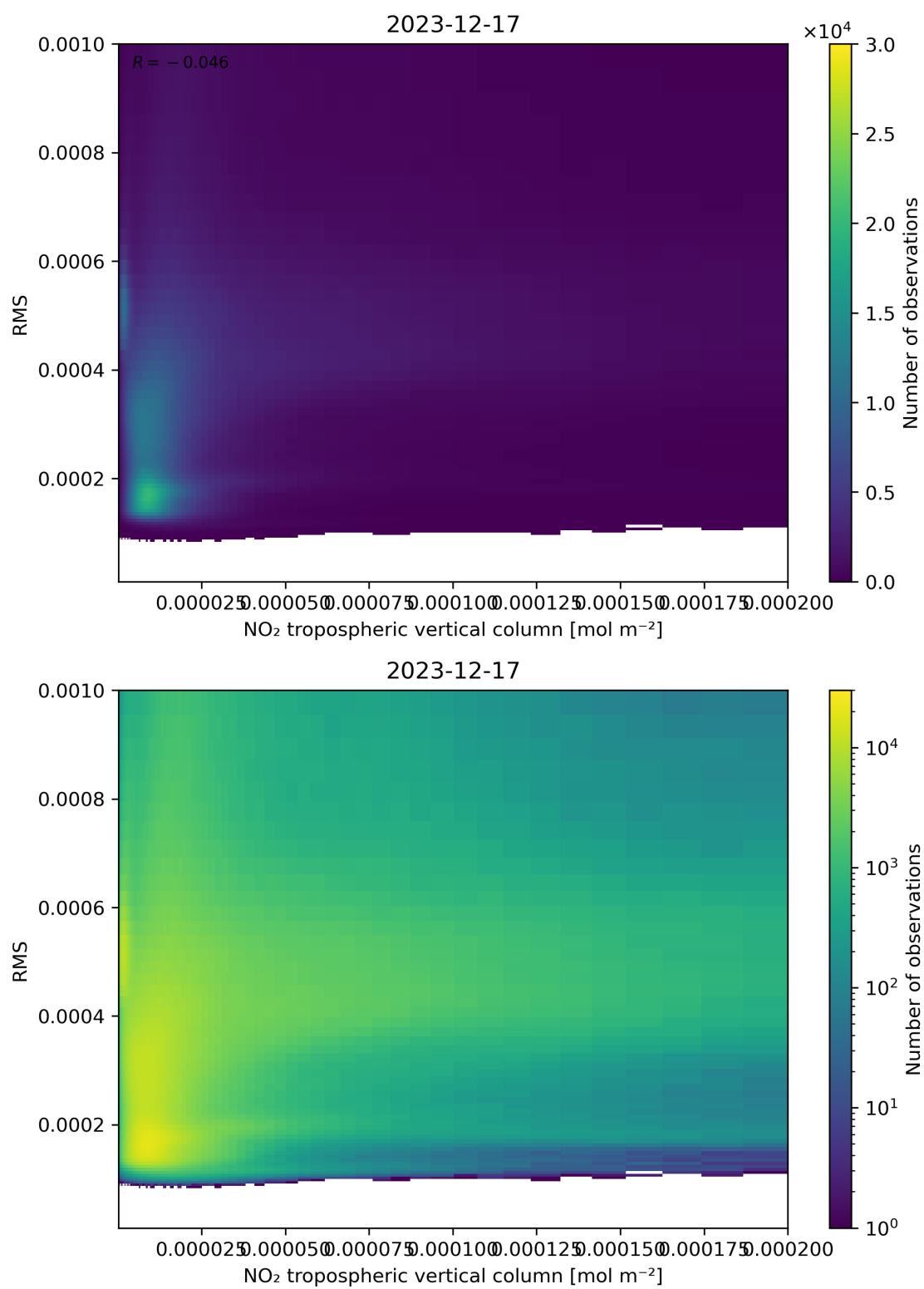
Figure 142: Scatter density plot of “NO 2 tropospheric vertical column” against “RMS” for 2023-12-16 to 2023-12-18.
