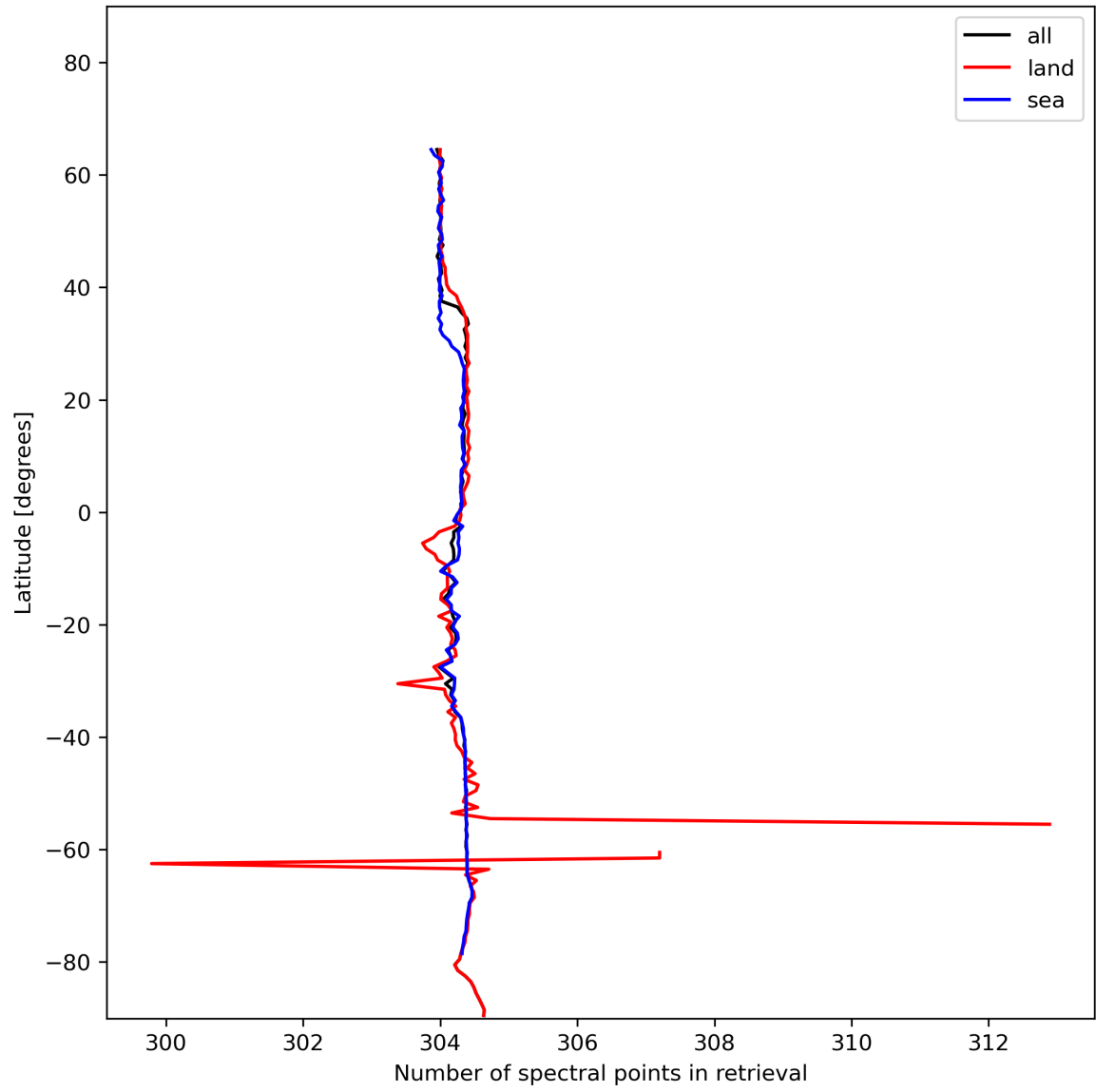
Figure 16: Zonal average of “Number of spectral points in retrieval” for 2023-12-16 to 2023-12-18.
