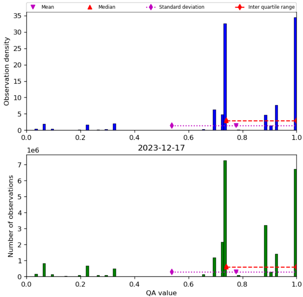
Figure 28: Histogram of “QA value” for 2023-12-16 to 2023-12-18
