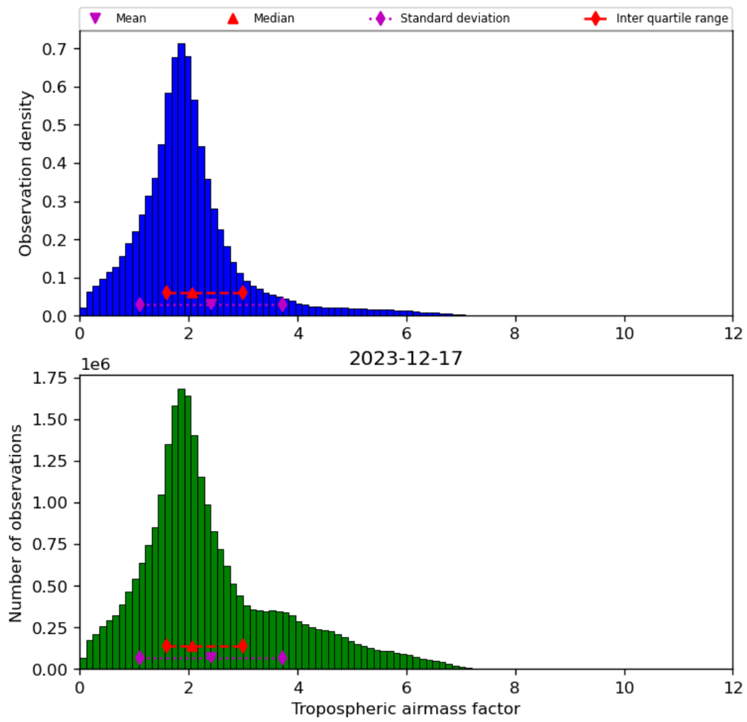
Figure 31: Histogram of “Tropospheric airmass factor” for 2023-12-16 to 2023-12-18
