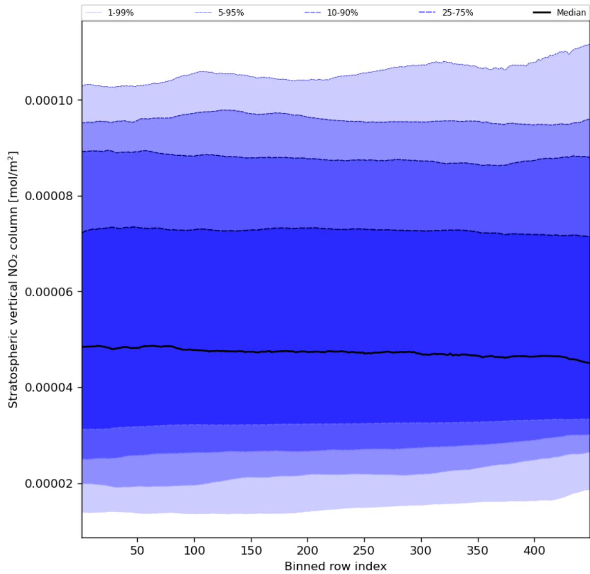
Figure 53: Along track statistics of “Stratospheric vertical NO 2 column” for 2023-12-16 to 2023-12-18
