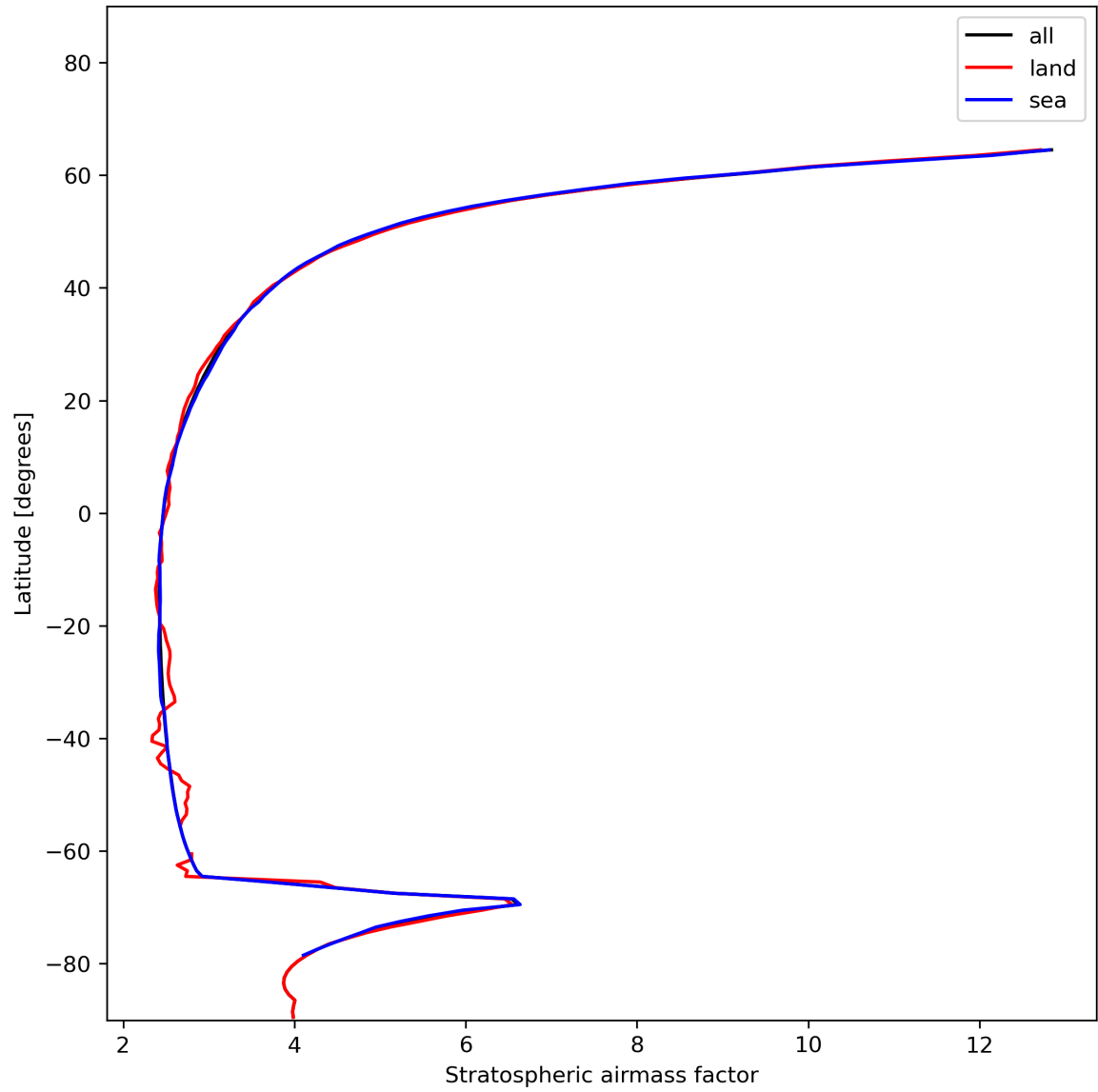
Figure 27: Zonal average of “Stratospheric airmass factor” for 2023-12-16 to 2023-12-18.
