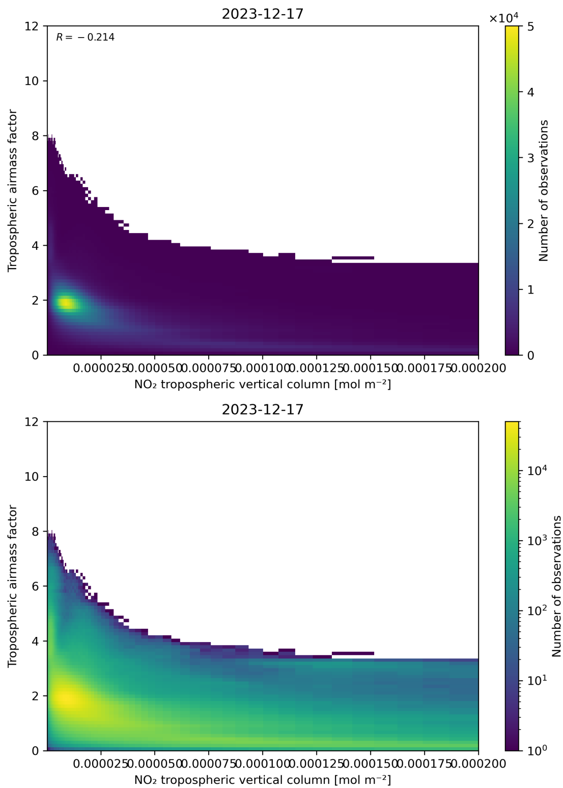
Figure 123: Scatter density plot of “NO 2 tropospheric vertical column” against “Tropospheric airmass factor” for 2023-12-16 to 2023-12-18.
