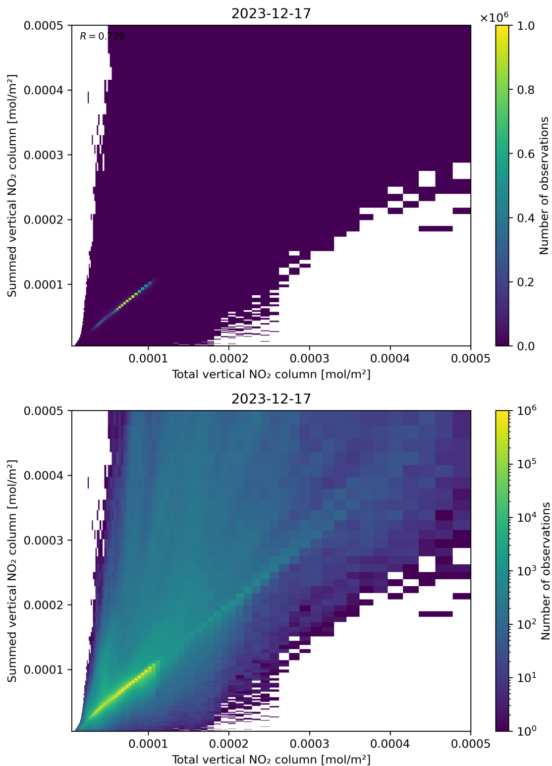
Figure 112: Scatter density plot of “Total vertical NO 2 column” against “Summed vertical NO 2 column” for 2023-12-16 to 2023-12-18.
