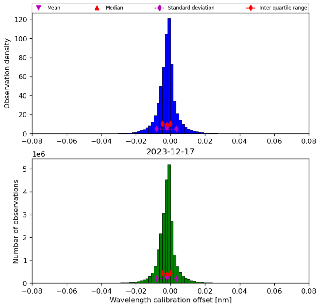
Figure 35: Histogram of “Wavelength calibration offset” for 2023-12-16 to 2023-12-18
