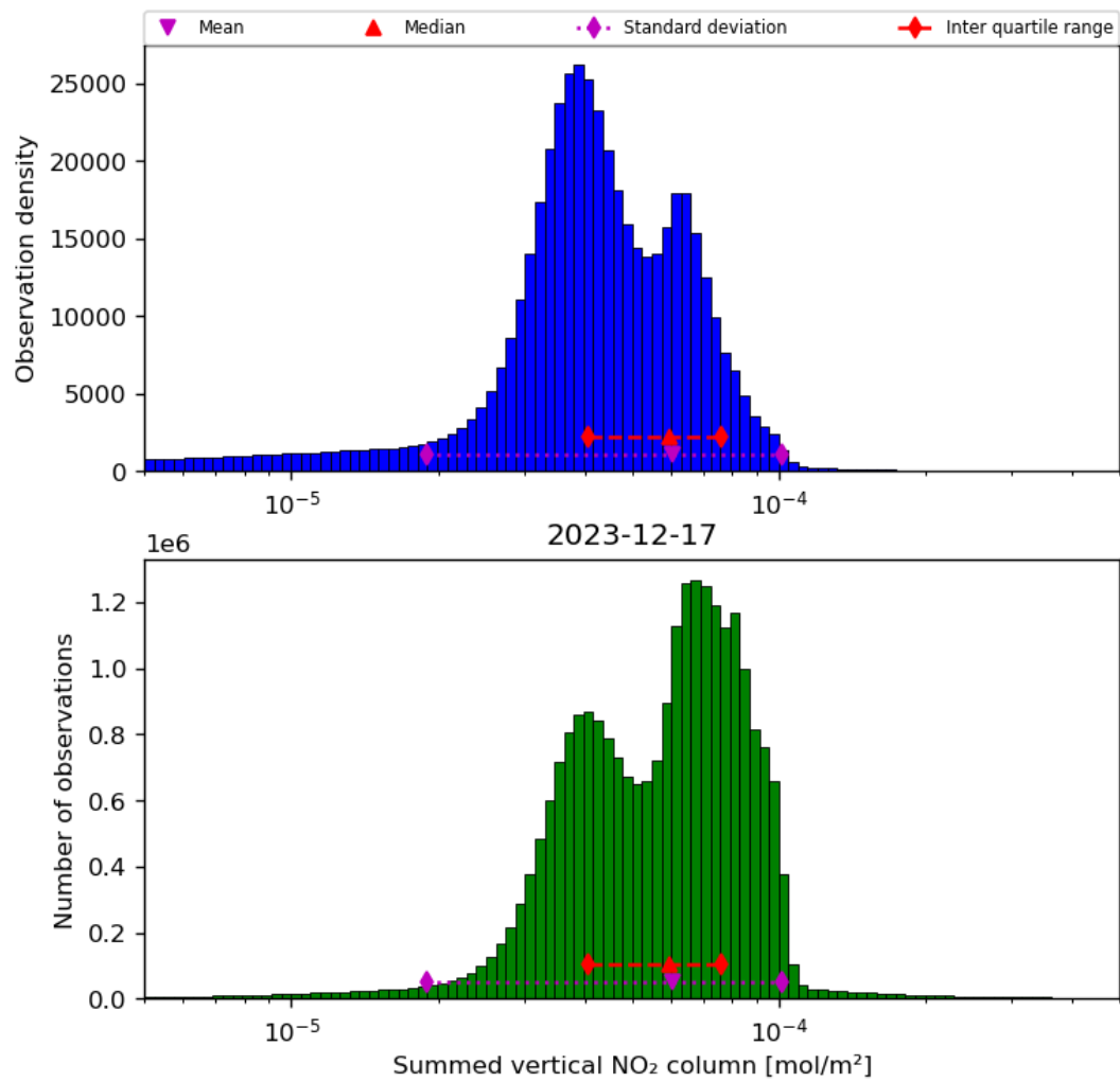
Figure 40: Histogram of “Summed vertical NO 2 column” for 2023-12-16 to 2023-12-18
