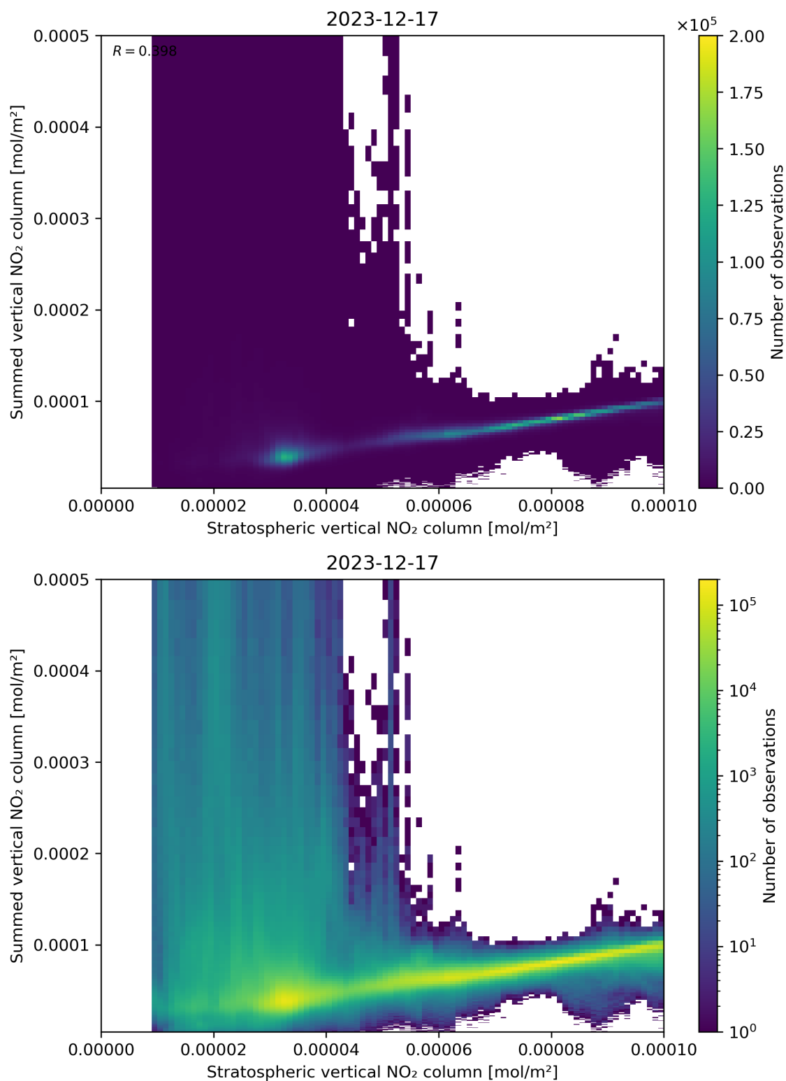
Figure 98: Scatter density plot of “Stratospheric vertical NO 2 column” against “Summed vertical NO 2 column” for 2023-12-16 to 2023-12-18.
