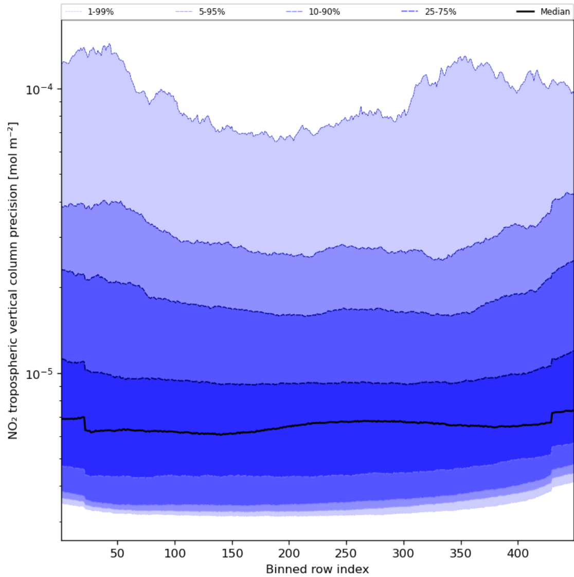
Figure 47: Along track statistics of “NO 2 tropospheric vertical column precision” for 2023-12-16 to 2023-12-18
