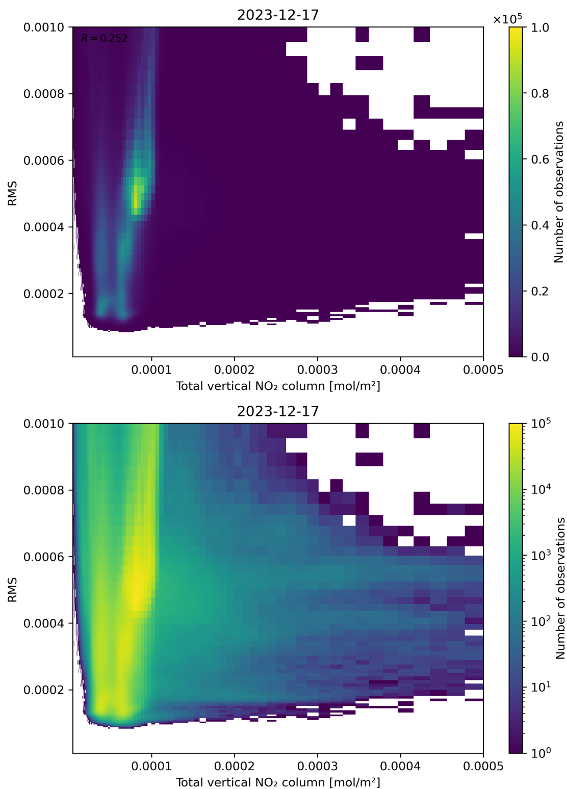
Figure 120: Scatter density plot of “Total vertical NO 2 column” against “RMS” for 2023-12-16 to 2023-12-18.
