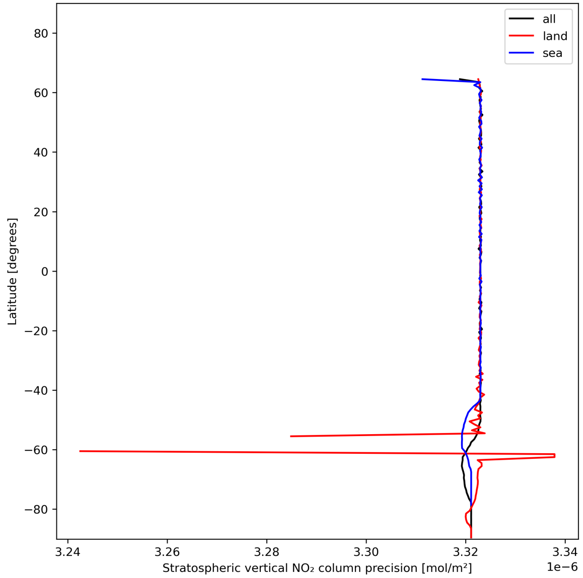
Figure 20: Zonal average of “Stratospheric vertical NO 2 column precision” for 2023-12-16 to 2023-12-18.
