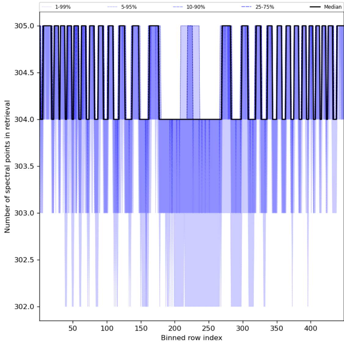
Figure 50: Along track statistics of “Number of spectral points in retrieval” for 2023-12-16 to 2023-12-18
