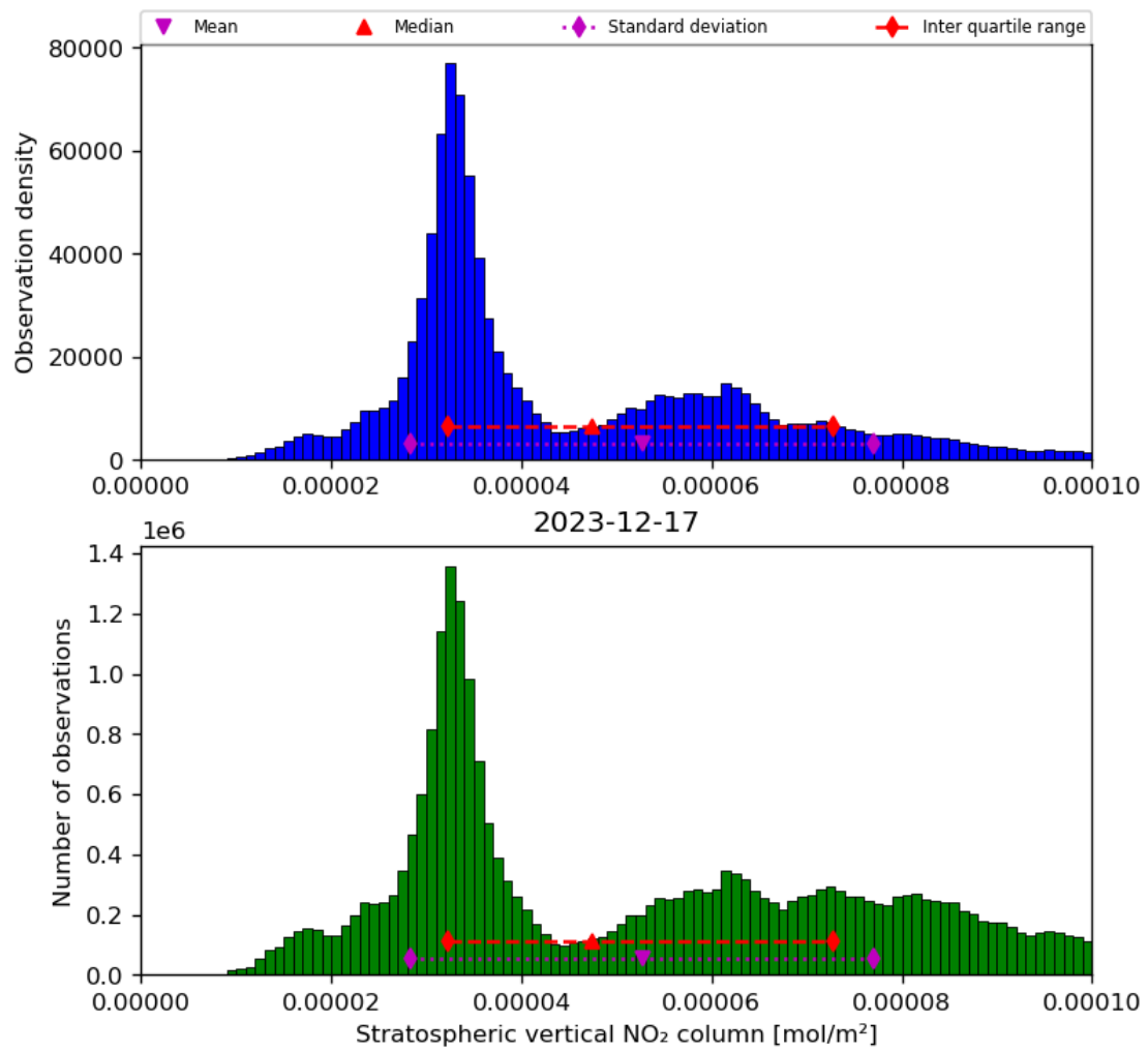
Figure 36: Histogram of “Stratospheric vertical NO 2 column” for 2023-12-16 to 2023-12-18
