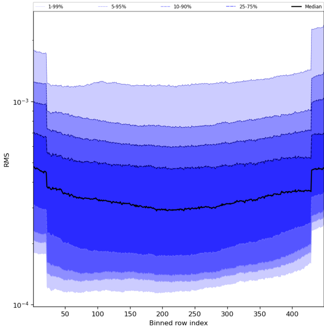
Figure 60: Along track statistics of “RMS” for 2023-12-16 to 2023-12-18
