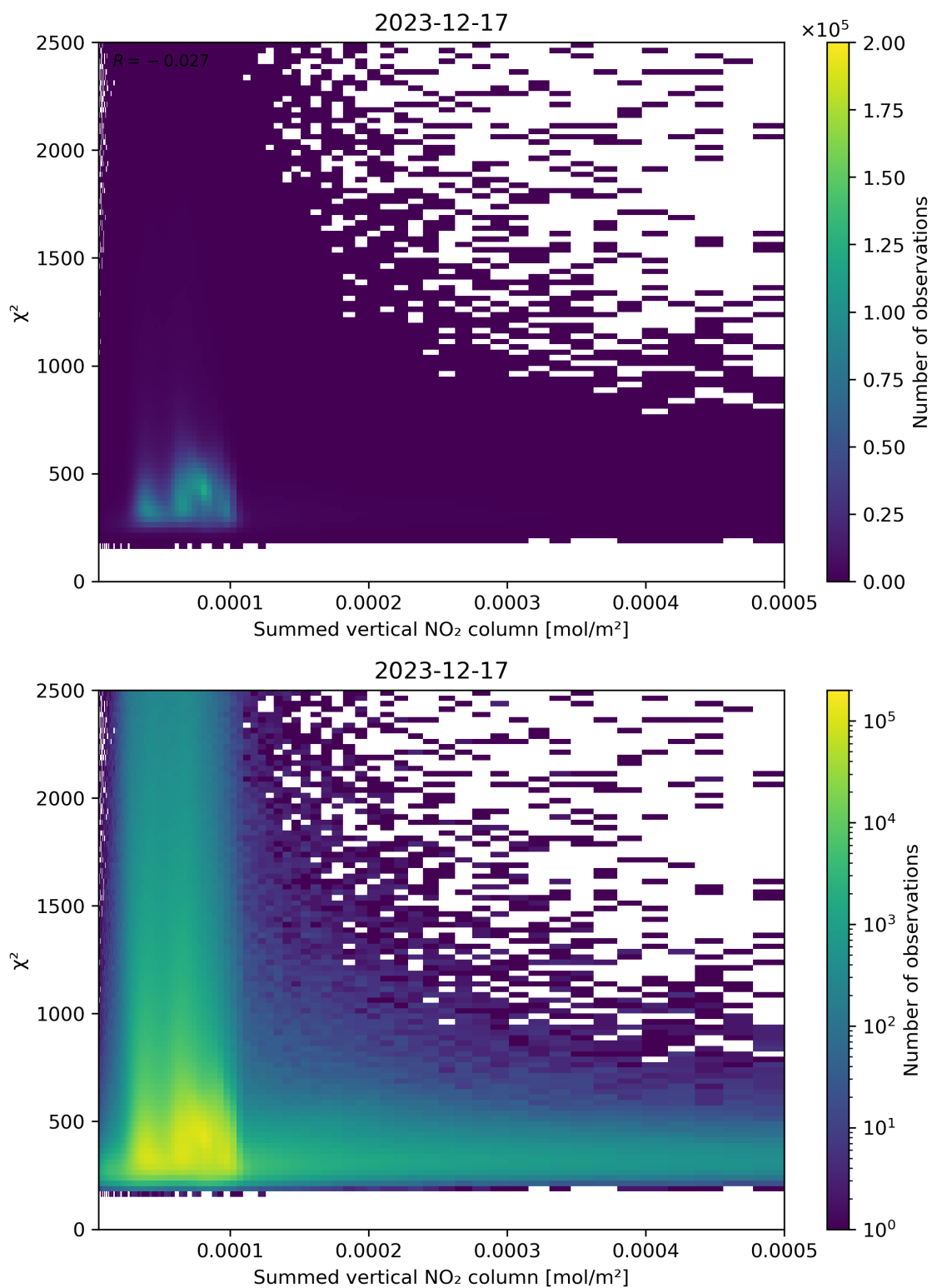
Figure 104: Scatter density plot of “Summed vertical NO 2 column” against “ \chi^2 ” for 2023-12-16 to 2023-12-18.
