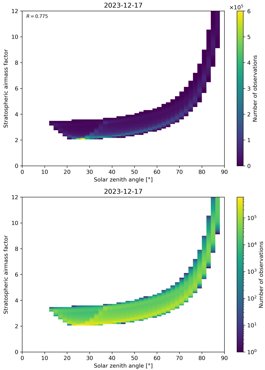
Figure 145: Scatter density plot of “Solar zenith angle” against “Stratospheric airmass factor” for 2023-12-16 to 2023-12-18.
