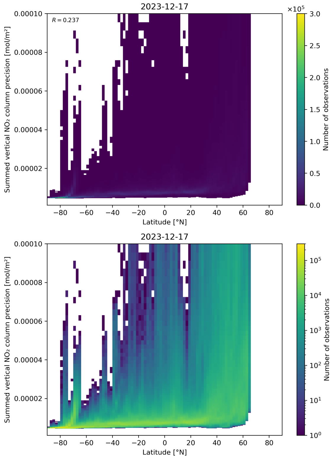
Figure 89: Scatter density plot of “Latitude” against “Summed vertical NO 2 column precision” for 2023-12-16 to 2023-12-18.
