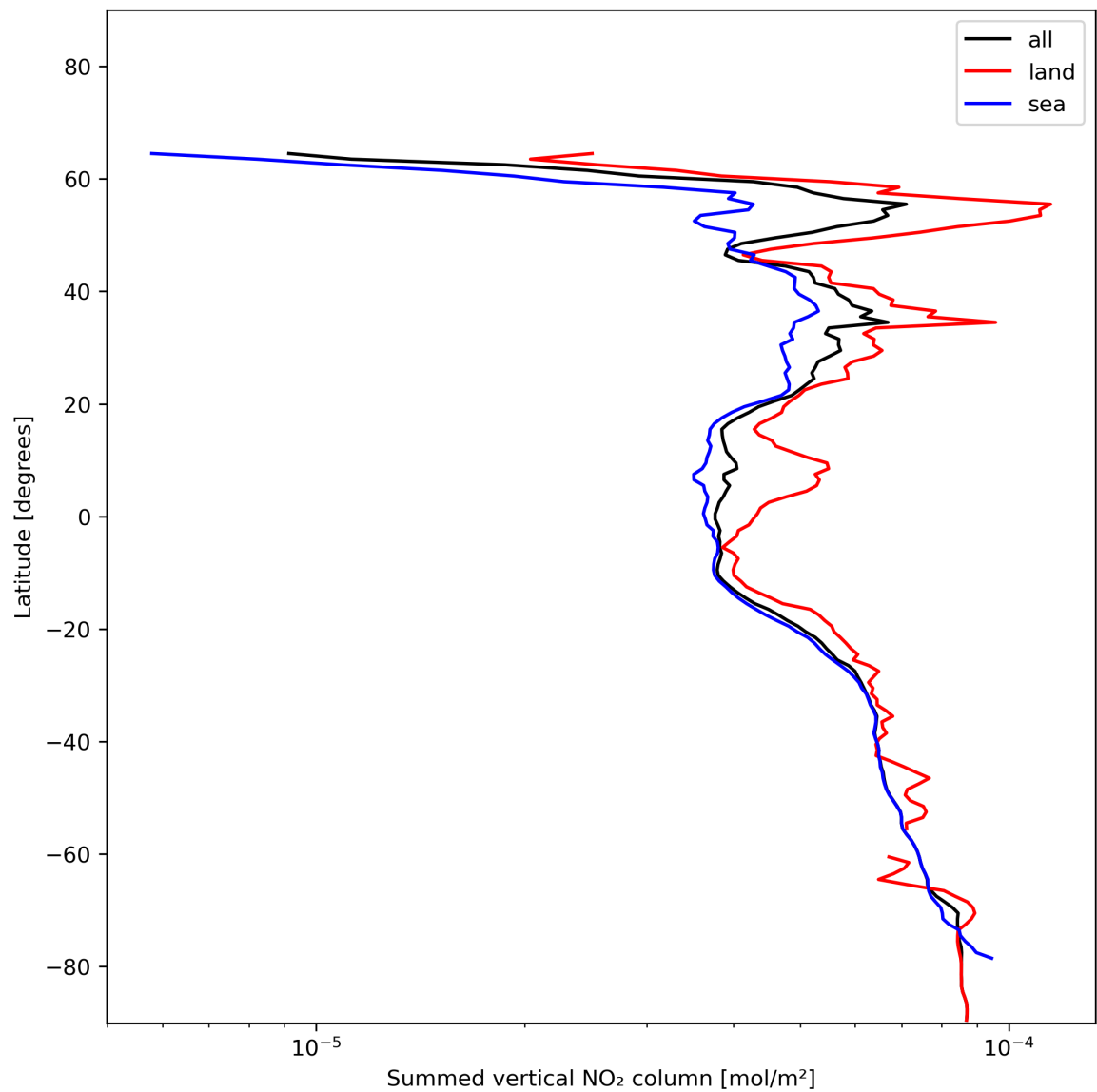
Figure 23: Zonal average of “Summed vertical NO 2 column” for 2023-12-16 to 2023-12-18.
