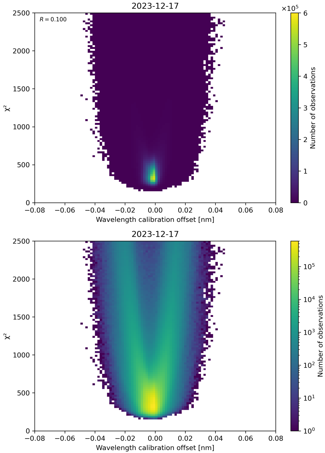
Figure 175: Scatter density plot of “Wavelength calibration offset” against “ \chi^2 ” for 2023-12-16 to 2023-12-18.
