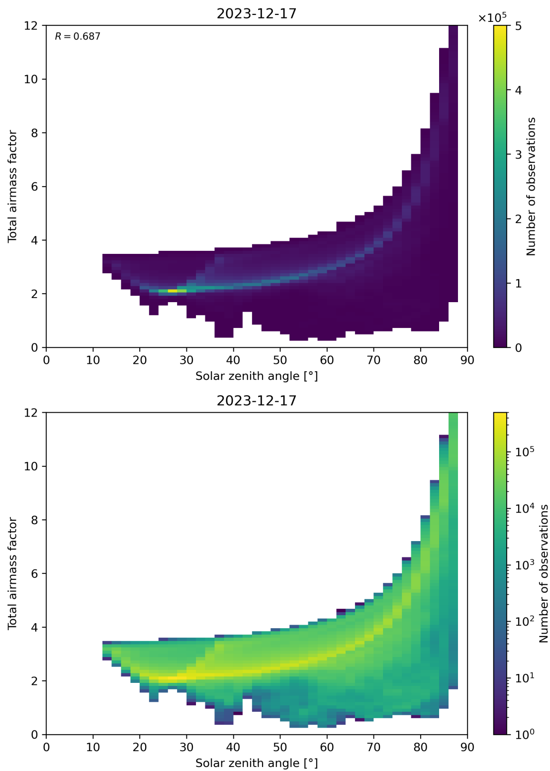
Figure 146: Scatter density plot of “Solar zenith angle” against “Total air mass factor” for 2023-12-16 to 2023-12-18.
