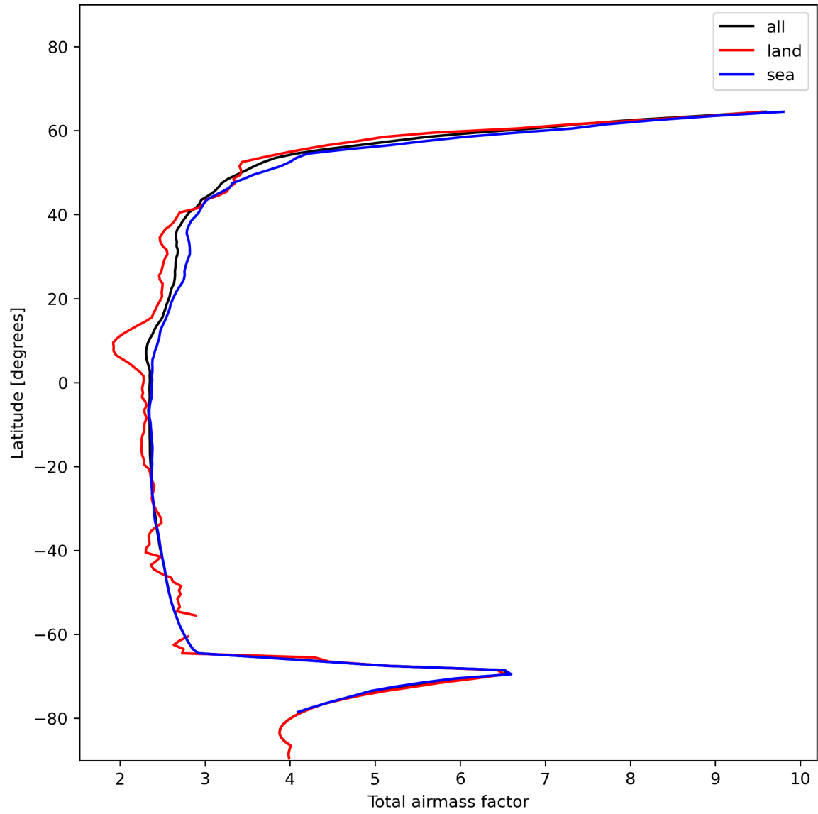
Figure 15: Zonal average of “Total airmass factor” for 2023-12-16 to 2023-12-18.
