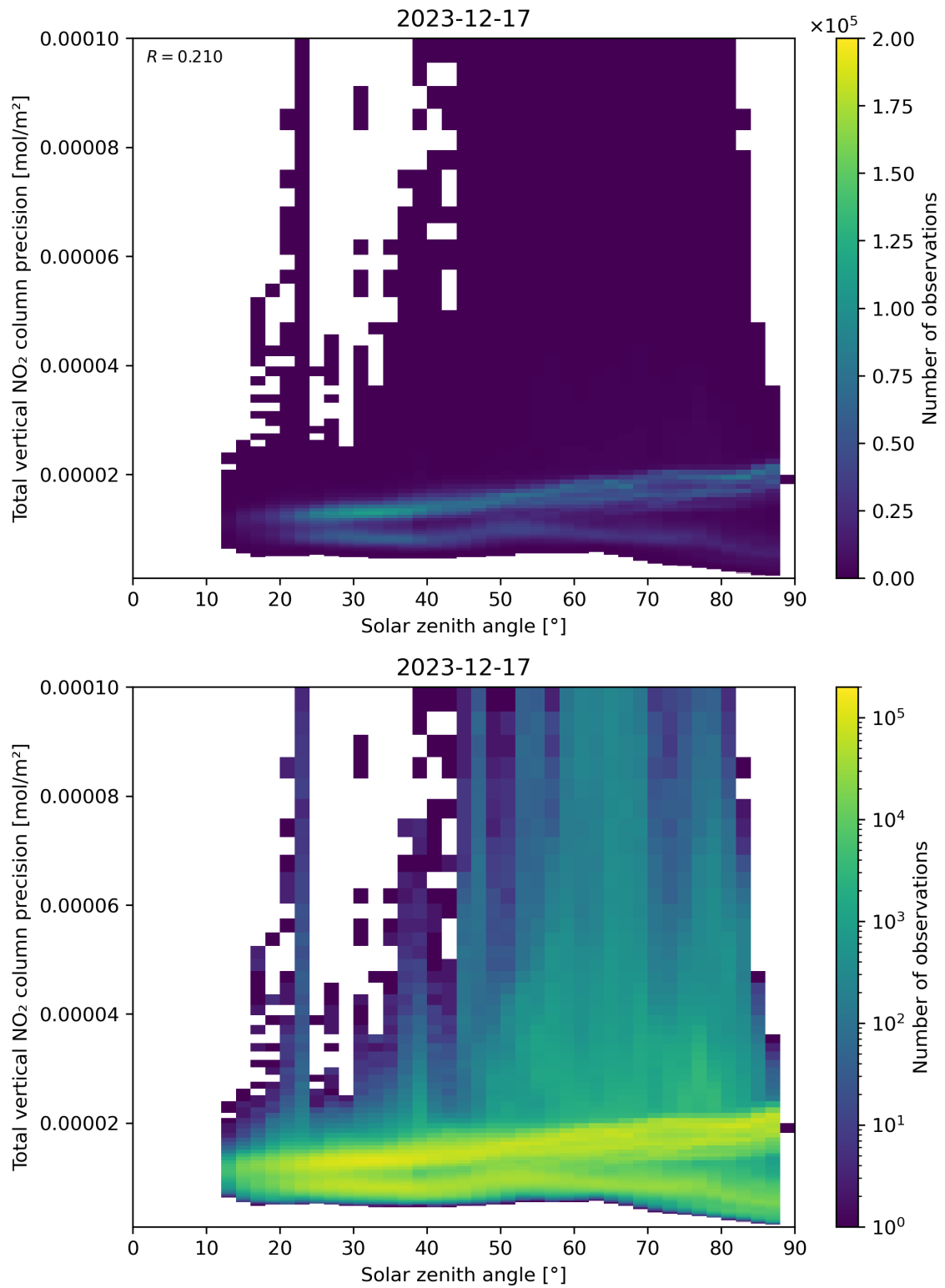
Figure 154: Scatter density plot of “Solar zenith angle” against “Total vertical NO 2 column precision” for 2023-12-16 to 2023-12-18.
