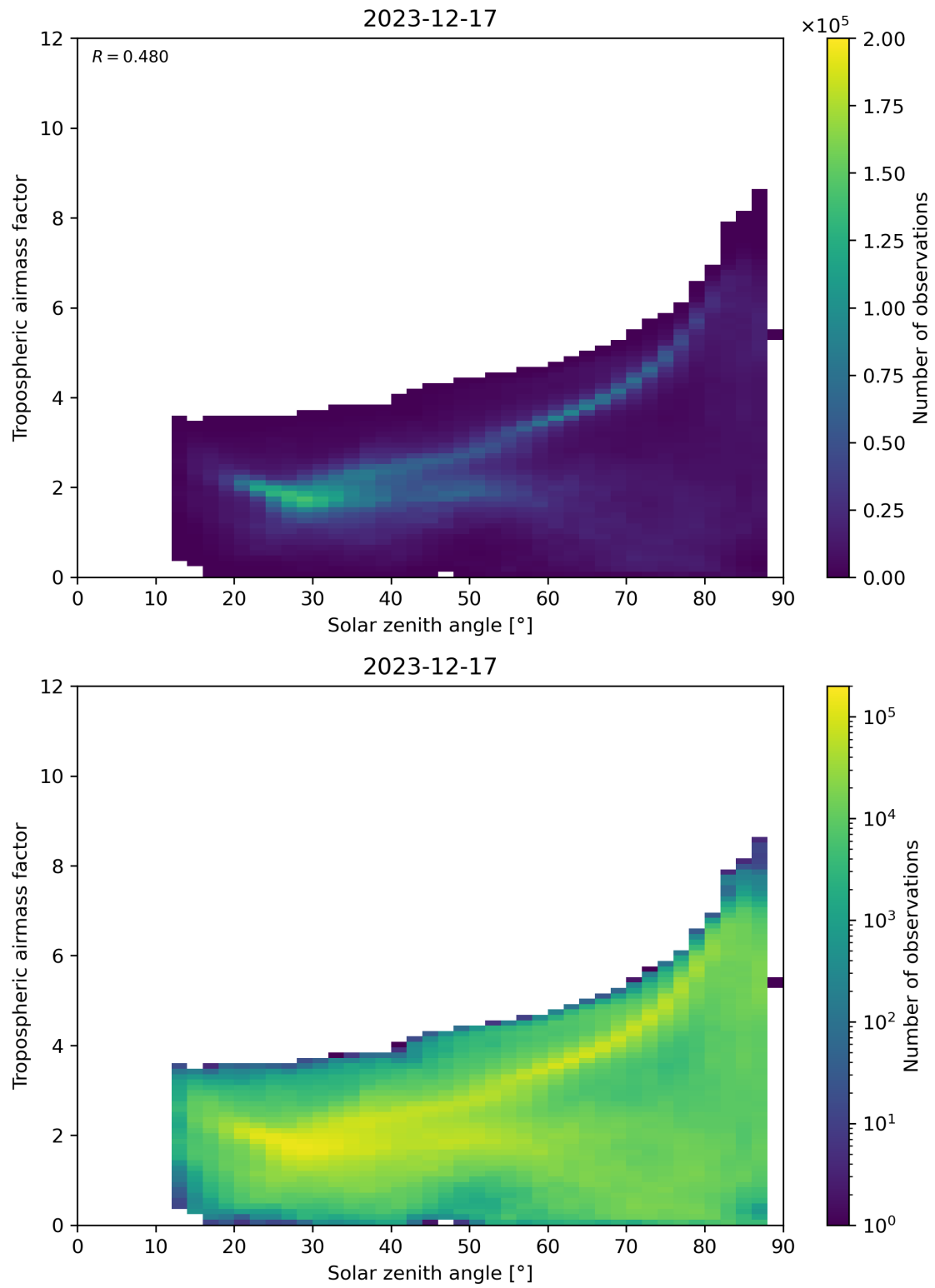
Figure 147: Scatter density plot of “Solar zenith angle” against “Tropospheric airmass factor” for 2023-12-16 to 2023-12-18.
