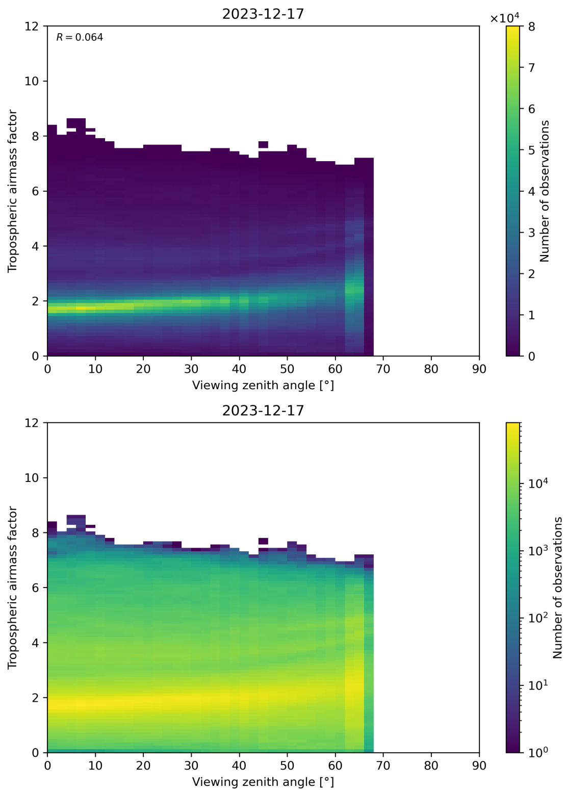
Figure 161: Scatter density plot of “Viewing zenith angle” against “Tropospheric airmass factor” for 2023-12-16 to 2023-12-18.
