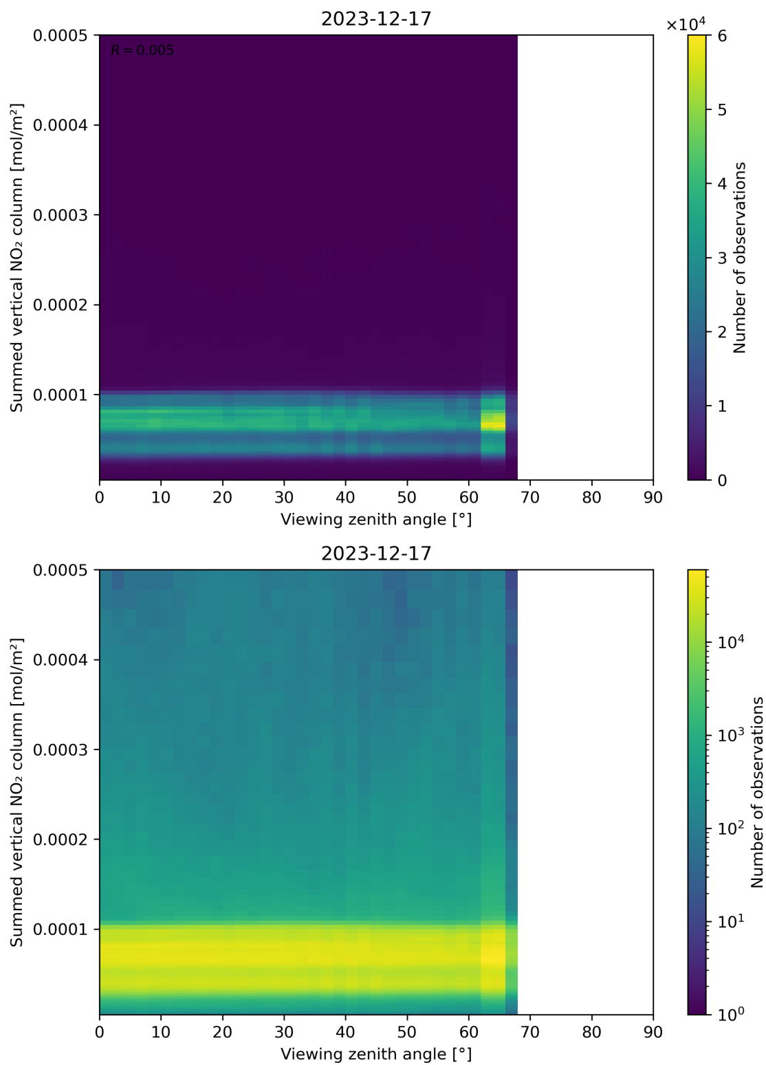
Figure 165: Scatter density plot of “Viewing zenith angle” against “Summed vertical NO 2 column” for 2023-12-16 to 2023-12-18.
