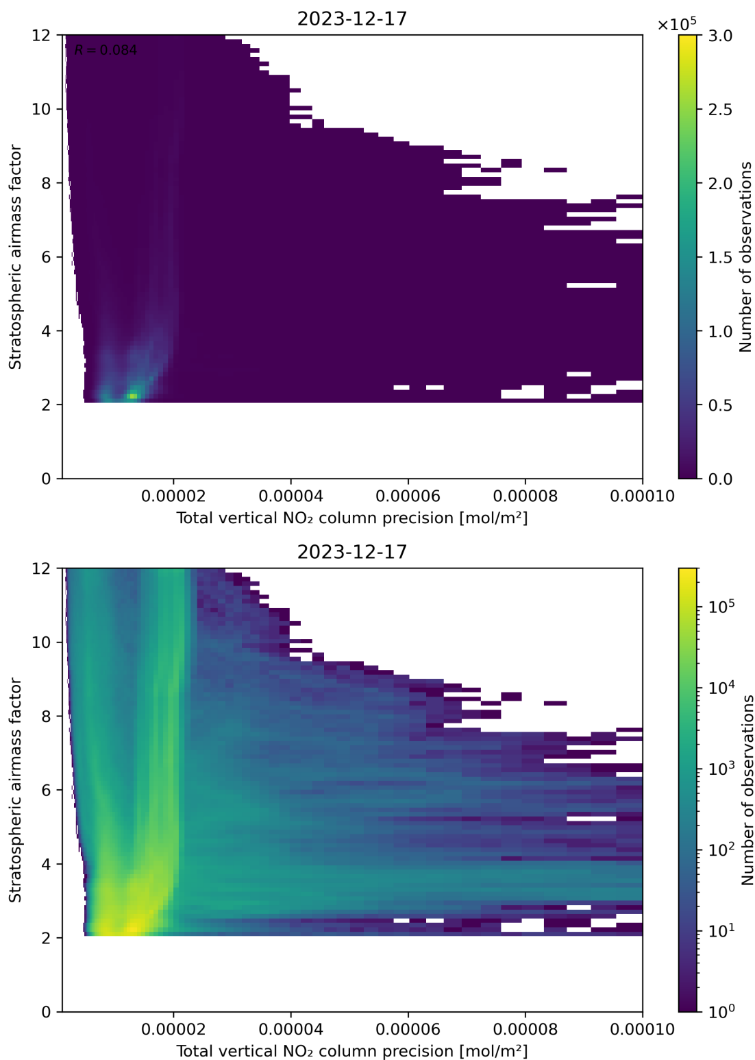
Figure 115: Scatter density plot of “Total vertical NO 2 column precision” against “Stratospheric air mass factor” for 2023-12-16 to 2023-12-18.
