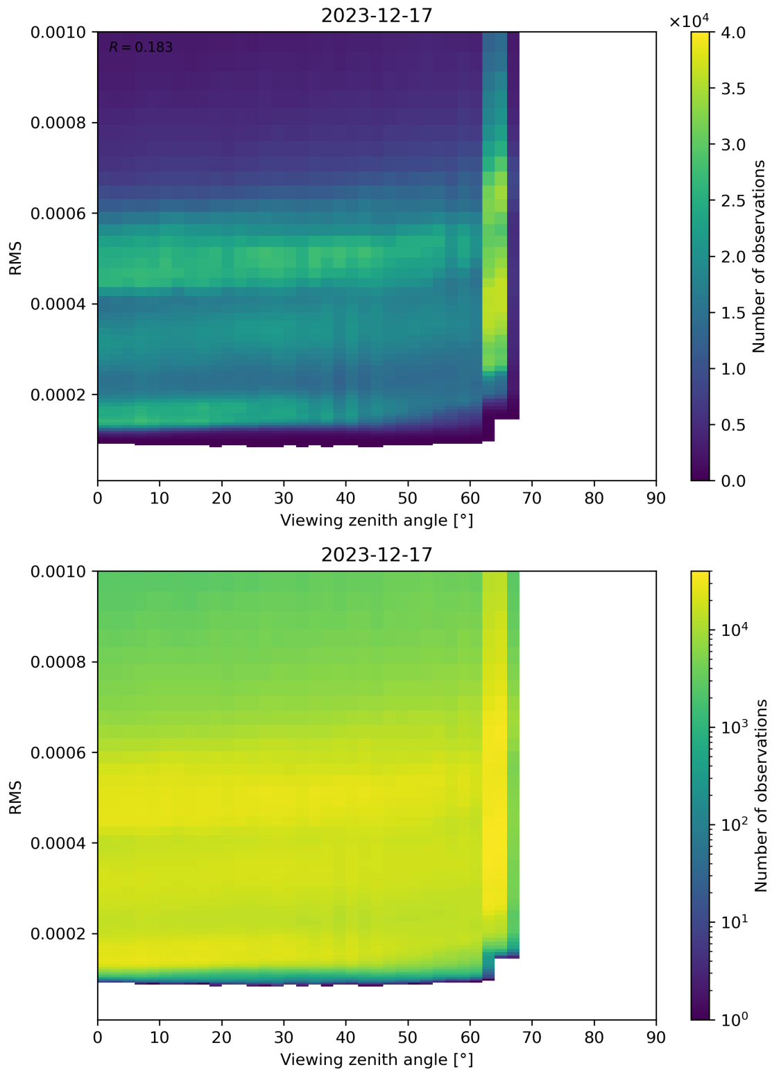
Figure 171: Scatter density plot of “Viewing zenith angle” against “RMS” for 2023-12-16 to 2023-12-18.
