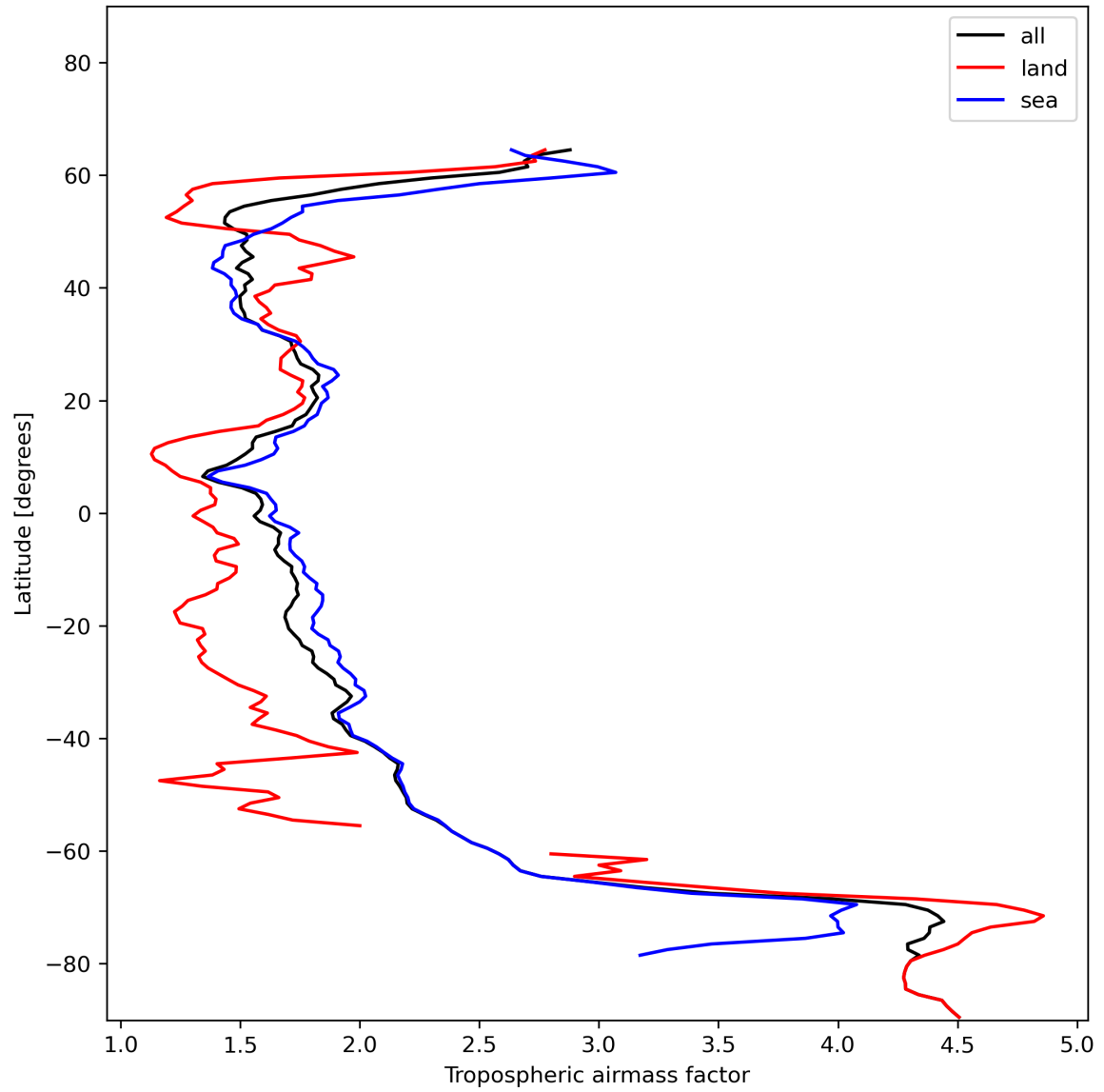
Figure 14: Zonal average of “Tropospheric airmass factor” for 2023-12-16 to 2023-12-18.
