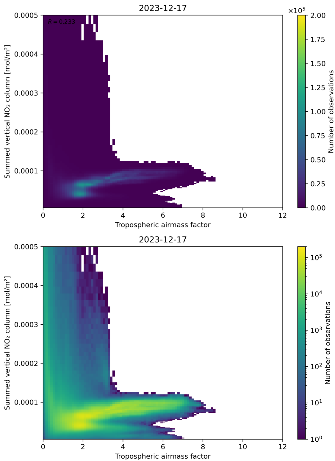
Figure 75: Scatter density plot of “Tropospheric airmass factor” against “Summed vertical NO 2 column” for 2023-12-16 to 2023-12-18.
