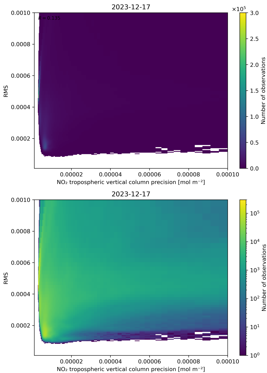
Figure 140: Scatter density plot of “NO 2 tropospheric vertical column precision” against “RMS” for 2023-12-16 to 2023-12-18.
