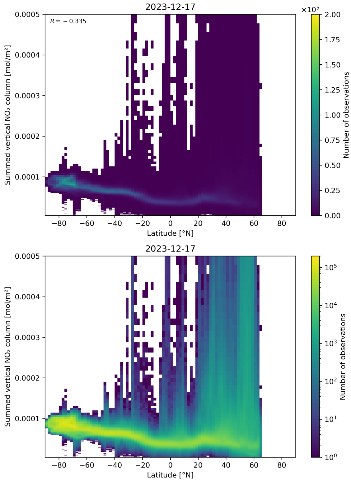
Figure 88: Scatter density plot of “Latitude” against “Summed vertical NO 2 column” for 2023-12-16 to 2023-12-18.
