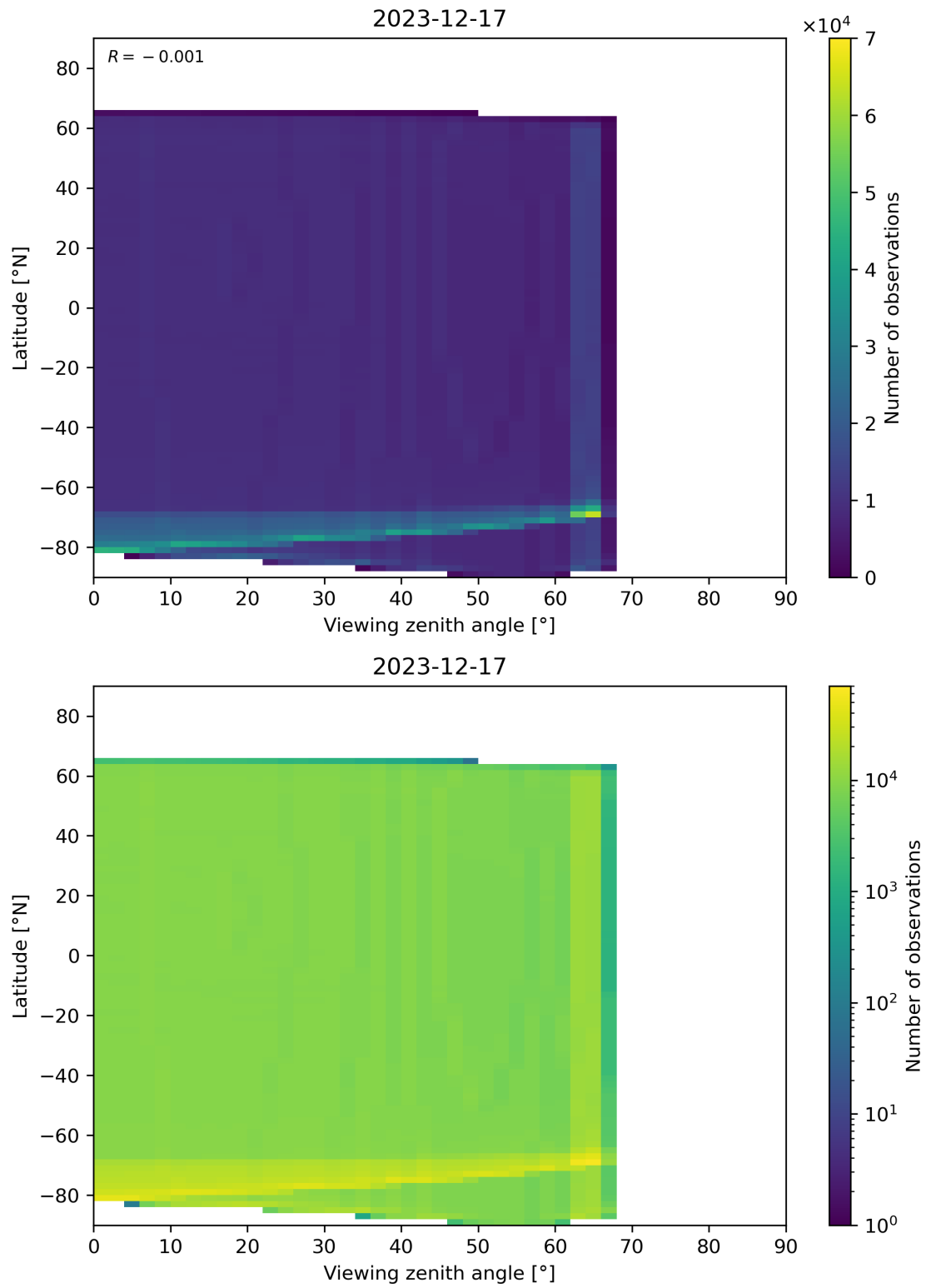
Figure 163: Scatter density plot of “Viewing zenith angle” against “Latitude” for 2023-12-16 to 2023-12-18.
