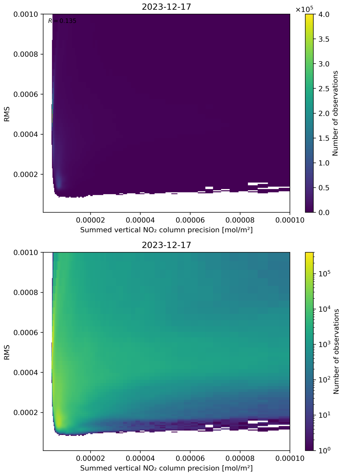
Figure 108: Scatter density plot of “Summed vertical NO 2 column precision” against “RMS” for 2023-12-16 to 2023-12-18.
