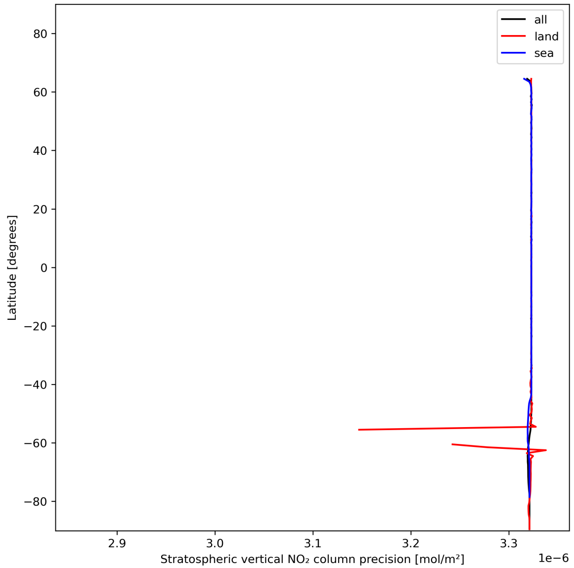
Figure 20: Zonal average of “Stratospheric vertical NO 2 column precision” for 2023-12-17 to 2023-12-19.
