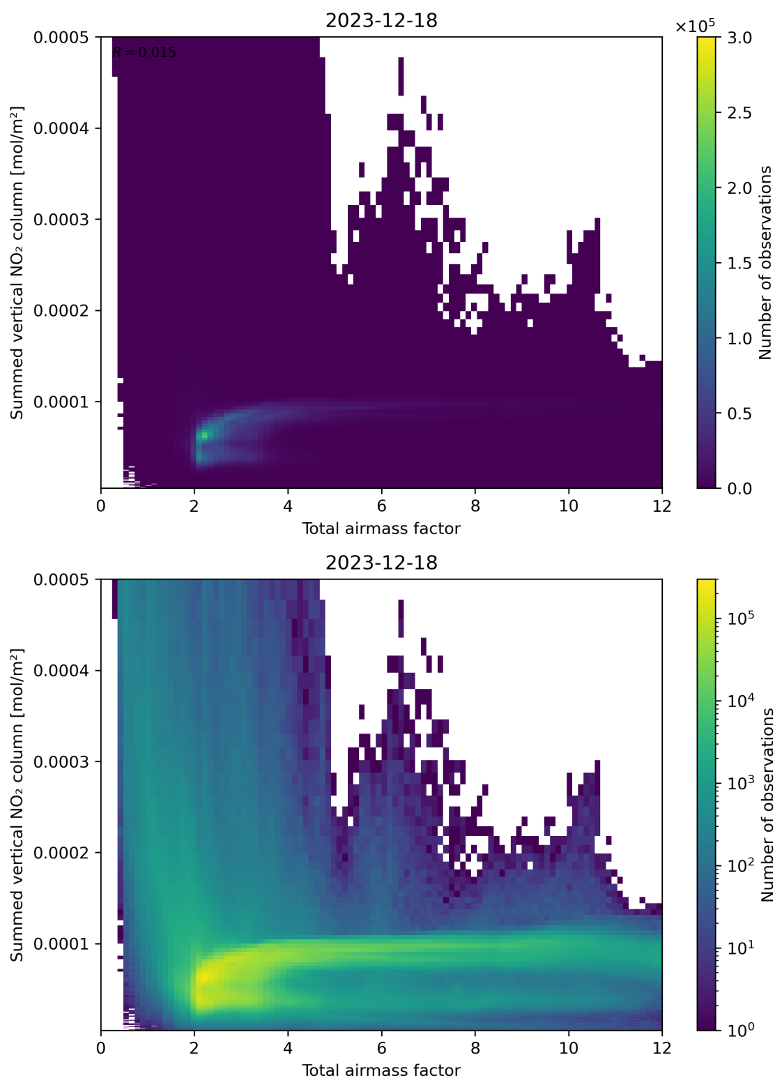
Figure 65: Scatter density plot of “Total airmass factor” against “Summed vertical NO 2 column” for 2023-12-17 to 2023-12-19.
