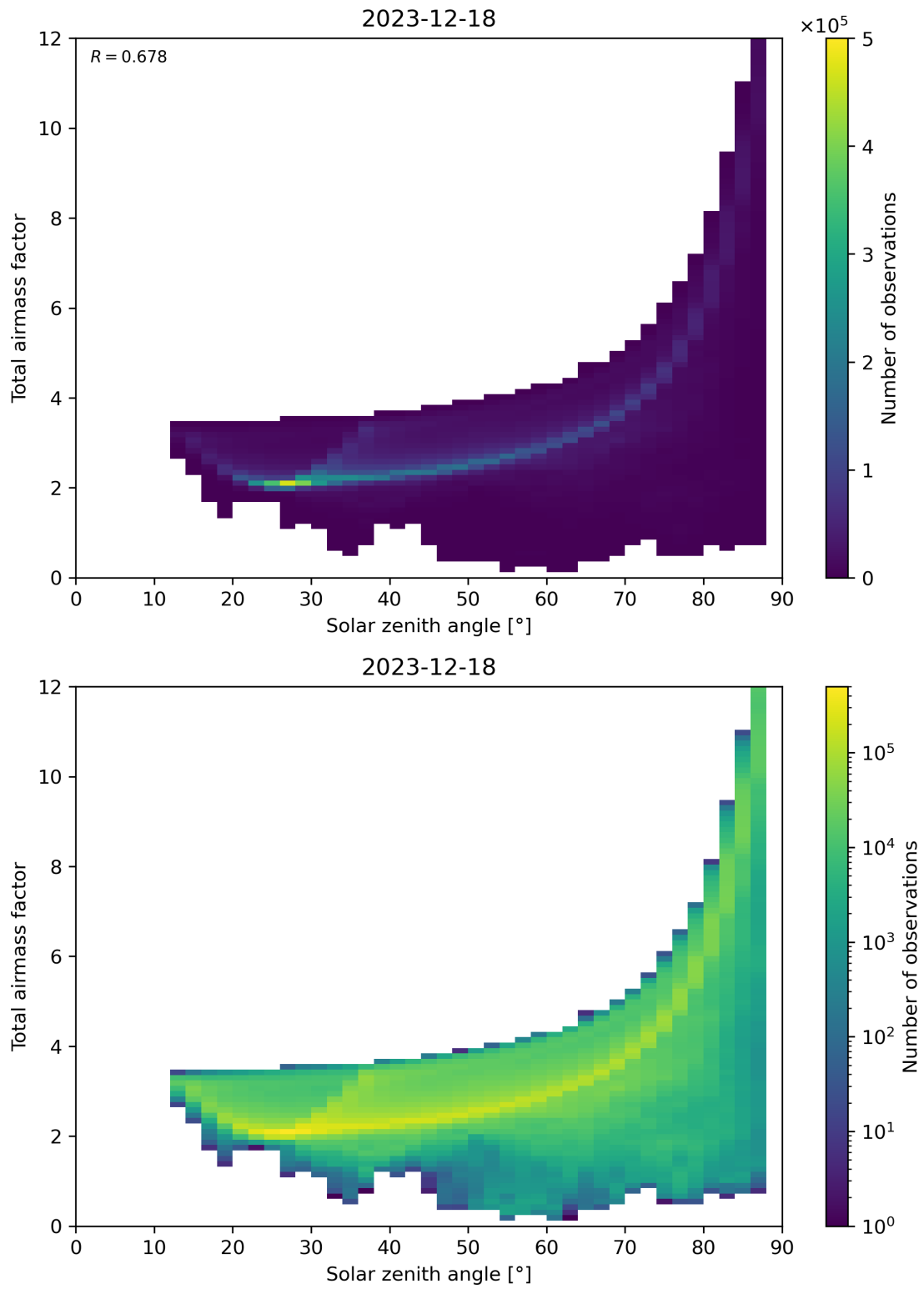
Figure 146: Scatter density plot of “Solar zenith angle” against “Total air mass factor” for 2023-12-17 to 2023-12-19.
