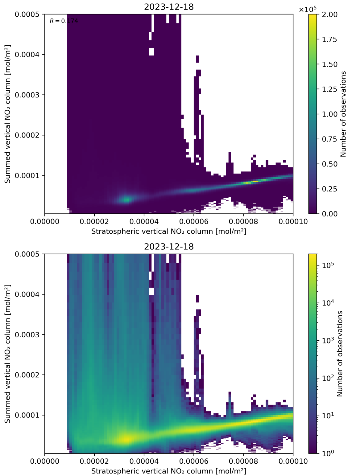
Figure 98: Scatter density plot of “Stratospheric vertical NO 2 column” against “Summed vertical NO 2 column” for 2023-12-17 to 2023-12-19.
