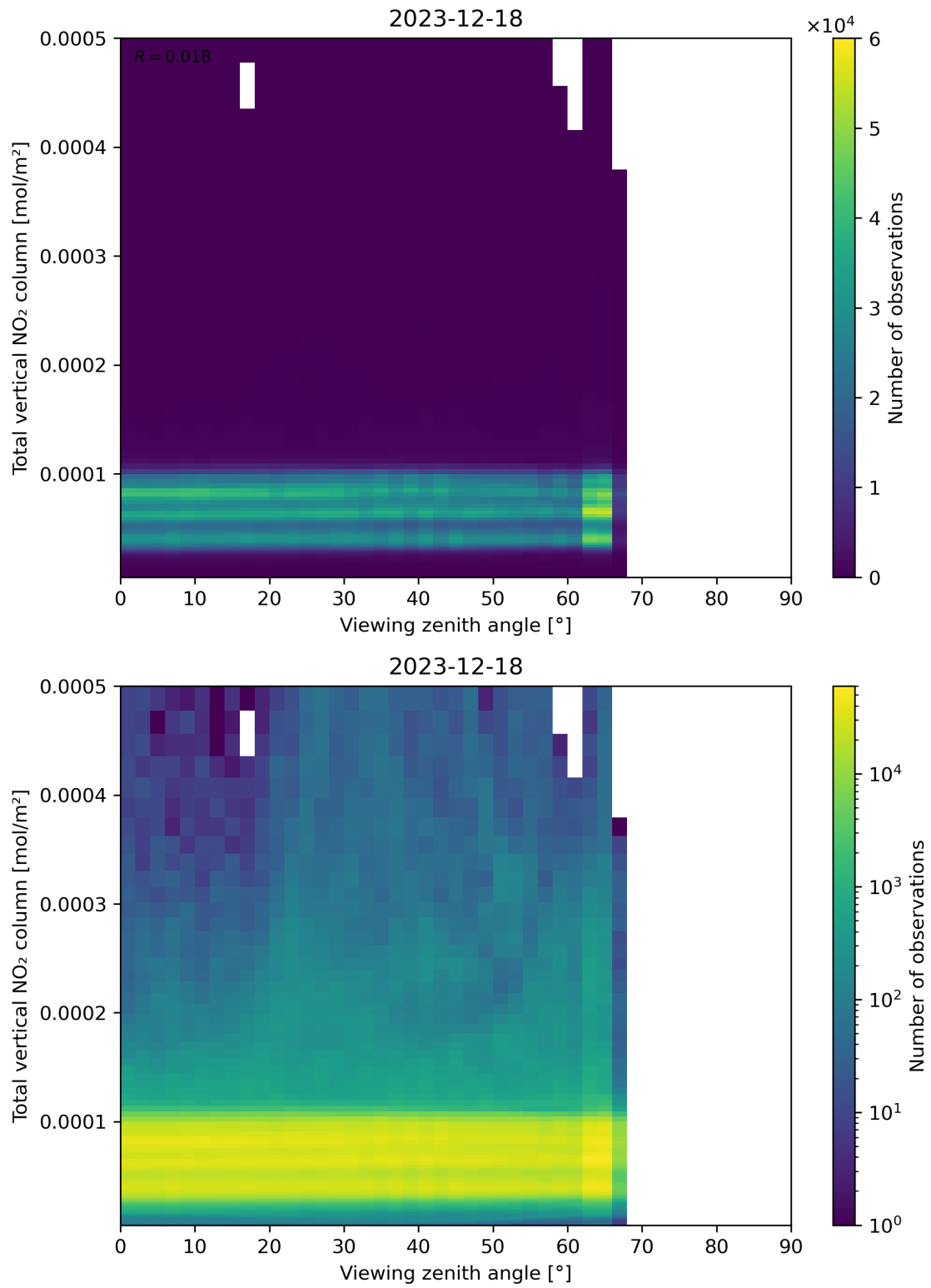
Figure 167: Scatter density plot of “Viewing zenith angle” against “Total vertical NO 2 column” for 2023-12-17 to 2023-12-19.
