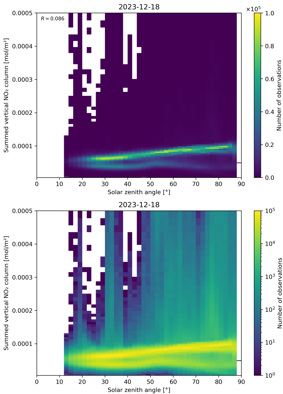
Figure 151: Scatter density plot of “Solar zenith angle” against “Summed vertical NO 2 column” for 2023-12-17 to 2023-12-19.
