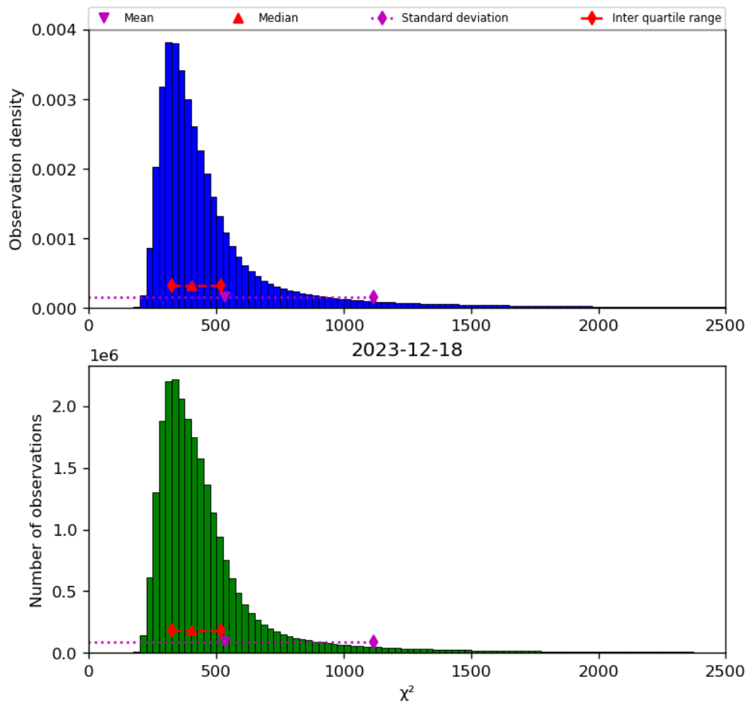
Figure 42: Histogram of “ \chi^2 ” for 2023-12-17 to 2023-12-19
