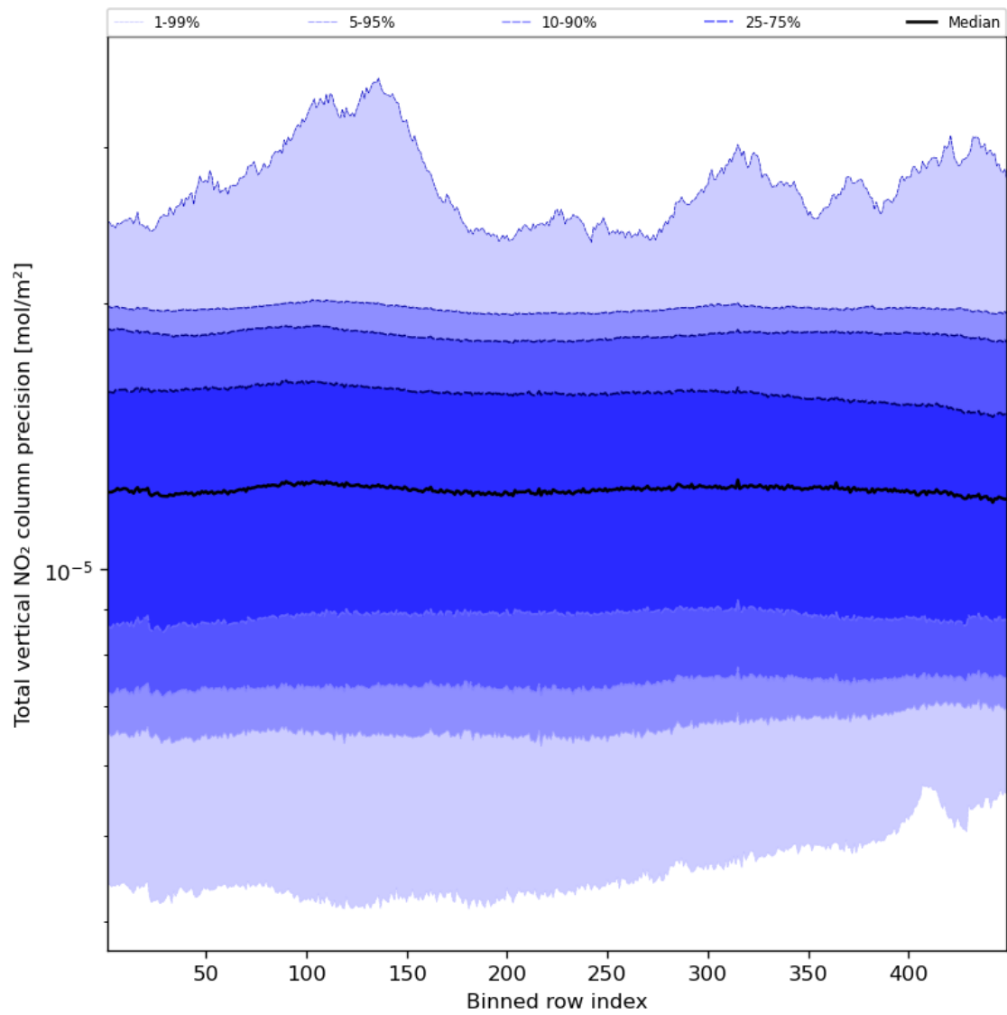
Figure 56: Along track statistics of “Total vertical NO 2 column precision” for 2023-12-17 to 2023-12-19
