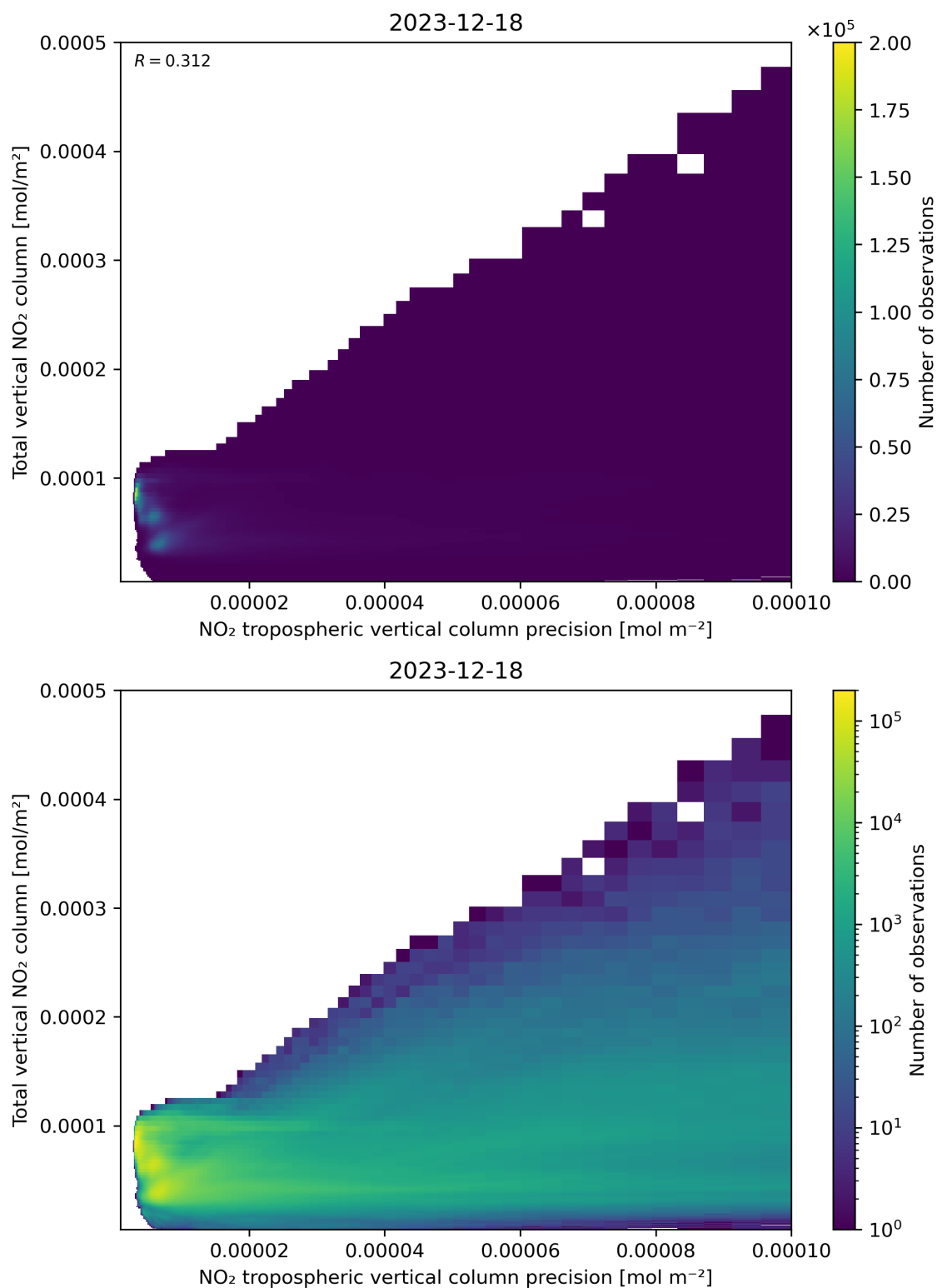
Figure 138: Scatter density plot of “NO 2 tropospheric vertical column precision” against “Total vertical NO 2 column” for 2023-12-17 to 2023-12-19.
