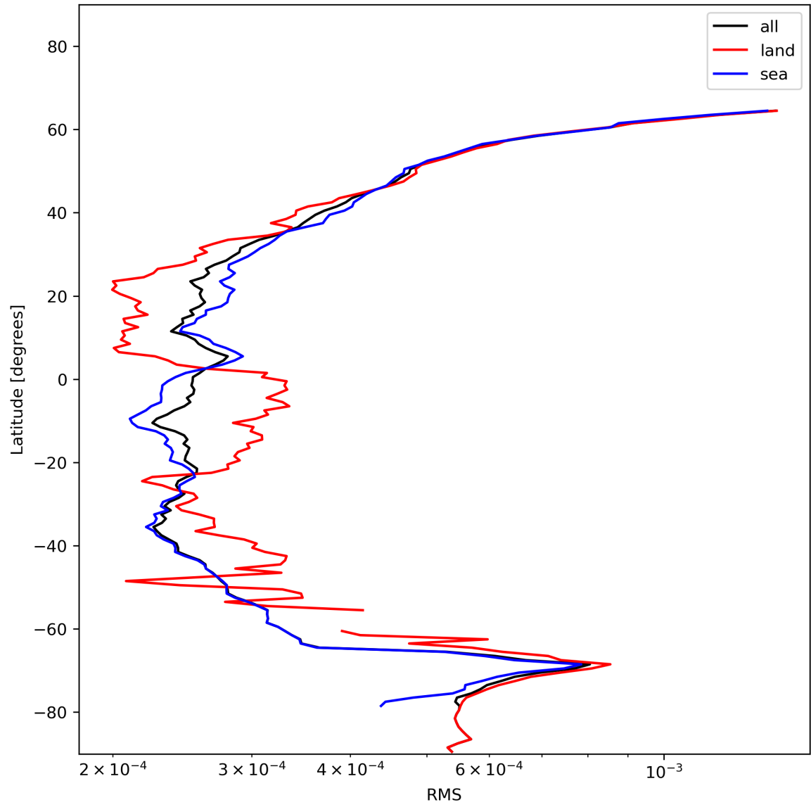
Figure 26: Zonal average of “RMS” for 2023-12-17 to 2023-12-19.
