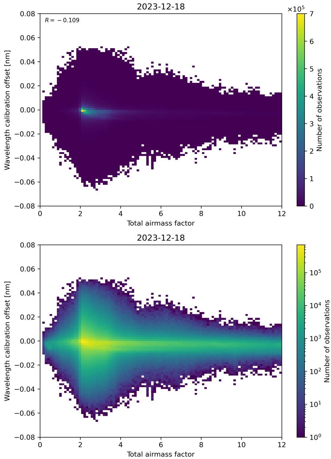
Figure 70: Scatter density plot of “Total airmass factor” against “Wavelength calibration offset” for 2023-12-17 to 2023-12-19.
