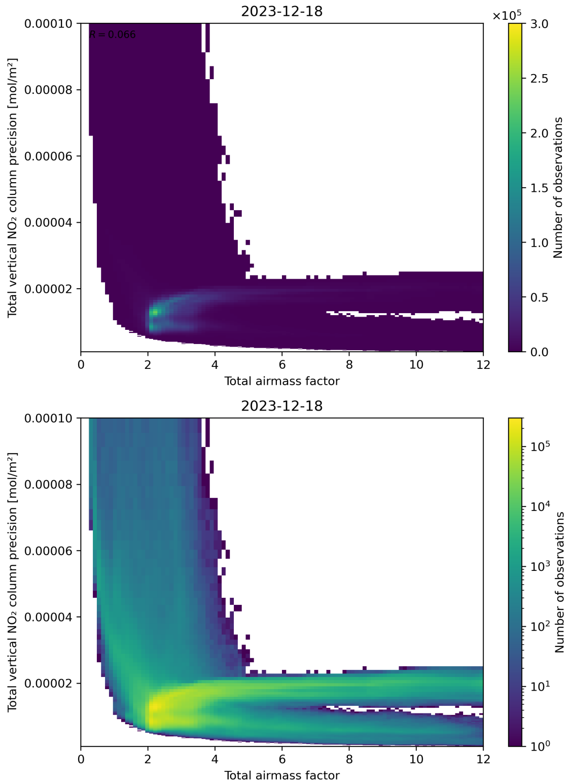
Figure 68: Scatter density plot of “Total airmass factor” against “Total vertical NO 2 column precision” for 2023-12-17 to 2023-12-19.
