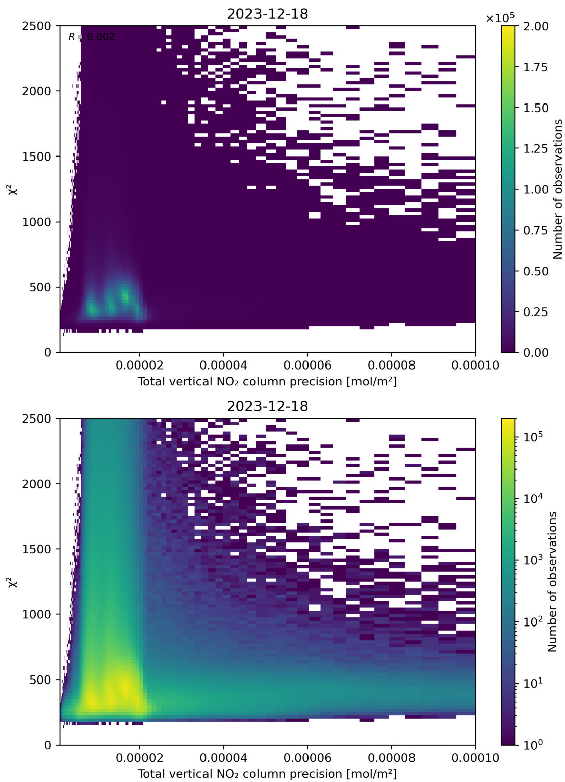
Figure 116: Scatter density plot of “Total vertical NO 2 column precision” against “ \chi^2 ” for 2023-12-17 to 2023-12-19.
