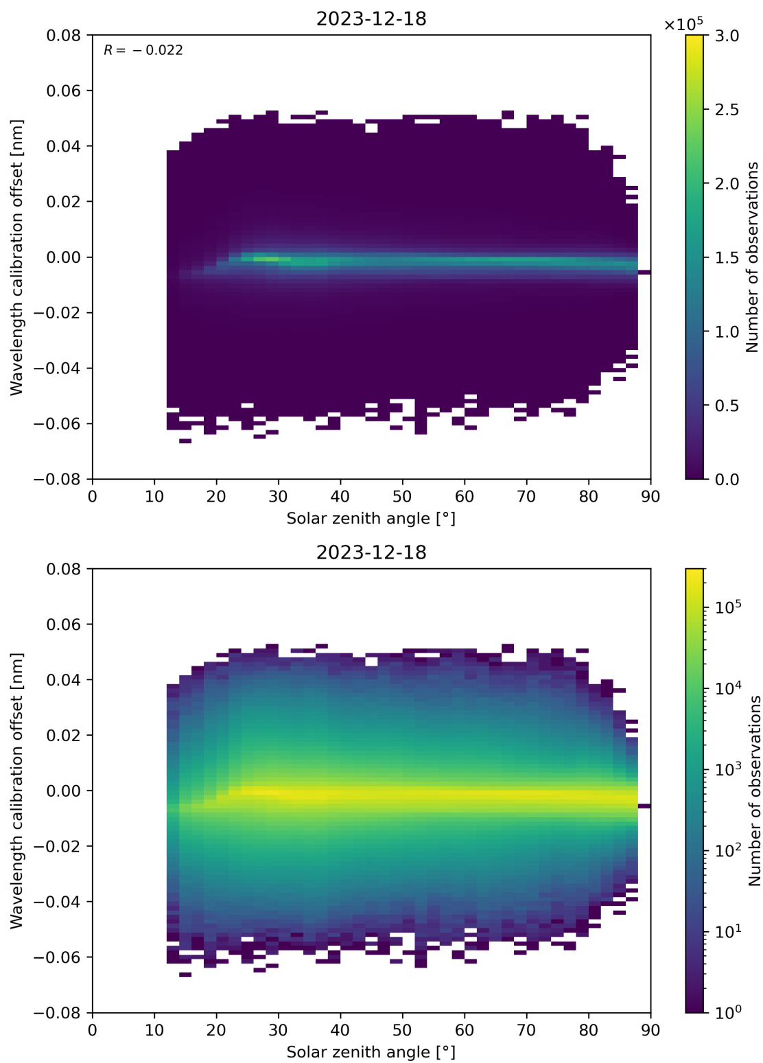
Figure 158: Scatter density plot of “Solar zenith angle” against “Wavelength calibration offset” for 2023-12-17 to 2023-12-19.
