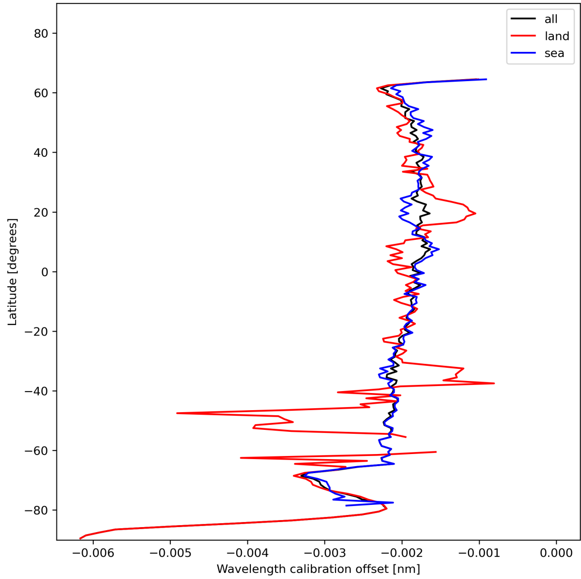
Figure 18: Zonal average of “Wavelength calibration offset” for 2023-12-17 to 2023-12-19.
