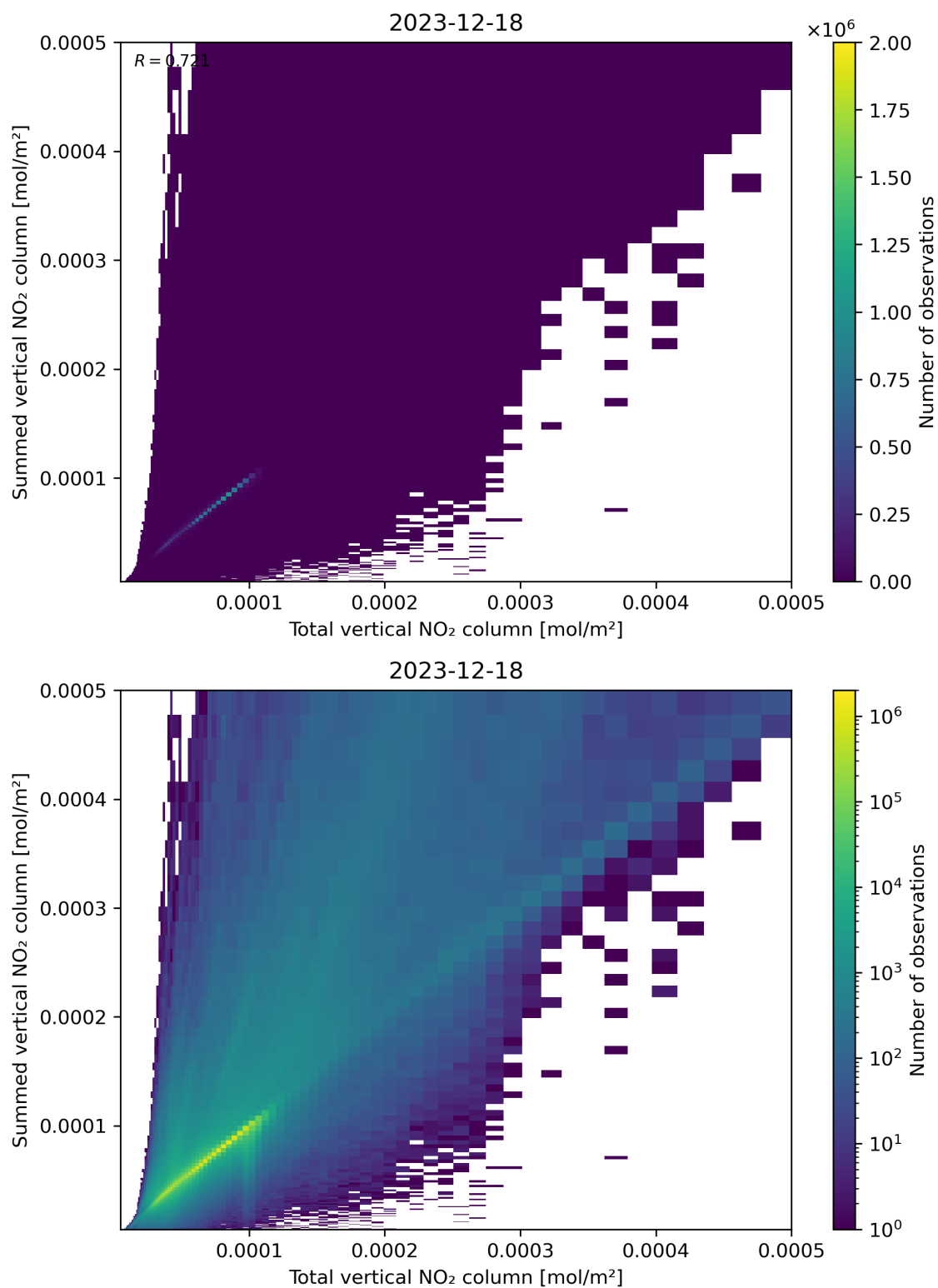
Figure 112: Scatter density plot of “Total vertical NO 2 column” against “Summed vertical NO 2 column” for 2023-12-17 to 2023-12-19.
