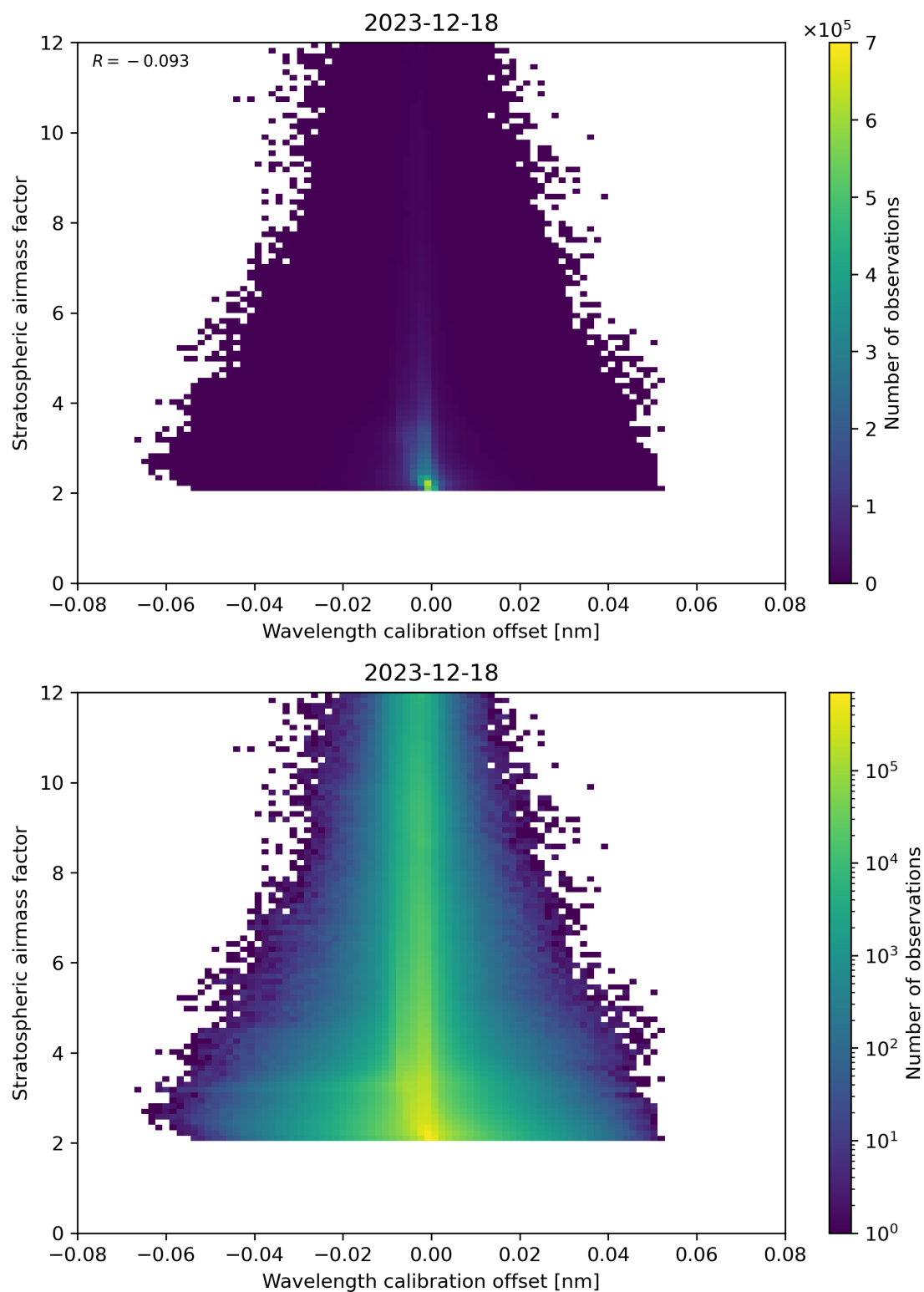
Figure 174: Scatter density plot of “Wavelength calibration offset” against “Stratospheric airmass factor” for 2023-12-17 to 2023-12-19.
