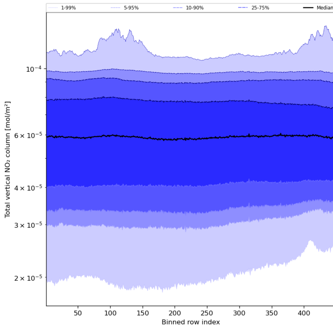
Figure 55: Along track statistics of “Total vertical NO 2 column” for 2023-12-17 to 2023-12-19
