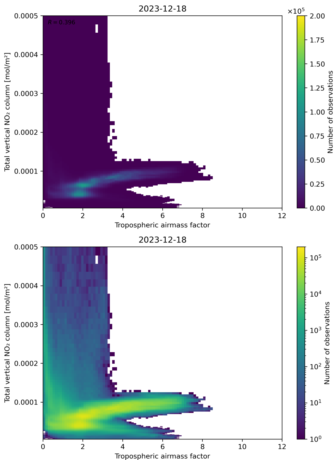
Figure 77: Scatter density plot of “Tropospheric airmass factor” against “Total vertical \text{NO}_2 column” for 2023-12-17 to 2023-12-19.
