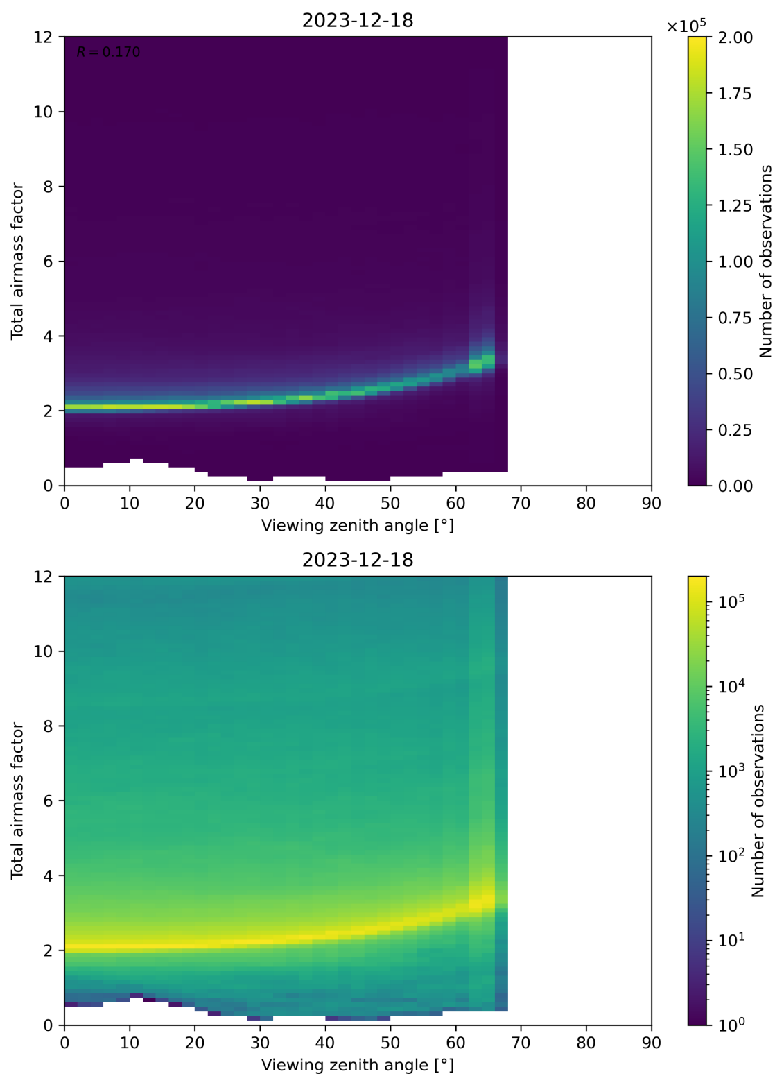
Figure 160: Scatter density plot of “Viewing zenith angle” against “Total airmass factor” for 2023-12-17 to 2023-12-19.
