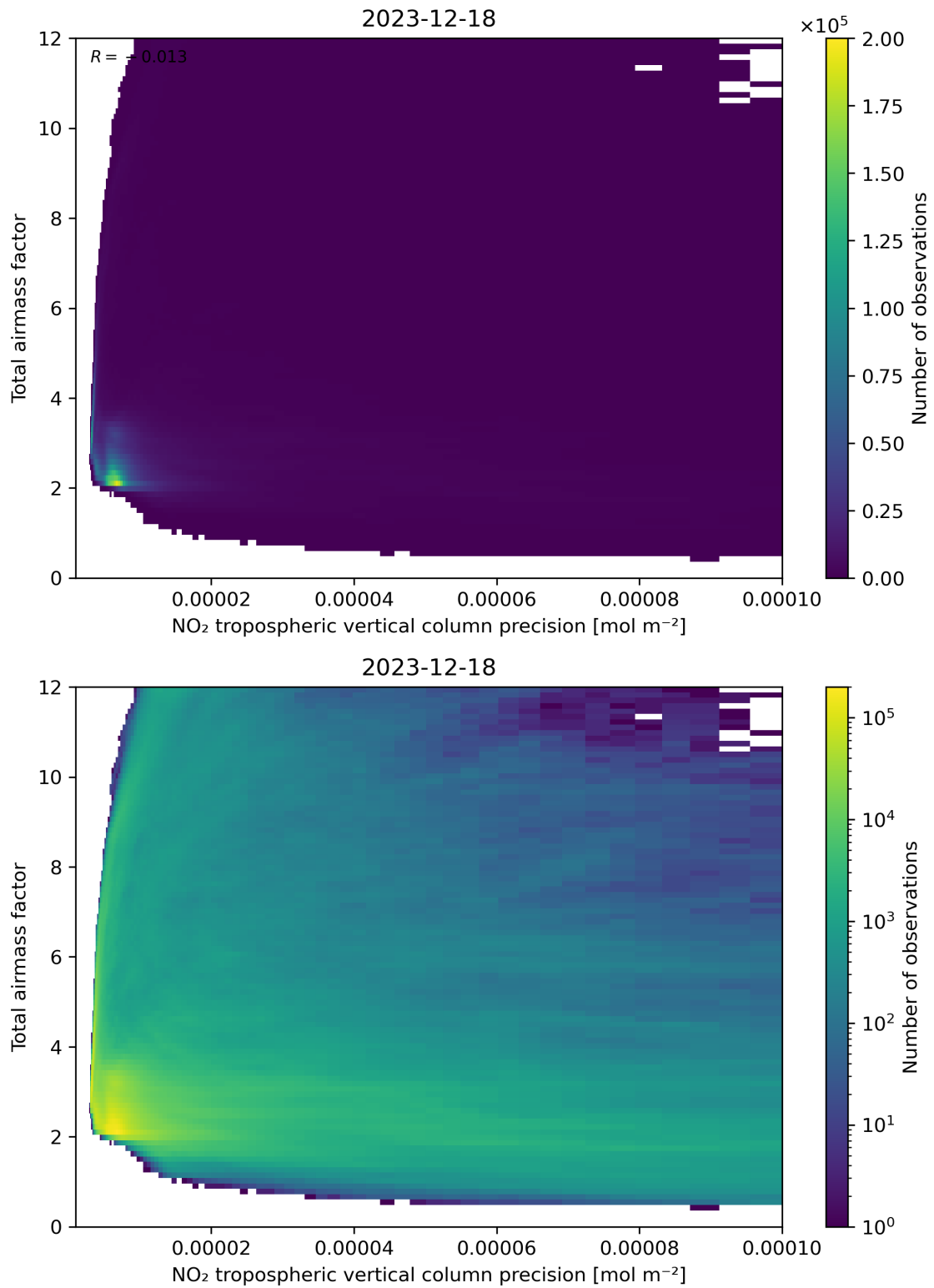
Figure 132: Scatter density plot of “NO 2 tropospheric vertical column precision” against “Total air mass factor” for 2023-12-17 to 2023-12-19.
