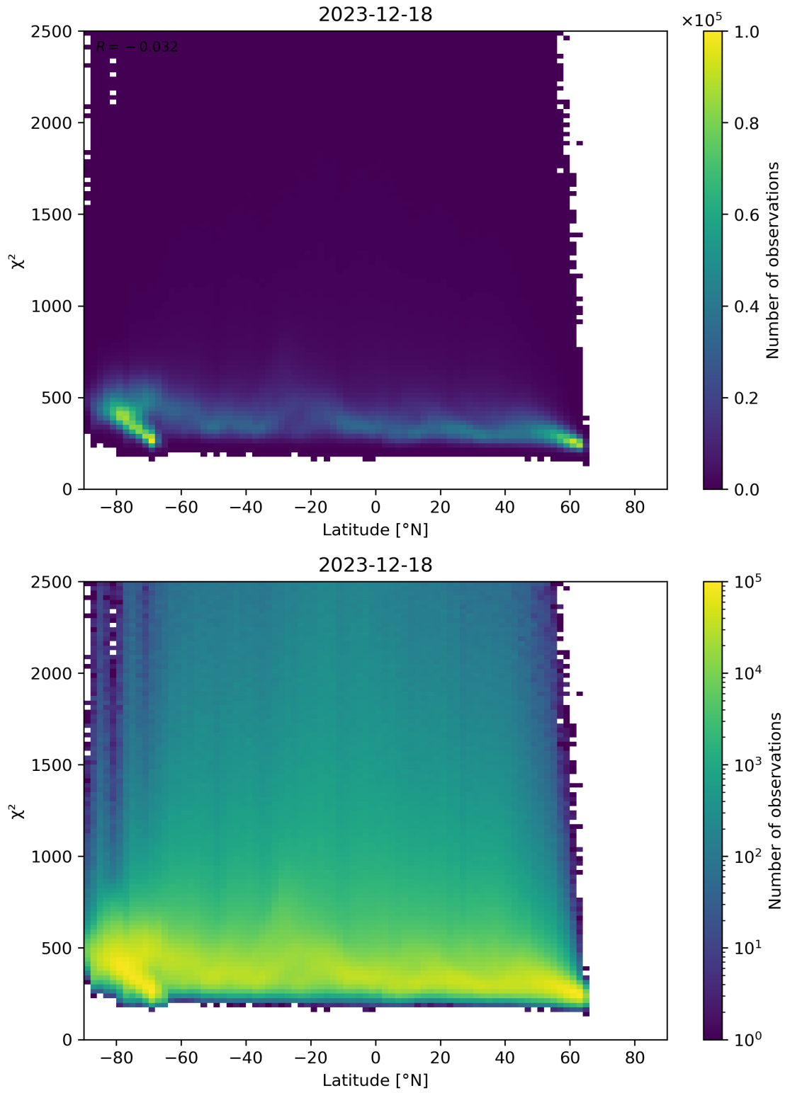
Figure 86: Scatter density plot of “Latitude” against “ \chi^2 ” for 2023-12-17 to 2023-12-19.
