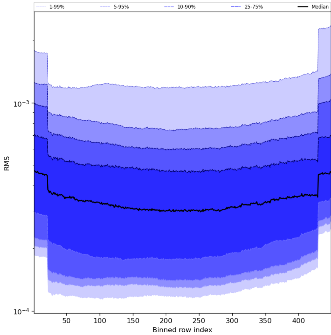
Figure 60: Along track statistics of “RMS” for 2023-12-17 to 2023-12-19
