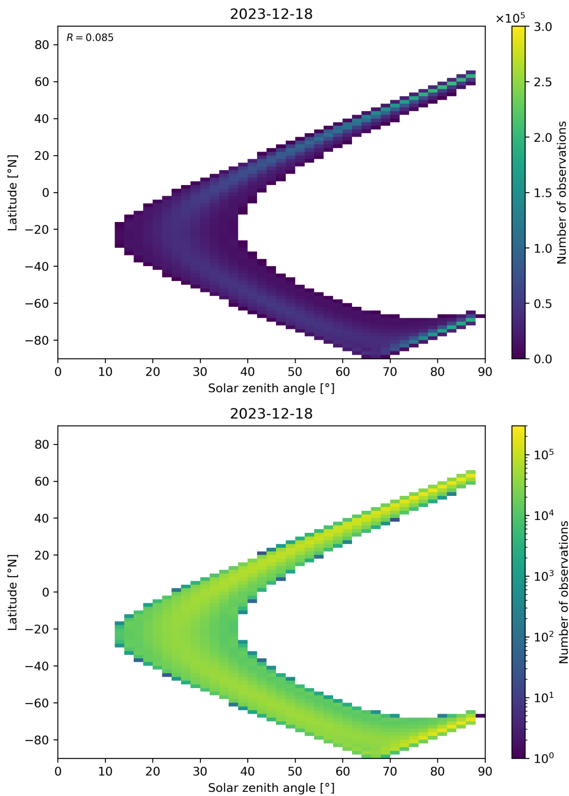
Figure 149: Scatter density plot of “Solar zenith angle” against “Latitude” for 2023-12-17 to 2023-12-19.
