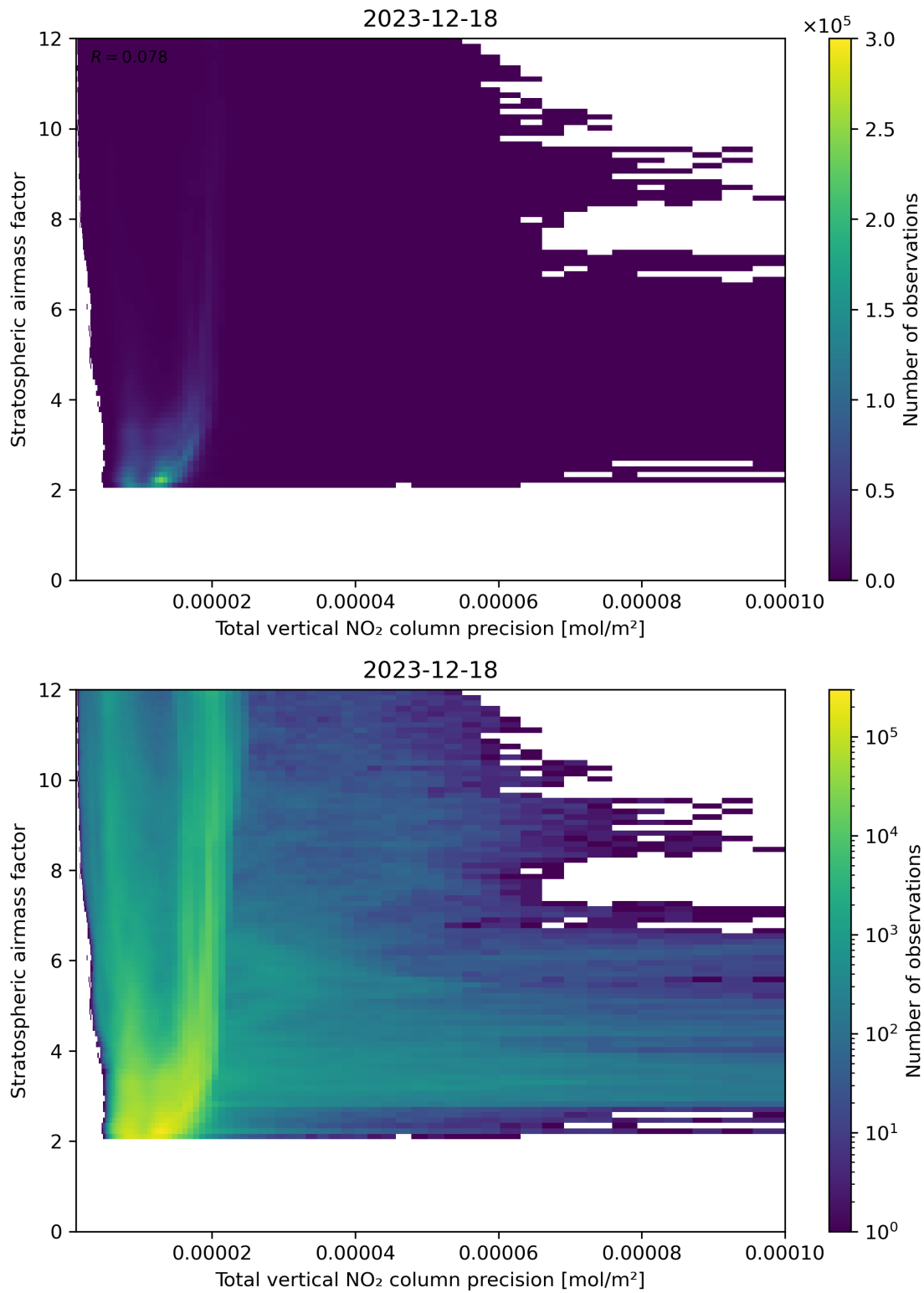
Figure 115: Scatter density plot of “Total vertical NO 2 column precision” against “Stratospheric airmass factor” for 2023-12-17 to 2023-12-19.
