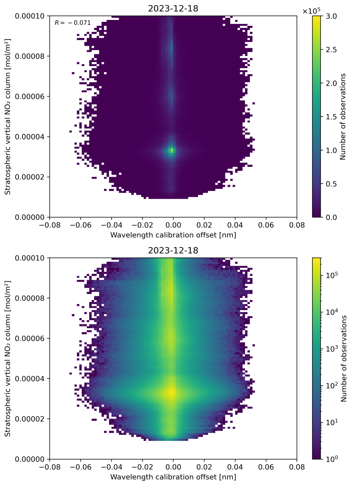
Figure 176: Scatter density plot of “Wavelength calibration offset” against “Stratospheric vertical NO 2 column” for 2023-12-17 to 2023-12-19.
