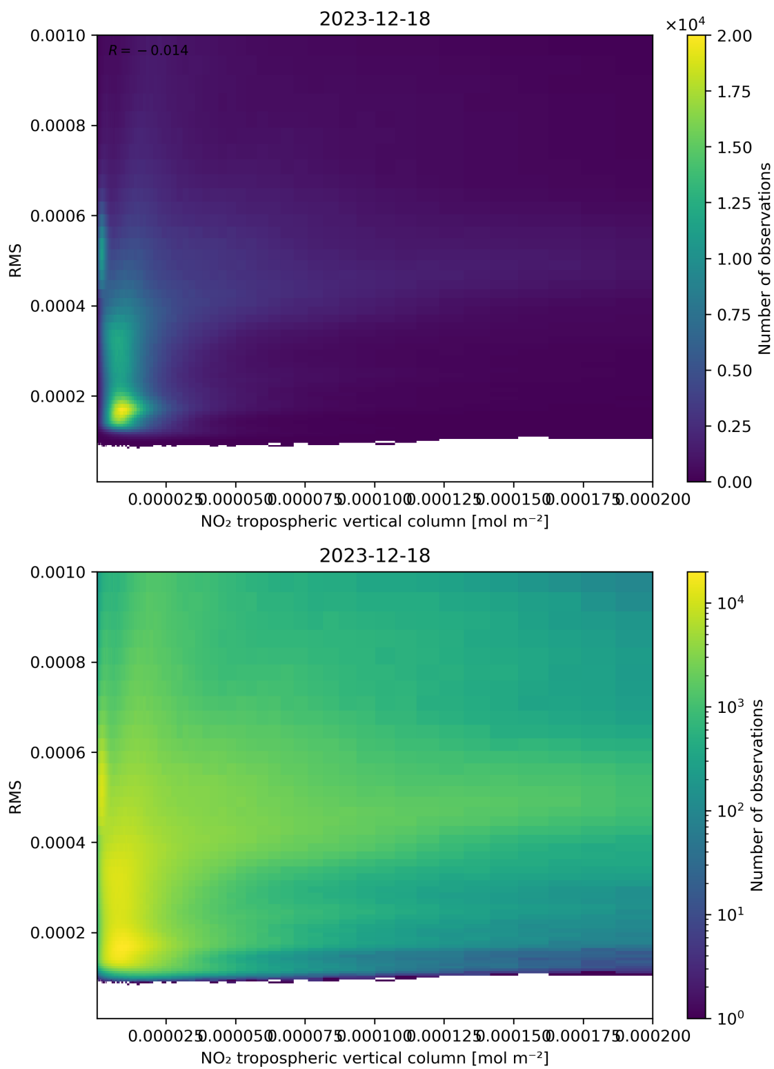
Figure 142: Scatter density plot of “NO 2 tropospheric vertical column” against “RMS” for 2023-12-17 to 2023-12-19.
