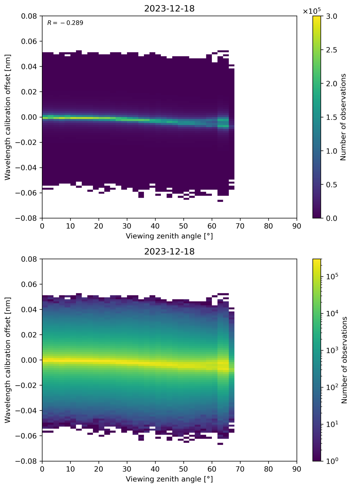
Figure 173: Scatter density plot of “Viewing zenith angle” against “Wavelength calibration offset” for 2023-12-17 to 2023-12-19.
