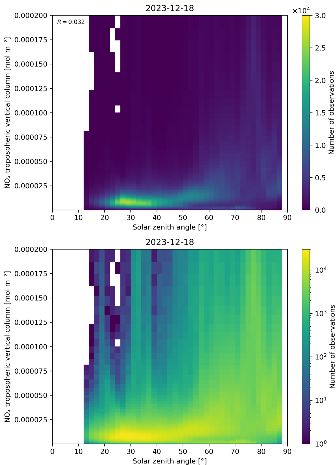
Figure 155: Scatter density plot of “Solar zenith angle” against “NO 2 tropospheric vertical column” for 2023-12-17 to 2023-12-19.
