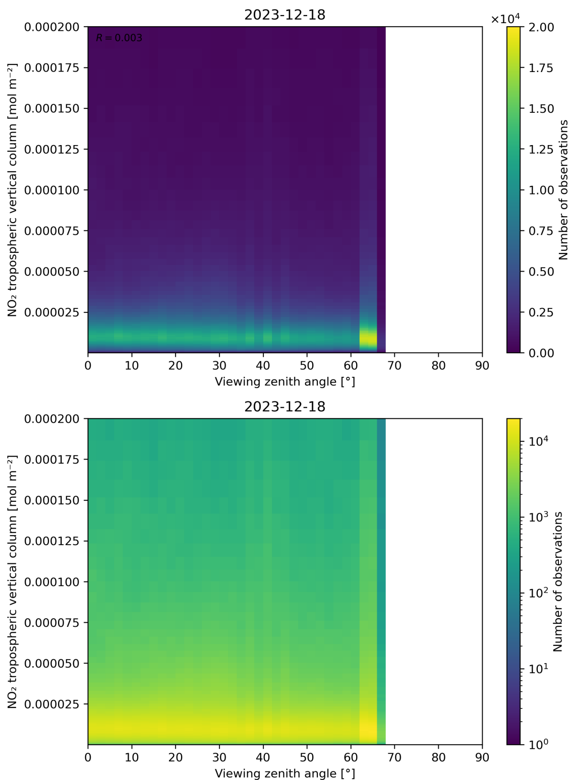
Figure 169: Scatter density plot of “Viewing zenith angle” against “NO 2 tropospheric vertical column” for 2023-12-17 to 2023-12-19.
