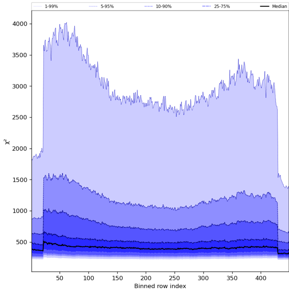
Figure 59: Along track statistics of “ \chi^2 ” for 2023-12-17 to 2023-12-19
