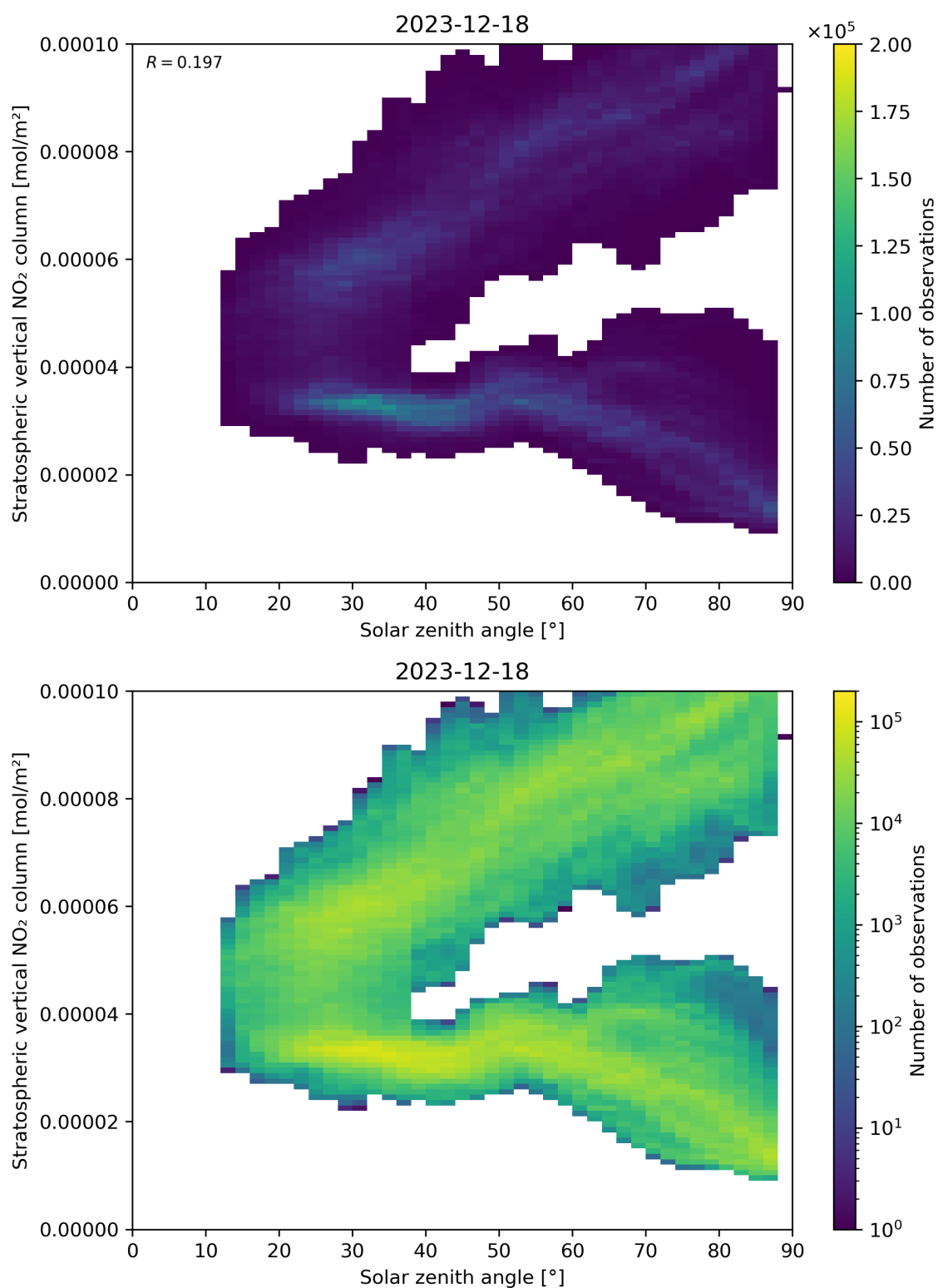
Figure 150: Scatter density plot of “Solar zenith angle” against “Stratospheric vertical NO 2 column” for 2023-12-17 to 2023-12-19.
