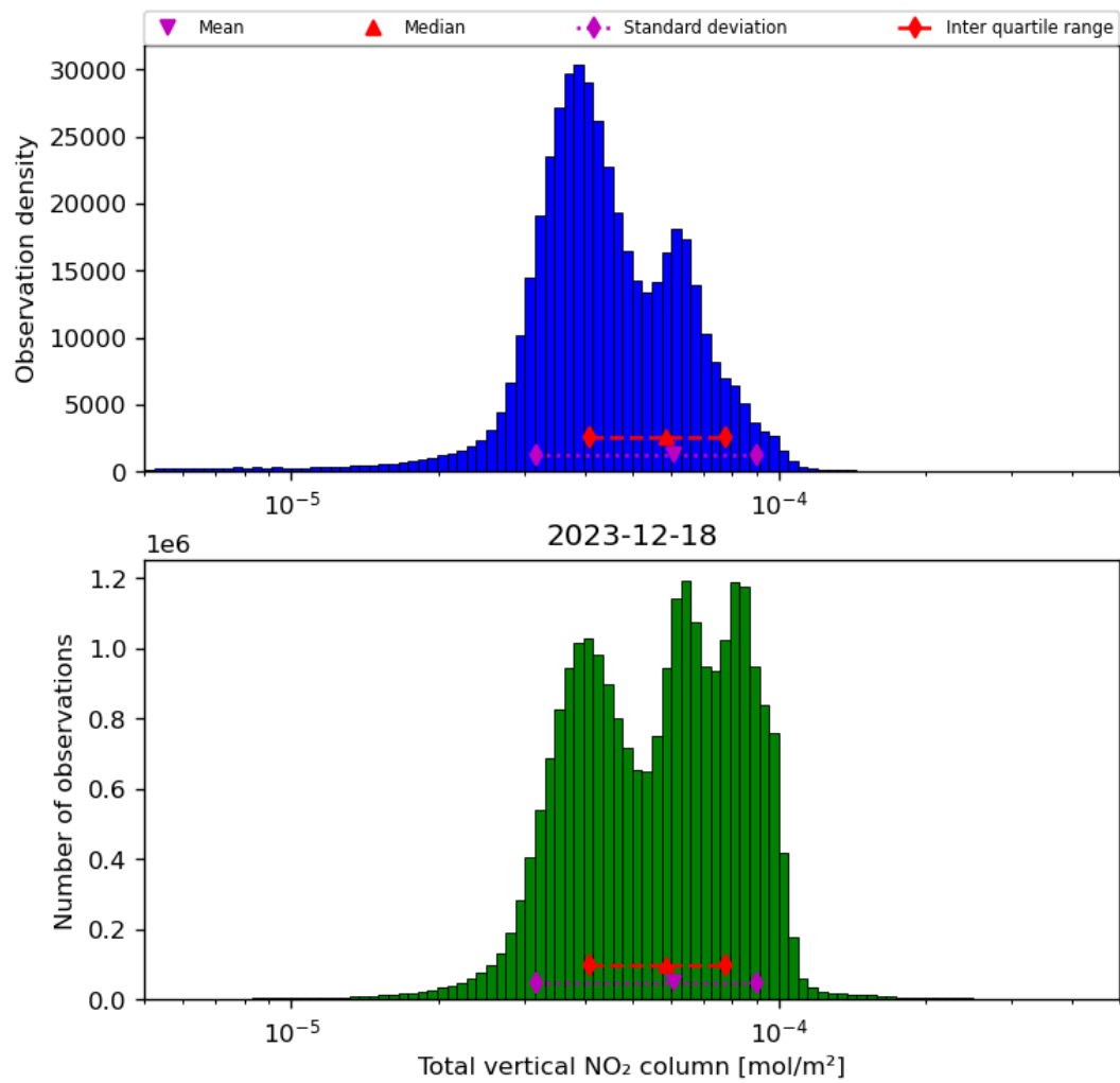
Figure 38: Histogram of “Total vertical NO 2 column” for 2023-12-17 to 2023-12-19
