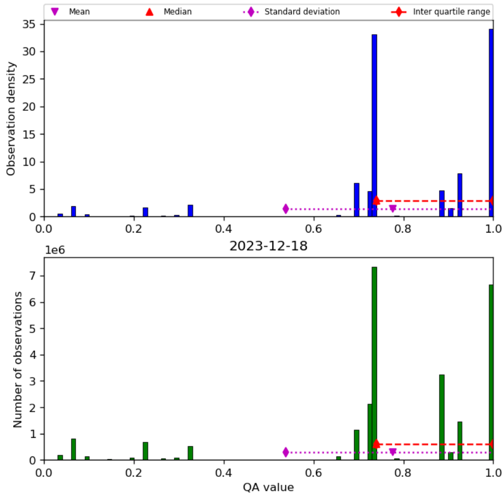
Figure 28: Histogram of “QA value” for 2023-12-17 to 2023-12-19
