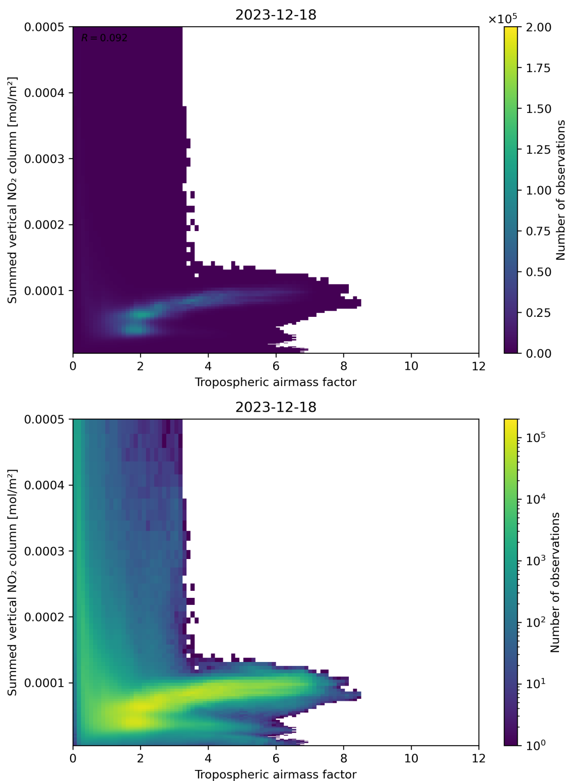
Figure 75: Scatter density plot of “Tropospheric airmass factor” against “Summed vertical NO 2 column” for 2023-12-17 to 2023-12-19.
