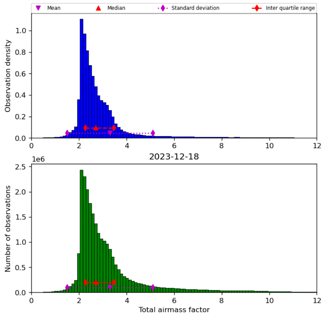
Figure 32: Histogram of “Total airmass factor” for 2023-12-17 to 2023-12-19
