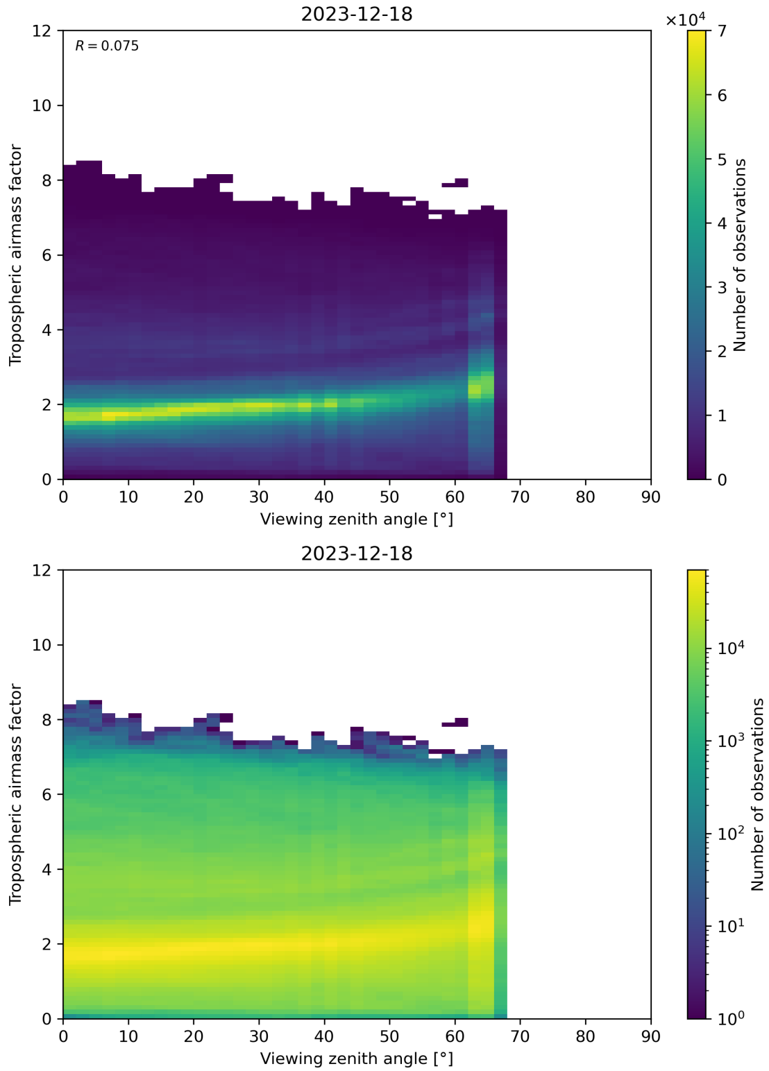
Figure 161: Scatter density plot of “Viewing zenith angle” against “Tropospheric airmass factor” for 2023-12-17 to 2023-12-19.
