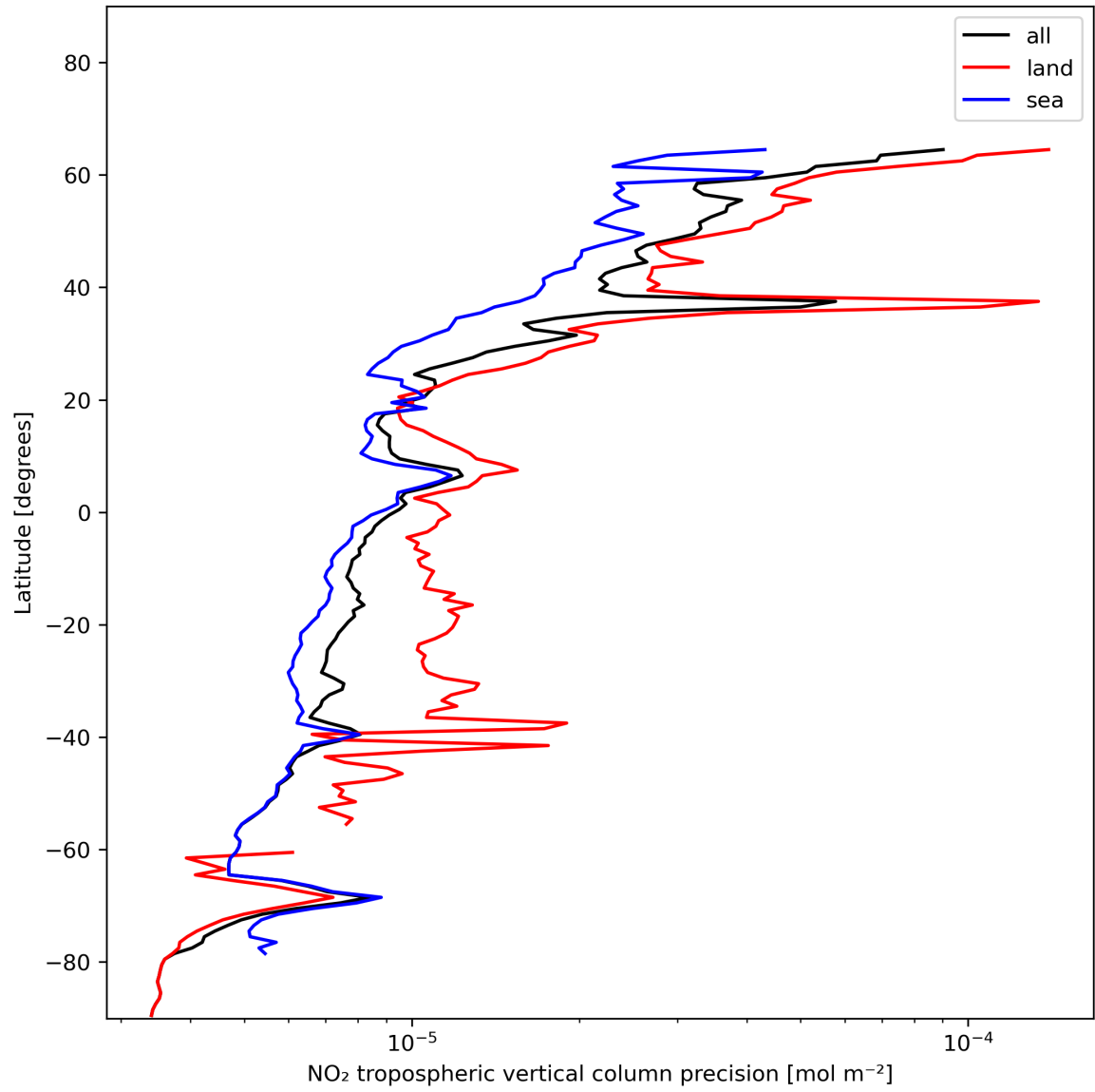
Figure 13: Zonal average of “NO 2 tropospheric vertical column precision” for 2023-12-17 to 2023-12-19.
