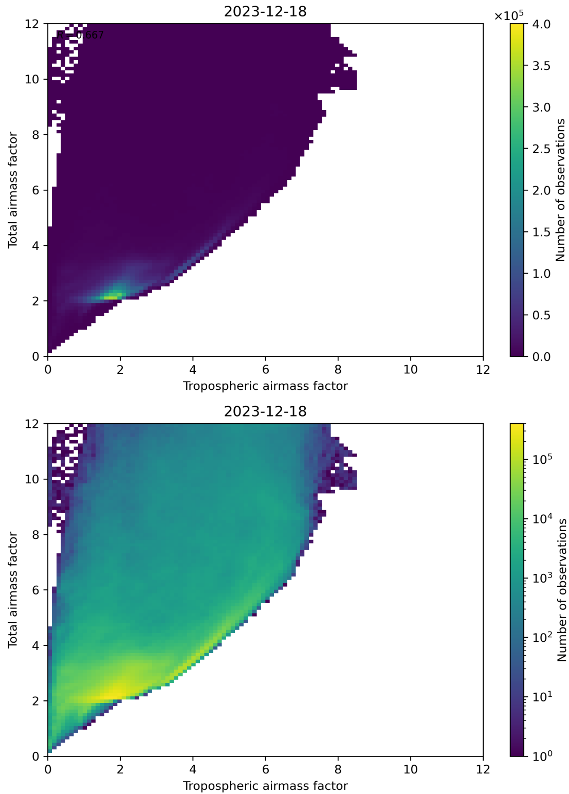
Figure 72: Scatter density plot of “Tropospheric airmass factor” against “Total airmass factor” for 2023-12-17 to 2023-12-19.
