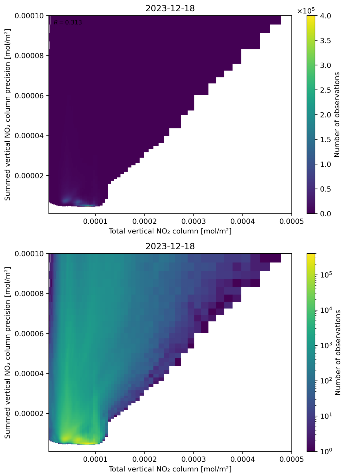
Figure 113: Scatter density plot of “Total vertical NO 2 column” against “Summed vertical NO 2 column precision” for 2023-12-17 to 2023-12-19.
