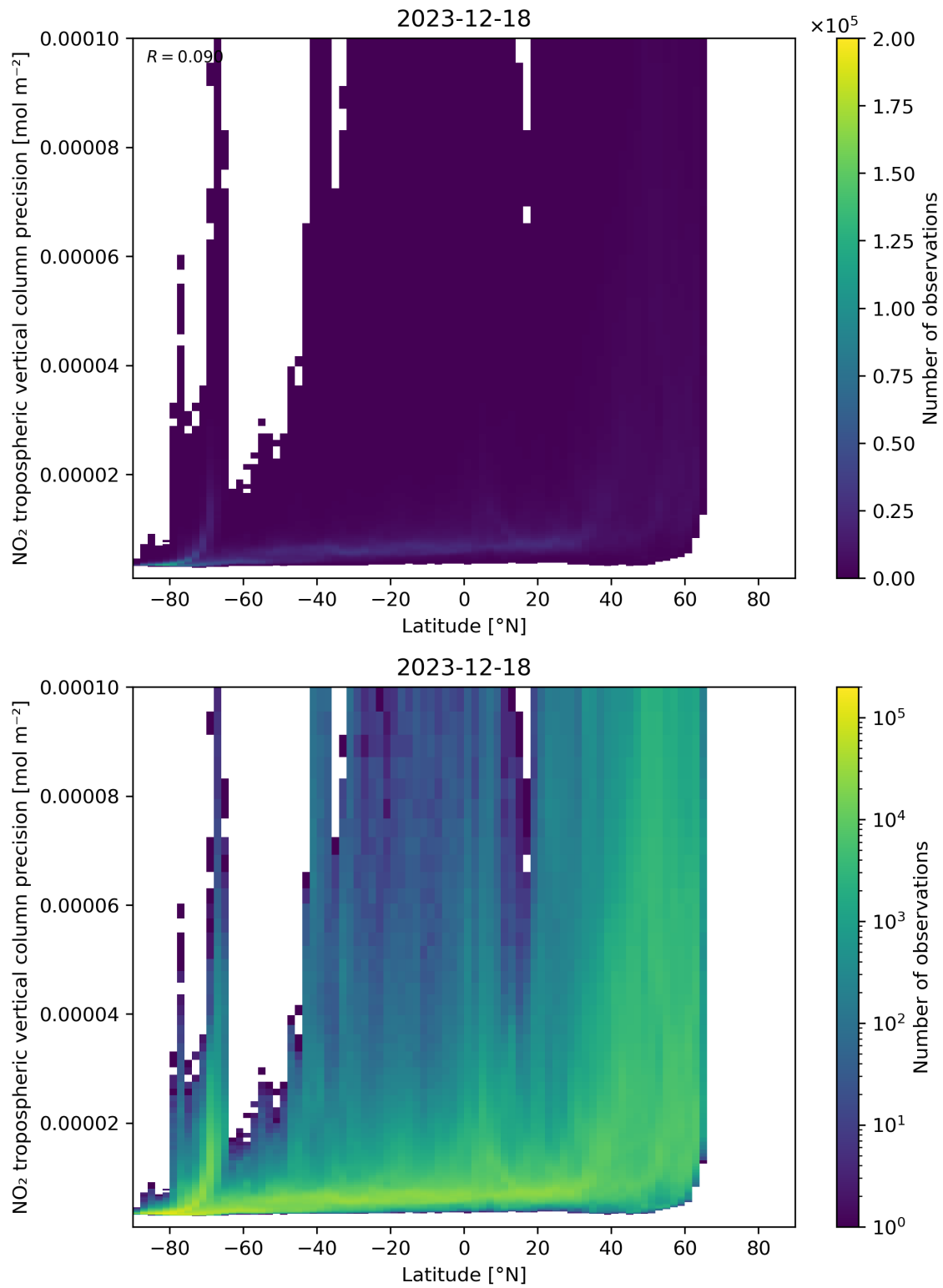
Figure 93: Scatter density plot of “Latitude” against “NO 2 tropospheric vertical column precision” for 2023-12-17 to 2023-12-19.
