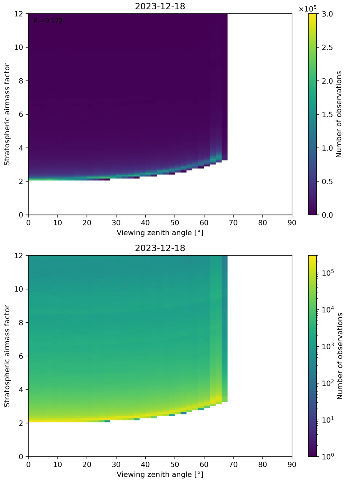
Figure 159: Scatter density plot of “Viewing zenith angle” against “Stratospheric airmass factor” for 2023-12-17 to 2023-12-19.
