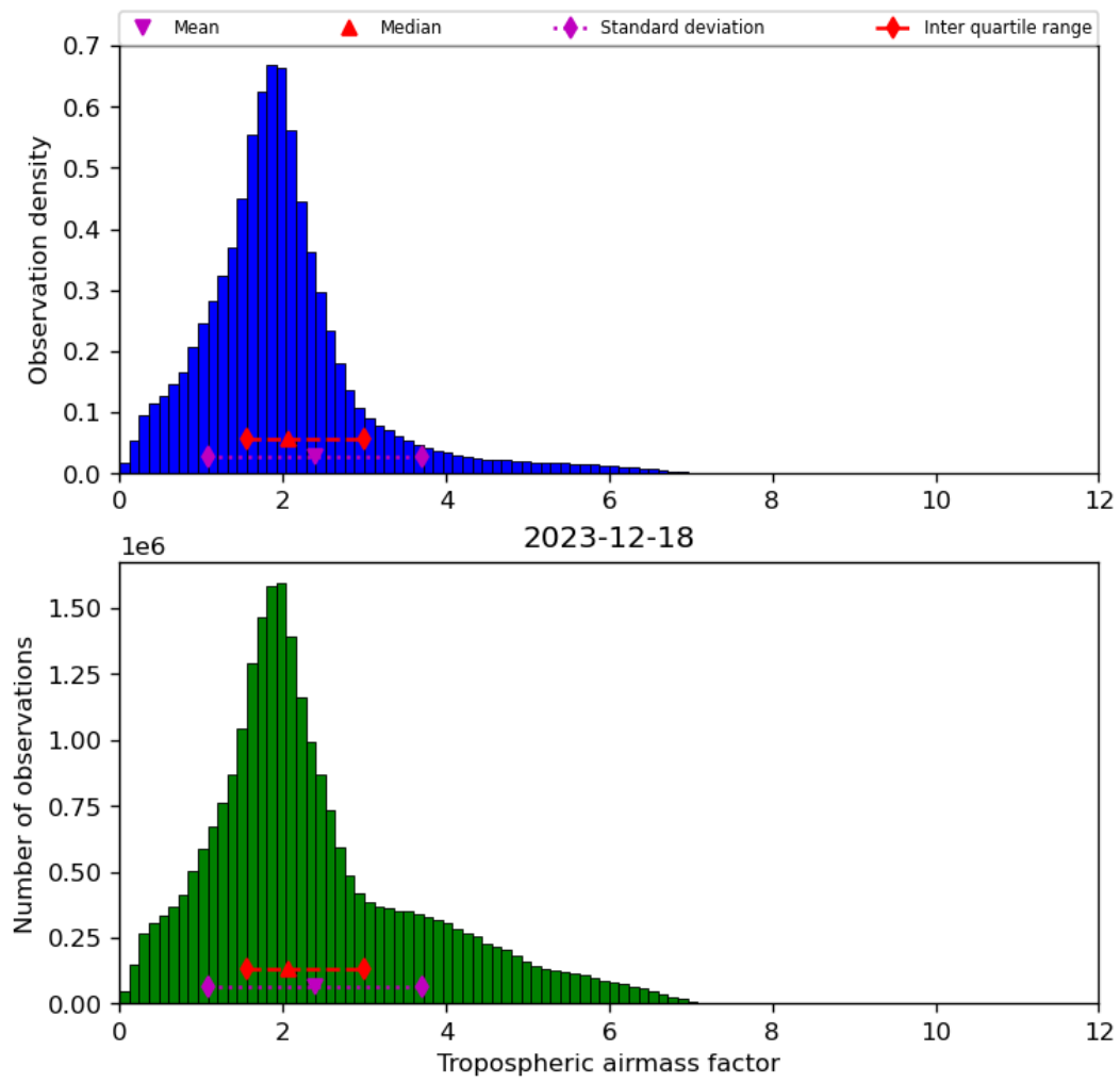
Figure 31: Histogram of “Tropospheric airmass factor” for 2023-12-17 to 2023-12-19
