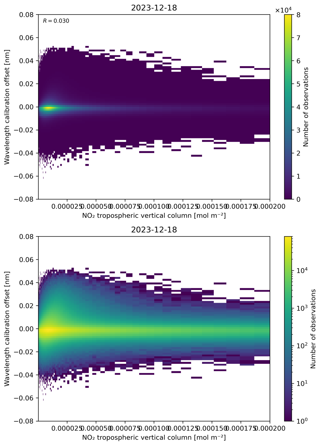
Figure 143: Scatter density plot of “NO 2 tropospheric vertical column” against “Wavelength calibration offset” for 2023-12-17 to 2023-12-19.
