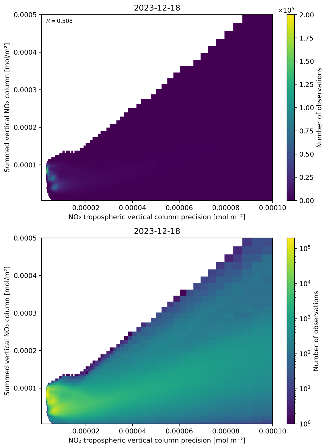
Figure 136: Scatter density plot of “NO 2 tropospheric vertical column precision” against “Summed vertical NO 2 column” for 2023-12-17 to 2023-12-19.
