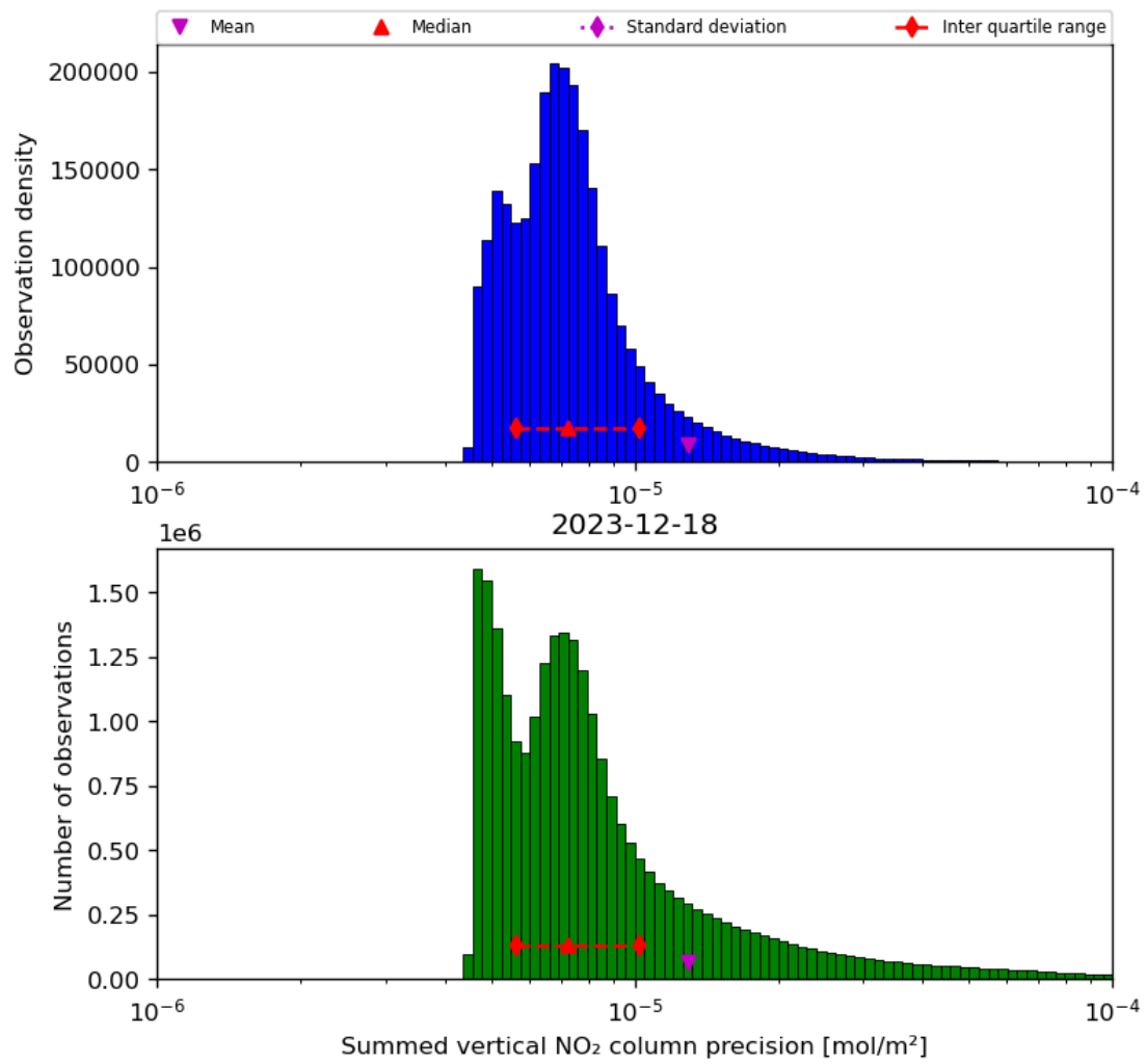
Figure 41: Histogram of "Summed vertical NO 2 column precision" for 2023-12-17 to 2023-12-19
