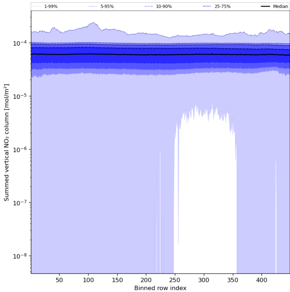
Figure 57: Along track statistics of “Summed vertical NO 2 column” for 2023-12-17 to 2023-12-19
