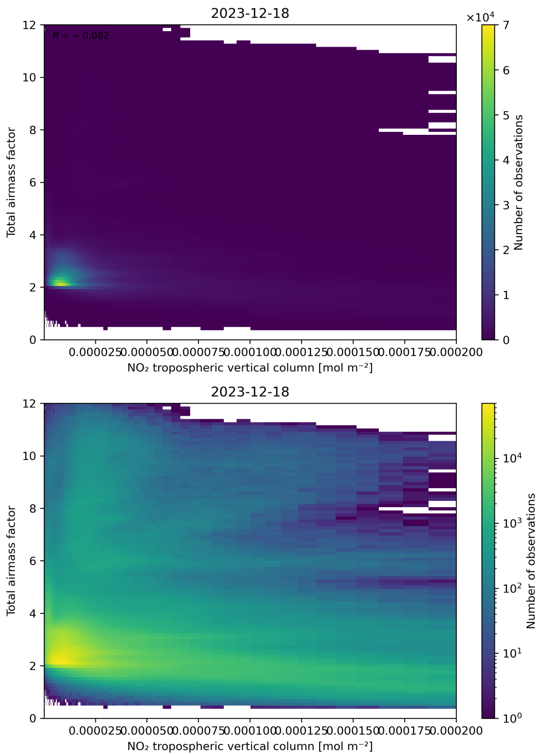
Figure 122: Scatter density plot of “NO 2 tropospheric vertical column” against “Total air mass factor” for 2023-12-17 to 2023-12-19.
