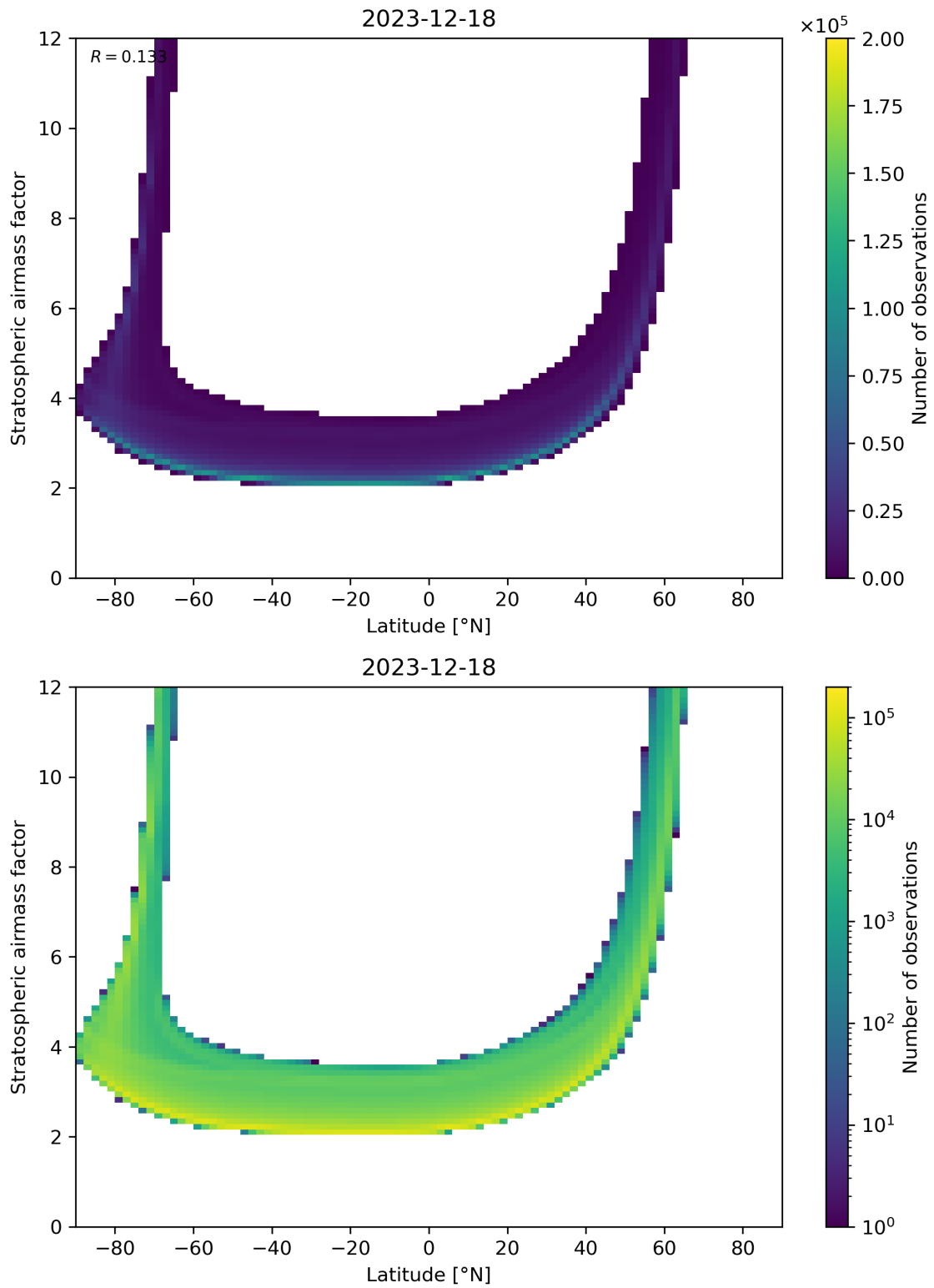
Figure 83: Scatter density plot of “Latitude” against “Stratospheric air mass factor” for 2023-12-17 to 2023-12-19.
