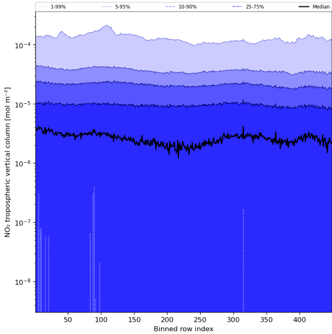
Figure 46: Along track statistics of “ \text{NO}_2 tropospheric vertical column” for 2023-12-17 to 2023-12-19
