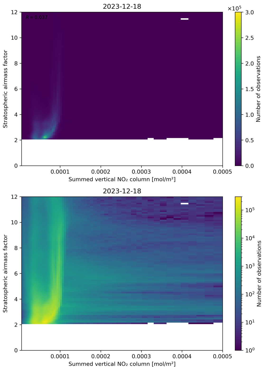
Figure 103: Scatter density plot of “Summed vertical NO 2 column” against “Stratospheric airmass factor” for 2023-12-17 to 2023-12-19.
