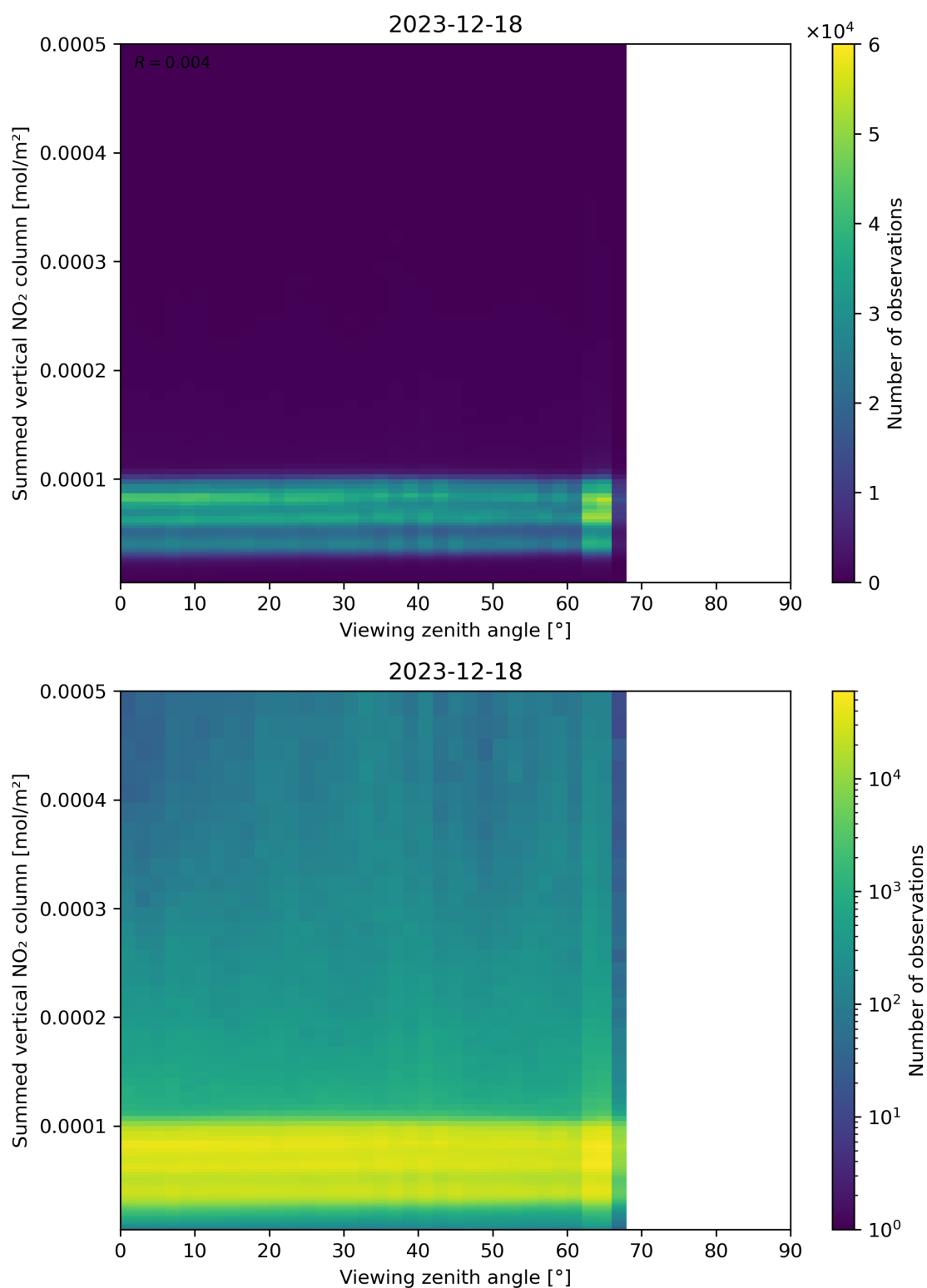
Figure 165: Scatter density plot of “Viewing zenith angle” against “Summed vertical NO 2 column” for 2023-12-17 to 2023-12-19.
