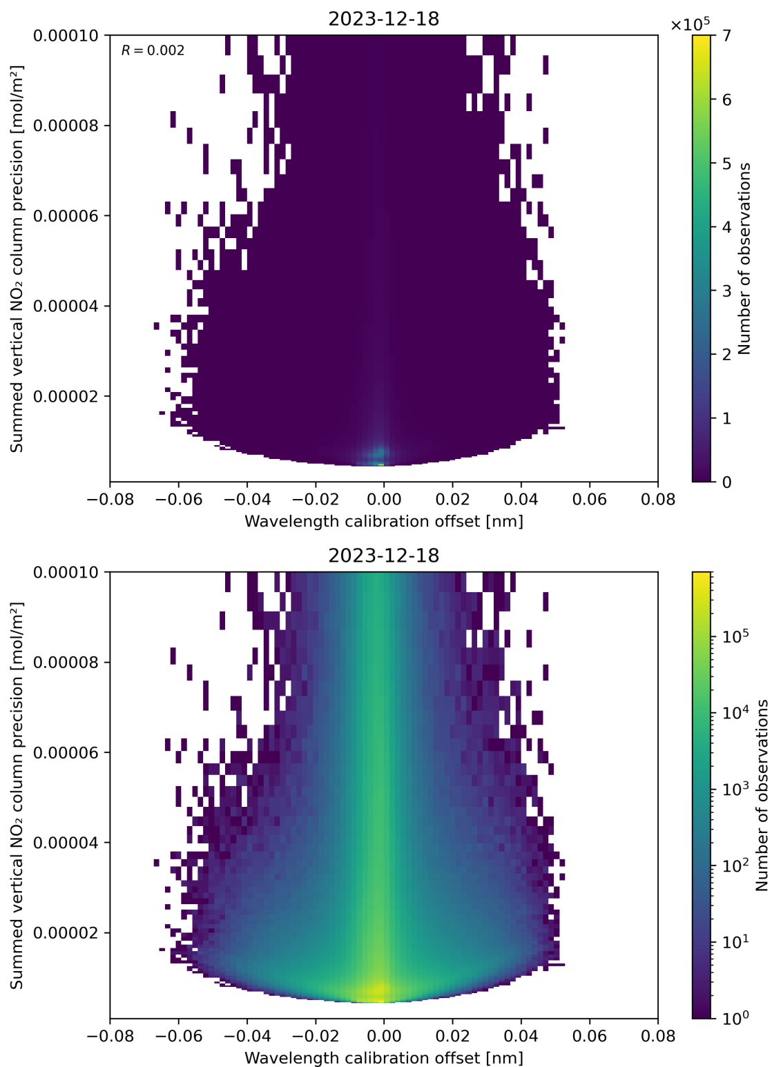
Figure 178: Scatter density plot of “Wavelength calibration offset” against “Summed vertical NO 2 column precision” for 2023-12-17 to 2023-12-19.
