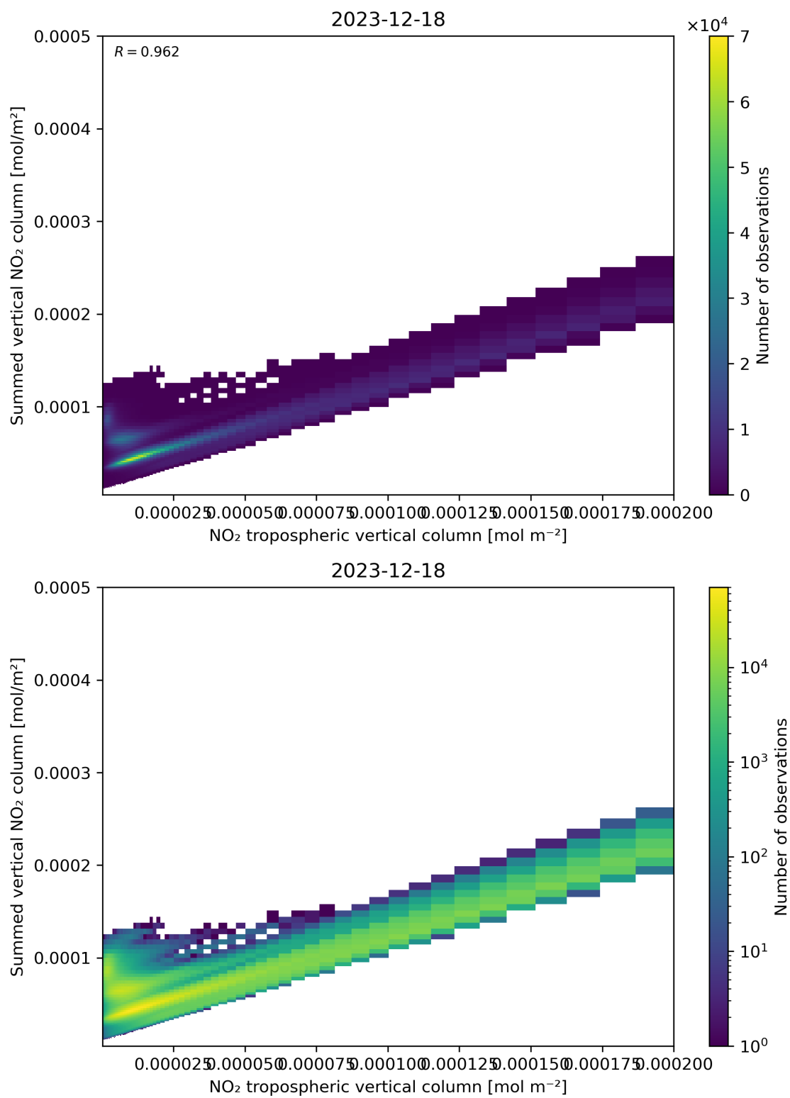
Figure 126: Scatter density plot of “NO 2 tropospheric vertical column” against “Summed vertical NO 2 column” for 2023-12-17 to 2023-12-19.
