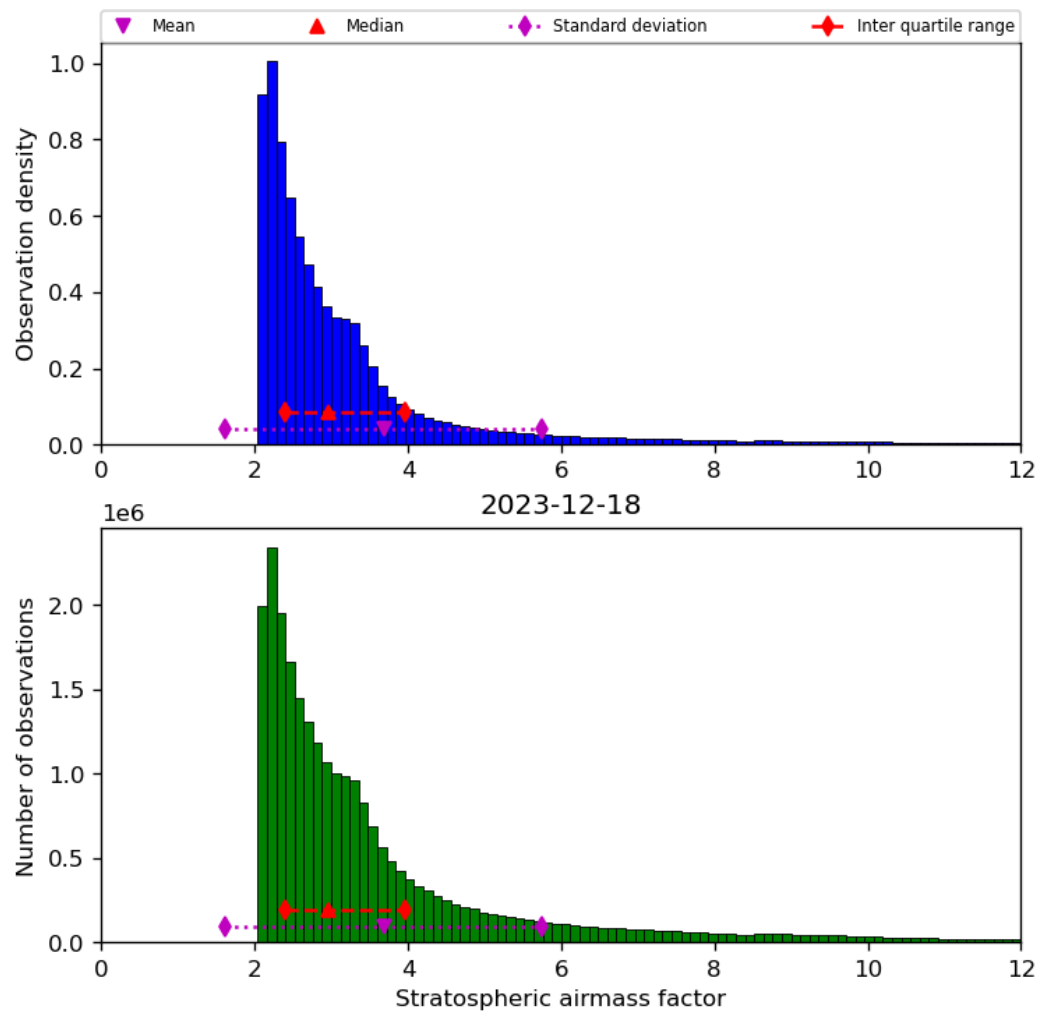
Figure 44: Histogram of “Stratospheric airmass factor” for 2023-12-17 to 2023-12-19
