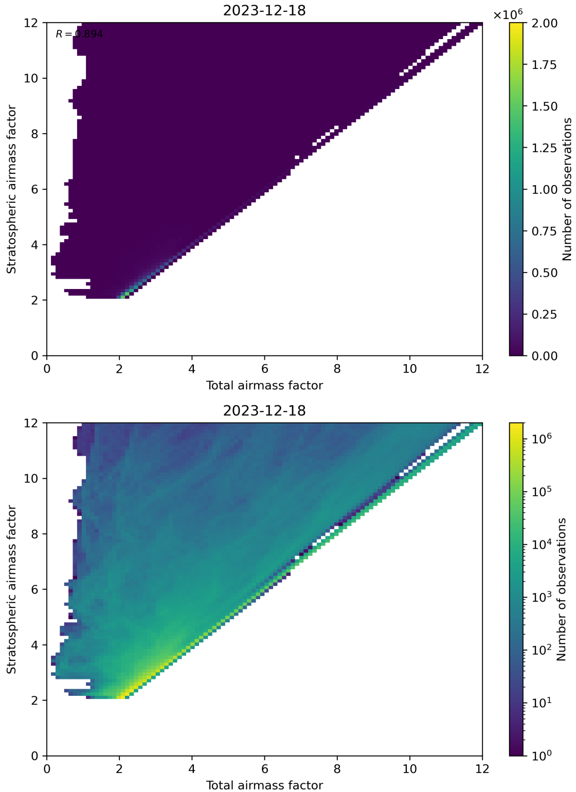
Figure 62: Scatter density plot of “Total airmass factor” against “Stratospheric airmass factor” for 2023-12-17 to 2023-12-19.
