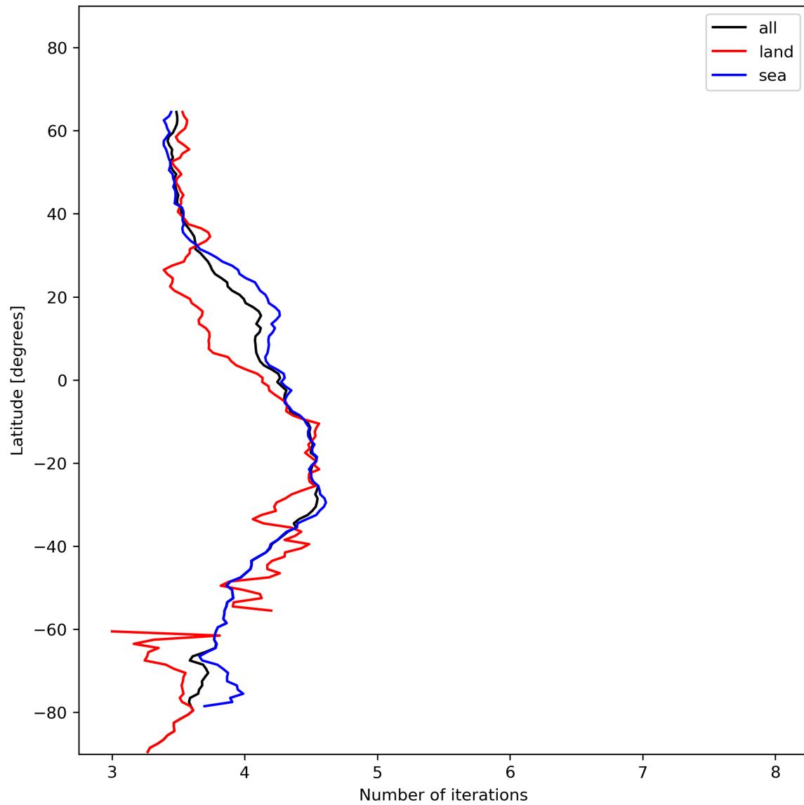
Figure 17: Zonal average of “Number of iterations” for 2023-12-17 to 2023-12-19.
