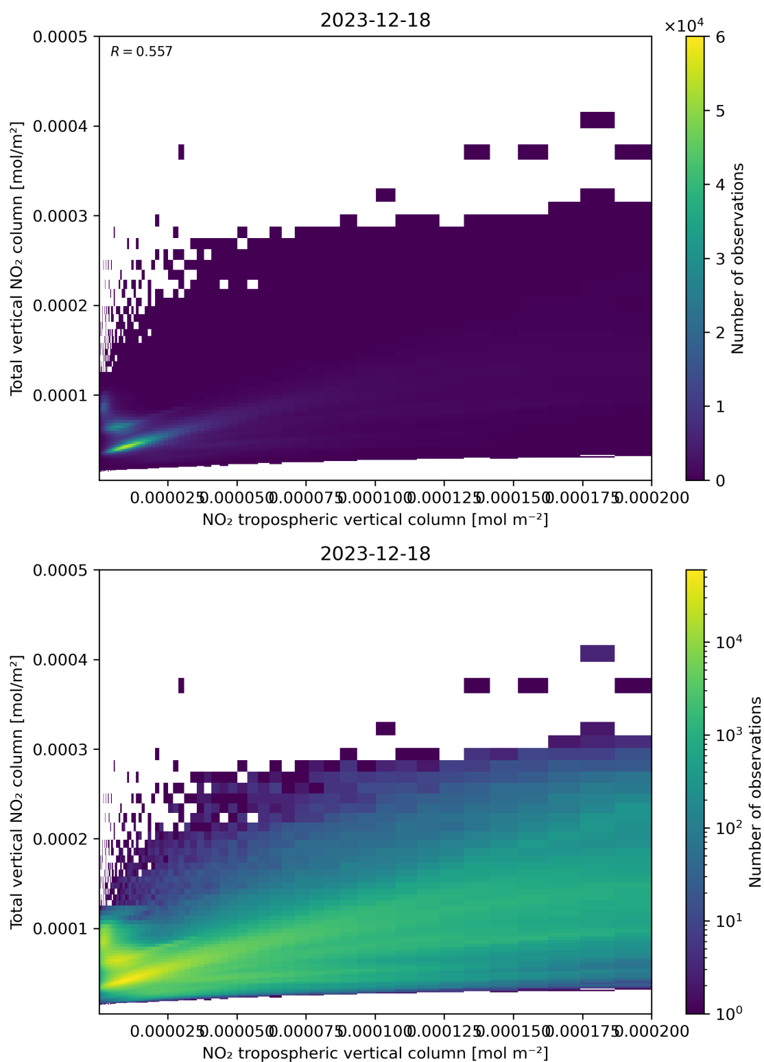
Figure 128: Scatter density plot of “NO 2 tropospheric vertical column” against “Total vertical NO 2 column” for 2023-12-17 to 2023-12-19.
