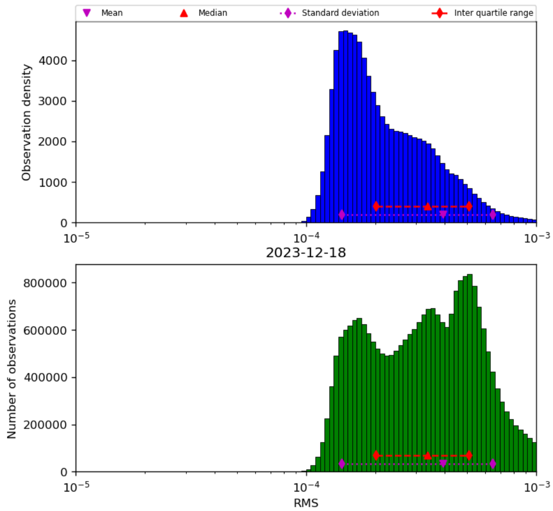
Figure 43: Histogram of “RMS” for 2023-12-17 to 2023-12-19
