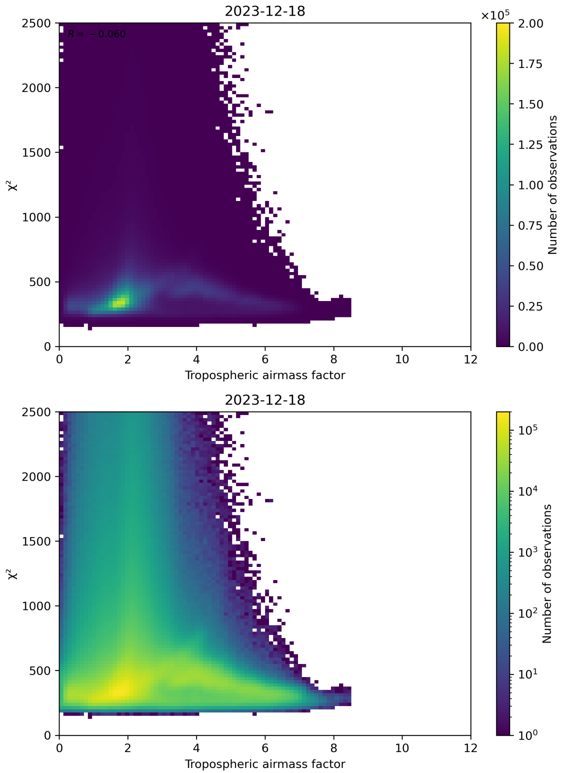
Figure 73: Scatter density plot of “Tropospheric airmass factor” against “ \chi^2 ” for 2023-12-17 to 2023-12-19.
