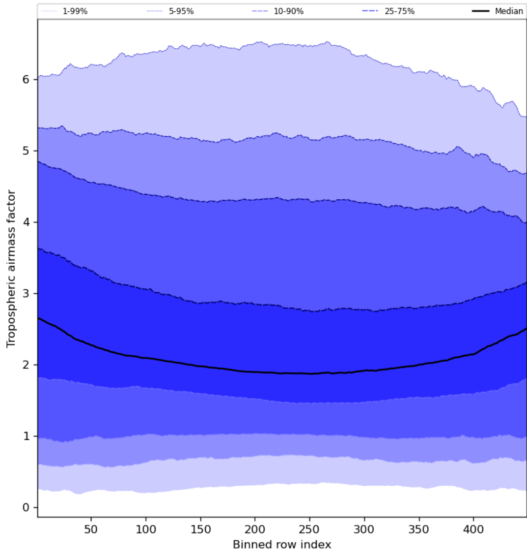
Figure 48: Along track statistics of “Tropospheric airmass factor” for 2023-12-17 to 2023-12-19
