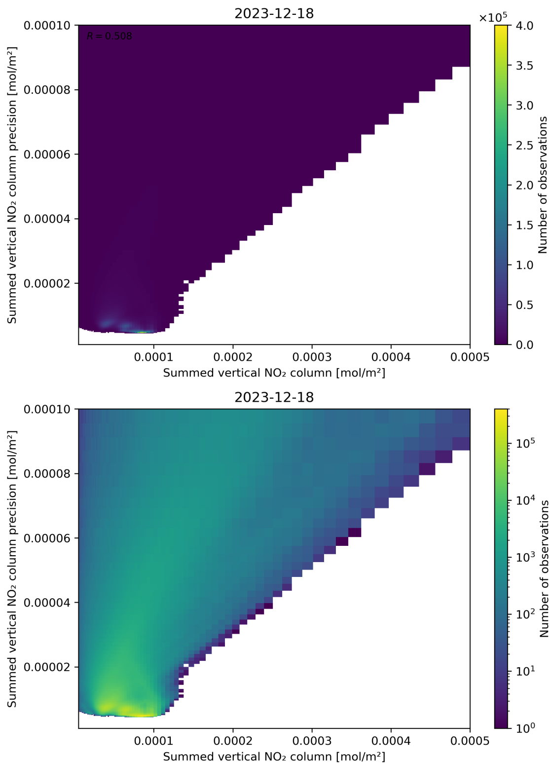
Figure 105: Scatter density plot of “Summed vertical NO 2 column” against “Summed vertical NO 2 column precision” for 2023-12-17 to 2023-12-19.
