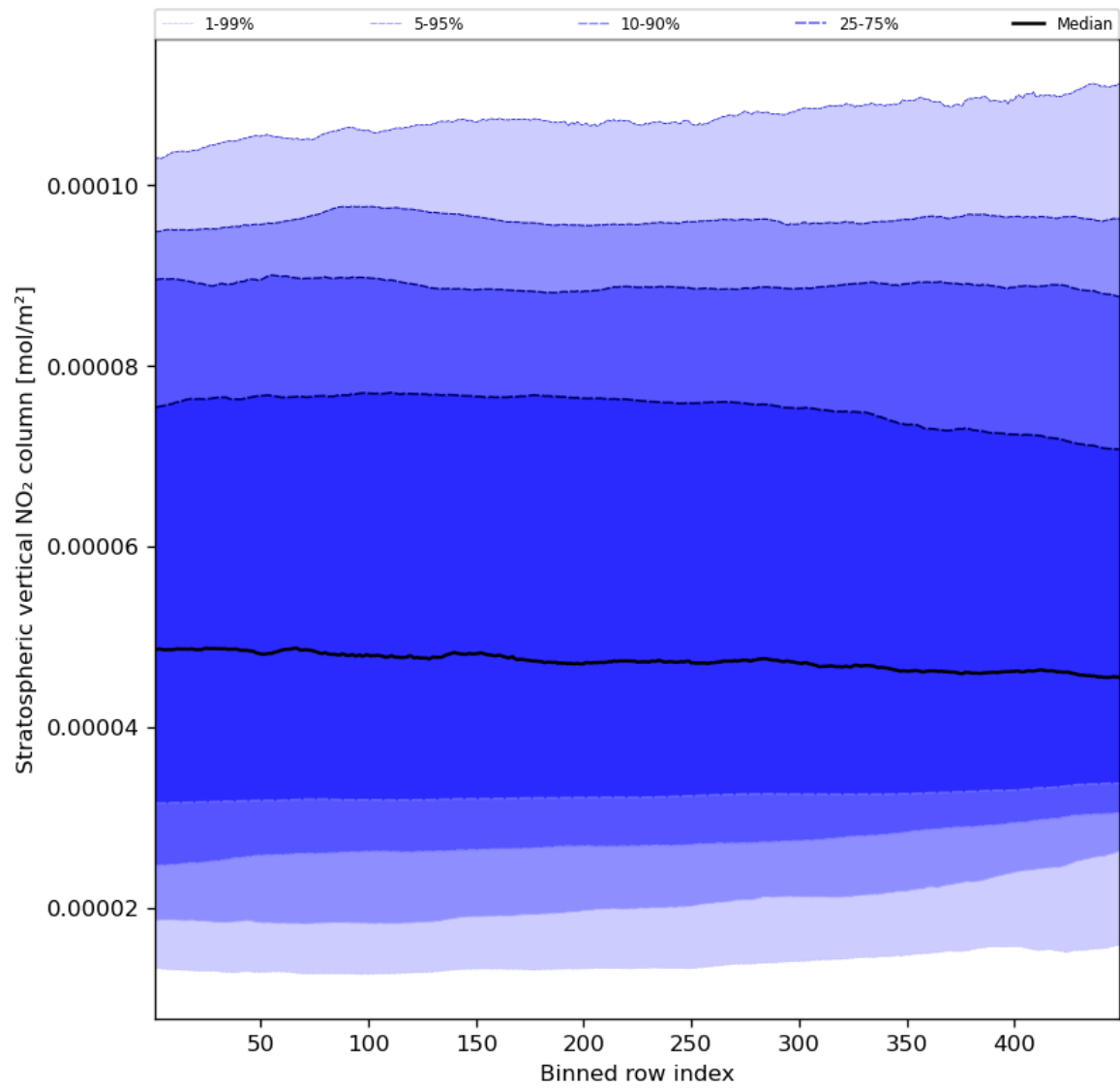
Figure 53: Along track statistics of “Stratospheric vertical NO 2 column” for 2023-12-17 to 2023-12-19
