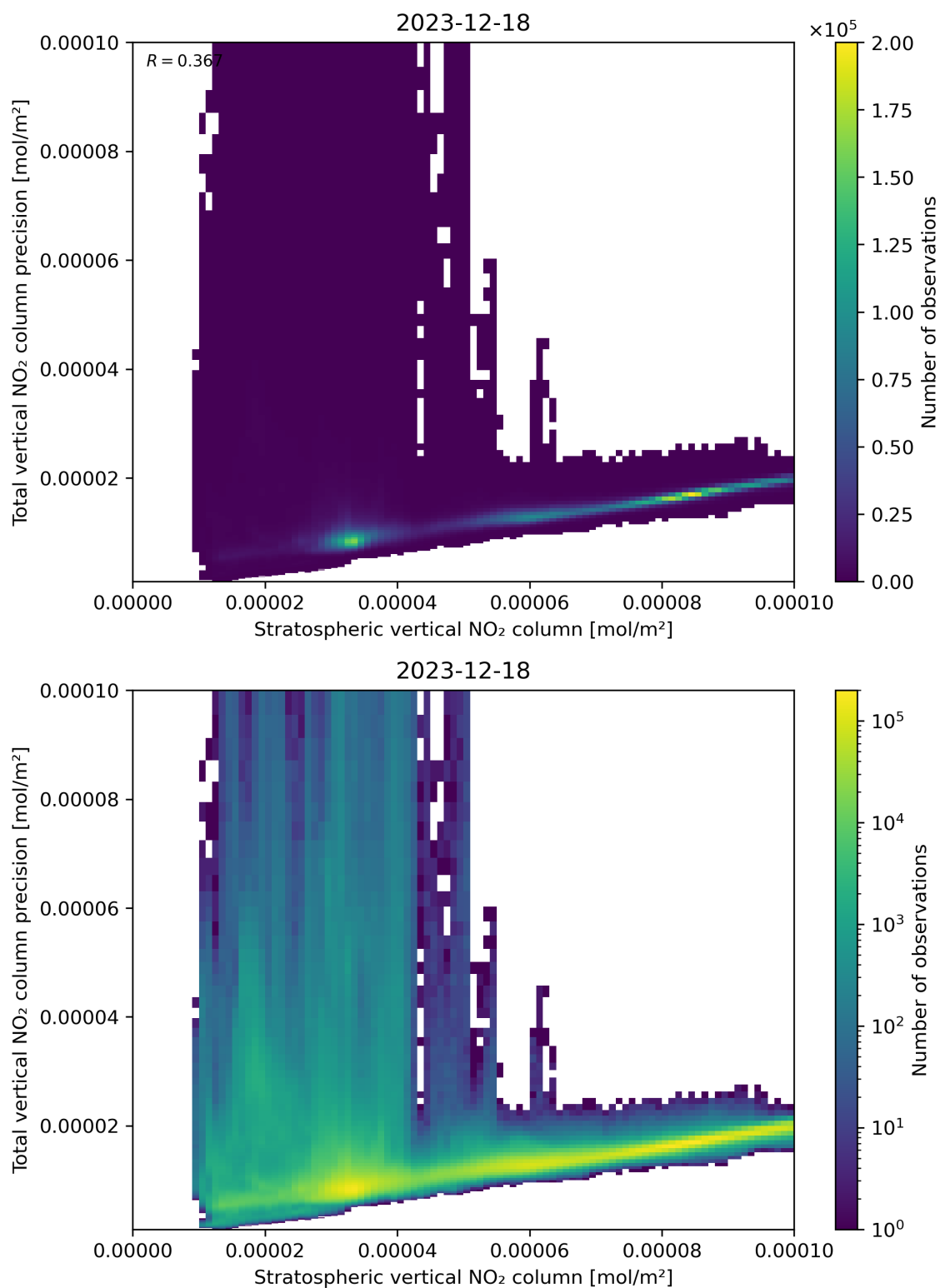
Figure 101: Scatter density plot of “Stratospheric vertical NO 2 column” against “Total vertical NO 2 column precision” for 2023-12-17 to 2023-12-19.
