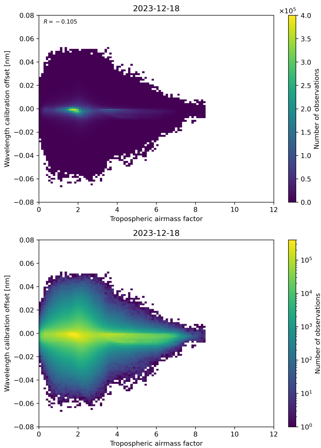
Figure 80: Scatter density plot of “Tropospheric airmass factor” against “Wavelength calibration offset” for 2023-12-17 to 2023-12-19.
