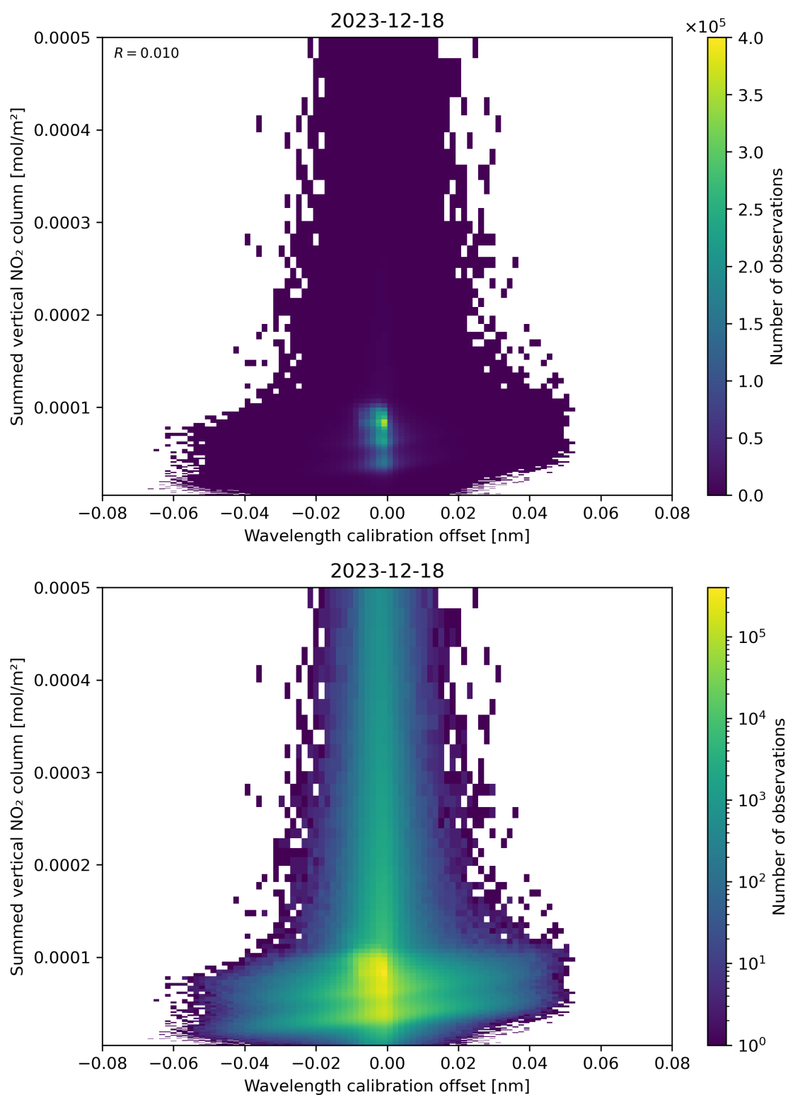
Figure 177: Scatter density plot of “Wavelength calibration offset” against “Summed vertical NO 2 column” for 2023-12-17 to 2023-12-19.
