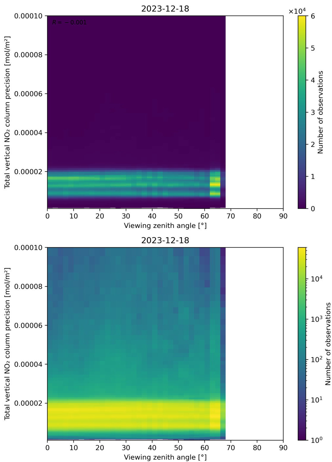
Figure 168: Scatter density plot of “Viewing zenith angle” against “Total vertical NO 2 column precision” for 2023-12-17 to 2023-12-19.
