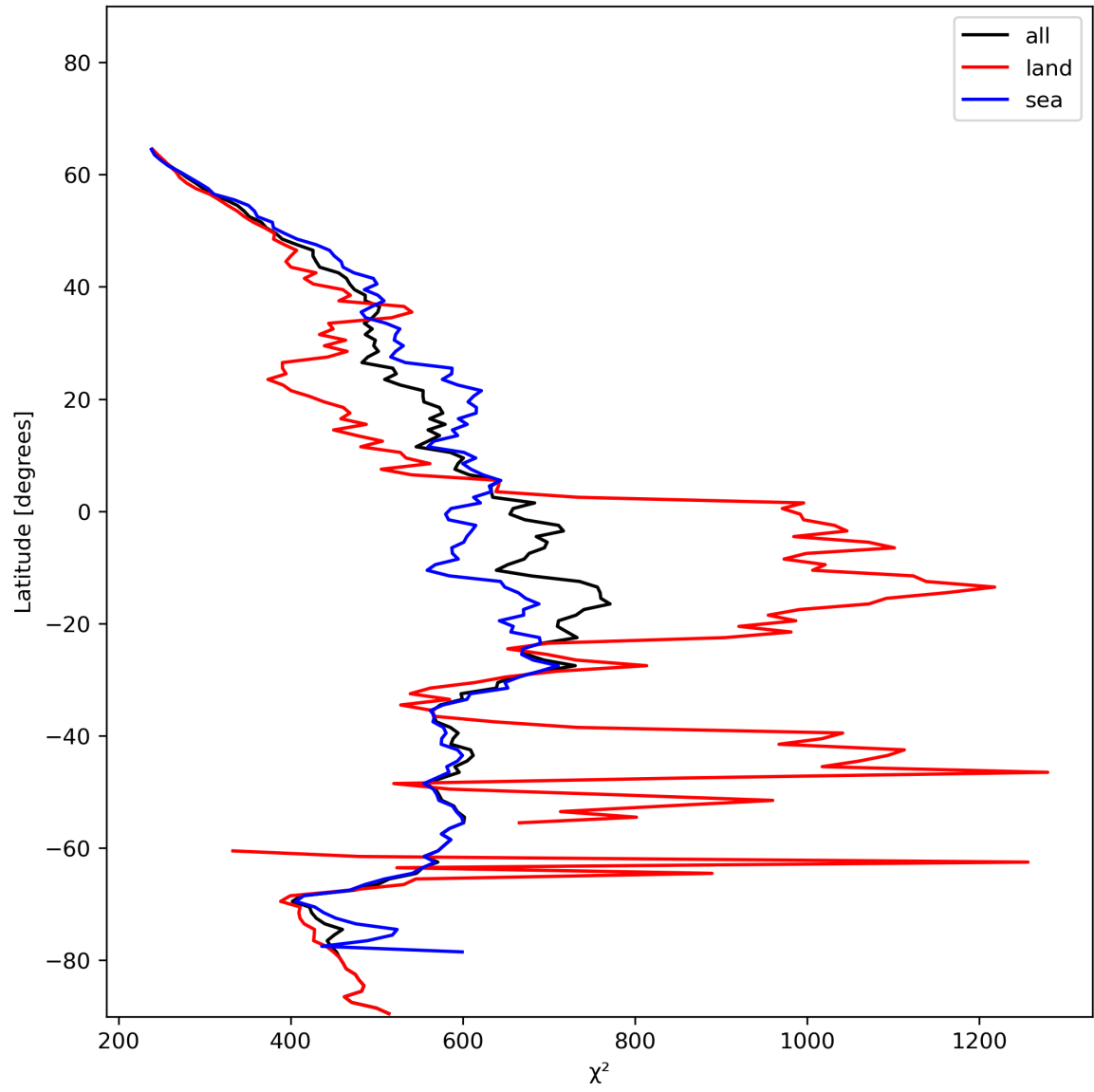
Figure 25: Zonal average of “ \chi^2 ” for 2023-12-17 to 2023-12-19.
