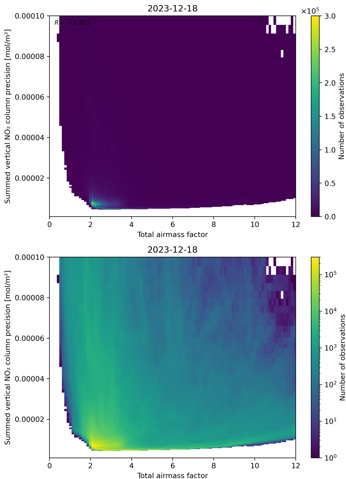
Figure 66: Scatter density plot of “Total airmass factor” against “Summed vertical NO 2 column precision” for 2023-12-17 to 2023-12-19.
