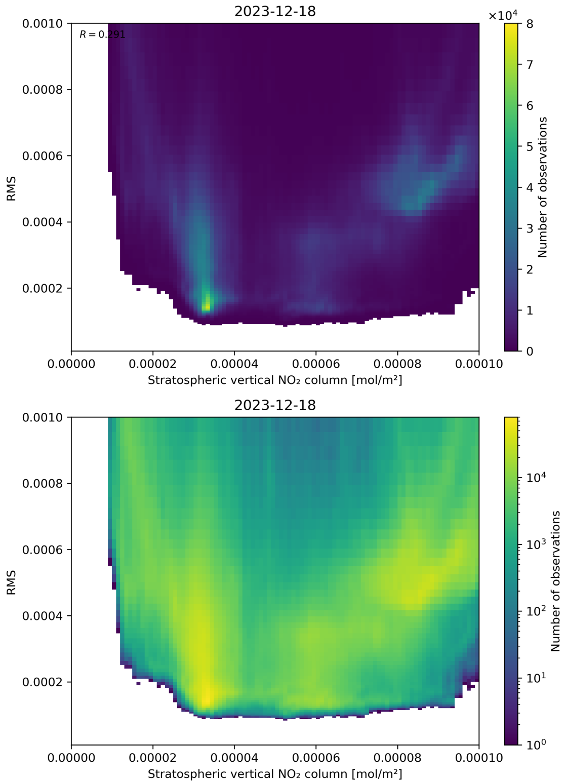
Figure 102: Scatter density plot of “Stratospheric vertical NO 2 column” against “RMS” for 2023-12-17 to 2023-12-19.
