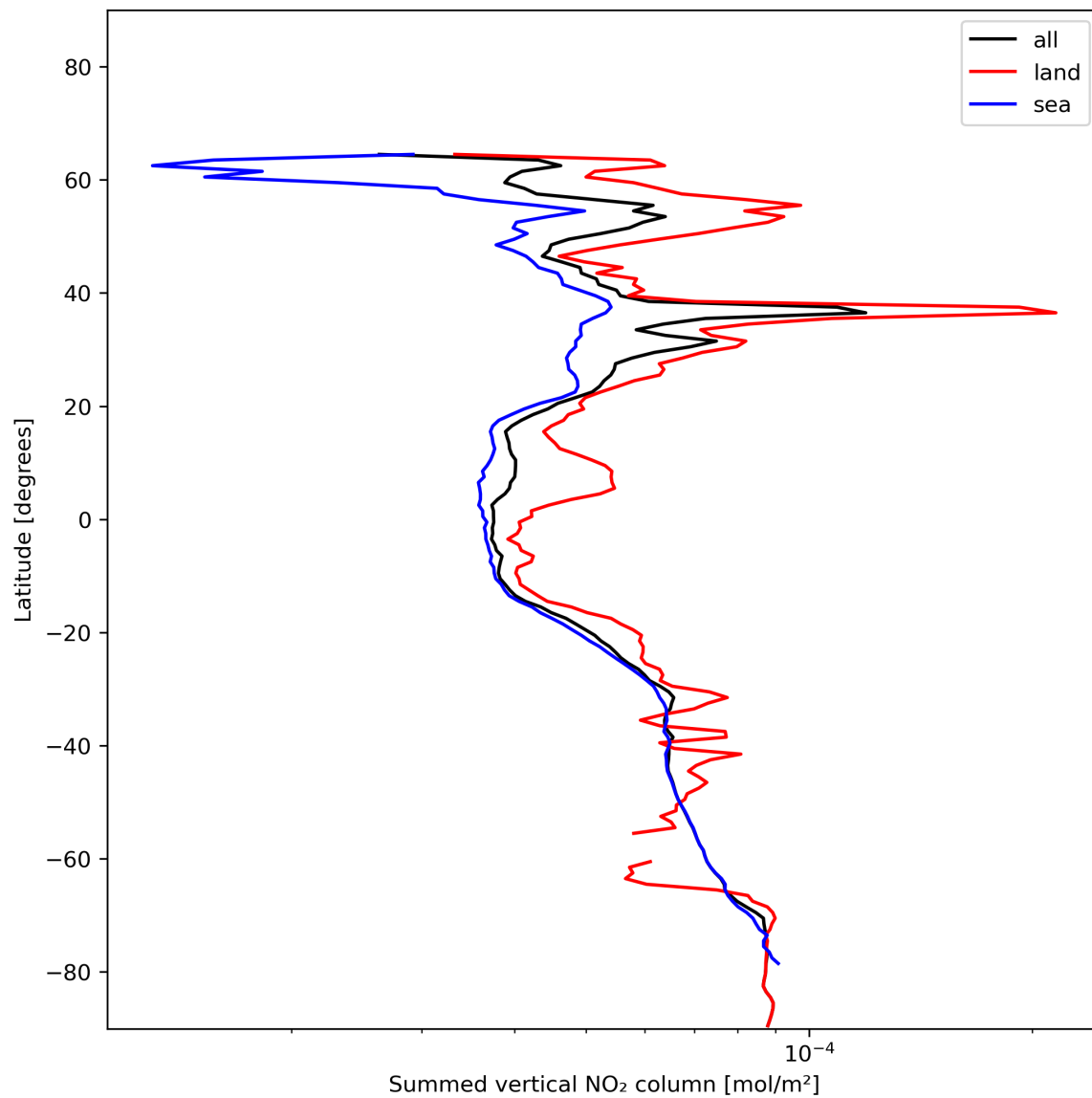
Figure 23: Zonal average of “Summed vertical NO 2 column” for 2023-12-17 to 2023-12-19.
