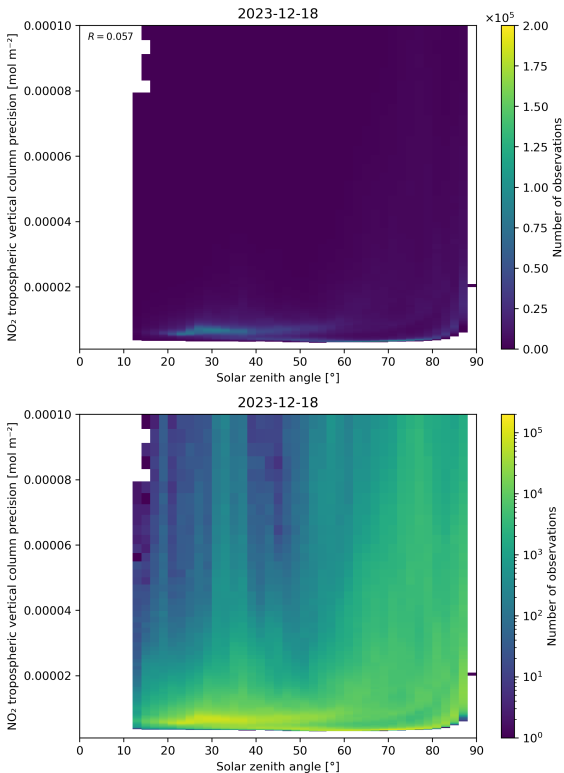
Figure 156: Scatter density plot of “Solar zenith angle” against “NO 2 tropospheric vertical column precision” for 2023-12-17 to 2023-12-19.
