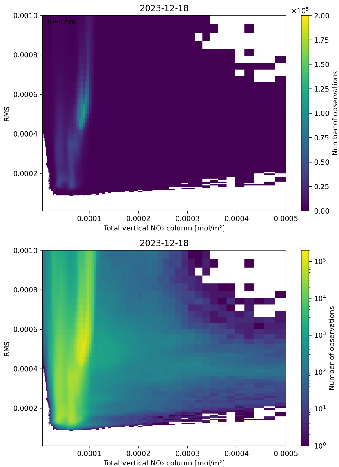
Figure 120: Scatter density plot of “Total vertical NO 2 column” against “RMS” for 2023-12-17 to 2023-12-19.
