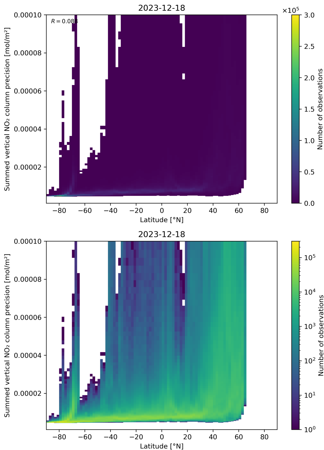
Figure 89: Scatter density plot of “Latitude” against “Summed vertical NO 2 column precision” for 2023-12-17 to 2023-12-19.
