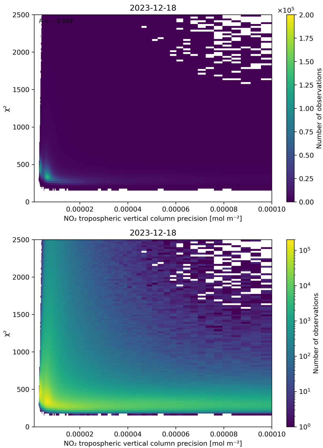
Figure 134: Scatter density plot of “NO 2 tropospheric vertical column precision” against “ \chi^2 ” for 2023-12-17 to 2023-12-19.
