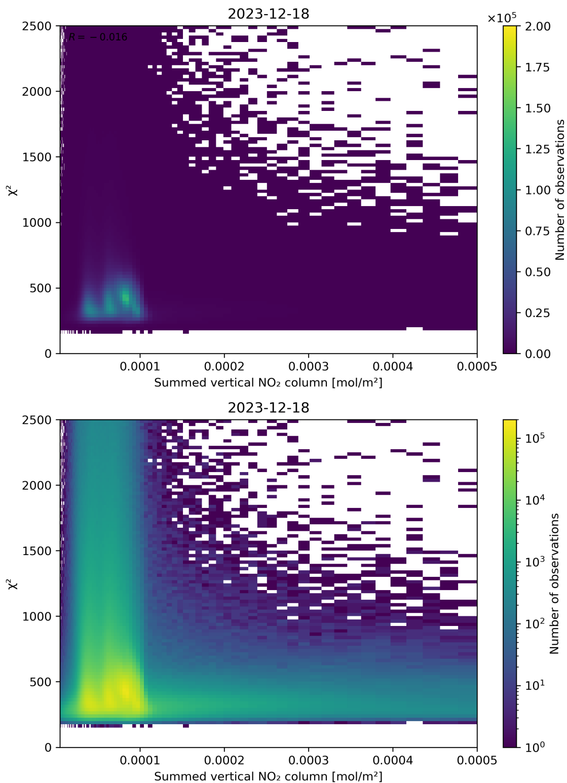
Figure 104: Scatter density plot of “Summed vertical NO 2 column” against “ \chi^2 ” for 2023-12-17 to 2023-12-19.
