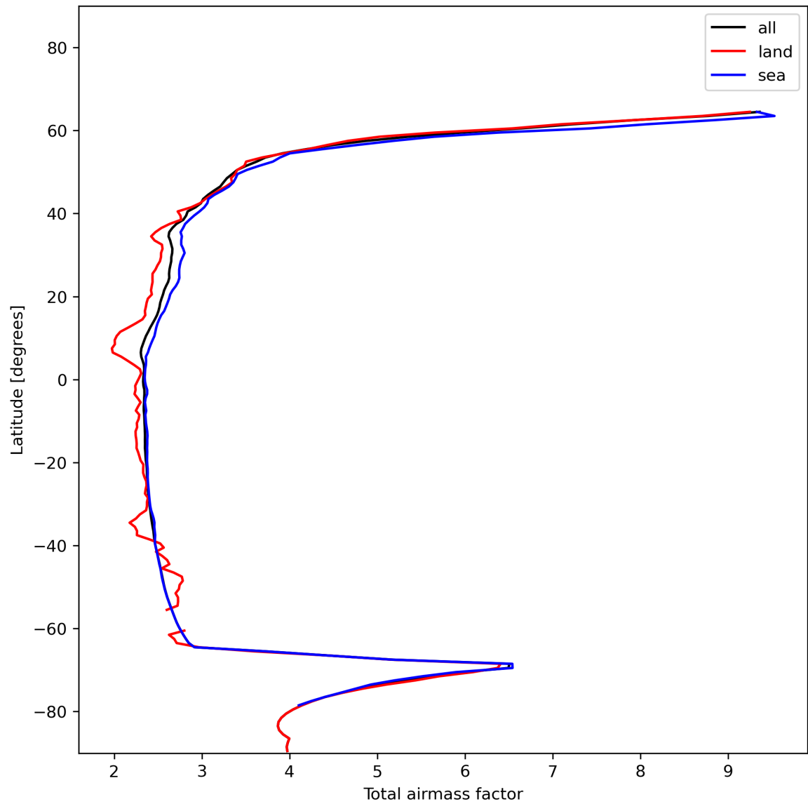
Figure 15: Zonal average of “Total airmass factor” for 2023-12-17 to 2023-12-19.
