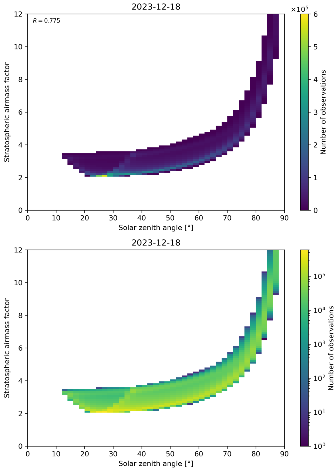
Figure 145: Scatter density plot of “Solar zenith angle” against “Stratospheric airmass factor” for 2023-12-17 to 2023-12-19.
