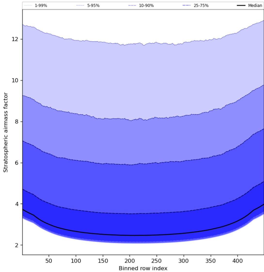
Figure 61: Along track statistics of “Stratospheric airmass factor” for 2023-12-17 to 2023-12-19
