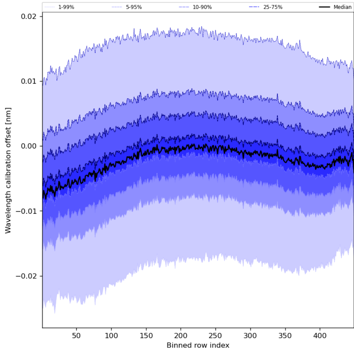
Figure 52: Along track statistics of “Wavelength calibration offset” for 2023-12-17 to 2023-12-19
