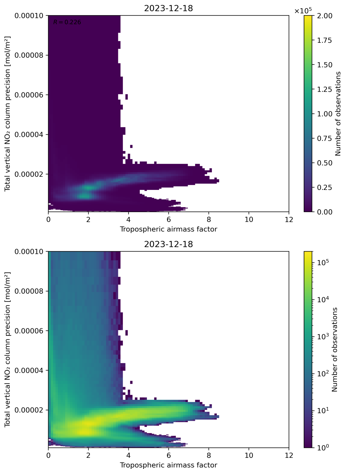
Figure 78: Scatter density plot of “Tropospheric air mass factor” against “Total vertical NO 2 column precision” for 2023-12-17 to 2023-12-19.
