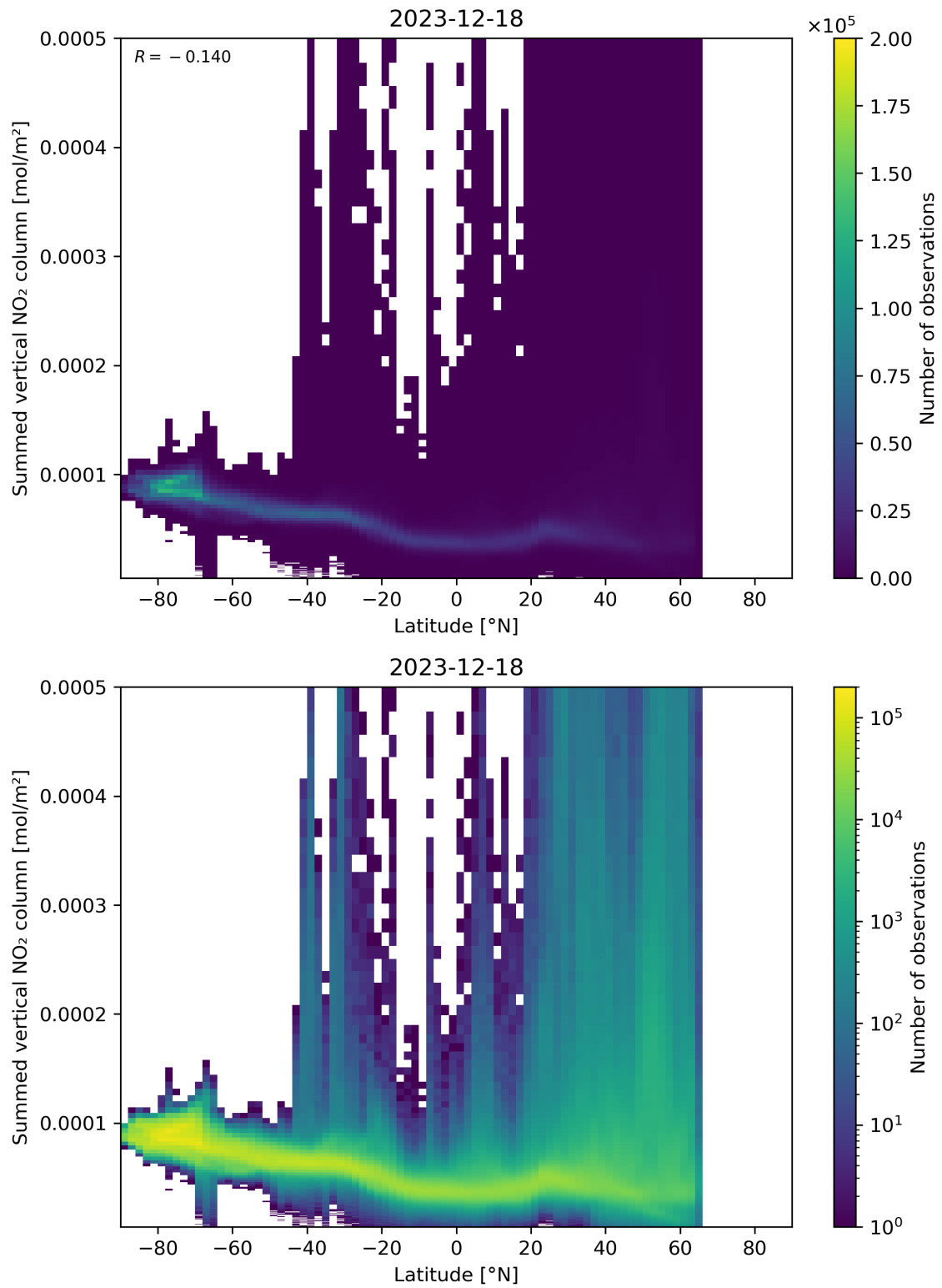
Figure 88: Scatter density plot of “Latitude” against “Summed vertical NO 2 column” for 2023-12-17 to 2023-12-19.
