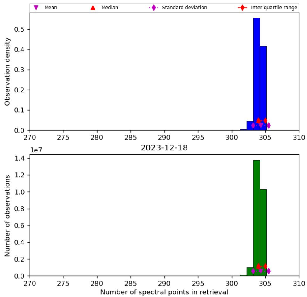
Figure 33: Histogram of “Number of spectral points in retrieval” for 2023-12-17 to 2023-12-19
