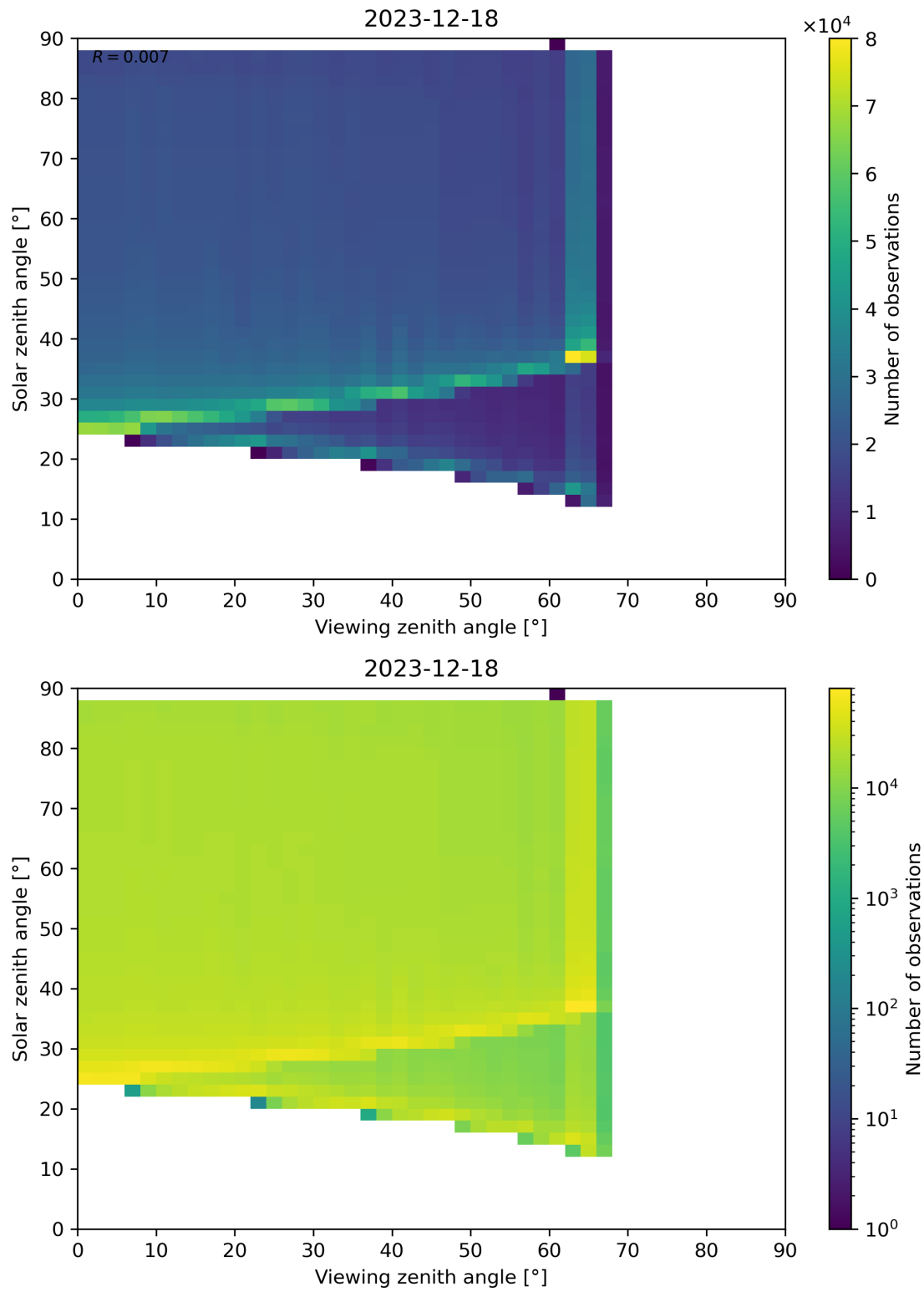
Figure 172: Scatter density plot of “Viewing zenith angle” against “Solar zenith angle” for 2023-12-17 to 2023-12-19.
