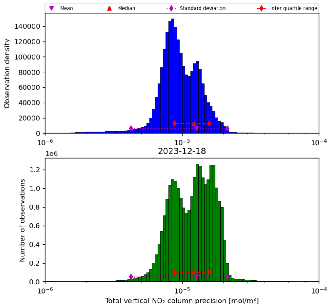
Figure 39: Histogram of “Total vertical NO 2 column precision” for 2023-12-17 to 2023-12-19
