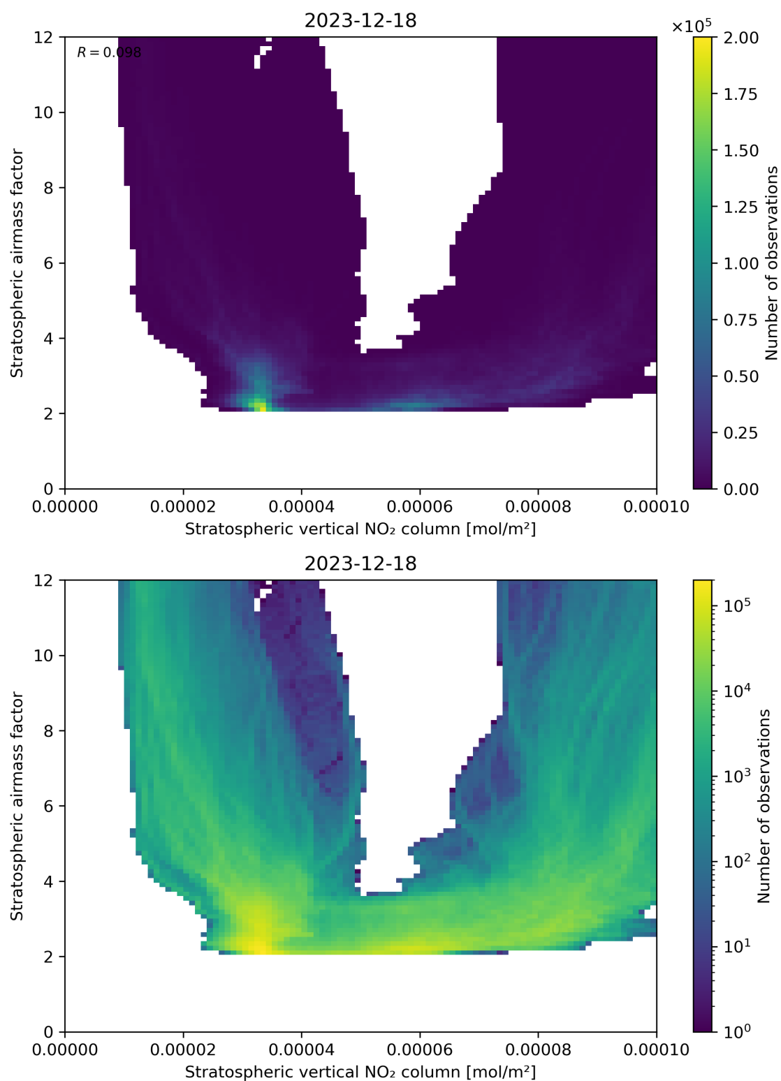
Figure 96: Scatter density plot of “Stratospheric vertical NO 2 column” against “Stratospheric airmass factor” for 2023-12-17 to 2023-12-19.
