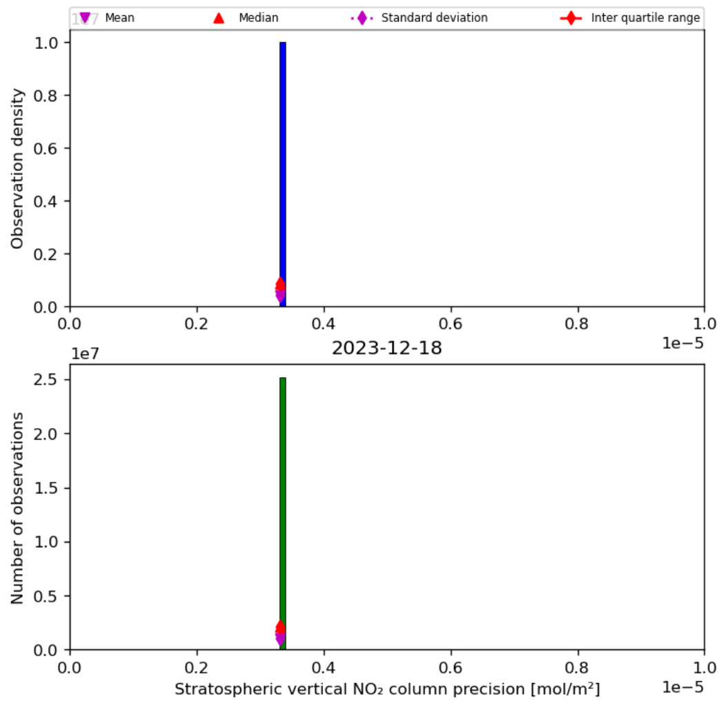
Figure 37: Histogram of “Stratospheric vertical NO 2 column precision” for 2023-12-17 to 2023-12-19
