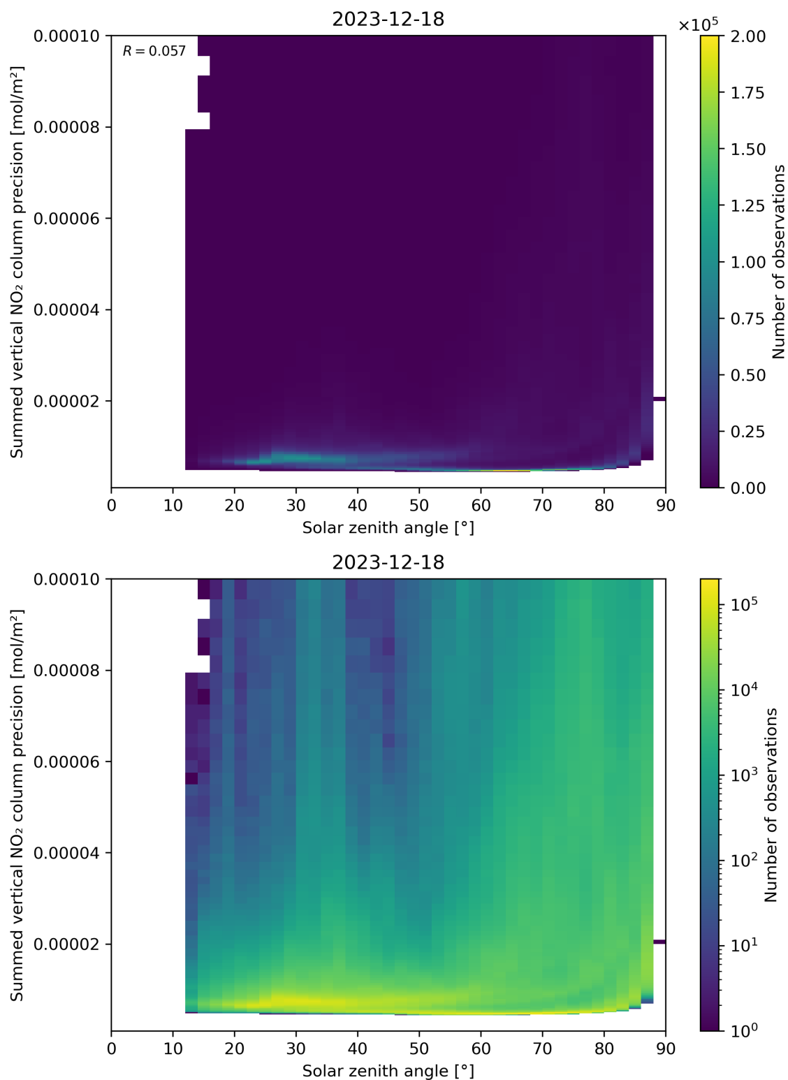
Figure 152: Scatter density plot of “Solar zenith angle” against “Summed vertical NO 2 column precision” for 2023-12-17 to 2023-12-19.
