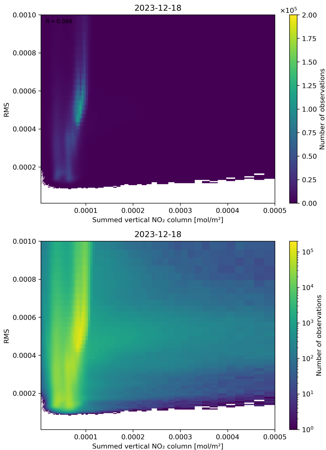
Figure 109: Scatter density plot of “Summed vertical NO 2 column” against “RMS” for 2023-12-17 to 2023-12-19.
