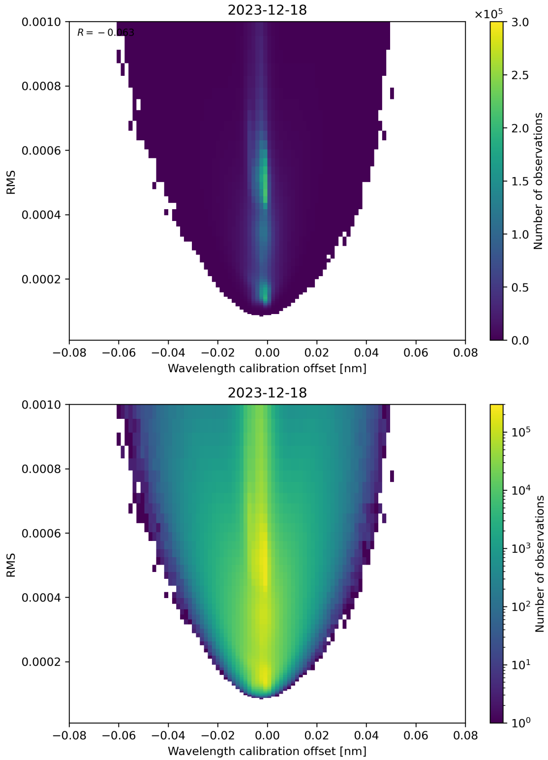
Figure 181: Scatter density plot of “Wavelength calibration offset” against “RMS” for 2023-12-17 to 2023-12-19.
