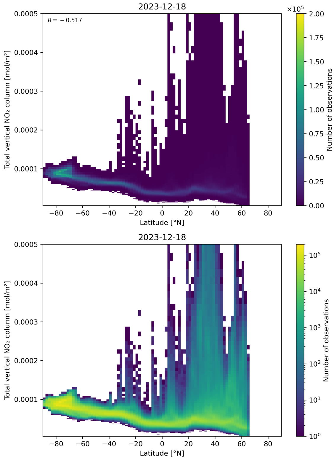
Figure 90: Scatter density plot of “Latitude” against “Total vertical NO 2 column” for 2023-12-17 to 2023-12-19.
