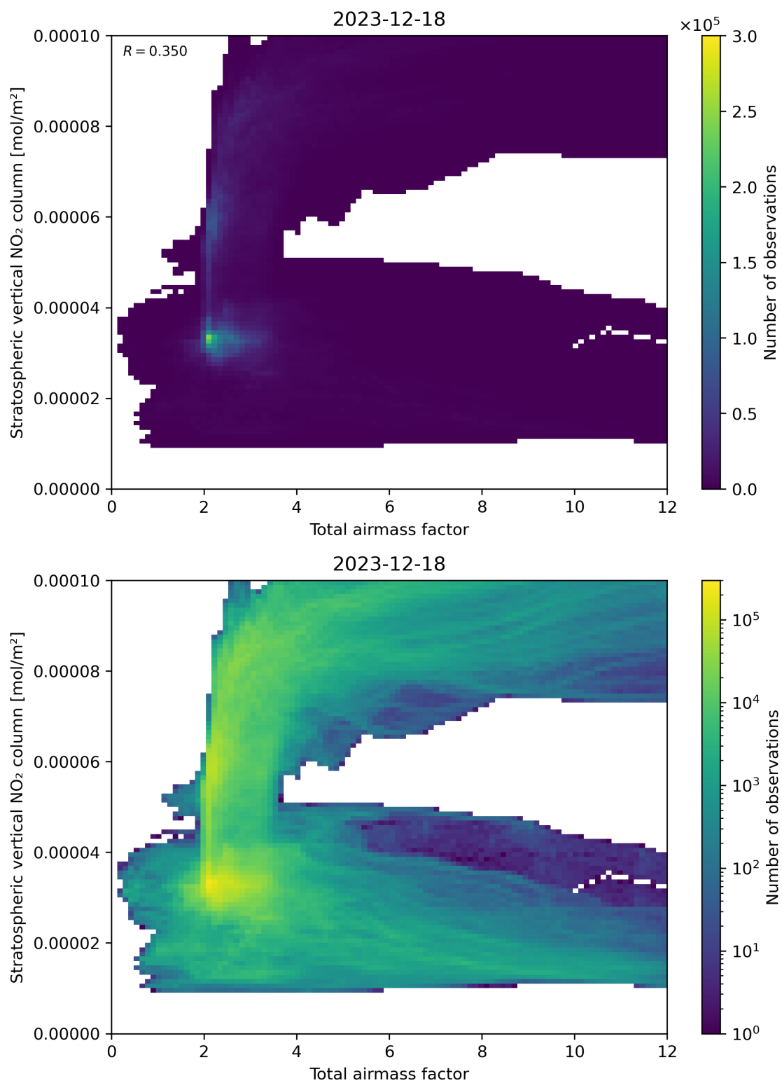
Figure 64: Scatter density plot of “Total airmass factor” against “Stratospheric vertical NO 2 column” for 2023-12-17 to 2023-12-19.
