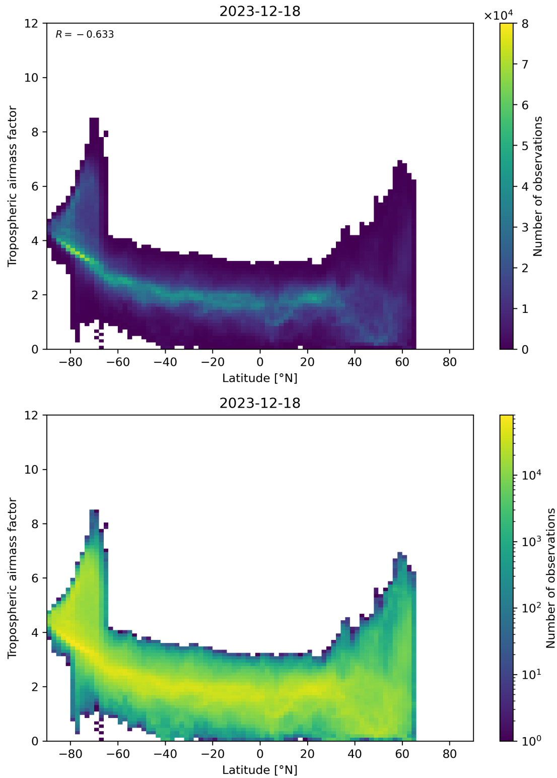
Figure 85: Scatter density plot of “Latitude” against “Tropospheric airmass factor” for 2023-12-17 to 2023-12-19.
