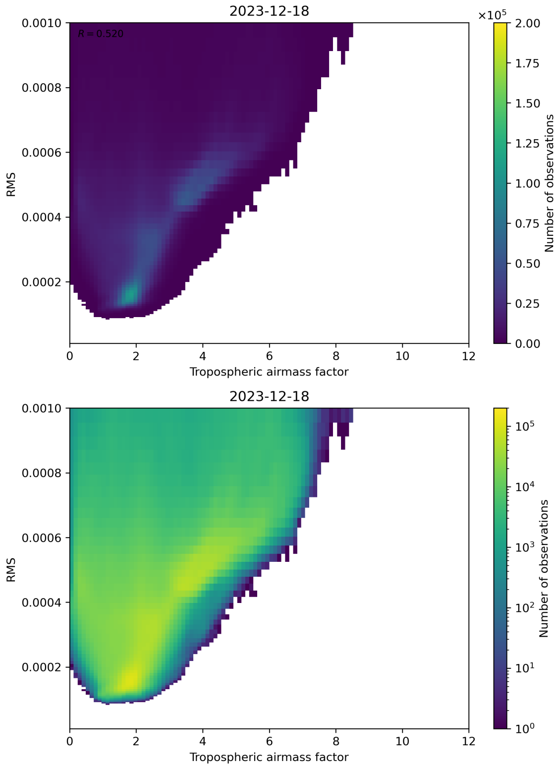
Figure 79: Scatter density plot of “Tropospheric airmass factor” against “RMS” for 2023-12-17 to 2023-12-19.
