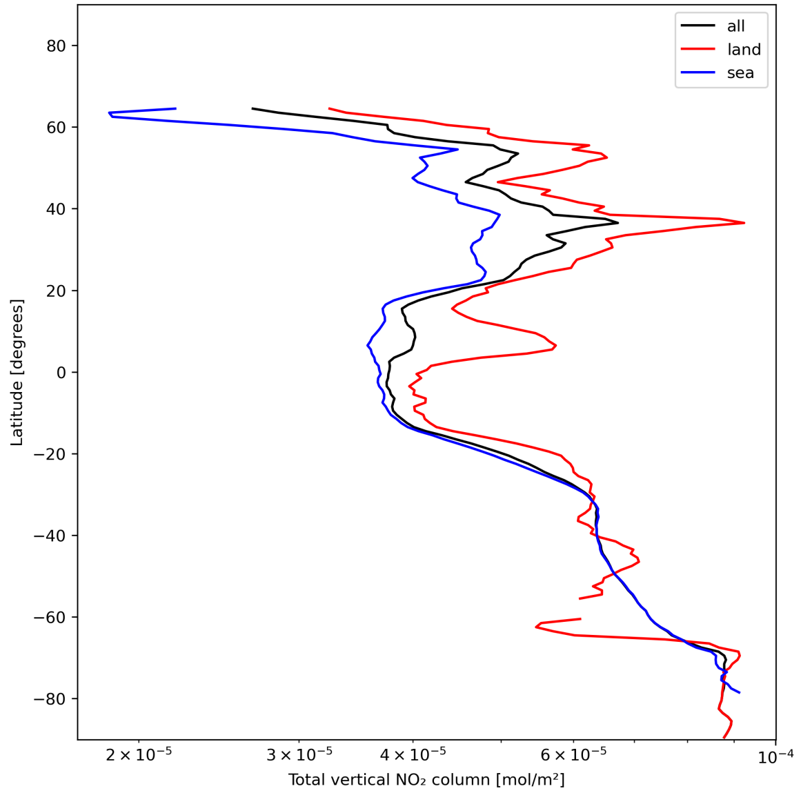
Figure 21: Zonal average of “Total vertical NO 2 column” for 2023-12-17 to 2023-12-19.
