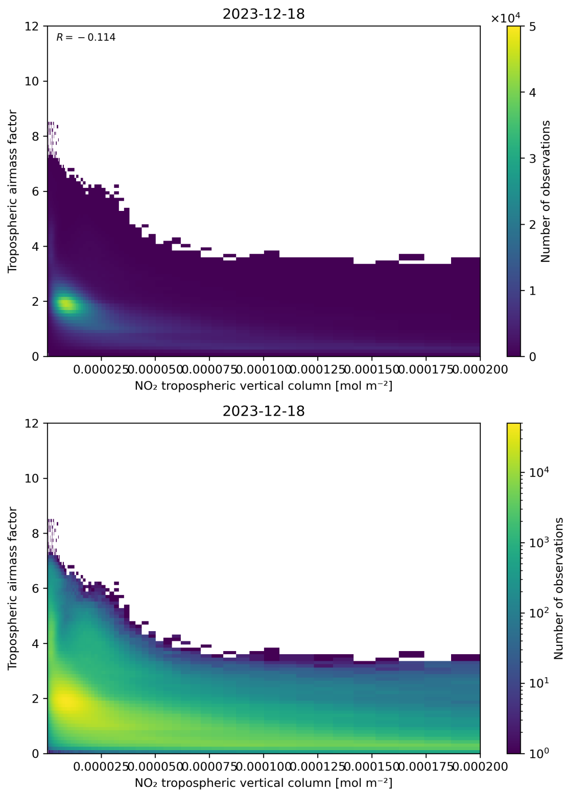
Figure 123: Scatter density plot of “NO 2 tropospheric vertical column” against “Tropospheric air mass factor” for 2023-12-17 to 2023-12-19.
