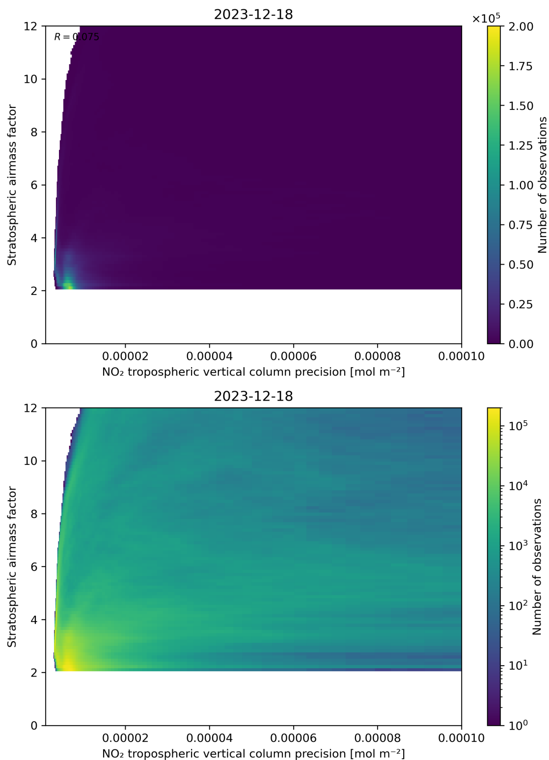
Figure 131: Scatter density plot of “NO 2 tropospheric vertical column precision” against “Stratospheric airmass factor” for 2023-12-17 to 2023-12-19.
