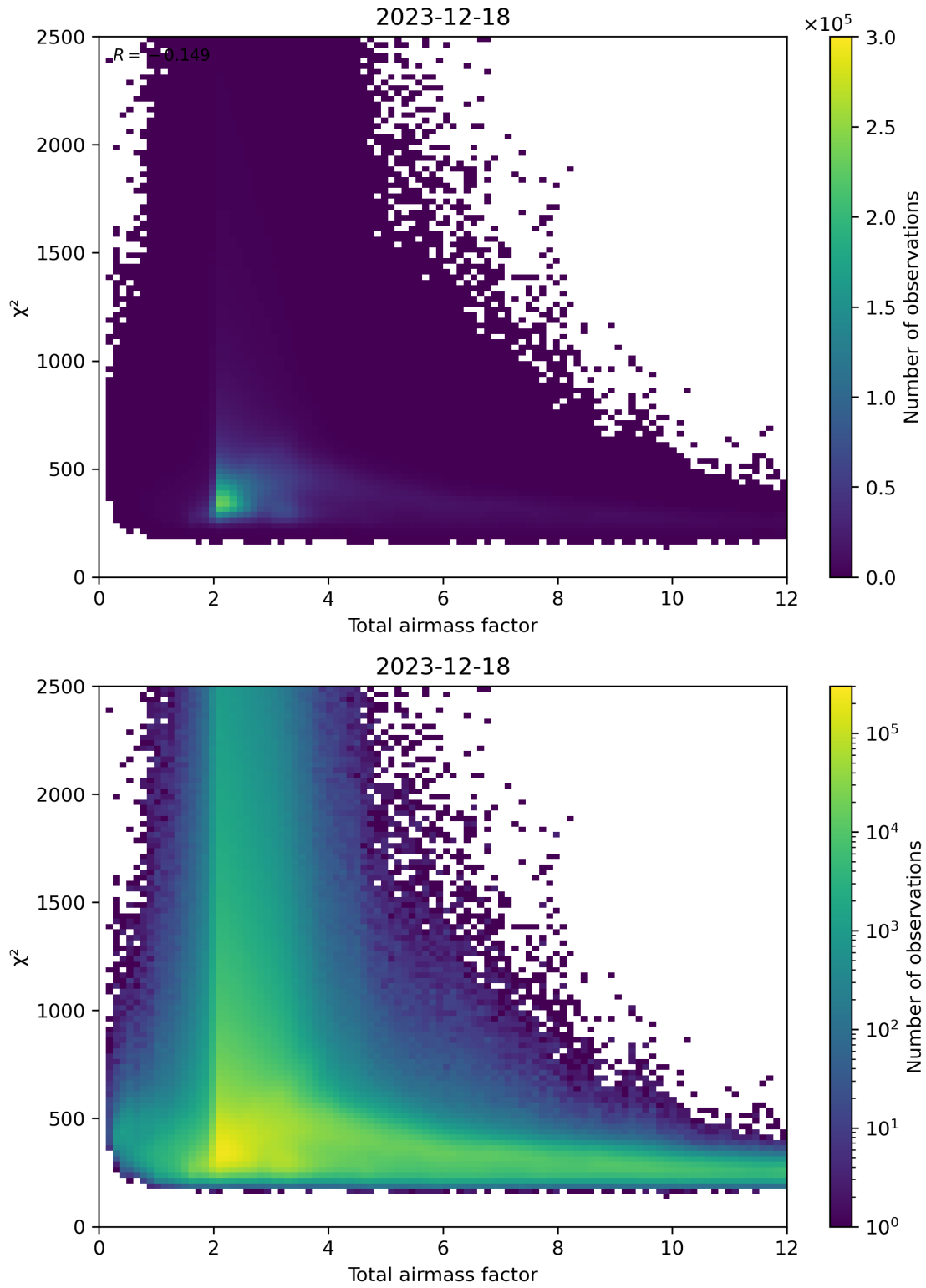
Figure 63: Scatter density plot of “Total airmass factor” against “ \chi^2 ” for 2023-12-17 to 2023-12-19.
