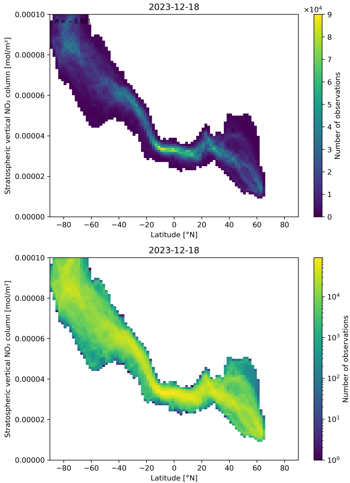
Figure 87: Scatter density plot of “Latitude” against “Stratospheric vertical NO 2 column” for 2023-12-17 to 2023-12-19.
