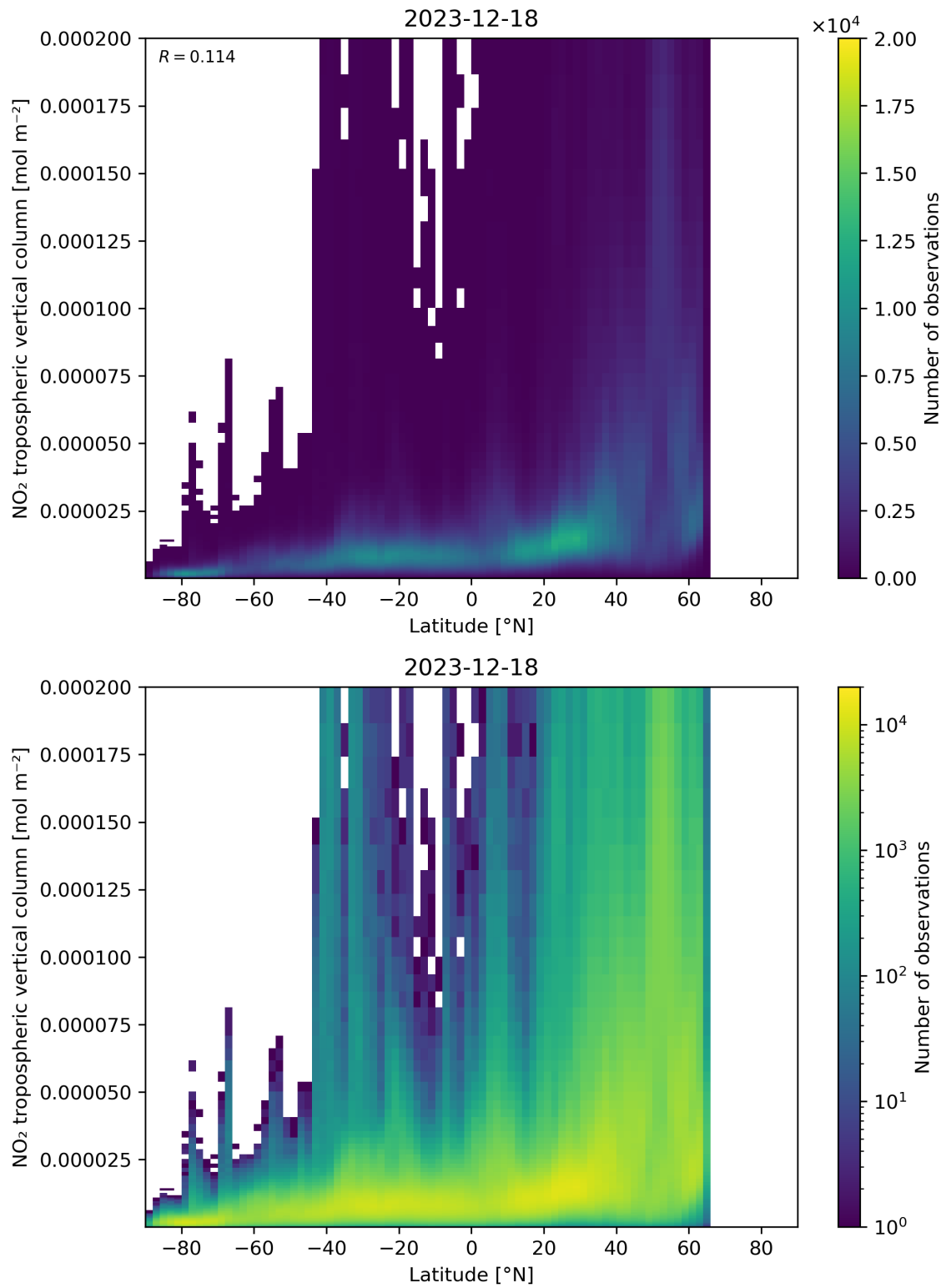
Figure 92: Scatter density plot of “Latitude” against “NO 2 tropospheric vertical column” for 2023-12-17 to 2023-12-19.
