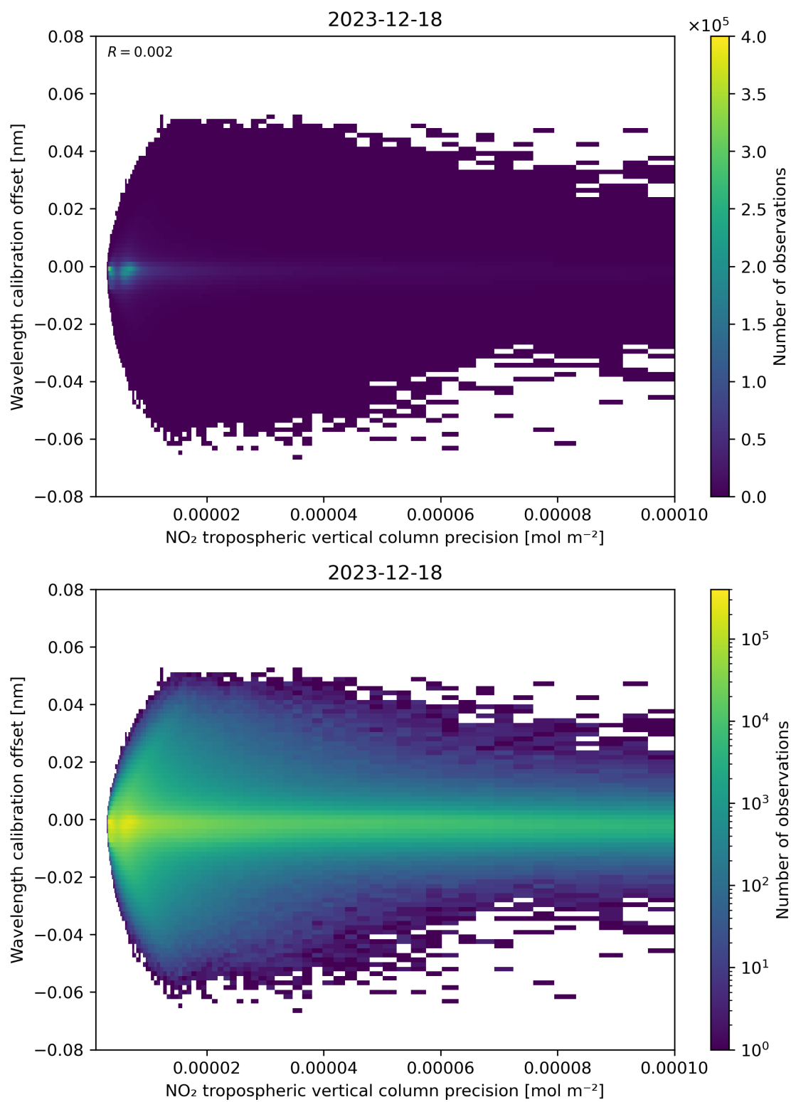
Figure 141: Scatter density plot of “NO 2 tropospheric vertical column precision” against “Wavelength calibration offset” for 2023-12-17 to 2023-12-19.
