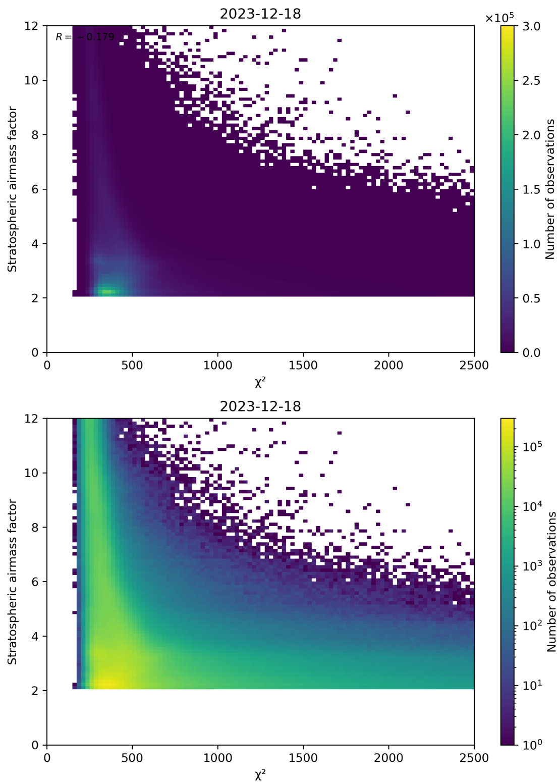
Figure 81: Scatter density plot of “ \chi^2 ” against “Stratospheric airmass factor” for 2023-12-17 to 2023-12-19.
