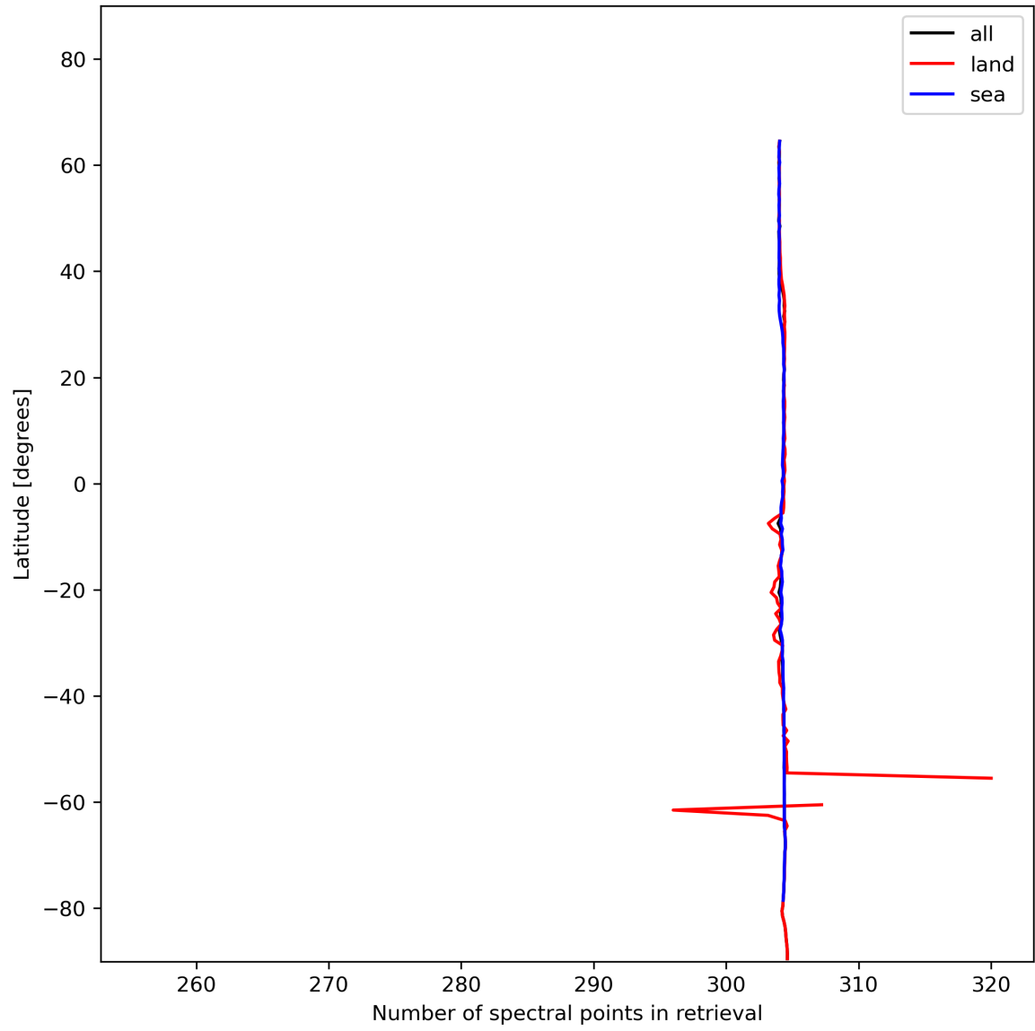
Figure 16: Zonal average of “Number of spectral points in retrieval” for 2023-12-17 to 2023-12-19.
