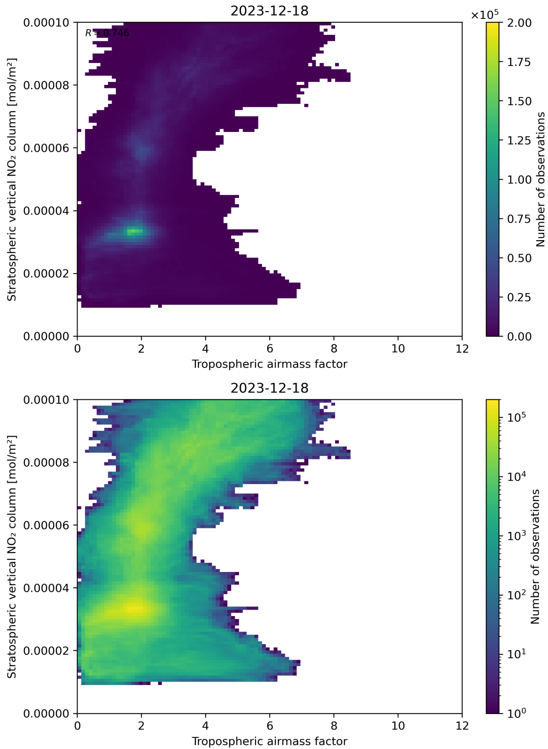
Figure 74: Scatter density plot of “Tropospheric air mass factor” against “Stratospheric vertical NO 2 column” for 2023-12-17 to 2023-12-19.
