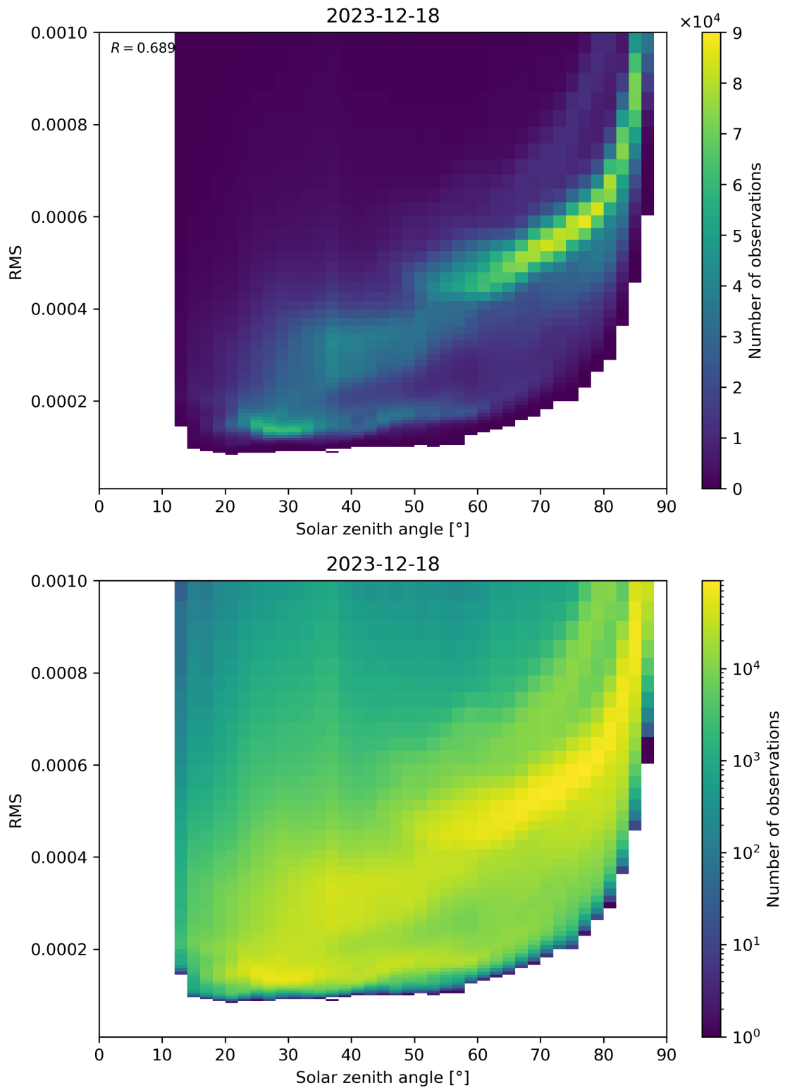
Figure 157: Scatter density plot of “Solar zenith angle” against “RMS” for 2023-12-17 to 2023-12-19.
