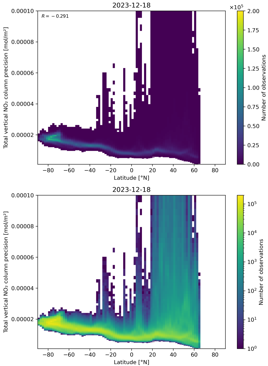
Figure 91: Scatter density plot of “Latitude” against “Total vertical NO 2 column precision” for 2023-12-17 to 2023-12-19.
