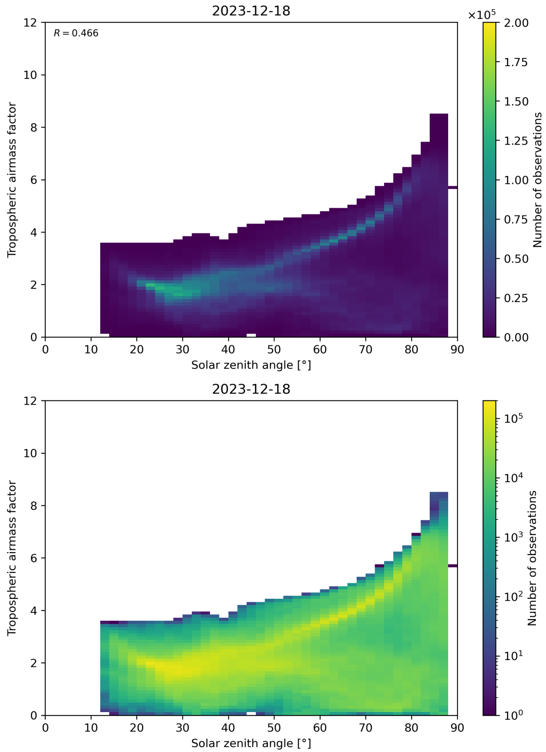
Figure 147: Scatter density plot of “Solar zenith angle” against “Tropospheric airmass factor” for 2023-12-17 to 2023-12-19.
