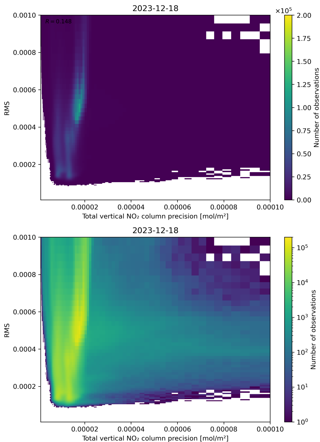
Figure 119: Scatter density plot of “Total vertical NO 2 column precision” against “RMS” for 2023-12-17 to 2023-12-19.
