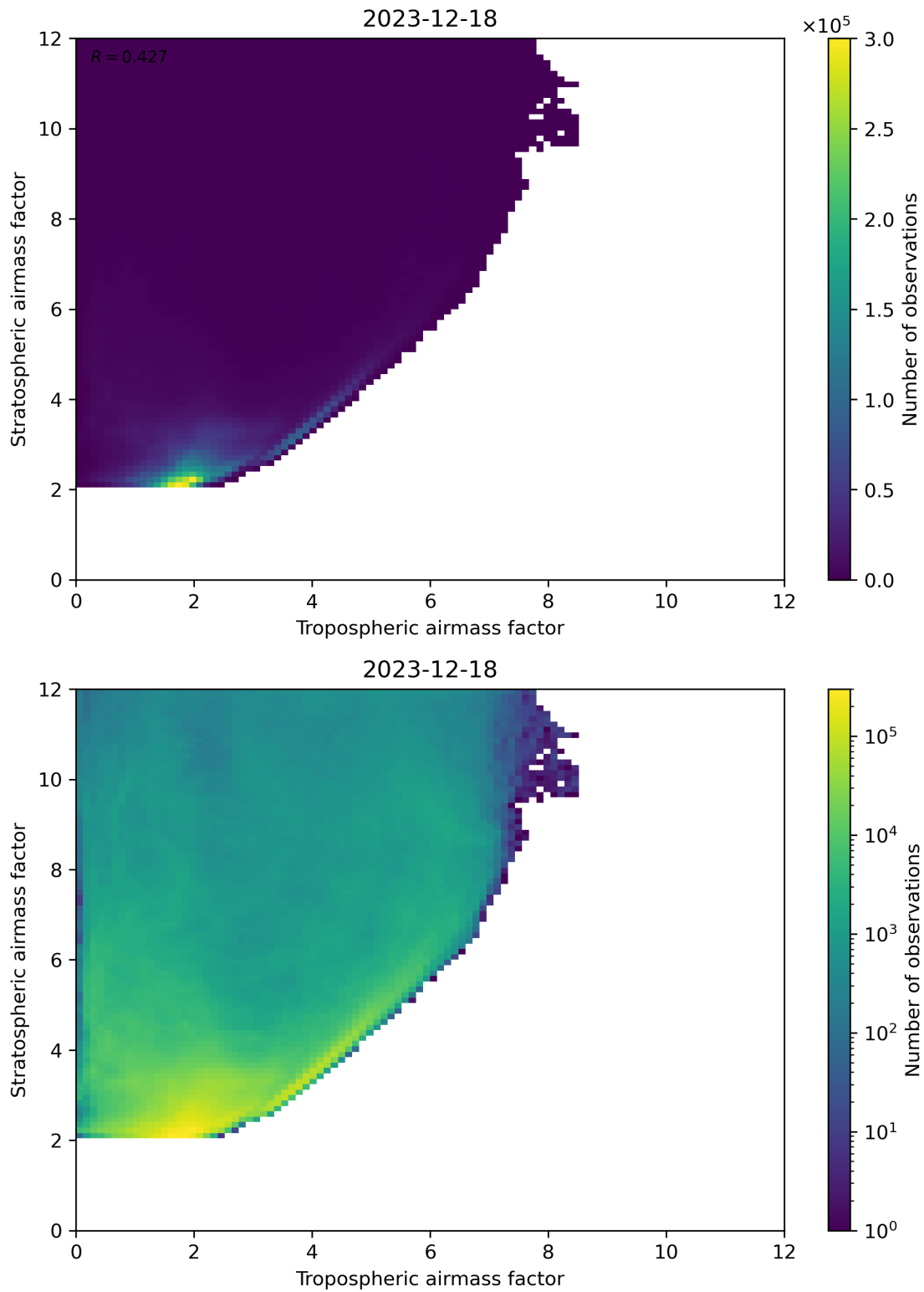
Figure 71: Scatter density plot of “Tropospheric airmass factor” against “Stratospheric airmass factor” for 2023-12-17 to 2023-12-19.
