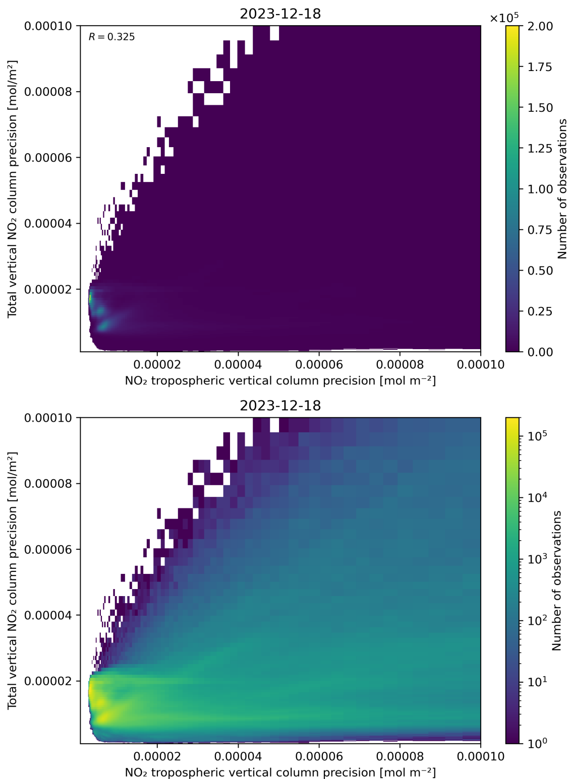
Figure 139: Scatter density plot of “NO 2 tropospheric vertical column precision” against “Total vertical NO 2 column precision” for 2023-12-17 to 2023-12-19.
