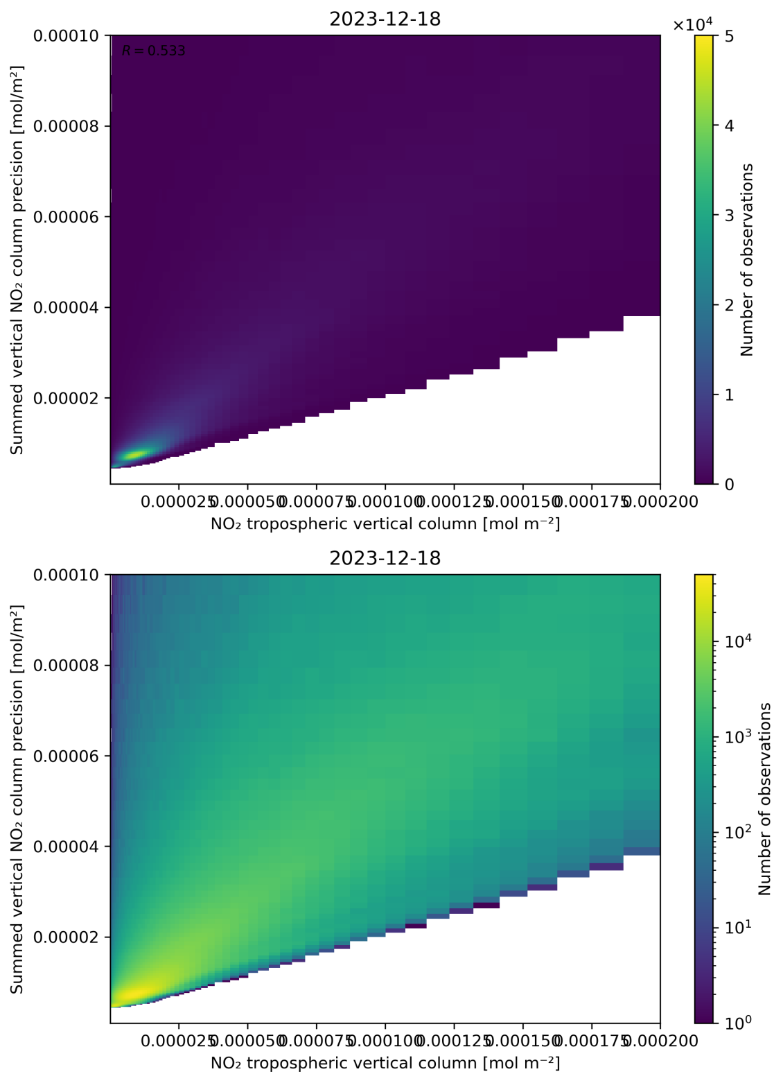
Figure 127: Scatter density plot of “NO 2 tropospheric vertical column” against “Summed vertical NO 2 column precision” for 2023-12-17 to 2023-12-19.
