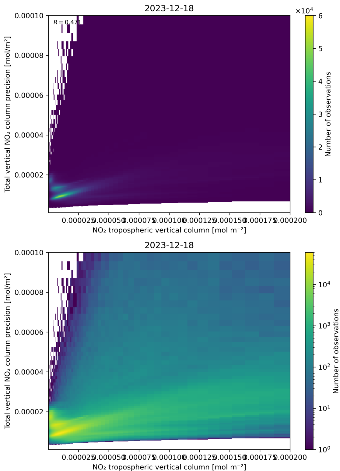
Figure 129: Scatter density plot of “NO 2 tropospheric vertical column” against “Total vertical NO 2 column precision” for 2023-12-17 to 2023-12-19.
