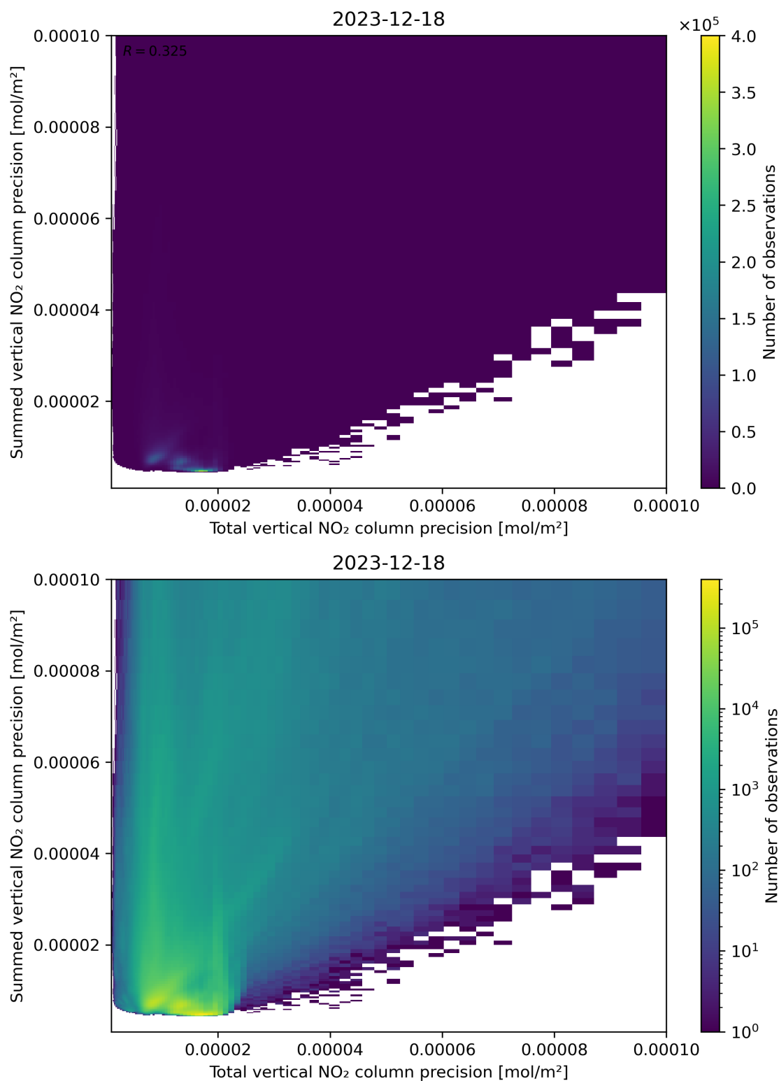
Figure 118: Scatter density plot of “Total vertical NO 2 column precision” against “Summed vertical NO 2 column precision” for 2023-12-17 to 2023-12-19.
