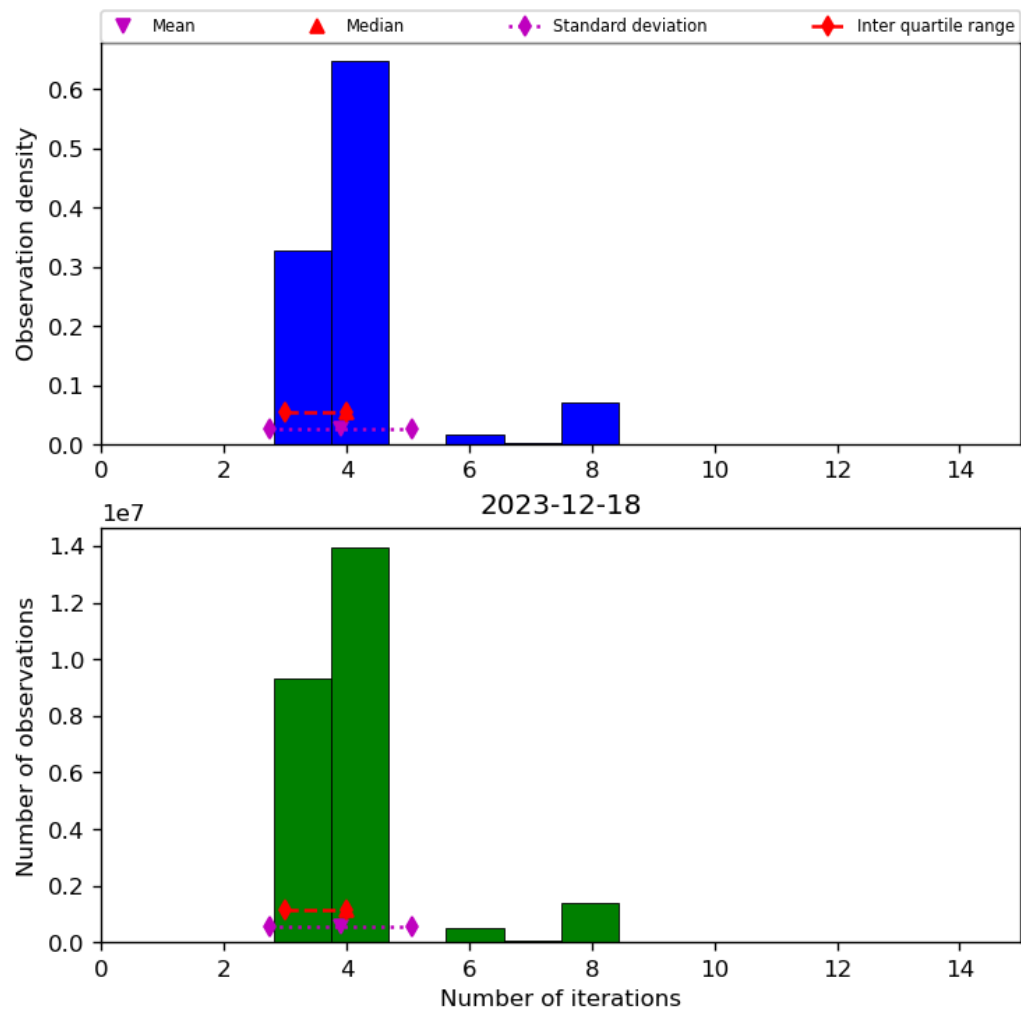
Figure 34: Histogram of “Number of iterations” for 2023-12-17 to 2023-12-19
