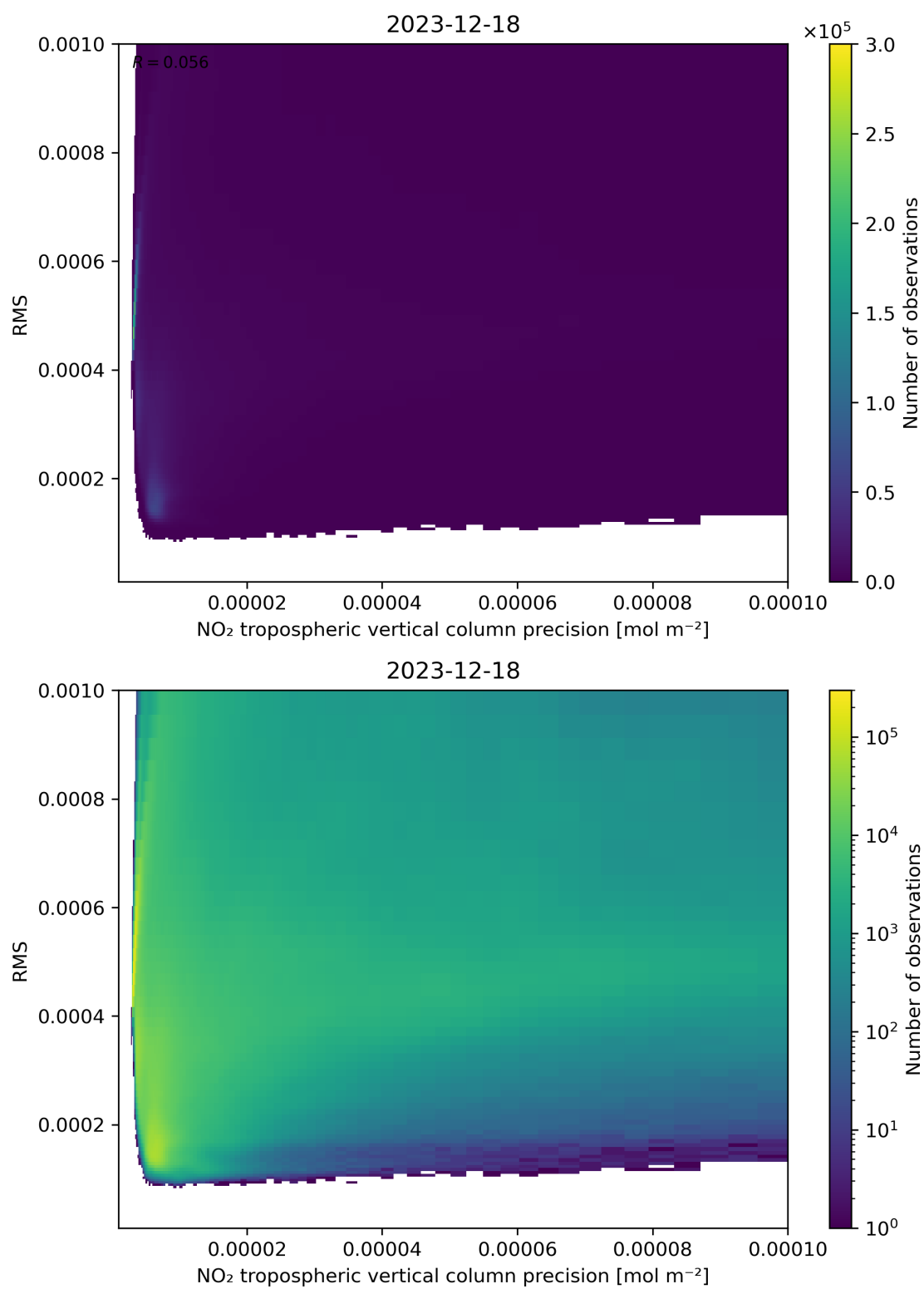
Figure 140: Scatter density plot of “NO 2 tropospheric vertical column precision” against “RMS” for 2023-12-17 to 2023-12-19.
