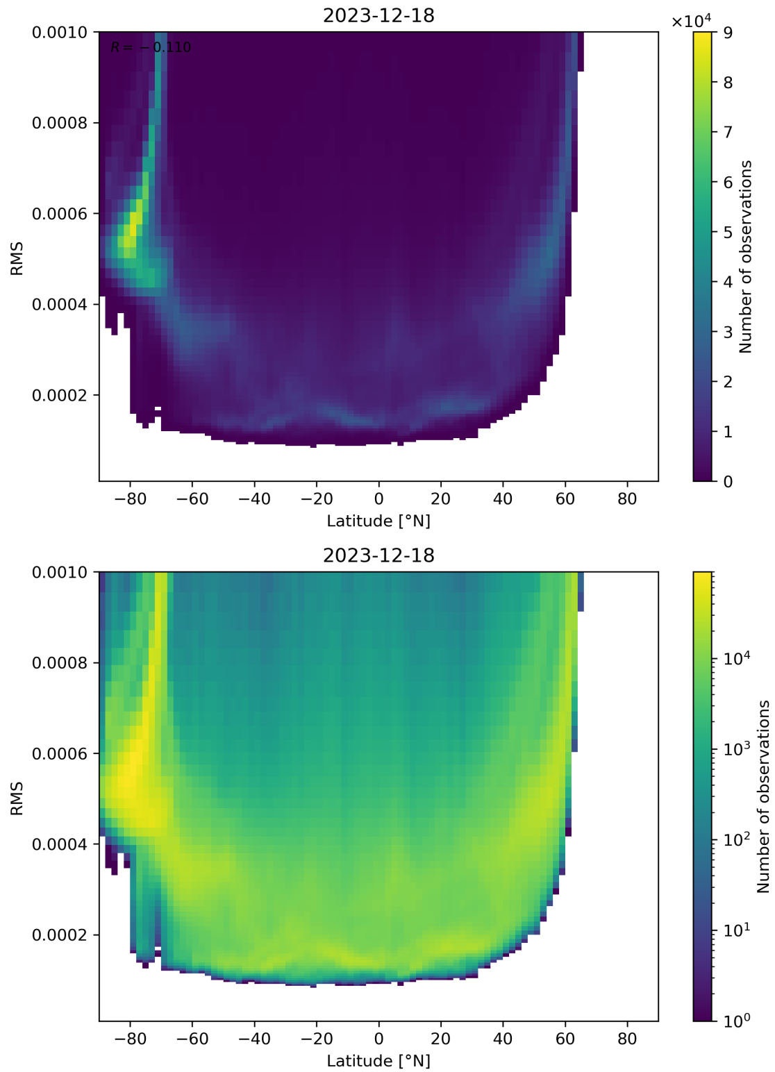
Figure 94: Scatter density plot of “Latitude” against “RMS” for 2023-12-17 to 2023-12-19.
