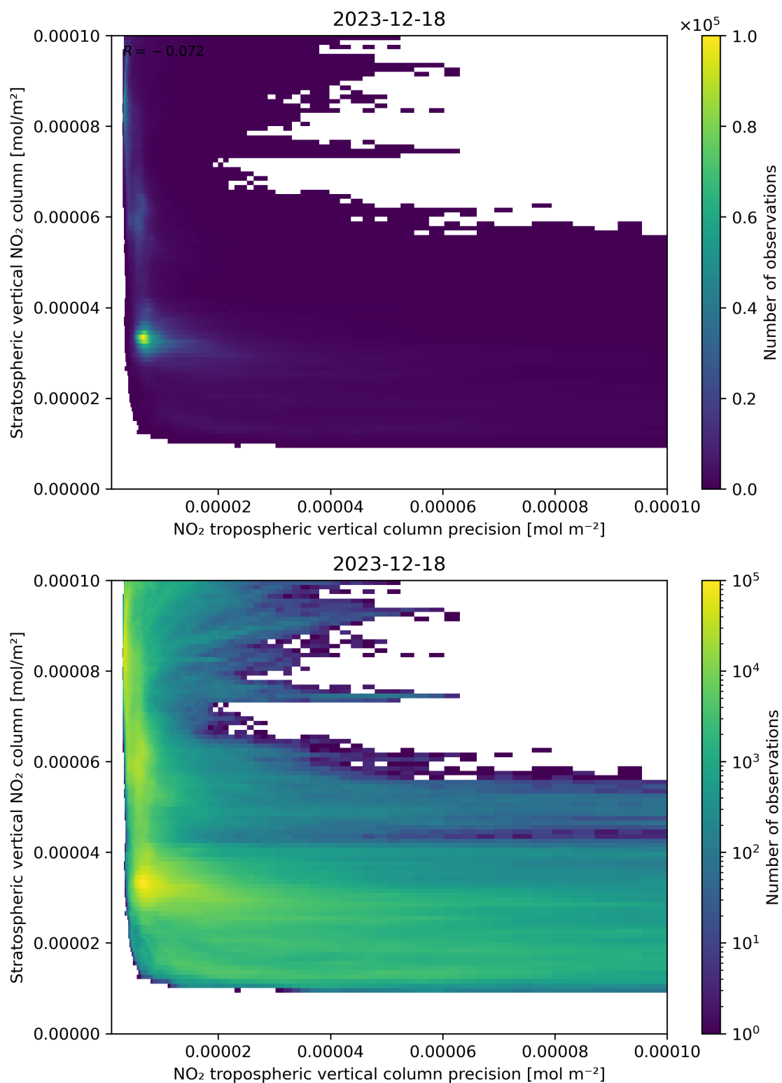
Figure 135: Scatter density plot of “NO 2 tropospheric vertical column precision” against “Stratospheric vertical NO 2 column” for 2023-12-17 to 2023-12-19.
