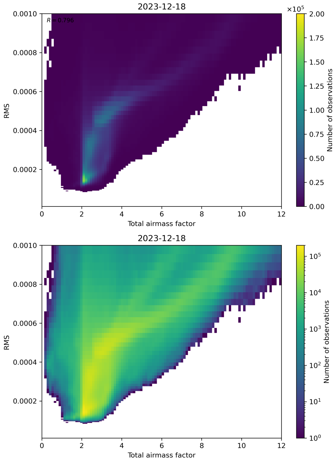
Figure 69: Scatter density plot of “Total airmass factor” against “RMS” for 2023-12-17 to 2023-12-19.
