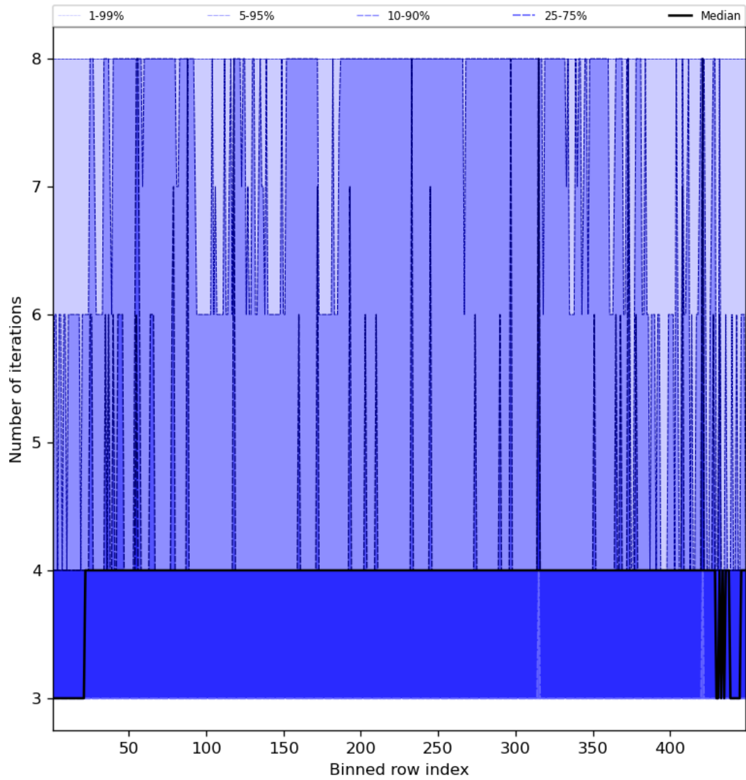
Figure 51: Along track statistics of “Number of iterations” for 2023-12-17 to 2023-12-19
