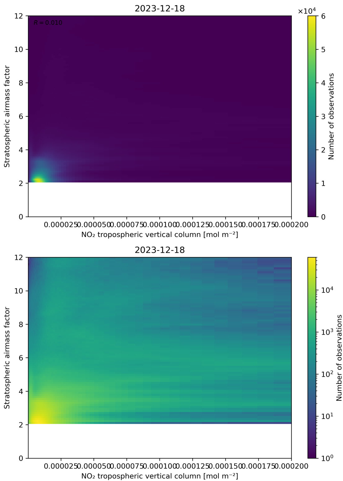
Figure 121: Scatter density plot of “NO 2 tropospheric vertical column” against “Stratospheric airmass factor” for 2023-12-17 to 2023-12-19.
