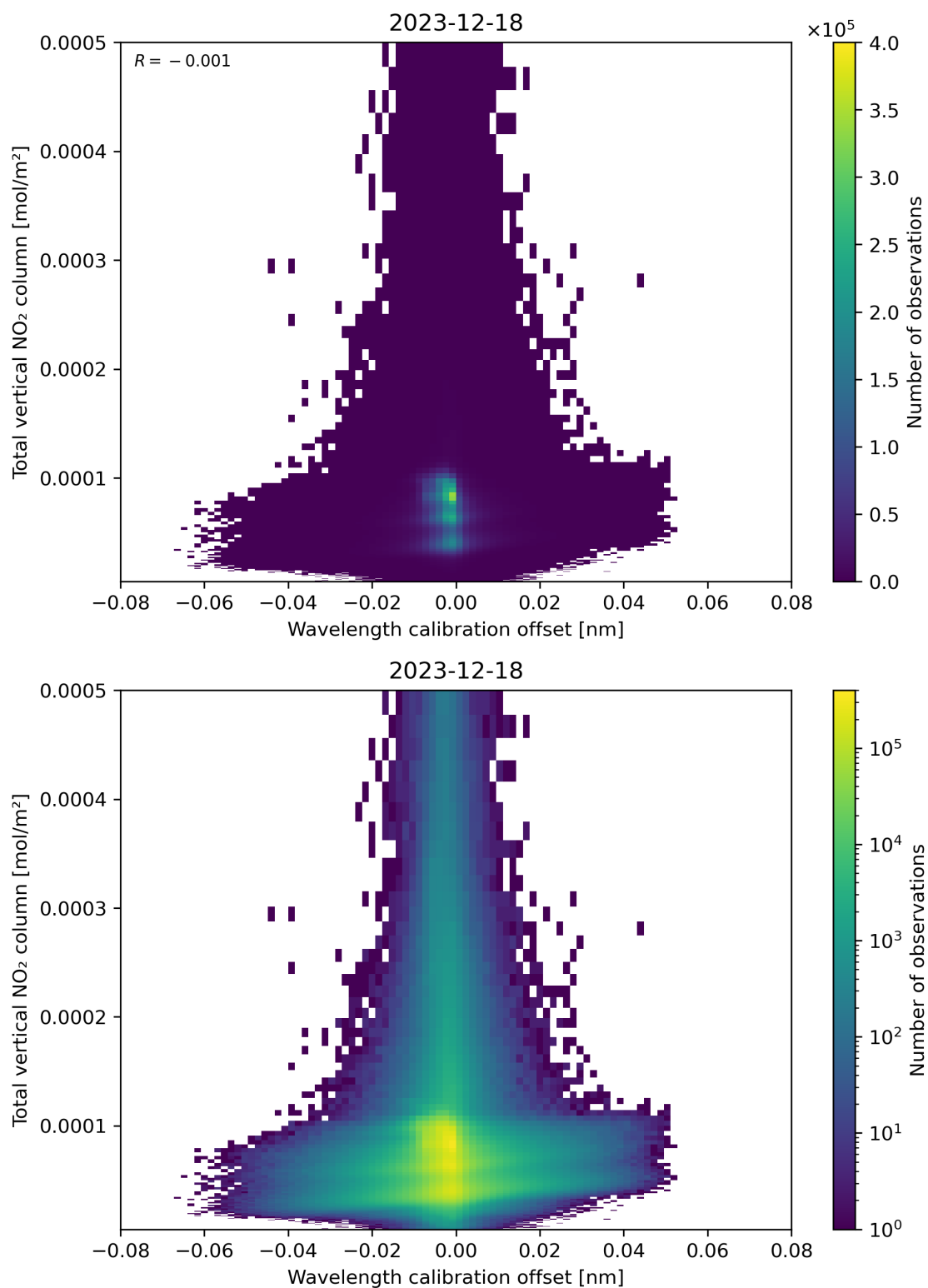
Figure 179: Scatter density plot of “Wavelength calibration offset” against “Total vertical NO 2 column” for 2023-12-17 to 2023-12-19.
