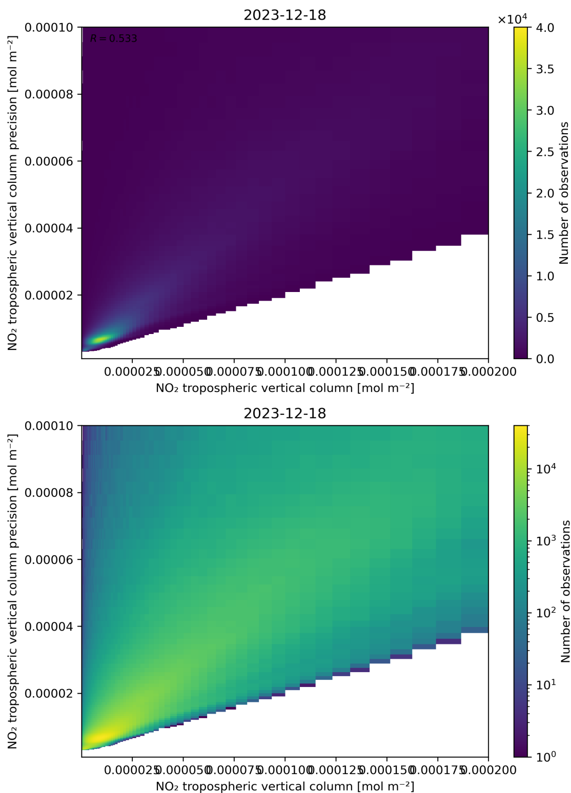
Figure 130: Scatter density plot of “NO 2 tropospheric vertical column” against “NO 2 tropospheric vertical column precision” for 2023-12-17 to 2023-12-19.
