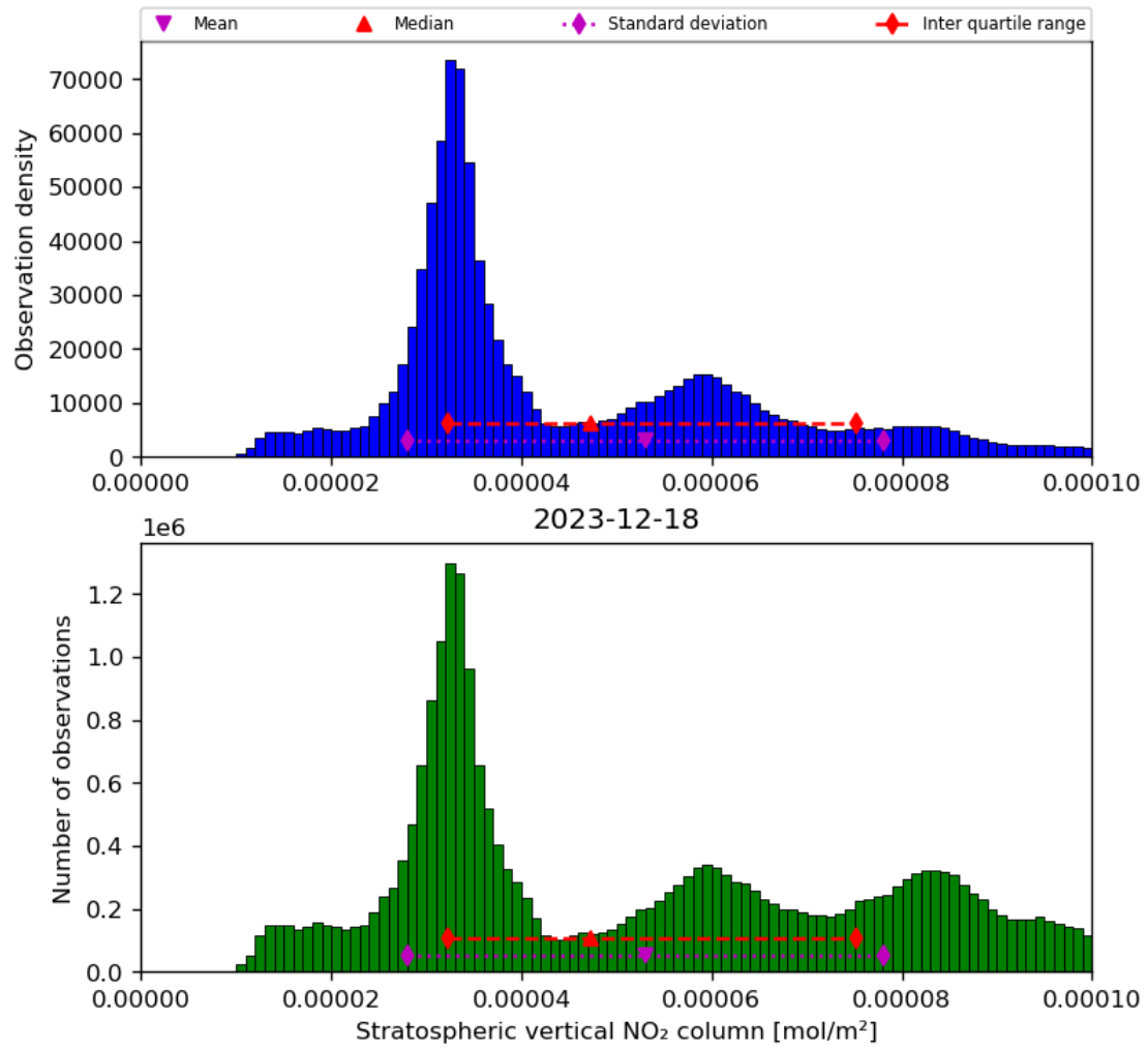
Figure 36: Histogram of “Stratospheric vertical NO 2 column” for 2023-12-17 to 2023-12-19
