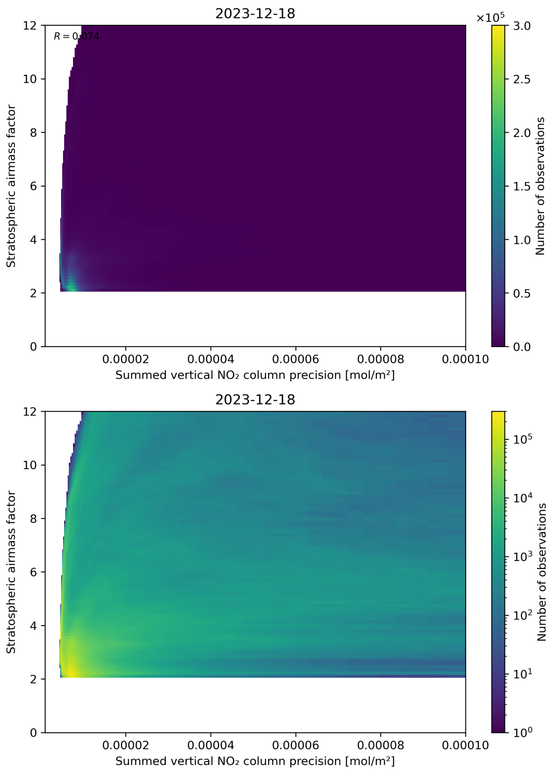
Figure 106: Scatter density plot of “Summed vertical NO 2 column precision” against “Stratospheric airmass factor” for 2023-12-17 to 2023-12-19.
