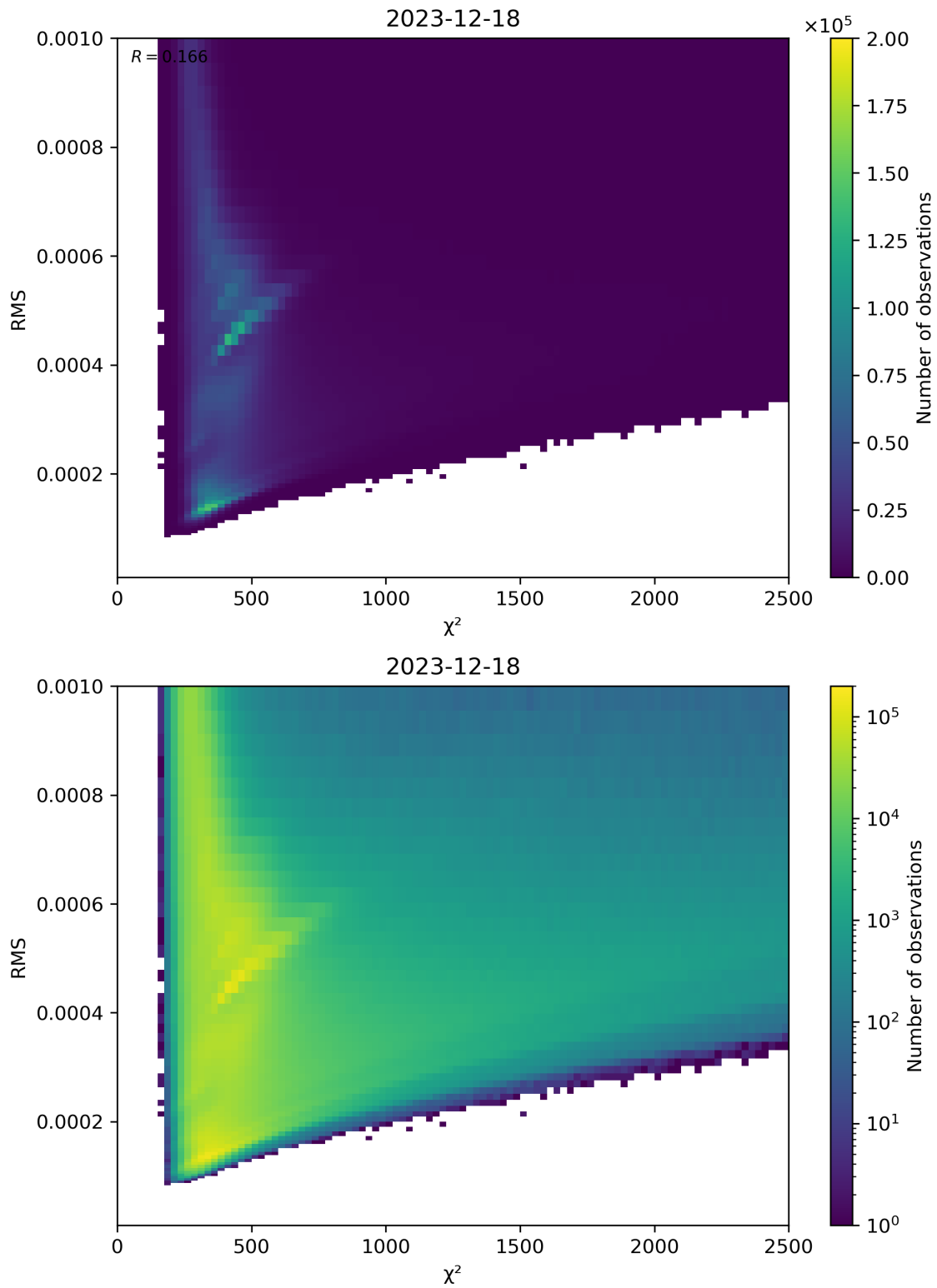
Figure 82: Scatter density plot of “ \chi^2 ” against “RMS” for 2023-12-17 to 2023-12-19.
