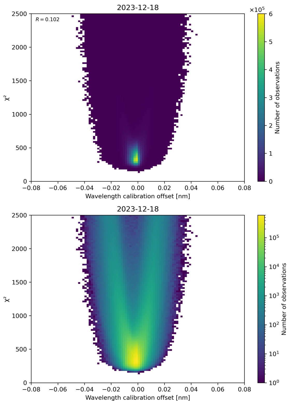
Figure 175: Scatter density plot of “Wavelength calibration offset” against “ \chi^2 ” for 2023-12-17 to 2023-12-19.
