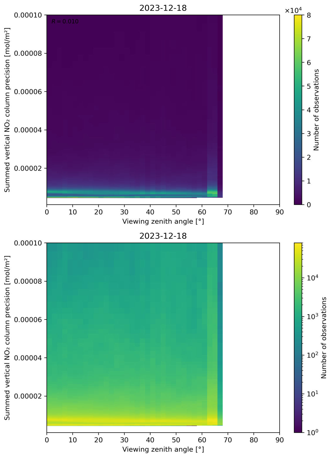
Figure 166: Scatter density plot of “Viewing zenith angle” against “Summed vertical NO 2 column precision” for 2023-12-17 to 2023-12-19.
