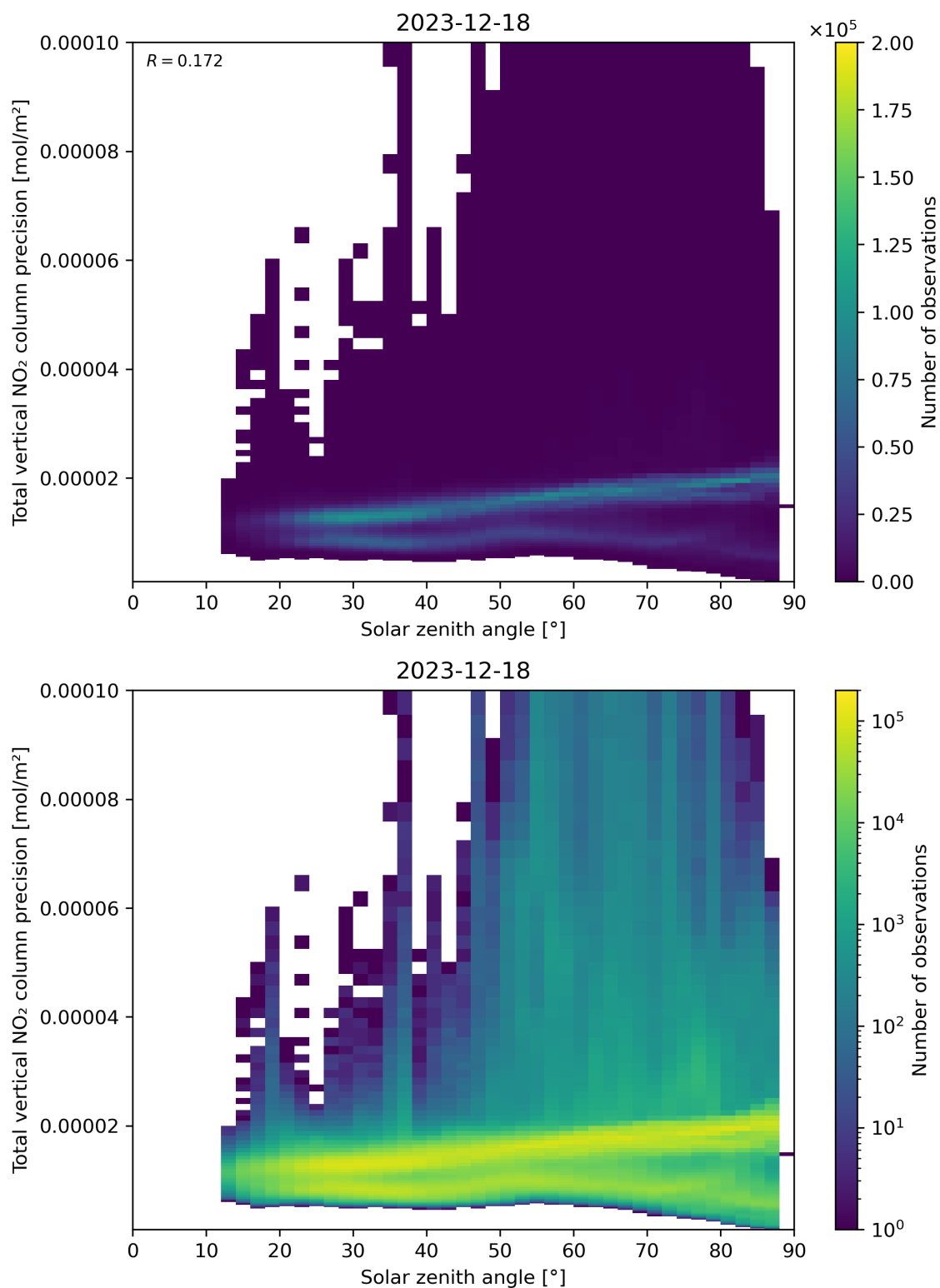
Figure 154: Scatter density plot of “Solar zenith angle” against “Total vertical NO 2 column precision” for 2023-12-17 to 2023-12-19.
