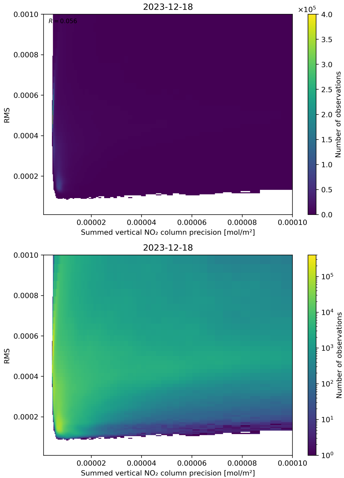
Figure 108: Scatter density plot of “Summed vertical NO 2 column precision” against “RMS” for 2023-12-17 to 2023-12-19.
