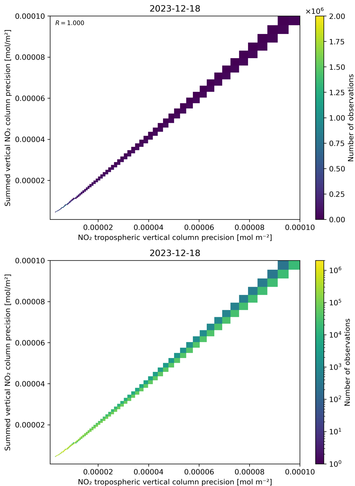
Figure 137: Scatter density plot of “NO 2 tropospheric vertical column precision” against “Summed vertical NO 2 column precision” for 2023-12-17 to 2023-12-19.
