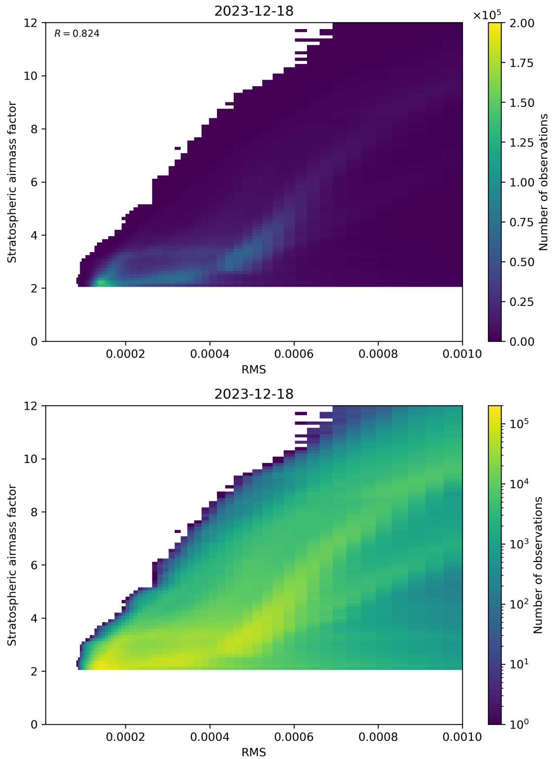
Figure 144: Scatter density plot of “RMS” against “Stratospheric airmass factor” for 2023-12-17 to 2023-12-19.
