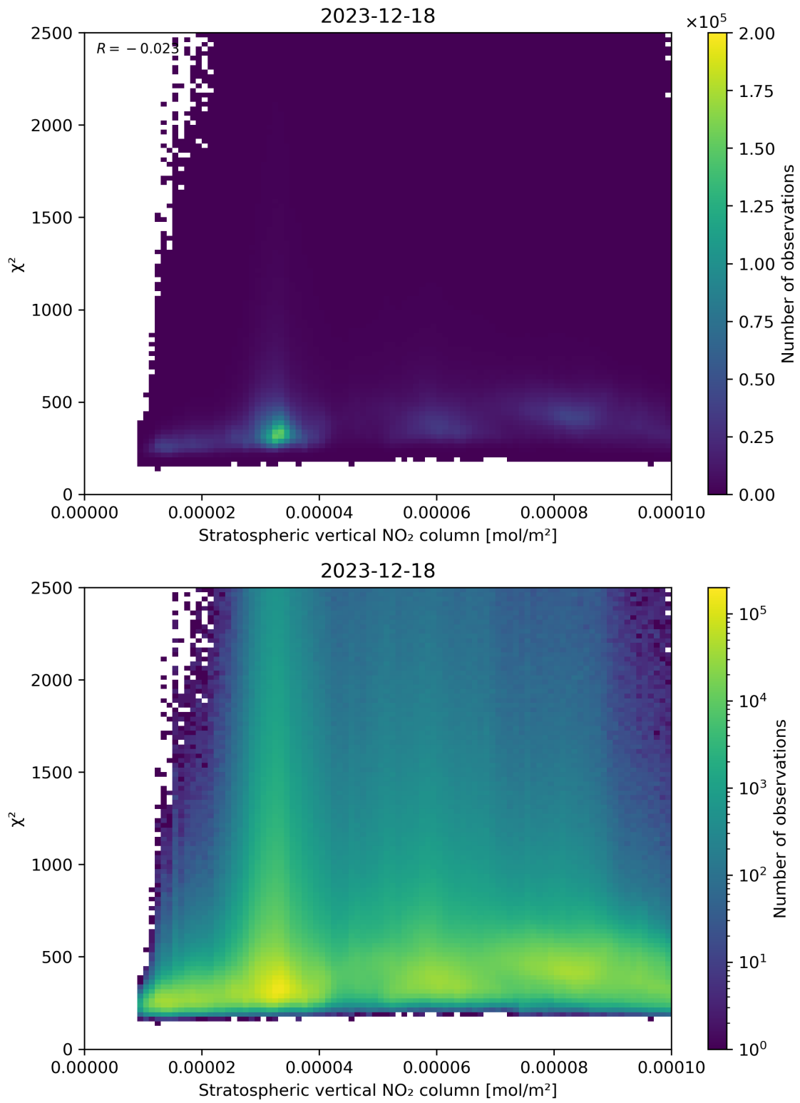
Figure 97: Scatter density plot of “Stratospheric vertical NO 2 column” against “ \chi^2 ” for 2023-12-17 to 2023-12-19.
