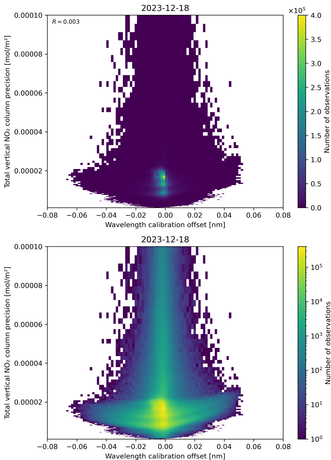
Figure 180: Scatter density plot of “Wavelength calibration offset” against “Total vertical NO 2 column precision” for 2023-12-17 to 2023-12-19.
