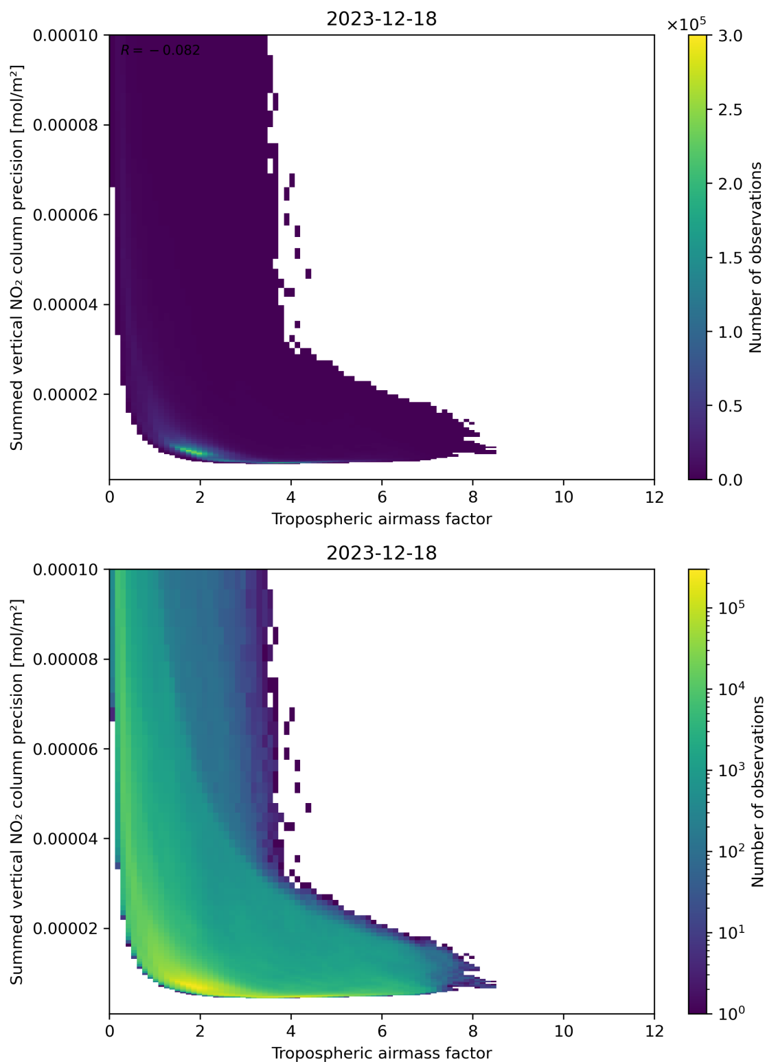
Figure 76: Scatter density plot of “Tropospheric air mass factor” against “Summed vertical NO 2 column precision” for 2023-12-17 to 2023-12-19.
