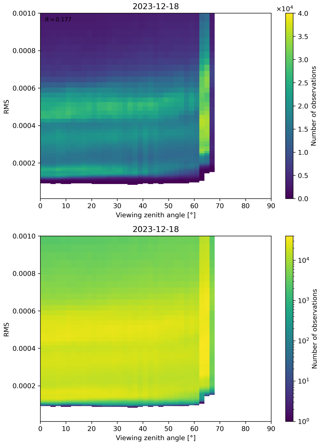
Figure 171: Scatter density plot of “Viewing zenith angle” against “RMS” for 2023-12-17 to 2023-12-19.
