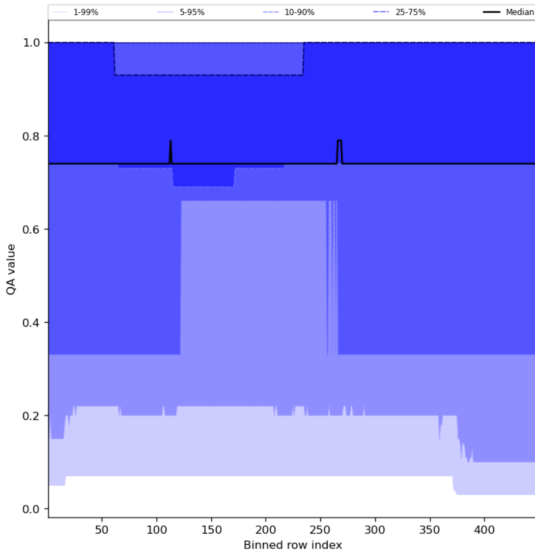
Figure 45: Along track statistics of “QA value” for 2023-12-17 to 2023-12-19
