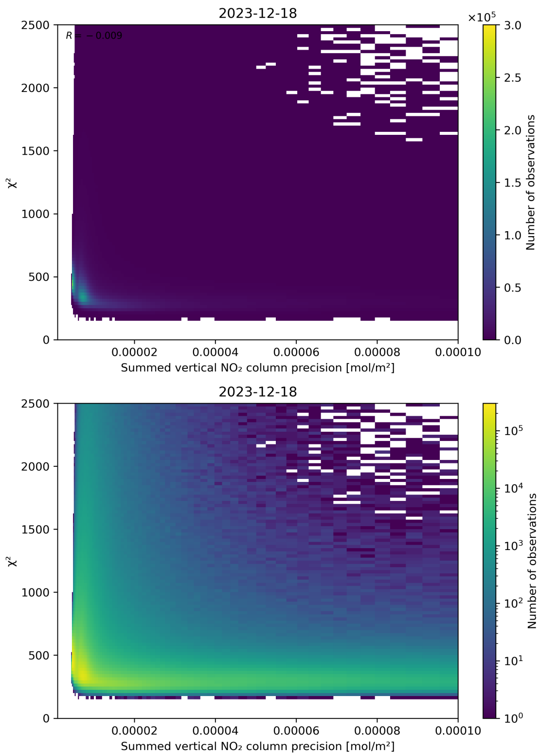
Figure 107: Scatter density plot of “Summed vertical NO 2 column precision” against “ \chi^2 ” for 2023-12-17 to 2023-12-19.
