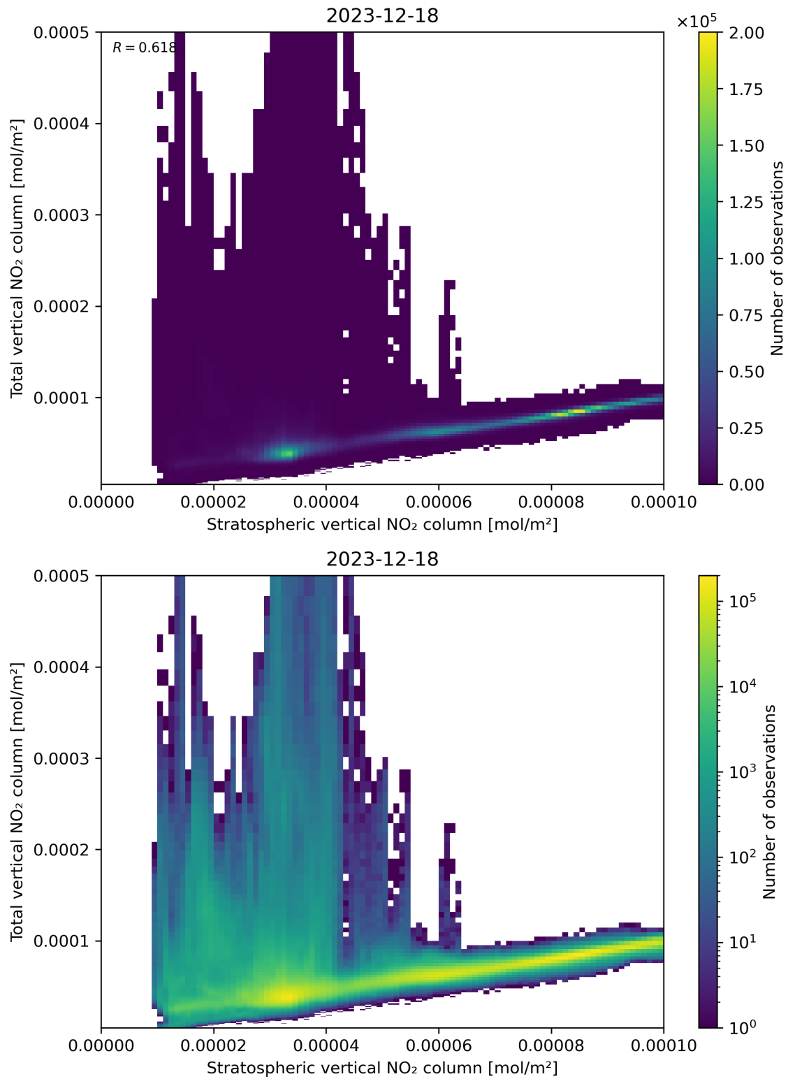
Figure 100: Scatter density plot of “Stratospheric vertical NO 2 column” against “Total vertical NO 2 column” for 2023-12-17 to 2023-12-19.
