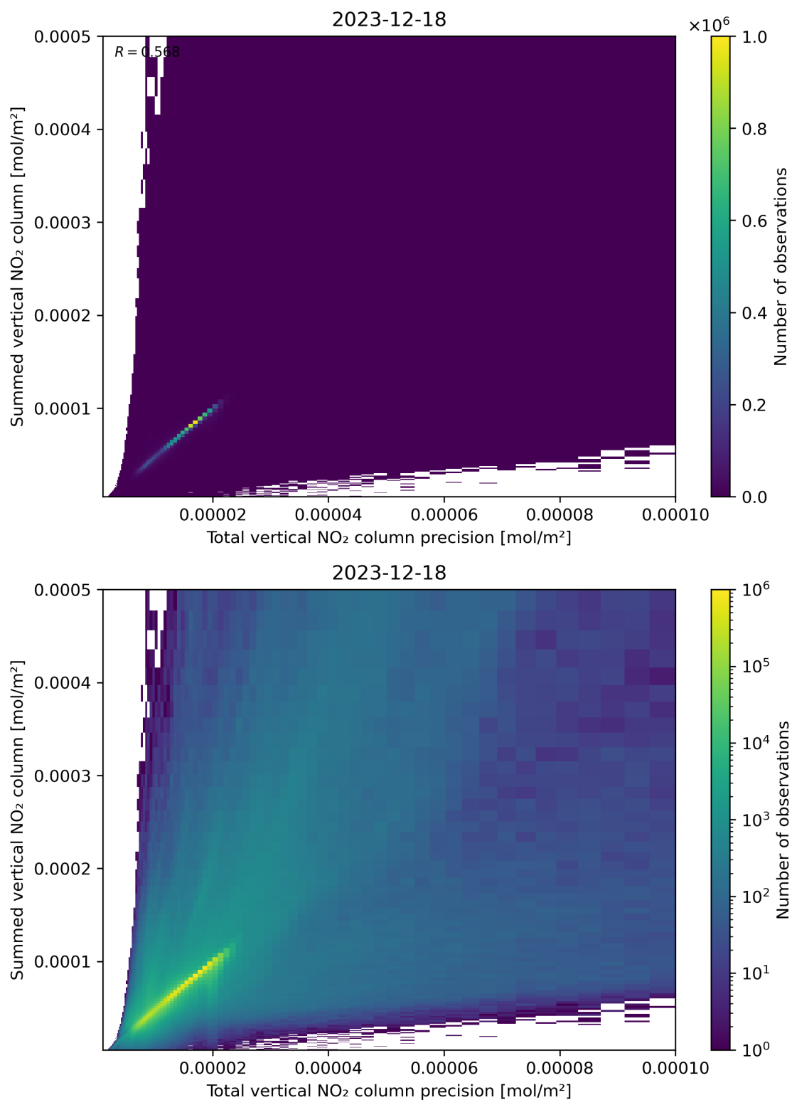
Figure 117: Scatter density plot of “Total vertical NO 2 column precision” against “Summed vertical NO 2 column” for 2023-12-17 to 2023-12-19.
