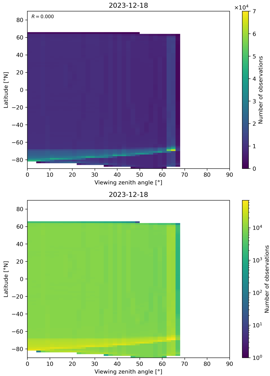
Figure 163: Scatter density plot of “Viewing zenith angle” against “Latitude” for 2023-12-17 to 2023-12-19.
