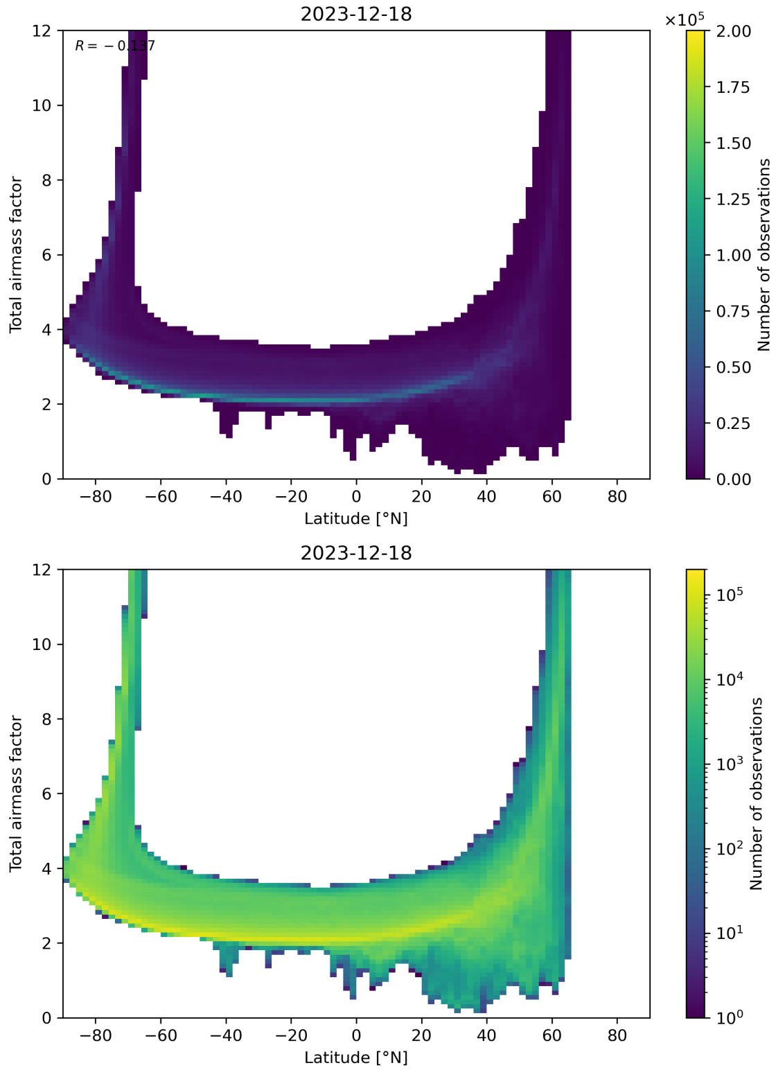
Figure 84: Scatter density plot of “Latitude” against “Total airmass factor” for 2023-12-17 to 2023-12-19.
