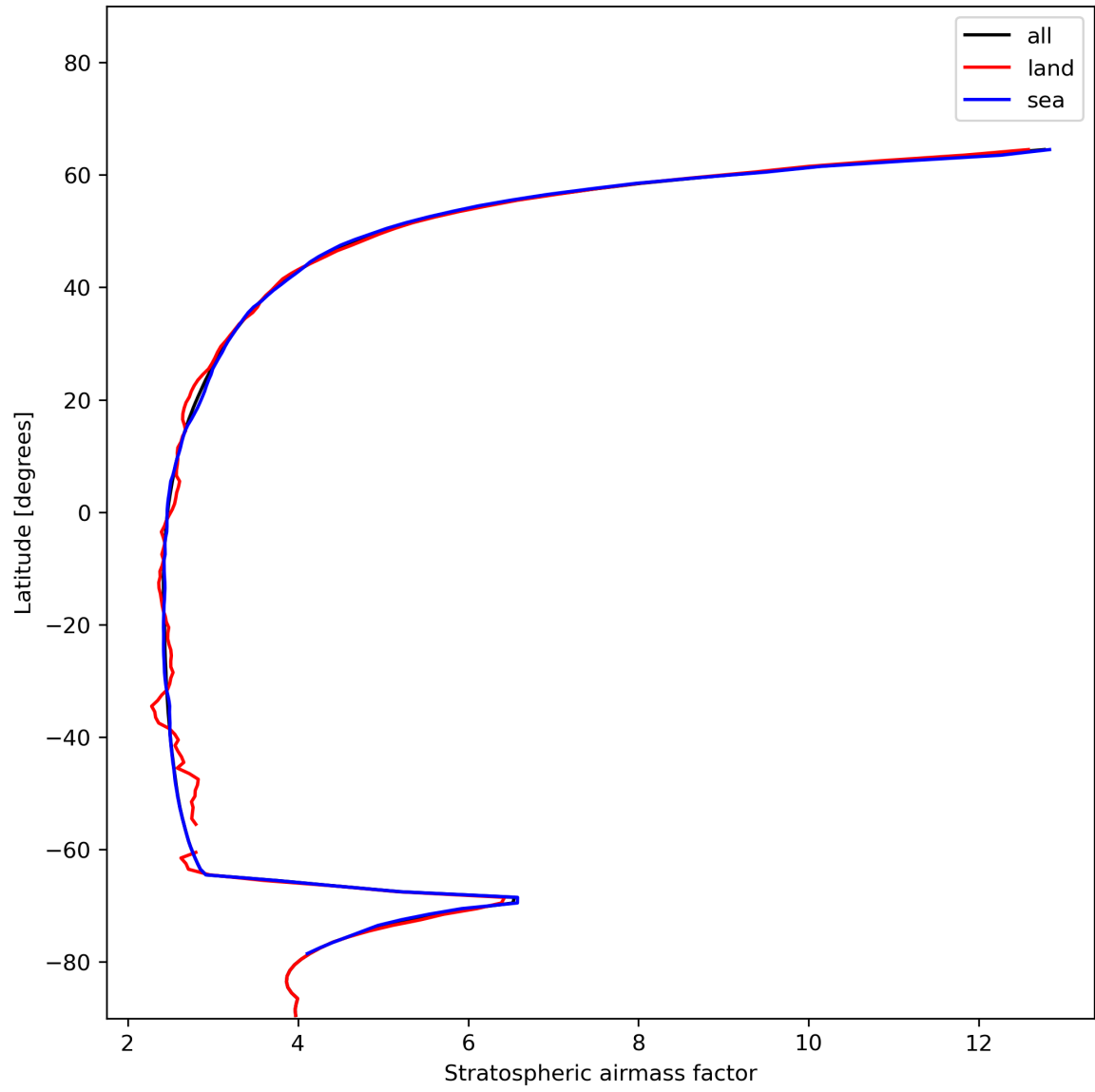
Figure 27: Zonal average of “Stratospheric airmass factor” for 2023-12-17 to 2023-12-19.
