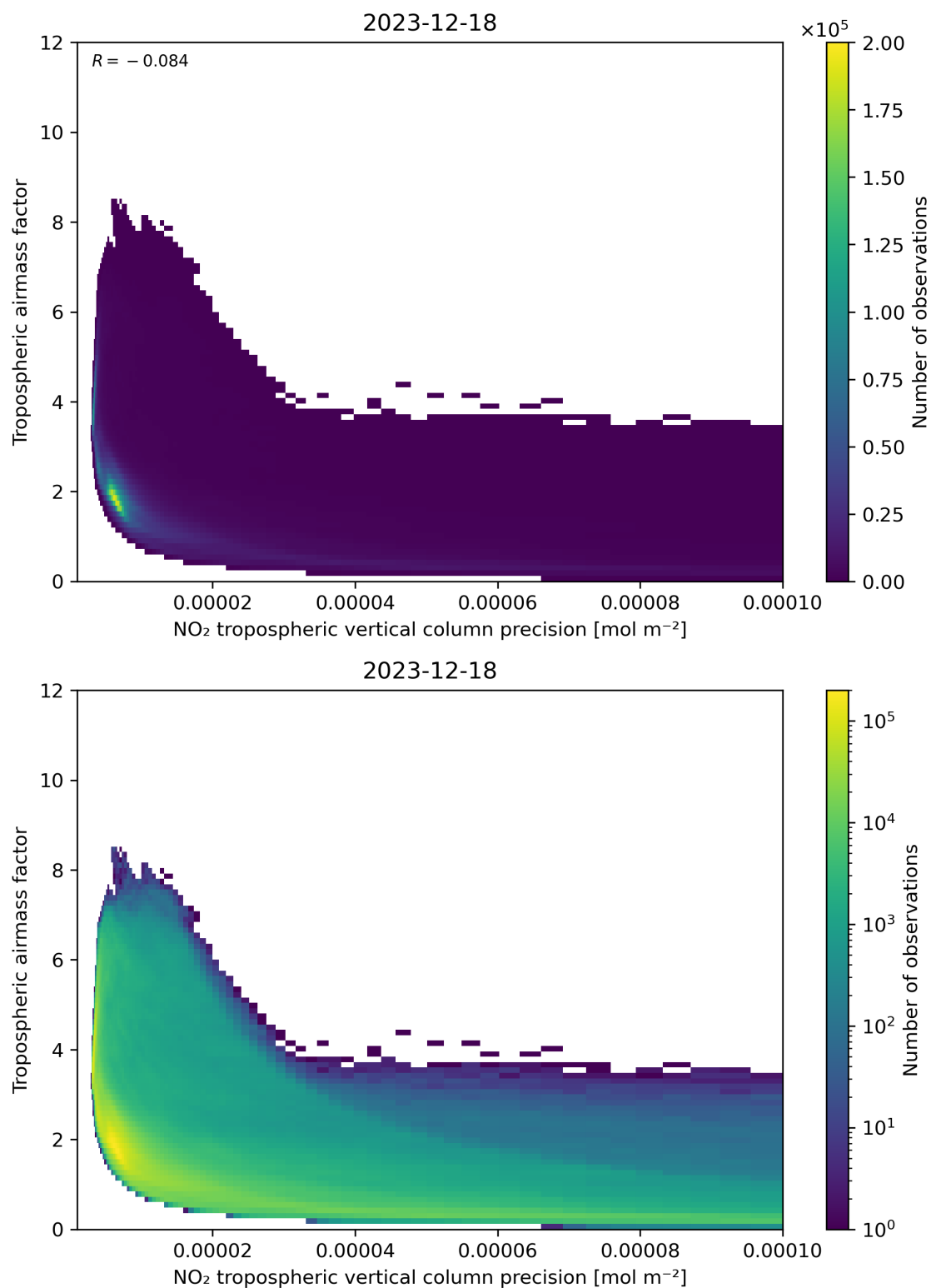
Figure 133: Scatter density plot of “NO 2 tropospheric vertical column precision” against “Tropospheric airmass factor” for 2023-12-17 to 2023-12-19.
