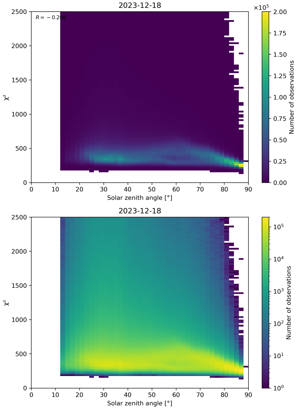
Figure 148: Scatter density plot of “Solar zenith angle” against “ \chi^2 ” for 2023-12-17 to 2023-12-19.
