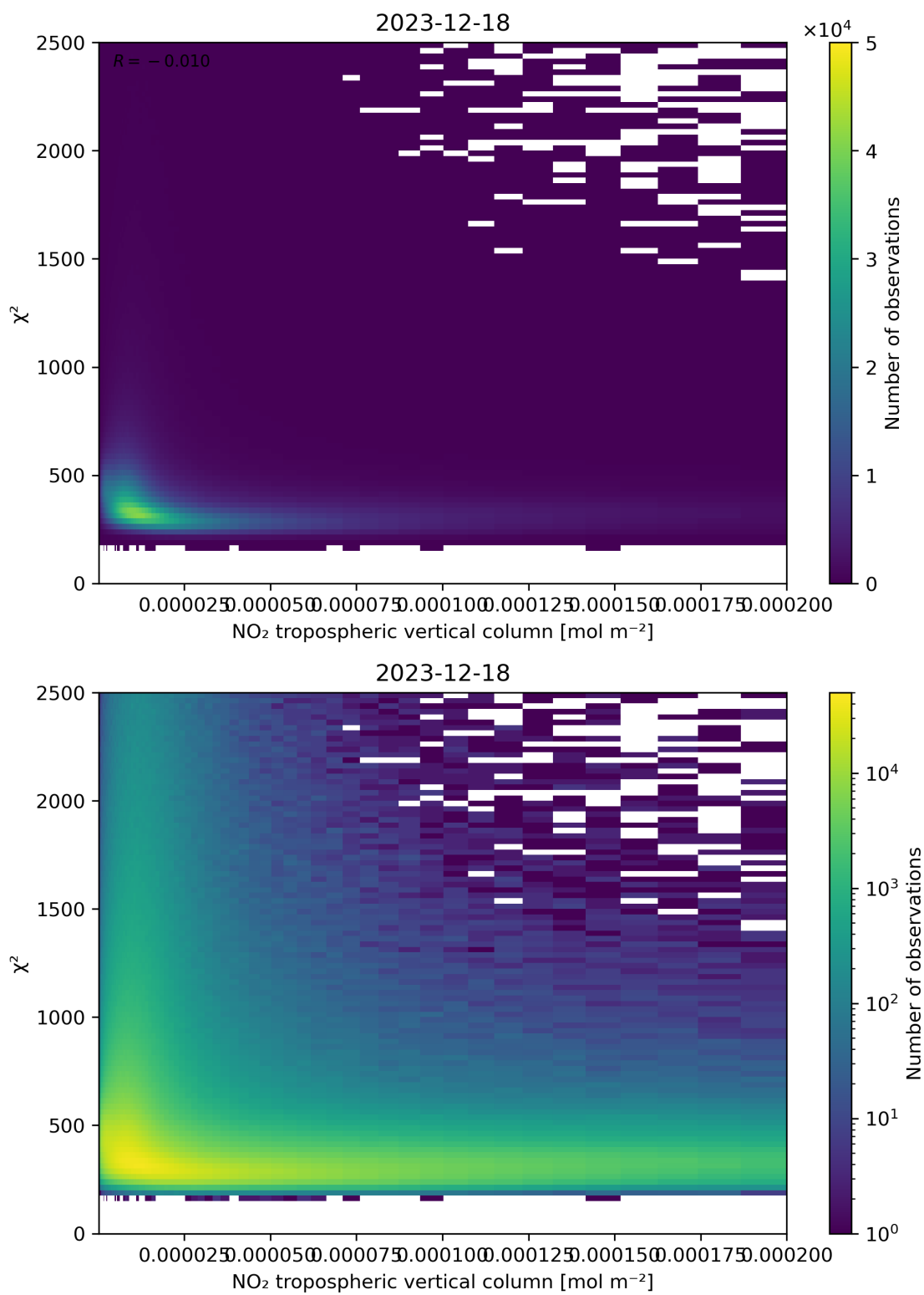
Figure 124: Scatter density plot of “NO 2 tropospheric vertical column” against “ \chi^2 ” for 2023-12-17 to 2023-12-19.
