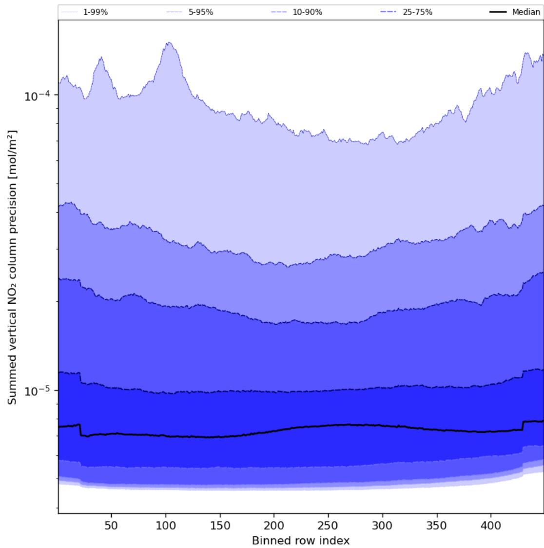
Figure 58: Along track statistics of “Summed vertical NO 2 column precision” for 2023-12-17 to 2023-12-19
