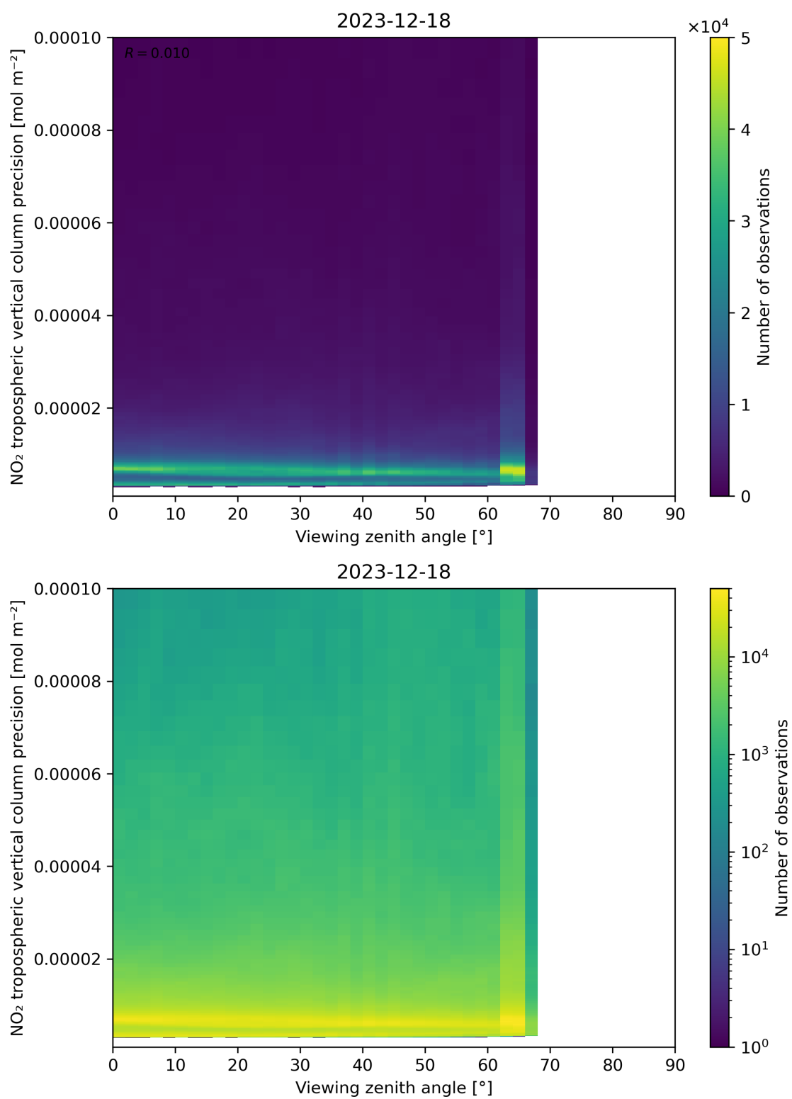
Figure 170: Scatter density plot of “Viewing zenith angle” against “NO 2 tropospheric vertical column precision” for 2023-12-17 to 2023-12-19.
