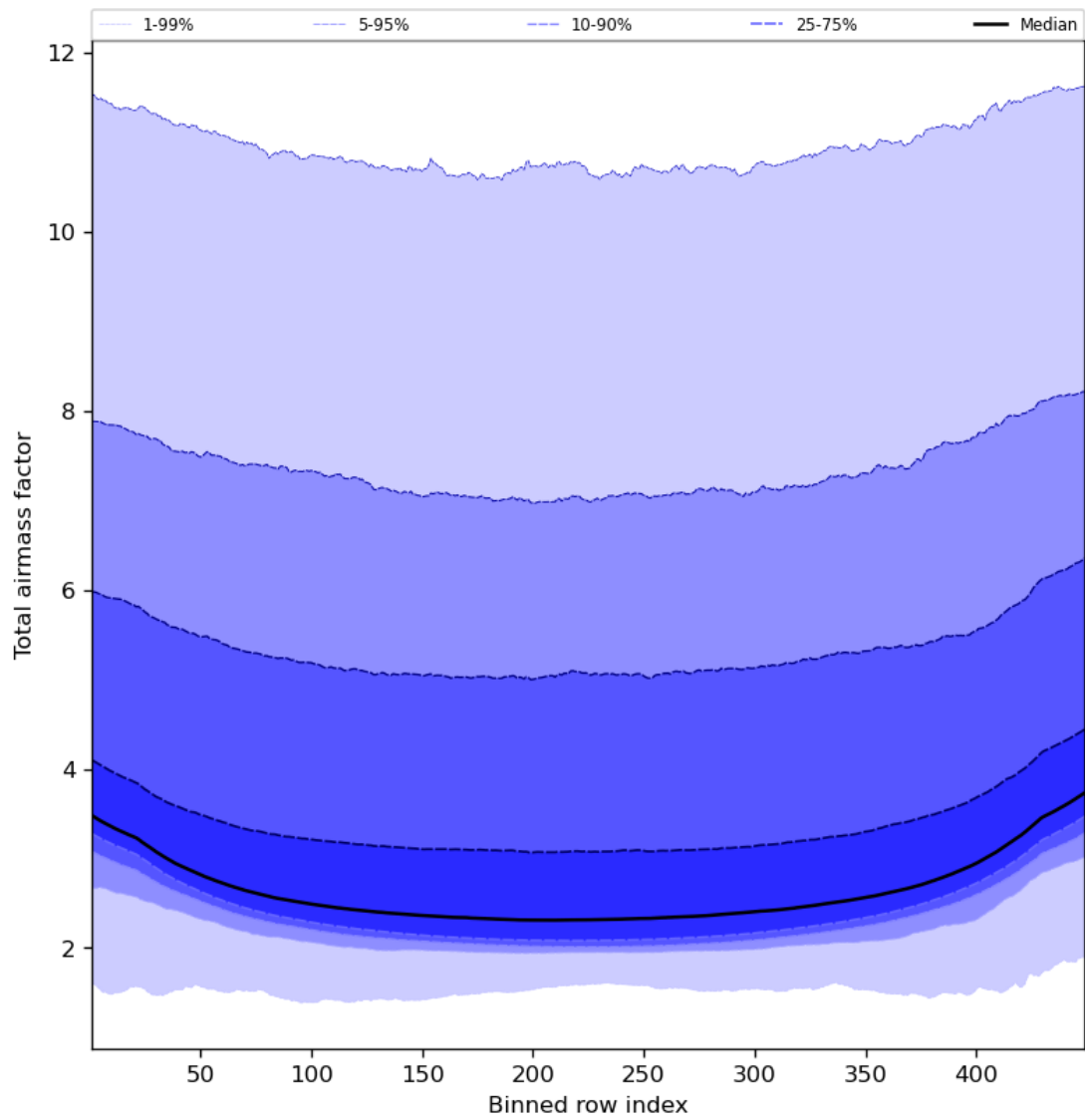
Figure 49: Along track statistics of “Total airmass factor” for 2023-12-17 to 2023-12-19
