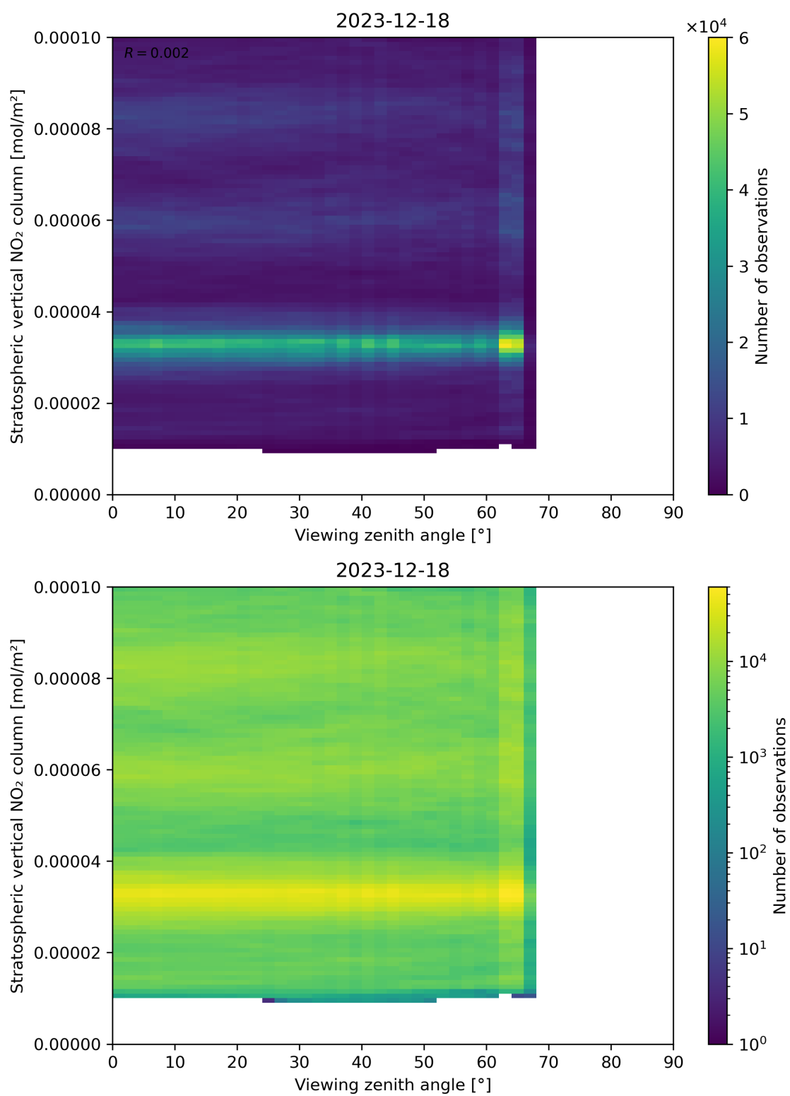
Figure 164: Scatter density plot of “Viewing zenith angle” against “Stratospheric vertical NO 2 column” for 2023-12-17 to 2023-12-19.
