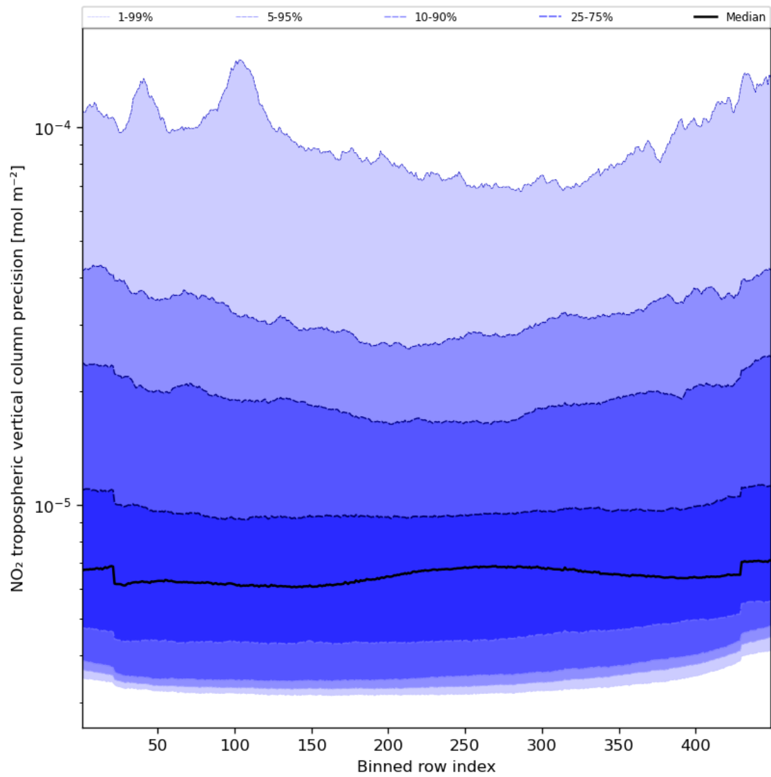
Figure 47: Along track statistics of “NO 2 tropospheric vertical column precision” for 2023-12-17 to 2023-12-19
