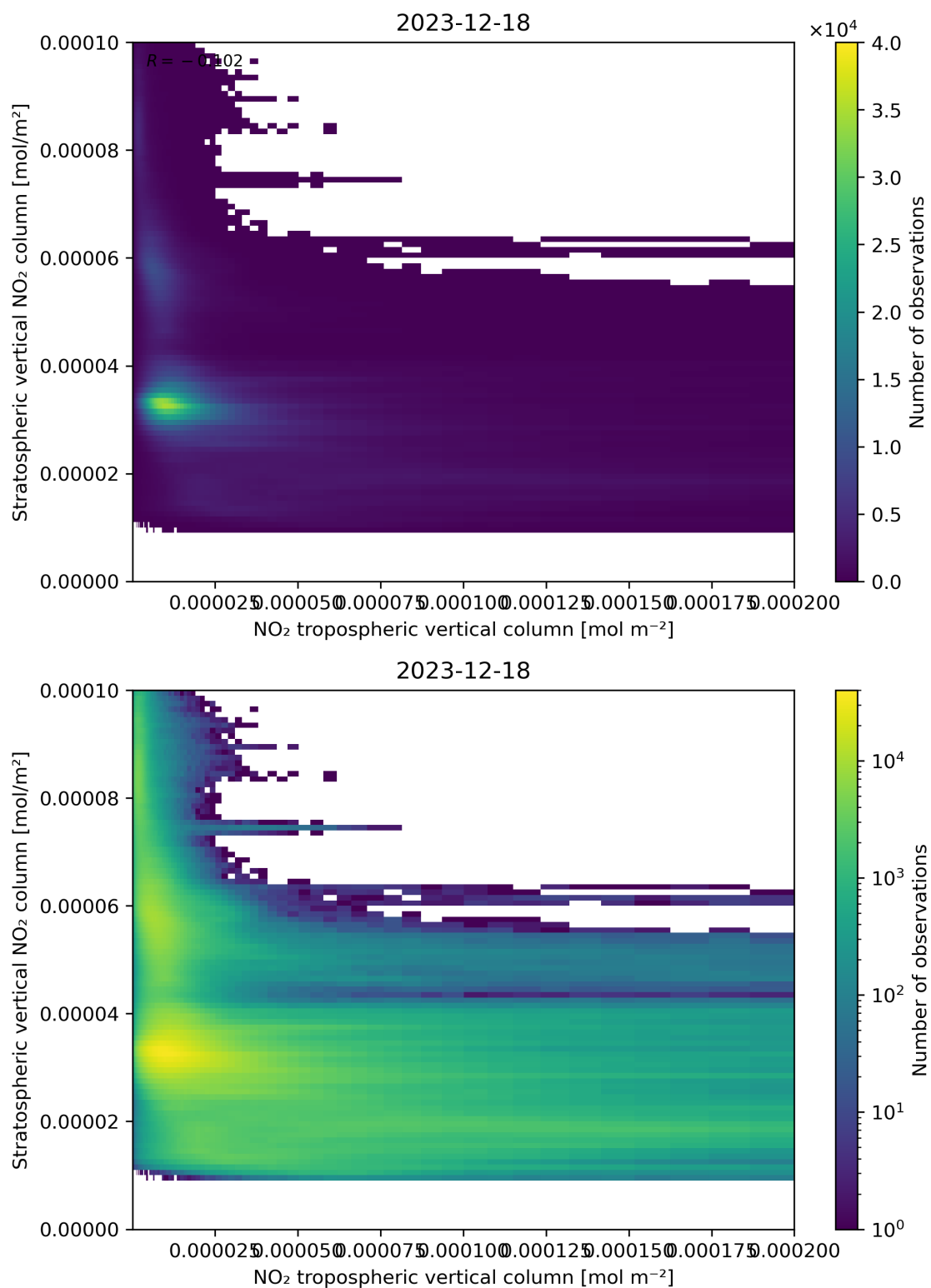
Figure 125: Scatter density plot of “NO 2 tropospheric vertical column” against “Stratospheric vertical NO 2 column” for 2023-12-17 to 2023-12-19.
