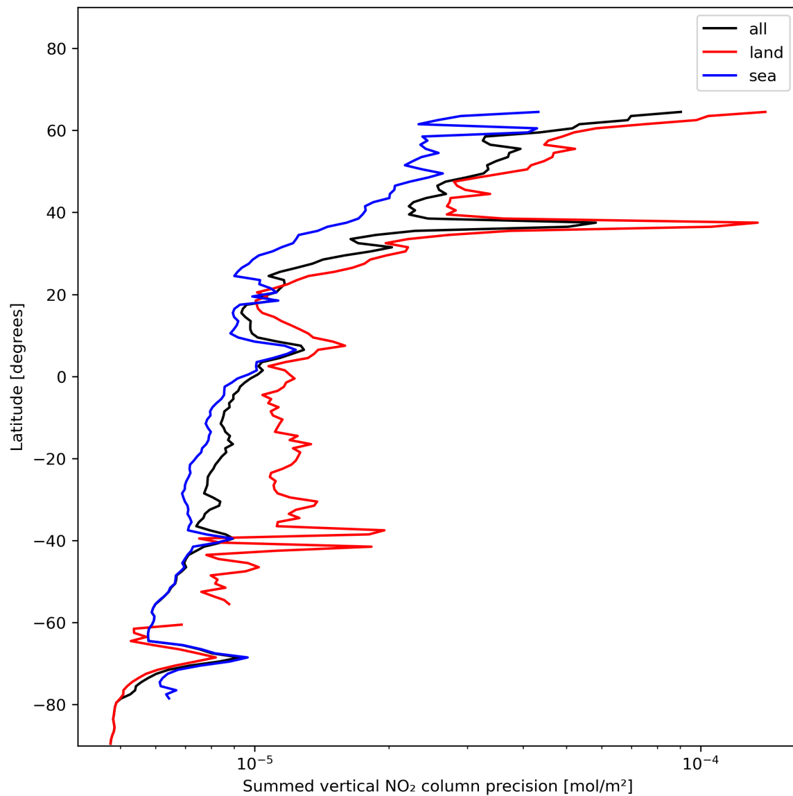
Figure 24: Zonal average of “Summed vertical NO 2 column precision” for 2023-12-17 to 2023-12-19.
