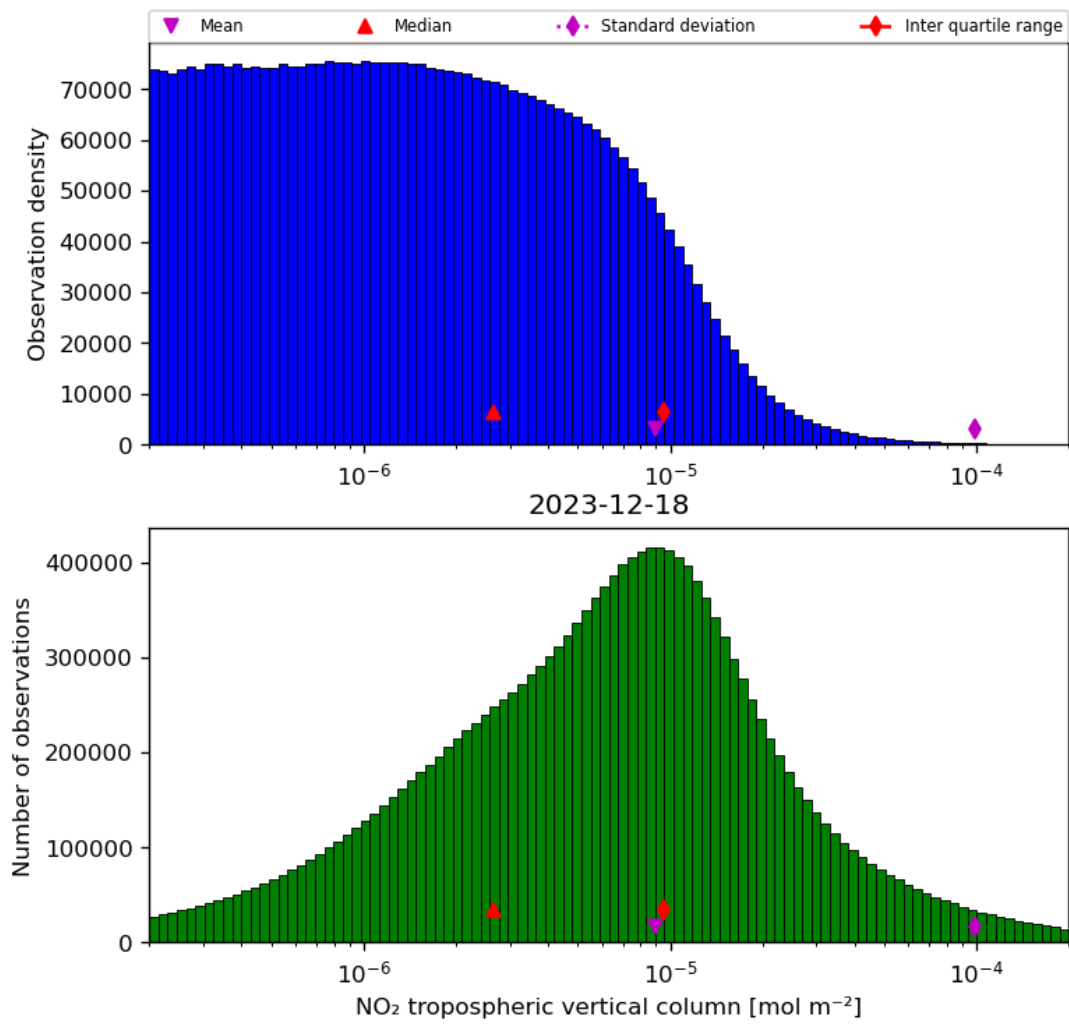
Figure 29: Histogram of “NO 2 tropospheric vertical column” for 2023-12-17 to 2023-12-19
