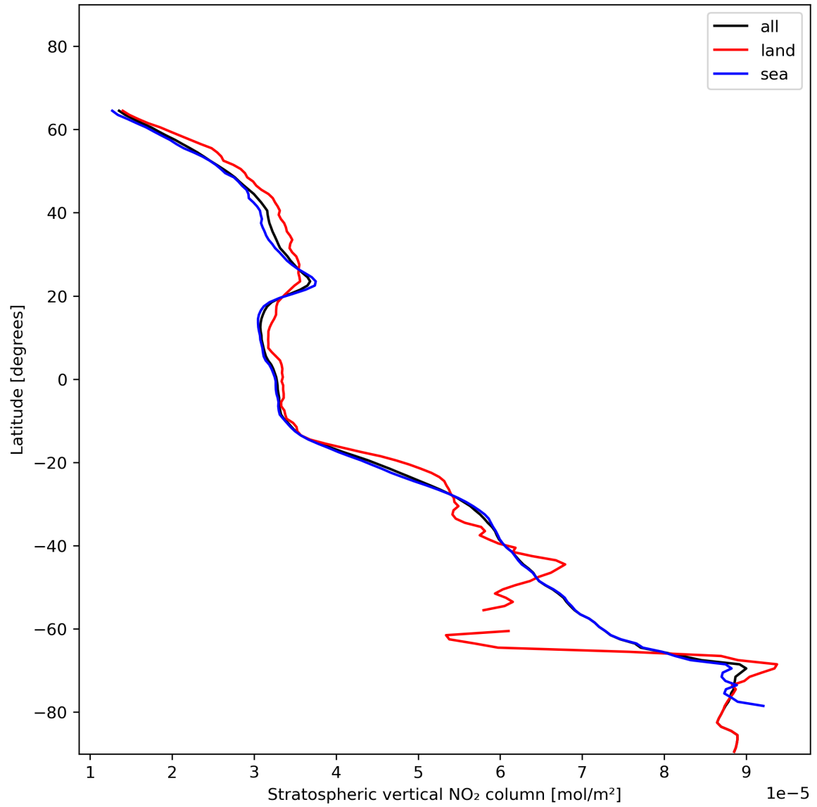
Figure 19: Zonal average of “Stratospheric vertical NO 2 column” for 2023-12-17 to 2023-12-19.
