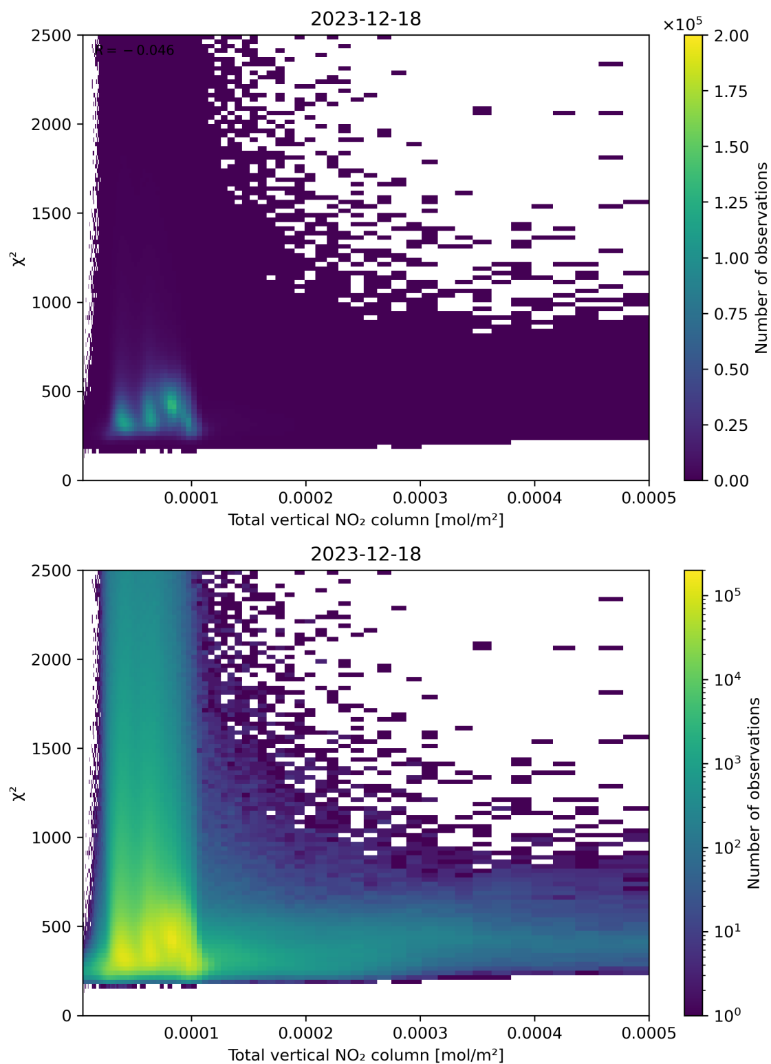
Figure 111: Scatter density plot of “Total vertical NO 2 column” against “ \chi^2 ” for 2023-12-17 to 2023-12-19.
