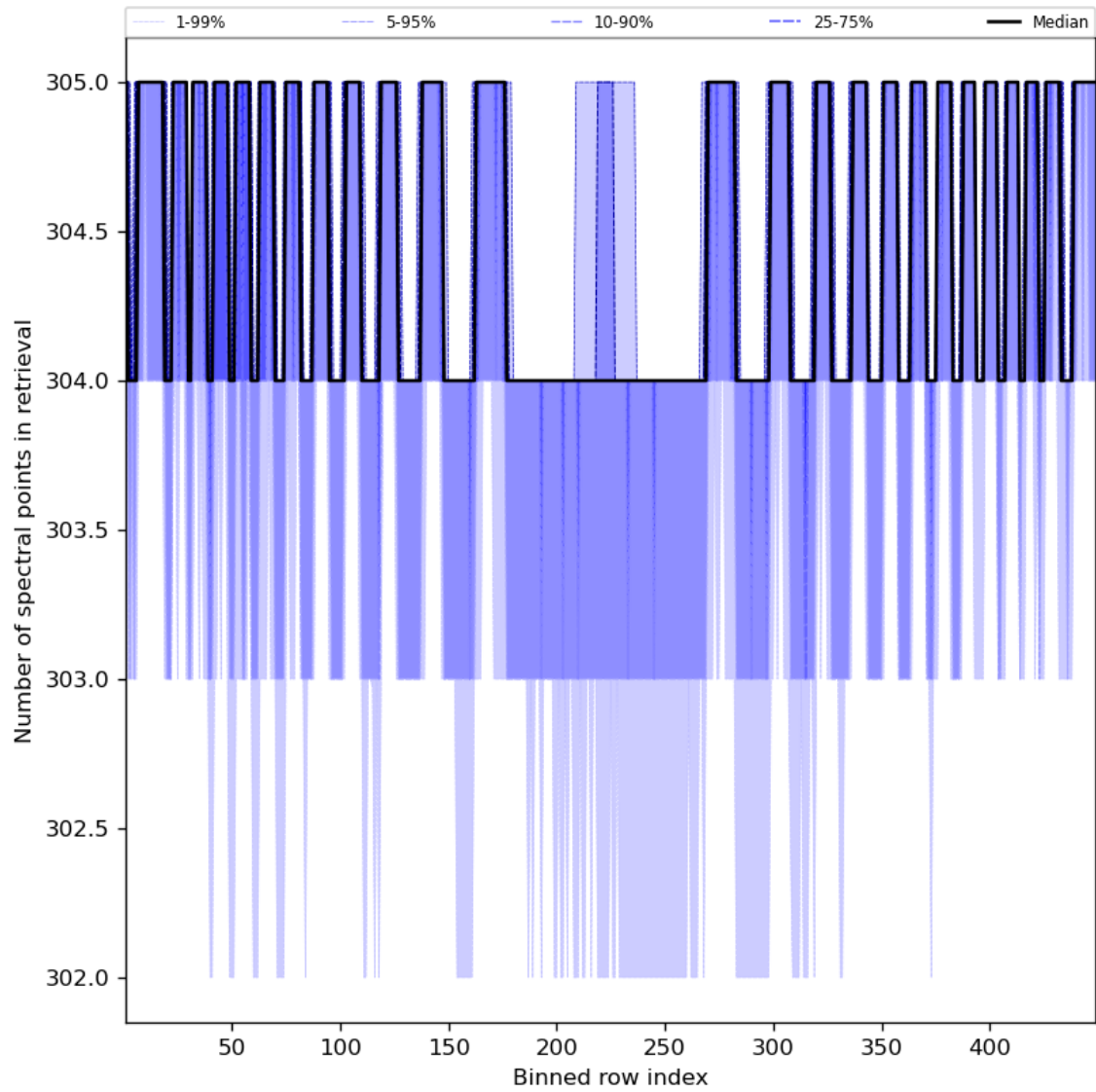
Figure 50: Along track statistics of “Number of spectral points in retrieval” for 2023-12-17 to 2023-12-19
