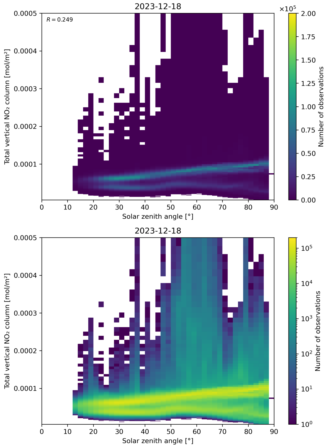
Figure 153: Scatter density plot of “Solar zenith angle” against “Total vertical NO 2 column” for 2023-12-17 to 2023-12-19.
