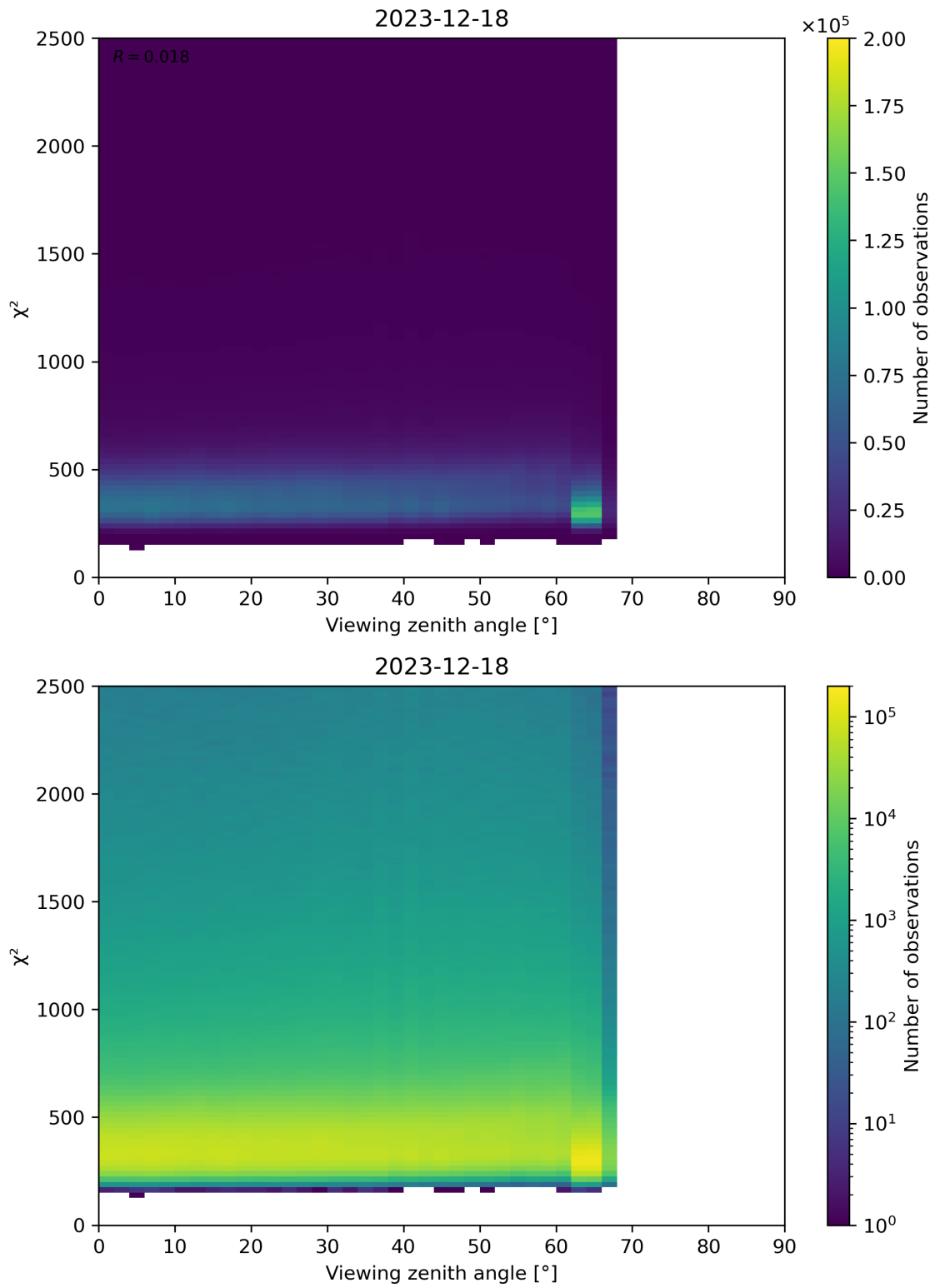
Figure 162: Scatter density plot of “Viewing zenith angle” against “ \chi^2 ” for 2023-12-17 to 2023-12-19.
