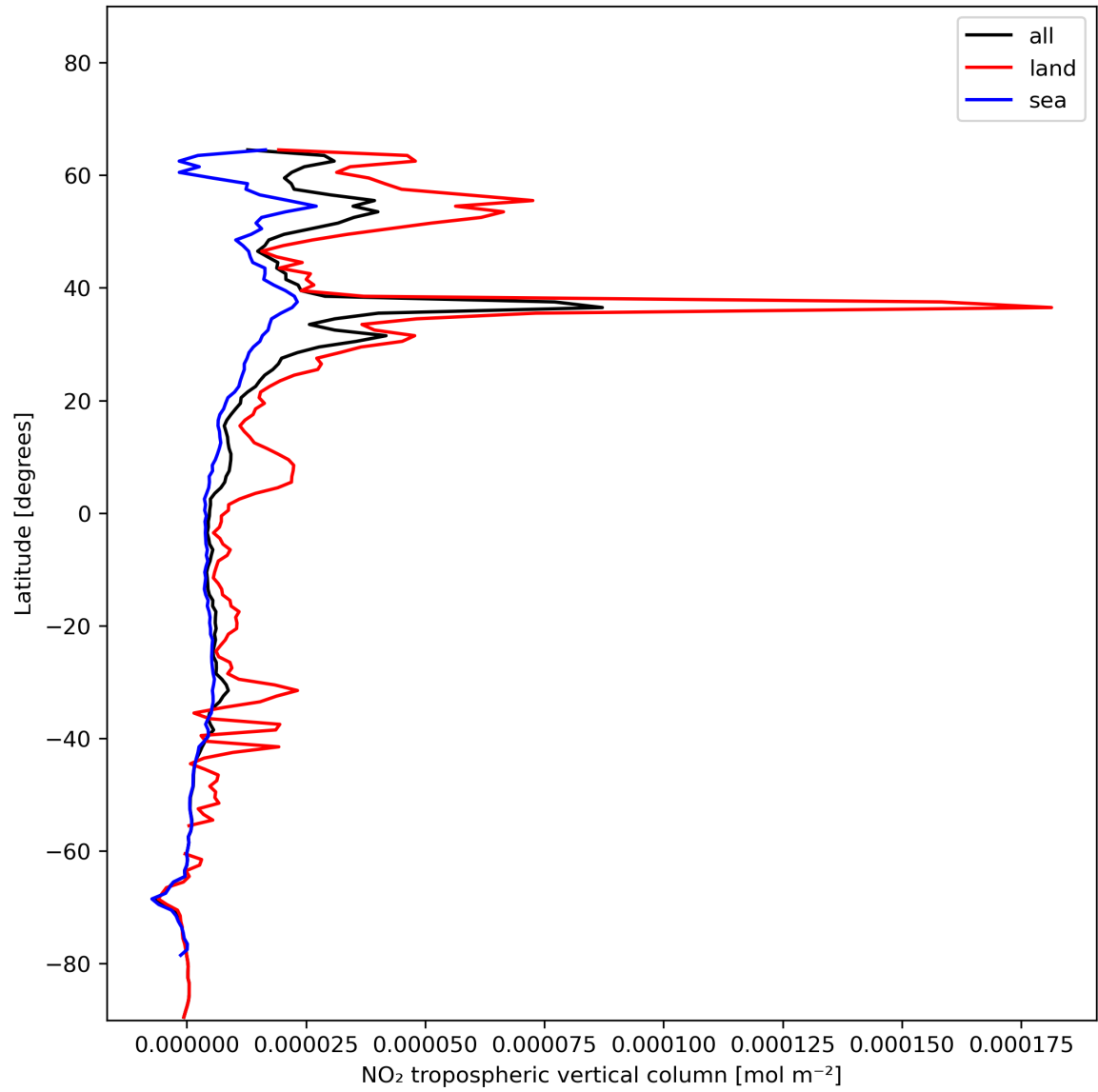
Figure 12: Zonal average of “NO 2 tropospheric vertical column” for 2023-12-17 to 2023-12-19.
