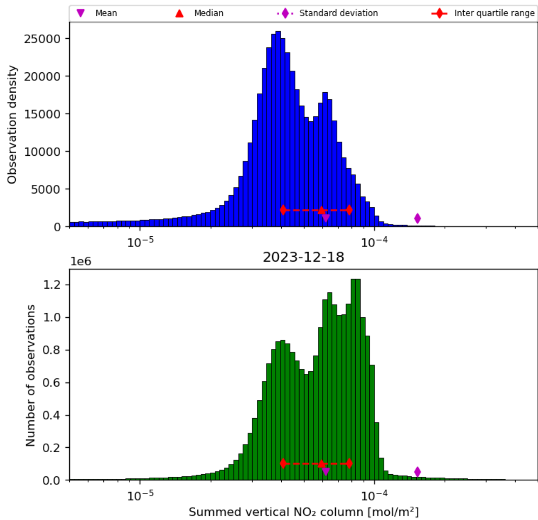
Figure 40: Histogram of “Summed vertical NO 2 column” for 2023-12-17 to 2023-12-19
