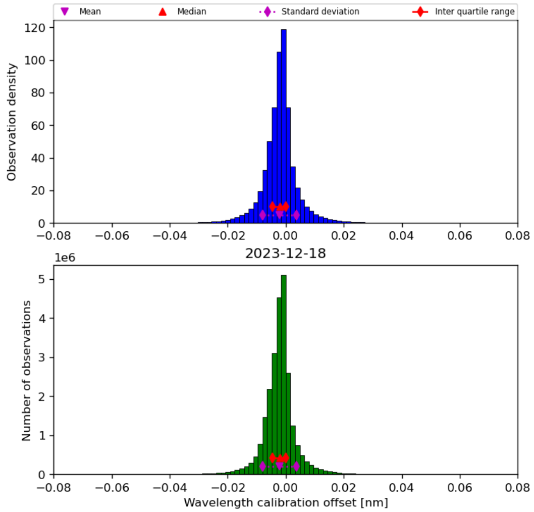
Figure 35: Histogram of “Wavelength calibration offset” for 2023-12-17 to 2023-12-19
