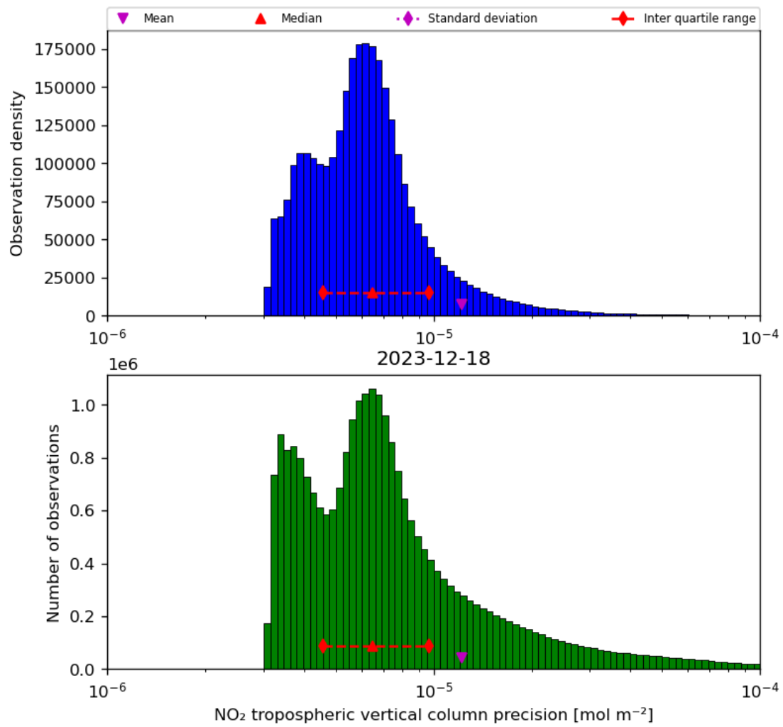
Figure 30: Histogram of “NO 2 tropospheric vertical column precision” for 2023-12-17 to 2023-12-19
