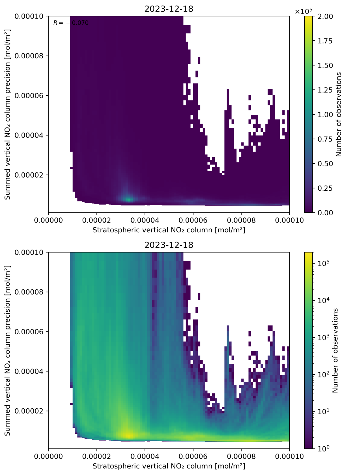
Figure 99: Scatter density plot of “Stratospheric vertical NO 2 column” against “Summed vertical NO 2 column precision” for 2023-12-17 to 2023-12-19.
