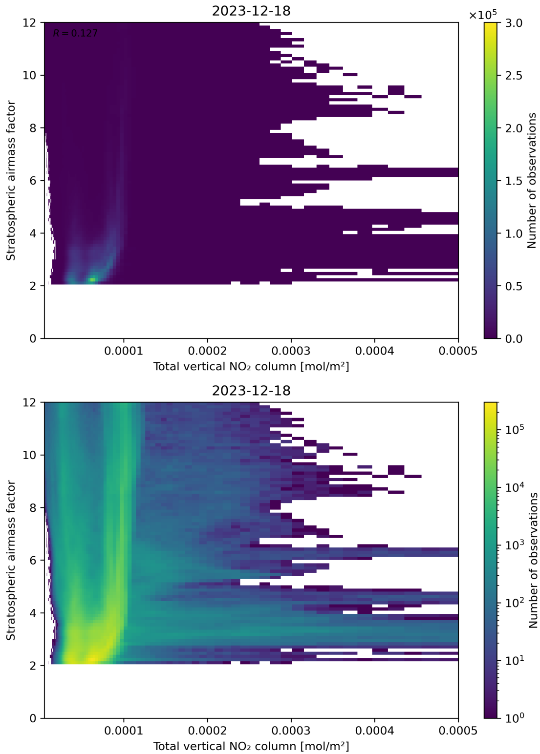
Figure 110: Scatter density plot of “Total vertical NO 2 column” against “Stratospheric airmass factor” for 2023-12-17 to 2023-12-19.
