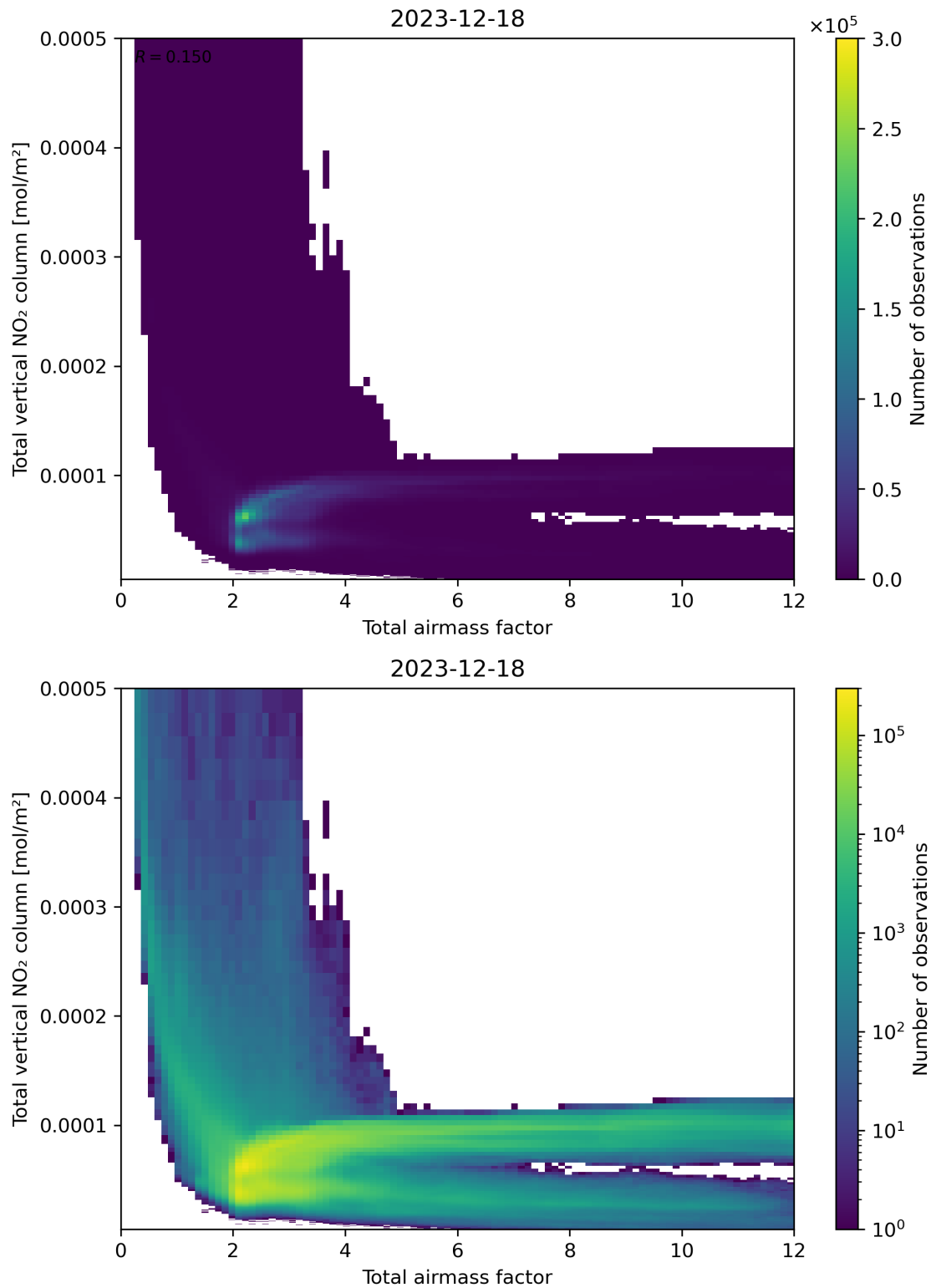
Figure 67: Scatter density plot of “Total airmass factor” against “Total vertical \text{NO}_2 column” for 2023-12-17 to 2023-12-19.
