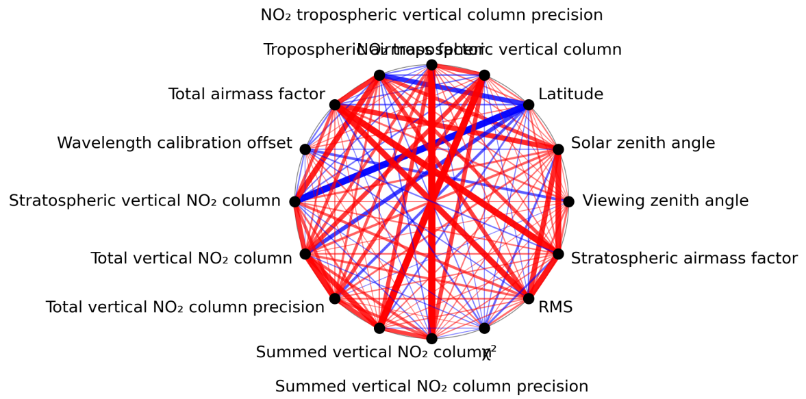
Figure 1: Map of correlation graph for 2023-12-17 to 2023-12-19.
