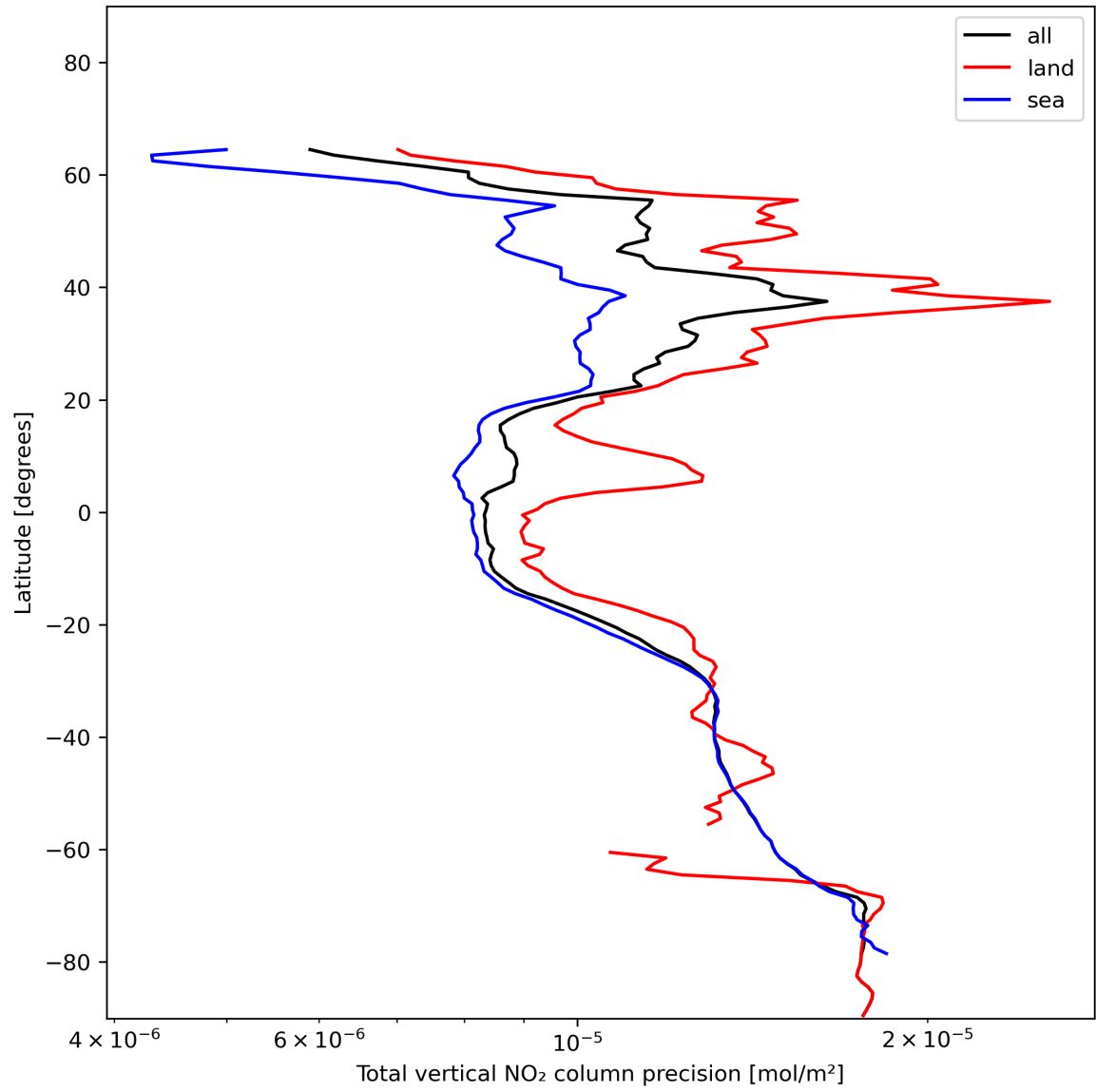
Figure 22: Zonal average of “Total vertical NO 2 column precision” for 2023-12-17 to 2023-12-19.
