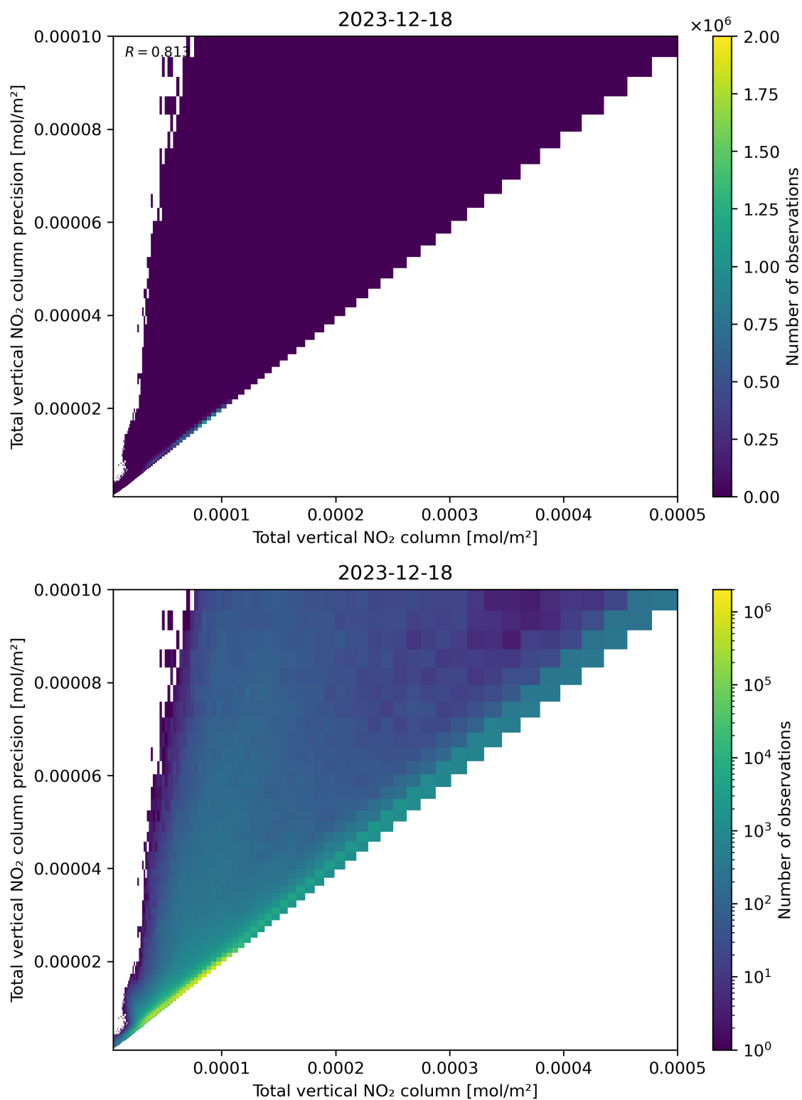
Figure 114: Scatter density plot of “Total vertical NO 2 column” against “Total vertical NO 2 column precision” for 2023-12-17 to 2023-12-19.
