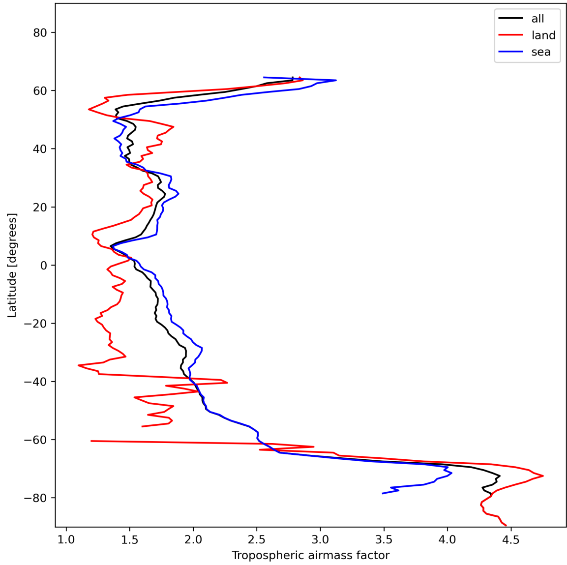
Figure 14: Zonal average of “Tropospheric airmass factor” for 2023-12-17 to 2023-12-19.
