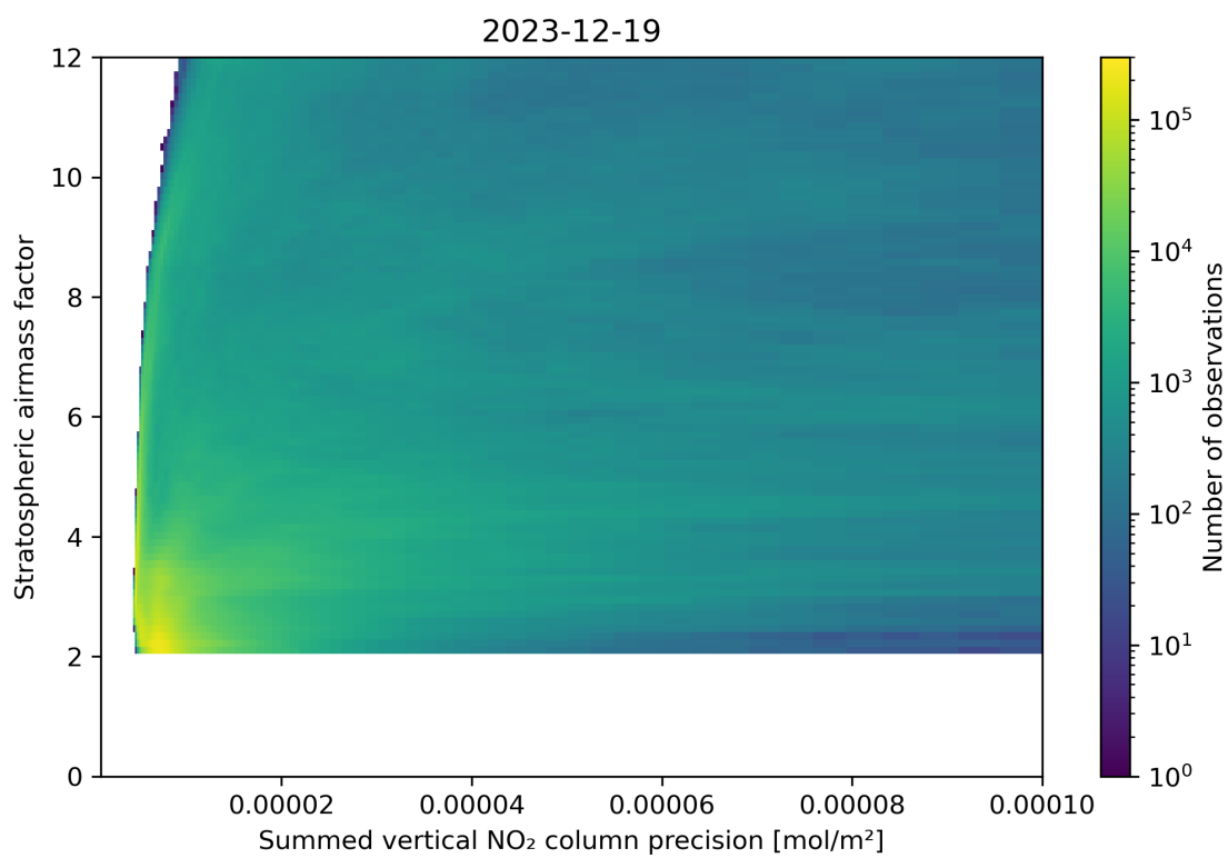
Figure 106: Scatter density plot of “Summed vertical NO 2 column precision” against “Stratospheric airmass factor” for 2023-12-18 to 2023-12-20.
