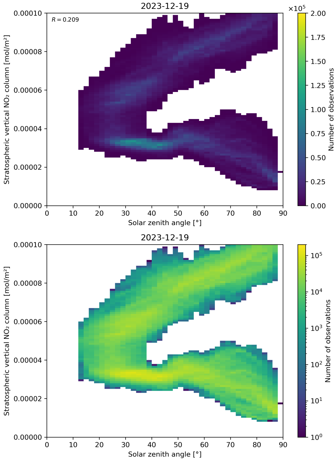
Figure 150: Scatter density plot of “Solar zenith angle” against “Stratospheric vertical NO 2 column” for 2023-12-18 to 2023-12-20.
