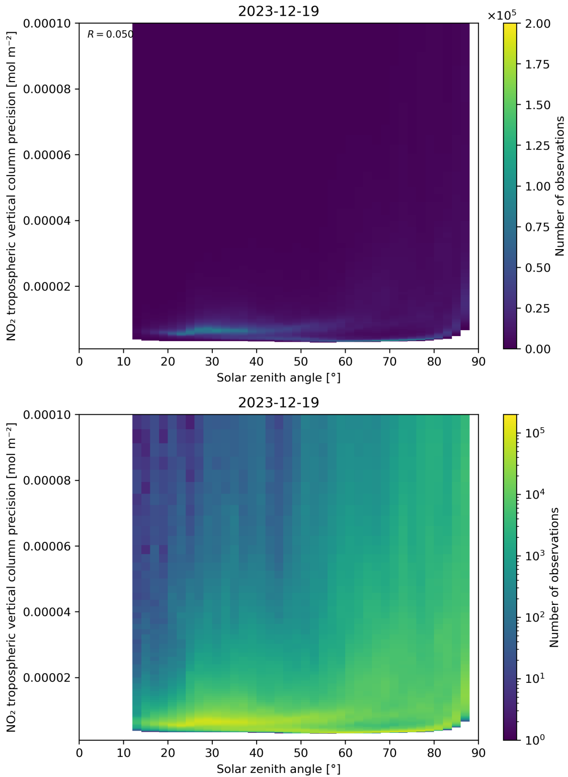
Figure 156: Scatter density plot of “Solar zenith angle” against “NO 2 tropospheric vertical column precision” for 2023-12-18 to 2023-12-20.
