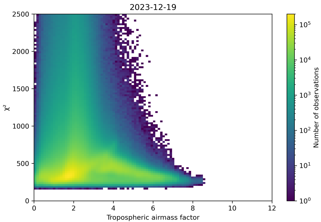
Figure 73: Scatter density plot of “Tropospheric airmass factor” against “ \chi^2 ” for 2023-12-18 to 2023-12-20.
