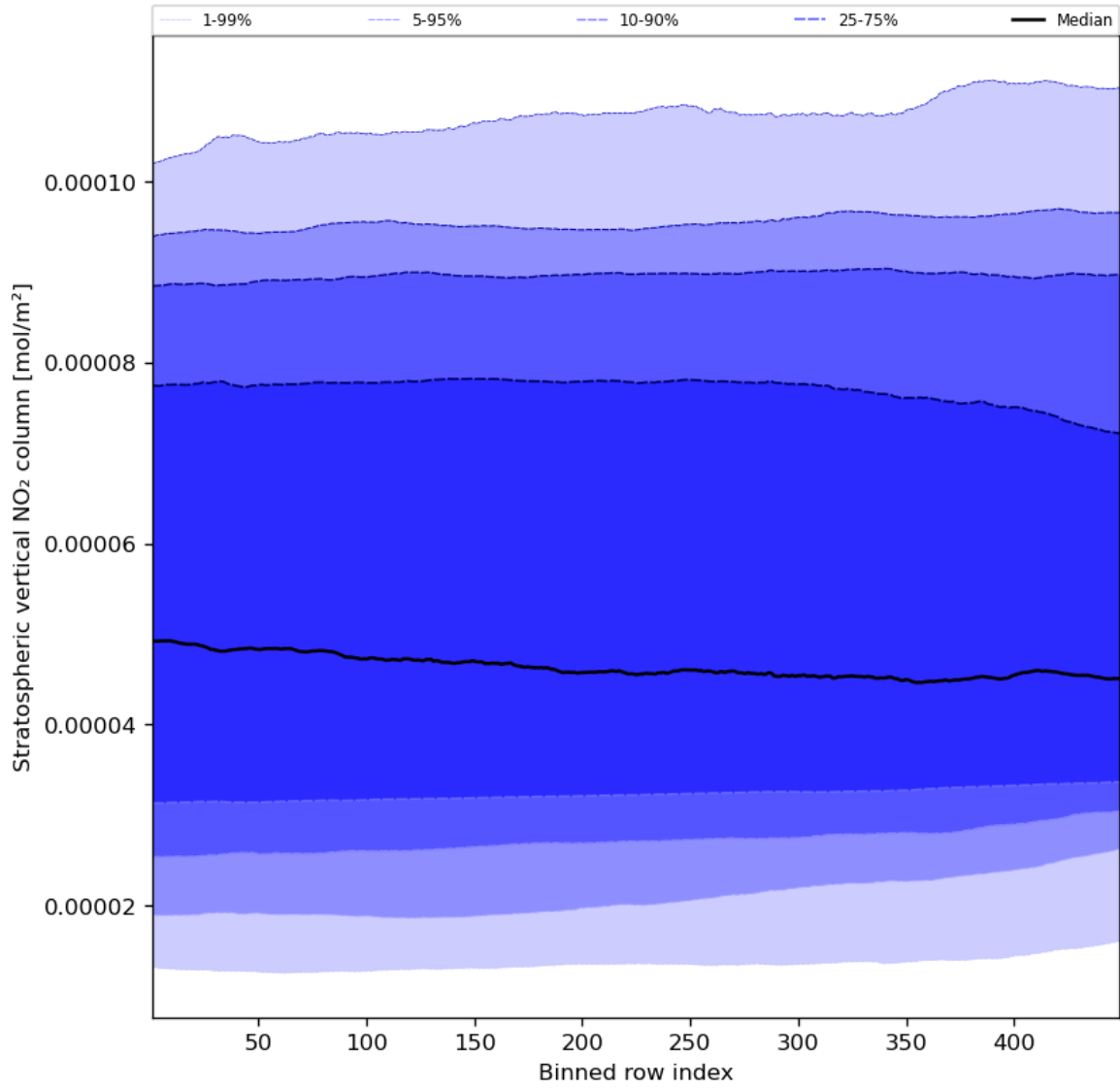
Figure 53: Along track statistics of “Stratospheric vertical NO 2 column” for 2023-12-18 to 2023-12-20
