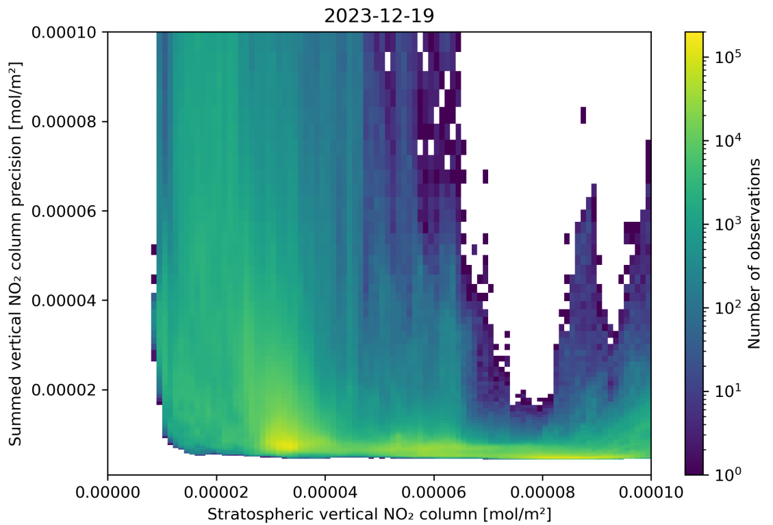
Figure 99: Scatter density plot of “Stratospheric vertical NO 2 column” against “Summed vertical NO 2 column precision” for 2023-12-18 to 2023-12-20.
