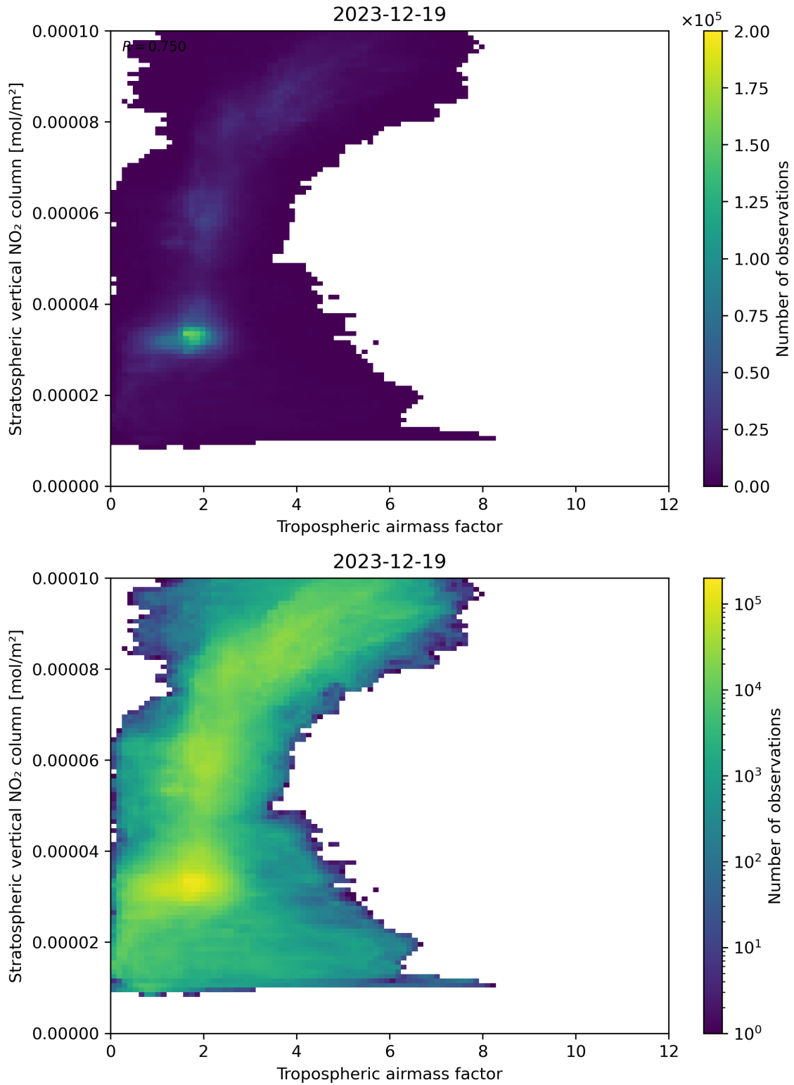
Figure 74: Scatter density plot of “Tropospheric airmass factor” against “Stratospheric vertical NO 2 column” for 2023-12-18 to 2023-12-20.
