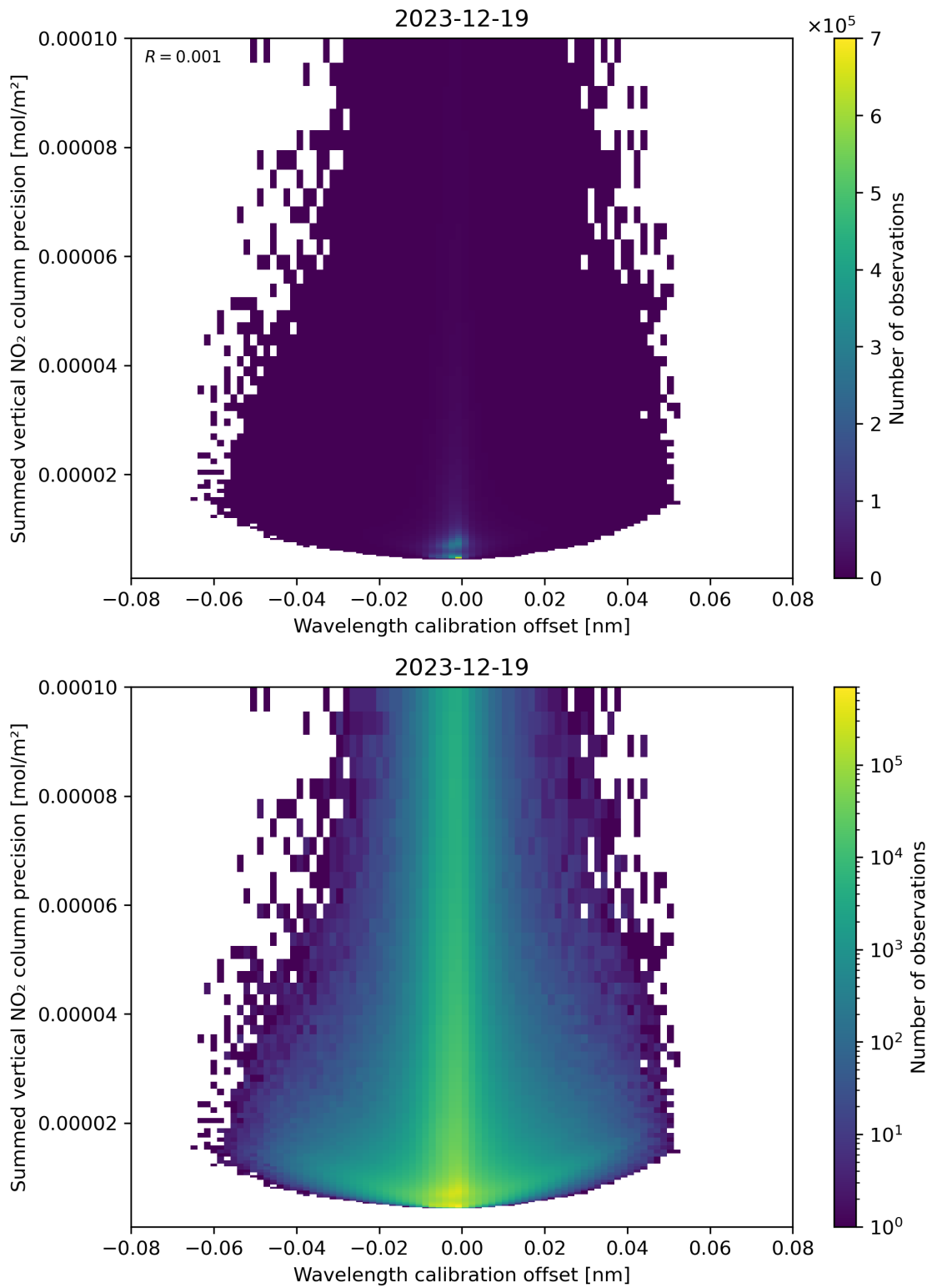
Figure 178: Scatter density plot of “Wavelength calibration offset” against “Summed vertical NO 2 column precision” for 2023-12-18 to 2023-12-20.
