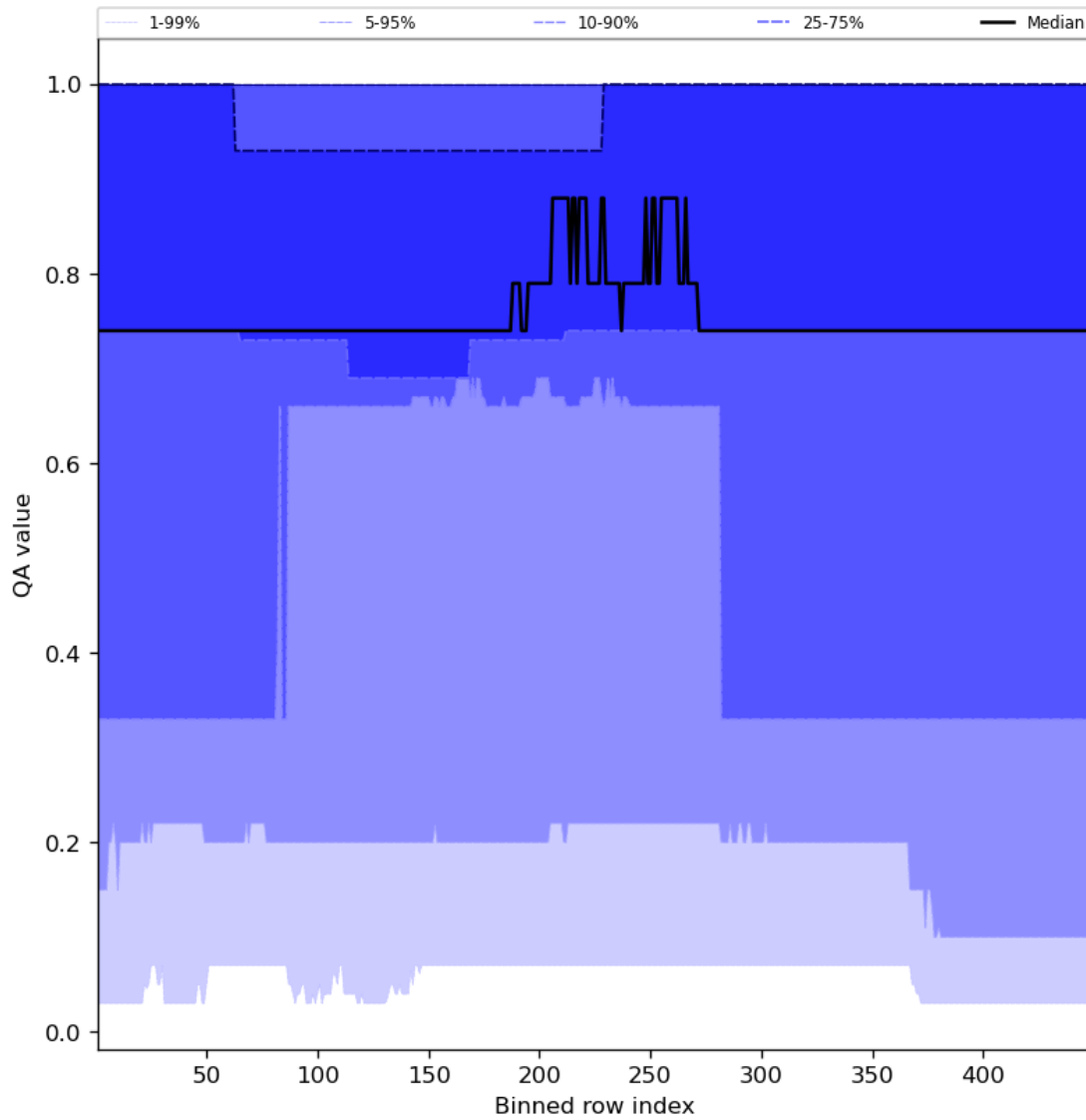
Figure 45: Along track statistics of “QA value” for 2023-12-18 to 2023-12-20
