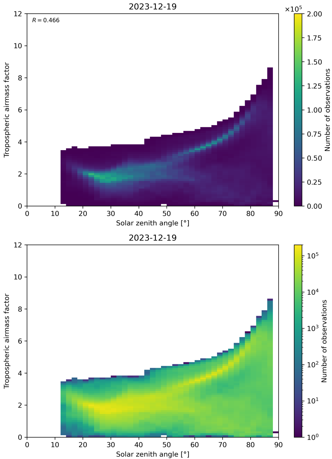
Figure 147: Scatter density plot of “Solar zenith angle” against “Tropospheric airmass factor” for 2023-12-18 to 2023-12-20.
