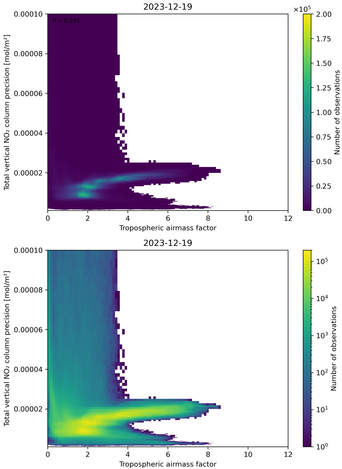
Figure 78: Scatter density plot of “Tropospheric airmass factor” against “Total vertical NO 2 column precision” for 2023-12-18 to 2023-12-20.
