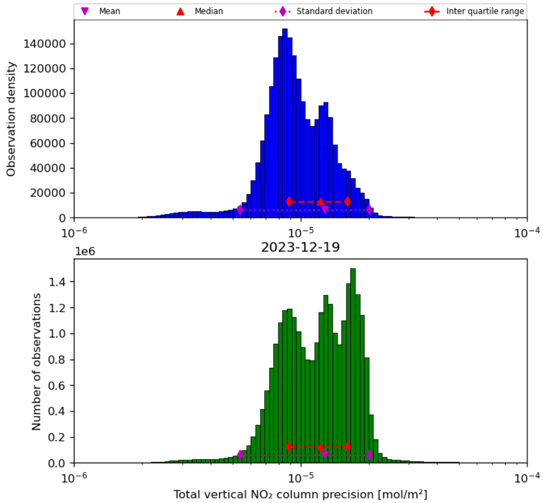
Figure 39: Histogram of “Total vertical NO 2 column precision” for 2023-12-18 to 2023-12-20
