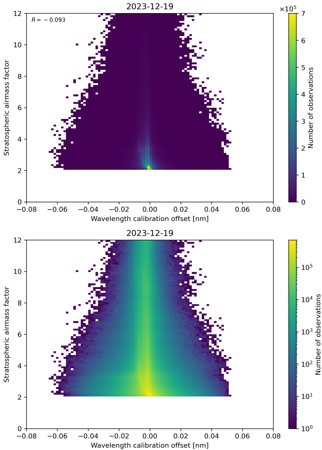
Figure 174: Scatter density plot of “Wavelength calibration offset” against “Stratospheric airmass factor” for 2023-12-18 to 2023-12-20.
