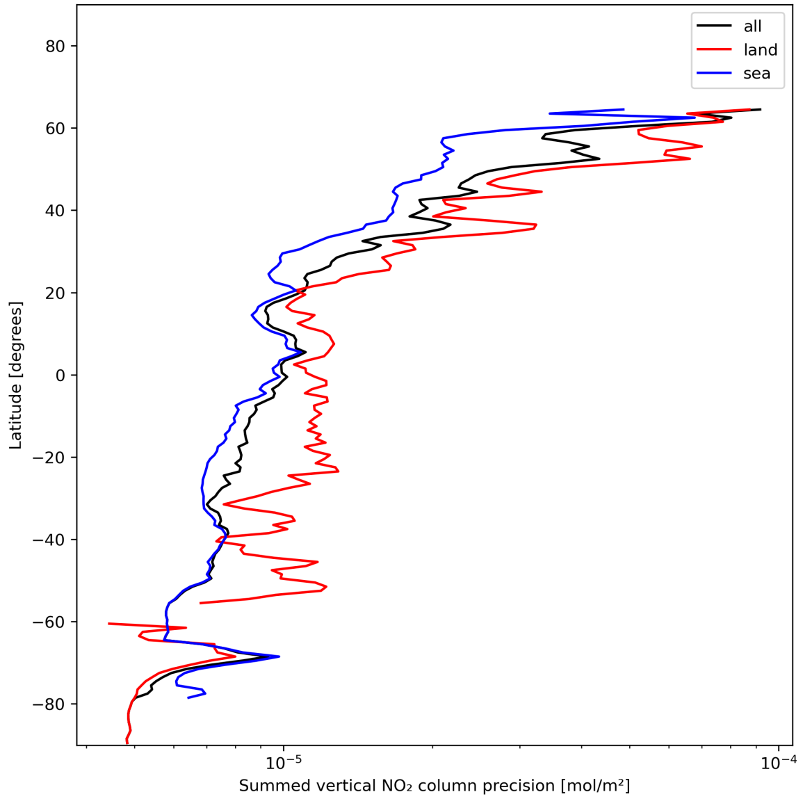
Figure 24: Zonal average of “Summed vertical NO 2 column precision” for 2023-12-18 to 2023-12-20.
