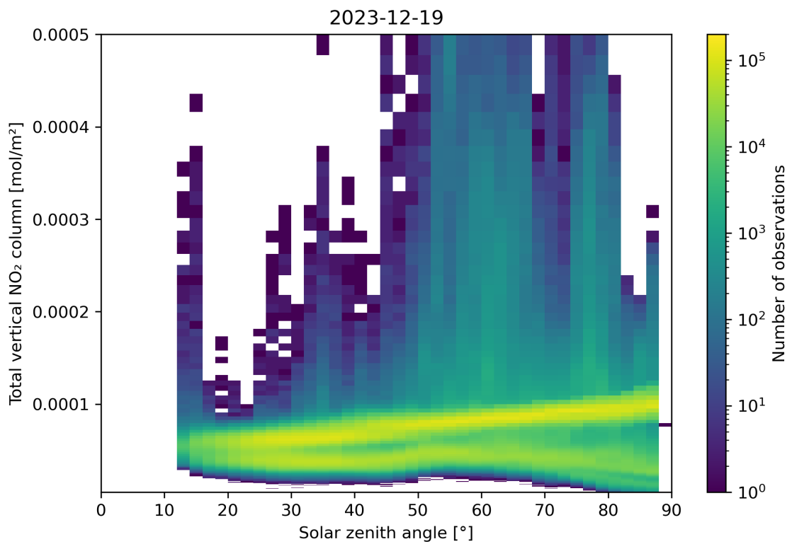
Figure 153: Scatter density plot of “Solar zenith angle” against “Total vertical NO 2 column” for 2023-12-18 to 2023-12-20.
