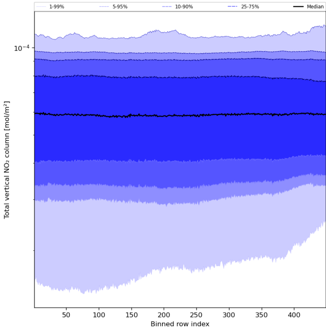
Figure 55: Along track statistics of “Total vertical NO 2 column” for 2023-12-18 to 2023-12-20
