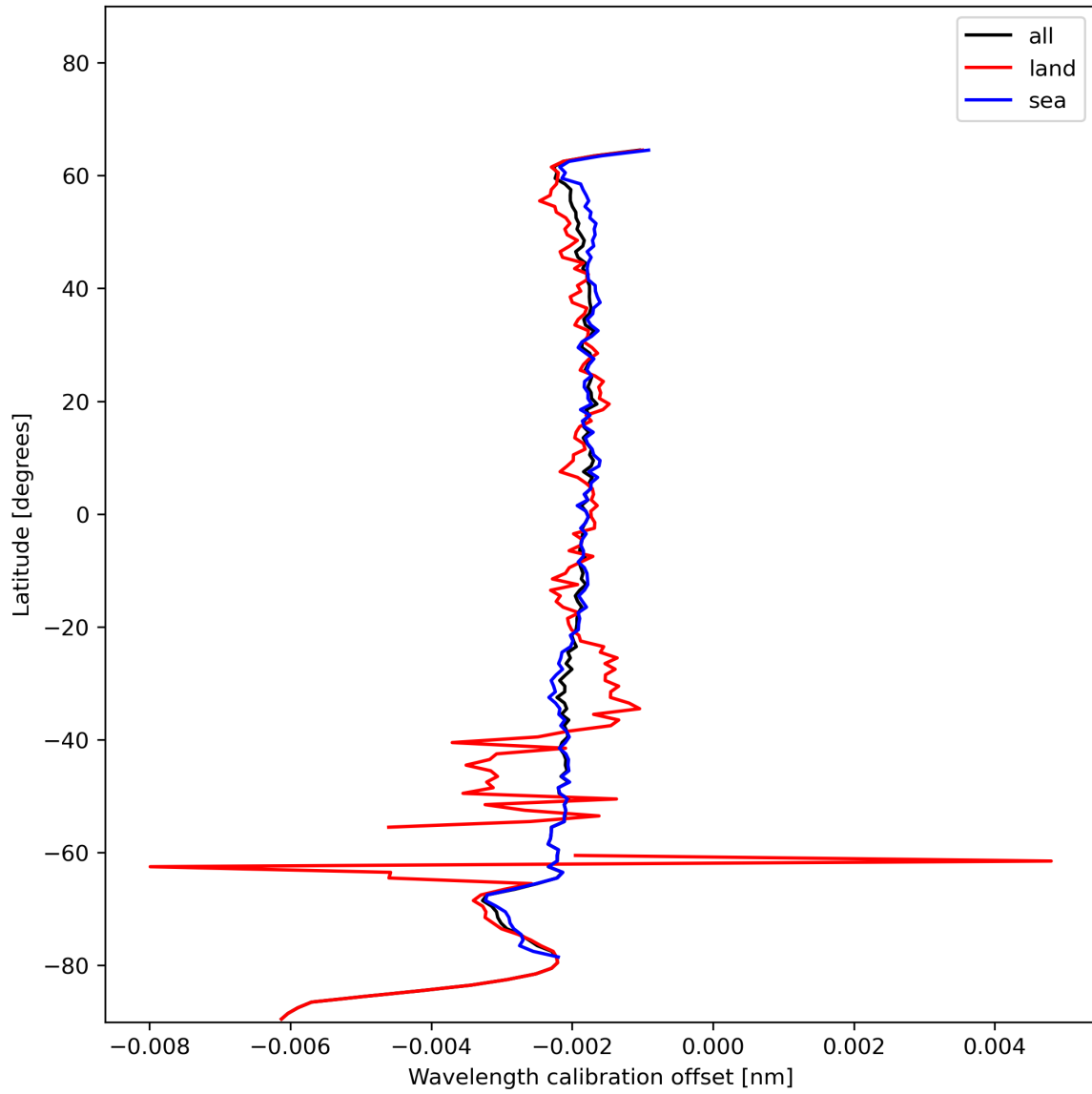
Figure 18: Zonal average of “Wavelength calibration offset” for 2023-12-18 to 2023-12-20.
