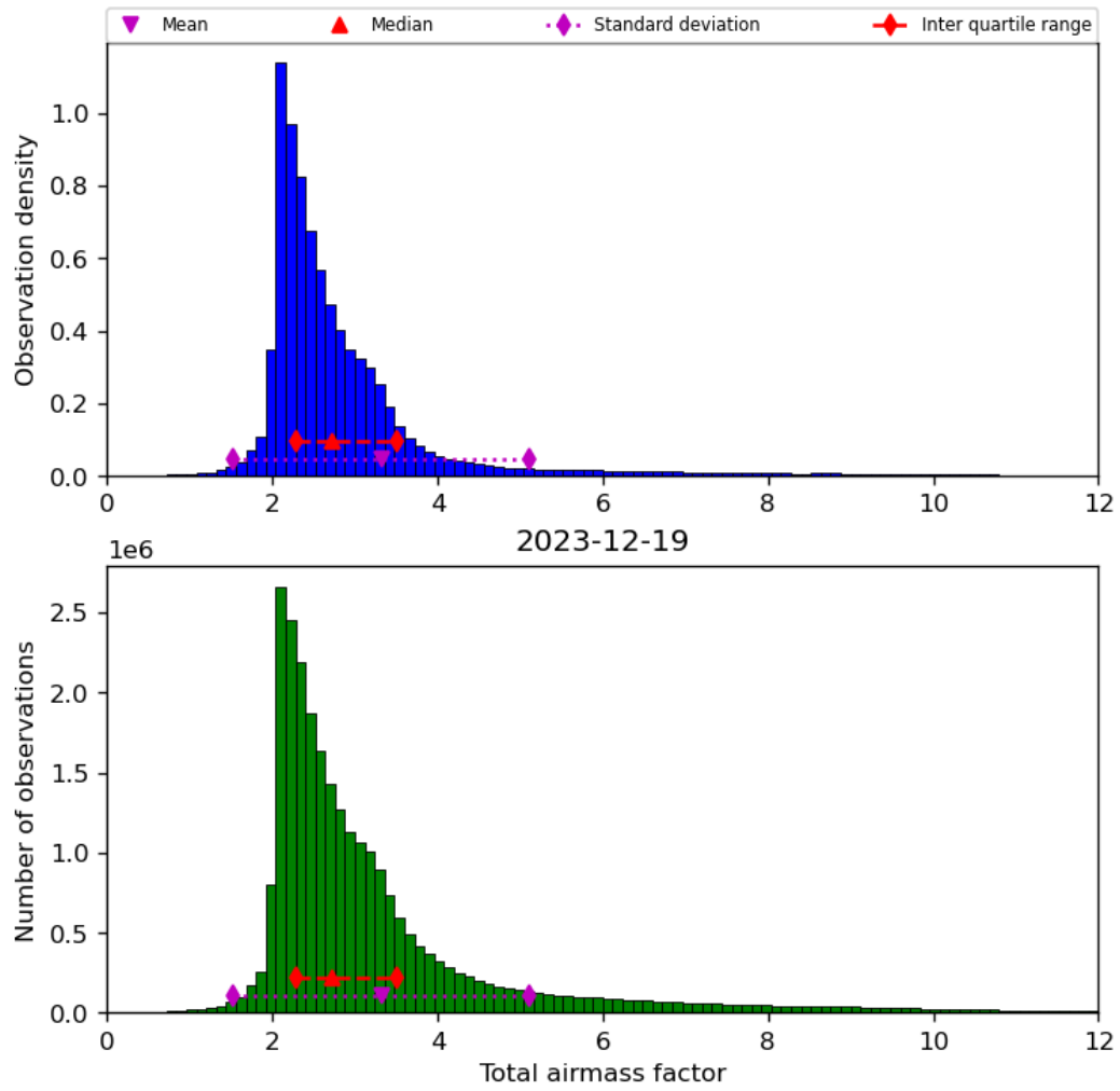
Figure 32: Histogram of “Total air mass factor” for 2023-12-18 to 2023-12-20
