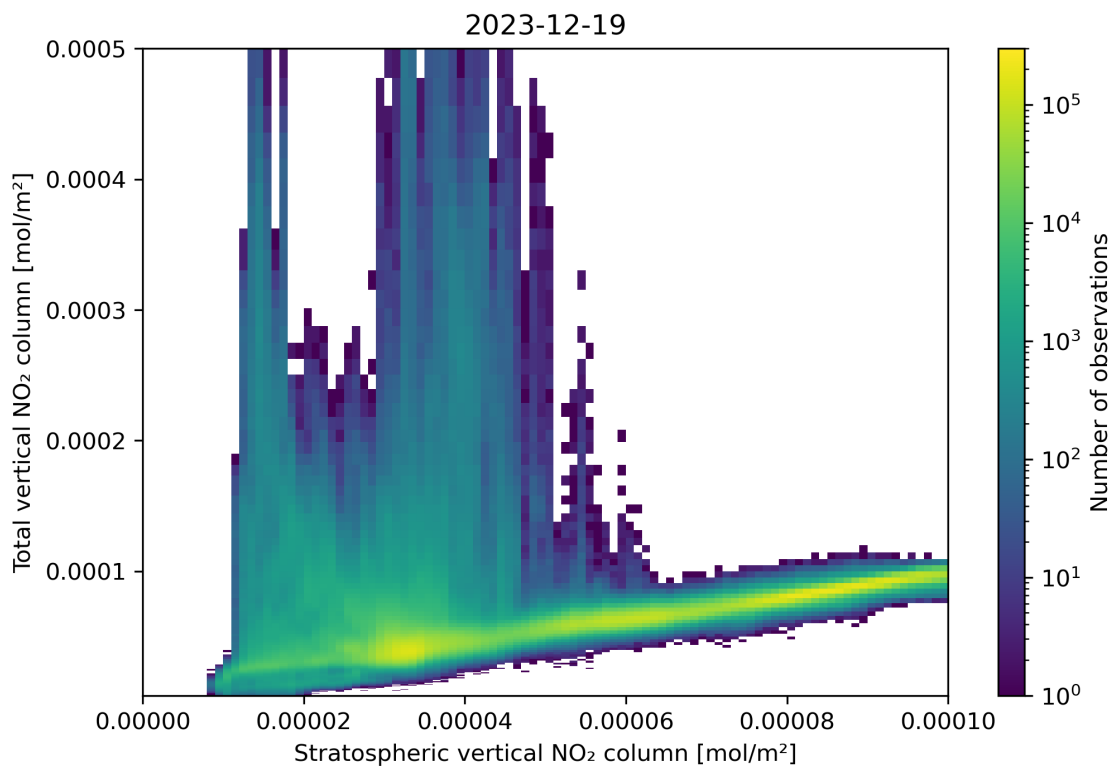
Figure 100: Scatter density plot of “Stratospheric vertical NO 2 column” against “Total vertical NO 2 column” for 2023-12-18 to 2023-12-20.
