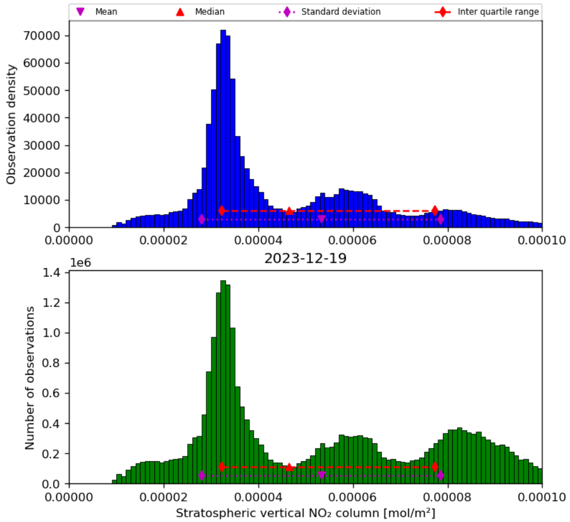
Figure 36: Histogram of “Stratospheric vertical NO 2 column” for 2023-12-18 to 2023-12-20
