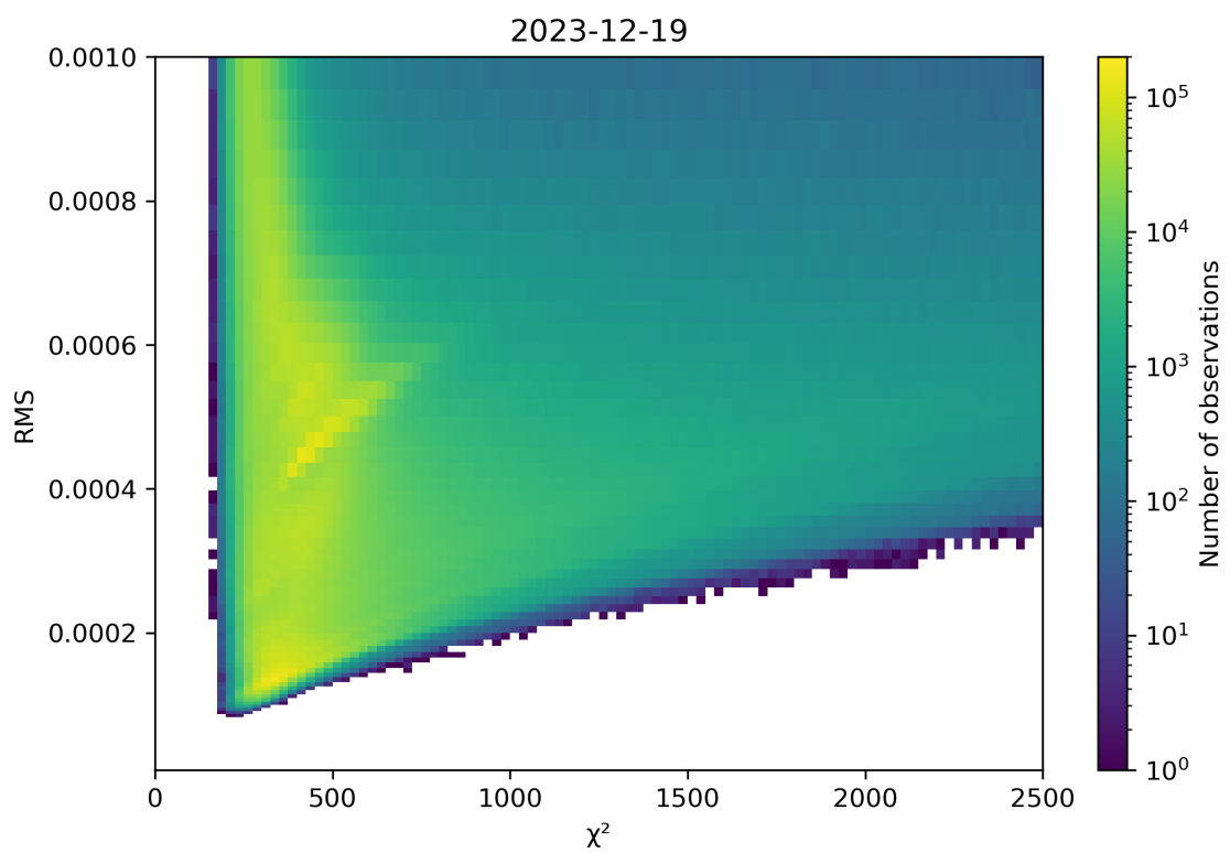
Figure 82: Scatter density plot of " \chi^2 " against "RMS" for 2023-12-18 to 2023-12-20.
