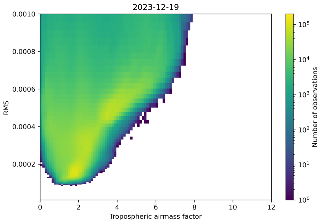
Figure 79: Scatter density plot of “Tropospheric airmass factor” against “RMS” for 2023-12-18 to 2023-12-20.
