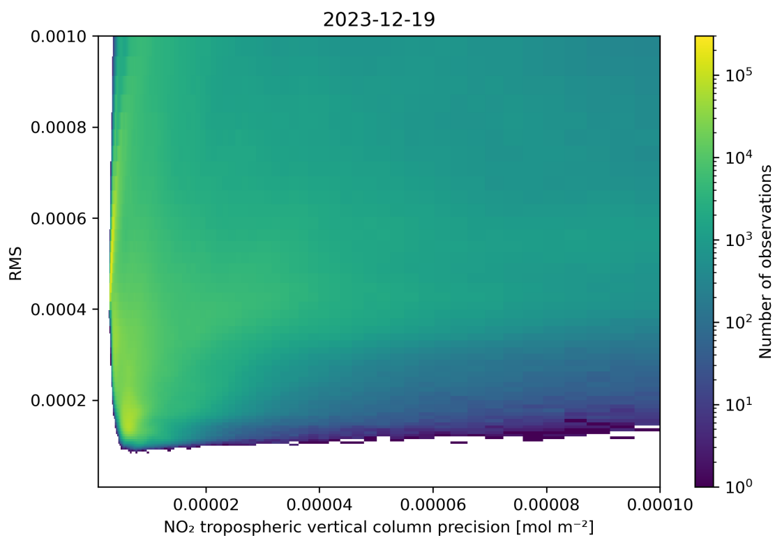
Figure 140: Scatter density plot of “NO 2 tropospheric vertical column precision” against “RMS” for 2023-12-18 to 2023-12-20.
