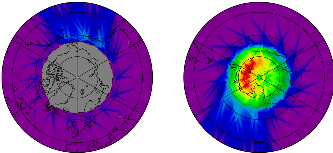
Figure 10: Map of the number of observations for 2023-12-18 to 2023-12-20
