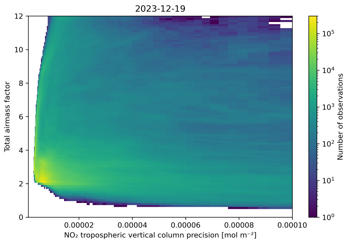
Figure 132: Scatter density plot of “NO 2 tropospheric vertical column precision” against “Total airmass factor” for 2023-12-18 to 2023-12-20.
