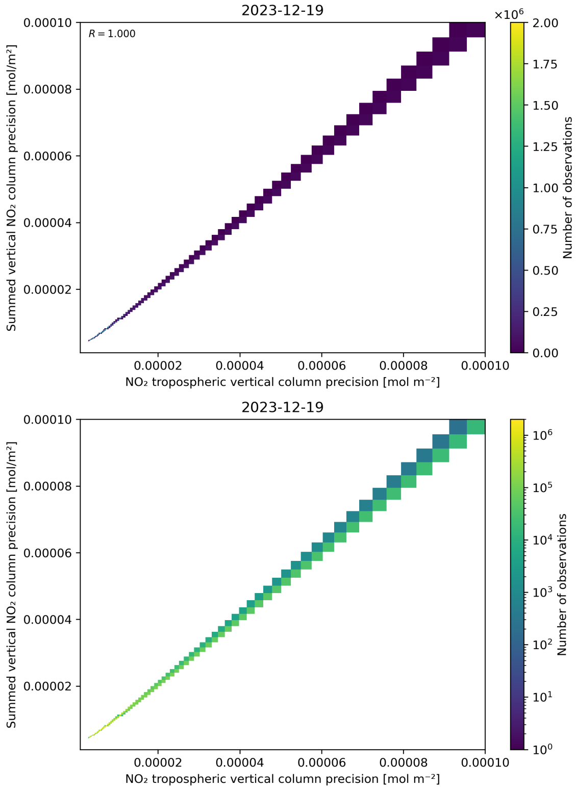
Figure 137: Scatter density plot of “NO 2 tropospheric vertical column precision” against “Summed vertical NO 2 column precision” for 2023-12-18 to 2023-12-20.
