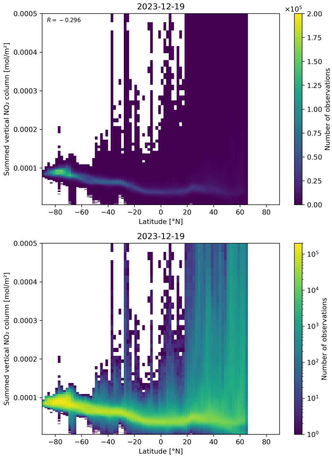
Figure 88: Scatter density plot of “Latitude” against “Summed vertical NO 2 column” for 2023-12-18 to 2023-12-20.
