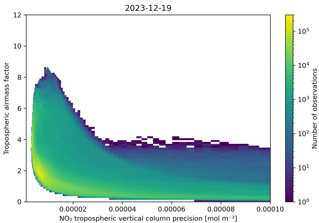
Figure 133: Scatter density plot of “NO 2 tropospheric vertical column precision” against “Tropospheric air mass factor” for 2023-12-18 to 2023-12-20.
