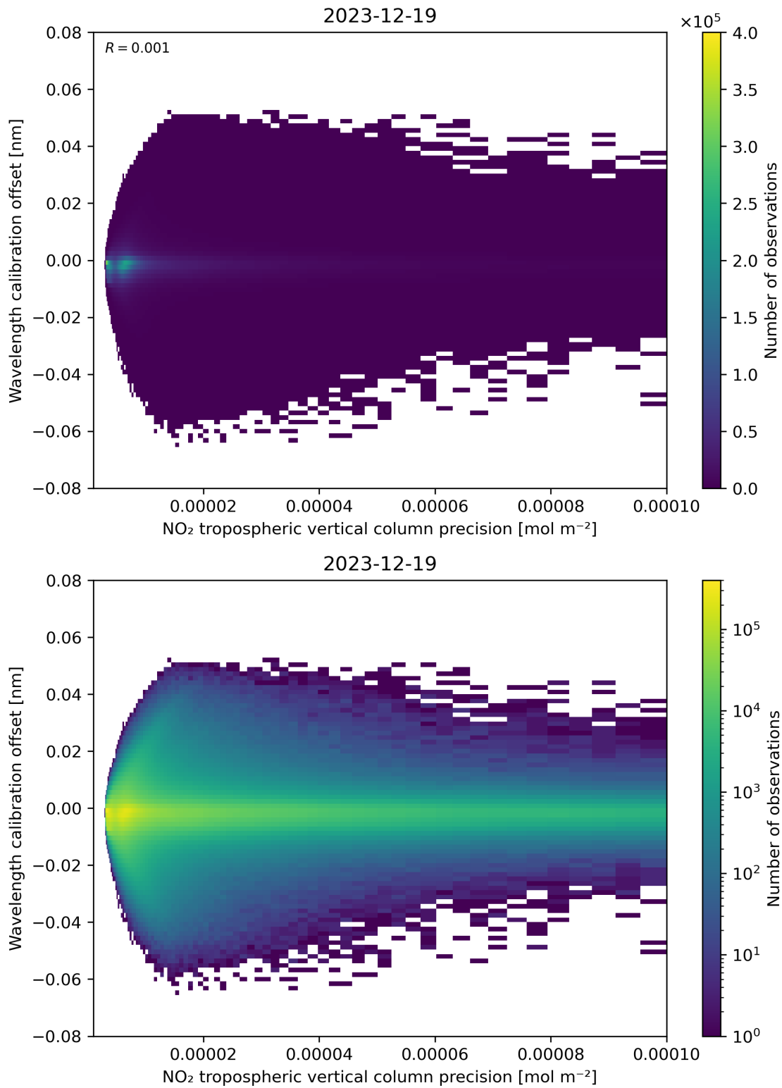
Figure 141: Scatter density plot of “NO 2 tropospheric vertical column precision” against “Wavelength calibration offset” for 2023-12-18 to 2023-12-20.
