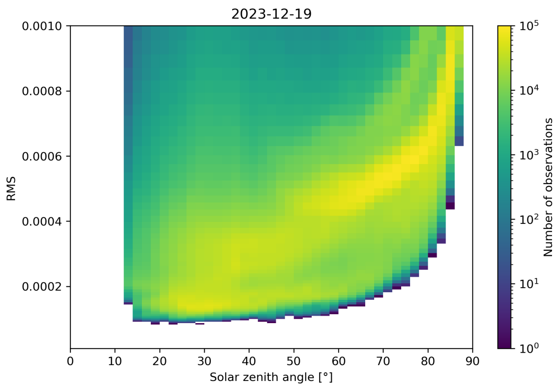
Figure 157: Scatter density plot of “Solar zenith angle” against “RMS” for 2023-12-18 to 2023-12-20.
