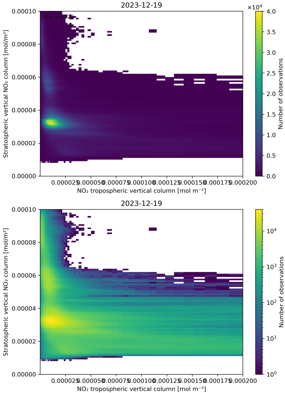
Figure 125: Scatter density plot of “NO 2 tropospheric vertical column” against “Stratospheric vertical NO 2 column” for 2023-12-18 to 2023-12-20.
