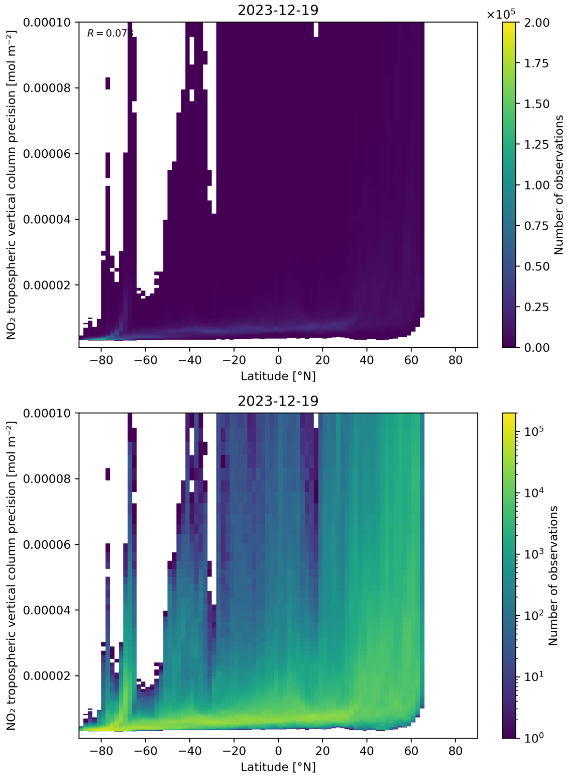
Figure 93: Scatter density plot of “Latitude” against “NO 2 tropospheric vertical column precision” for 2023-12-18 to 2023-12-20.
