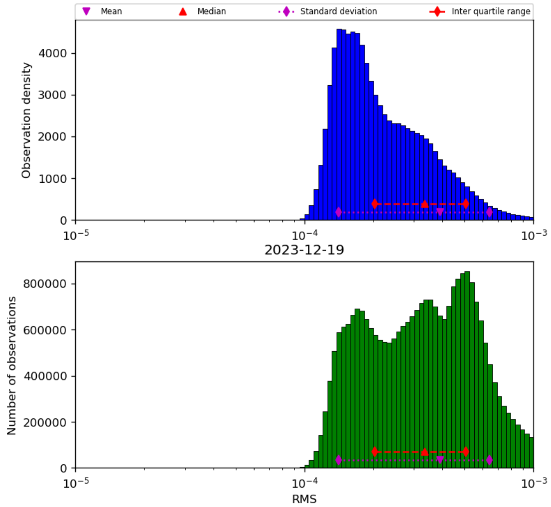
Figure 43: Histogram of “RMS” for 2023-12-18 to 2023-12-20
