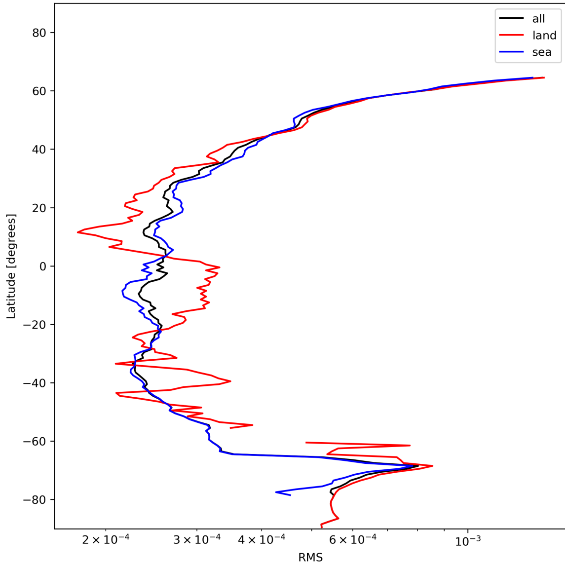
Figure 26: Zonal average of “RMS” for 2023-12-18 to 2023-12-20.
