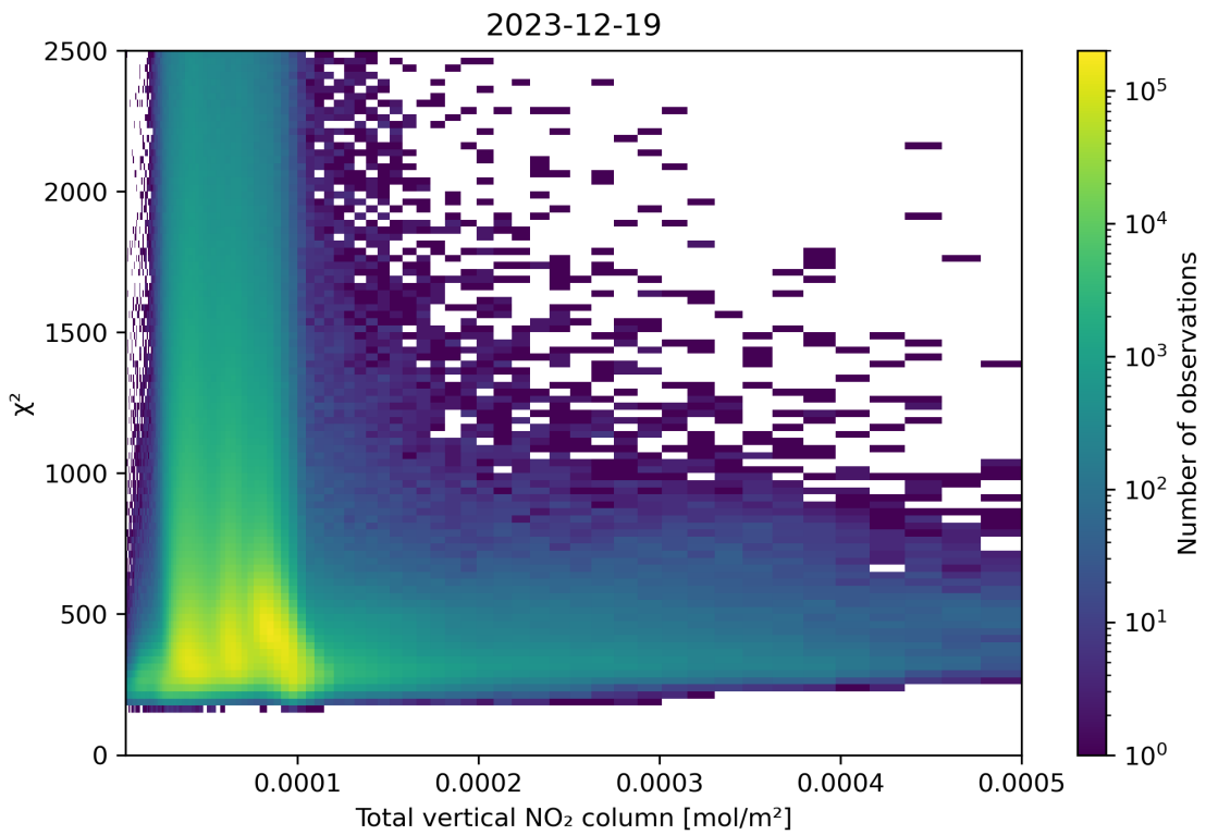
Figure 111: Scatter density plot of “Total vertical NO 2 column” against “ \chi^2 ” for 2023-12-18 to 2023-12-20.
