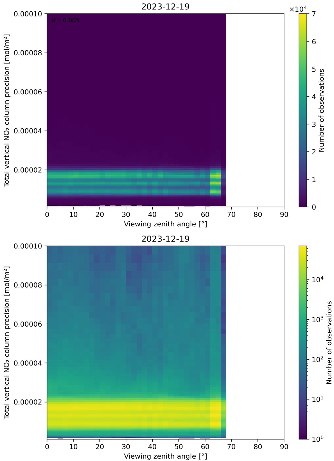
Figure 168: Scatter density plot of “Viewing zenith angle” against “Total vertical NO 2 column precision” for 2023-12-18 to 2023-12-20.
