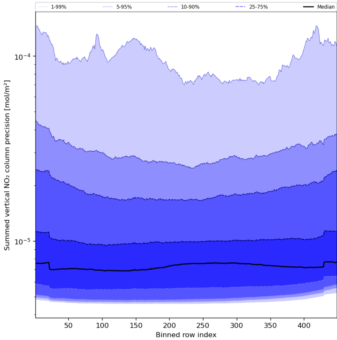
Figure 58: Along track statistics of “Summed vertical NO 2 column precision” for 2023-12-18 to 2023-12-20
