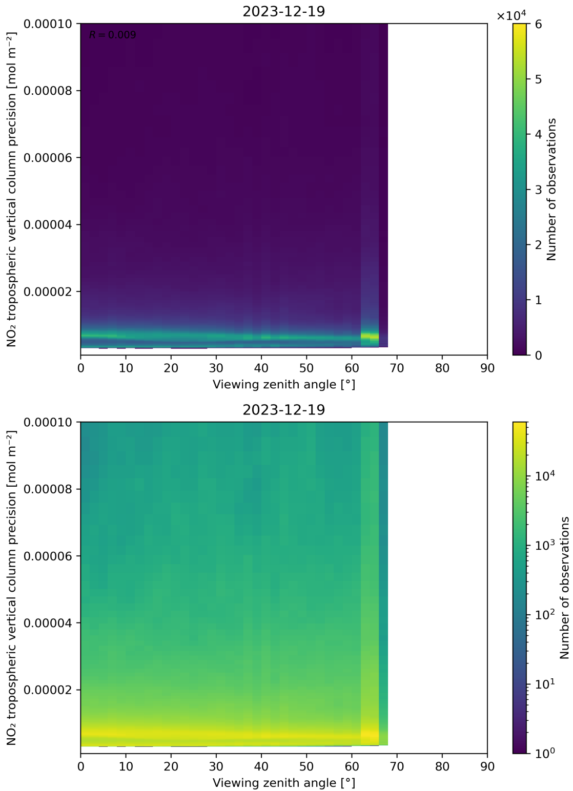
Figure 170: Scatter density plot of “Viewing zenith angle” against “NO 2 tropospheric vertical column precision” for 2023-12-18 to 2023-12-20.
