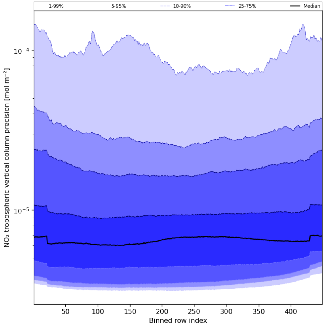
Figure 47: Along track statistics of “NO 2 tropospheric vertical column precision” for 2023-12-18 to 2023-12-20
