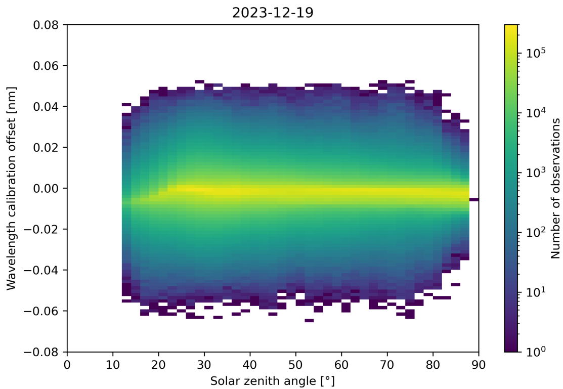
Figure 158: Scatter density plot of “Solar zenith angle” against “Wavelength calibration offset” for 2023-12-18 to 2023-12-20.
