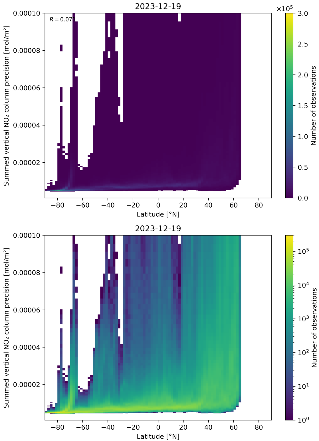
Figure 89: Scatter density plot of “Latitude” against “Summed vertical NO 2 column precision” for 2023-12-18 to 2023-12-20.
