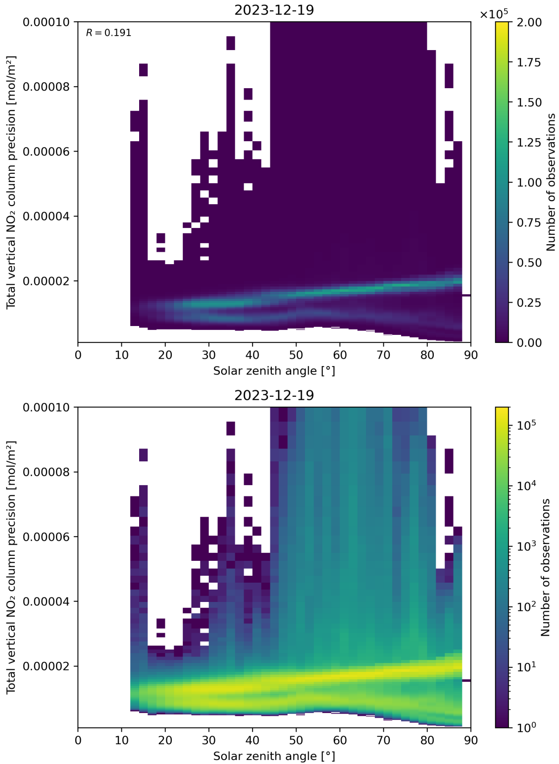
Figure 154: Scatter density plot of “Solar zenith angle” against “Total vertical NO 2 column precision” for 2023-12-18 to 2023-12-20.
