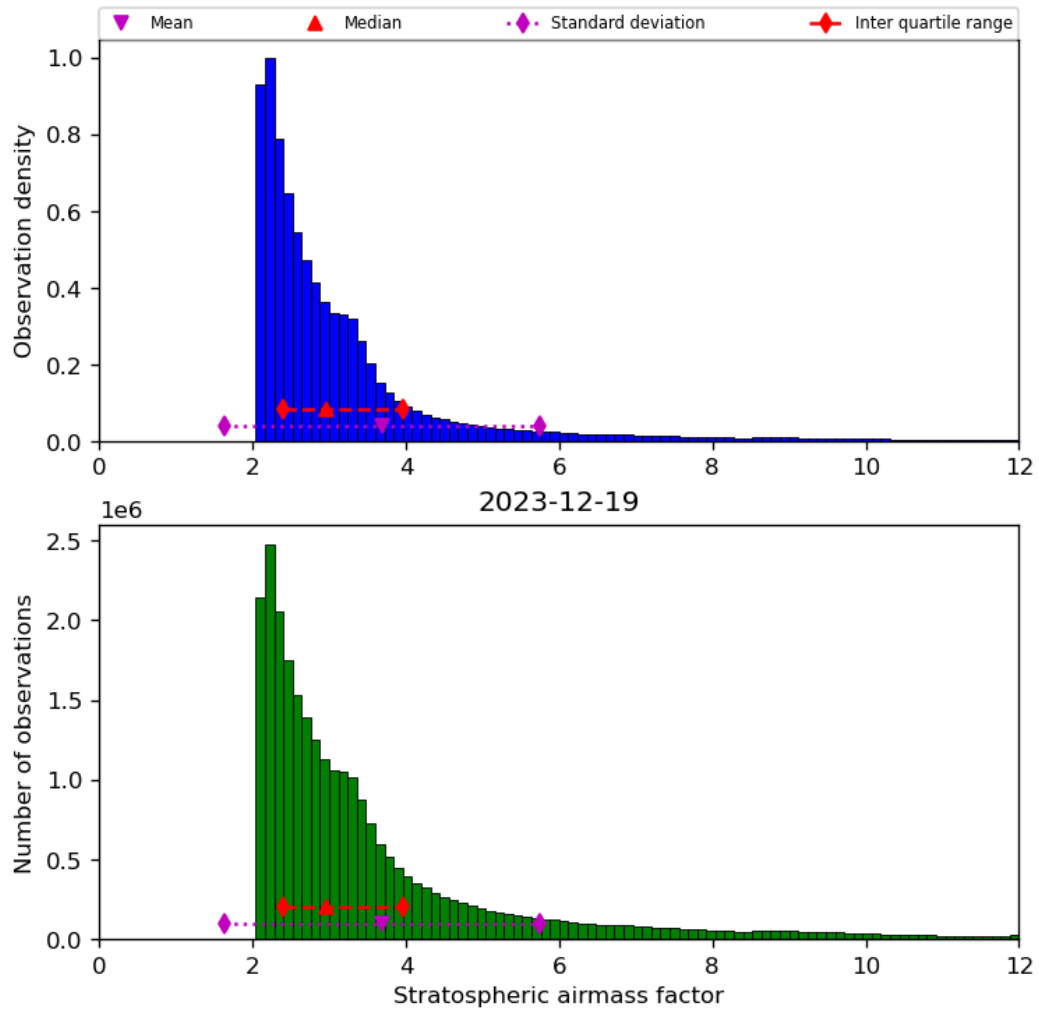
Figure 44: Histogram of “Stratospheric airmass factor” for 2023-12-18 to 2023-12-20
