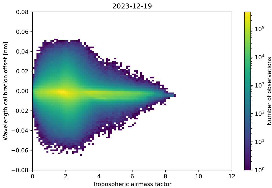
Figure 80: Scatter density plot of “Tropospheric airmass factor” against “Wavelength calibration offset” for 2023-12-18 to 2023-12-20.
