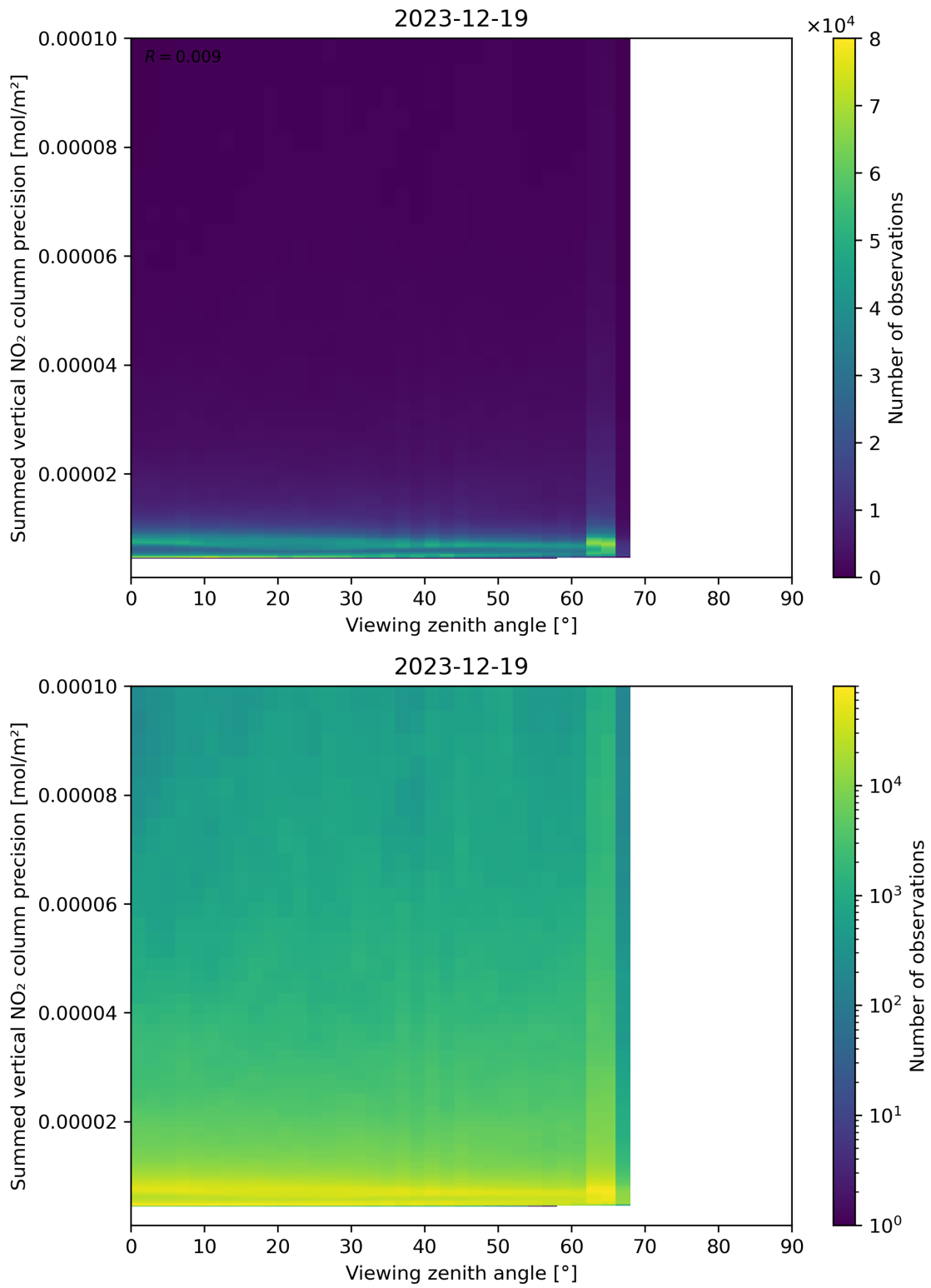
Figure 166: Scatter density plot of “Viewing zenith angle” against “Summed vertical NO 2 column precision” for 2023-12-18 to 2023-12-20.
