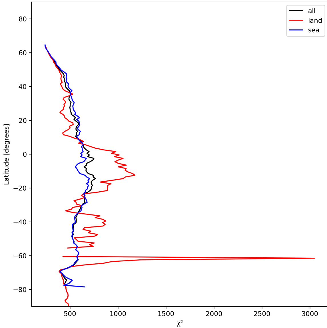
Figure 25: Zonal average of " \chi^2 " for 2023-12-18 to 2023-12-20.
