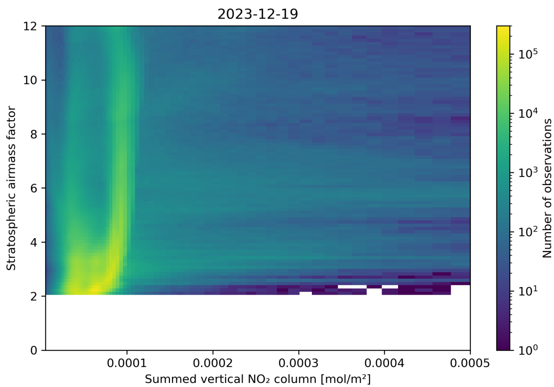
Figure 103: Scatter density plot of “Summed vertical NO 2 column” against “Stratospheric airmass factor” for 2023-12-18 to 2023-12-20.
