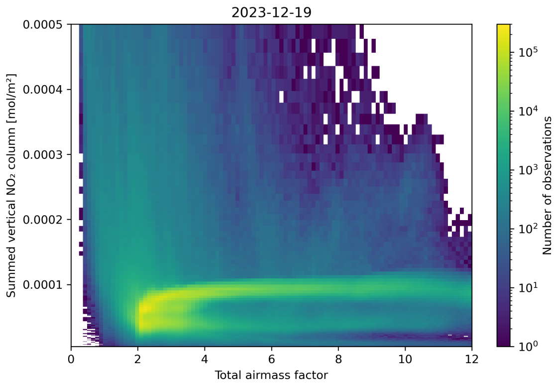
Figure 65: Scatter density plot of “Total airmass factor” against “Summed vertical NO 2 column” for 2023-12-18 to 2023-12-20.
