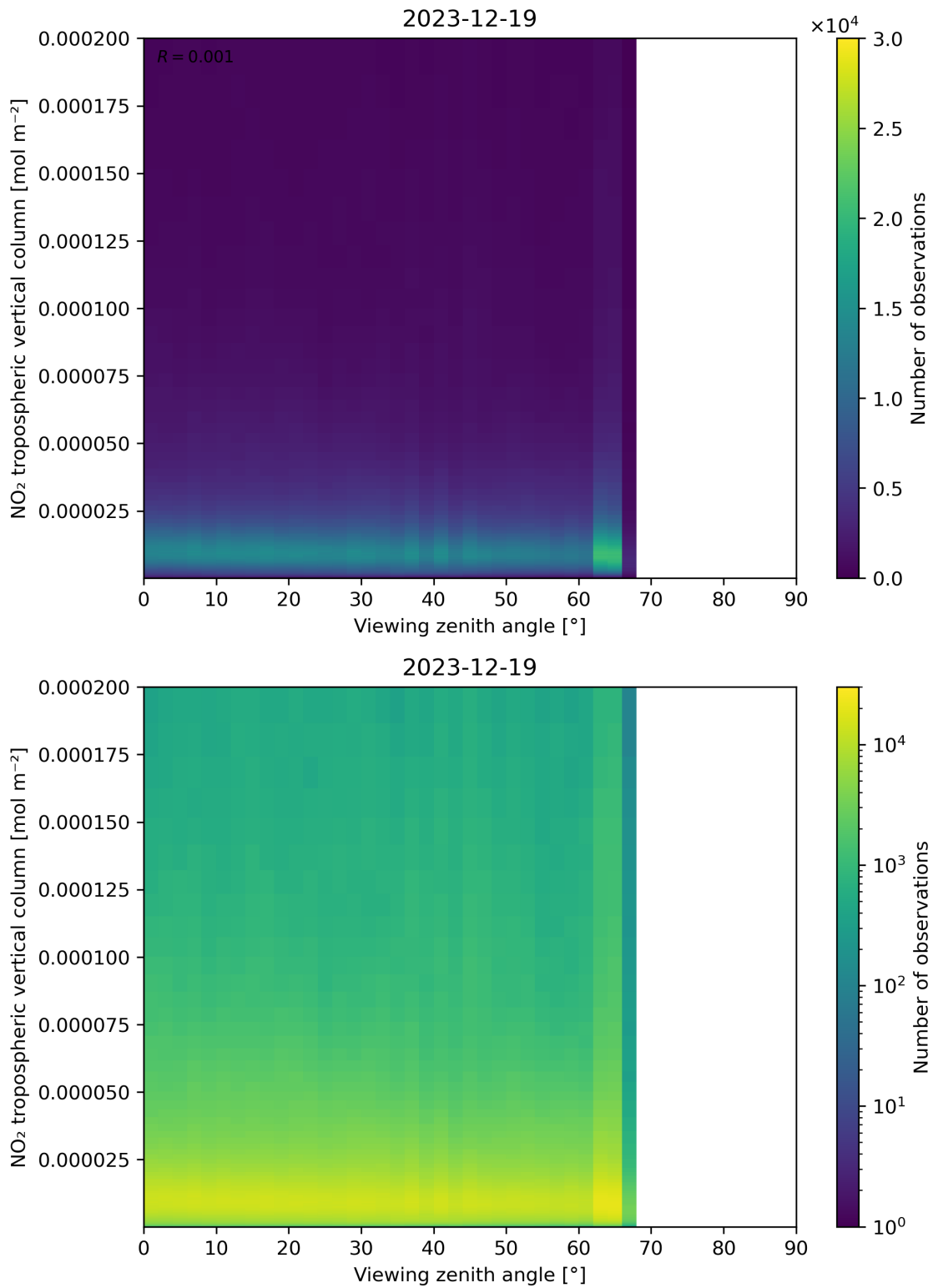
Figure 169: Scatter density plot of “Viewing zenith angle” against “NO 2 tropospheric vertical column” for 2023-12-18 to 2023-12-20.
