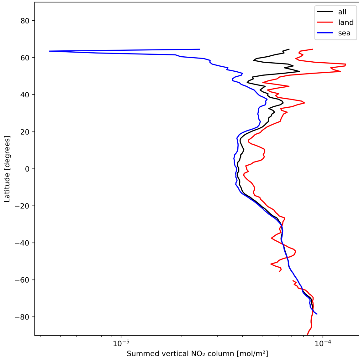
Figure 23: Zonal average of “Summed vertical NO 2 column” for 2023-12-18 to 2023-12-20.
