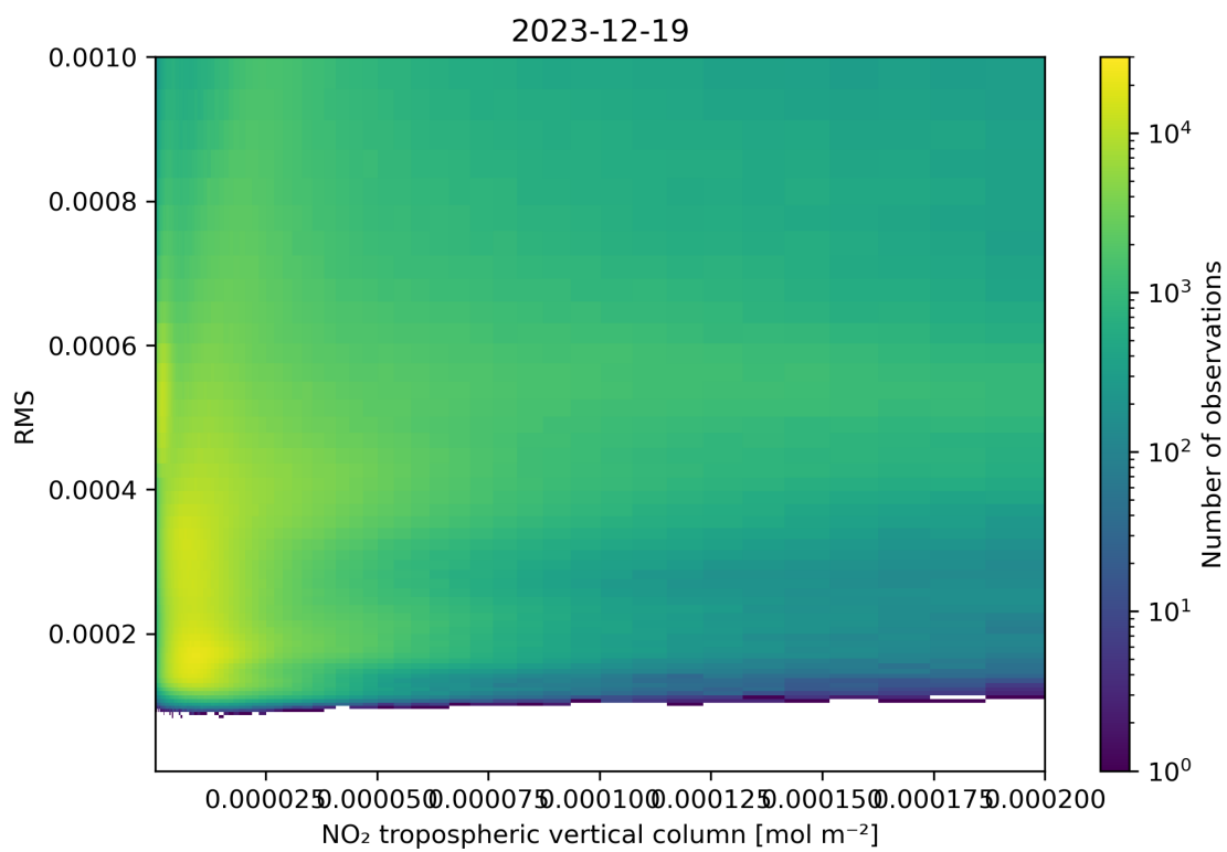
Figure 142: Scatter density plot of “NO 2 tropospheric vertical column” against “RMS” for 2023-12-18 to 2023-12-20.
