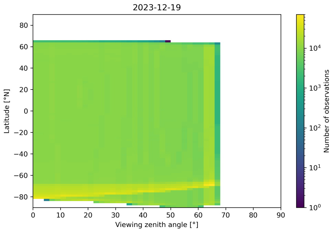
Figure 163: Scatter density plot of “Viewing zenith angle” against “Latitude” for 2023-12-18 to 2023-12-20.
