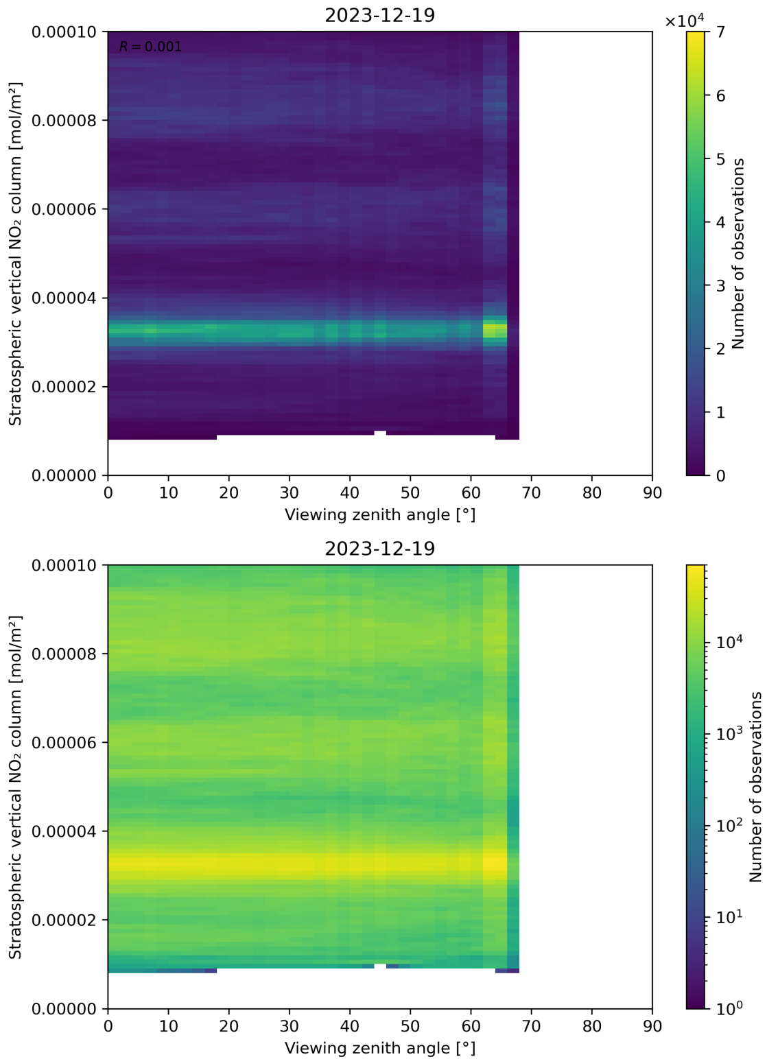
Figure 164: Scatter density plot of “Viewing zenith angle” against “Stratospheric vertical NO 2 column” for 2023-12-18 to 2023-12-20.
