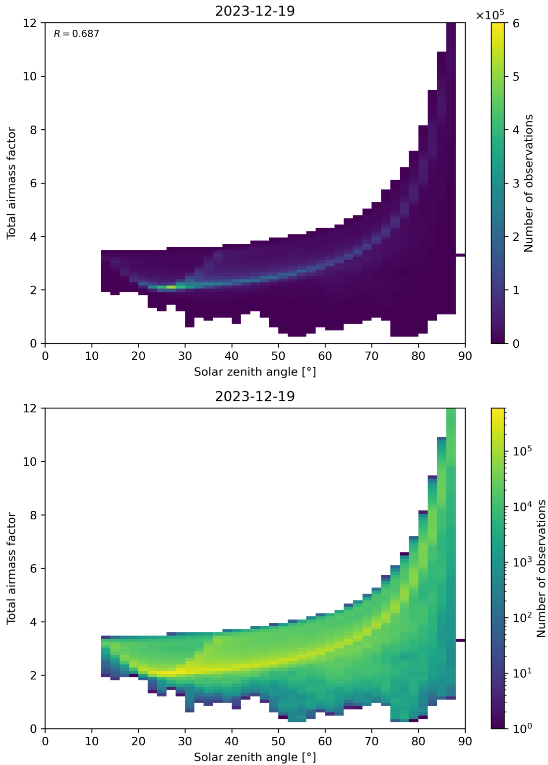
Figure 146: Scatter density plot of “Solar zenith angle” against “Total airmass factor” for 2023-12-18 to 2023-12-20.
