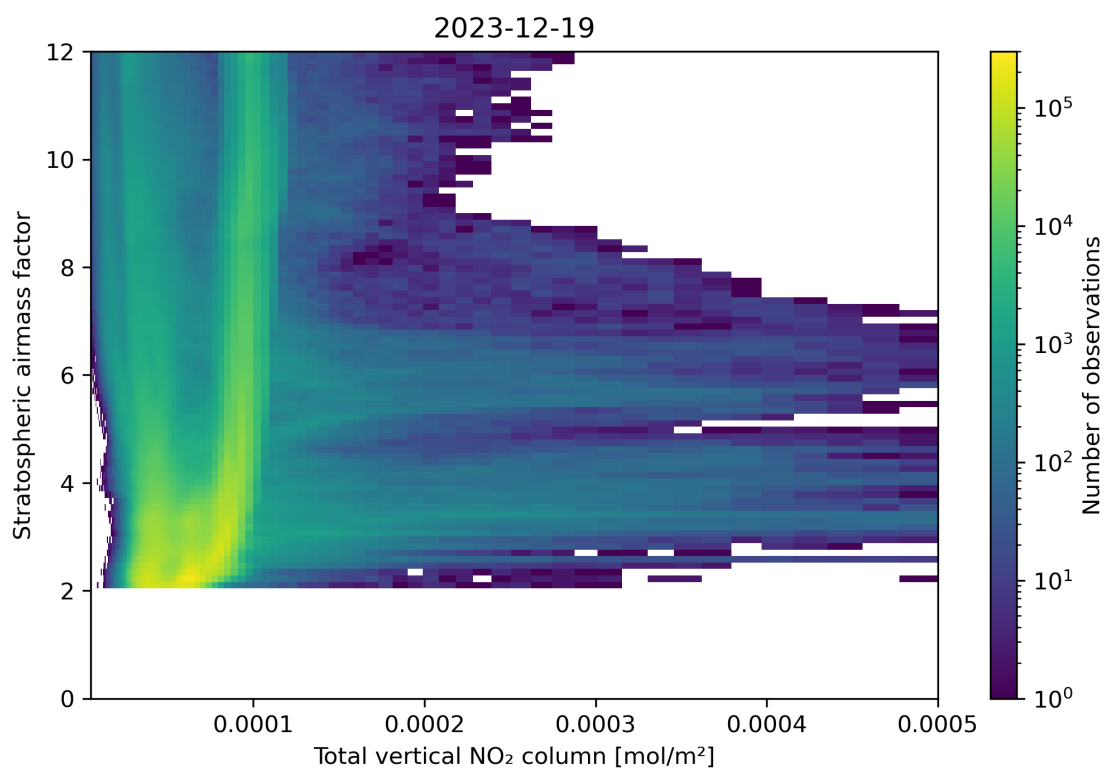
Figure 110: Scatter density plot of “Total vertical NO 2 column” against “Stratospheric airmass factor” for 2023-12-18 to 2023-12-20.
