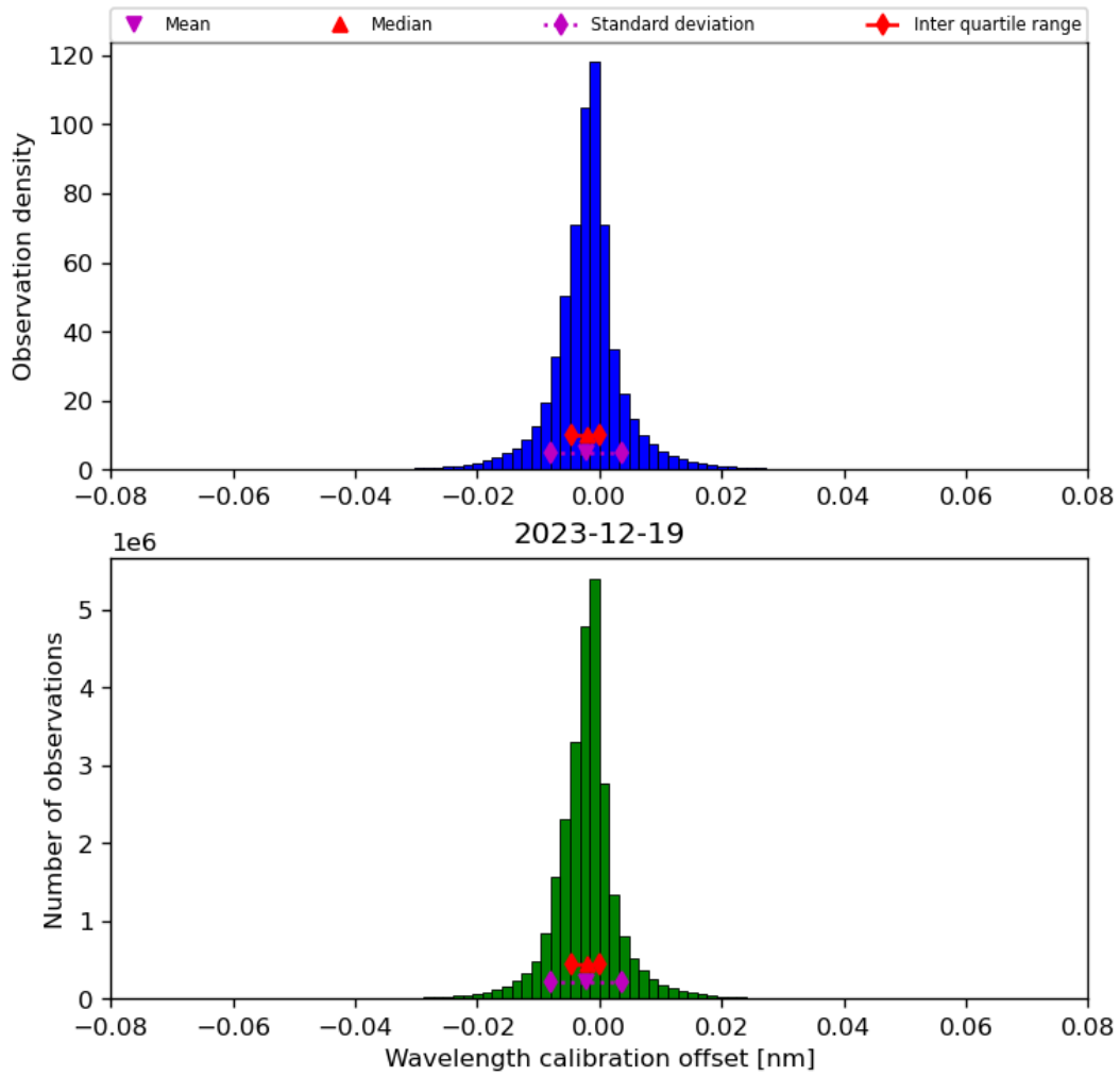
Figure 35: Histogram of “Wavelength calibration offset” for 2023-12-18 to 2023-12-20
