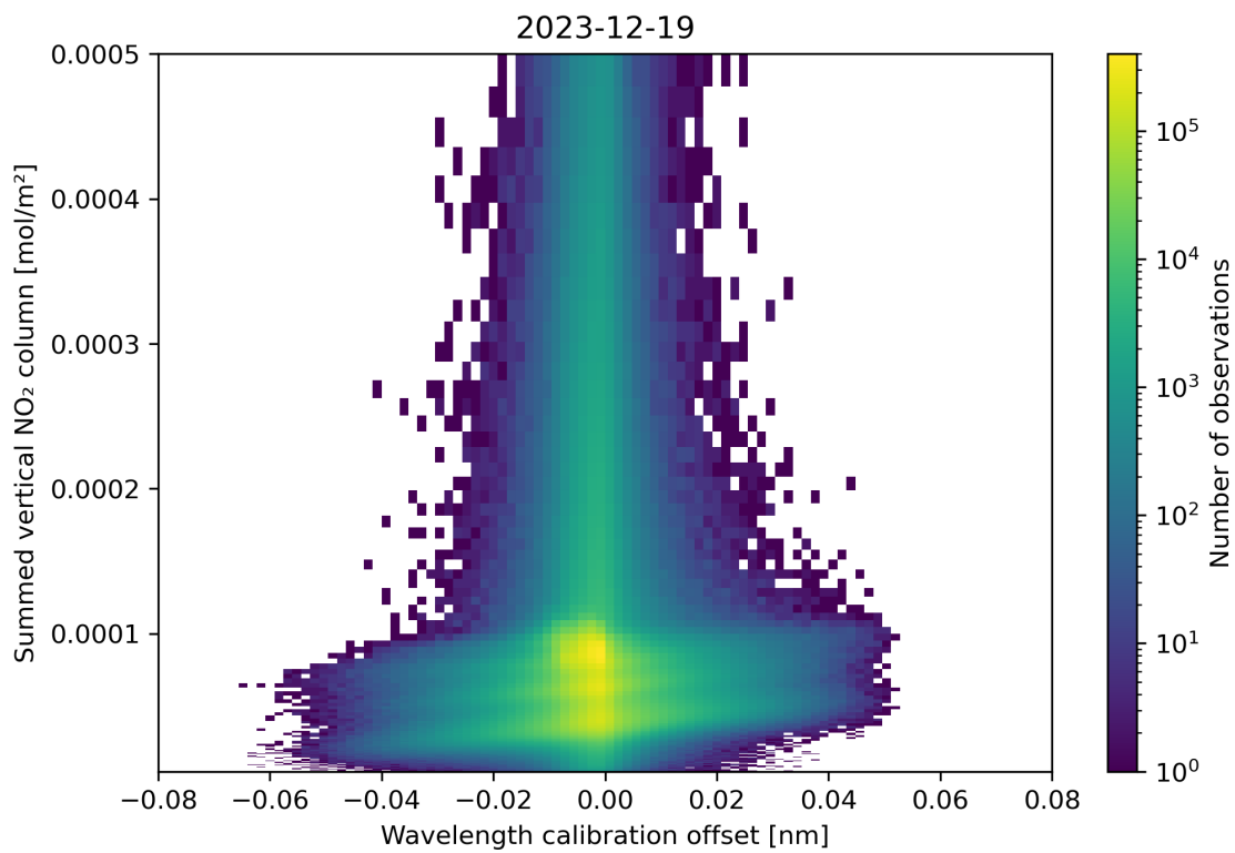
Figure 177: Scatter density plot of “Wavelength calibration offset” against “Summed vertical NO 2 column” for 2023-12-18 to 2023-12-20.
