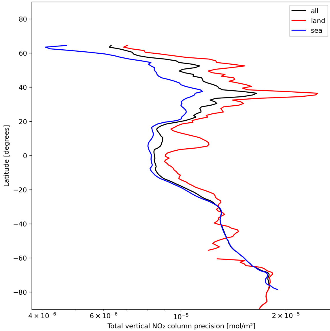
Figure 22: Zonal average of “Total vertical NO 2 column precision” for 2023-12-18 to 2023-12-20.
