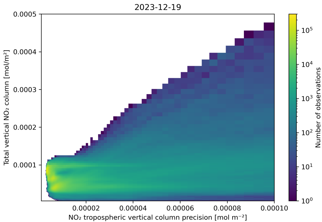
Figure 138: Scatter density plot of “NO 2 tropospheric vertical column precision” against “Total vertical NO 2 column” for 2023-12-18 to 2023-12-20.
