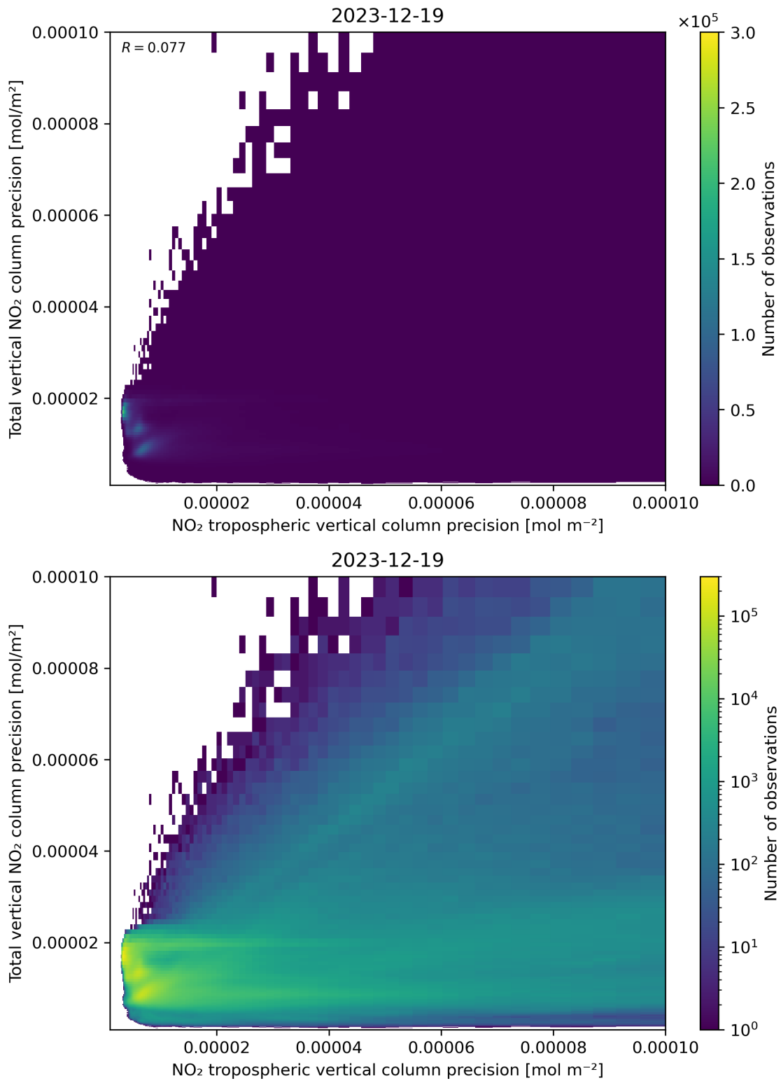
Figure 139: Scatter density plot of “NO 2 tropospheric vertical column precision” against “Total vertical NO 2 column precision” for 2023-12-18 to 2023-12-20.
