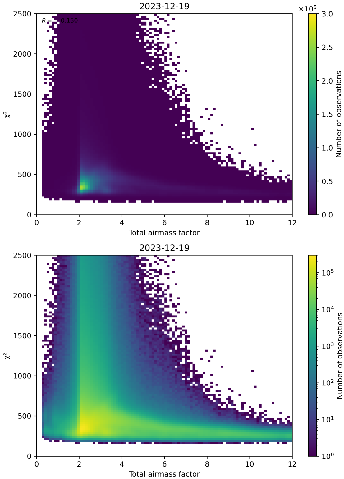
Figure 63: Scatter density plot of “Total airmass factor” against “ \chi^2 ” for 2023-12-18 to 2023-12-20.
