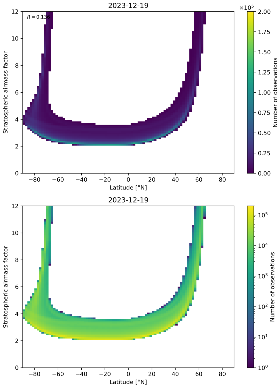
Figure 83: Scatter density plot of “Latitude” against “Stratospheric airmass factor” for 2023-12-18 to 2023-12-20.
