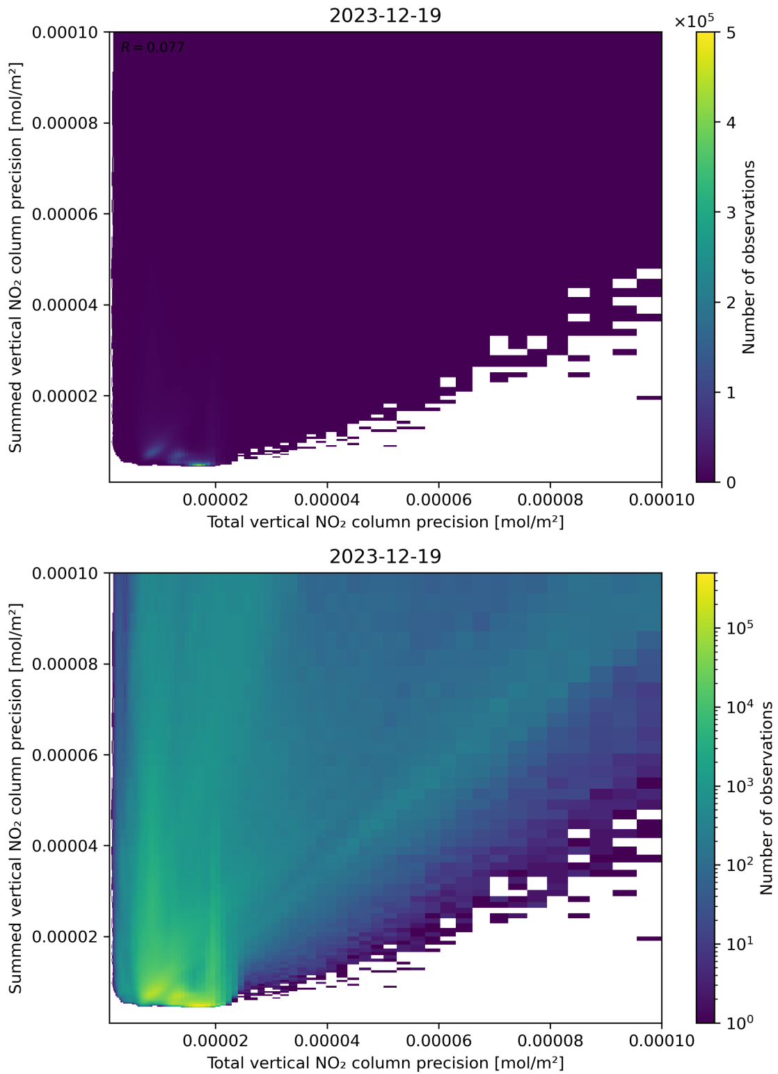
Figure 118: Scatter density plot of “Total vertical NO 2 column precision” against “Summed vertical NO 2 column precision” for 2023-12-18 to 2023-12-20.
