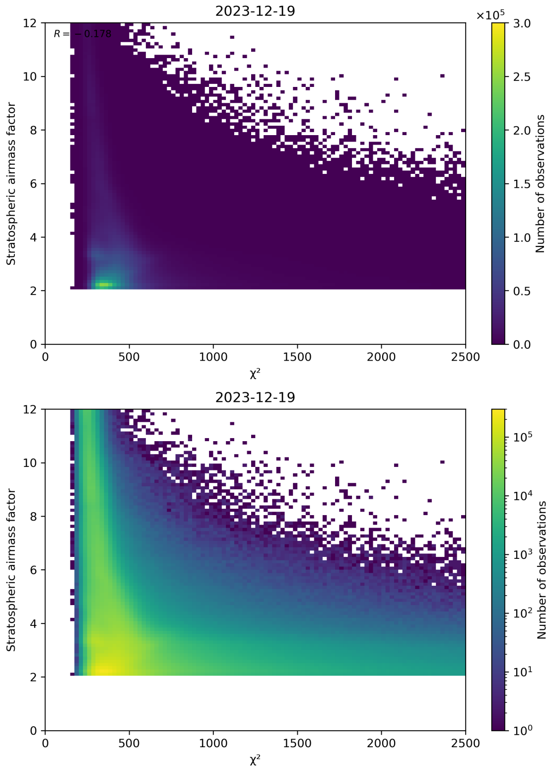
Figure 81: Scatter density plot of “ \chi^2 ” against “Stratospheric airmass factor” for 2023-12-18 to 2023-12-20.
