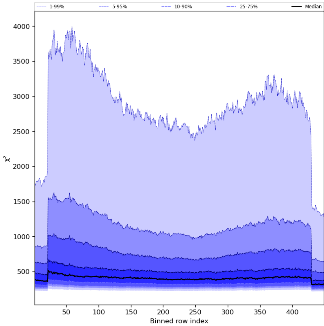
Figure 59: Along track statistics of " \chi^2 " for 2023-12-18 to 2023-12-20
