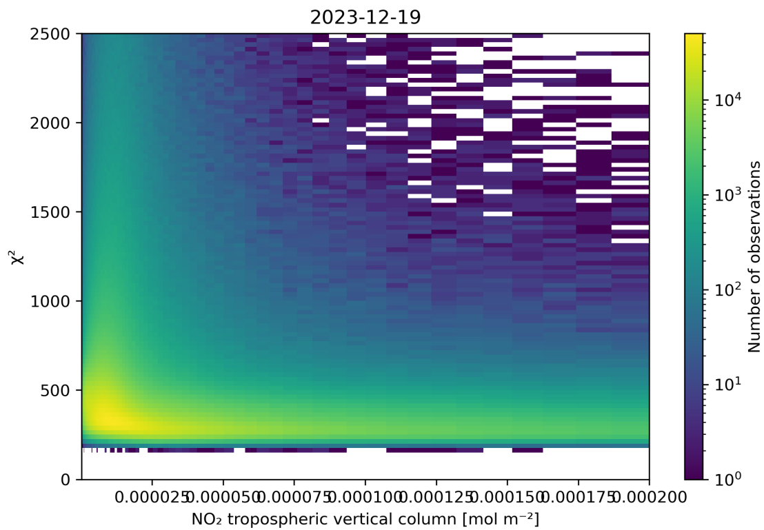
Figure 124: Scatter density plot of “NO 2 tropospheric vertical column” against “ \chi^2 ” for 2023-12-18 to 2023-12-20.
