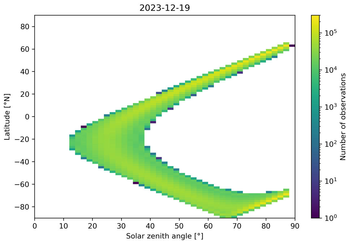
Figure 149: Scatter density plot of “Solar zenith angle” against “Latitude” for 2023-12-18 to 2023-12-20.
