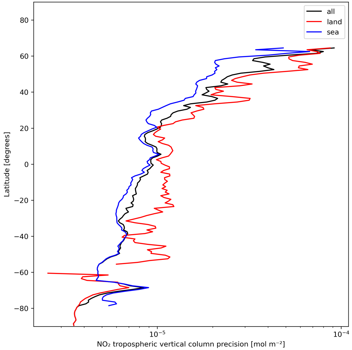
Figure 13: Zonal average of “NO 2 tropospheric vertical column precision” for 2023-12-18 to 2023-12-20.
