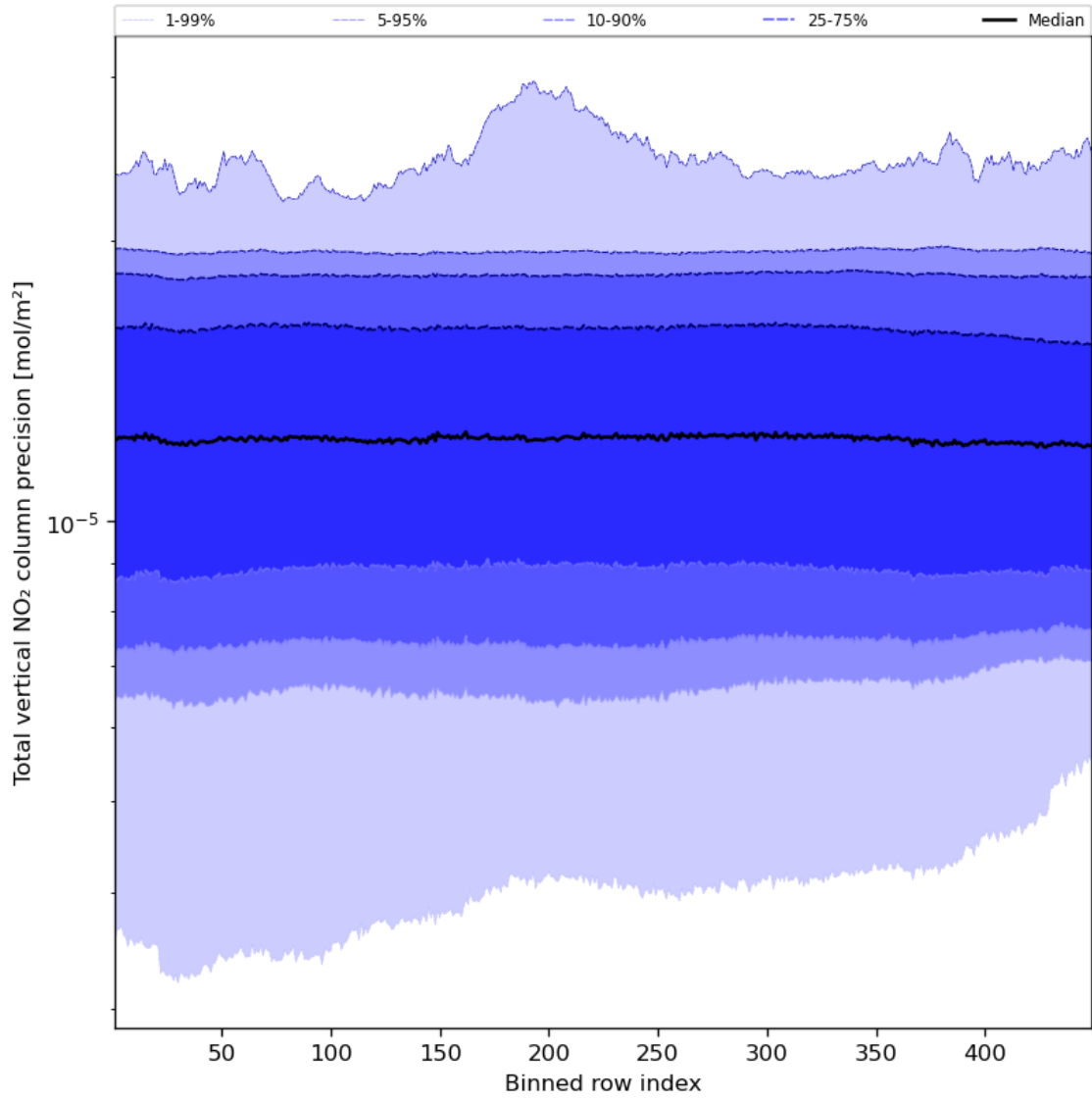
Figure 56: Along track statistics of “Total vertical NO 2 column precision” for 2023-12-18 to 2023-12-20
