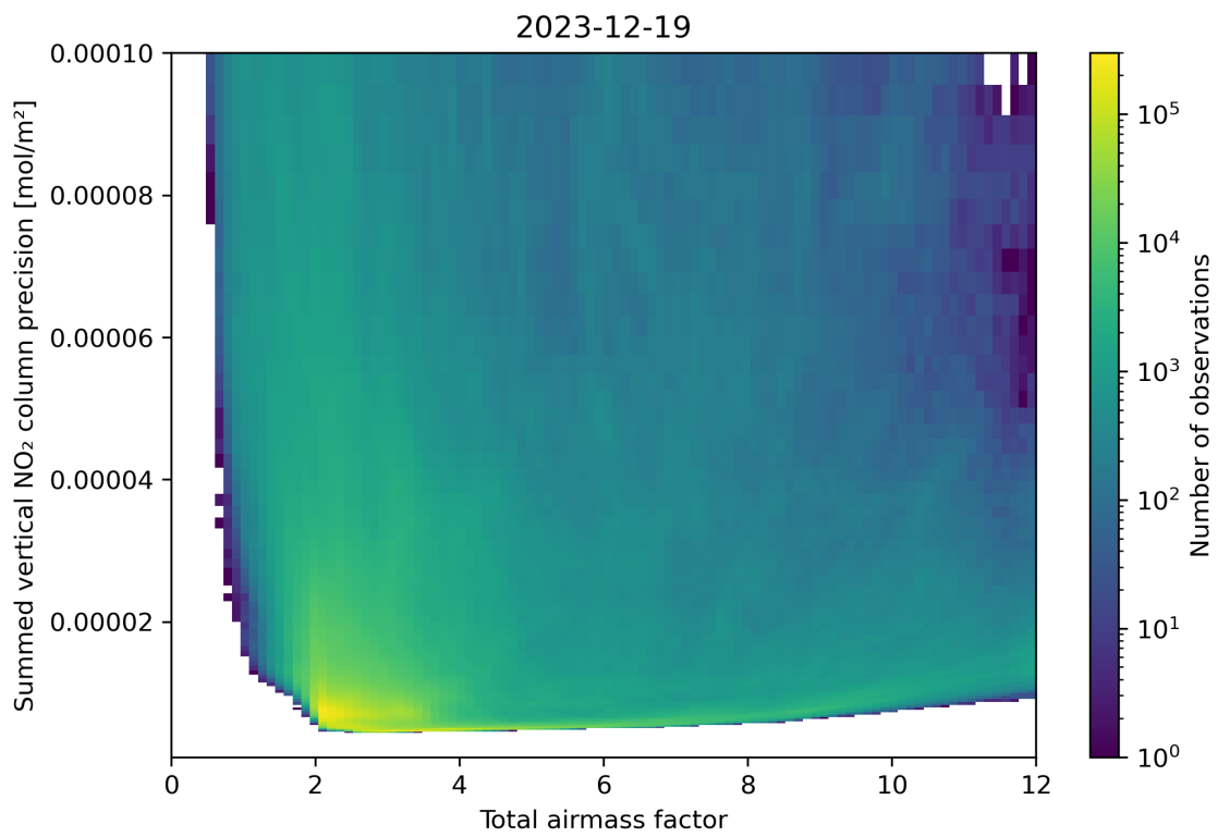
Figure 66: Scatter density plot of “Total airmass factor” against “Summed vertical NO 2 column precision” for 2023-12-18 to 2023-12-20.
