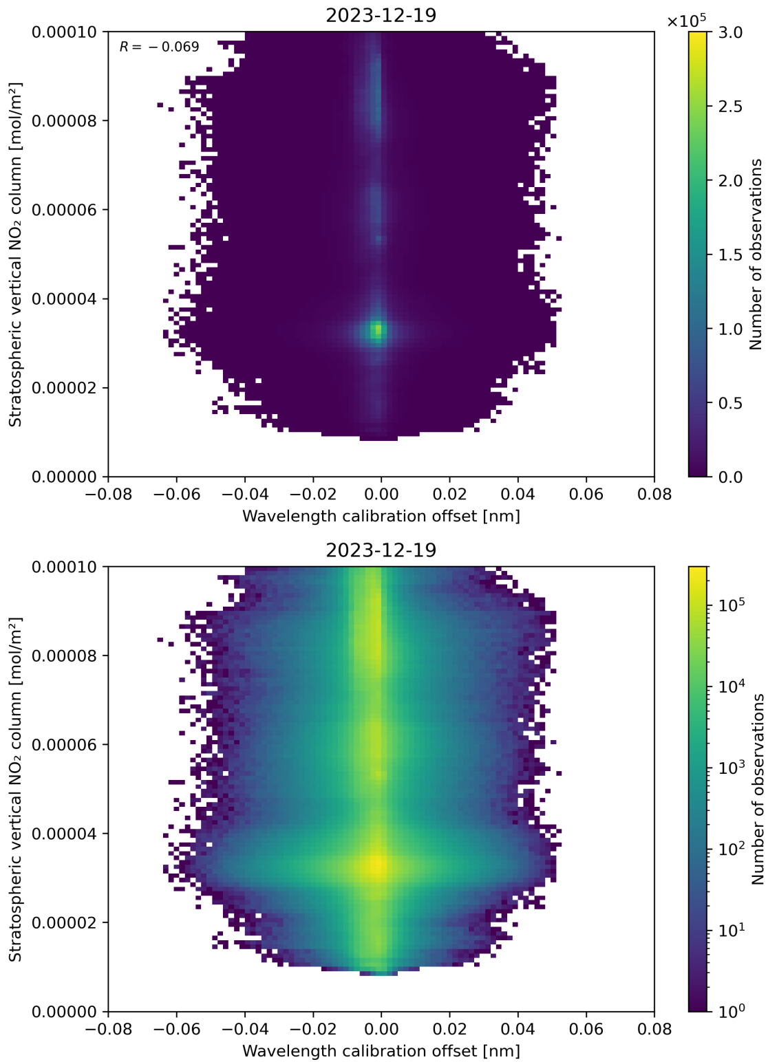
Figure 176: Scatter density plot of “Wavelength calibration offset” against “Stratospheric vertical NO 2 column” for 2023-12-18 to 2023-12-20.
