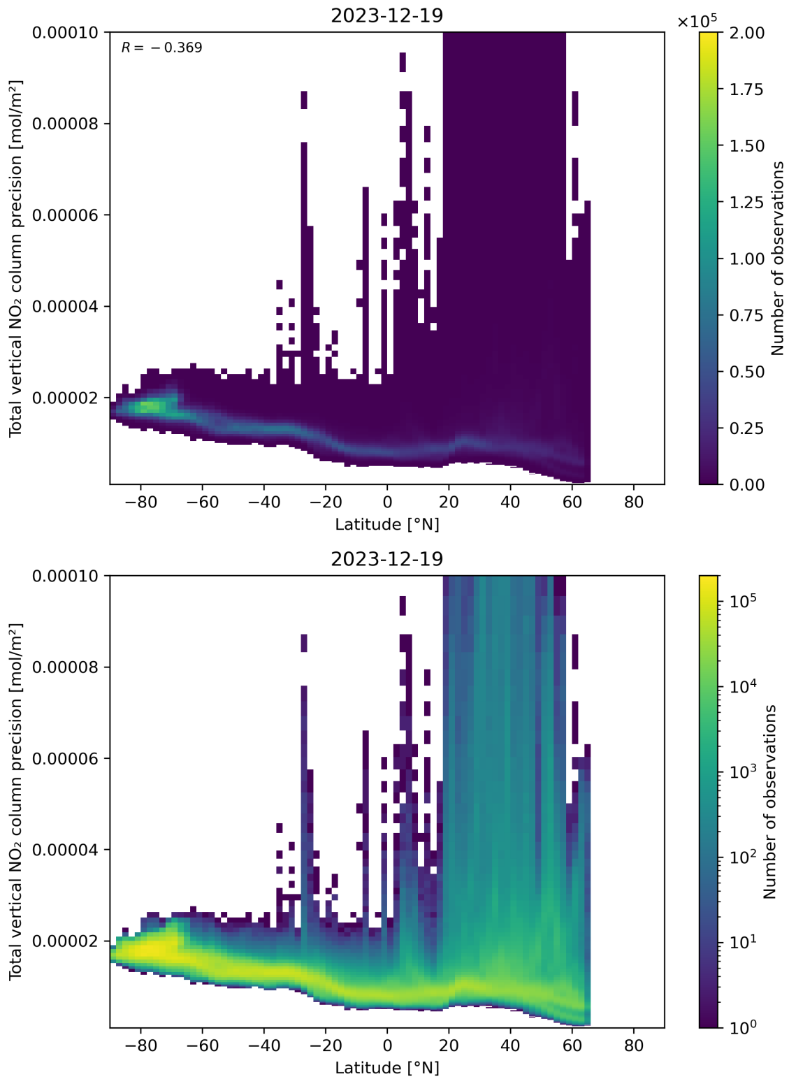
Figure 91: Scatter density plot of “Latitude” against “Total vertical NO 2 column precision” for 2023-12-18 to 2023-12-20.
