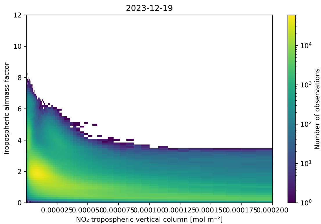
Figure 123: Scatter density plot of “NO 2 tropospheric vertical column” against “Tropospheric air mass factor” for 2023-12-18 to 2023-12-20.
