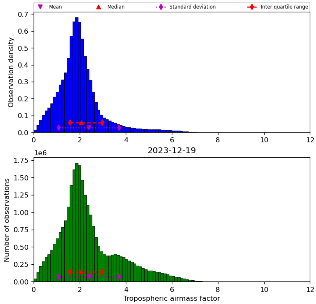
Figure 31: Histogram of “Tropospheric airmass factor” for 2023-12-18 to 2023-12-20
