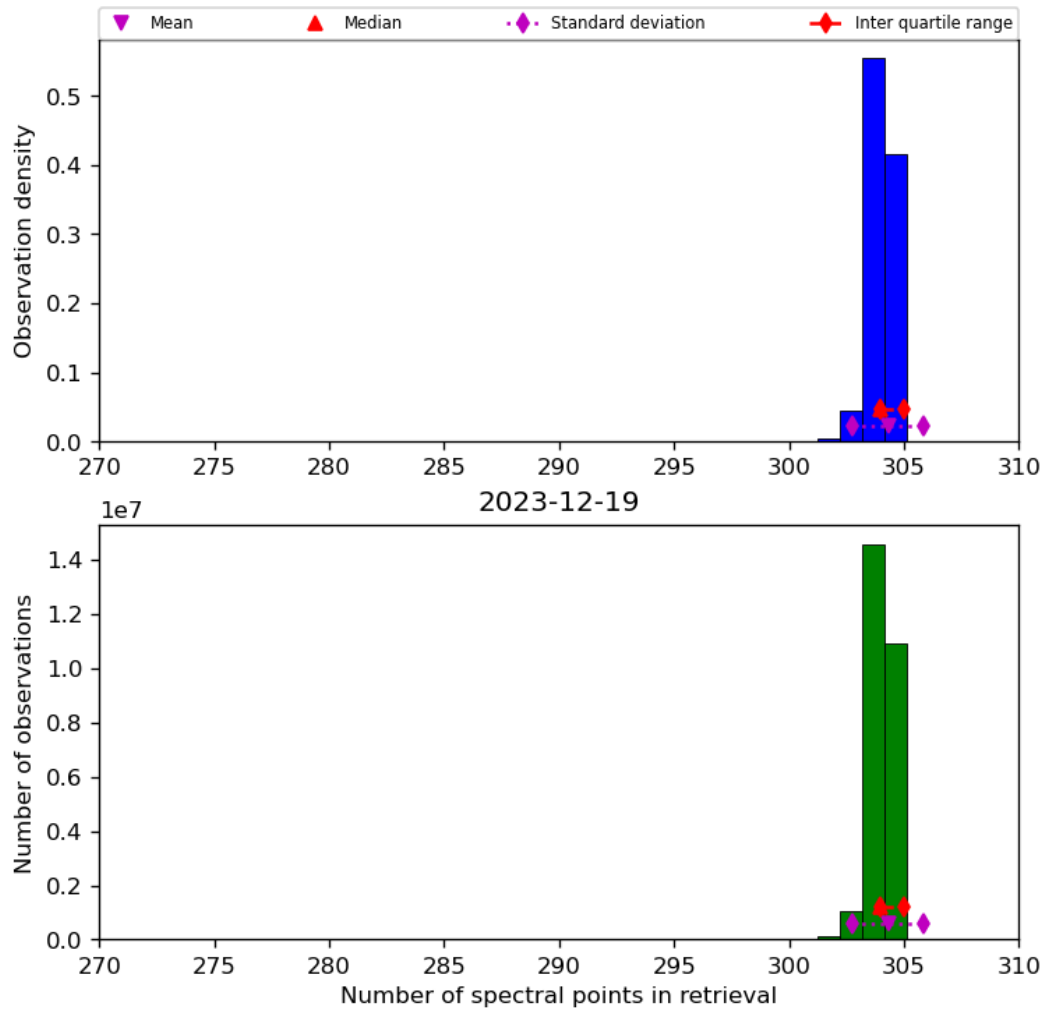
Figure 33: Histogram of “Number of spectral points in retrieval” for 2023-12-18 to 2023-12-20
