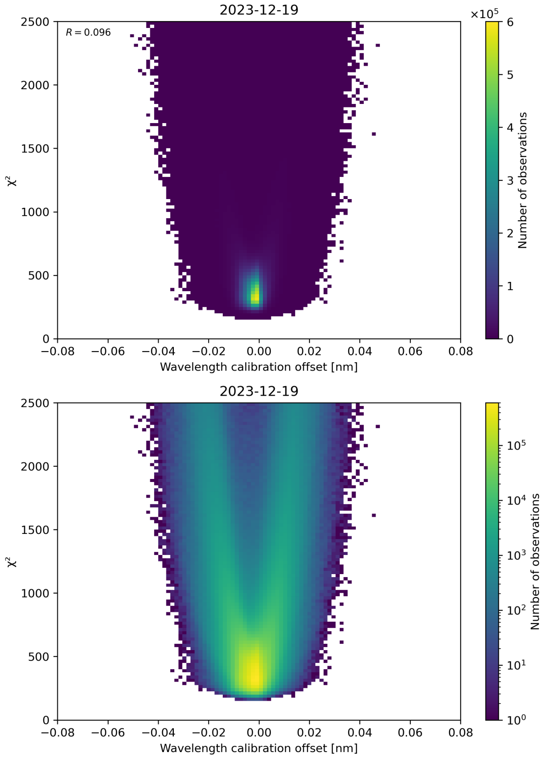
Figure 175: Scatter density plot of “Wavelength calibration offset” against “ \chi^2 ” for 2023-12-18 to 2023-12-20.
