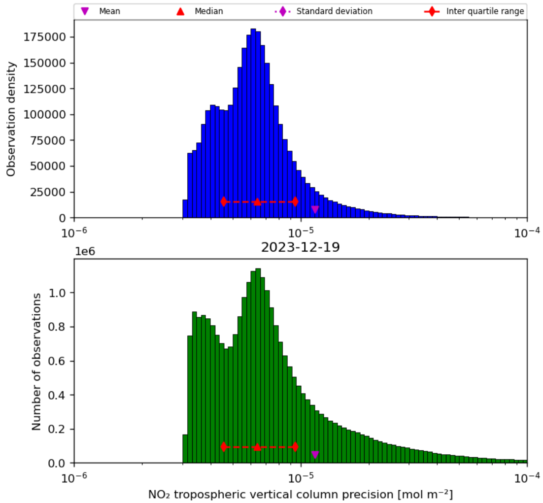
Figure 30: Histogram of “NO 2 tropospheric vertical column precision” for 2023-12-18 to 2023-12-20
