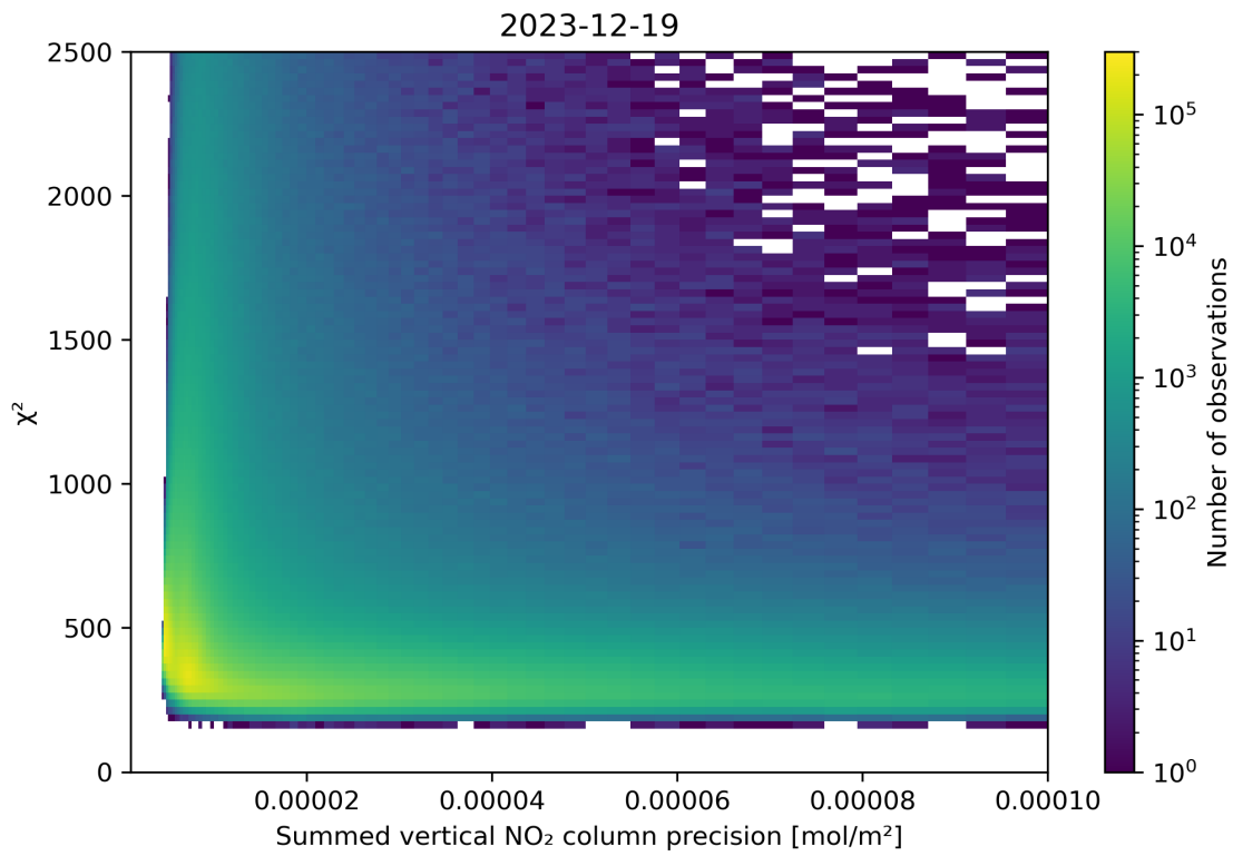
Figure 107: Scatter density plot of “Summed vertical NO 2 column precision” against “ \chi^2 ” for 2023-12-18 to 2023-12-20.
