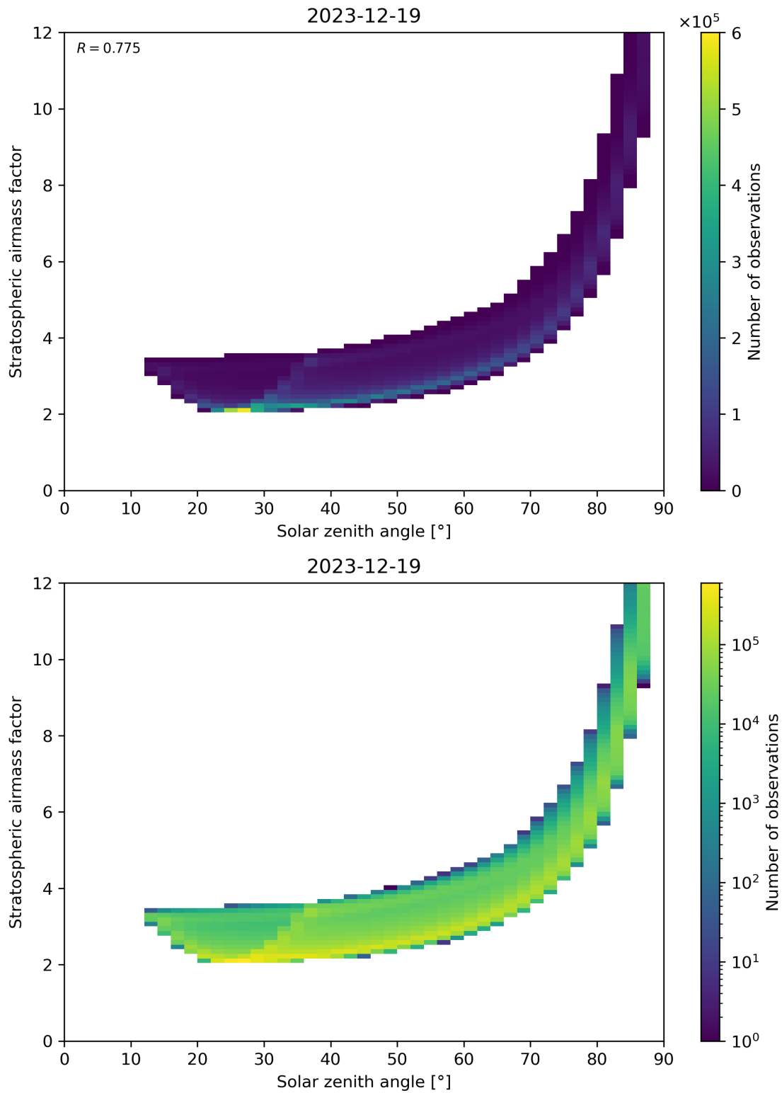
Figure 145: Scatter density plot of “Solar zenith angle” against “Stratospheric airmass factor” for 2023-12-18 to 2023-12-20.
