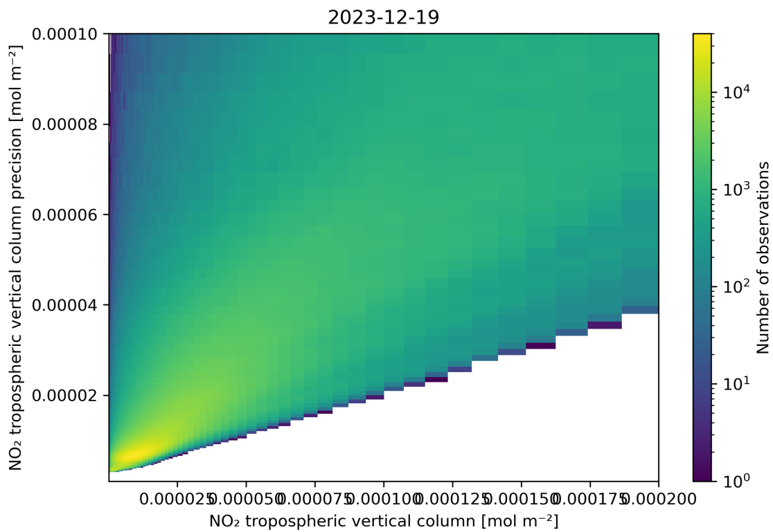
Figure 130: Scatter density plot of “NO 2 tropospheric vertical column” against “NO 2 tropospheric vertical column precision” for 2023-12-18 to 2023-12-20.
