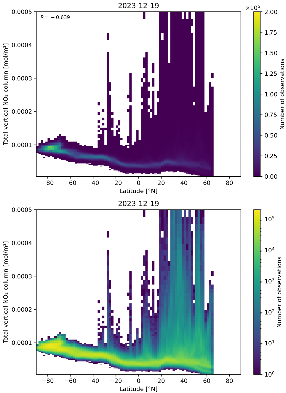
Figure 90: Scatter density plot of “Latitude” against “Total vertical NO 2 column” for 2023-12-18 to 2023-12-20.
