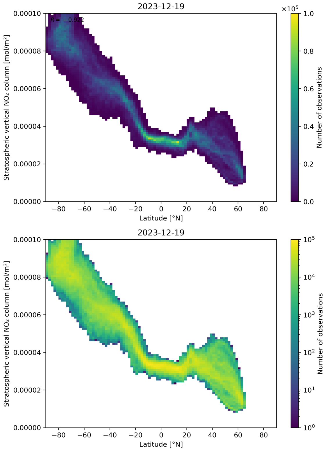
Figure 87: Scatter density plot of “Latitude” against “Stratospheric vertical NO 2 column” for 2023-12-18 to 2023-12-20.
