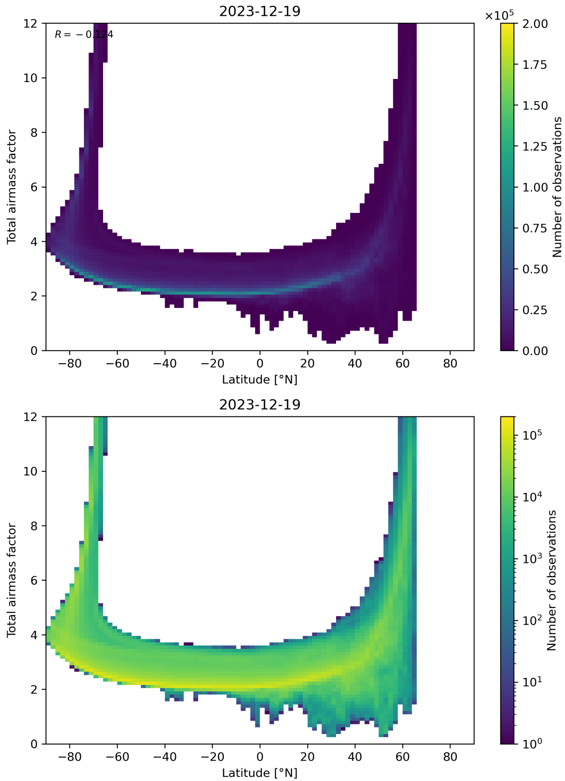
Figure 84: Scatter density plot of “Latitude” against “Total airmass factor” for 2023-12-18 to 2023-12-20.
