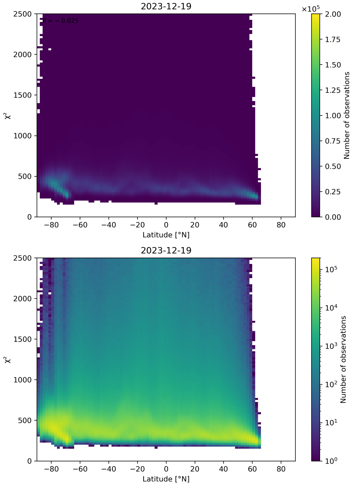
Figure 86: Scatter density plot of “Latitude” against “ \chi^2 ” for 2023-12-18 to 2023-12-20.
