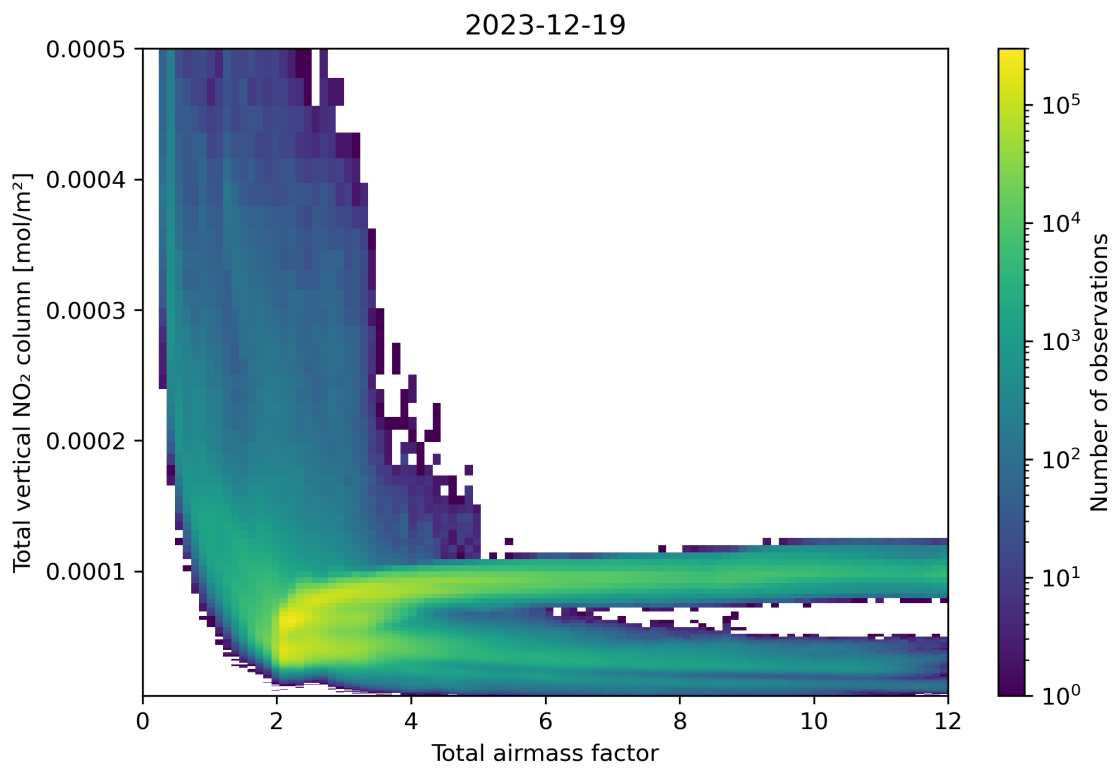
Figure 67: Scatter density plot of “Total airmass factor” against “Total vertical NO 2 column” for 2023-12-18 to 2023-12-20.
