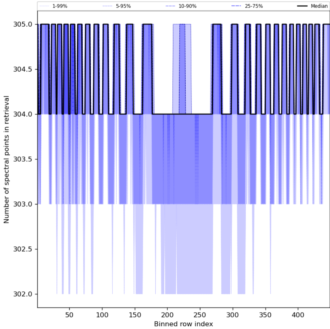
Figure 50: Along track statistics of “Number of spectral points in retrieval” for 2023-12-18 to 2023-12-20
