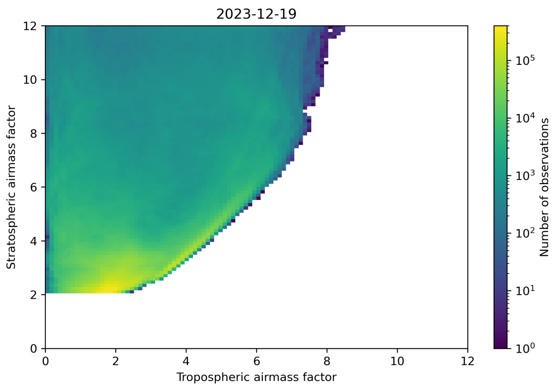
Figure 71: Scatter density plot of “Tropospheric airmass factor” against “Stratospheric airmass factor” for 2023-12-18 to 2023-12-20.
