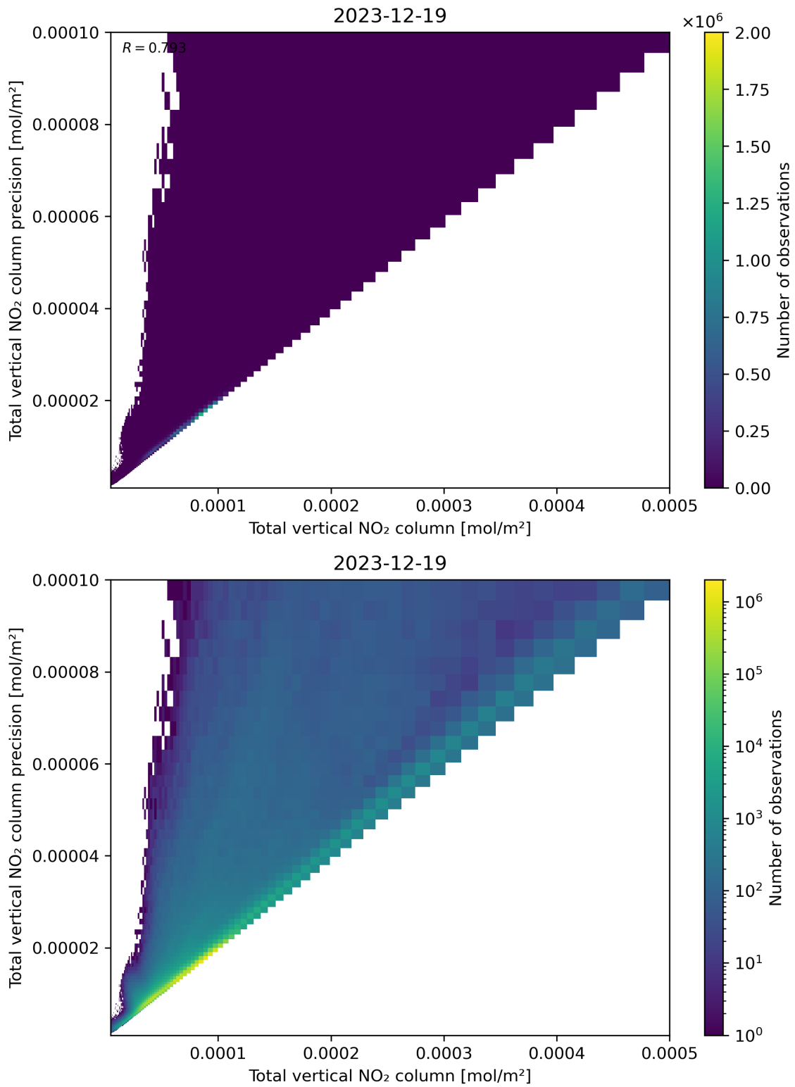
Figure 114: Scatter density plot of “Total vertical NO 2 column” against “Total vertical NO 2 column precision” for 2023-12-18 to 2023-12-20.
