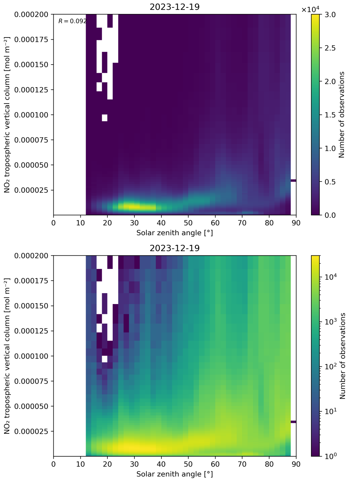
Figure 155: Scatter density plot of “Solar zenith angle” against “NO 2 tropospheric vertical column” for 2023-12-18 to 2023-12-20.
