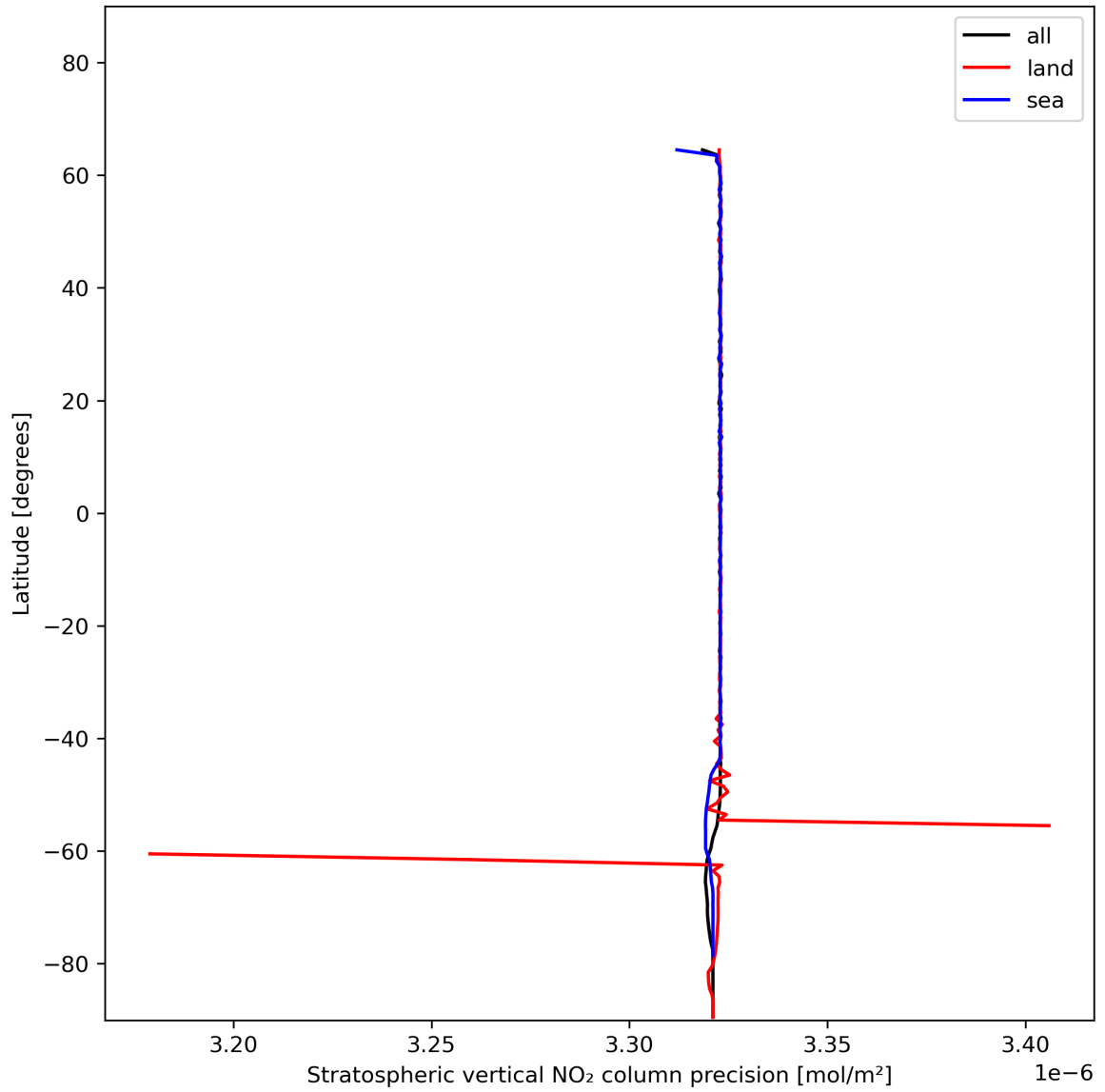
Figure 20: Zonal average of “Stratospheric vertical NO 2 column precision” for 2023-12-18 to 2023-12-20.
