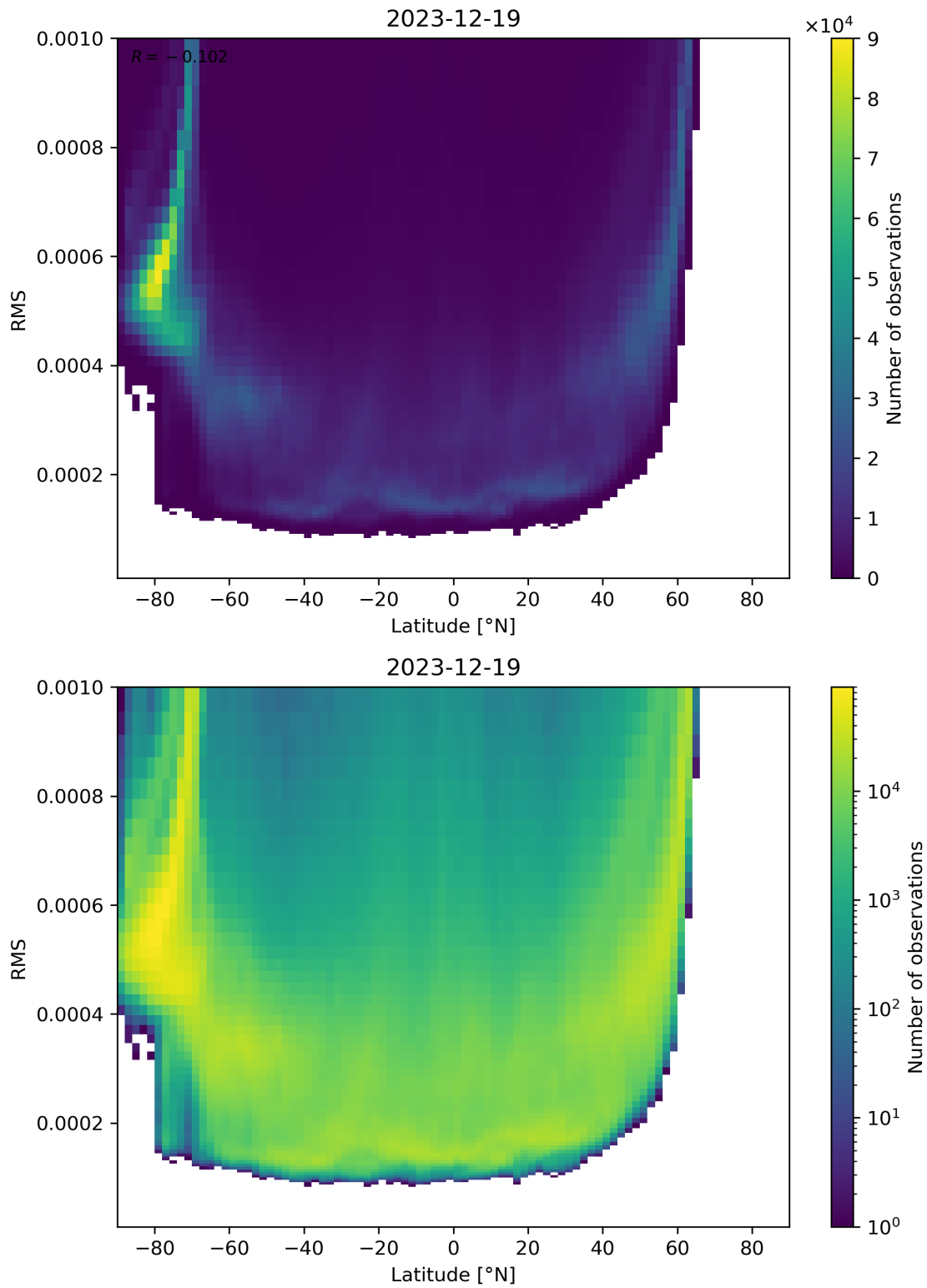
Figure 94: Scatter density plot of “Latitude” against “RMS” for 2023-12-18 to 2023-12-20.
