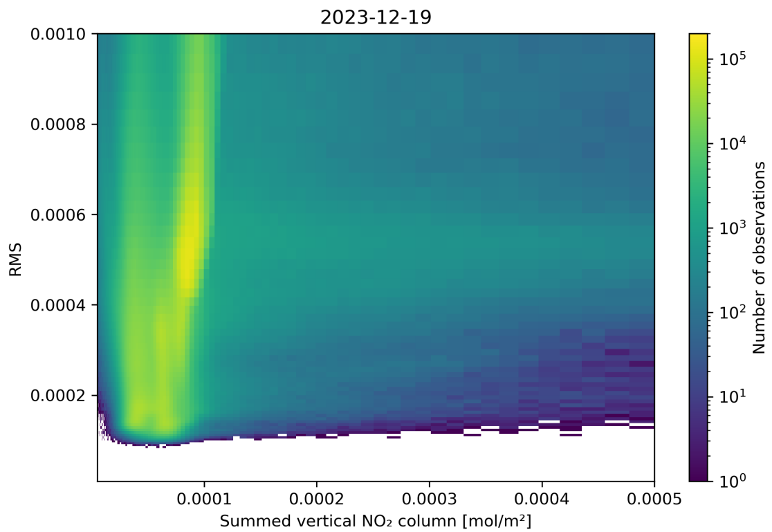
Figure 109: Scatter density plot of “Summed vertical NO 2 column” against “RMS” for 2023-12-18 to 2023-12-20.
