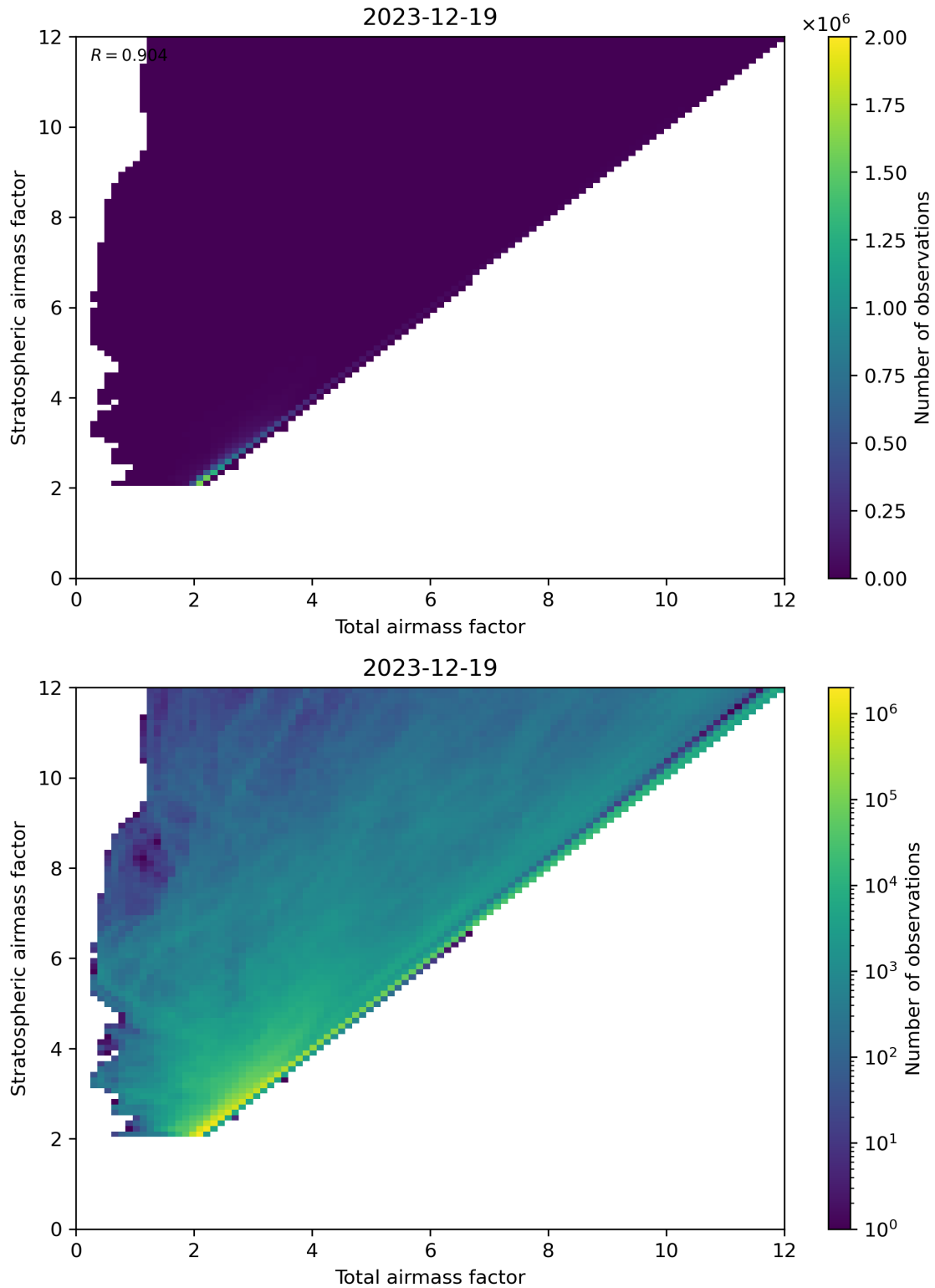
Figure 62: Scatter density plot of “Total airmass factor” against “Stratospheric airmass factor” for 2023-12-18 to 2023-12-20.
