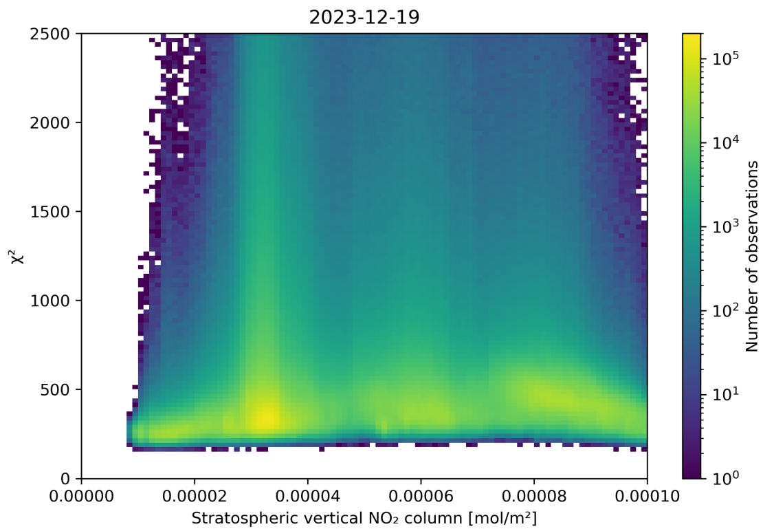
Figure 97: Scatter density plot of “Stratospheric vertical NO 2 column” against “ \chi^2 ” for 2023-12-18 to 2023-12-20.
