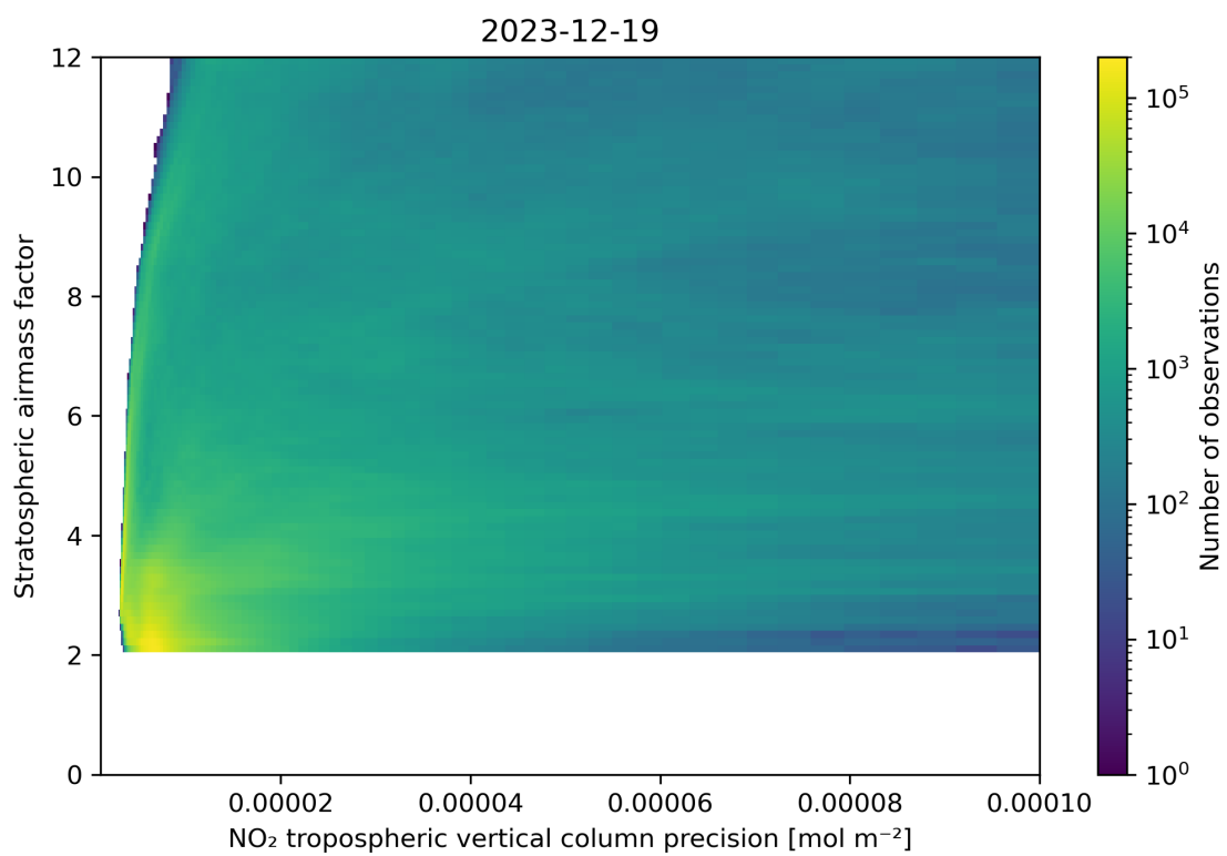
Figure 131: Scatter density plot of “NO 2 tropospheric vertical column precision” against “Stratospheric airmass factor” for 2023-12-18 to 2023-12-20.
