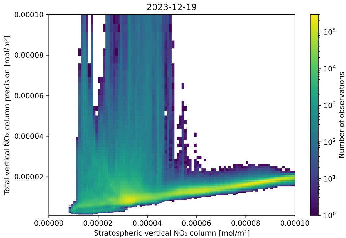
Figure 101: Scatter density plot of “Stratospheric vertical NO 2 column” against “Total vertical NO 2 column precision” for 2023-12-18 to 2023-12-20.
