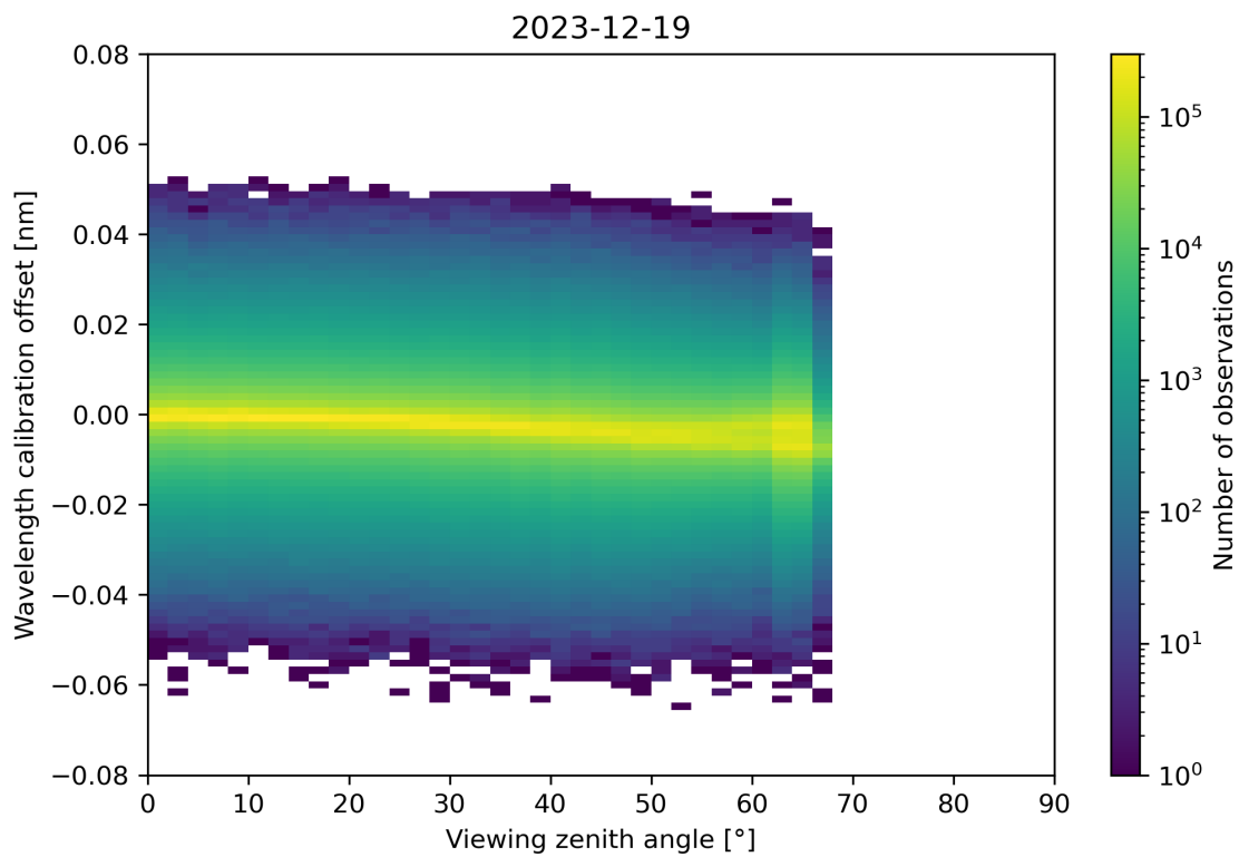
Figure 173: Scatter density plot of “Viewing zenith angle” against “Wavelength calibration offset” for 2023-12-18 to 2023-12-20.
