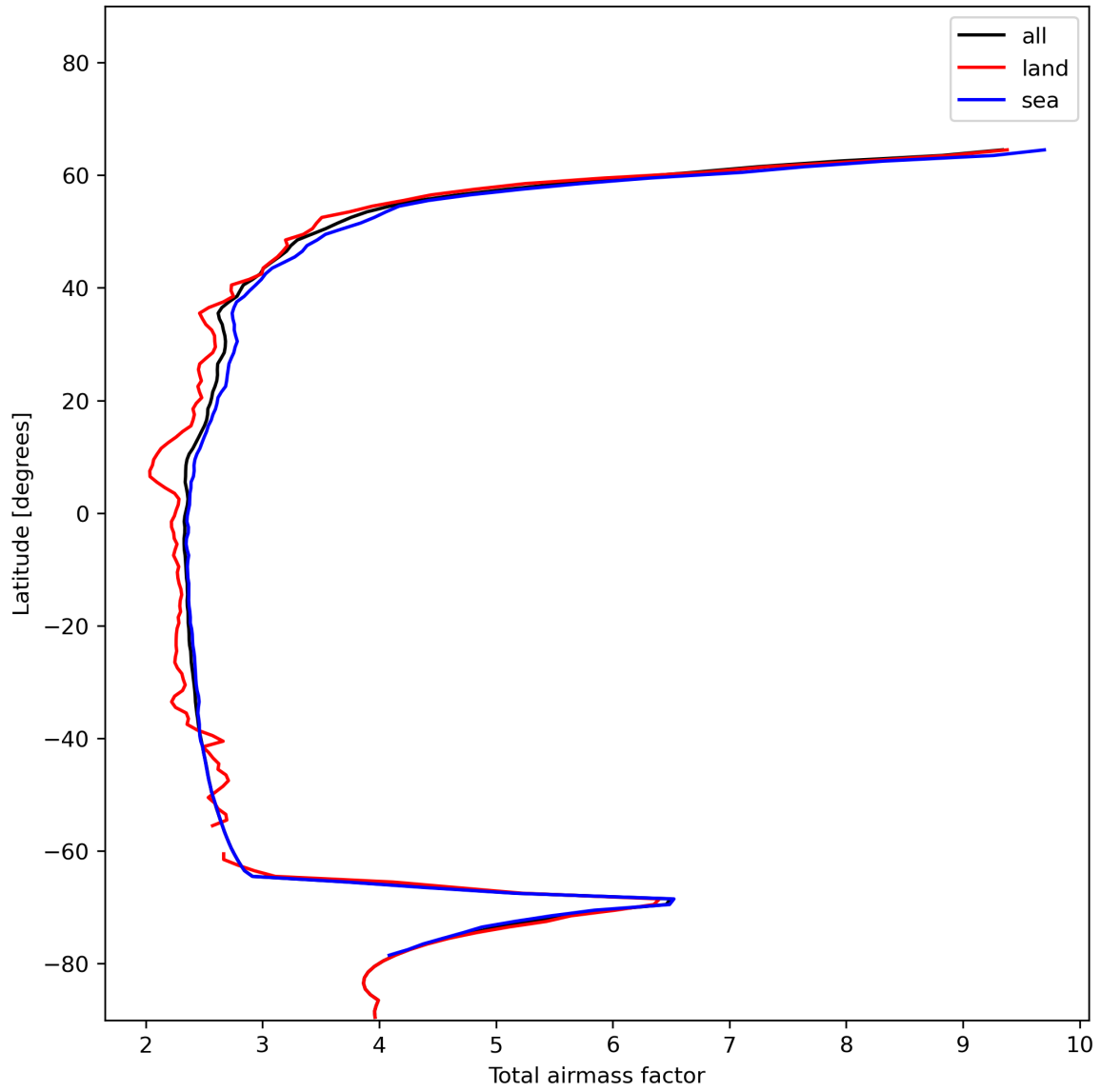
Figure 15: Zonal average of “Total airmass factor” for 2023-12-18 to 2023-12-20.
