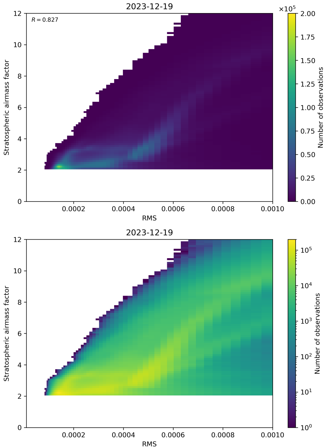
Figure 144: Scatter density plot of “RMS” against “Stratospheric airmass factor” for 2023-12-18 to 2023-12-20.
