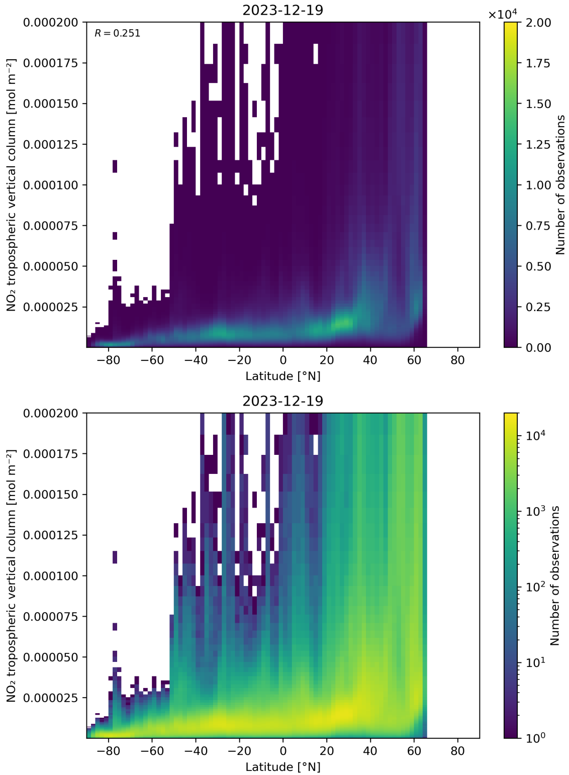
Figure 92: Scatter density plot of “Latitude” against “NO 2 tropospheric vertical column” for 2023-12-18 to 2023-12-20.
