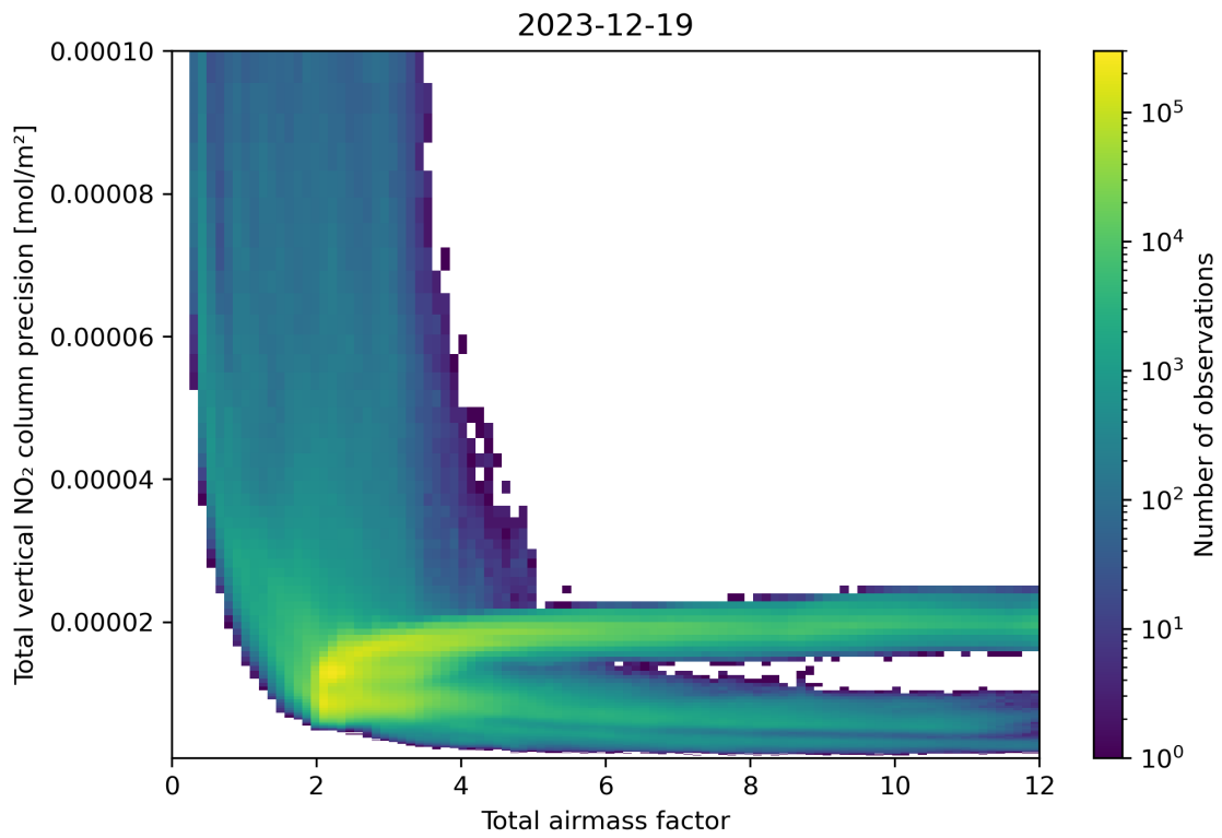
Figure 68: Scatter density plot of “Total airmass factor” against “Total vertical NO 2 column precision” for 2023-12-18 to 2023-12-20.
