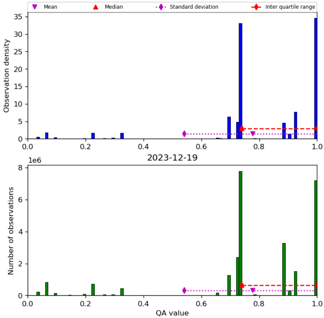
Figure 28: Histogram of “QA value” for 2023-12-18 to 2023-12-20
