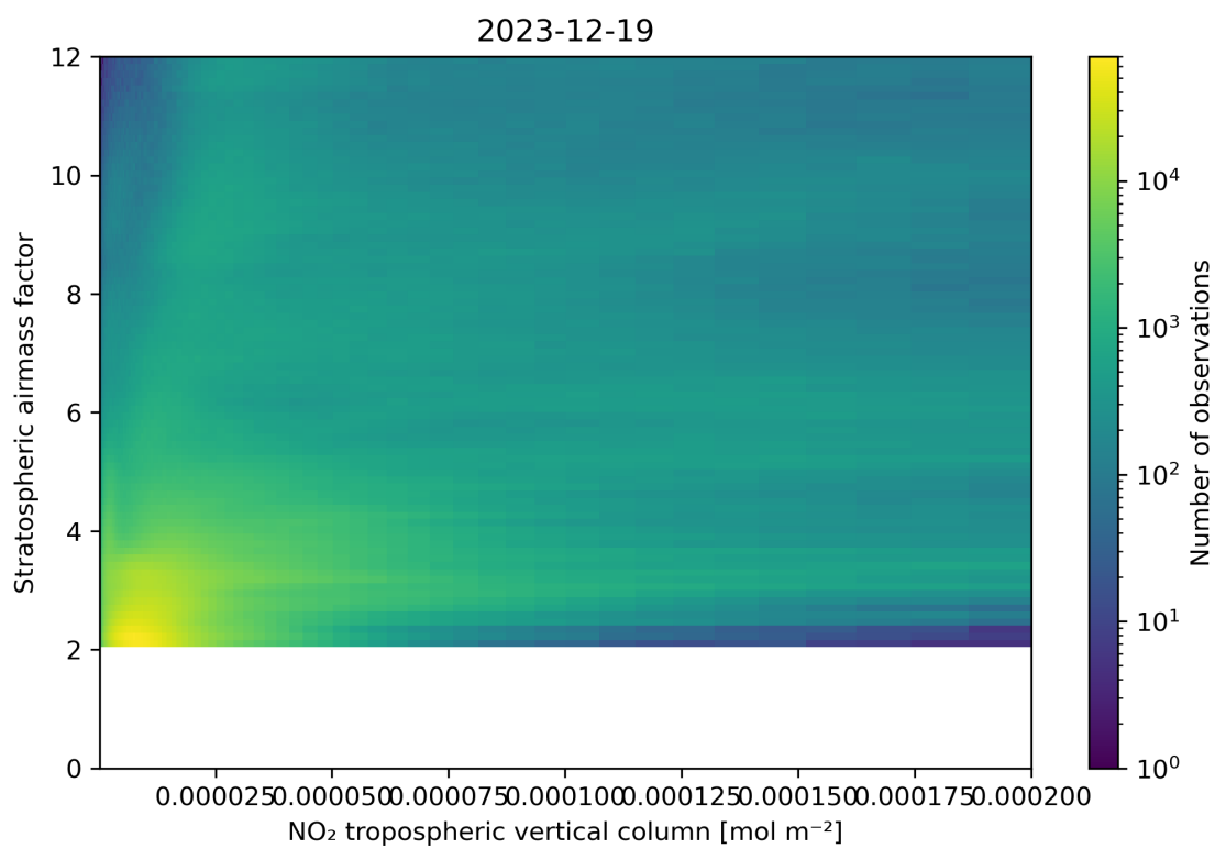
Figure 121: Scatter density plot of “NO 2 tropospheric vertical column” against “Stratospheric airmass factor” for 2023-12-18 to 2023-12-20.
