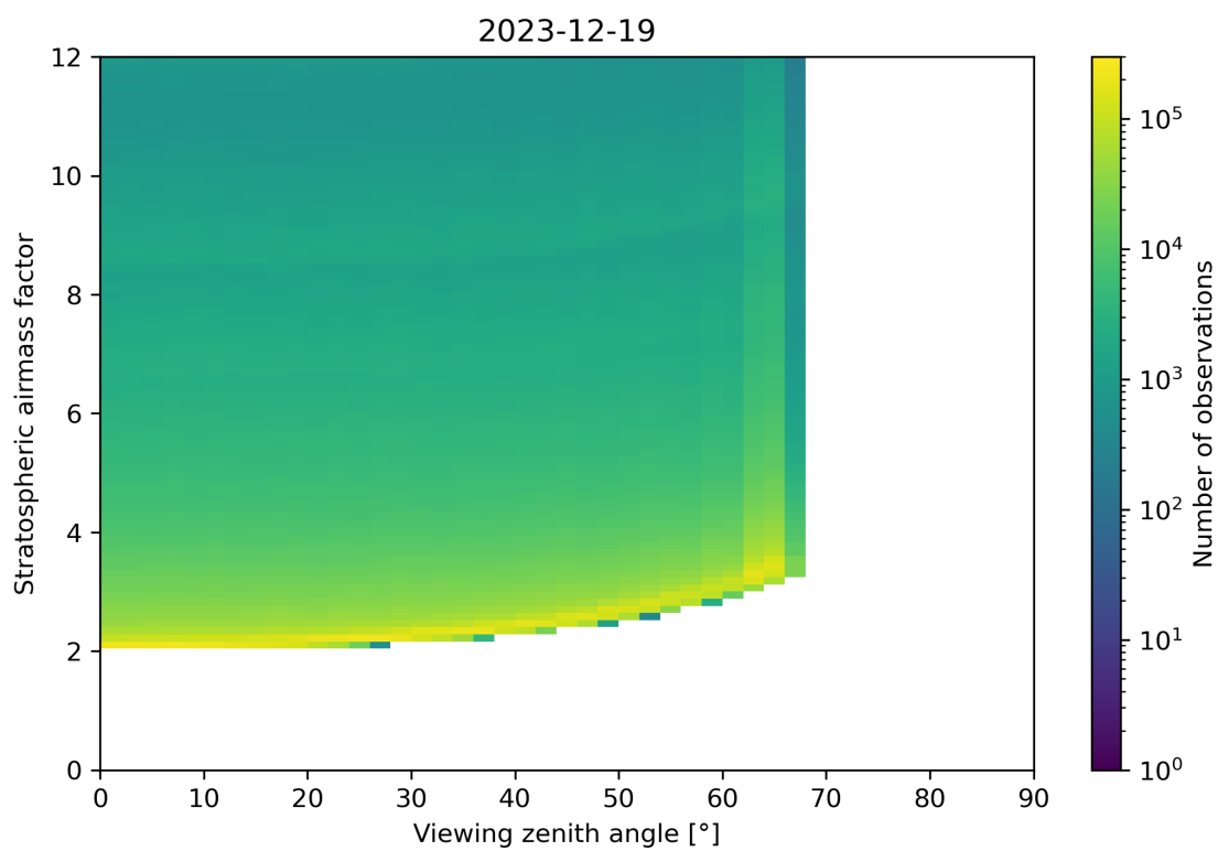
Figure 159: Scatter density plot of “Viewing zenith angle” against “Stratospheric airmass factor” for 2023-12-18 to 2023-12-20.
