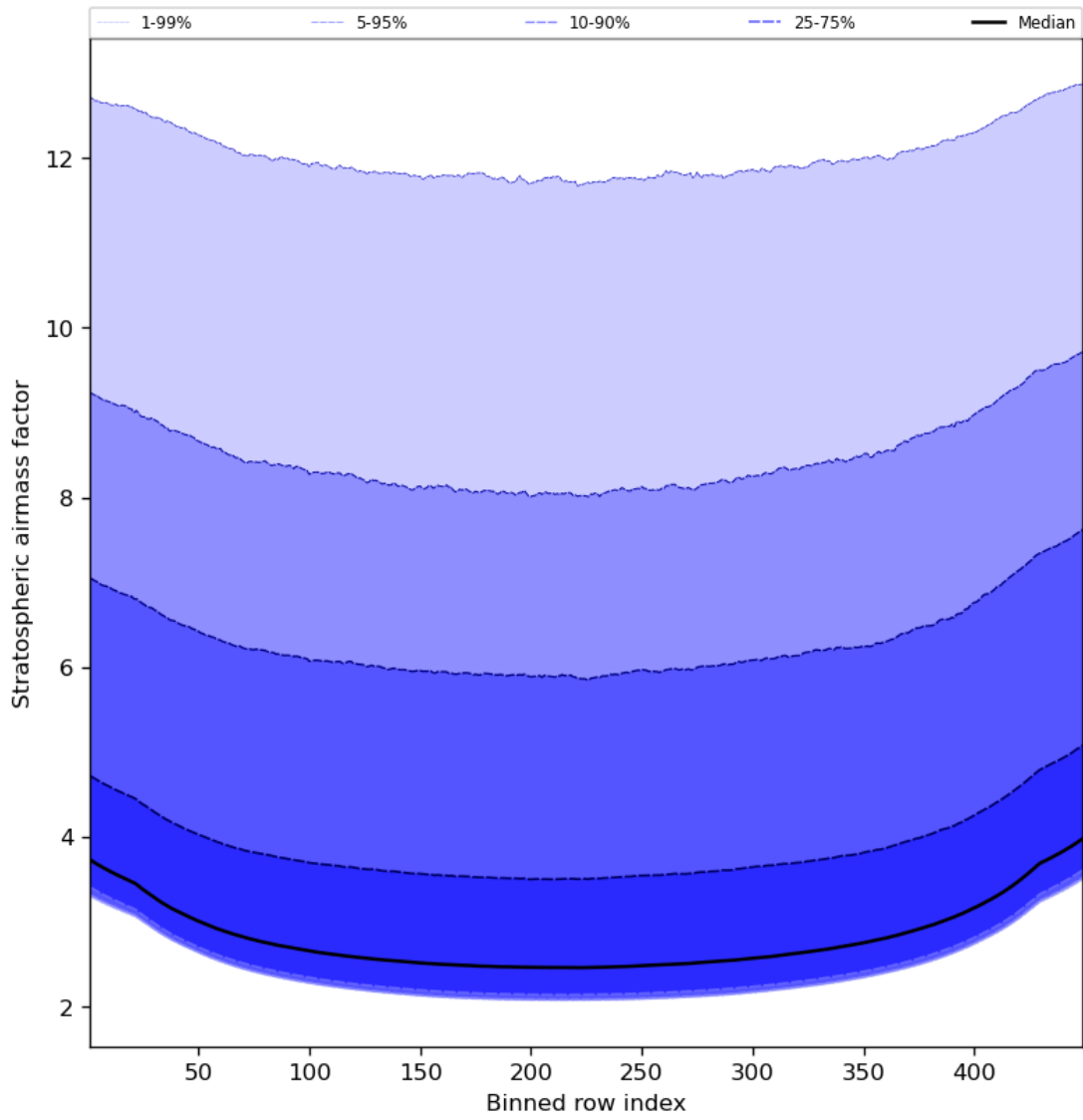
Figure 61: Along track statistics of “Stratospheric airmass factor” for 2023-12-18 to 2023-12-20
