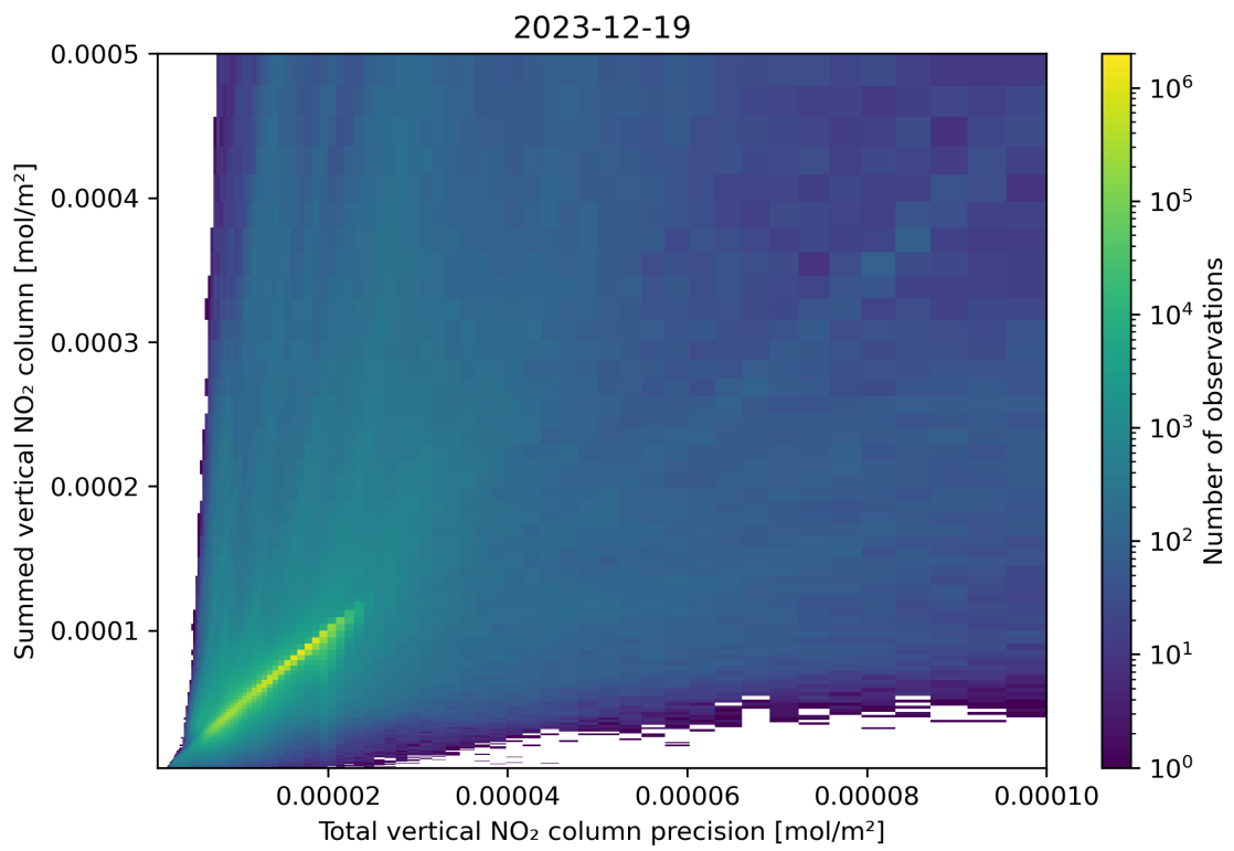
Figure 117: Scatter density plot of “Total vertical NO 2 column precision” against “Summed vertical NO 2 column” for 2023-12-18 to 2023-12-20.
