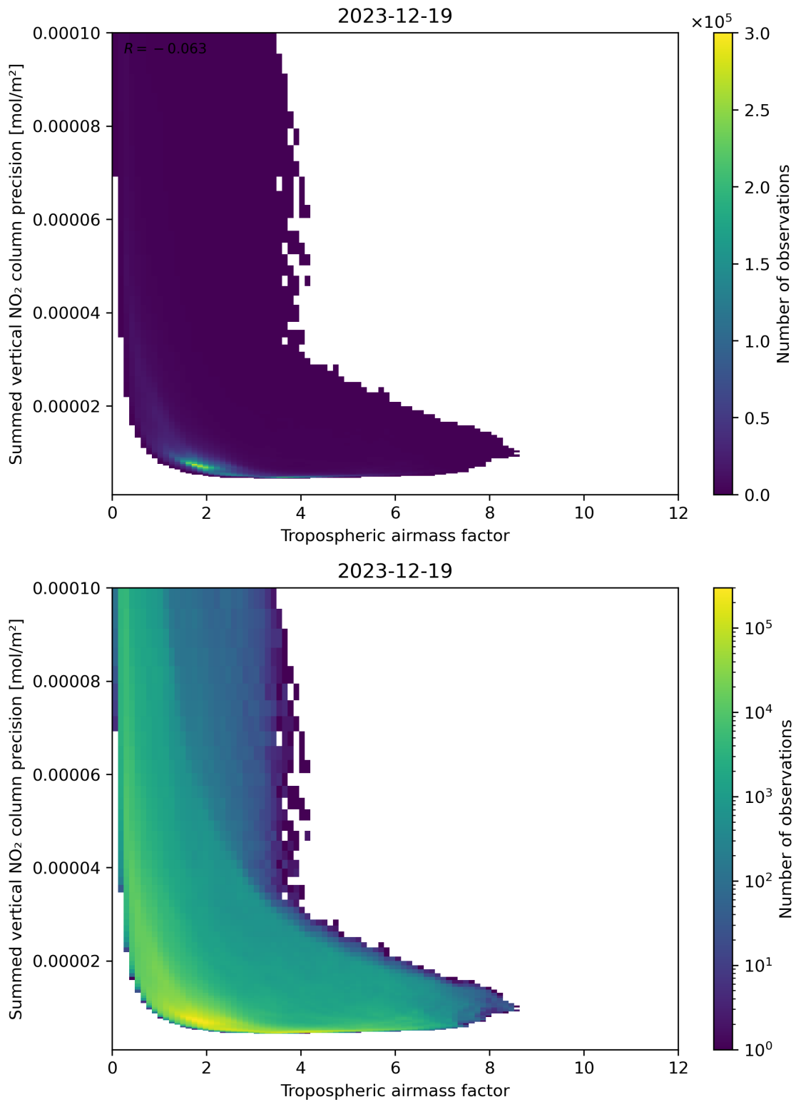
Figure 76: Scatter density plot of “Tropospheric airmass factor” against “Summed vertical NO 2 column precision” for 2023-12-18 to 2023-12-20.
