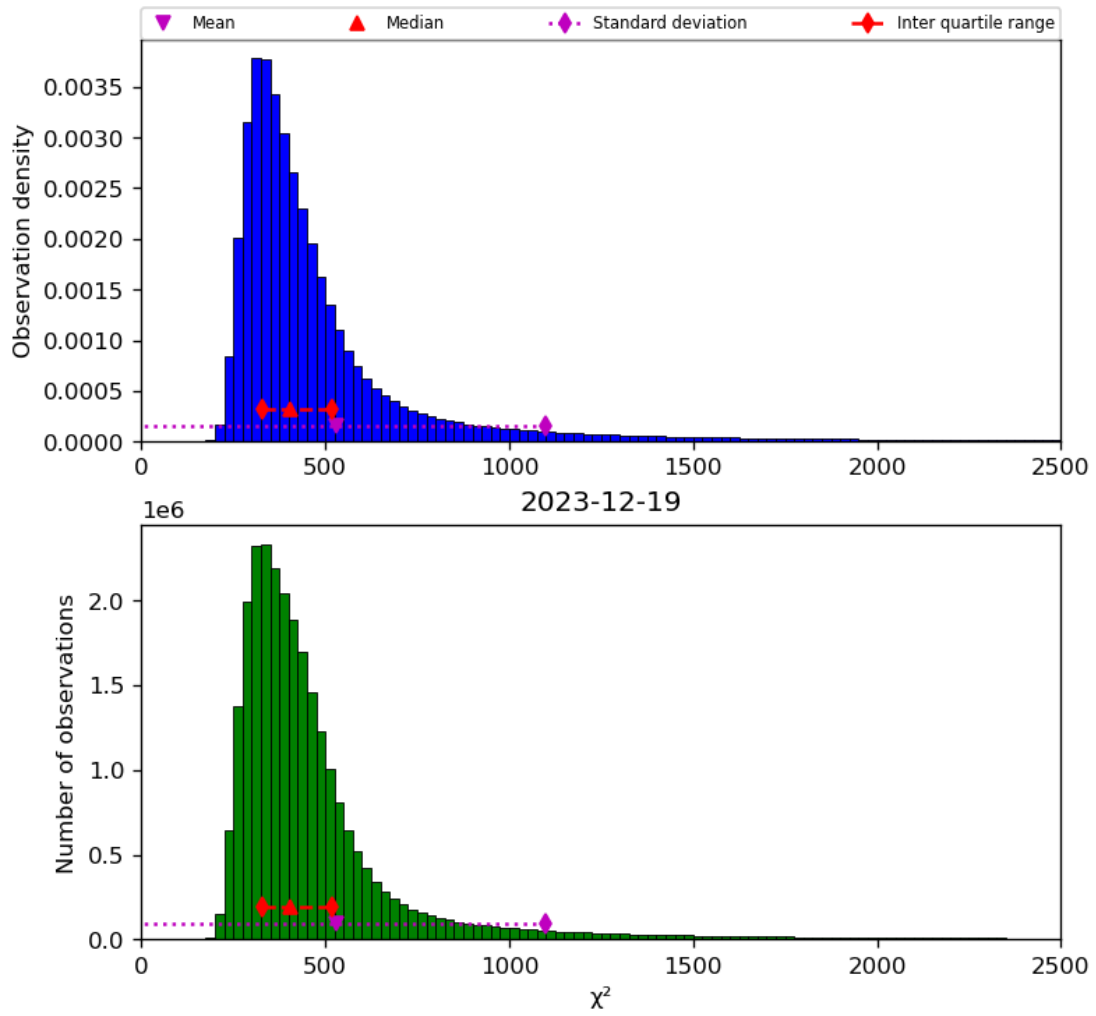
Figure 42: Histogram of " \chi^2 " for 2023-12-18 to 2023-12-20
