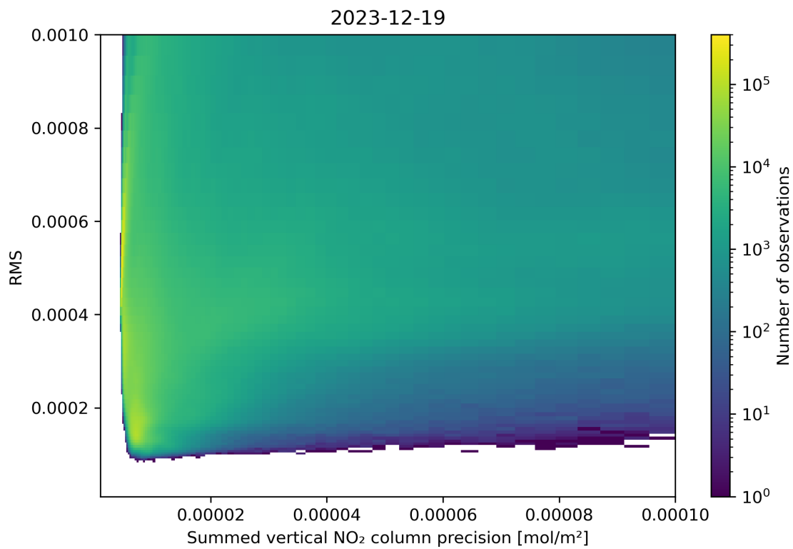
Figure 108: Scatter density plot of “Summed vertical NO 2 column precision” against “RMS” for 2023-12-18 to 2023-12-20.
