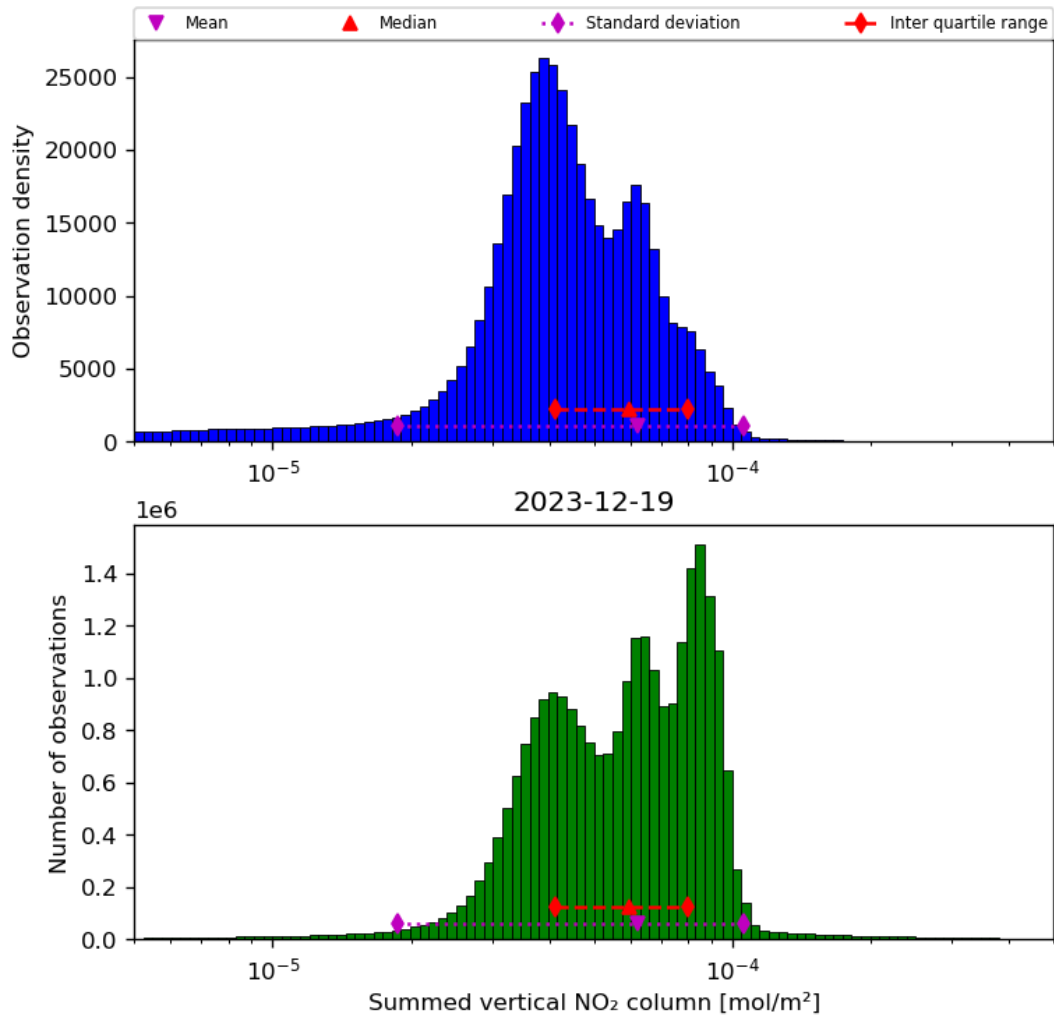
Figure 40: Histogram of “Summed vertical NO 2 column” for 2023-12-18 to 2023-12-20
