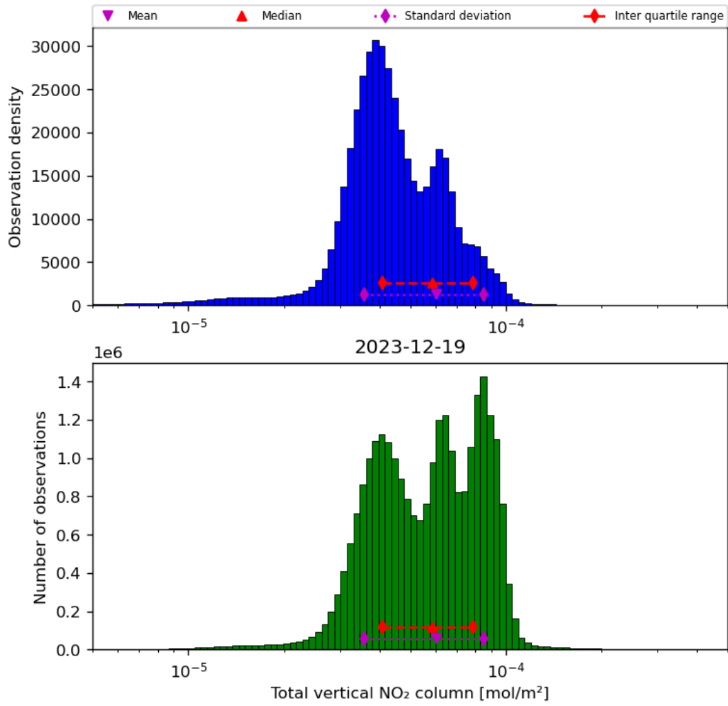
Figure 38: Histogram of “Total vertical NO 2 column” for 2023-12-18 to 2023-12-20
