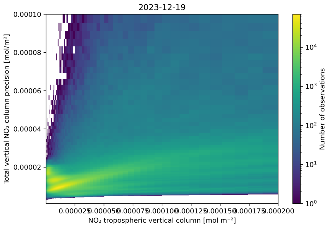
Figure 129: Scatter density plot of “NO 2 tropospheric vertical column” against “Total vertical NO 2 column precision” for 2023-12-18 to 2023-12-20.
