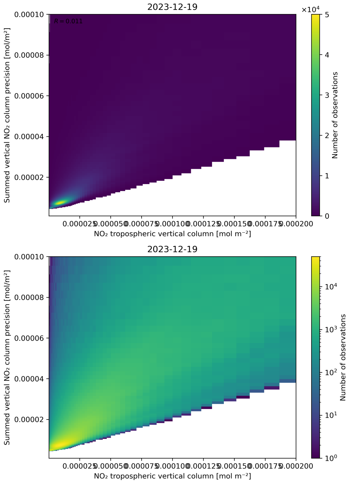
Figure 127: Scatter density plot of “NO 2 tropospheric vertical column” against “Summed vertical NO 2 column precision” for 2023-12-18 to 2023-12-20.
