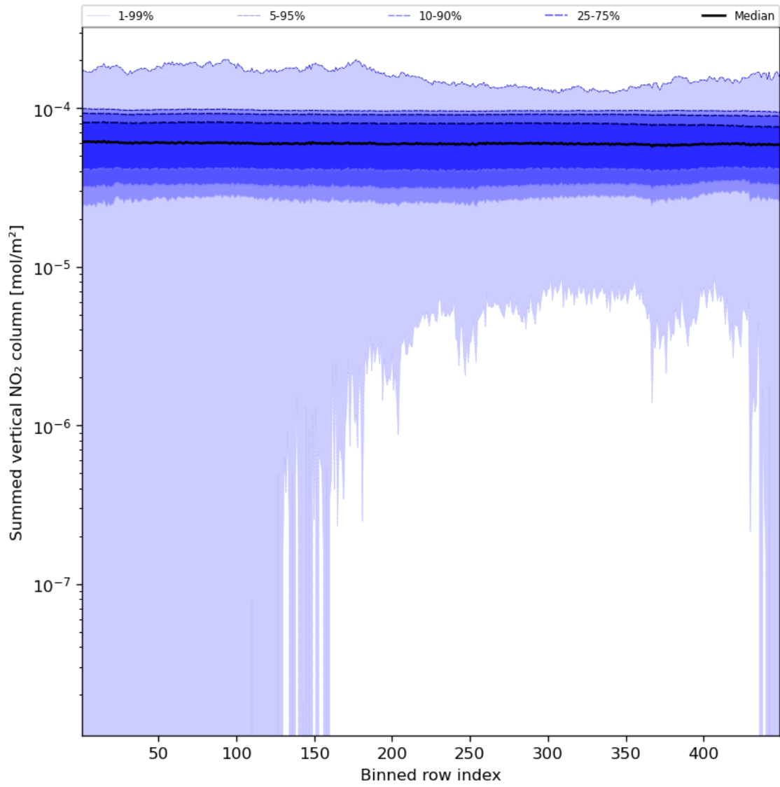
Figure 57: Along track statistics of “Summed vertical NO 2 column” for 2023-12-18 to 2023-12-20
