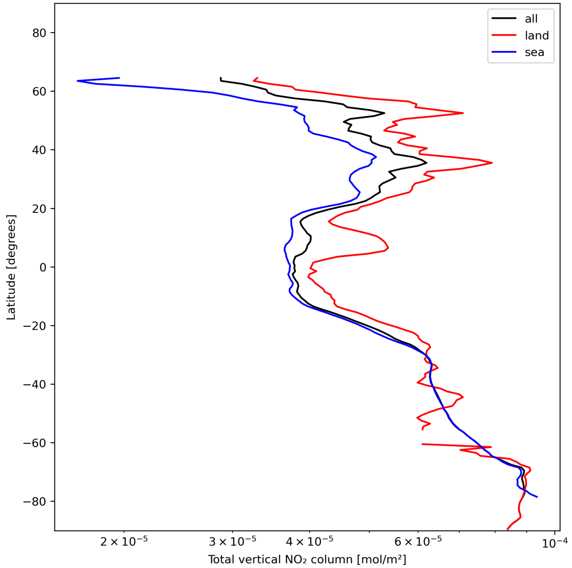
Figure 21: Zonal average of “Total vertical NO 2 column” for 2023-12-18 to 2023-12-20.
