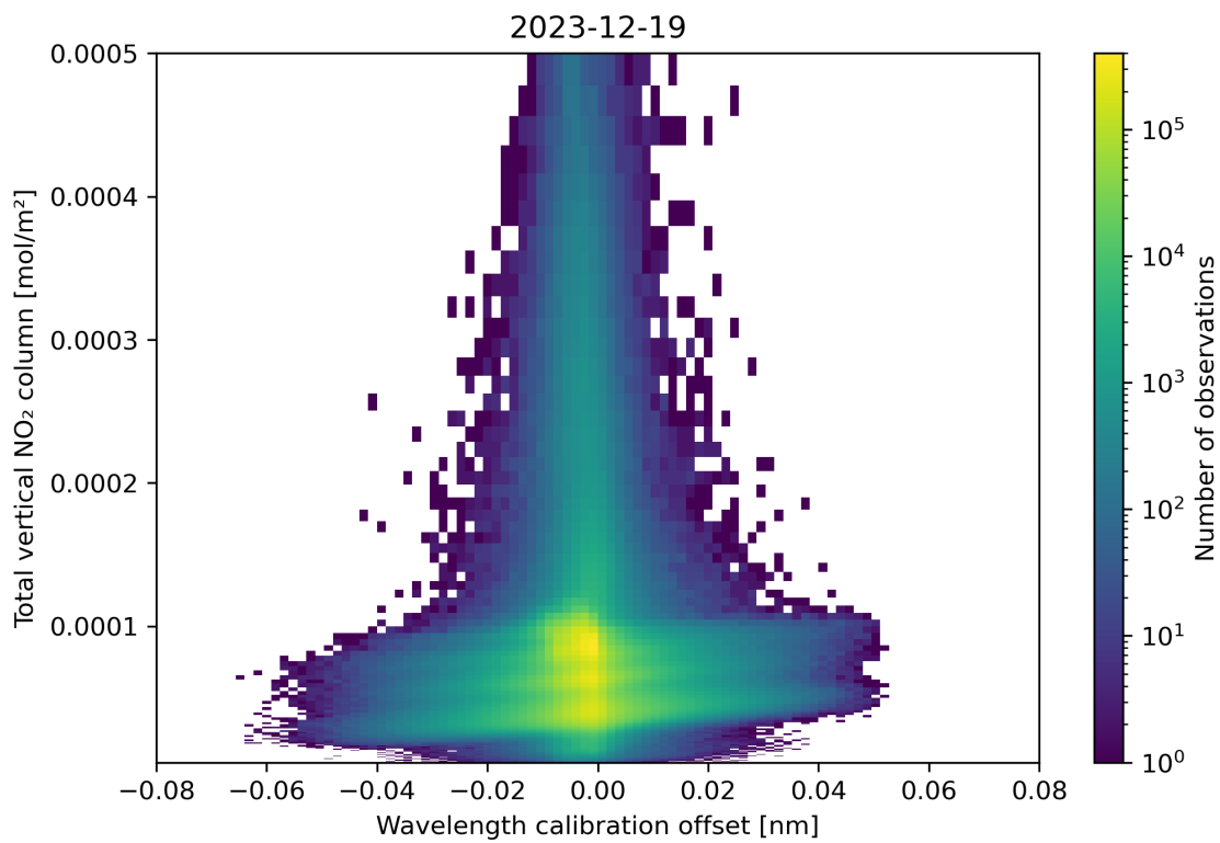
Figure 179: Scatter density plot of “Wavelength calibration offset” against “Total vertical NO 2 column” for 2023-12-18 to 2023-12-20.
