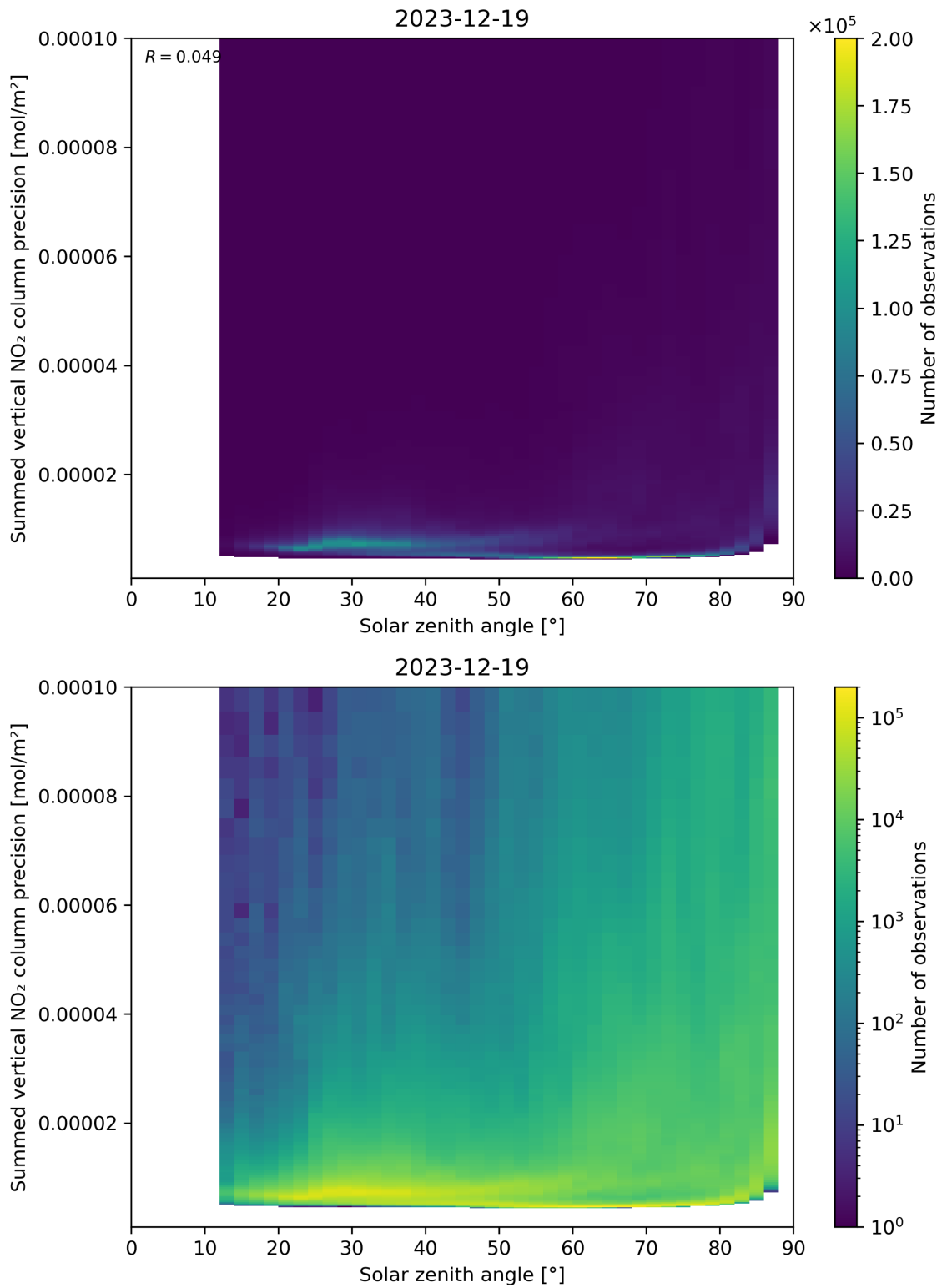
Figure 152: Scatter density plot of “Solar zenith angle” against “Summed vertical NO 2 column precision” for 2023-12-18 to 2023-12-20.
