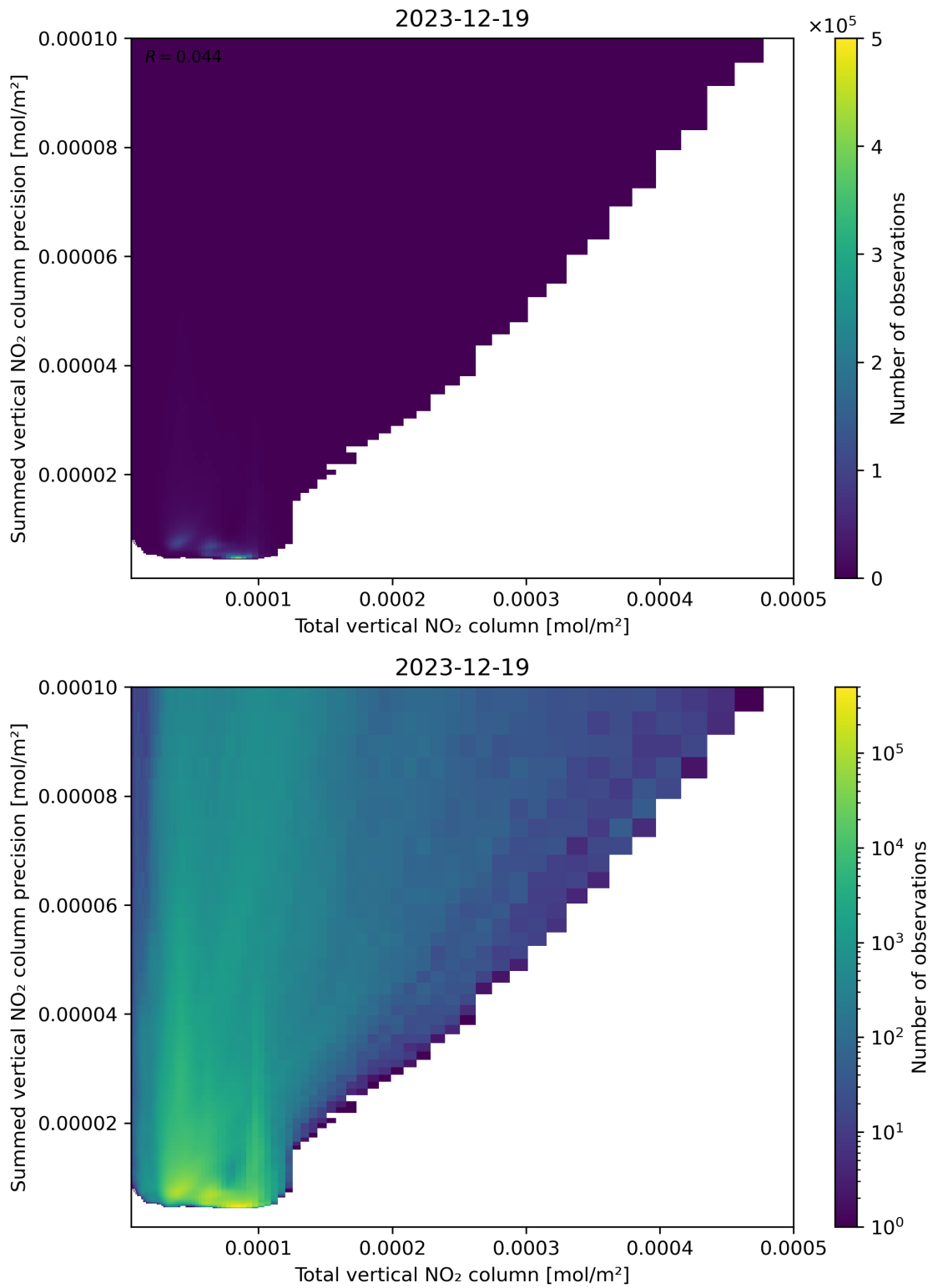
Figure 113: Scatter density plot of “Total vertical NO 2 column” against “Summed vertical NO 2 column precision” for 2023-12-18 to 2023-12-20.
