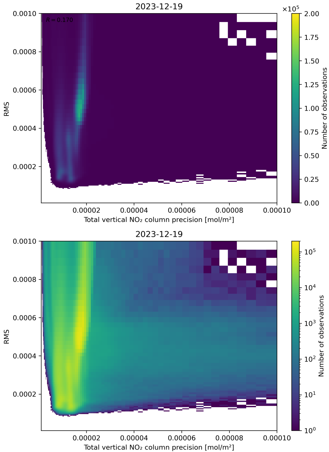
Figure 119: Scatter density plot of “Total vertical NO 2 column precision” against “RMS” for 2023-12-18 to 2023-12-20.
