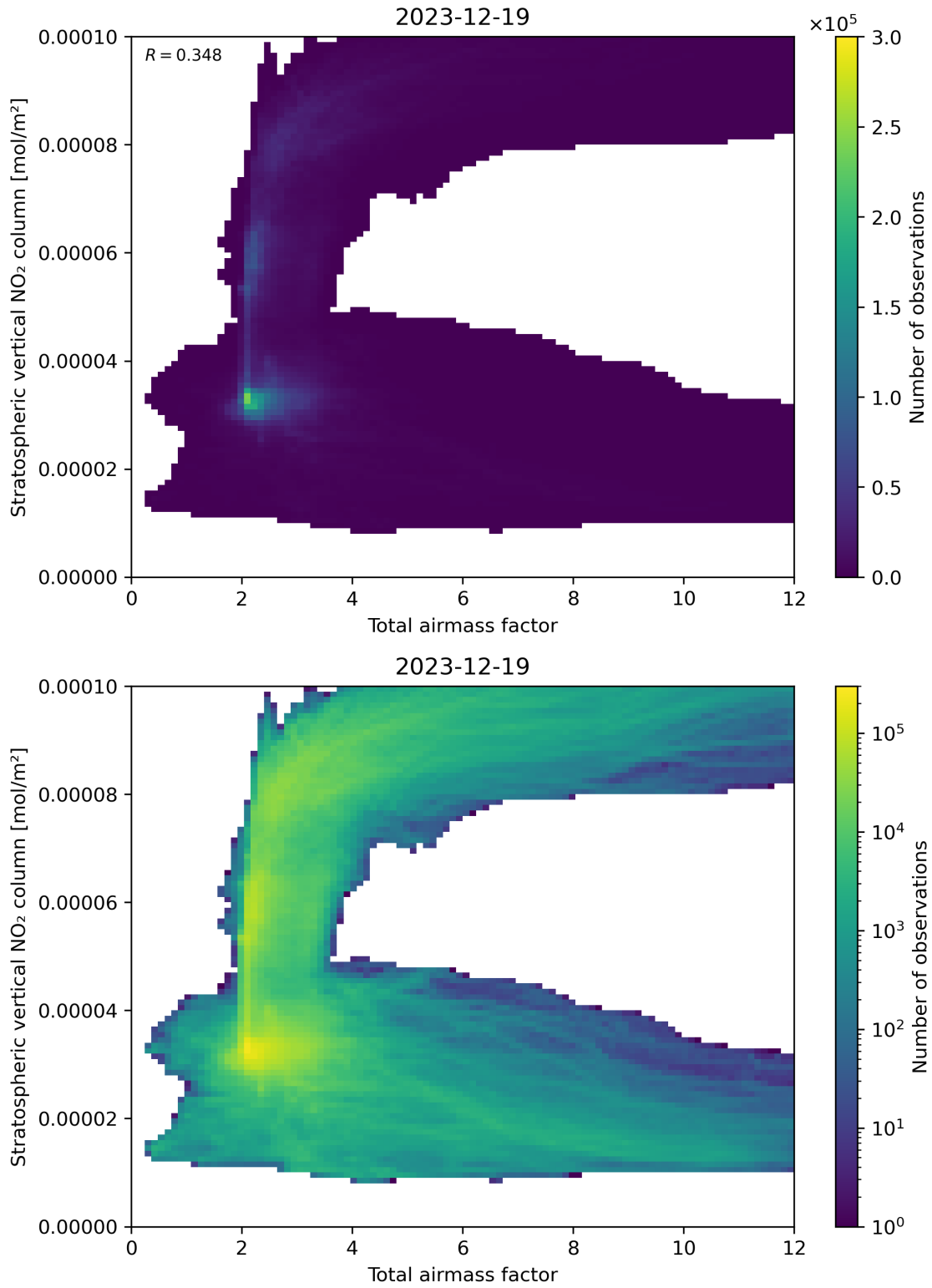
Figure 64: Scatter density plot of “Total airmass factor” against “Stratospheric vertical NO 2 column” for 2023-12-18 to 2023-12-20.
