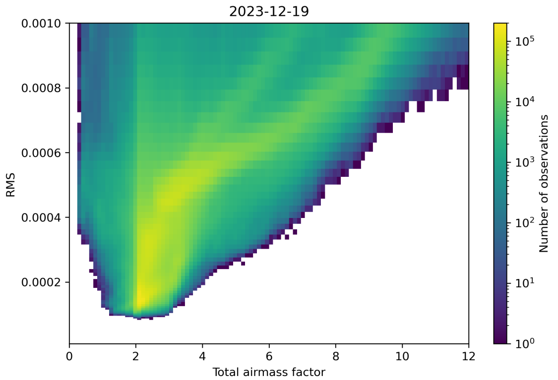
Figure 69: Scatter density plot of “Total airmass factor” against “RMS” for 2023-12-18 to 2023-12-20.
