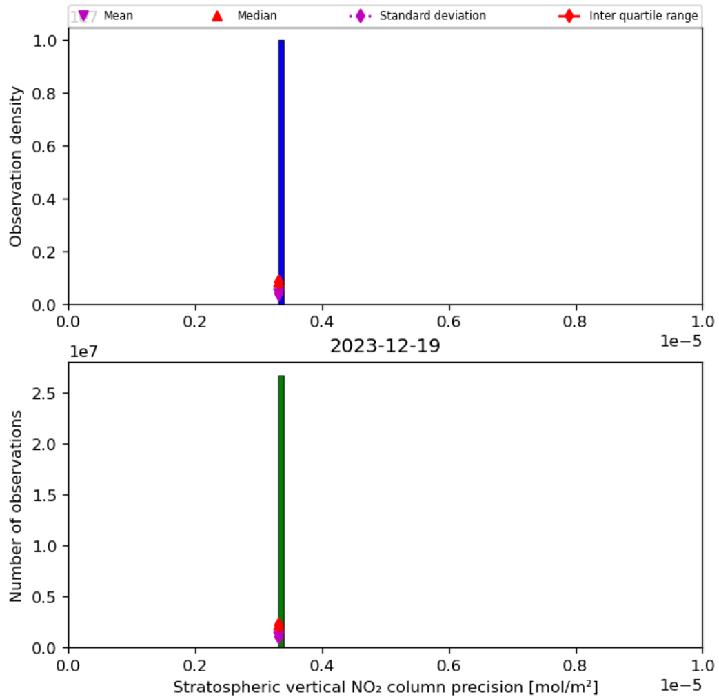
Figure 37: Histogram of “Stratospheric vertical NO 2 column precision” for 2023-12-18 to 2023-12-20
