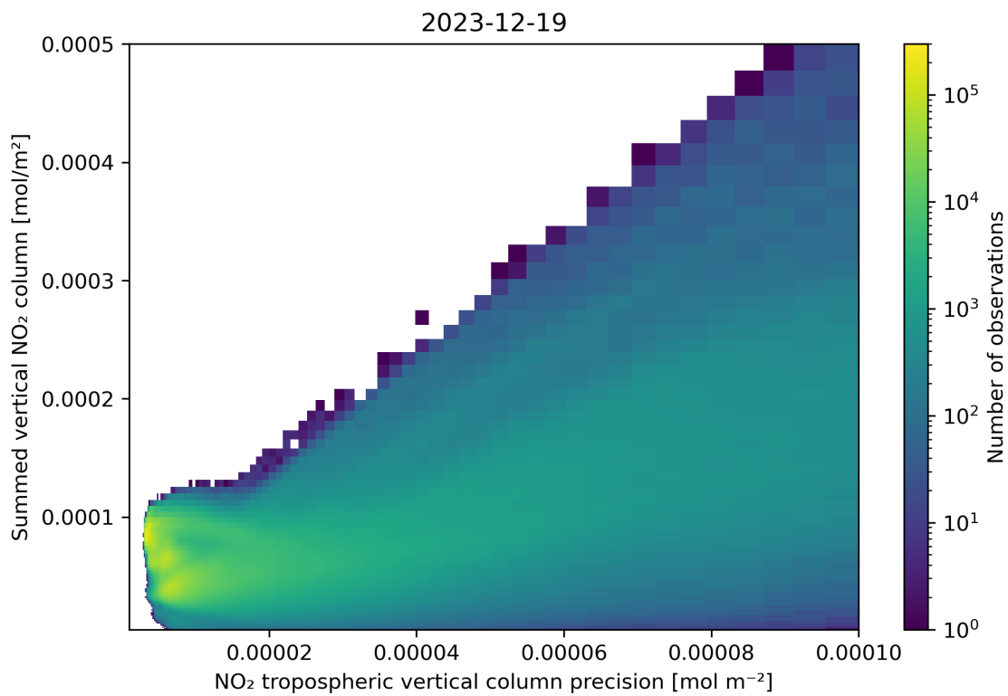
Figure 136: Scatter density plot of “NO 2 tropospheric vertical column precision” against “Summed vertical NO 2 column” for 2023-12-18 to 2023-12-20.
