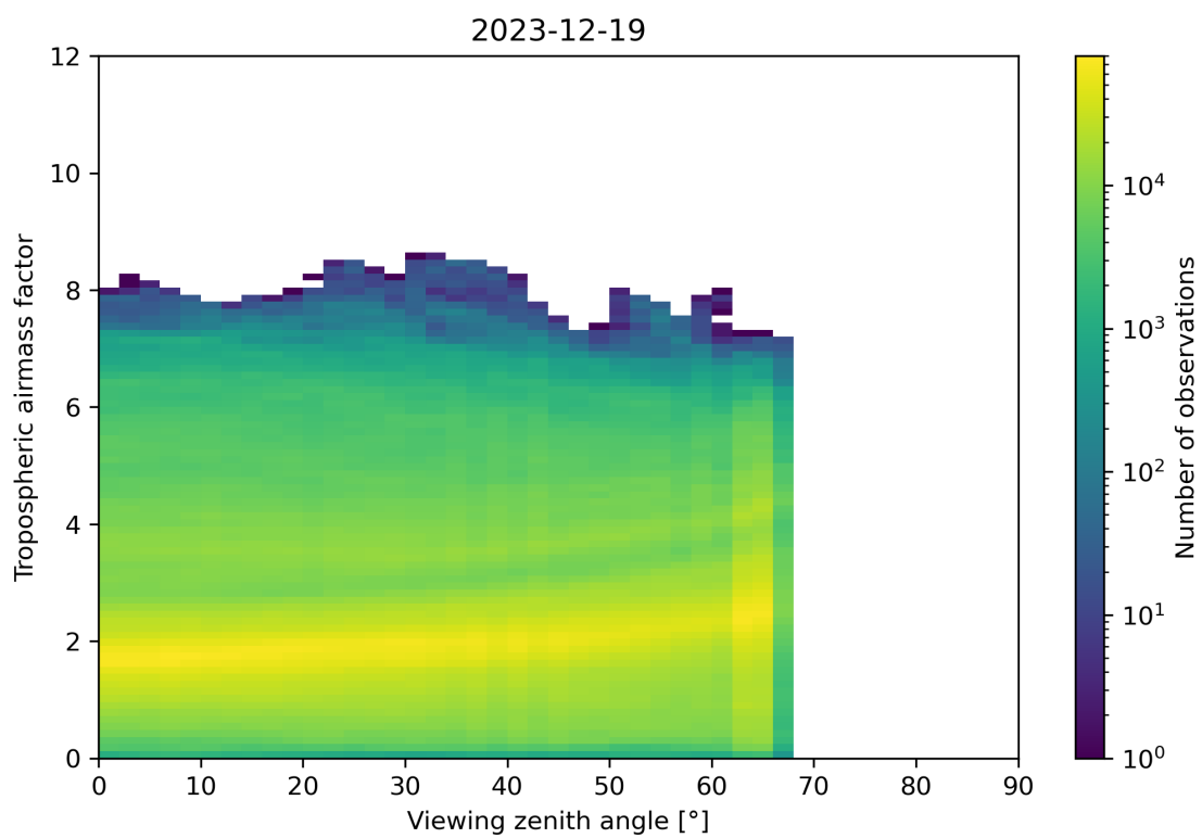
Figure 161: Scatter density plot of “Viewing zenith angle” against “Tropospheric airmass factor” for 2023-12-18 to 2023-12-20.
