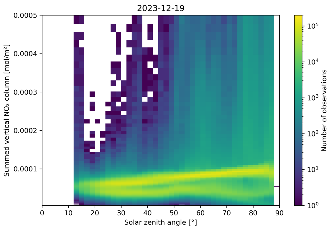
Figure 151: Scatter density plot of “Solar zenith angle” against “Summed vertical NO 2 column” for 2023-12-18 to 2023-12-20.
