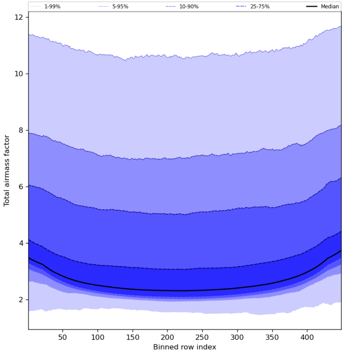
Figure 49: Along track statistics of “Total airmass factor” for 2023-12-18 to 2023-12-20
