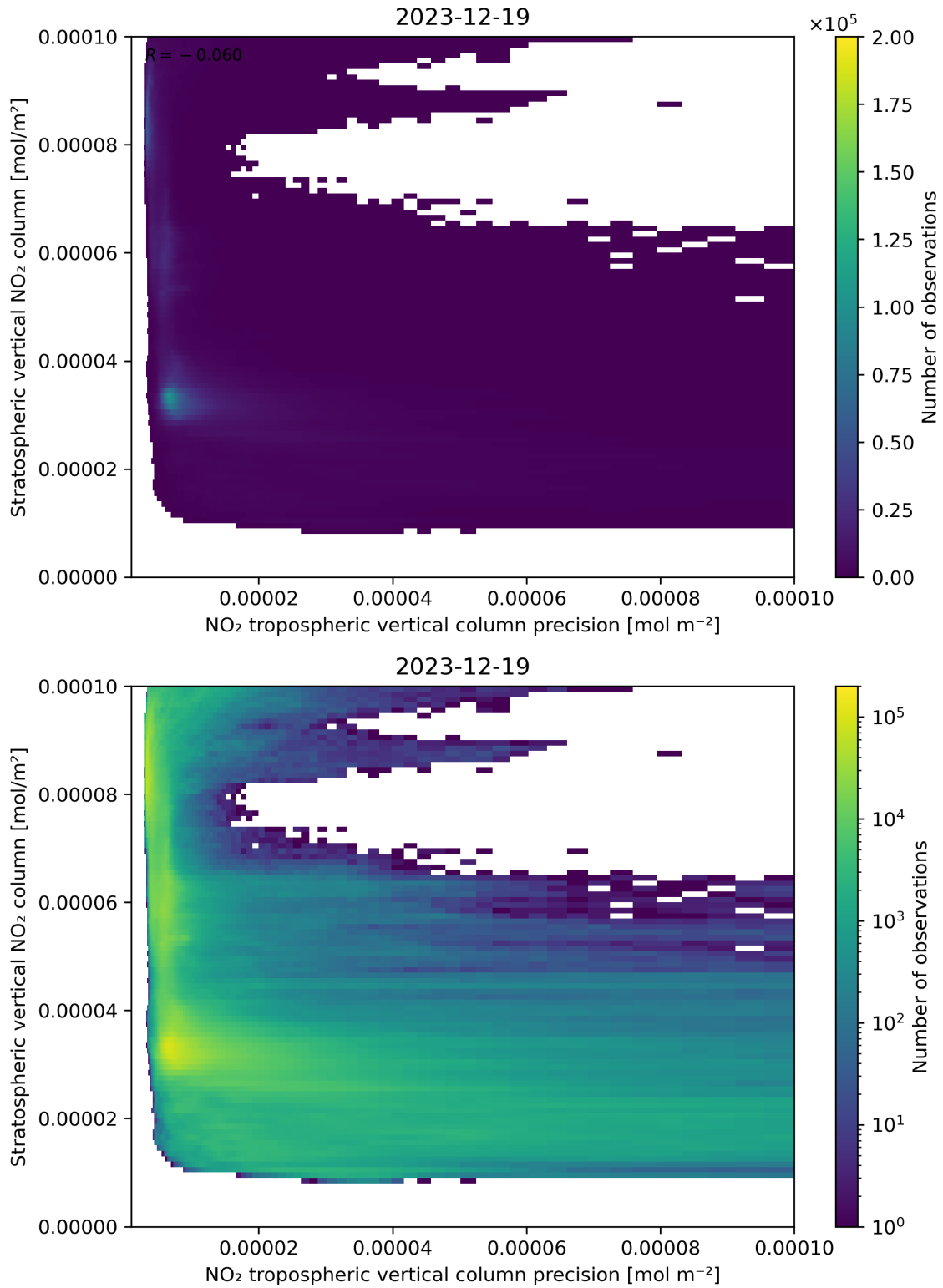
Figure 135: Scatter density plot of “NO 2 tropospheric vertical column precision” against “Stratospheric vertical NO 2 column” for 2023-12-18 to 2023-12-20.
