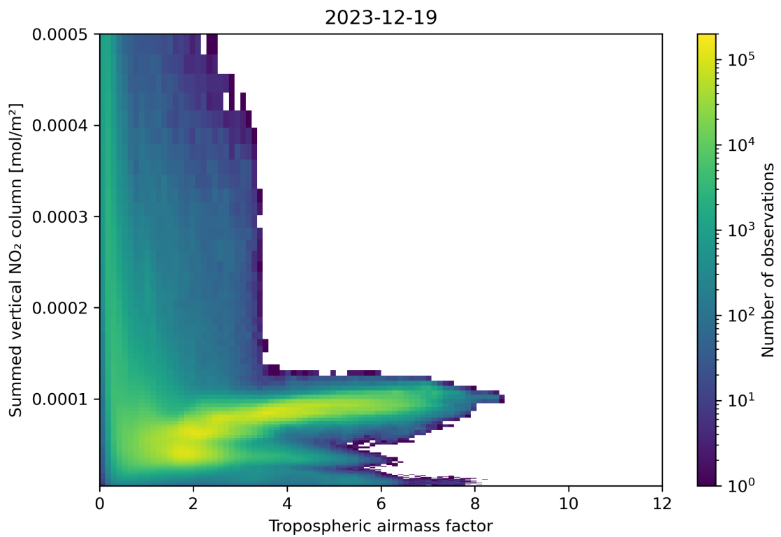
Figure 75: Scatter density plot of “Tropospheric airmass factor” against “Summed vertical NO 2 column” for 2023-12-18 to 2023-12-20.
