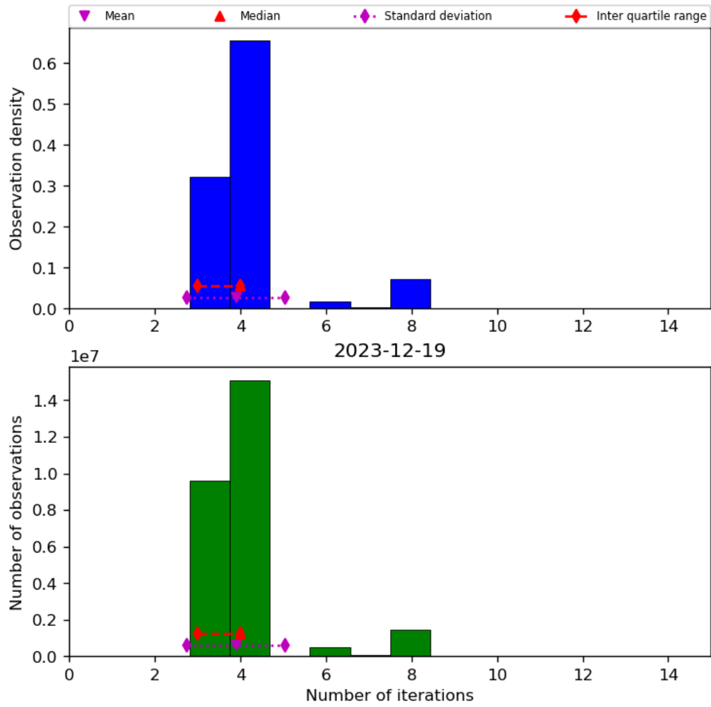
Figure 34: Histogram of “Number of iterations” for 2023-12-18 to 2023-12-20
