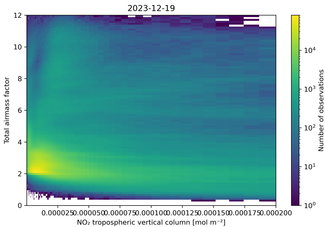
Figure 122: Scatter density plot of “NO 2 tropospheric vertical column” against “Total airmass factor” for 2023-12-18 to 2023-12-20.
