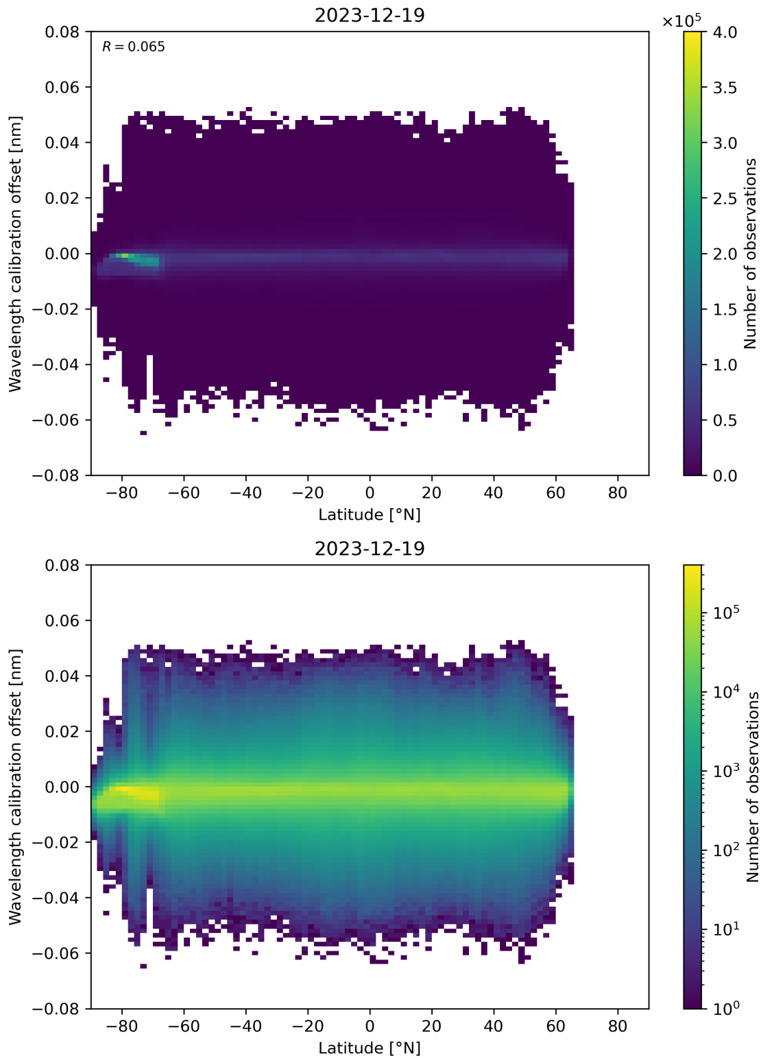
Figure 95: Scatter density plot of “Latitude” against “Wavelength calibration offset” for 2023-12-18 to 2023-12-20.
