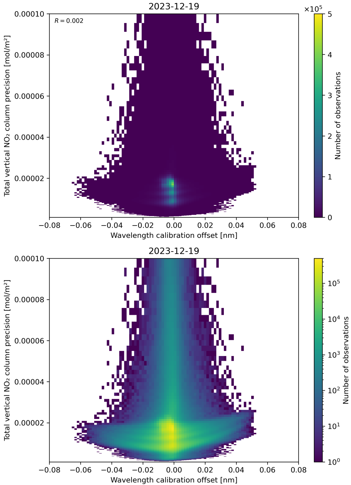
Figure 180: Scatter density plot of “Wavelength calibration offset” against “Total vertical NO 2 column precision” for 2023-12-18 to 2023-12-20.
