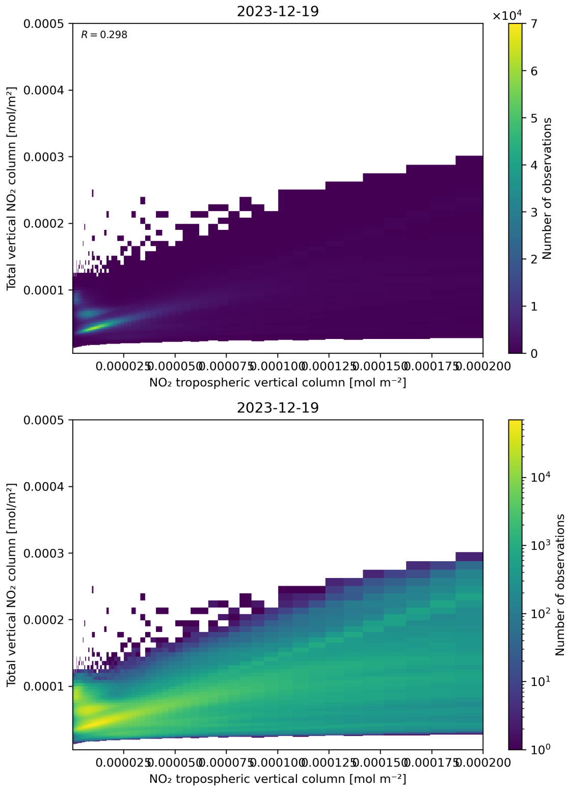
Figure 128: Scatter density plot of “NO 2 tropospheric vertical column” against “Total vertical NO 2 column” for 2023-12-18 to 2023-12-20.
