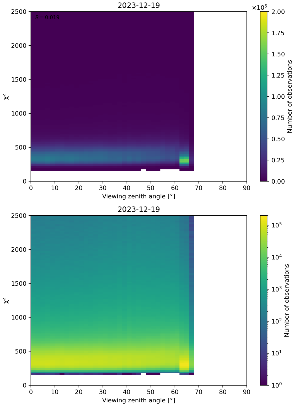
Figure 162: Scatter density plot of “Viewing zenith angle” against “ \chi^2 ” for 2023-12-18 to 2023-12-20.
