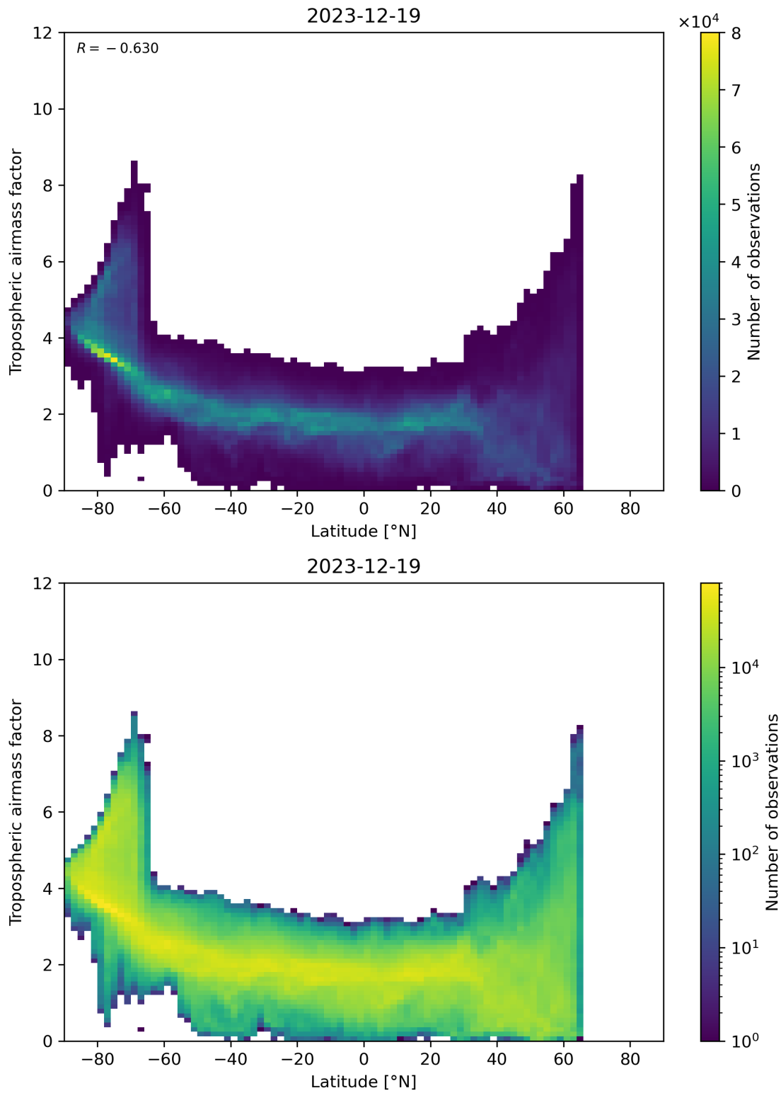
Figure 85: Scatter density plot of “Latitude” against “Tropospheric airmass factor” for 2023-12-18 to 2023-12-20.
