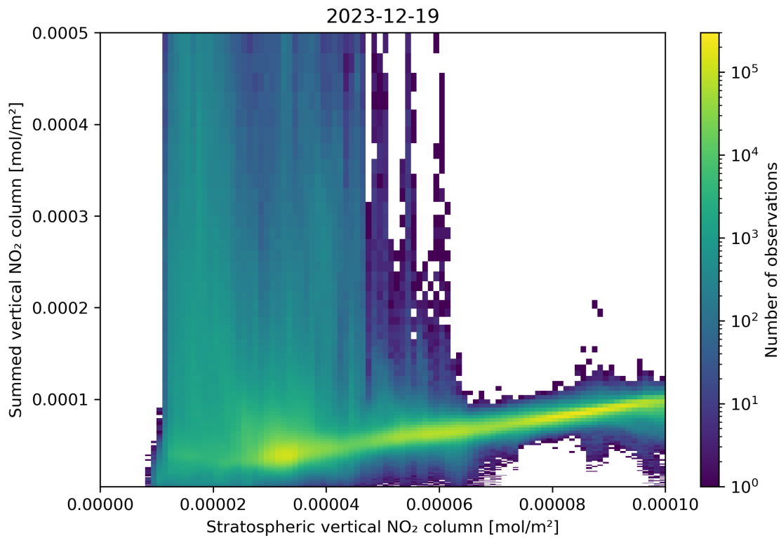
Figure 98: Scatter density plot of “Stratospheric vertical NO 2 column” against “Summed vertical NO 2 column” for 2023-12-18 to 2023-12-20.
