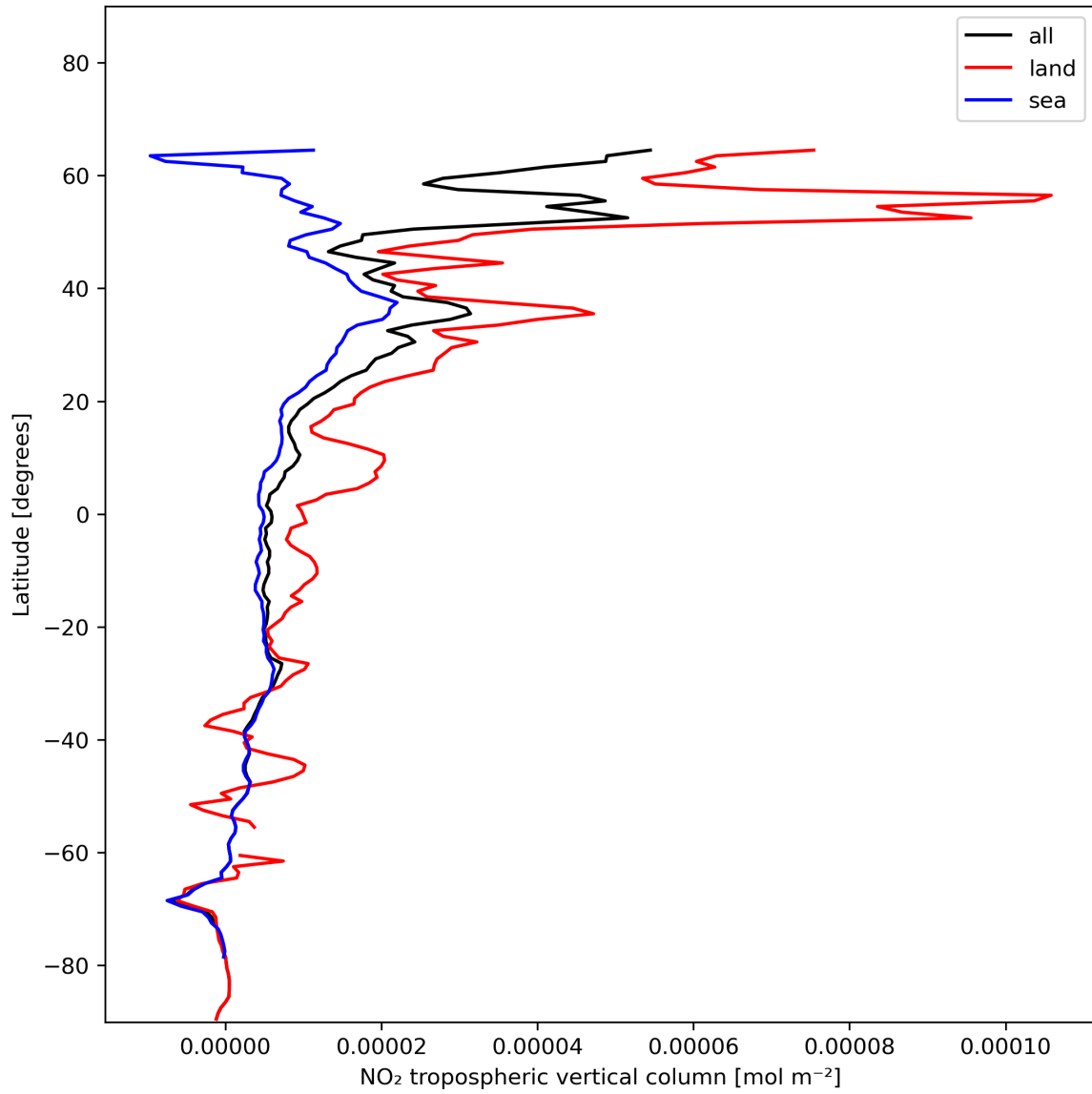
Figure 12: Zonal average of “NO 2 tropospheric vertical column” for 2023-12-18 to 2023-12-20.
