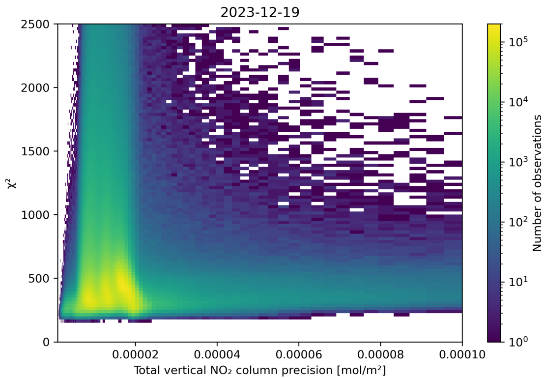
Figure 116: Scatter density plot of “Total vertical NO 2 column precision” against “ \chi^2 ” for 2023-12-18 to 2023-12-20.
