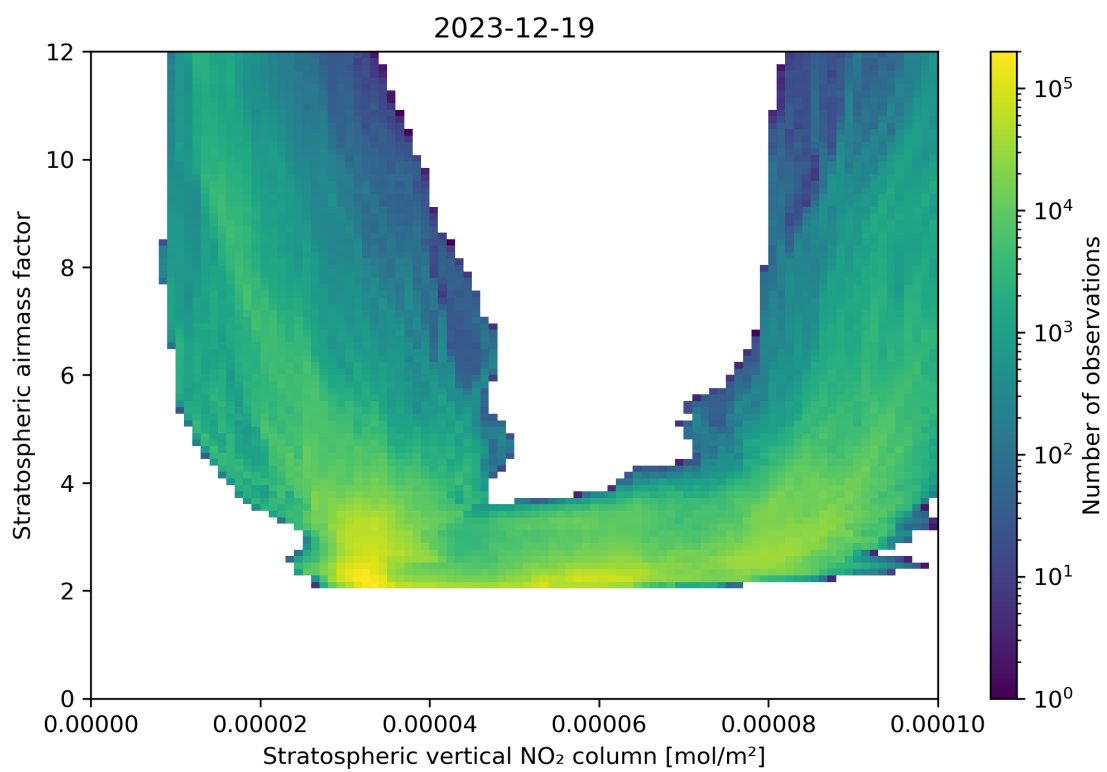
Figure 96: Scatter density plot of “Stratospheric vertical NO 2 column” against “Stratospheric airmass factor” for 2023-12-18 to 2023-12-20.
