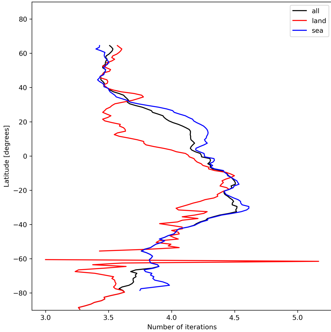
Figure 17: Zonal average of “Number of iterations” for 2023-12-18 to 2023-12-20.
