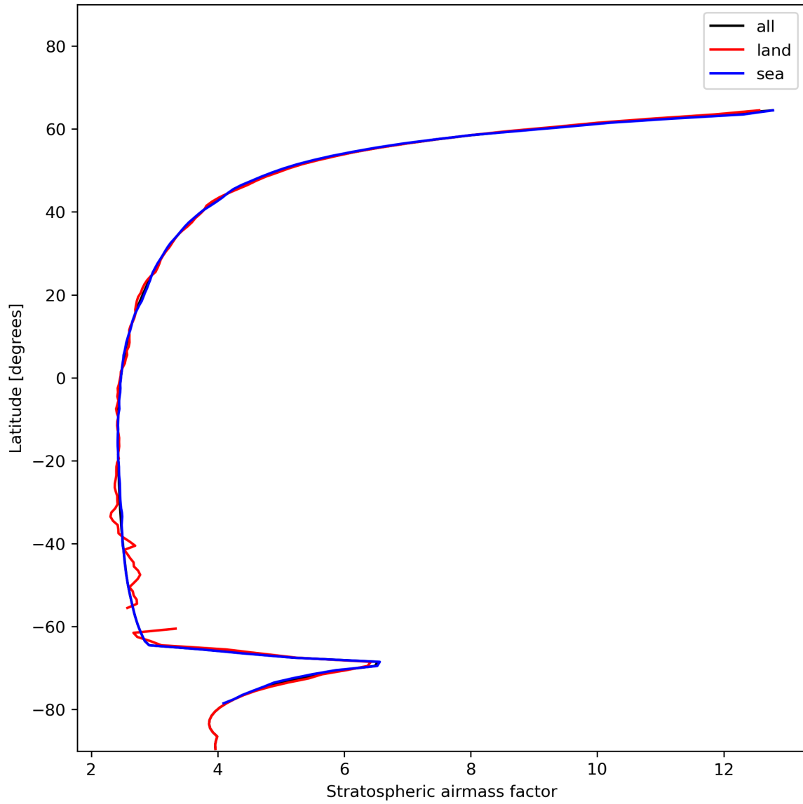
Figure 27: Zonal average of “Stratospheric air mass factor” for 2023-12-18 to 2023-12-20.
