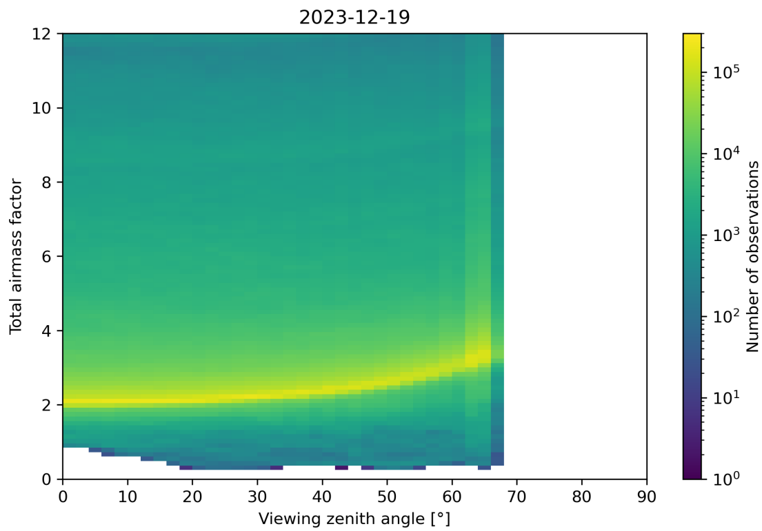
Figure 160: Scatter density plot of “Viewing zenith angle” against “Total airmass factor” for 2023-12-18 to 2023-12-20.
