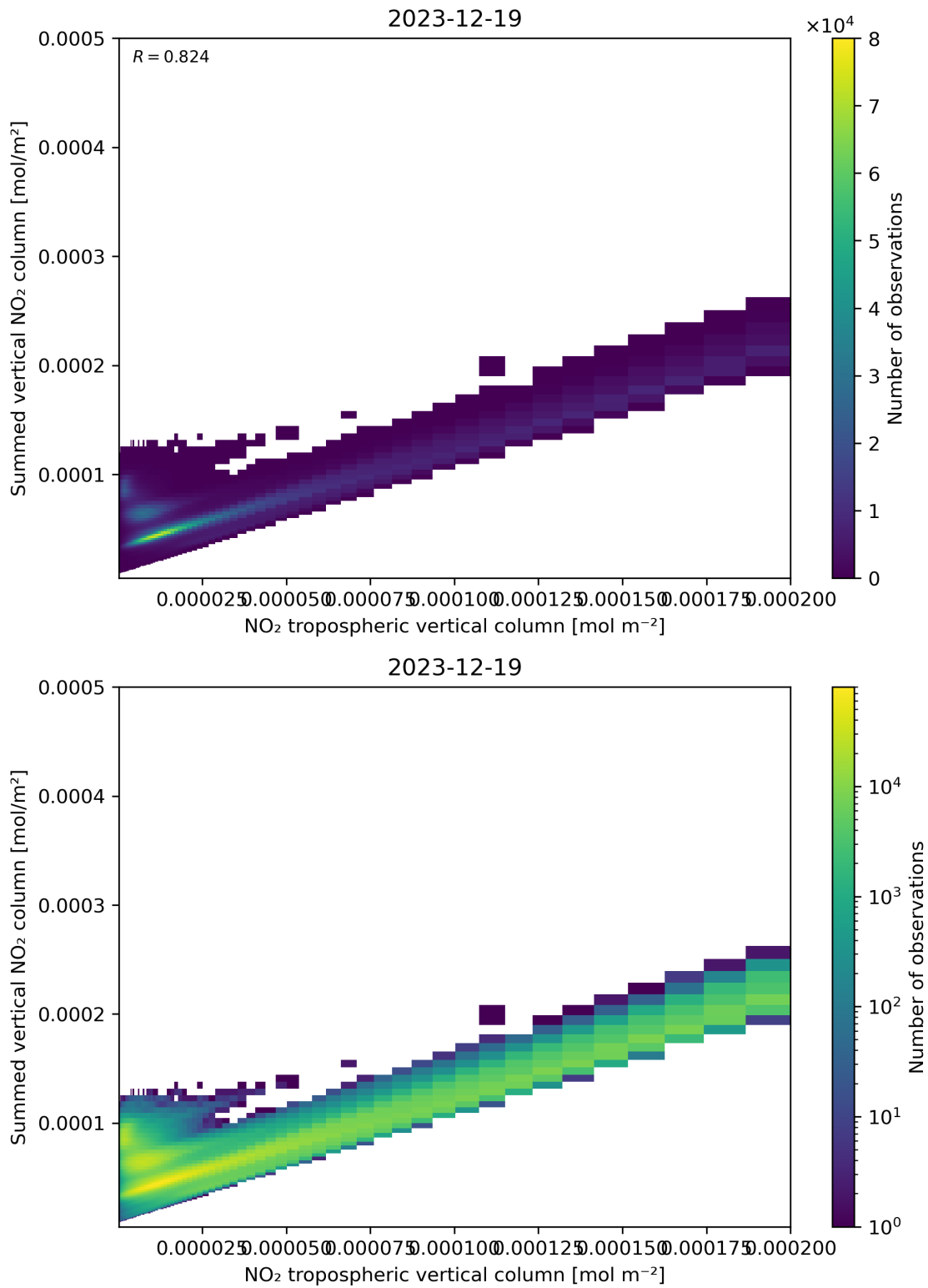
Figure 126: Scatter density plot of “NO 2 tropospheric vertical column” against “Summed vertical NO 2 column” for 2023-12-18 to 2023-12-20.
