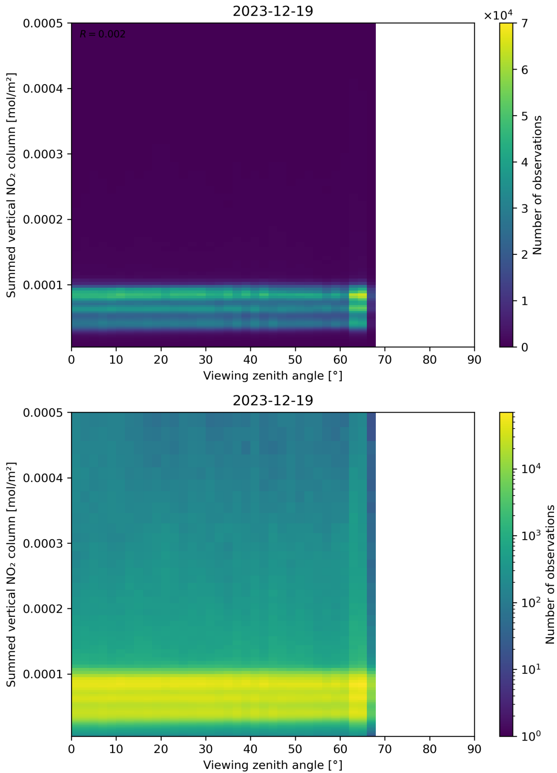
Figure 165: Scatter density plot of “Viewing zenith angle” against “Summed vertical NO 2 column” for 2023-12-18 to 2023-12-20.
