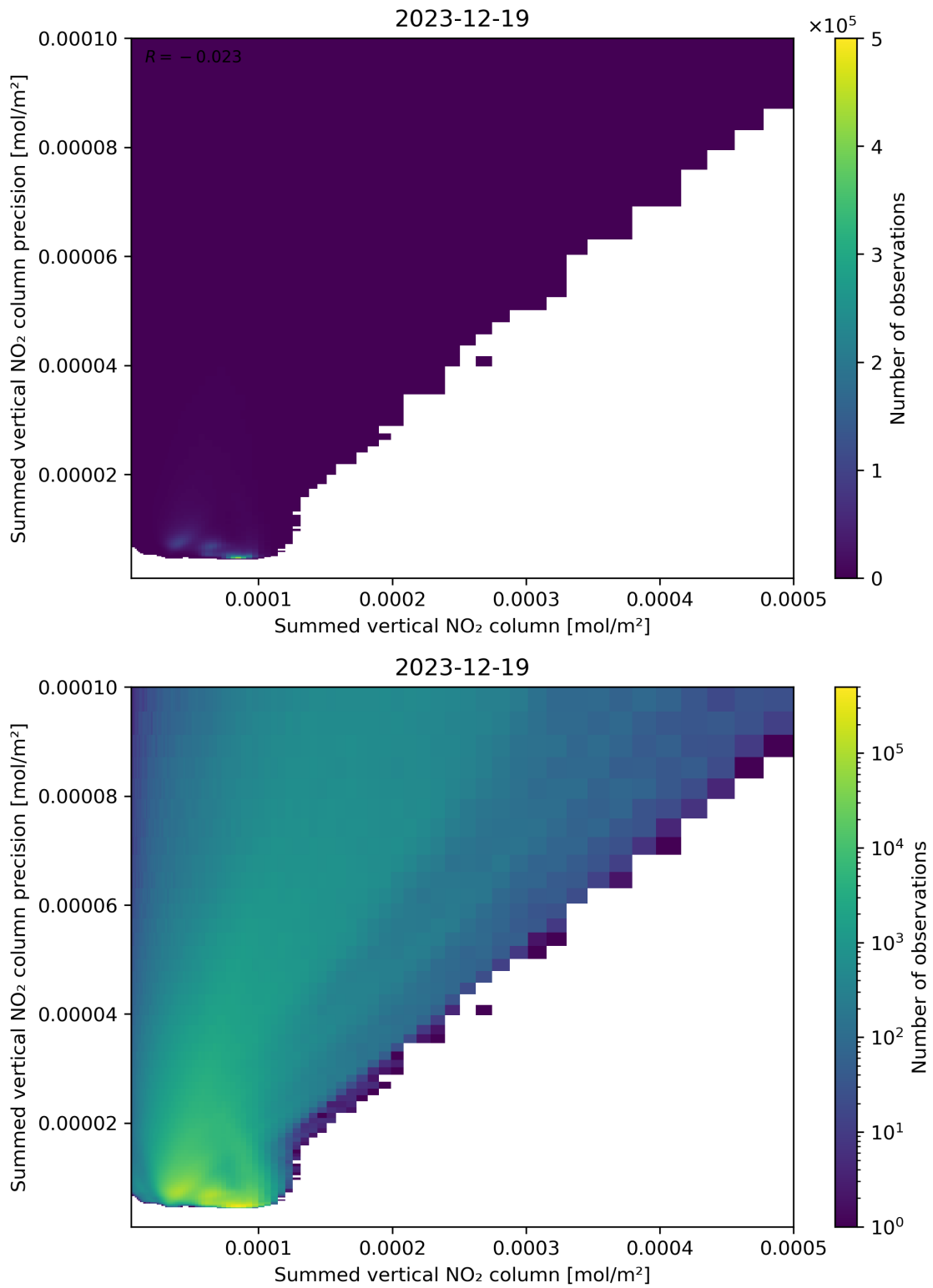
Figure 105: Scatter density plot of “Summed vertical NO 2 column” against “Summed vertical NO 2 column precision” for 2023-12-18 to 2023-12-20.
