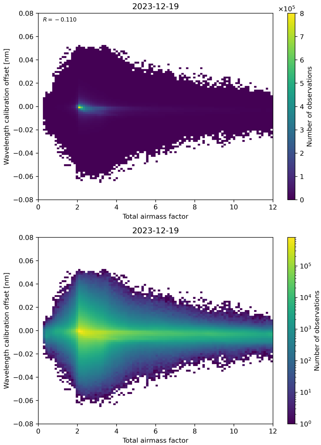
Figure 70: Scatter density plot of “Total airmass factor” against “Wavelength calibration offset” for 2023-12-18 to 2023-12-20.
