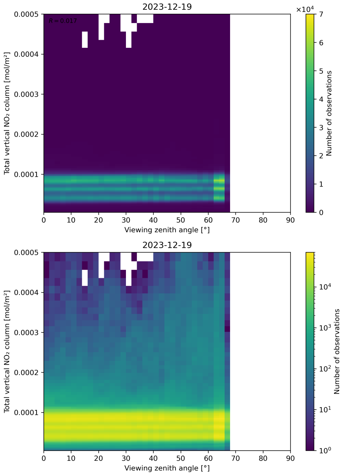
Figure 167: Scatter density plot of “Viewing zenith angle” against “Total vertical NO 2 column” for 2023-12-18 to 2023-12-20.
