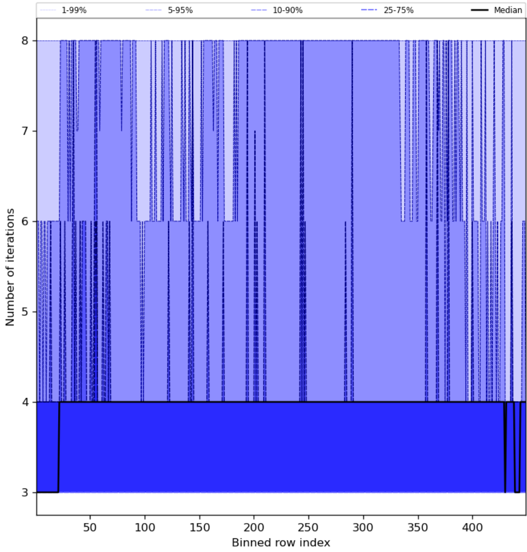
Figure 51: Along track statistics of “Number of iterations” for 2023-12-18 to 2023-12-20
