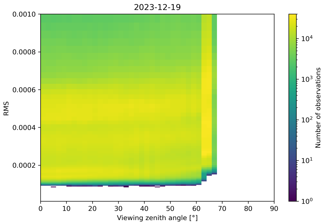
Figure 171: Scatter density plot of “Viewing zenith angle” against “RMS” for 2023-12-18 to 2023-12-20.
