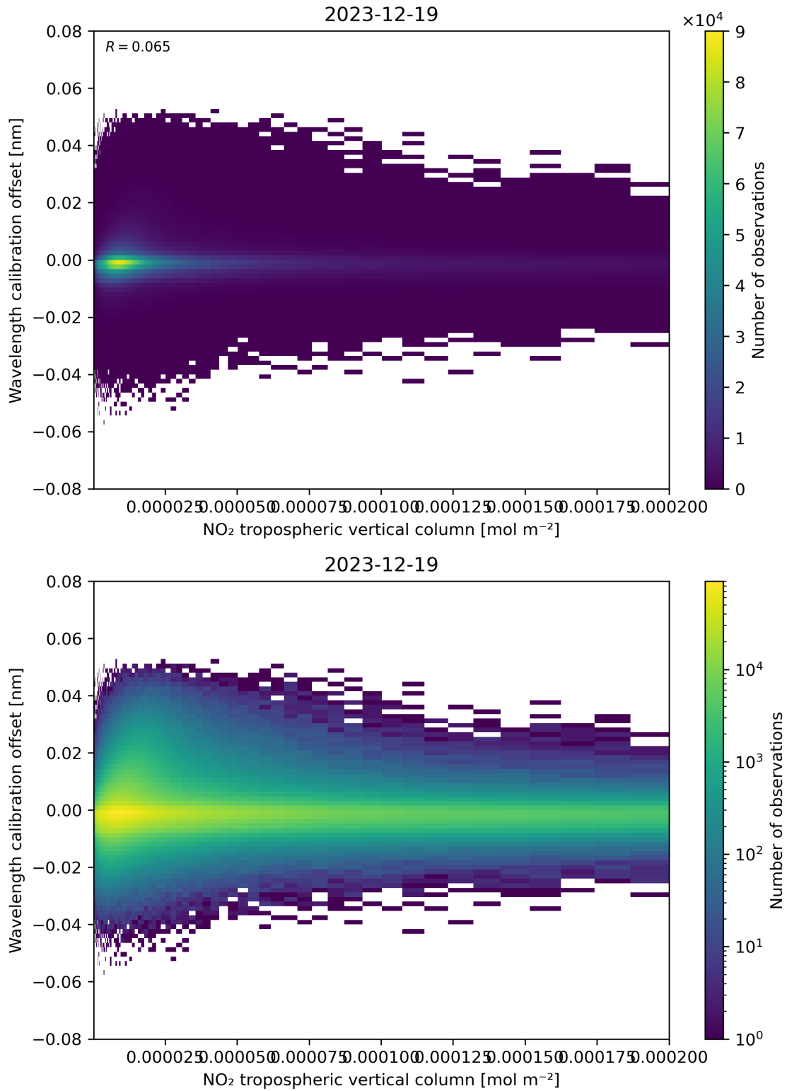
Figure 143: Scatter density plot of “NO 2 tropospheric vertical column” against “Wavelength calibration offset” for 2023-12-18 to 2023-12-20.
