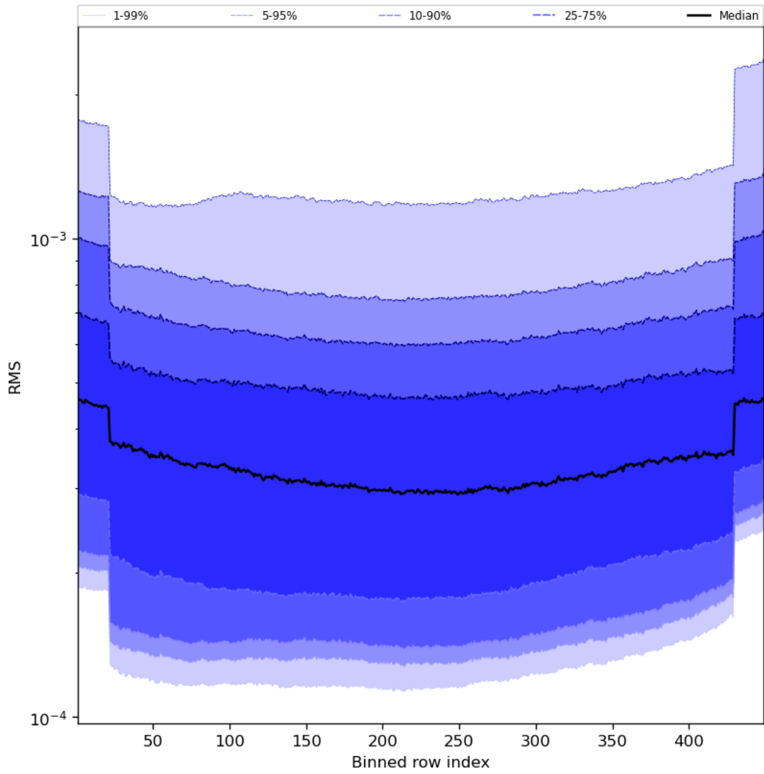
Figure 60: Along track statistics of “RMS” for 2023-12-18 to 2023-12-20
