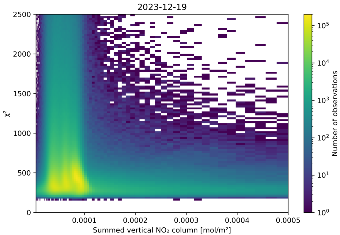
Figure 104: Scatter density plot of “Summed vertical NO 2 column” against “ \chi^2 ” for 2023-12-18 to 2023-12-20.
