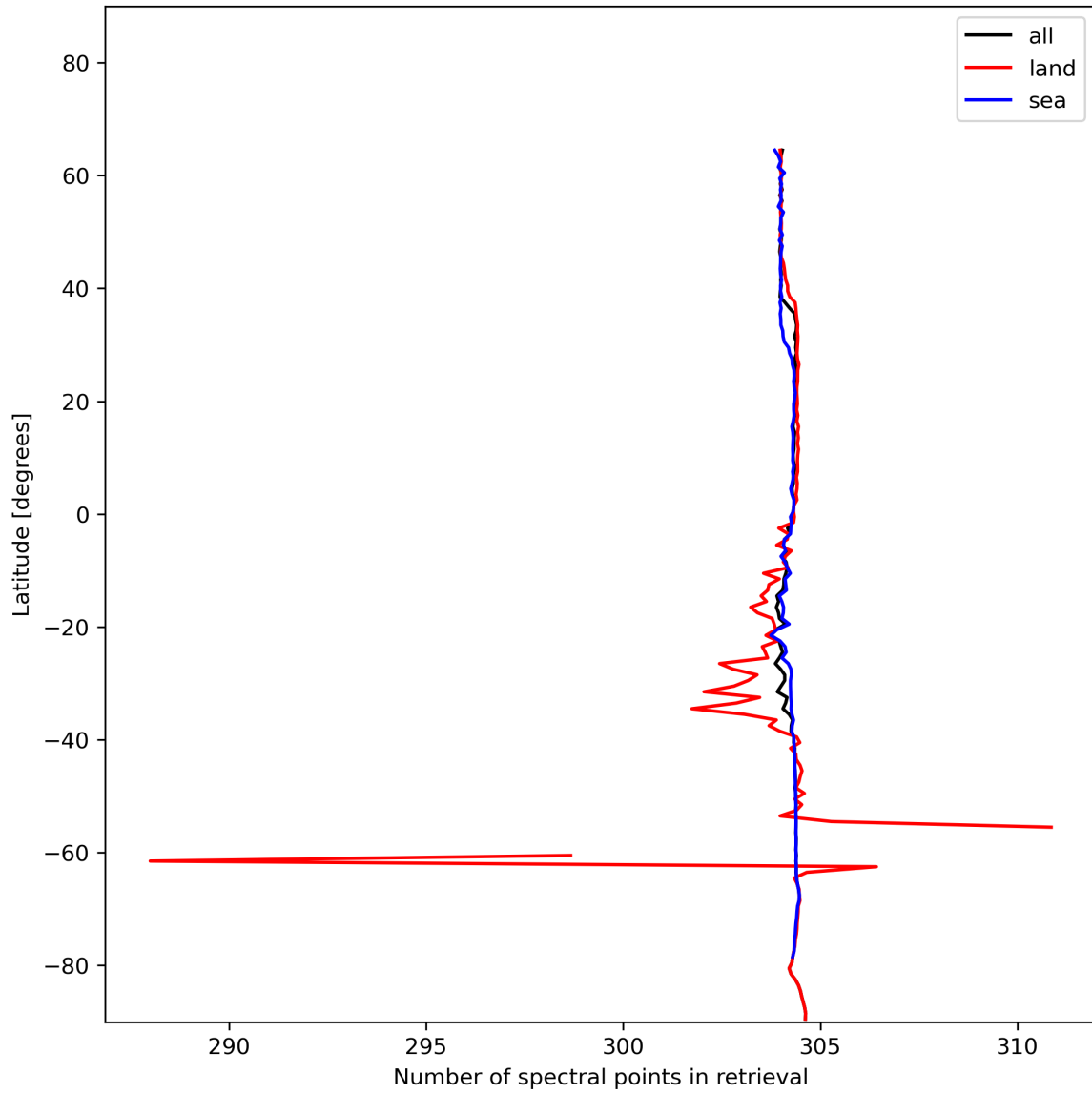
Figure 16: Zonal average of “Number of spectral points in retrieval” for 2023-12-18 to 2023-12-20.
