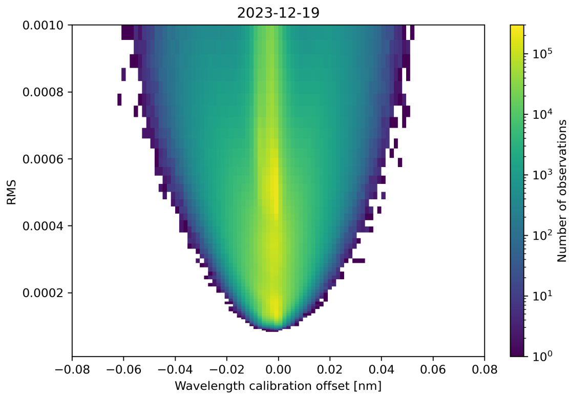
Figure 181: Scatter density plot of “Wavelength calibration offset” against “RMS” for 2023-12-18 to 2023-12-20.
