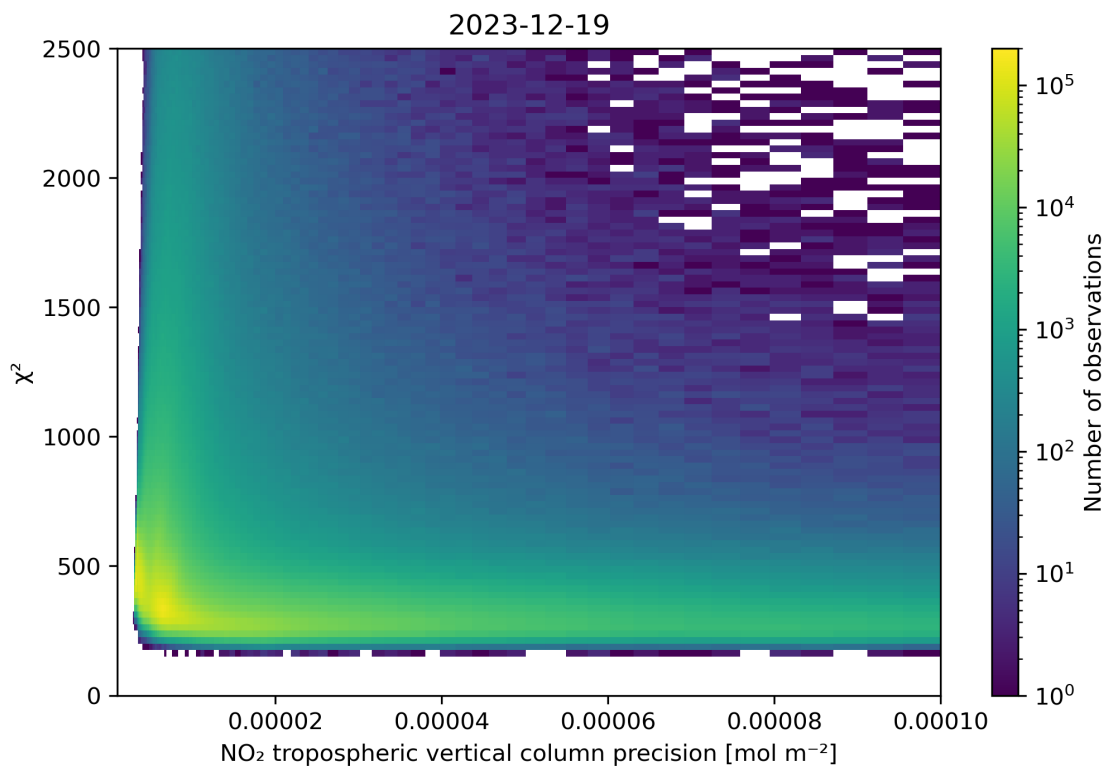
Figure 134: Scatter density plot of “NO 2 tropospheric vertical column precision” against “ \chi^2 ” for 2023-12-18 to 2023-12-20.
