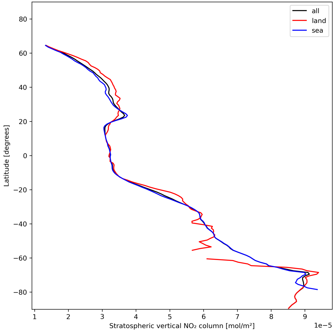
Figure 19: Zonal average of “Stratospheric vertical NO 2 column” for 2023-12-18 to 2023-12-20.
