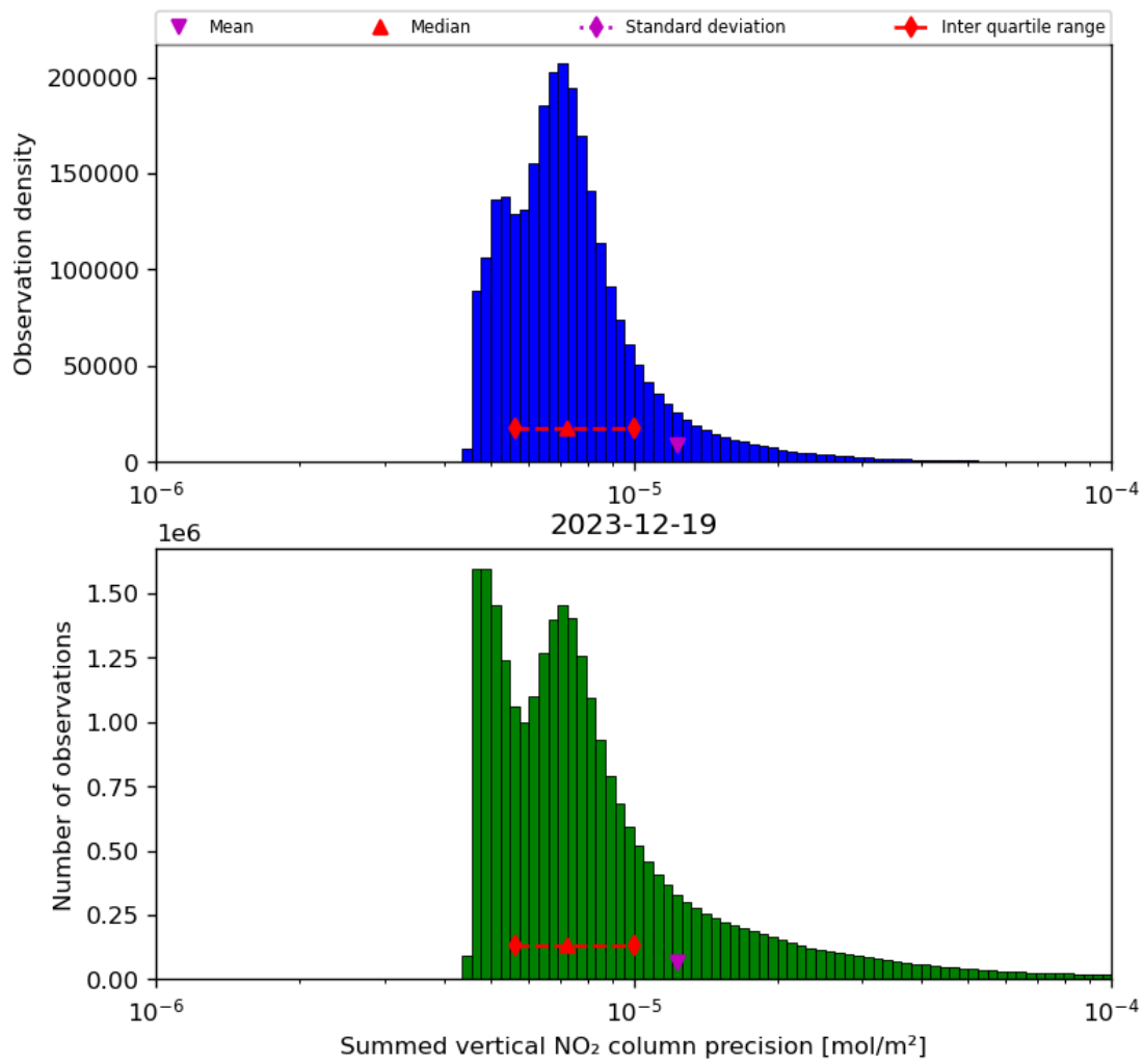
Figure 41: Histogram of “Summed vertical NO 2 column precision” for 2023-12-18 to 2023-12-20
