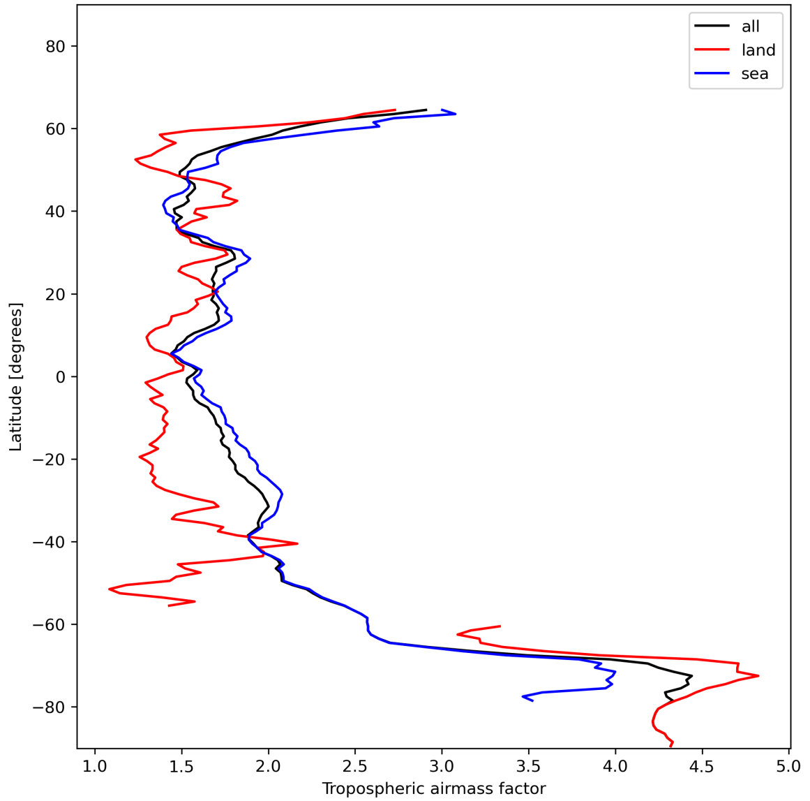
Figure 14: Zonal average of “Tropospheric airmass factor” for 2023-12-18 to 2023-12-20.
