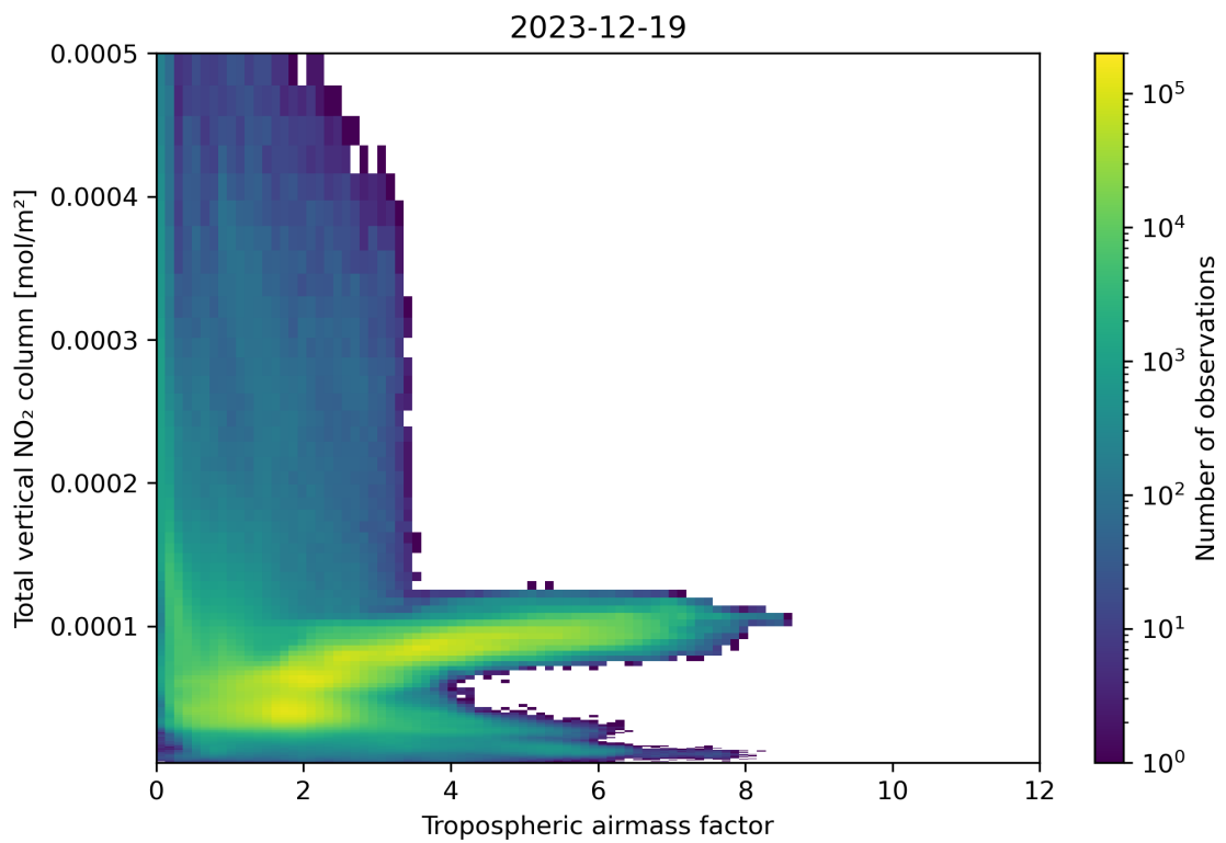
Figure 77: Scatter density plot of “Tropospheric airmass factor” against “Total vertical NO 2 column” for 2023-12-18 to 2023-12-20.
