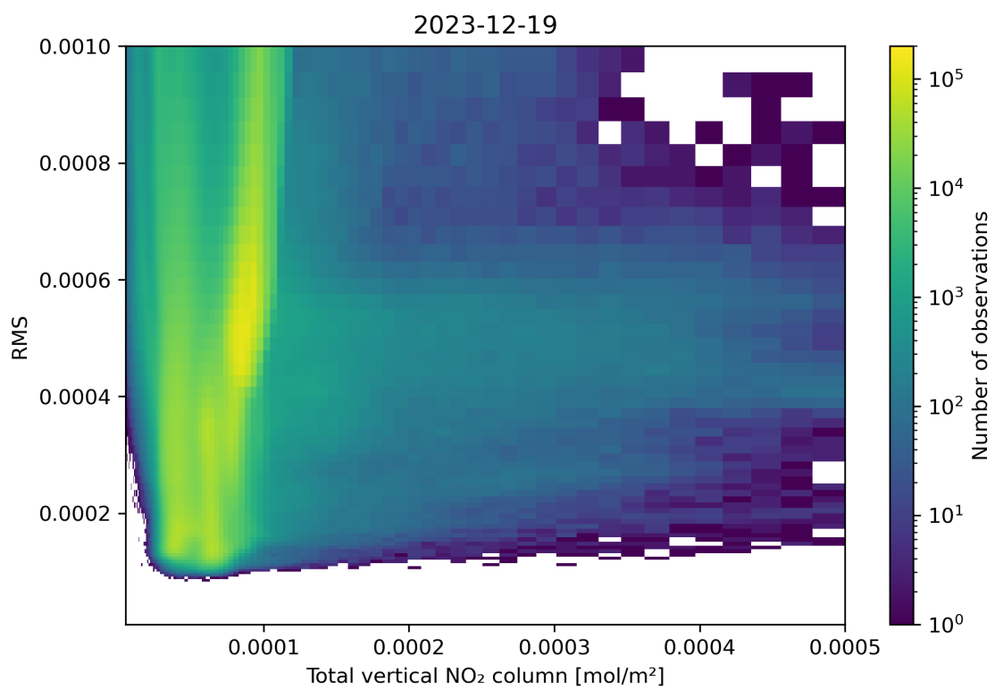
Figure 120: Scatter density plot of “Total vertical NO 2 column” against “RMS” for 2023-12-18 to 2023-12-20.
