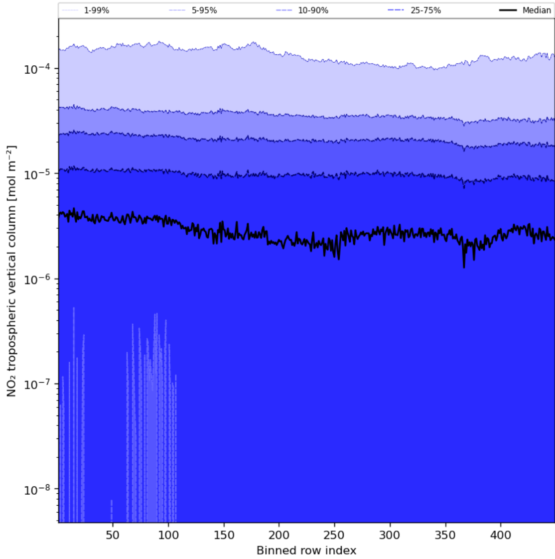
Figure 46: Along track statistics of “NO 2 tropospheric vertical column” for 2023-12-18 to 2023-12-20
