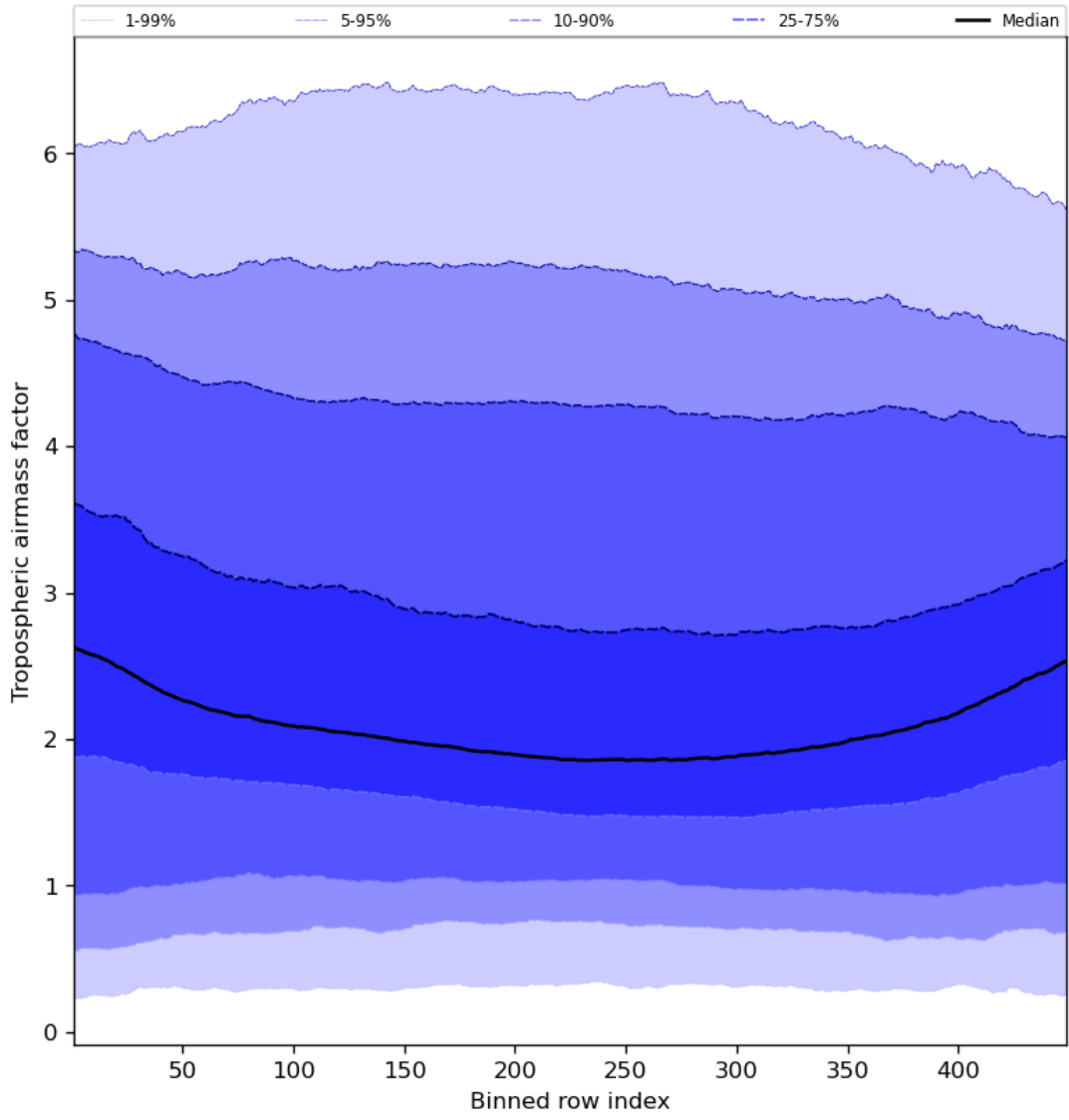
Figure 48: Along track statistics of “Tropospheric airmass factor” for 2023-12-18 to 2023-12-20
