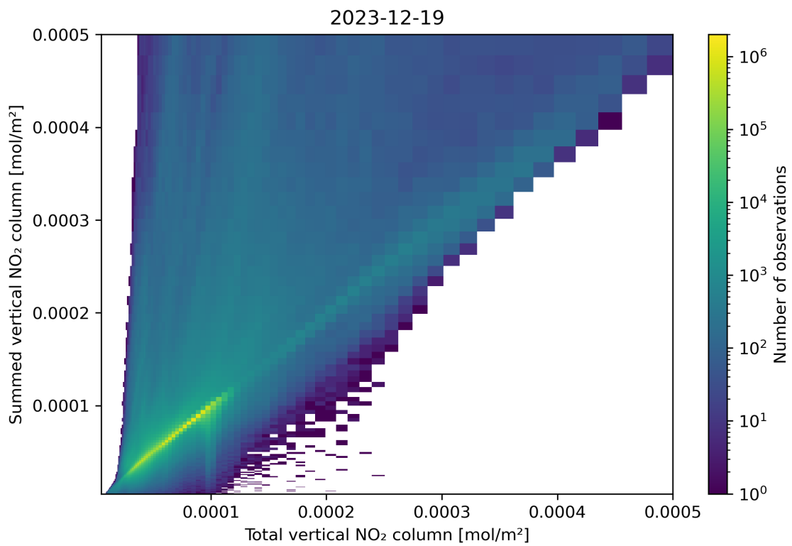
Figure 112: Scatter density plot of “Total vertical NO 2 column” against “Summed vertical NO 2 column” for 2023-12-18 to 2023-12-20.
