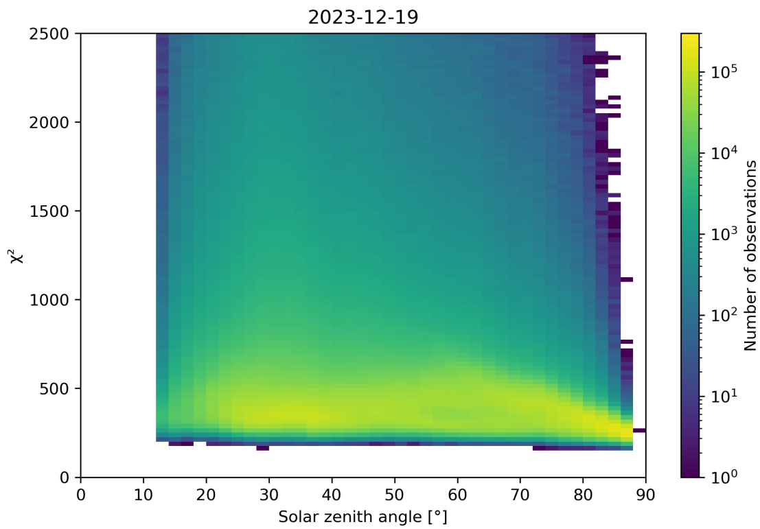
Figure 148: Scatter density plot of “Solar zenith angle” against “ \chi^2 ” for 2023-12-18 to 2023-12-20.
