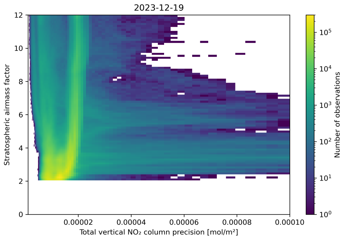
Figure 115: Scatter density plot of “Total vertical NO 2 column precision” against “Stratospheric airmass factor” for 2023-12-18 to 2023-12-20.
