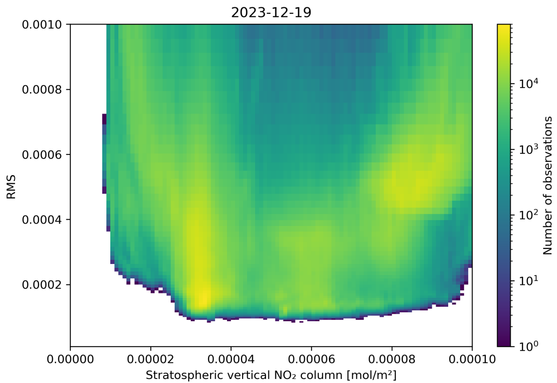
Figure 102: Scatter density plot of “Stratospheric vertical NO 2 column” against “RMS” for 2023-12-18 to 2023-12-20.
