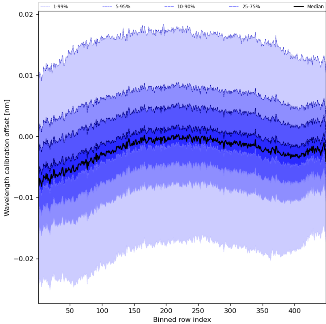
Figure 52: Along track statistics of “Wavelength calibration offset” for 2023-12-18 to 2023-12-20
