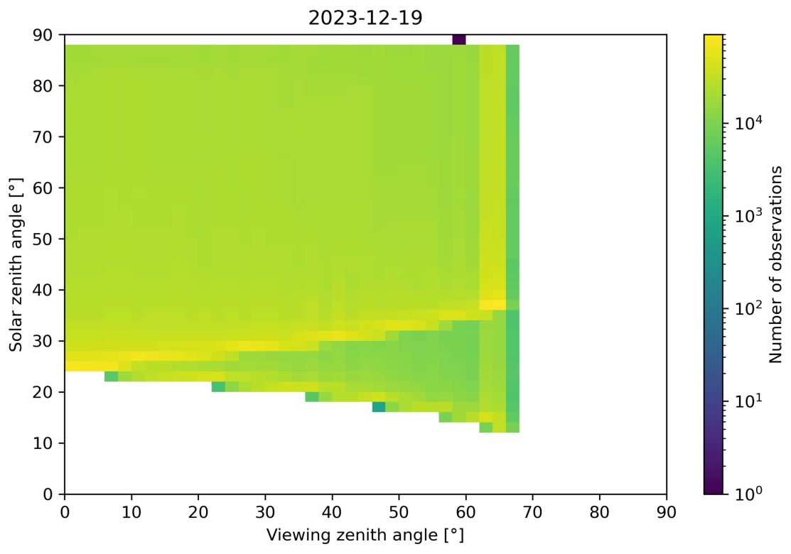
Figure 172: Scatter density plot of “Viewing zenith angle” against “Solar zenith angle” for 2023-12-18 to 2023-12-20.
