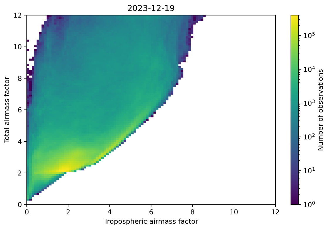
Figure 72: Scatter density plot of “Tropospheric airmass factor” against “Total airmass factor” for 2023-12-18 to 2023-12-20.
