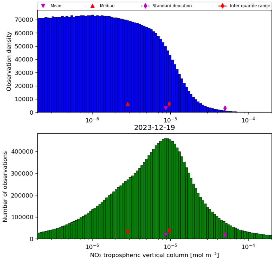
Figure 29: Histogram of “NO 2 tropospheric vertical column” for 2023-12-18 to 2023-12-20
