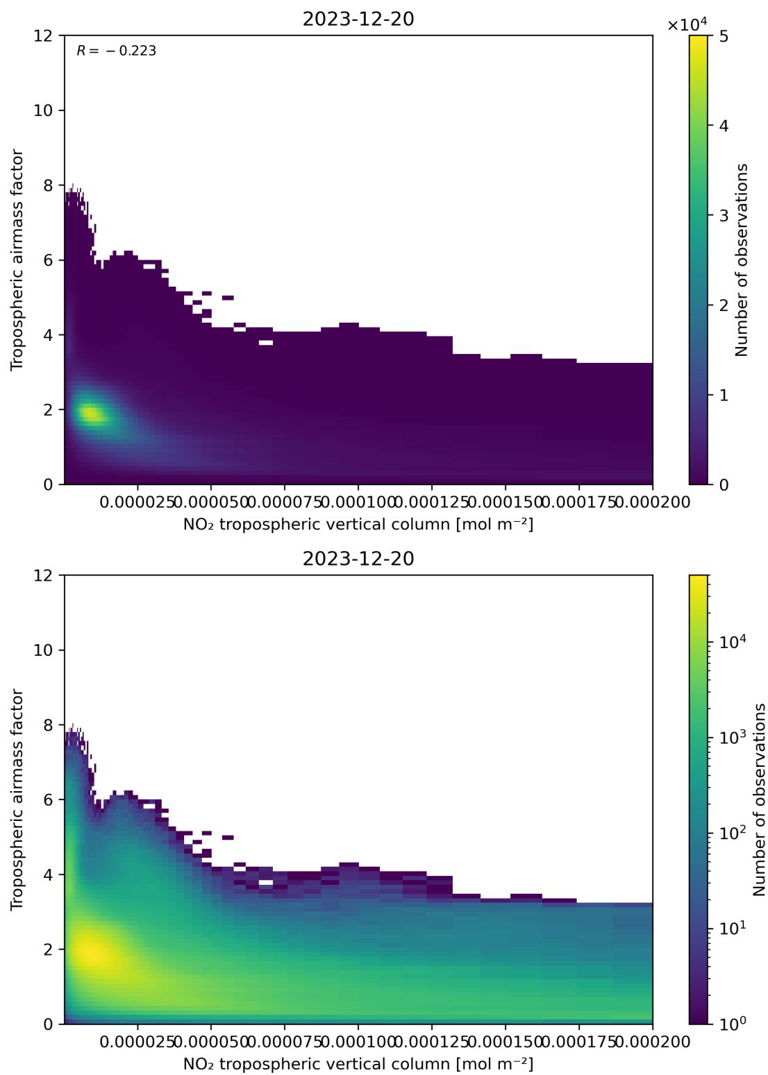
Figure 123: Scatter density plot of “NO 2 tropospheric vertical column” against “Tropospheric airmass factor” for 2023-12-20 to 2023-12-21.
