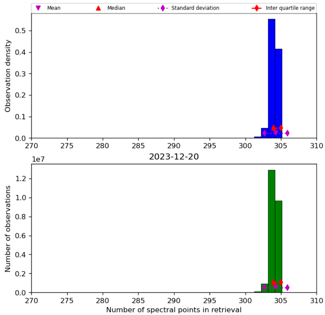
Figure 33: Histogram of “Number of spectral points in retrieval” for 2023-12-20 to 2023-12-21
