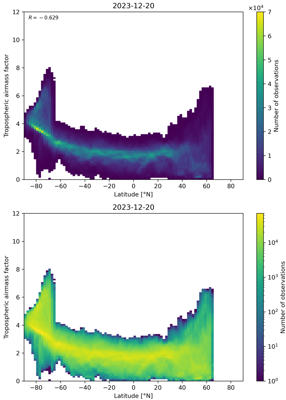
Figure 85: Scatter density plot of “Latitude” against “Tropospheric airmass factor” for 2023-12-20 to 2023-12-21.
