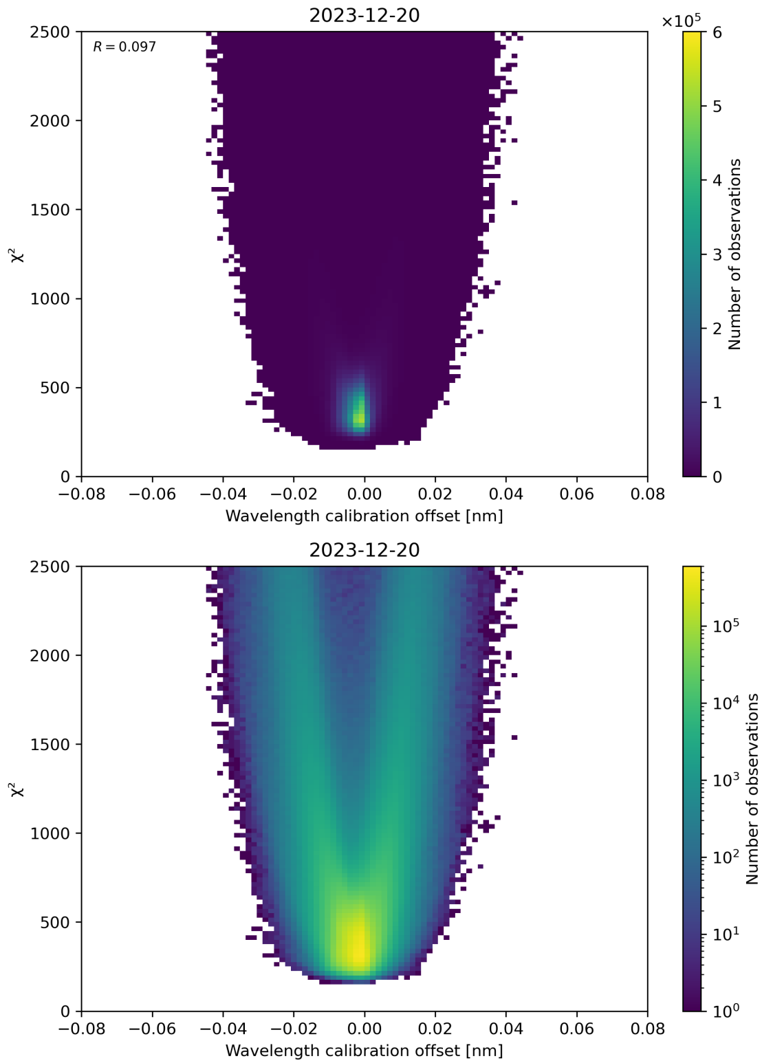
Figure 175: Scatter density plot of “Wavelength calibration offset” against “ \chi^2 ” for 2023-12-20 to 2023-12-21.
