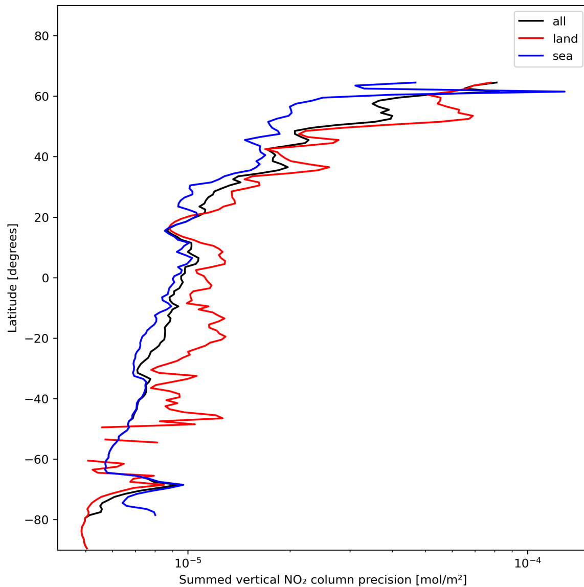
Figure 24: Zonal average of “Summed vertical NO 2 column precision” for 2023-12-20 to 2023-12-21.
