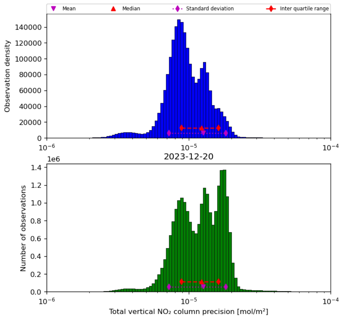
Figure 39: Histogram of “Total vertical NO 2 column precision” for 2023-12-20 to 2023-12-21
