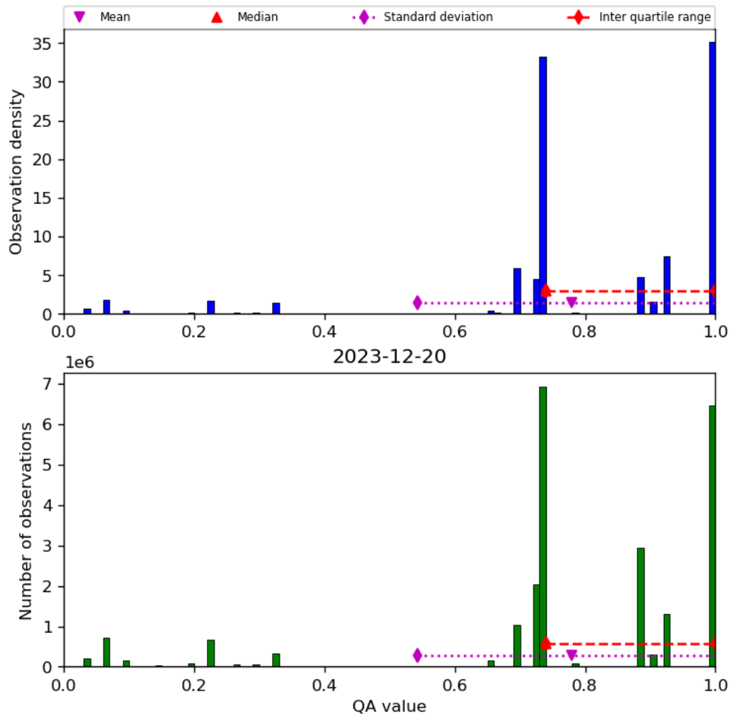
Figure 28: Histogram of “QA value” for 2023-12-20 to 2023-12-21
