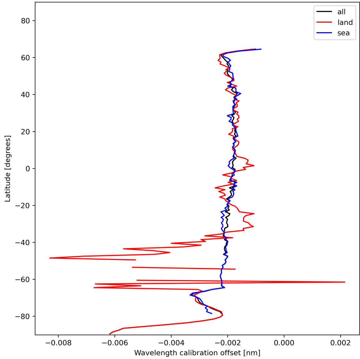
Figure 18: Zonal average of “Wavelength calibration offset” for 2023-12-20 to 2023-12-21.
