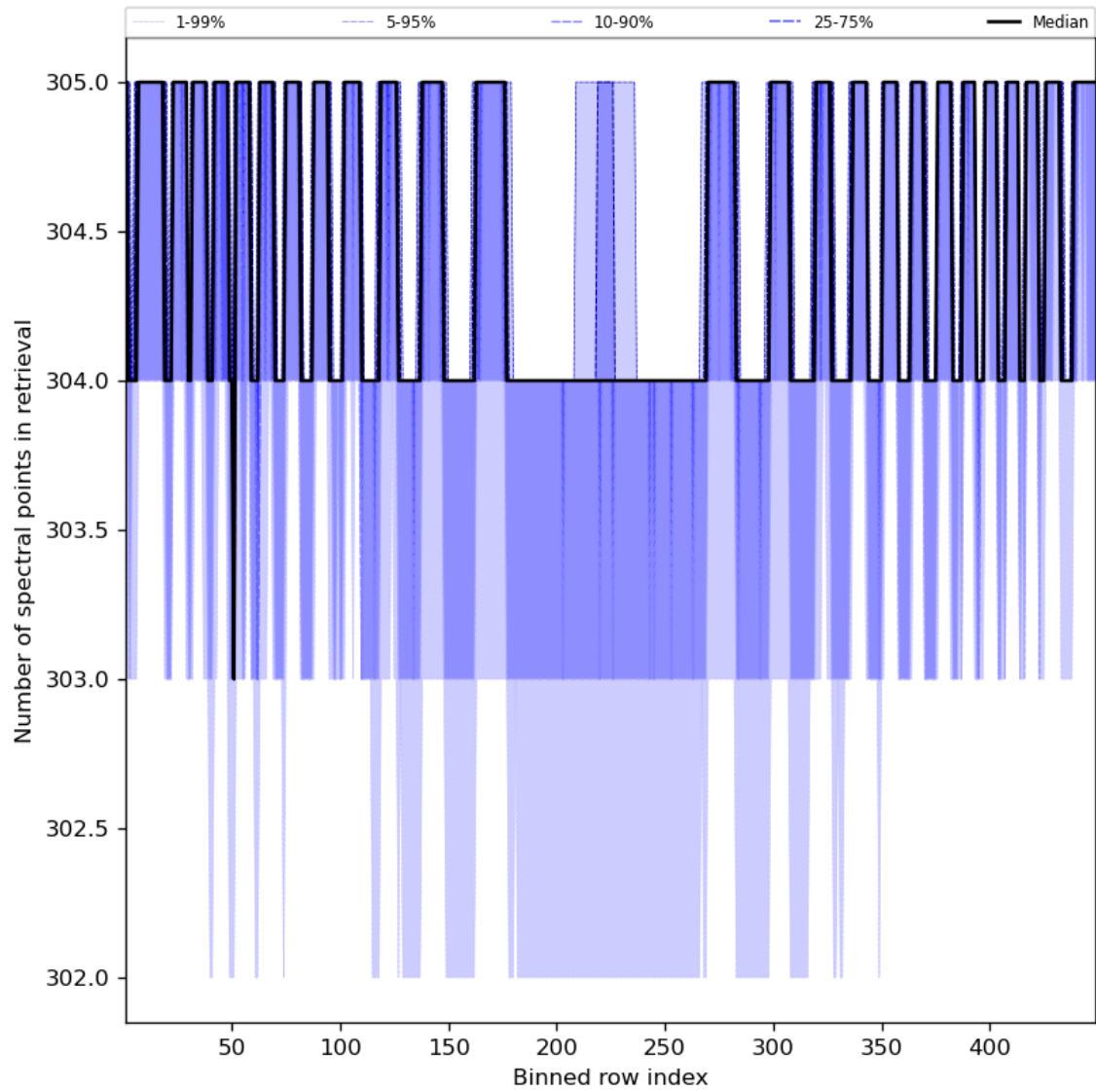
Figure 50: Along track statistics of “Number of spectral points in retrieval” for 2023-12-20 to 2023-12-21
