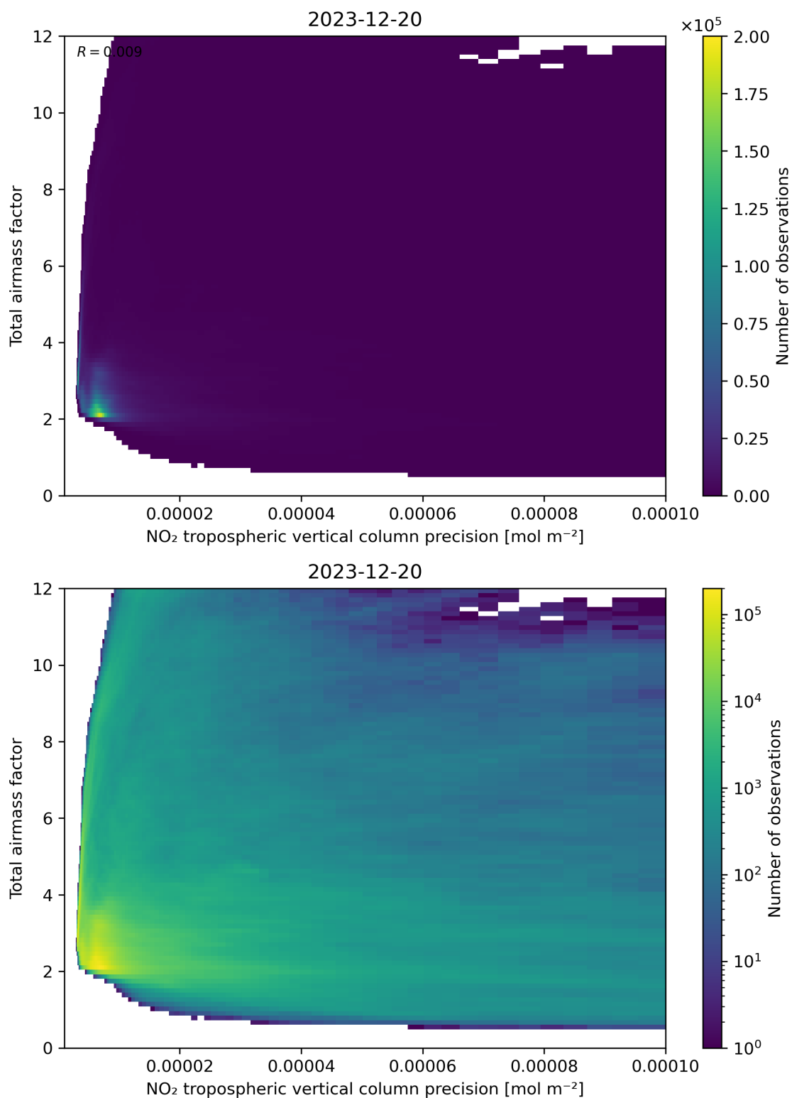
Figure 132: Scatter density plot of “NO 2 tropospheric vertical column precision” against “Total air mass factor” for 2023-12-20 to 2023-12-21.
