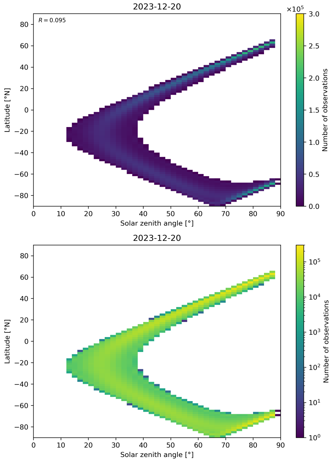
Figure 149: Scatter density plot of “Solar zenith angle” against “Latitude” for 2023-12-20 to 2023-12-21.
