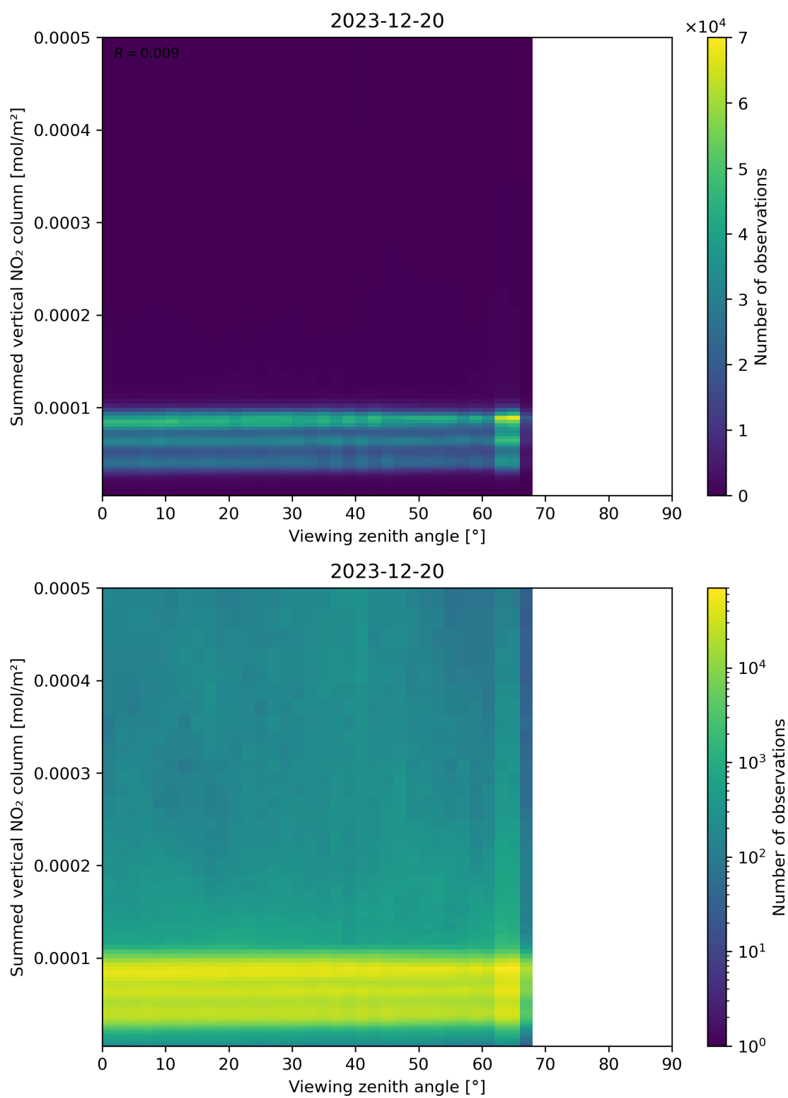
Figure 165: Scatter density plot of “Viewing zenith angle” against “Summed vertical NO 2 column” for 2023-12-20 to 2023-12-21.
