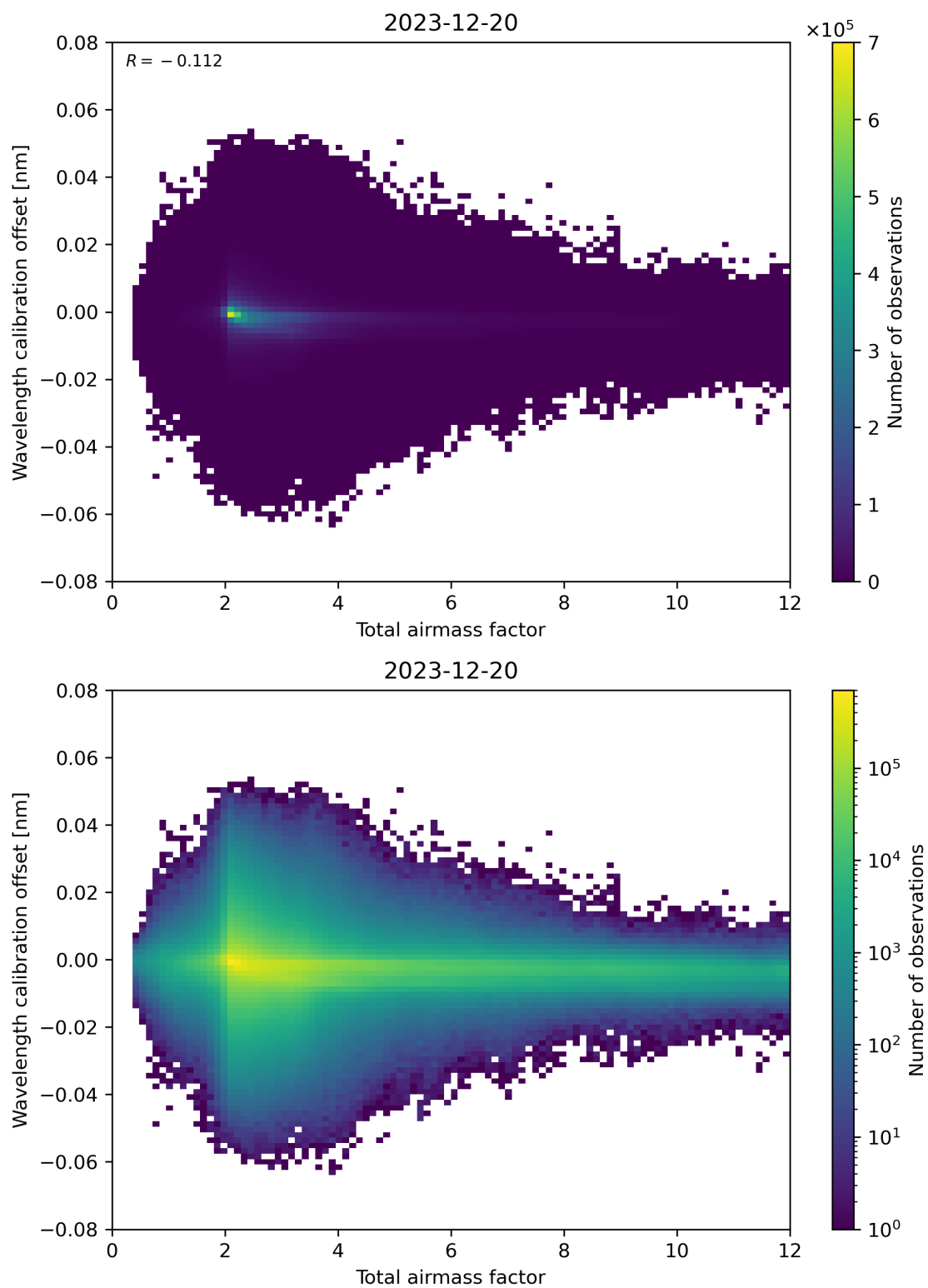
Figure 70: Scatter density plot of “Total airmass factor” against “Wavelength calibration offset” for 2023-12-20 to 2023-12-21.
