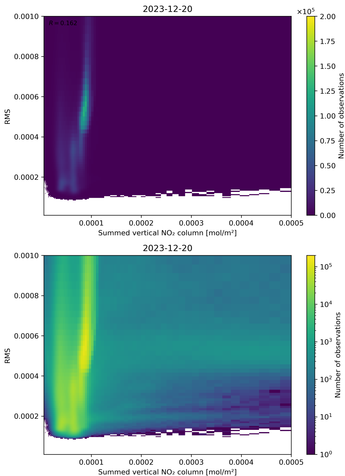
Figure 109: Scatter density plot of “Summed vertical NO 2 column” against “RMS” for 2023-12-20 to 2023-12-21.
