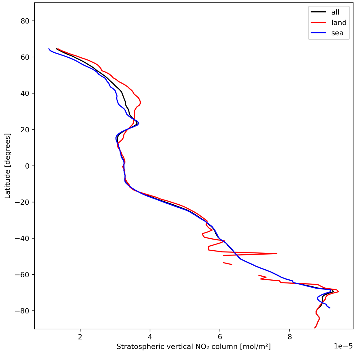
Figure 19: Zonal average of “Stratospheric vertical NO 2 column” for 2023-12-20 to 2023-12-21.
