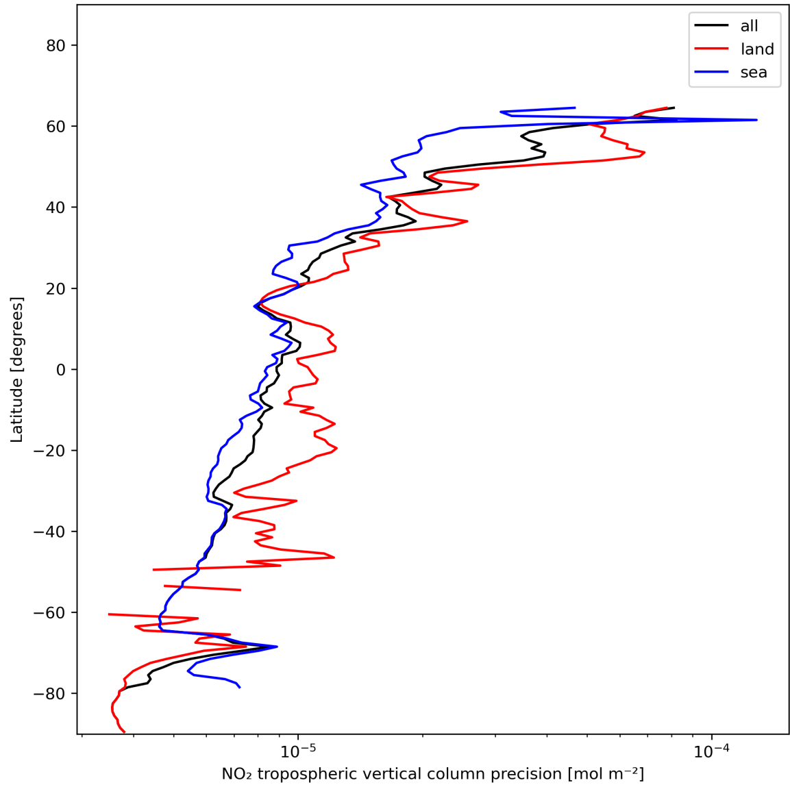
Figure 13: Zonal average of “NO 2 tropospheric vertical column precision” for 2023-12-20 to 2023-12-21.
