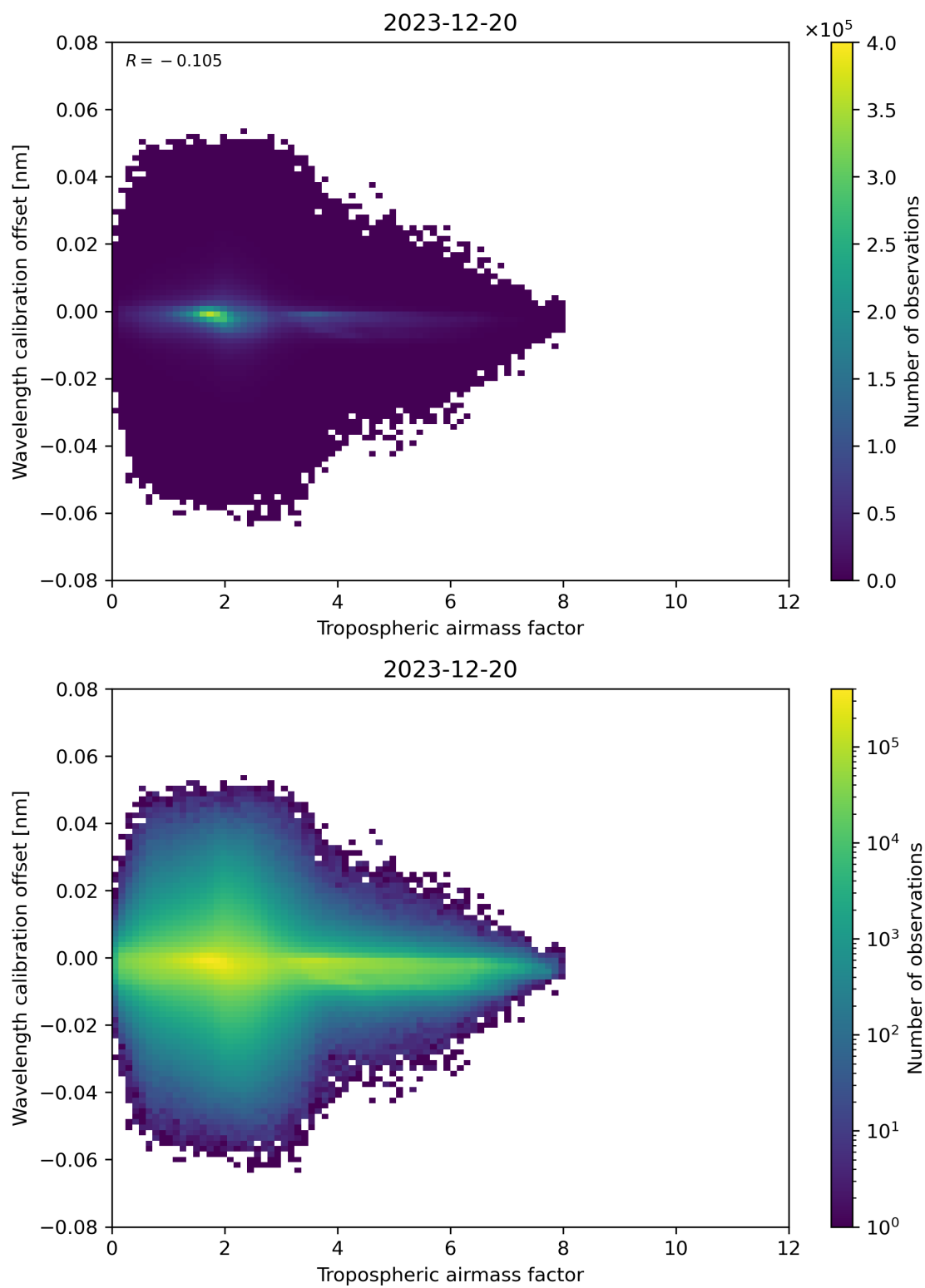
Figure 80: Scatter density plot of “Tropospheric airmass factor” against “Wavelength calibration offset” for 2023-12-20 to 2023-12-21.
