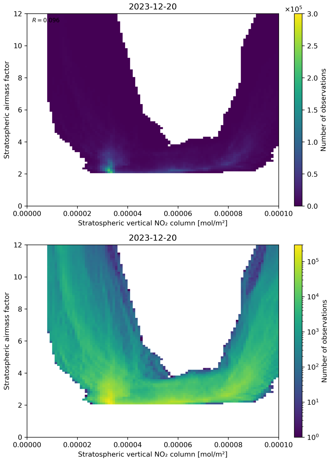
Figure 96: Scatter density plot of “Stratospheric vertical NO 2 column” against “Stratospheric airmass factor” for 2023-12-20 to 2023-12-21.
