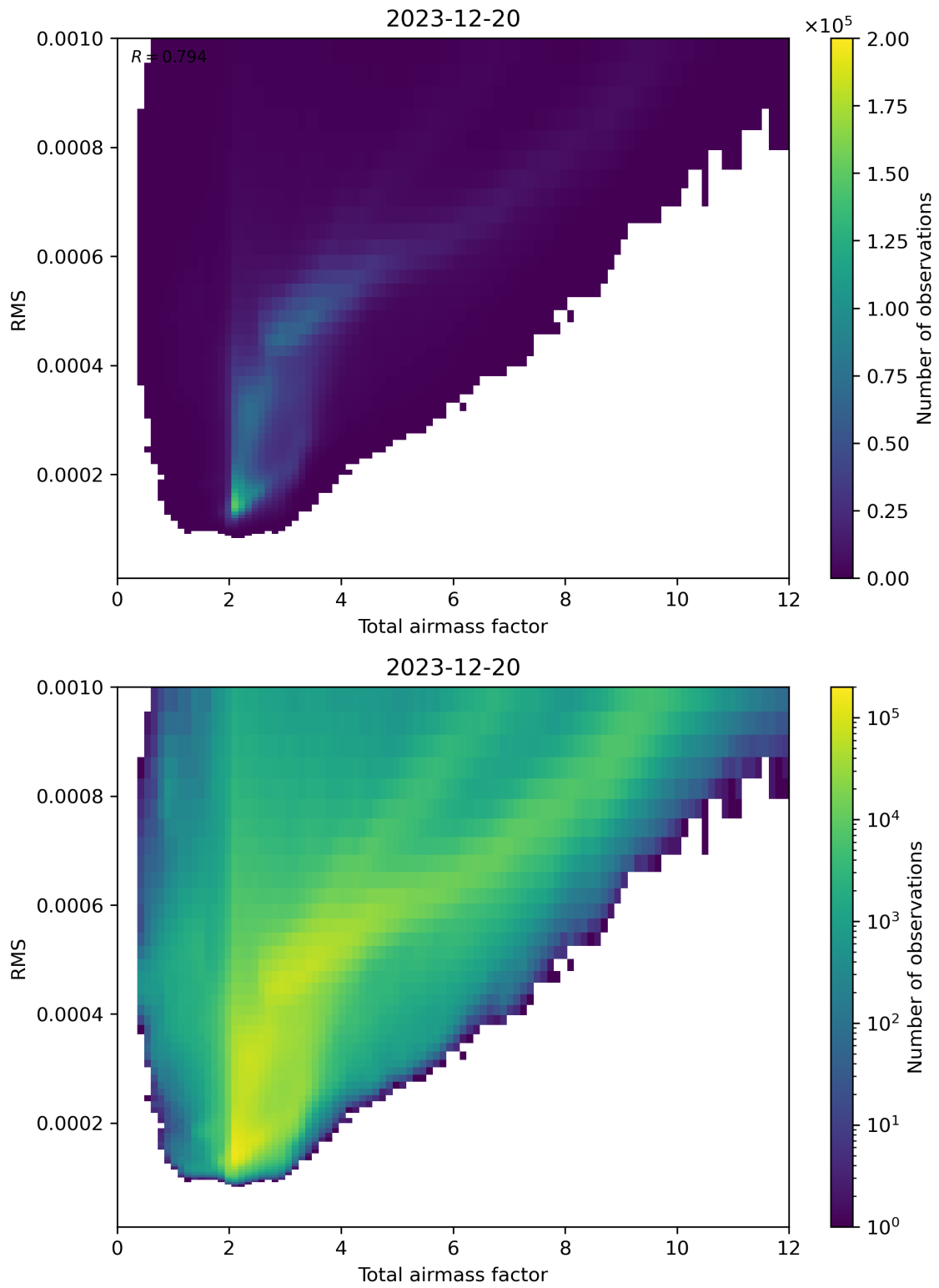
Figure 69: Scatter density plot of “Total airmass factor” against “RMS” for 2023-12-20 to 2023-12-21.
