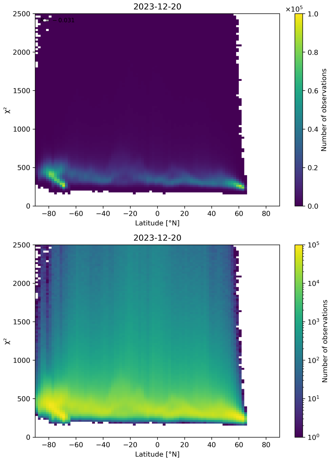
Figure 86: Scatter density plot of “Latitude” against “ \chi^2 ” for 2023-12-20 to 2023-12-21.
