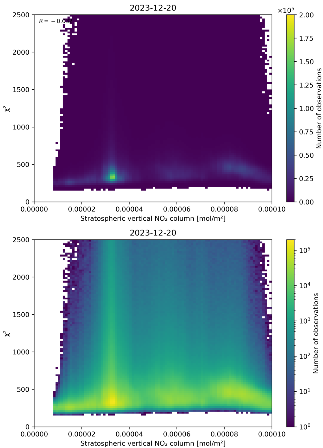
Figure 97: Scatter density plot of “Stratospheric vertical NO 2 column” against “ \chi^2 ” for 2023-12-20 to 2023-12-21.
