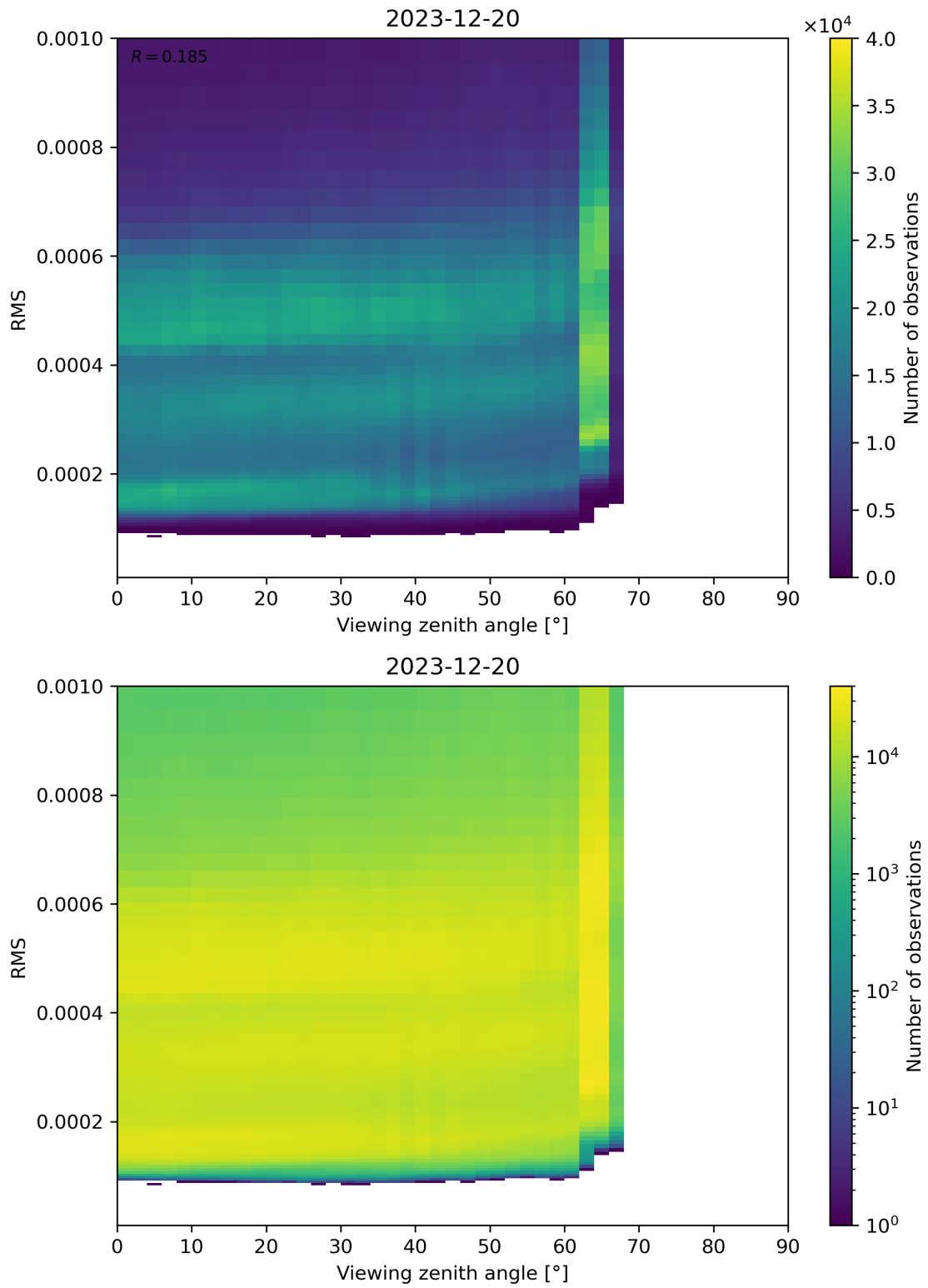
Figure 171: Scatter density plot of “Viewing zenith angle” against “RMS” for 2023-12-20 to 2023-12-21.
