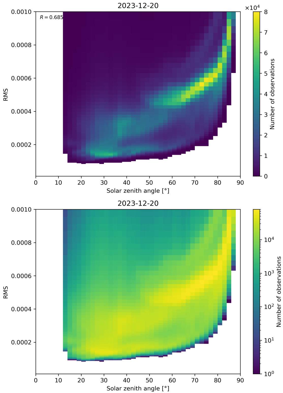
Figure 157: Scatter density plot of “Solar zenith angle” against “RMS” for 2023-12-20 to 2023-12-21.
