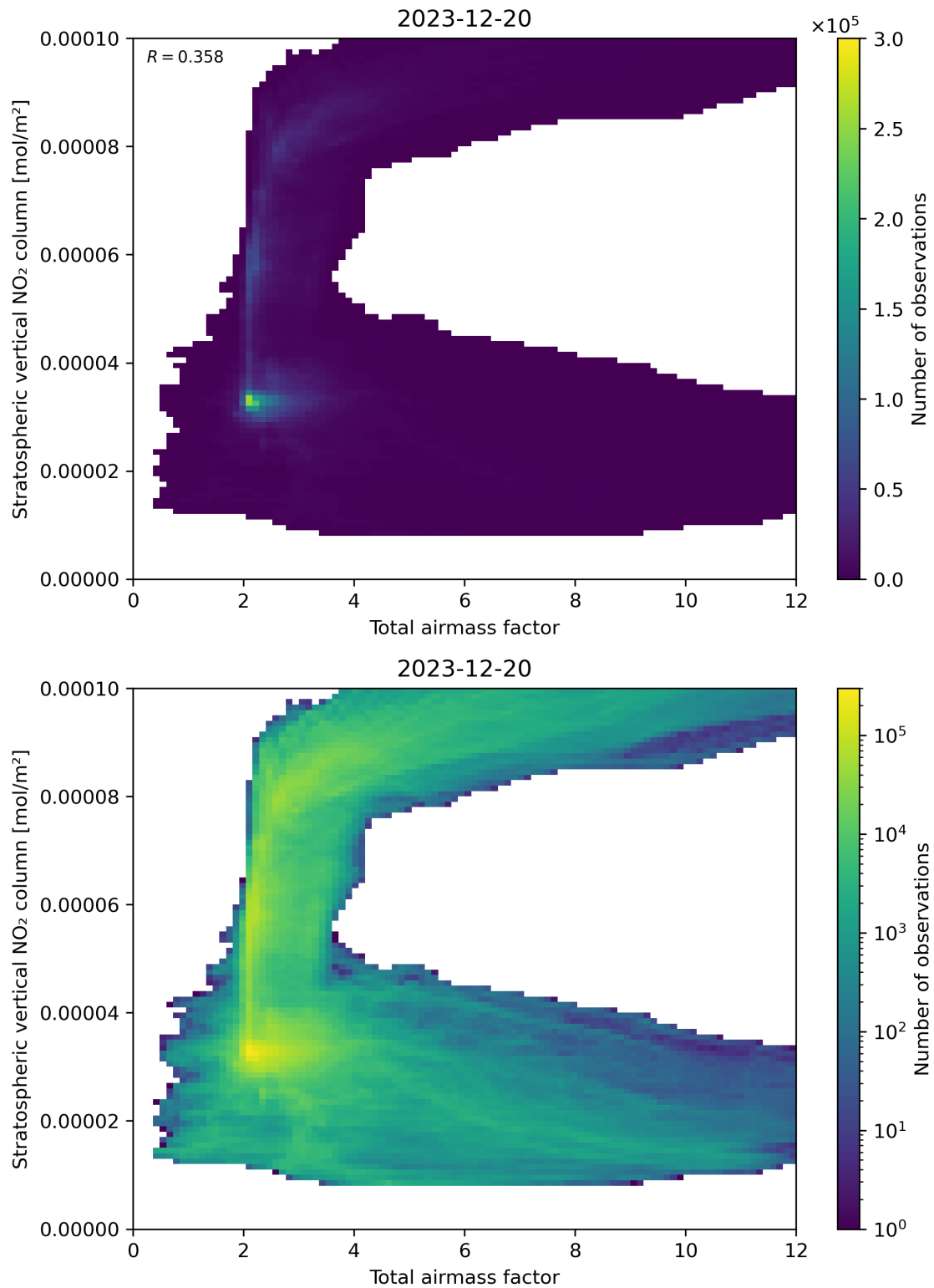
Figure 64: Scatter density plot of “Total airmass factor” against “Stratospheric vertical \text{NO}_2 column” for 2023-12-20 to 2023-12-21.
