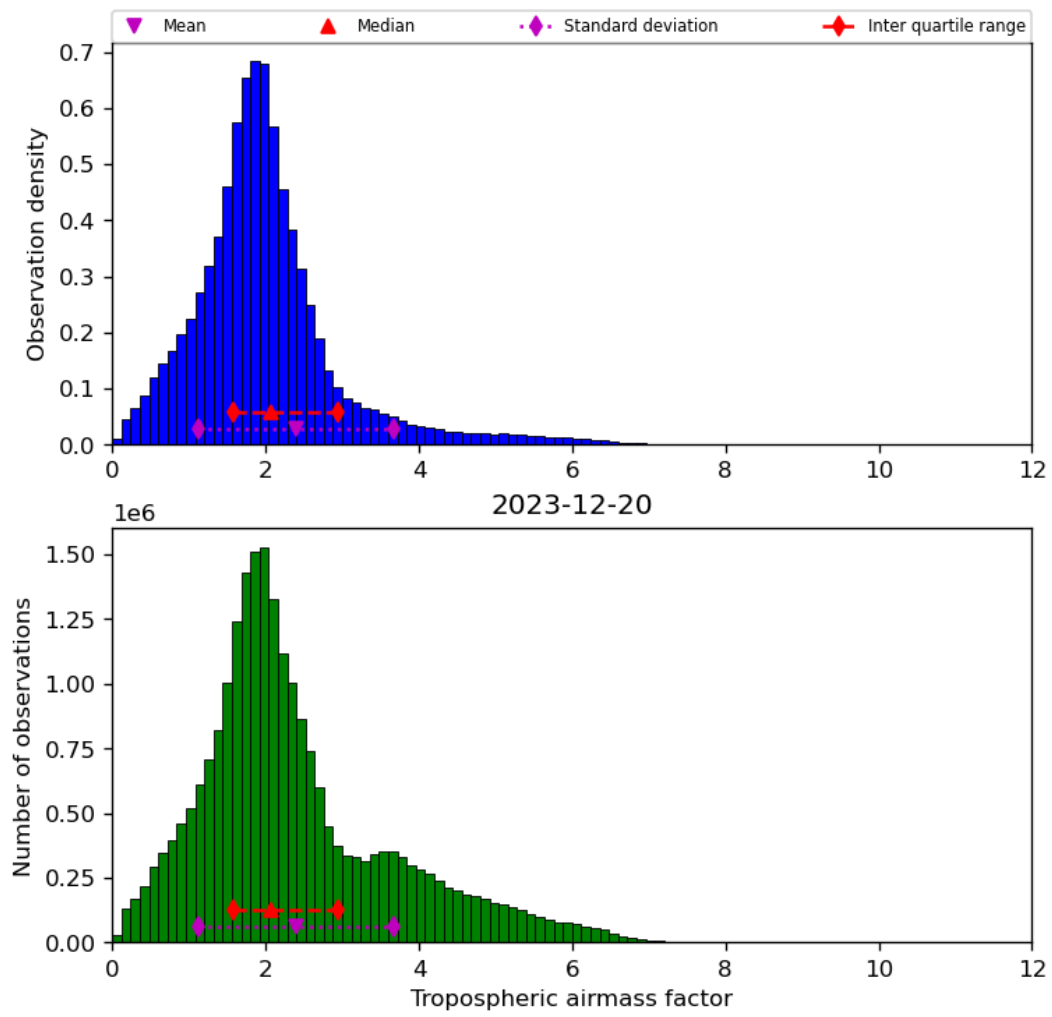
Figure 31: Histogram of “Tropospheric airmass factor” for 2023-12-20 to 2023-12-21
