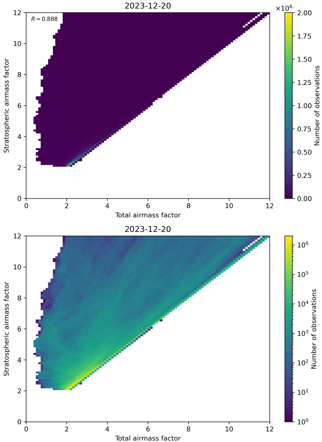
Figure 62: Scatter density plot of “Total airmass factor” against “Stratospheric airmass factor” for 2023-12-20 to 2023-12-21.
