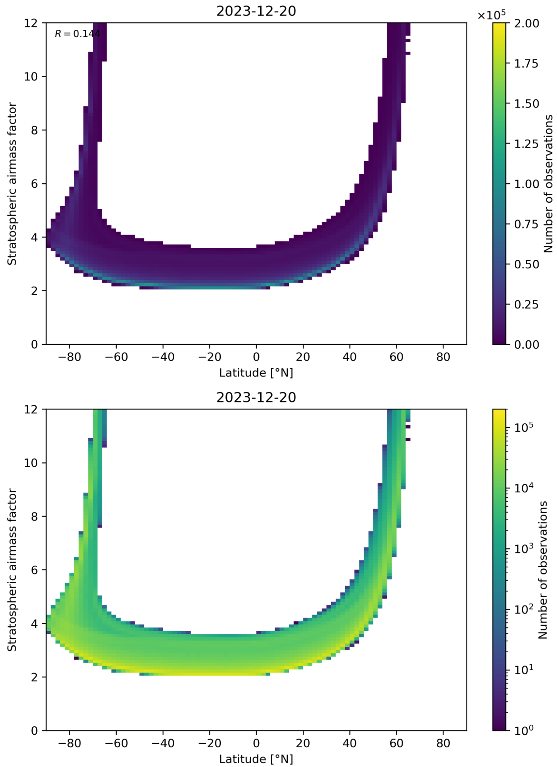
Figure 83: Scatter density plot of “Latitude” against “Stratospheric air mass factor” for 2023-12-20 to 2023-12-21.
