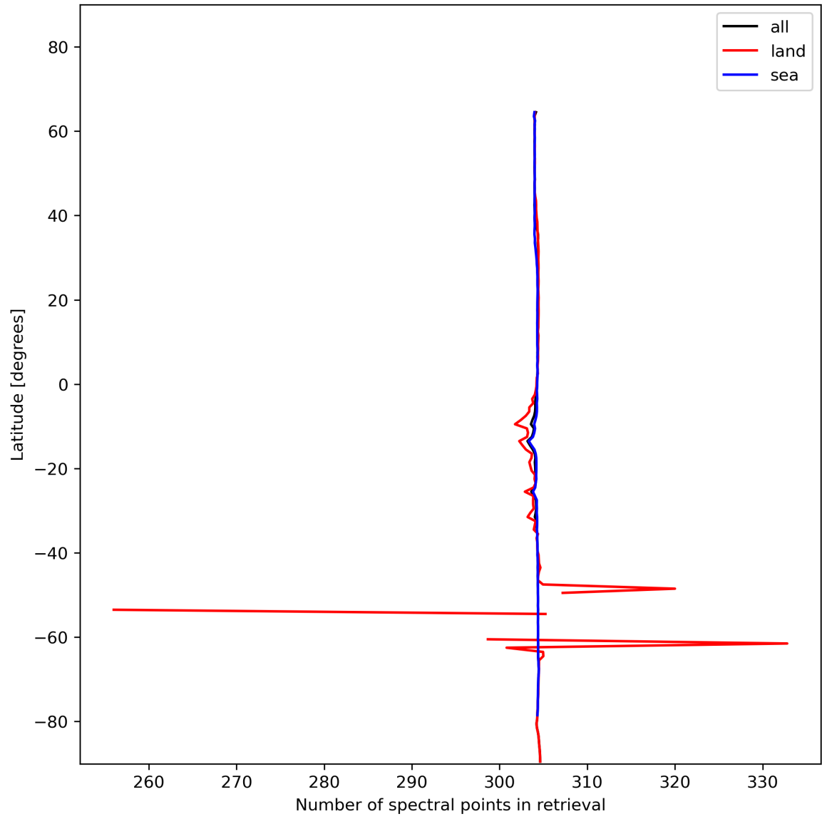
Figure 16: Zonal average of “Number of spectral points in retrieval” for 2023-12-20 to 2023-12-21.
