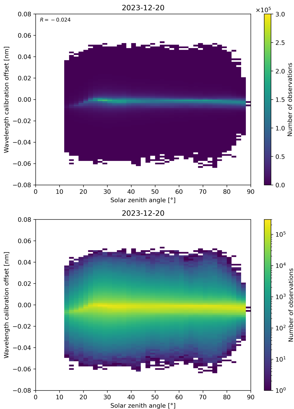
Figure 158: Scatter density plot of “Solar zenith angle” against “Wavelength calibration offset” for 2023-12-20 to 2023-12-21.
