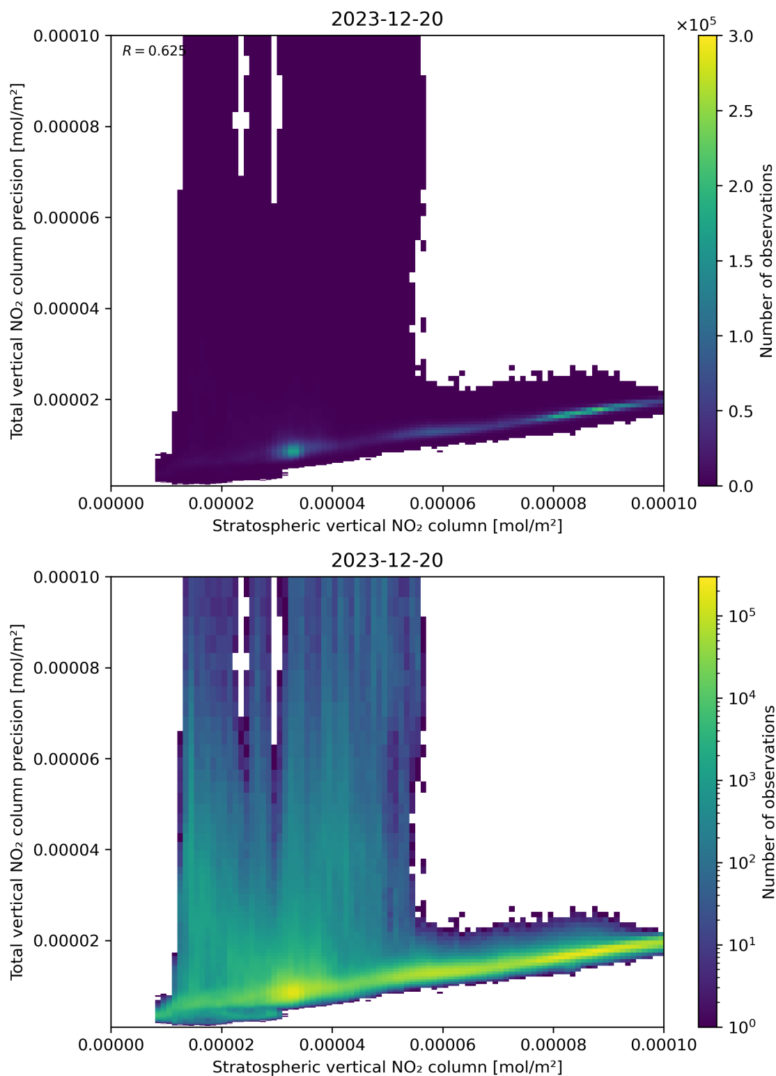
Figure 101: Scatter density plot of “Stratospheric vertical NO 2 column” against “Total vertical NO 2 column precision” for 2023-12-20 to 2023-12-21.
