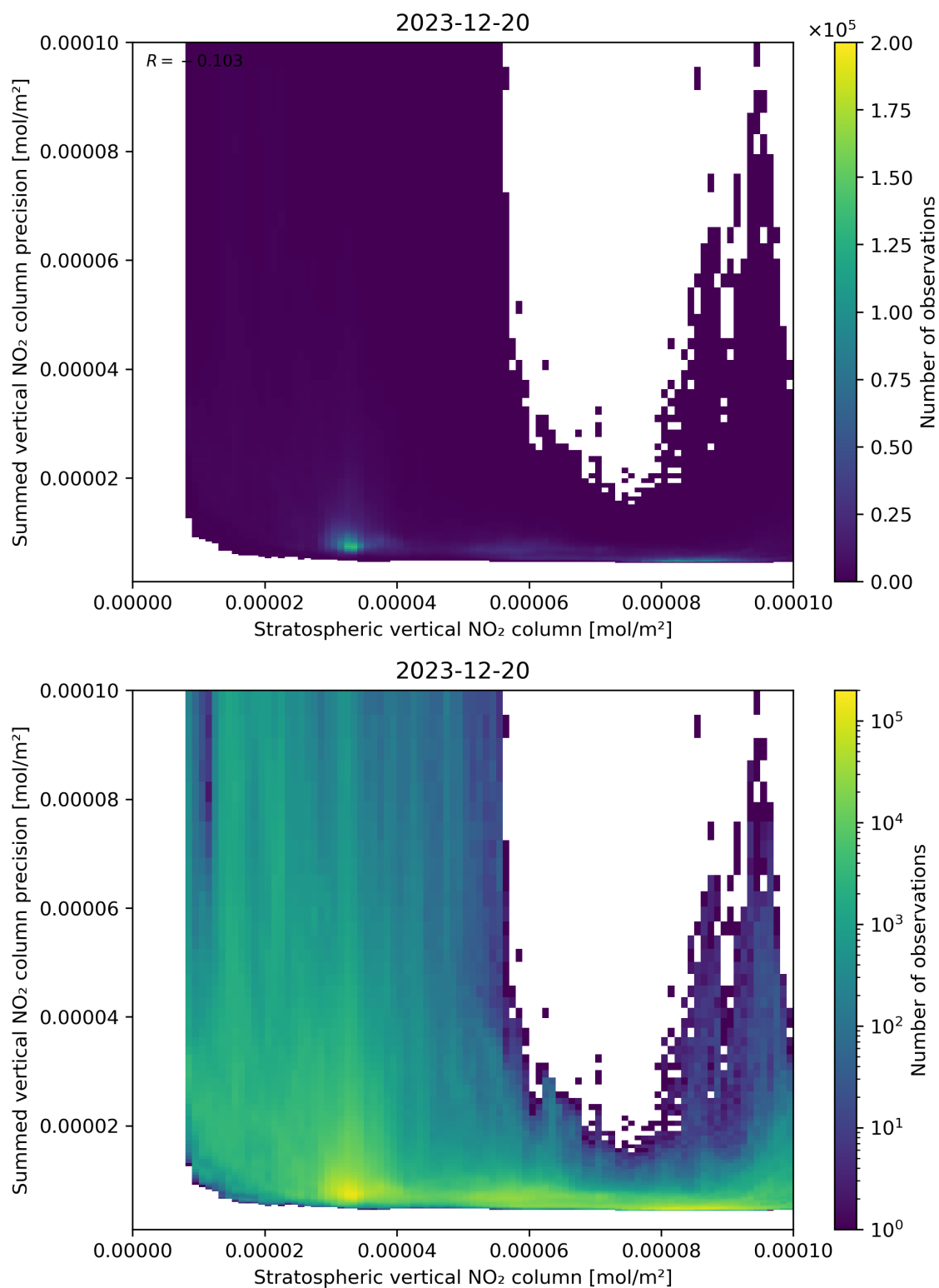
Figure 99: Scatter density plot of “Stratospheric vertical NO 2 column” against “Summed vertical NO 2 column precision” for 2023-12-20 to 2023-12-21.
