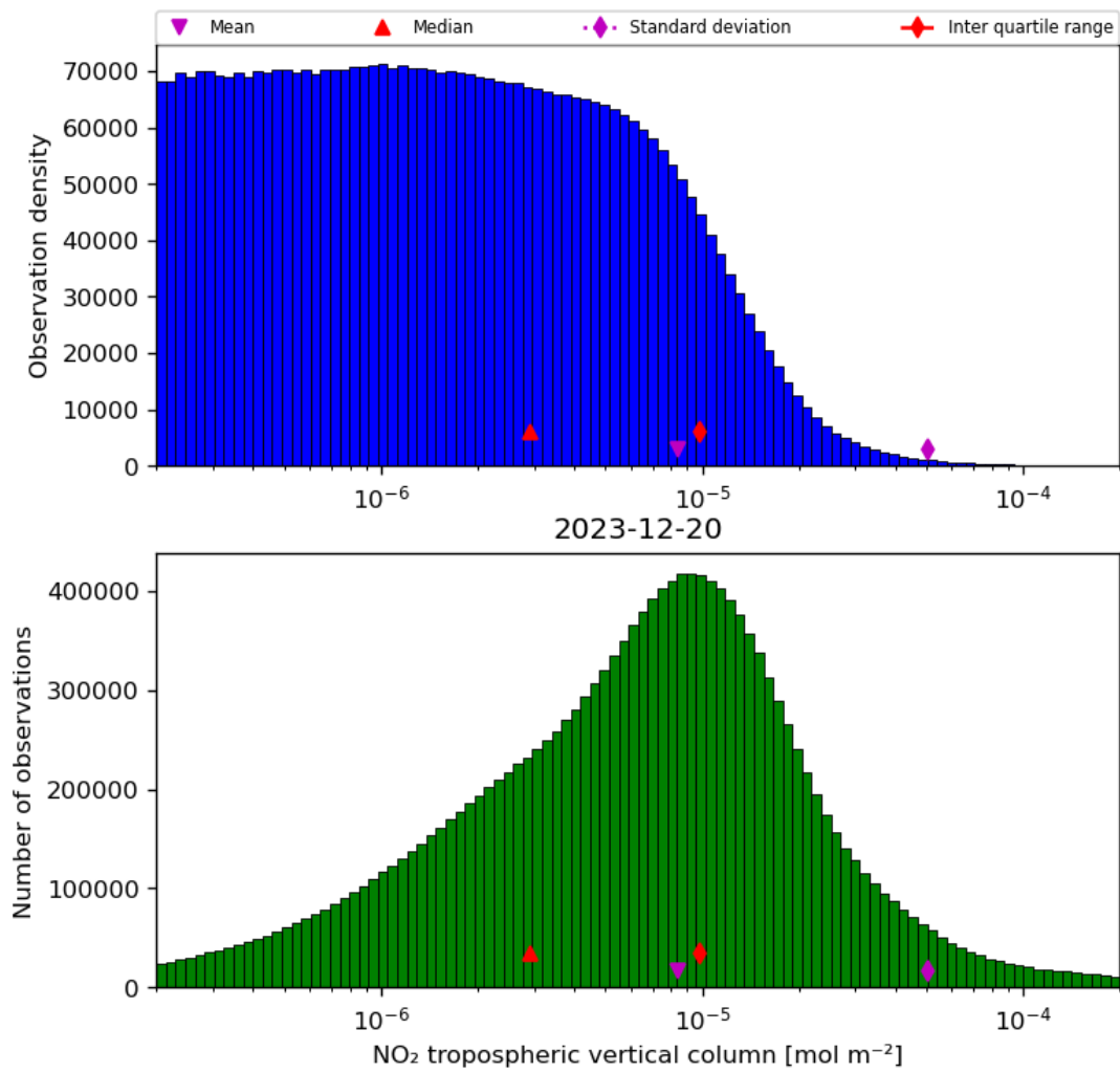
Figure 29: Histogram of “NO 2 tropospheric vertical column” for 2023-12-20 to 2023-12-21
