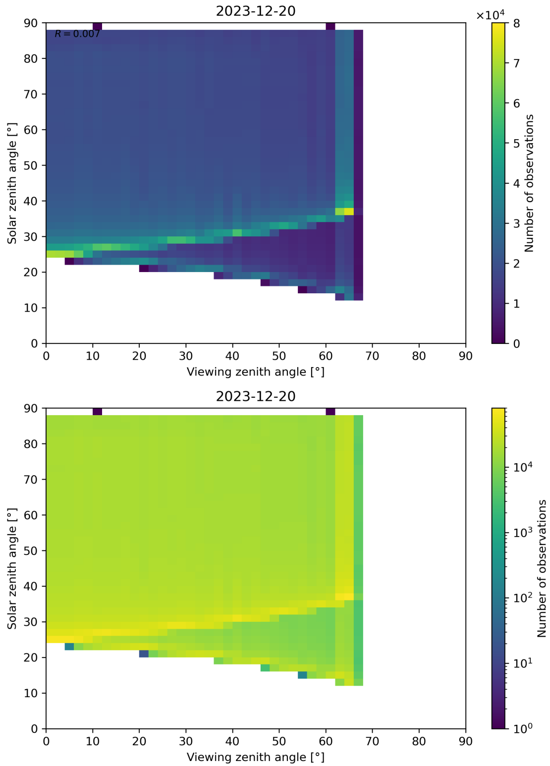
Figure 172: Scatter density plot of “Viewing zenith angle” against “Solar zenith angle” for 2023-12-20 to 2023-12-21.
