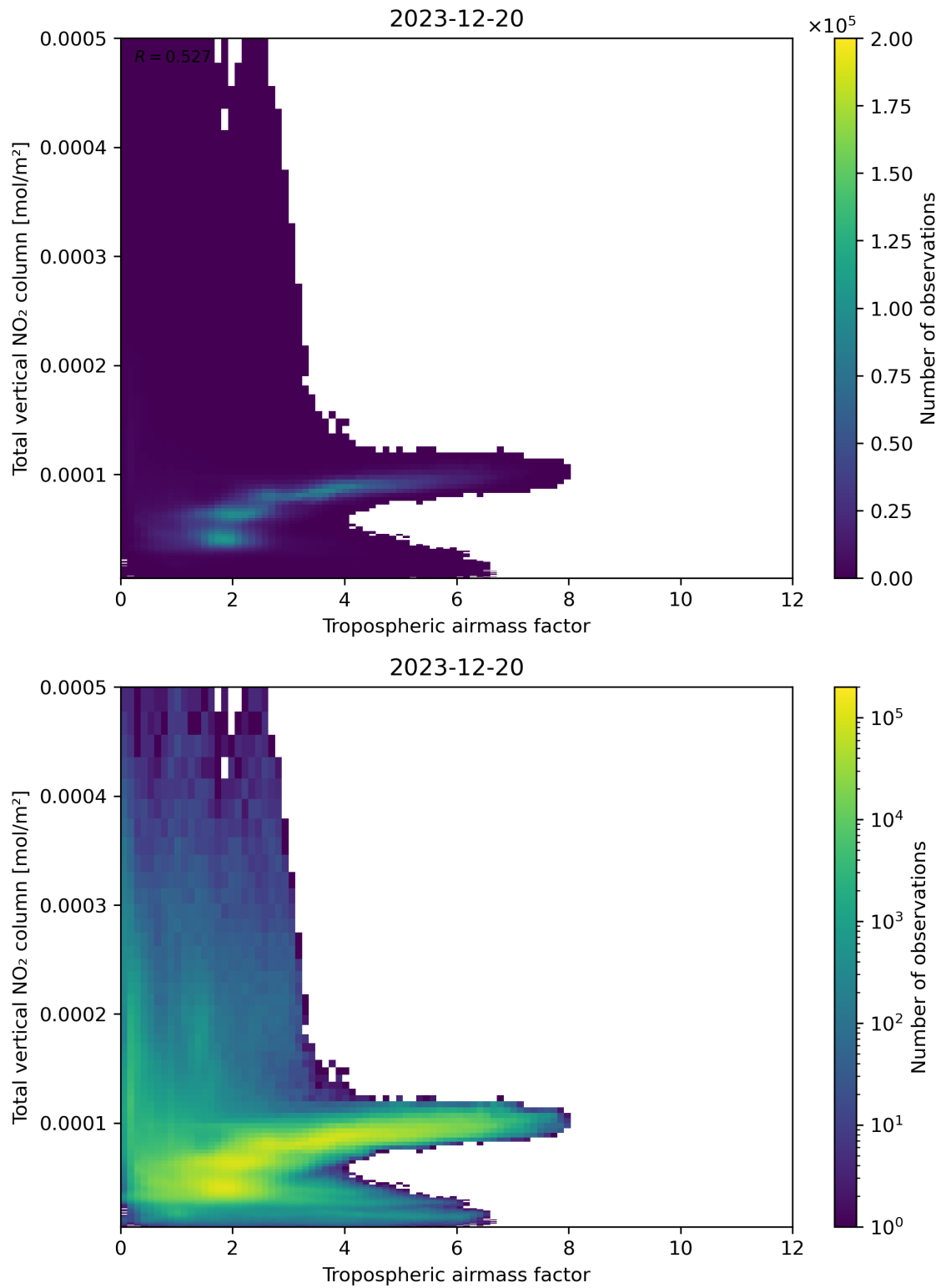
Figure 77: Scatter density plot of “Tropospheric airmass factor” against “Total vertical NO 2 column” for 2023-12-20 to 2023-12-21.
