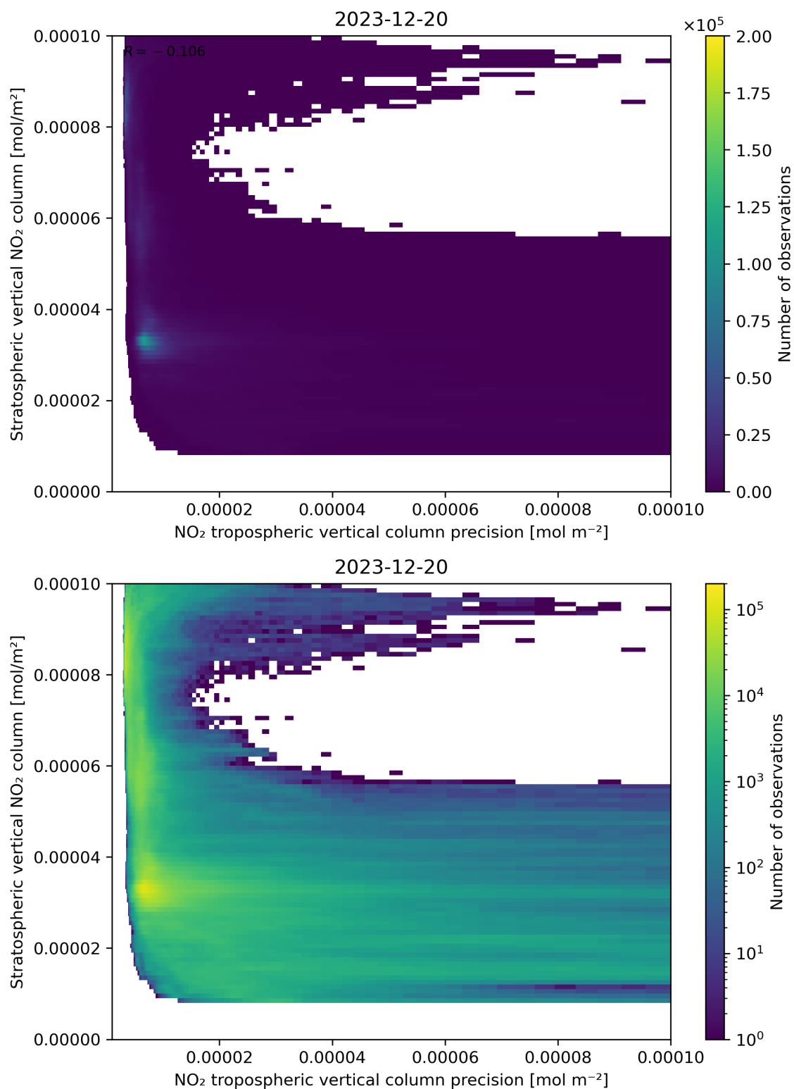
Figure 135: Scatter density plot of “NO 2 tropospheric vertical column precision” against “Stratospheric vertical NO 2 column” for 2023-12-20 to 2023-12-21.
