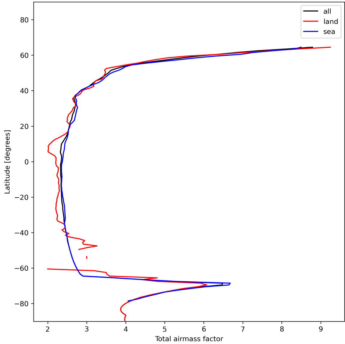
Figure 15: Zonal average of “Total airmass factor” for 2023-12-20 to 2023-12-21.
