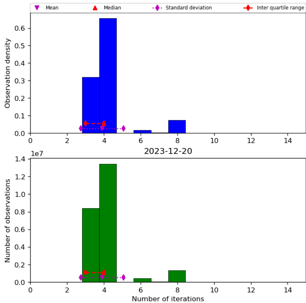
Figure 34: Histogram of “Number of iterations” for 2023-12-20 to 2023-12-21
