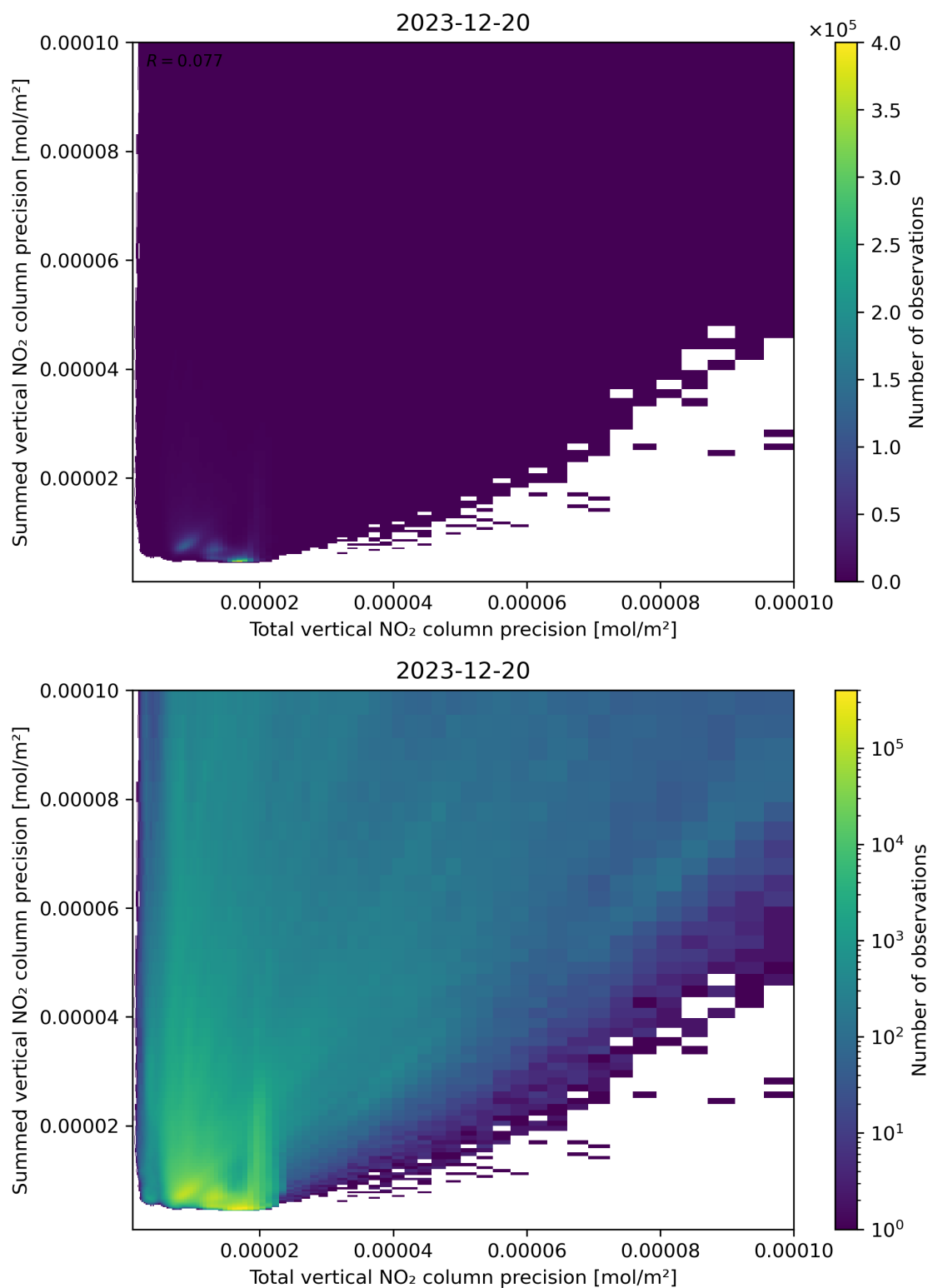
Figure 118: Scatter density plot of “Total vertical NO 2 column precision” against “Summed vertical NO 2 column precision” for 2023-12-20 to 2023-12-21.
