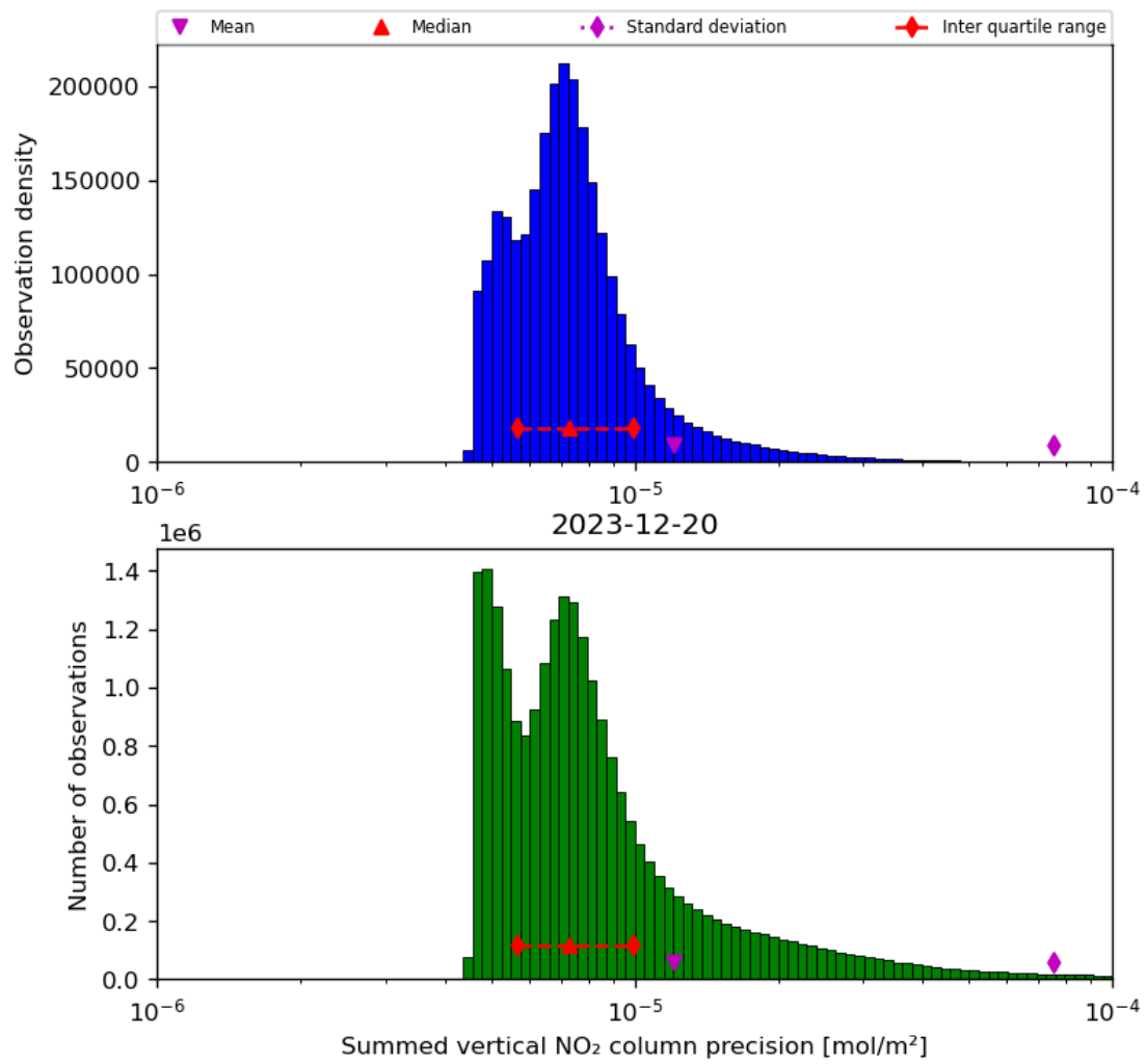
Figure 41: Histogram of “Summed vertical NO 2 column precision” for 2023-12-20 to 2023-12-21
