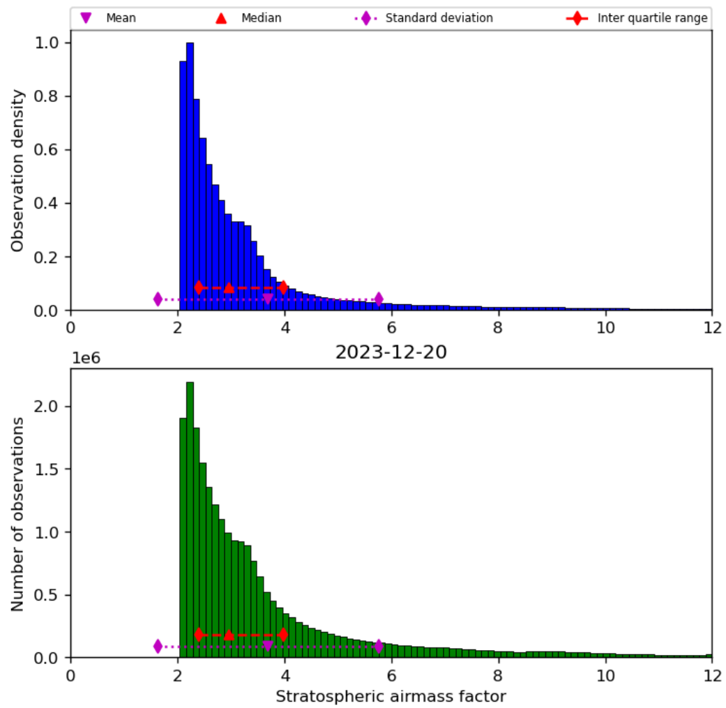
Figure 44: Histogram of “Stratospheric airmass factor” for 2023-12-20 to 2023-12-21
