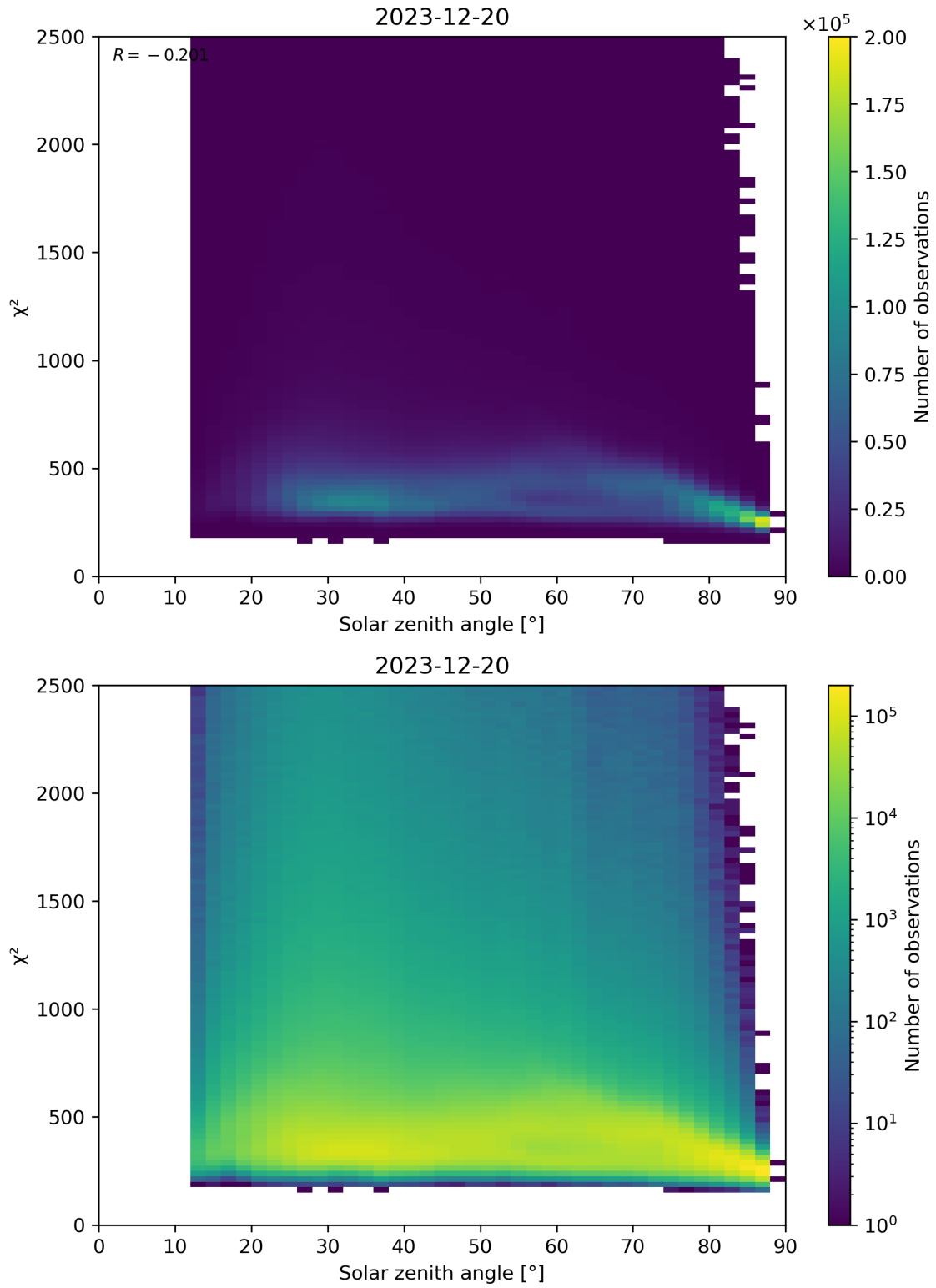
Figure 148: Scatter density plot of “Solar zenith angle” against “ \chi^2 ” for 2023-12-20 to 2023-12-21.
