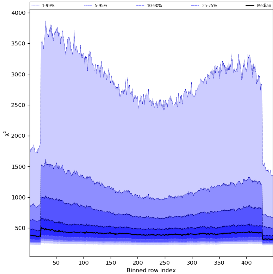
Figure 59: Along track statistics of “ \chi^2 ” for 2023-12-20 to 2023-12-21
