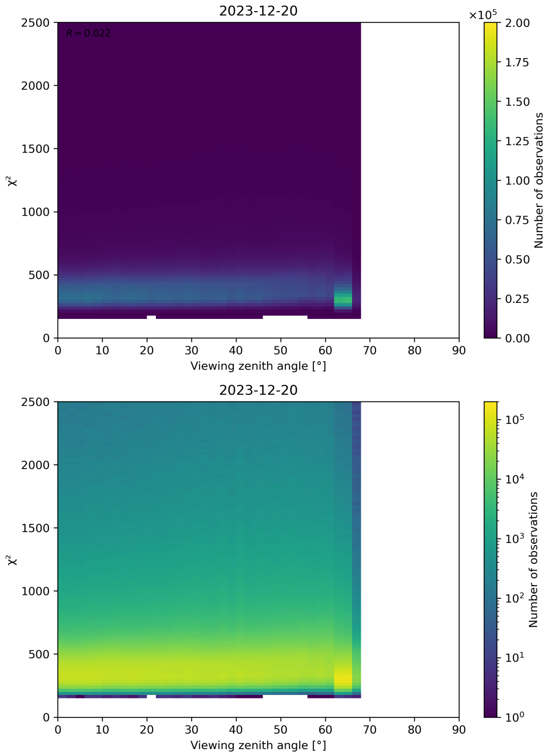
Figure 162: Scatter density plot of “Viewing zenith angle” against “ \chi^2 ” for 2023-12-20 to 2023-12-21.
