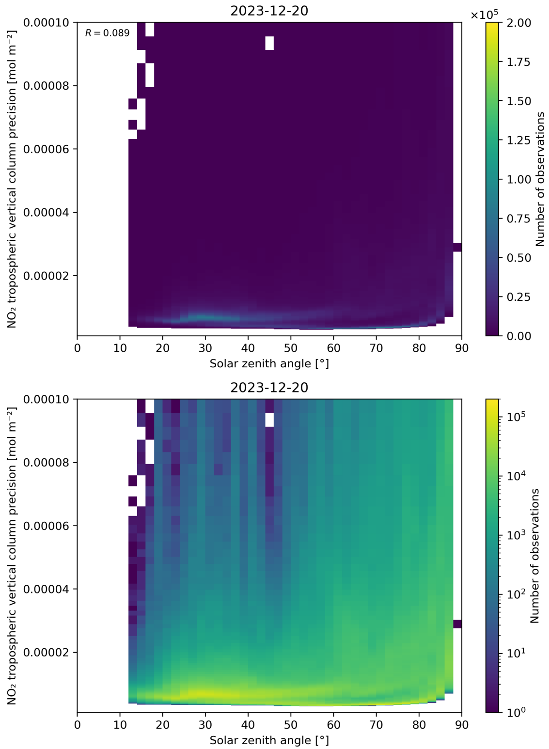
Figure 156: Scatter density plot of “Solar zenith angle” against “NO 2 tropospheric vertical column precision” for 2023-12-20 to 2023-12-21.
