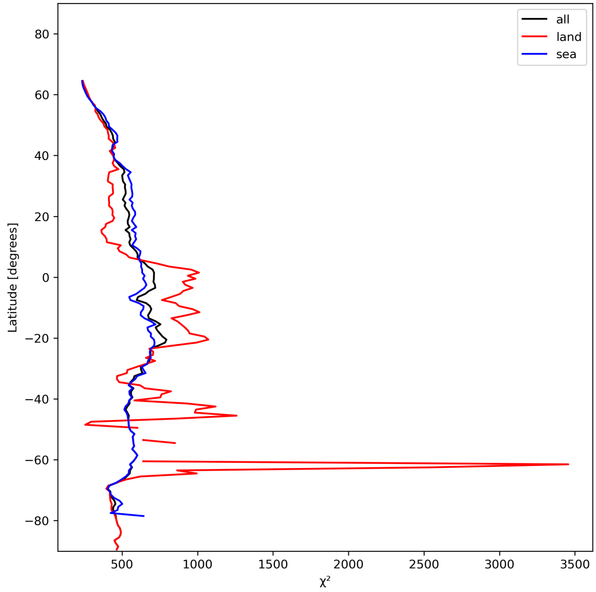
Figure 25: Zonal average of “ \chi^2 ” for 2023-12-20 to 2023-12-21.
