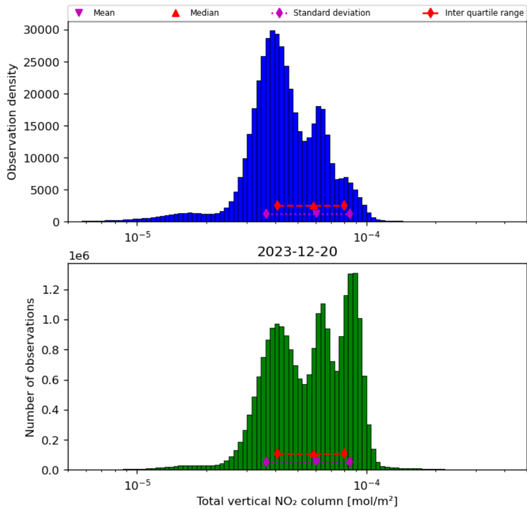
Figure 38: Histogram of “Total vertical NO 2 column” for 2023-12-20 to 2023-12-21
