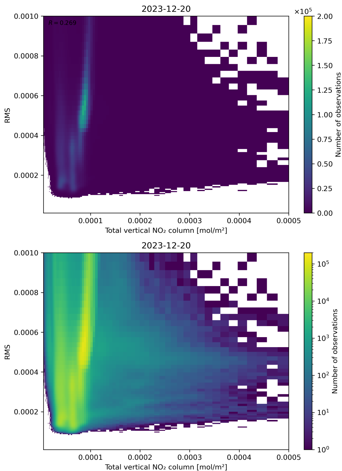
Figure 120: Scatter density plot of “Total vertical NO 2 column” against “RMS” for 2023-12-20 to 2023-12-21.
