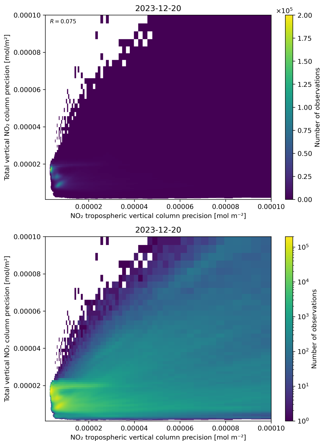
Figure 139: Scatter density plot of “NO 2 tropospheric vertical column precision” against “Total vertical NO 2 column precision” for 2023-12-20 to 2023-12-21.
