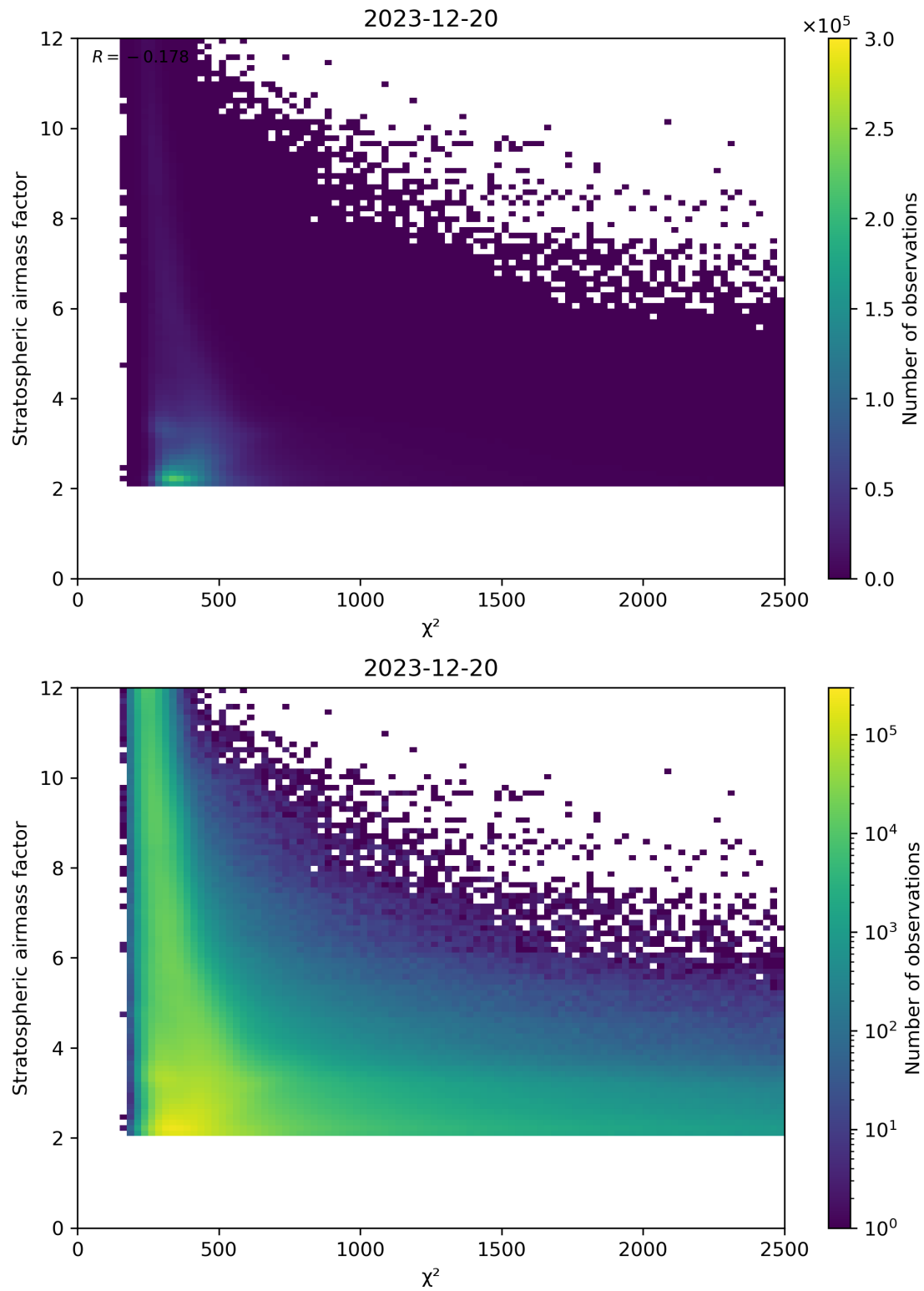
Figure 81: Scatter density plot of “ \chi^2 ” against “Stratospheric airmass factor” for 2023-12-20 to 2023-12-21.
