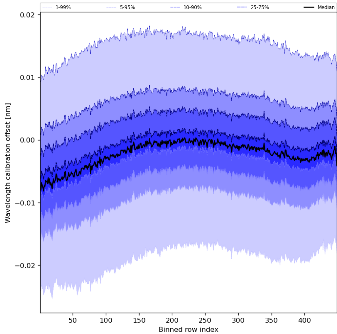
Figure 52: Along track statistics of “Wavelength calibration offset” for 2023-12-20 to 2023-12-21
