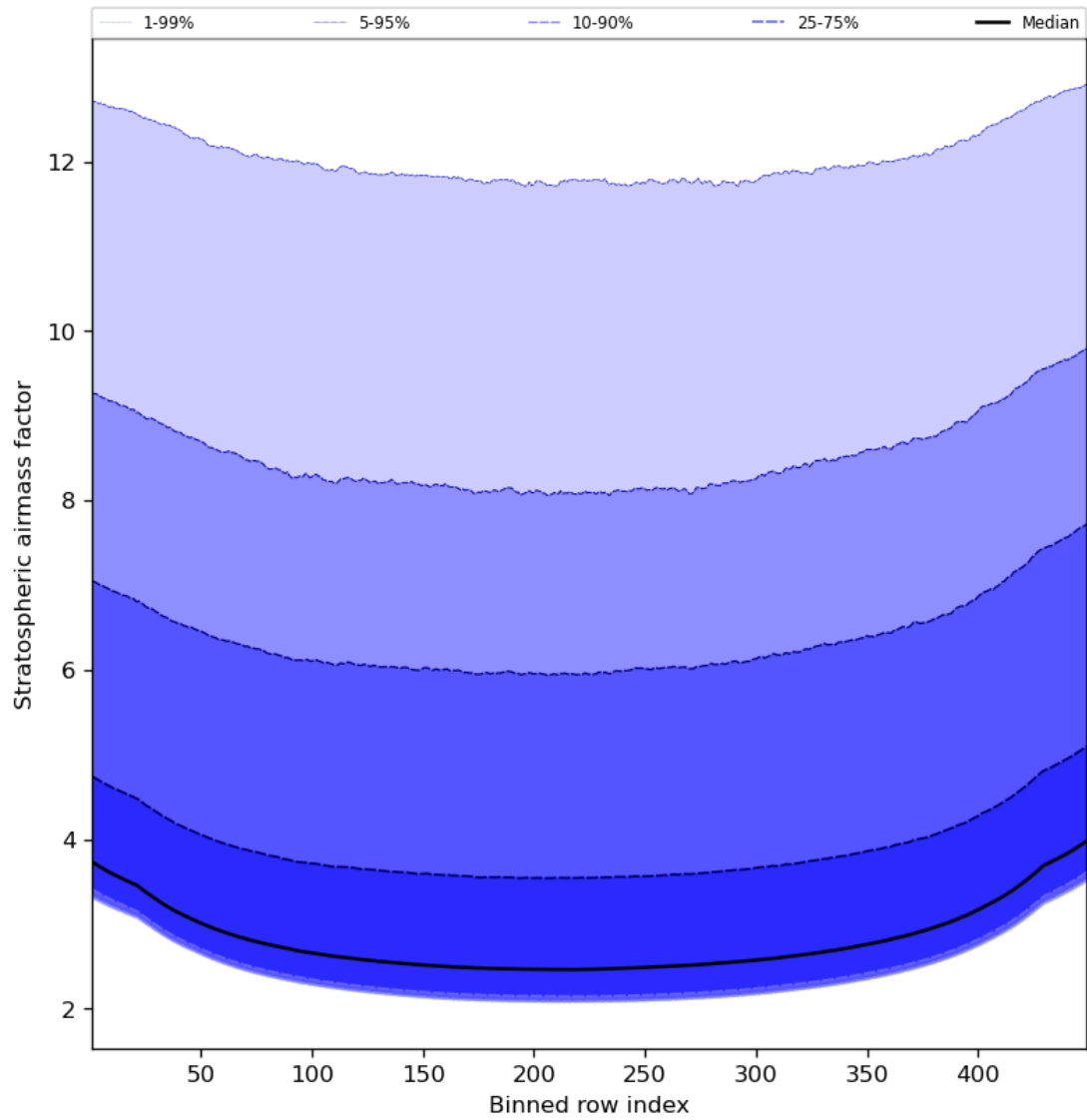
Figure 61: Along track statistics of “Stratospheric airmass factor” for 2023-12-20 to 2023-12-21
