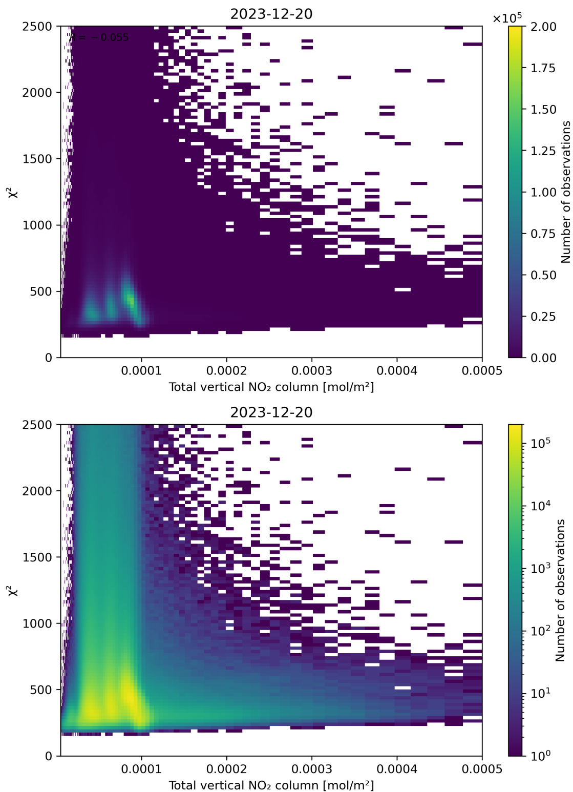
Figure 111: Scatter density plot of “Total vertical NO 2 column” against “ \chi^2 ” for 2023-12-20 to 2023-12-21.
