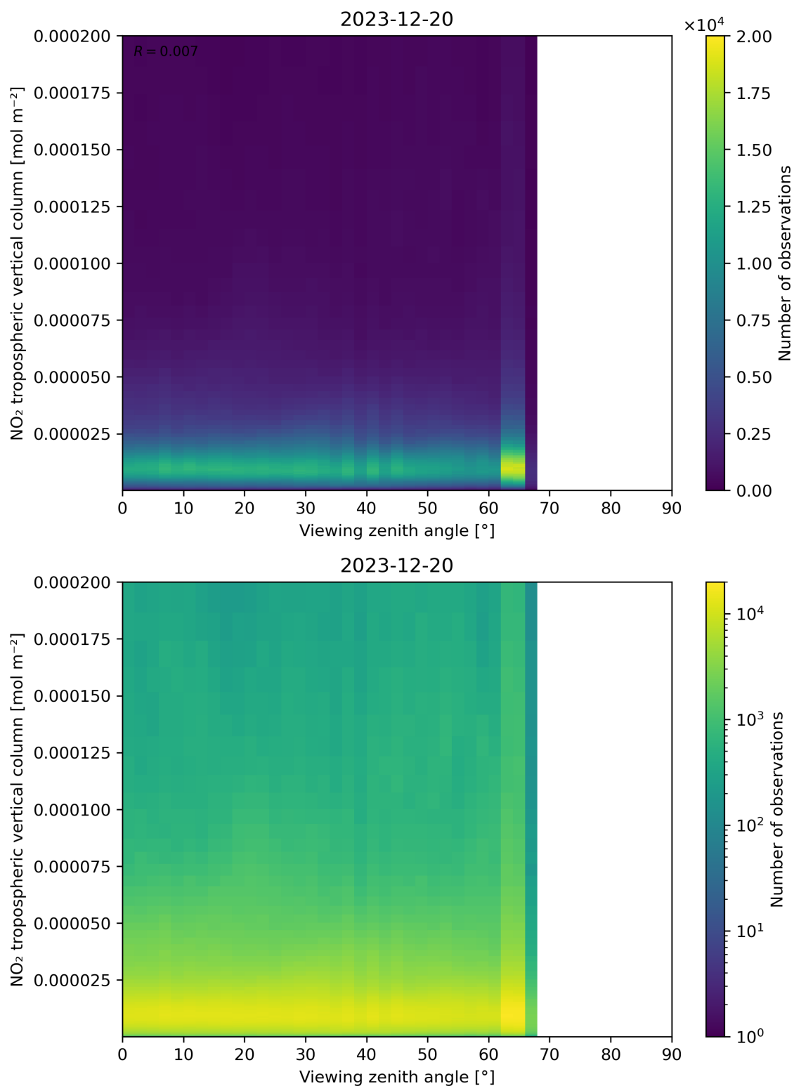
Figure 169: Scatter density plot of “Viewing zenith angle” against “NO 2 tropospheric vertical column” for 2023-12-20 to 2023-12-21.
