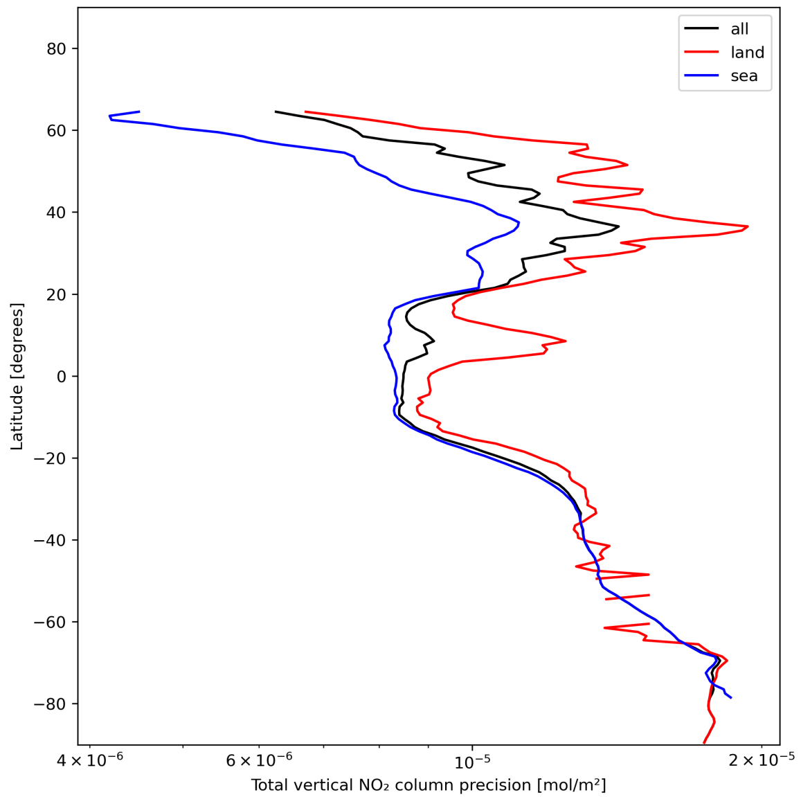
Figure 22: Zonal average of "Total vertical NO 2 column precision" for 2023-12-20 to 2023-12-21.
