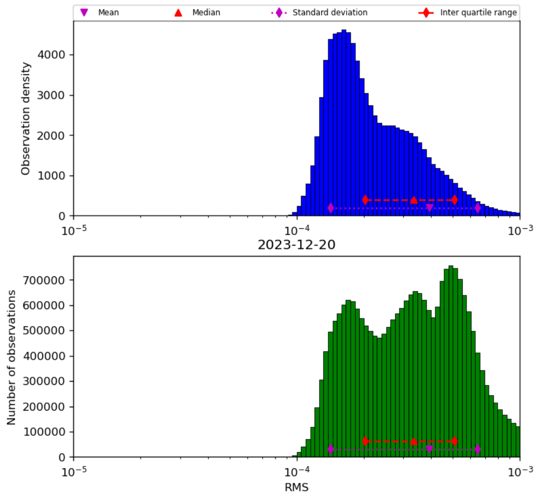
Figure 43: Histogram of “RMS” for 2023-12-20 to 2023-12-21
