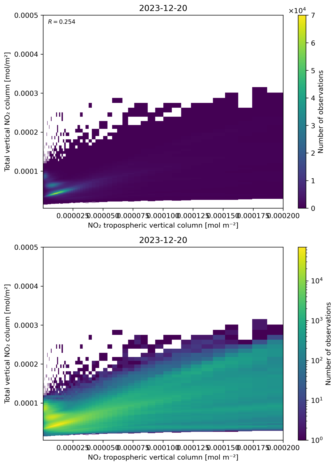
Figure 128: Scatter density plot of “NO 2 tropospheric vertical column” against “Total vertical NO 2 column” for 2023-12-20 to 2023-12-21.
