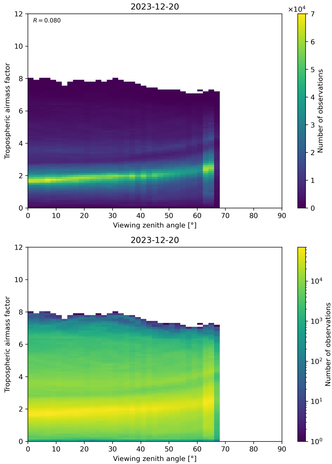
Figure 161: Scatter density plot of “Viewing zenith angle” against “Tropospheric airmass factor” for 2023-12-20 to 2023-12-21.
