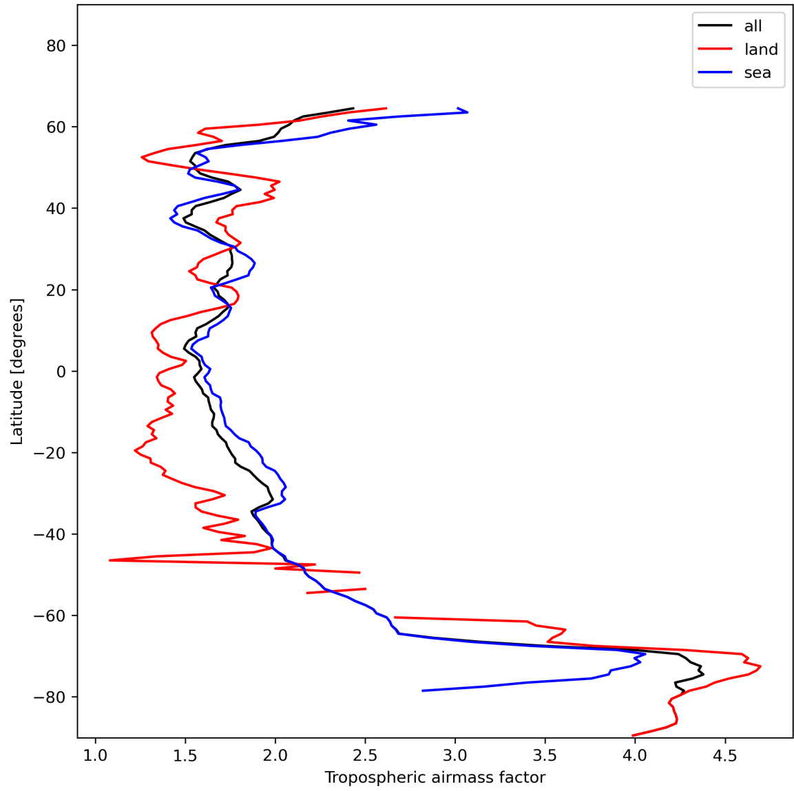
Figure 14: Zonal average of “Tropospheric airmass factor” for 2023-12-20 to 2023-12-21.
