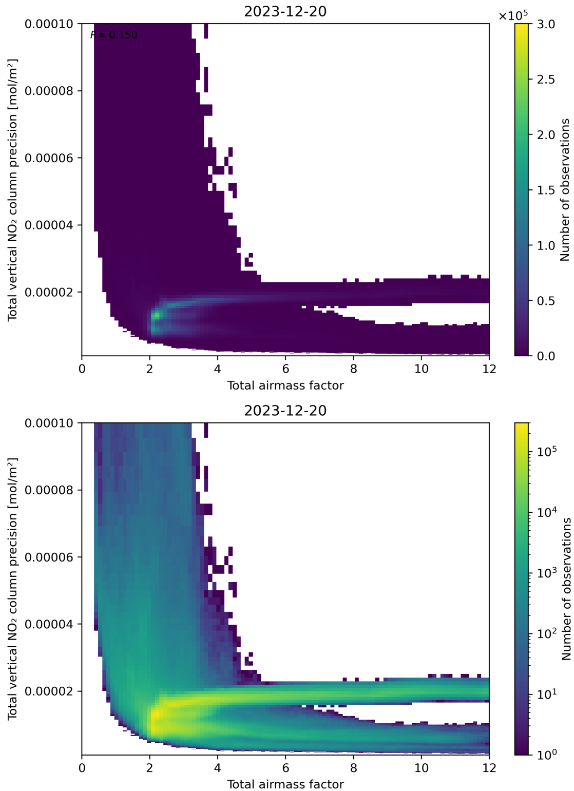
Figure 68: Scatter density plot of “Total airmass factor” against “Total vertical NO 2 column precision” for 2023-12-20 to 2023-12-21.
