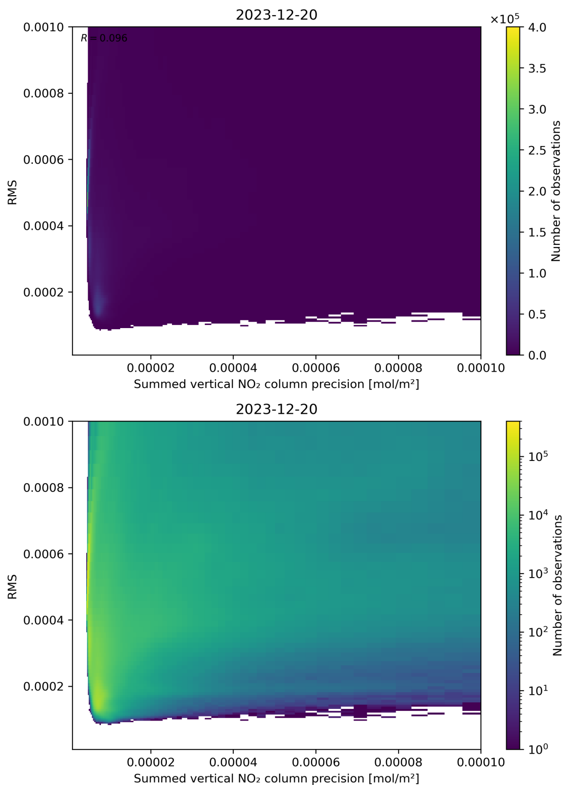
Figure 108: Scatter density plot of “Summed vertical NO 2 column precision” against “RMS” for 2023-12-20 to 2023-12-21.
