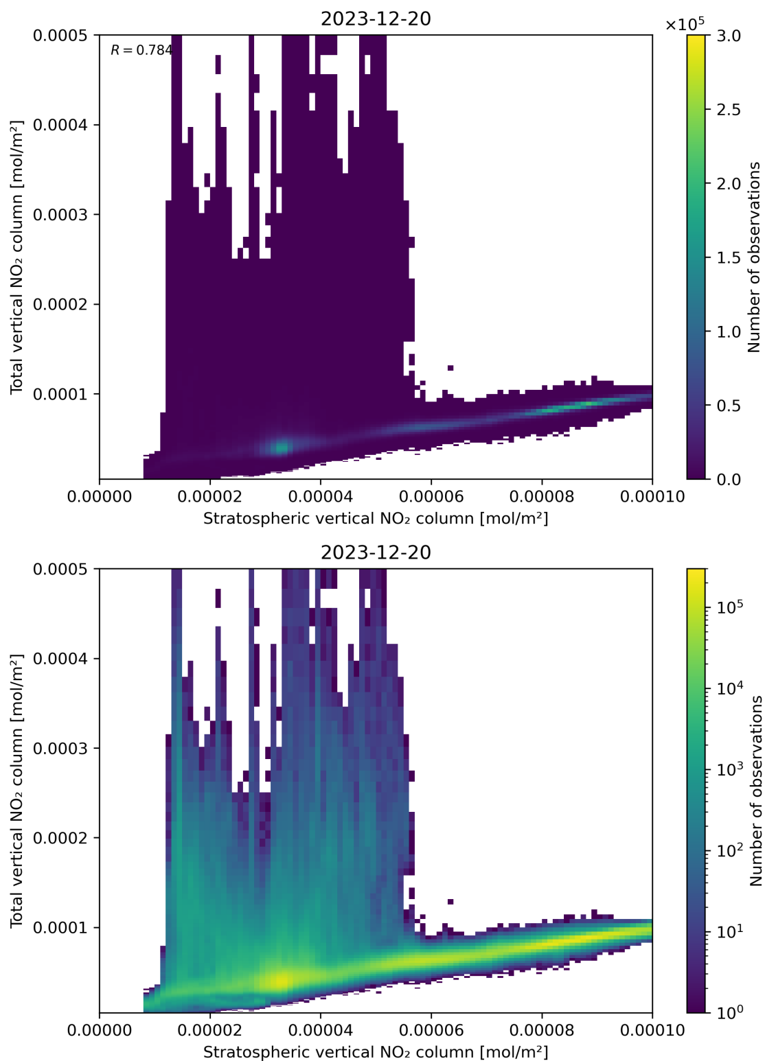
Figure 100: Scatter density plot of “Stratospheric vertical NO 2 column” against “Total vertical NO 2 column” for 2023-12-20 to 2023-12-21.
