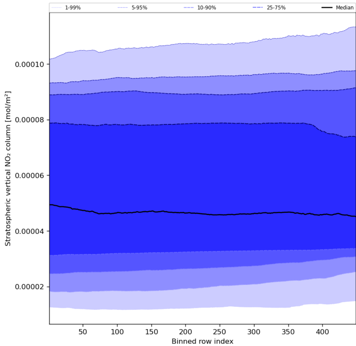
Figure 53: Along track statistics of “Stratospheric vertical NO 2 column” for 2023-12-20 to 2023-12-21
