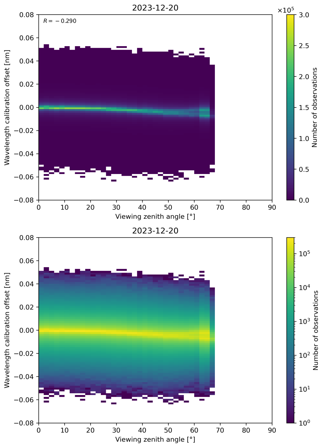
Figure 173: Scatter density plot of “Viewing zenith angle” against “Wavelength calibration offset” for 2023-12-20 to 2023-12-21.
