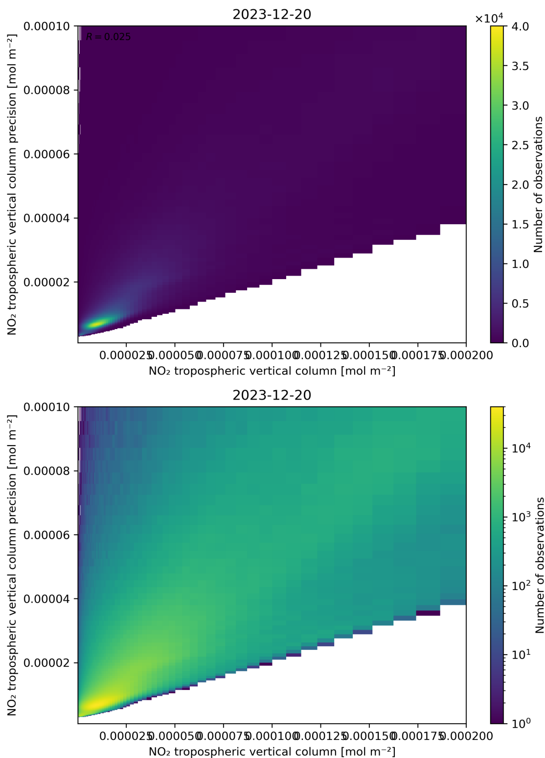
Figure 130: Scatter density plot of “NO 2 tropospheric vertical column” against “NO 2 tropospheric vertical column precision” for 2023-12-20 to 2023-12-21.
