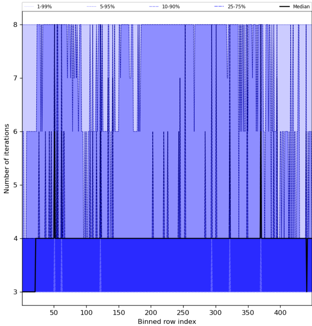
Figure 51: Along track statistics of “Number of iterations” for 2023-12-20 to 2023-12-21
