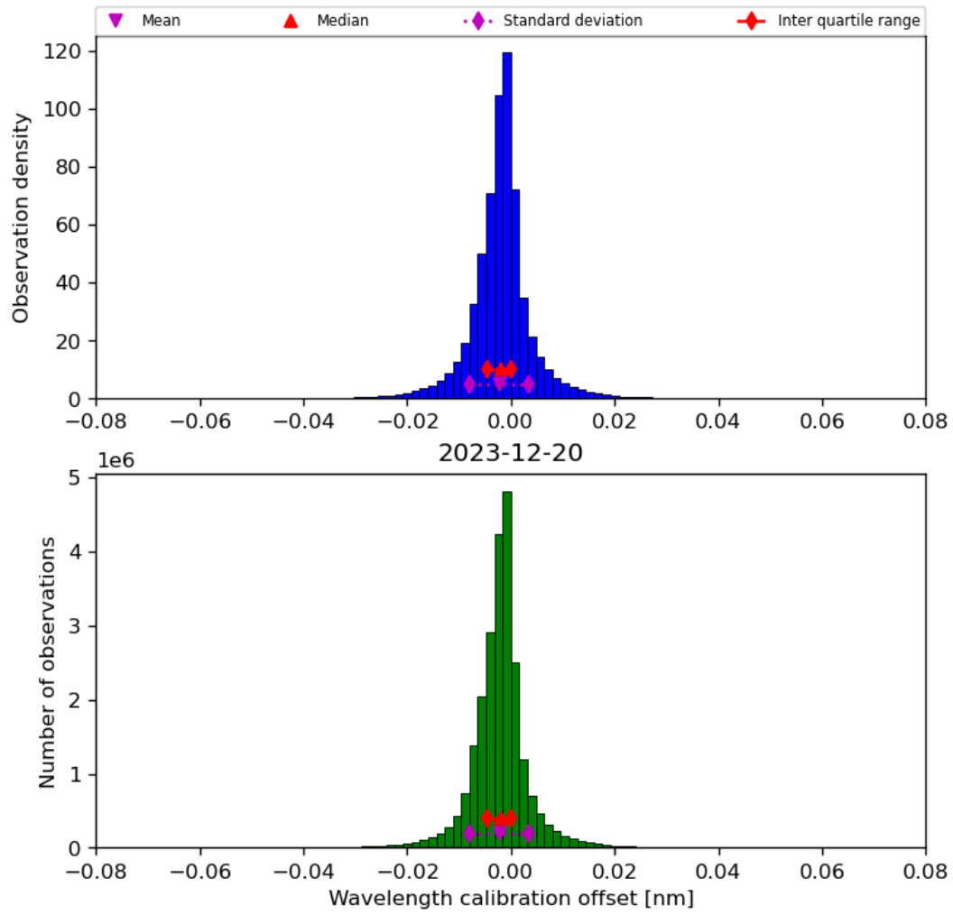
Figure 35: Histogram of “Wavelength calibration offset” for 2023-12-20 to 2023-12-21
