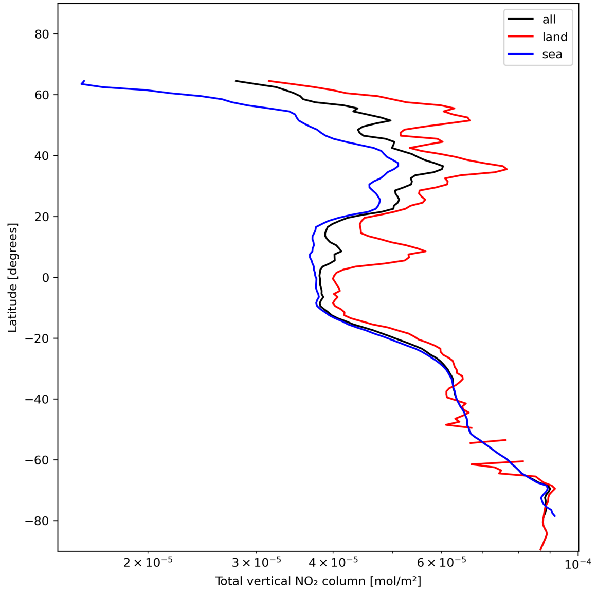
Figure 21: Zonal average of “Total vertical NO 2 column” for 2023-12-20 to 2023-12-21.
