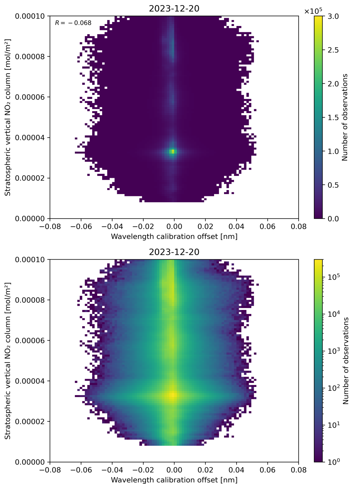
Figure 176: Scatter density plot of “Wavelength calibration offset” against “Stratospheric vertical NO 2 column” for 2023-12-20 to 2023-12-21.
