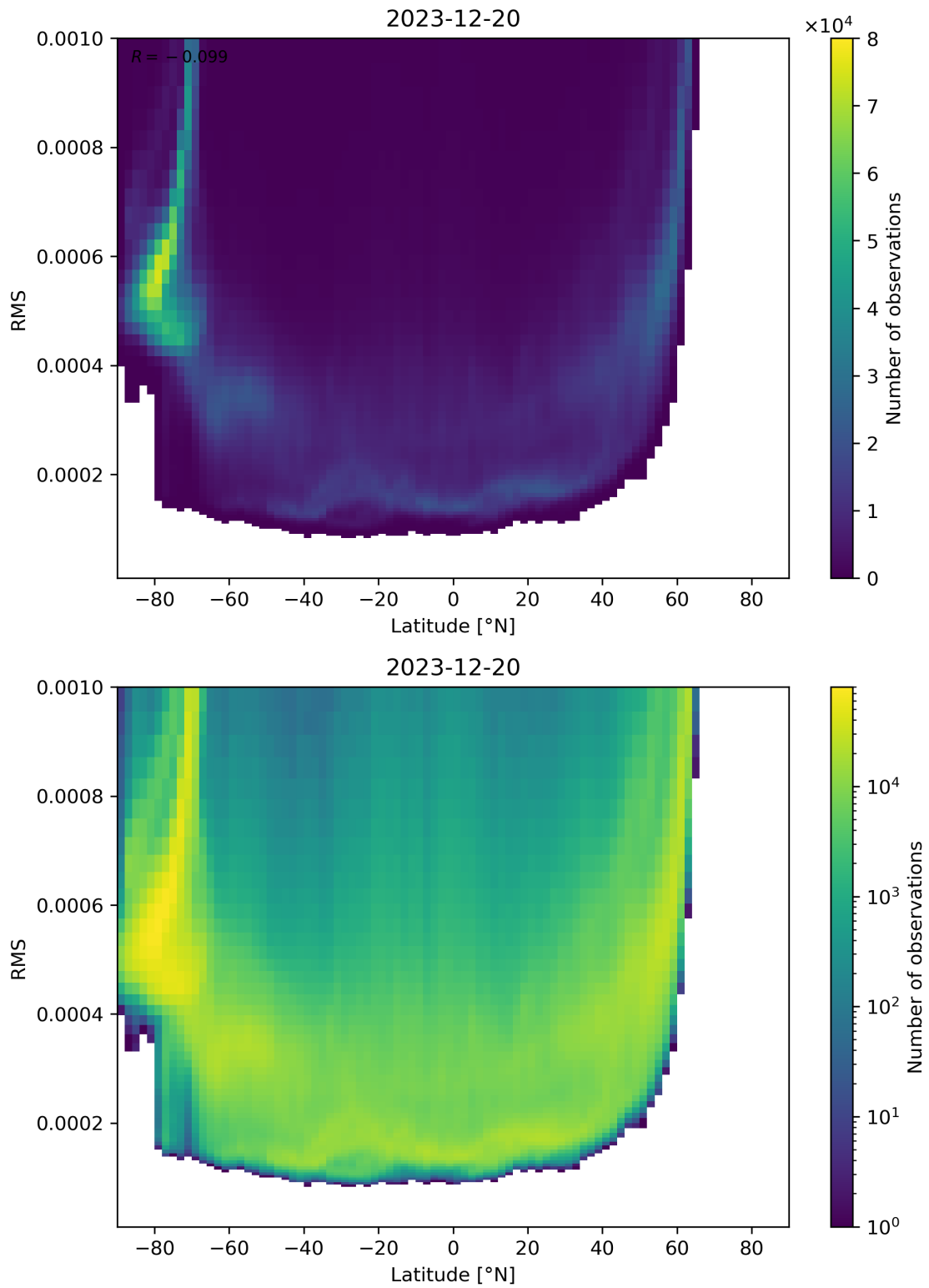
Figure 94: Scatter density plot of “Latitude” against “RMS” for 2023-12-20 to 2023-12-21.
