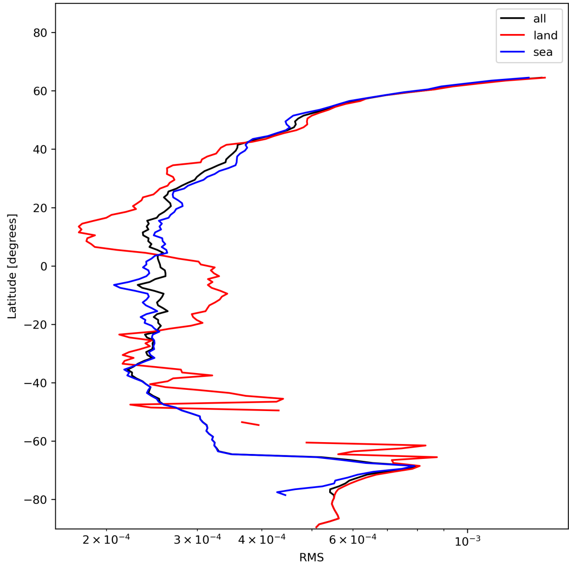
Figure 26: Zonal average of “RMS” for 2023-12-20 to 2023-12-21.
