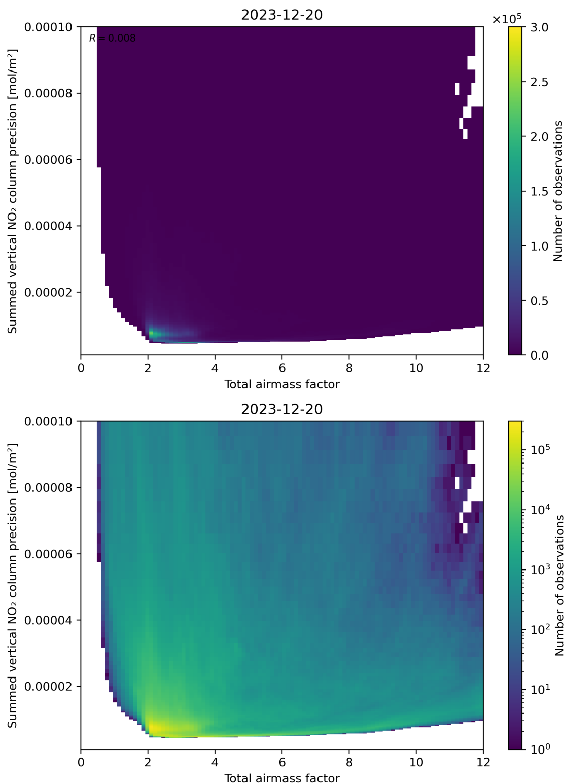
Figure 66: Scatter density plot of “Total airmass factor” against “Summed vertical NO 2 column precision” for 2023-12-20 to 2023-12-21.
