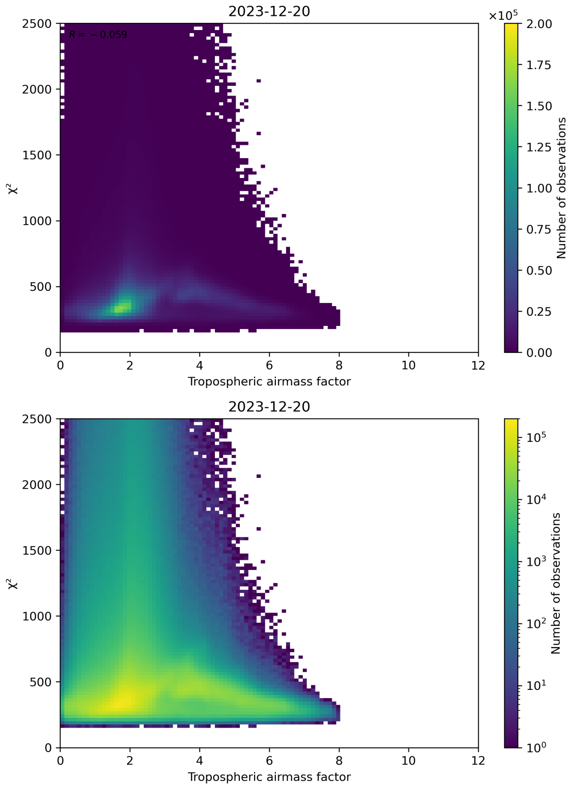
Figure 73: Scatter density plot of “Tropospheric airmass factor” against “ \chi^2 ” for 2023-12-20 to 2023-12-21.
