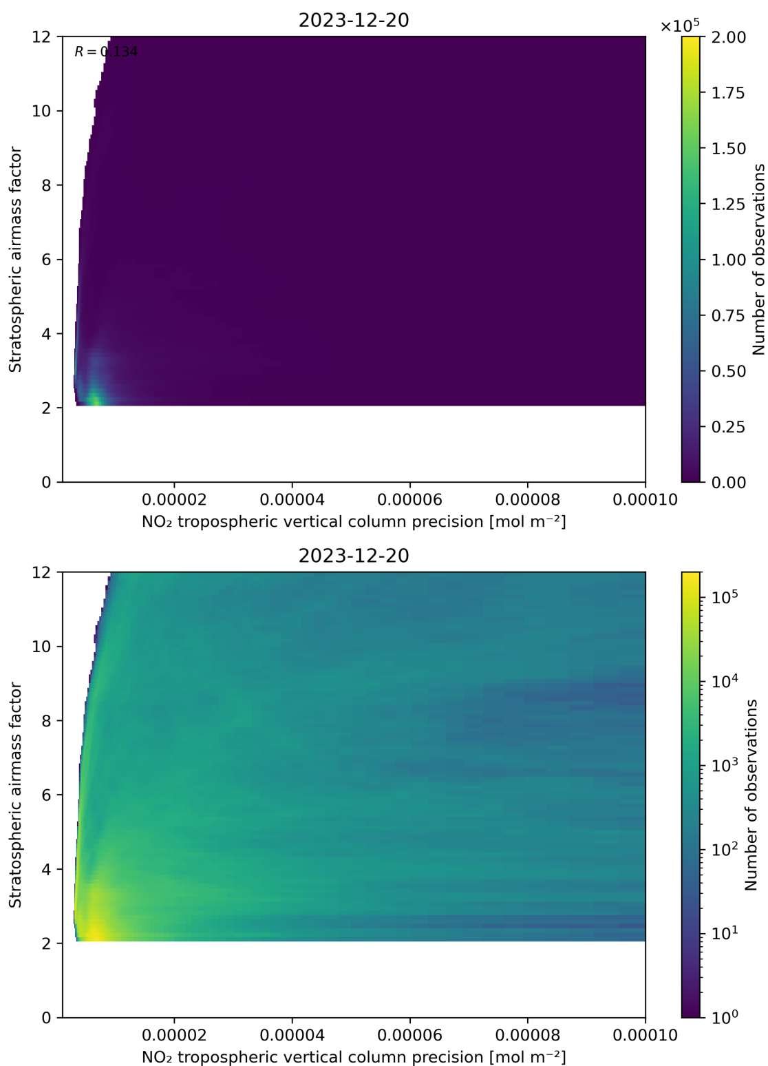
Figure 131: Scatter density plot of “NO 2 tropospheric vertical column precision” against “Stratospheric airmass factor” for 2023-12-20 to 2023-12-21.
