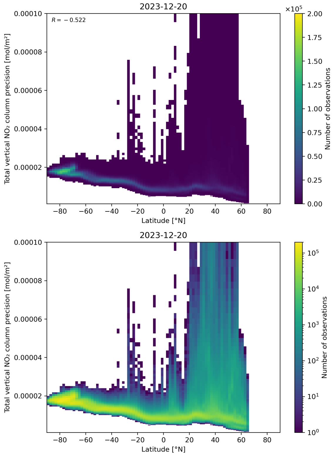
Figure 91: Scatter density plot of “Latitude” against “Total vertical NO 2 column precision” for 2023-12-20 to 2023-12-21.
