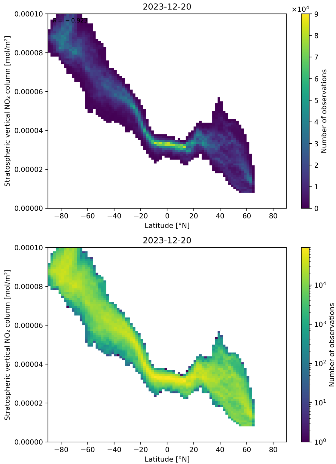
Figure 87: Scatter density plot of “Latitude” against “Stratospheric vertical NO 2 column” for 2023-12-20 to 2023-12-21.
