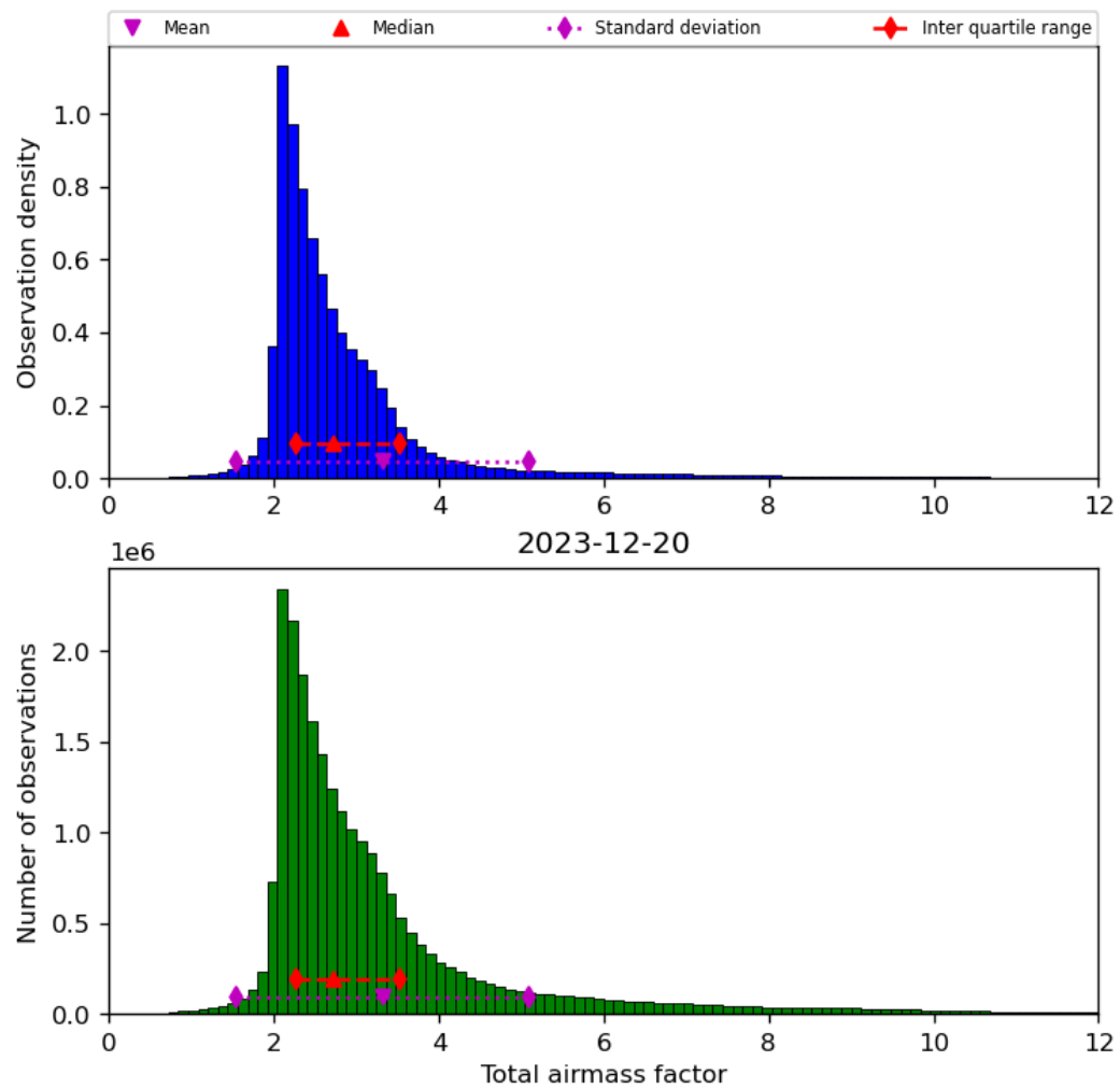
Figure 32: Histogram of “Total airmass factor” for 2023-12-20 to 2023-12-21
