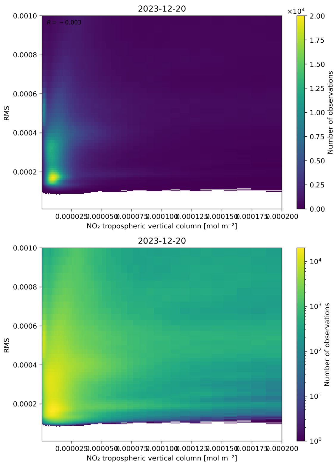
Figure 142: Scatter density plot of “NO 2 tropospheric vertical column” against “RMS” for 2023-12-20 to 2023-12-21.
