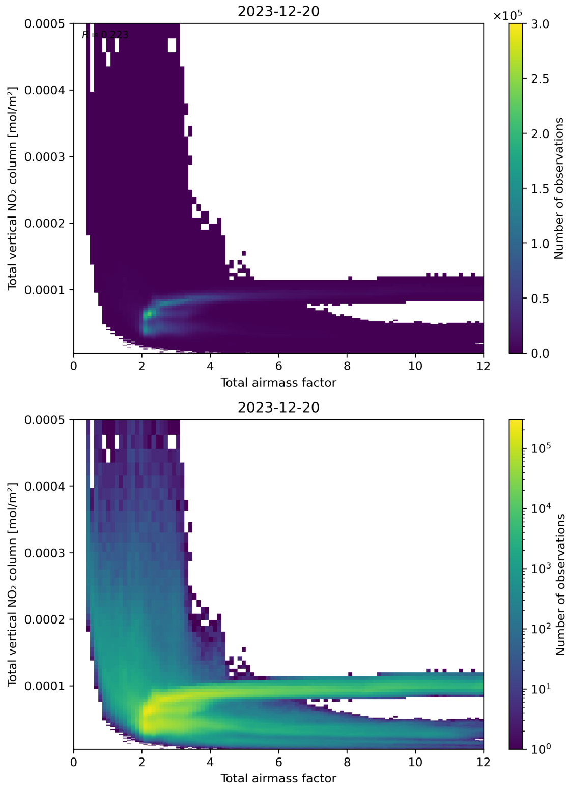
Figure 67: Scatter density plot of “Total airmass factor” against “Total vertical NO 2 column” for 2023-12-20 to 2023-12-21.
