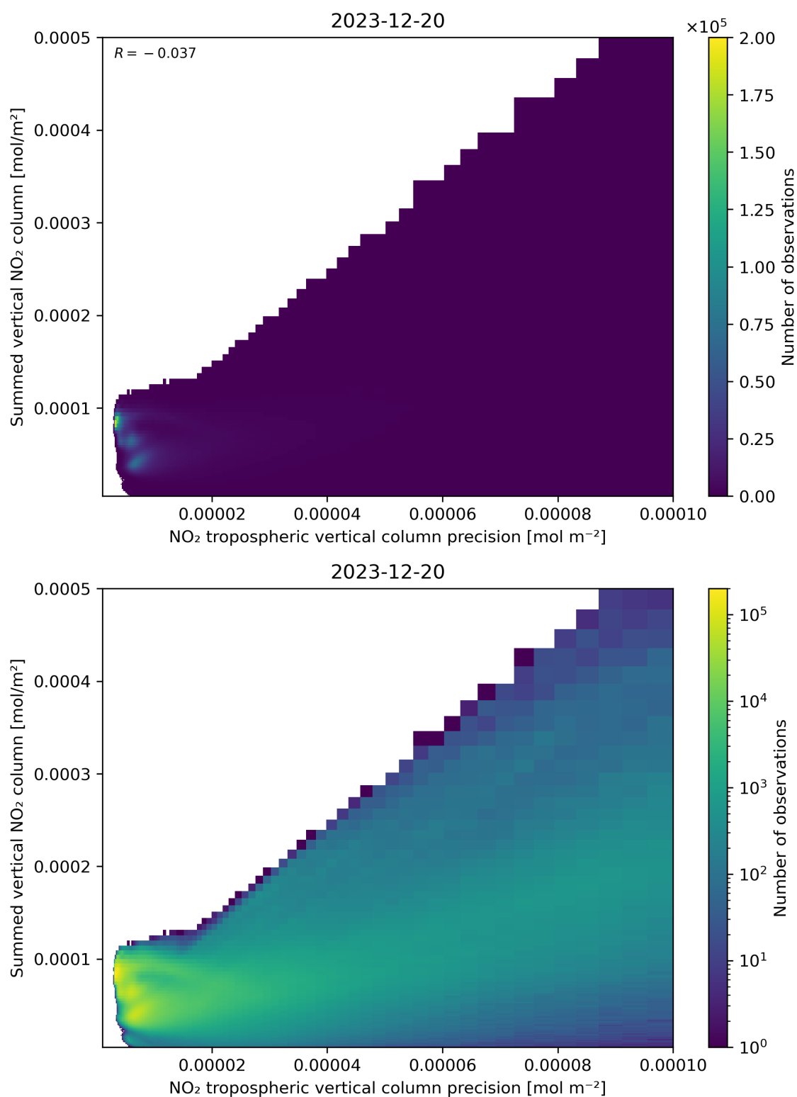
Figure 136: Scatter density plot of “NO 2 tropospheric vertical column precision” against “Summed vertical NO 2 column” for 2023-12-20 to 2023-12-21.
