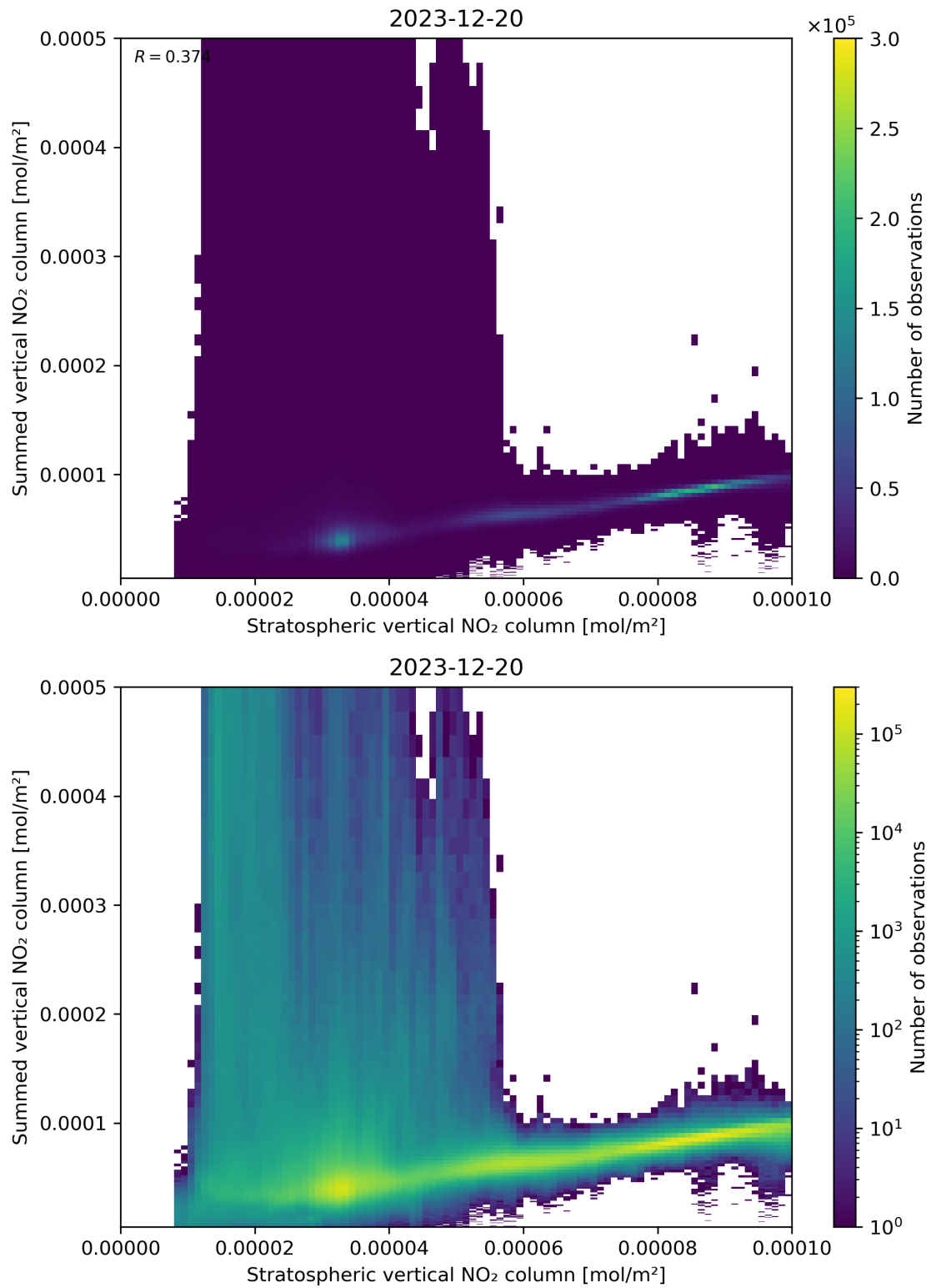
Figure 98: Scatter density plot of “Stratospheric vertical NO 2 column” against “Summed vertical NO 2 column” for 2023-12-20 to 2023-12-21.
