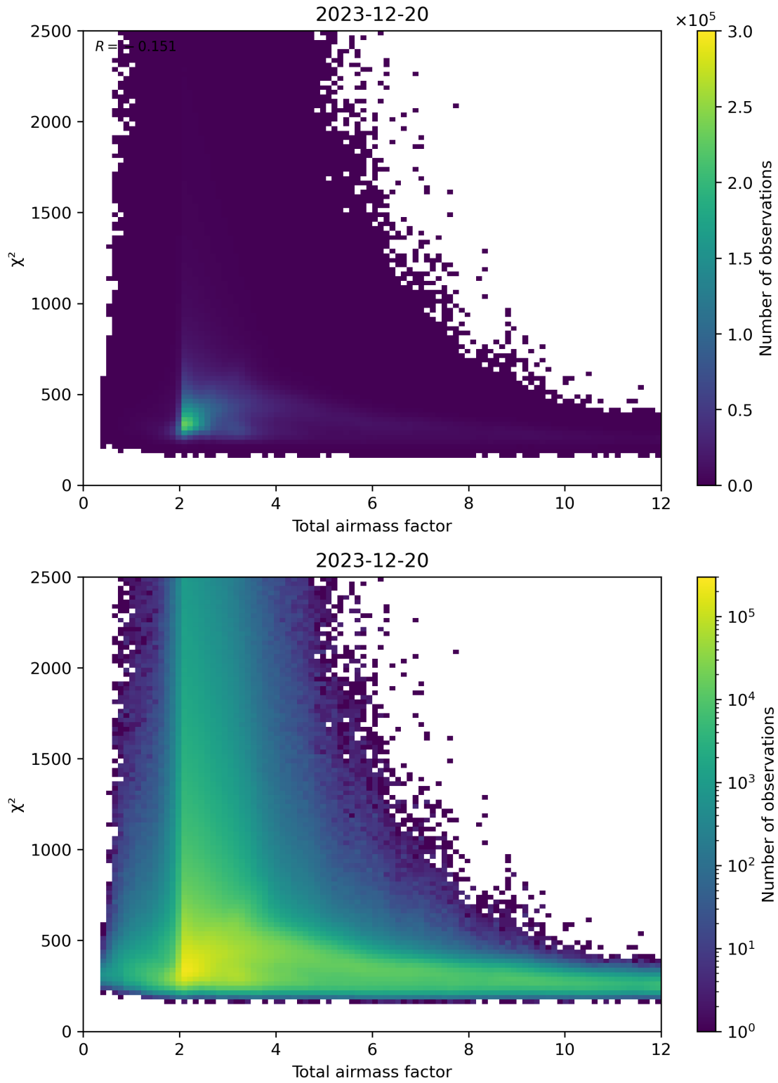
Figure 63: Scatter density plot of “Total airmass factor” against “ \chi^2 ” for 2023-12-20 to 2023-12-21.
