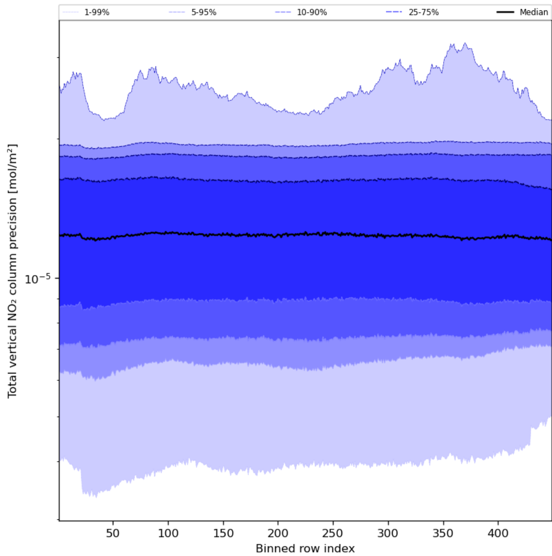
Figure 56: Along track statistics of “Total vertical NO 2 column precision” for 2023-12-20 to 2023-12-21
