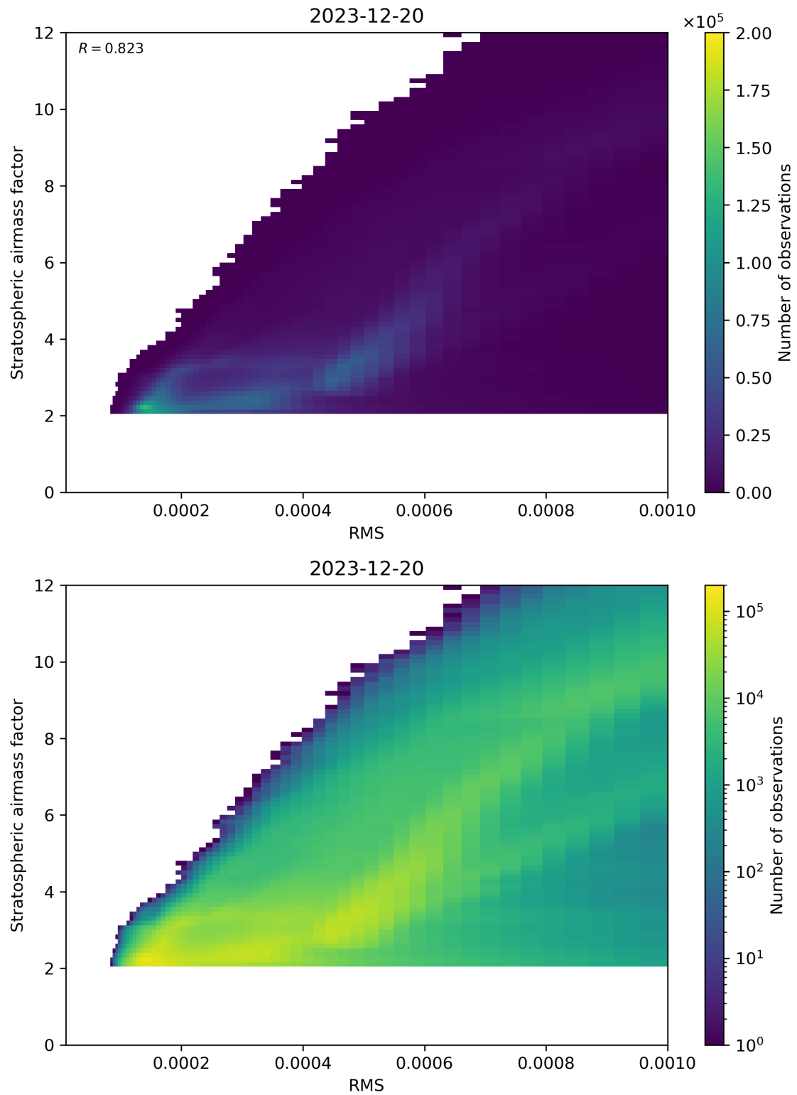
Figure 144: Scatter density plot of “RMS” against “Stratospheric airmass factor” for 2023-12-20 to 2023-12-21.
