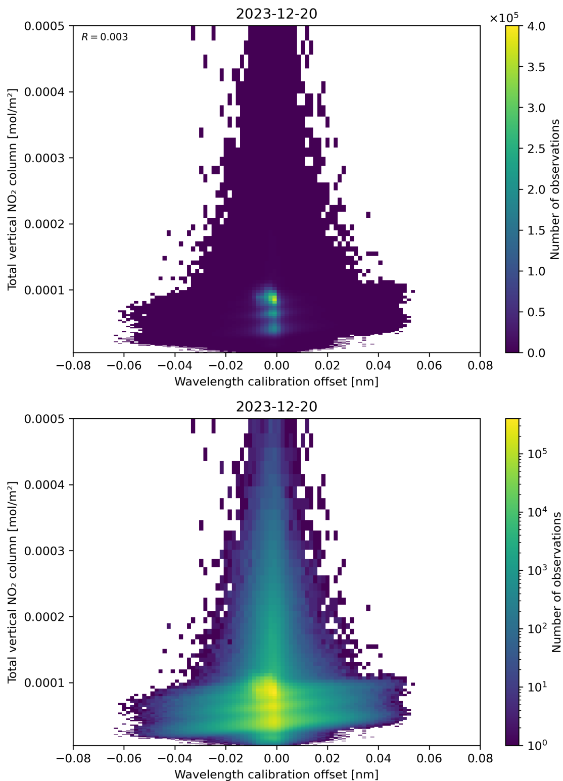
Figure 179: Scatter density plot of “Wavelength calibration offset” against “Total vertical NO 2 column” for 2023-12-20 to 2023-12-21.
