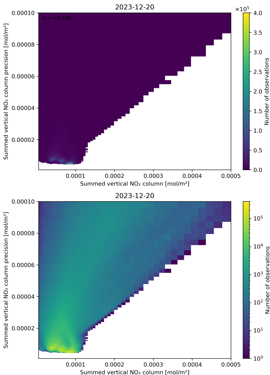
Figure 105: Scatter density plot of “Summed vertical NO 2 column” against “Summed vertical NO 2 column precision” for 2023-12-20 to 2023-12-21.
