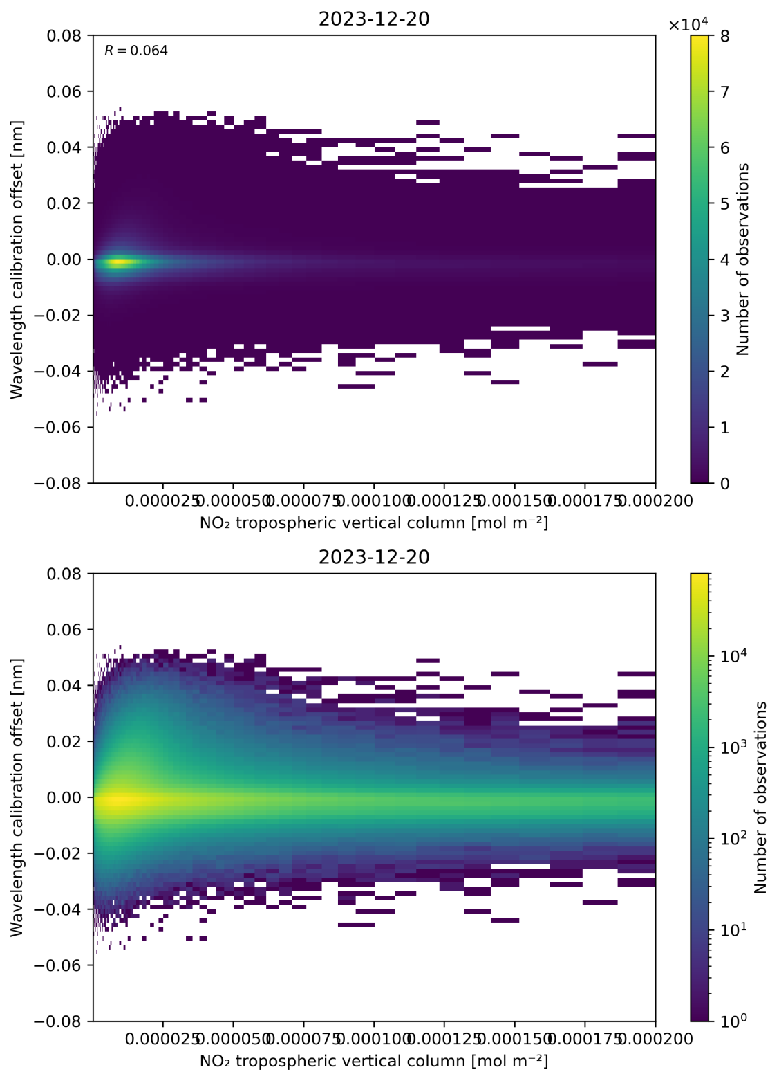
Figure 143: Scatter density plot of “NO 2 tropospheric vertical column” against “Wavelength calibration offset” for 2023-12-20 to 2023-12-21.
