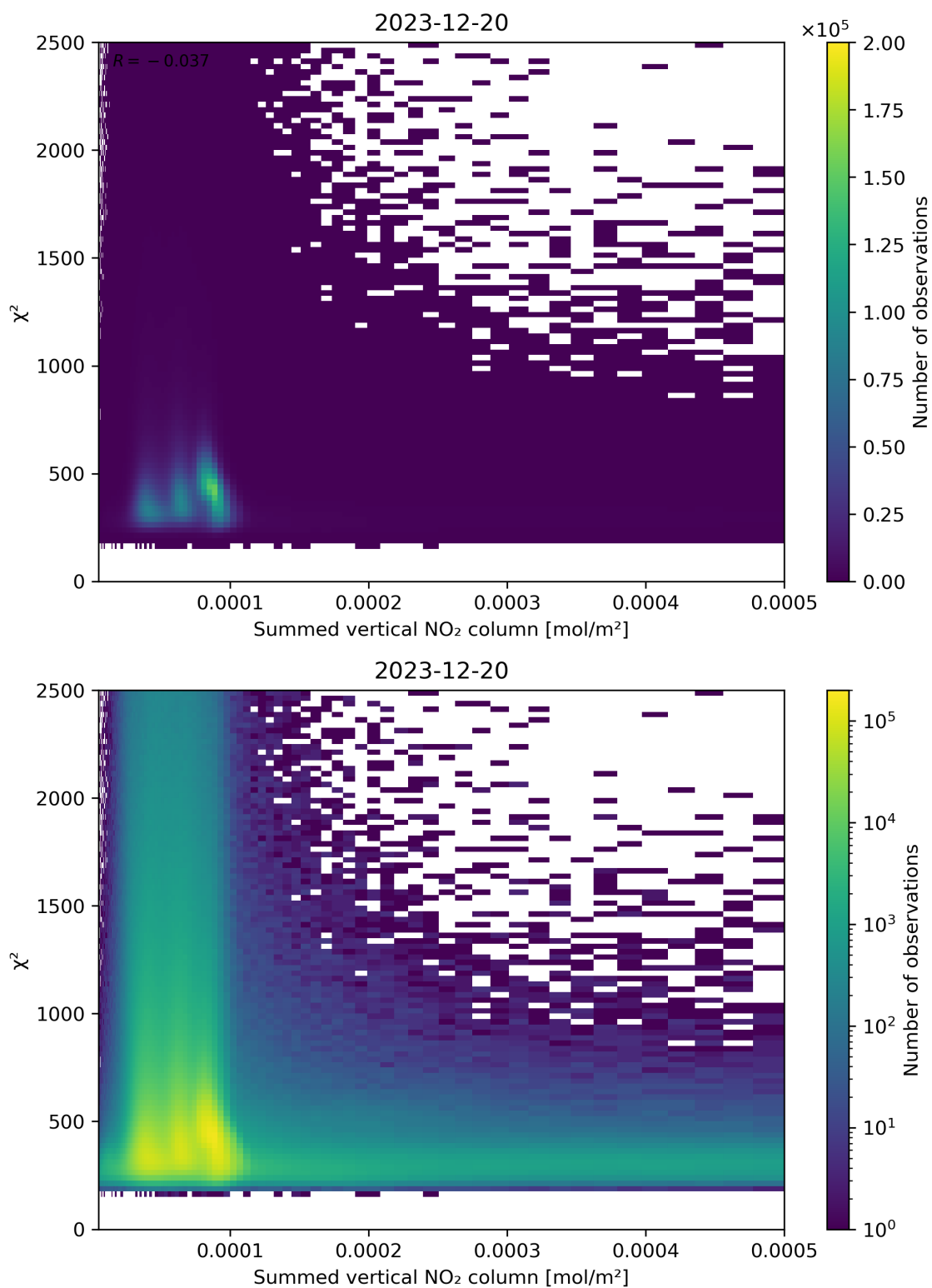
Figure 104: Scatter density plot of “Summed vertical NO 2 column” against “ \chi^2 ” for 2023-12-20 to 2023-12-21.
