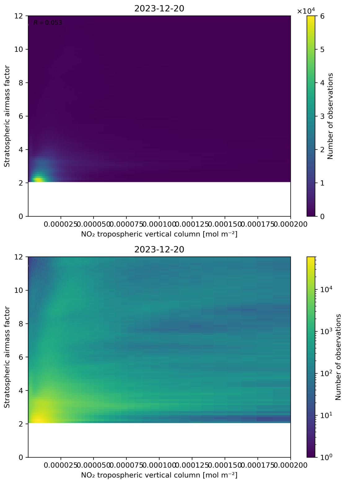
Figure 121: Scatter density plot of “NO 2 tropospheric vertical column” against “Stratospheric airmass factor” for 2023-12-20 to 2023-12-21.
