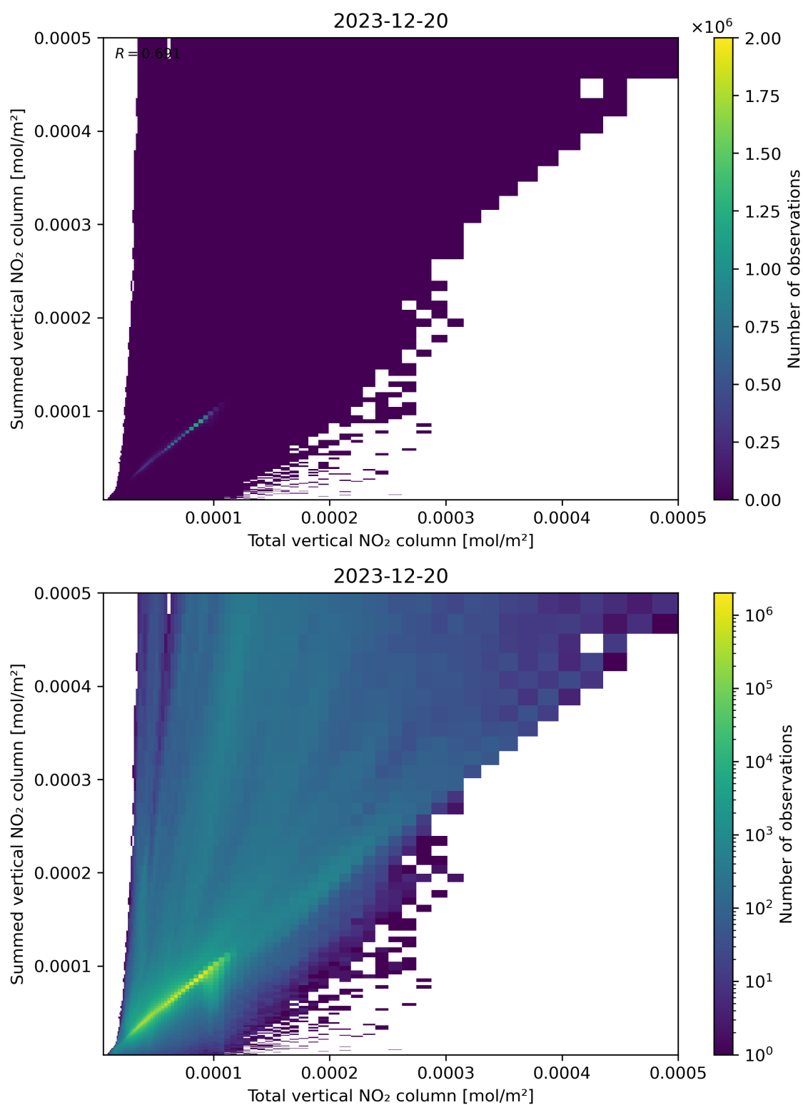
Figure 112: Scatter density plot of “Total vertical NO 2 column” against “Summed vertical NO 2 column” for 2023-12-20 to 2023-12-21.
