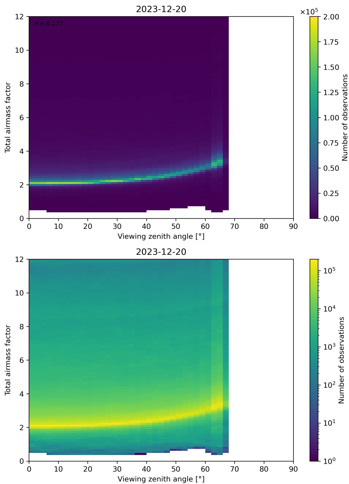
Figure 160: Scatter density plot of “Viewing zenith angle” against “Total airmass factor” for 2023-12-20 to 2023-12-21.
