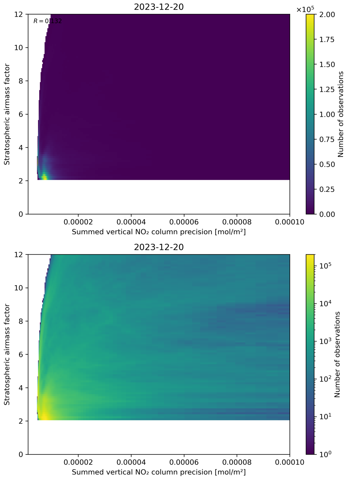
Figure 106: Scatter density plot of “Summed vertical NO 2 column precision” against “Stratospheric airmass factor” for 2023-12-20 to 2023-12-21.
