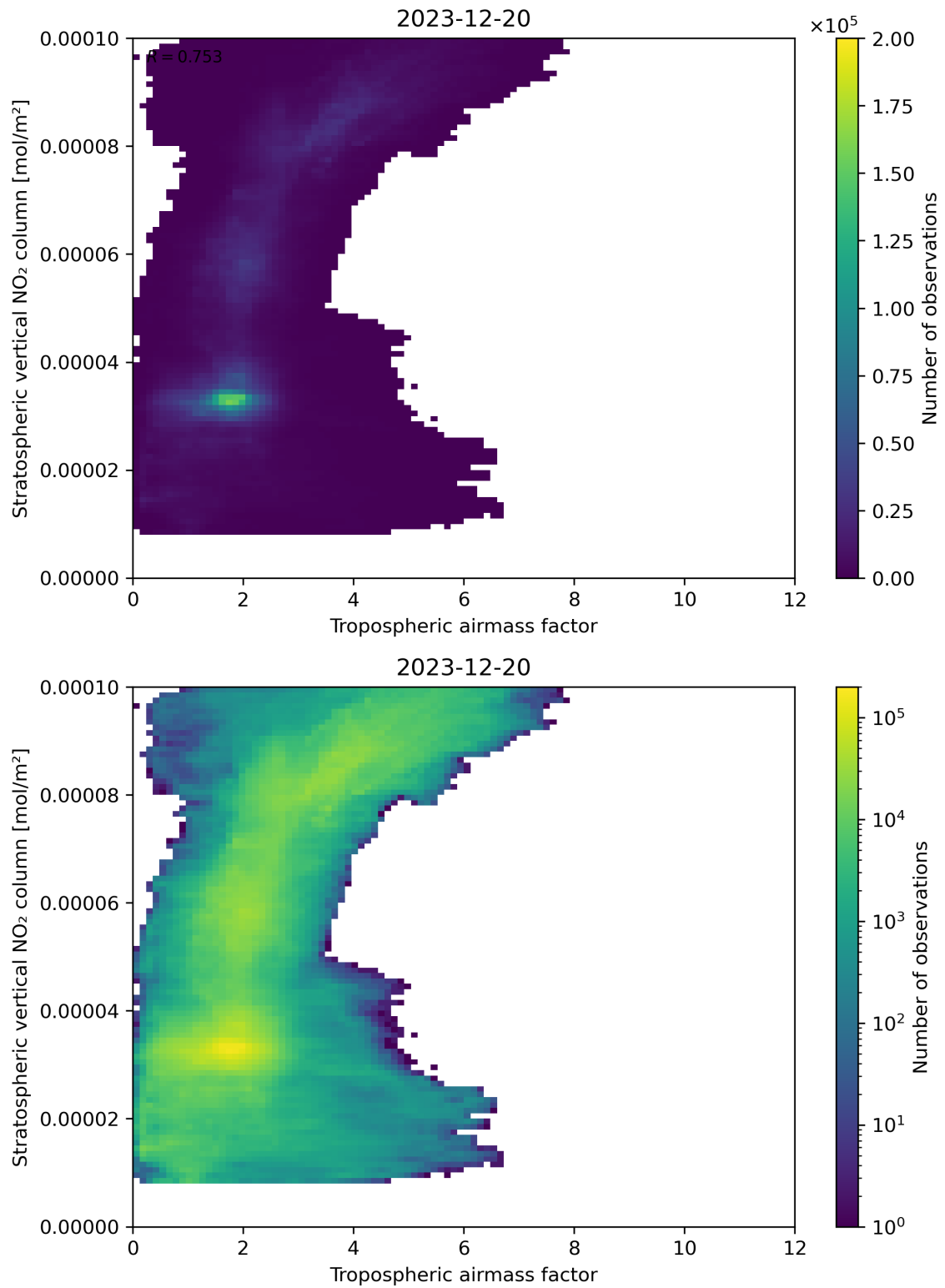
Figure 74: Scatter density plot of “Tropospheric air mass factor” against “Stratospheric vertical NO 2 column” for 2023-12-20 to 2023-12-21.
