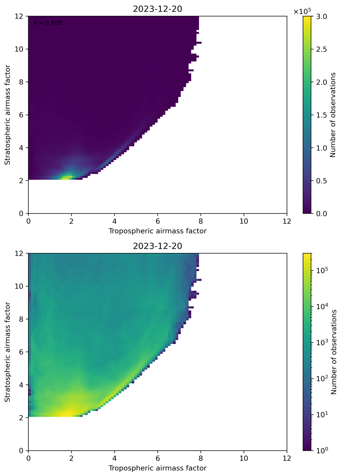
Figure 71: Scatter density plot of “Tropospheric airmass factor” against “Stratospheric airmass factor” for 2023-12-20 to 2023-12-21.
