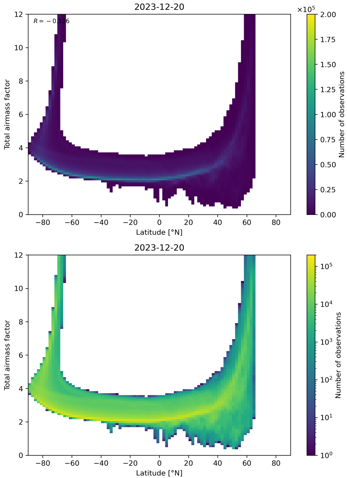
Figure 84: Scatter density plot of “Latitude” against “Total airmass factor” for 2023-12-20 to 2023-12-21.
