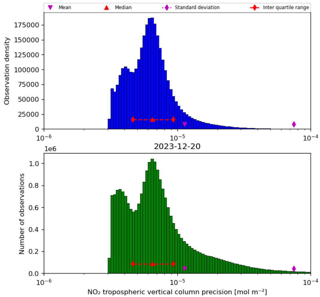
Figure 30: Histogram of “NO 2 tropospheric vertical column precision” for 2023-12-20 to 2023-12-21
