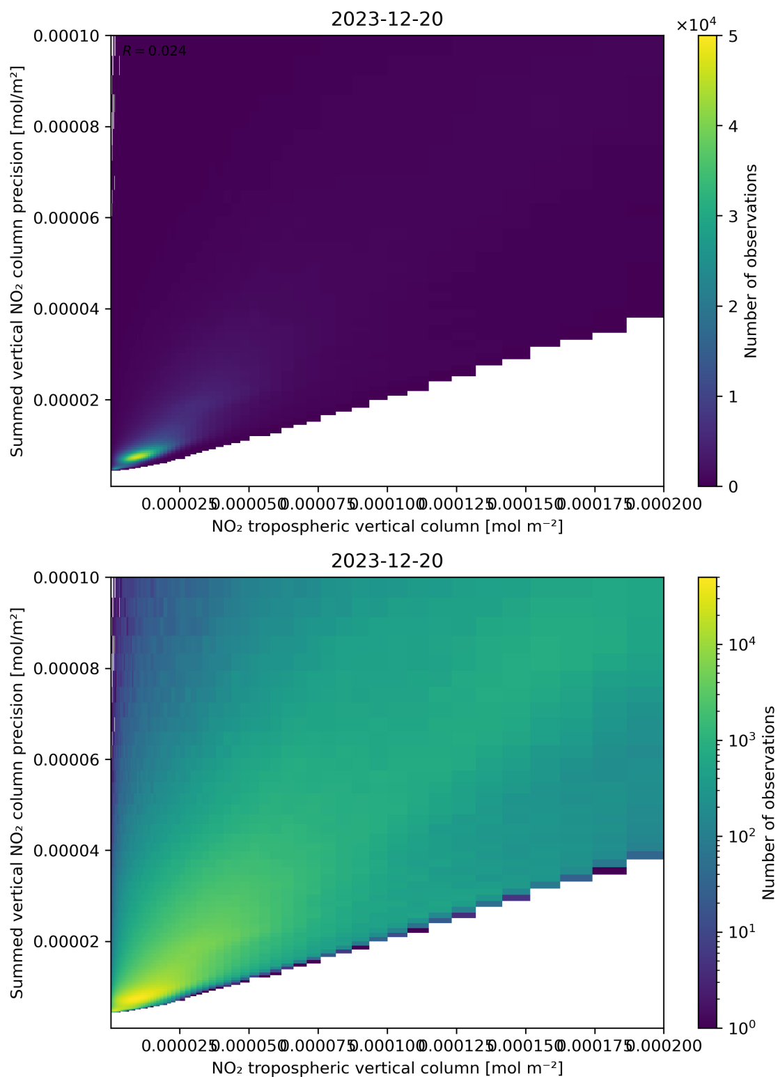
Figure 127: Scatter density plot of “NO 2 tropospheric vertical column” against “Summed vertical NO 2 column precision” for 2023-12-20 to 2023-12-21.
