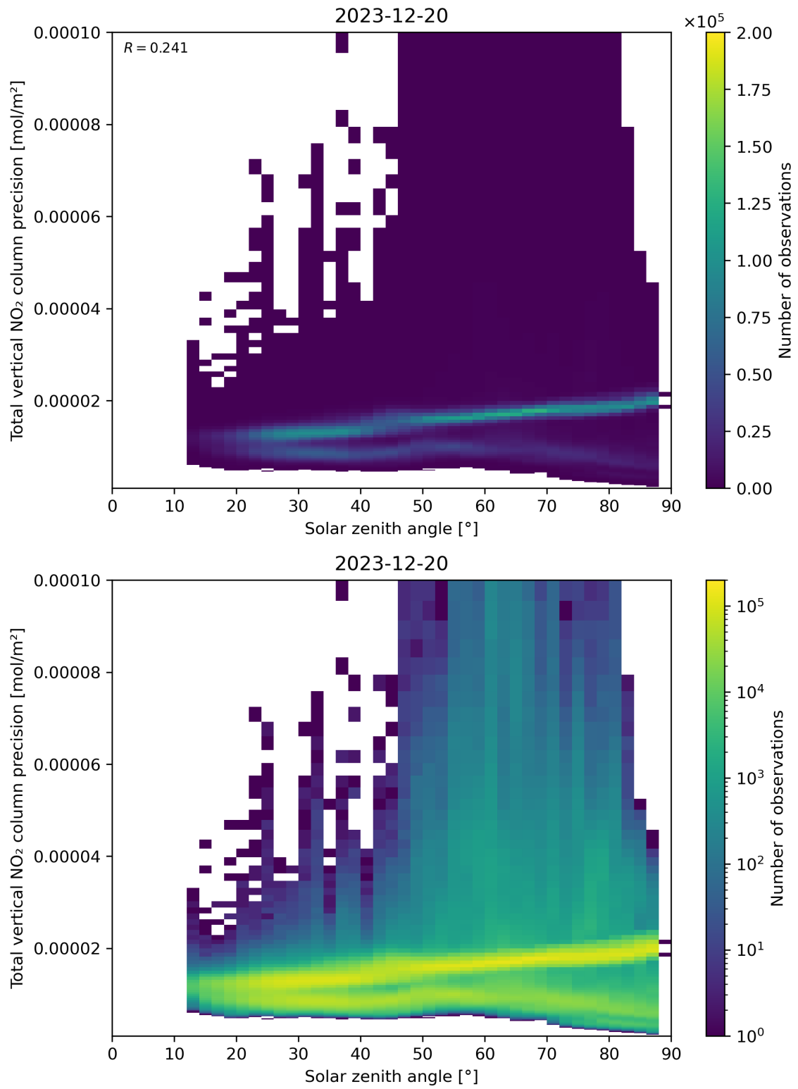
Figure 154: Scatter density plot of “Solar zenith angle” against “Total vertical NO 2 column precision” for 2023-12-20 to 2023-12-21.
