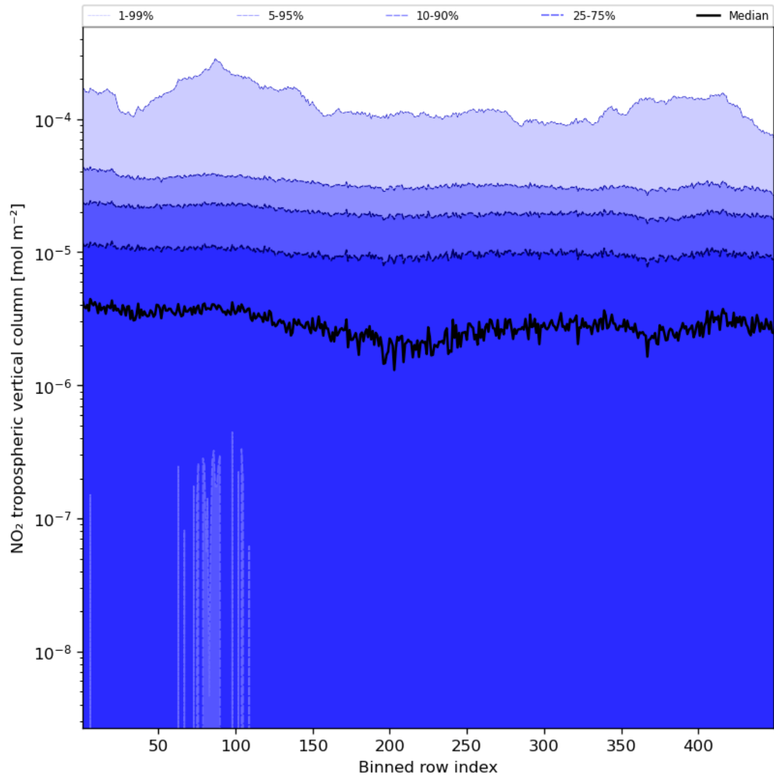
Figure 46: Along track statistics of “NO 2 tropospheric vertical column” for 2023-12-20 to 2023-12-21
