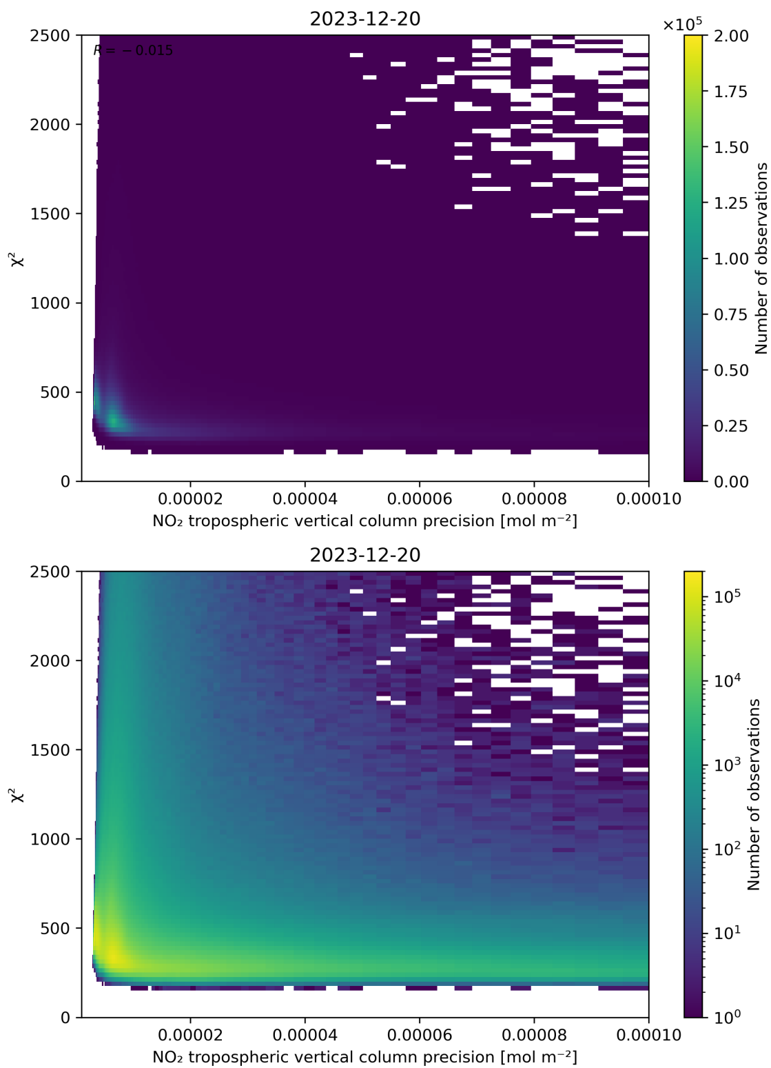
Figure 134: Scatter density plot of “NO 2 tropospheric vertical column precision” against “ \chi^2 ” for 2023-12-20 to 2023-12-21.
