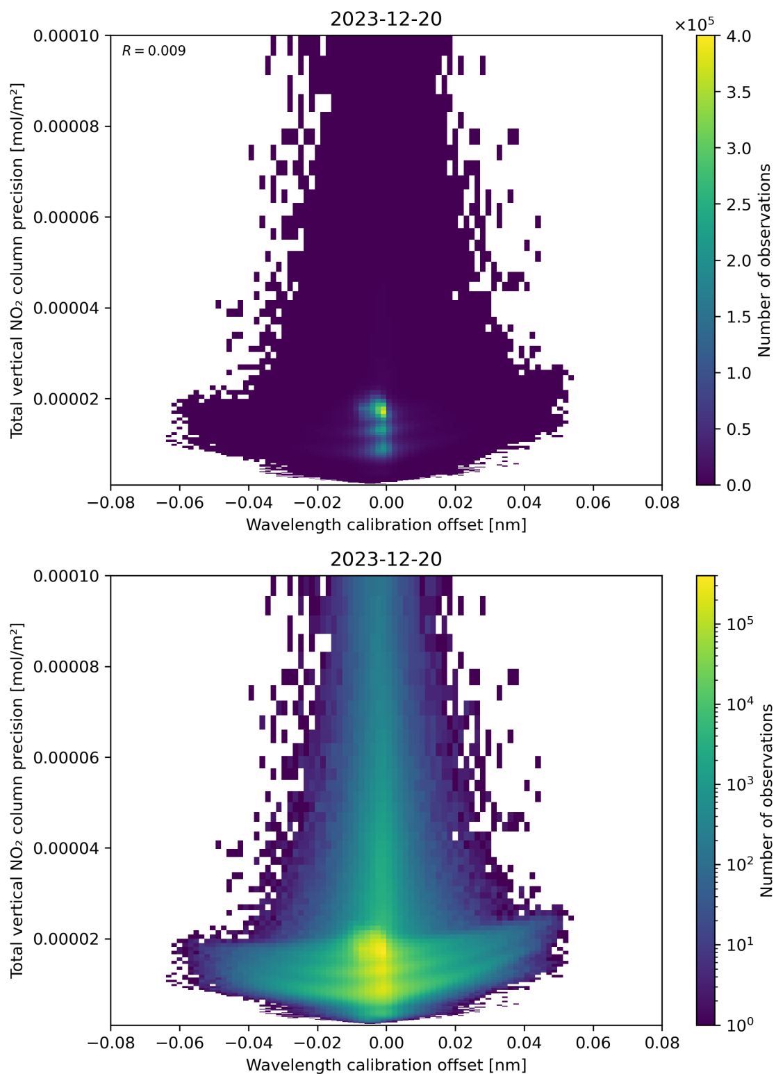
Figure 180: Scatter density plot of “Wavelength calibration offset” against “Total vertical NO 2 column precision” for 2023-12-20 to 2023-12-21.
