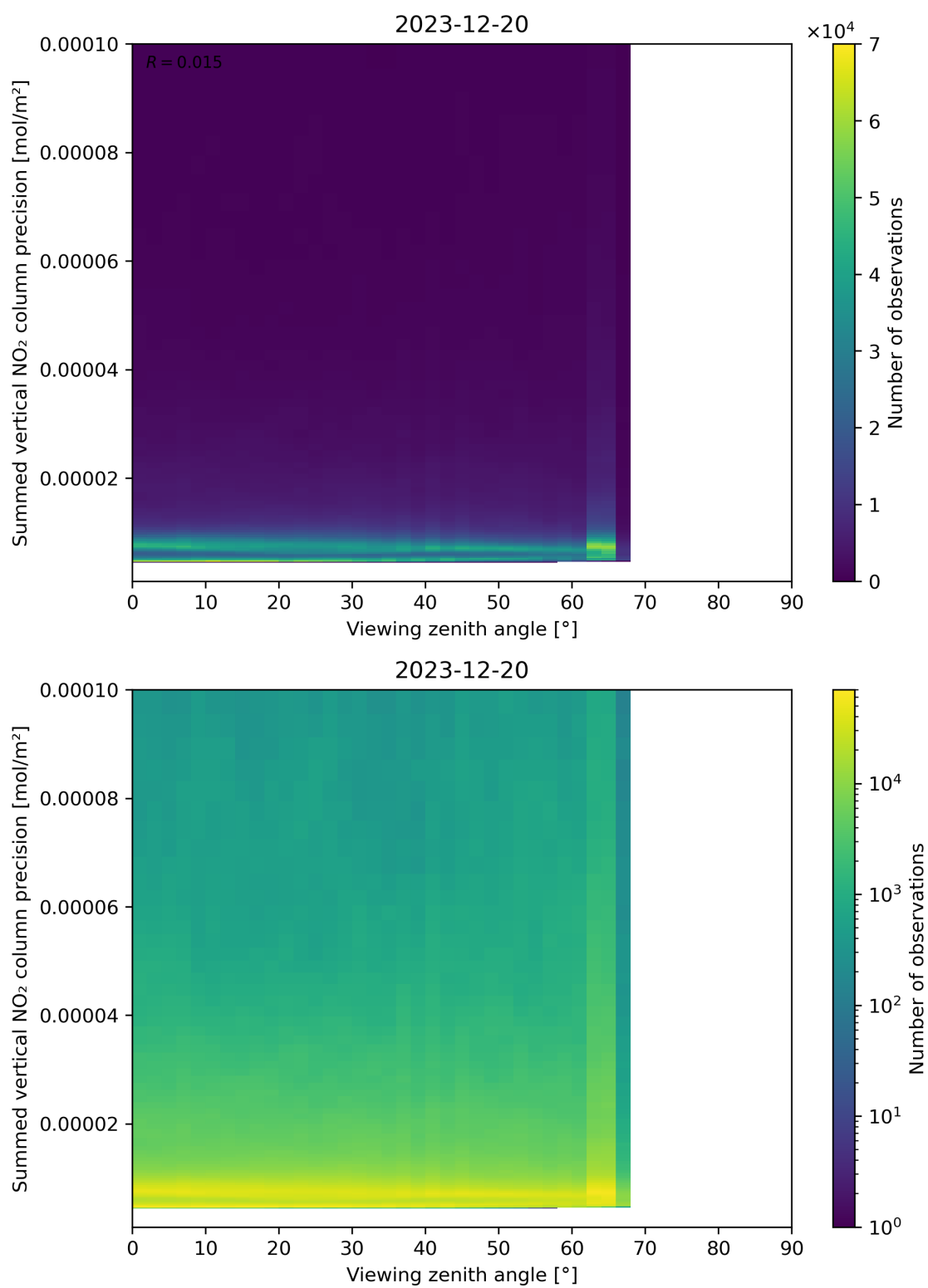
Figure 166: Scatter density plot of “Viewing zenith angle” against “Summed vertical NO 2 column precision” for 2023-12-20 to 2023-12-21.
