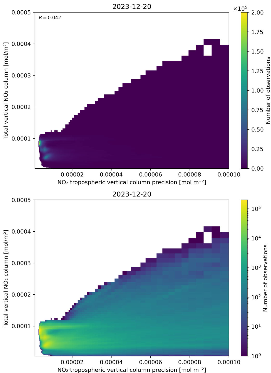
Figure 138: Scatter density plot of “NO 2 tropospheric vertical column precision” against “Total vertical NO 2 column” for 2023-12-20 to 2023-12-21.
