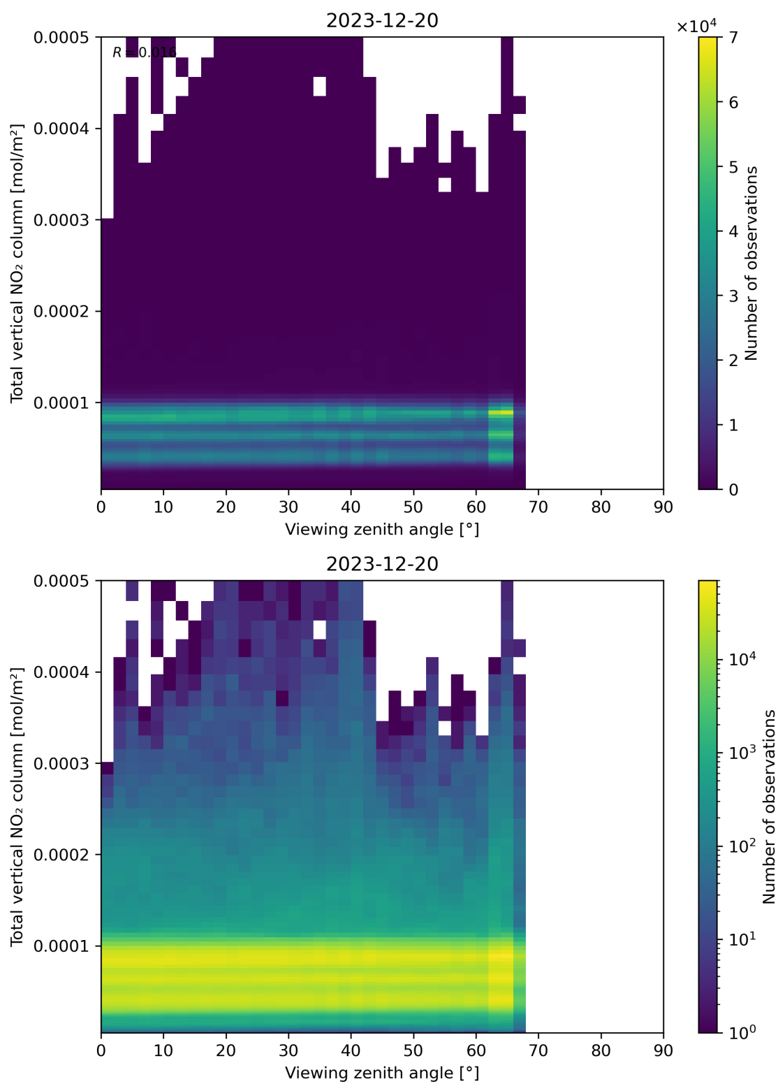
Figure 167: Scatter density plot of “Viewing zenith angle” against “Total vertical NO 2 column” for 2023-12-20 to 2023-12-21.
