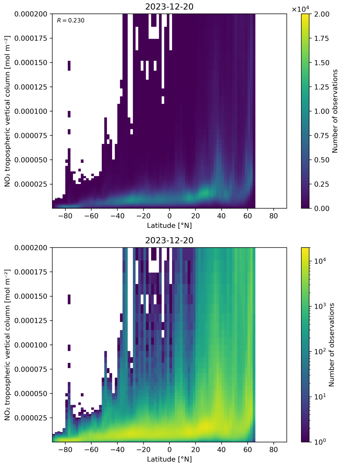
Figure 92: Scatter density plot of “Latitude” against “NO 2 tropospheric vertical column” for 2023-12-20 to 2023-12-21.
