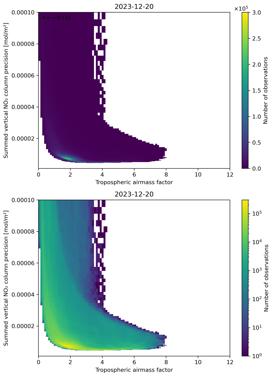
Figure 76: Scatter density plot of “Tropospheric air mass factor” against “Summed vertical NO 2 column precision” for 2023-12-20 to 2023-12-21.
