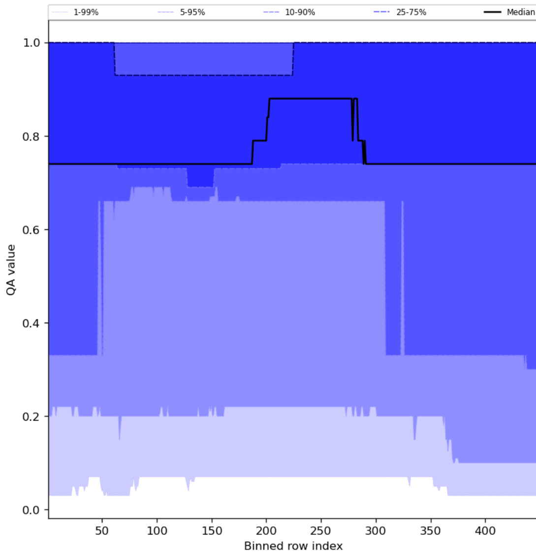
Figure 45: Along track statistics of “QA value” for 2023-12-20 to 2023-12-21
