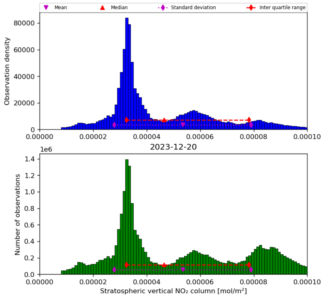
Figure 36: Histogram of “Stratospheric vertical NO 2 column” for 2023-12-20 to 2023-12-21
