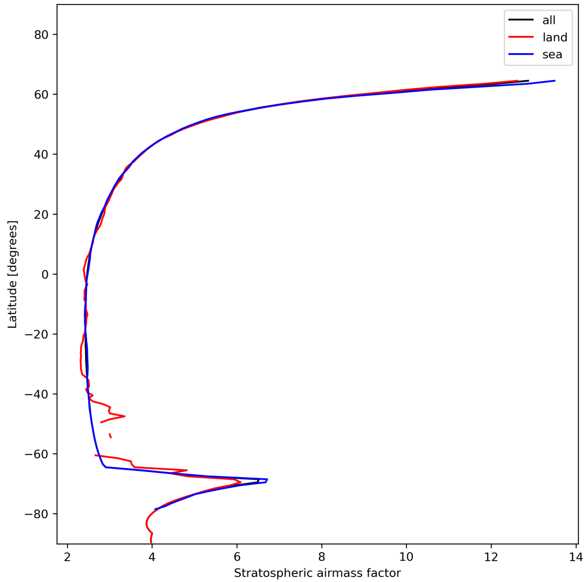
Figure 27: Zonal average of “Stratospheric airmass factor” for 2023-12-20 to 2023-12-21.
