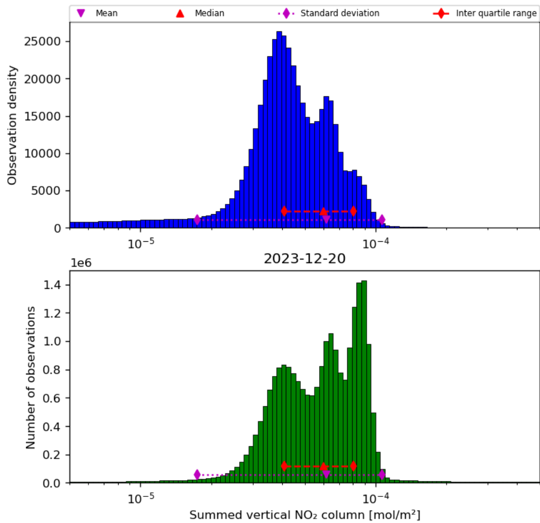
Figure 40: Histogram of “Summed vertical NO 2 column” for 2023-12-20 to 2023-12-21
