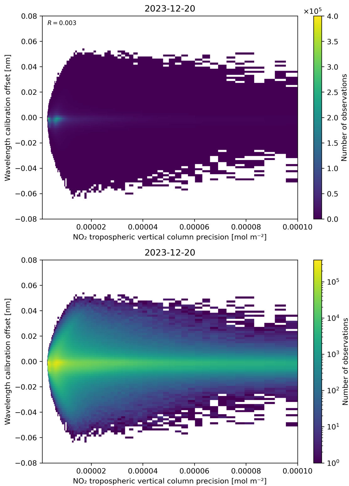
Figure 141: Scatter density plot of “NO 2 tropospheric vertical column precision” against “Wavelength calibration offset” for 2023-12-20 to 2023-12-21.
