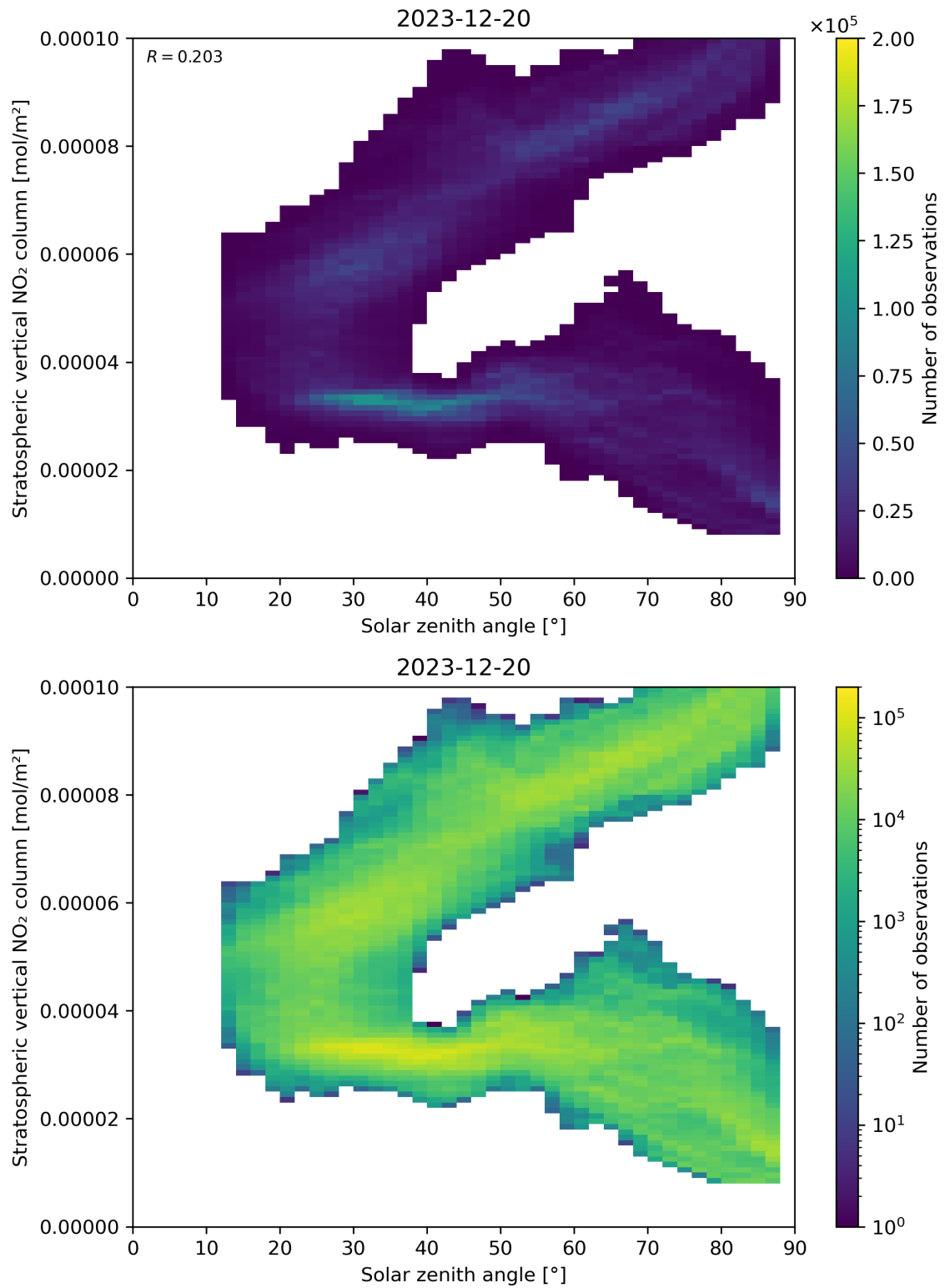
Figure 150: Scatter density plot of “Solar zenith angle” against “Stratospheric vertical NO 2 column” for 2023-12-20 to 2023-12-21.
