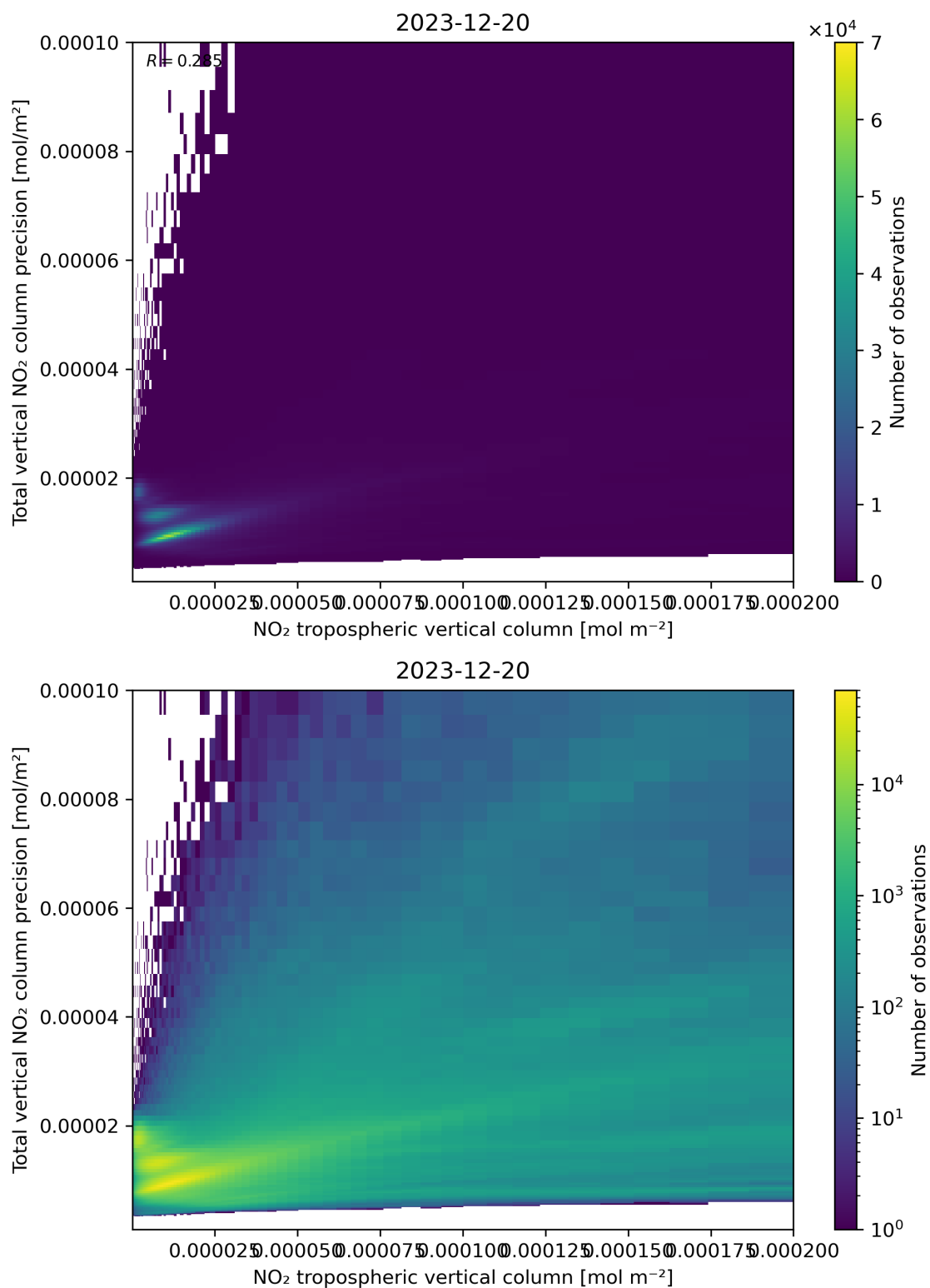
Figure 129: Scatter density plot of “NO 2 tropospheric vertical column” against “Total vertical NO 2 column precision” for 2023-12-20 to 2023-12-21.
