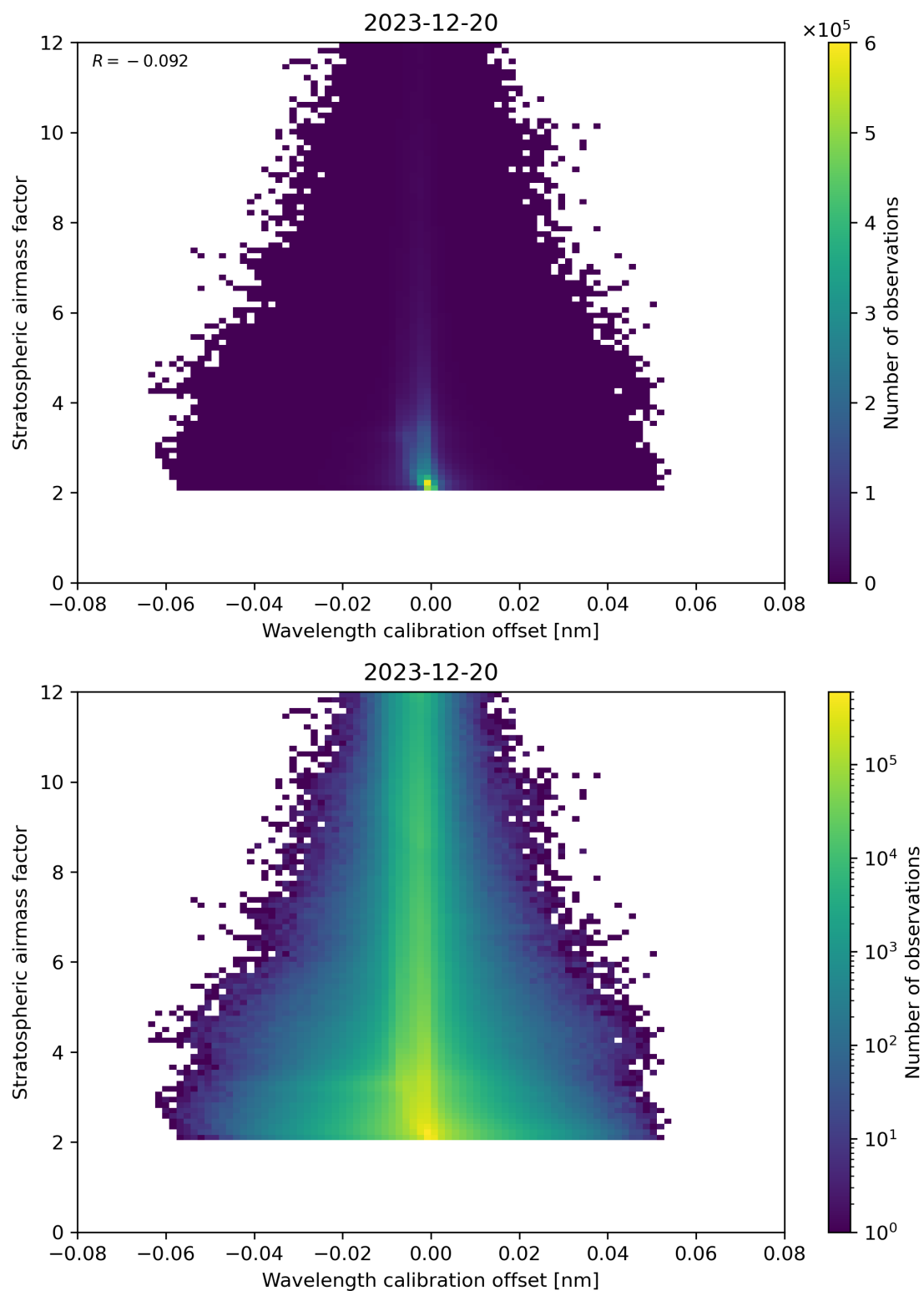
Figure 174: Scatter density plot of “Wavelength calibration offset” against “Stratospheric airmass factor” for 2023-12-20 to 2023-12-21.
