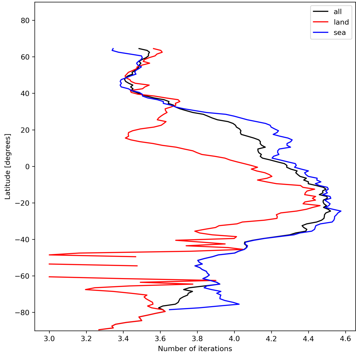
Figure 17: Zonal average of “Number of iterations” for 2023-12-20 to 2023-12-21.
