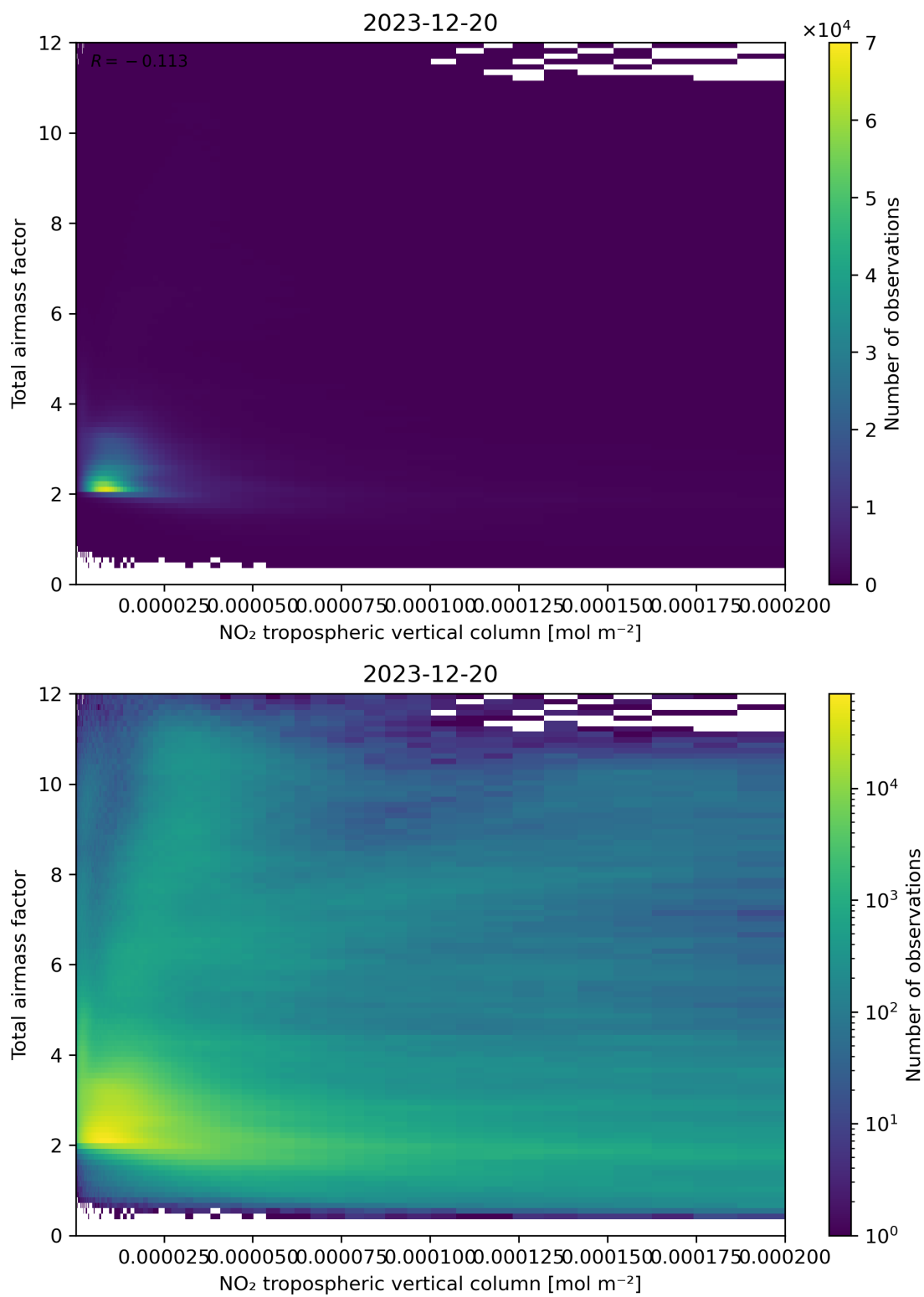
Figure 122: Scatter density plot of “NO 2 tropospheric vertical column” against “Total air mass factor” for 2023-12-20 to 2023-12-21.
