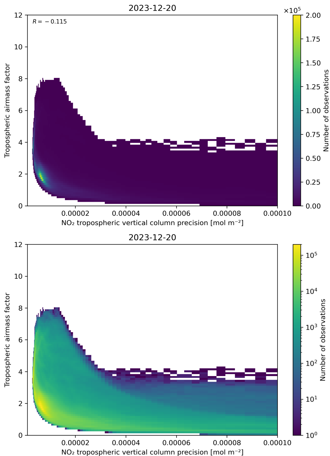
Figure 133: Scatter density plot of “NO 2 tropospheric vertical column precision” against “Tropospheric airmass factor” for 2023-12-20 to 2023-12-21.
