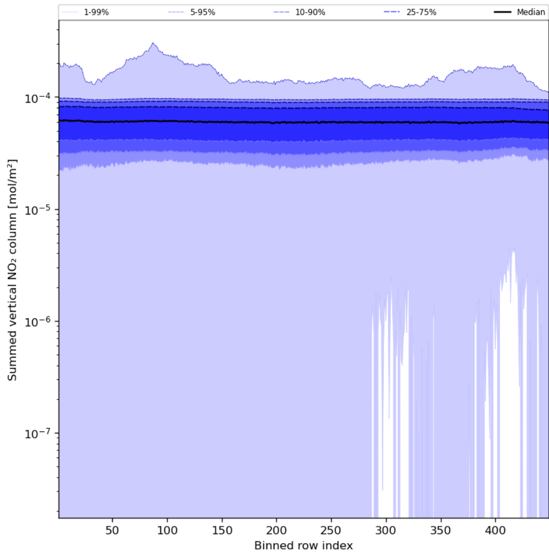
Figure 57: Along track statistics of “Summed vertical NO 2 column” for 2023-12-20 to 2023-12-21
