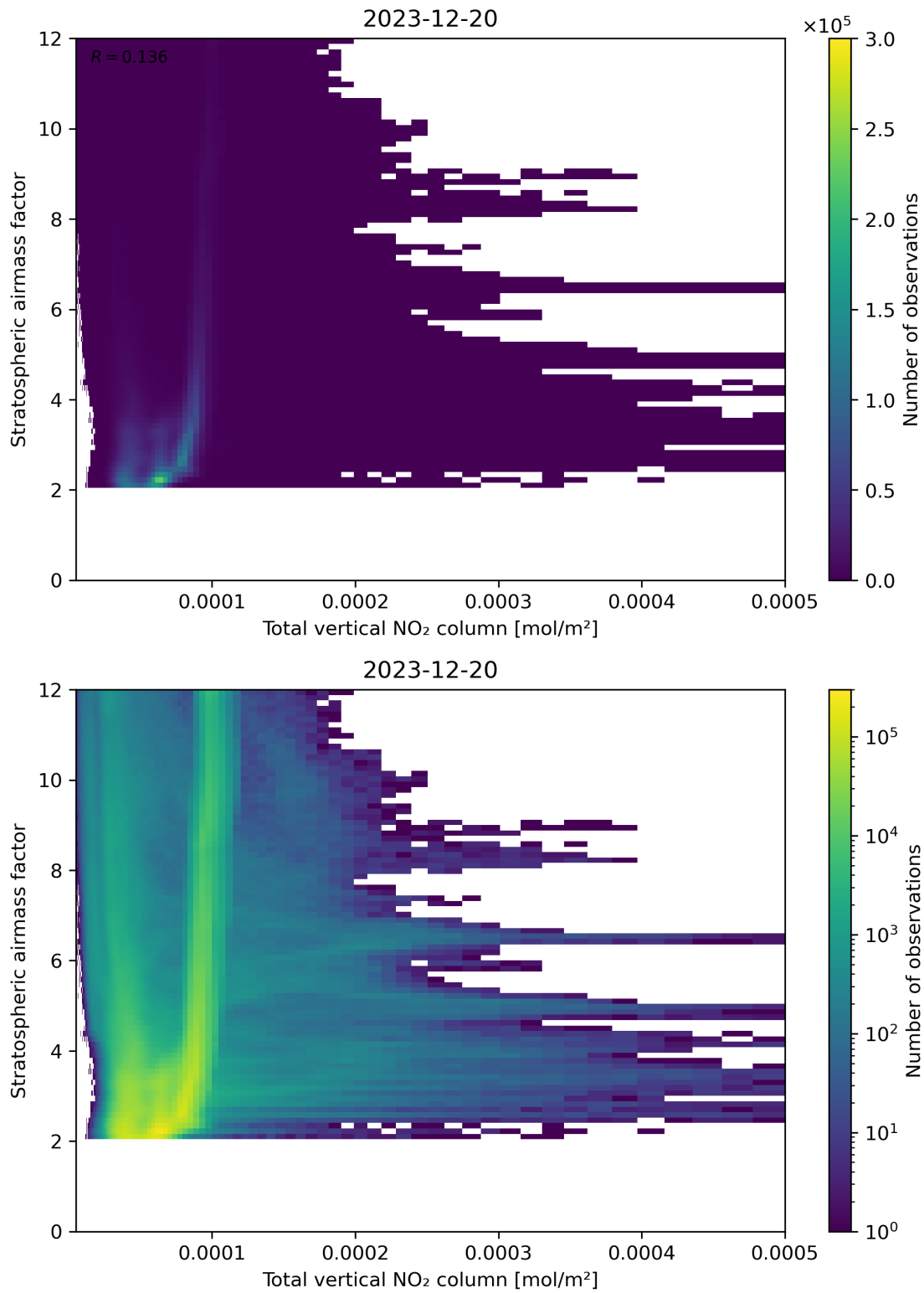
Figure 110: Scatter density plot of “Total vertical NO 2 column” against “Stratospheric air mass factor” for 2023-12-20 to 2023-12-21.
