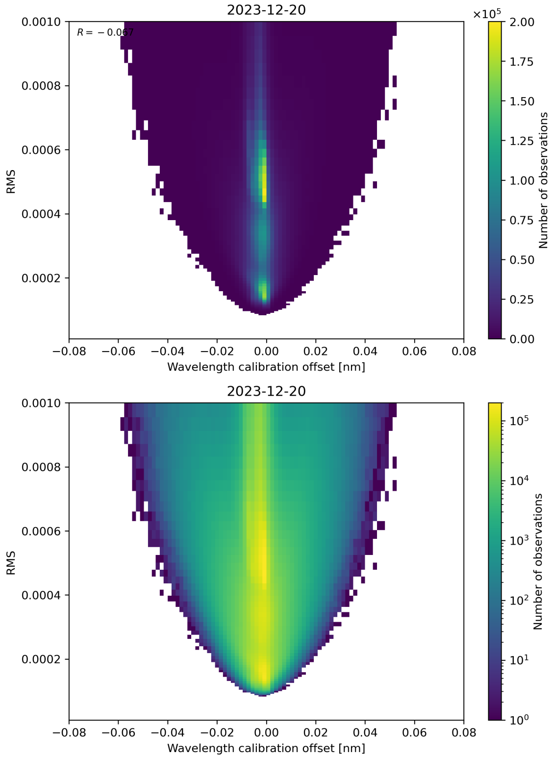
Figure 181: Scatter density plot of “Wavelength calibration offset” against “RMS” for 2023-12-20 to 2023-12-21.
