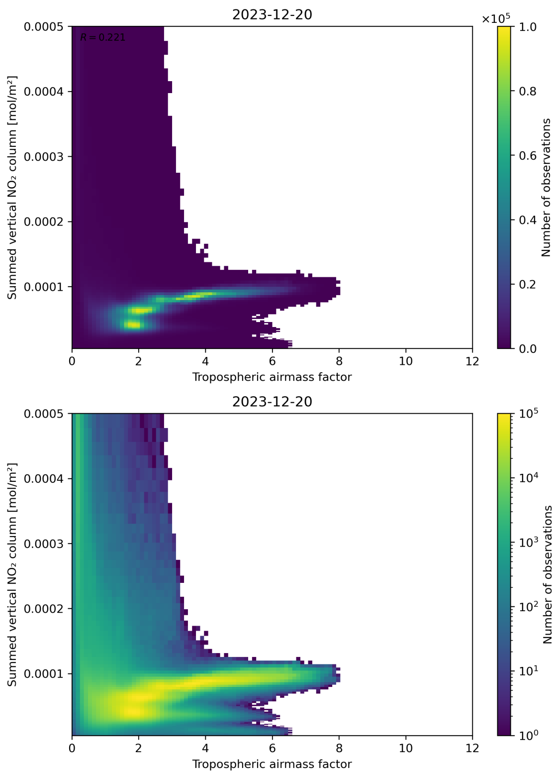
Figure 75: Scatter density plot of “Tropospheric airmass factor” against “Summed vertical NO 2 column” for 2023-12-20 to 2023-12-21.
