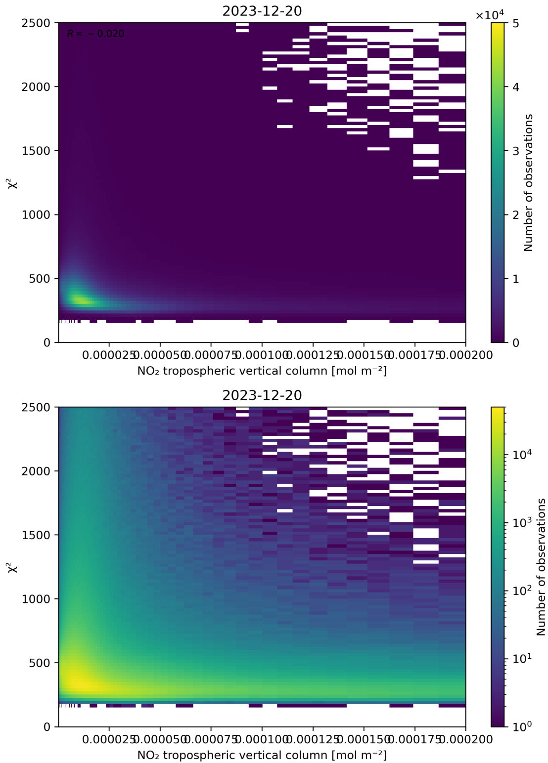
Figure 124: Scatter density plot of “NO 2 tropospheric vertical column” against “ \chi^2 ” for 2023-12-20 to 2023-12-21.
