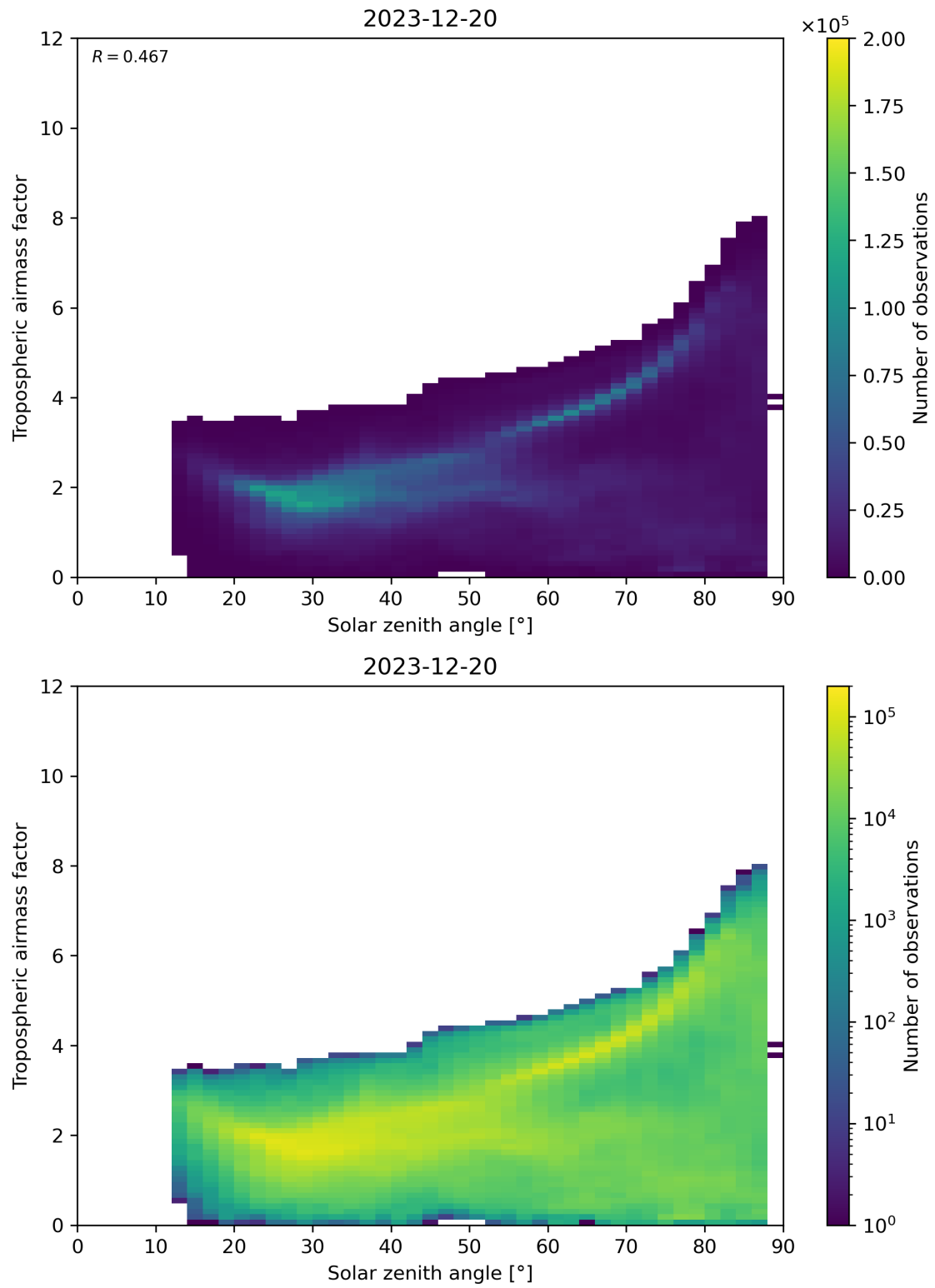
Figure 147: Scatter density plot of “Solar zenith angle” against “Tropospheric airmass factor” for 2023-12-20 to 2023-12-21.
