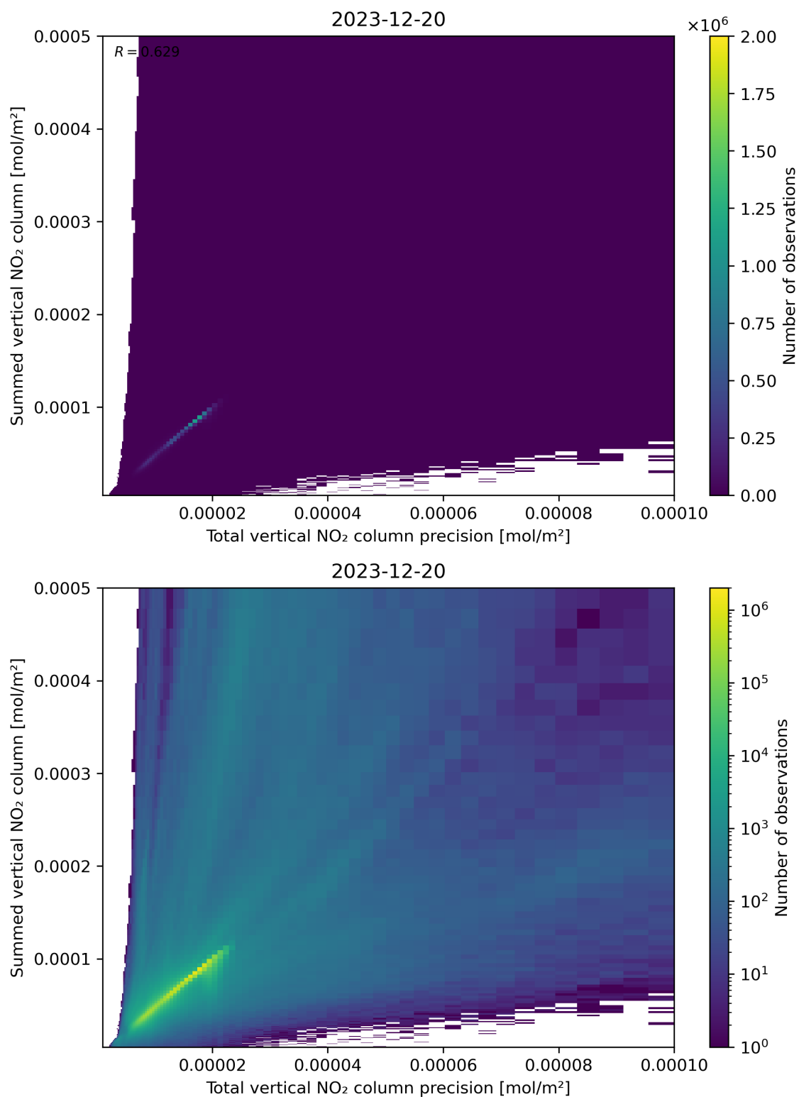
Figure 117: Scatter density plot of “Total vertical NO 2 column precision” against “Summed vertical NO 2 column” for 2023-12-20 to 2023-12-21.
