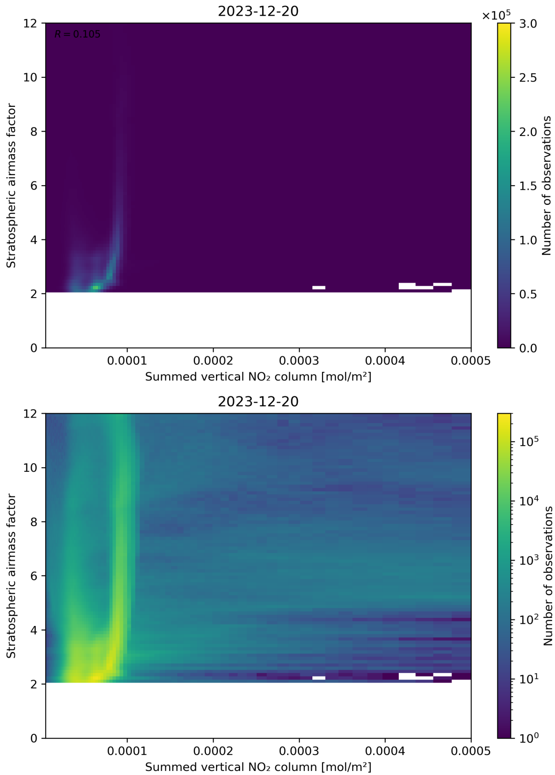
Figure 103: Scatter density plot of “Summed vertical NO 2 column” against “Stratospheric airmass factor” for 2023-12-20 to 2023-12-21.
