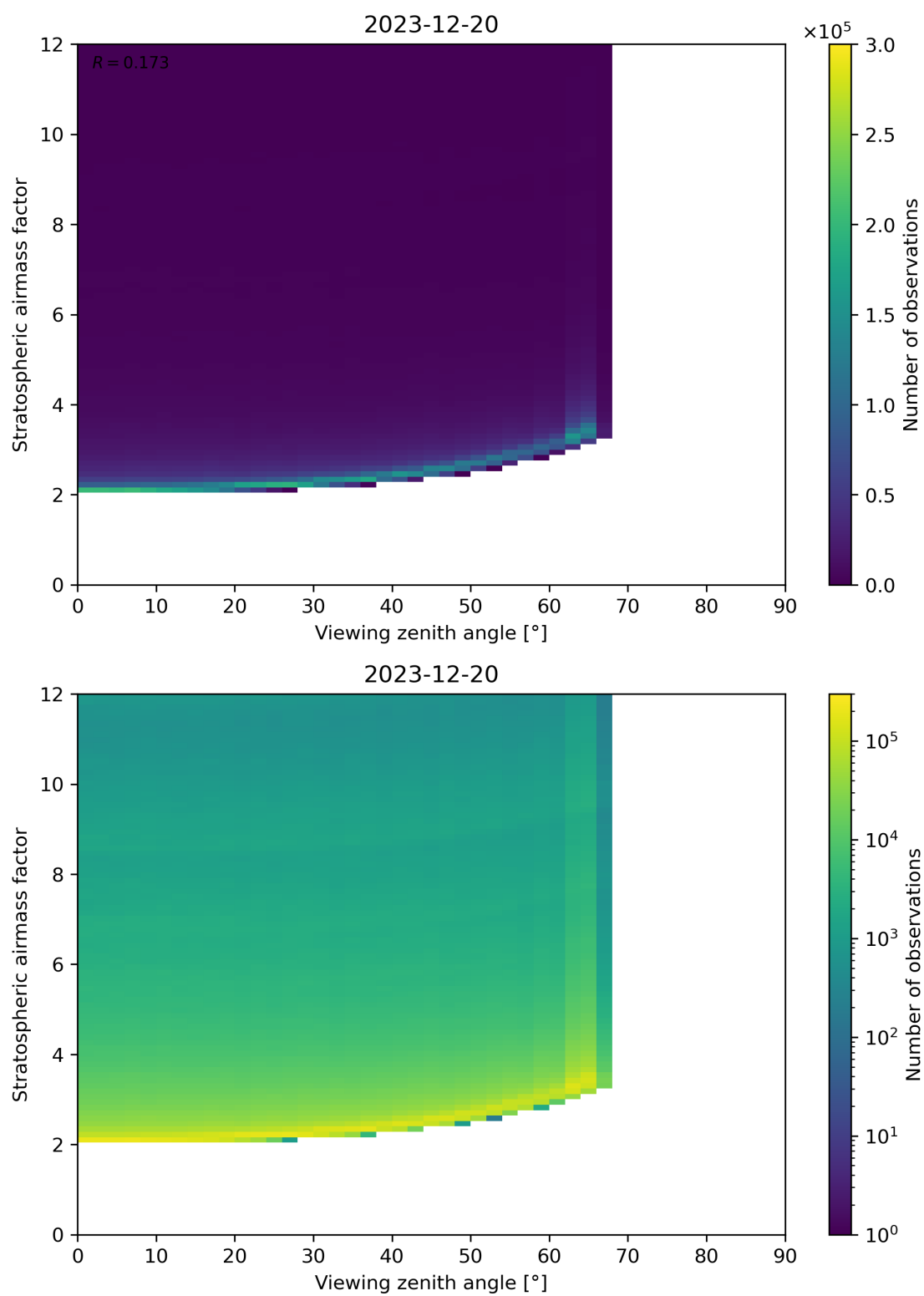
Figure 159: Scatter density plot of “Viewing zenith angle” against “Stratospheric airmass factor” for 2023-12-20 to 2023-12-21.
