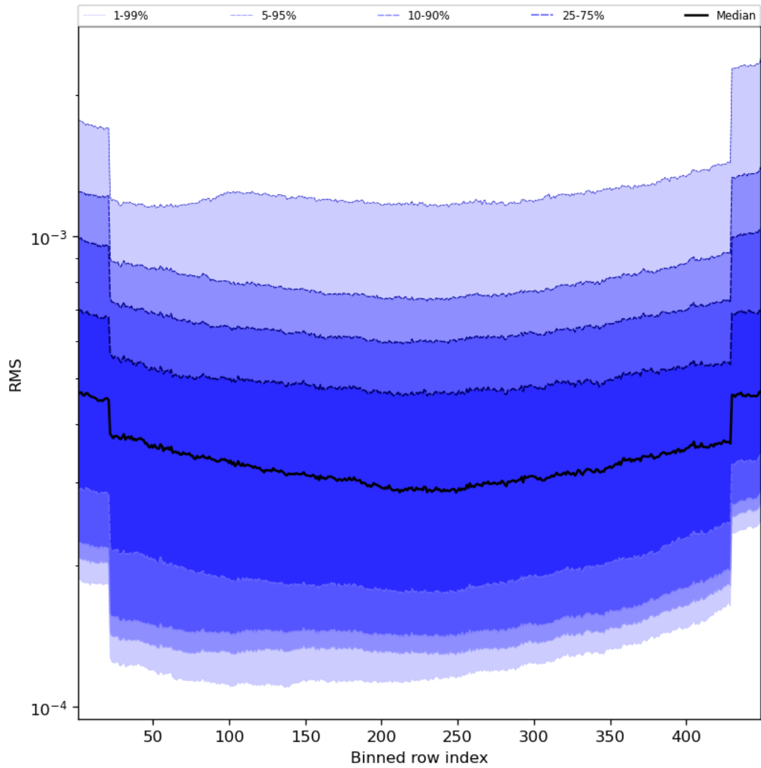
Figure 60: Along track statistics of “RMS” for 2023-12-20 to 2023-12-21
