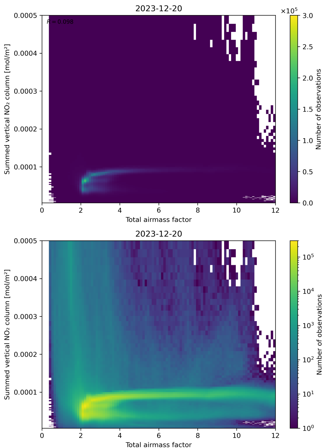
Figure 65: Scatter density plot of “Total airmass factor” against “Summed vertical NO 2 column” for 2023-12-20 to 2023-12-21.
