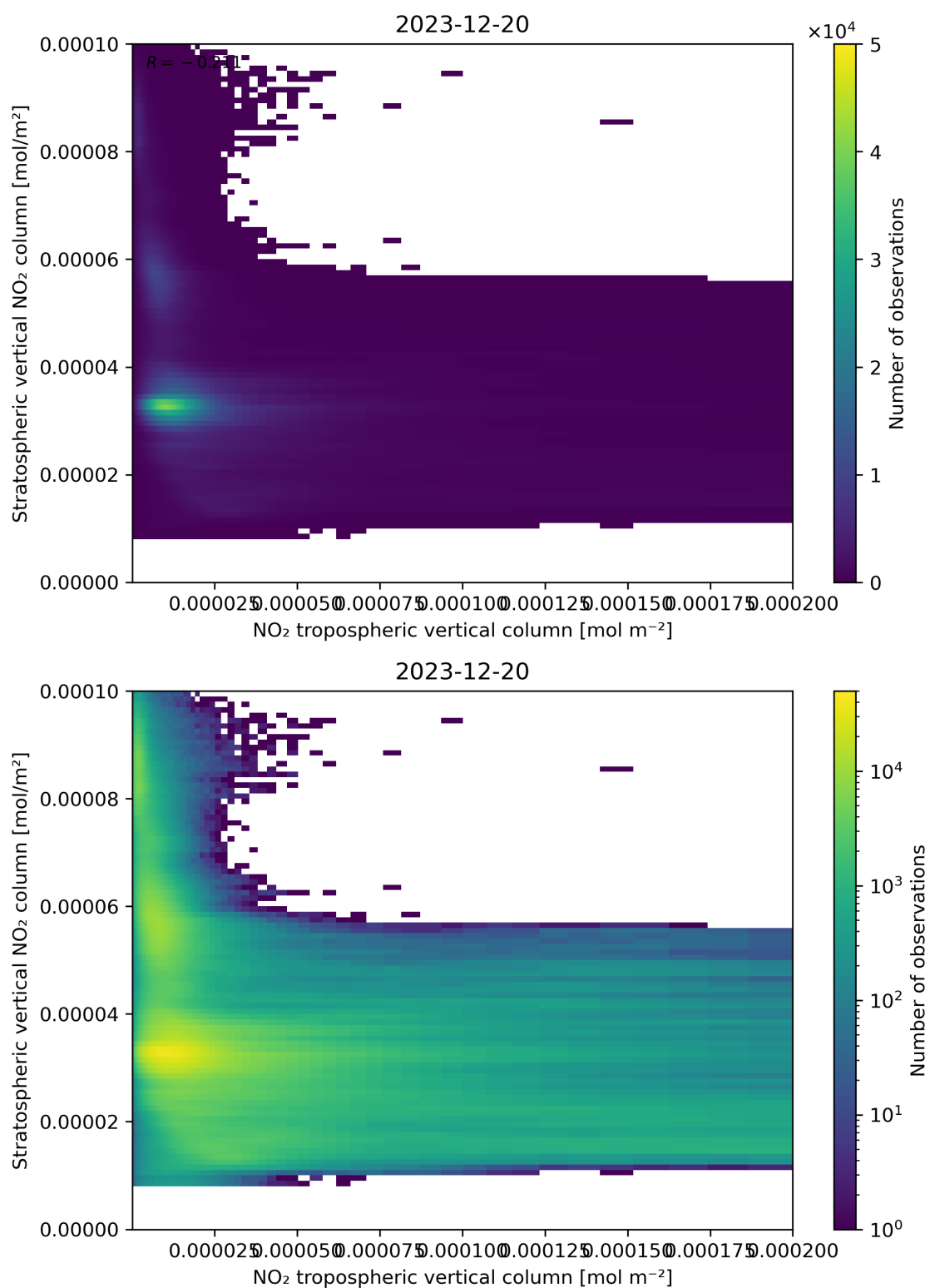
Figure 125: Scatter density plot of “NO 2 tropospheric vertical column” against “Stratospheric vertical NO 2 column” for 2023-12-20 to 2023-12-21.
