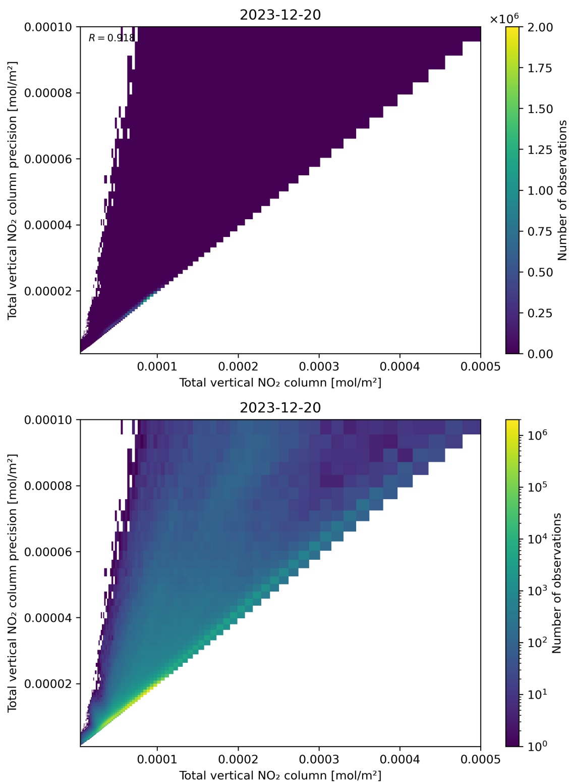
Figure 114: Scatter density plot of “Total vertical NO 2 column” against “Total vertical NO 2 column precision” for 2023-12-20 to 2023-12-21.
