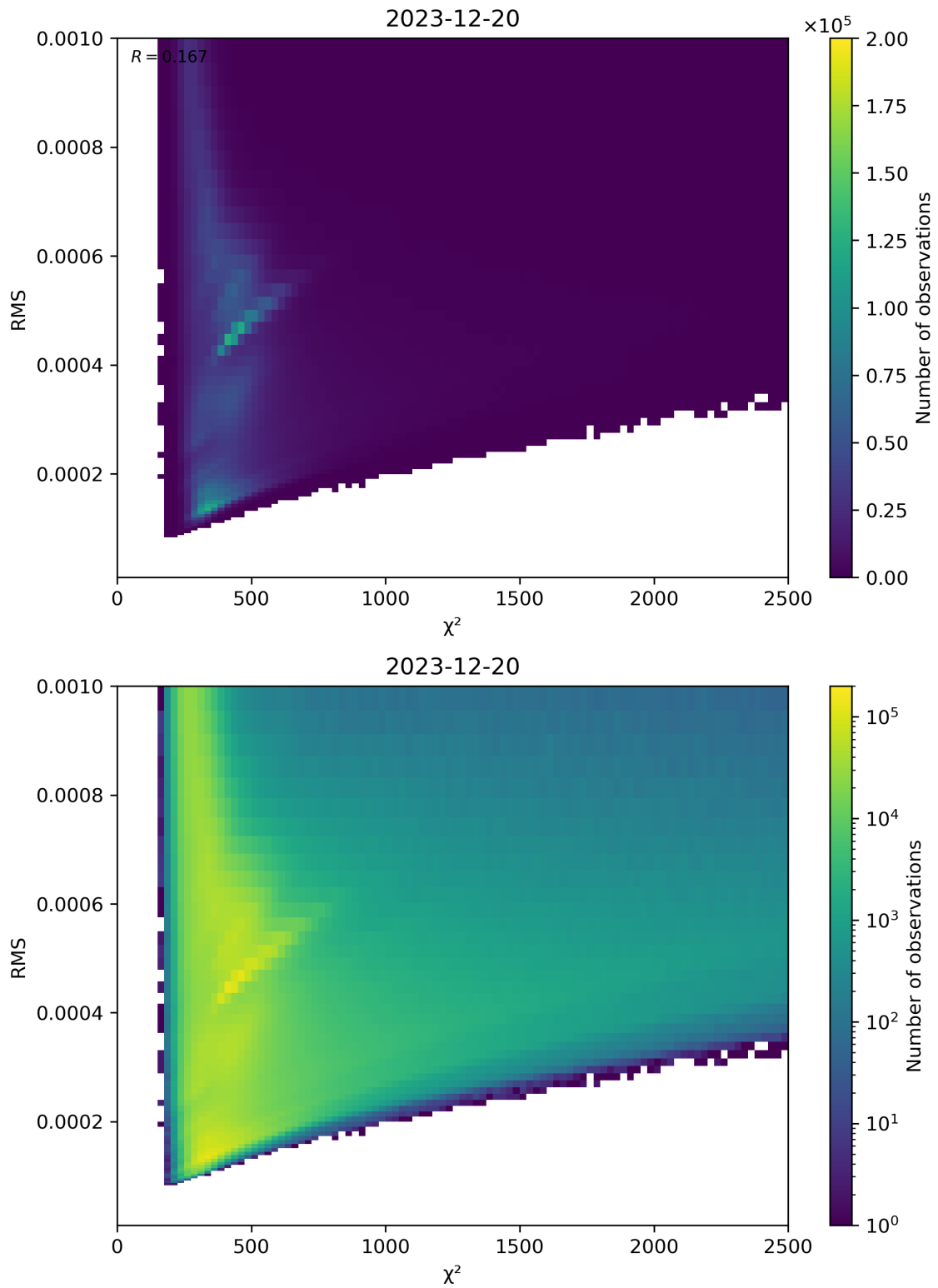
Figure 82: Scatter density plot of “ \chi^2 ” against “RMS” for 2023-12-20 to 2023-12-21.
