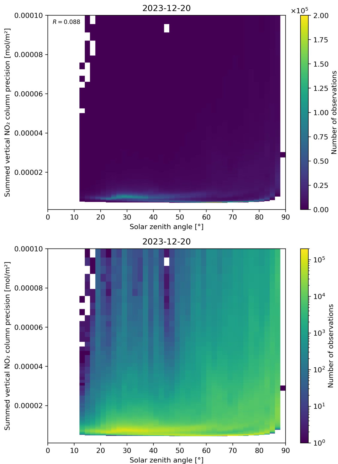
Figure 152: Scatter density plot of “Solar zenith angle” against “Summed vertical NO 2 column precision” for 2023-12-20 to 2023-12-21.
