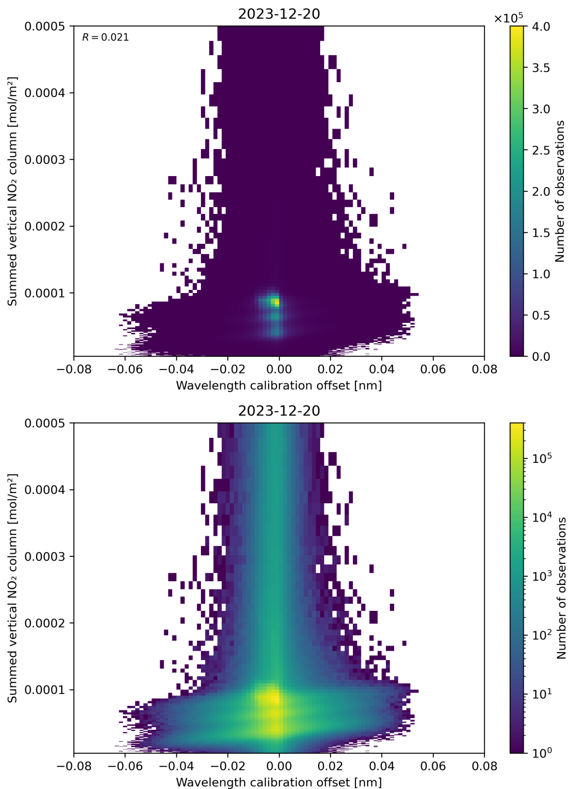
Figure 177: Scatter density plot of “Wavelength calibration offset” against “Summed vertical NO 2 column” for 2023-12-20 to 2023-12-21.
