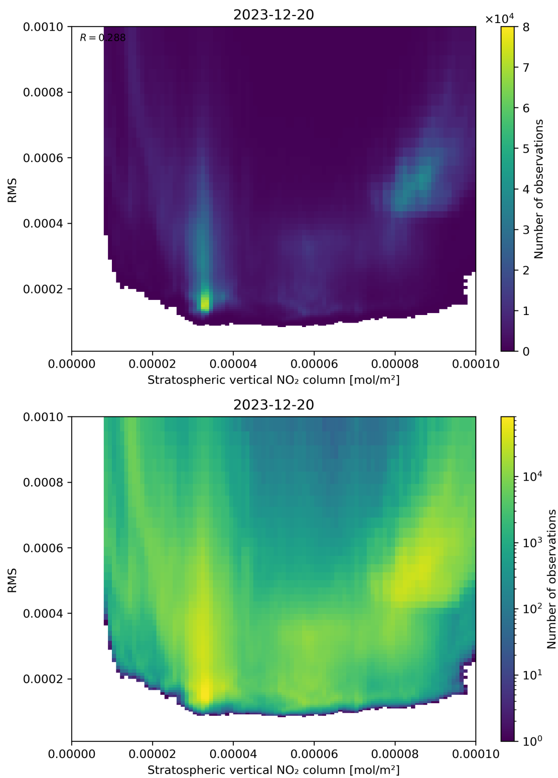
Figure 102: Scatter density plot of “Stratospheric vertical NO 2 column” against “RMS” for 2023-12-20 to 2023-12-21.
