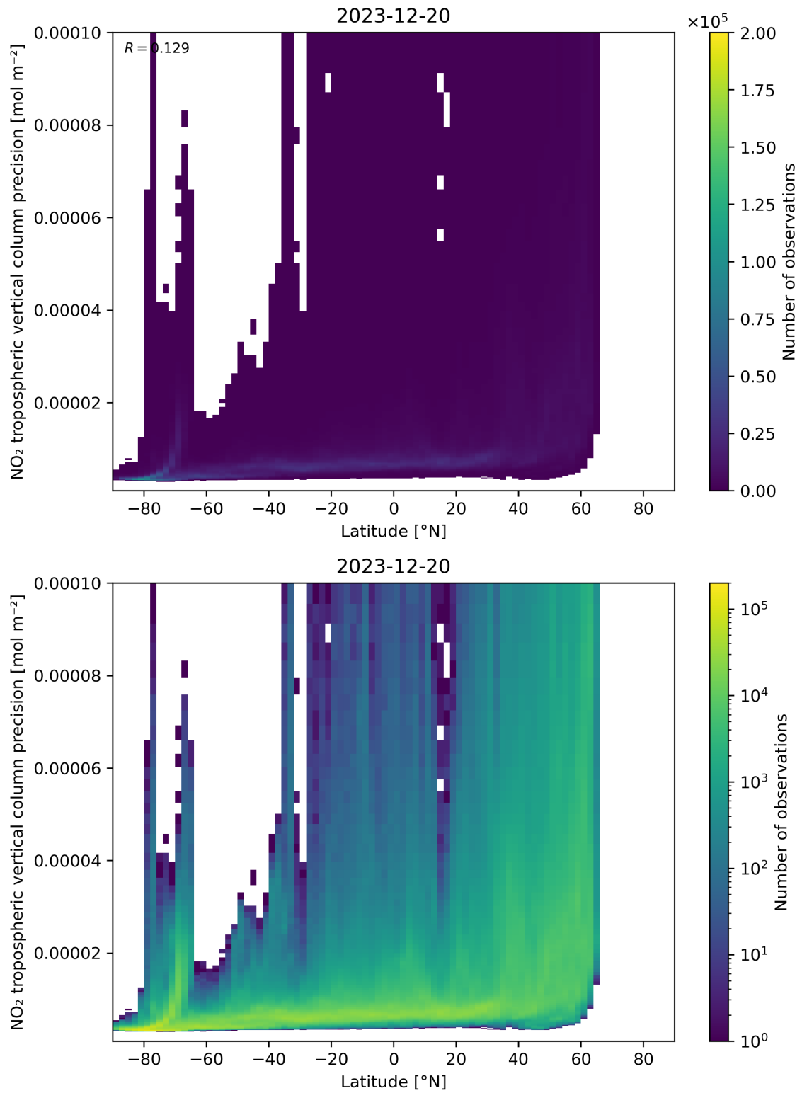
Figure 93: Scatter density plot of “Latitude” against “NO 2 tropospheric vertical column precision” for 2023-12-20 to 2023-12-21.
