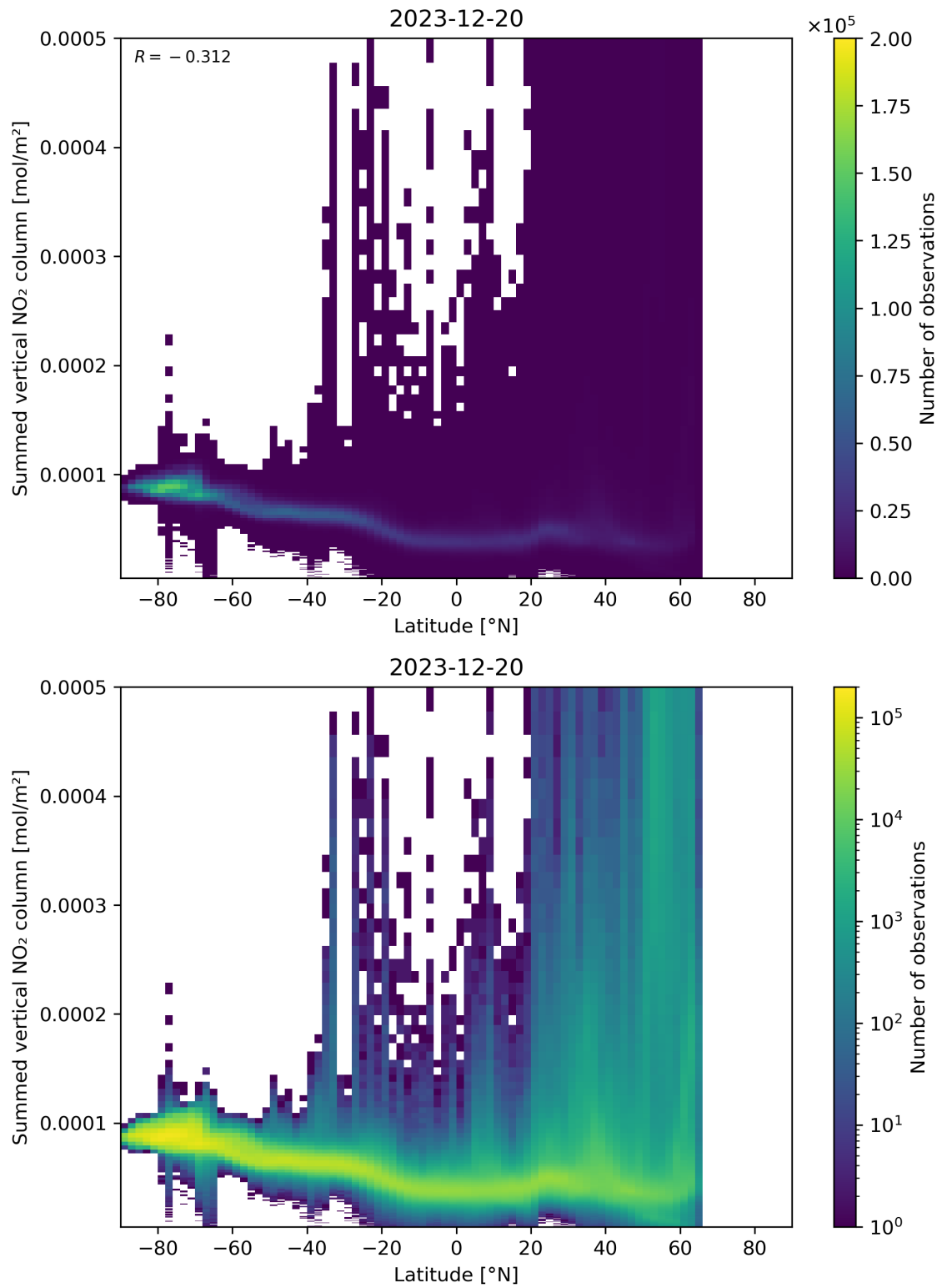
Figure 88: Scatter density plot of “Latitude” against “Summed vertical NO 2 column” for 2023-12-20 to 2023-12-21.
