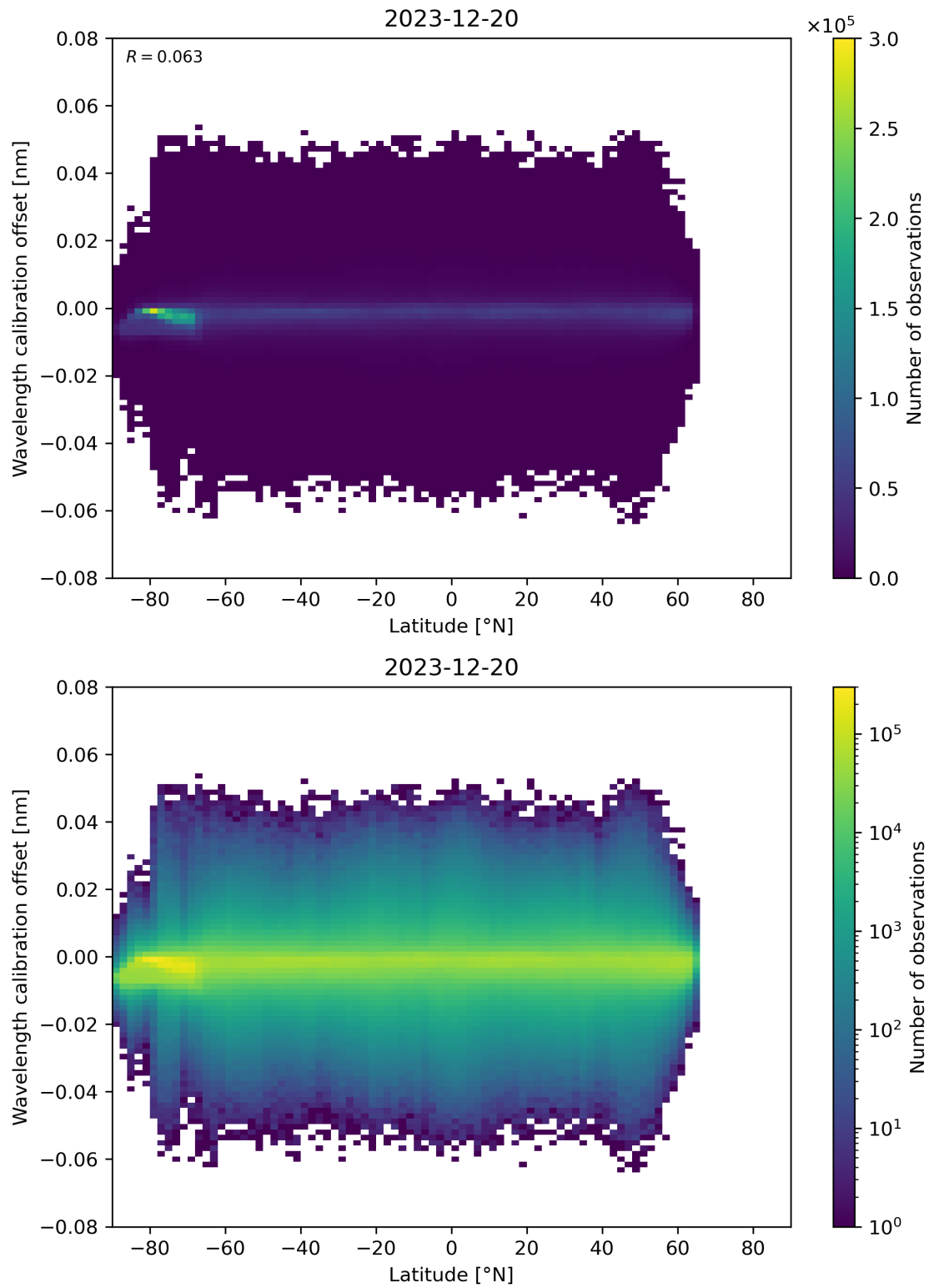
Figure 95: Scatter density plot of “Latitude” against “Wavelength calibration offset” for 2023-12-20 to 2023-12-21.
