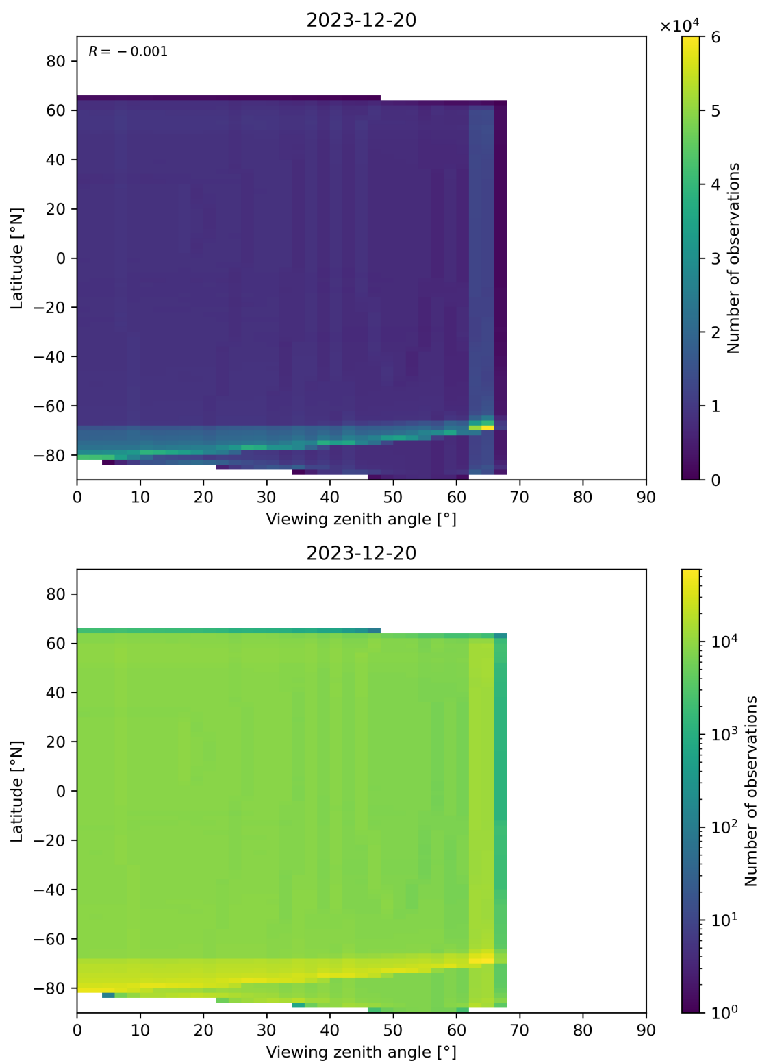
Figure 163: Scatter density plot of “Viewing zenith angle” against “Latitude” for 2023-12-20 to 2023-12-21.
