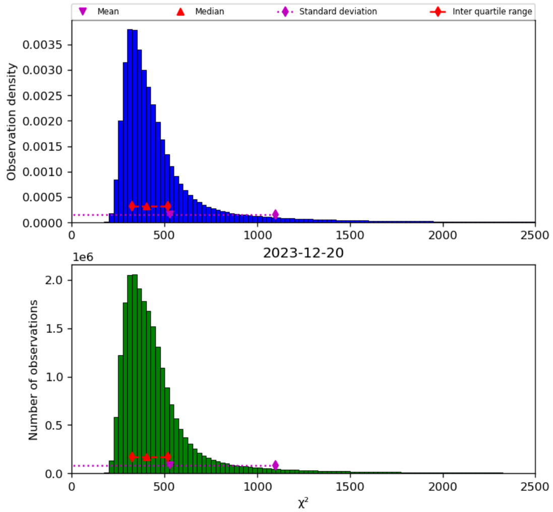
Figure 42: Histogram of " \chi^2 " for 2023-12-20 to 2023-12-21
