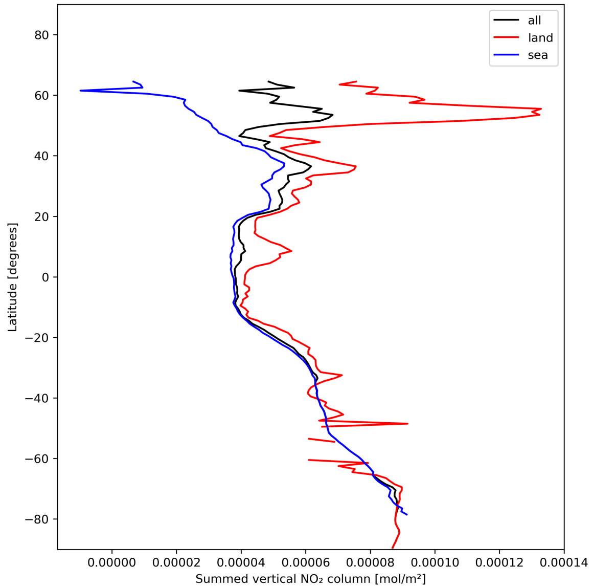
Figure 23: Zonal average of “Summed vertical NO 2 column” for 2023-12-20 to 2023-12-21.
