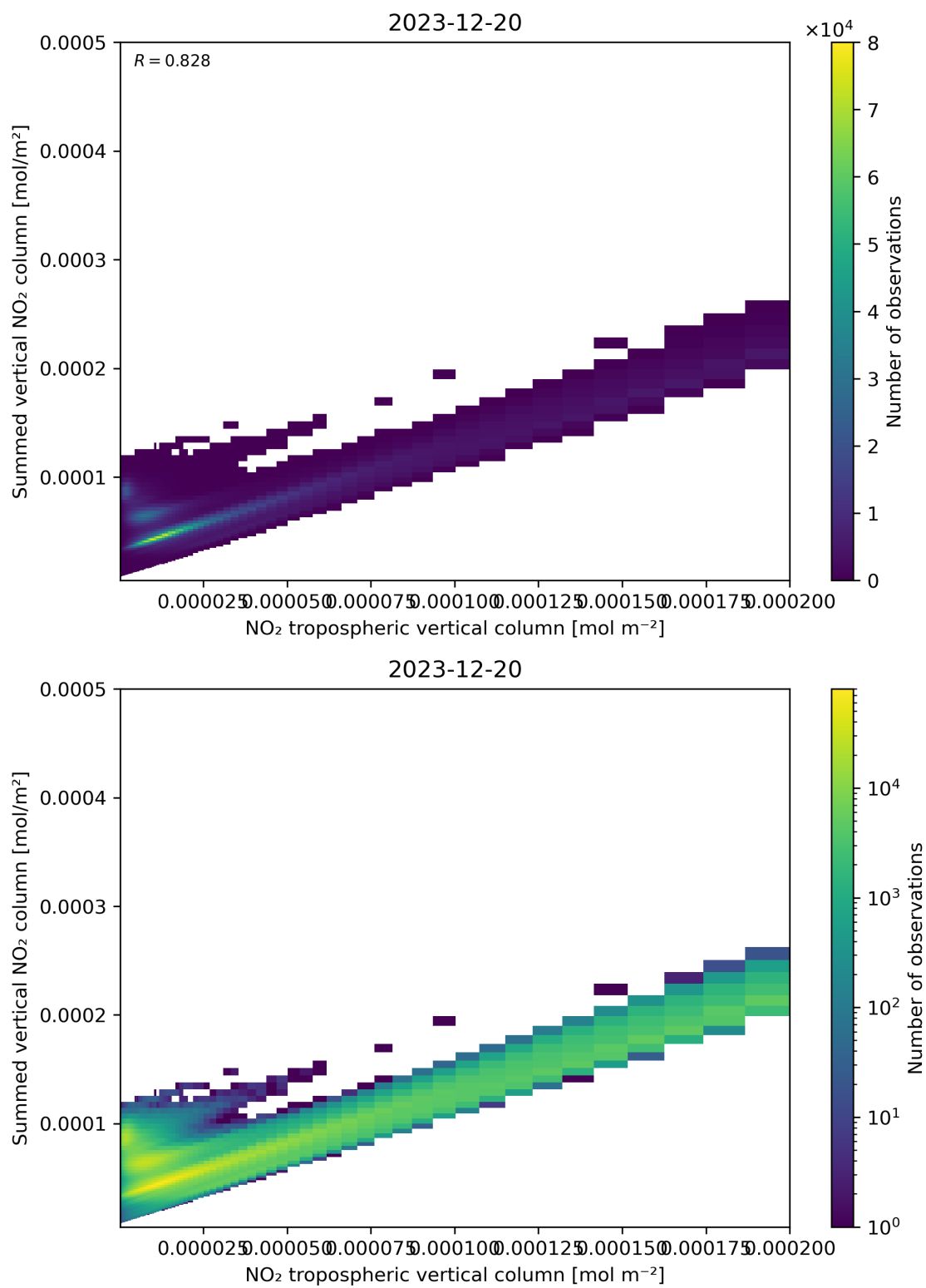
Figure 126: Scatter density plot of “NO 2 tropospheric vertical column” against “Summed vertical NO 2 column” for 2023-12-20 to 2023-12-21.
