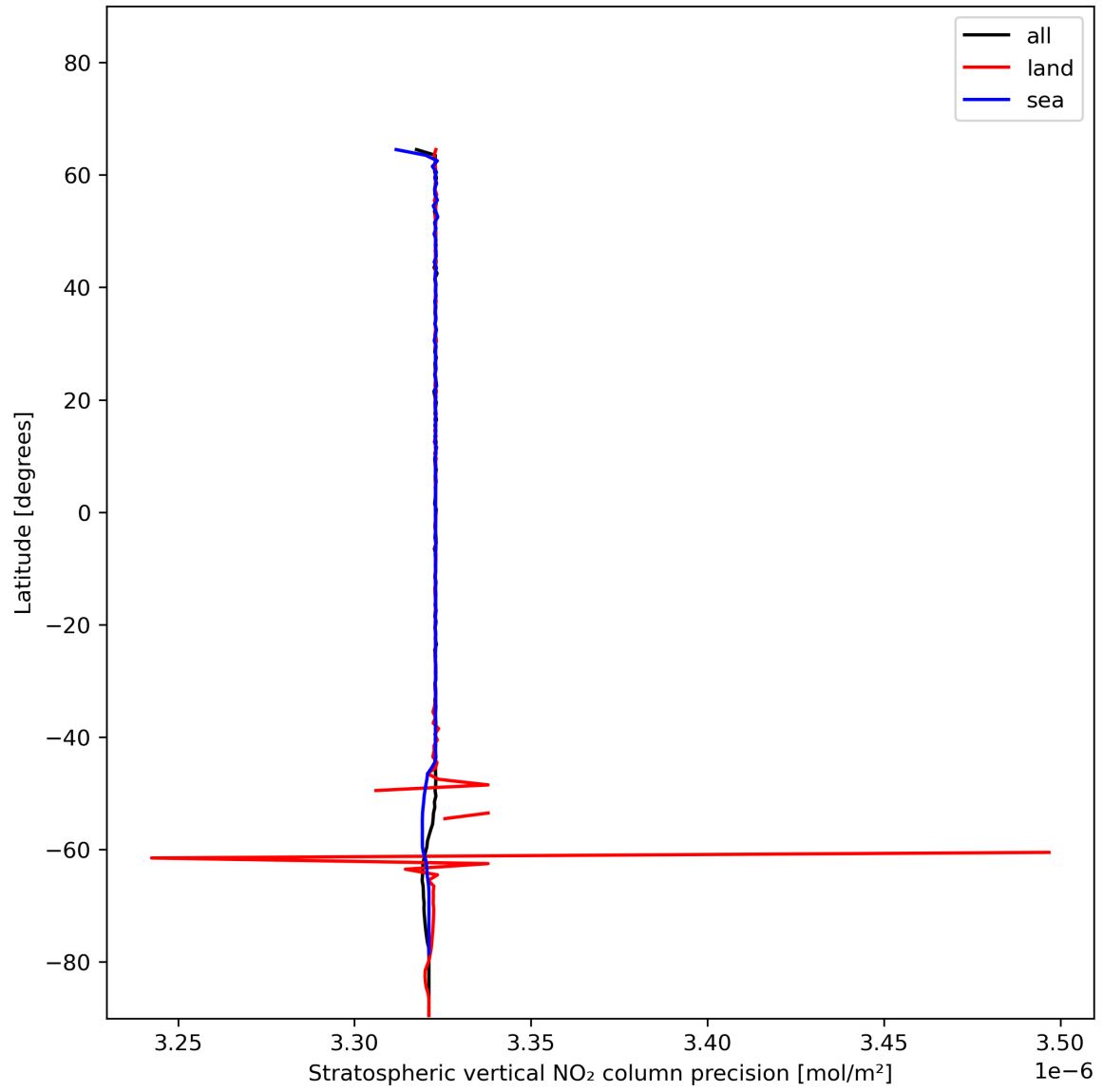
Figure 20: Zonal average of “Stratospheric vertical NO 2 column precision” for 2023-12-20 to 2023-12-21.
