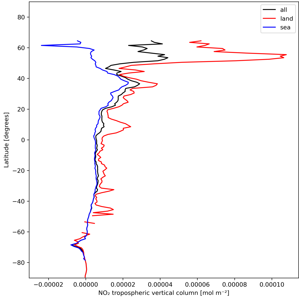
Figure 12: Zonal average of “NO 2 tropospheric vertical column” for 2023-12-20 to 2023-12-21.
