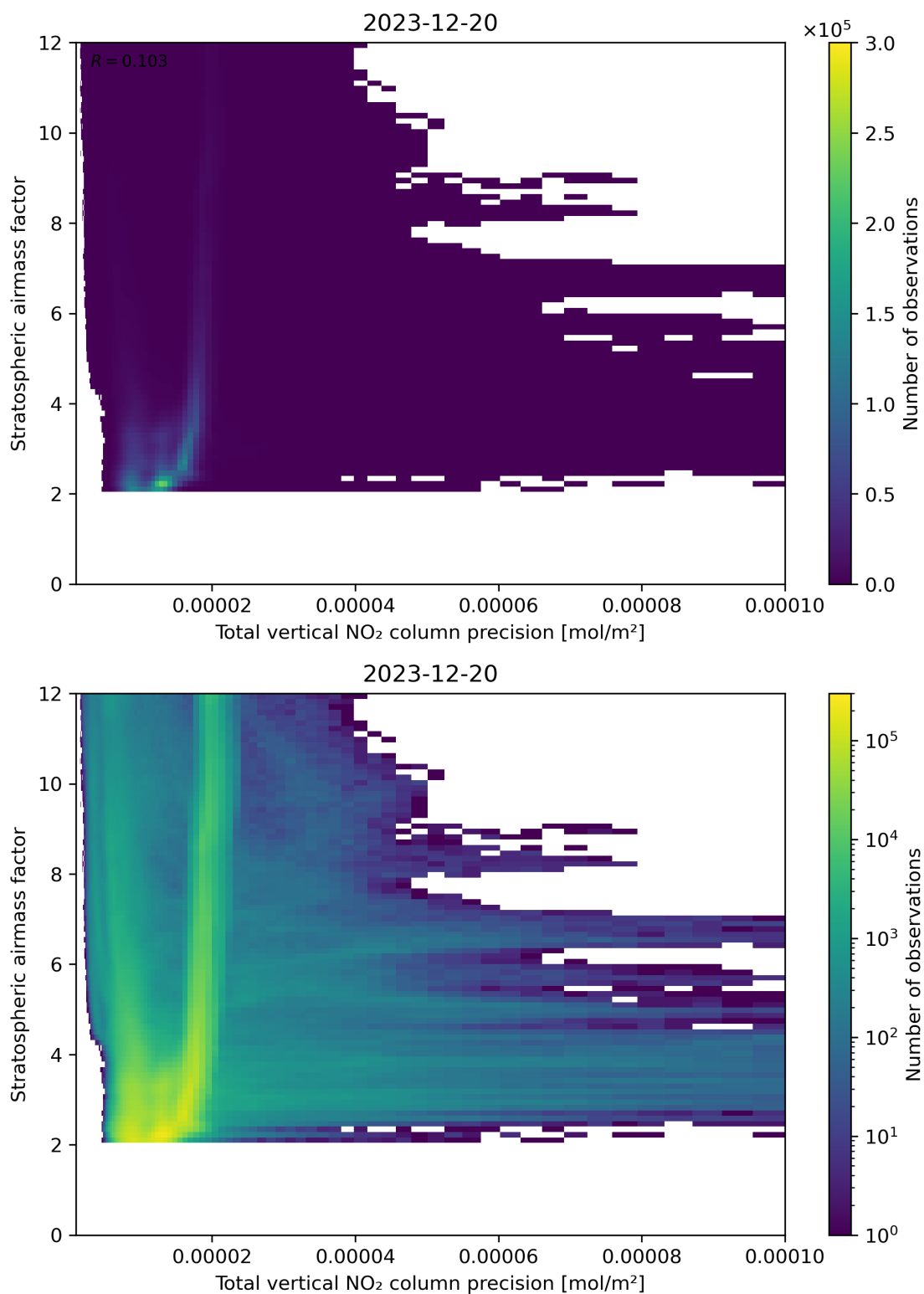
Figure 115: Scatter density plot of “Total vertical NO 2 column precision” against “Stratospheric air mass factor” for 2023-12-20 to 2023-12-21.
