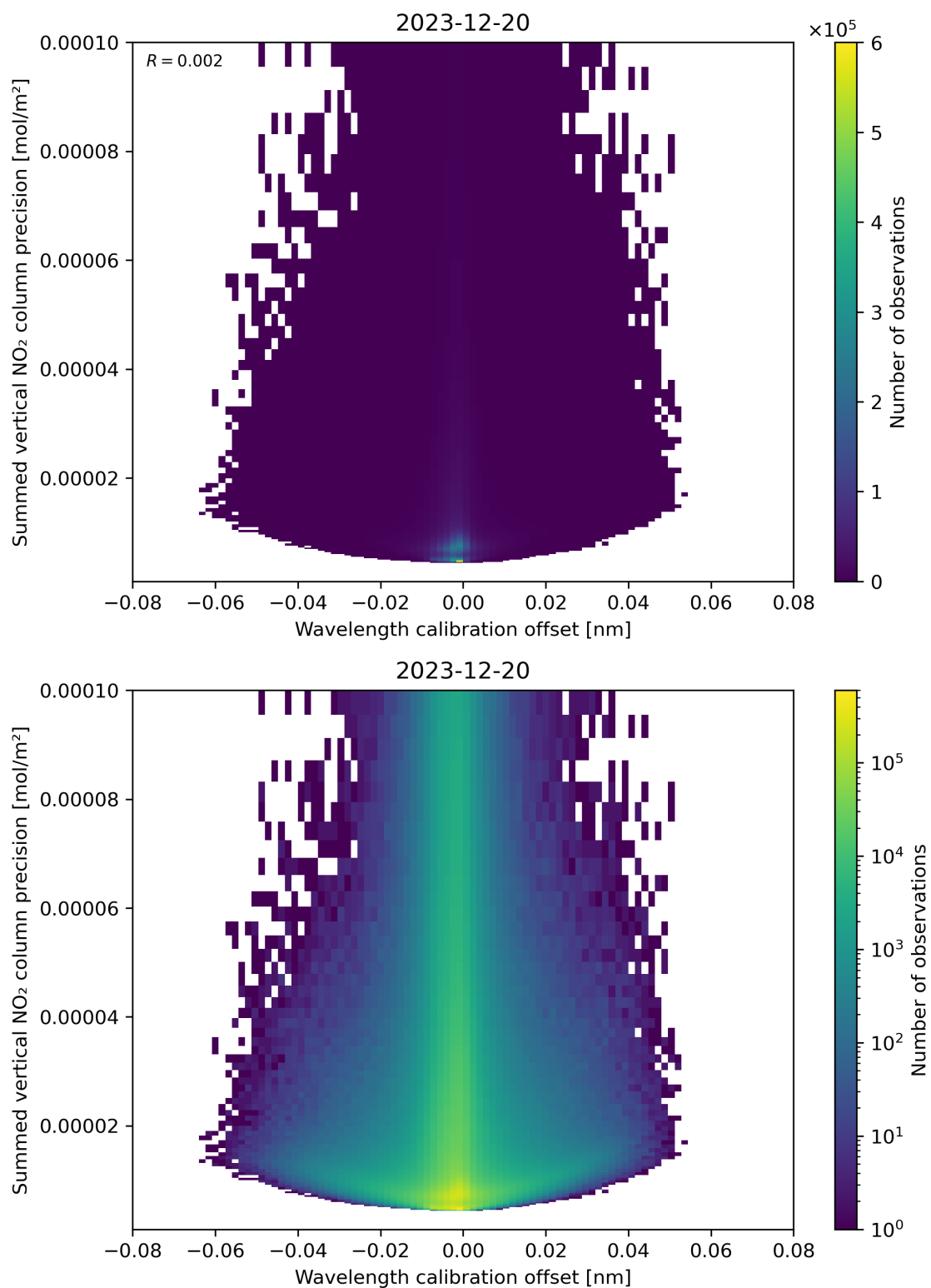
Figure 178: Scatter density plot of “Wavelength calibration offset” against “Summed vertical NO 2 column precision” for 2023-12-20 to 2023-12-21.
