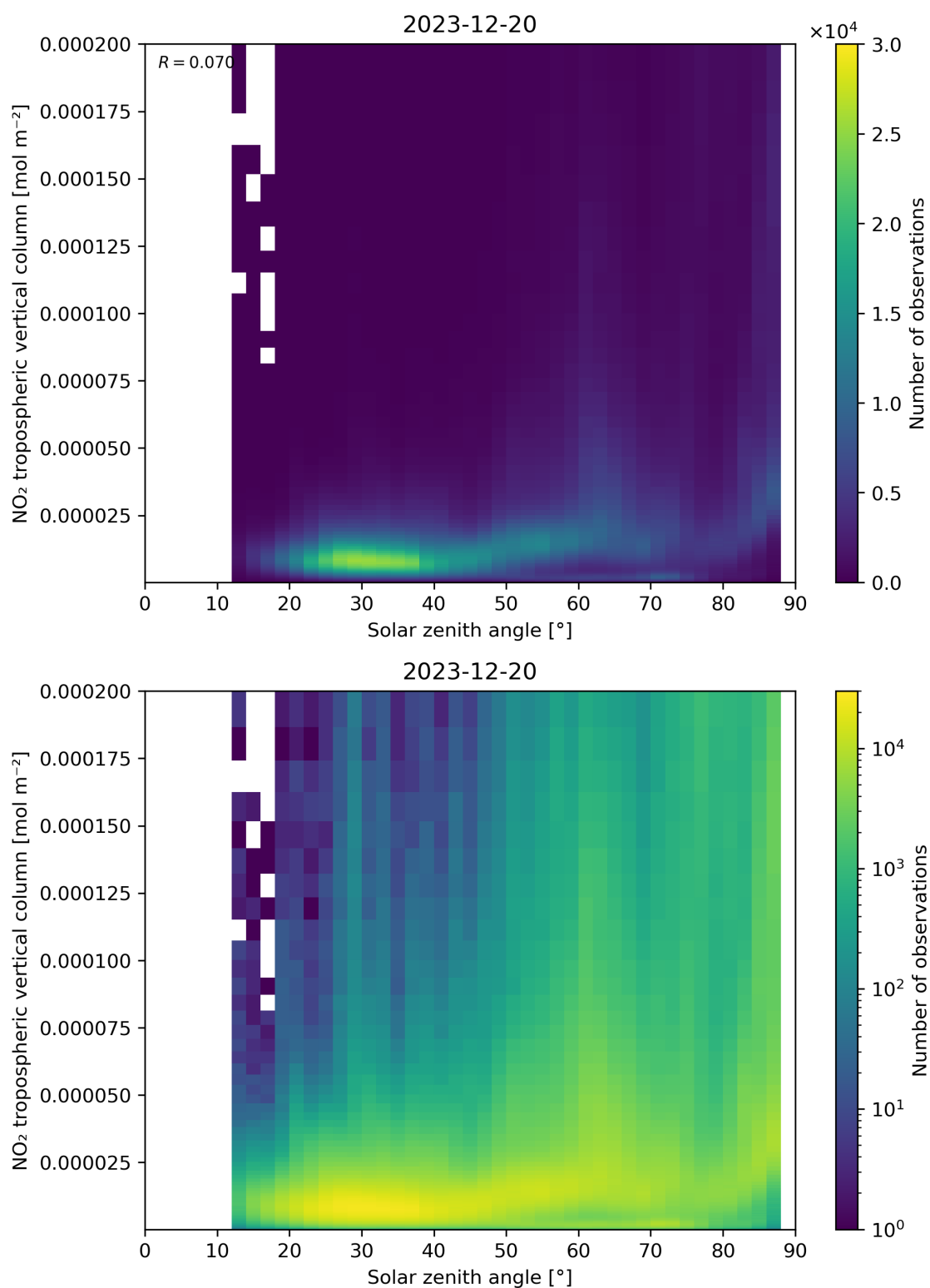
Figure 155: Scatter density plot of “Solar zenith angle” against “NO 2 tropospheric vertical column” for 2023-12-20 to 2023-12-21.
