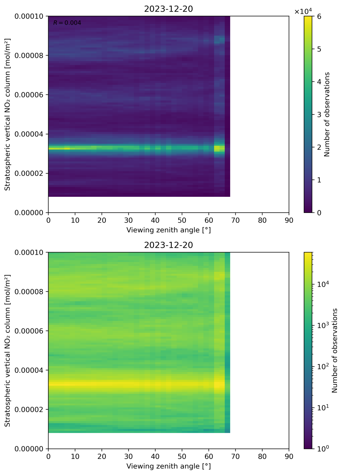
Figure 164: Scatter density plot of “Viewing zenith angle” against “Stratospheric vertical NO 2 column” for 2023-12-20 to 2023-12-21.
