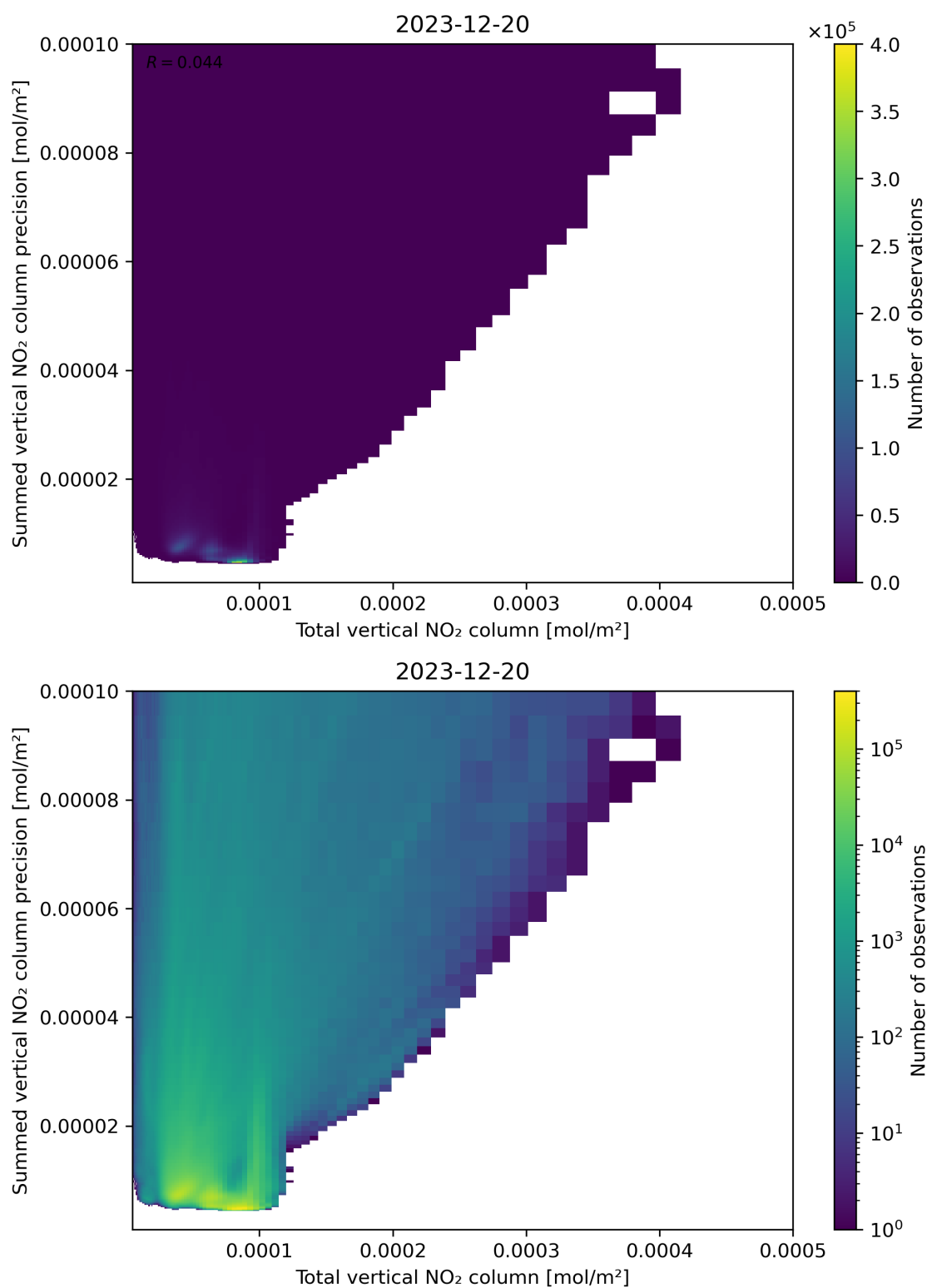
Figure 113: Scatter density plot of “Total vertical NO 2 column” against “Summed vertical NO 2 column precision” for 2023-12-20 to 2023-12-21.
