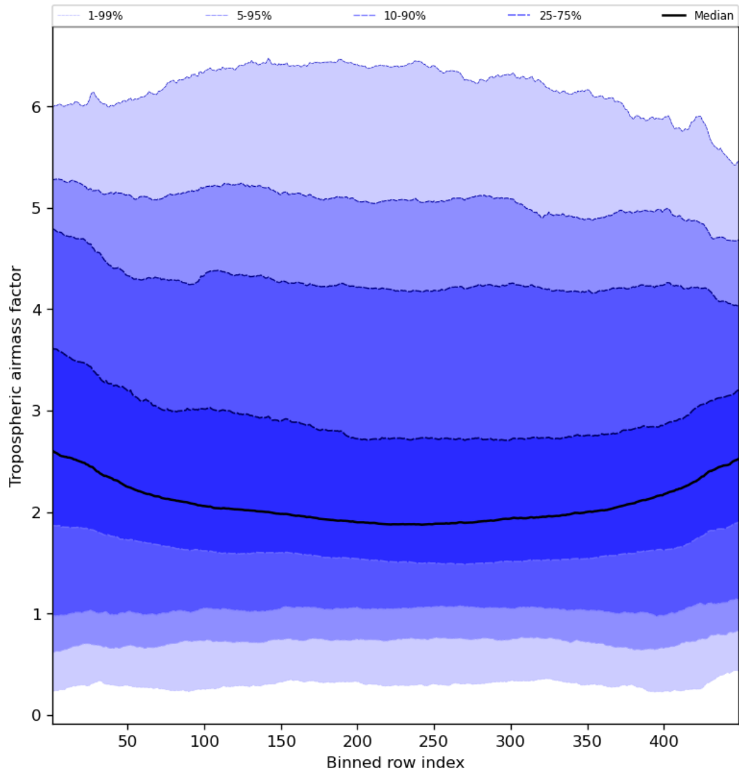
Figure 48: Along track statistics of “Tropospheric airmass factor” for 2023-12-20 to 2023-12-21
