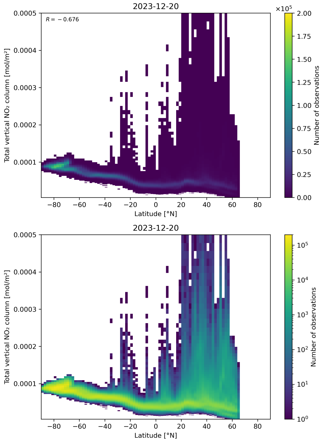
Figure 90: Scatter density plot of “Latitude” against “Total vertical NO 2 column” for 2023-12-20 to 2023-12-21.
