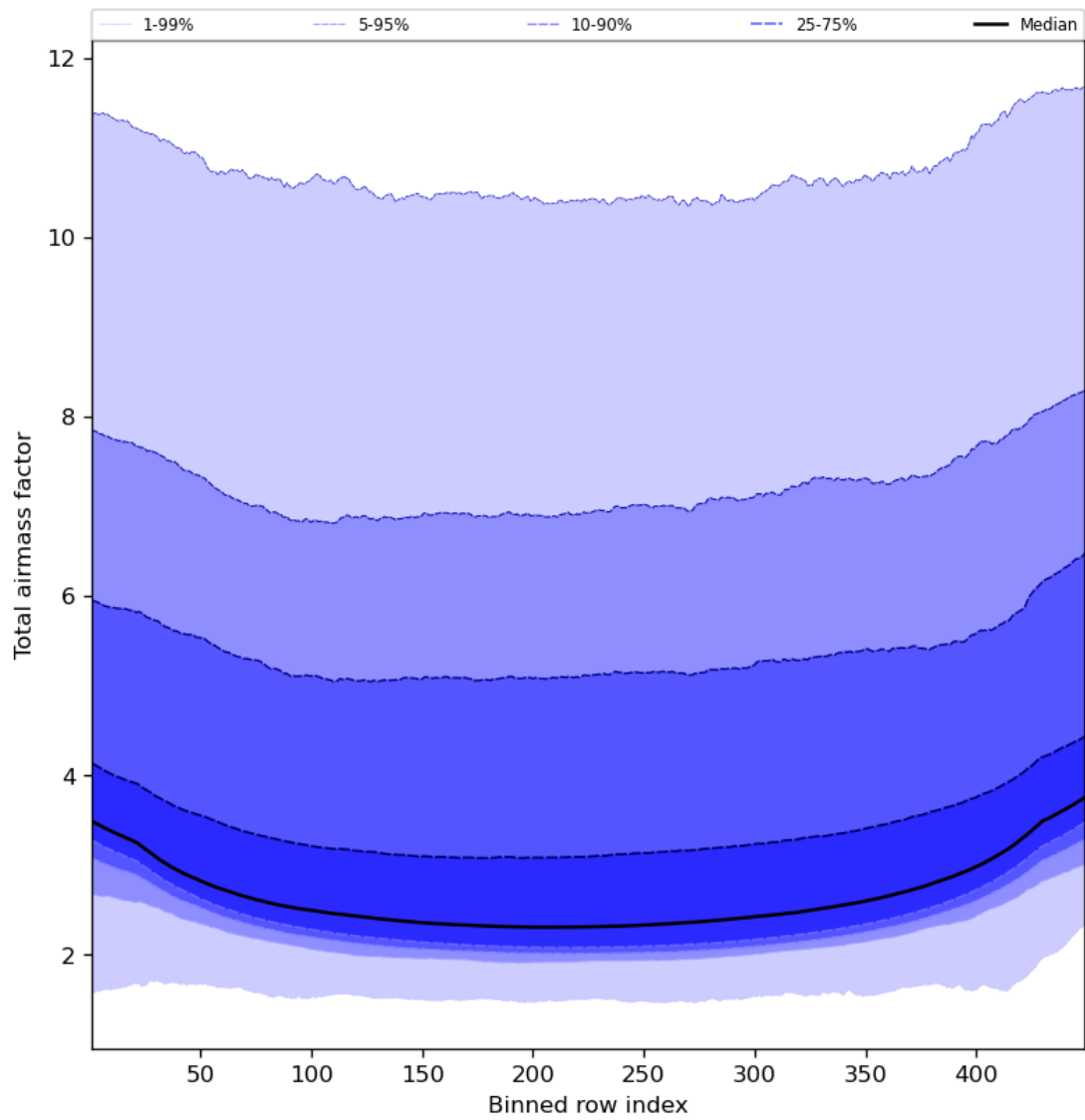
Figure 49: Along track statistics of “Total airmass factor” for 2023-12-20 to 2023-12-21
