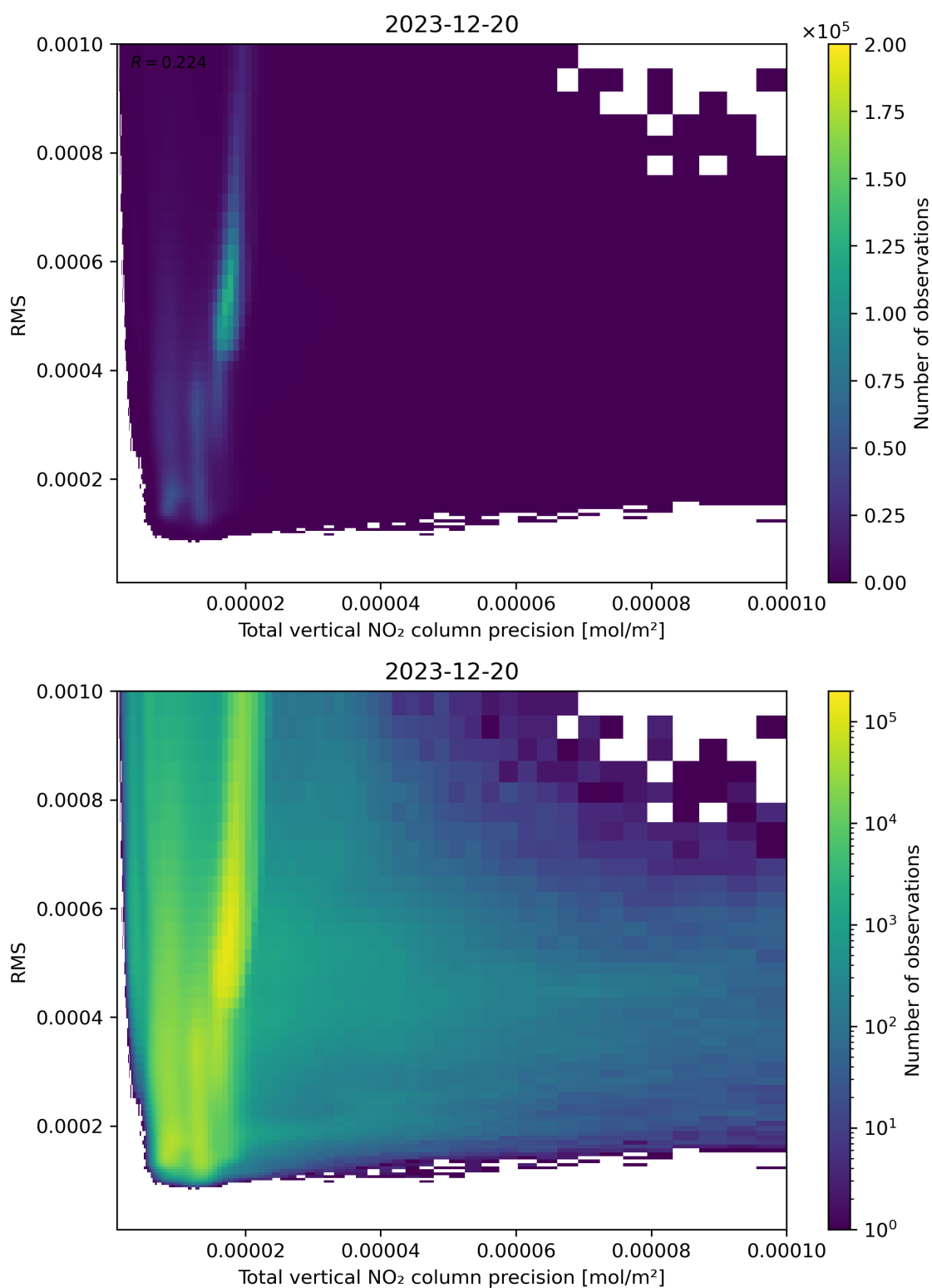
Figure 119: Scatter density plot of “Total vertical NO 2 column precision” against “RMS” for 2023-12-20 to 2023-12-21.
