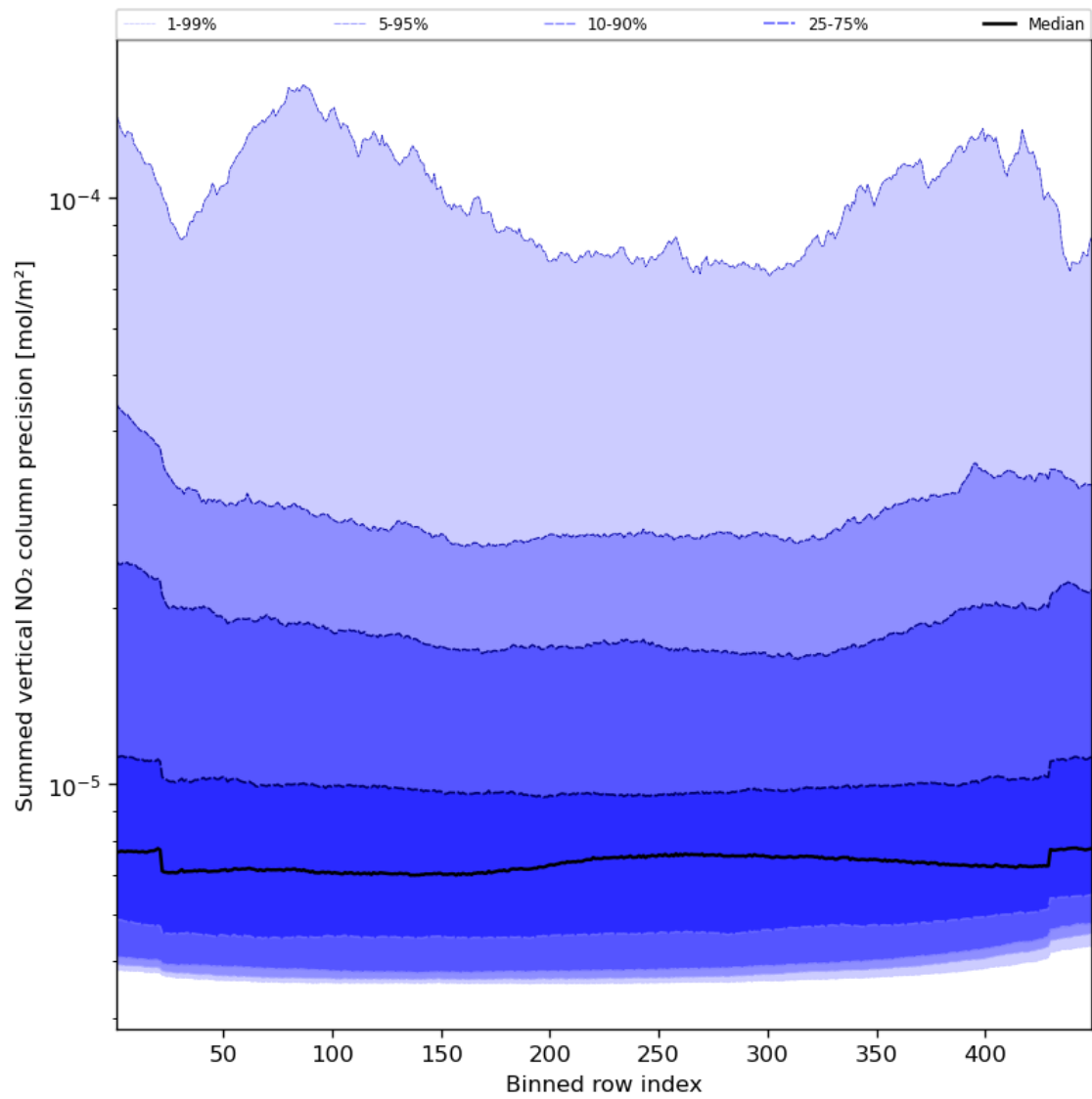
Figure 58: Along track statistics of “Summed vertical NO 2 column precision” for 2023-12-20 to 2023-12-21
