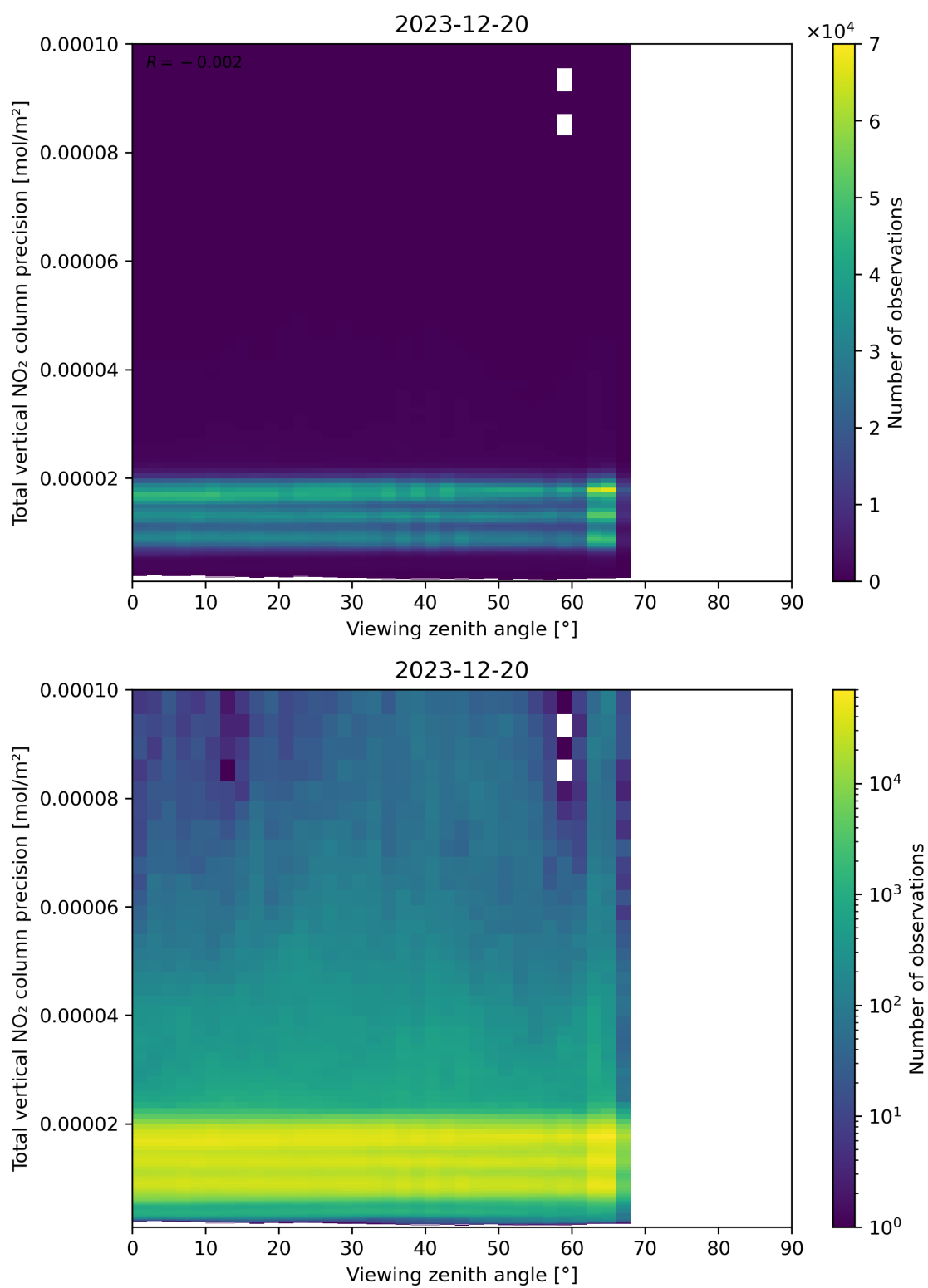
Figure 168: Scatter density plot of “Viewing zenith angle” against “Total vertical NO 2 column precision” for 2023-12-20 to 2023-12-21.
