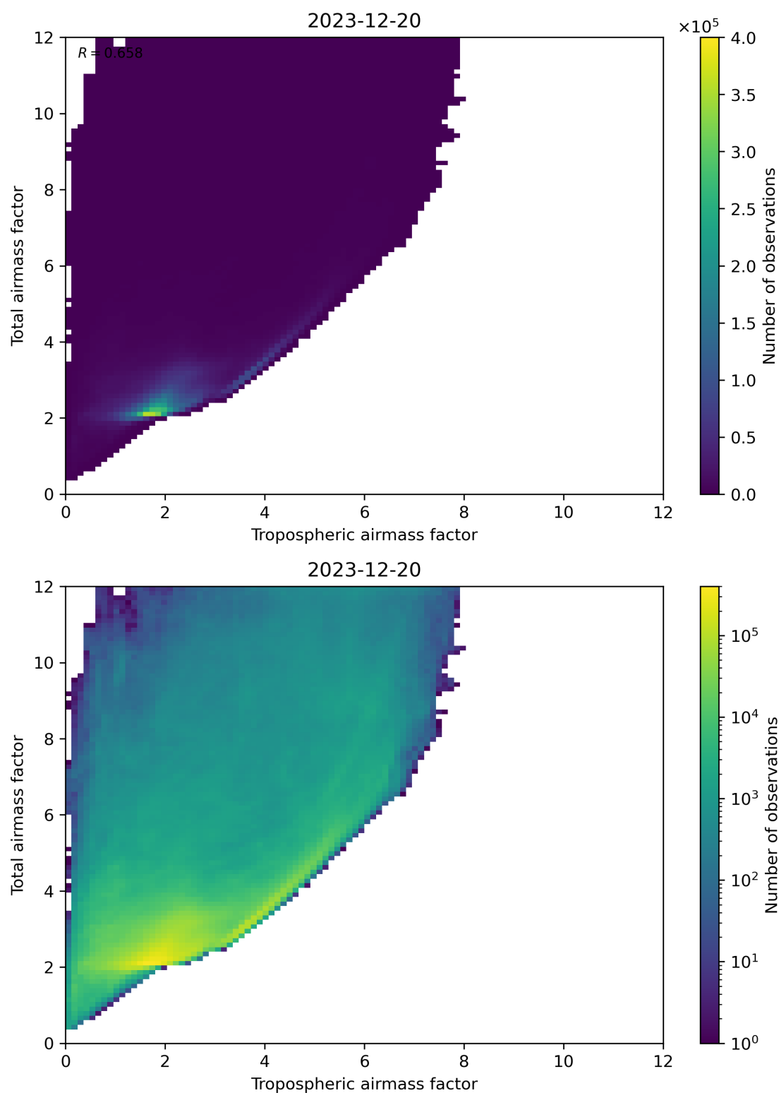
Figure 72: Scatter density plot of “Tropospheric airmass factor” against “Total airmass factor” for 2023-12-20 to 2023-12-21.
