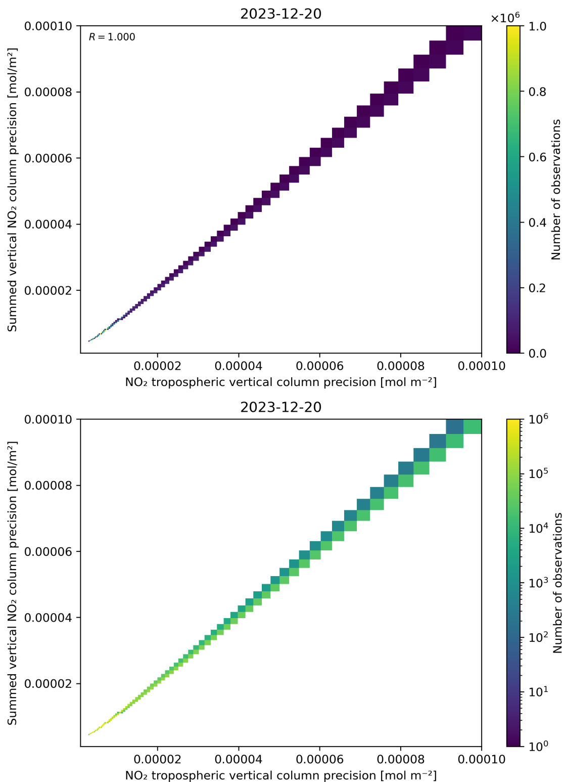
Figure 137: Scatter density plot of “NO 2 tropospheric vertical column precision” against “Summed vertical NO 2 column precision” for 2023-12-20 to 2023-12-21.
