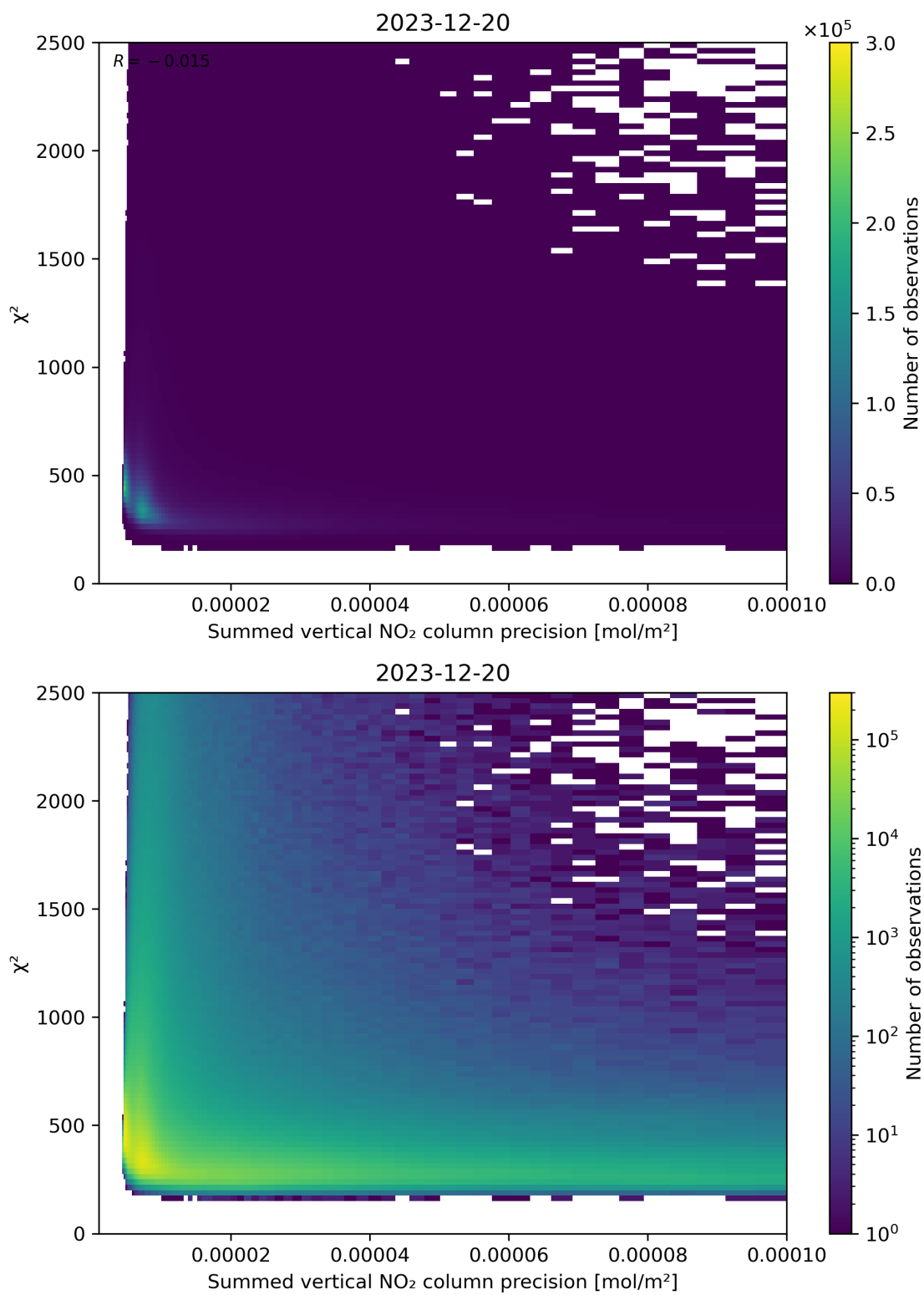
Figure 107: Scatter density plot of “Summed vertical NO 2 column precision” against “ \chi^2 ” for 2023-12-20 to 2023-12-21.
