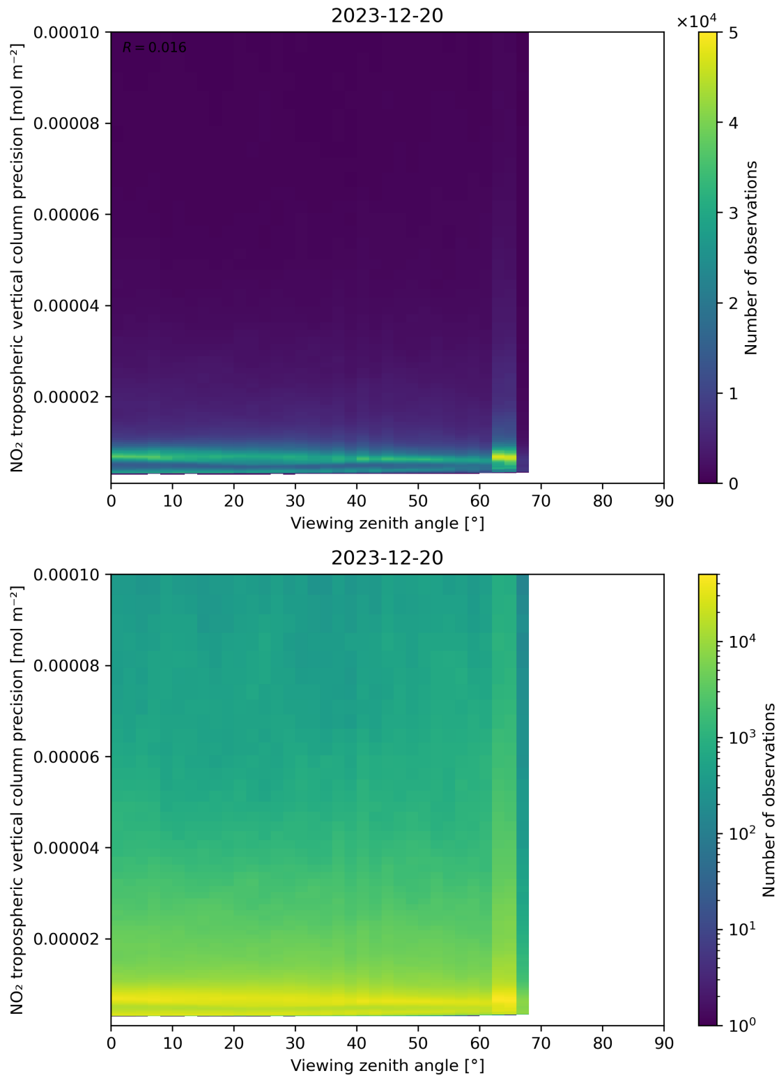
Figure 170: Scatter density plot of “Viewing zenith angle” against “NO 2 tropospheric vertical column precision” for 2023-12-20 to 2023-12-21.
