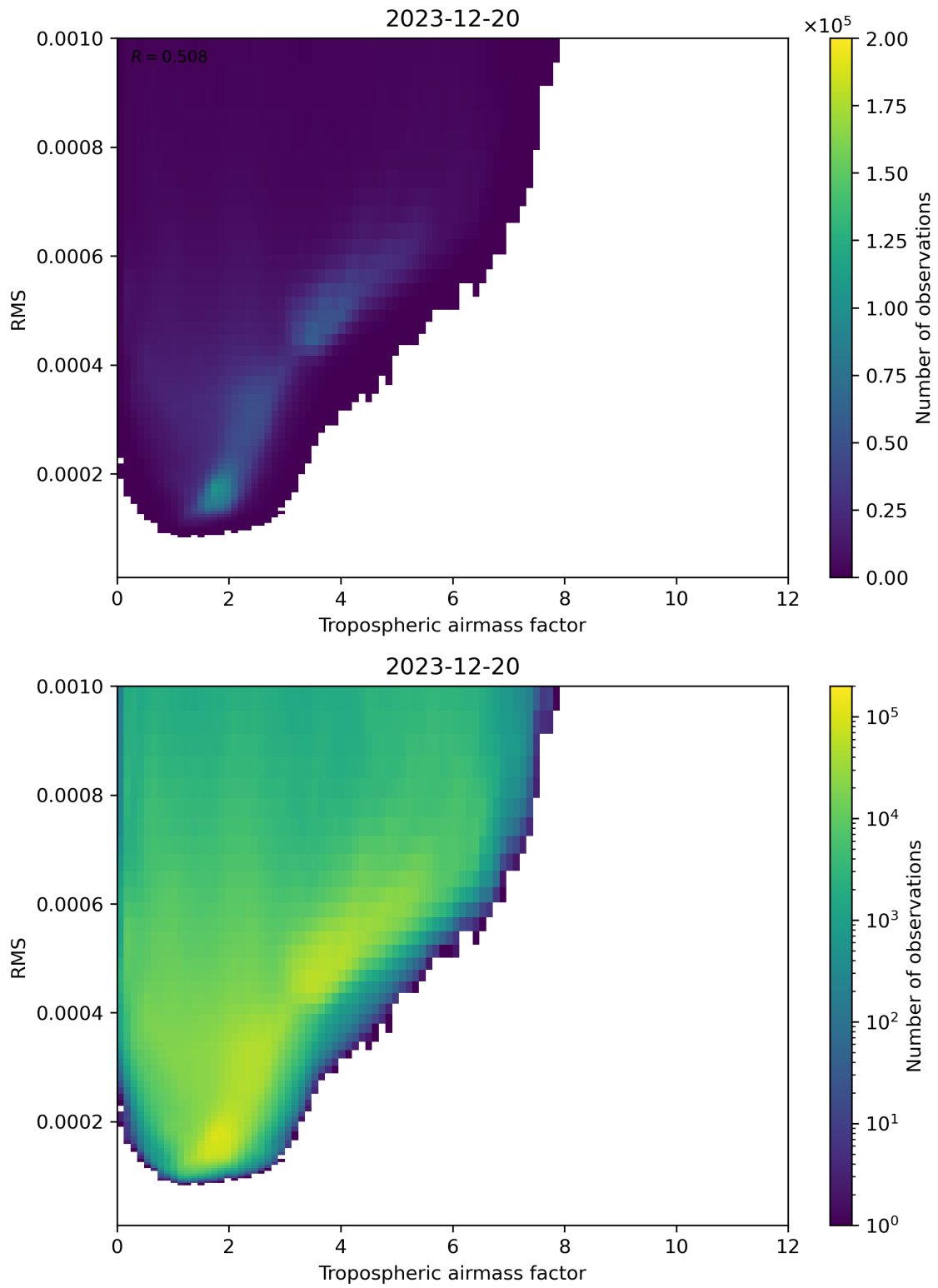
Figure 79: Scatter density plot of “Tropospheric airmass factor” against “RMS” for 2023-12-20 to 2023-12-21.
