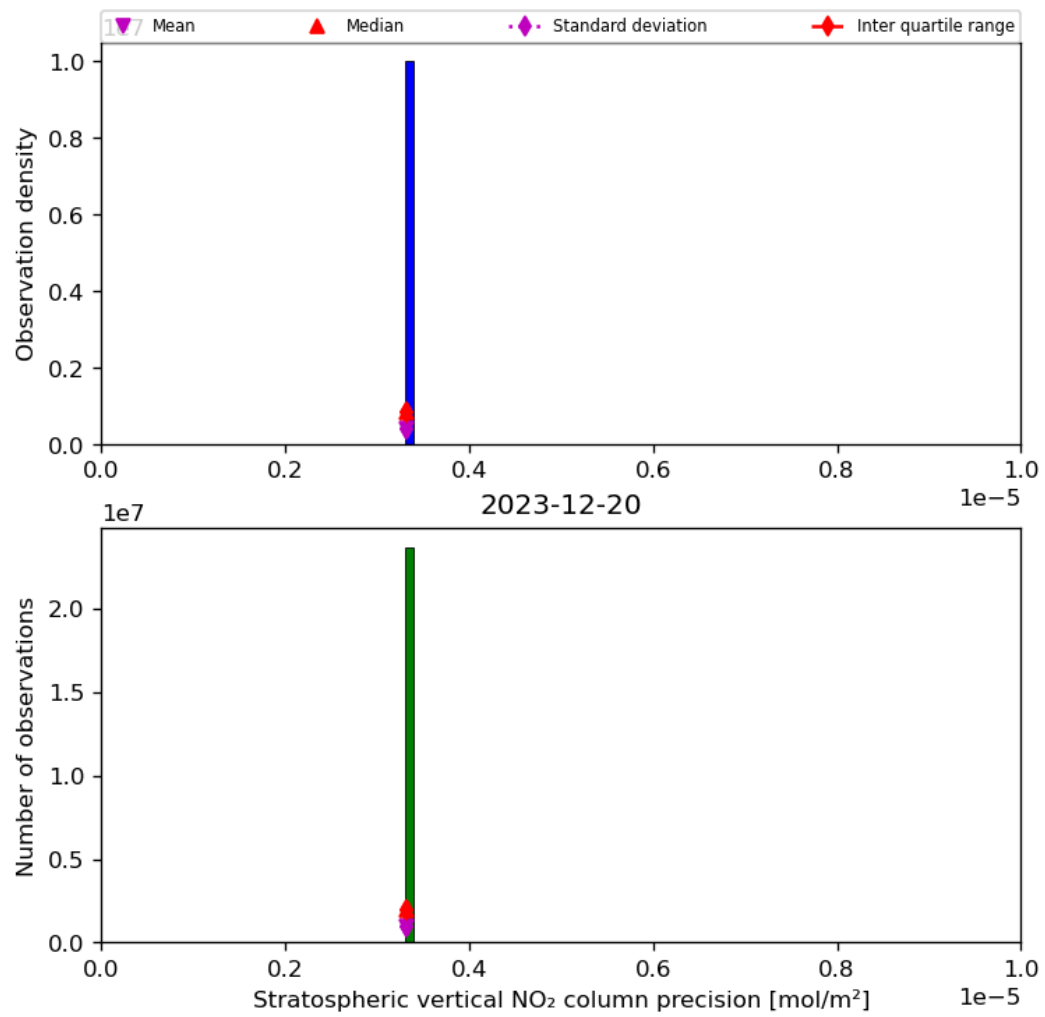
Figure 37: Histogram of “Stratospheric vertical NO 2 column precision” for 2023-12-20 to 2023-12-21
