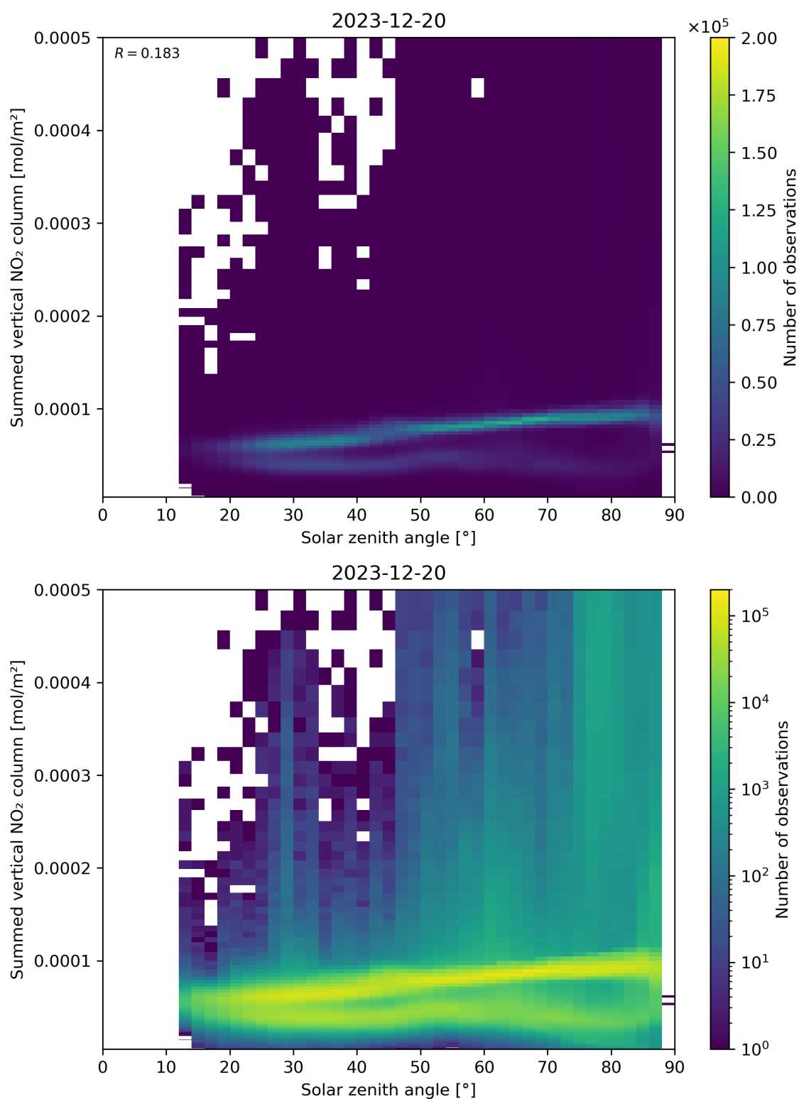
Figure 151: Scatter density plot of “Solar zenith angle” against “Summed vertical NO 2 column” for 2023-12-20 to 2023-12-21.
