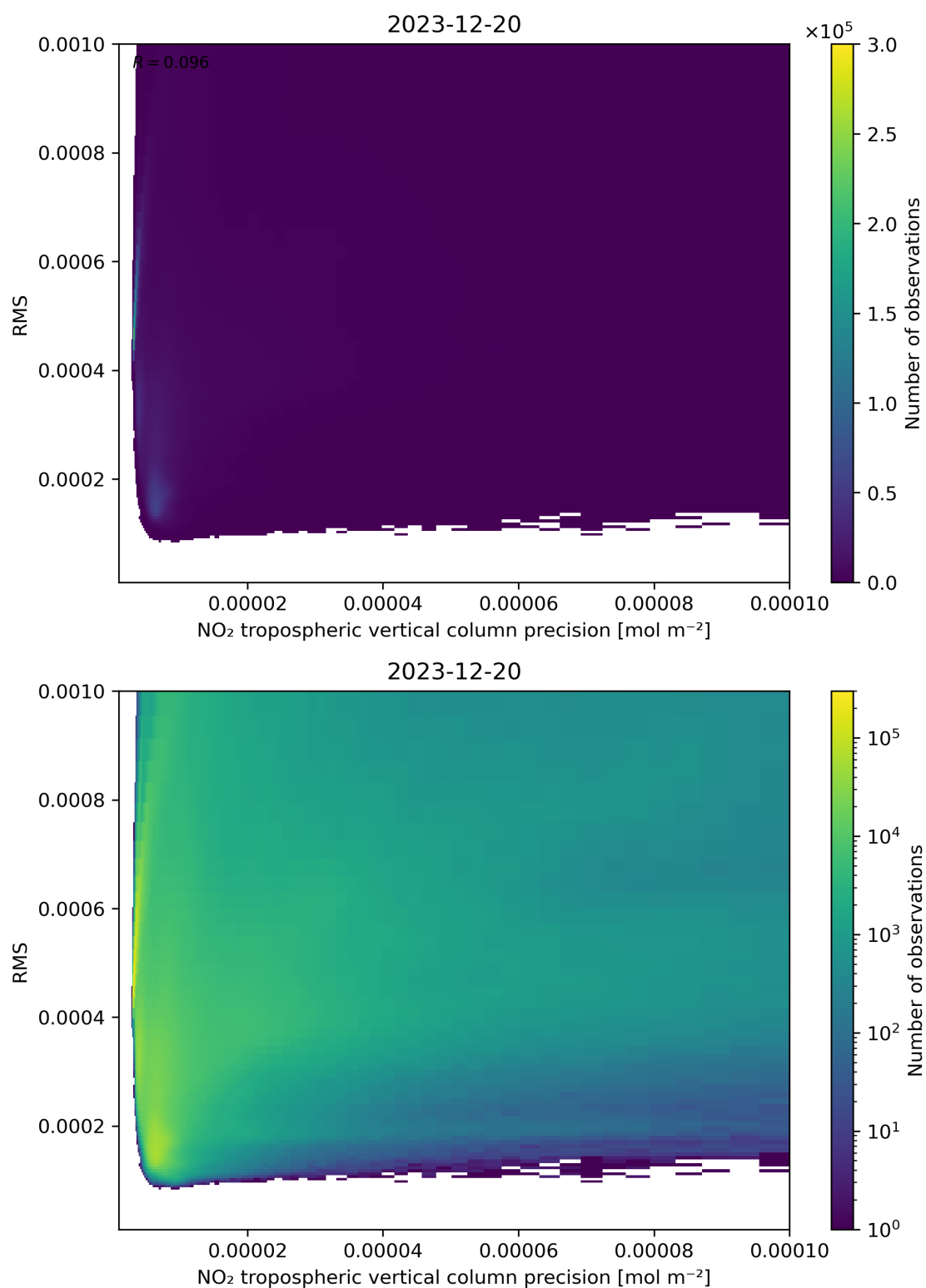
Figure 140: Scatter density plot of “NO 2 tropospheric vertical column precision” against “RMS” for 2023-12-20 to 2023-12-21.
