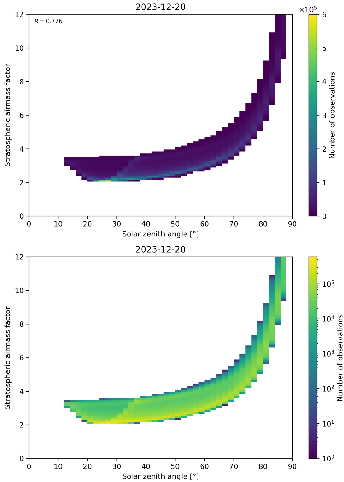
Figure 145: Scatter density plot of “Solar zenith angle” against “Stratospheric airmass factor” for 2023-12-20 to 2023-12-21.
