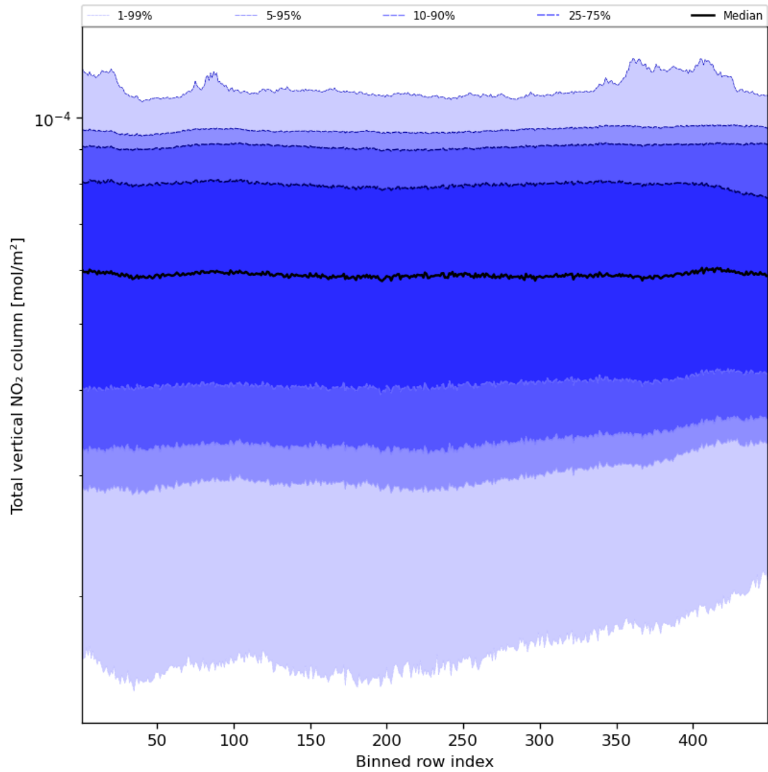
Figure 55: Along track statistics of “Total vertical NO 2 column” for 2023-12-20 to 2023-12-21
