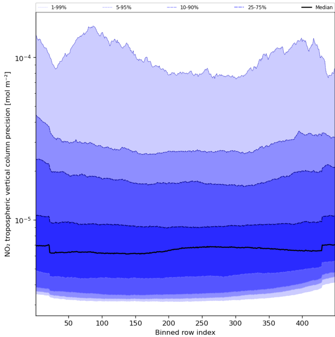
Figure 47: Along track statistics of “NO 2 tropospheric vertical column precision” for 2023-12-20 to 2023-12-21
