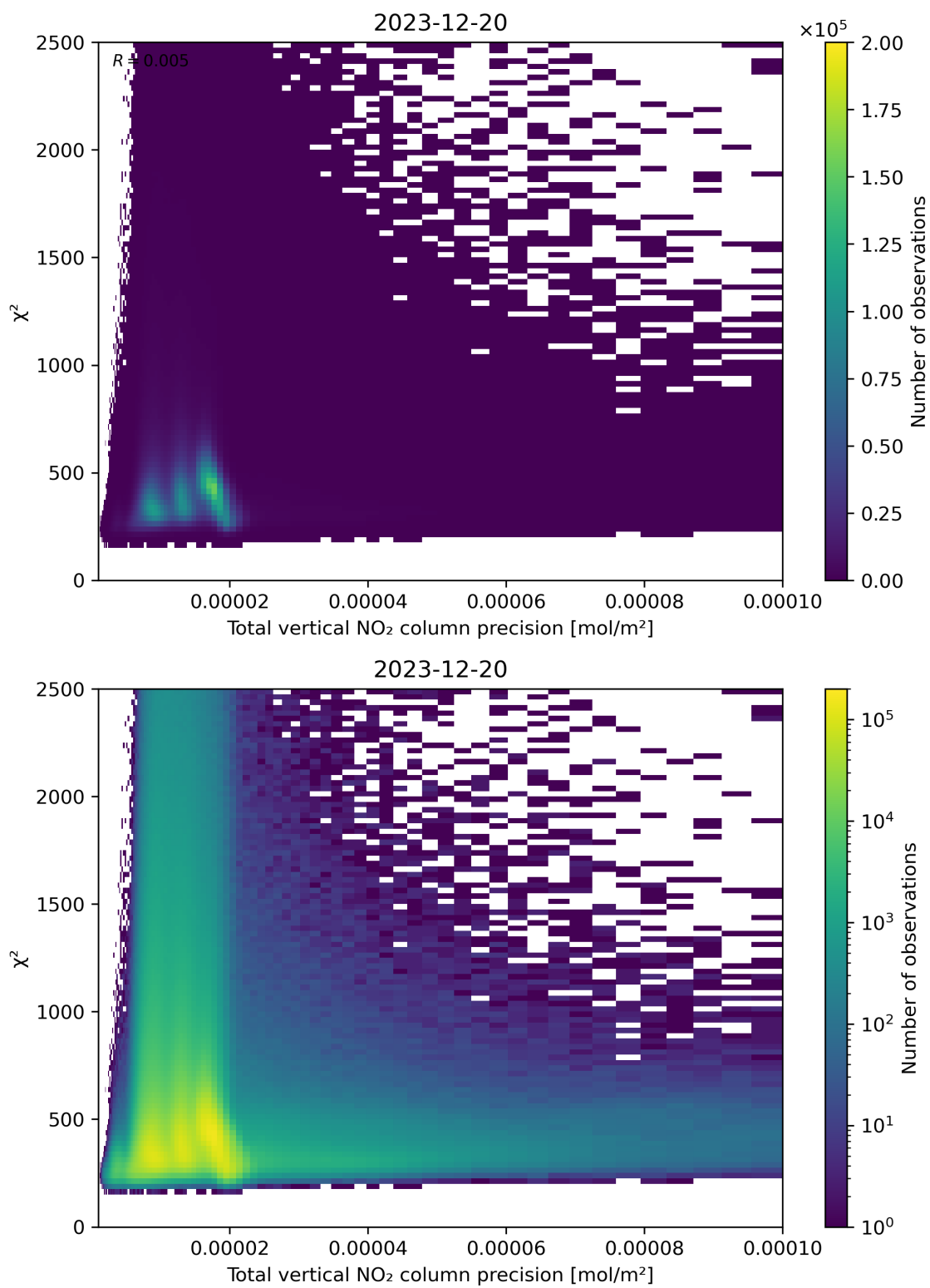
Figure 116: Scatter density plot of “Total vertical NO 2 column precision” against “ \chi^2 ” for 2023-12-20 to 2023-12-21.
