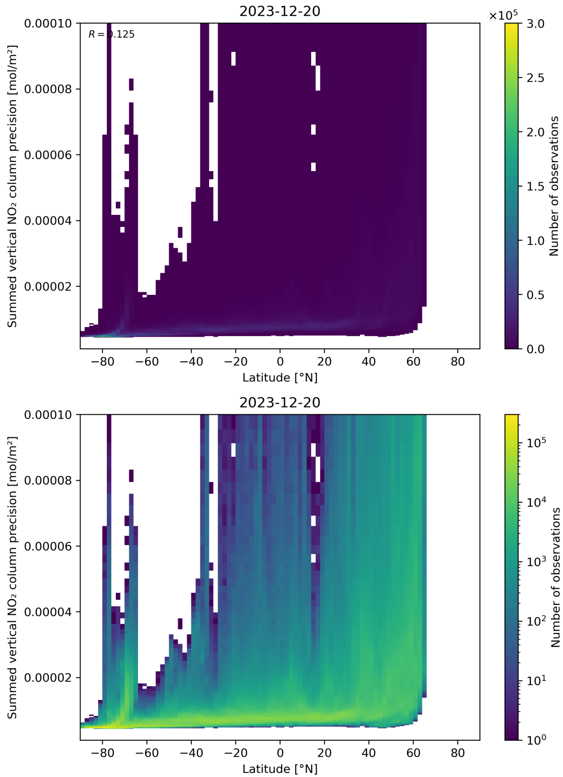
Figure 89: Scatter density plot of “Latitude” against “Summed vertical NO 2 column precision” for 2023-12-20 to 2023-12-21.
