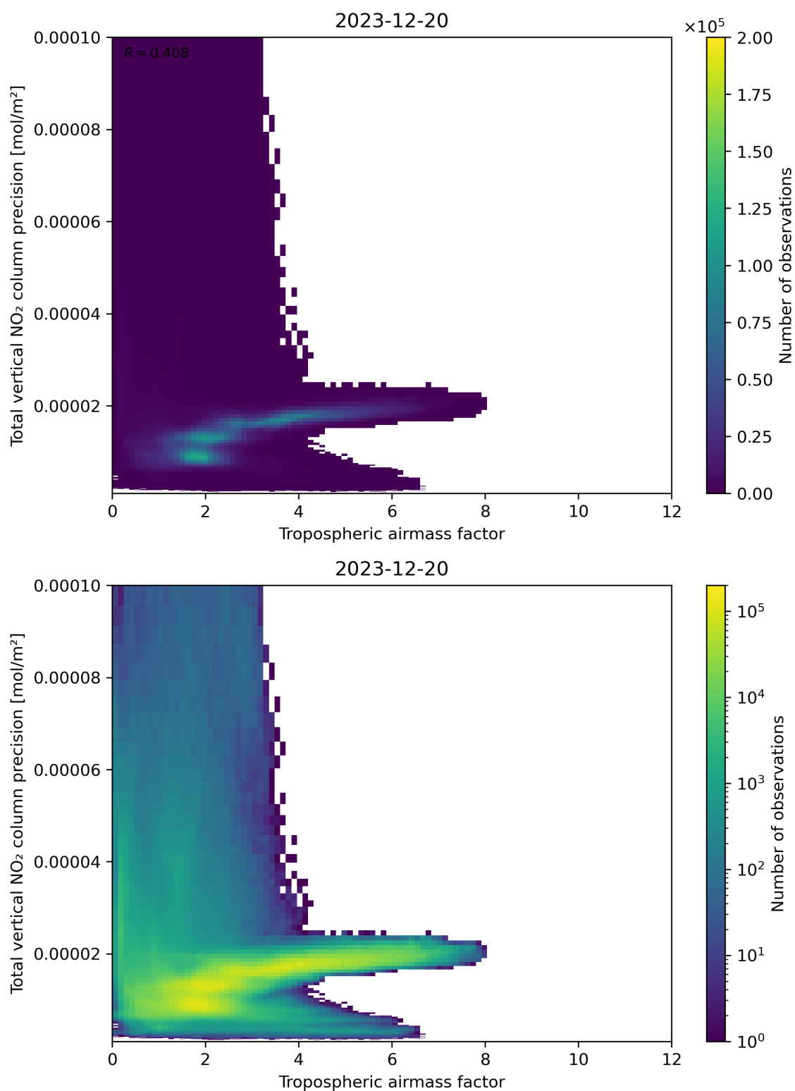
Figure 78: Scatter density plot of “Tropospheric air mass factor” against “Total vertical NO 2 column precision” for 2023-12-20 to 2023-12-21.
