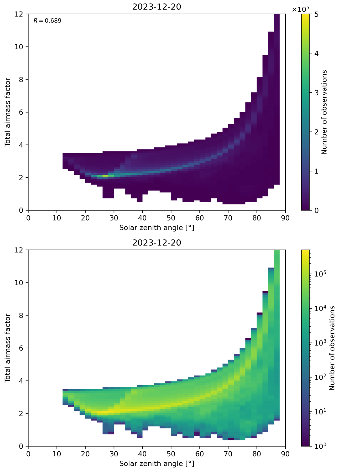
Figure 146: Scatter density plot of “Solar zenith angle” against “Total air mass factor” for 2023-12-20 to 2023-12-21.
