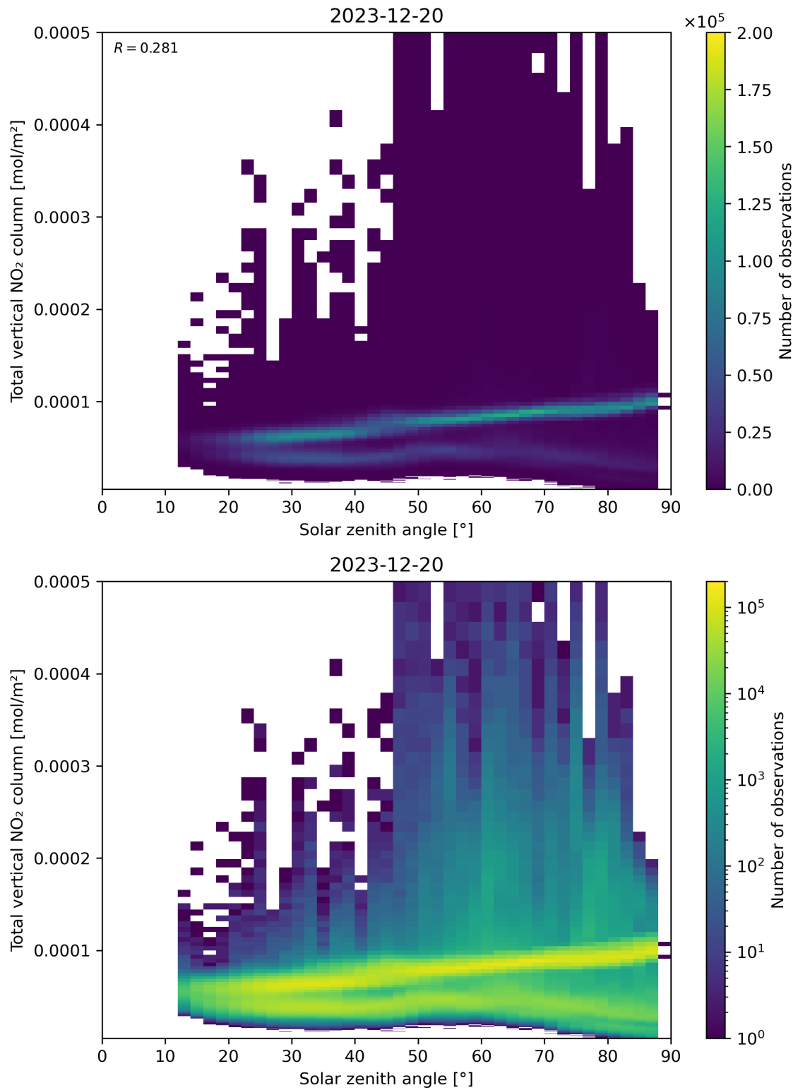
Figure 153: Scatter density plot of “Solar zenith angle” against “Total vertical \text{NO}_2 column” for 2023-12-20 to 2023-12-21.
