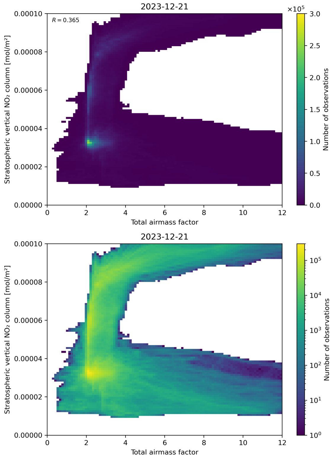
Figure 64: Scatter density plot of “Total airmass factor” against “Stratospheric vertical NO 2 column” for 2023-12-20 to 2023-12-22.
