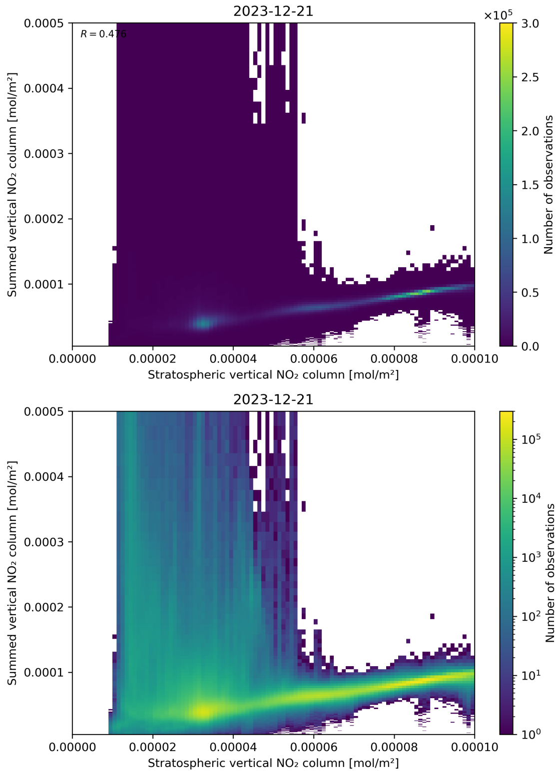
Figure 98: Scatter density plot of “Stratospheric vertical NO 2 column” against “Summed vertical NO 2 column” for 2023-12-20 to 2023-12-22.
