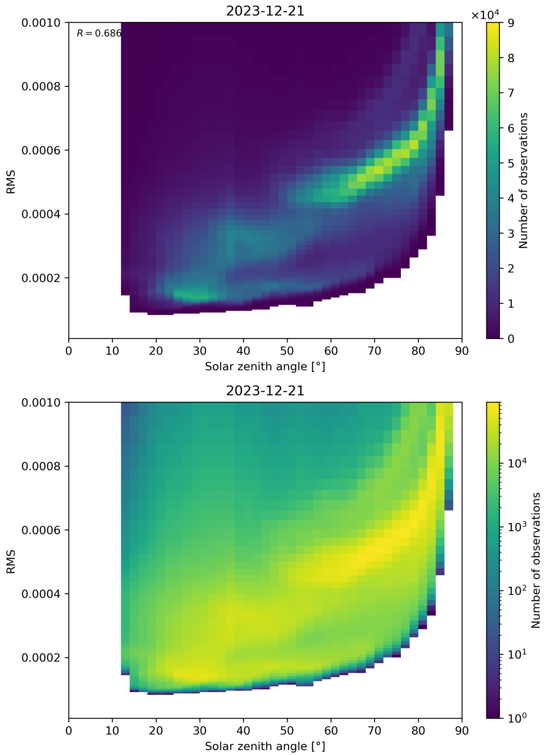
Figure 157: Scatter density plot of “Solar zenith angle” against “RMS” for 2023-12-20 to 2023-12-22.
