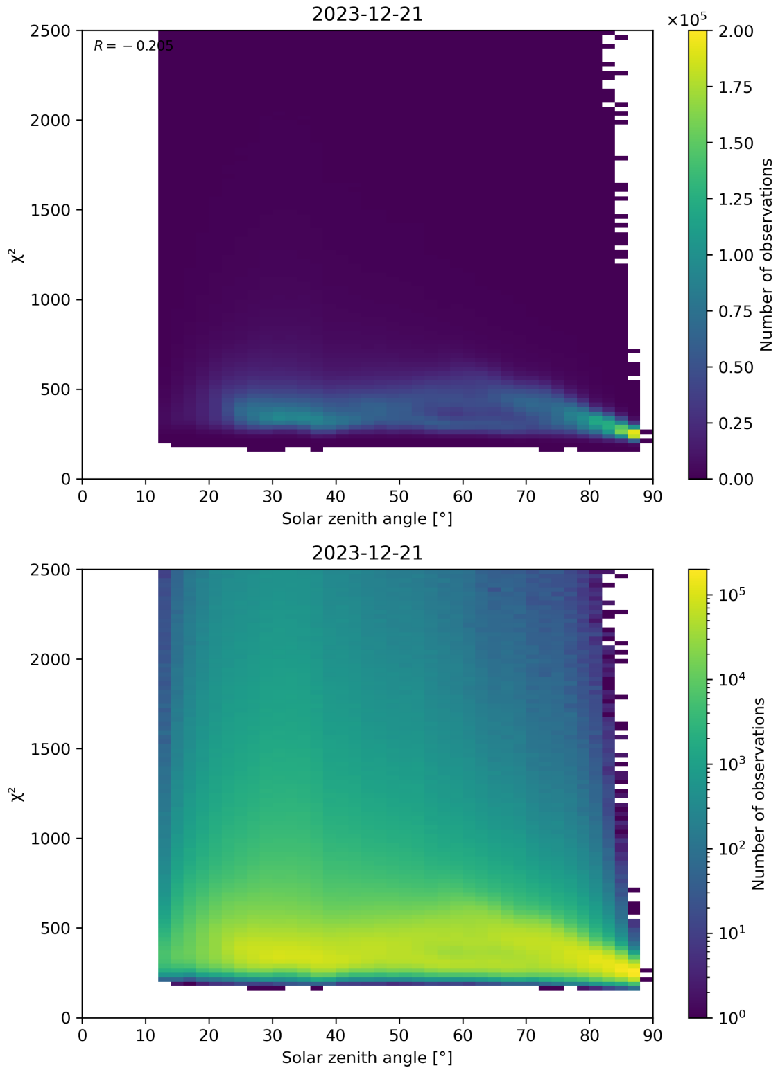
Figure 148: Scatter density plot of “Solar zenith angle” against “ \chi^2 ” for 2023-12-20 to 2023-12-22.
