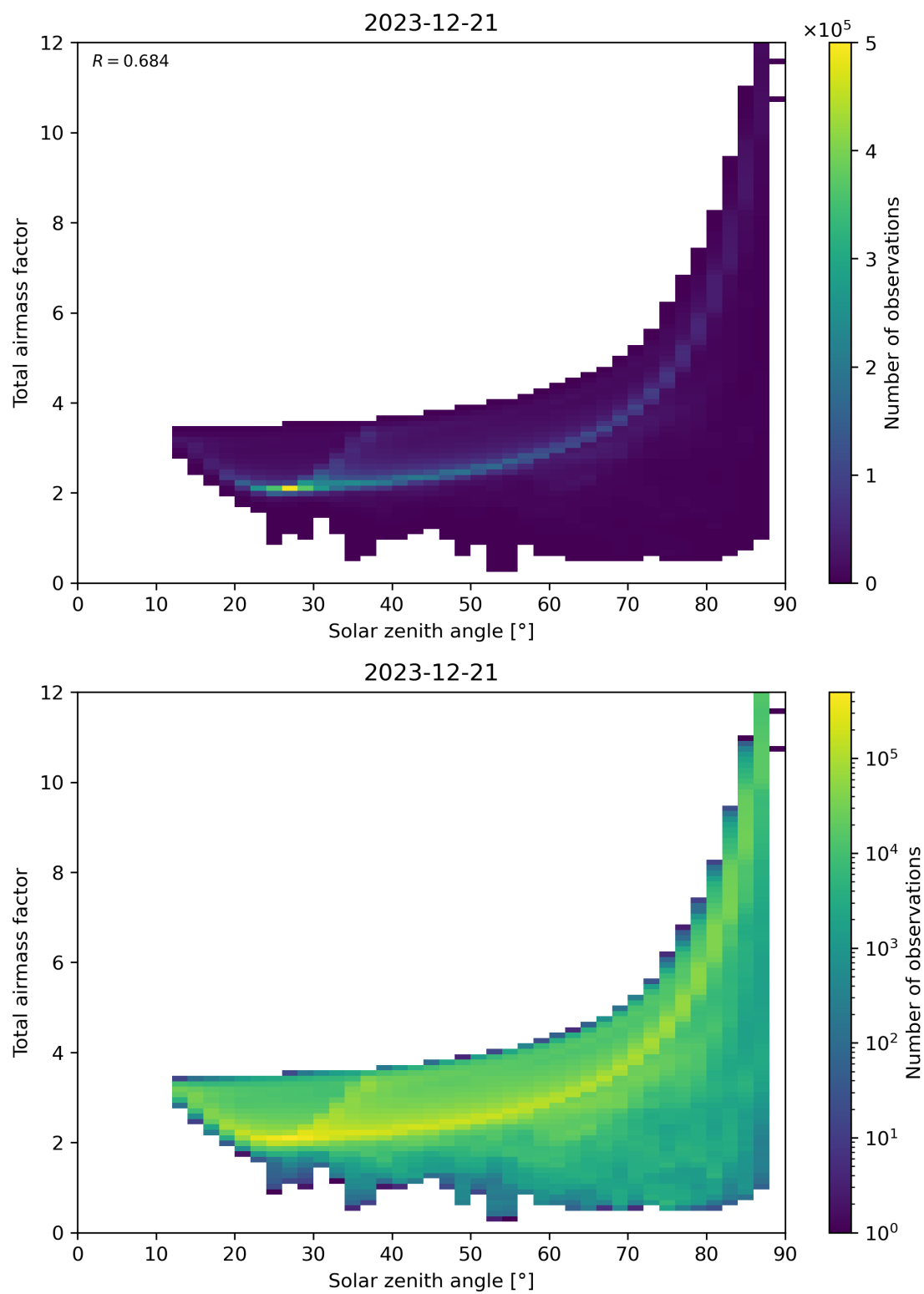
Figure 146: Scatter density plot of “Solar zenith angle” against “Total air mass factor” for 2023-12-20 to 2023-12-22.
