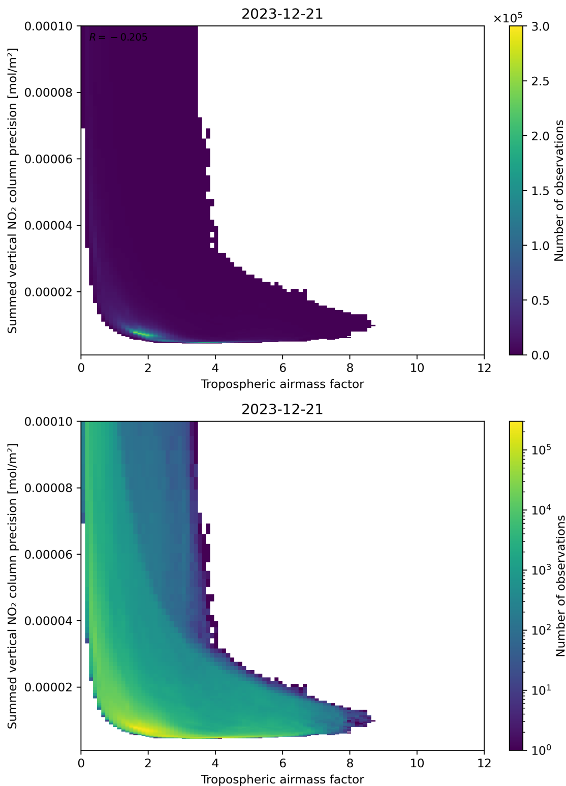
Figure 76: Scatter density plot of “Tropospheric air mass factor” against “Summed vertical NO 2 column precision” for 2023-12-20 to 2023-12-22.
