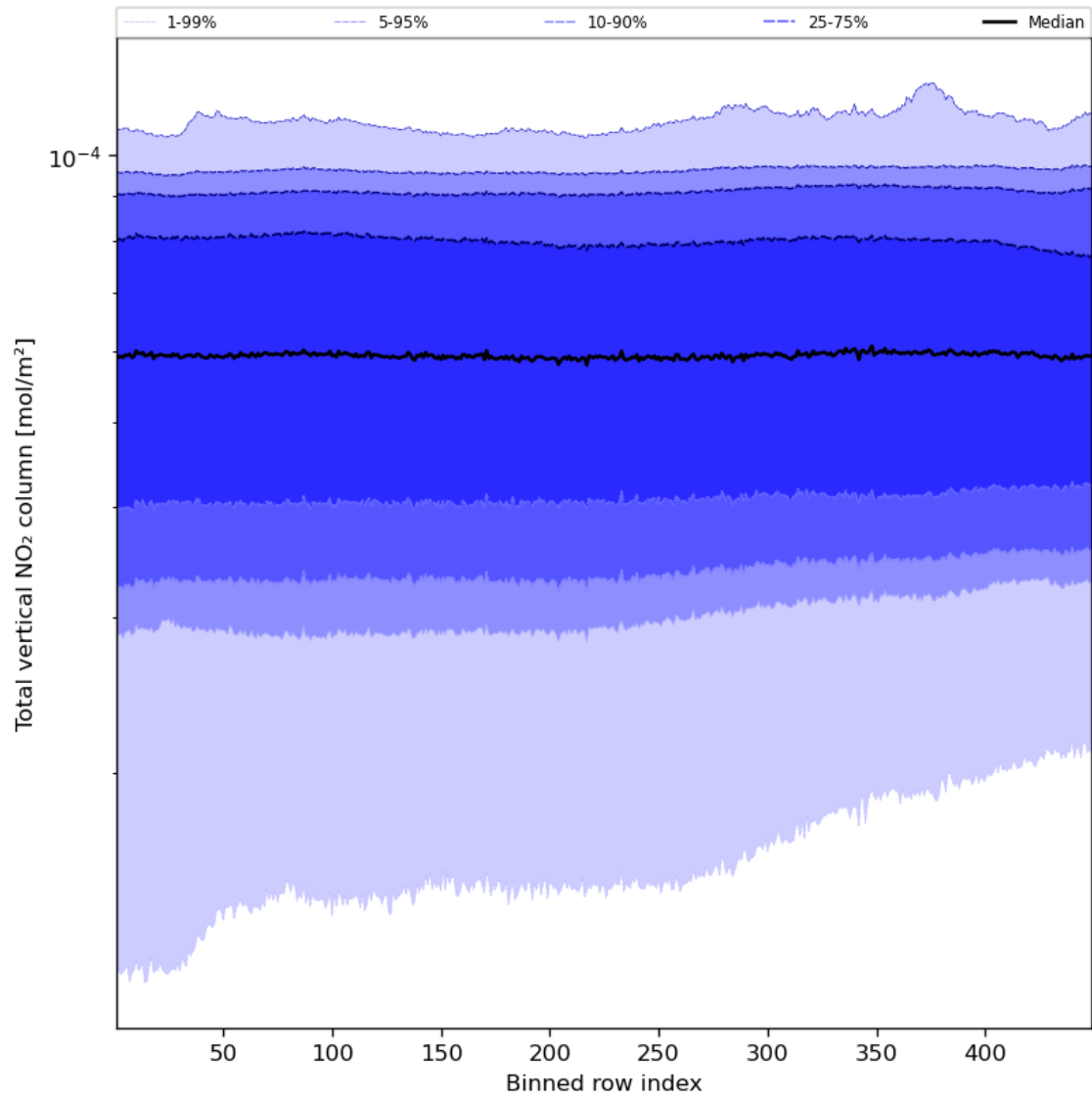
Figure 55: Along track statistics of “Total vertical NO 2 column” for 2023-12-20 to 2023-12-22
