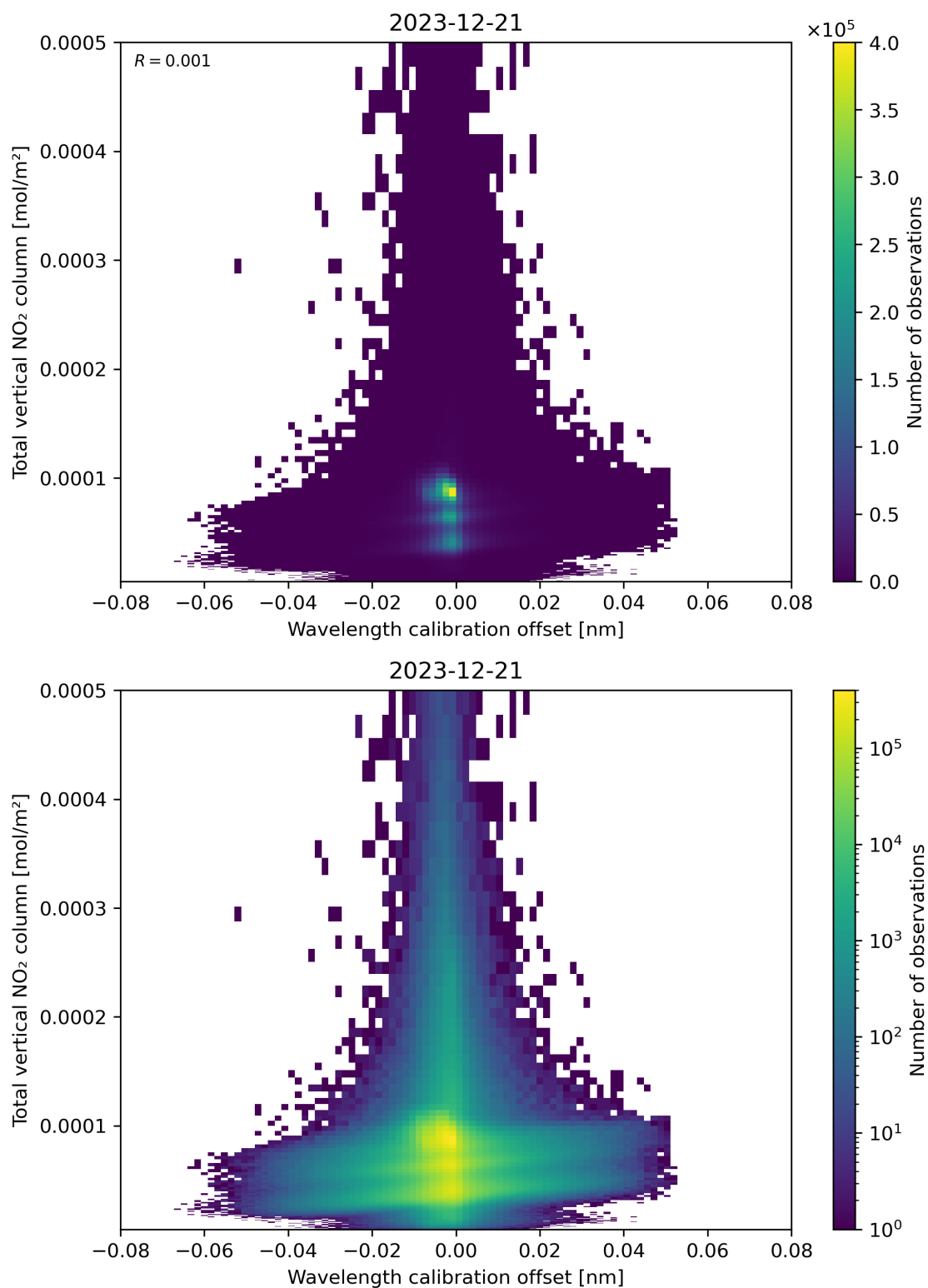
Figure 179: Scatter density plot of “Wavelength calibration offset” against “Total vertical NO 2 column” for 2023-12-20 to 2023-12-22.
