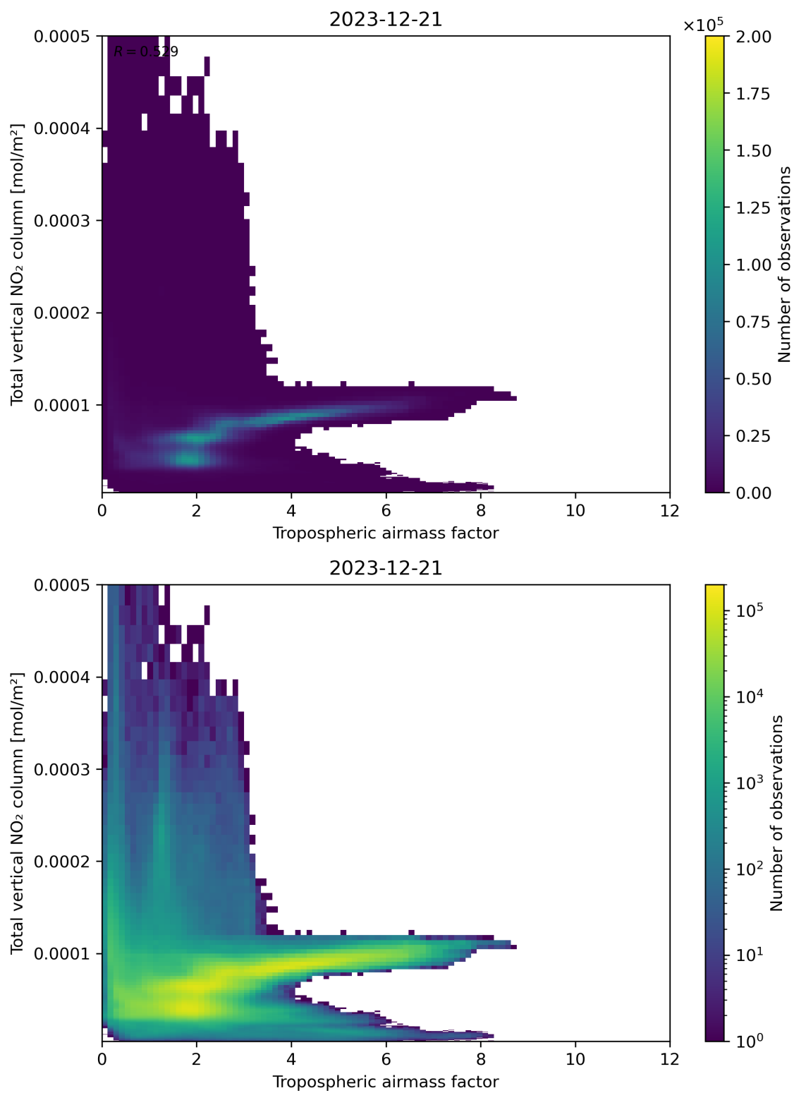
Figure 77: Scatter density plot of “Tropospheric airmass factor” against “Total vertical NO 2 column” for 2023-12-20 to 2023-12-22.
