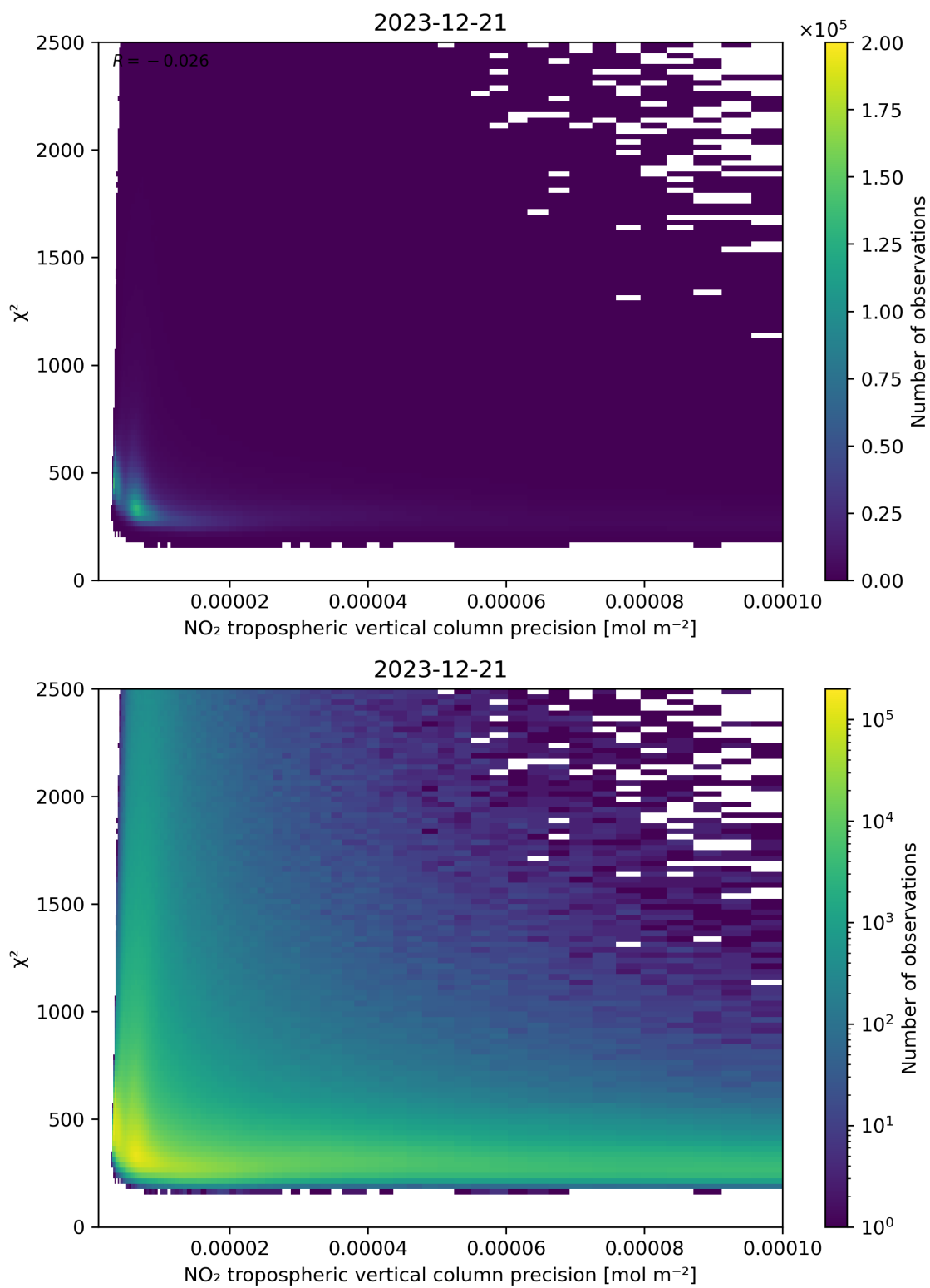
Figure 134: Scatter density plot of “NO 2 tropospheric vertical column precision” against “ \chi^2 ” for 2023-12-20 to 2023-12-22.
