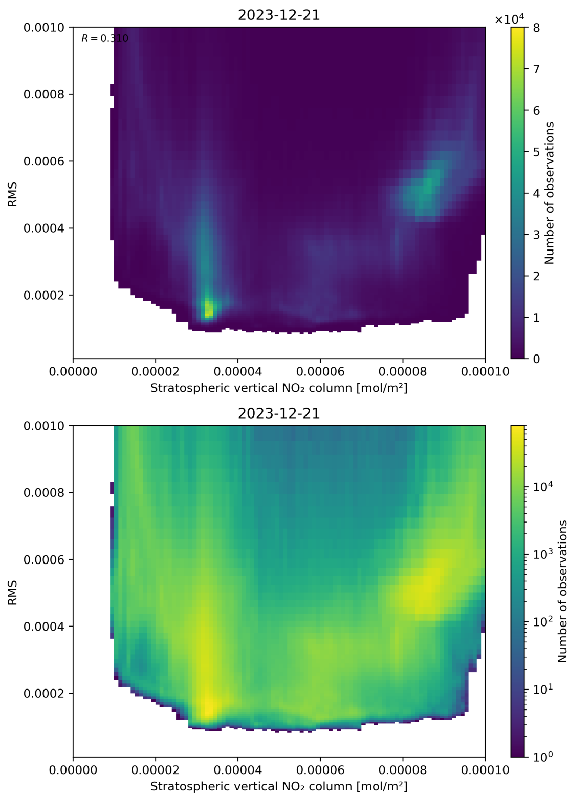
Figure 102: Scatter density plot of “Stratospheric vertical NO 2 column” against “RMS” for 2023-12-20 to 2023-12-22.
