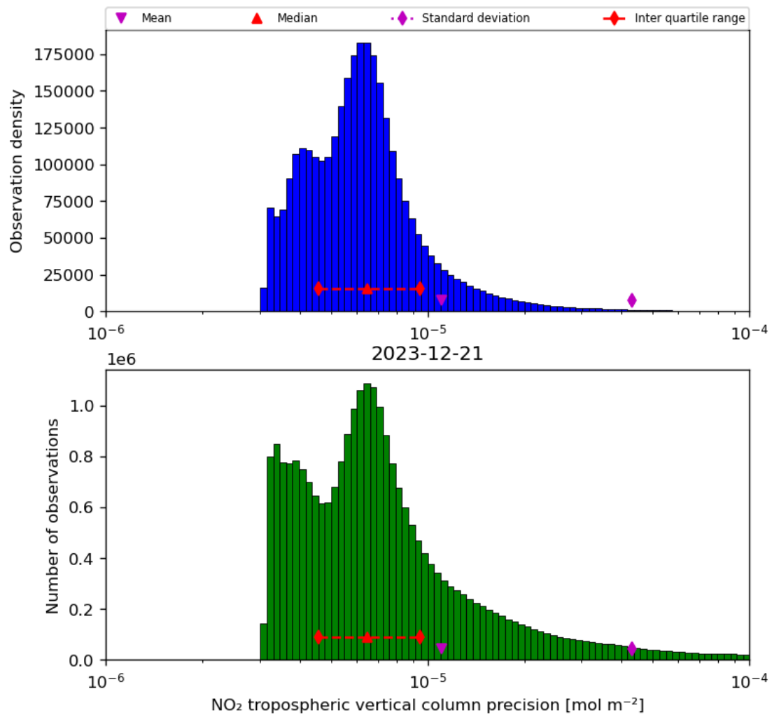
Figure 30: Histogram of “NO 2 tropospheric vertical column precision” for 2023-12-20 to 2023-12-22
