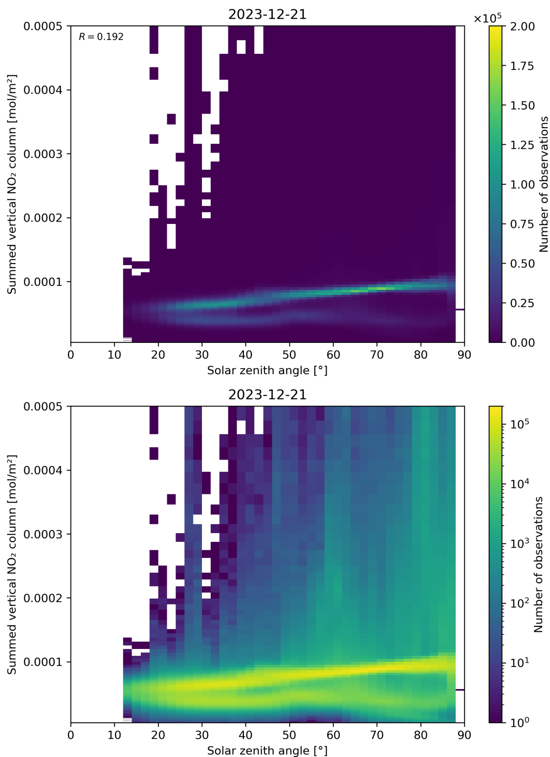
Figure 151: Scatter density plot of “Solar zenith angle” against “Summed vertical NO 2 column” for 2023-12-20 to 2023-12-22.
