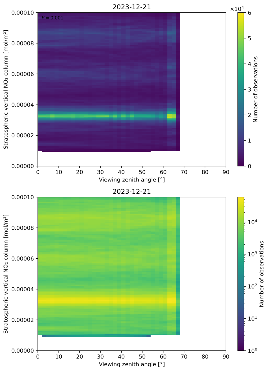
Figure 164: Scatter density plot of “Viewing zenith angle” against “Stratospheric vertical NO 2 column” for 2023-12-20 to 2023-12-22.
