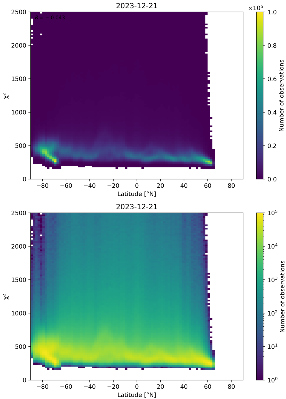
Figure 86: Scatter density plot of “Latitude” against “ \chi^2 ” for 2023-12-20 to 2023-12-22.
