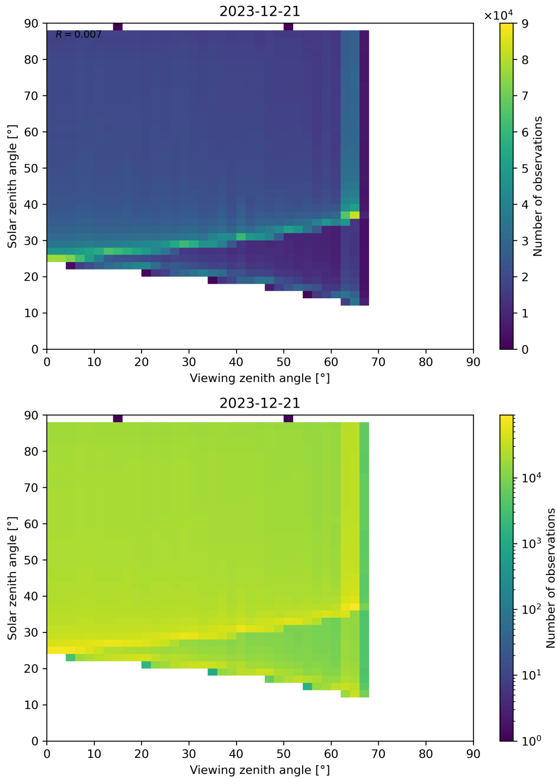
Figure 172: Scatter density plot of “Viewing zenith angle” against “Solar zenith angle” for 2023-12-20 to 2023-12-22.
