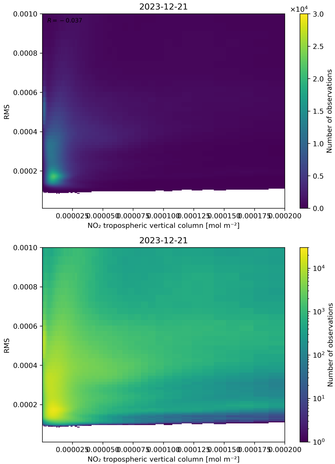
Figure 142: Scatter density plot of “NO 2 tropospheric vertical column” against “RMS” for 2023-12-20 to 2023-12-22.
