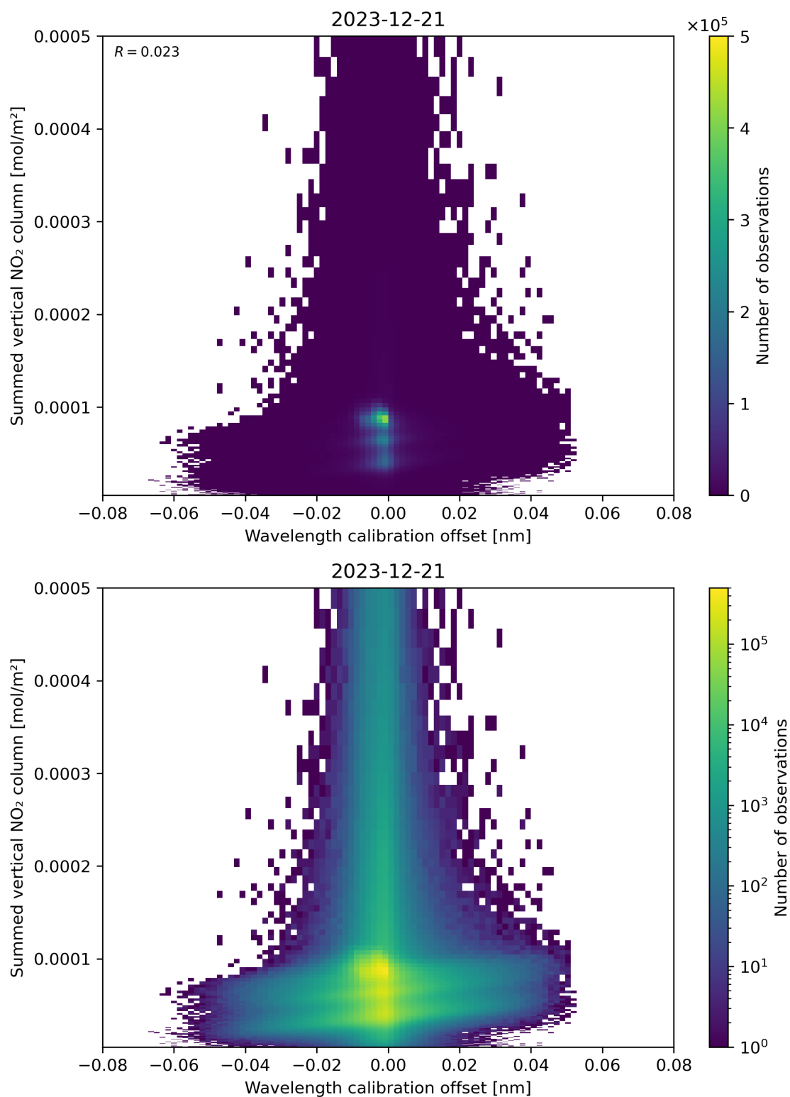
Figure 177: Scatter density plot of “Wavelength calibration offset” against “Summed vertical NO 2 column” for 2023-12-20 to 2023-12-22.
