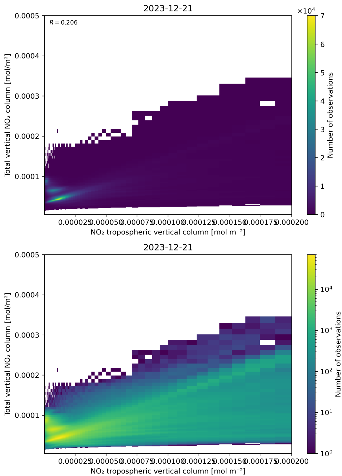
Figure 128: Scatter density plot of “NO 2 tropospheric vertical column” against “Total vertical NO 2 column” for 2023-12-20 to 2023-12-22.
