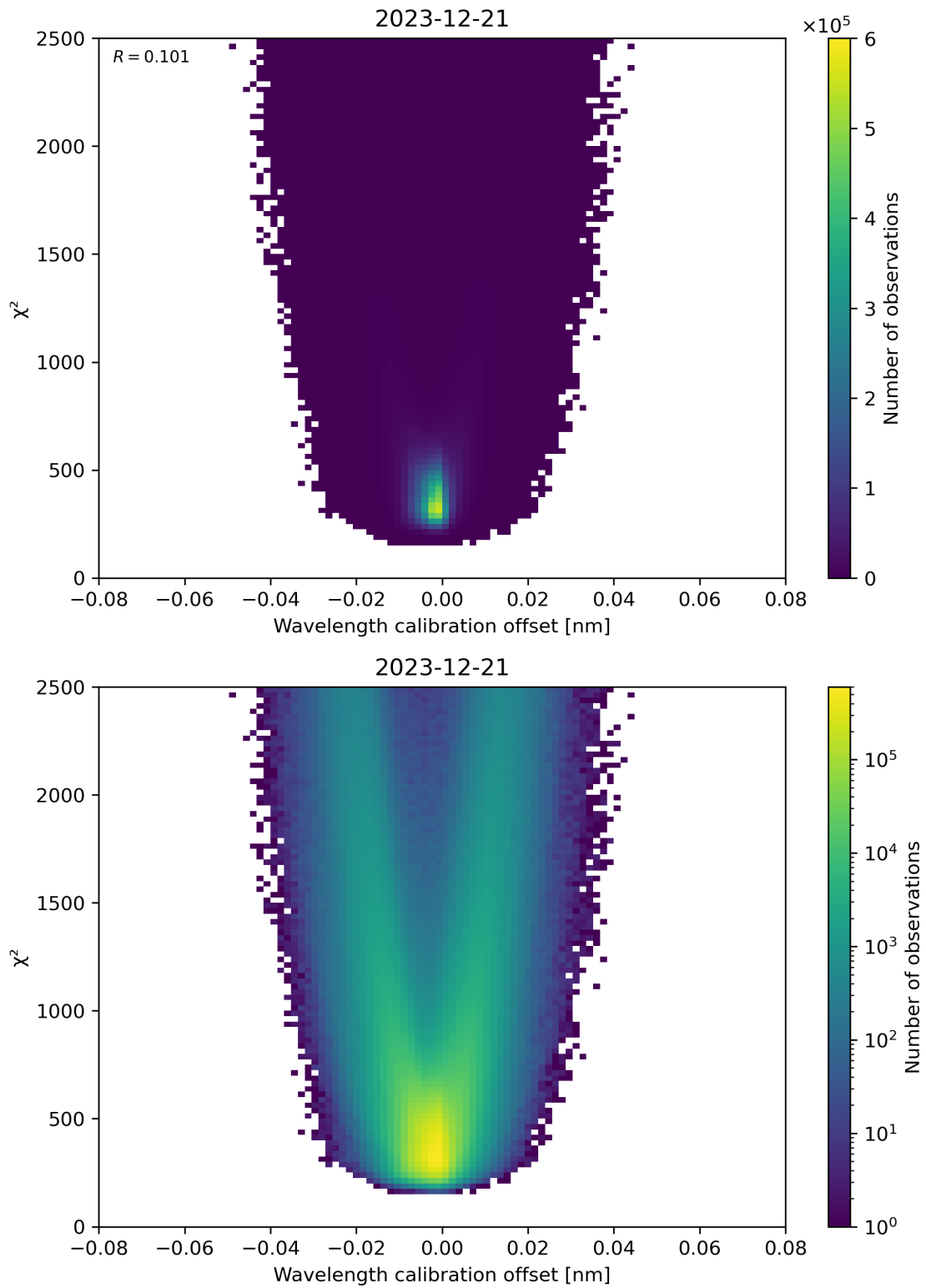
Figure 175: Scatter density plot of “Wavelength calibration offset” against “ \chi^2 ” for 2023-12-20 to 2023-12-22.
