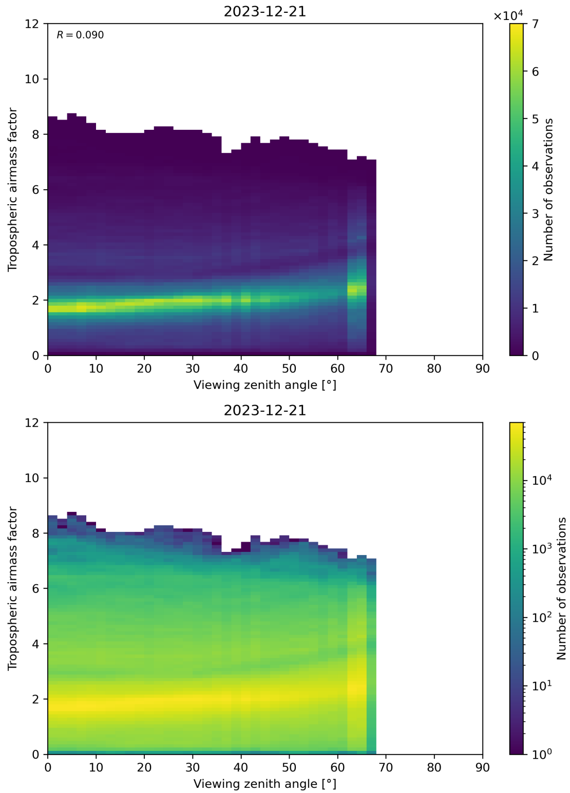
Figure 161: Scatter density plot of “Viewing zenith angle” against “Tropospheric airmass factor” for 2023-12-20 to 2023-12-22.
