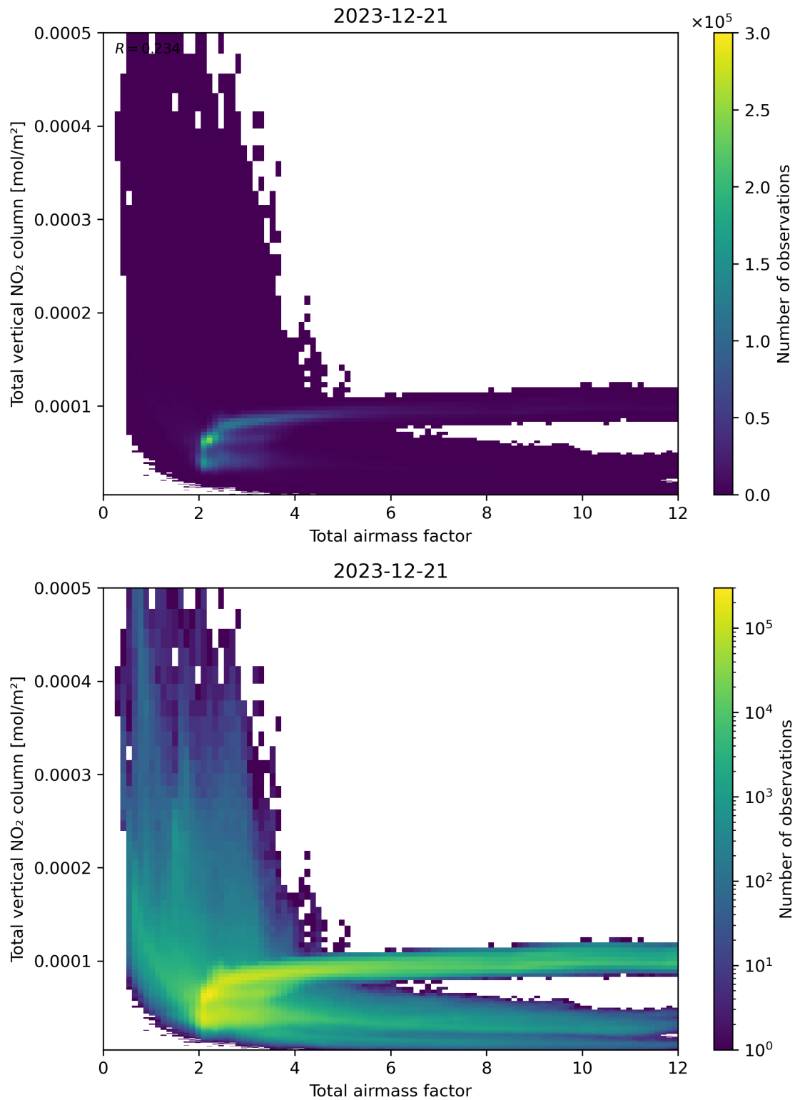
Figure 67: Scatter density plot of “Total airmass factor” against “Total vertical NO 2 column” for 2023-12-20 to 2023-12-22.
