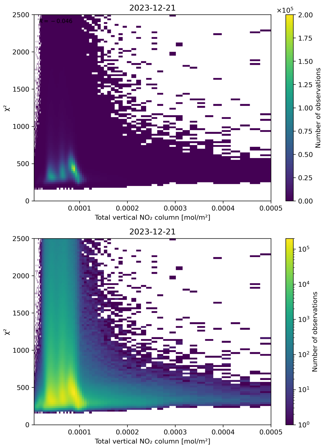
Figure 111: Scatter density plot of “Total vertical NO 2 column” against “ \chi^2 ” for 2023-12-20 to 2023-12-22.
