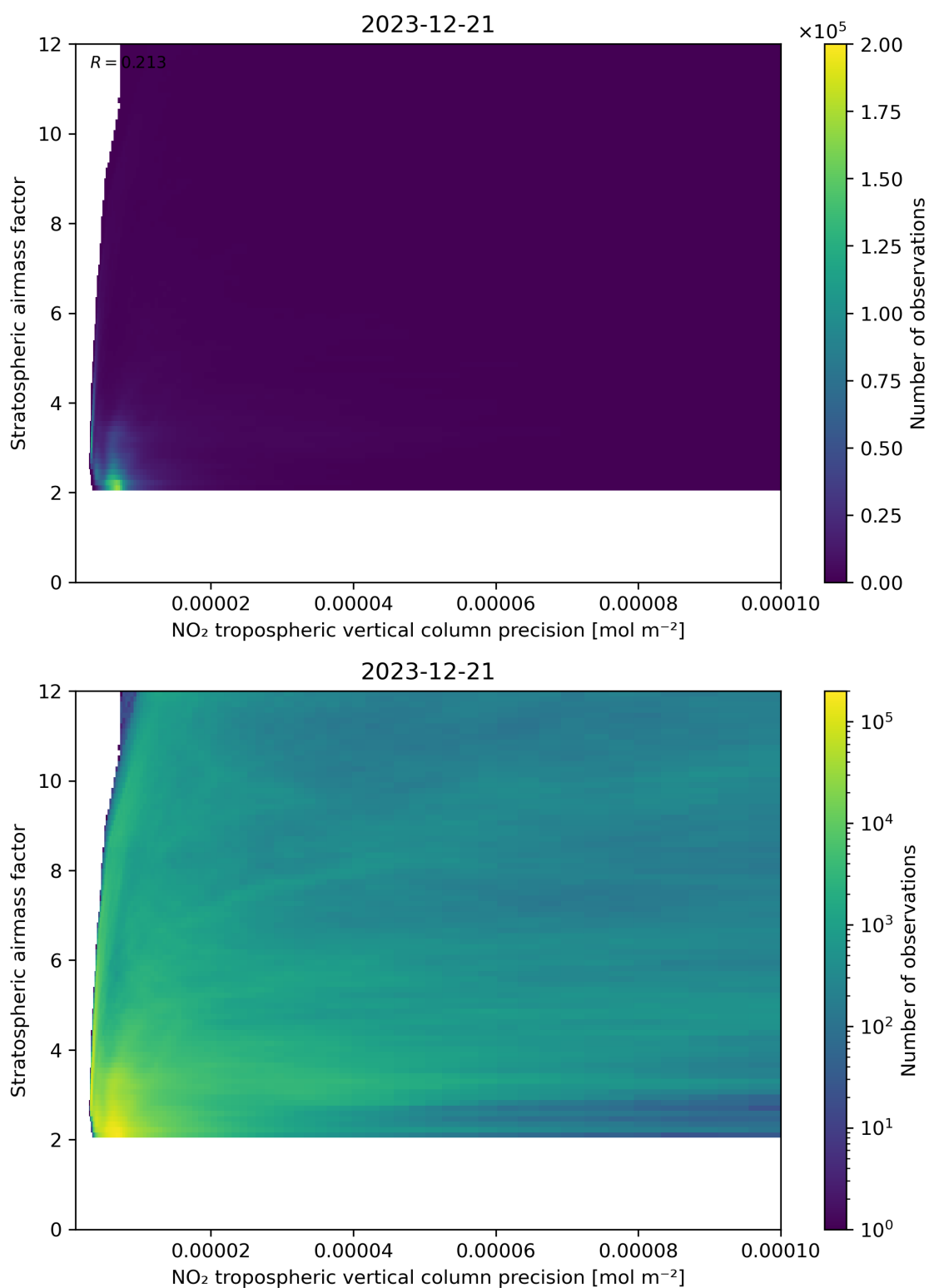
Figure 131: Scatter density plot of “NO 2 tropospheric vertical column precision” against “Stratospheric airmass factor” for 2023-12-20 to 2023-12-22.
