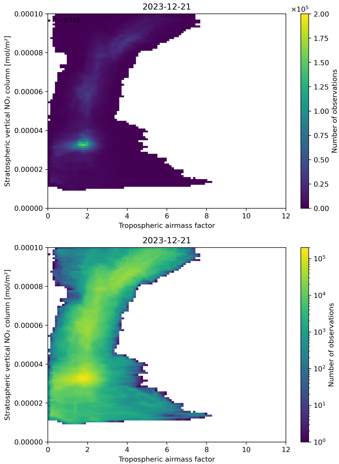
Figure 74: Scatter density plot of “Tropospheric air mass factor” against “Stratospheric vertical NO 2 column” for 2023-12-20 to 2023-12-22.
