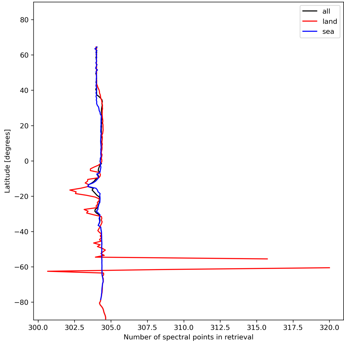
Figure 16: Zonal average of “Number of spectral points in retrieval” for 2023-12-20 to 2023-12-22.
