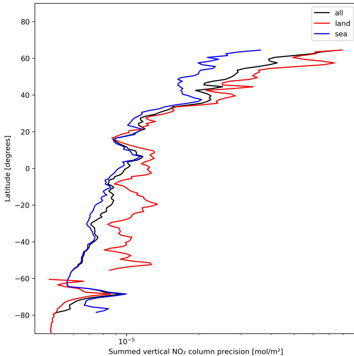
Figure 24: Zonal average of “Summed vertical NO 2 column precision” for 2023-12-20 to 2023-12-22.
