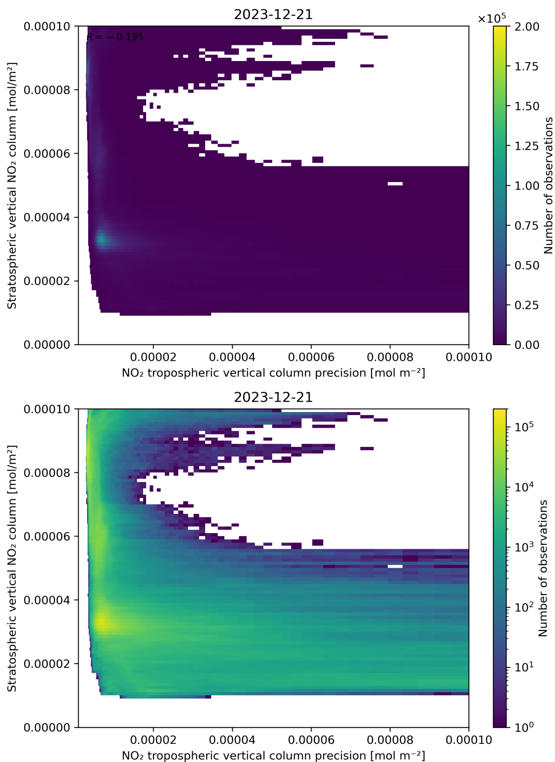
Figure 135: Scatter density plot of “NO 2 tropospheric vertical column precision” against “Stratospheric vertical NO 2 column” for 2023-12-20 to 2023-12-22.
