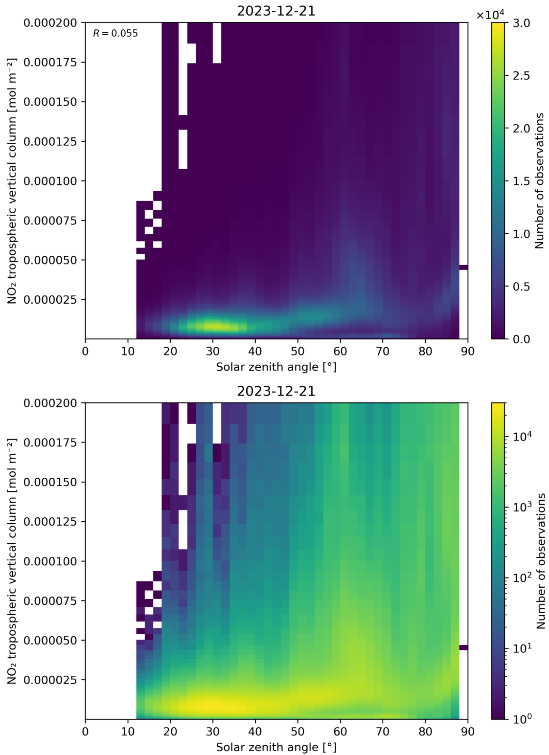
Figure 155: Scatter density plot of “Solar zenith angle” against “NO 2 tropospheric vertical column” for 2023-12-20 to 2023-12-22.
