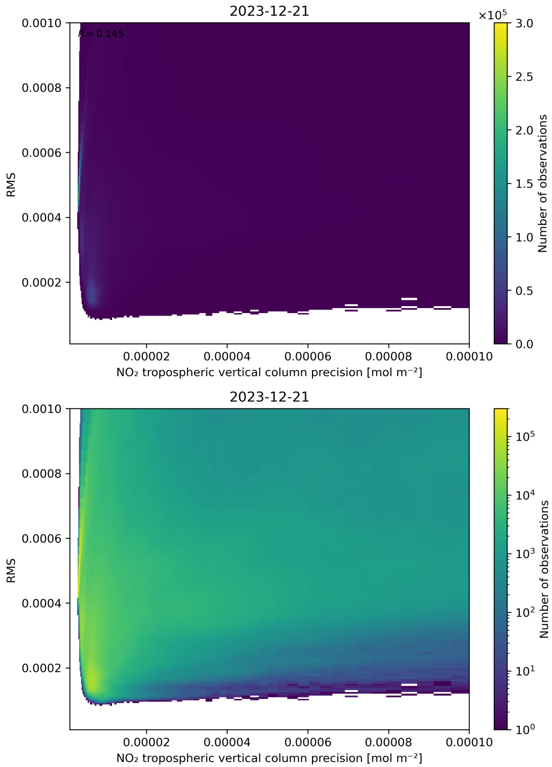
Figure 140: Scatter density plot of “NO 2 tropospheric vertical column precision” against “RMS” for 2023-12-20 to 2023-12-22.
