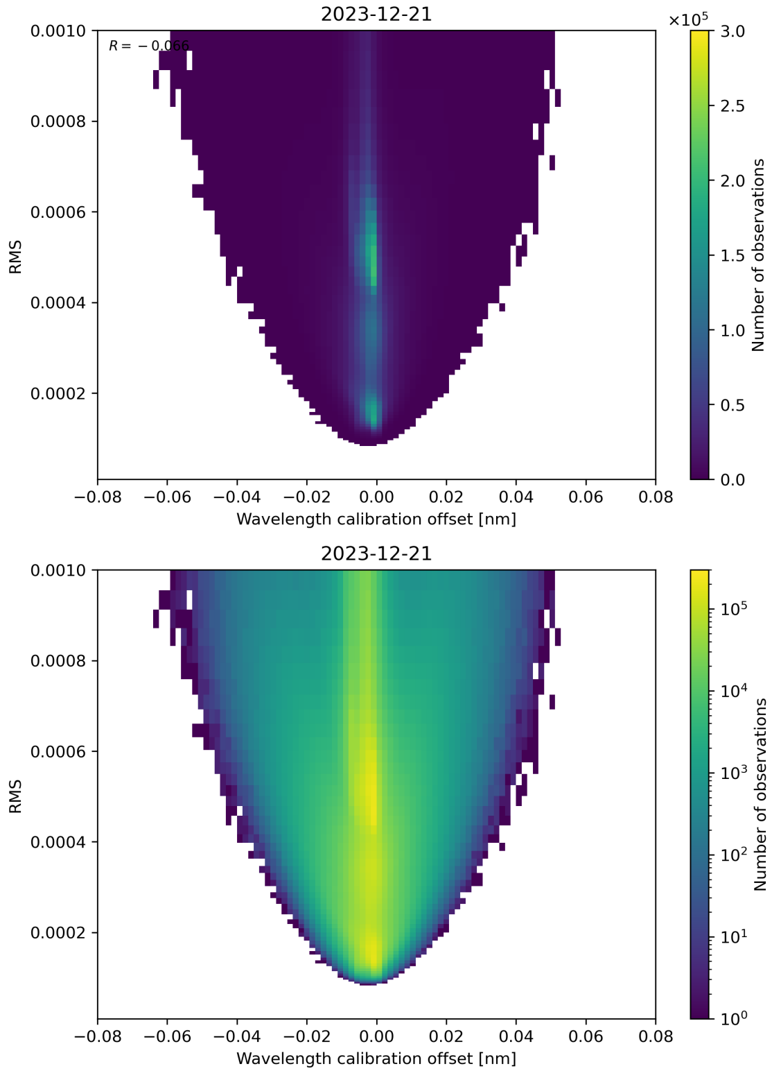
Figure 181: Scatter density plot of “Wavelength calibration offset” against “RMS” for 2023-12-20 to 2023-12-22.
