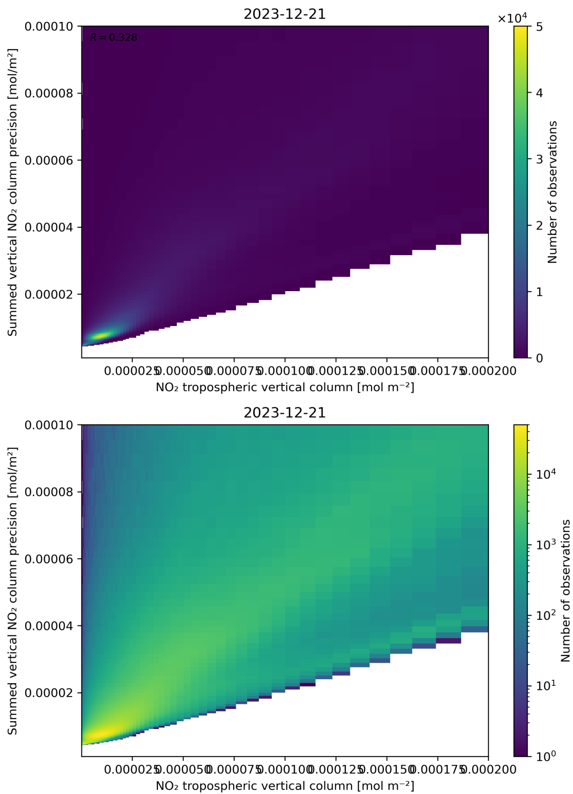
Figure 127: Scatter density plot of “NO 2 tropospheric vertical column” against “Summed vertical NO 2 column precision” for 2023-12-20 to 2023-12-22.
