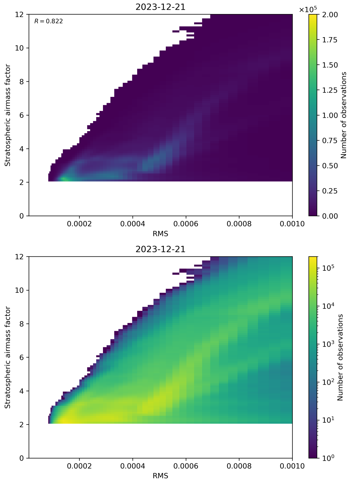
Figure 144: Scatter density plot of “RMS” against “Stratospheric airmass factor” for 2023-12-20 to 2023-12-22.
