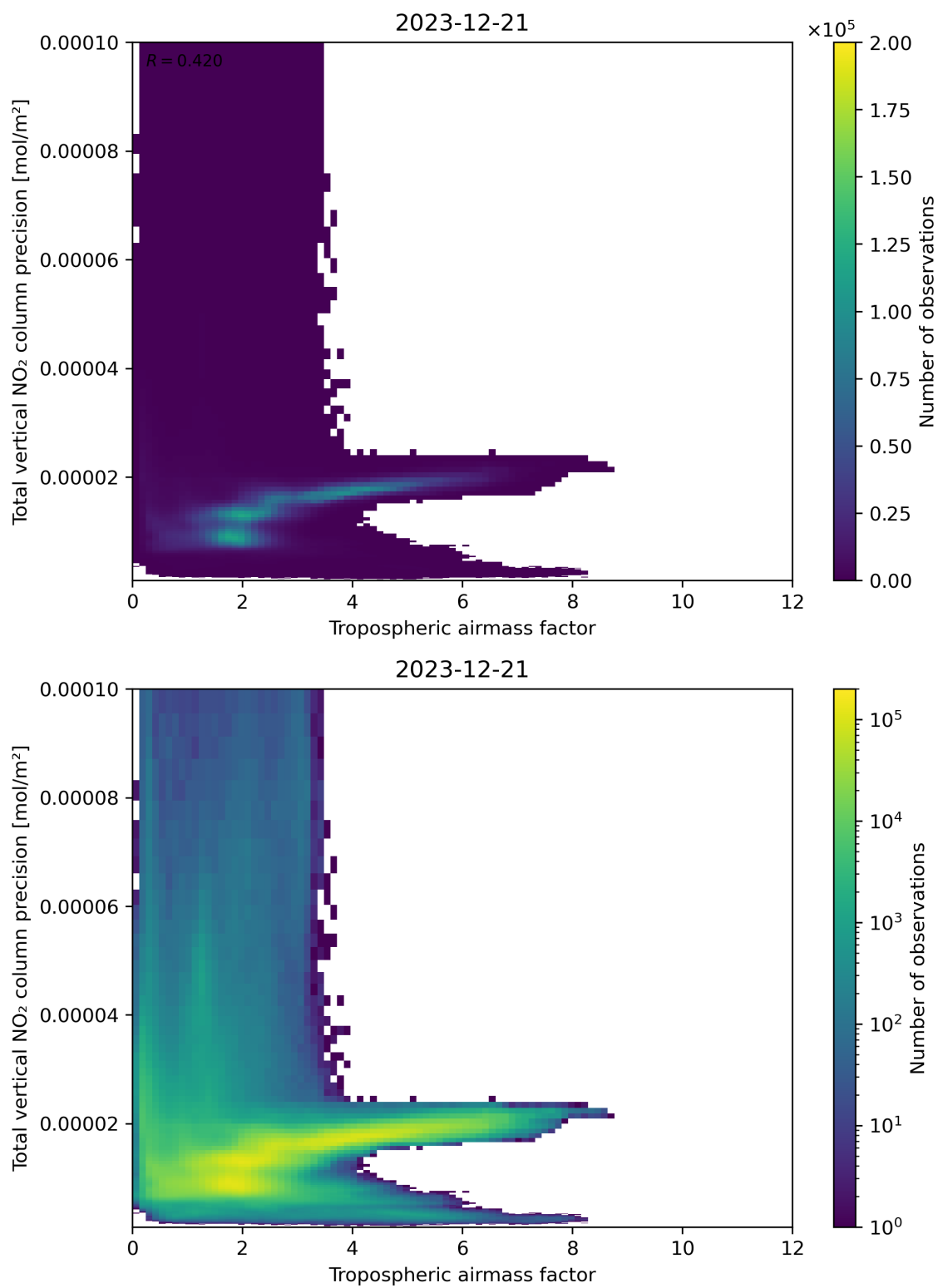
Figure 78: Scatter density plot of “Tropospheric air mass factor” against “Total vertical NO 2 column precision” for 2023-12-20 to 2023-12-22.
