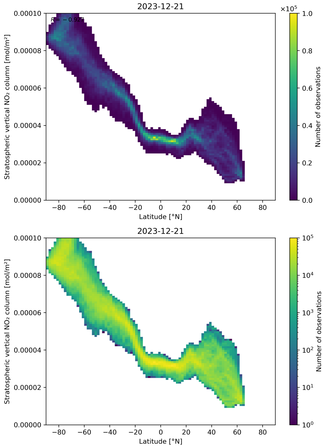
Figure 87: Scatter density plot of “Latitude” against “Stratospheric vertical NO 2 column” for 2023-12-20 to 2023-12-22.
