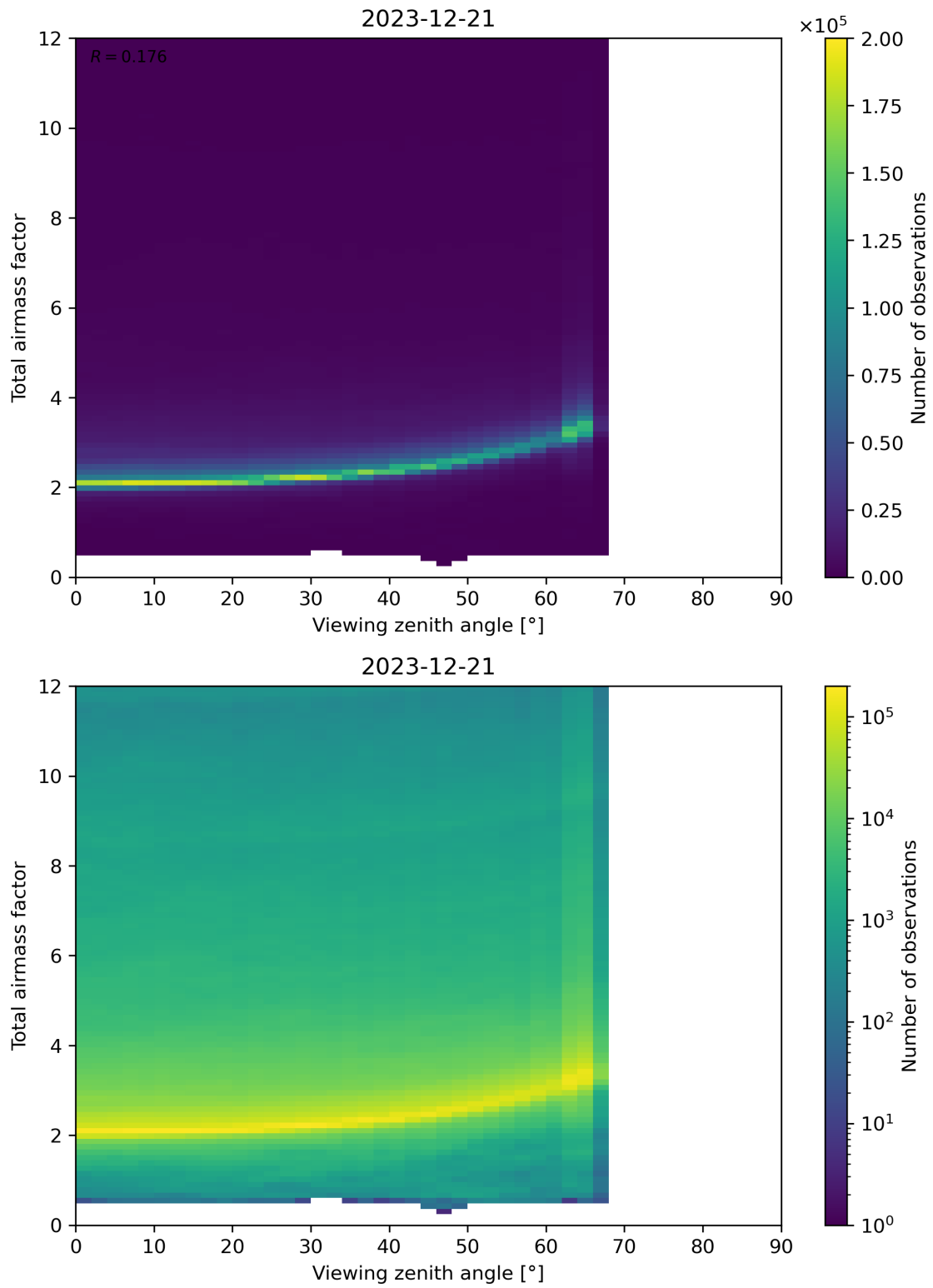
Figure 160: Scatter density plot of “Viewing zenith angle” against “Total airmass factor” for 2023-12-20 to 2023-12-22.
