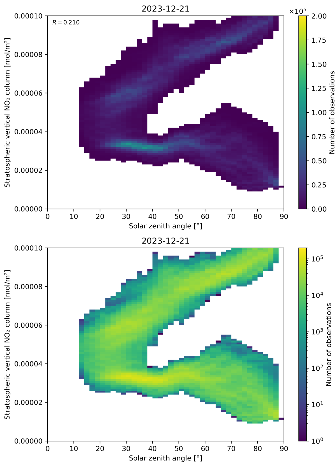
Figure 150: Scatter density plot of “Solar zenith angle” against “Stratospheric vertical NO 2 column” for 2023-12-20 to 2023-12-22.
