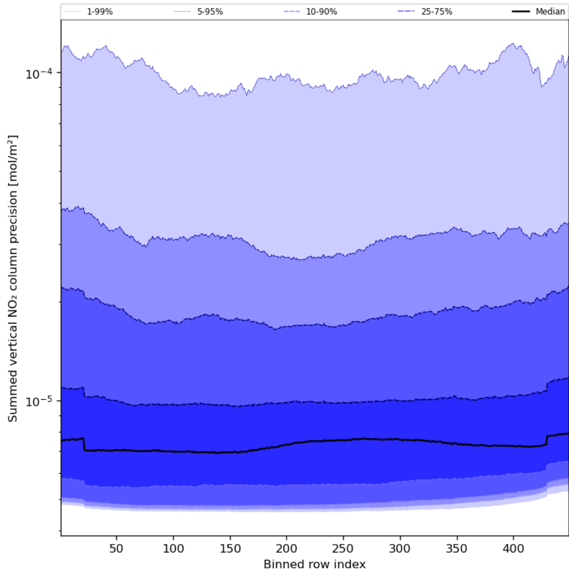
Figure 58: Along track statistics of “Summed vertical NO 2 column precision” for 2023-12-20 to 2023-12-22
