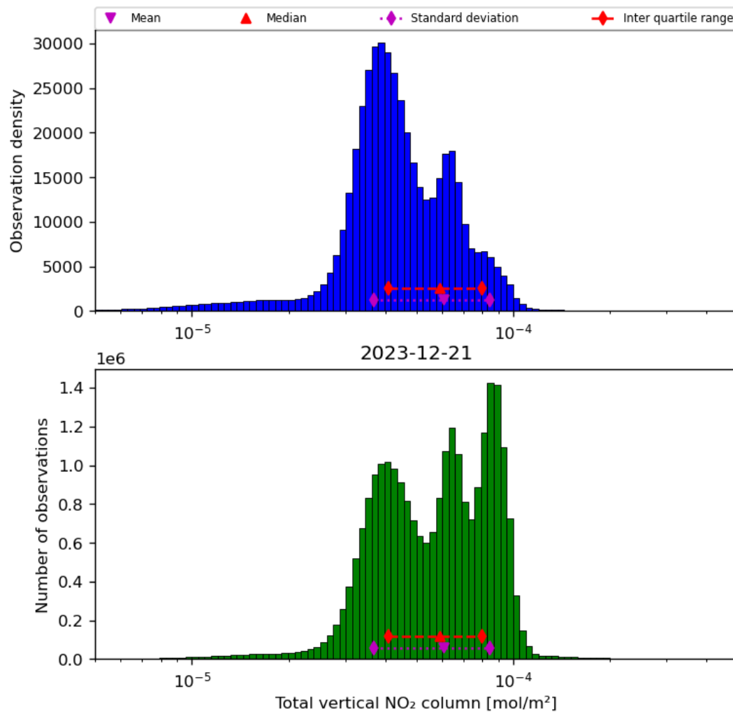
Figure 38: Histogram of “Total vertical NO 2 column” for 2023-12-20 to 2023-12-22
