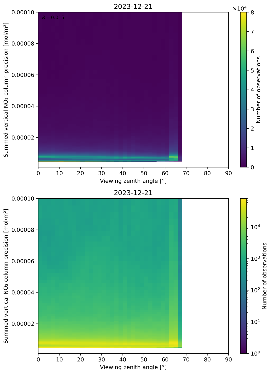
Figure 166: Scatter density plot of “Viewing zenith angle” against “Summed vertical NO 2 column precision” for 2023-12-20 to 2023-12-22.
