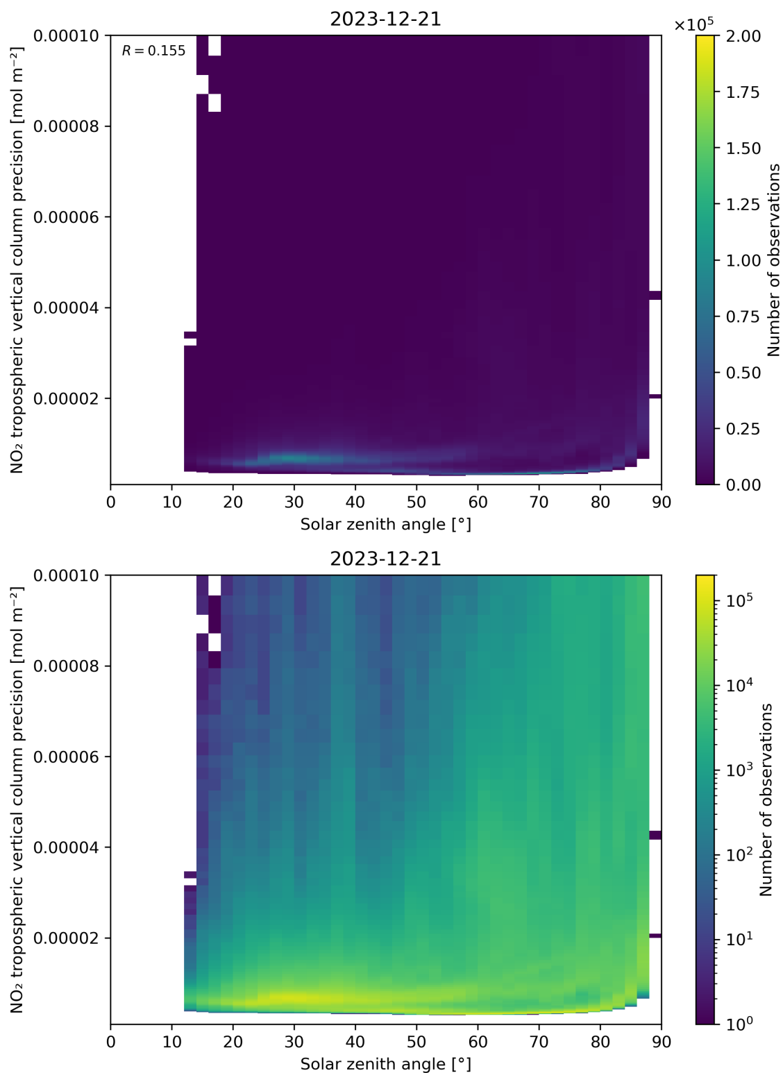
Figure 156: Scatter density plot of “Solar zenith angle” against “NO 2 tropospheric vertical column precision” for 2023-12-20 to 2023-12-22.
