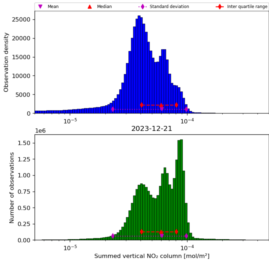
Figure 40: Histogram of “Summed vertical NO 2 column” for 2023-12-20 to 2023-12-22
