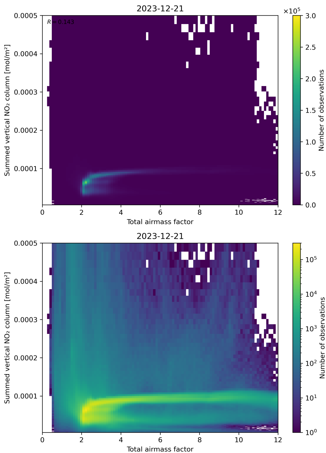
Figure 65: Scatter density plot of “Total airmass factor” against “Summed vertical NO 2 column” for 2023-12-20 to 2023-12-22.
