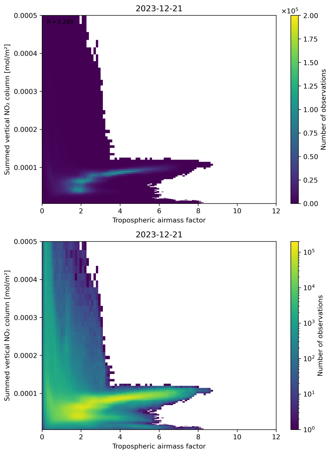
Figure 75: Scatter density plot of “Tropospheric airmass factor” against “Summed vertical NO 2 column” for 2023-12-20 to 2023-12-22.
