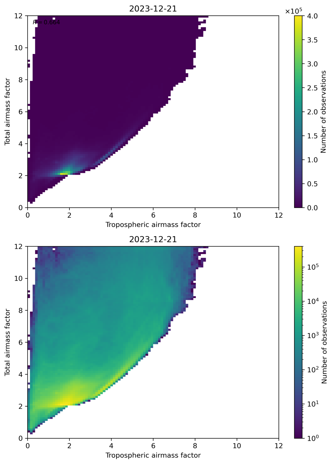
Figure 72: Scatter density plot of “Tropospheric airmass factor” against “Total airmass factor” for 2023-12-20 to 2023-12-22.
