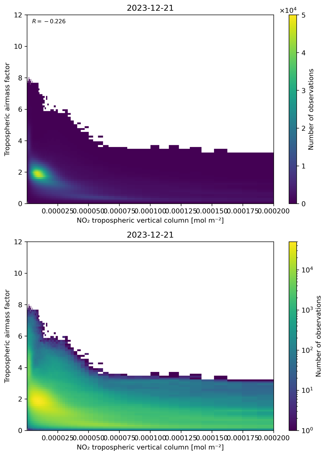
Figure 123: Scatter density plot of “NO 2 tropospheric vertical column” against “Tropospheric airmass factor” for 2023-12-20 to 2023-12-22.
