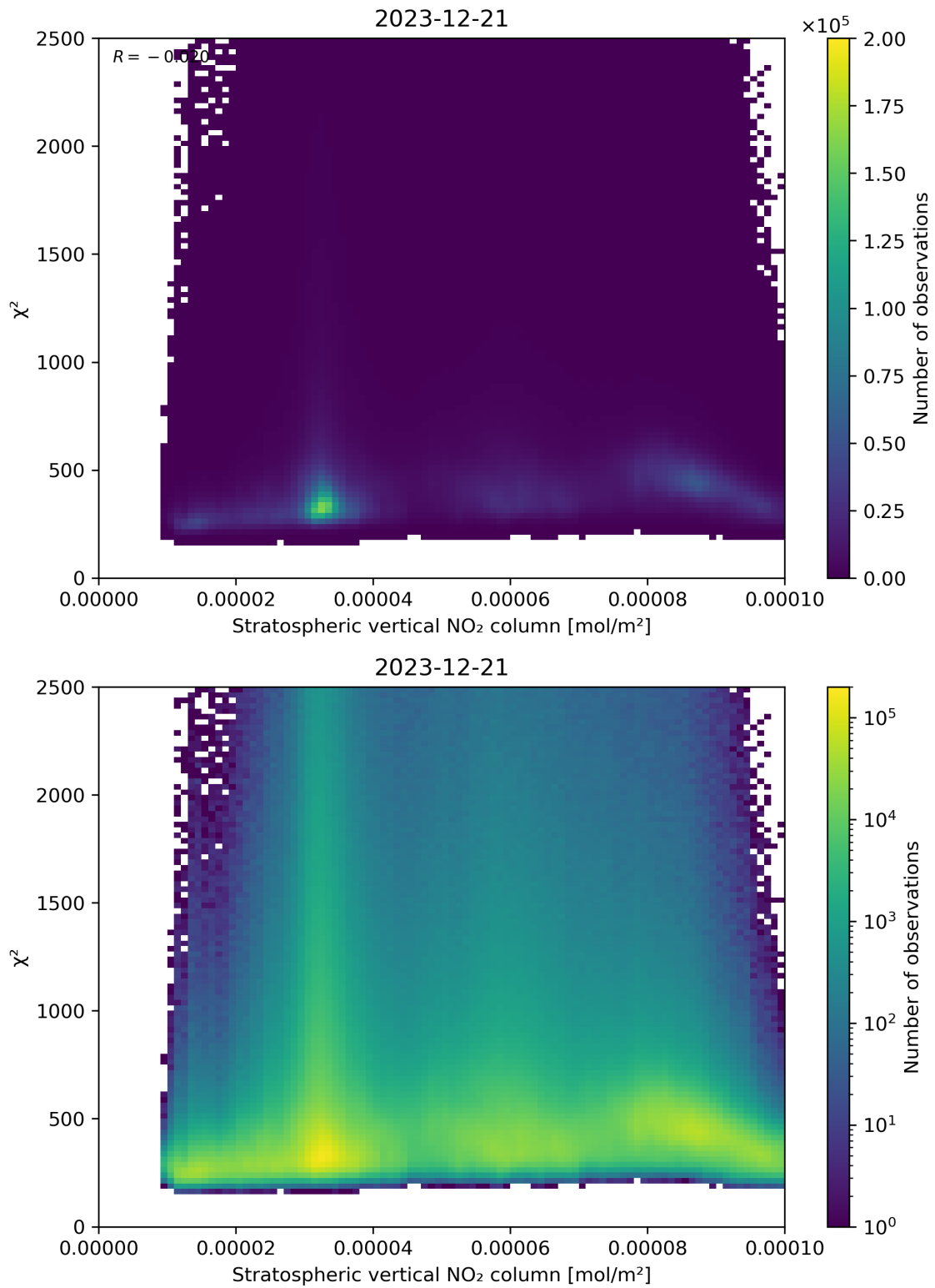
Figure 97: Scatter density plot of “Stratospheric vertical NO 2 column” against “ \chi^2 ” for 2023-12-20 to 2023-12-22.
