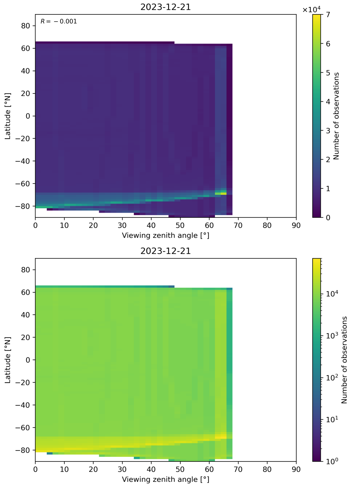
Figure 163: Scatter density plot of “Viewing zenith angle” against “Latitude” for 2023-12-20 to 2023-12-22.
