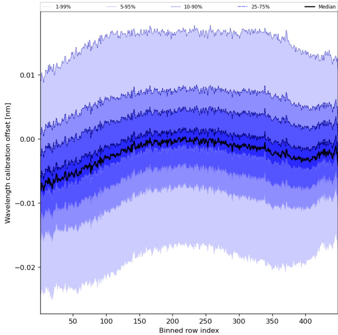
Figure 52: Along track statistics of “Wavelength calibration offset” for 2023-12-20 to 2023-12-22
