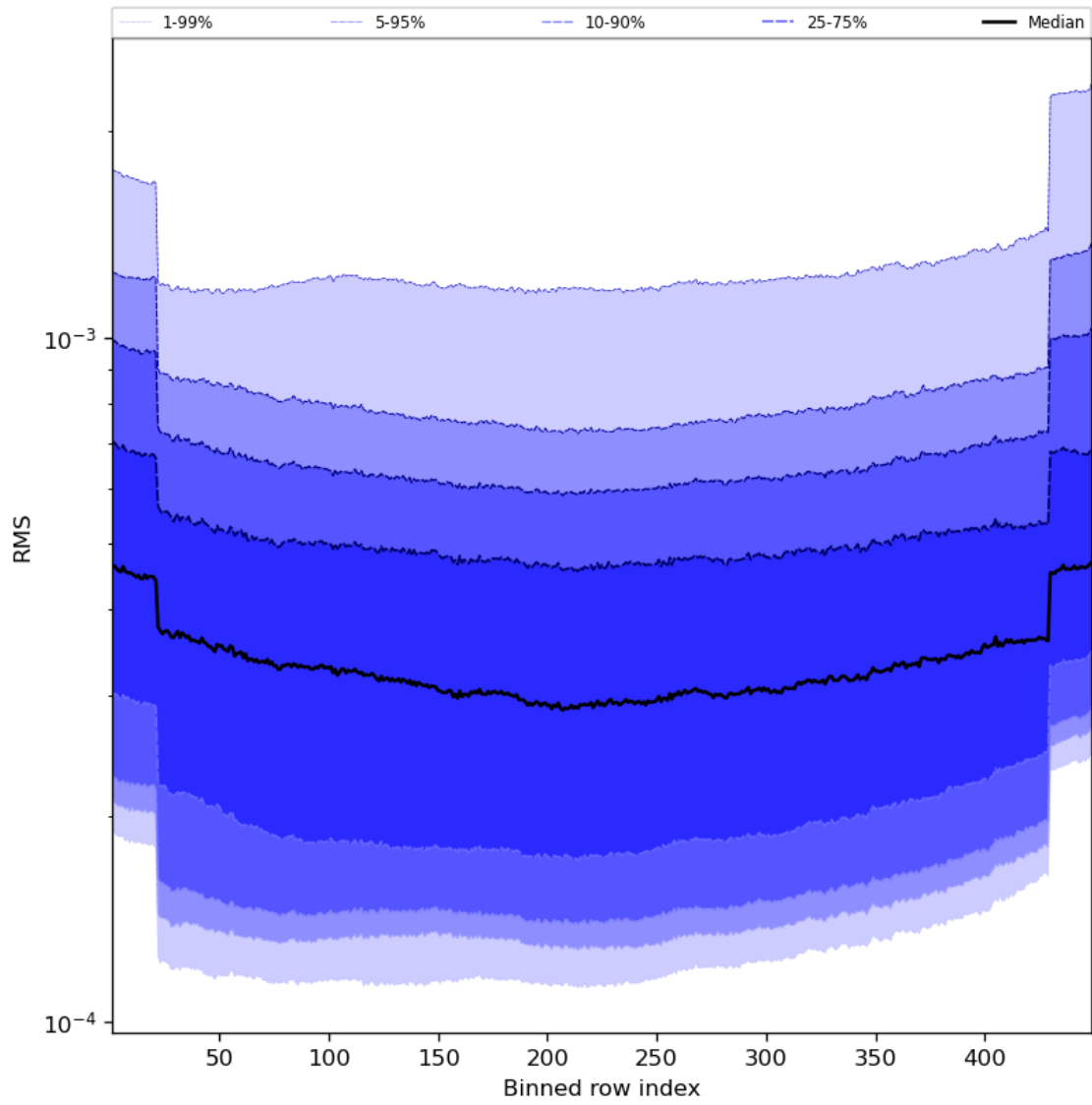
Figure 60: Along track statistics of “RMS” for 2023-12-20 to 2023-12-22
