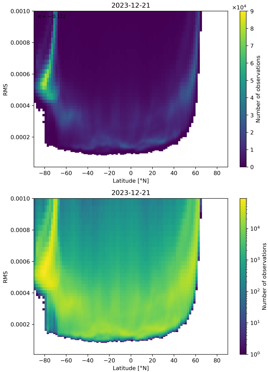
Figure 94: Scatter density plot of “Latitude” against “RMS” for 2023-12-20 to 2023-12-22.
