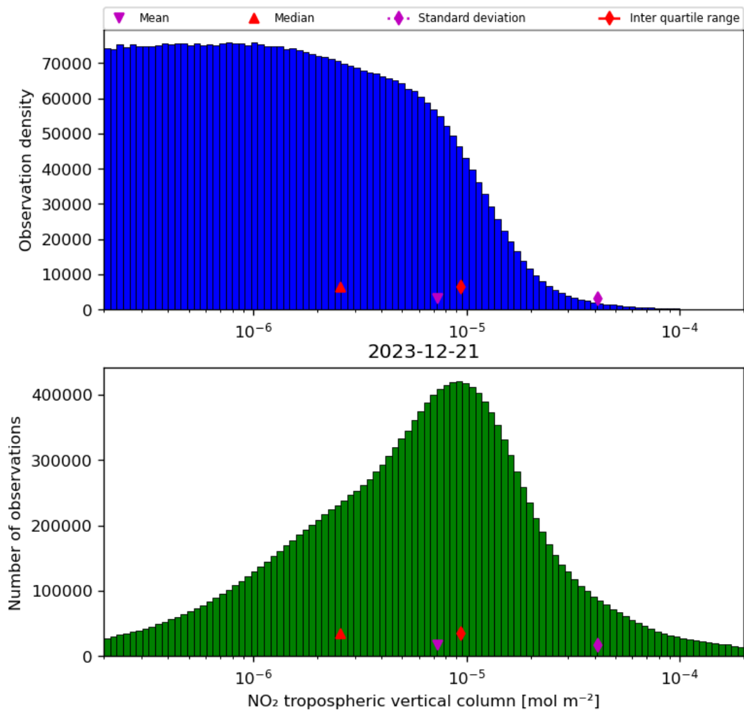
Figure 29: Histogram of “NO 2 tropospheric vertical column” for 2023-12-20 to 2023-12-22
