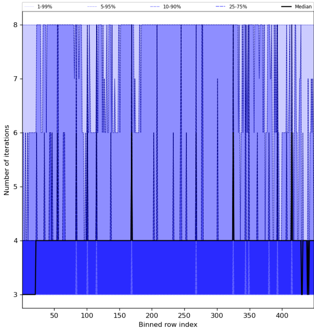
Figure 51: Along track statistics of “Number of iterations” for 2023-12-20 to 2023-12-22
