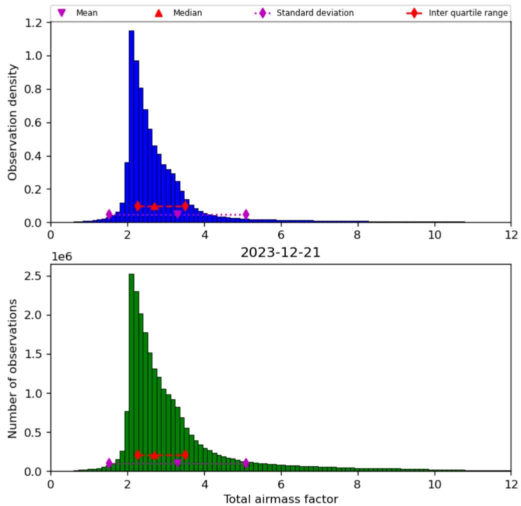
Figure 32: Histogram of “Total airmass factor” for 2023-12-20 to 2023-12-22
