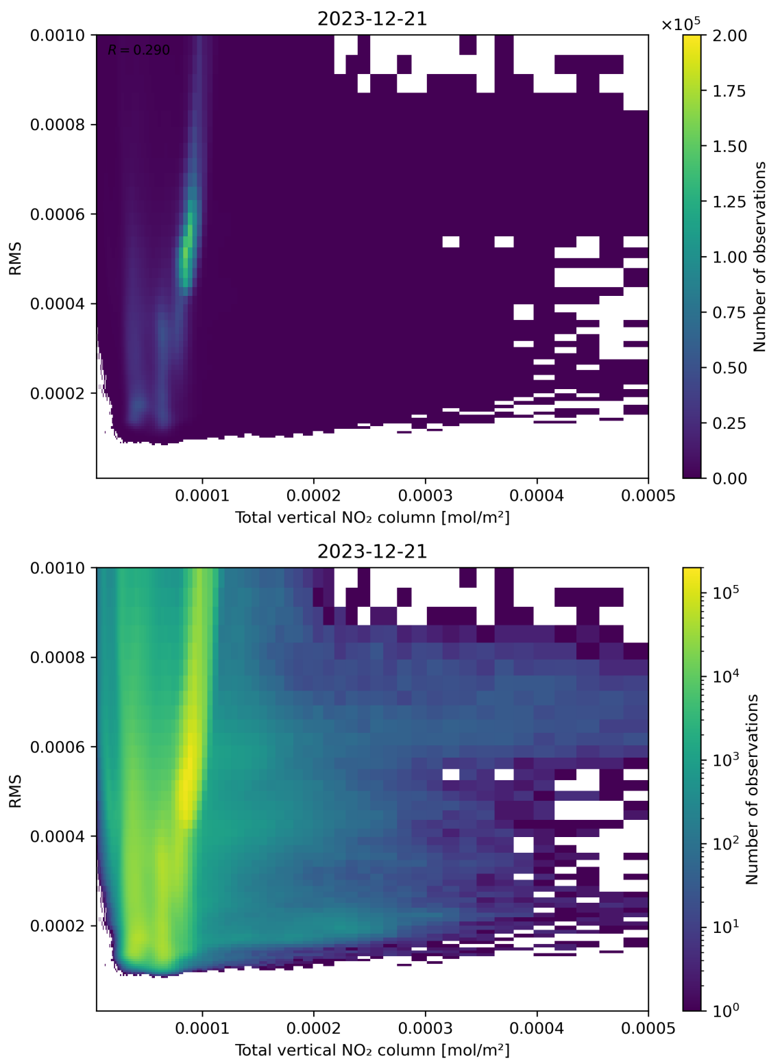
Figure 120: Scatter density plot of “Total vertical NO 2 column” against “RMS” for 2023-12-20 to 2023-12-22.
