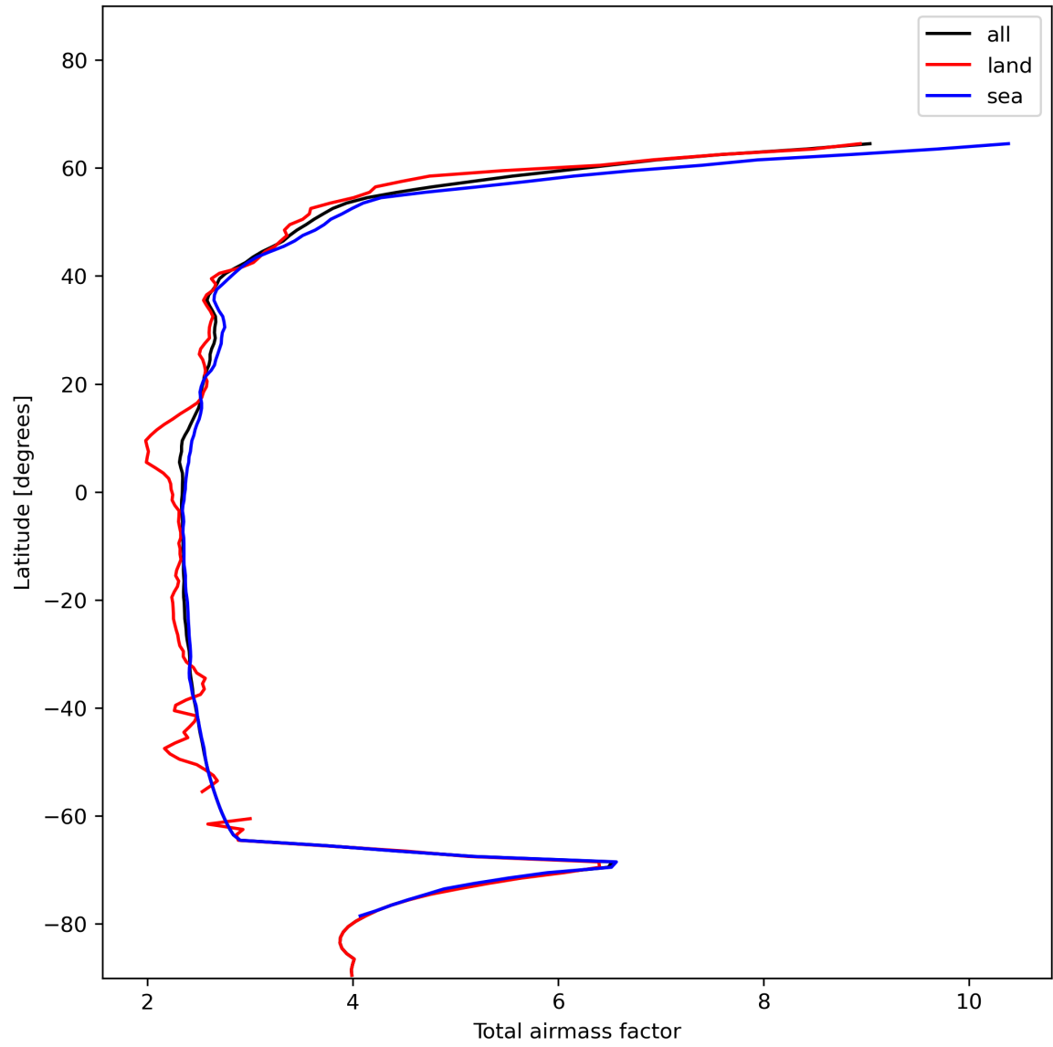
Figure 15: Zonal average of “Total airmass factor” for 2023-12-20 to 2023-12-22.
