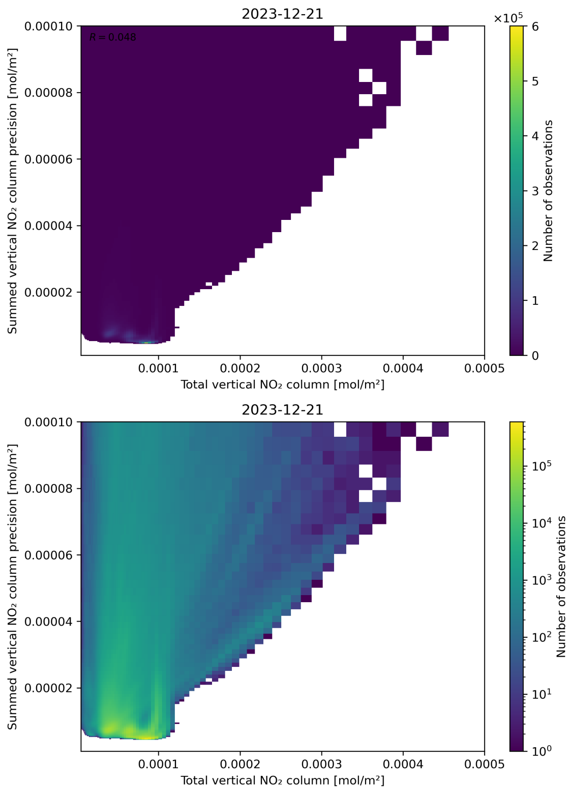
Figure 113: Scatter density plot of “Total vertical NO 2 column” against “Summed vertical NO 2 column precision” for 2023-12-20 to 2023-12-22.
