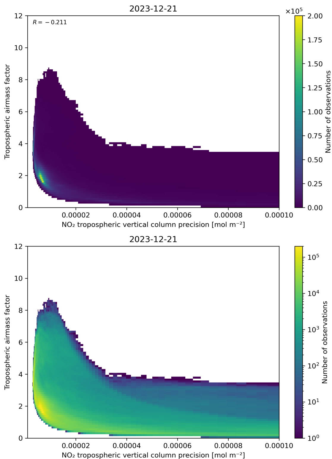
Figure 133: Scatter density plot of “NO 2 tropospheric vertical column precision” against “Tropospheric airmass factor” for 2023-12-20 to 2023-12-22.
