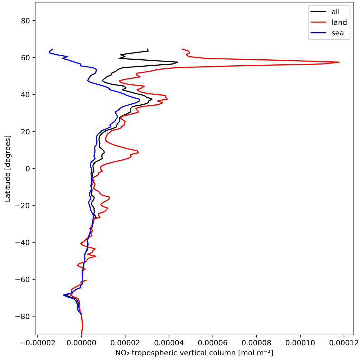
Figure 12: Zonal average of “NO 2 tropospheric vertical column” for 2023-12-20 to 2023-12-22.
