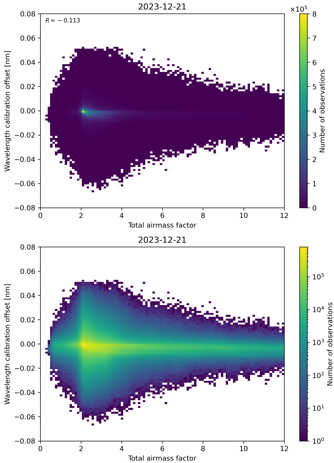
Figure 70: Scatter density plot of “Total airmass factor” against “Wavelength calibration offset” for 2023-12-20 to 2023-12-22.
