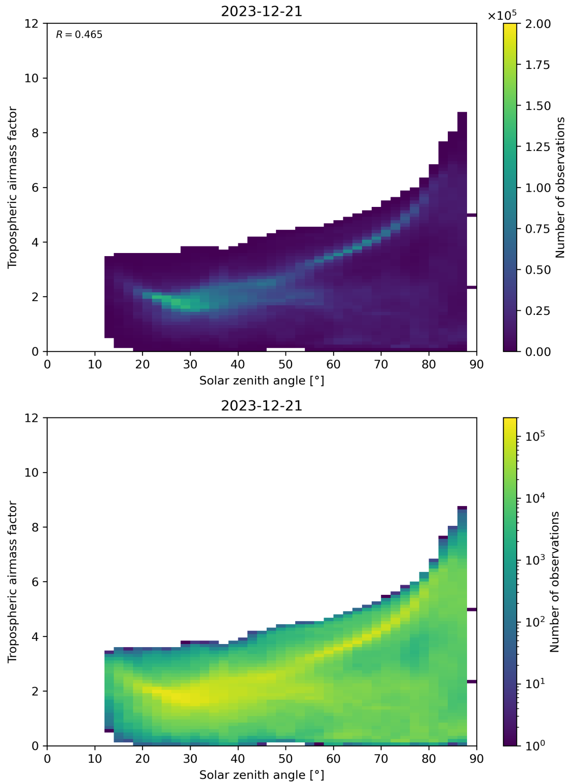
Figure 147: Scatter density plot of “Solar zenith angle” against “Tropospheric airmass factor” for 2023-12-20 to 2023-12-22.
