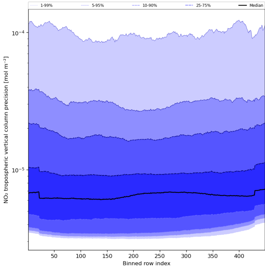
Figure 47: Along track statistics of “NO 2 tropospheric vertical column precision” for 2023-12-20 to 2023-12-22
