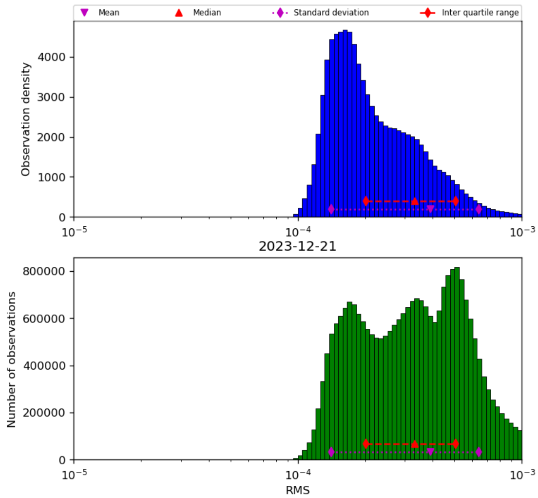
Figure 43: Histogram of “RMS” for 2023-12-20 to 2023-12-22
