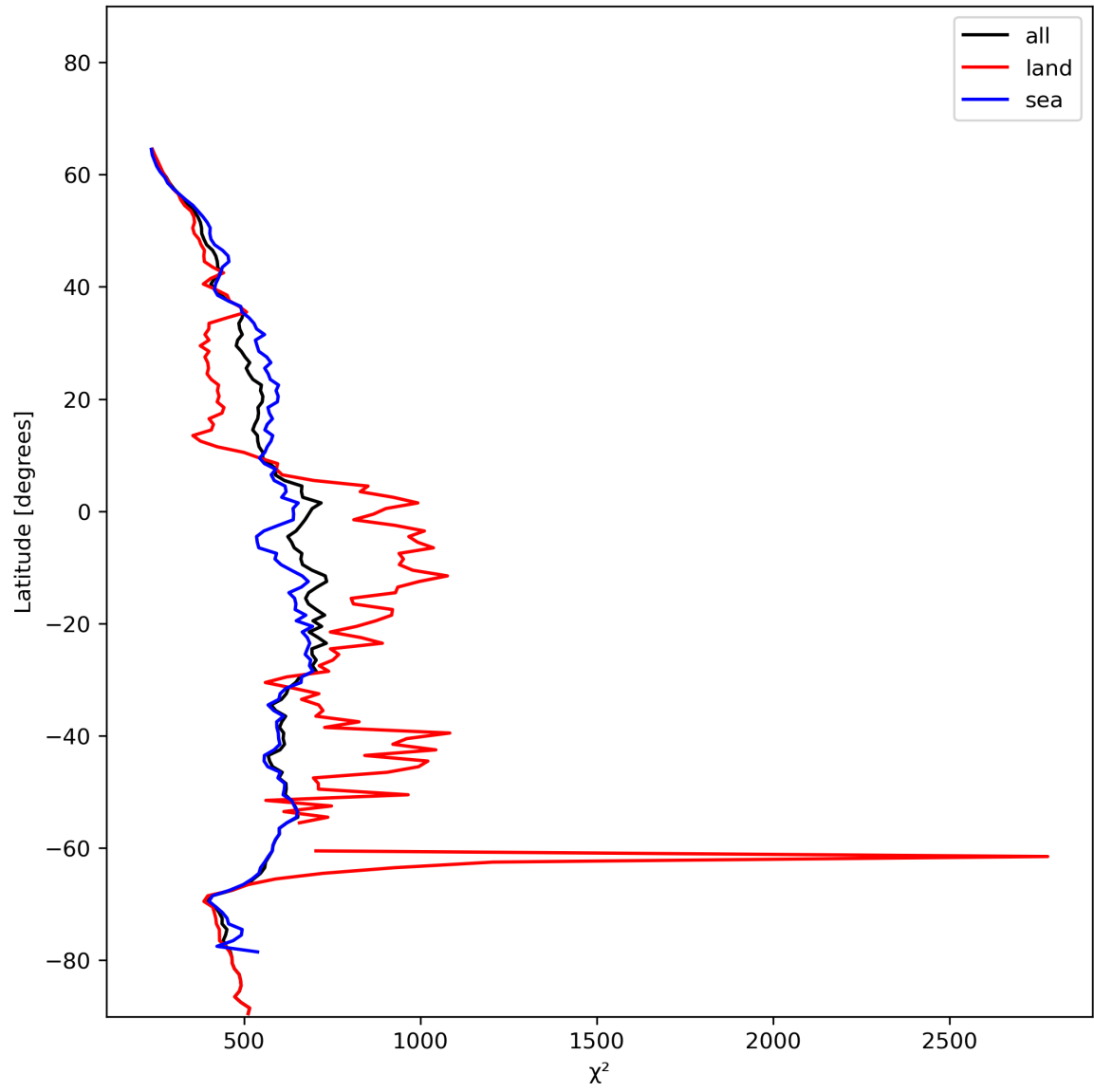
Figure 25: Zonal average of “ \chi^2 ” for 2023-12-20 to 2023-12-22.
