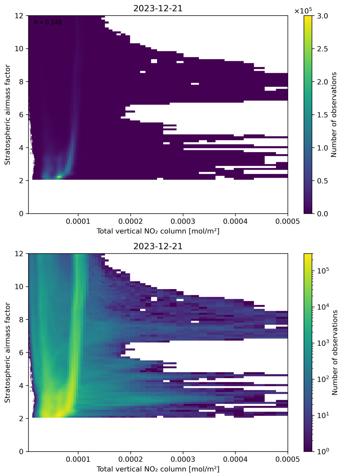
Figure 110: Scatter density plot of “Total vertical NO 2 column” against “Stratospheric airmass factor” for 2023-12-20 to 2023-12-22.
