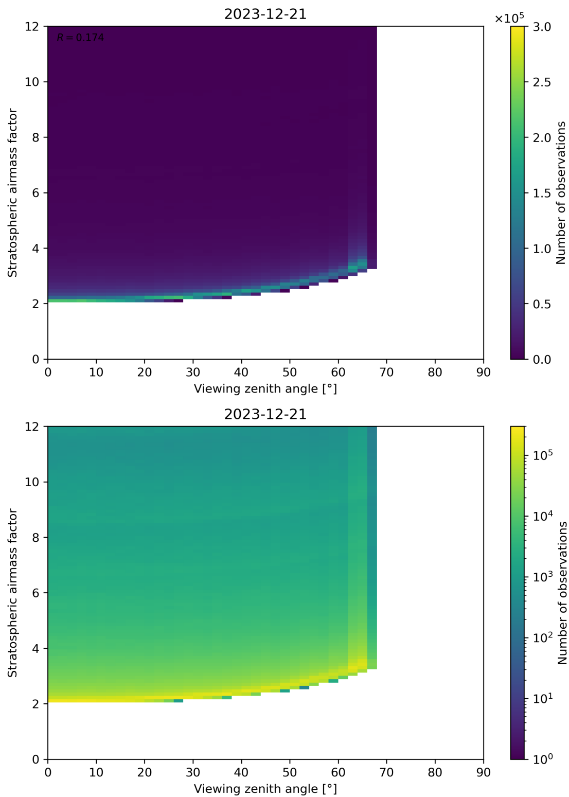
Figure 159: Scatter density plot of “Viewing zenith angle” against “Stratospheric airmass factor” for 2023-12-20 to 2023-12-22.
