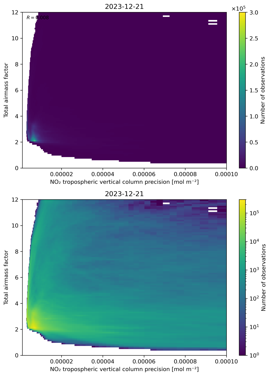
Figure 132: Scatter density plot of “NO 2 tropospheric vertical column precision” against “Total air mass factor” for 2023-12-20 to 2023-12-22.
