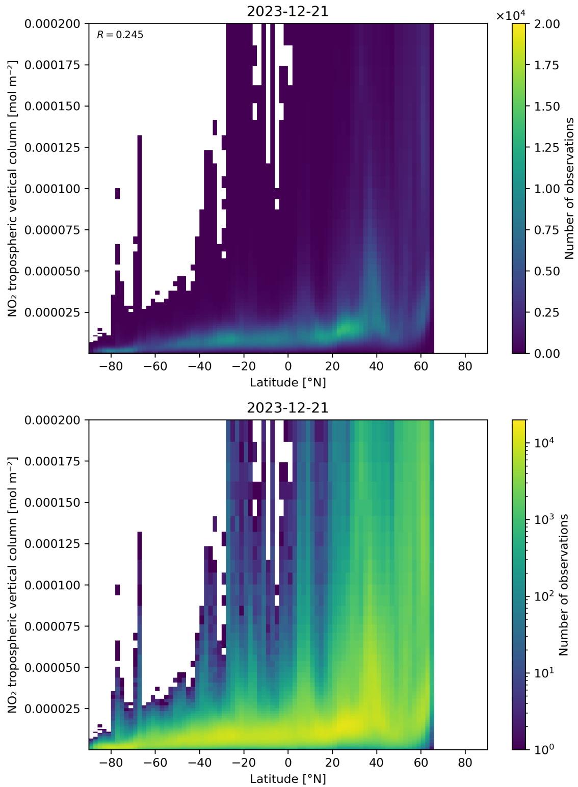
Figure 92: Scatter density plot of “Latitude” against “NO 2 tropospheric vertical column” for 2023-12-20 to 2023-12-22.
