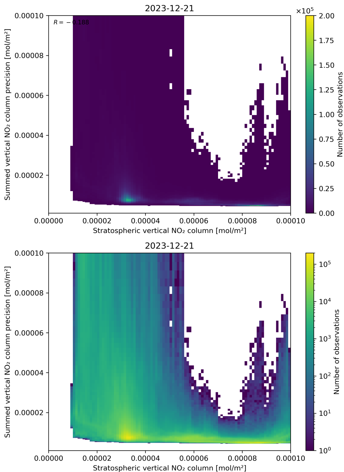
Figure 99: Scatter density plot of “Stratospheric vertical NO 2 column” against “Summed vertical NO 2 column precision” for 2023-12-20 to 2023-12-22.
