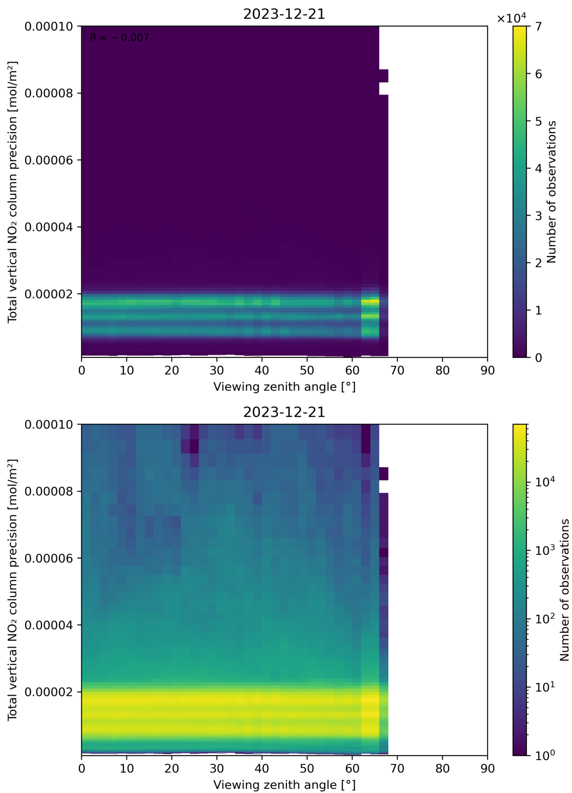
Figure 168: Scatter density plot of “Viewing zenith angle” against “Total vertical NO 2 column precision” for 2023-12-20 to 2023-12-22.
