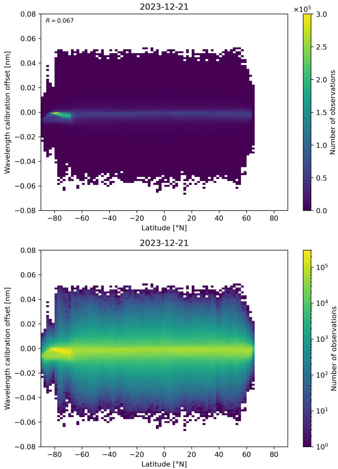
Figure 95: Scatter density plot of “Latitude” against “Wavelength calibration offset” for 2023-12-20 to 2023-12-22.
