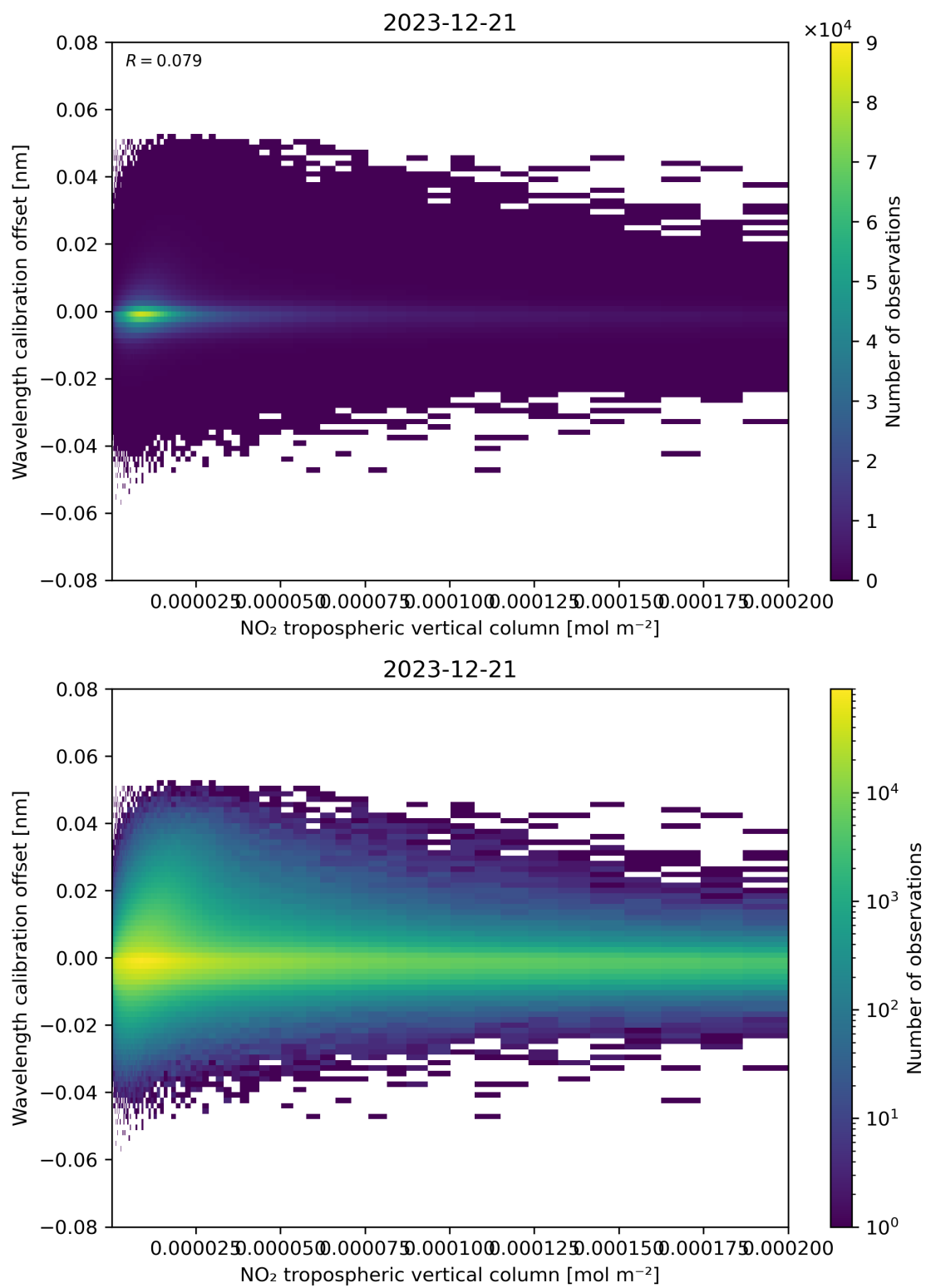
Figure 143: Scatter density plot of “NO 2 tropospheric vertical column” against “Wavelength calibration offset” for 2023-12-20 to 2023-12-22.
