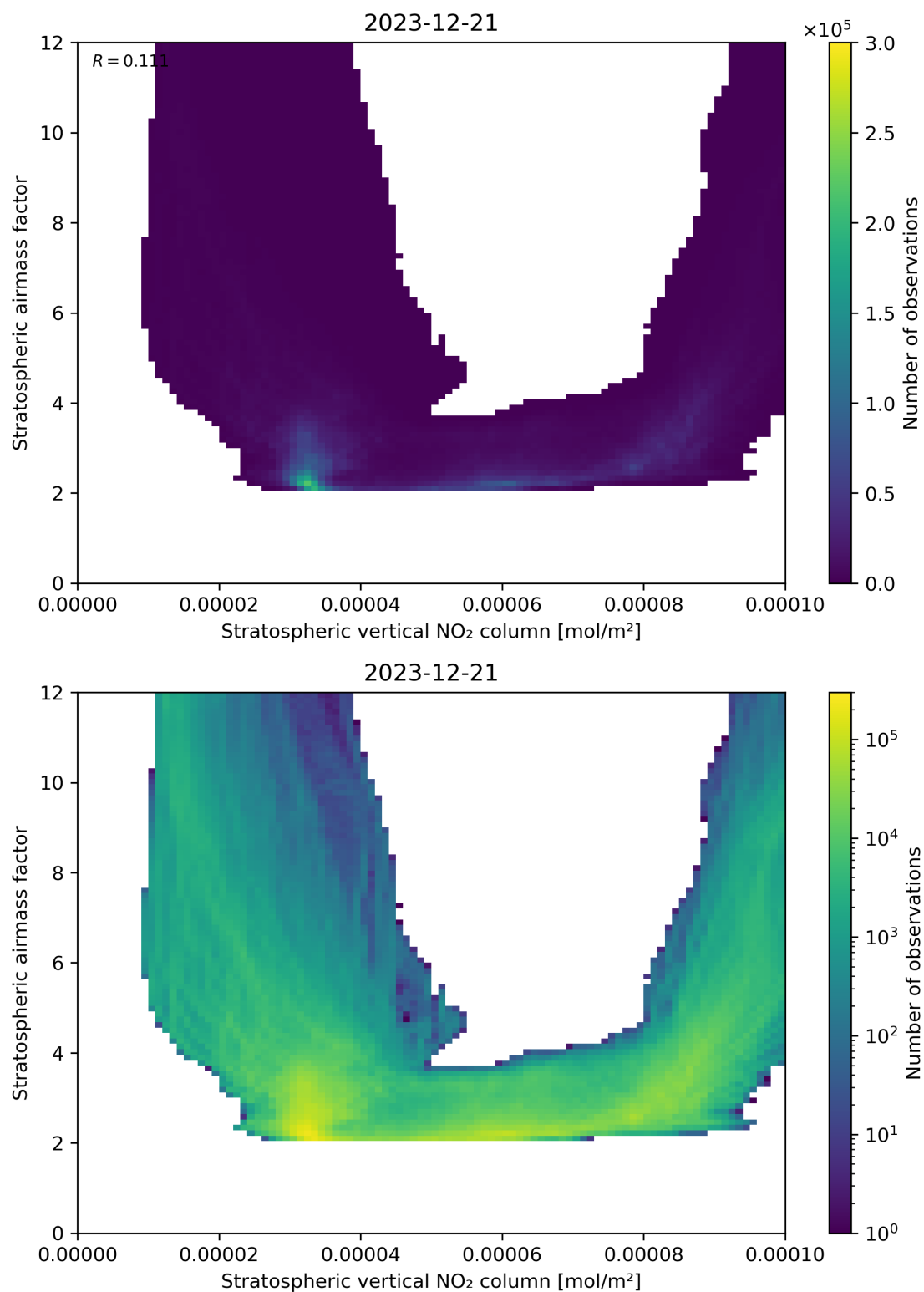
Figure 96: Scatter density plot of “Stratospheric vertical NO 2 column” against “Stratospheric airmass factor” for 2023-12-20 to 2023-12-22.
