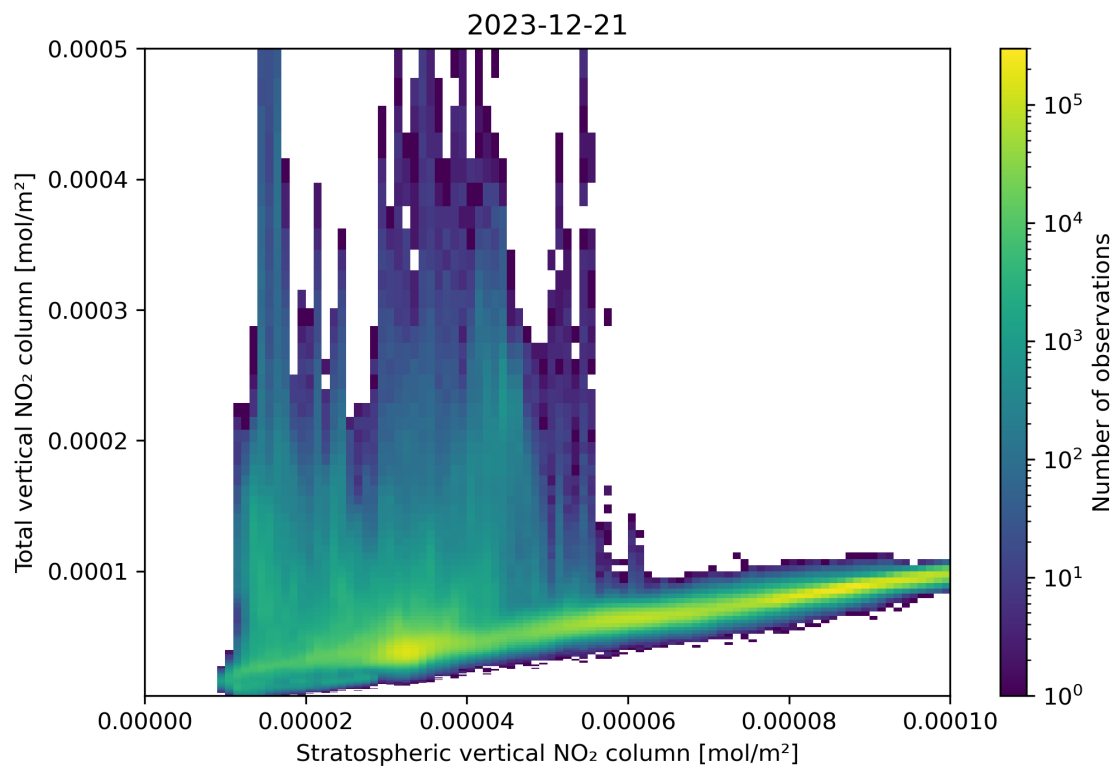
Figure 100: Scatter density plot of “Stratospheric vertical NO 2 column” against “Total vertical NO 2 column” for 2023-12-20 to 2023-12-22.
