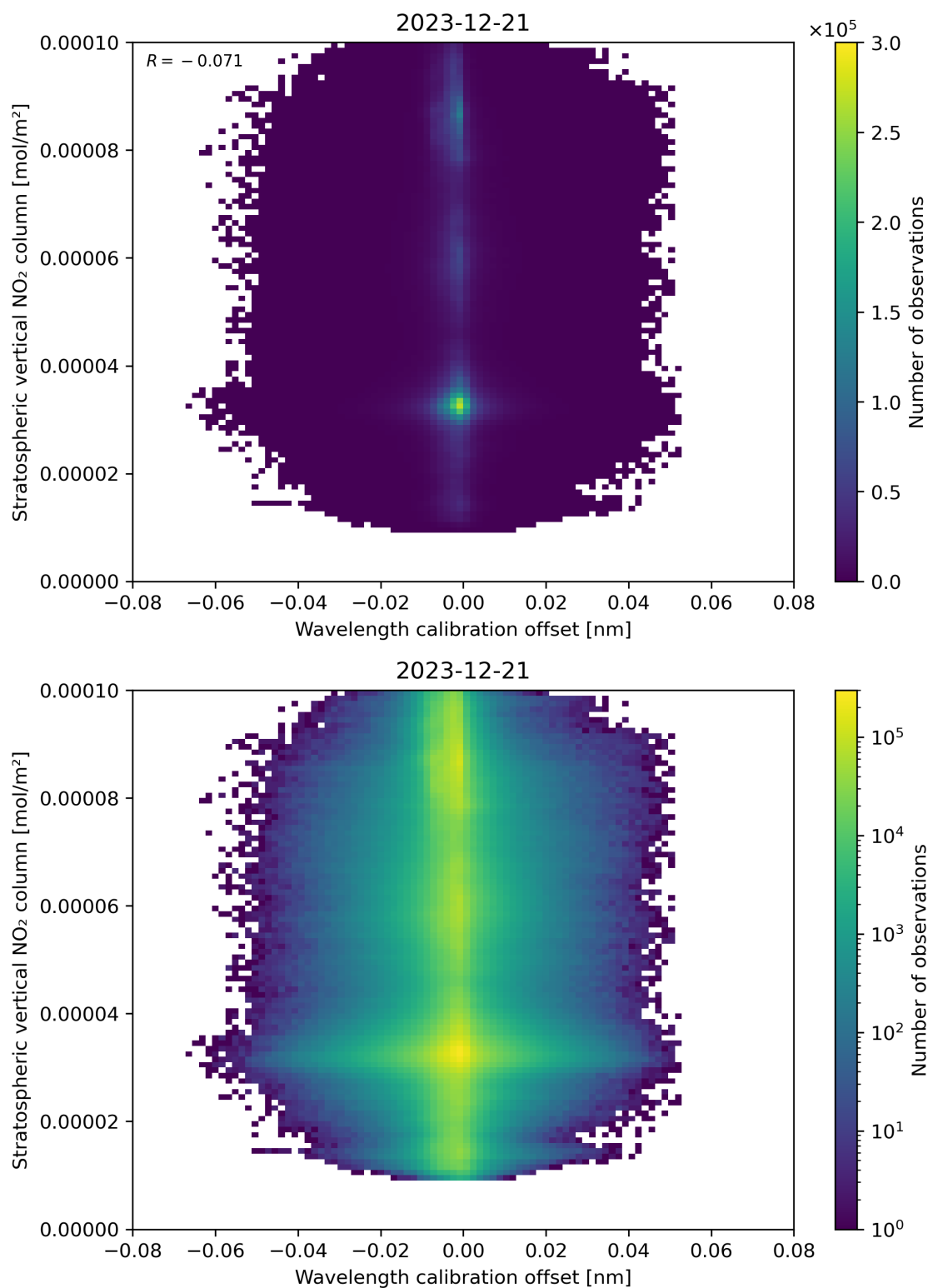
Figure 176: Scatter density plot of “Wavelength calibration offset” against “Stratospheric vertical NO 2 column” for 2023-12-20 to 2023-12-22.
