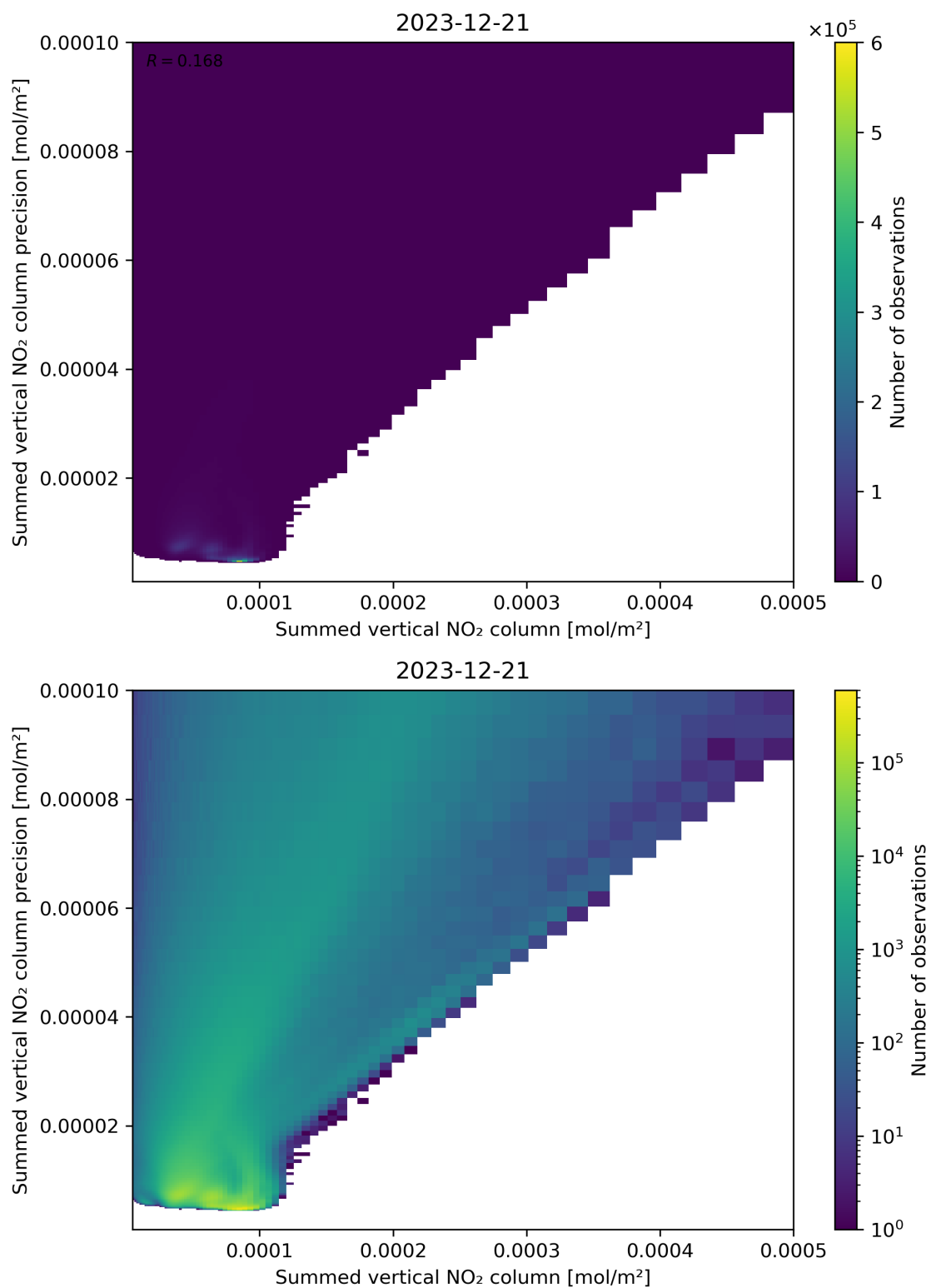
Figure 105: Scatter density plot of “Summed vertical NO 2 column” against “Summed vertical NO 2 column precision” for 2023-12-20 to 2023-12-22.
