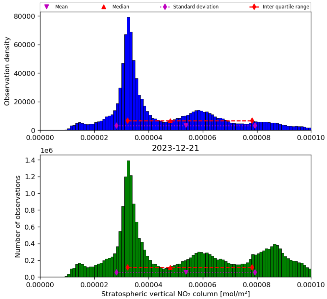
Figure 36: Histogram of “Stratospheric vertical NO 2 column” for 2023-12-20 to 2023-12-22
