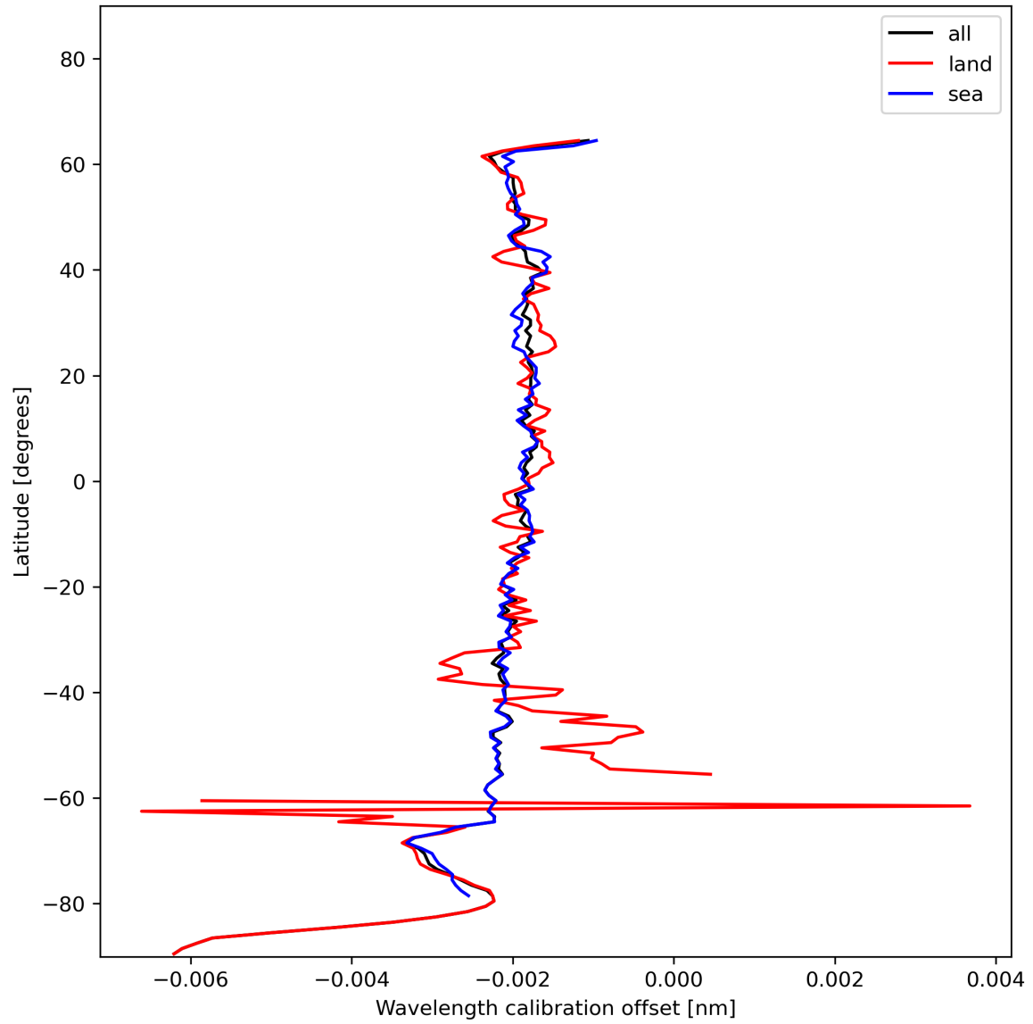
Figure 18: Zonal average of “Wavelength calibration offset” for 2023-12-20 to 2023-12-22.
