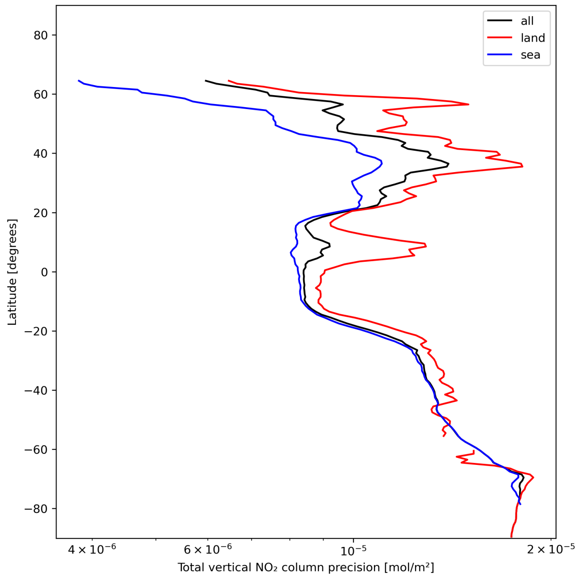
Figure 22: Zonal average of “Total vertical NO 2 column precision” for 2023-12-20 to 2023-12-22.
