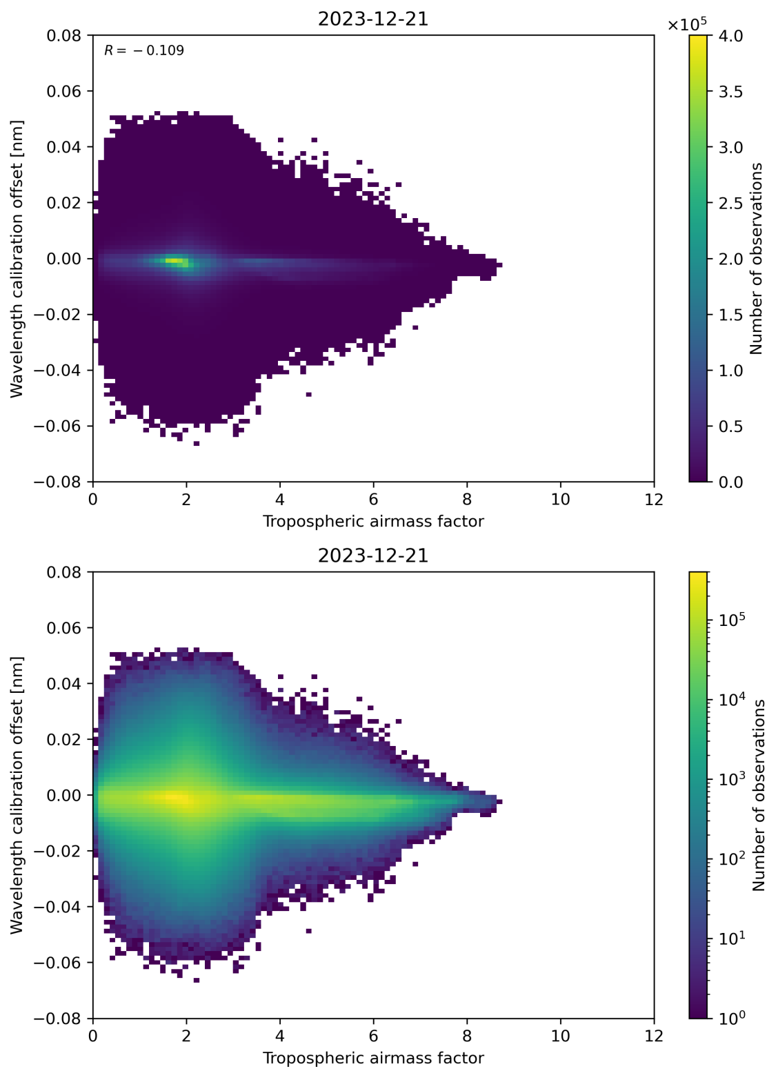
Figure 80: Scatter density plot of “Tropospheric airmass factor” against “Wavelength calibration offset” for 2023-12-20 to 2023-12-22.
