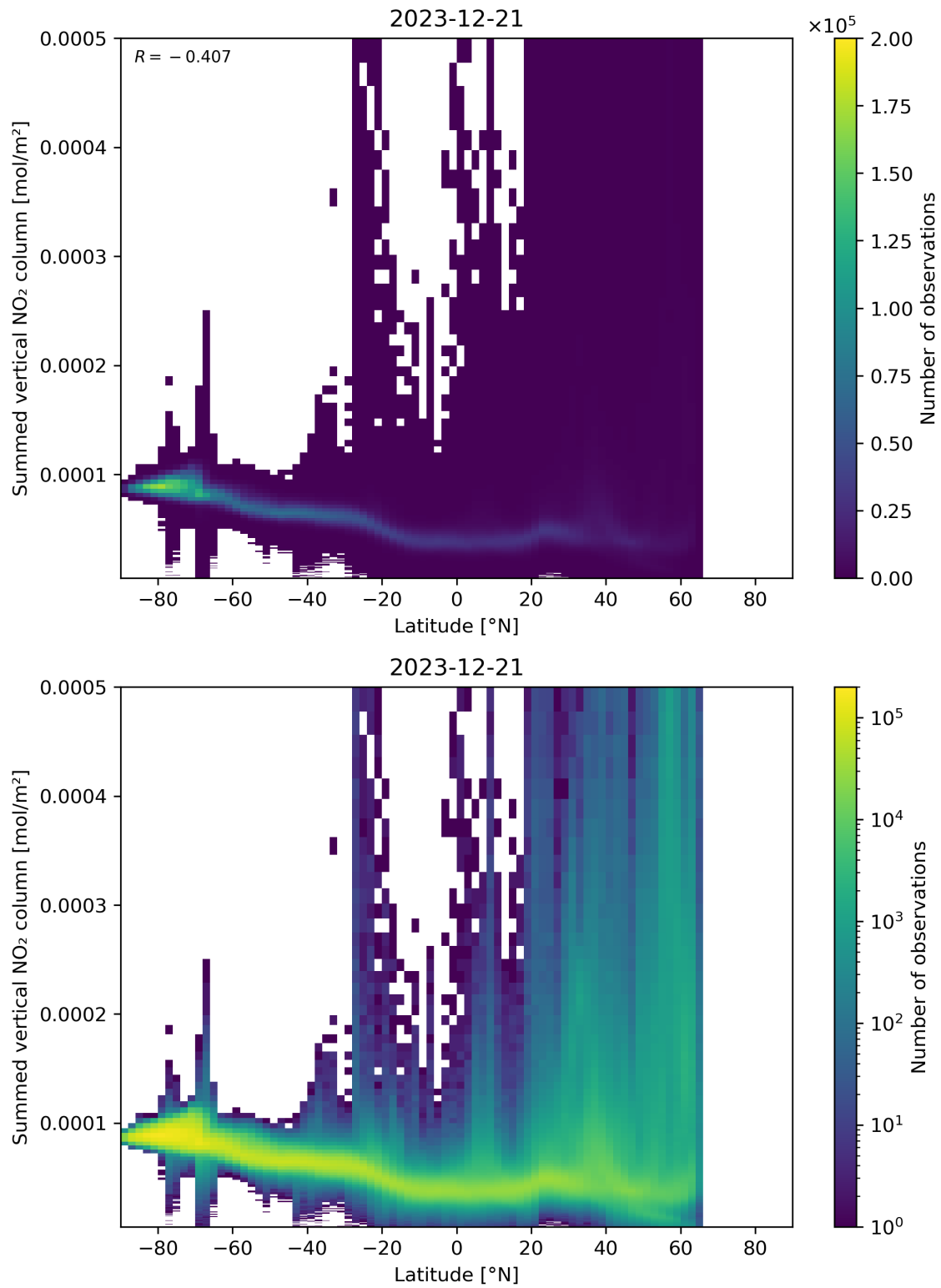
Figure 88: Scatter density plot of “Latitude” against “Summed vertical NO 2 column” for 2023-12-20 to 2023-12-22.
