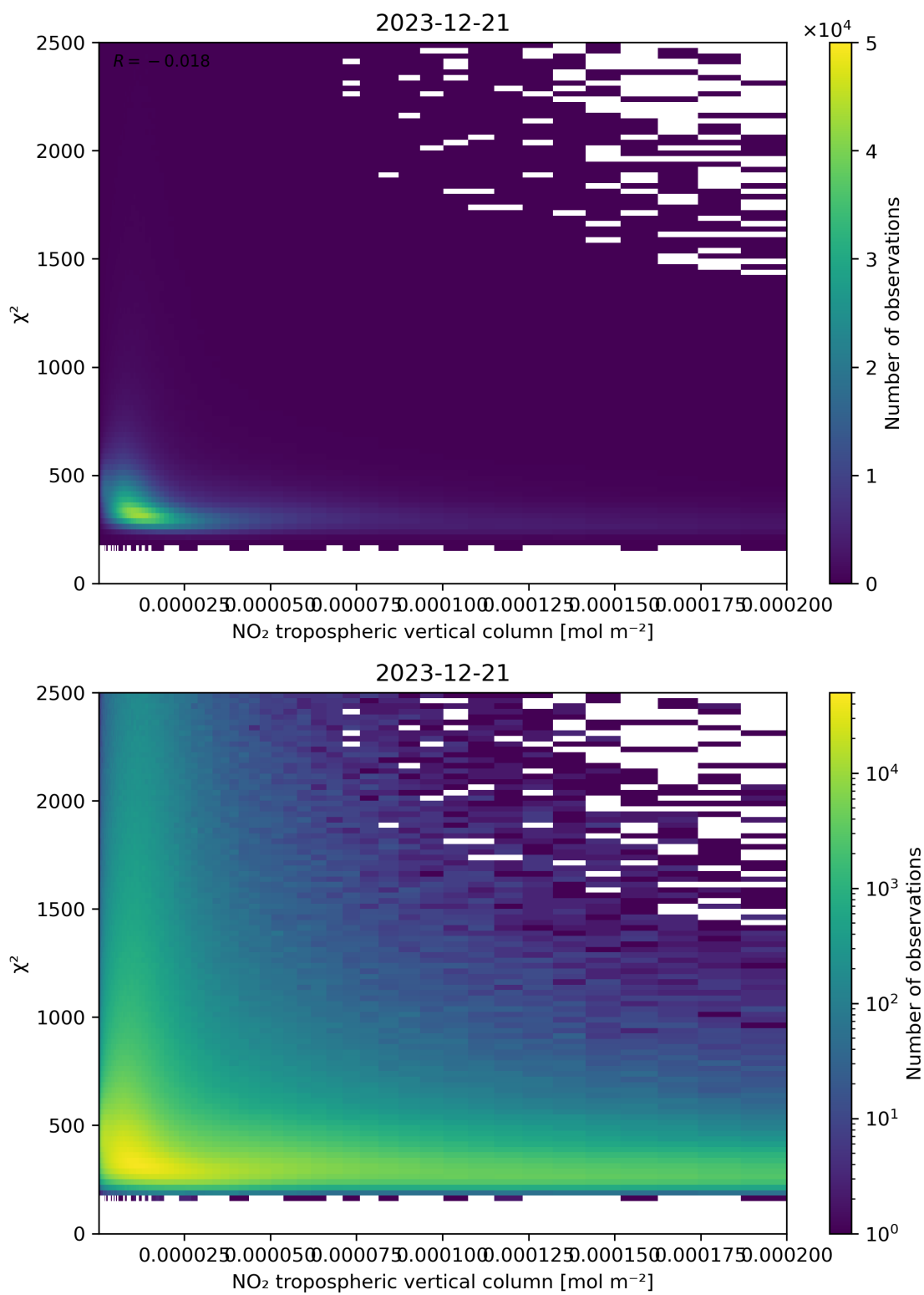
Figure 124: Scatter density plot of “NO 2 tropospheric vertical column” against “ \chi^2 ” for 2023-12-20 to 2023-12-22.
