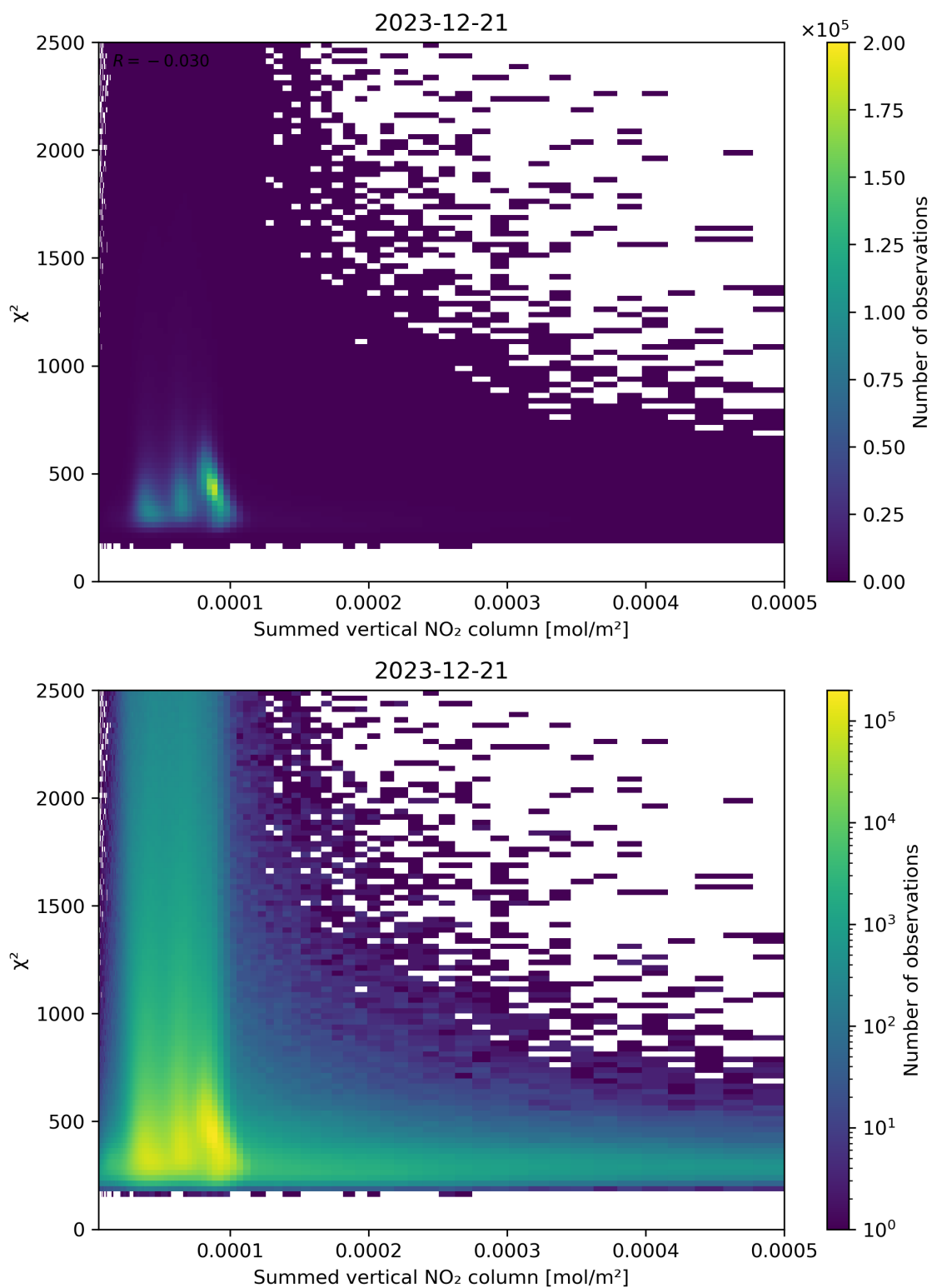
Figure 104: Scatter density plot of “Summed vertical NO 2 column” against “ \chi^2 ” for 2023-12-20 to 2023-12-22.
