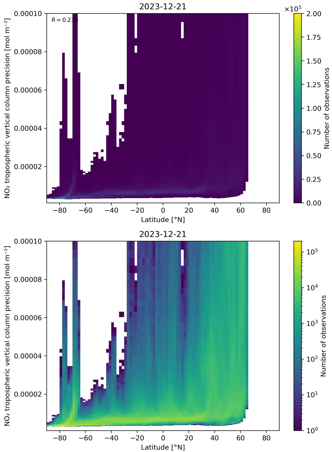
Figure 93: Scatter density plot of “Latitude” against “NO 2 tropospheric vertical column precision” for 2023-12-20 to 2023-12-22.
