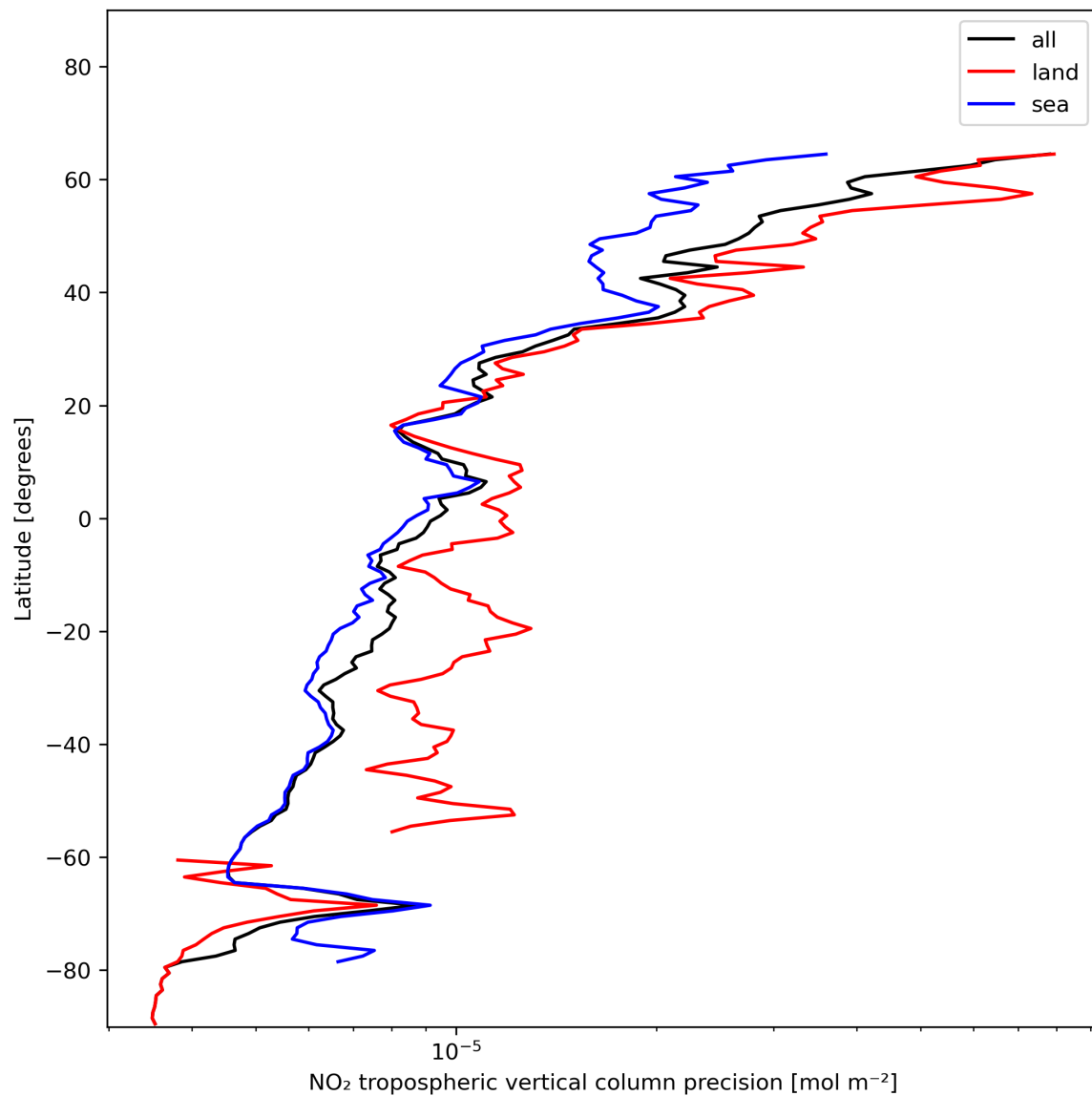
Figure 13: Zonal average of “NO 2 tropospheric vertical column precision” for 2023-12-20 to 2023-12-22.
