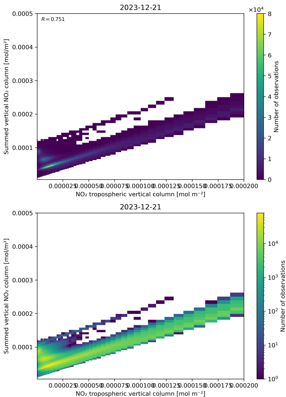
Figure 126: Scatter density plot of “NO 2 tropospheric vertical column” against “Summed vertical NO 2 column” for 2023-12-20 to 2023-12-22.
