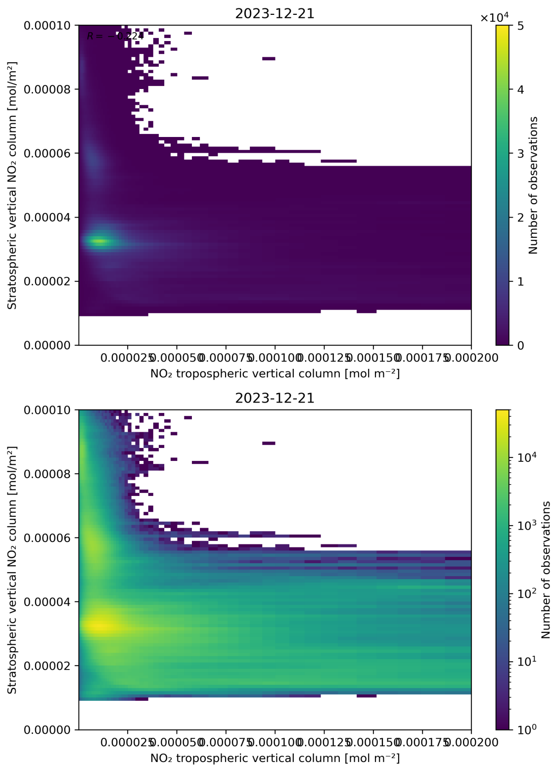
Figure 125: Scatter density plot of “NO 2 tropospheric vertical column” against “Stratospheric vertical NO 2 column” for 2023-12-20 to 2023-12-22.
