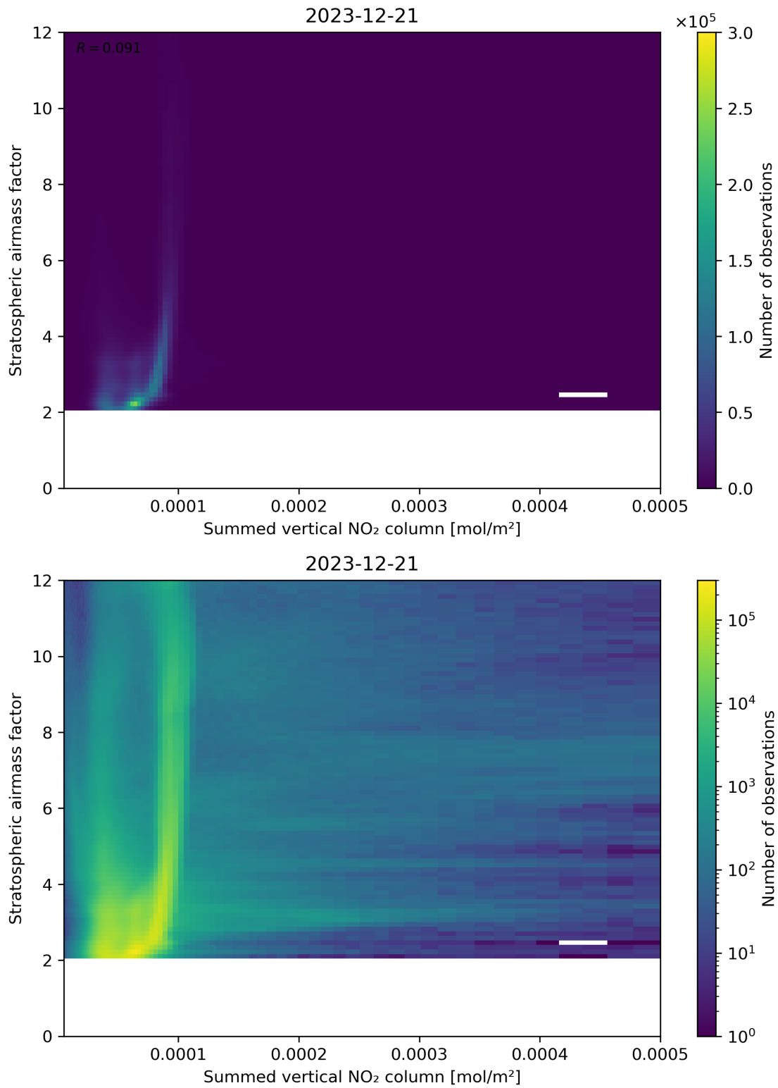
Figure 103: Scatter density plot of “Summed vertical NO 2 column” against “Stratospheric airmass factor” for 2023-12-20 to 2023-12-22.
