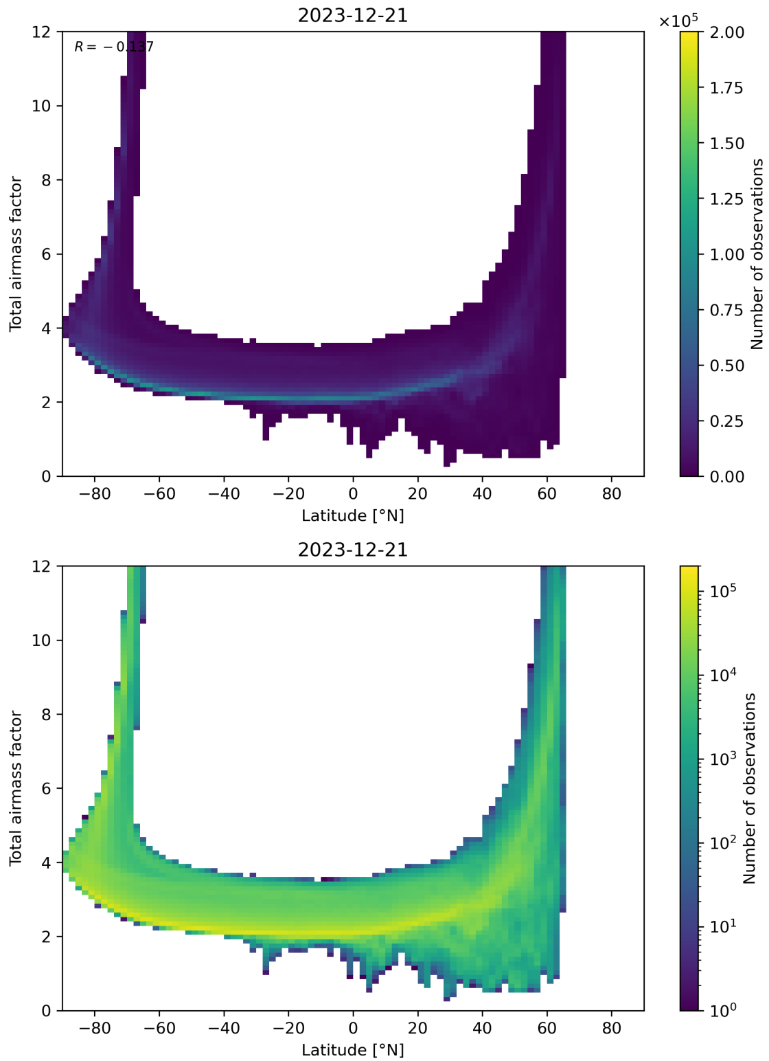
Figure 84: Scatter density plot of “Latitude” against “Total airmass factor” for 2023-12-20 to 2023-12-22.
