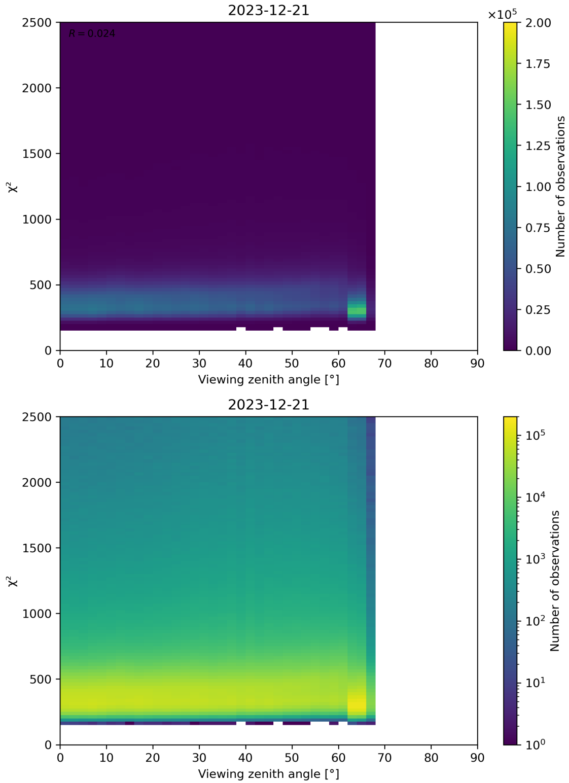
Figure 162: Scatter density plot of “Viewing zenith angle” against “ \chi^2 ” for 2023-12-20 to 2023-12-22.
