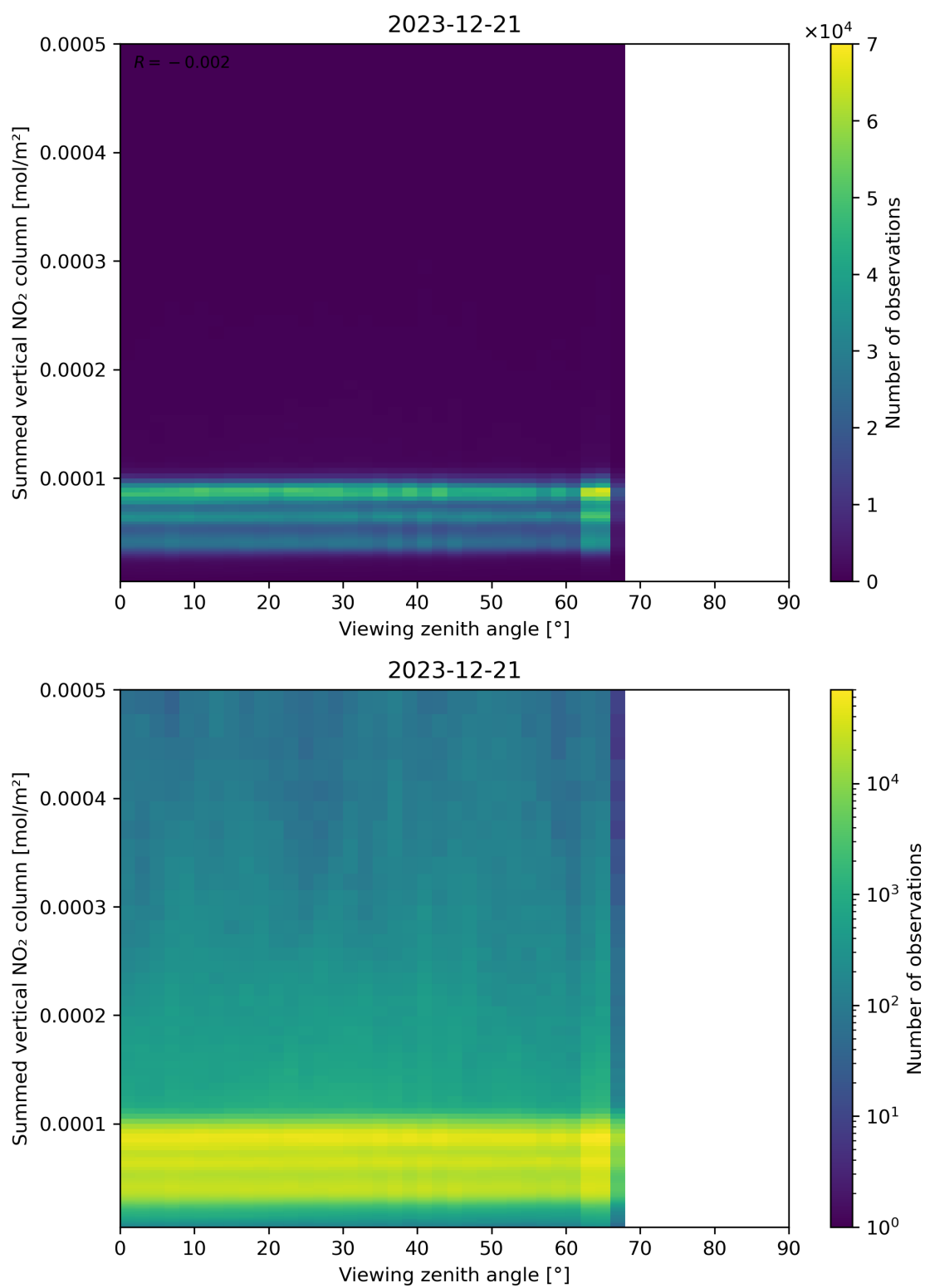
Figure 165: Scatter density plot of “Viewing zenith angle” against “Summed vertical NO 2 column” for 2023-12-20 to 2023-12-22.
