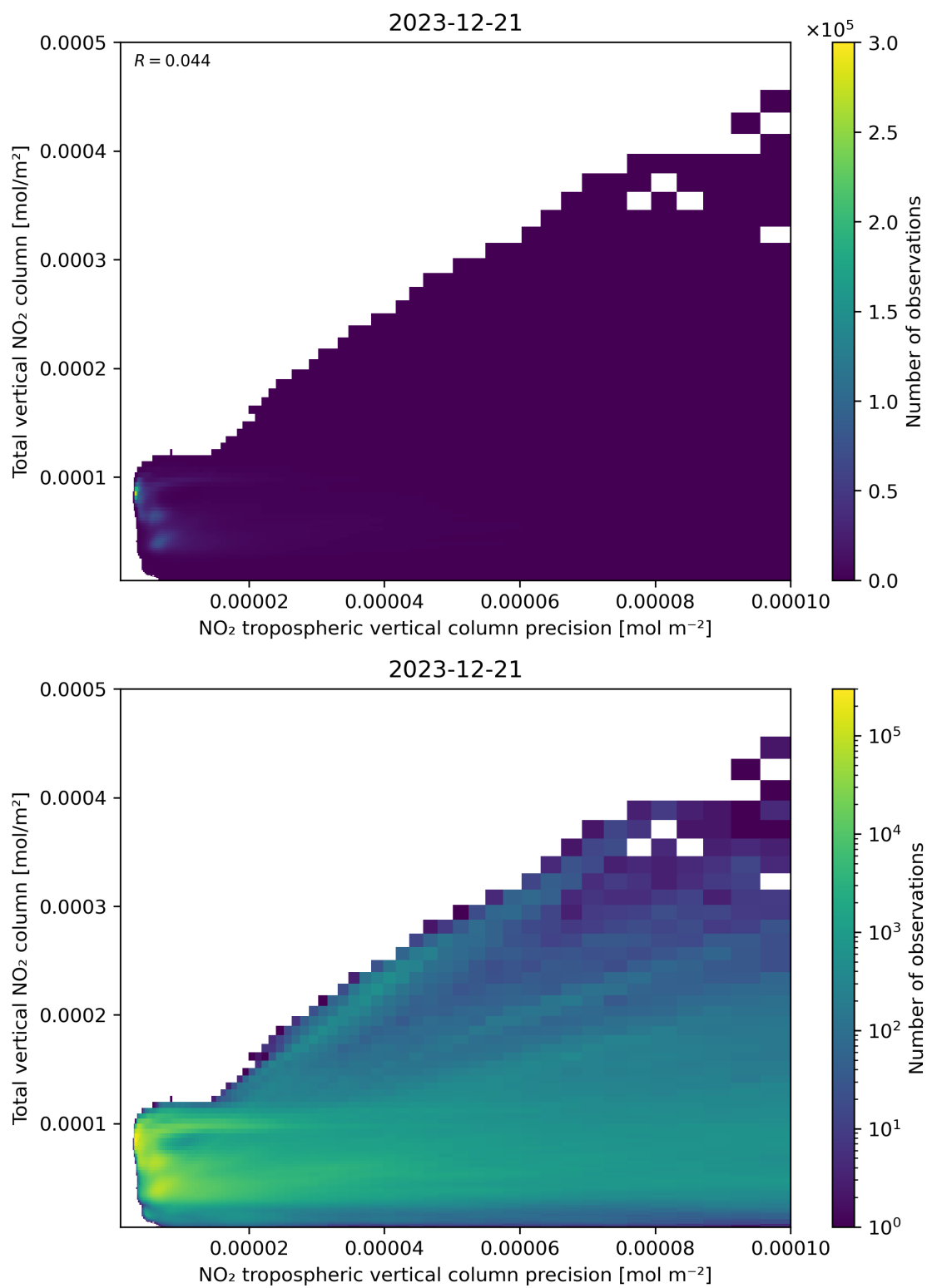
Figure 138: Scatter density plot of “NO 2 tropospheric vertical column precision” against “Total vertical NO 2 column” for 2023-12-20 to 2023-12-22.
