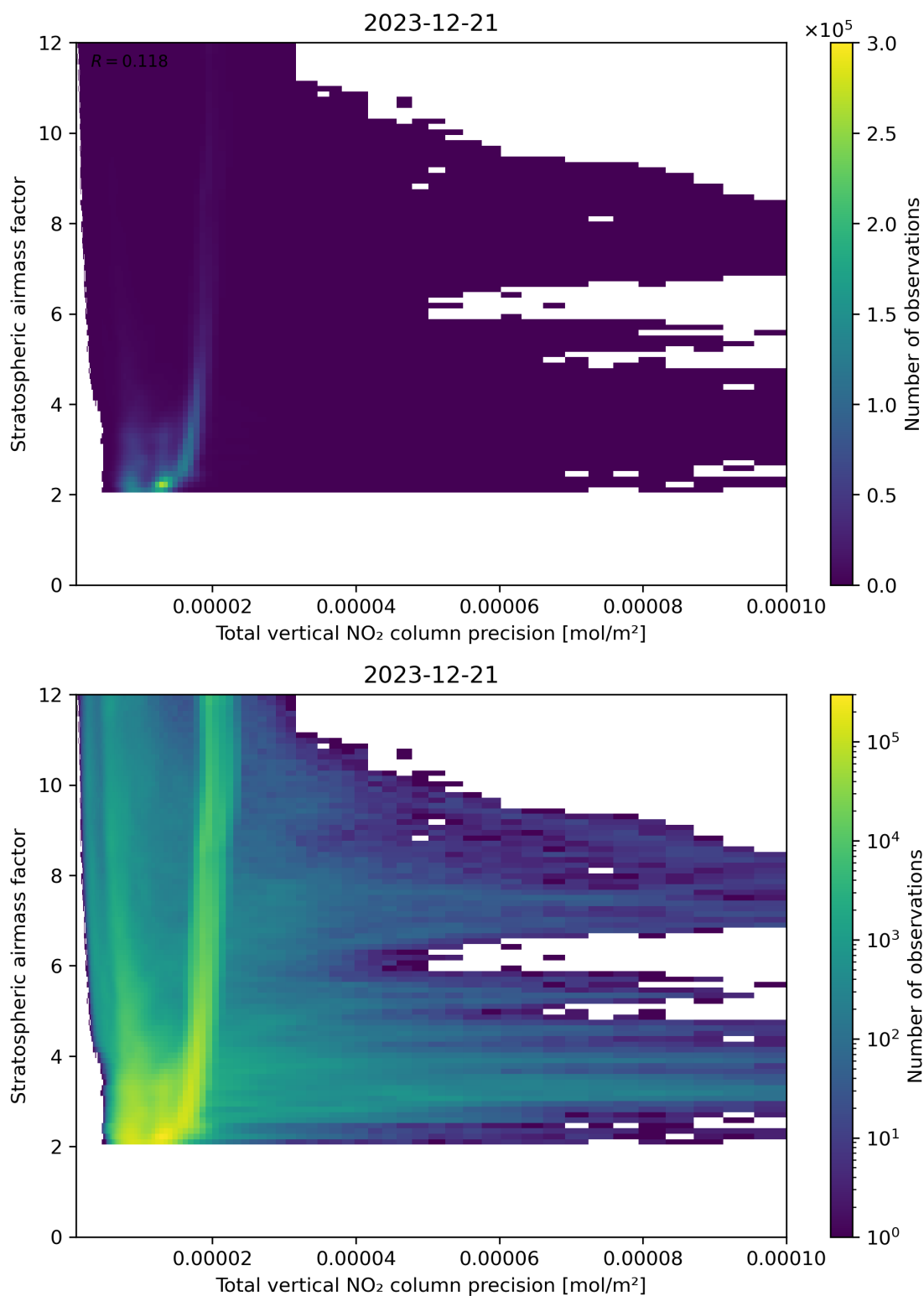
Figure 115: Scatter density plot of “Total vertical NO 2 column precision” against “Stratospheric air mass factor” for 2023-12-20 to 2023-12-22.
