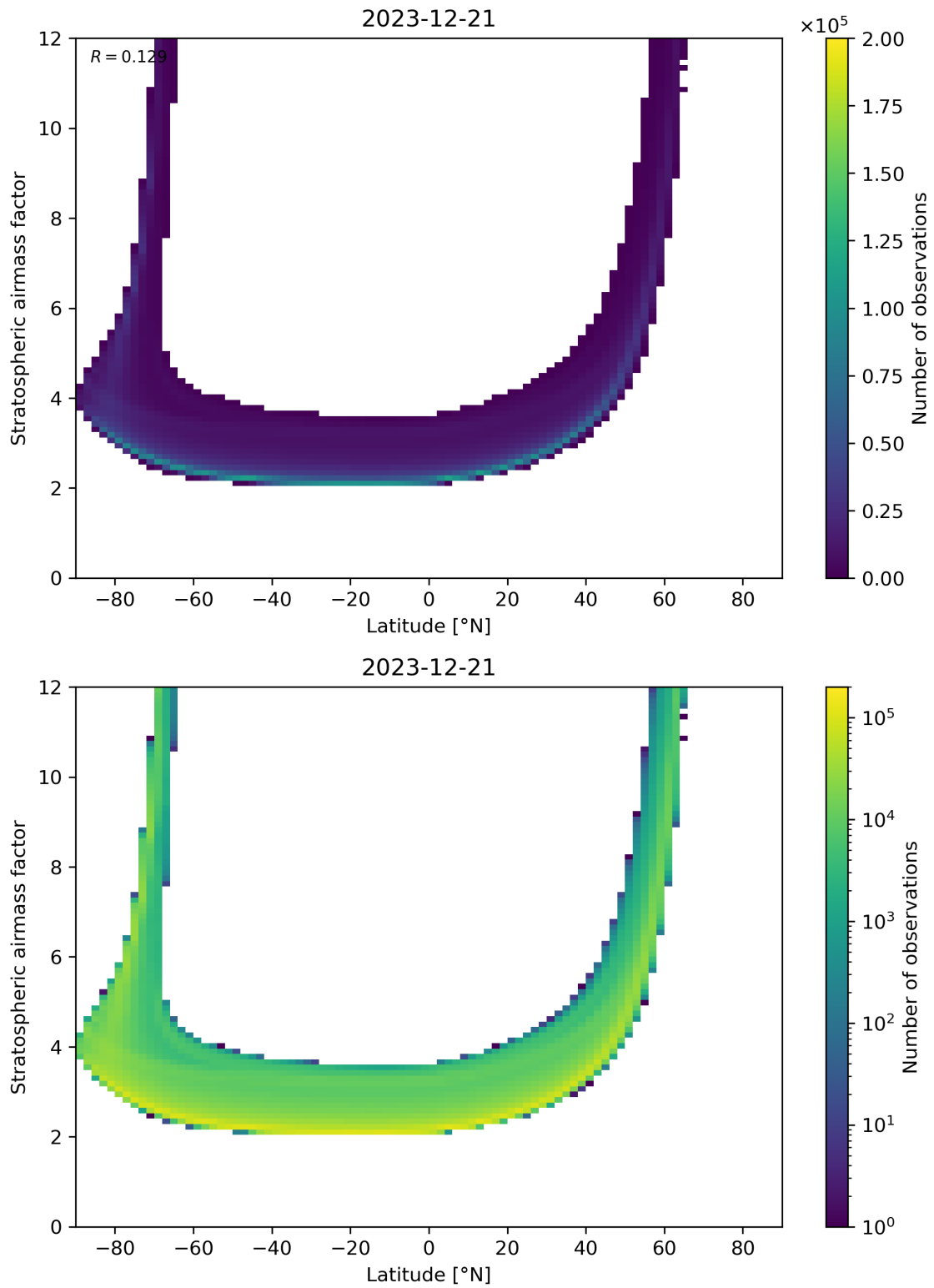
Figure 83: Scatter density plot of “Latitude” against “Stratospheric airmass factor” for 2023-12-20 to 2023-12-22.
