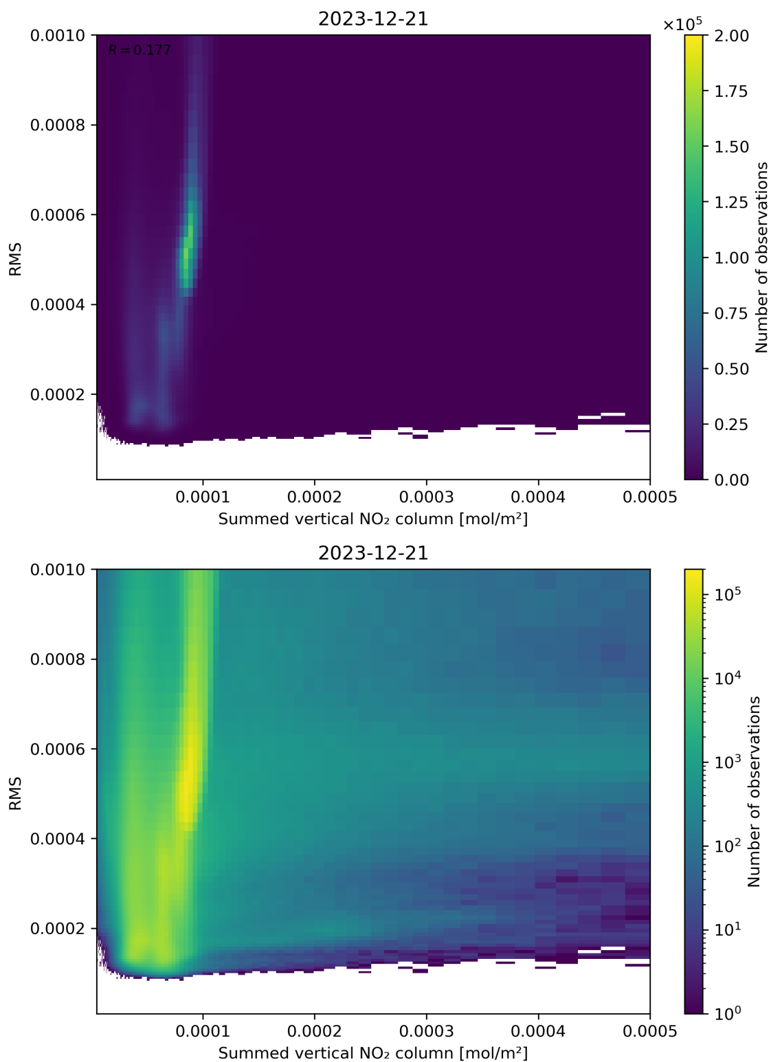
Figure 109: Scatter density plot of “Summed vertical NO 2 column” against “RMS” for 2023-12-20 to 2023-12-22.
