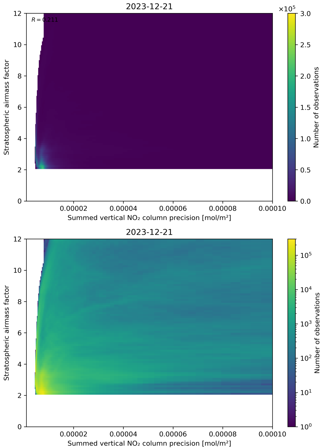
Figure 106: Scatter density plot of “Summed vertical NO 2 column precision” against “Stratospheric airmass factor” for 2023-12-20 to 2023-12-22.
