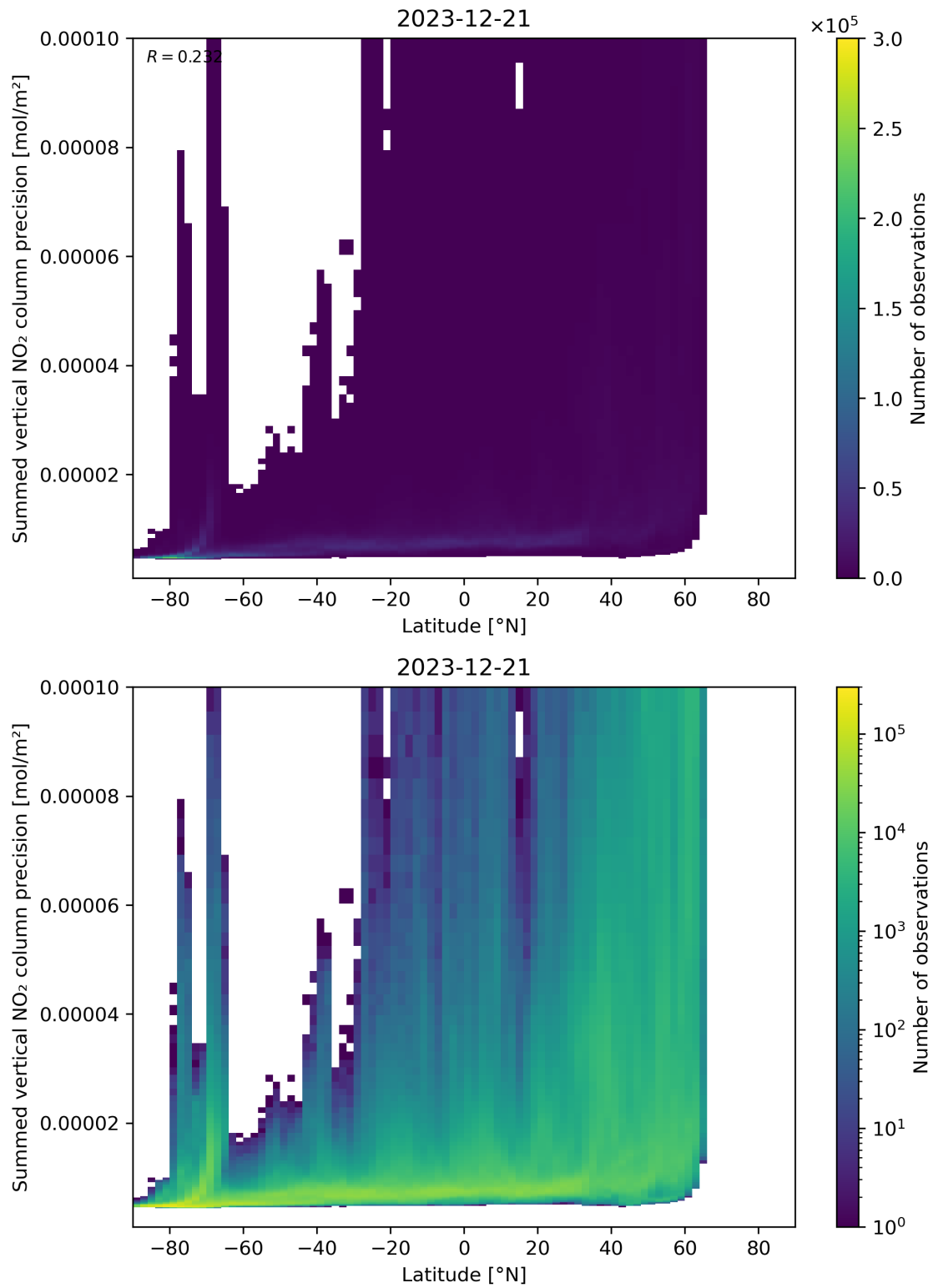
Figure 89: Scatter density plot of “Latitude” against “Summed vertical NO 2 column precision” for 2023-12-20 to 2023-12-22.
