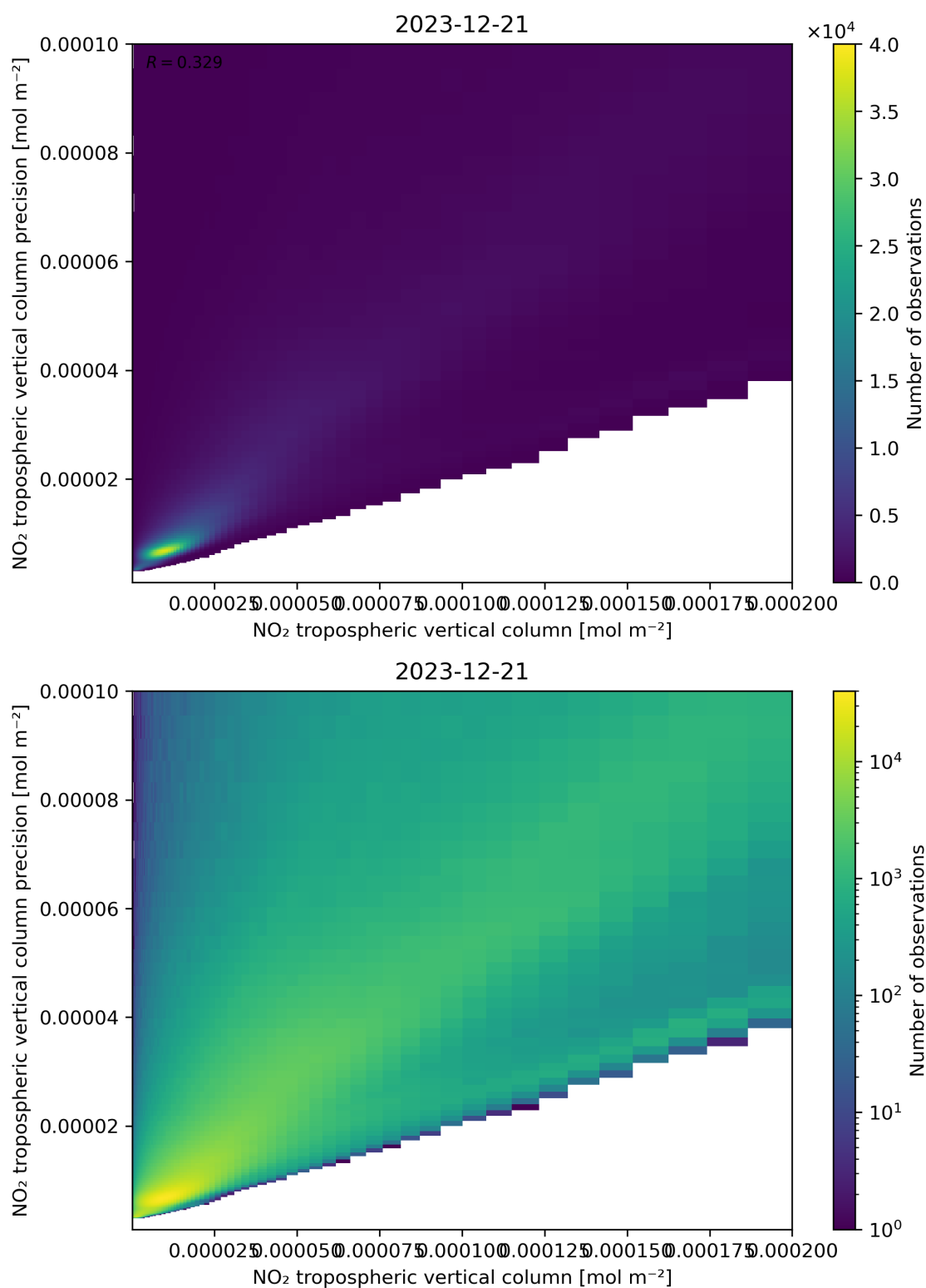
Figure 130: Scatter density plot of “NO 2 tropospheric vertical column” against “NO 2 tropospheric vertical column precision” for 2023-12-20 to 2023-12-22.
