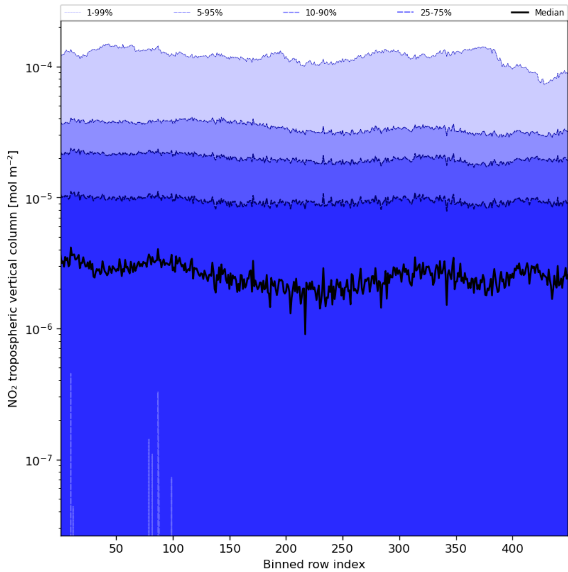
Figure 46: Along track statistics of “NO 2 tropospheric vertical column” for 2023-12-20 to 2023-12-22
