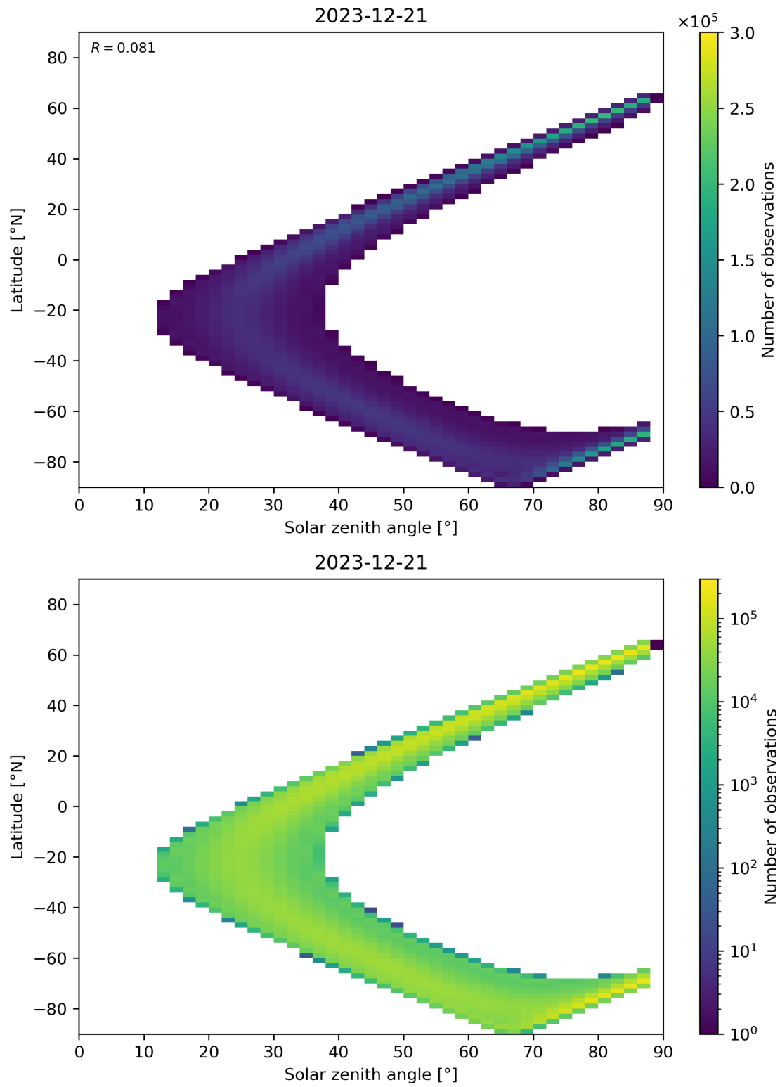
Figure 149: Scatter density plot of “Solar zenith angle” against “Latitude” for 2023-12-20 to 2023-12-22.
