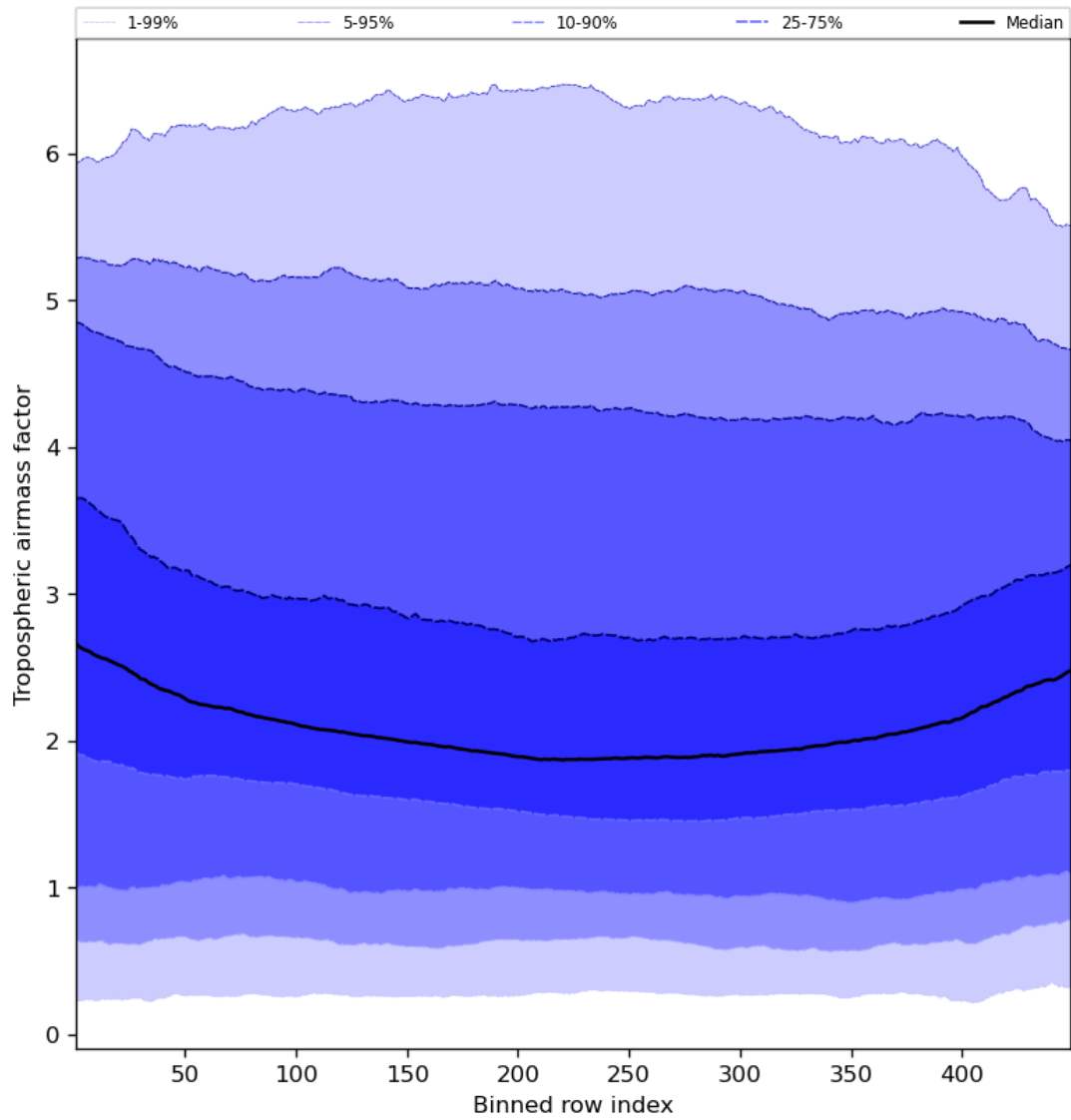
Figure 48: Along track statistics of “Tropospheric airmass factor” for 2023-12-20 to 2023-12-22
