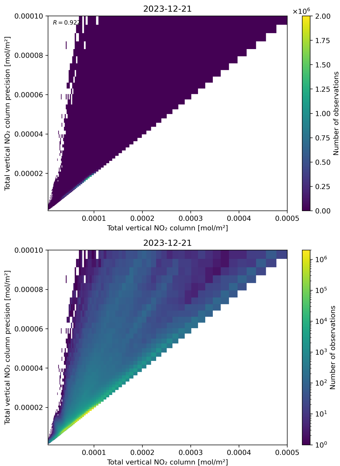
Figure 114: Scatter density plot of “Total vertical NO 2 column” against “Total vertical NO 2 column precision” for 2023-12-20 to 2023-12-22.
