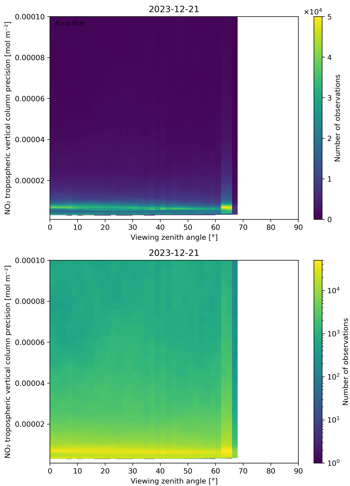
Figure 170: Scatter density plot of “Viewing zenith angle” against “NO 2 tropospheric vertical column precision” for 2023-12-20 to 2023-12-22.
