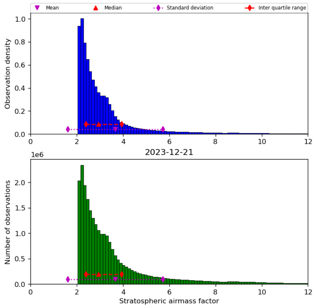
Figure 44: Histogram of “Stratospheric airmass factor” for 2023-12-20 to 2023-12-22
