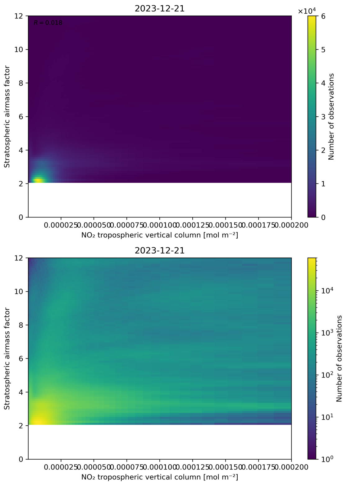
Figure 121: Scatter density plot of “NO 2 tropospheric vertical column” against “Stratospheric airmass factor” for 2023-12-20 to 2023-12-22.
