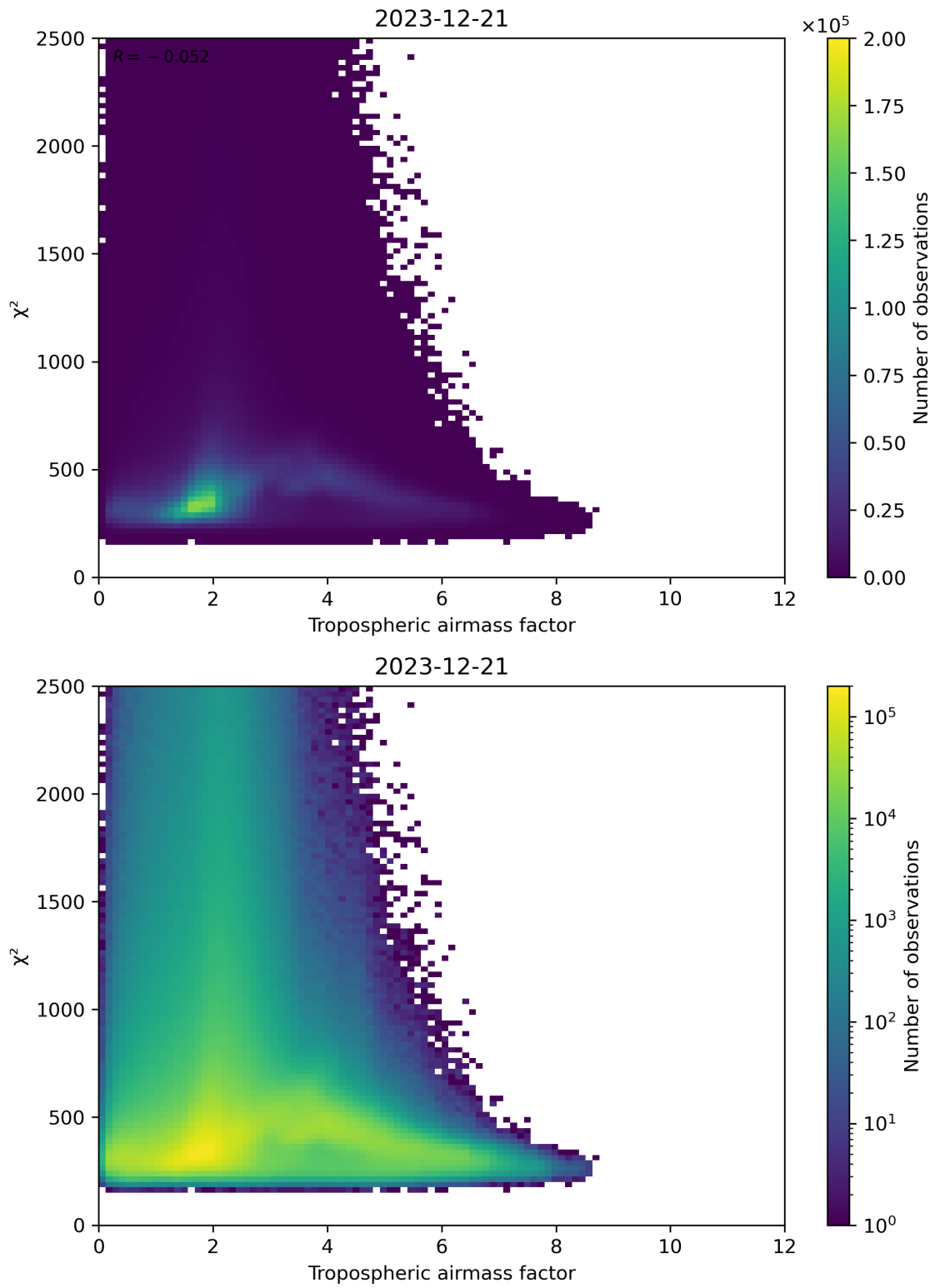
Figure 73: Scatter density plot of “Tropospheric airmass factor” against “ \chi^2 ” for 2023-12-20 to 2023-12-22.
