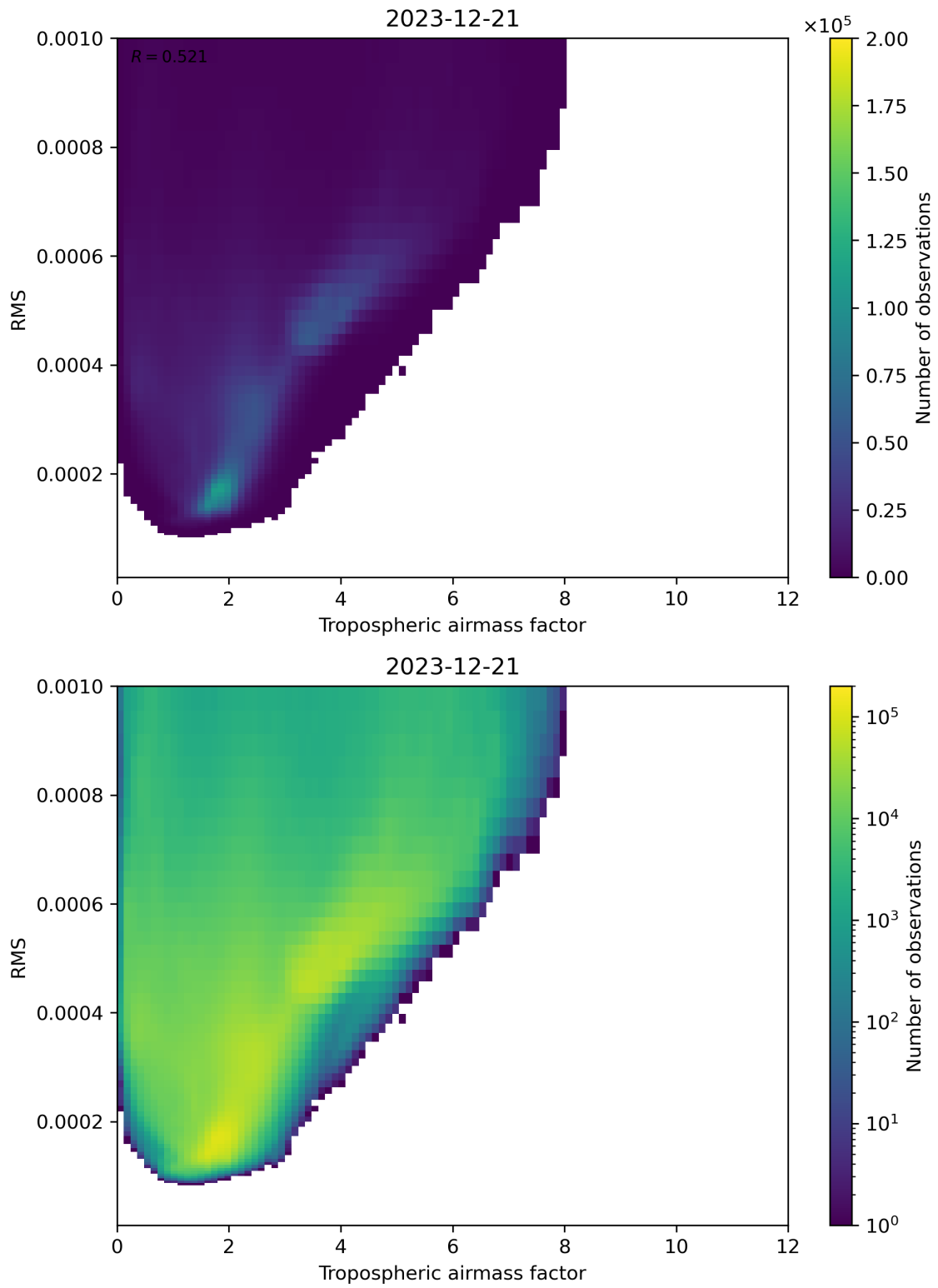
Figure 79: Scatter density plot of “Tropospheric airmass factor” against “RMS” for 2023-12-20 to 2023-12-22.
