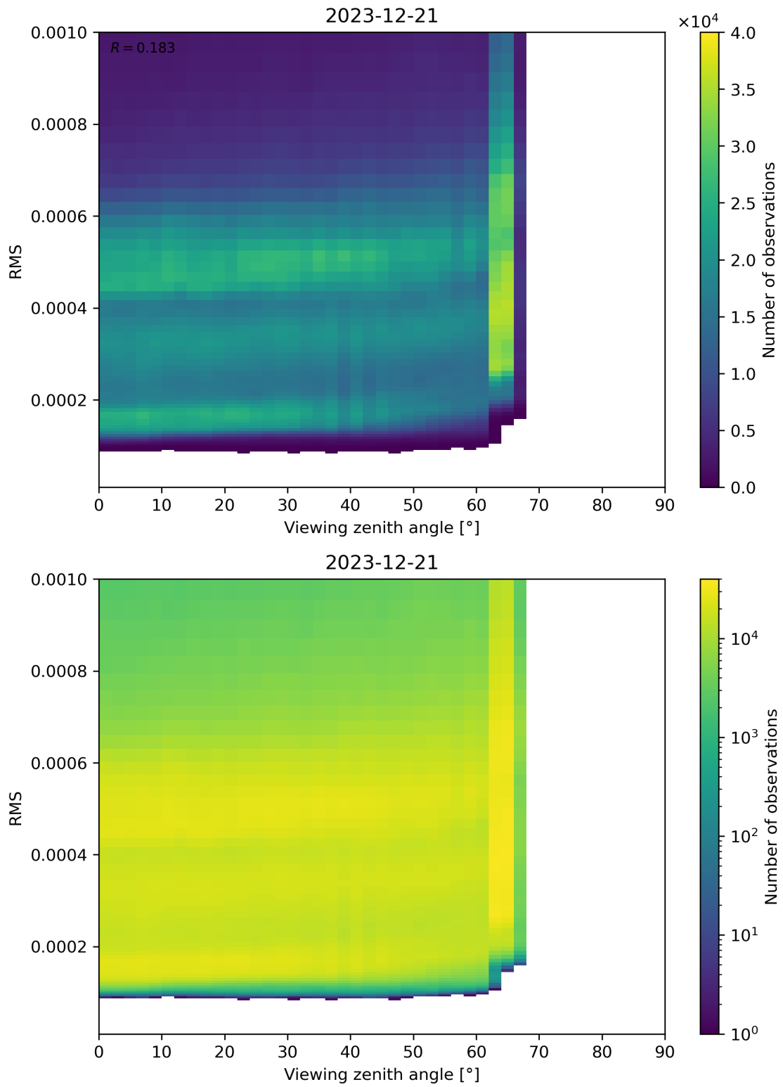
Figure 171: Scatter density plot of “Viewing zenith angle” against “RMS” for 2023-12-20 to 2023-12-22.
