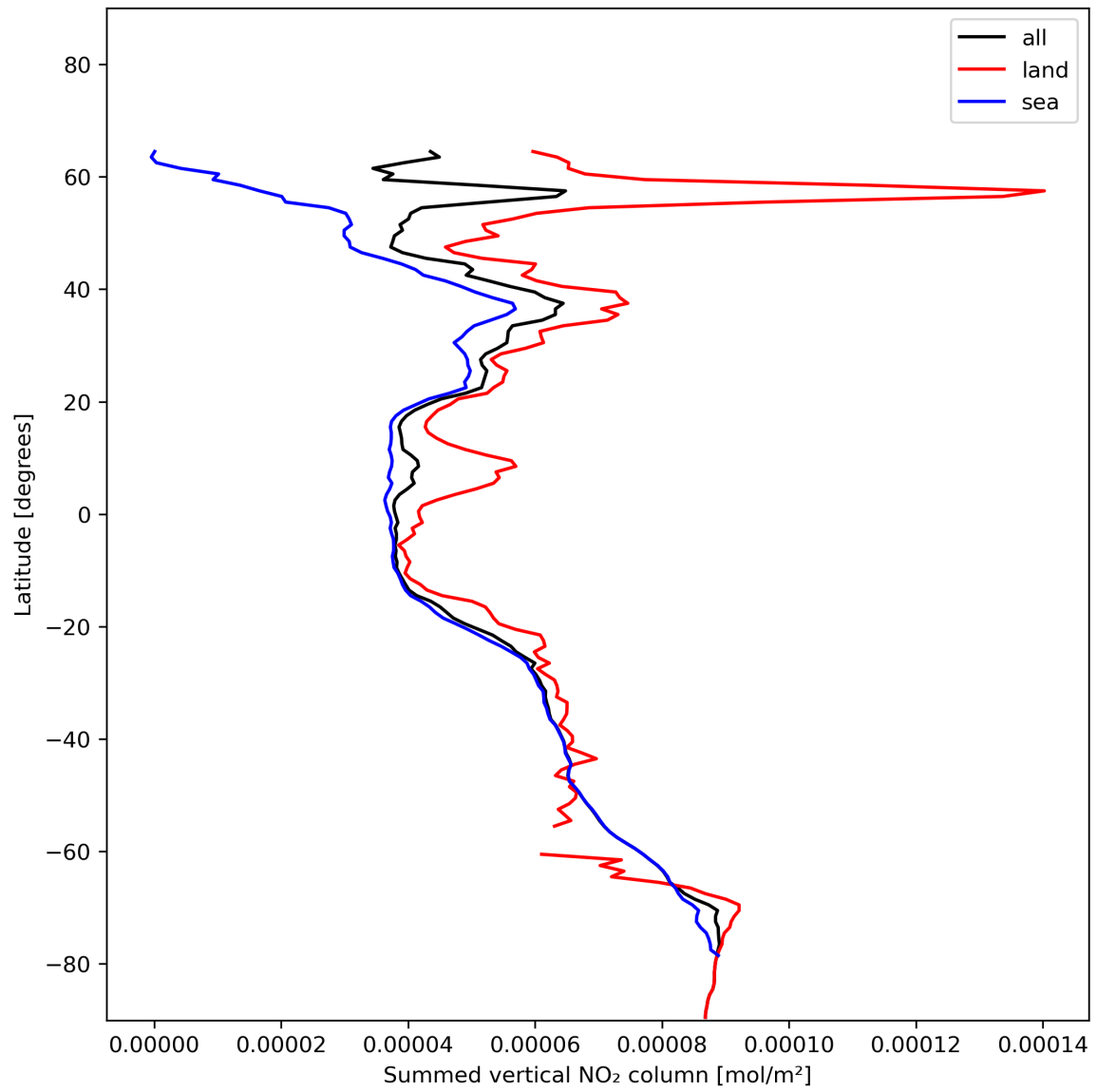
Figure 23: Zonal average of “Summed vertical NO 2 column” for 2023-12-20 to 2023-12-22.
