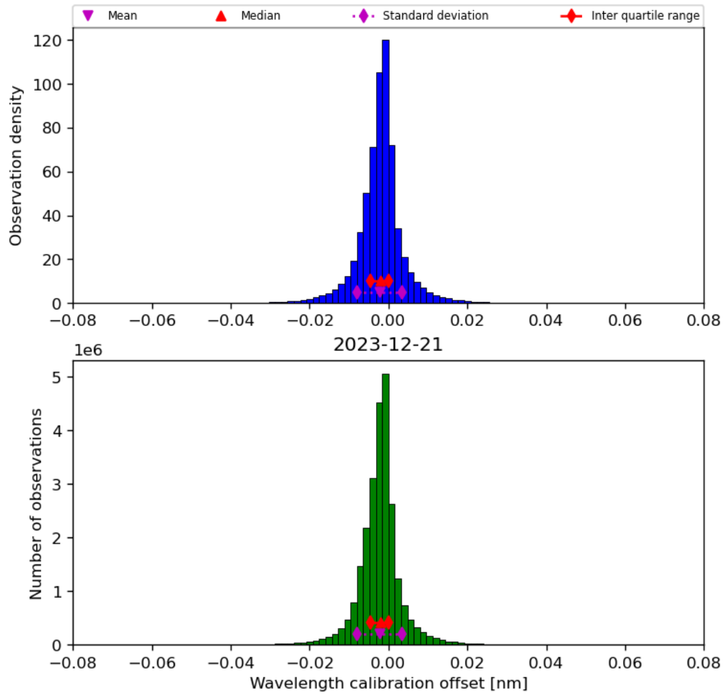
Figure 35: Histogram of “Wavelength calibration offset” for 2023-12-20 to 2023-12-22
