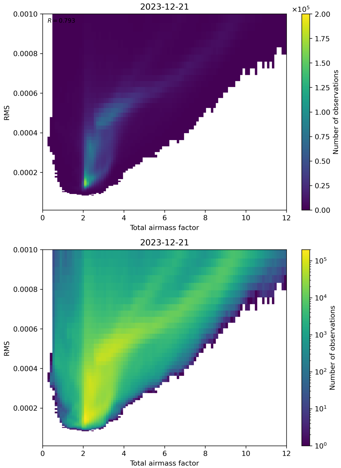
Figure 69: Scatter density plot of “Total airmass factor” against “RMS” for 2023-12-20 to 2023-12-22.
