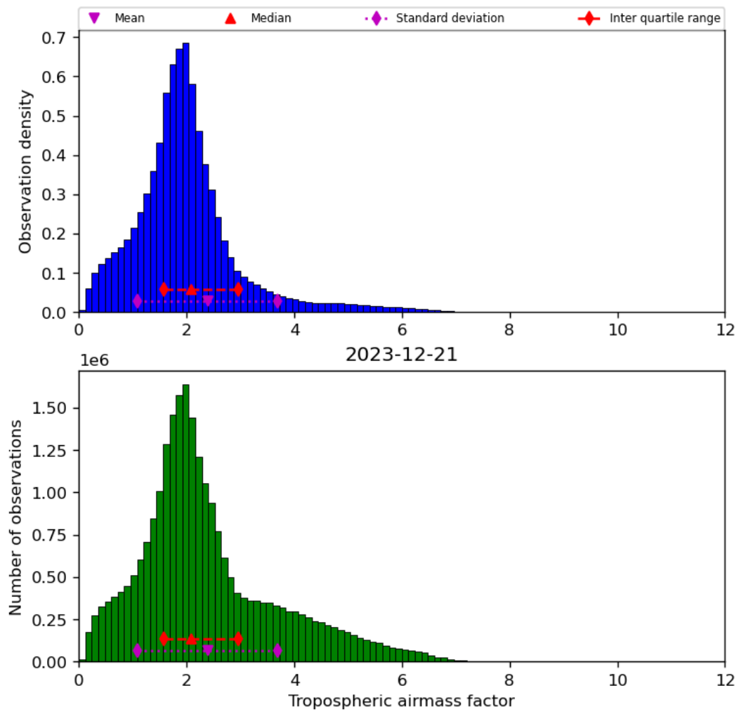
Figure 31: Histogram of “Tropospheric airmass factor” for 2023-12-20 to 2023-12-22
