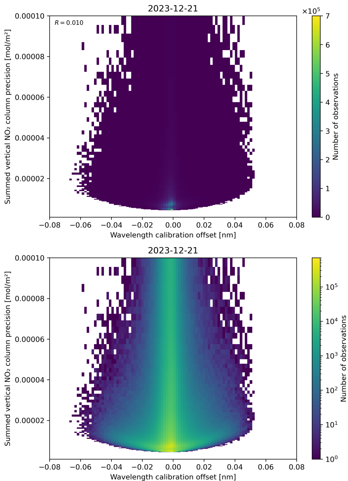
Figure 178: Scatter density plot of “Wavelength calibration offset” against “Summed vertical NO 2 column precision” for 2023-12-20 to 2023-12-22.
