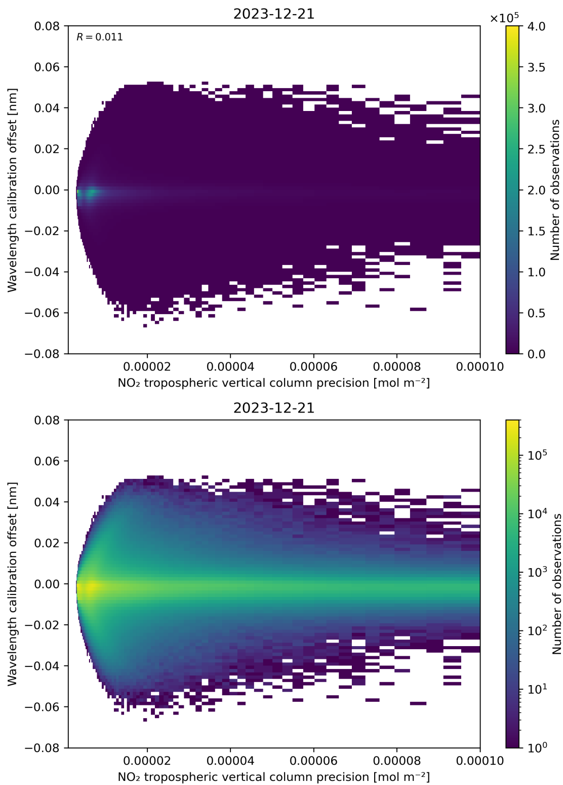
Figure 141: Scatter density plot of “NO 2 tropospheric vertical column precision” against “Wavelength calibration offset” for 2023-12-20 to 2023-12-22.
