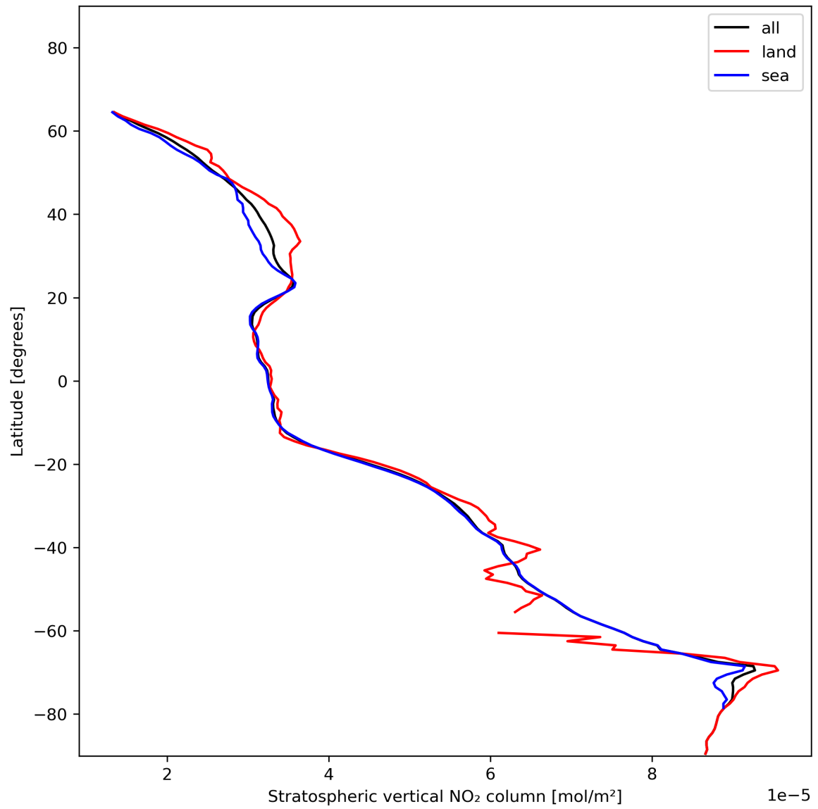
Figure 19: Zonal average of “Stratospheric vertical NO 2 column” for 2023-12-20 to 2023-12-22.
