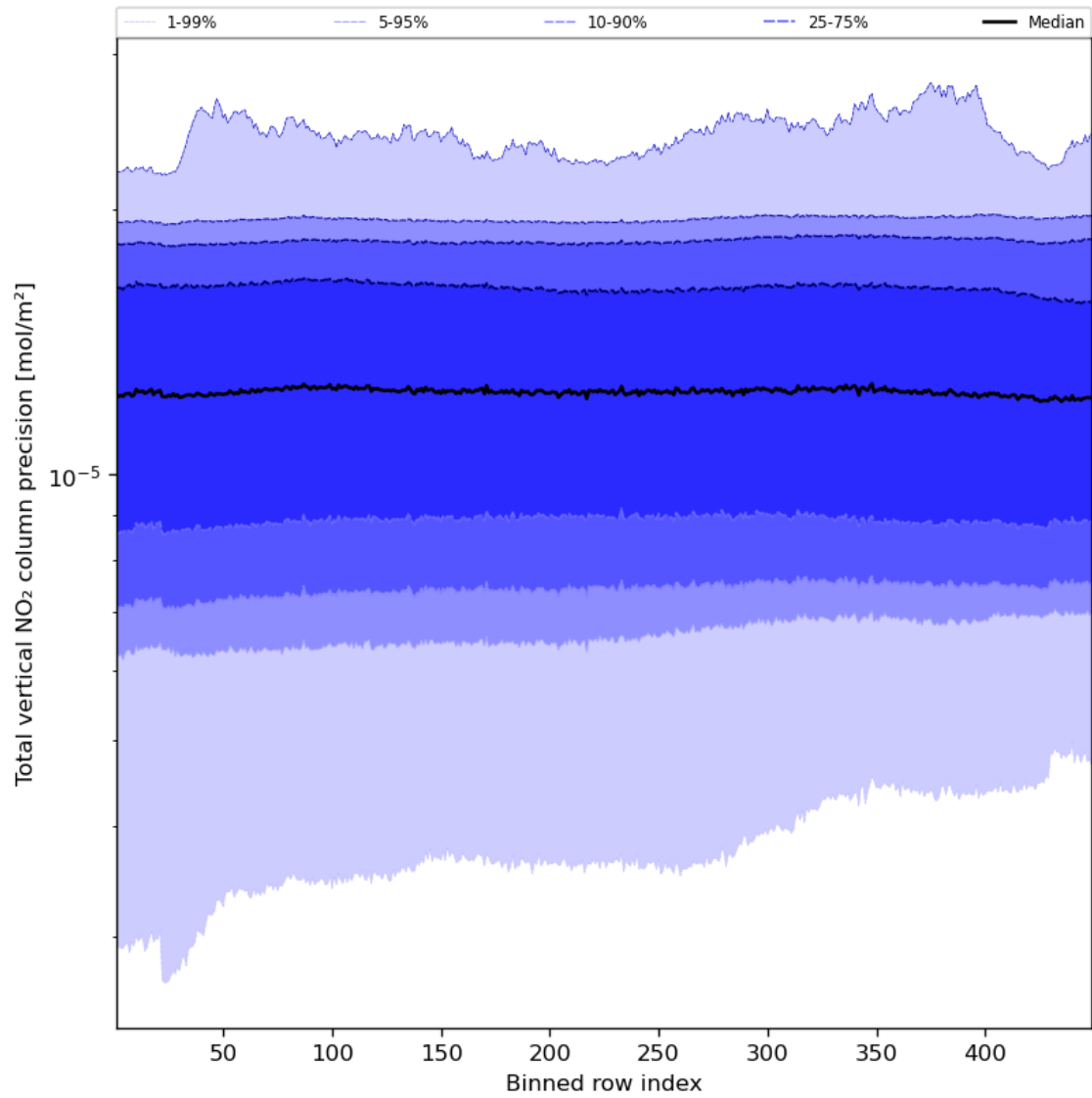
Figure 56: Along track statistics of “Total vertical NO 2 column precision” for 2023-12-20 to 2023-12-22
