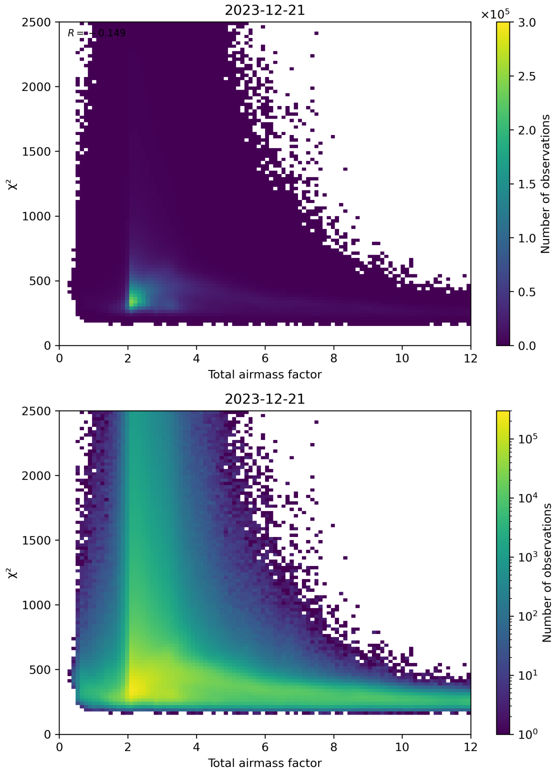
Figure 63: Scatter density plot of “Total airmass factor” against “ \chi^2 ” for 2023-12-20 to 2023-12-22.
