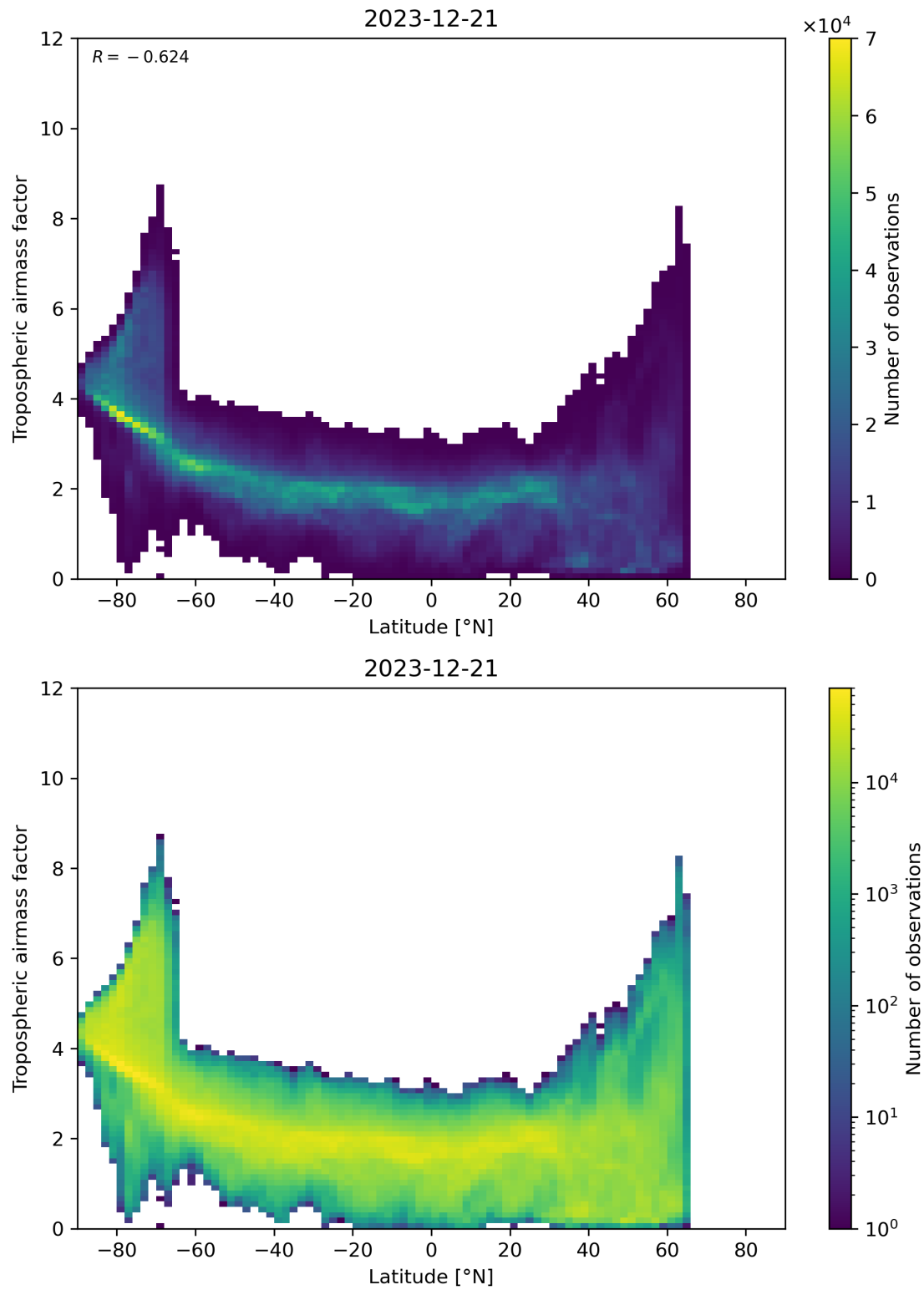
Figure 85: Scatter density plot of “Latitude” against “Tropospheric airmass factor” for 2023-12-20 to 2023-12-22.
