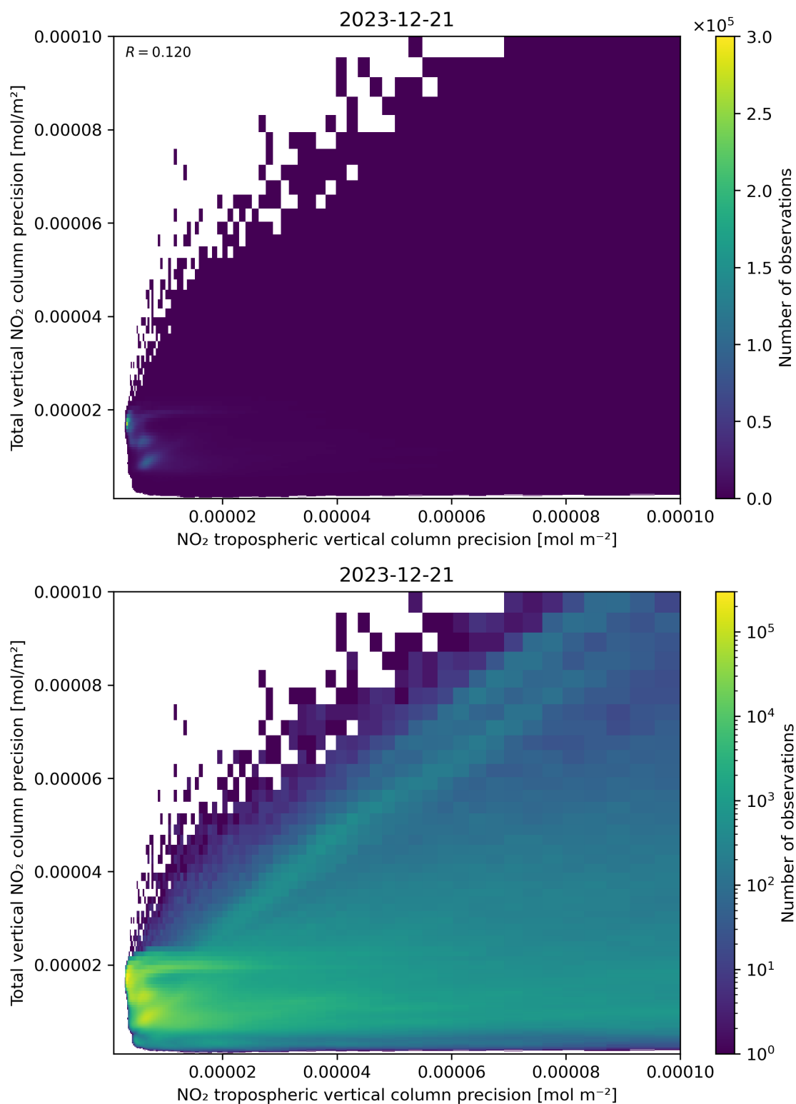
Figure 139: Scatter density plot of “NO 2 tropospheric vertical column precision” against “Total vertical NO 2 column precision” for 2023-12-20 to 2023-12-22.
