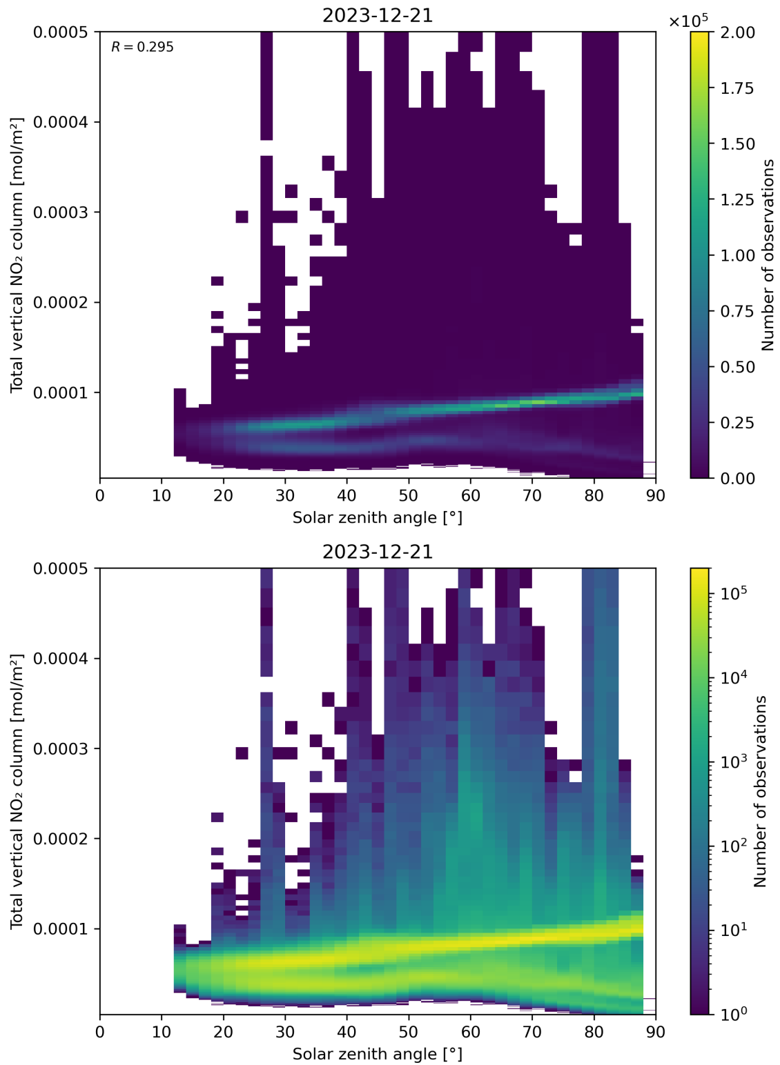
Figure 153: Scatter density plot of “Solar zenith angle” against “Total vertical NO 2 column” for 2023-12-20 to 2023-12-22.
