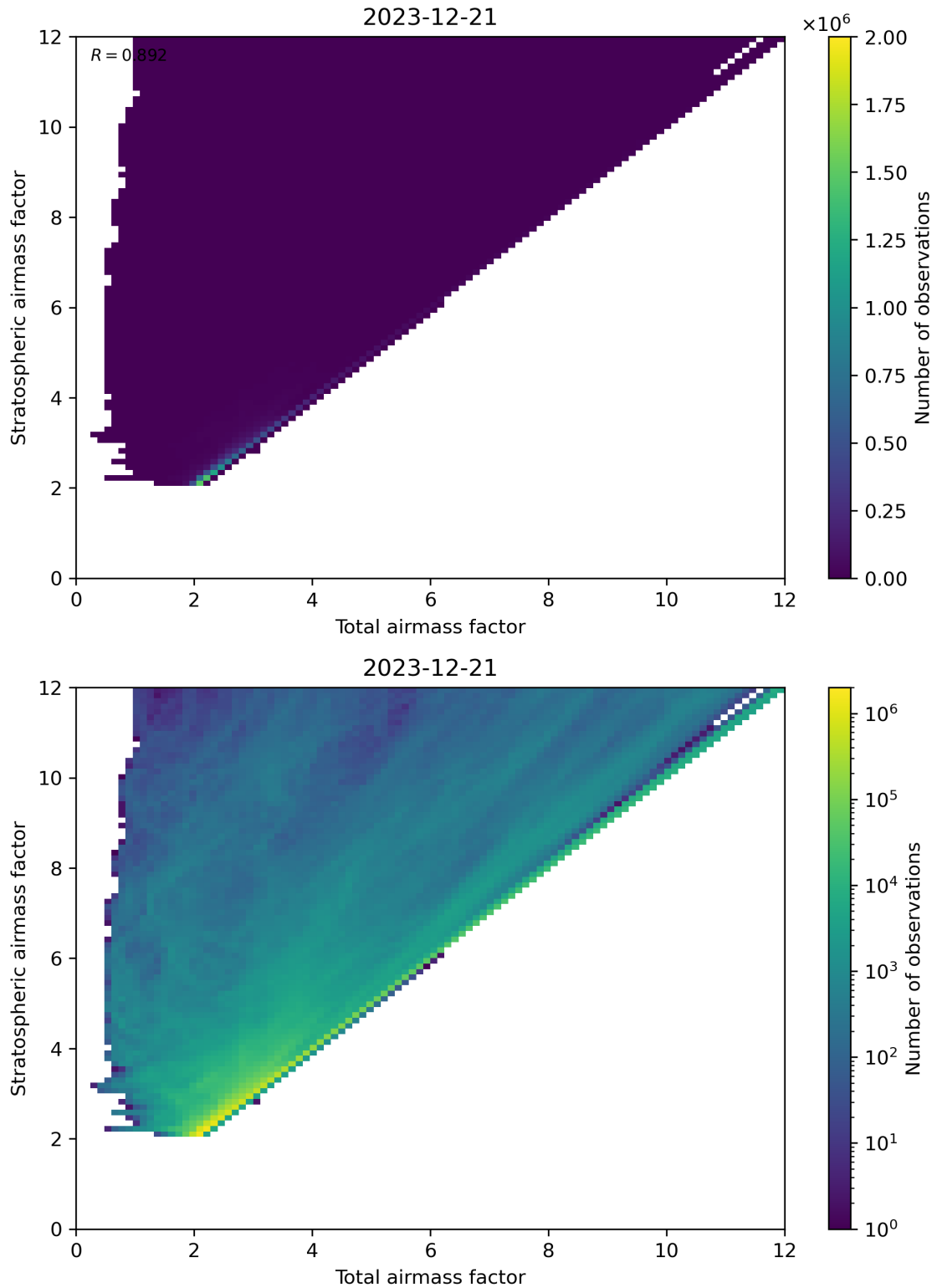
Figure 62: Scatter density plot of “Total airmass factor” against “Stratospheric airmass factor” for 2023-12-20 to 2023-12-22.
