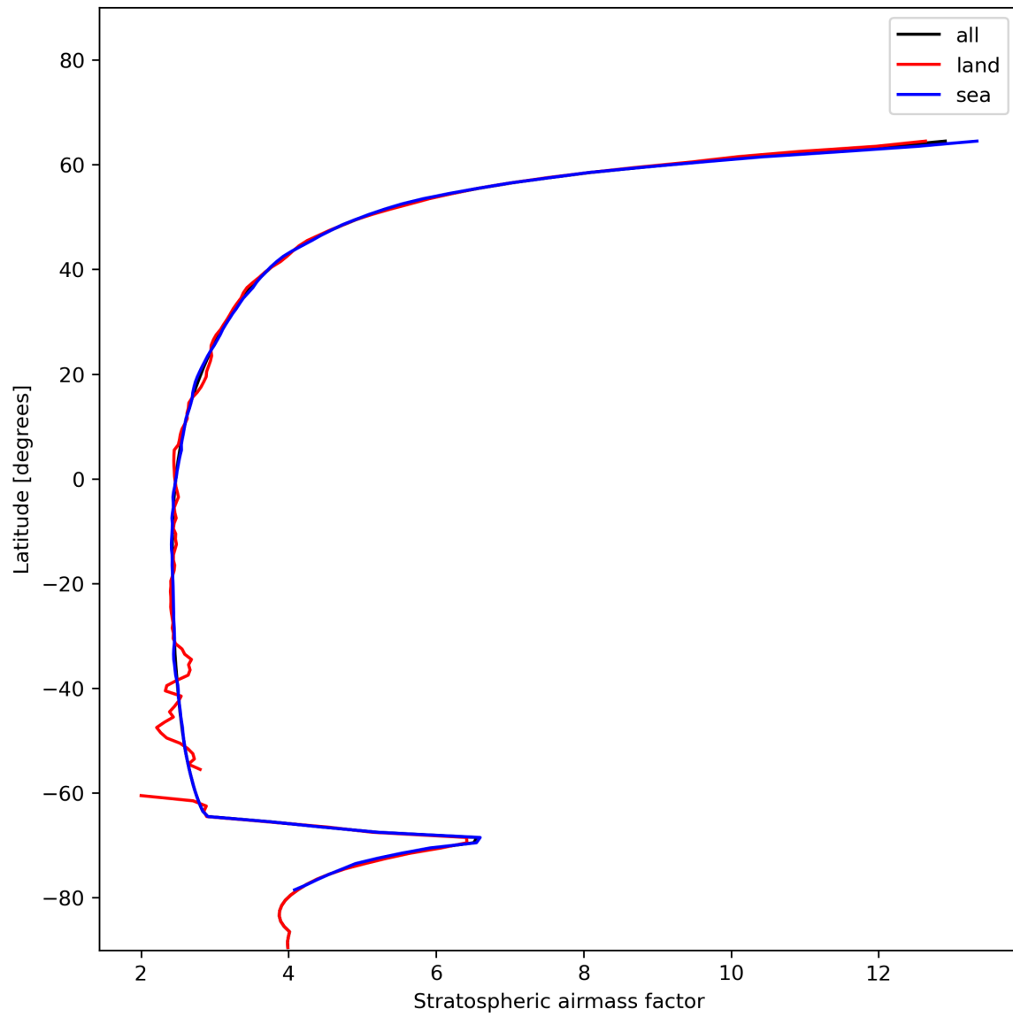
Figure 27: Zonal average of “Stratospheric air mass factor” for 2023-12-20 to 2023-12-22.
