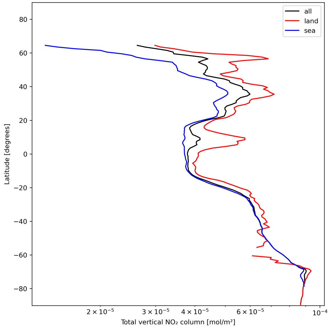
Figure 21: Zonal average of “Total vertical NO 2 column” for 2023-12-20 to 2023-12-22.
