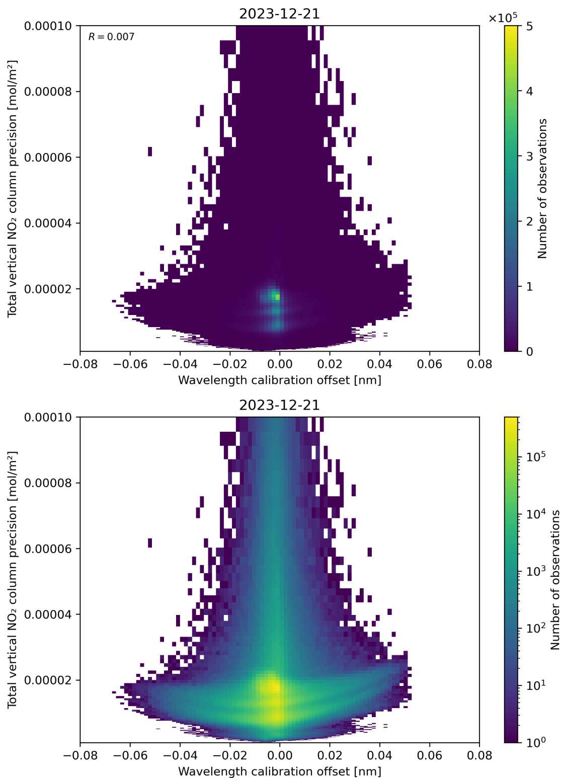
Figure 180: Scatter density plot of “Wavelength calibration offset” against “Total vertical NO 2 column precision” for 2023-12-20 to 2023-12-22.
