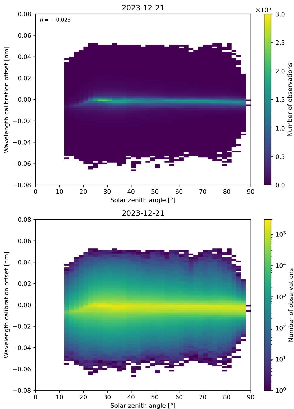
Figure 158: Scatter density plot of “Solar zenith angle” against “Wavelength calibration offset” for 2023-12-20 to 2023-12-22.
