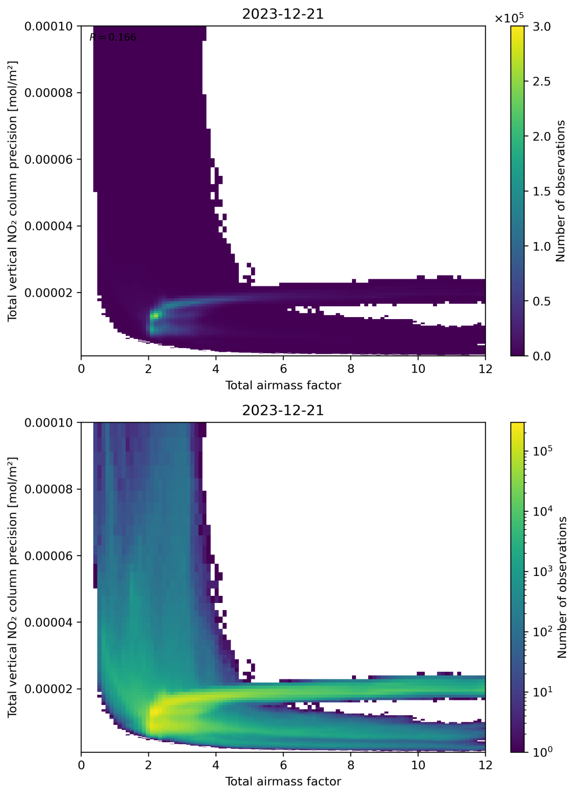
Figure 68: Scatter density plot of “Total airmass factor” against “Total vertical NO 2 column precision” for 2023-12-20 to 2023-12-22.
