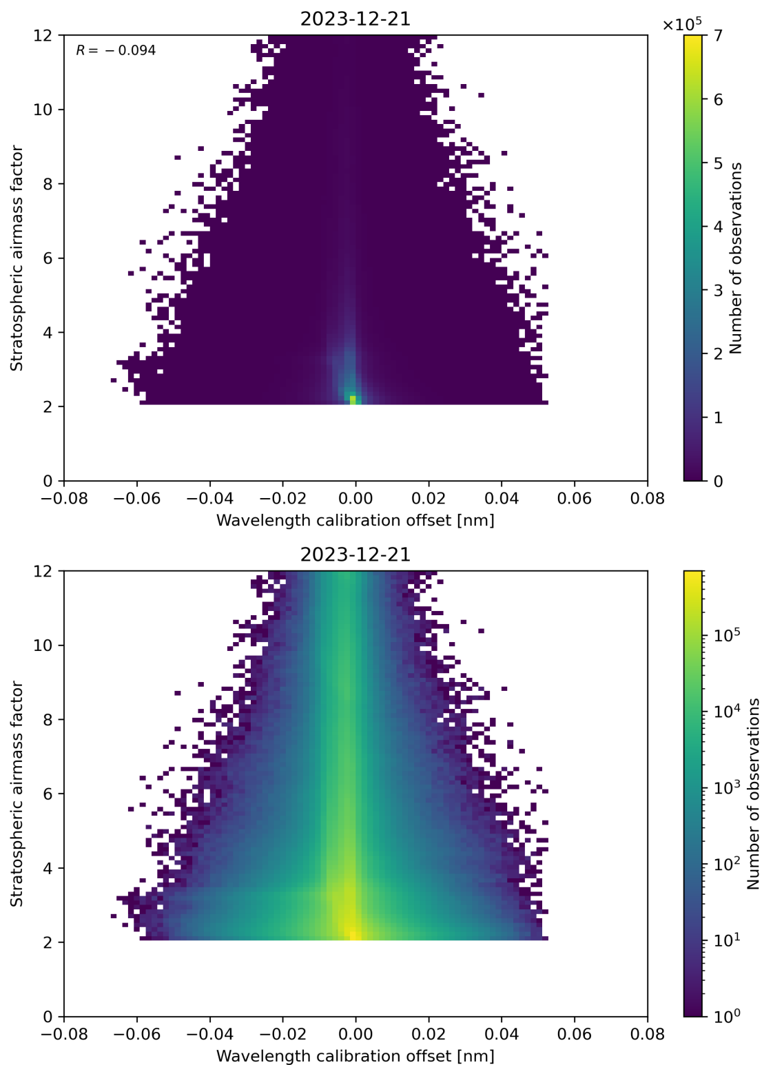
Figure 174: Scatter density plot of “Wavelength calibration offset” against “Stratospheric airmass factor” for 2023-12-20 to 2023-12-22.
