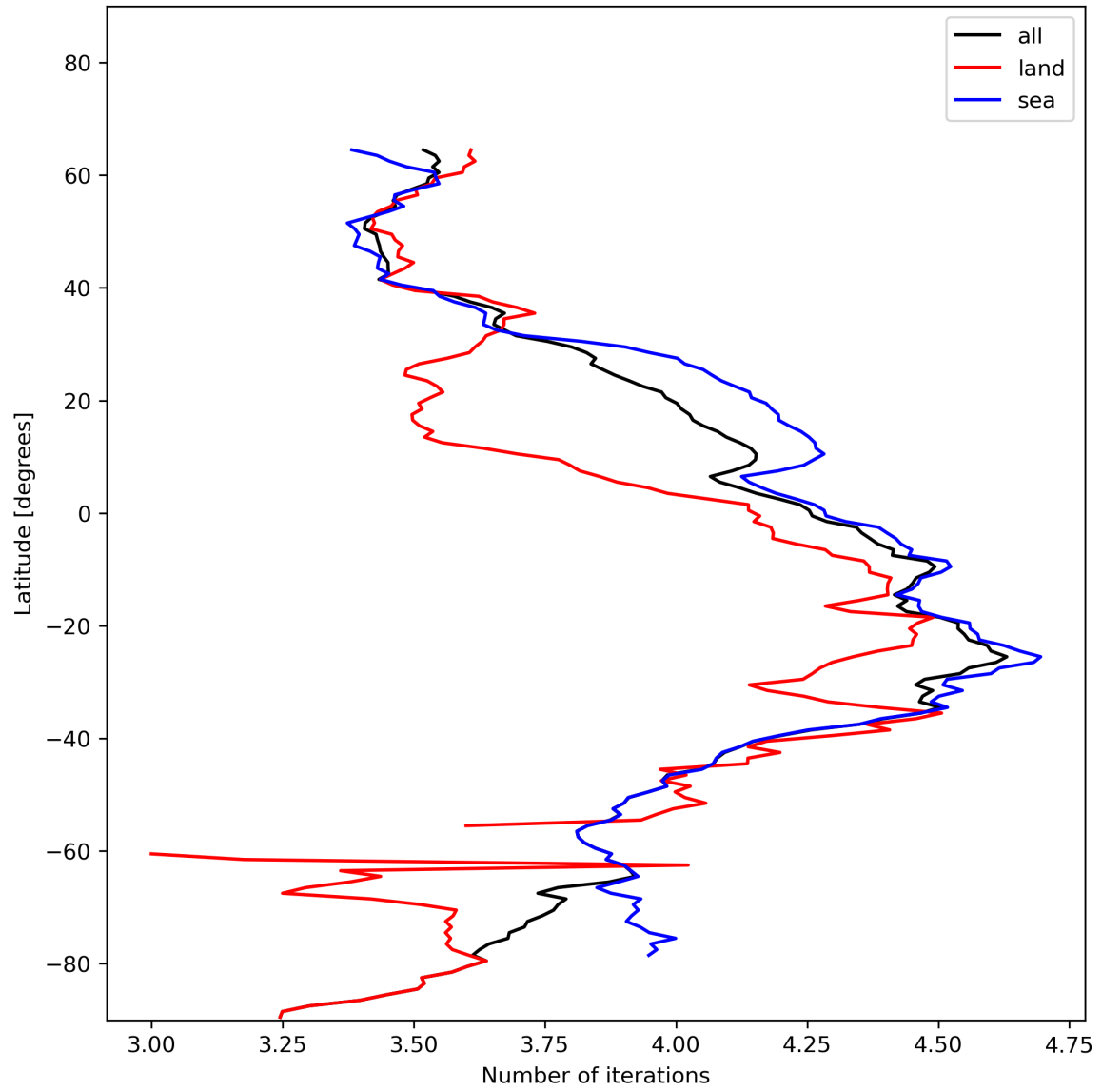
Figure 17: Zonal average of “Number of iterations” for 2023-12-20 to 2023-12-22.
