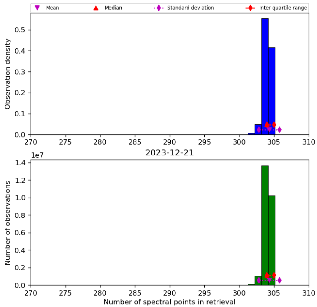
Figure 33: Histogram of “Number of spectral points in retrieval” for 2023-12-20 to 2023-12-22
