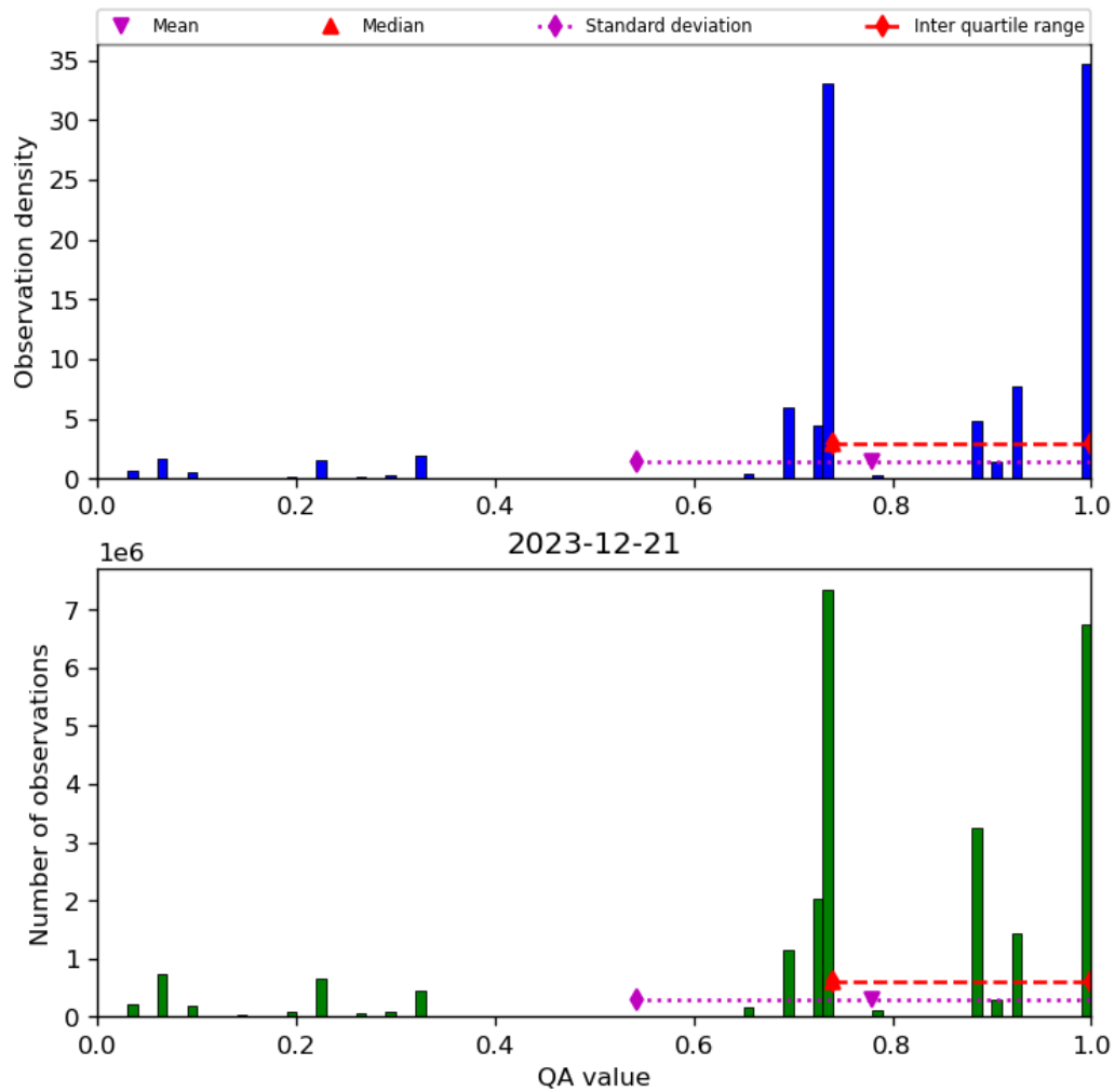
Figure 28: Histogram of “QA value” for 2023-12-20 to 2023-12-22
