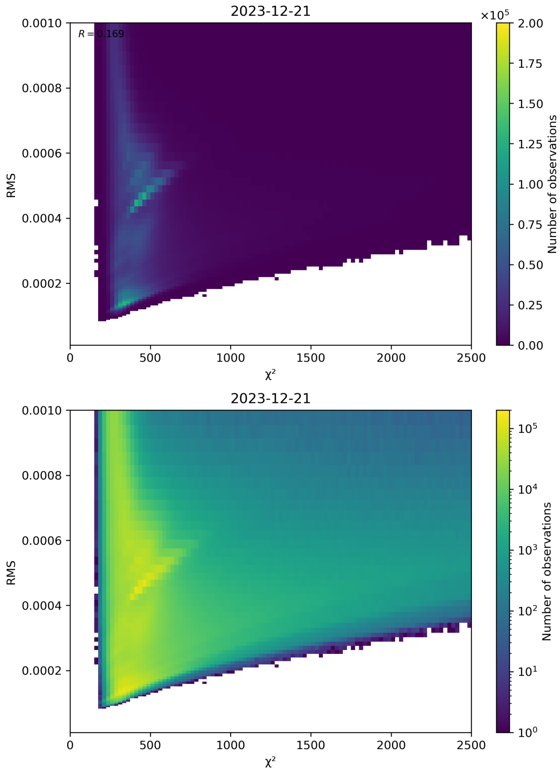
Figure 82: Scatter density plot of “ \chi^2 ” against “RMS” for 2023-12-20 to 2023-12-22.
