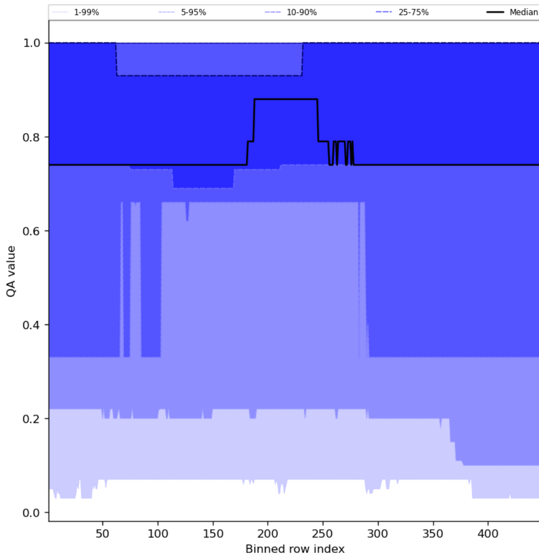
Figure 45: Along track statistics of “QA value” for 2023-12-20 to 2023-12-22
