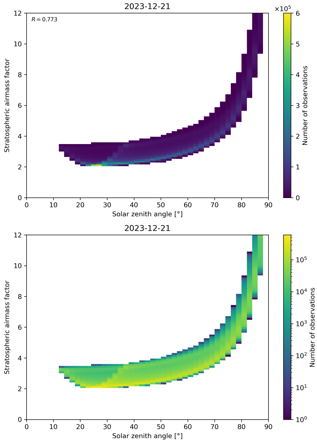
Figure 145: Scatter density plot of “Solar zenith angle” against “Stratospheric airmass factor” for 2023-12-20 to 2023-12-22.
