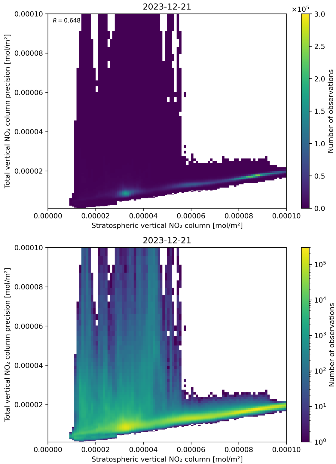
Figure 101: Scatter density plot of “Stratospheric vertical NO 2 column” against “Total vertical NO 2 column precision” for 2023-12-20 to 2023-12-22.
