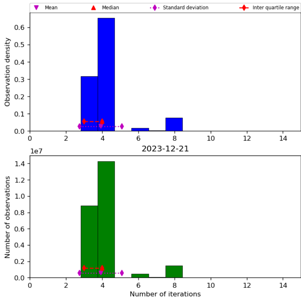
Figure 34: Histogram of “Number of iterations” for 2023-12-20 to 2023-12-22
