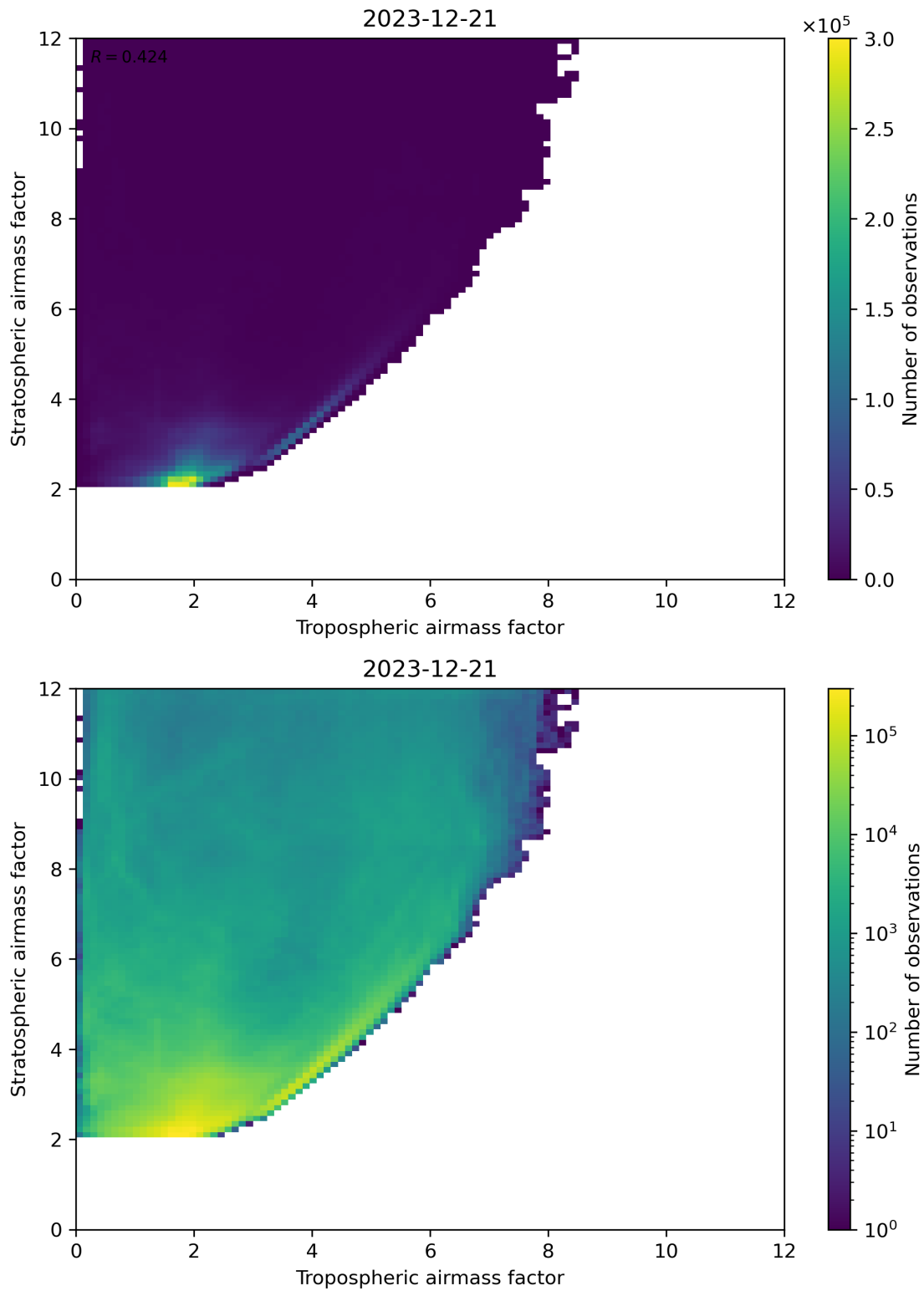
Figure 71: Scatter density plot of “Tropospheric airmass factor” against “Stratospheric airmass factor” for 2023-12-20 to 2023-12-22.
