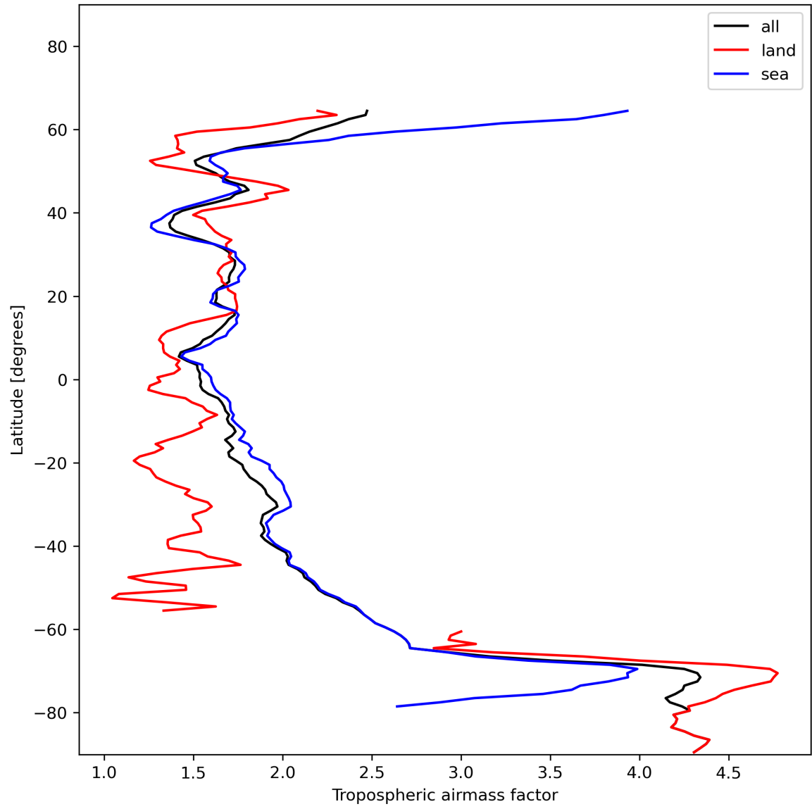
Figure 14: Zonal average of “Tropospheric airmass factor” for 2023-12-20 to 2023-12-22.
