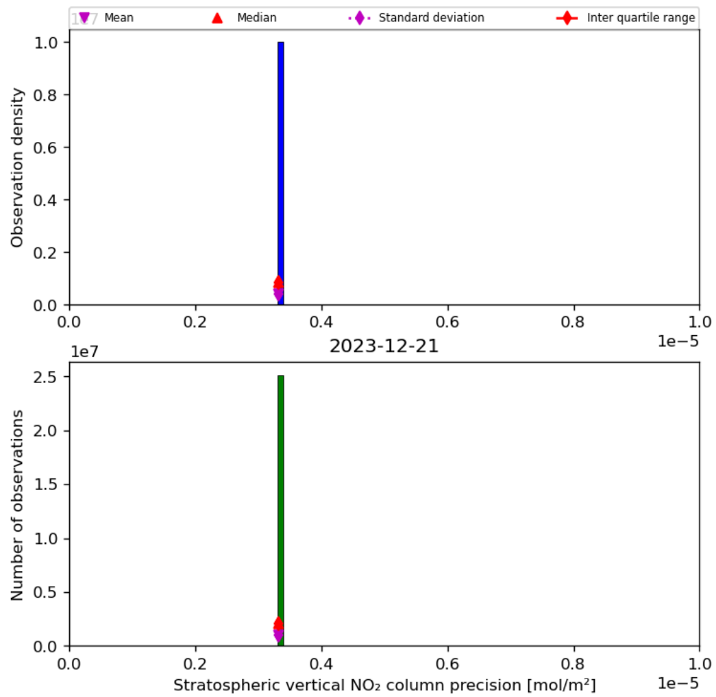
Figure 37: Histogram of “Stratospheric vertical NO 2 column precision” for 2023-12-20 to 2023-12-22
