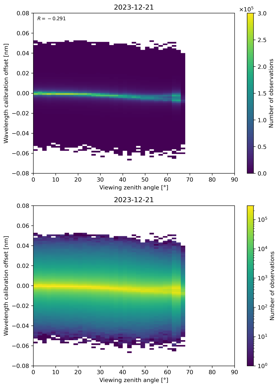
Figure 173: Scatter density plot of “Viewing zenith angle” against “Wavelength calibration offset” for 2023-12-20 to 2023-12-22.
