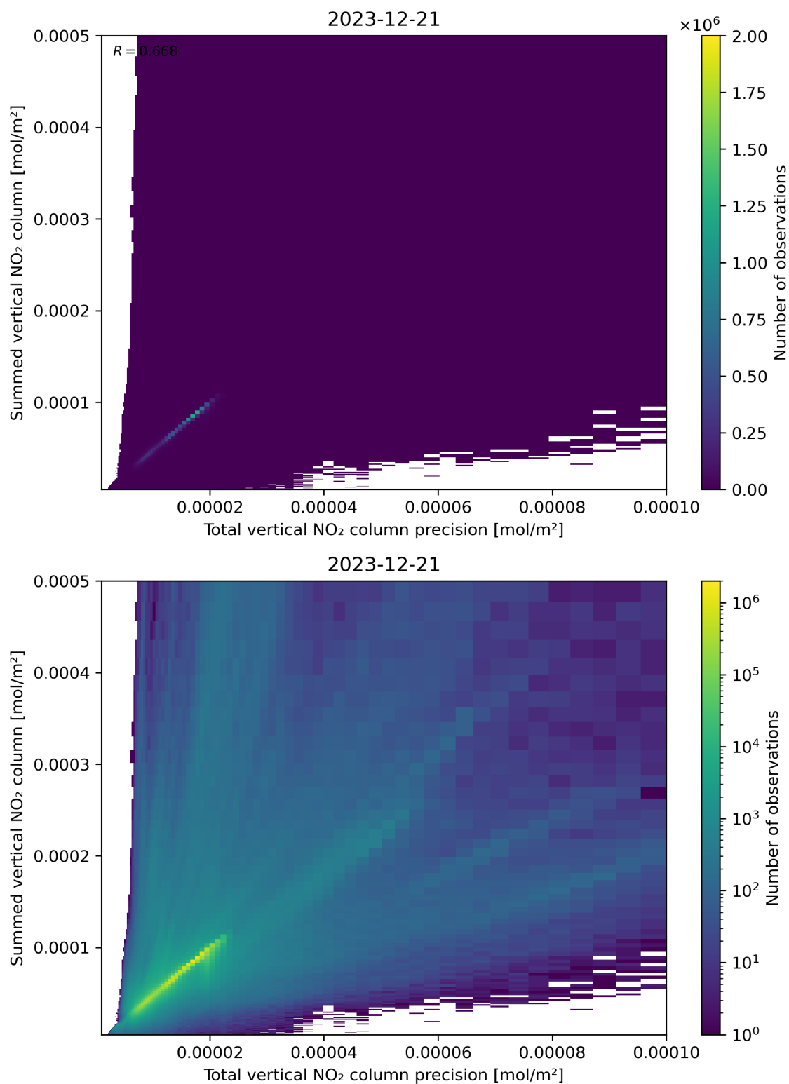
Figure 117: Scatter density plot of “Total vertical NO 2 column precision” against “Summed vertical NO 2 column” for 2023-12-20 to 2023-12-22.
