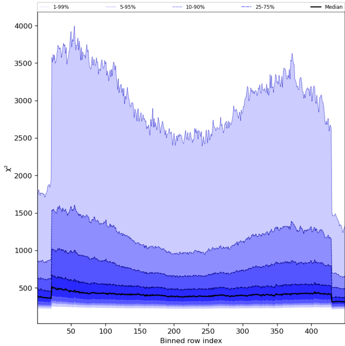
Figure 59: Along track statistics of “ \chi^2 ” for 2023-12-20 to 2023-12-22
