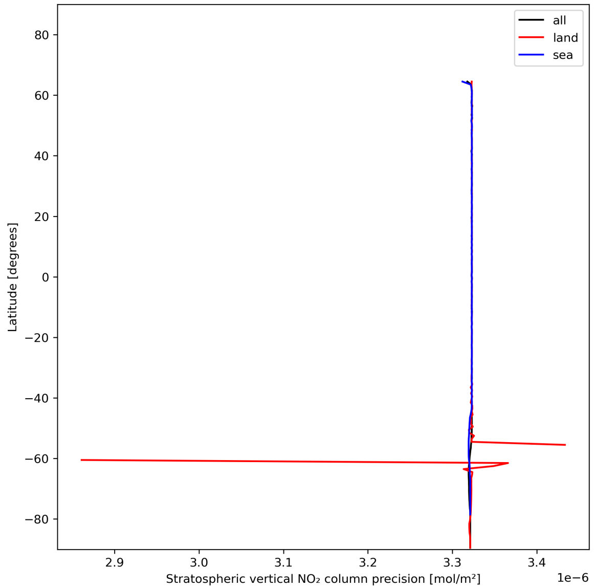
Figure 20: Zonal average of “Stratospheric vertical NO 2 column precision” for 2023-12-20 to 2023-12-22.
