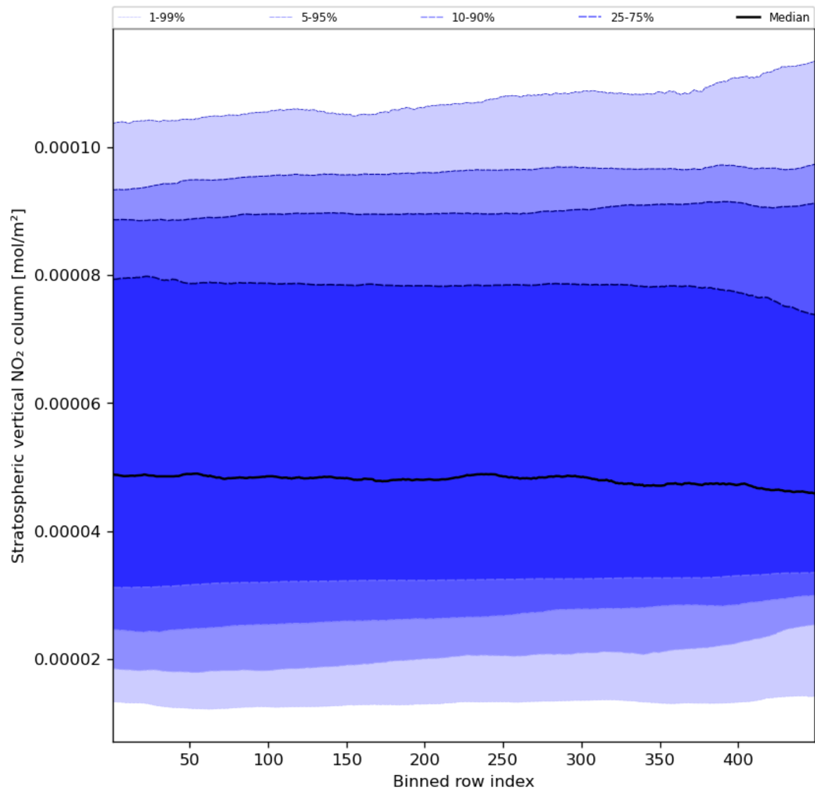
Figure 53: Along track statistics of “Stratospheric vertical NO 2 column” for 2023-12-20 to 2023-12-22
