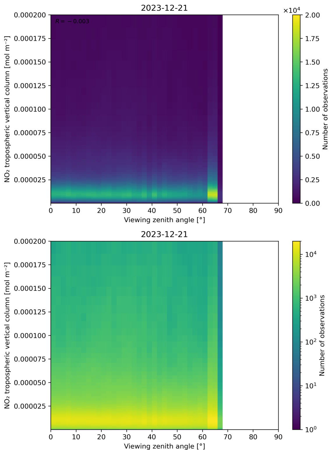
Figure 169: Scatter density plot of “Viewing zenith angle” against “NO 2 tropospheric vertical column” for 2023-12-20 to 2023-12-22.
