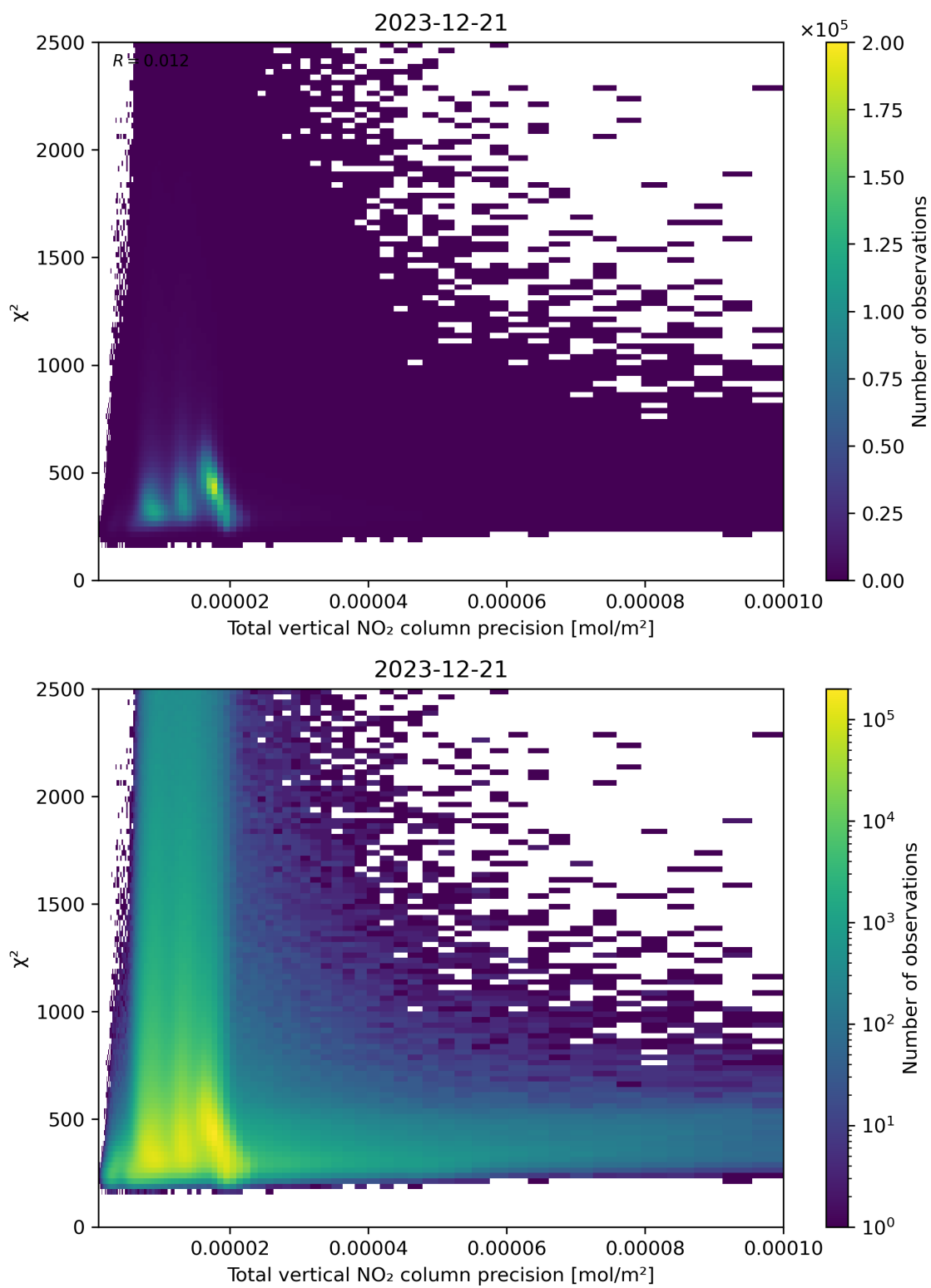
Figure 116: Scatter density plot of “Total vertical NO 2 column precision” against “ \chi^2 ” for 2023-12-20 to 2023-12-22.
