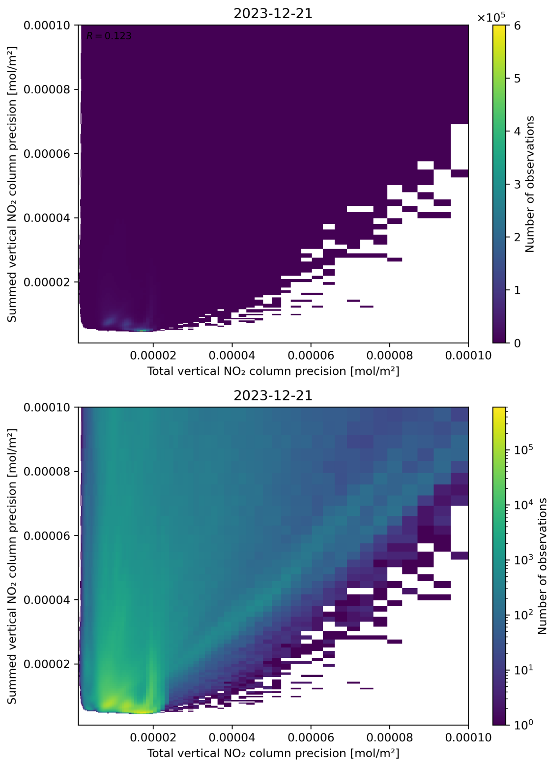
Figure 118: Scatter density plot of “Total vertical NO 2 column precision” against “Summed vertical NO 2 column precision” for 2023-12-20 to 2023-12-22.
