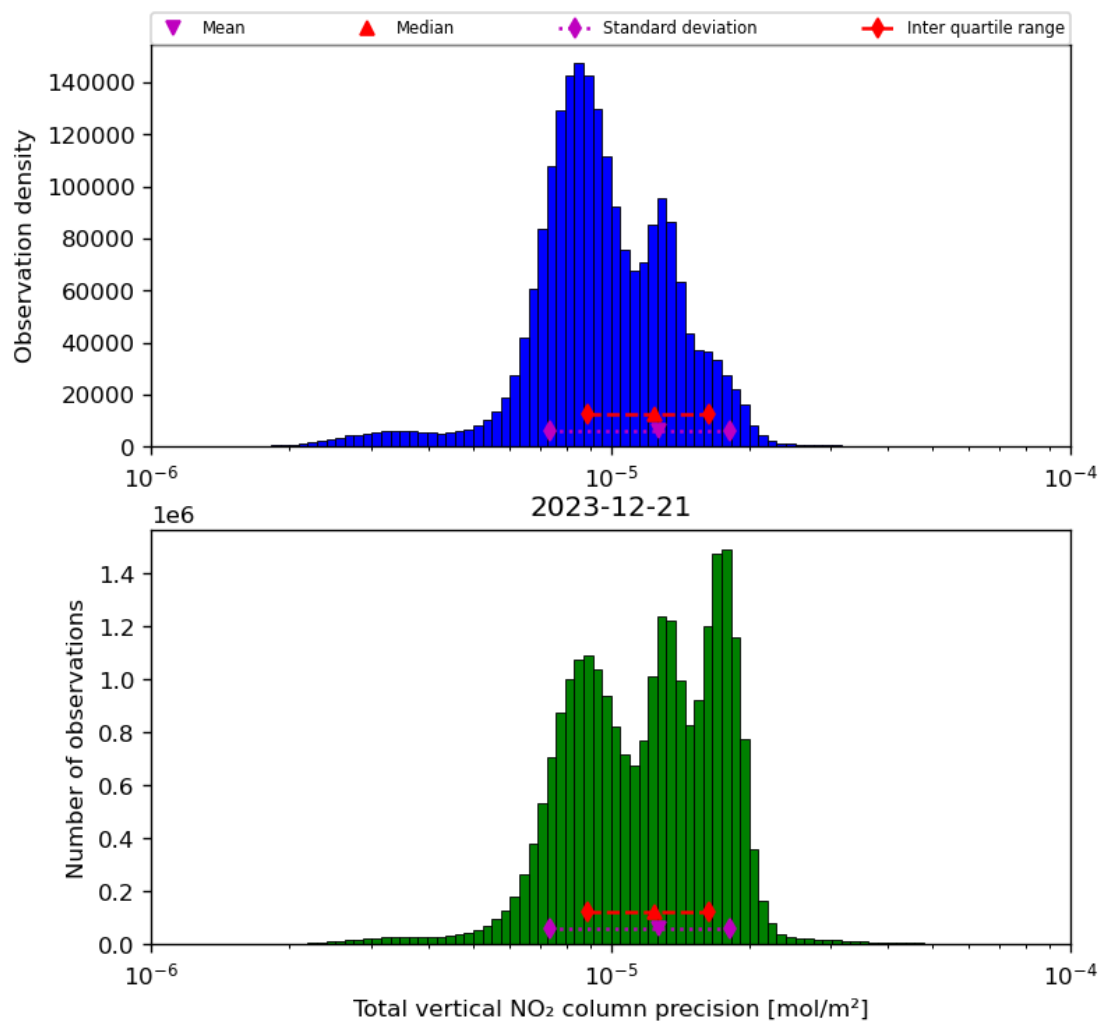
Figure 39: Histogram of “Total vertical NO 2 column precision” for 2023-12-20 to 2023-12-22
