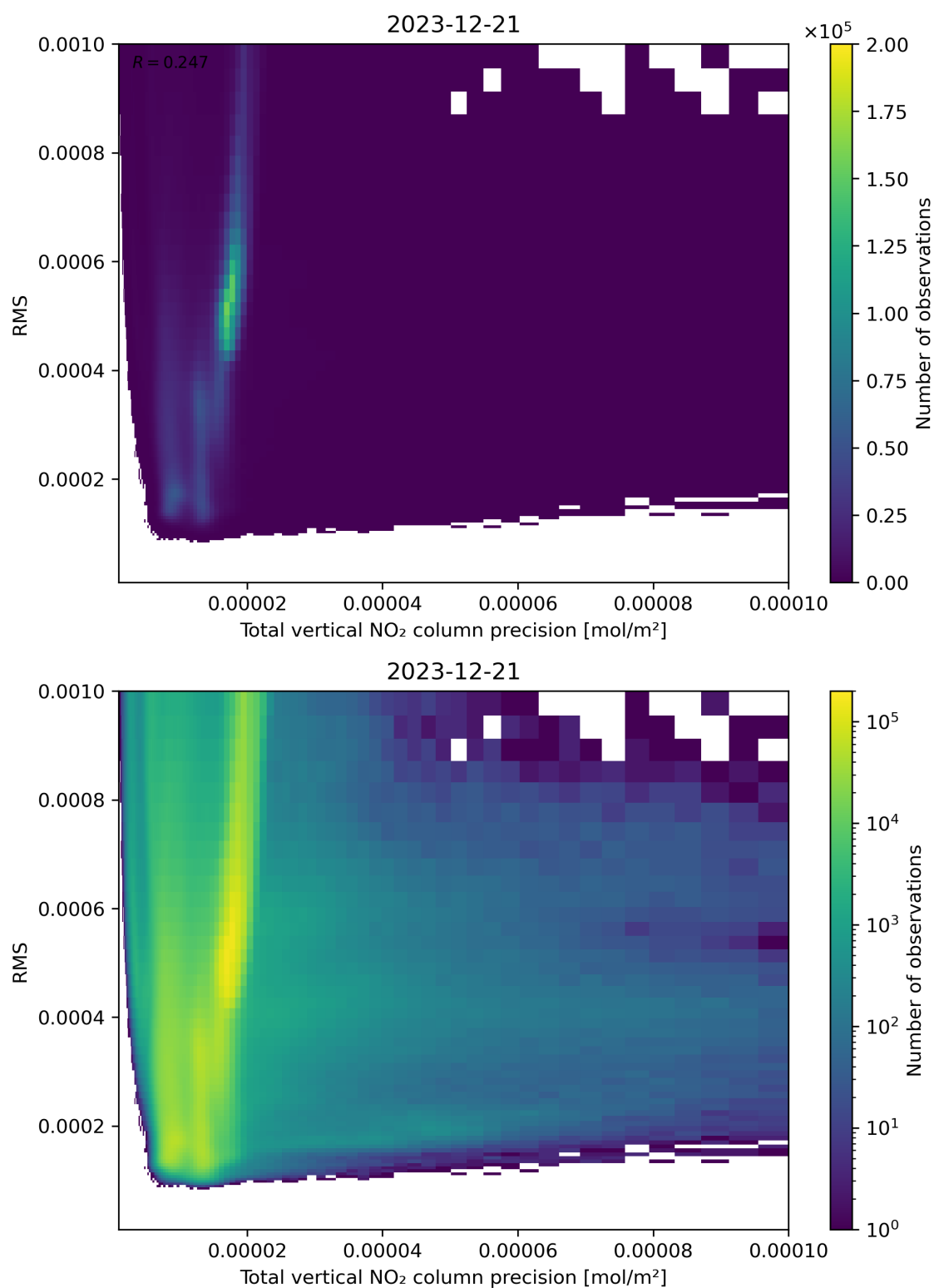
Figure 119: Scatter density plot of “Total vertical NO 2 column precision” against “RMS” for 2023-12-20 to 2023-12-22.
