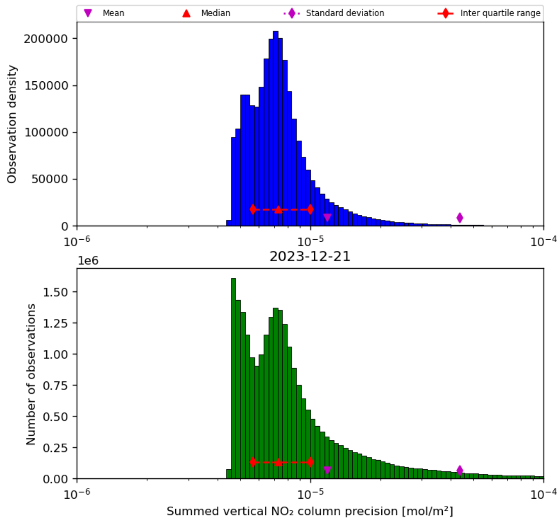
Figure 41: Histogram of “Summed vertical NO 2 column precision” for 2023-12-20 to 2023-12-22
