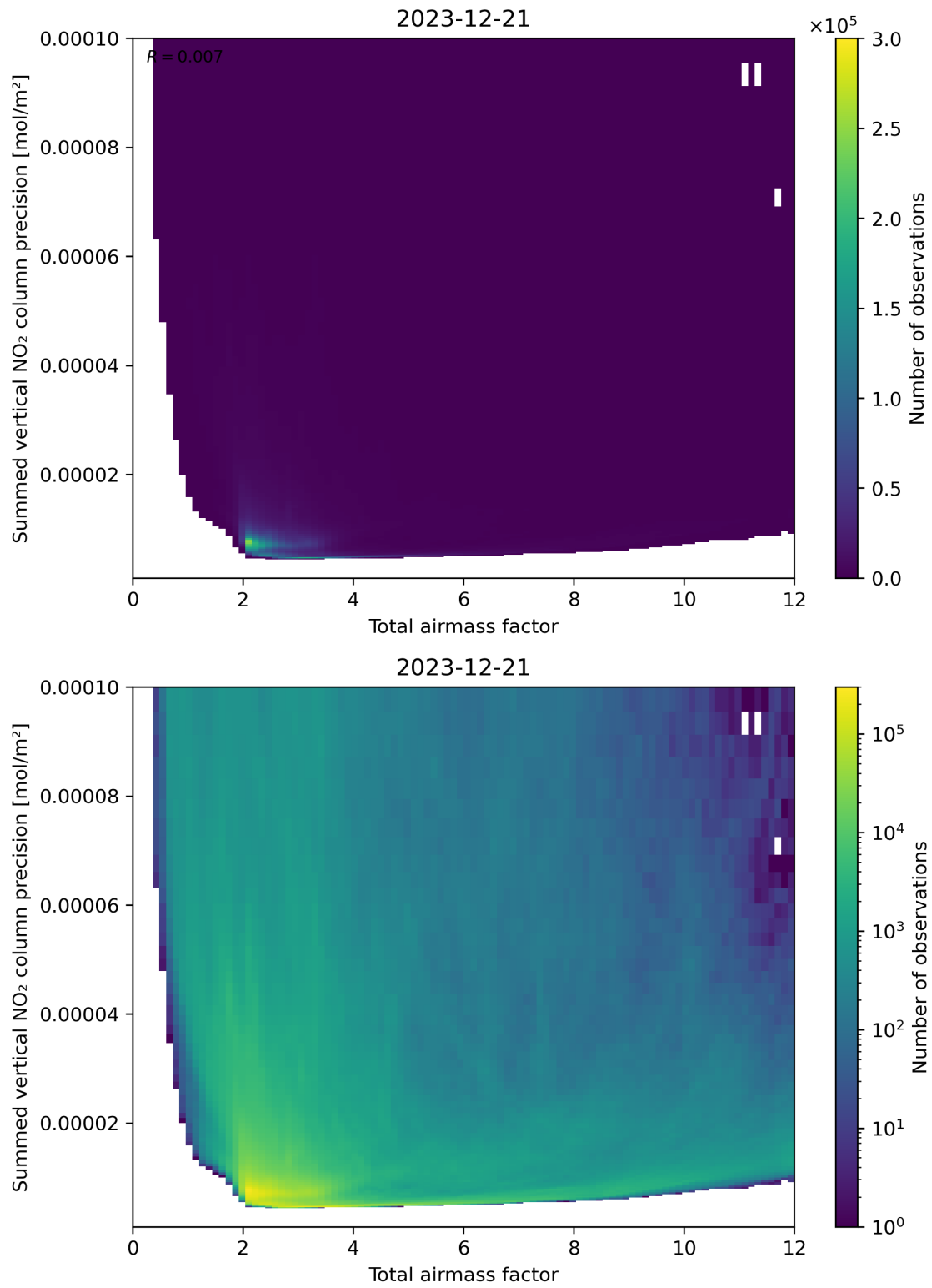
Figure 66: Scatter density plot of “Total airmass factor” against “Summed vertical NO 2 column precision” for 2023-12-20 to 2023-12-22.
