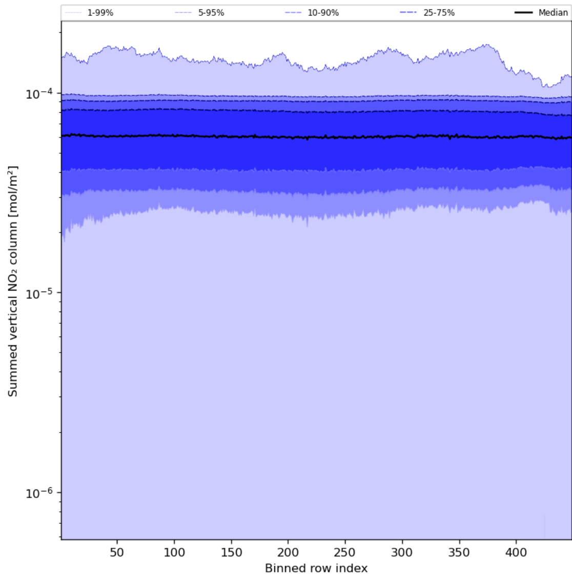
Figure 57: Along track statistics of “Summed vertical NO 2 column” for 2023-12-20 to 2023-12-22
