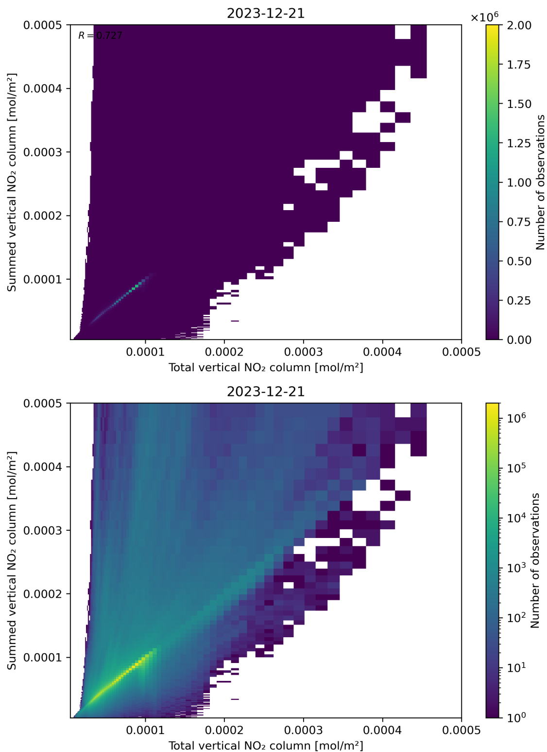
Figure 112: Scatter density plot of “Total vertical NO 2 column” against “Summed vertical NO 2 column” for 2023-12-20 to 2023-12-22.
