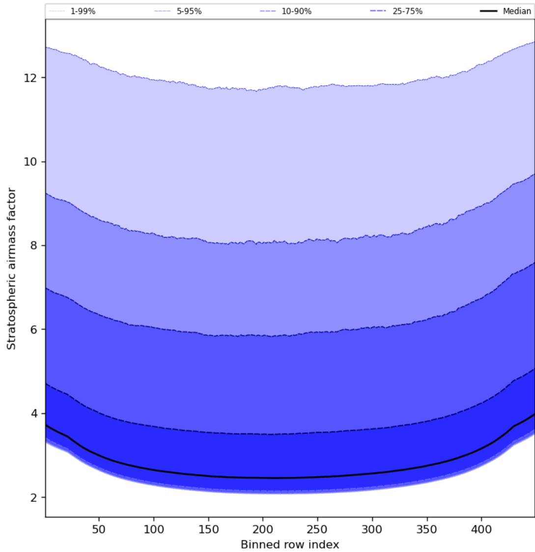
Figure 61: Along track statistics of “Stratospheric airmass factor” for 2023-12-20 to 2023-12-22
