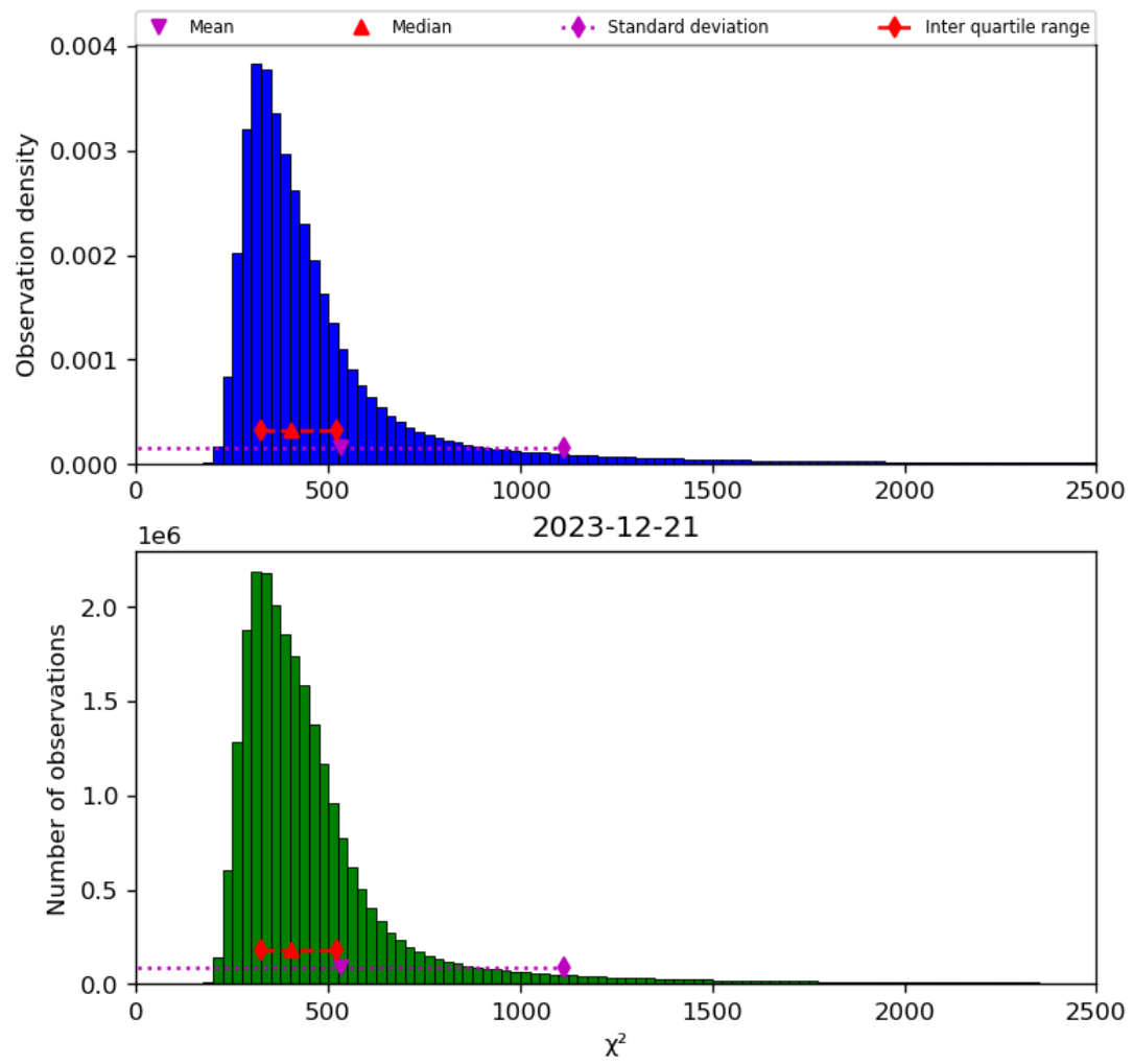
Figure 42: Histogram of “ \chi^2 ” for 2023-12-20 to 2023-12-22
