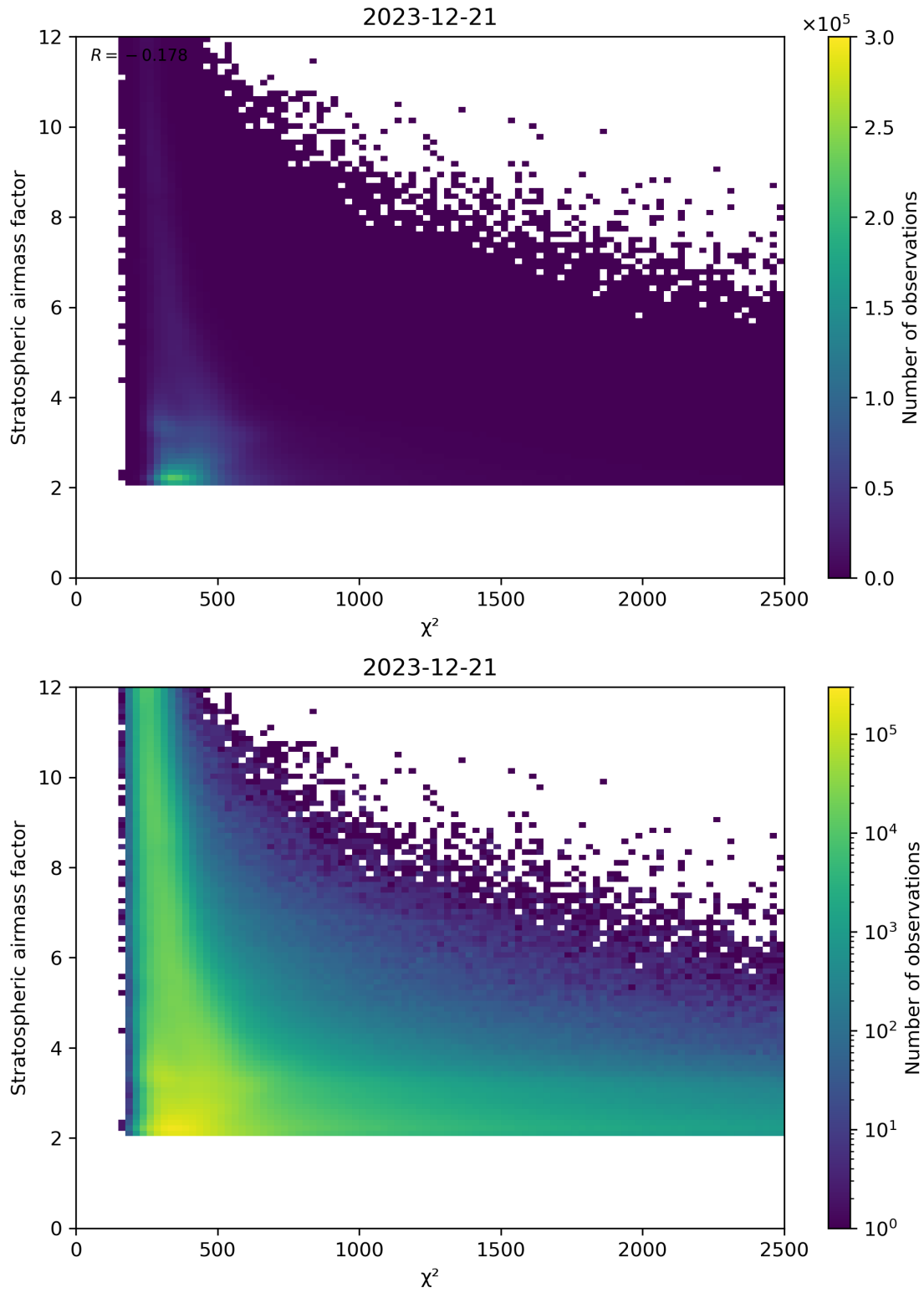
Figure 81: Scatter density plot of “ \chi^2 ” against “Stratospheric airmass factor” for 2023-12-20 to 2023-12-22.
