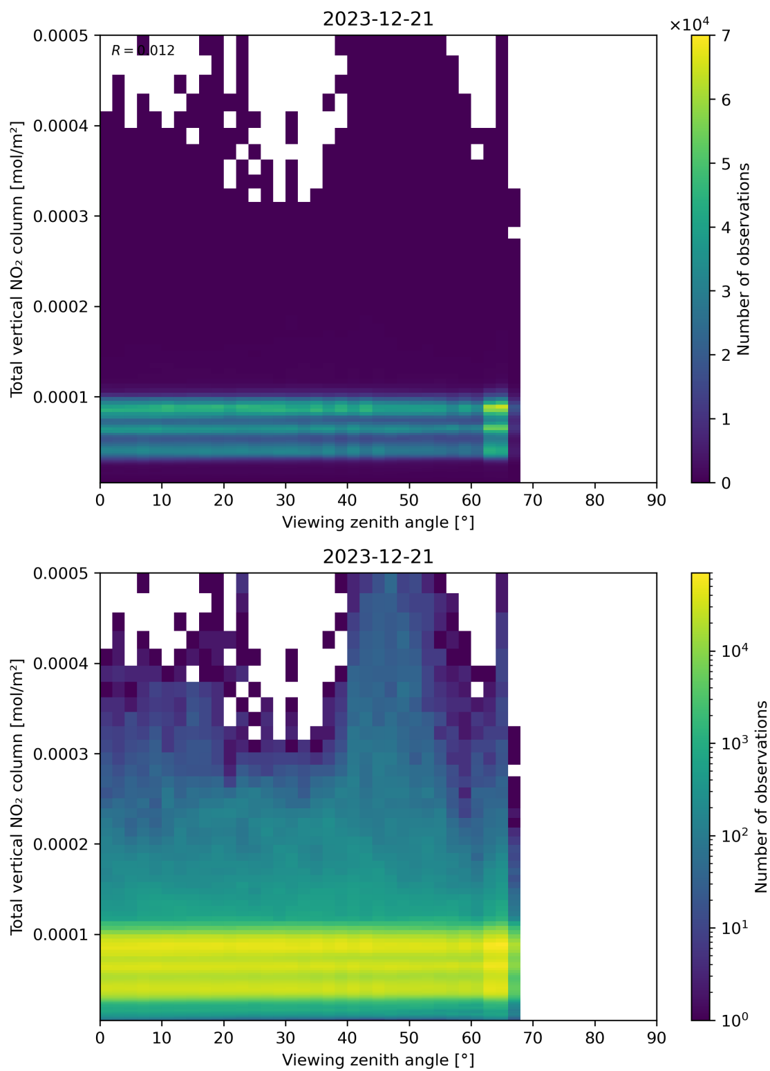
Figure 167: Scatter density plot of “Viewing zenith angle” against “Total vertical NO 2 column” for 2023-12-20 to 2023-12-22.
