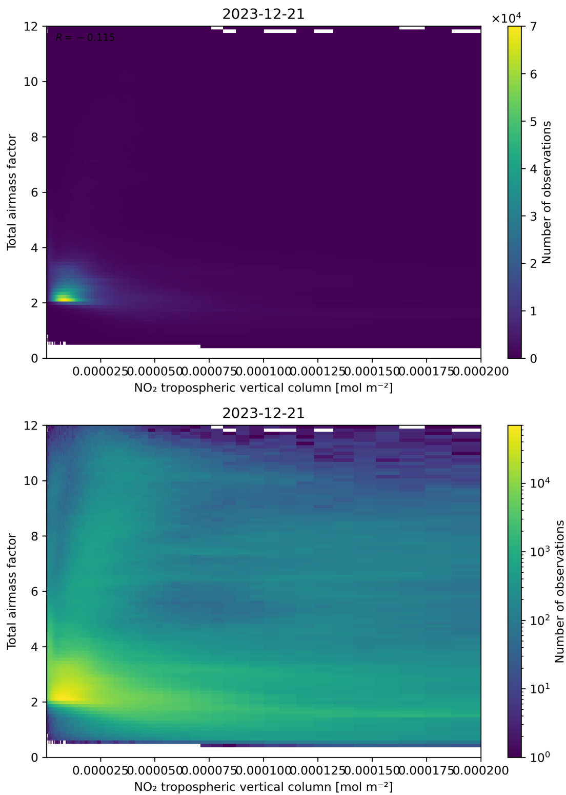
Figure 122: Scatter density plot of “NO 2 tropospheric vertical column” against “Total air mass factor” for 2023-12-20 to 2023-12-22.
