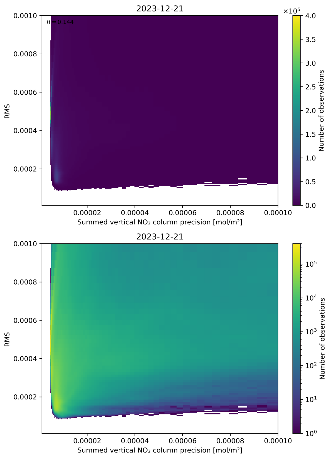
Figure 108: Scatter density plot of “Summed vertical NO 2 column precision” against “RMS” for 2023-12-20 to 2023-12-22.
