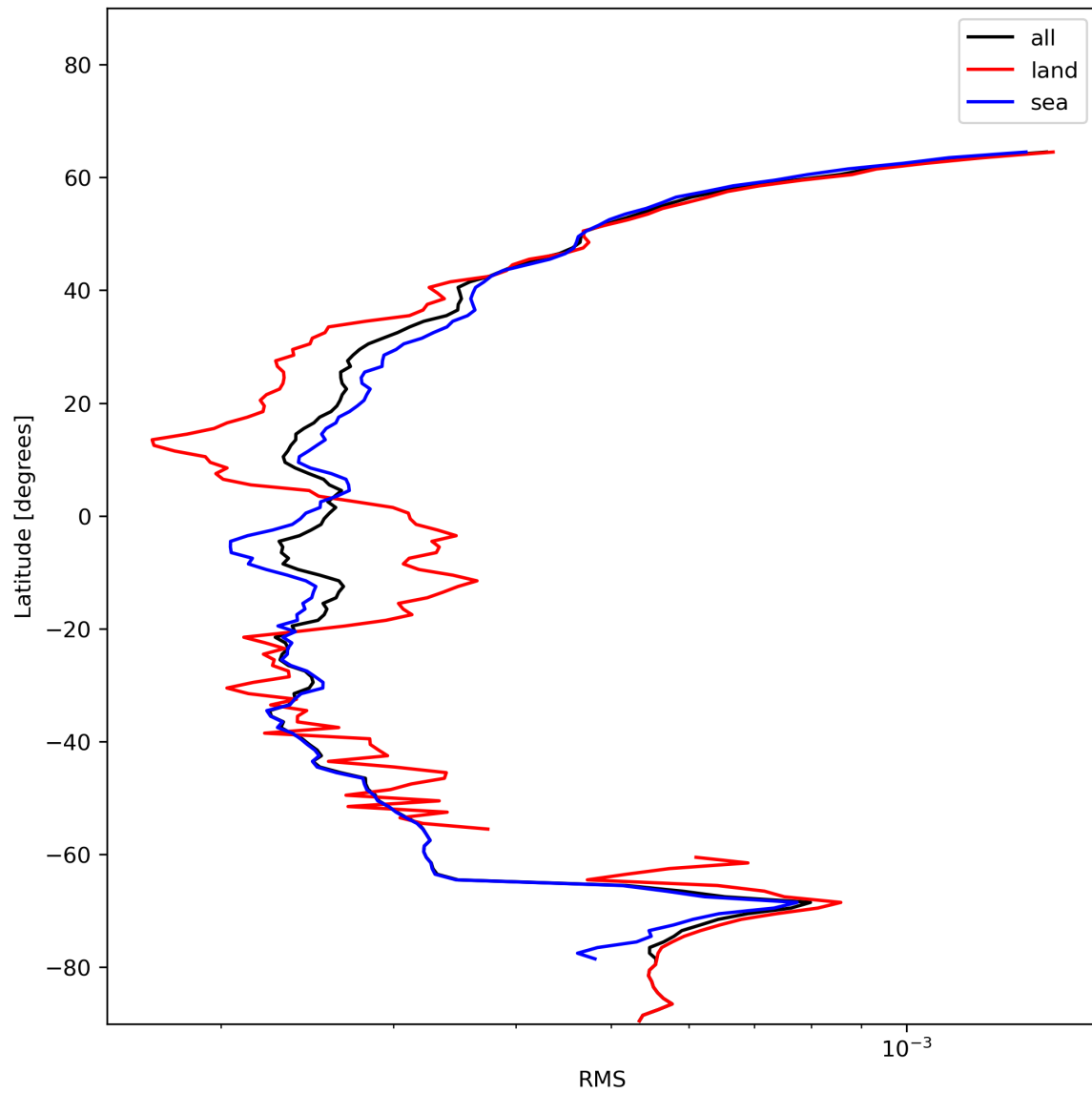
Figure 26: Zonal average of “RMS” for 2023-12-20 to 2023-12-22.
