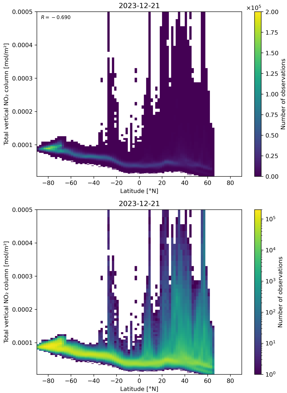
Figure 90: Scatter density plot of “Latitude” against “Total vertical NO 2 column” for 2023-12-20 to 2023-12-22.
