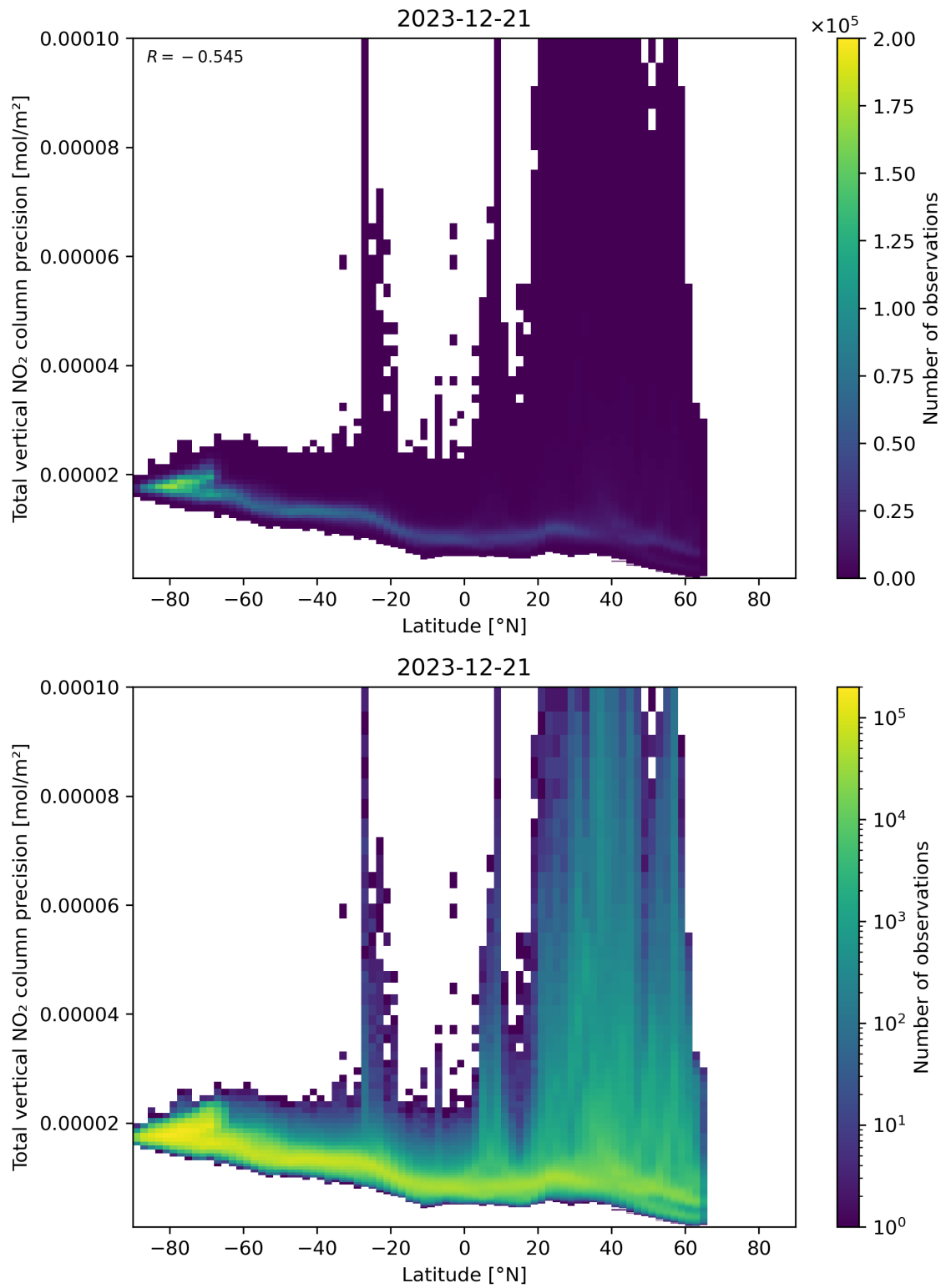
Figure 91: Scatter density plot of “Latitude” against “Total vertical NO 2 column precision” for 2023-12-20 to 2023-12-22.
