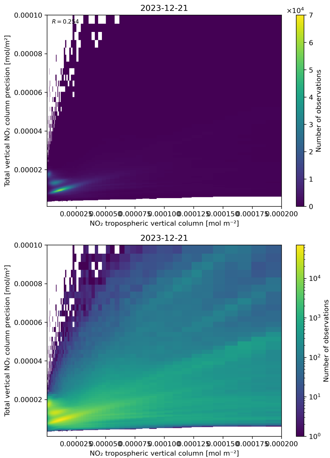
Figure 129: Scatter density plot of “NO 2 tropospheric vertical column” against “Total vertical NO 2 column precision” for 2023-12-20 to 2023-12-22.
