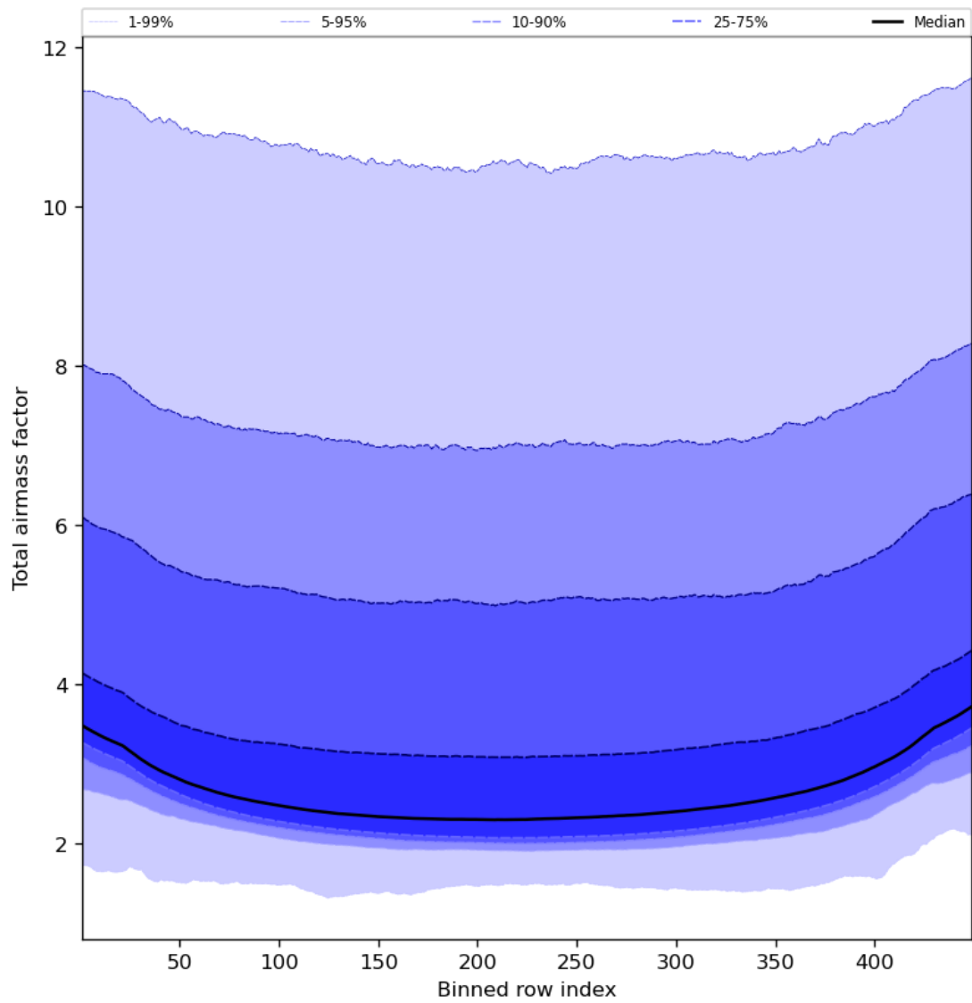
Figure 49: Along track statistics of “Total airmass factor” for 2023-12-20 to 2023-12-22
