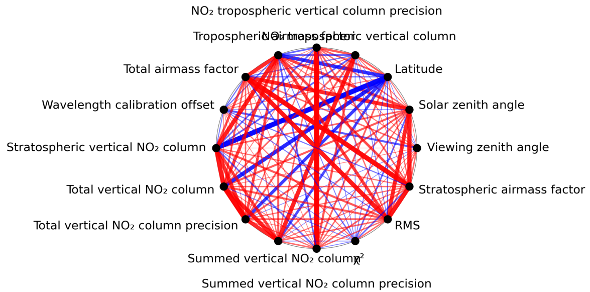
Figure 1: Map of correlation graph for 2023-12-20 to 2023-12-22.
