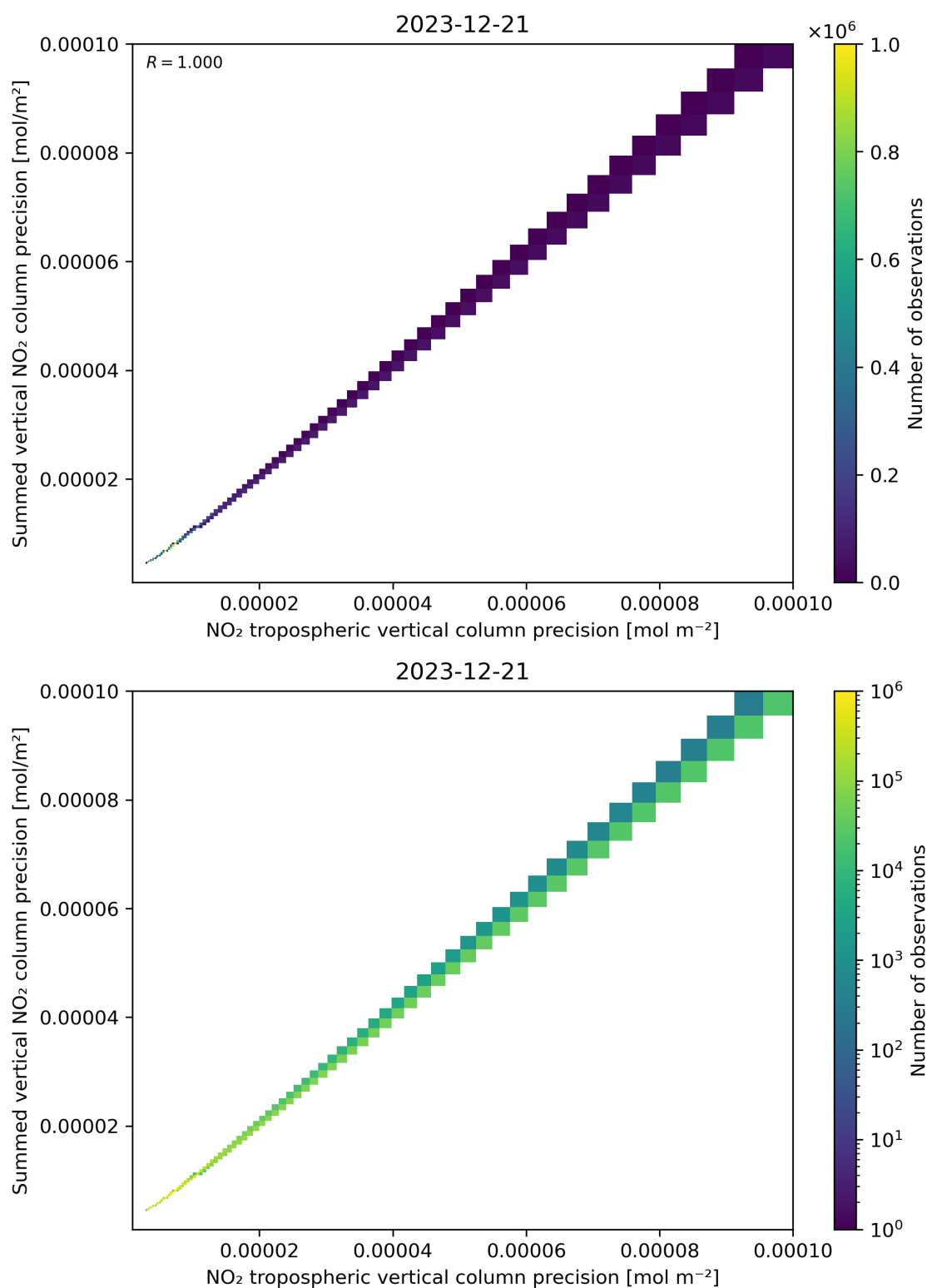
Figure 137: Scatter density plot of “NO 2 tropospheric vertical column precision” against “Summed vertical NO 2 column precision” for 2023-12-20 to 2023-12-22.
