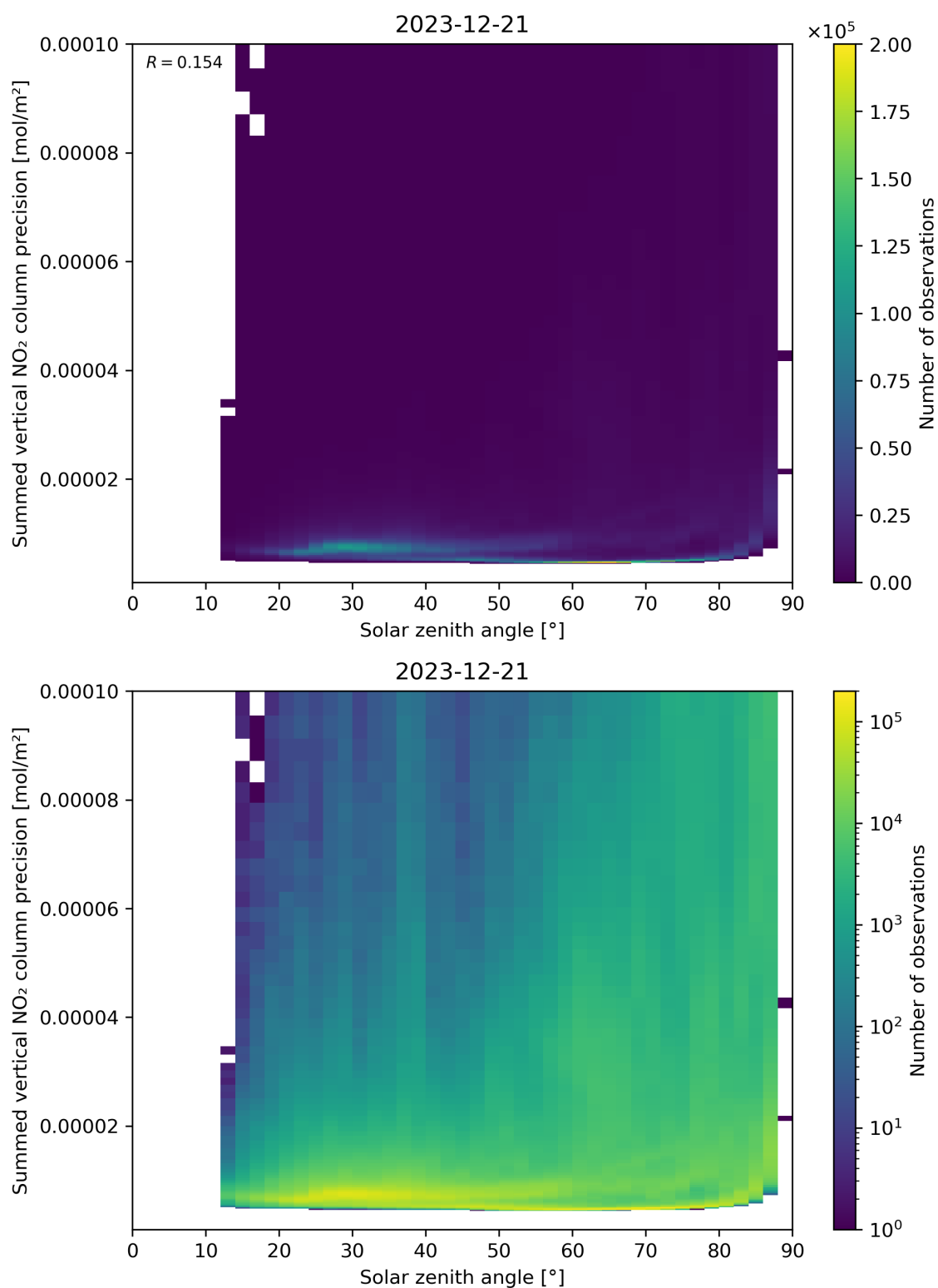
Figure 152: Scatter density plot of “Solar zenith angle” against “Summed vertical NO 2 column precision” for 2023-12-20 to 2023-12-22.
