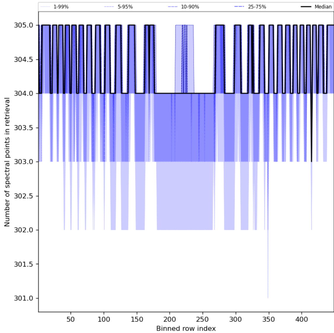
Figure 50: Along track statistics of “Number of spectral points in retrieval” for 2023-12-20 to 2023-12-22
