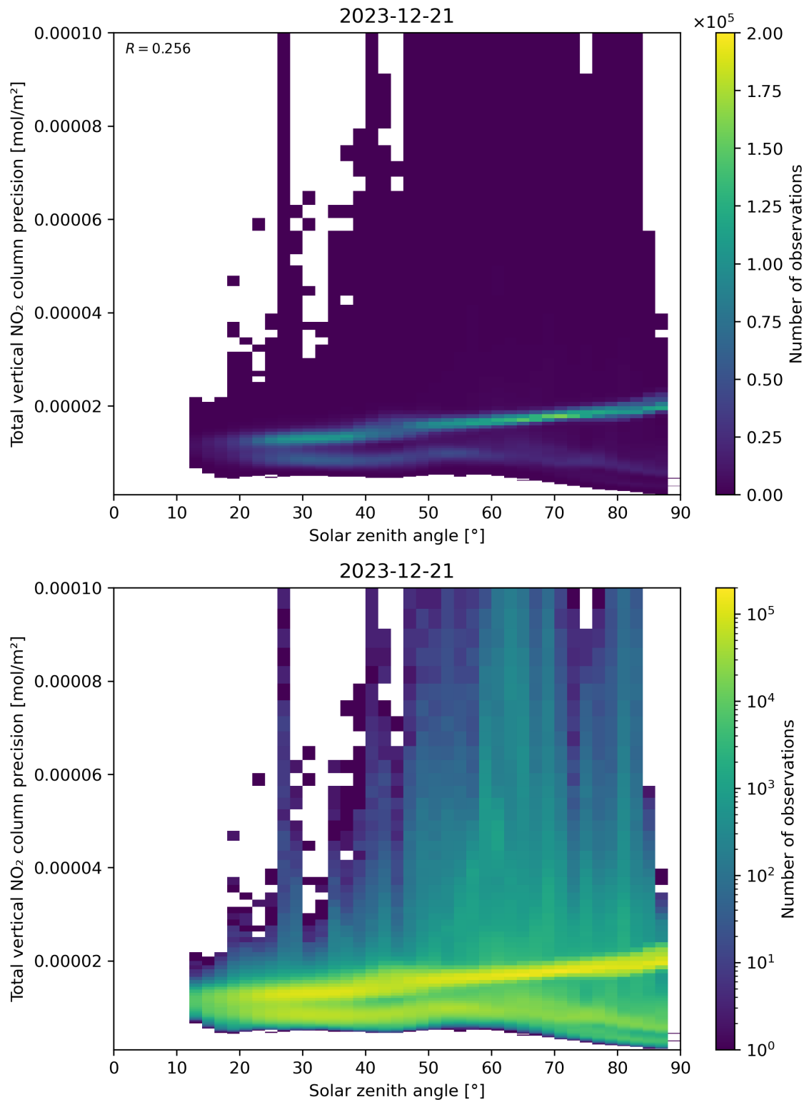
Figure 154: Scatter density plot of “Solar zenith angle” against “Total vertical NO 2 column precision” for 2023-12-20 to 2023-12-22.
