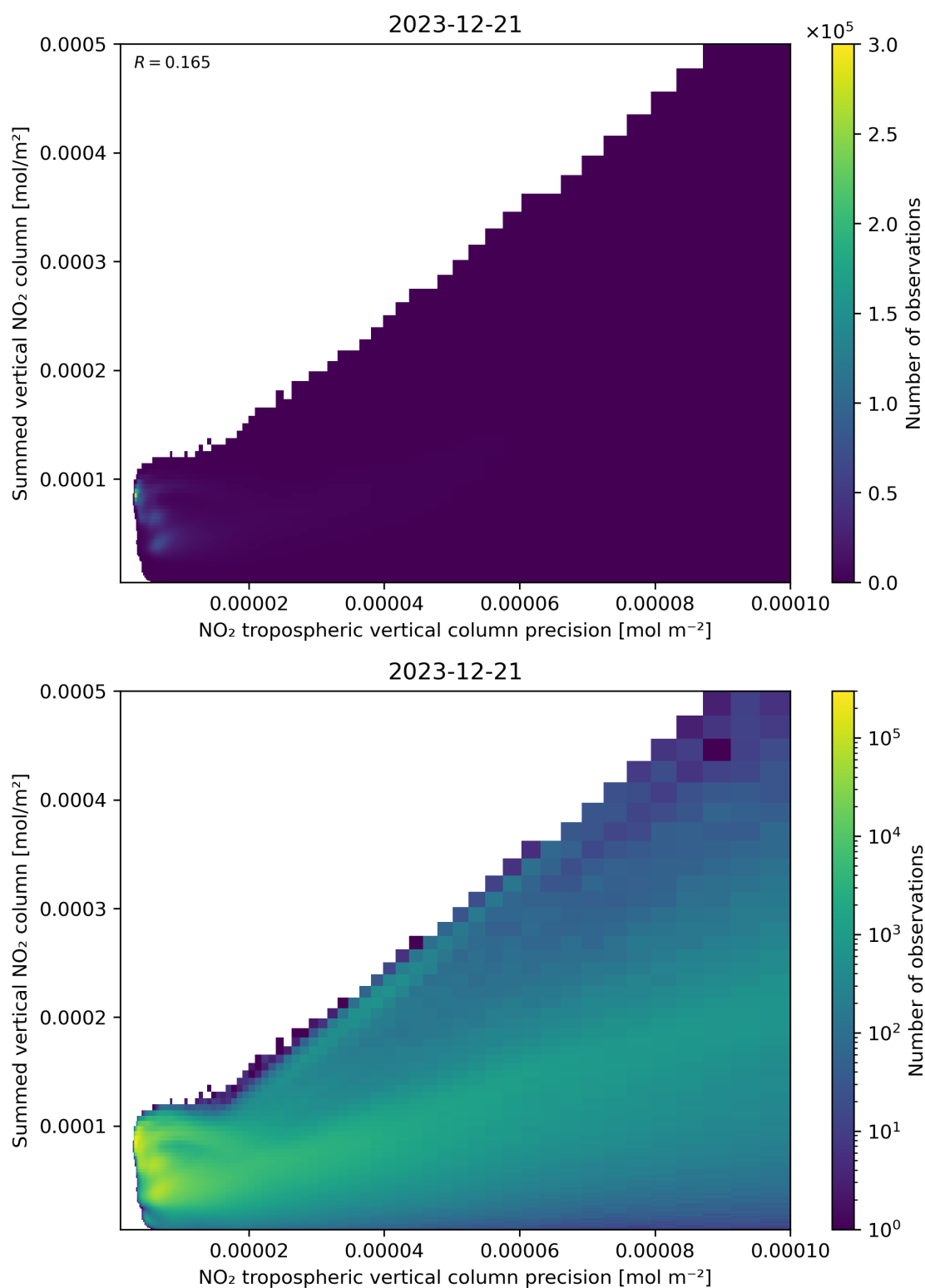
Figure 136: Scatter density plot of “NO 2 tropospheric vertical column precision” against “Summed vertical NO 2 column” for 2023-12-20 to 2023-12-22.
