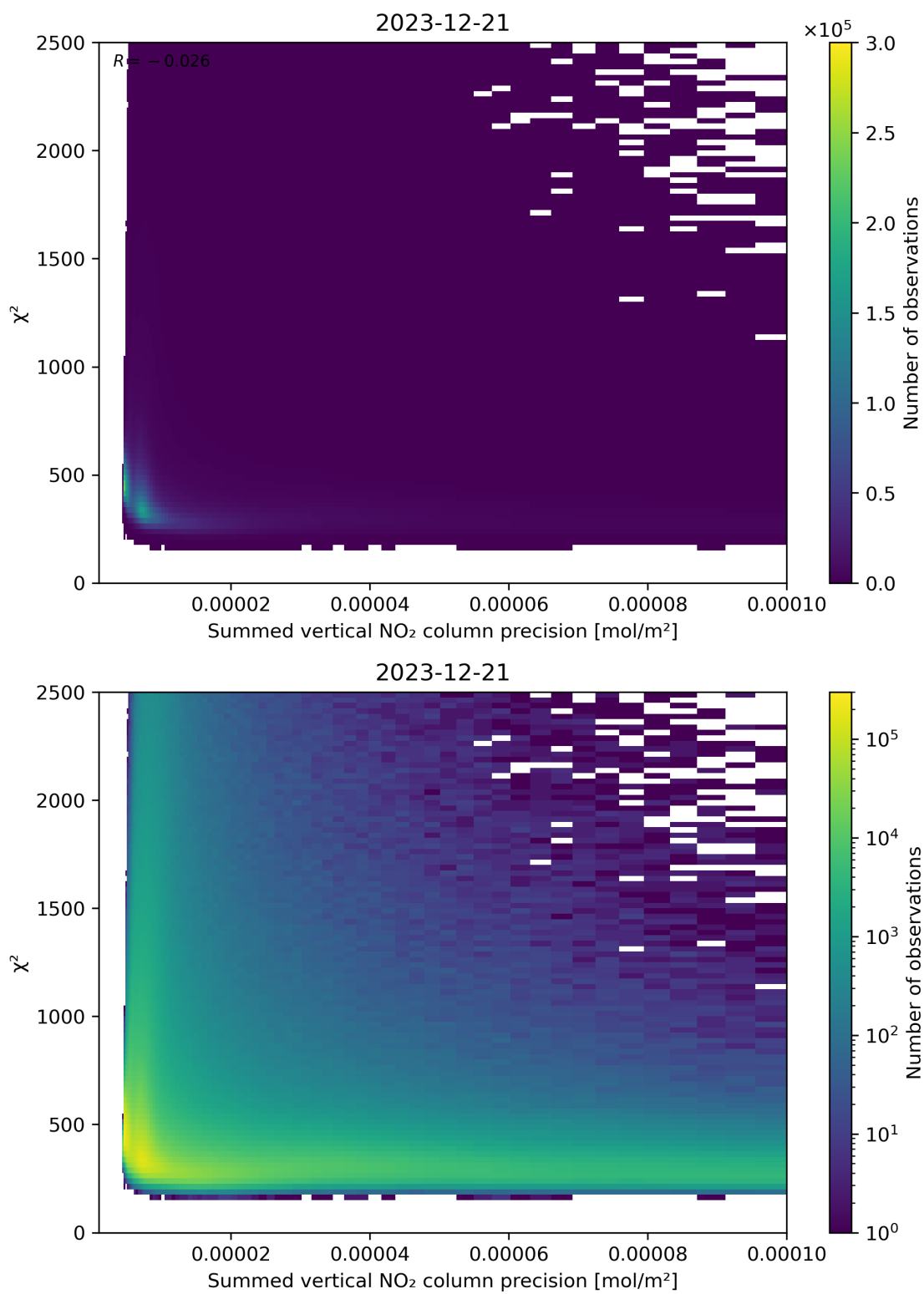
Figure 107: Scatter density plot of “Summed vertical NO 2 column precision” against “ \chi^2 ” for 2023-12-20 to 2023-12-22.
