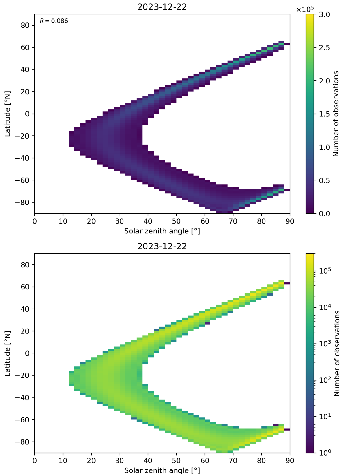
Figure 149: Scatter density plot of “Solar zenith angle” against “Latitude” for 2023-12-21 to 2023-12-23.
