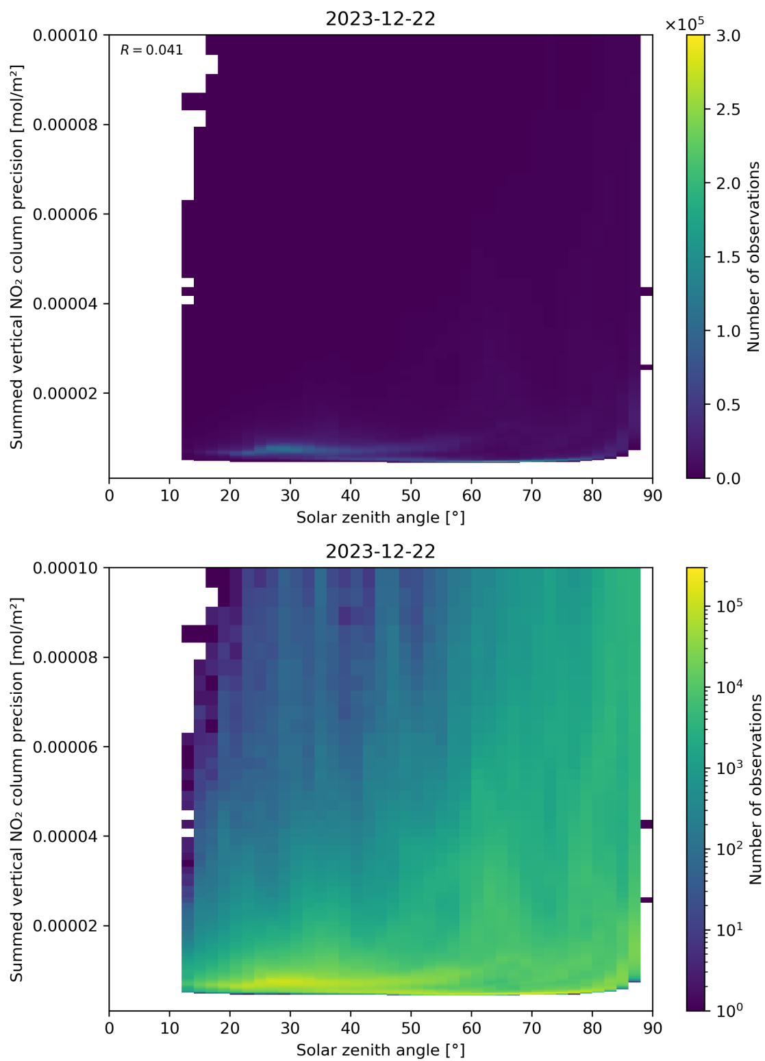
Figure 152: Scatter density plot of “Solar zenith angle” against “Summed vertical NO 2 column precision” for 2023-12-21 to 2023-12-23.
