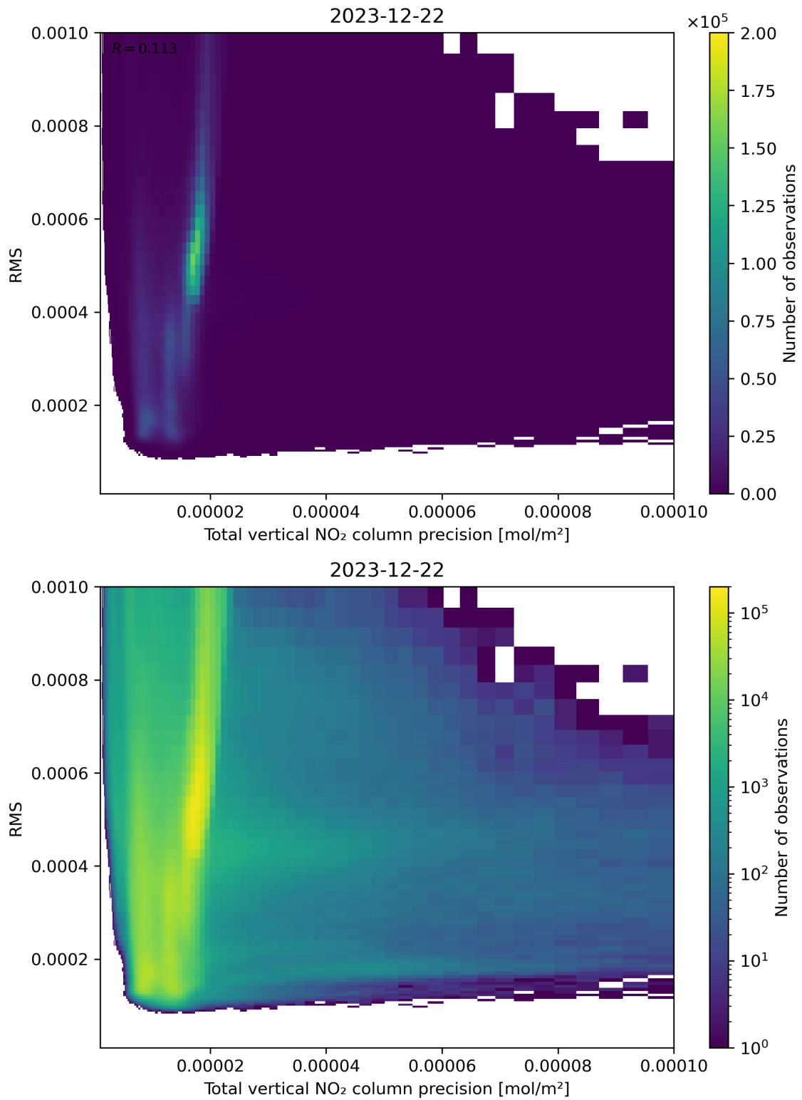
Figure 119: Scatter density plot of “Total vertical NO 2 column precision” against “RMS” for 2023-12-21 to 2023-12-23.
