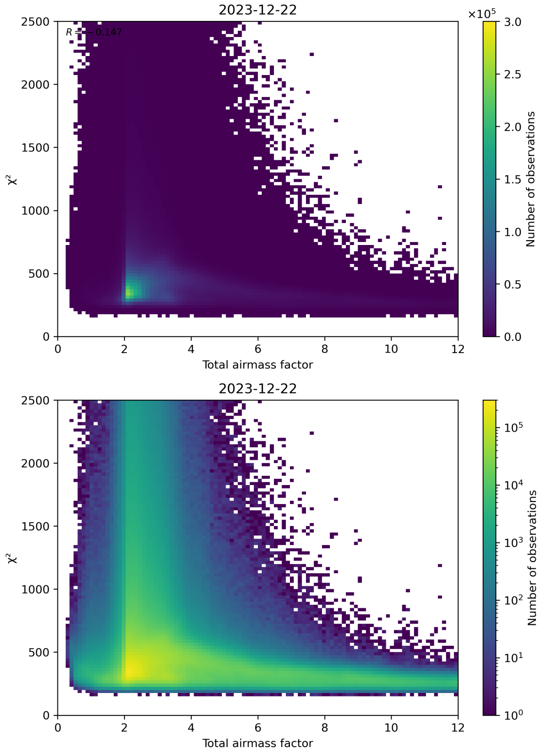
Figure 63: Scatter density plot of “Total airmass factor” against “ \chi^2 ” for 2023-12-21 to 2023-12-23.
