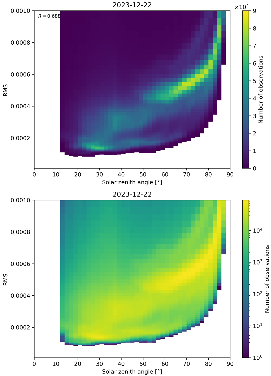
Figure 157: Scatter density plot of “Solar zenith angle” against “RMS” for 2023-12-21 to 2023-12-23.
