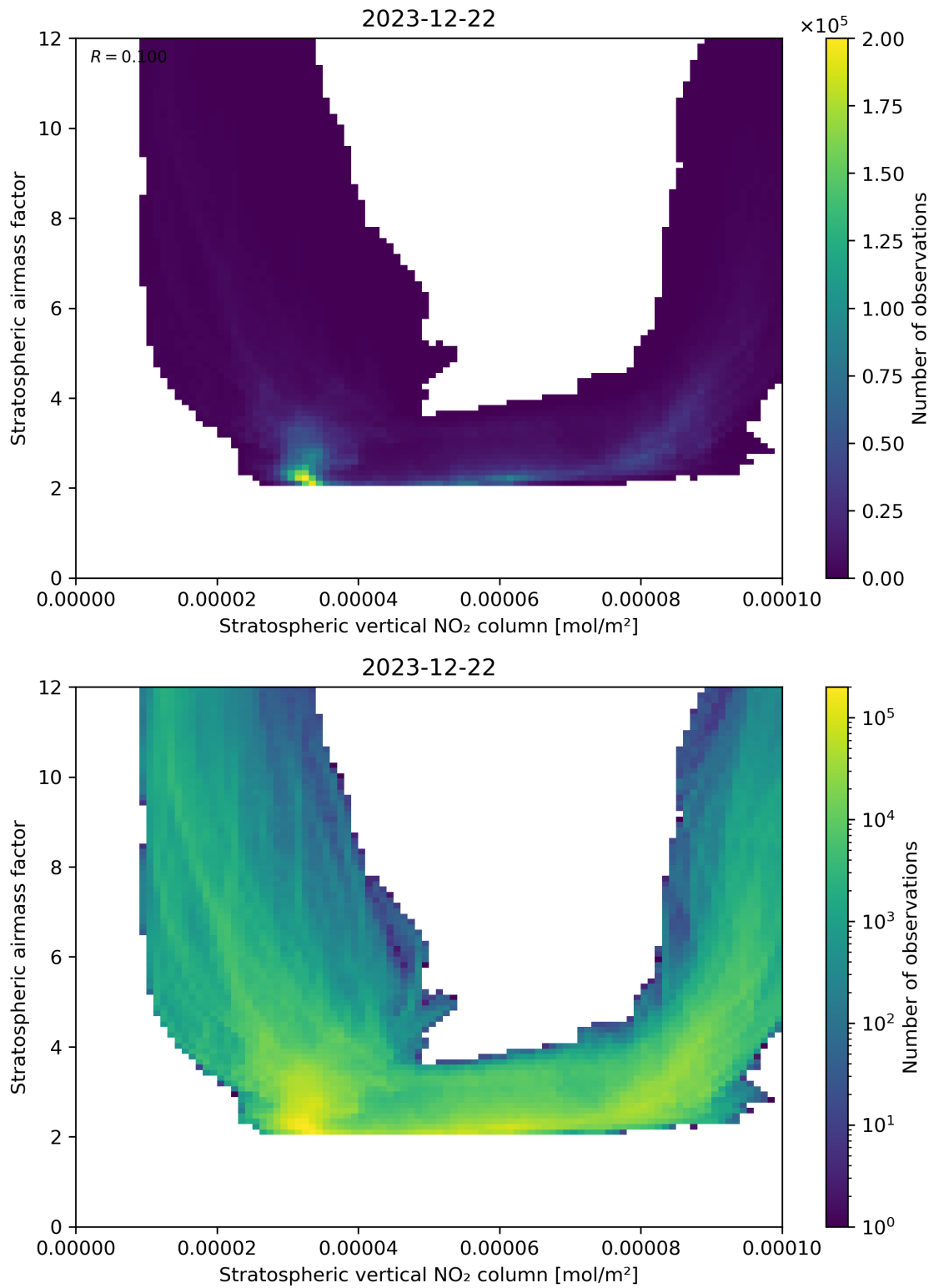
Figure 96: Scatter density plot of “Stratospheric vertical NO 2 column” against “Stratospheric airmass factor” for 2023-12-21 to 2023-12-23.
