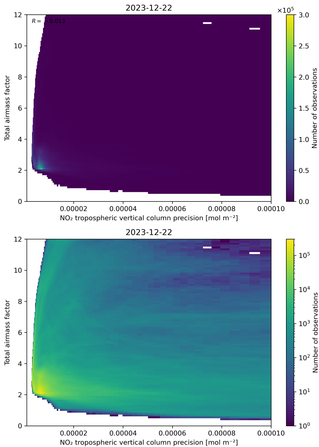
Figure 132: Scatter density plot of “NO 2 tropospheric vertical column precision” against “Total airmass factor” for 2023-12-21 to 2023-12-23.
