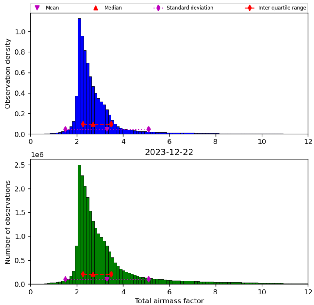
Figure 32: Histogram of “Total airmass factor” for 2023-12-21 to 2023-12-23
