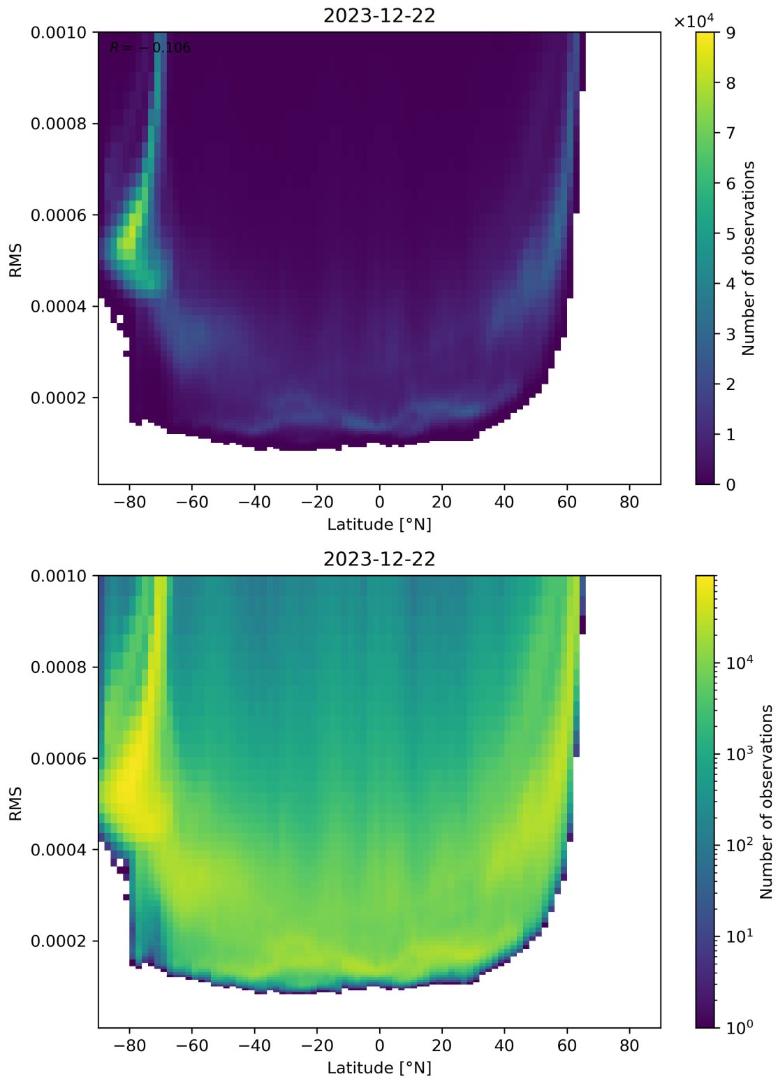
Figure 94: Scatter density plot of “Latitude” against “RMS” for 2023-12-21 to 2023-12-23.
