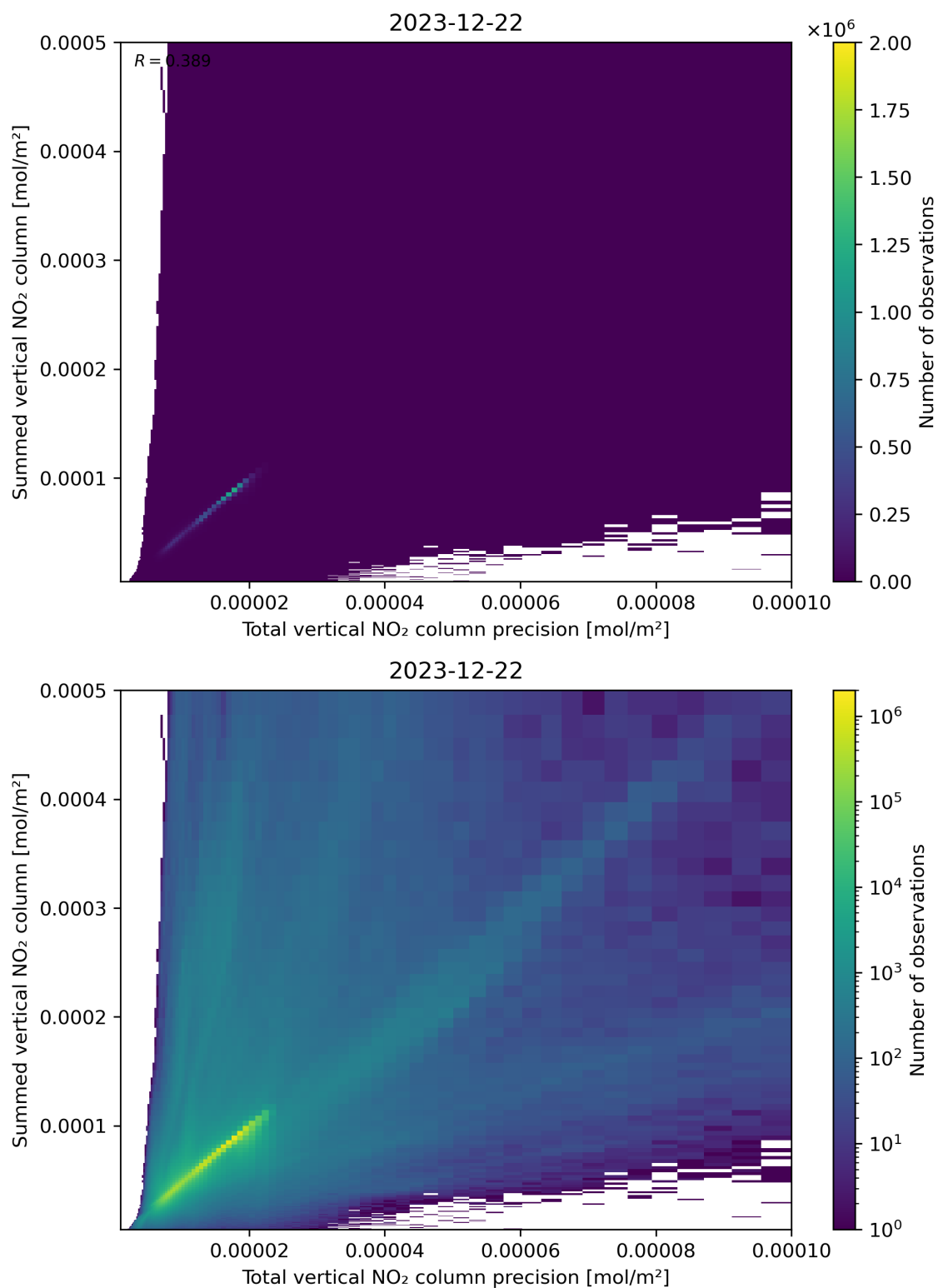
Figure 117: Scatter density plot of “Total vertical NO 2 column precision” against “Summed vertical NO 2 column” for 2023-12-21 to 2023-12-23.
