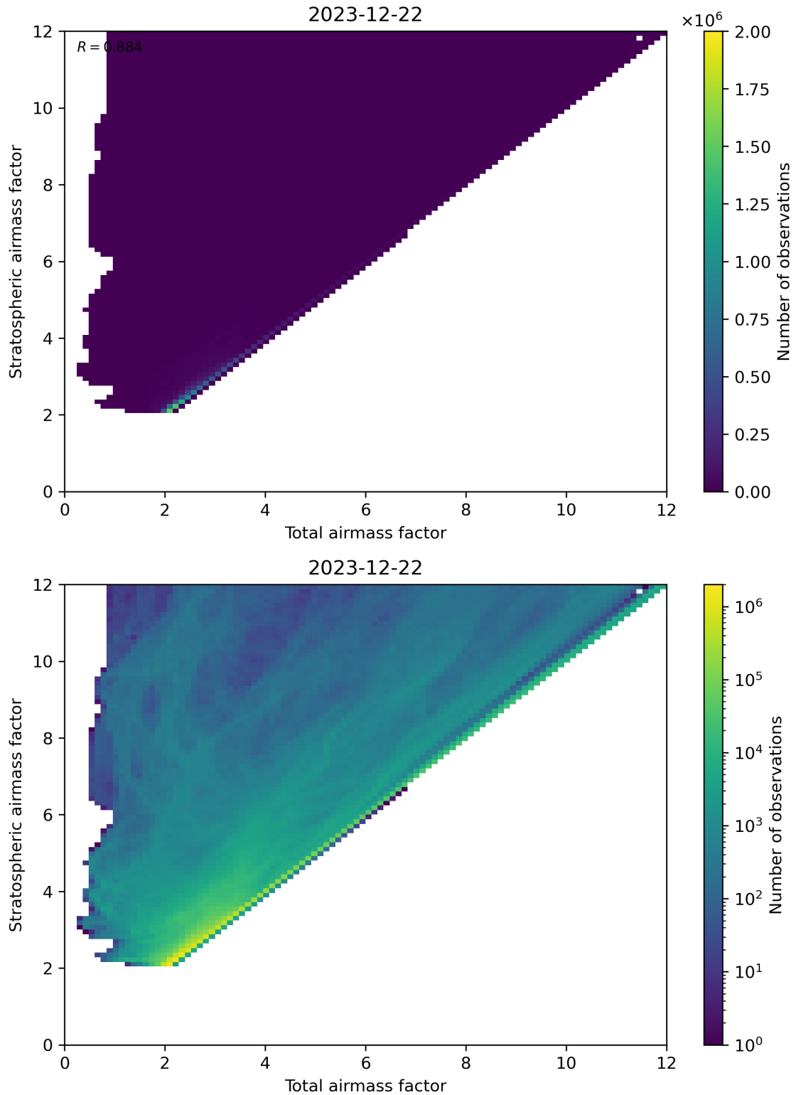
Figure 62: Scatter density plot of “Total airmass factor” against “Stratospheric airmass factor” for 2023-12-21 to 2023-12-23.
