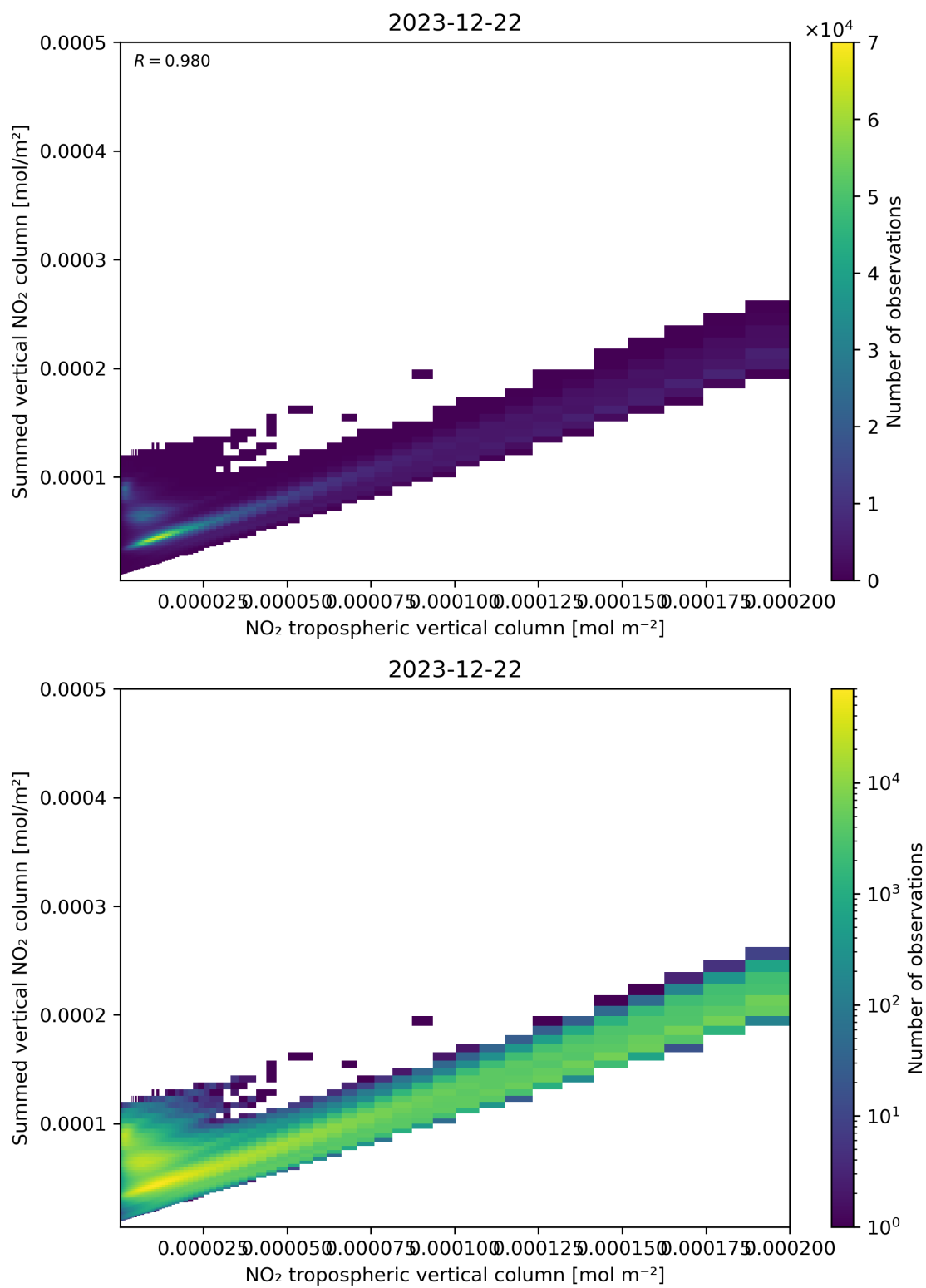
Figure 126: Scatter density plot of “NO 2 tropospheric vertical column” against “Summed vertical NO 2 column” for 2023-12-21 to 2023-12-23.
