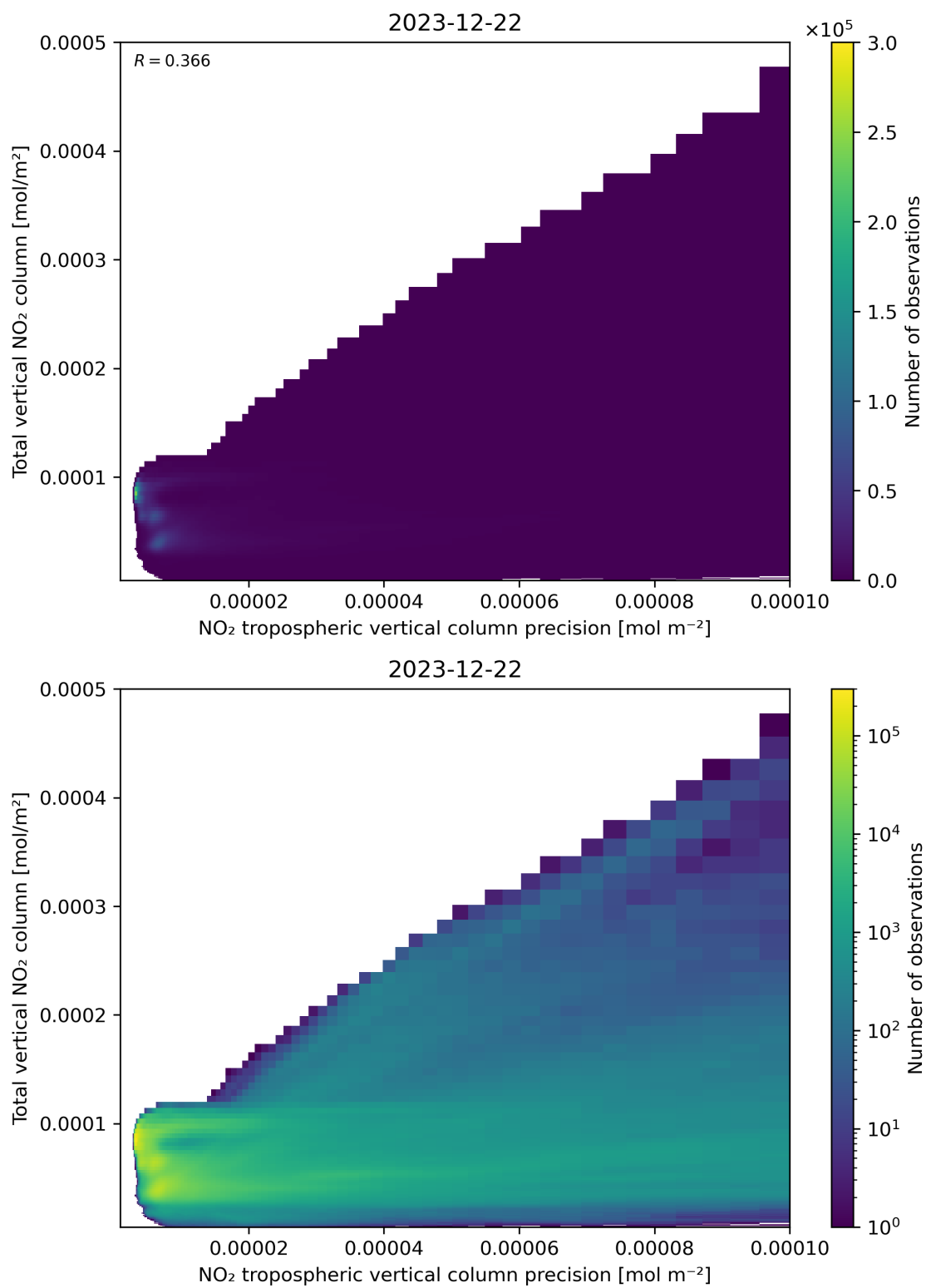
Figure 138: Scatter density plot of “NO 2 tropospheric vertical column precision” against “Total vertical NO 2 column” for 2023-12-21 to 2023-12-23.
