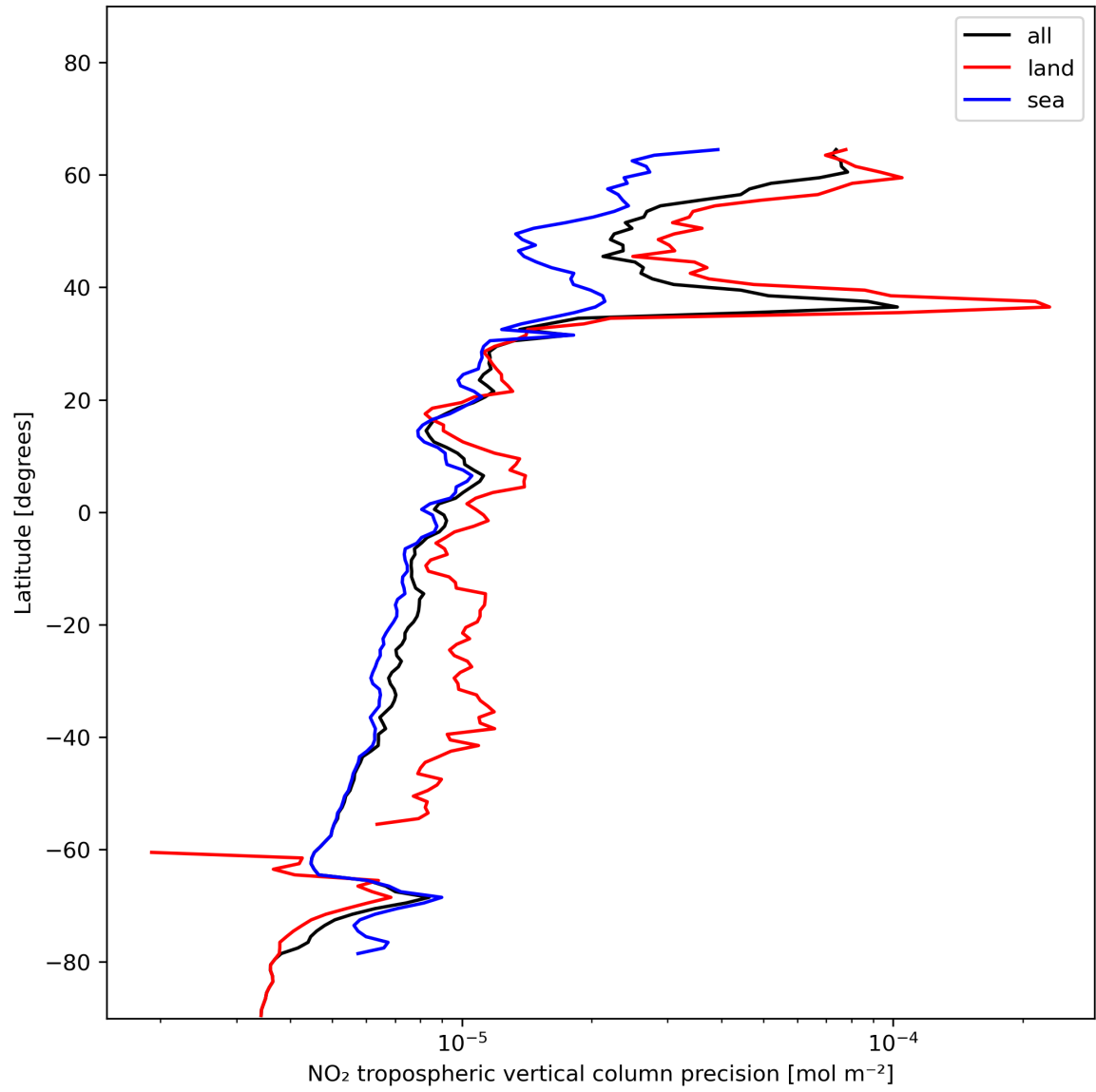
Figure 13: Zonal average of “NO 2 tropospheric vertical column precision” for 2023-12-21 to 2023-12-23.
