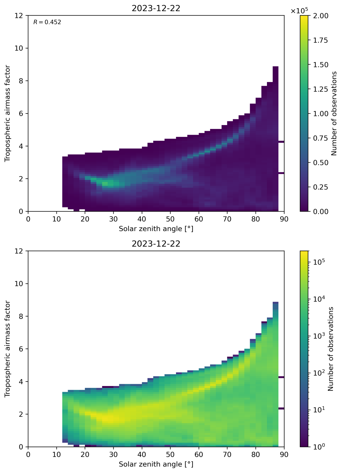
Figure 147: Scatter density plot of “Solar zenith angle” against “Tropospheric airmass factor” for 2023-12-21 to 2023-12-23.
