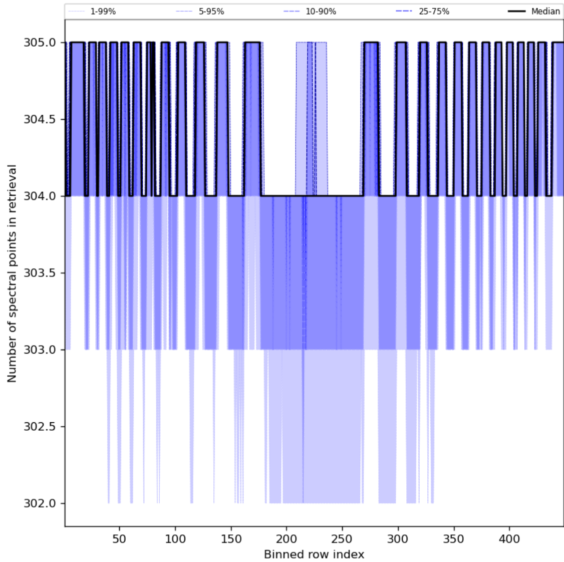
Figure 50: Along track statistics of “Number of spectral points in retrieval” for 2023-12-21 to 2023-12-23
