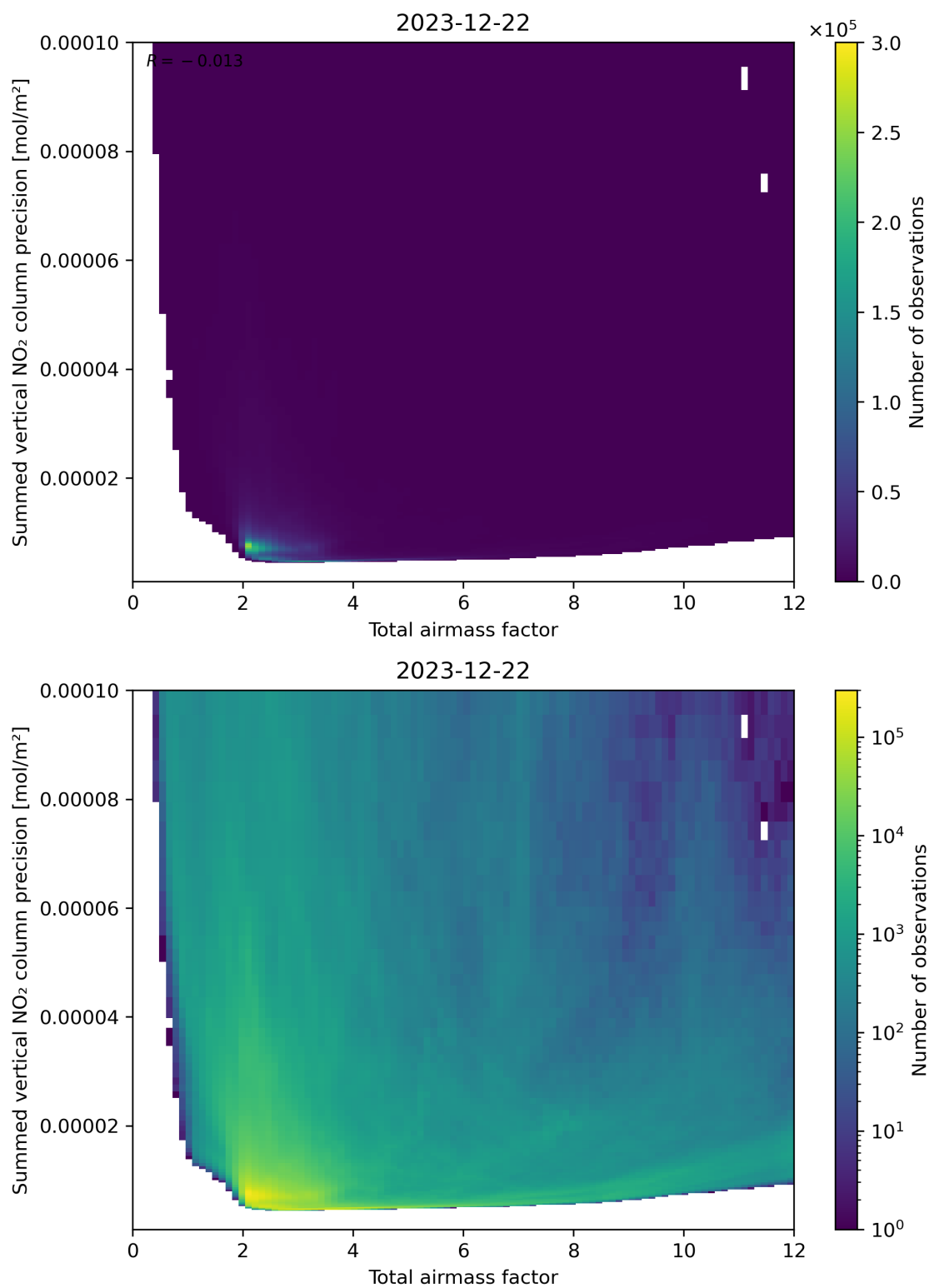
Figure 66: Scatter density plot of “Total airmass factor” against “Summed vertical NO 2 column precision” for 2023-12-21 to 2023-12-23.
