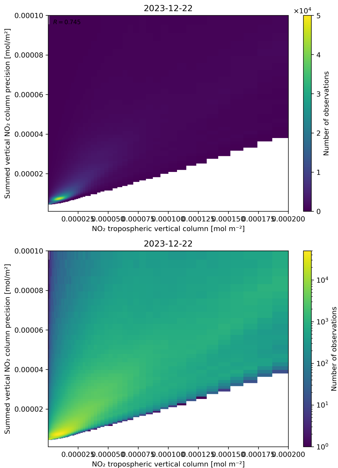
Figure 127: Scatter density plot of “NO 2 tropospheric vertical column” against “Summed vertical NO 2 column precision” for 2023-12-21 to 2023-12-23.
