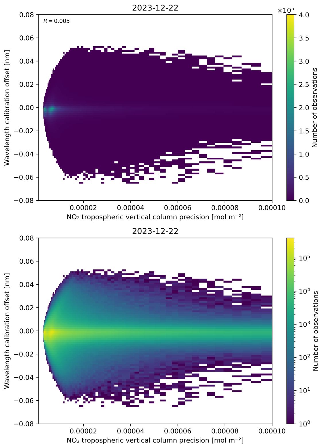
Figure 141: Scatter density plot of “NO 2 tropospheric vertical column precision” against “Wavelength calibration offset” for 2023-12-21 to 2023-12-23.
