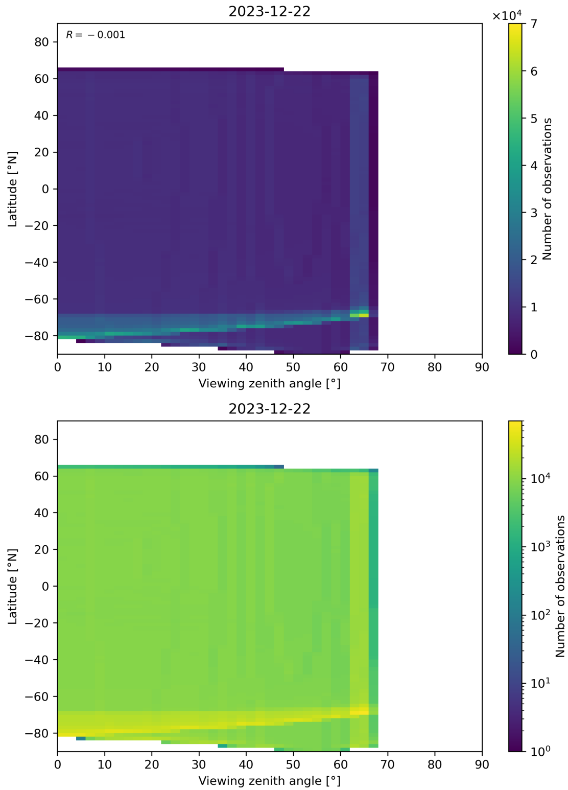
Figure 163: Scatter density plot of “Viewing zenith angle” against “Latitude” for 2023-12-21 to 2023-12-23.
