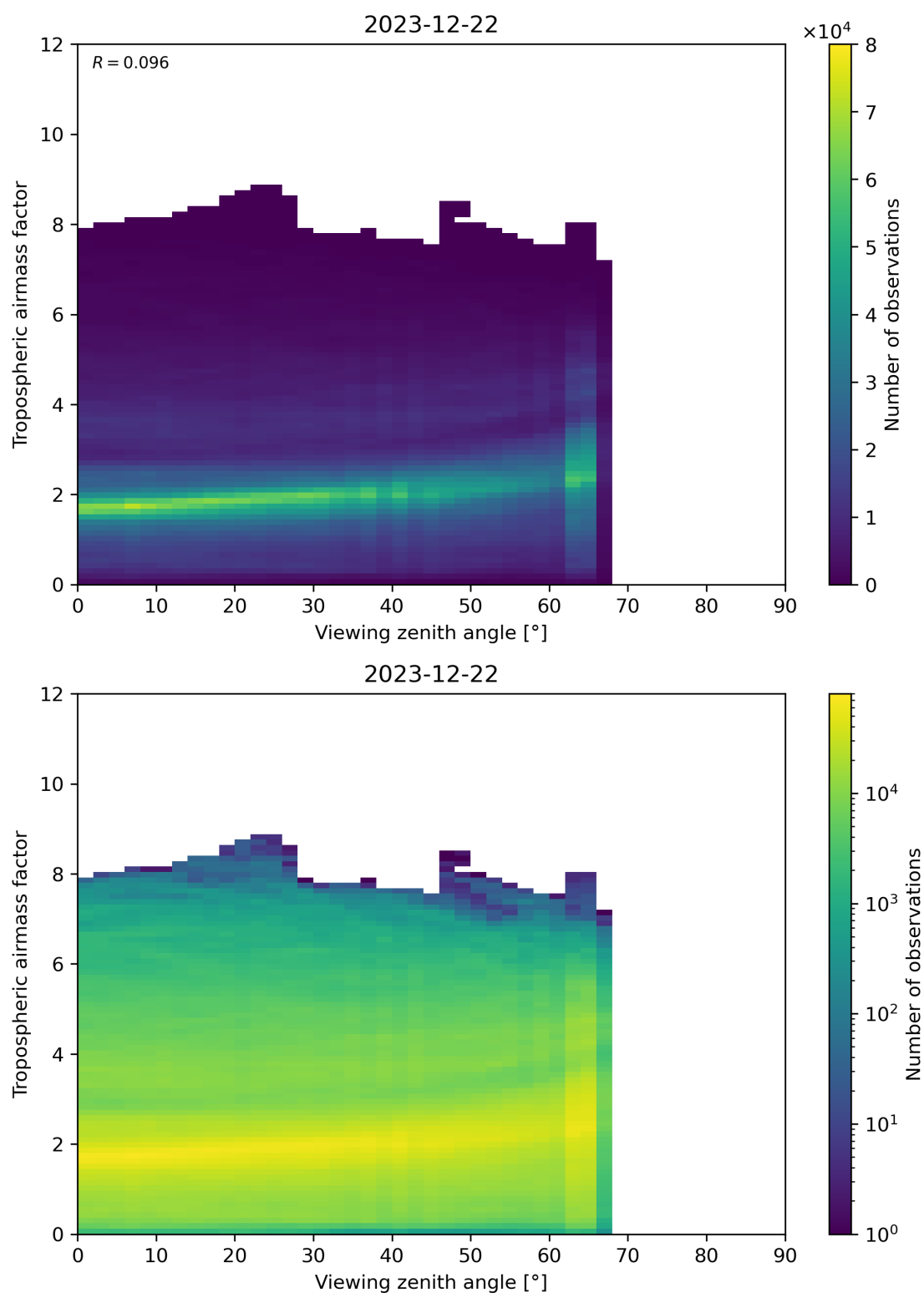
Figure 161: Scatter density plot of “Viewing zenith angle” against “Tropospheric airmass factor” for 2023-12-21 to 2023-12-23.
