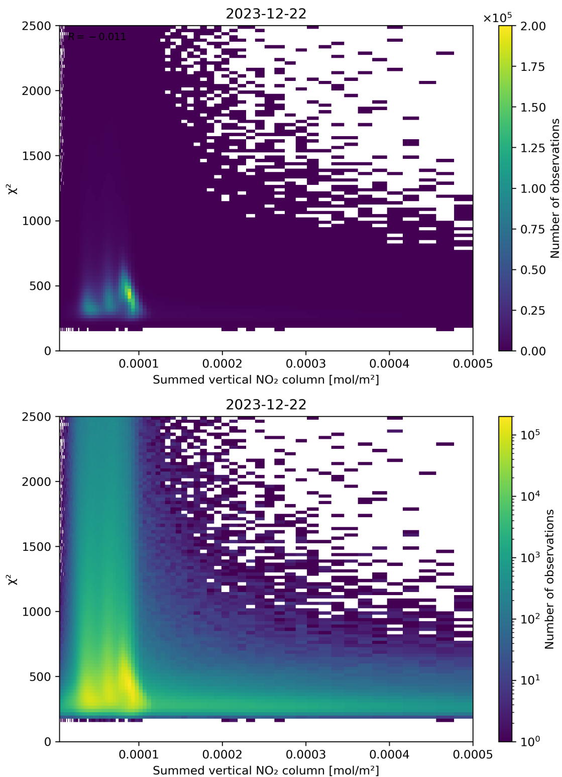
Figure 104: Scatter density plot of “Summed vertical NO 2 column” against “ \chi^2 ” for 2023-12-21 to 2023-12-23.
