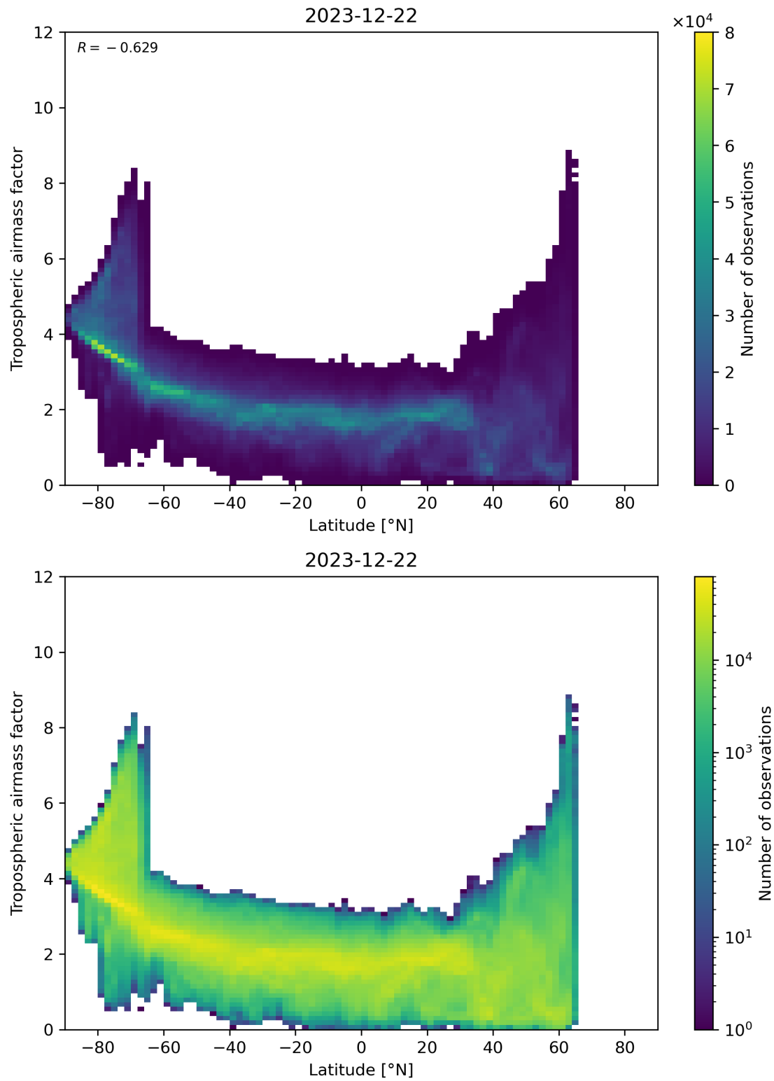
Figure 85: Scatter density plot of “Latitude” against “Tropospheric airmass factor” for 2023-12-21 to 2023-12-23.
