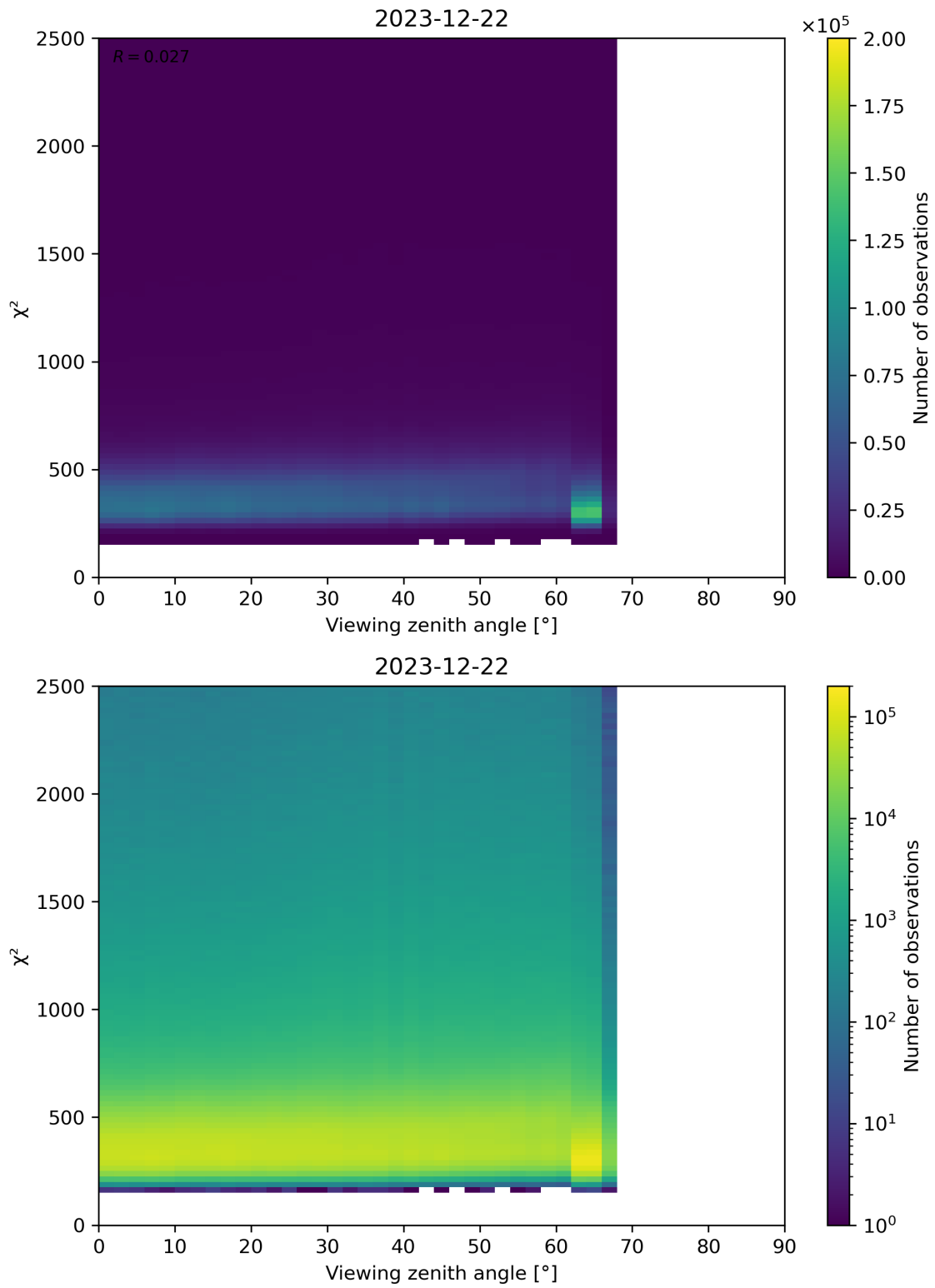
Figure 162: Scatter density plot of “Viewing zenith angle” against “ \chi^2 ” for 2023-12-21 to 2023-12-23.
