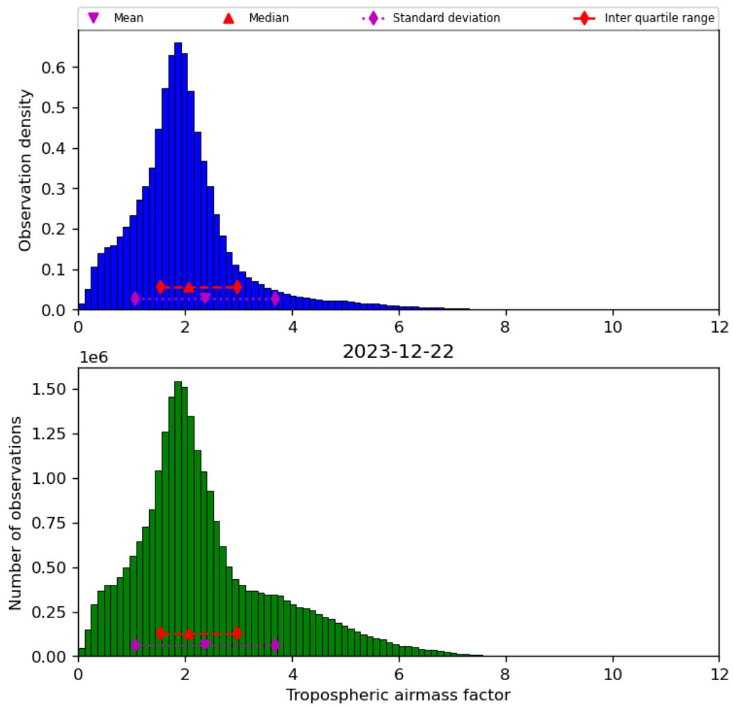
Figure 31: Histogram of “Tropospheric airmass factor” for 2023-12-21 to 2023-12-23
