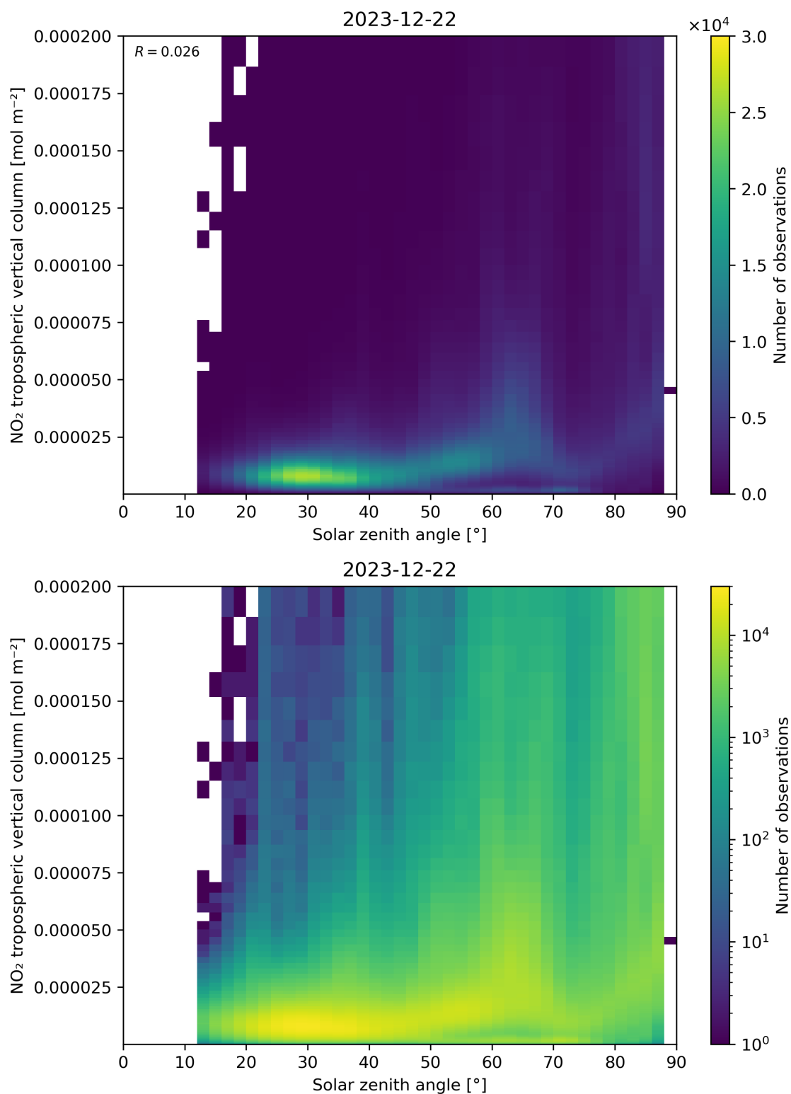
Figure 155: Scatter density plot of “Solar zenith angle” against “NO 2 tropospheric vertical column” for 2023-12-21 to 2023-12-23.
