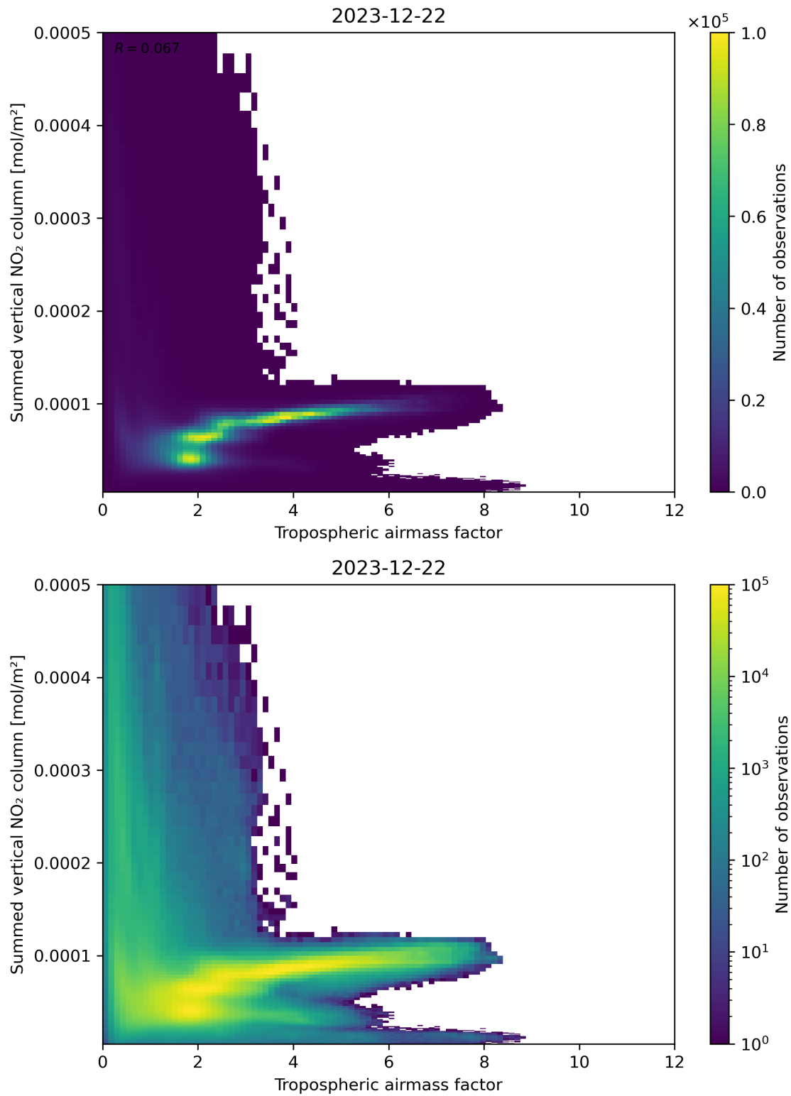
Figure 75: Scatter density plot of “Tropospheric airmass factor” against “Summed vertical NO 2 column” for 2023-12-21 to 2023-12-23.
