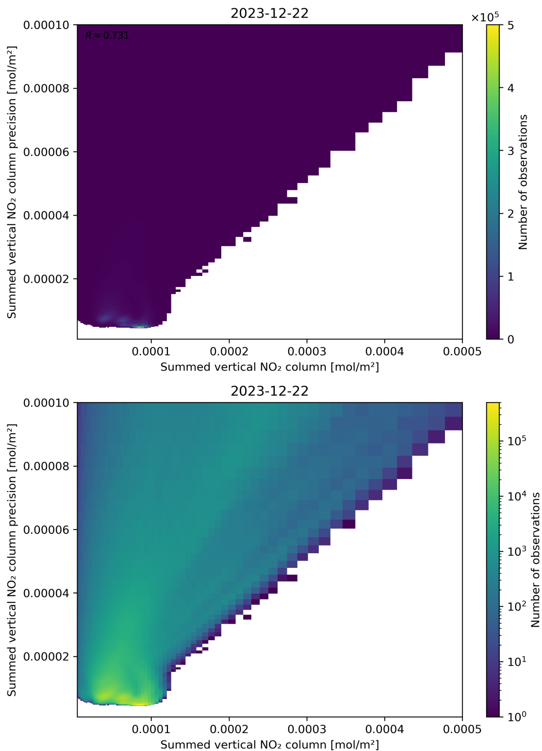
Figure 105: Scatter density plot of “Summed vertical NO 2 column” against “Summed vertical NO 2 column precision” for 2023-12-21 to 2023-12-23.
