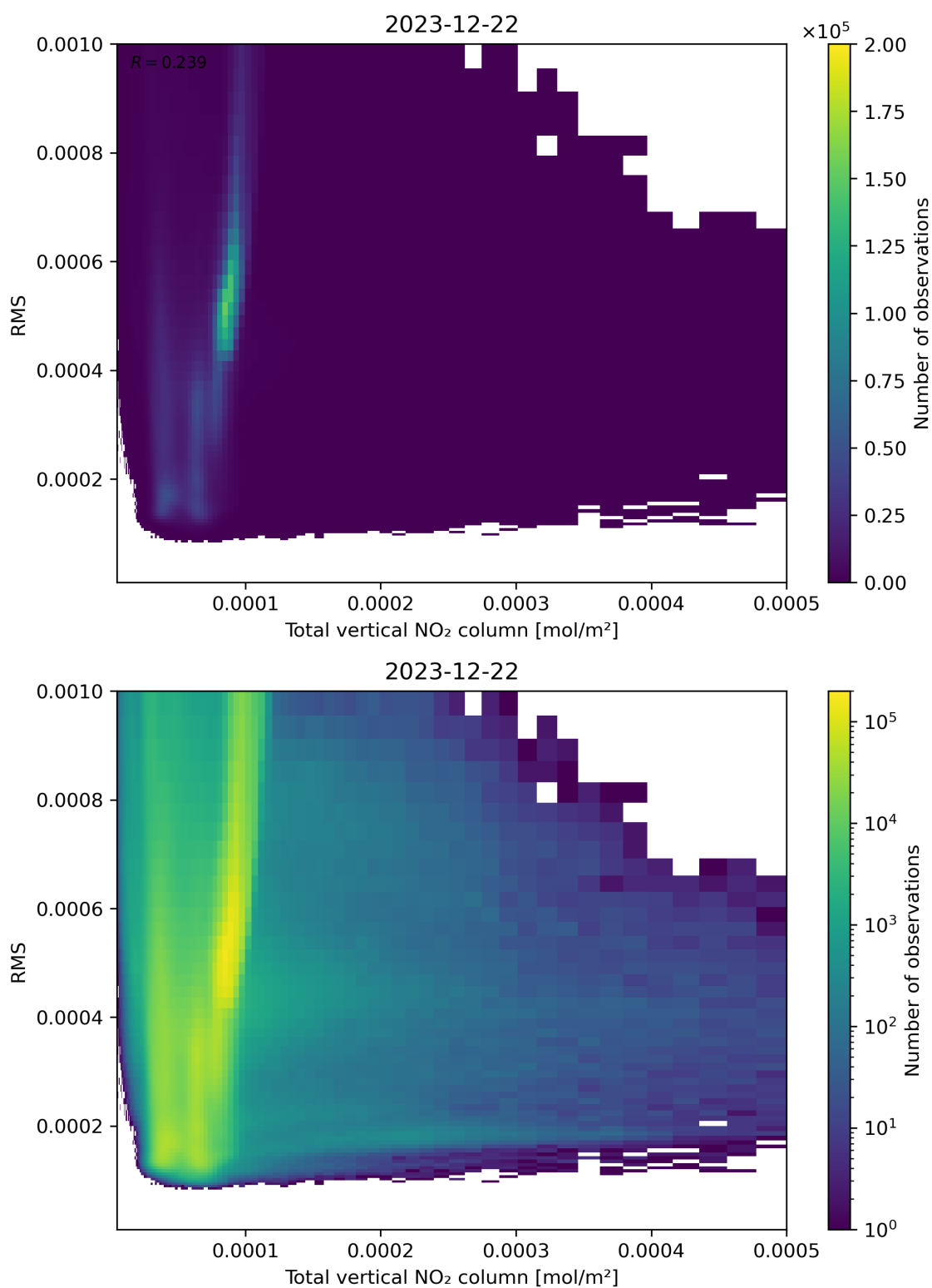
Figure 120: Scatter density plot of “Total vertical NO 2 column” against “RMS” for 2023-12-21 to 2023-12-23.
