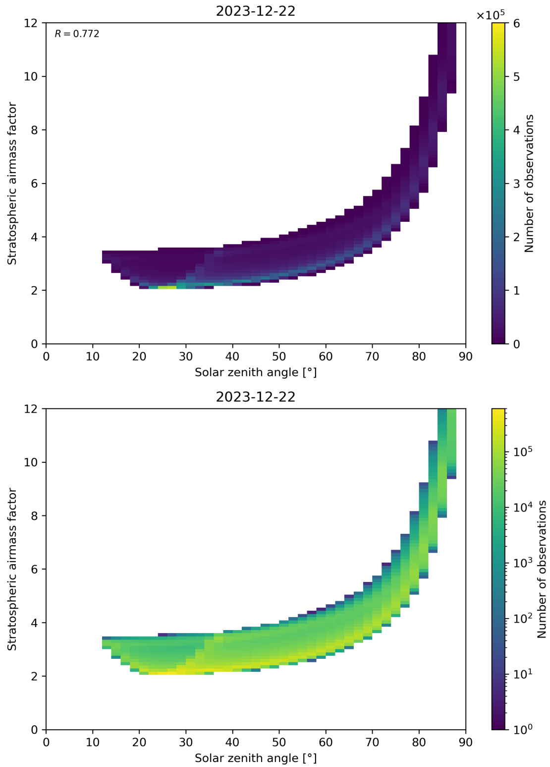
Figure 145: Scatter density plot of “Solar zenith angle” against “Stratospheric airmass factor” for 2023-12-21 to 2023-12-23.
