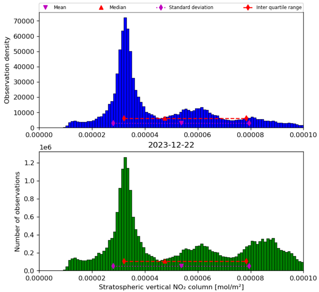
Figure 36: Histogram of “Stratospheric vertical NO 2 column” for 2023-12-21 to 2023-12-23
