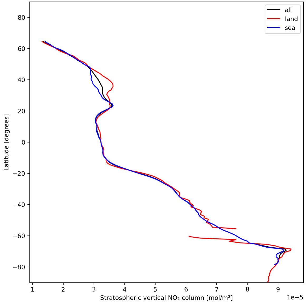
Figure 19: Zonal average of “Stratospheric vertical NO 2 column” for 2023-12-21 to 2023-12-23.
