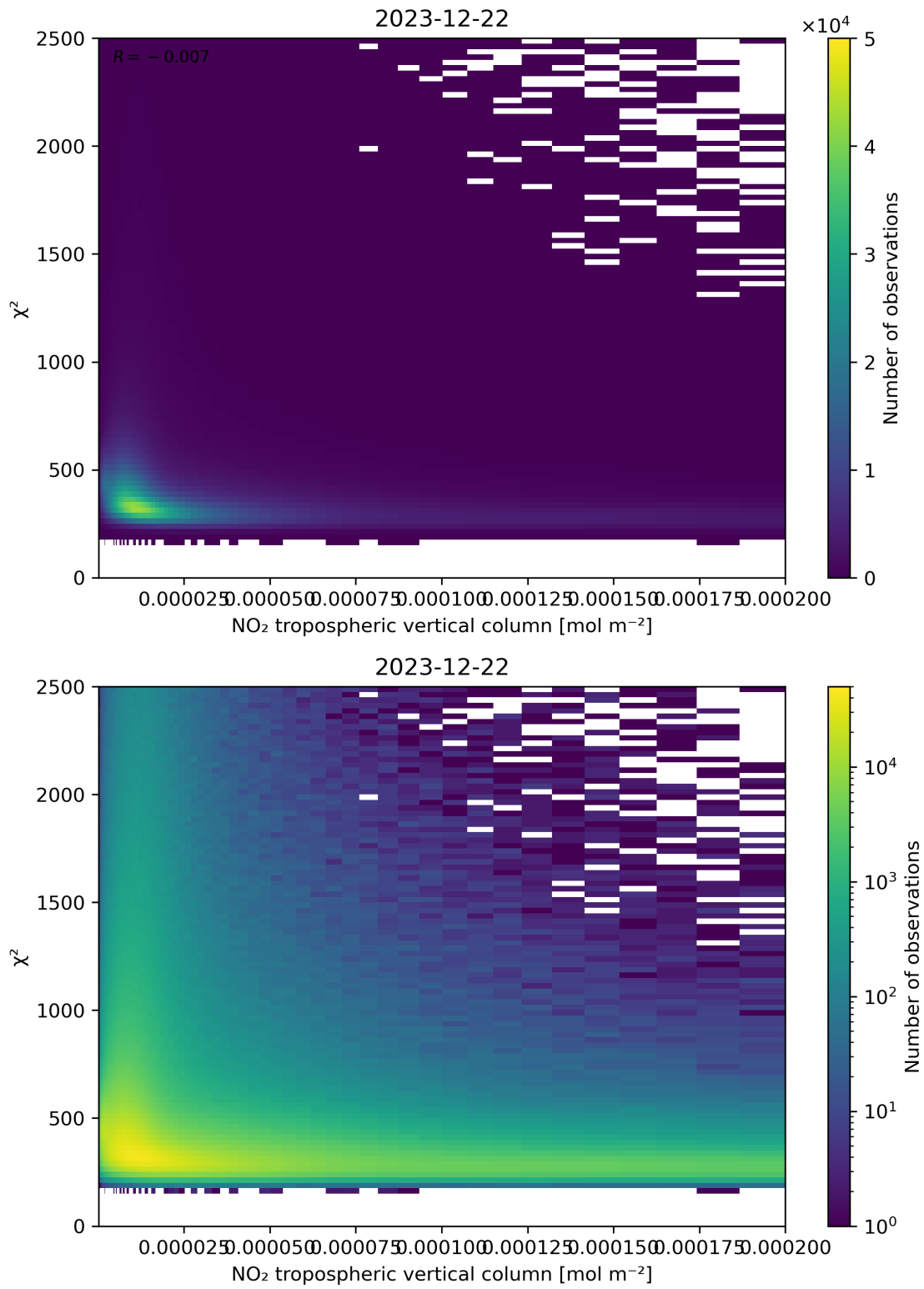
Figure 124: Scatter density plot of “NO 2 tropospheric vertical column” against “ \chi^2 ” for 2023-12-21 to 2023-12-23.
