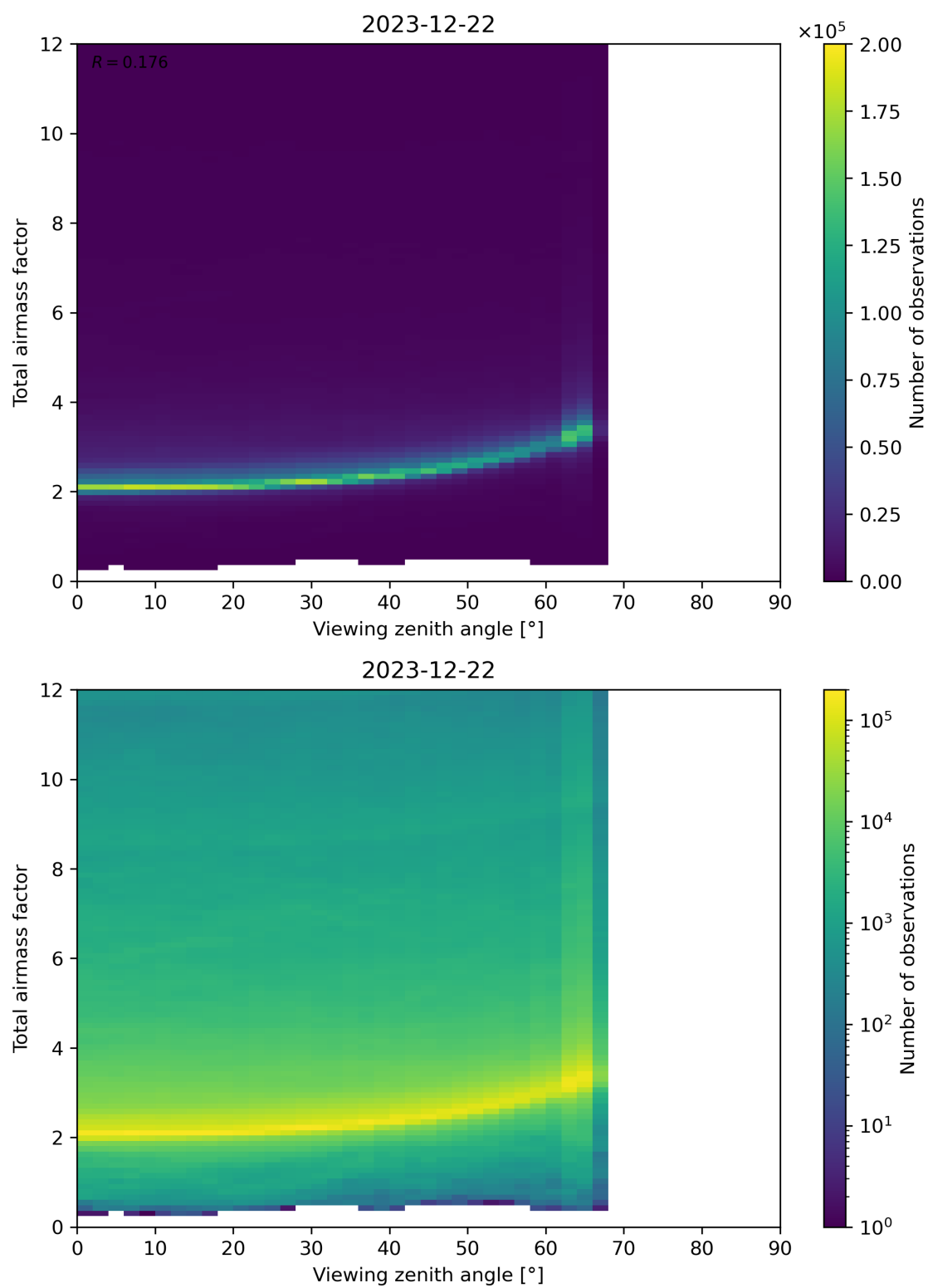
Figure 160: Scatter density plot of “Viewing zenith angle” against “Total airmass factor” for 2023-12-21 to 2023-12-23.
