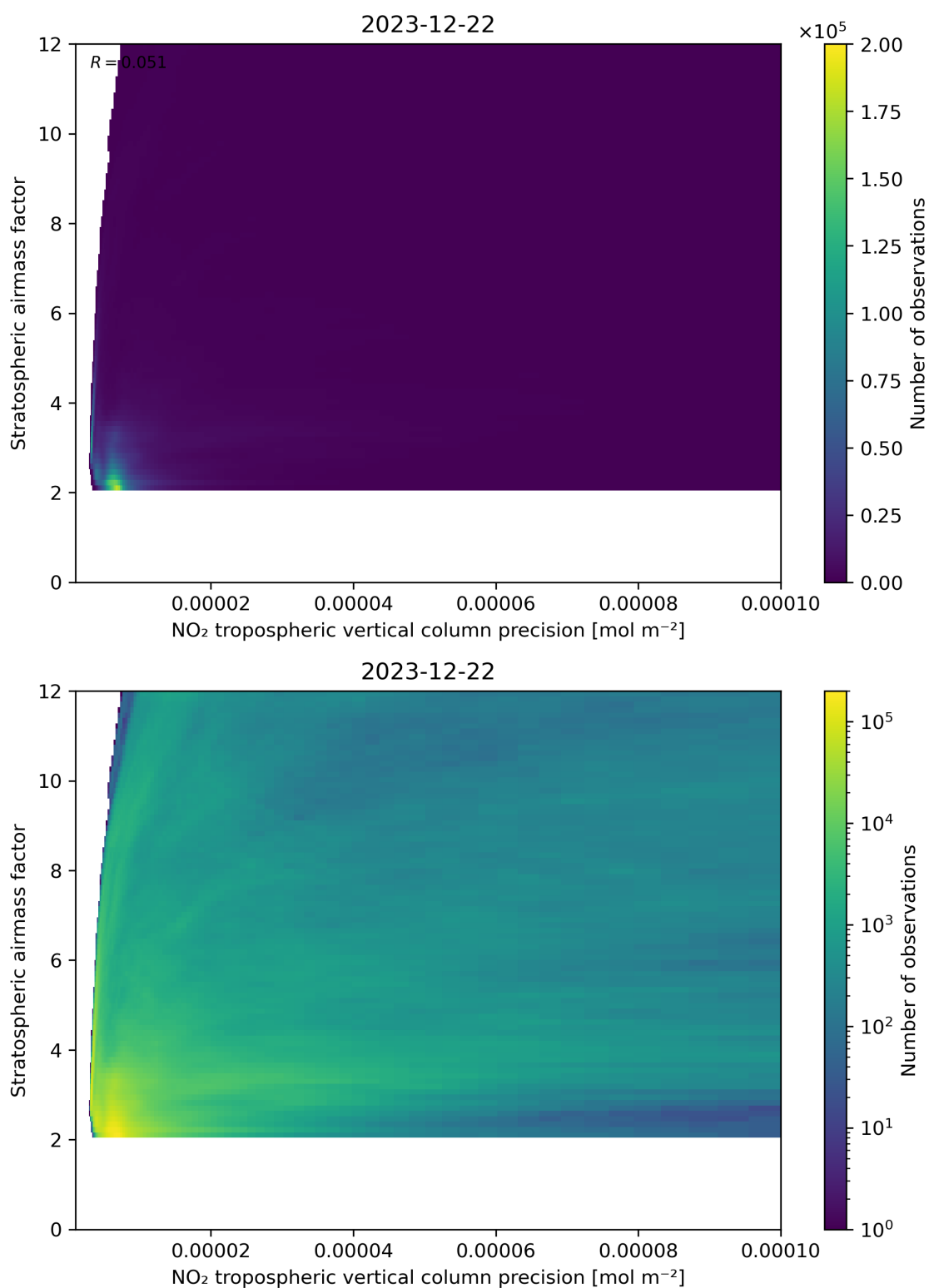
Figure 131: Scatter density plot of “NO 2 tropospheric vertical column precision” against “Stratospheric airmass factor” for 2023-12-21 to 2023-12-23.
