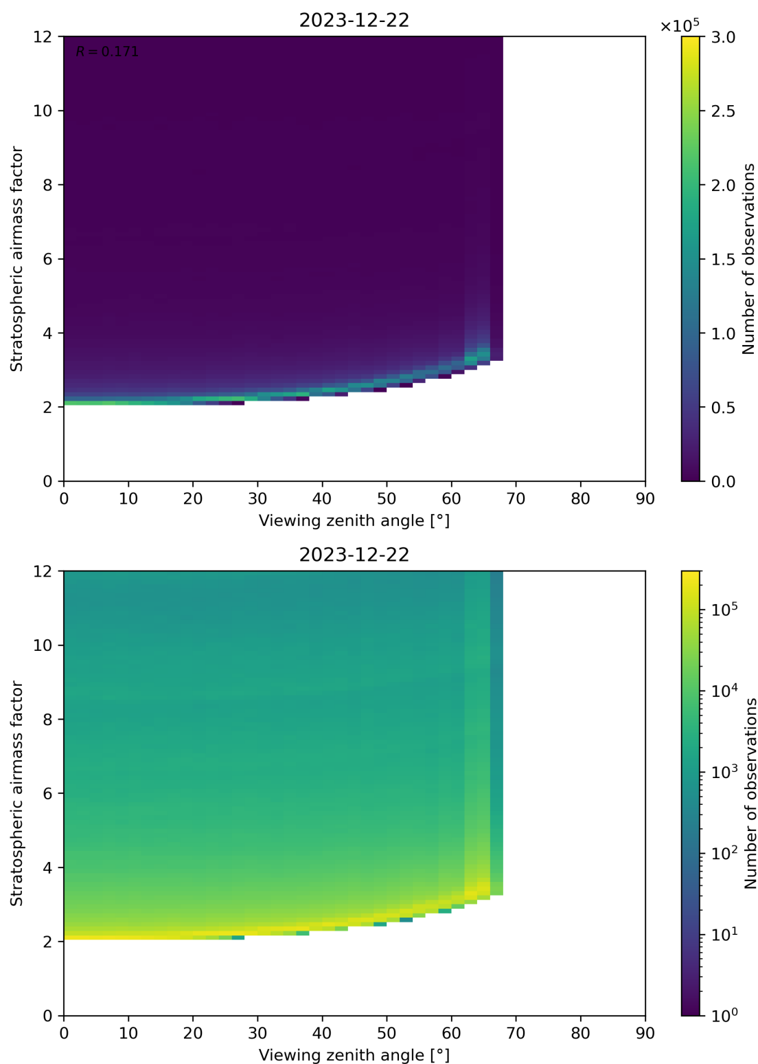
Figure 159: Scatter density plot of “Viewing zenith angle” against “Stratospheric airmass factor” for 2023-12-21 to 2023-12-23.
