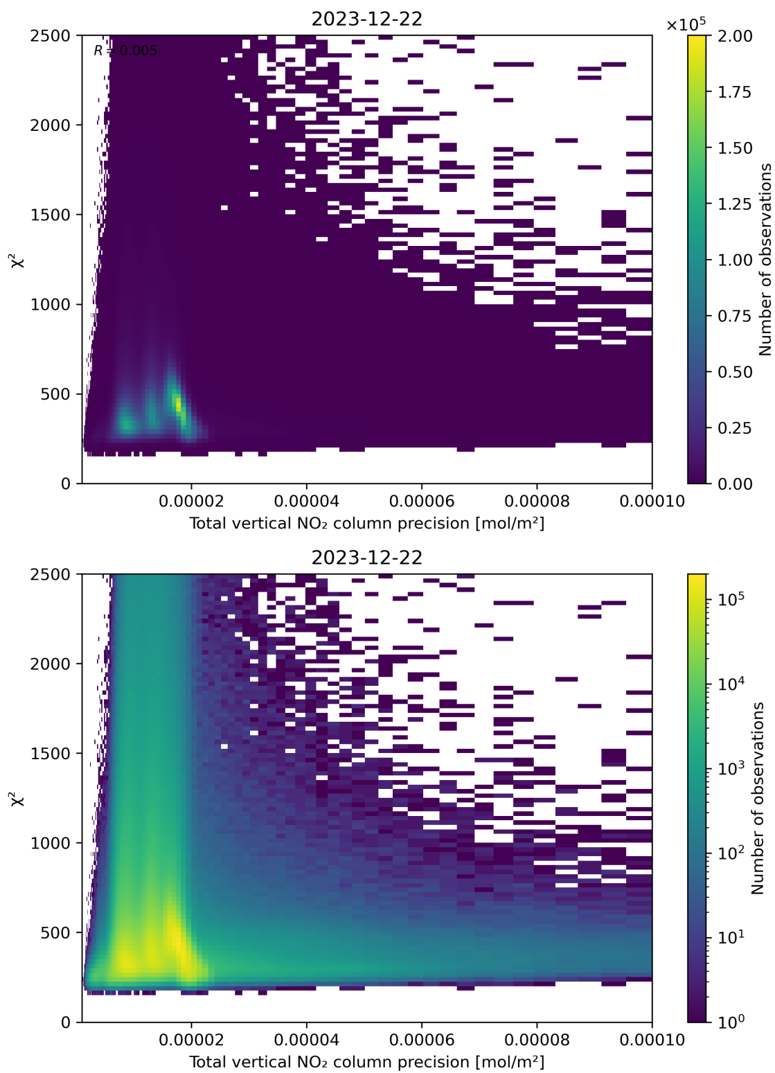
Figure 116: Scatter density plot of “Total vertical NO 2 column precision” against “ \chi^2 ” for 2023-12-21 to 2023-12-23.
