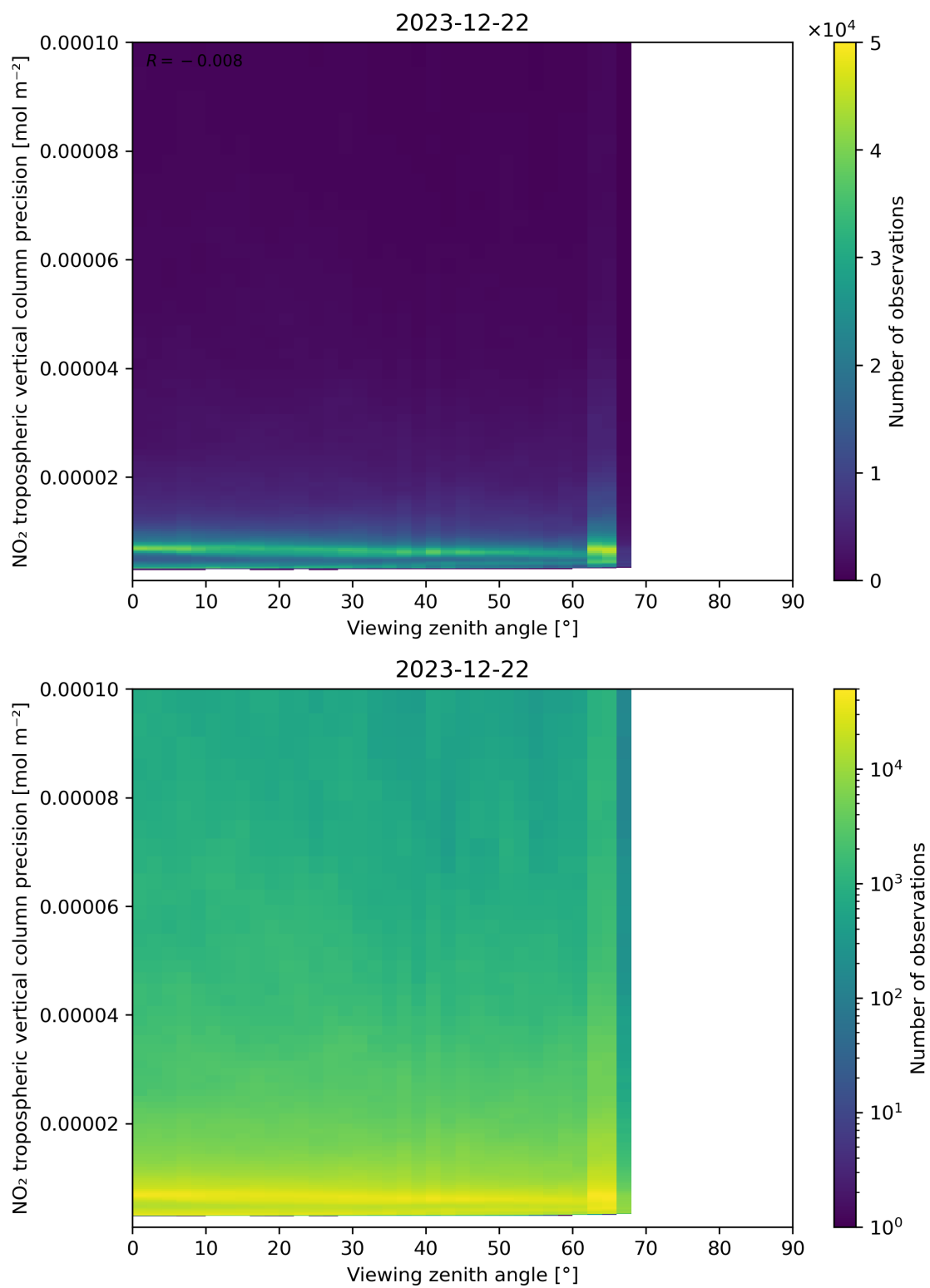
Figure 170: Scatter density plot of “Viewing zenith angle” against “NO 2 tropospheric vertical column precision” for 2023-12-21 to 2023-12-23.
