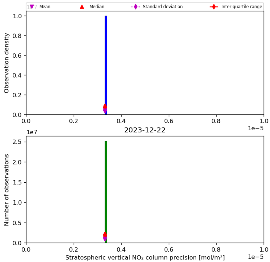
Figure 37: Histogram of “Stratospheric vertical NO 2 column precision” for 2023-12-21 to 2023-12-23
