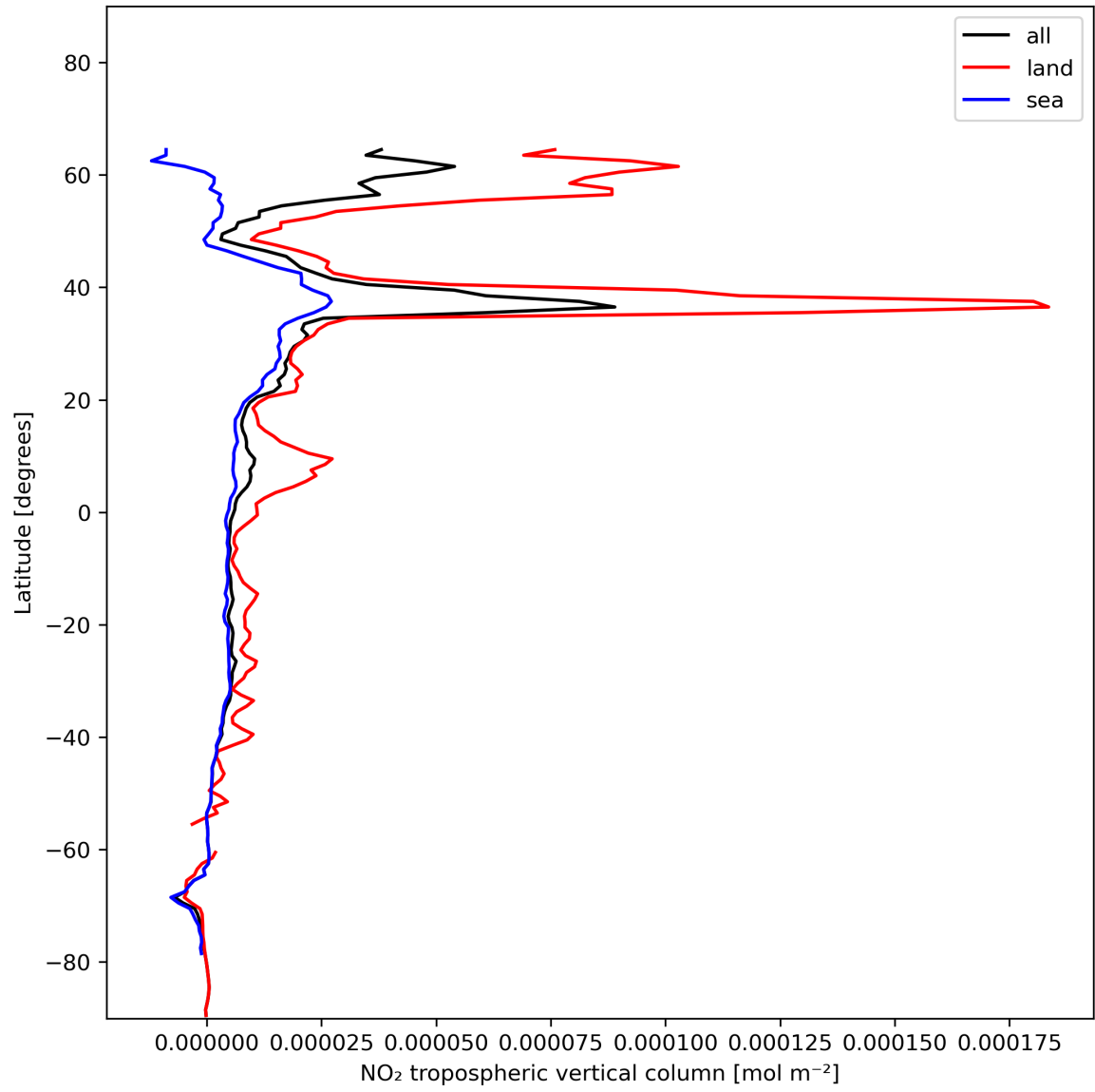
Figure 12: Zonal average of “NO 2 tropospheric vertical column” for 2023-12-21 to 2023-12-23.
