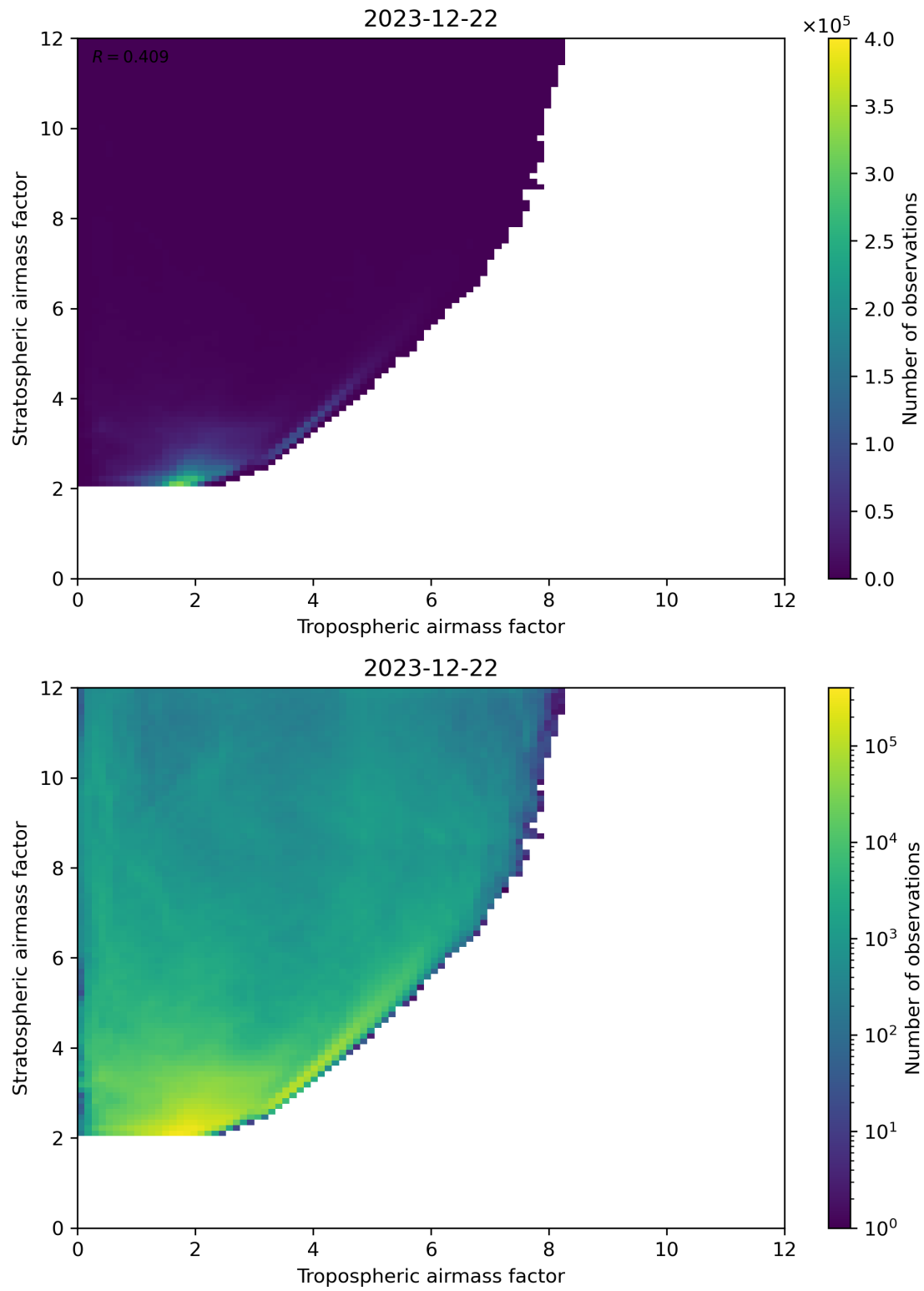
Figure 71: Scatter density plot of “Tropospheric airmass factor” against “Stratospheric airmass factor” for 2023-12-21 to 2023-12-23.
