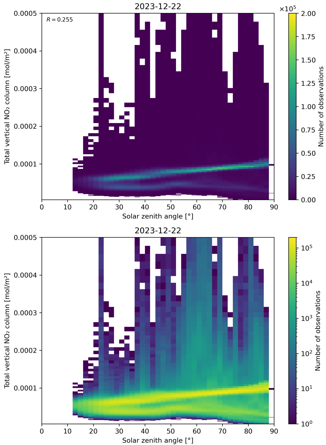
Figure 153: Scatter density plot of “Solar zenith angle” against “Total vertical NO 2 column” for 2023-12-21 to 2023-12-23.
