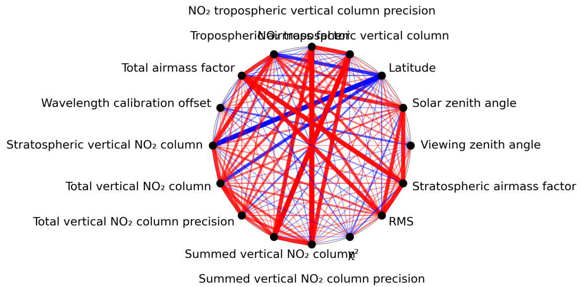
Figure 1: Map of correlation graph for 2023-12-21 to 2023-12-23.
