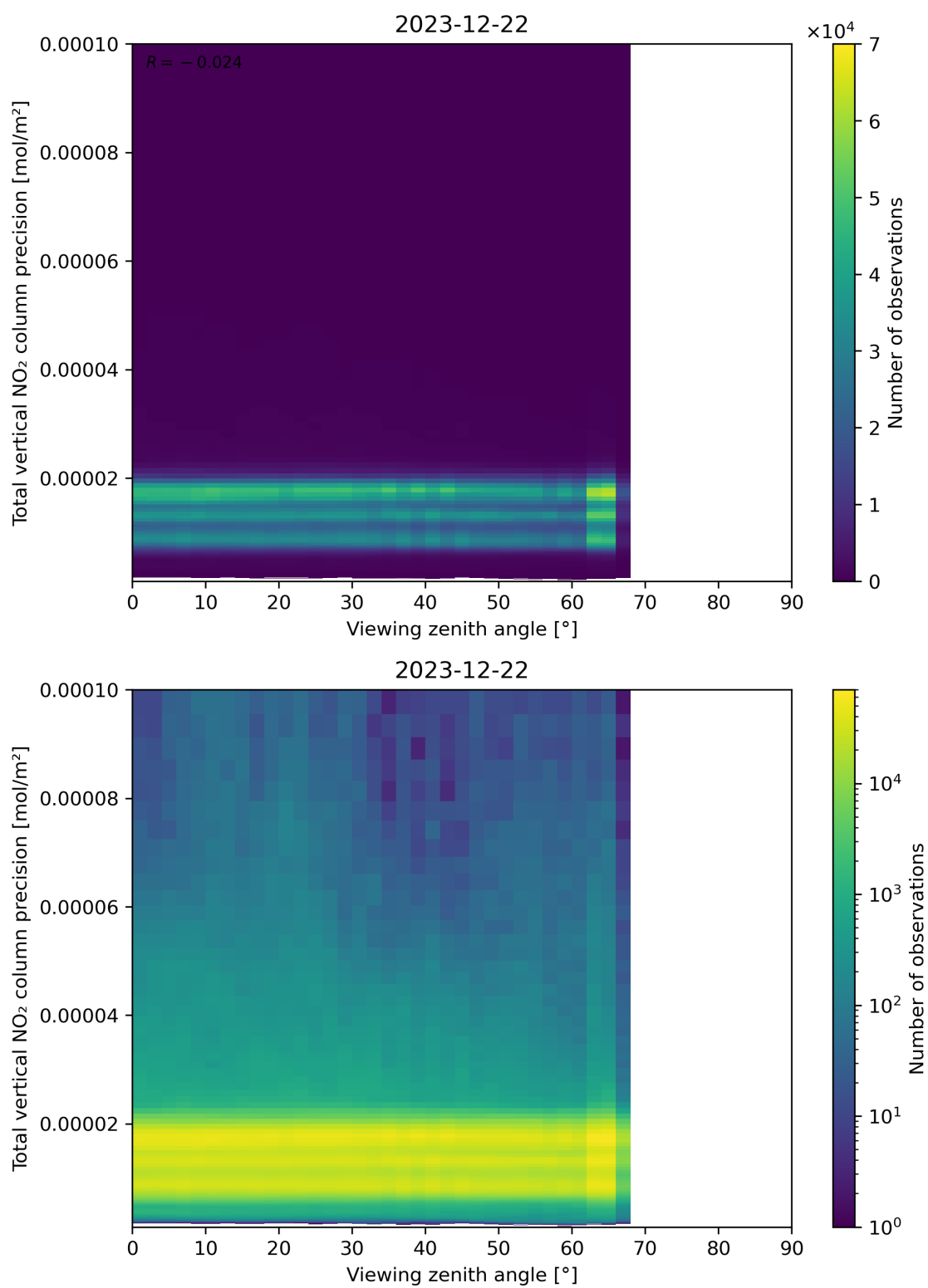
Figure 168: Scatter density plot of “Viewing zenith angle” against “Total vertical NO 2 column precision” for 2023-12-21 to 2023-12-23.
