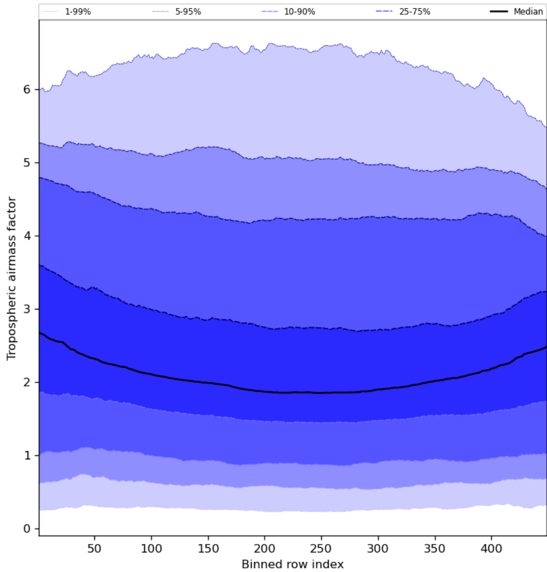
Figure 48: Along track statistics of “Tropospheric air mass factor” for 2023-12-21 to 2023-12-23
