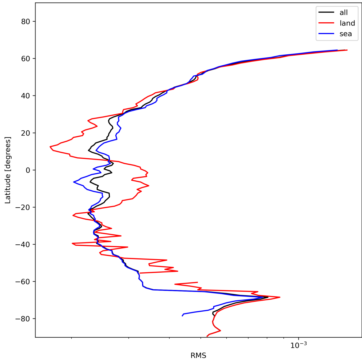
Figure 26: Zonal average of “RMS” for 2023-12-21 to 2023-12-23.
