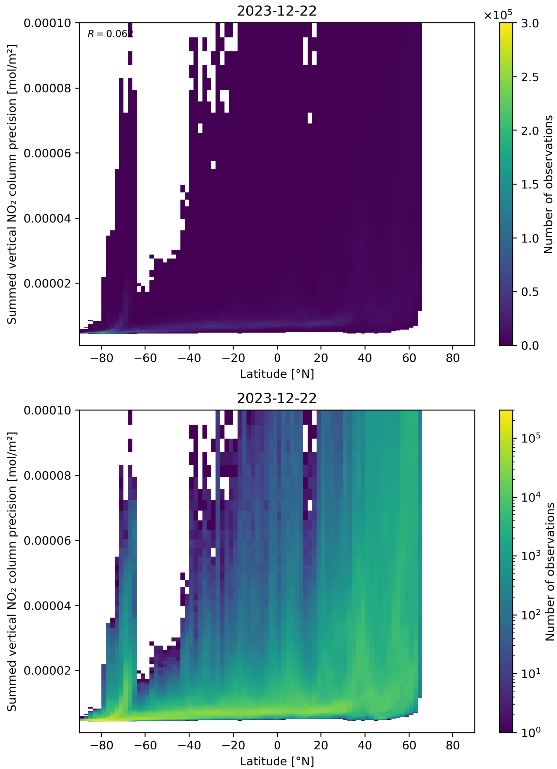
Figure 89: Scatter density plot of “Latitude” against “Summed vertical NO 2 column precision” for 2023-12-21 to 2023-12-23.
