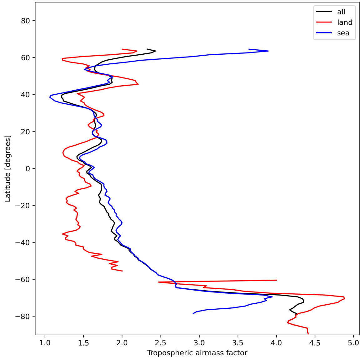
Figure 14: Zonal average of “Tropospheric airmass factor” for 2023-12-21 to 2023-12-23.
