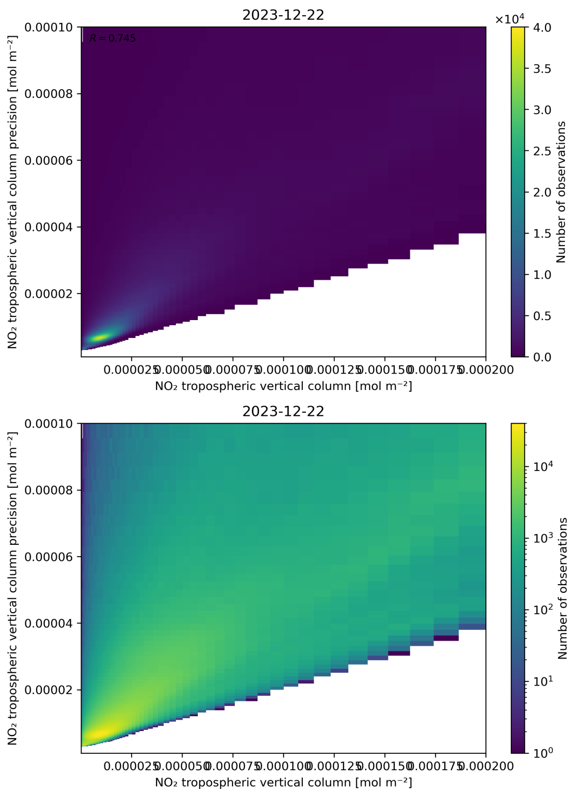
Figure 130: Scatter density plot of “NO 2 tropospheric vertical column” against “NO 2 tropospheric vertical column precision” for 2023-12-21 to 2023-12-23.
