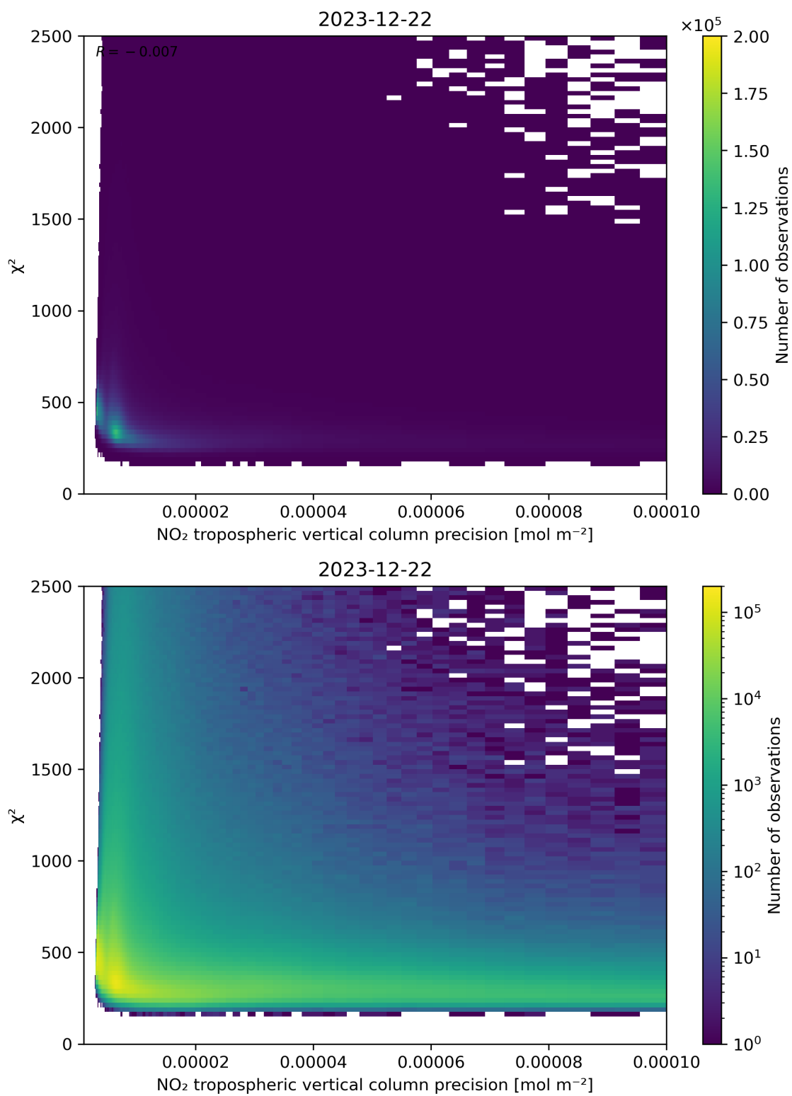
Figure 134: Scatter density plot of “NO 2 tropospheric vertical column precision” against “ \chi^2 ” for 2023-12-21 to 2023-12-23.
