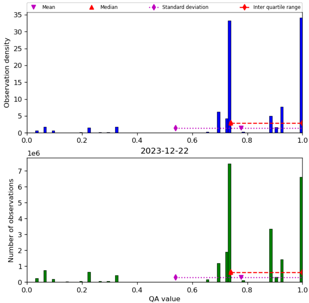
Figure 28: Histogram of “QA value” for 2023-12-21 to 2023-12-23
