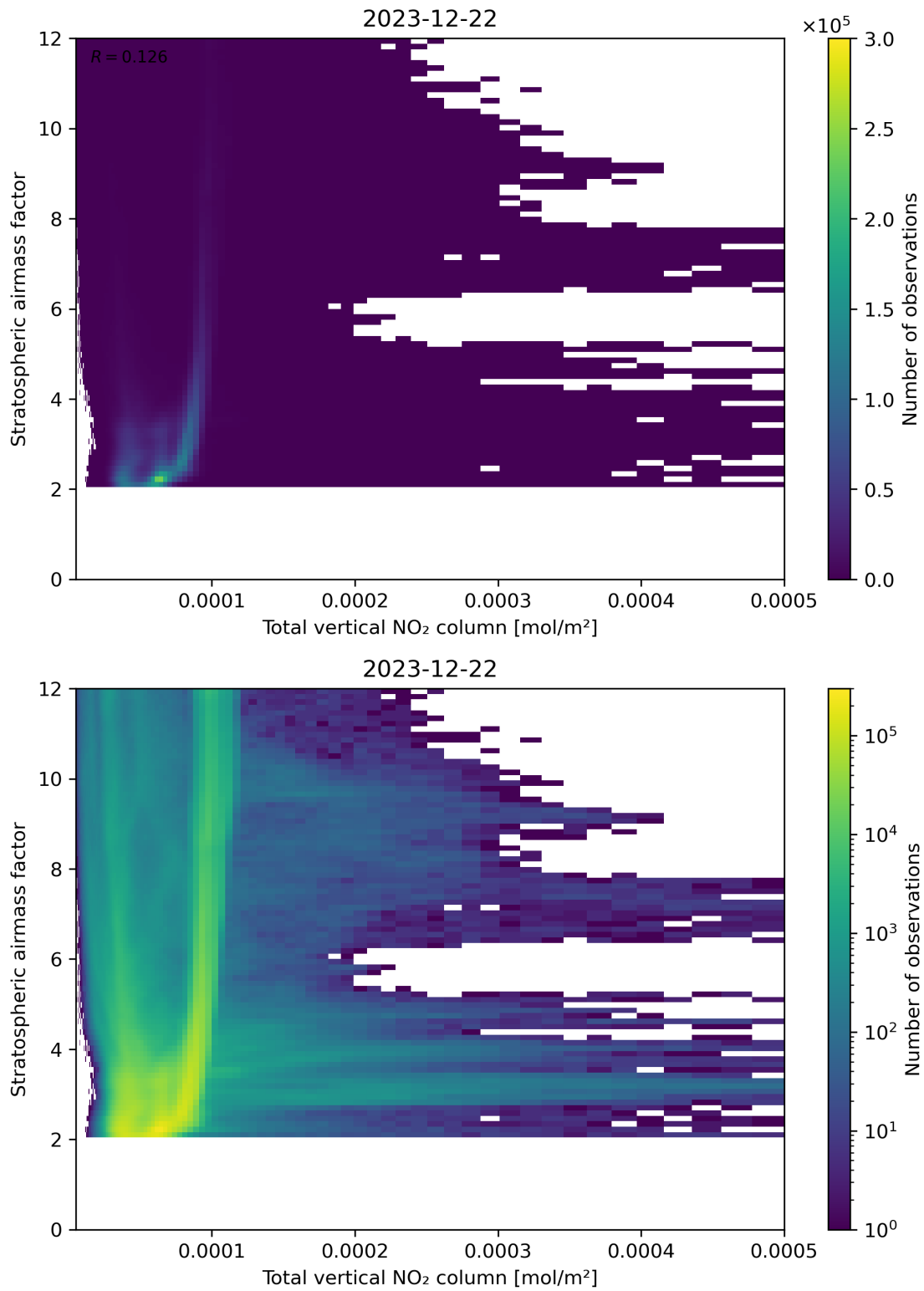
Figure 110: Scatter density plot of “Total vertical NO 2 column” against “Stratospheric air mass factor” for 2023-12-21 to 2023-12-23.
