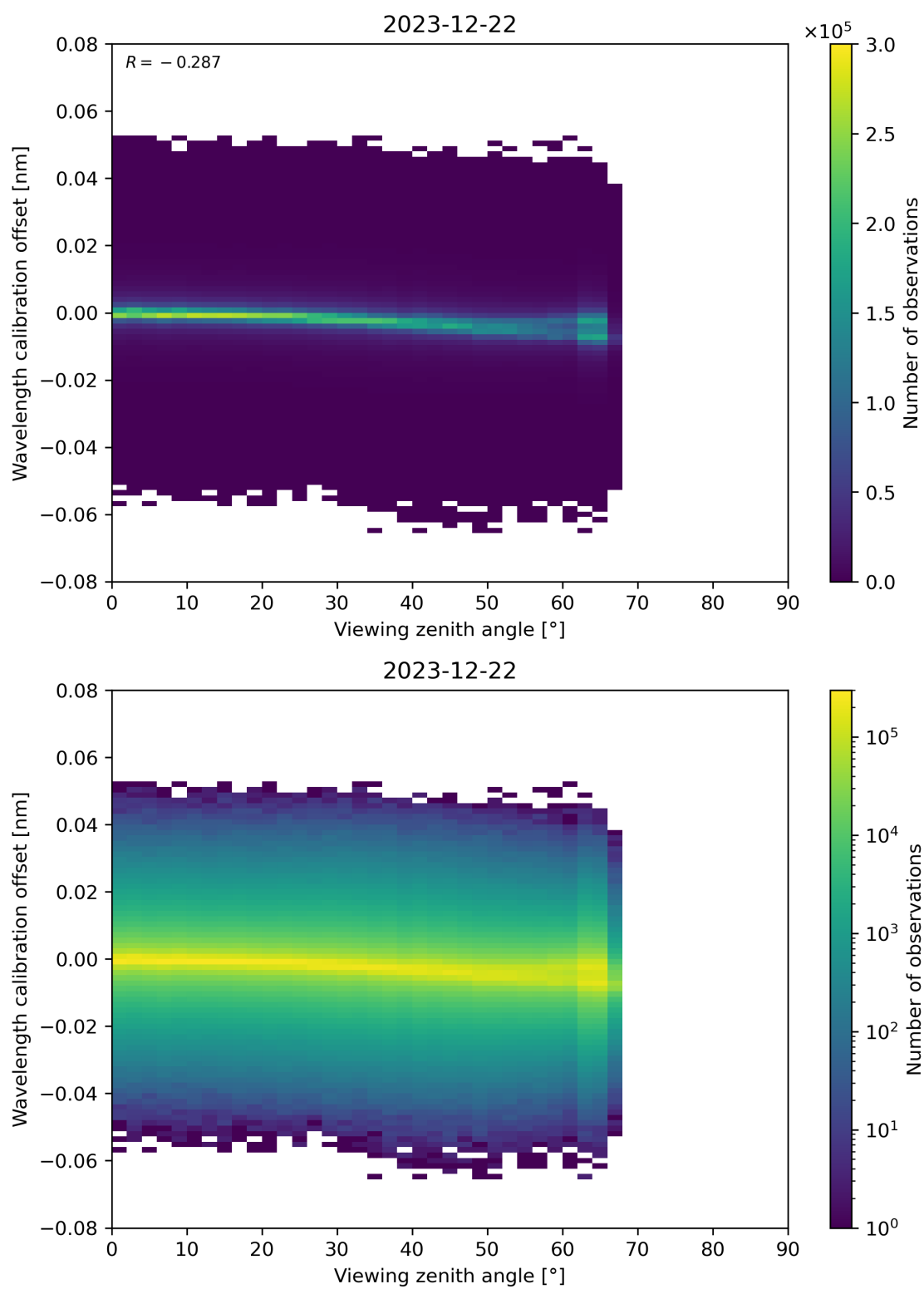
Figure 173: Scatter density plot of “Viewing zenith angle” against “Wavelength calibration offset” for 2023-12-21 to 2023-12-23.
