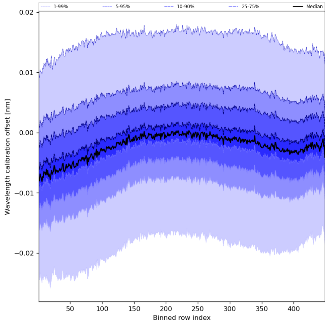
Figure 52: Along track statistics of “Wavelength calibration offset” for 2023-12-21 to 2023-12-23
