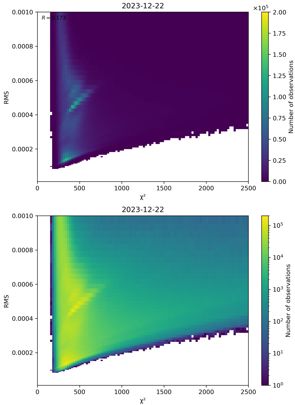
Figure 82: Scatter density plot of “ \chi^2 ” against “RMS” for 2023-12-21 to 2023-12-23.
