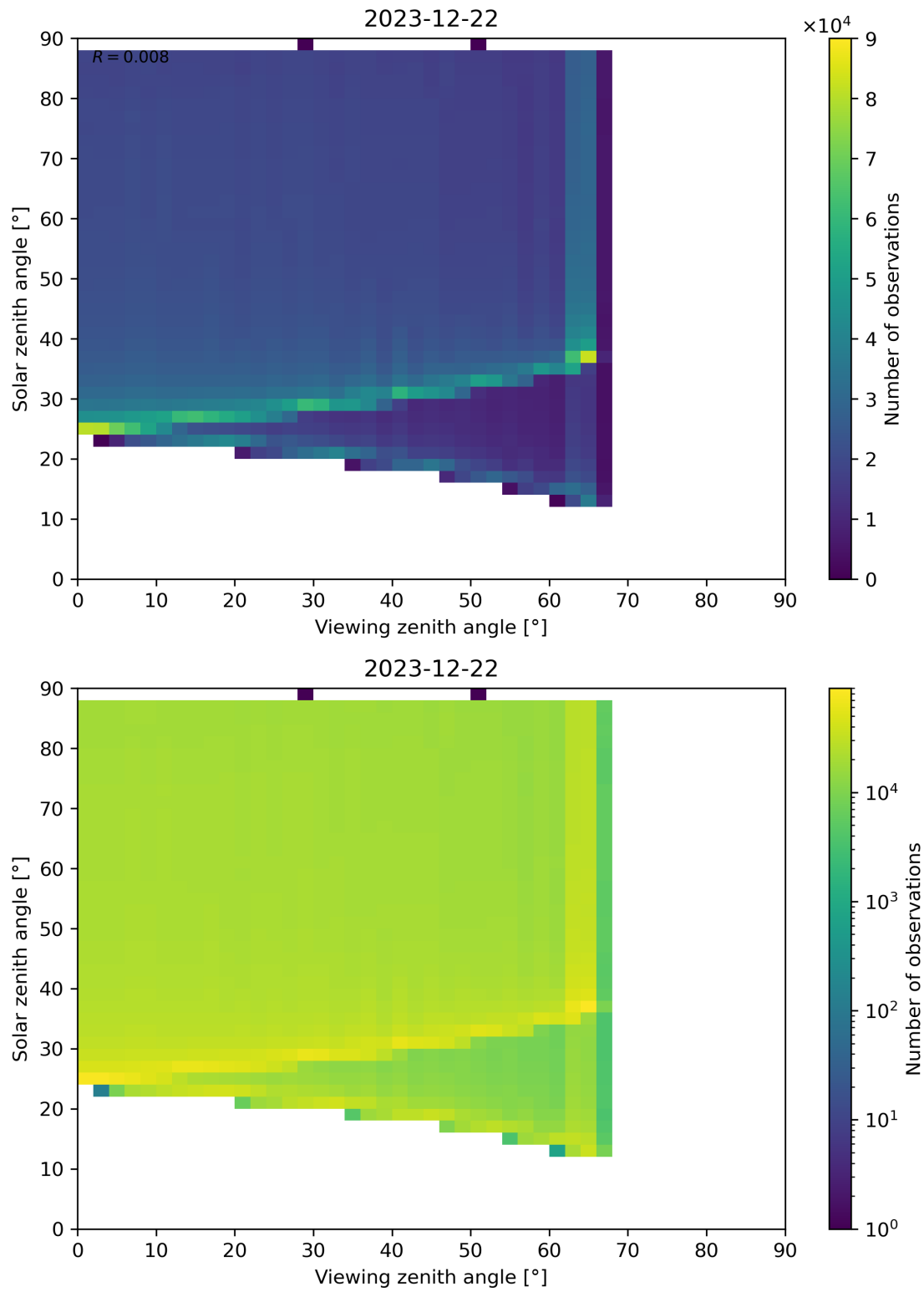
Figure 172: Scatter density plot of “Viewing zenith angle” against “Solar zenith angle” for 2023-12-21 to 2023-12-23.
