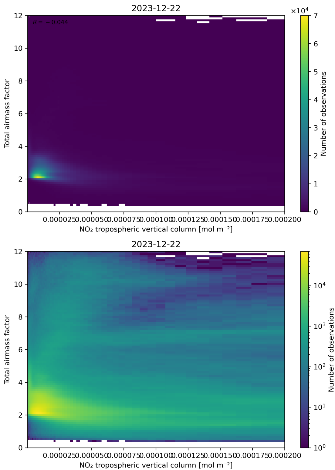
Figure 122: Scatter density plot of “NO 2 tropospheric vertical column” against “Total air mass factor” for 2023-12-21 to 2023-12-23.
