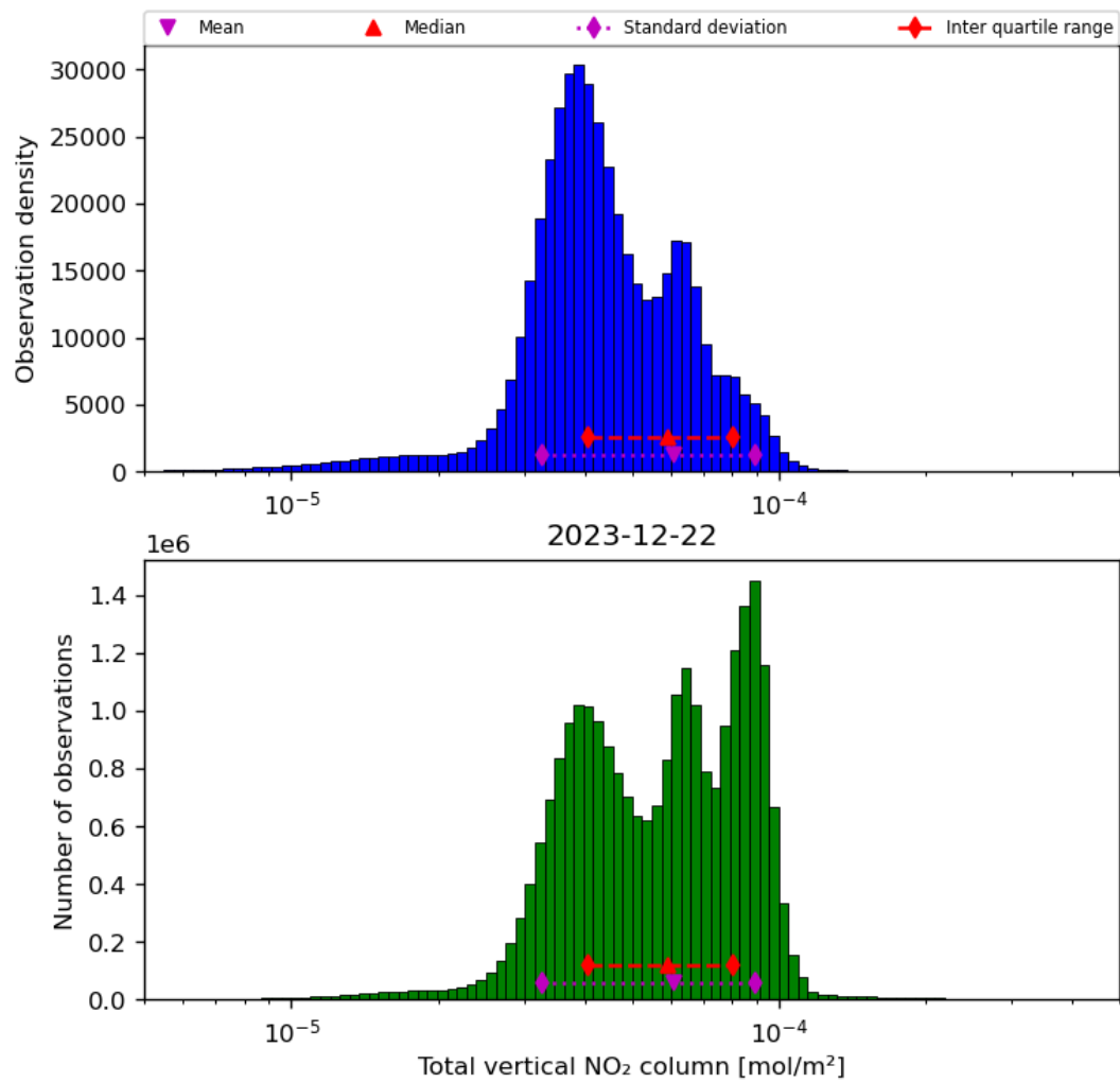
Figure 38: Histogram of “Total vertical NO 2 column” for 2023-12-21 to 2023-12-23
