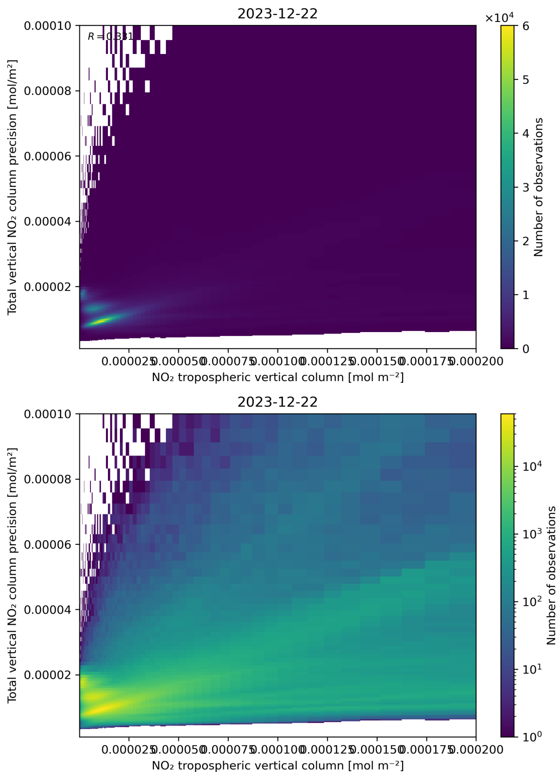
Figure 129: Scatter density plot of “NO 2 tropospheric vertical column” against “Total vertical NO 2 column precision” for 2023-12-21 to 2023-12-23.
