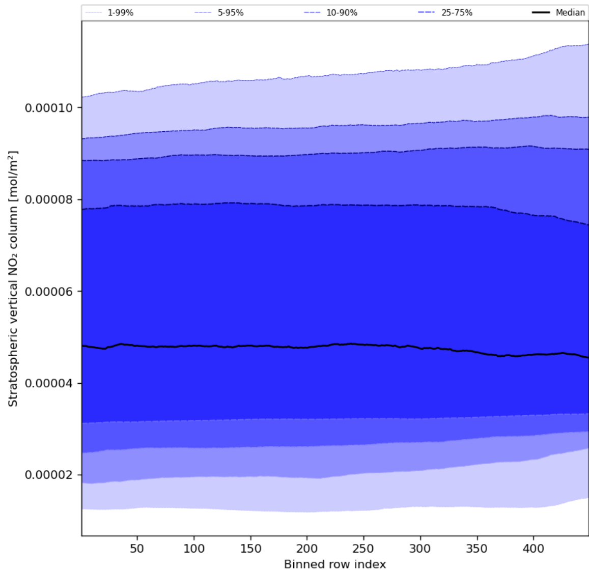
Figure 53: Along track statistics of “Stratospheric vertical NO 2 column” for 2023-12-21 to 2023-12-23
