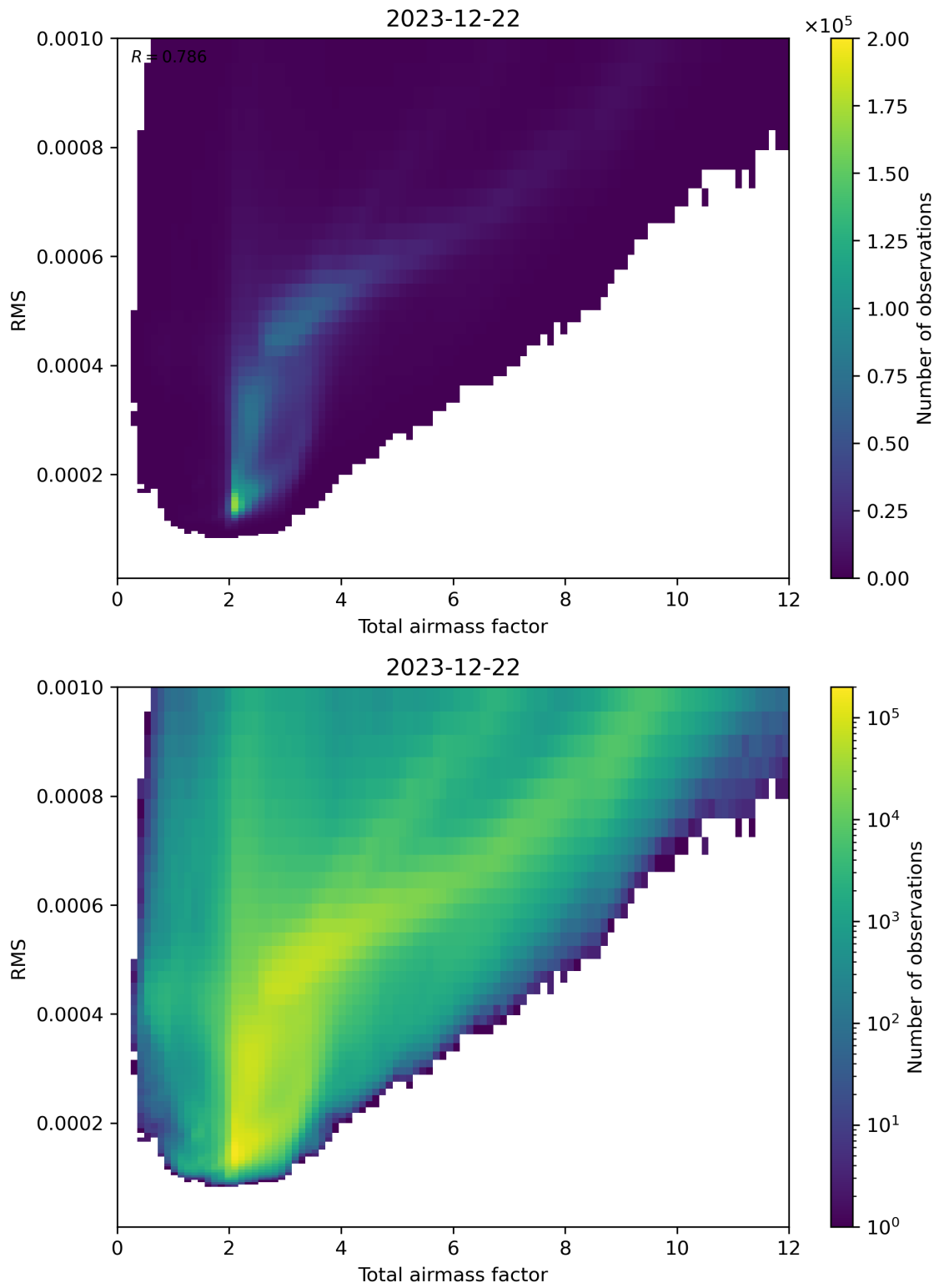
Figure 69: Scatter density plot of “Total airmass factor” against “RMS” for 2023-12-21 to 2023-12-23.
