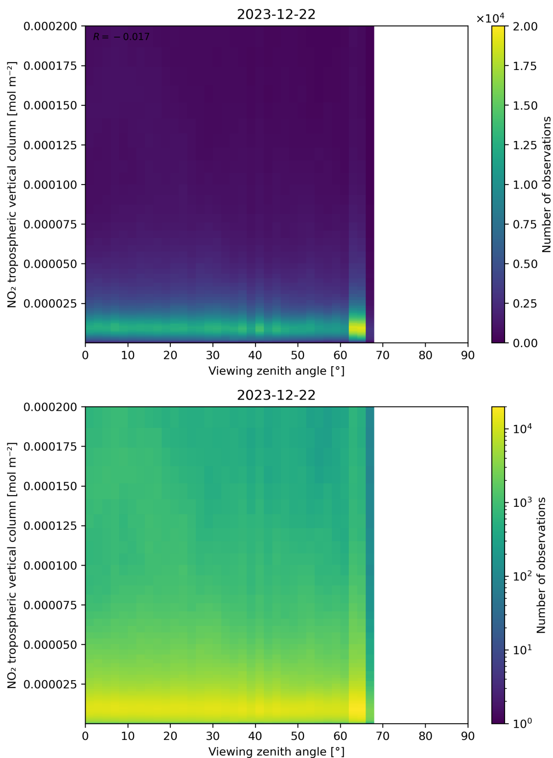
Figure 169: Scatter density plot of “Viewing zenith angle” against “NO 2 tropospheric vertical column” for 2023-12-21 to 2023-12-23.
