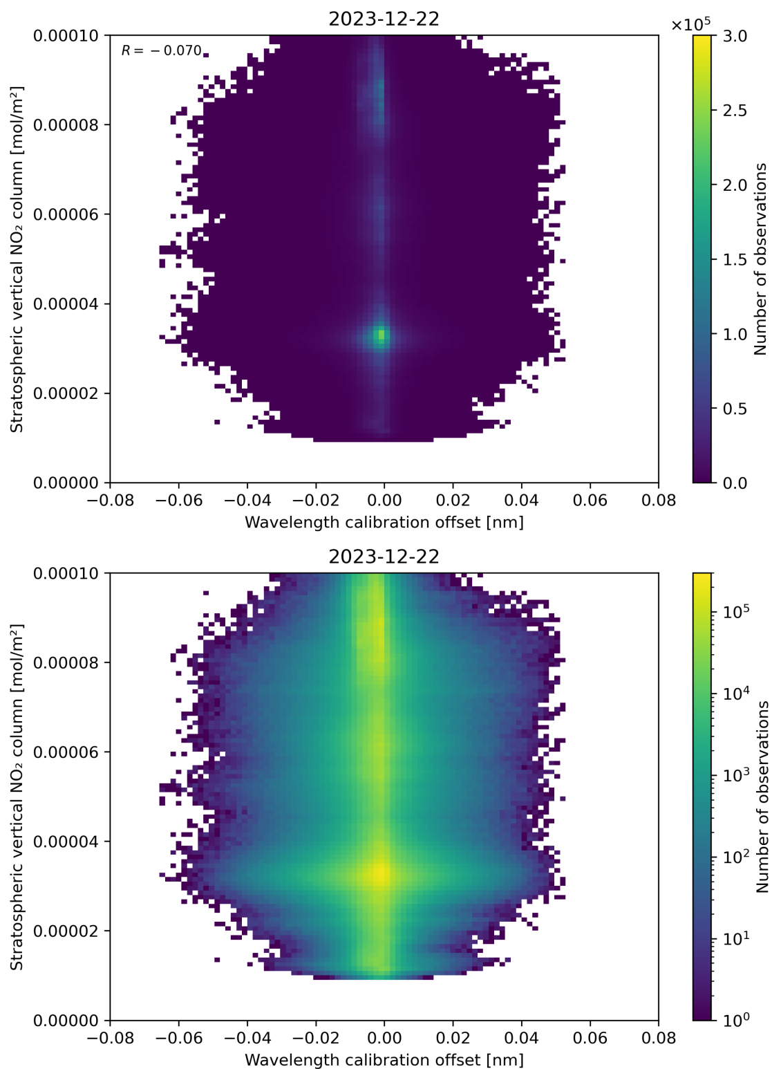
Figure 176: Scatter density plot of “Wavelength calibration offset” against “Stratospheric vertical NO 2 column” for 2023-12-21 to 2023-12-23.
