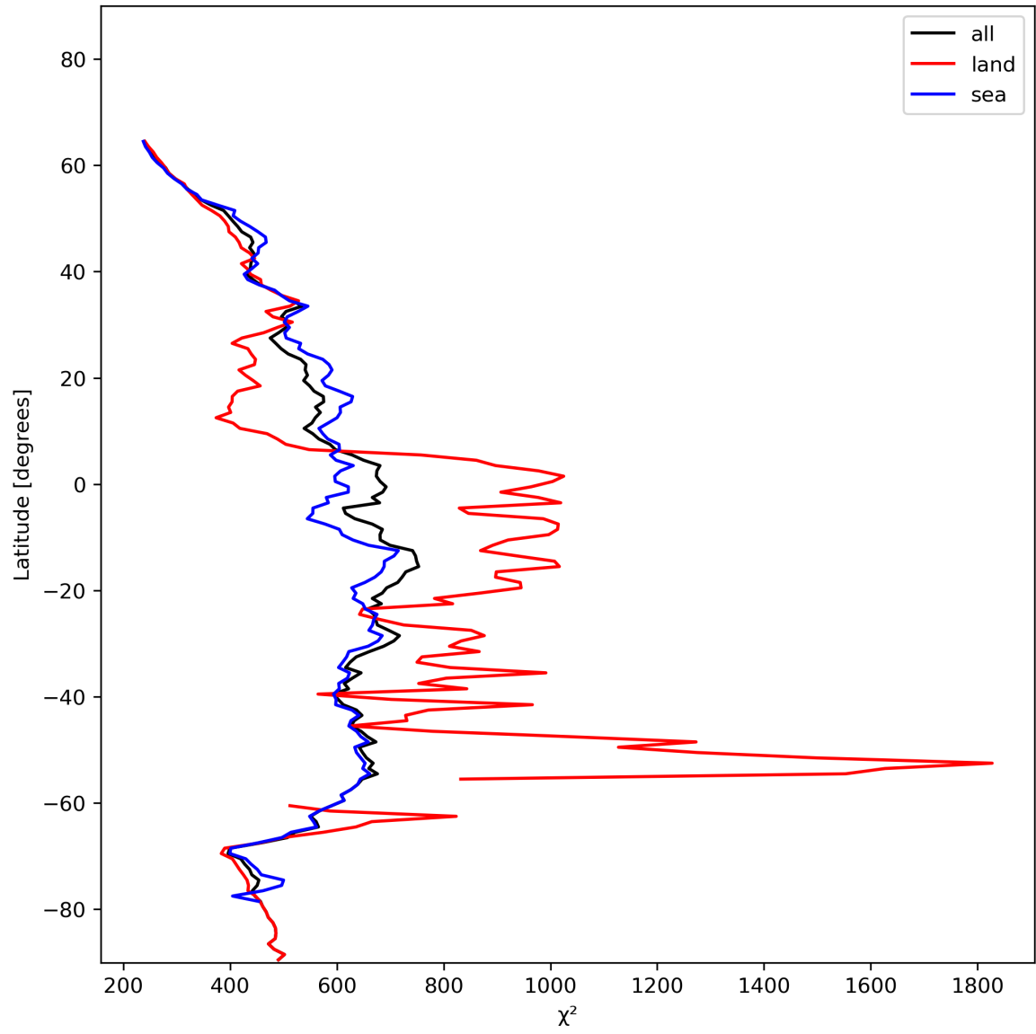
Figure 25: Zonal average of “ \chi^2 ” for 2023-12-21 to 2023-12-23.
