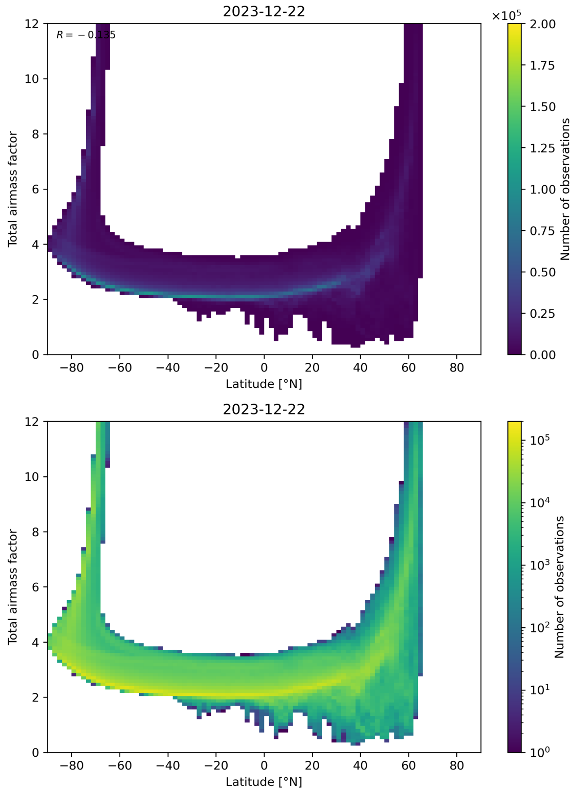
Figure 84: Scatter density plot of “Latitude” against “Total airmass factor” for 2023-12-21 to 2023-12-23.
