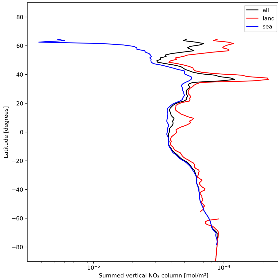
Figure 23: Zonal average of “Summed vertical NO 2 column” for 2023-12-21 to 2023-12-23.
