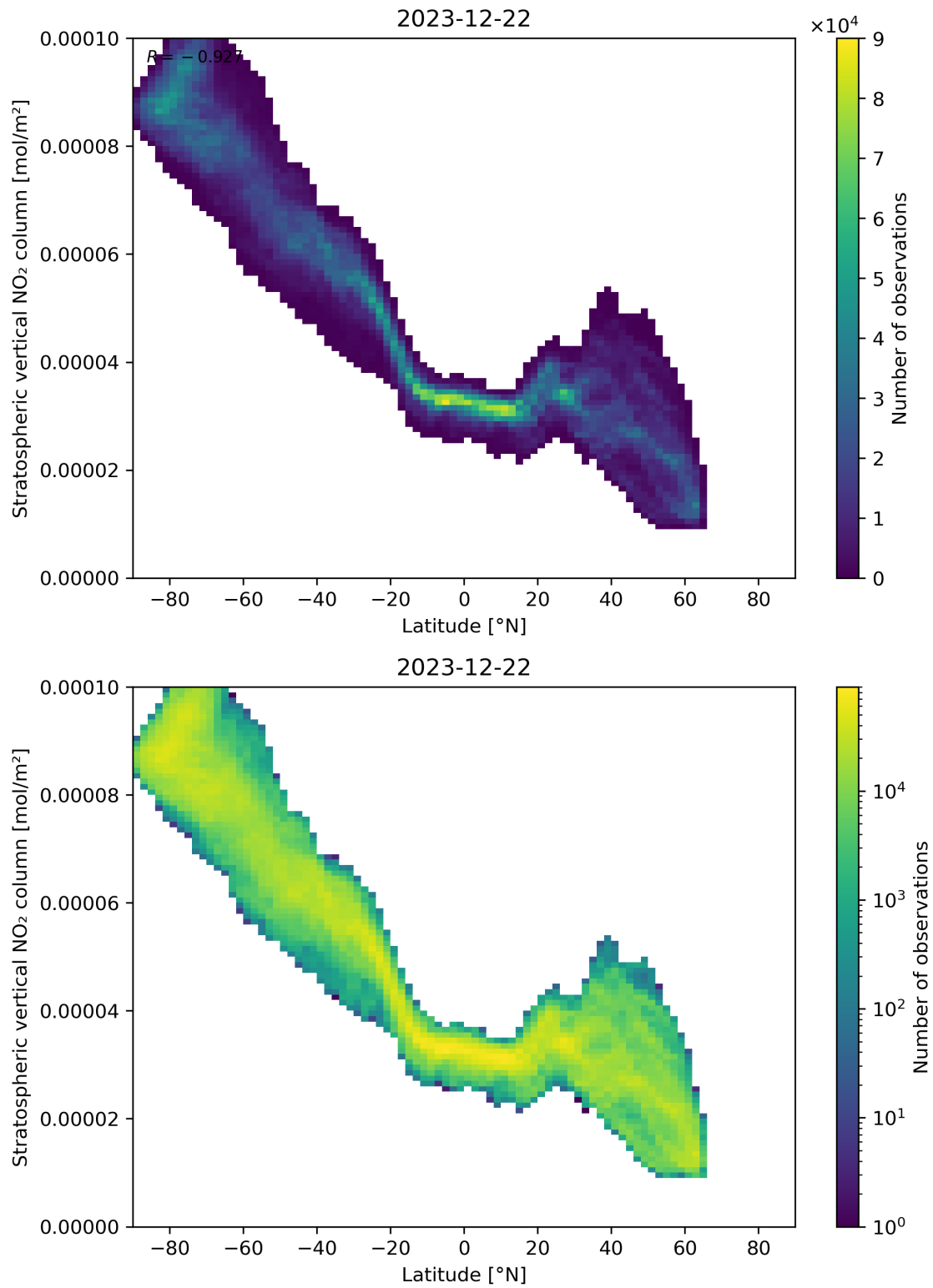
Figure 87: Scatter density plot of “Latitude” against “Stratospheric vertical NO 2 column” for 2023-12-21 to 2023-12-23.
