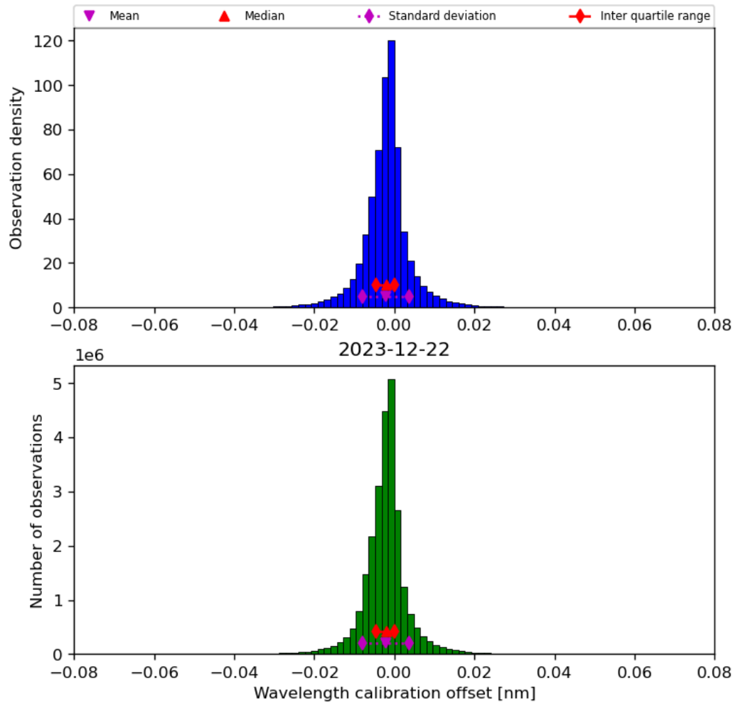
Figure 35: Histogram of “Wavelength calibration offset” for 2023-12-21 to 2023-12-23
