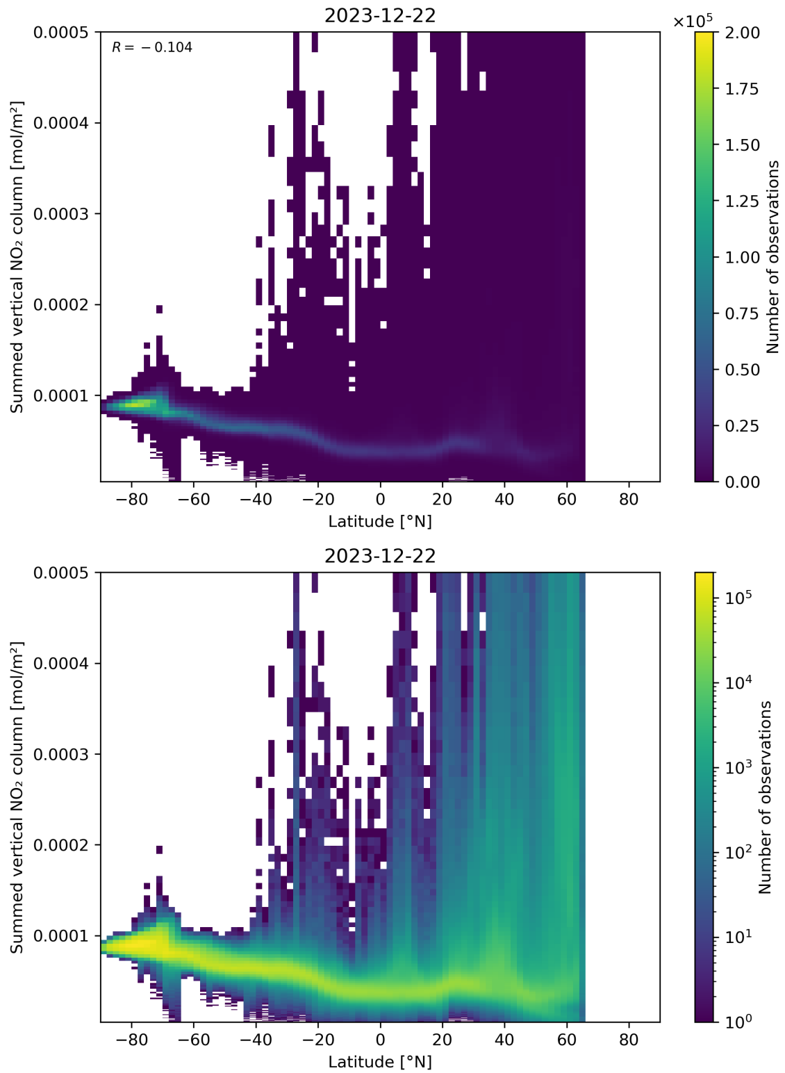
Figure 88: Scatter density plot of “Latitude” against “Summed vertical NO 2 column” for 2023-12-21 to 2023-12-23.
