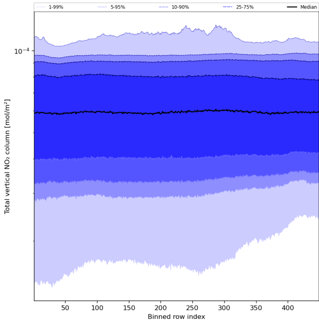
Figure 55: Along track statistics of “Total vertical NO 2 column” for 2023-12-21 to 2023-12-23
