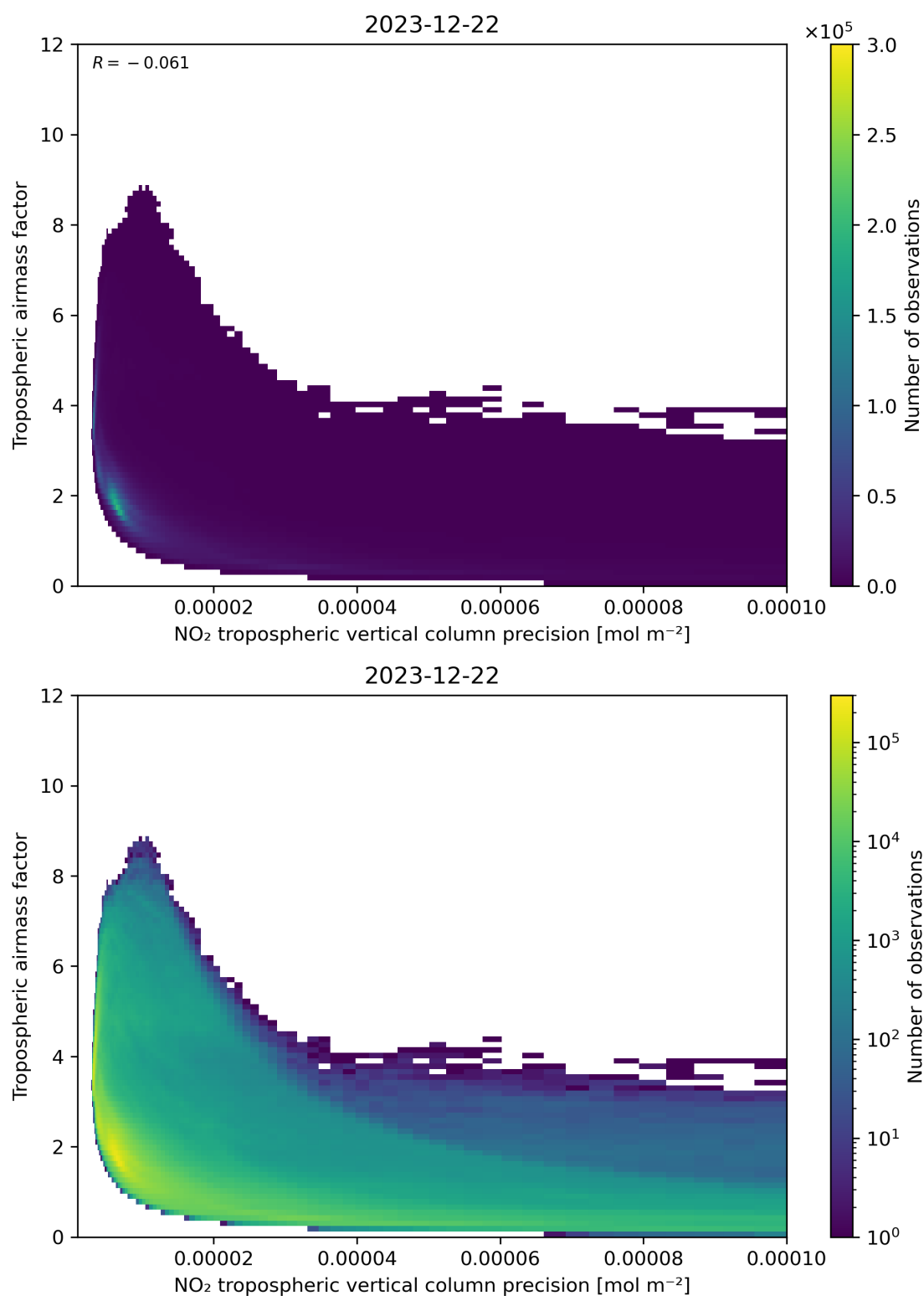
Figure 133: Scatter density plot of “NO 2 tropospheric vertical column precision” against “Tropospheric airmass factor” for 2023-12-21 to 2023-12-23.
