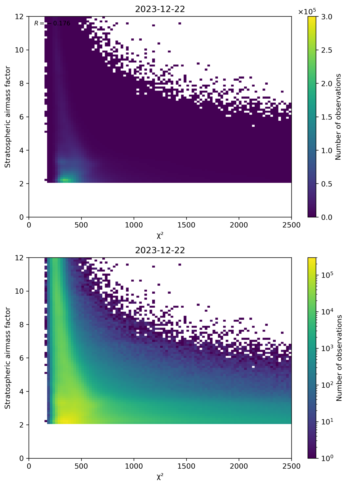
Figure 81: Scatter density plot of “ \chi^2 ” against “Stratospheric airmass factor” for 2023-12-21 to 2023-12-23.
