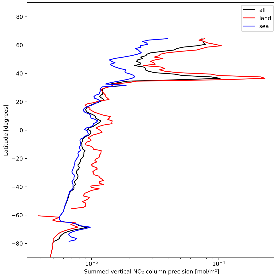
Figure 24: Zonal average of “Summed vertical NO 2 column precision” for 2023-12-21 to 2023-12-23.
