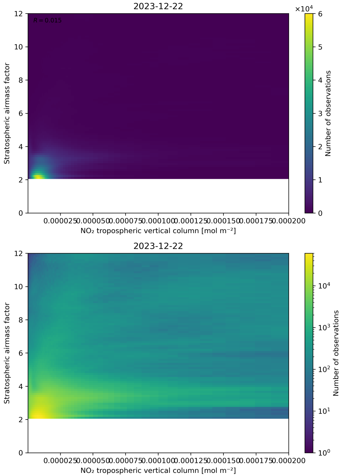
Figure 121: Scatter density plot of “NO 2 tropospheric vertical column” against “Stratospheric airmass factor” for 2023-12-21 to 2023-12-23.
