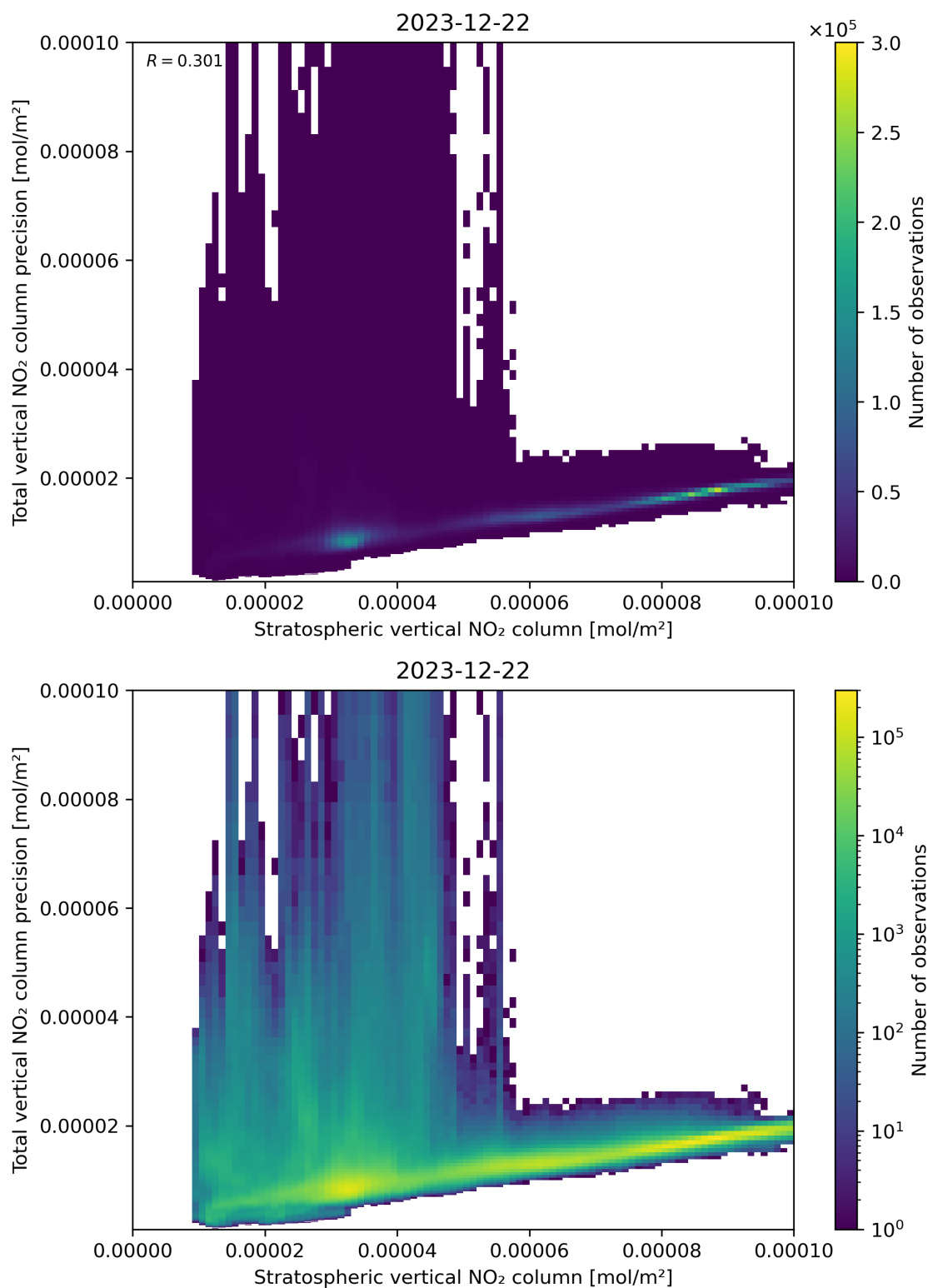
Figure 101: Scatter density plot of “Stratospheric vertical NO 2 column” against “Total vertical NO 2 column precision” for 2023-12-21 to 2023-12-23.
