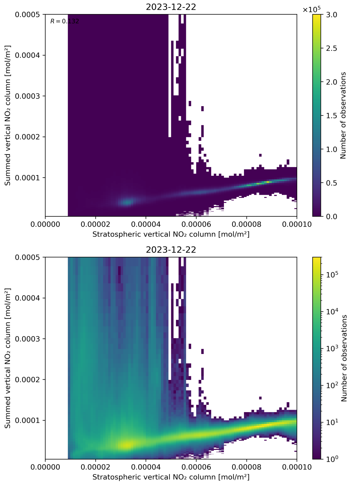
Figure 98: Scatter density plot of “Stratospheric vertical NO 2 column” against “Summed vertical NO 2 column” for 2023-12-21 to 2023-12-23.
