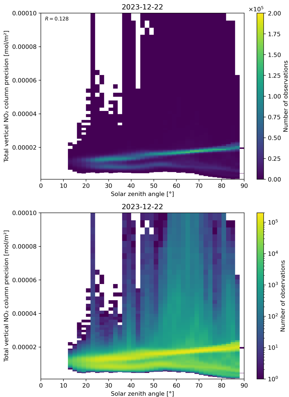
Figure 154: Scatter density plot of “Solar zenith angle” against “Total vertical NO 2 column precision” for 2023-12-21 to 2023-12-23.
