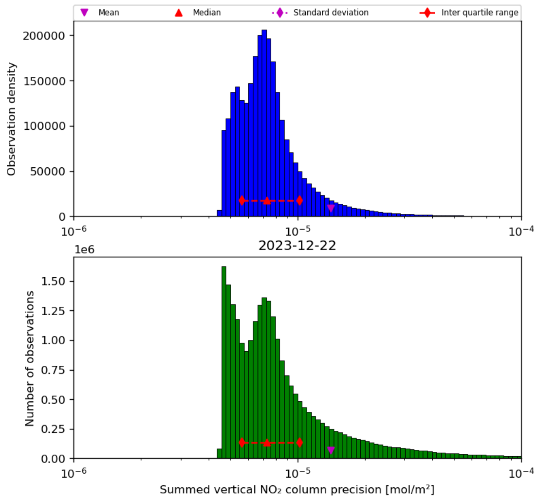
Figure 41: Histogram of “Summed vertical NO 2 column precision” for 2023-12-21 to 2023-12-23
