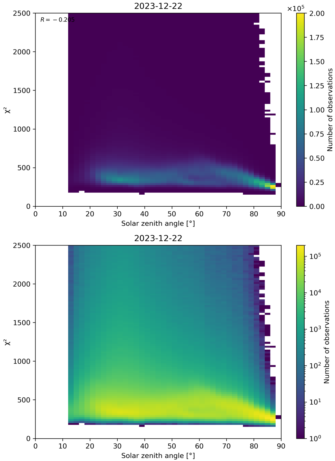
Figure 148: Scatter density plot of “Solar zenith angle” against “ \chi^2 ” for 2023-12-21 to 2023-12-23.
