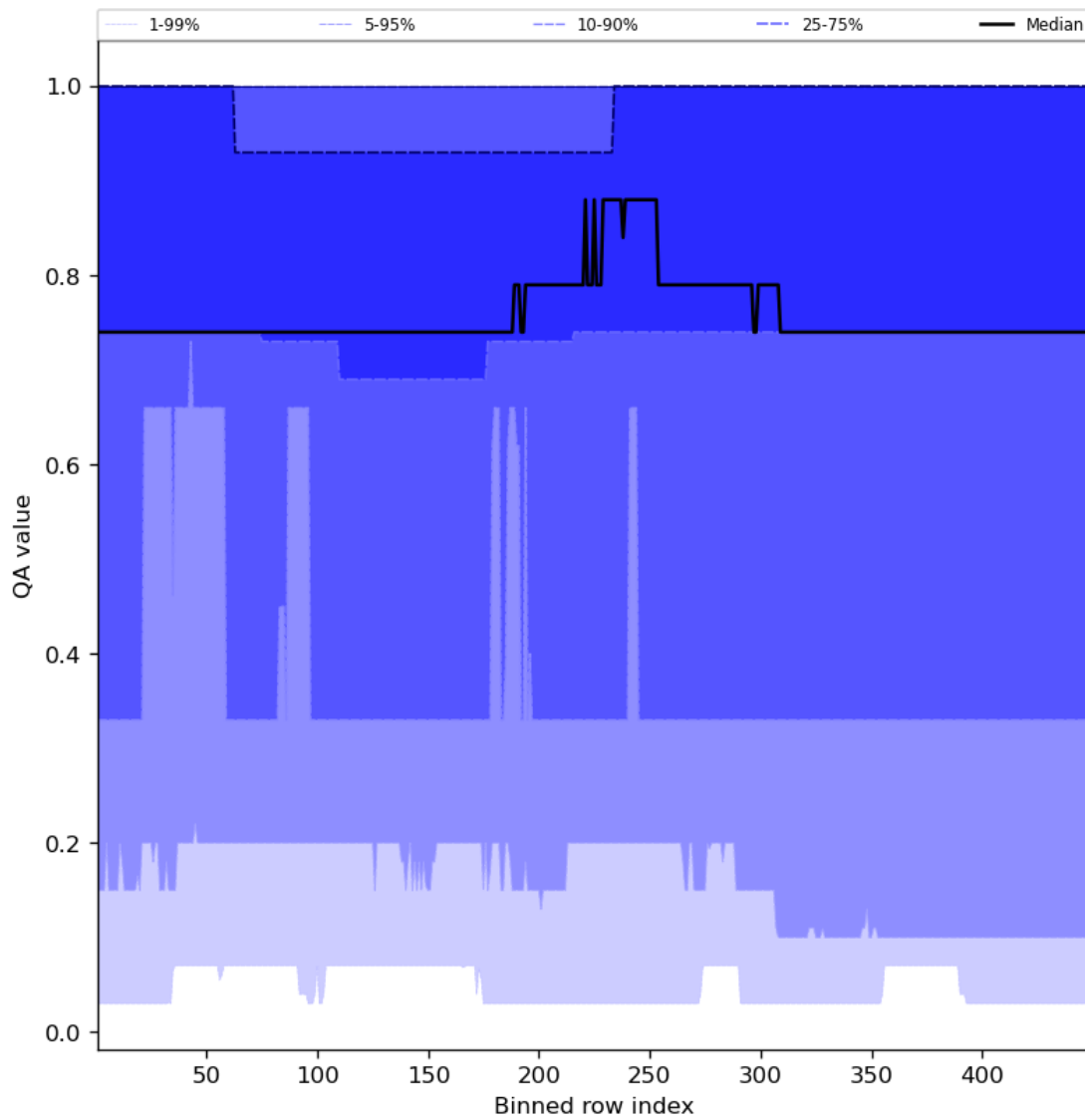
Figure 45: Along track statistics of “QA value” for 2023-12-21 to 2023-12-23
