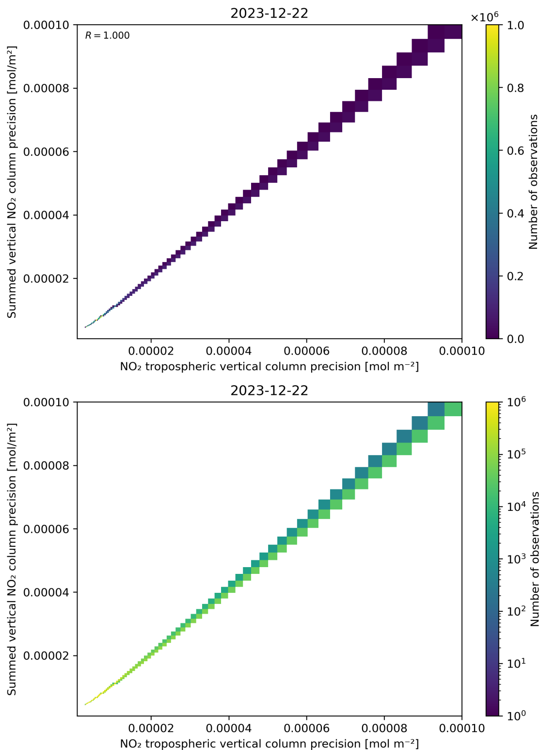
Figure 137: Scatter density plot of “NO 2 tropospheric vertical column precision” against “Summed vertical NO 2 column precision” for 2023-12-21 to 2023-12-23.
