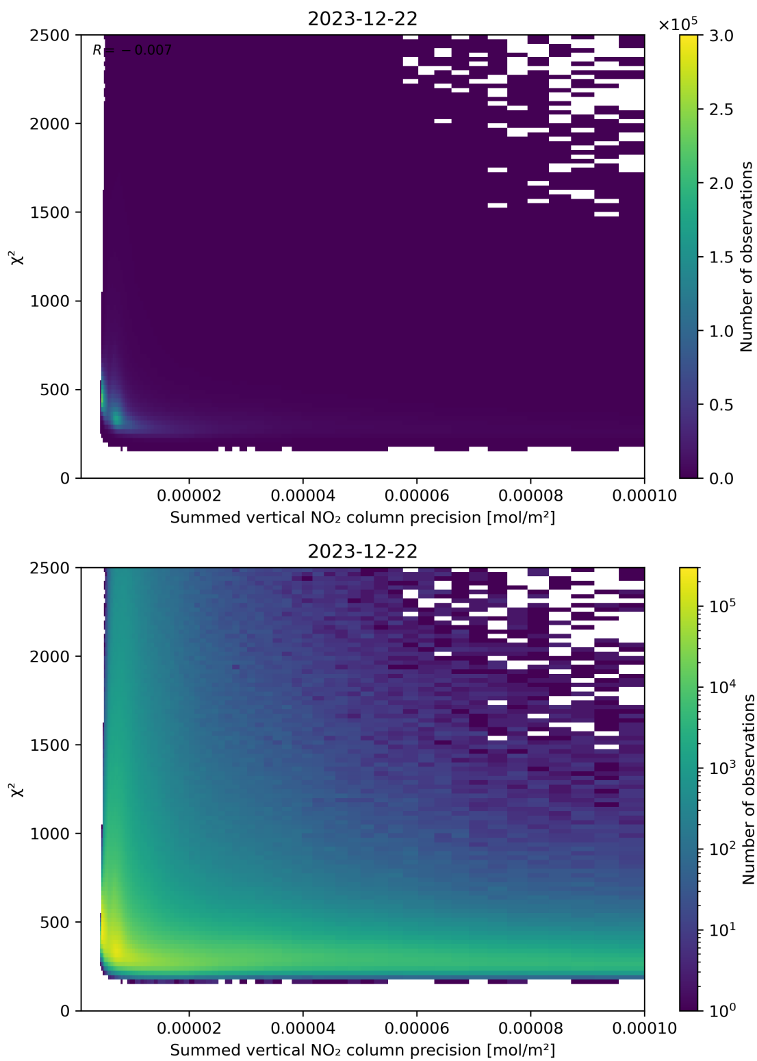
Figure 107: Scatter density plot of “Summed vertical NO 2 column precision” against “ \chi^2 ” for 2023-12-21 to 2023-12-23.
