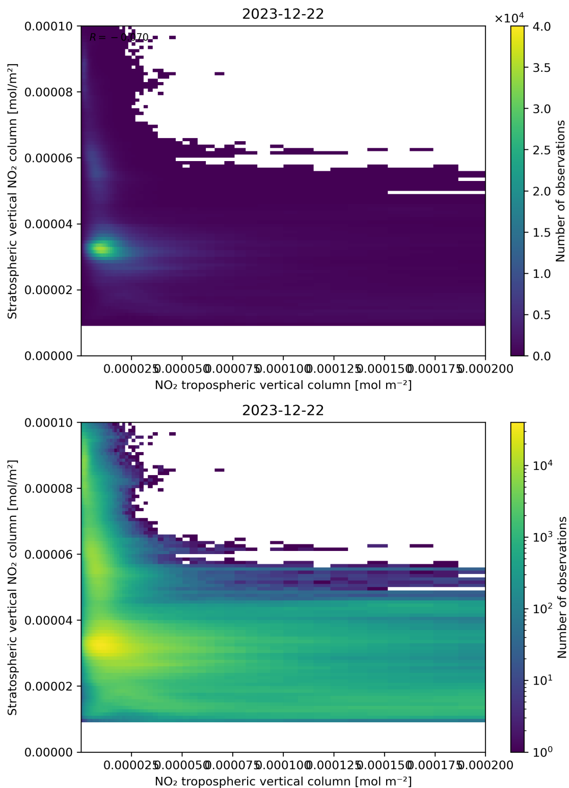
Figure 125: Scatter density plot of “NO 2 tropospheric vertical column” against “Stratospheric vertical NO 2 column” for 2023-12-21 to 2023-12-23.
