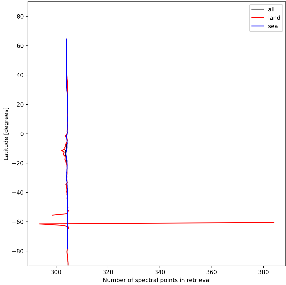
Figure 16: Zonal average of “Number of spectral points in retrieval” for 2023-12-21 to 2023-12-23.
