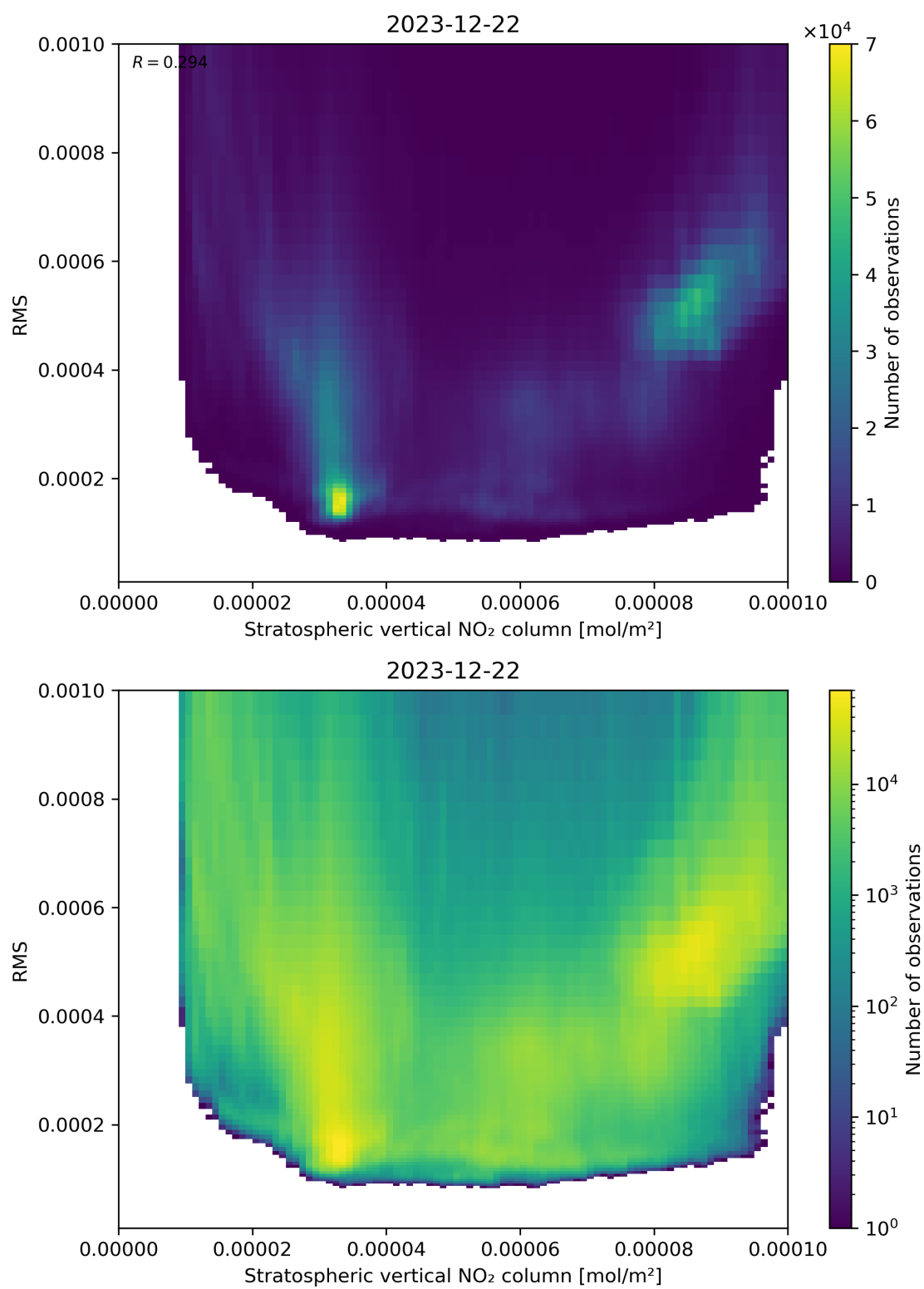
Figure 102: Scatter density plot of “Stratospheric vertical NO 2 column” against “RMS” for 2023-12-21 to 2023-12-23.
