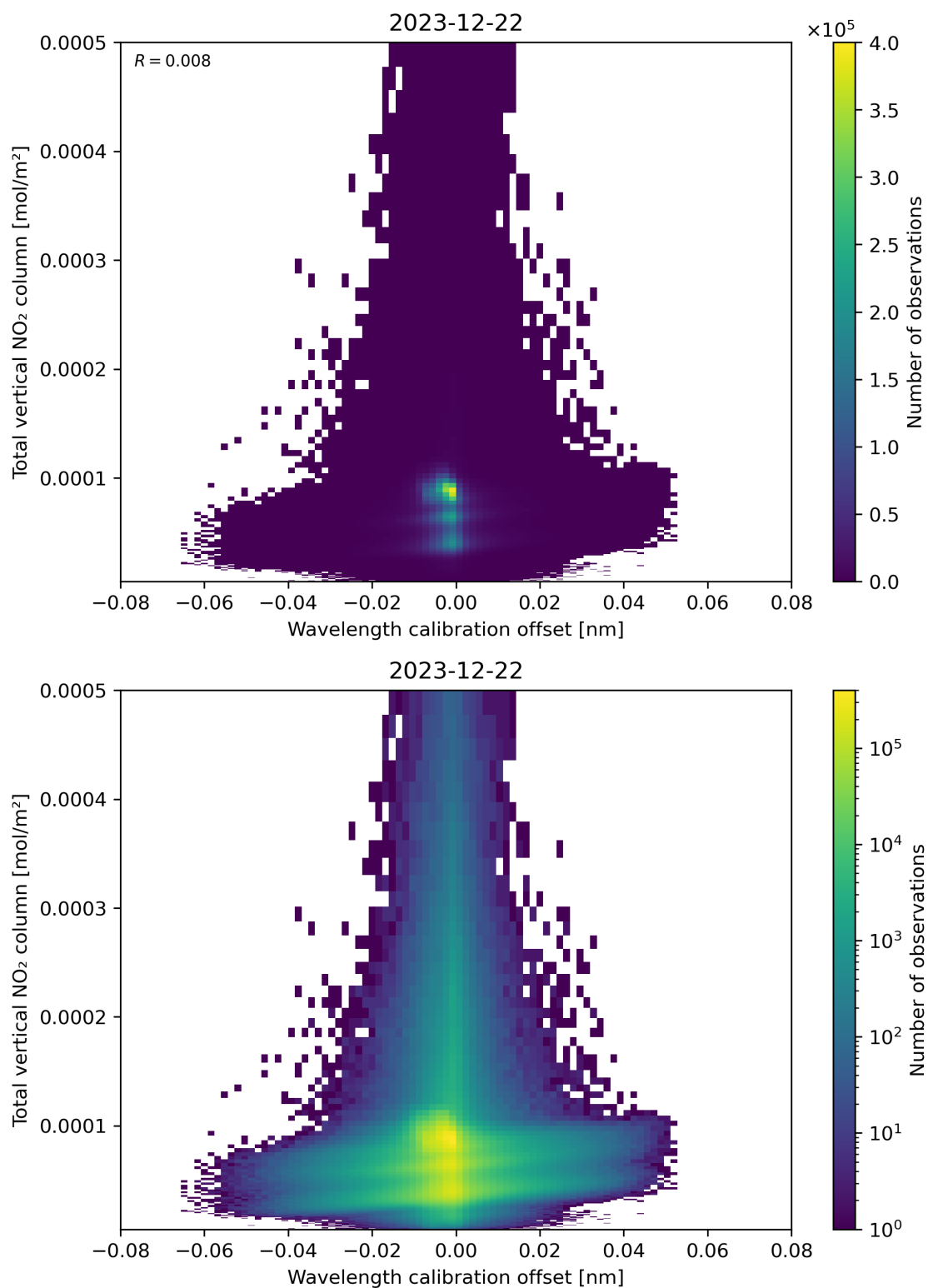
Figure 179: Scatter density plot of “Wavelength calibration offset” against “Total vertical NO 2 column” for 2023-12-21 to 2023-12-23.
