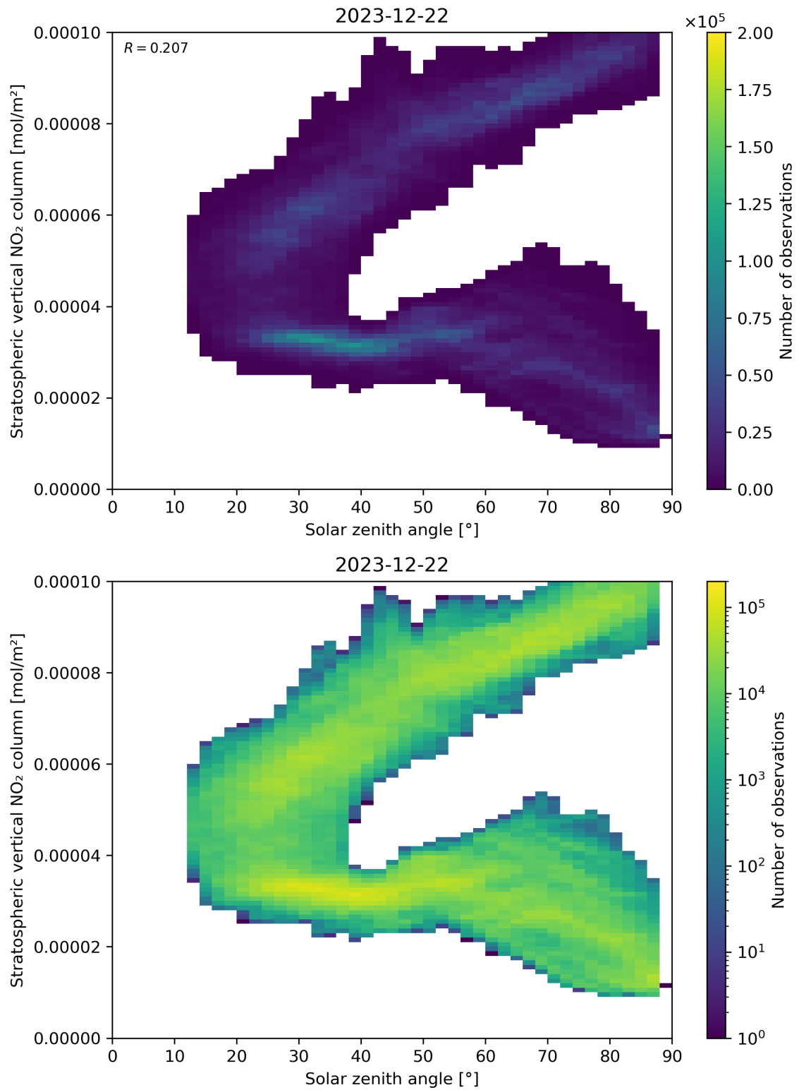
Figure 150: Scatter density plot of “Solar zenith angle” against “Stratospheric vertical NO 2 column” for 2023-12-21 to 2023-12-23.
