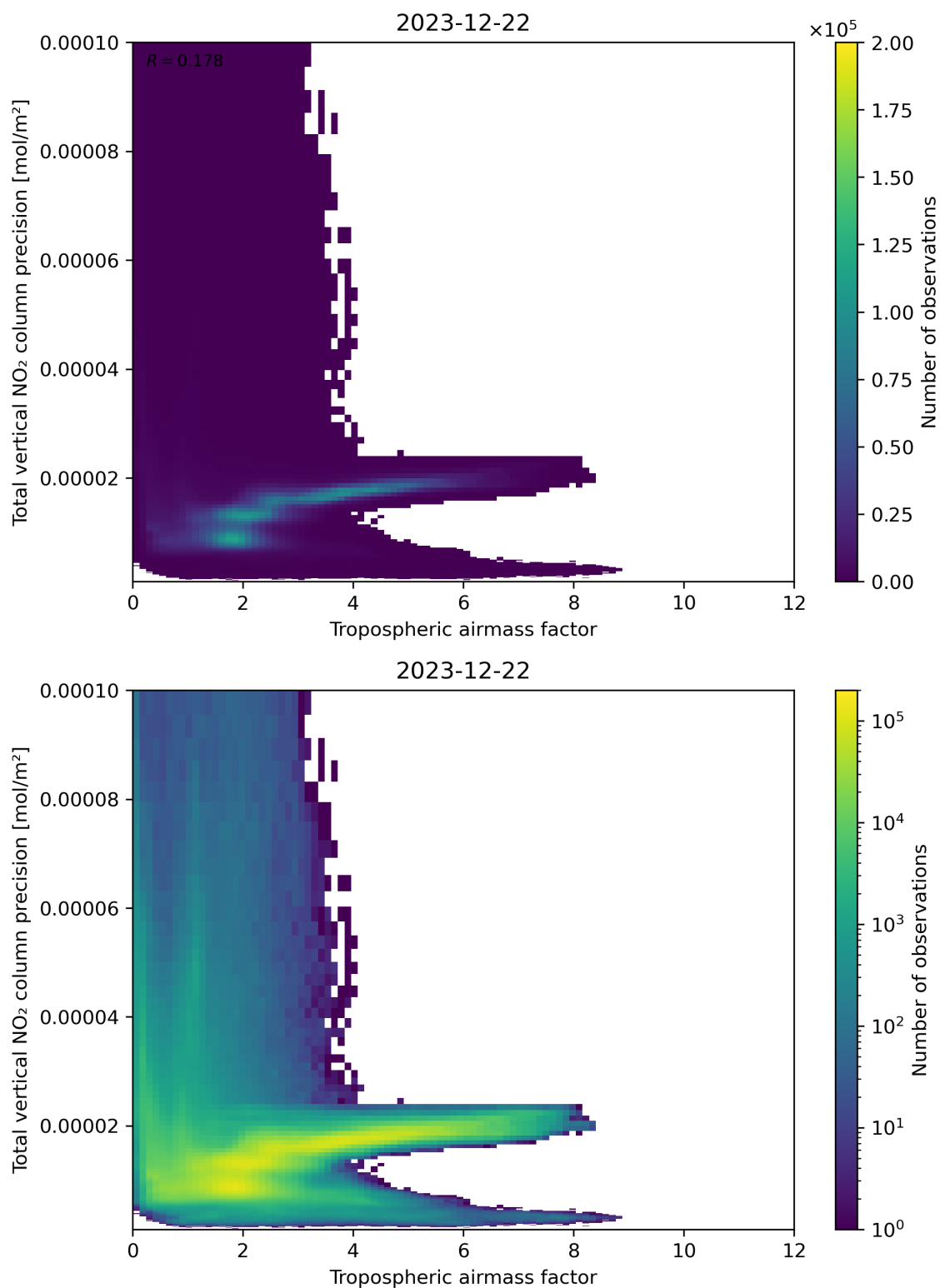
Figure 78: Scatter density plot of “Tropospheric air mass factor” against “Total vertical NO 2 column precision” for 2023-12-21 to 2023-12-23.
