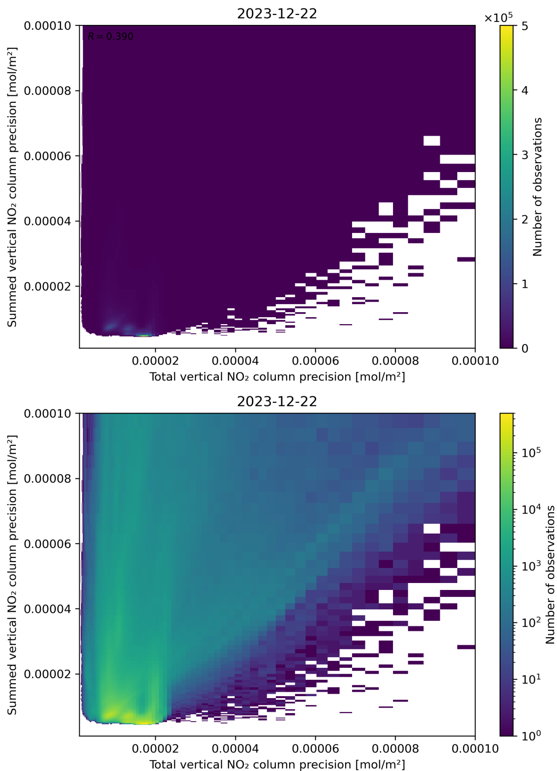
Figure 118: Scatter density plot of “Total vertical NO 2 column precision” against “Summed vertical NO 2 column precision” for 2023-12-21 to 2023-12-23.
