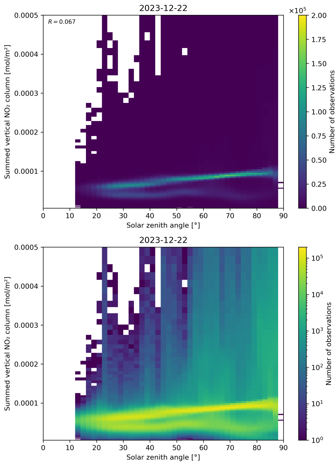
Figure 151: Scatter density plot of “Solar zenith angle” against “Summed vertical NO 2 column” for 2023-12-21 to 2023-12-23.
