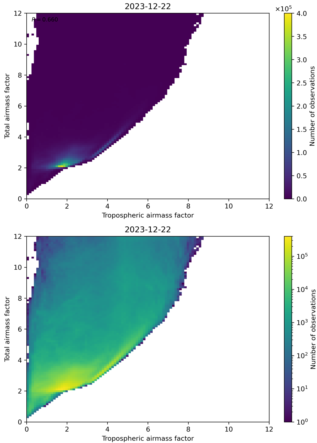
Figure 72: Scatter density plot of “Tropospheric airmass factor” against “Total airmass factor” for 2023-12-21 to 2023-12-23.
