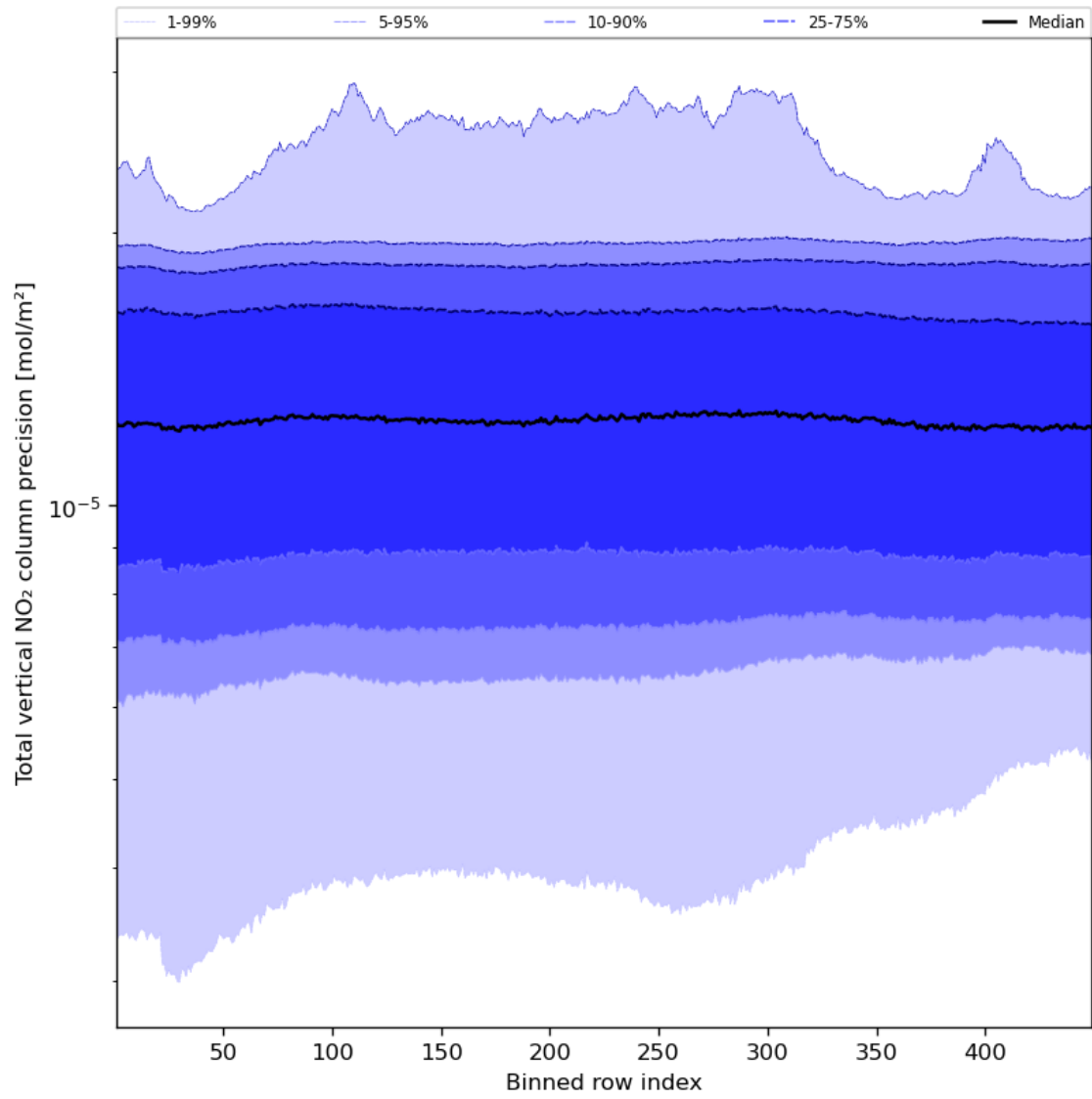
Figure 56: Along track statistics of “Total vertical NO 2 column precision” for 2023-12-21 to 2023-12-23
