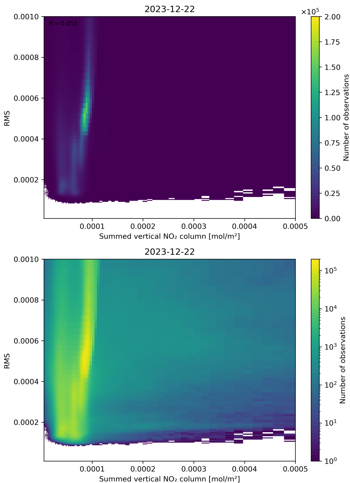
Figure 109: Scatter density plot of “Summed vertical NO 2 column” against “RMS” for 2023-12-21 to 2023-12-23.
