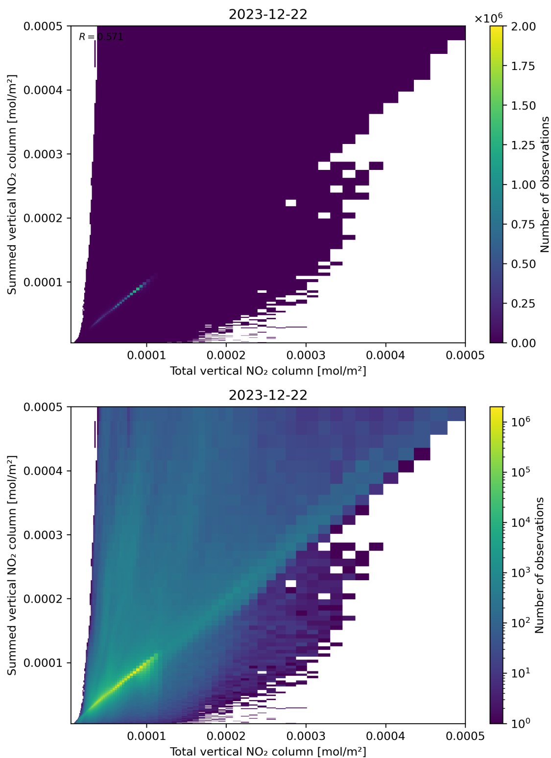
Figure 112: Scatter density plot of “Total vertical NO 2 column” against “Summed vertical NO 2 column” for 2023-12-21 to 2023-12-23.
