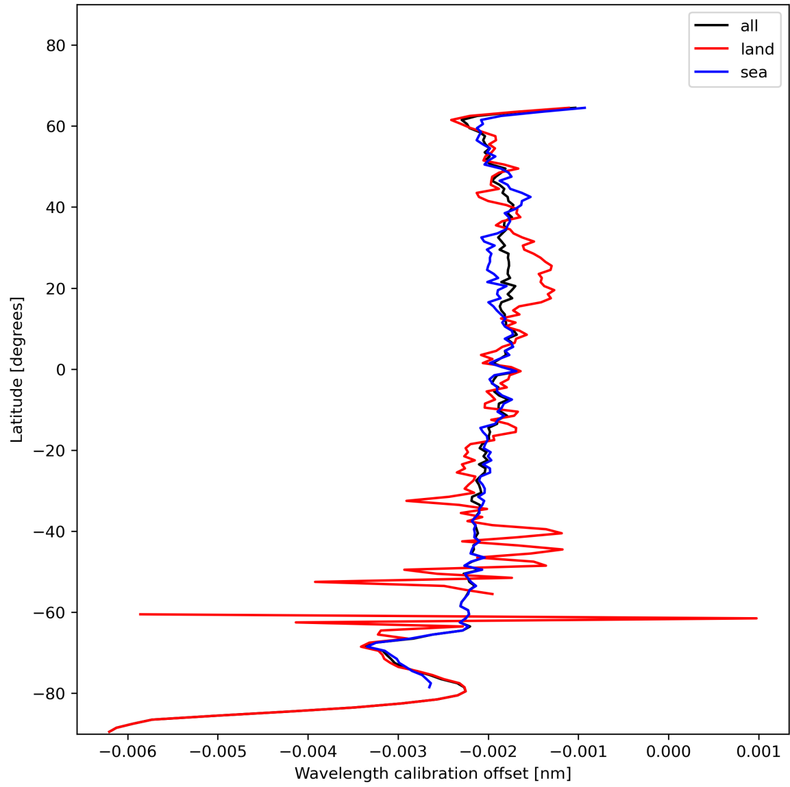
Figure 18: Zonal average of “Wavelength calibration offset” for 2023-12-21 to 2023-12-23.
