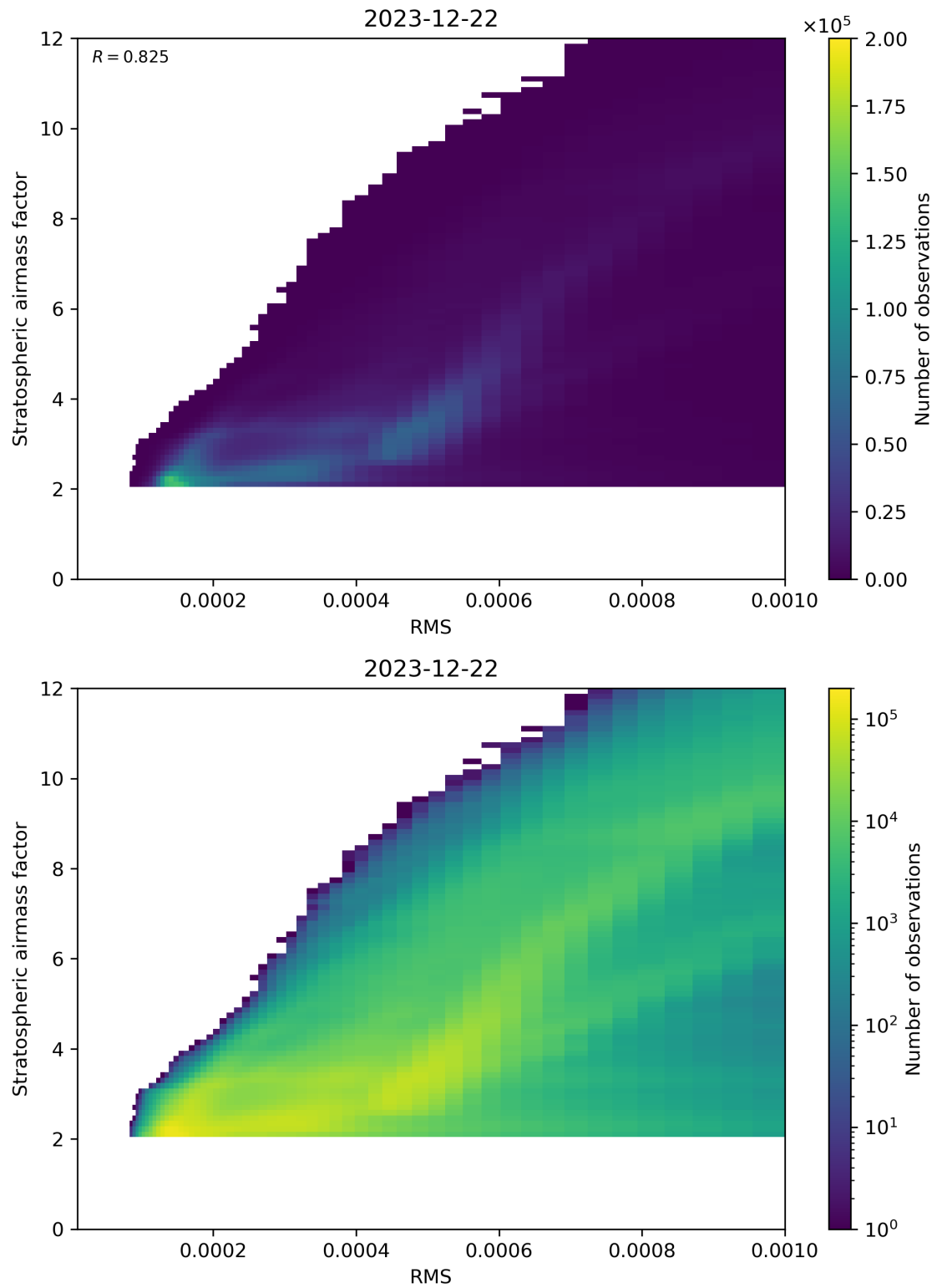
Figure 144: Scatter density plot of “RMS” against “Stratospheric airmass factor” for 2023-12-21 to 2023-12-23.
