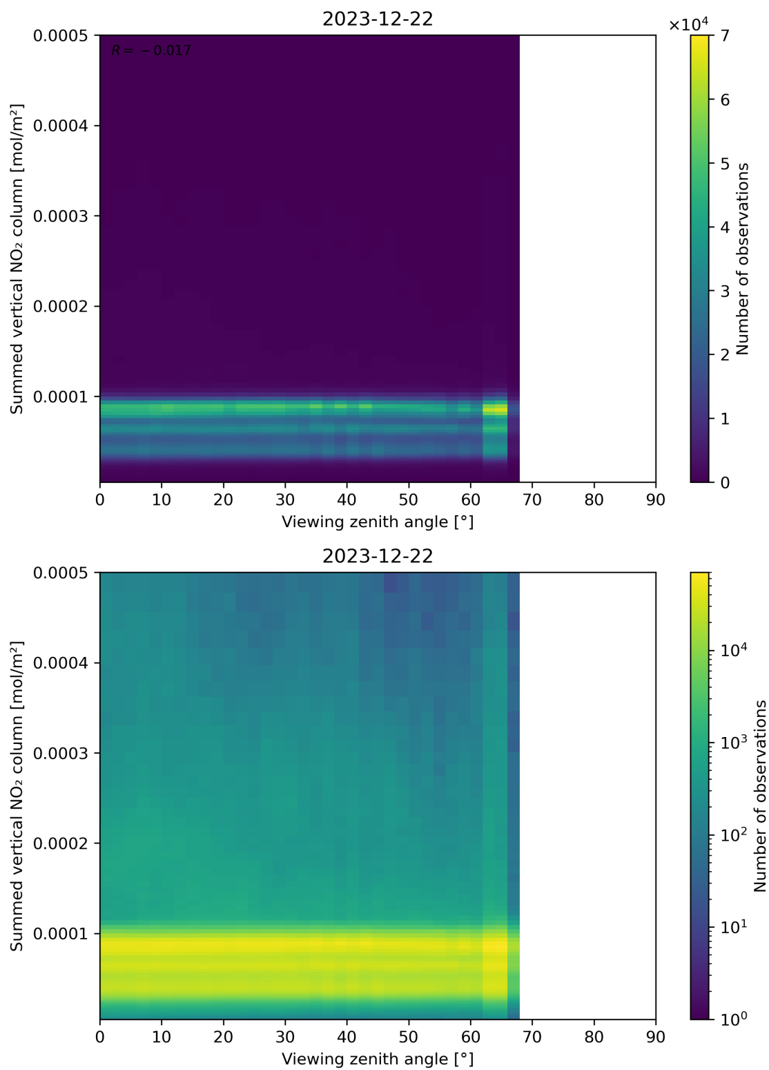
Figure 165: Scatter density plot of “Viewing zenith angle” against “Summed vertical NO 2 column” for 2023-12-21 to 2023-12-23.
