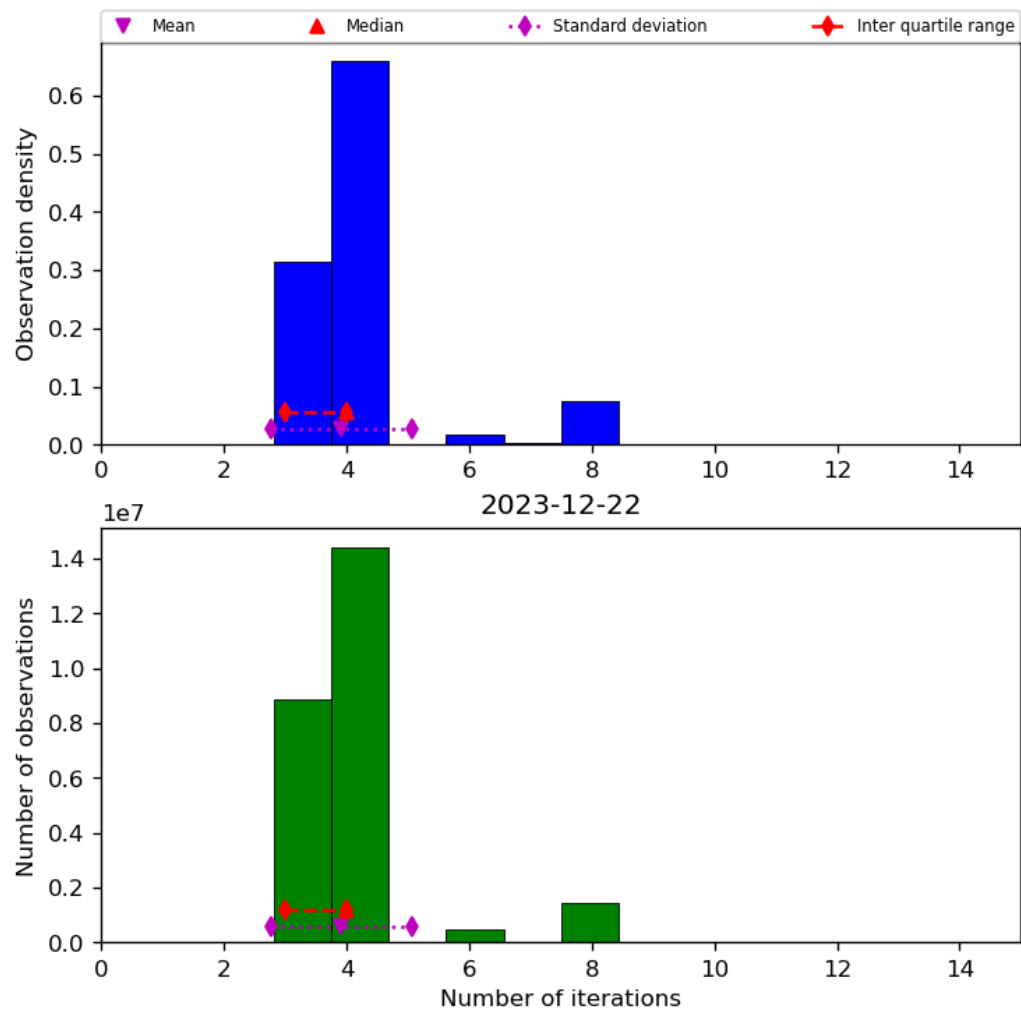
Figure 34: Histogram of “Number of iterations” for 2023-12-21 to 2023-12-23
