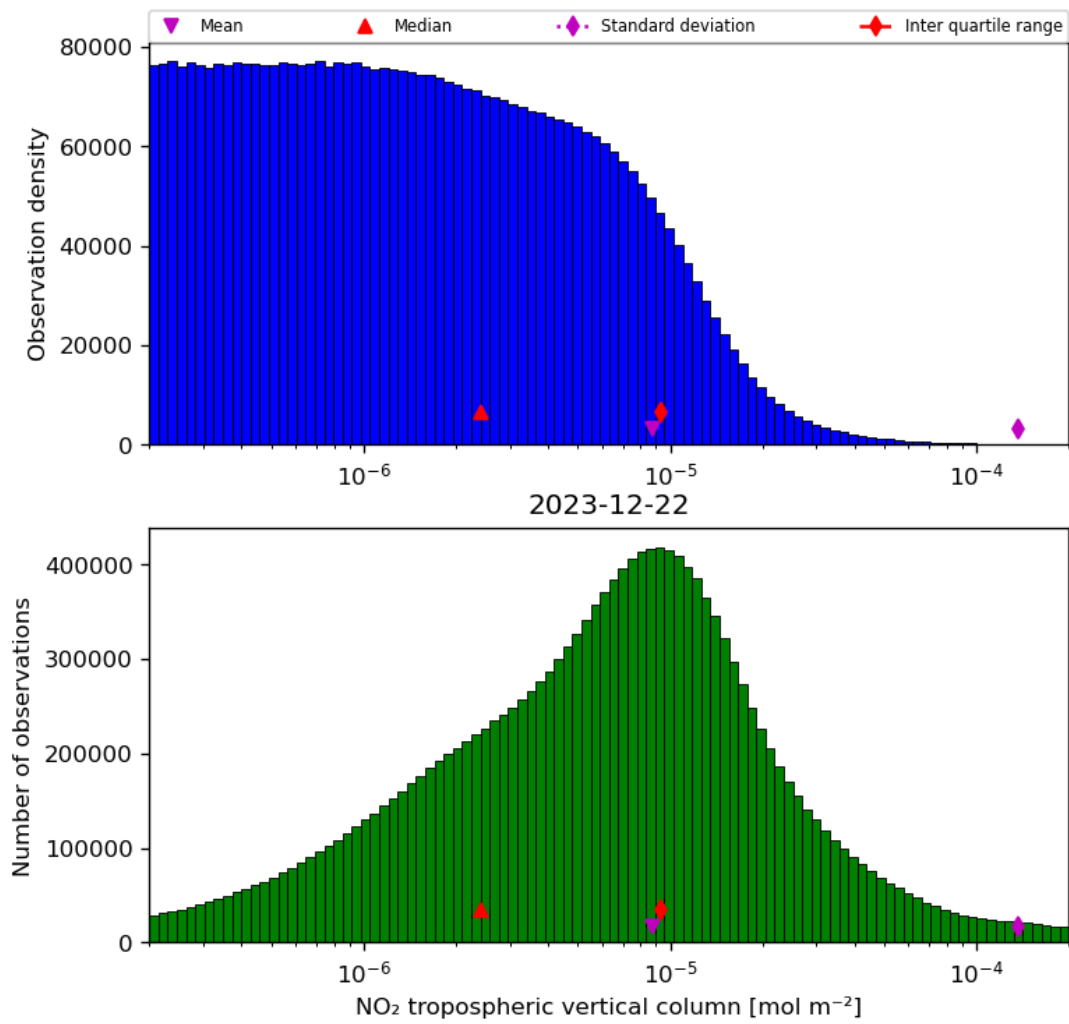
Figure 29: Histogram of “ \text{NO}_2 tropospheric vertical column” for 2023-12-21 to 2023-12-23
