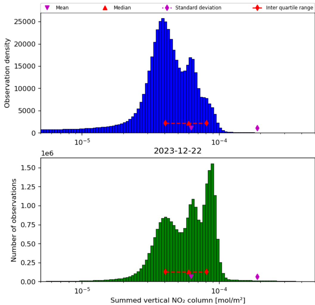
Figure 40: Histogram of “Summed vertical NO 2 column” for 2023-12-21 to 2023-12-23
