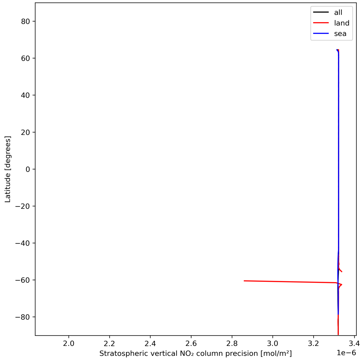
Figure 20: Zonal average of “Stratospheric vertical NO 2 column precision” for 2023-12-21 to 2023-12-23.
