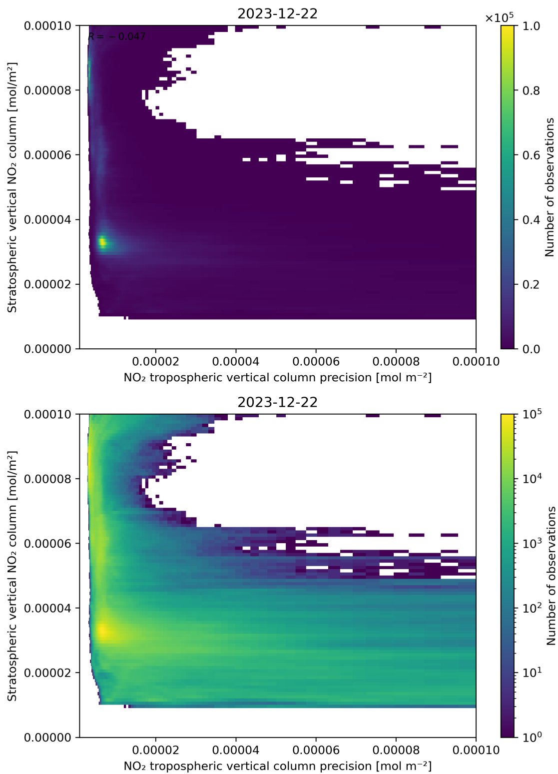
Figure 135: Scatter density plot of “NO 2 tropospheric vertical column precision” against “Stratospheric vertical NO 2 column” for 2023-12-21 to 2023-12-23.
