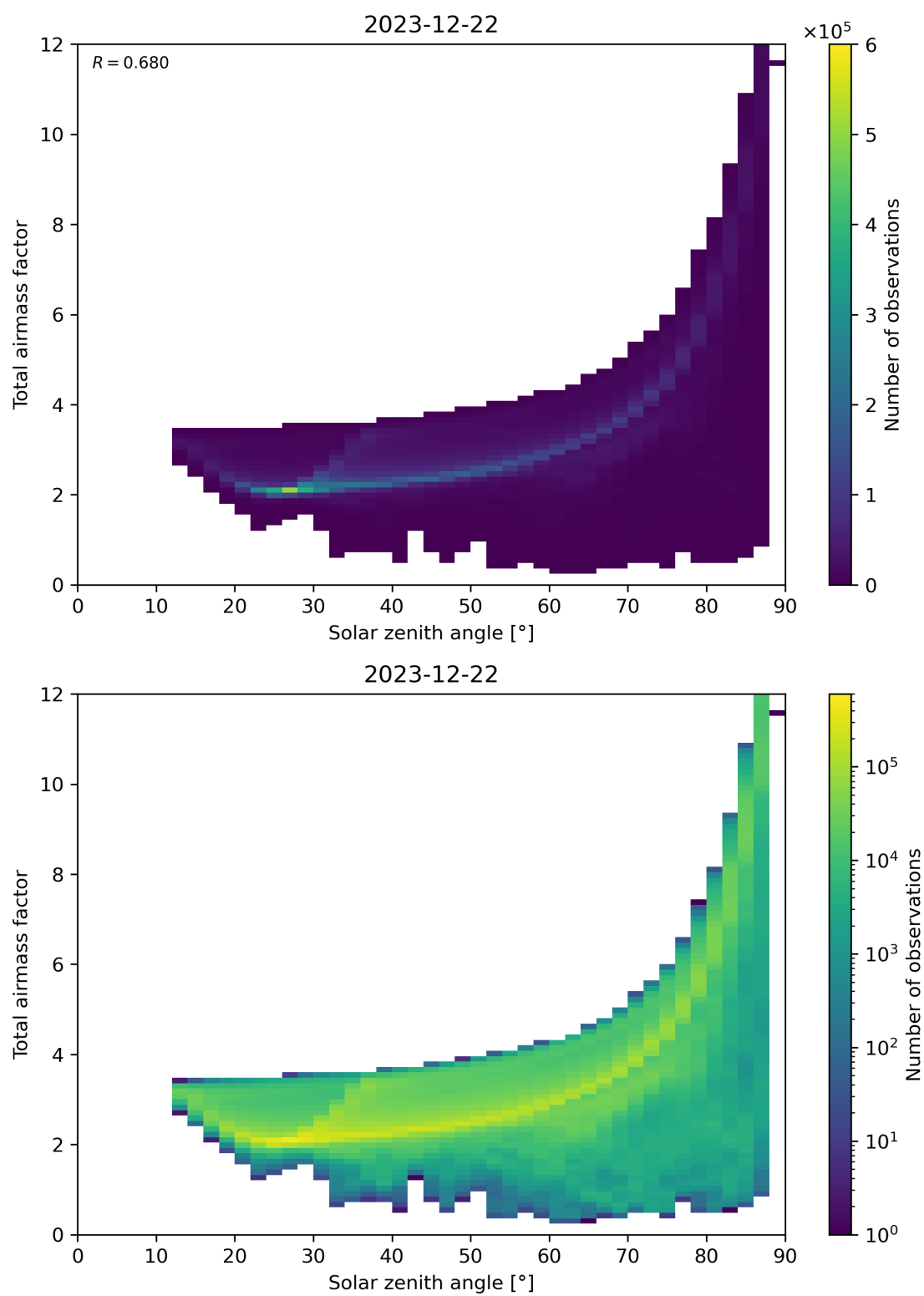
Figure 146: Scatter density plot of “Solar zenith angle” against “Total air mass factor” for 2023-12-21 to 2023-12-23.
