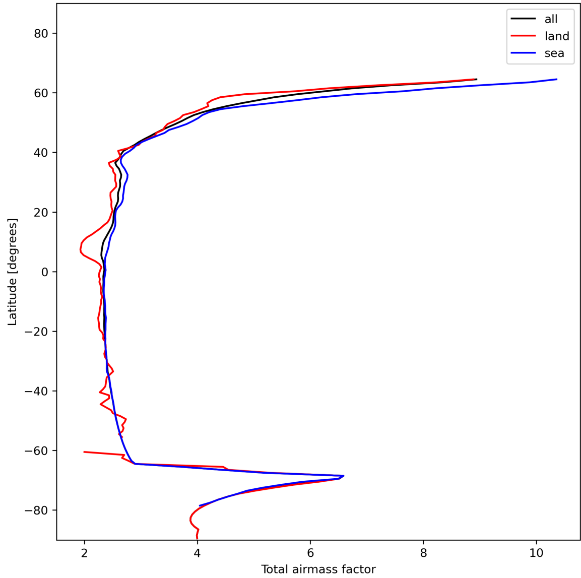
Figure 15: Zonal average of “Total airmass factor” for 2023-12-21 to 2023-12-23.
