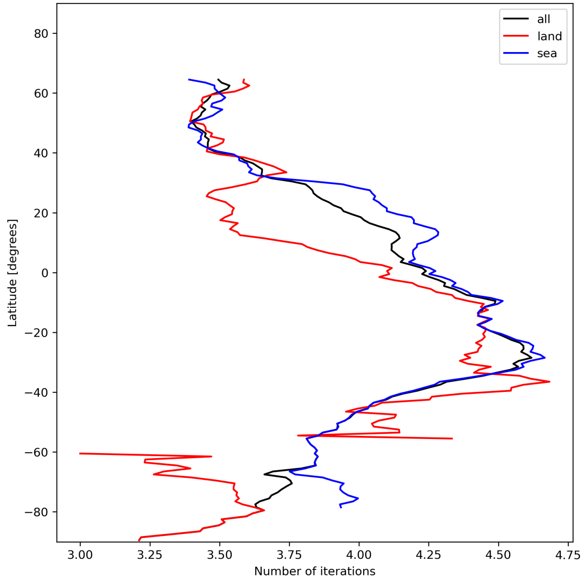
Figure 17: Zonal average of “Number of iterations” for 2023-12-21 to 2023-12-23.
