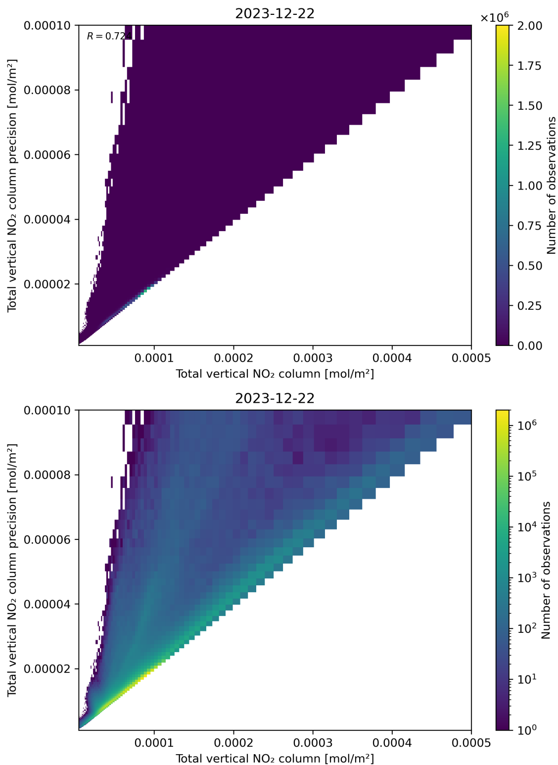
Figure 114: Scatter density plot of “Total vertical NO 2 column” against “Total vertical NO 2 column precision” for 2023-12-21 to 2023-12-23.
