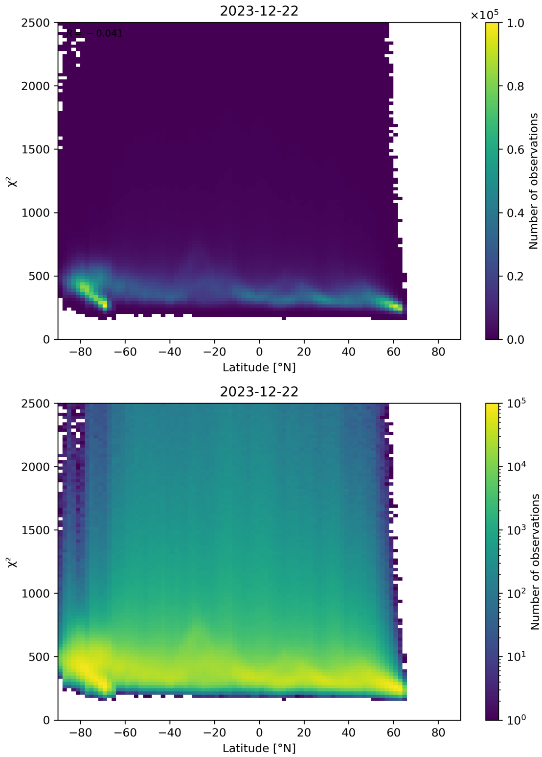
Figure 86: Scatter density plot of “Latitude” against “ \chi^2 ” for 2023-12-21 to 2023-12-23.
