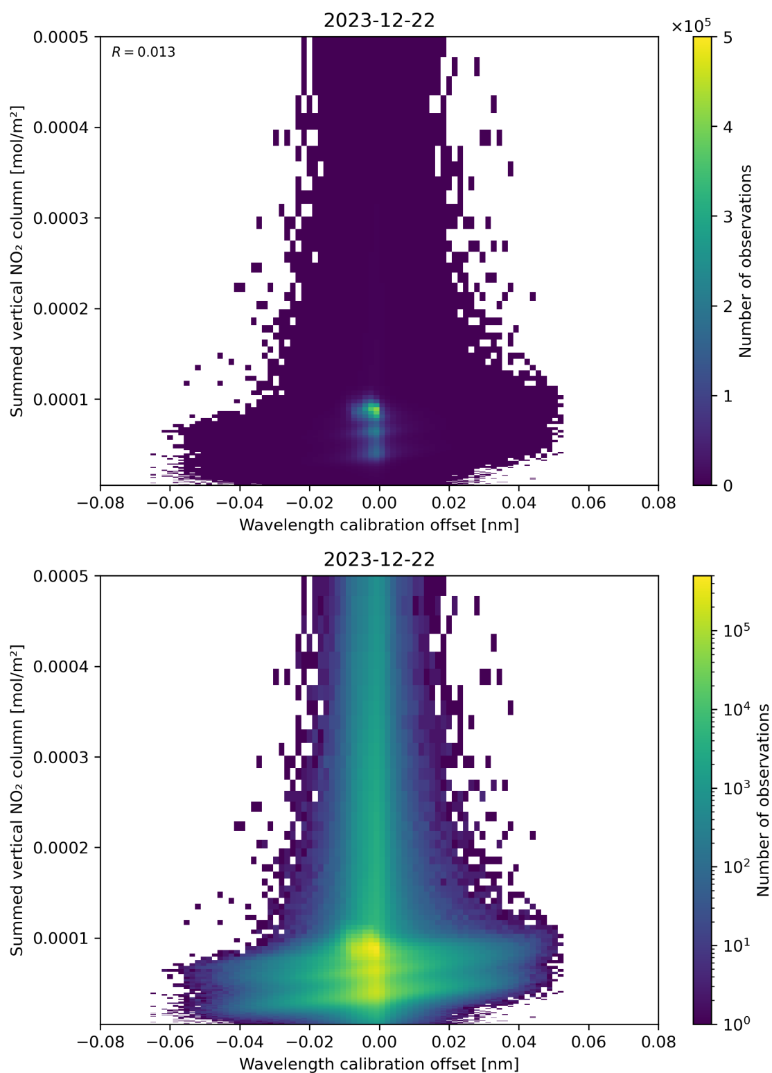
Figure 177: Scatter density plot of “Wavelength calibration offset” against “Summed vertical NO 2 column” for 2023-12-21 to 2023-12-23.
