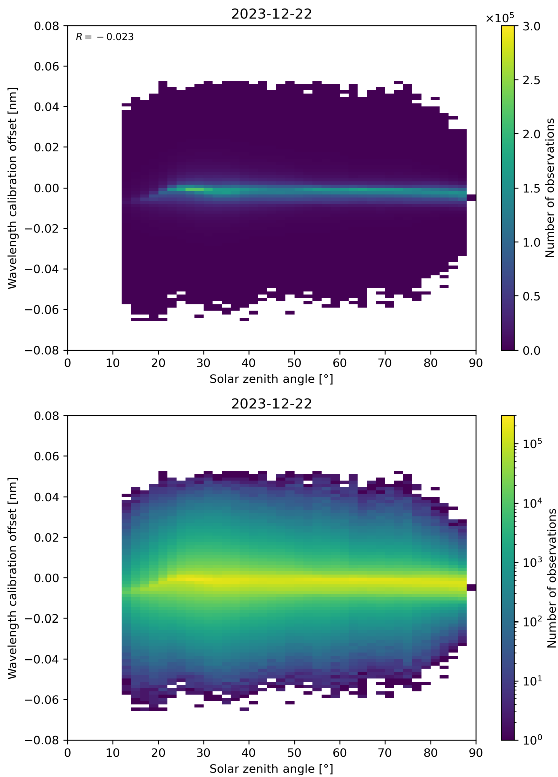
Figure 158: Scatter density plot of “Solar zenith angle” against “Wavelength calibration offset” for 2023-12-21 to 2023-12-23.
