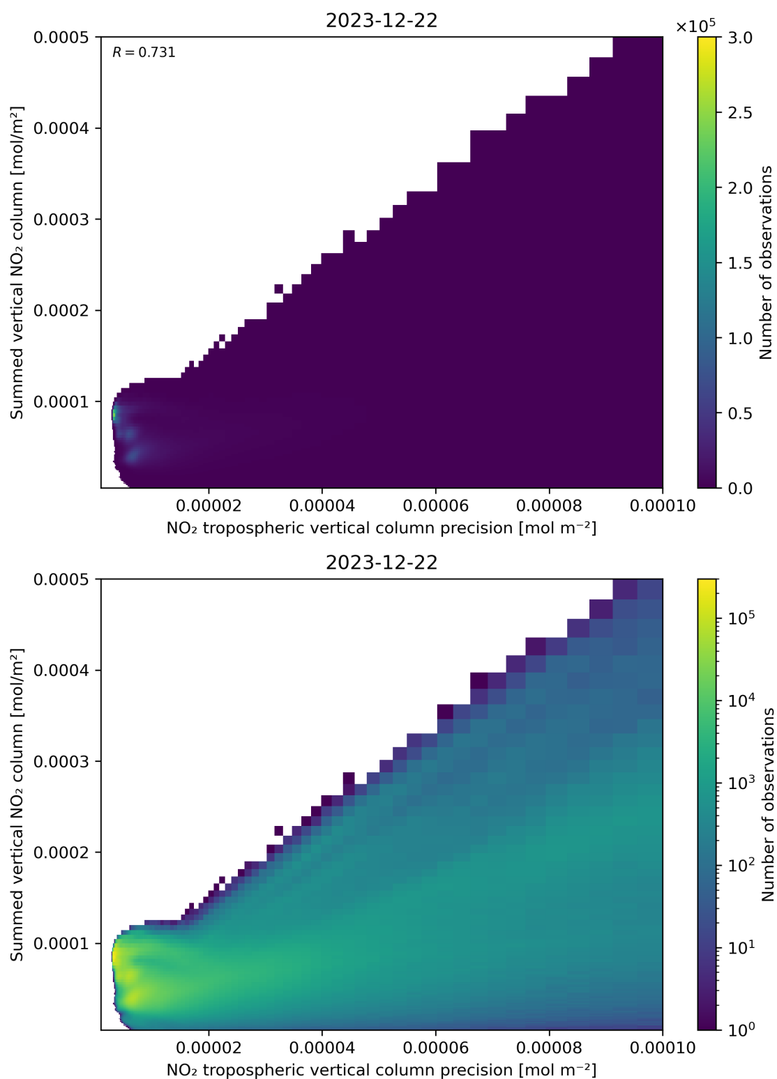
Figure 136: Scatter density plot of “NO 2 tropospheric vertical column precision” against “Summed vertical NO 2 column” for 2023-12-21 to 2023-12-23.
