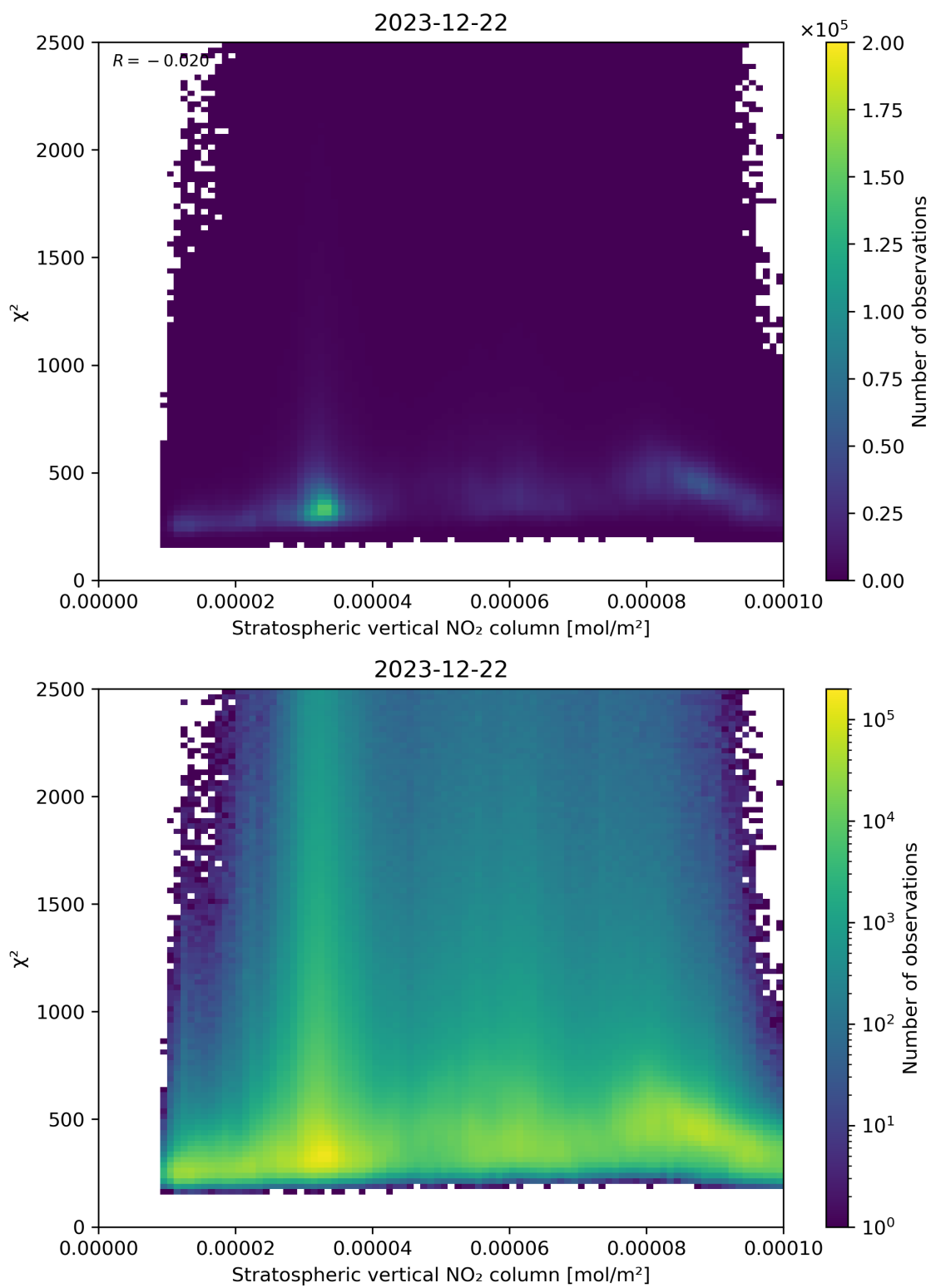
Figure 97: Scatter density plot of “Stratospheric vertical NO 2 column” against “ \chi^2 ” for 2023-12-21 to 2023-12-23.
