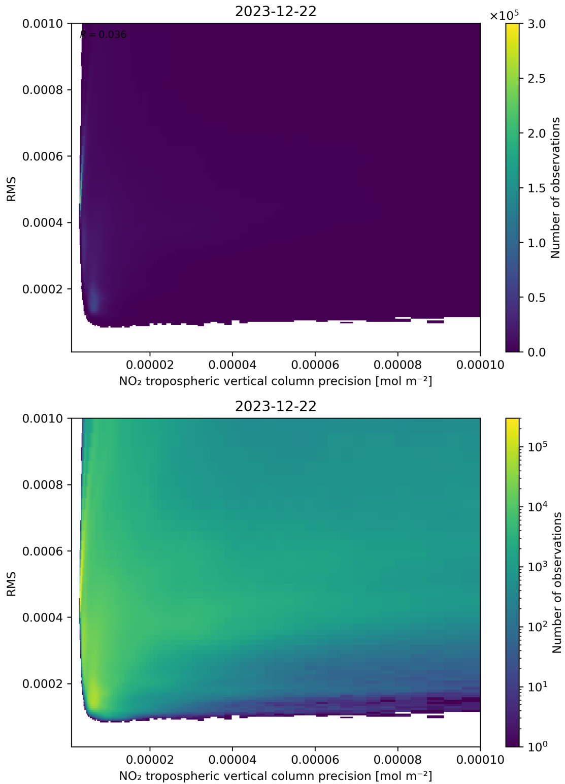
Figure 140: Scatter density plot of “NO 2 tropospheric vertical column precision” against “RMS” for 2023-12-21 to 2023-12-23.
