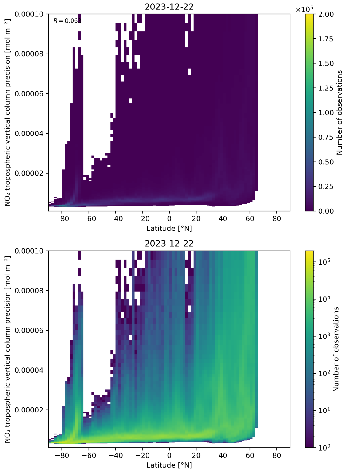
Figure 93: Scatter density plot of “Latitude” against “NO 2 tropospheric vertical column precision” for 2023-12-21 to 2023-12-23.
