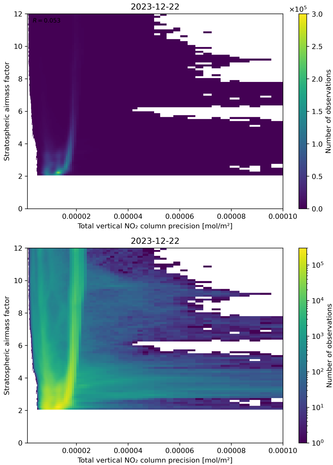
Figure 115: Scatter density plot of “Total vertical NO 2 column precision” against “Stratospheric air mass factor” for 2023-12-21 to 2023-12-23.
