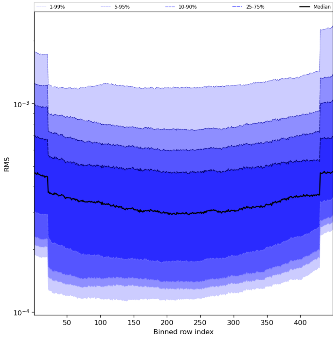
Figure 60: Along track statistics of “RMS” for 2023-12-21 to 2023-12-23
