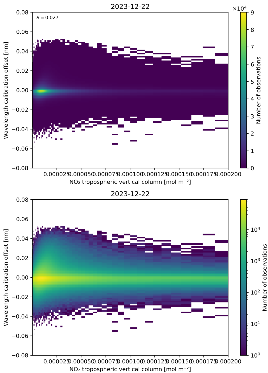
Figure 143: Scatter density plot of “NO 2 tropospheric vertical column” against “Wavelength calibration offset” for 2023-12-21 to 2023-12-23.
