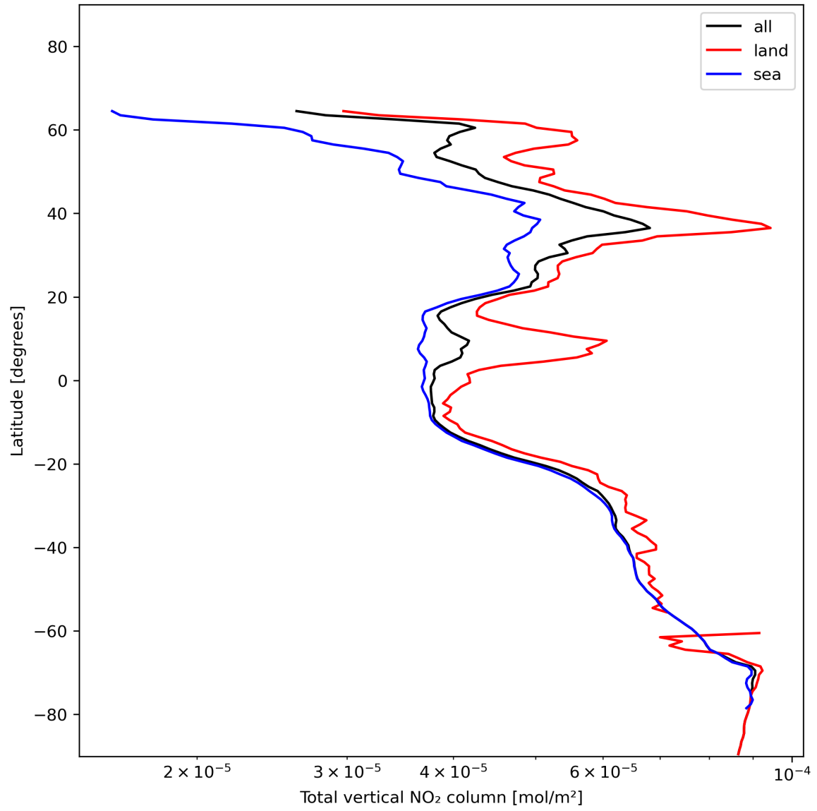
Figure 21: Zonal average of “Total vertical NO 2 column” for 2023-12-21 to 2023-12-23.
