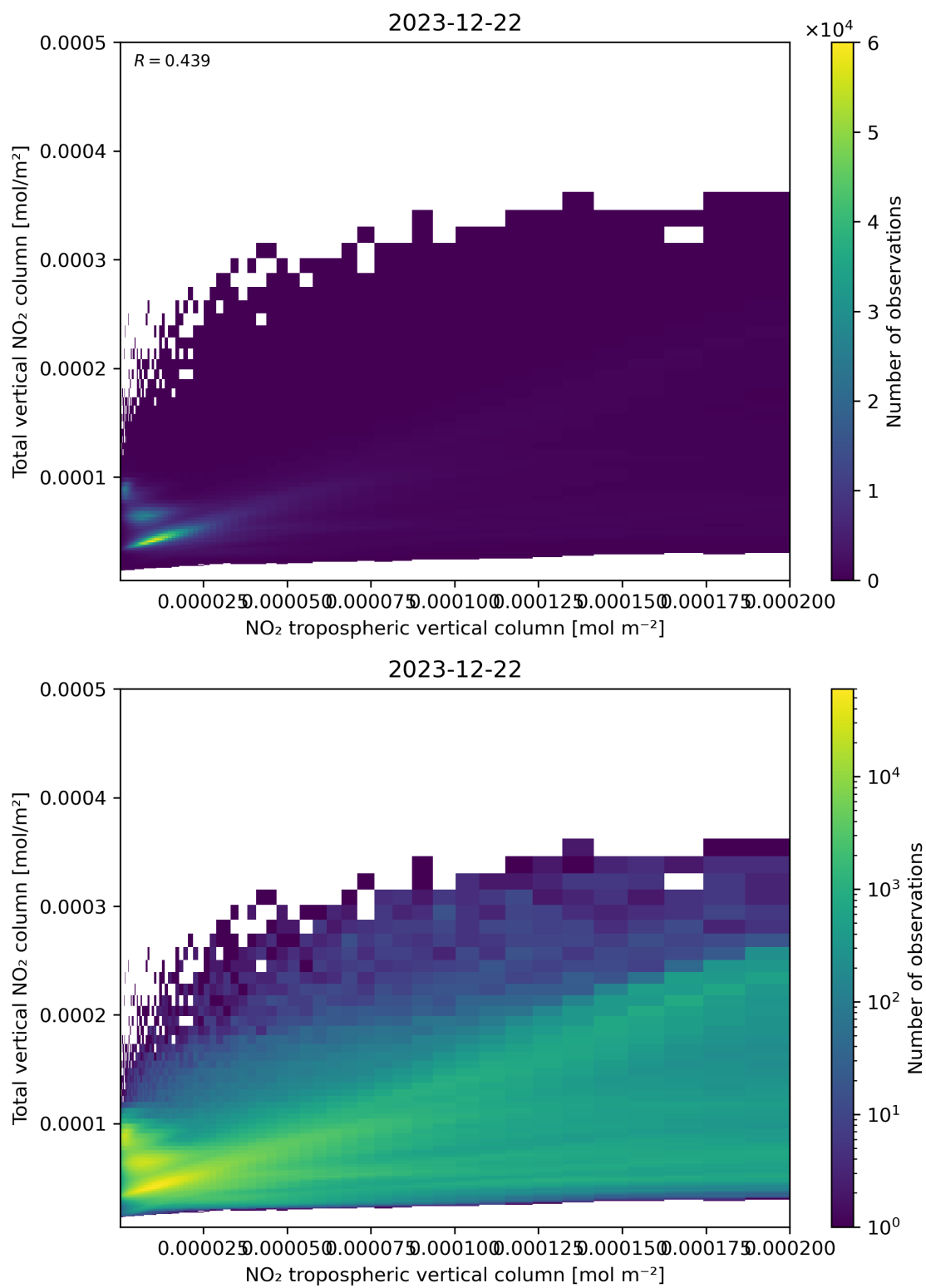
Figure 128: Scatter density plot of “NO 2 tropospheric vertical column” against “Total vertical NO 2 column” for 2023-12-21 to 2023-12-23.
