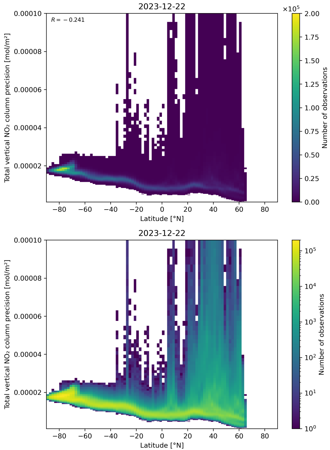
Figure 91: Scatter density plot of “Latitude” against “Total vertical NO 2 column precision” for 2023-12-21 to 2023-12-23.
