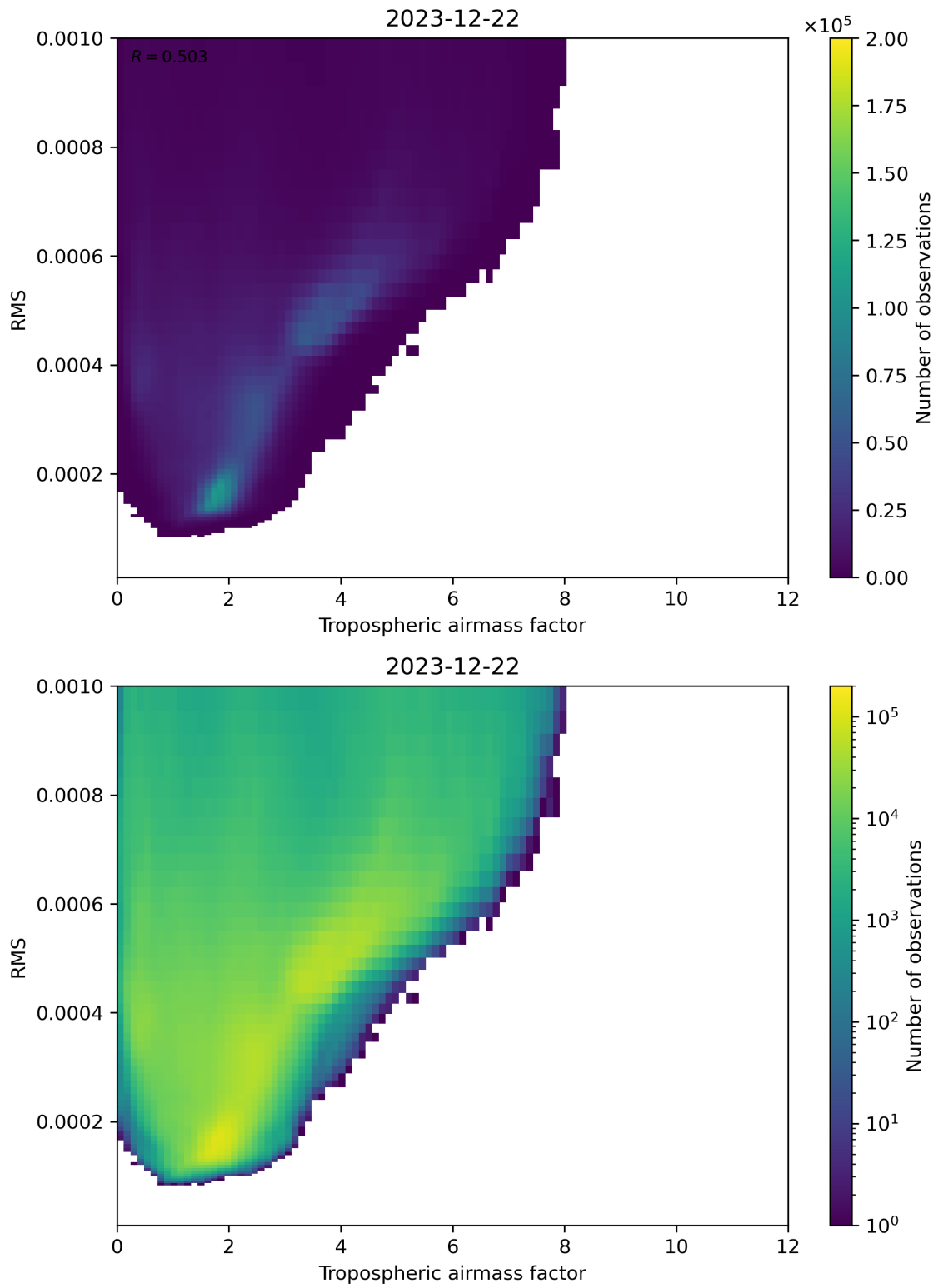
Figure 79: Scatter density plot of “Tropospheric airmass factor” against “RMS” for 2023-12-21 to 2023-12-23.
