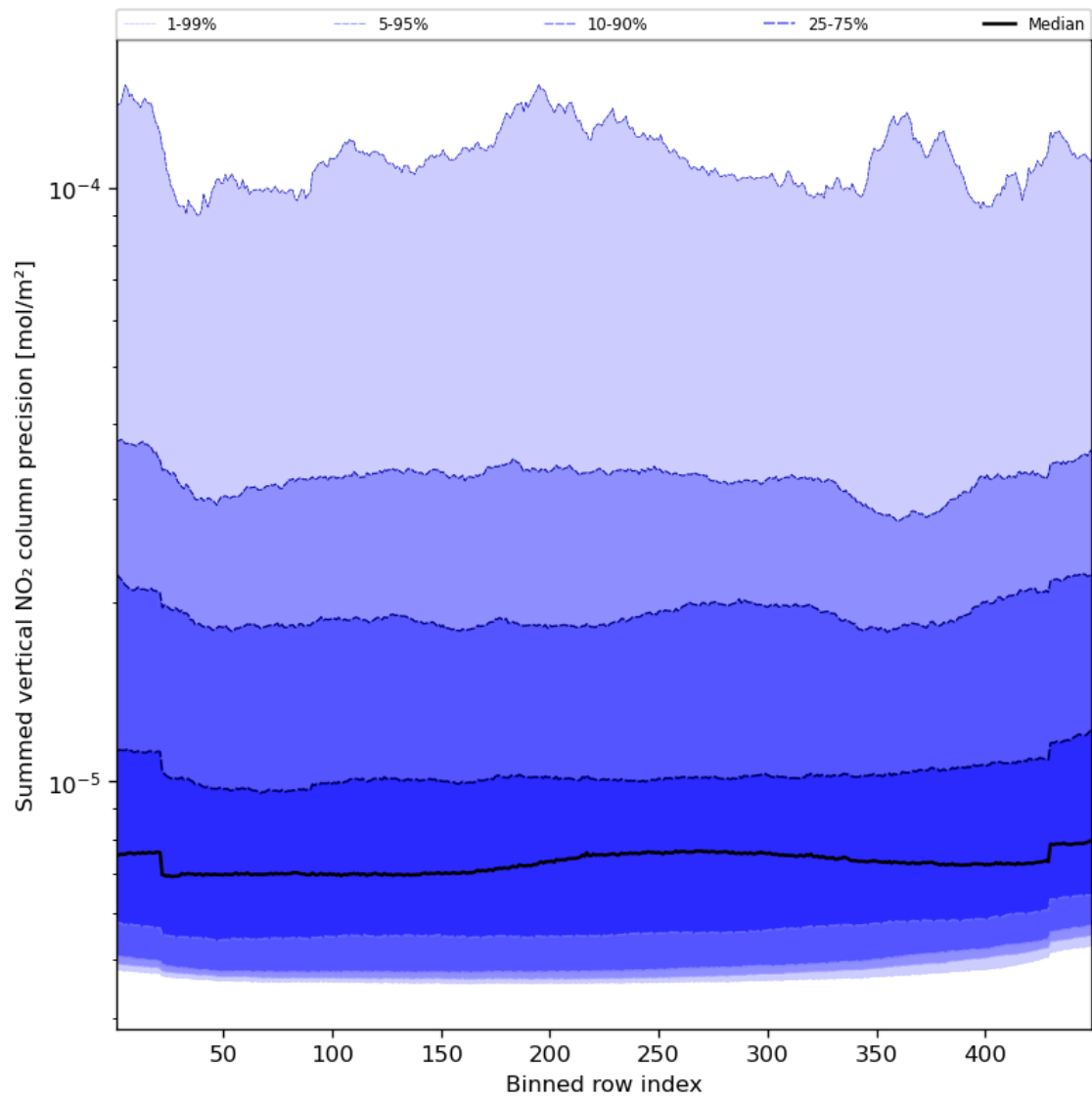
Figure 58: Along track statistics of “Summed vertical NO 2 column precision” for 2023-12-21 to 2023-12-23
