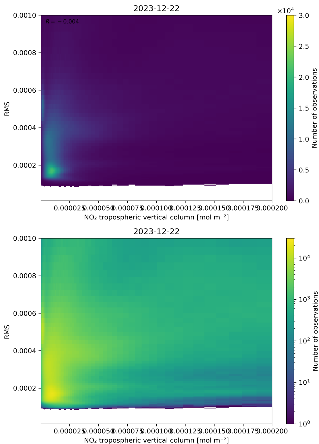
Figure 142: Scatter density plot of “NO 2 tropospheric vertical column” against “RMS” for 2023-12-21 to 2023-12-23.
