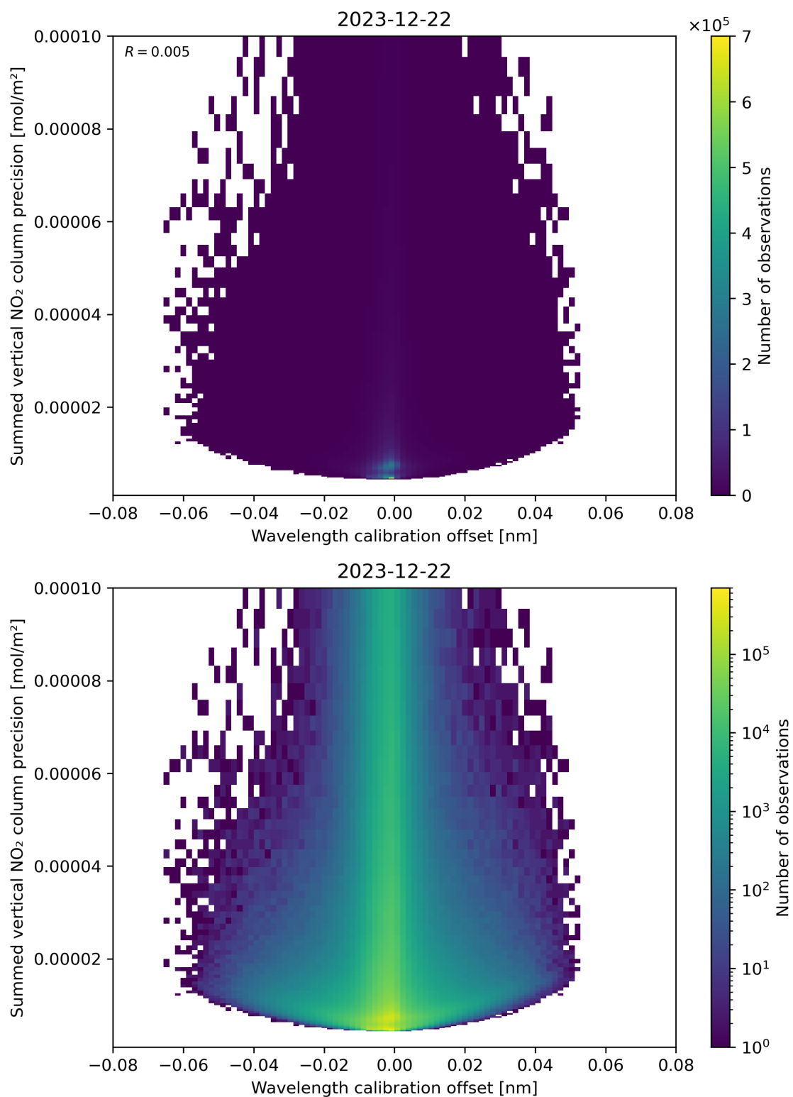
Figure 178: Scatter density plot of “Wavelength calibration offset” against “Summed vertical NO 2 column precision” for 2023-12-21 to 2023-12-23.
