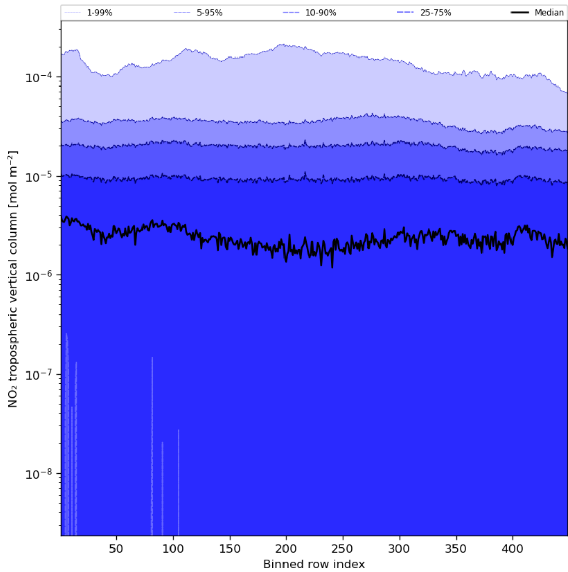
Figure 46: Along track statistics of “NO 2 tropospheric vertical column” for 2023-12-21 to 2023-12-23
