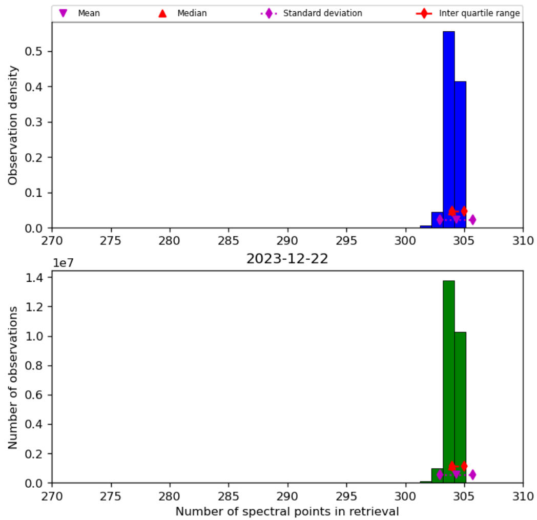
Figure 33: Histogram of “Number of spectral points in retrieval” for 2023-12-21 to 2023-12-23
