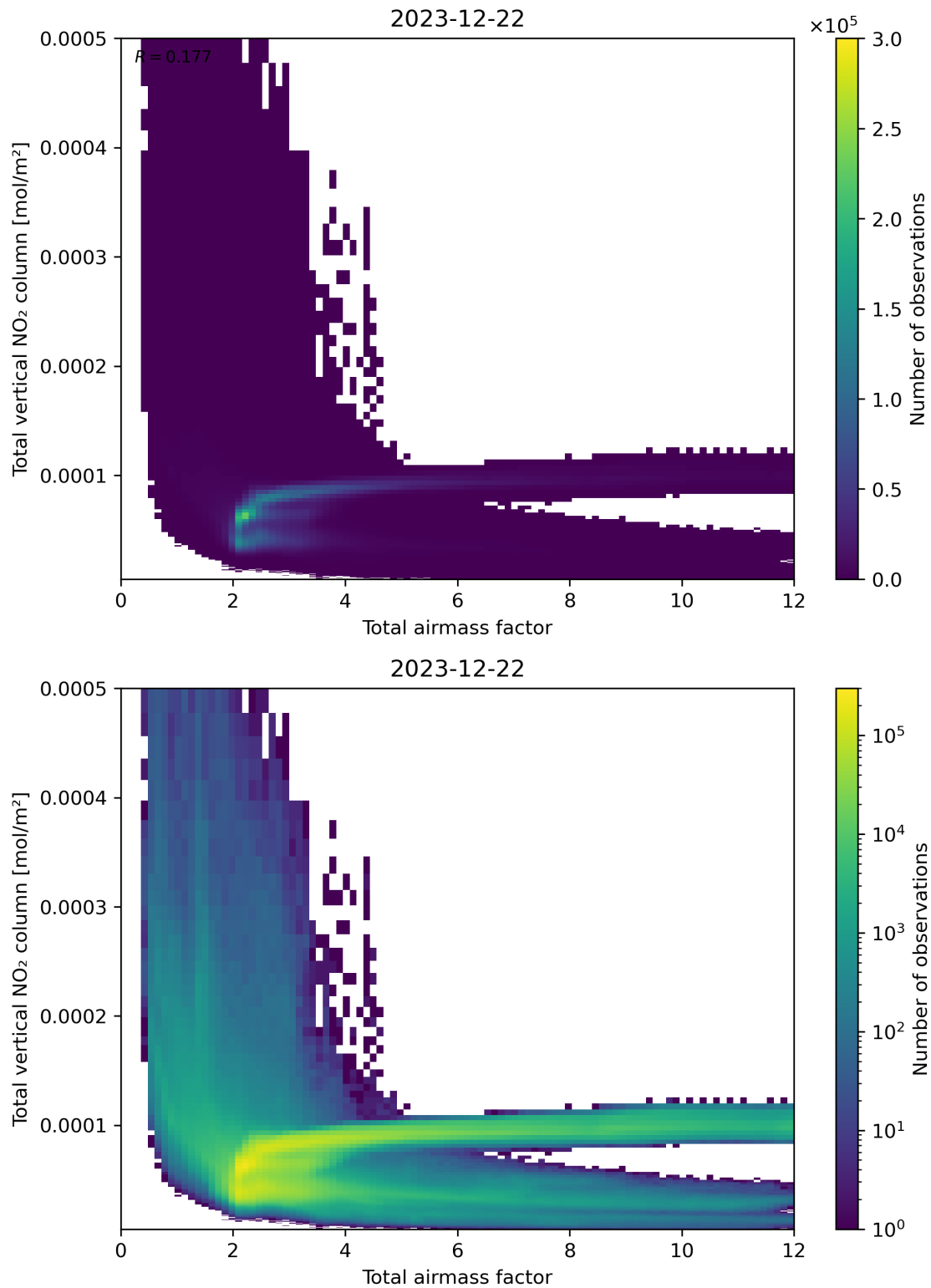
Figure 67: Scatter density plot of “Total airmass factor” against “Total vertical NO 2 column” for 2023-12-21 to 2023-12-23.
