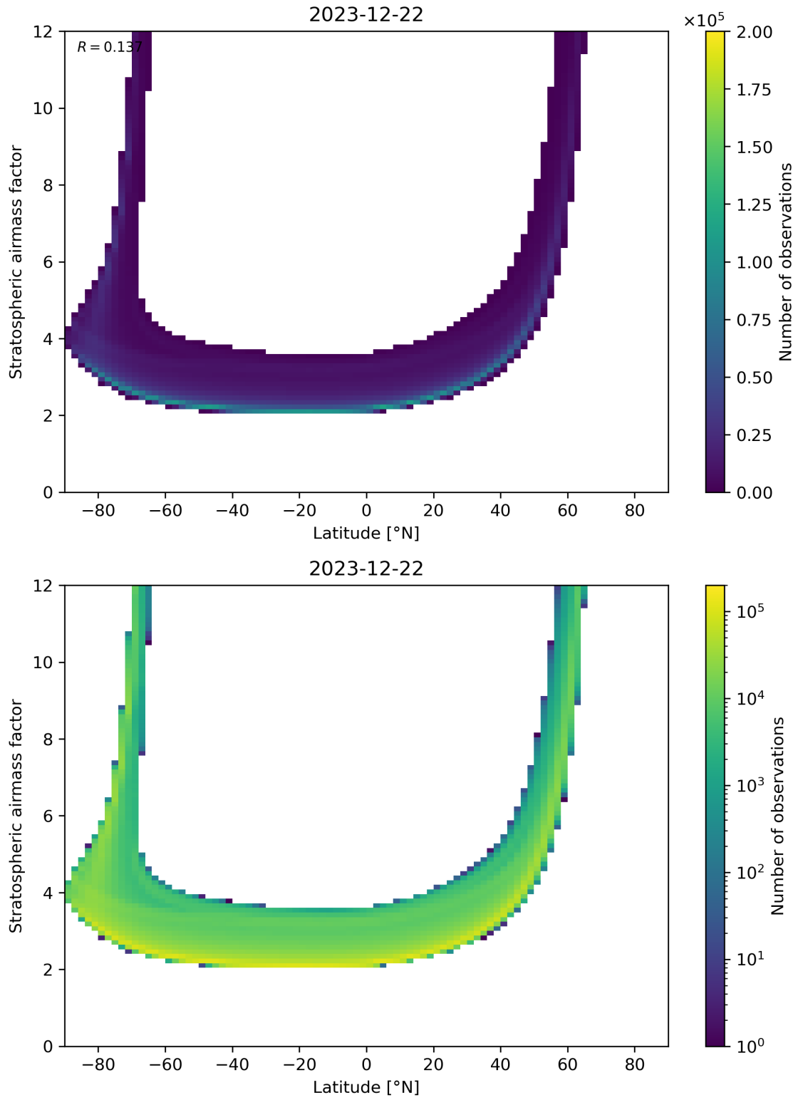
Figure 83: Scatter density plot of “Latitude” against “Stratospheric air mass factor” for 2023-12-21 to 2023-12-23.
