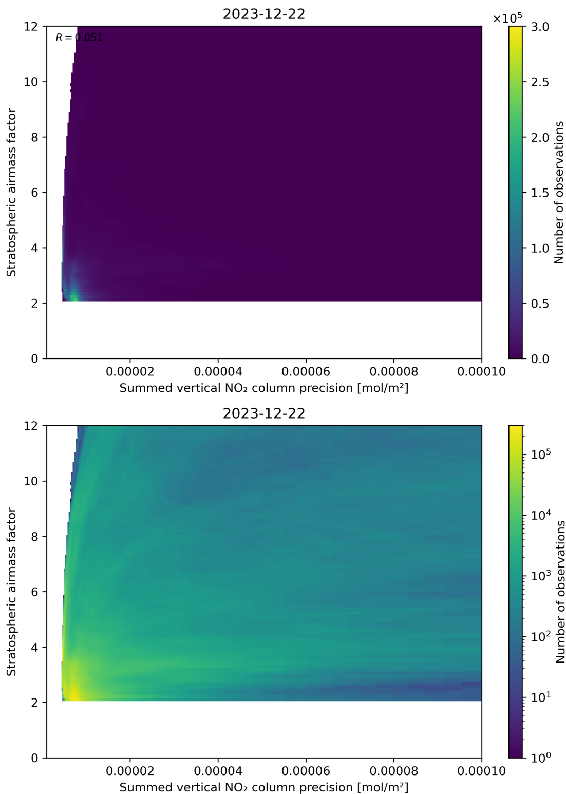
Figure 106: Scatter density plot of “Summed vertical NO 2 column precision” against “Stratospheric airmass factor” for 2023-12-21 to 2023-12-23.
