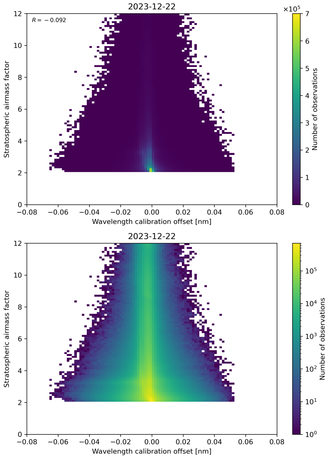
Figure 174: Scatter density plot of “Wavelength calibration offset” against “Stratospheric airmass factor” for 2023-12-21 to 2023-12-23.
