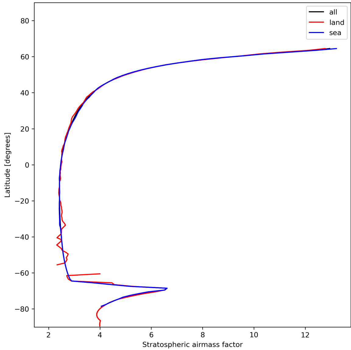
Figure 27: Zonal average of “Stratospheric airmass factor” for 2023-12-21 to 2023-12-23.
