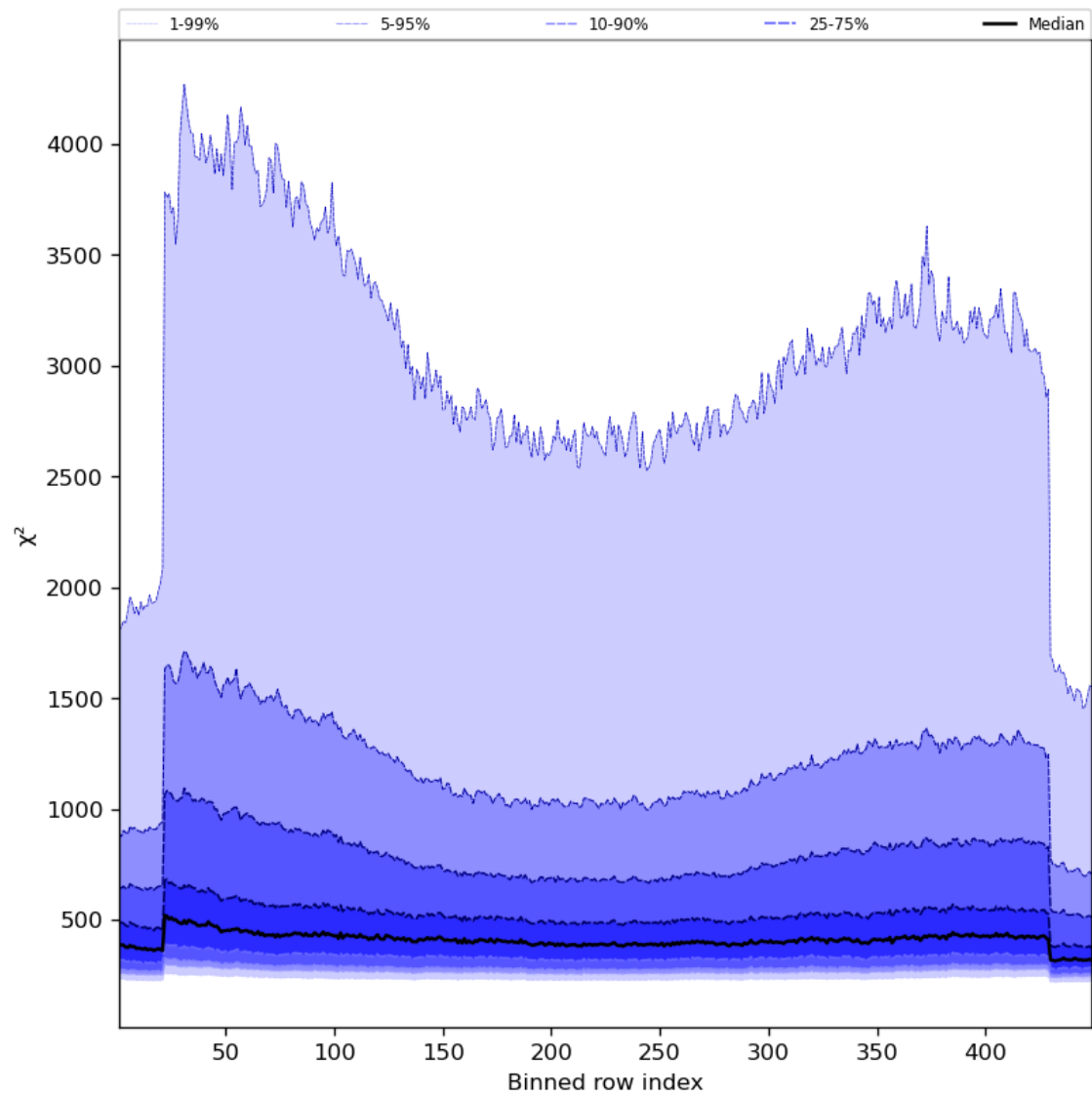
Figure 59: Along track statistics of “ \chi^2 ” for 2023-12-21 to 2023-12-23
