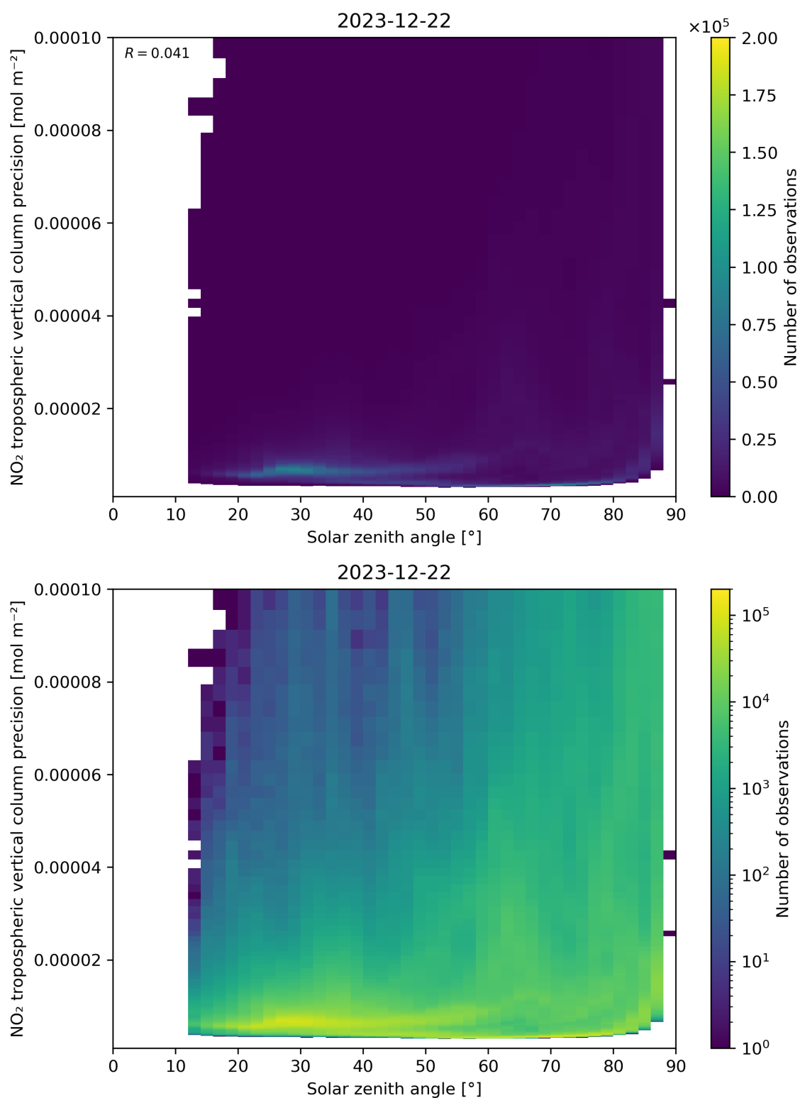
Figure 156: Scatter density plot of “Solar zenith angle” against “NO 2 tropospheric vertical column precision” for 2023-12-21 to 2023-12-23.
