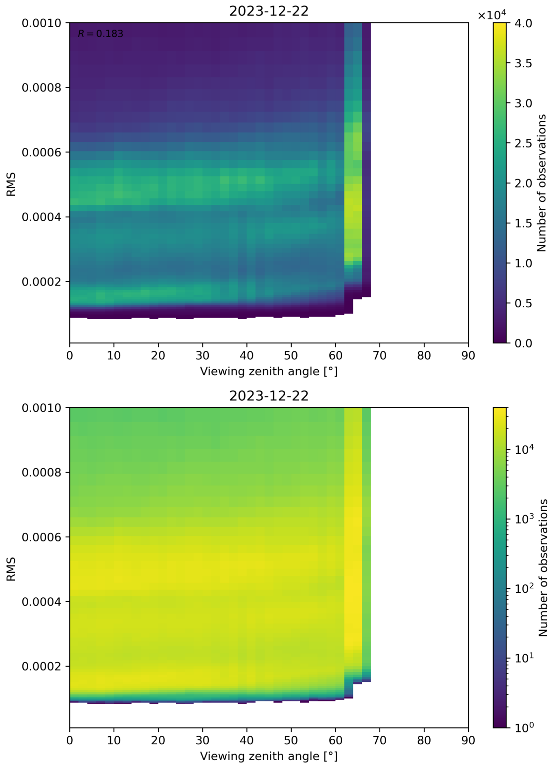
Figure 171: Scatter density plot of “Viewing zenith angle” against “RMS” for 2023-12-21 to 2023-12-23.
