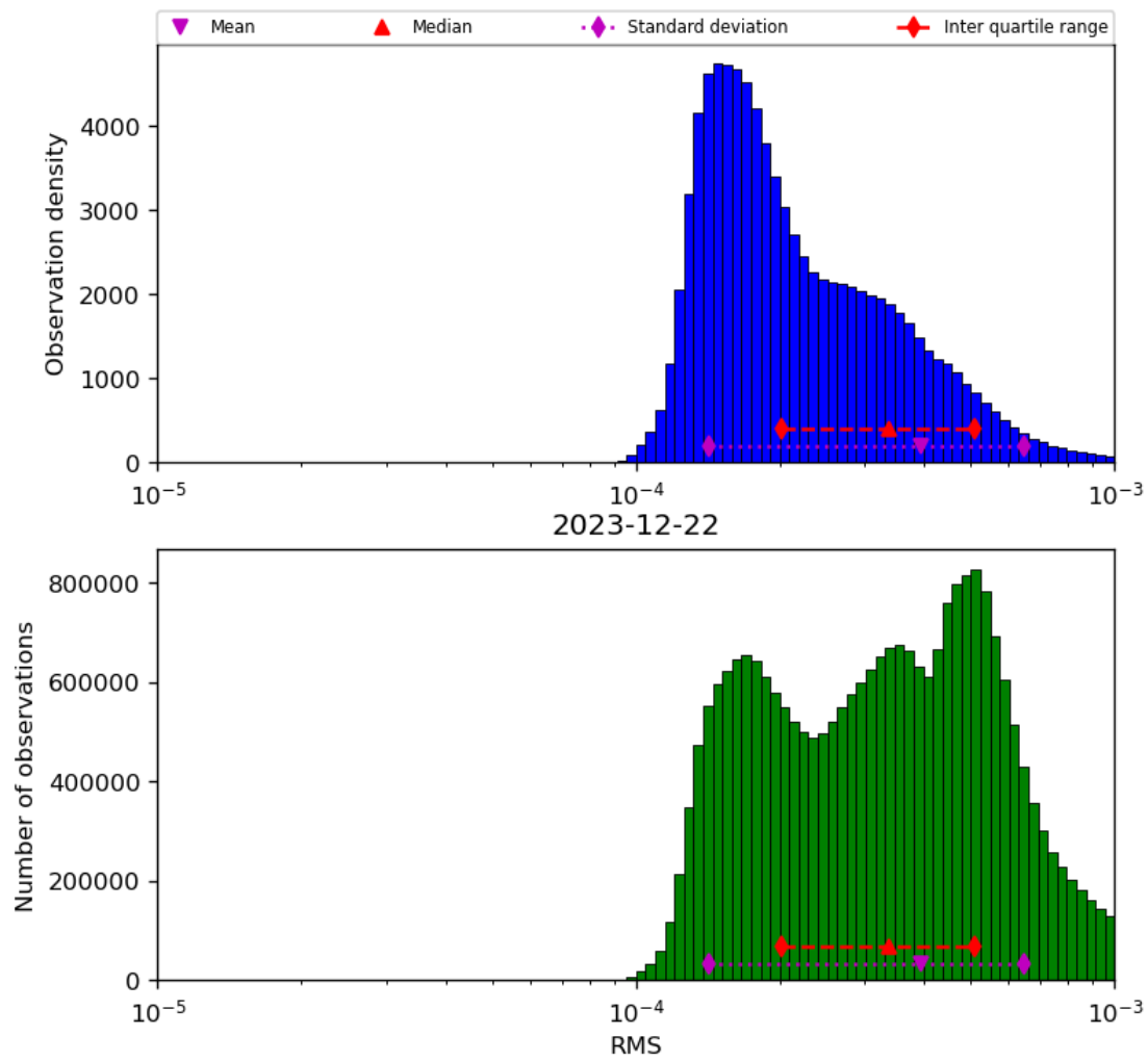
Figure 43: Histogram of “RMS” for 2023-12-21 to 2023-12-23
