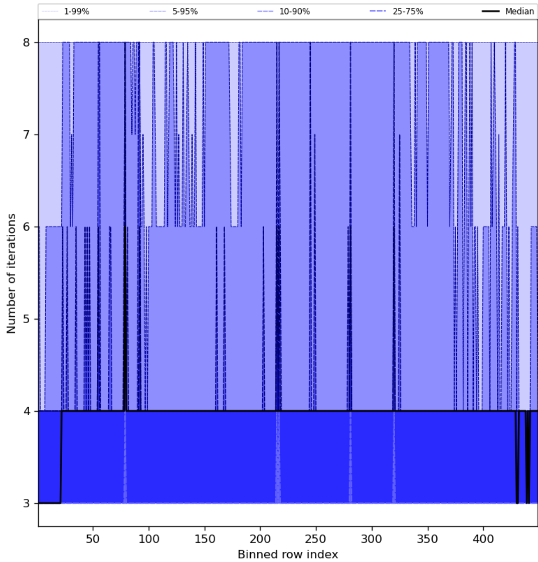
Figure 51: Along track statistics of “Number of iterations” for 2023-12-21 to 2023-12-23
