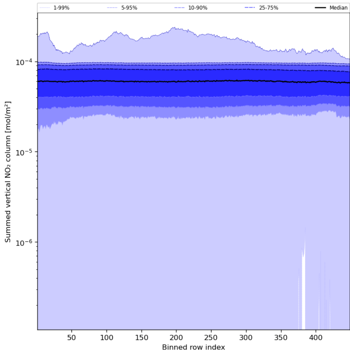
Figure 57: Along track statistics of “Summed vertical NO 2 column” for 2023-12-21 to 2023-12-23
