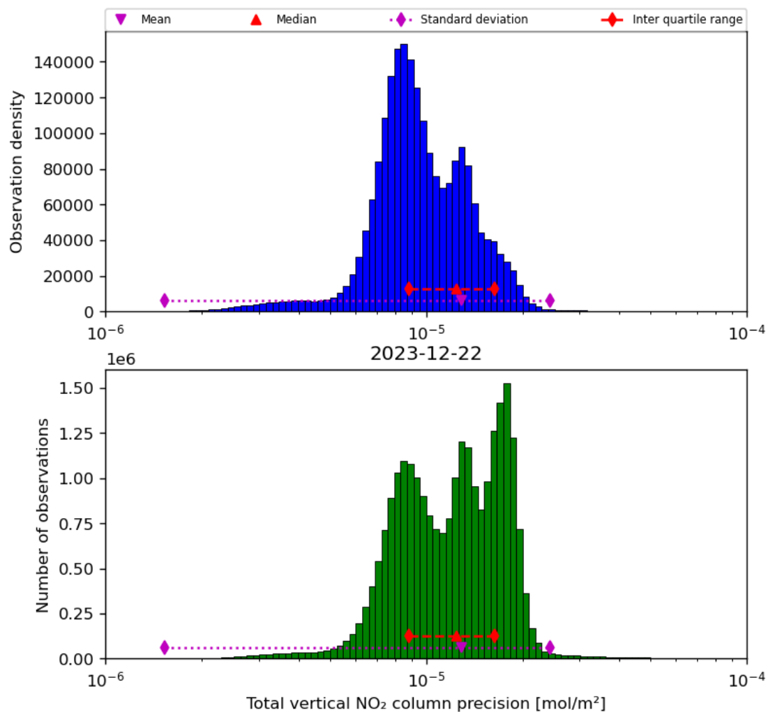
Figure 39: Histogram of “Total vertical NO 2 column precision” for 2023-12-21 to 2023-12-23
