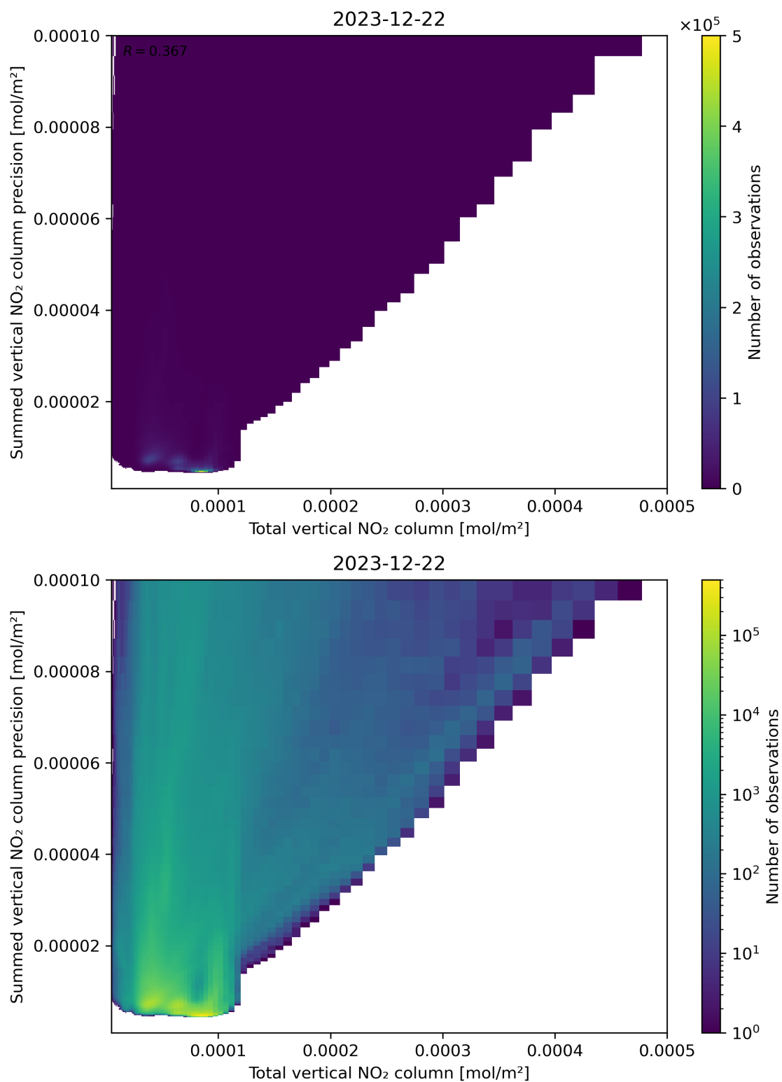
Figure 113: Scatter density plot of “Total vertical NO 2 column” against “Summed vertical NO 2 column precision” for 2023-12-21 to 2023-12-23.
