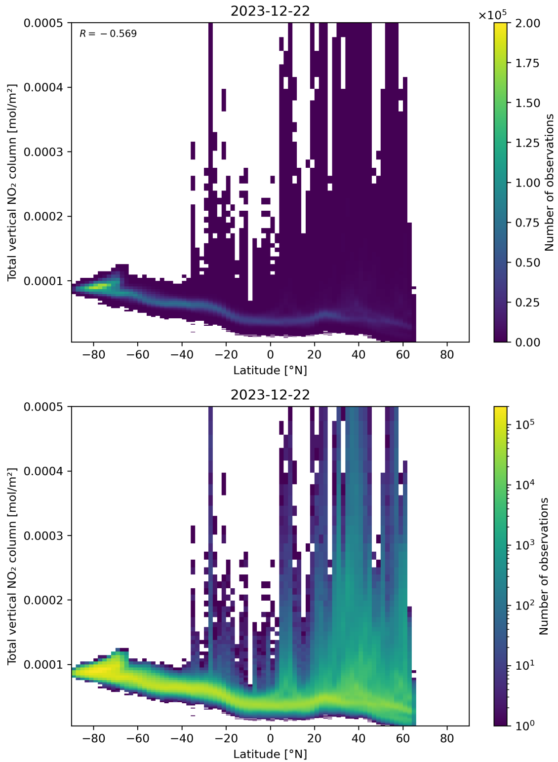
Figure 90: Scatter density plot of “Latitude” against “Total vertical NO 2 column” for 2023-12-21 to 2023-12-23.
