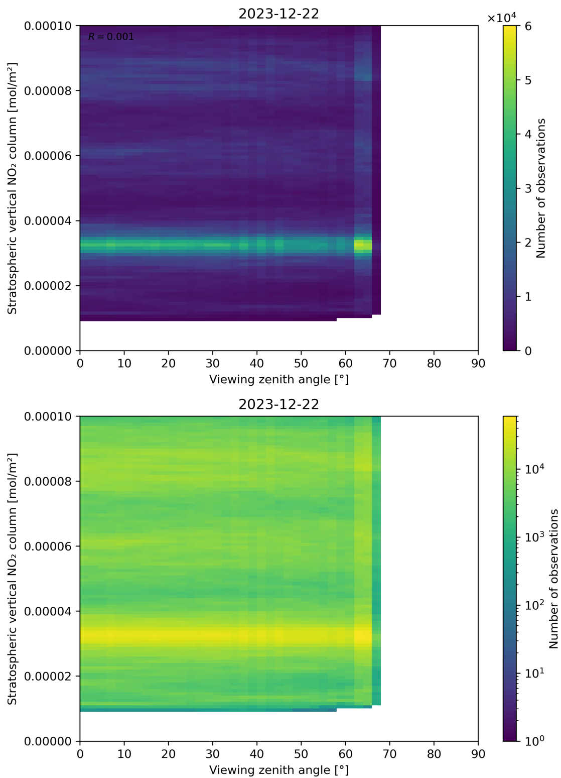
Figure 164: Scatter density plot of “Viewing zenith angle” against “Stratospheric vertical NO 2 column” for 2023-12-21 to 2023-12-23.
