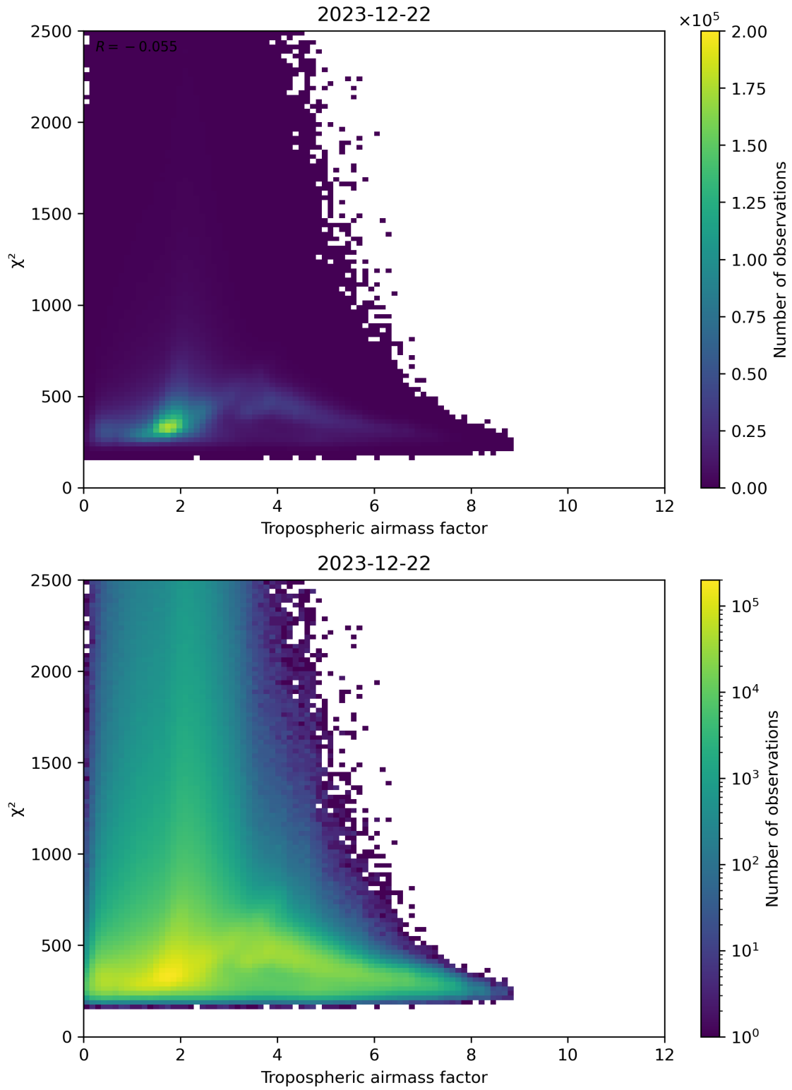
Figure 73: Scatter density plot of “Tropospheric airmass factor” against “ \chi^2 ” for 2023-12-21 to 2023-12-23.
