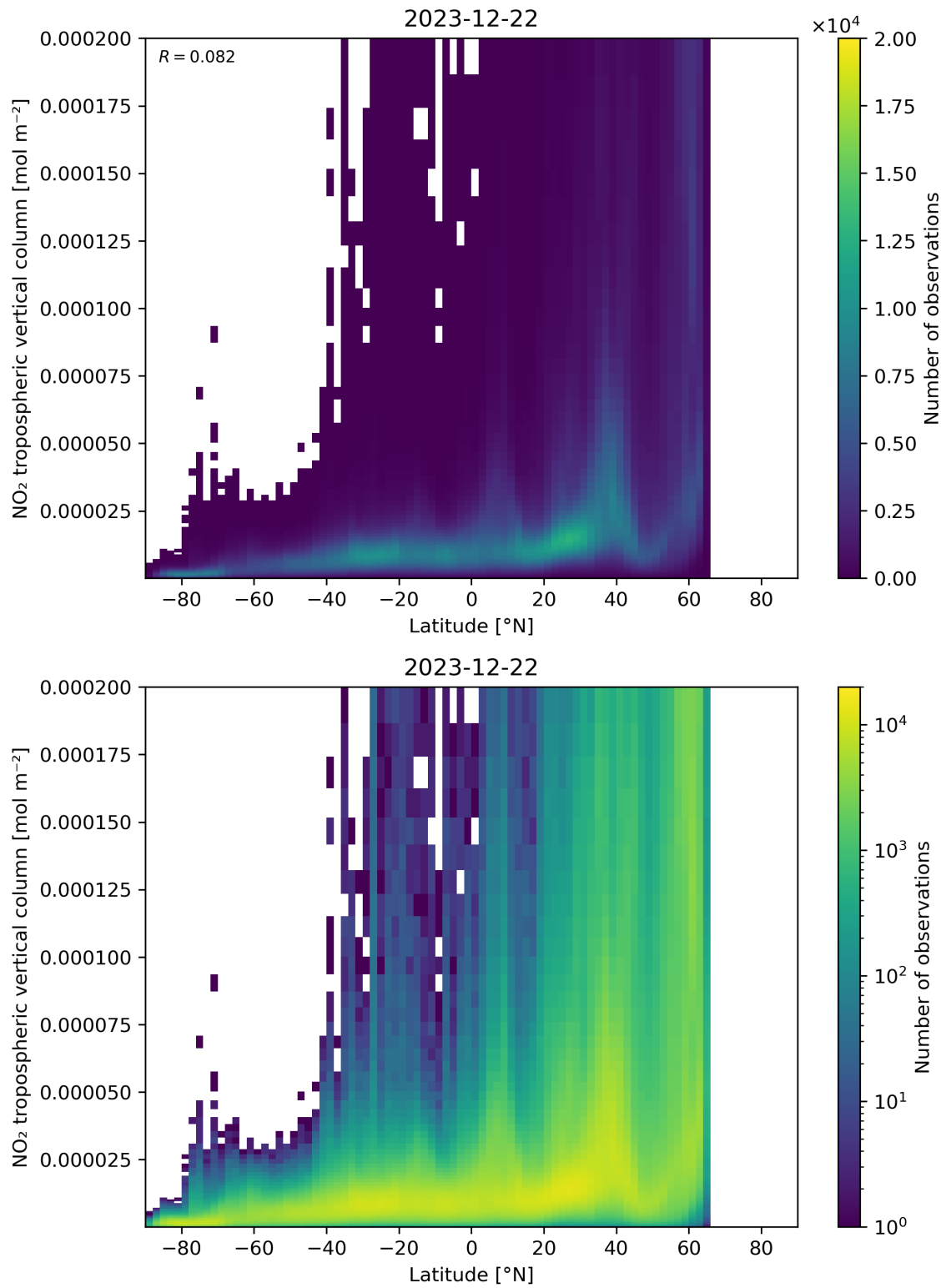
Figure 92: Scatter density plot of “Latitude” against “NO 2 tropospheric vertical column” for 2023-12-21 to 2023-12-23.
