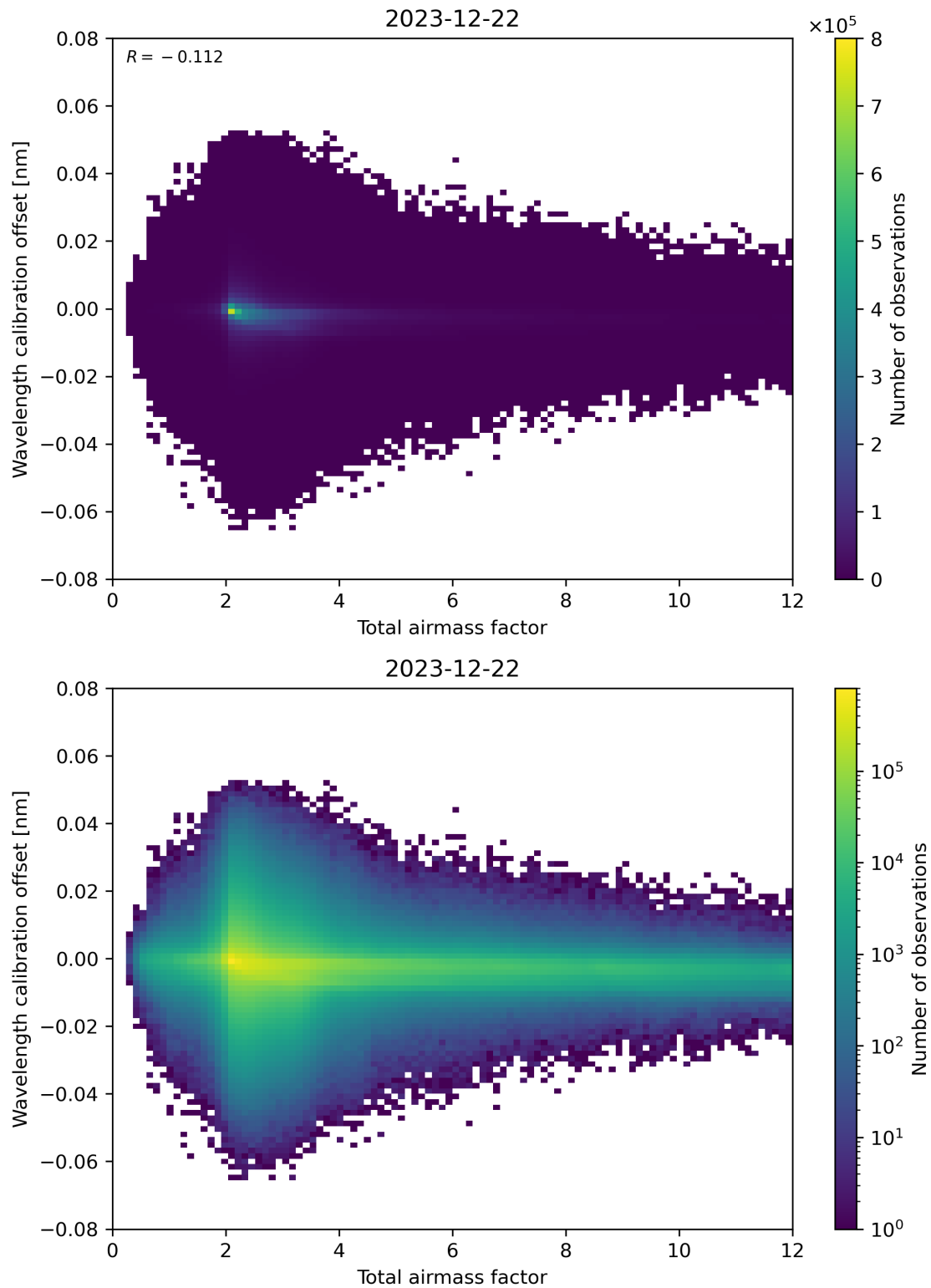
Figure 70: Scatter density plot of “Total airmass factor” against “Wavelength calibration offset” for 2023-12-21 to 2023-12-23.
