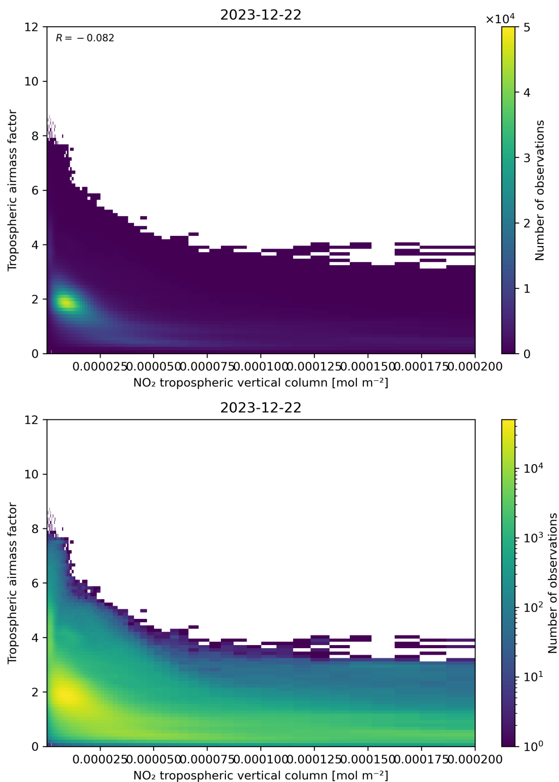
Figure 123: Scatter density plot of “NO 2 tropospheric vertical column” against “Tropospheric air mass factor” for 2023-12-21 to 2023-12-23.
