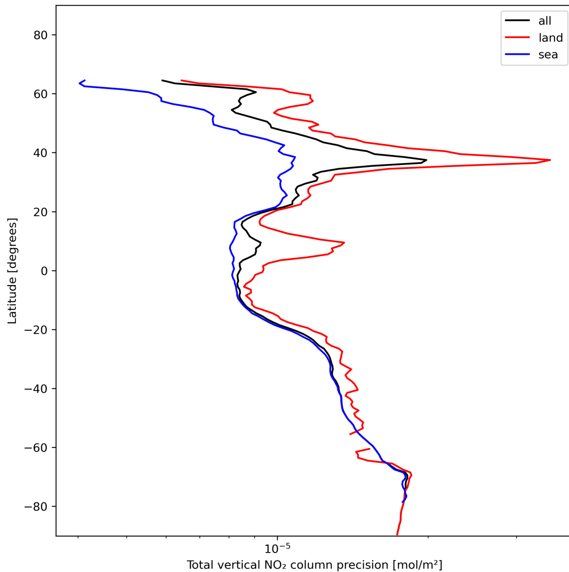
Figure 22: Zonal average of “Total vertical NO 2 column precision” for 2023-12-21 to 2023-12-23.
