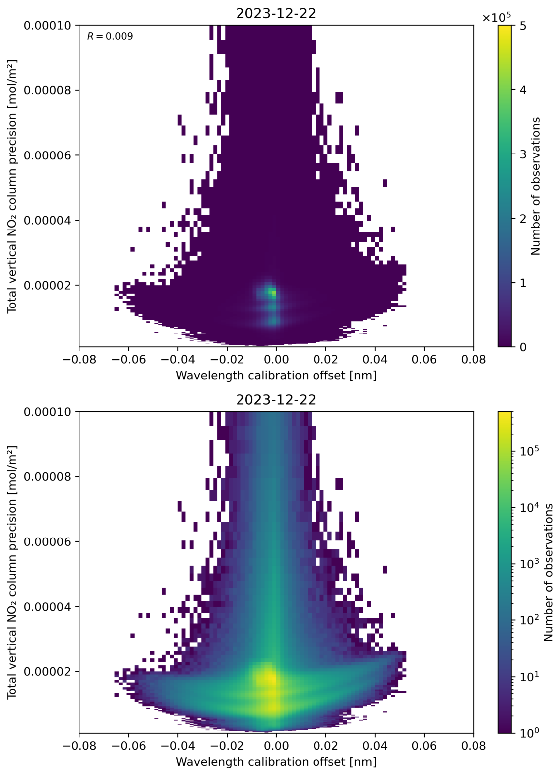
Figure 180: Scatter density plot of “Wavelength calibration offset” against “Total vertical NO 2 column precision” for 2023-12-21 to 2023-12-23.
