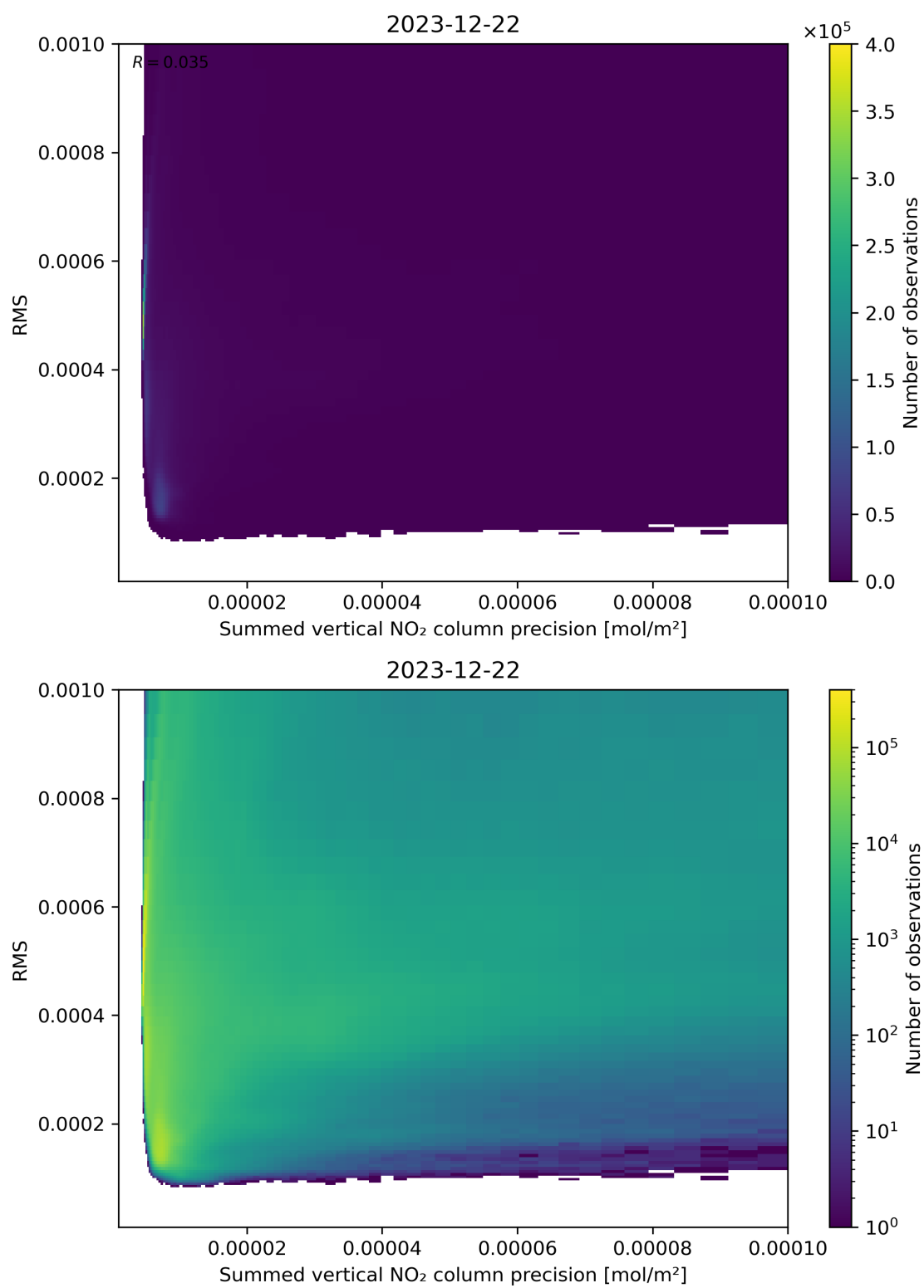
Figure 108: Scatter density plot of “Summed vertical NO 2 column precision” against “RMS” for 2023-12-21 to 2023-12-23.
