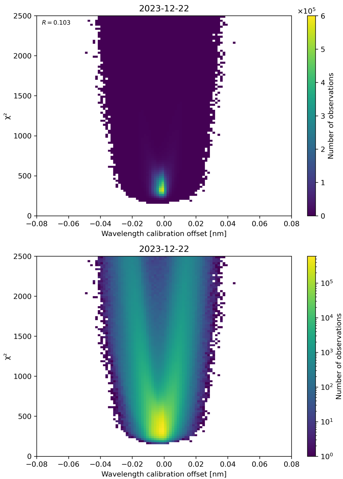
Figure 175: Scatter density plot of “Wavelength calibration offset” against “ \chi^2 ” for 2023-12-21 to 2023-12-23.
