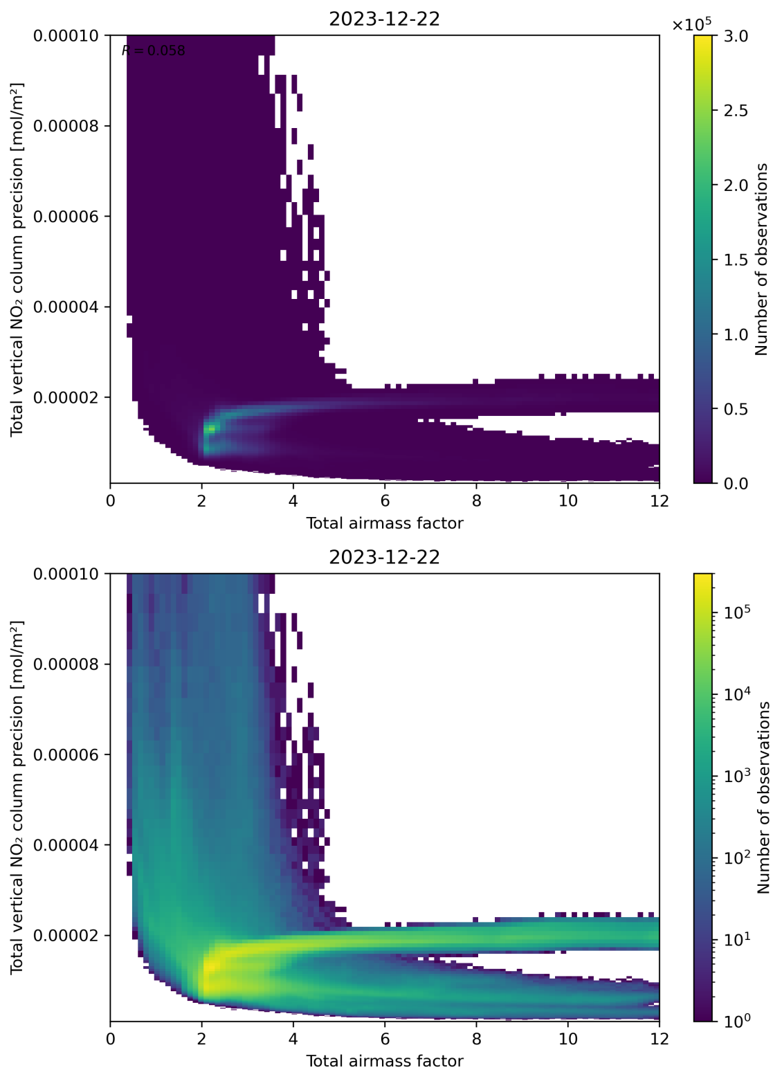
Figure 68: Scatter density plot of “Total airmass factor” against “Total vertical NO 2 column precision” for 2023-12-21 to 2023-12-23.
