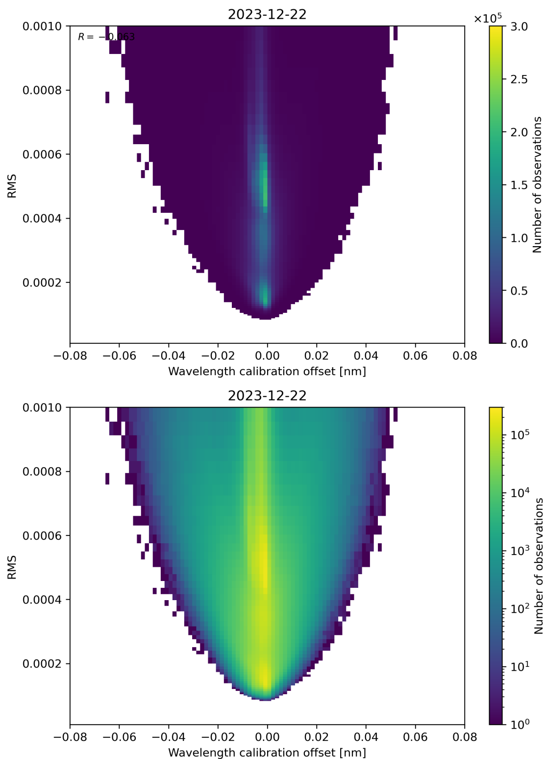
Figure 181: Scatter density plot of “Wavelength calibration offset” against “RMS” for 2023-12-21 to 2023-12-23.
