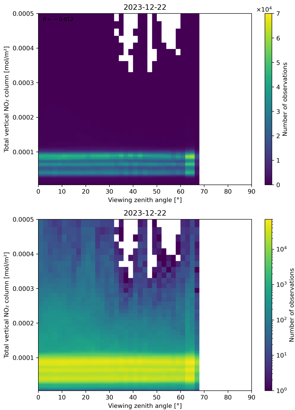
Figure 167: Scatter density plot of “Viewing zenith angle” against “Total vertical NO 2 column” for 2023-12-21 to 2023-12-23.
