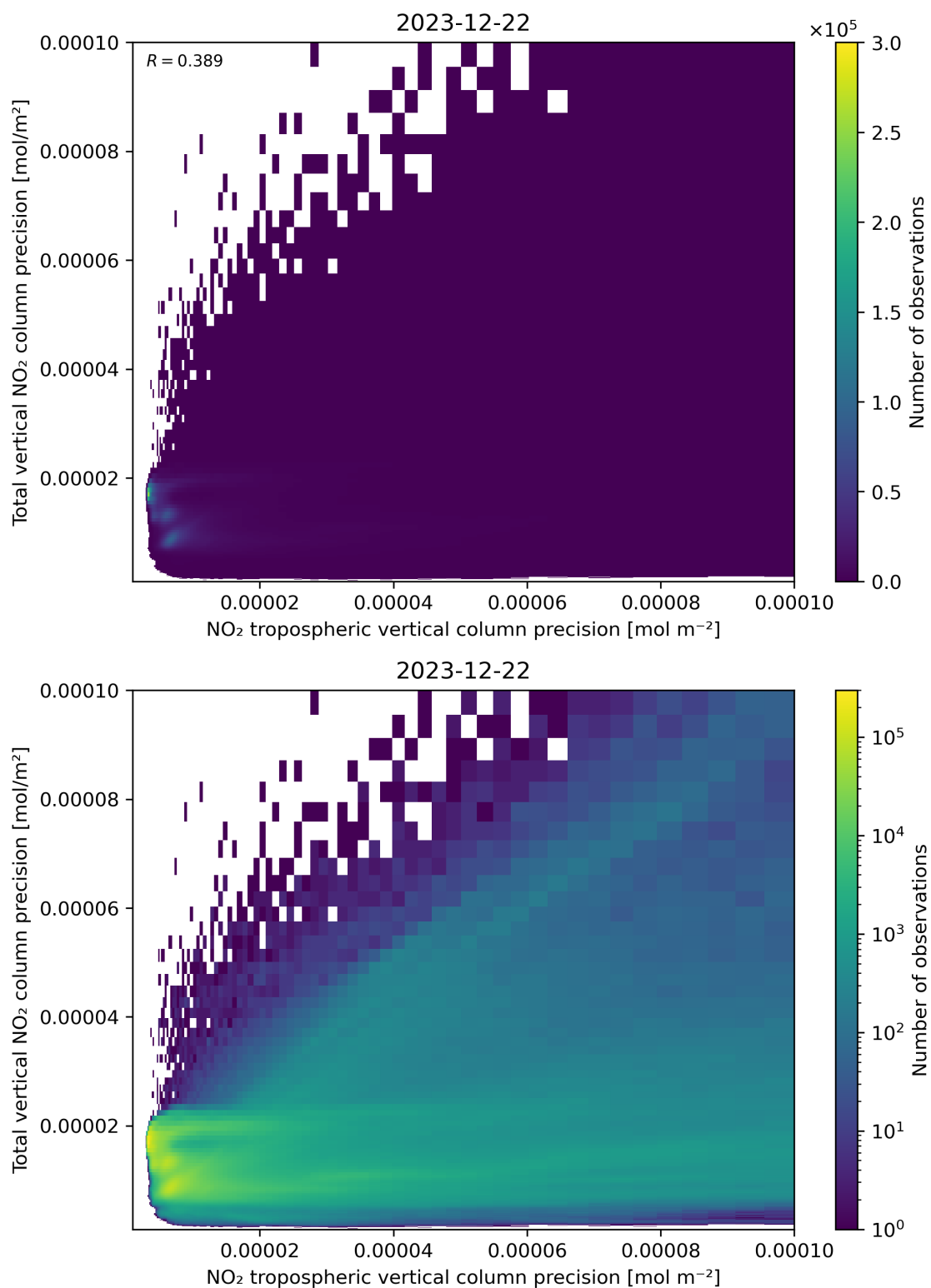
Figure 139: Scatter density plot of “NO 2 tropospheric vertical column precision” against “Total vertical NO 2 column precision” for 2023-12-21 to 2023-12-23.
