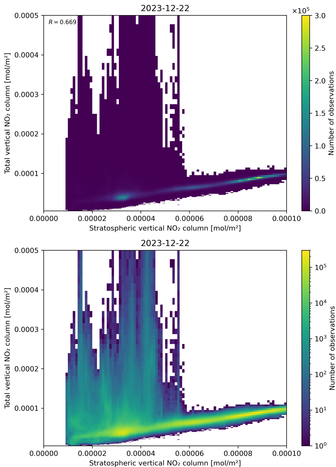
Figure 100: Scatter density plot of “Stratospheric vertical NO 2 column” against “Total vertical NO 2 column” for 2023-12-21 to 2023-12-23.
