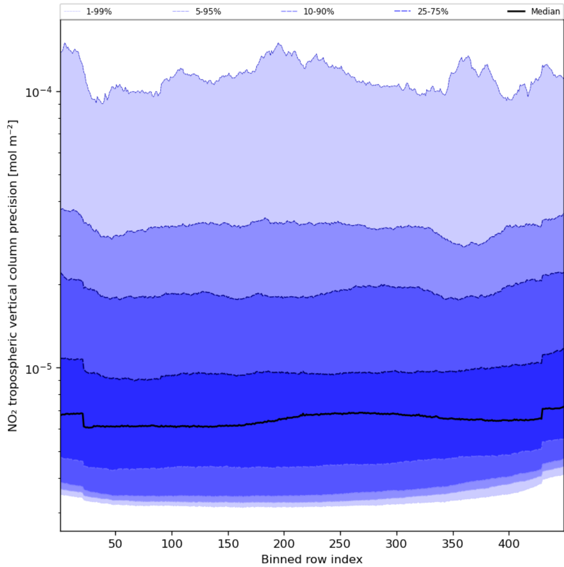
Figure 47: Along track statistics of “NO 2 tropospheric vertical column precision” for 2023-12-21 to 2023-12-23
