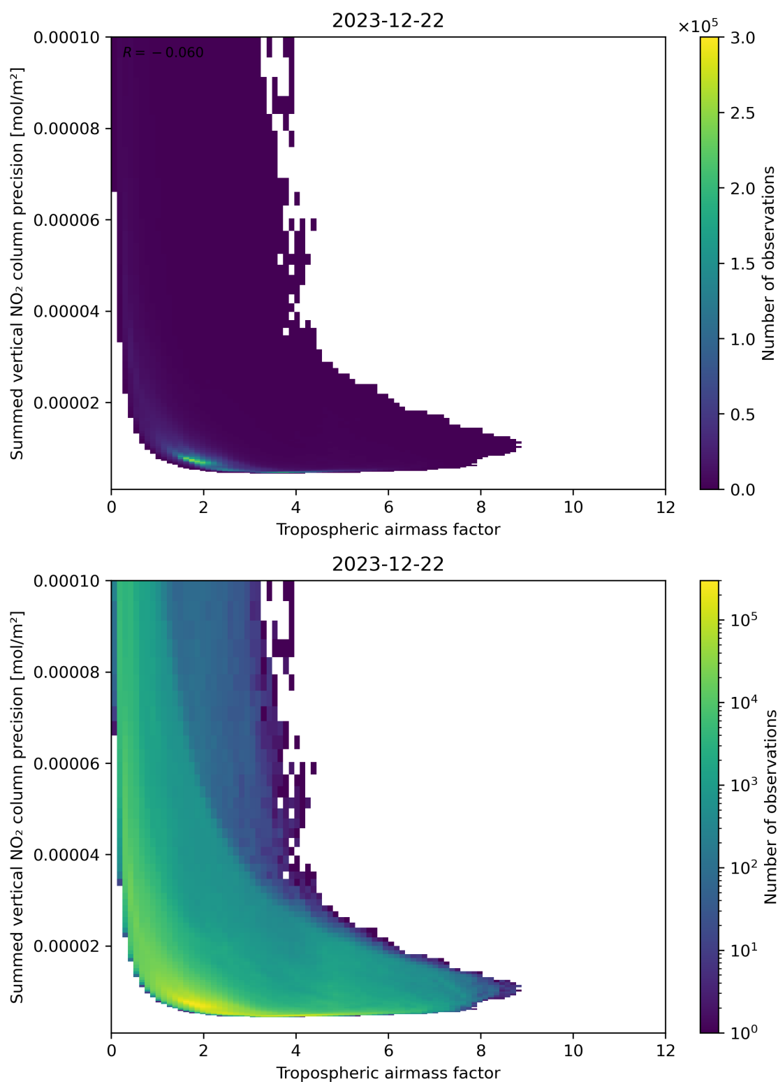
Figure 76: Scatter density plot of “Tropospheric air mass factor” against “Summed vertical NO 2 column precision” for 2023-12-21 to 2023-12-23.
