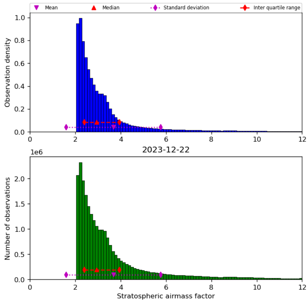
Figure 44: Histogram of “Stratospheric airmass factor” for 2023-12-21 to 2023-12-23
