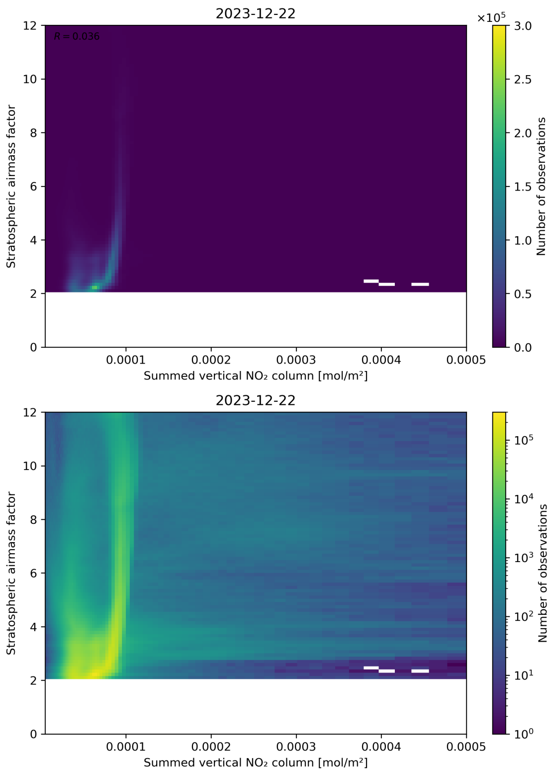
Figure 103: Scatter density plot of “Summed vertical NO 2 column” against “Stratospheric airmass factor” for 2023-12-21 to 2023-12-23.
