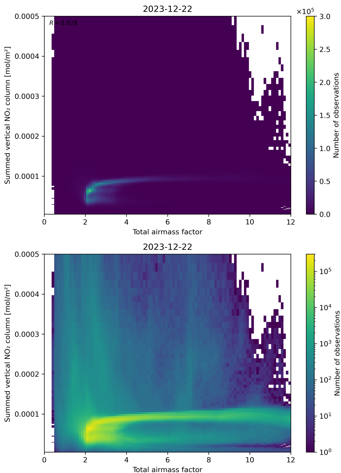
Figure 65: Scatter density plot of “Total airmass factor” against “Summed vertical NO 2 column” for 2023-12-21 to 2023-12-23.
