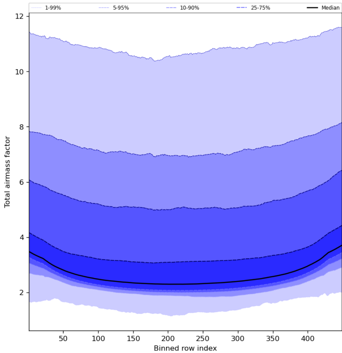
Figure 49: Along track statistics of “Total airmass factor” for 2023-12-21 to 2023-12-23
