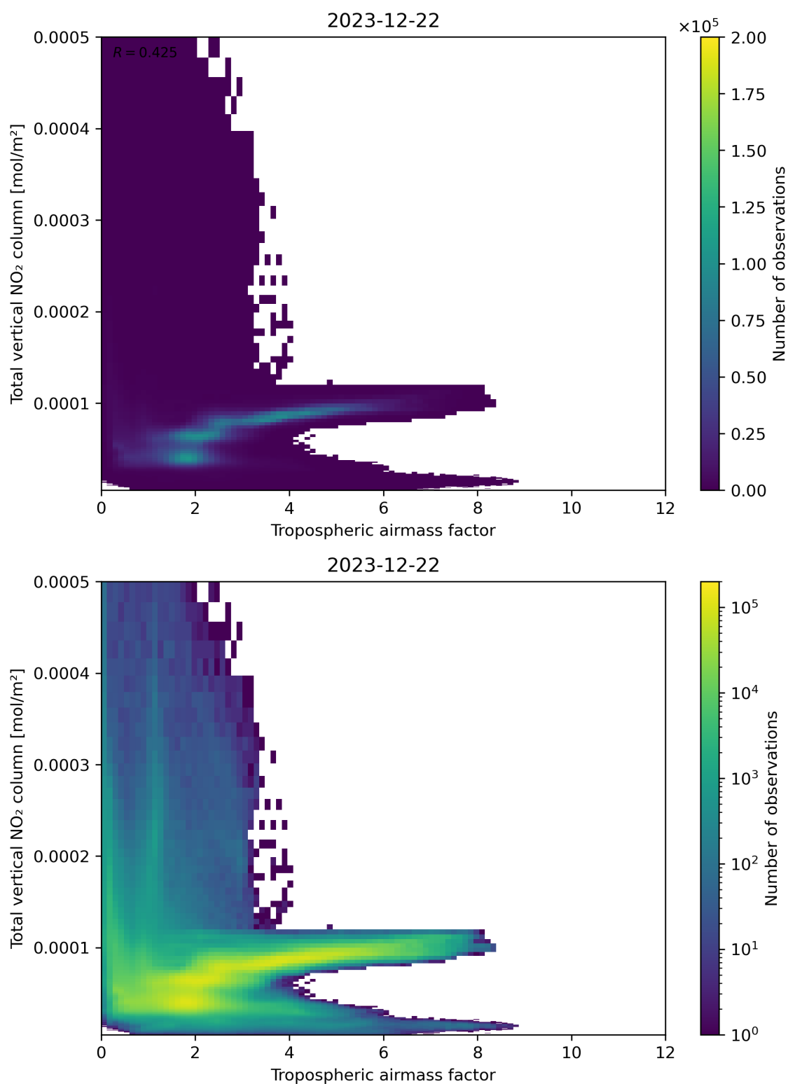
Figure 77: Scatter density plot of “Tropospheric airmass factor” against “Total vertical NO 2 column” for 2023-12-21 to 2023-12-23.
