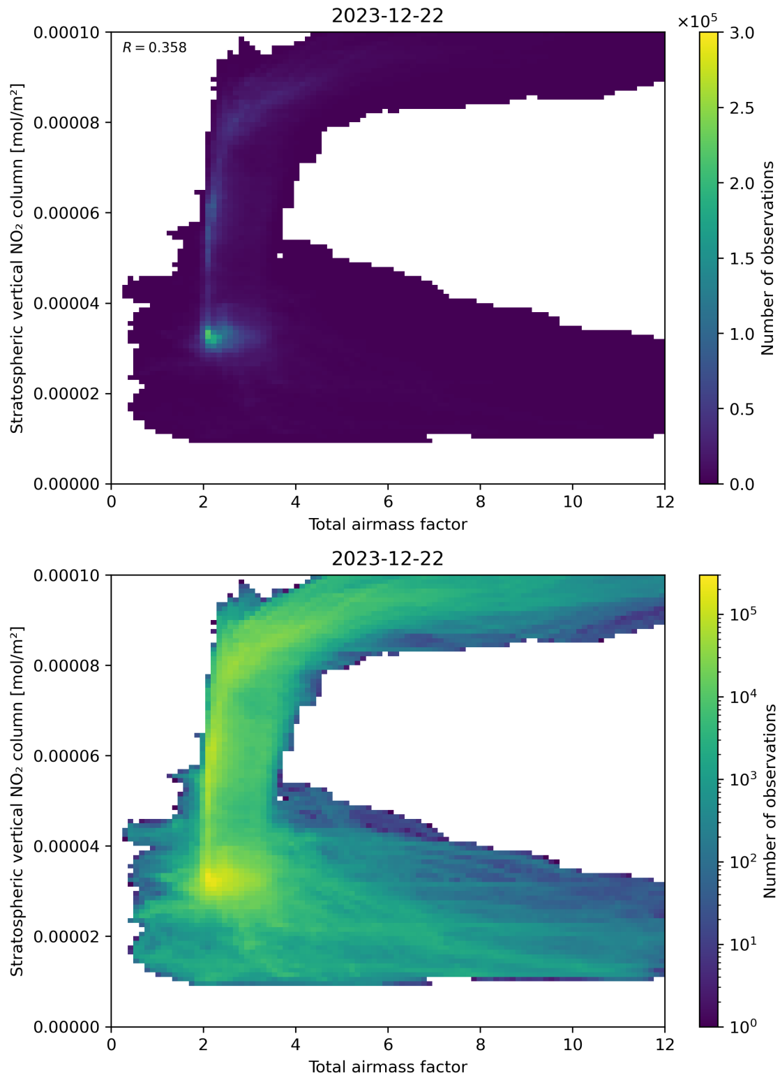
Figure 64: Scatter density plot of “Total airmass factor” against “Stratospheric vertical NO 2 column” for 2023-12-21 to 2023-12-23.
