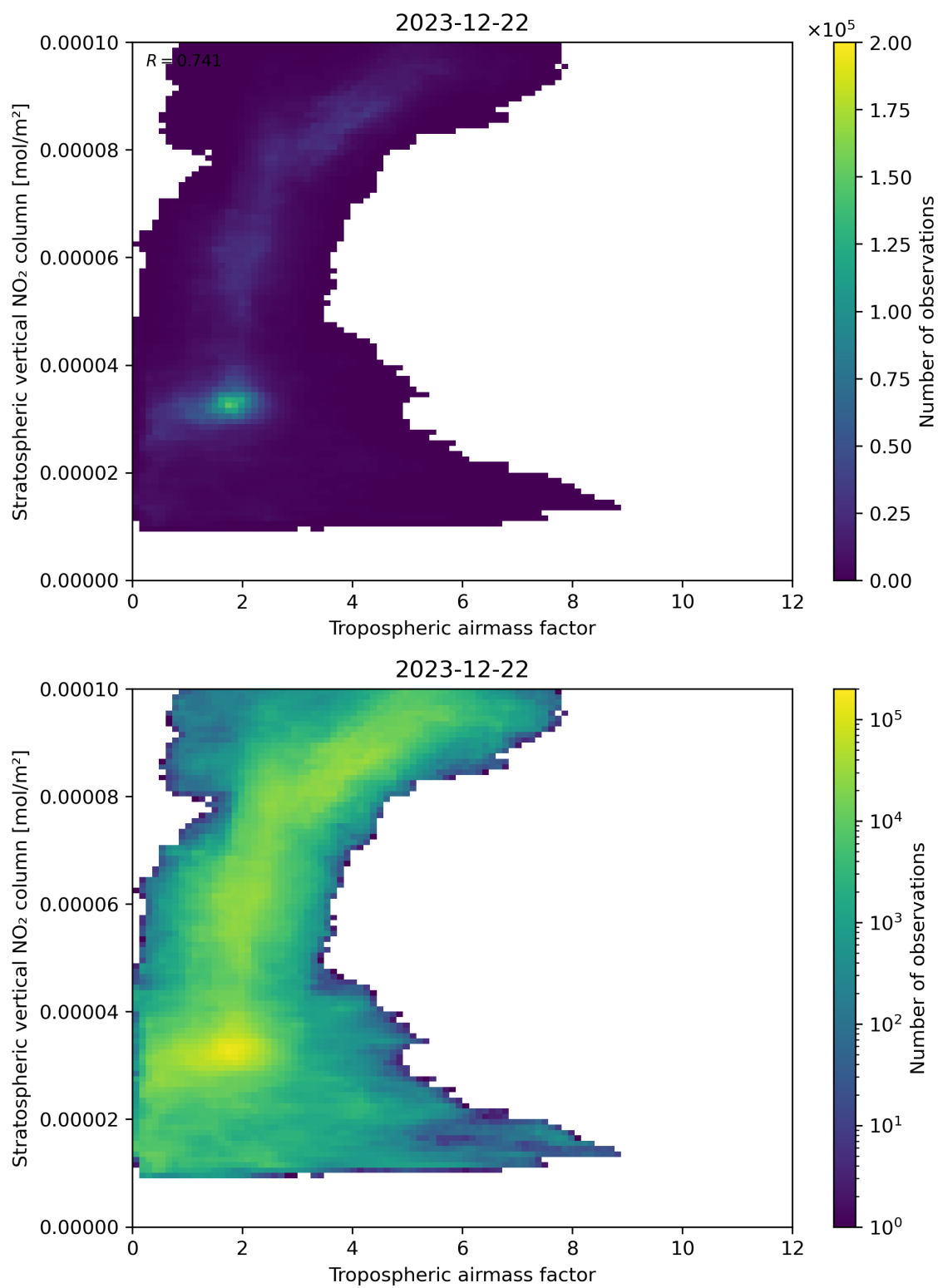
Figure 74: Scatter density plot of “Tropospheric air mass factor” against “Stratospheric vertical NO 2 column” for 2023-12-21 to 2023-12-23.
