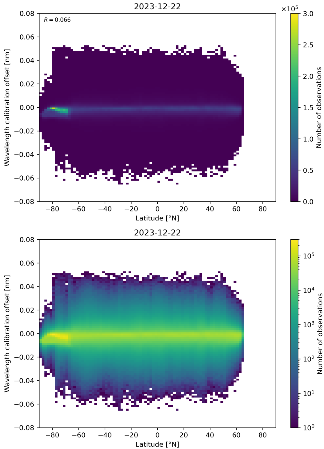
Figure 95: Scatter density plot of “Latitude” against “Wavelength calibration offset” for 2023-12-21 to 2023-12-23.
