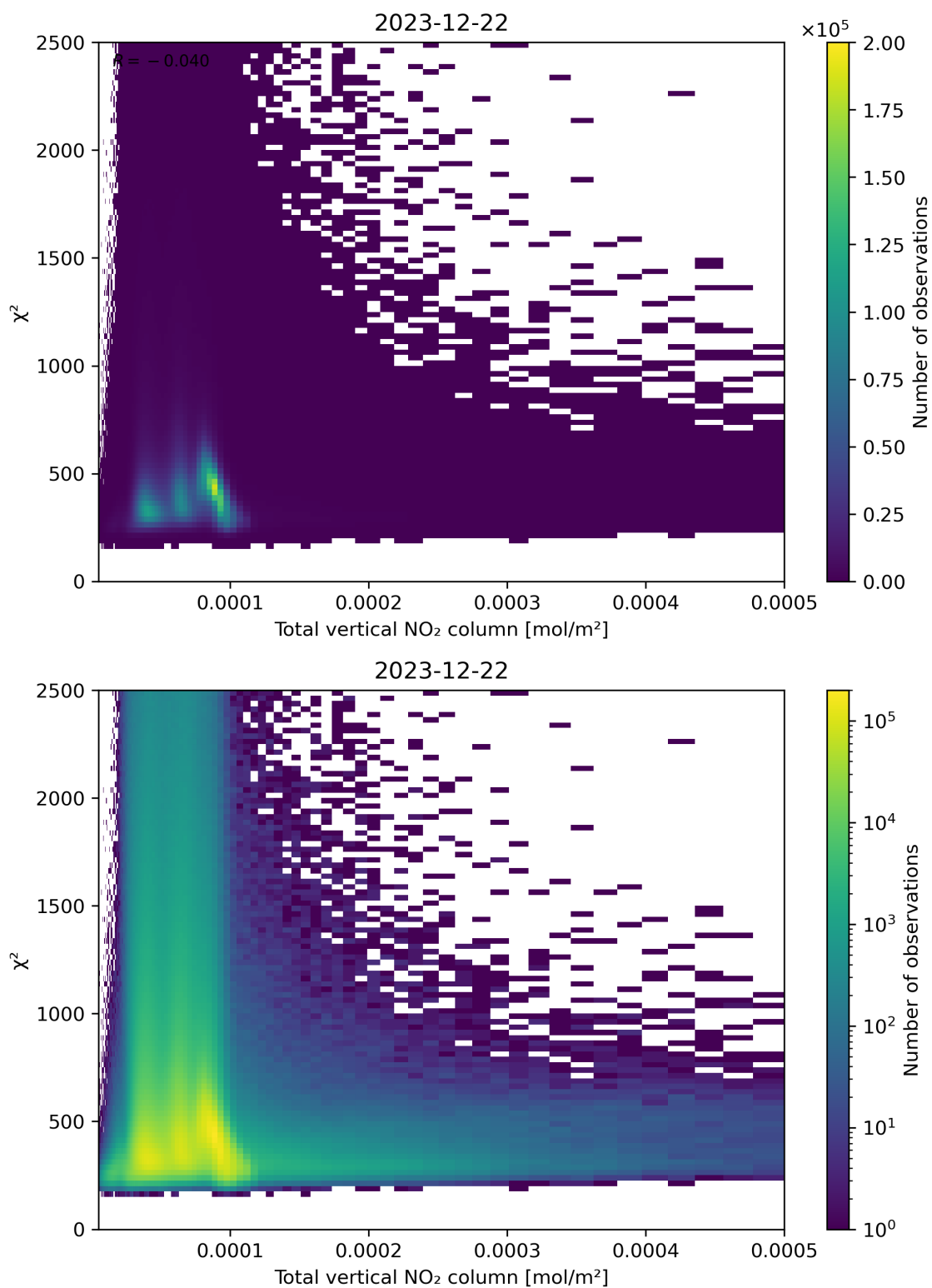
Figure 111: Scatter density plot of “Total vertical NO 2 column” against “ \chi^2 ” for 2023-12-21 to 2023-12-23.
