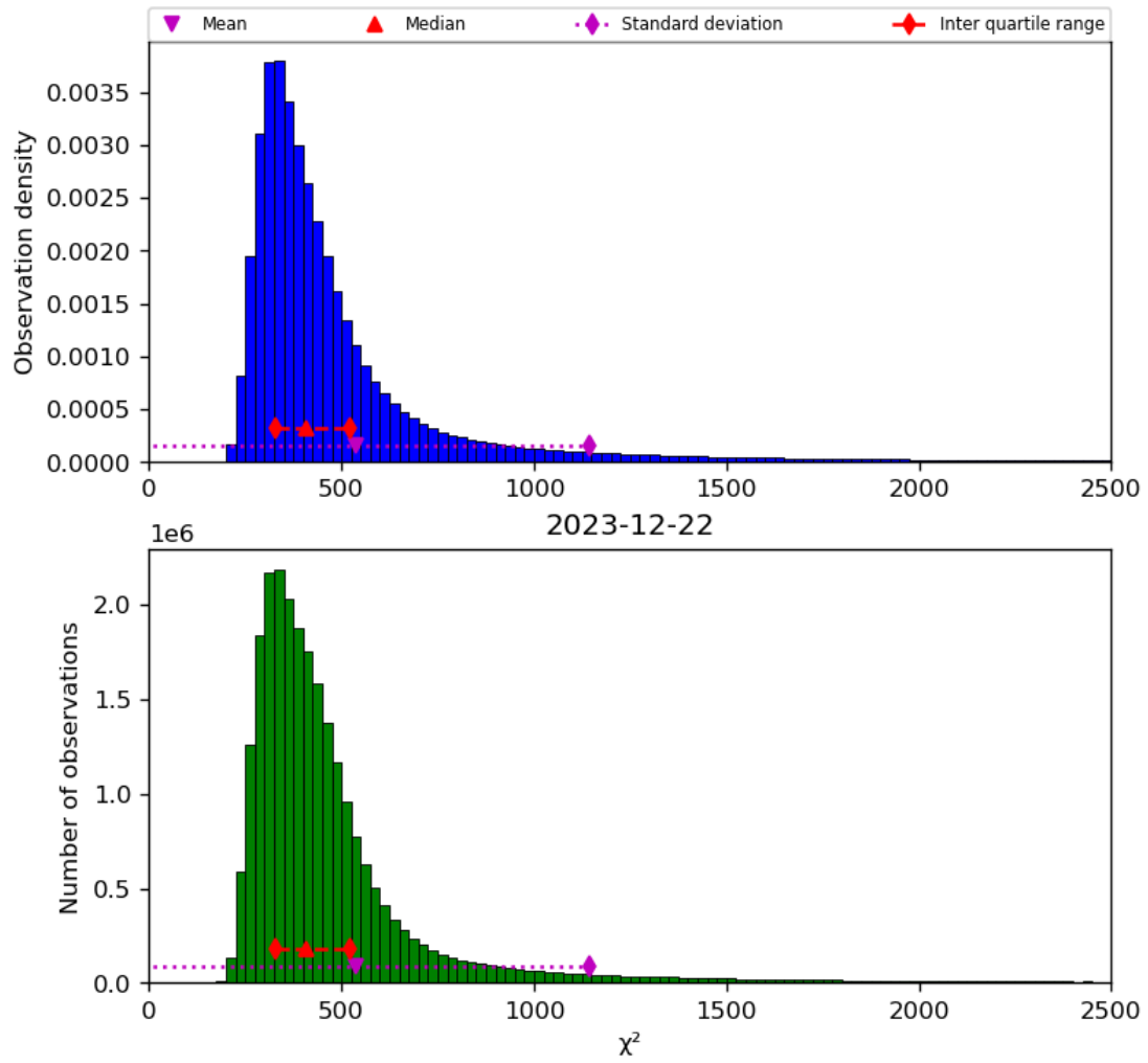
Figure 42: Histogram of “ \chi^2 ” for 2023-12-21 to 2023-12-23
