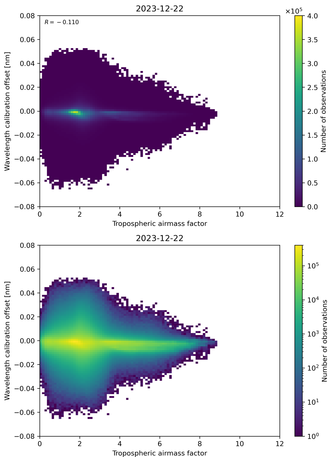
Figure 80: Scatter density plot of “Tropospheric air mass factor” against “Wavelength calibration offset” for 2023-12-21 to 2023-12-23.
