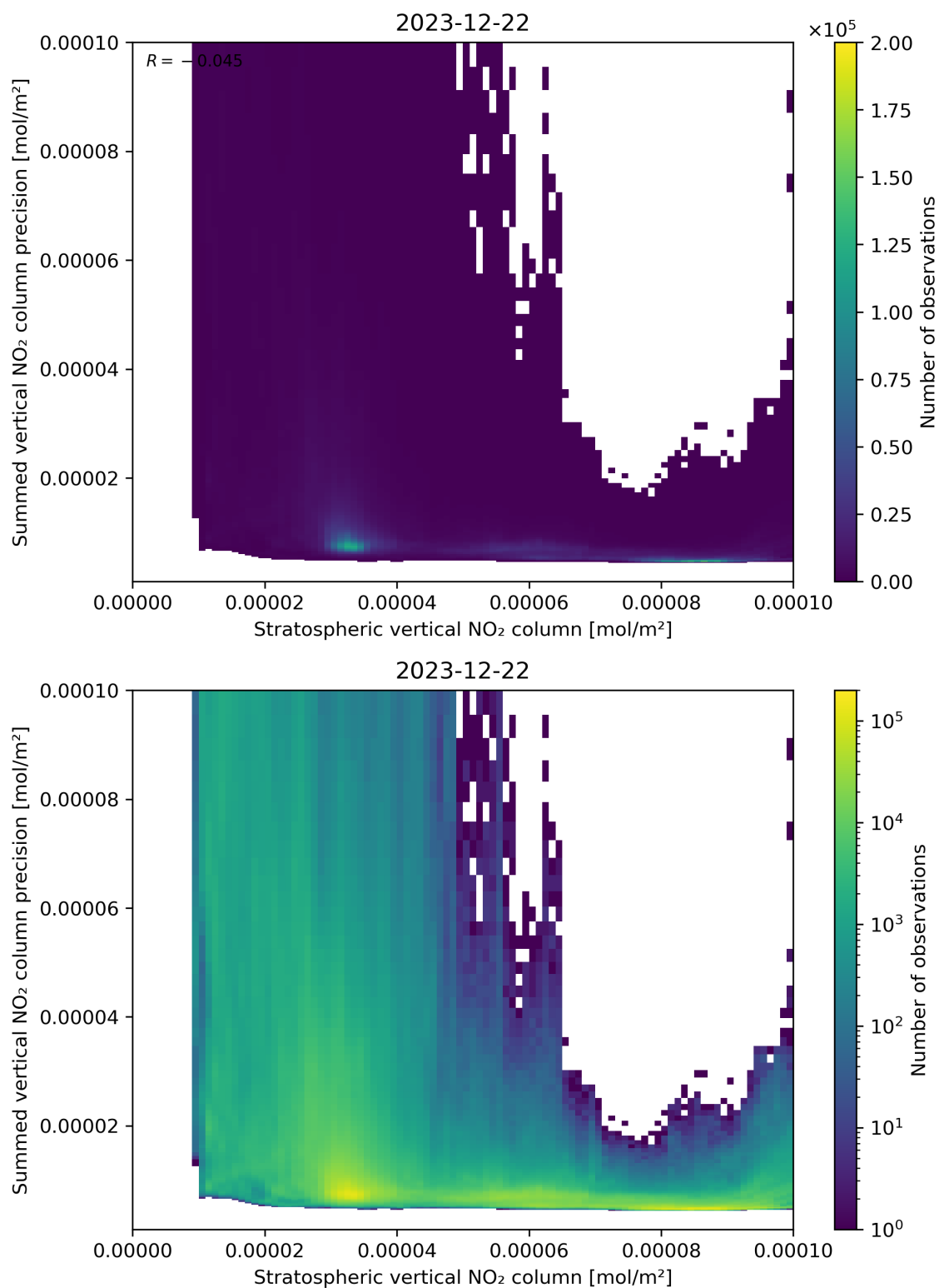
Figure 99: Scatter density plot of “Stratospheric vertical NO 2 column” against “Summed vertical NO 2 column precision” for 2023-12-21 to 2023-12-23.
