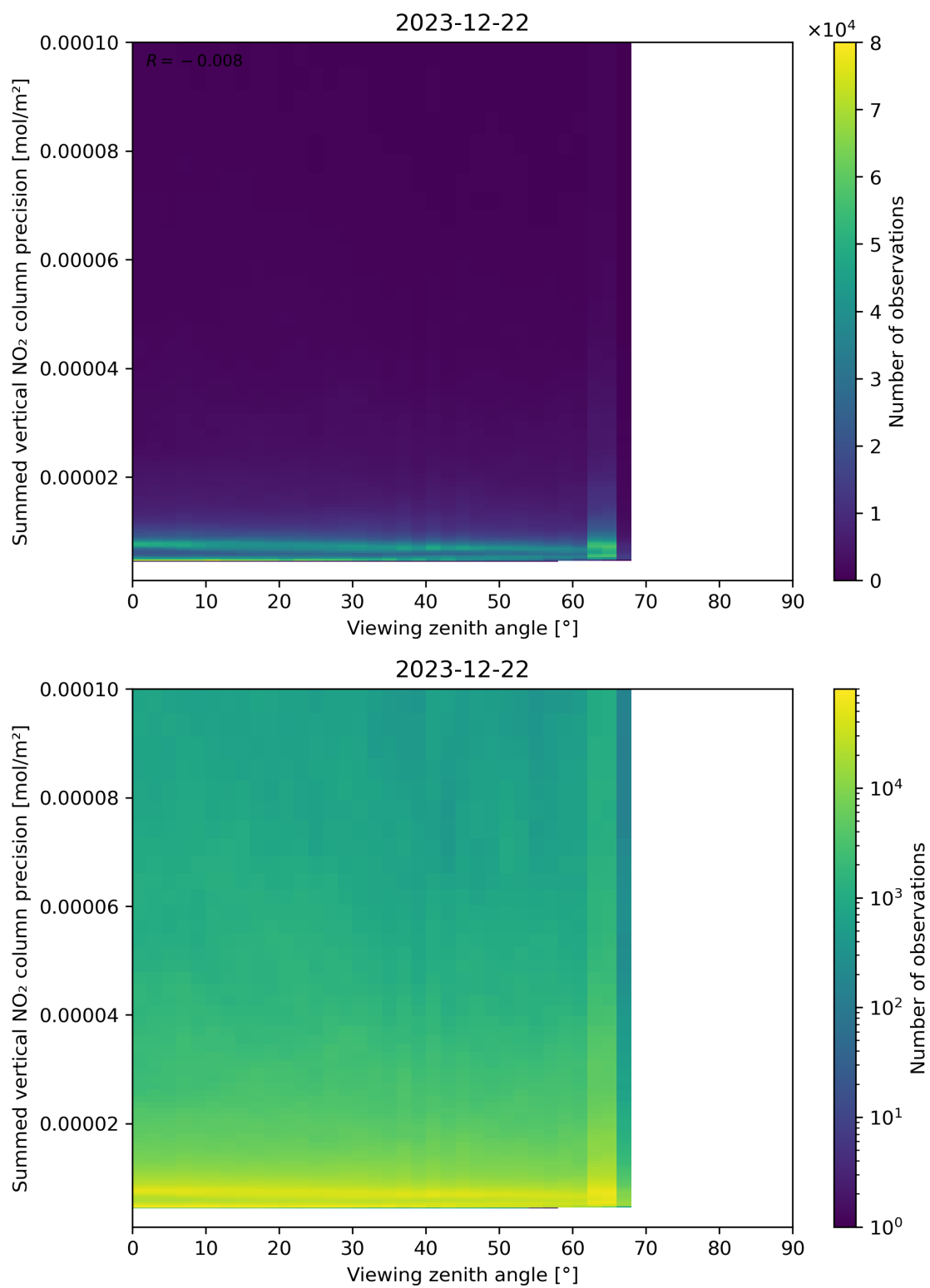
Figure 166: Scatter density plot of “Viewing zenith angle” against “Summed vertical NO 2 column precision” for 2023-12-21 to 2023-12-23.
