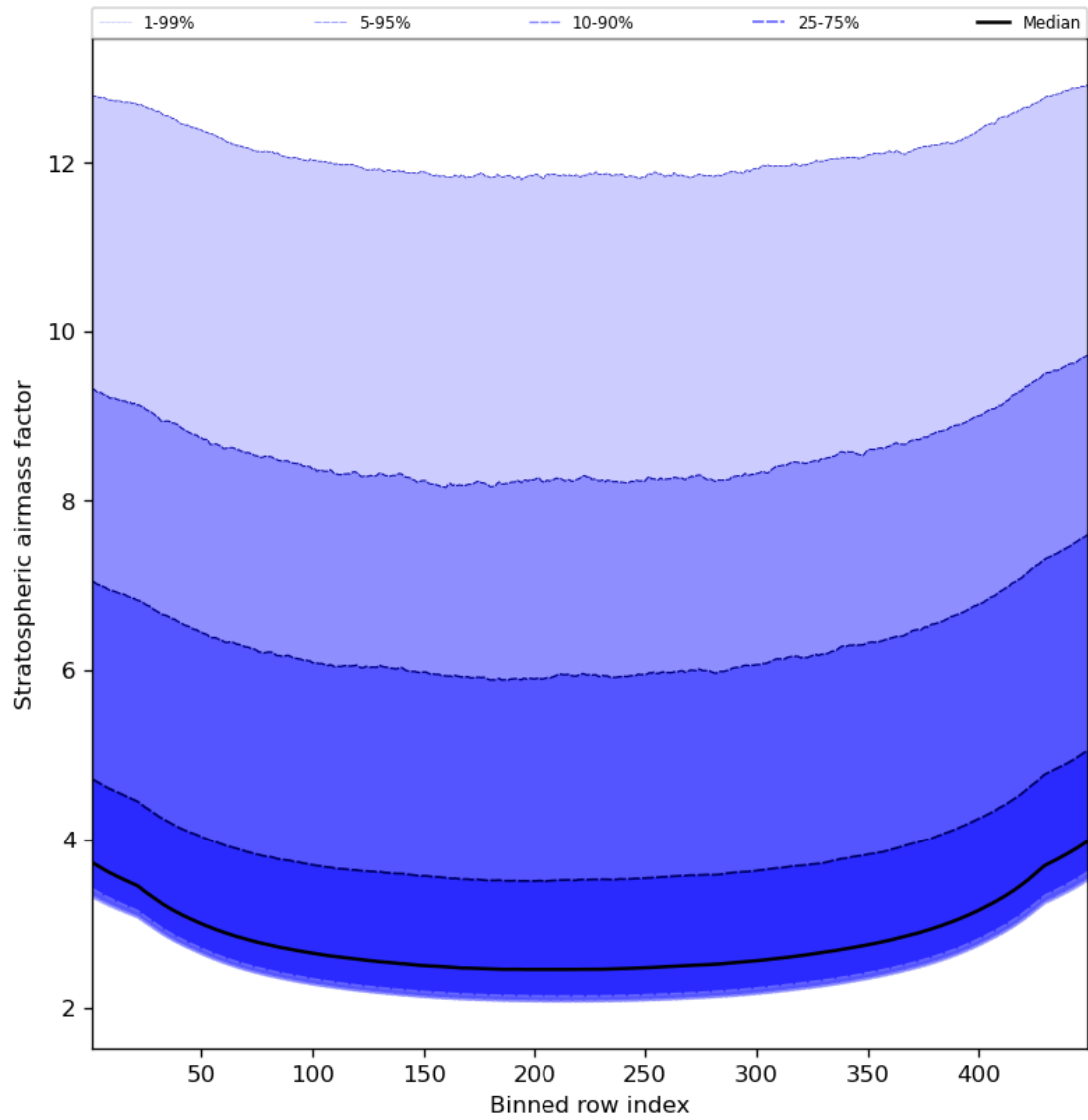
Figure 61: Along track statistics of “Stratospheric air mass factor” for 2023-12-21 to 2023-12-23
