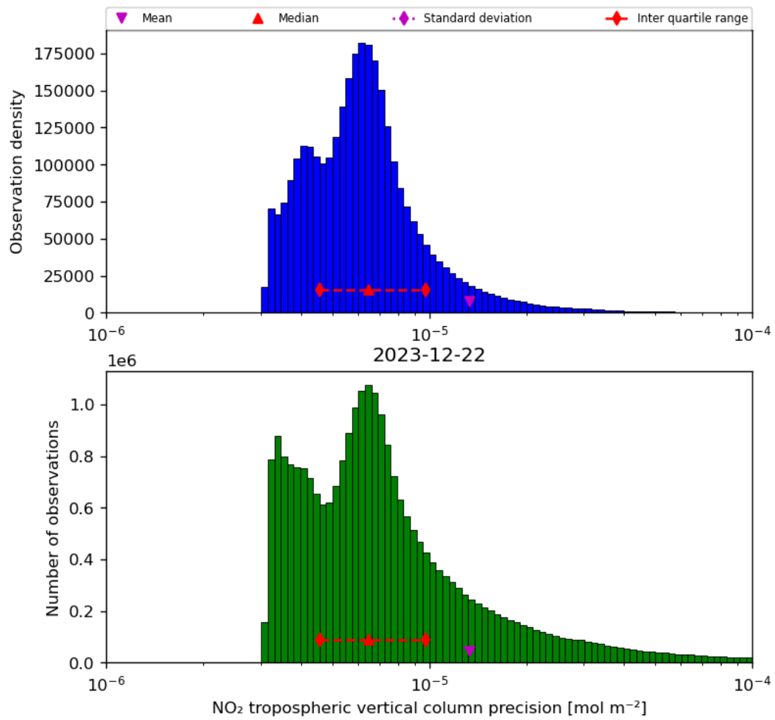
Figure 30: Histogram of “NO 2 tropospheric vertical column precision” for 2023-12-21 to 2023-12-23
