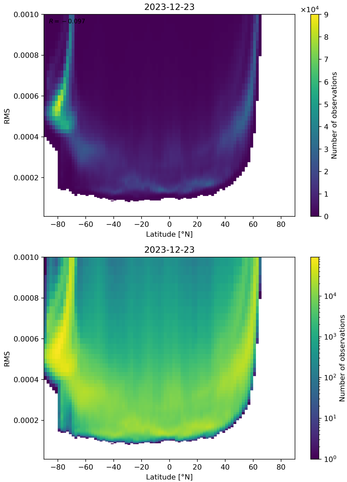
Figure 94: Scatter density plot of “Latitude” against “RMS” for 2023-12-22 to 2023-12-24.
