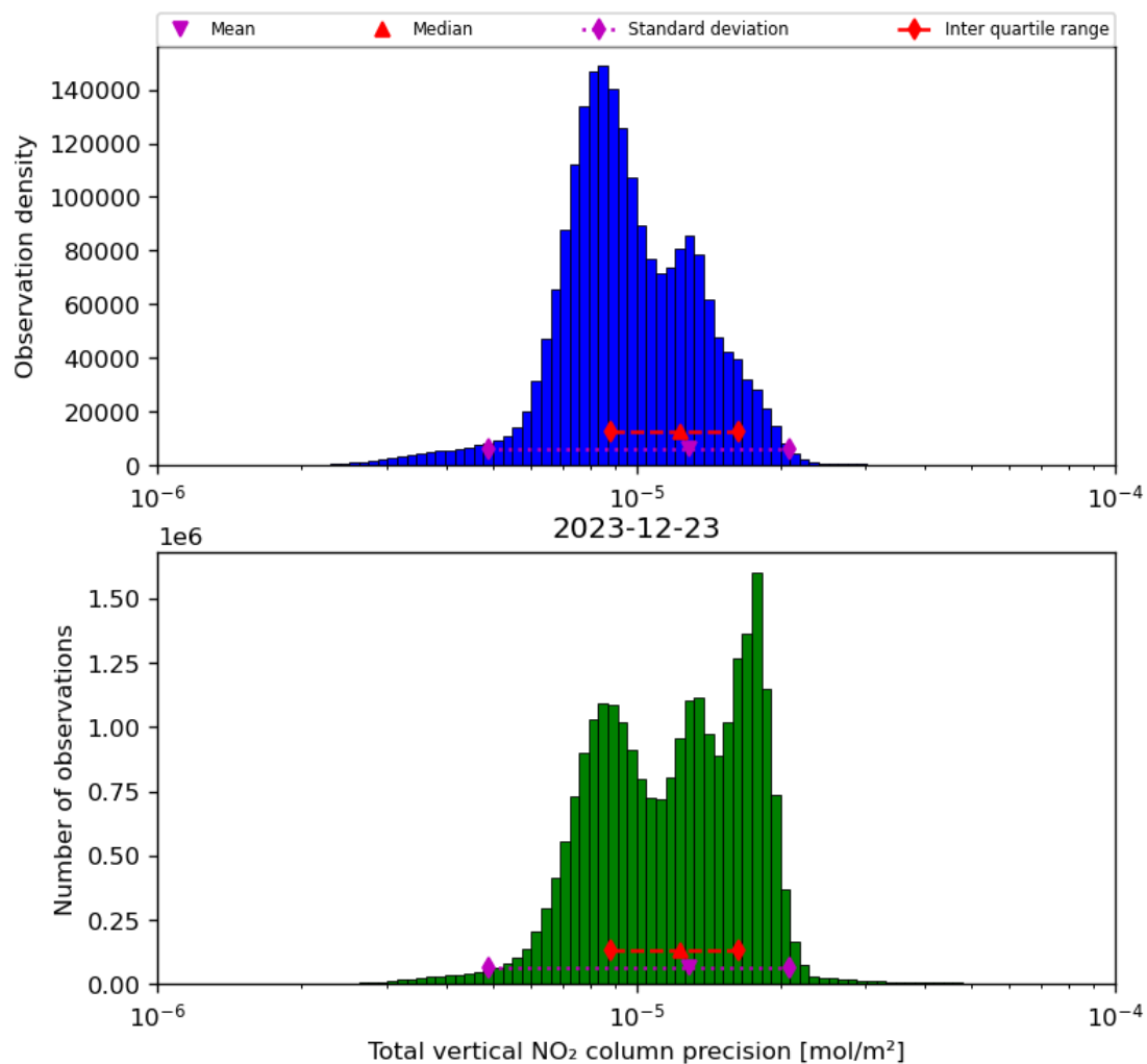
Figure 39: Histogram of “Total vertical NO 2 column precision” for 2023-12-22 to 2023-12-24
