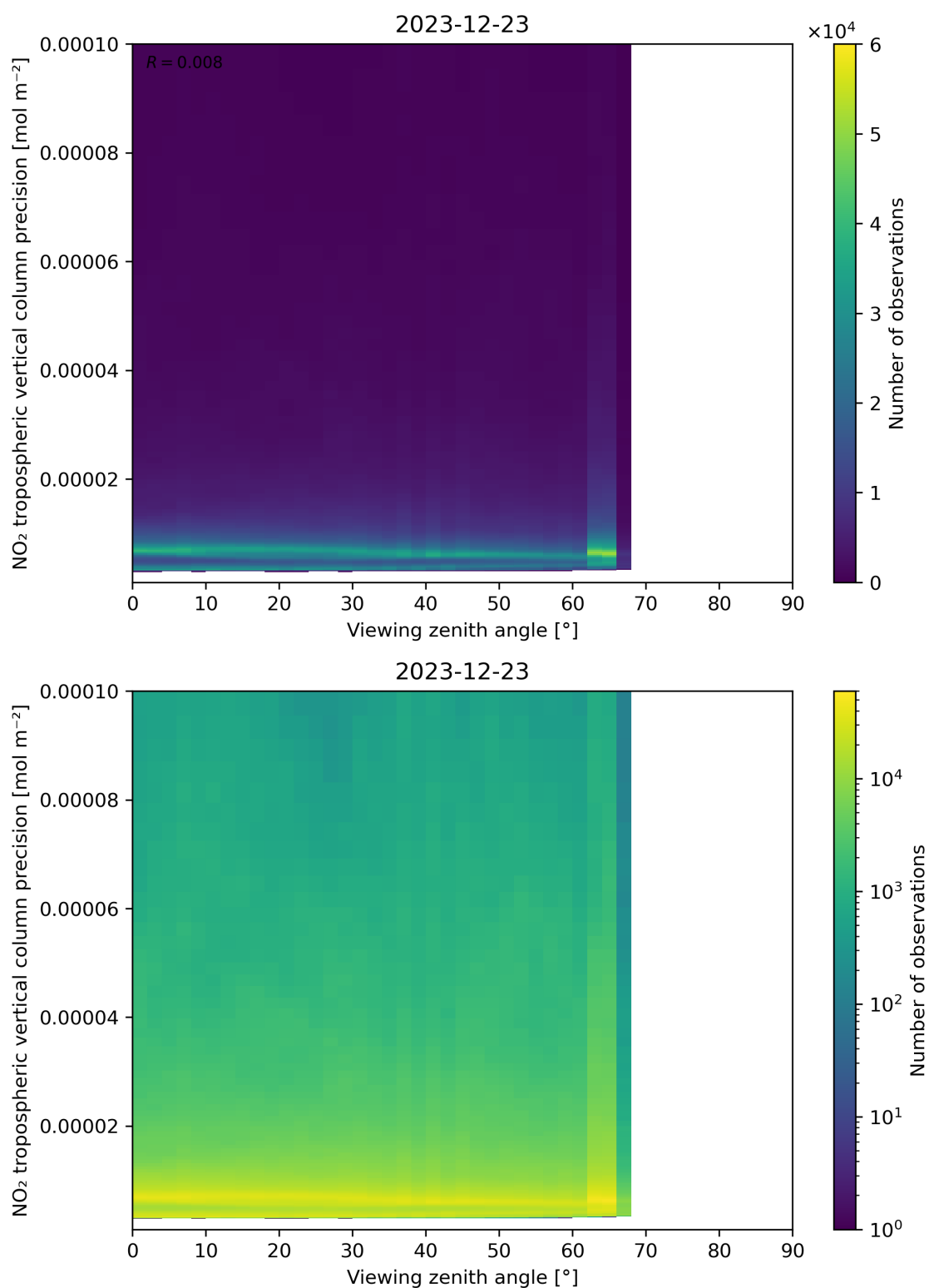
Figure 170: Scatter density plot of “Viewing zenith angle” against “NO 2 tropospheric vertical column precision” for 2023-12-22 to 2023-12-24.
