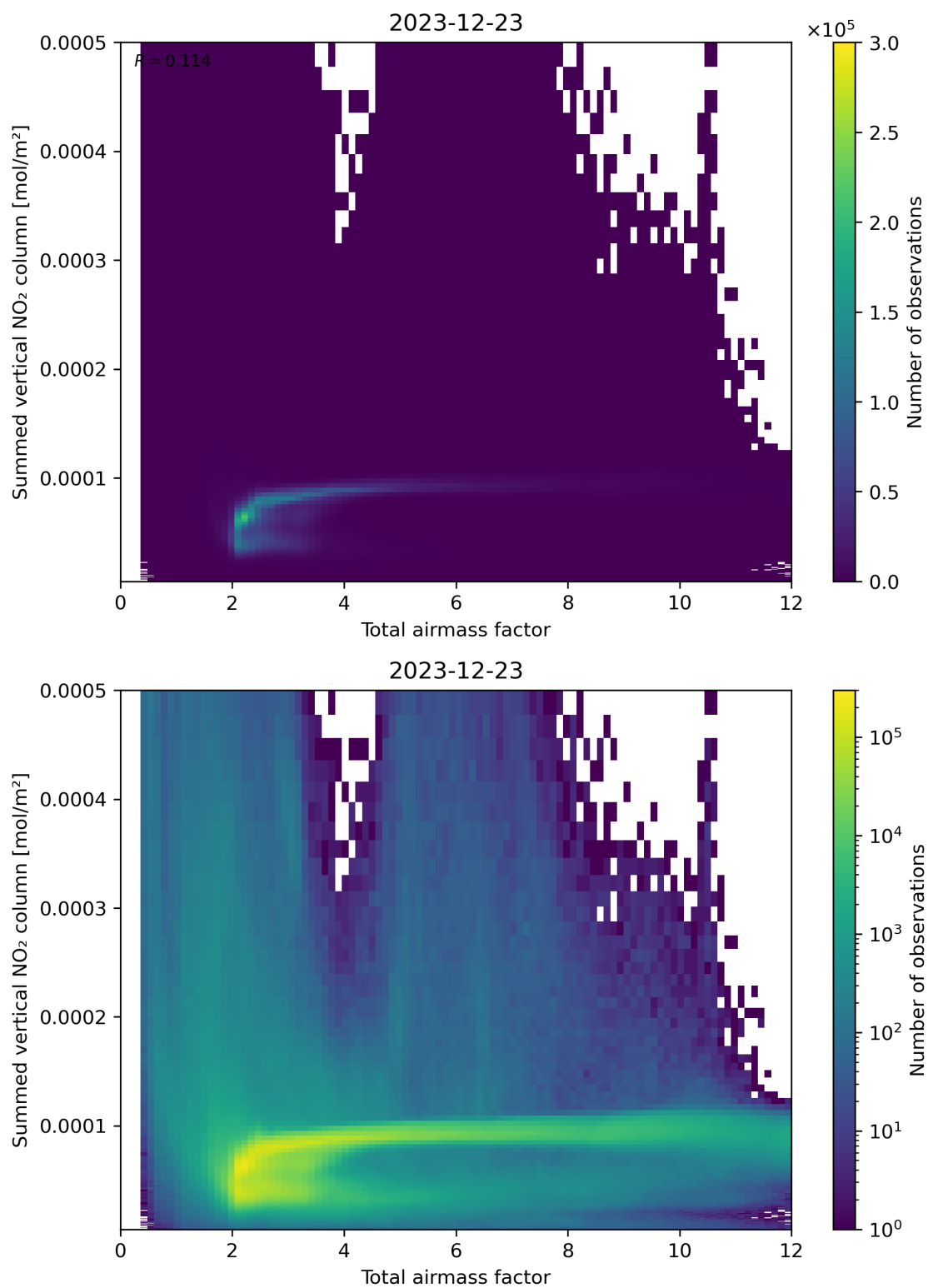
Figure 65: Scatter density plot of “Total airmass factor” against “Summed vertical NO 2 column” for 2023-12-22 to 2023-12-24.
