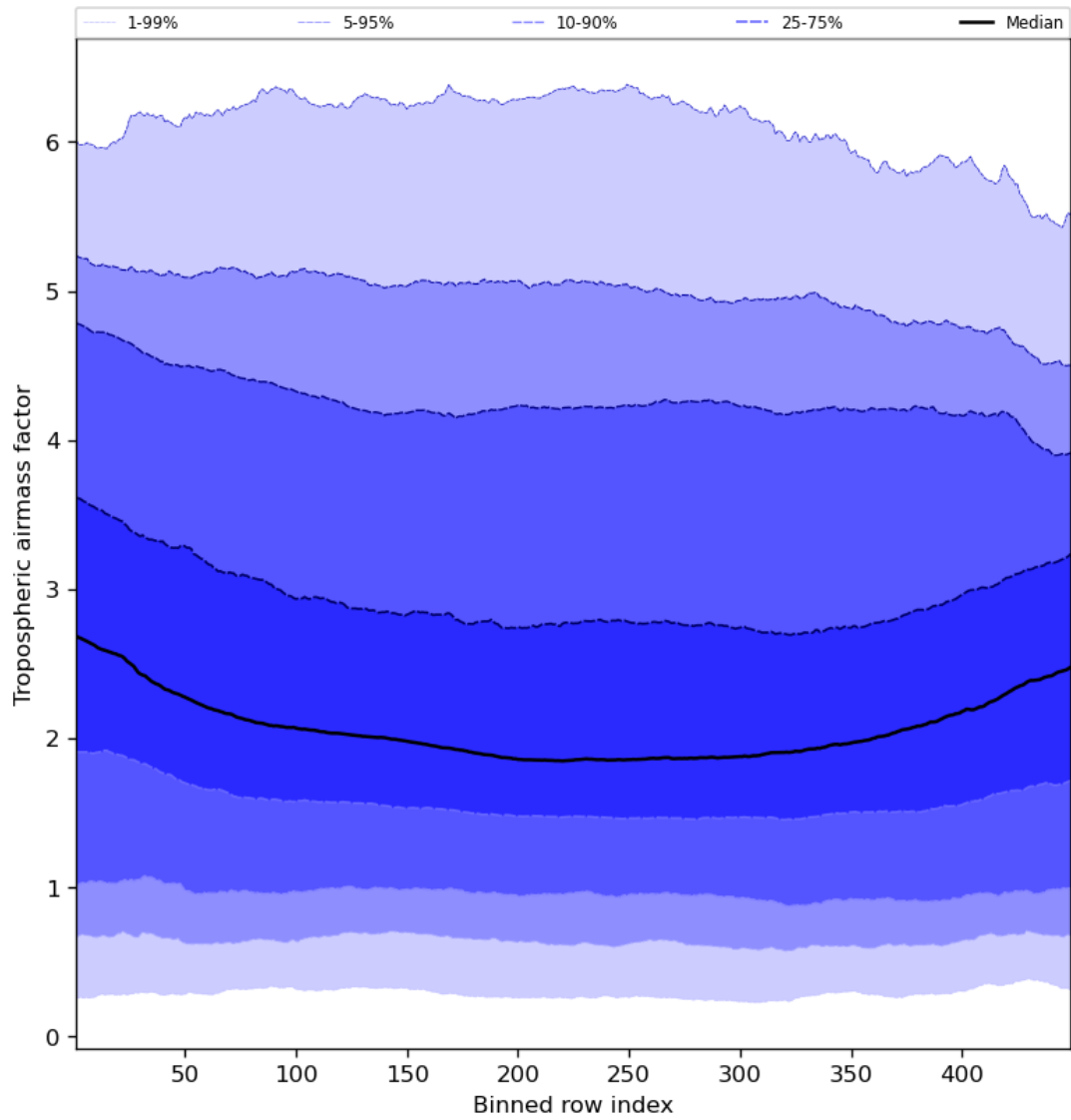
Figure 48: Along track statistics of “Tropospheric airmass factor” for 2023-12-22 to 2023-12-24
