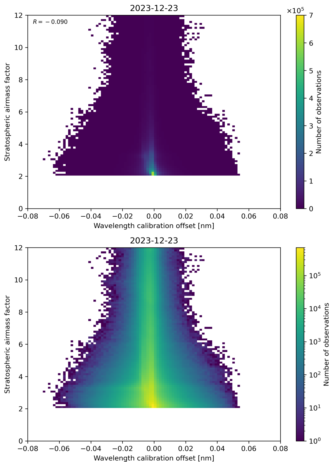
Figure 174: Scatter density plot of “Wavelength calibration offset” against “Stratospheric airmass factor” for 2023-12-22 to 2023-12-24.
