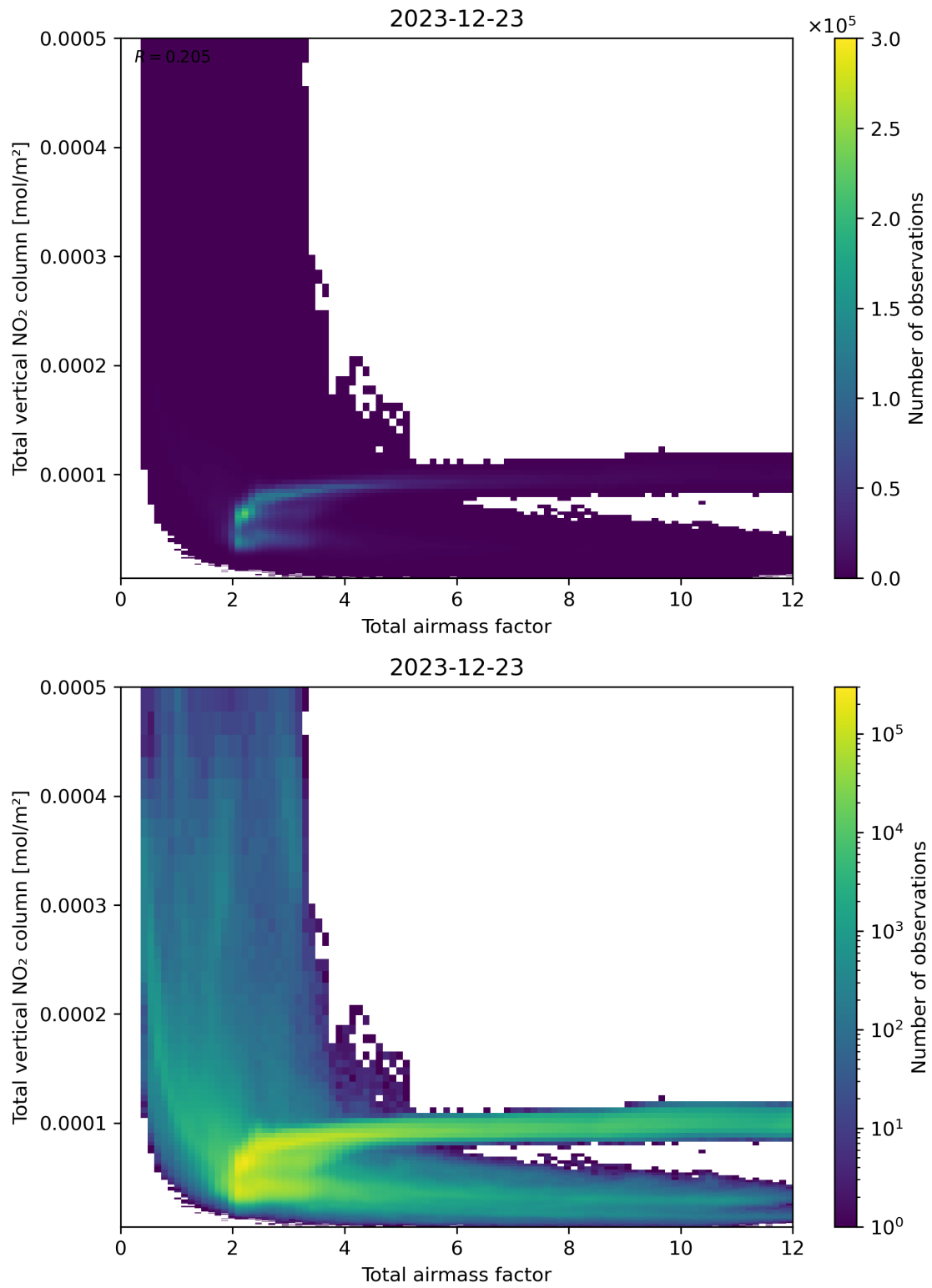
Figure 67: Scatter density plot of “Total air mass factor” against “Total vertical NO 2 column” for 2023-12-22 to 2023-12-24.
