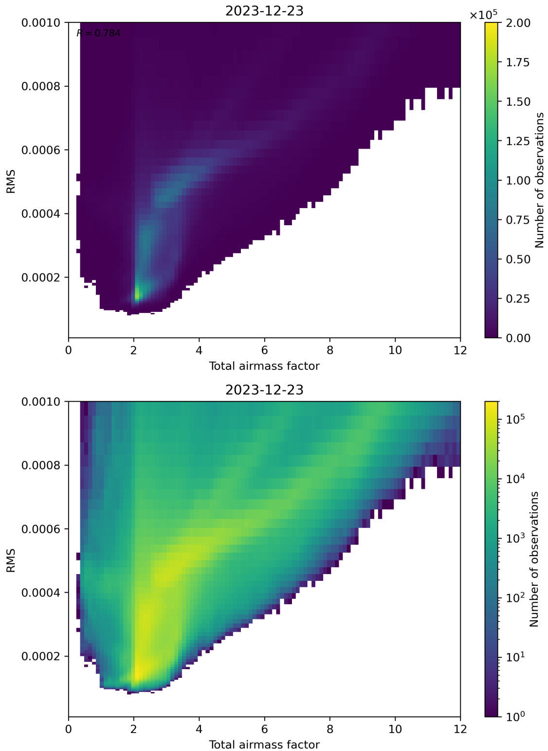
Figure 69: Scatter density plot of “Total airmass factor” against “RMS” for 2023-12-22 to 2023-12-24.
