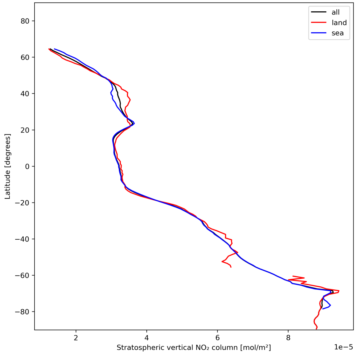
Figure 19: Zonal average of “Stratospheric vertical NO 2 column” for 2023-12-22 to 2023-12-24.
