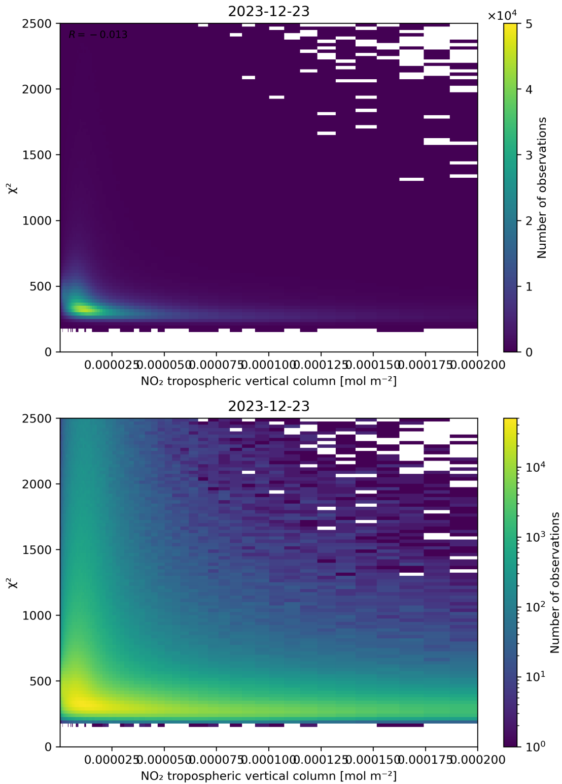
Figure 124: Scatter density plot of “NO 2 tropospheric vertical column” against “ \chi^2 ” for 2023-12-22 to 2023-12-24.
