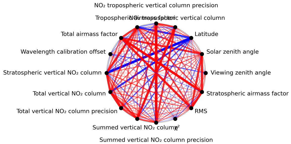
Figure 1: Map of correlation graph for 2023-12-22 to 2023-12-24.
