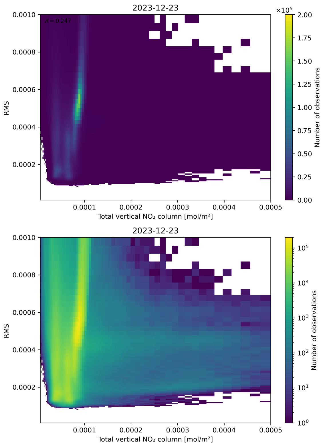
Figure 120: Scatter density plot of “Total vertical NO 2 column” against “RMS” for 2023-12-22 to 2023-12-24.
