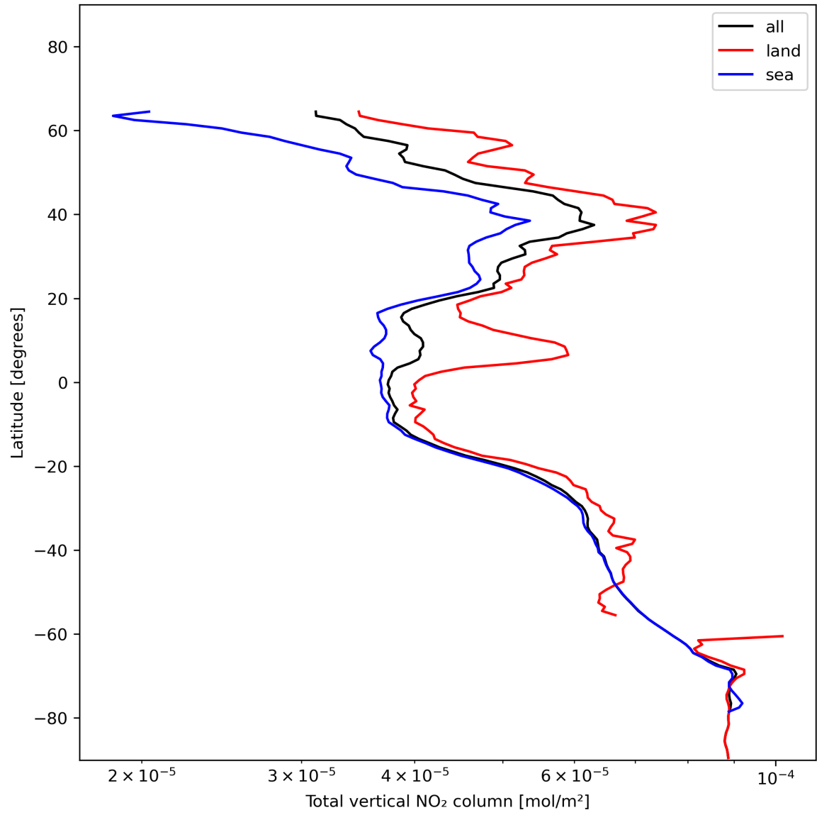
Figure 21: Zonal average of “Total vertical NO 2 column” for 2023-12-22 to 2023-12-24.
