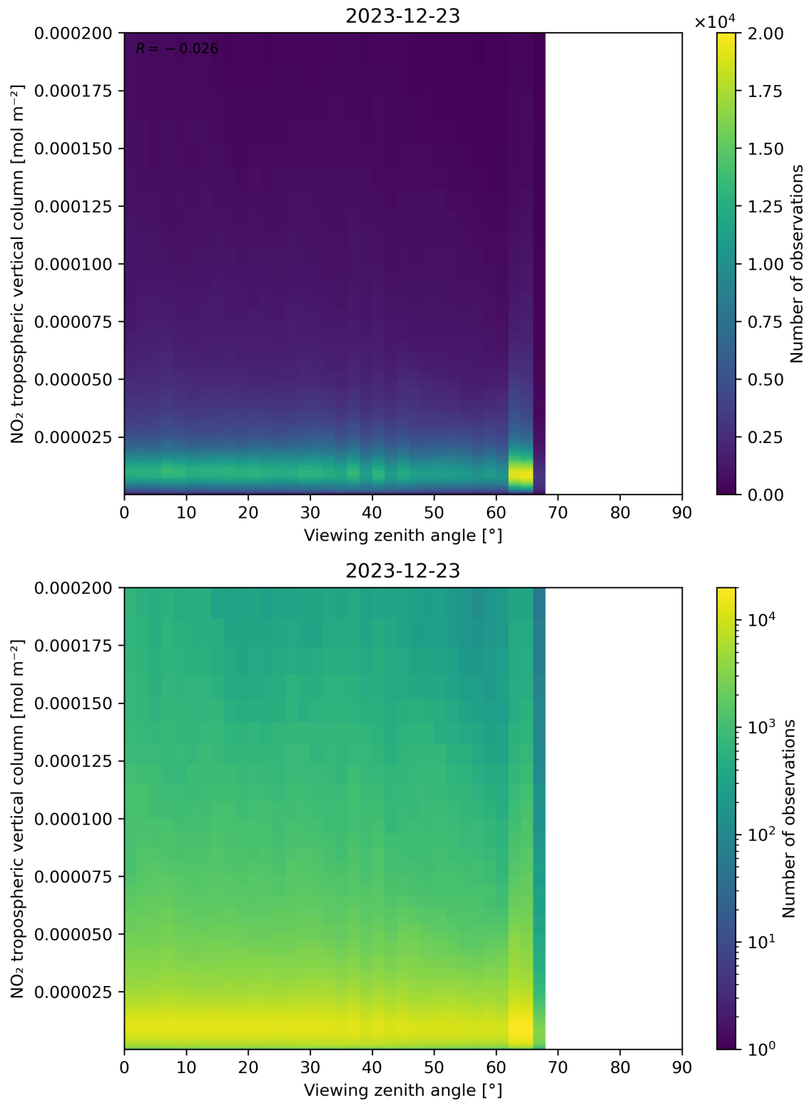
Figure 169: Scatter density plot of “Viewing zenith angle” against “NO 2 tropospheric vertical column” for 2023-12-22 to 2023-12-24.
