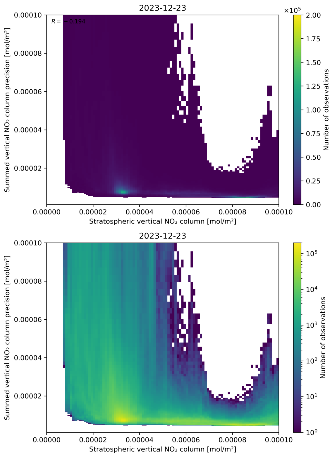
Figure 99: Scatter density plot of “Stratospheric vertical NO 2 column” against “Summed vertical NO 2 column precision” for 2023-12-22 to 2023-12-24.
