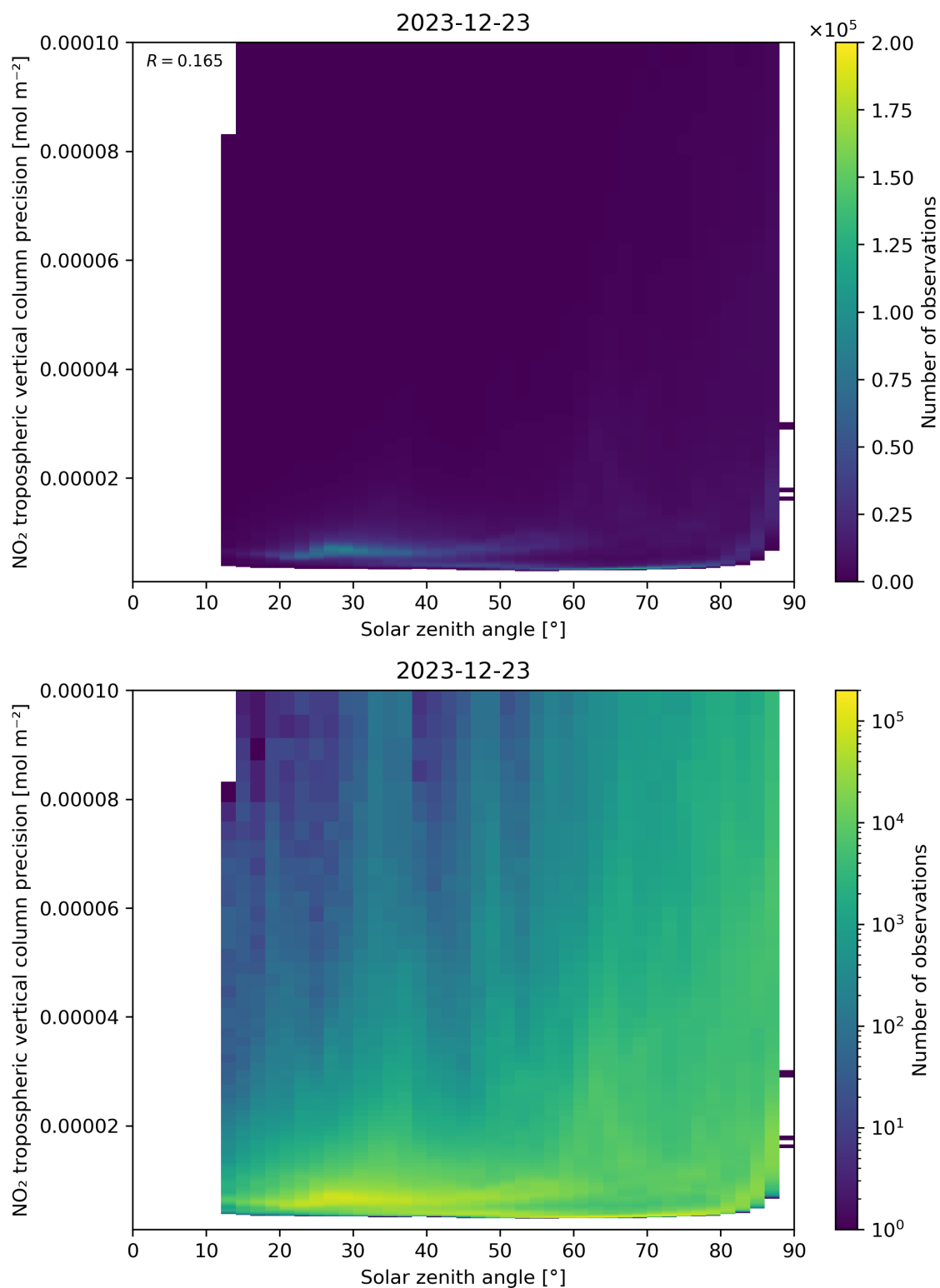
Figure 156: Scatter density plot of “Solar zenith angle” against “NO 2 tropospheric vertical column precision” for 2023-12-22 to 2023-12-24.
