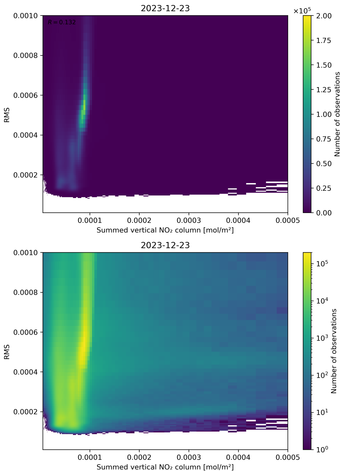
Figure 109: Scatter density plot of “Summed vertical NO 2 column” against “RMS” for 2023-12-22 to 2023-12-24.
