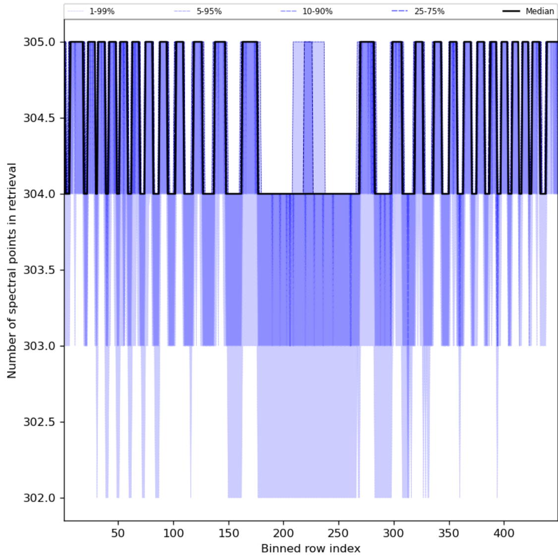
Figure 50: Along track statistics of “Number of spectral points in retrieval” for 2023-12-22 to 2023-12-24
