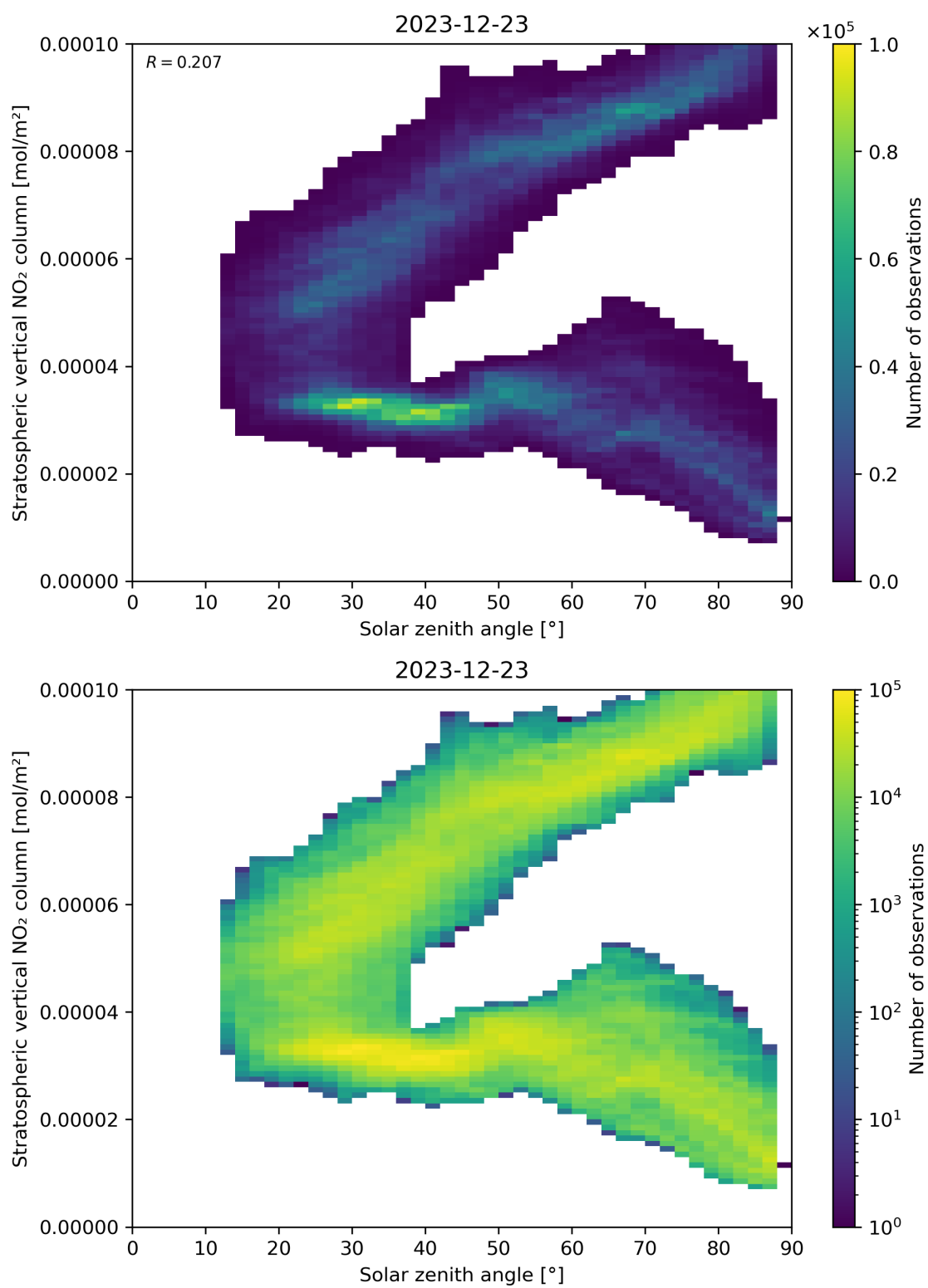
Figure 150: Scatter density plot of “Solar zenith angle” against “Stratospheric vertical NO 2 column” for 2023-12-22 to 2023-12-24.
