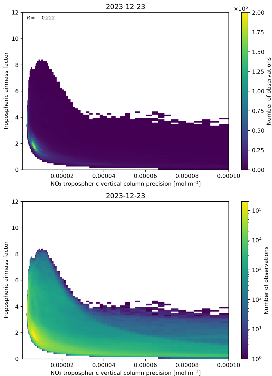
Figure 133: Scatter density plot of “NO 2 tropospheric vertical column precision” against “Tropospheric airmass factor” for 2023-12-22 to 2023-12-24.
