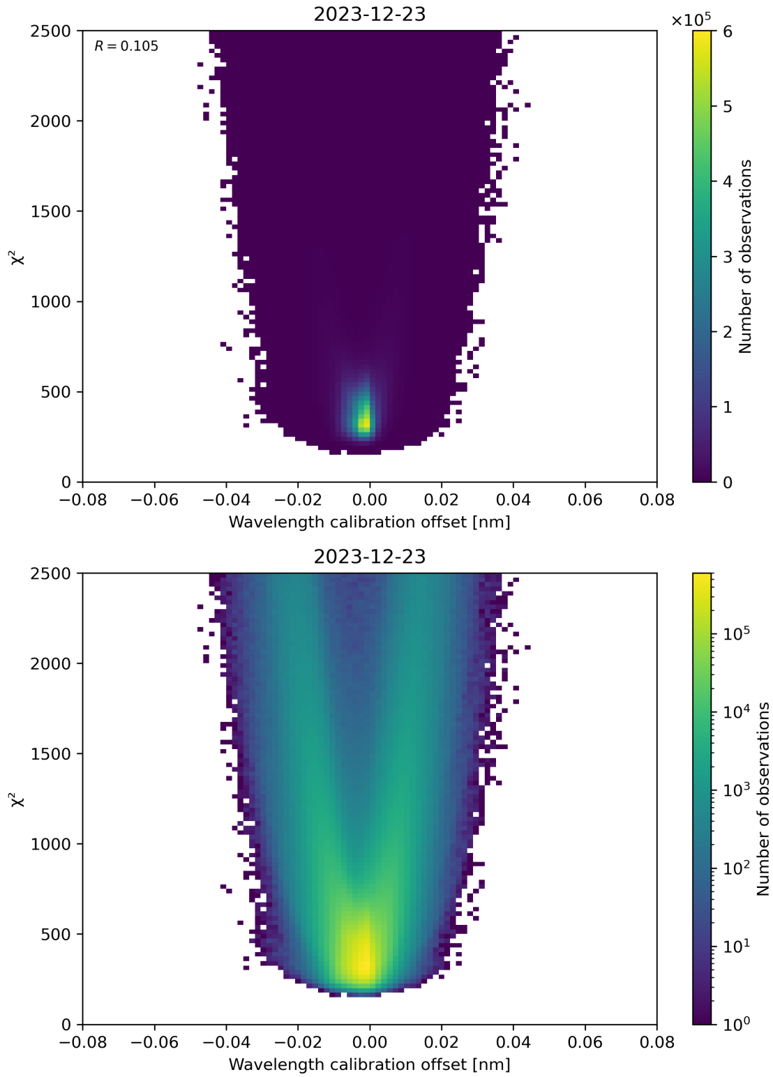
Figure 175: Scatter density plot of “Wavelength calibration offset” against “ \chi^2 ” for 2023-12-22 to 2023-12-24.
