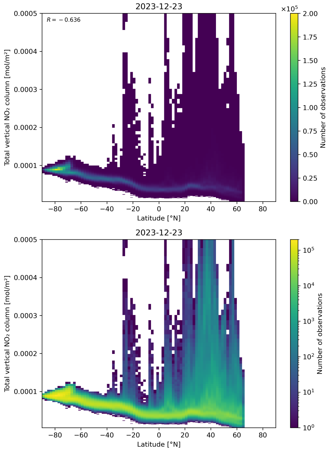
Figure 90: Scatter density plot of “Latitude” against “Total vertical NO 2 column” for 2023-12-22 to 2023-12-24.
