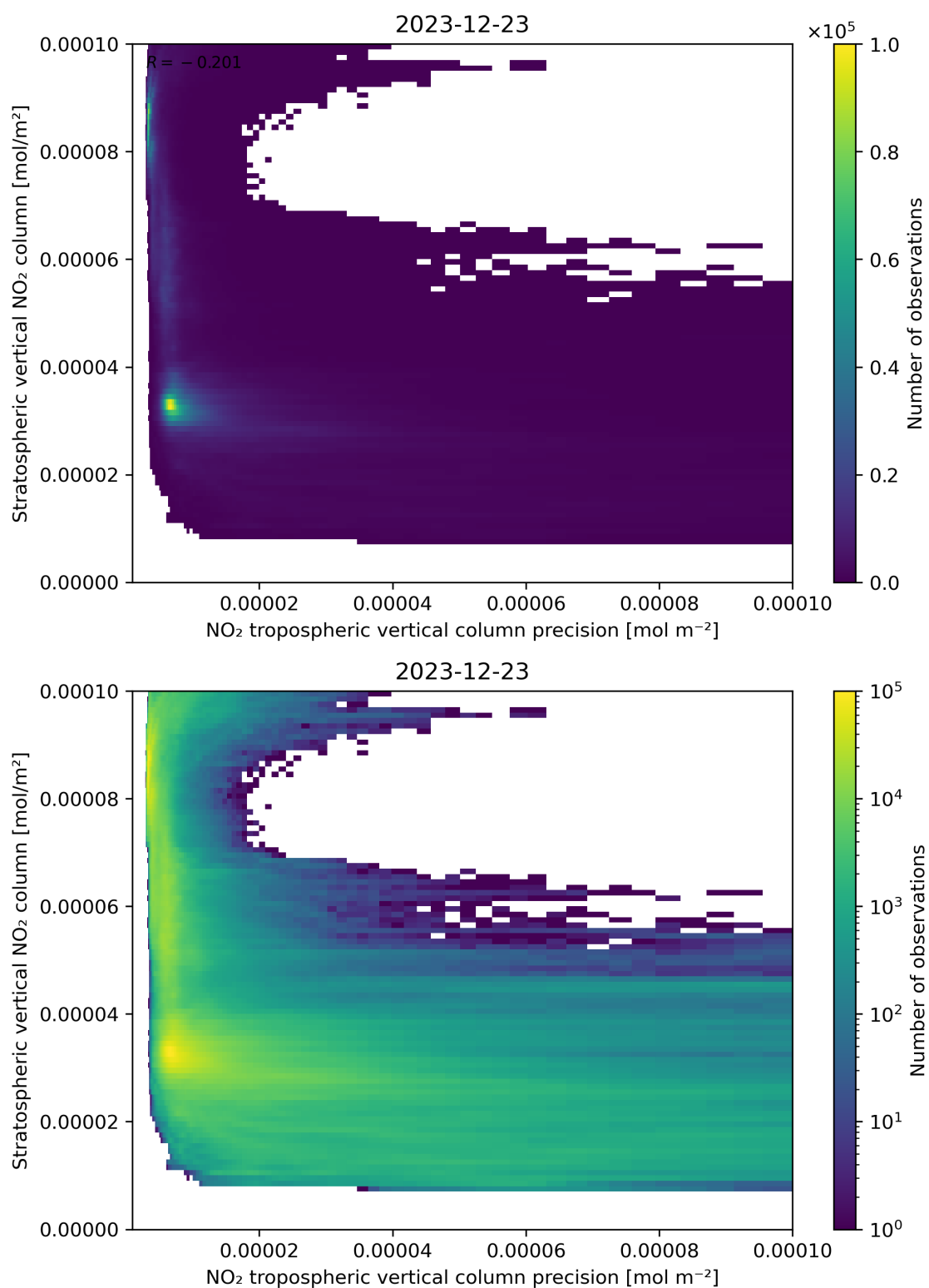
Figure 135: Scatter density plot of “NO 2 tropospheric vertical column precision” against “Stratospheric vertical NO 2 column” for 2023-12-22 to 2023-12-24.
