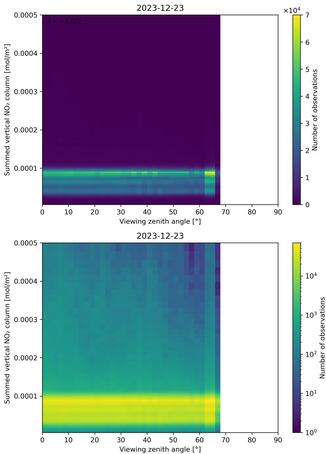
Figure 165: Scatter density plot of “Viewing zenith angle” against “Summed vertical NO 2 column” for 2023-12-22 to 2023-12-24.
