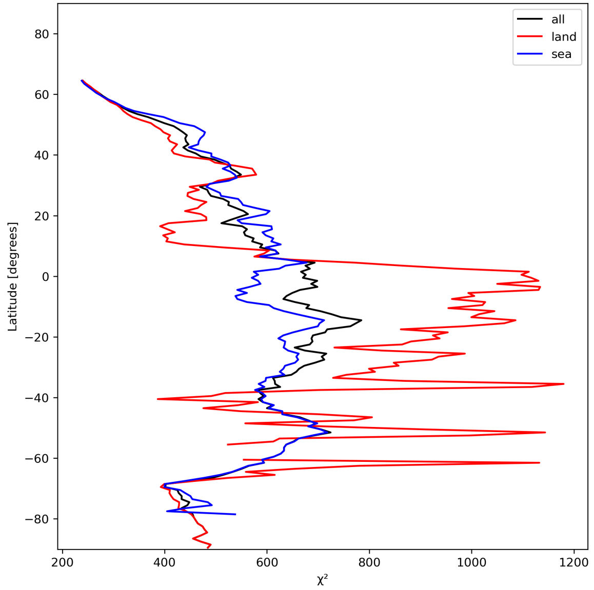
Figure 25: Zonal average of “ \chi^2 ” for 2023-12-22 to 2023-12-24.
