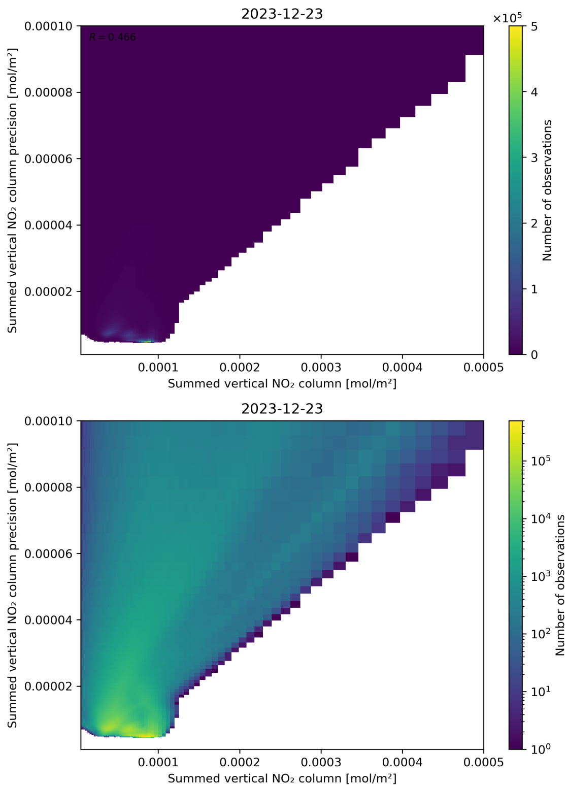
Figure 105: Scatter density plot of “Summed vertical NO 2 column” against “Summed vertical NO 2 column precision” for 2023-12-22 to 2023-12-24.
