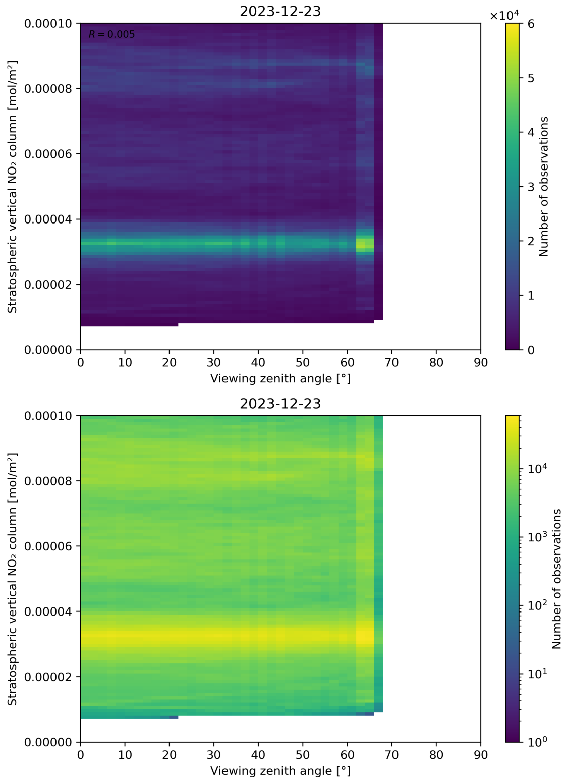
Figure 164: Scatter density plot of “Viewing zenith angle” against “Stratospheric vertical NO 2 column” for 2023-12-22 to 2023-12-24.
