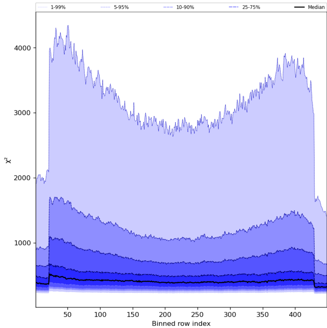
Figure 59: Along track statistics of “ \chi^2 ” for 2023-12-22 to 2023-12-24
