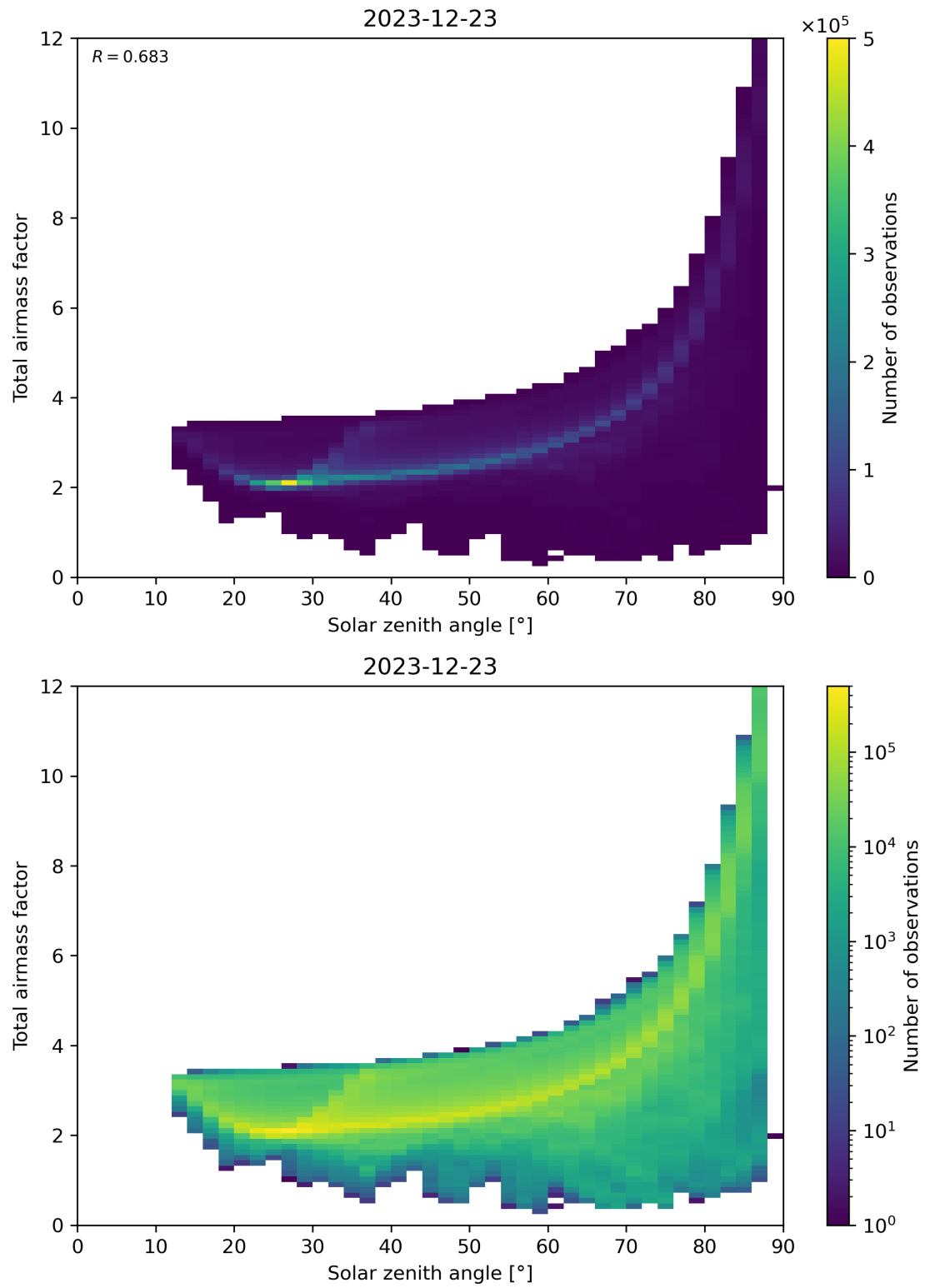
Figure 146: Scatter density plot of “Solar zenith angle” against “Total air mass factor” for 2023-12-22 to 2023-12-24.
