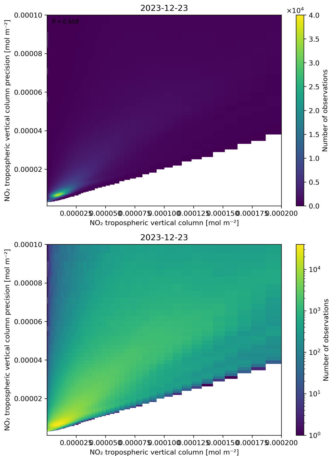
Figure 130: Scatter density plot of “NO 2 tropospheric vertical column” against “NO 2 tropospheric vertical column precision” for 2023-12-22 to 2023-12-24.
