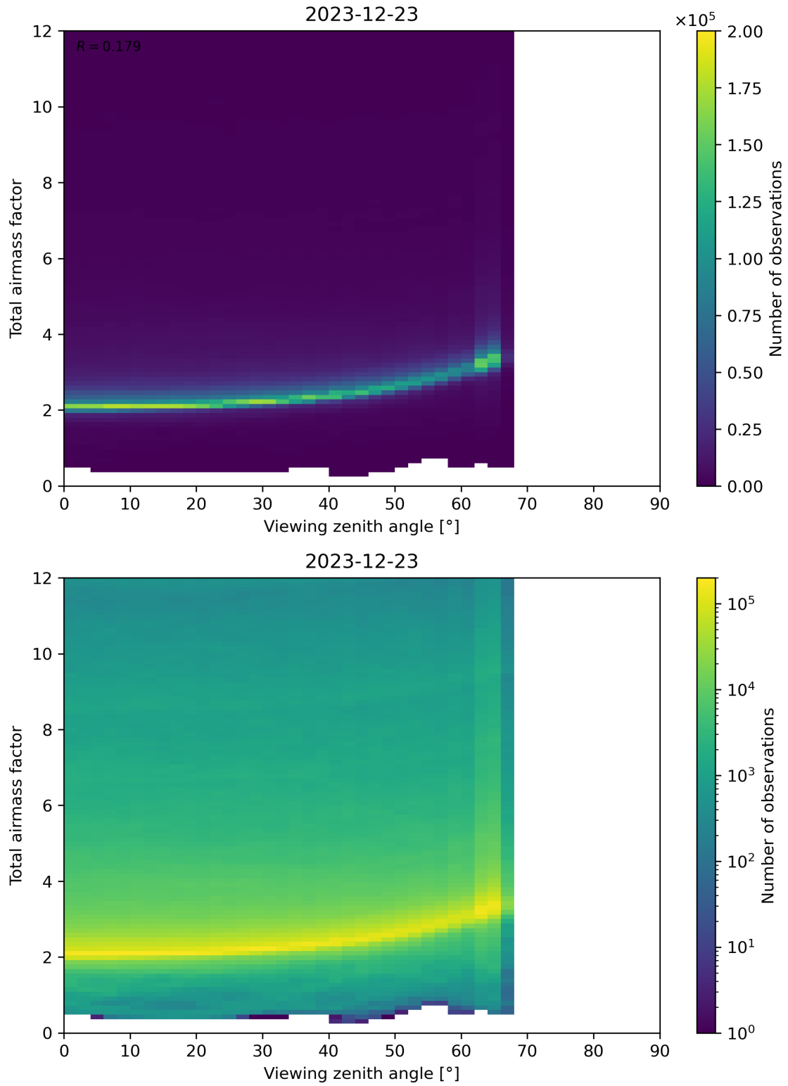
Figure 160: Scatter density plot of “Viewing zenith angle” against “Total airmass factor” for 2023-12-22 to 2023-12-24.
