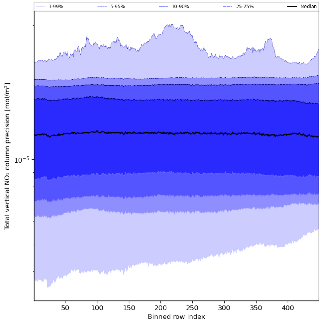
Figure 56: Along track statistics of “Total vertical NO 2 column precision” for 2023-12-22 to 2023-12-24
