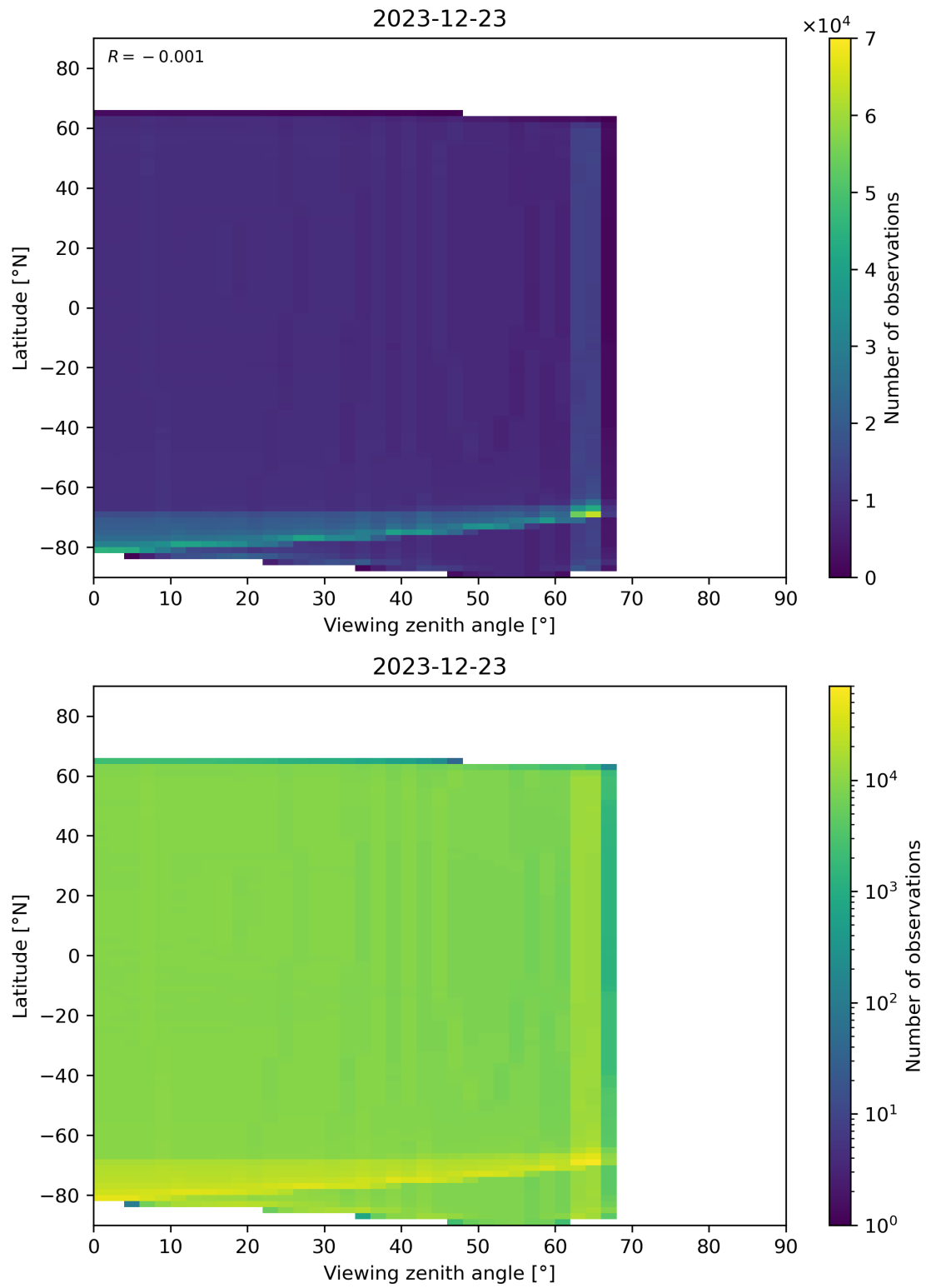
Figure 163: Scatter density plot of “Viewing zenith angle” against “Latitude” for 2023-12-22 to 2023-12-24.
