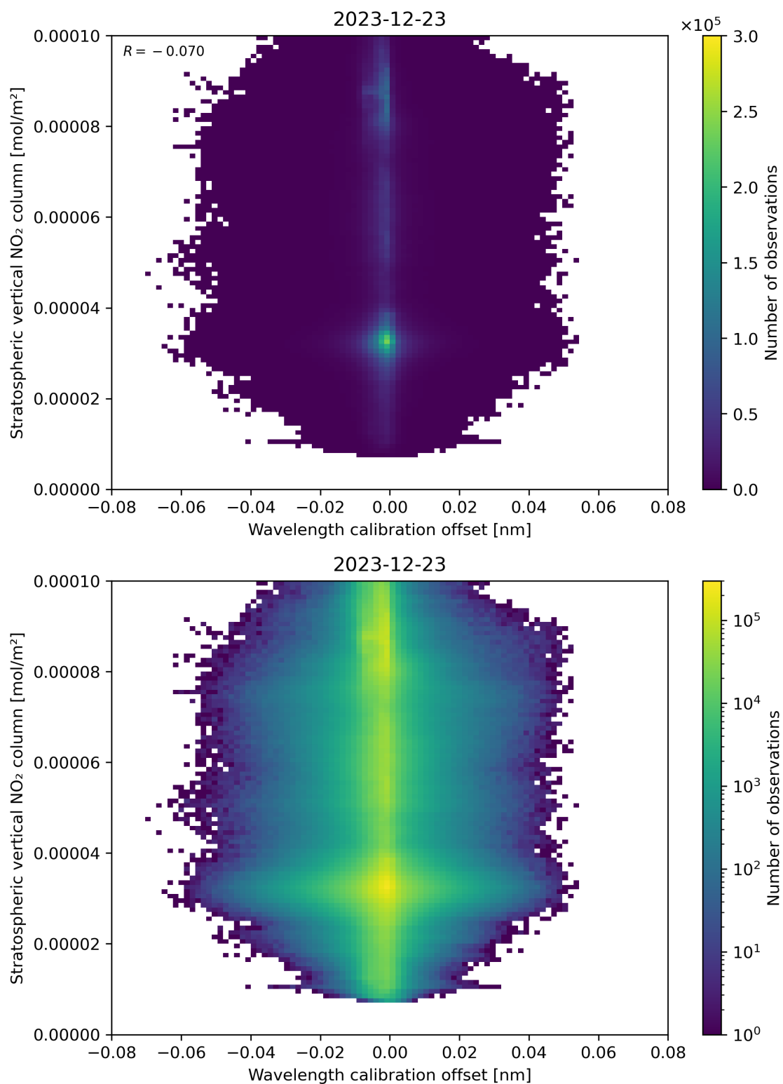
Figure 176: Scatter density plot of “Wavelength calibration offset” against “Stratospheric vertical NO 2 column” for 2023-12-22 to 2023-12-24.
