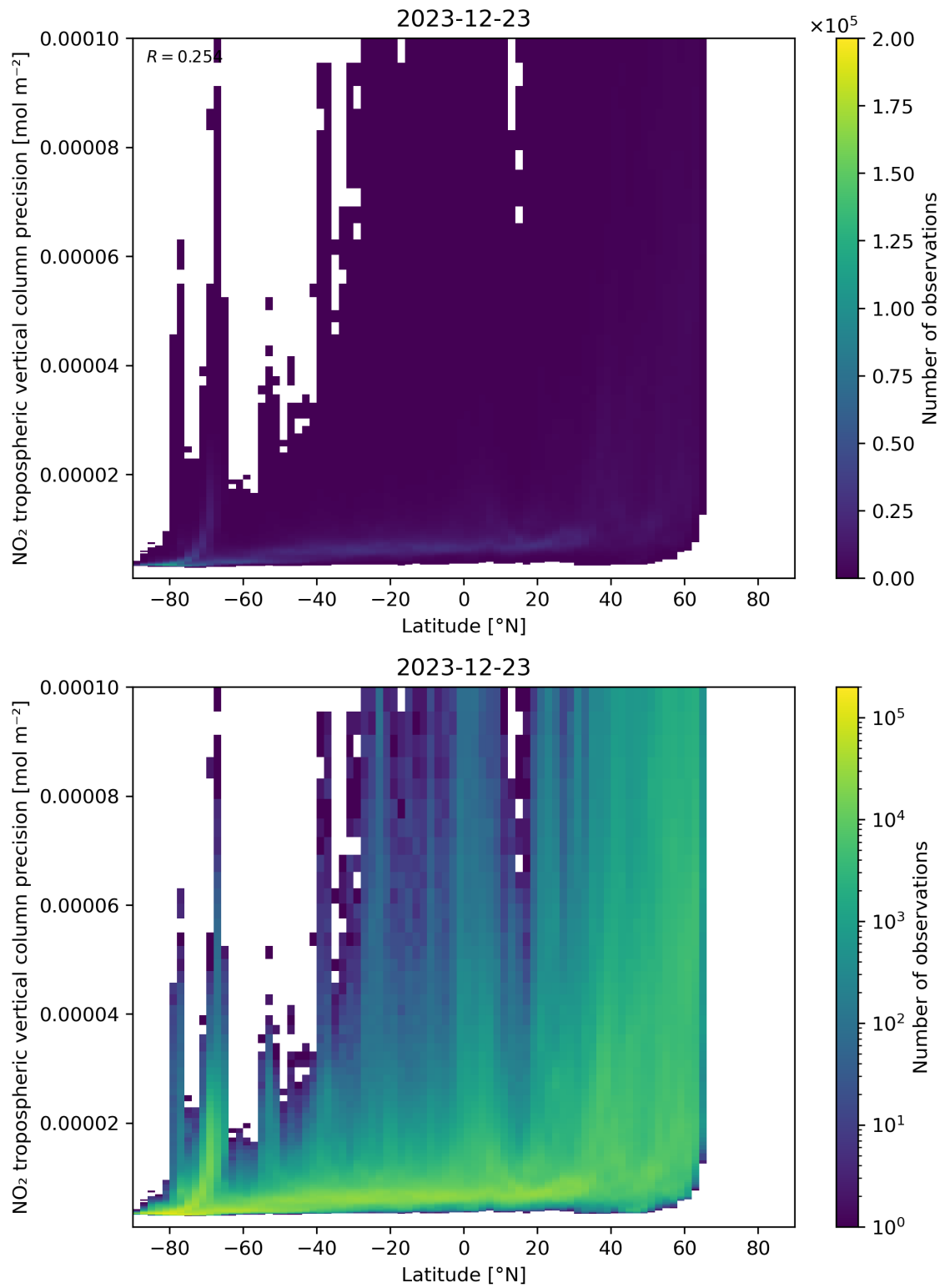
Figure 93: Scatter density plot of “Latitude” against “NO 2 tropospheric vertical column precision” for 2023-12-22 to 2023-12-24.
