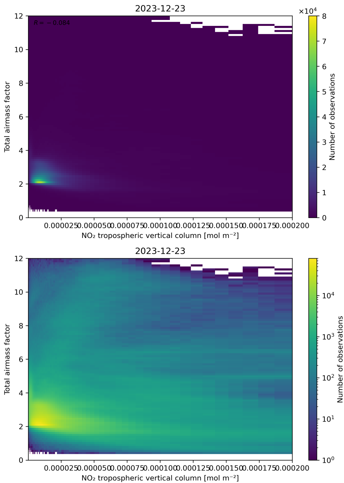
Figure 122: Scatter density plot of “NO 2 tropospheric vertical column” against “Total air mass factor” for 2023-12-22 to 2023-12-24.
