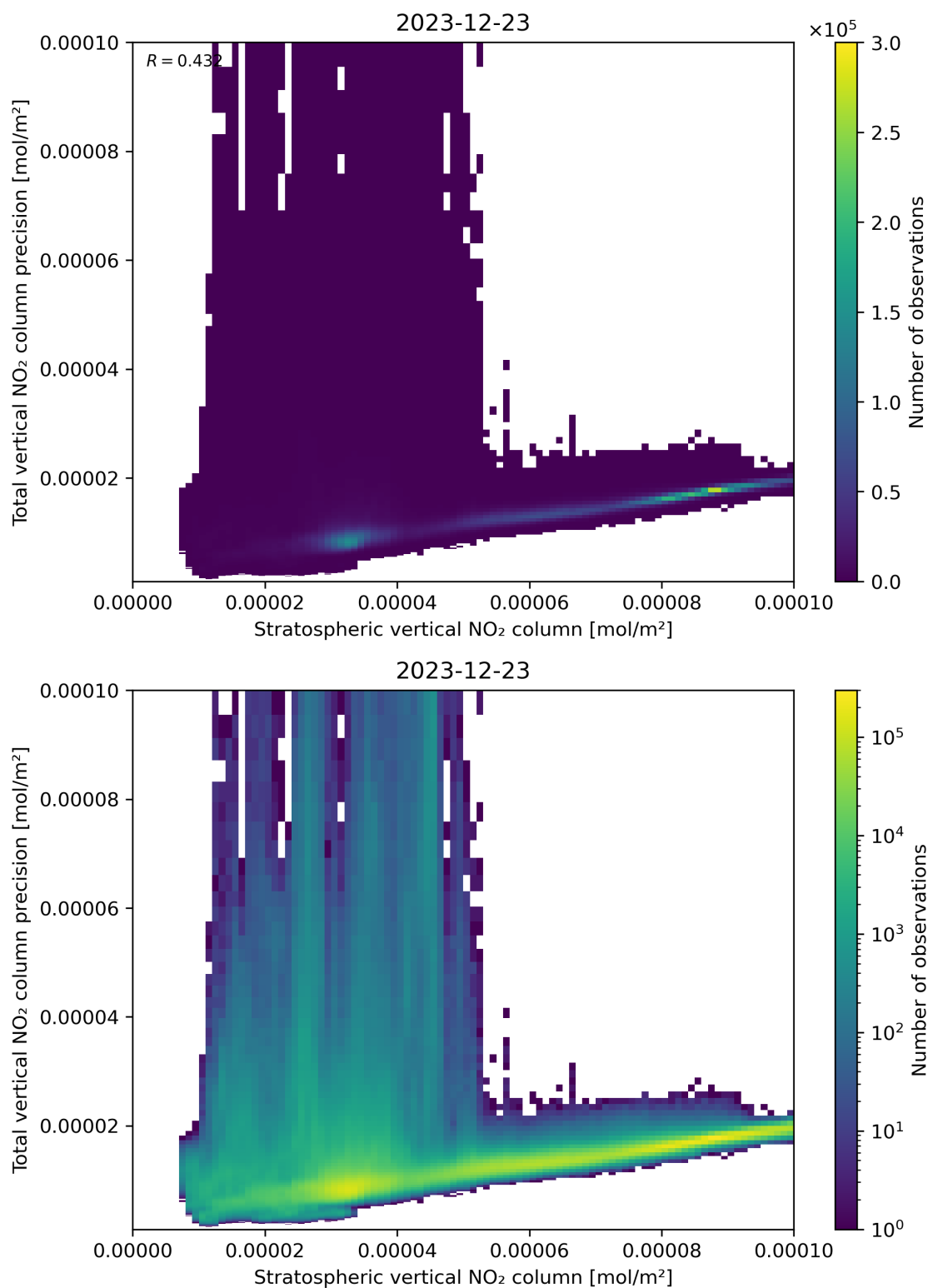
Figure 101: Scatter density plot of “Stratospheric vertical NO 2 column” against “Total vertical NO 2 column precision” for 2023-12-22 to 2023-12-24.
