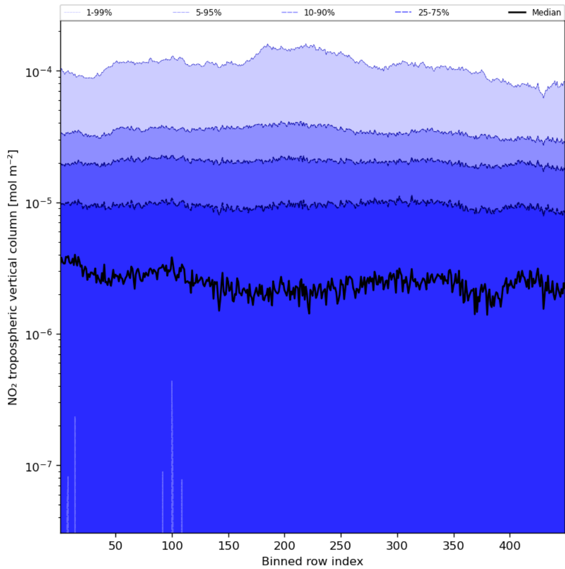
Figure 46: Along track statistics of “NO 2 tropospheric vertical column” for 2023-12-22 to 2023-12-24
