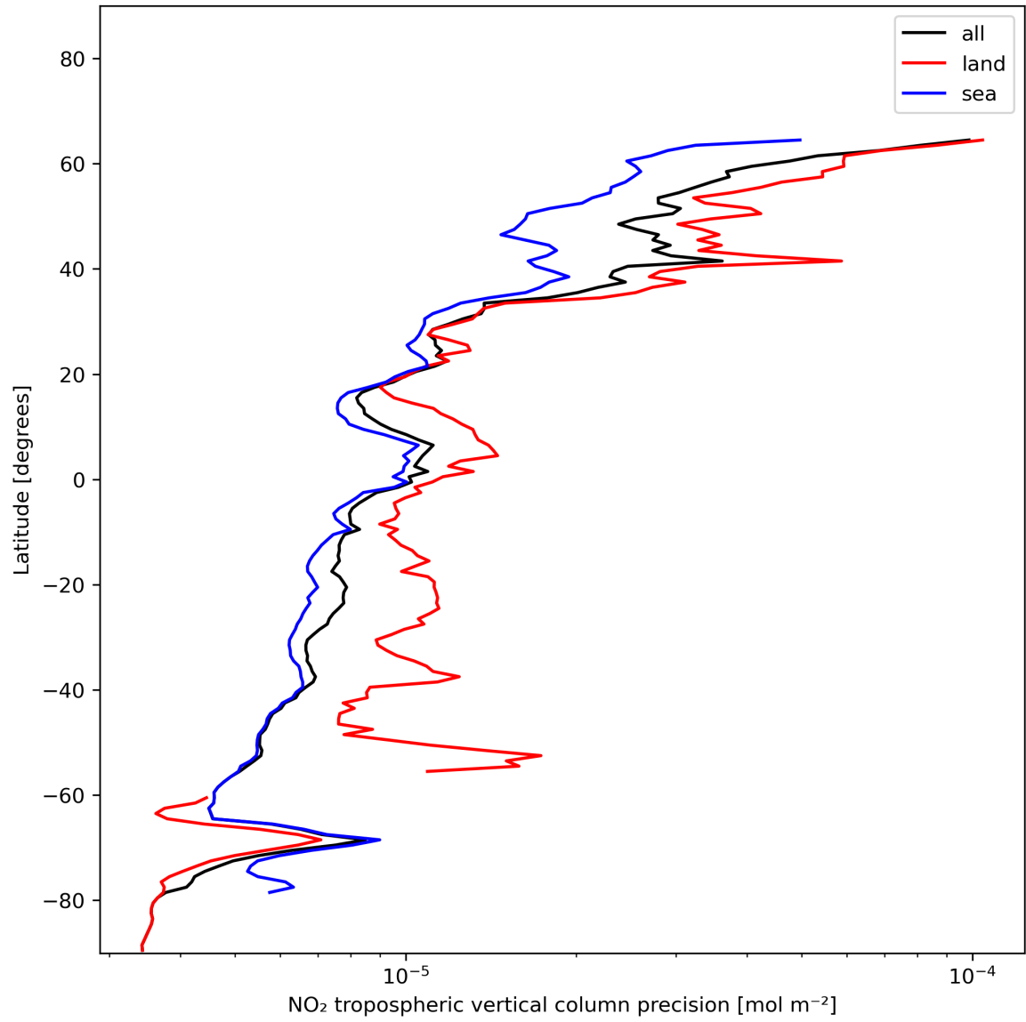
Figure 13: Zonal average of “NO 2 tropospheric vertical column precision” for 2023-12-22 to 2023-12-24.
