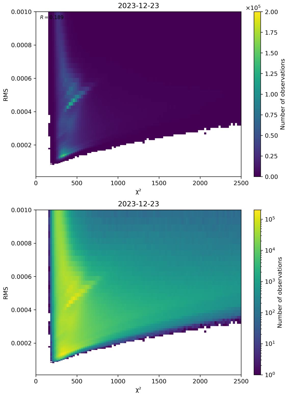
Figure 82: Scatter density plot of “ \chi^2 ” against “RMS” for 2023-12-22 to 2023-12-24.
