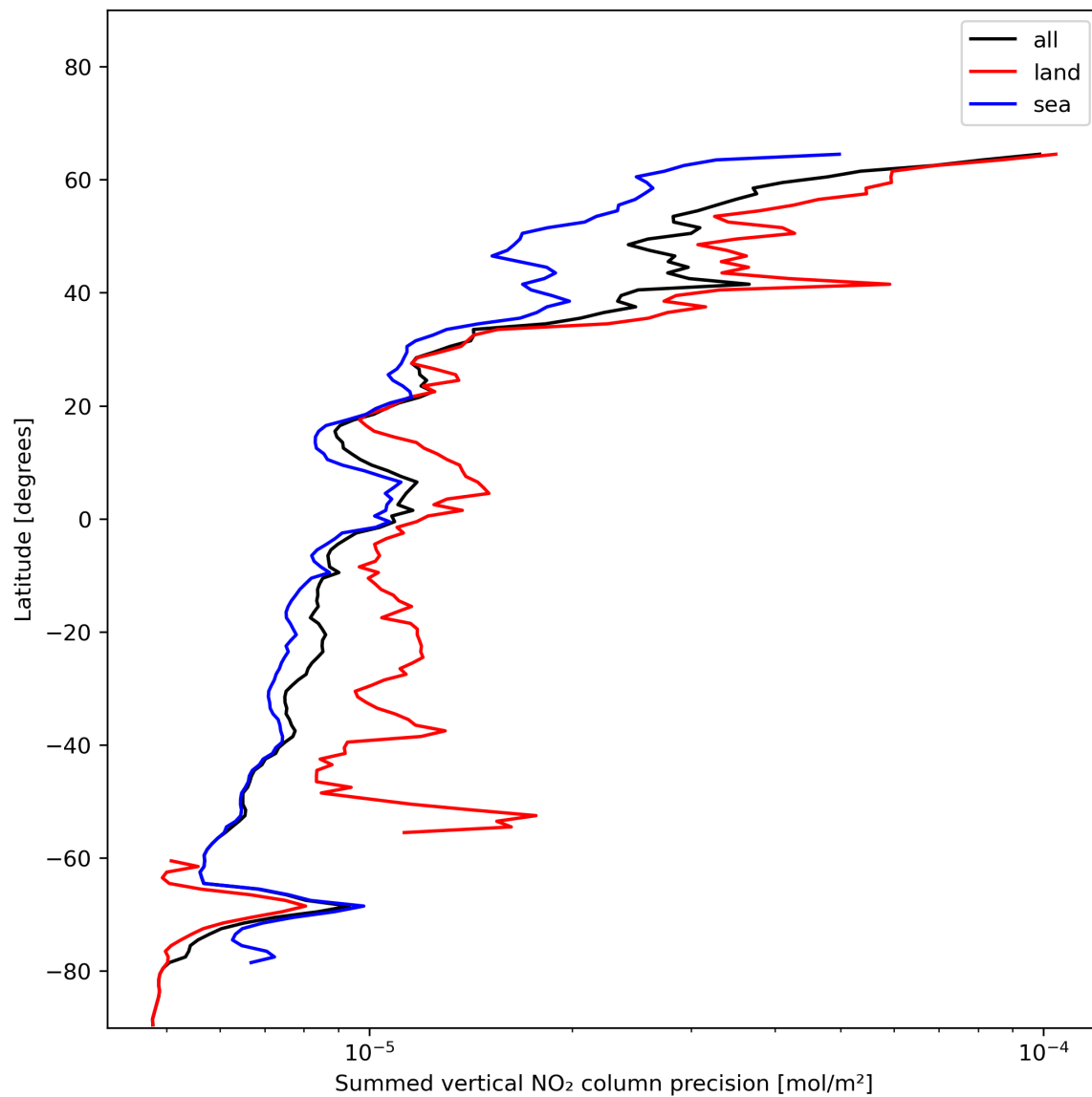
Figure 24: Zonal average of “Summed vertical NO 2 column precision” for 2023-12-22 to 2023-12-24.
