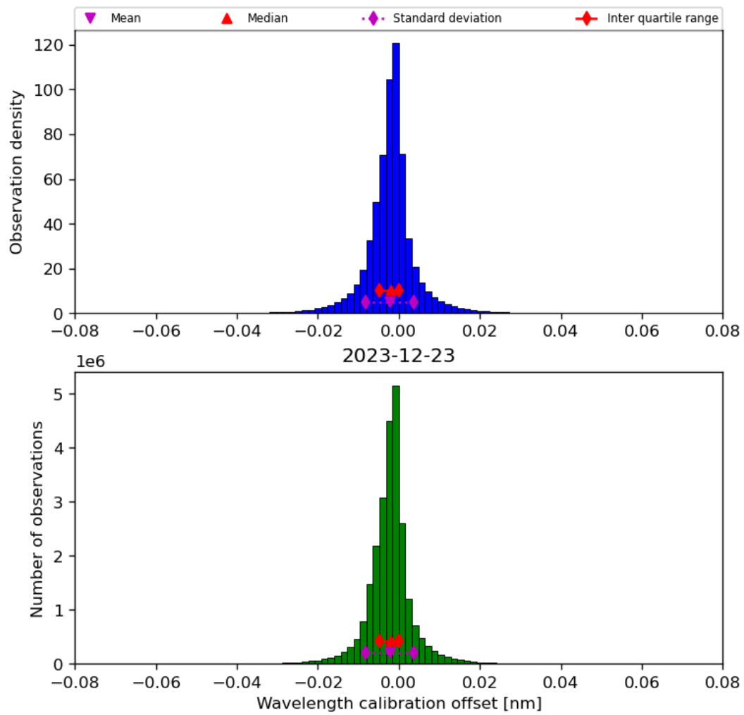
Figure 35: Histogram of “Wavelength calibration offset” for 2023-12-22 to 2023-12-24
