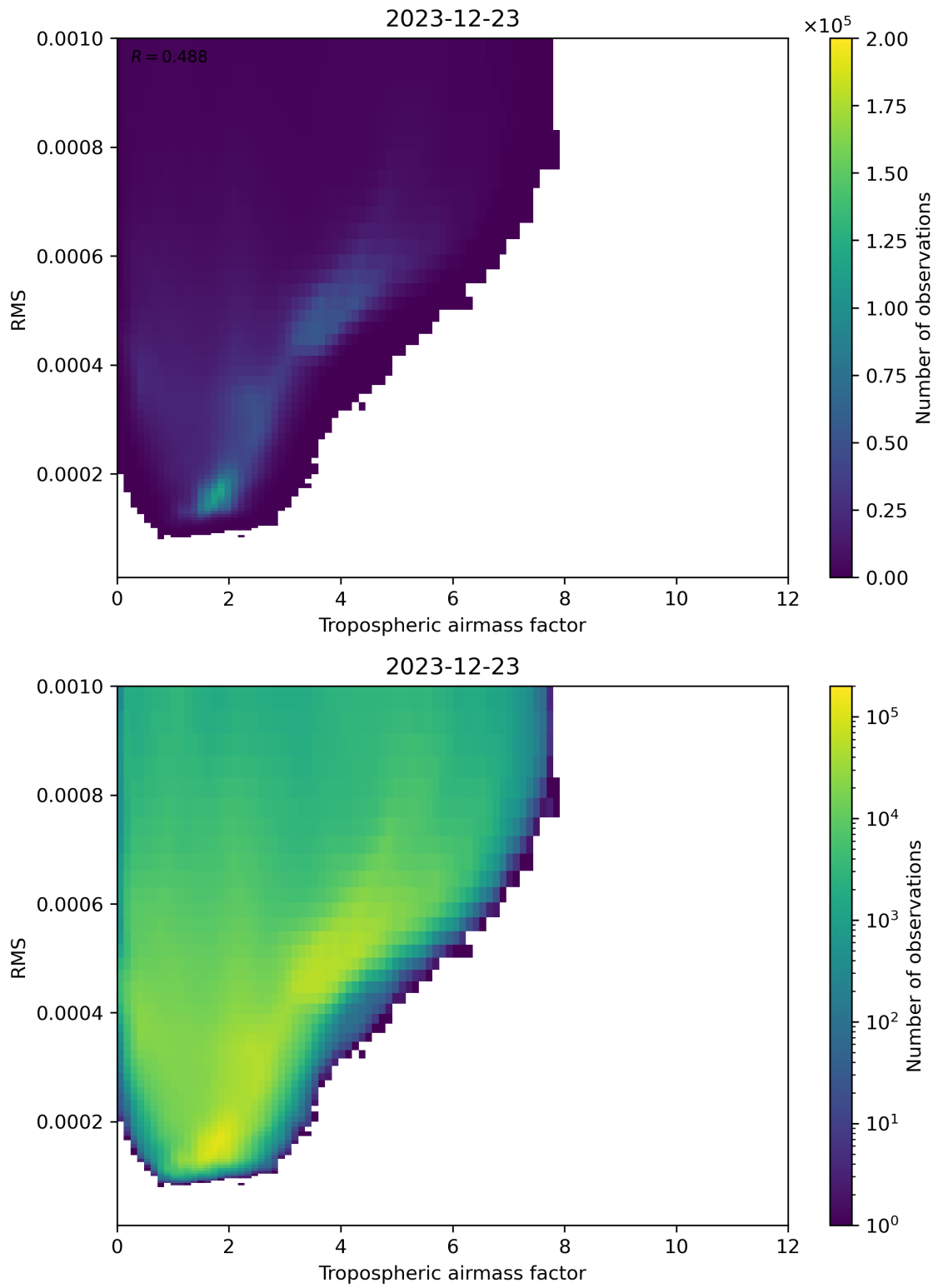
Figure 79: Scatter density plot of “Tropospheric airmass factor” against “RMS” for 2023-12-22 to 2023-12-24.
