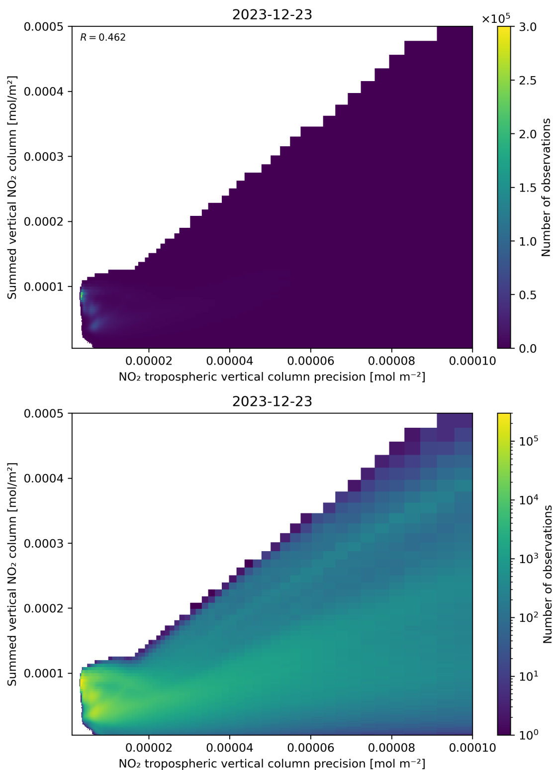
Figure 136: Scatter density plot of “NO 2 tropospheric vertical column precision” against “Summed vertical NO 2 column” for 2023-12-22 to 2023-12-24.
