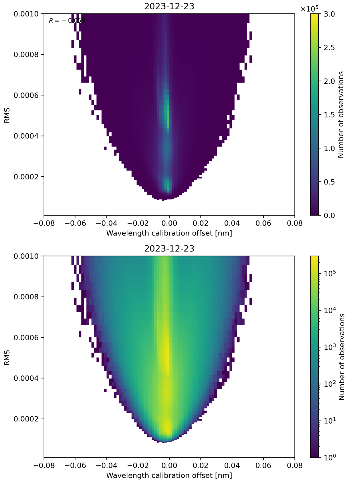
Figure 181: Scatter density plot of “Wavelength calibration offset” against “RMS” for 2023-12-22 to 2023-12-24.
