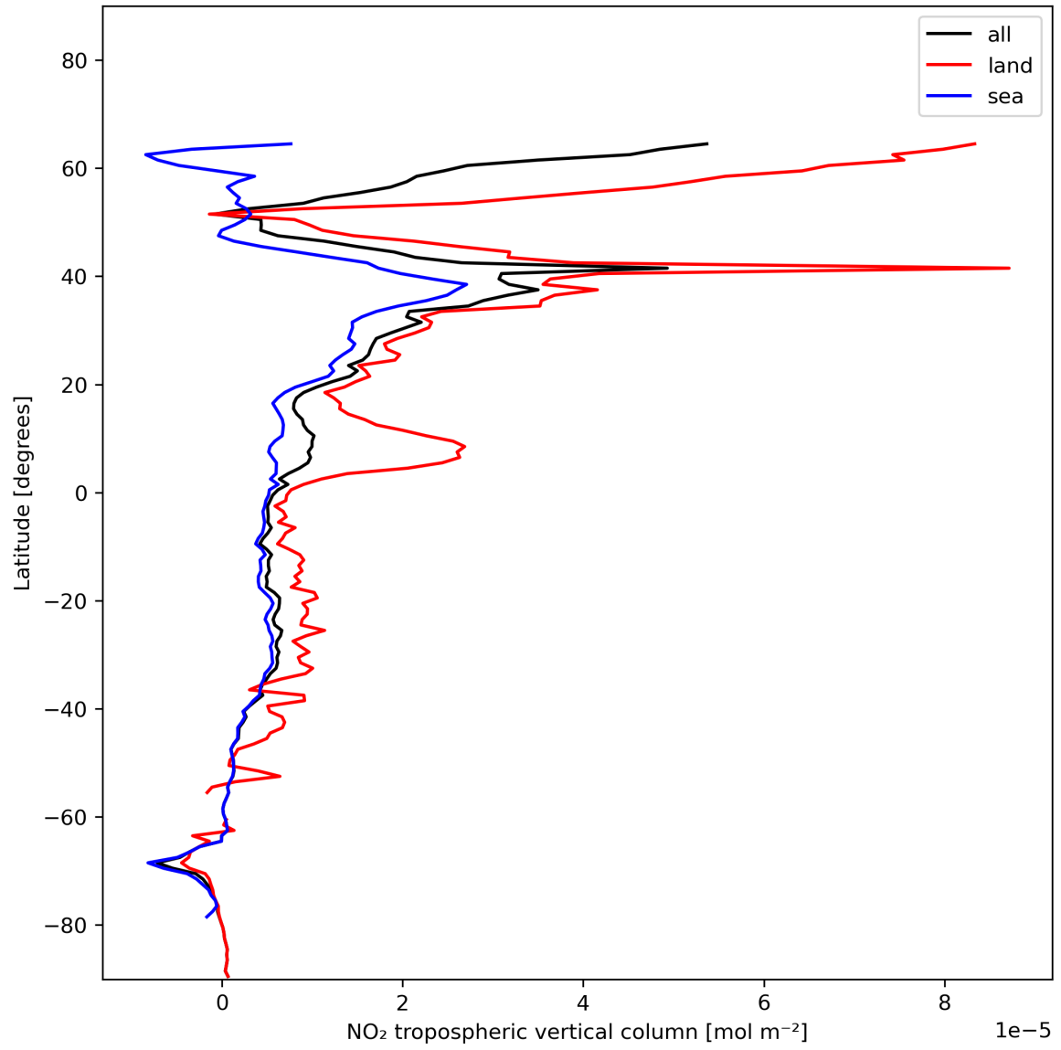
Figure 12: Zonal average of “NO 2 tropospheric vertical column” for 2023-12-22 to 2023-12-24.
