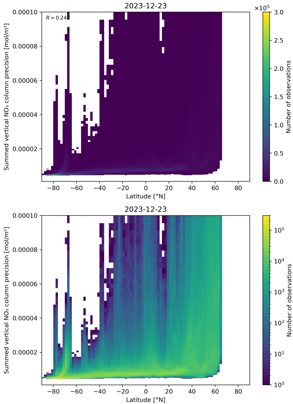
Figure 89: Scatter density plot of “Latitude” against “Summed vertical NO 2 column precision” for 2023-12-22 to 2023-12-24.
