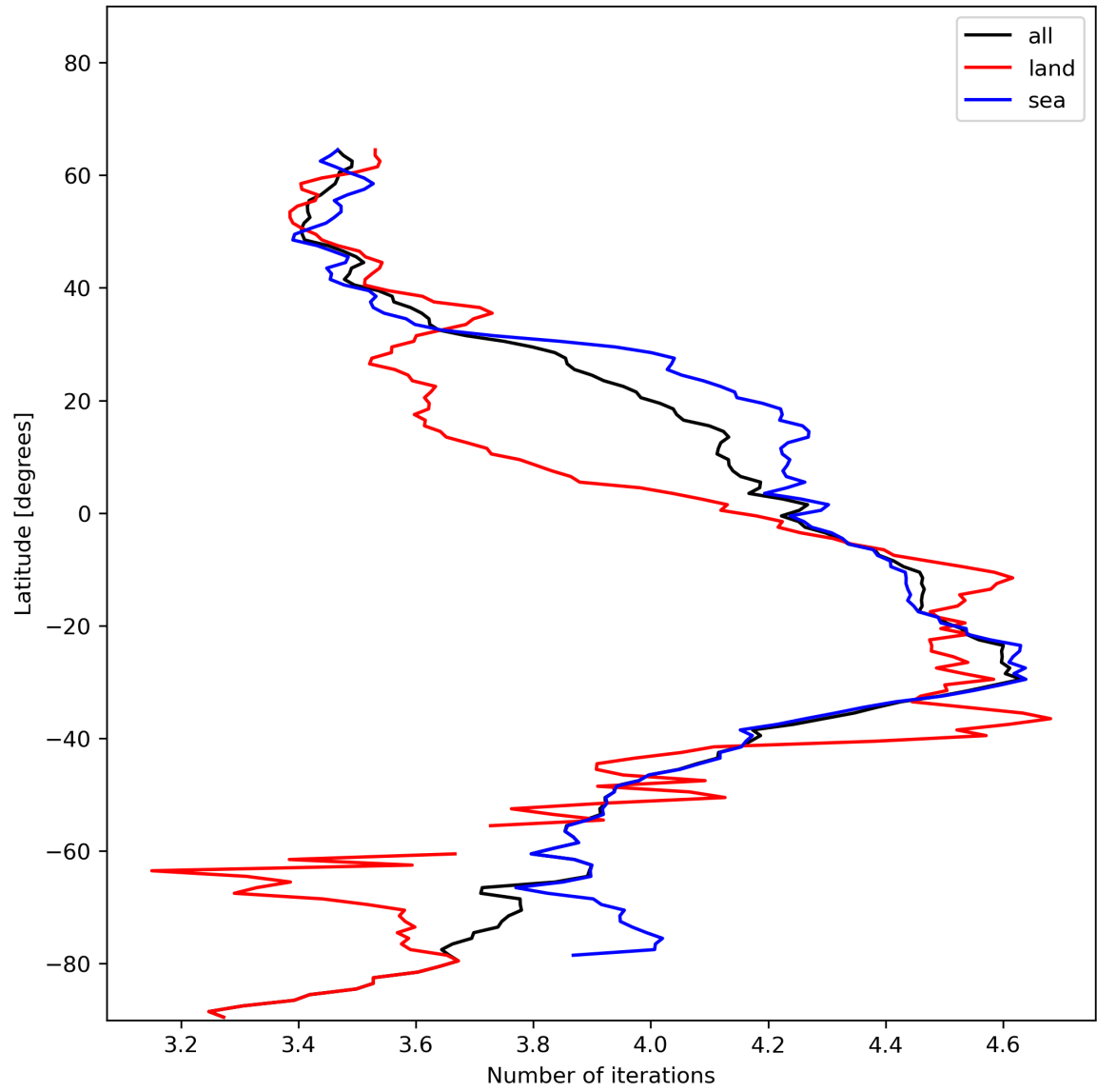
Figure 17: Zonal average of “Number of iterations” for 2023-12-22 to 2023-12-24.
