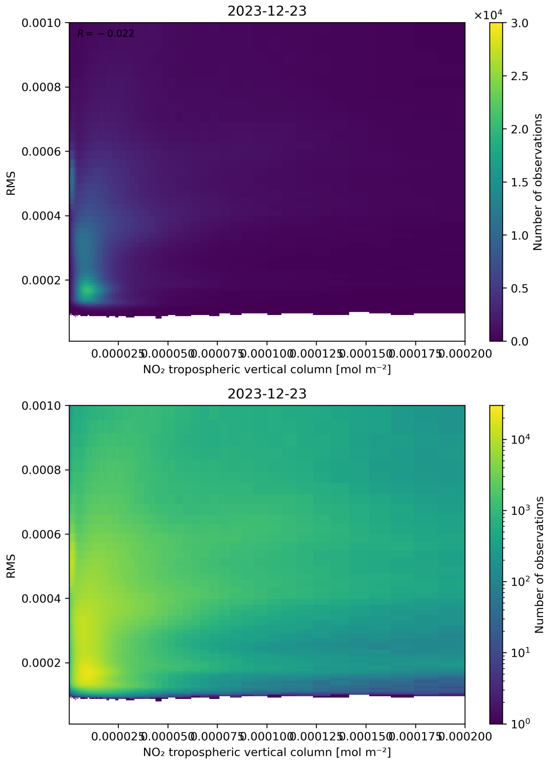
Figure 142: Scatter density plot of “NO 2 tropospheric vertical column” against “RMS” for 2023-12-22 to 2023-12-24.
