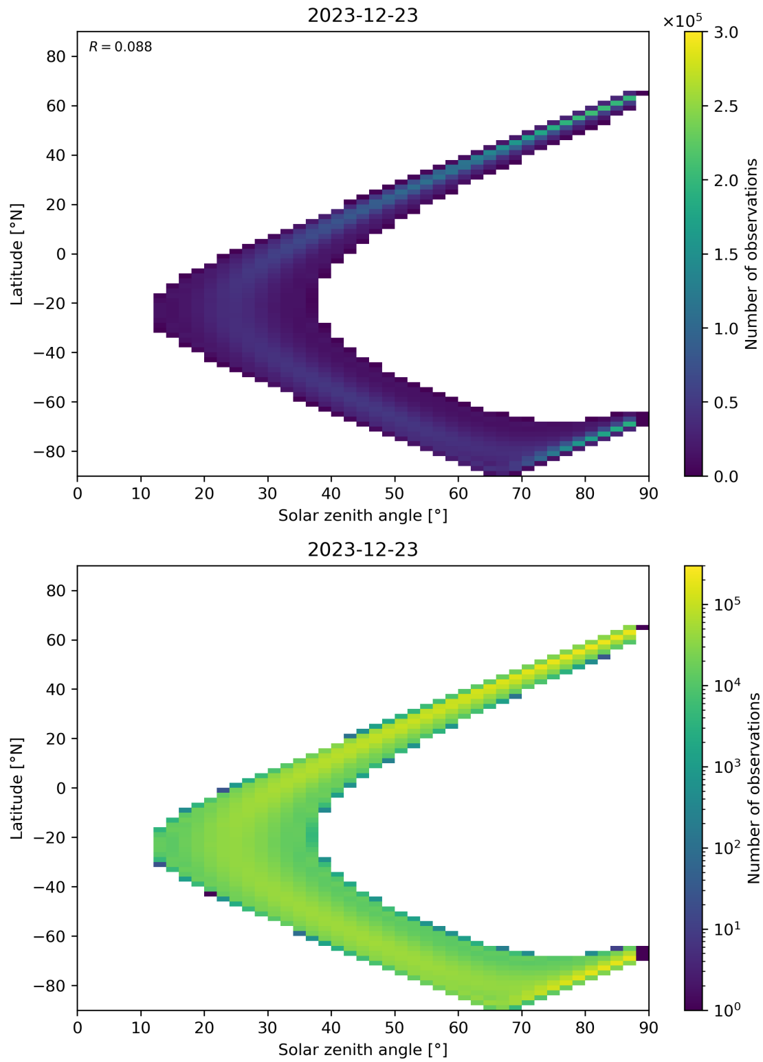
Figure 149: Scatter density plot of “Solar zenith angle” against “Latitude” for 2023-12-22 to 2023-12-24.
