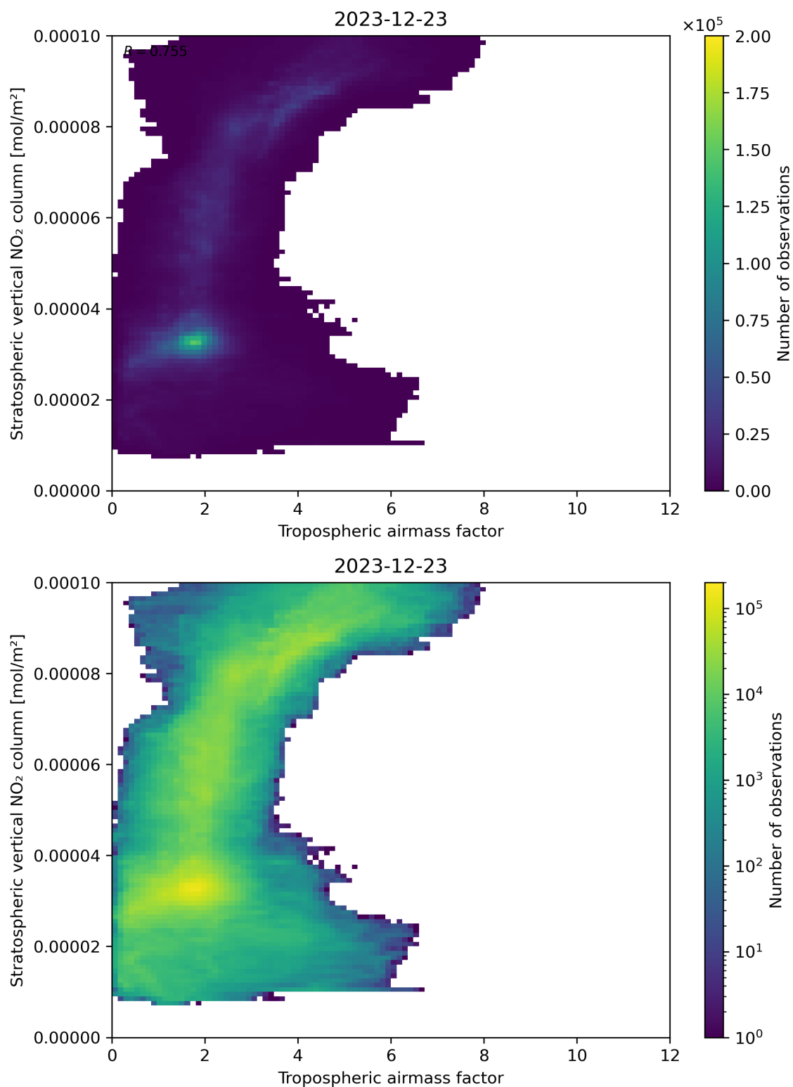
Figure 74: Scatter density plot of “Tropospheric air mass factor” against “Stratospheric vertical NO 2 column” for 2023-12-22 to 2023-12-24.
