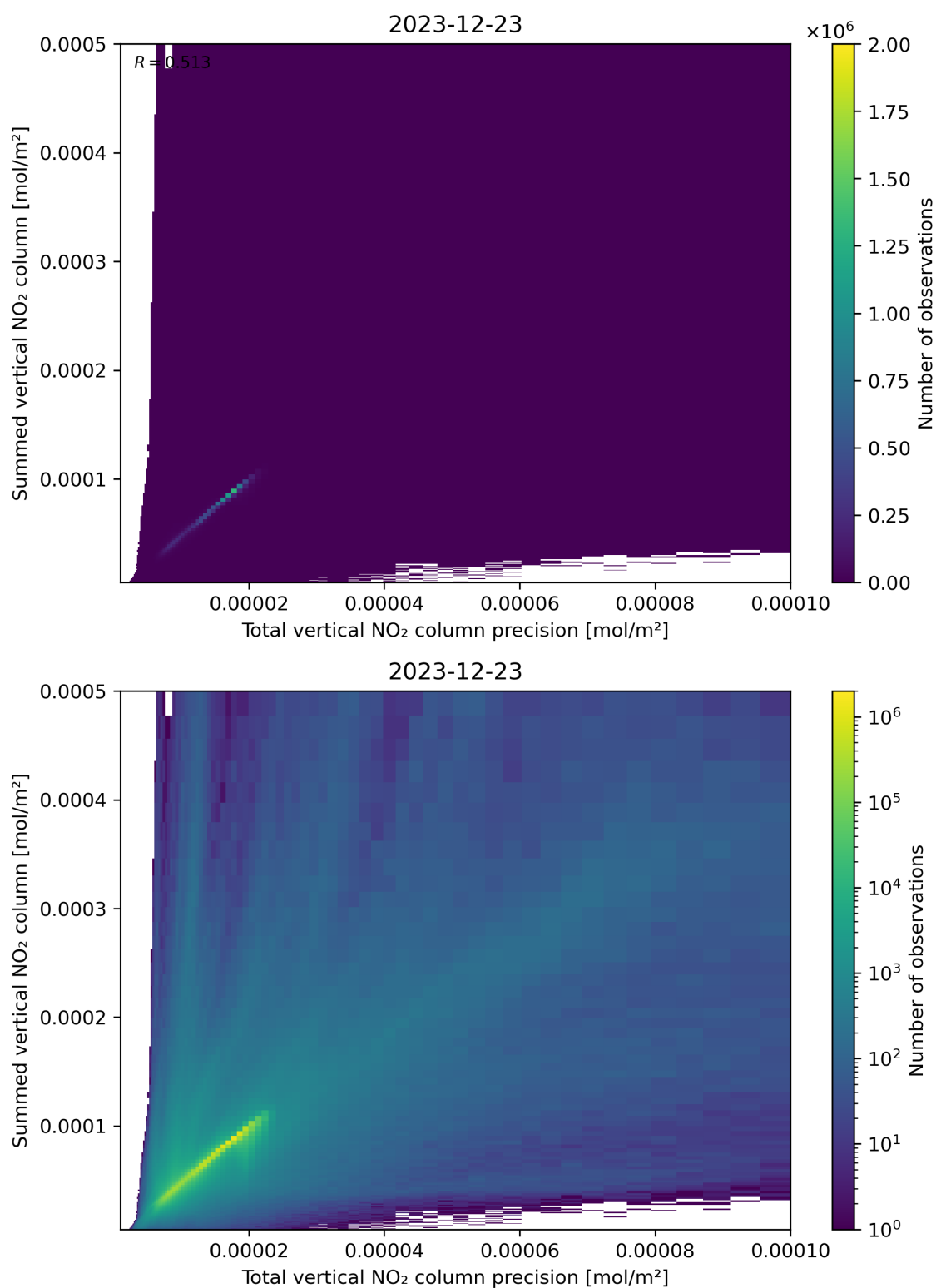
Figure 117: Scatter density plot of “Total vertical NO 2 column precision” against “Summed vertical NO 2 column” for 2023-12-22 to 2023-12-24.
