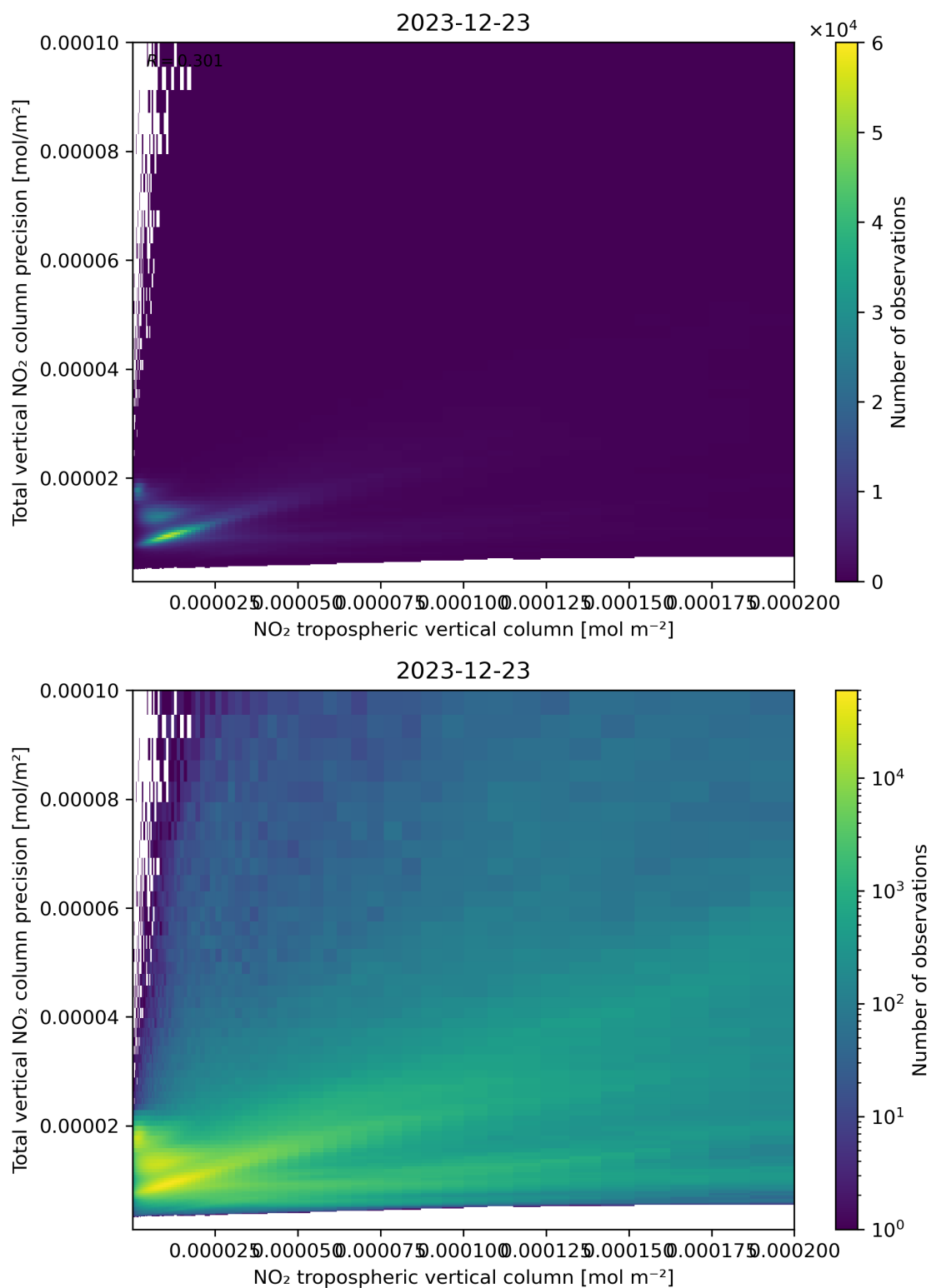
Figure 129: Scatter density plot of “NO 2 tropospheric vertical column” against “Total vertical NO 2 column precision” for 2023-12-22 to 2023-12-24.
