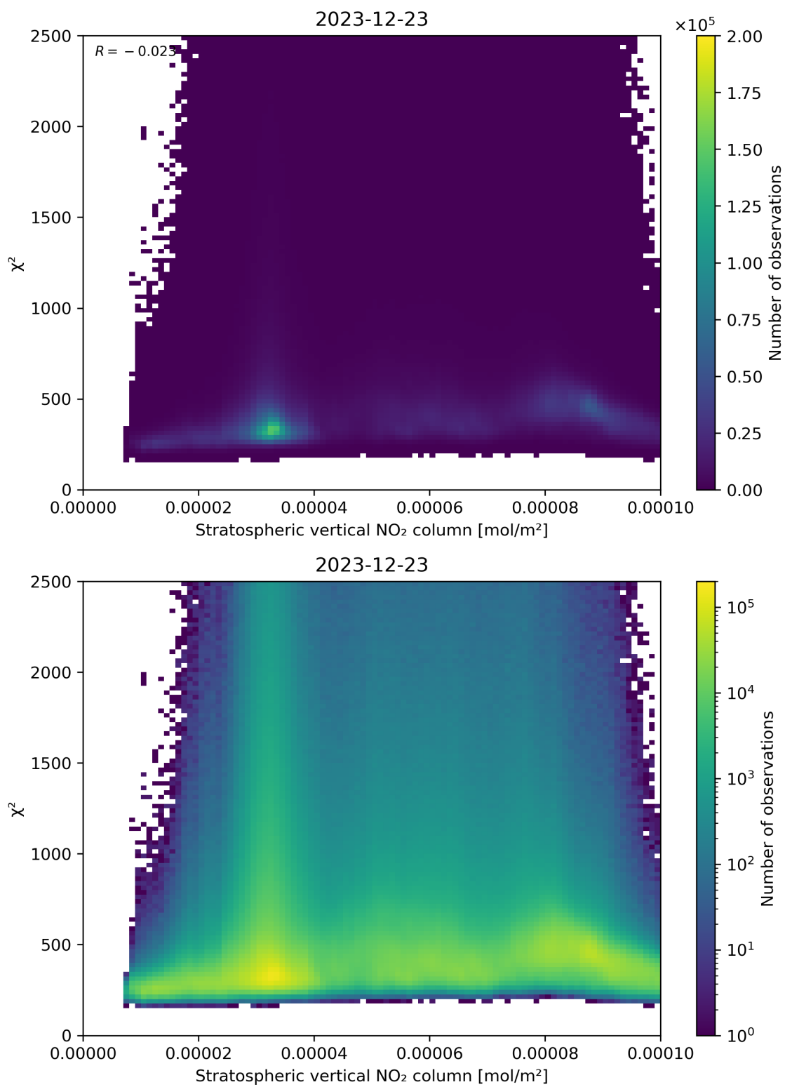
Figure 97: Scatter density plot of “Stratospheric vertical NO 2 column” against “ \chi^2 ” for 2023-12-22 to 2023-12-24.
