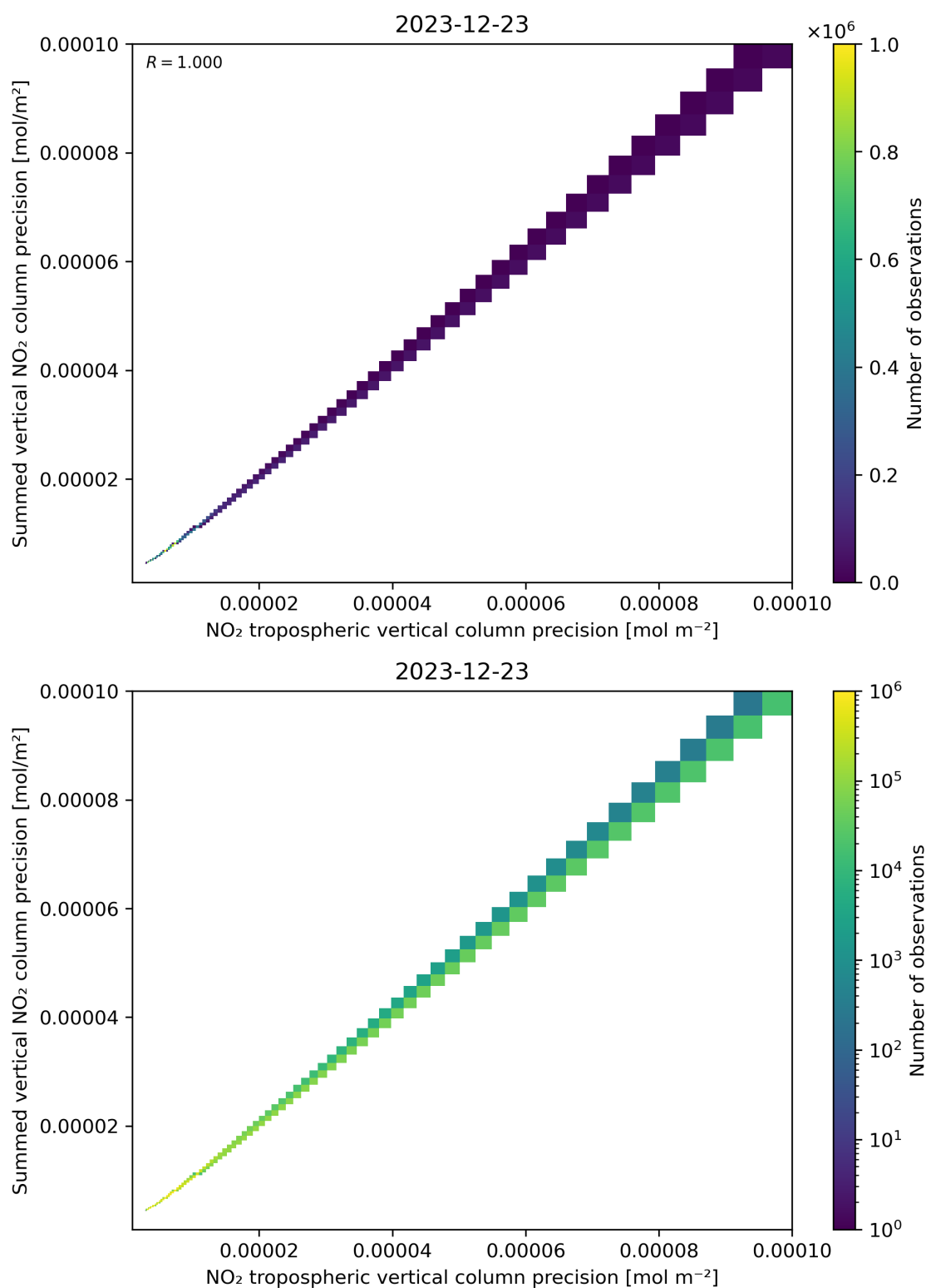
Figure 137: Scatter density plot of “NO 2 tropospheric vertical column precision” against “Summed vertical NO 2 column precision” for 2023-12-22 to 2023-12-24.
