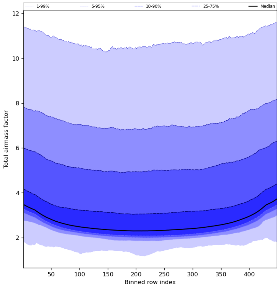
Figure 49: Along track statistics of “Total airmass factor” for 2023-12-22 to 2023-12-24
