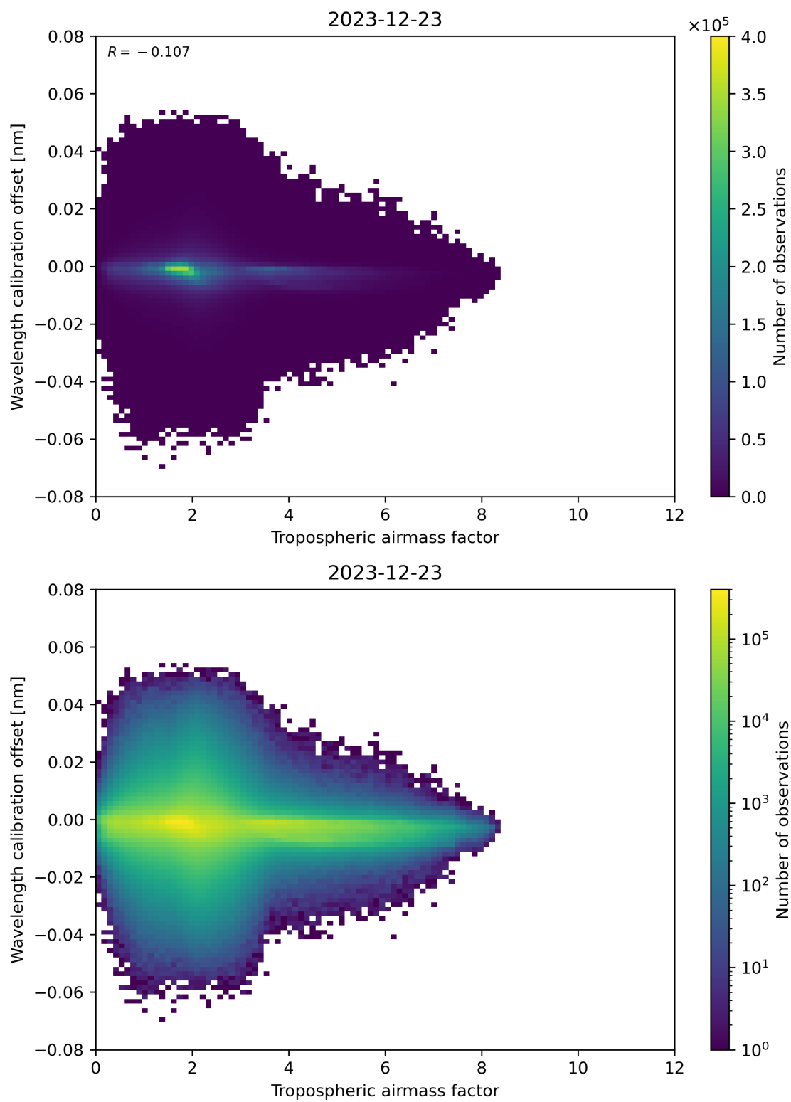
Figure 80: Scatter density plot of “Tropospheric airmass factor” against “Wavelength calibration offset” for 2023-12-22 to 2023-12-24.
