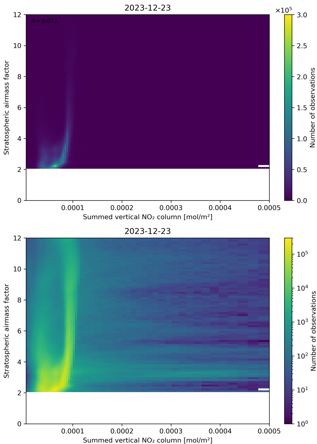
Figure 103: Scatter density plot of “Summed vertical NO 2 column” against “Stratospheric airmass factor” for 2023-12-22 to 2023-12-24.
