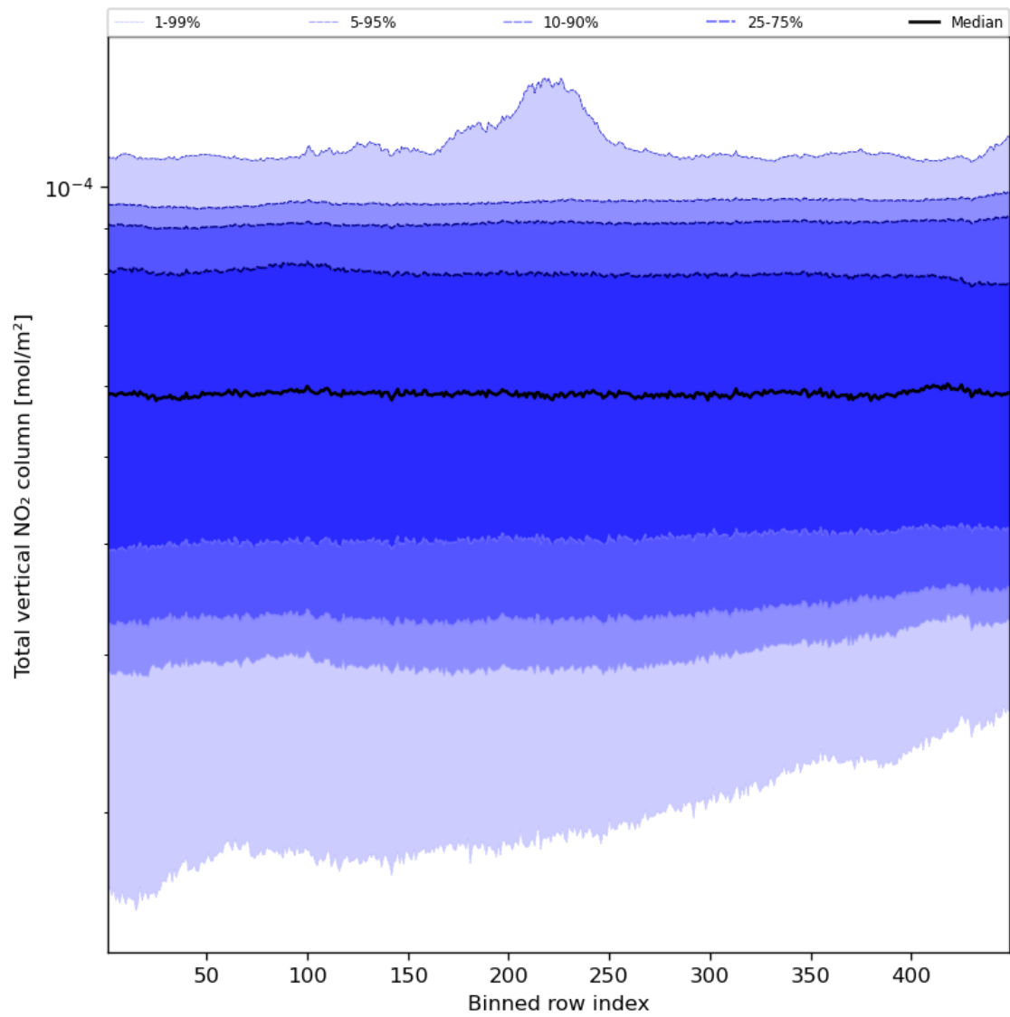
Figure 55: Along track statistics of “Total vertical NO 2 column” for 2023-12-22 to 2023-12-24
