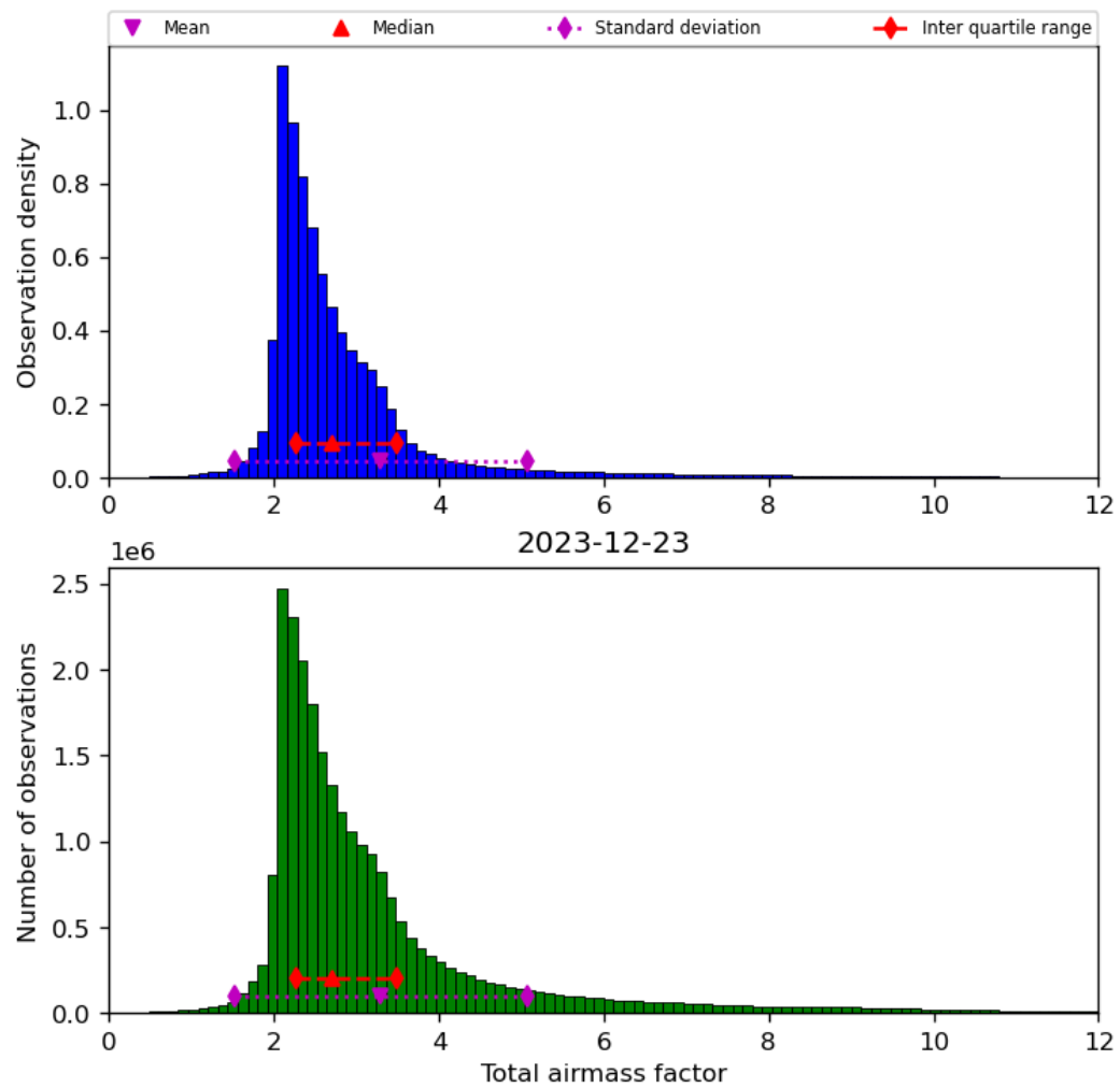
Figure 32: Histogram of “Total airmass factor” for 2023-12-22 to 2023-12-24
