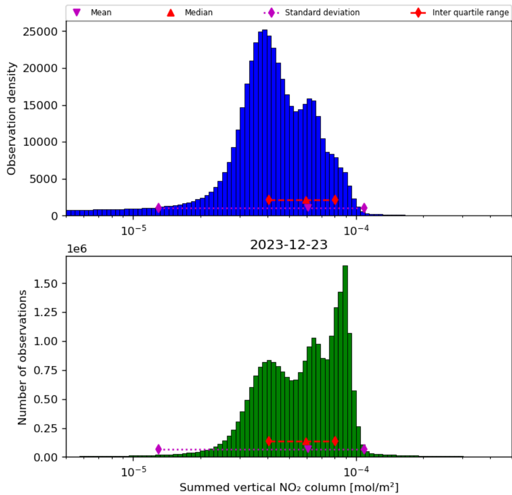
Figure 40: Histogram of “Summed vertical NO 2 column” for 2023-12-22 to 2023-12-24
