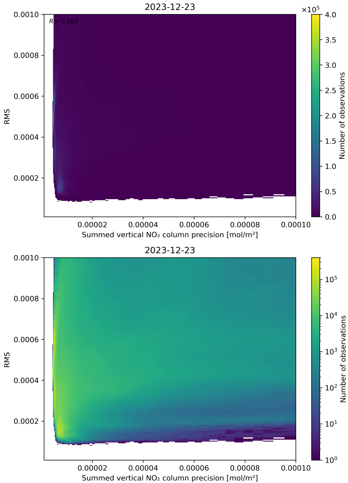
Figure 108: Scatter density plot of “Summed vertical NO 2 column precision” against “RMS” for 2023-12-22 to 2023-12-24.
