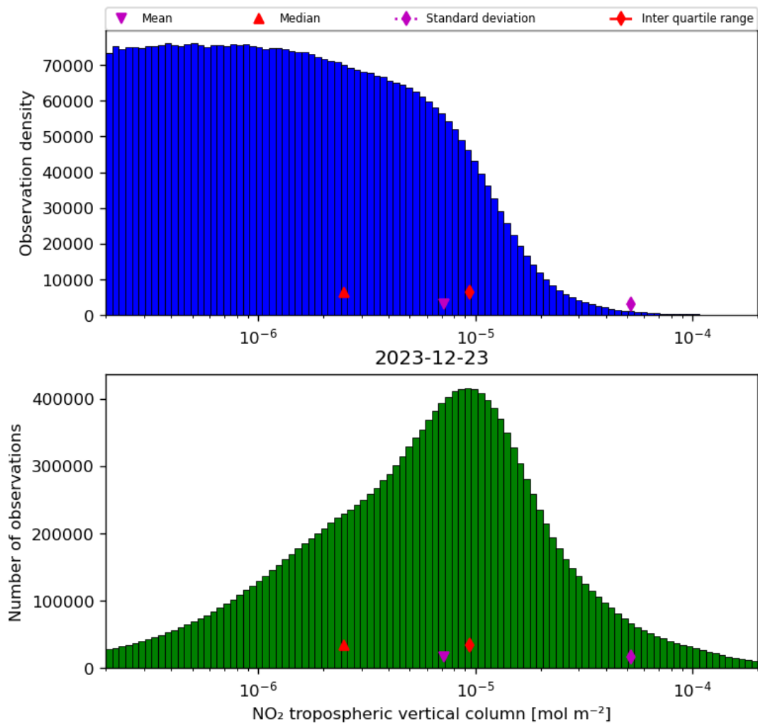
Figure 29: Histogram of “NO 2 tropospheric vertical column” for 2023-12-22 to 2023-12-24
