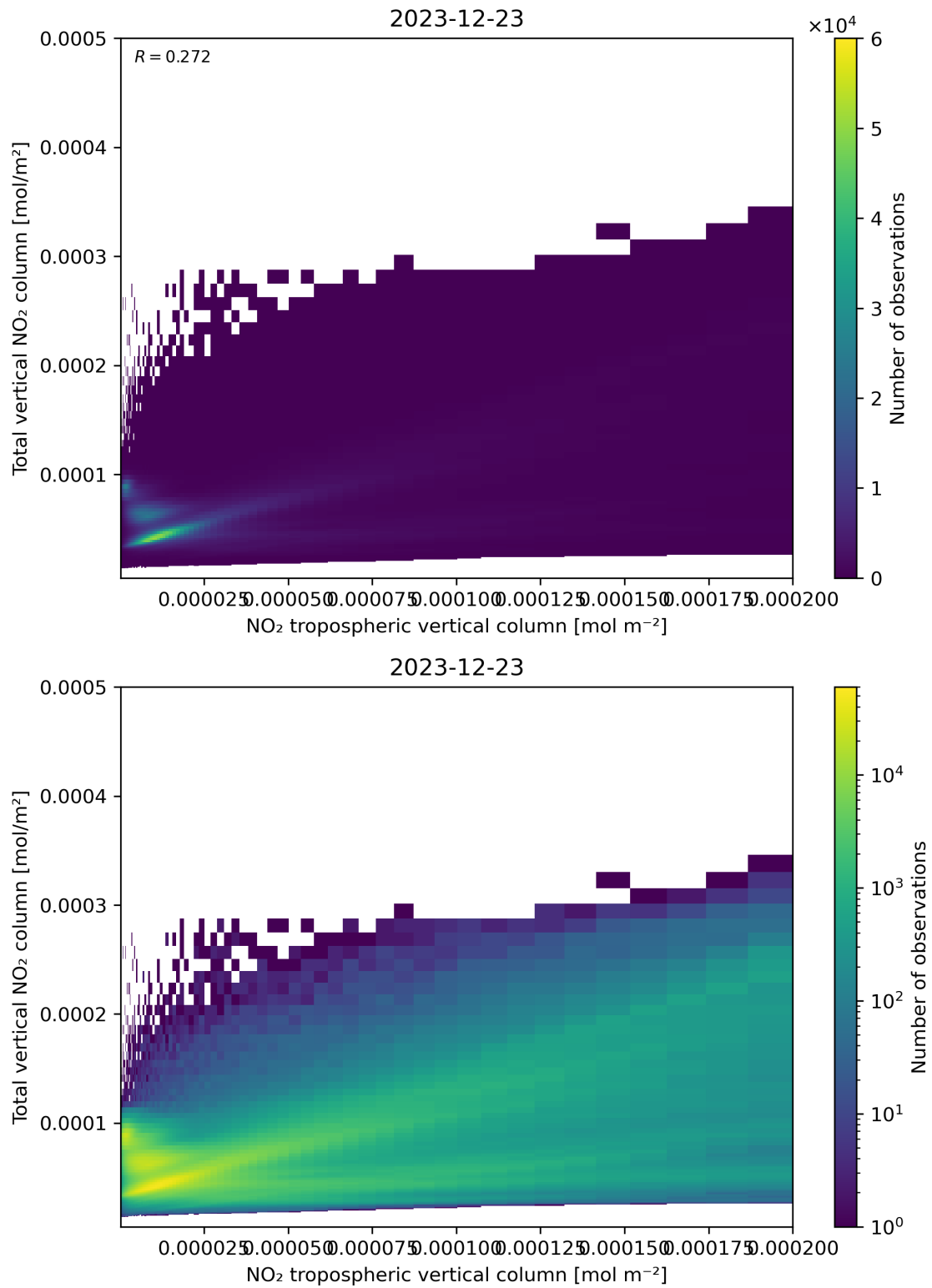
Figure 128: Scatter density plot of “NO 2 tropospheric vertical column” against “Total vertical NO 2 column” for 2023-12-22 to 2023-12-24.
