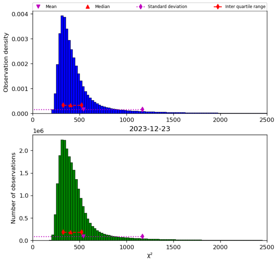
Figure 42: Histogram of “ \chi^2 ” for 2023-12-22 to 2023-12-24
