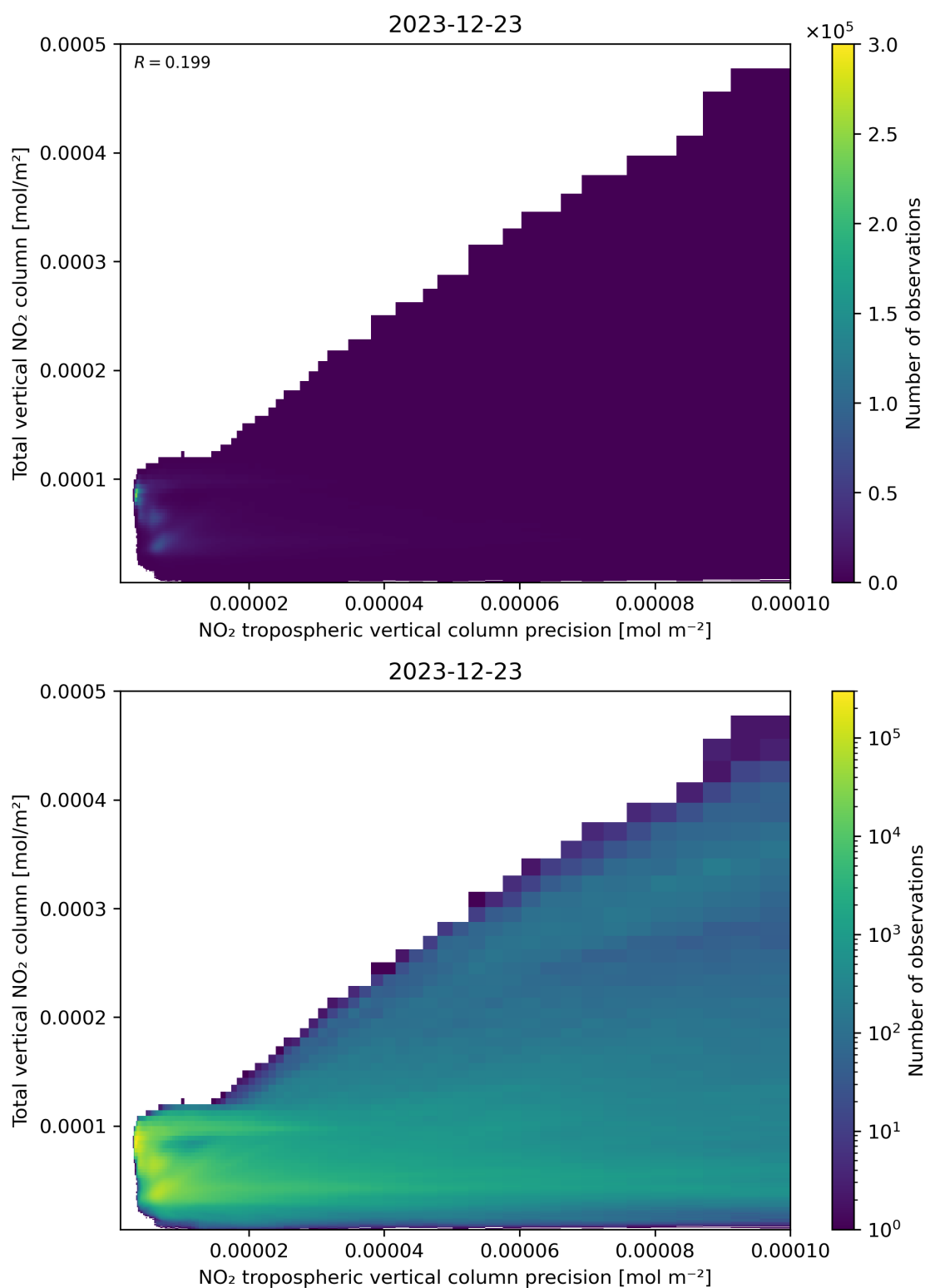
Figure 138: Scatter density plot of “NO 2 tropospheric vertical column precision” against “Total vertical NO 2 column” for 2023-12-22 to 2023-12-24.
