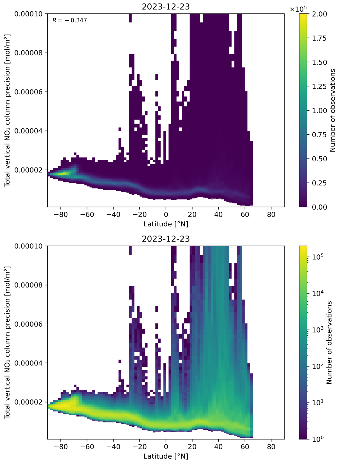
Figure 91: Scatter density plot of “Latitude” against “Total vertical NO 2 column precision” for 2023-12-22 to 2023-12-24.
