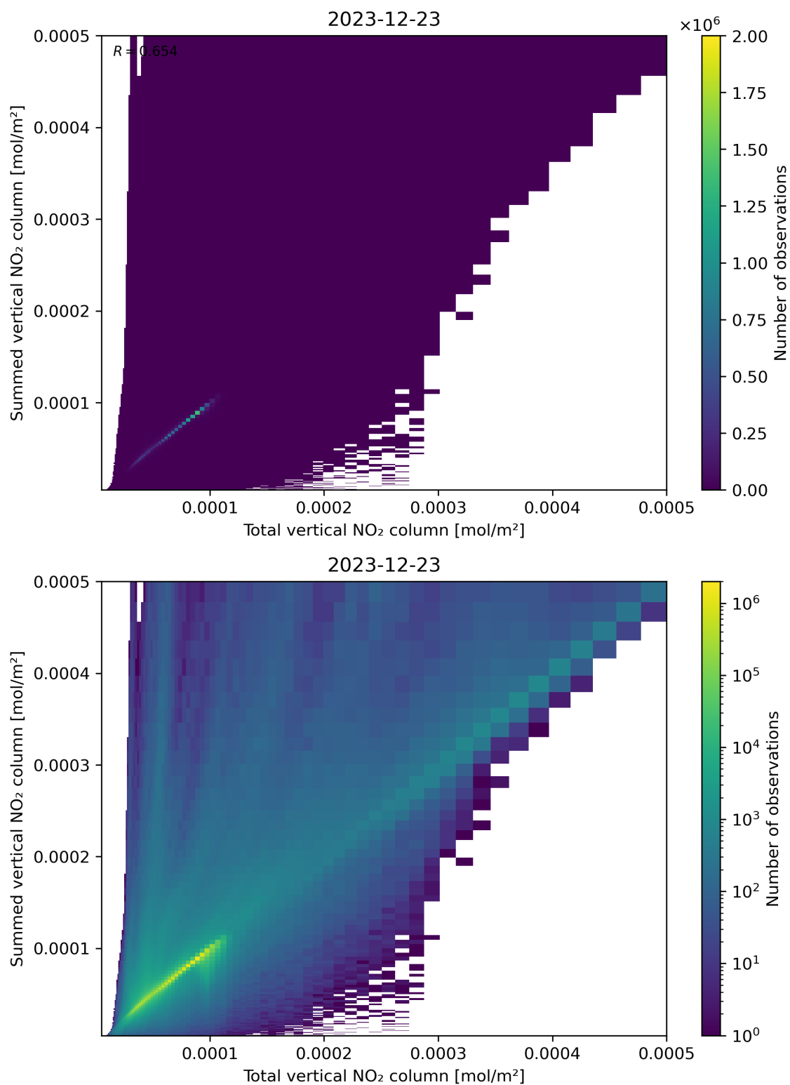
Figure 112: Scatter density plot of “Total vertical NO 2 column” against “Summed vertical NO 2 column” for 2023-12-22 to 2023-12-24.
