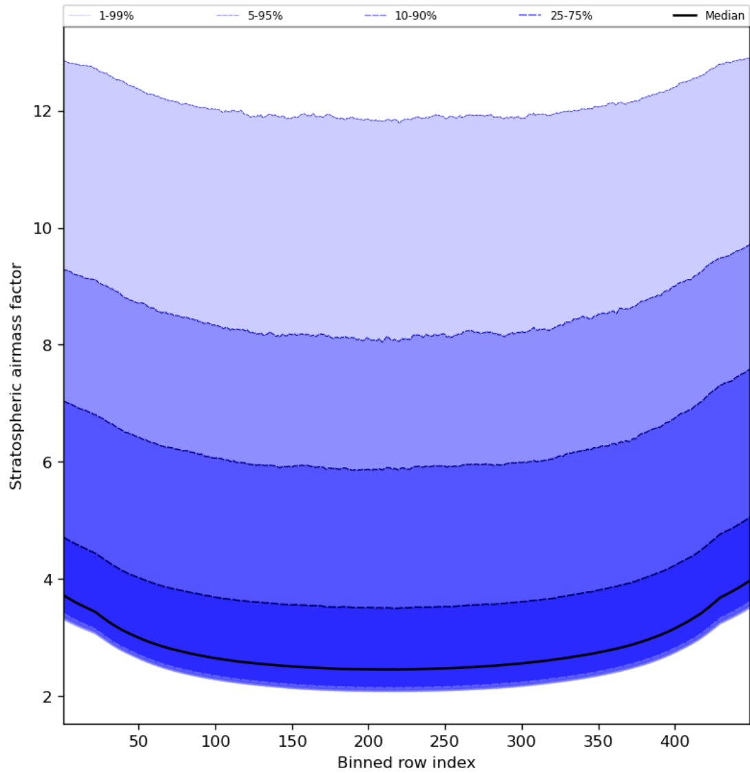
Figure 61: Along track statistics of “Stratospheric airmass factor” for 2023-12-22 to 2023-12-24
