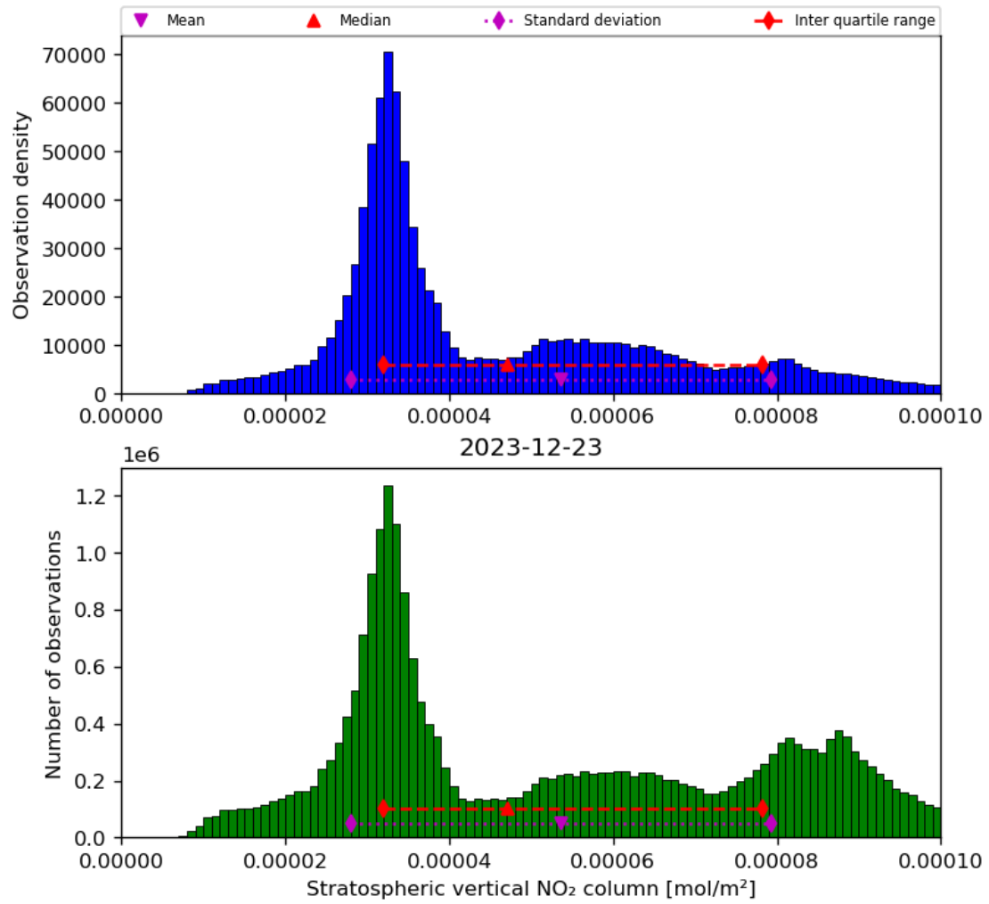
Figure 36: Histogram of “Stratospheric vertical NO 2 column” for 2023-12-22 to 2023-12-24
