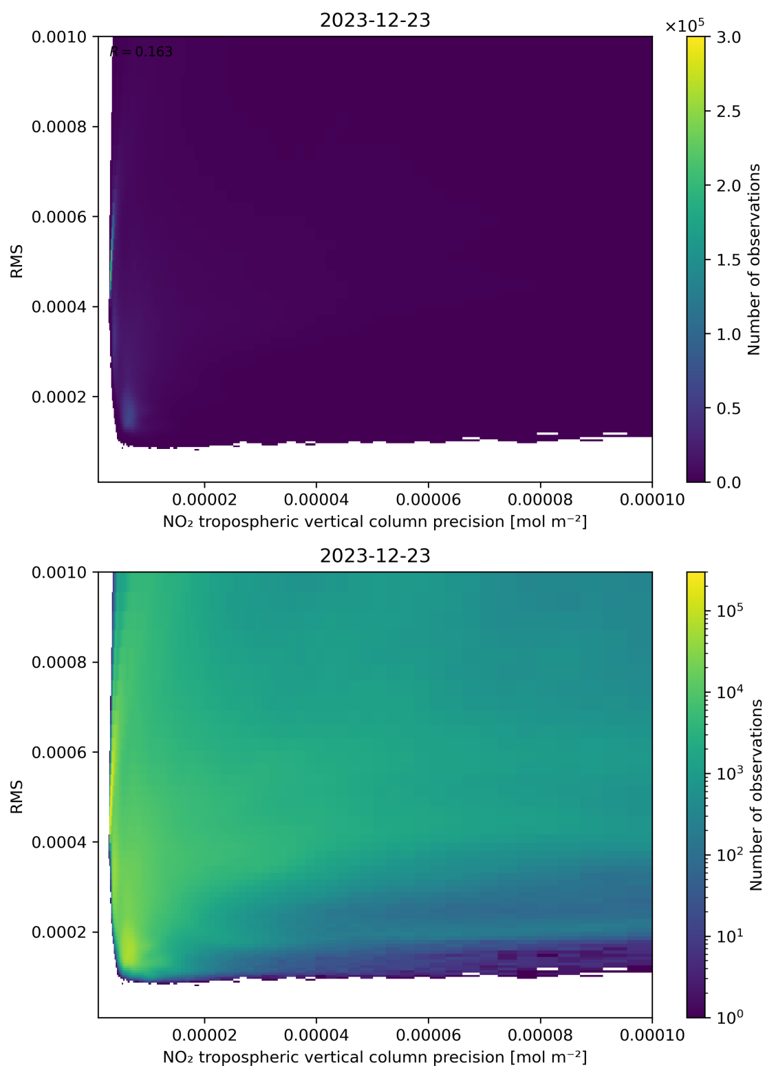
Figure 140: Scatter density plot of “NO 2 tropospheric vertical column precision” against “RMS” for 2023-12-22 to 2023-12-24.
