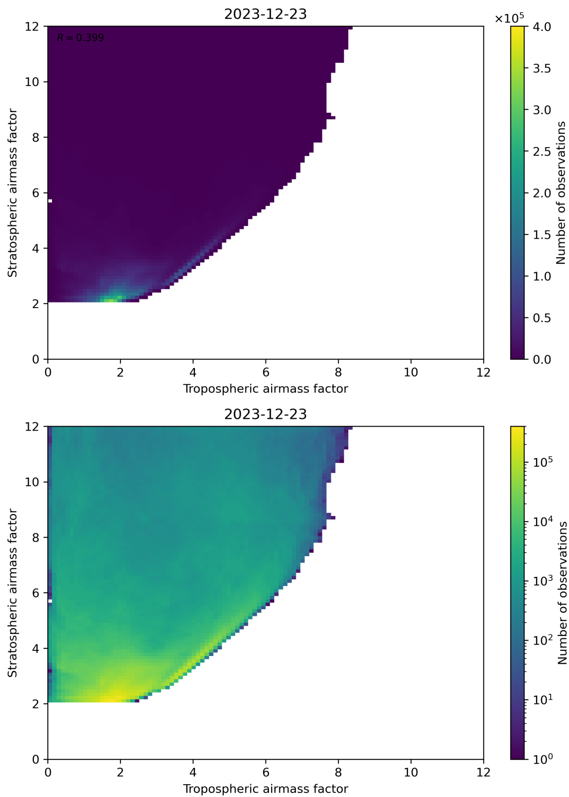
Figure 71: Scatter density plot of “Tropospheric airmass factor” against “Stratospheric airmass factor” for 2023-12-22 to 2023-12-24.
