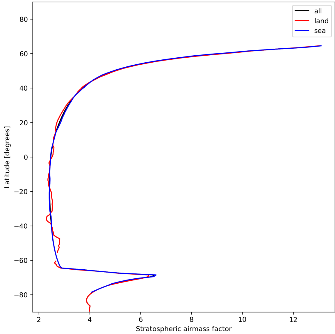
Figure 27: Zonal average of “Stratospheric air mass factor” for 2023-12-22 to 2023-12-24.
