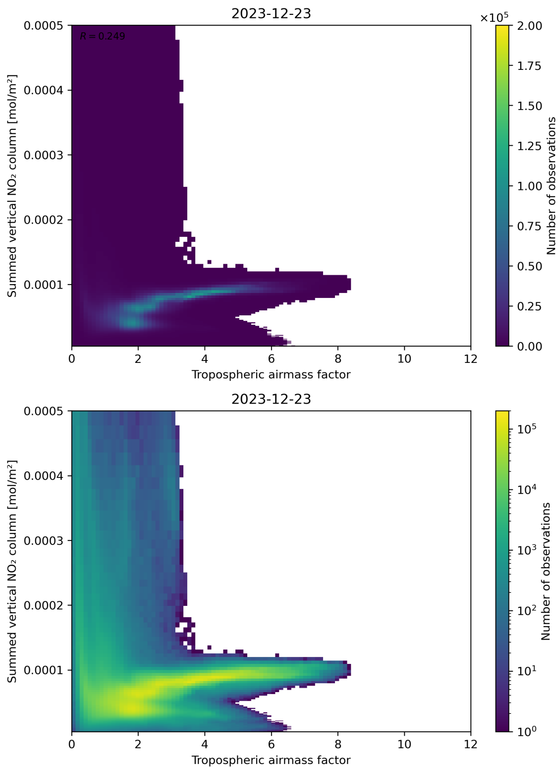
Figure 75: Scatter density plot of “Tropospheric airmass factor” against “Summed vertical NO 2 column” for 2023-12-22 to 2023-12-24.
