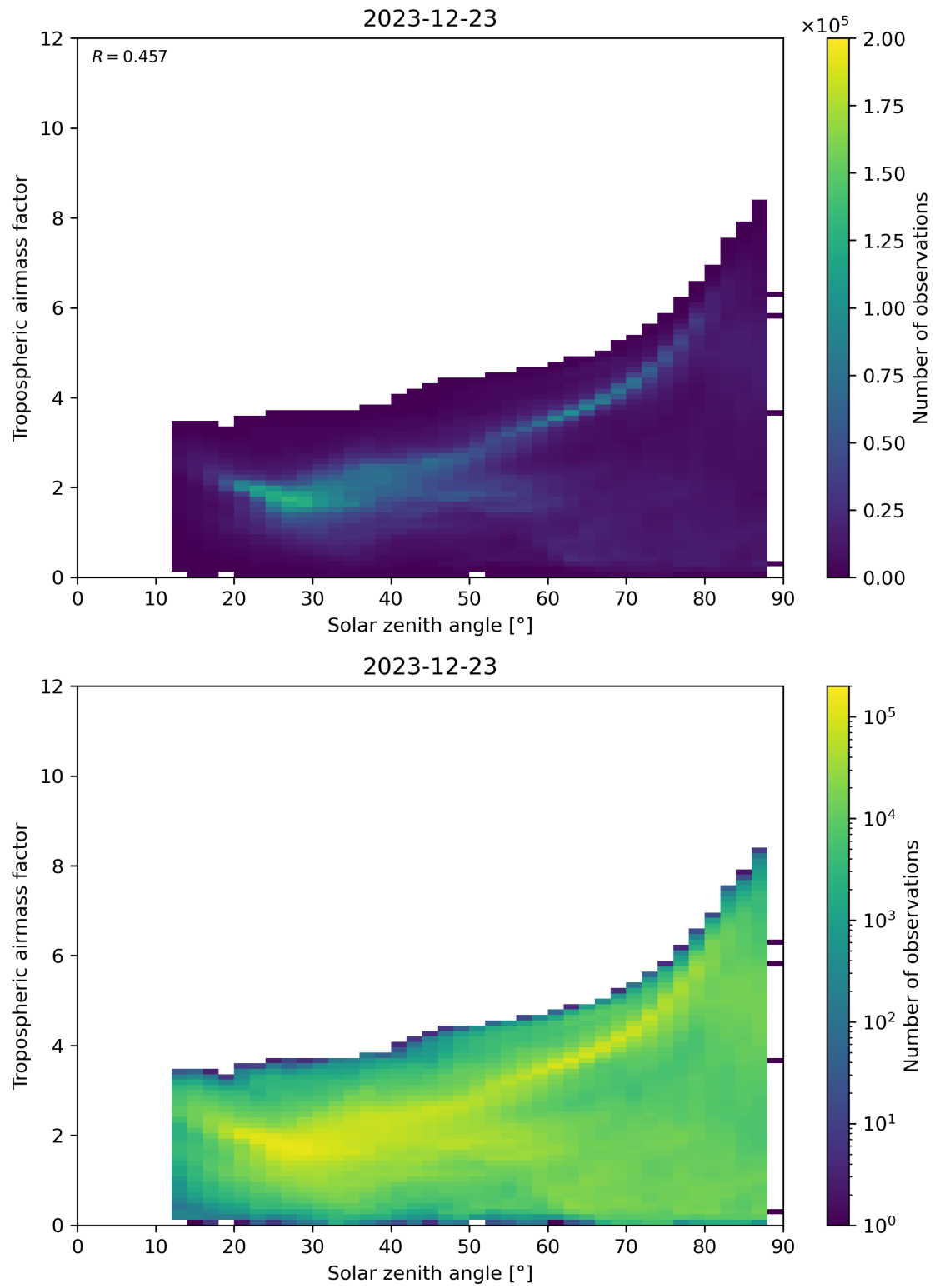
Figure 147: Scatter density plot of “Solar zenith angle” against “Tropospheric airmass factor” for 2023-12-22 to 2023-12-24.
