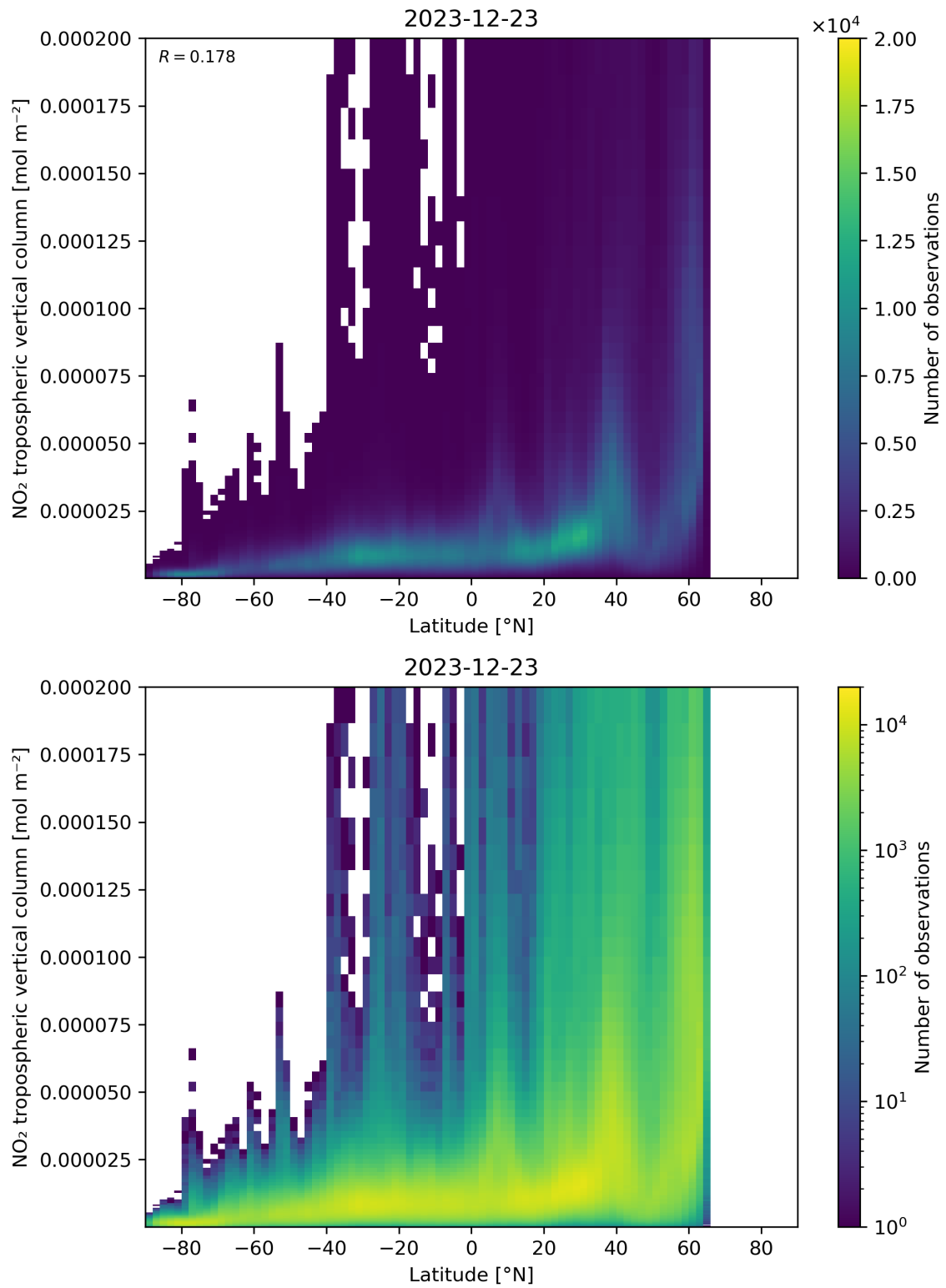
Figure 92: Scatter density plot of “Latitude” against “NO 2 tropospheric vertical column” for 2023-12-22 to 2023-12-24.
