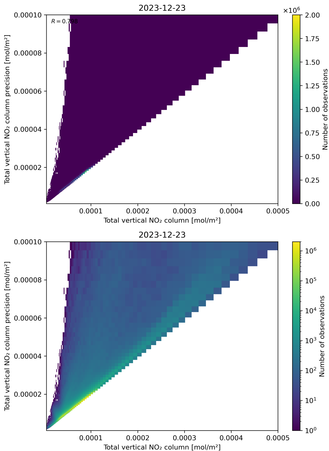
Figure 114: Scatter density plot of “Total vertical NO 2 column” against “Total vertical NO 2 column precision” for 2023-12-22 to 2023-12-24.
