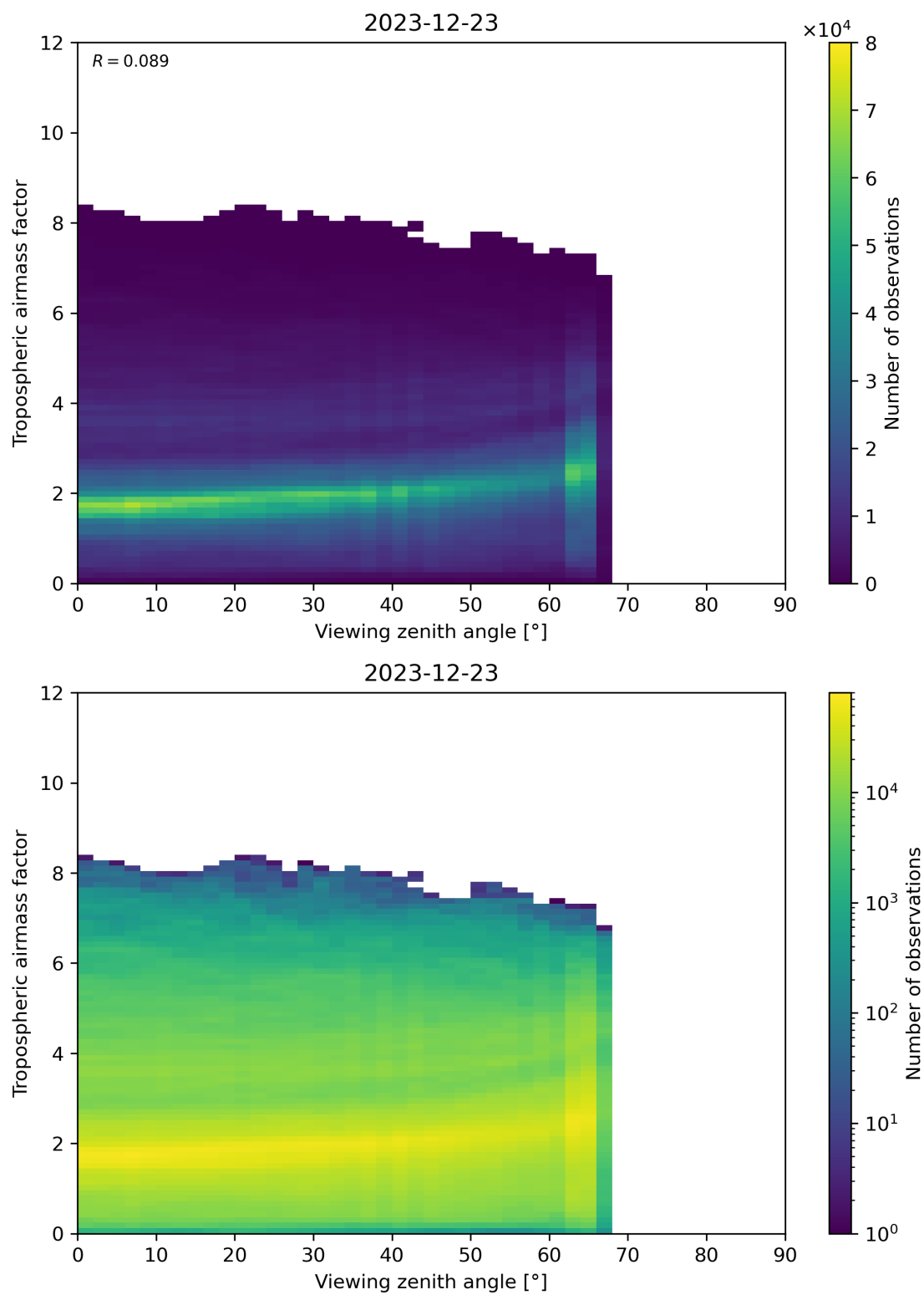
Figure 161: Scatter density plot of “Viewing zenith angle” against “Tropospheric airmass factor” for 2023-12-22 to 2023-12-24.
