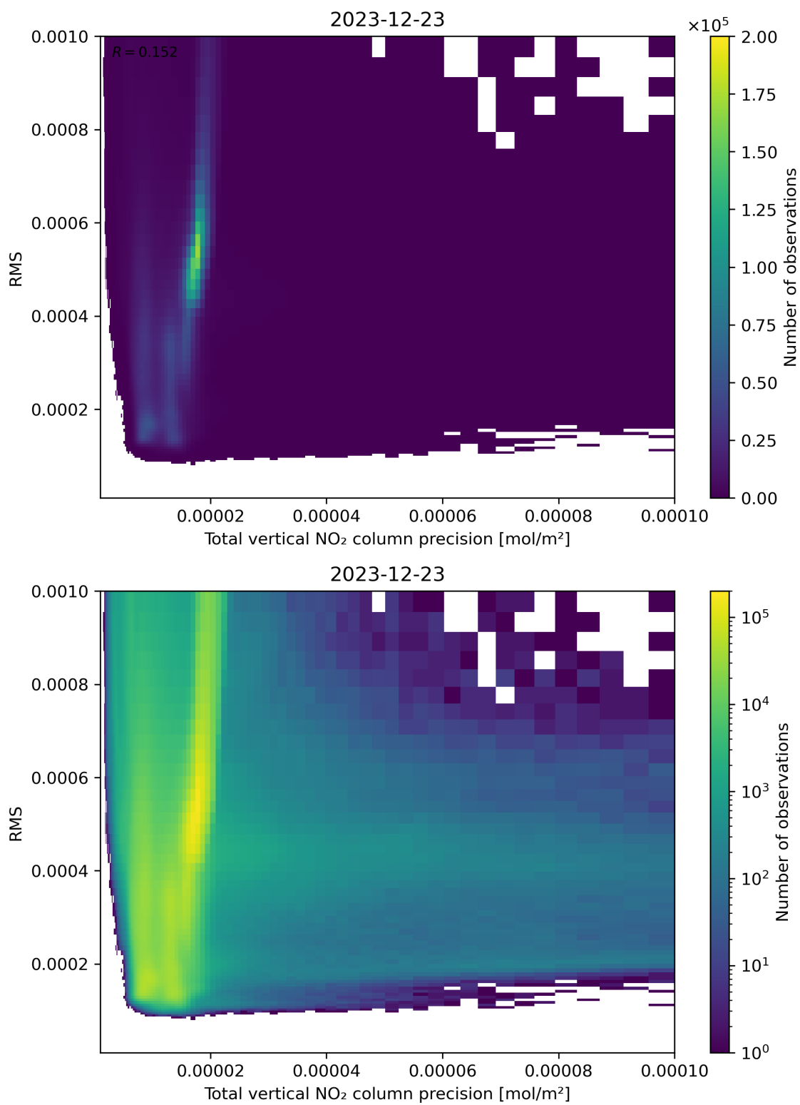
Figure 119: Scatter density plot of “Total vertical NO 2 column precision” against “RMS” for 2023-12-22 to 2023-12-24.
