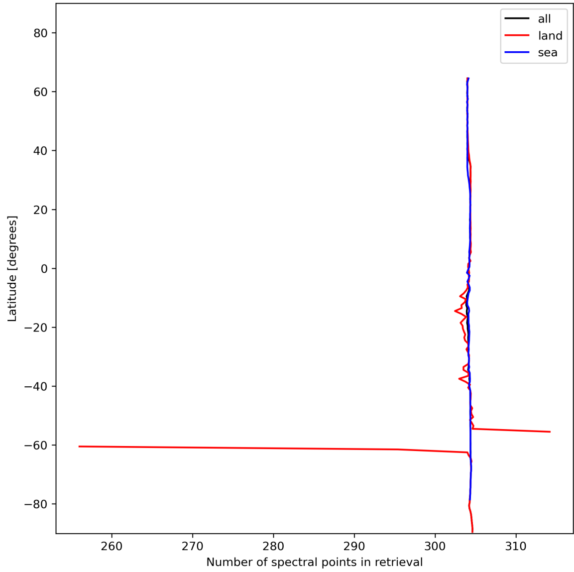
Figure 16: Zonal average of “Number of spectral points in retrieval” for 2023-12-22 to 2023-12-24.
