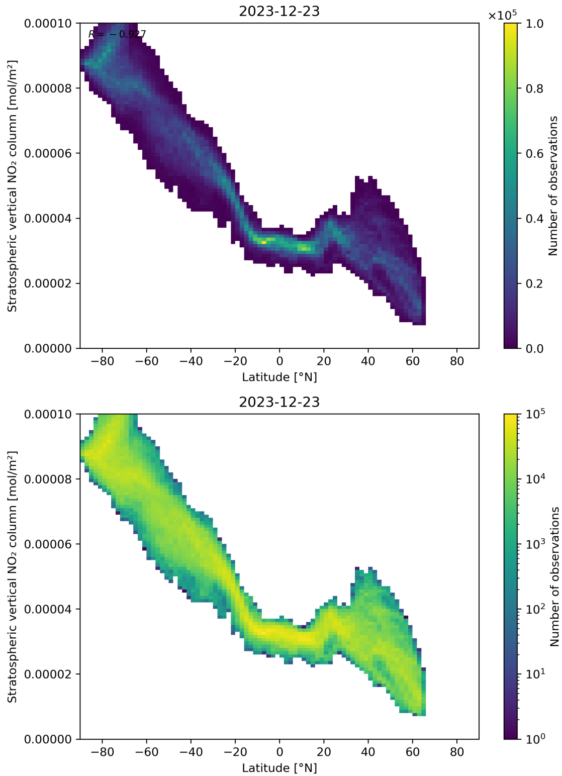
Figure 87: Scatter density plot of “Latitude” against “Stratospheric vertical NO 2 column” for 2023-12-22 to 2023-12-24.
