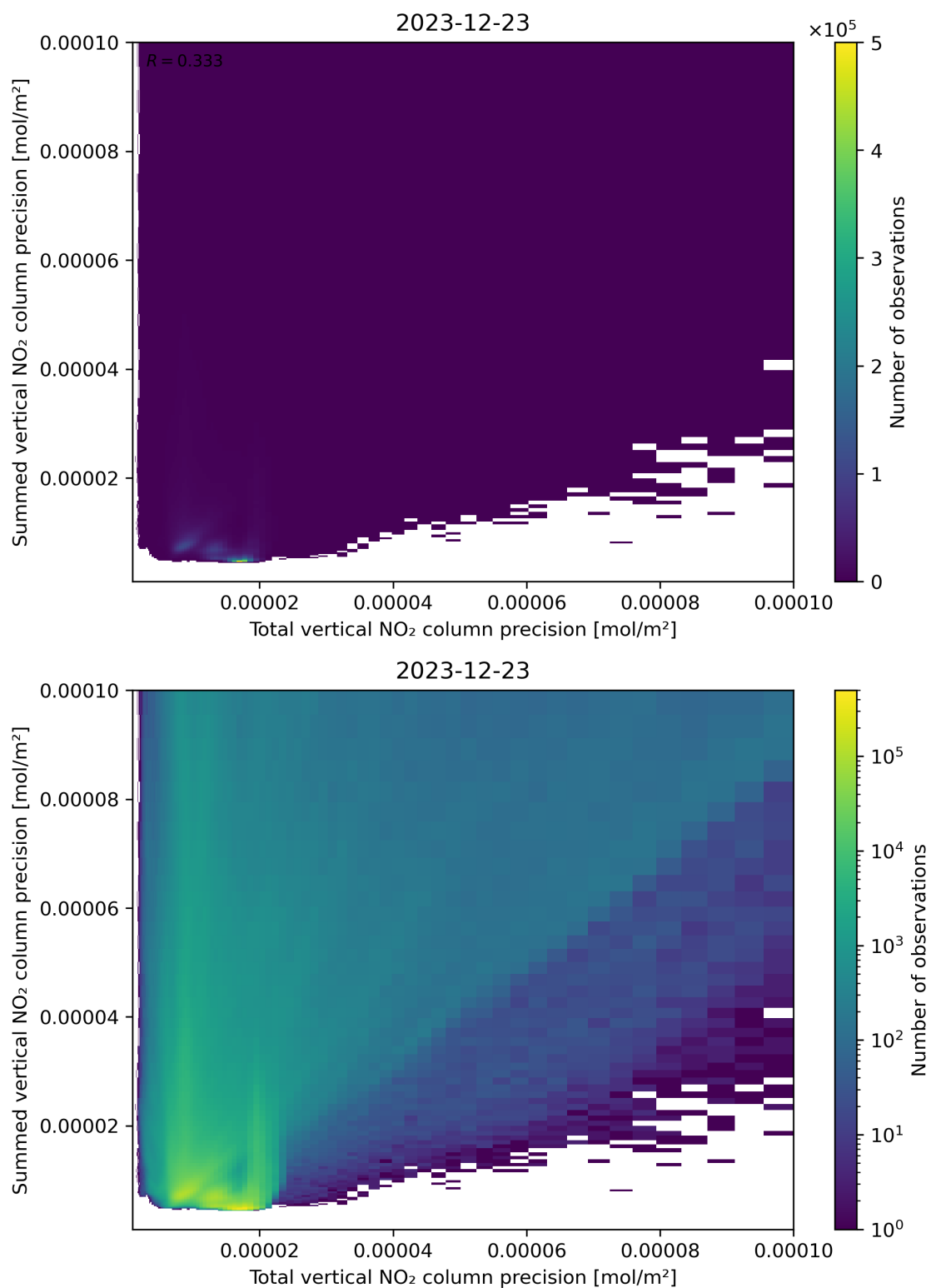
Figure 118: Scatter density plot of “Total vertical NO 2 column precision” against “Summed vertical NO 2 column precision” for 2023-12-22 to 2023-12-24.
