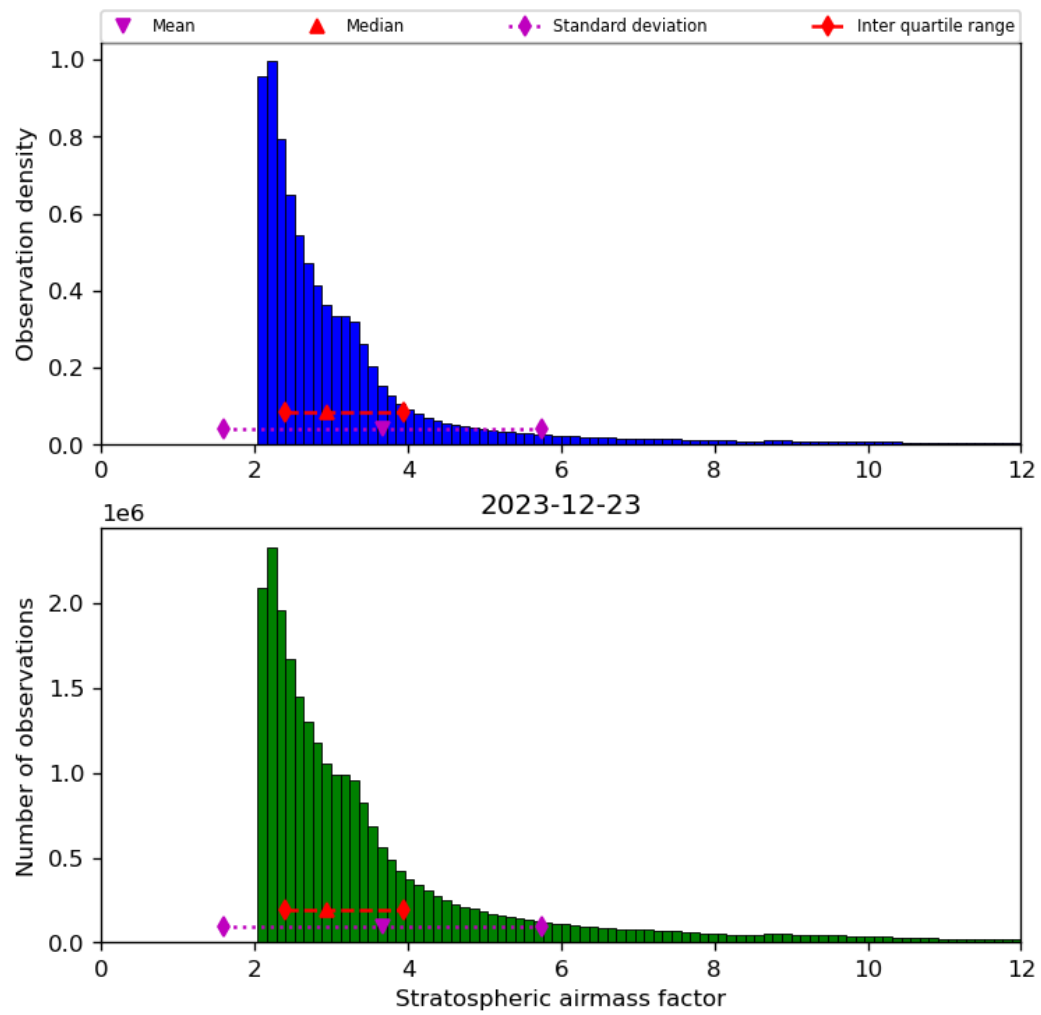
Figure 44: Histogram of “Stratospheric airmass factor” for 2023-12-22 to 2023-12-24
