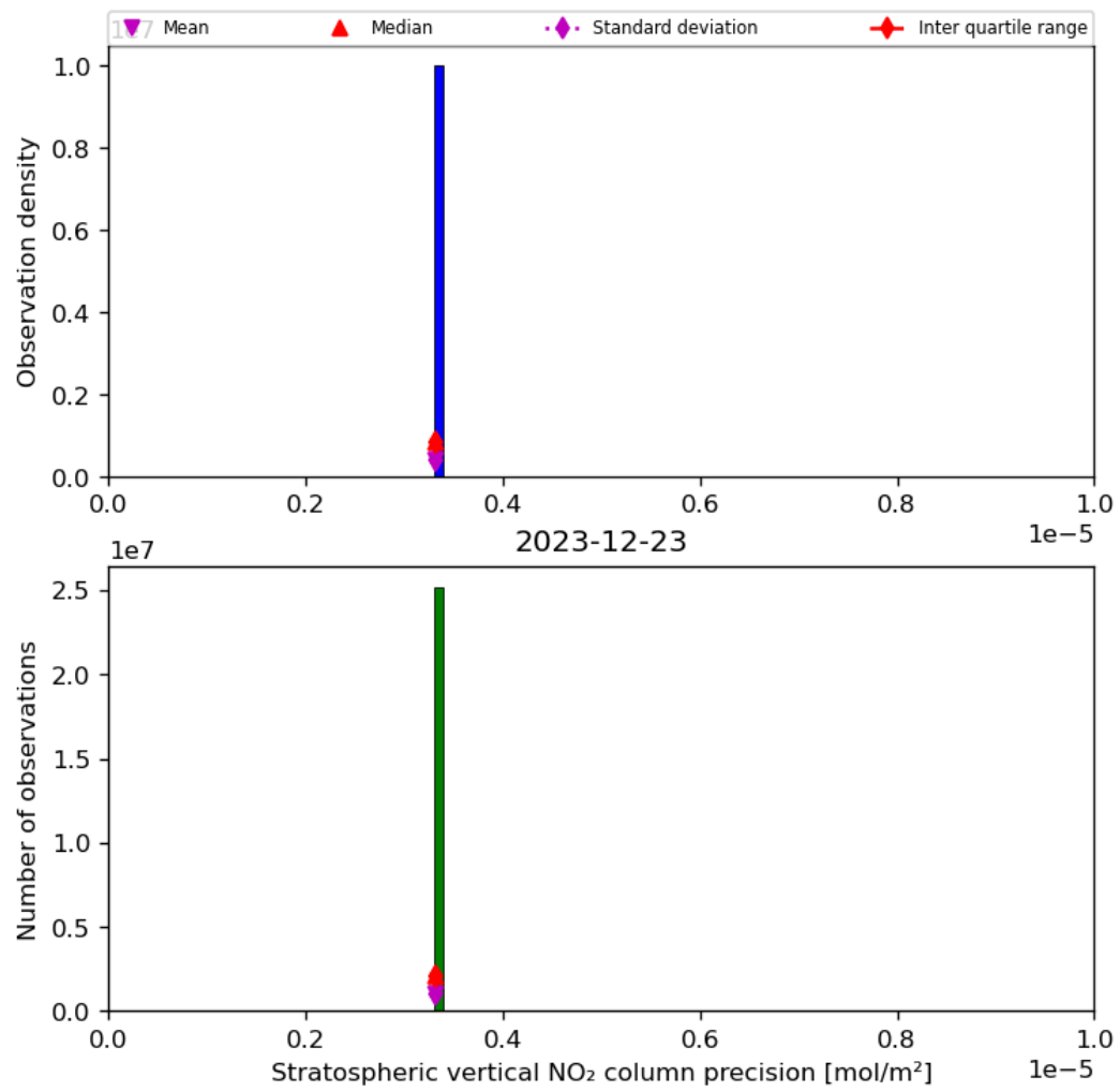
Figure 37: Histogram of “Stratospheric vertical NO 2 column precision” for 2023-12-22 to 2023-12-24
