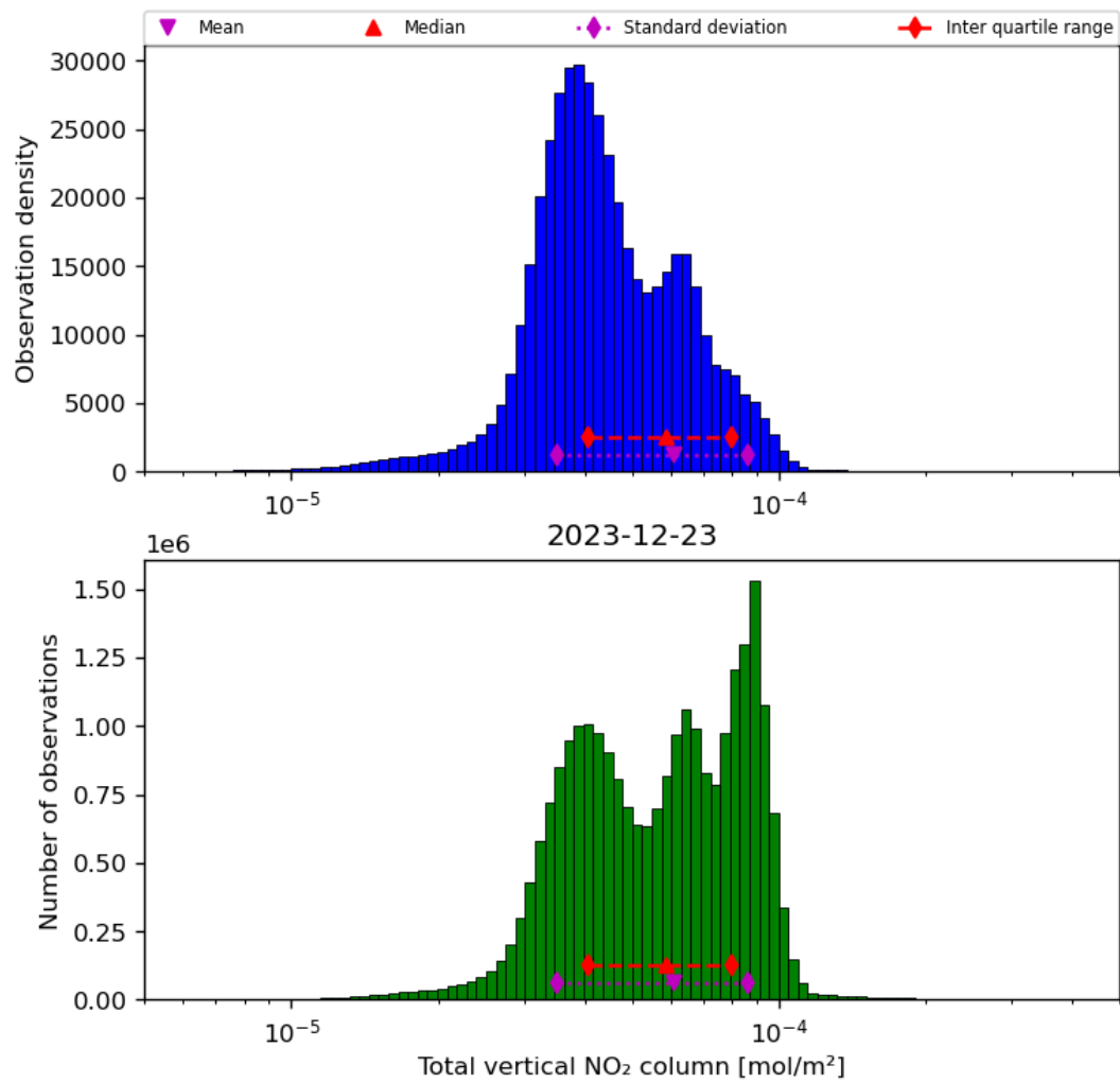
Figure 38: Histogram of “Total vertical NO 2 column” for 2023-12-22 to 2023-12-24
