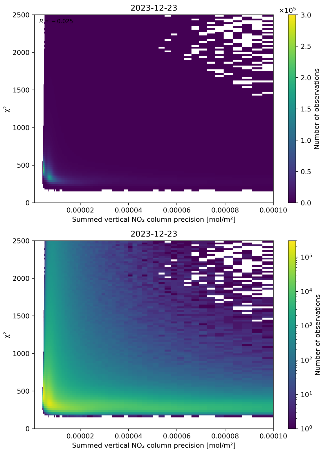
Figure 107: Scatter density plot of “Summed vertical NO 2 column precision” against “ \chi^2 ” for 2023-12-22 to 2023-12-24.
