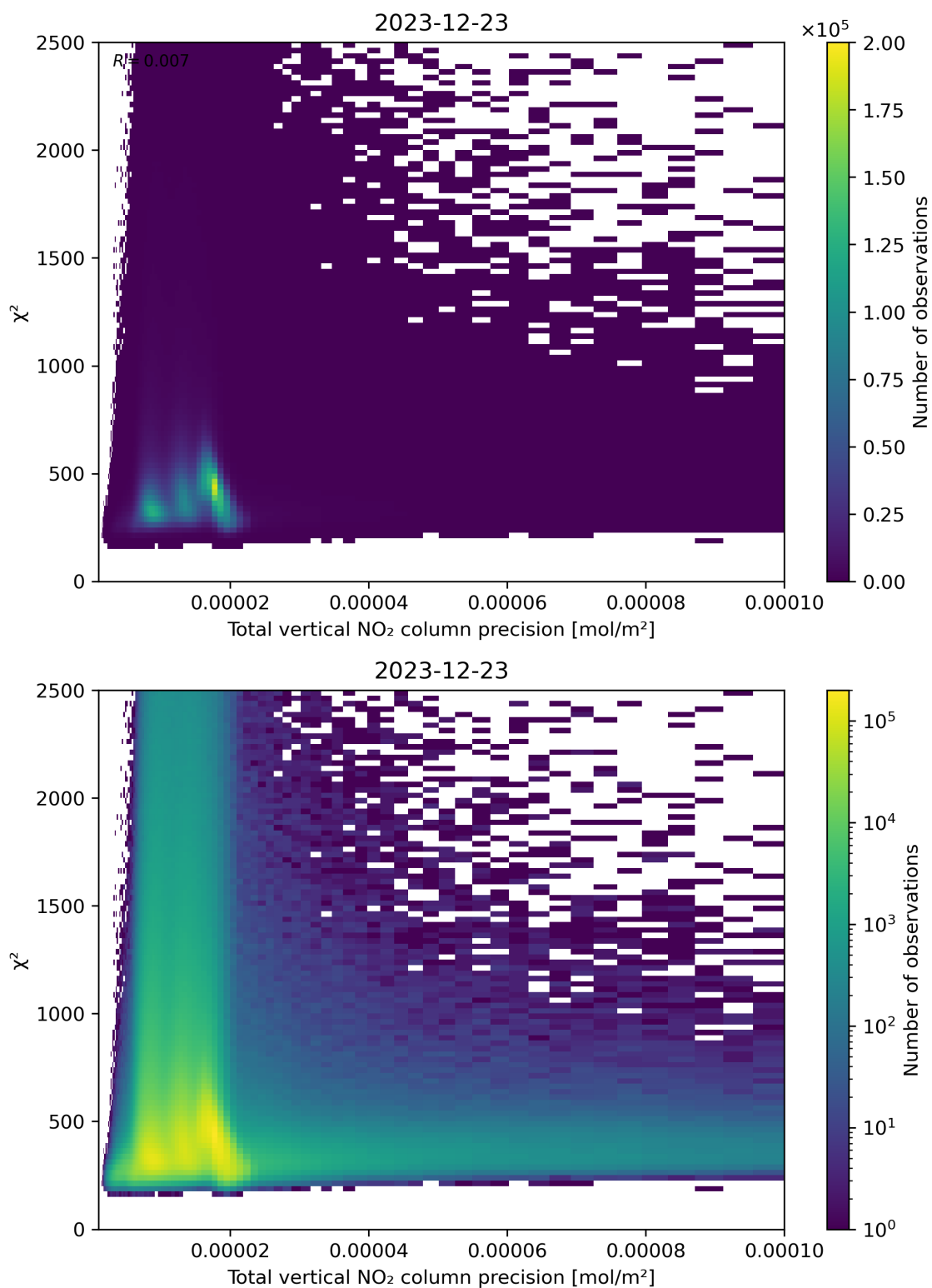
Figure 116: Scatter density plot of “Total vertical NO 2 column precision” against “ \chi^2 ” for 2023-12-22 to 2023-12-24.
