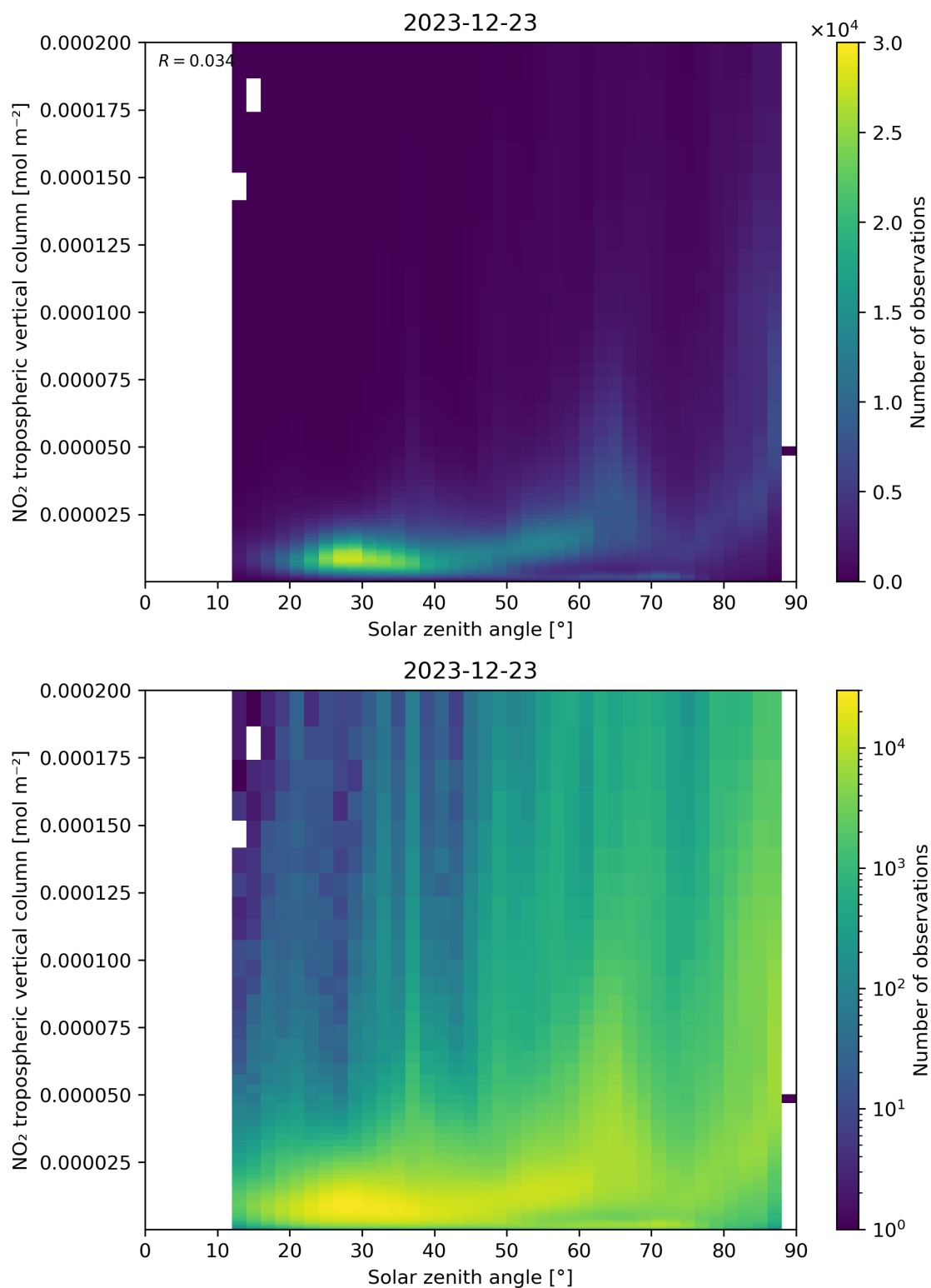
Figure 155: Scatter density plot of “Solar zenith angle” against “NO 2 tropospheric vertical column” for 2023-12-22 to 2023-12-24.
