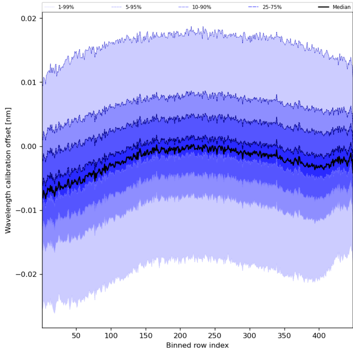
Figure 52: Along track statistics of “Wavelength calibration offset” for 2023-12-22 to 2023-12-24
