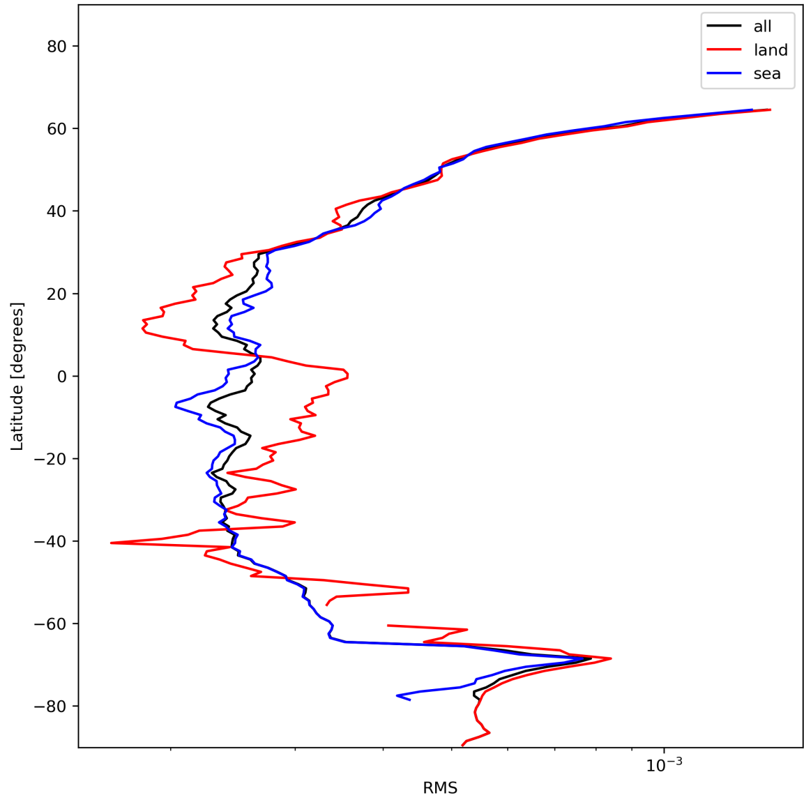
Figure 26: Zonal average of “RMS” for 2023-12-22 to 2023-12-24.
