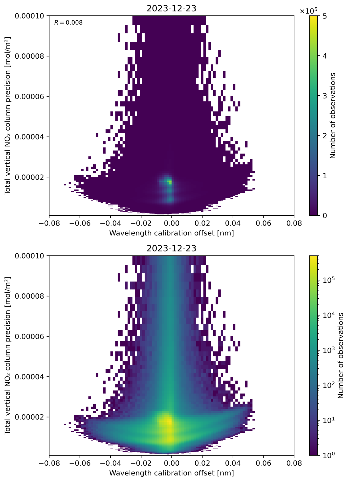
Figure 180: Scatter density plot of “Wavelength calibration offset” against “Total vertical NO 2 column precision” for 2023-12-22 to 2023-12-24.
