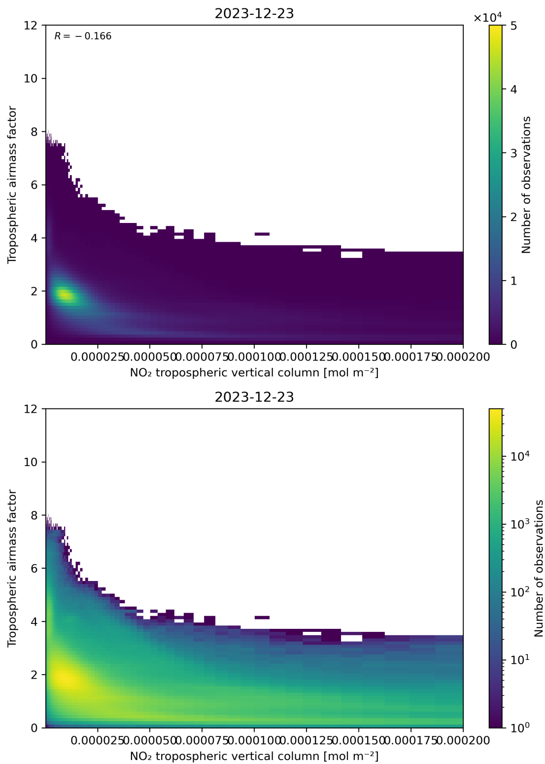
Figure 123: Scatter density plot of “NO 2 tropospheric vertical column” against “Tropospheric air mass factor” for 2023-12-22 to 2023-12-24.
