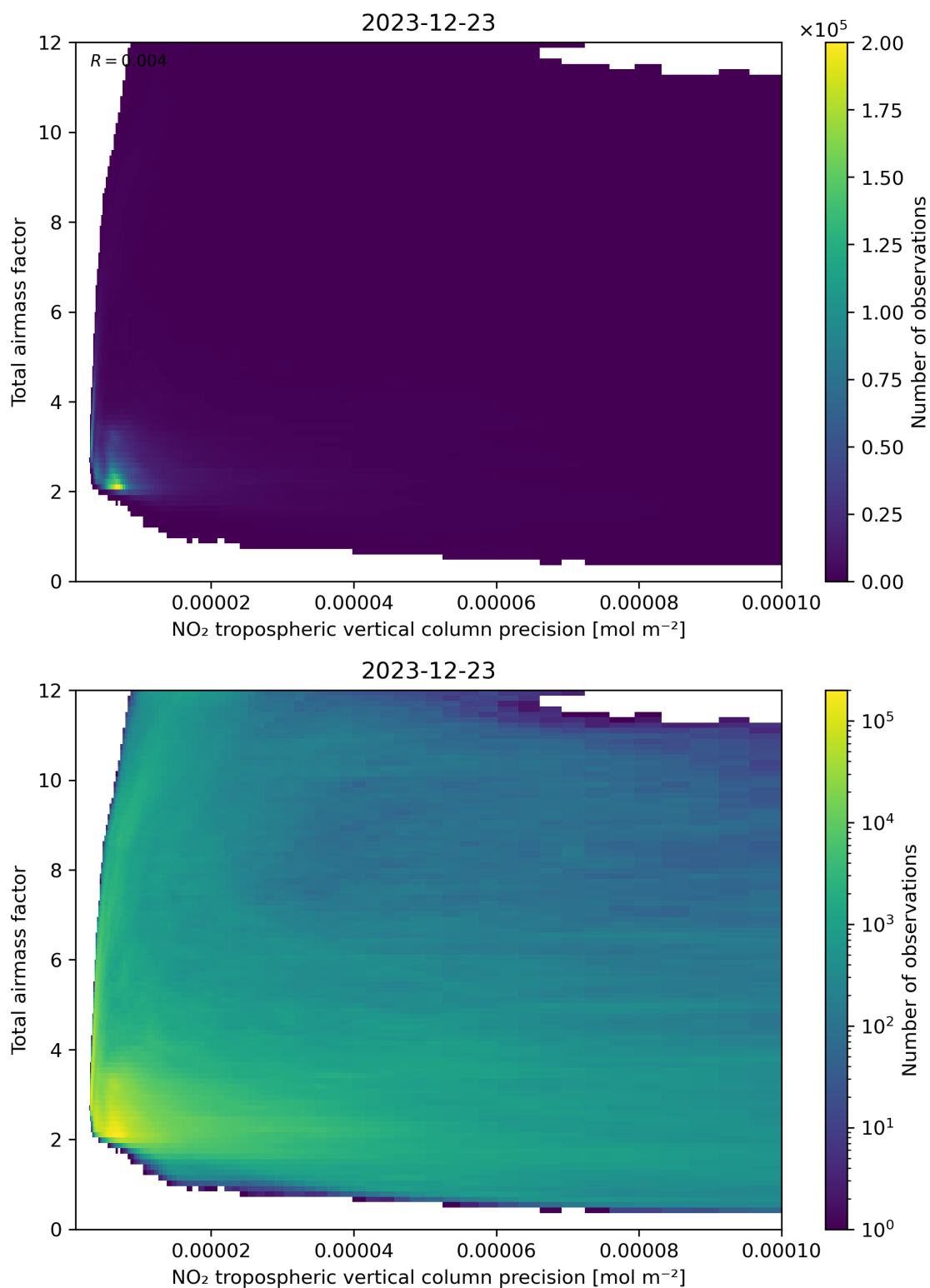
Figure 132: Scatter density plot of “NO 2 tropospheric vertical column precision” against “Total airmass factor” for 2023-12-22 to 2023-12-24.
