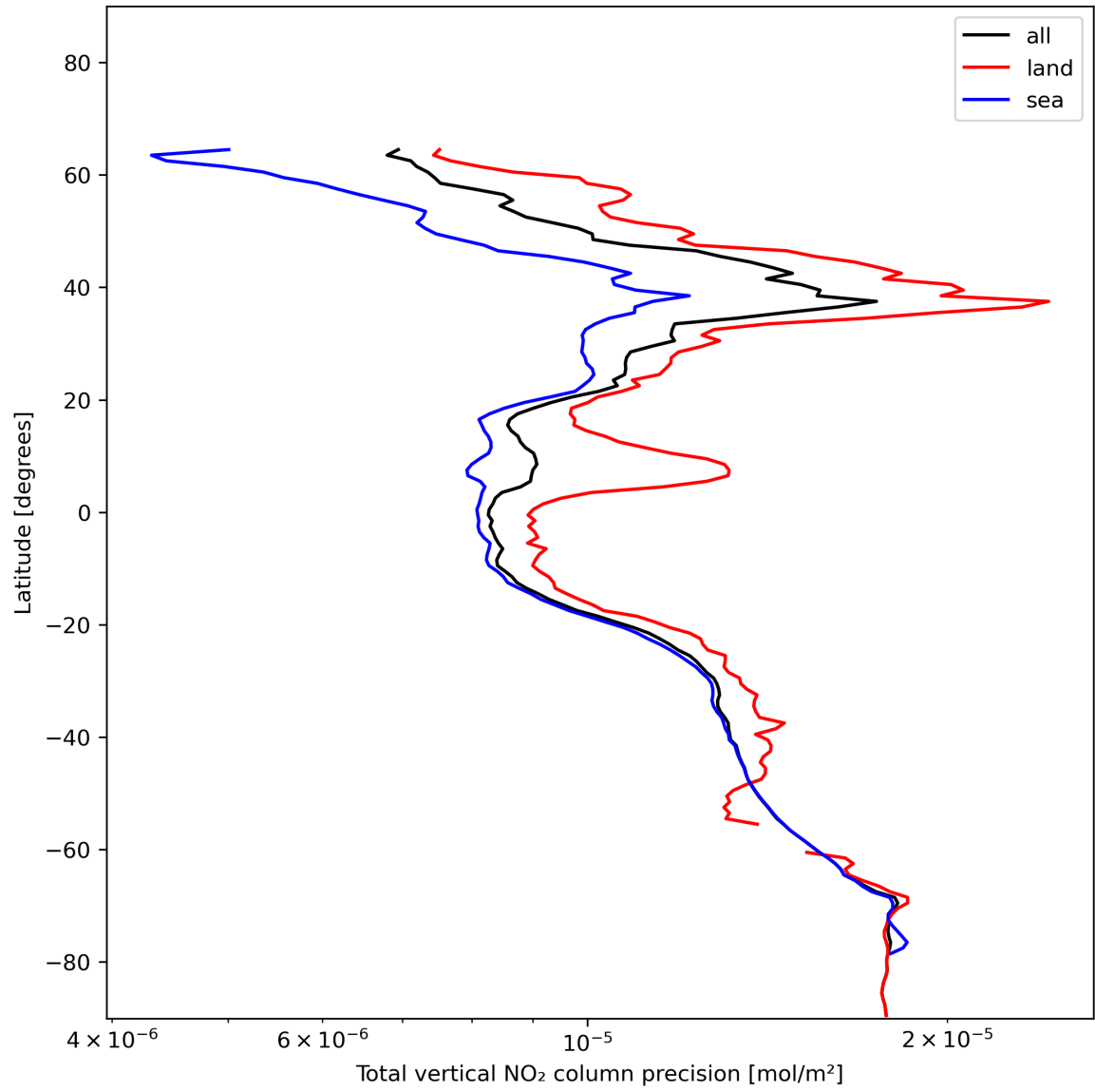
Figure 22: Zonal average of “Total vertical NO 2 column precision” for 2023-12-22 to 2023-12-24.
