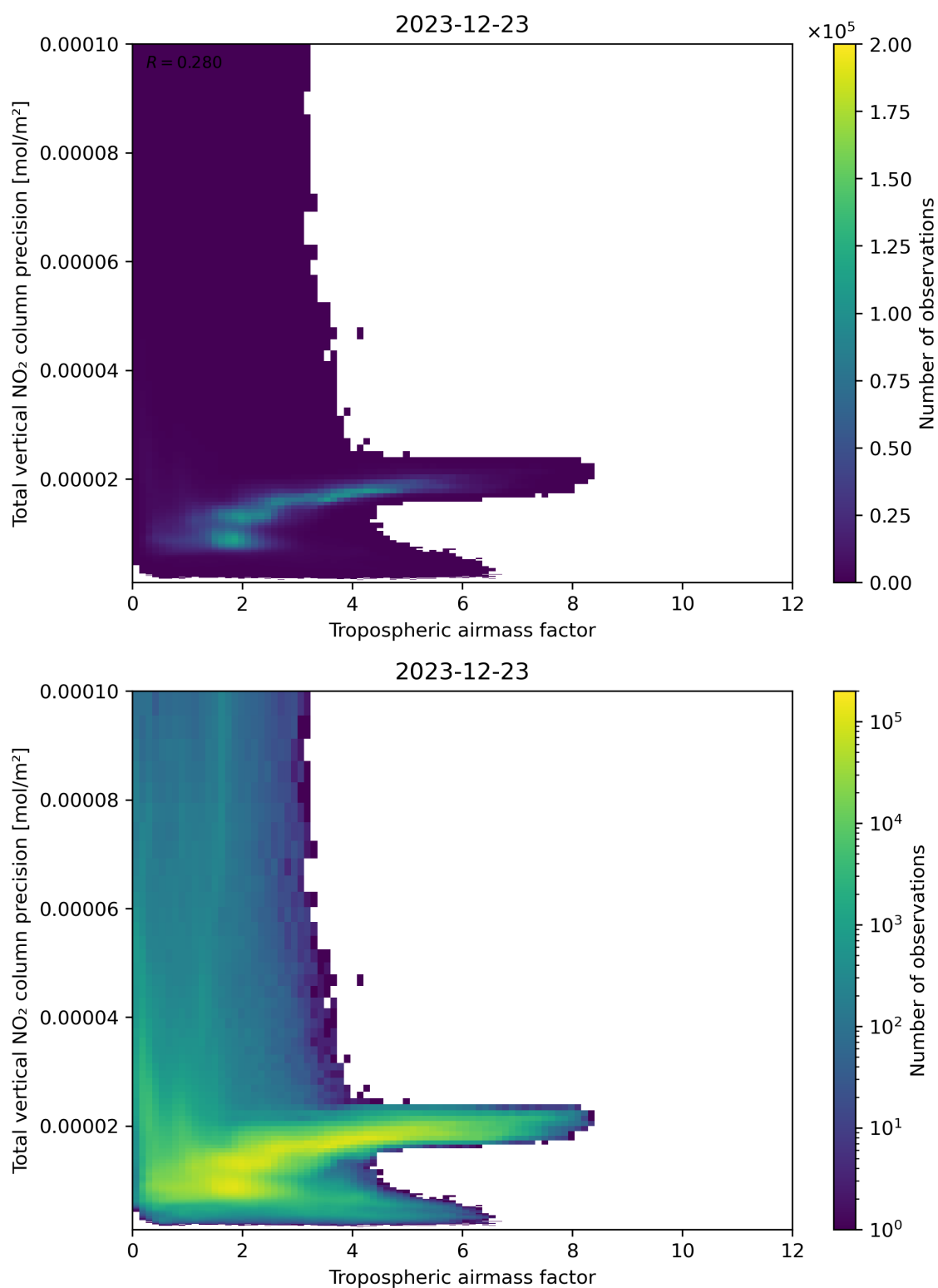
Figure 78: Scatter density plot of “Tropospheric air mass factor” against “Total vertical NO 2 column precision” for 2023-12-22 to 2023-12-24.
