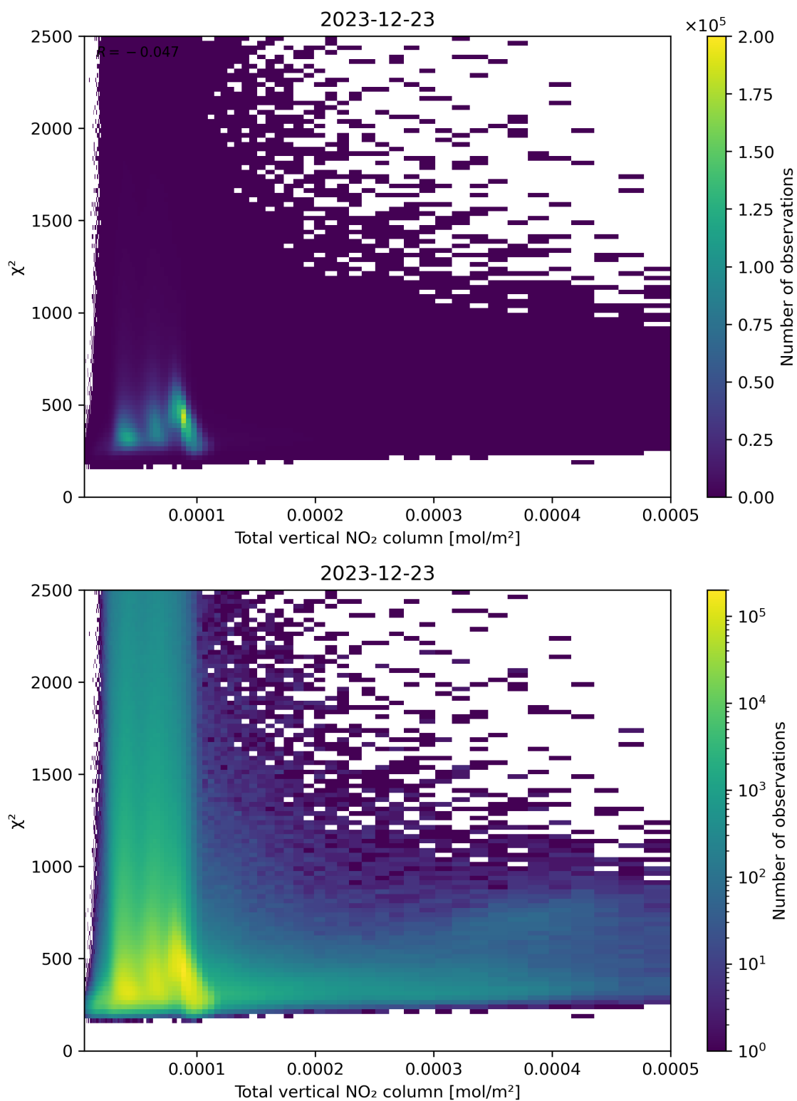
Figure 111: Scatter density plot of “Total vertical NO 2 column” against “ \chi^2 ” for 2023-12-22 to 2023-12-24.
