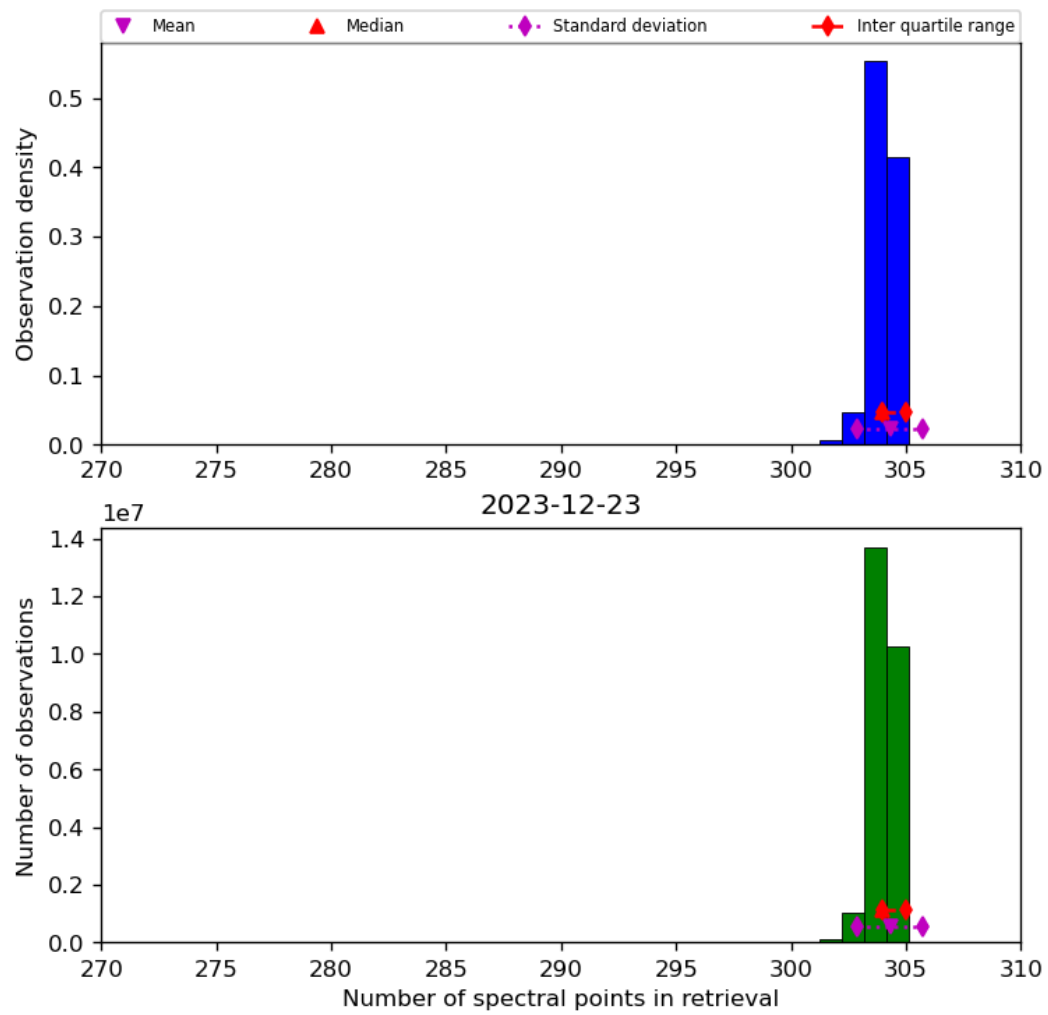
Figure 33: Histogram of “Number of spectral points in retrieval” for 2023-12-22 to 2023-12-24
