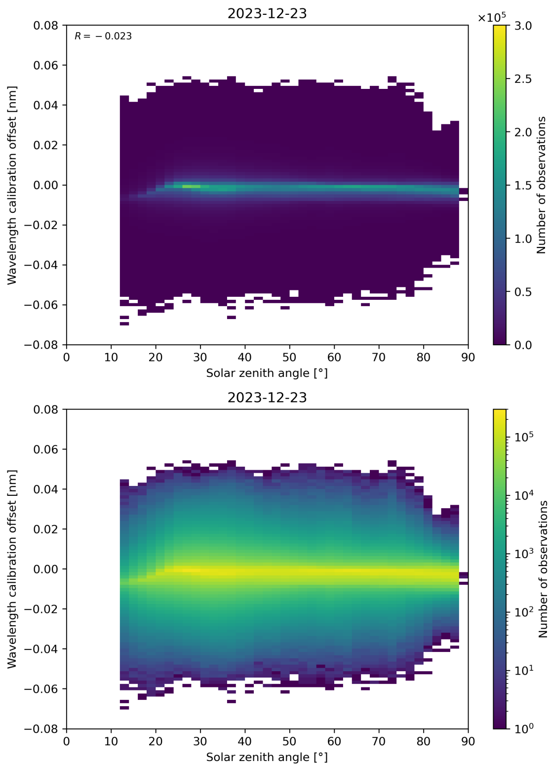
Figure 158: Scatter density plot of “Solar zenith angle” against “Wavelength calibration offset” for 2023-12-22 to 2023-12-24.
