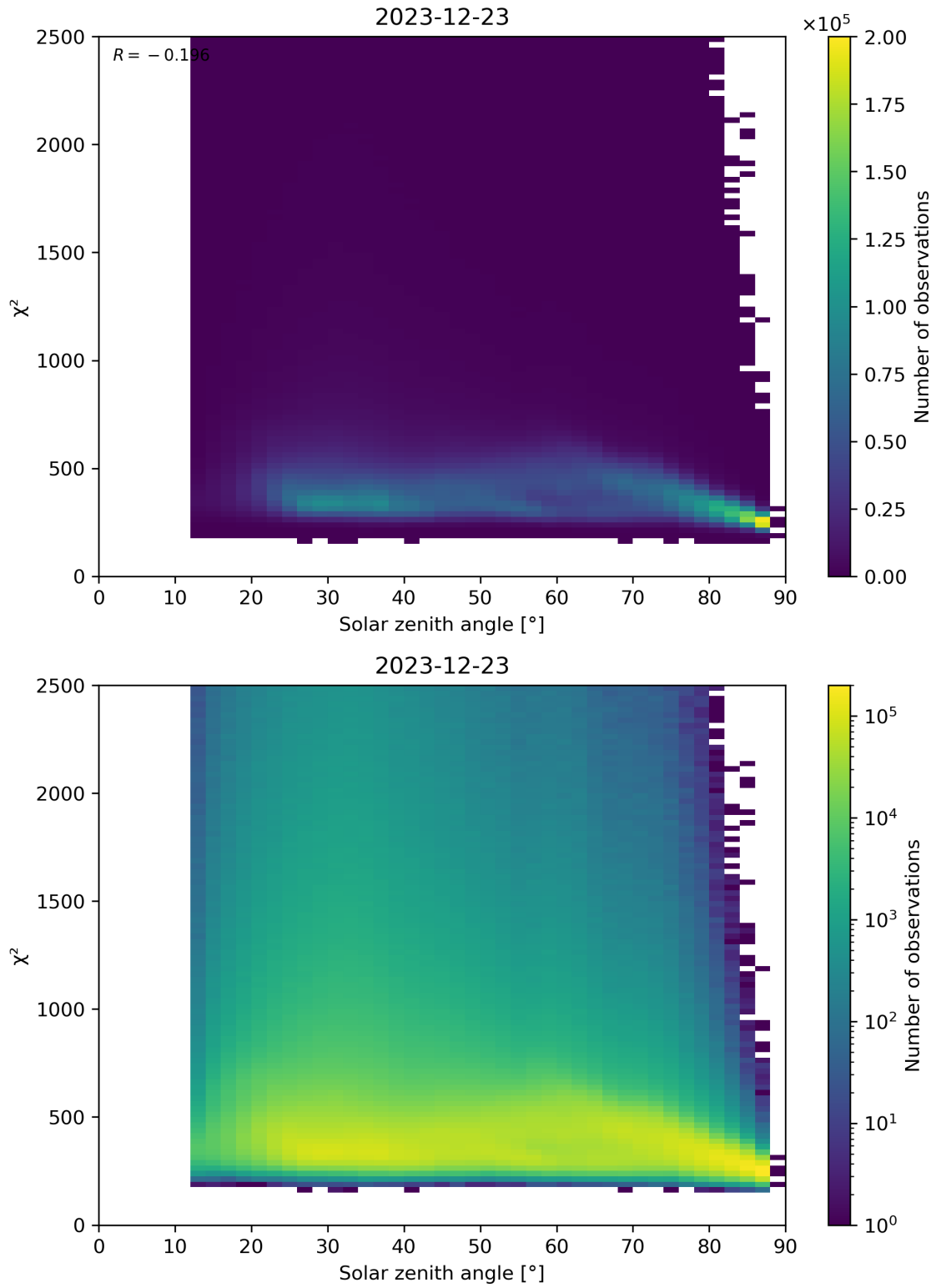
Figure 148: Scatter density plot of “Solar zenith angle” against “ \chi^2 ” for 2023-12-22 to 2023-12-24.
