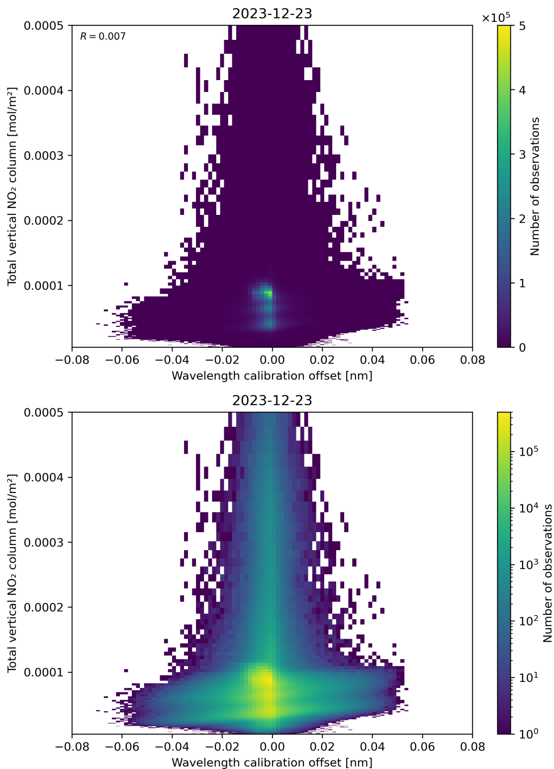
Figure 179: Scatter density plot of “Wavelength calibration offset” against “Total vertical NO 2 column” for 2023-12-22 to 2023-12-24.
