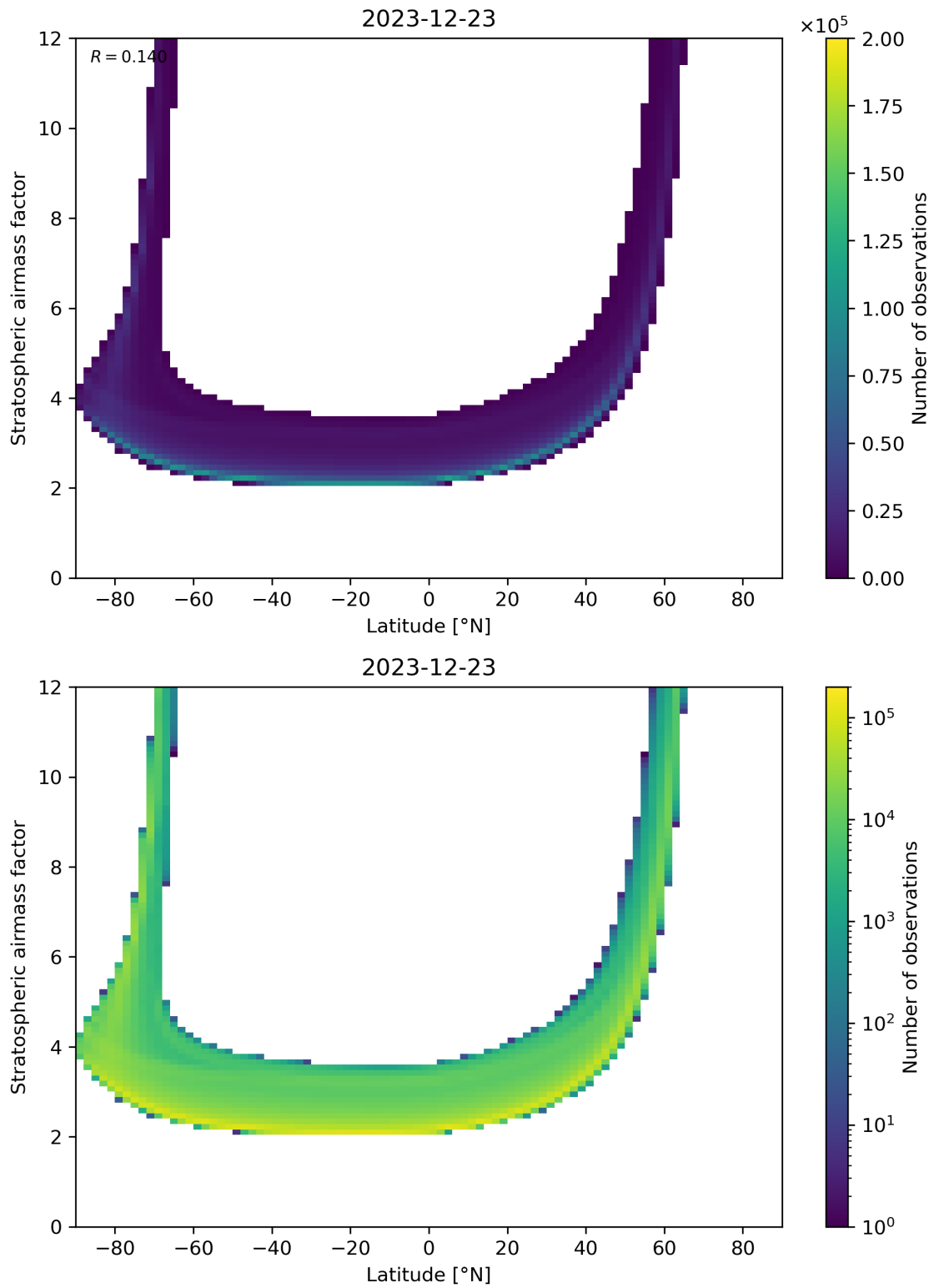
Figure 83: Scatter density plot of “Latitude” against “Stratospheric air mass factor” for 2023-12-22 to 2023-12-24.
