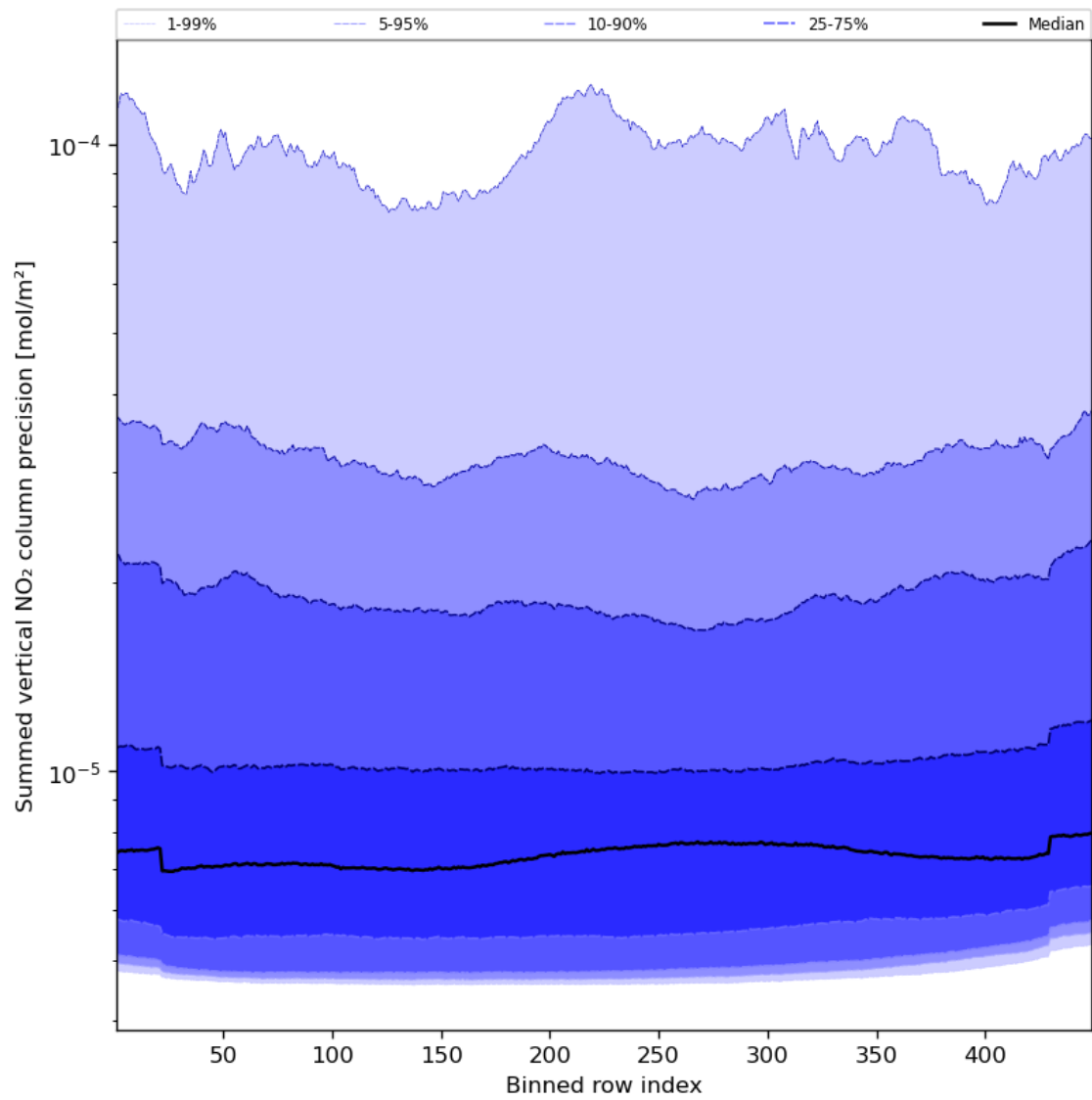
Figure 58: Along track statistics of “Summed vertical NO 2 column precision” for 2023-12-22 to 2023-12-24
