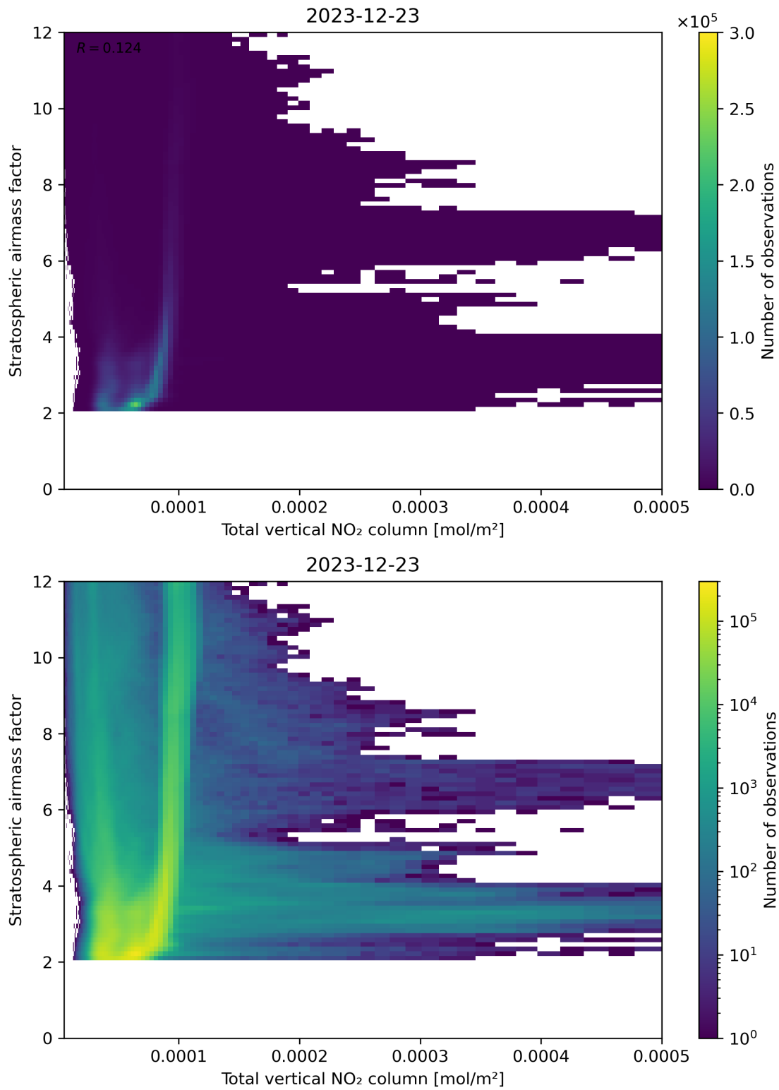
Figure 110: Scatter density plot of “Total vertical NO 2 column” against “Stratospheric air mass factor” for 2023-12-22 to 2023-12-24.
