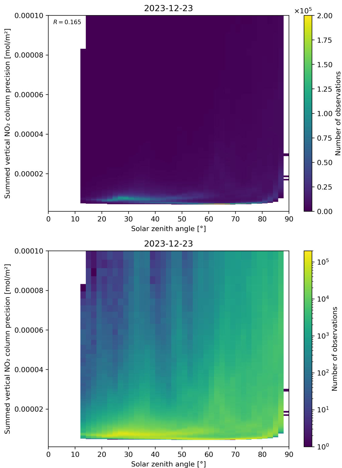
Figure 152: Scatter density plot of “Solar zenith angle” against “Summed vertical NO 2 column precision” for 2023-12-22 to 2023-12-24.
