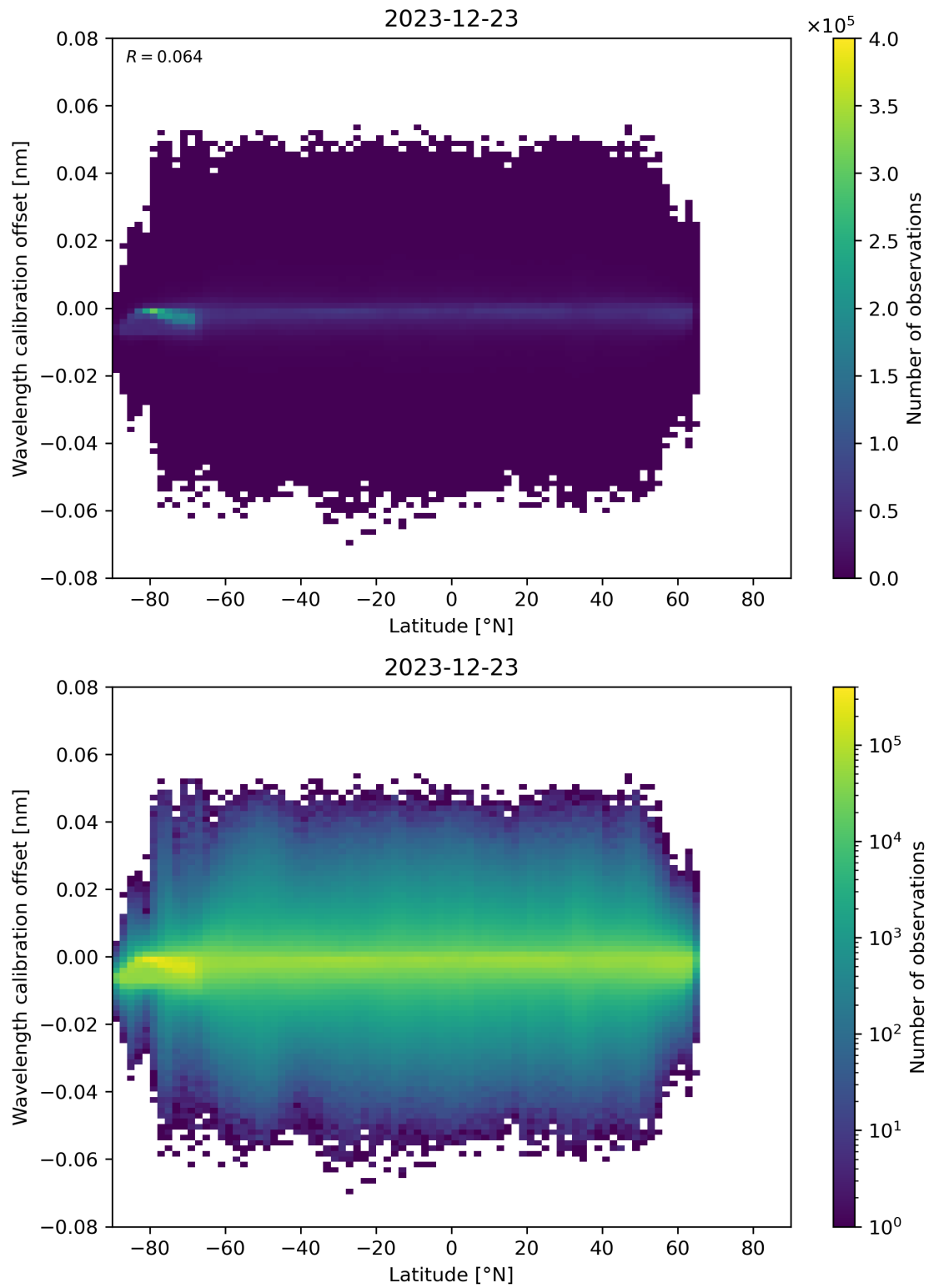
Figure 95: Scatter density plot of “Latitude” against “Wavelength calibration offset” for 2023-12-22 to 2023-12-24.
