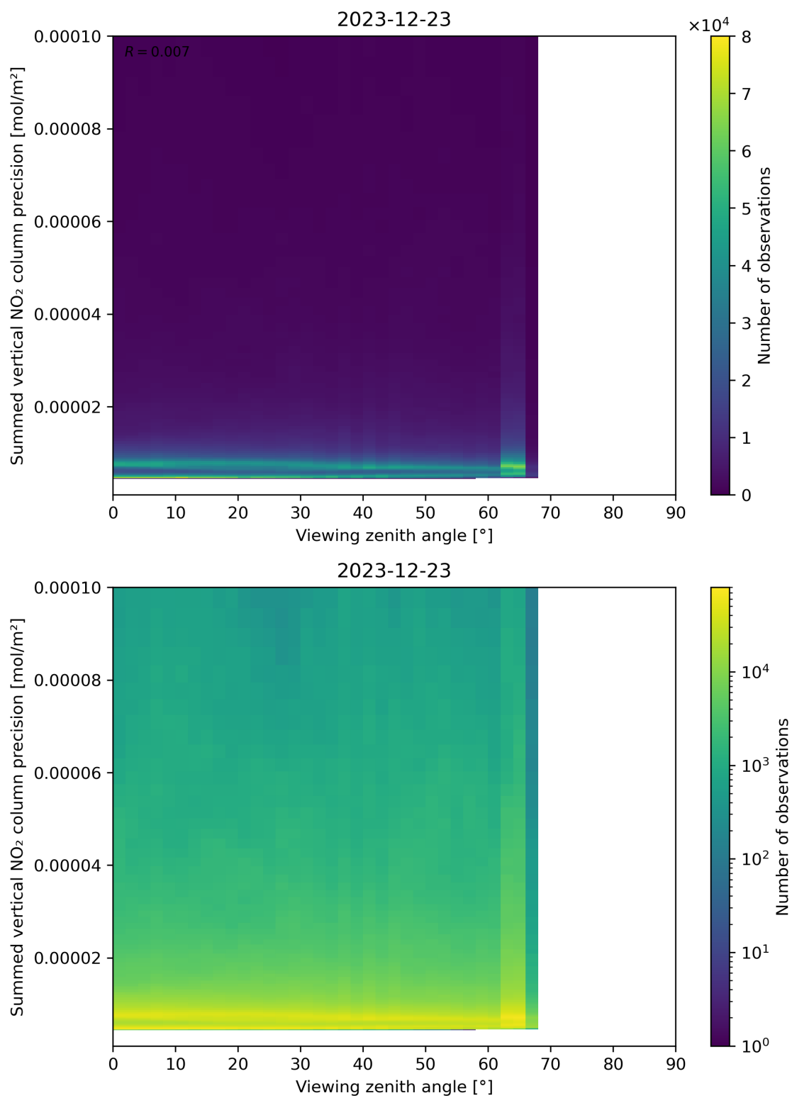
Figure 166: Scatter density plot of “Viewing zenith angle” against “Summed vertical NO 2 column precision” for 2023-12-22 to 2023-12-24.
