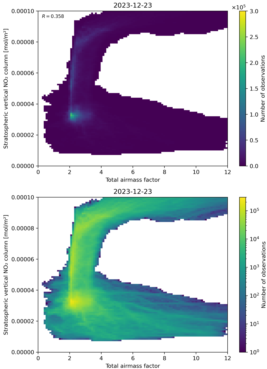
Figure 64: Scatter density plot of “Total airmass factor” against “Stratospheric vertical \text{NO}_2 column” for 2023-12-22 to 2023-12-24.
