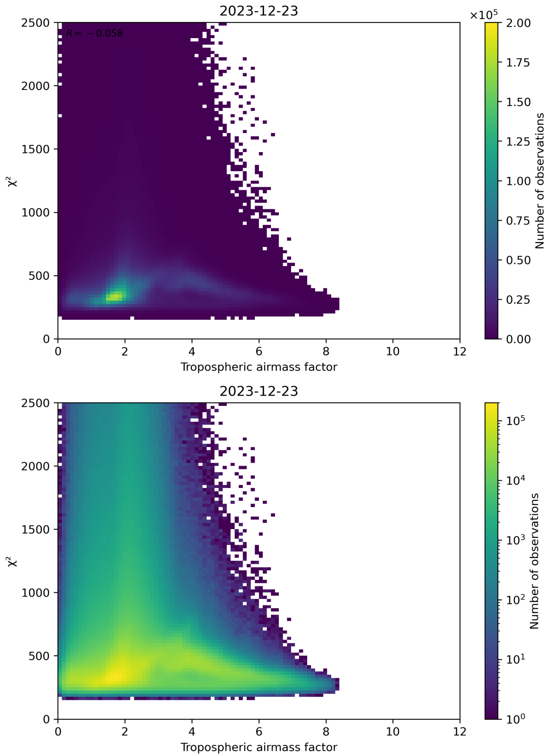
Figure 73: Scatter density plot of “Tropospheric airmass factor” against “ \chi^2 ” for 2023-12-22 to 2023-12-24.
