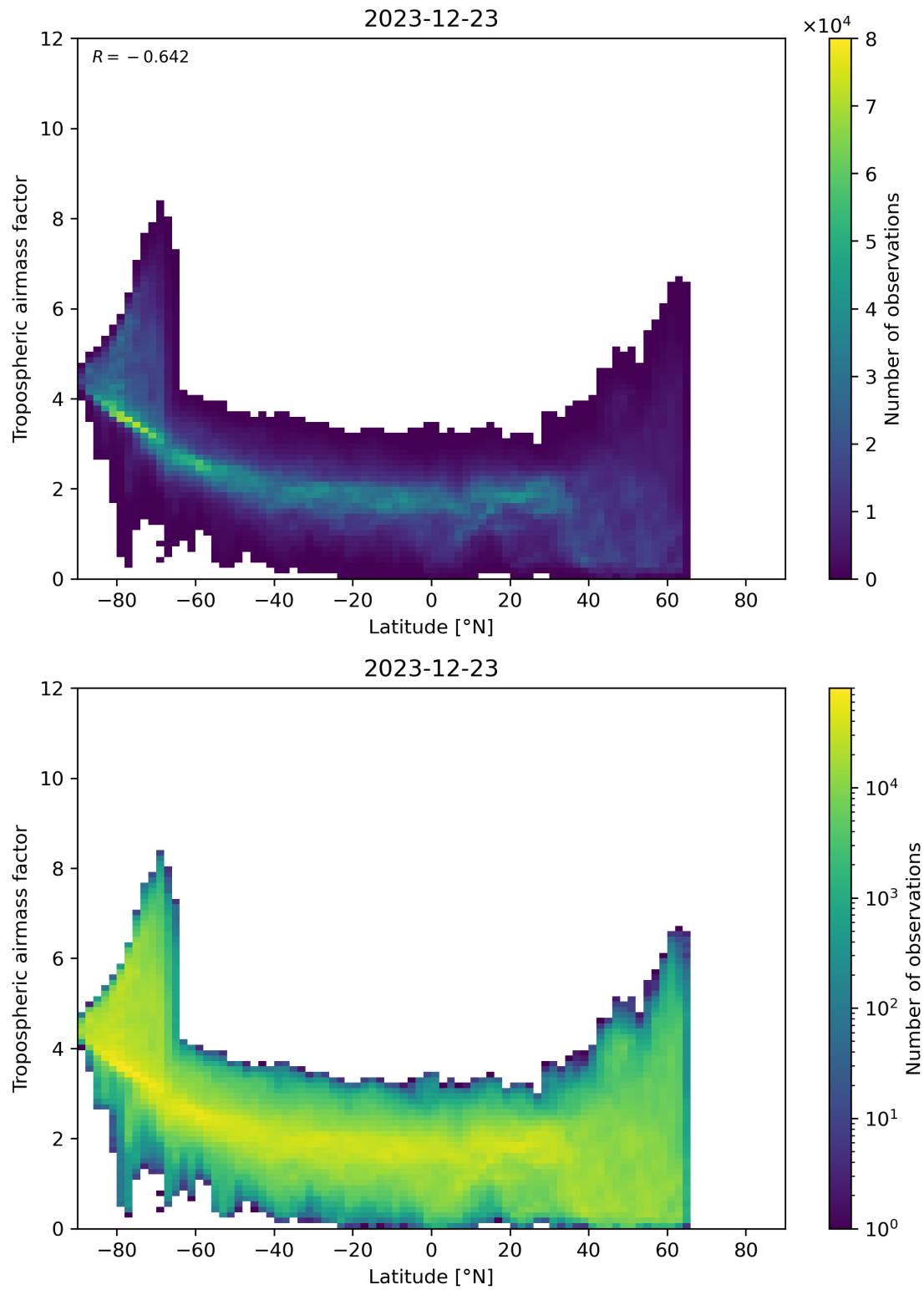
Figure 85: Scatter density plot of “Latitude” against “Tropospheric airmass factor” for 2023-12-22 to 2023-12-24.
