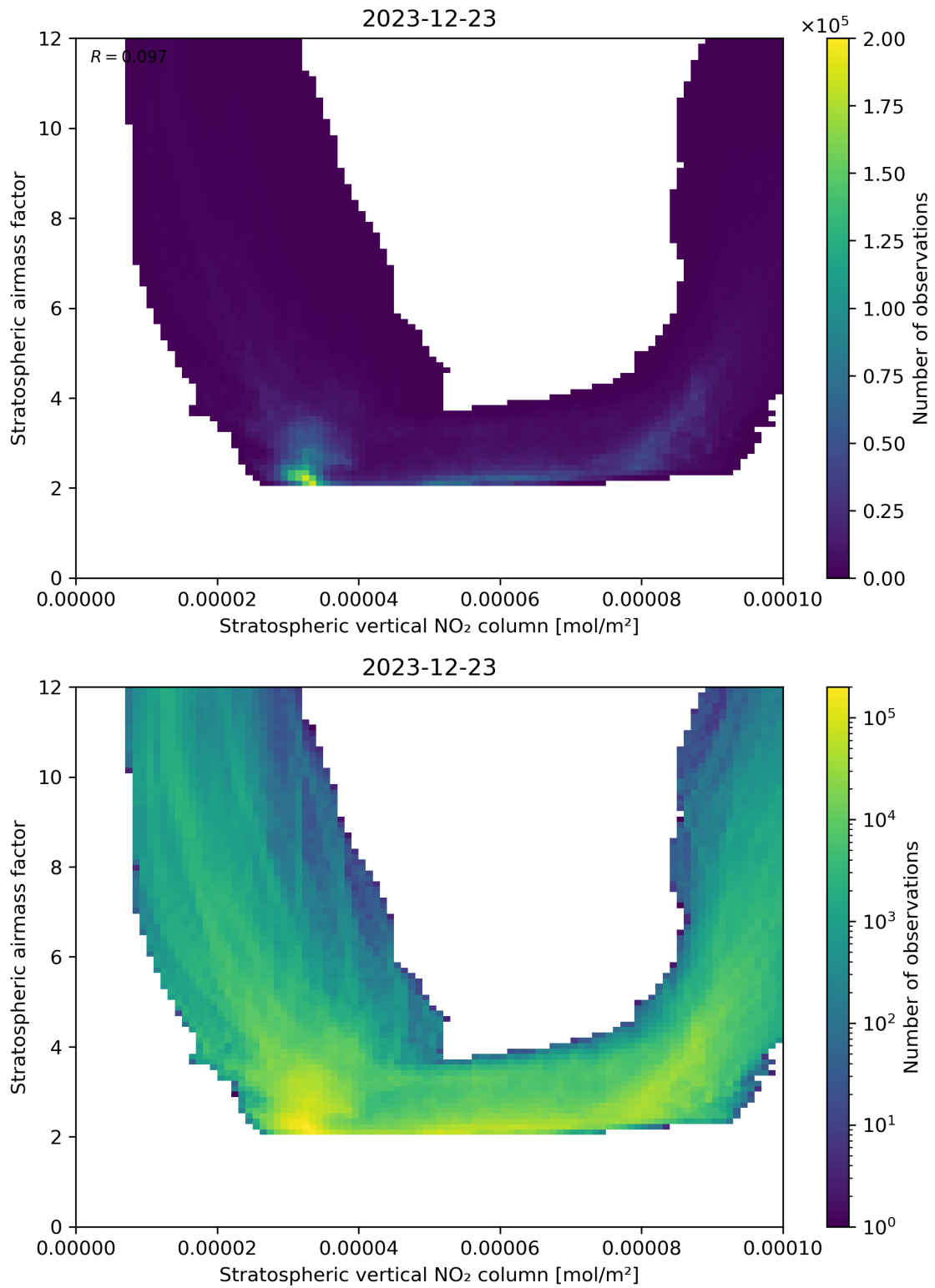
Figure 96: Scatter density plot of “Stratospheric vertical NO 2 column” against “Stratospheric airmass factor” for 2023-12-22 to 2023-12-24.
