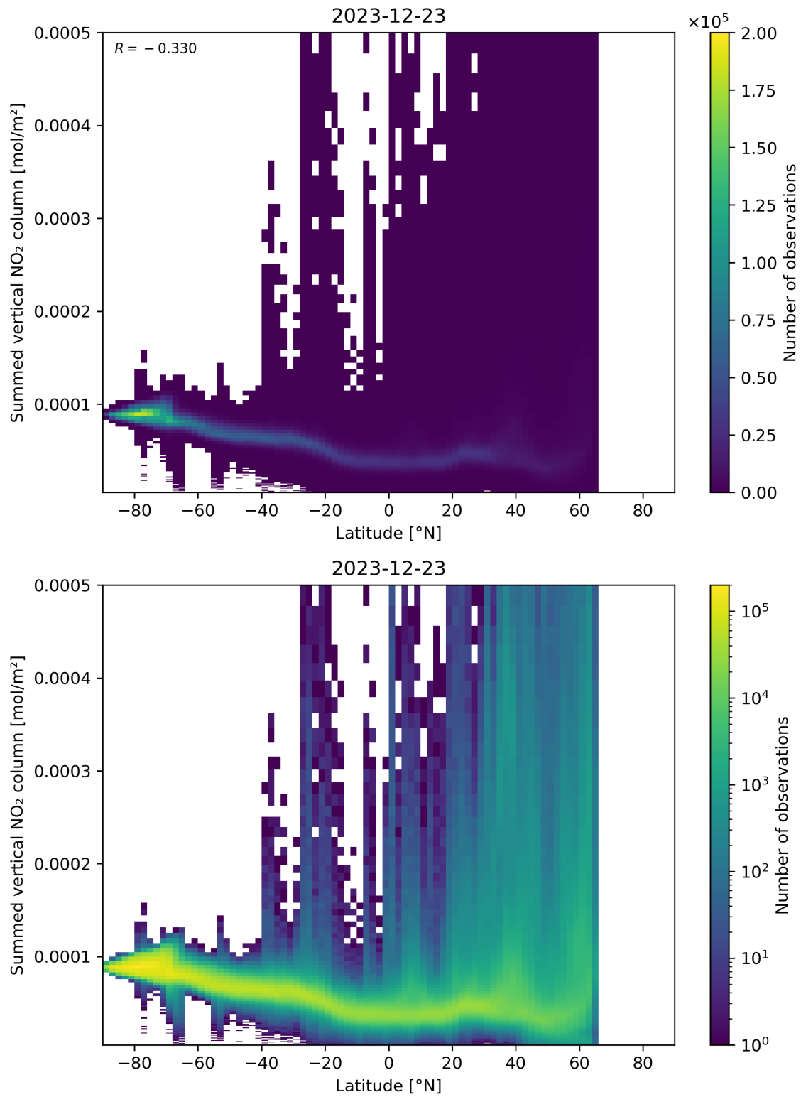
Figure 88: Scatter density plot of “Latitude” against “Summed vertical NO 2 column” for 2023-12-22 to 2023-12-24.
