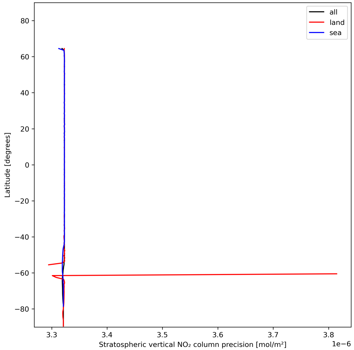
Figure 20: Zonal average of “Stratospheric vertical NO 2 column precision” for 2023-12-22 to 2023-12-24.
