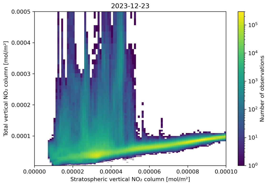
Figure 100: Scatter density plot of “Stratospheric vertical NO 2 column” against “Total vertical NO 2 column” for 2023-12-22 to 2023-12-24.
