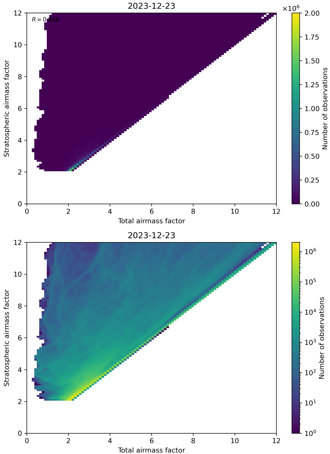
Figure 62: Scatter density plot of “Total airmass factor” against “Stratospheric airmass factor” for 2023-12-22 to 2023-12-24.
