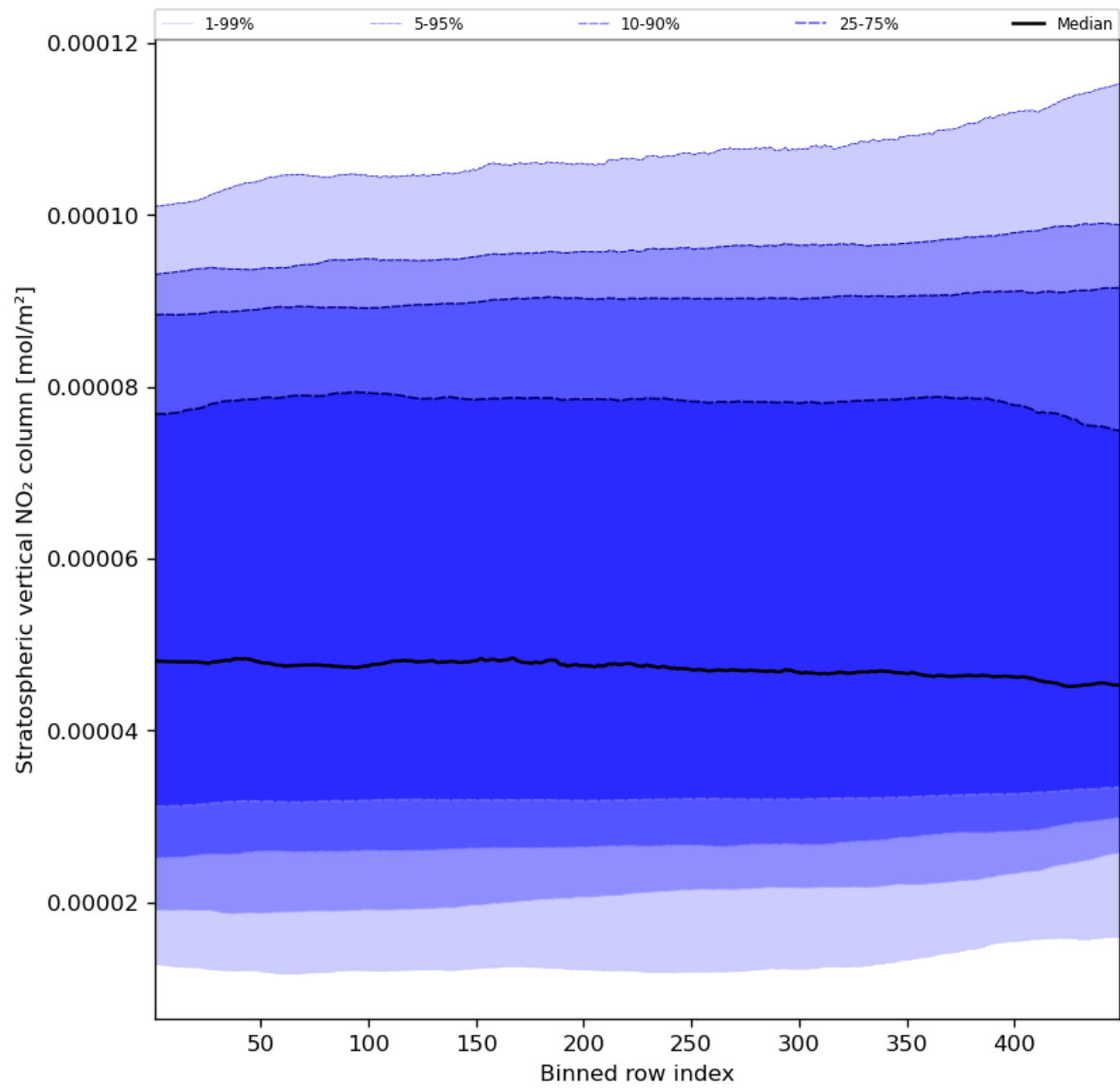
Figure 53: Along track statistics of “Stratospheric vertical NO 2 column” for 2023-12-22 to 2023-12-24
