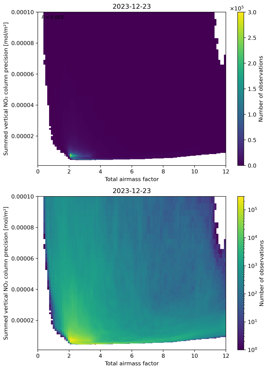
Figure 66: Scatter density plot of “Total airmass factor” against “Summed vertical NO 2 column precision” for 2023-12-22 to 2023-12-24.
