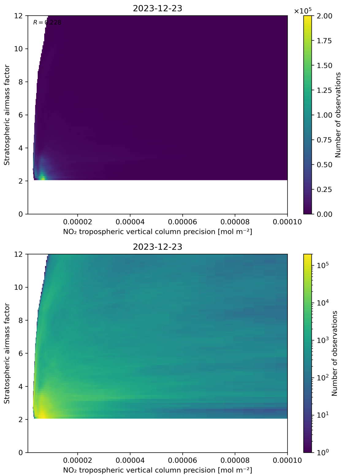
Figure 131: Scatter density plot of “NO 2 tropospheric vertical column precision” against “Stratospheric airmass factor” for 2023-12-22 to 2023-12-24.
