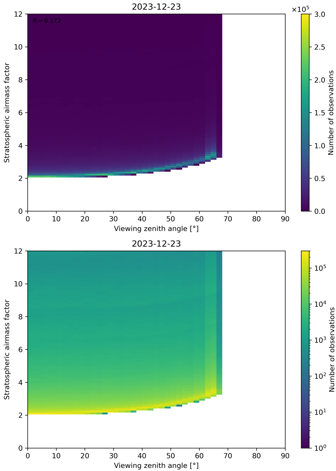
Figure 159: Scatter density plot of “Viewing zenith angle” against “Stratospheric airmass factor” for 2023-12-22 to 2023-12-24.
