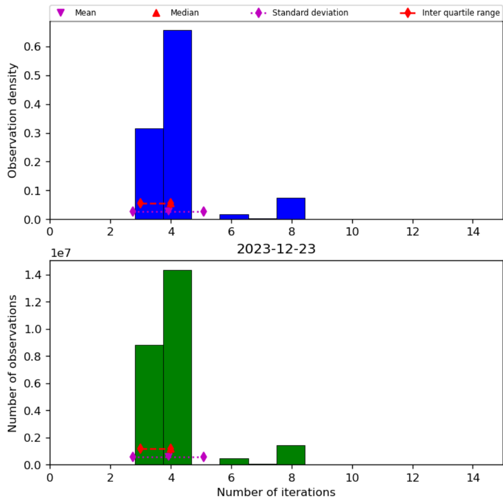
Figure 34: Histogram of “Number of iterations” for 2023-12-22 to 2023-12-24
