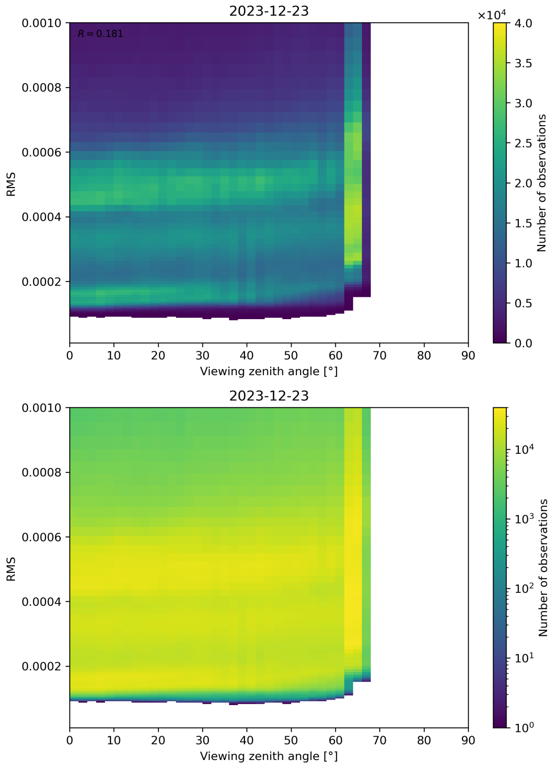
Figure 171: Scatter density plot of “Viewing zenith angle” against “RMS” for 2023-12-22 to 2023-12-24.
