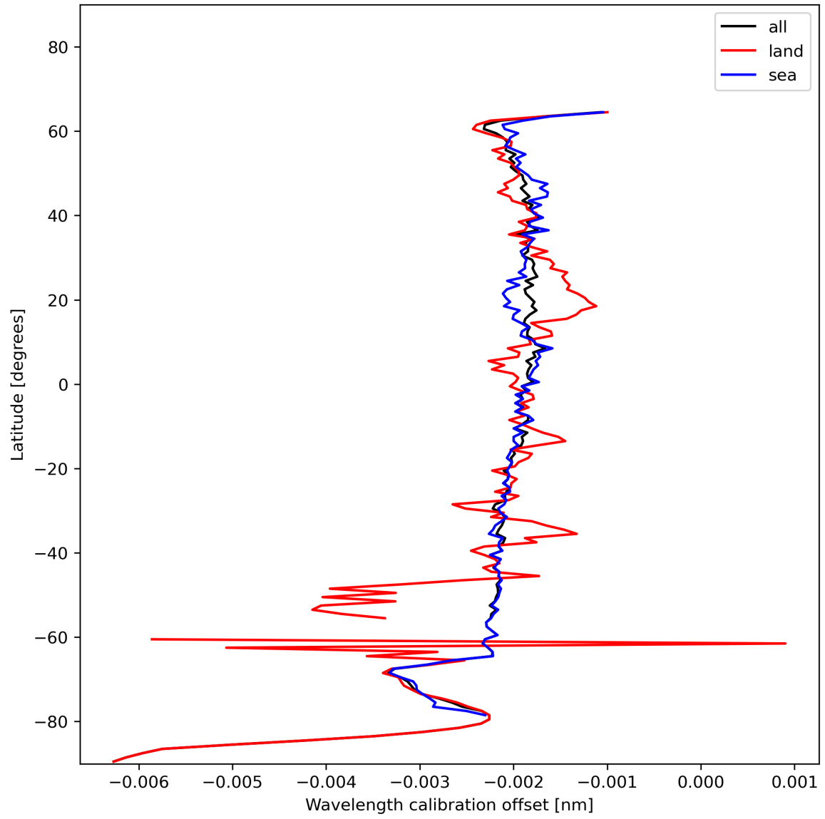
Figure 18: Zonal average of “Wavelength calibration offset” for 2023-12-22 to 2023-12-24.
