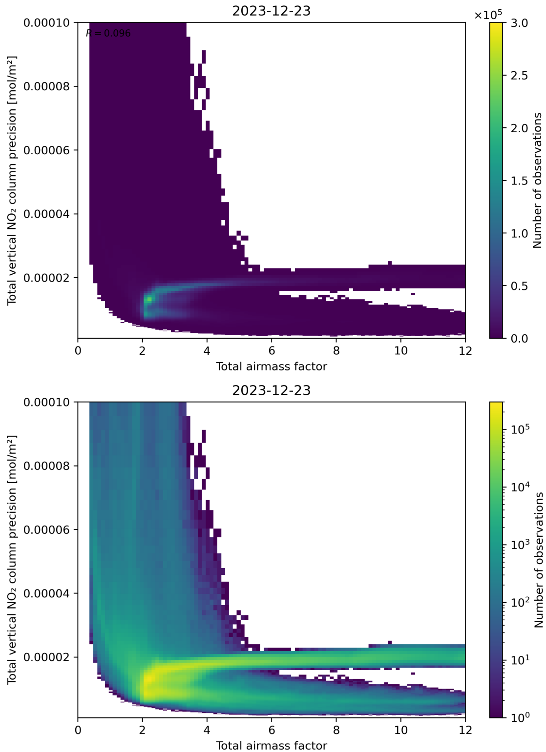
Figure 68: Scatter density plot of “Total airmass factor” against “Total vertical NO 2 column precision” for 2023-12-22 to 2023-12-24.
