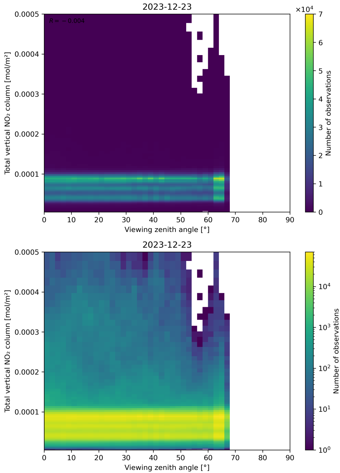
Figure 167: Scatter density plot of “Viewing zenith angle” against “Total vertical NO 2 column” for 2023-12-22 to 2023-12-24.
