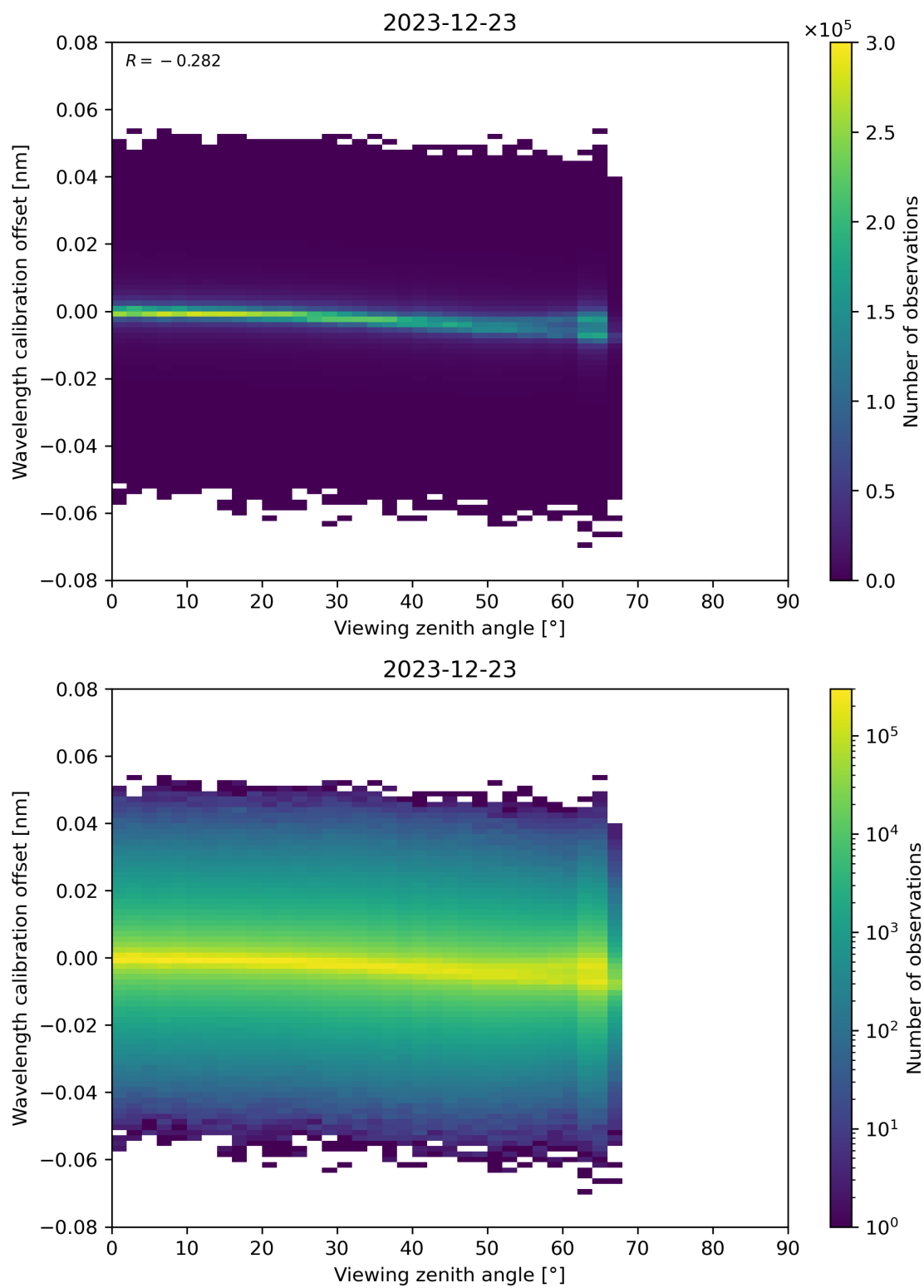
Figure 173: Scatter density plot of “Viewing zenith angle” against “Wavelength calibration offset” for 2023-12-22 to 2023-12-24.
