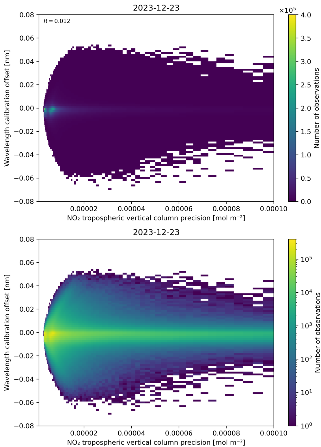
Figure 141: Scatter density plot of “NO 2 tropospheric vertical column precision” against “Wavelength calibration offset” for 2023-12-22 to 2023-12-24.
