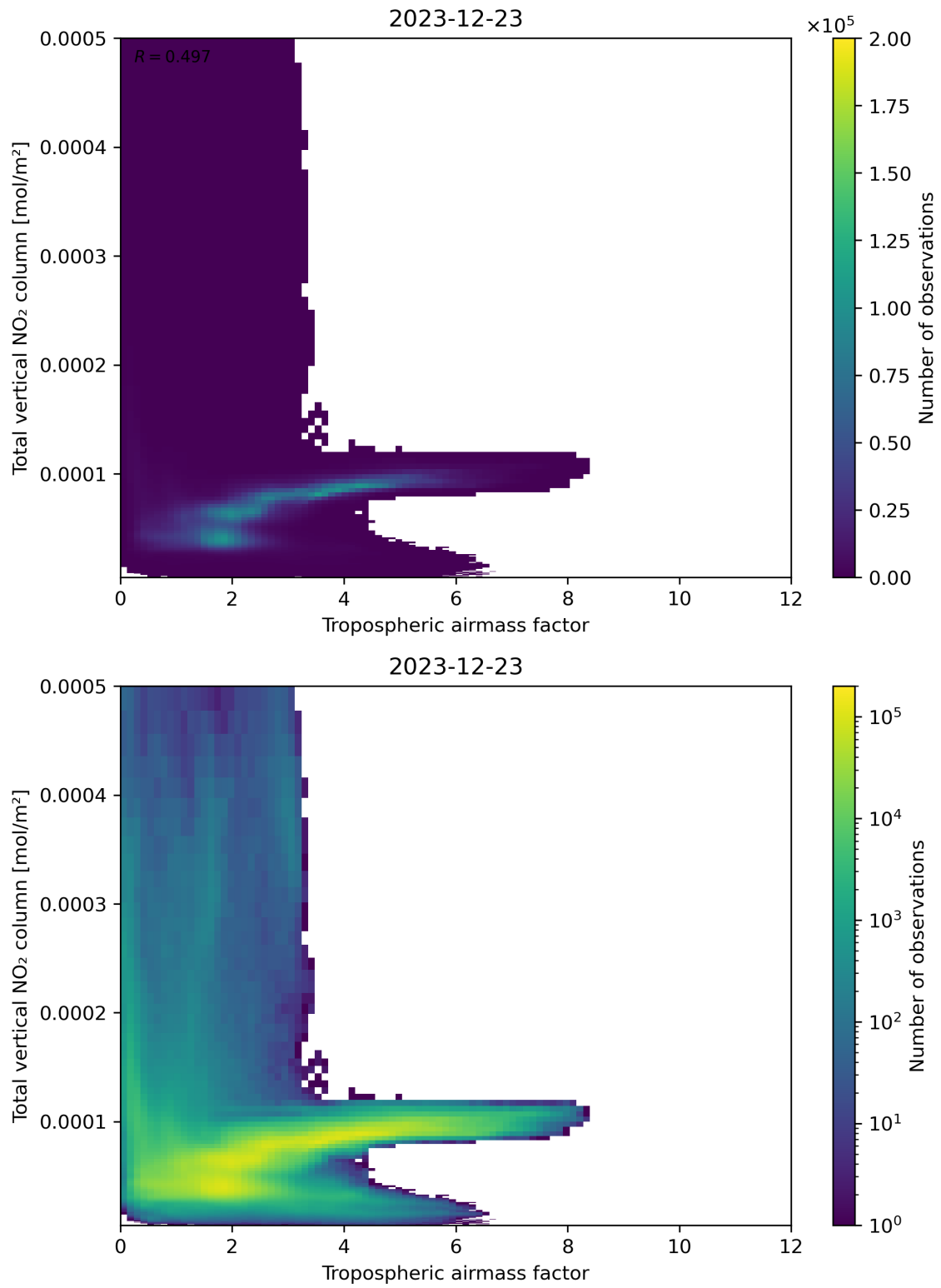
Figure 77: Scatter density plot of “Tropospheric airmass factor” against “Total vertical NO 2 column” for 2023-12-22 to 2023-12-24.
