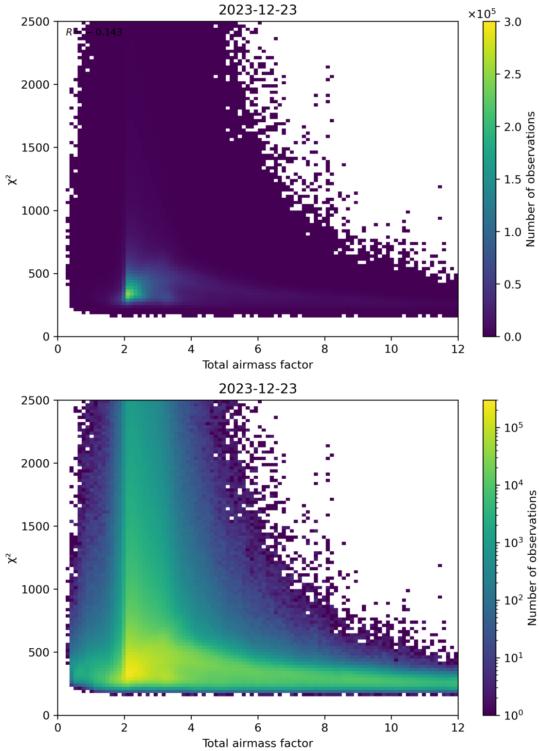
Figure 63: Scatter density plot of “Total airmass factor” against “ \chi^2 ” for 2023-12-22 to 2023-12-24.
