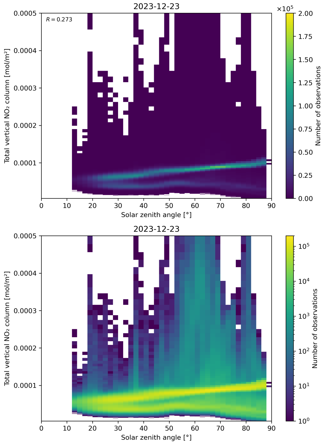
Figure 153: Scatter density plot of “Solar zenith angle” against “Total vertical NO 2 column” for 2023-12-22 to 2023-12-24.
