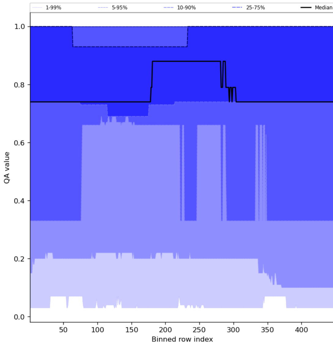
Figure 45: Along track statistics of “QA value” for 2023-12-22 to 2023-12-24
