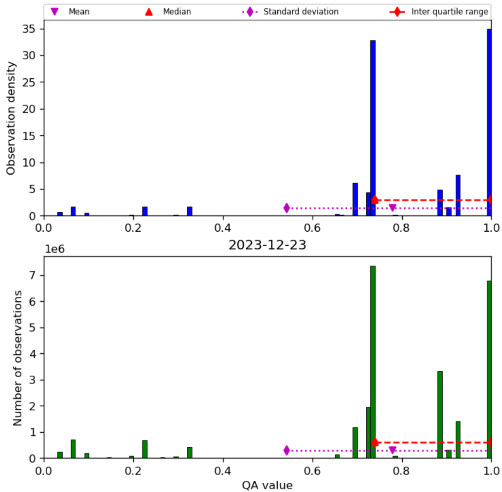
Figure 28: Histogram of “QA value” for 2023-12-22 to 2023-12-24
