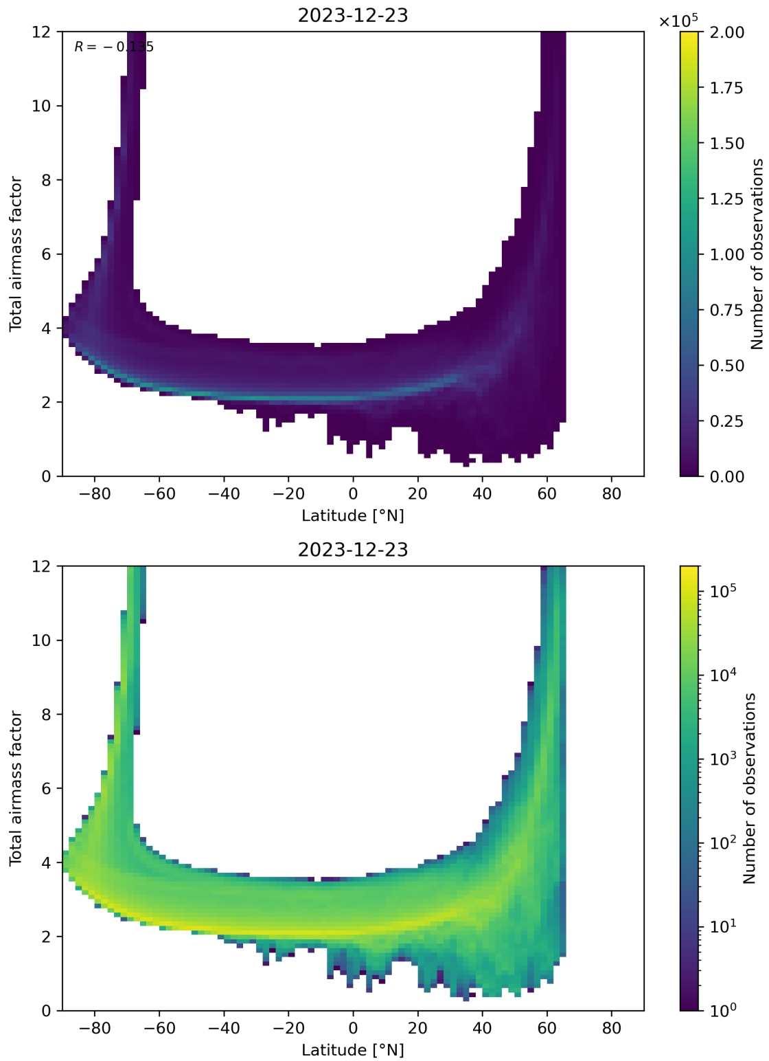
Figure 84: Scatter density plot of “Latitude” against “Total airmass factor” for 2023-12-22 to 2023-12-24.
