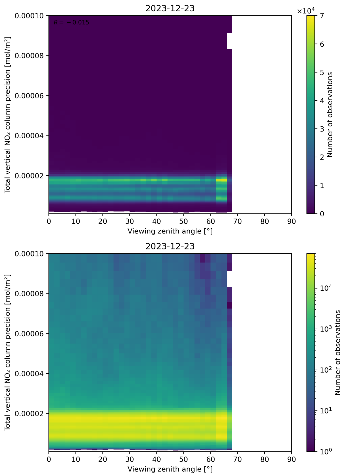
Figure 168: Scatter density plot of “Viewing zenith angle” against “Total vertical NO 2 column precision” for 2023-12-22 to 2023-12-24.
