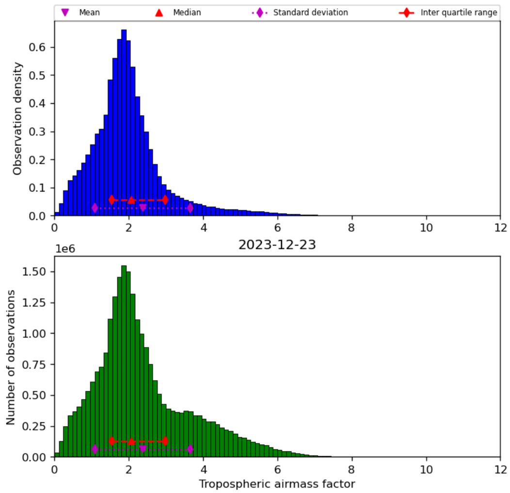
Figure 31: Histogram of “Tropospheric airmass factor” for 2023-12-22 to 2023-12-24
