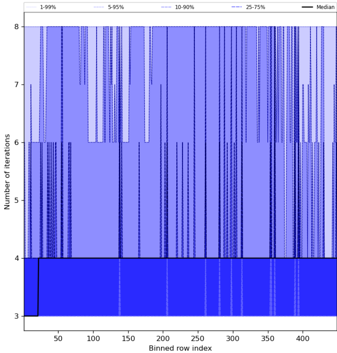
Figure 51: Along track statistics of “Number of iterations” for 2023-12-22 to 2023-12-24
