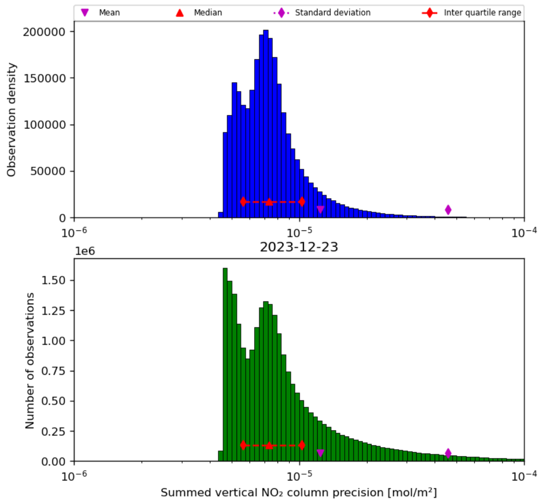
Figure 41: Histogram of “Summed vertical NO 2 column precision” for 2023-12-22 to 2023-12-24
