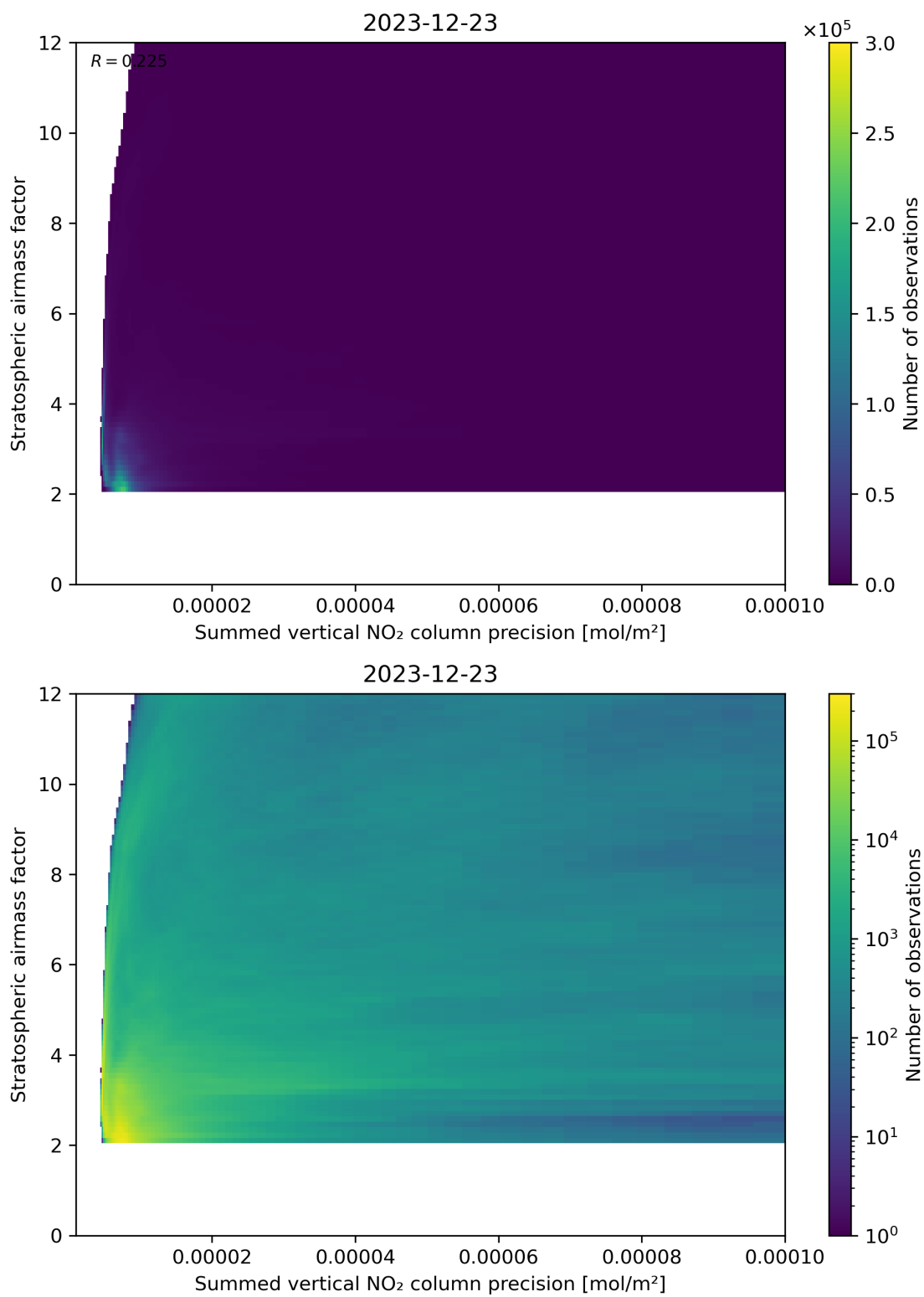
Figure 106: Scatter density plot of “Summed vertical NO 2 column precision” against “Stratospheric airmass factor” for 2023-12-22 to 2023-12-24.
