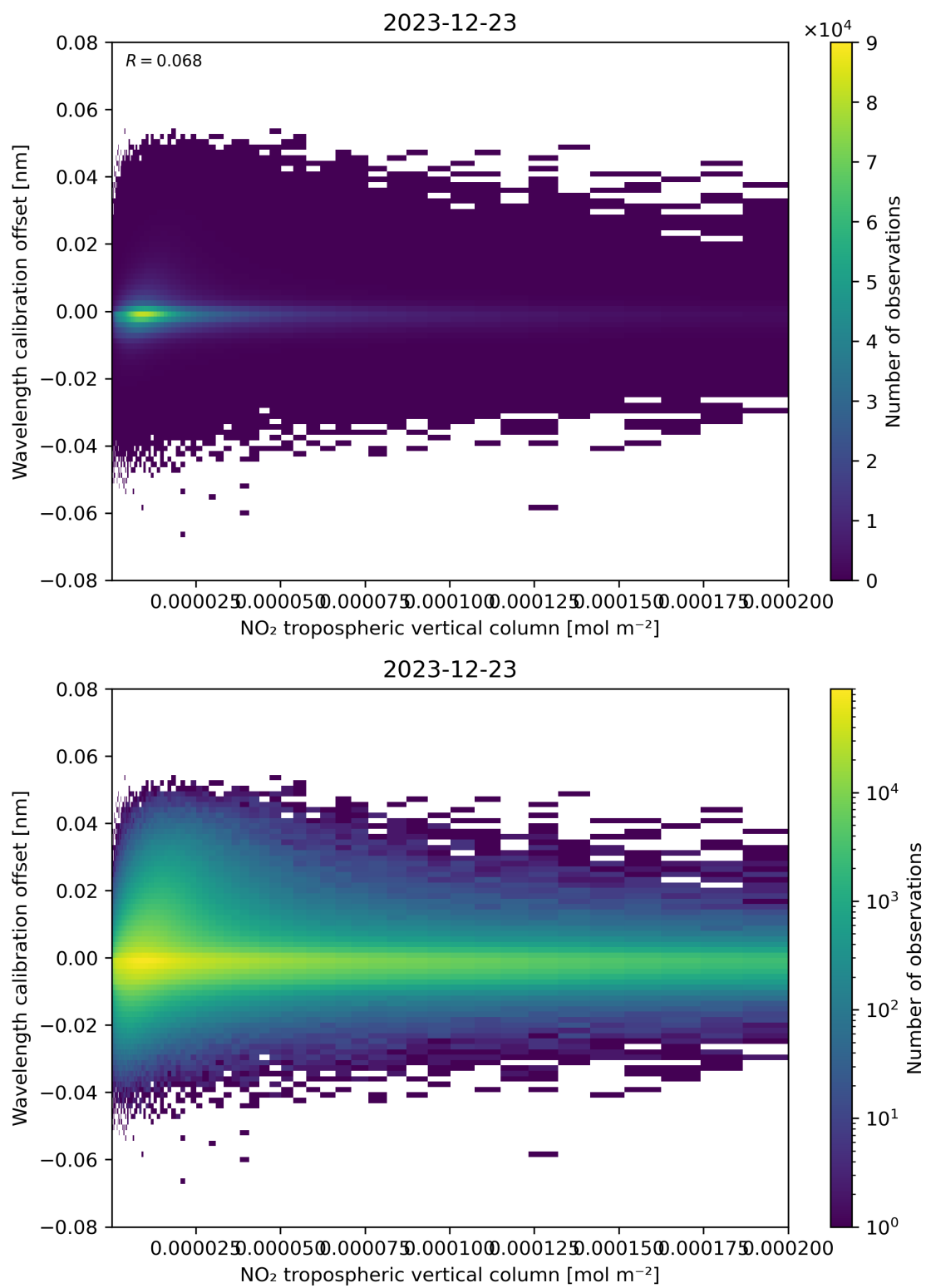
Figure 143: Scatter density plot of “NO 2 tropospheric vertical column” against “Wavelength calibration offset” for 2023-12-22 to 2023-12-24.
