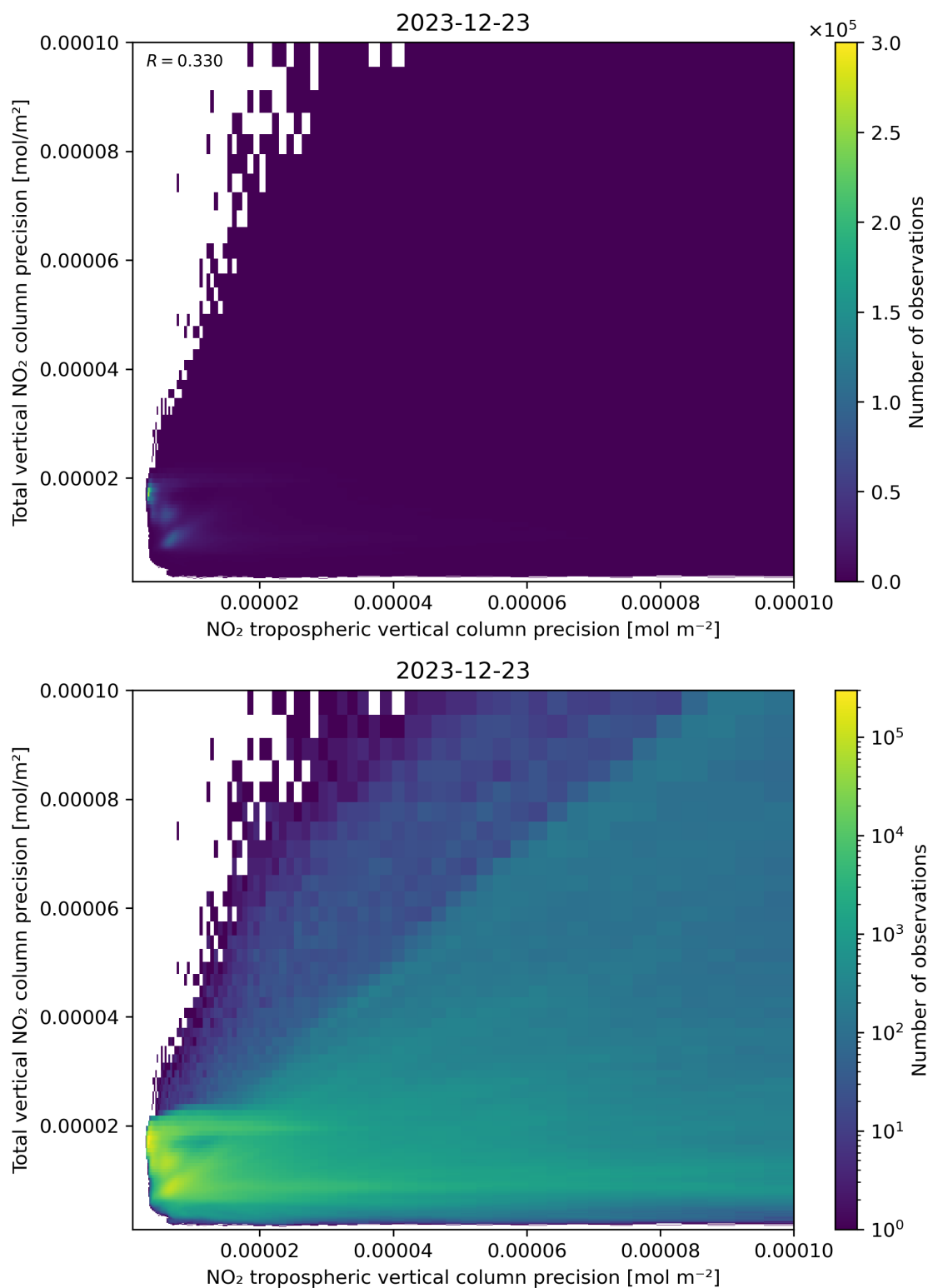
Figure 139: Scatter density plot of “NO 2 tropospheric vertical column precision” against “Total vertical NO 2 column precision” for 2023-12-22 to 2023-12-24.
