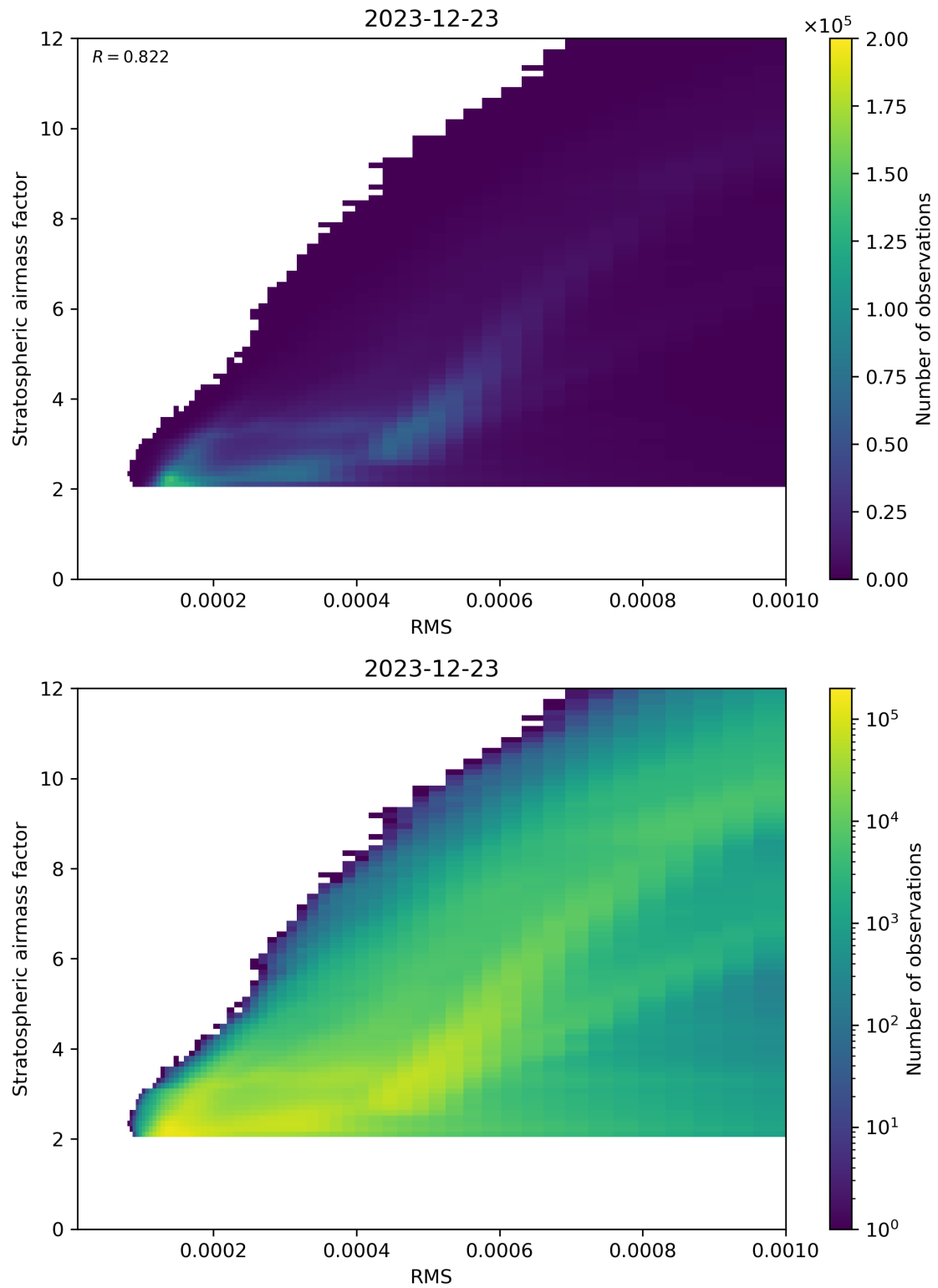
Figure 144: Scatter density plot of “RMS” against “Stratospheric airmass factor” for 2023-12-22 to 2023-12-24.
