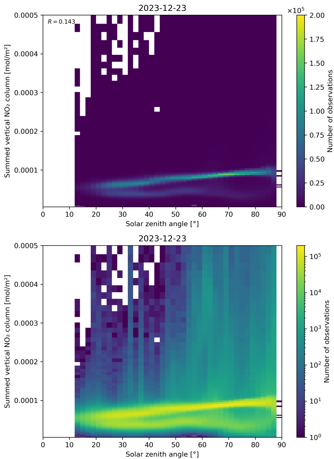
Figure 151: Scatter density plot of “Solar zenith angle” against “Summed vertical NO 2 column” for 2023-12-22 to 2023-12-24.
