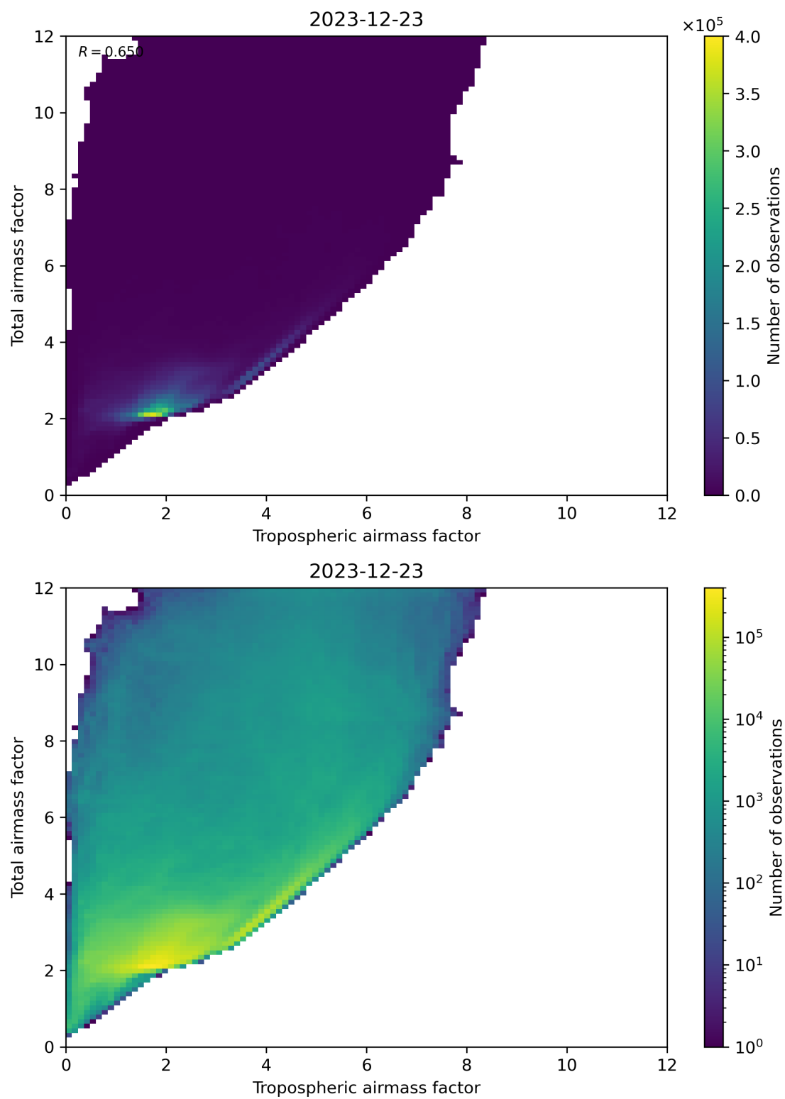
Figure 72: Scatter density plot of “Tropospheric airmass factor” against “Total airmass factor” for 2023-12-22 to 2023-12-24.
