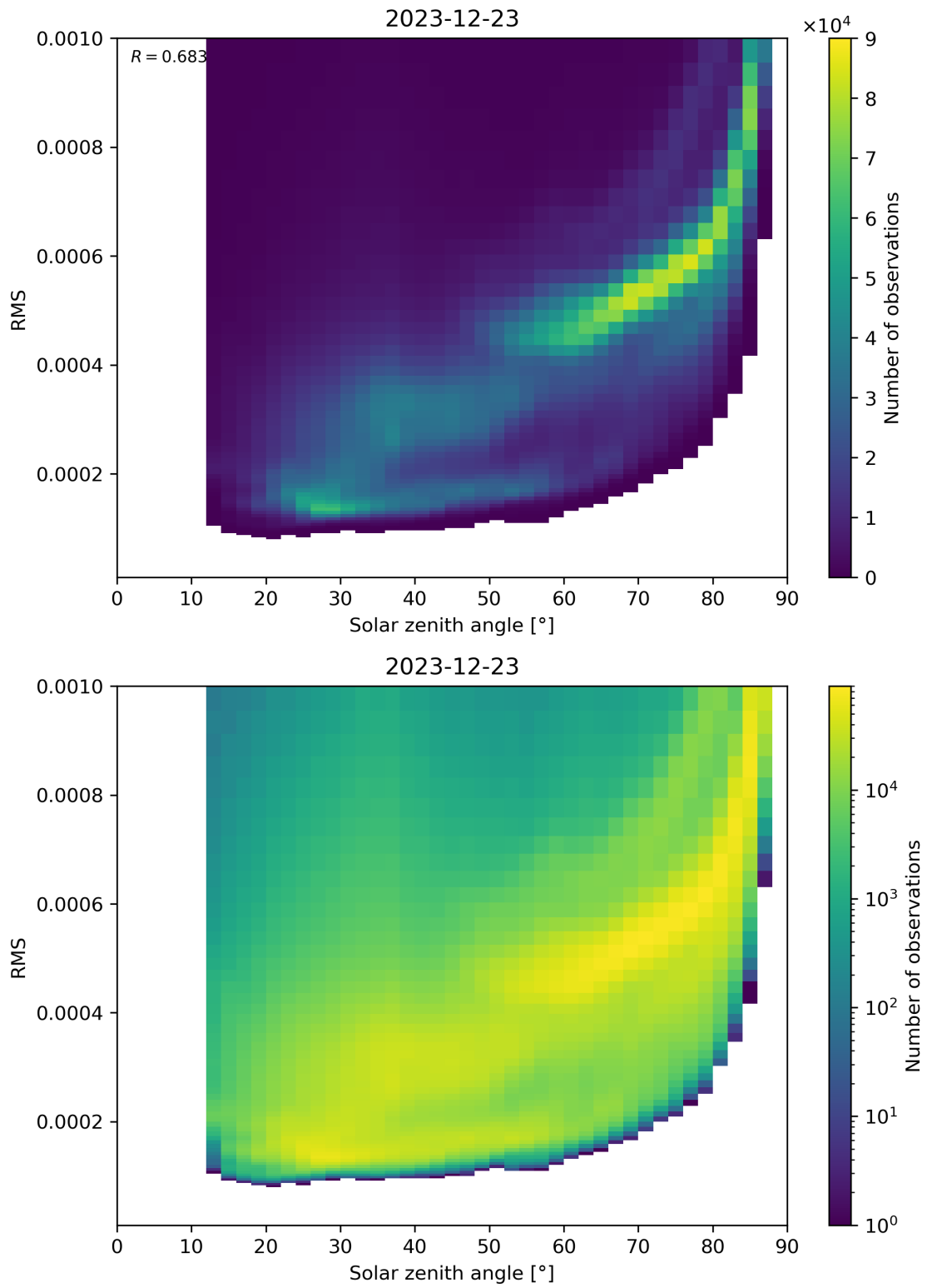
Figure 157: Scatter density plot of “Solar zenith angle” against “RMS” for 2023-12-22 to 2023-12-24.
