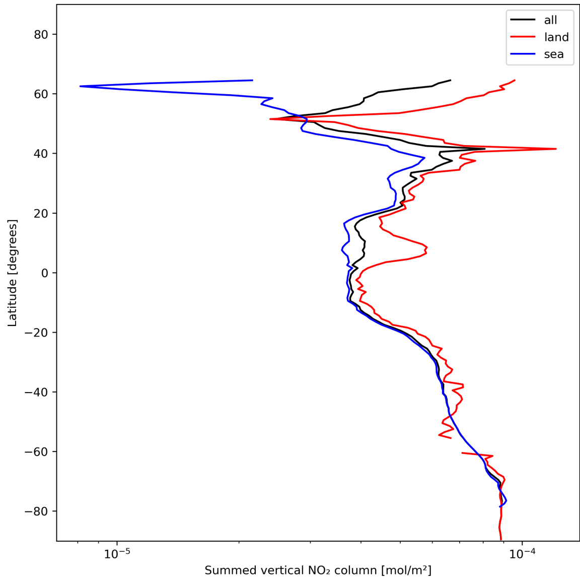
Figure 23: Zonal average of “Summed vertical NO 2 column” for 2023-12-22 to 2023-12-24.
