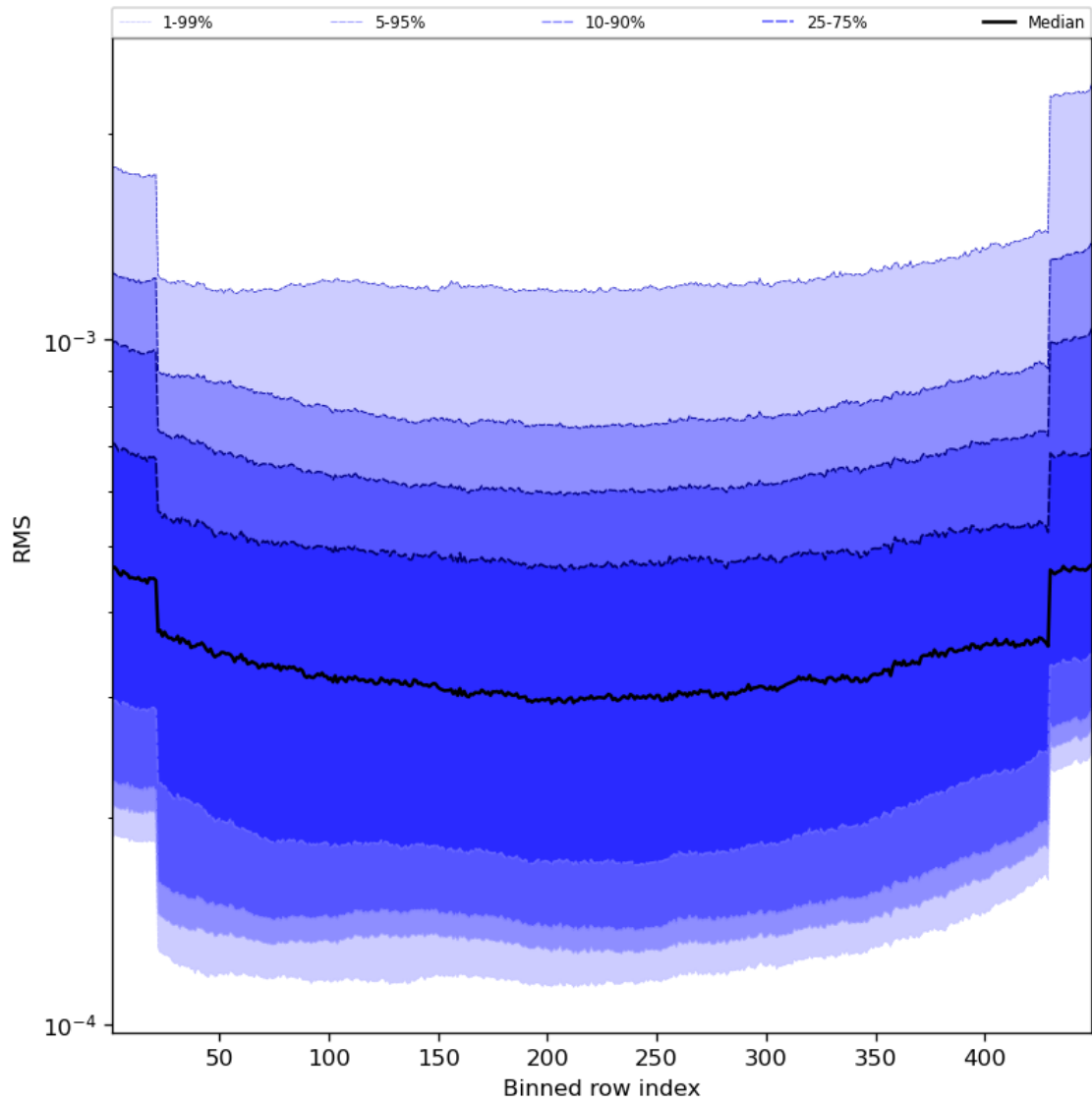
Figure 60: Along track statistics of “RMS” for 2023-12-22 to 2023-12-24
