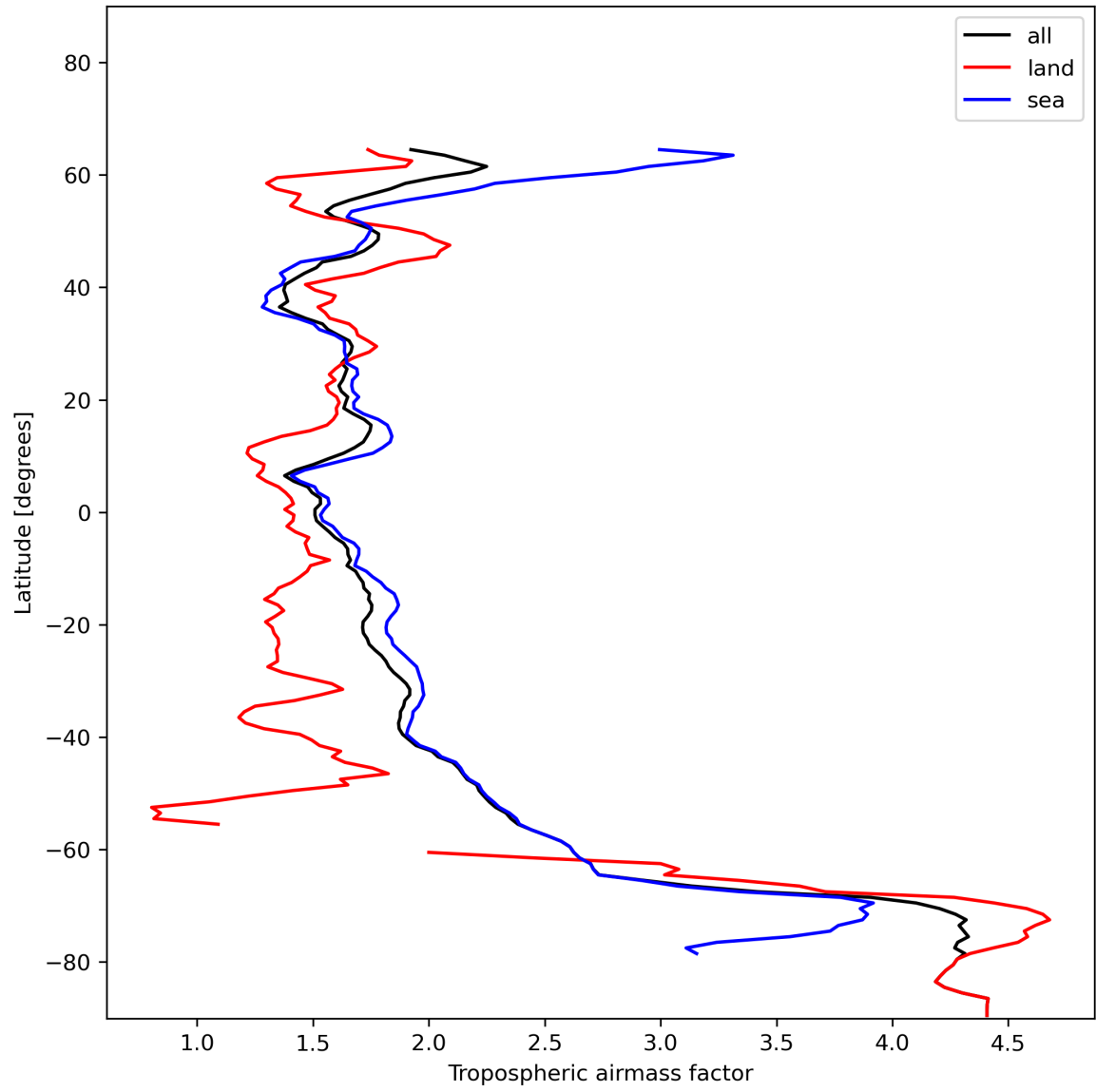
Figure 14: Zonal average of “Tropospheric airmass factor” for 2023-12-22 to 2023-12-24.
