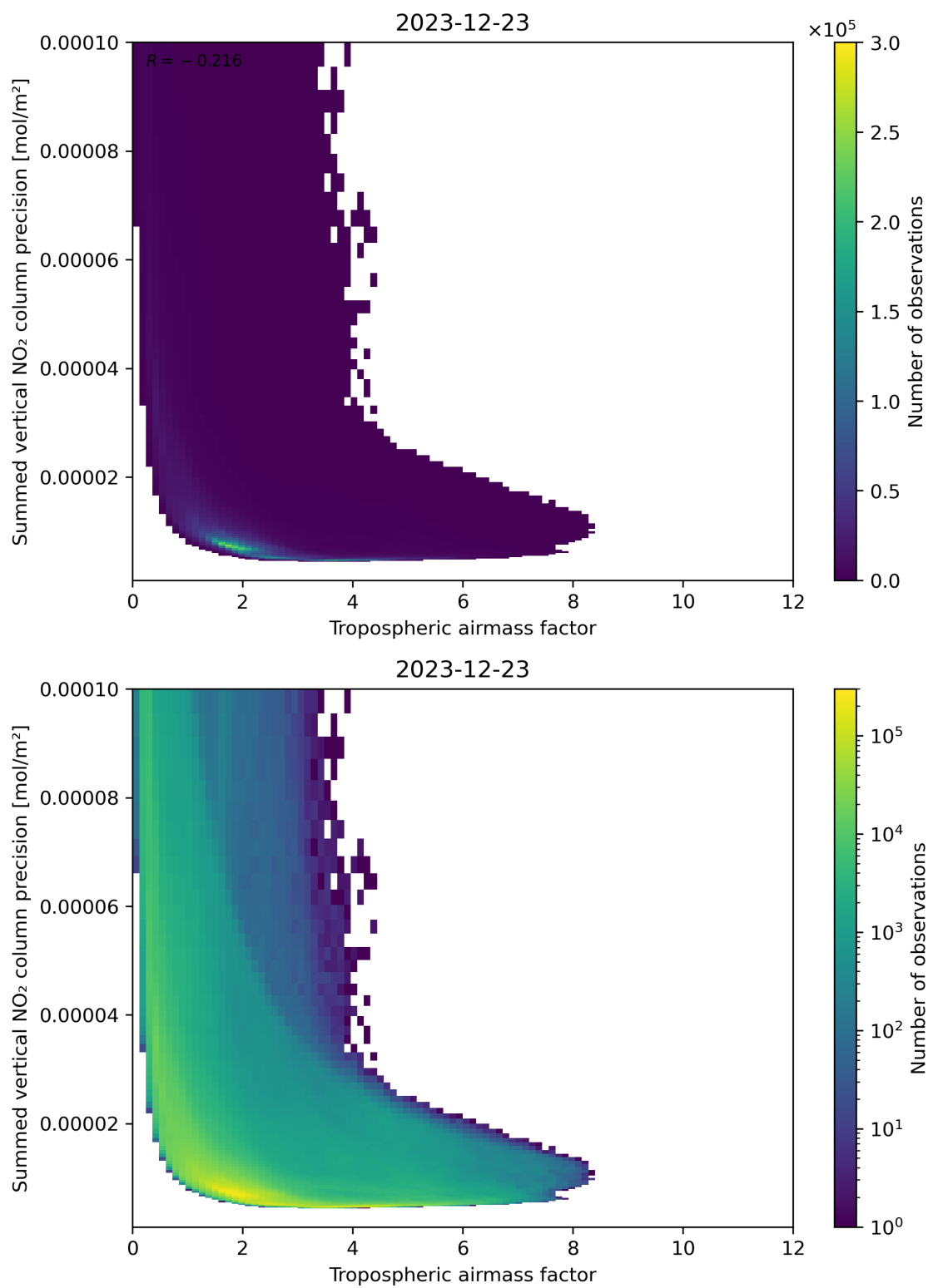
Figure 76: Scatter density plot of “Tropospheric air mass factor” against “Summed vertical NO 2 column precision” for 2023-12-22 to 2023-12-24.
