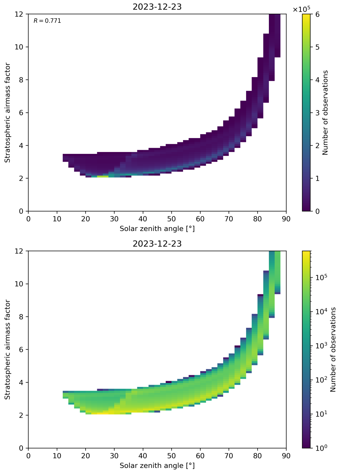
Figure 145: Scatter density plot of “Solar zenith angle” against “Stratospheric airmass factor” for 2023-12-22 to 2023-12-24.
