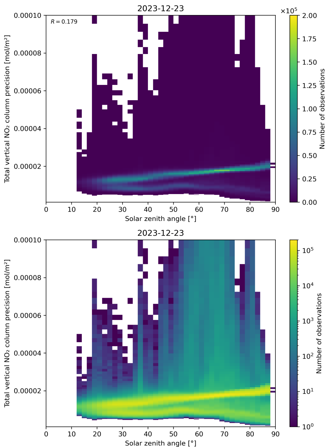
Figure 154: Scatter density plot of “Solar zenith angle” against “Total vertical NO 2 column precision” for 2023-12-22 to 2023-12-24.
