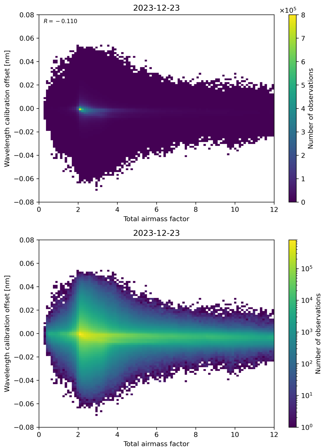
Figure 70: Scatter density plot of “Total airmass factor” against “Wavelength calibration offset” for 2023-12-22 to 2023-12-24.
