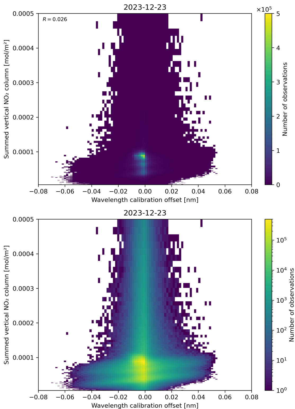
Figure 177: Scatter density plot of “Wavelength calibration offset” against “Summed vertical NO 2 column” for 2023-12-22 to 2023-12-24.
