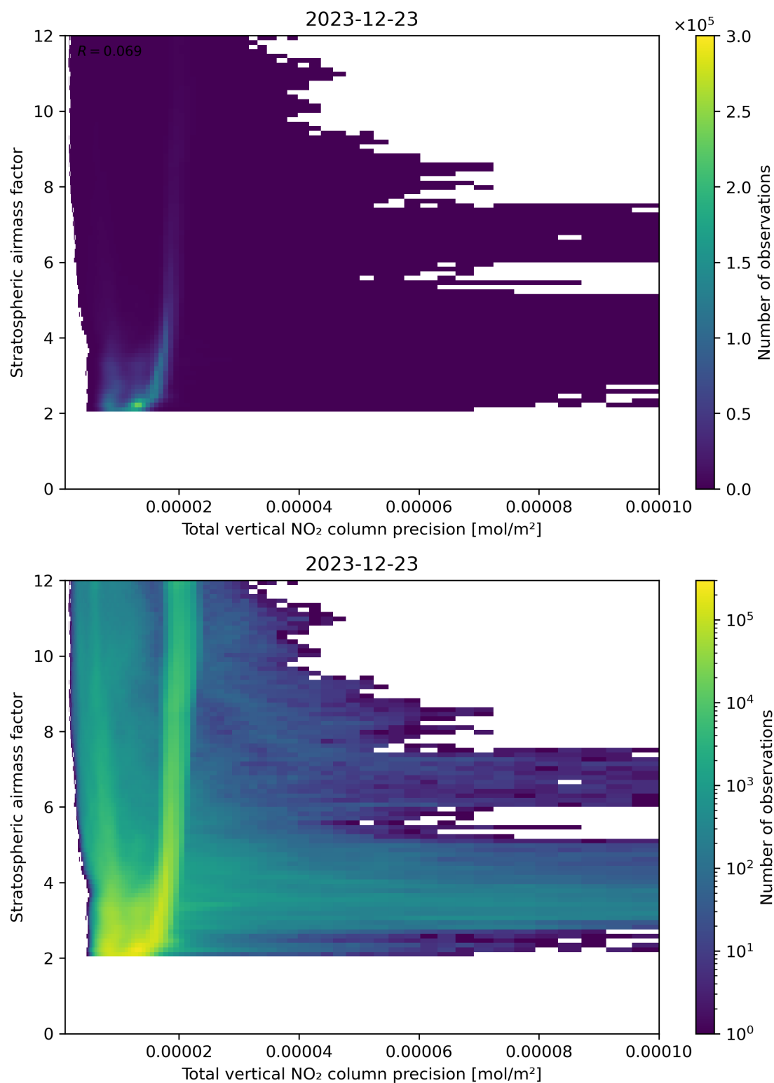
Figure 115: Scatter density plot of “Total vertical NO 2 column precision” against “Stratospheric air mass factor” for 2023-12-22 to 2023-12-24.
