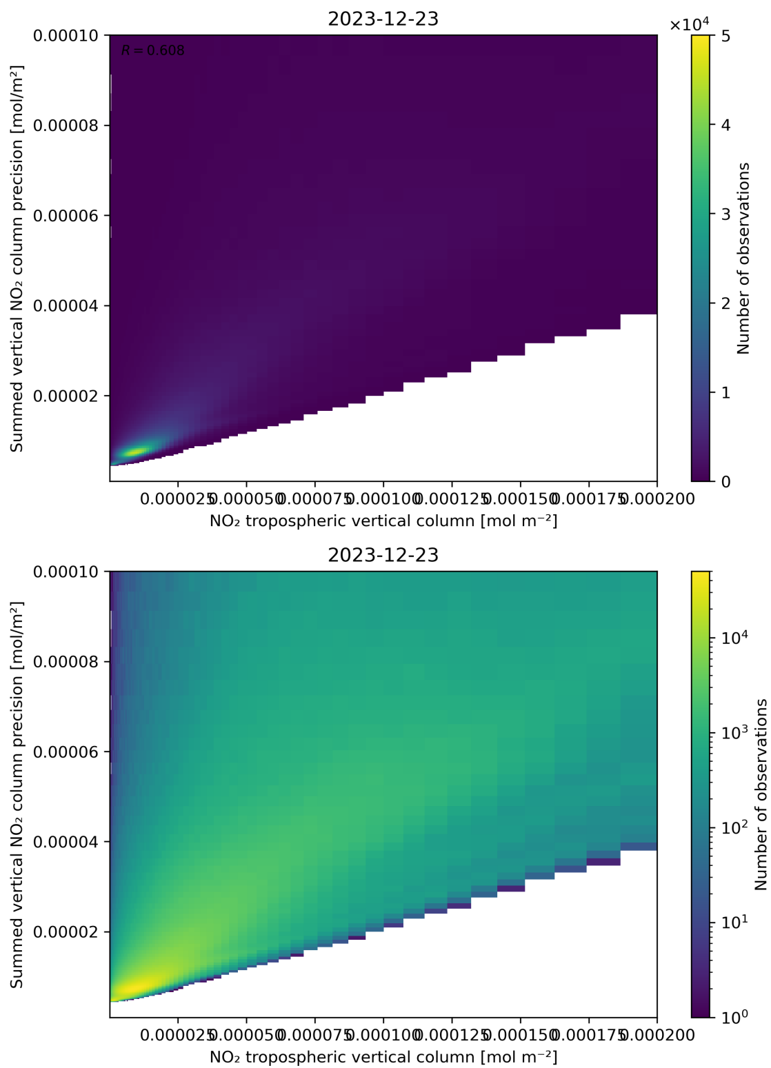
Figure 127: Scatter density plot of “NO 2 tropospheric vertical column” against “Summed vertical NO 2 column precision” for 2023-12-22 to 2023-12-24.
