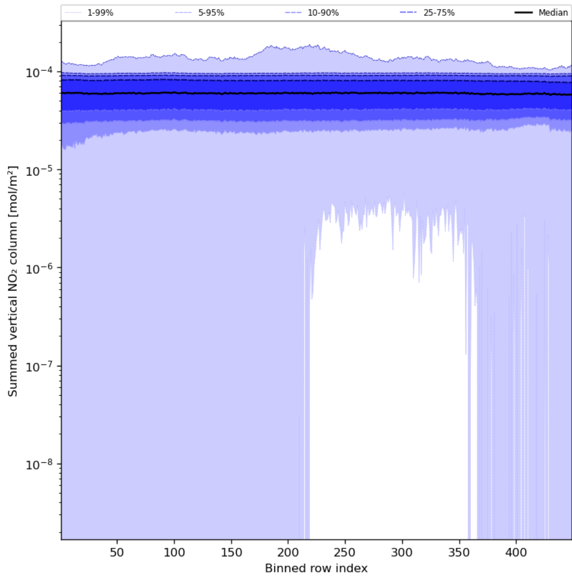
Figure 57: Along track statistics of “Summed vertical NO 2 column” for 2023-12-22 to 2023-12-24
