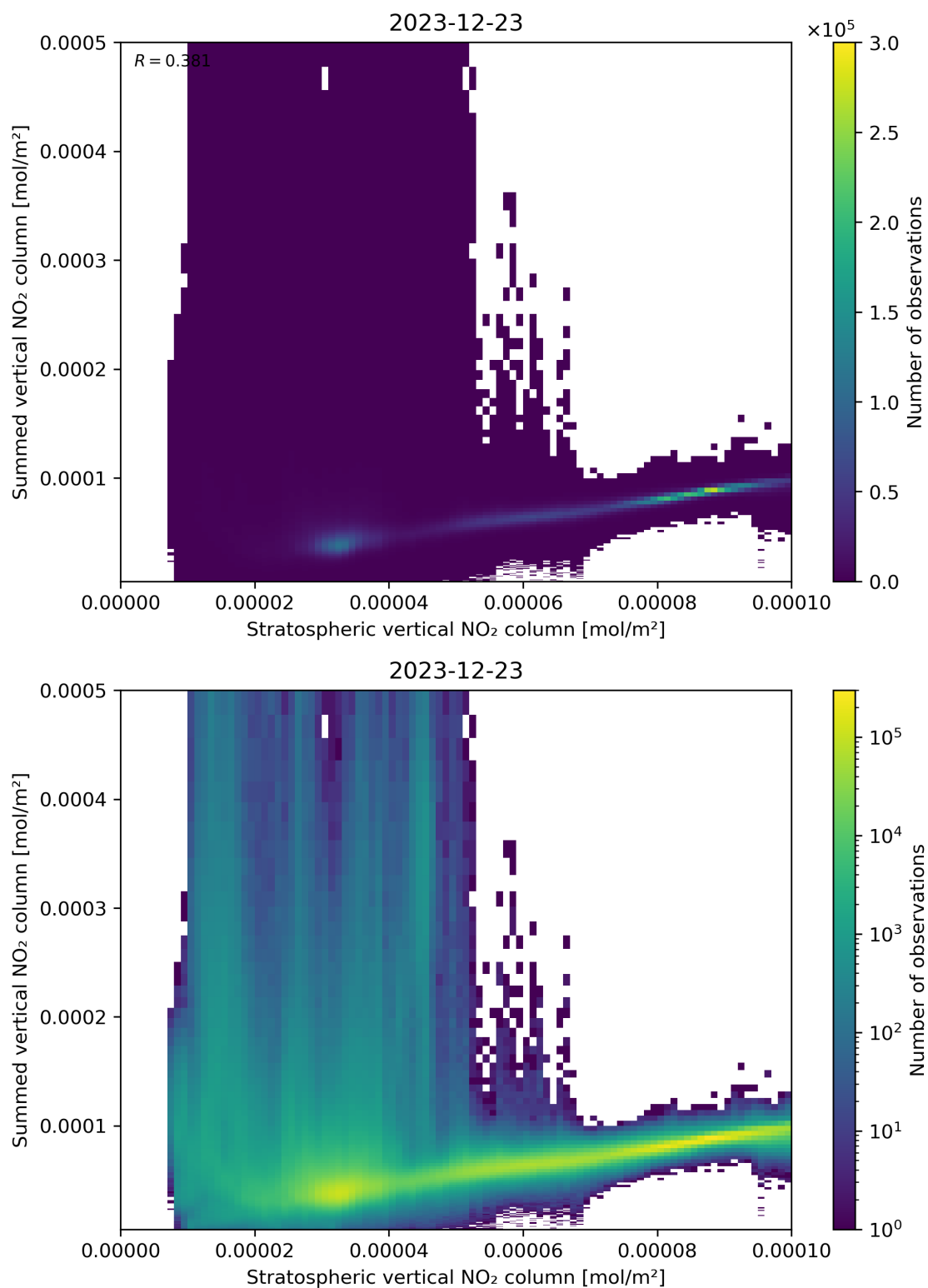
Figure 98: Scatter density plot of “Stratospheric vertical NO 2 column” against “Summed vertical NO 2 column” for 2023-12-22 to 2023-12-24.
