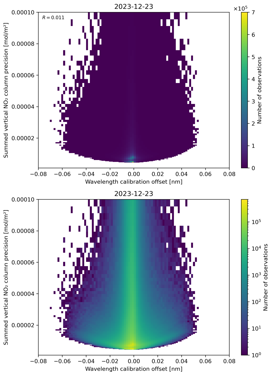
Figure 178: Scatter density plot of “Wavelength calibration offset” against “Summed vertical NO 2 column precision” for 2023-12-22 to 2023-12-24.
