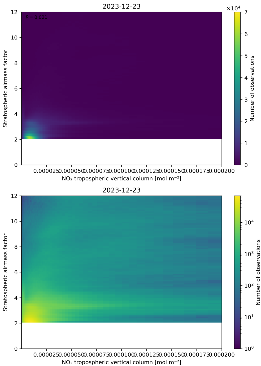
Figure 121: Scatter density plot of “NO 2 tropospheric vertical column” against “Stratospheric airmass factor” for 2023-12-22 to 2023-12-24.
