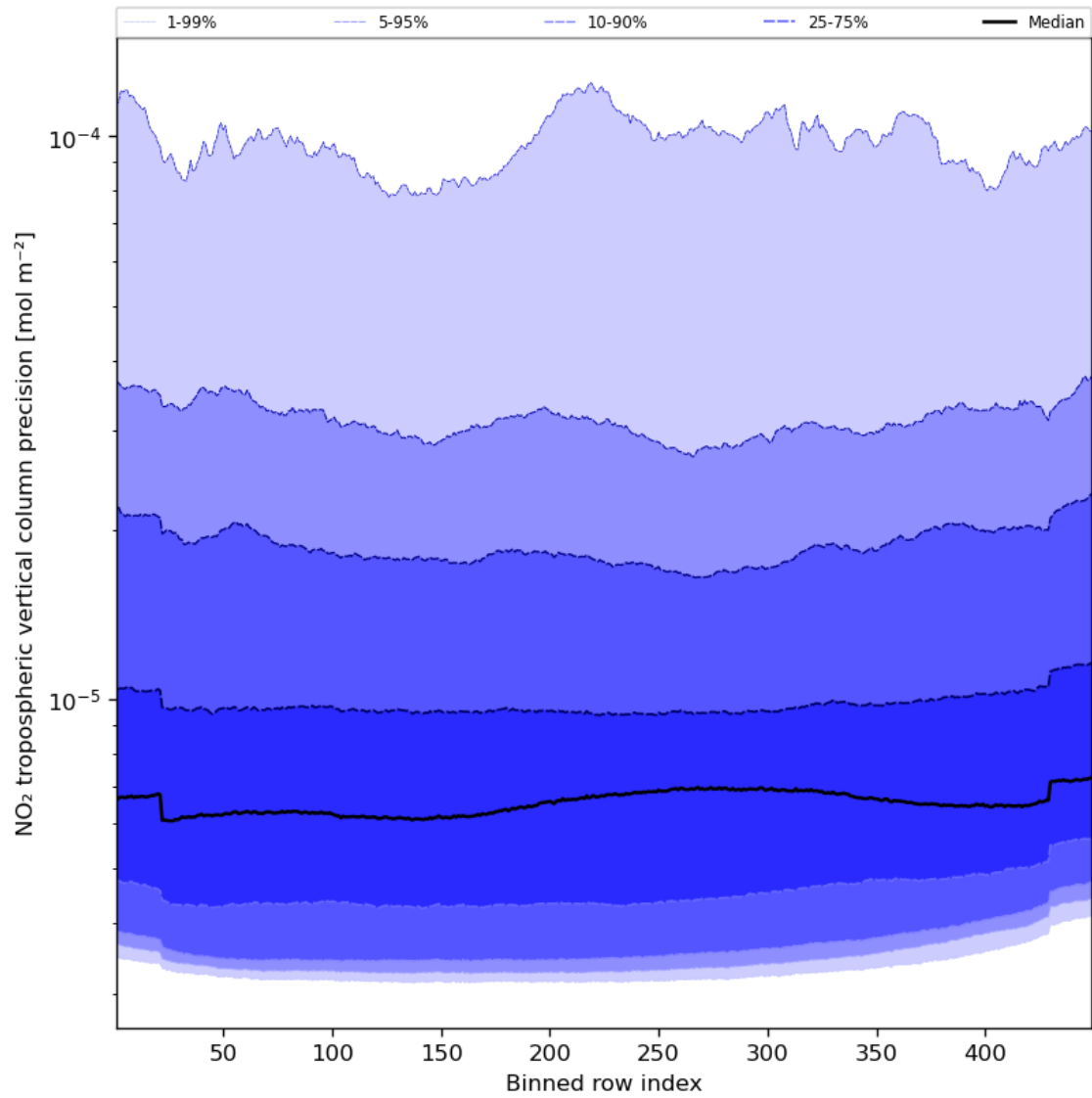
Figure 47: Along track statistics of “NO 2 tropospheric vertical column precision” for 2023-12-22 to 2023-12-24
