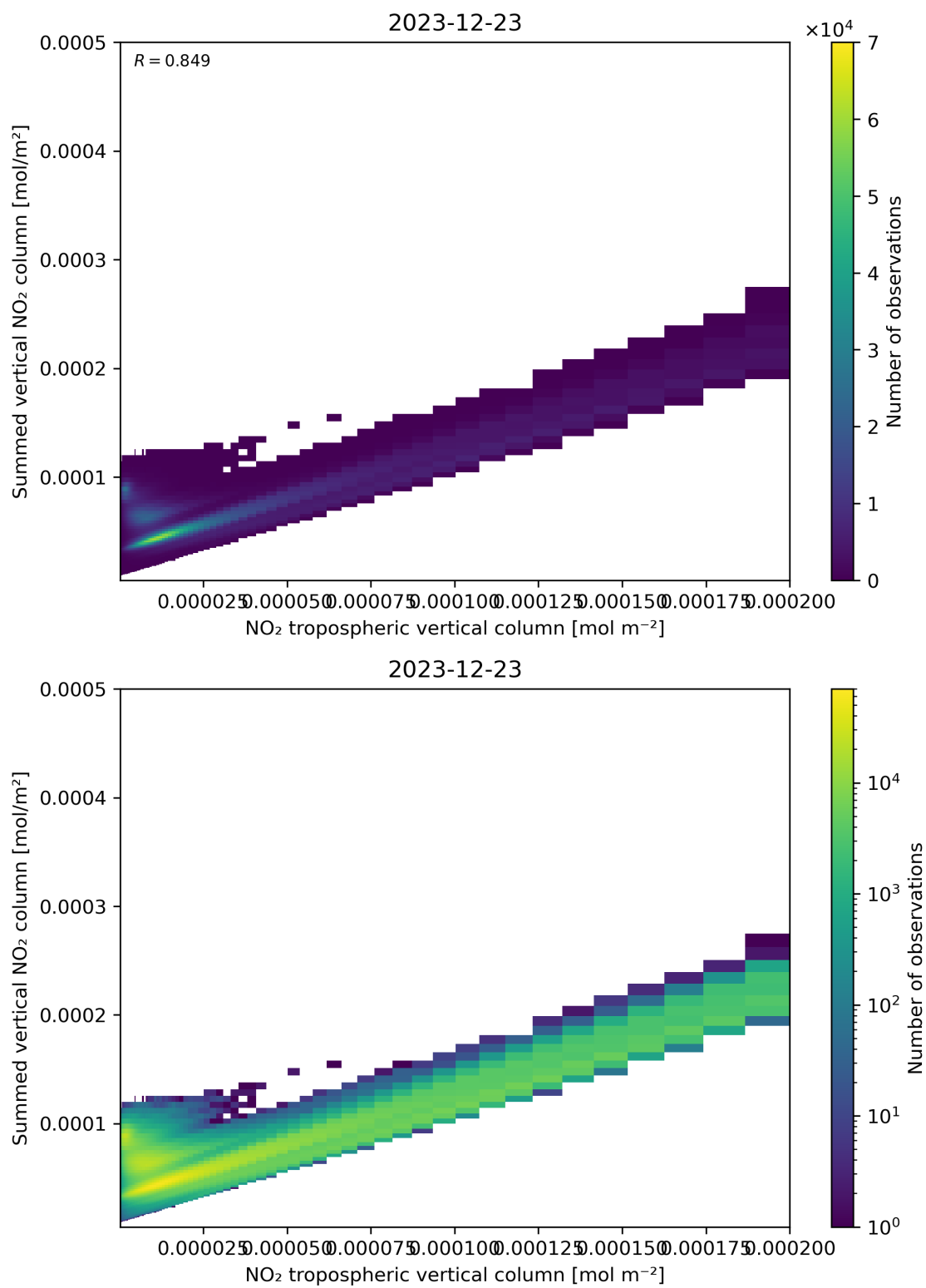
Figure 126: Scatter density plot of “NO 2 tropospheric vertical column” against “Summed vertical NO 2 column” for 2023-12-22 to 2023-12-24.
