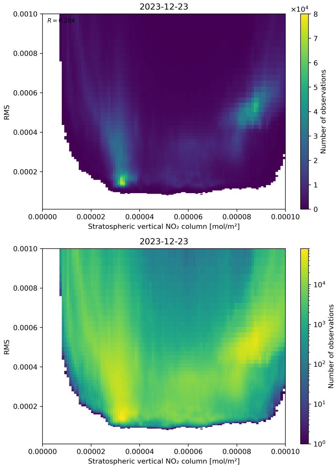
Figure 102: Scatter density plot of “Stratospheric vertical NO 2 column” against “RMS” for 2023-12-22 to 2023-12-24.
