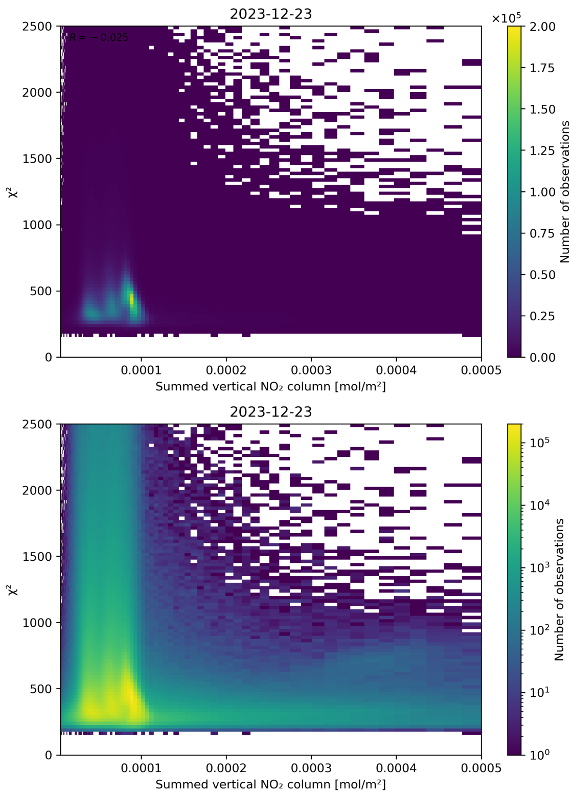
Figure 104: Scatter density plot of “Summed vertical NO 2 column” against “ \chi^2 ” for 2023-12-22 to 2023-12-24.
