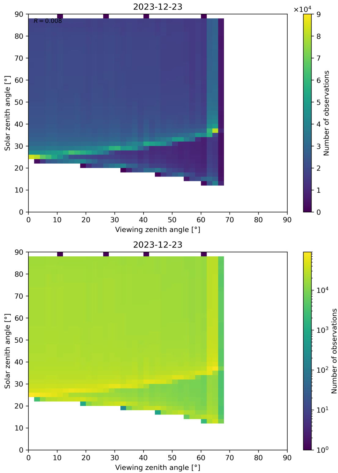
Figure 172: Scatter density plot of “Viewing zenith angle” against “Solar zenith angle” for 2023-12-22 to 2023-12-24.
