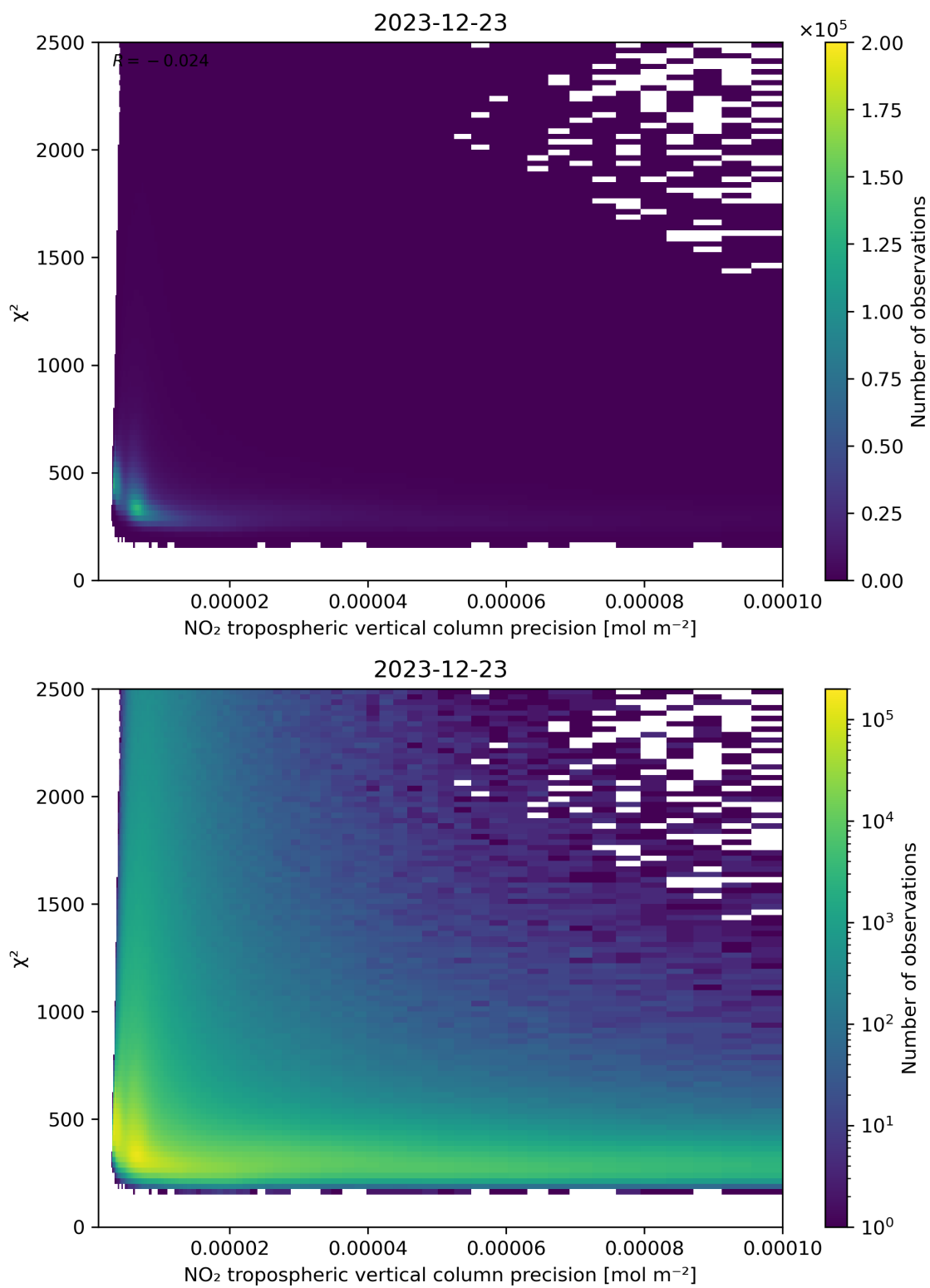
Figure 134: Scatter density plot of “NO 2 tropospheric vertical column precision” against “ \chi^2 ” for 2023-12-22 to 2023-12-24.
