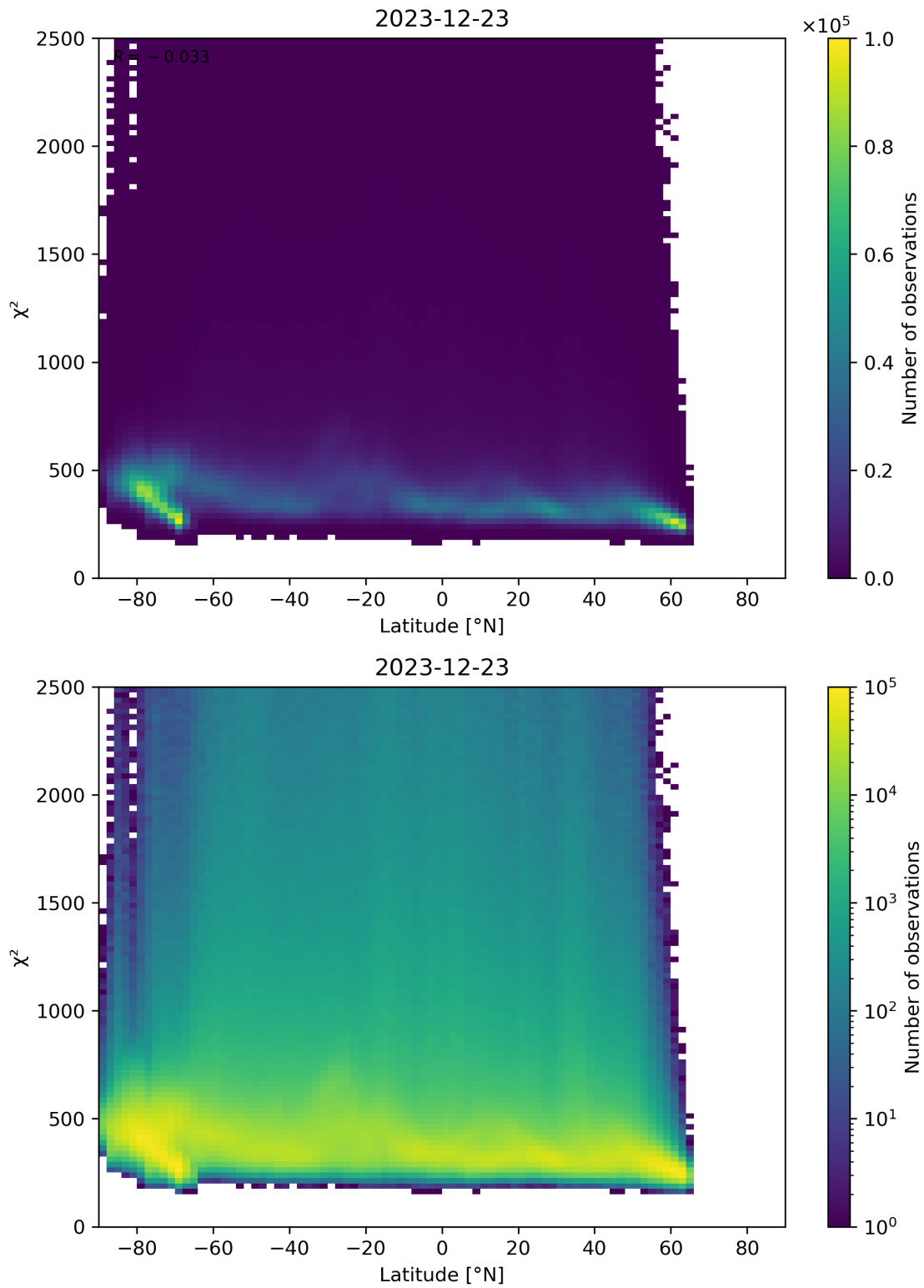
Figure 86: Scatter density plot of “Latitude” against “ \chi^2 ” for 2023-12-22 to 2023-12-24.
