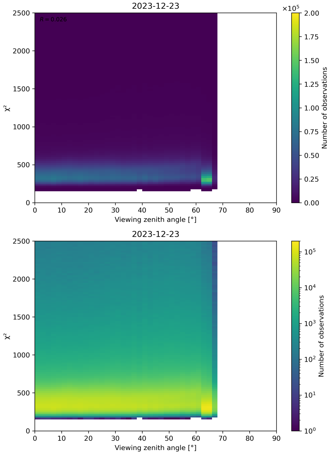
Figure 162: Scatter density plot of “Viewing zenith angle” against “ \chi^2 ” for 2023-12-22 to 2023-12-24.
