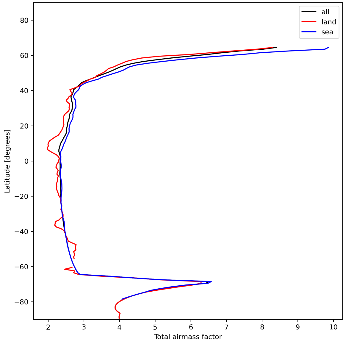
Figure 15: Zonal average of “Total airmass factor” for 2023-12-22 to 2023-12-24.
