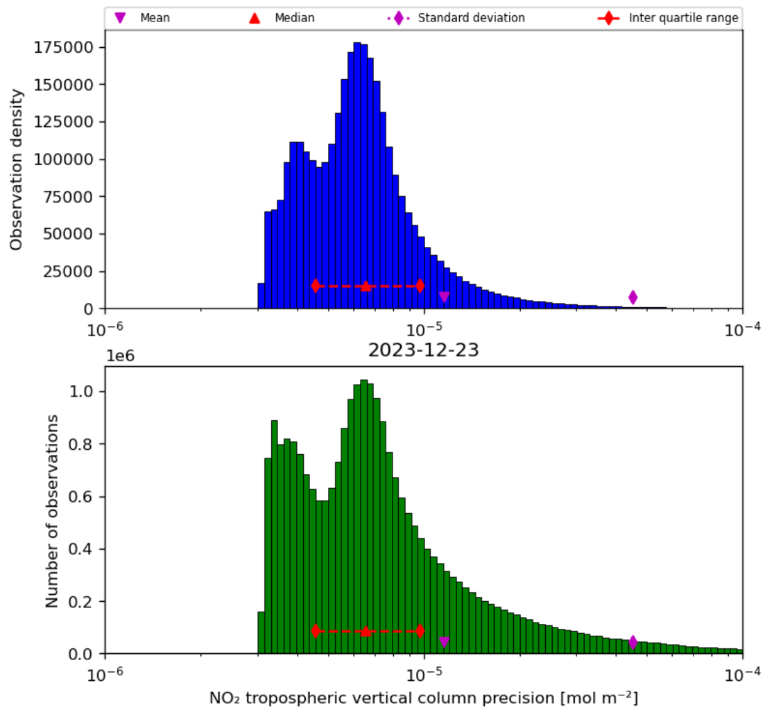
Figure 30: Histogram of “NO 2 tropospheric vertical column precision” for 2023-12-22 to 2023-12-24
