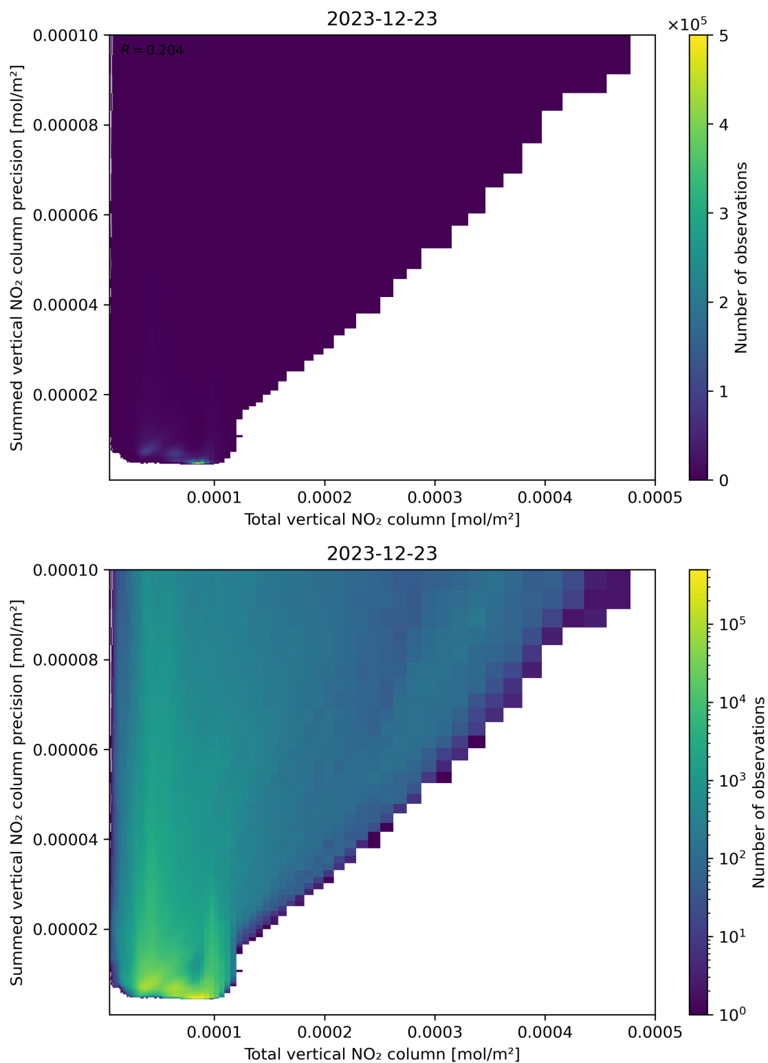
Figure 113: Scatter density plot of “Total vertical NO 2 column” against “Summed vertical NO 2 column precision” for 2023-12-22 to 2023-12-24.
