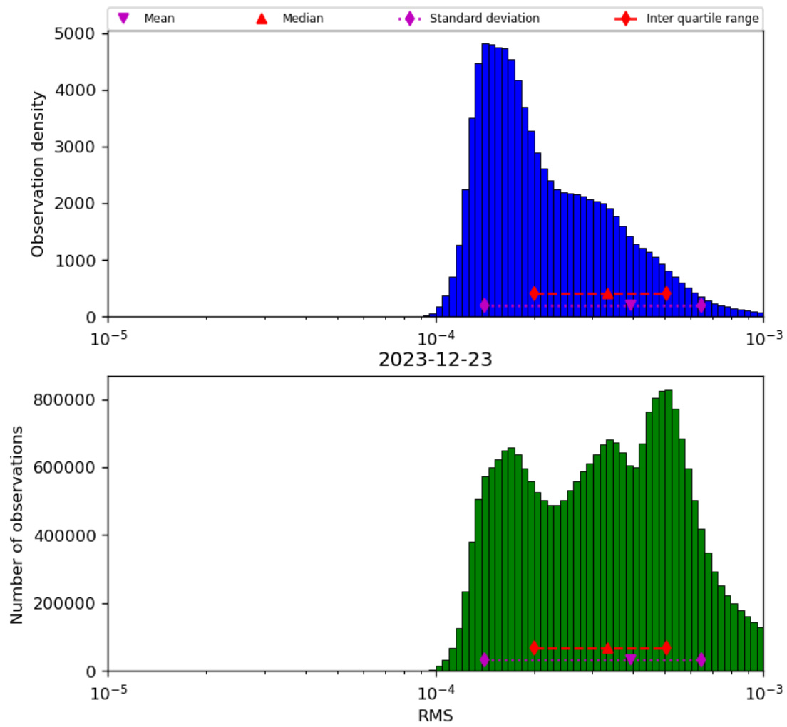
Figure 43: Histogram of “RMS” for 2023-12-22 to 2023-12-24
