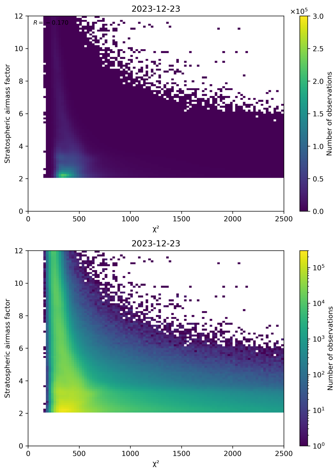
Figure 81: Scatter density plot of “ \chi^2 ” against “Stratospheric airmass factor” for 2023-12-22 to 2023-12-24.
