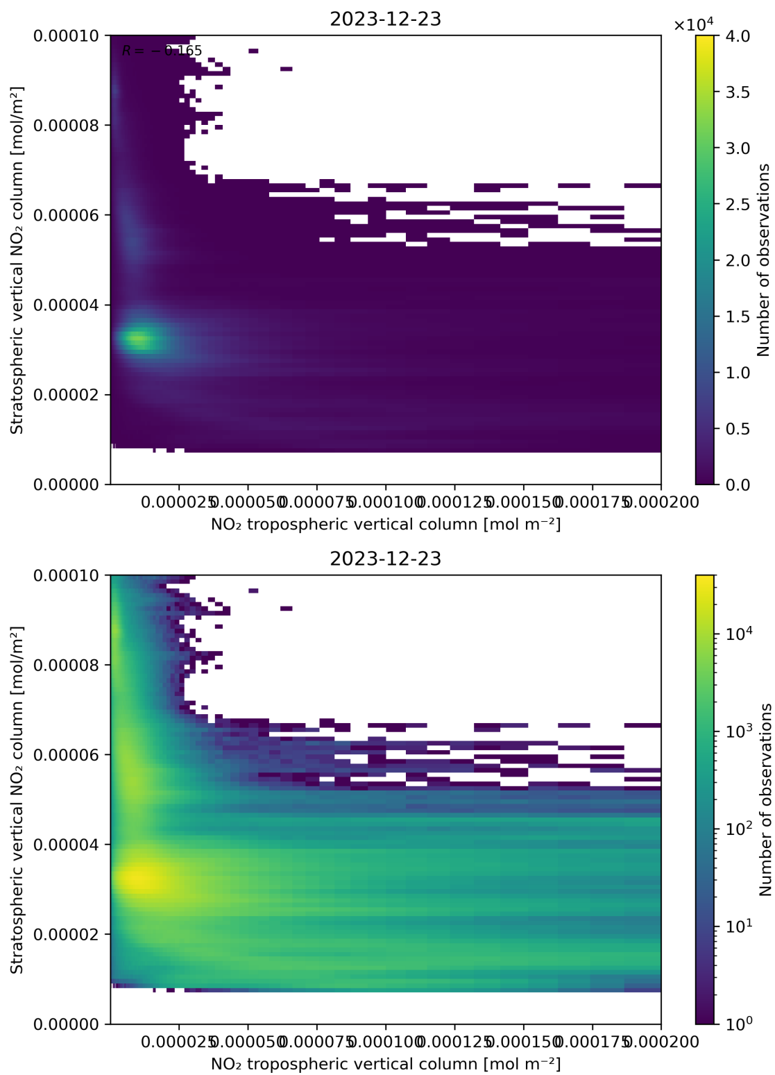
Figure 125: Scatter density plot of “NO 2 tropospheric vertical column” against “Stratospheric vertical NO 2 column” for 2023-12-22 to 2023-12-24.
