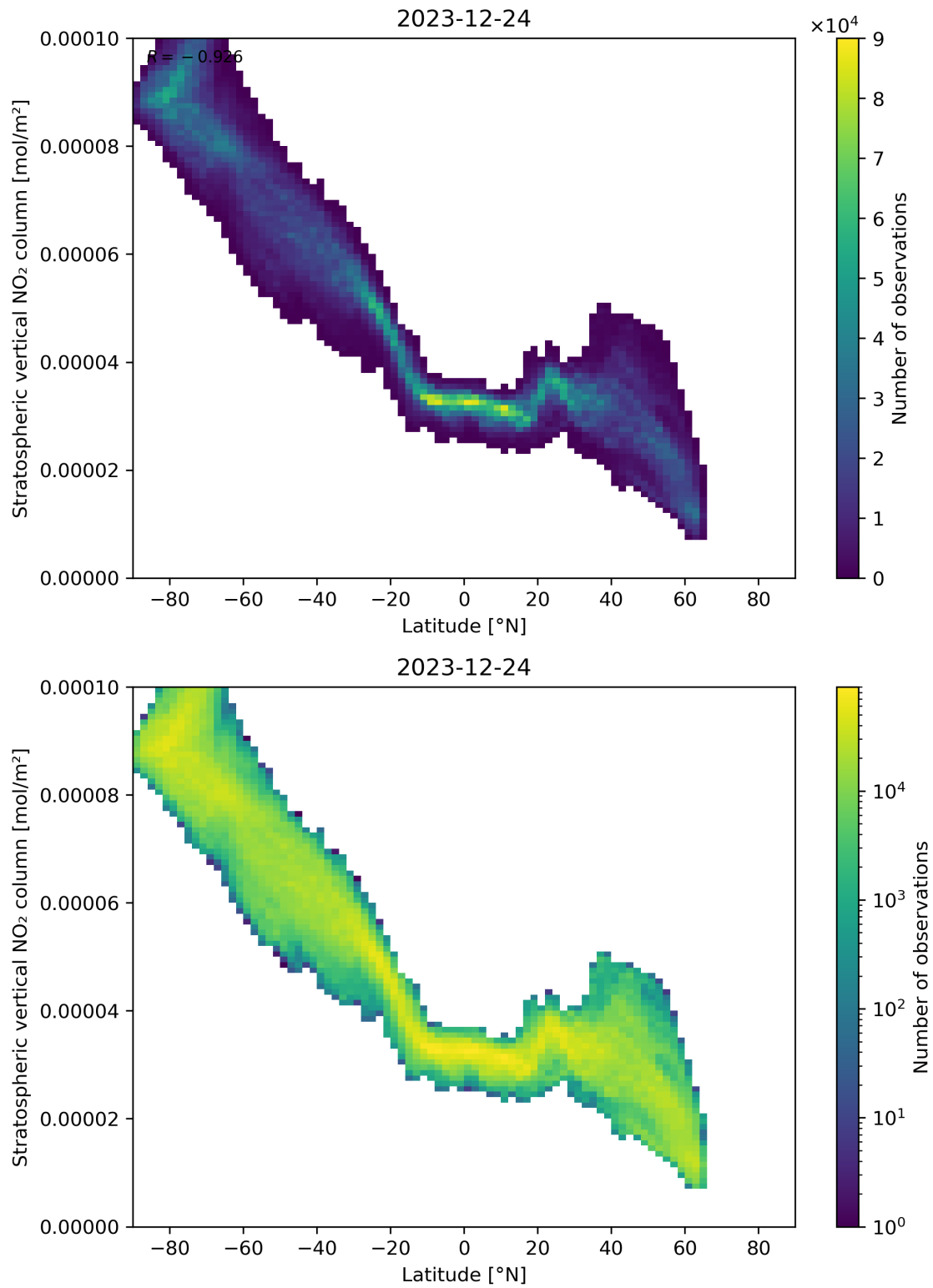
Figure 87: Scatter density plot of “Latitude” against “Stratospheric vertical NO 2 column” for 2023-12-23 to 2023-12-25.
