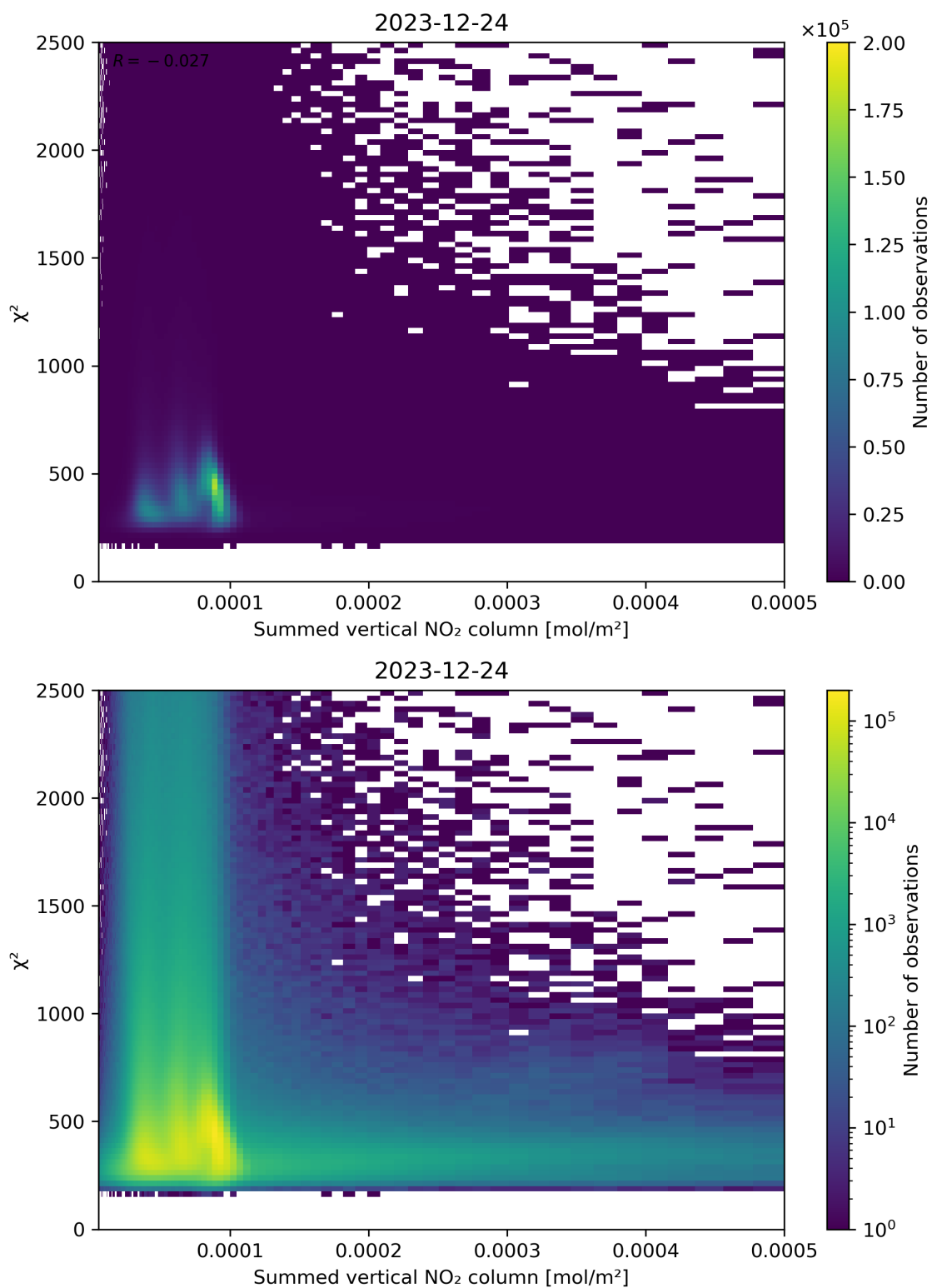
Figure 104: Scatter density plot of “Summed vertical NO 2 column” against “ \chi^2 ” for 2023-12-23 to 2023-12-25.
