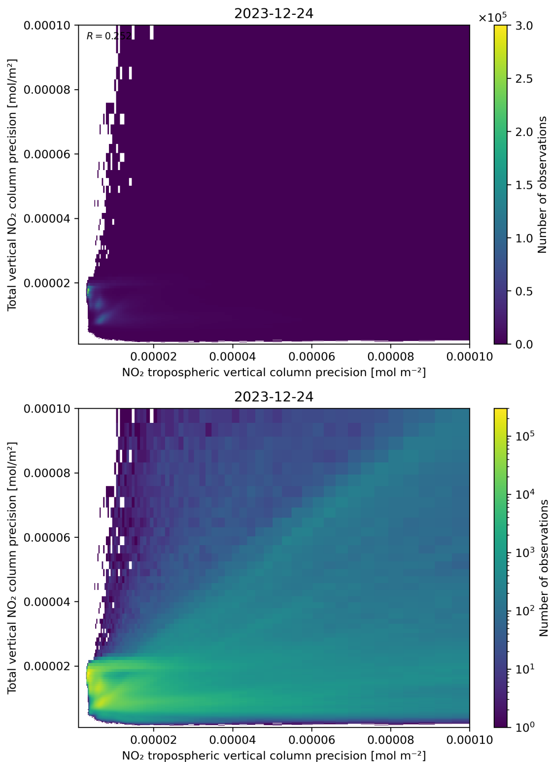
Figure 139: Scatter density plot of “NO 2 tropospheric vertical column precision” against “Total vertical NO 2 column precision” for 2023-12-23 to 2023-12-25.
