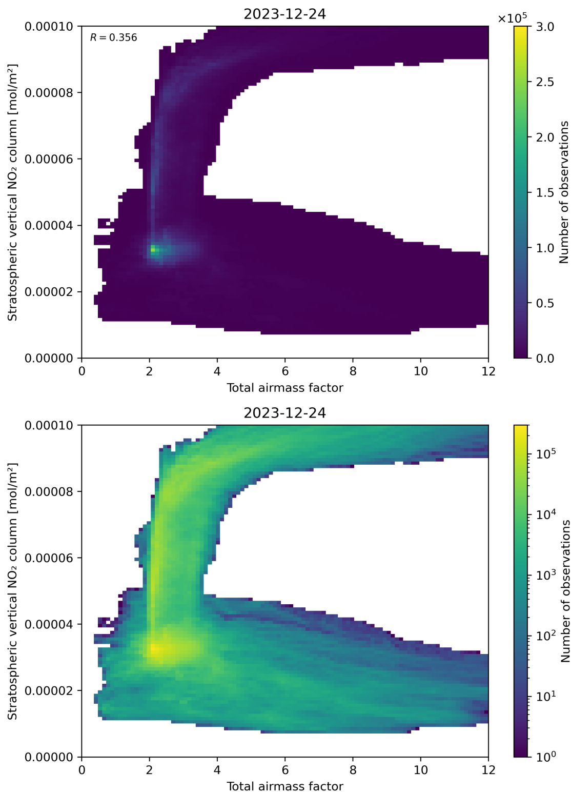
Figure 64: Scatter density plot of “Total airmass factor” against “Stratospheric vertical \text{NO}_2 column” for 2023-12-23 to 2023-12-25.
