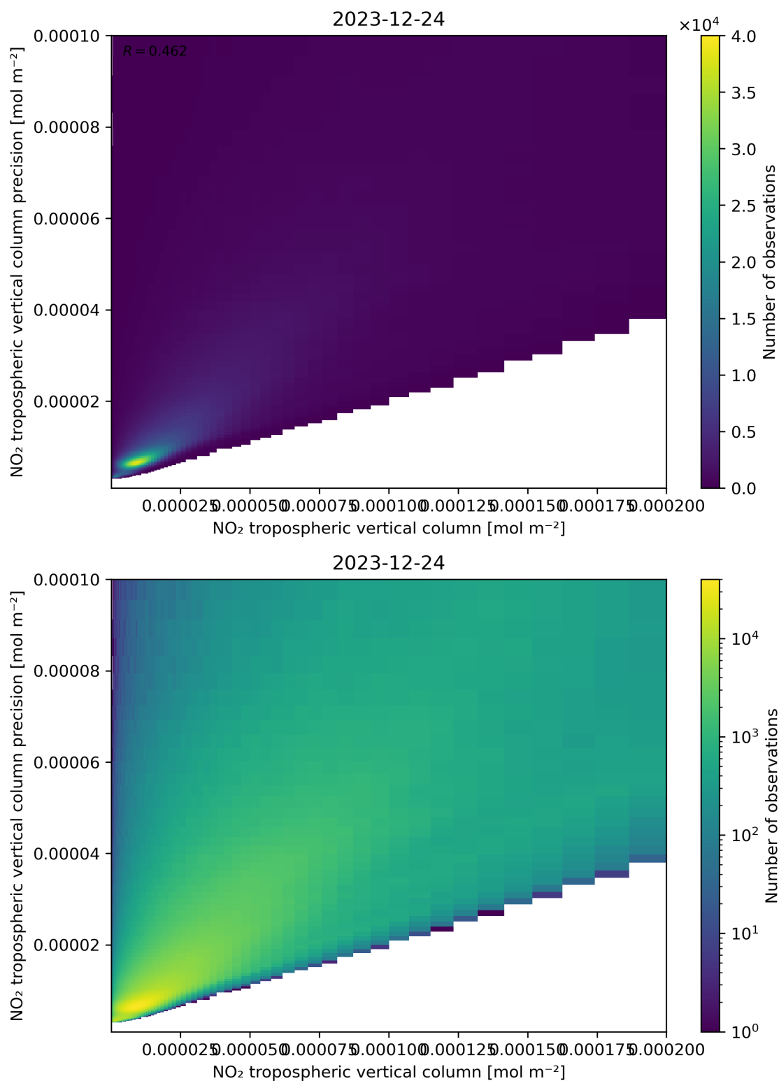
Figure 130: Scatter density plot of “NO 2 tropospheric vertical column” against “NO 2 tropospheric vertical column precision” for 2023-12-23 to 2023-12-25.
