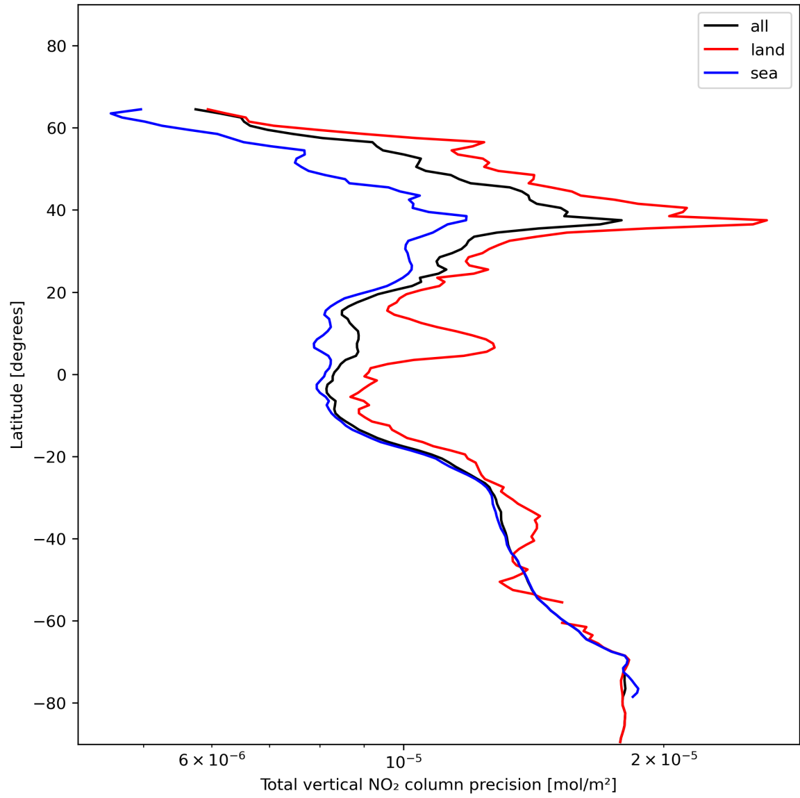
Figure 22: Zonal average of “Total vertical NO 2 column precision” for 2023-12-23 to 2023-12-25.
