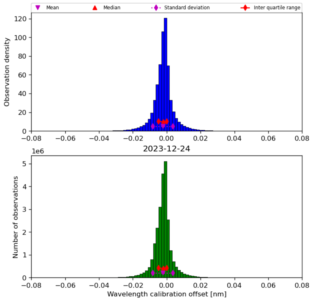
Figure 35: Histogram of “Wavelength calibration offset” for 2023-12-23 to 2023-12-25
