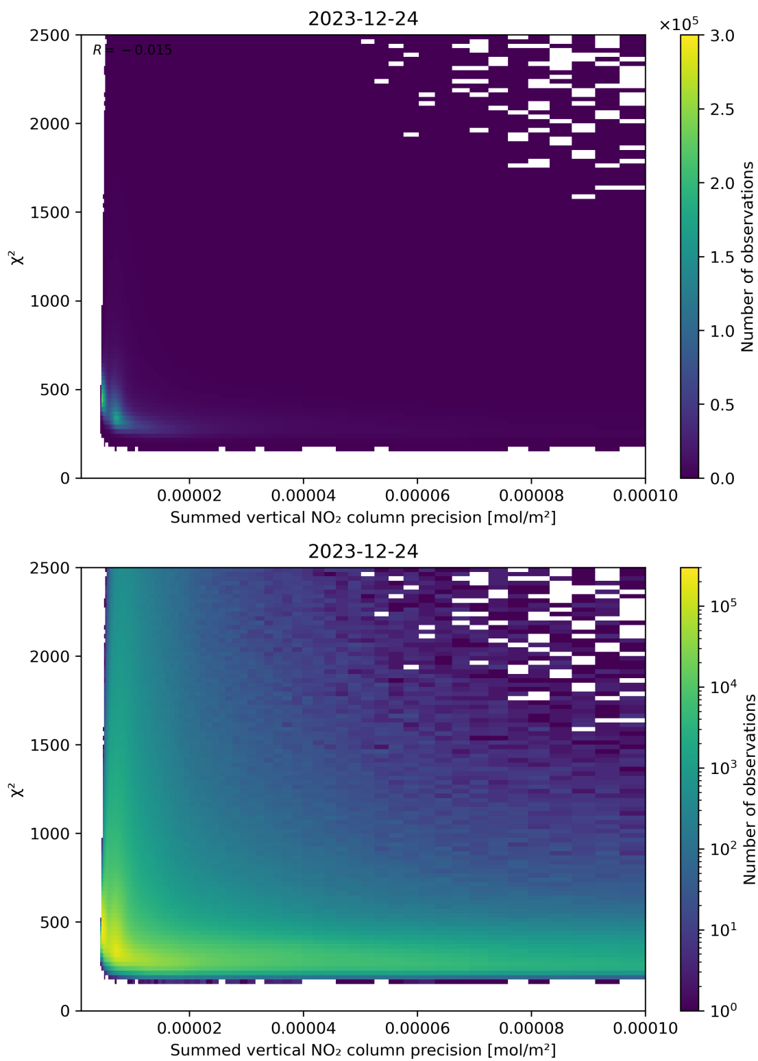
Figure 107: Scatter density plot of “Summed vertical NO 2 column precision” against “ \chi^2 ” for 2023-12-23 to 2023-12-25.
