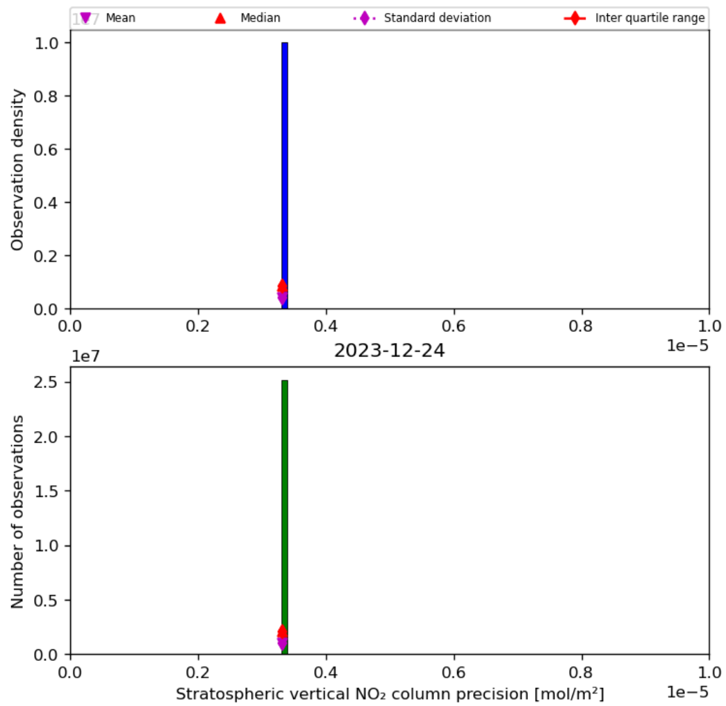
Figure 37: Histogram of “Stratospheric vertical NO 2 column precision” for 2023-12-23 to 2023-12-25
