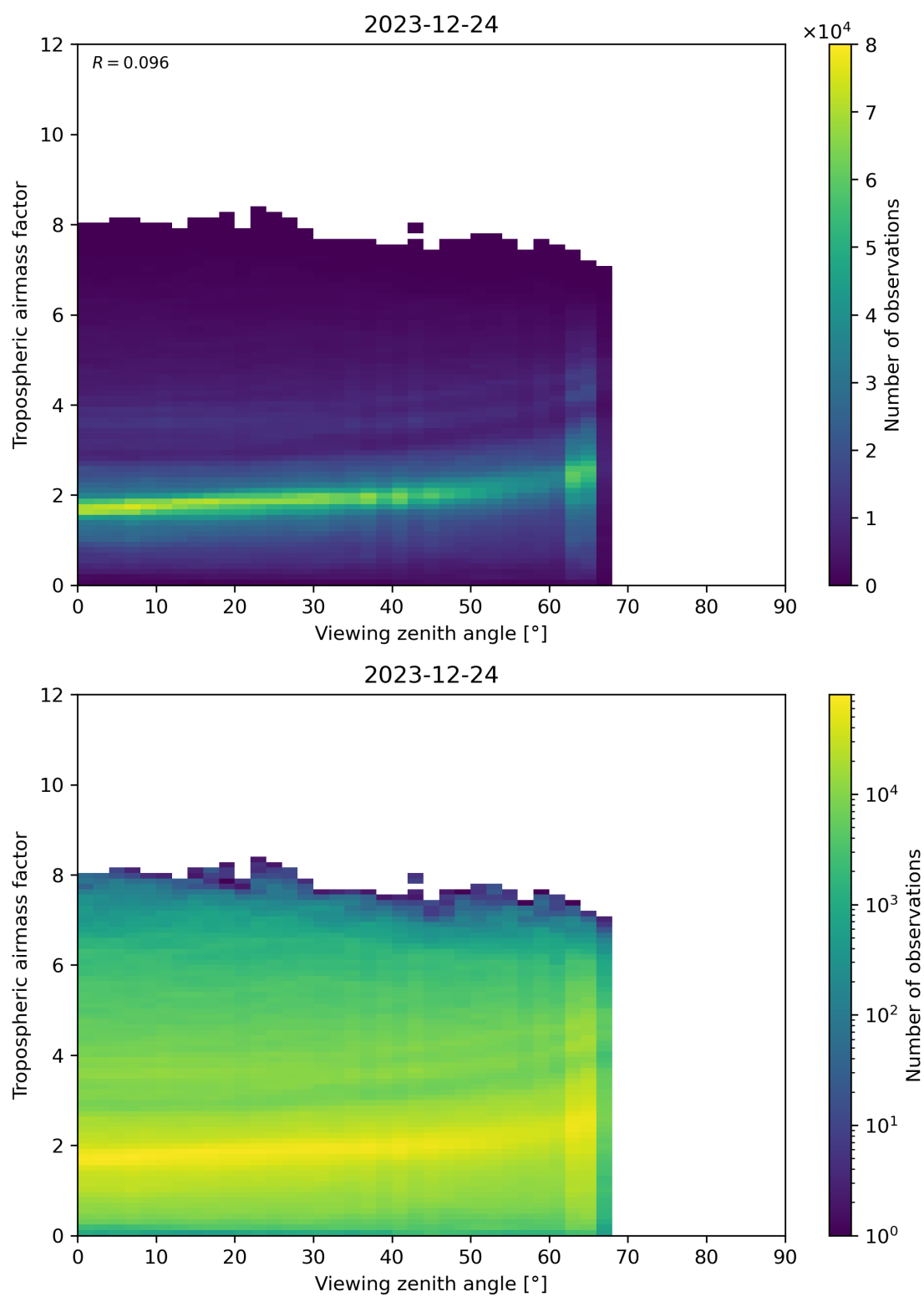
Figure 161: Scatter density plot of “Viewing zenith angle” against “Tropospheric airmass factor” for 2023-12-23 to 2023-12-25.
