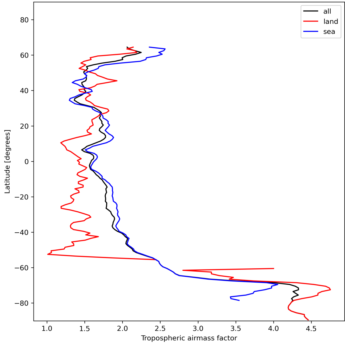
Figure 14: Zonal average of “Tropospheric airmass factor” for 2023-12-23 to 2023-12-25.
