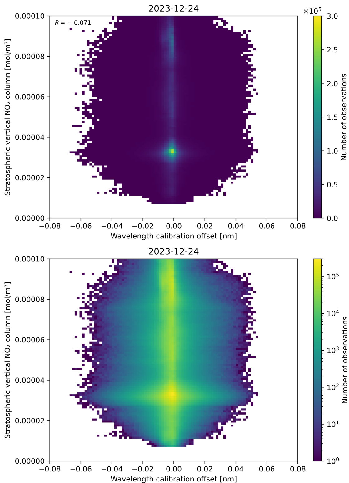
Figure 176: Scatter density plot of “Wavelength calibration offset” against “Stratospheric vertical NO 2 column” for 2023-12-23 to 2023-12-25.
