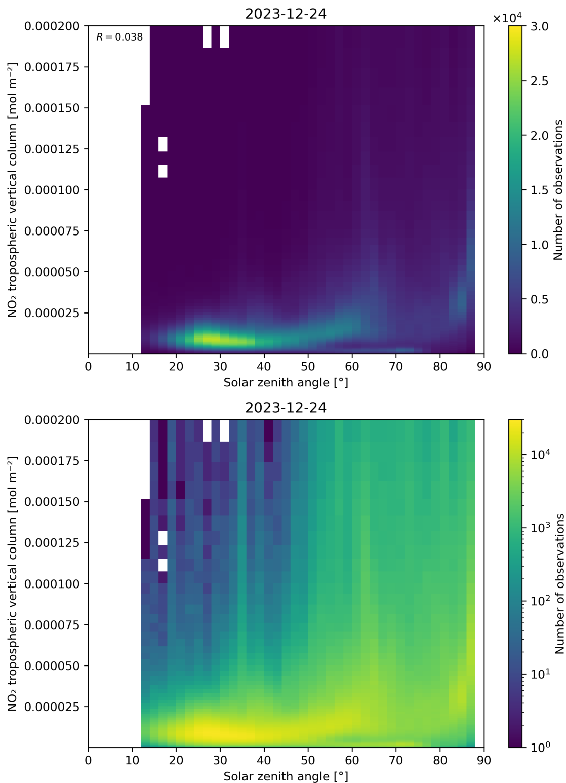
Figure 155: Scatter density plot of “Solar zenith angle” against “NO 2 tropospheric vertical column” for 2023-12-23 to 2023-12-25.
