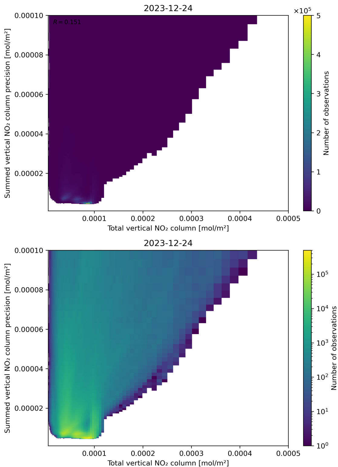
Figure 113: Scatter density plot of “Total vertical NO 2 column” against “Summed vertical NO 2 column precision” for 2023-12-23 to 2023-12-25.
