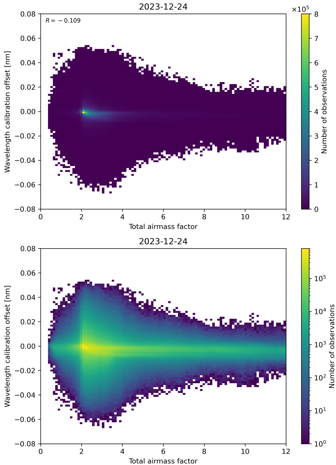
Figure 70: Scatter density plot of “Total airmass factor” against “Wavelength calibration offset” for 2023-12-23 to 2023-12-25.
