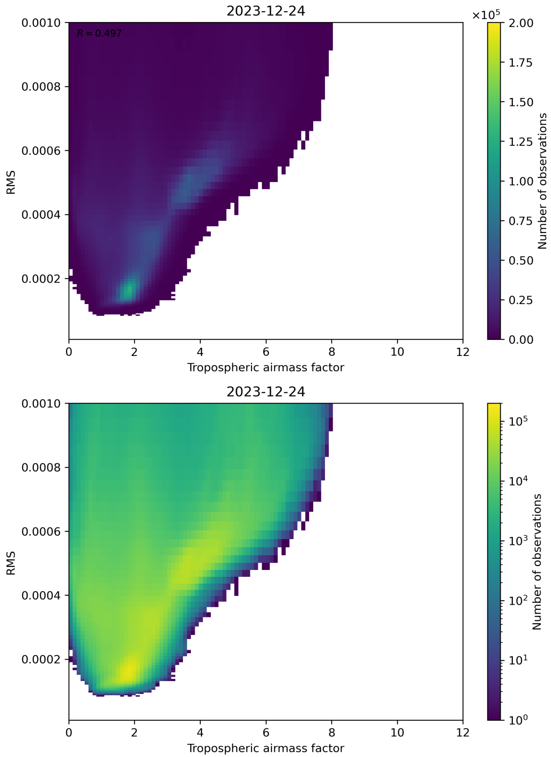
Figure 79: Scatter density plot of “Tropospheric airmass factor” against “RMS” for 2023-12-23 to 2023-12-25.
