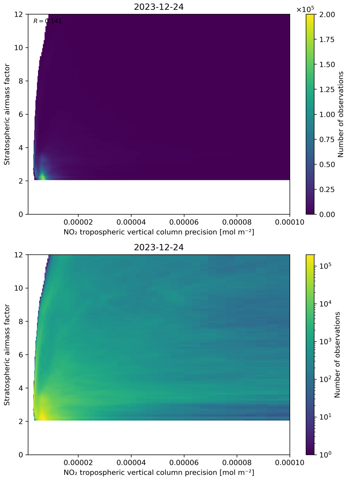
Figure 131: Scatter density plot of “NO 2 tropospheric vertical column precision” against “Stratospheric airmass factor” for 2023-12-23 to 2023-12-25.
