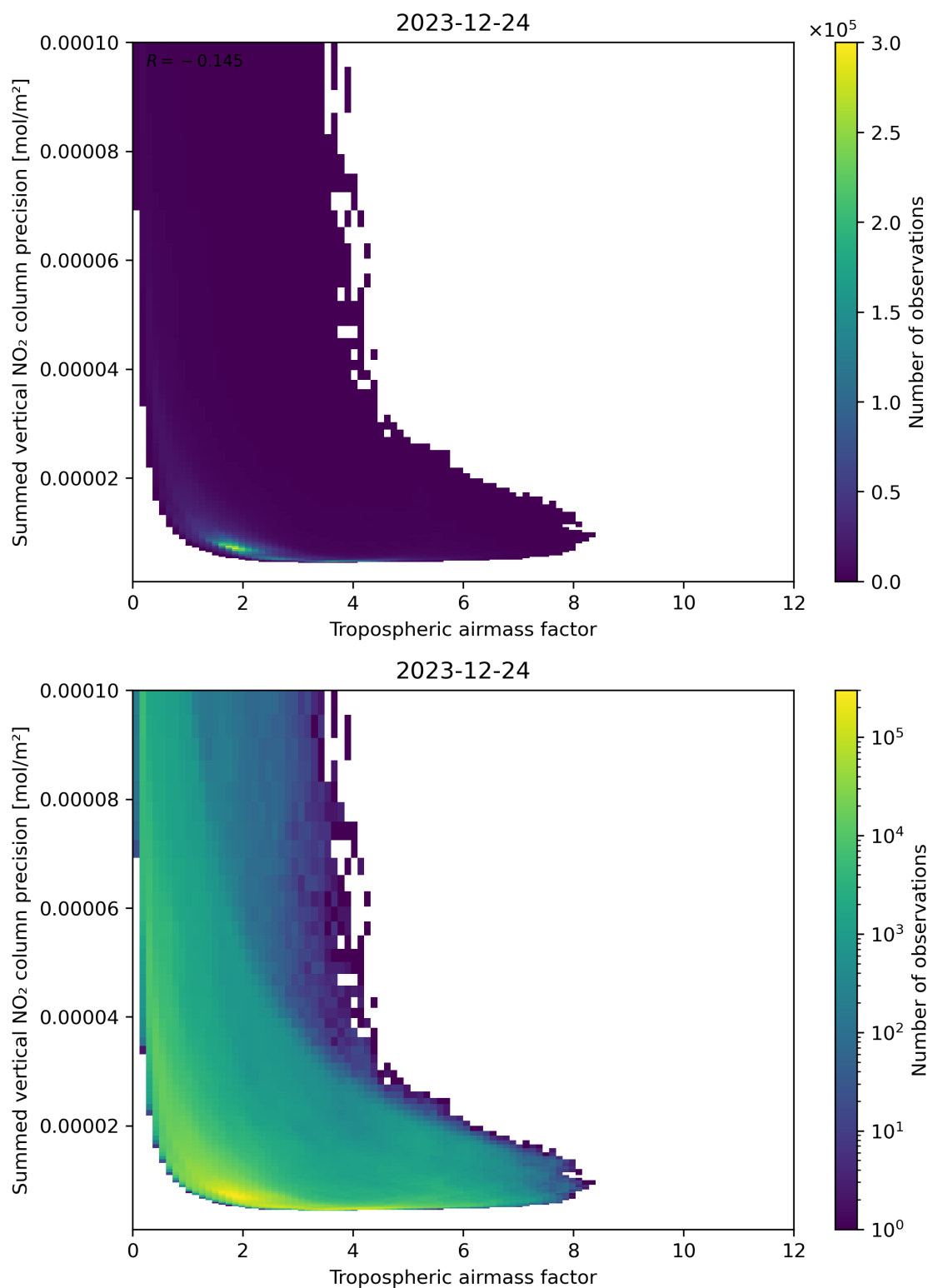
Figure 76: Scatter density plot of “Tropospheric air mass factor” against “Summed vertical NO 2 column precision” for 2023-12-23 to 2023-12-25.
