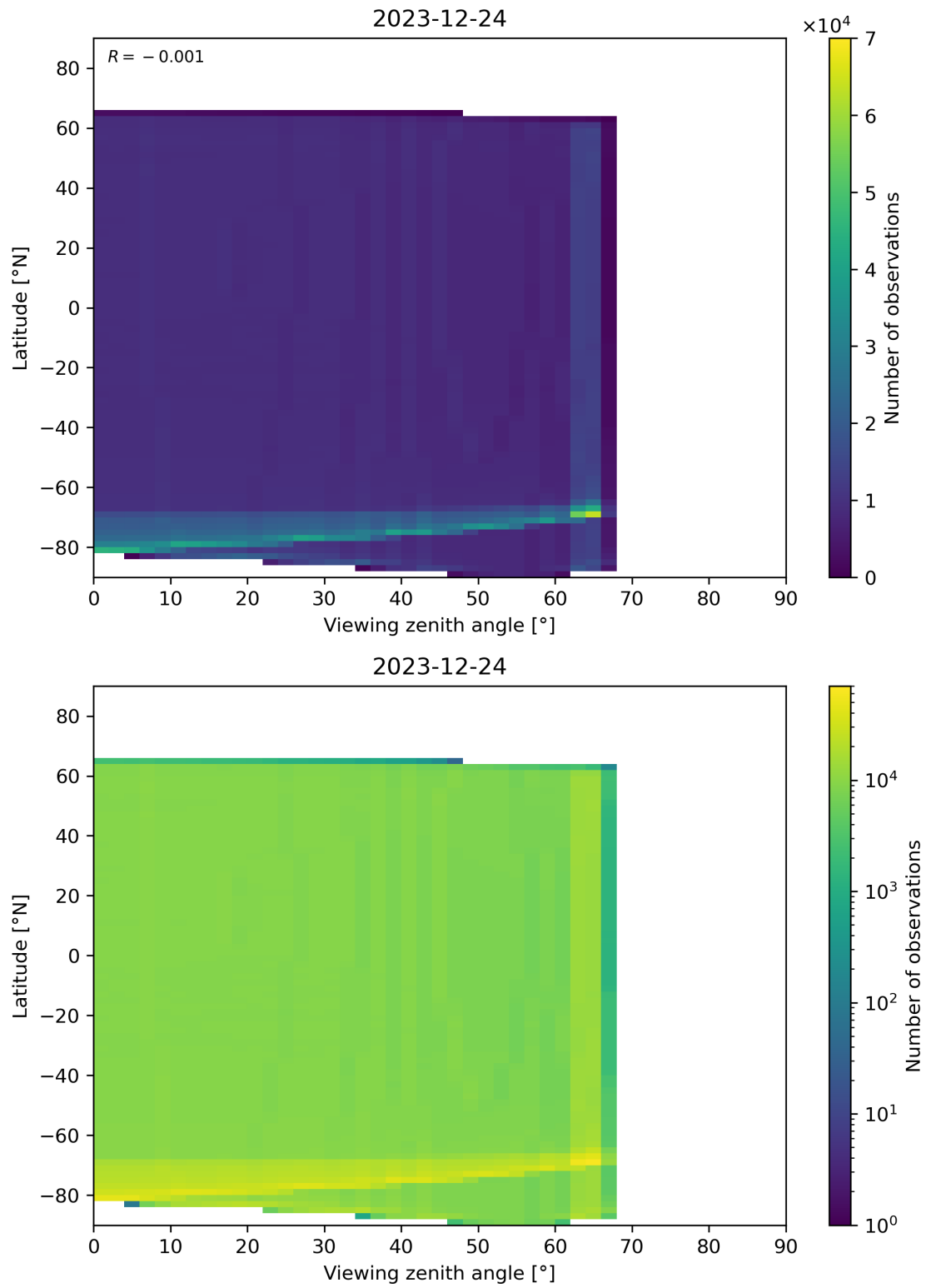
Figure 163: Scatter density plot of “Viewing zenith angle” against “Latitude” for 2023-12-23 to 2023-12-25.
