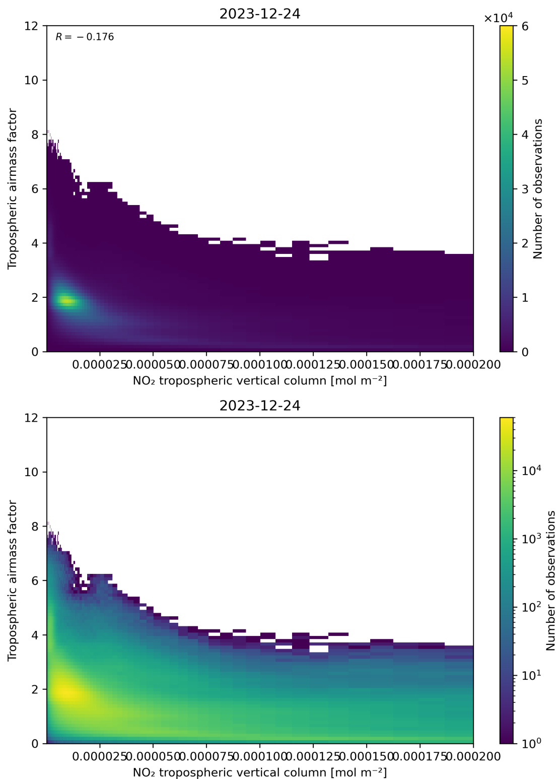
Figure 123: Scatter density plot of “NO 2 tropospheric vertical column” against “Tropospheric airmass factor” for 2023-12-23 to 2023-12-25.
