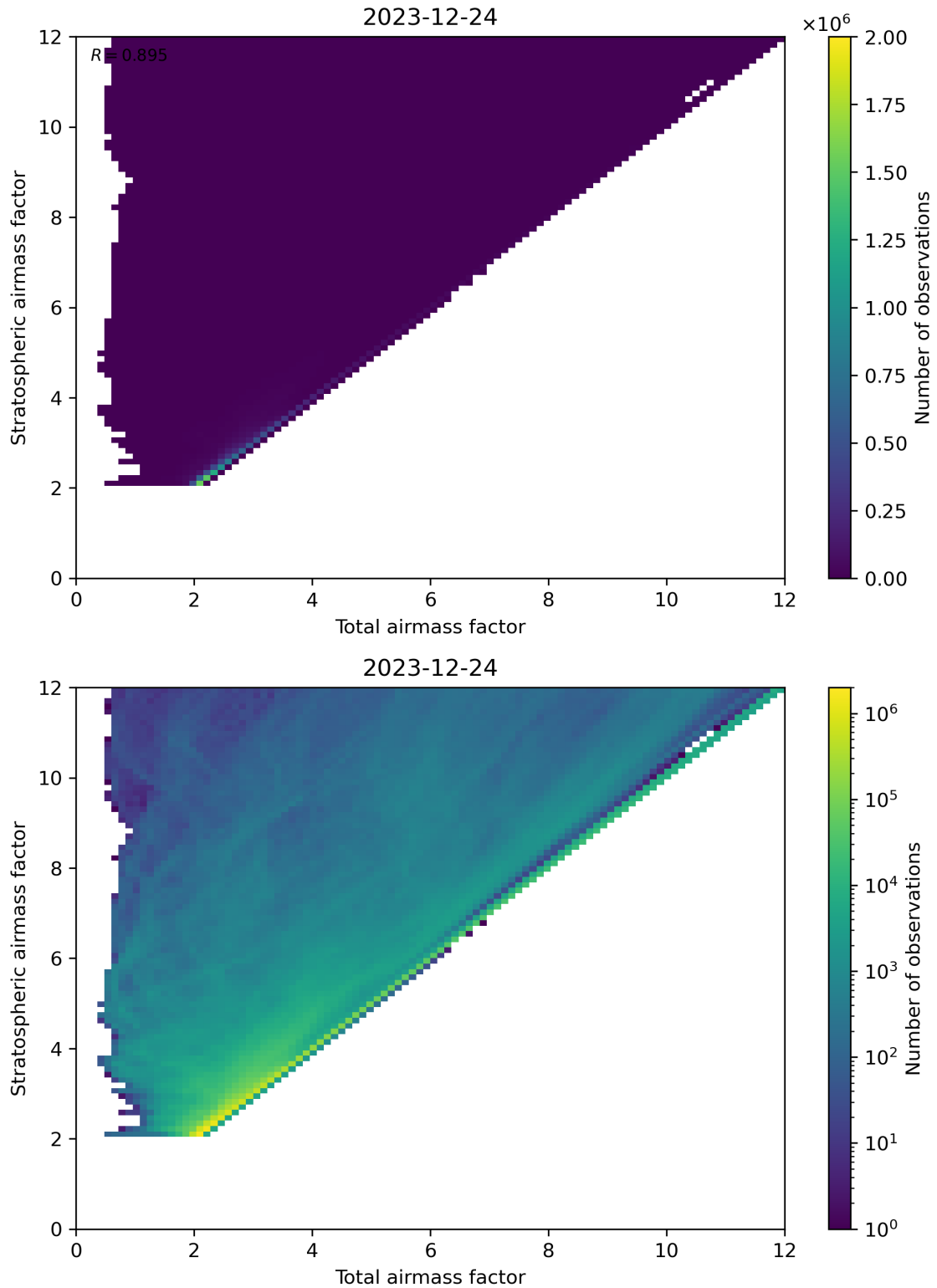
Figure 62: Scatter density plot of “Total airmass factor” against “Stratospheric airmass factor” for 2023-12-23 to 2023-12-25.
