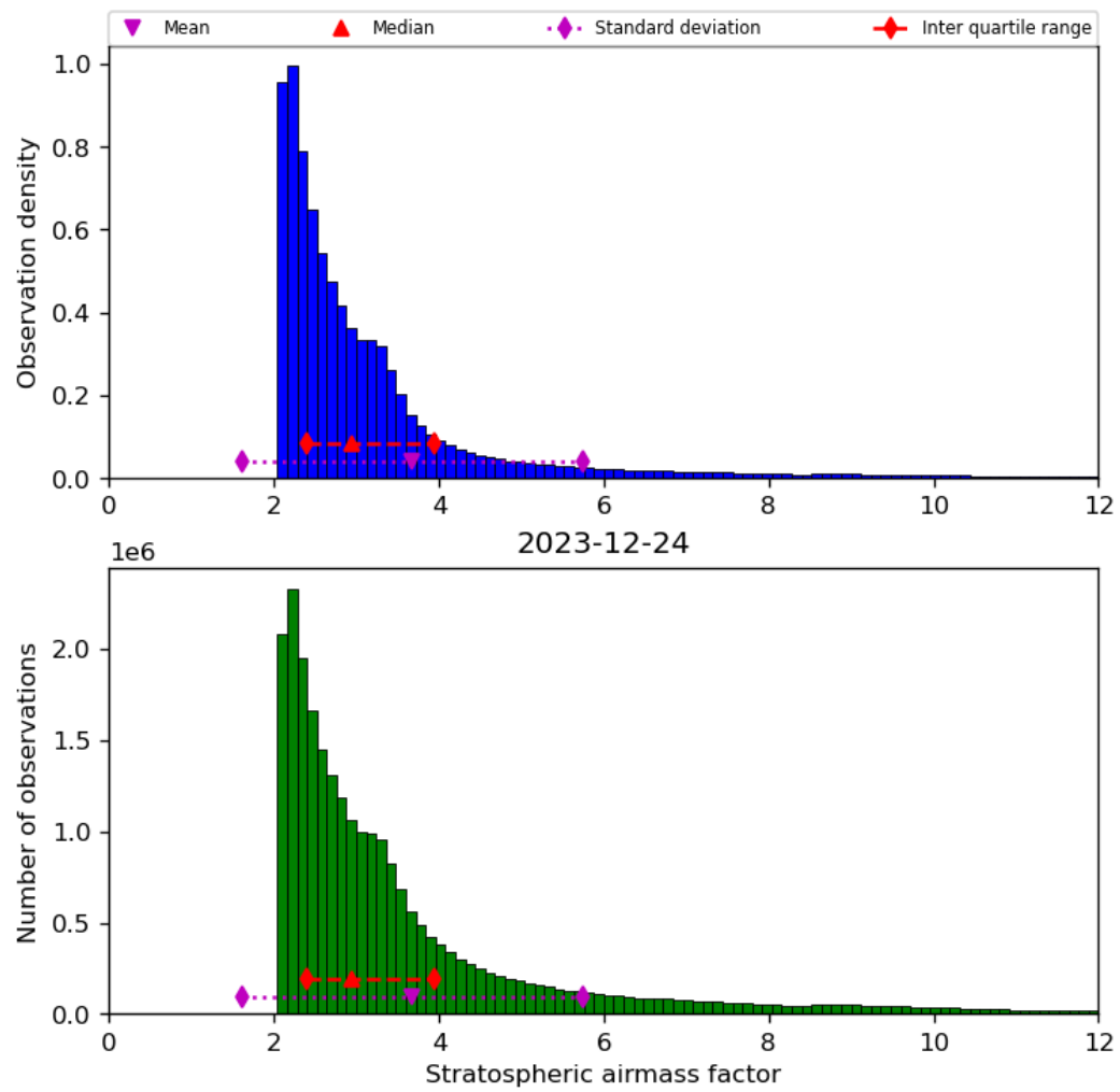
Figure 44: Histogram of “Stratospheric airmass factor” for 2023-12-23 to 2023-12-25
