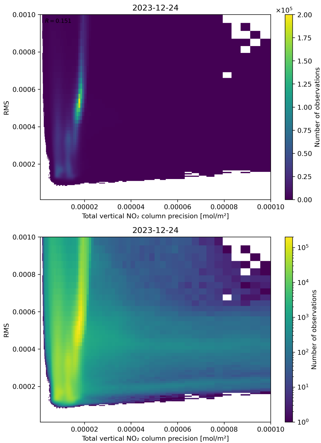
Figure 119: Scatter density plot of “Total vertical NO 2 column precision” against “RMS” for 2023-12-23 to 2023-12-25.
