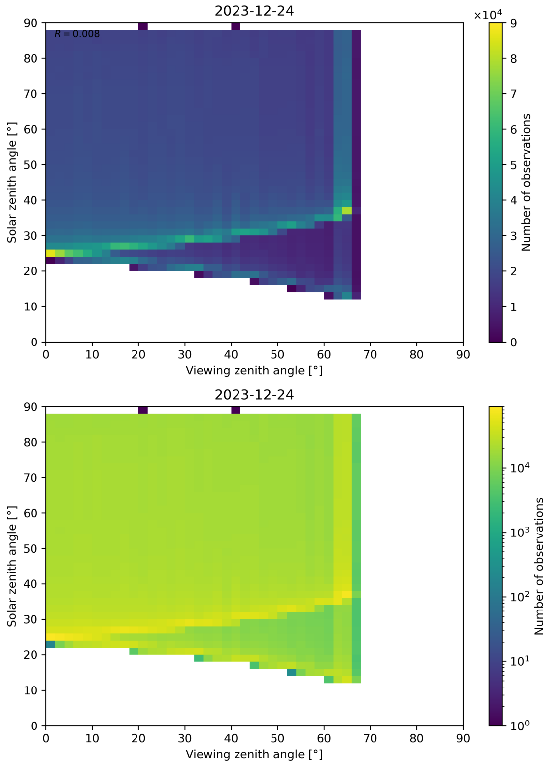
Figure 172: Scatter density plot of “Viewing zenith angle” against “Solar zenith angle” for 2023-12-23 to 2023-12-25.
