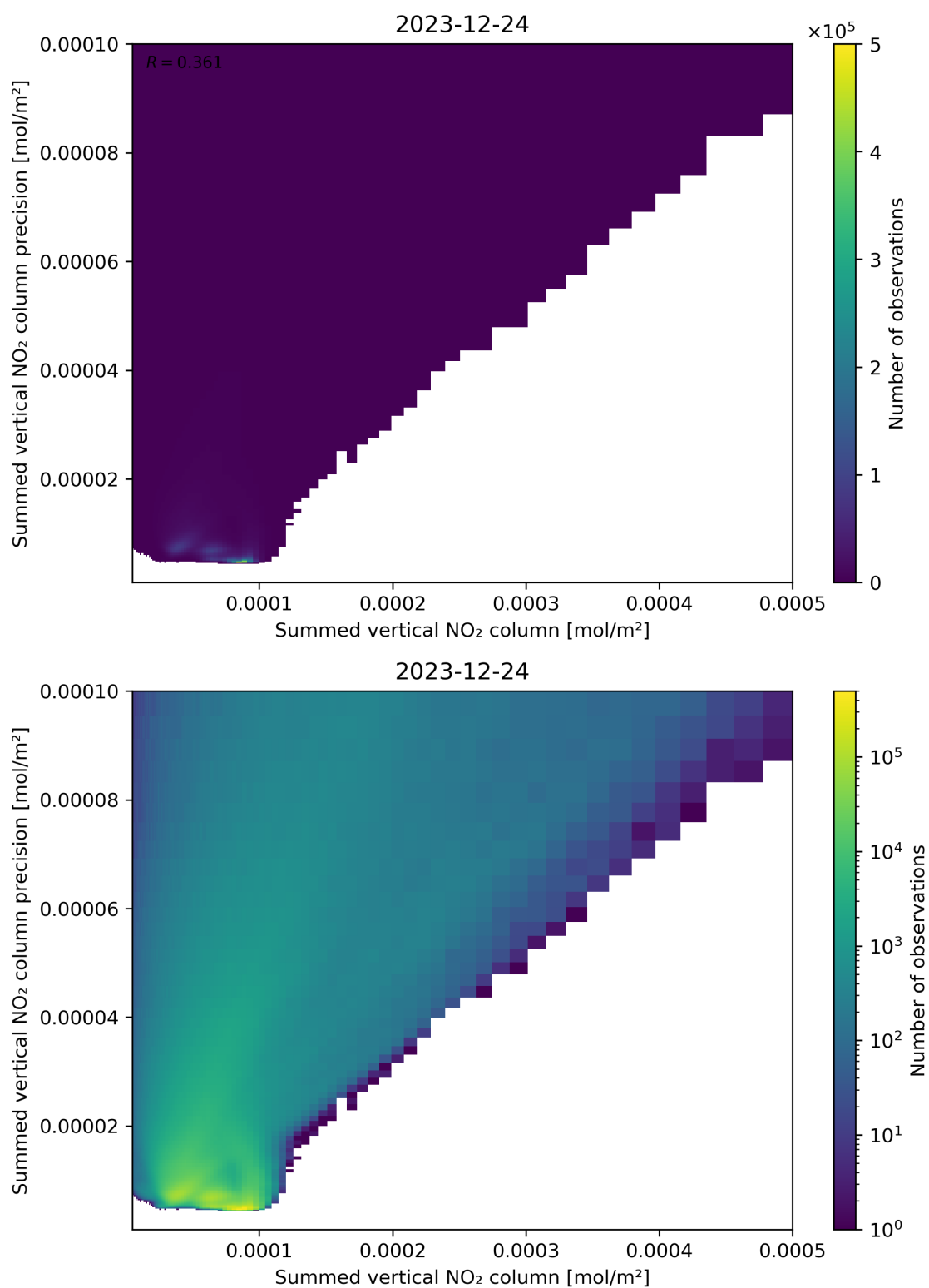
Figure 105: Scatter density plot of “Summed vertical NO 2 column” against “Summed vertical NO 2 column precision” for 2023-12-23 to 2023-12-25.
