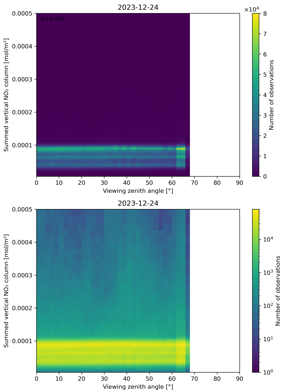
Figure 165: Scatter density plot of “Viewing zenith angle” against “Summed vertical NO 2 column” for 2023-12-23 to 2023-12-25.
