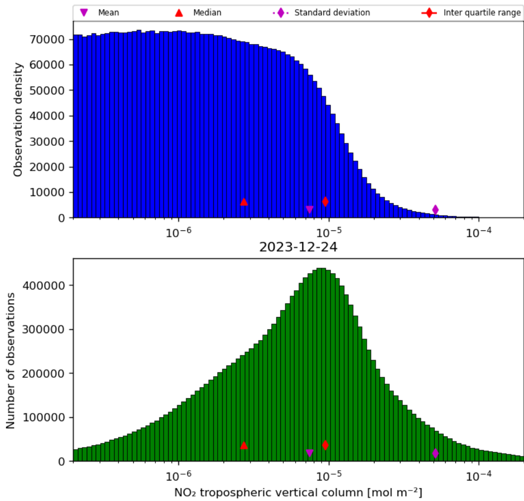
Figure 29: Histogram of “NO 2 tropospheric vertical column” for 2023-12-23 to 2023-12-25
