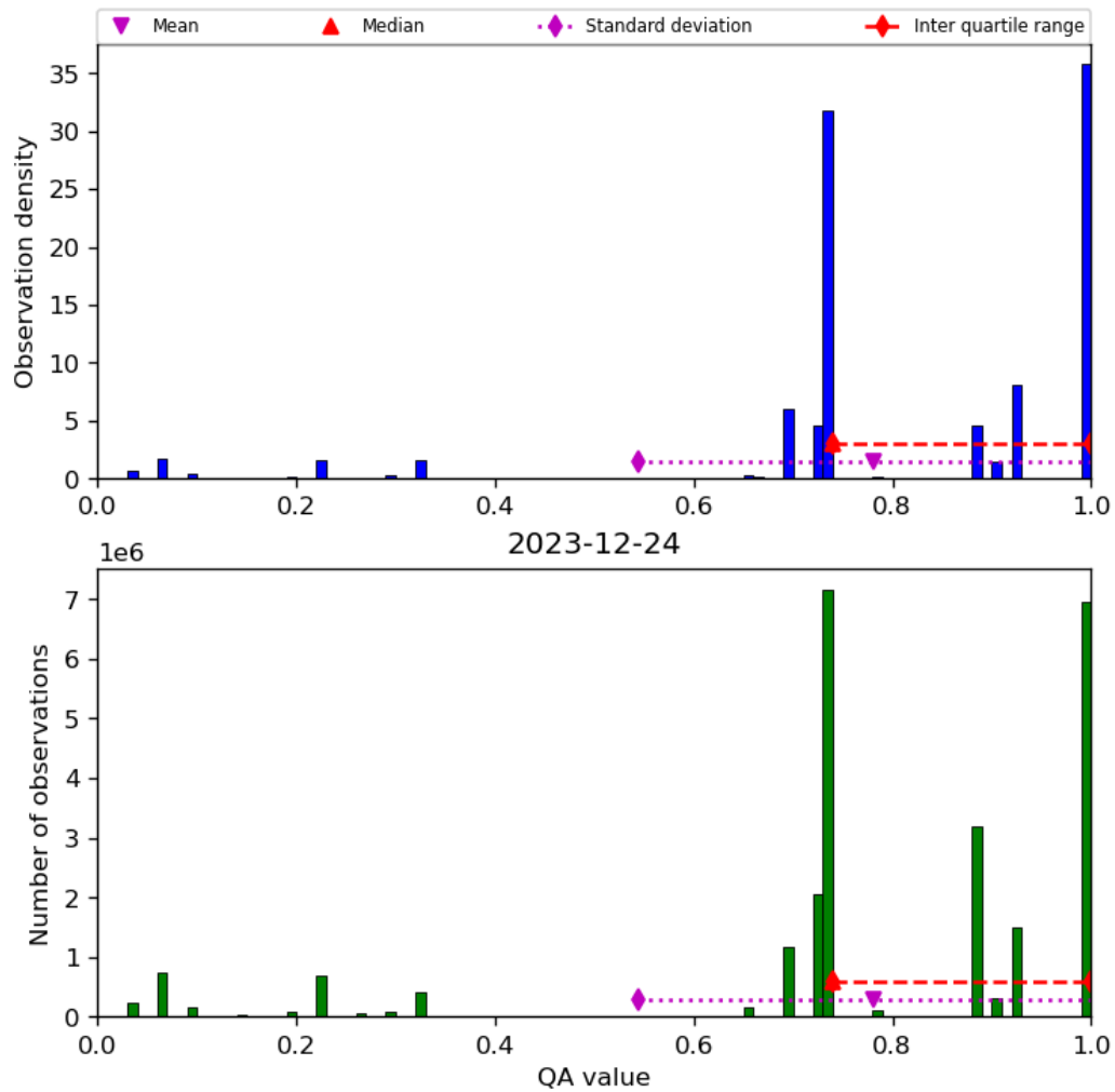
Figure 28: Histogram of “QA value” for 2023-12-23 to 2023-12-25
