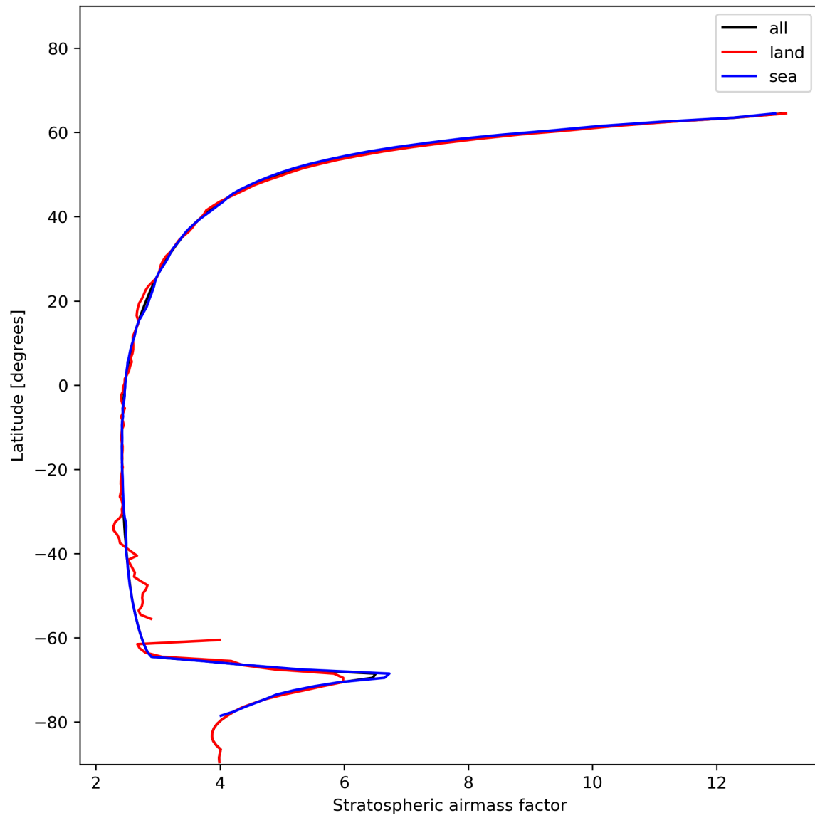
Figure 27: Zonal average of “Stratospheric airmass factor” for 2023-12-23 to 2023-12-25.
