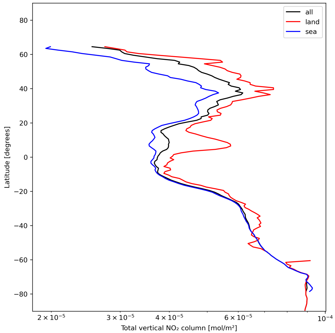
Figure 21: Zonal average of “Total vertical NO 2 column” for 2023-12-23 to 2023-12-25.
