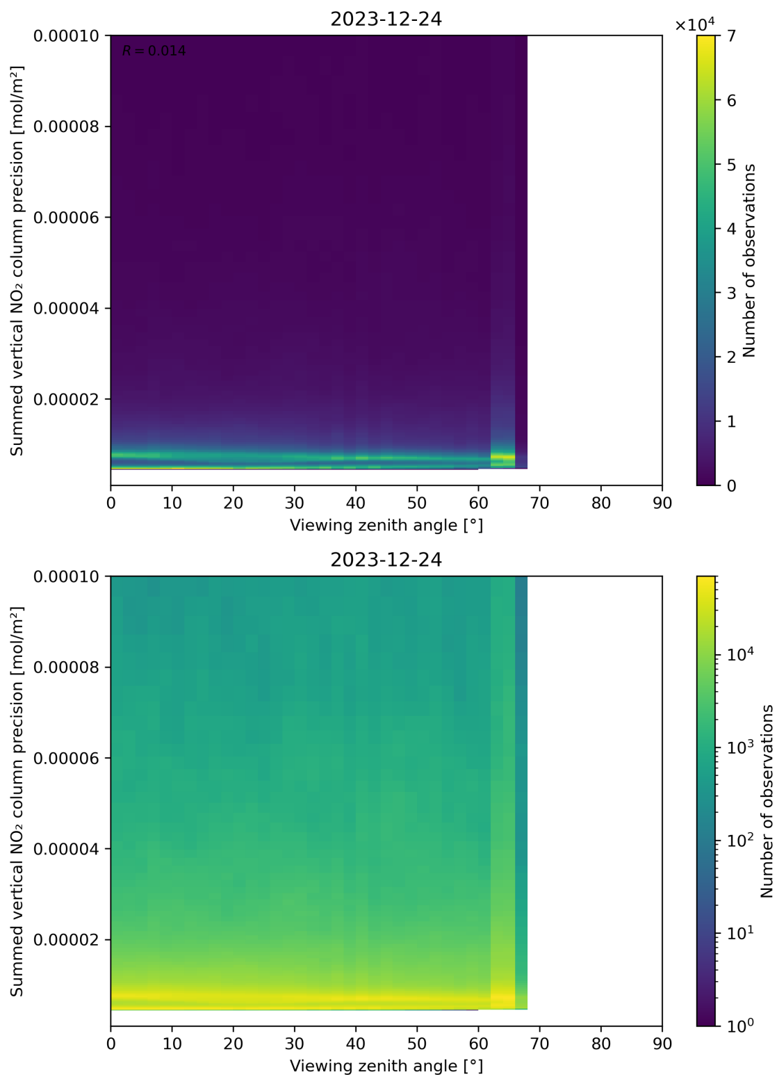
Figure 166: Scatter density plot of “Viewing zenith angle” against “Summed vertical NO 2 column precision” for 2023-12-23 to 2023-12-25.
