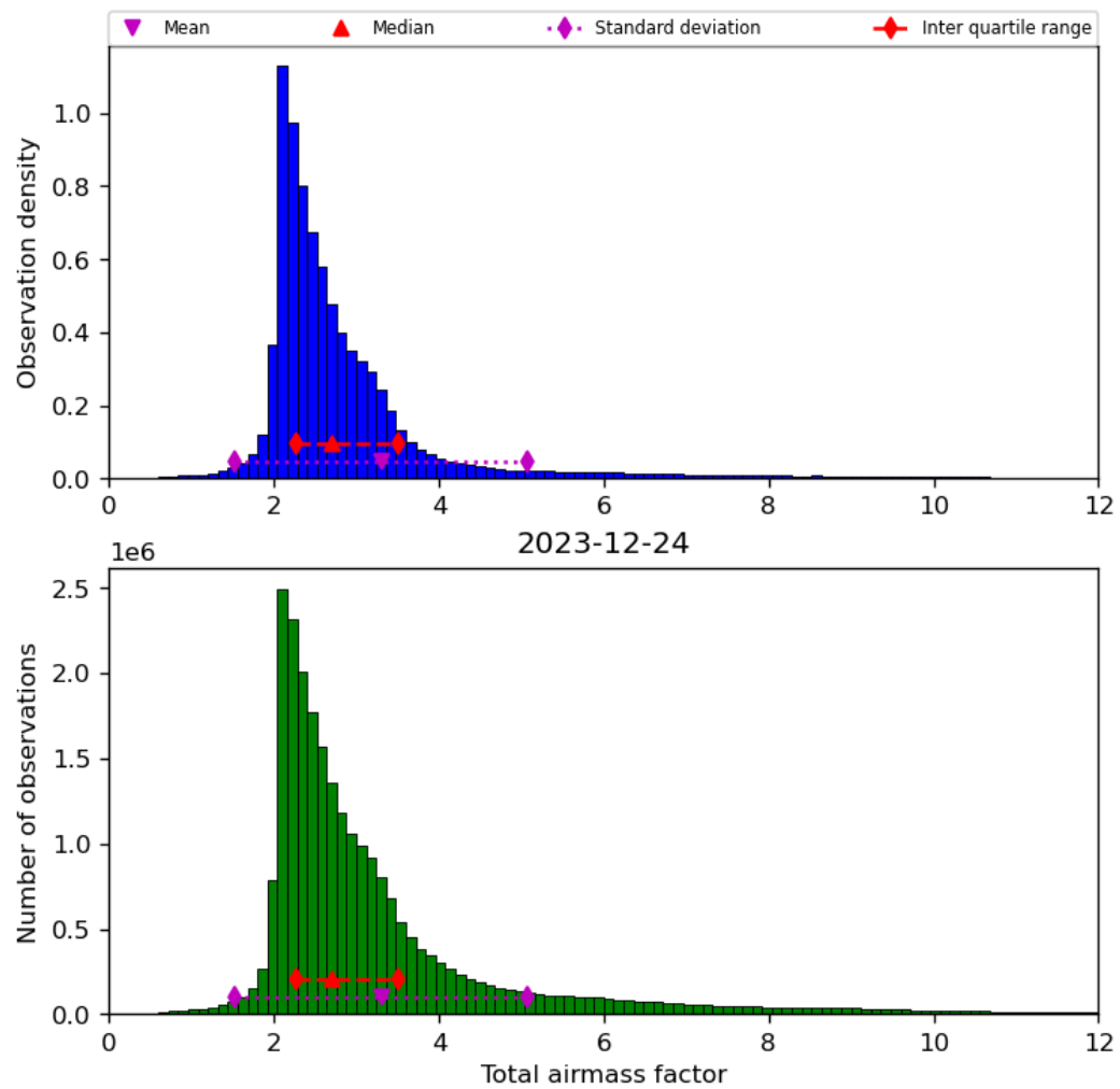
Figure 32: Histogram of “Total airmass factor” for 2023-12-23 to 2023-12-25
