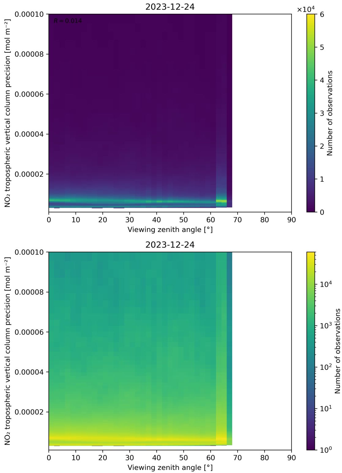
Figure 170: Scatter density plot of “Viewing zenith angle” against “NO 2 tropospheric vertical column precision” for 2023-12-23 to 2023-12-25.
