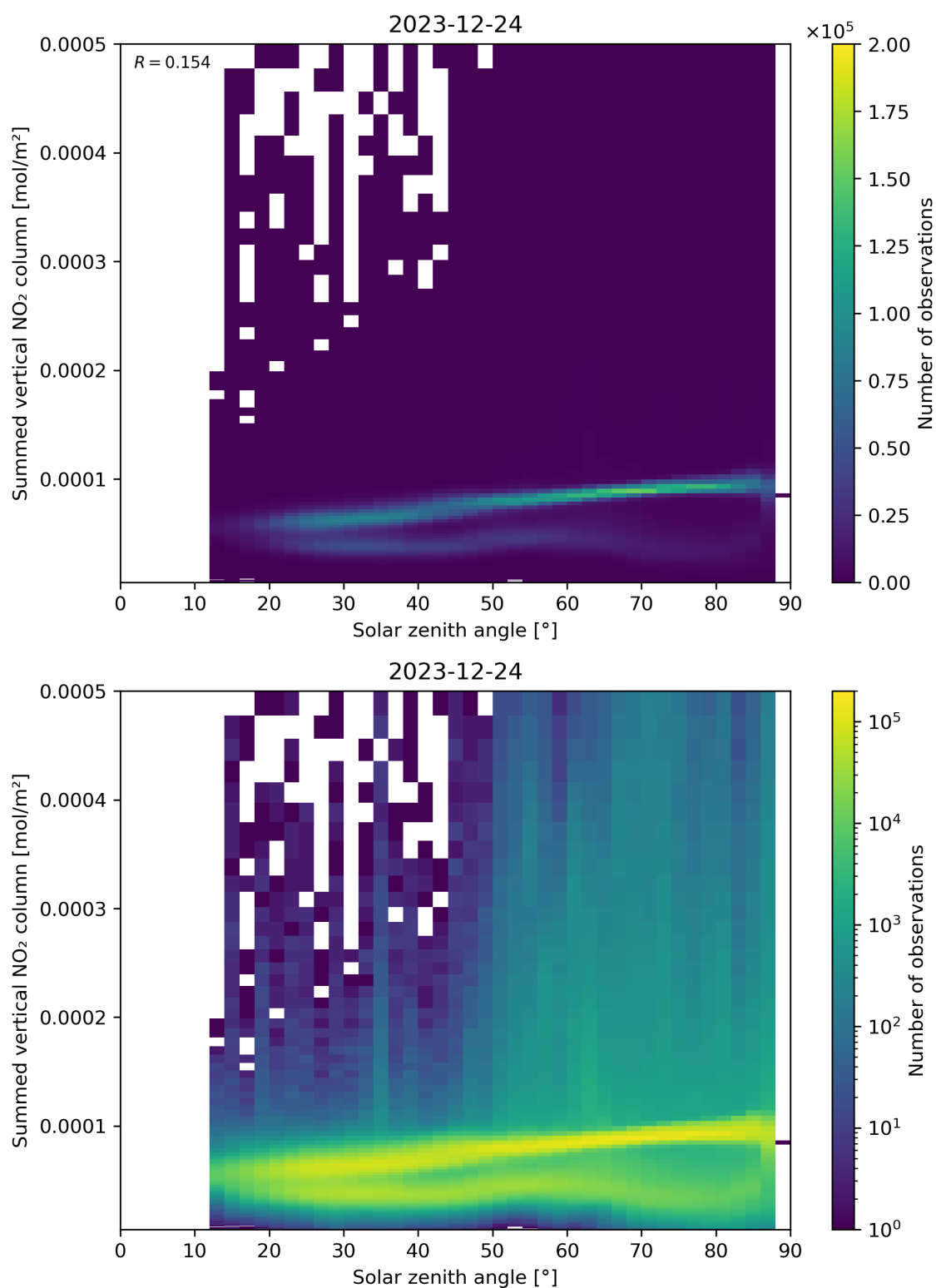
Figure 151: Scatter density plot of “Solar zenith angle” against “Summed vertical NO 2 column” for 2023-12-23 to 2023-12-25.
