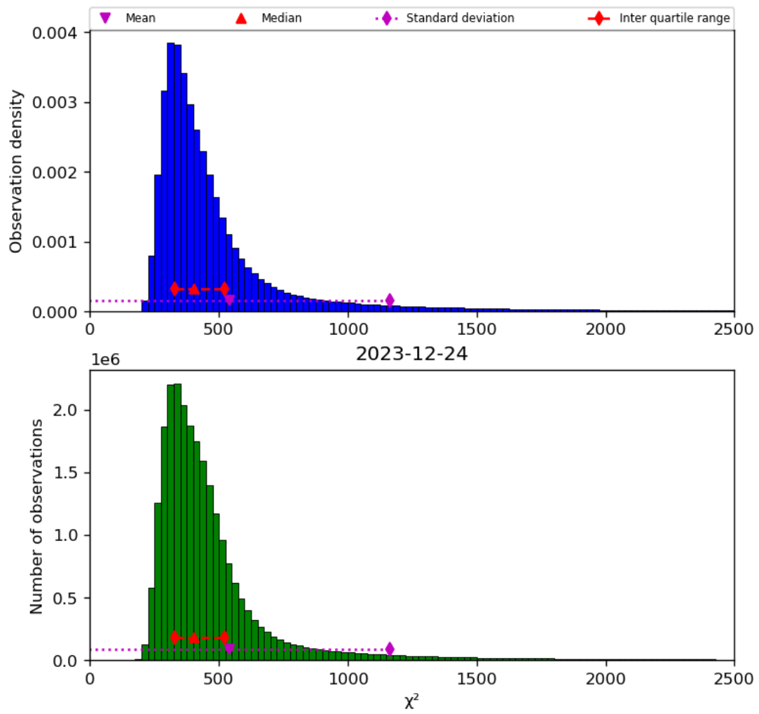
Figure 42: Histogram of “ \chi^2 ” for 2023-12-23 to 2023-12-25
