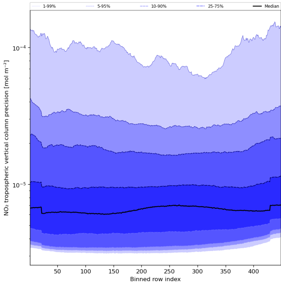
Figure 47: Along track statistics of “NO 2 tropospheric vertical column precision” for 2023-12-23 to 2023-12-25
