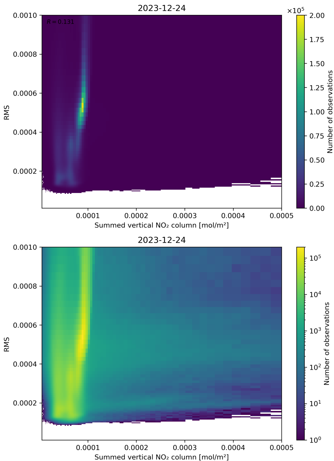
Figure 109: Scatter density plot of “Summed vertical NO 2 column” against “RMS” for 2023-12-23 to 2023-12-25.
