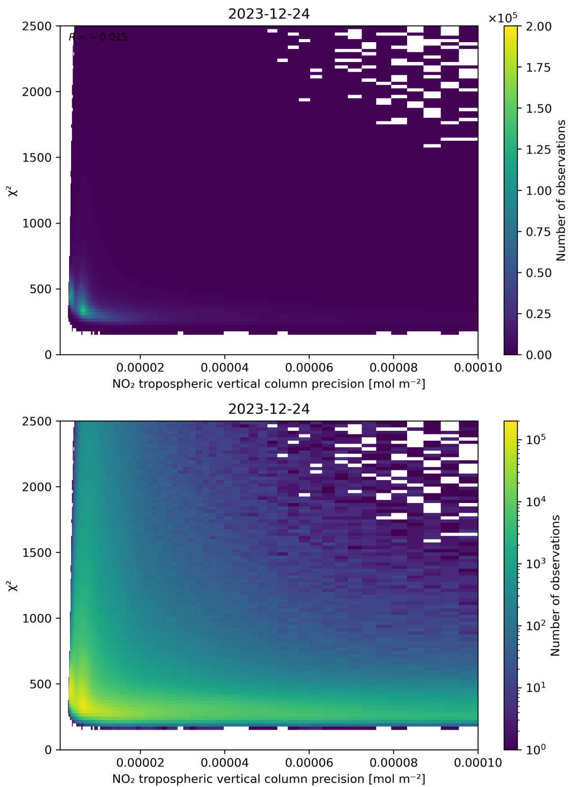
Figure 134: Scatter density plot of “NO 2 tropospheric vertical column precision” against “ \chi^2 ” for 2023-12-23 to 2023-12-25.
