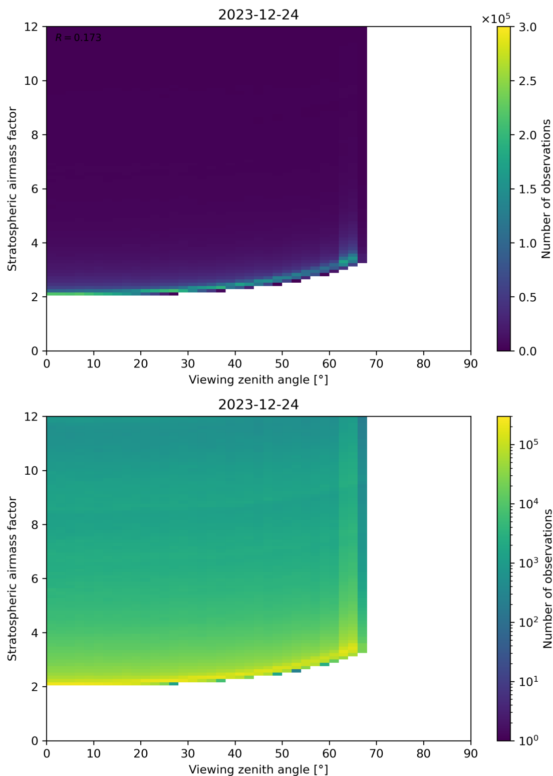
Figure 159: Scatter density plot of “Viewing zenith angle” against “Stratospheric airmass factor” for 2023-12-23 to 2023-12-25.
