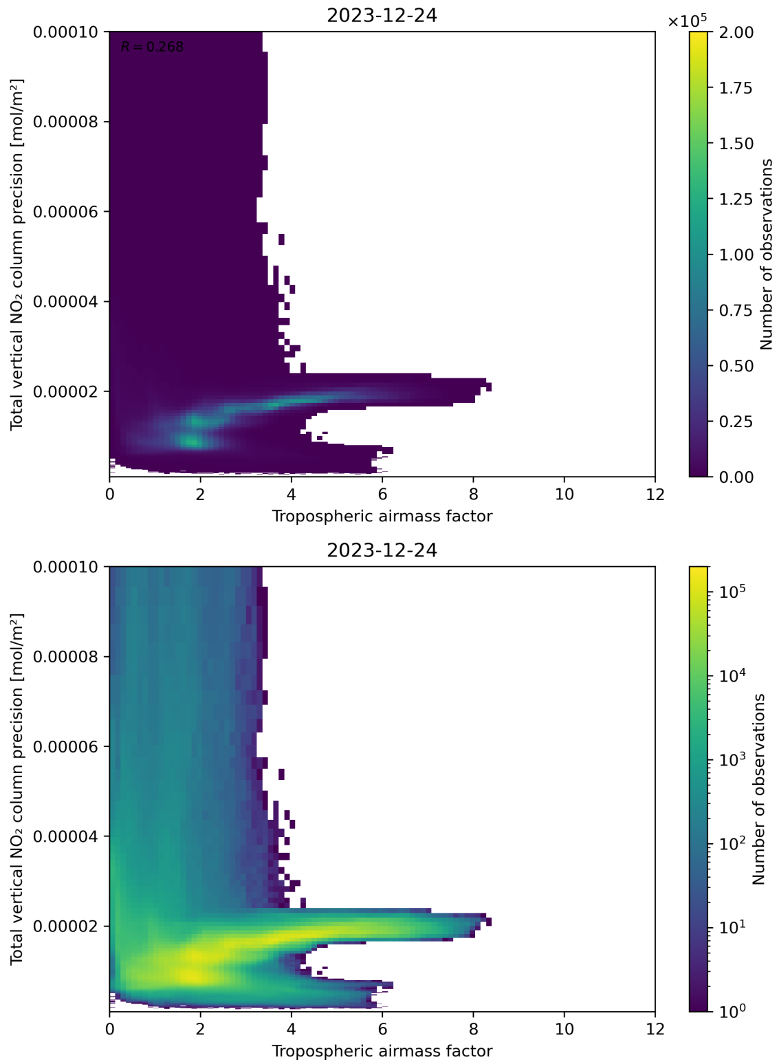
Figure 78: Scatter density plot of “Tropospheric air mass factor” against “Total vertical NO 2 column precision” for 2023-12-23 to 2023-12-25.
