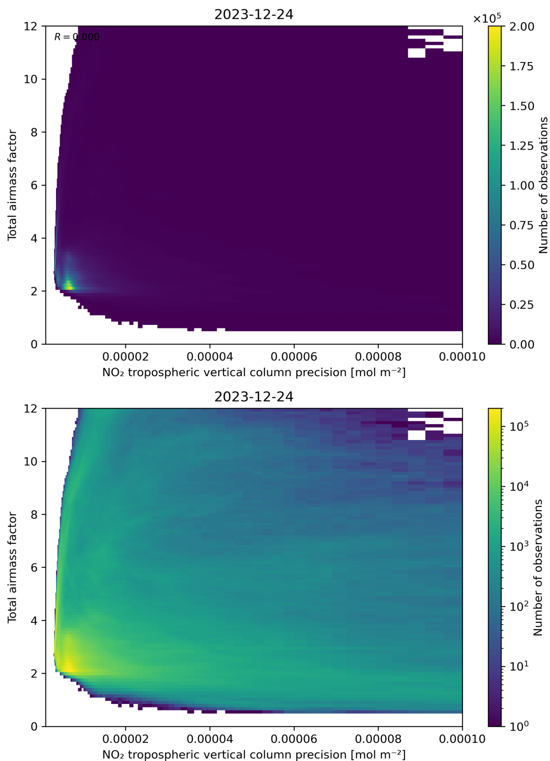
Figure 132: Scatter density plot of “NO 2 tropospheric vertical column precision” against “Total air mass factor” for 2023-12-23 to 2023-12-25.
