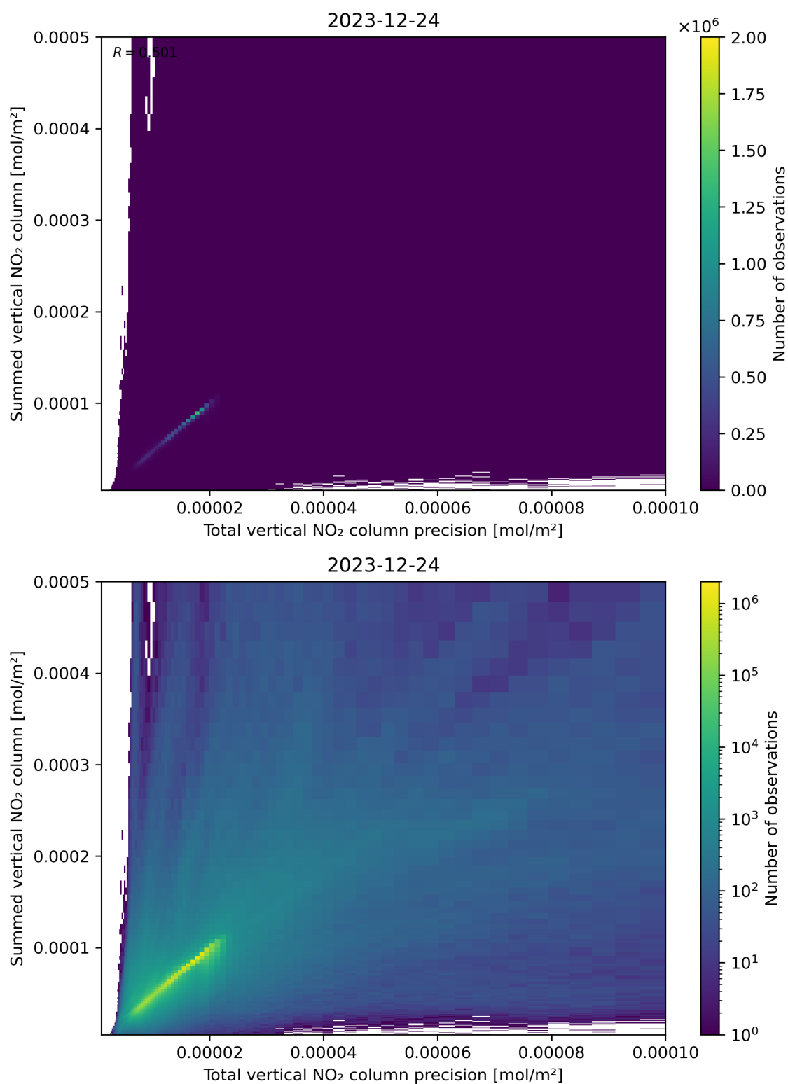
Figure 117: Scatter density plot of “Total vertical NO 2 column precision” against “Summed vertical NO 2 column” for 2023-12-23 to 2023-12-25.
