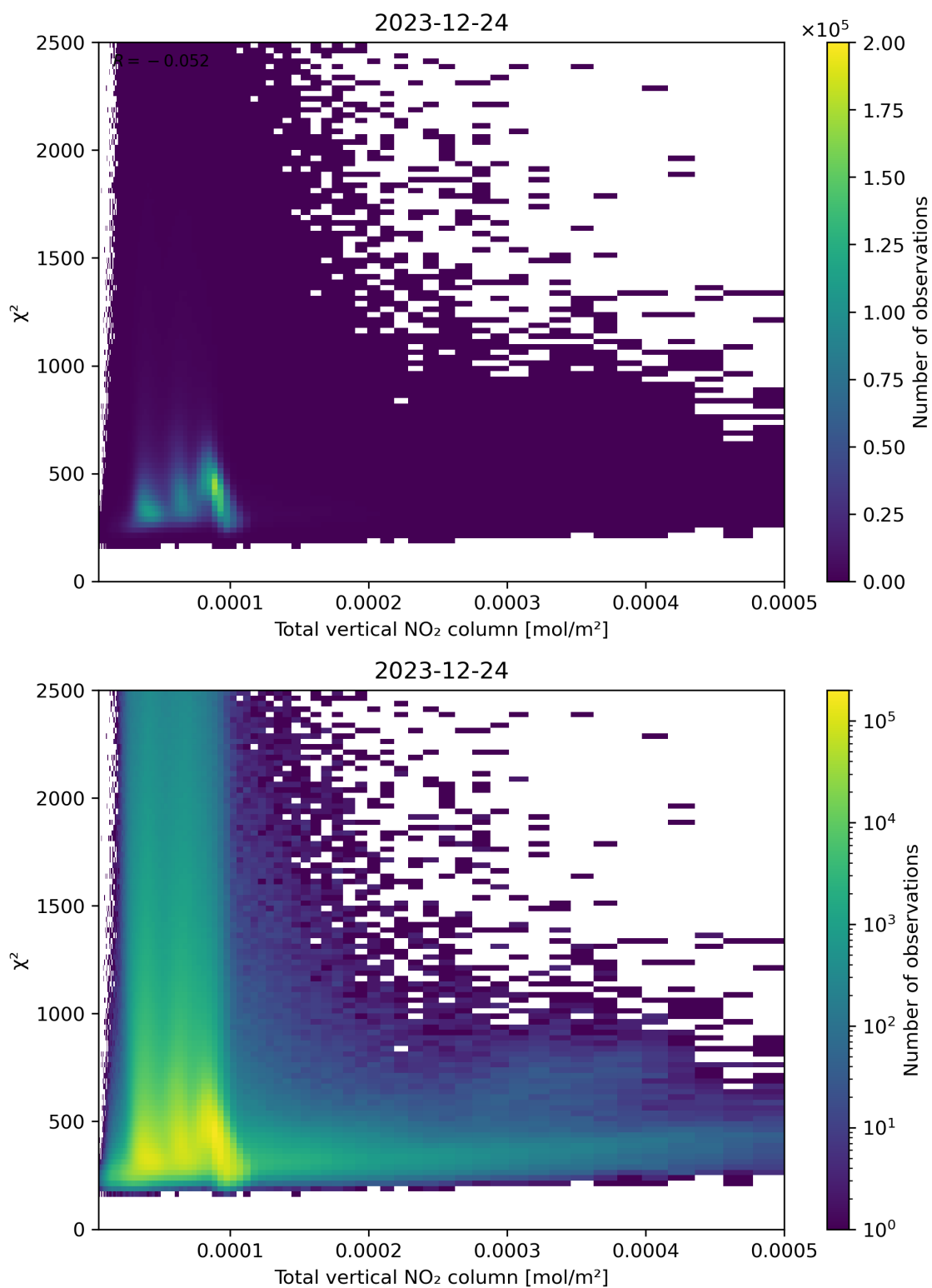
Figure 111: Scatter density plot of “Total vertical NO 2 column” against “ \chi^2 ” for 2023-12-23 to 2023-12-25.
