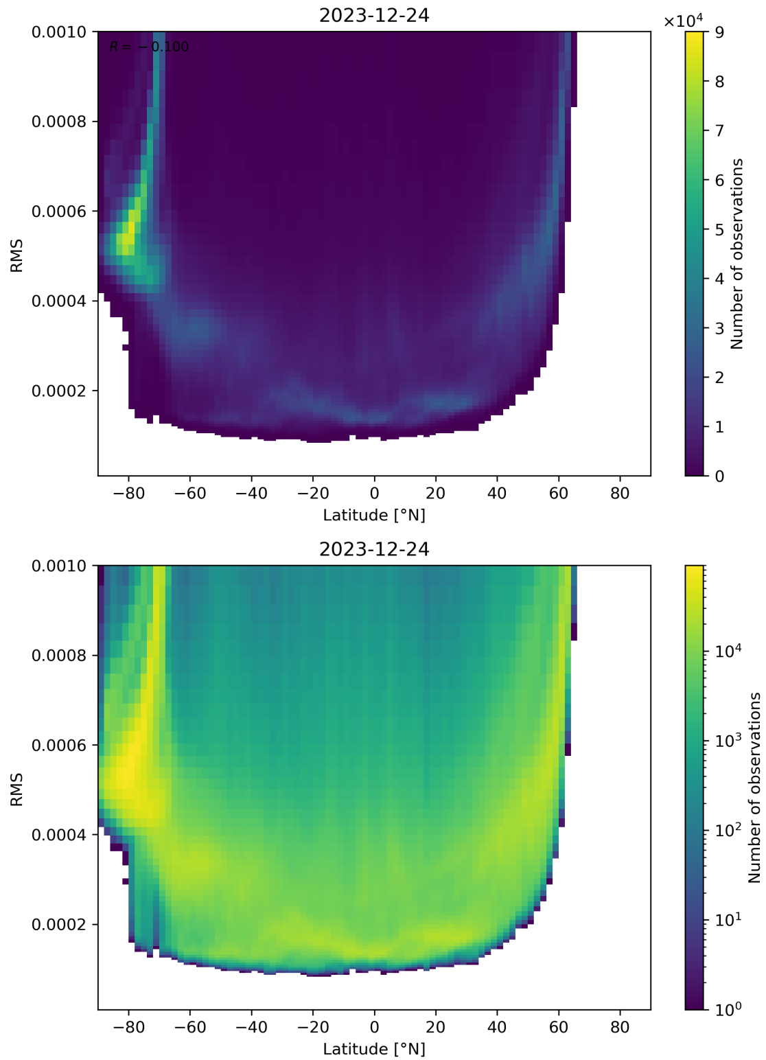
Figure 94: Scatter density plot of “Latitude” against “RMS” for 2023-12-23 to 2023-12-25.
