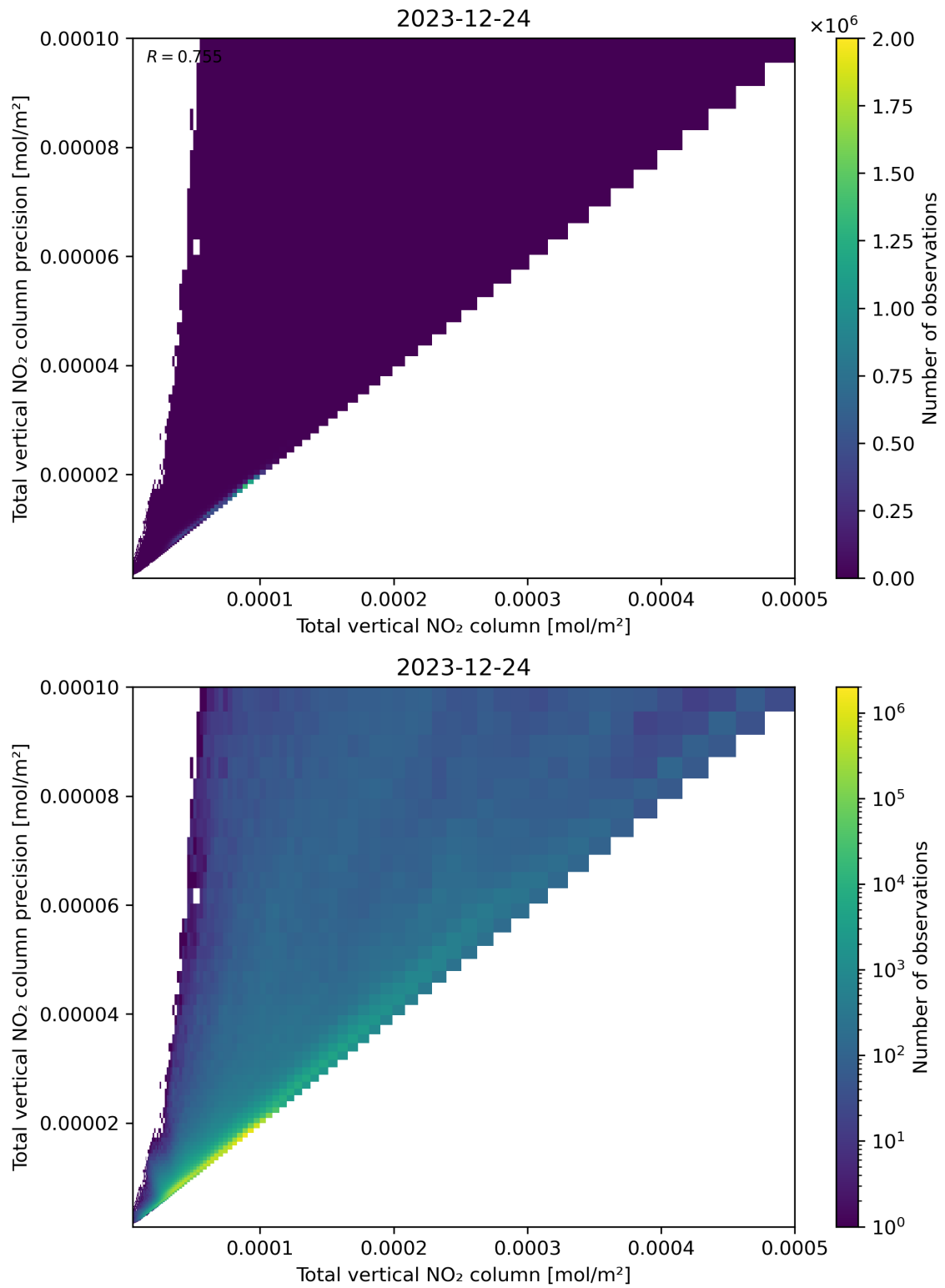
Figure 114: Scatter density plot of “Total vertical NO 2 column” against “Total vertical NO 2 column precision” for 2023-12-23 to 2023-12-25.
