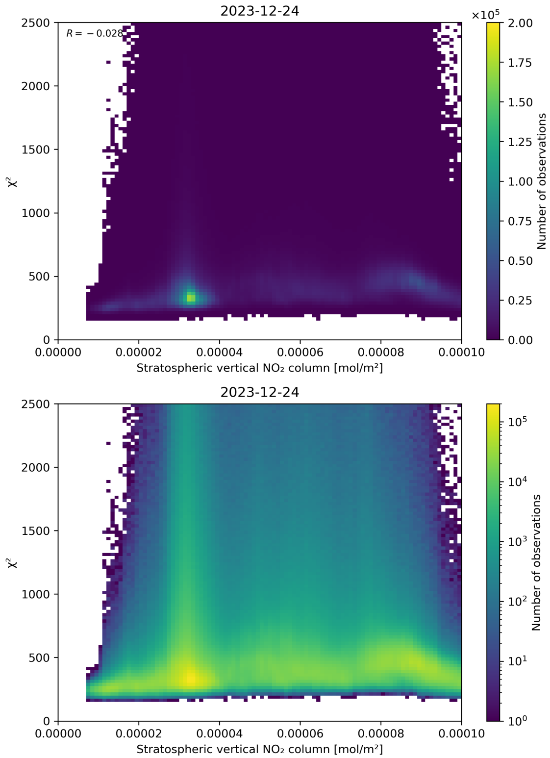
Figure 97: Scatter density plot of “Stratospheric vertical NO 2 column” against “ \chi^2 ” for 2023-12-23 to 2023-12-25.
