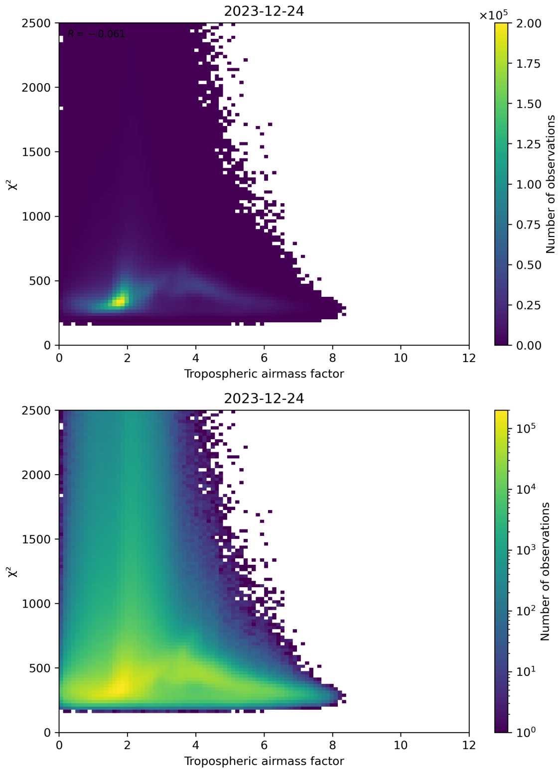
Figure 73: Scatter density plot of “Tropospheric airmass factor” against “ \chi^2 ” for 2023-12-23 to 2023-12-25.
