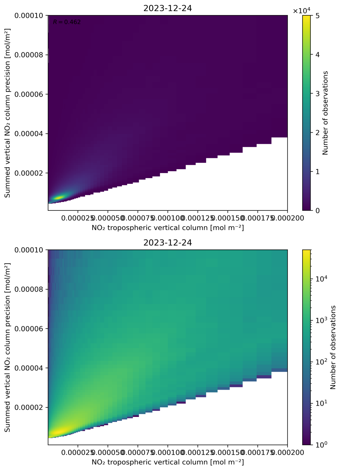
Figure 127: Scatter density plot of “NO 2 tropospheric vertical column” against “Summed vertical NO 2 column precision” for 2023-12-23 to 2023-12-25.
