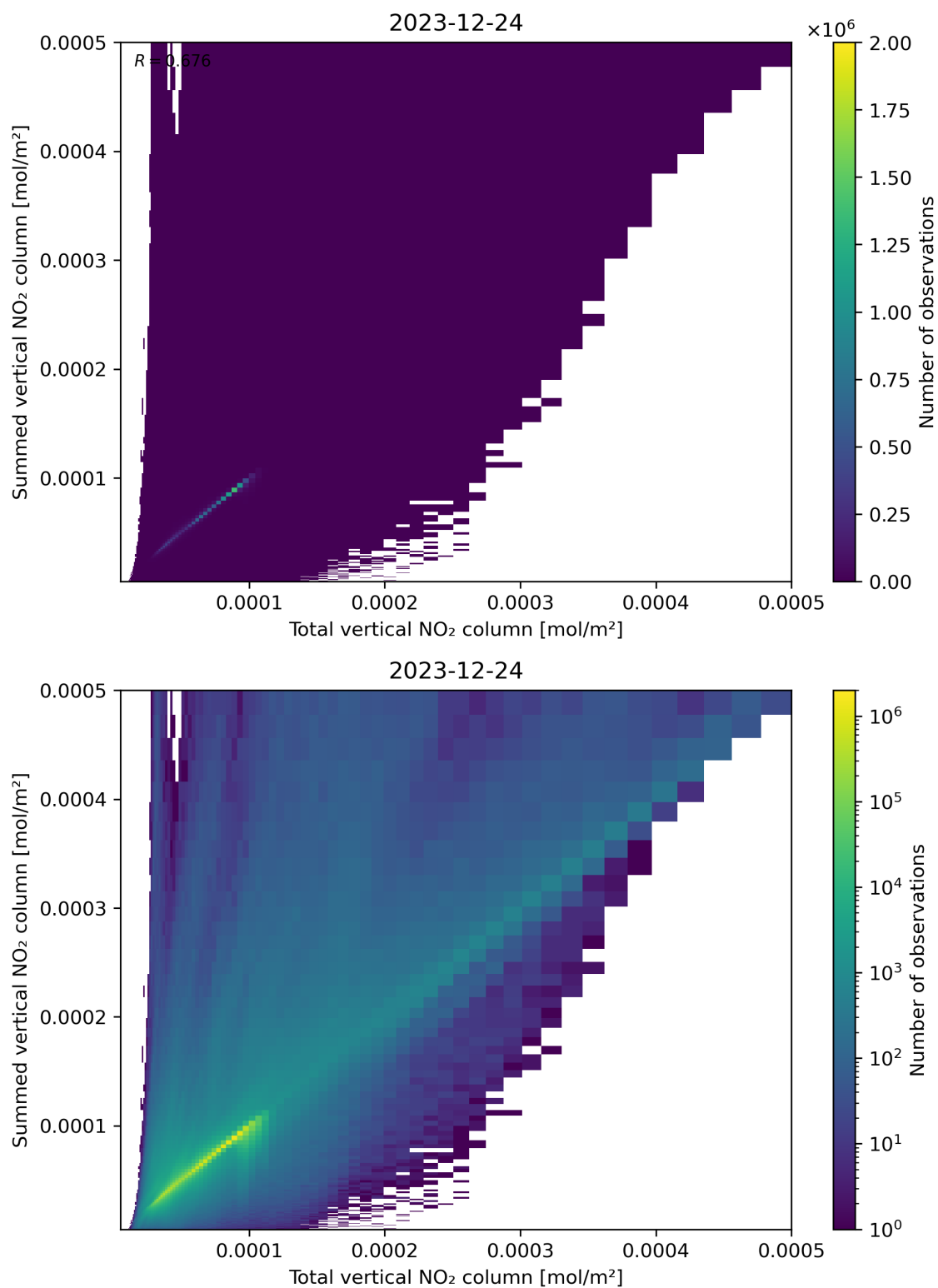
Figure 112: Scatter density plot of “Total vertical NO 2 column” against “Summed vertical NO 2 column” for 2023-12-23 to 2023-12-25.
