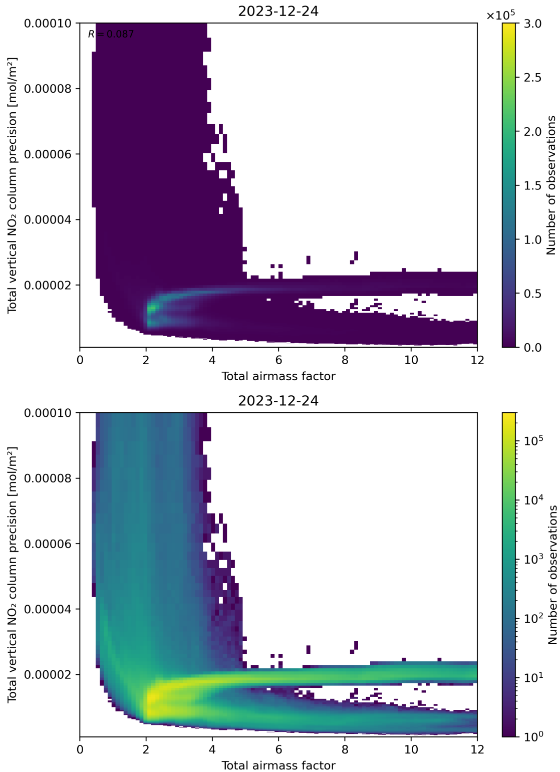
Figure 68: Scatter density plot of “Total airmass factor” against “Total vertical NO 2 column precision” for 2023-12-23 to 2023-12-25.
