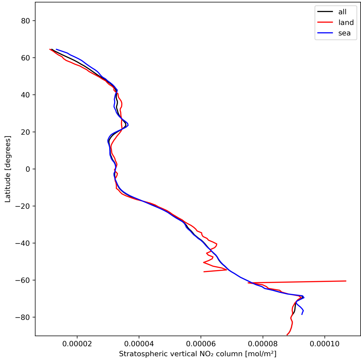
Figure 19: Zonal average of “Stratospheric vertical NO 2 column” for 2023-12-23 to 2023-12-25.
