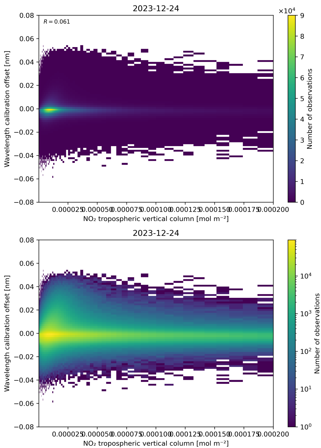
Figure 143: Scatter density plot of “NO 2 tropospheric vertical column” against “Wavelength calibration offset” for 2023-12-23 to 2023-12-25.
