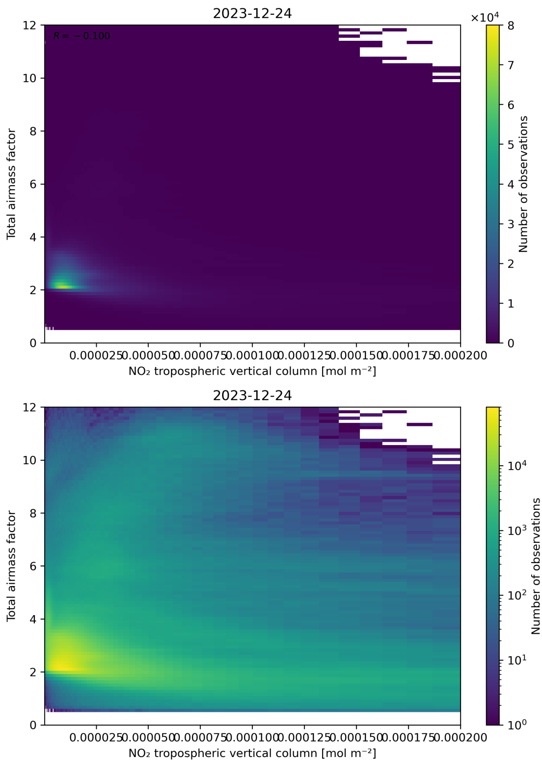
Figure 122: Scatter density plot of “NO 2 tropospheric vertical column” against “Total air mass factor” for 2023-12-23 to 2023-12-25.
