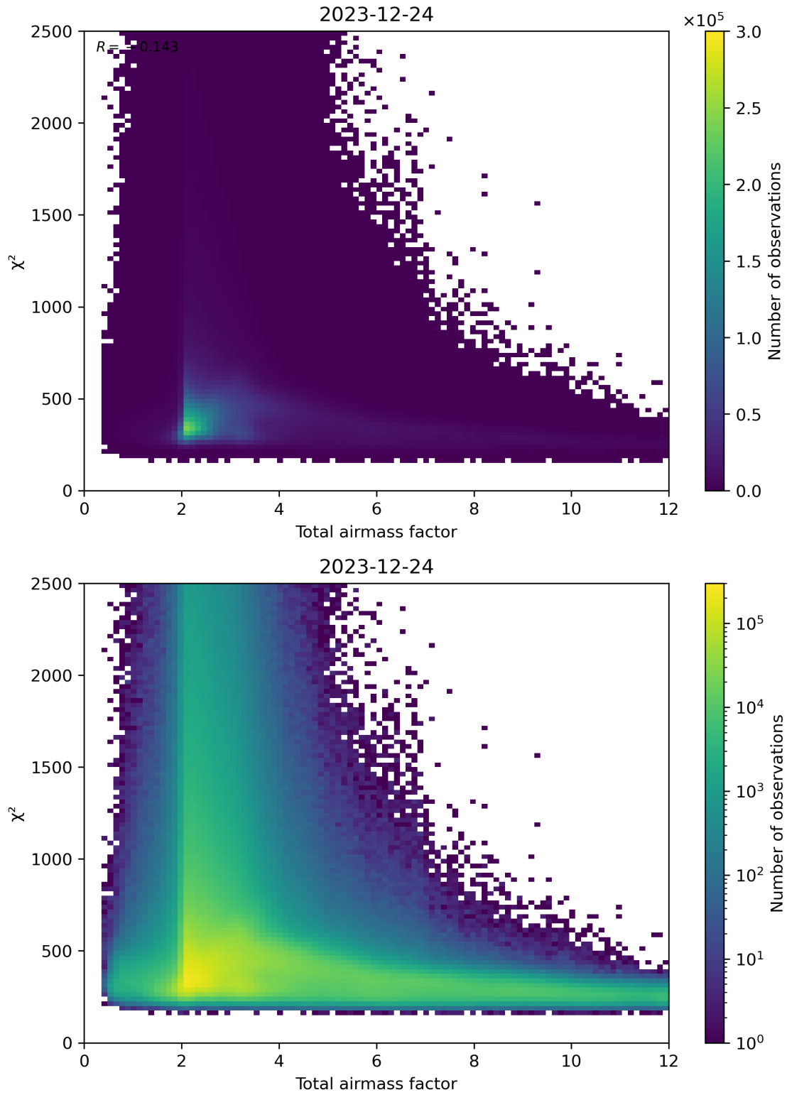
Figure 63: Scatter density plot of “Total airmass factor” against “ \chi^2 ” for 2023-12-23 to 2023-12-25.
