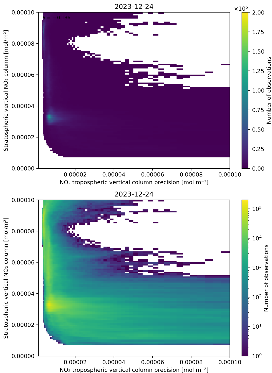
Figure 135: Scatter density plot of “NO 2 tropospheric vertical column precision” against “Stratospheric vertical NO 2 column” for 2023-12-23 to 2023-12-25.
