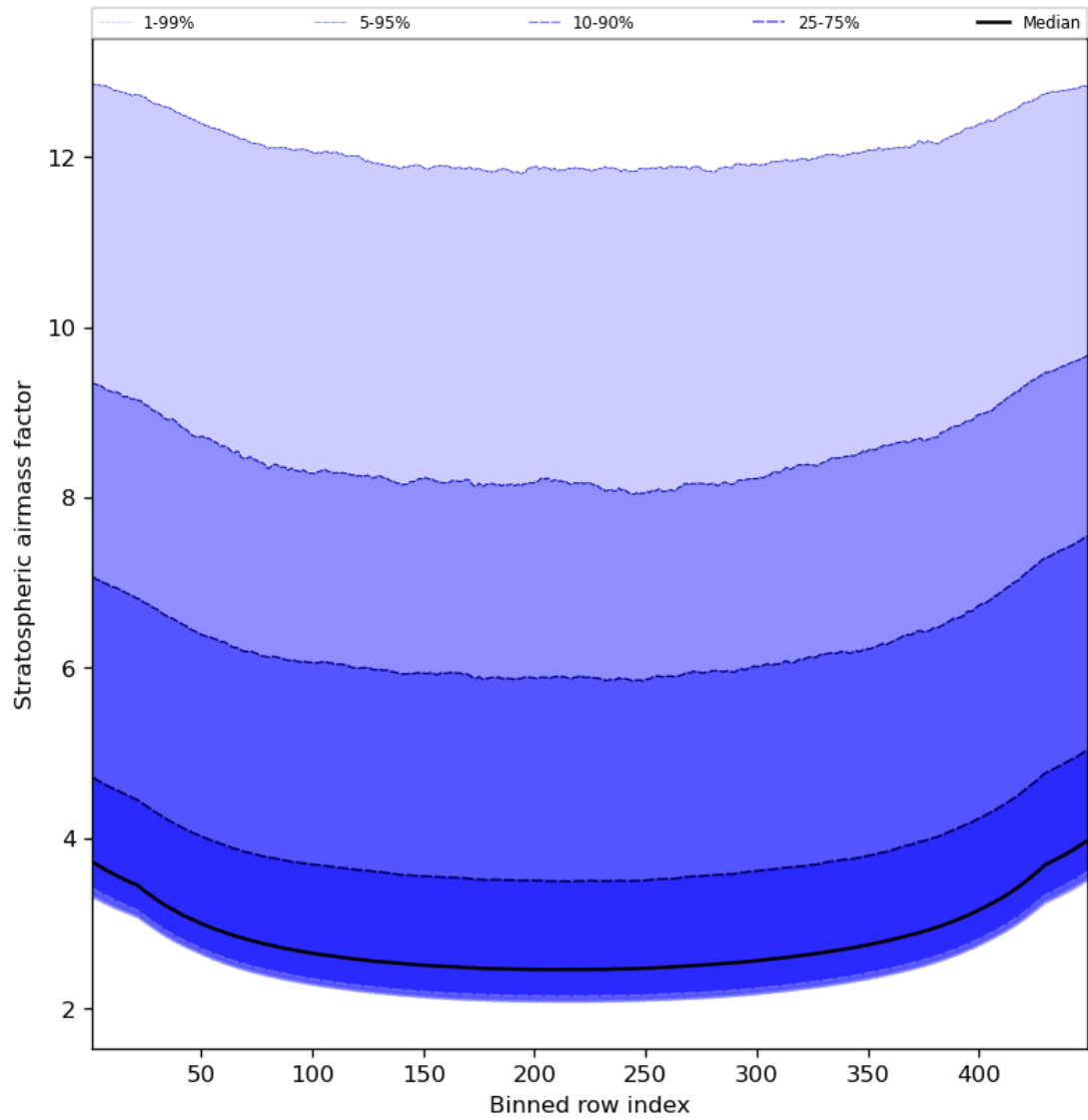
Figure 61: Along track statistics of “Stratospheric airmass factor” for 2023-12-23 to 2023-12-25
