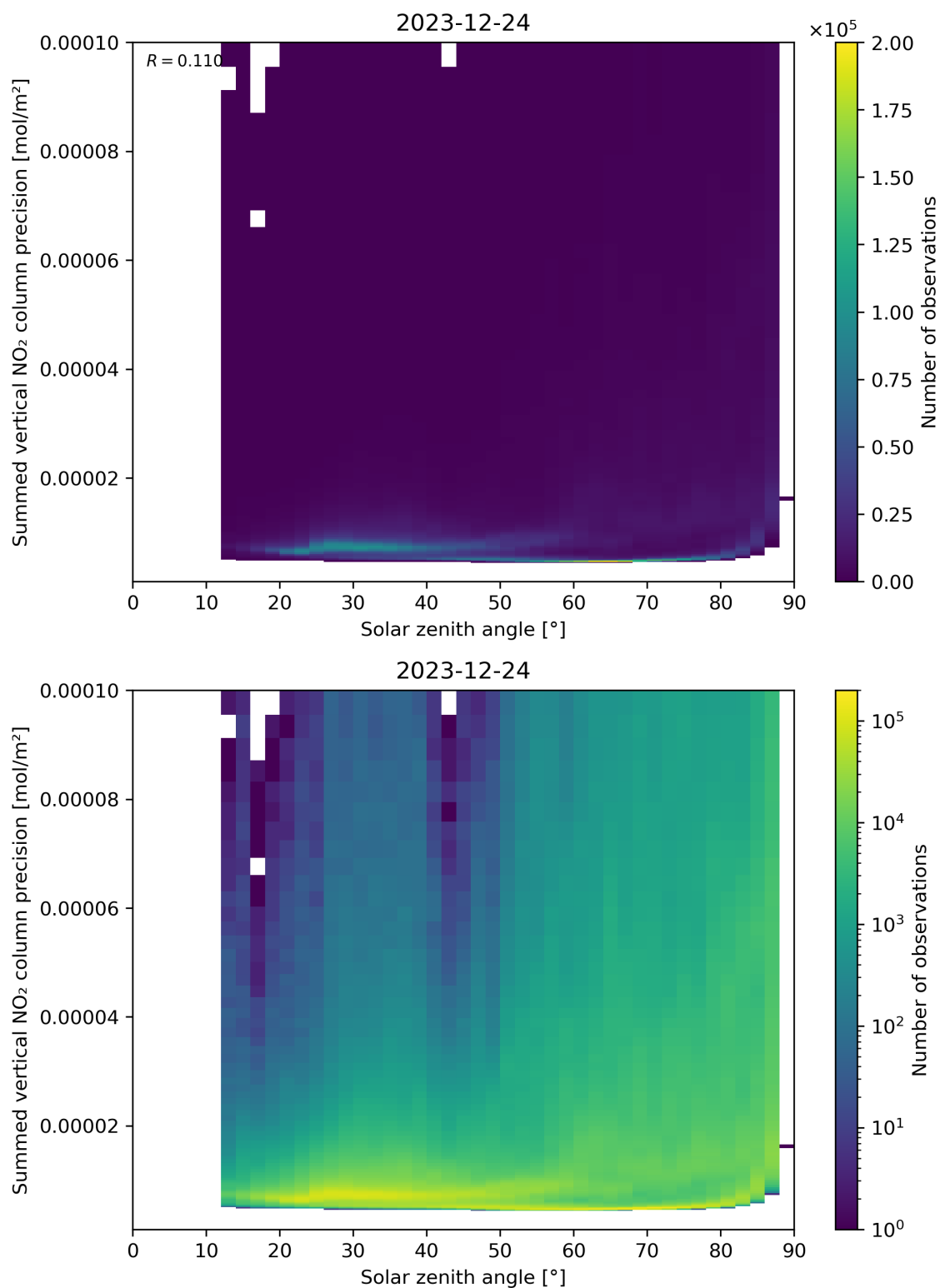
Figure 152: Scatter density plot of “Solar zenith angle” against “Summed vertical NO 2 column precision” for 2023-12-23 to 2023-12-25.
