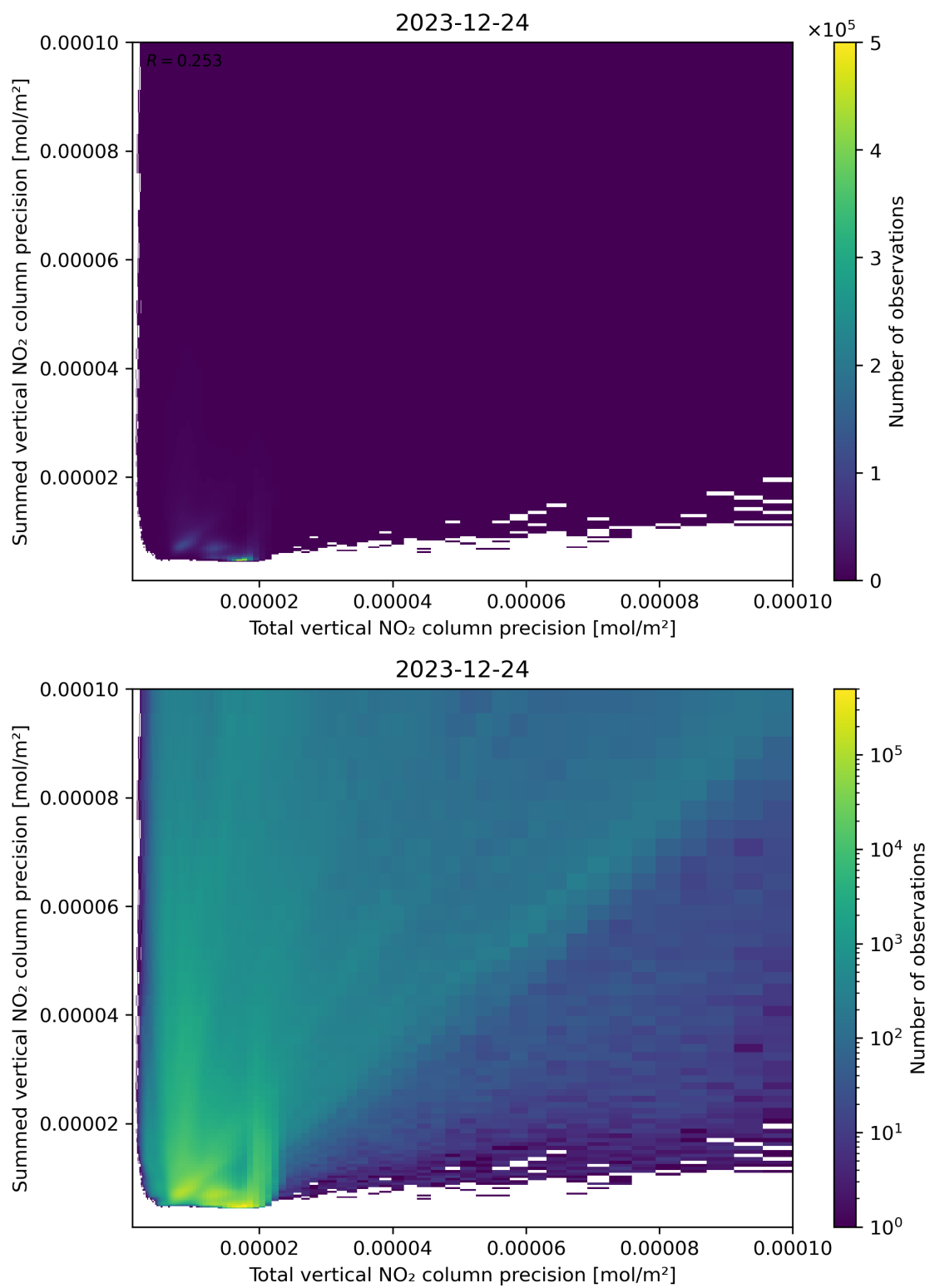
Figure 118: Scatter density plot of “Total vertical NO 2 column precision” against “Summed vertical NO 2 column precision” for 2023-12-23 to 2023-12-25.
