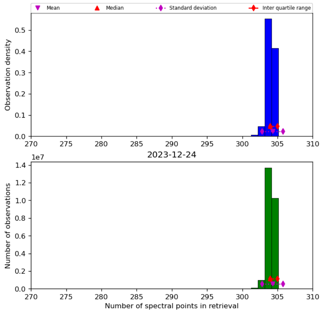
Figure 33: Histogram of “Number of spectral points in retrieval” for 2023-12-23 to 2023-12-25
