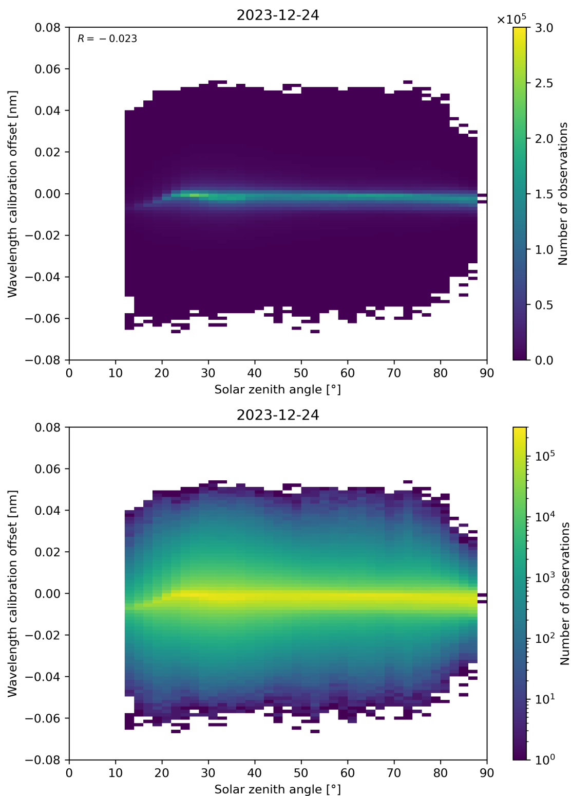
Figure 158: Scatter density plot of “Solar zenith angle” against “Wavelength calibration offset” for 2023-12-23 to 2023-12-25.
