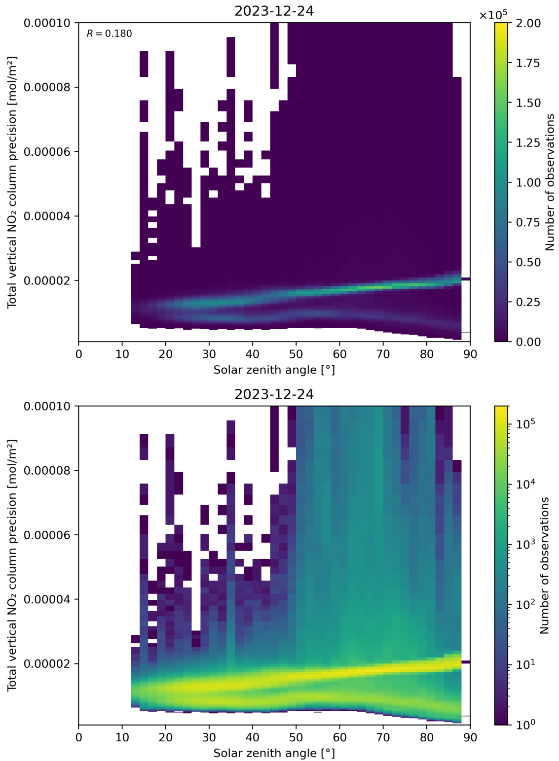
Figure 154: Scatter density plot of “Solar zenith angle” against “Total vertical NO 2 column precision” for 2023-12-23 to 2023-12-25.
