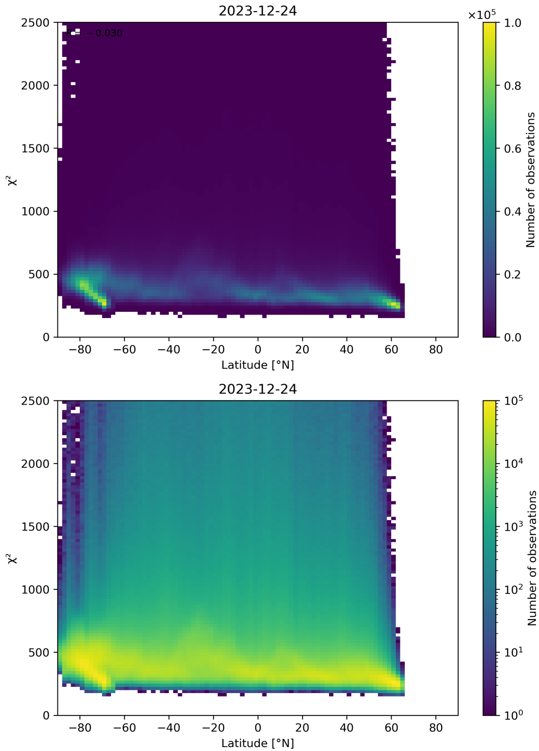
Figure 86: Scatter density plot of “Latitude” against “ \chi^2 ” for 2023-12-23 to 2023-12-25.
