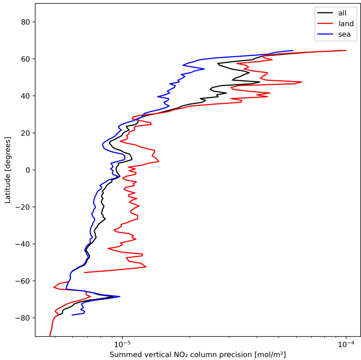
Figure 24: Zonal average of “Summed vertical NO 2 column precision” for 2023-12-23 to 2023-12-25.
