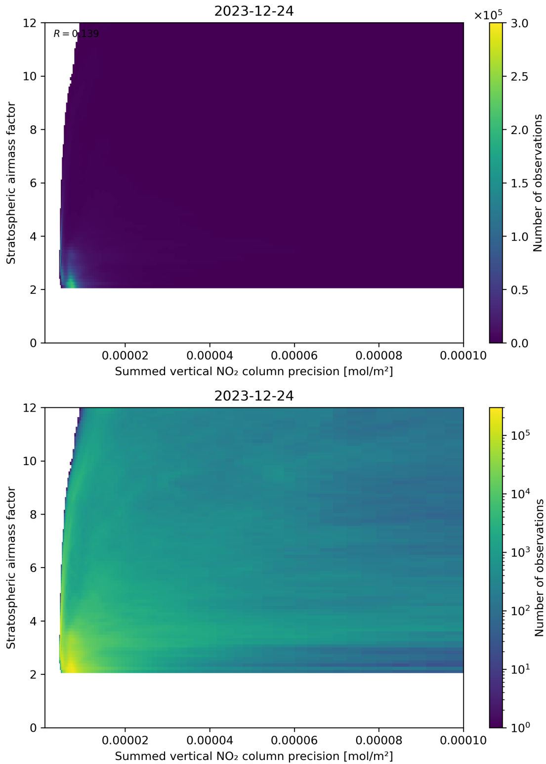
Figure 106: Scatter density plot of “Summed vertical NO 2 column precision” against “Stratospheric airmass factor” for 2023-12-23 to 2023-12-25.
