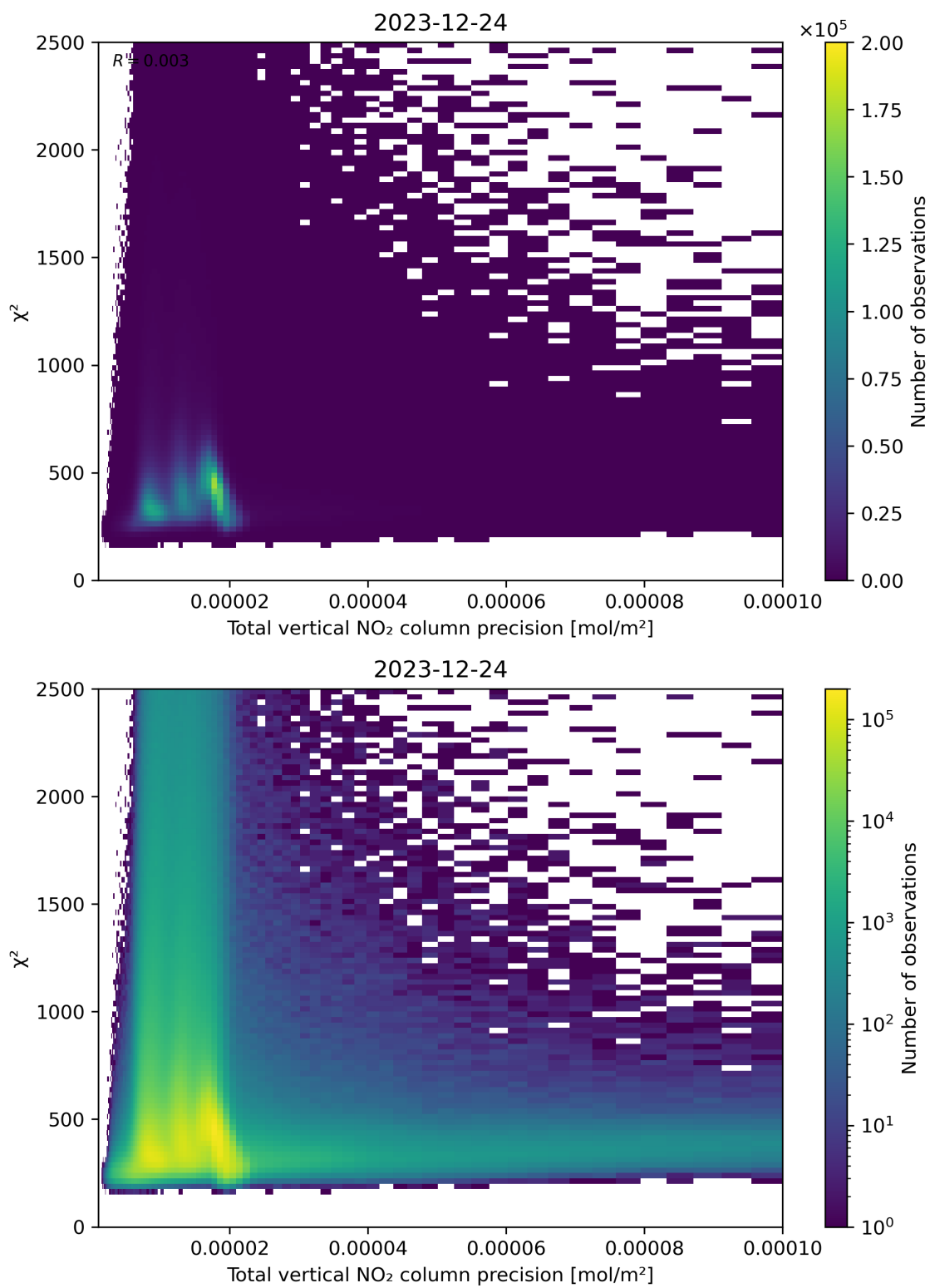
Figure 116: Scatter density plot of “Total vertical NO 2 column precision” against “ \chi^2 ” for 2023-12-23 to 2023-12-25.
