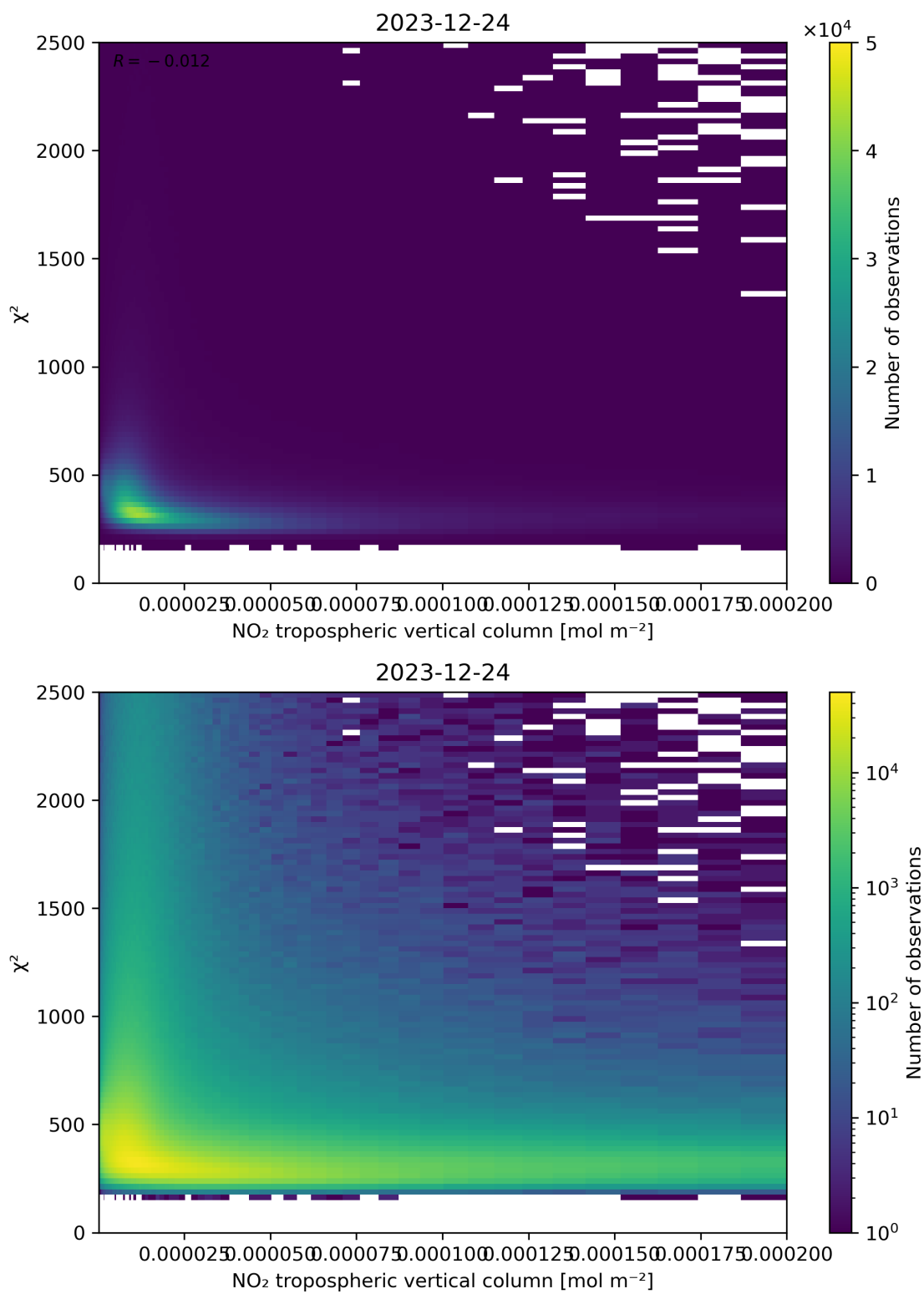
Figure 124: Scatter density plot of “NO 2 tropospheric vertical column” against “ \chi^2 ” for 2023-12-23 to 2023-12-25.
