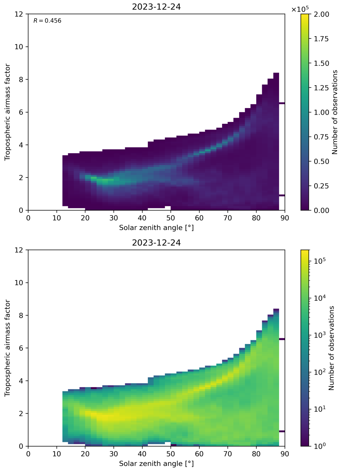
Figure 147: Scatter density plot of “Solar zenith angle” against “Tropospheric airmass factor” for 2023-12-23 to 2023-12-25.
