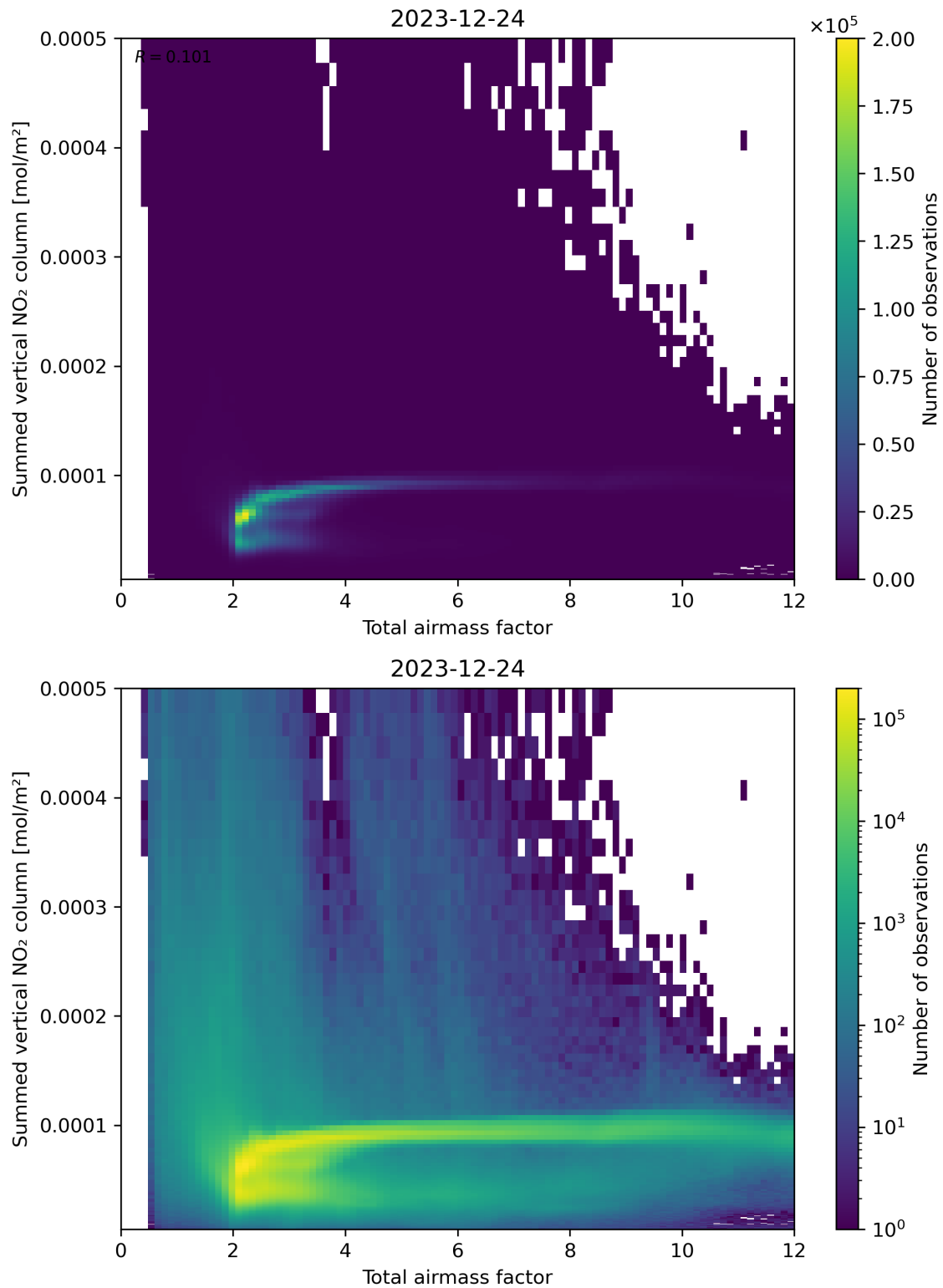
Figure 65: Scatter density plot of “Total airmass factor” against “Summed vertical NO 2 column” for 2023-12-23 to 2023-12-25.
