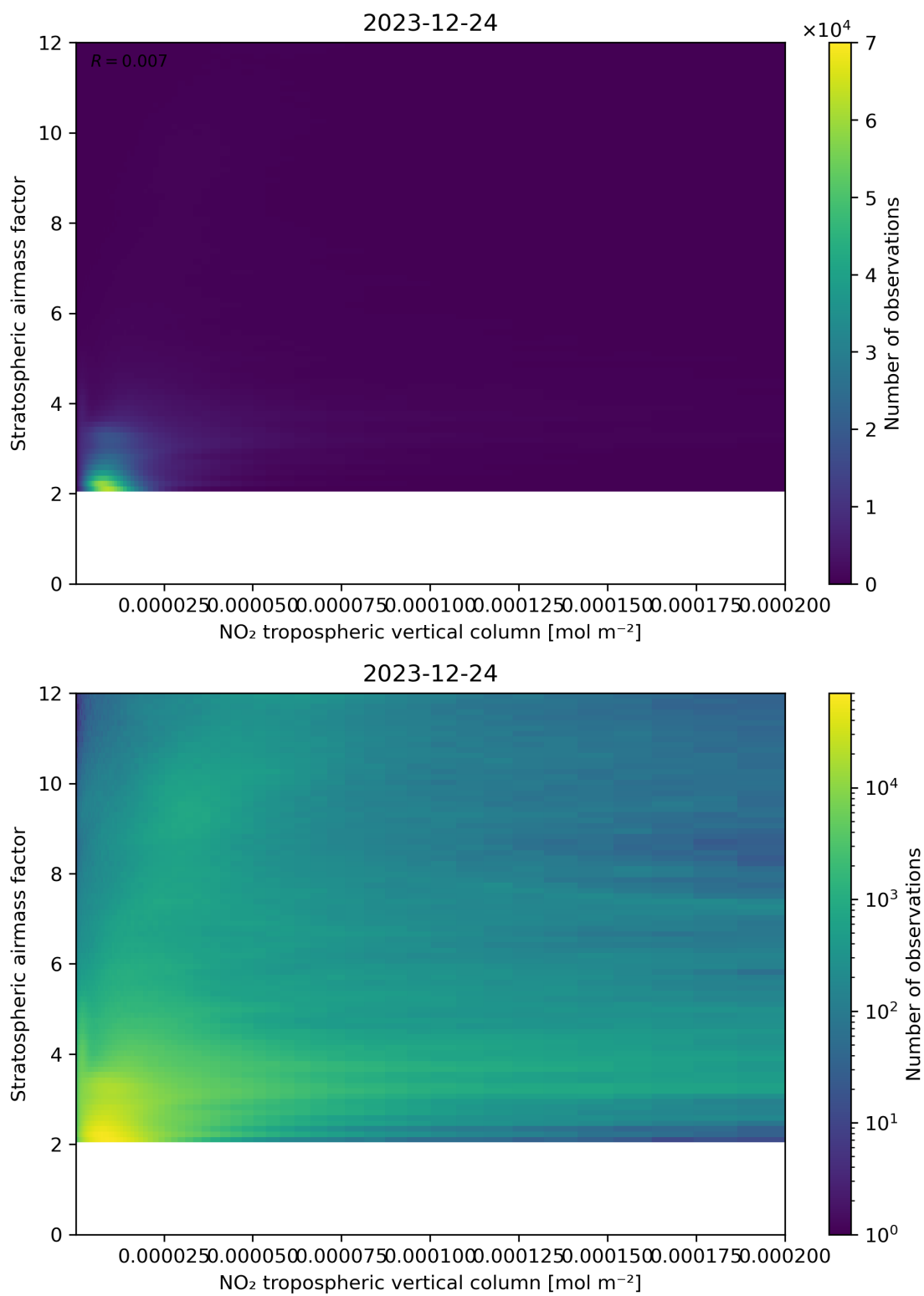
Figure 121: Scatter density plot of “NO 2 tropospheric vertical column” against “Stratospheric airmass factor” for 2023-12-23 to 2023-12-25.
