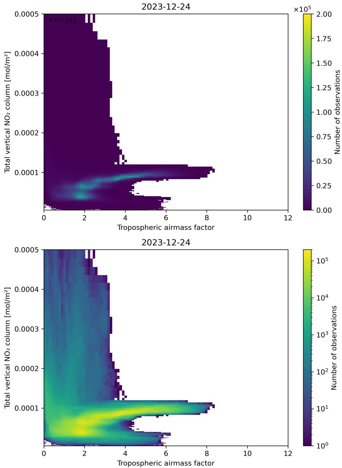
Figure 77: Scatter density plot of “Tropospheric airmass factor” against “Total vertical NO 2 column” for 2023-12-23 to 2023-12-25.
