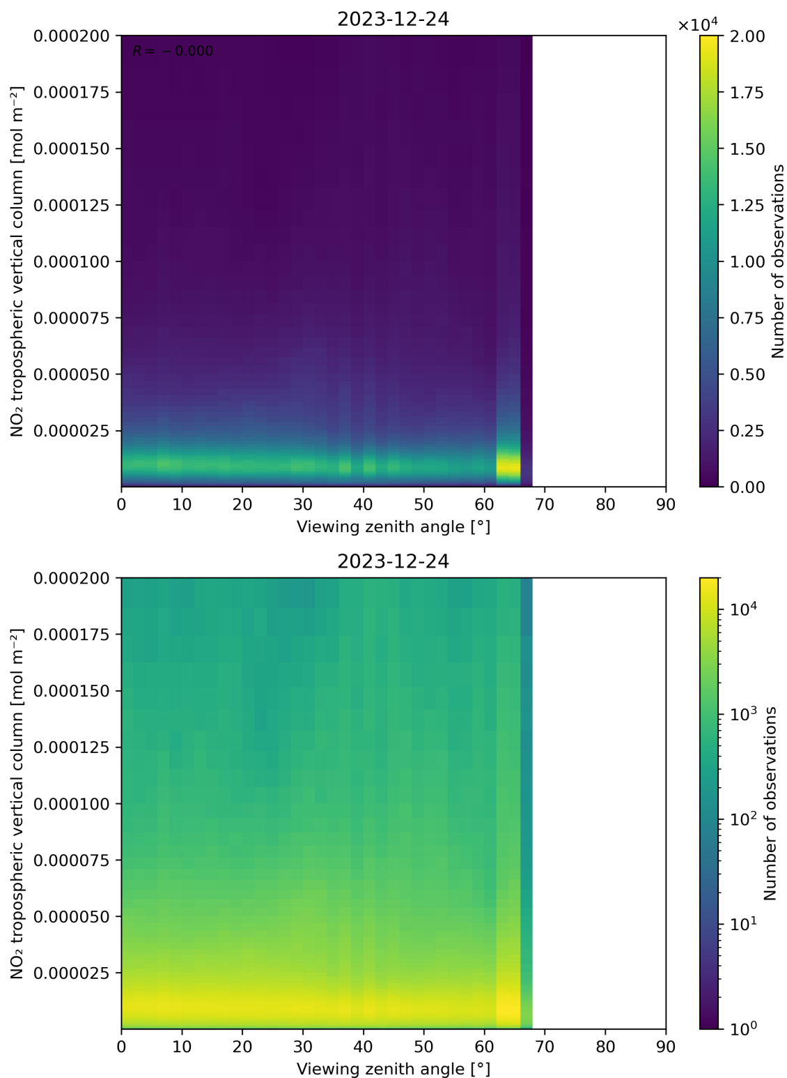
Figure 169: Scatter density plot of “Viewing zenith angle” against “NO 2 tropospheric vertical column” for 2023-12-23 to 2023-12-25.
