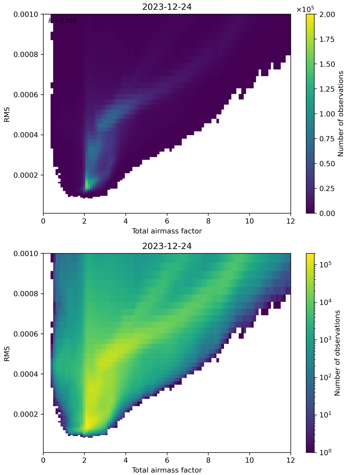
Figure 69: Scatter density plot of “Total airmass factor” against “RMS” for 2023-12-23 to 2023-12-25.
