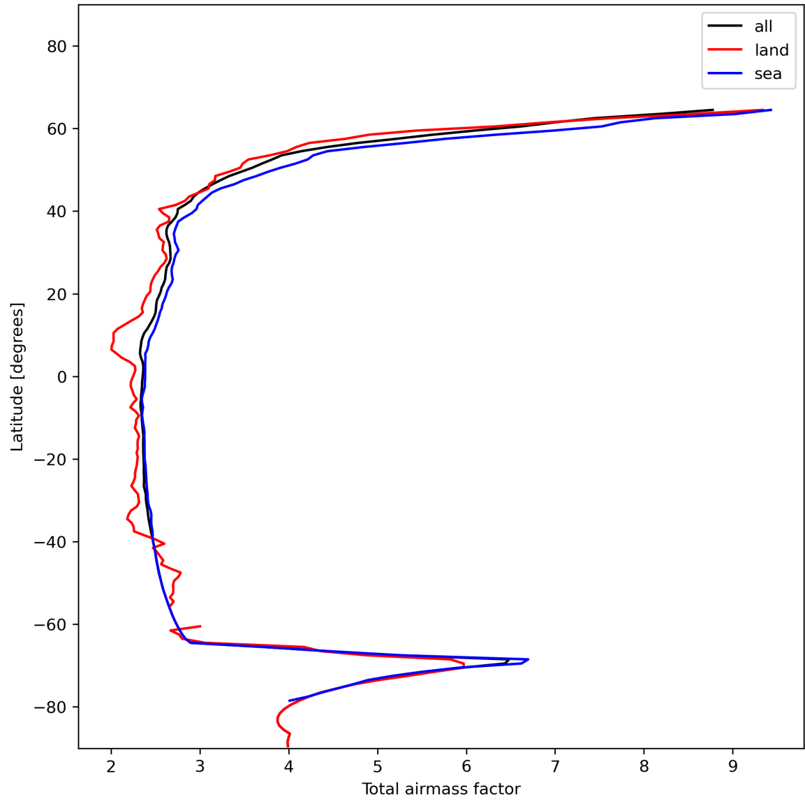
Figure 15: Zonal average of “Total airmass factor” for 2023-12-23 to 2023-12-25.
