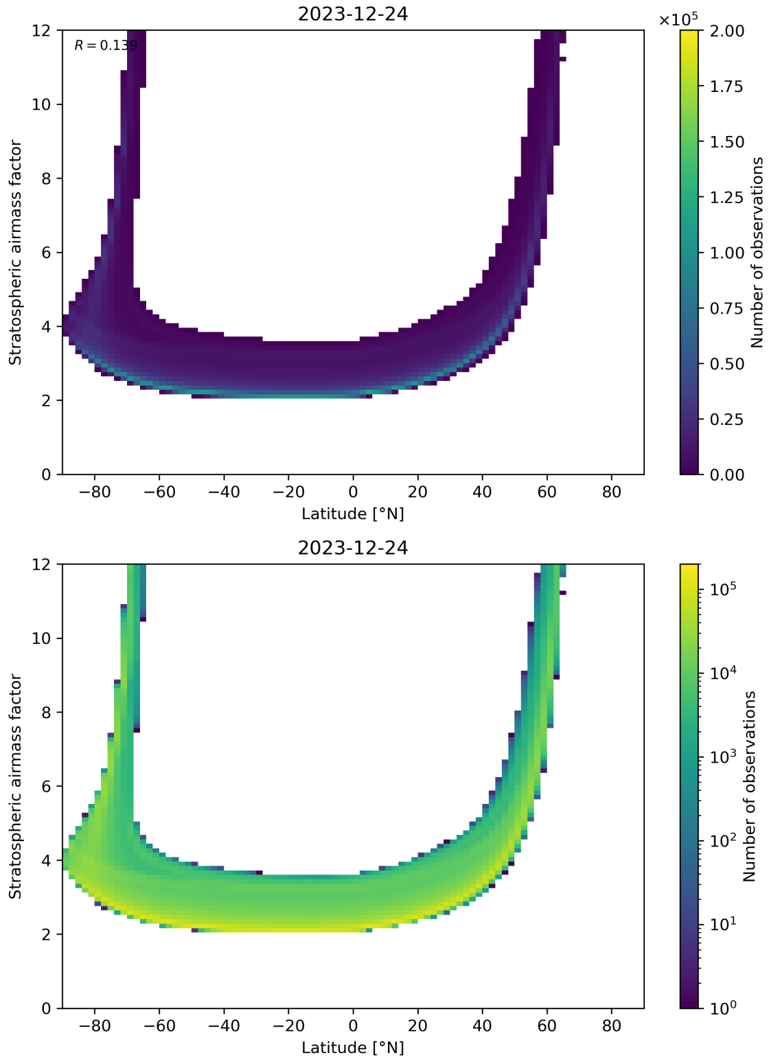
Figure 83: Scatter density plot of “Latitude” against “Stratospheric airmass factor” for 2023-12-23 to 2023-12-25.
