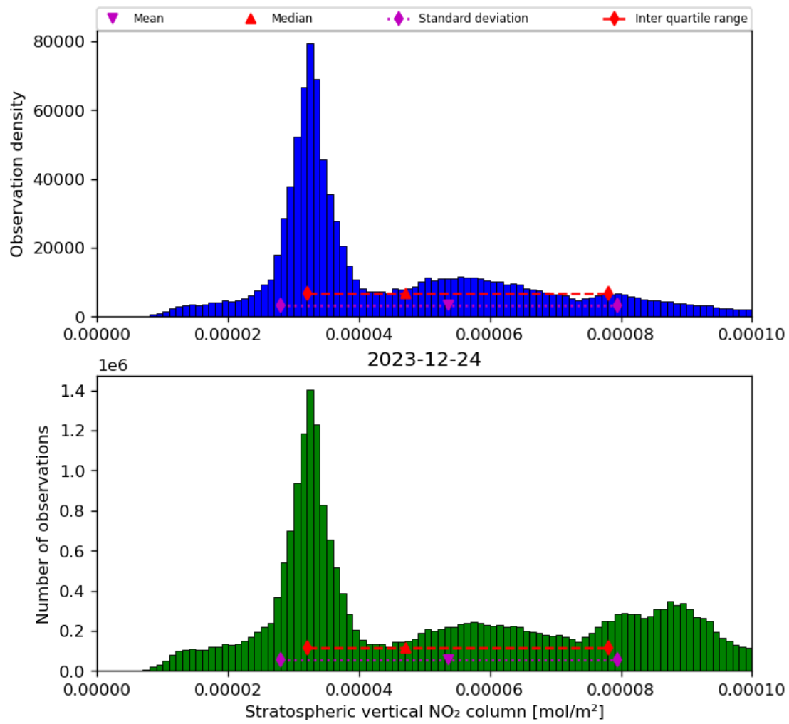
Figure 36: Histogram of “Stratospheric vertical NO 2 column” for 2023-12-23 to 2023-12-25
