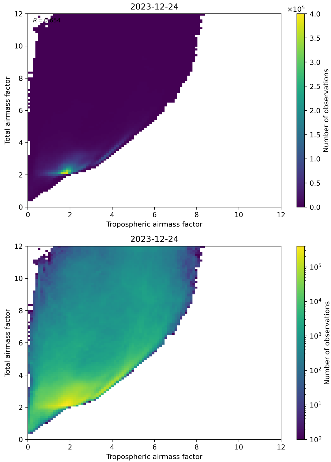
Figure 72: Scatter density plot of “Tropospheric airmass factor” against “Total airmass factor” for 2023-12-23 to 2023-12-25.
