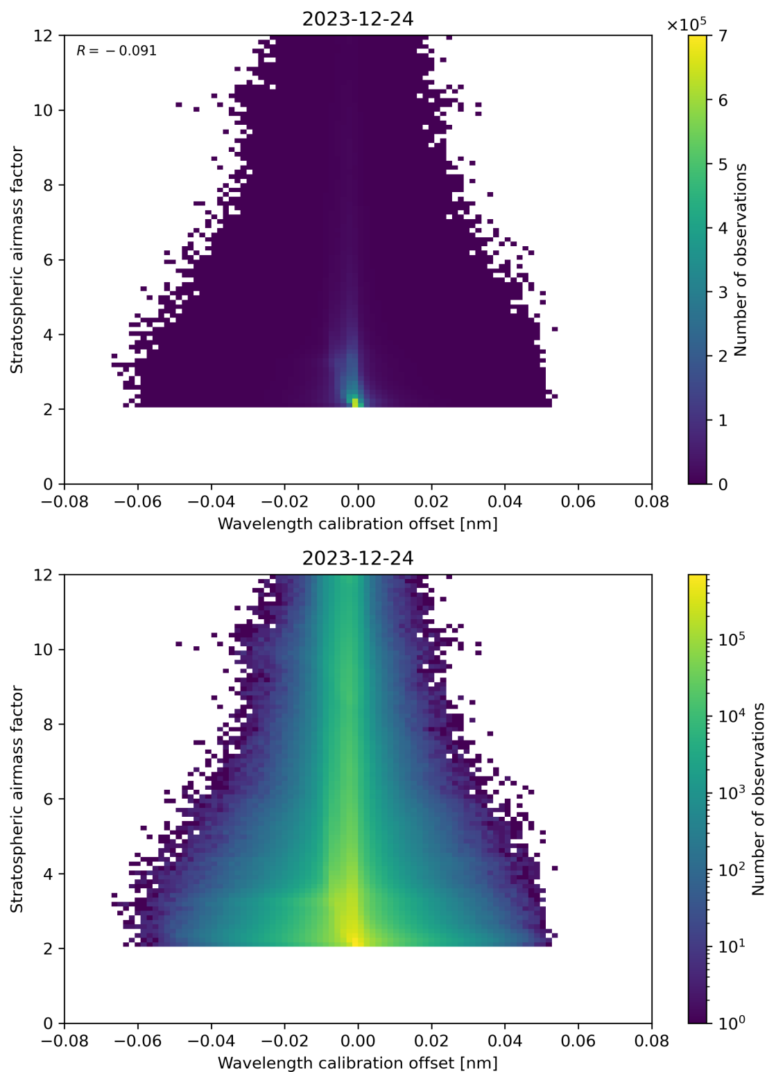
Figure 174: Scatter density plot of “Wavelength calibration offset” against “Stratospheric air mass factor” for 2023-12-23 to 2023-12-25.
