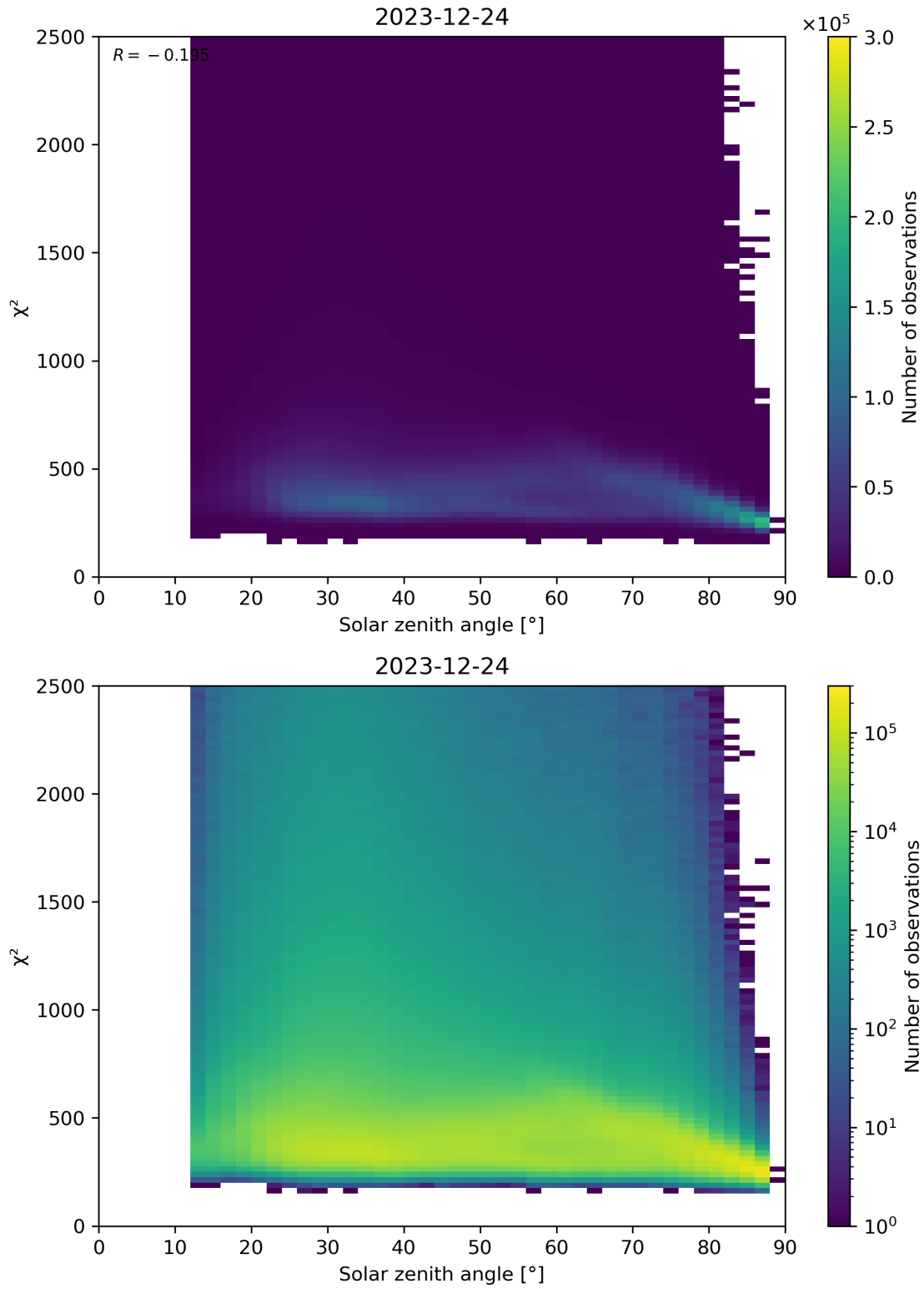
Figure 148: Scatter density plot of “Solar zenith angle” against “ \chi^2 ” for 2023-12-23 to 2023-12-25.
