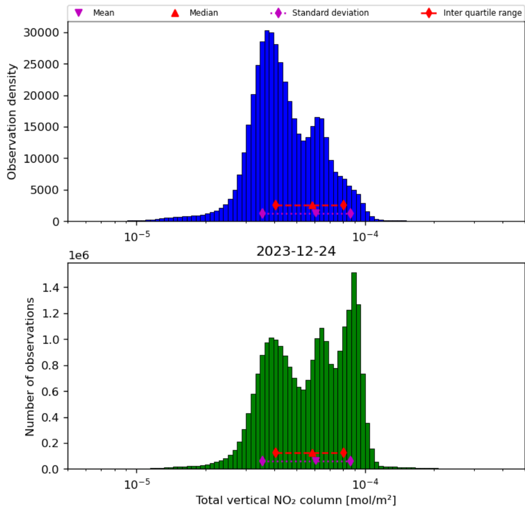
Figure 38: Histogram of “Total vertical NO 2 column” for 2023-12-23 to 2023-12-25
