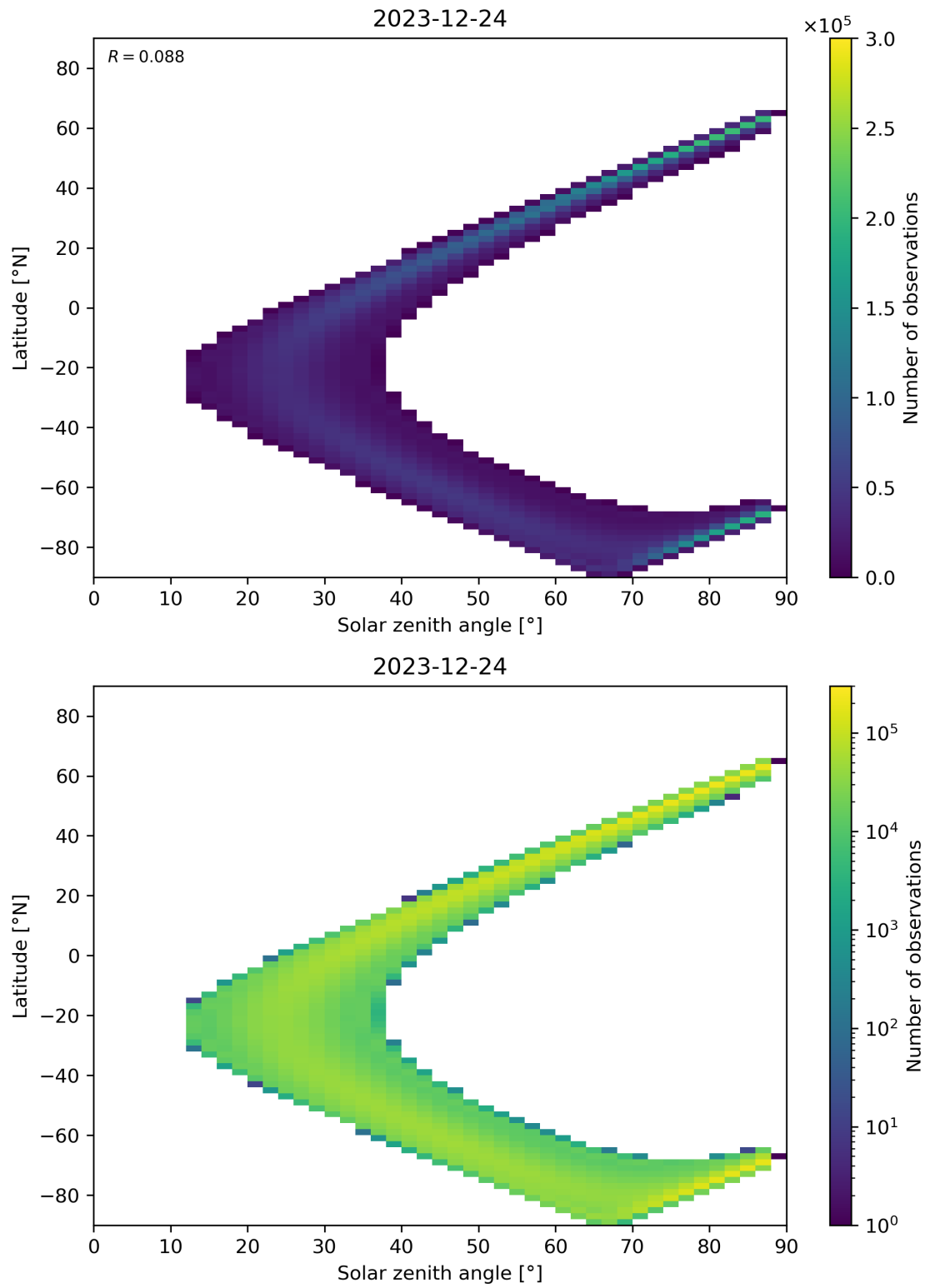
Figure 149: Scatter density plot of “Solar zenith angle” against “Latitude” for 2023-12-23 to 2023-12-25.
