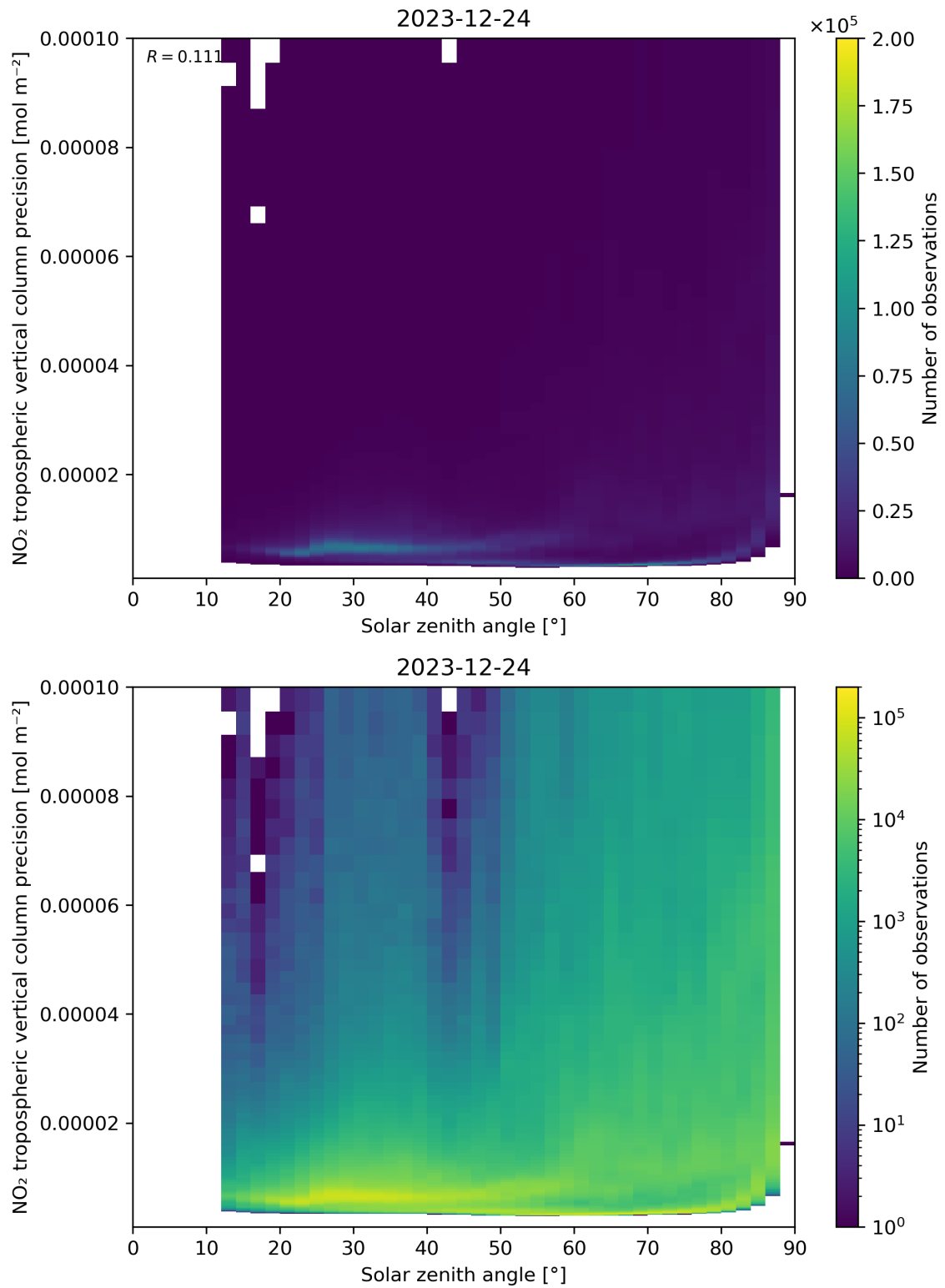
Figure 156: Scatter density plot of “Solar zenith angle” against “NO 2 tropospheric vertical column precision” for 2023-12-23 to 2023-12-25.
