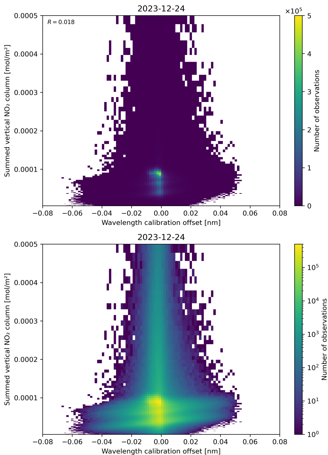
Figure 177: Scatter density plot of “Wavelength calibration offset” against “Summed vertical NO 2 column” for 2023-12-23 to 2023-12-25.
