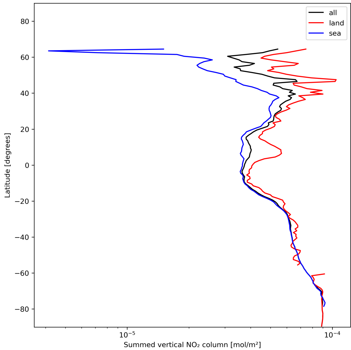
Figure 23: Zonal average of “Summed vertical NO 2 column” for 2023-12-23 to 2023-12-25.
