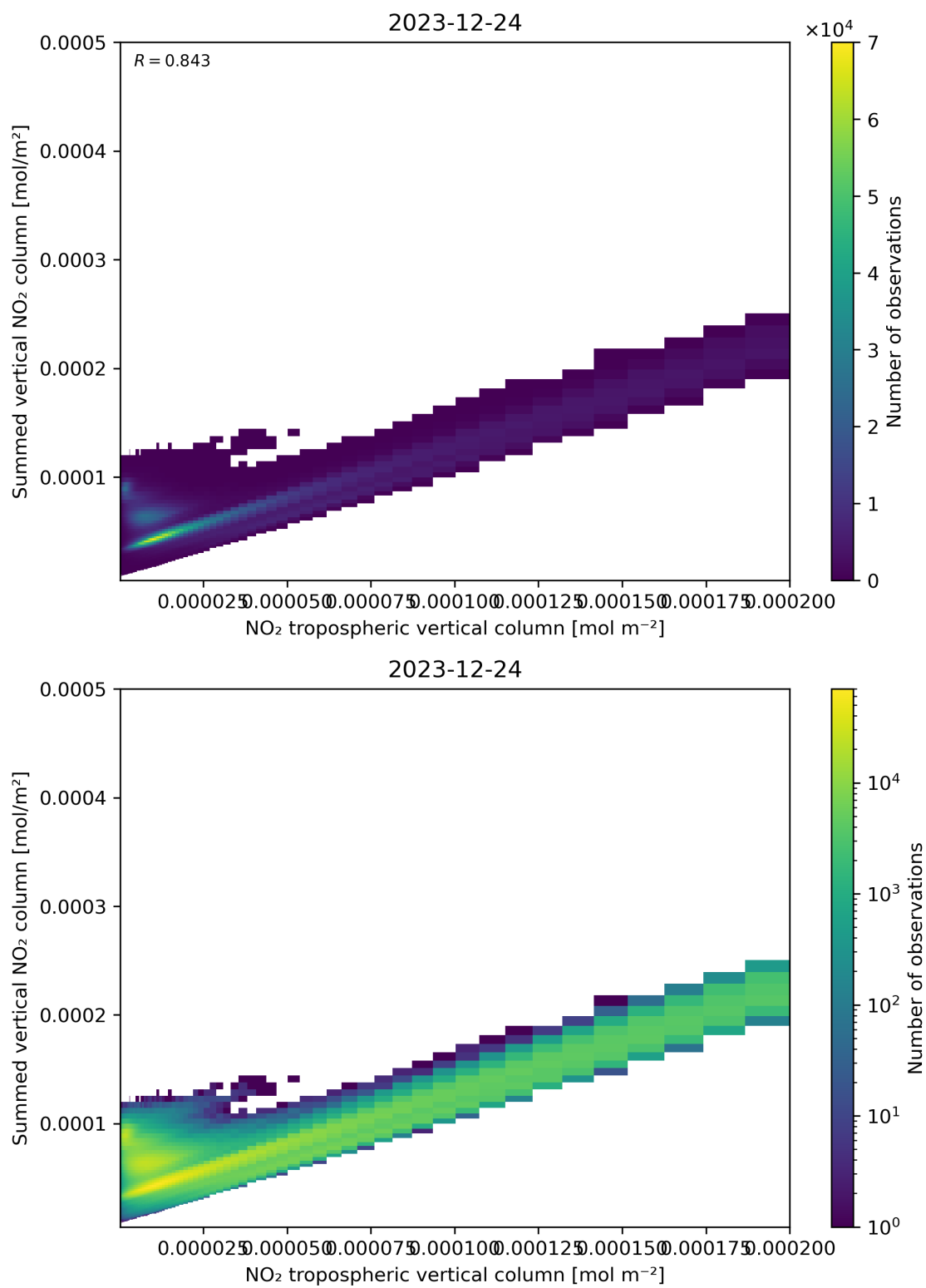
Figure 126: Scatter density plot of “NO 2 tropospheric vertical column” against “Summed vertical NO 2 column” for 2023-12-23 to 2023-12-25.
