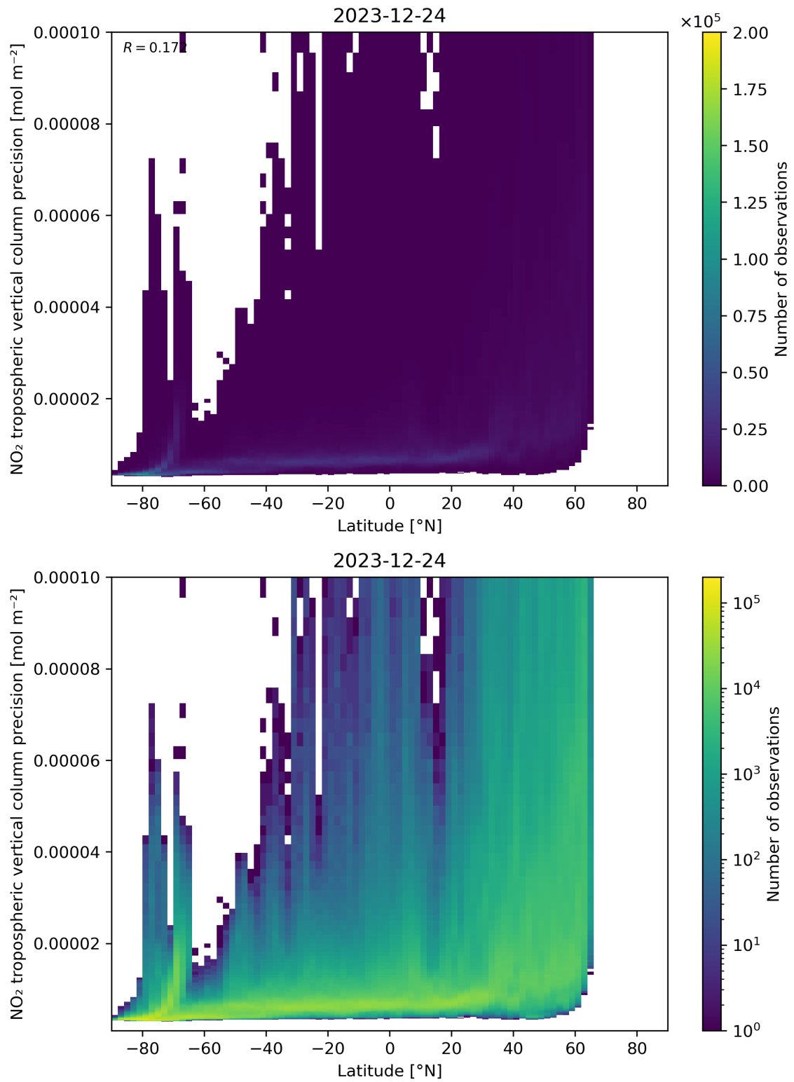
Figure 93: Scatter density plot of “Latitude” against “NO 2 tropospheric vertical column precision” for 2023-12-23 to 2023-12-25.
