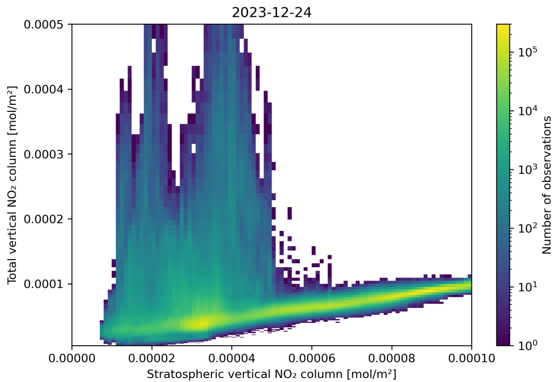
Figure 100: Scatter density plot of “Stratospheric vertical NO 2 column” against “Total vertical NO 2 column” for 2023-12-23 to 2023-12-25.
