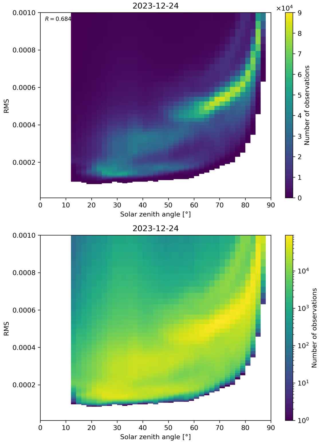
Figure 157: Scatter density plot of “Solar zenith angle” against “RMS” for 2023-12-23 to 2023-12-25.
