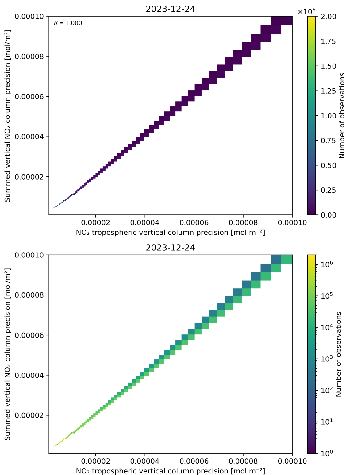
Figure 137: Scatter density plot of “NO 2 tropospheric vertical column precision” against “Summed vertical NO 2 column precision” for 2023-12-23 to 2023-12-25.
