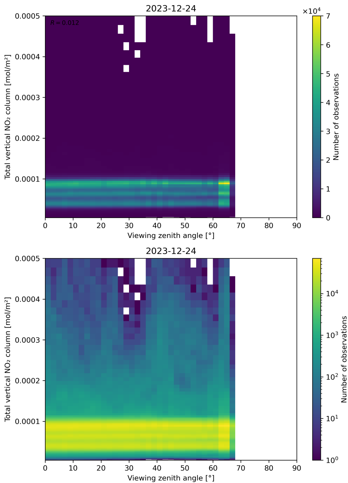
Figure 167: Scatter density plot of “Viewing zenith angle” against “Total vertical NO 2 column” for 2023-12-23 to 2023-12-25.
