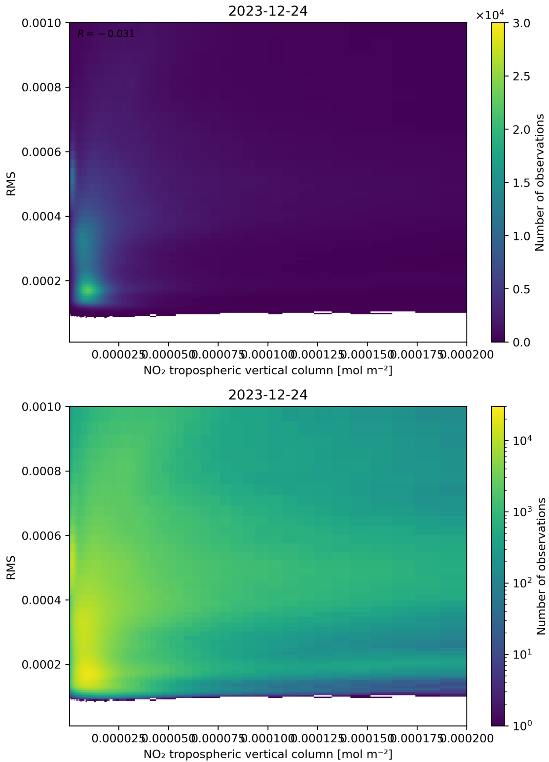
Figure 142: Scatter density plot of “NO 2 tropospheric vertical column” against “RMS” for 2023-12-23 to 2023-12-25.
