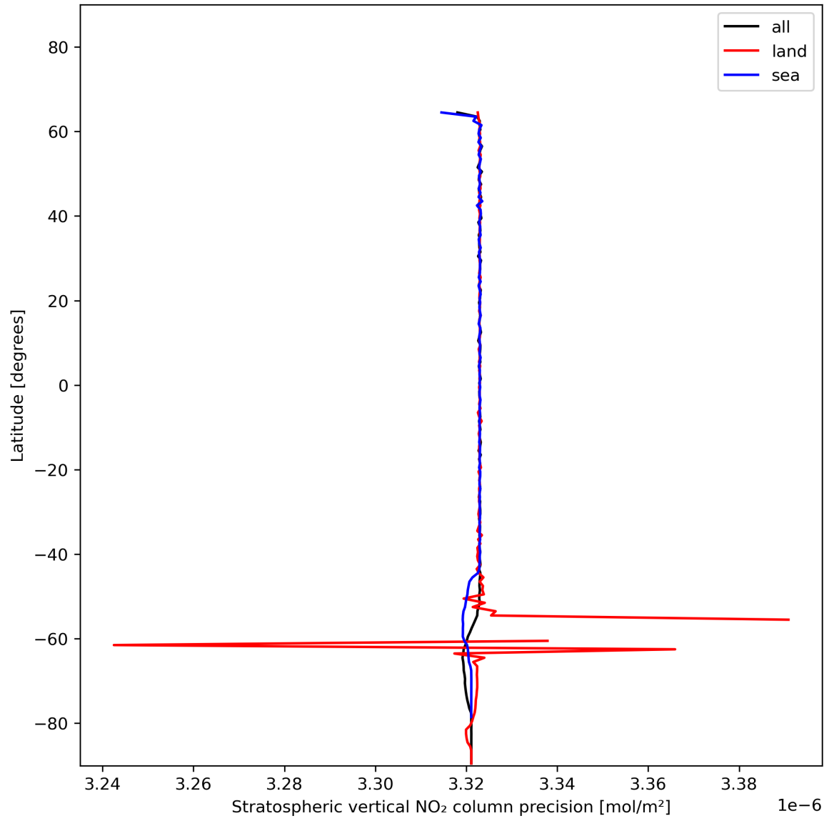
Figure 20: Zonal average of “Stratospheric vertical NO 2 column precision” for 2023-12-23 to 2023-12-25.
