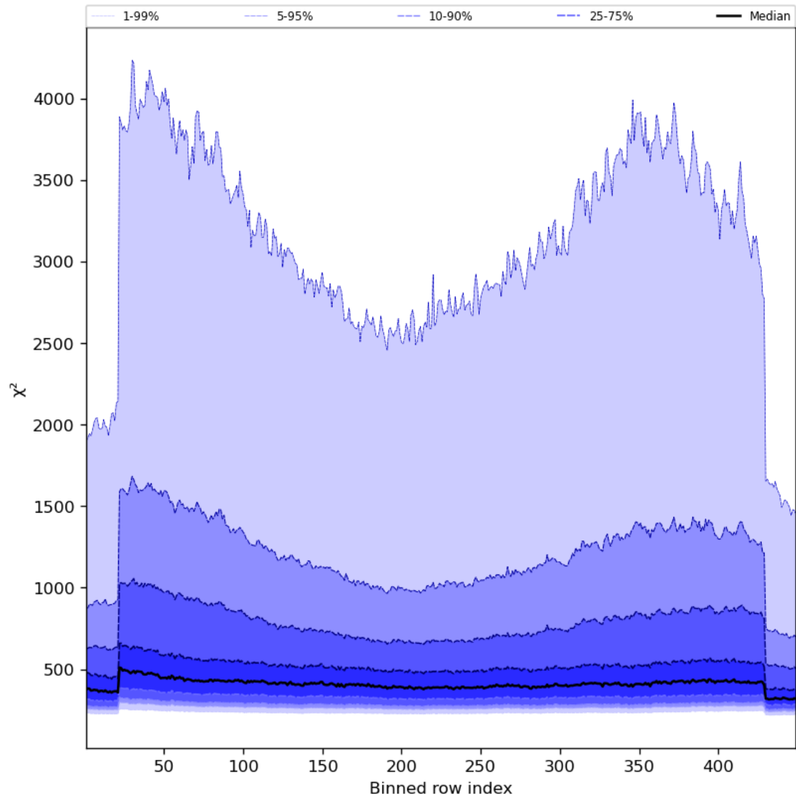
Figure 59: Along track statistics of “ \chi^2 ” for 2023-12-23 to 2023-12-25
