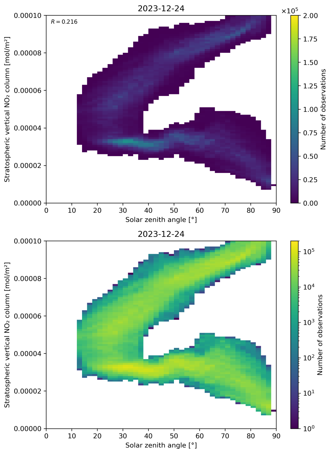
Figure 150: Scatter density plot of “Solar zenith angle” against “Stratospheric vertical NO 2 column” for 2023-12-23 to 2023-12-25.
