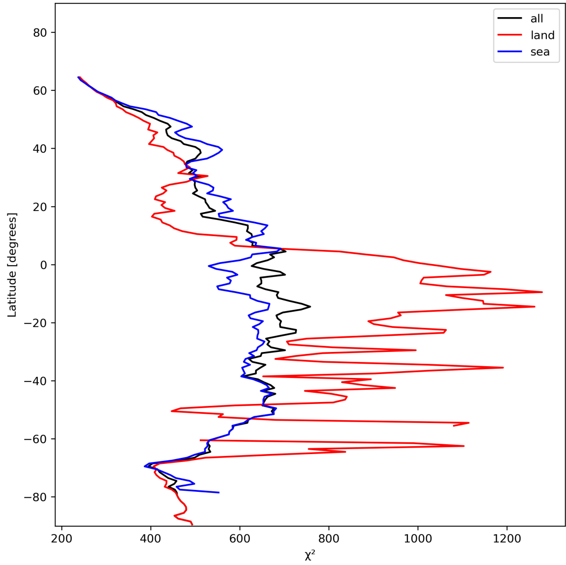
Figure 25: Zonal average of “ \chi^2 ” for 2023-12-23 to 2023-12-25.
