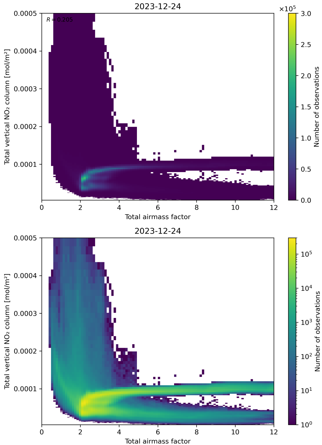
Figure 67: Scatter density plot of “Total airmass factor” against “Total vertical NO 2 column” for 2023-12-23 to 2023-12-25.
