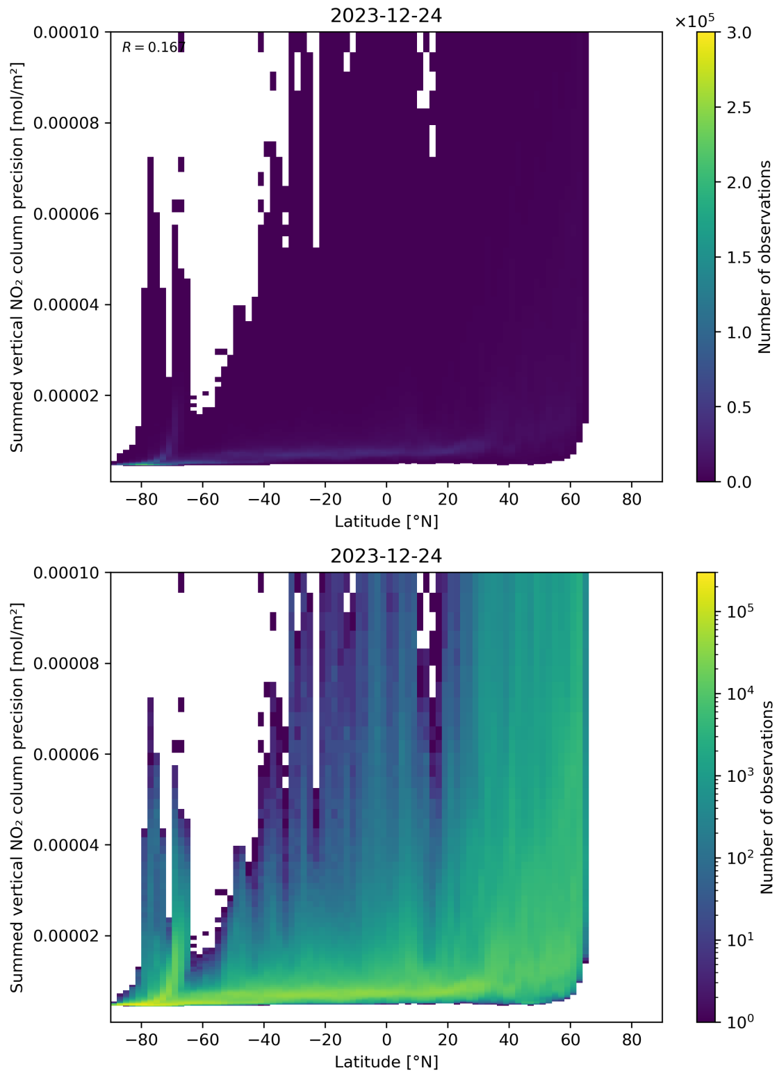
Figure 89: Scatter density plot of “Latitude” against “Summed vertical NO 2 column precision” for 2023-12-23 to 2023-12-25.
