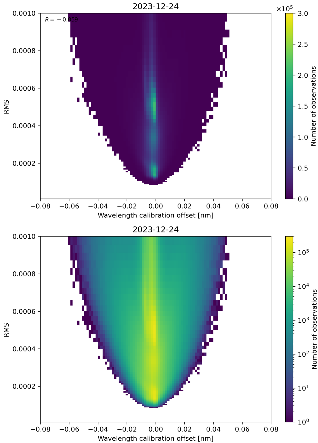
Figure 181: Scatter density plot of “Wavelength calibration offset” against “RMS” for 2023-12-23 to 2023-12-25.
