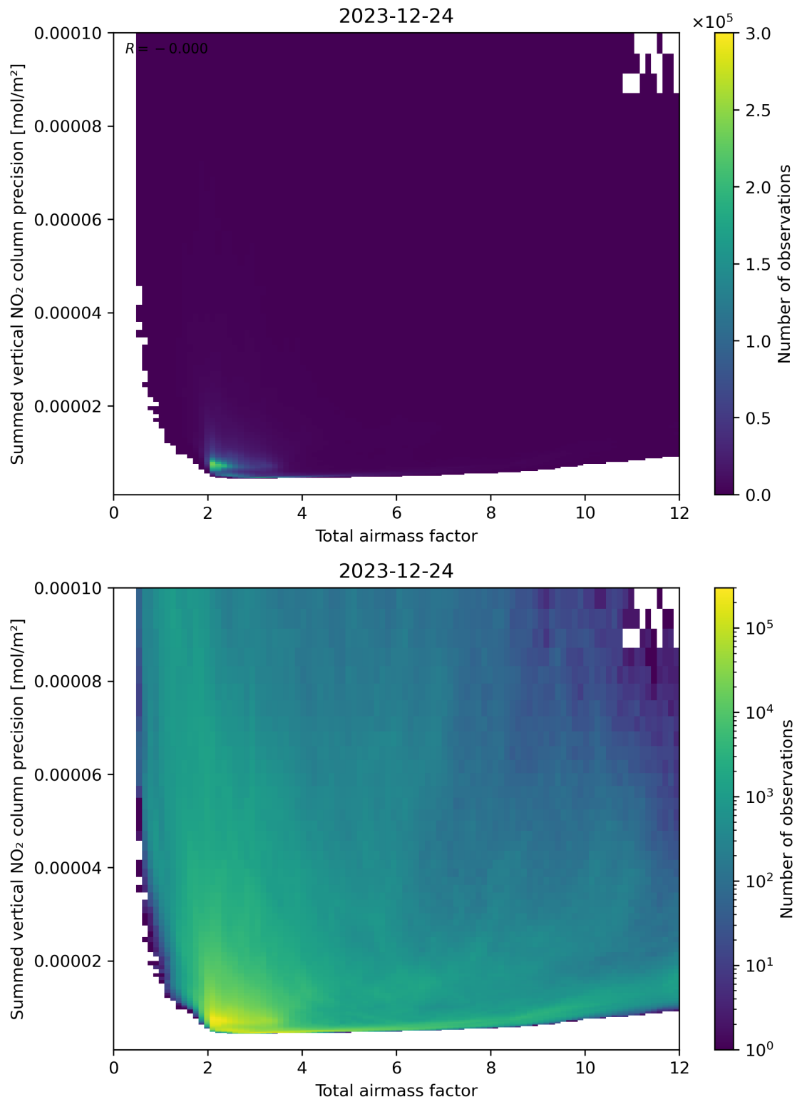
Figure 66: Scatter density plot of “Total airmass factor” against “Summed vertical NO 2 column precision” for 2023-12-23 to 2023-12-25.
