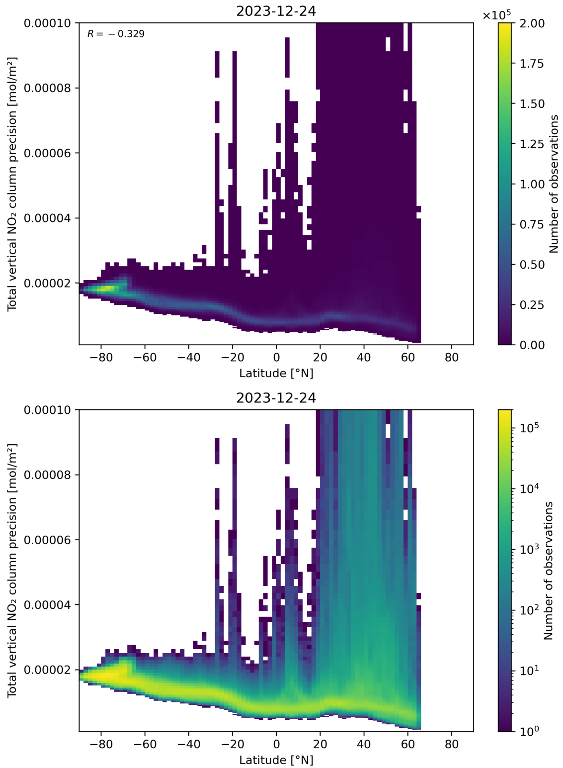
Figure 91: Scatter density plot of “Latitude” against “Total vertical NO 2 column precision” for 2023-12-23 to 2023-12-25.
