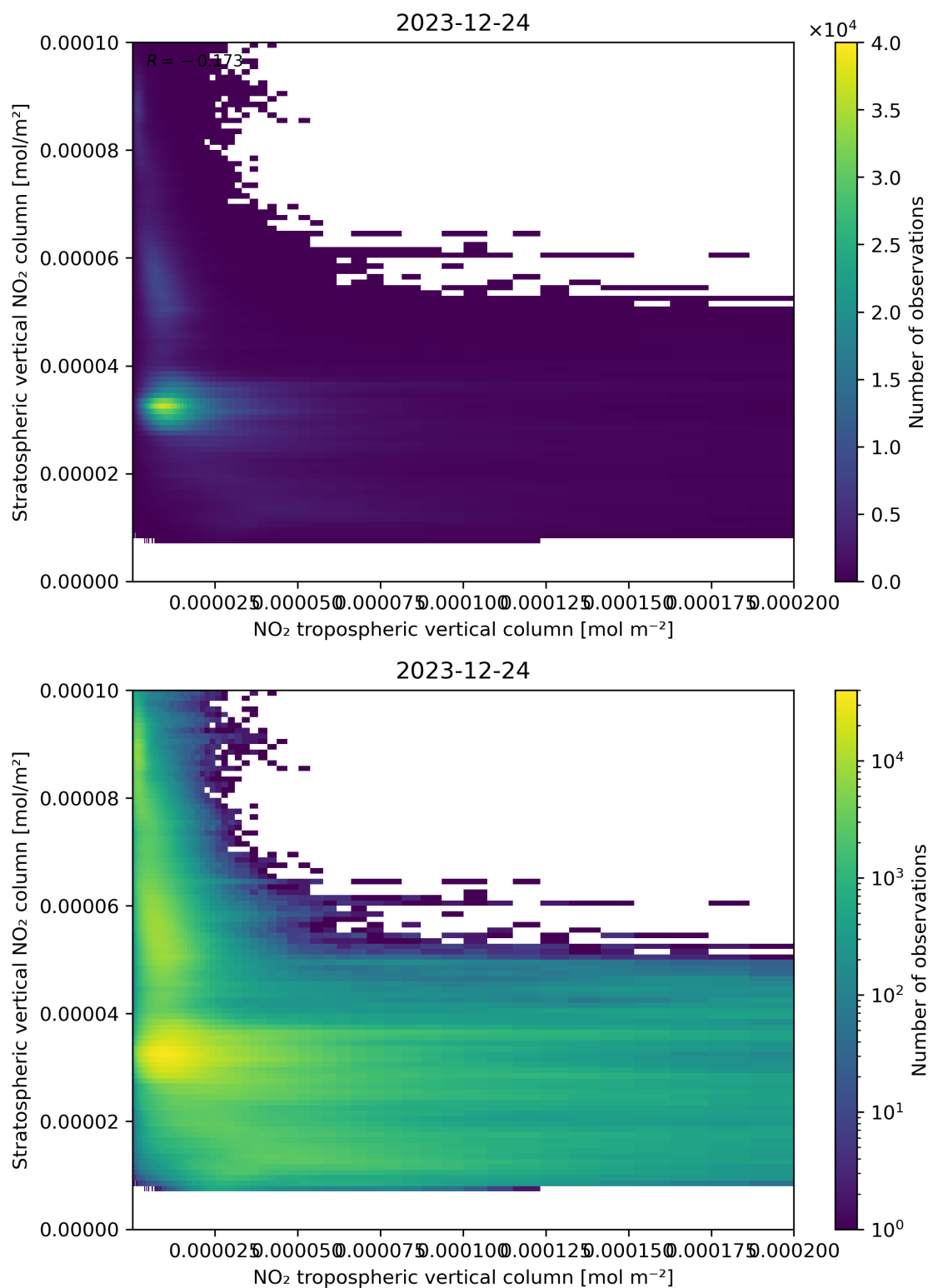
Figure 125: Scatter density plot of “NO 2 tropospheric vertical column” against “Stratospheric vertical NO 2 column” for 2023-12-23 to 2023-12-25.
