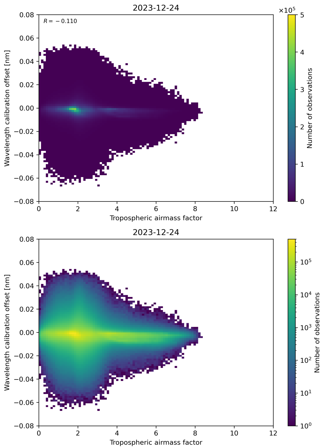
Figure 80: Scatter density plot of “Tropospheric airmass factor” against “Wavelength calibration offset” for 2023-12-23 to 2023-12-25.
