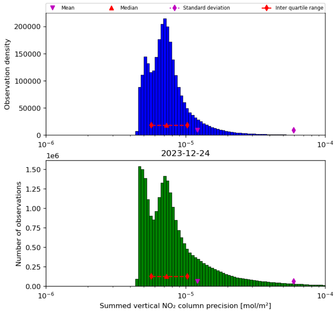
Figure 41: Histogram of “Summed vertical NO 2 column precision” for 2023-12-23 to 2023-12-25
