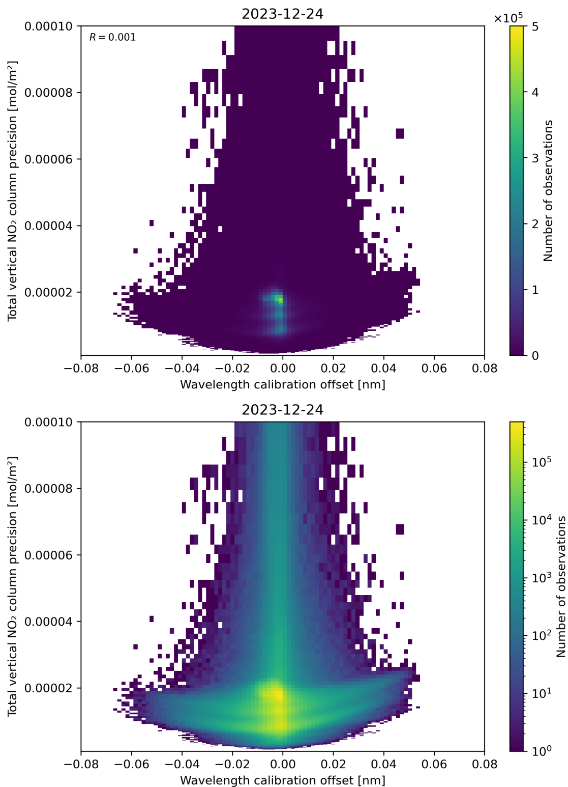
Figure 180: Scatter density plot of “Wavelength calibration offset” against “Total vertical NO 2 column precision” for 2023-12-23 to 2023-12-25.
