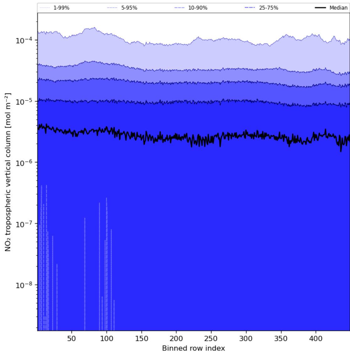
Figure 46: Along track statistics of “NO 2 tropospheric vertical column” for 2023-12-23 to 2023-12-25
