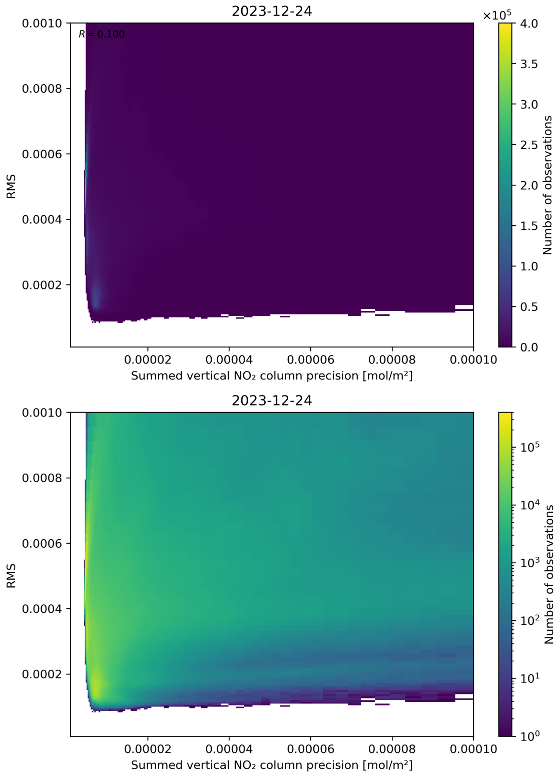
Figure 108: Scatter density plot of “Summed vertical NO 2 column precision” against “RMS” for 2023-12-23 to 2023-12-25.
