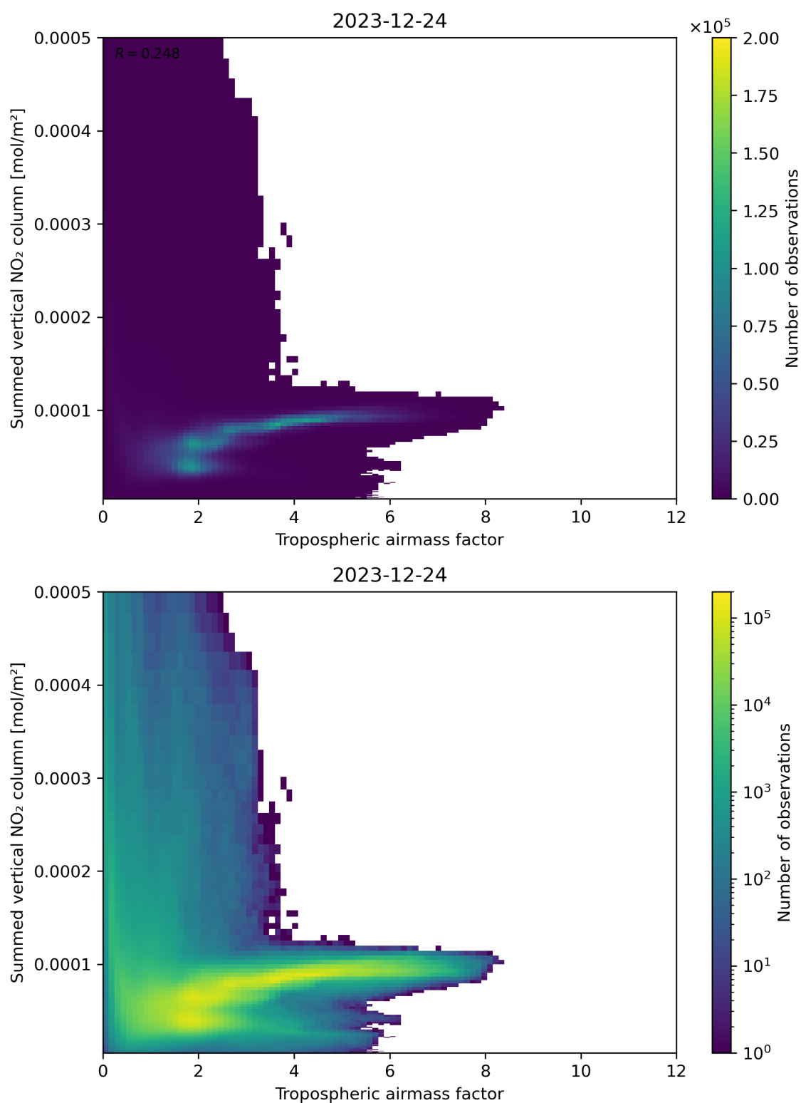
Figure 75: Scatter density plot of “Tropospheric airmass factor” against “Summed vertical NO 2 column” for 2023-12-23 to 2023-12-25.
