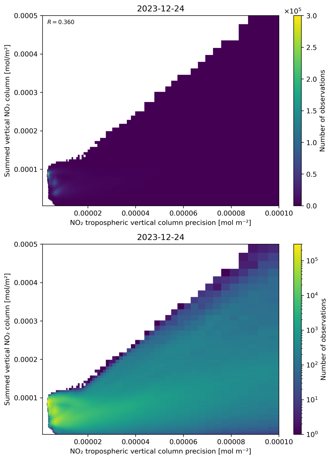
Figure 136: Scatter density plot of “NO 2 tropospheric vertical column precision” against “Summed vertical NO 2 column” for 2023-12-23 to 2023-12-25.
