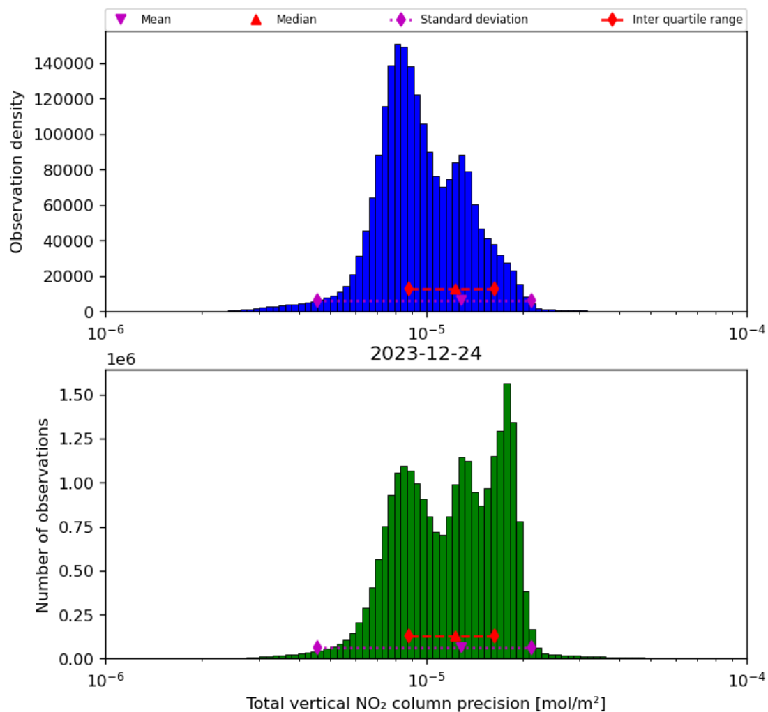
Figure 39: Histogram of “Total vertical NO 2 column precision” for 2023-12-23 to 2023-12-25
