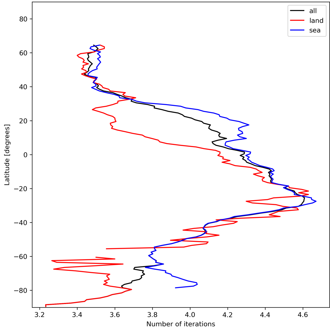
Figure 17: Zonal average of “Number of iterations” for 2023-12-23 to 2023-12-25.
