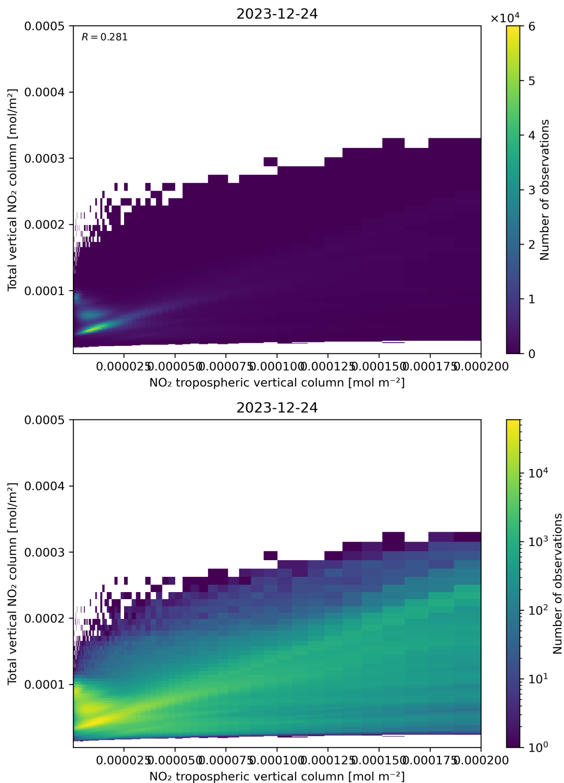
Figure 128: Scatter density plot of “NO 2 tropospheric vertical column” against “Total vertical NO 2 column” for 2023-12-23 to 2023-12-25.
