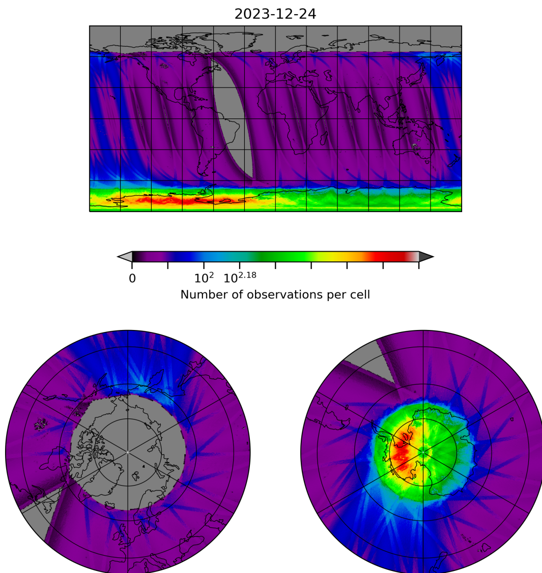
Figure 10: Map of the number of observations for 2023-12-23 to 2023-12-25
