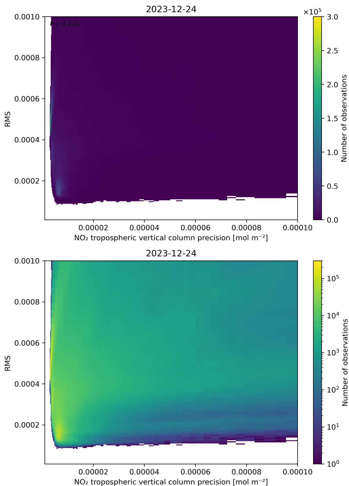
Figure 140: Scatter density plot of “NO 2 tropospheric vertical column precision” against “RMS” for 2023-12-23 to 2023-12-25.
