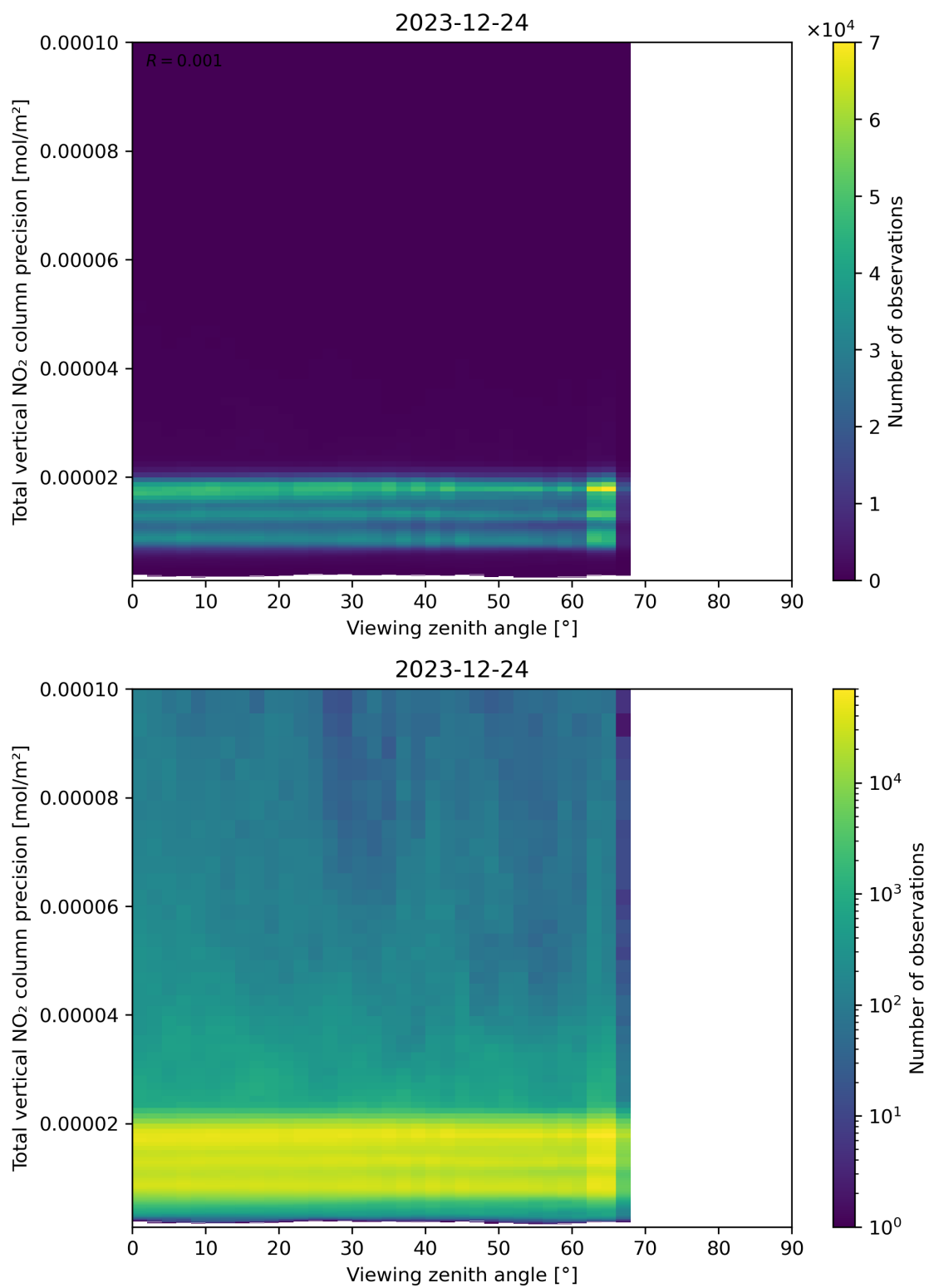
Figure 168: Scatter density plot of “Viewing zenith angle” against “Total vertical NO 2 column precision” for 2023-12-23 to 2023-12-25.
