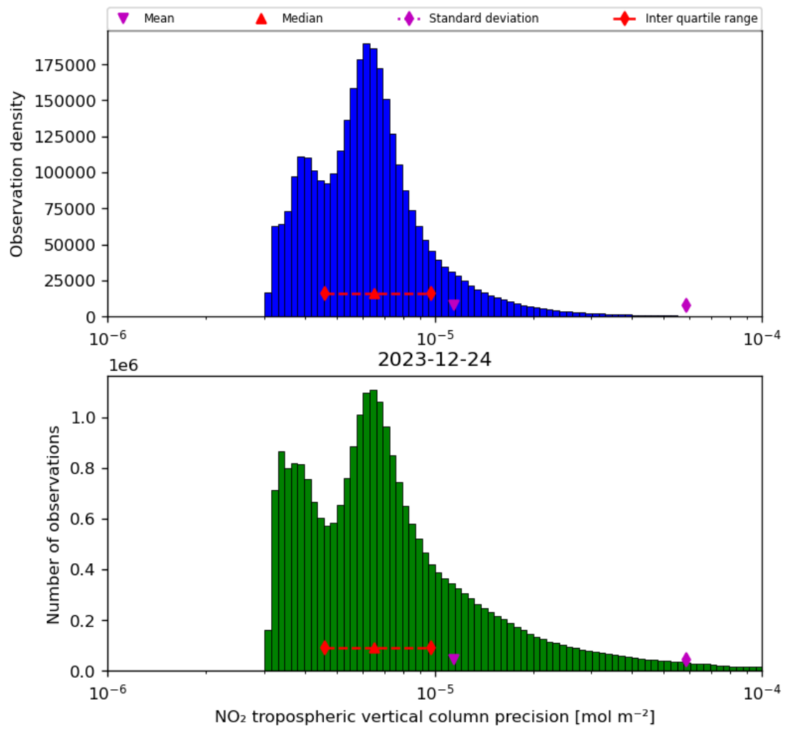
Figure 30: Histogram of “NO 2 tropospheric vertical column precision” for 2023-12-23 to 2023-12-25
