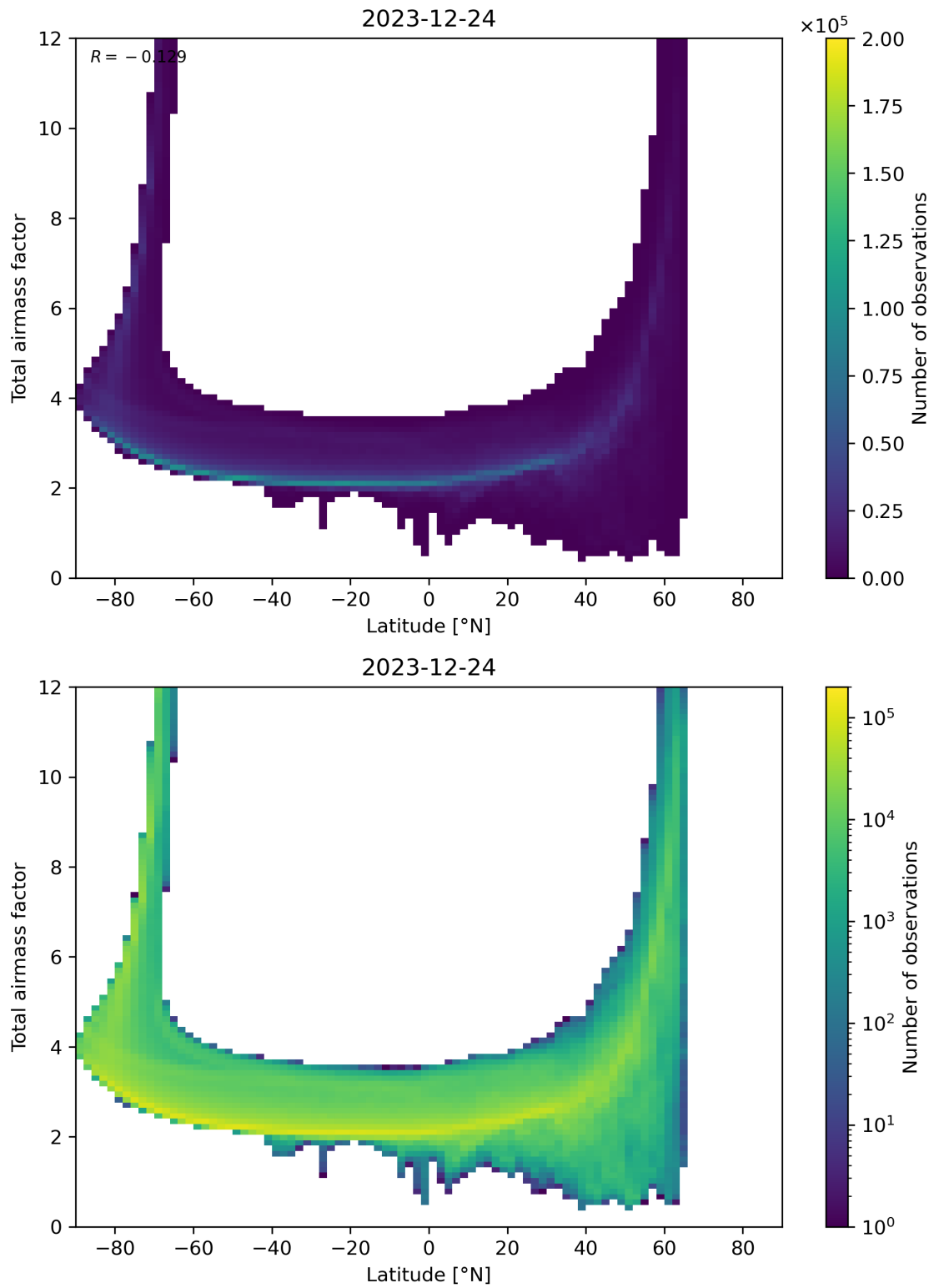
Figure 84: Scatter density plot of “Latitude” against “Total airmass factor” for 2023-12-23 to 2023-12-25.
