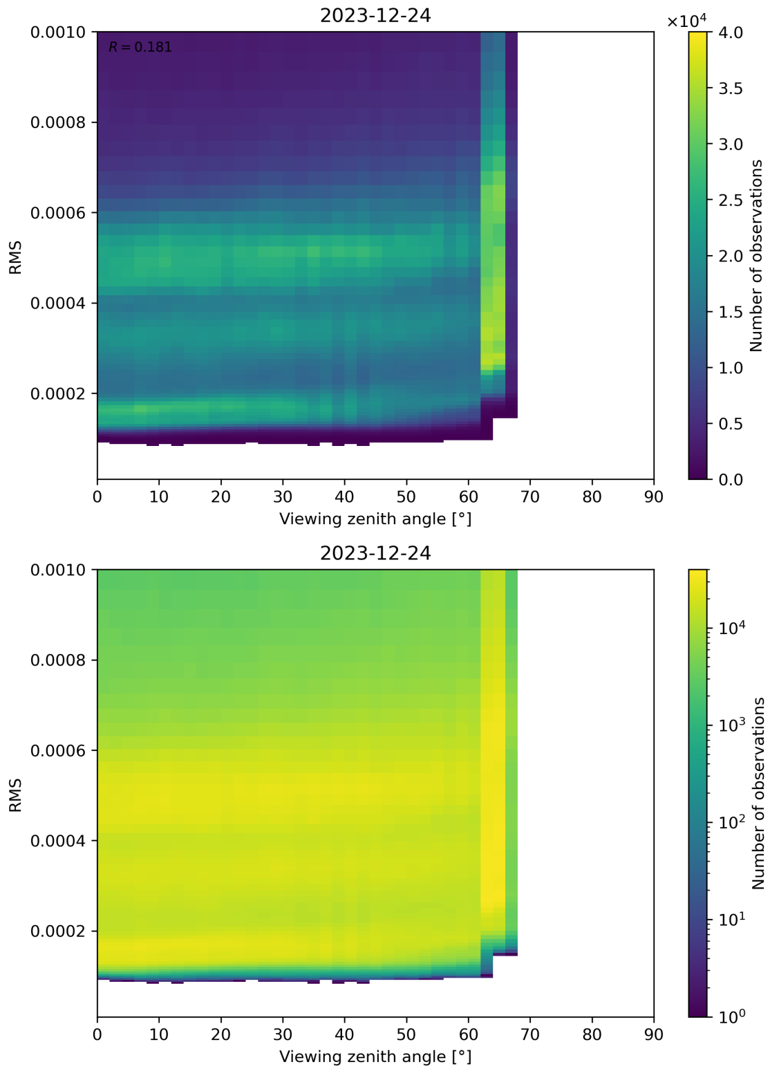
Figure 171: Scatter density plot of “Viewing zenith angle” against “RMS” for 2023-12-23 to 2023-12-25.
