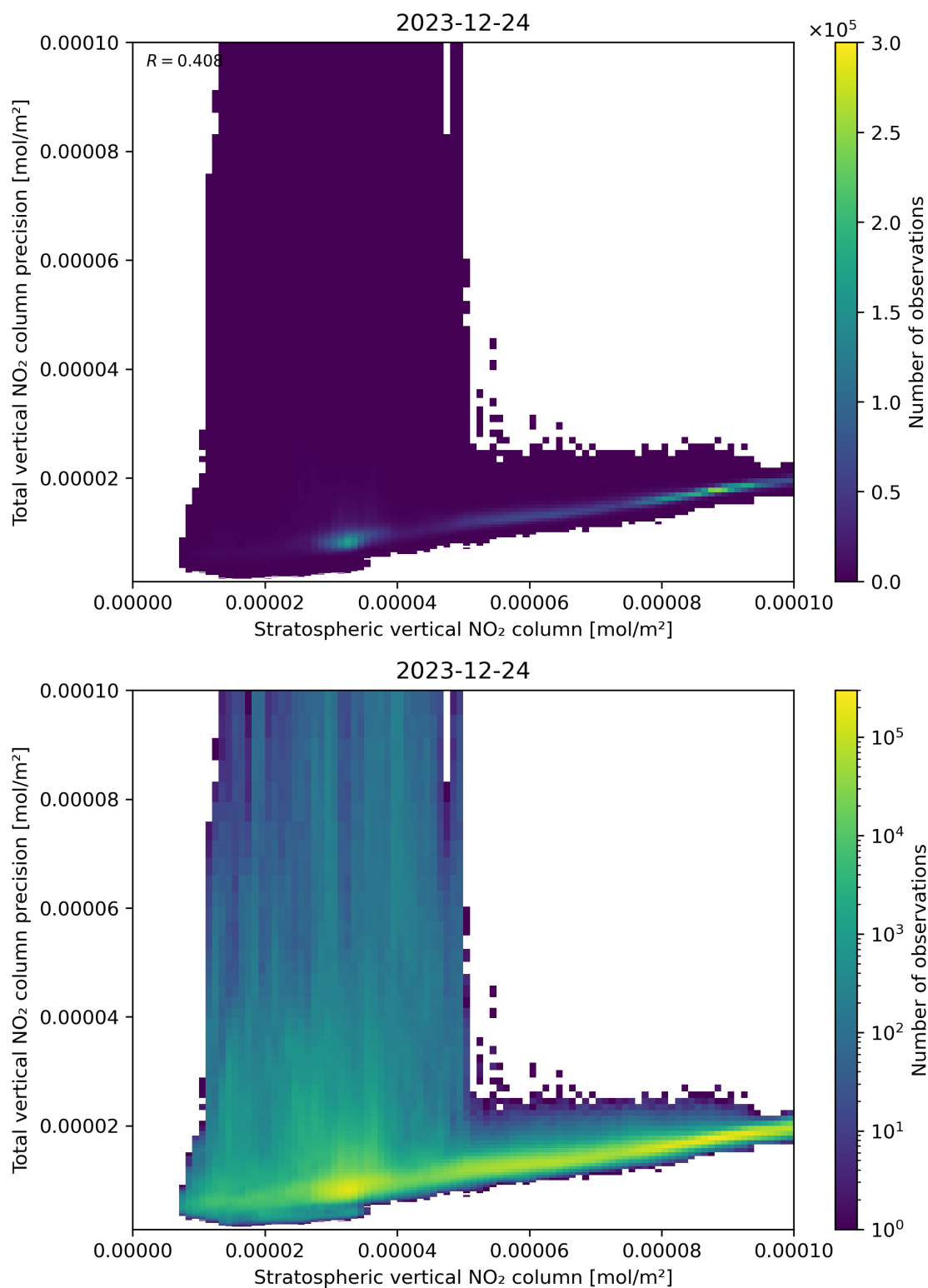
Figure 101: Scatter density plot of “Stratospheric vertical NO 2 column” against “Total vertical NO 2 column precision” for 2023-12-23 to 2023-12-25.
