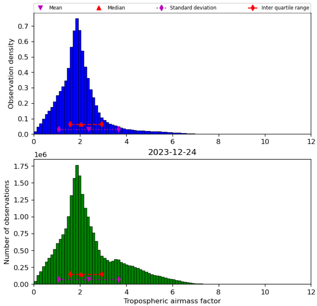
Figure 31: Histogram of “Tropospheric airmass factor” for 2023-12-23 to 2023-12-25
