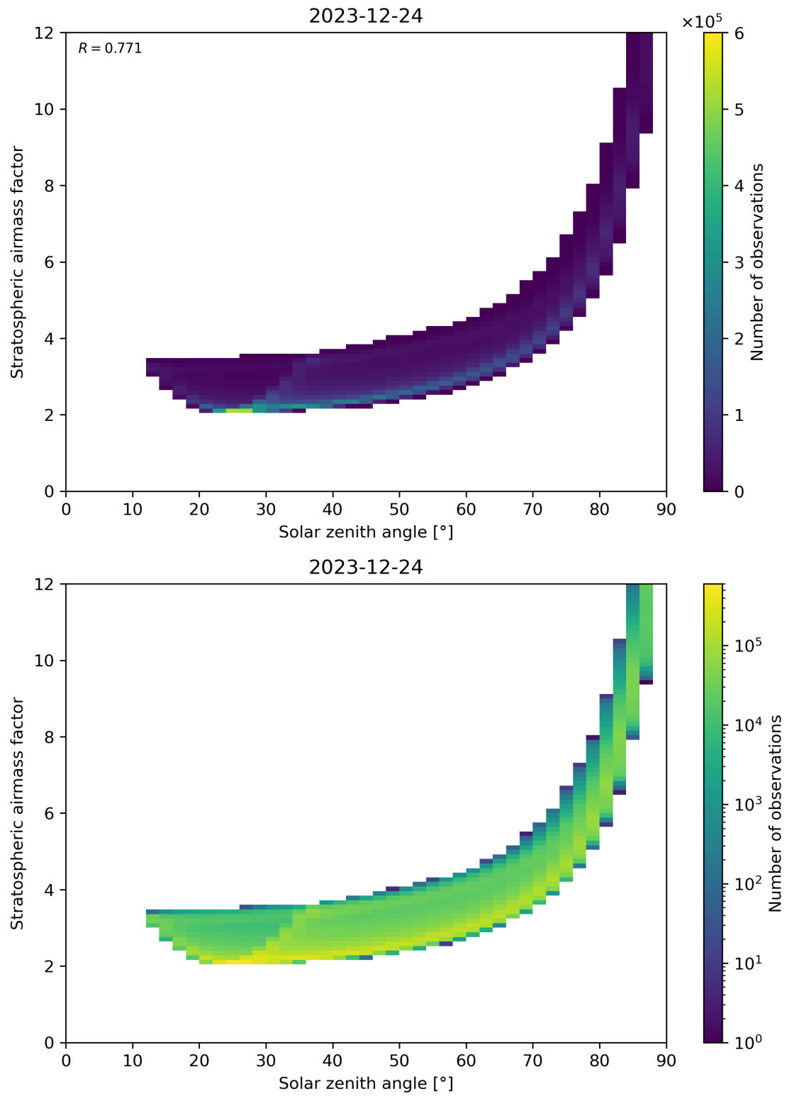
Figure 145: Scatter density plot of “Solar zenith angle” against “Stratospheric airmass factor” for 2023-12-23 to 2023-12-25.
