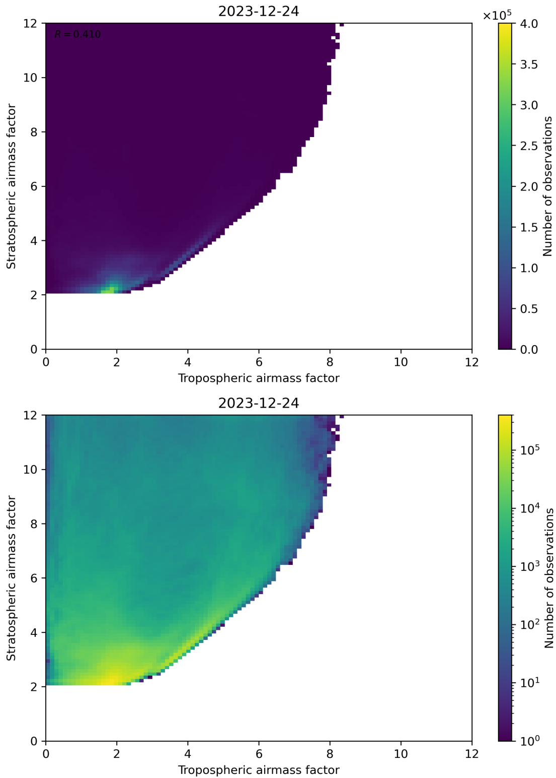
Figure 71: Scatter density plot of “Tropospheric airmass factor” against “Stratospheric airmass factor” for 2023-12-23 to 2023-12-25.
