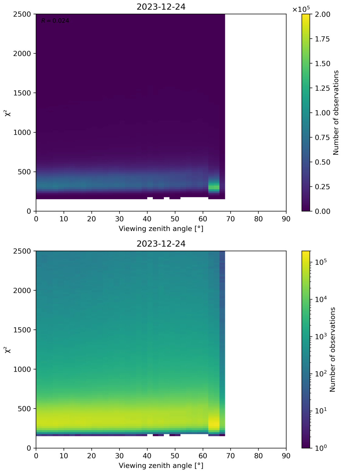
Figure 162: Scatter density plot of “Viewing zenith angle” against “ \chi^2 ” for 2023-12-23 to 2023-12-25.
