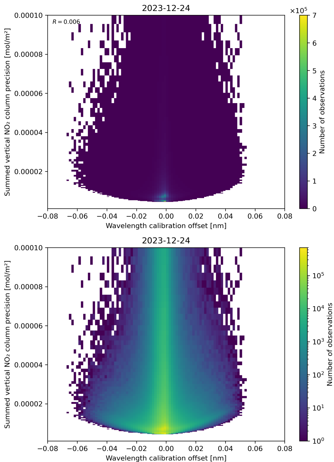
Figure 178: Scatter density plot of “Wavelength calibration offset” against “Summed vertical NO 2 column precision” for 2023-12-23 to 2023-12-25.
