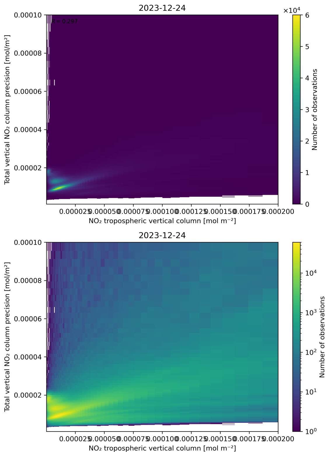
Figure 129: Scatter density plot of “NO 2 tropospheric vertical column” against “Total vertical NO 2 column precision” for 2023-12-23 to 2023-12-25.
