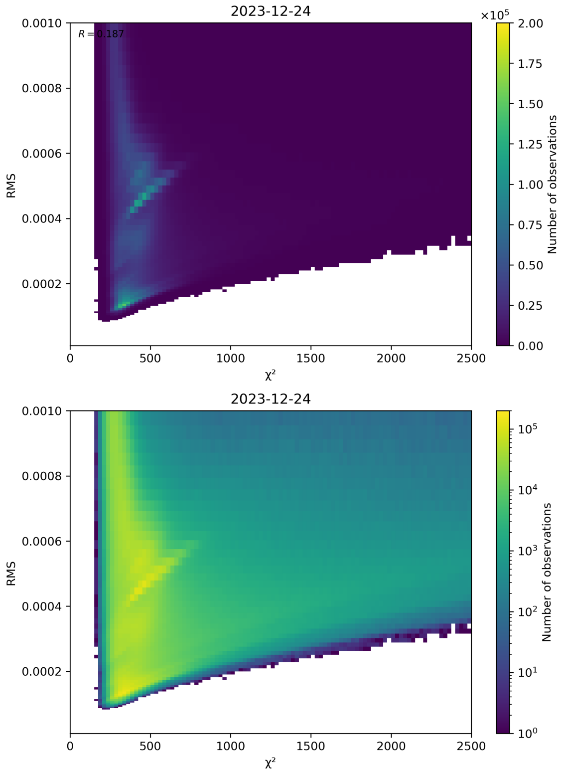
Figure 82: Scatter density plot of “ \chi^2 ” against “RMS” for 2023-12-23 to 2023-12-25.
