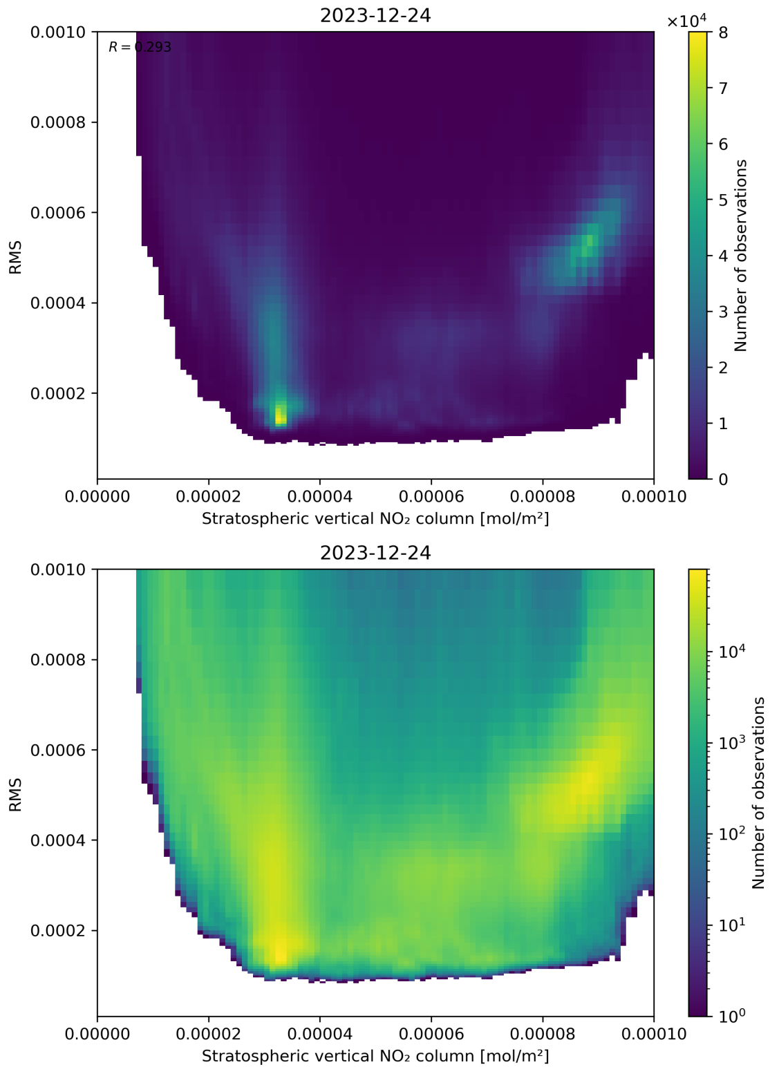
Figure 102: Scatter density plot of “Stratospheric vertical NO 2 column” against “RMS” for 2023-12-23 to 2023-12-25.
