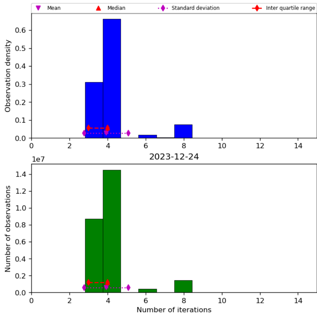
Figure 34: Histogram of “Number of iterations” for 2023-12-23 to 2023-12-25
