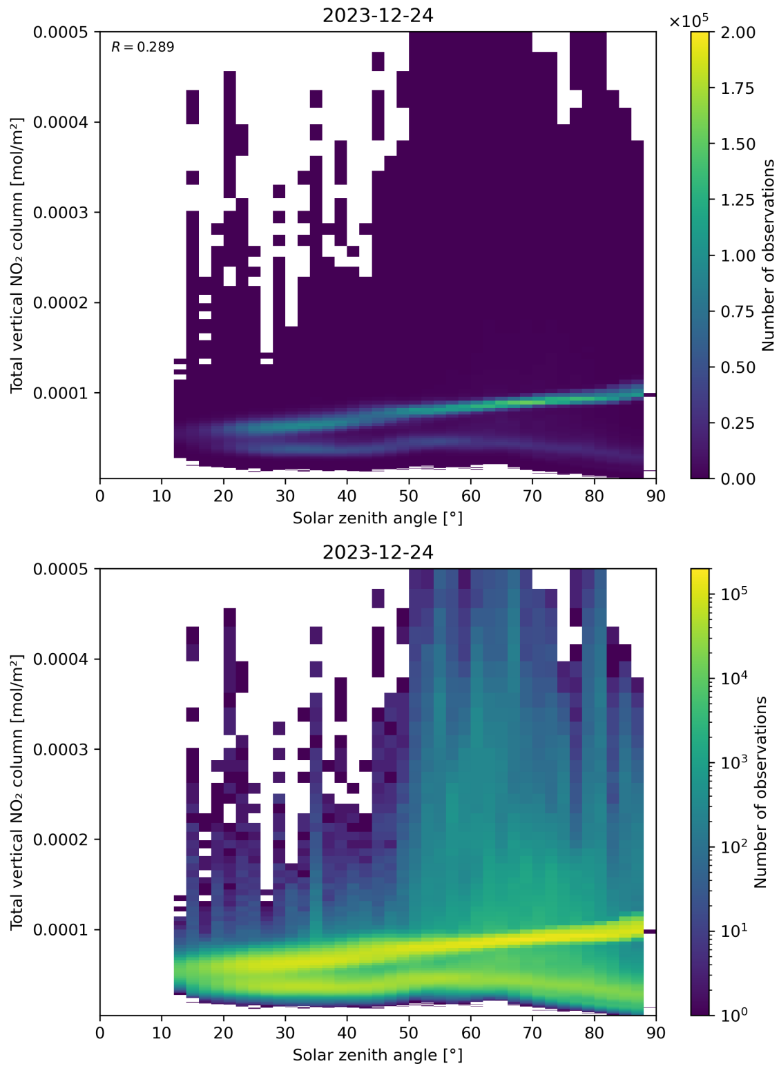
Figure 153: Scatter density plot of “Solar zenith angle” against “Total vertical NO 2 column” for 2023-12-23 to 2023-12-25.
