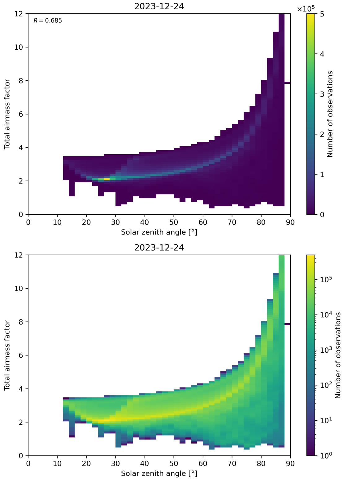
Figure 146: Scatter density plot of “Solar zenith angle” against “Total air mass factor” for 2023-12-23 to 2023-12-25.
