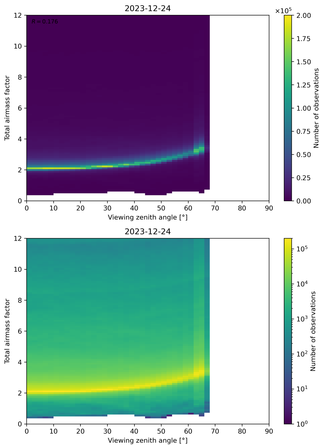
Figure 160: Scatter density plot of “Viewing zenith angle” against “Total airmass factor” for 2023-12-23 to 2023-12-25.
