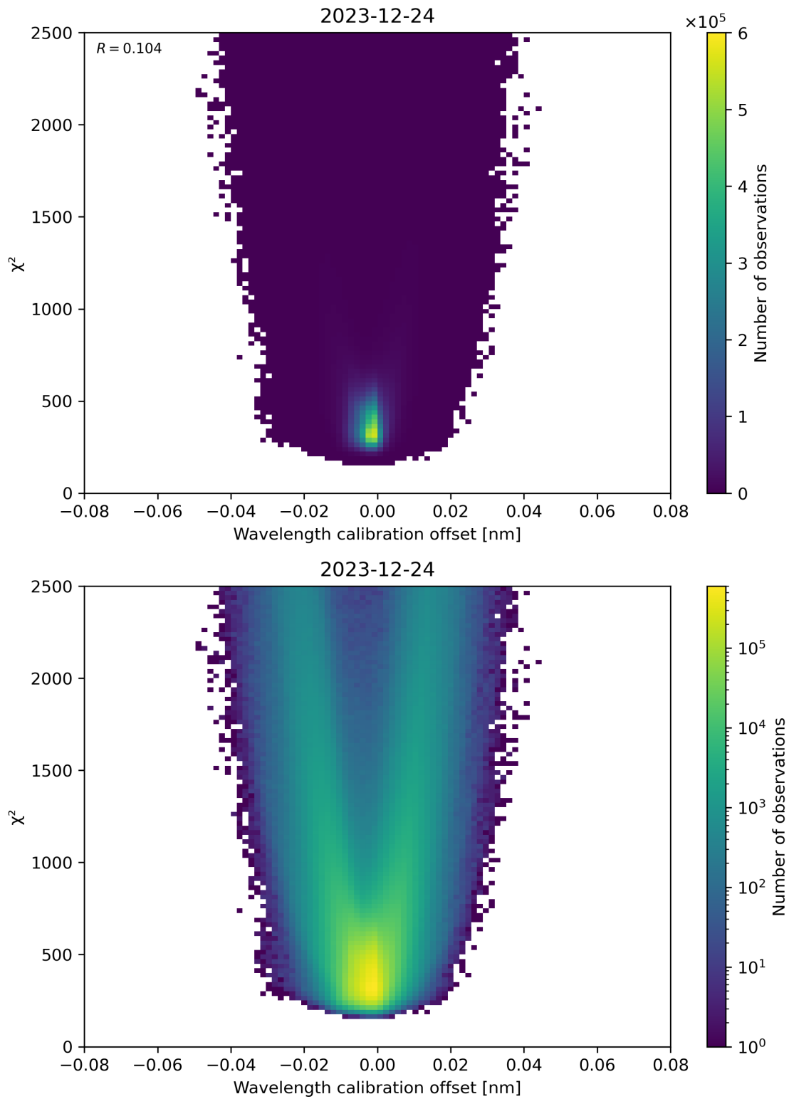
Figure 175: Scatter density plot of “Wavelength calibration offset” against “ \chi^2 ” for 2023-12-23 to 2023-12-25.
