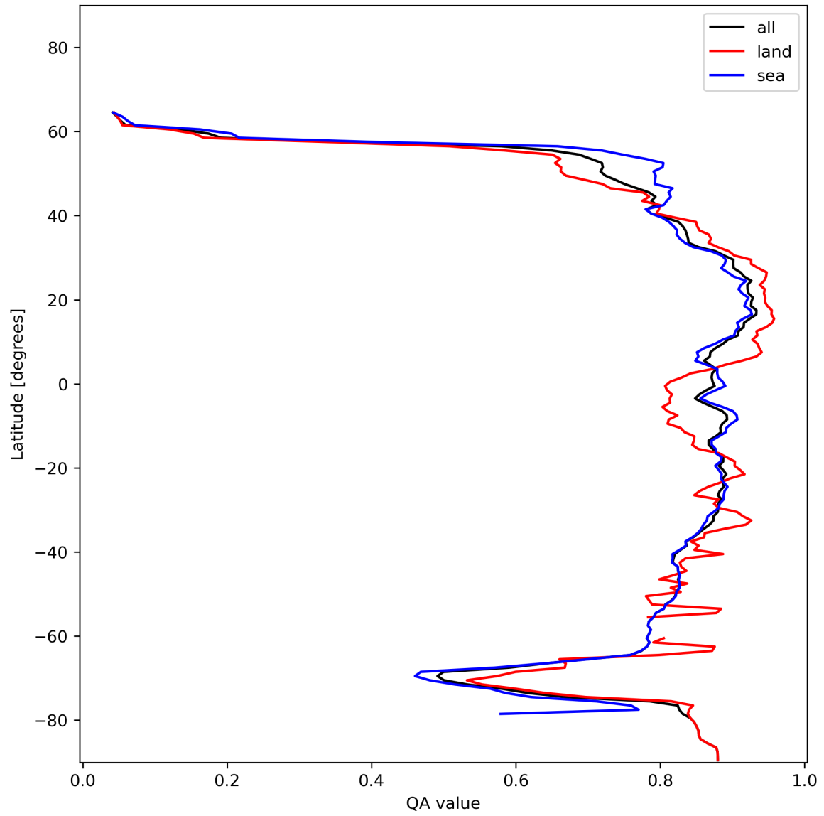
Figure 11: Zonal average of “QA value” for 2023-12-23 to 2023-12-25.
