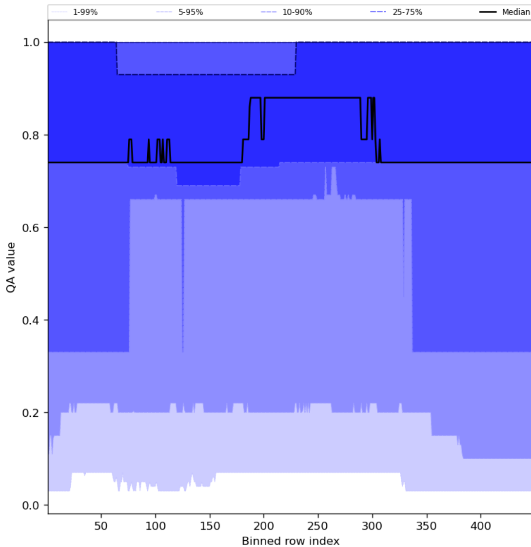
Figure 45: Along track statistics of “QA value” for 2023-12-23 to 2023-12-25
