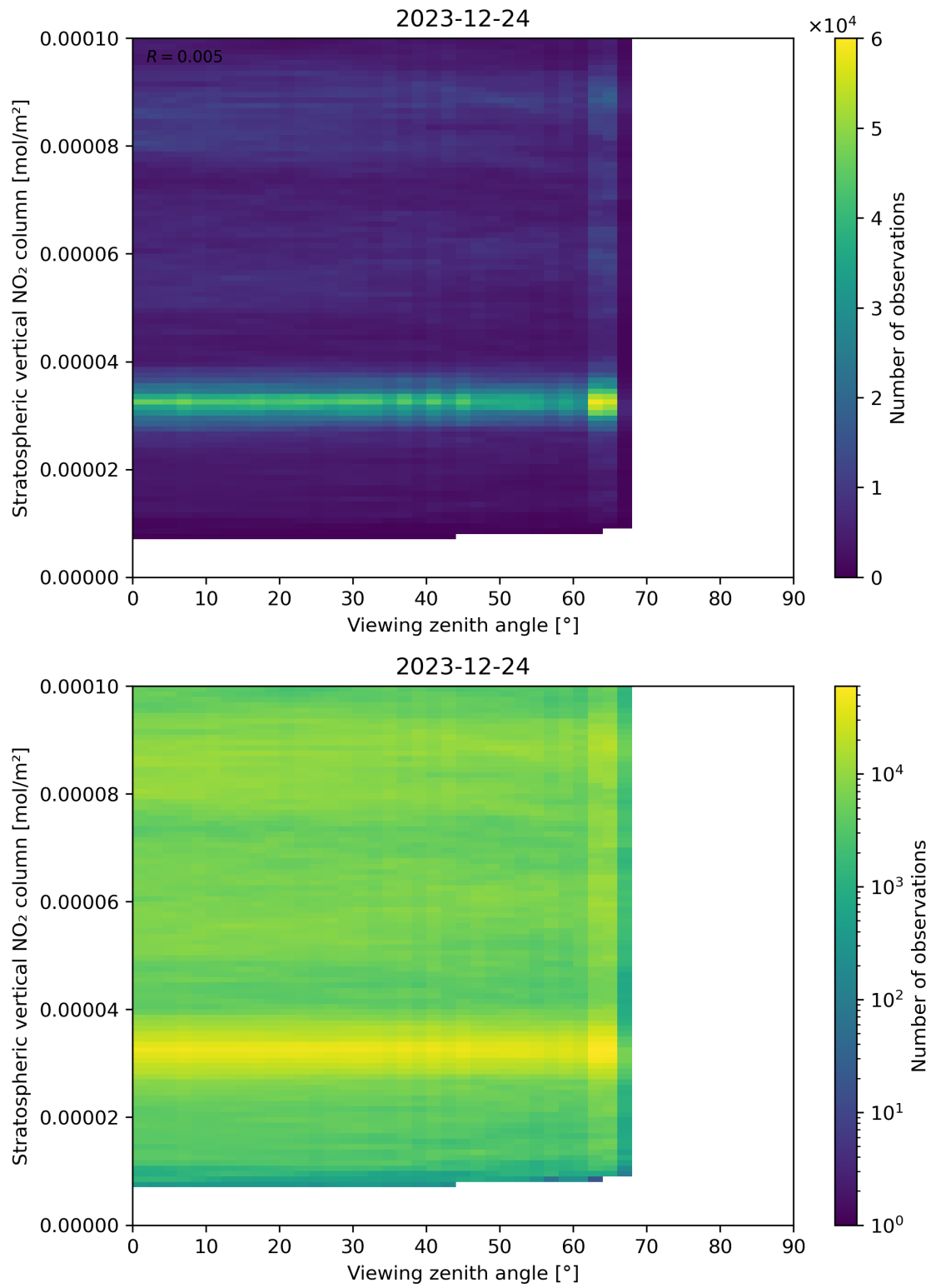
Figure 164: Scatter density plot of “Viewing zenith angle” against “Stratospheric vertical NO 2 column” for 2023-12-23 to 2023-12-25.
