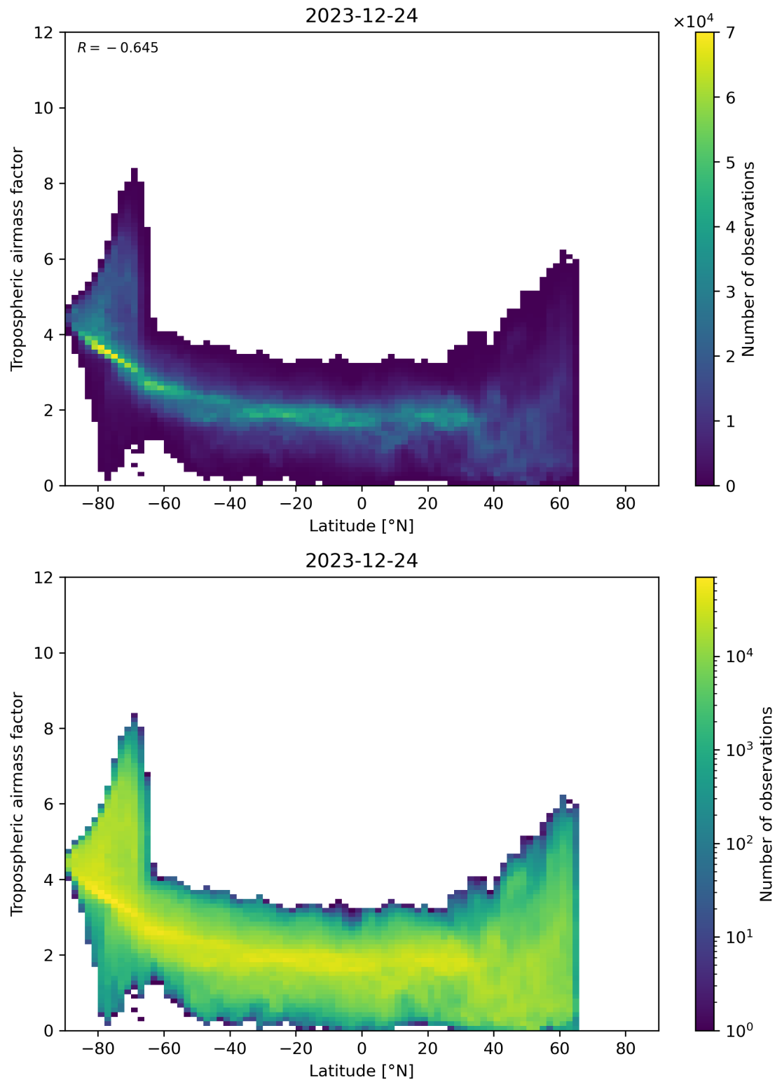
Figure 85: Scatter density plot of “Latitude” against “Tropospheric air mass factor” for 2023-12-23 to 2023-12-25.
