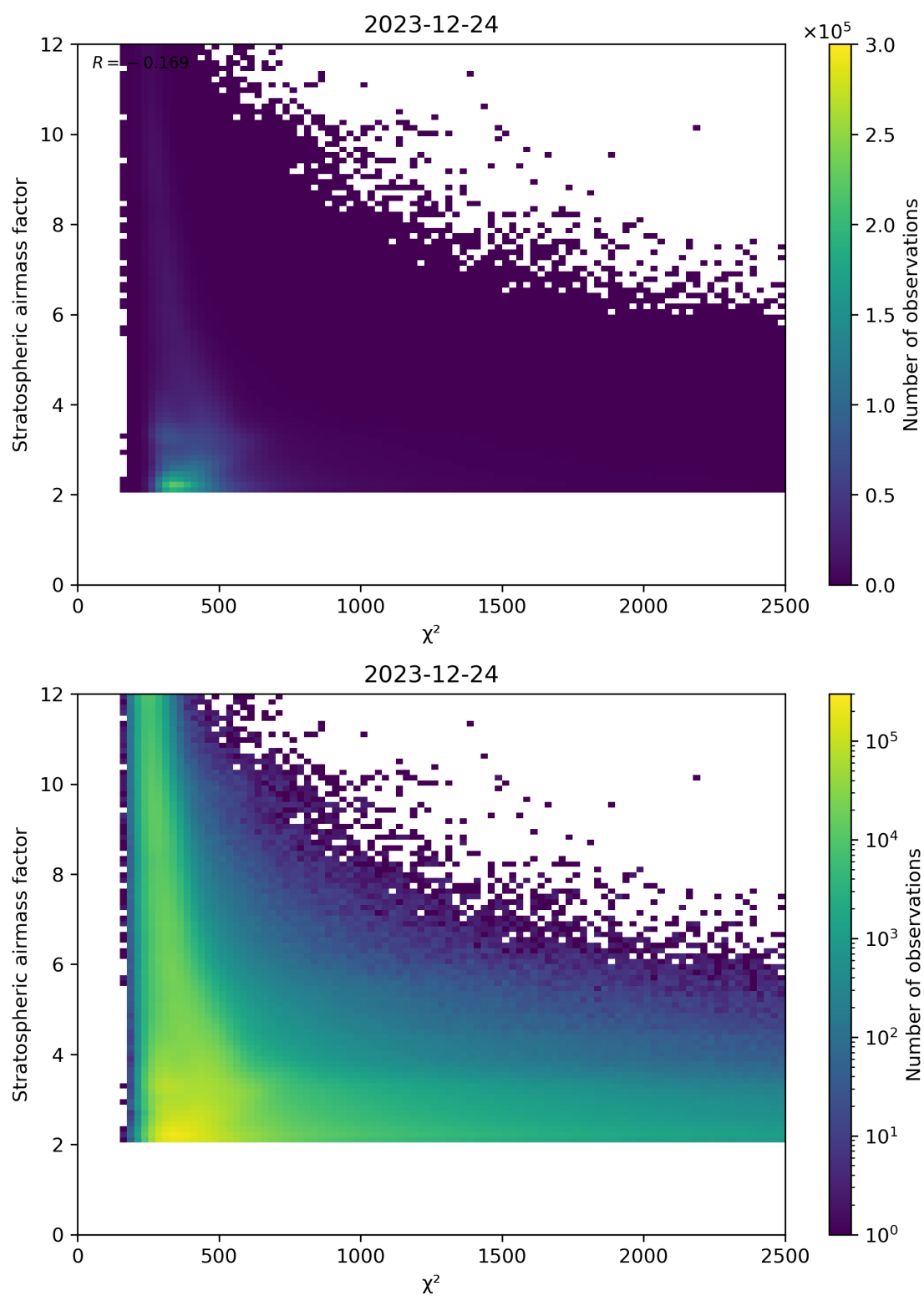
Figure 81: Scatter density plot of “ \chi^2 ” against “Stratospheric airmass factor” for 2023-12-23 to 2023-12-25.
