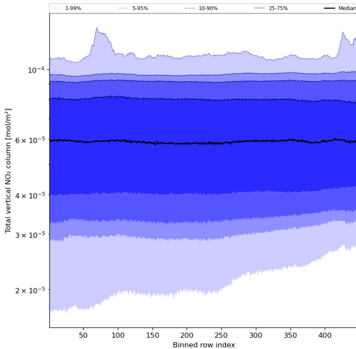
Figure 55: Along track statistics of “Total vertical NO 2 column” for 2023-12-23 to 2023-12-25
