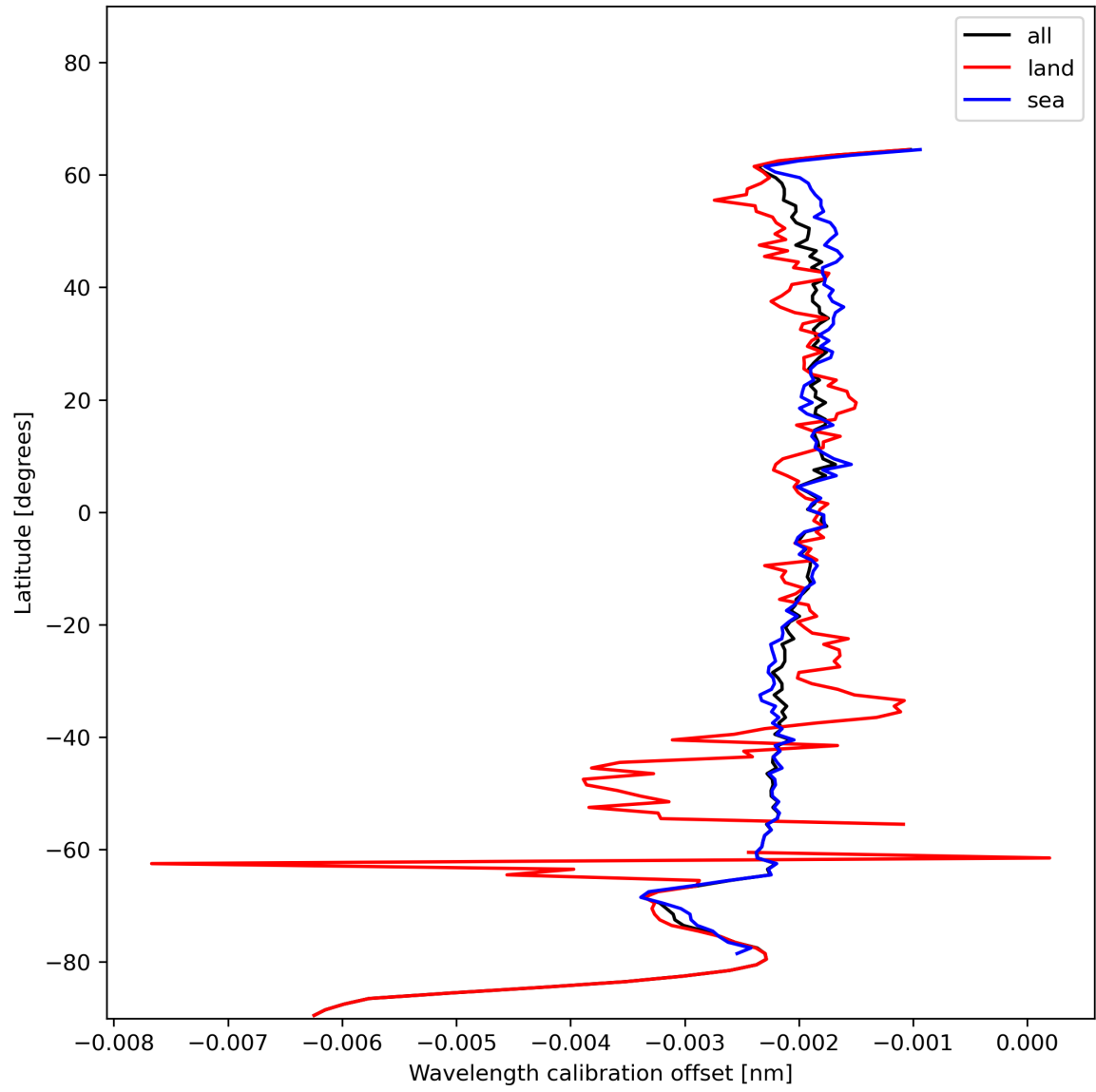
Figure 18: Zonal average of “Wavelength calibration offset” for 2023-12-23 to 2023-12-25.
