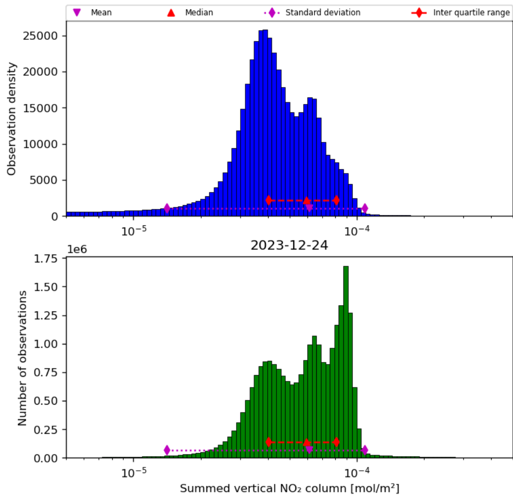
Figure 40: Histogram of “Summed vertical NO 2 column” for 2023-12-23 to 2023-12-25
