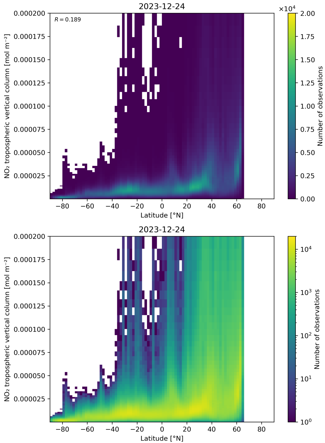
Figure 92: Scatter density plot of “Latitude” against “NO 2 tropospheric vertical column” for 2023-12-23 to 2023-12-25.
