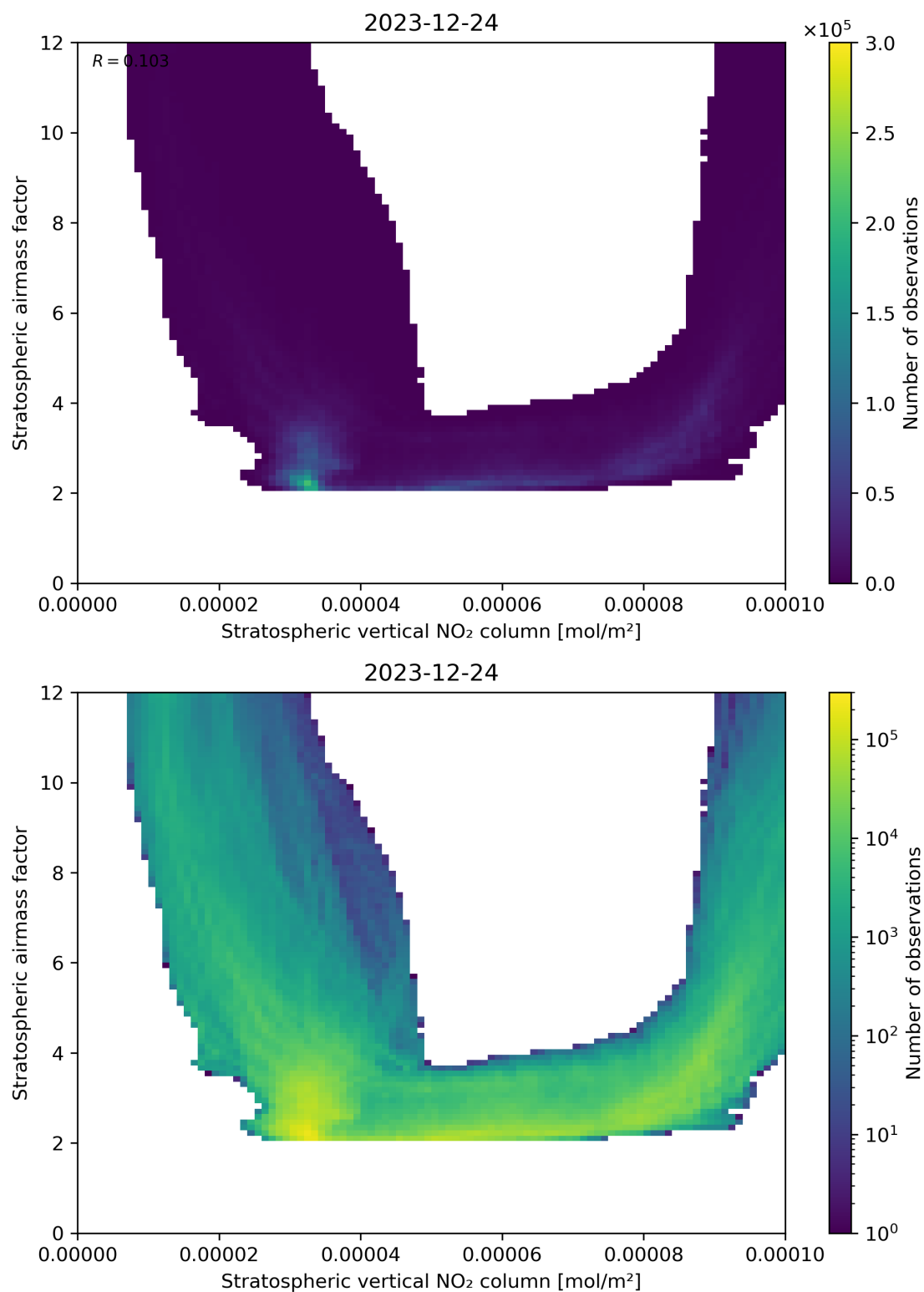
Figure 96: Scatter density plot of “Stratospheric vertical NO 2 column” against “Stratospheric airmass factor” for 2023-12-23 to 2023-12-25.
