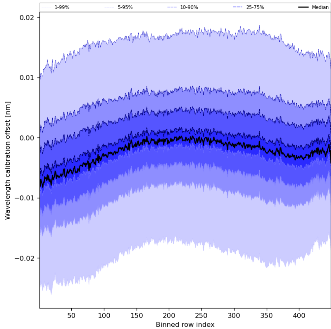
Figure 52: Along track statistics of “Wavelength calibration offset” for 2023-12-23 to 2023-12-25
