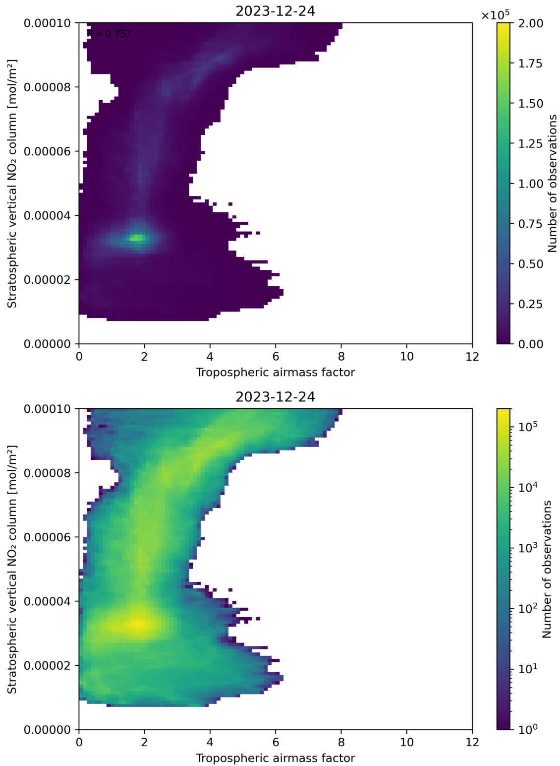
Figure 74: Scatter density plot of “Tropospheric air mass factor” against “Stratospheric vertical NO 2 column” for 2023-12-23 to 2023-12-25.
