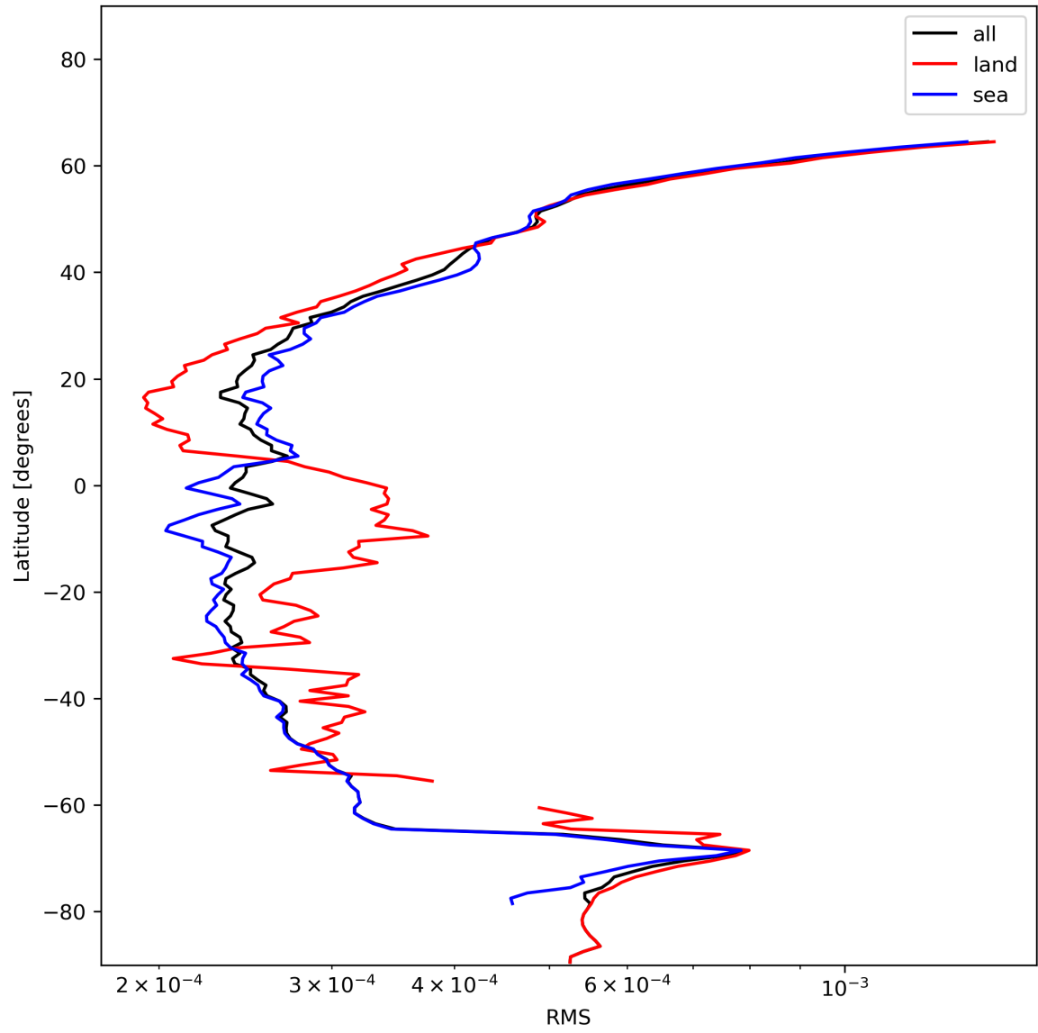
Figure 26: Zonal average of “RMS” for 2023-12-23 to 2023-12-25.
