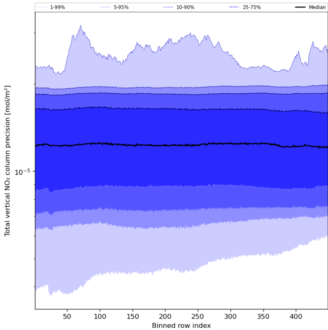
Figure 56: Along track statistics of “Total vertical NO 2 column precision” for 2023-12-23 to 2023-12-25
