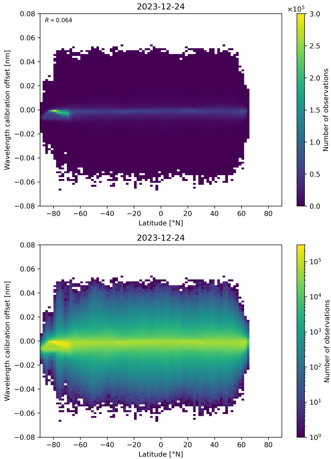
Figure 95: Scatter density plot of “Latitude” against “Wavelength calibration offset” for 2023-12-23 to 2023-12-25.
