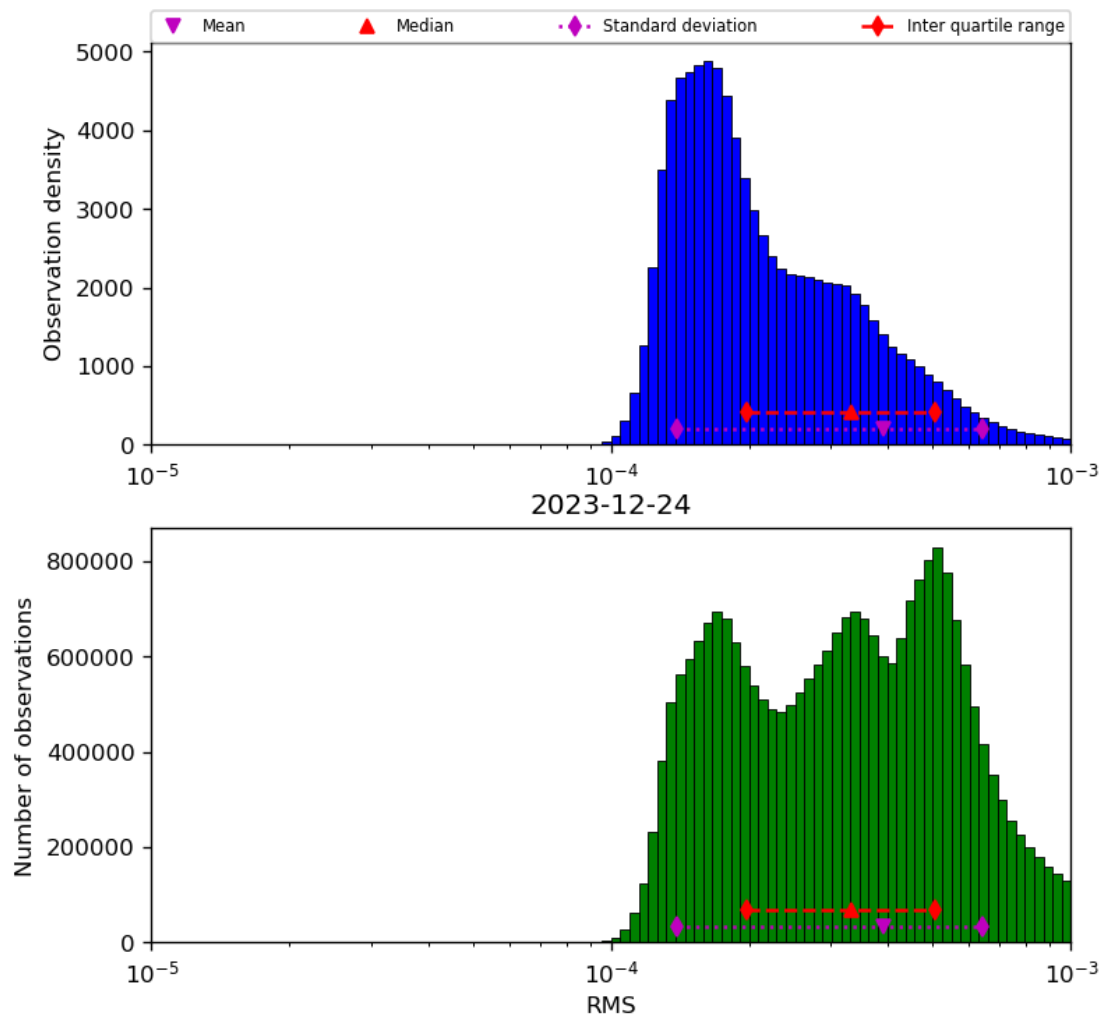
Figure 43: Histogram of “RMS” for 2023-12-23 to 2023-12-25
