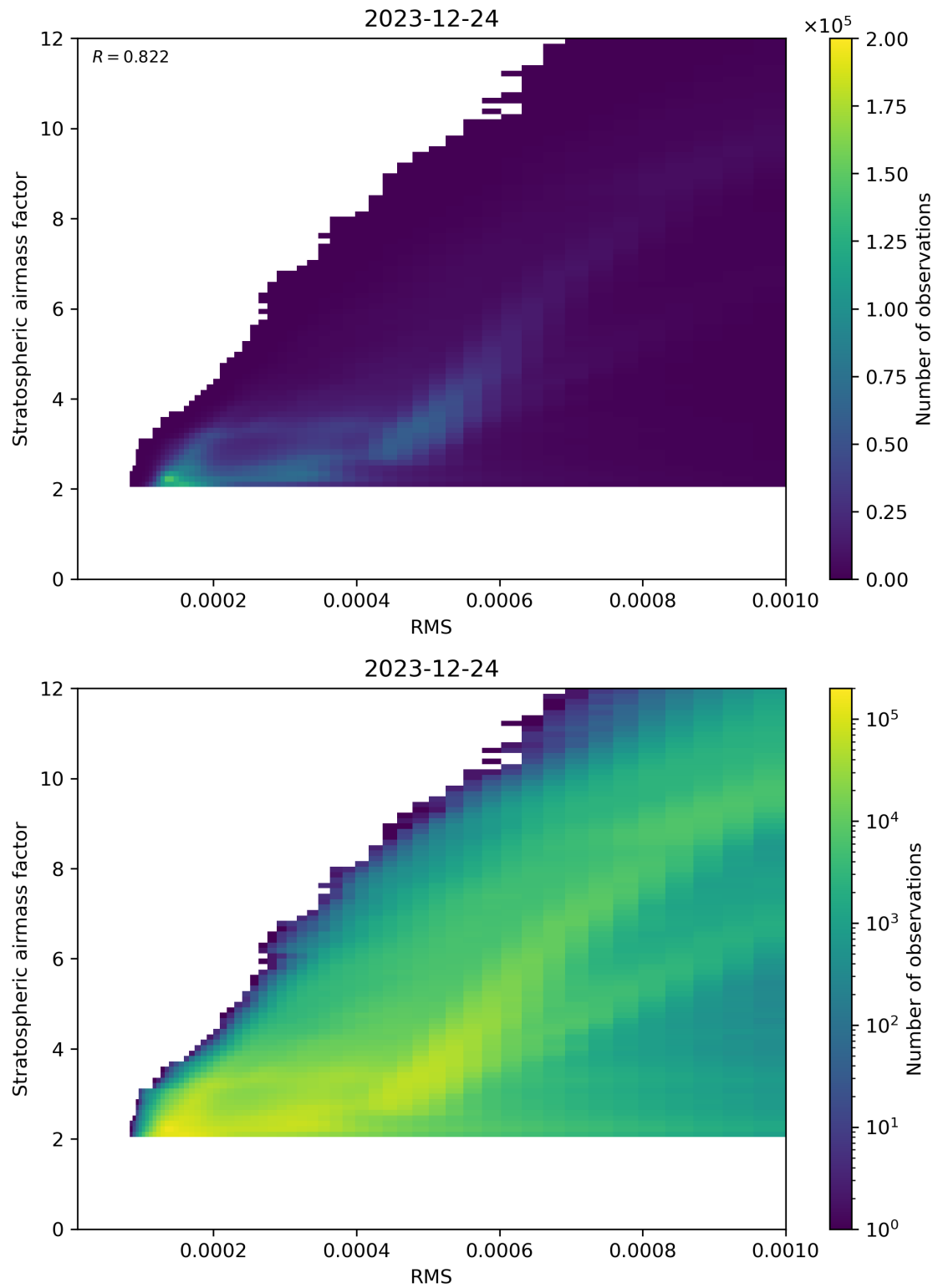
Figure 144: Scatter density plot of “RMS” against “Stratospheric airmass factor” for 2023-12-23 to 2023-12-25.
