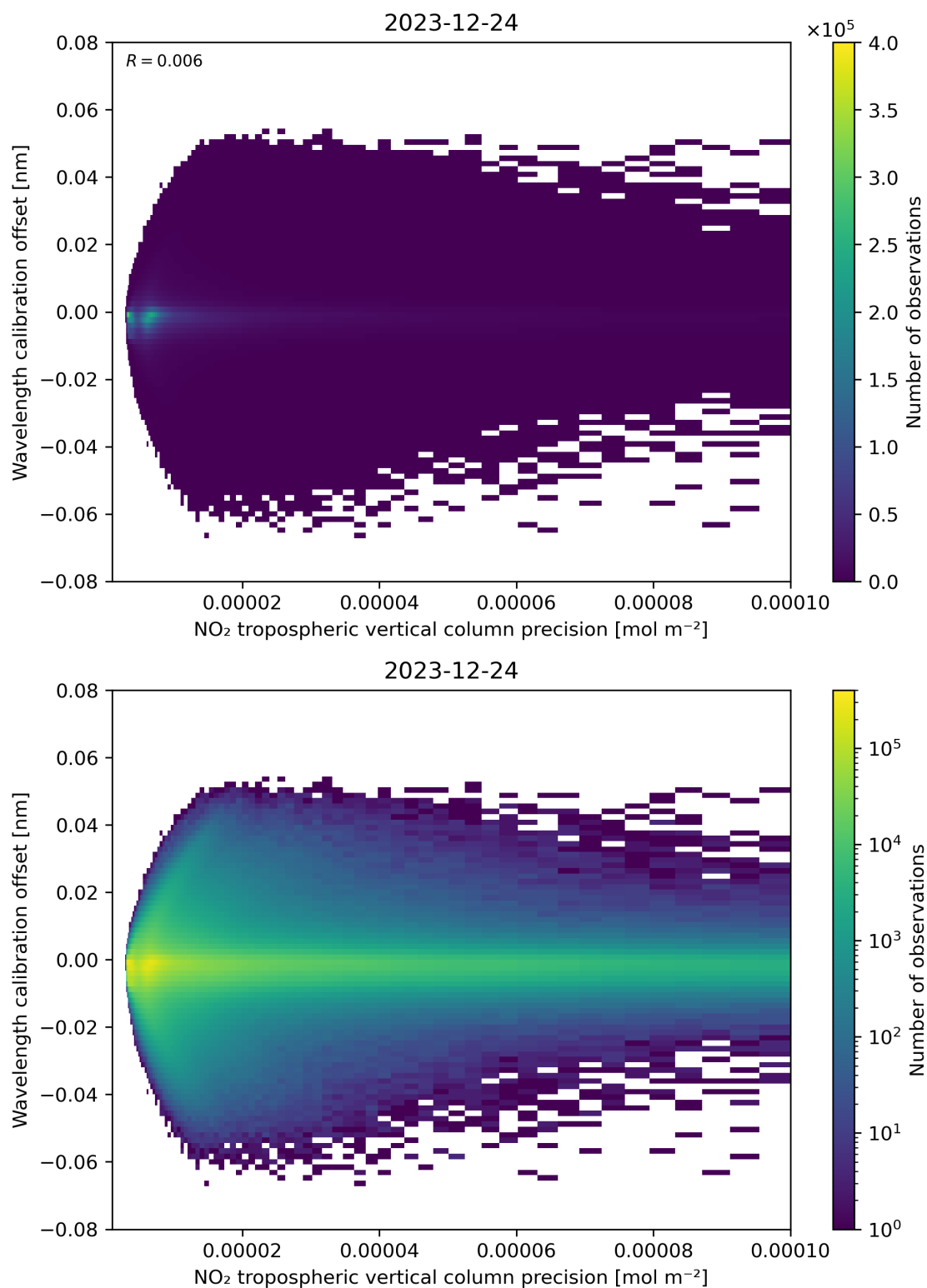
Figure 141: Scatter density plot of “NO 2 tropospheric vertical column precision” against “Wavelength calibration offset” for 2023-12-23 to 2023-12-25.
