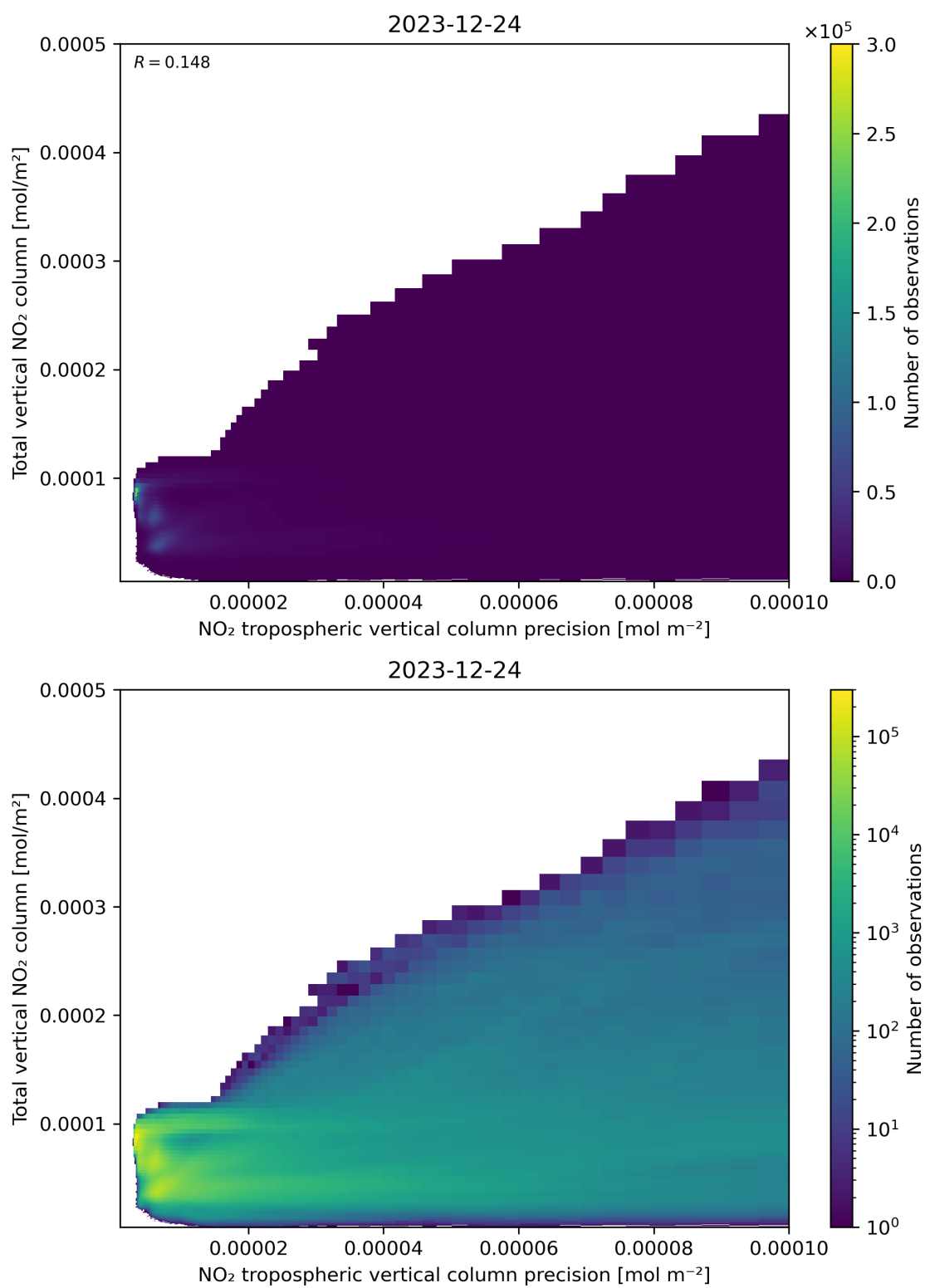
Figure 138: Scatter density plot of “NO 2 tropospheric vertical column precision” against “Total vertical NO 2 column” for 2023-12-23 to 2023-12-25.
