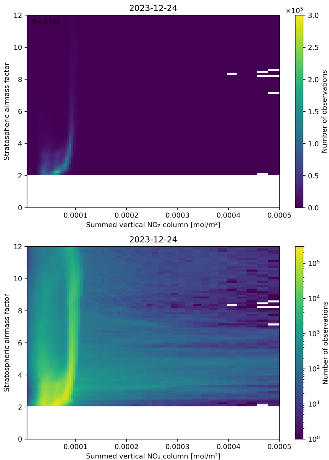
Figure 103: Scatter density plot of “Summed vertical NO 2 column” against “Stratospheric airmass factor” for 2023-12-23 to 2023-12-25.
