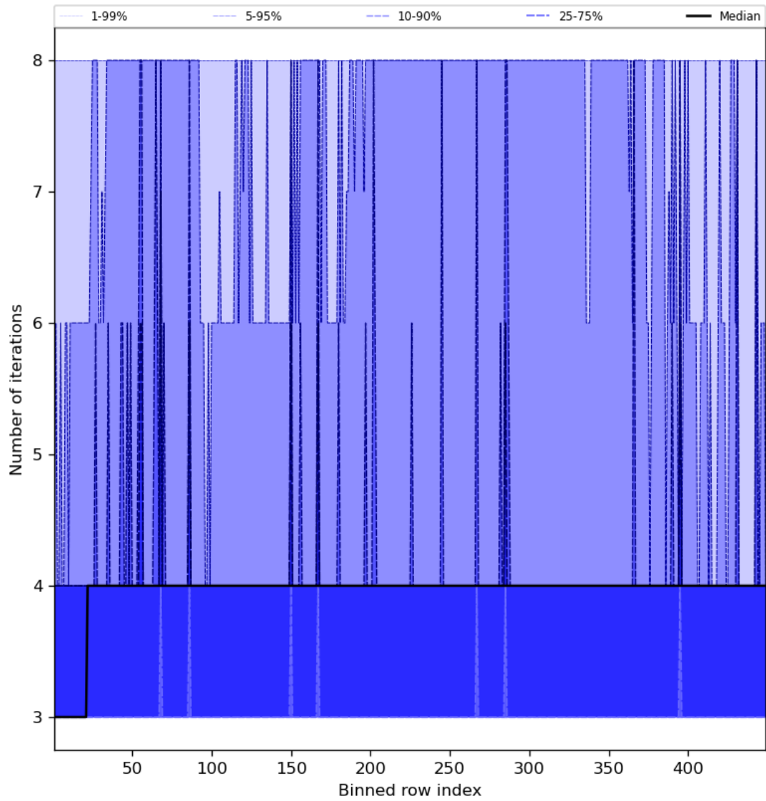
Figure 51: Along track statistics of “Number of iterations” for 2023-12-23 to 2023-12-25
