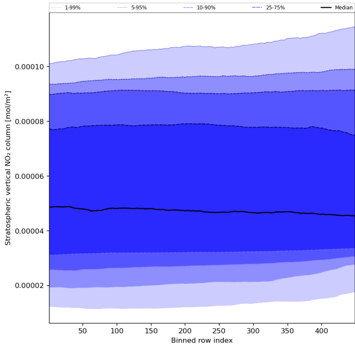
Figure 53: Along track statistics of “Stratospheric vertical NO 2 column” for 2023-12-23 to 2023-12-25
