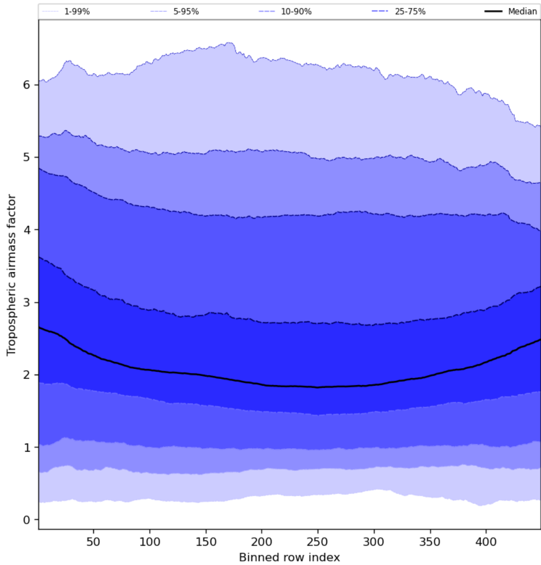
Figure 48: Along track statistics of “Tropospheric air mass factor” for 2023-12-23 to 2023-12-25
