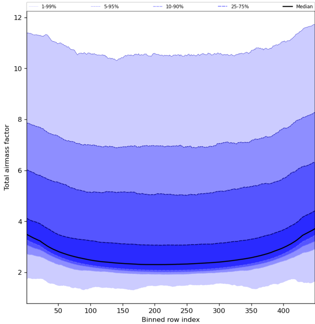
Figure 49: Along track statistics of “Total airmass factor” for 2023-12-23 to 2023-12-25
