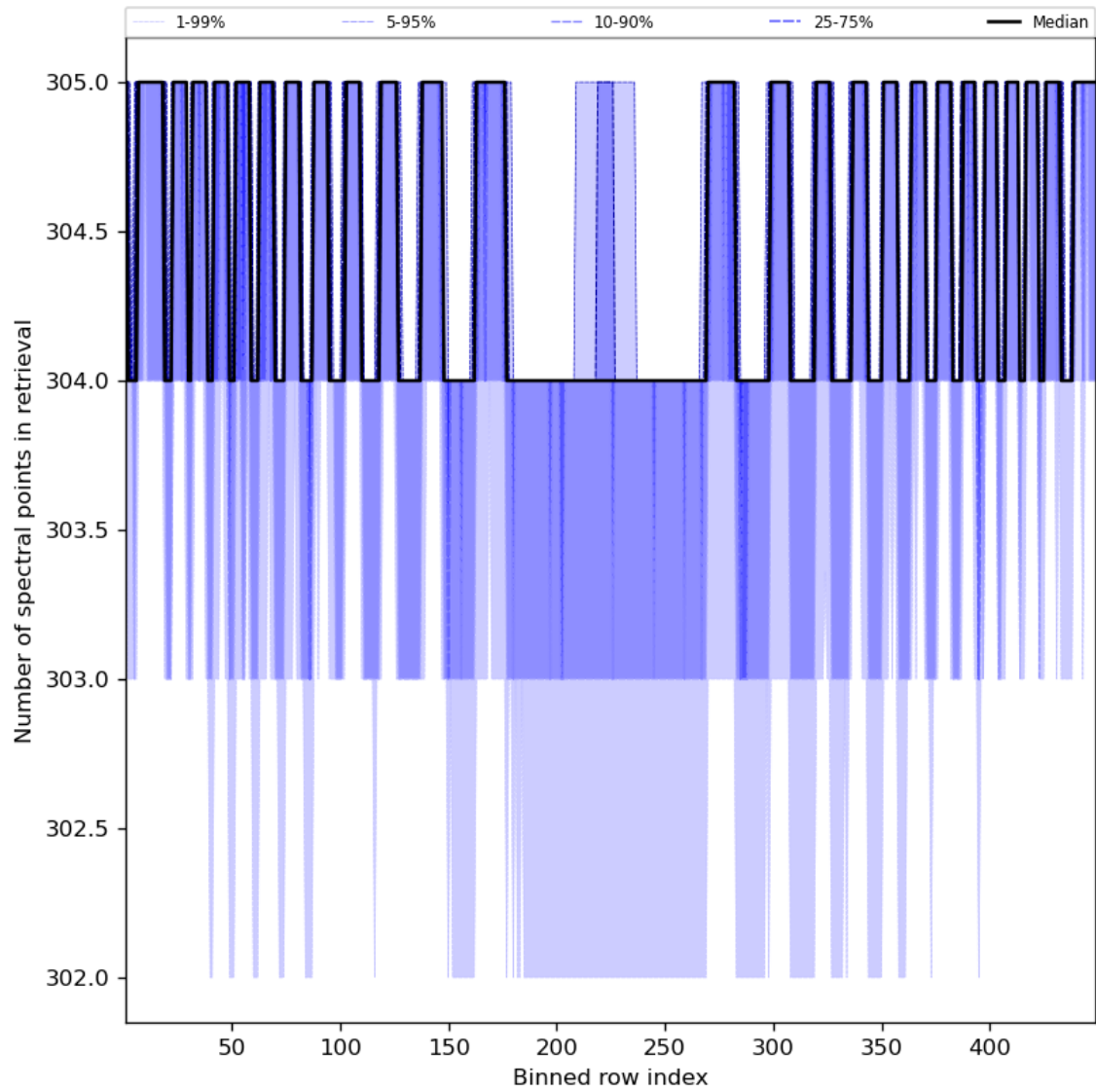
Figure 50: Along track statistics of “Number of spectral points in retrieval” for 2023-12-23 to 2023-12-25
