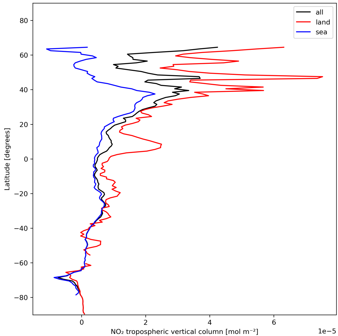
Figure 12: Zonal average of “NO 2 tropospheric vertical column” for 2023-12-23 to 2023-12-25.
