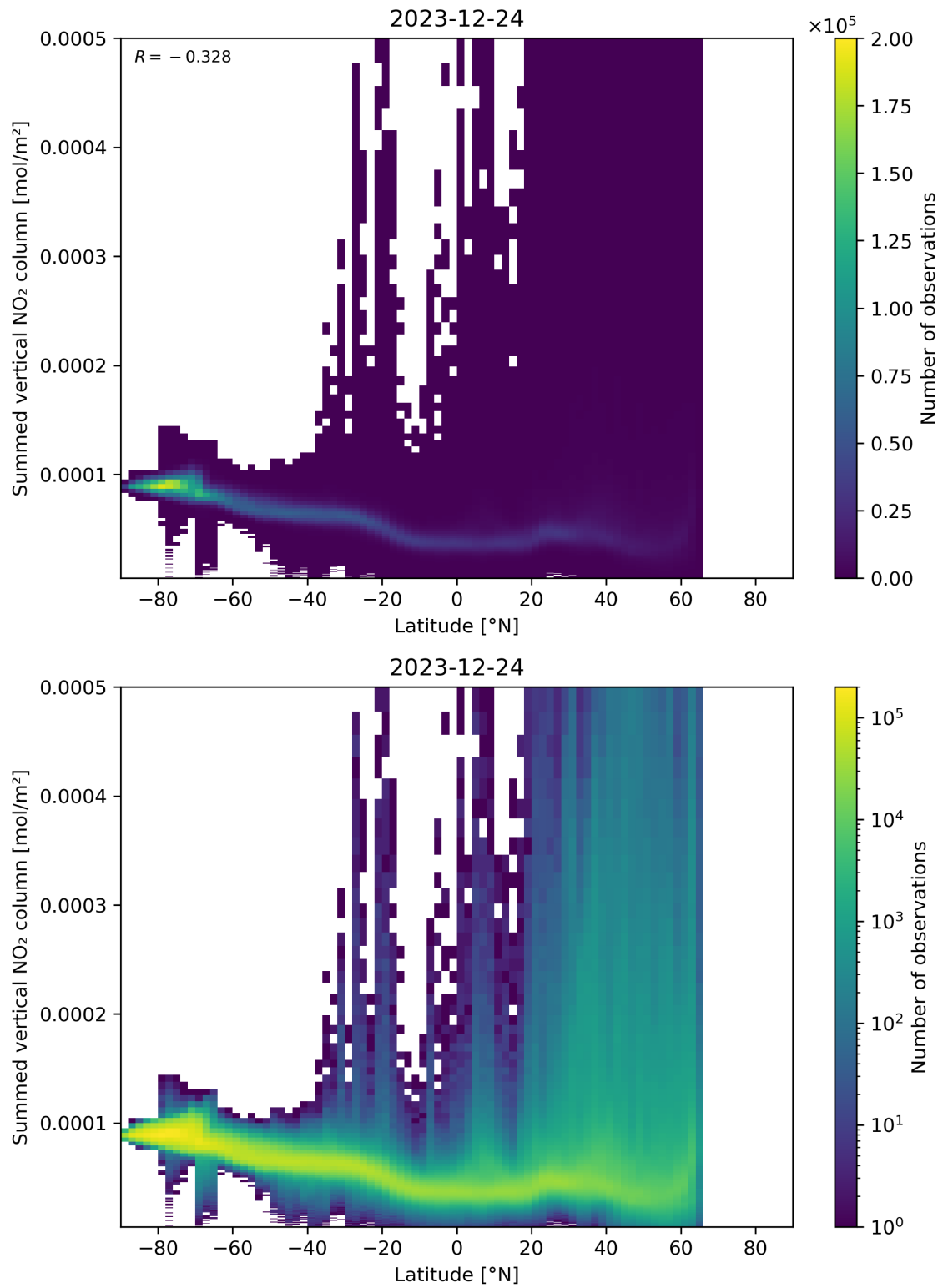
Figure 88: Scatter density plot of “Latitude” against “Summed vertical NO 2 column” for 2023-12-23 to 2023-12-25.
