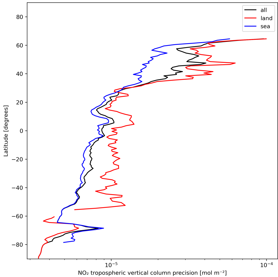
Figure 13: Zonal average of “NO 2 tropospheric vertical column precision” for 2023-12-23 to 2023-12-25.
