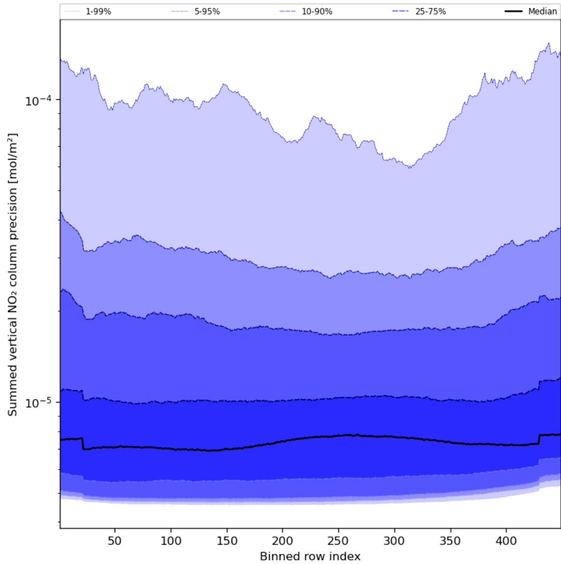
Figure 58: Along track statistics of “Summed vertical NO 2 column precision” for 2023-12-23 to 2023-12-25
