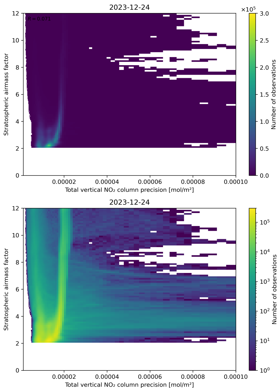
Figure 115: Scatter density plot of “Total vertical NO 2 column precision” against “Stratospheric air mass factor” for 2023-12-23 to 2023-12-25.
