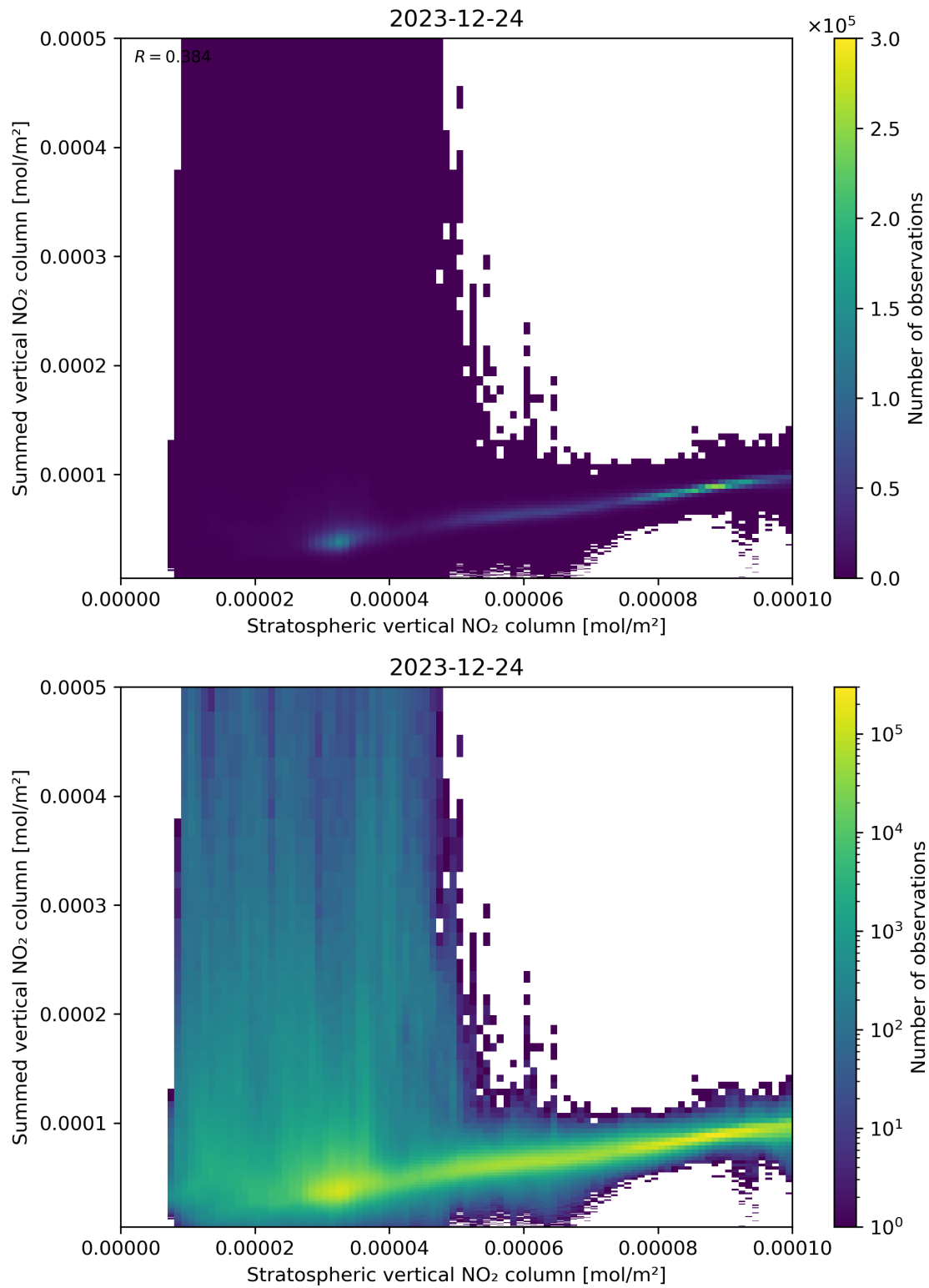
Figure 98: Scatter density plot of “Stratospheric vertical NO 2 column” against “Summed vertical NO 2 column” for 2023-12-23 to 2023-12-25.
