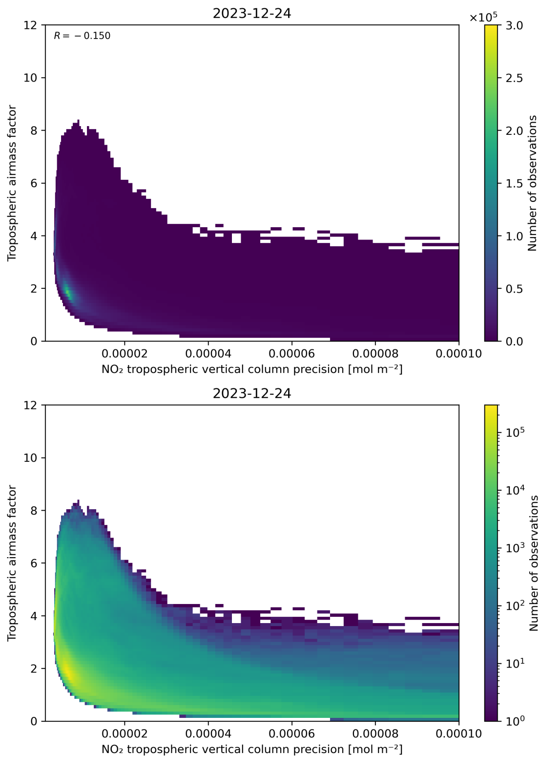
Figure 133: Scatter density plot of “NO 2 tropospheric vertical column precision” against “Tropospheric airmass factor” for 2023-12-23 to 2023-12-25.
