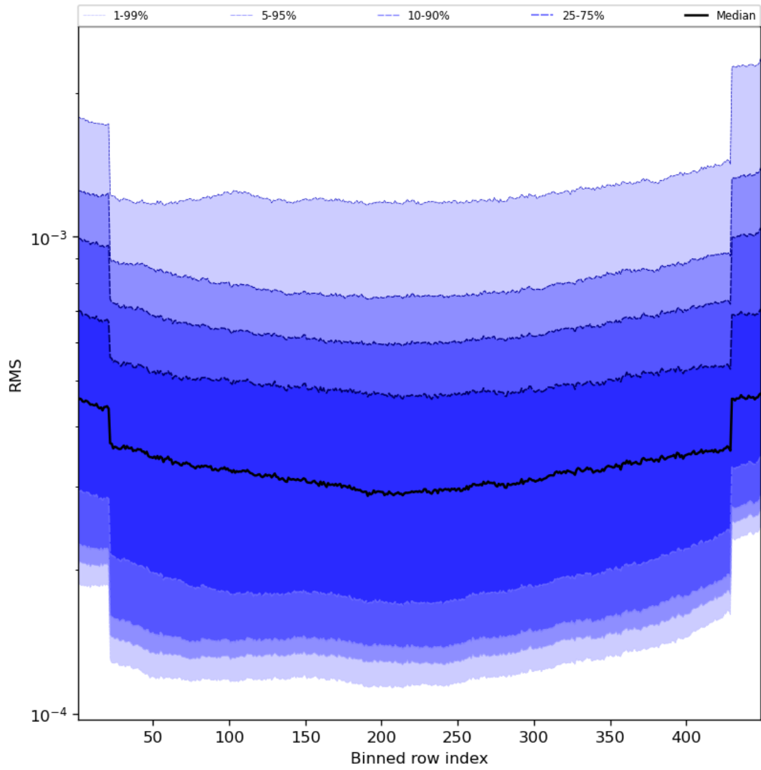
Figure 60: Along track statistics of “RMS” for 2023-12-23 to 2023-12-25
