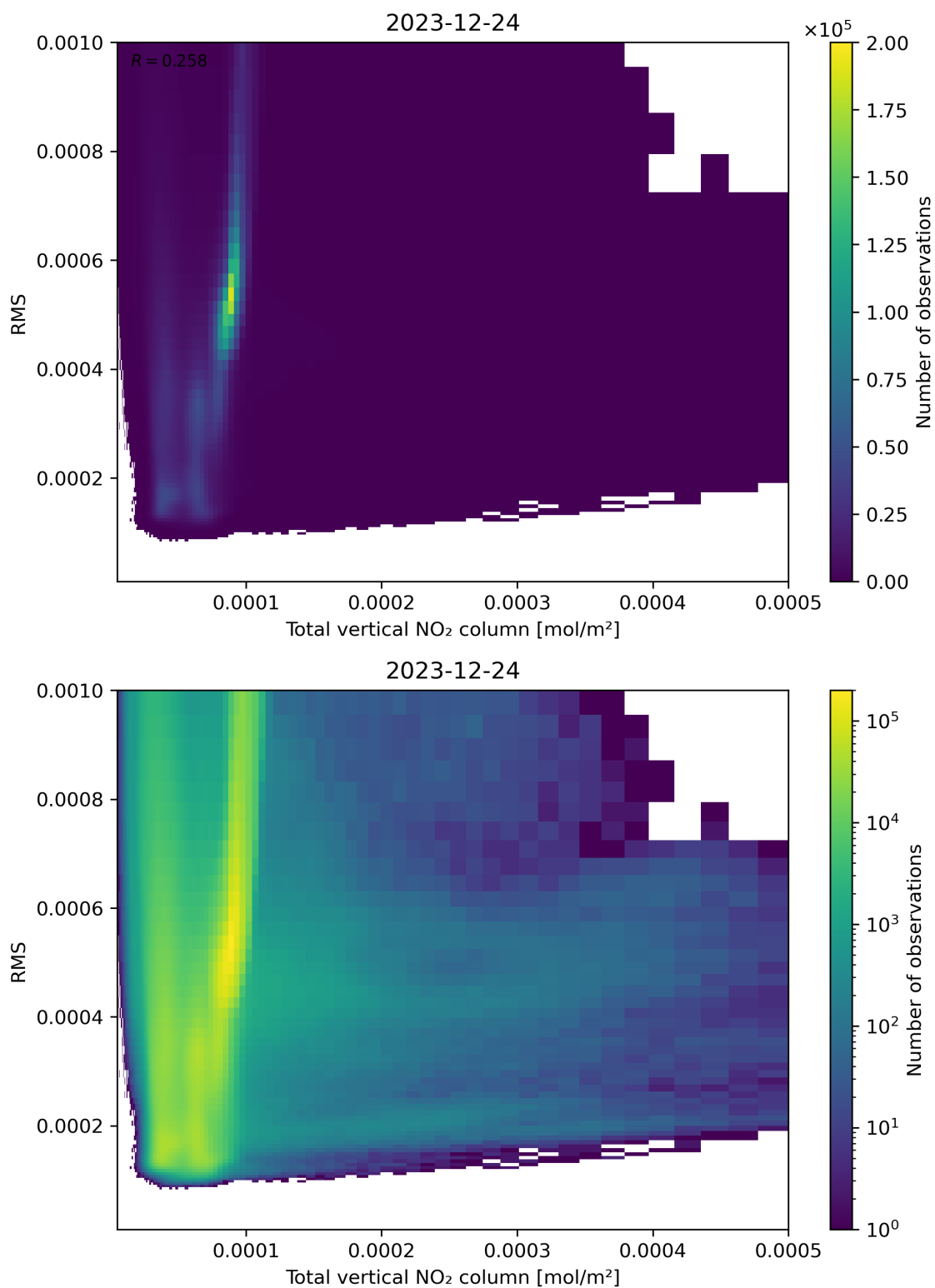
Figure 120: Scatter density plot of “Total vertical NO 2 column” against “RMS” for 2023-12-23 to 2023-12-25.
