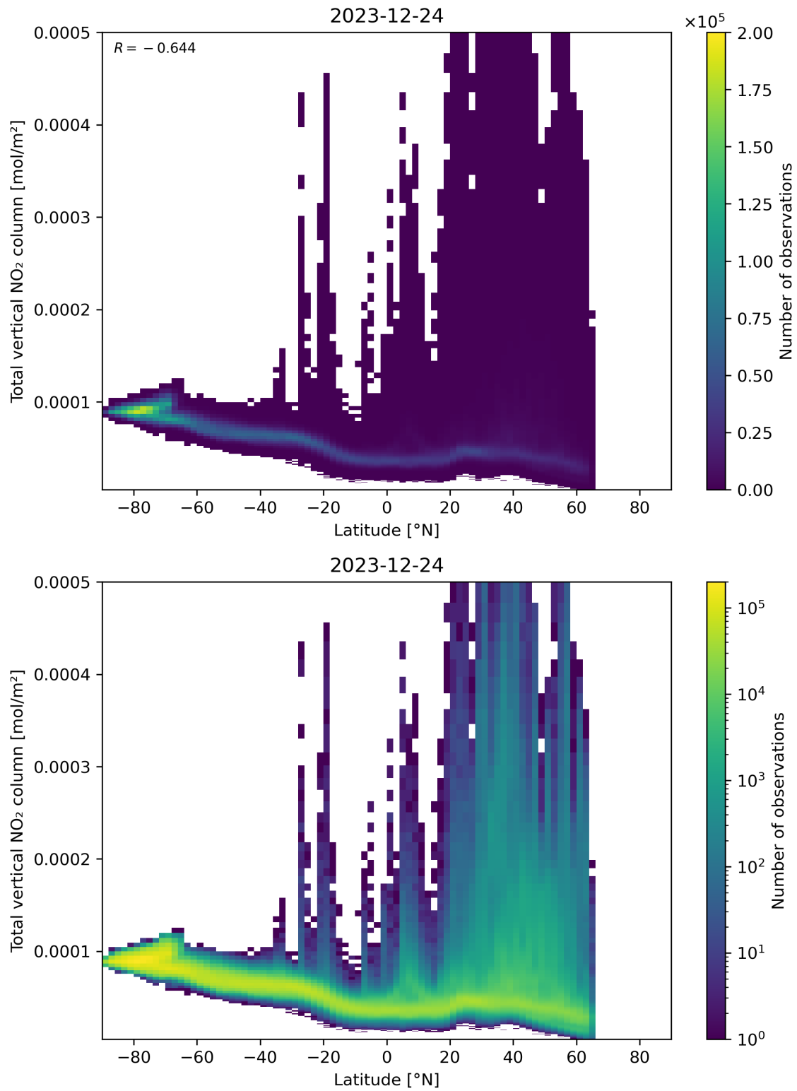
Figure 90: Scatter density plot of “Latitude” against “Total vertical NO 2 column” for 2023-12-23 to 2023-12-25.
