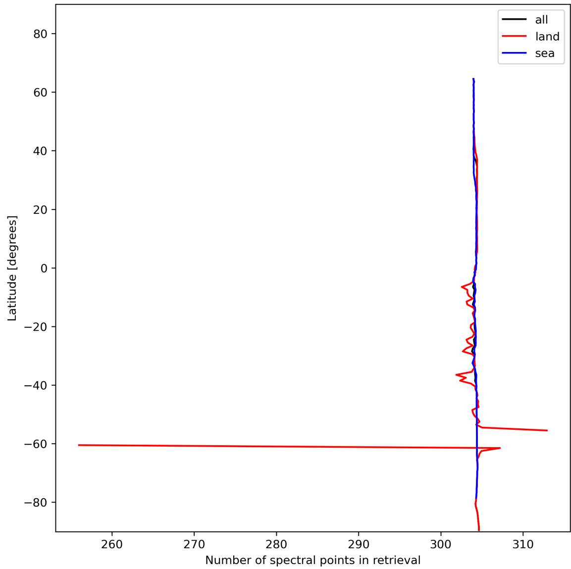
Figure 16: Zonal average of “Number of spectral points in retrieval” for 2023-12-23 to 2023-12-25.
