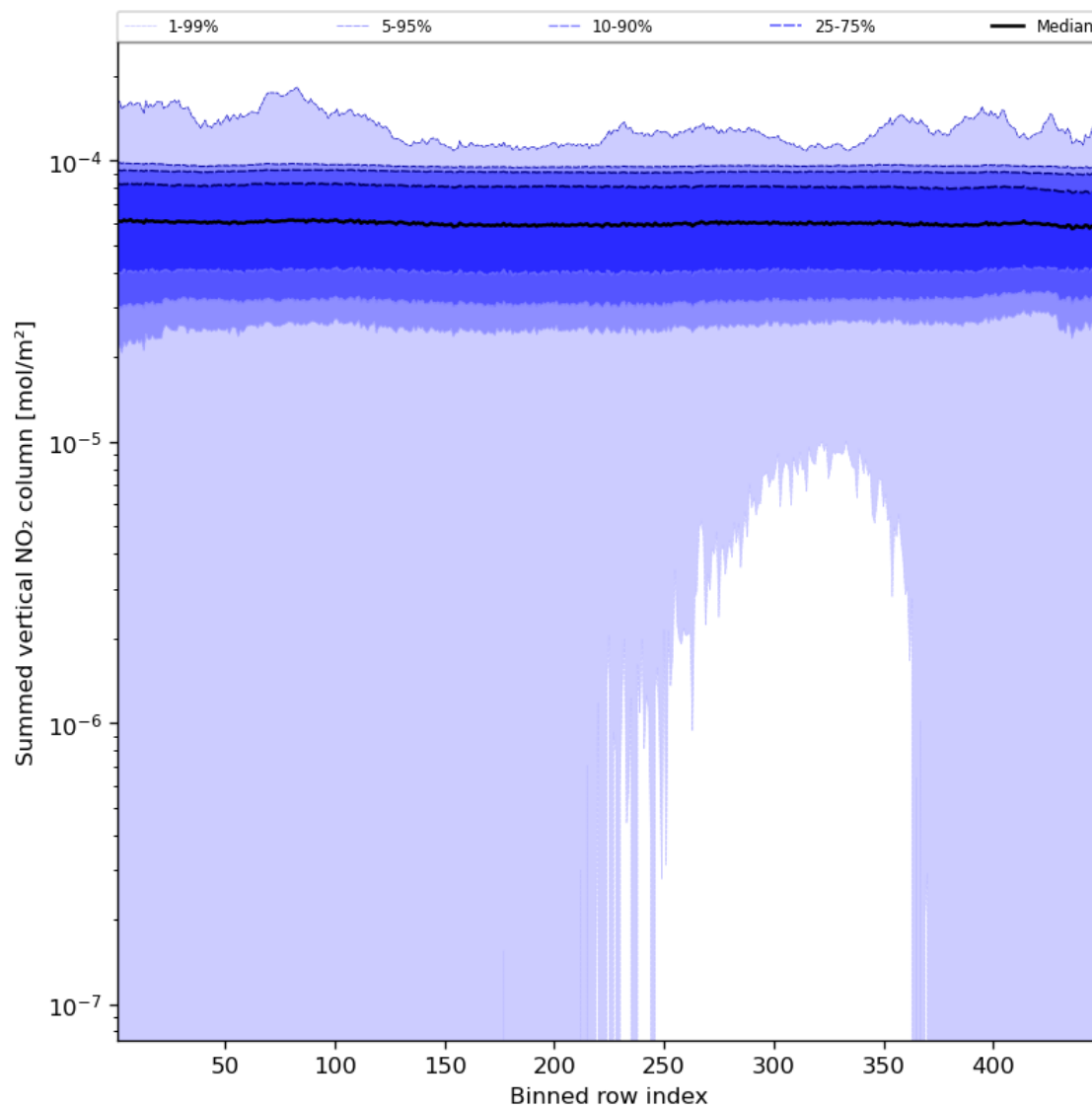
Figure 57: Along track statistics of “Summed vertical NO 2 column” for 2023-12-23 to 2023-12-25
