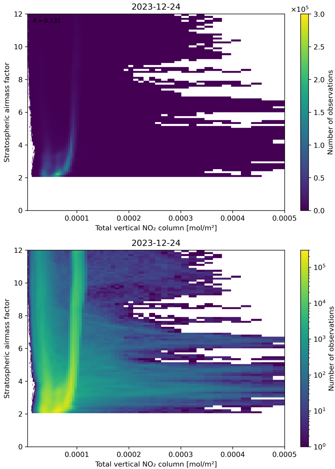
Figure 110: Scatter density plot of “Total vertical NO 2 column” against “Stratospheric air mass factor” for 2023-12-23 to 2023-12-25.
