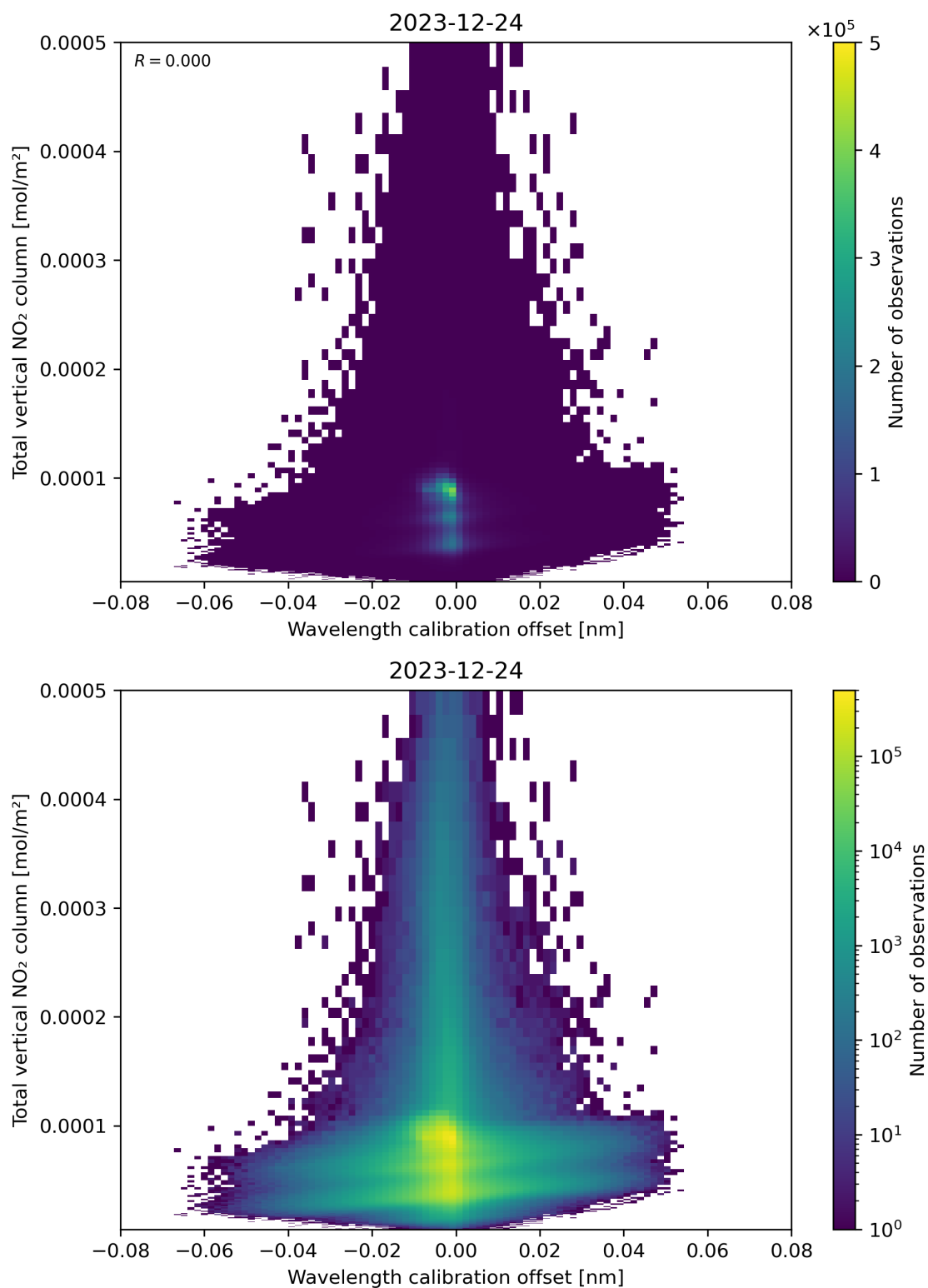
Figure 179: Scatter density plot of “Wavelength calibration offset” against “Total vertical NO 2 column” for 2023-12-23 to 2023-12-25.
