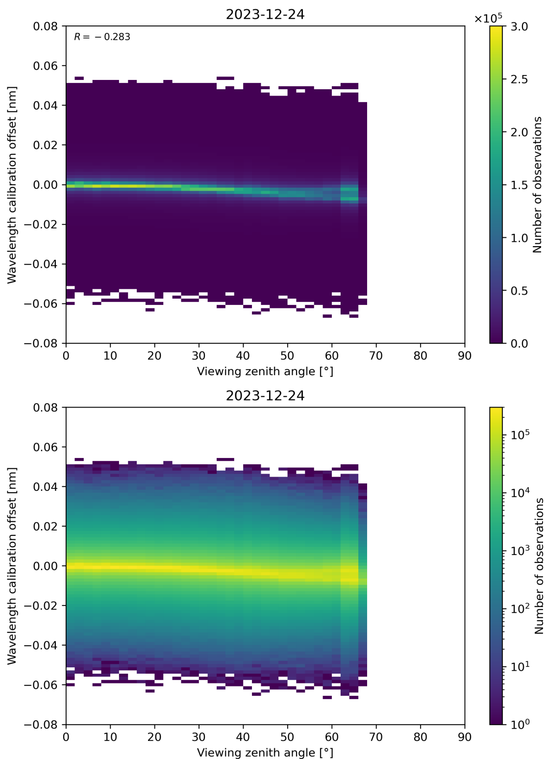
Figure 173: Scatter density plot of “Viewing zenith angle” against “Wavelength calibration offset” for 2023-12-23 to 2023-12-25.
