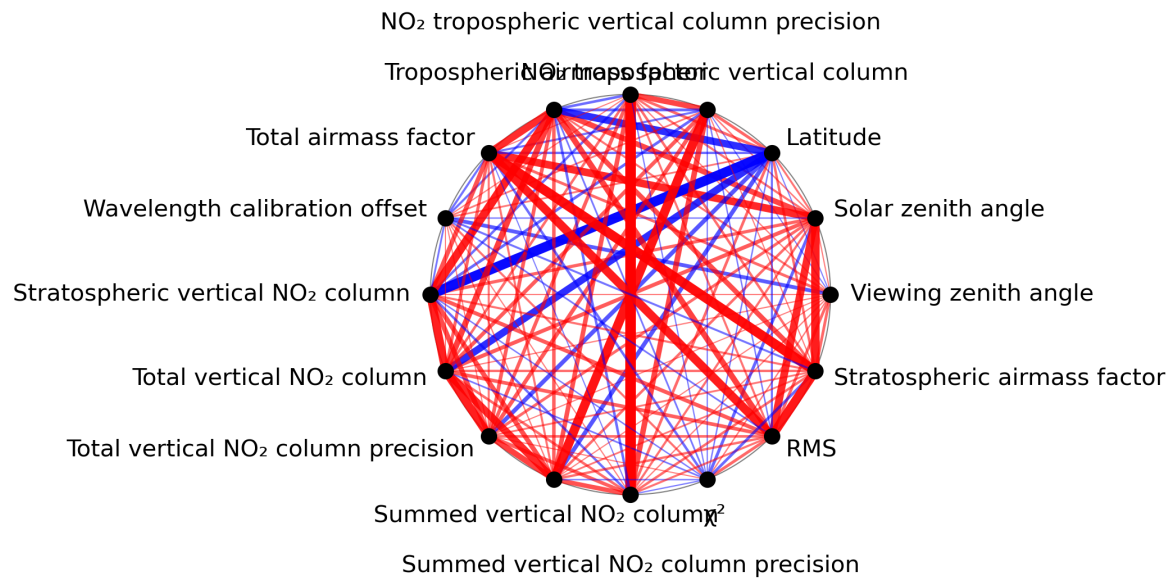
Figure 1: Map of correlation graph for 2023-12-23 to 2023-12-25.
