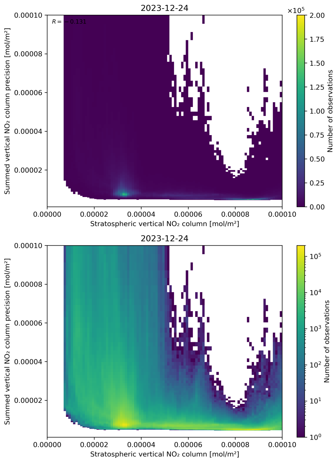
Figure 99: Scatter density plot of “Stratospheric vertical NO 2 column” against “Summed vertical NO 2 column precision” for 2023-12-23 to 2023-12-25.
