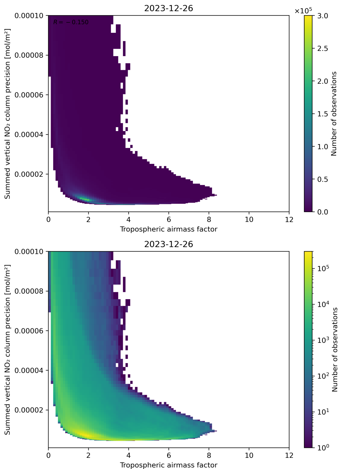
Figure 76: Scatter density plot of “Tropospheric air mass factor” against “Summed vertical NO 2 column precision” for 2023-12-25 to 2023-12-27.
