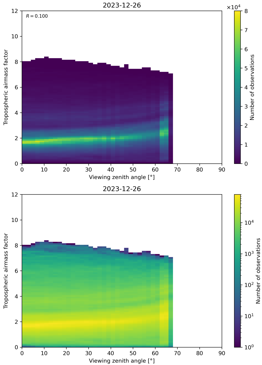
Figure 161: Scatter density plot of “Viewing zenith angle” against “Tropospheric airmass factor” for 2023-12-25 to 2023-12-27.
