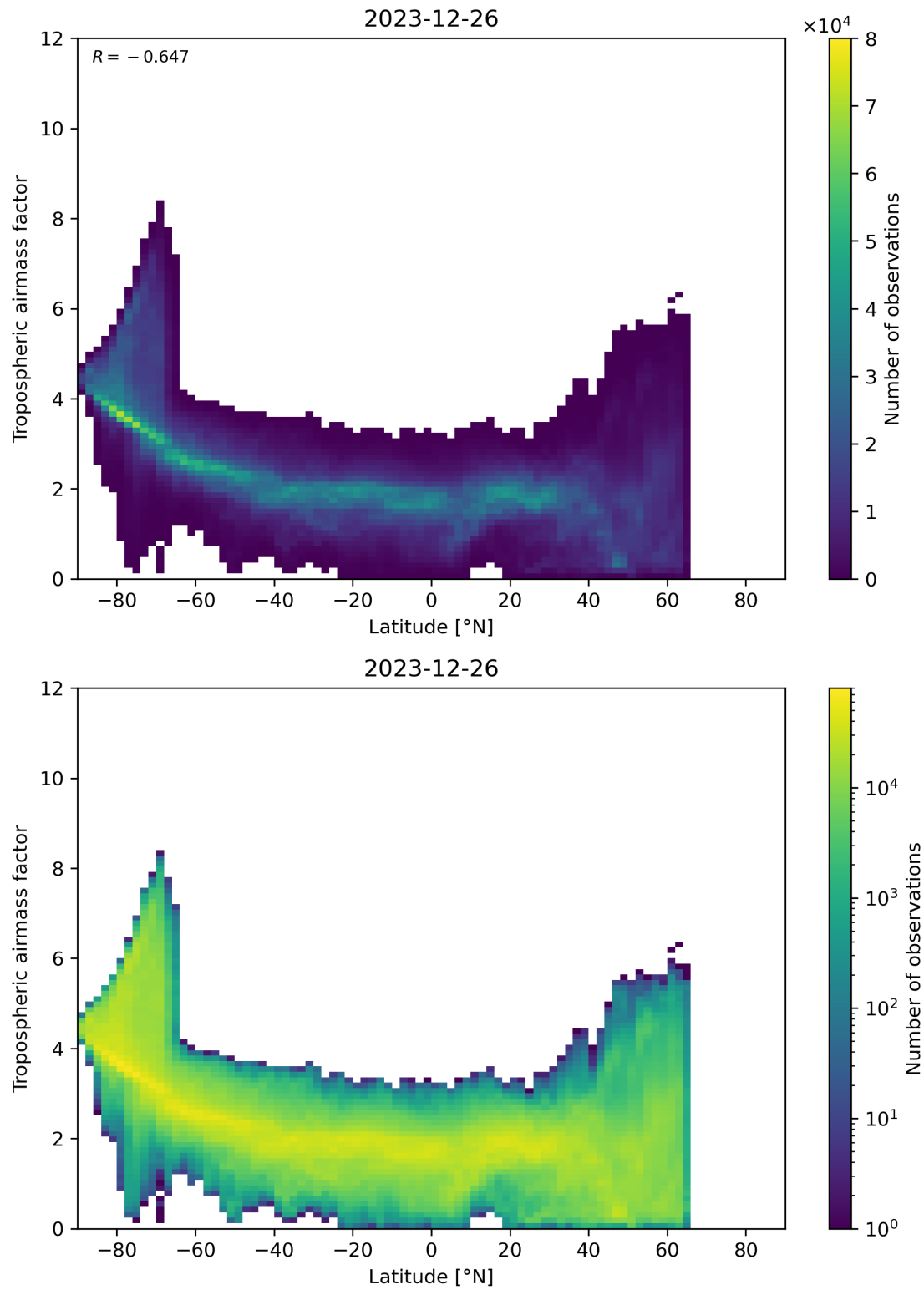
Figure 85: Scatter density plot of “Latitude” against “Tropospheric air mass factor” for 2023-12-25 to 2023-12-27.
