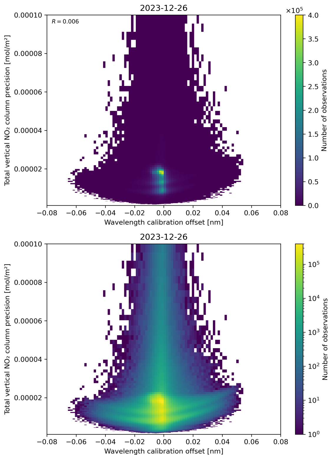
Figure 180: Scatter density plot of “Wavelength calibration offset” against “Total vertical NO 2 column precision” for 2023-12-25 to 2023-12-27.
