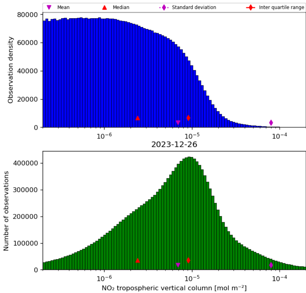
Figure 29: Histogram of “NO 2 tropospheric vertical column” for 2023-12-25 to 2023-12-27
