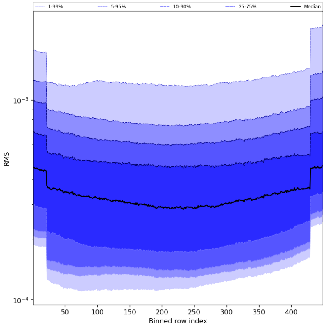
Figure 60: Along track statistics of “RMS” for 2023-12-25 to 2023-12-27
