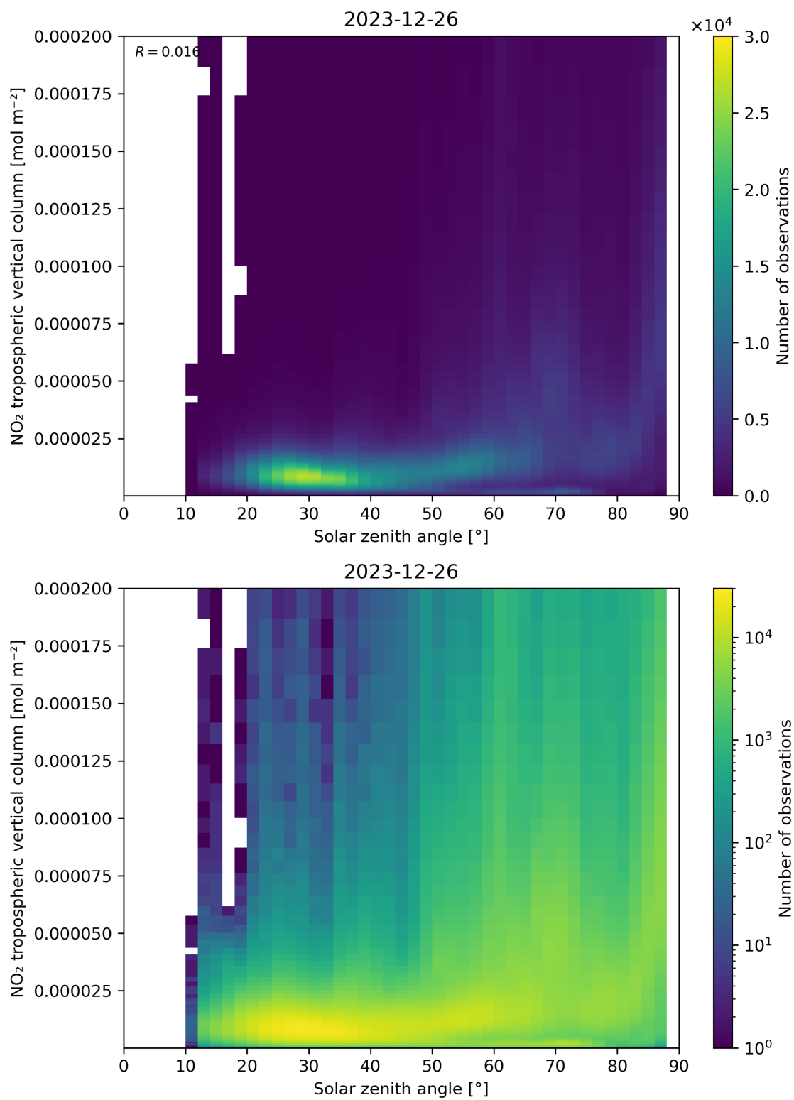
Figure 155: Scatter density plot of “Solar zenith angle” against “NO 2 tropospheric vertical column” for 2023-12-25 to 2023-12-27.
