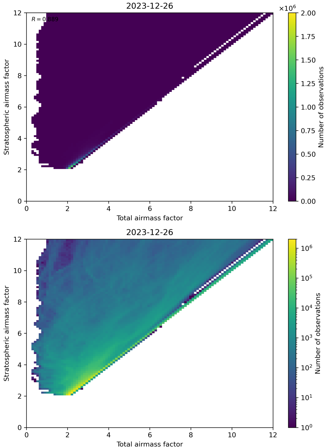
Figure 62: Scatter density plot of “Total airmass factor” against “Stratospheric airmass factor” for 2023-12-25 to 2023-12-27.
