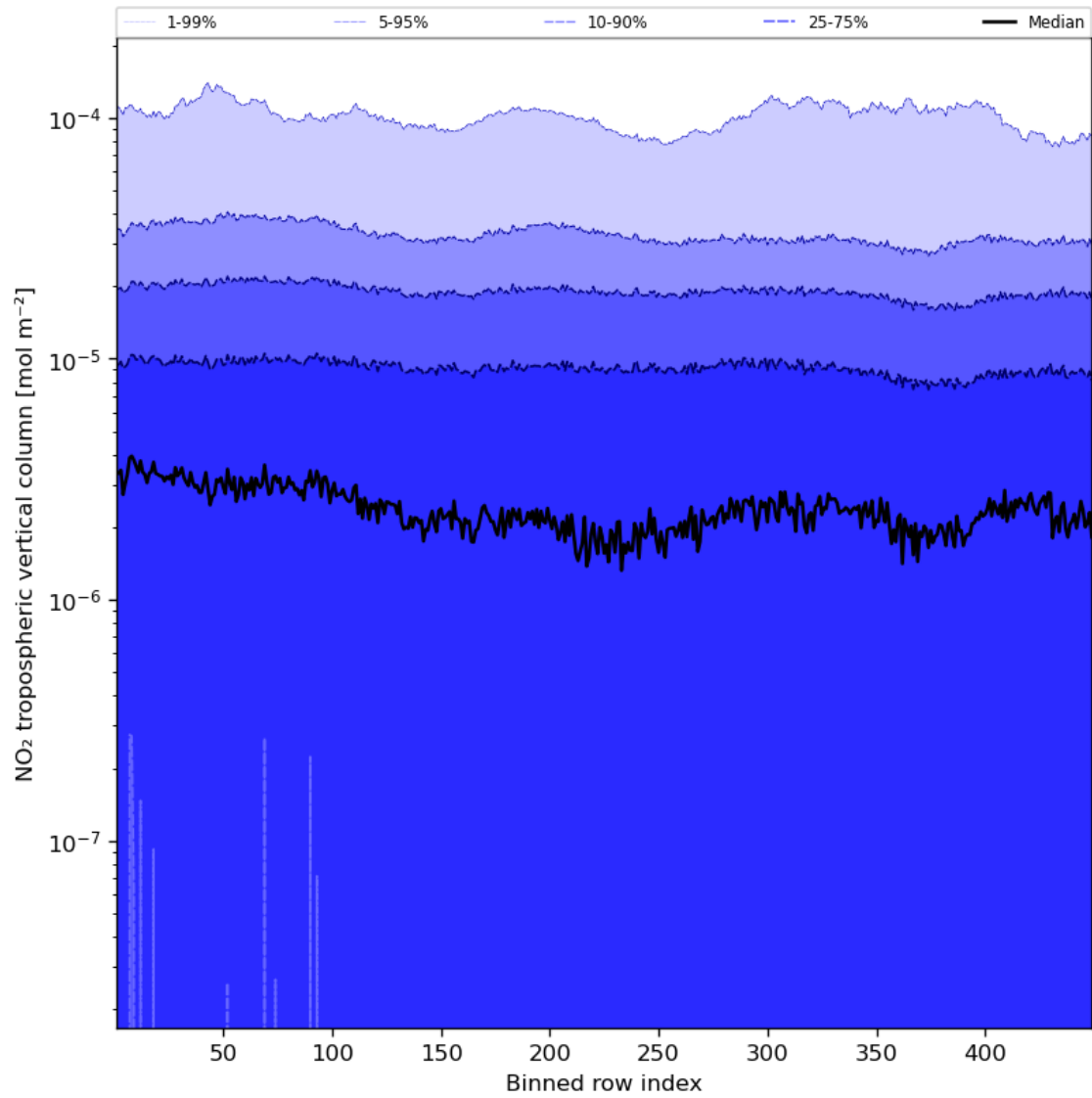
Figure 46: Along track statistics of “NO 2 tropospheric vertical column” for 2023-12-25 to 2023-12-27
