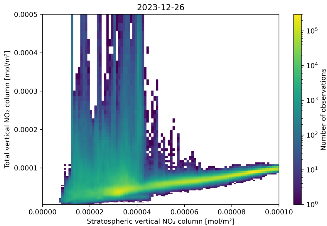
Figure 100: Scatter density plot of “Stratospheric vertical NO 2 column” against “Total vertical NO 2 column” for 2023-12-25 to 2023-12-27.
