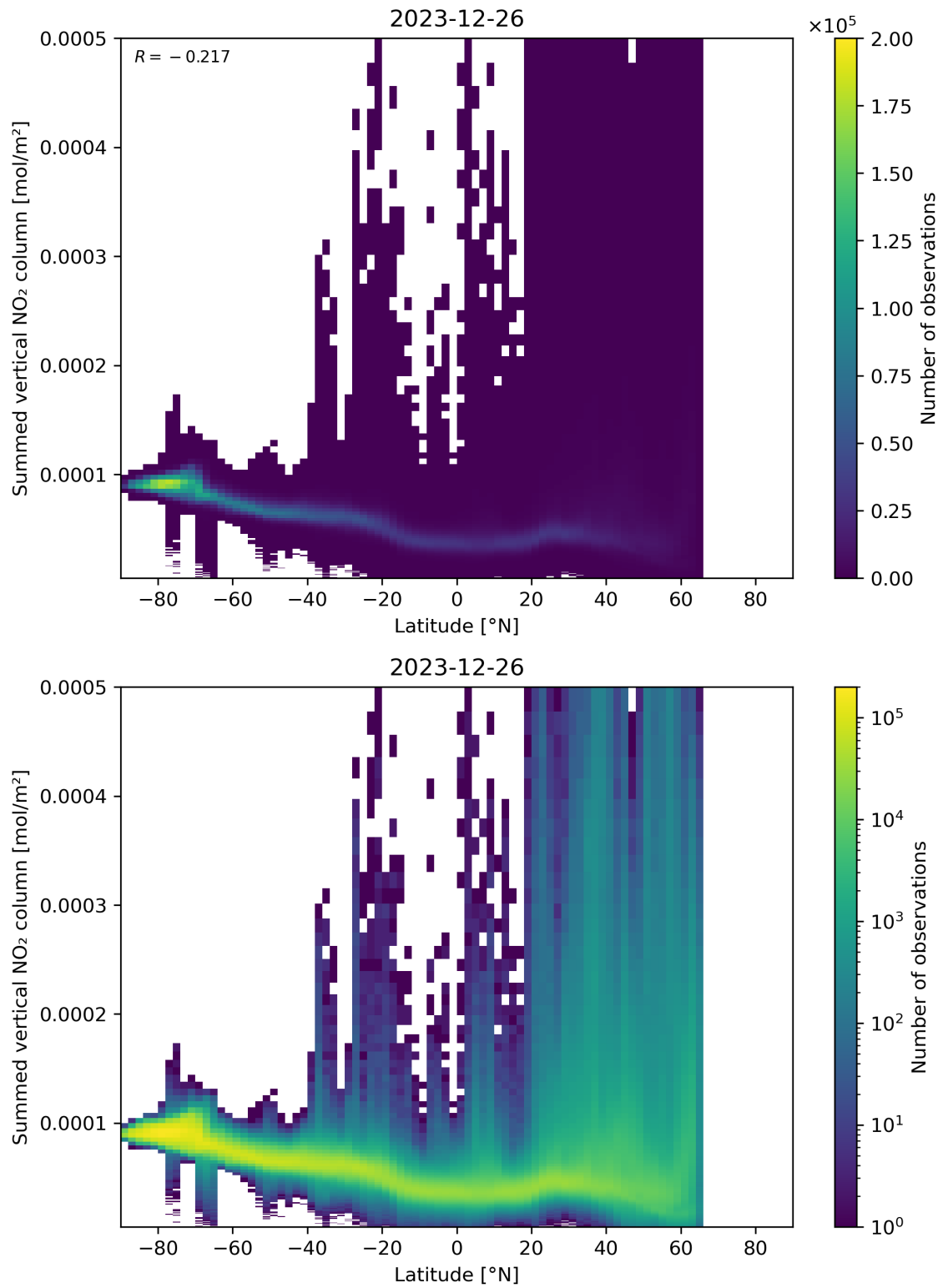
Figure 88: Scatter density plot of “Latitude” against “Summed vertical NO 2 column” for 2023-12-25 to 2023-12-27.
