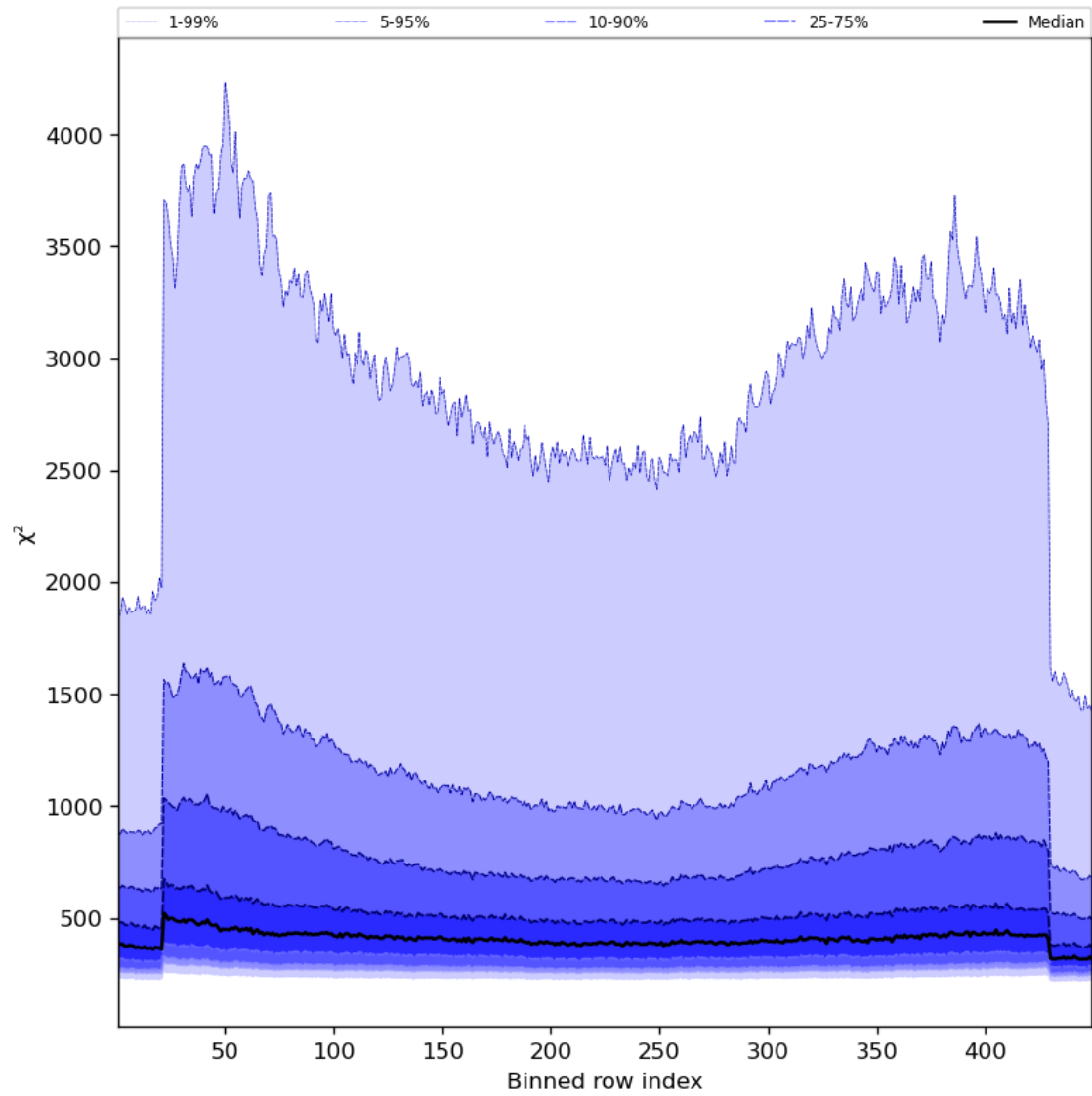
Figure 59: Along track statistics of “ \chi^2 ” for 2023-12-25 to 2023-12-27
