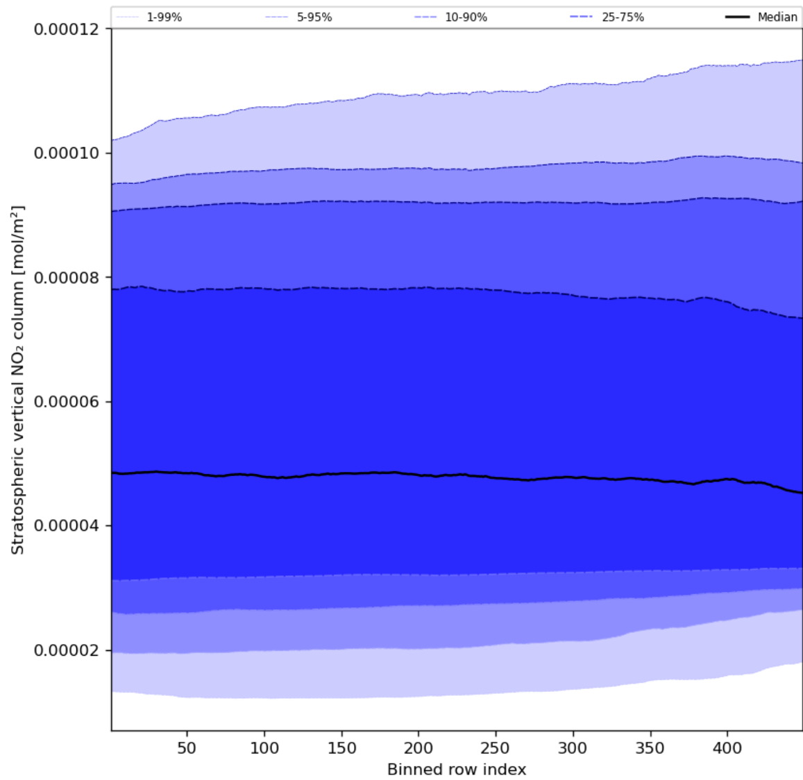
Figure 53: Along track statistics of “Stratospheric vertical NO 2 column” for 2023-12-25 to 2023-12-27
