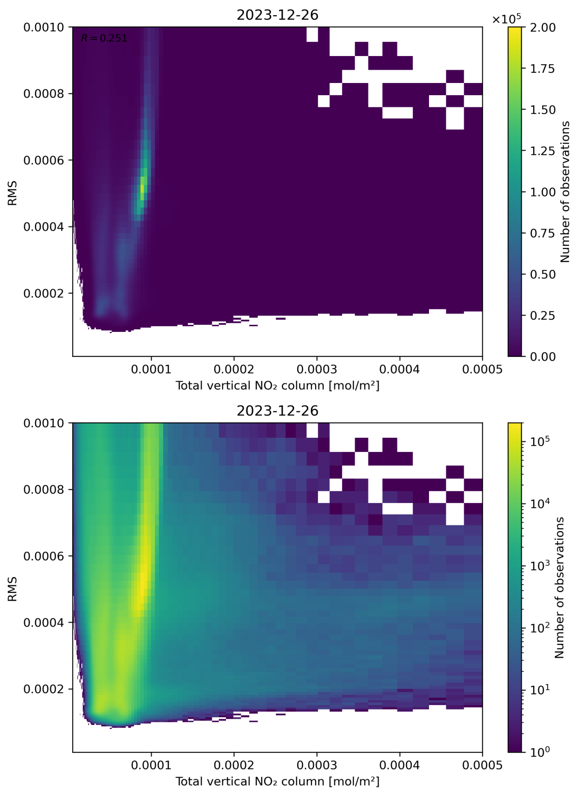
Figure 120: Scatter density plot of “Total vertical NO 2 column” against “RMS” for 2023-12-25 to 2023-12-27.
