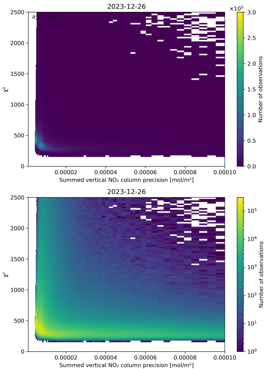
Figure 107: Scatter density plot of “Summed vertical NO 2 column precision” against “ \chi^2 ” for 2023-12-25 to 2023-12-27.
