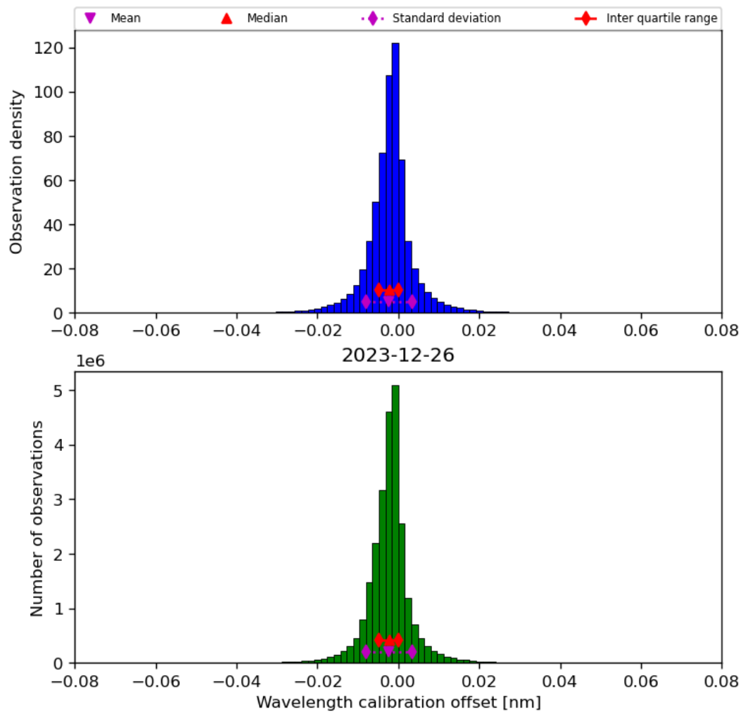
Figure 35: Histogram of “Wavelength calibration offset” for 2023-12-25 to 2023-12-27
