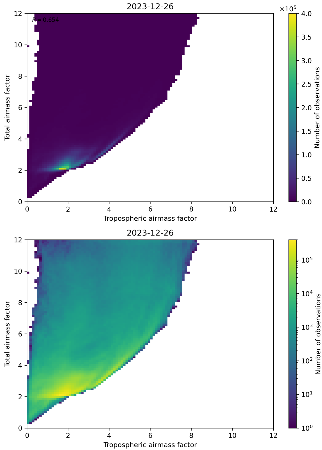
Figure 72: Scatter density plot of “Tropospheric airmass factor” against “Total airmass factor” for 2023-12-25 to 2023-12-27.
