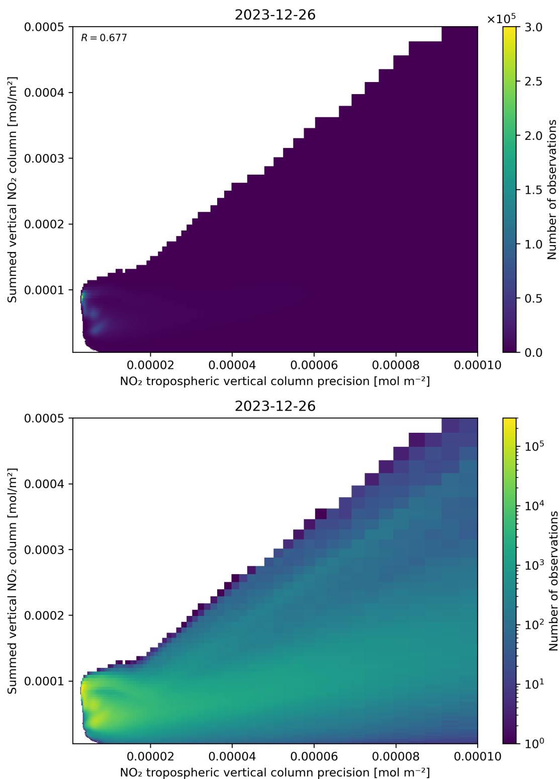
Figure 136: Scatter density plot of “NO 2 tropospheric vertical column precision” against “Summed vertical NO 2 column” for 2023-12-25 to 2023-12-27.
