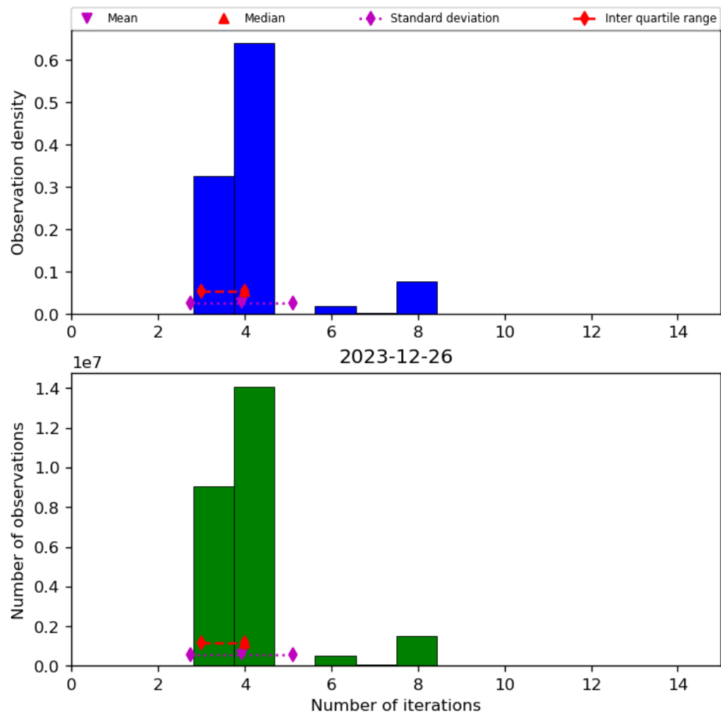
Figure 34: Histogram of “Number of iterations” for 2023-12-25 to 2023-12-27
