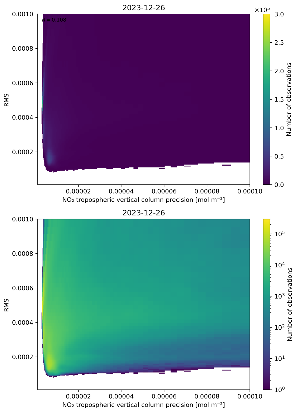
Figure 140: Scatter density plot of “NO 2 tropospheric vertical column precision” against “RMS” for 2023-12-25 to 2023-12-27.
