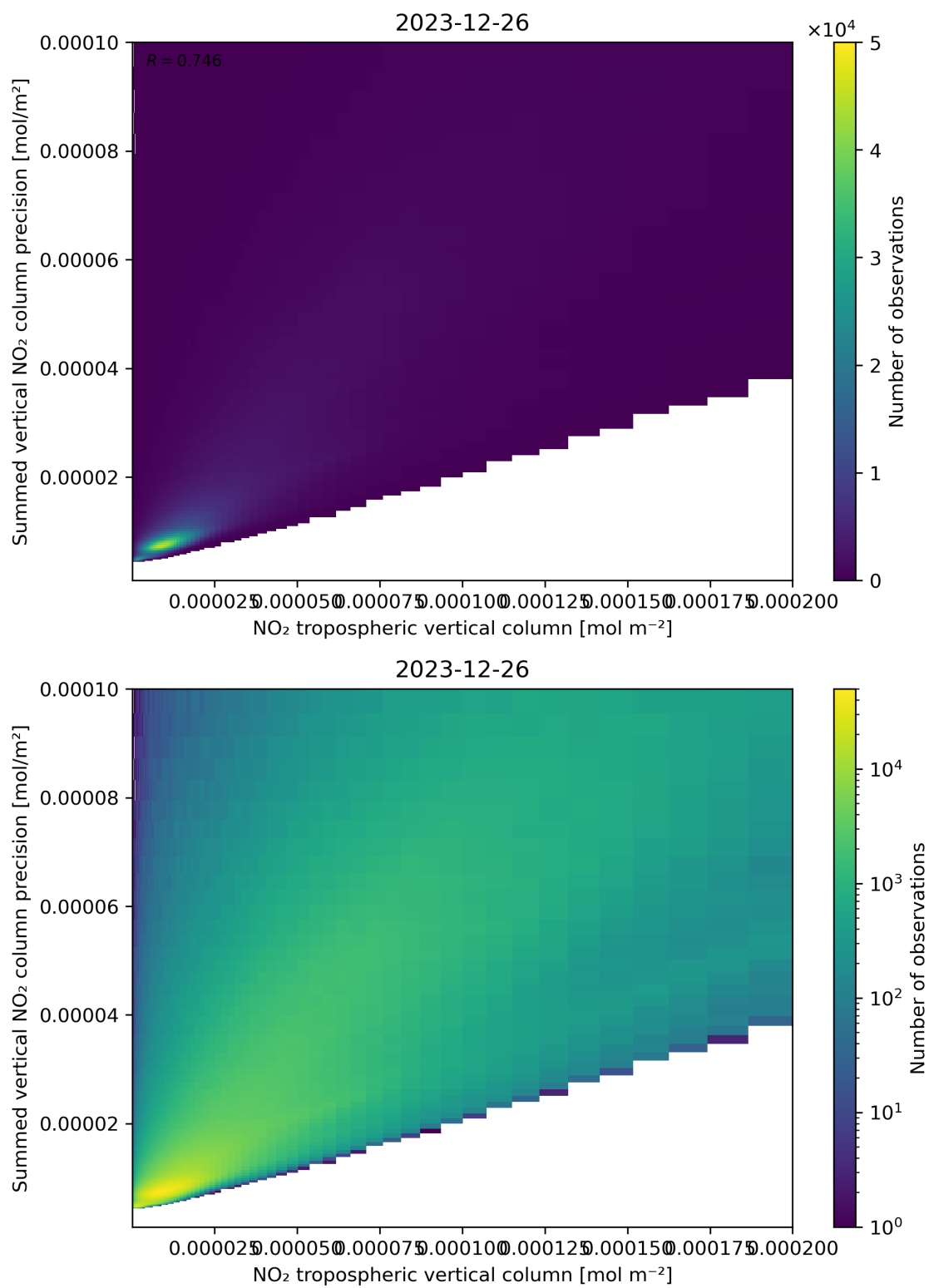
Figure 127: Scatter density plot of “NO 2 tropospheric vertical column” against “Summed vertical NO 2 column precision” for 2023-12-25 to 2023-12-27.
