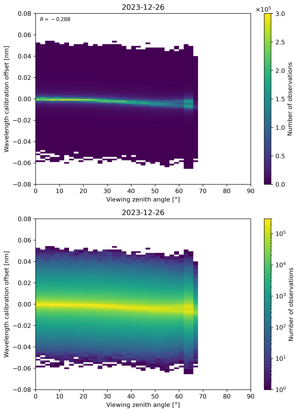
Figure 173: Scatter density plot of “Viewing zenith angle” against “Wavelength calibration offset” for 2023-12-25 to 2023-12-27.
