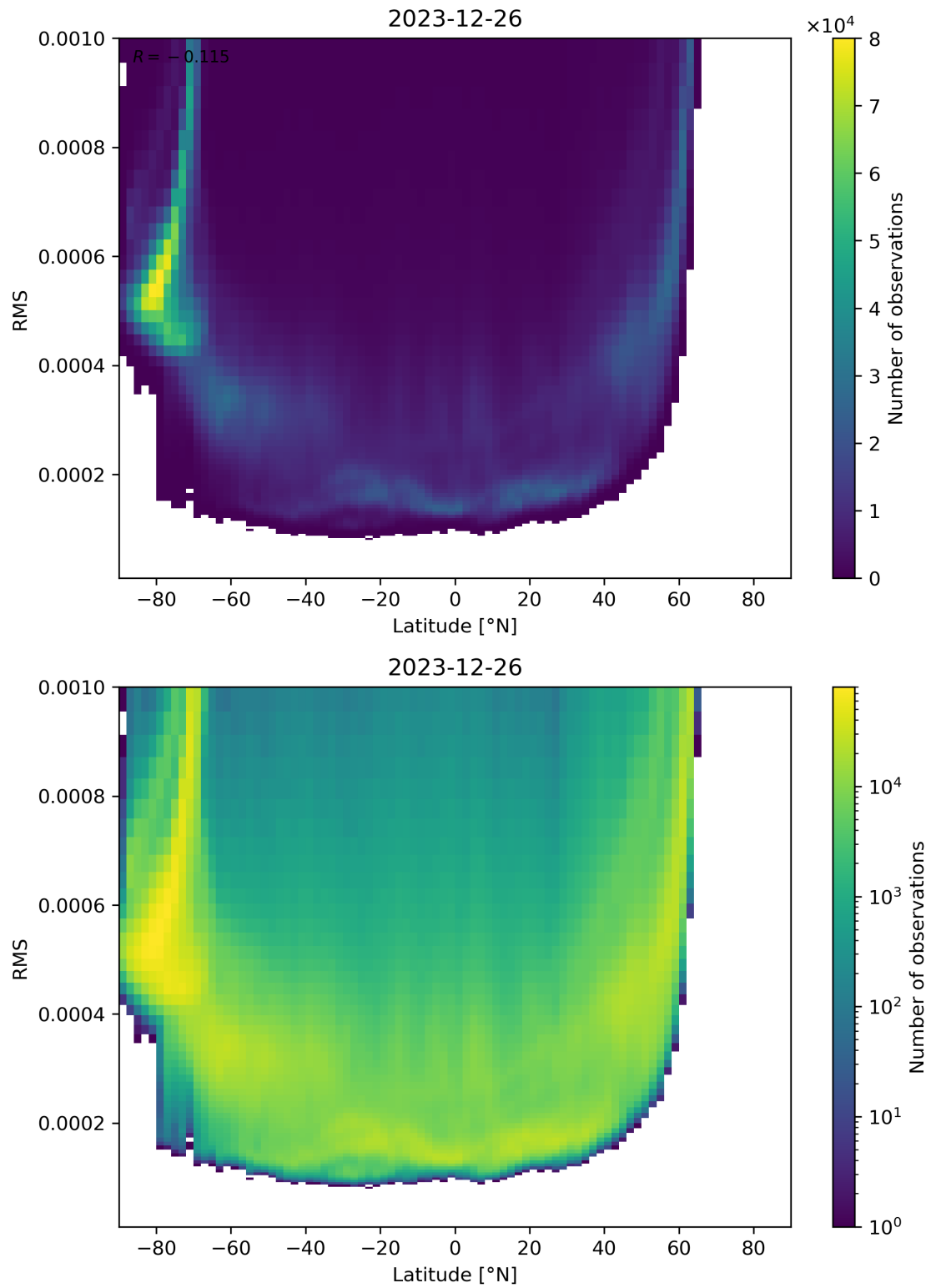
Figure 94: Scatter density plot of “Latitude” against “RMS” for 2023-12-25 to 2023-12-27.
