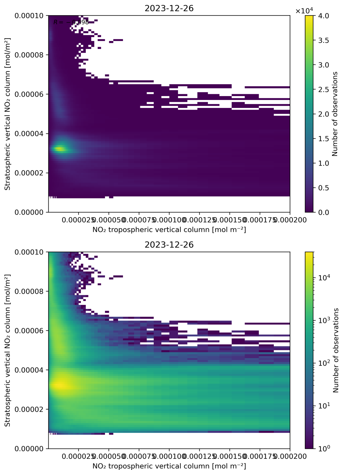
Figure 125: Scatter density plot of “NO 2 tropospheric vertical column” against “Stratospheric vertical NO 2 column” for 2023-12-25 to 2023-12-27.
