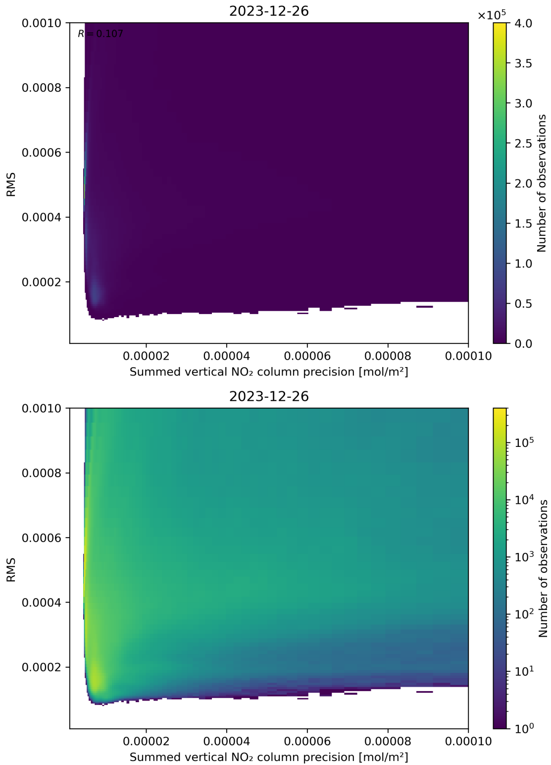
Figure 108: Scatter density plot of “Summed vertical NO 2 column precision” against “RMS” for 2023-12-25 to 2023-12-27.
