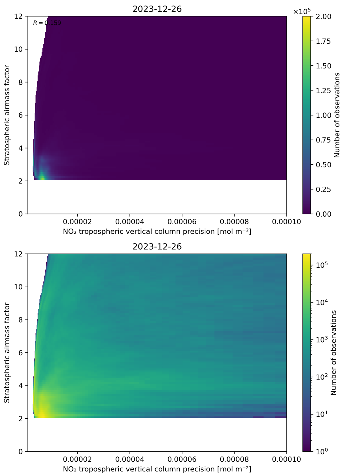
Figure 131: Scatter density plot of “NO 2 tropospheric vertical column precision” against “Stratospheric airmass factor” for 2023-12-25 to 2023-12-27.
