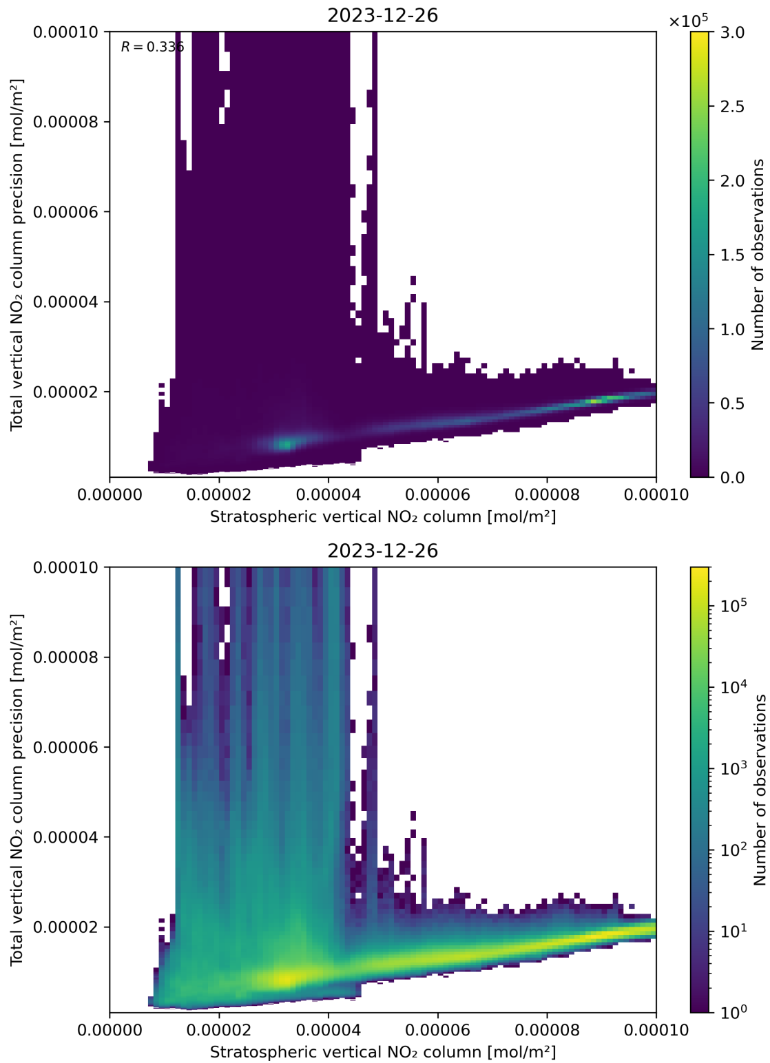
Figure 101: Scatter density plot of “Stratospheric vertical NO 2 column” against “Total vertical NO 2 column precision” for 2023-12-25 to 2023-12-27.
