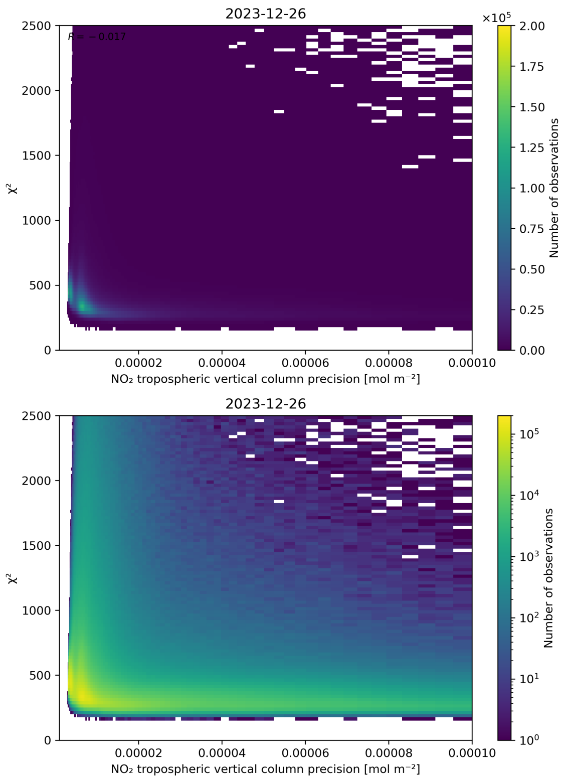
Figure 134: Scatter density plot of “NO 2 tropospheric vertical column precision” against “ \chi^2 ” for 2023-12-25 to 2023-12-27.
