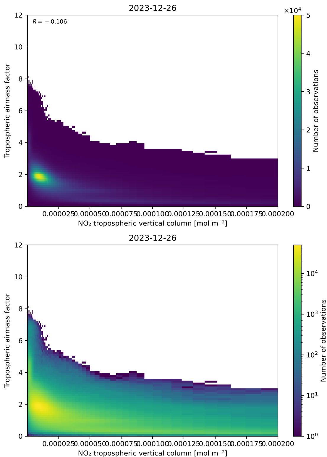
Figure 123: Scatter density plot of “NO 2 tropospheric vertical column” against “Tropospheric air mass factor” for 2023-12-25 to 2023-12-27.
