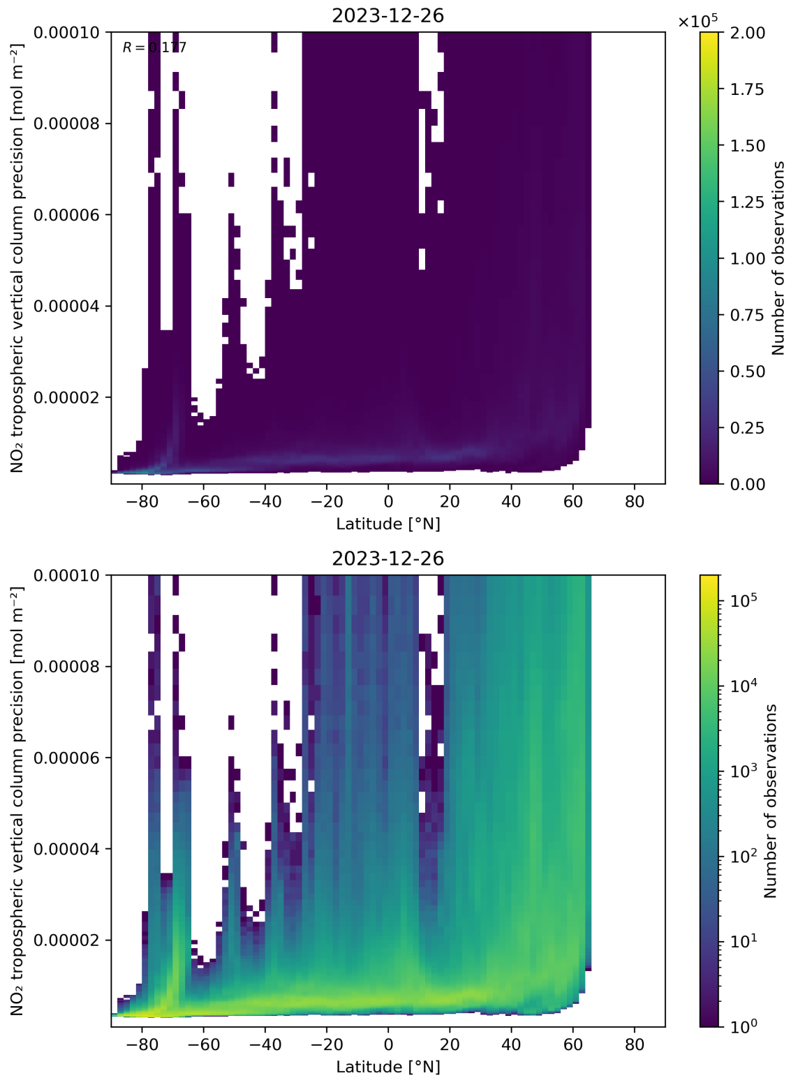
Figure 93: Scatter density plot of “Latitude” against “NO 2 tropospheric vertical column precision” for 2023-12-25 to 2023-12-27.
