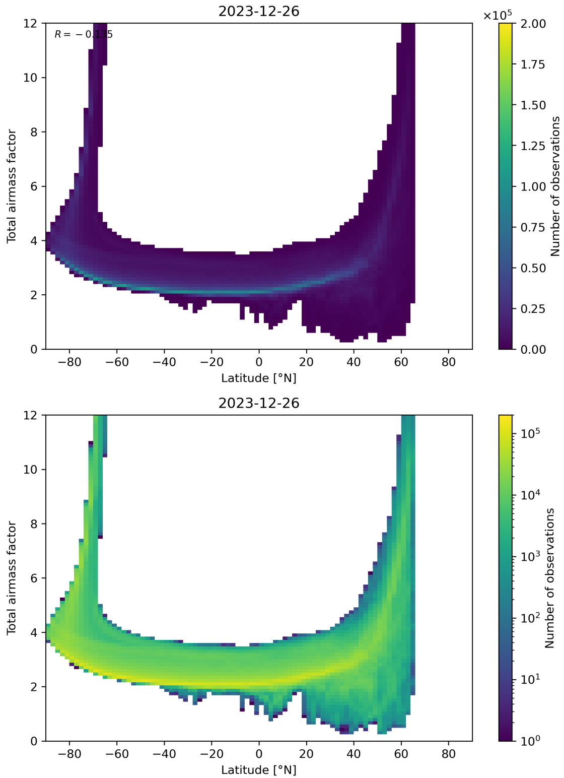
Figure 84: Scatter density plot of “Latitude” against “Total airmass factor” for 2023-12-25 to 2023-12-27.
