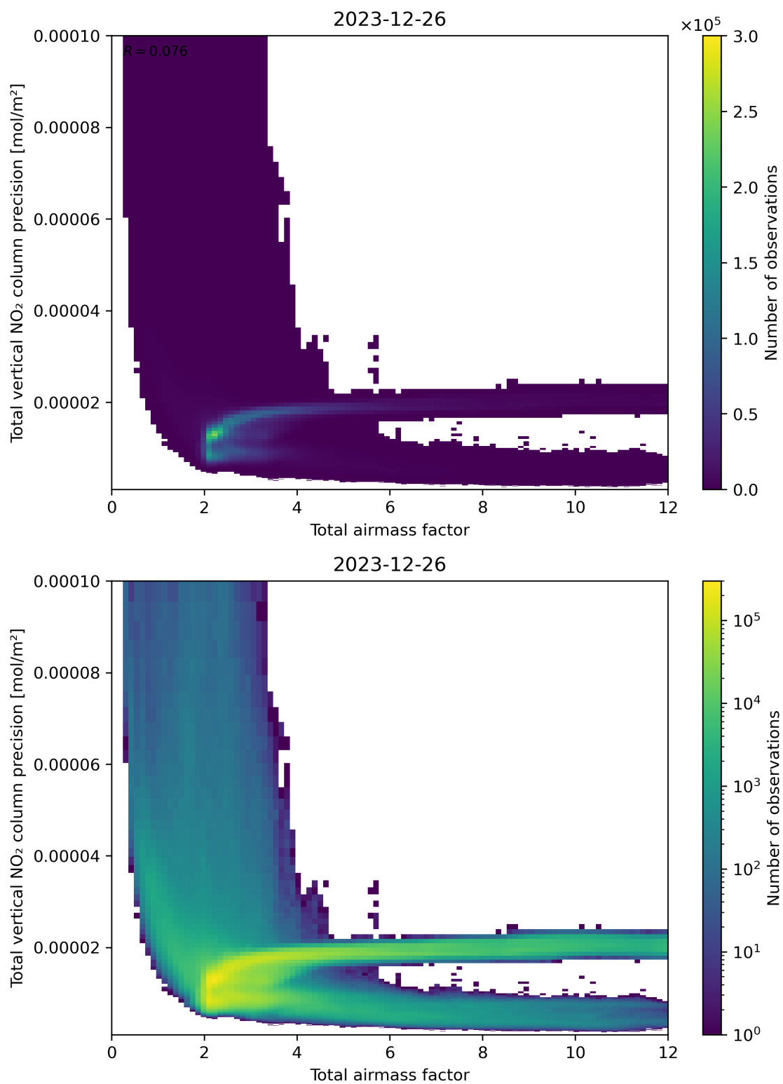
Figure 68: Scatter density plot of “Total airmass factor” against “Total vertical NO 2 column precision” for 2023-12-25 to 2023-12-27.
