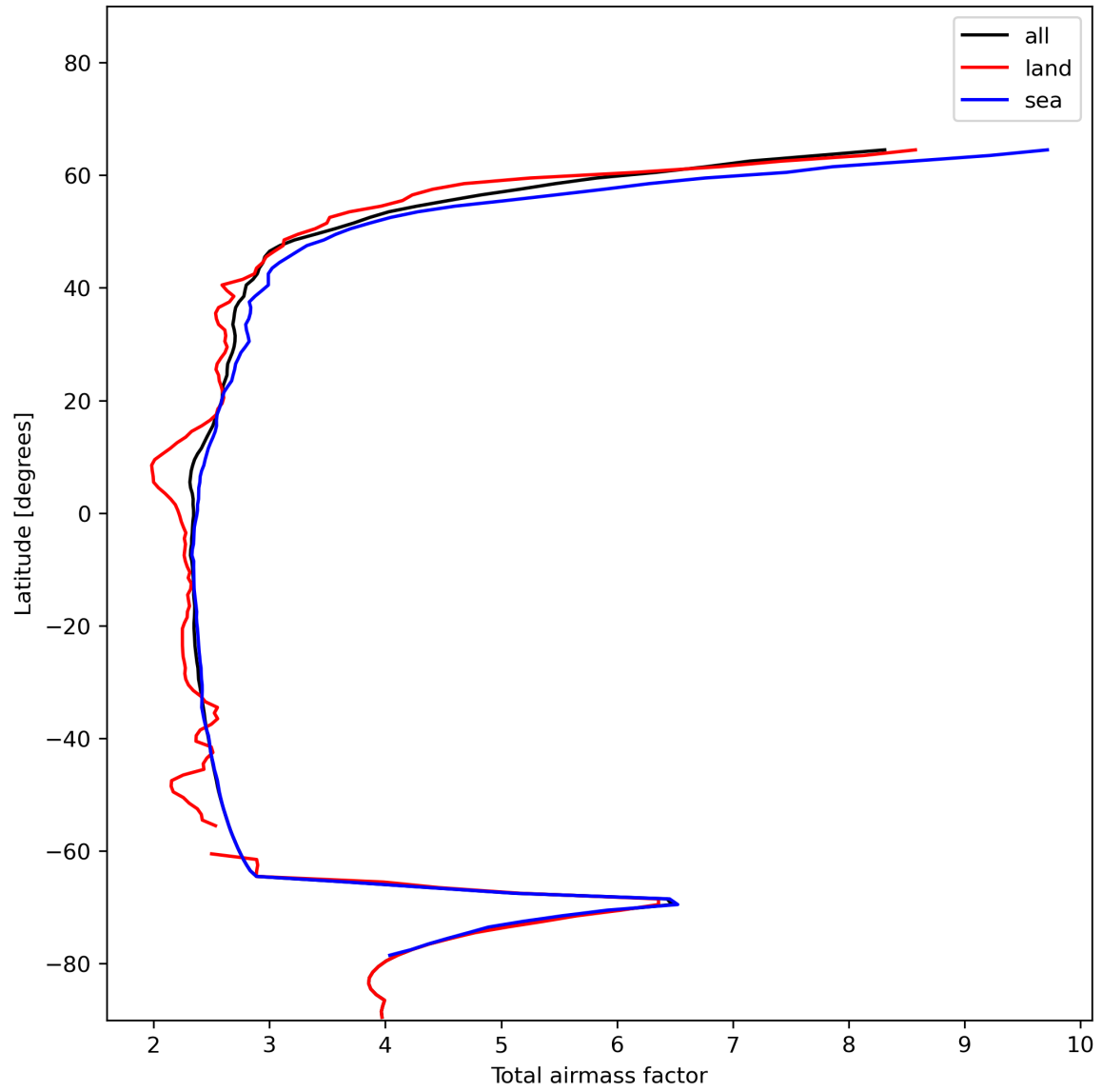
Figure 15: Zonal average of “Total airmass factor” for 2023-12-25 to 2023-12-27.
