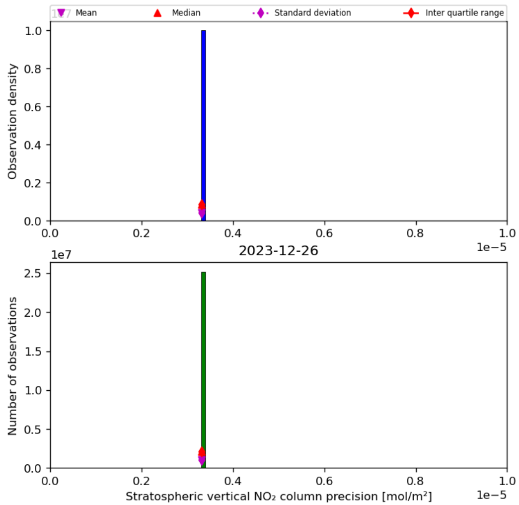
Figure 37: Histogram of “Stratospheric vertical NO 2 column precision” for 2023-12-25 to 2023-12-27
