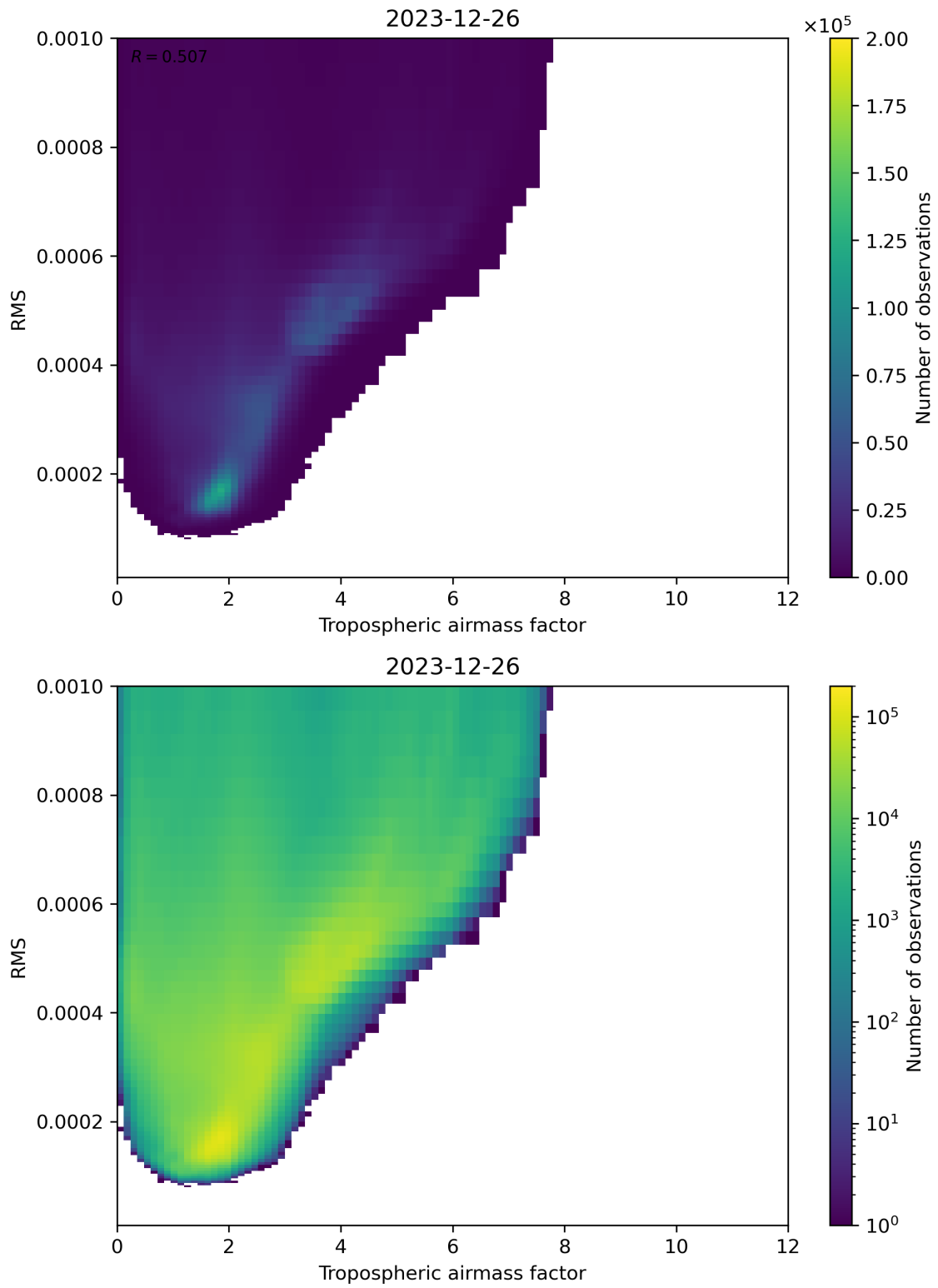
Figure 79: Scatter density plot of “Tropospheric airmass factor” against “RMS” for 2023-12-25 to 2023-12-27.
