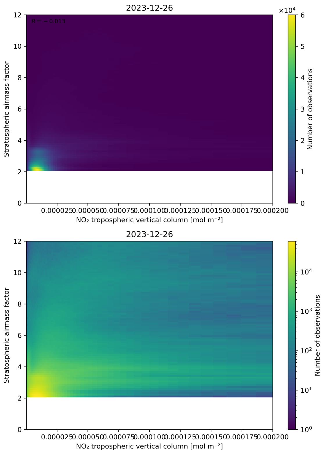
Figure 121: Scatter density plot of “NO 2 tropospheric vertical column” against “Stratospheric airmass factor” for 2023-12-25 to 2023-12-27.
