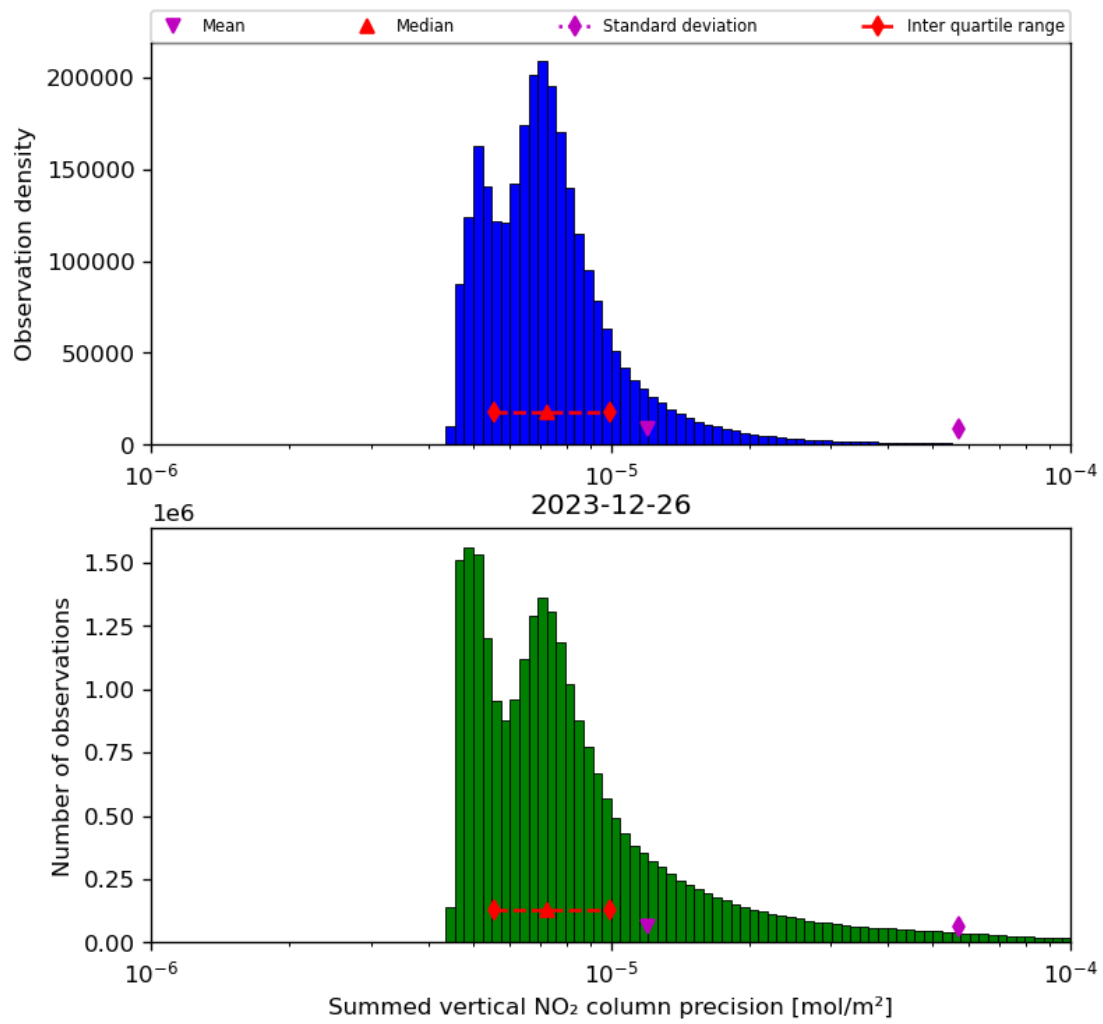
Figure 41: Histogram of “Summed vertical NO 2 column precision” for 2023-12-25 to 2023-12-27
