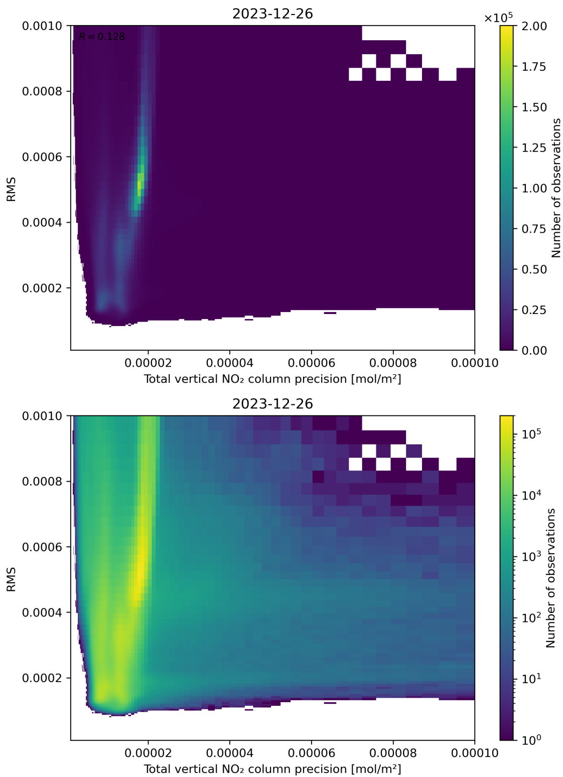
Figure 119: Scatter density plot of “Total vertical NO 2 column precision” against “RMS” for 2023-12-25 to 2023-12-27.
