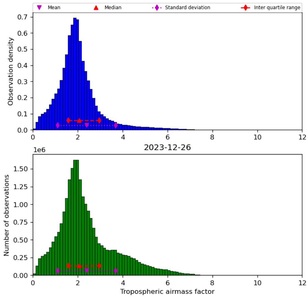
Figure 31: Histogram of “Tropospheric airmass factor” for 2023-12-25 to 2023-12-27
