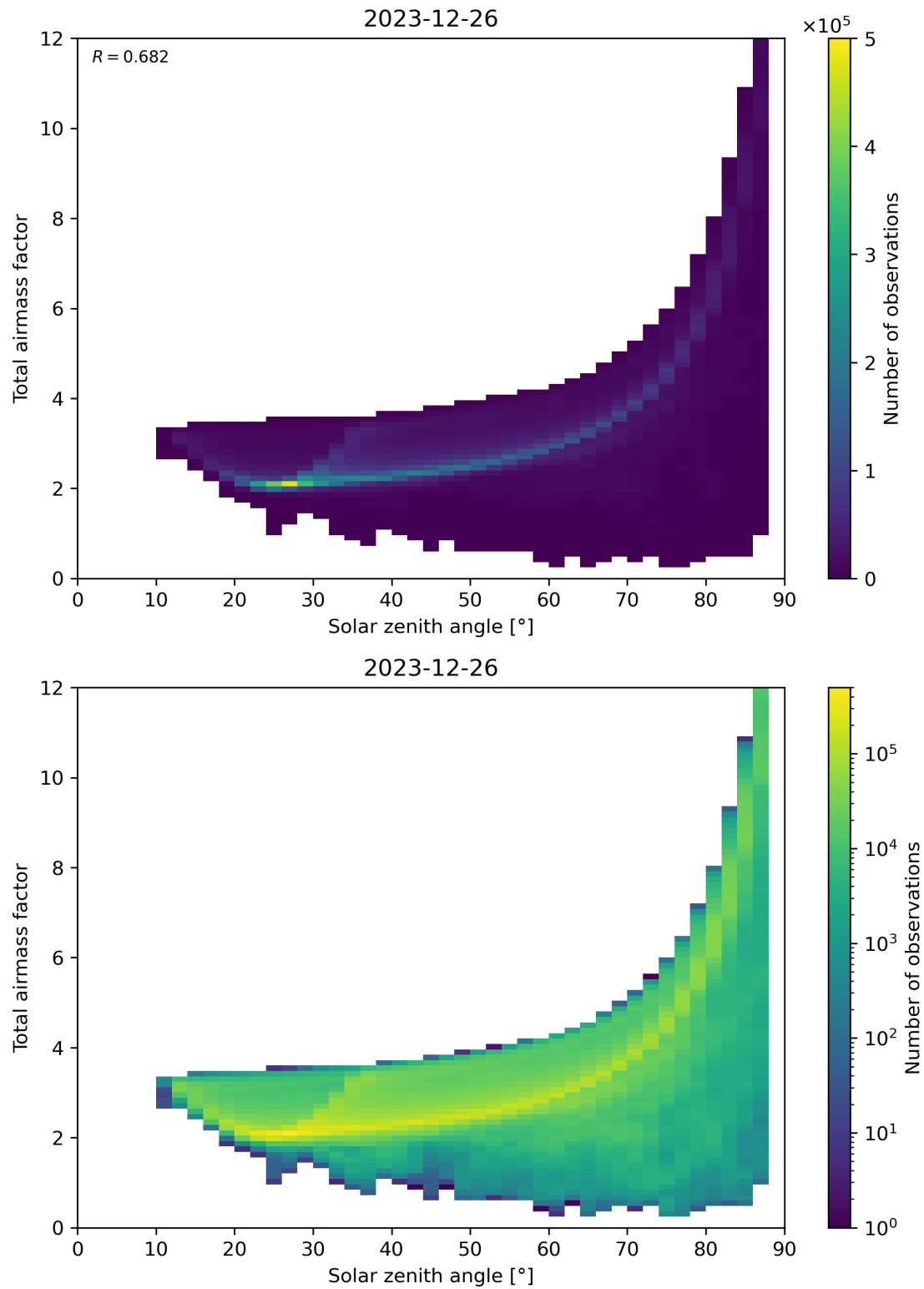
Figure 146: Scatter density plot of “Solar zenith angle” against “Total air mass factor” for 2023-12-25 to 2023-12-27.
