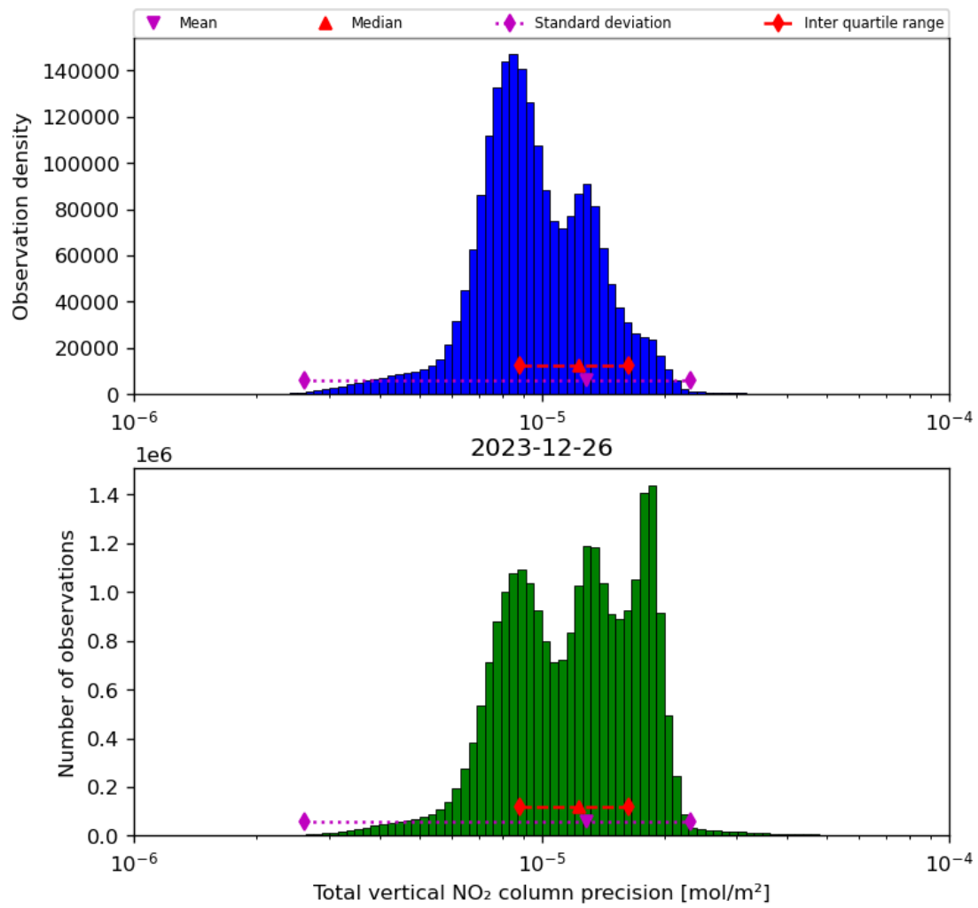
Figure 39: Histogram of “Total vertical NO 2 column precision” for 2023-12-25 to 2023-12-27
