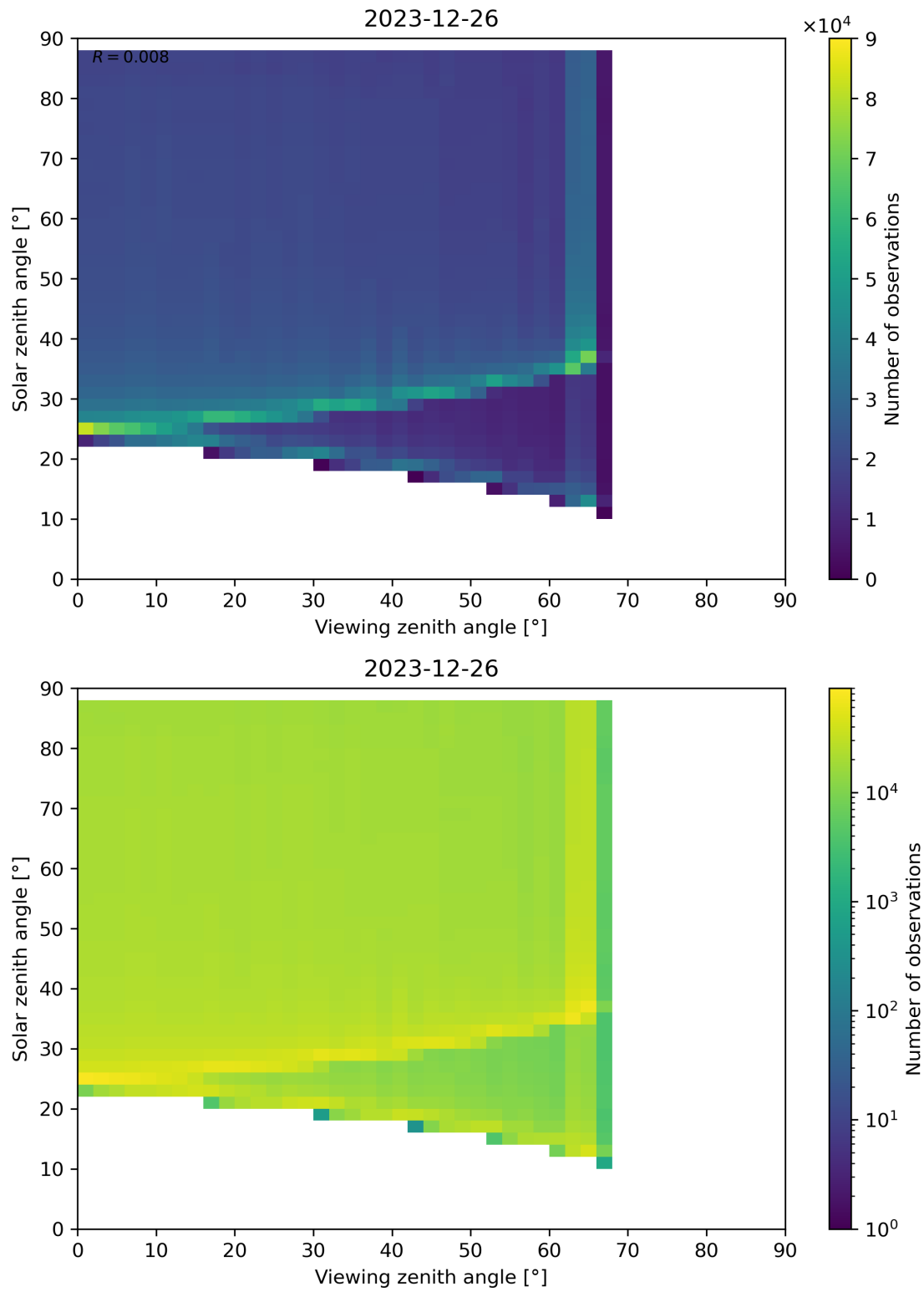
Figure 172: Scatter density plot of “Viewing zenith angle” against “Solar zenith angle” for 2023-12-25 to 2023-12-27.
