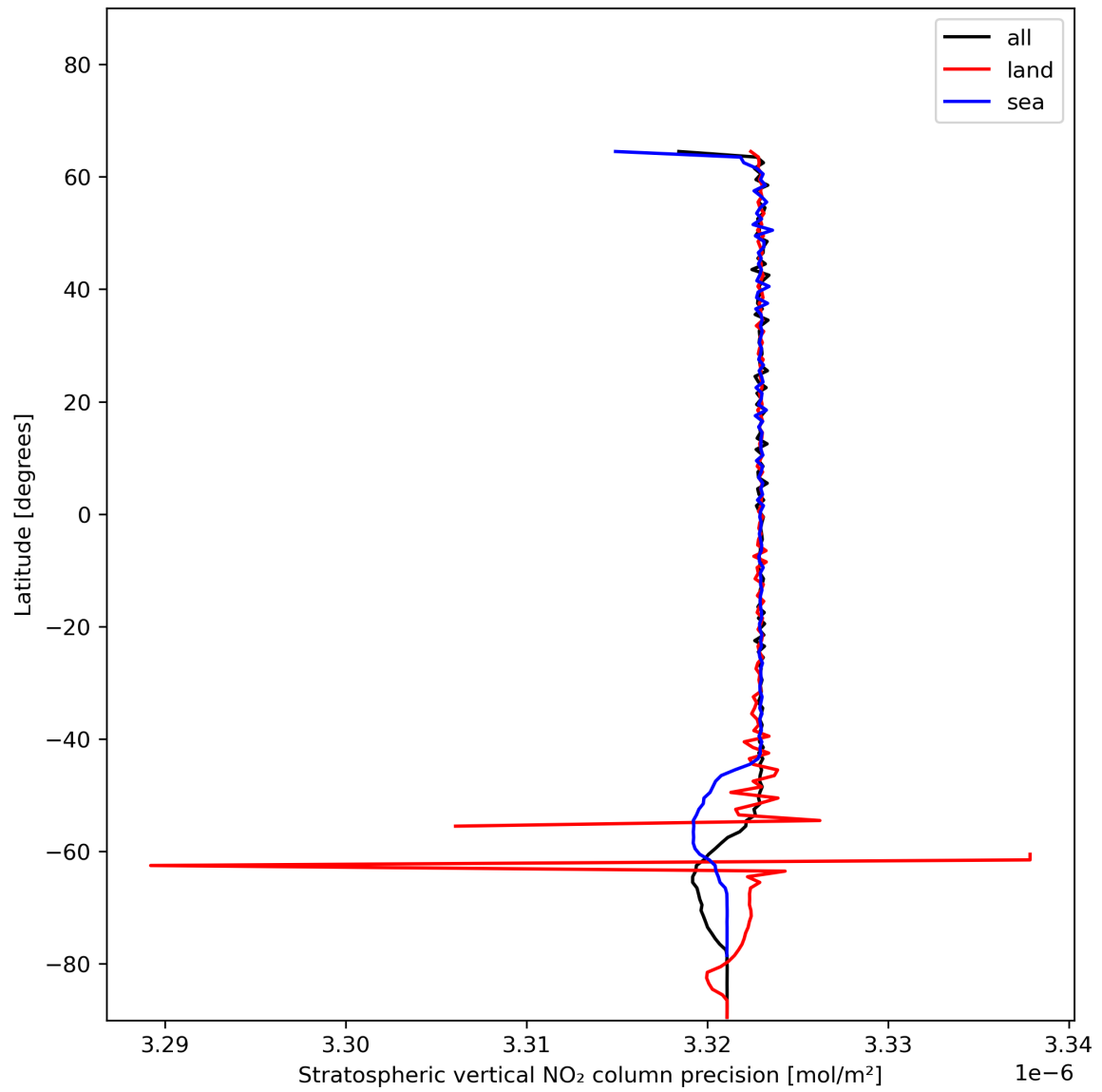
Figure 20: Zonal average of “Stratospheric vertical NO 2 column precision” for 2023-12-25 to 2023-12-27.
