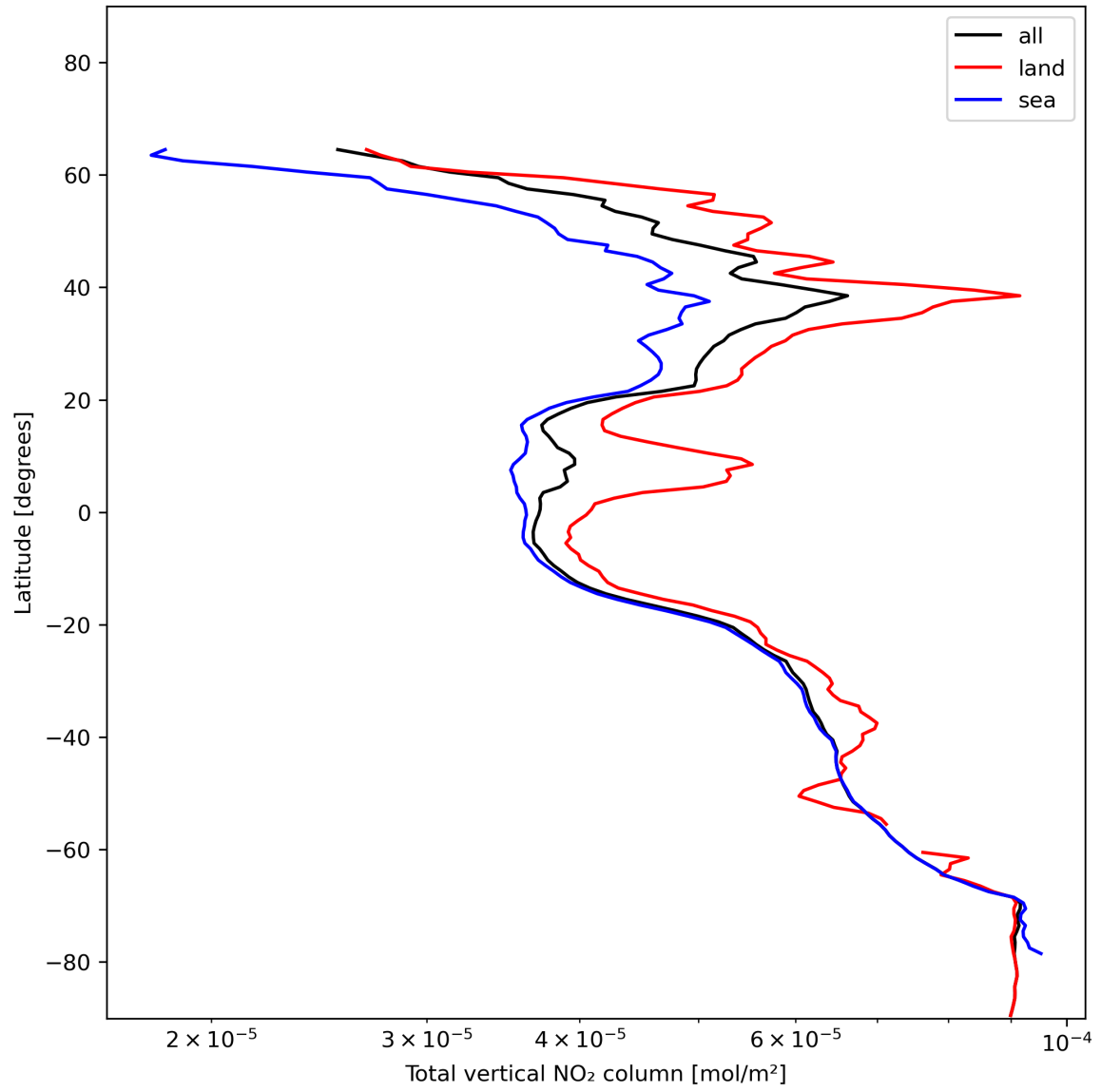
Figure 21: Zonal average of “Total vertical NO 2 column” for 2023-12-25 to 2023-12-27.
