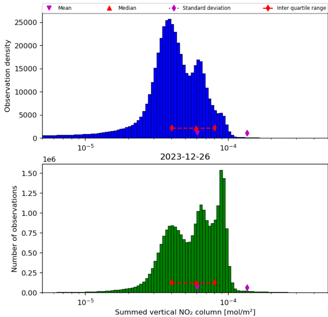
Figure 40: Histogram of “Summed vertical NO 2 column” for 2023-12-25 to 2023-12-27
