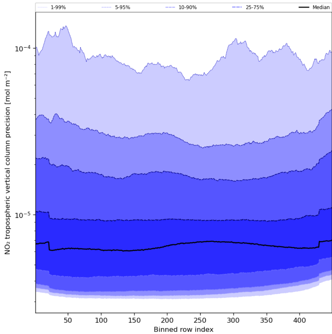
Figure 47: Along track statistics of “NO 2 tropospheric vertical column precision” for 2023-12-25 to 2023-12-27
