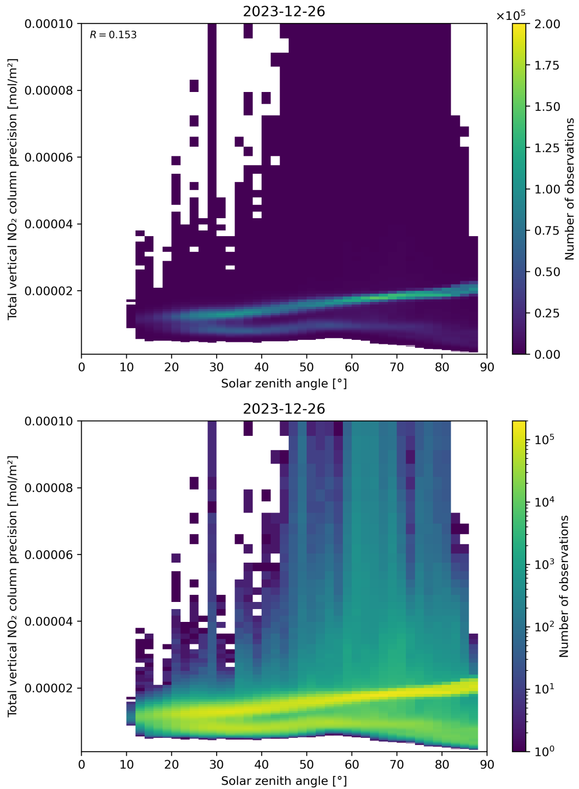
Figure 154: Scatter density plot of “Solar zenith angle” against “Total vertical NO 2 column precision” for 2023-12-25 to 2023-12-27.
