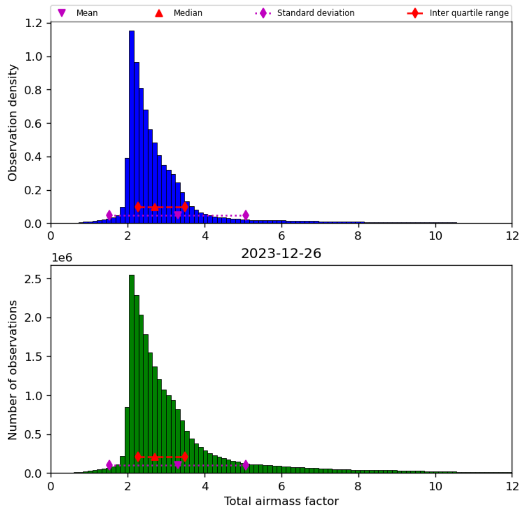
Figure 32: Histogram of “Total airmass factor” for 2023-12-25 to 2023-12-27
