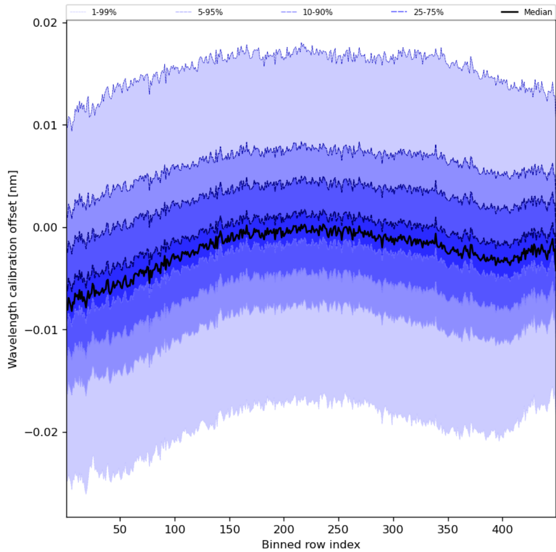
Figure 52: Along track statistics of “Wavelength calibration offset” for 2023-12-25 to 2023-12-27
