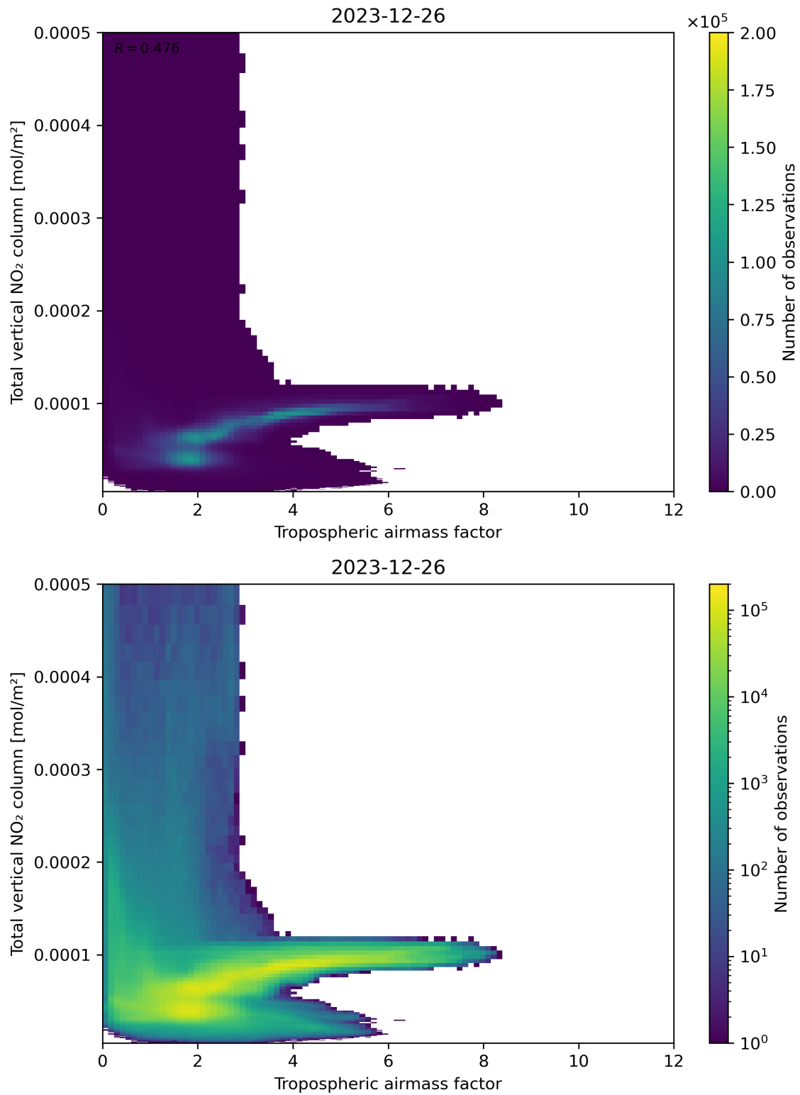
Figure 77: Scatter density plot of “Tropospheric airmass factor” against “Total vertical \text{NO}_2 column” for 2023-12-25 to 2023-12-27.
