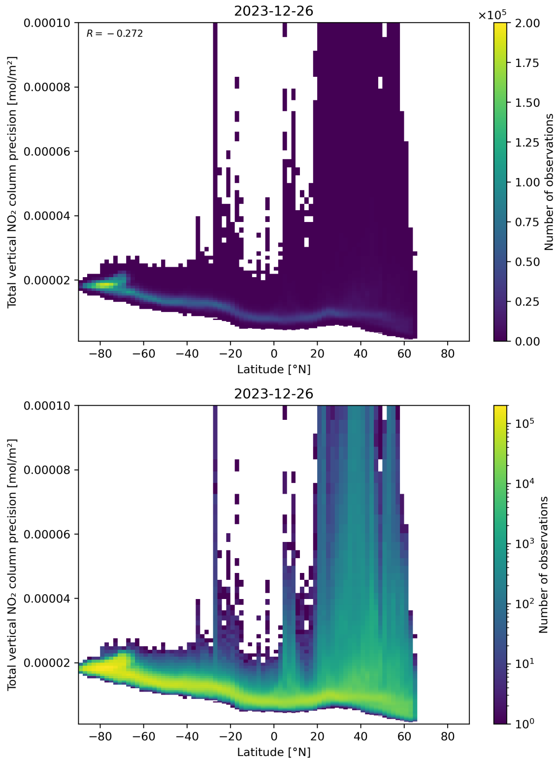
Figure 91: Scatter density plot of “Latitude” against “Total vertical NO 2 column precision” for 2023-12-25 to 2023-12-27.
