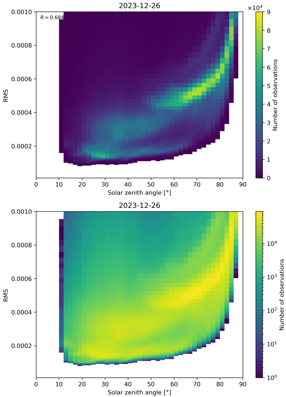
Figure 157: Scatter density plot of “Solar zenith angle” against “RMS” for 2023-12-25 to 2023-12-27.
