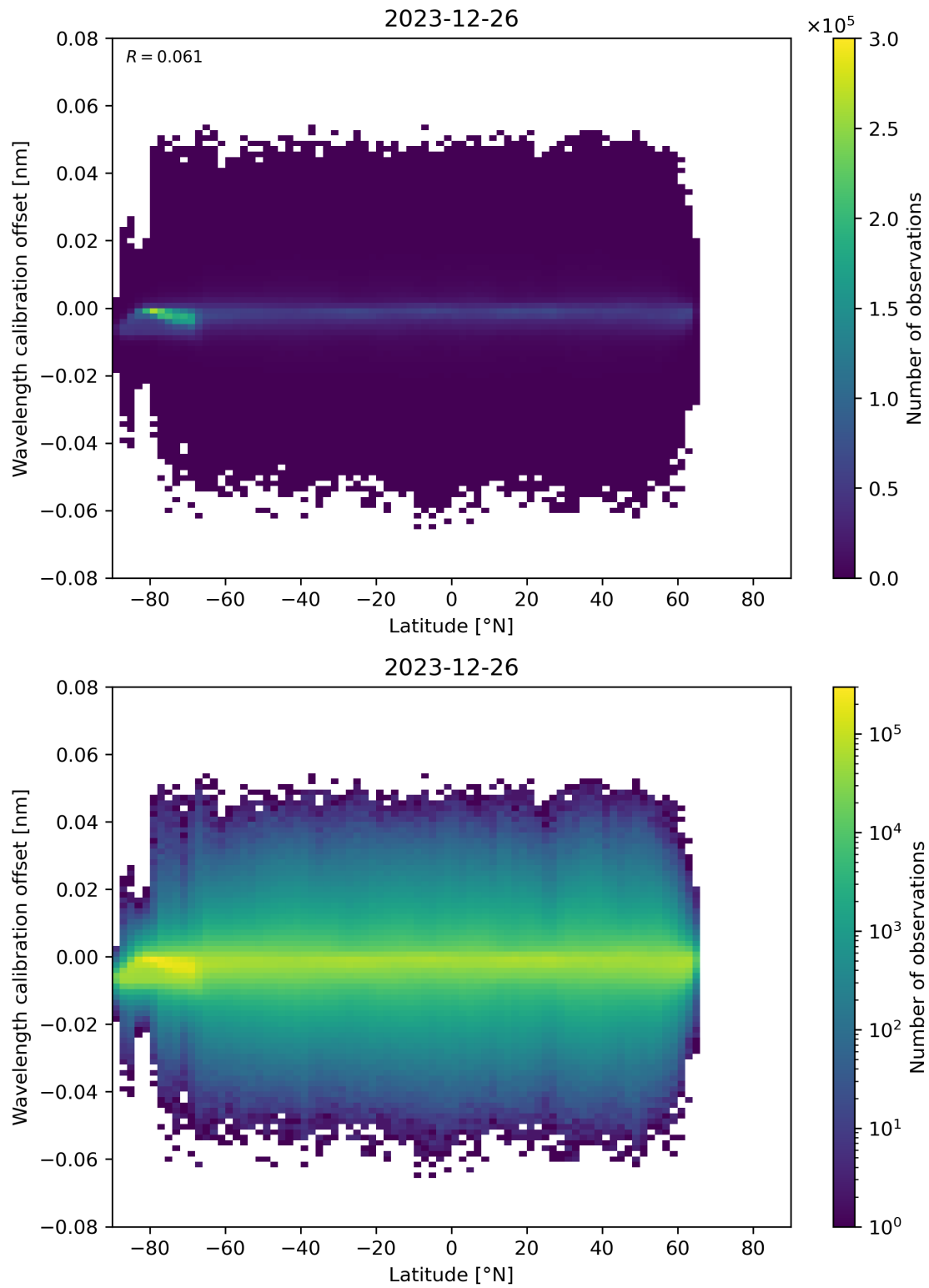
Figure 95: Scatter density plot of “Latitude” against “Wavelength calibration offset” for 2023-12-25 to 2023-12-27.
