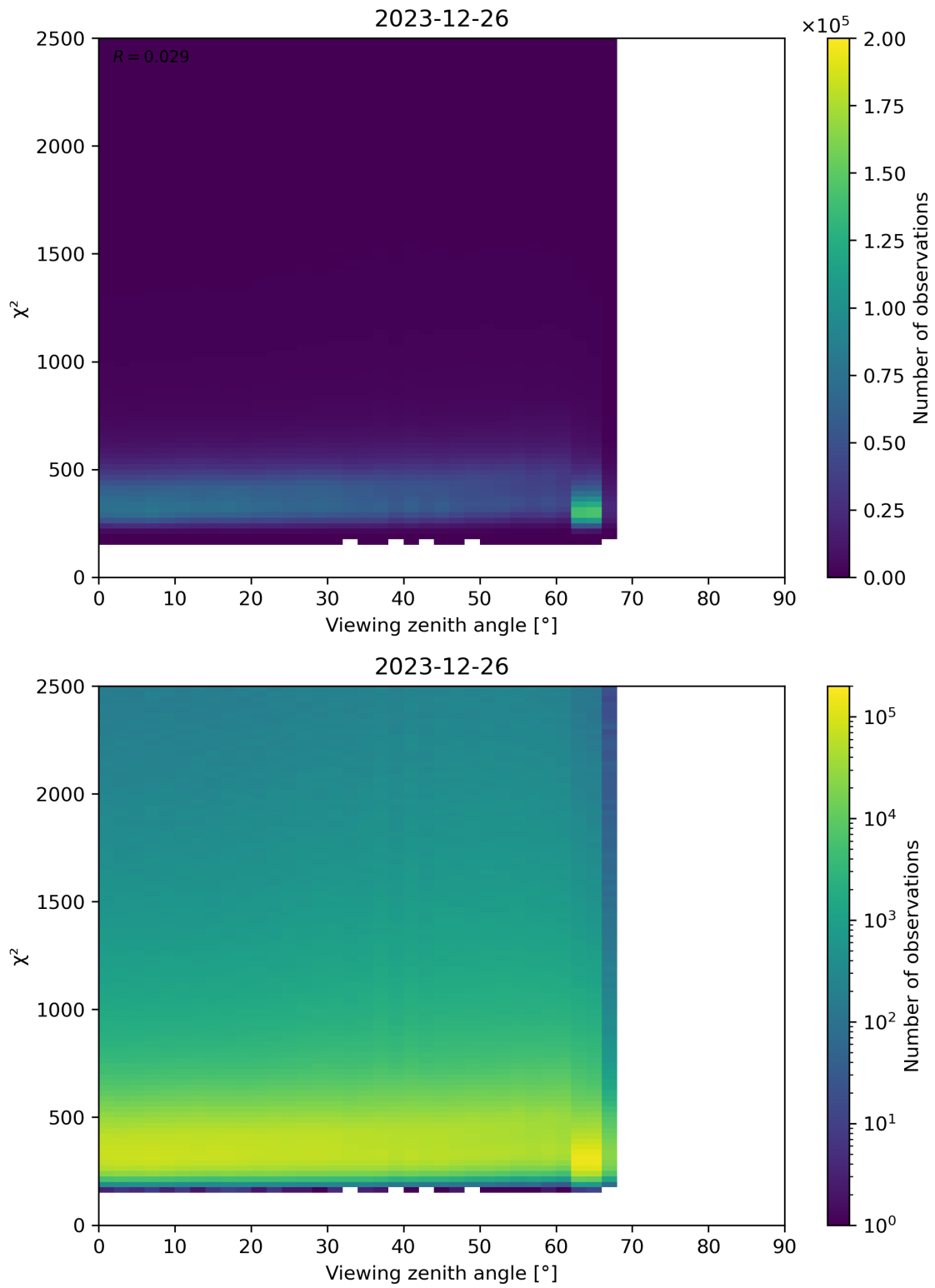
Figure 162: Scatter density plot of “Viewing zenith angle” against “ \chi^2 ” for 2023-12-25 to 2023-12-27.
