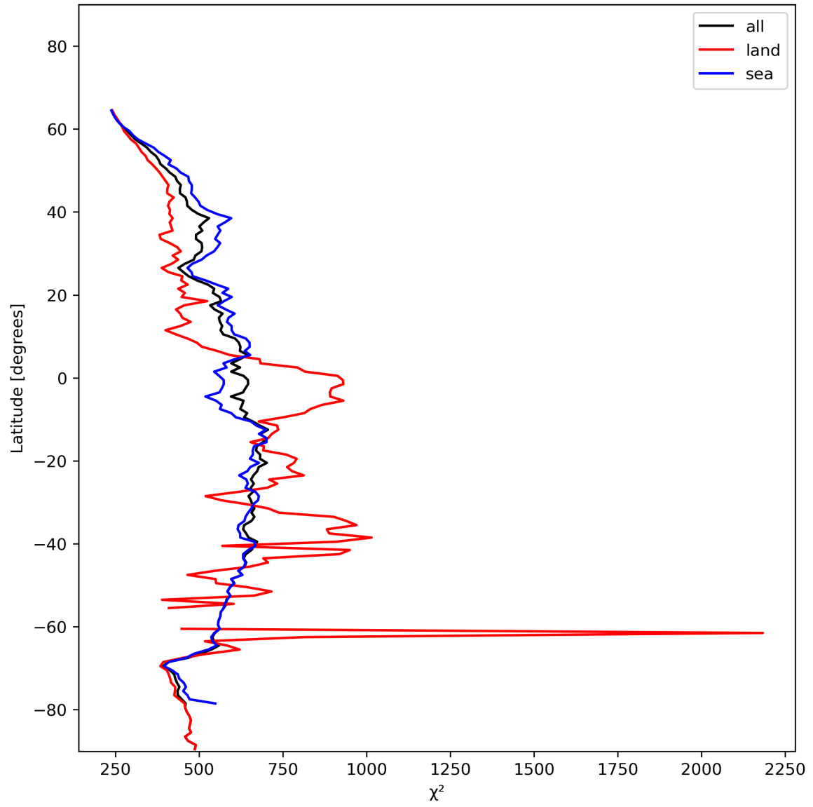
Figure 25: Zonal average of “ \chi^2 ” for 2023-12-25 to 2023-12-27.
