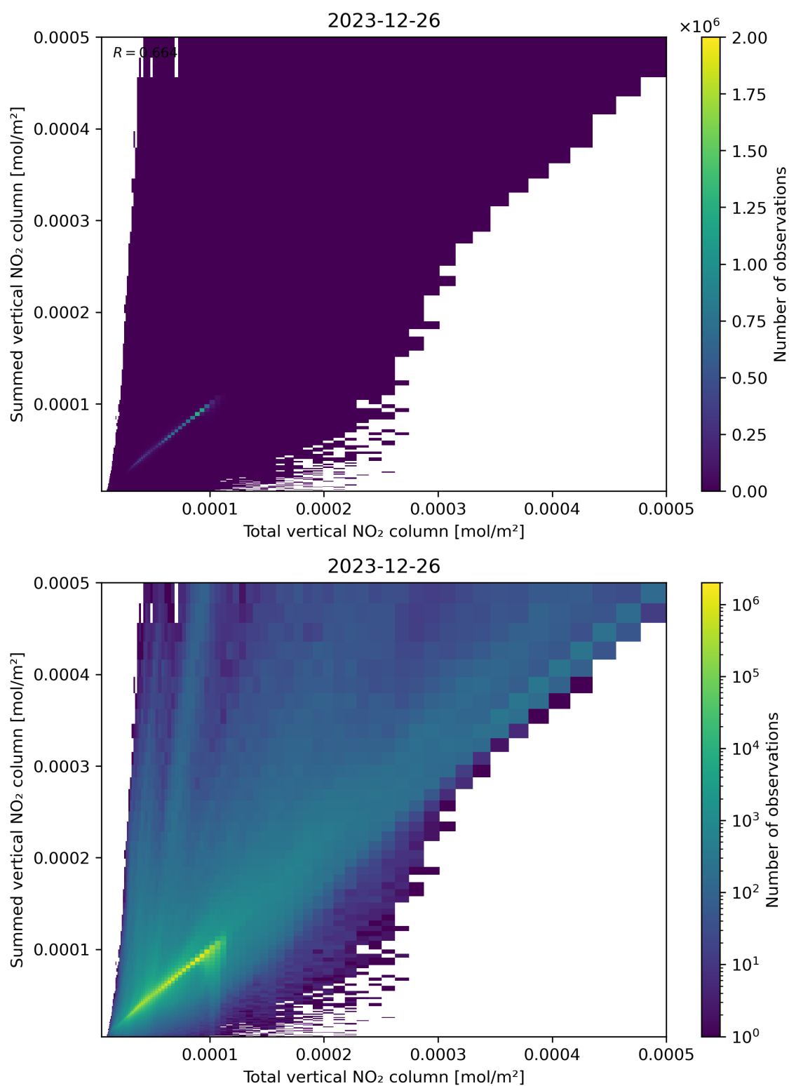
Figure 112: Scatter density plot of “Total vertical NO 2 column” against “Summed vertical NO 2 column” for 2023-12-25 to 2023-12-27.
