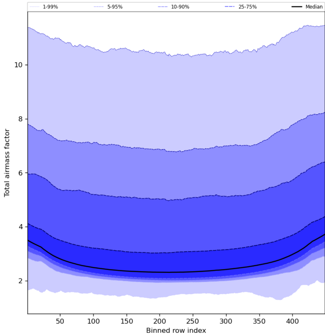
Figure 49: Along track statistics of “Total airmass factor” for 2023-12-25 to 2023-12-27
