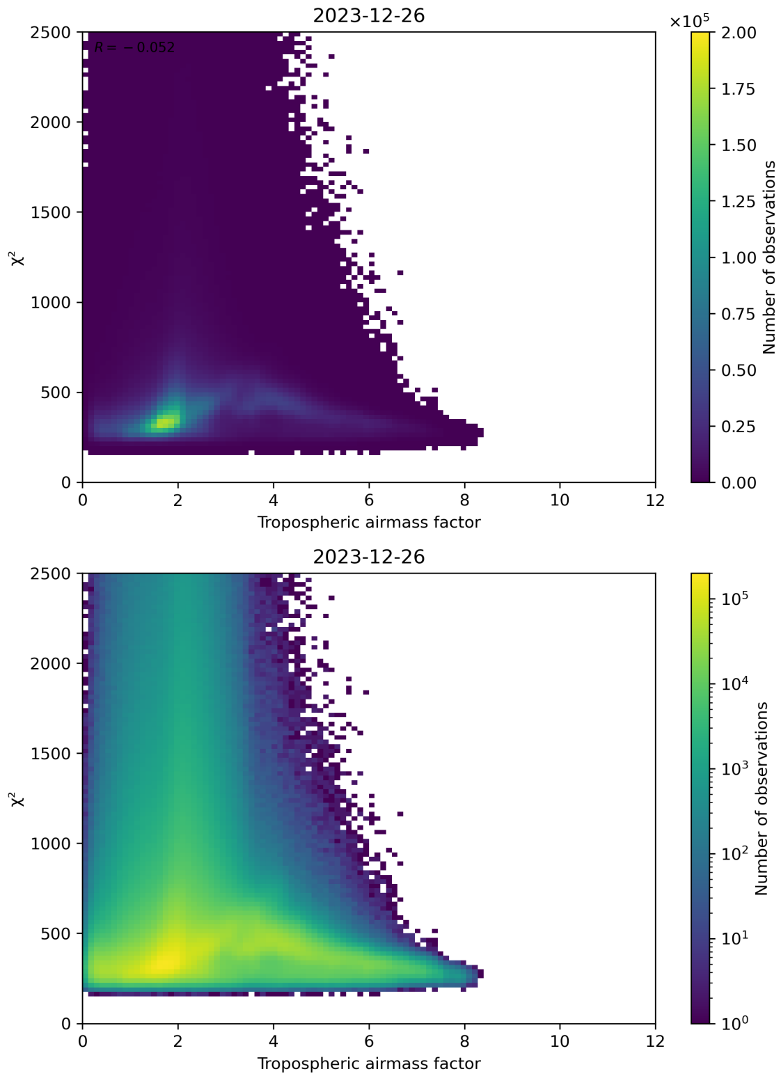
Figure 73: Scatter density plot of “Tropospheric airmass factor” against “ \chi^2 ” for 2023-12-25 to 2023-12-27.
