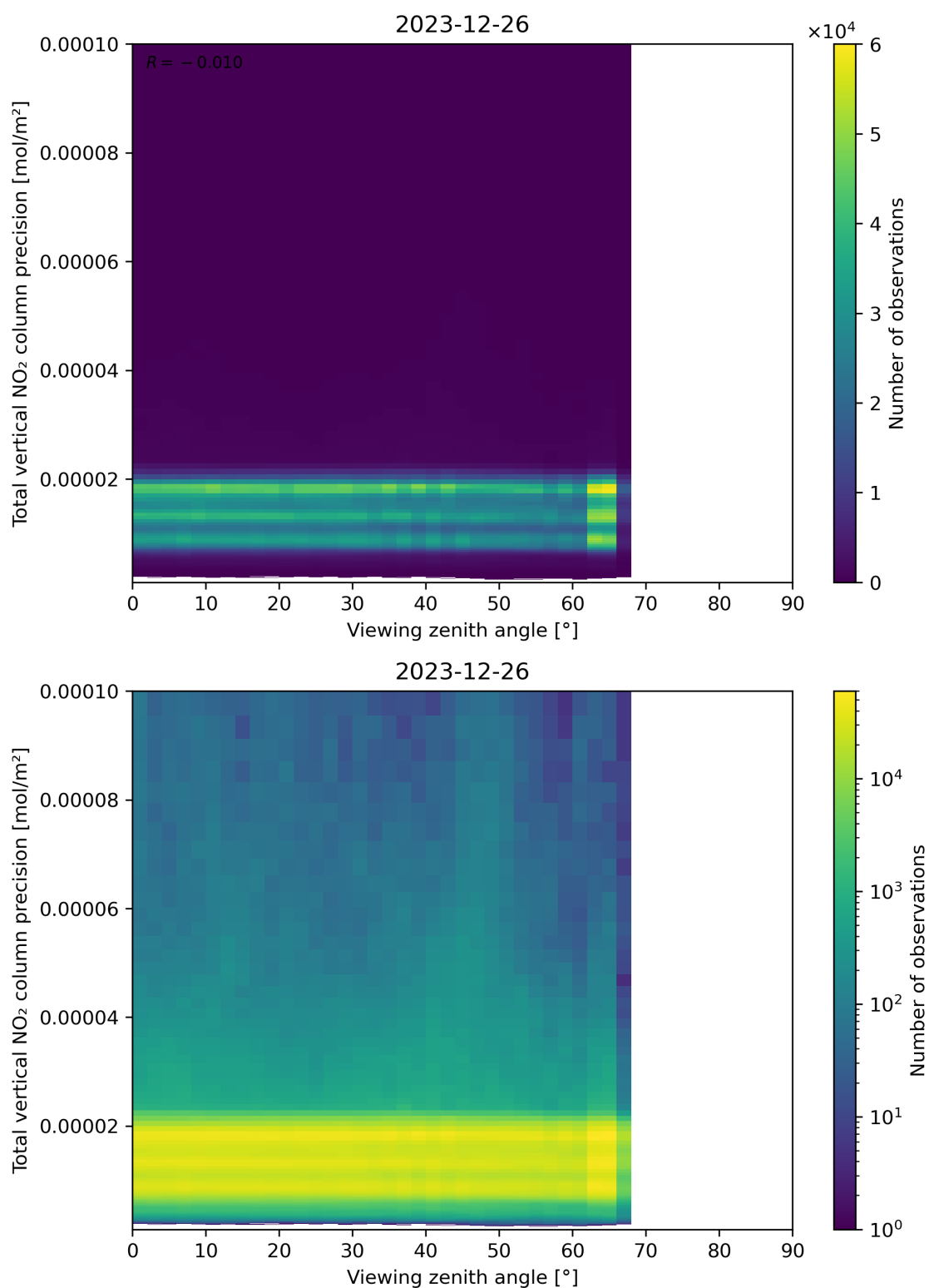
Figure 168: Scatter density plot of “Viewing zenith angle” against “Total vertical NO 2 column precision” for 2023-12-25 to 2023-12-27.
