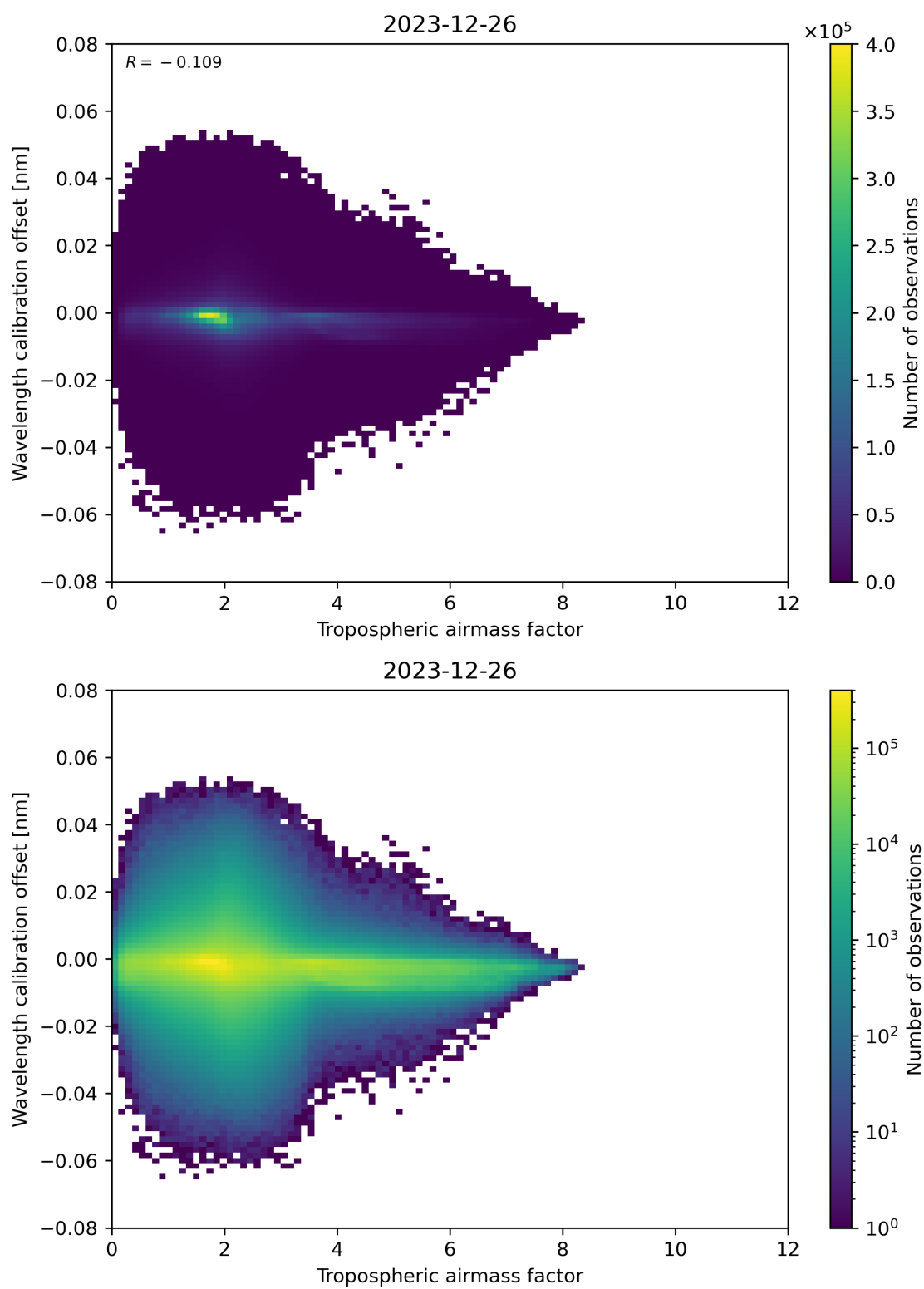
Figure 80: Scatter density plot of “Tropospheric airmass factor” against “Wavelength calibration offset” for 2023-12-25 to 2023-12-27.
