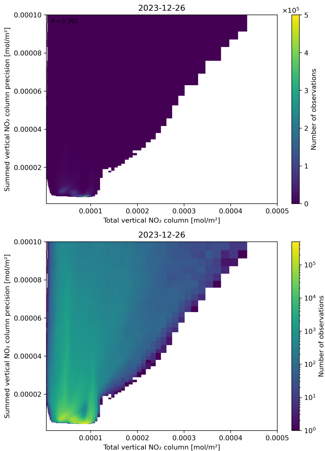
Figure 113: Scatter density plot of “Total vertical NO 2 column” against “Summed vertical NO 2 column precision” for 2023-12-25 to 2023-12-27.
