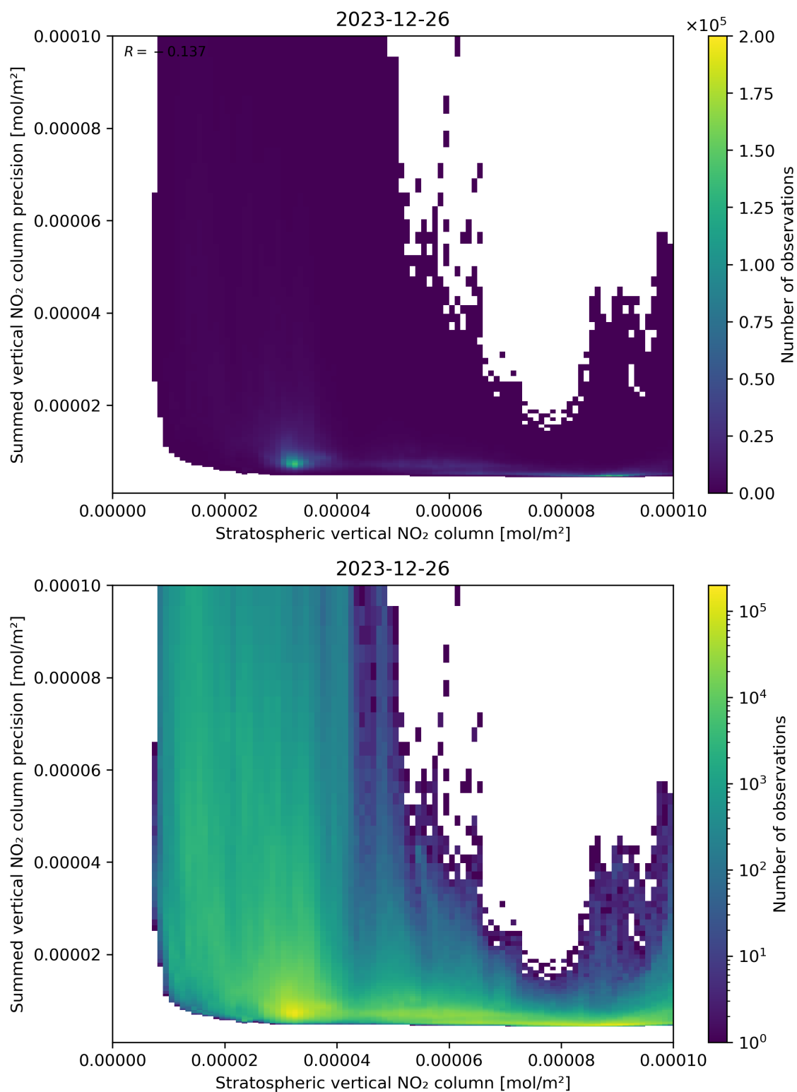
Figure 99: Scatter density plot of “Stratospheric vertical NO 2 column” against “Summed vertical NO 2 column precision” for 2023-12-25 to 2023-12-27.
