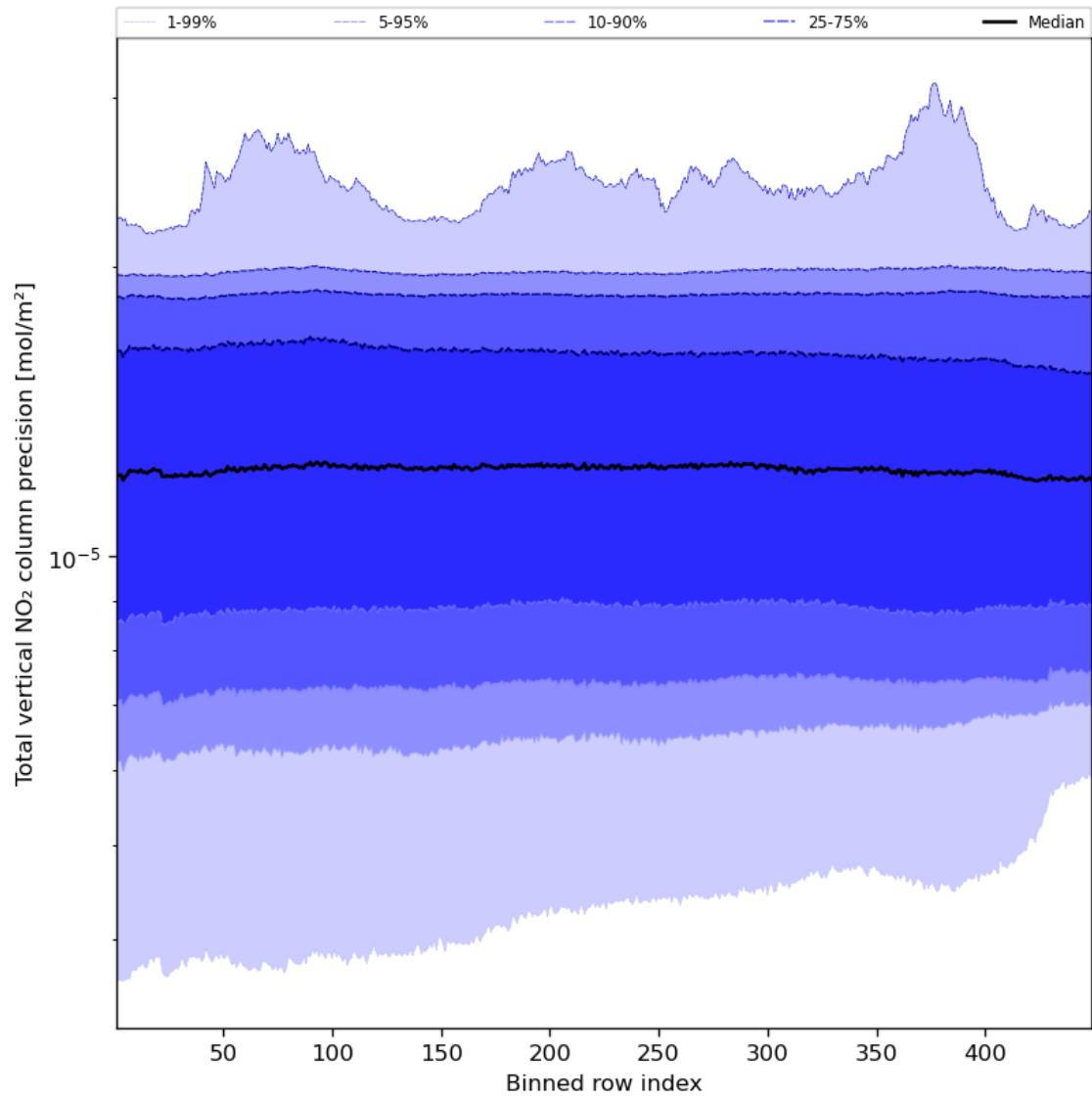
Figure 56: Along track statistics of “Total vertical NO 2 column precision” for 2023-12-25 to 2023-12-27
