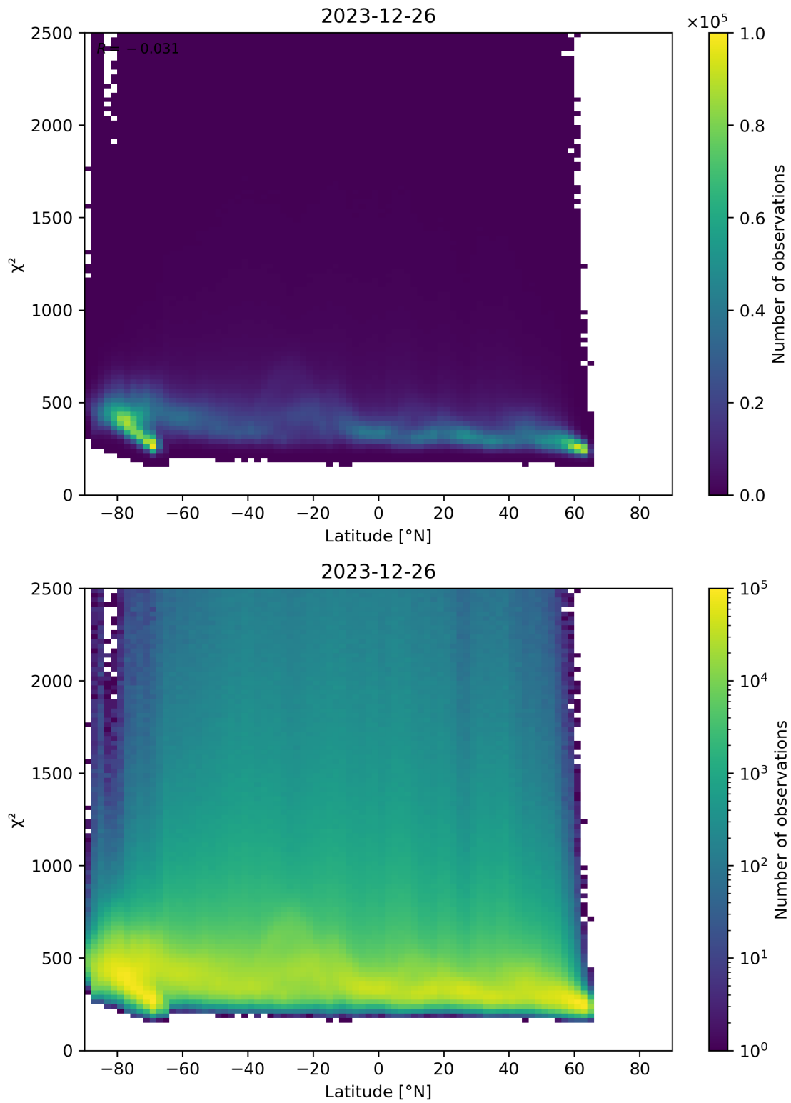
Figure 86: Scatter density plot of “Latitude” against “ \chi^2 ” for 2023-12-25 to 2023-12-27.
