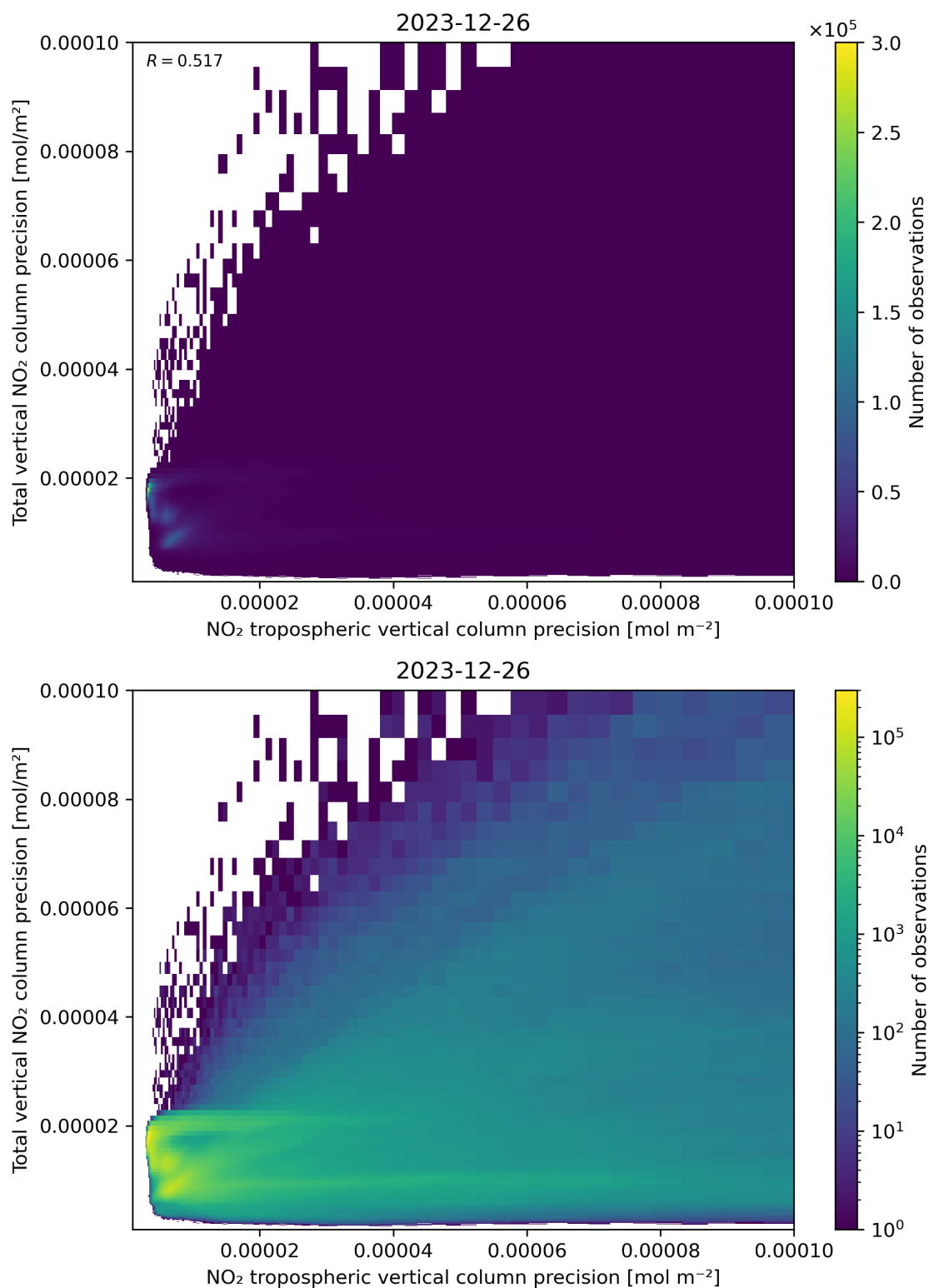
Figure 139: Scatter density plot of “NO 2 tropospheric vertical column precision” against “Total vertical NO 2 column precision” for 2023-12-25 to 2023-12-27.
