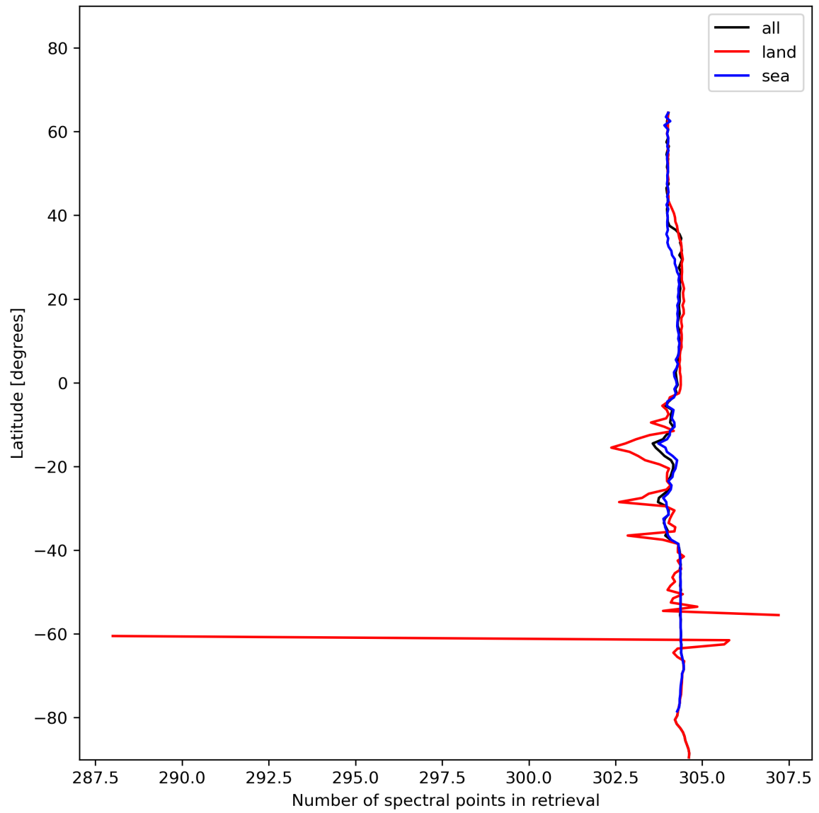
Figure 16: Zonal average of “Number of spectral points in retrieval” for 2023-12-25 to 2023-12-27.
