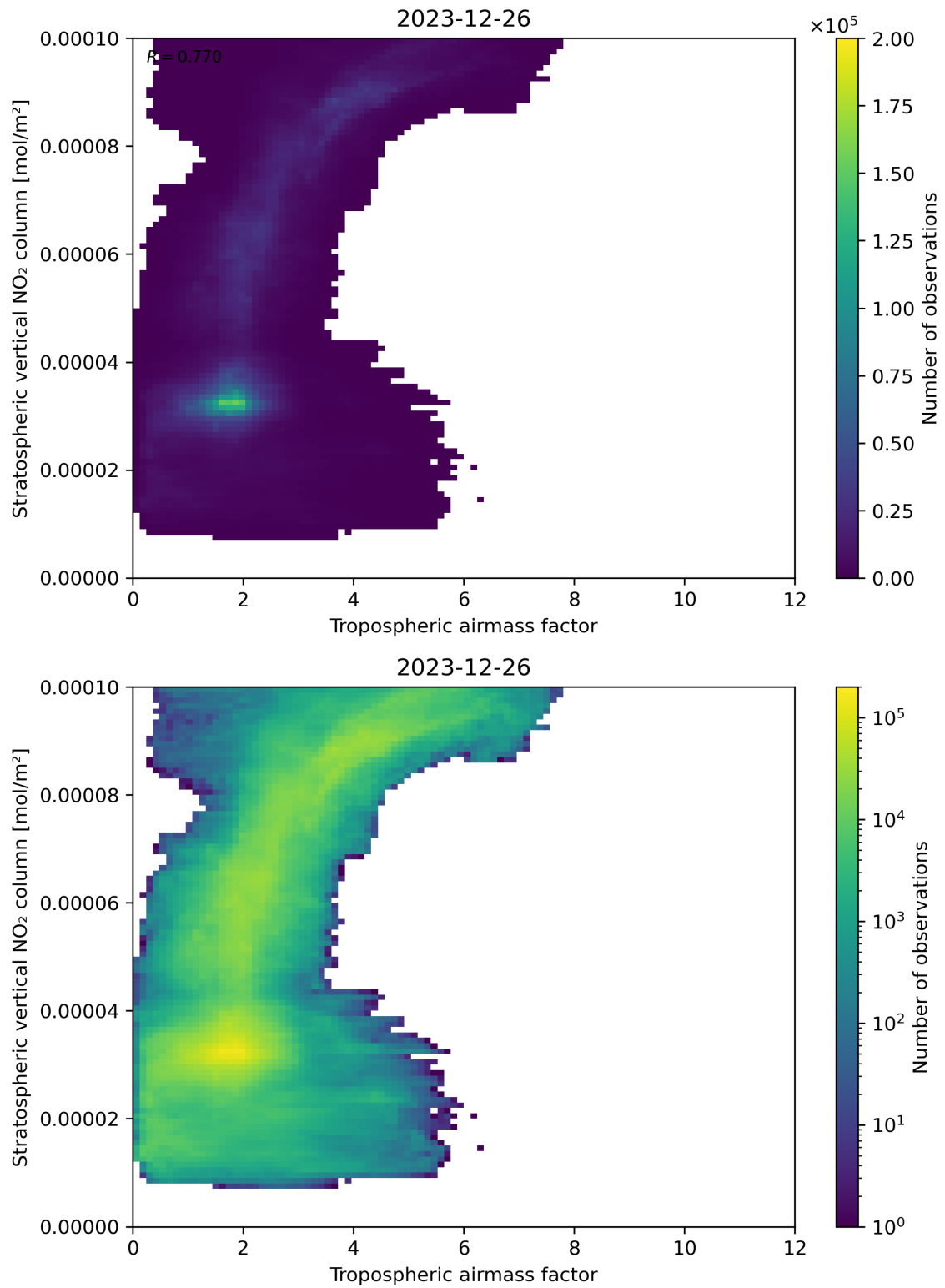
Figure 74: Scatter density plot of “Tropospheric air mass factor” against “Stratospheric vertical NO 2 column” for 2023-12-25 to 2023-12-27.
