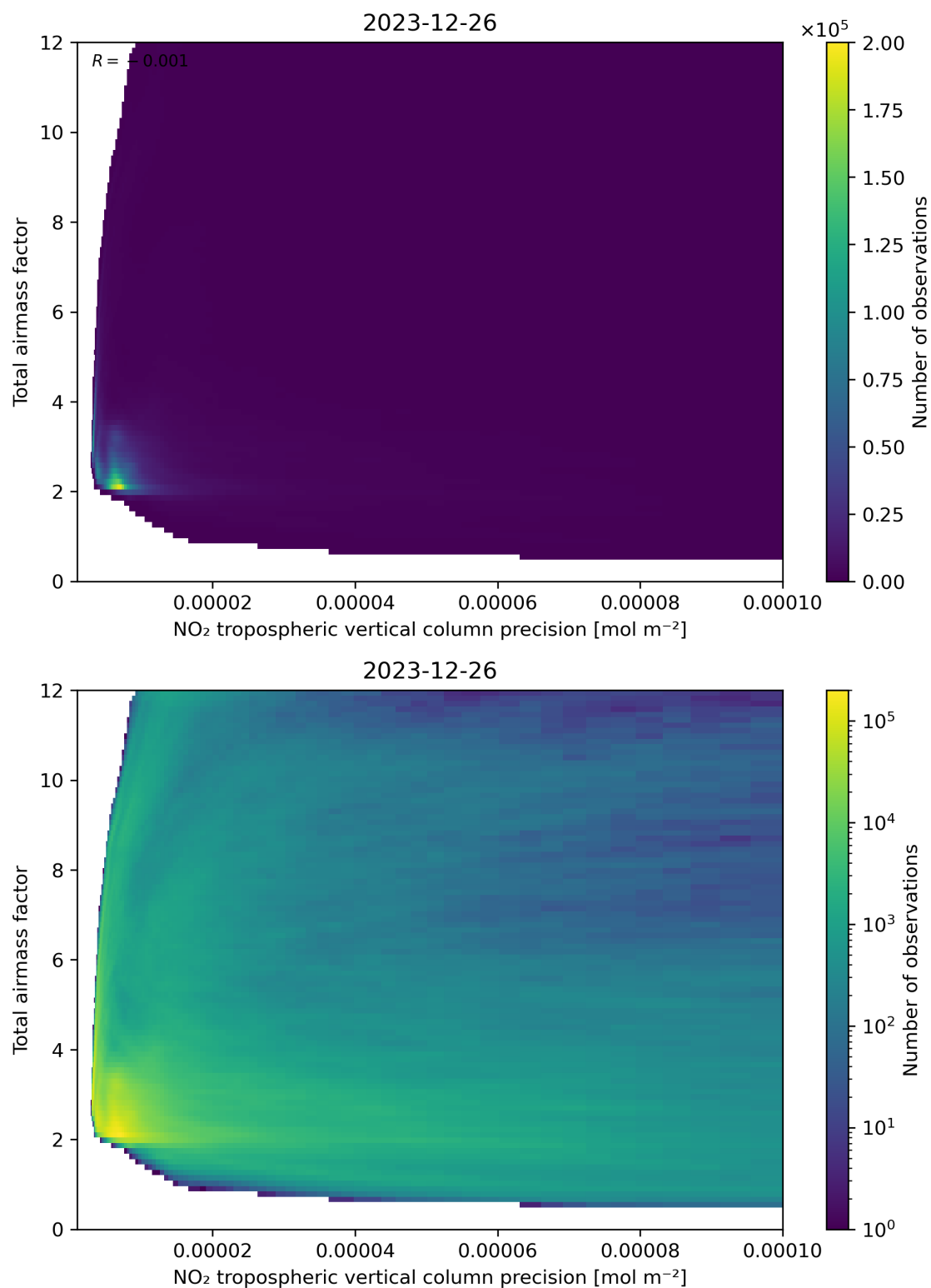
Figure 132: Scatter density plot of “NO 2 tropospheric vertical column precision” against “Total air mass factor” for 2023-12-25 to 2023-12-27.
