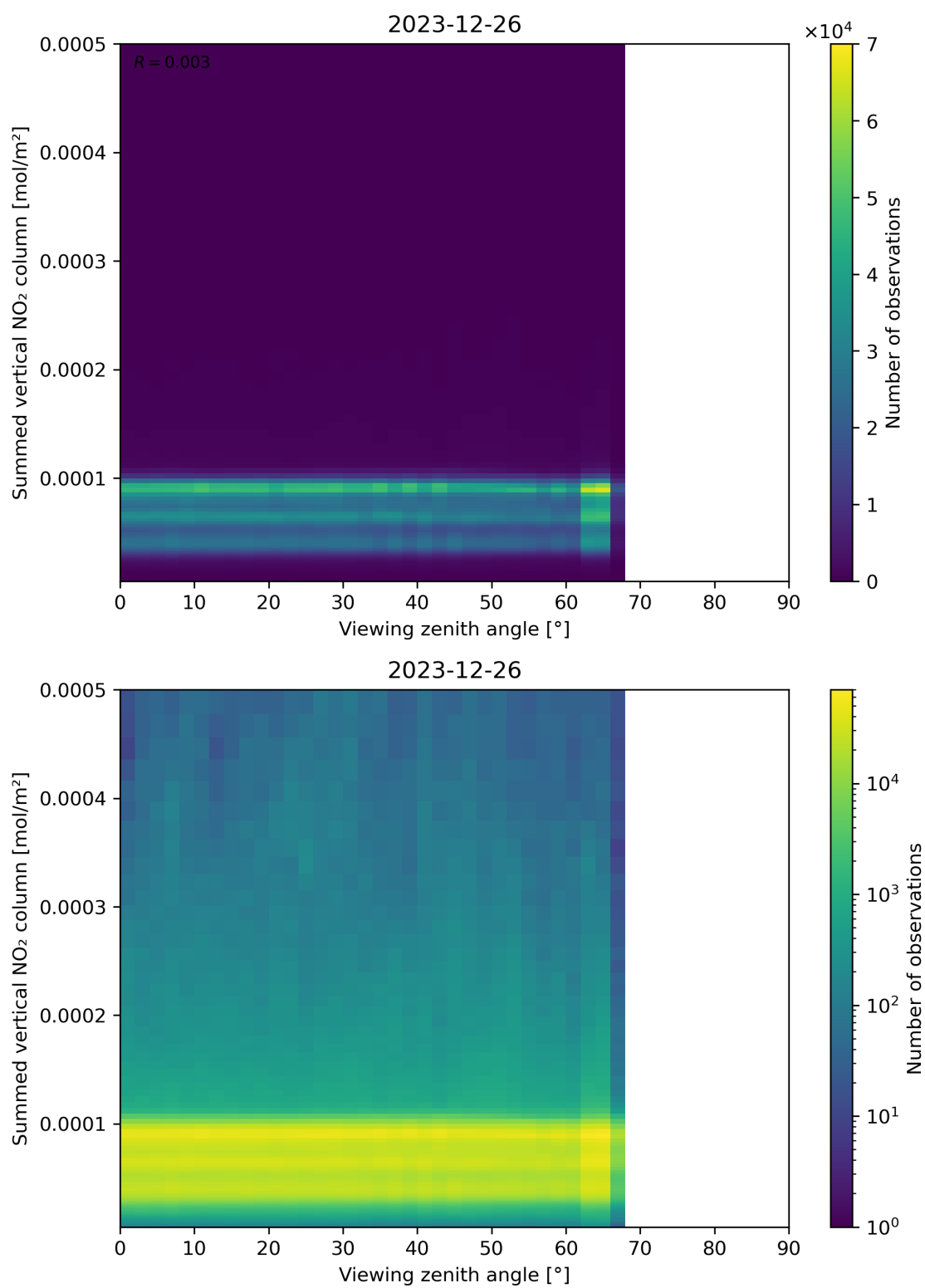
Figure 165: Scatter density plot of “Viewing zenith angle” against “Summed vertical NO 2 column” for 2023-12-25 to 2023-12-27.
