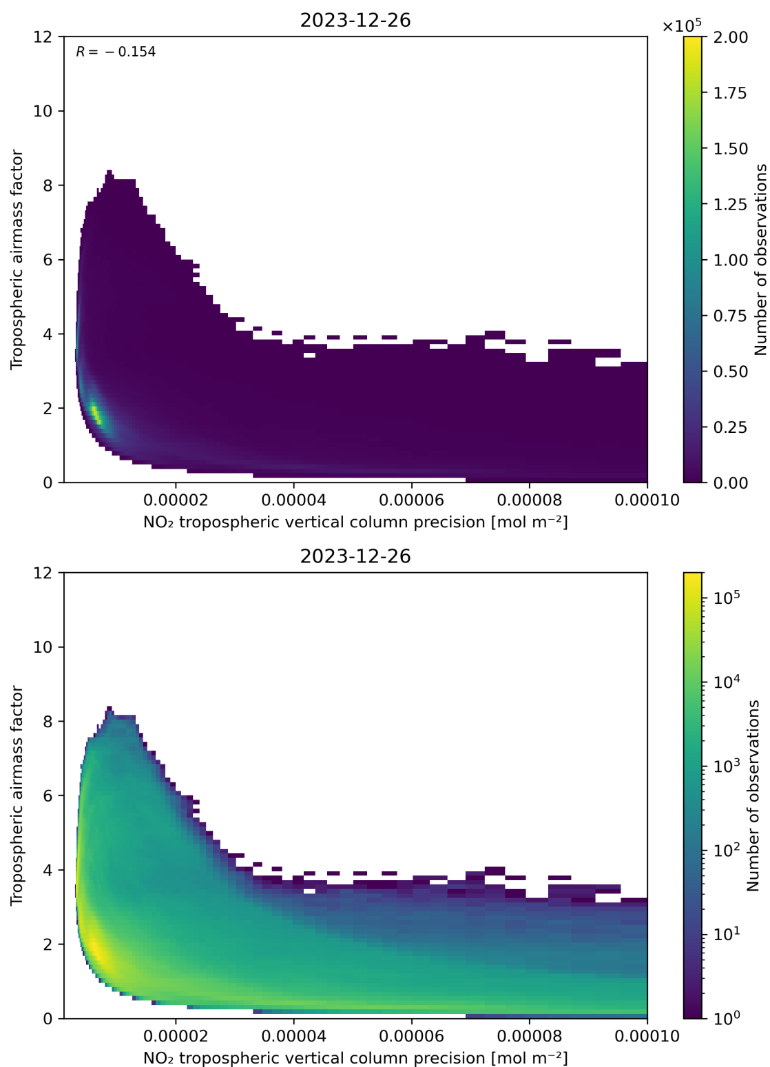
Figure 133: Scatter density plot of “NO 2 tropospheric vertical column precision” against “Tropospheric airmass factor” for 2023-12-25 to 2023-12-27.
