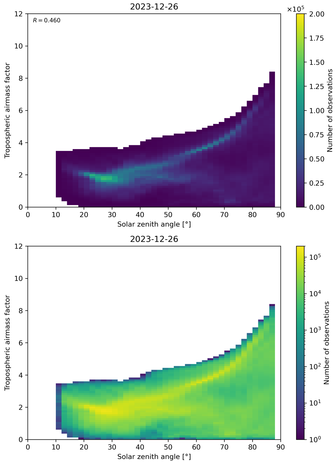
Figure 147: Scatter density plot of “Solar zenith angle” against “Tropospheric airmass factor” for 2023-12-25 to 2023-12-27.
