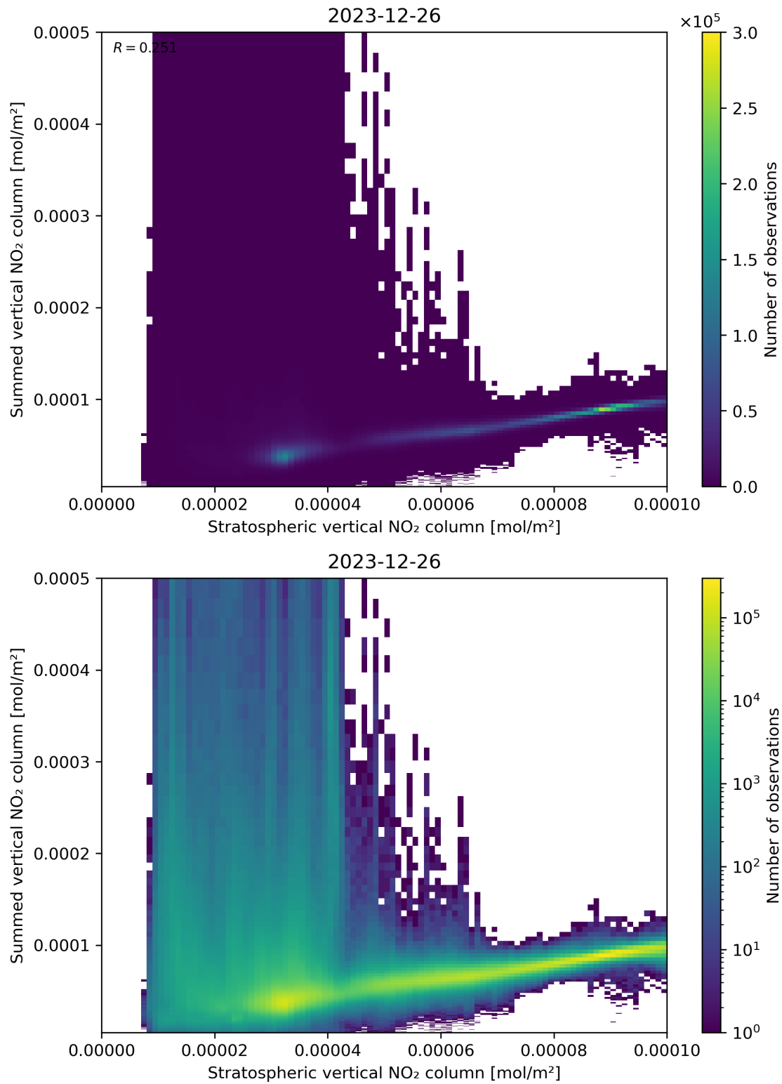
Figure 98: Scatter density plot of “Stratospheric vertical NO 2 column” against “Summed vertical NO 2 column” for 2023-12-25 to 2023-12-27.
