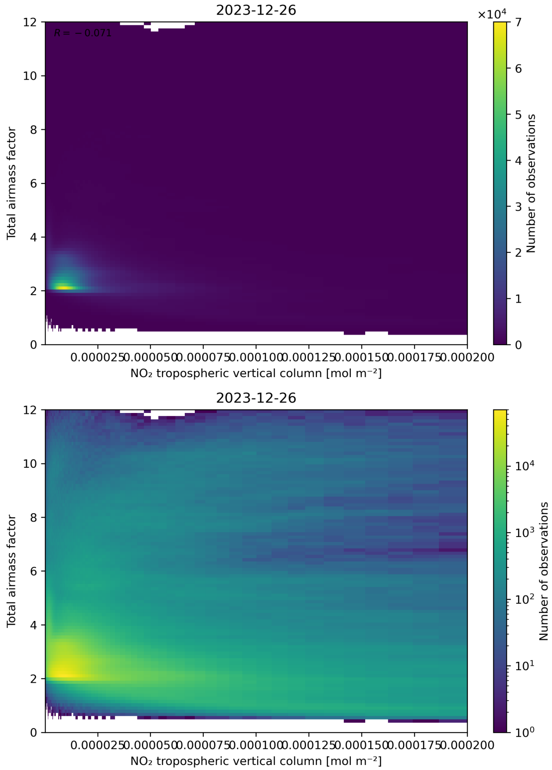
Figure 122: Scatter density plot of “NO 2 tropospheric vertical column” against “Total air mass factor” for 2023-12-25 to 2023-12-27.
