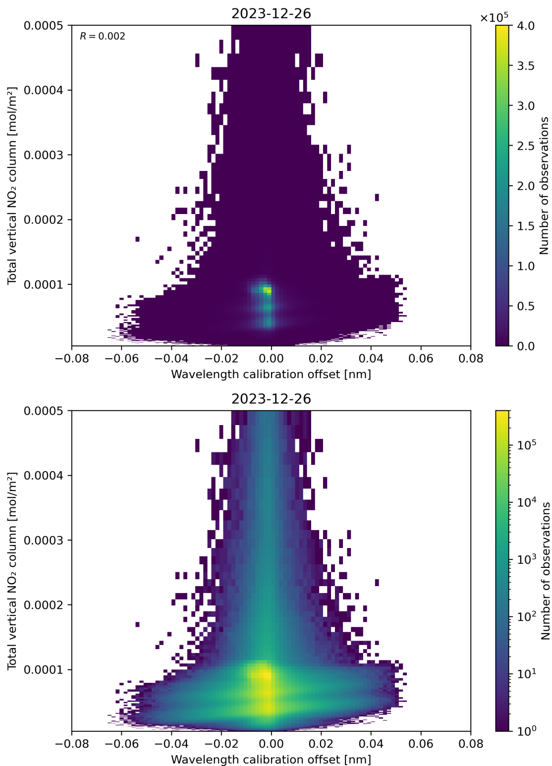
Figure 179: Scatter density plot of “Wavelength calibration offset” against “Total vertical NO 2 column” for 2023-12-25 to 2023-12-27.
