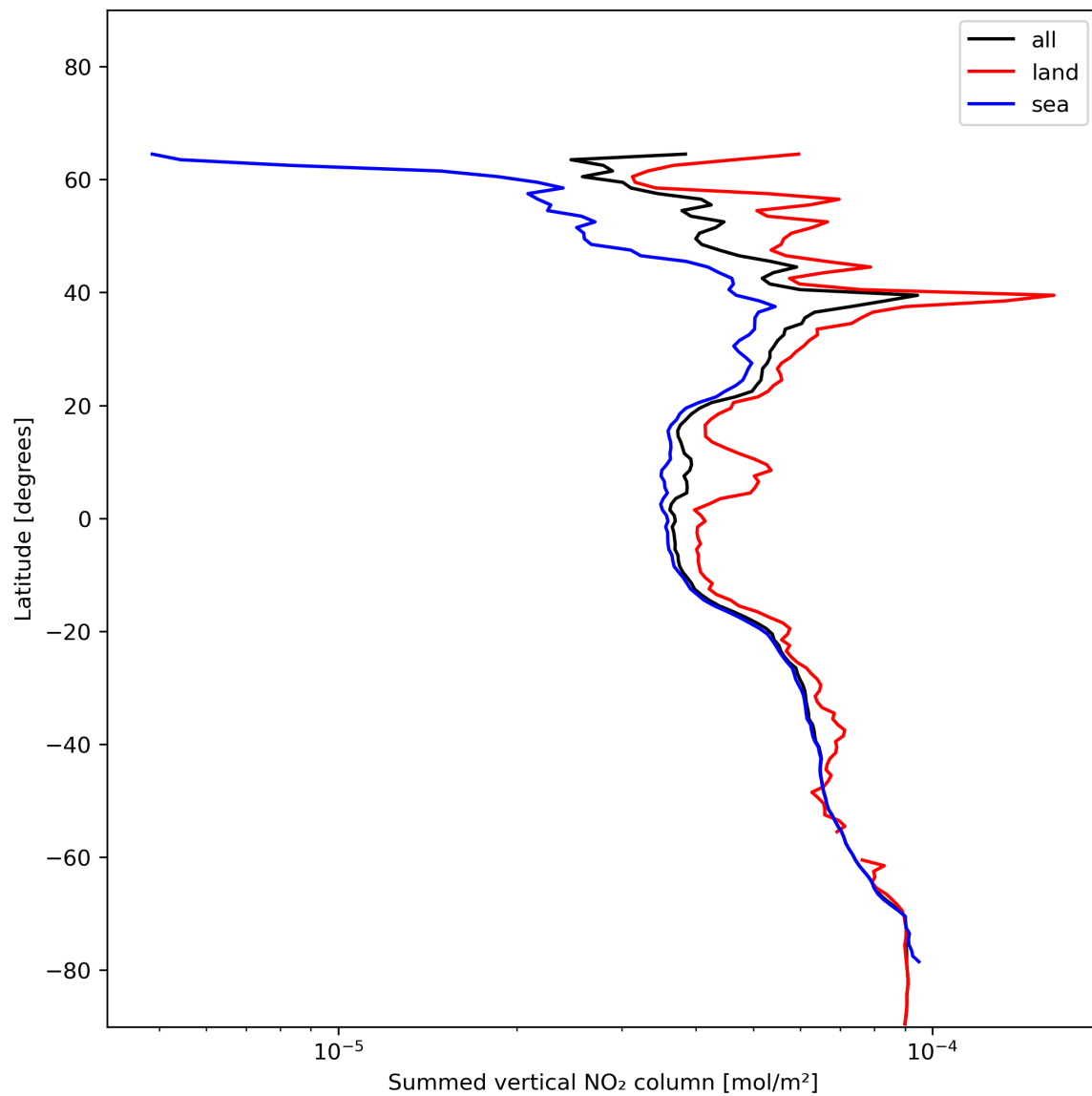
Figure 23: Zonal average of “Summed vertical NO 2 column” for 2023-12-25 to 2023-12-27.
