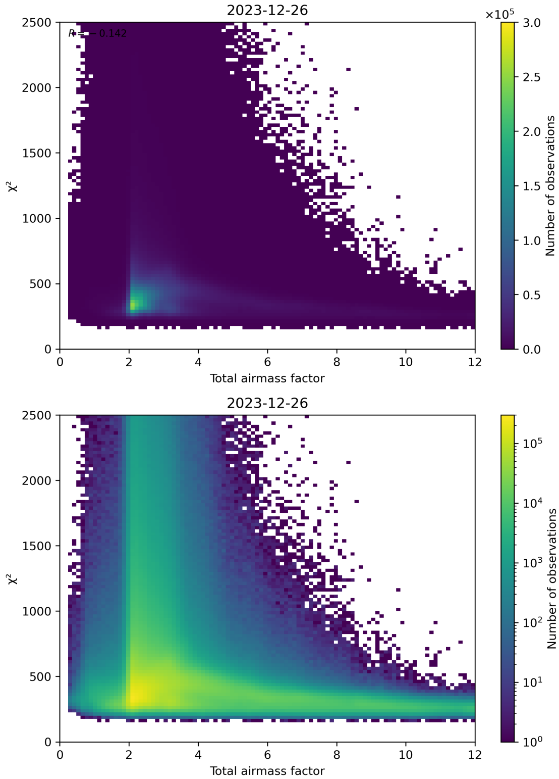
Figure 63: Scatter density plot of “Total airmass factor” against “ \chi^2 ” for 2023-12-25 to 2023-12-27.
