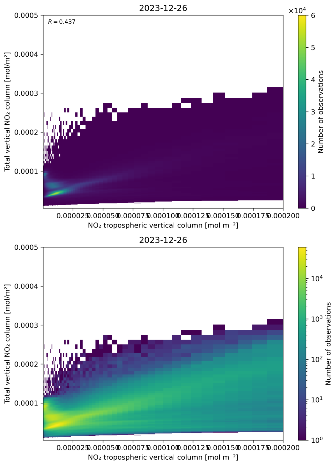
Figure 128: Scatter density plot of “NO 2 tropospheric vertical column” against “Total vertical NO 2 column” for 2023-12-25 to 2023-12-27.
