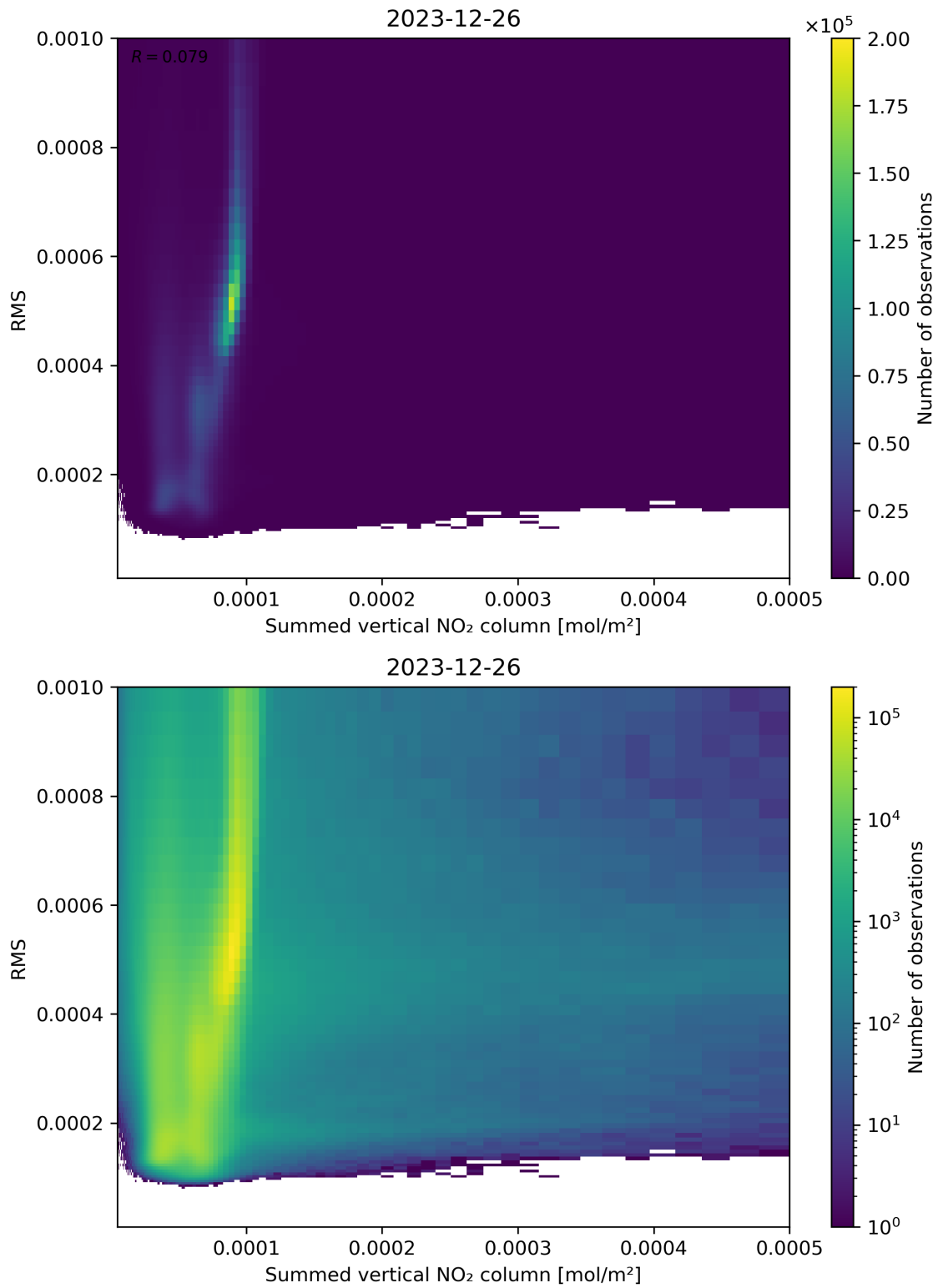
Figure 109: Scatter density plot of “Summed vertical NO 2 column” against “RMS” for 2023-12-25 to 2023-12-27.
