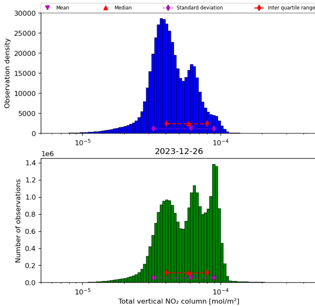
Figure 38: Histogram of “Total vertical NO 2 column” for 2023-12-25 to 2023-12-27
