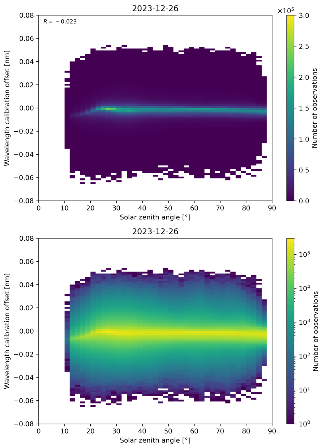
Figure 158: Scatter density plot of “Solar zenith angle” against “Wavelength calibration offset” for 2023-12-25 to 2023-12-27.
