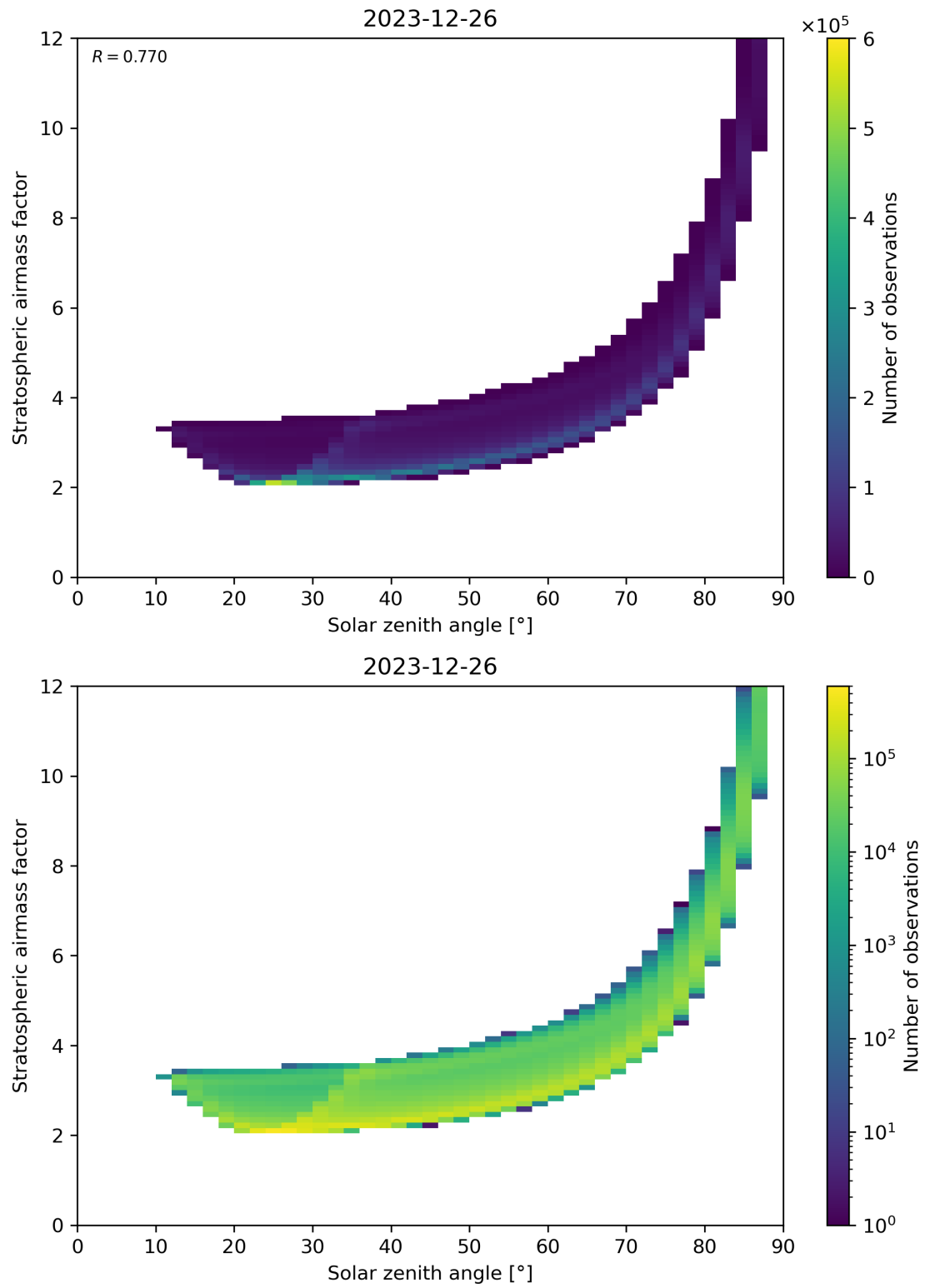
Figure 145: Scatter density plot of “Solar zenith angle” against “Stratospheric airmass factor” for 2023-12-25 to 2023-12-27.
