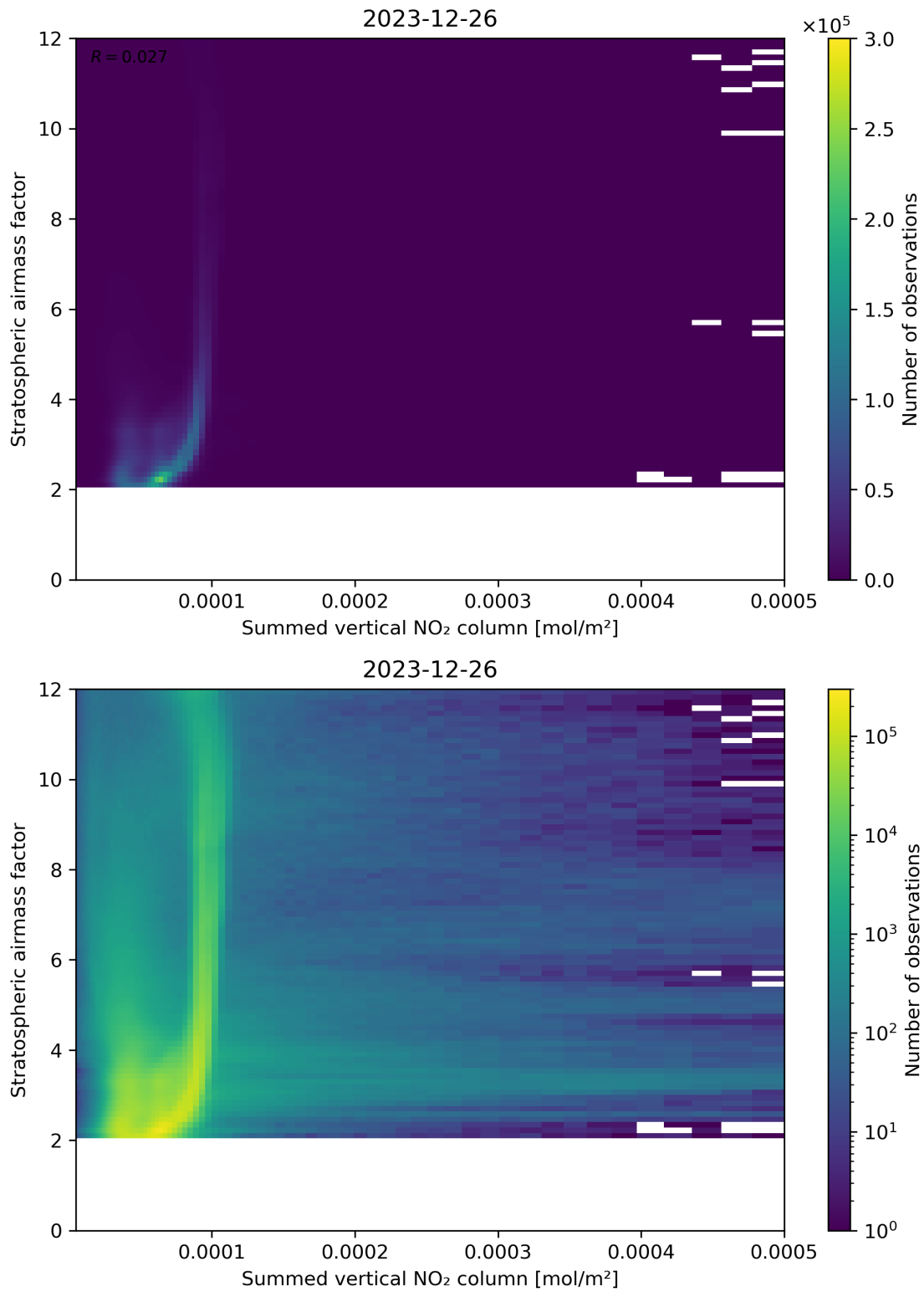
Figure 103: Scatter density plot of “Summed vertical NO 2 column” against “Stratospheric air mass factor” for 2023-12-25 to 2023-12-27.
