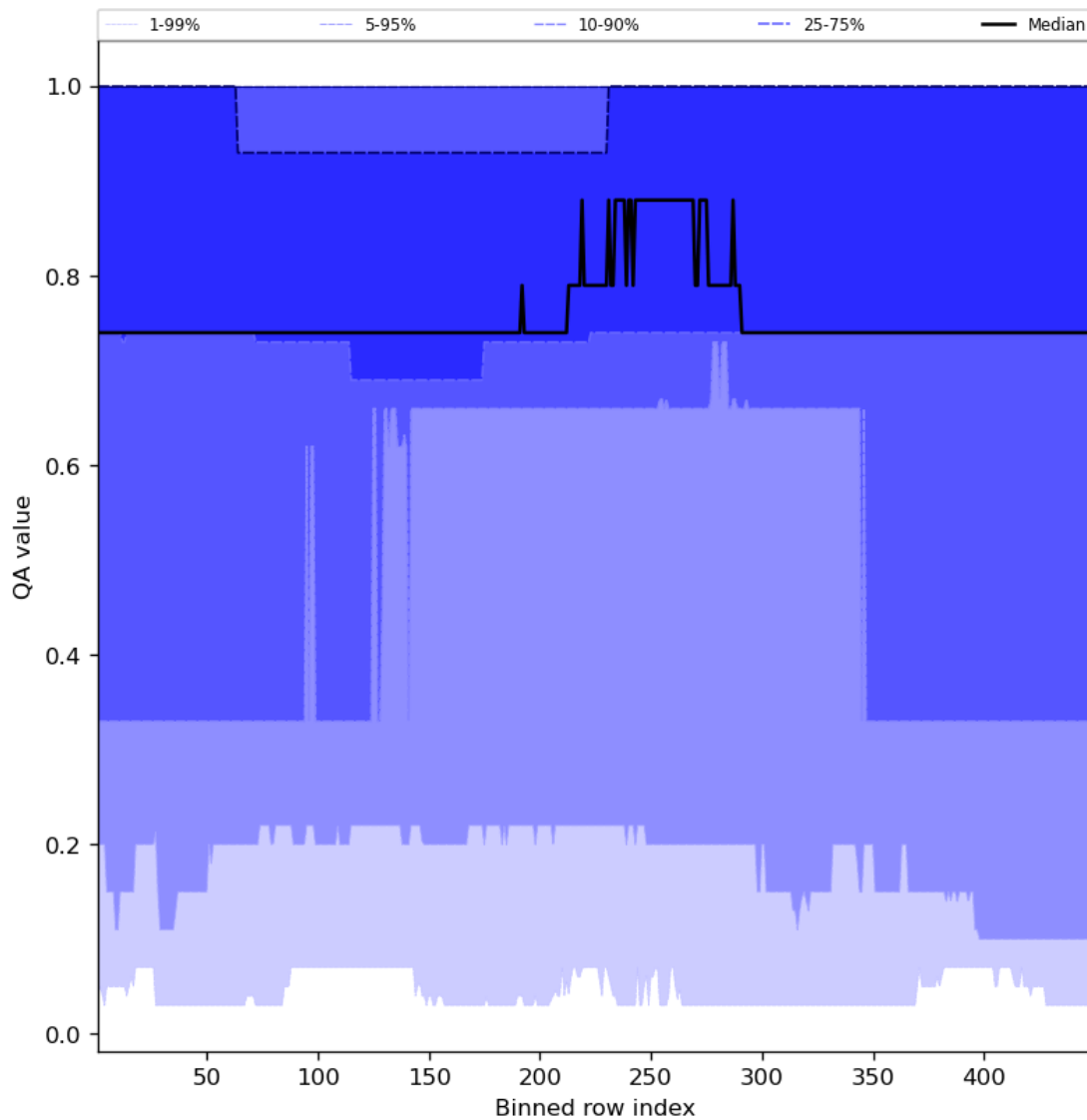
Figure 45: Along track statistics of “QA value” for 2023-12-25 to 2023-12-27
