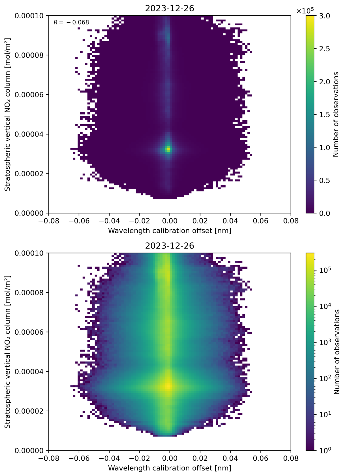
Figure 176: Scatter density plot of “Wavelength calibration offset” against “Stratospheric vertical NO 2 column” for 2023-12-25 to 2023-12-27.
