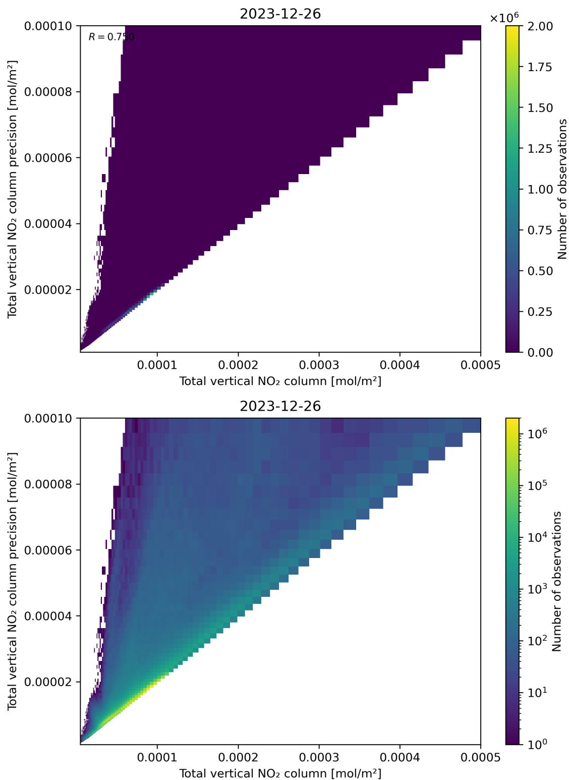
Figure 114: Scatter density plot of “Total vertical NO 2 column” against “Total vertical NO 2 column precision” for 2023-12-25 to 2023-12-27.
