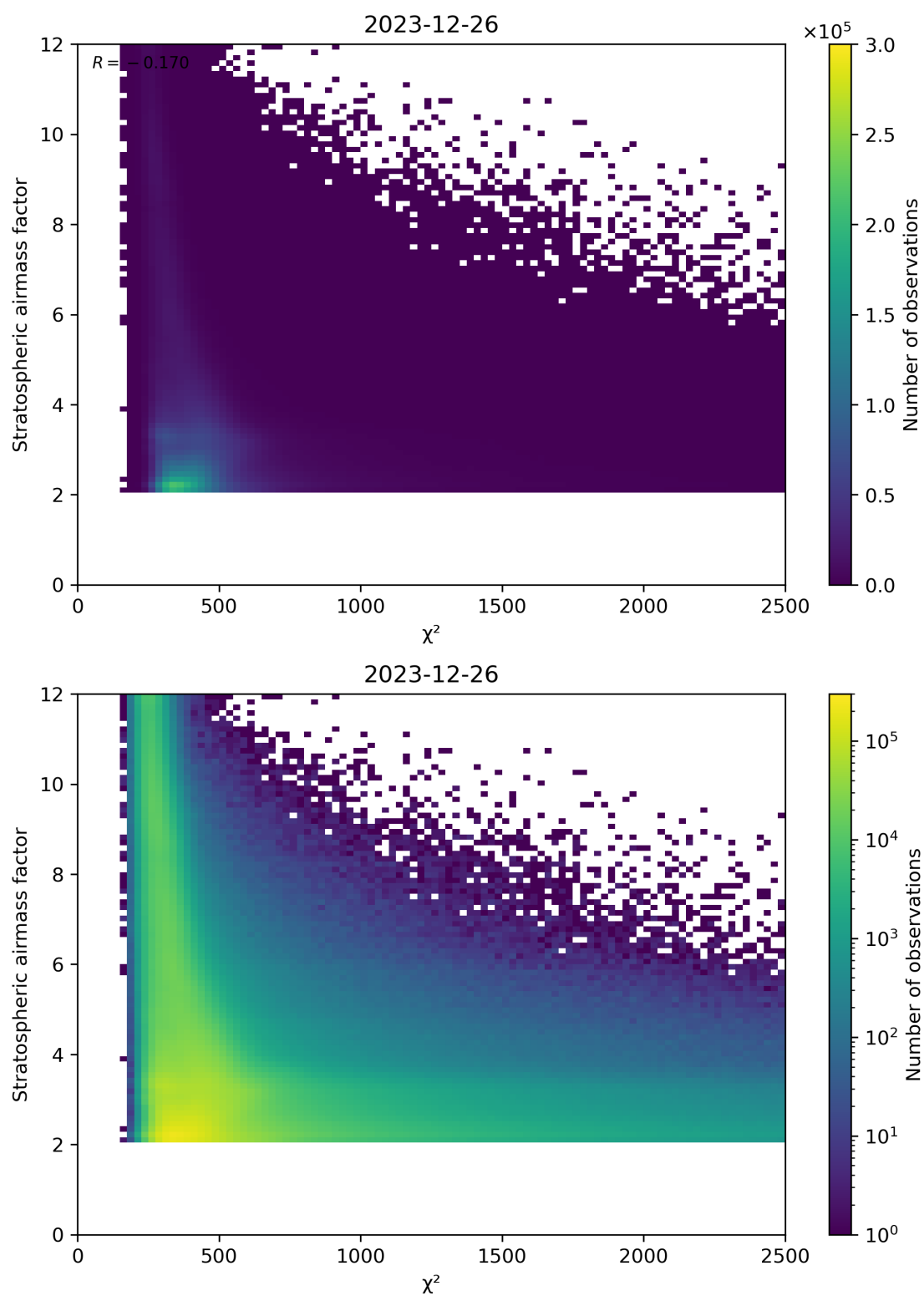
Figure 81: Scatter density plot of “ \chi^2 ” against “Stratospheric airmass factor” for 2023-12-25 to 2023-12-27.
