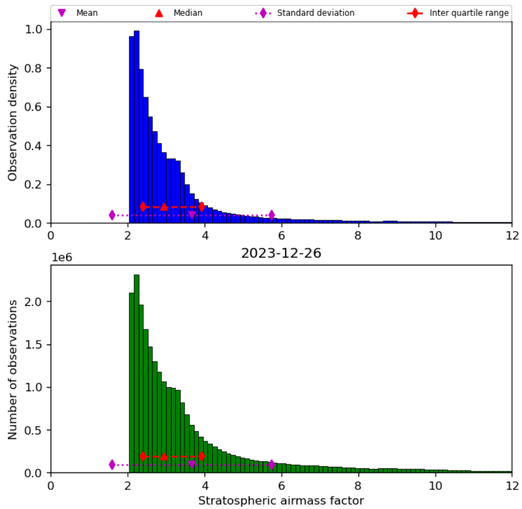
Figure 44: Histogram of “Stratospheric airmass factor” for 2023-12-25 to 2023-12-27
