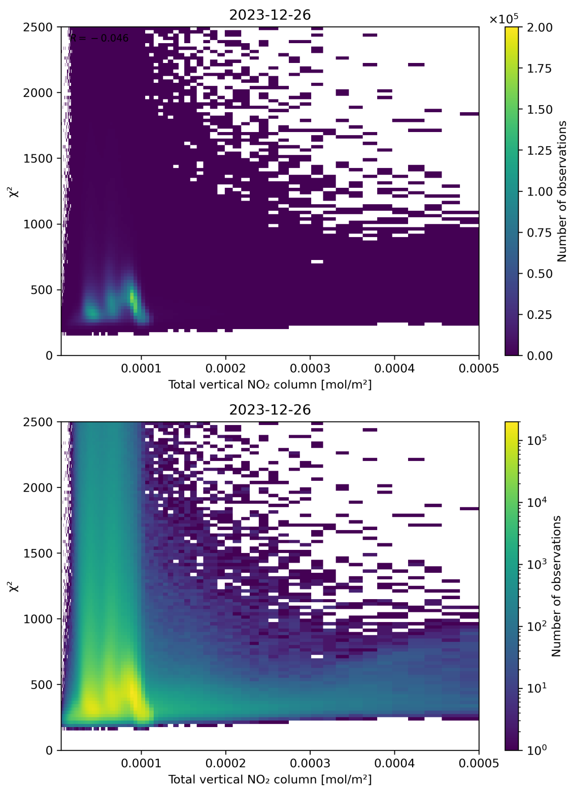
Figure 111: Scatter density plot of “Total vertical NO 2 column” against “ \chi^2 ” for 2023-12-25 to 2023-12-27.
