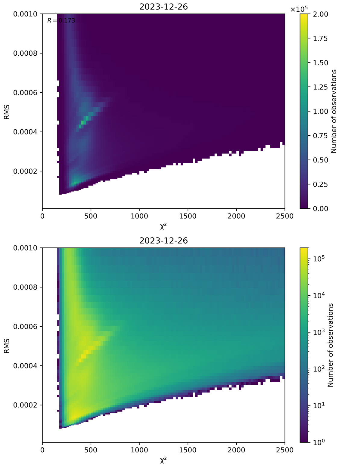
Figure 82: Scatter density plot of “ \chi^2 ” against “RMS” for 2023-12-25 to 2023-12-27.
