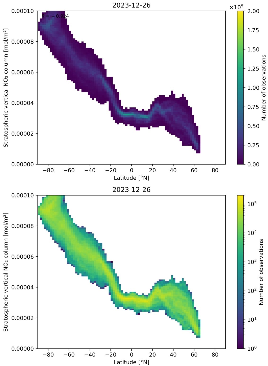
Figure 87: Scatter density plot of “Latitude” against “Stratospheric vertical NO 2 column” for 2023-12-25 to 2023-12-27.
