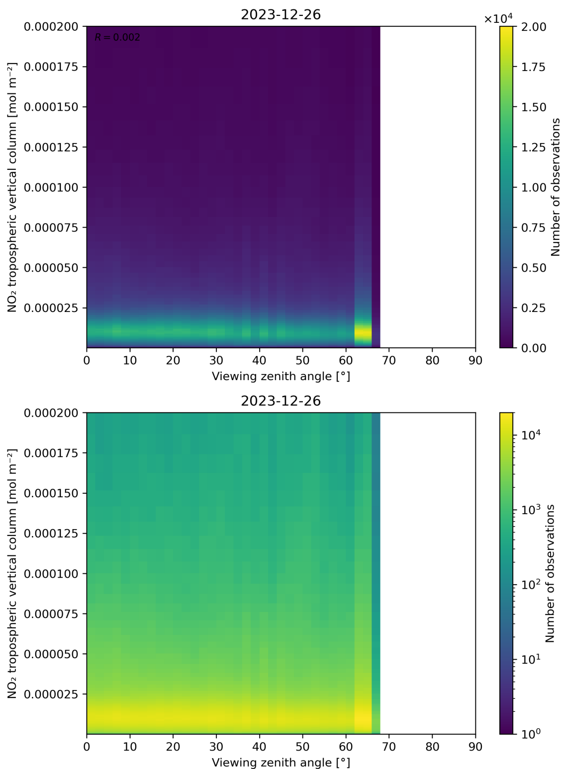
Figure 169: Scatter density plot of “Viewing zenith angle” against “NO 2 tropospheric vertical column” for 2023-12-25 to 2023-12-27.
