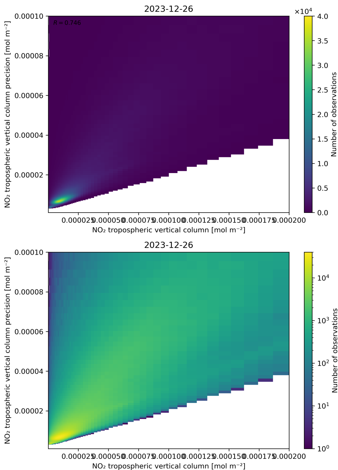
Figure 130: Scatter density plot of “NO 2 tropospheric vertical column” against “NO 2 tropospheric vertical column precision” for 2023-12-25 to 2023-12-27.
