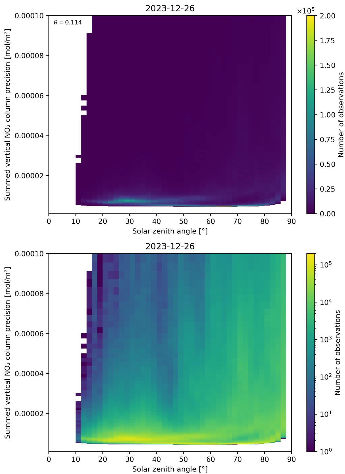
Figure 152: Scatter density plot of “Solar zenith angle” against “Summed vertical NO 2 column precision” for 2023-12-25 to 2023-12-27.
