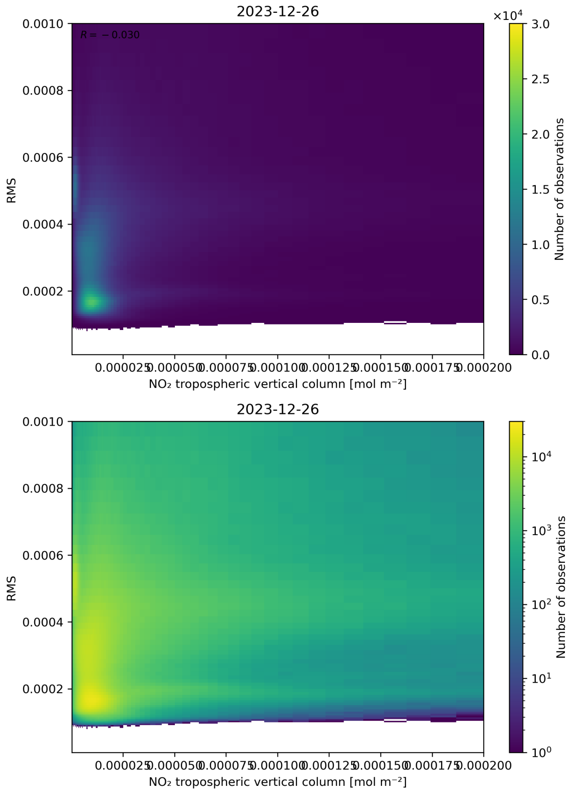
Figure 142: Scatter density plot of “NO 2 tropospheric vertical column” against “RMS” for 2023-12-25 to 2023-12-27.
