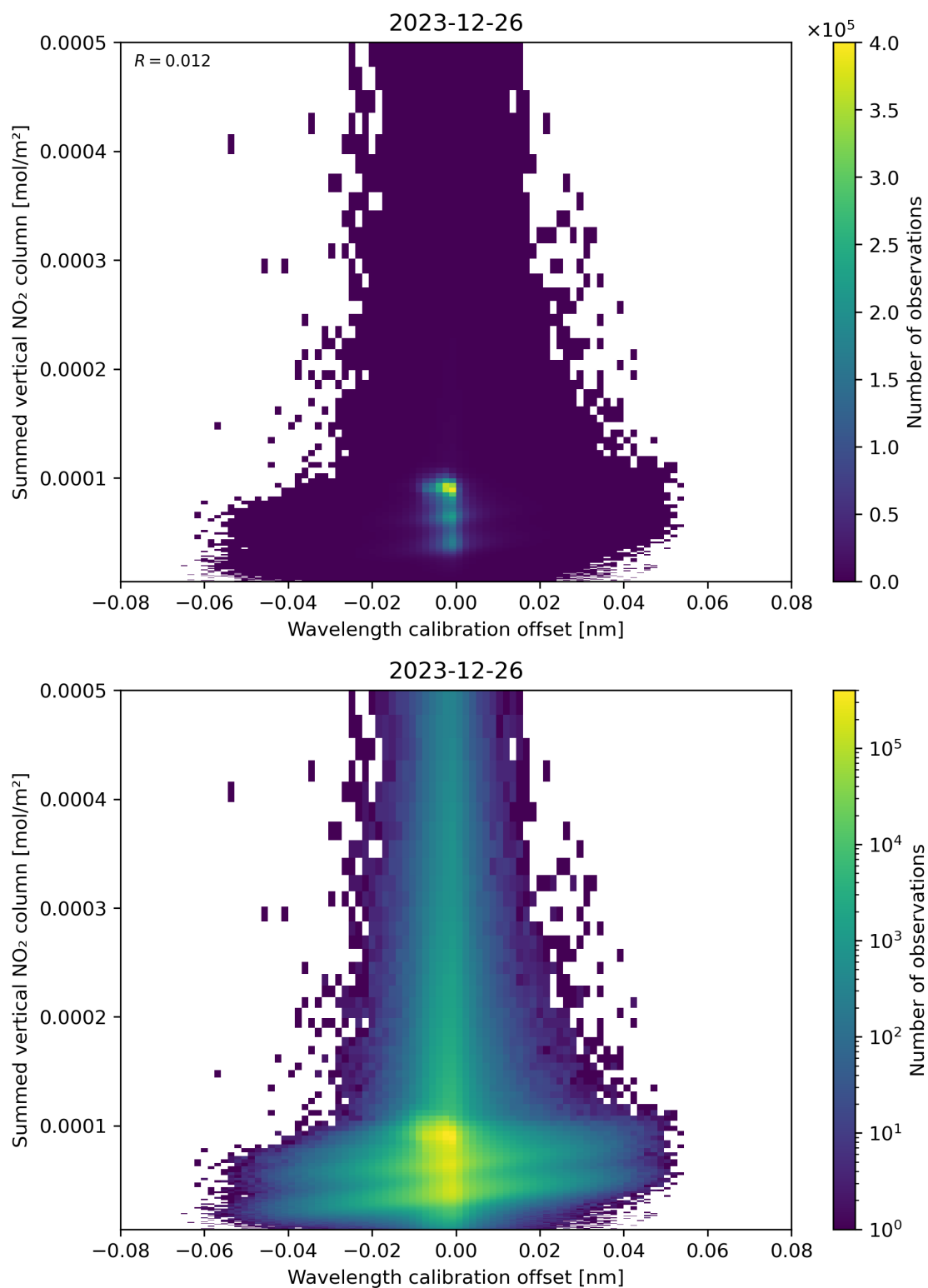
Figure 177: Scatter density plot of “Wavelength calibration offset” against “Summed vertical NO 2 column” for 2023-12-25 to 2023-12-27.
