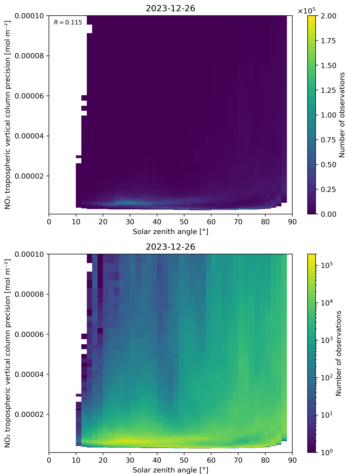
Figure 156: Scatter density plot of “Solar zenith angle” against “NO 2 tropospheric vertical column precision” for 2023-12-25 to 2023-12-27.
