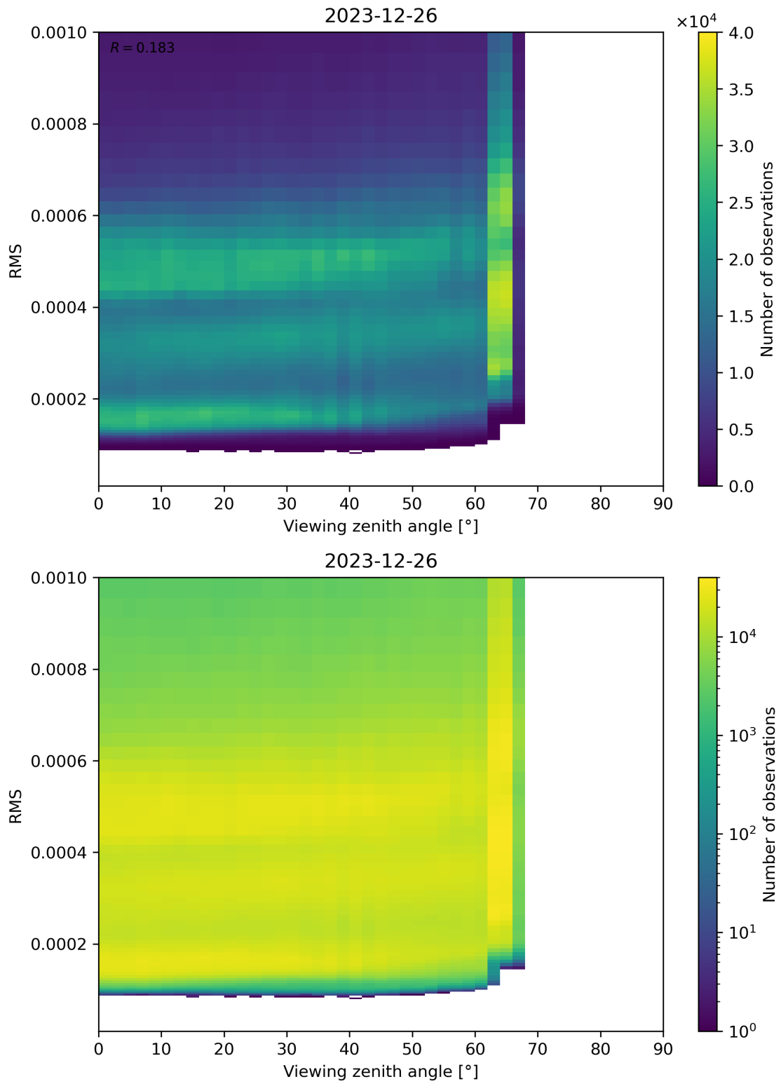
Figure 171: Scatter density plot of “Viewing zenith angle” against “RMS” for 2023-12-25 to 2023-12-27.
