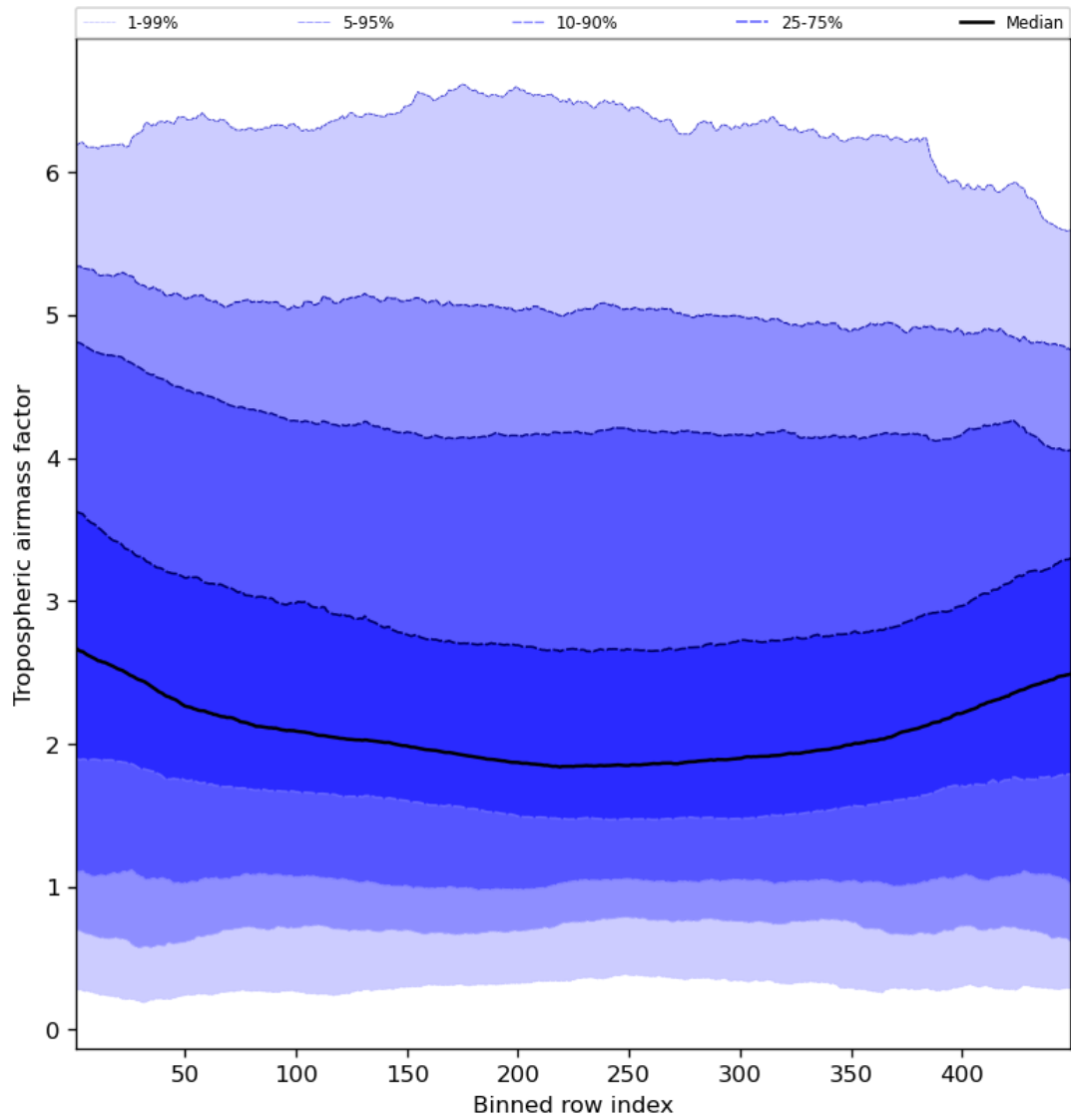
Figure 48: Along track statistics of “Tropospheric air mass factor” for 2023-12-25 to 2023-12-27
