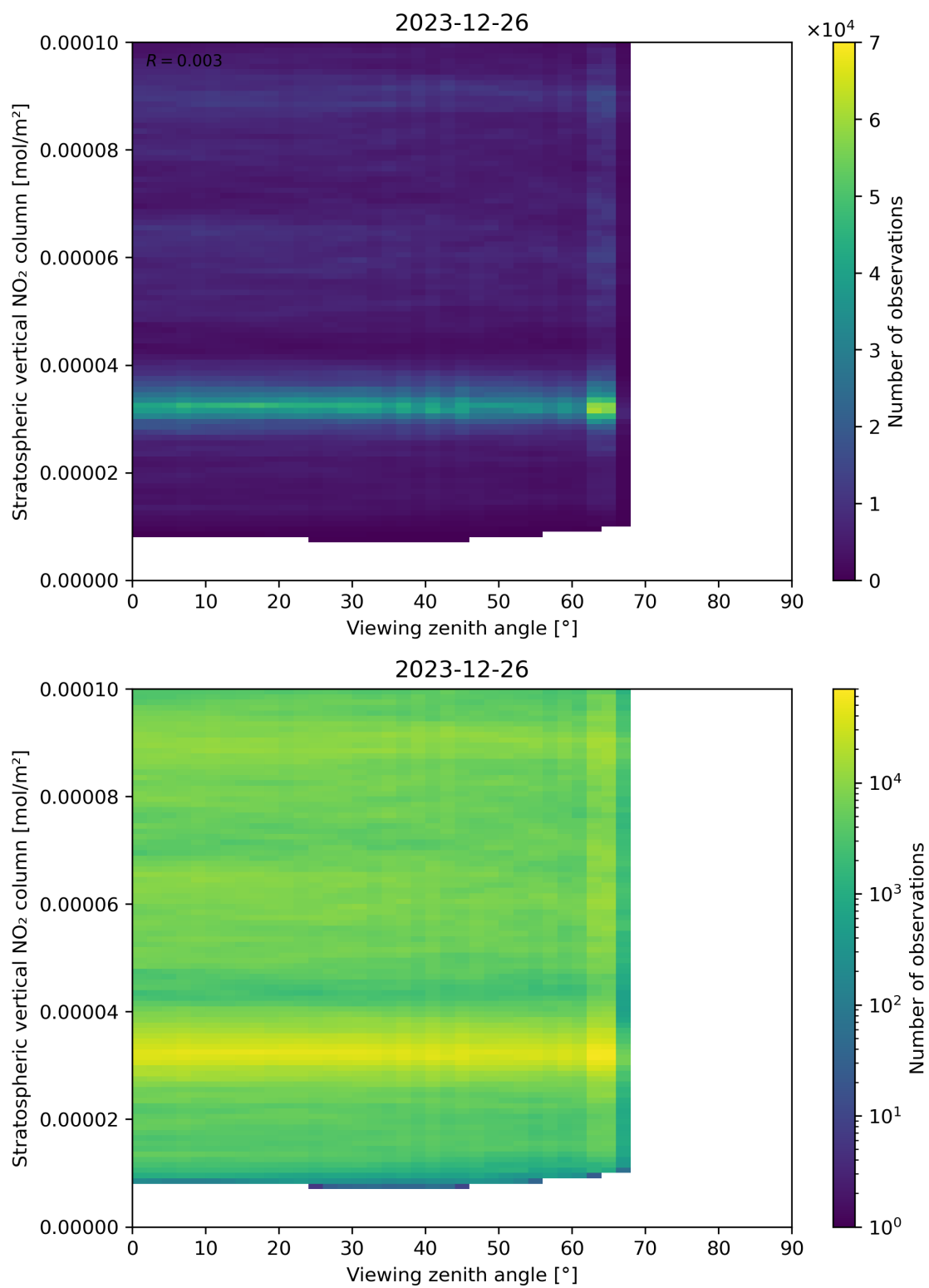
Figure 164: Scatter density plot of “Viewing zenith angle” against “Stratospheric vertical NO 2 column” for 2023-12-25 to 2023-12-27.
