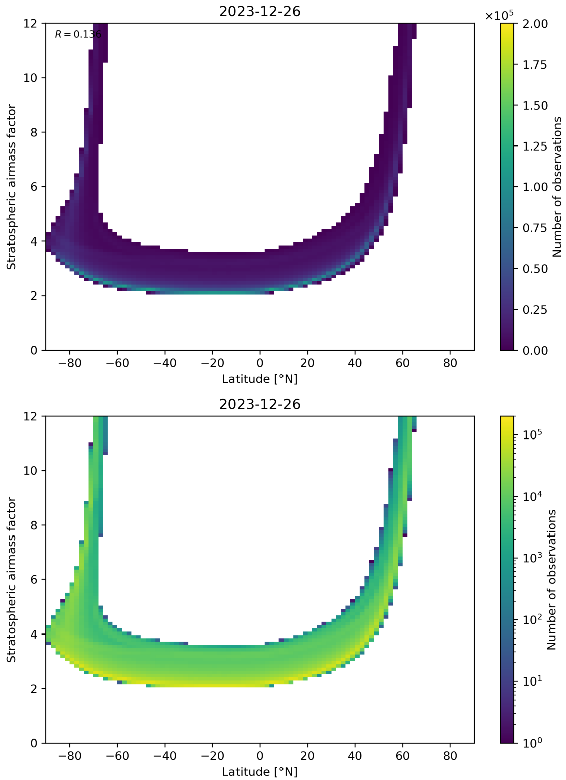
Figure 83: Scatter density plot of “Latitude” against “Stratospheric airmass factor” for 2023-12-25 to 2023-12-27.
