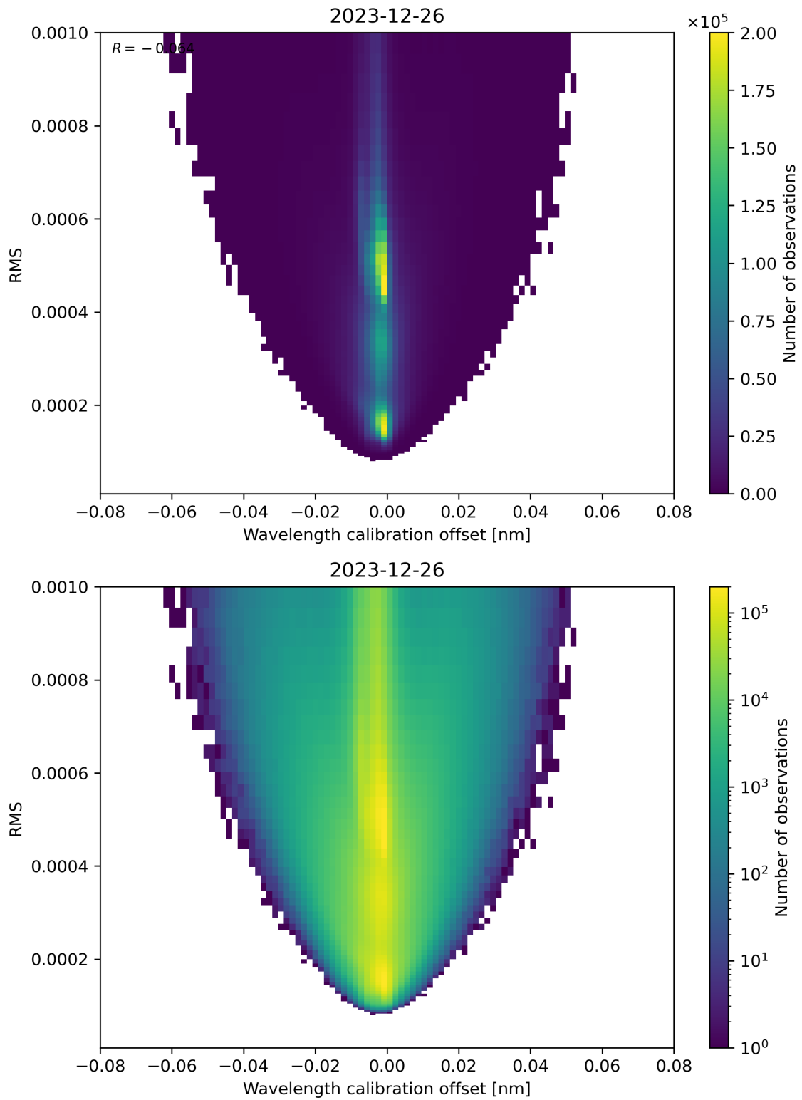
Figure 181: Scatter density plot of “Wavelength calibration offset” against “RMS” for 2023-12-25 to 2023-12-27.
