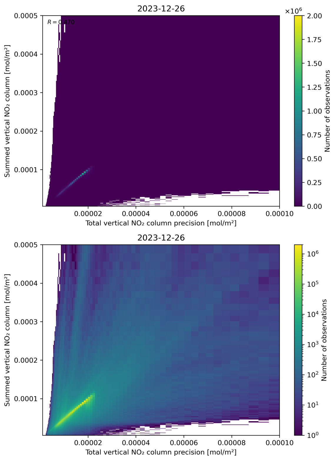
Figure 117: Scatter density plot of “Total vertical NO 2 column precision” against “Summed vertical NO 2 column” for 2023-12-25 to 2023-12-27.
