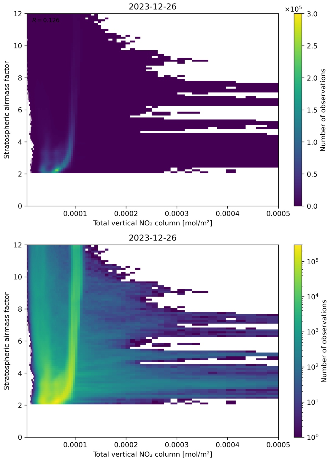
Figure 110: Scatter density plot of “Total vertical NO 2 column” against “Stratospheric air mass factor” for 2023-12-25 to 2023-12-27.
