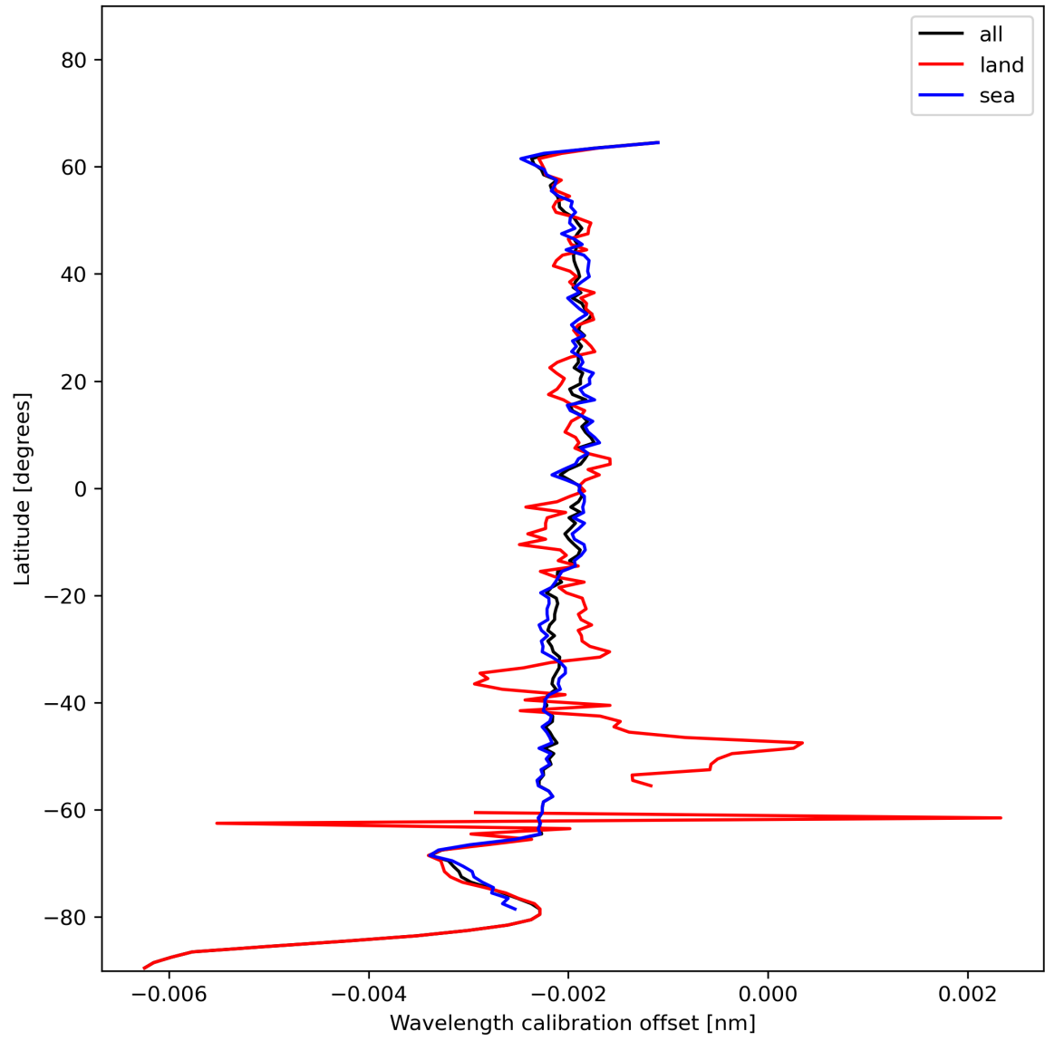
Figure 18: Zonal average of “Wavelength calibration offset” for 2023-12-25 to 2023-12-27.
