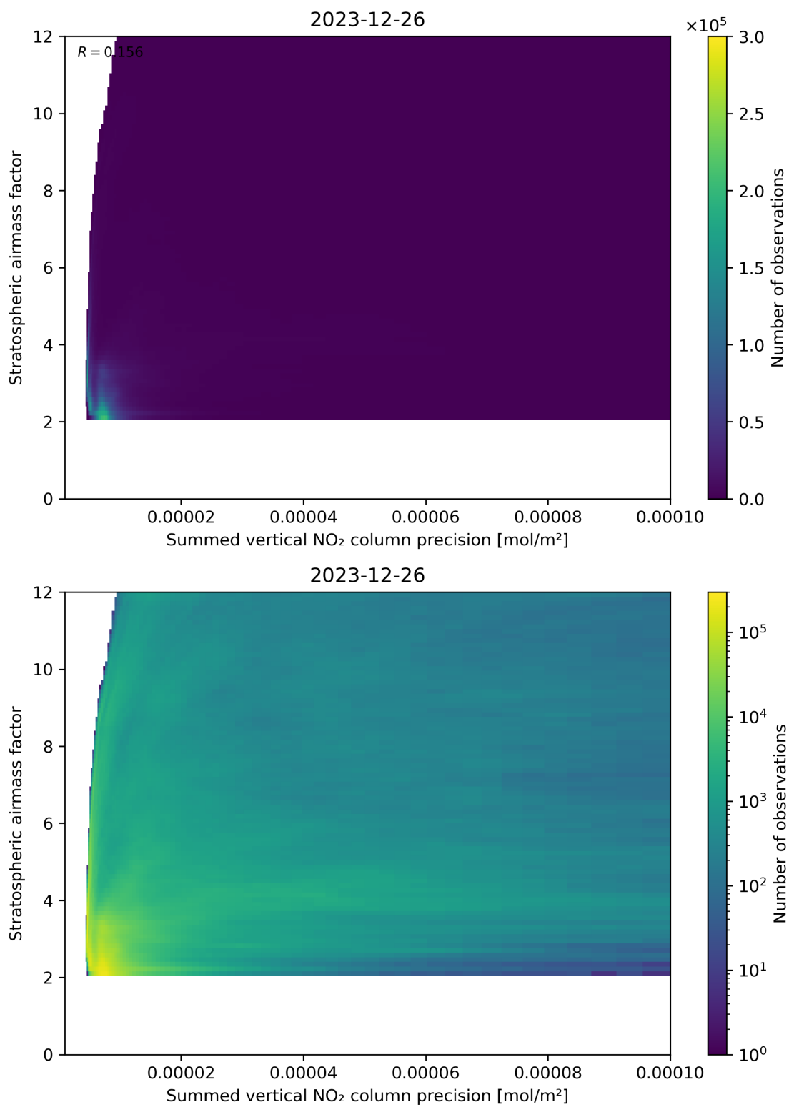
Figure 106: Scatter density plot of “Summed vertical NO 2 column precision” against “Stratospheric airmass factor” for 2023-12-25 to 2023-12-27.
