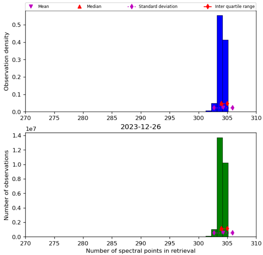
Figure 33: Histogram of “Number of spectral points in retrieval” for 2023-12-25 to 2023-12-27
