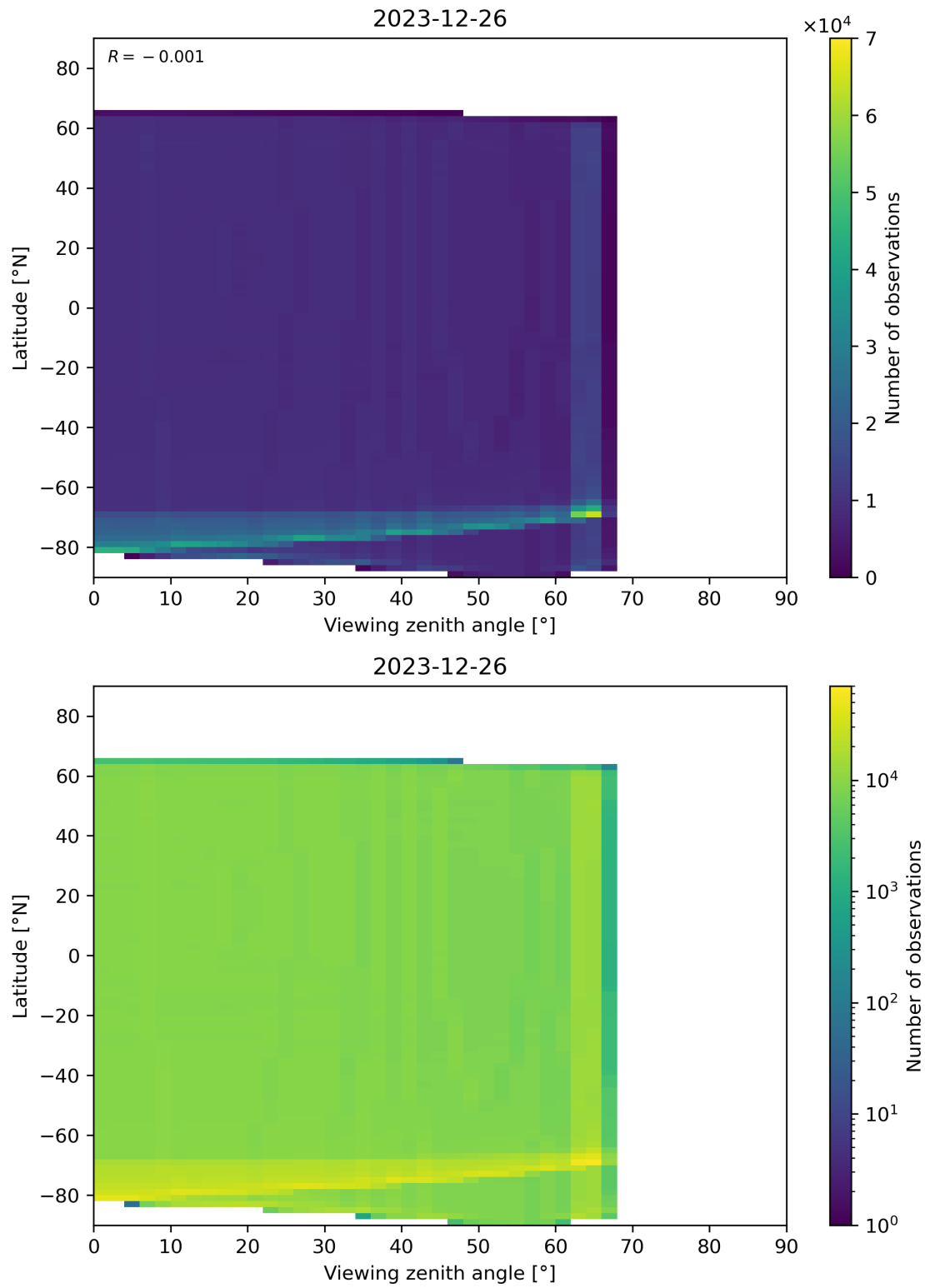
Figure 163: Scatter density plot of “Viewing zenith angle” against “Latitude” for 2023-12-25 to 2023-12-27.
