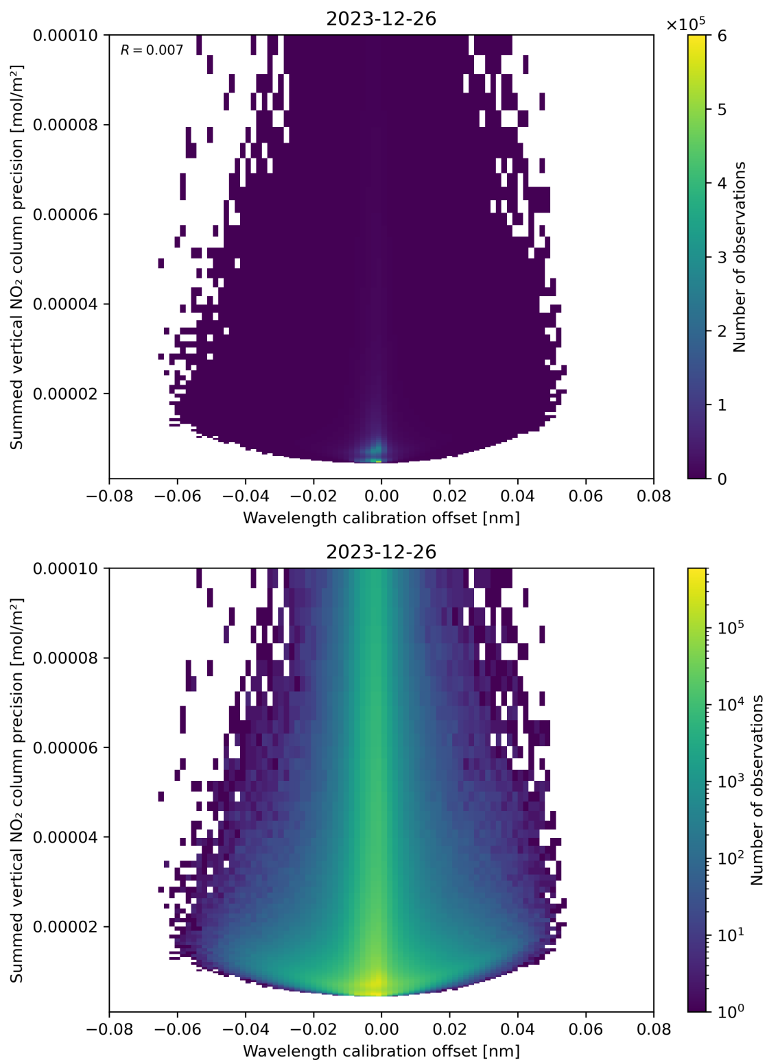
Figure 178: Scatter density plot of “Wavelength calibration offset” against “Summed vertical NO 2 column precision” for 2023-12-25 to 2023-12-27.
