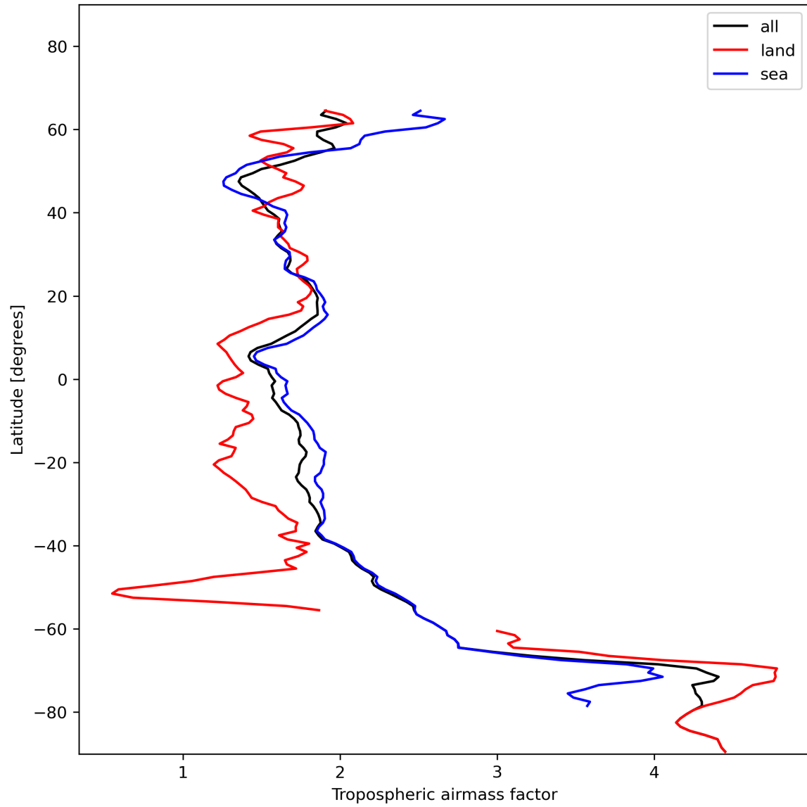
Figure 14: Zonal average of “Tropospheric airmass factor” for 2023-12-25 to 2023-12-27.
