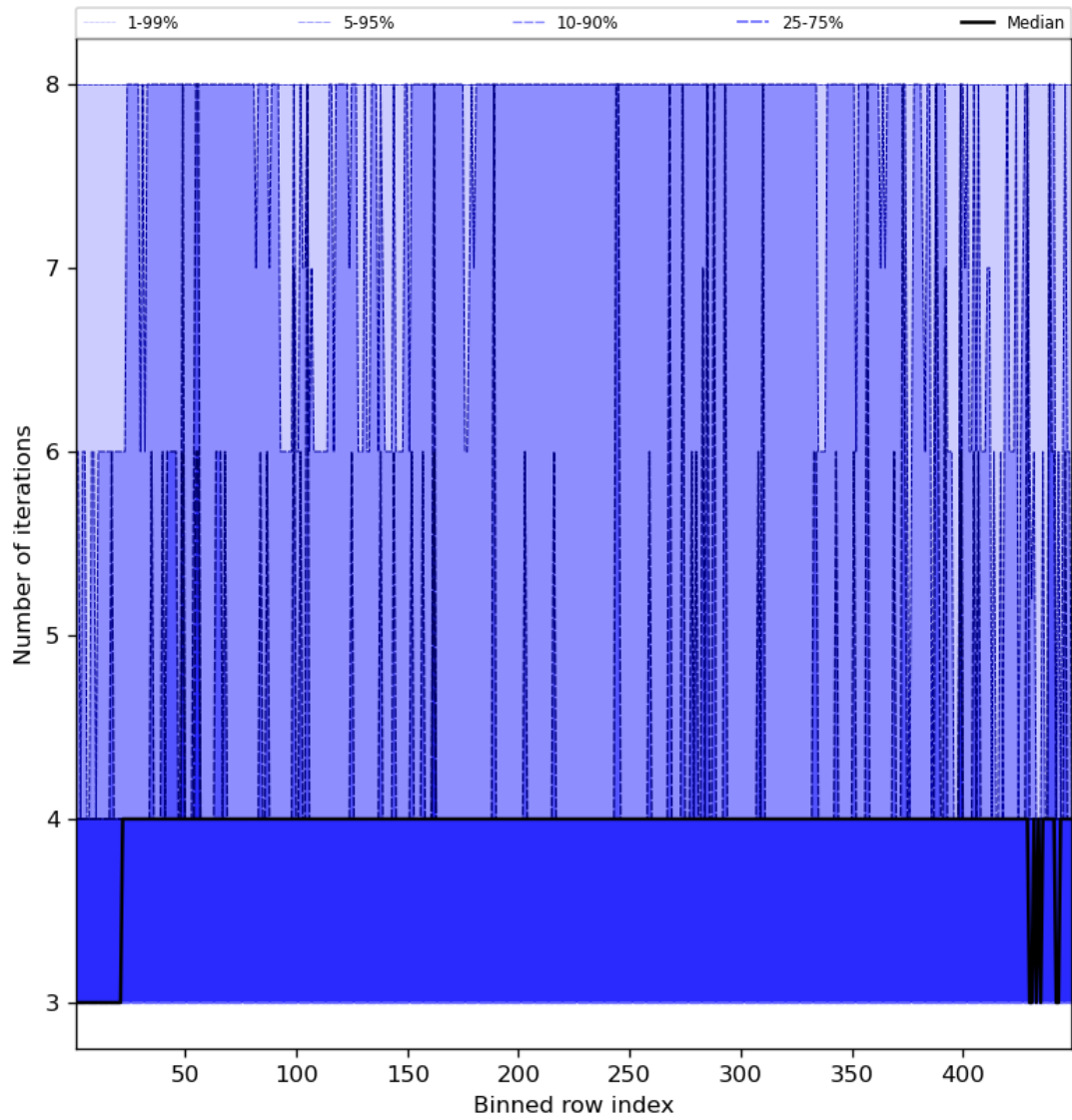
Figure 51: Along track statistics of “Number of iterations” for 2023-12-25 to 2023-12-27
