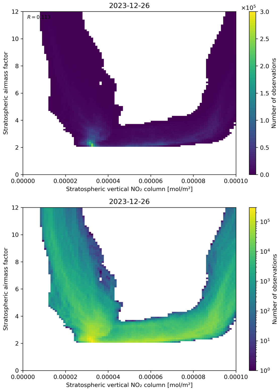
Figure 96: Scatter density plot of “Stratospheric vertical NO 2 column” against “Stratospheric airmass factor” for 2023-12-25 to 2023-12-27.
