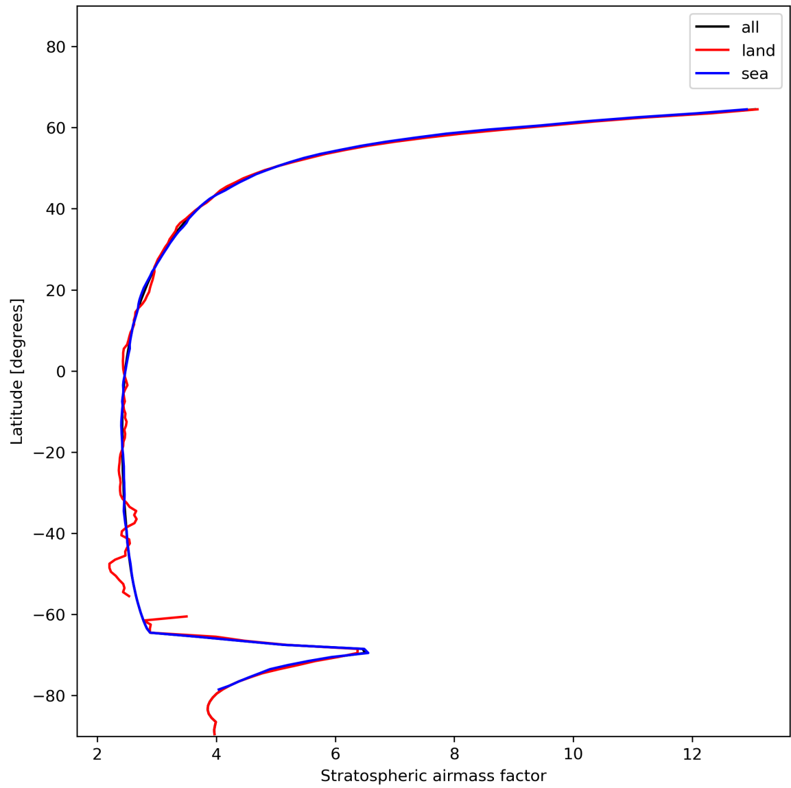
Figure 27: Zonal average of “Stratospheric air mass factor” for 2023-12-25 to 2023-12-27.
