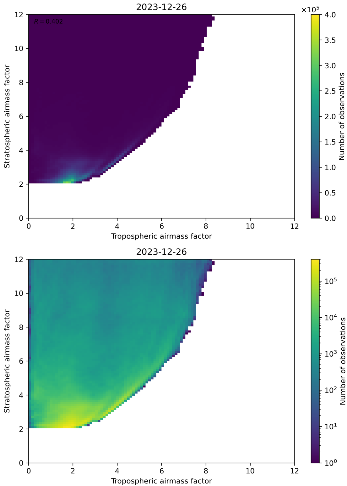
Figure 71: Scatter density plot of “Tropospheric airmass factor” against “Stratospheric airmass factor” for 2023-12-25 to 2023-12-27.
