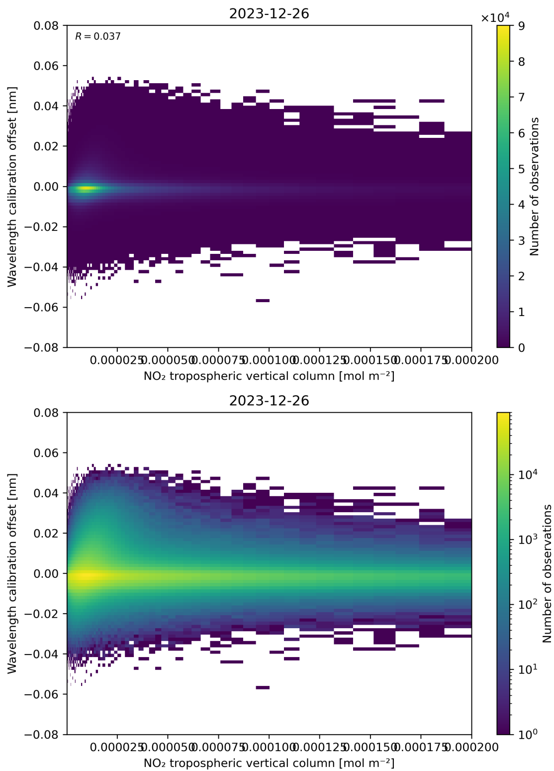
Figure 143: Scatter density plot of “NO 2 tropospheric vertical column” against “Wavelength calibration offset” for 2023-12-25 to 2023-12-27.
