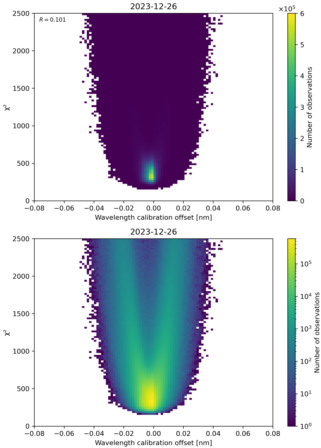
Figure 175: Scatter density plot of “Wavelength calibration offset” against “ \chi^2 ” for 2023-12-25 to 2023-12-27.
