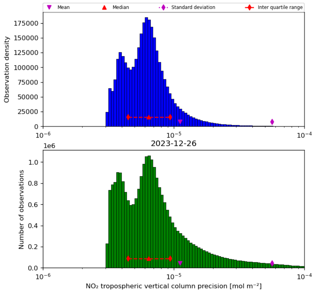
Figure 30: Histogram of “NO 2 tropospheric vertical column precision” for 2023-12-25 to 2023-12-27
