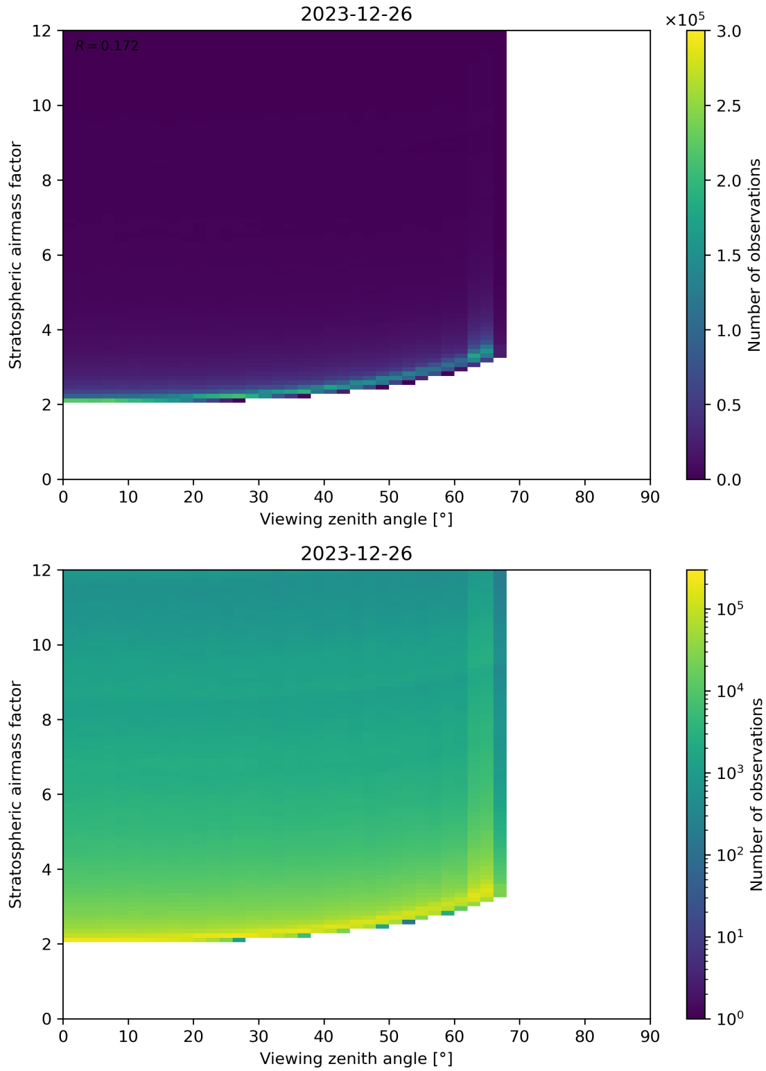
Figure 159: Scatter density plot of “Viewing zenith angle” against “Stratospheric airmass factor” for 2023-12-25 to 2023-12-27.
