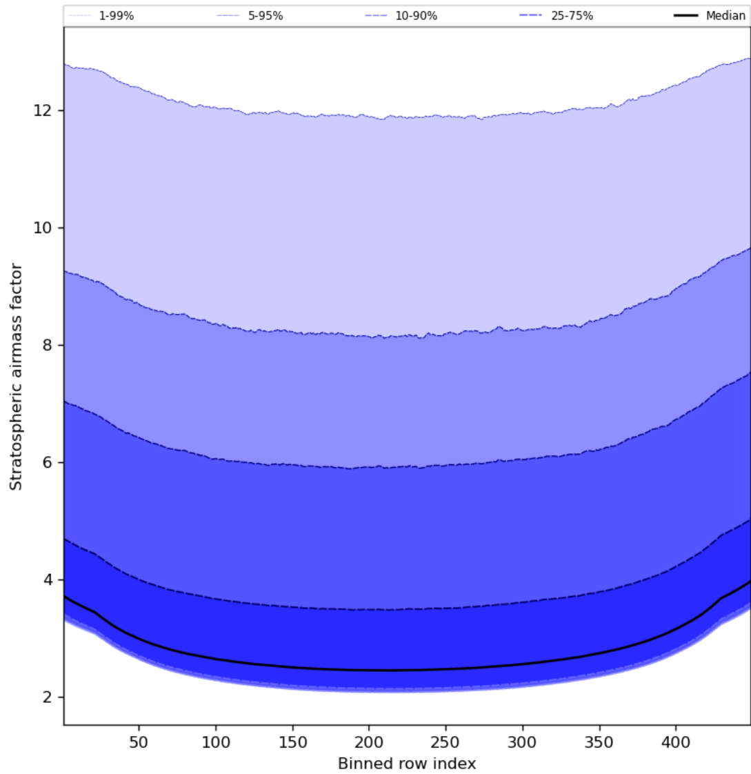
Figure 61: Along track statistics of “Stratospheric airmass factor” for 2023-12-25 to 2023-12-27
