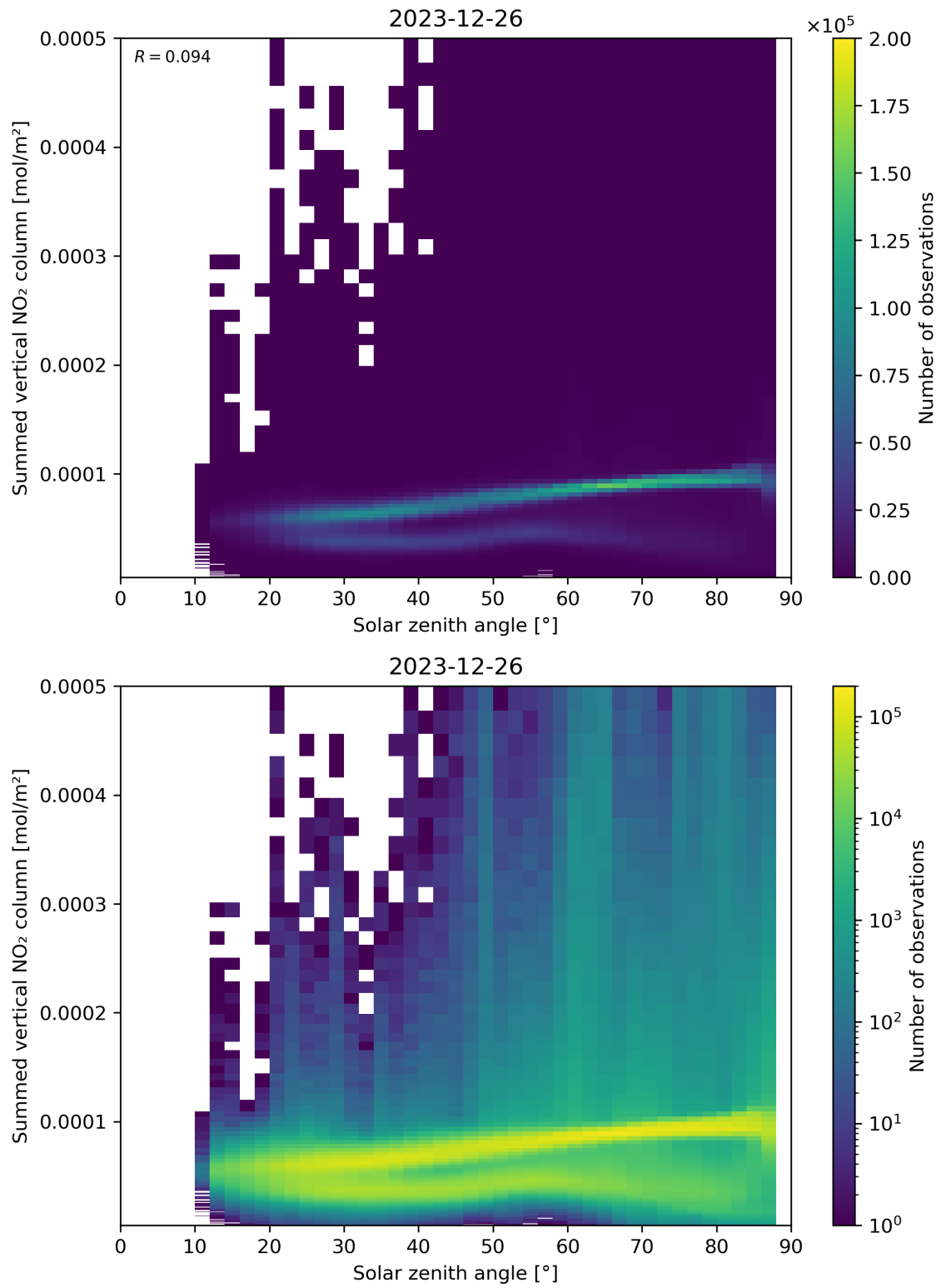
Figure 151: Scatter density plot of “Solar zenith angle” against “Summed vertical NO 2 column” for 2023-12-25 to 2023-12-27.
