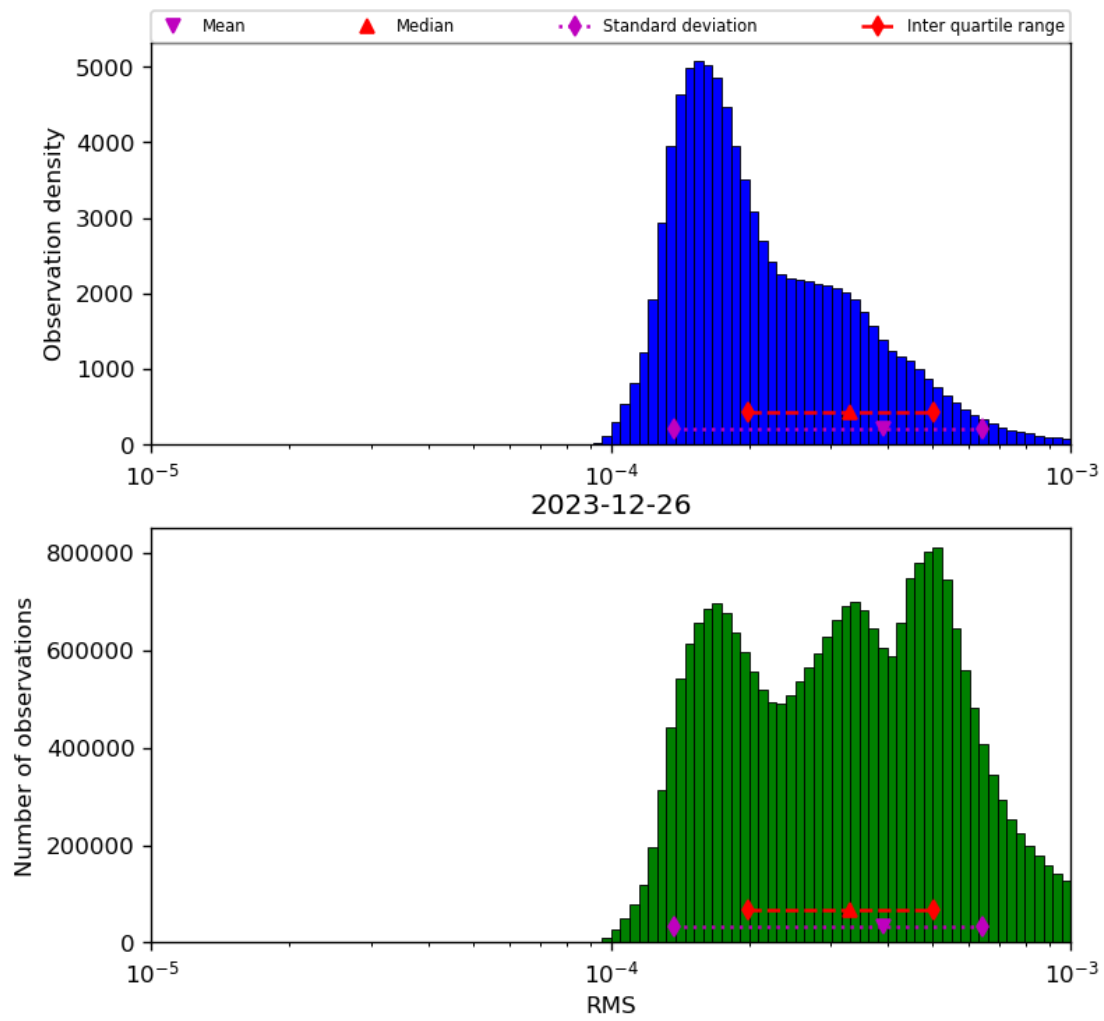
Figure 43: Histogram of “RMS” for 2023-12-25 to 2023-12-27
