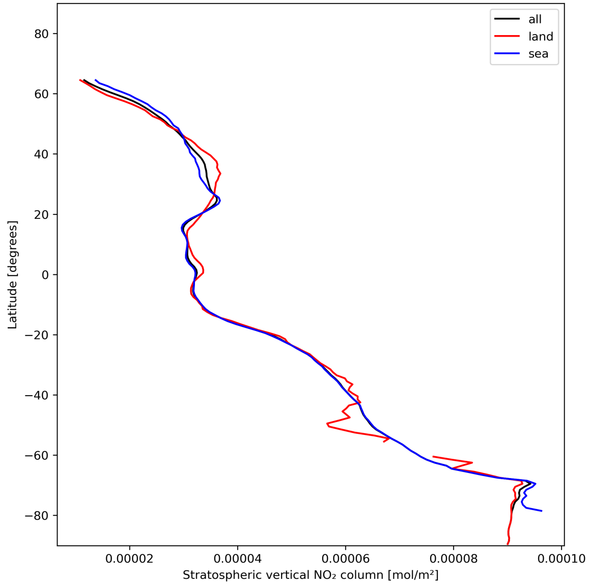
Figure 19: Zonal average of “Stratospheric vertical NO 2 column” for 2023-12-25 to 2023-12-27.
