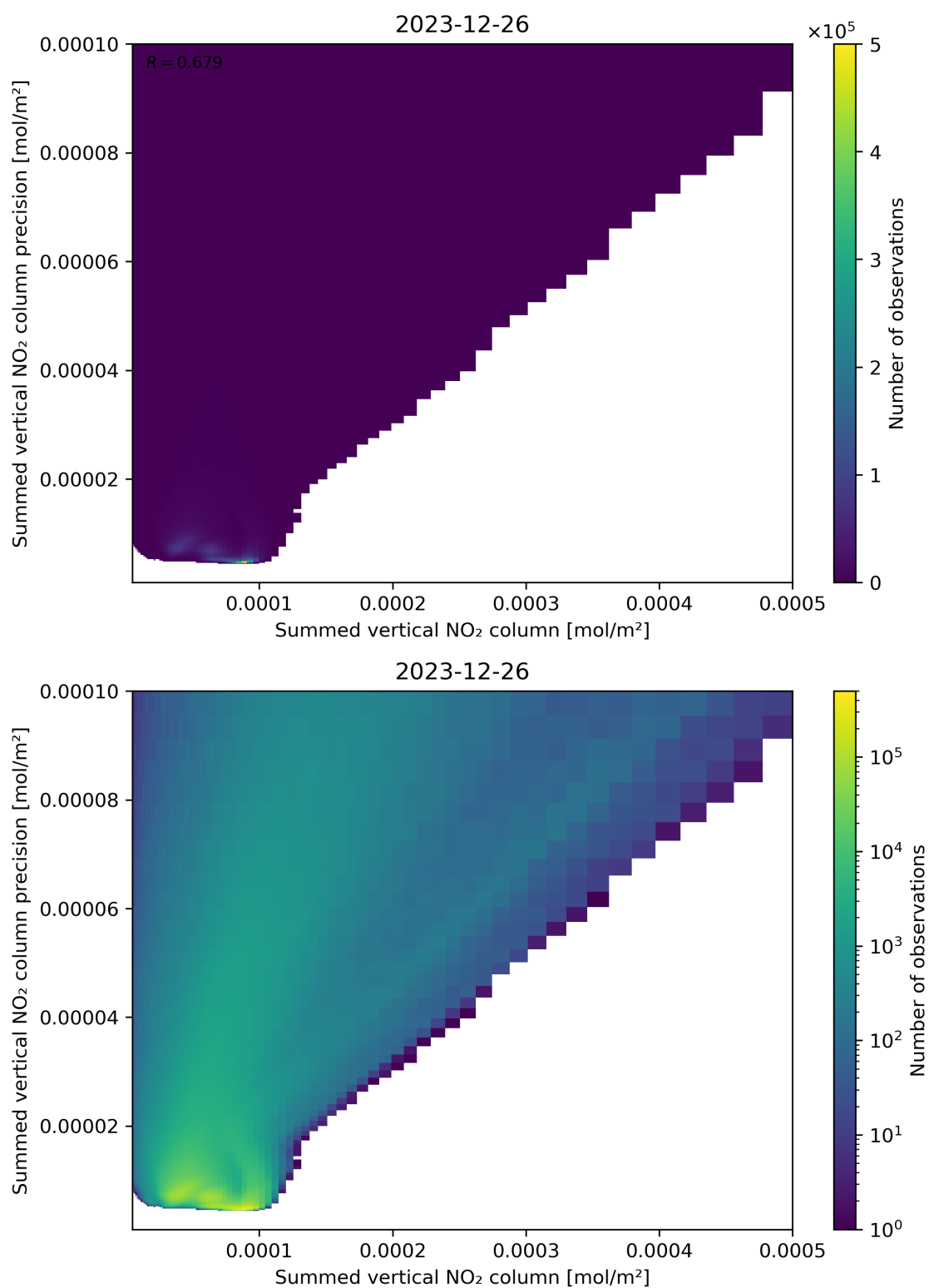
Figure 105: Scatter density plot of “Summed vertical NO 2 column” against “Summed vertical NO 2 column precision” for 2023-12-25 to 2023-12-27.
