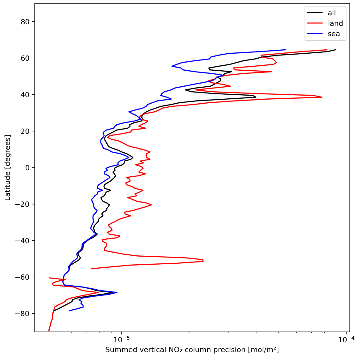
Figure 24: Zonal average of “Summed vertical NO 2 column precision” for 2023-12-25 to 2023-12-27.
