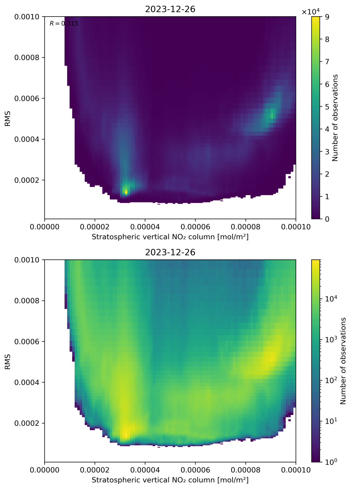
Figure 102: Scatter density plot of “Stratospheric vertical NO 2 column” against “RMS” for 2023-12-25 to 2023-12-27.
