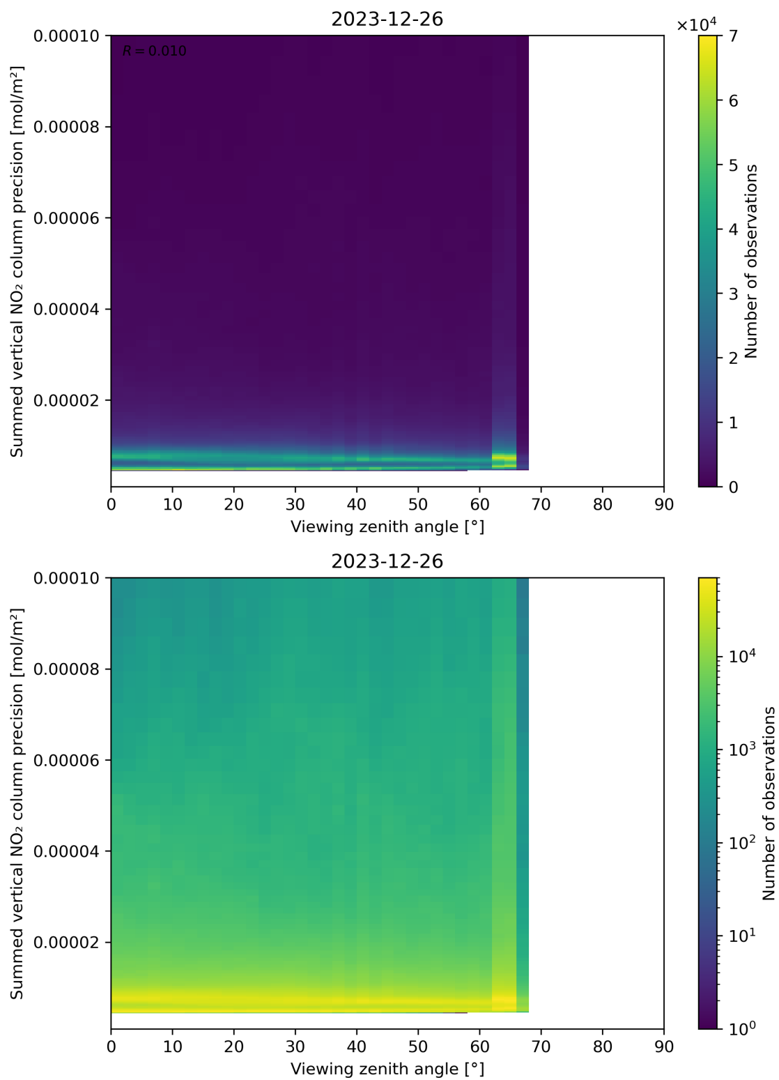
Figure 166: Scatter density plot of “Viewing zenith angle” against “Summed vertical NO 2 column precision” for 2023-12-25 to 2023-12-27.
