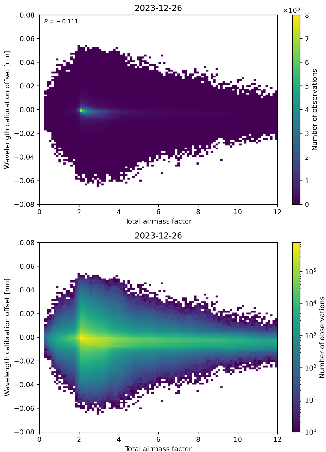
Figure 70: Scatter density plot of “Total airmass factor” against “Wavelength calibration offset” for 2023-12-25 to 2023-12-27.
