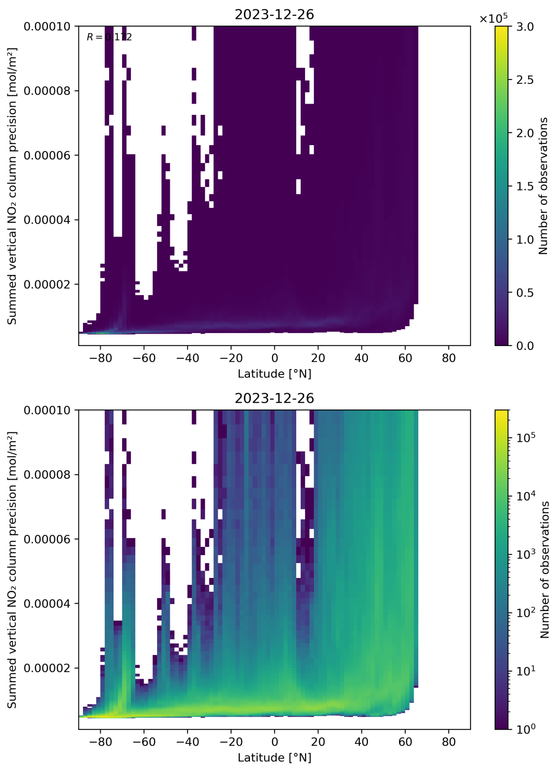
Figure 89: Scatter density plot of “Latitude” against “Summed vertical NO 2 column precision” for 2023-12-25 to 2023-12-27.
