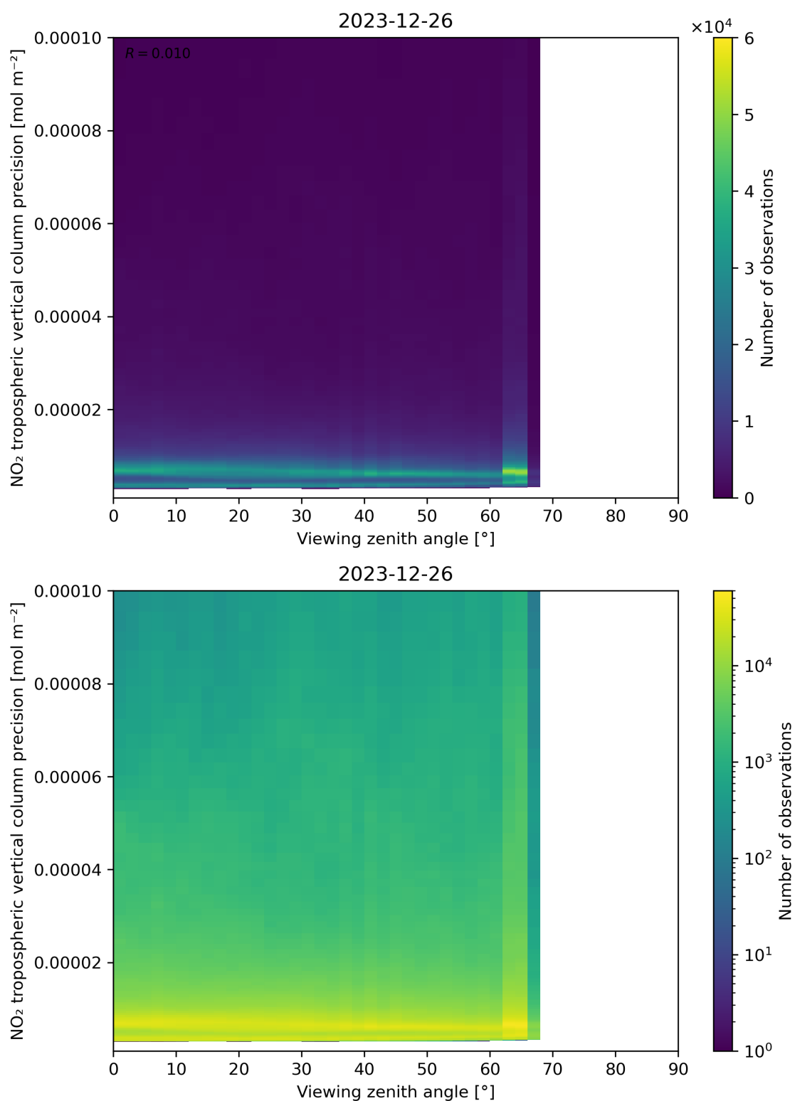
Figure 170: Scatter density plot of “Viewing zenith angle” against “NO 2 tropospheric vertical column precision” for 2023-12-25 to 2023-12-27.
