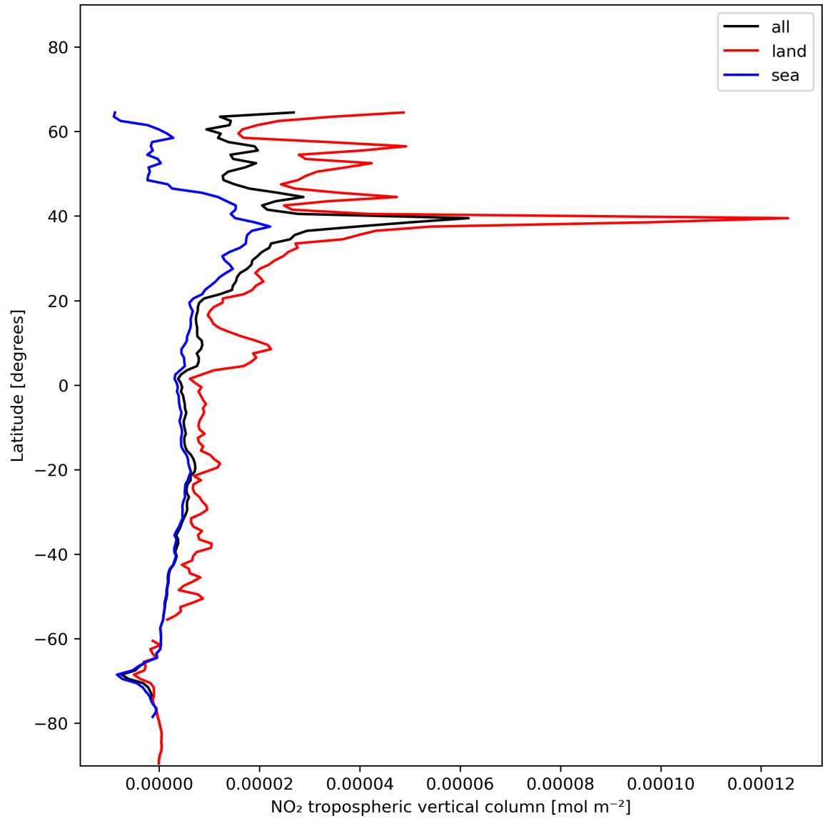
Figure 12: Zonal average of “NO 2 tropospheric vertical column” for 2023-12-25 to 2023-12-27.
