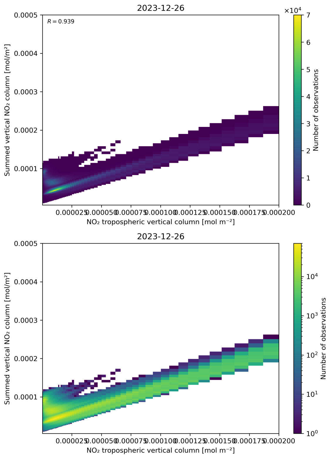
Figure 126: Scatter density plot of “NO 2 tropospheric vertical column” against “Summed vertical NO 2 column” for 2023-12-25 to 2023-12-27.
