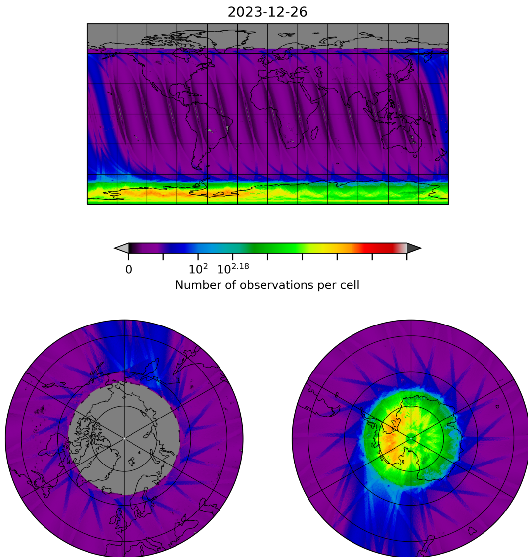
Figure 10: Map of the number of observations for 2023-12-25 to 2023-12-27
