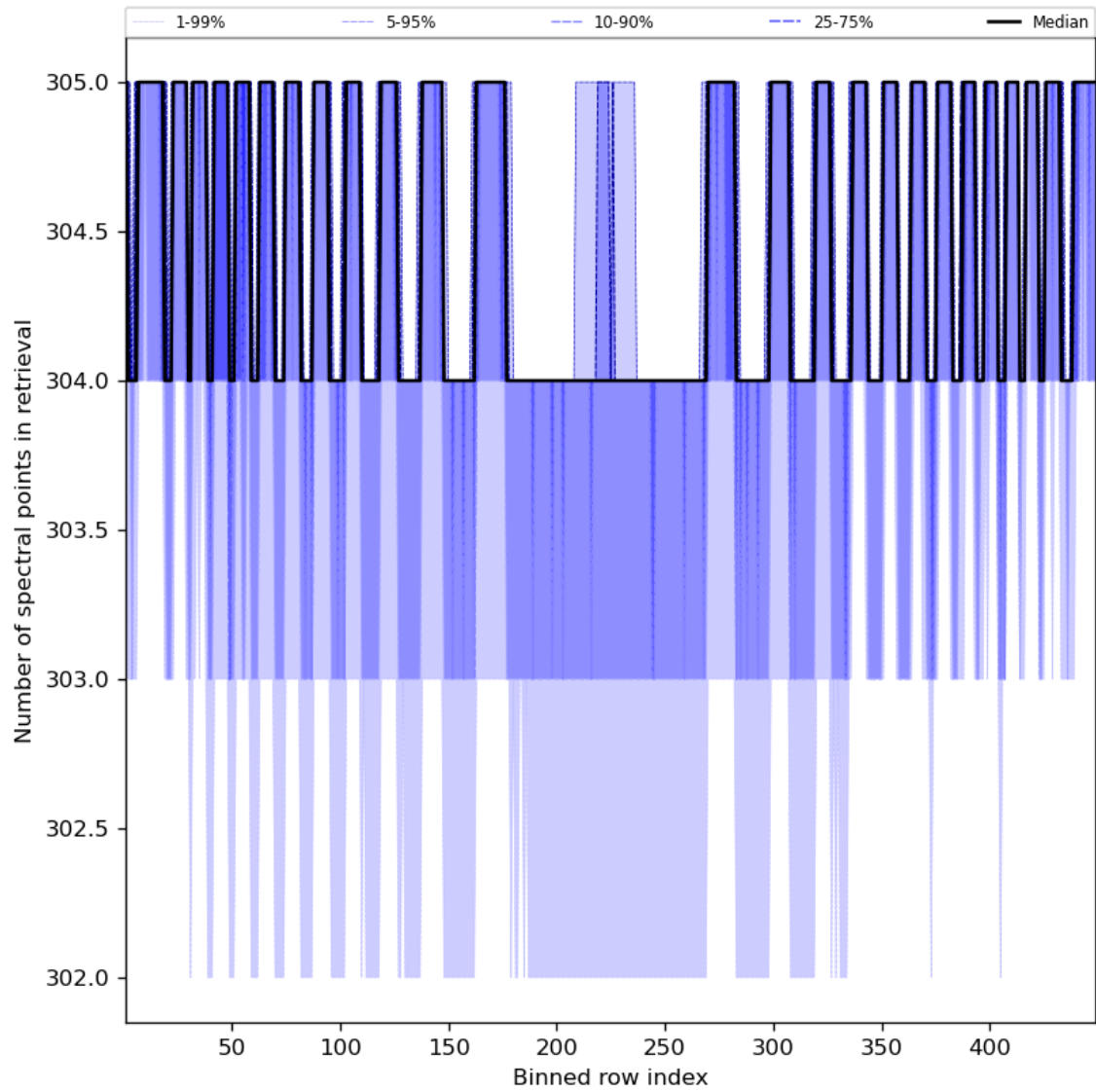
Figure 50: Along track statistics of “Number of spectral points in retrieval” for 2023-12-25 to 2023-12-27
