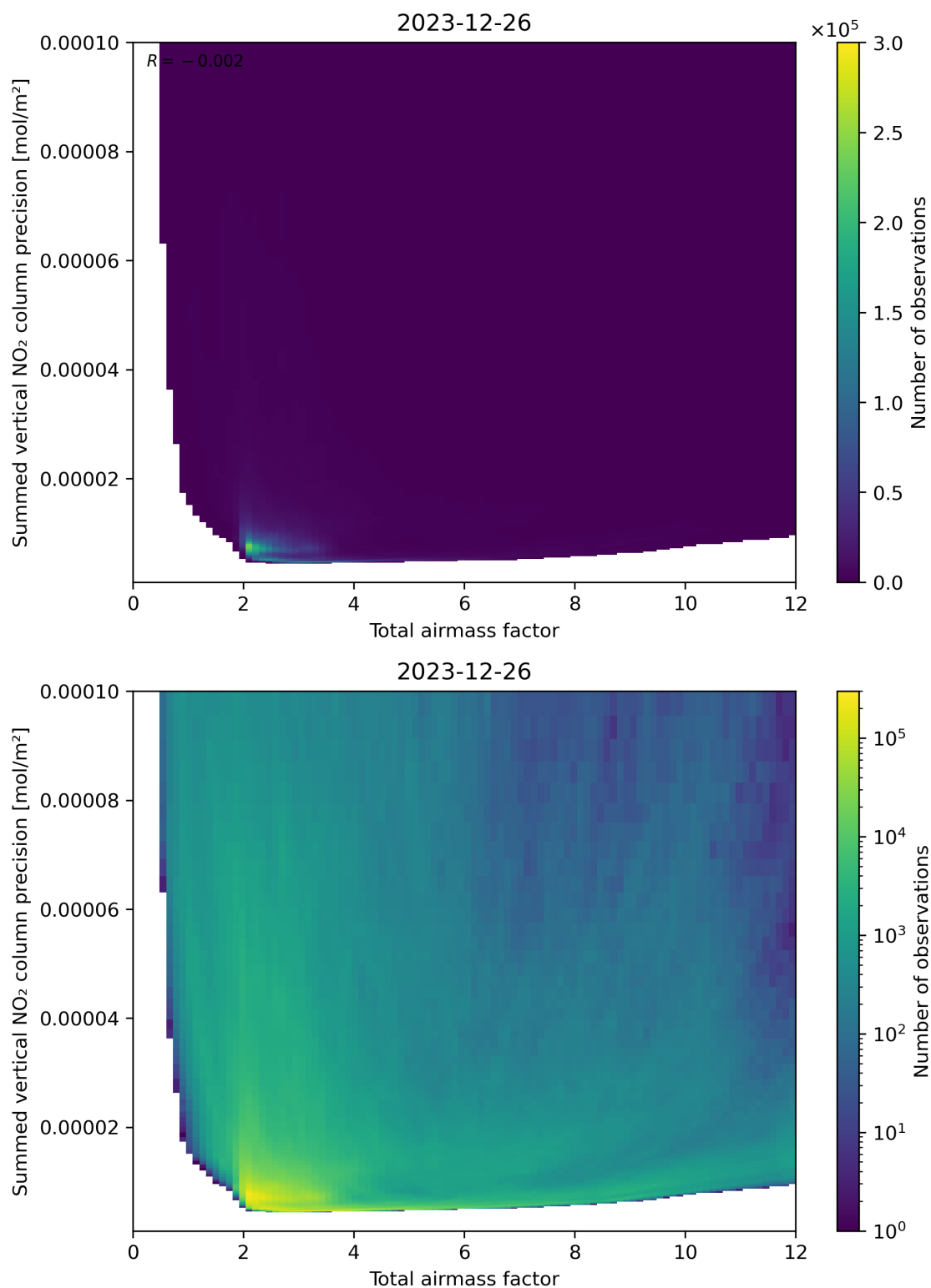
Figure 66: Scatter density plot of “Total airmass factor” against “Summed vertical NO 2 column precision” for 2023-12-25 to 2023-12-27.
