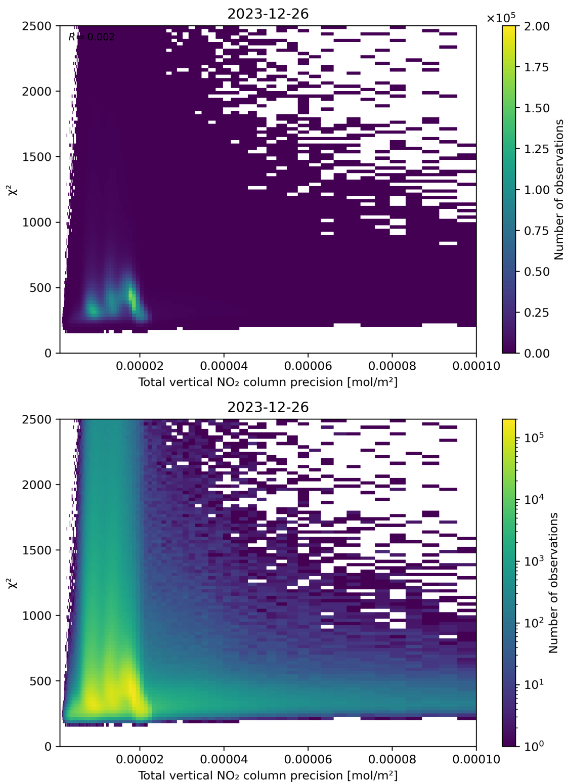
Figure 116: Scatter density plot of “Total vertical NO 2 column precision” against “ \chi^2 ” for 2023-12-25 to 2023-12-27.
