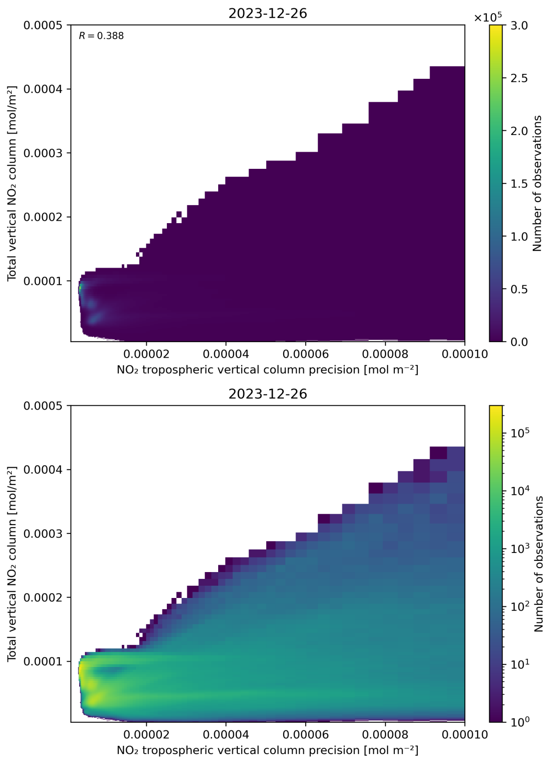
Figure 138: Scatter density plot of “NO 2 tropospheric vertical column precision” against “Total vertical NO 2 column” for 2023-12-25 to 2023-12-27.
