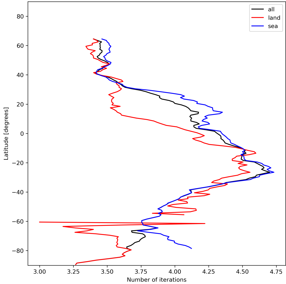
Figure 17: Zonal average of “Number of iterations” for 2023-12-25 to 2023-12-27.
