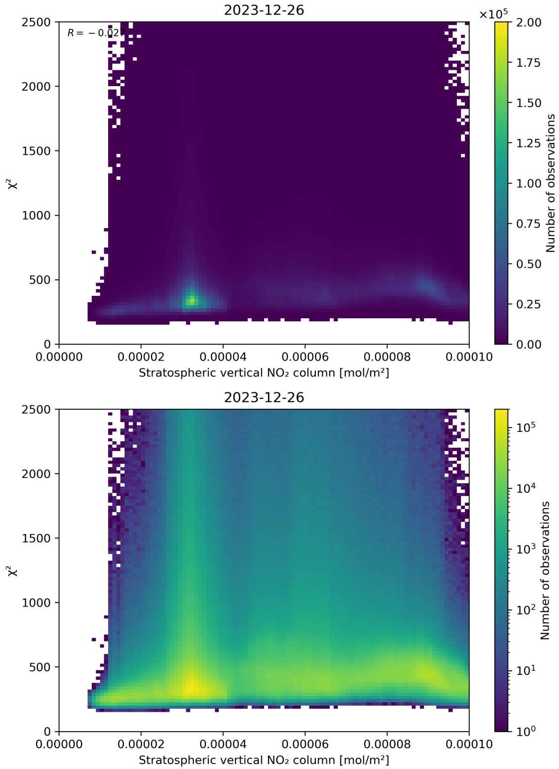
Figure 97: Scatter density plot of “Stratospheric vertical NO 2 column” against “ \chi^2 ” for 2023-12-25 to 2023-12-27.
