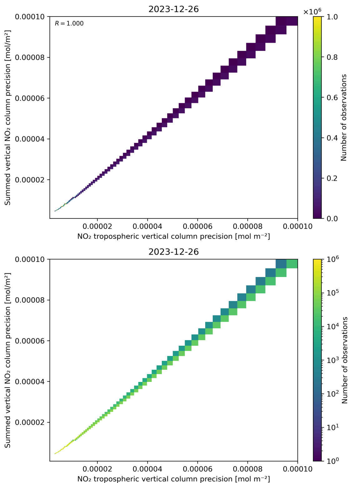
Figure 137: Scatter density plot of “NO 2 tropospheric vertical column precision” against “Summed vertical NO 2 column precision” for 2023-12-25 to 2023-12-27.
