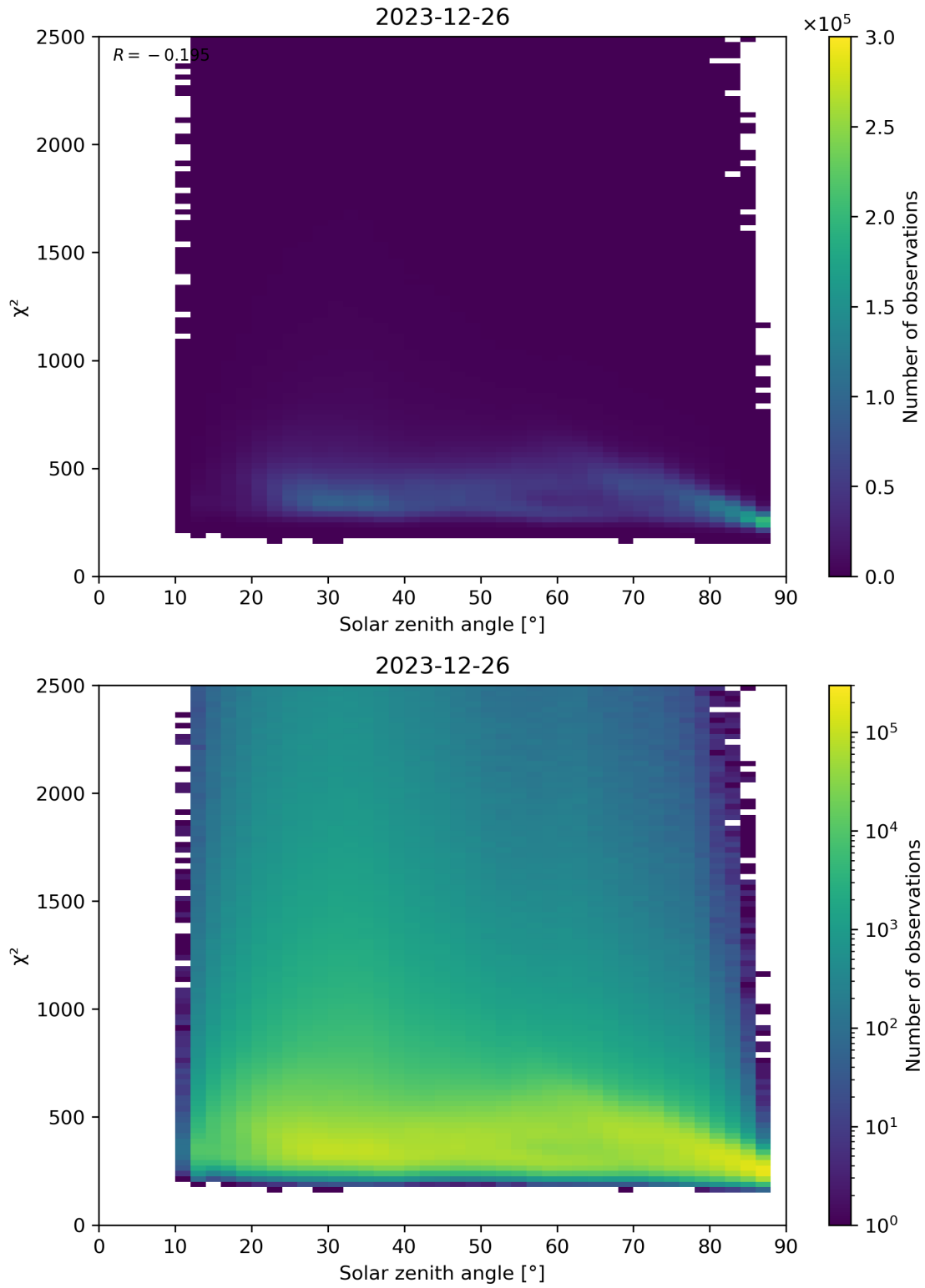
Figure 148: Scatter density plot of “Solar zenith angle” against “ \chi^2 ” for 2023-12-25 to 2023-12-27.
