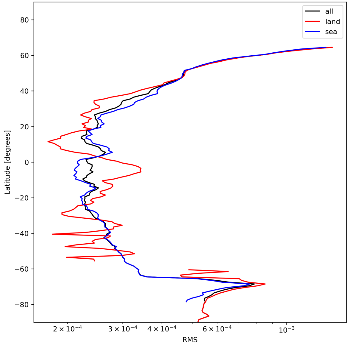
Figure 26: Zonal average of “RMS” for 2023-12-25 to 2023-12-27.
