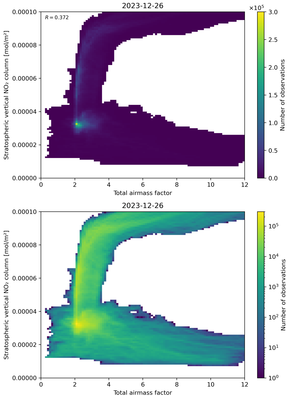
Figure 64: Scatter density plot of “Total airmass factor” against “Stratospheric vertical \text{NO}_2 column” for 2023-12-25 to 2023-12-27.
