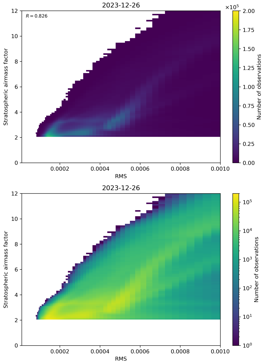
Figure 144: Scatter density plot of “RMS” against “Stratospheric airmass factor” for 2023-12-25 to 2023-12-27.
