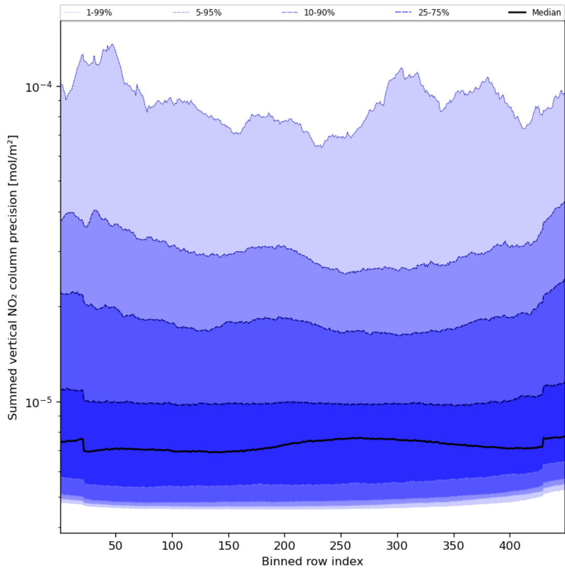
Figure 58: Along track statistics of “Summed vertical NO 2 column precision” for 2023-12-25 to 2023-12-27
