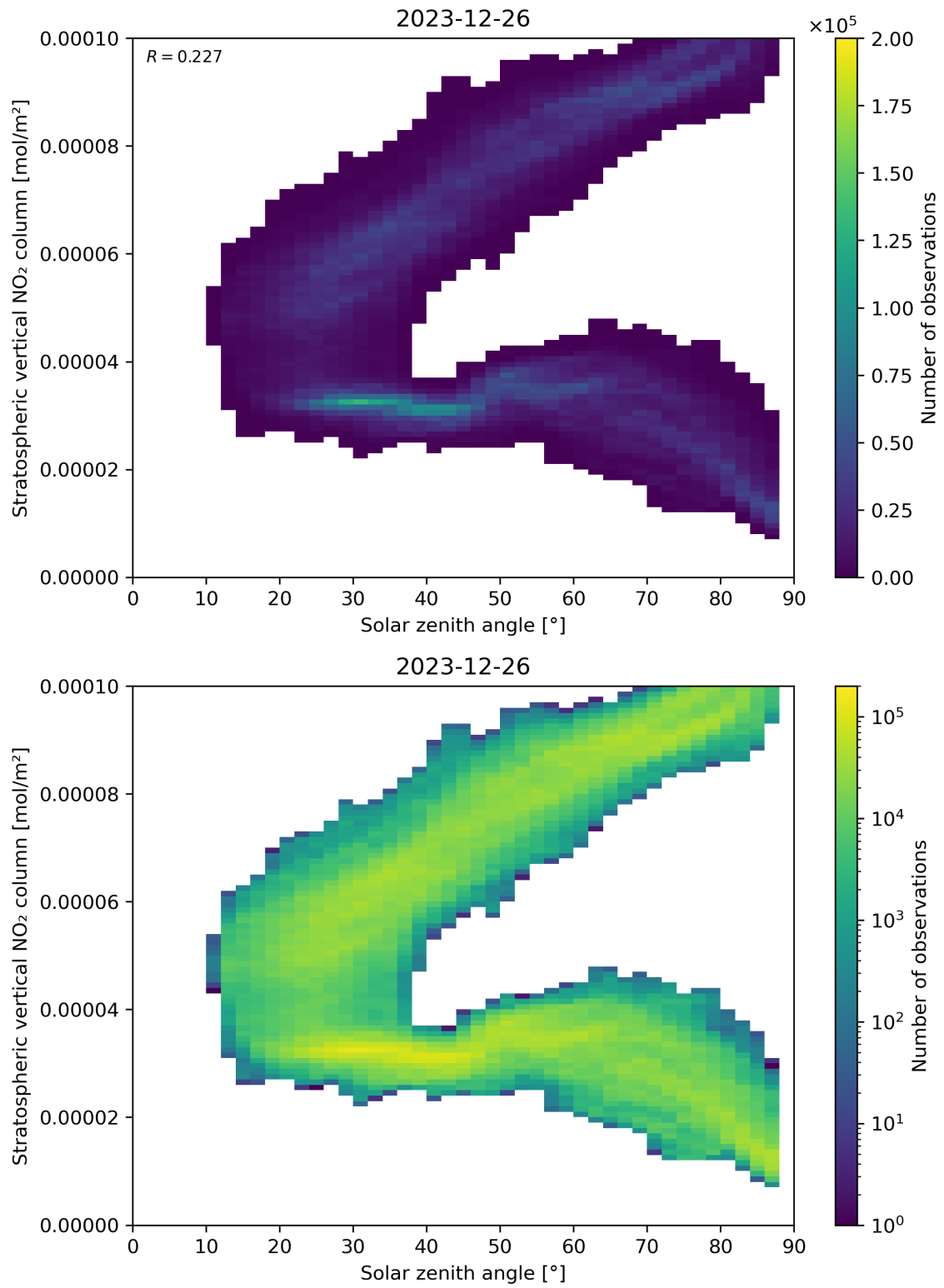
Figure 150: Scatter density plot of “Solar zenith angle” against “Stratospheric vertical NO 2 column” for 2023-12-25 to 2023-12-27.
