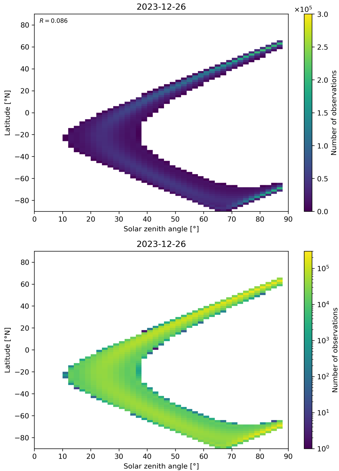
Figure 149: Scatter density plot of “Solar zenith angle” against “Latitude” for 2023-12-25 to 2023-12-27.
