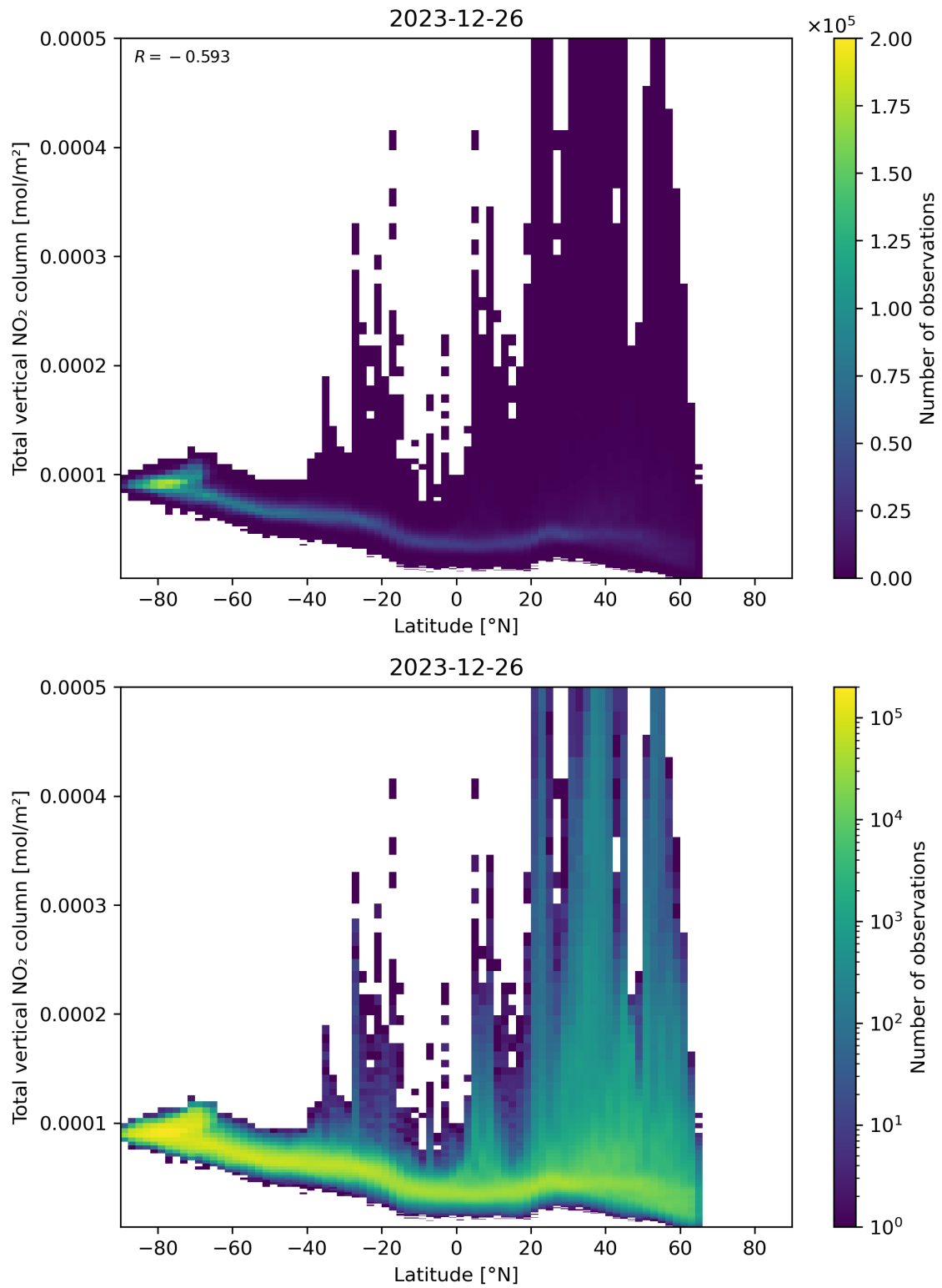
Figure 90: Scatter density plot of “Latitude” against “Total vertical NO 2 column” for 2023-12-25 to 2023-12-27.
