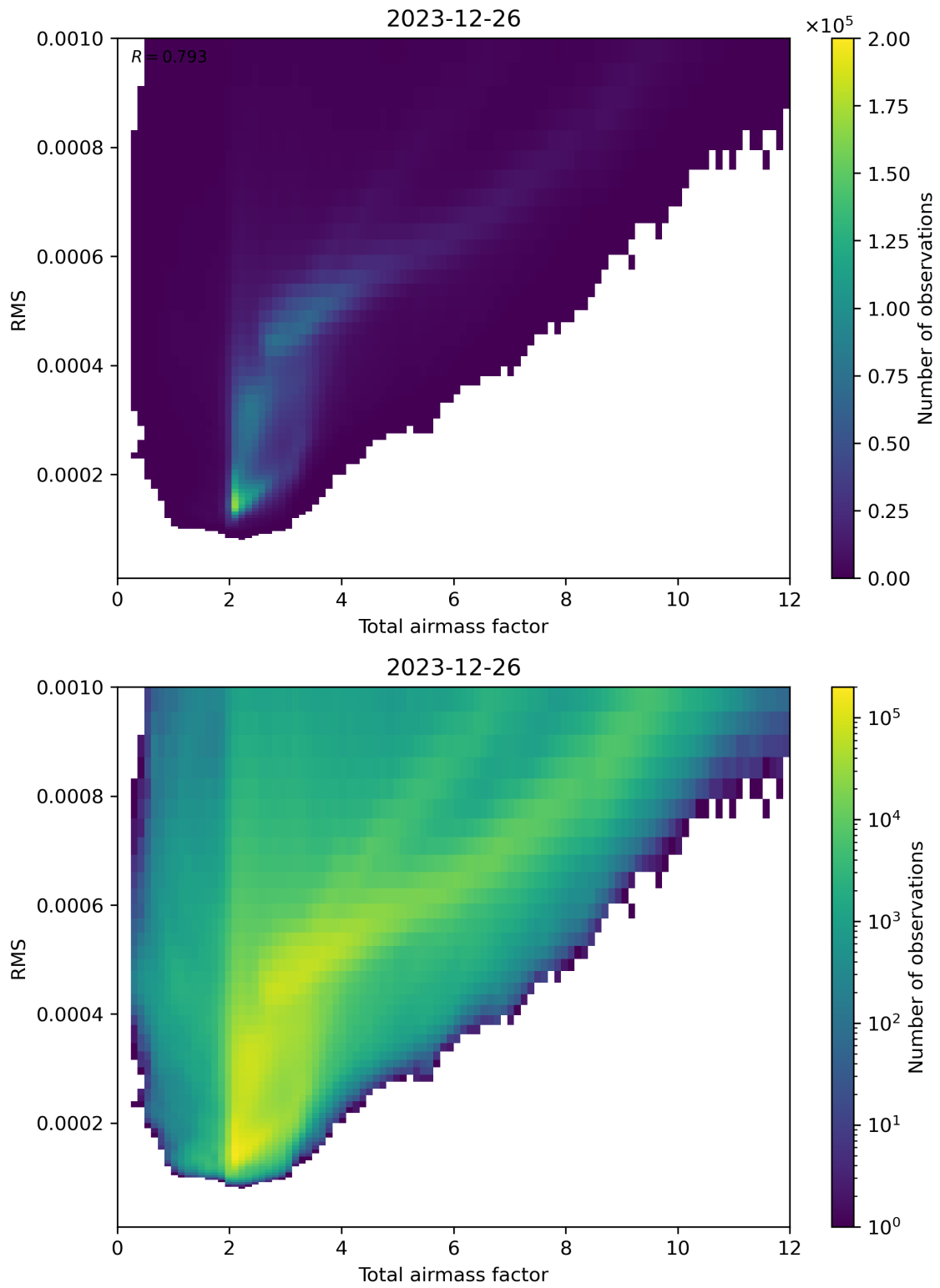
Figure 69: Scatter density plot of “Total airmass factor” against “RMS” for 2023-12-25 to 2023-12-27.
