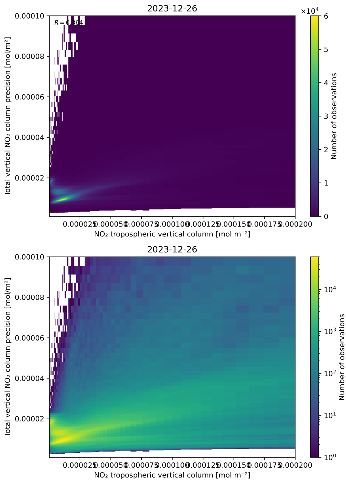
Figure 129: Scatter density plot of “NO 2 tropospheric vertical column” against “Total vertical NO 2 column precision” for 2023-12-25 to 2023-12-27.
