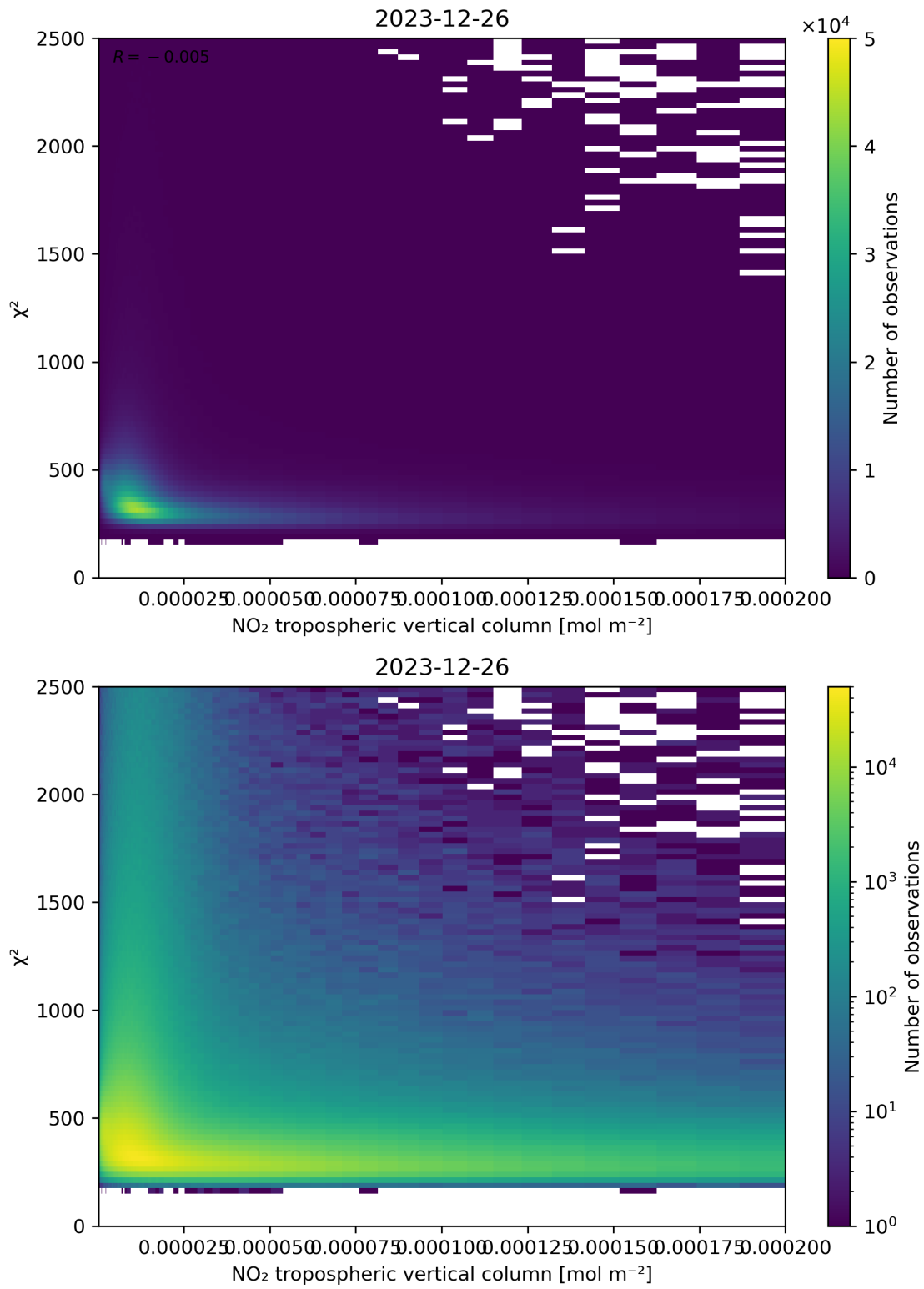
Figure 124: Scatter density plot of “NO 2 tropospheric vertical column” against “ \chi^2 ” for 2023-12-25 to 2023-12-27.
