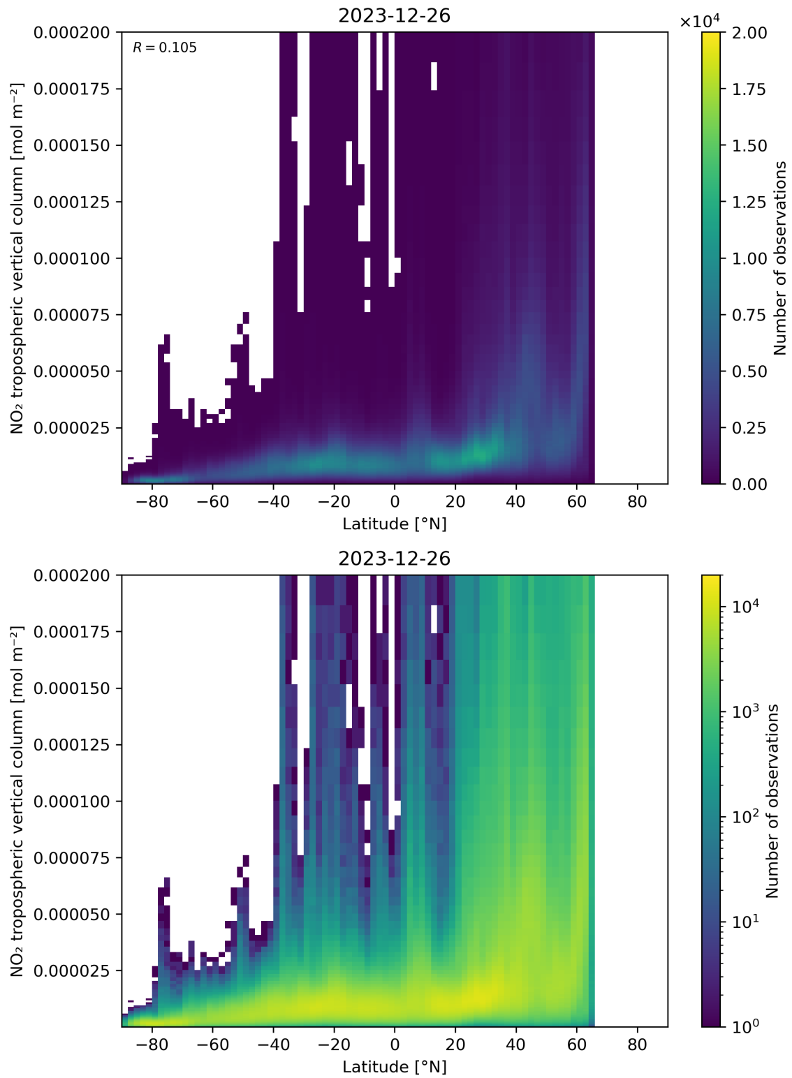
Figure 92: Scatter density plot of “Latitude” against “NO 2 tropospheric vertical column” for 2023-12-25 to 2023-12-27.
