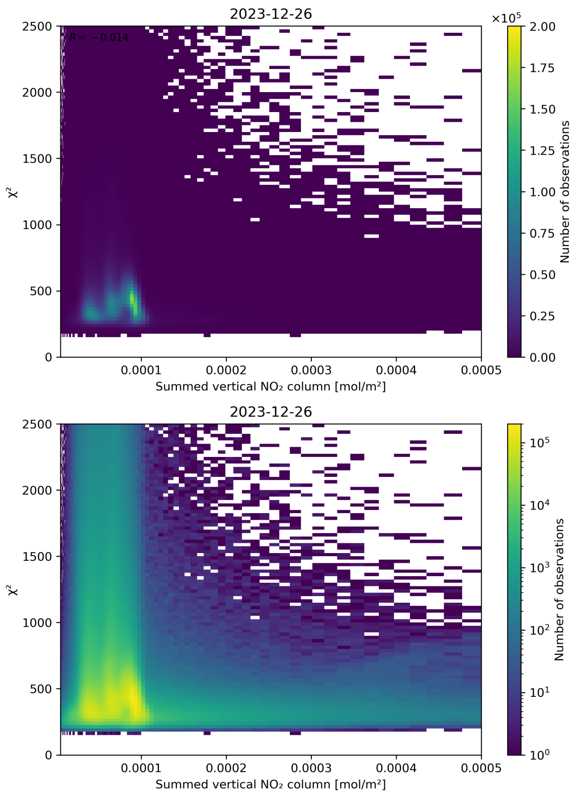
Figure 104: Scatter density plot of “Summed vertical NO 2 column” against “ \chi^2 ” for 2023-12-25 to 2023-12-27.
