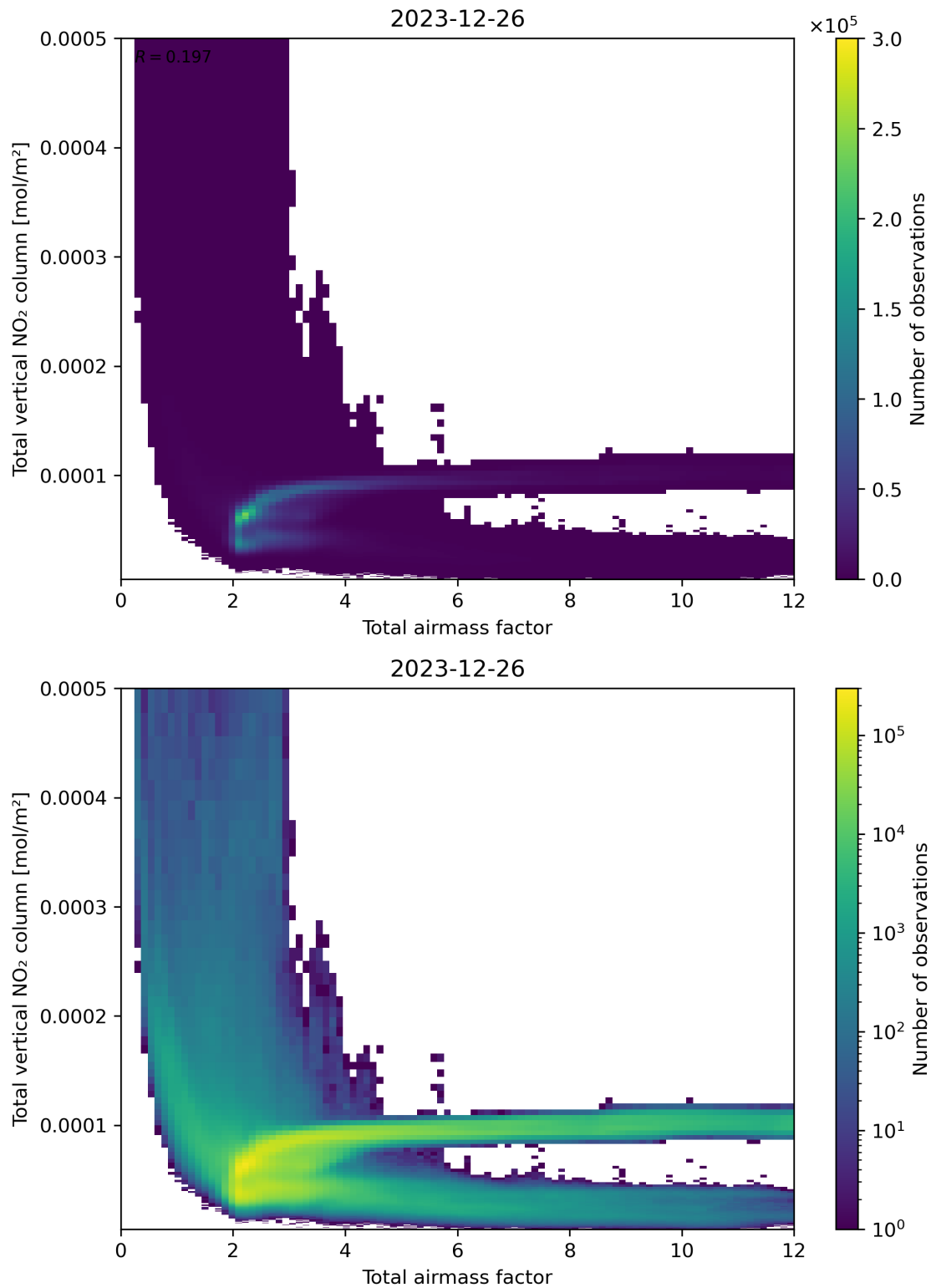
Figure 67: Scatter density plot of “Total airmass factor” against “Total vertical NO 2 column” for 2023-12-25 to 2023-12-27.
