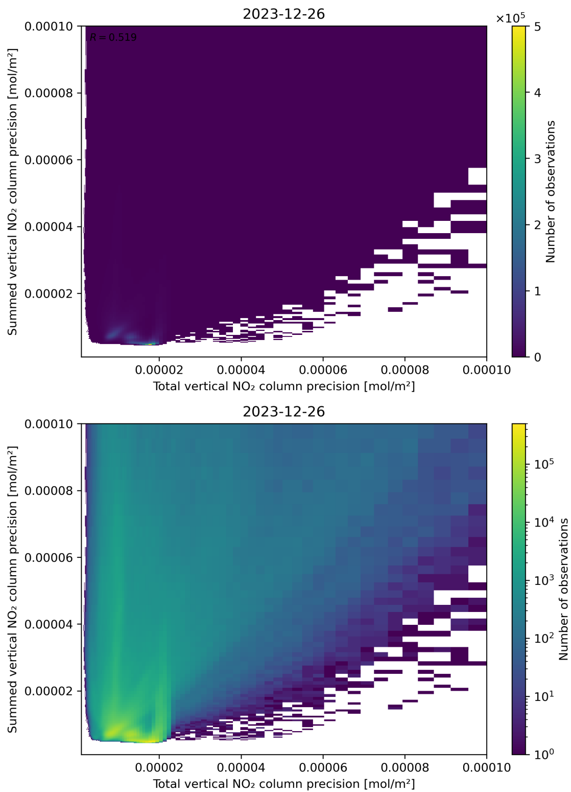
Figure 118: Scatter density plot of “Total vertical NO 2 column precision” against “Summed vertical NO 2 column precision” for 2023-12-25 to 2023-12-27.
