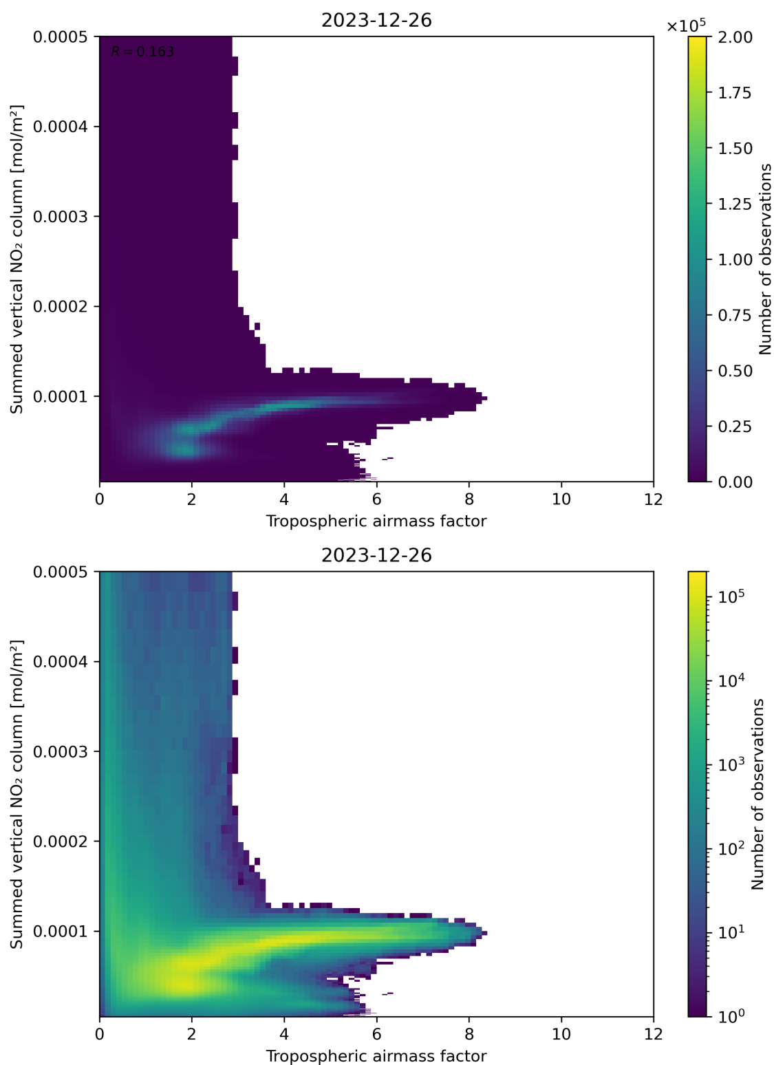
Figure 75: Scatter density plot of “Tropospheric airmass factor” against “Summed vertical NO 2 column” for 2023-12-25 to 2023-12-27.
