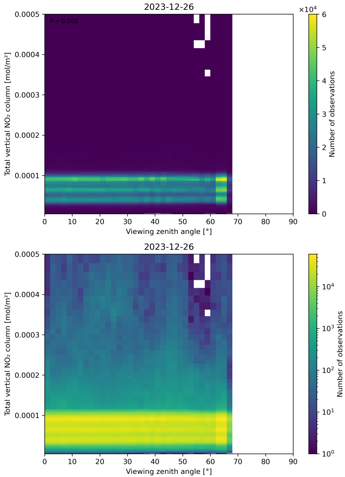
Figure 167: Scatter density plot of “Viewing zenith angle” against “Total vertical NO 2 column” for 2023-12-25 to 2023-12-27.
