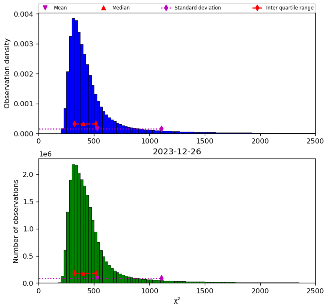
Figure 42: Histogram of “ \chi^2 ” for 2023-12-25 to 2023-12-27
