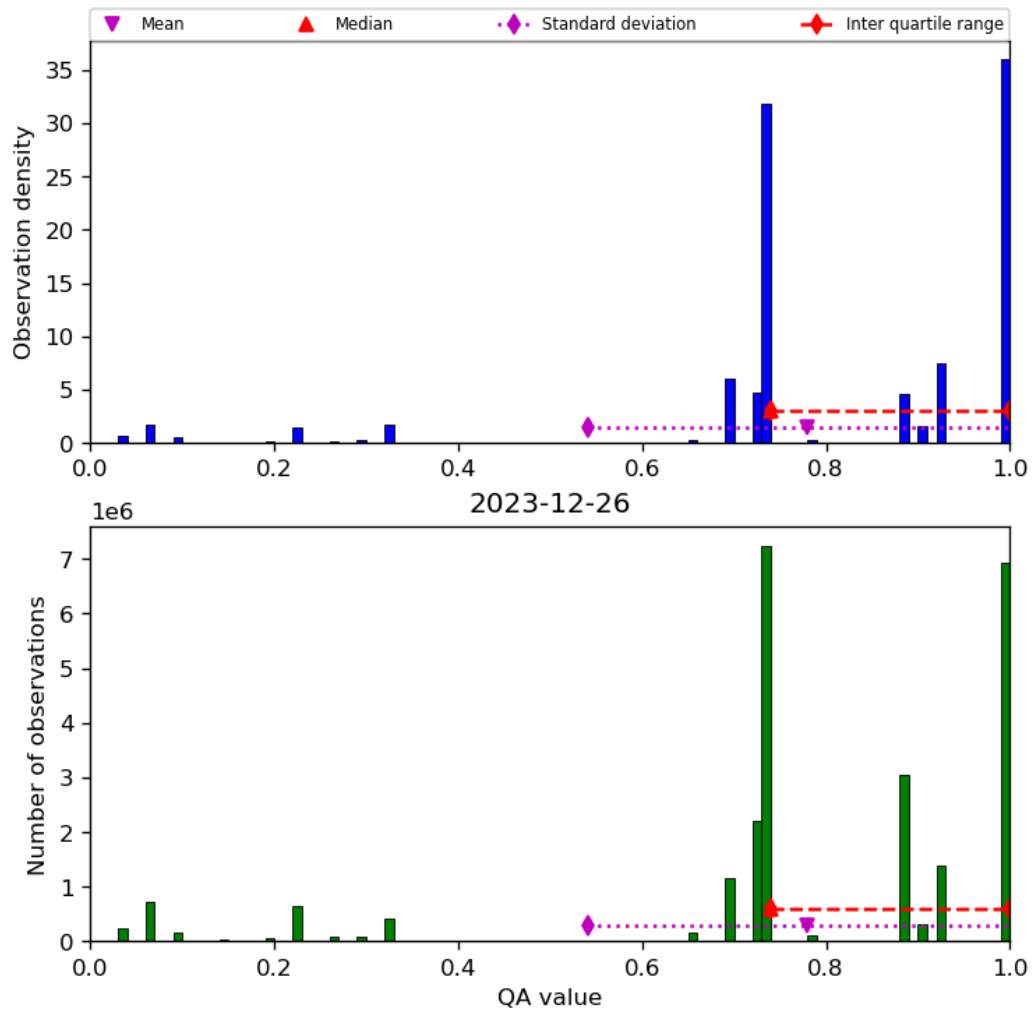
Figure 28: Histogram of “QA value” for 2023-12-25 to 2023-12-27
