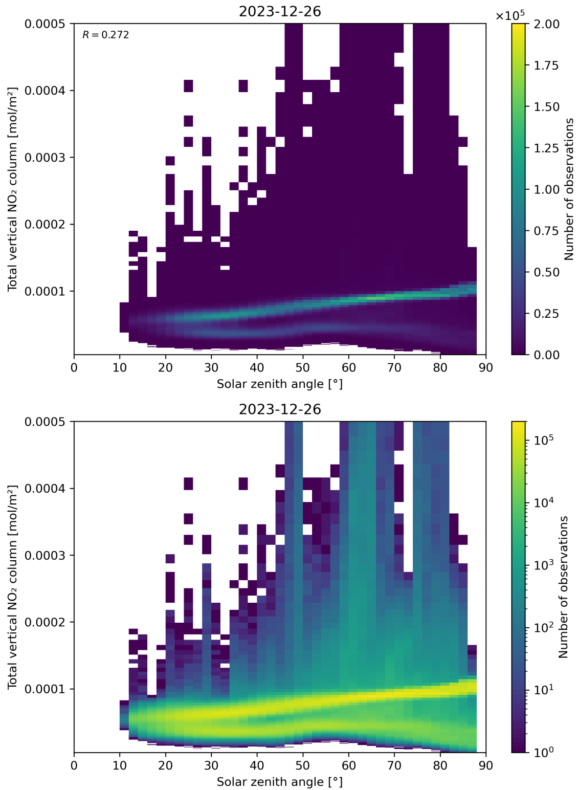
Figure 153: Scatter density plot of “Solar zenith angle” against “Total vertical NO 2 column” for 2023-12-25 to 2023-12-27.
