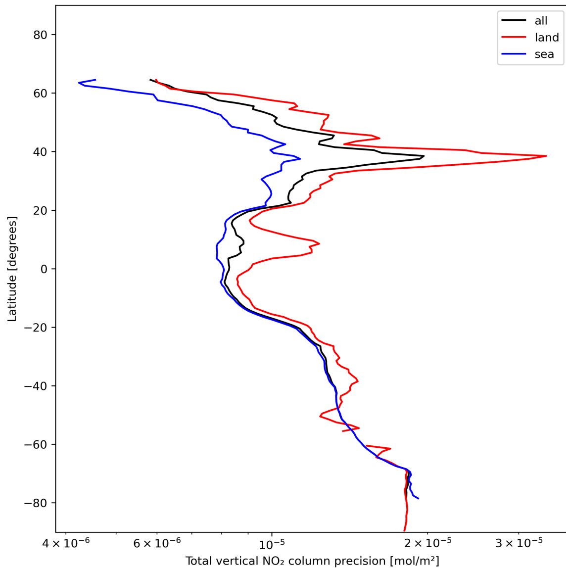
Figure 22: Zonal average of “Total vertical NO 2 column precision” for 2023-12-25 to 2023-12-27.
