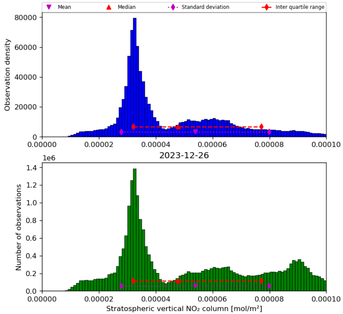
Figure 36: Histogram of “Stratospheric vertical NO 2 column” for 2023-12-25 to 2023-12-27
