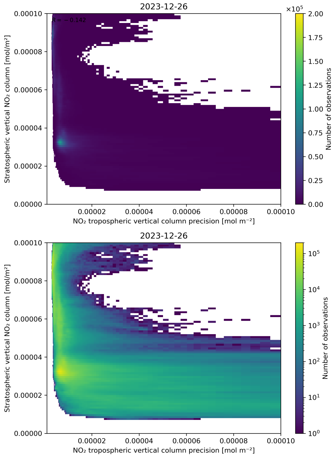
Figure 135: Scatter density plot of “NO 2 tropospheric vertical column precision” against “Stratospheric vertical NO 2 column” for 2023-12-25 to 2023-12-27.
