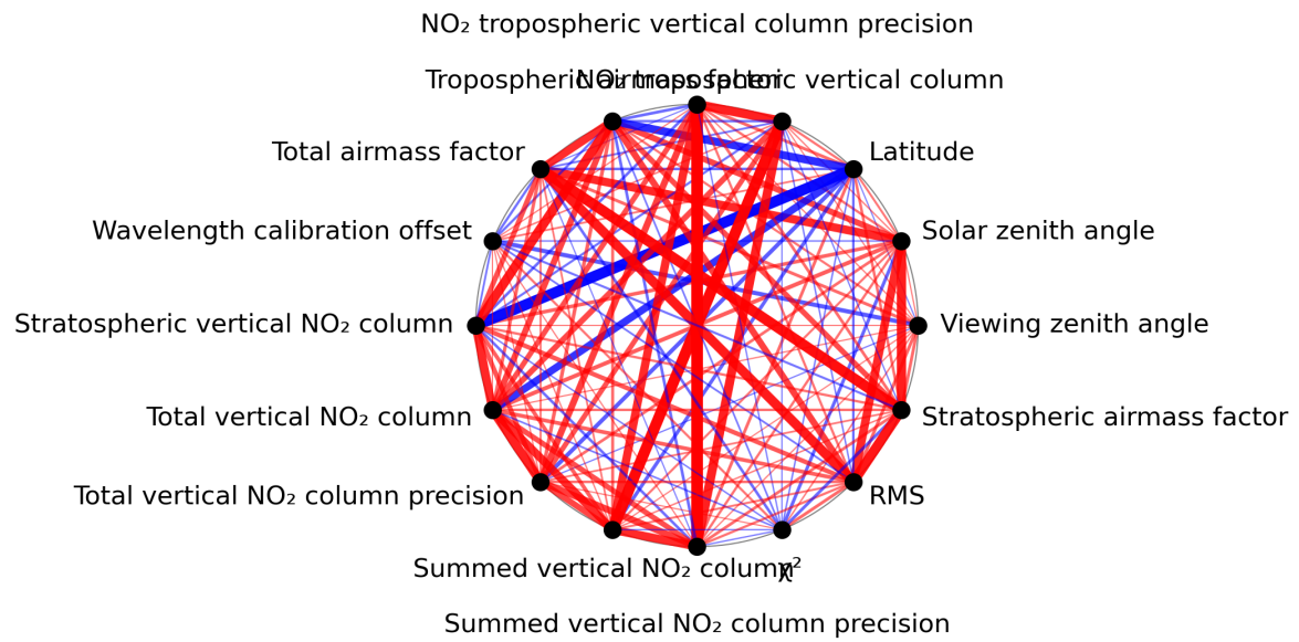
Figure 1: Map of correlation graph for 2023-12-25 to 2023-12-27.
