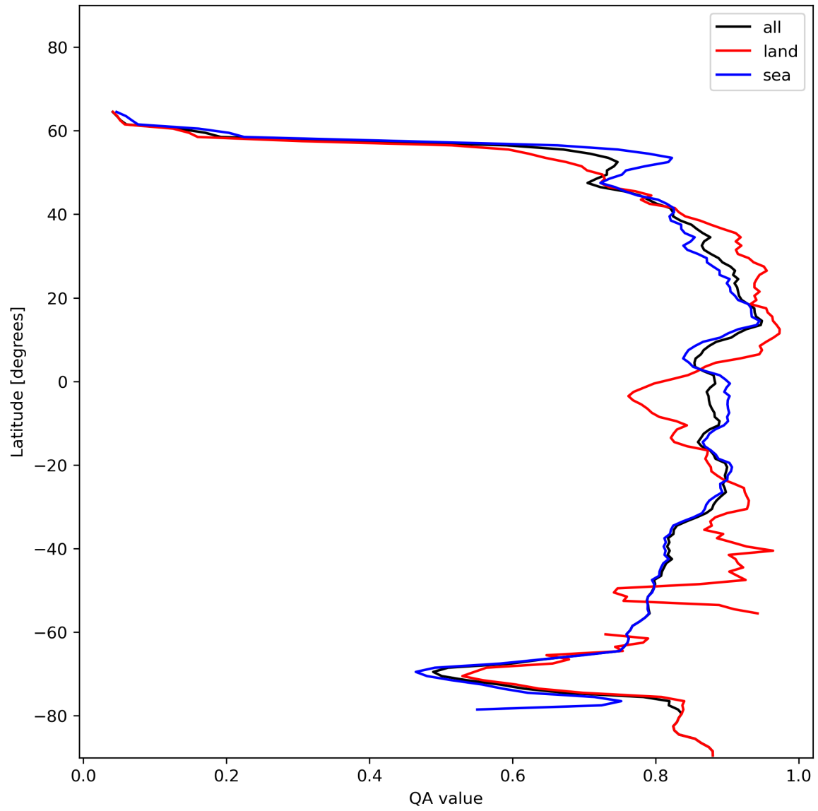
Figure 11: Zonal average of “QA value” for 2023-12-25 to 2023-12-27.
