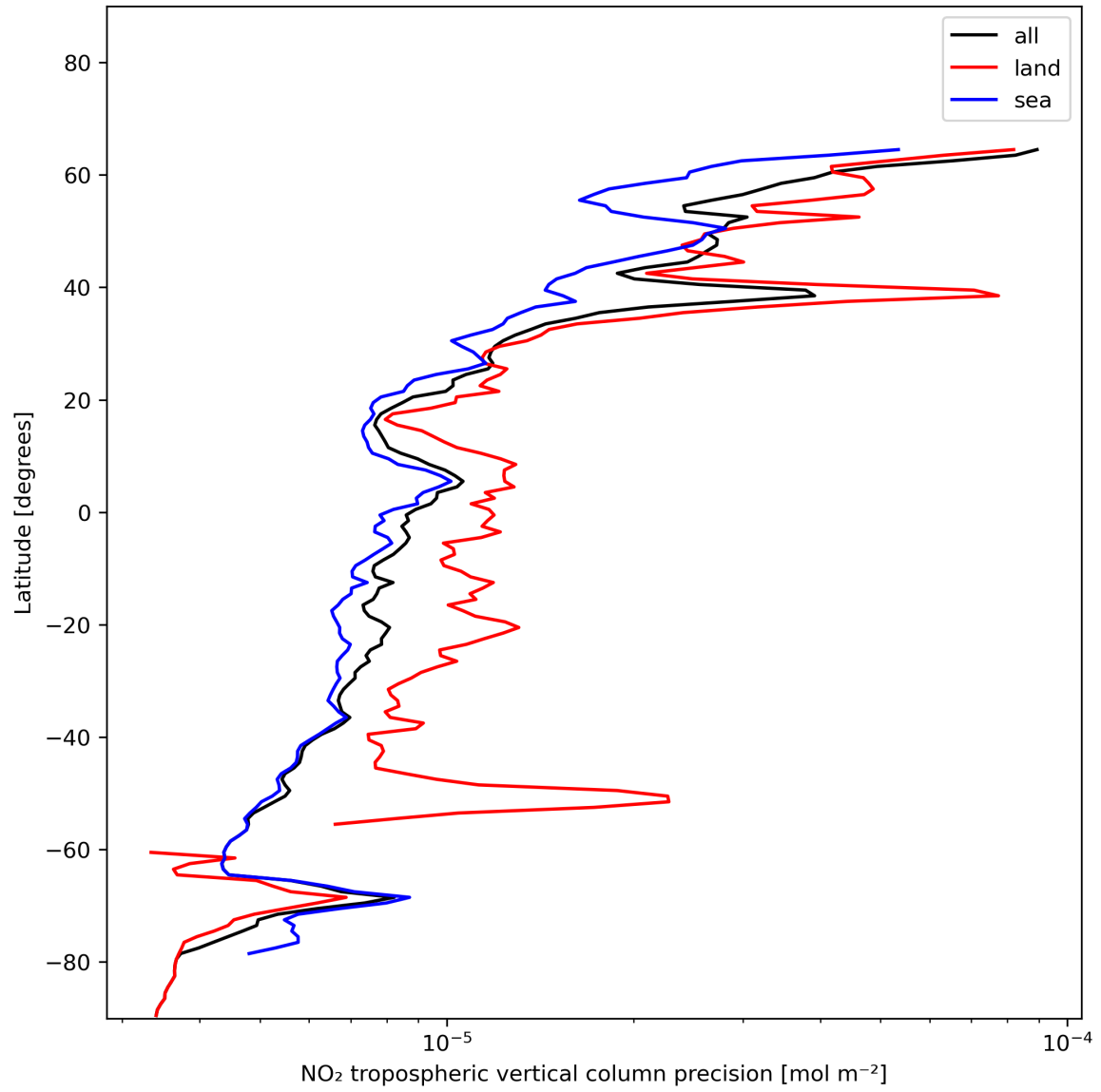
Figure 13: Zonal average of “NO 2 tropospheric vertical column precision” for 2023-12-25 to 2023-12-27.
