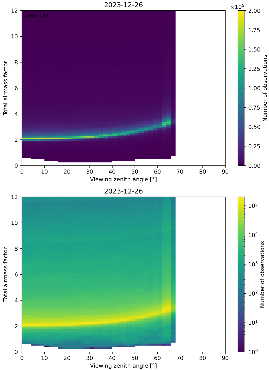
Figure 160: Scatter density plot of “Viewing zenith angle” against “Total airmass factor” for 2023-12-25 to 2023-12-27.
