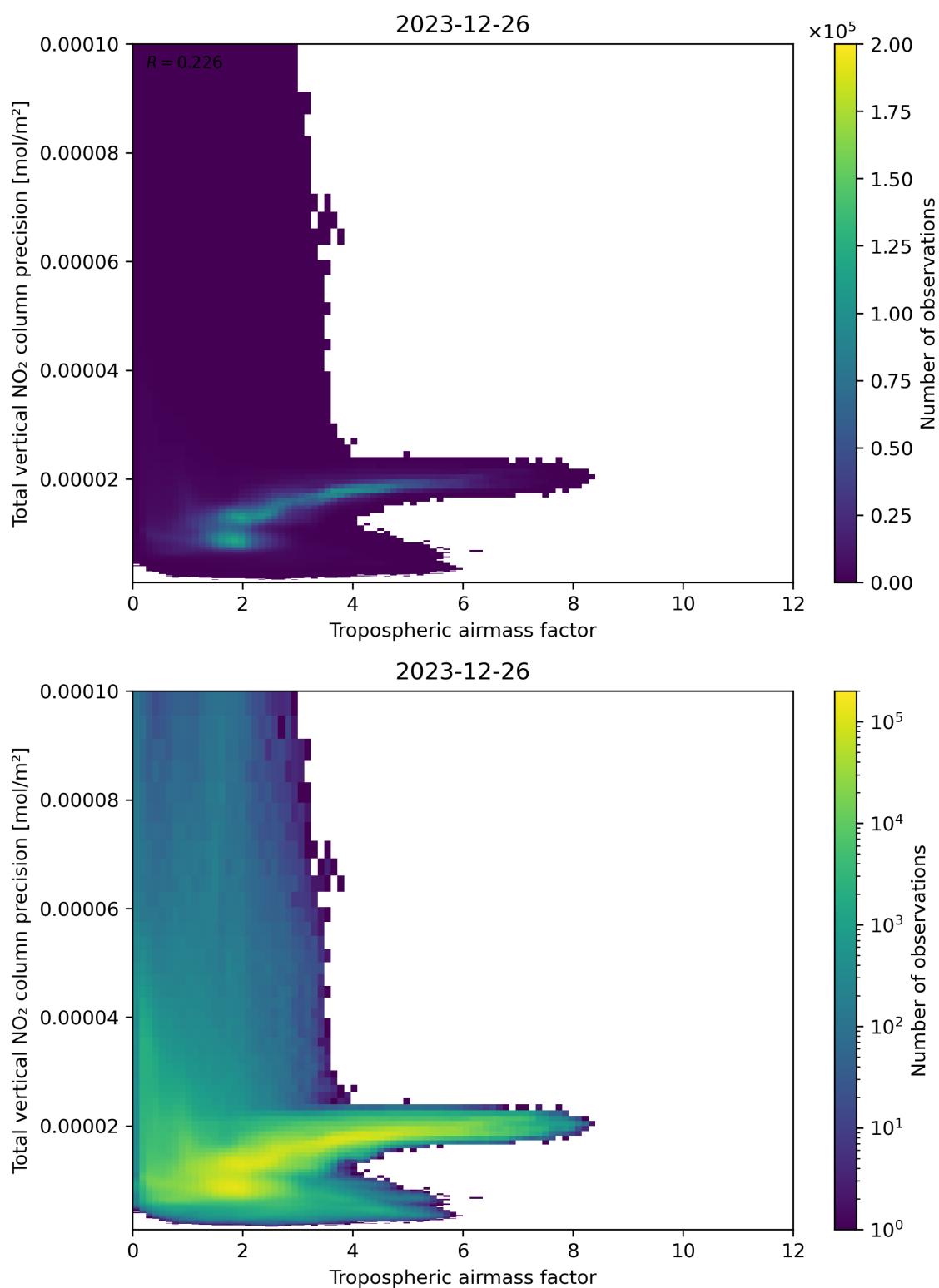
Figure 78: Scatter density plot of “Tropospheric air mass factor” against “Total vertical NO 2 column precision” for 2023-12-25 to 2023-12-27.
