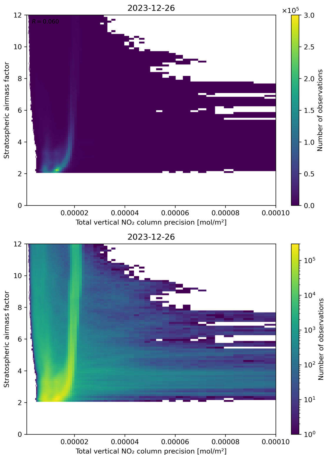
Figure 115: Scatter density plot of “Total vertical NO 2 column precision” against “Stratospheric air mass factor” for 2023-12-25 to 2023-12-27.
