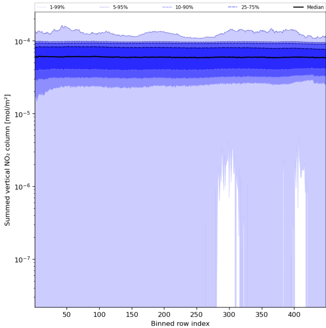
Figure 57: Along track statistics of “Summed vertical NO 2 column” for 2023-12-25 to 2023-12-27
