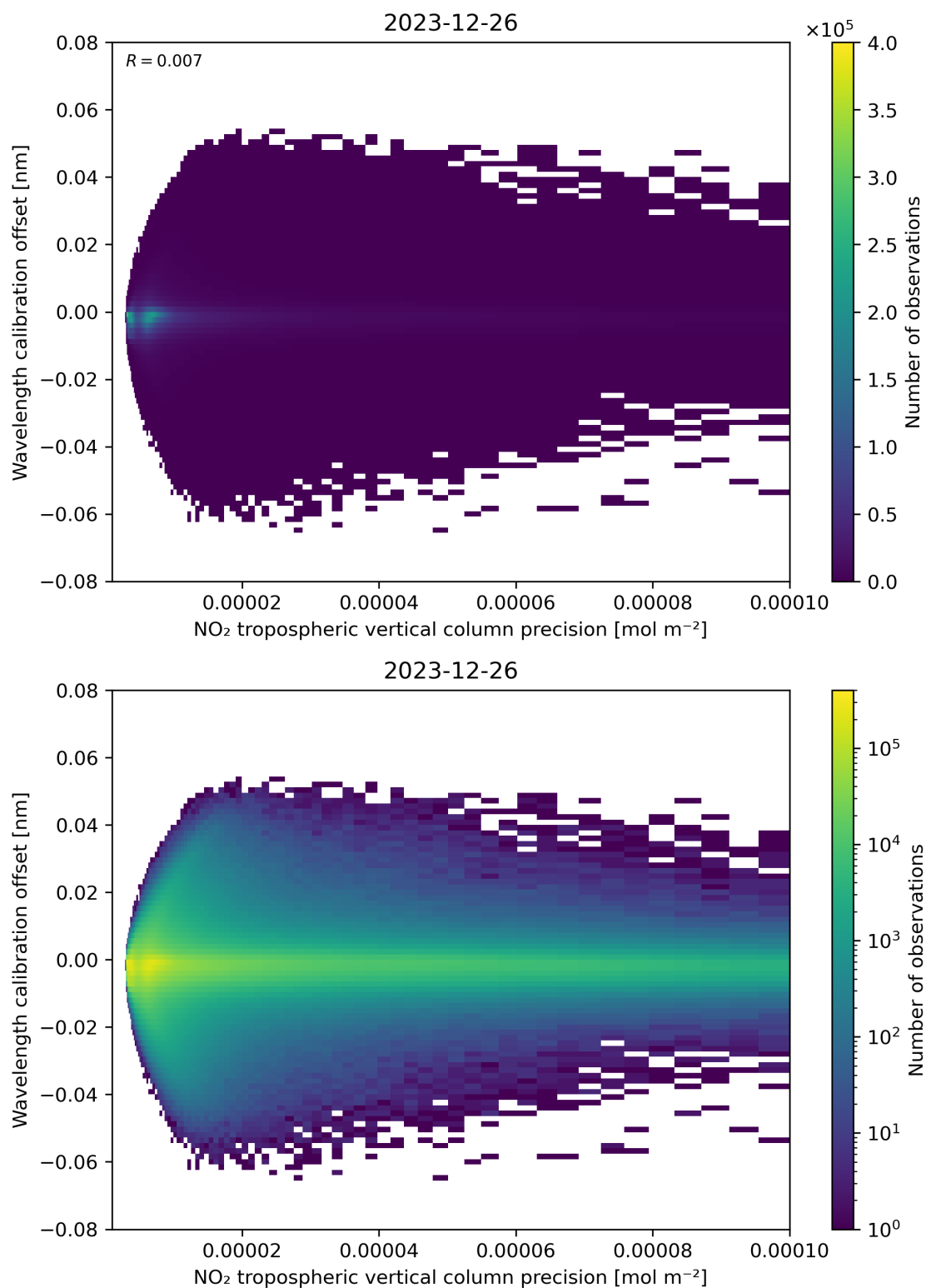
Figure 141: Scatter density plot of “NO 2 tropospheric vertical column precision” against “Wavelength calibration offset” for 2023-12-25 to 2023-12-27.
