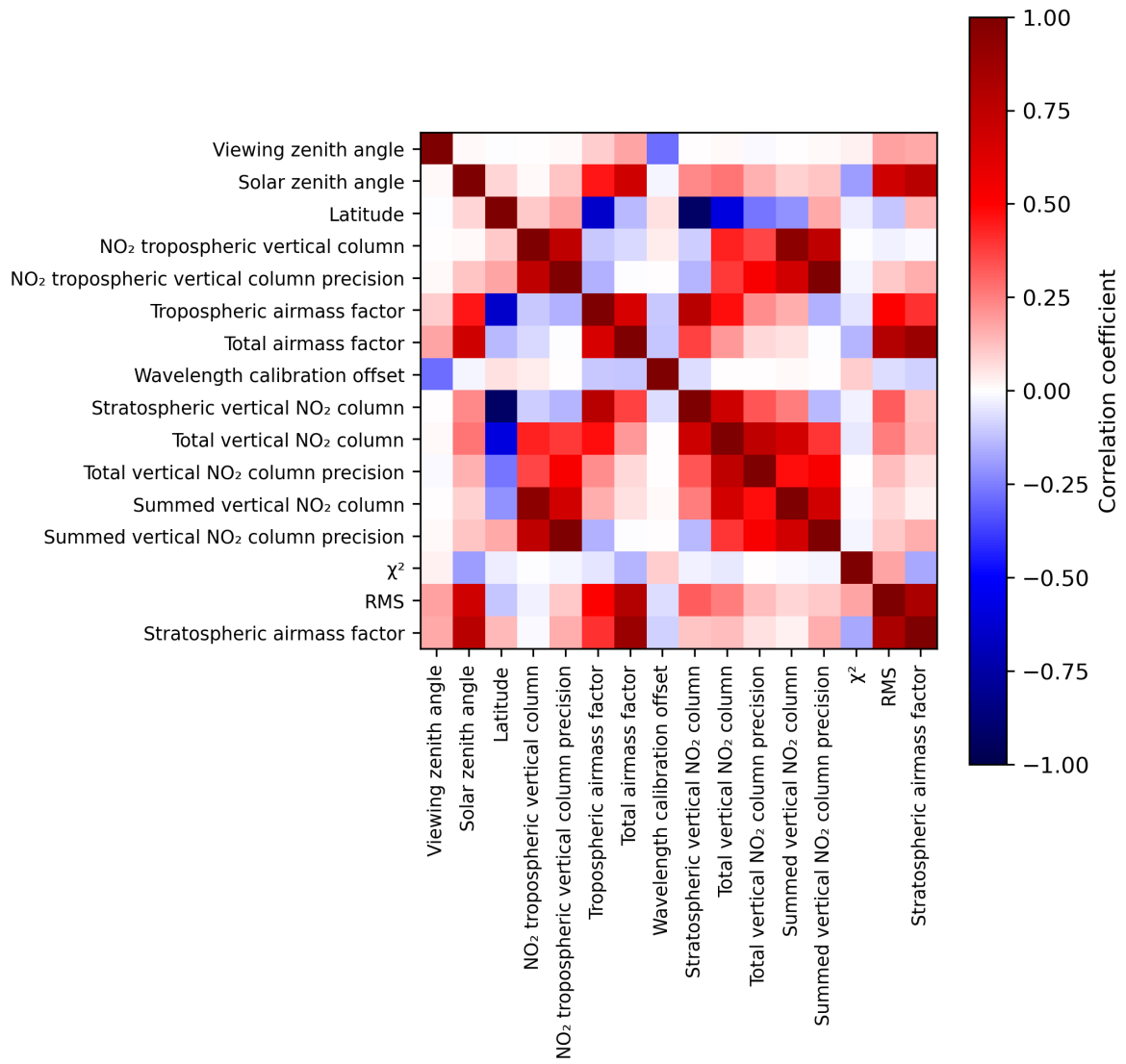
Figure 2: Map of correlation matrix for 2023-12-25 to 2023-12-27.
