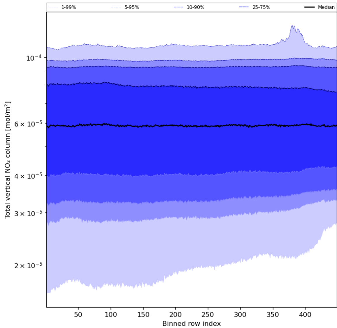
Figure 55: Along track statistics of “Total vertical NO 2 column” for 2023-12-25 to 2023-12-27
