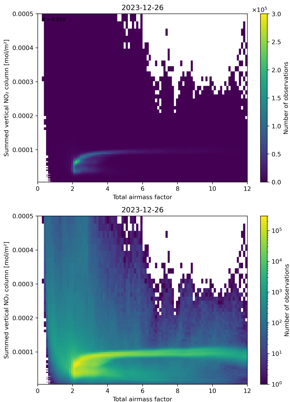
Figure 65: Scatter density plot of “Total airmass factor” against “Summed vertical NO 2 column” for 2023-12-25 to 2023-12-27.
