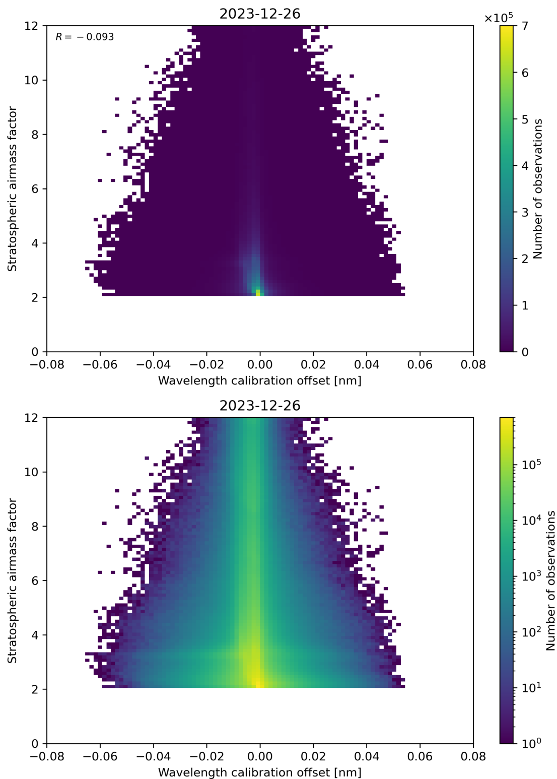
Figure 174: Scatter density plot of “Wavelength calibration offset” against “Stratospheric airmass factor” for 2023-12-25 to 2023-12-27.
