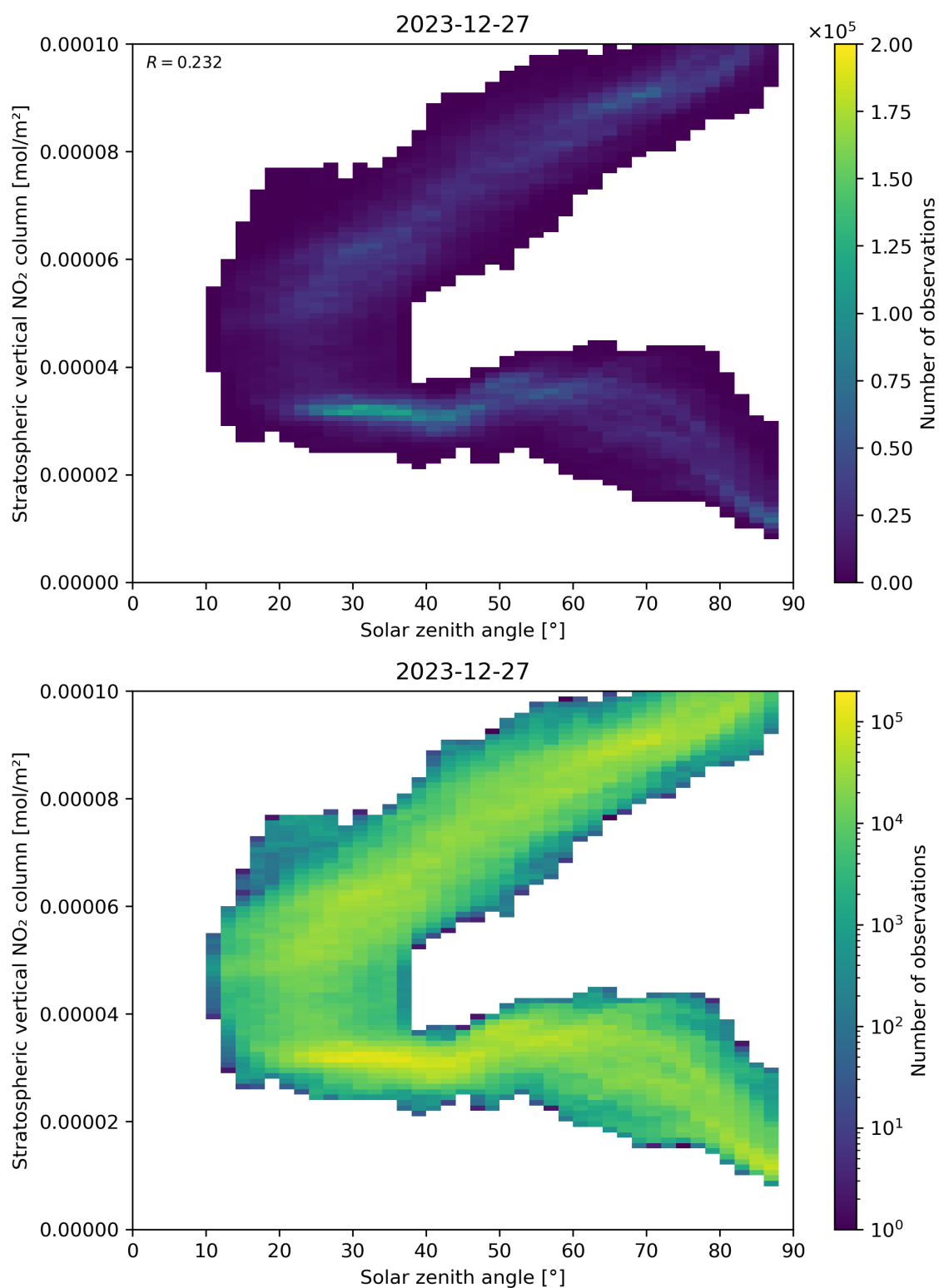
Figure 150: Scatter density plot of “Solar zenith angle” against “Stratospheric vertical NO 2 column” for 2023-12-26 to 2023-12-28.
