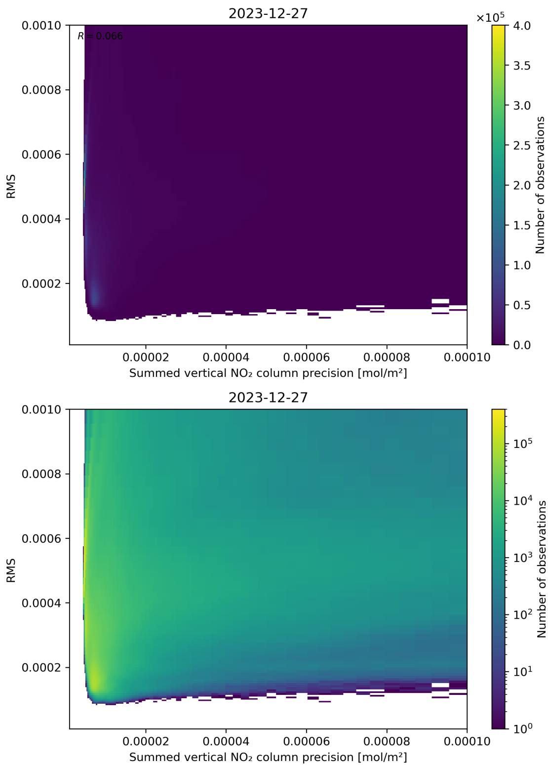
Figure 108: Scatter density plot of “Summed vertical NO 2 column precision” against “RMS” for 2023-12-26 to 2023-12-28.
