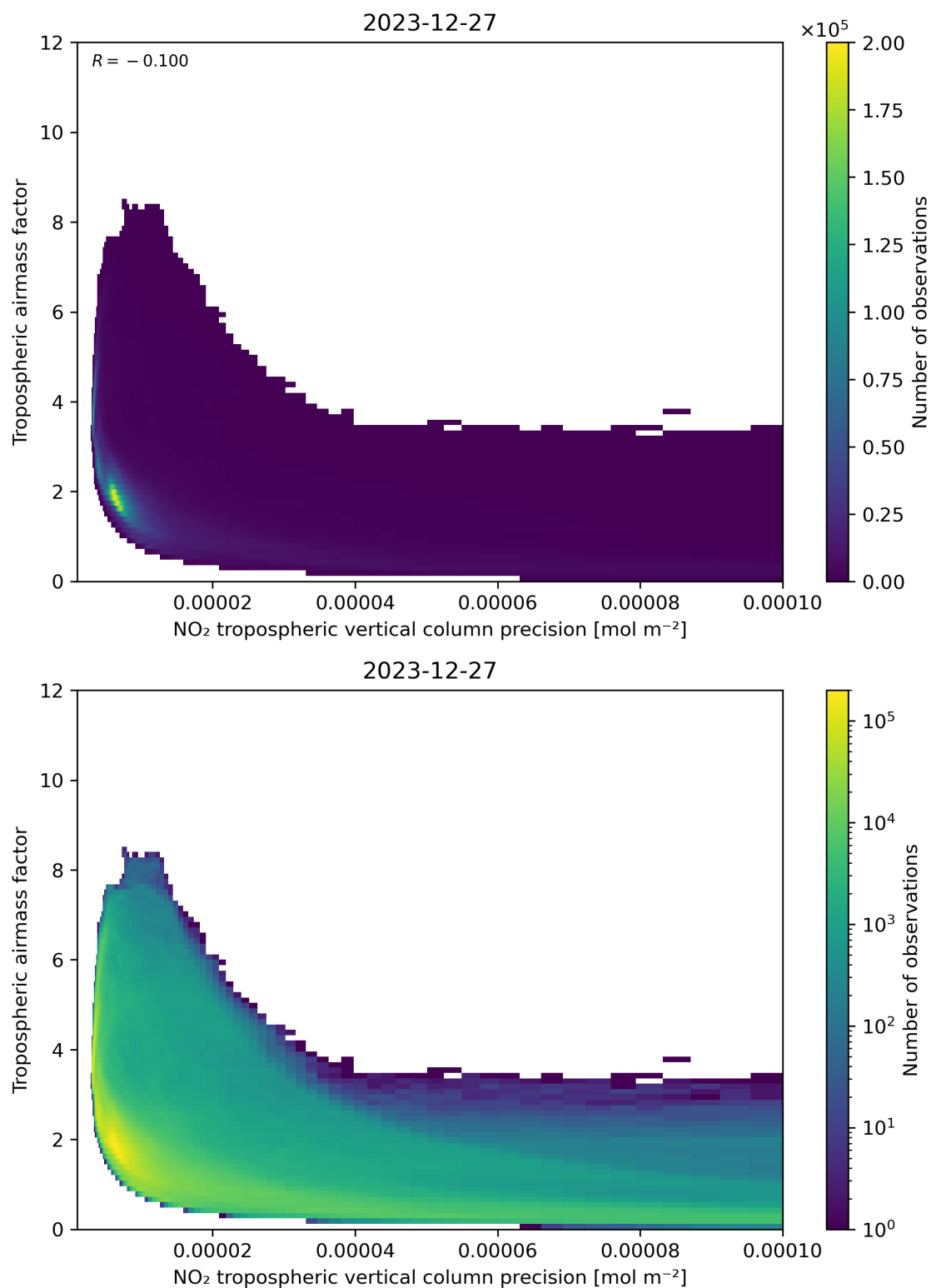
Figure 133: Scatter density plot of “NO 2 tropospheric vertical column precision” against “Tropospheric airmass factor” for 2023-12-26 to 2023-12-28.
