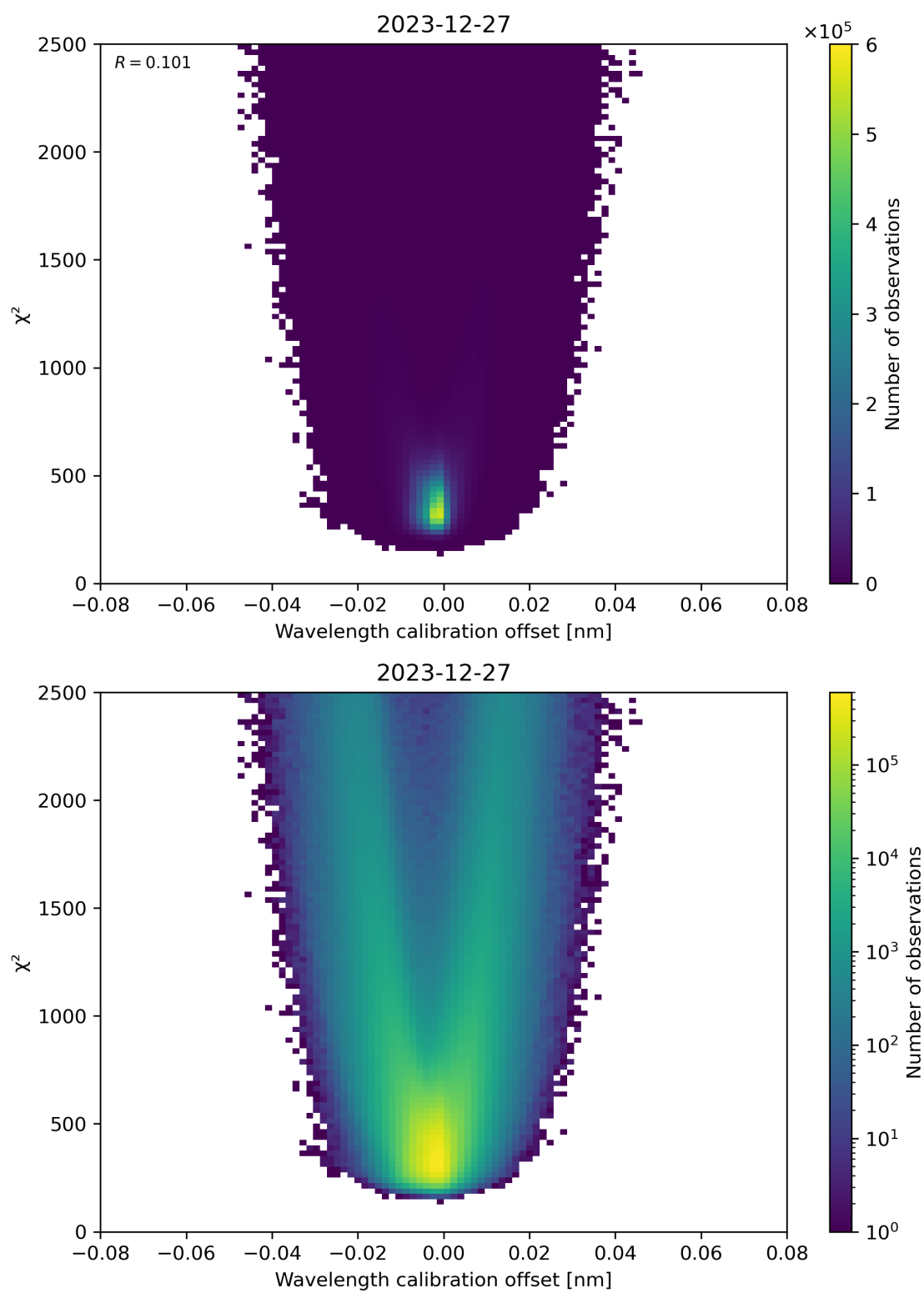
Figure 175: Scatter density plot of “Wavelength calibration offset” against “ \chi^2 ” for 2023-12-26 to 2023-12-28.
