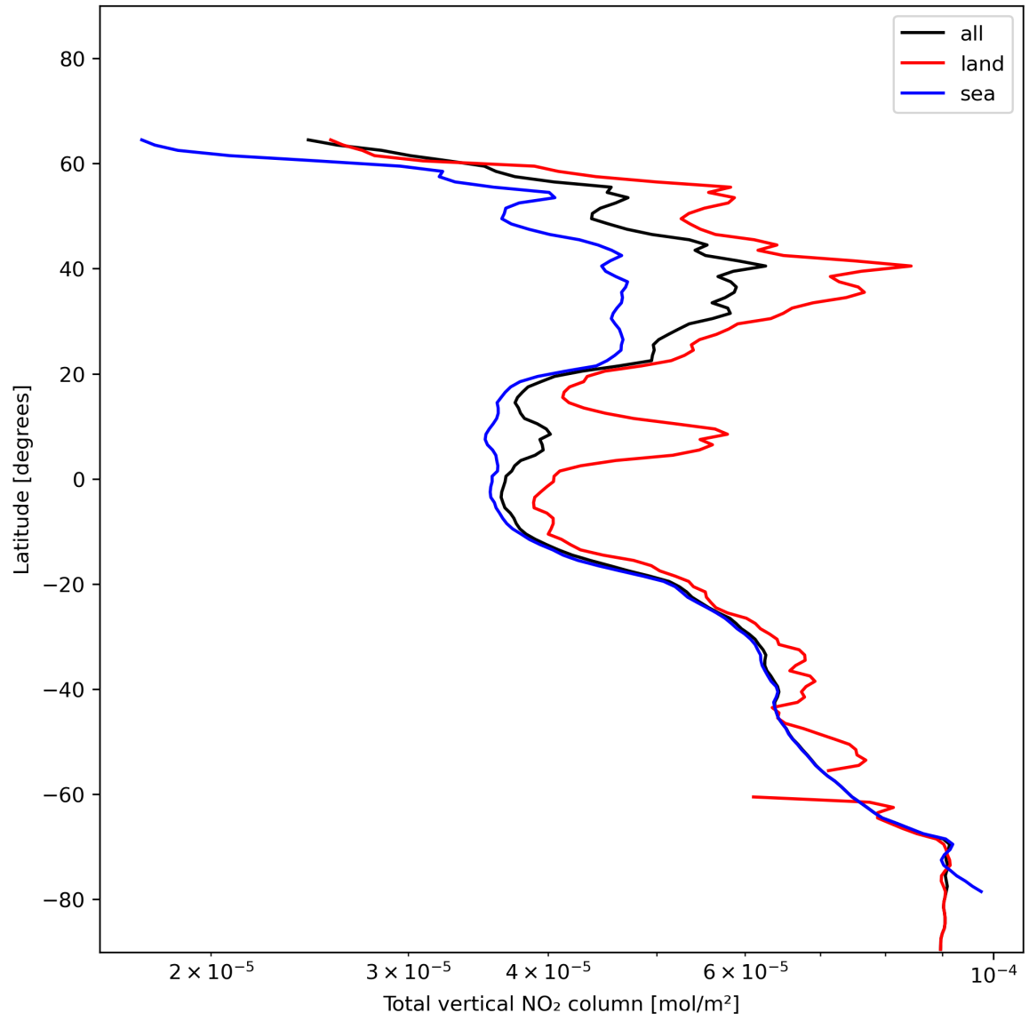
Figure 21: Zonal average of “Total vertical NO 2 column” for 2023-12-26 to 2023-12-28.
