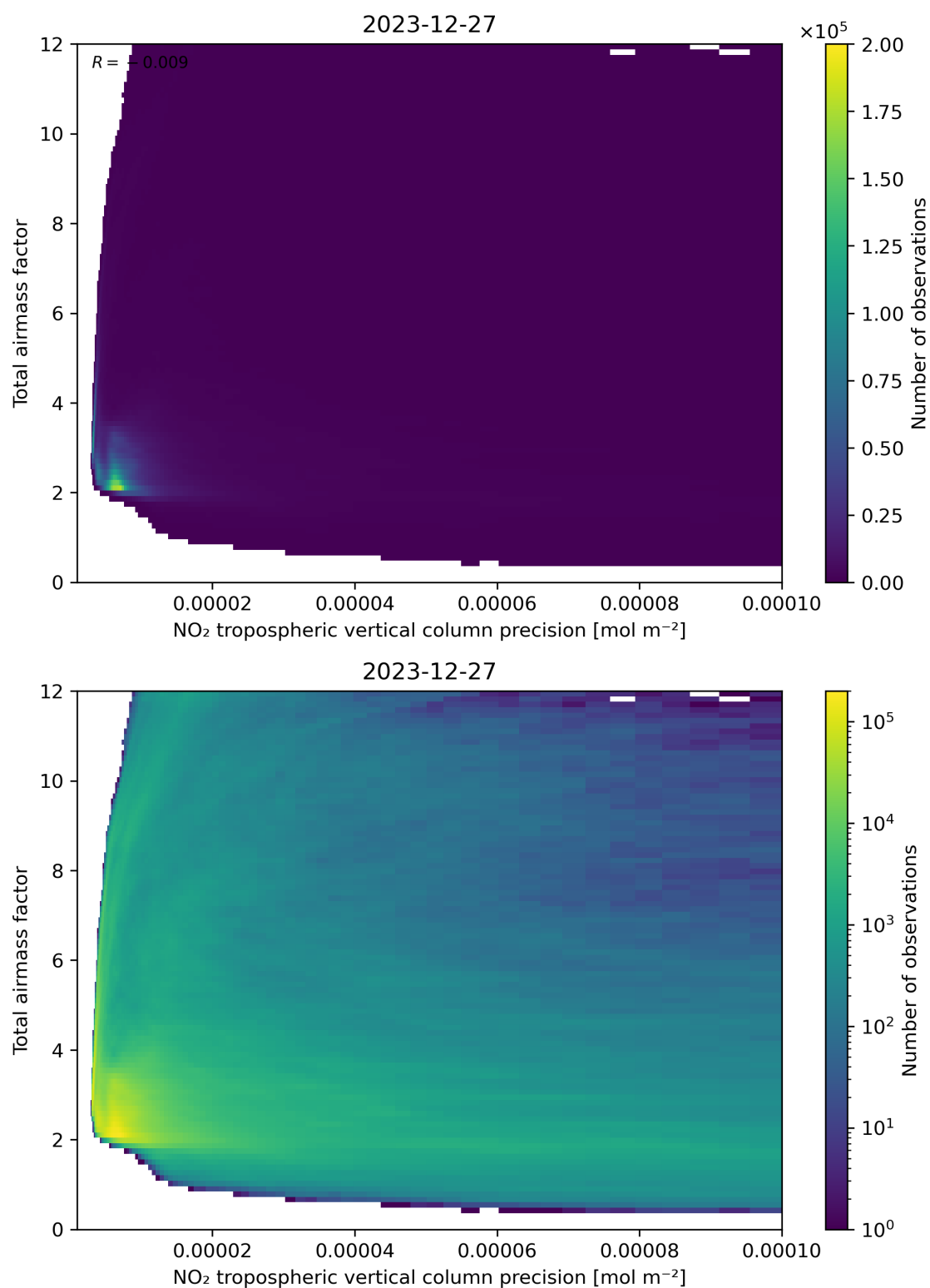
Figure 132: Scatter density plot of “NO 2 tropospheric vertical column precision” against “Total air mass factor” for 2023-12-26 to 2023-12-28.
