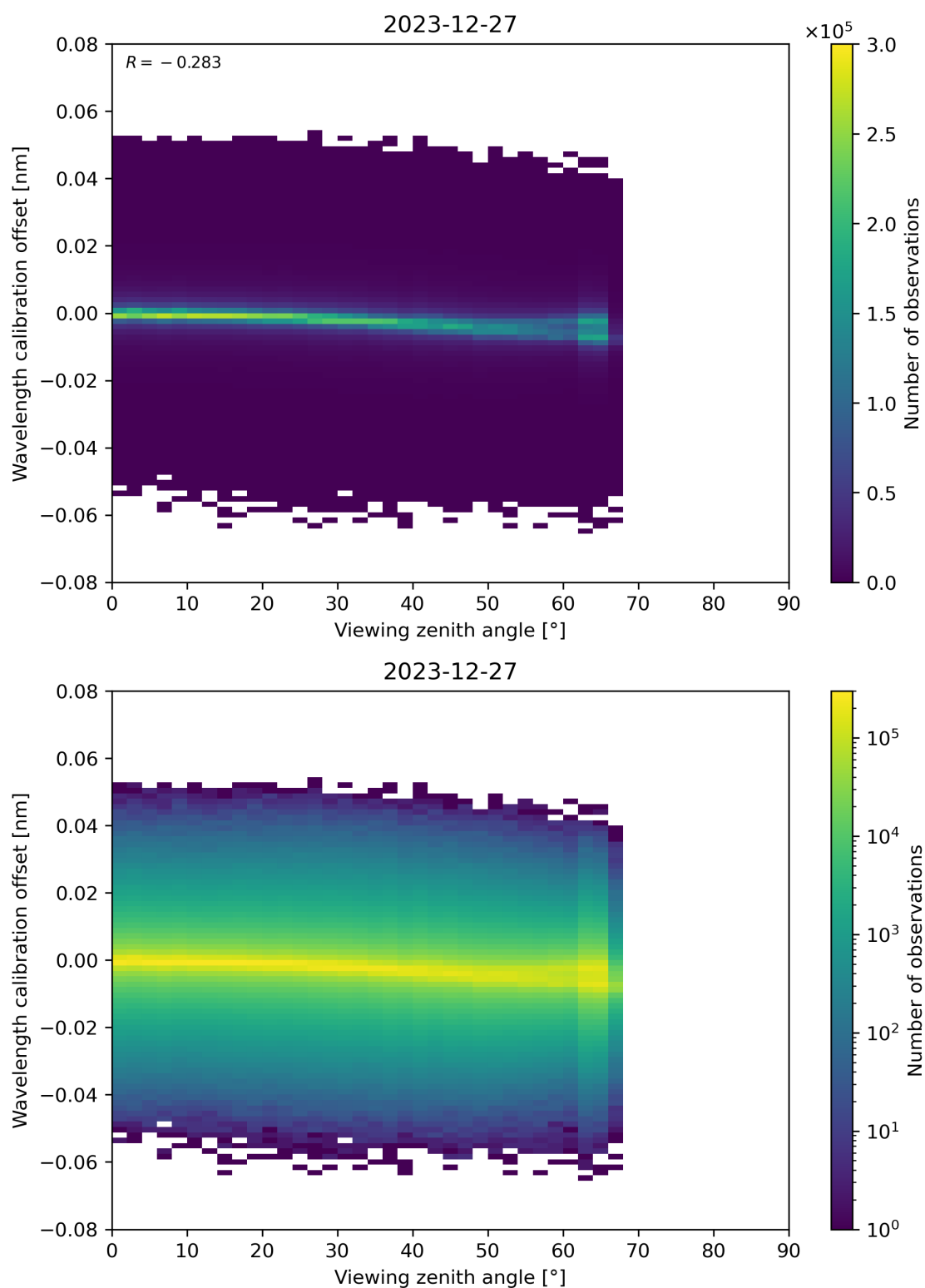
Figure 173: Scatter density plot of “Viewing zenith angle” against “Wavelength calibration offset” for 2023-12-26 to 2023-12-28.
