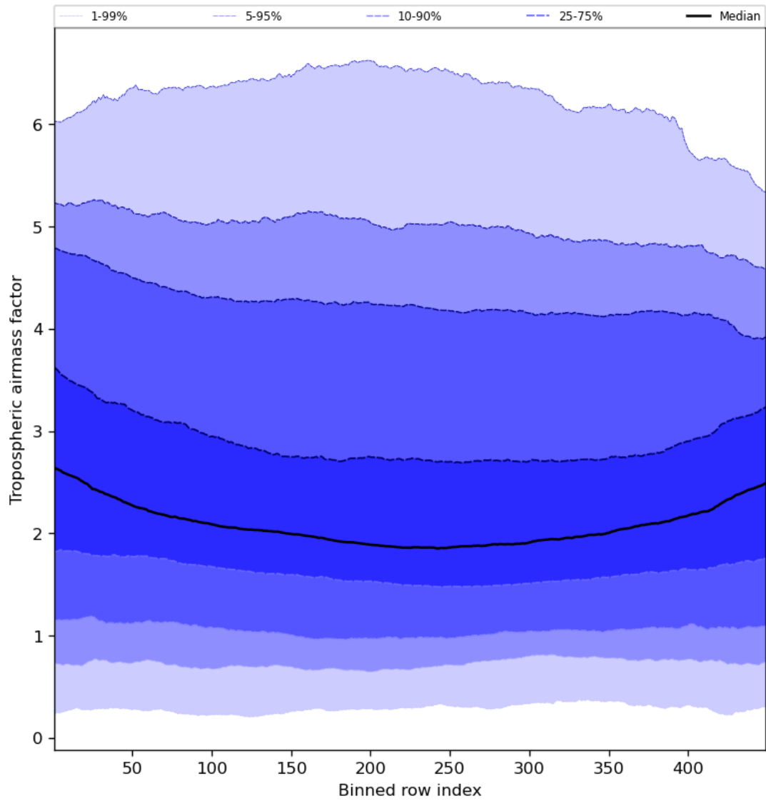
Figure 48: Along track statistics of “Tropospheric airmass factor” for 2023-12-26 to 2023-12-28
