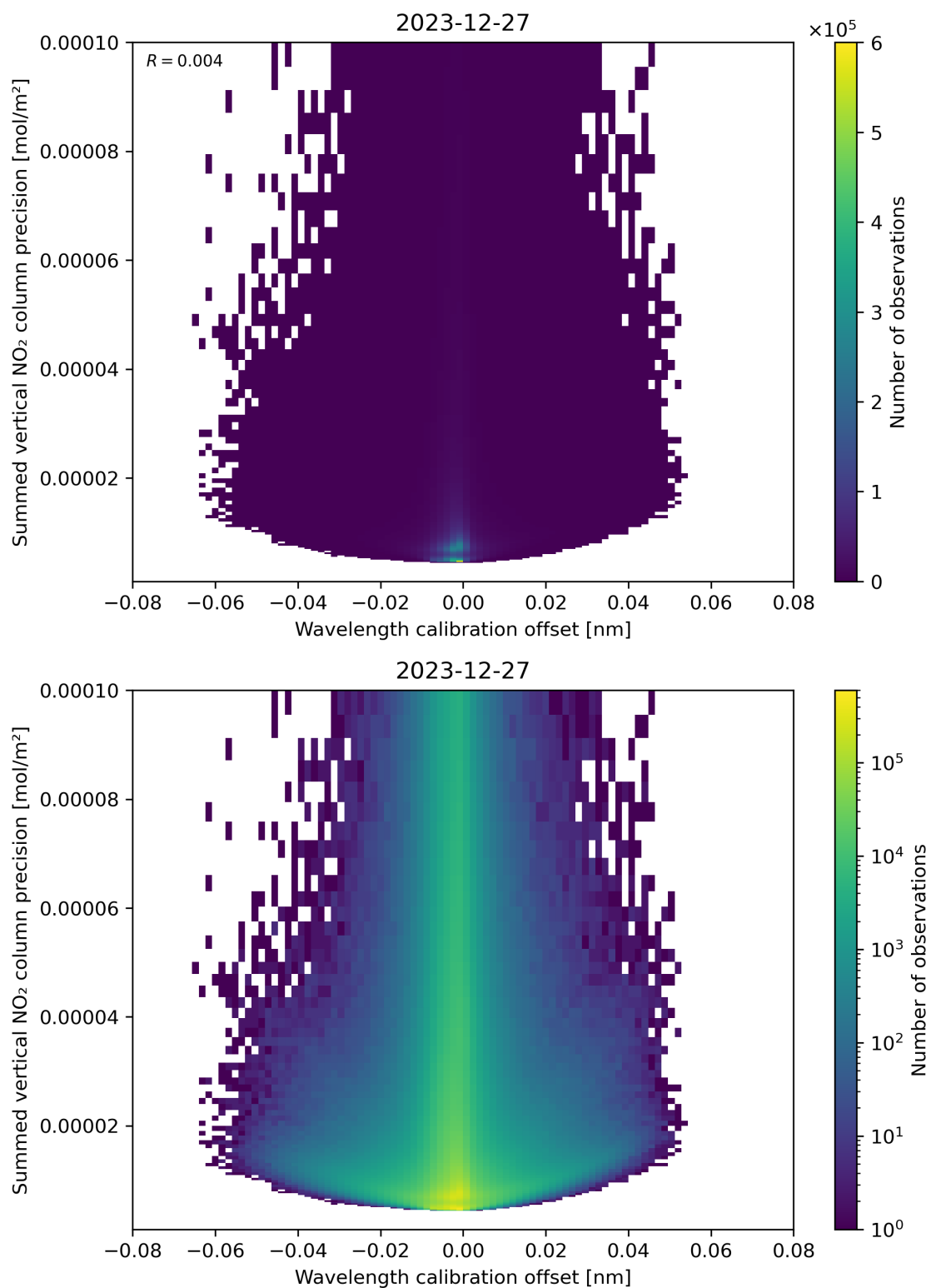
Figure 178: Scatter density plot of “Wavelength calibration offset” against “Summed vertical NO 2 column precision” for 2023-12-26 to 2023-12-28.
