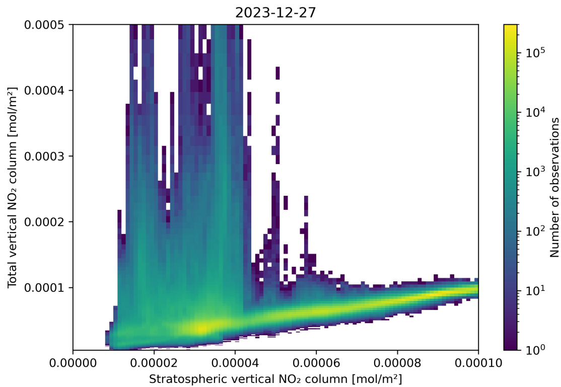
Figure 100: Scatter density plot of “Stratospheric vertical NO 2 column” against “Total vertical NO 2 column” for 2023-12-26 to 2023-12-28.
