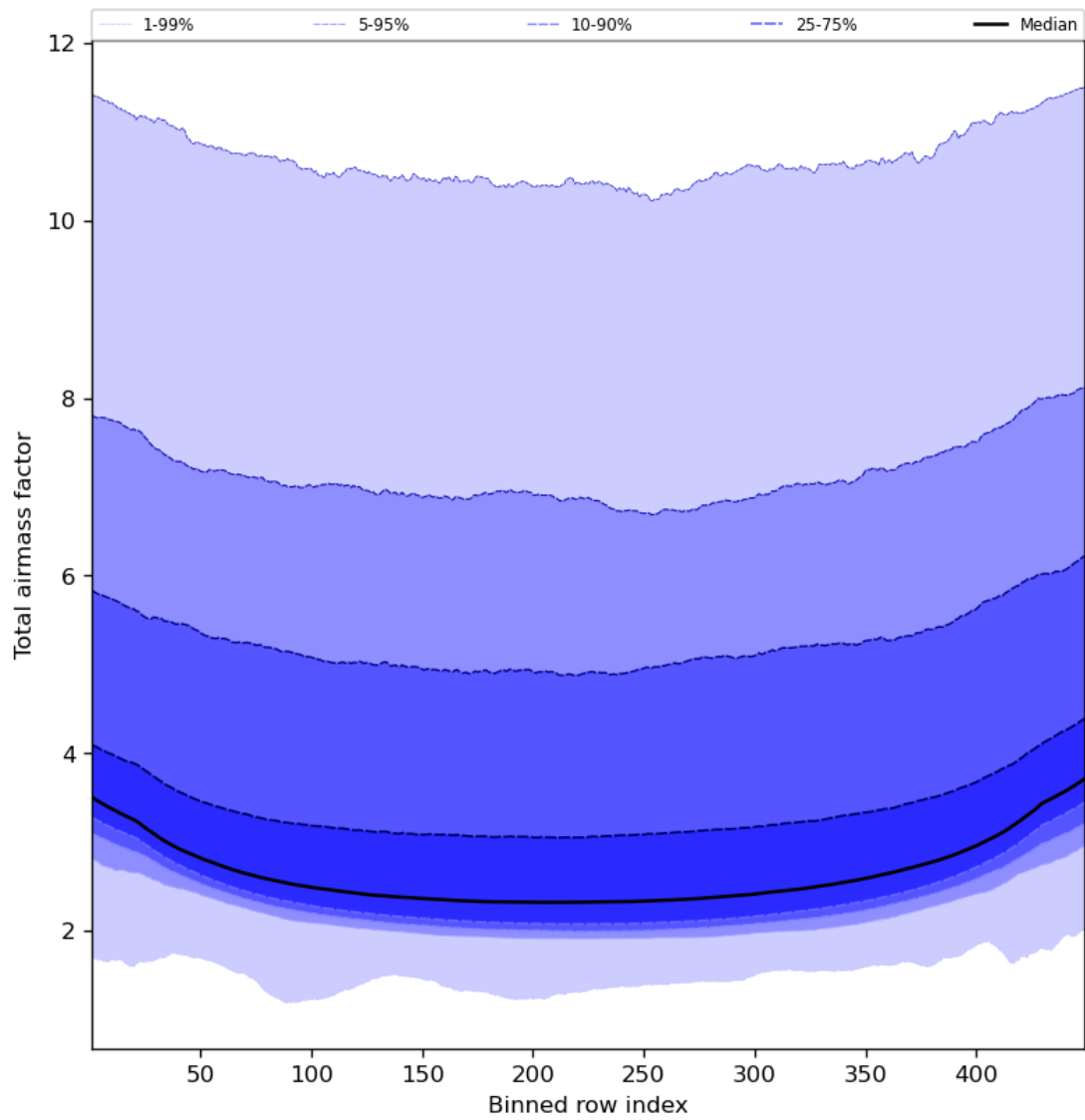
Figure 49: Along track statistics of “Total airmass factor” for 2023-12-26 to 2023-12-28
