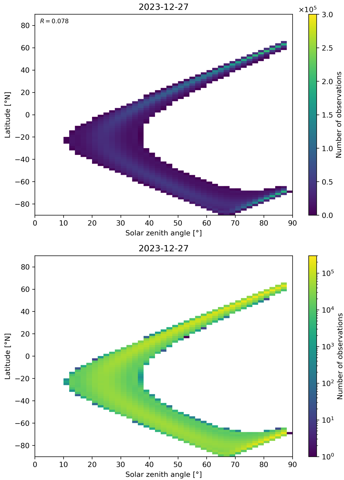
Figure 149: Scatter density plot of “Solar zenith angle” against “Latitude” for 2023-12-26 to 2023-12-28.
