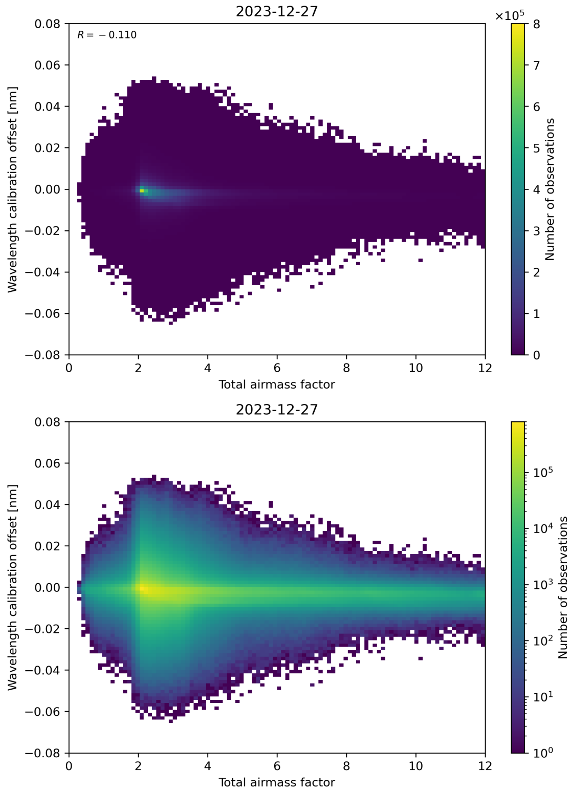
Figure 70: Scatter density plot of “Total airmass factor” against “Wavelength calibration offset” for 2023-12-26 to 2023-12-28.
