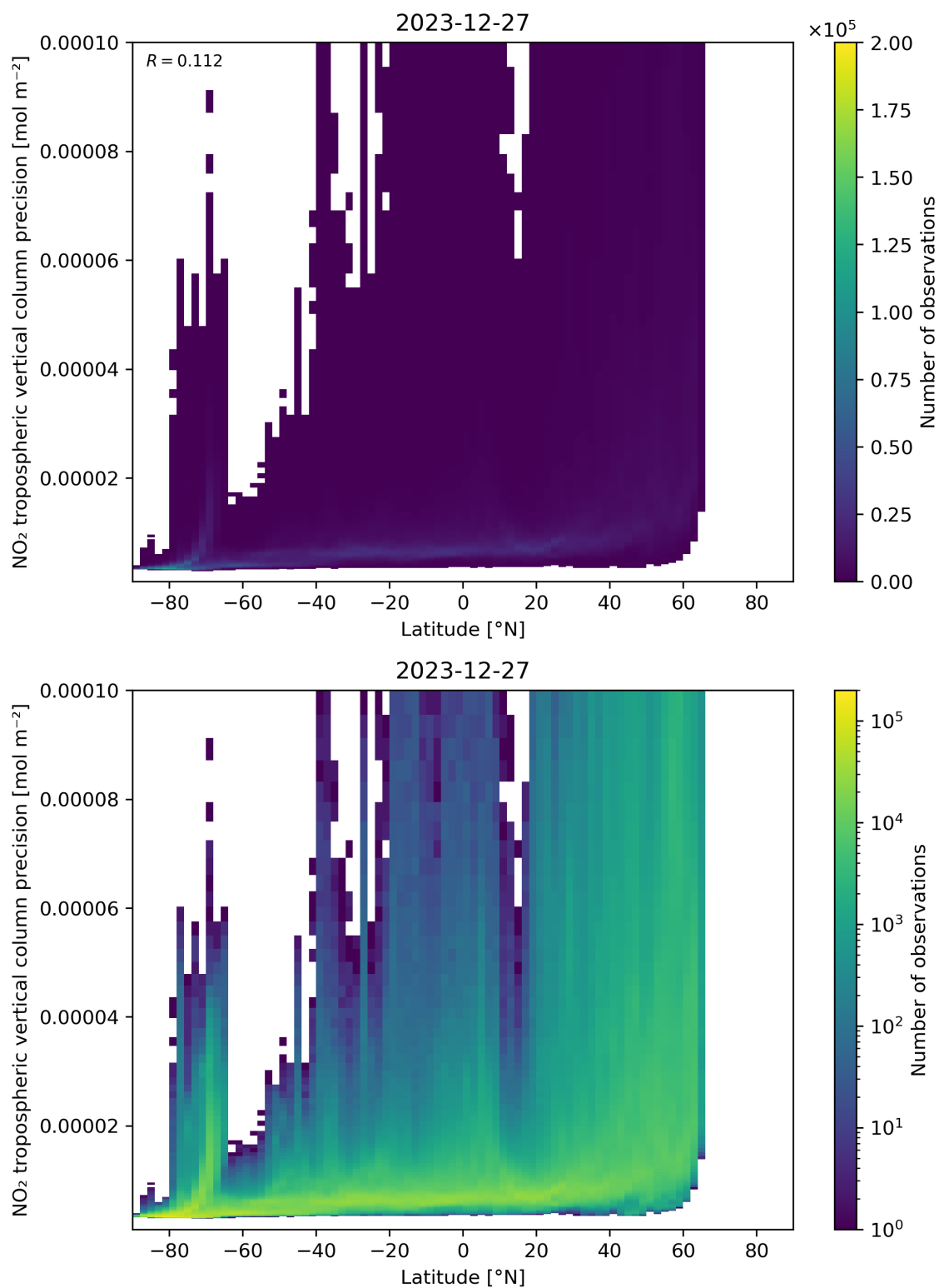
Figure 93: Scatter density plot of “Latitude” against “NO 2 tropospheric vertical column precision” for 2023-12-26 to 2023-12-28.
