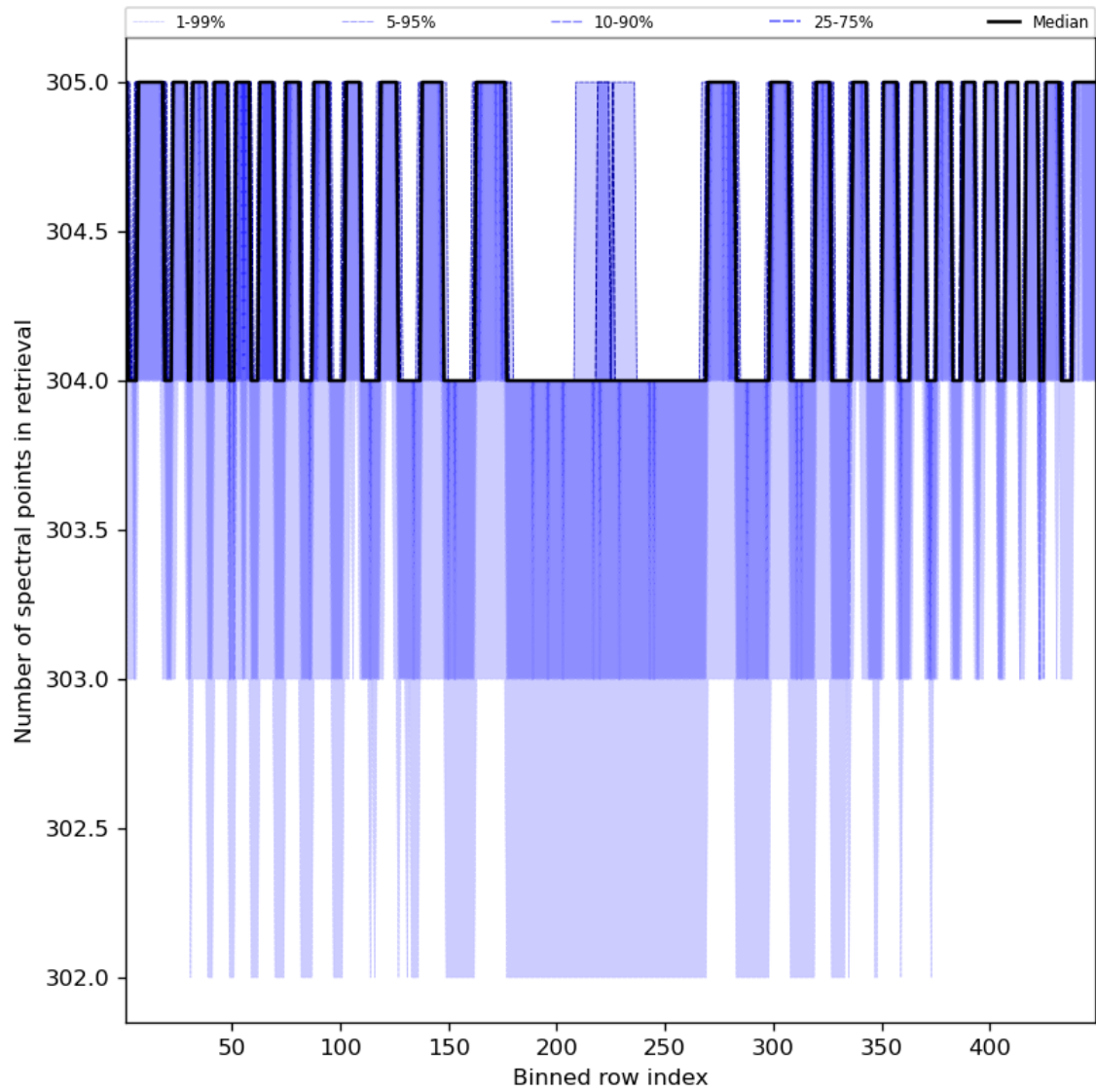
Figure 50: Along track statistics of “Number of spectral points in retrieval” for 2023-12-26 to 2023-12-28
