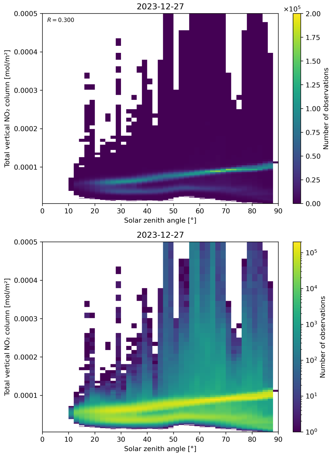
Figure 153: Scatter density plot of “Solar zenith angle” against “Total vertical NO 2 column” for 2023-12-26 to 2023-12-28.
