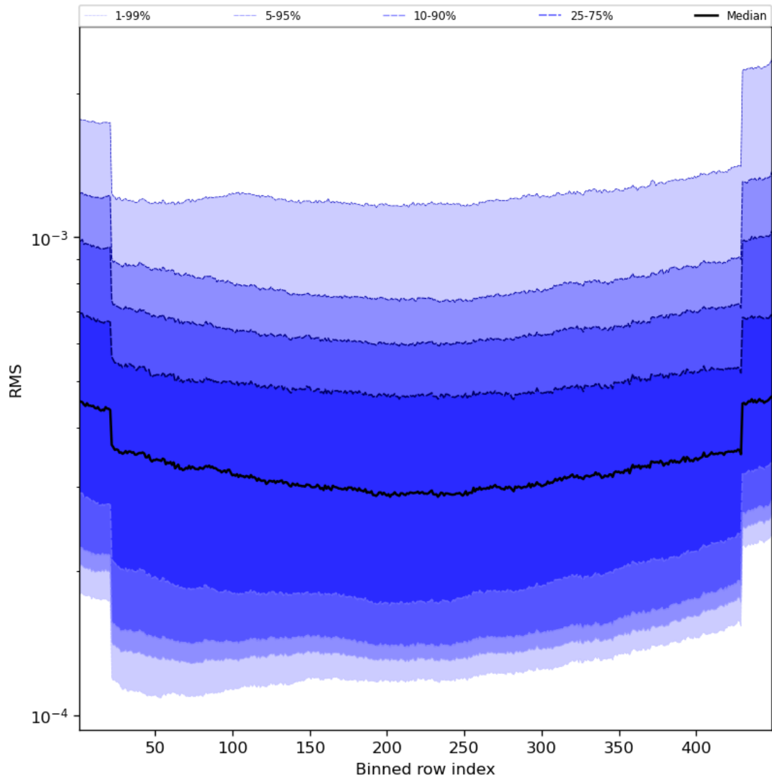
Figure 60: Along track statistics of “RMS” for 2023-12-26 to 2023-12-28
