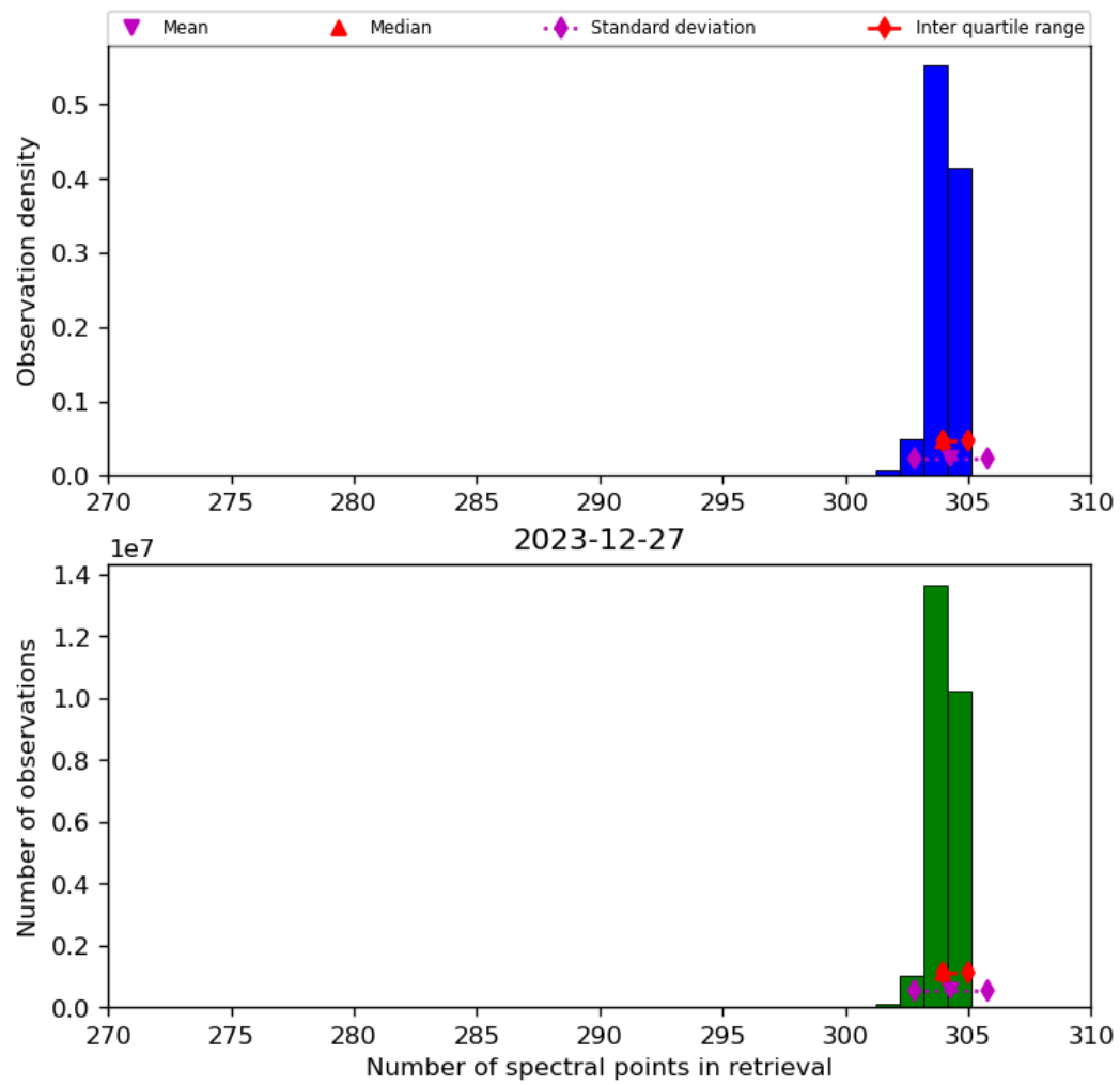
Figure 33: Histogram of “Number of spectral points in retrieval” for 2023-12-26 to 2023-12-28
