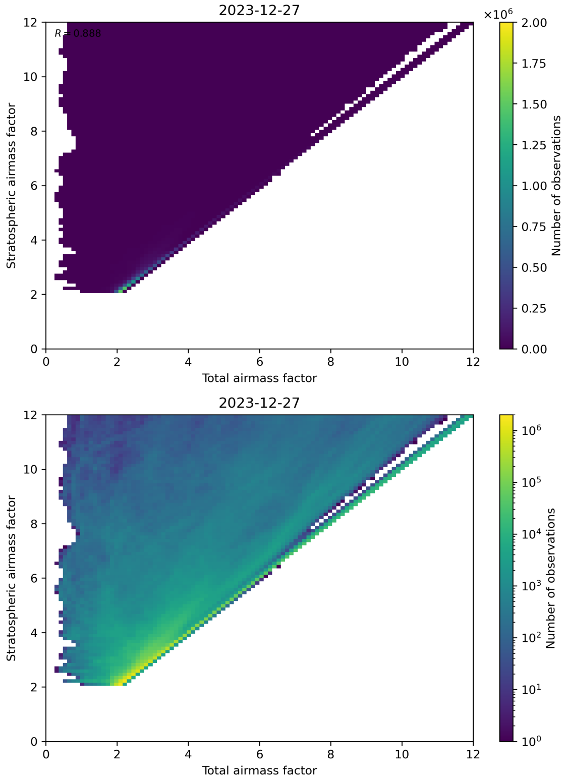
Figure 62: Scatter density plot of “Total airmass factor” against “Stratospheric airmass factor” for 2023-12-26 to 2023-12-28.
