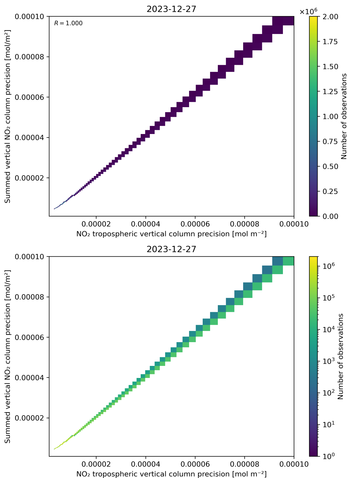
Figure 137: Scatter density plot of “NO 2 tropospheric vertical column precision” against “Summed vertical NO 2 column precision” for 2023-12-26 to 2023-12-28.
