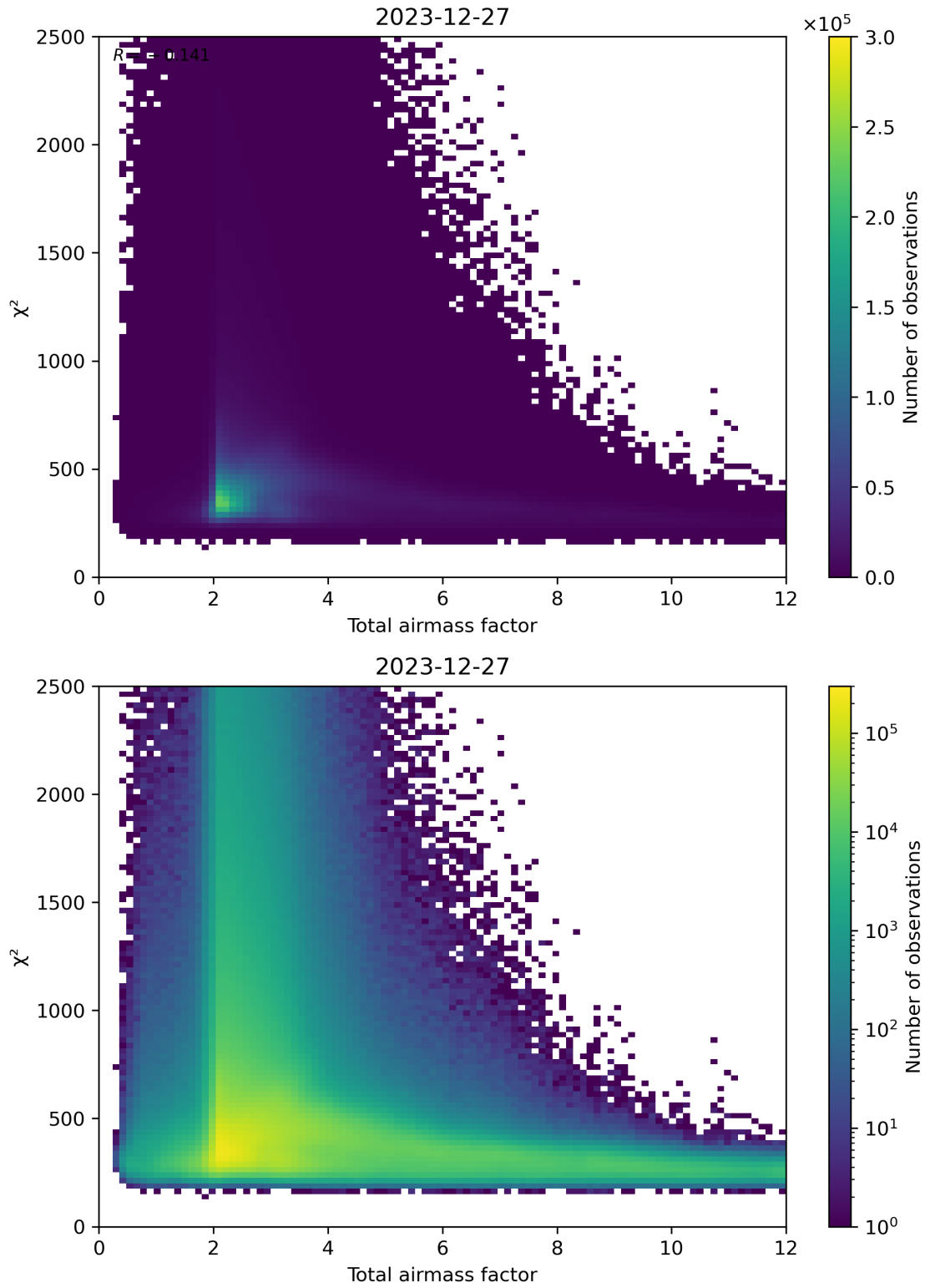
Figure 63: Scatter density plot of “Total airmass factor” against “ \chi^2 ” for 2023-12-26 to 2023-12-28.
