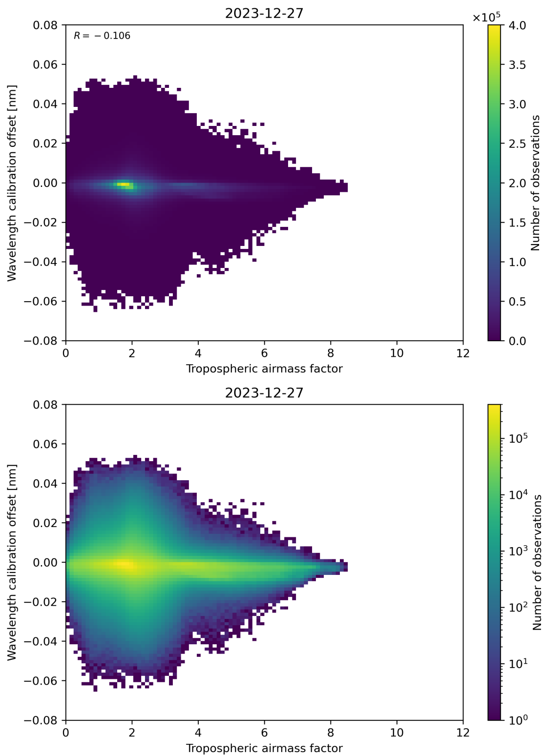
Figure 80: Scatter density plot of “Tropospheric airmass factor” against “Wavelength calibration offset” for 2023-12-26 to 2023-12-28.
