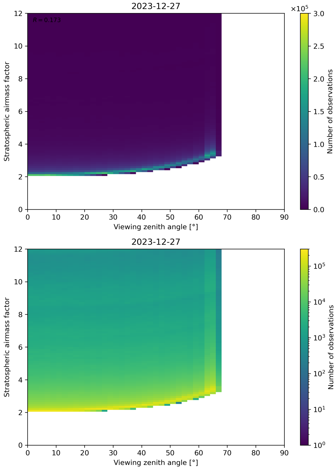
Figure 159: Scatter density plot of “Viewing zenith angle” against “Stratospheric airmass factor” for 2023-12-26 to 2023-12-28.
