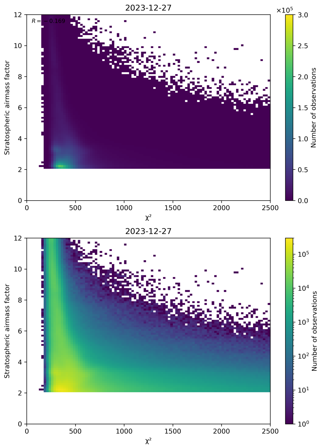
Figure 81: Scatter density plot of “ \chi^2 ” against “Stratospheric airmass factor” for 2023-12-26 to 2023-12-28.
