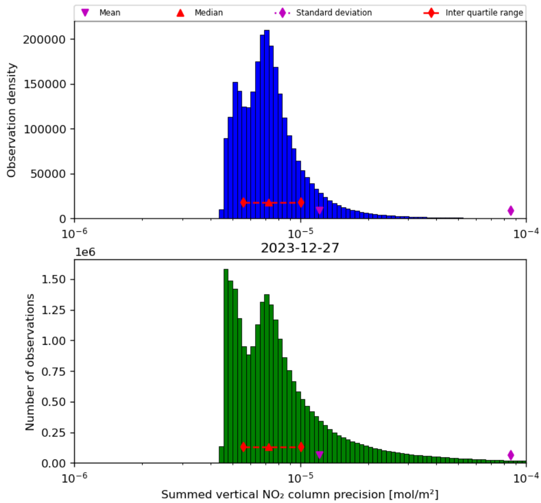
Figure 41: Histogram of “Summed vertical NO 2 column precision” for 2023-12-26 to 2023-12-28
