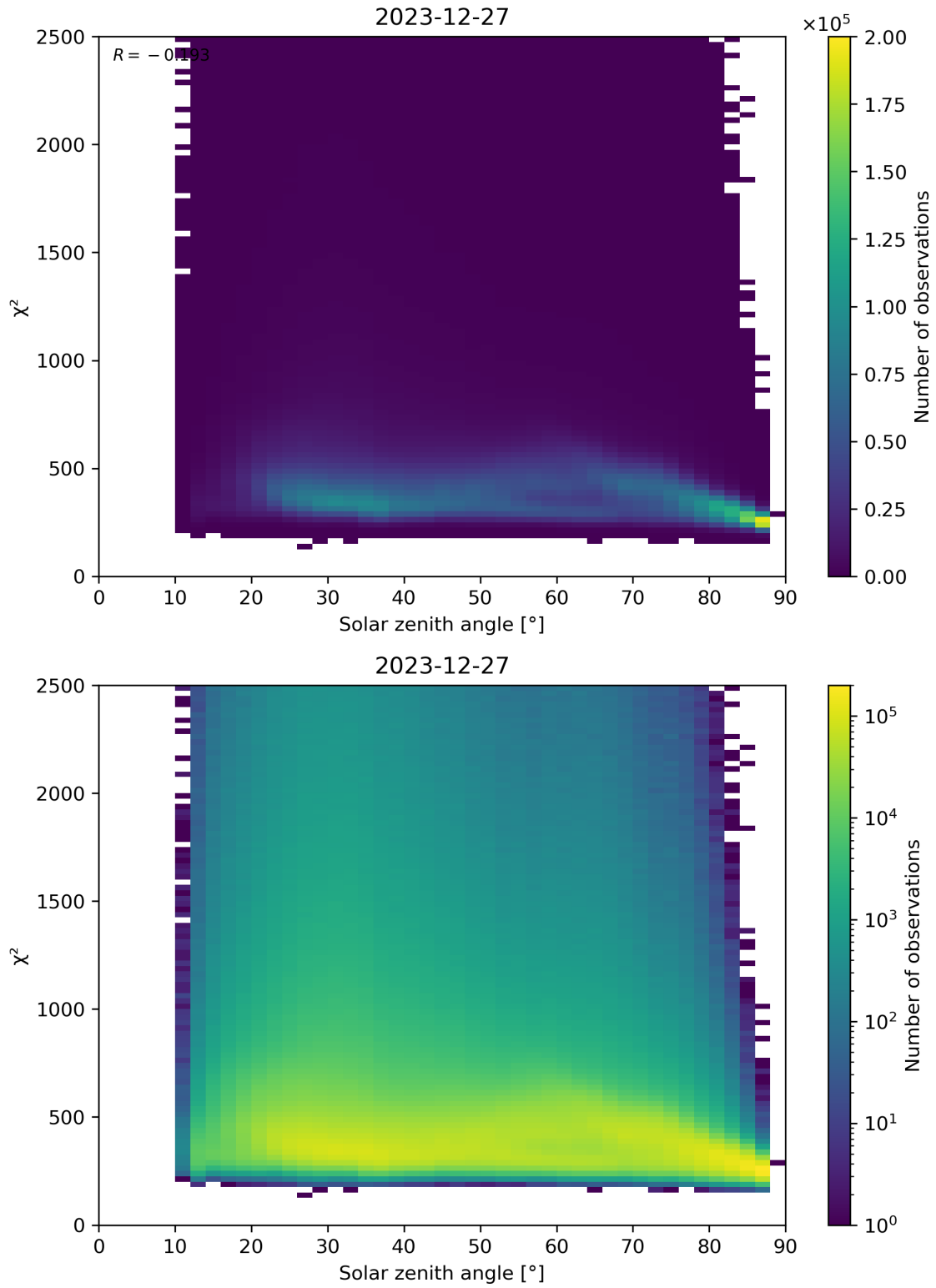
Figure 148: Scatter density plot of “Solar zenith angle” against “ \chi^2 ” for 2023-12-26 to 2023-12-28.
