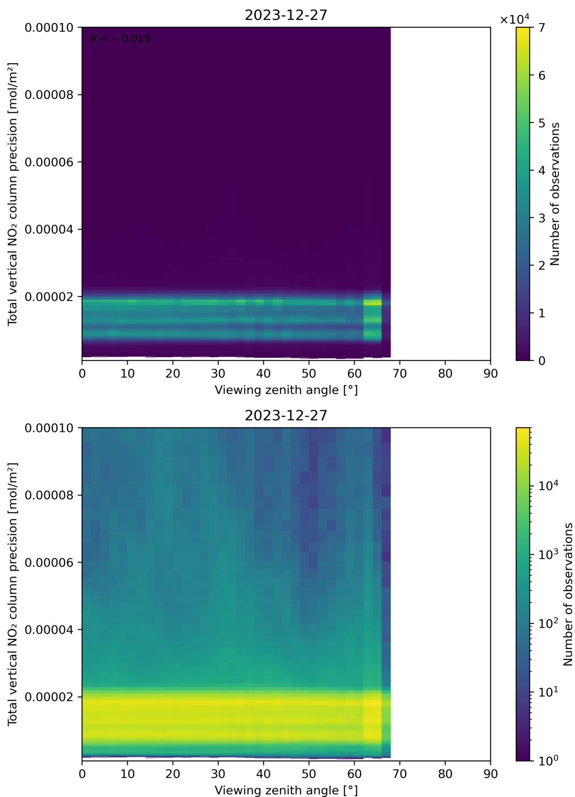
Figure 168: Scatter density plot of “Viewing zenith angle” against “Total vertical NO 2 column precision” for 2023-12-26 to 2023-12-28.
