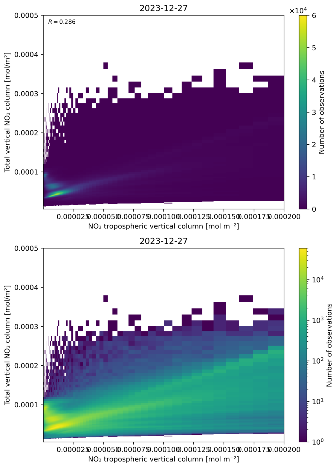
Figure 128: Scatter density plot of “NO 2 tropospheric vertical column” against “Total vertical NO 2 column” for 2023-12-26 to 2023-12-28.
