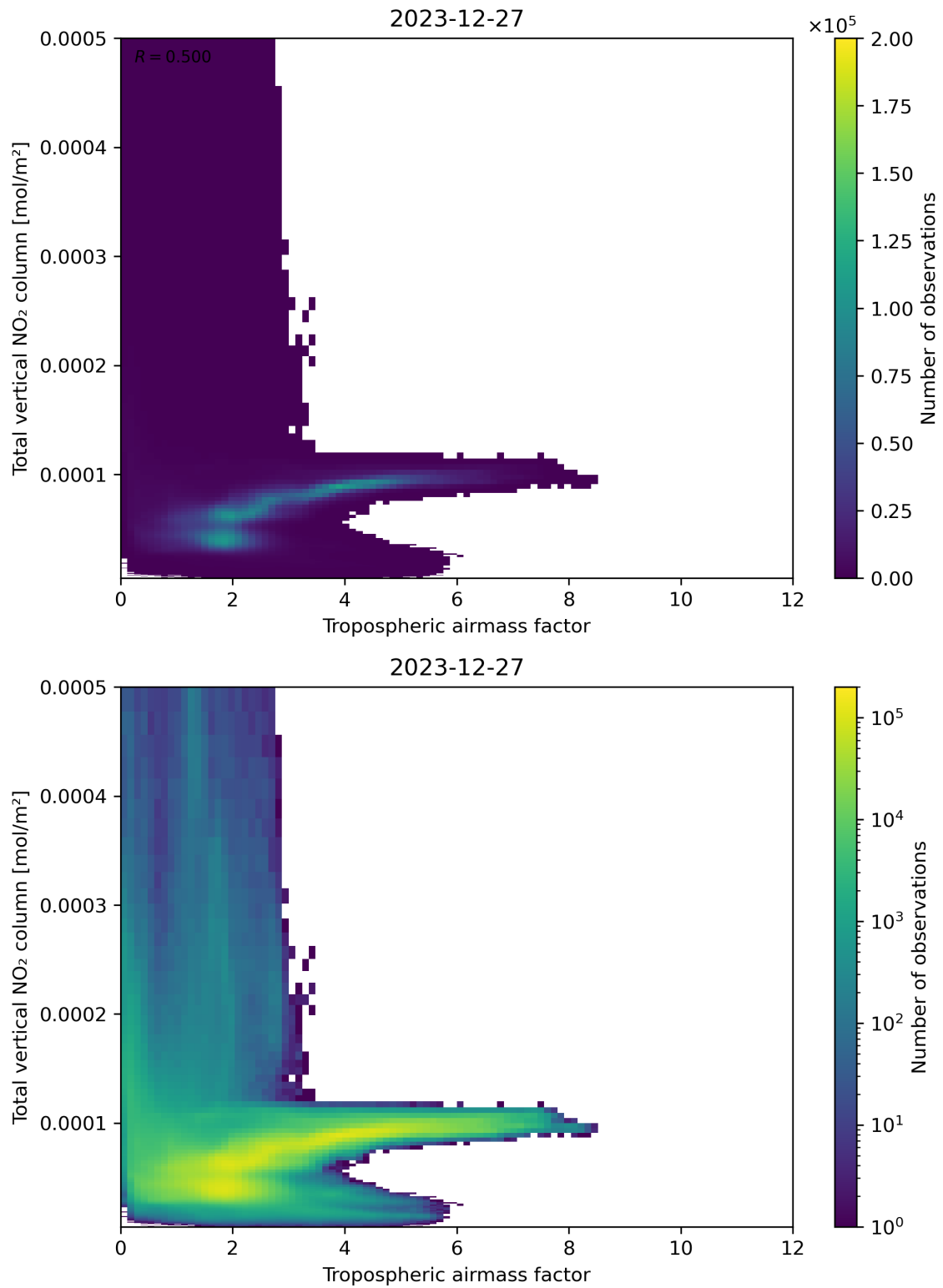
Figure 77: Scatter density plot of “Tropospheric airmass factor” against “Total vertical NO 2 column” for 2023-12-26 to 2023-12-28.
