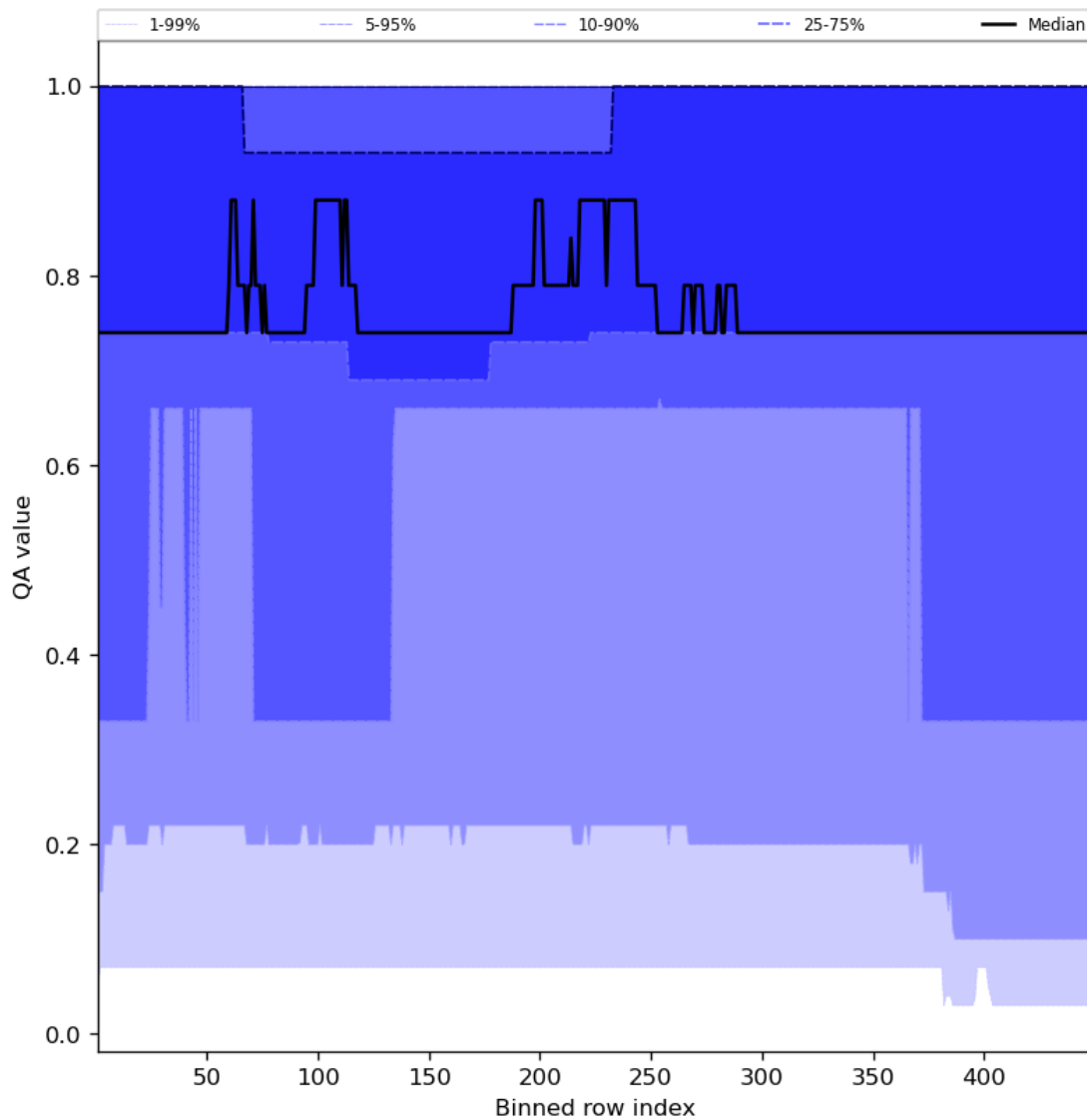
Figure 45: Along track statistics of “QA value” for 2023-12-26 to 2023-12-28
