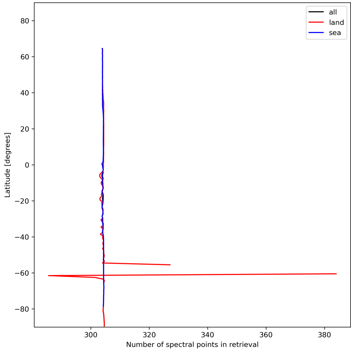
Figure 16: Zonal average of “Number of spectral points in retrieval” for 2023-12-26 to 2023-12-28.
