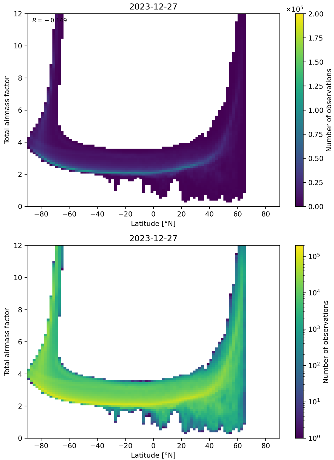
Figure 84: Scatter density plot of “Latitude” against “Total airmass factor” for 2023-12-26 to 2023-12-28.
