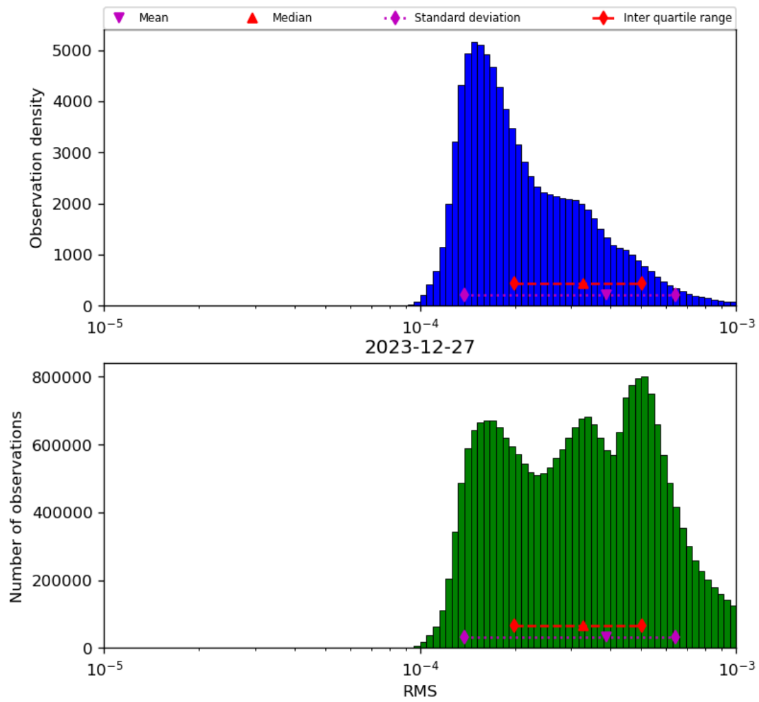
Figure 43: Histogram of “RMS” for 2023-12-26 to 2023-12-28
