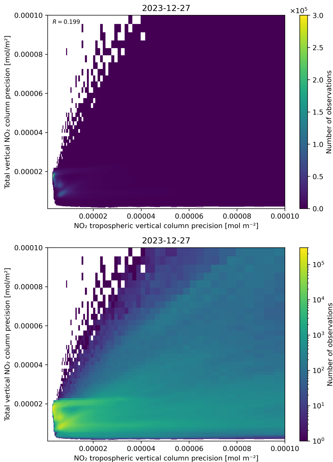
Figure 139: Scatter density plot of “NO 2 tropospheric vertical column precision” against “Total vertical NO 2 column precision” for 2023-12-26 to 2023-12-28.
