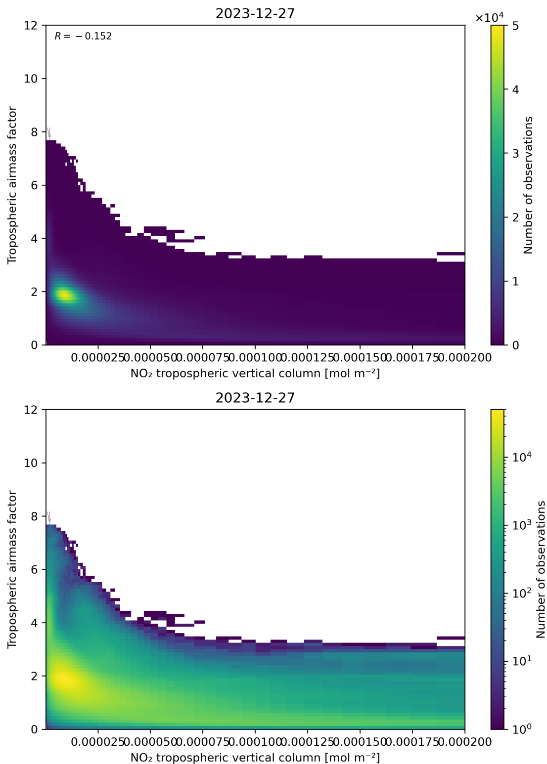
Figure 123: Scatter density plot of “NO 2 tropospheric vertical column” against “Tropospheric air mass factor” for 2023-12-26 to 2023-12-28.
