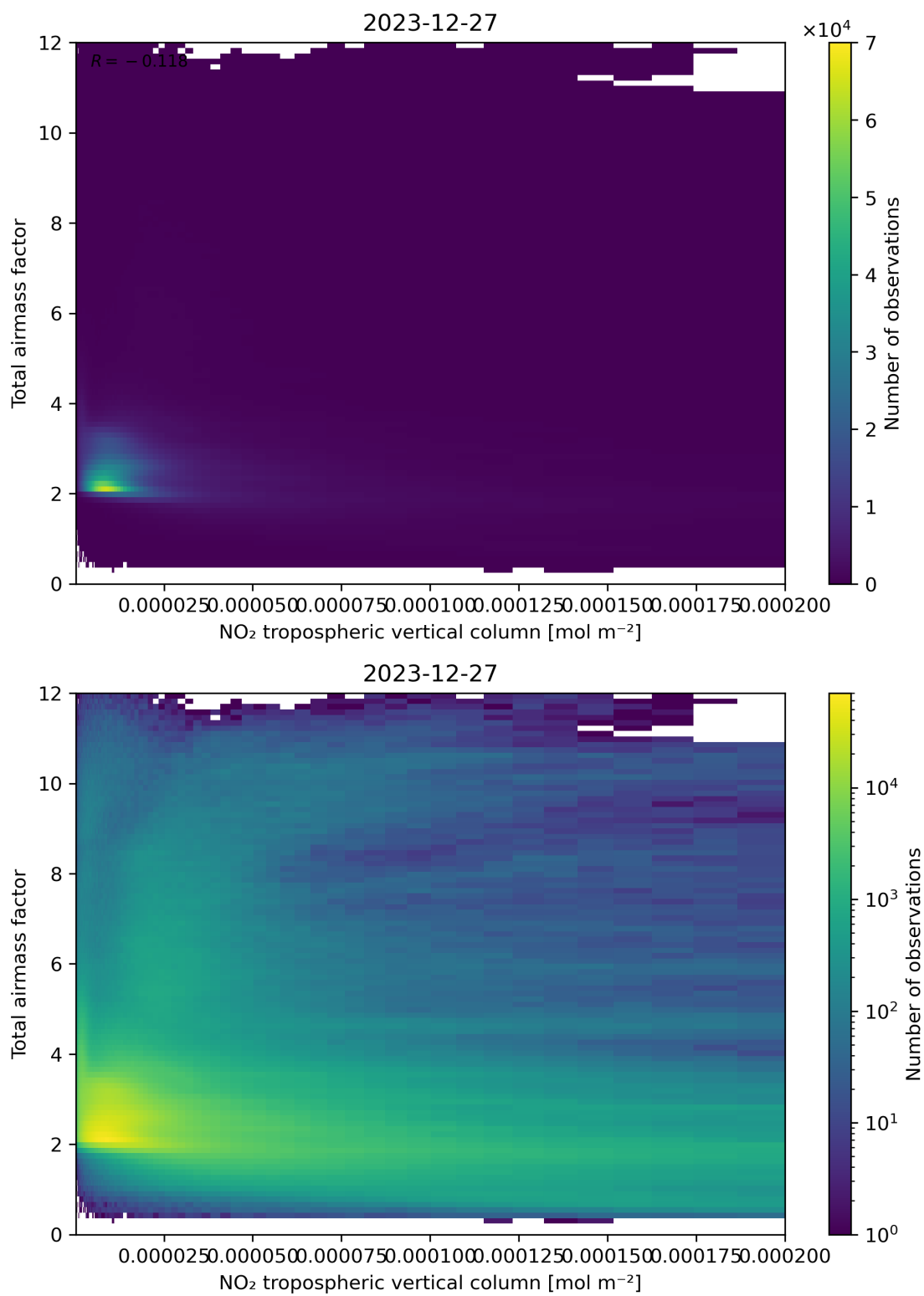
Figure 122: Scatter density plot of “NO 2 tropospheric vertical column” against “Total air mass factor” for 2023-12-26 to 2023-12-28.
