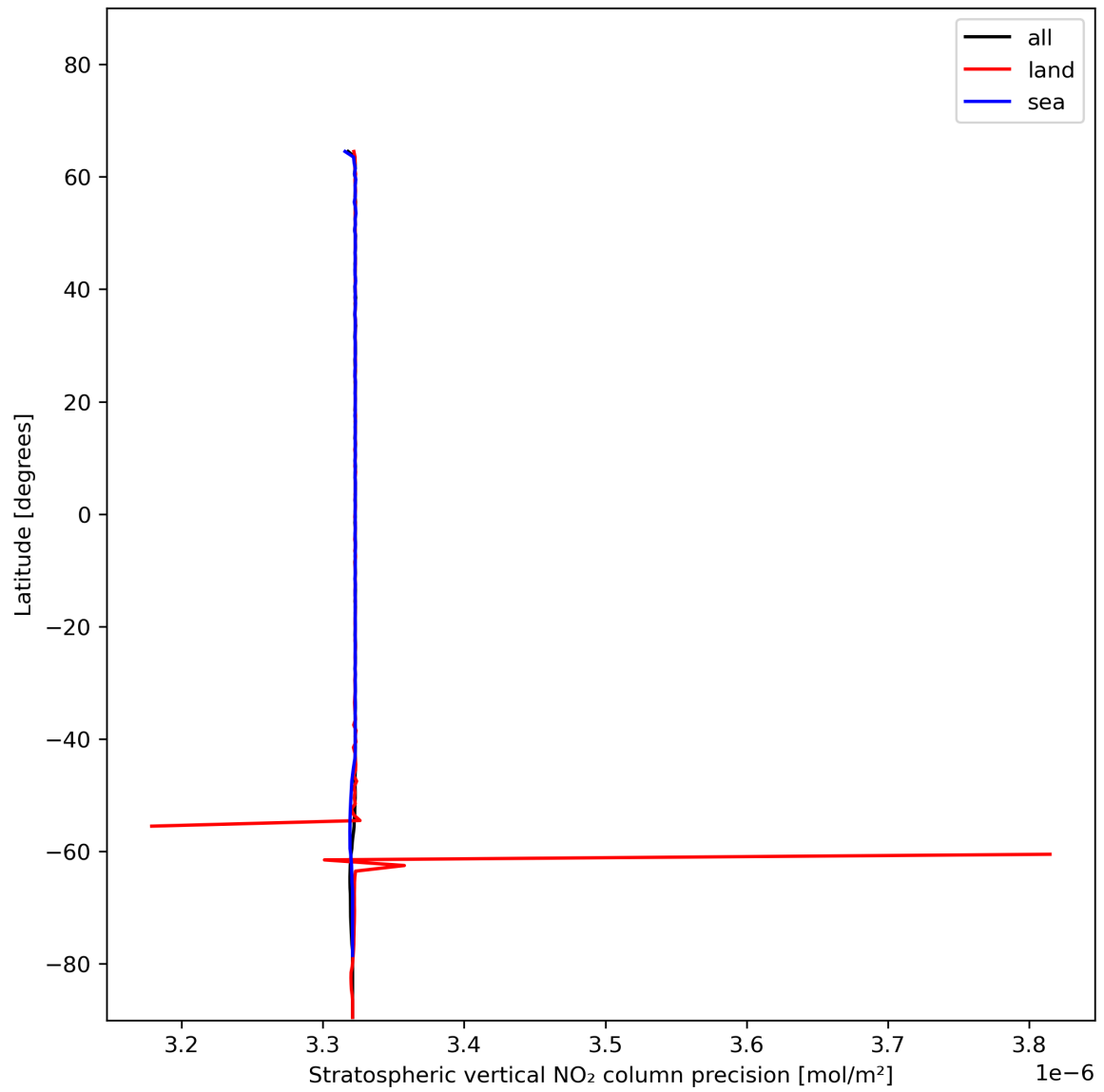
Figure 20: Zonal average of “Stratospheric vertical NO 2 column precision” for 2023-12-26 to 2023-12-28.
