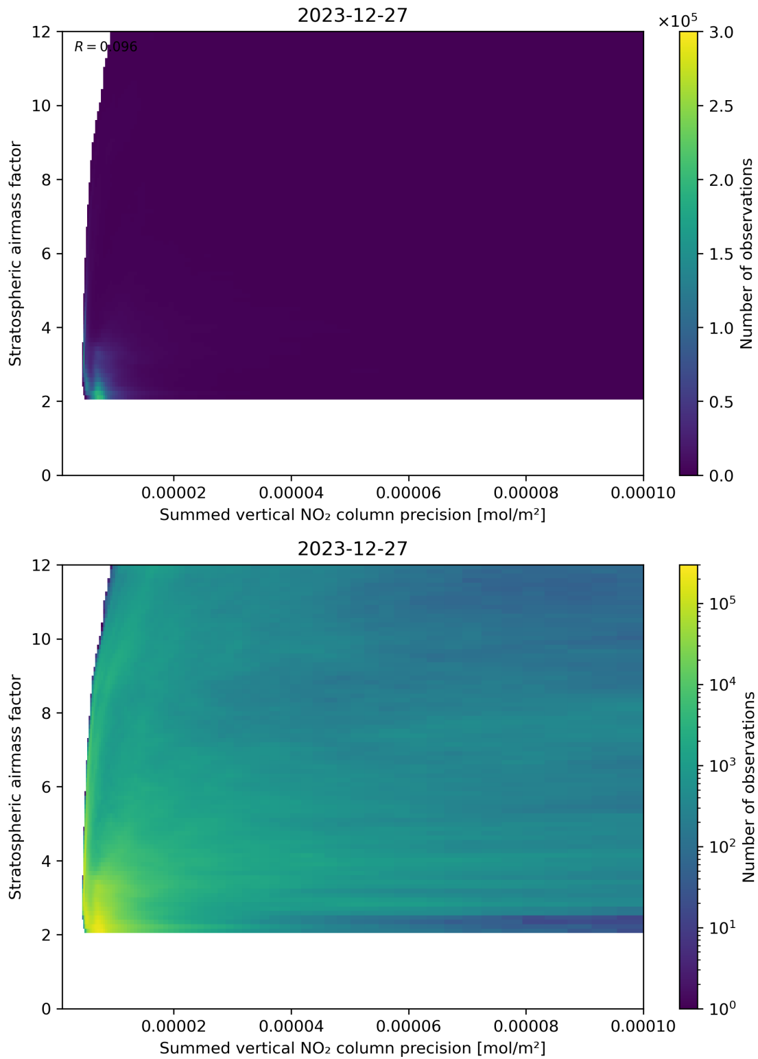
Figure 106: Scatter density plot of “Summed vertical NO 2 column precision” against “Stratospheric airmass factor” for 2023-12-26 to 2023-12-28.
