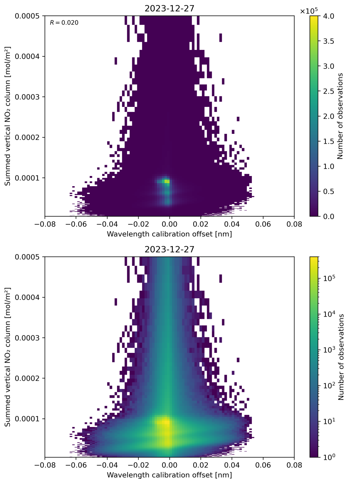
Figure 177: Scatter density plot of “Wavelength calibration offset” against “Summed vertical NO 2 column” for 2023-12-26 to 2023-12-28.
