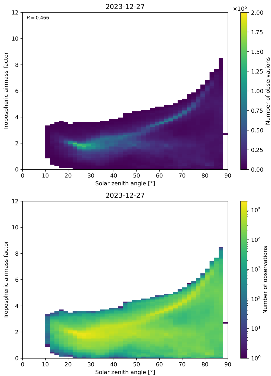
Figure 147: Scatter density plot of “Solar zenith angle” against “Tropospheric airmass factor” for 2023-12-26 to 2023-12-28.
