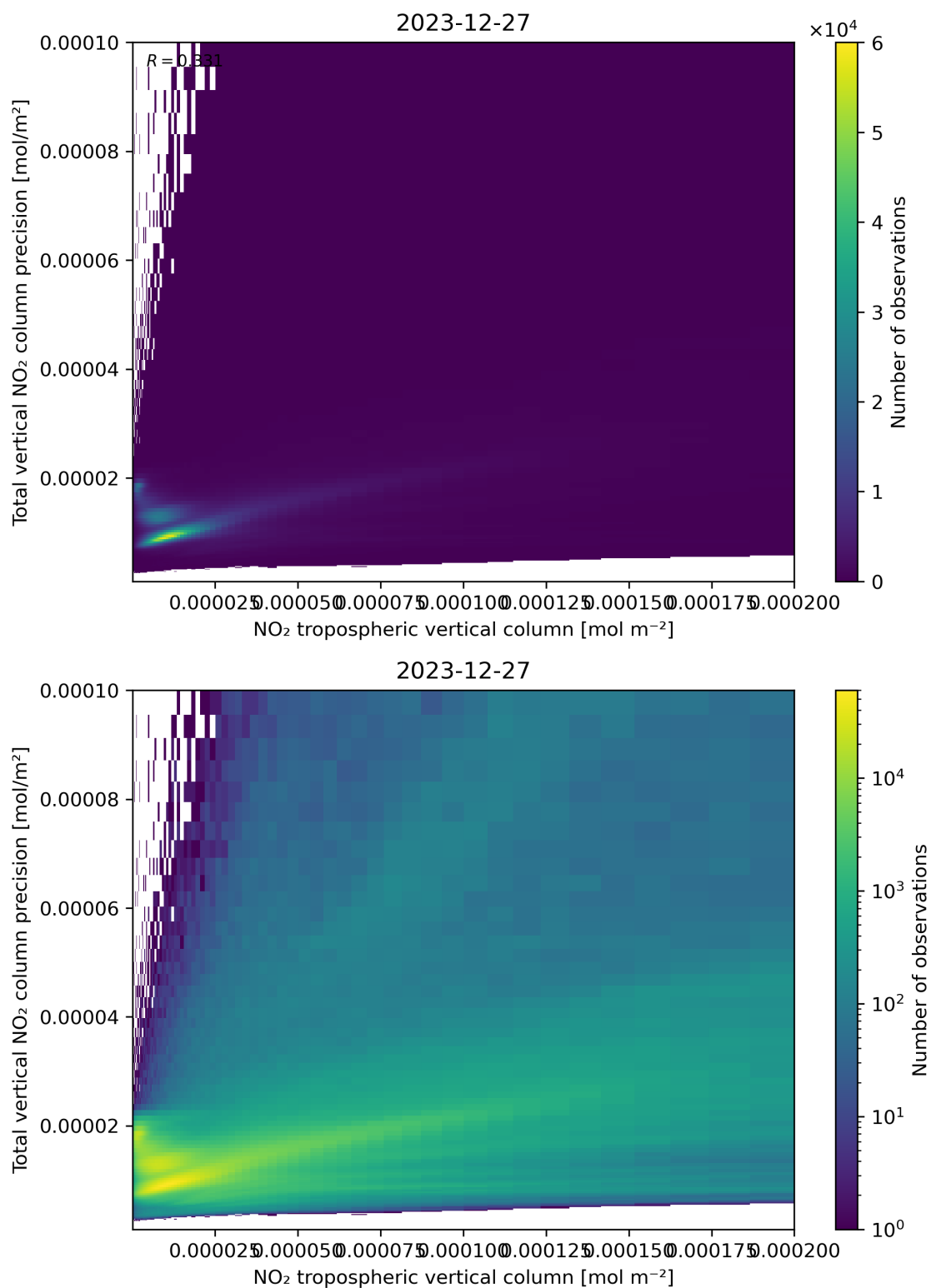
Figure 129: Scatter density plot of “NO 2 tropospheric vertical column” against “Total vertical NO 2 column precision” for 2023-12-26 to 2023-12-28.
