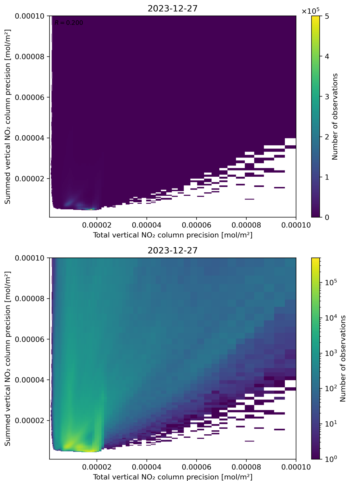
Figure 118: Scatter density plot of “Total vertical NO 2 column precision” against “Summed vertical NO 2 column precision” for 2023-12-26 to 2023-12-28.
