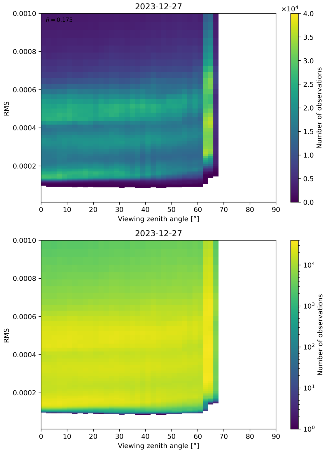
Figure 171: Scatter density plot of “Viewing zenith angle” against “RMS” for 2023-12-26 to 2023-12-28.
