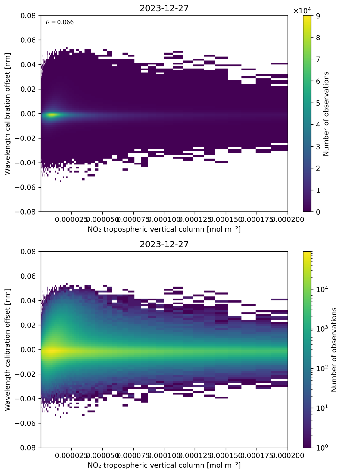
Figure 143: Scatter density plot of “NO 2 tropospheric vertical column” against “Wavelength calibration offset” for 2023-12-26 to 2023-12-28.
