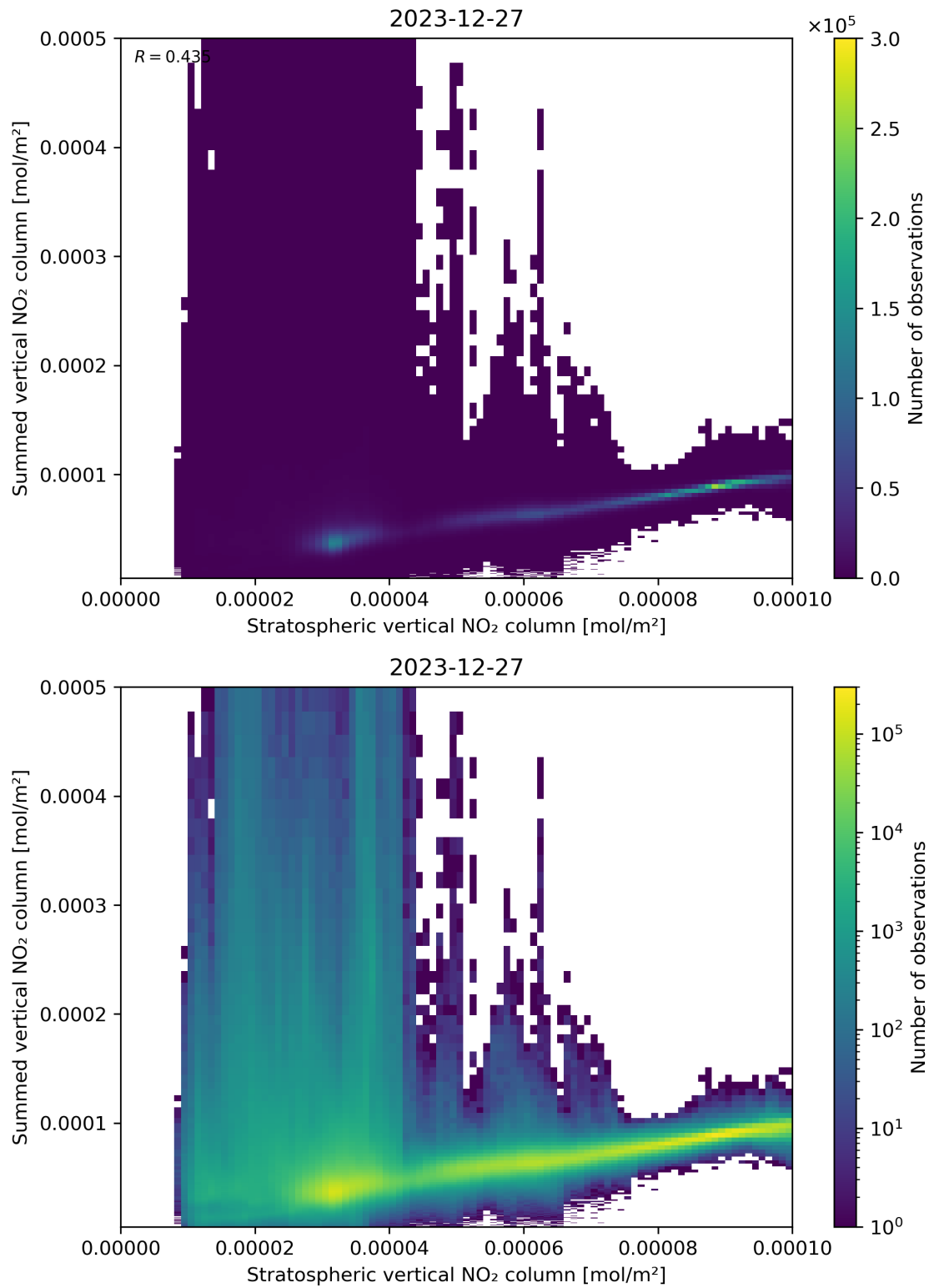
Figure 98: Scatter density plot of “Stratospheric vertical NO 2 column” against “Summed vertical NO 2 column” for 2023-12-26 to 2023-12-28.
