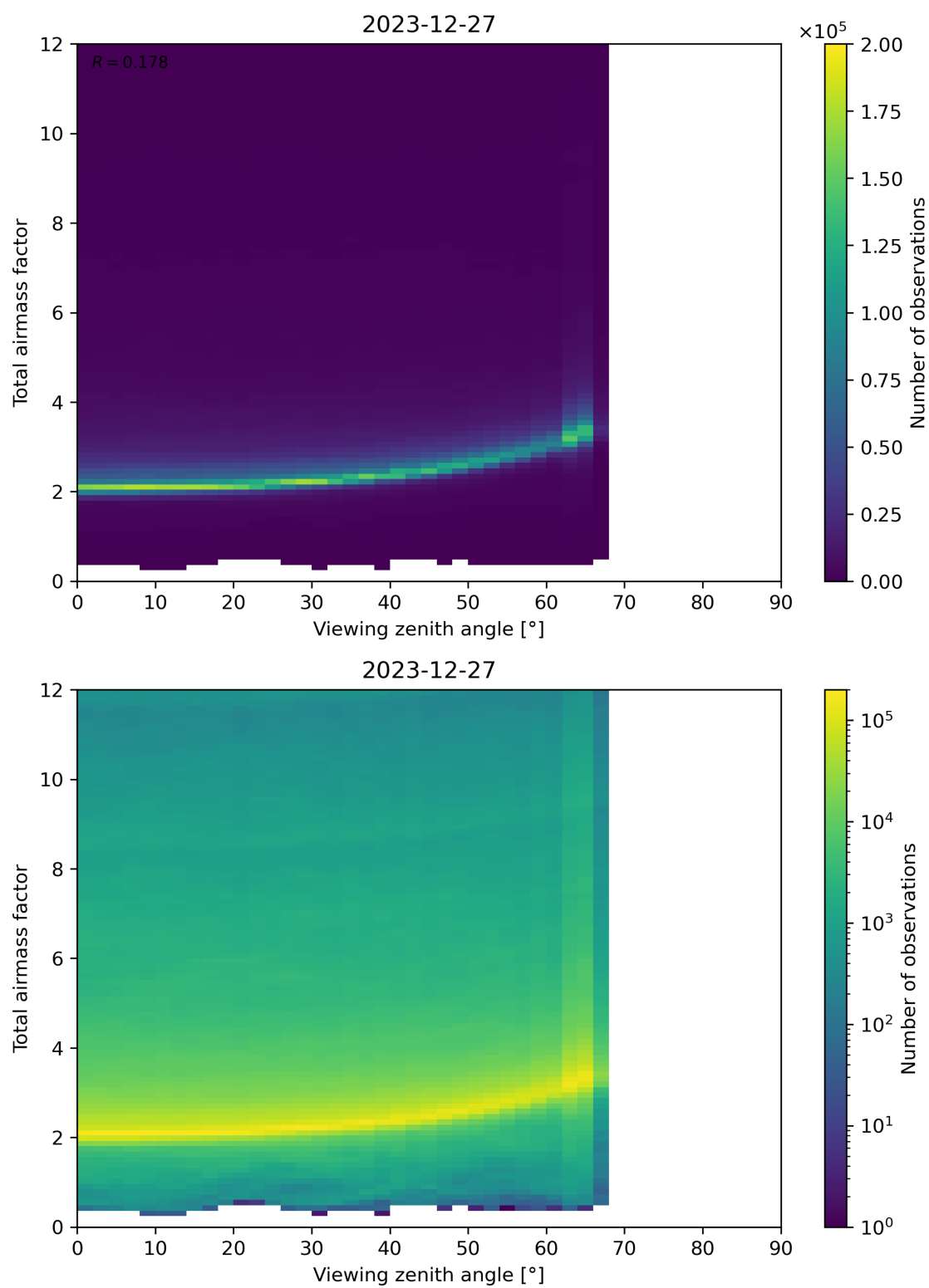
Figure 160: Scatter density plot of “Viewing zenith angle” against “Total airmass factor” for 2023-12-26 to 2023-12-28.
