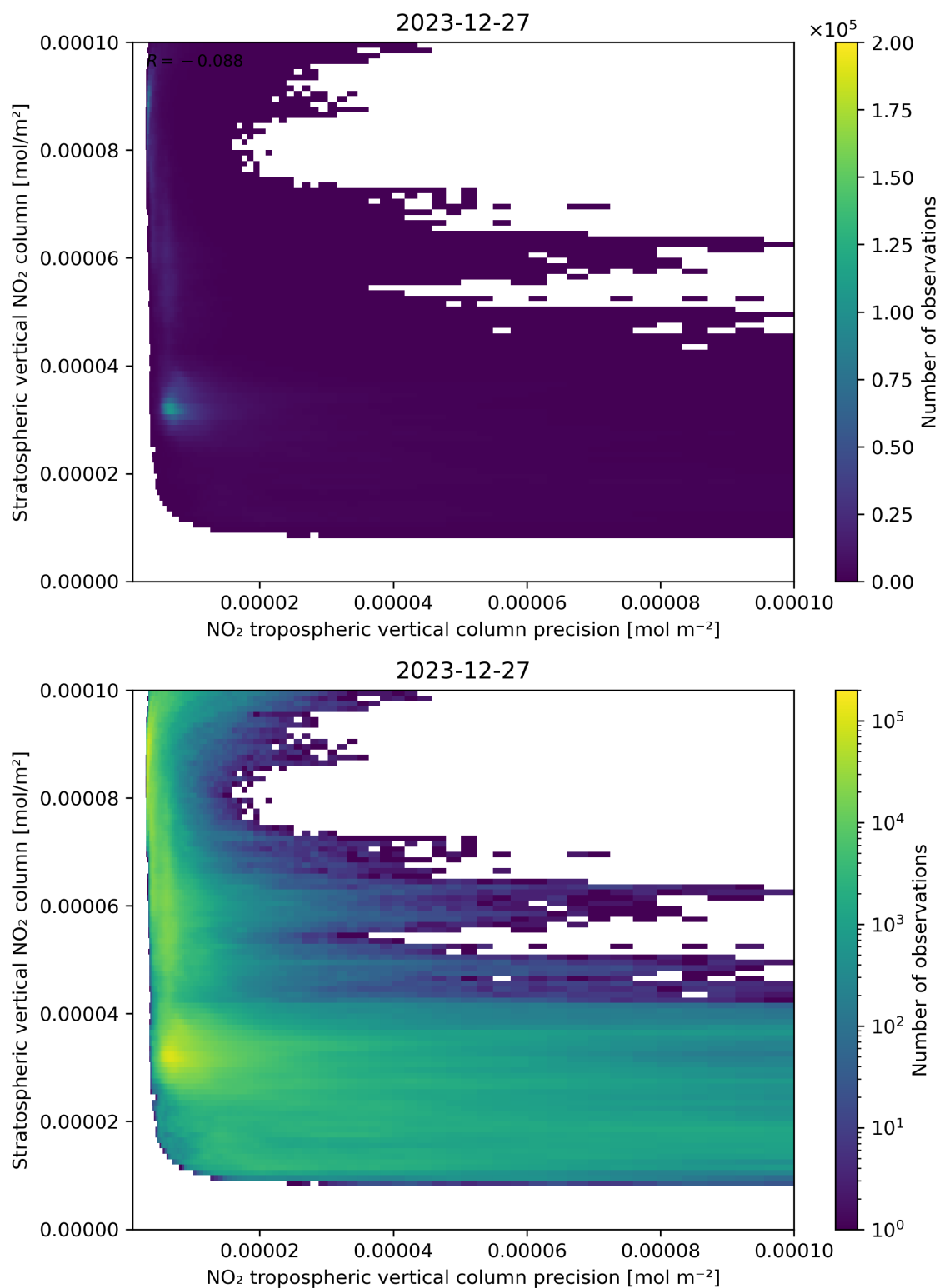
Figure 135: Scatter density plot of “NO 2 tropospheric vertical column precision” against “Stratospheric vertical NO 2 column” for 2023-12-26 to 2023-12-28.
