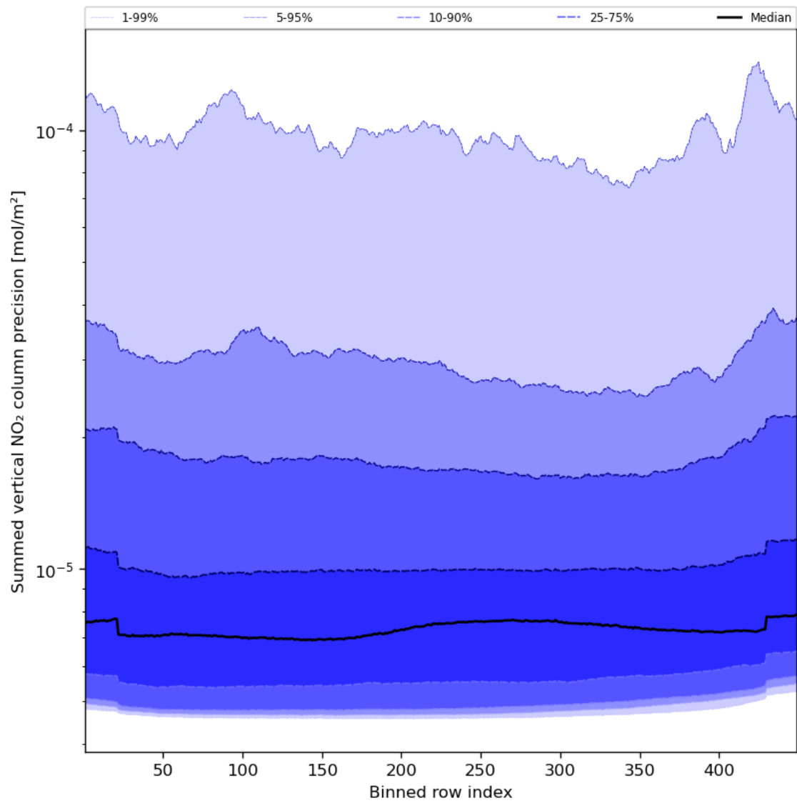
Figure 58: Along track statistics of “Summed vertical NO 2 column precision” for 2023-12-26 to 2023-12-28
