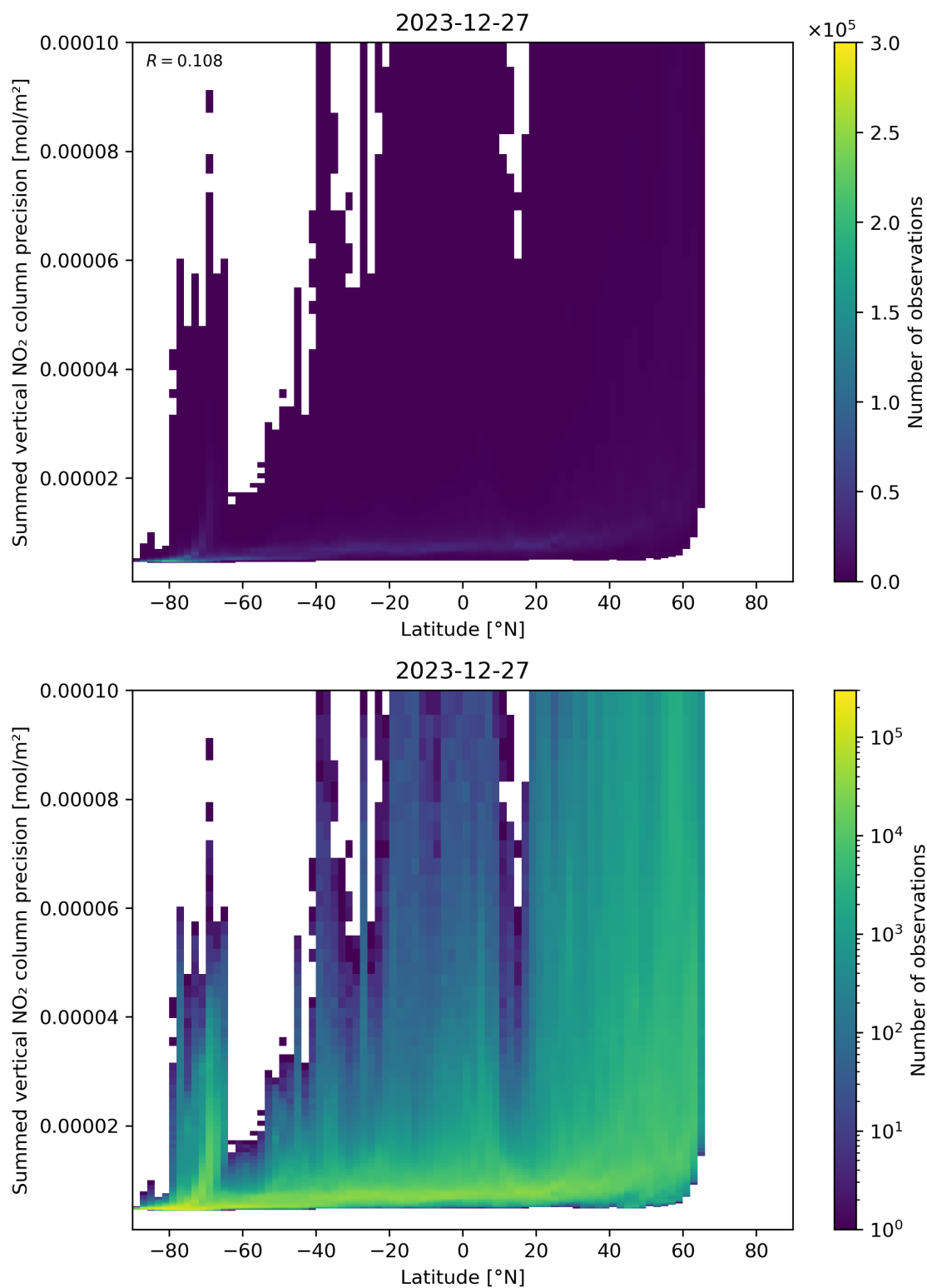
Figure 89: Scatter density plot of “Latitude” against “Summed vertical NO 2 column precision” for 2023-12-26 to 2023-12-28.
