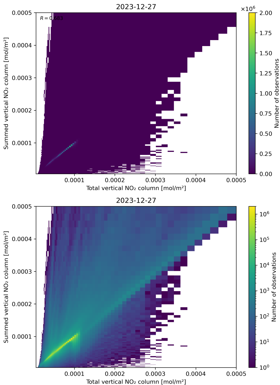
Figure 112: Scatter density plot of “Total vertical NO 2 column” against “Summed vertical NO 2 column” for 2023-12-26 to 2023-12-28.
