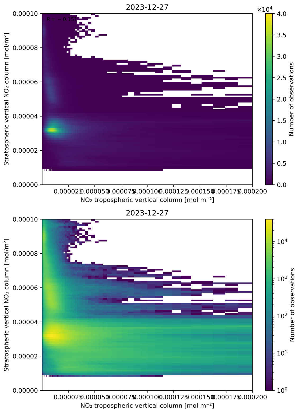
Figure 125: Scatter density plot of “NO 2 tropospheric vertical column” against “Stratospheric vertical NO 2 column” for 2023-12-26 to 2023-12-28.
