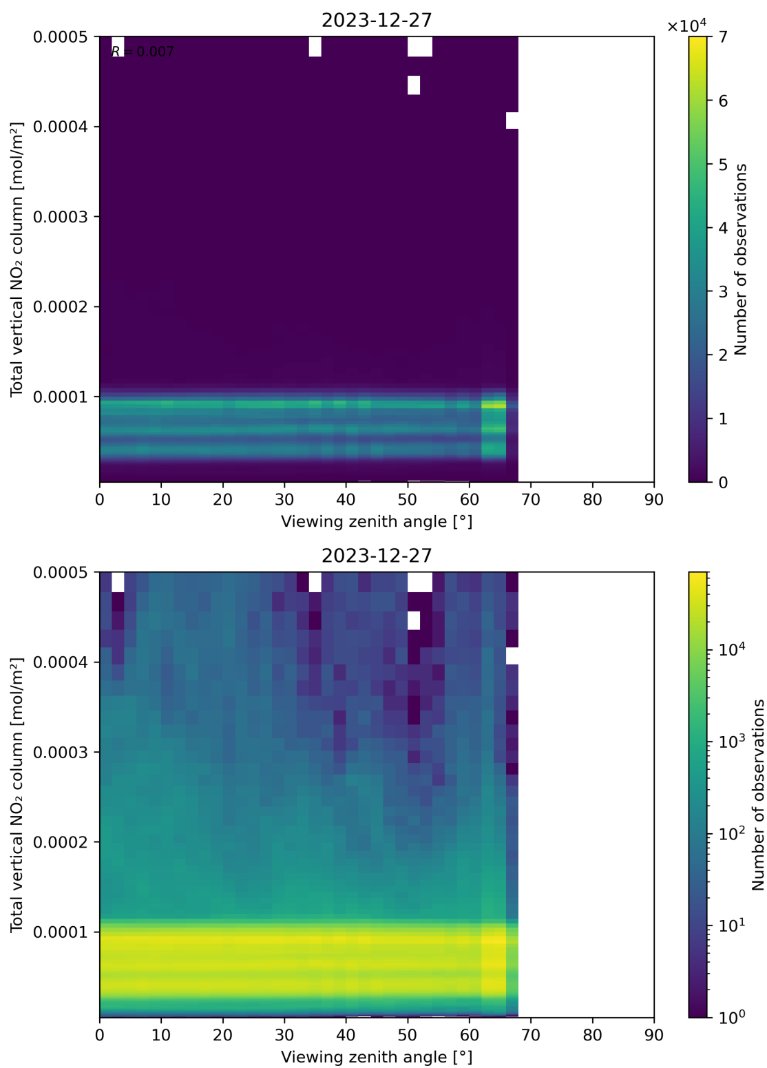
Figure 167: Scatter density plot of “Viewing zenith angle” against “Total vertical NO 2 column” for 2023-12-26 to 2023-12-28.
