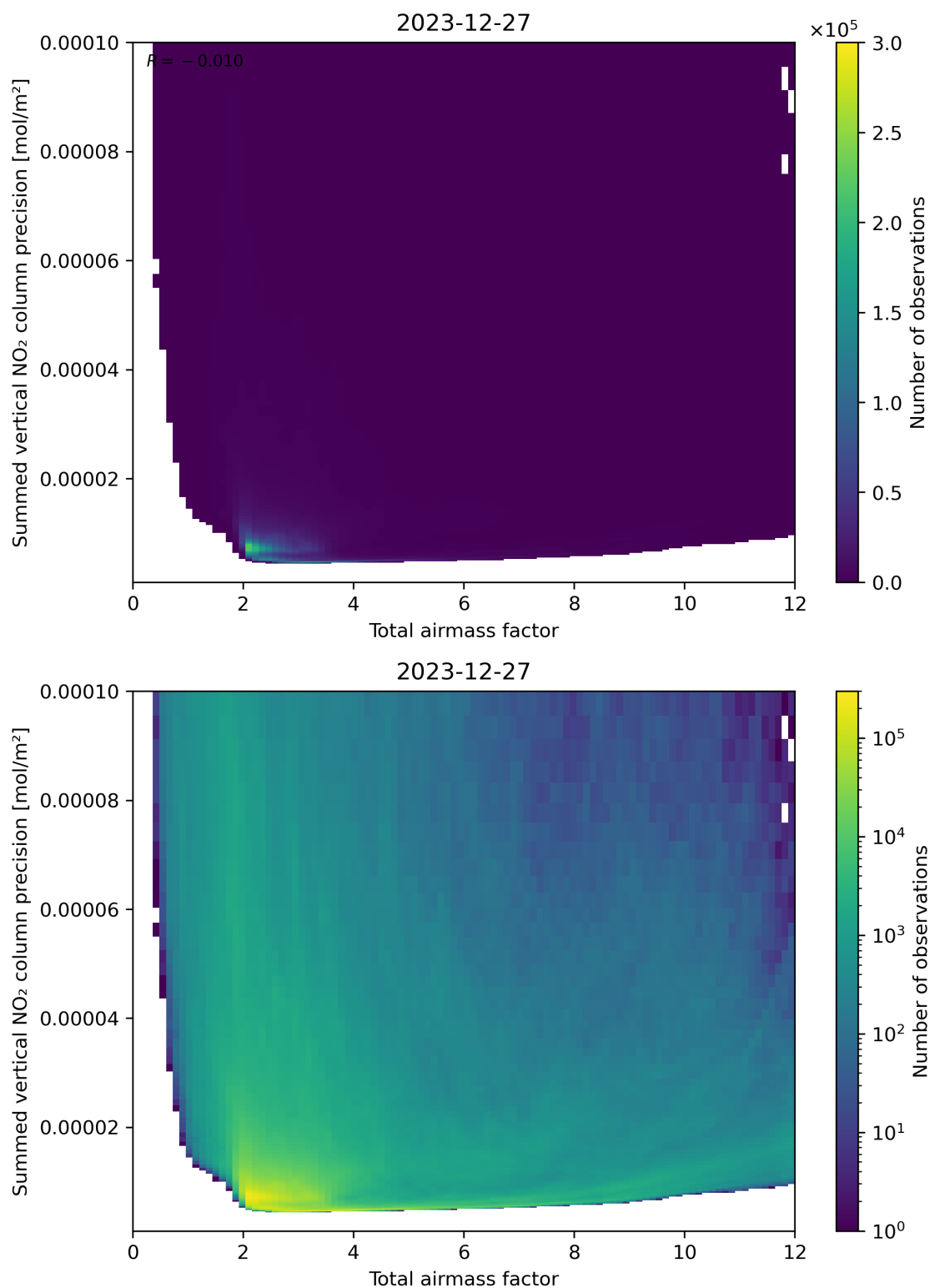
Figure 66: Scatter density plot of “Total airmass factor” against “Summed vertical NO 2 column precision” for 2023-12-26 to 2023-12-28.
