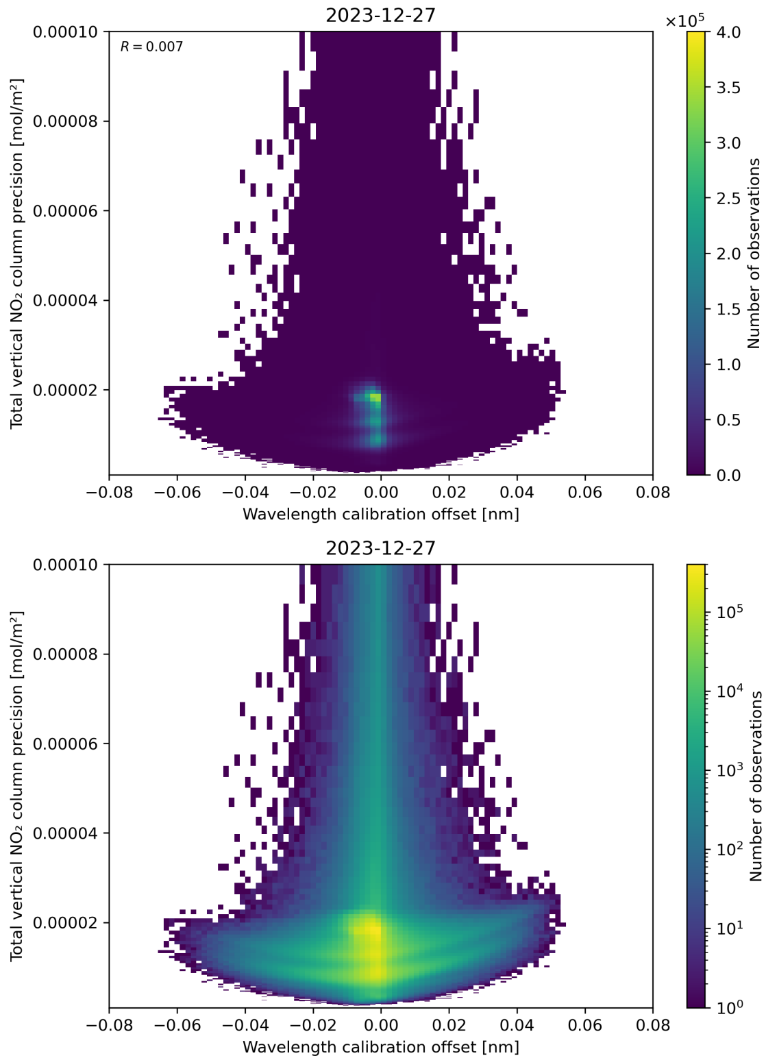
Figure 180: Scatter density plot of “Wavelength calibration offset” against “Total vertical NO 2 column precision” for 2023-12-26 to 2023-12-28.
