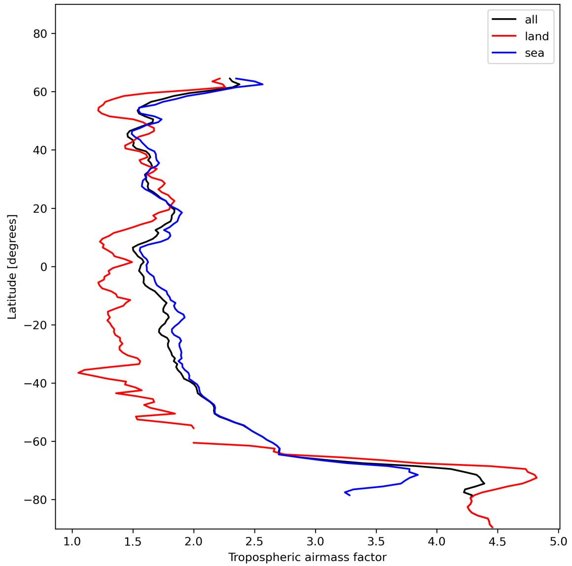
Figure 14: Zonal average of “Tropospheric airmass factor” for 2023-12-26 to 2023-12-28.
