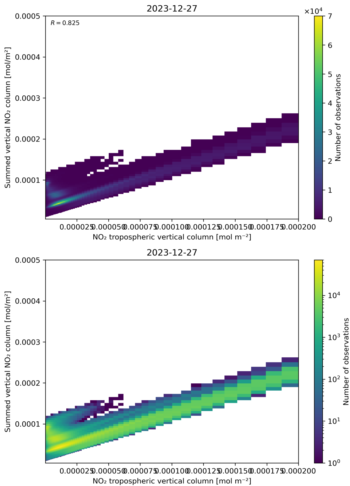
Figure 126: Scatter density plot of “NO 2 tropospheric vertical column” against “Summed vertical NO 2 column” for 2023-12-26 to 2023-12-28.
