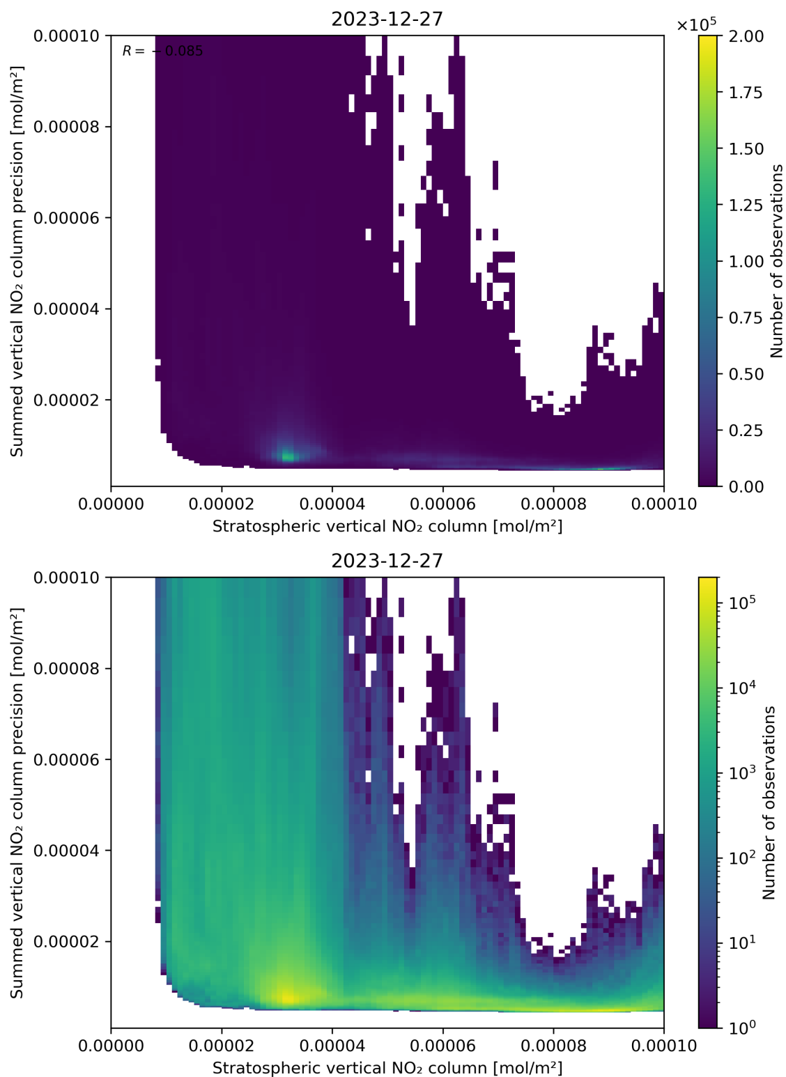
Figure 99: Scatter density plot of “Stratospheric vertical NO 2 column” against “Summed vertical NO 2 column precision” for 2023-12-26 to 2023-12-28.
