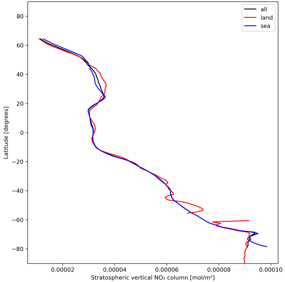
Figure 19: Zonal average of “Stratospheric vertical NO 2 column” for 2023-12-26 to 2023-12-28.
