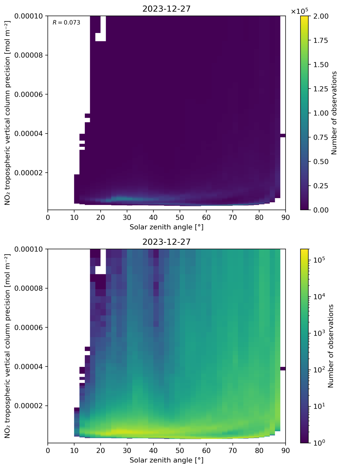
Figure 156: Scatter density plot of “Solar zenith angle” against “NO 2 tropospheric vertical column precision” for 2023-12-26 to 2023-12-28.
