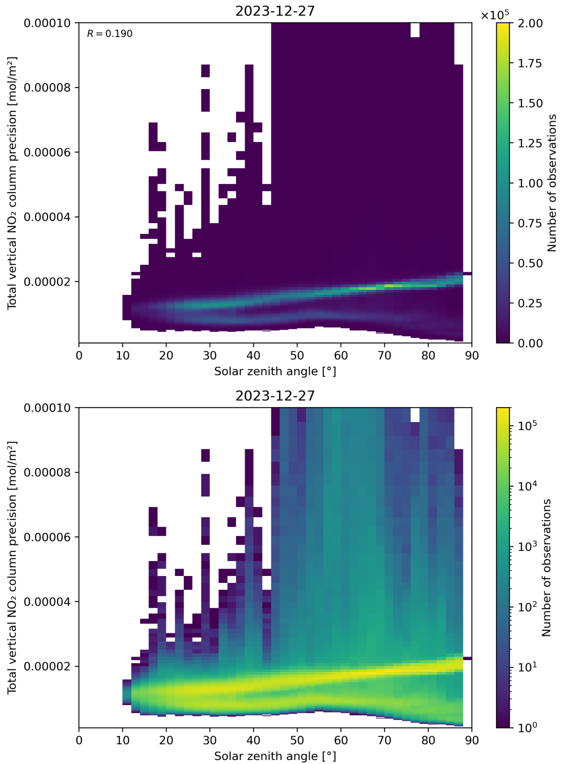
Figure 154: Scatter density plot of “Solar zenith angle” against “Total vertical NO 2 column precision” for 2023-12-26 to 2023-12-28.
