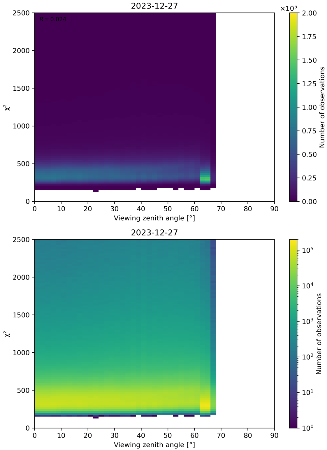
Figure 162: Scatter density plot of “Viewing zenith angle” against “ \chi^2 ” for 2023-12-26 to 2023-12-28.
