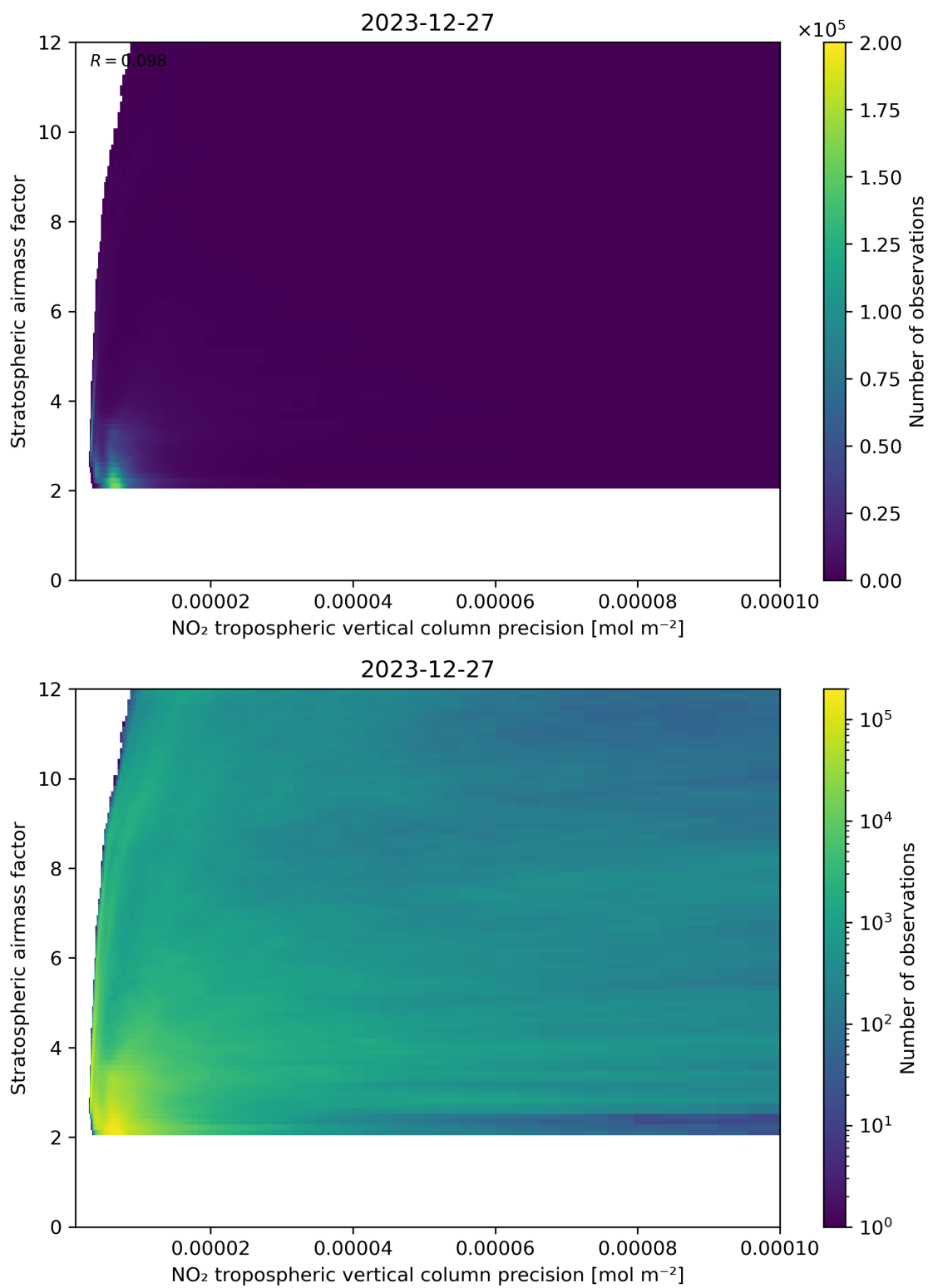
Figure 131: Scatter density plot of “NO 2 tropospheric vertical column precision” against “Stratospheric airmass factor” for 2023-12-26 to 2023-12-28.
