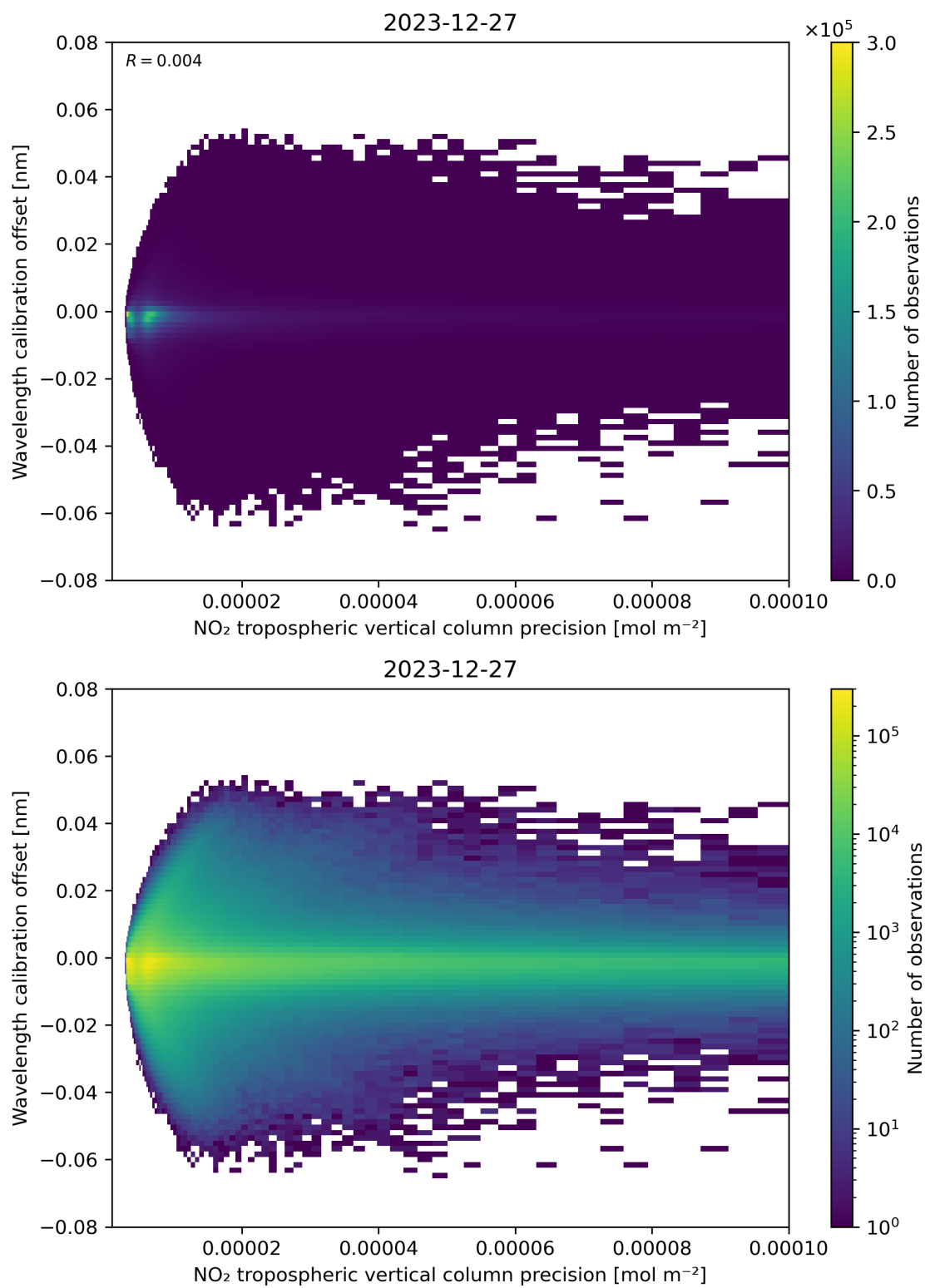
Figure 141: Scatter density plot of “NO 2 tropospheric vertical column precision” against “Wavelength calibration offset” for 2023-12-26 to 2023-12-28.
