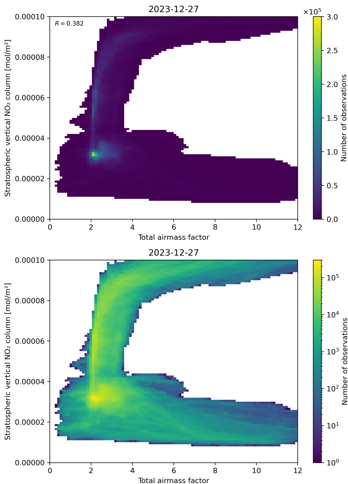
Figure 64: Scatter density plot of “Total airmass factor” against “Stratospheric vertical \text{NO}_2 column” for 2023-12-26 to 2023-12-28.
