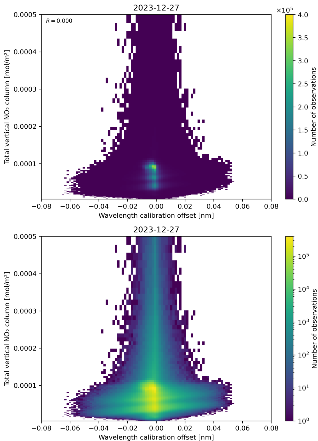
Figure 179: Scatter density plot of “Wavelength calibration offset” against “Total vertical NO 2 column” for 2023-12-26 to 2023-12-28.
