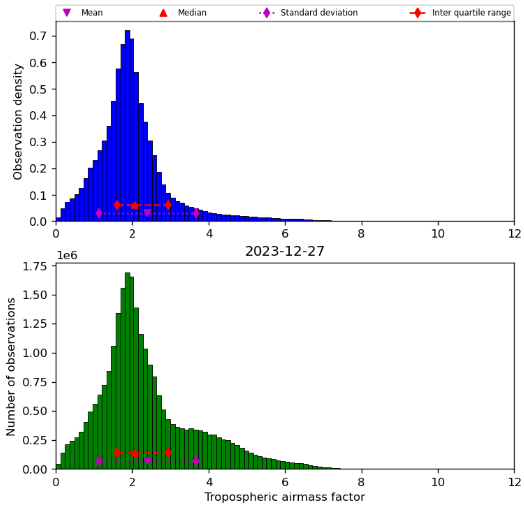
Figure 31: Histogram of “Tropospheric airmass factor” for 2023-12-26 to 2023-12-28
