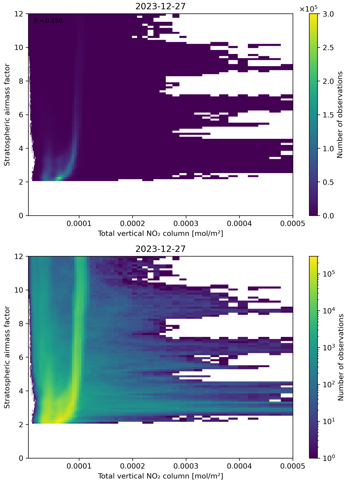
Figure 110: Scatter density plot of “Total vertical NO 2 column” against “Stratospheric airmass factor” for 2023-12-26 to 2023-12-28.
