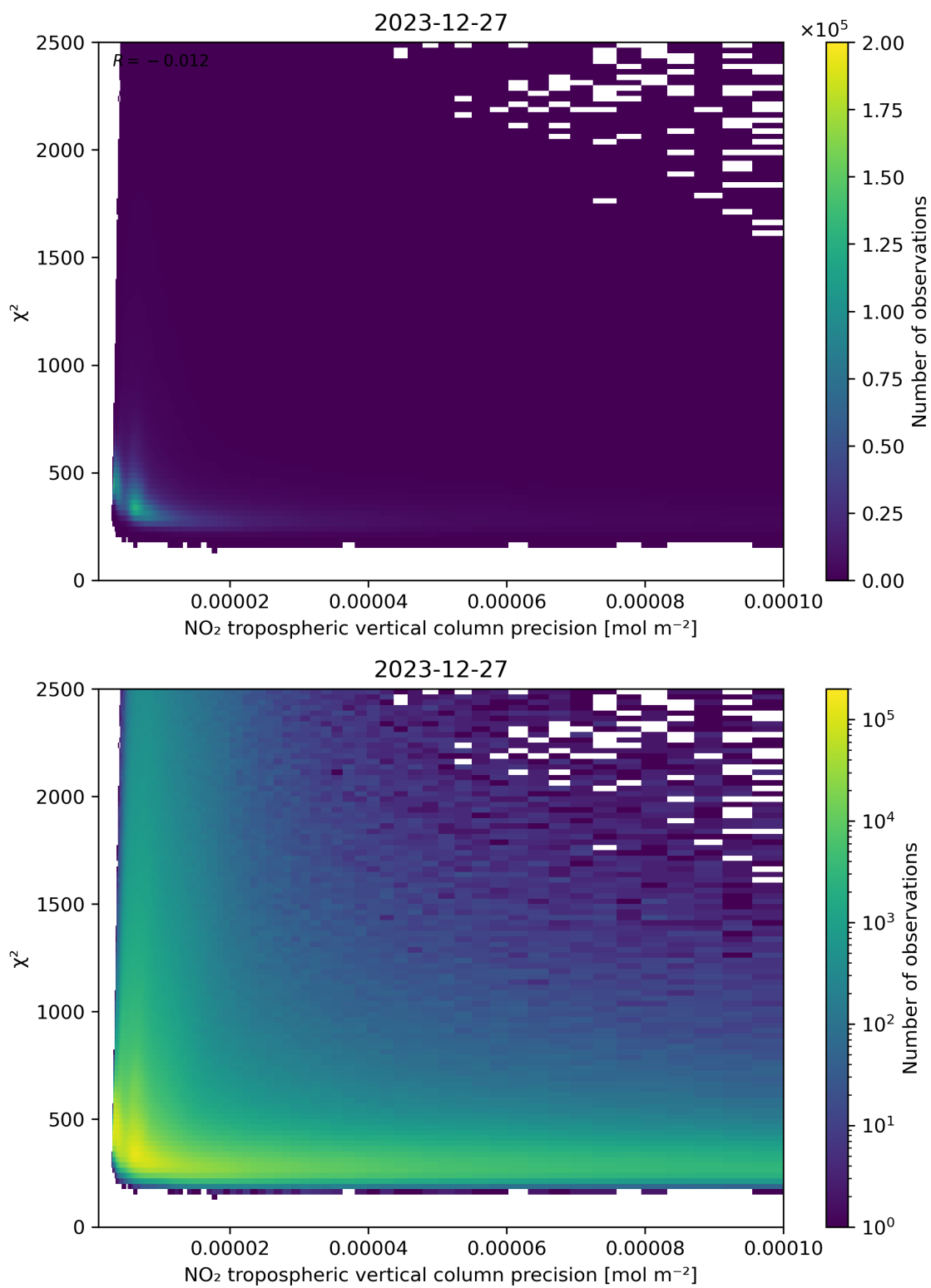
Figure 134: Scatter density plot of “NO 2 tropospheric vertical column precision” against “ \chi^2 ” for 2023-12-26 to 2023-12-28.
