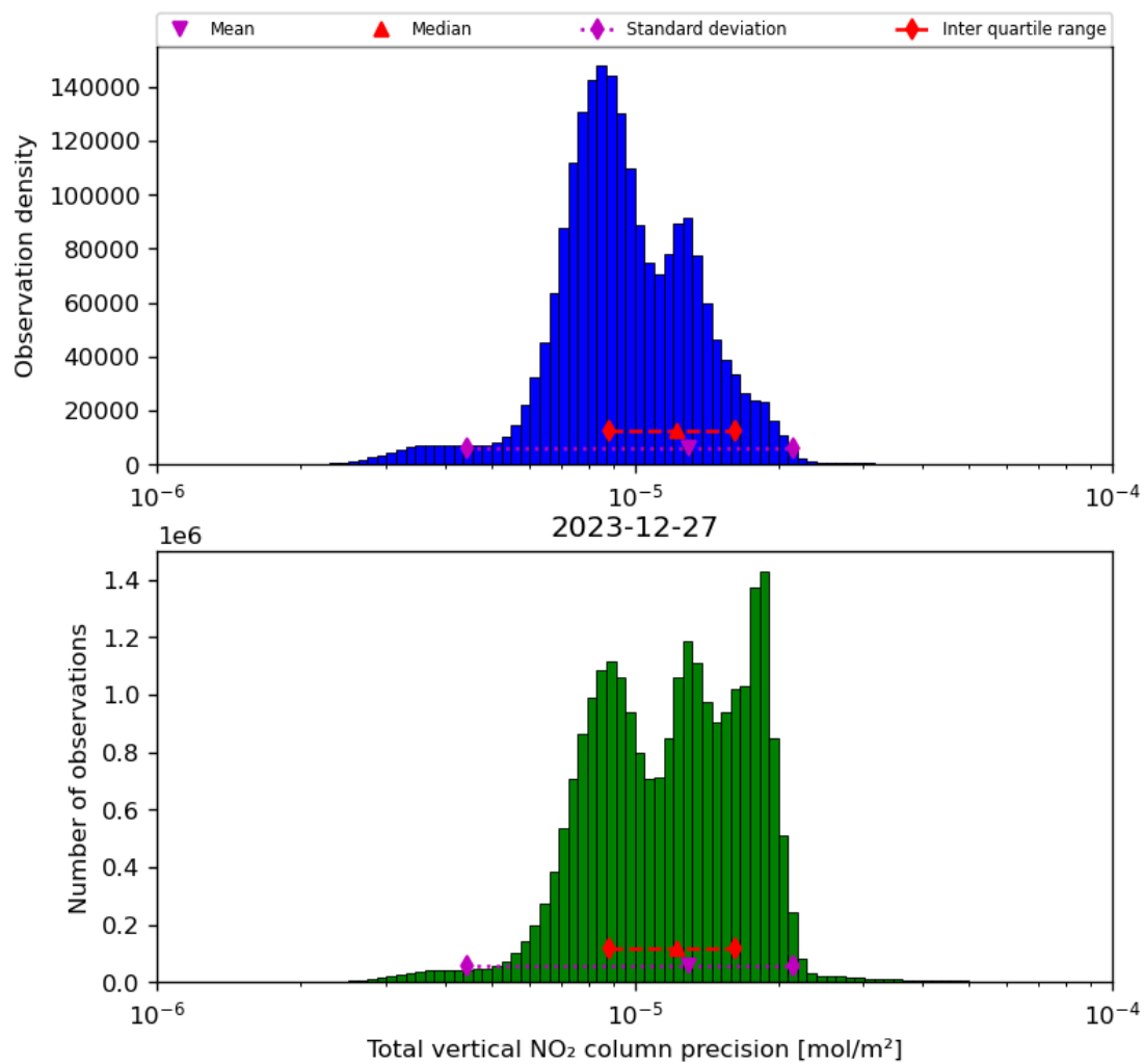
Figure 39: Histogram of “Total vertical NO 2 column precision” for 2023-12-26 to 2023-12-28
