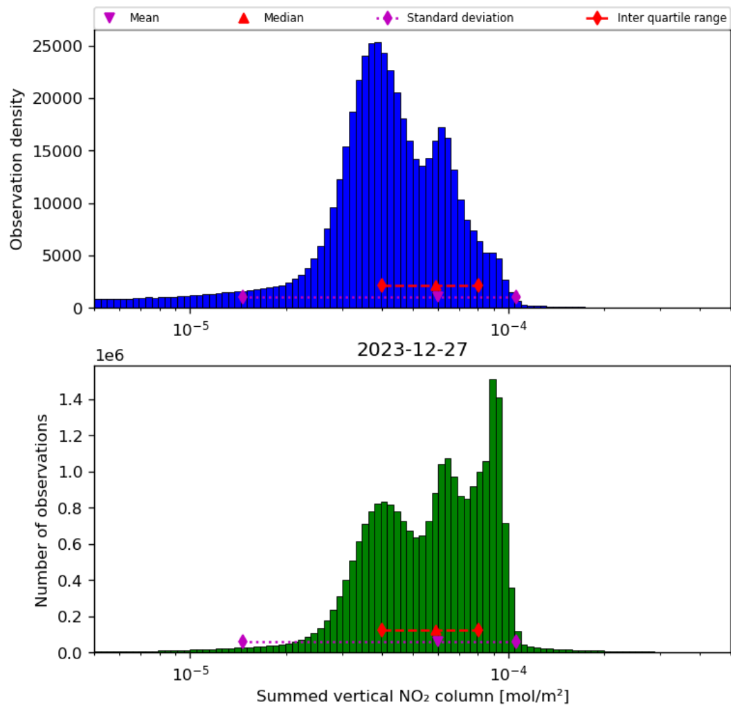
Figure 40: Histogram of “Summed vertical NO 2 column” for 2023-12-26 to 2023-12-28
