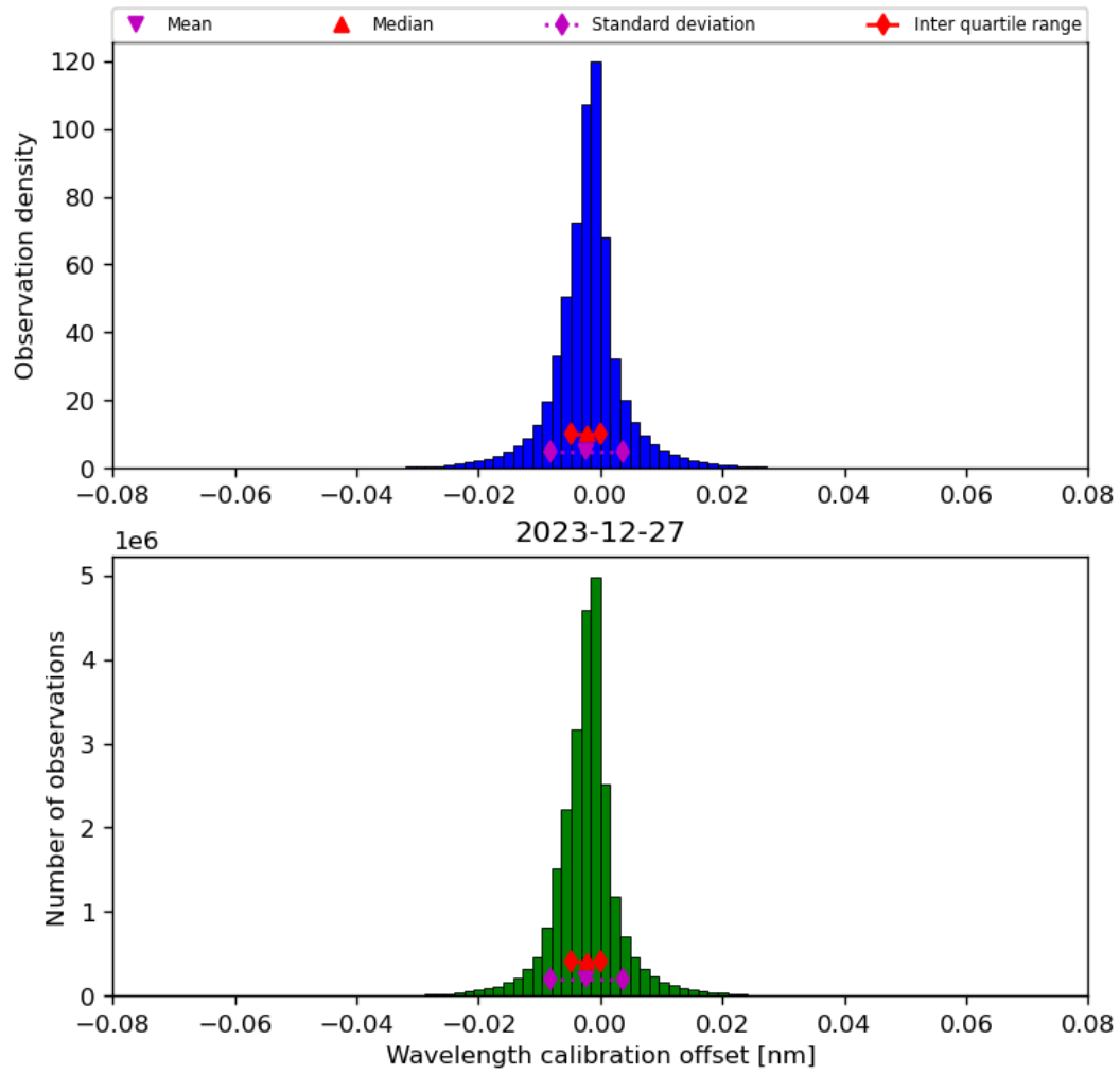
Figure 35: Histogram of “Wavelength calibration offset” for 2023-12-26 to 2023-12-28
