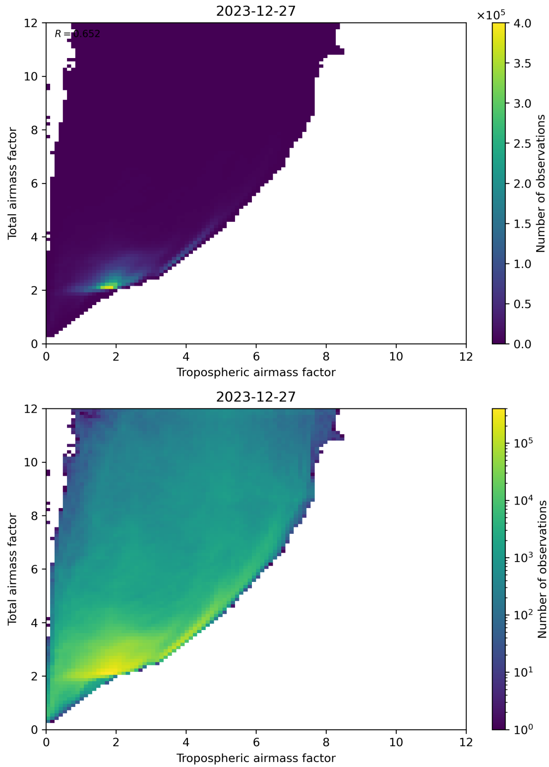
Figure 72: Scatter density plot of “Tropospheric airmass factor” against “Total airmass factor” for 2023-12-26 to 2023-12-28.
