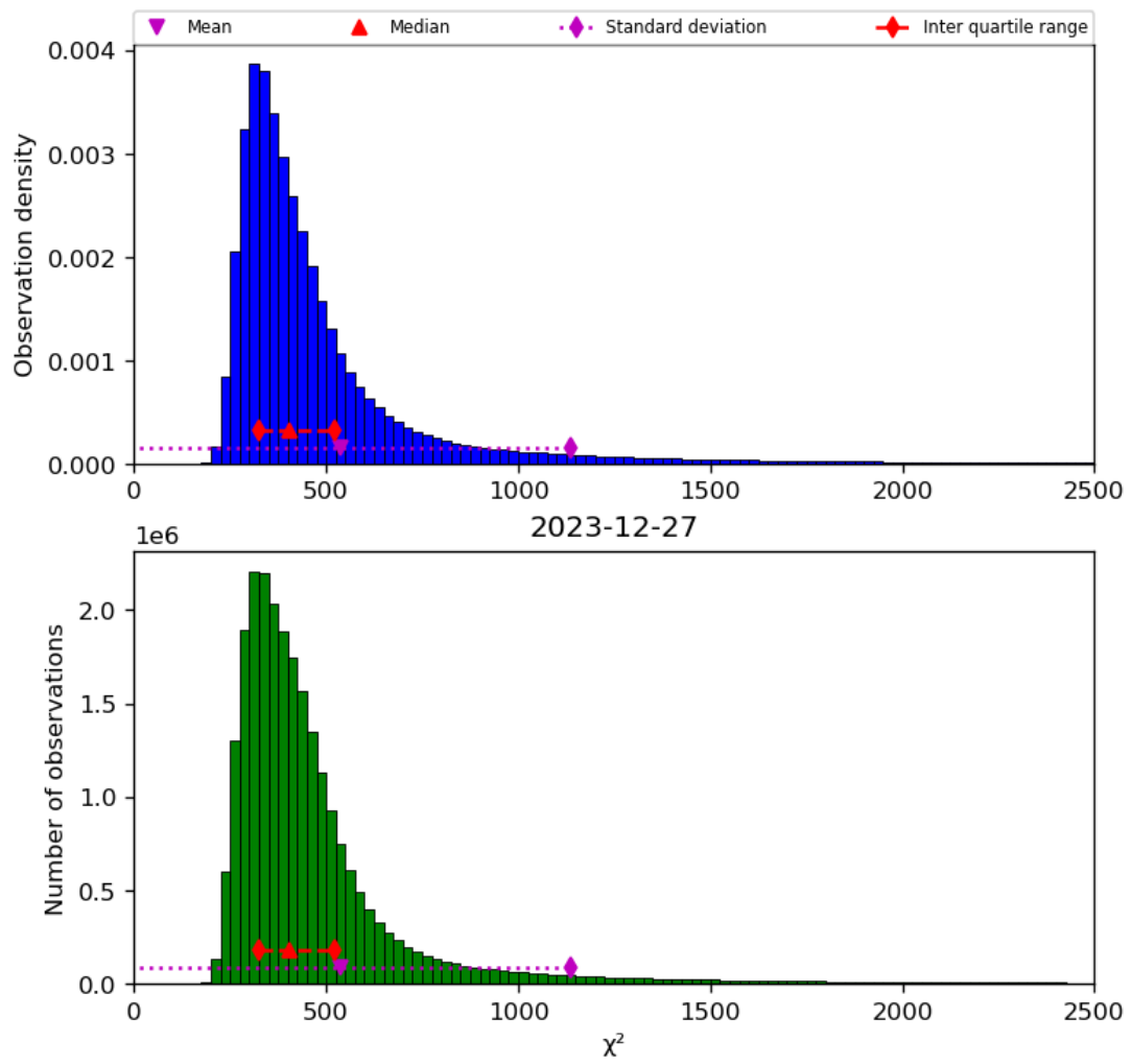
Figure 42: Histogram of " \chi^2 " for 2023-12-26 to 2023-12-28
