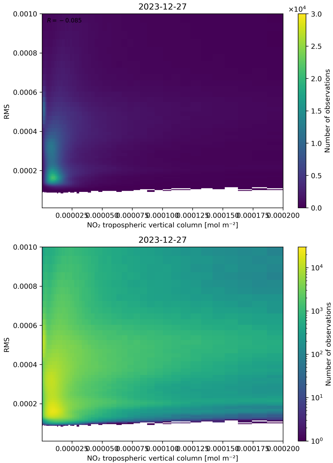
Figure 142: Scatter density plot of “NO 2 tropospheric vertical column” against “RMS” for 2023-12-26 to 2023-12-28.
