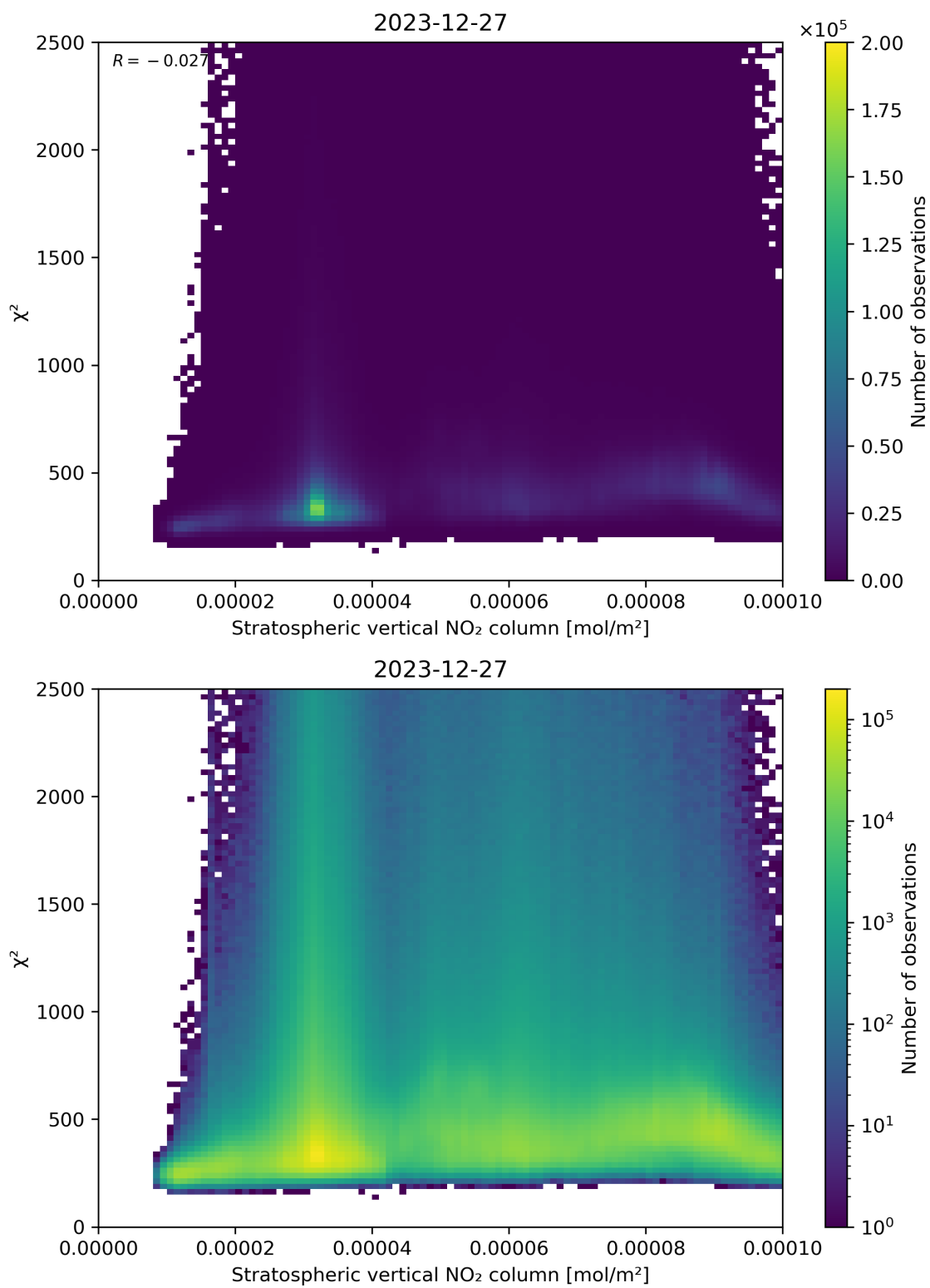
Figure 97: Scatter density plot of “Stratospheric vertical NO 2 column” against “ \chi^2 ” for 2023-12-26 to 2023-12-28.
