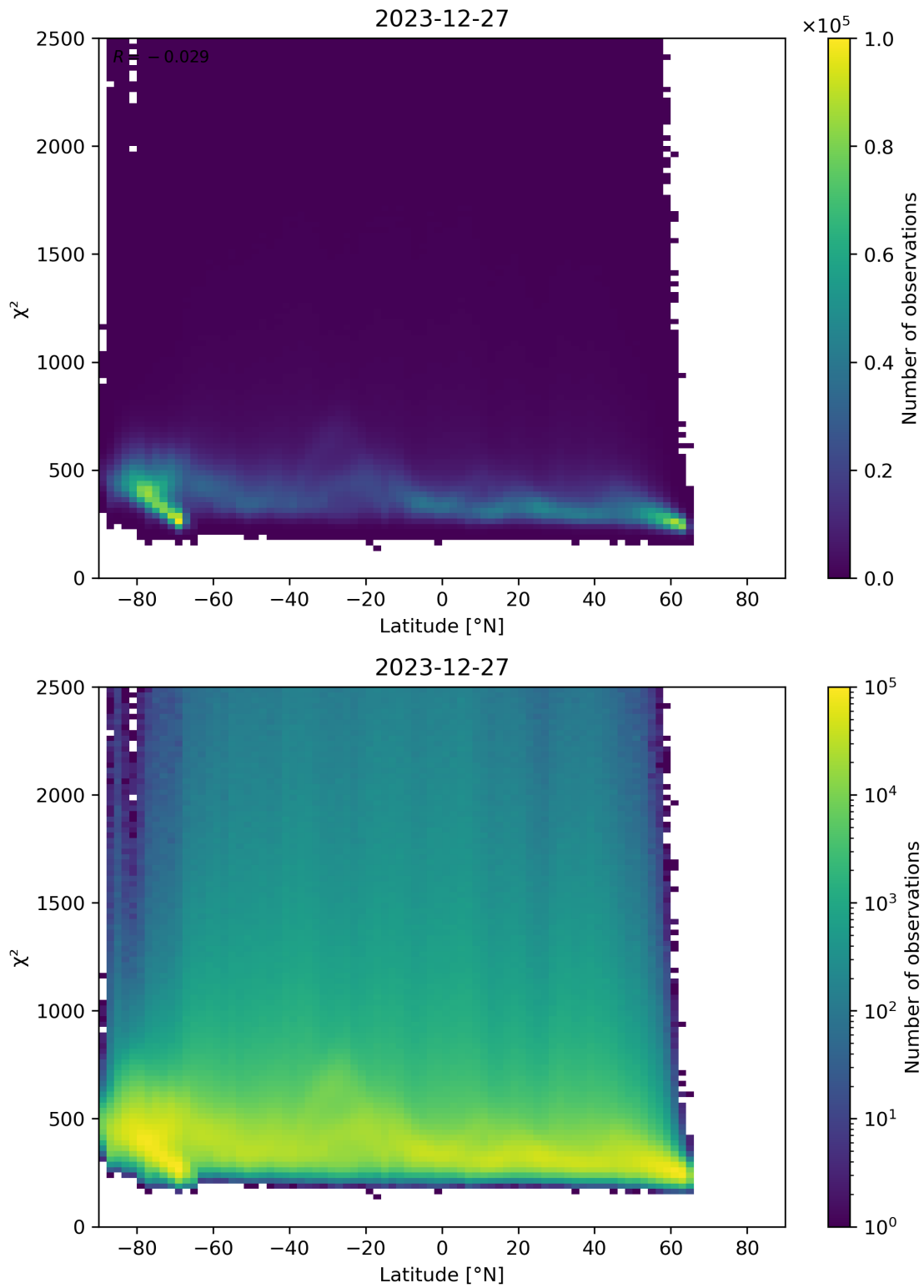
Figure 86: Scatter density plot of “Latitude” against “ \chi^2 ” for 2023-12-26 to 2023-12-28.
