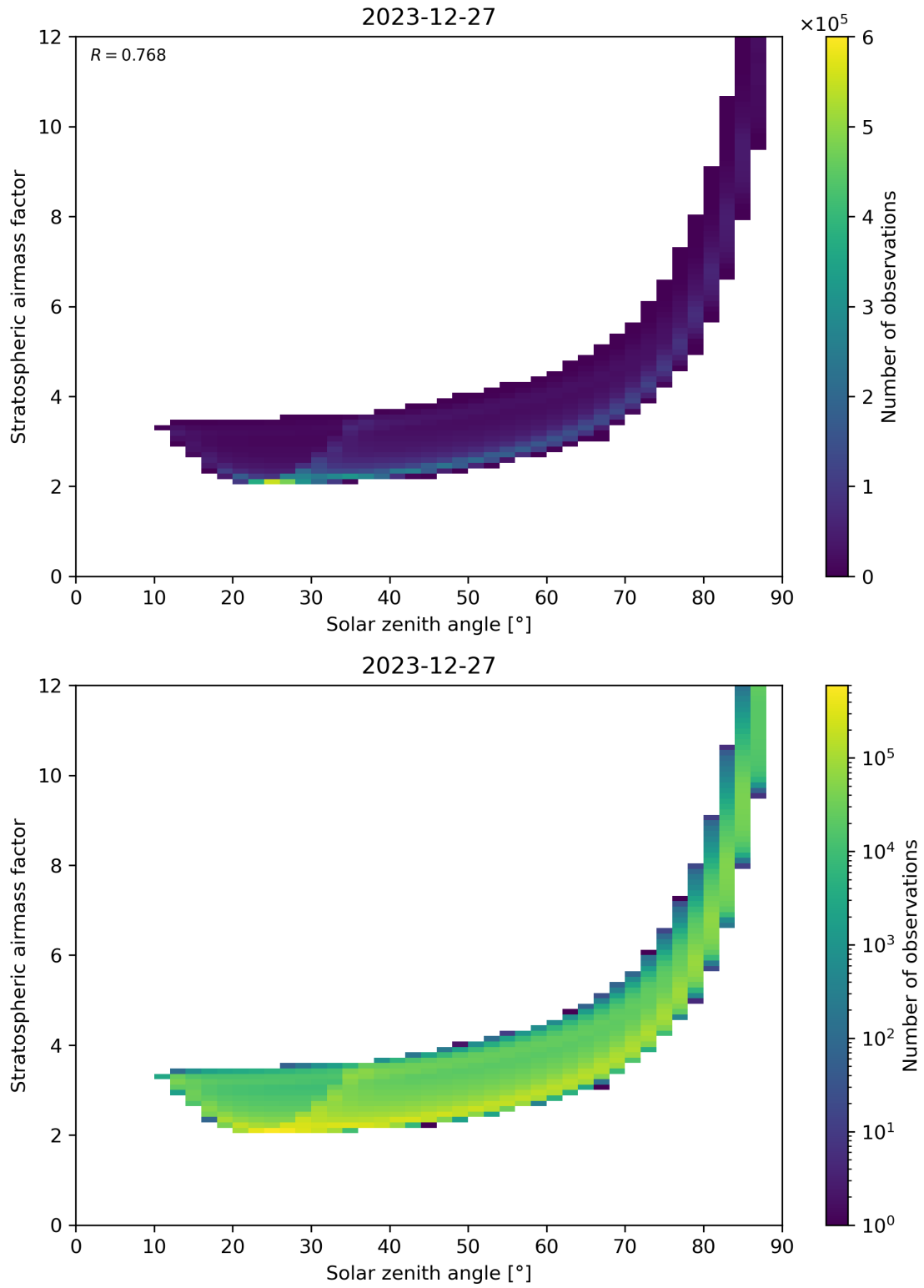
Figure 145: Scatter density plot of “Solar zenith angle” against “Stratospheric airmass factor” for 2023-12-26 to 2023-12-28.
