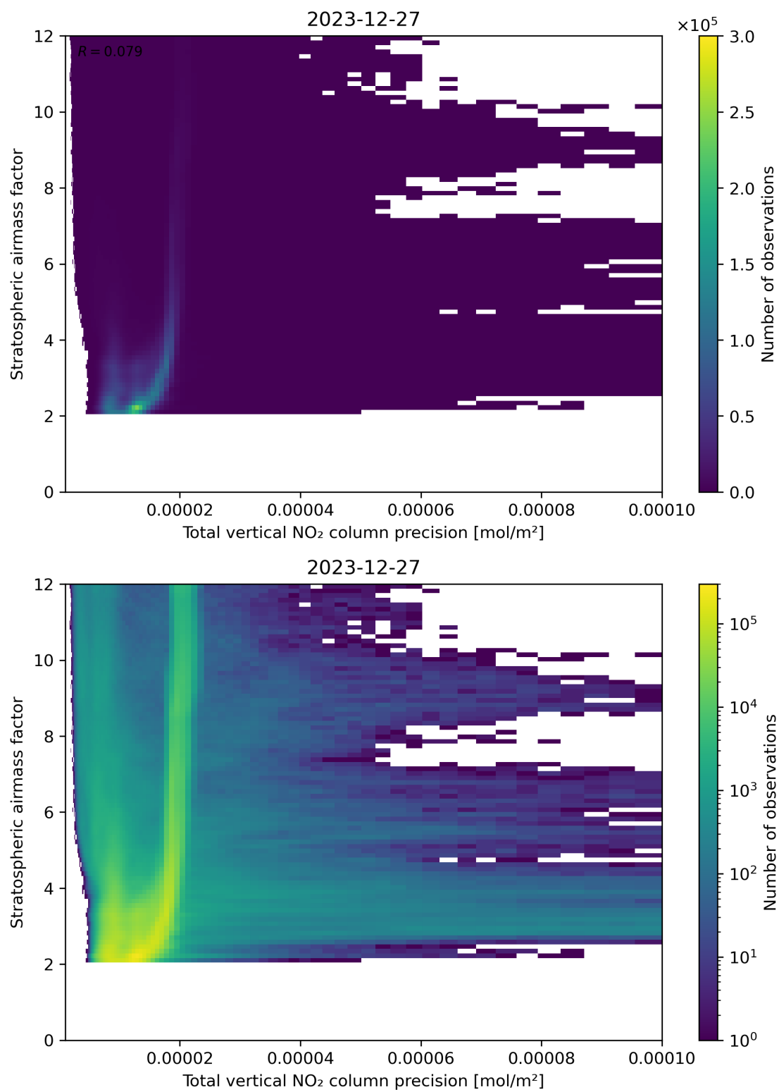
Figure 115: Scatter density plot of “Total vertical NO 2 column precision” against “Stratospheric air mass factor” for 2023-12-26 to 2023-12-28.
