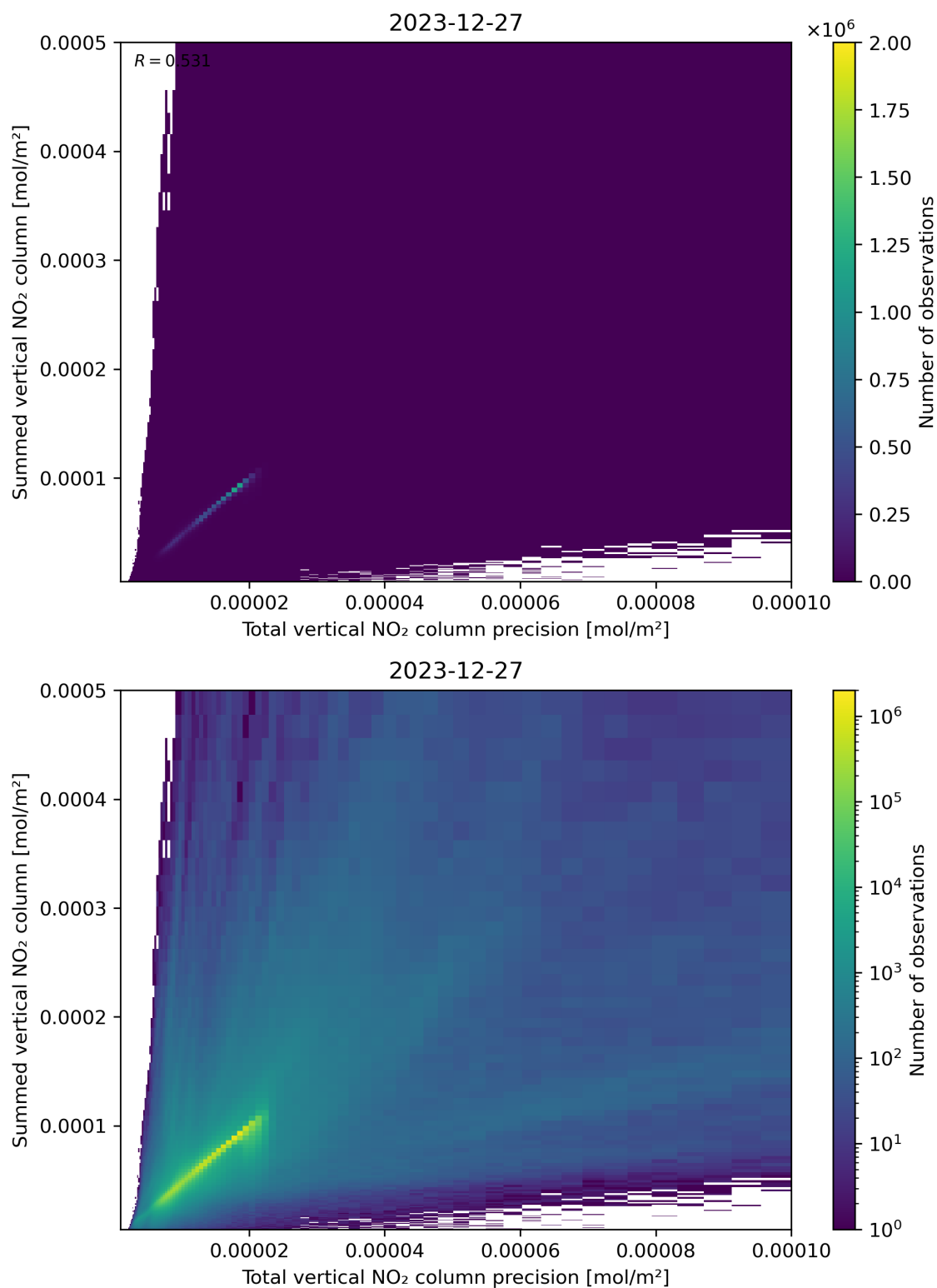
Figure 117: Scatter density plot of “Total vertical NO 2 column precision” against “Summed vertical NO 2 column” for 2023-12-26 to 2023-12-28.
