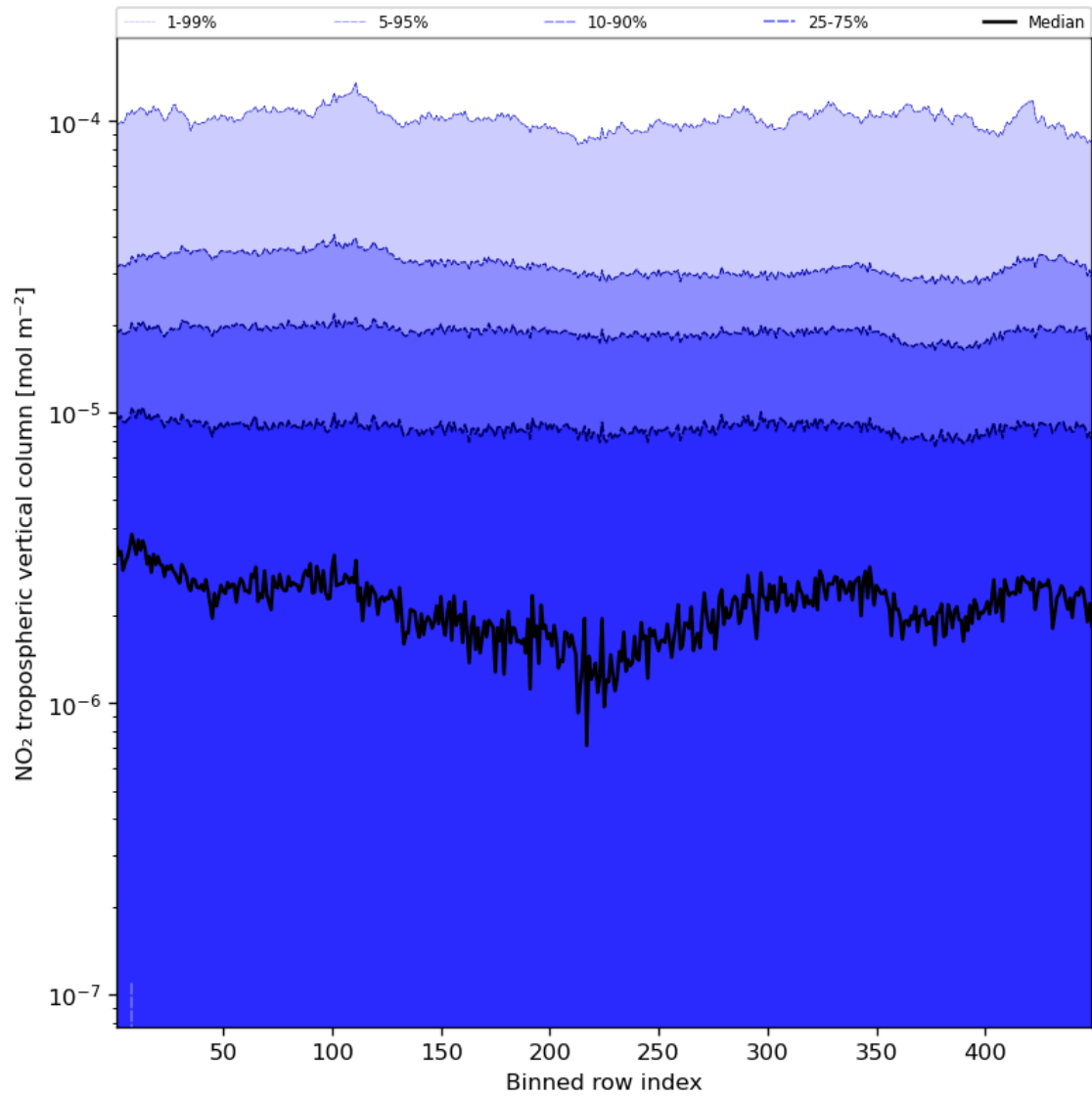
Figure 46: Along track statistics of “NO 2 tropospheric vertical column” for 2023-12-26 to 2023-12-28
