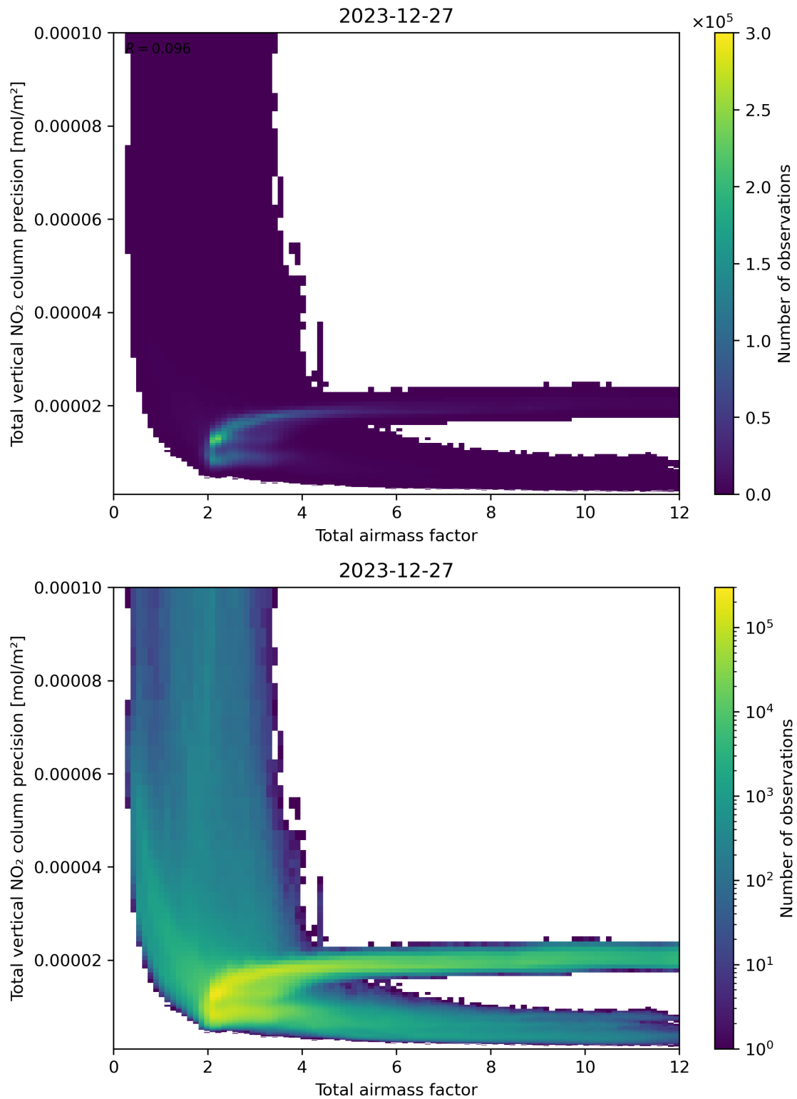
Figure 68: Scatter density plot of “Total airmass factor” against “Total vertical NO 2 column precision” for 2023-12-26 to 2023-12-28.
