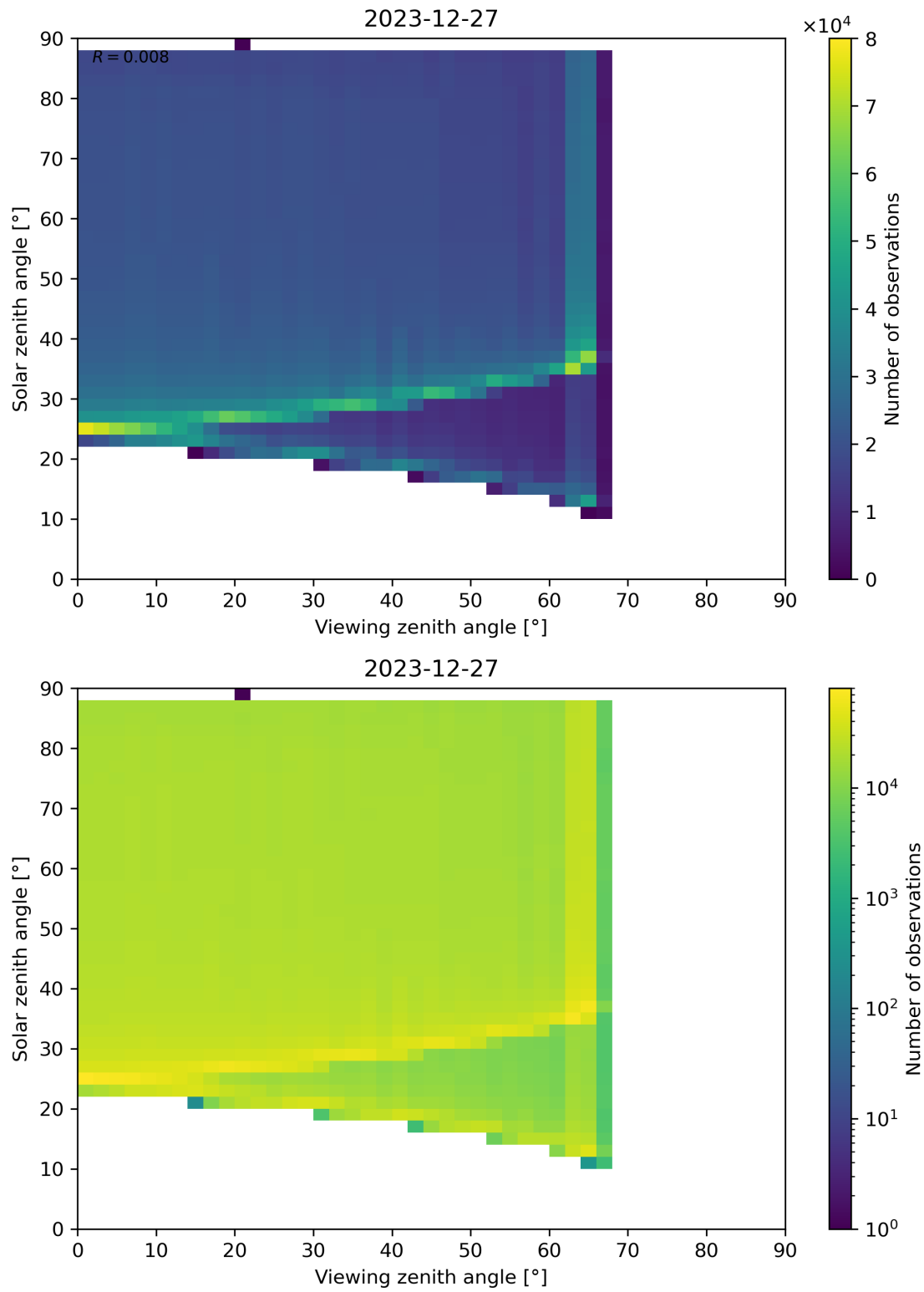
Figure 172: Scatter density plot of “Viewing zenith angle” against “Solar zenith angle” for 2023-12-26 to 2023-12-28.
