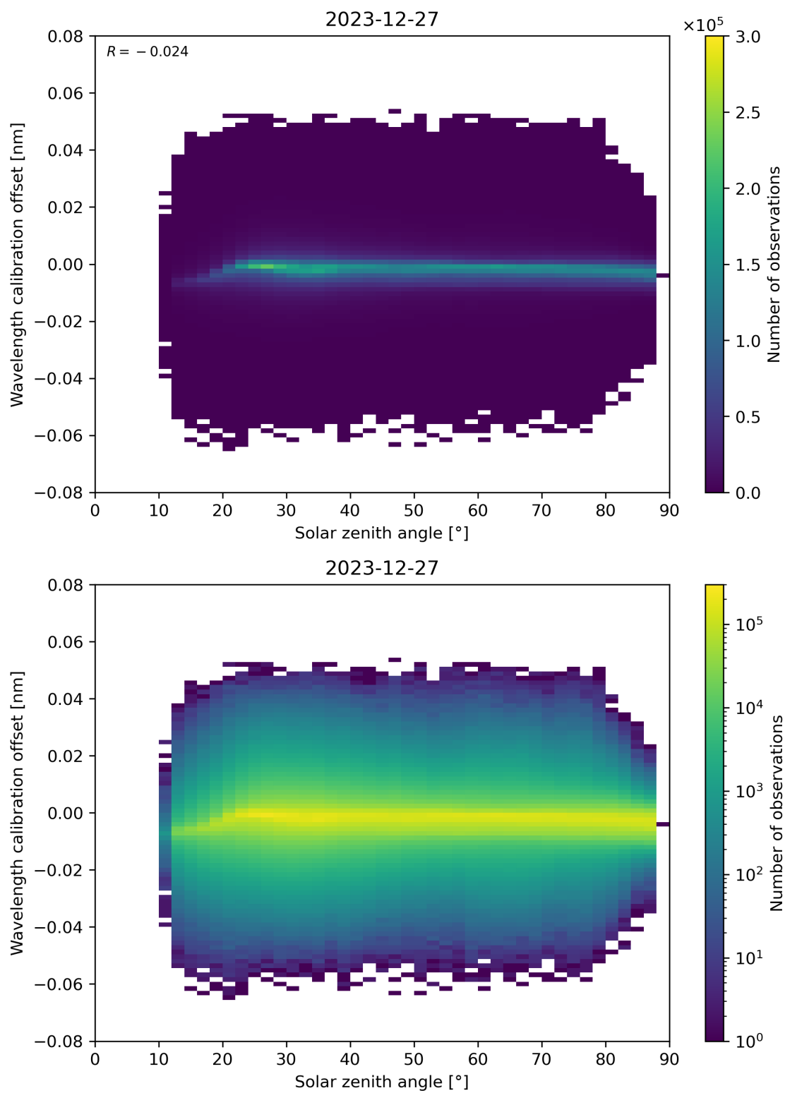
Figure 158: Scatter density plot of “Solar zenith angle” against “Wavelength calibration offset” for 2023-12-26 to 2023-12-28.
