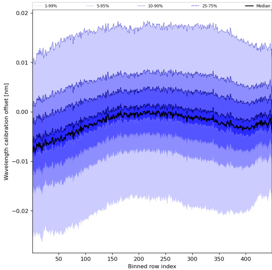
Figure 52: Along track statistics of “Wavelength calibration offset” for 2023-12-26 to 2023-12-28
