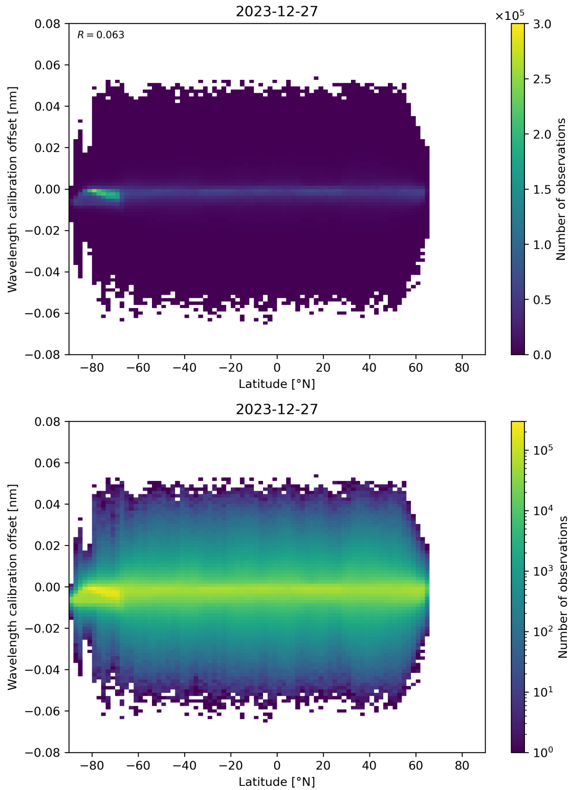
Figure 95: Scatter density plot of “Latitude” against “Wavelength calibration offset” for 2023-12-26 to 2023-12-28.
