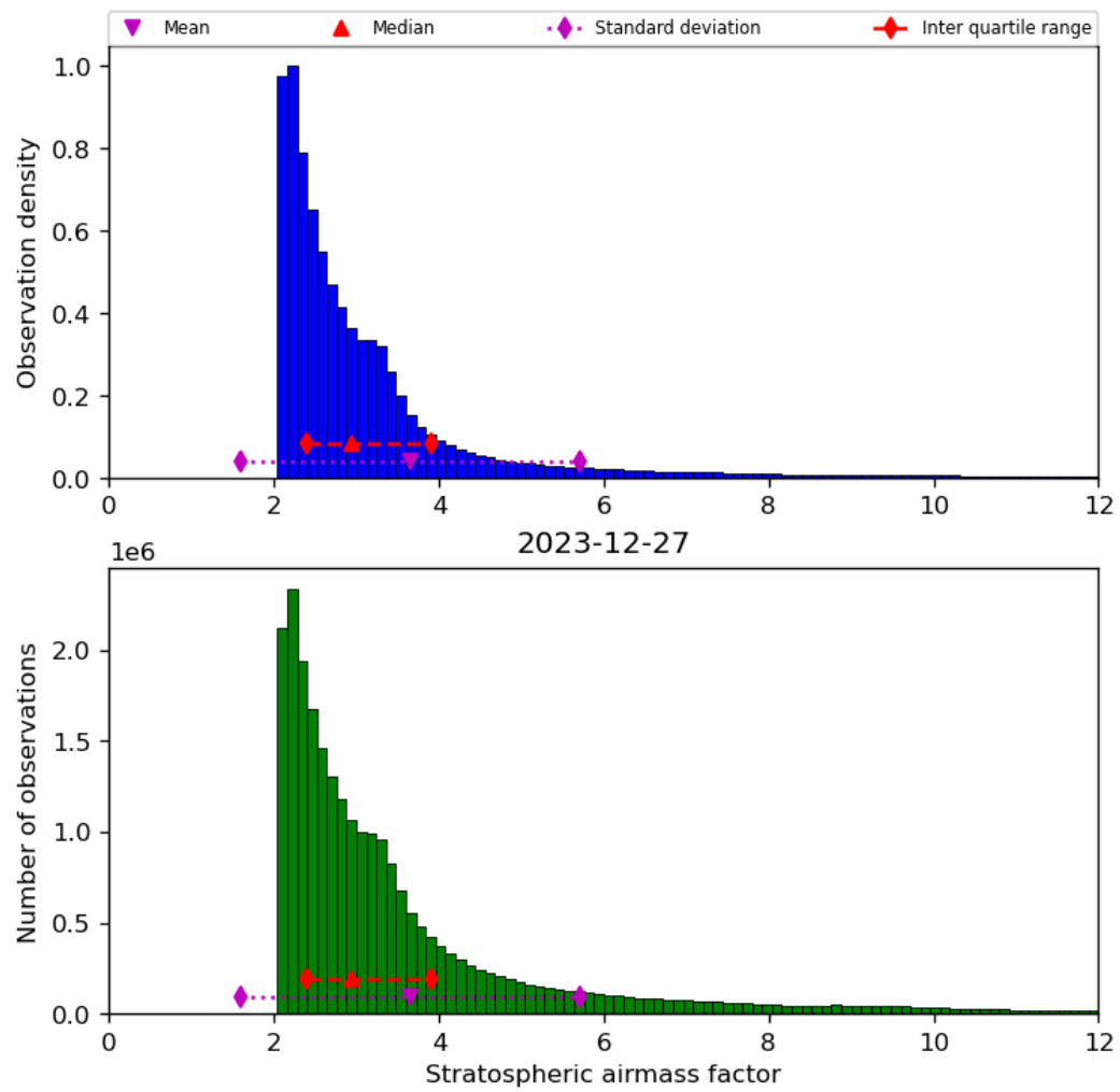
Figure 44: Histogram of “Stratospheric airmass factor” for 2023-12-26 to 2023-12-28
