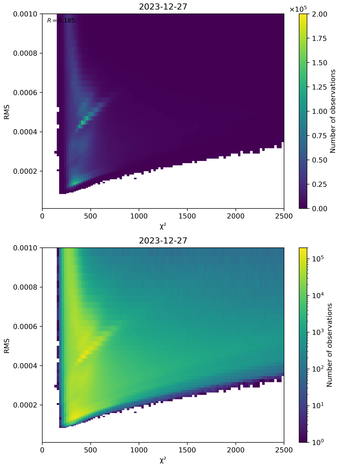
Figure 82: Scatter density plot of “ \chi^2 ” against “RMS” for 2023-12-26 to 2023-12-28.
