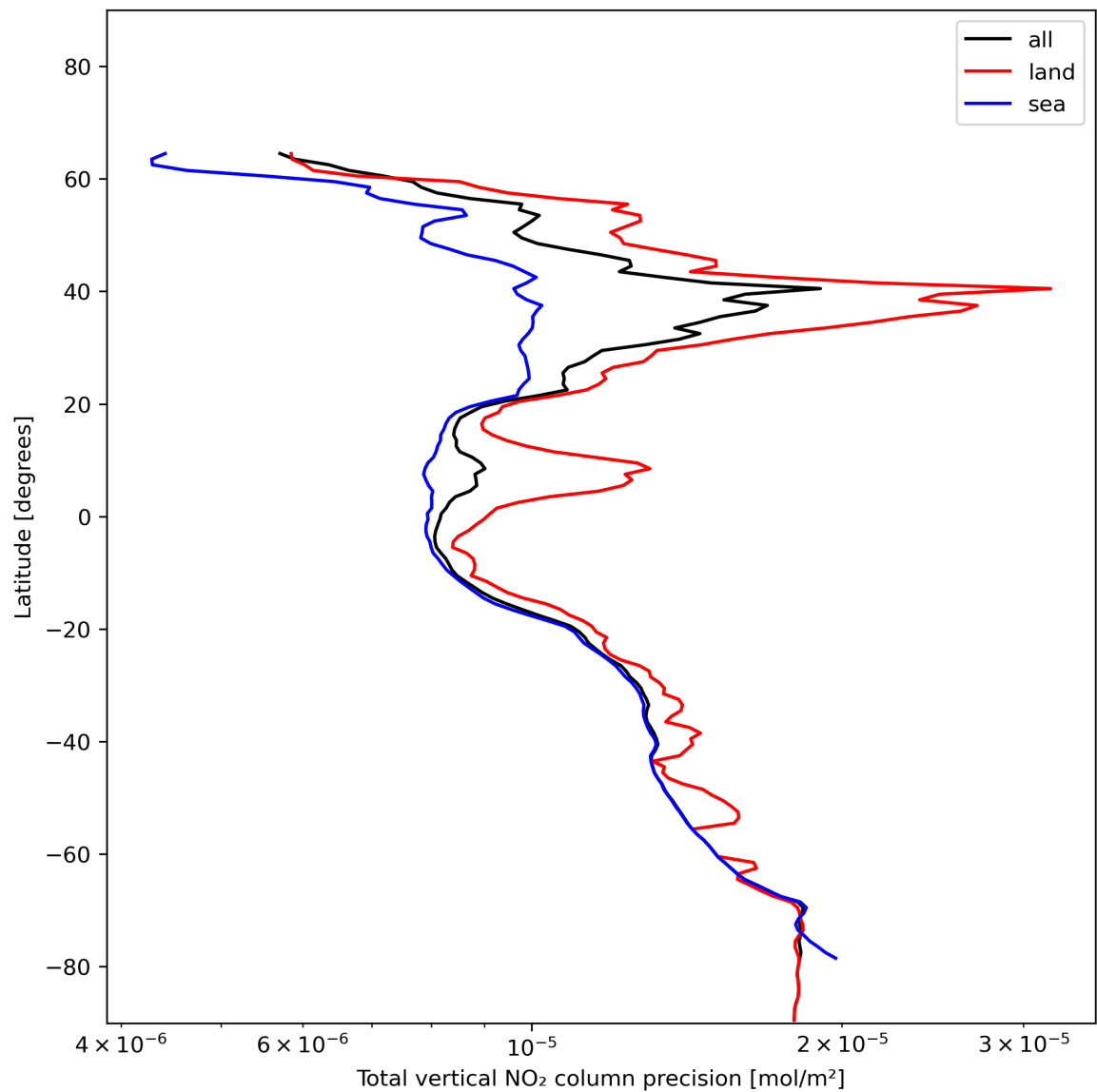
Figure 22: Zonal average of “Total vertical NO 2 column precision” for 2023-12-26 to 2023-12-28.
