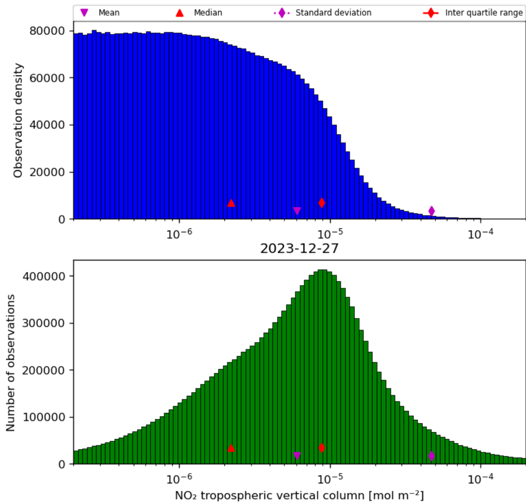
Figure 29: Histogram of “NO 2 tropospheric vertical column” for 2023-12-26 to 2023-12-28
