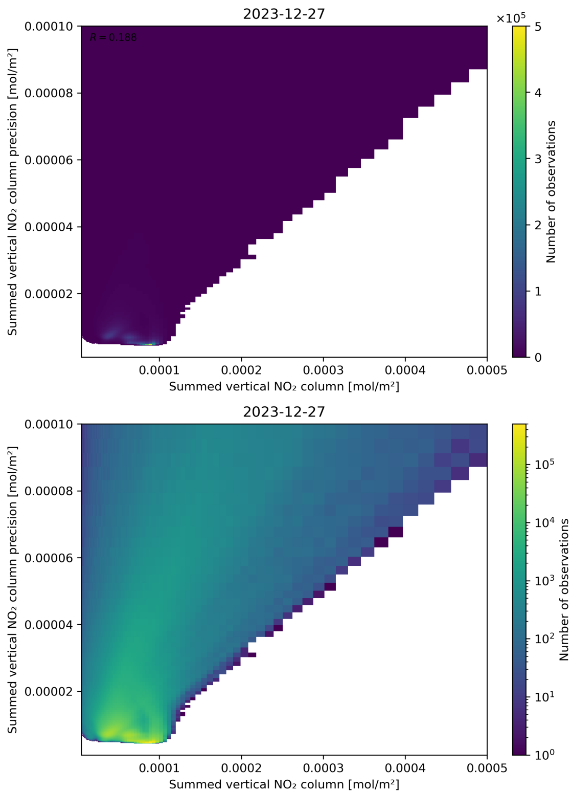
Figure 105: Scatter density plot of “Summed vertical NO 2 column” against “Summed vertical NO 2 column precision” for 2023-12-26 to 2023-12-28.
