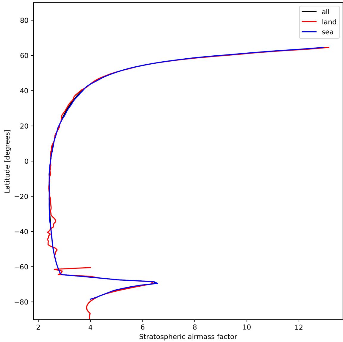
Figure 27: Zonal average of “Stratospheric airmass factor” for 2023-12-26 to 2023-12-28.
