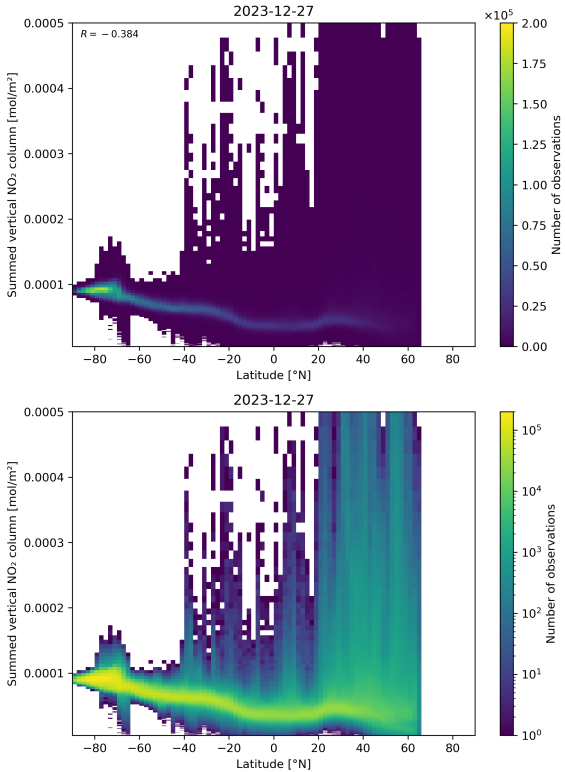
Figure 88: Scatter density plot of “Latitude” against “Summed vertical NO 2 column” for 2023-12-26 to 2023-12-28.
