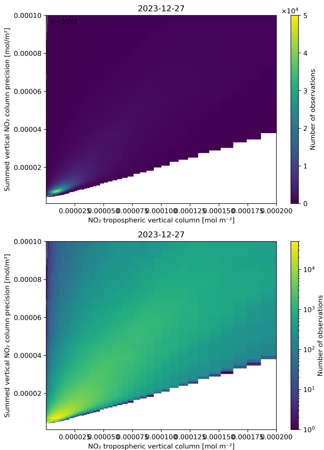
Figure 127: Scatter density plot of “NO 2 tropospheric vertical column” against “Summed vertical NO 2 column precision” for 2023-12-26 to 2023-12-28.
