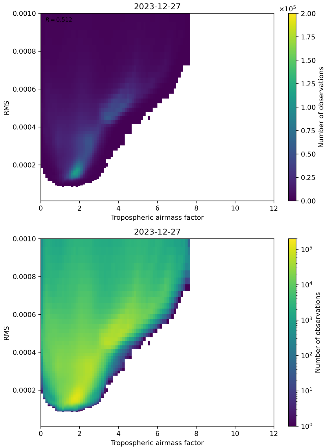
Figure 79: Scatter density plot of “Tropospheric airmass factor” against “RMS” for 2023-12-26 to 2023-12-28.
