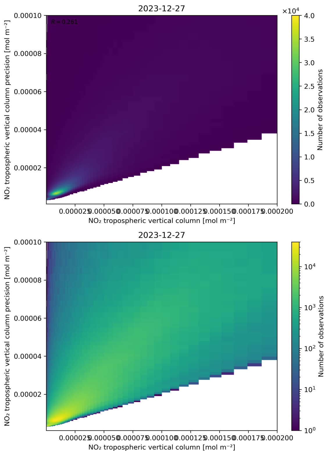
Figure 130: Scatter density plot of “NO 2 tropospheric vertical column” against “NO 2 tropospheric vertical column precision” for 2023-12-26 to 2023-12-28.
