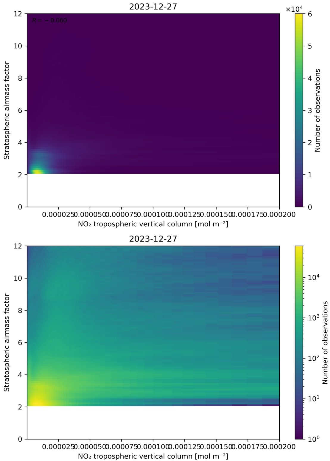
Figure 121: Scatter density plot of “NO 2 tropospheric vertical column” against “Stratospheric airmass factor” for 2023-12-26 to 2023-12-28.
