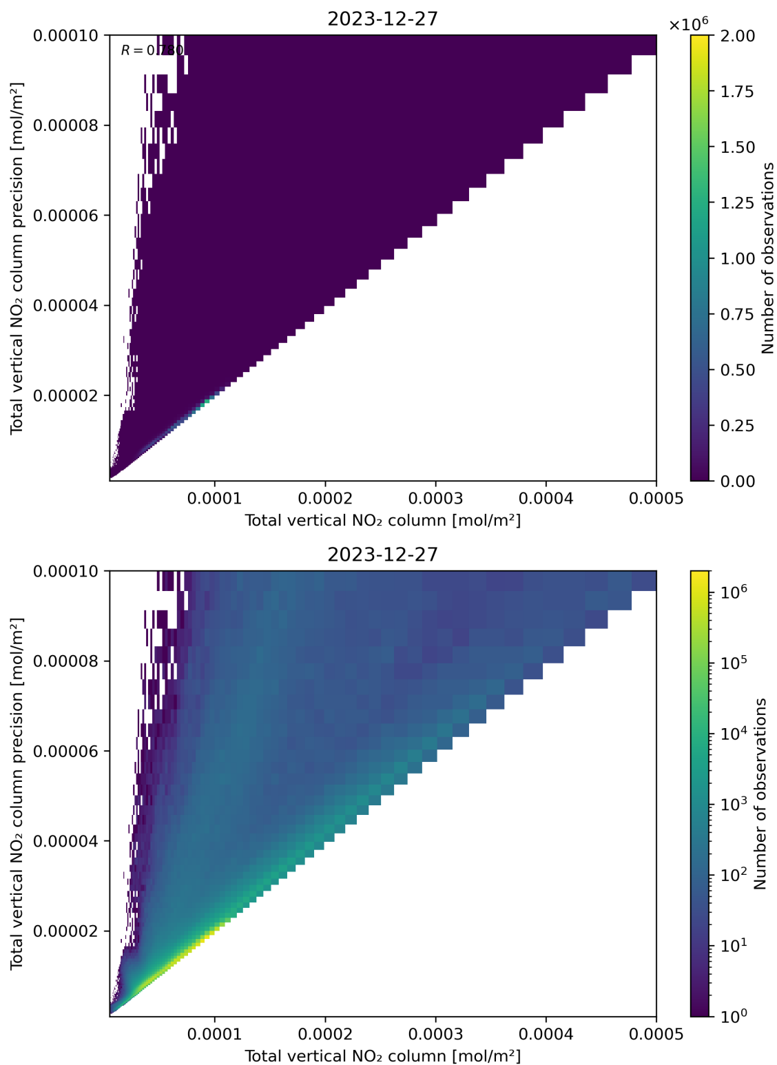
Figure 114: Scatter density plot of “Total vertical NO 2 column” against “Total vertical NO 2 column precision” for 2023-12-26 to 2023-12-28.
