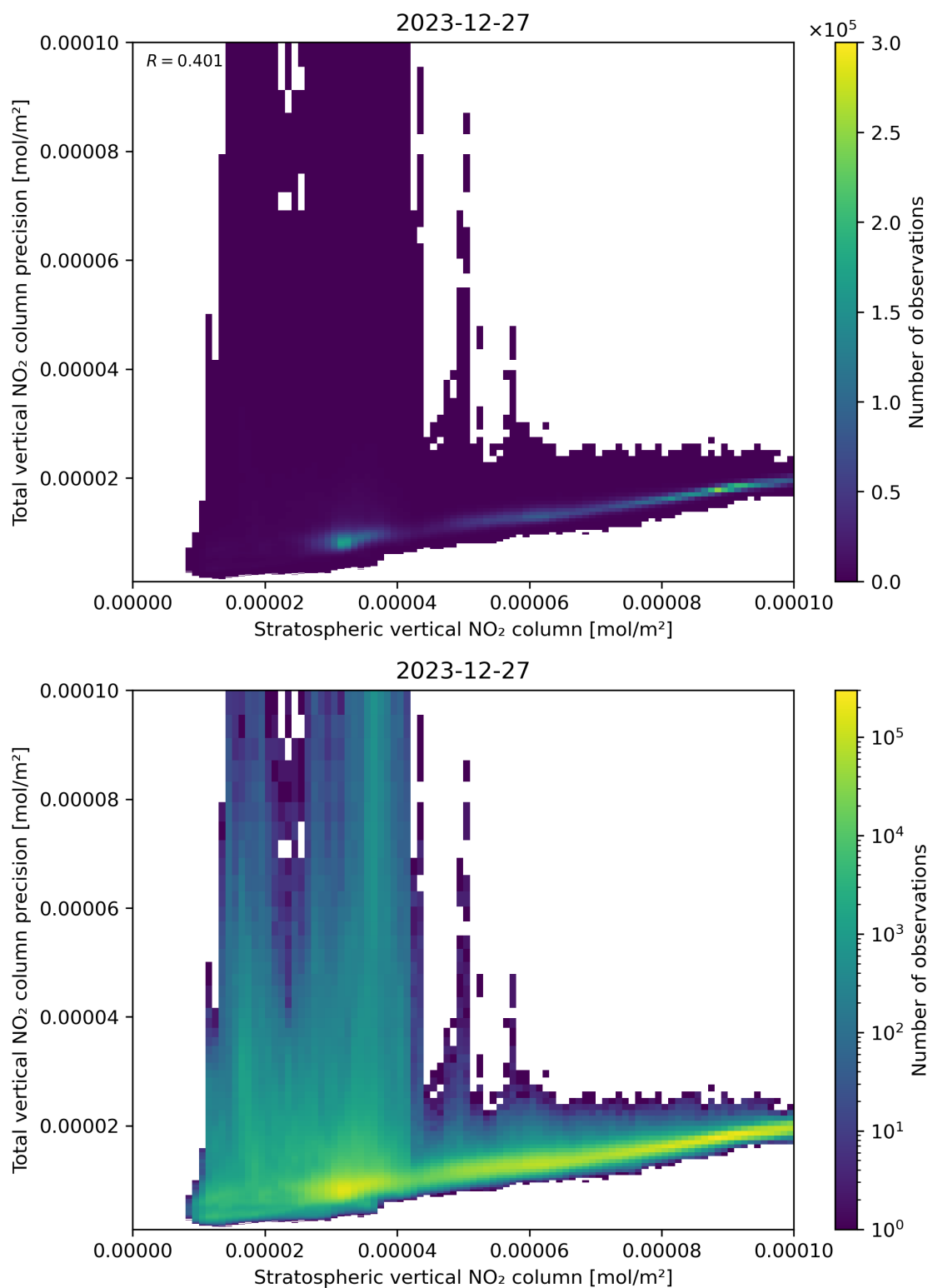
Figure 101: Scatter density plot of “Stratospheric vertical NO 2 column” against “Total vertical NO 2 column precision” for 2023-12-26 to 2023-12-28.
