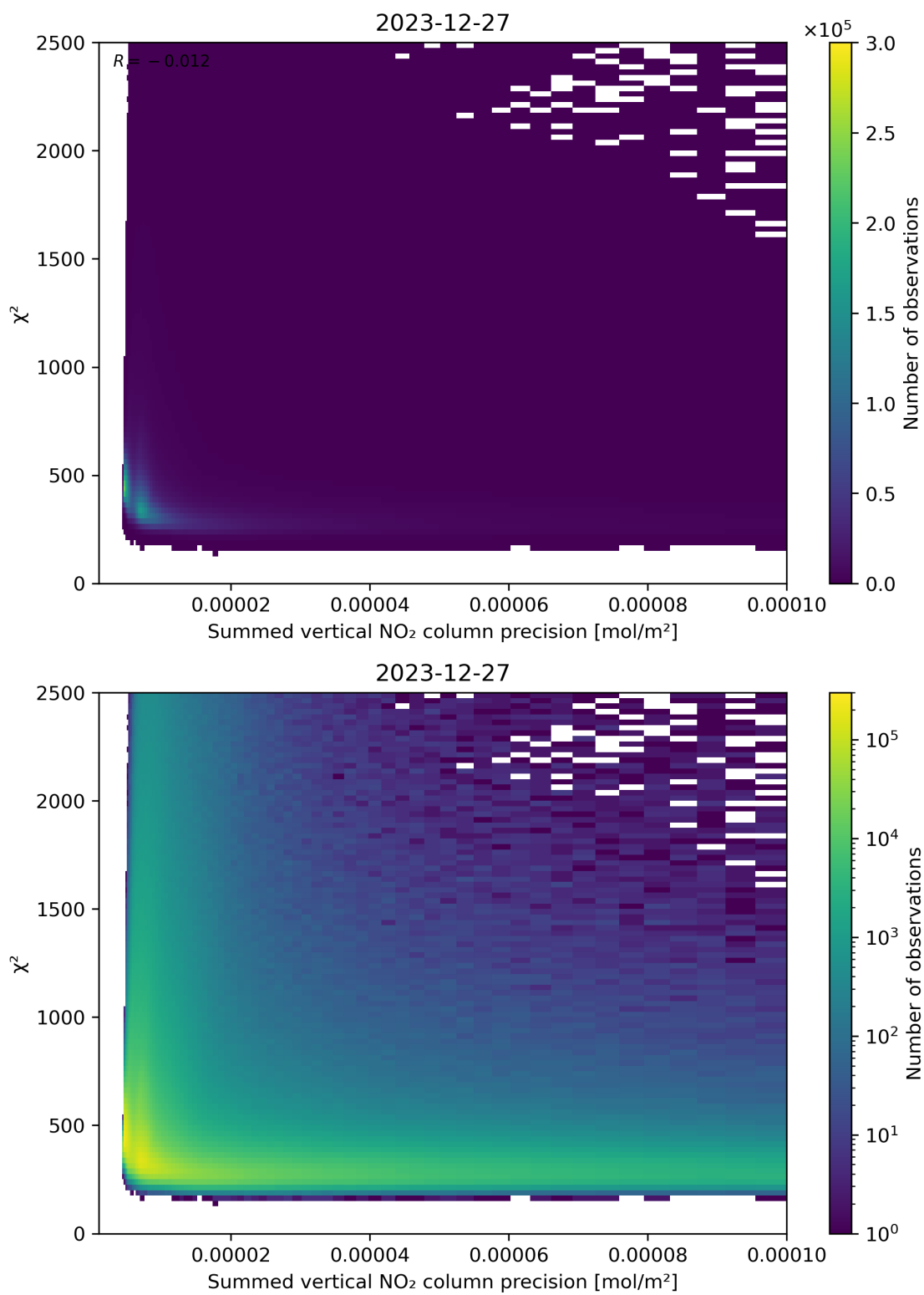
Figure 107: Scatter density plot of “Summed vertical NO 2 column precision” against “ \chi^2 ” for 2023-12-26 to 2023-12-28.
