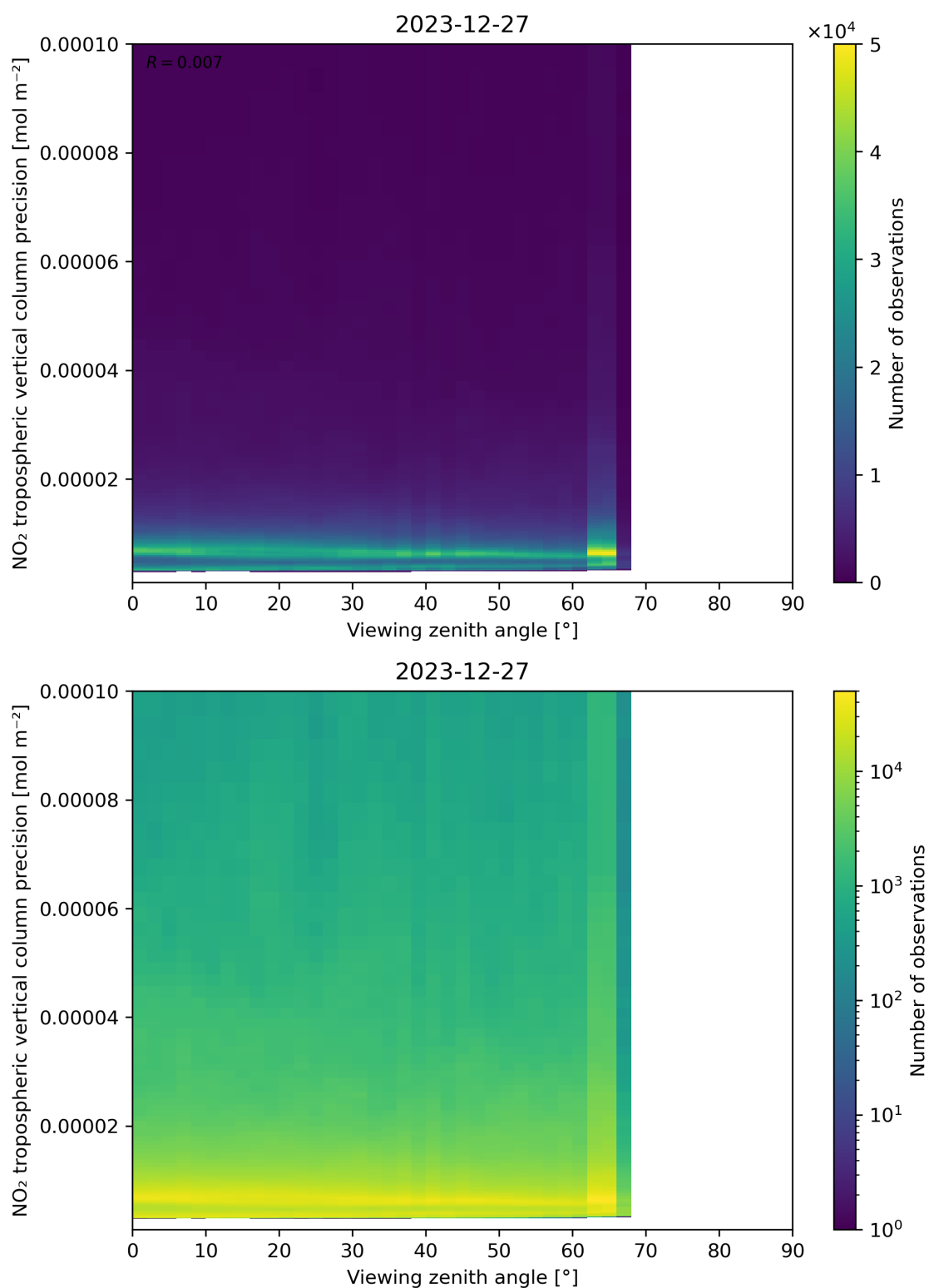
Figure 170: Scatter density plot of “Viewing zenith angle” against “NO 2 tropospheric vertical column precision” for 2023-12-26 to 2023-12-28.
