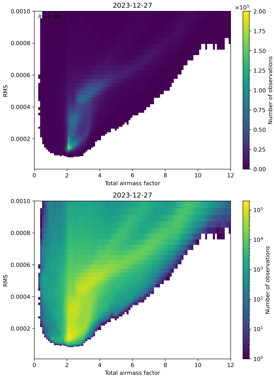
Figure 69: Scatter density plot of “Total airmass factor” against “RMS” for 2023-12-26 to 2023-12-28.
