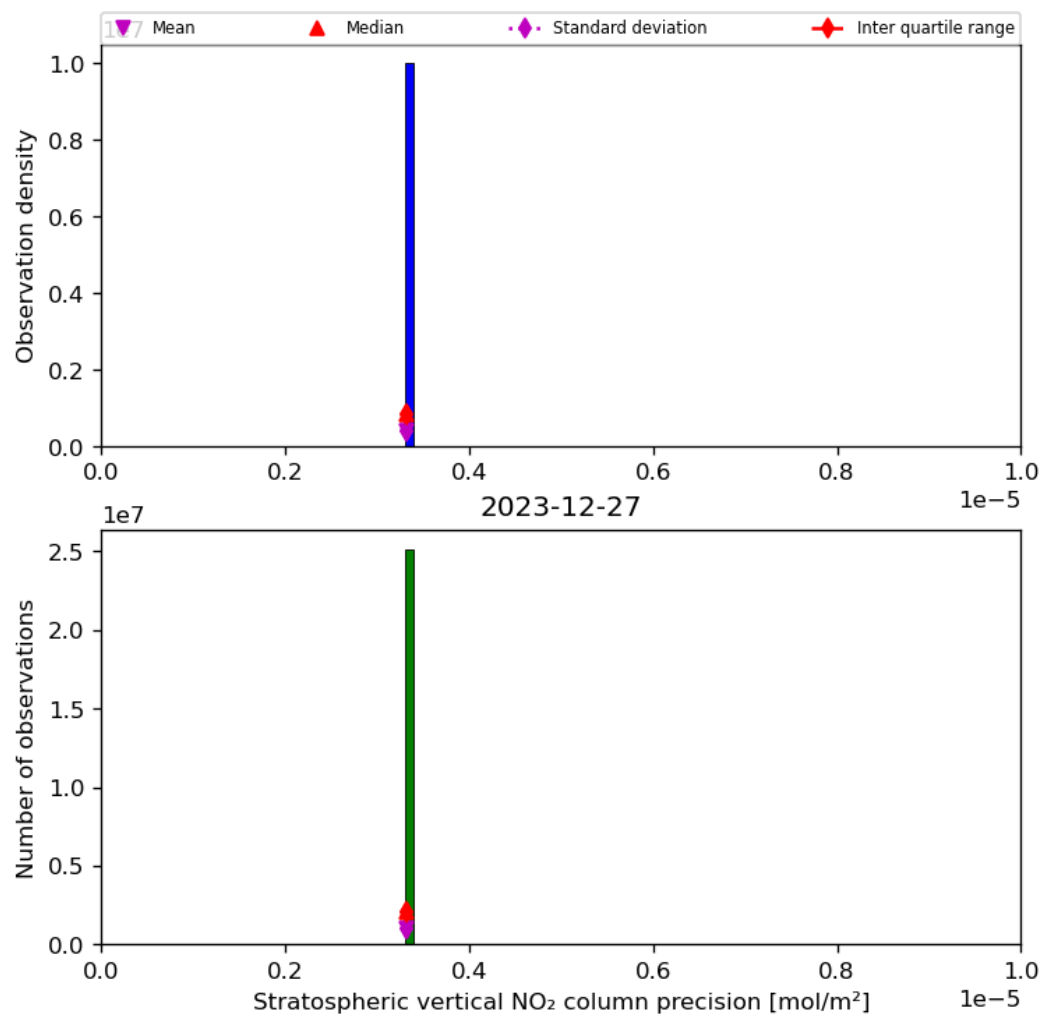
Figure 37: Histogram of “Stratospheric vertical NO 2 column precision” for 2023-12-26 to 2023-12-28
