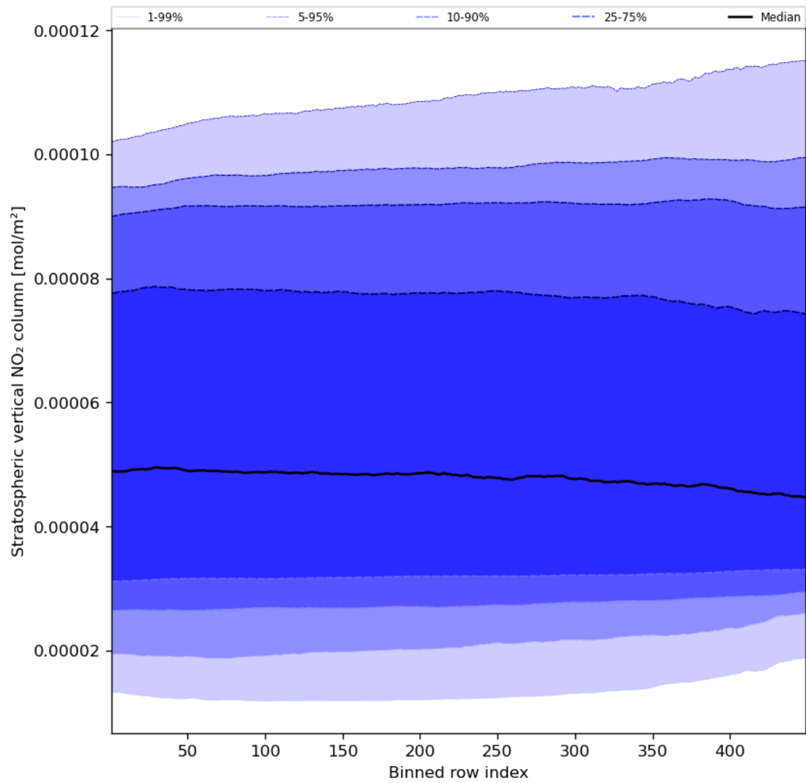
Figure 53: Along track statistics of “Stratospheric vertical NO 2 column” for 2023-12-26 to 2023-12-28
