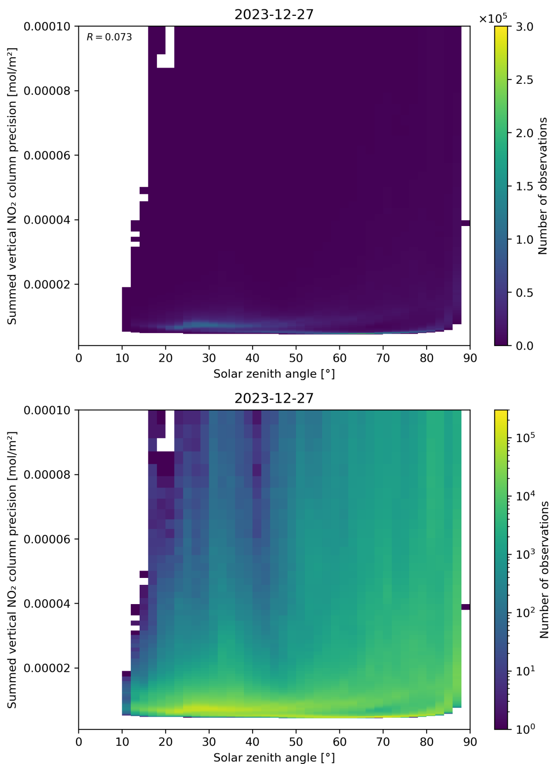
Figure 152: Scatter density plot of “Solar zenith angle” against “Summed vertical NO 2 column precision” for 2023-12-26 to 2023-12-28.
