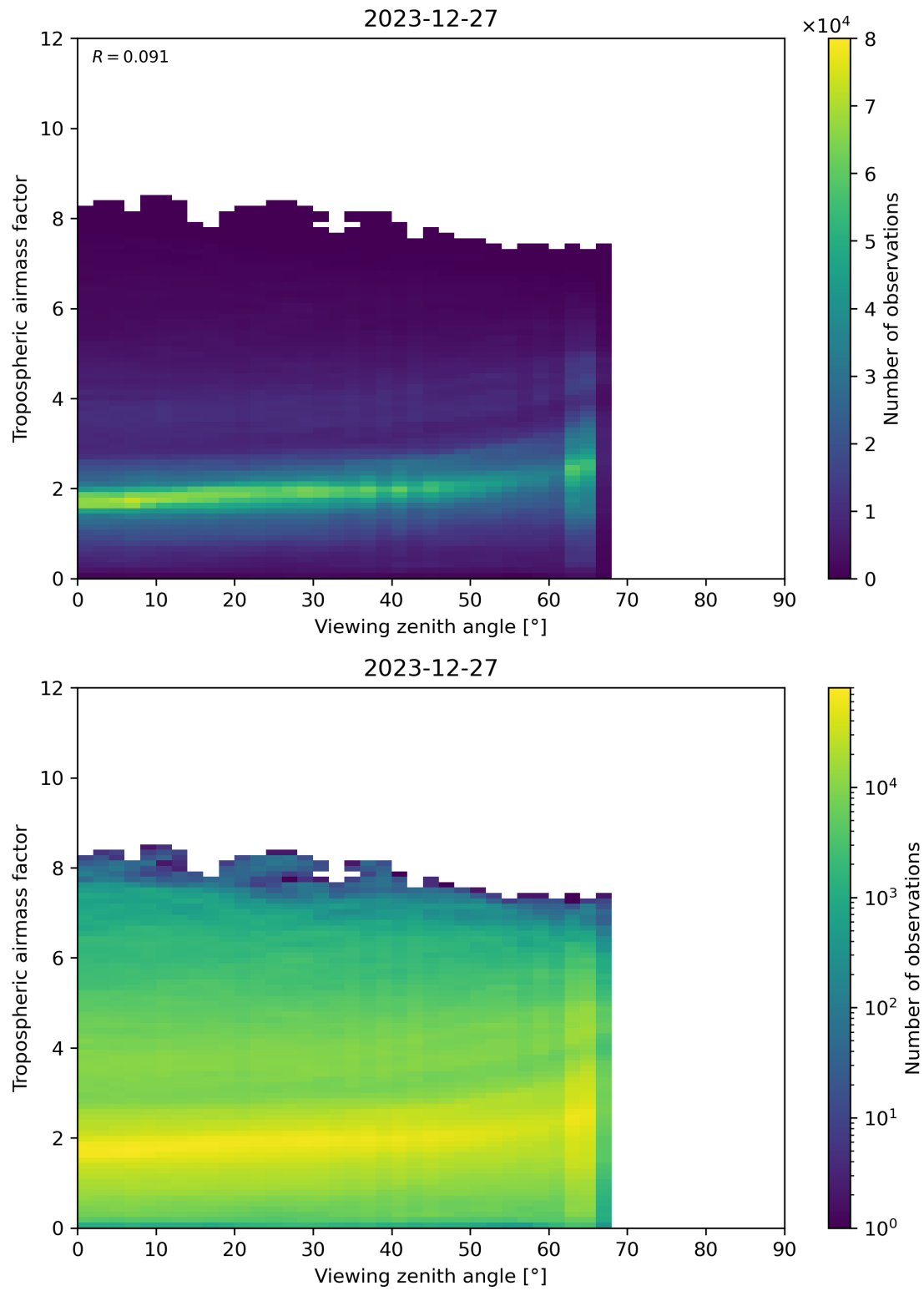
Figure 161: Scatter density plot of “Viewing zenith angle” against “Tropospheric airmass factor” for 2023-12-26 to 2023-12-28.
