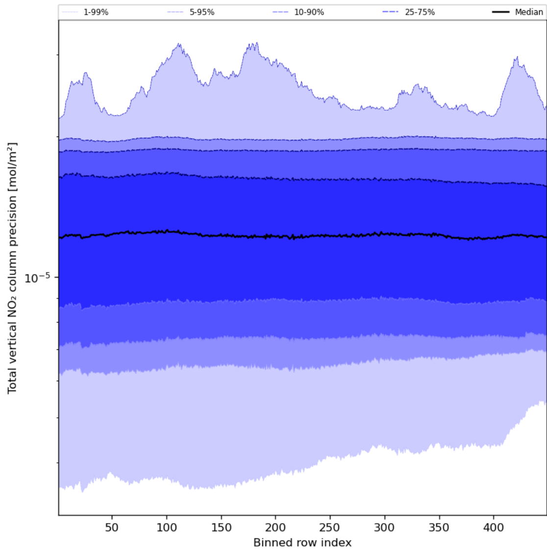
Figure 56: Along track statistics of “Total vertical NO 2 column precision” for 2023-12-26 to 2023-12-28
