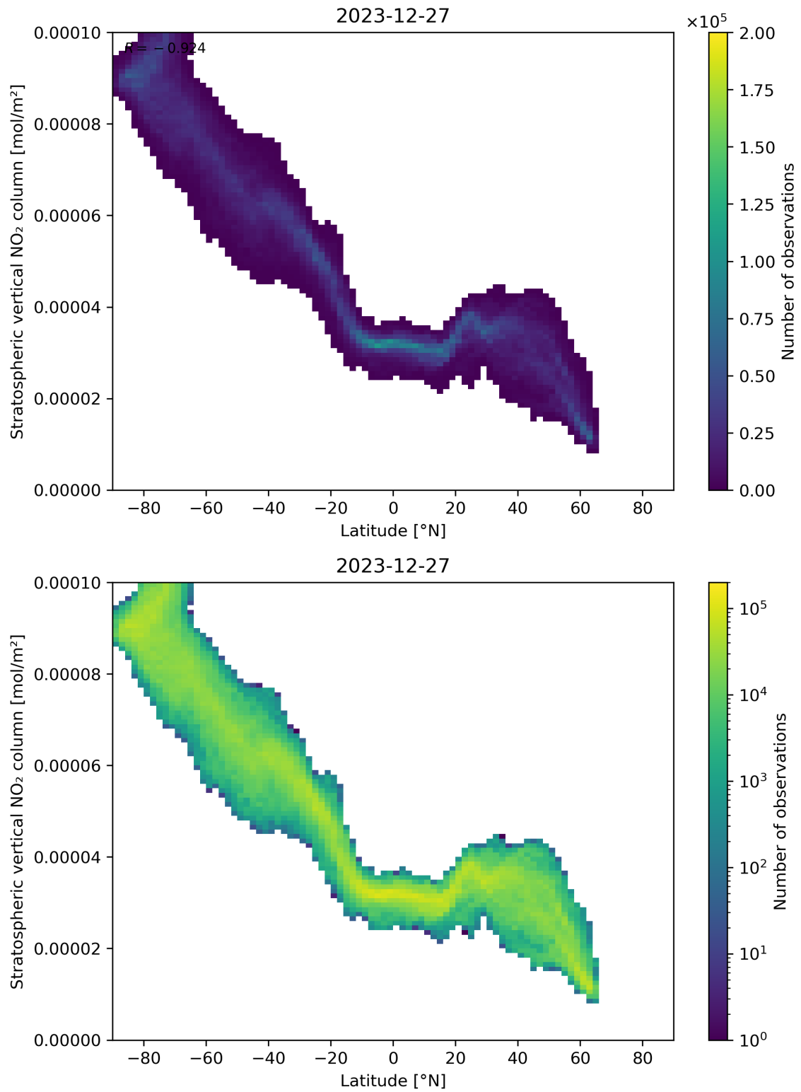
Figure 87: Scatter density plot of “Latitude” against “Stratospheric vertical NO 2 column” for 2023-12-26 to 2023-12-28.
