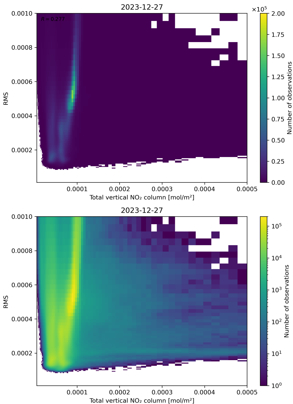
Figure 120: Scatter density plot of “Total vertical NO 2 column” against “RMS” for 2023-12-26 to 2023-12-28.
