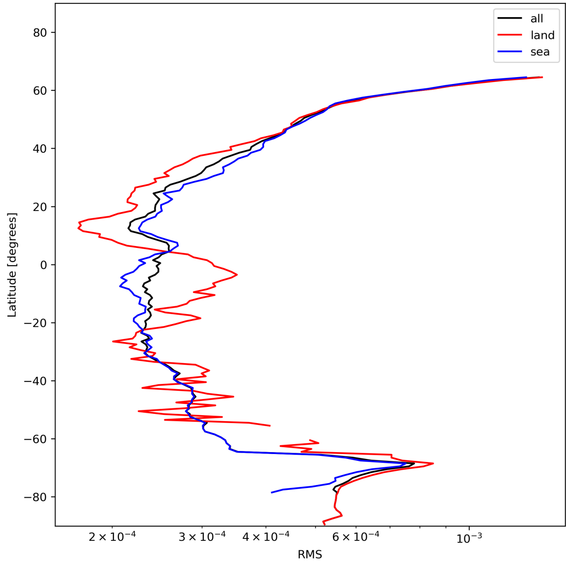
Figure 26: Zonal average of “RMS” for 2023-12-26 to 2023-12-28.
