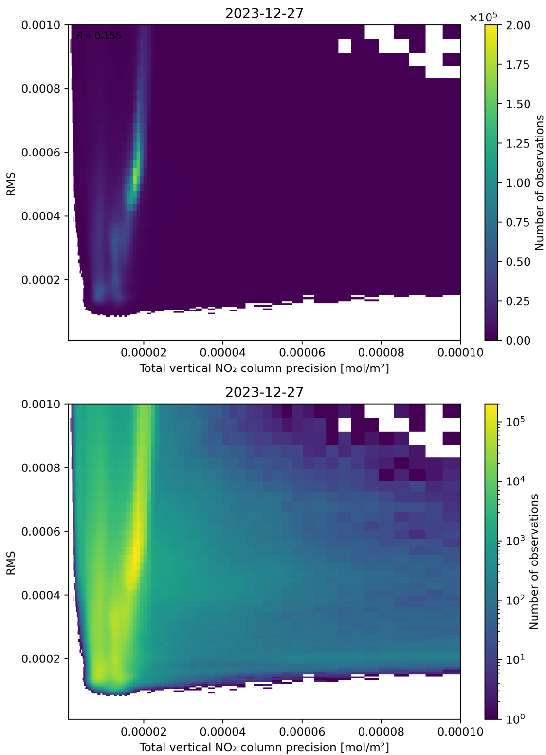
Figure 119: Scatter density plot of “Total vertical NO 2 column precision” against “RMS” for 2023-12-26 to 2023-12-28.
