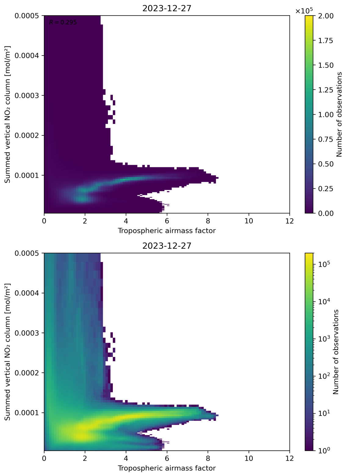
Figure 75: Scatter density plot of “Tropospheric airmass factor” against “Summed vertical NO 2 column” for 2023-12-26 to 2023-12-28.
