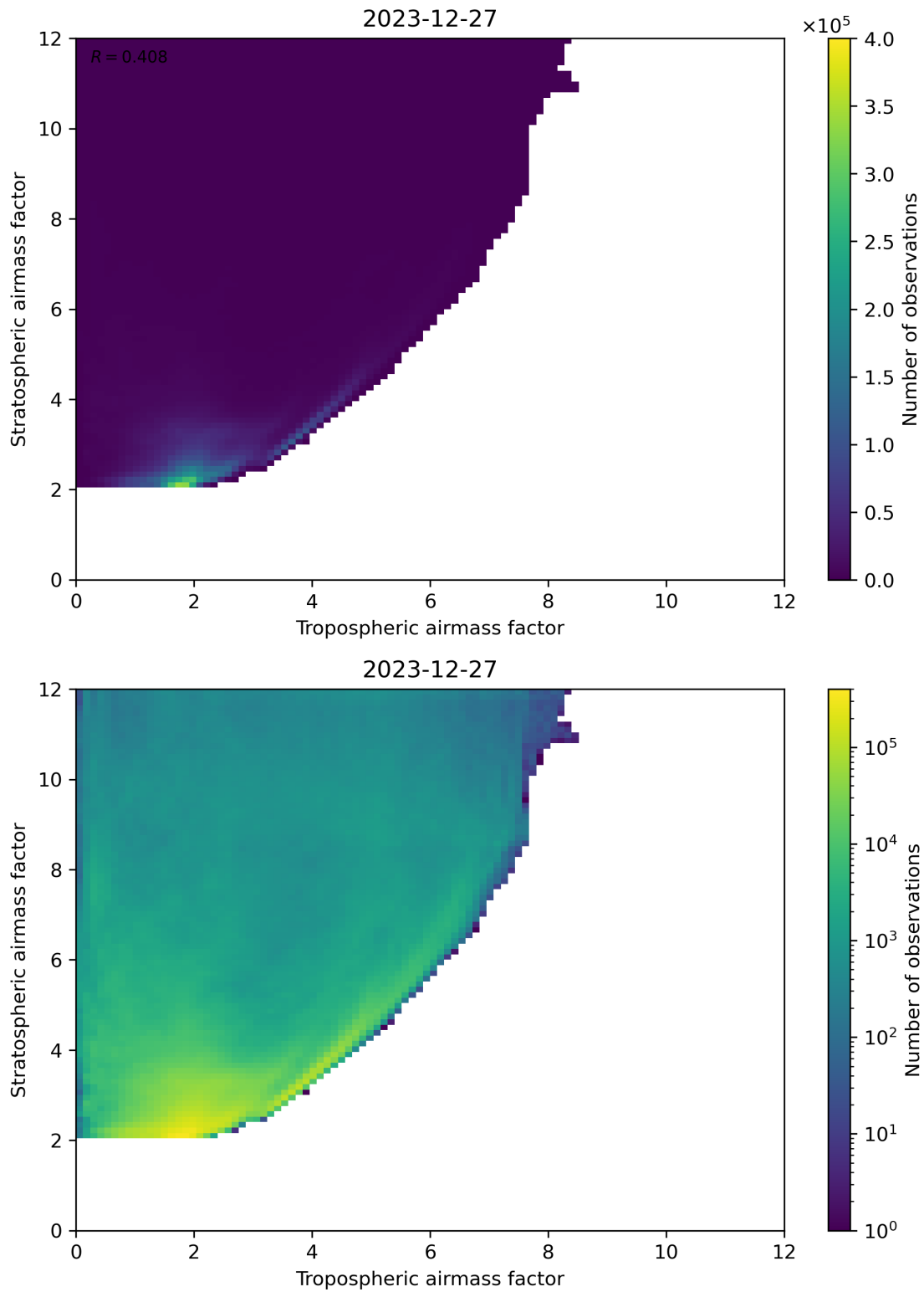
Figure 71: Scatter density plot of “Tropospheric airmass factor” against “Stratospheric airmass factor” for 2023-12-26 to 2023-12-28.
