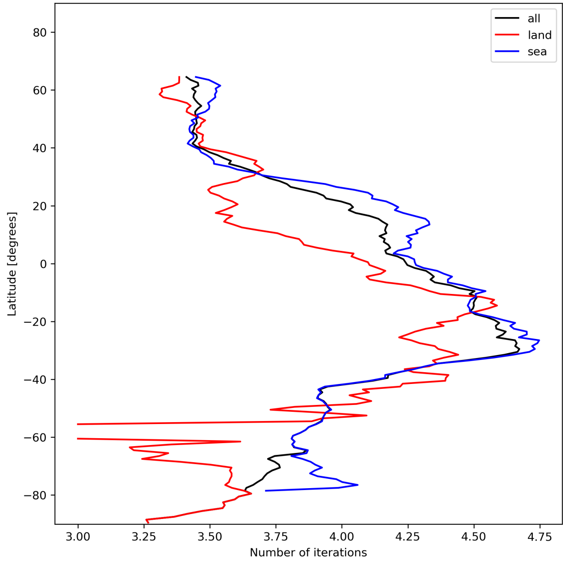
Figure 17: Zonal average of “Number of iterations” for 2023-12-26 to 2023-12-28.
