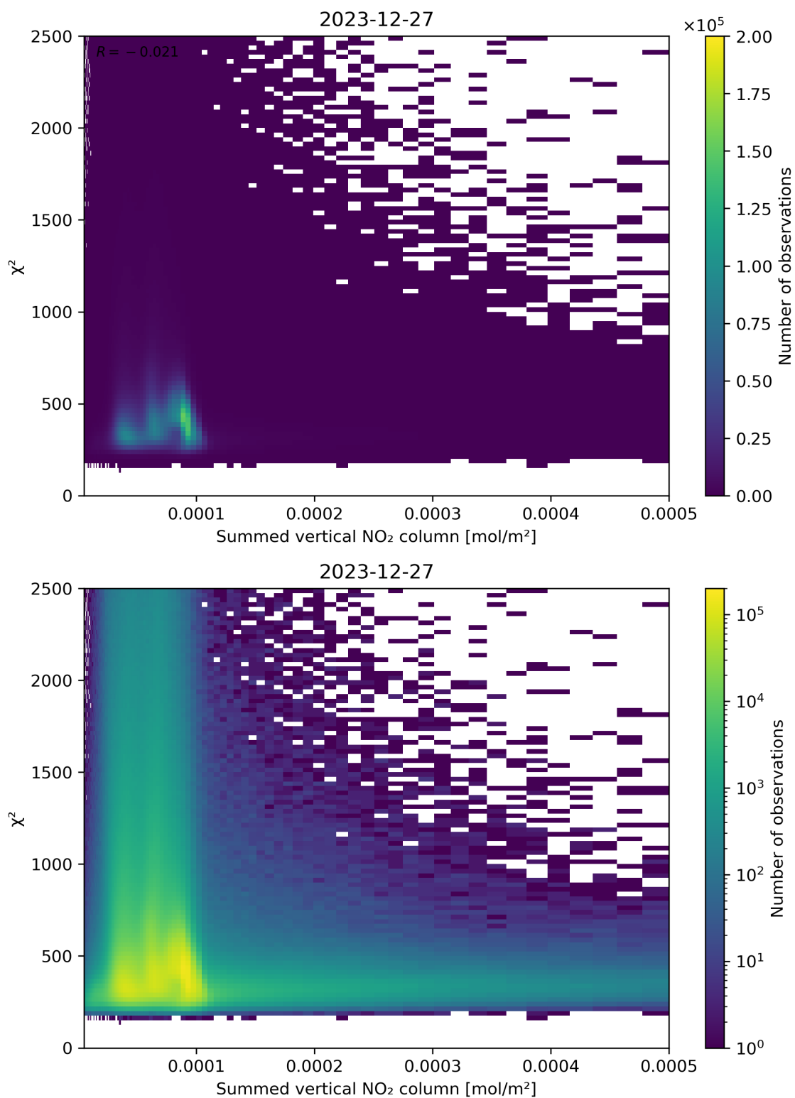
Figure 104: Scatter density plot of “Summed vertical NO 2 column” against “ \chi^2 ” for 2023-12-26 to 2023-12-28.
