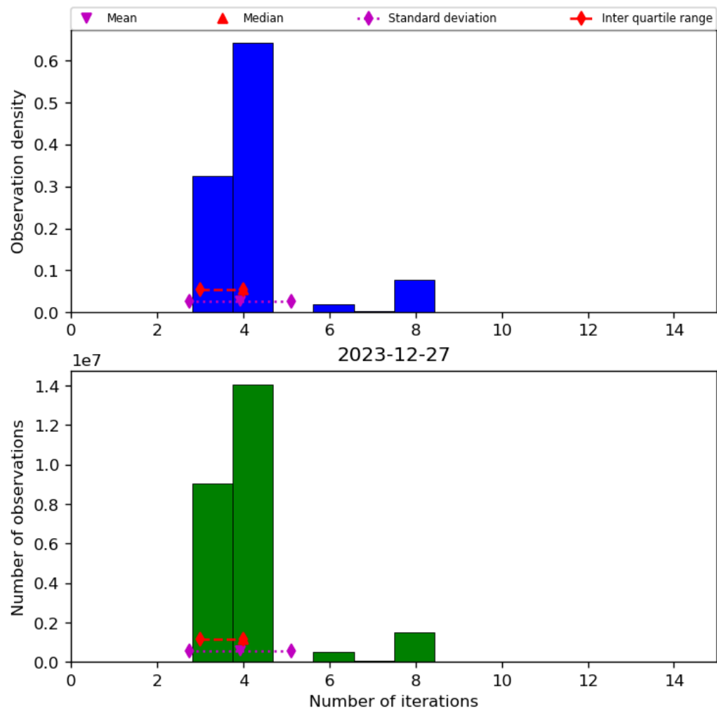
Figure 34: Histogram of “Number of iterations” for 2023-12-26 to 2023-12-28
