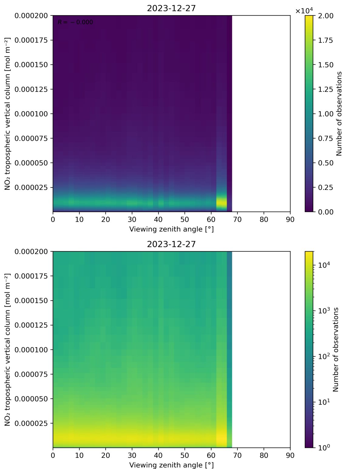
Figure 169: Scatter density plot of “Viewing zenith angle” against “NO 2 tropospheric vertical column” for 2023-12-26 to 2023-12-28.
