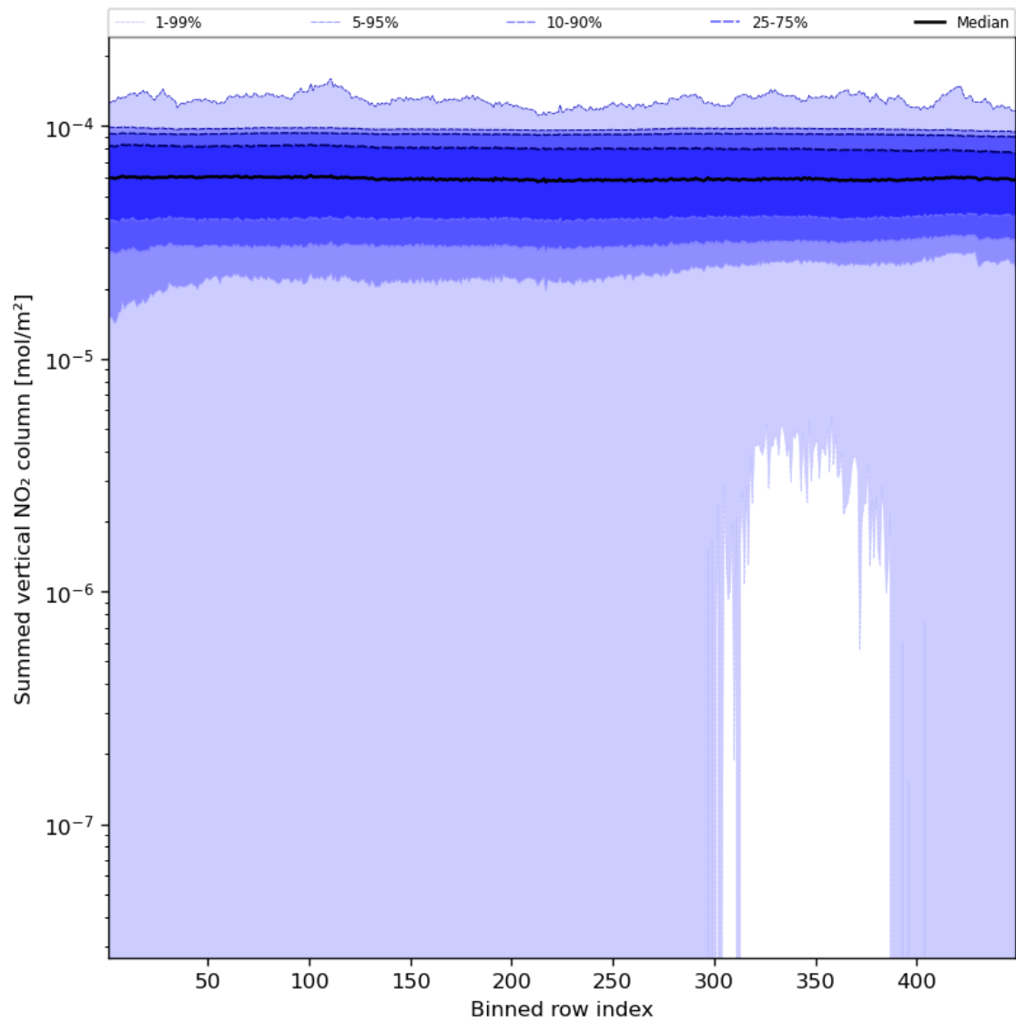
Figure 57: Along track statistics of “Summed vertical NO 2 column” for 2023-12-26 to 2023-12-28
