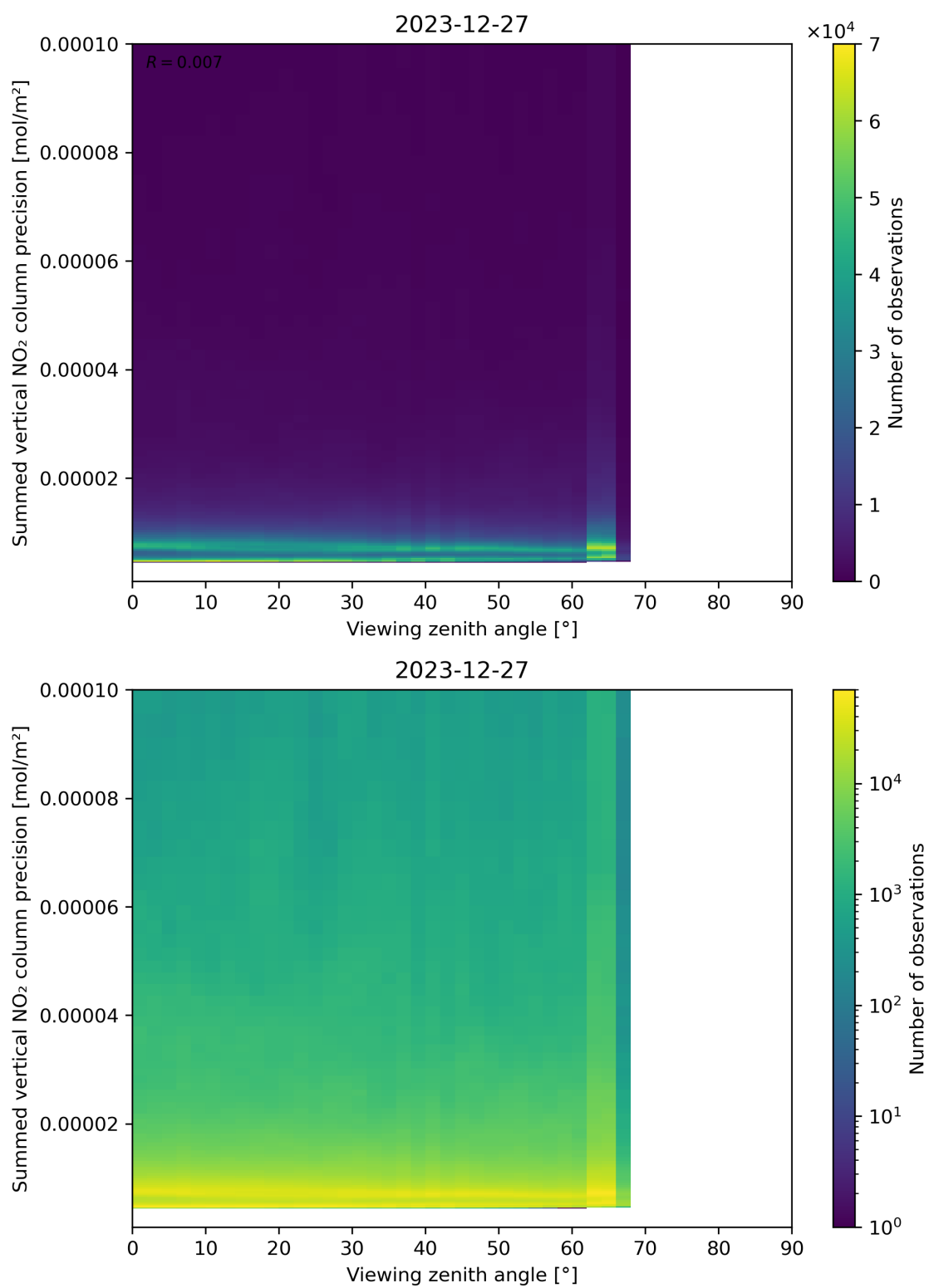
Figure 166: Scatter density plot of “Viewing zenith angle” against “Summed vertical NO 2 column precision” for 2023-12-26 to 2023-12-28.
