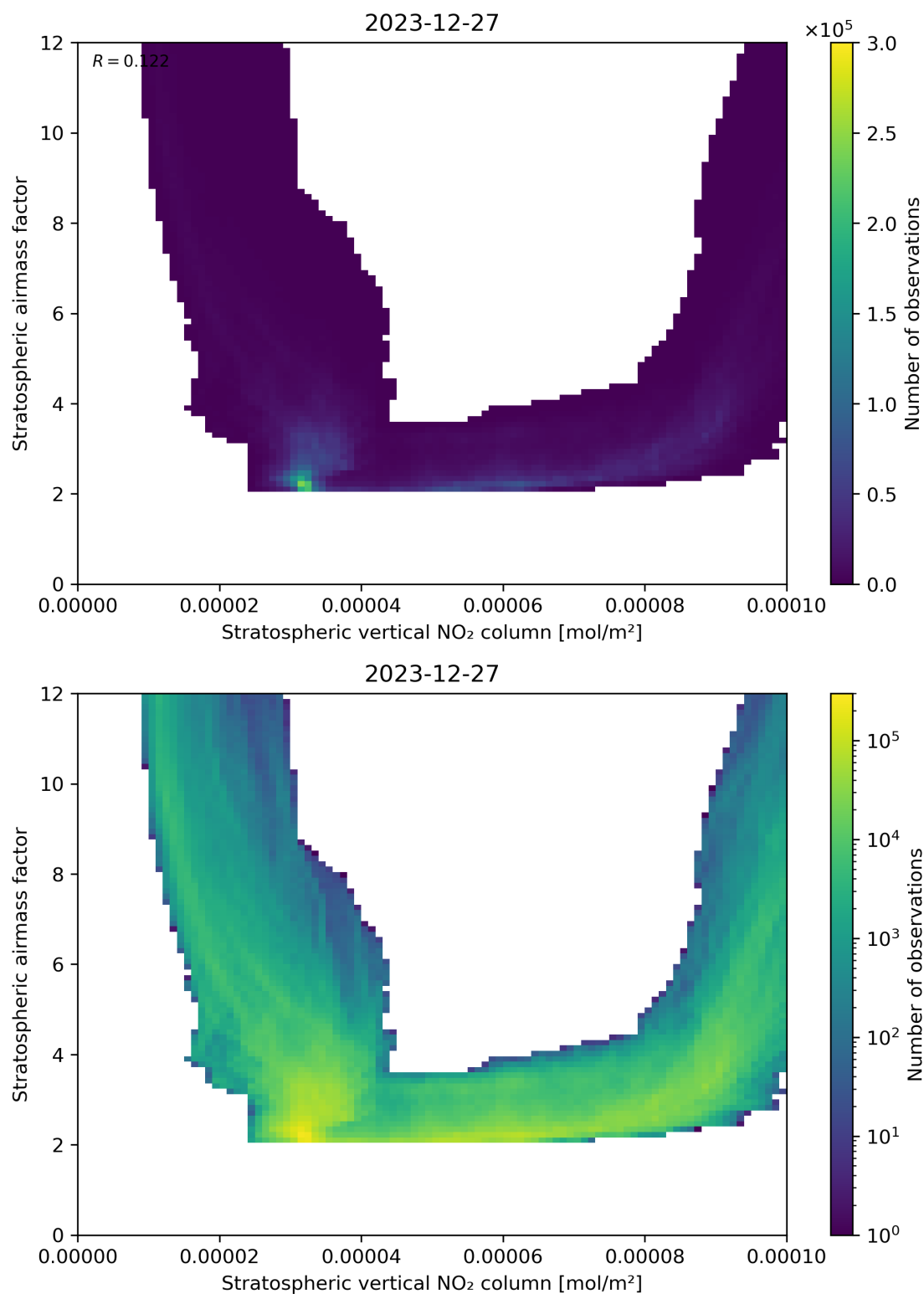
Figure 96: Scatter density plot of “Stratospheric vertical NO 2 column” against “Stratospheric airmass factor” for 2023-12-26 to 2023-12-28.
