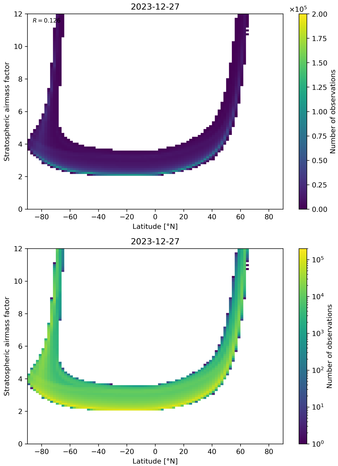
Figure 83: Scatter density plot of “Latitude” against “Stratospheric air mass factor” for 2023-12-26 to 2023-12-28.
