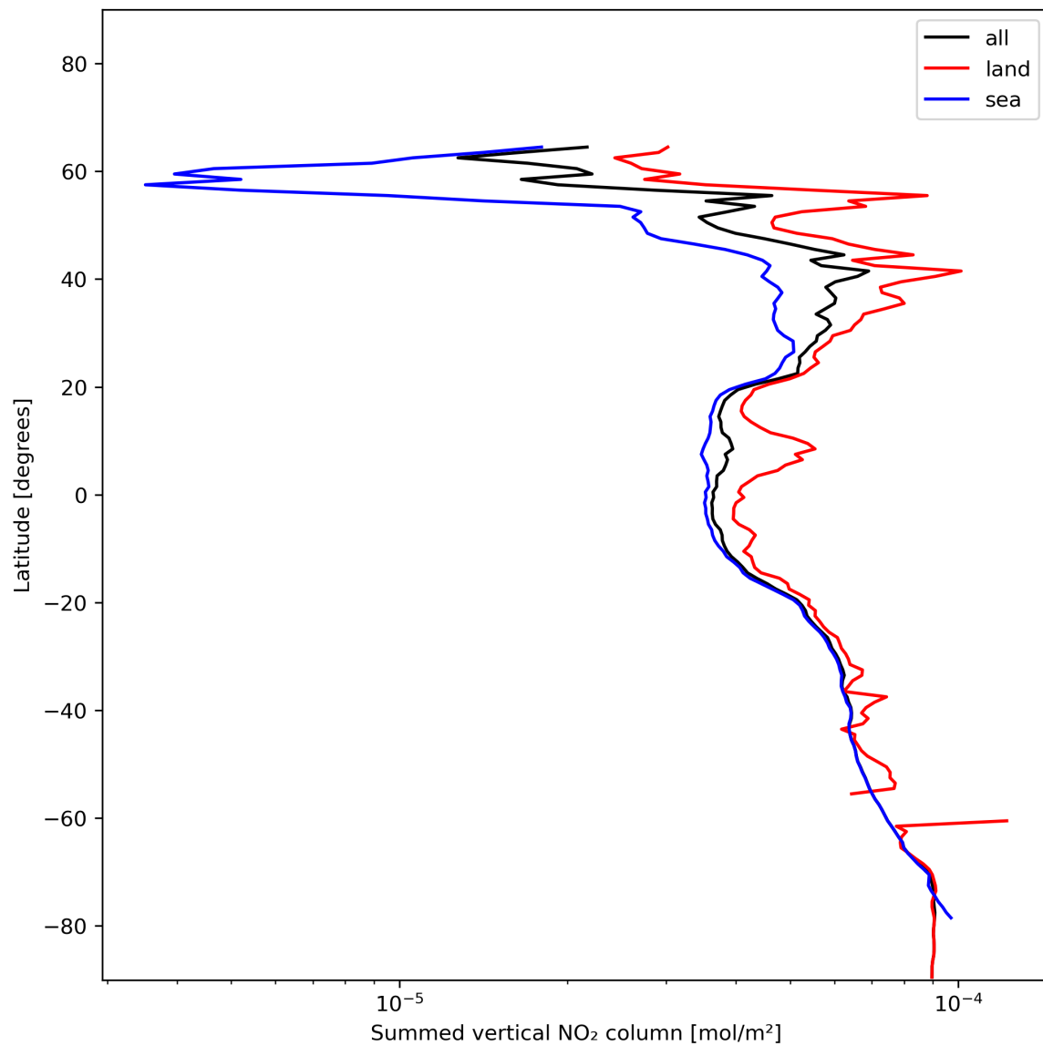
Figure 23: Zonal average of “Summed vertical NO 2 column” for 2023-12-26 to 2023-12-28.
