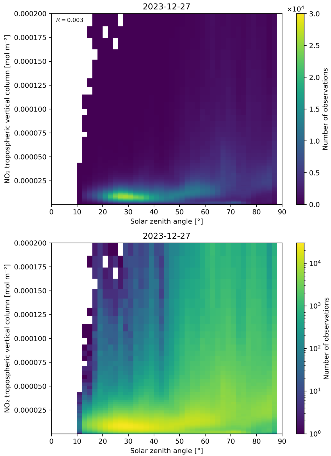
Figure 155: Scatter density plot of “Solar zenith angle” against “NO 2 tropospheric vertical column” for 2023-12-26 to 2023-12-28.
