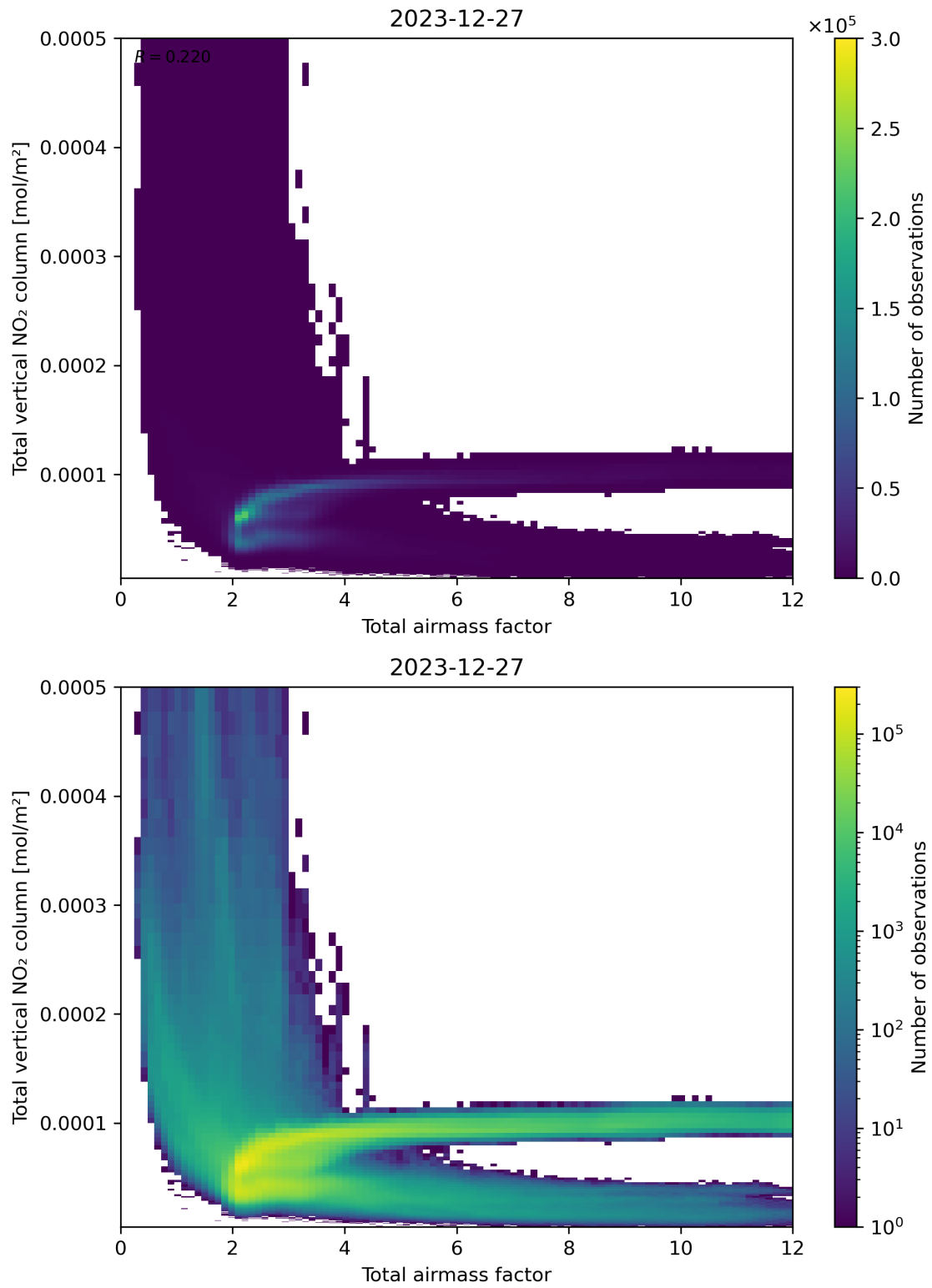
Figure 67: Scatter density plot of “Total airmass factor” against “Total vertical NO 2 column” for 2023-12-26 to 2023-12-28.
