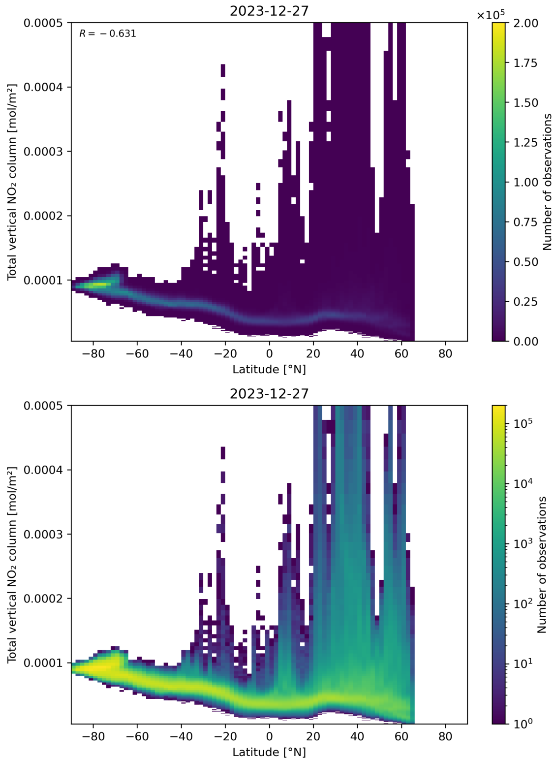
Figure 90: Scatter density plot of “Latitude” against “Total vertical NO 2 column” for 2023-12-26 to 2023-12-28.
