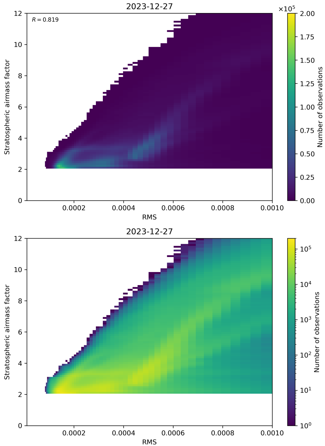
Figure 144: Scatter density plot of “RMS” against “Stratospheric airmass factor” for 2023-12-26 to 2023-12-28.
