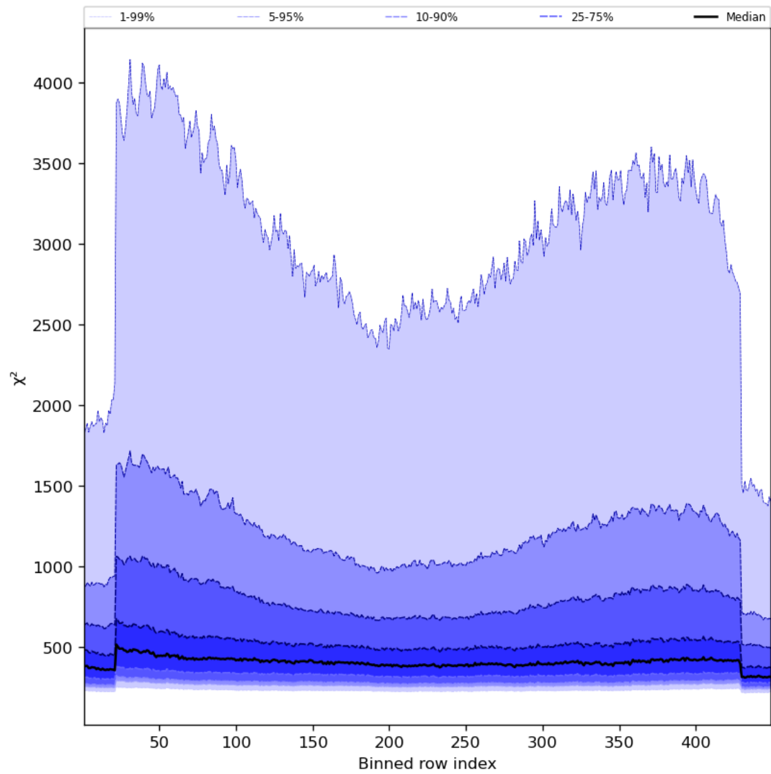
Figure 59: Along track statistics of “ \chi^2 ” for 2023-12-26 to 2023-12-28
