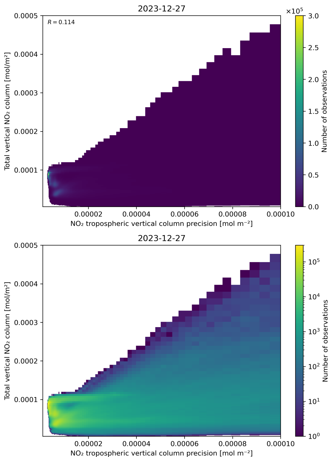
Figure 138: Scatter density plot of “NO 2 tropospheric vertical column precision” against “Total vertical NO 2 column” for 2023-12-26 to 2023-12-28.
