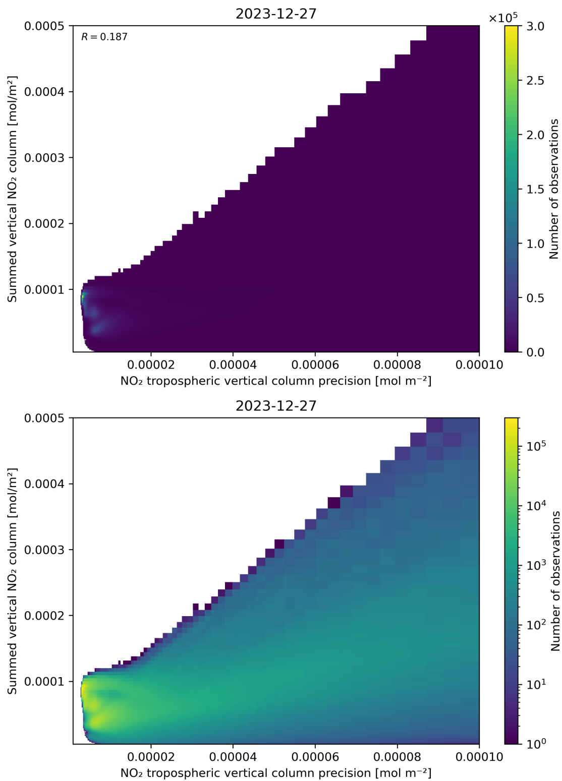
Figure 136: Scatter density plot of “NO 2 tropospheric vertical column precision” against “Summed vertical NO 2 column” for 2023-12-26 to 2023-12-28.
