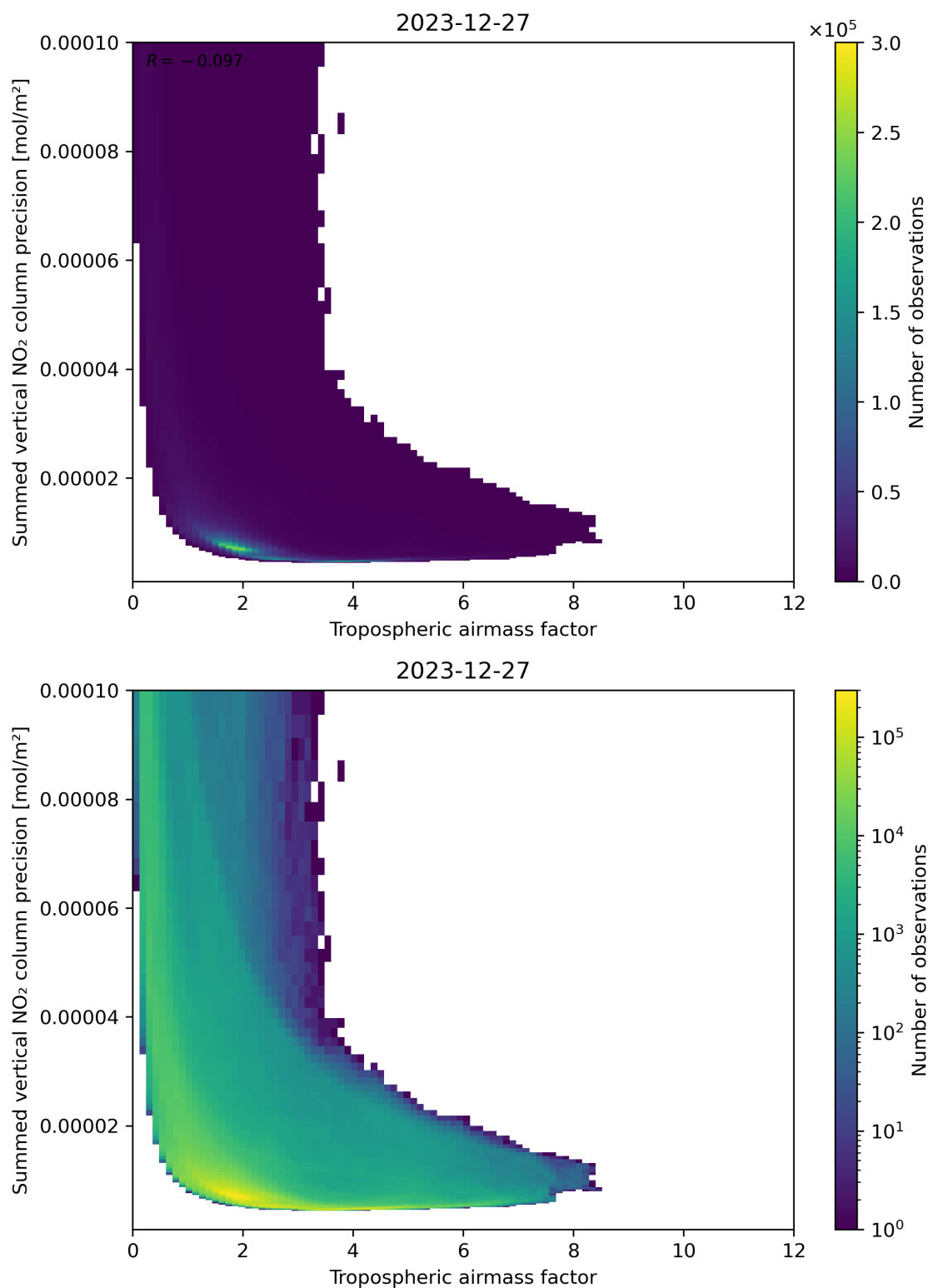
Figure 76: Scatter density plot of “Tropospheric air mass factor” against “Summed vertical NO 2 column precision” for 2023-12-26 to 2023-12-28.
