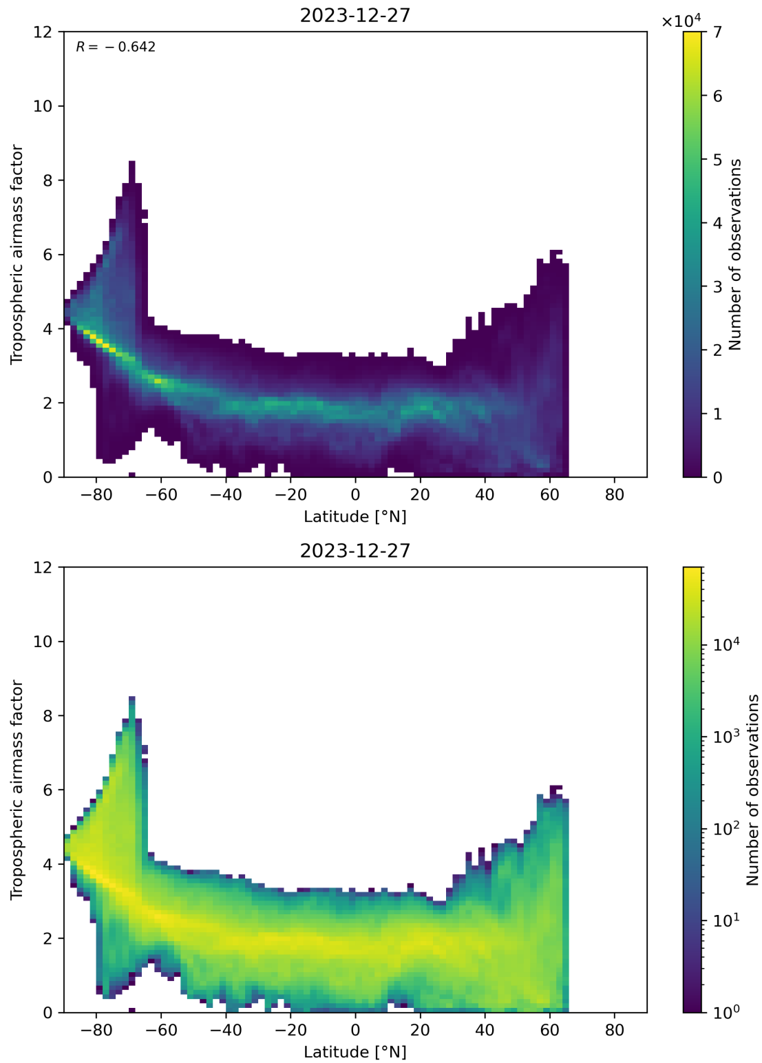
Figure 85: Scatter density plot of “Latitude” against “Tropospheric airmass factor” for 2023-12-26 to 2023-12-28.
