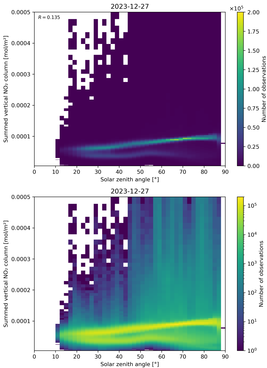
Figure 151: Scatter density plot of “Solar zenith angle” against “Summed vertical NO 2 column” for 2023-12-26 to 2023-12-28.
