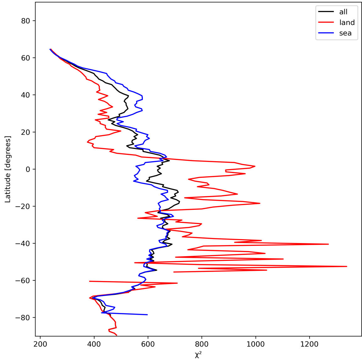
Figure 25: Zonal average of “ \chi^2 ” for 2023-12-26 to 2023-12-28.
