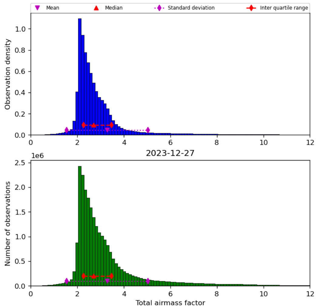
Figure 32: Histogram of “Total airmass factor” for 2023-12-26 to 2023-12-28
