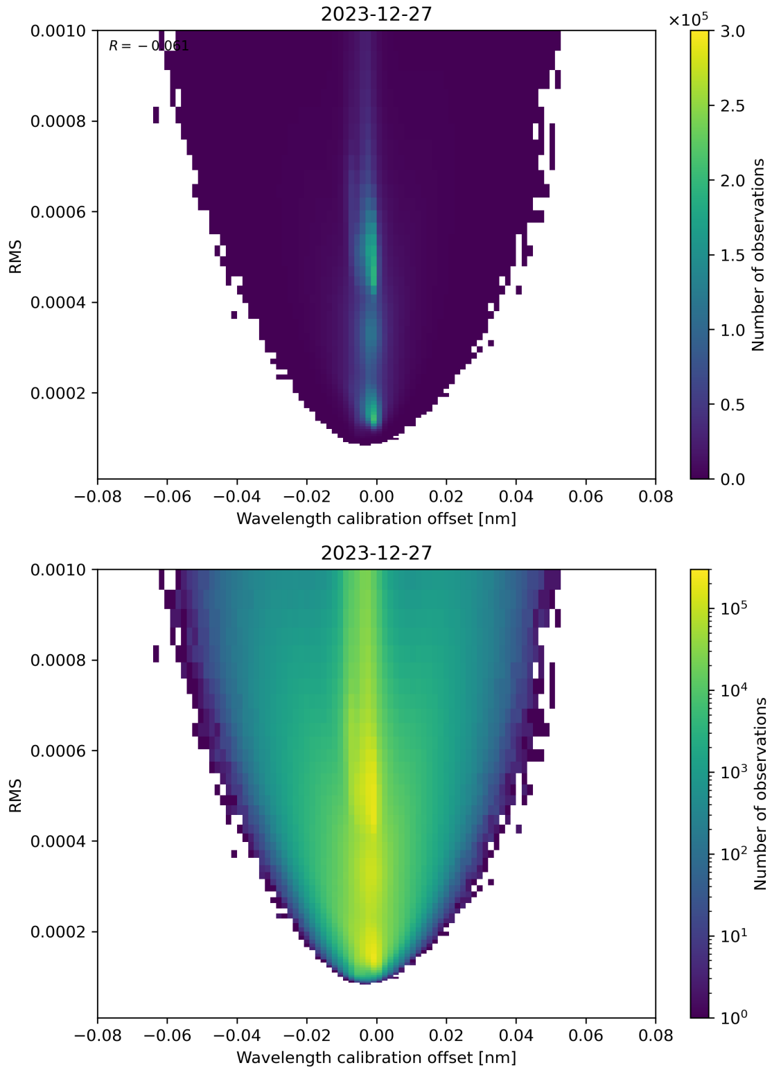
Figure 181: Scatter density plot of “Wavelength calibration offset” against “RMS” for 2023-12-26 to 2023-12-28.
