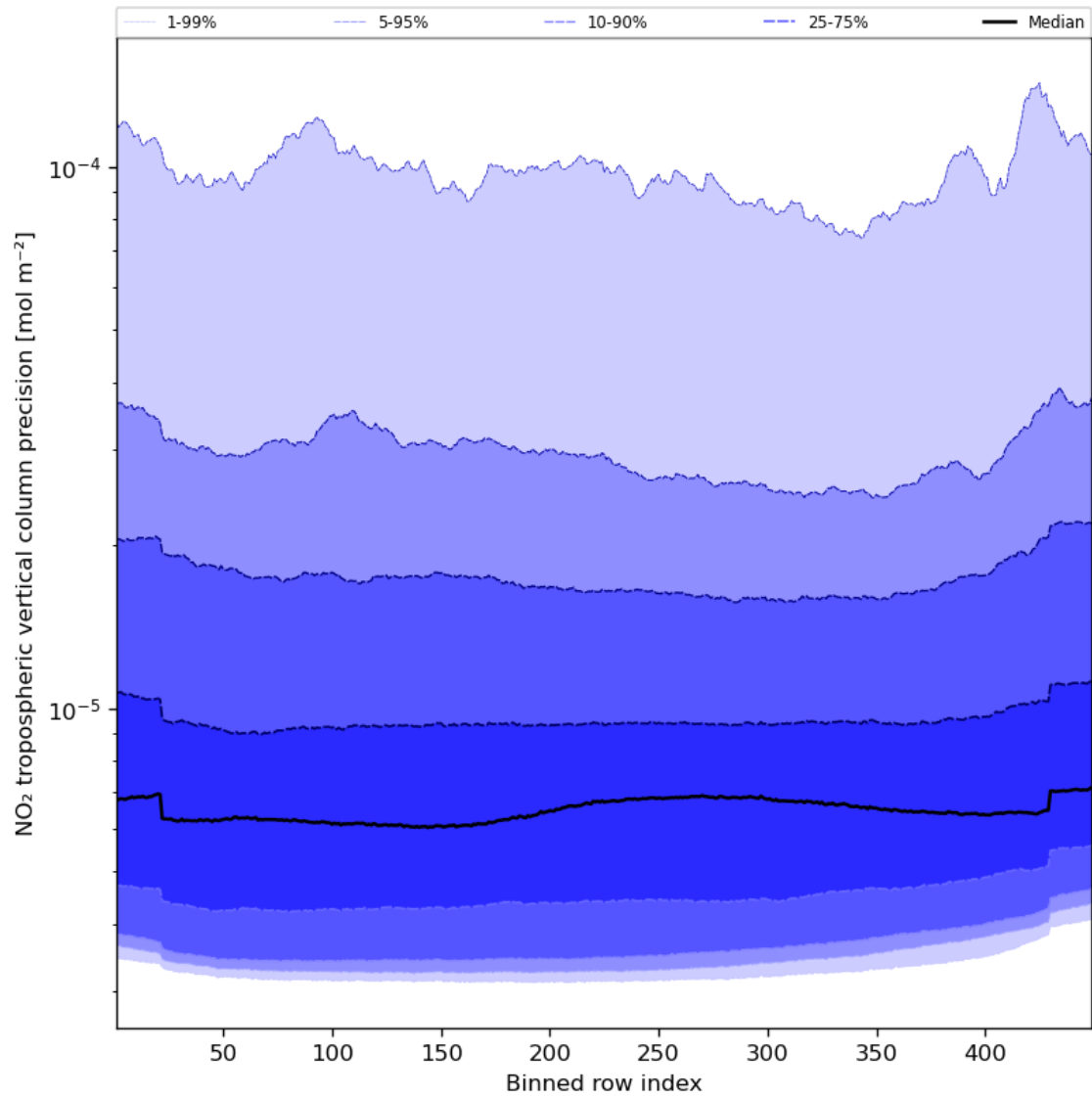
Figure 47: Along track statistics of “NO 2 tropospheric vertical column precision” for 2023-12-26 to 2023-12-28
