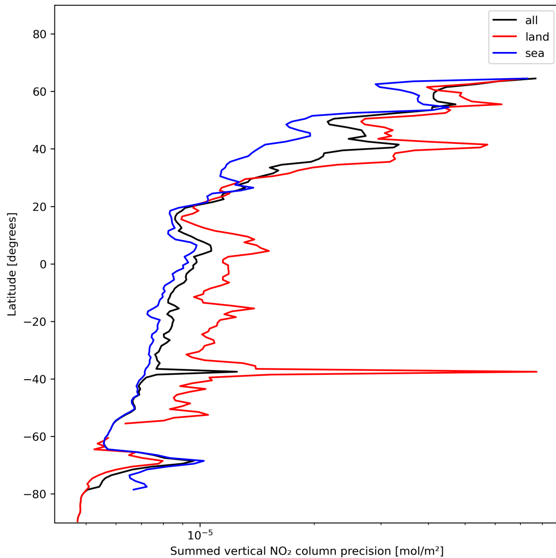
Figure 24: Zonal average of “Summed vertical NO 2 column precision” for 2023-12-26 to 2023-12-28.
