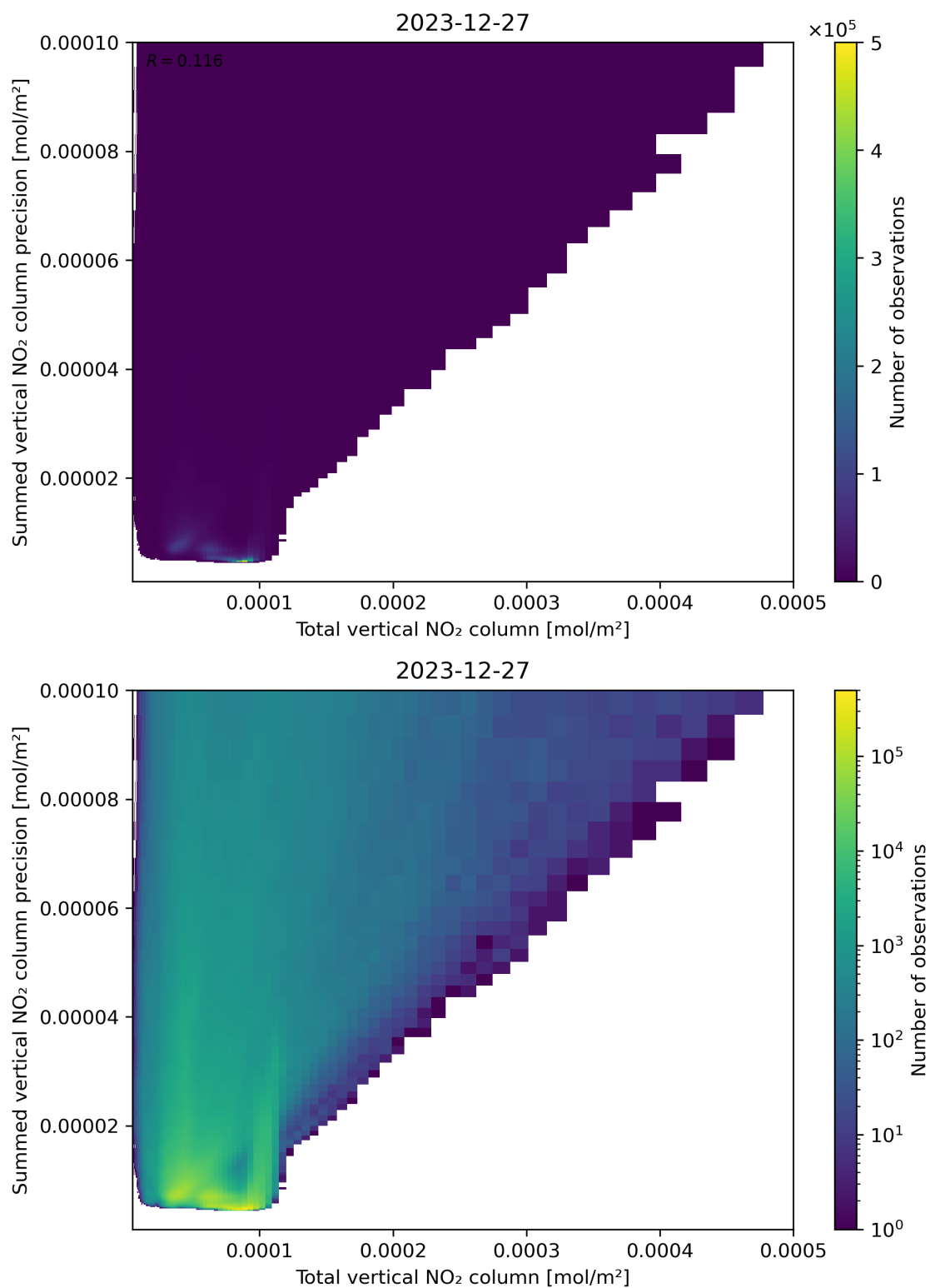
Figure 113: Scatter density plot of “Total vertical NO 2 column” against “Summed vertical NO 2 column precision” for 2023-12-26 to 2023-12-28.
