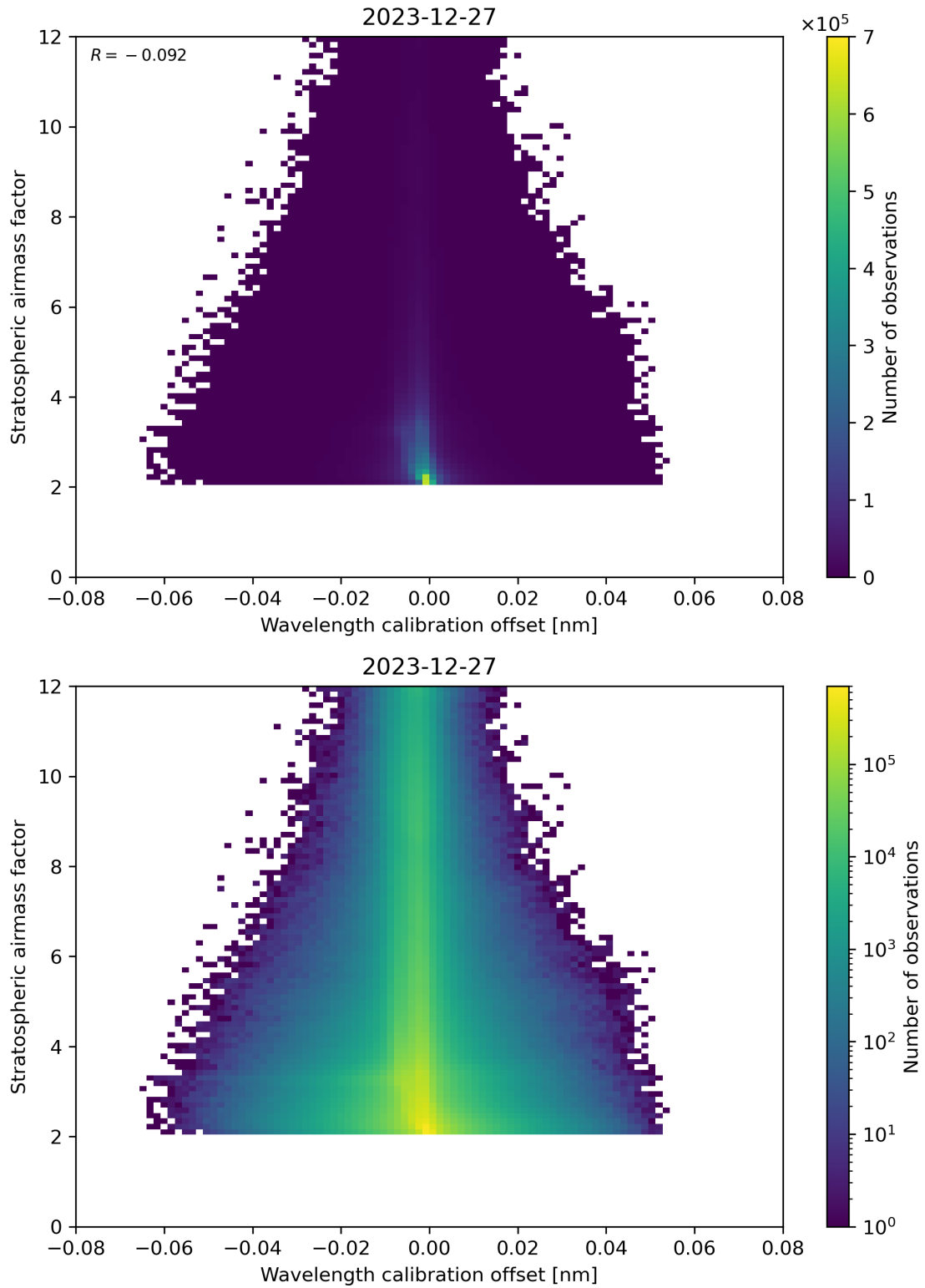
Figure 174: Scatter density plot of “Wavelength calibration offset” against “Stratospheric air mass factor” for 2023-12-26 to 2023-12-28.
