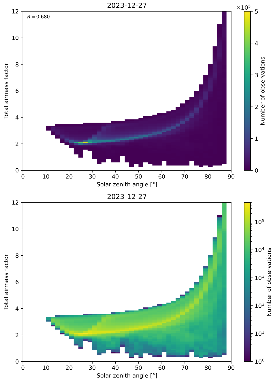
Figure 146: Scatter density plot of “Solar zenith angle” against “Total air mass factor” for 2023-12-26 to 2023-12-28.
