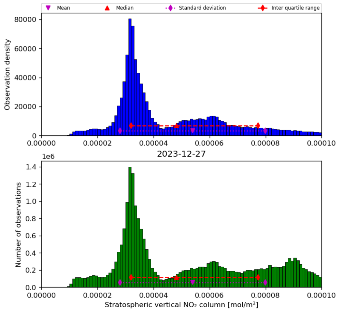
Figure 36: Histogram of “Stratospheric vertical NO 2 column” for 2023-12-26 to 2023-12-28
