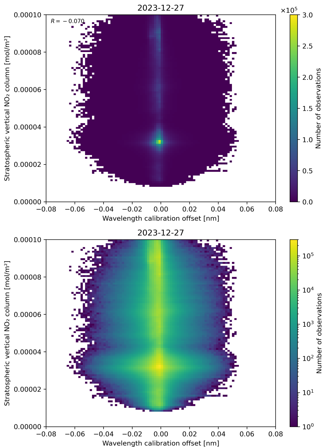
Figure 176: Scatter density plot of “Wavelength calibration offset” against “Stratospheric vertical NO 2 column” for 2023-12-26 to 2023-12-28.
