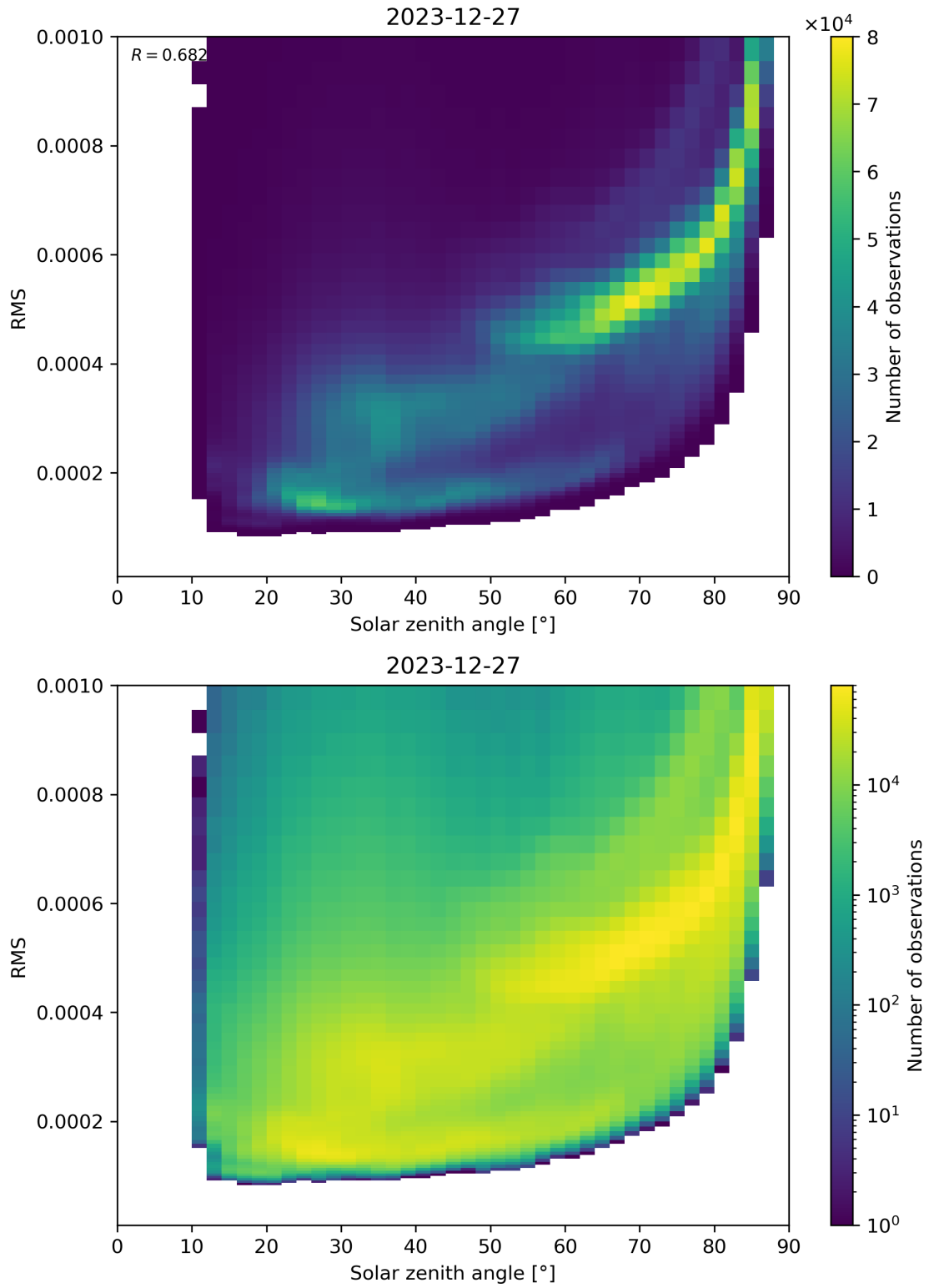
Figure 157: Scatter density plot of “Solar zenith angle” against “RMS” for 2023-12-26 to 2023-12-28.
