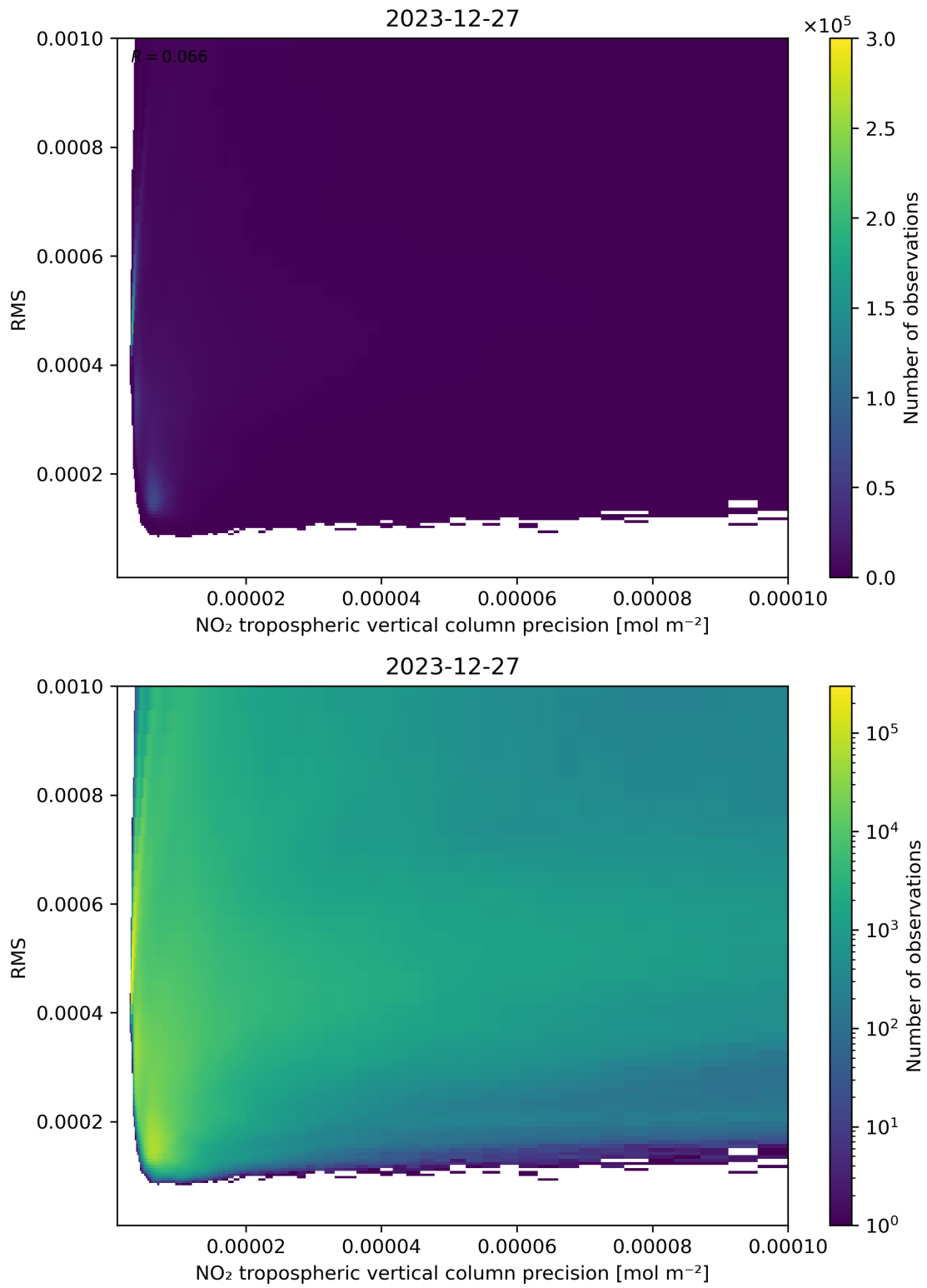
Figure 140: Scatter density plot of “NO 2 tropospheric vertical column precision” against “RMS” for 2023-12-26 to 2023-12-28.
