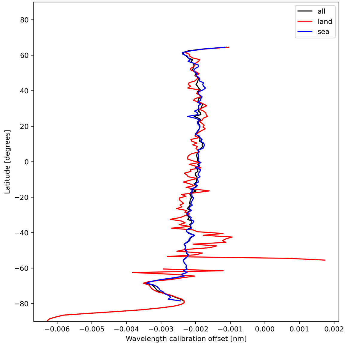
Figure 18: Zonal average of “Wavelength calibration offset” for 2023-12-26 to 2023-12-28.
