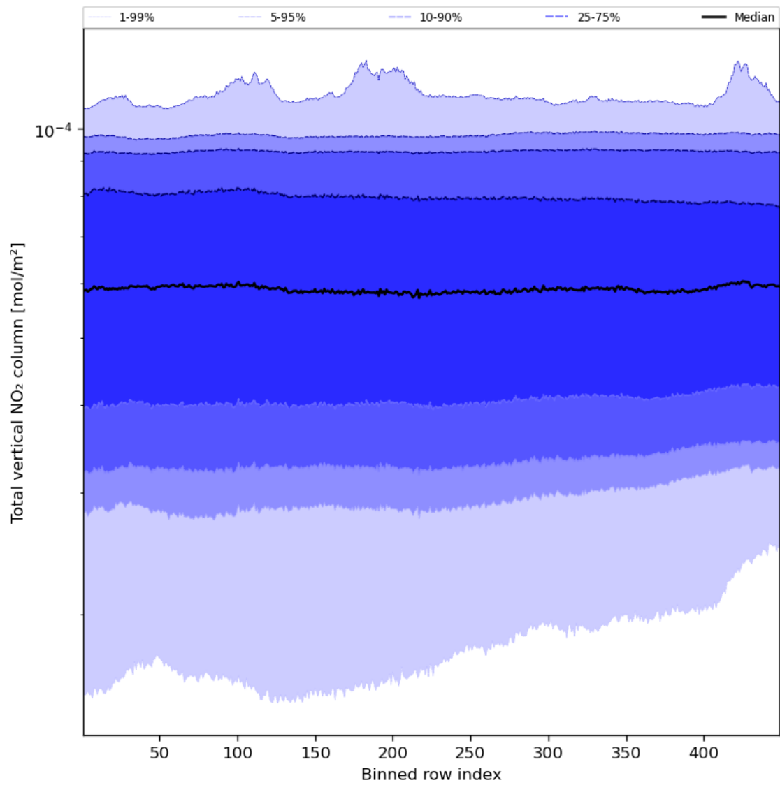
Figure 55: Along track statistics of “Total vertical NO 2 column” for 2023-12-26 to 2023-12-28
