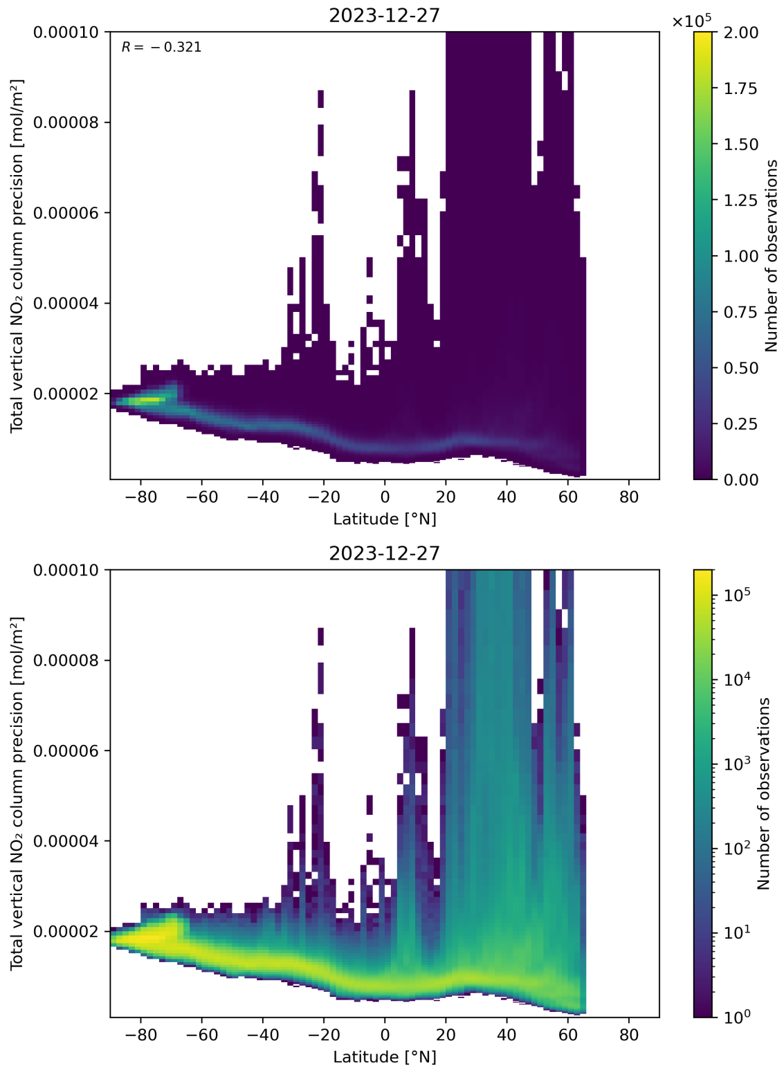
Figure 91: Scatter density plot of “Latitude” against “Total vertical NO 2 column precision” for 2023-12-26 to 2023-12-28.
