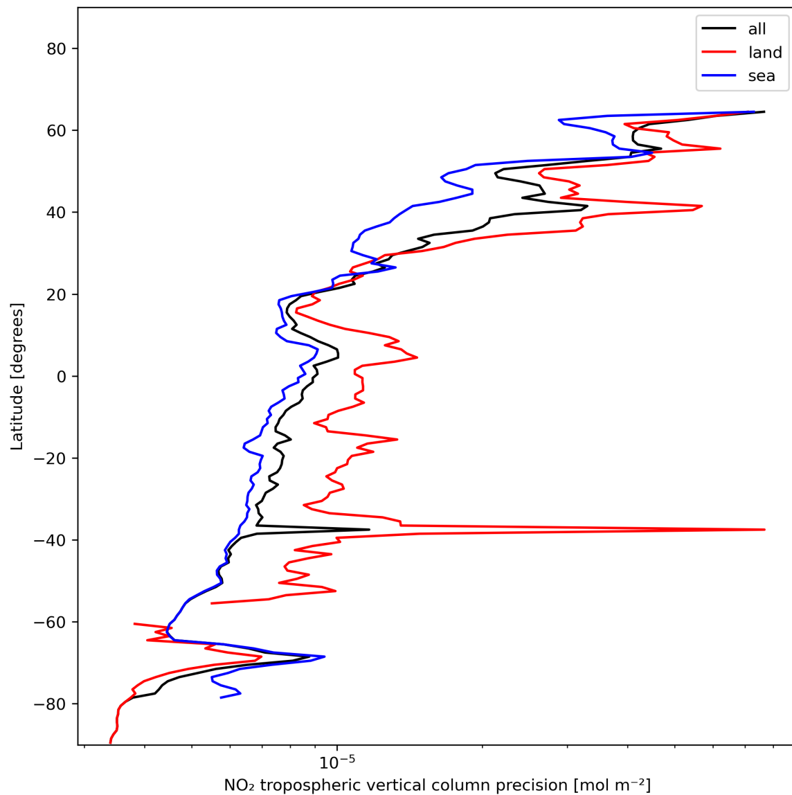
Figure 13: Zonal average of “NO 2 tropospheric vertical column precision” for 2023-12-26 to 2023-12-28.
