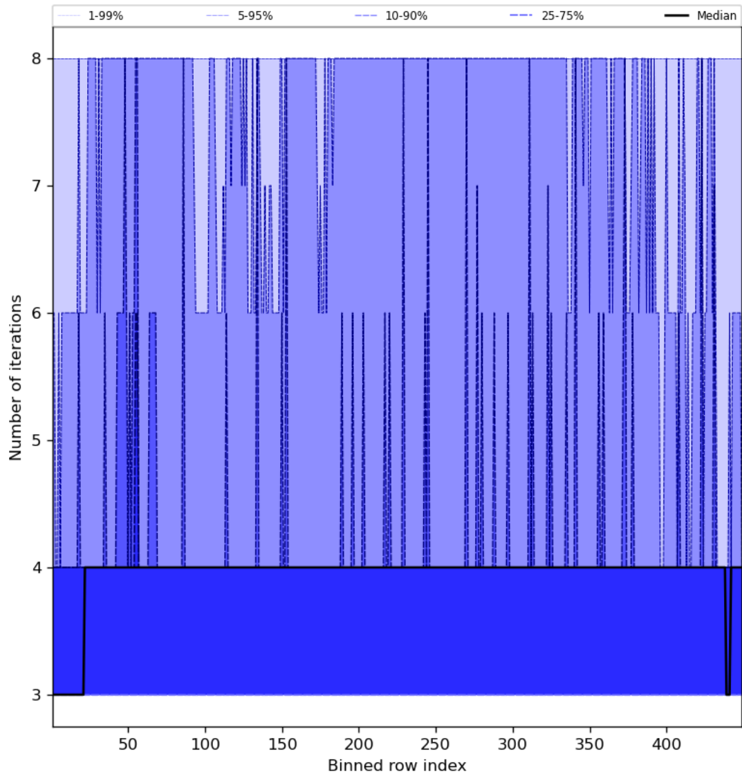
Figure 51: Along track statistics of “Number of iterations” for 2023-12-26 to 2023-12-28
