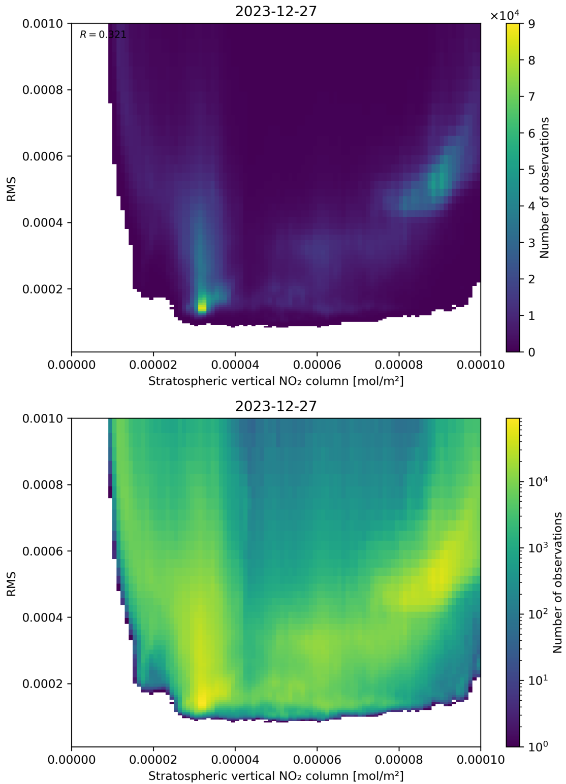
Figure 102: Scatter density plot of “Stratospheric vertical NO 2 column” against “RMS” for 2023-12-26 to 2023-12-28.
