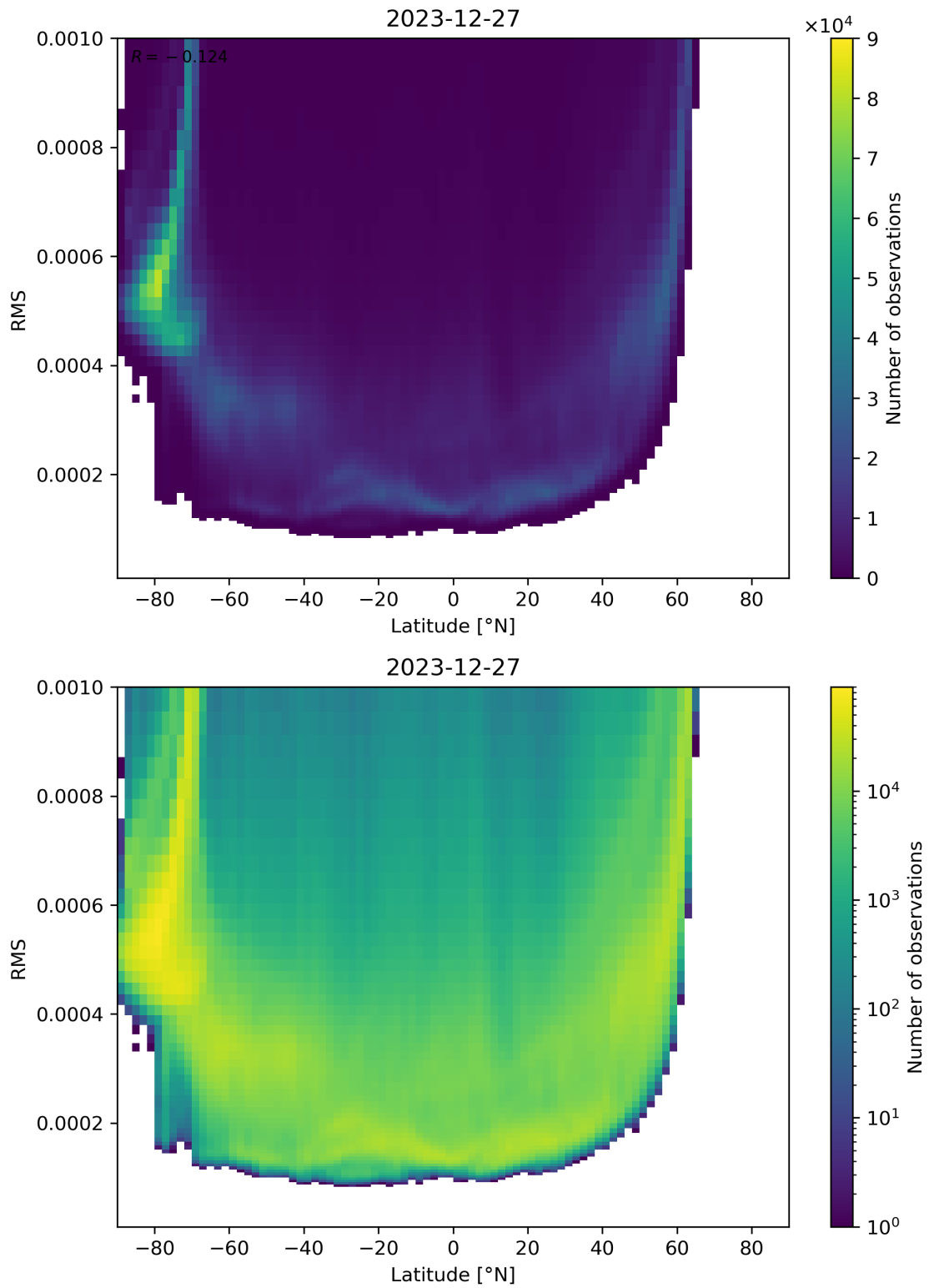
Figure 94: Scatter density plot of “Latitude” against “RMS” for 2023-12-26 to 2023-12-28.
