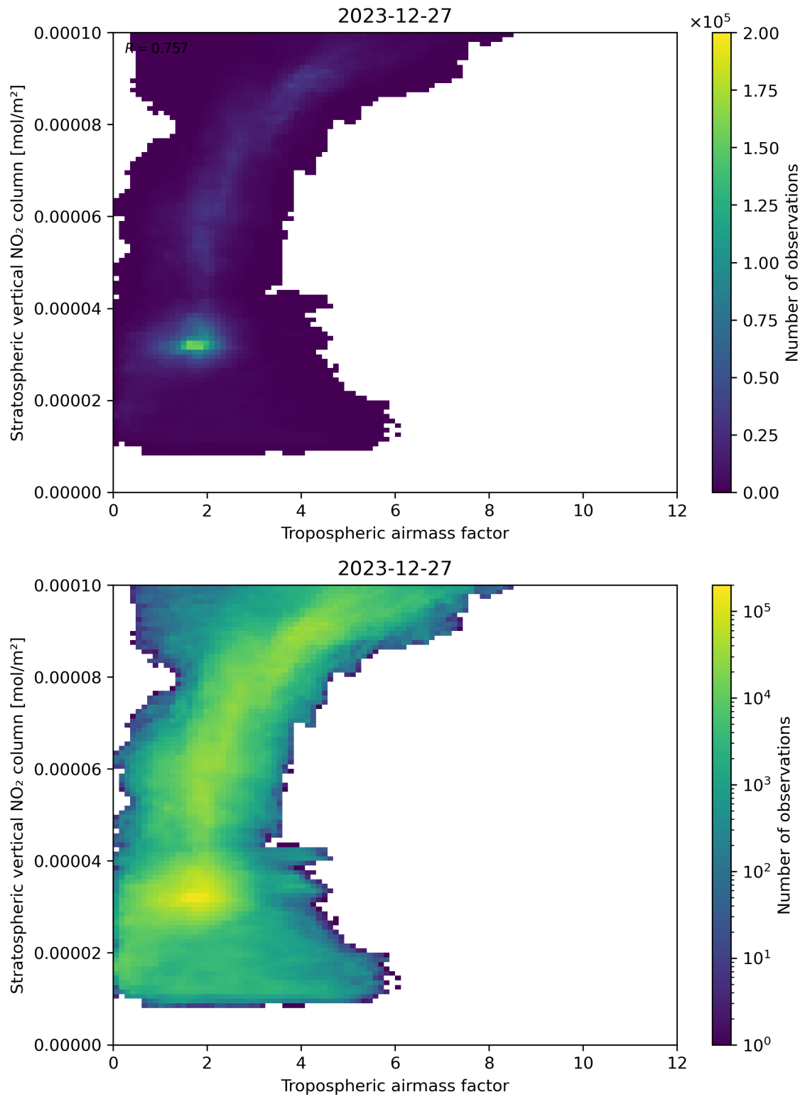
Figure 74: Scatter density plot of “Tropospheric air mass factor” against “Stratospheric vertical NO 2 column” for 2023-12-26 to 2023-12-28.
