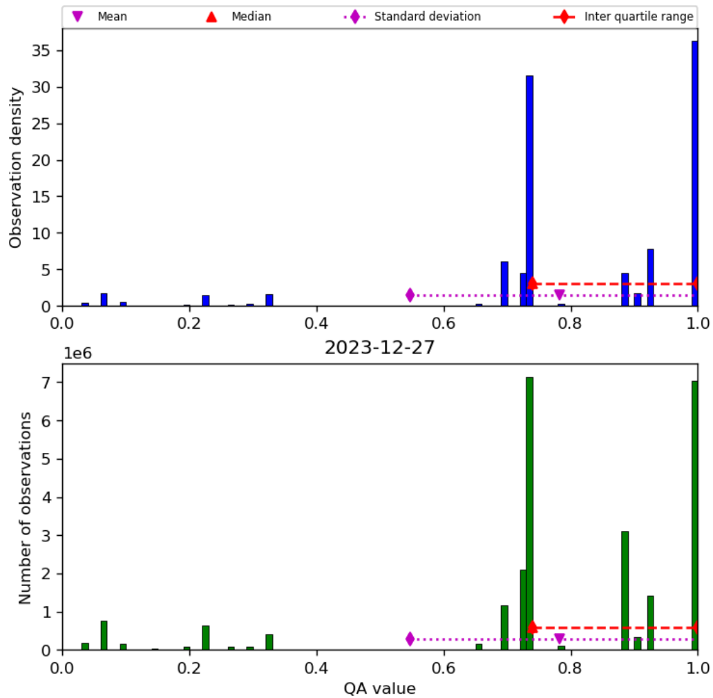
Figure 28: Histogram of “QA value” for 2023-12-26 to 2023-12-28
