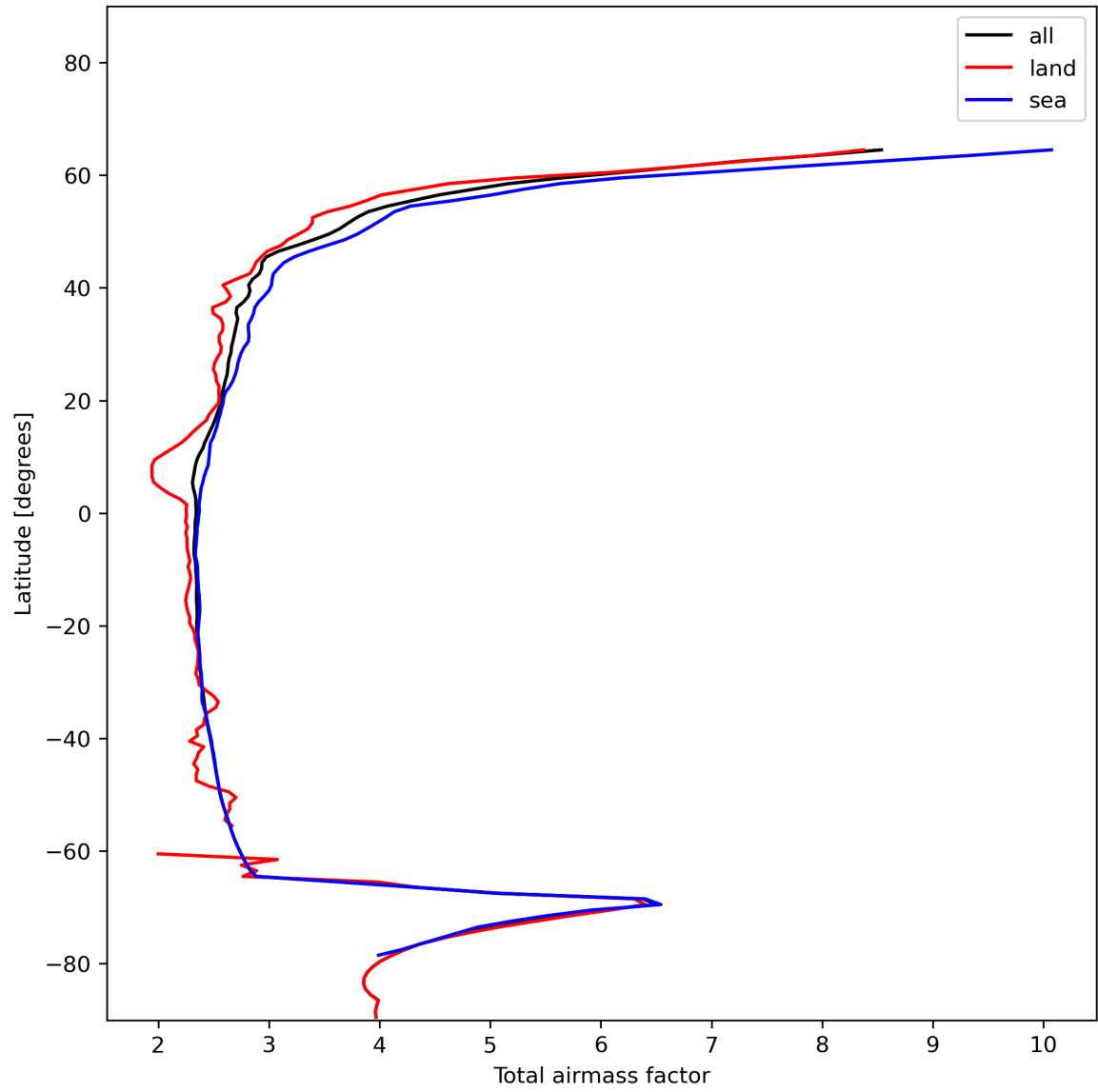
Figure 15: Zonal average of “Total airmass factor” for 2023-12-26 to 2023-12-28.
