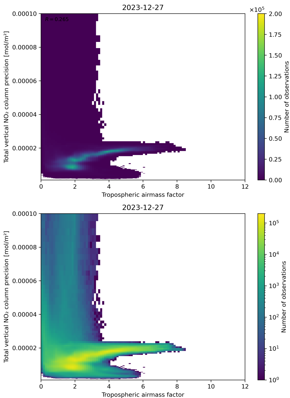
Figure 78: Scatter density plot of “Tropospheric air mass factor” against “Total vertical NO 2 column precision” for 2023-12-26 to 2023-12-28.
