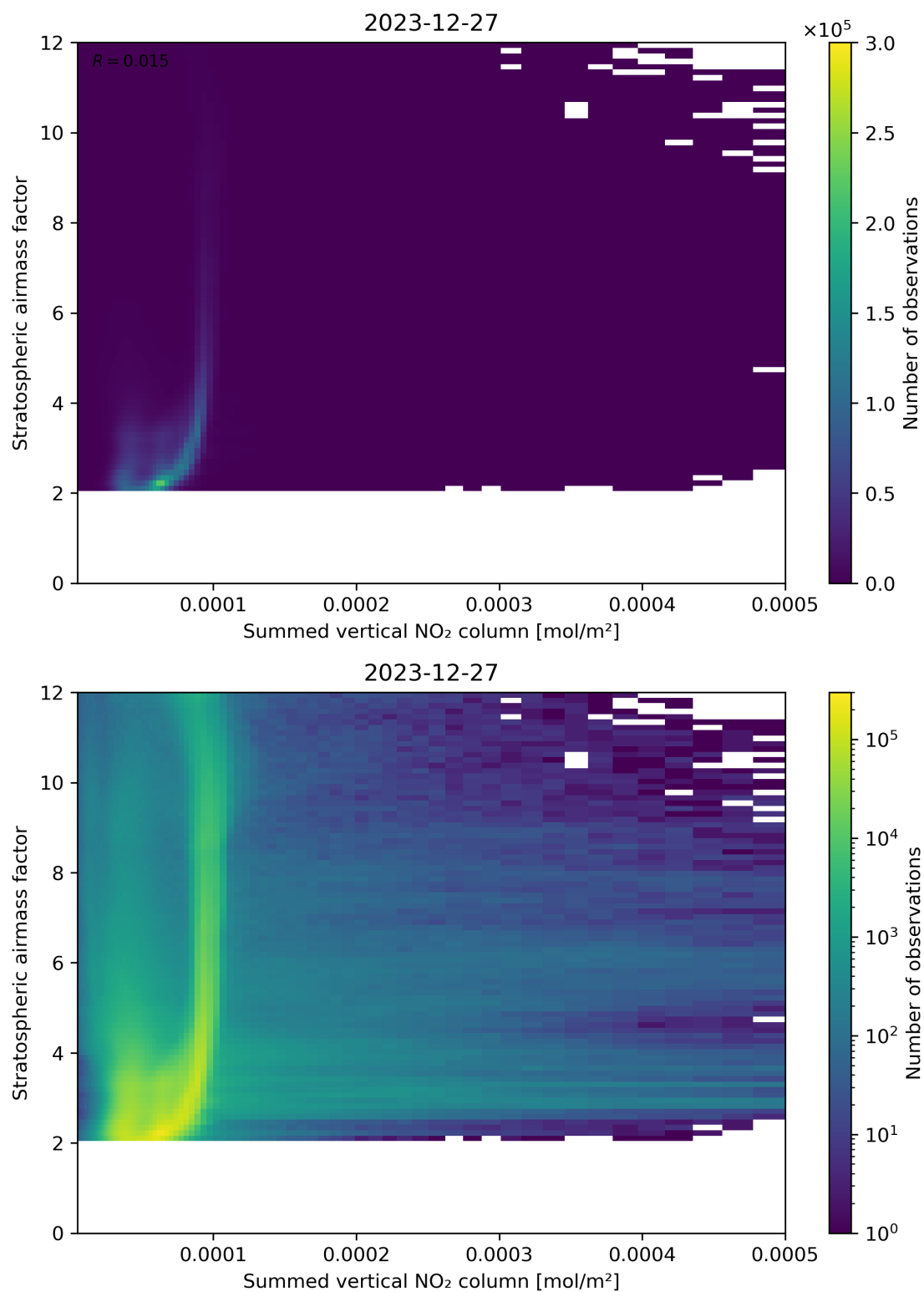
Figure 103: Scatter density plot of “Summed vertical NO 2 column” against “Stratospheric air mass factor” for 2023-12-26 to 2023-12-28.
