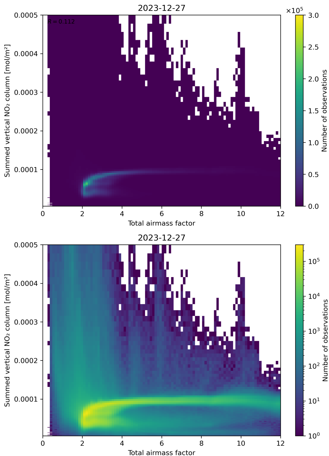
Figure 65: Scatter density plot of “Total airmass factor” against “Summed vertical NO 2 column” for 2023-12-26 to 2023-12-28.
