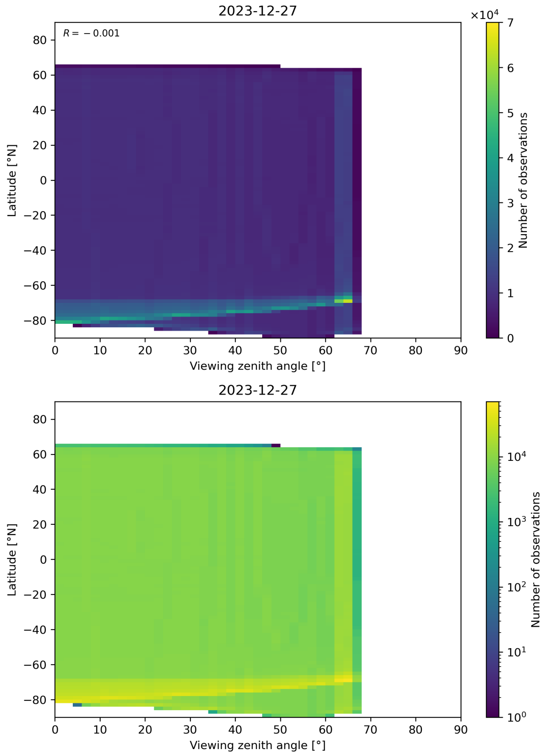
Figure 163: Scatter density plot of “Viewing zenith angle” against “Latitude” for 2023-12-26 to 2023-12-28.
