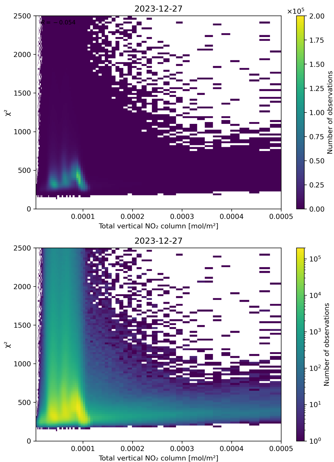
Figure 111: Scatter density plot of “Total vertical NO 2 column” against “ \chi^2 ” for 2023-12-26 to 2023-12-28.
