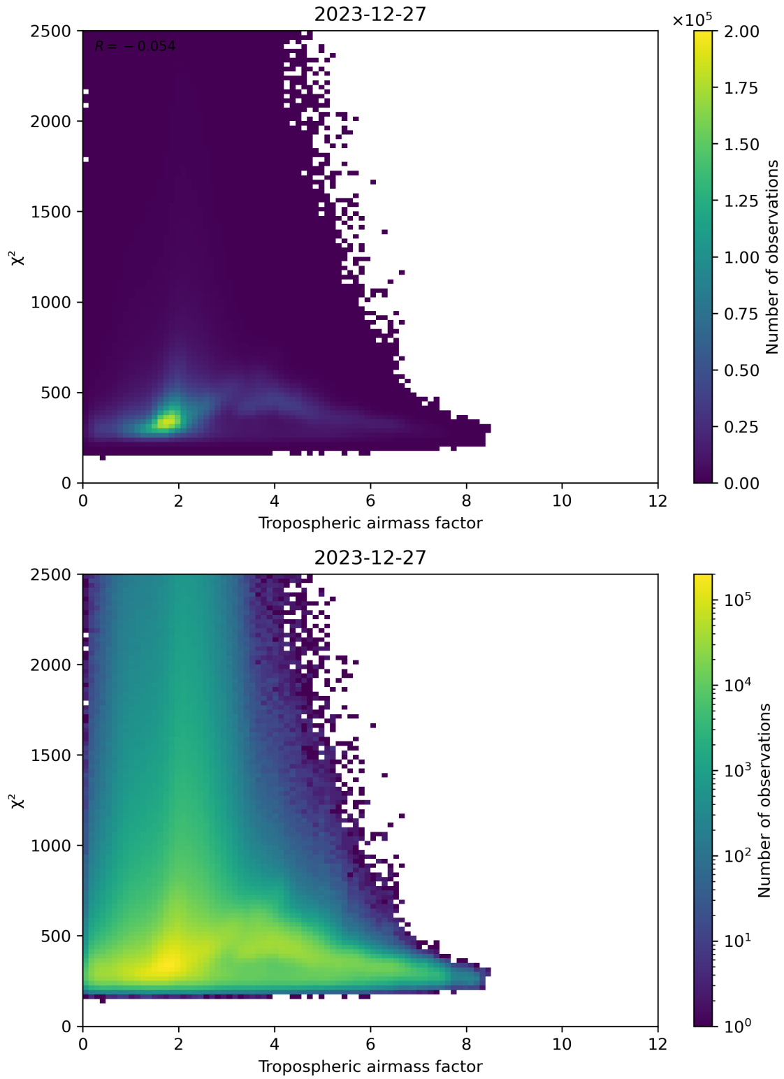
Figure 73: Scatter density plot of “Tropospheric airmass factor” against “ \chi^2 ” for 2023-12-26 to 2023-12-28.
