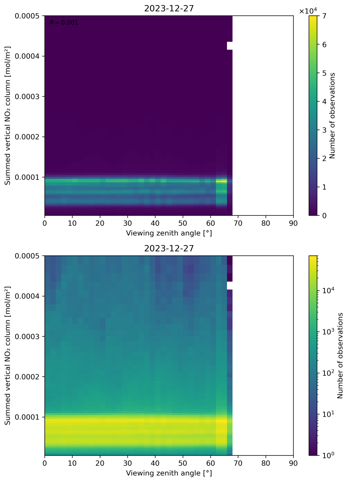
Figure 165: Scatter density plot of “Viewing zenith angle” against “Summed vertical NO 2 column” for 2023-12-26 to 2023-12-28.
