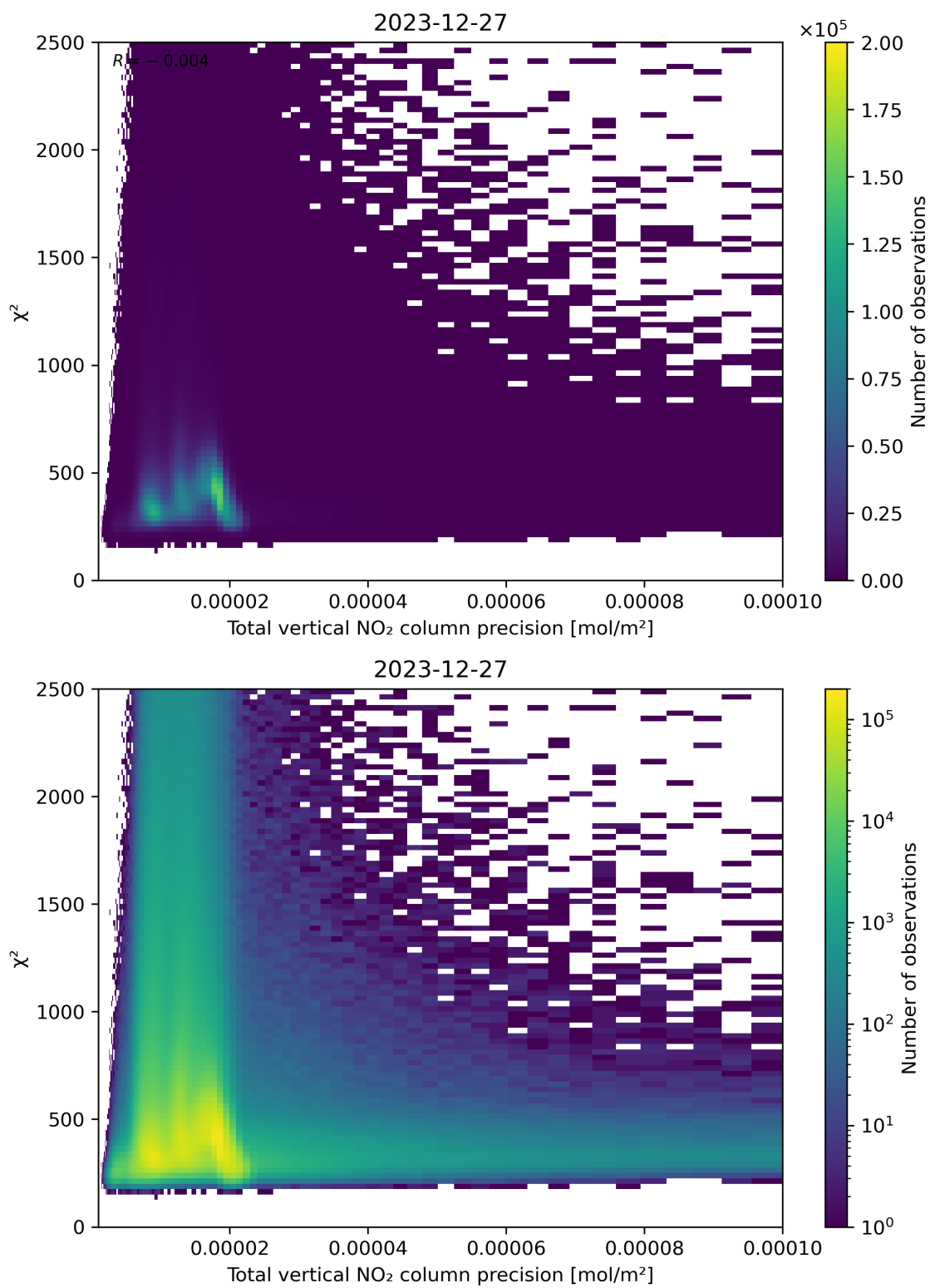
Figure 116: Scatter density plot of “Total vertical NO 2 column precision” against “ \chi^2 ” for 2023-12-26 to 2023-12-28.
