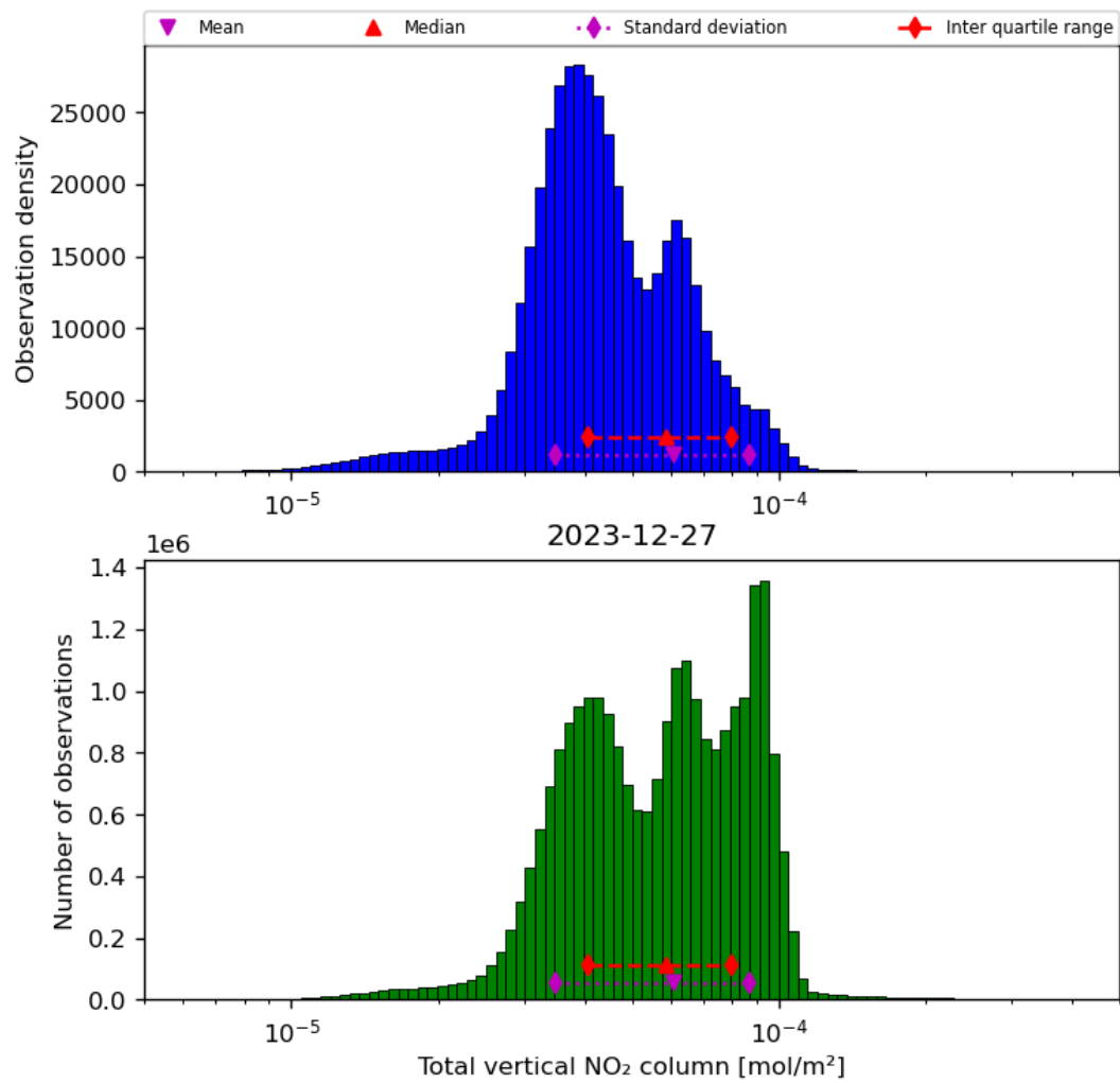
Figure 38: Histogram of “Total vertical NO 2 column” for 2023-12-26 to 2023-12-28
