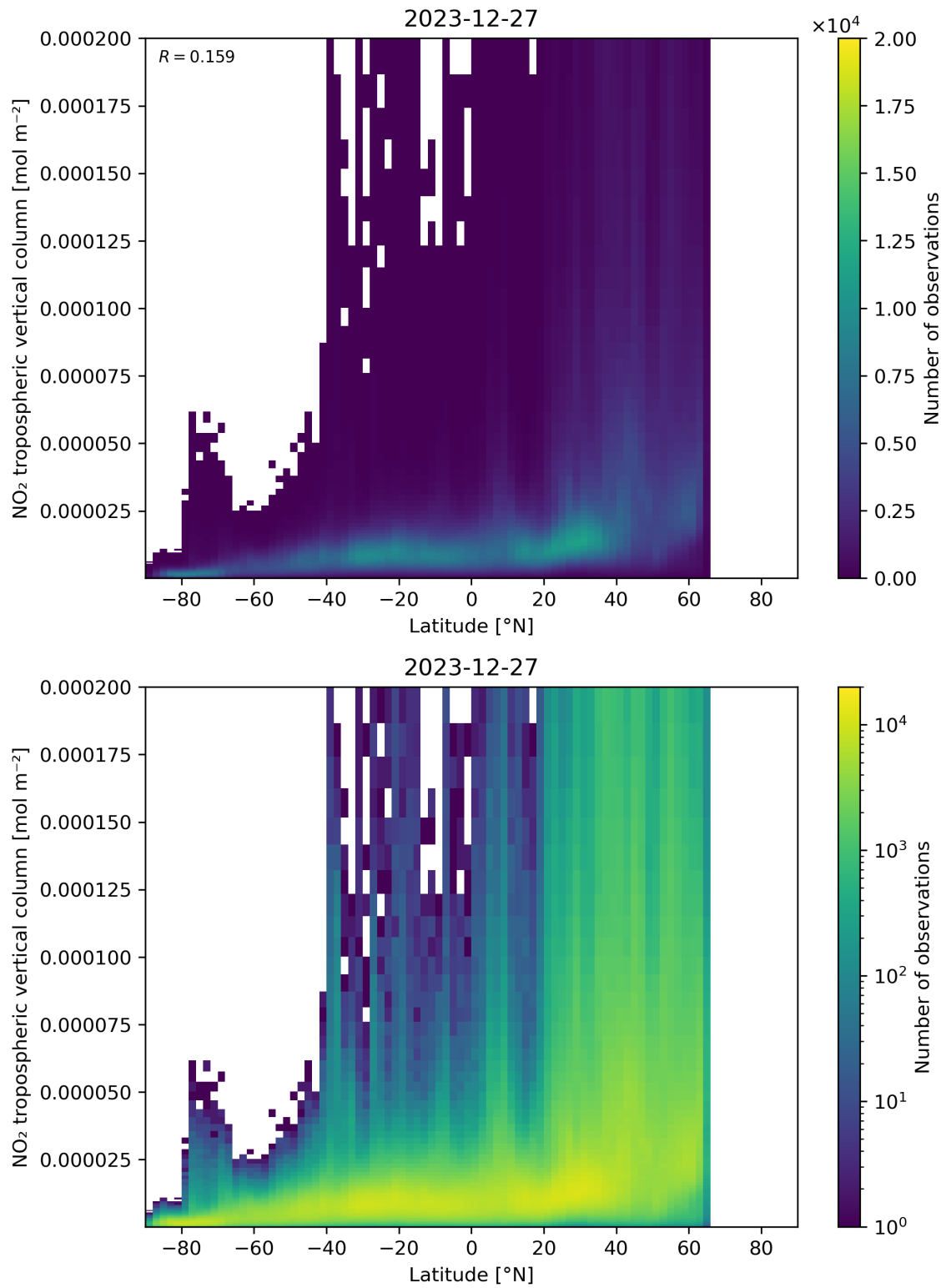
Figure 92: Scatter density plot of “Latitude” against “NO 2 tropospheric vertical column” for 2023-12-26 to 2023-12-28.
