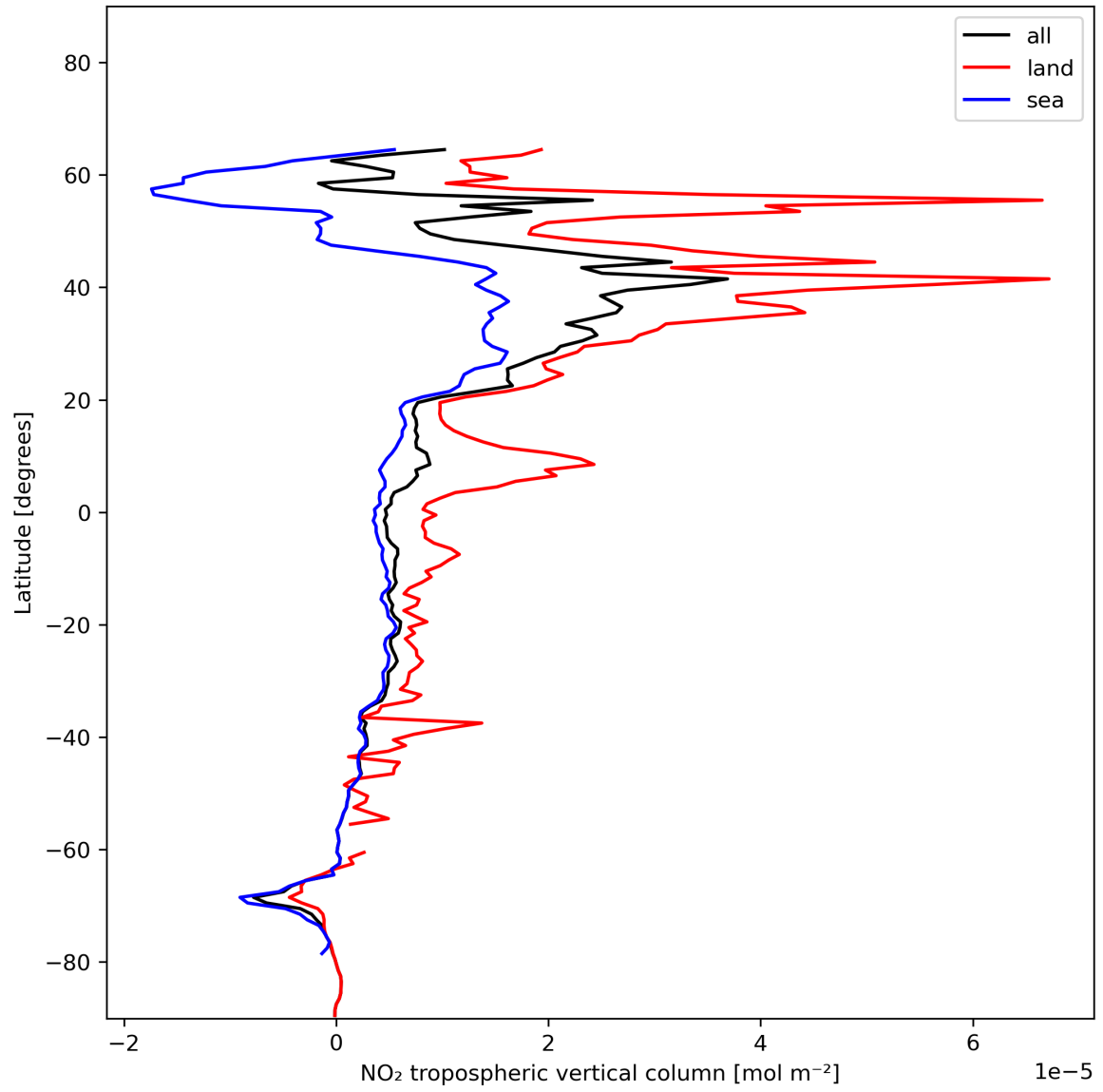
Figure 12: Zonal average of “NO 2 tropospheric vertical column” for 2023-12-26 to 2023-12-28.
