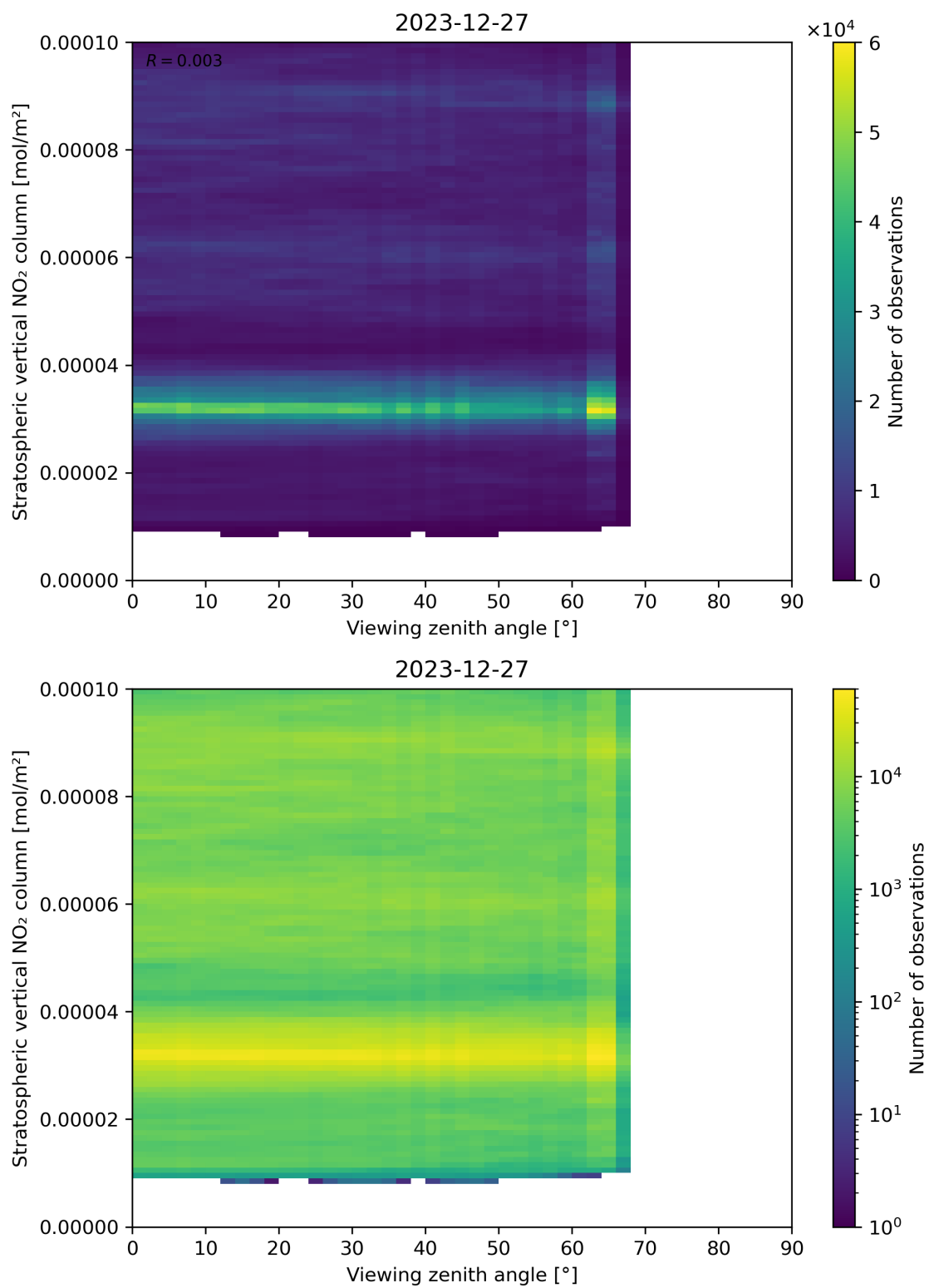
Figure 164: Scatter density plot of “Viewing zenith angle” against “Stratospheric vertical NO 2 column” for 2023-12-26 to 2023-12-28.
