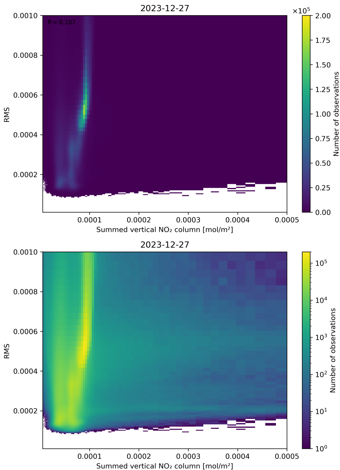
Figure 109: Scatter density plot of “Summed vertical NO 2 column” against “RMS” for 2023-12-26 to 2023-12-28.
