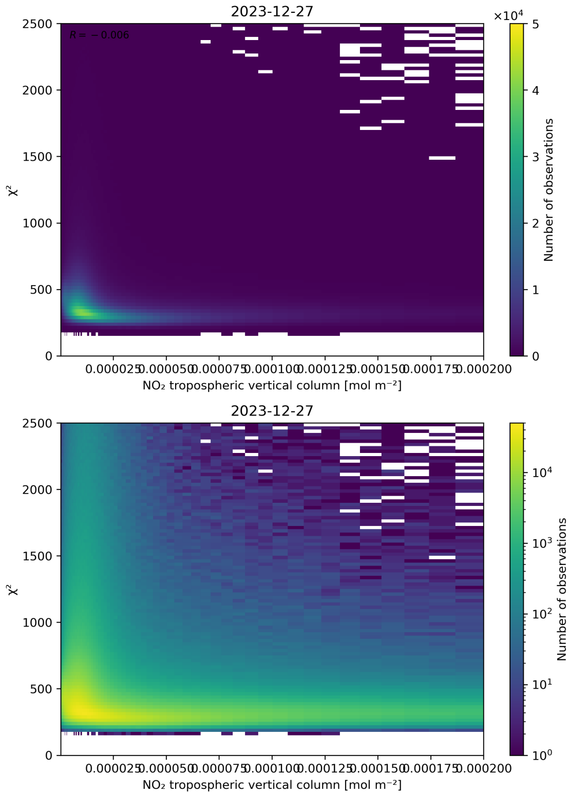
Figure 124: Scatter density plot of “NO 2 tropospheric vertical column” against “ \chi^2 ” for 2023-12-26 to 2023-12-28.
