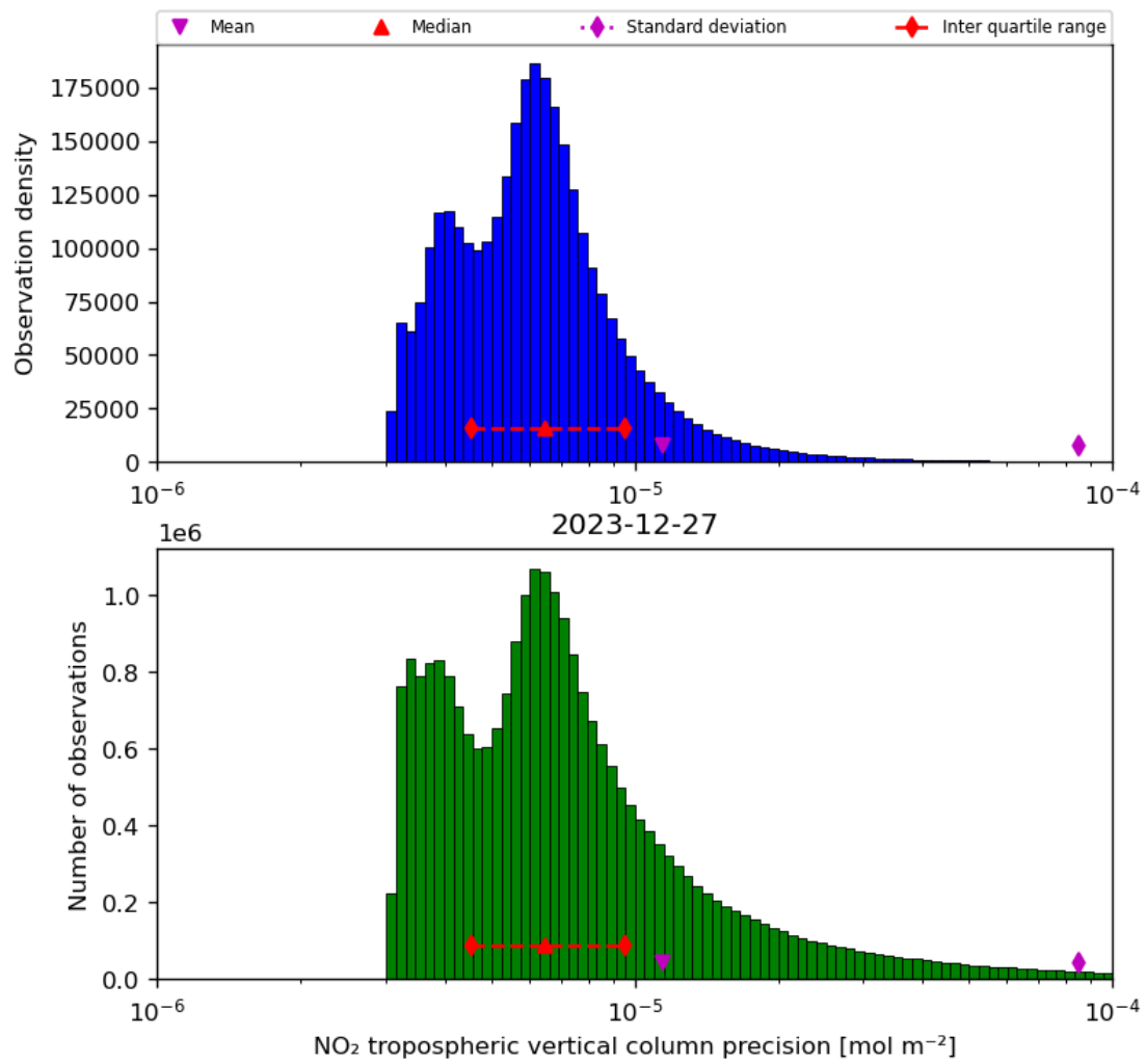
Figure 30: Histogram of “NO 2 tropospheric vertical column precision” for 2023-12-26 to 2023-12-28
