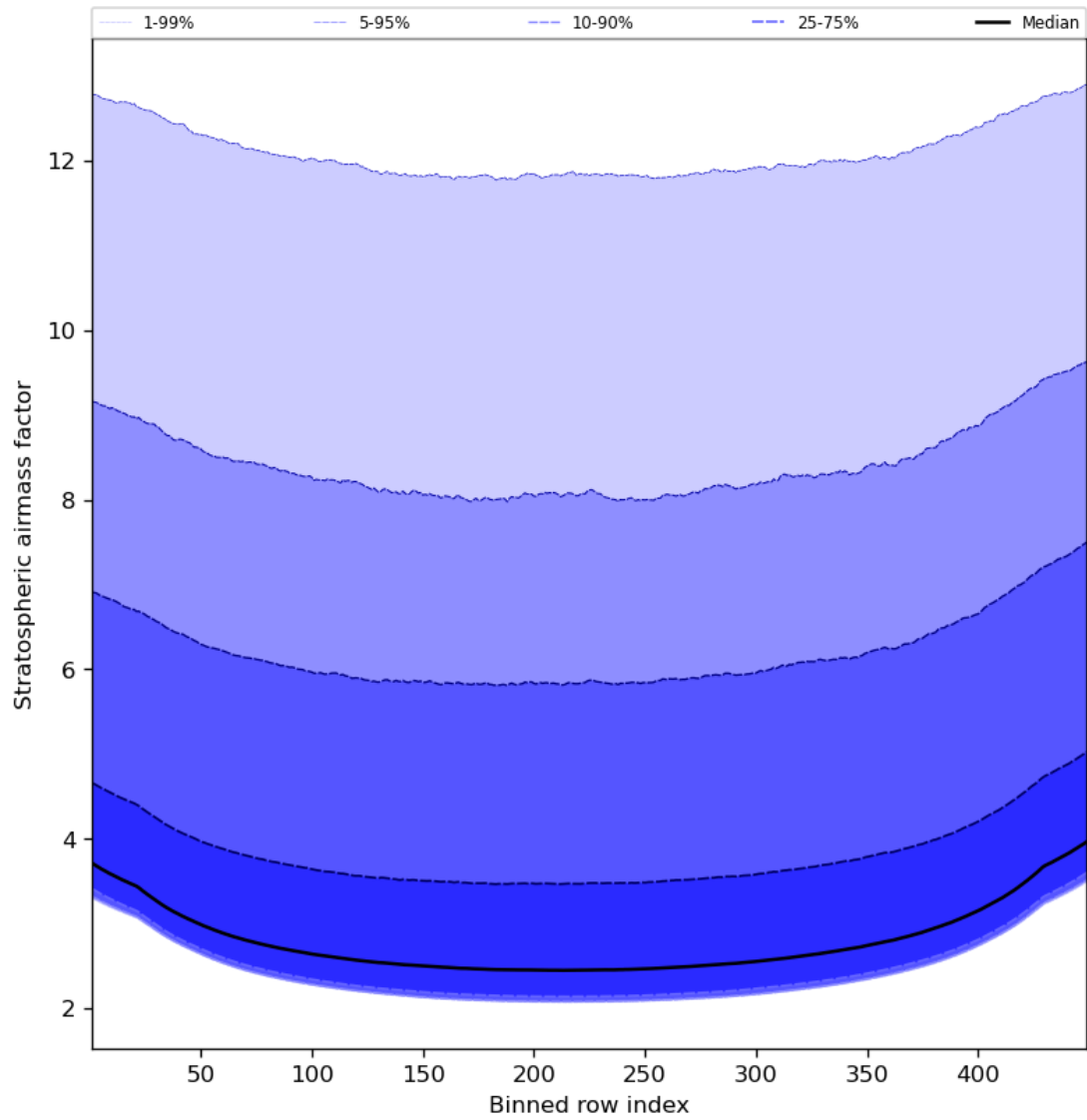
Figure 61: Along track statistics of “Stratospheric airmass factor” for 2023-12-26 to 2023-12-28
