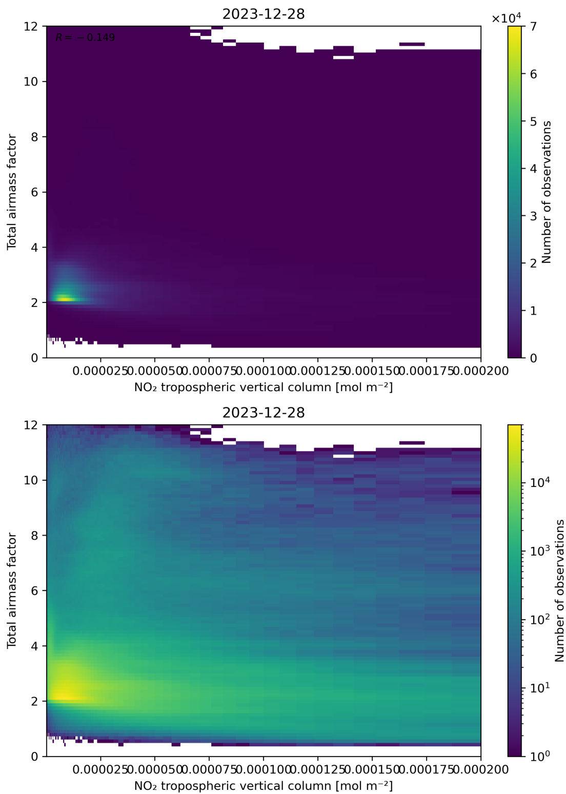
Figure 122: Scatter density plot of “NO 2 tropospheric vertical column” against “Total air mass factor” for 2023-12-27 to 2023-12-29.
