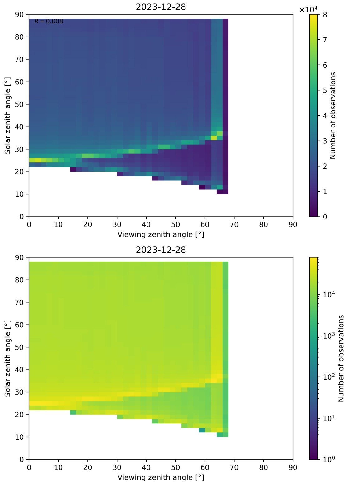
Figure 172: Scatter density plot of “Viewing zenith angle” against “Solar zenith angle” for 2023-12-27 to 2023-12-29.
