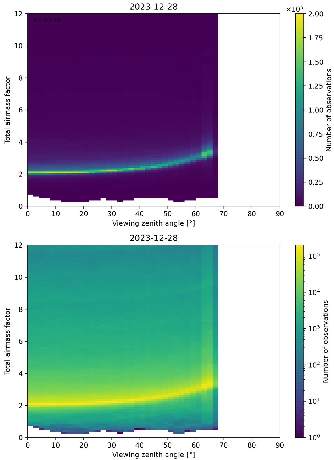
Figure 160: Scatter density plot of “Viewing zenith angle” against “Total airmass factor” for 2023-12-27 to 2023-12-29.
