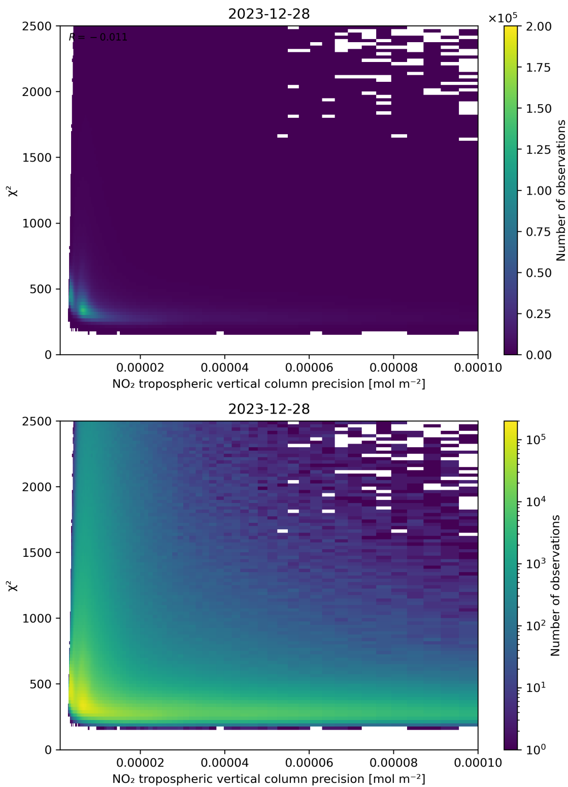
Figure 134: Scatter density plot of “NO 2 tropospheric vertical column precision” against “ \chi^2 ” for 2023-12-27 to 2023-12-29.
