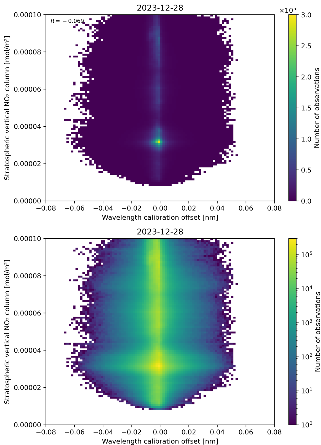
Figure 176: Scatter density plot of “Wavelength calibration offset” against “Stratospheric vertical NO 2 column” for 2023-12-27 to 2023-12-29.
