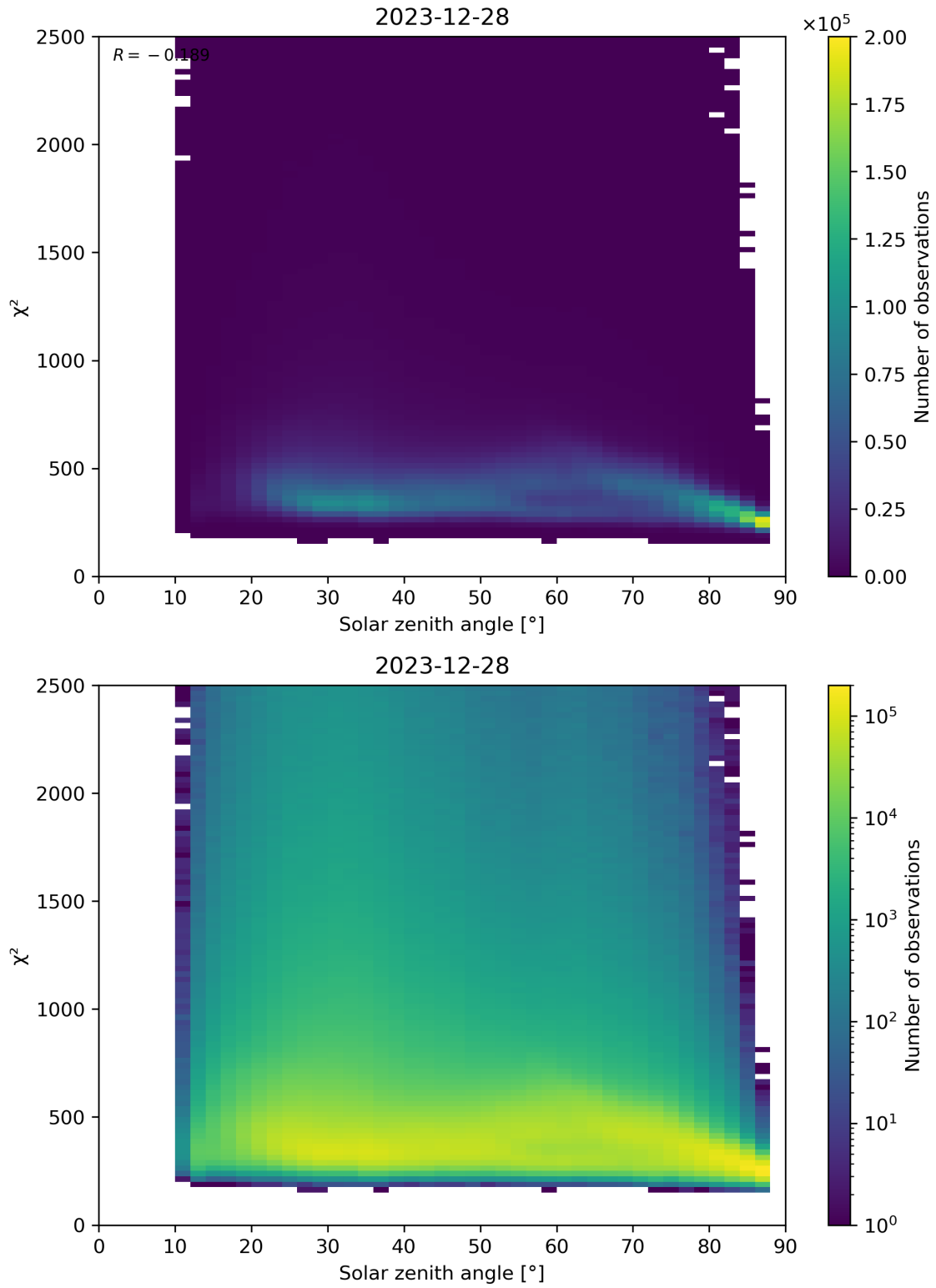
Figure 148: Scatter density plot of “Solar zenith angle” against “ \chi^2 ” for 2023-12-27 to 2023-12-29.
