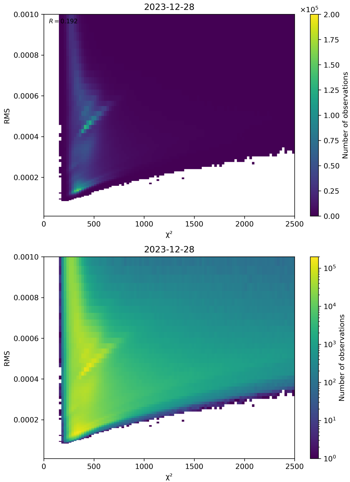
Figure 82: Scatter density plot of “ \chi^2 ” against “RMS” for 2023-12-27 to 2023-12-29.
