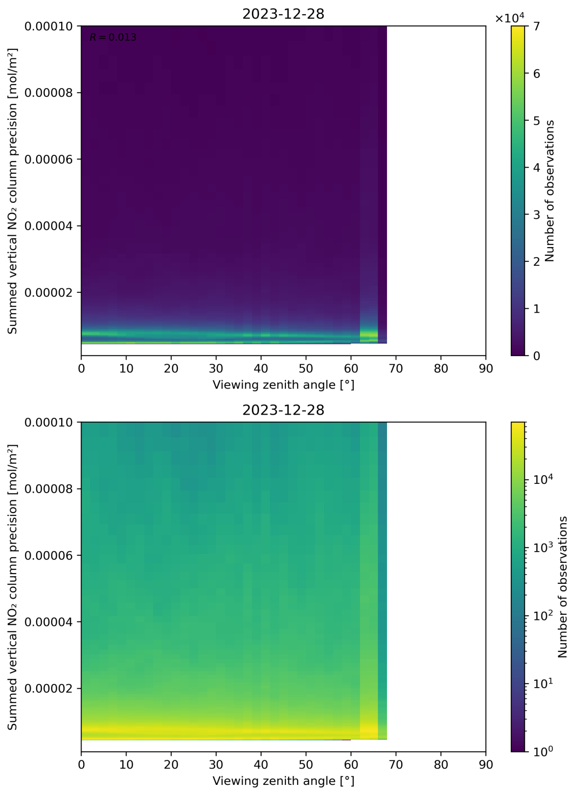
Figure 166: Scatter density plot of “Viewing zenith angle” against “Summed vertical NO 2 column precision” for 2023-12-27 to 2023-12-29.
