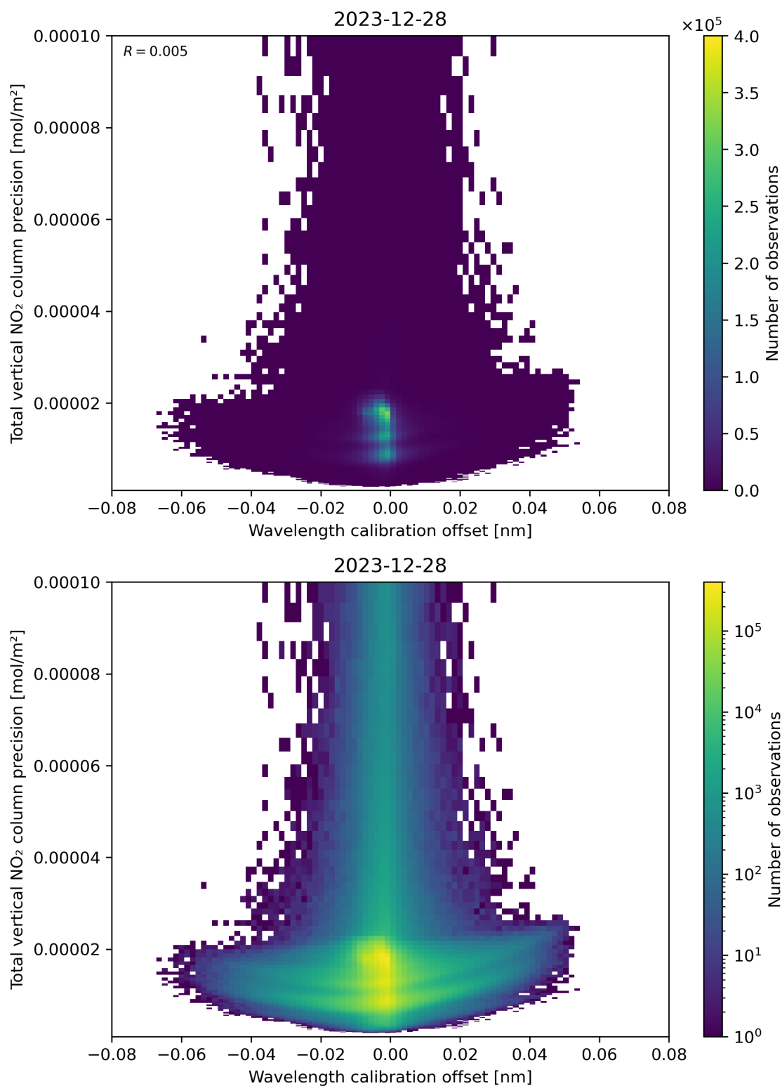
Figure 180: Scatter density plot of “Wavelength calibration offset” against “Total vertical NO 2 column precision” for 2023-12-27 to 2023-12-29.
