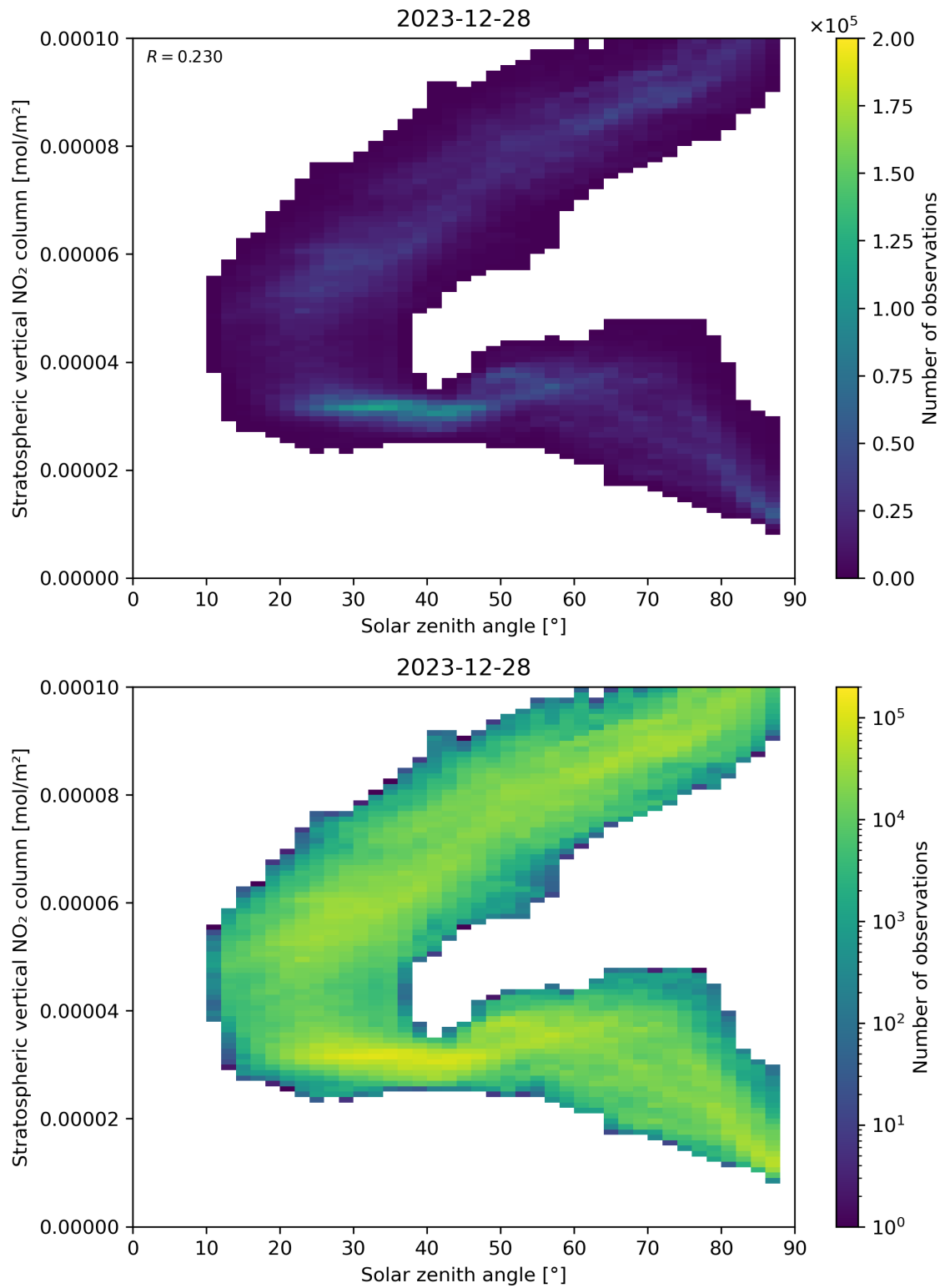
Figure 150: Scatter density plot of “Solar zenith angle” against “Stratospheric vertical NO 2 column” for 2023-12-27 to 2023-12-29.
