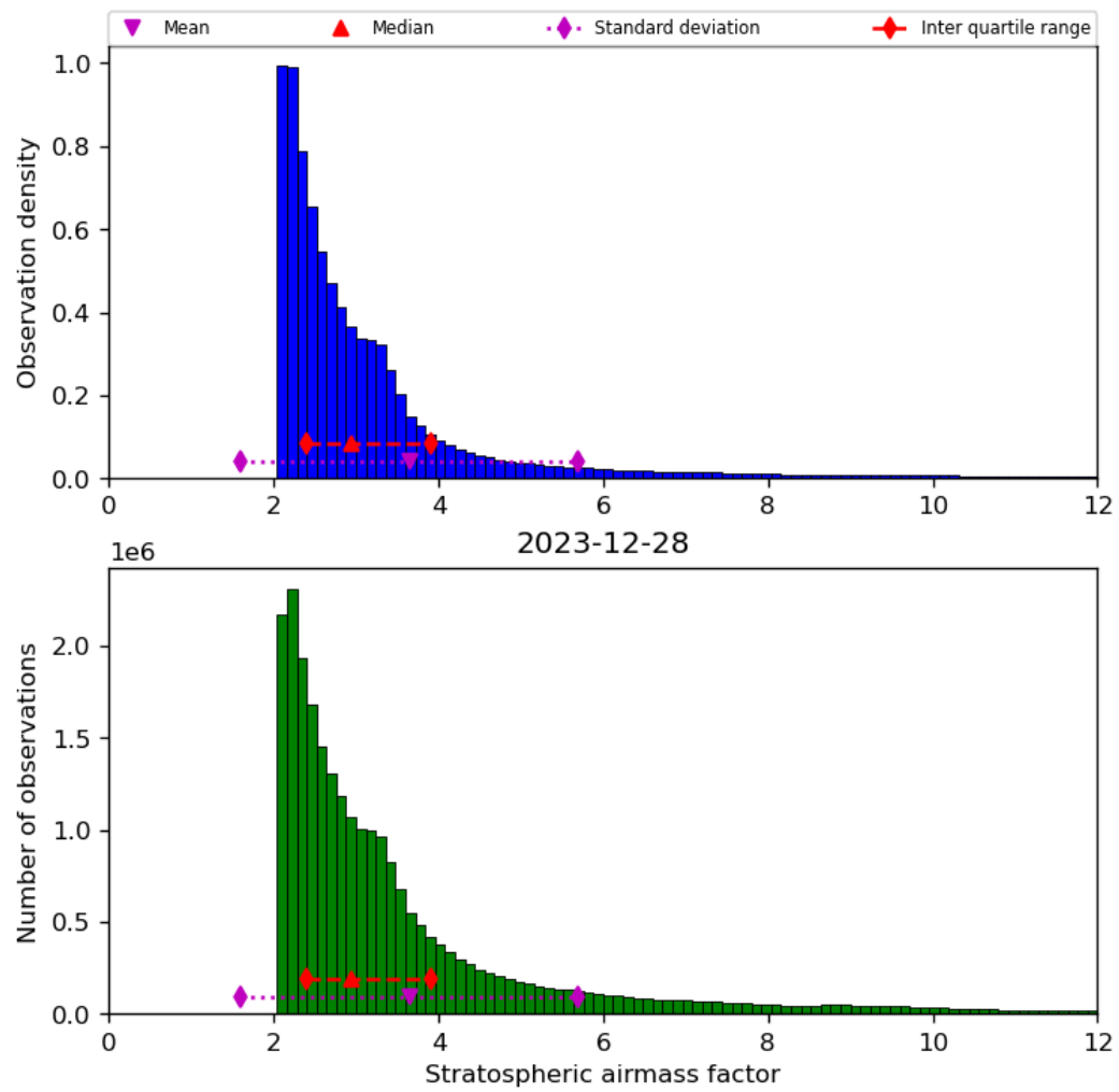
Figure 44: Histogram of “Stratospheric airmass factor” for 2023-12-27 to 2023-12-29
