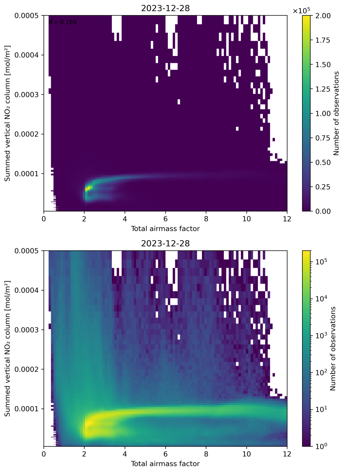
Figure 65: Scatter density plot of “Total airmass factor” against “Summed vertical NO 2 column” for 2023-12-27 to 2023-12-29.
