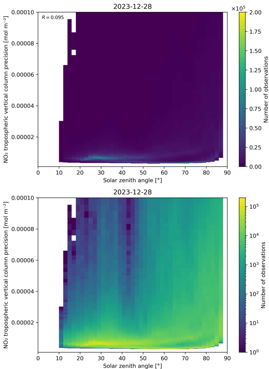
Figure 156: Scatter density plot of “Solar zenith angle” against “NO 2 tropospheric vertical column precision” for 2023-12-27 to 2023-12-29.
