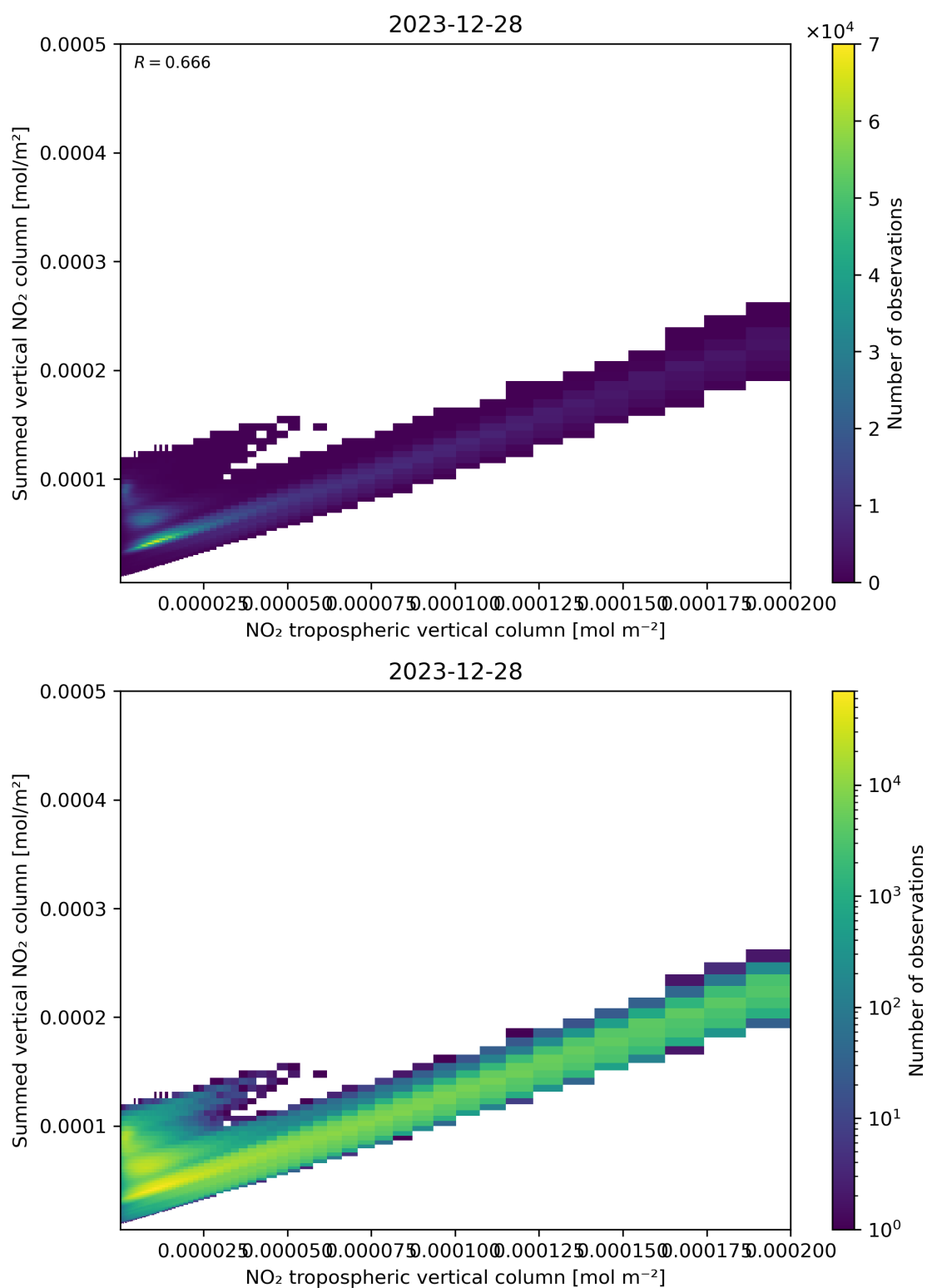
Figure 126: Scatter density plot of “NO 2 tropospheric vertical column” against “Summed vertical NO 2 column” for 2023-12-27 to 2023-12-29.
