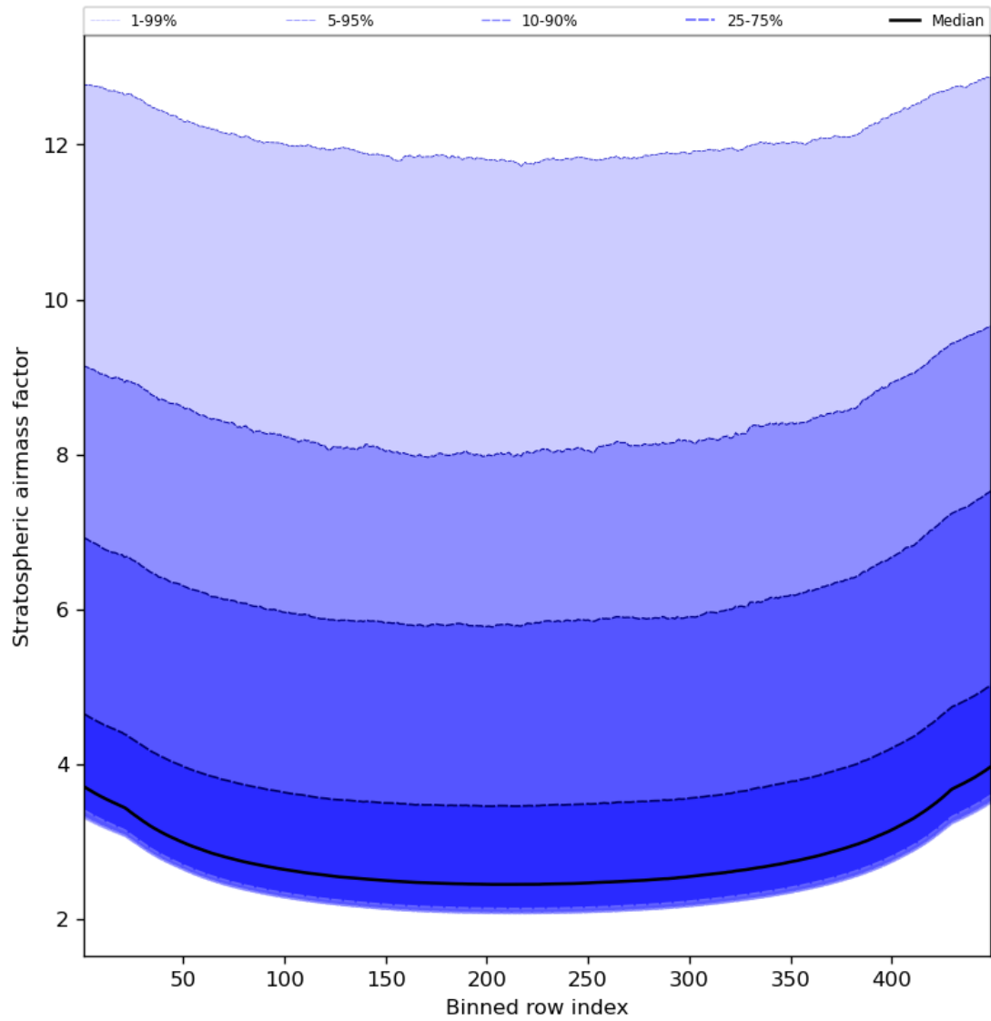
Figure 61: Along track statistics of “Stratospheric airmass factor” for 2023-12-27 to 2023-12-29
