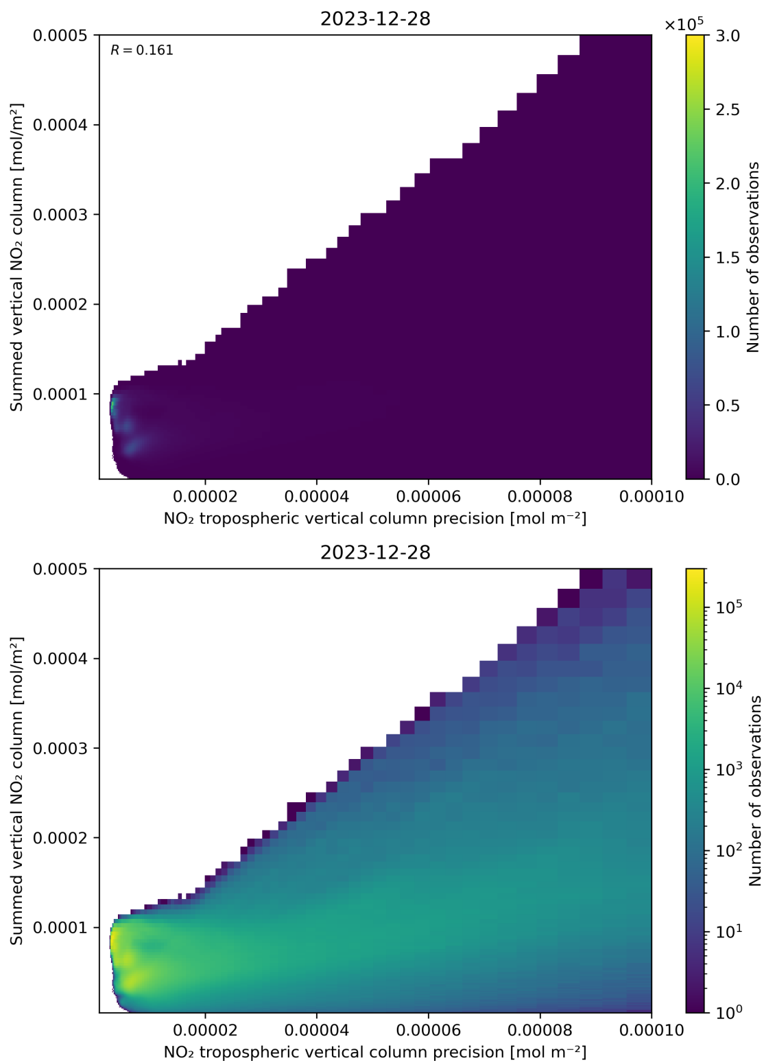
Figure 136: Scatter density plot of “NO 2 tropospheric vertical column precision” against “Summed vertical NO 2 column” for 2023-12-27 to 2023-12-29.
