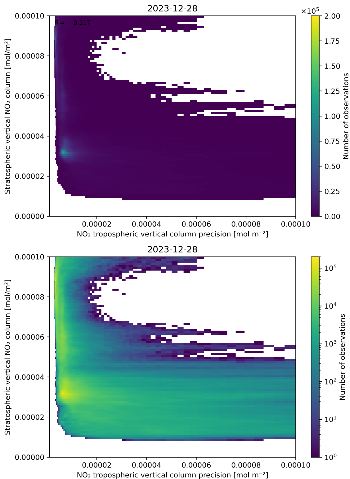
Figure 135: Scatter density plot of “NO 2 tropospheric vertical column precision” against “Stratospheric vertical NO 2 column” for 2023-12-27 to 2023-12-29.
