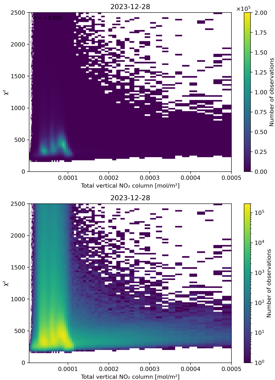
Figure 111: Scatter density plot of “Total vertical NO 2 column” against “ \chi^2 ” for 2023-12-27 to 2023-12-29.
