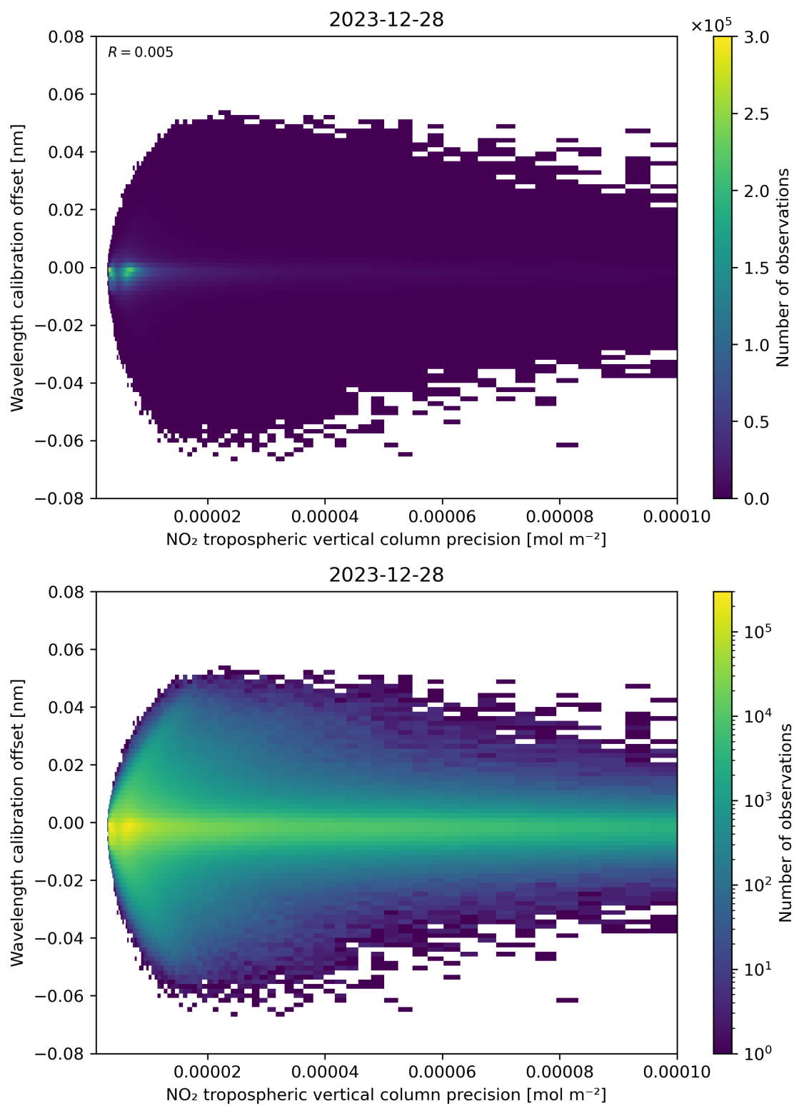
Figure 141: Scatter density plot of “NO 2 tropospheric vertical column precision” against “Wavelength calibration offset” for 2023-12-27 to 2023-12-29.
