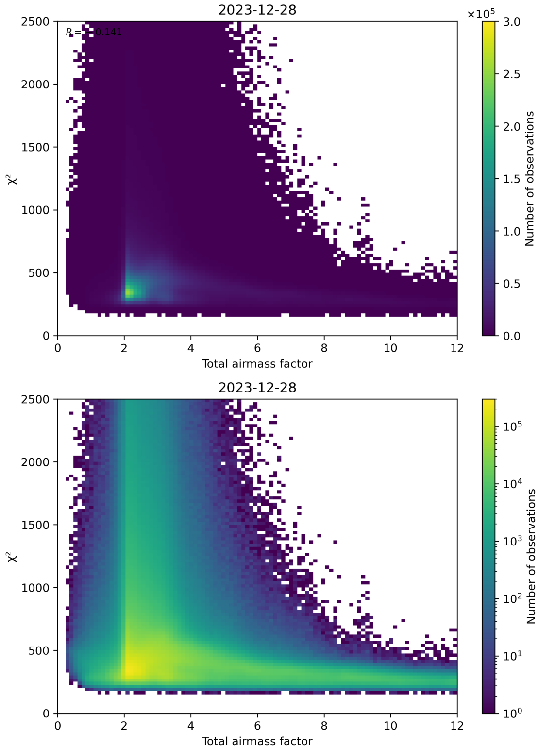
Figure 63: Scatter density plot of “Total airmass factor” against “ \chi^2 ” for 2023-12-27 to 2023-12-29.
