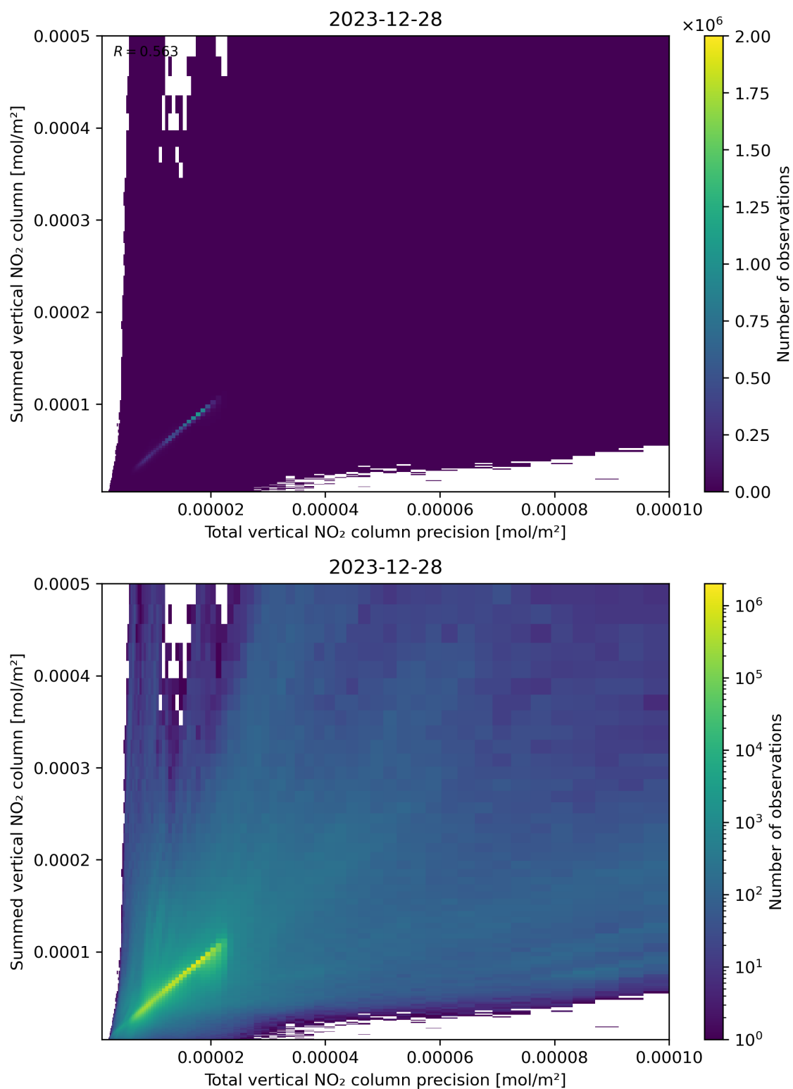
Figure 117: Scatter density plot of “Total vertical NO 2 column precision” against “Summed vertical NO 2 column” for 2023-12-27 to 2023-12-29.
