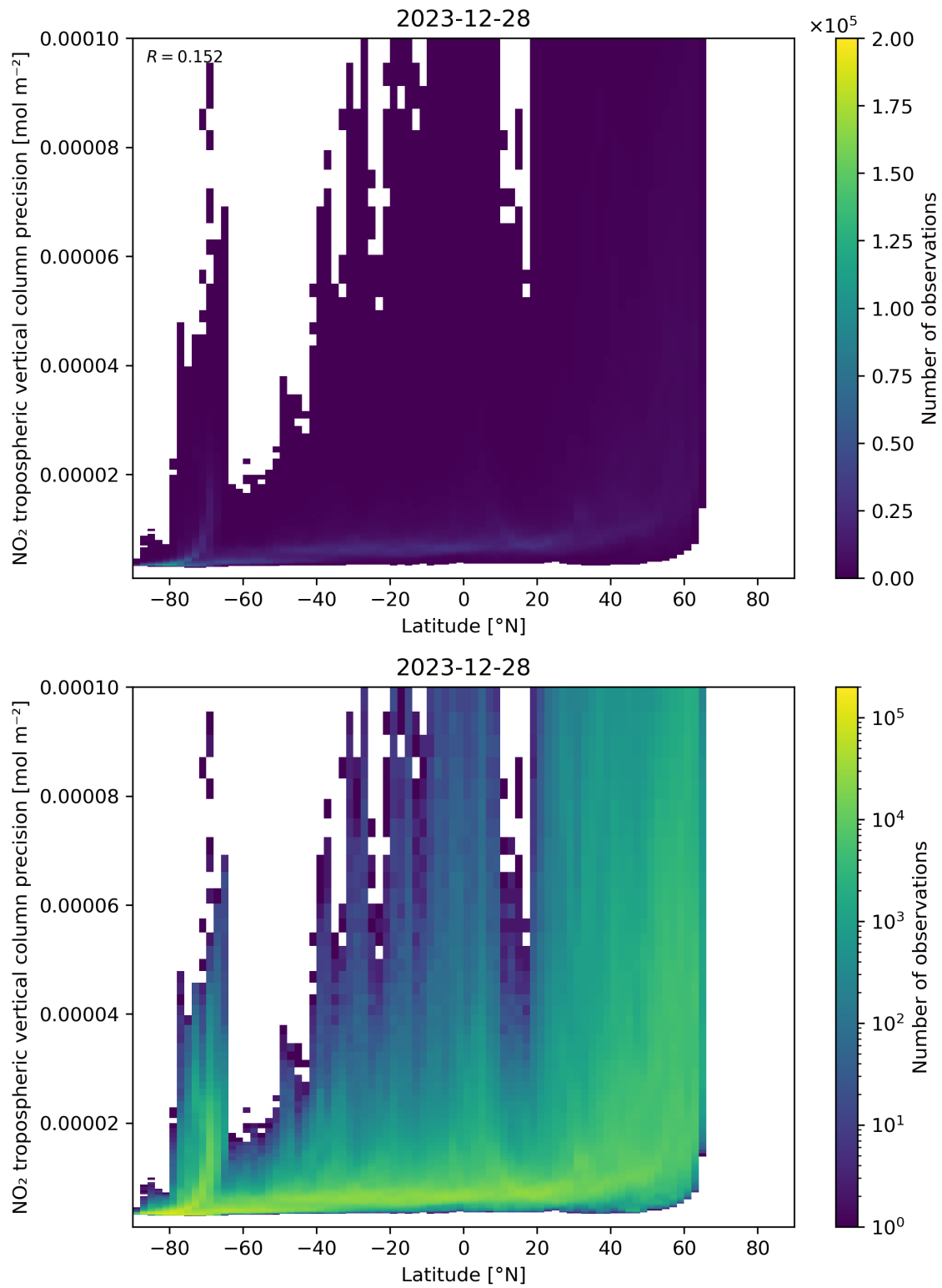
Figure 93: Scatter density plot of “Latitude” against “NO 2 tropospheric vertical column precision” for 2023-12-27 to 2023-12-29.
