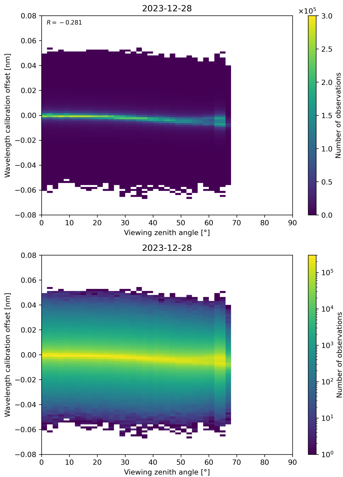
Figure 173: Scatter density plot of “Viewing zenith angle” against “Wavelength calibration offset” for 2023-12-27 to 2023-12-29.
