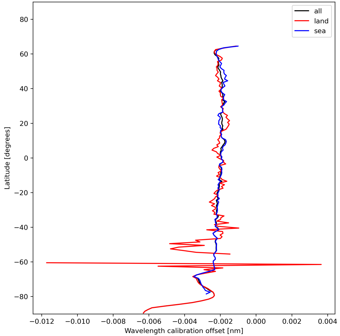
Figure 18: Zonal average of “Wavelength calibration offset” for 2023-12-27 to 2023-12-29.
