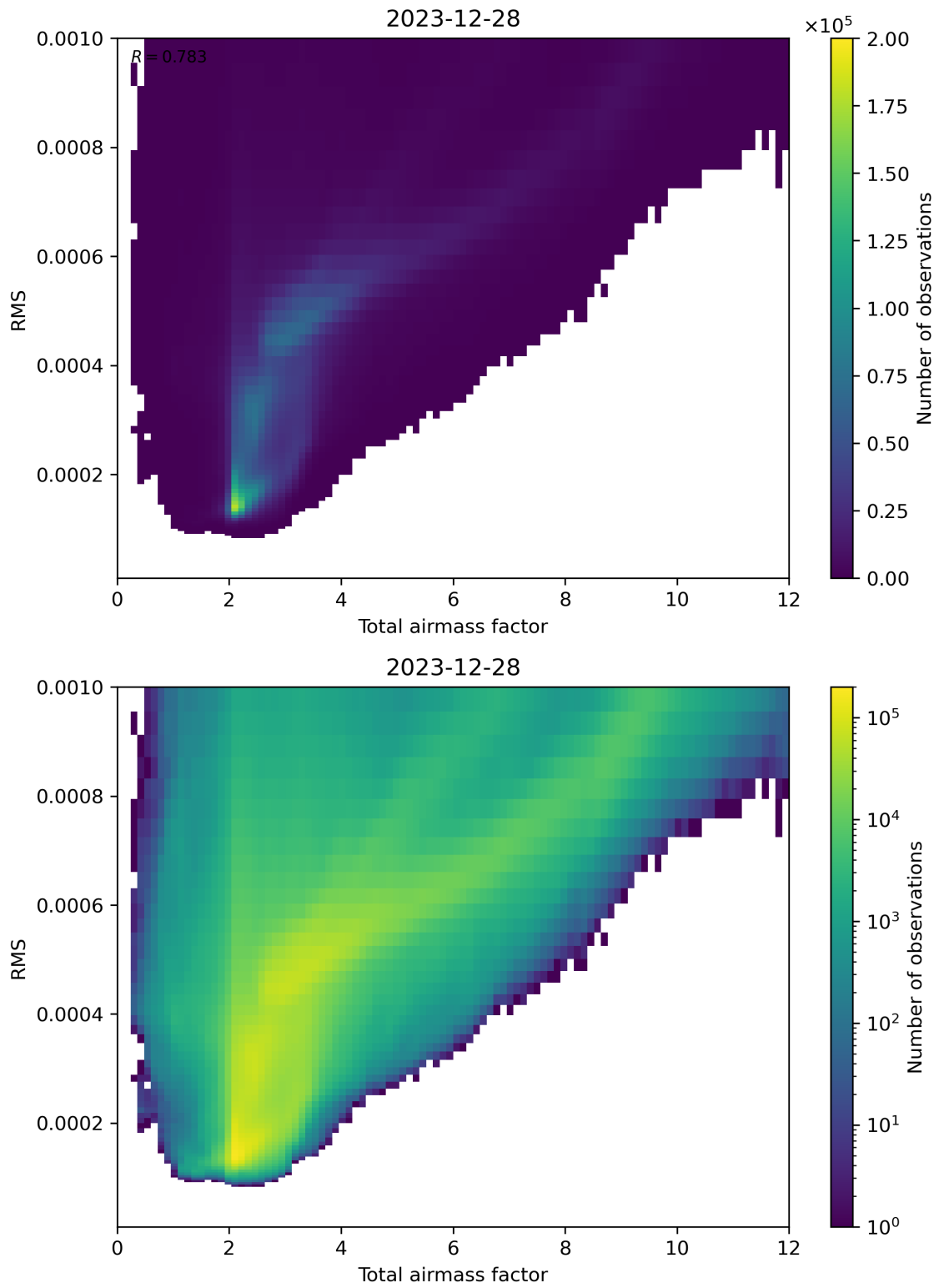
Figure 69: Scatter density plot of “Total airmass factor” against “RMS” for 2023-12-27 to 2023-12-29.
