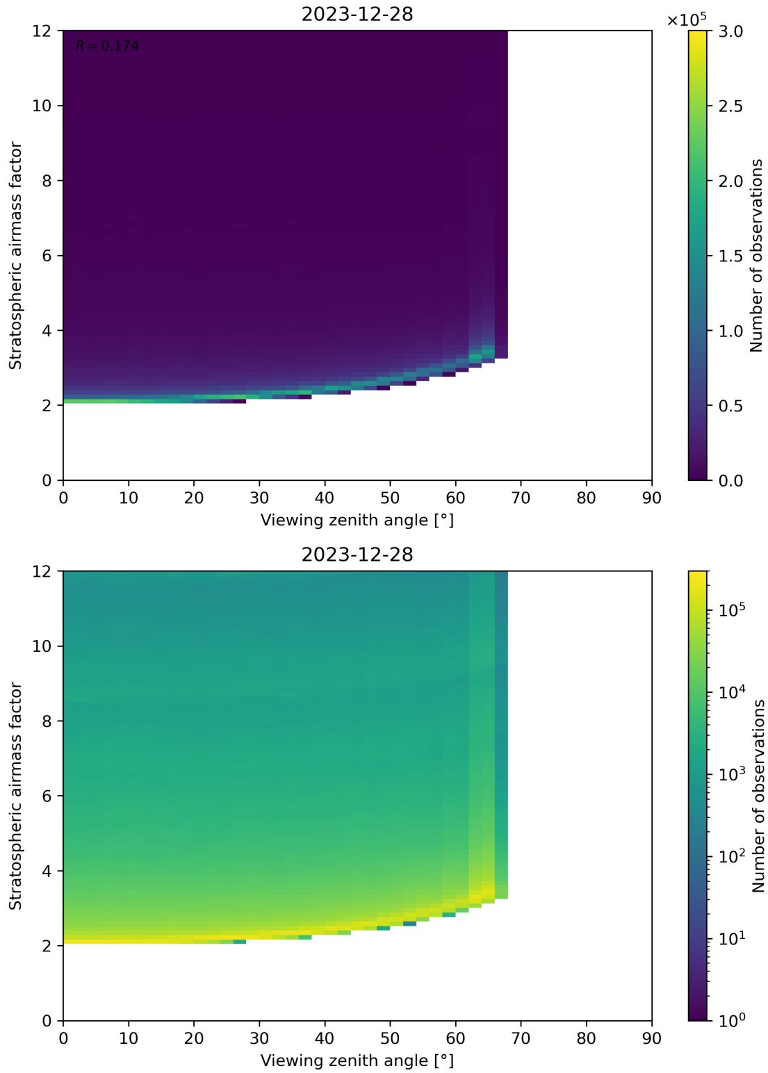
Figure 159: Scatter density plot of “Viewing zenith angle” against “Stratospheric airmass factor” for 2023-12-27 to 2023-12-29.
