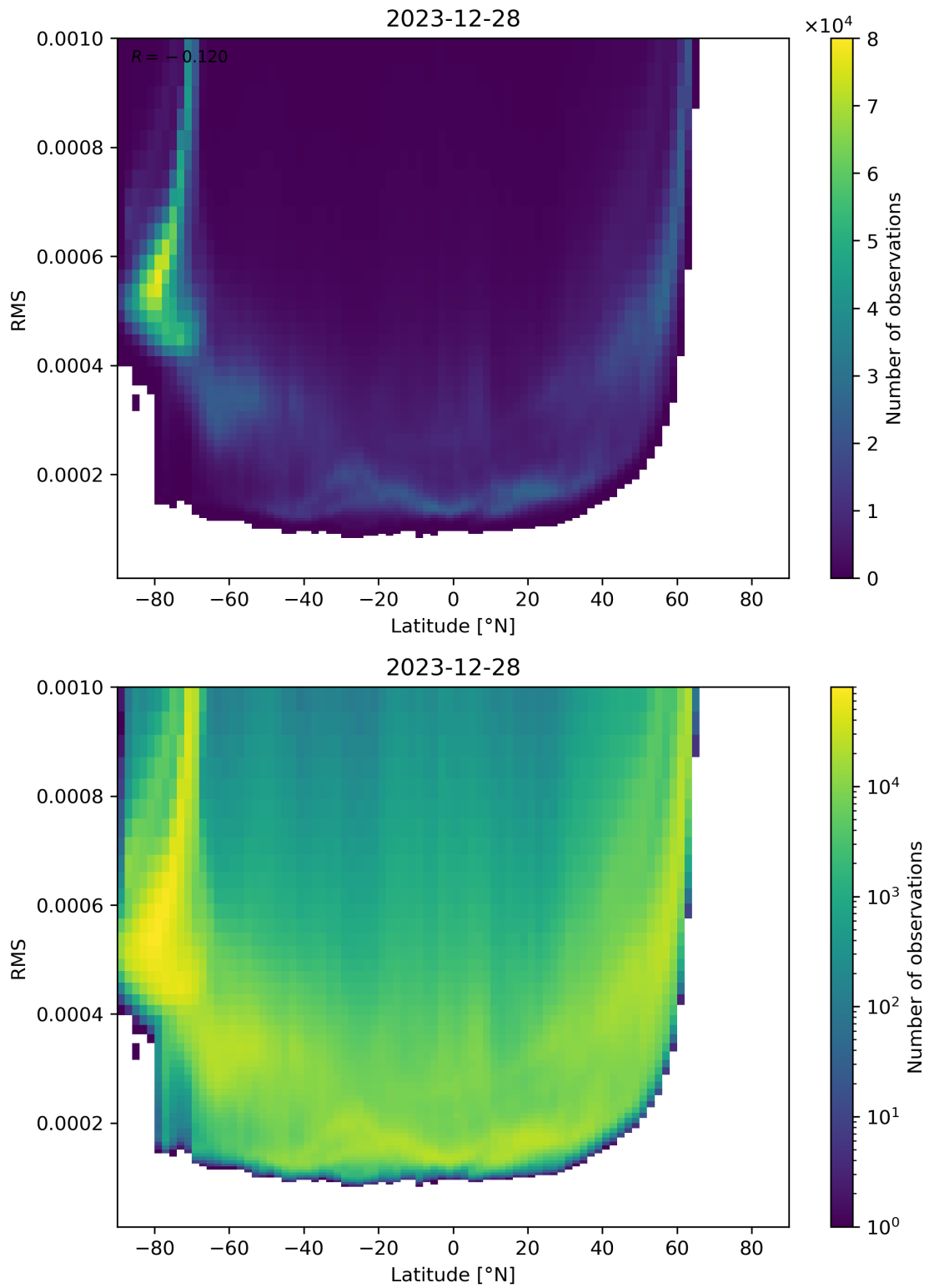
Figure 94: Scatter density plot of “Latitude” against “RMS” for 2023-12-27 to 2023-12-29.
