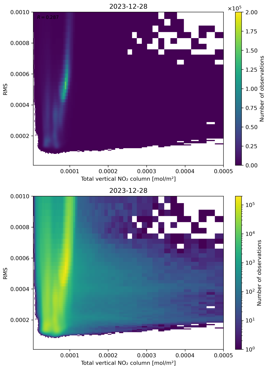
Figure 120: Scatter density plot of “Total vertical NO 2 column” against “RMS” for 2023-12-27 to 2023-12-29.
