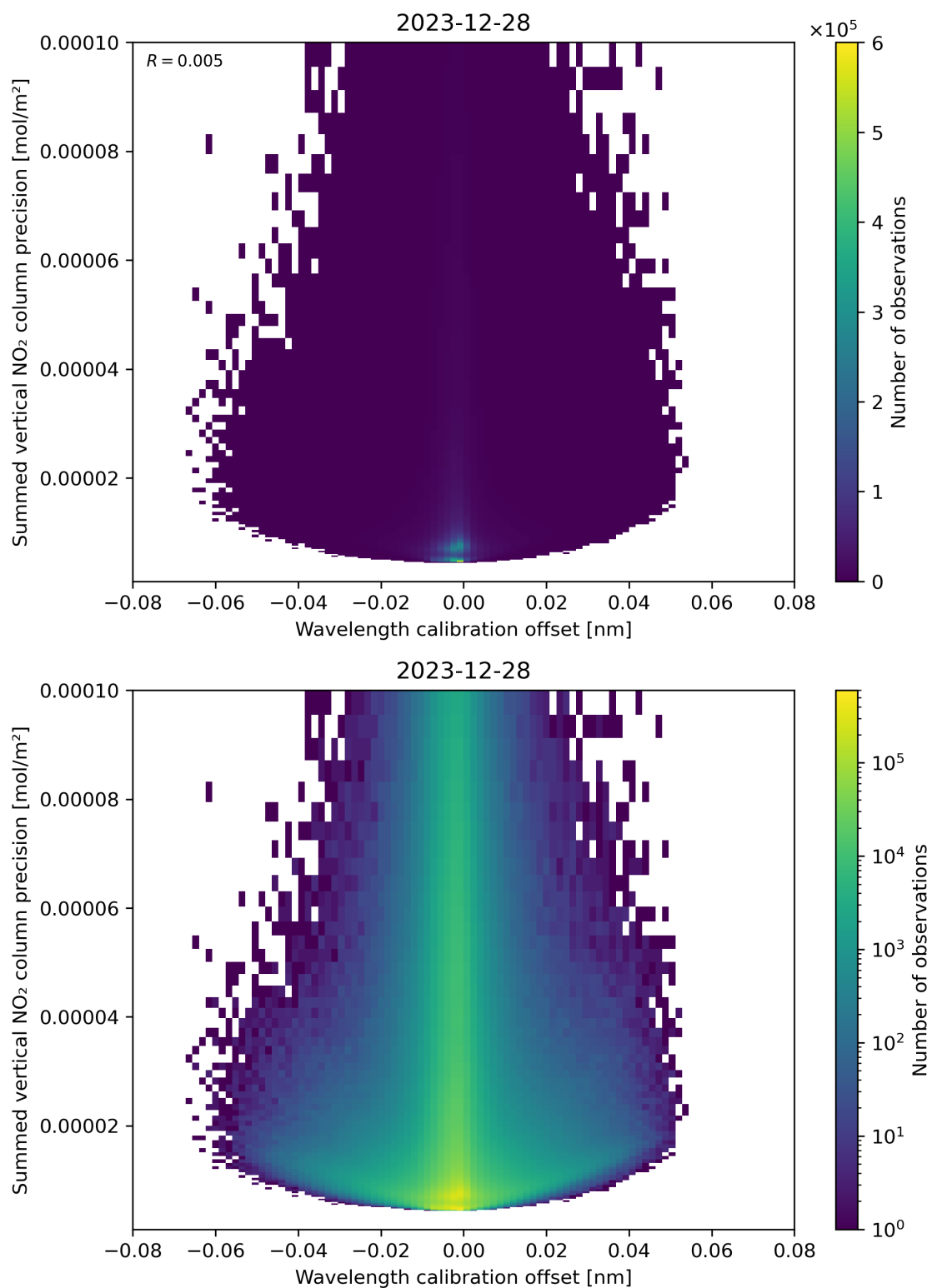
Figure 178: Scatter density plot of “Wavelength calibration offset” against “Summed vertical NO 2 column precision” for 2023-12-27 to 2023-12-29.
