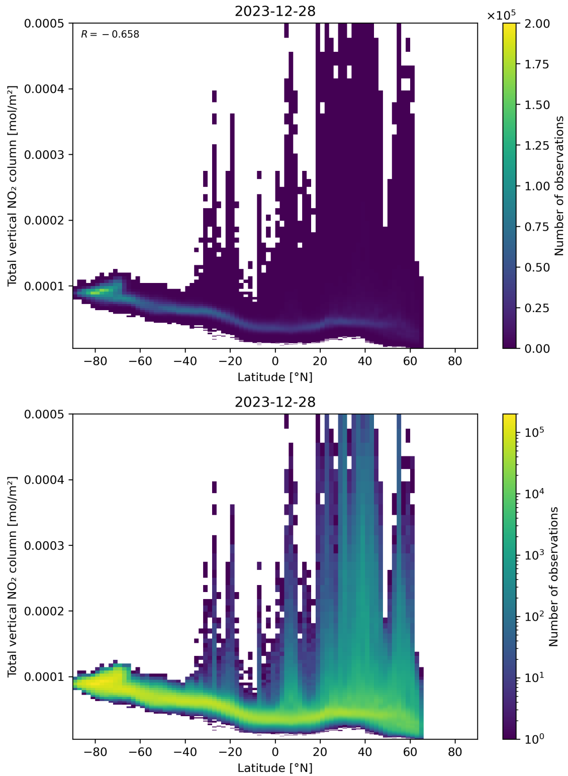
Figure 90: Scatter density plot of “Latitude” against “Total vertical NO 2 column” for 2023-12-27 to 2023-12-29.
