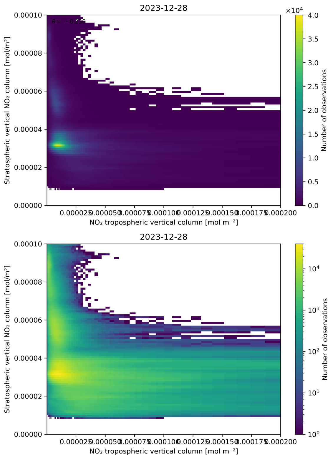
Figure 125: Scatter density plot of “NO 2 tropospheric vertical column” against “Stratospheric vertical NO 2 column” for 2023-12-27 to 2023-12-29.
