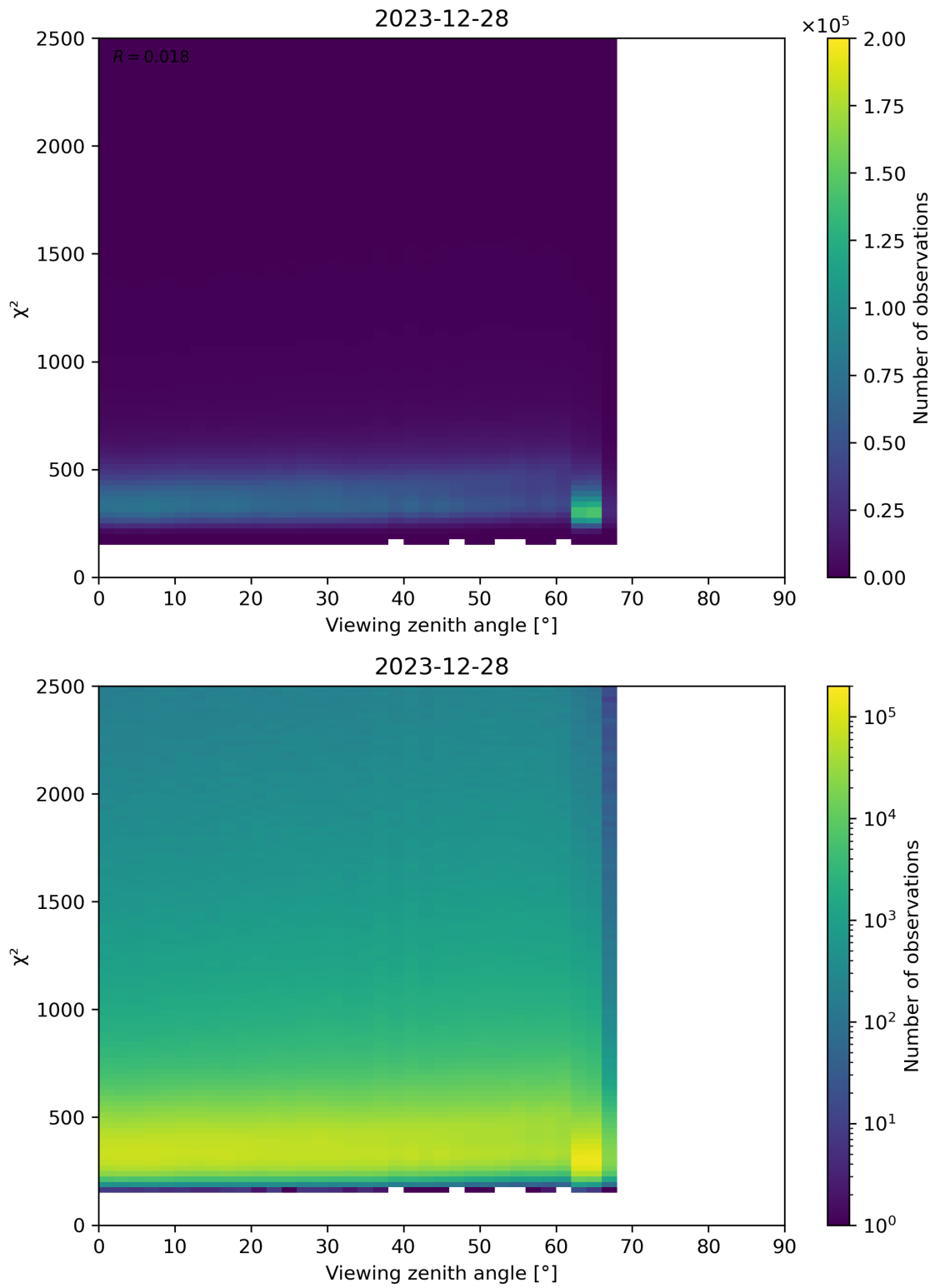
Figure 162: Scatter density plot of “Viewing zenith angle” against “ \chi^2 ” for 2023-12-27 to 2023-12-29.
