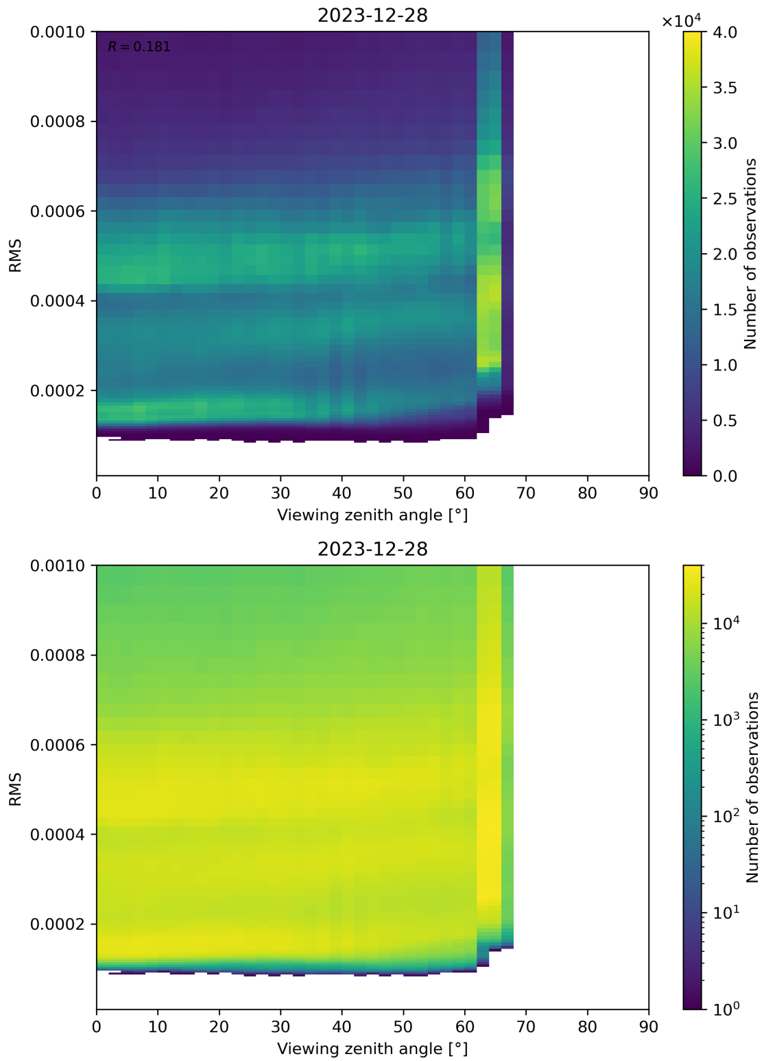
Figure 171: Scatter density plot of “Viewing zenith angle” against “RMS” for 2023-12-27 to 2023-12-29.
