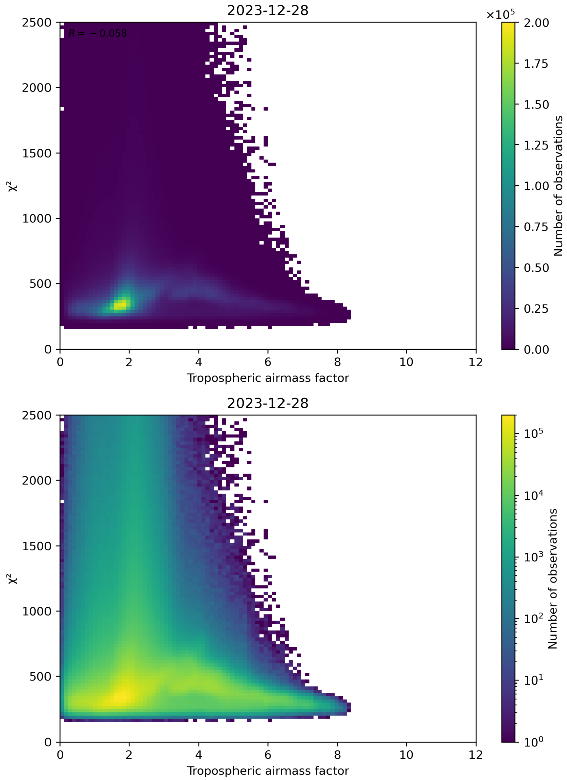
Figure 73: Scatter density plot of “Tropospheric airmass factor” against “ \chi^2 ” for 2023-12-27 to 2023-12-29.
