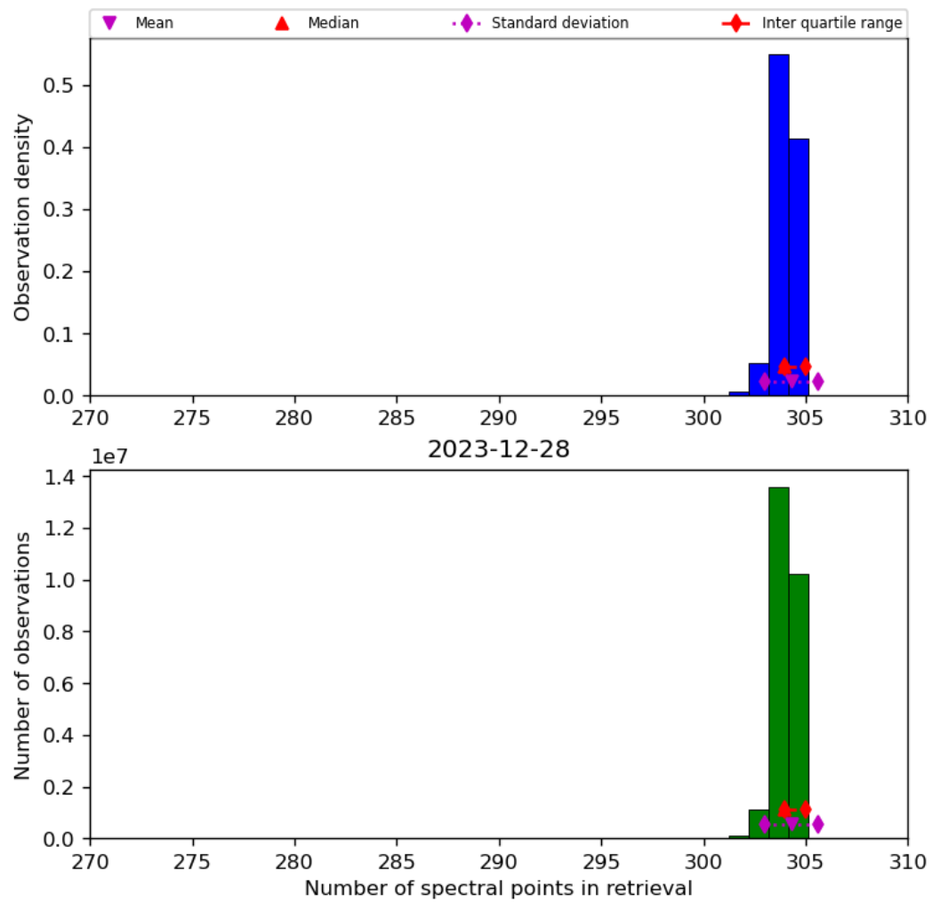
Figure 33: Histogram of “Number of spectral points in retrieval” for 2023-12-27 to 2023-12-29
