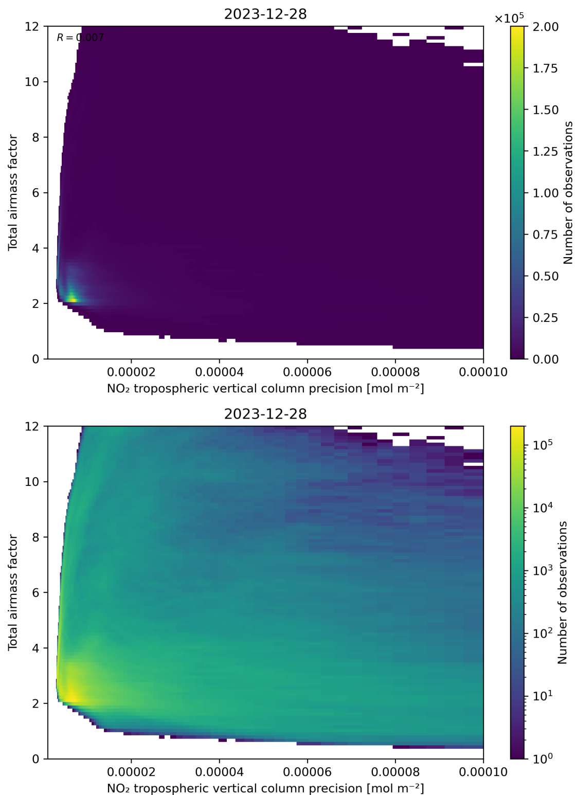
Figure 132: Scatter density plot of “NO 2 tropospheric vertical column precision” against “Total air mass factor” for 2023-12-27 to 2023-12-29.
