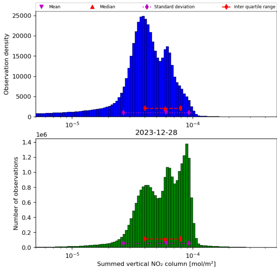
Figure 40: Histogram of “Summed vertical NO 2 column” for 2023-12-27 to 2023-12-29
