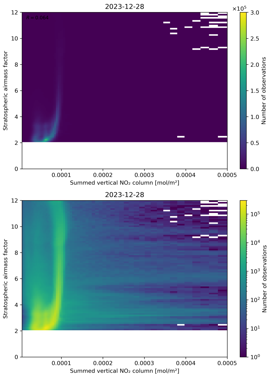
Figure 103: Scatter density plot of “Summed vertical NO 2 column” against “Stratospheric air mass factor” for 2023-12-27 to 2023-12-29.
