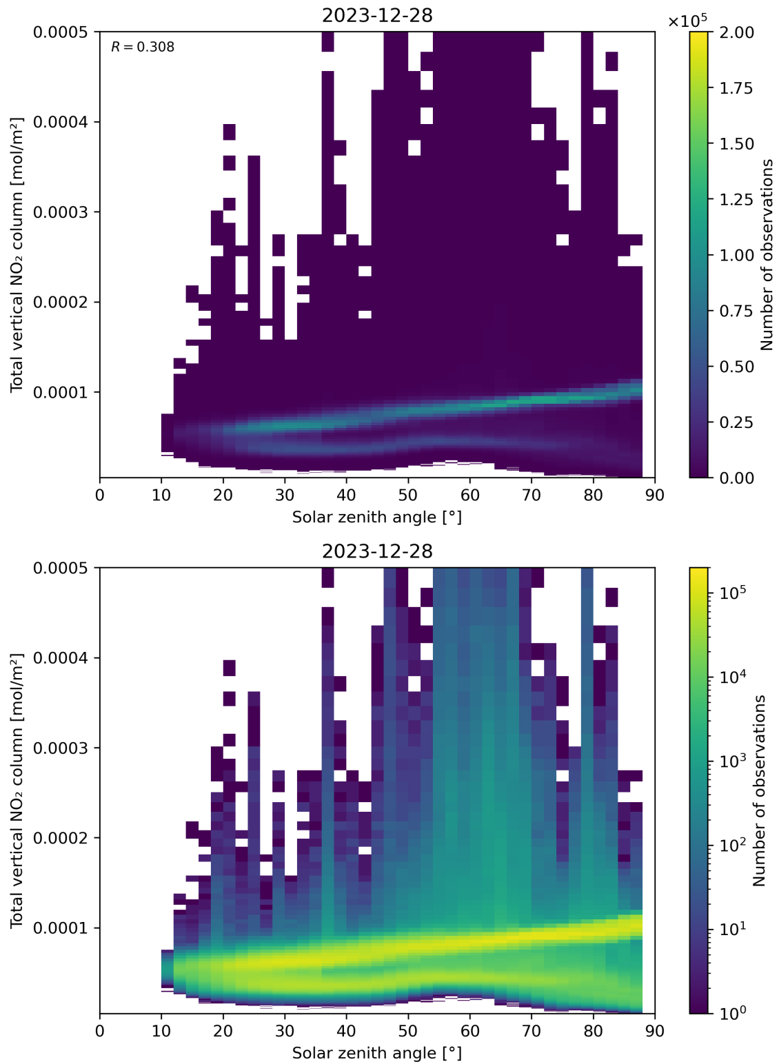
Figure 153: Scatter density plot of “Solar zenith angle” against “Total vertical NO 2 column” for 2023-12-27 to 2023-12-29.
