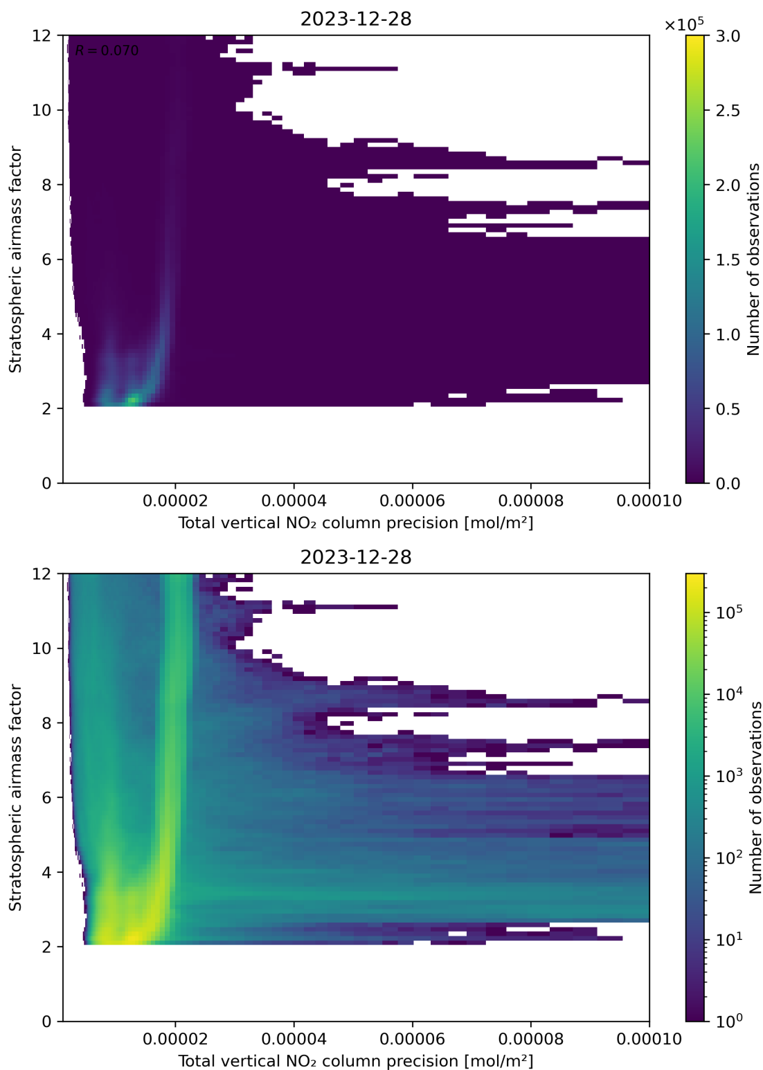
Figure 115: Scatter density plot of “Total vertical NO 2 column precision” against “Stratospheric airmass factor” for 2023-12-27 to 2023-12-29.
