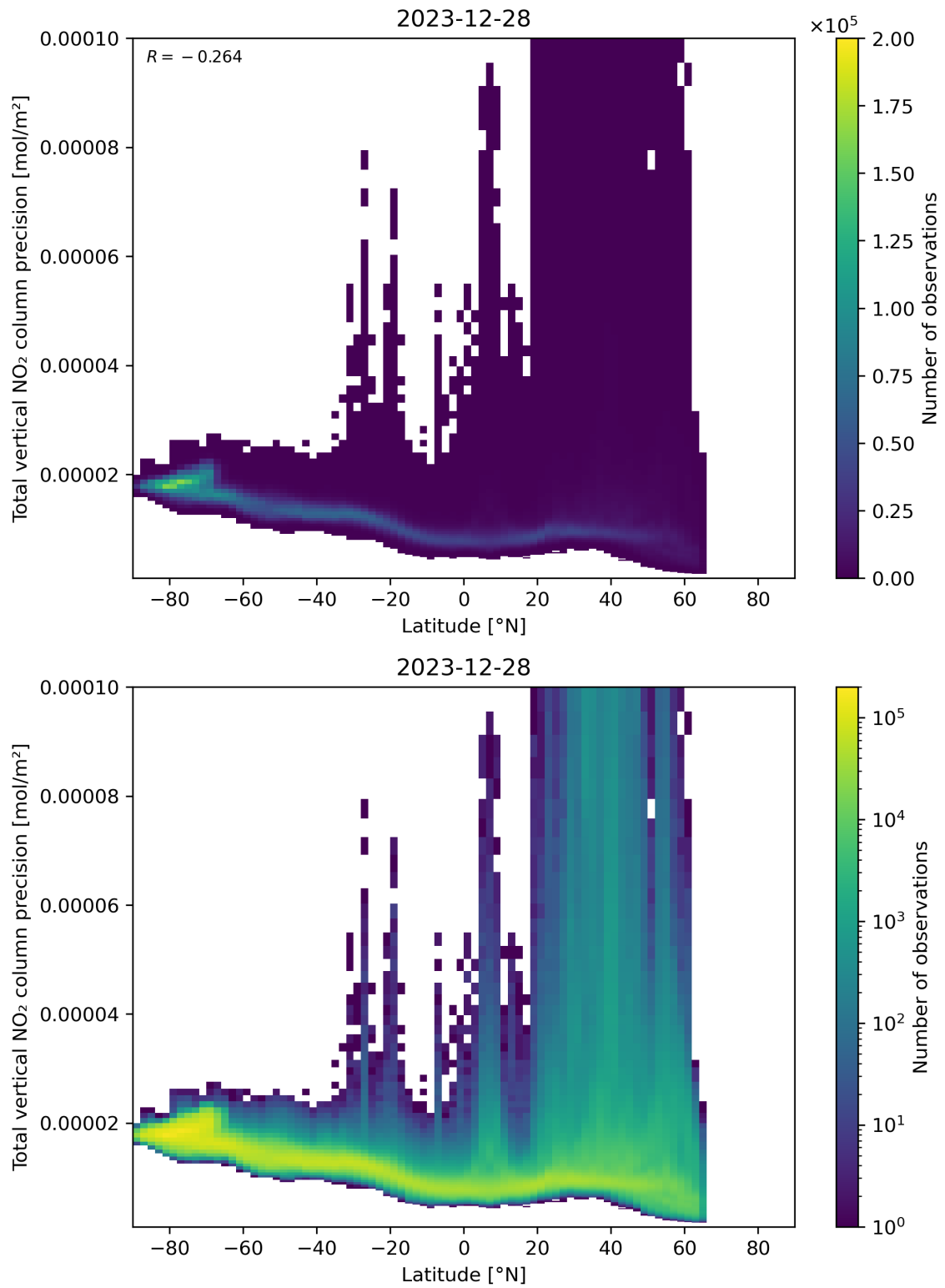
Figure 91: Scatter density plot of “Latitude” against “Total vertical NO 2 column precision” for 2023-12-27 to 2023-12-29.
