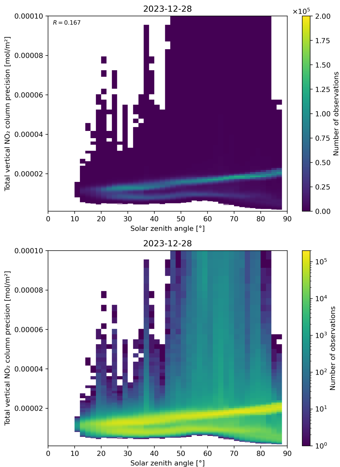
Figure 154: Scatter density plot of “Solar zenith angle” against “Total vertical NO 2 column precision” for 2023-12-27 to 2023-12-29.
