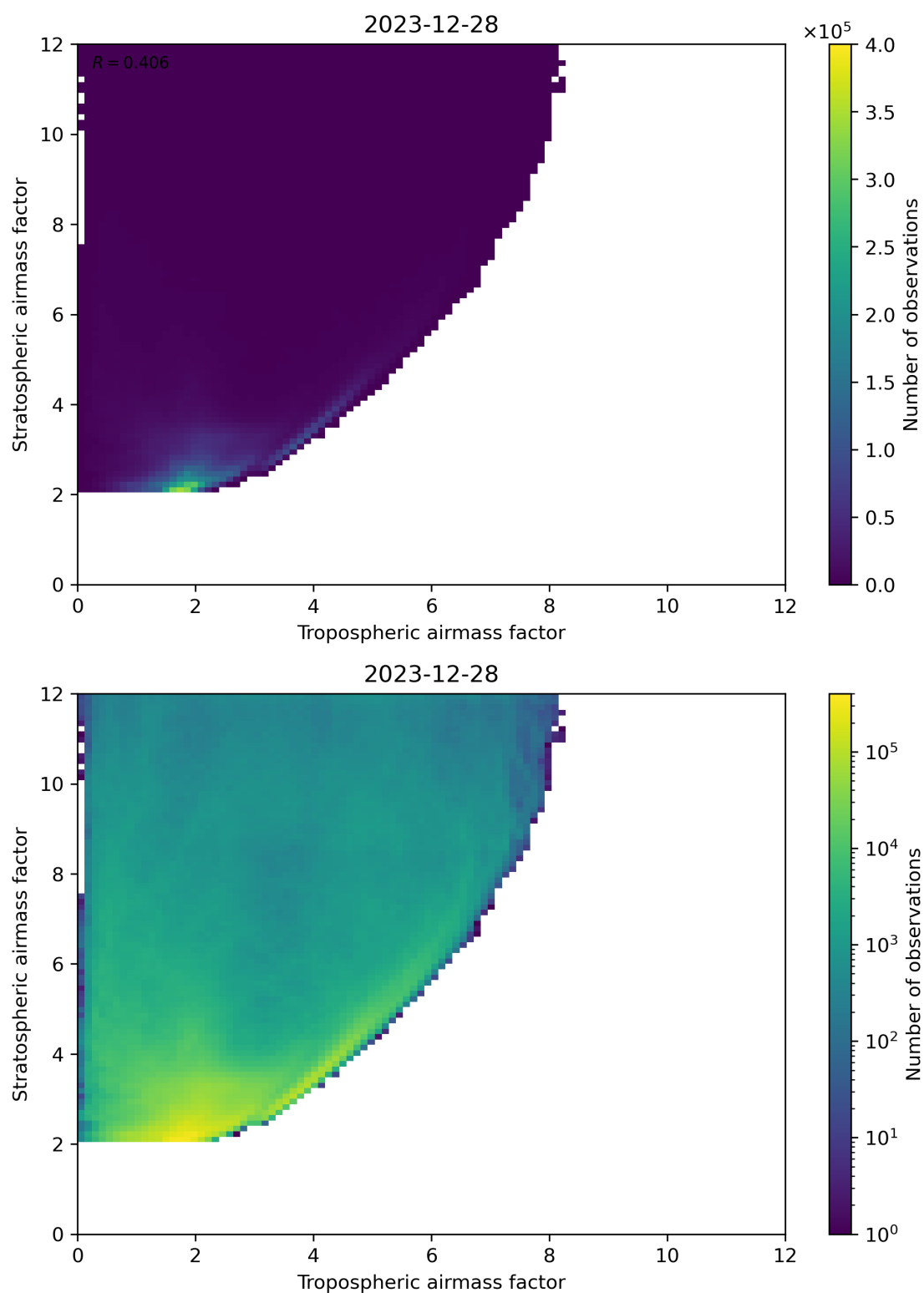
Figure 71: Scatter density plot of “Tropospheric airmass factor” against “Stratospheric airmass factor” for 2023-12-27 to 2023-12-29.
