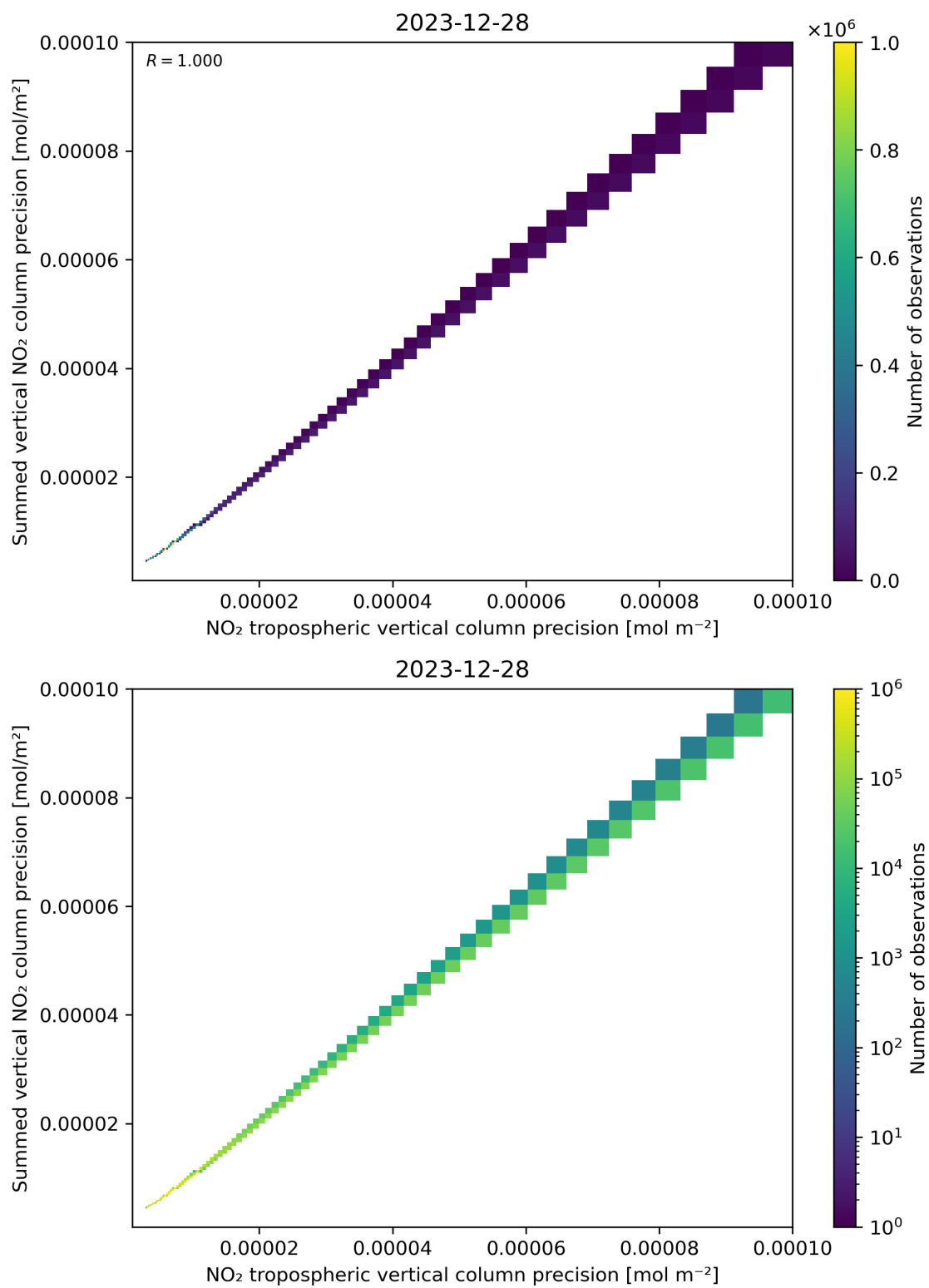
Figure 137: Scatter density plot of “NO 2 tropospheric vertical column precision” against “Summed vertical NO 2 column precision” for 2023-12-27 to 2023-12-29.
