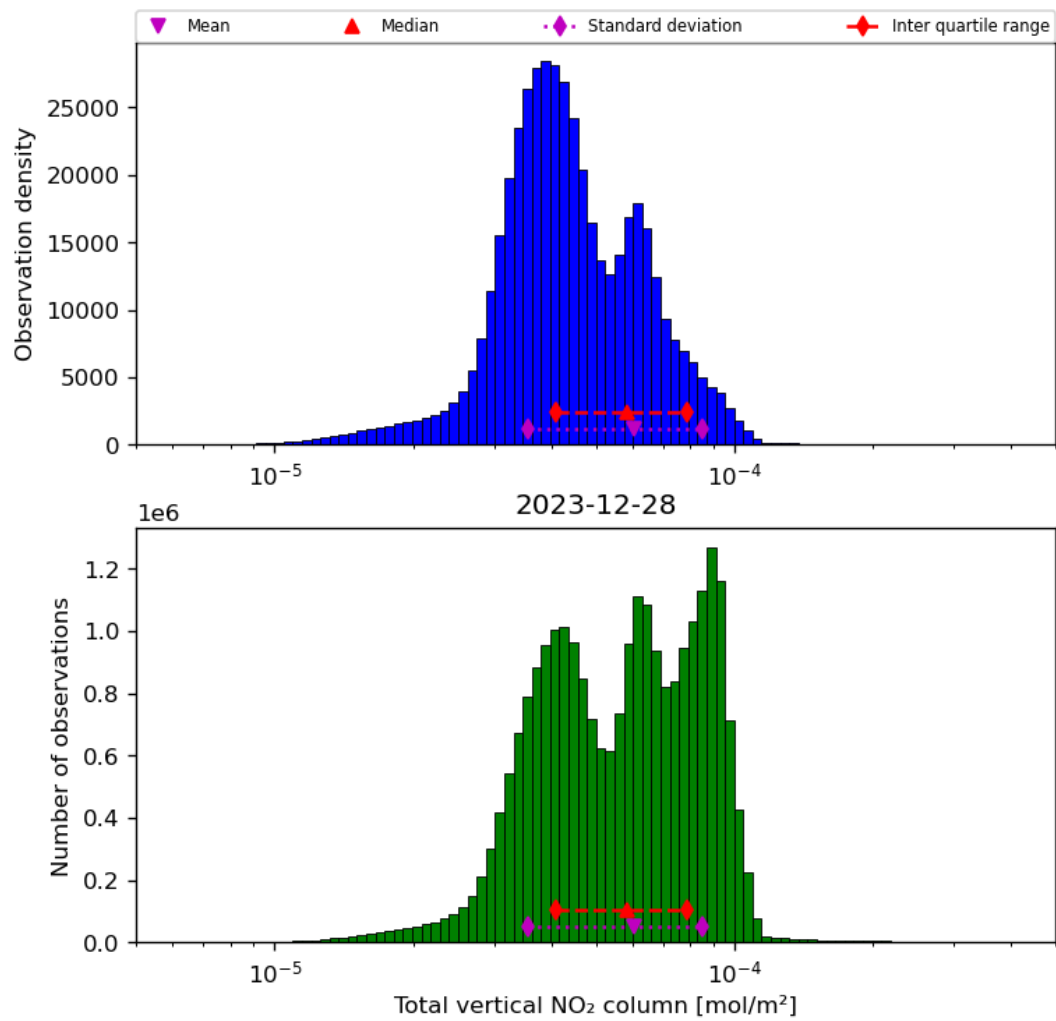
Figure 38: Histogram of “Total vertical NO 2 column” for 2023-12-27 to 2023-12-29
