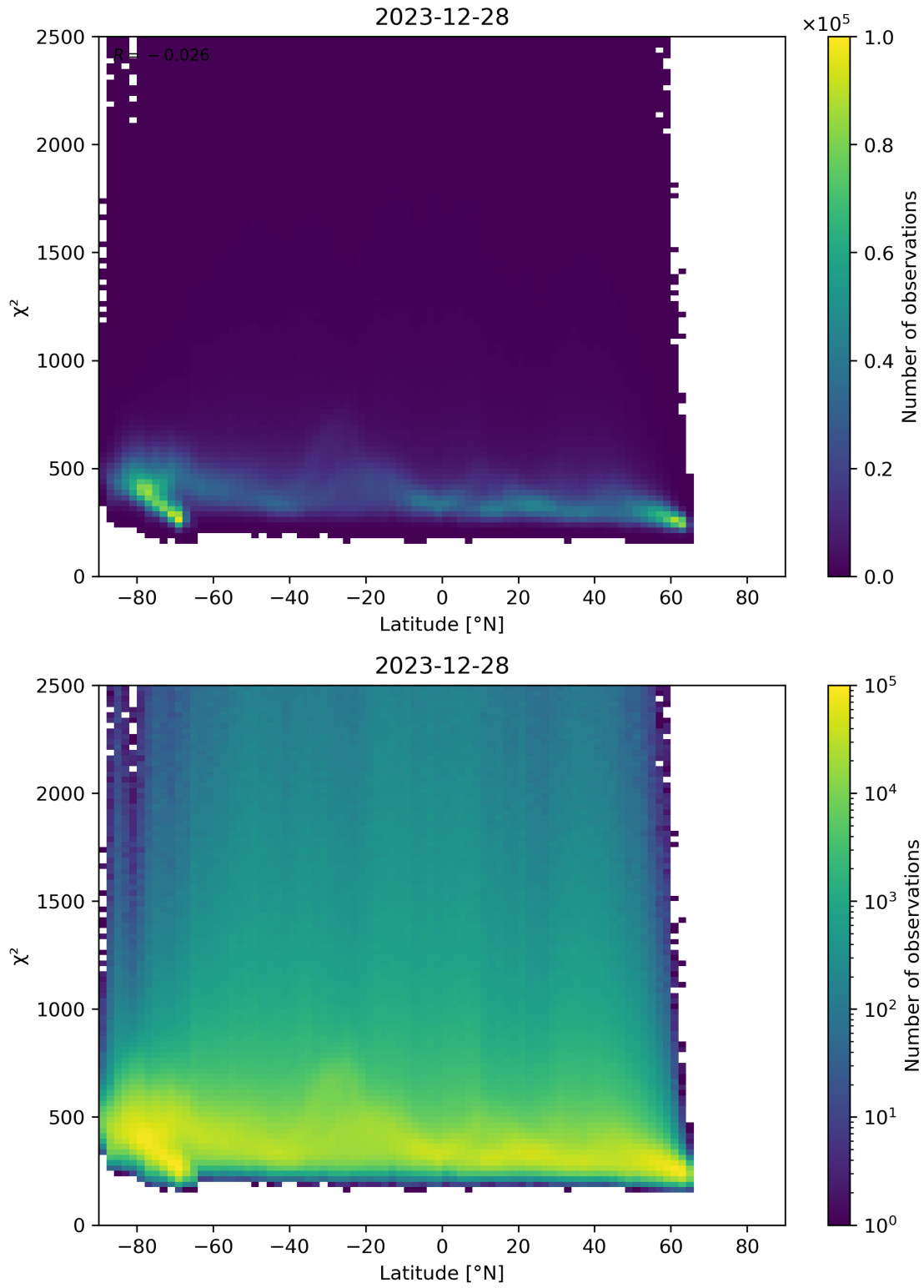
Figure 86: Scatter density plot of “Latitude” against “ \chi^2 ” for 2023-12-27 to 2023-12-29.
