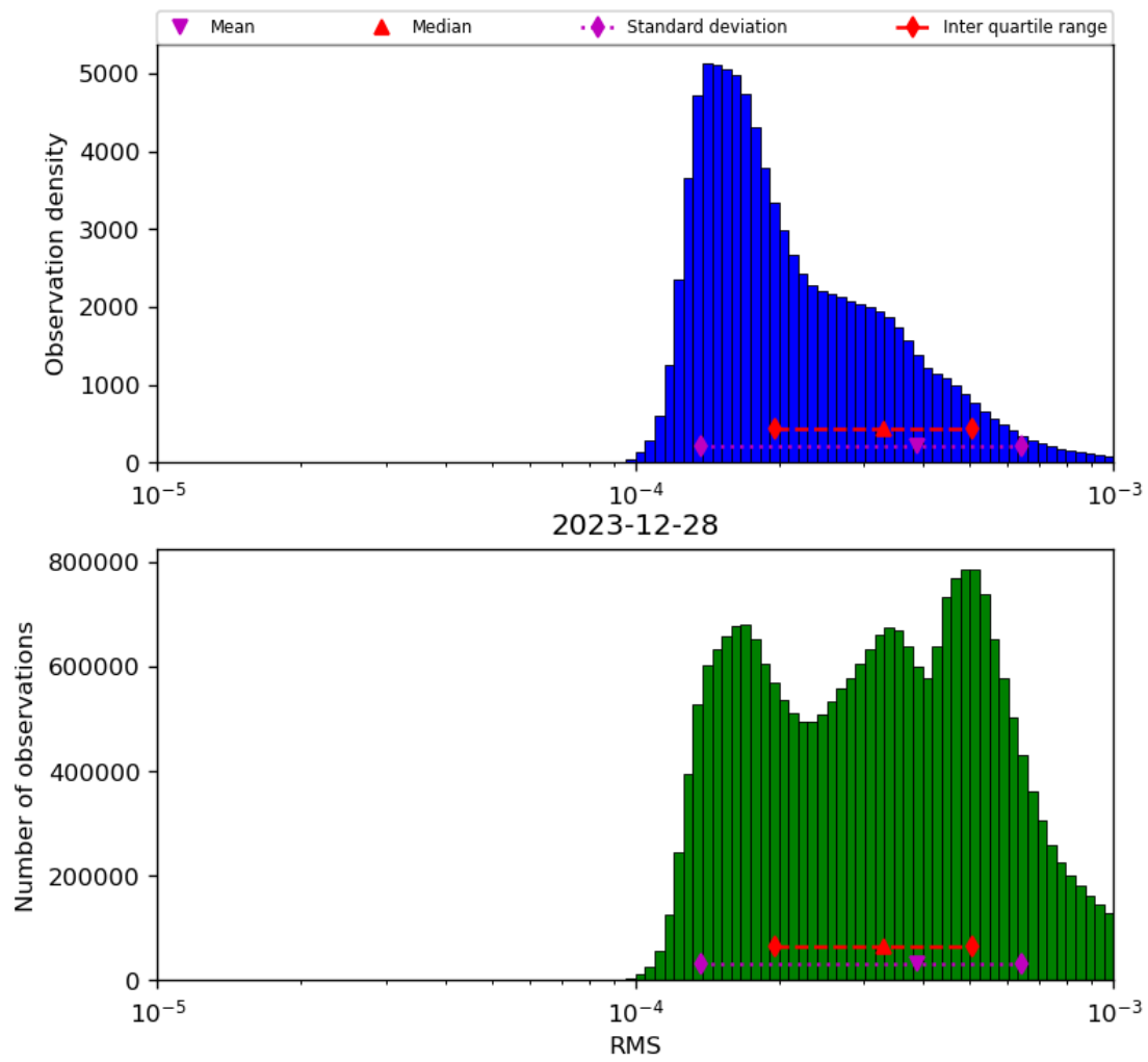
Figure 43: Histogram of “RMS” for 2023-12-27 to 2023-12-29
