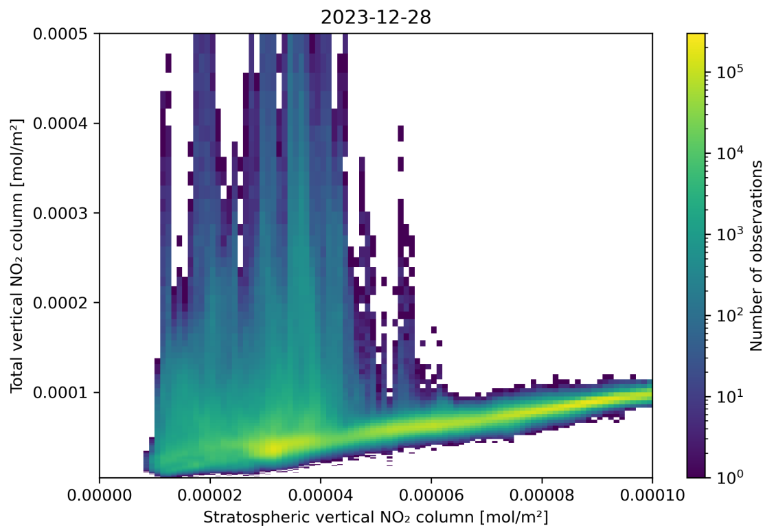
Figure 100: Scatter density plot of “Stratospheric vertical NO 2 column” against “Total vertical NO 2 column” for 2023-12-27 to 2023-12-29.
