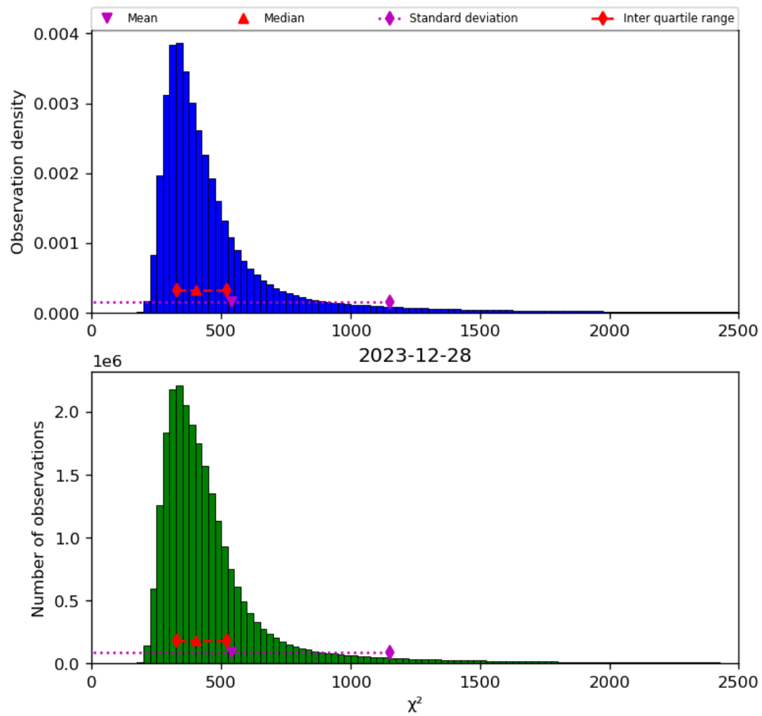
Figure 42: Histogram of “ \chi^2 ” for 2023-12-27 to 2023-12-29
