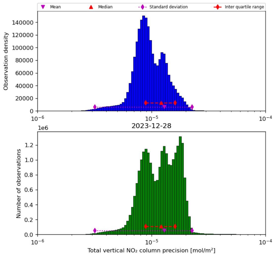
Figure 39: Histogram of “Total vertical NO 2 column precision” for 2023-12-27 to 2023-12-29
