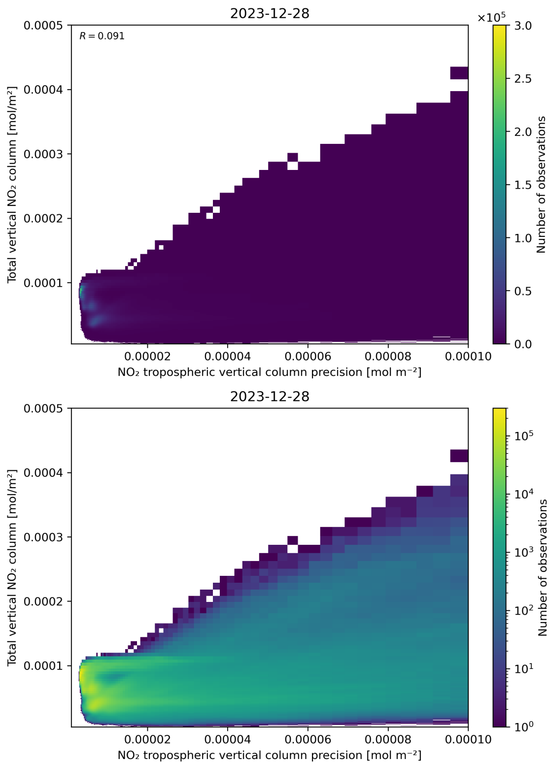
Figure 138: Scatter density plot of “NO 2 tropospheric vertical column precision” against “Total vertical NO 2 column” for 2023-12-27 to 2023-12-29.
