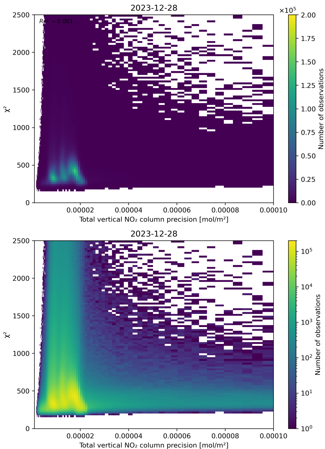
Figure 116: Scatter density plot of “Total vertical NO 2 column precision” against “ \chi^2 ” for 2023-12-27 to 2023-12-29.
