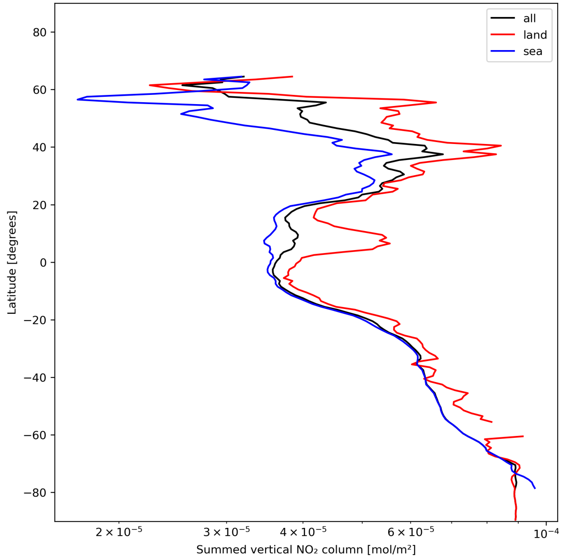
Figure 23: Zonal average of “Summed vertical NO 2 column” for 2023-12-27 to 2023-12-29.
