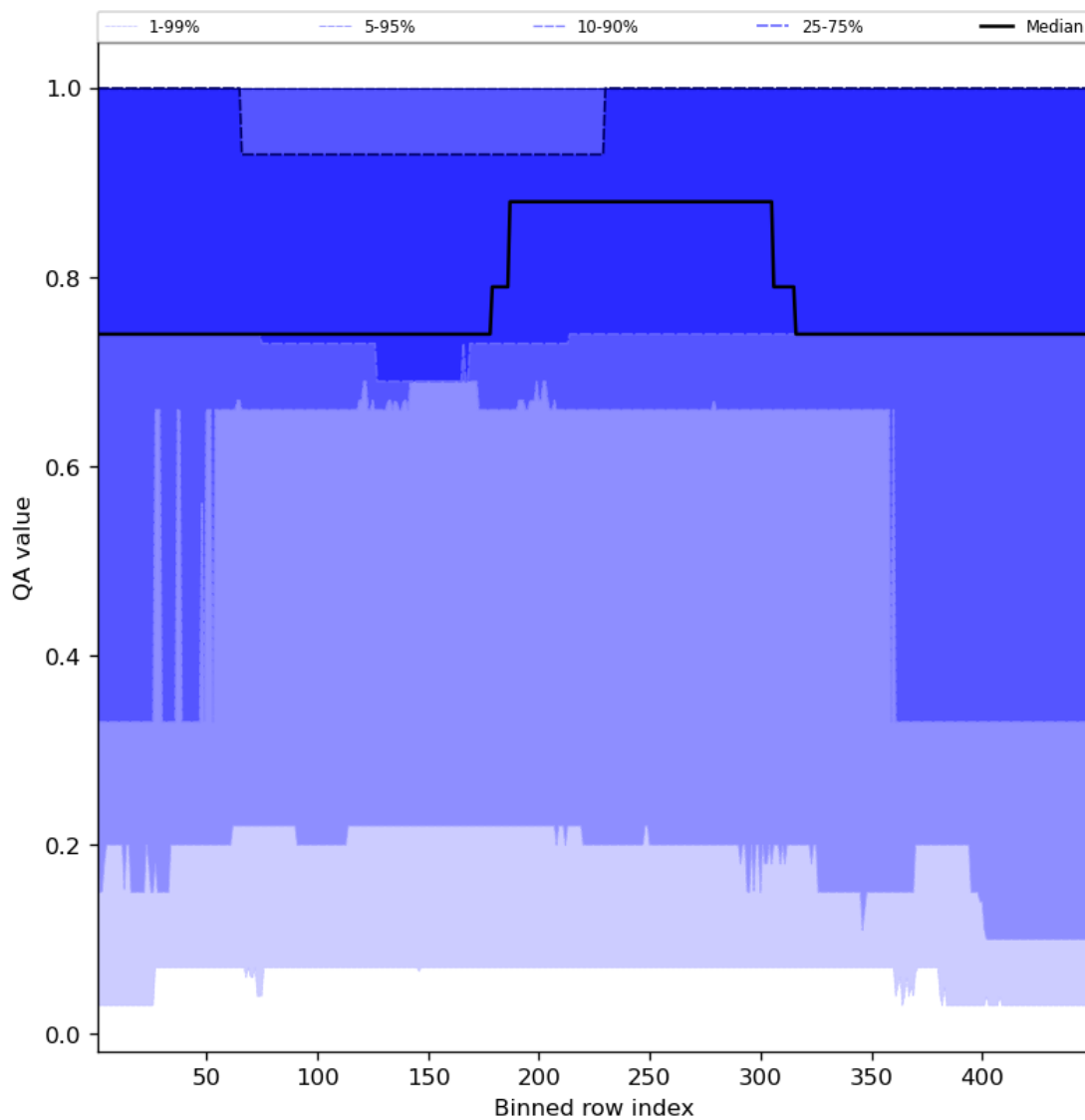
Figure 45: Along track statistics of “QA value” for 2023-12-27 to 2023-12-29
