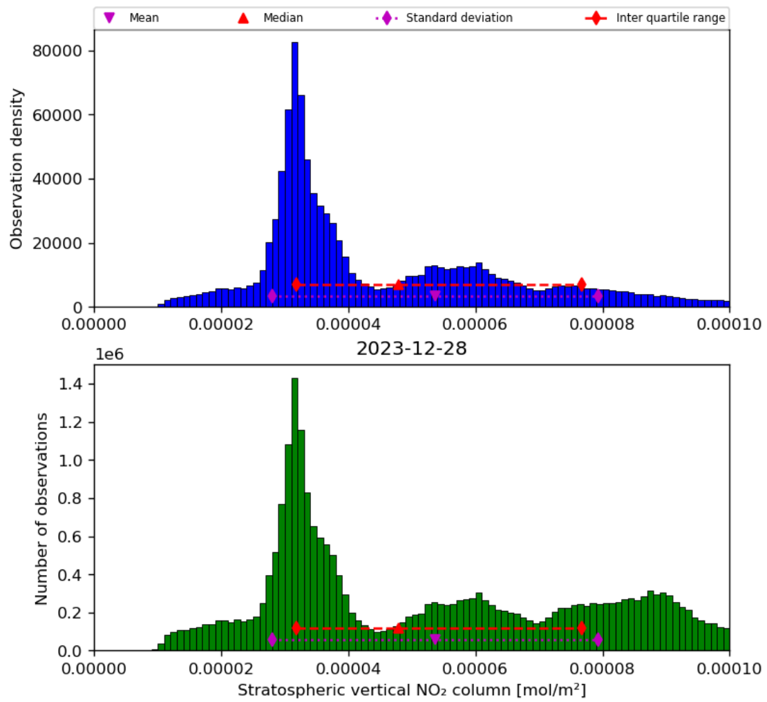
Figure 36: Histogram of “Stratospheric vertical NO 2 column” for 2023-12-27 to 2023-12-29
