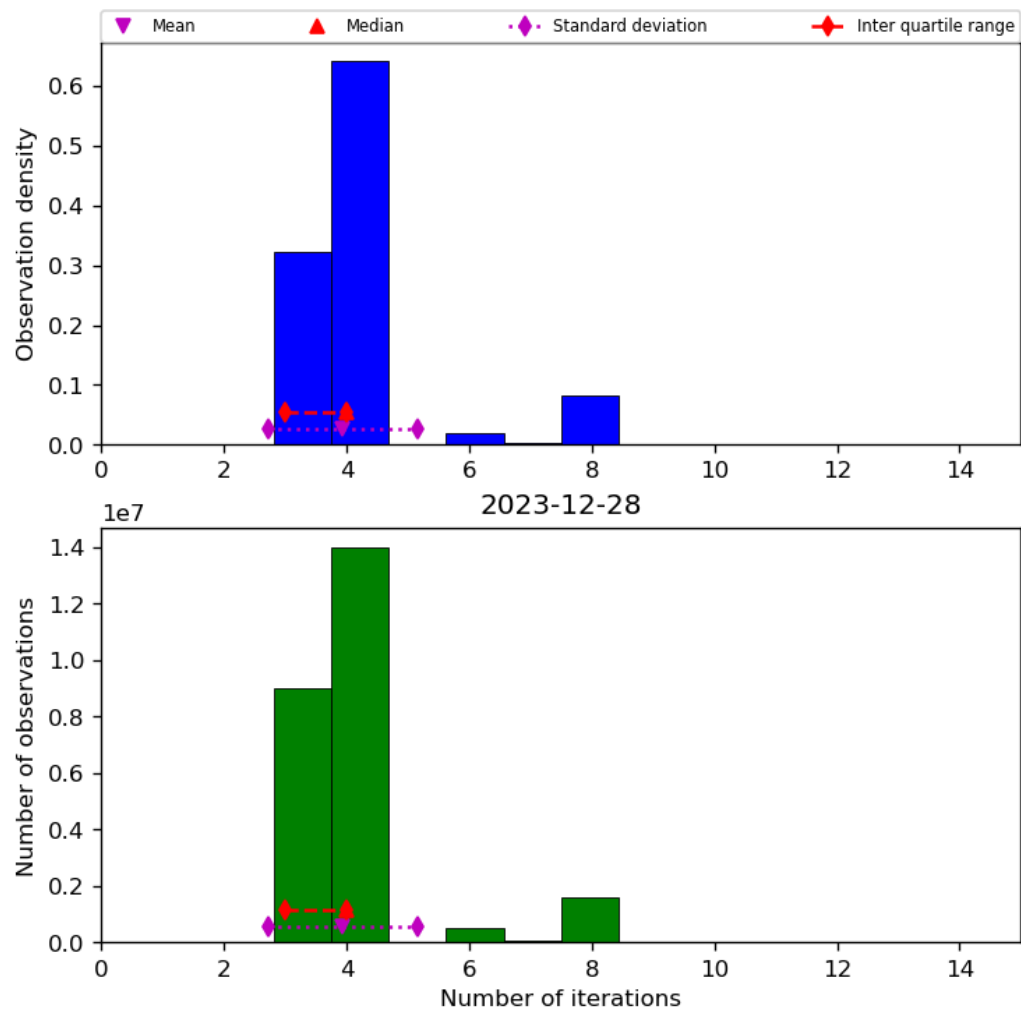
Figure 34: Histogram of “Number of iterations” for 2023-12-27 to 2023-12-29
