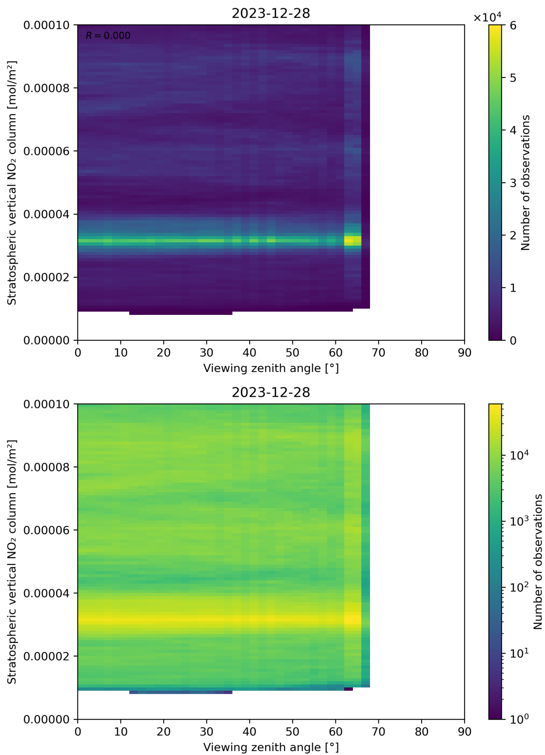
Figure 164: Scatter density plot of “Viewing zenith angle” against “Stratospheric vertical NO 2 column” for 2023-12-27 to 2023-12-29.
