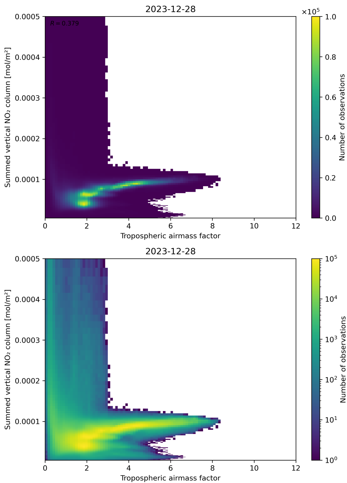
Figure 75: Scatter density plot of “Tropospheric airmass factor” against “Summed vertical NO 2 column” for 2023-12-27 to 2023-12-29.
