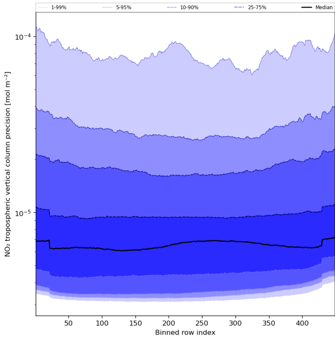
Figure 47: Along track statistics of “NO 2 tropospheric vertical column precision” for 2023-12-27 to 2023-12-29
