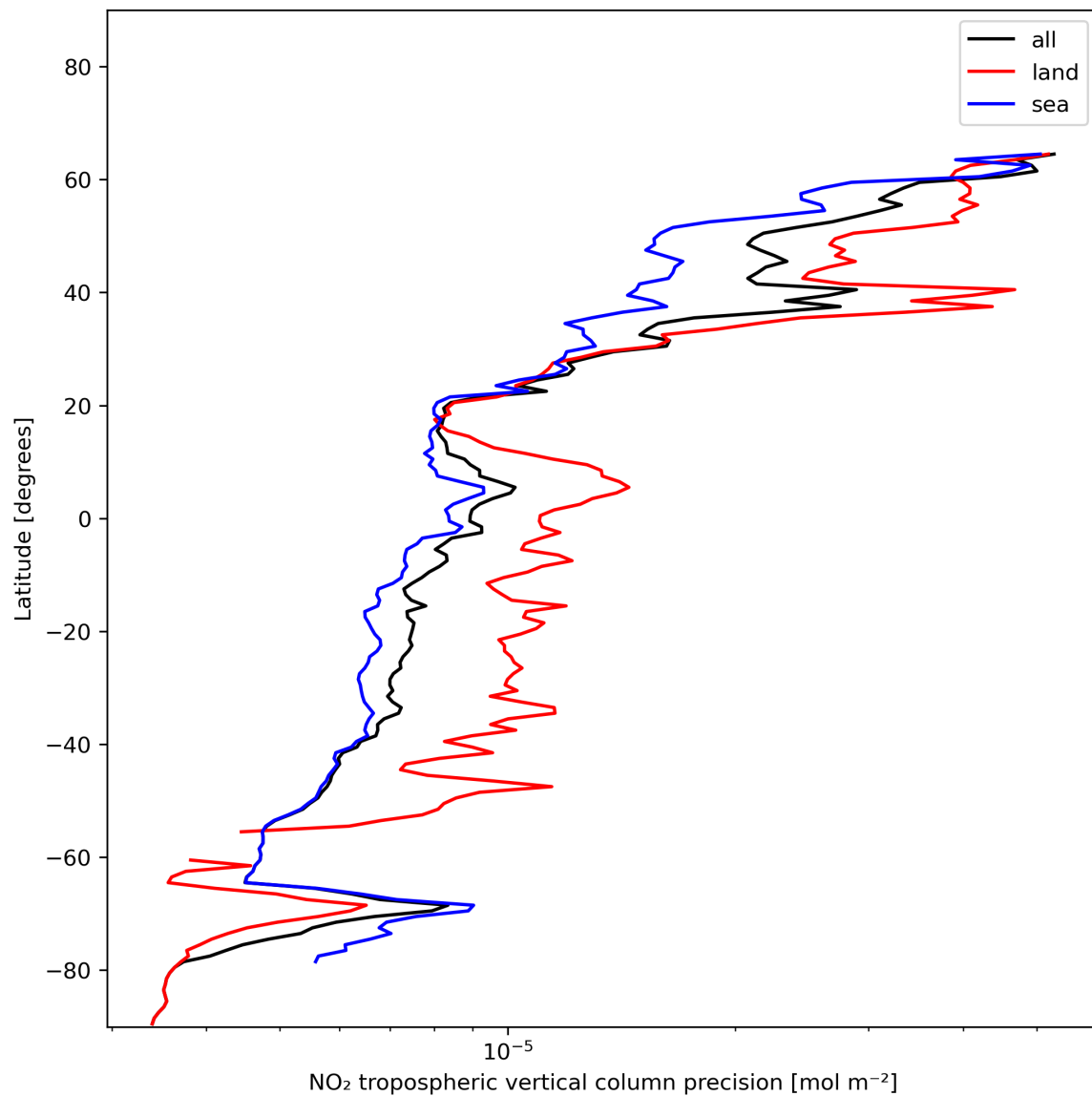
Figure 13: Zonal average of “NO 2 tropospheric vertical column precision” for 2023-12-27 to 2023-12-29.
