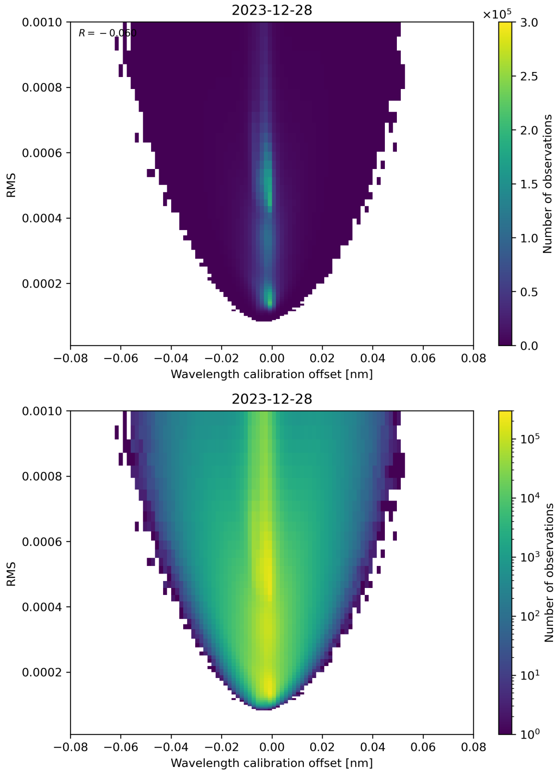
Figure 181: Scatter density plot of “Wavelength calibration offset” against “RMS” for 2023-12-27 to 2023-12-29.
