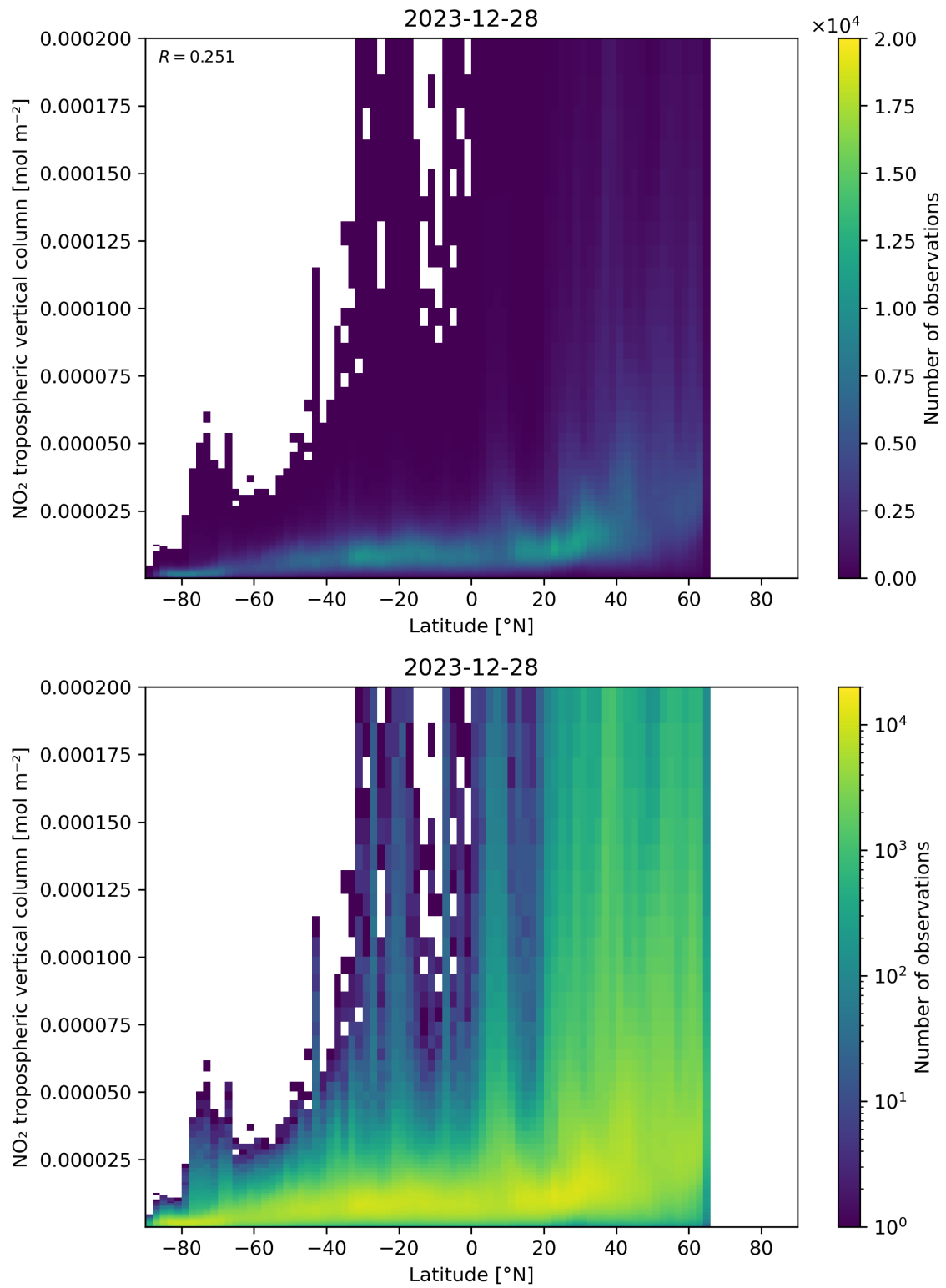
Figure 92: Scatter density plot of “Latitude” against “NO 2 tropospheric vertical column” for 2023-12-27 to 2023-12-29.
