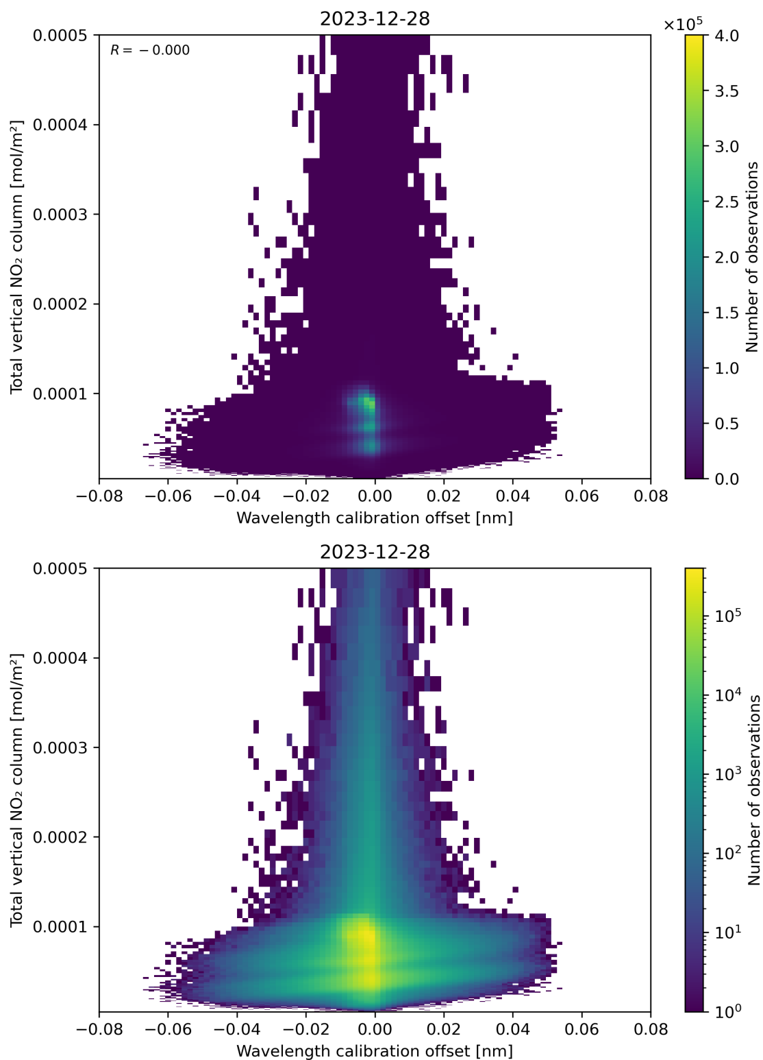
Figure 179: Scatter density plot of “Wavelength calibration offset” against “Total vertical NO 2 column” for 2023-12-27 to 2023-12-29.
