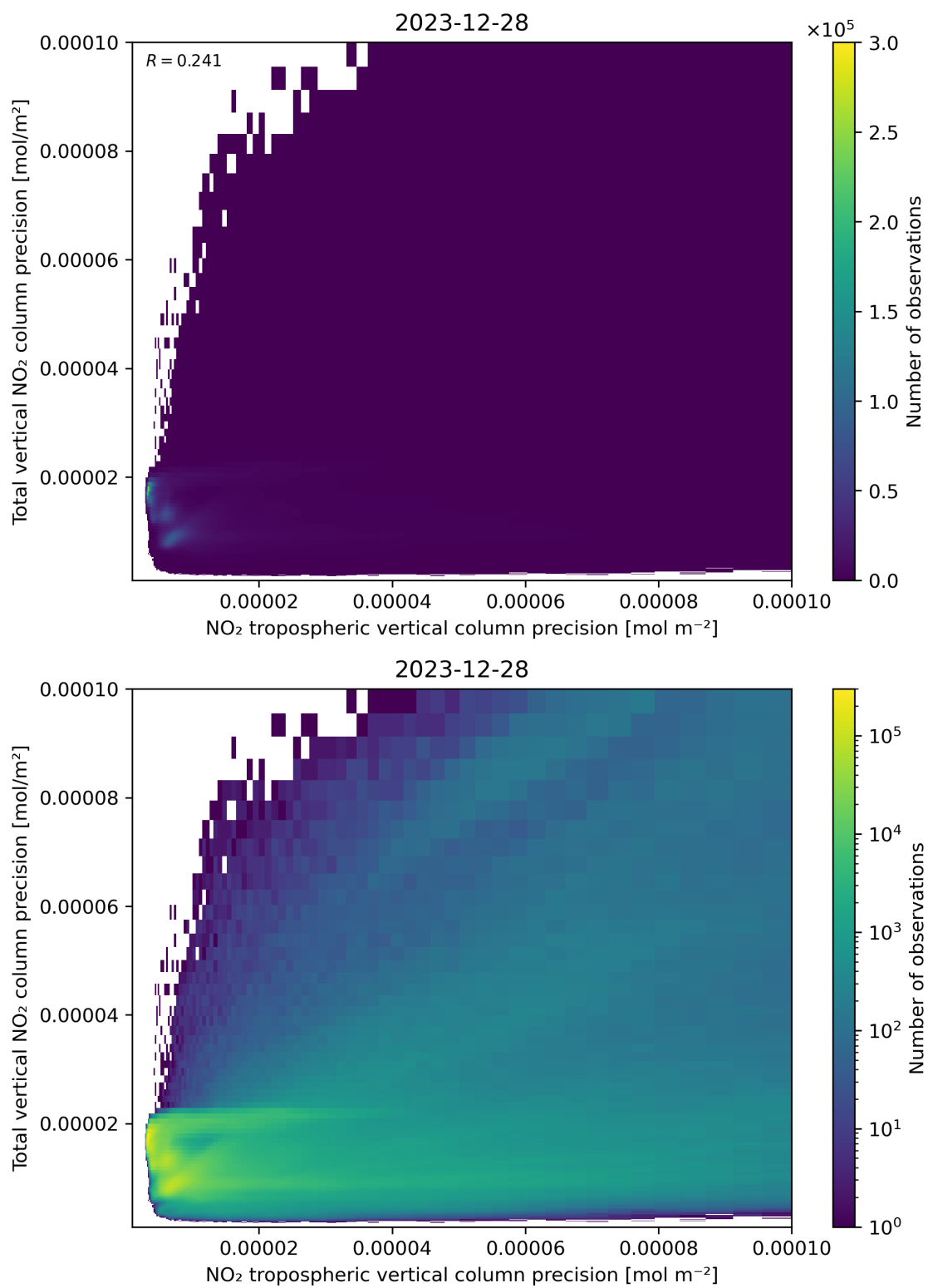
Figure 139: Scatter density plot of “NO 2 tropospheric vertical column precision” against “Total vertical NO 2 column precision” for 2023-12-27 to 2023-12-29.
