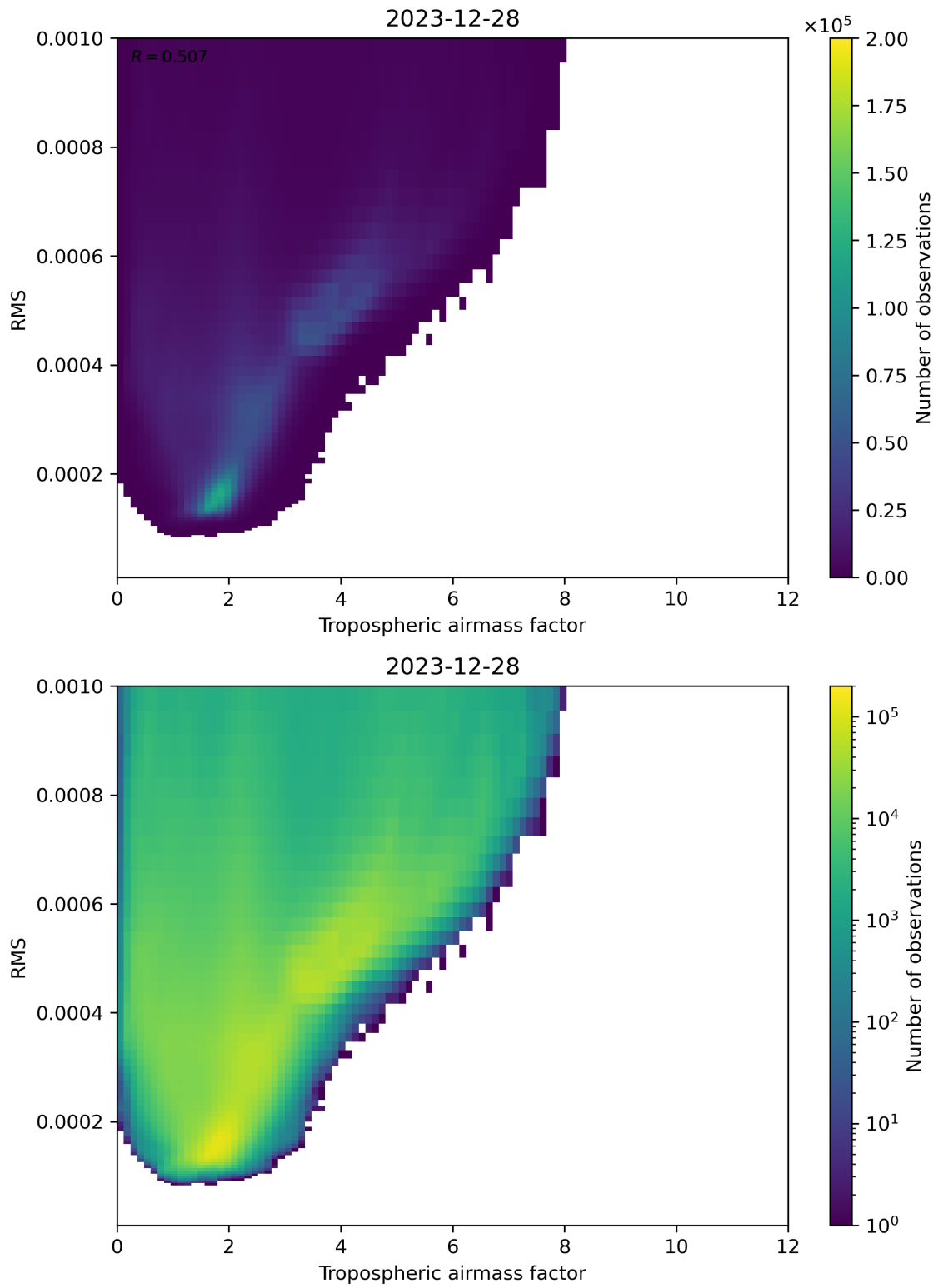
Figure 79: Scatter density plot of “Tropospheric airmass factor” against “RMS” for 2023-12-27 to 2023-12-29.
