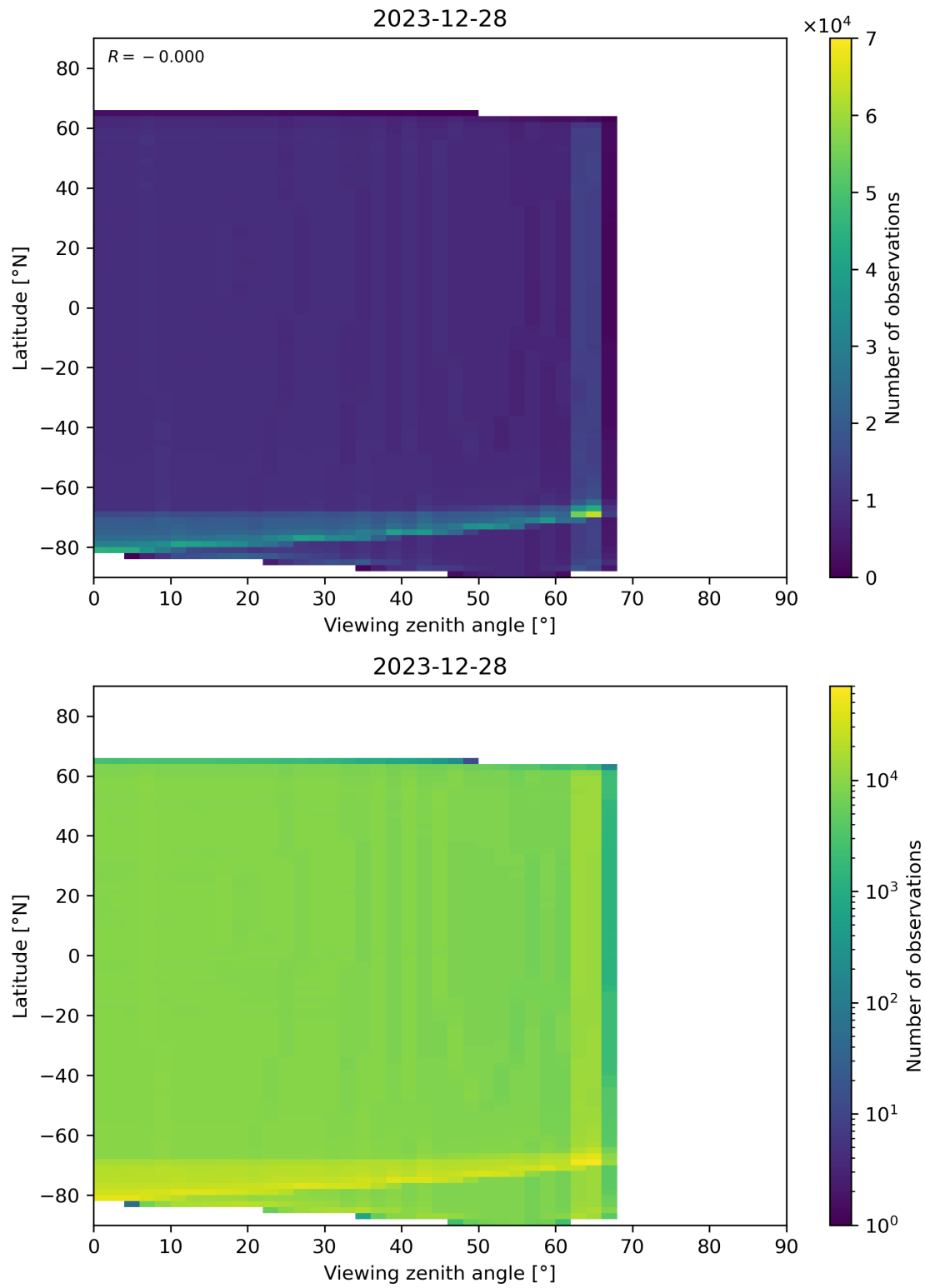
Figure 163: Scatter density plot of “Viewing zenith angle” against “Latitude” for 2023-12-27 to 2023-12-29.
