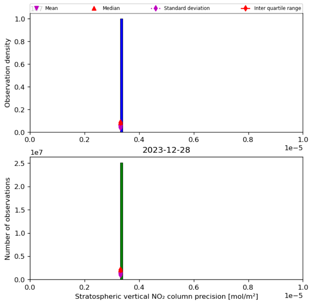
Figure 37: Histogram of “Stratospheric vertical NO 2 column precision” for 2023-12-27 to 2023-12-29
