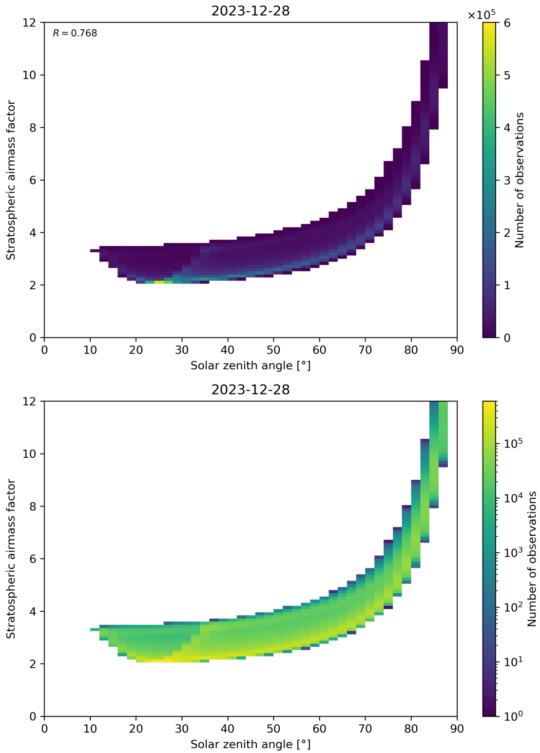
Figure 145: Scatter density plot of “Solar zenith angle” against “Stratospheric airmass factor” for 2023-12-27 to 2023-12-29.
