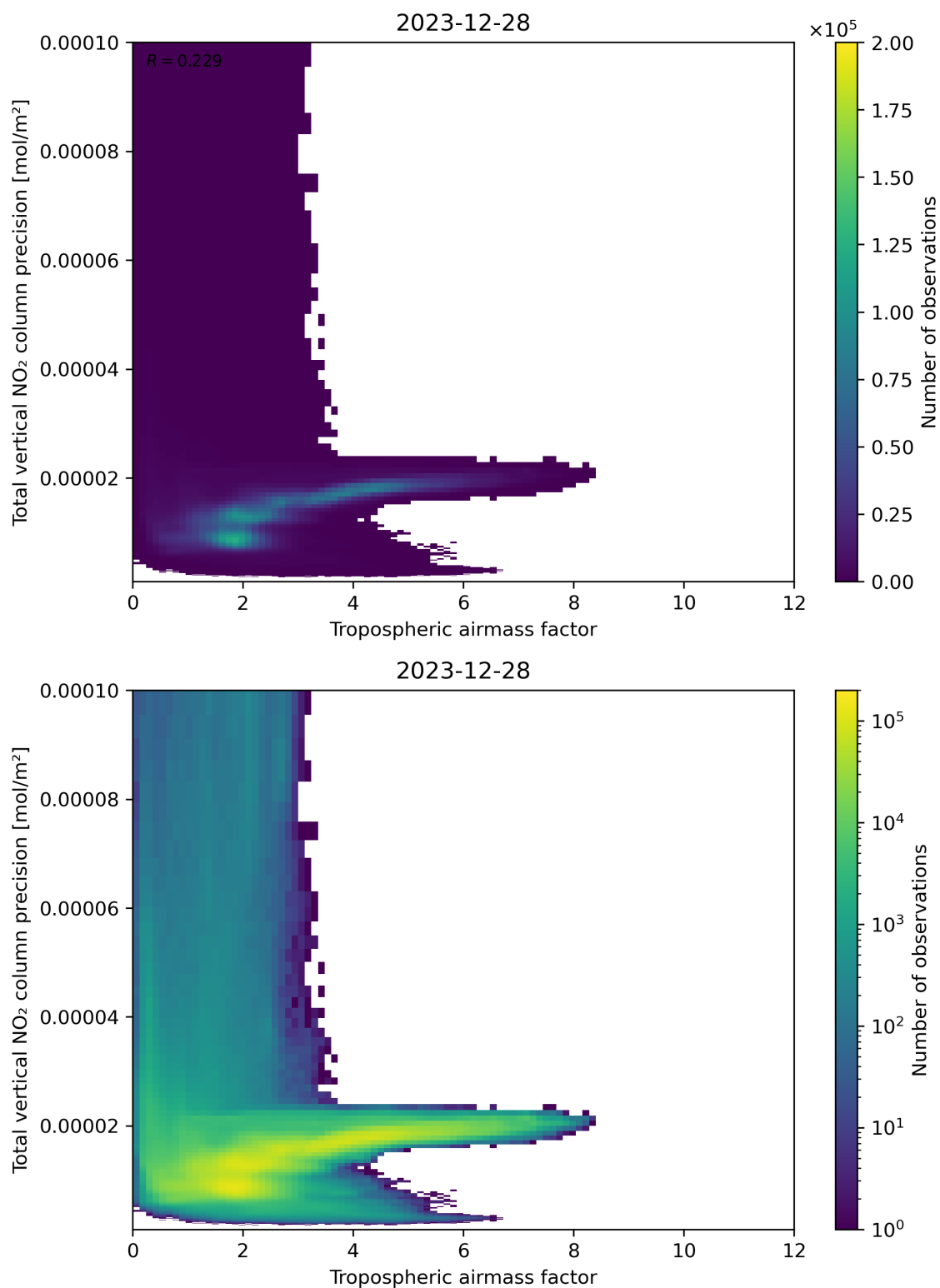
Figure 78: Scatter density plot of “Tropospheric air mass factor” against “Total vertical NO 2 column precision” for 2023-12-27 to 2023-12-29.
