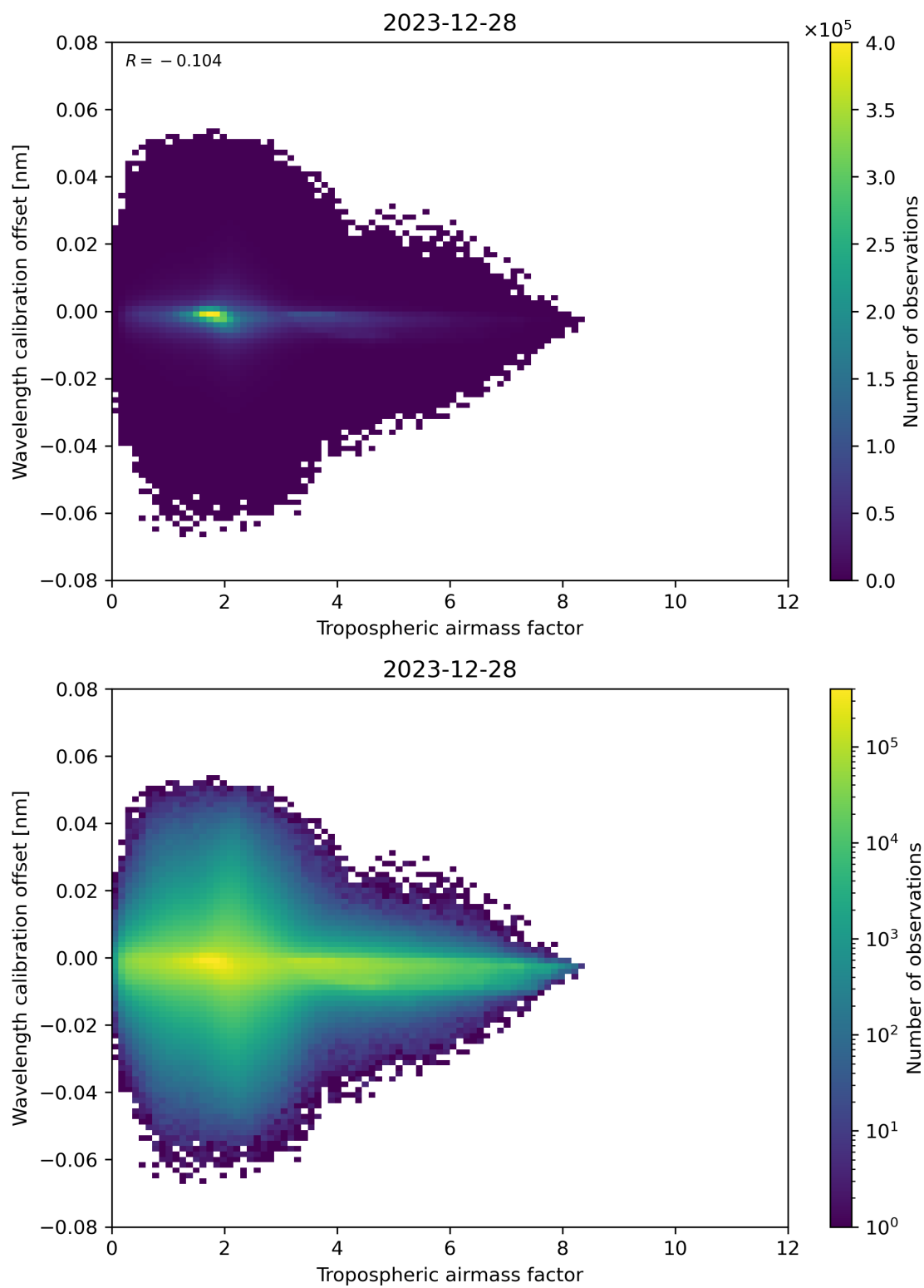
Figure 80: Scatter density plot of “Tropospheric airmass factor” against “Wavelength calibration offset” for 2023-12-27 to 2023-12-29.
