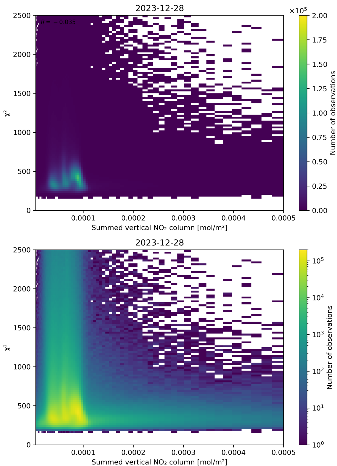
Figure 104: Scatter density plot of “Summed vertical NO 2 column” against “ \chi^2 ” for 2023-12-27 to 2023-12-29.
