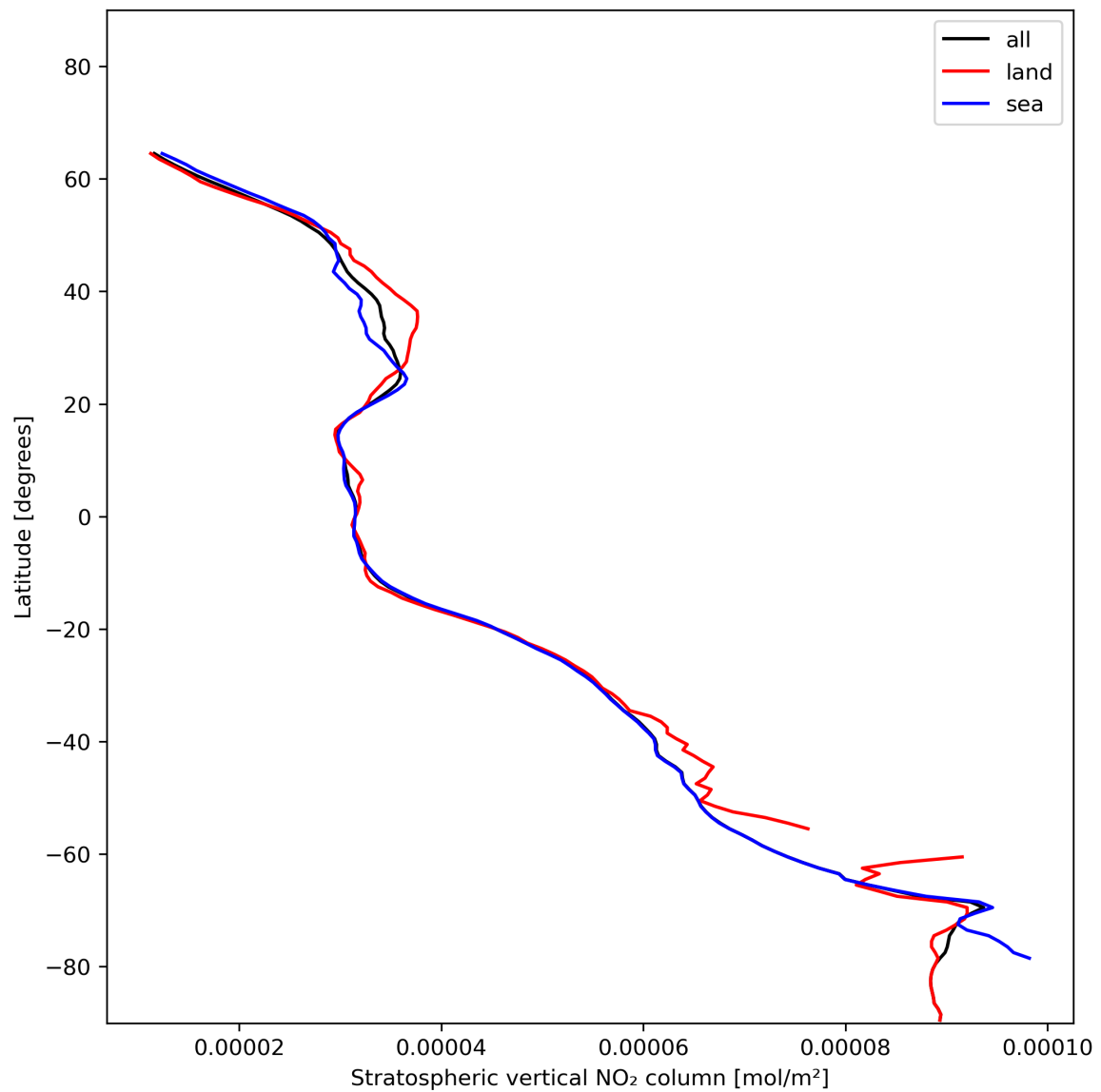
Figure 19: Zonal average of “Stratospheric vertical NO 2 column” for 2023-12-27 to 2023-12-29.
