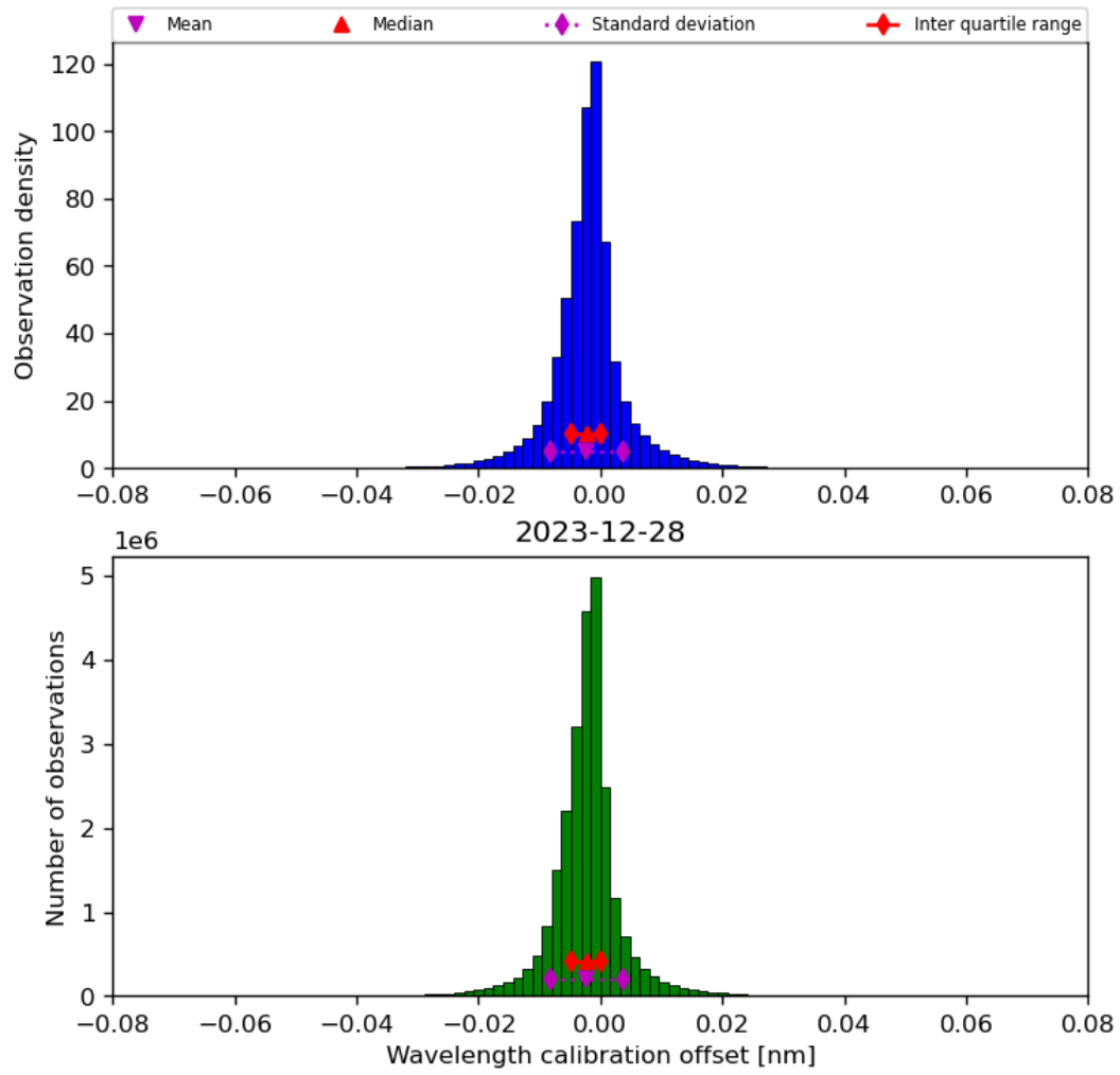
Figure 35: Histogram of “Wavelength calibration offset” for 2023-12-27 to 2023-12-29
