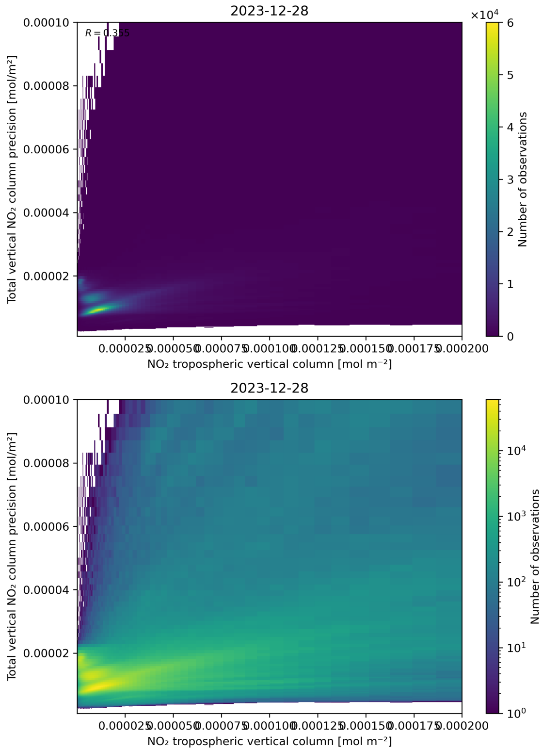
Figure 129: Scatter density plot of “NO 2 tropospheric vertical column” against “Total vertical NO 2 column precision” for 2023-12-27 to 2023-12-29.
