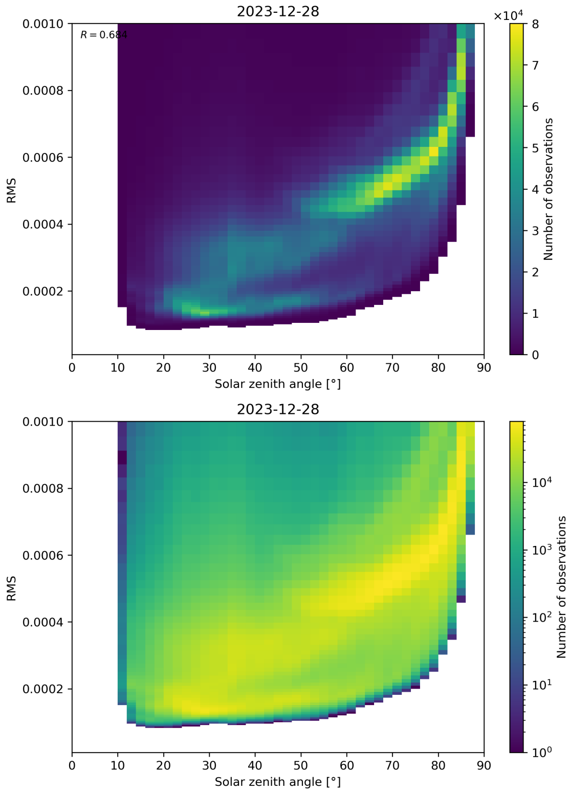
Figure 157: Scatter density plot of “Solar zenith angle” against “RMS” for 2023-12-27 to 2023-12-29.
