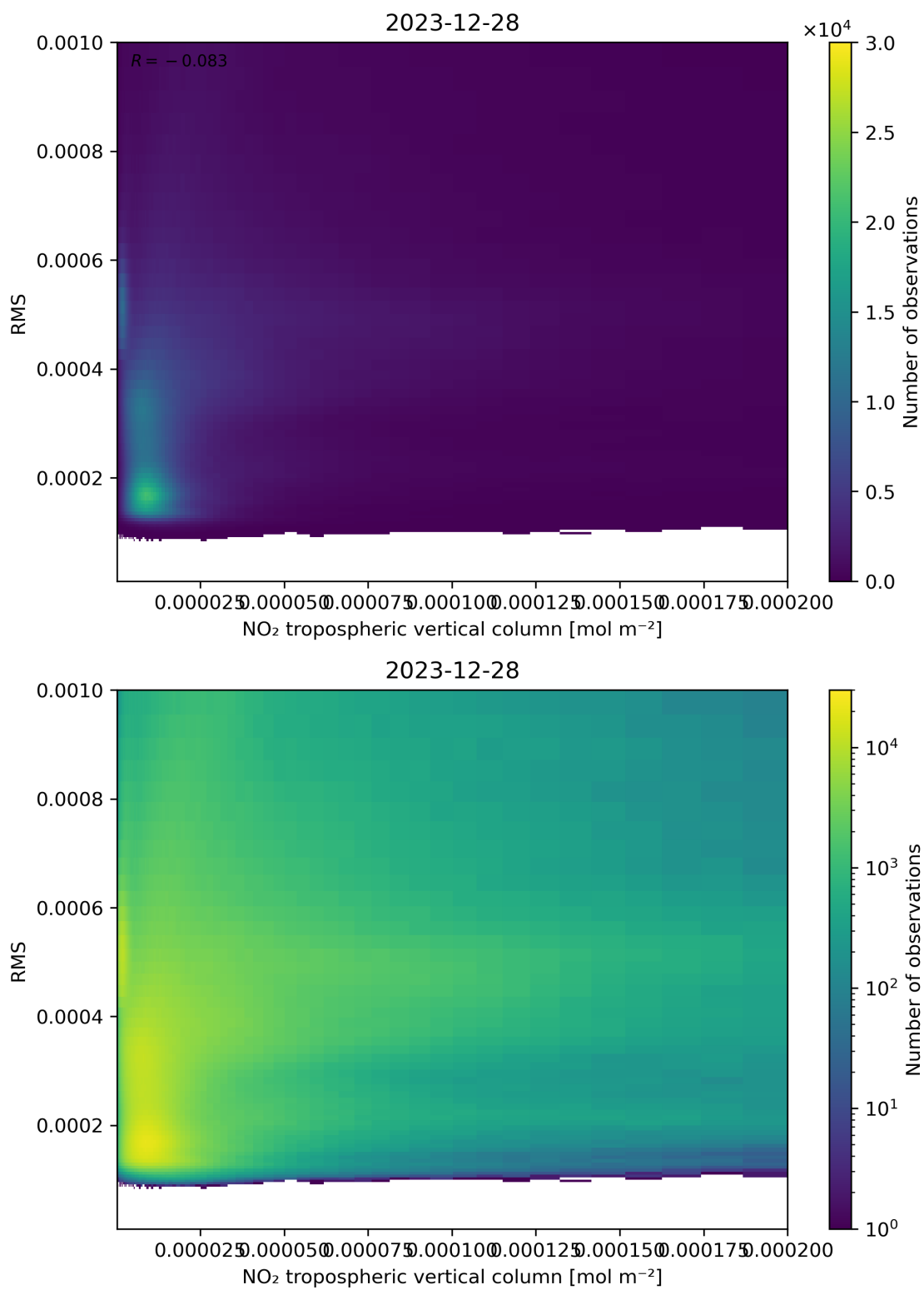
Figure 142: Scatter density plot of “NO 2 tropospheric vertical column” against “RMS” for 2023-12-27 to 2023-12-29.
