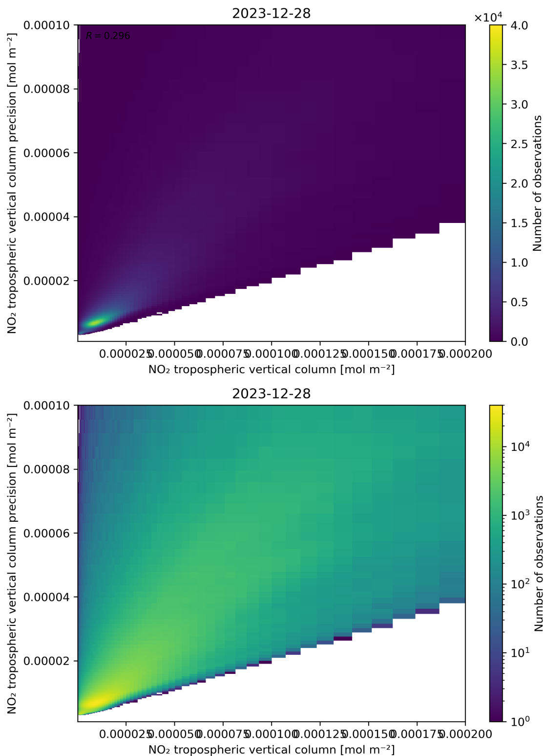
Figure 130: Scatter density plot of “NO 2 tropospheric vertical column” against “NO 2 tropospheric vertical column precision” for 2023-12-27 to 2023-12-29.
