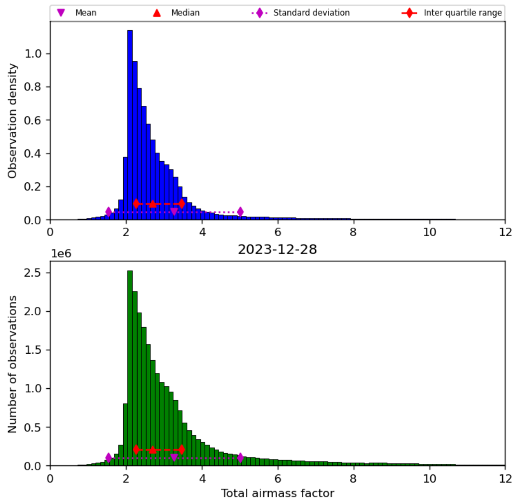
Figure 32: Histogram of “Total airmass factor” for 2023-12-27 to 2023-12-29
