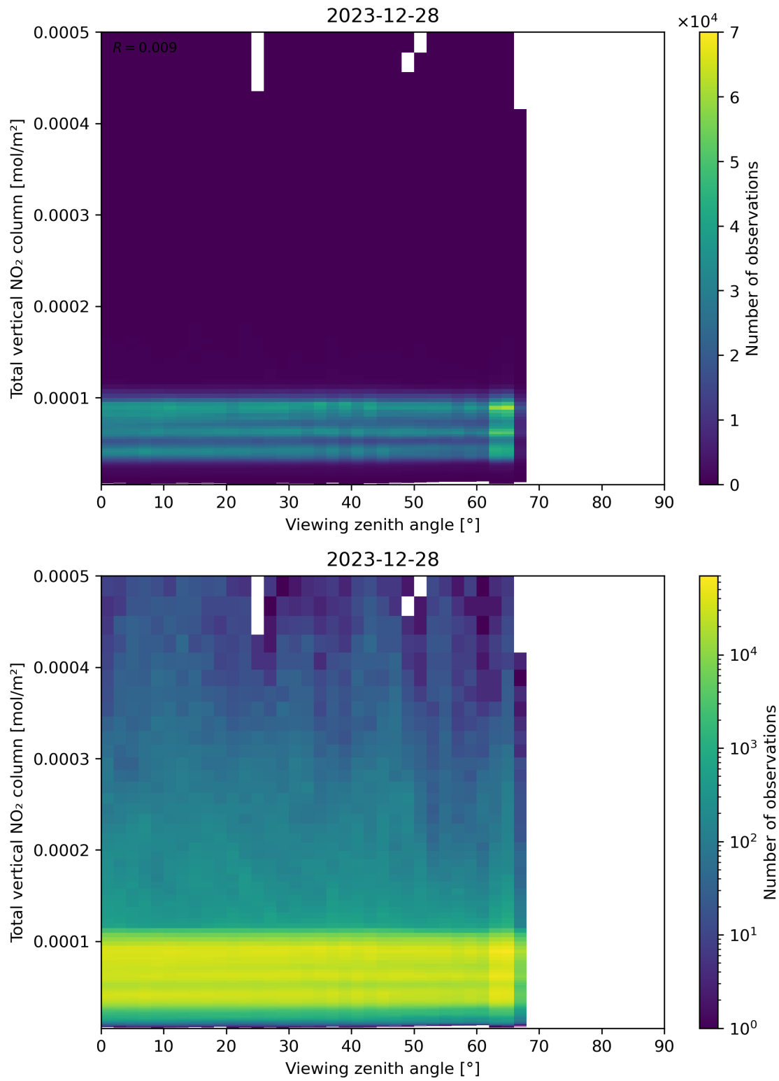
Figure 167: Scatter density plot of “Viewing zenith angle” against “Total vertical NO 2 column” for 2023-12-27 to 2023-12-29.
