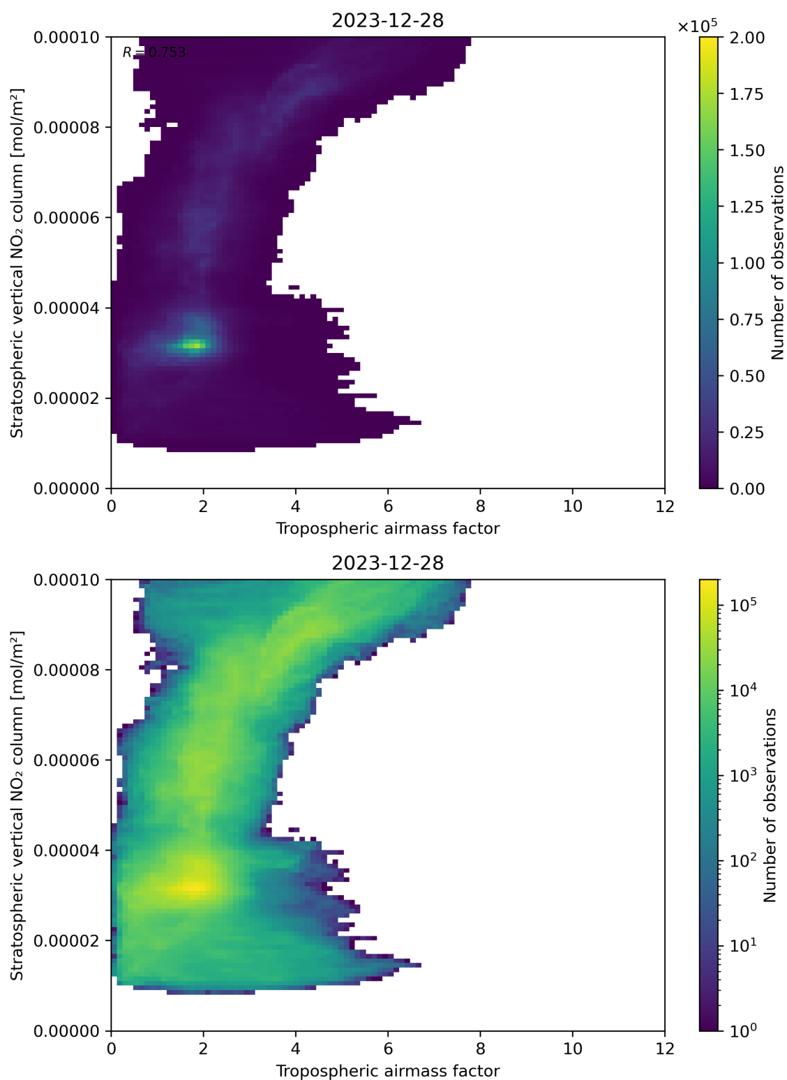
Figure 74: Scatter density plot of “Tropospheric air mass factor” against “Stratospheric vertical NO 2 column” for 2023-12-27 to 2023-12-29.
