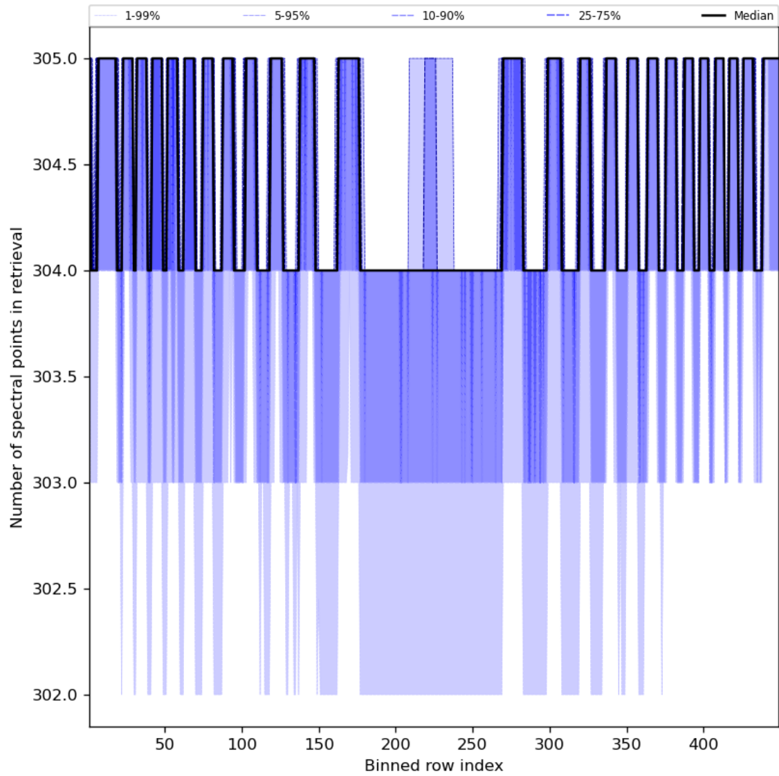
Figure 50: Along track statistics of “Number of spectral points in retrieval” for 2023-12-27 to 2023-12-29
