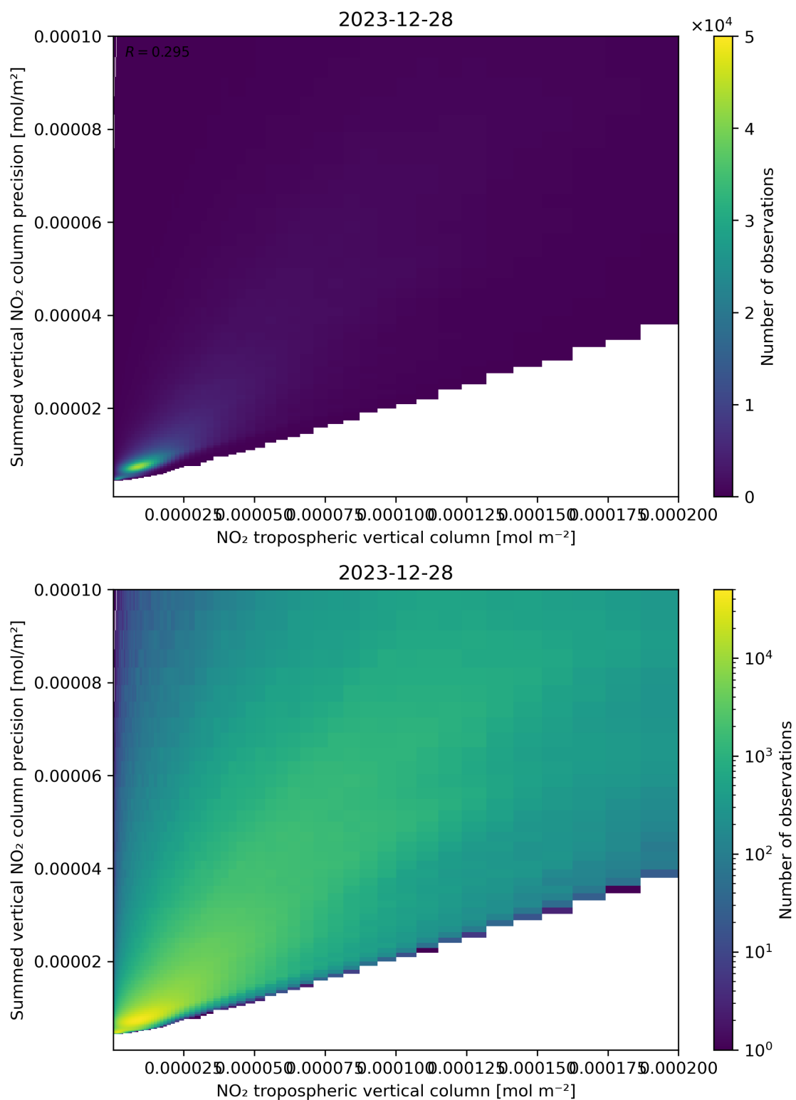
Figure 127: Scatter density plot of “NO 2 tropospheric vertical column” against “Summed vertical NO 2 column precision” for 2023-12-27 to 2023-12-29.
