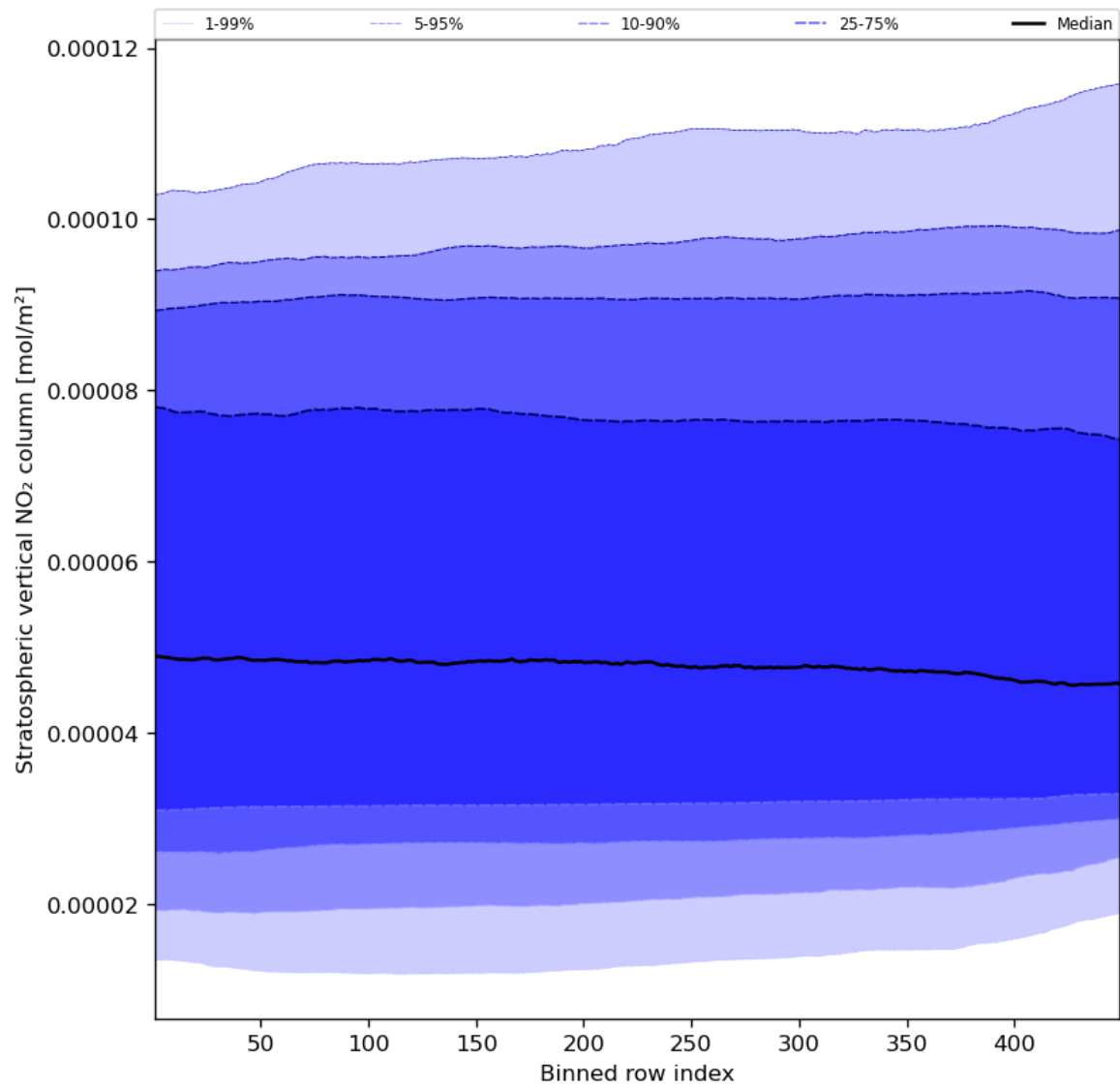
Figure 53: Along track statistics of “Stratospheric vertical NO 2 column” for 2023-12-27 to 2023-12-29
