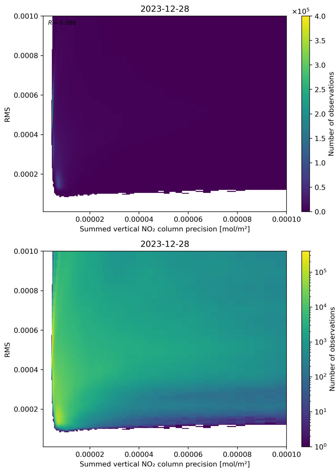
Figure 108: Scatter density plot of “Summed vertical NO 2 column precision” against “RMS” for 2023-12-27 to 2023-12-29.
