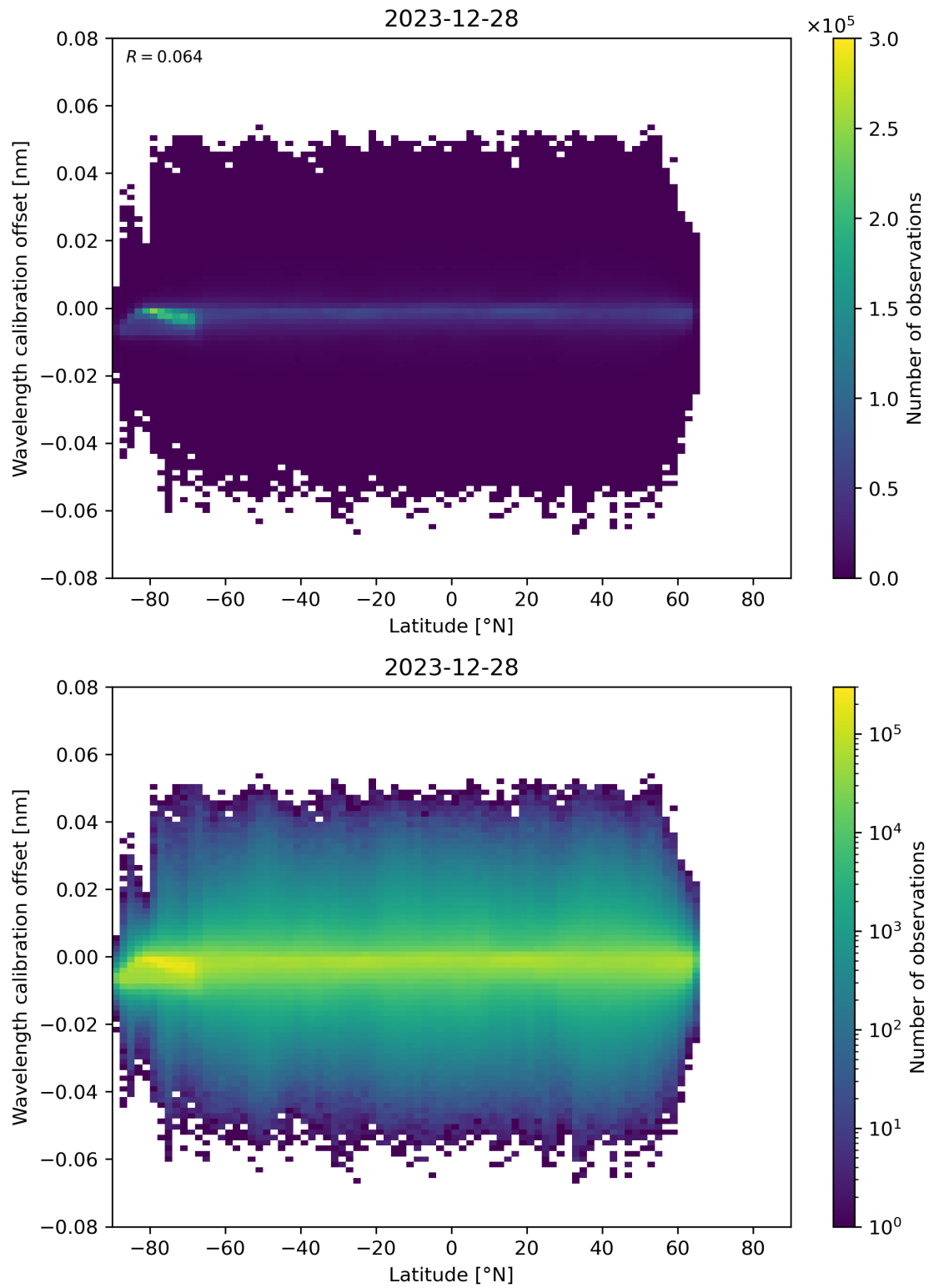
Figure 95: Scatter density plot of “Latitude” against “Wavelength calibration offset” for 2023-12-27 to 2023-12-29.
