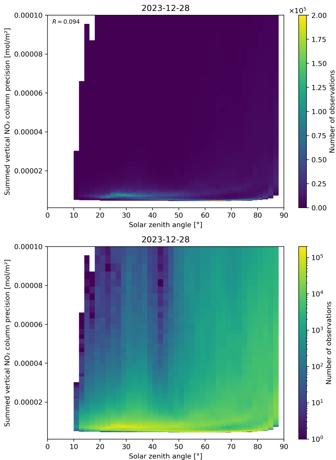
Figure 152: Scatter density plot of “Solar zenith angle” against “Summed vertical NO 2 column precision” for 2023-12-27 to 2023-12-29.
