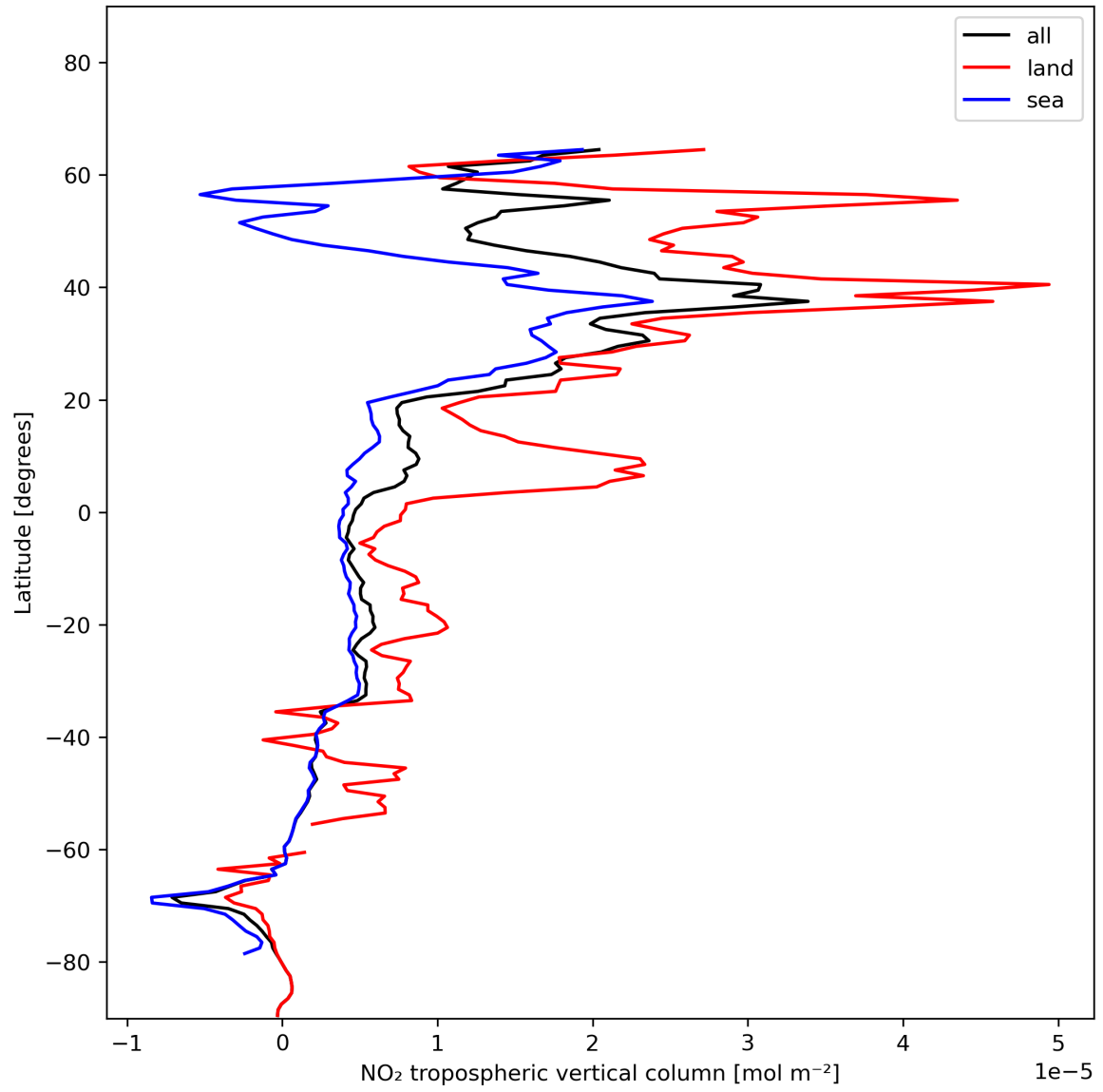
Figure 12: Zonal average of “NO 2 tropospheric vertical column” for 2023-12-27 to 2023-12-29.
