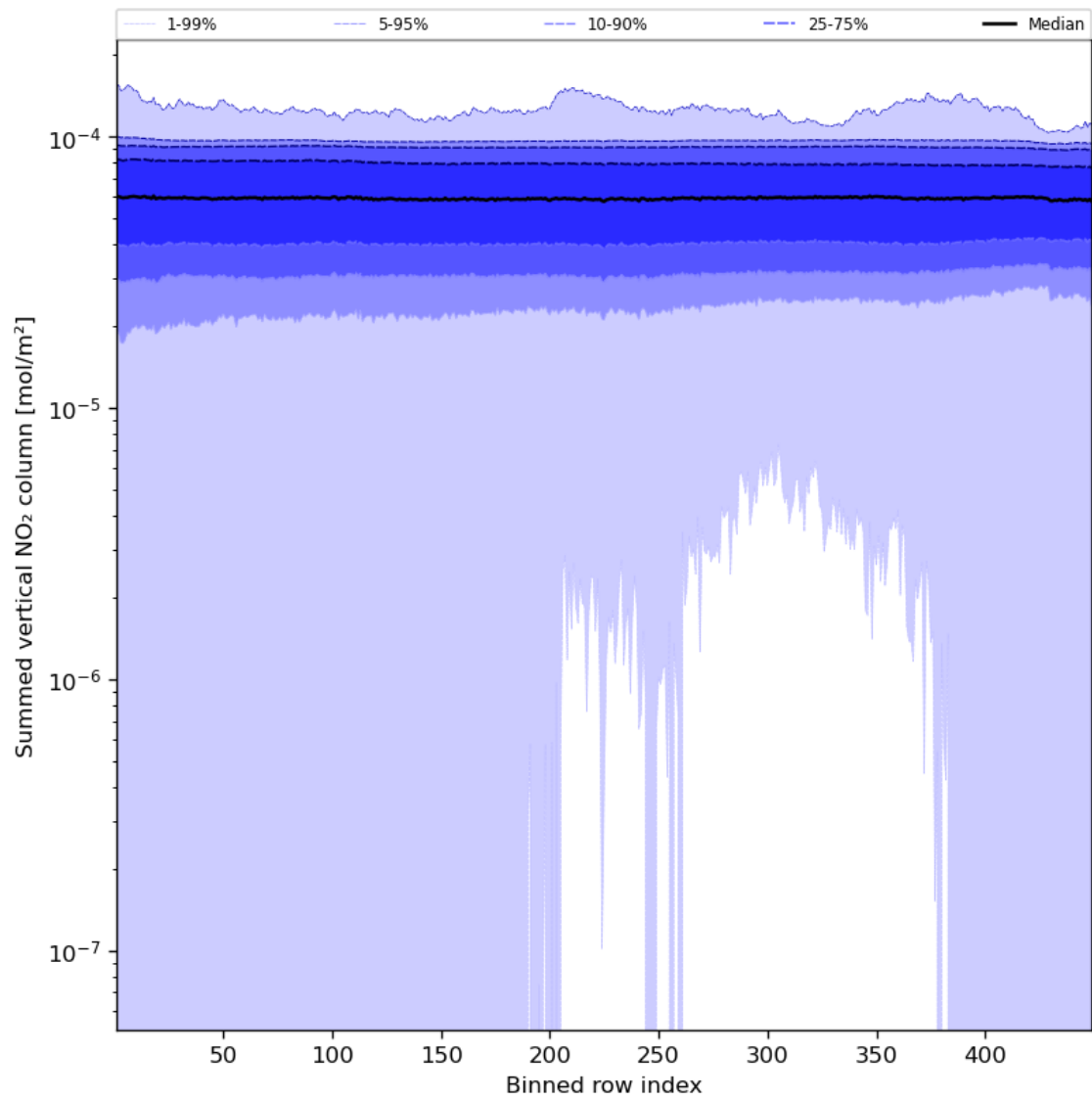
Figure 57: Along track statistics of “Summed vertical NO 2 column” for 2023-12-27 to 2023-12-29
