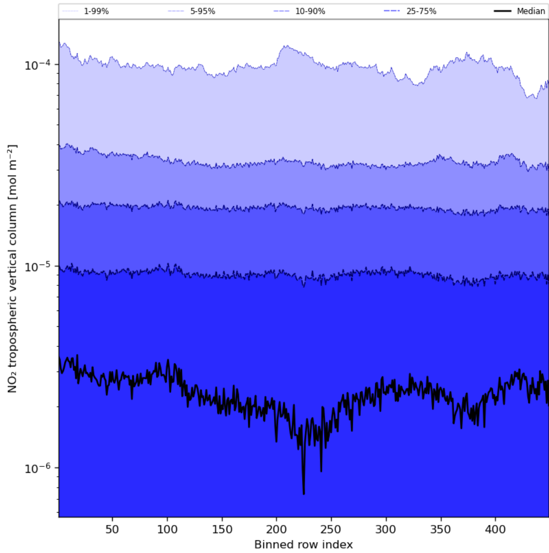
Figure 46: Along track statistics of “NO 2 tropospheric vertical column” for 2023-12-27 to 2023-12-29
