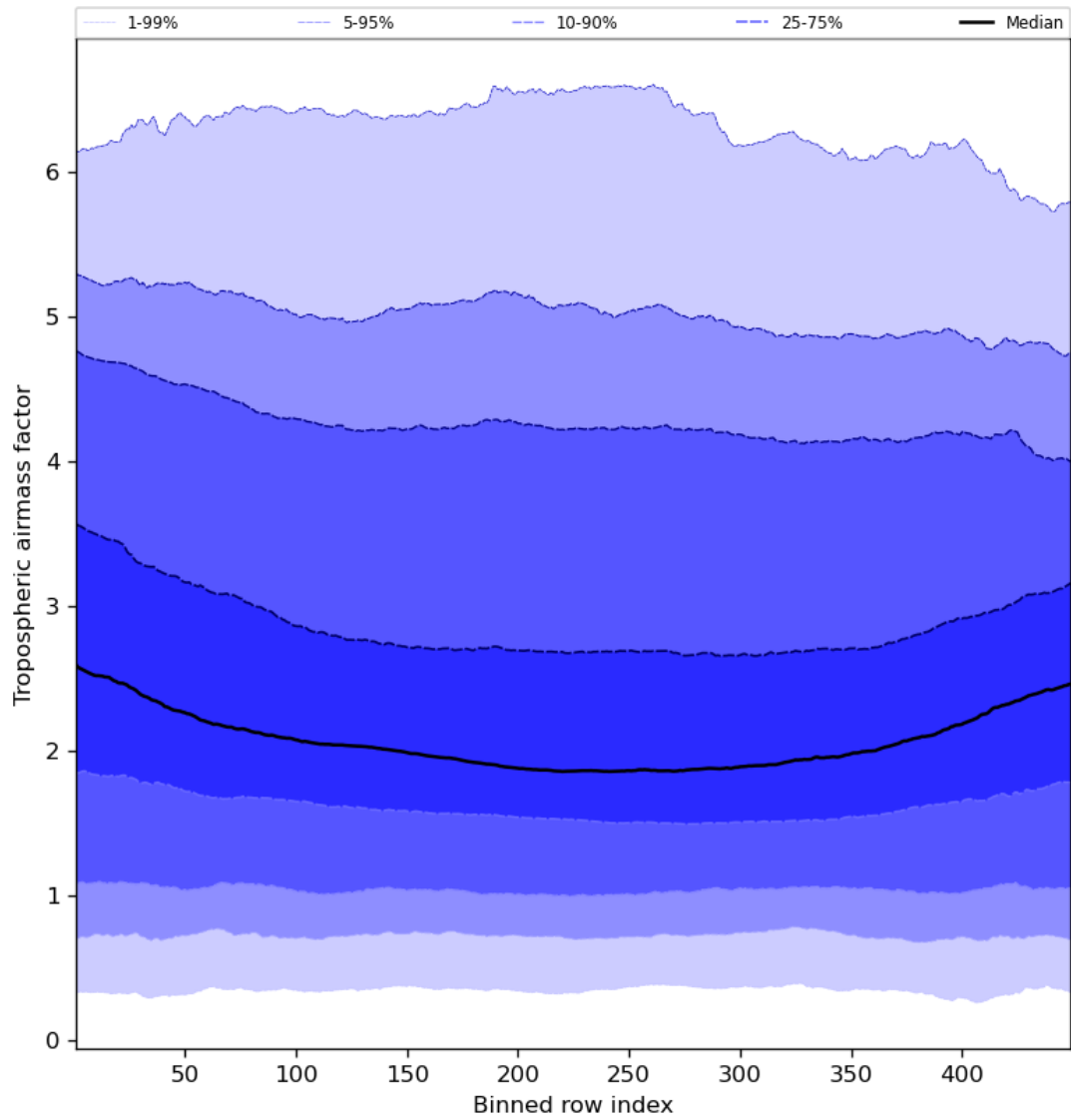
Figure 48: Along track statistics of “Tropospheric airmass factor” for 2023-12-27 to 2023-12-29
