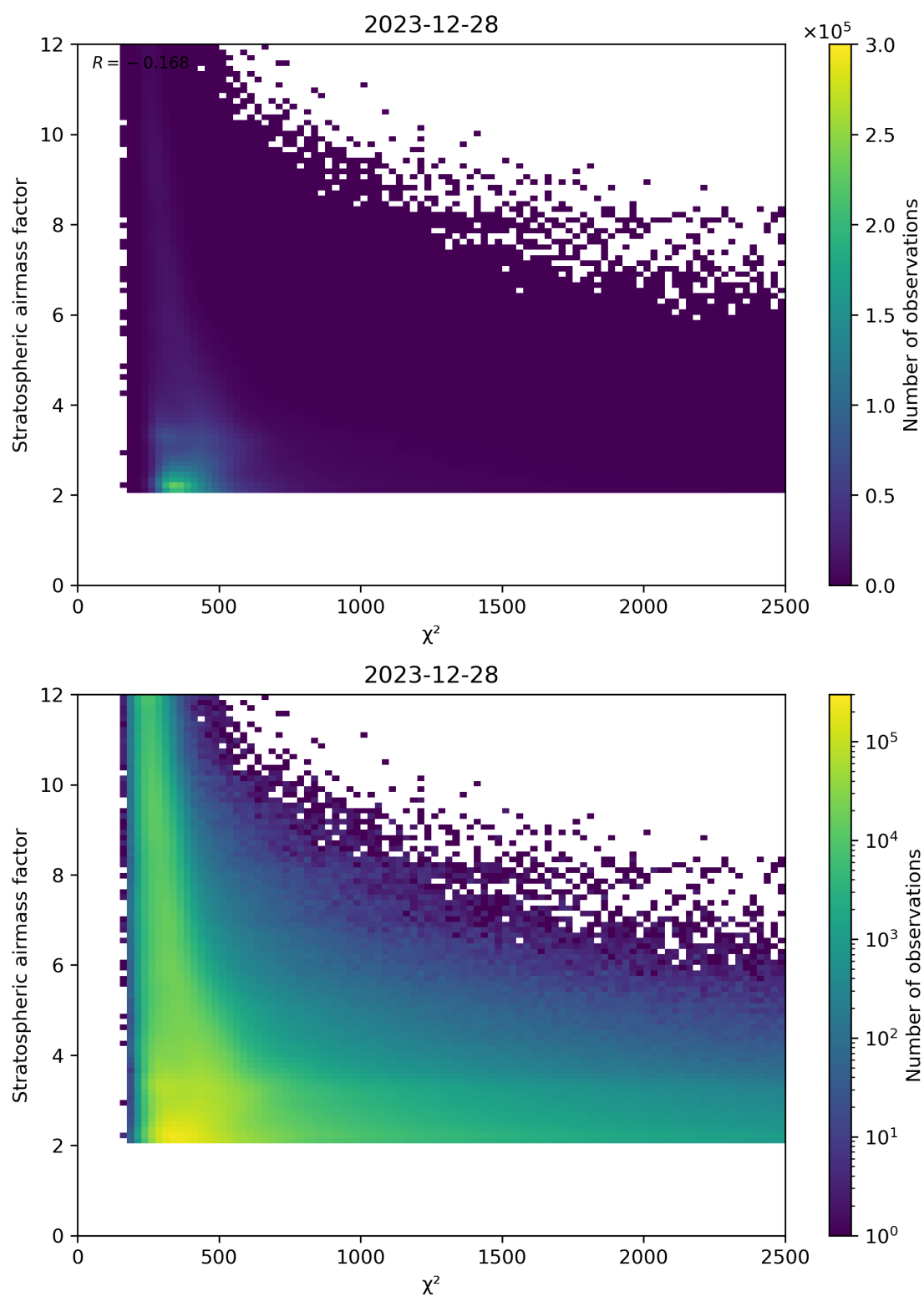
Figure 81: Scatter density plot of “ \chi^2 ” against “Stratospheric airmass factor” for 2023-12-27 to 2023-12-29.
