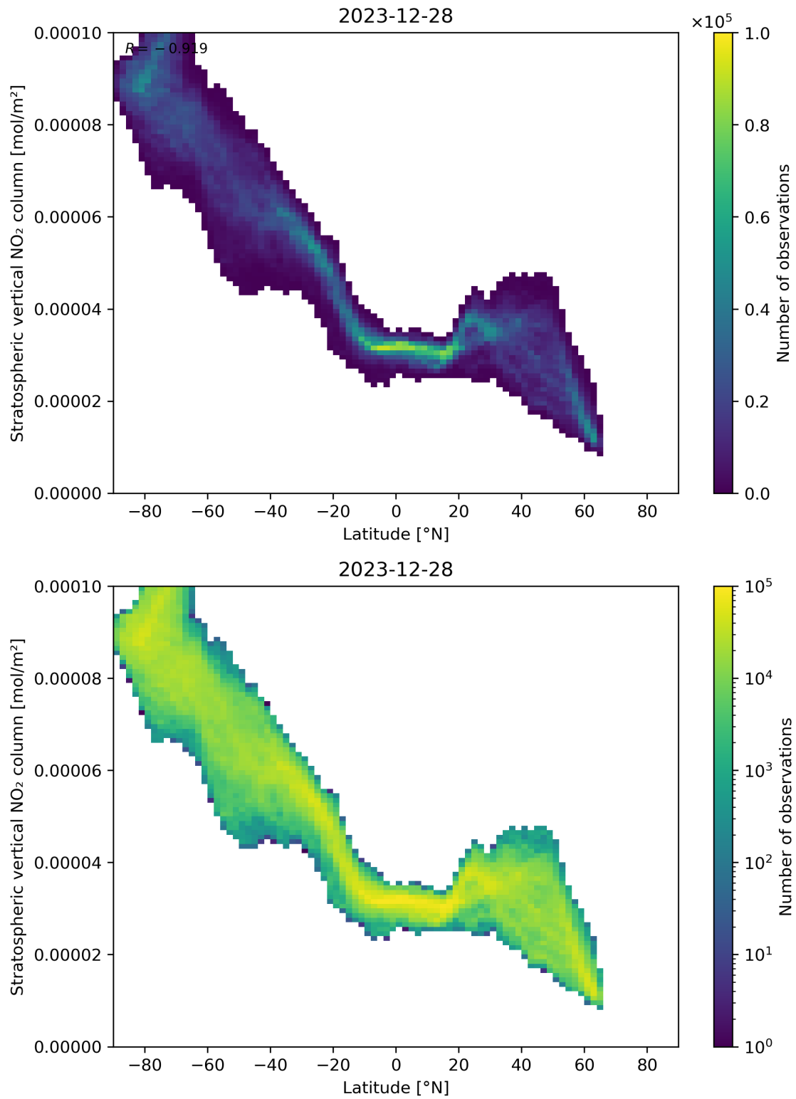
Figure 87: Scatter density plot of “Latitude” against “Stratospheric vertical NO 2 column” for 2023-12-27 to 2023-12-29.
