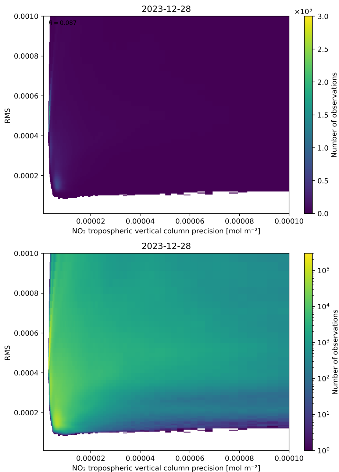
Figure 140: Scatter density plot of “NO 2 tropospheric vertical column precision” against “RMS” for 2023-12-27 to 2023-12-29.
