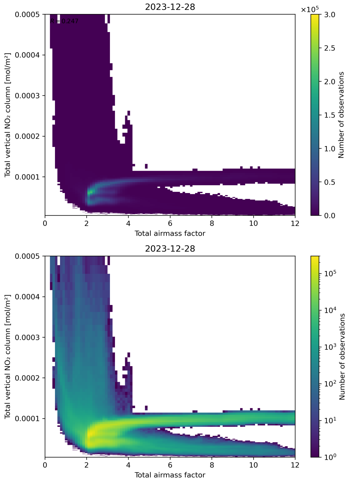
Figure 67: Scatter density plot of “Total airmass factor” against “Total vertical NO 2 column” for 2023-12-27 to 2023-12-29.
