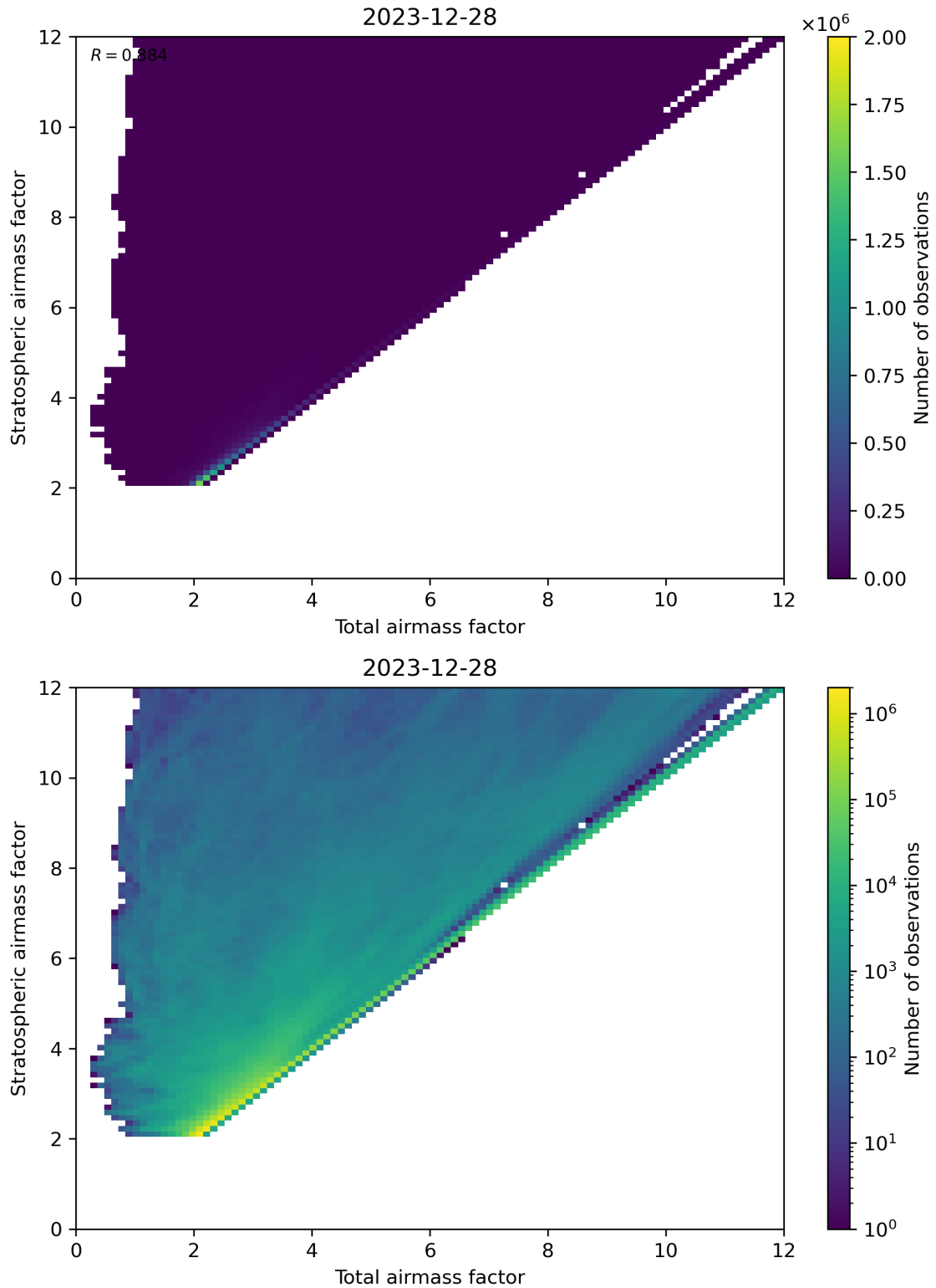
Figure 62: Scatter density plot of “Total airmass factor” against “Stratospheric airmass factor” for 2023-12-27 to 2023-12-29.
