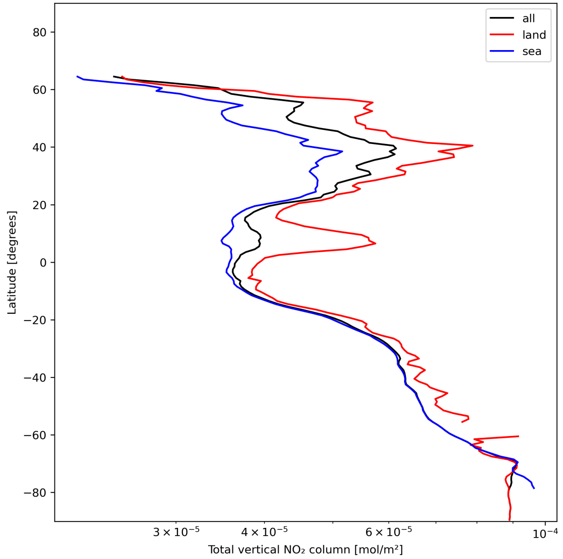
Figure 21: Zonal average of “Total vertical NO 2 column” for 2023-12-27 to 2023-12-29.
