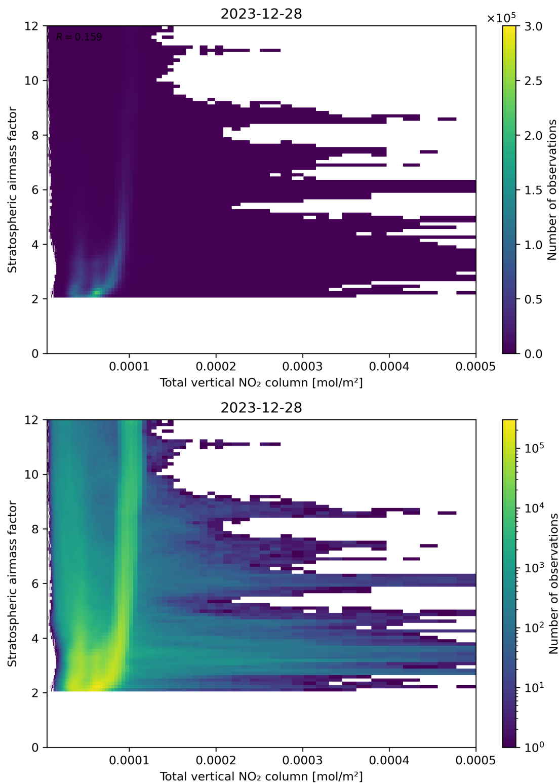
Figure 110: Scatter density plot of “Total vertical NO 2 column” against “Stratospheric airmass factor” for 2023-12-27 to 2023-12-29.
