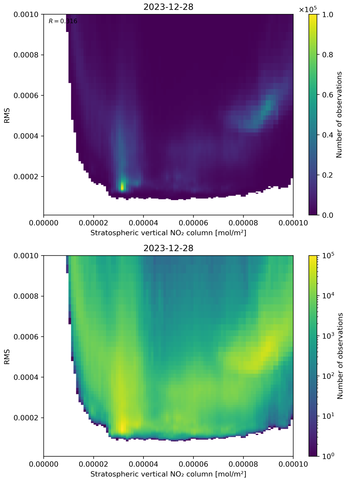
Figure 102: Scatter density plot of “Stratospheric vertical NO 2 column” against “RMS” for 2023-12-27 to 2023-12-29.
