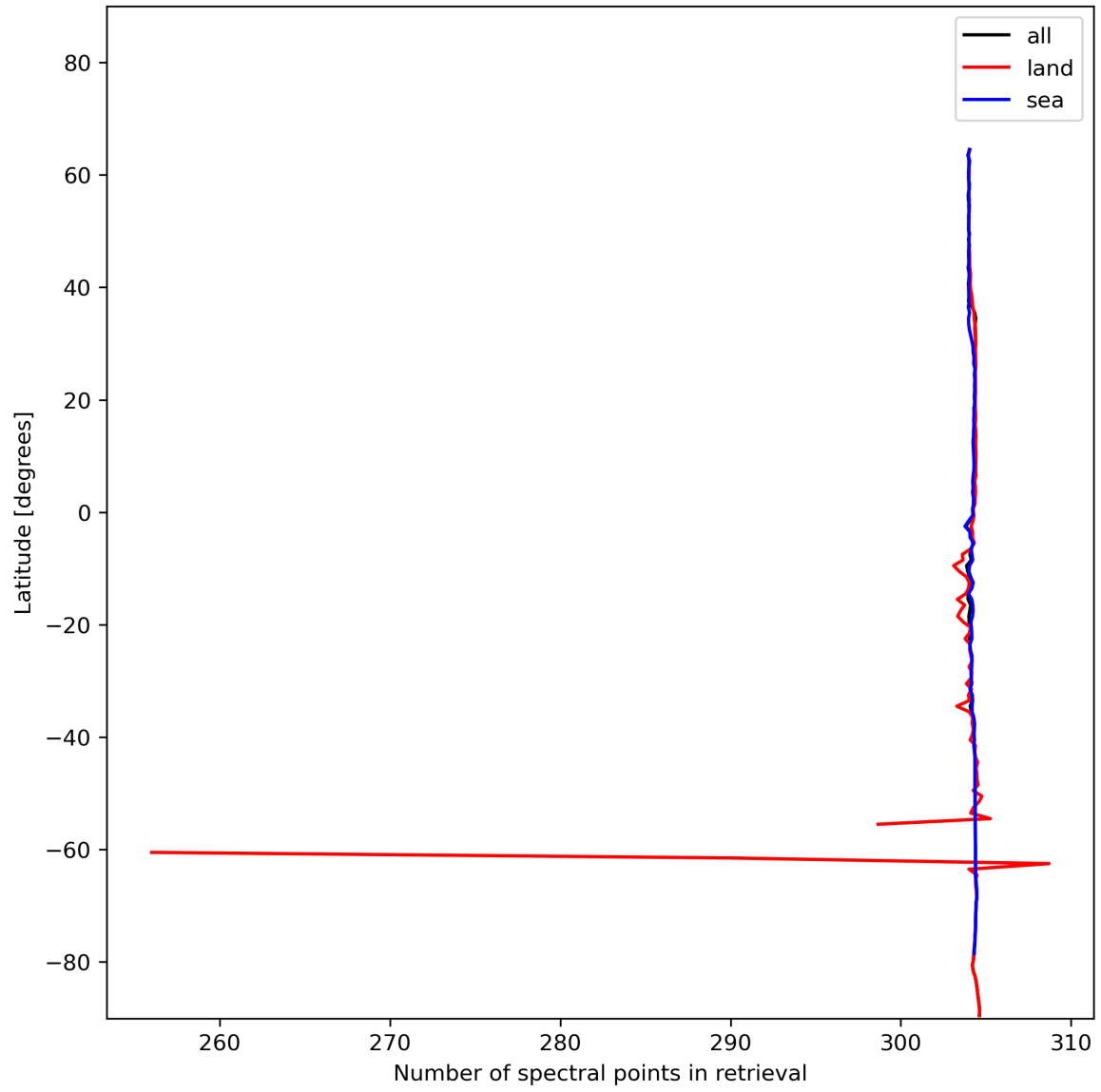
Figure 16: Zonal average of “Number of spectral points in retrieval” for 2023-12-27 to 2023-12-29.
