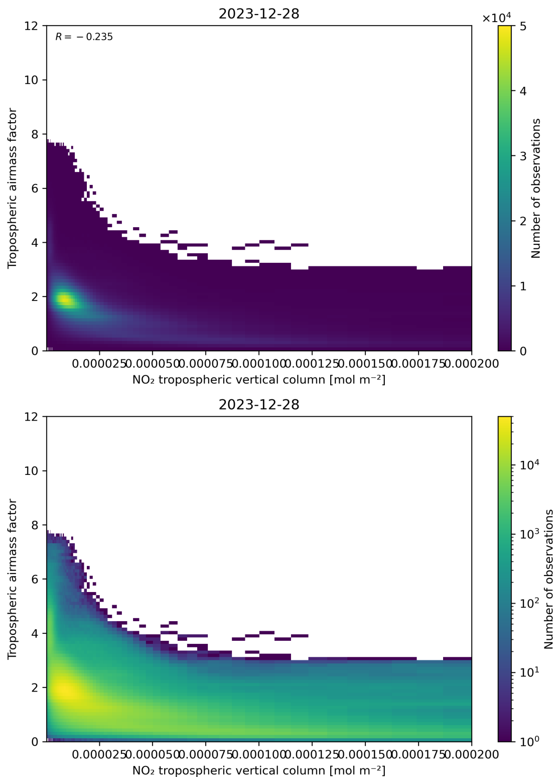
Figure 123: Scatter density plot of “NO 2 tropospheric vertical column” against “Tropospheric air mass factor” for 2023-12-27 to 2023-12-29.
