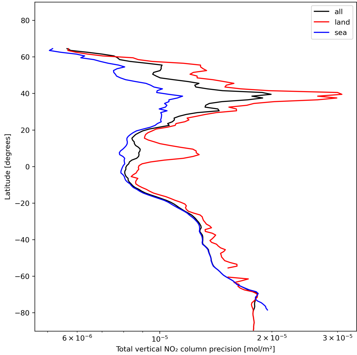
Figure 22: Zonal average of “Total vertical NO 2 column precision” for 2023-12-27 to 2023-12-29.
