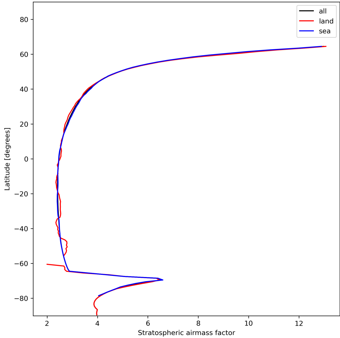
Figure 27: Zonal average of “Stratospheric air mass factor” for 2023-12-27 to 2023-12-29.
