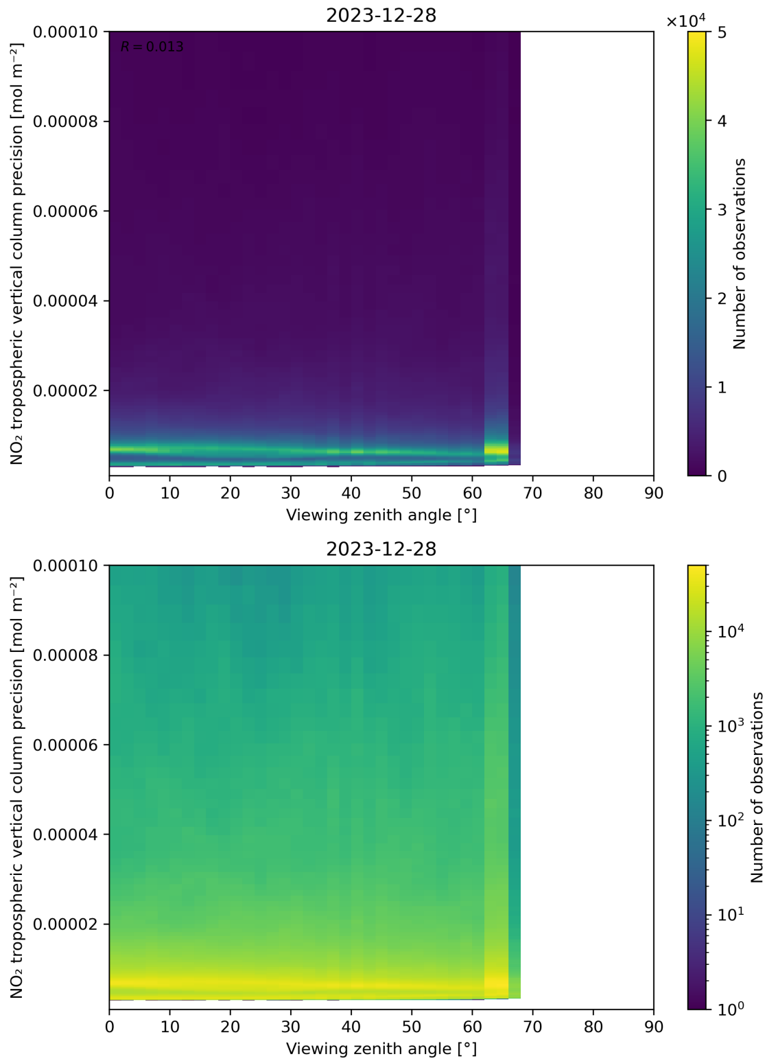
Figure 170: Scatter density plot of “Viewing zenith angle” against “NO 2 tropospheric vertical column precision” for 2023-12-27 to 2023-12-29.
