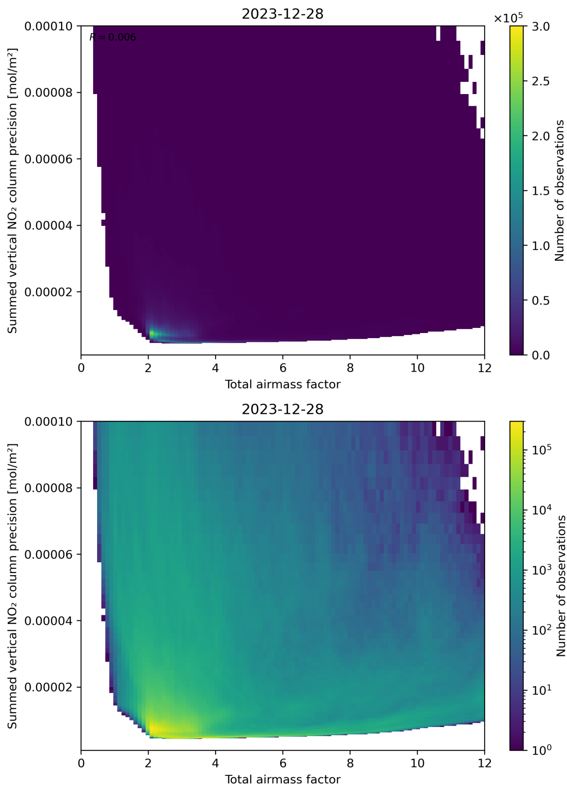
Figure 66: Scatter density plot of “Total airmass factor” against “Summed vertical NO 2 column precision” for 2023-12-27 to 2023-12-29.
