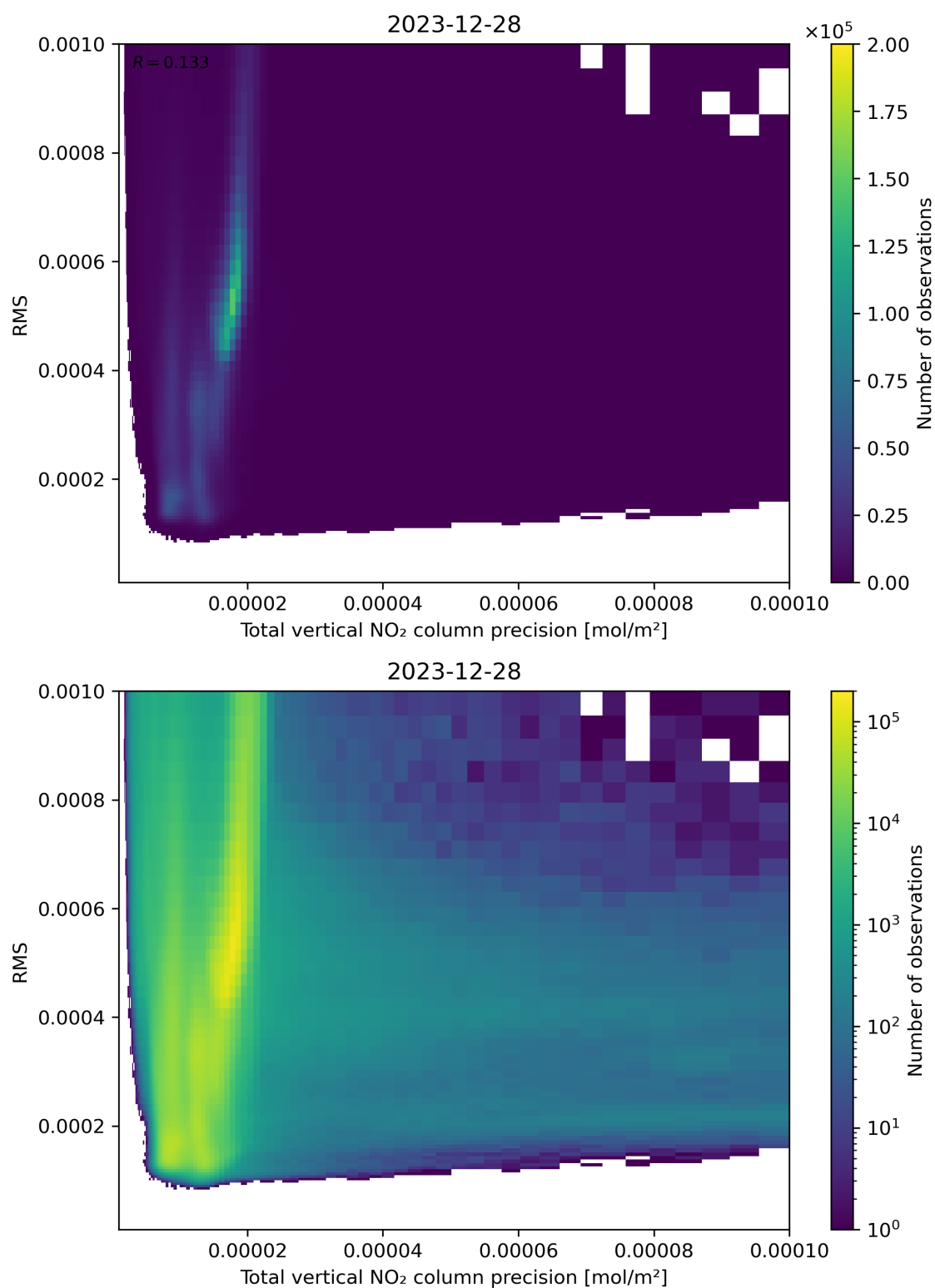
Figure 119: Scatter density plot of “Total vertical NO 2 column precision” against “RMS” for 2023-12-27 to 2023-12-29.
