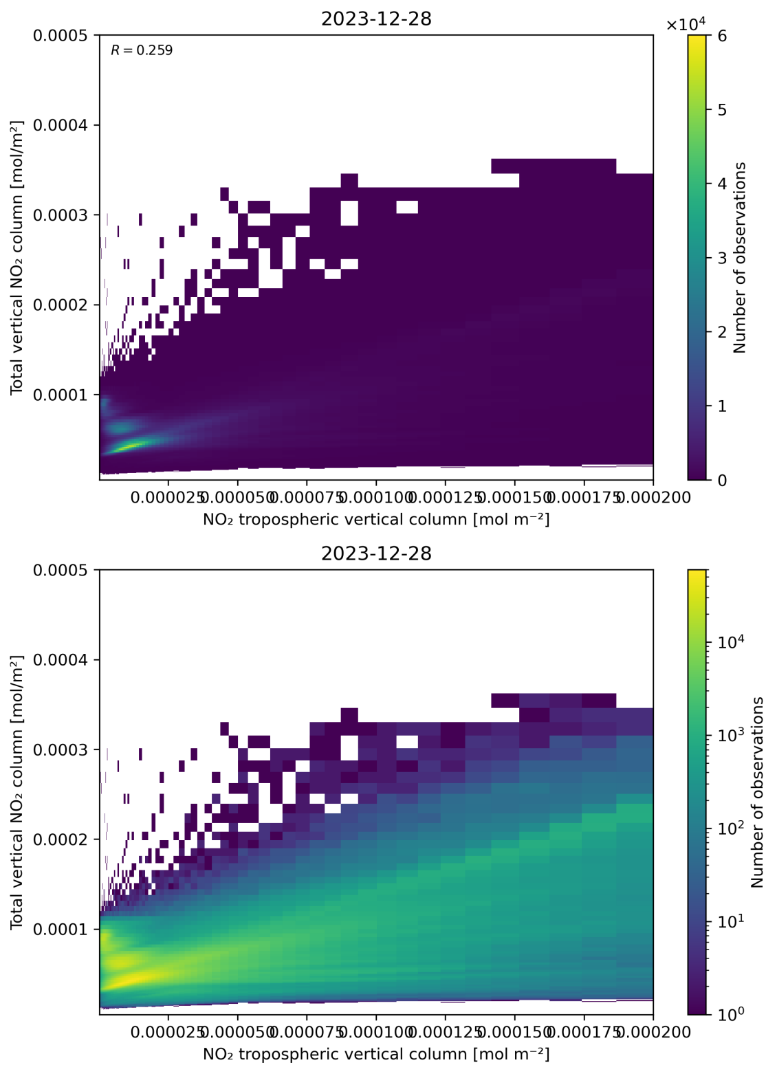
Figure 128: Scatter density plot of “NO 2 tropospheric vertical column” against “Total vertical NO 2 column” for 2023-12-27 to 2023-12-29.
