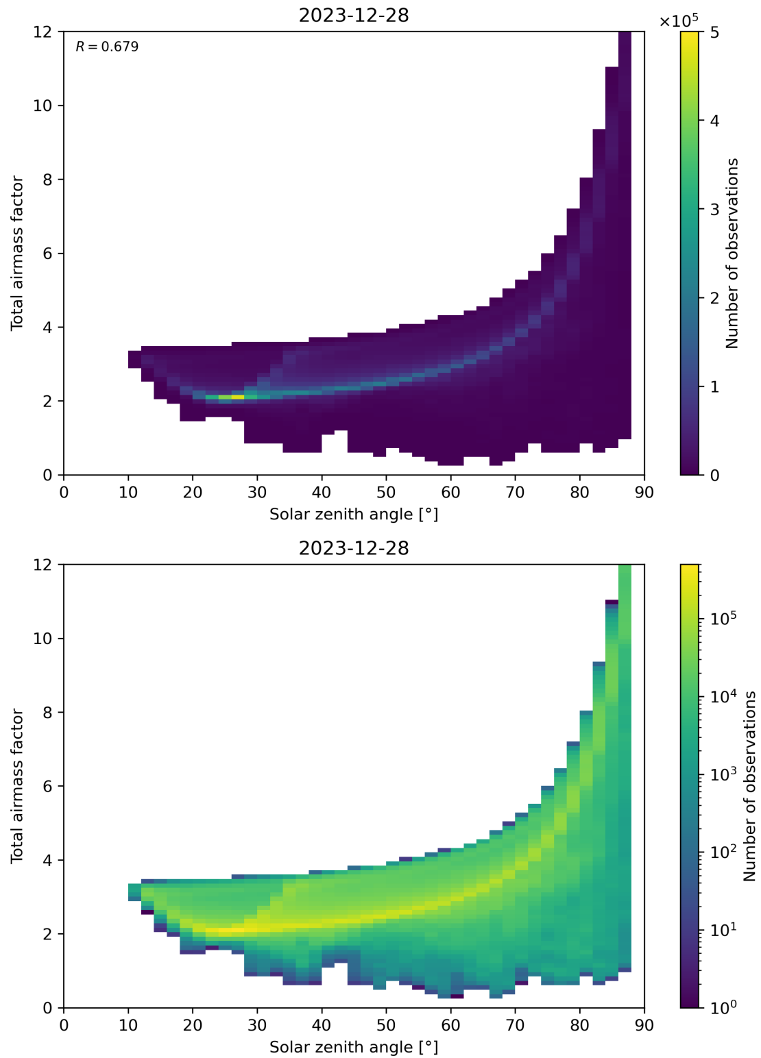
Figure 146: Scatter density plot of “Solar zenith angle” against “Total air mass factor” for 2023-12-27 to 2023-12-29.
