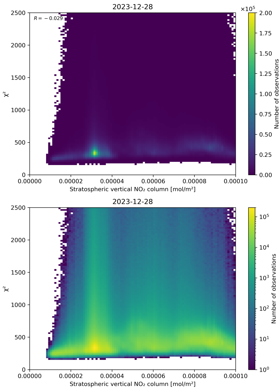
Figure 97: Scatter density plot of “Stratospheric vertical NO 2 column” against “ \chi^2 ” for 2023-12-27 to 2023-12-29.
