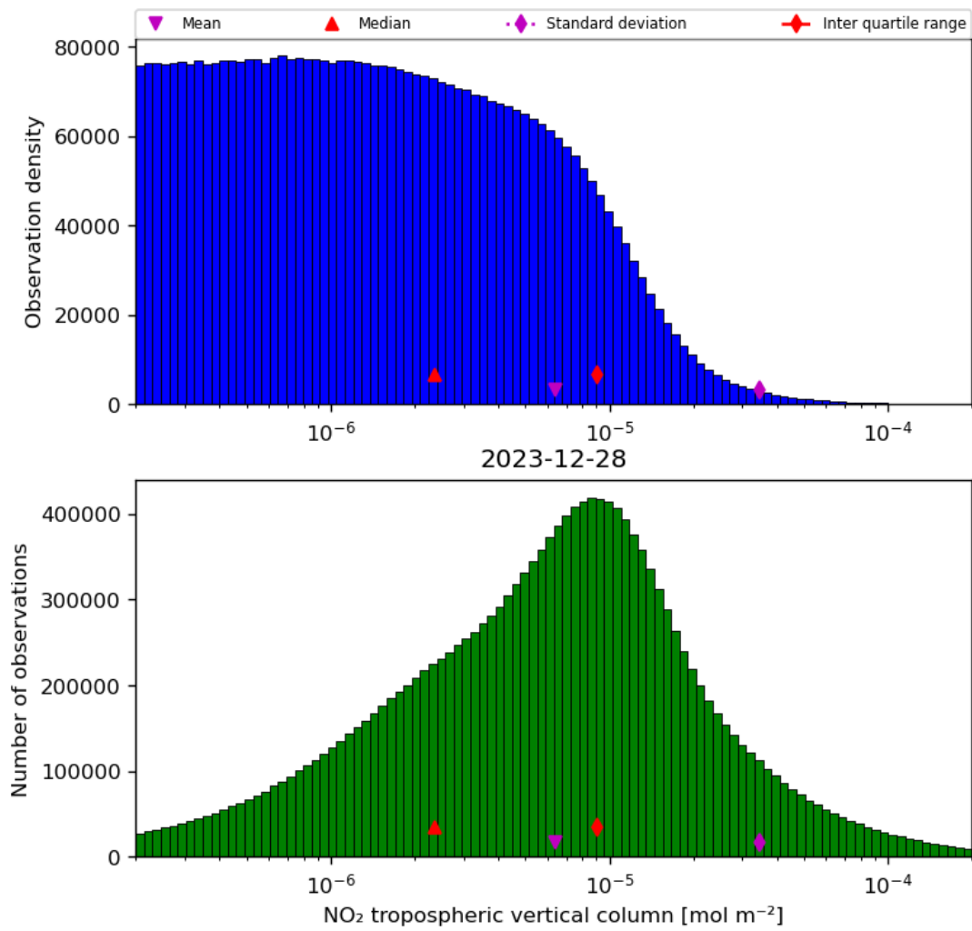
Figure 29: Histogram of “NO 2 tropospheric vertical column” for 2023-12-27 to 2023-12-29
