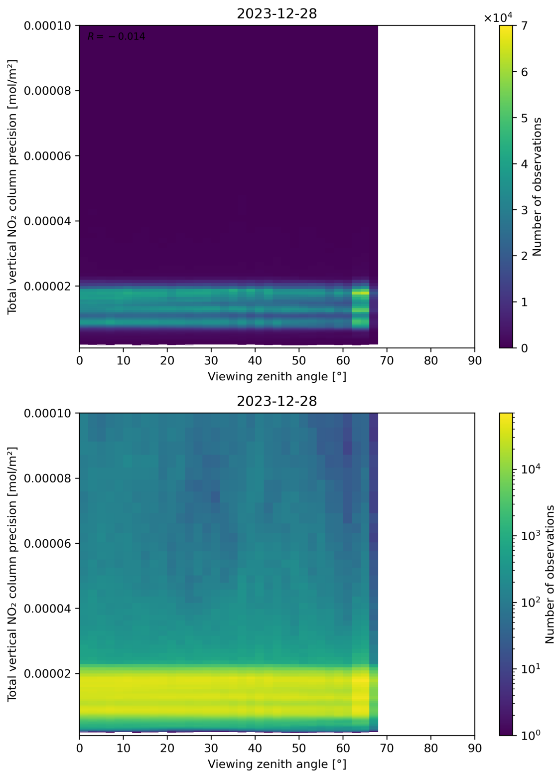
Figure 168: Scatter density plot of “Viewing zenith angle” against “Total vertical NO 2 column precision” for 2023-12-27 to 2023-12-29.
