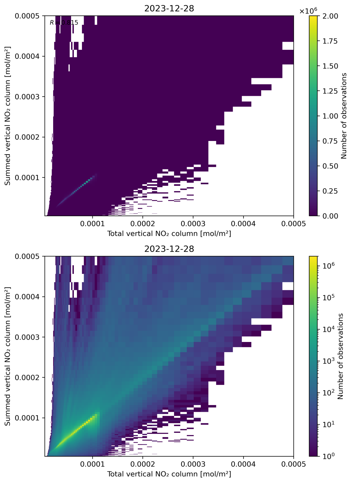
Figure 112: Scatter density plot of “Total vertical NO 2 column” against “Summed vertical NO 2 column” for 2023-12-27 to 2023-12-29.
