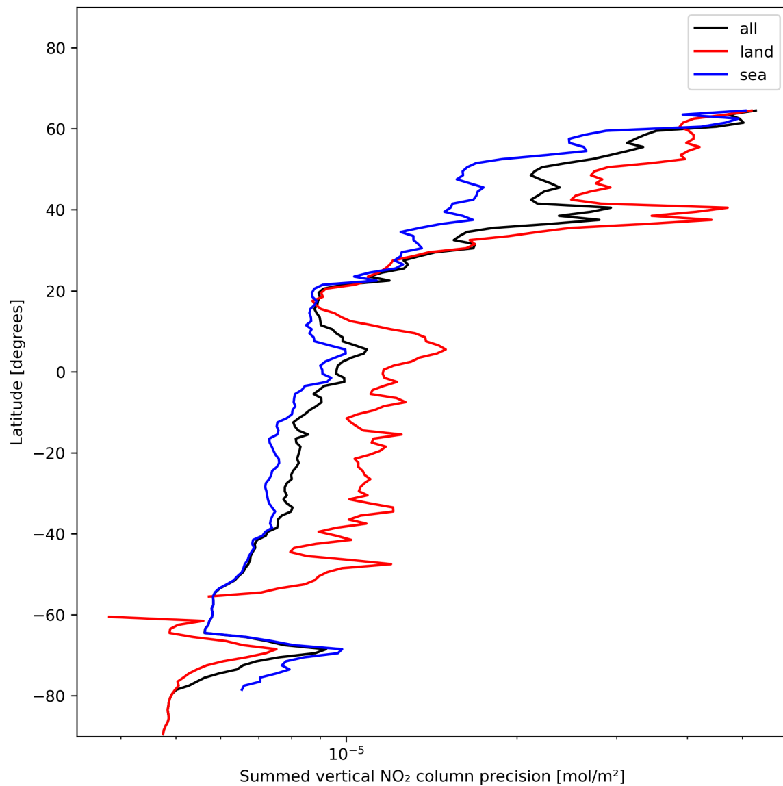
Figure 24: Zonal average of “Summed vertical NO 2 column precision” for 2023-12-27 to 2023-12-29.
