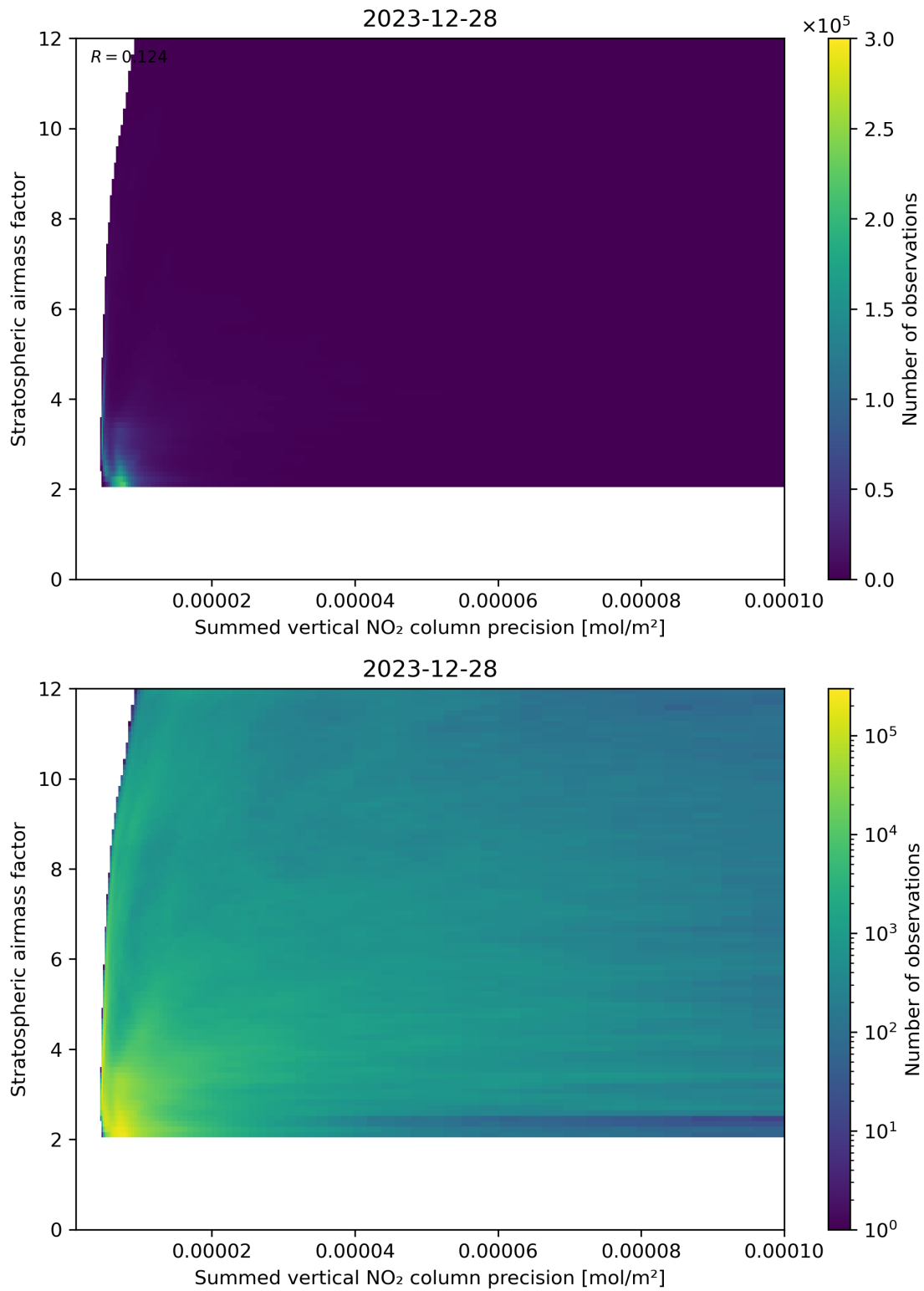
Figure 106: Scatter density plot of “Summed vertical NO 2 column precision” against “Stratospheric airmass factor” for 2023-12-27 to 2023-12-29.
