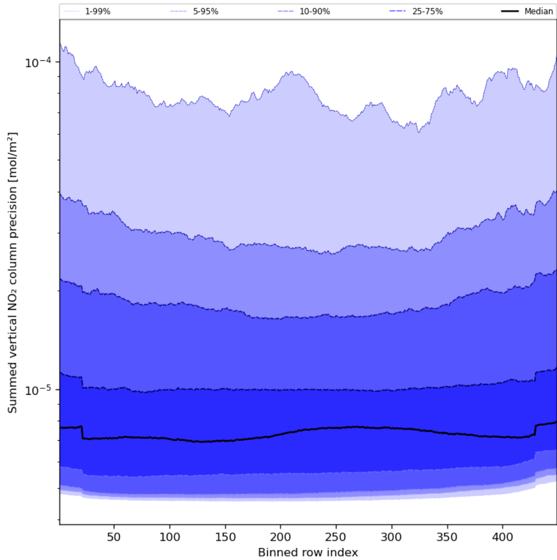
Figure 58: Along track statistics of “Summed vertical NO 2 column precision” for 2023-12-27 to 2023-12-29
