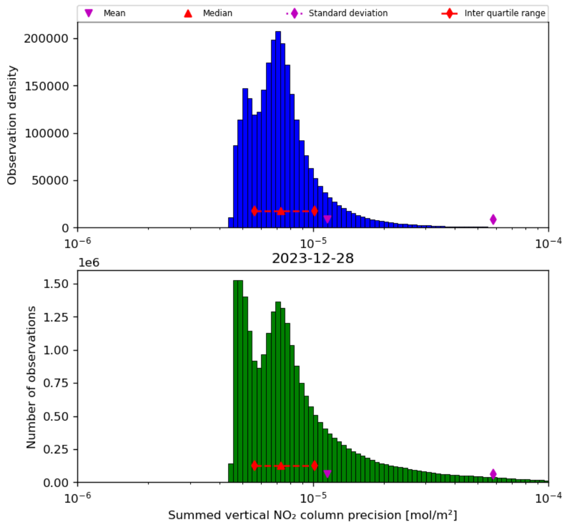
Figure 41: Histogram of “Summed vertical NO 2 column precision” for 2023-12-27 to 2023-12-29
