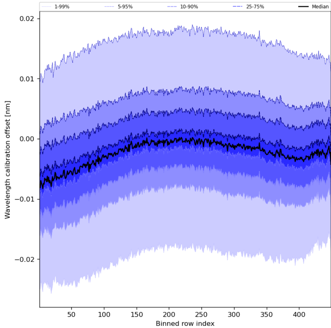
Figure 52: Along track statistics of “Wavelength calibration offset” for 2023-12-27 to 2023-12-29
