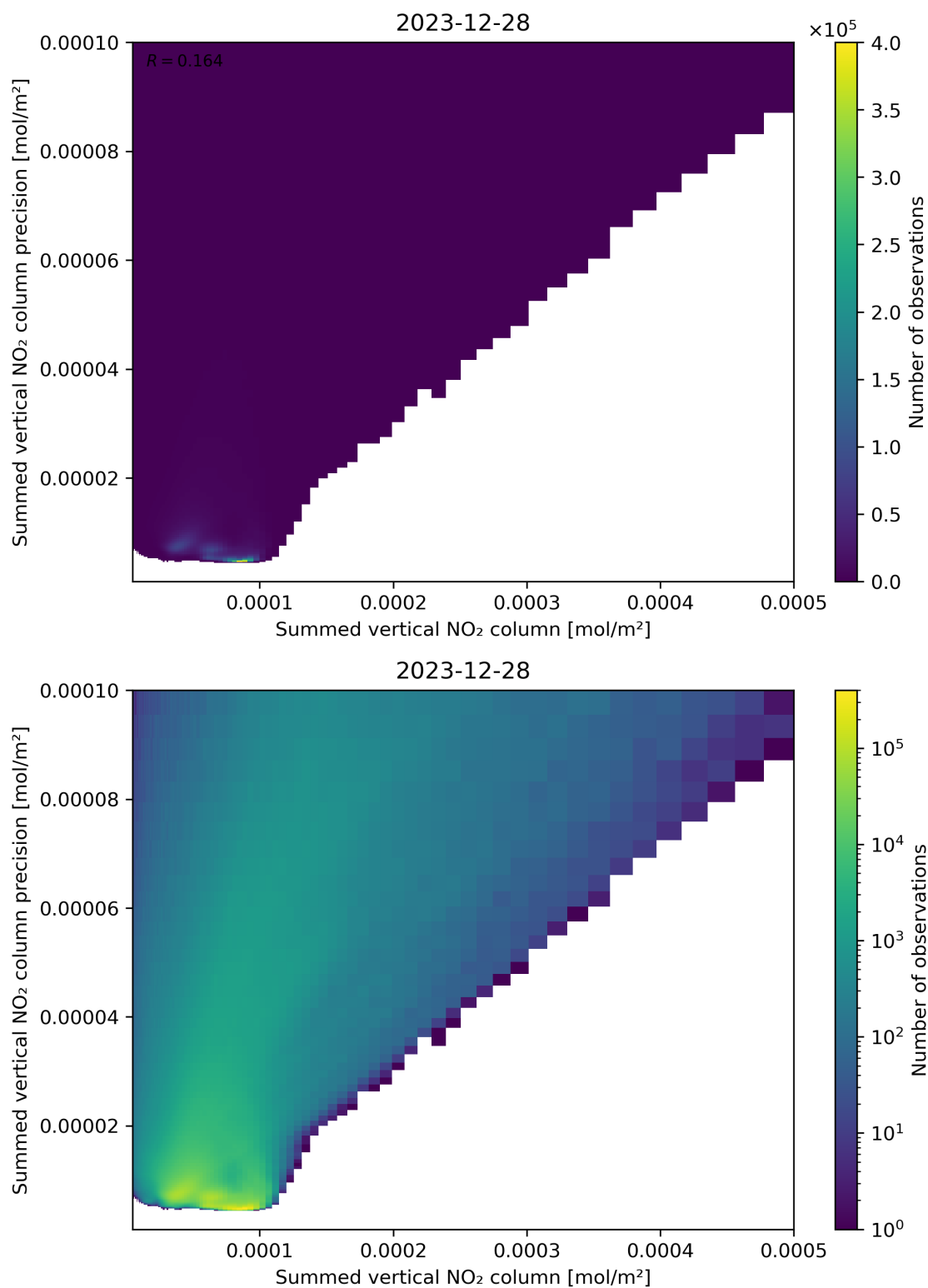
Figure 105: Scatter density plot of “Summed vertical NO 2 column” against “Summed vertical NO 2 column precision” for 2023-12-27 to 2023-12-29.
