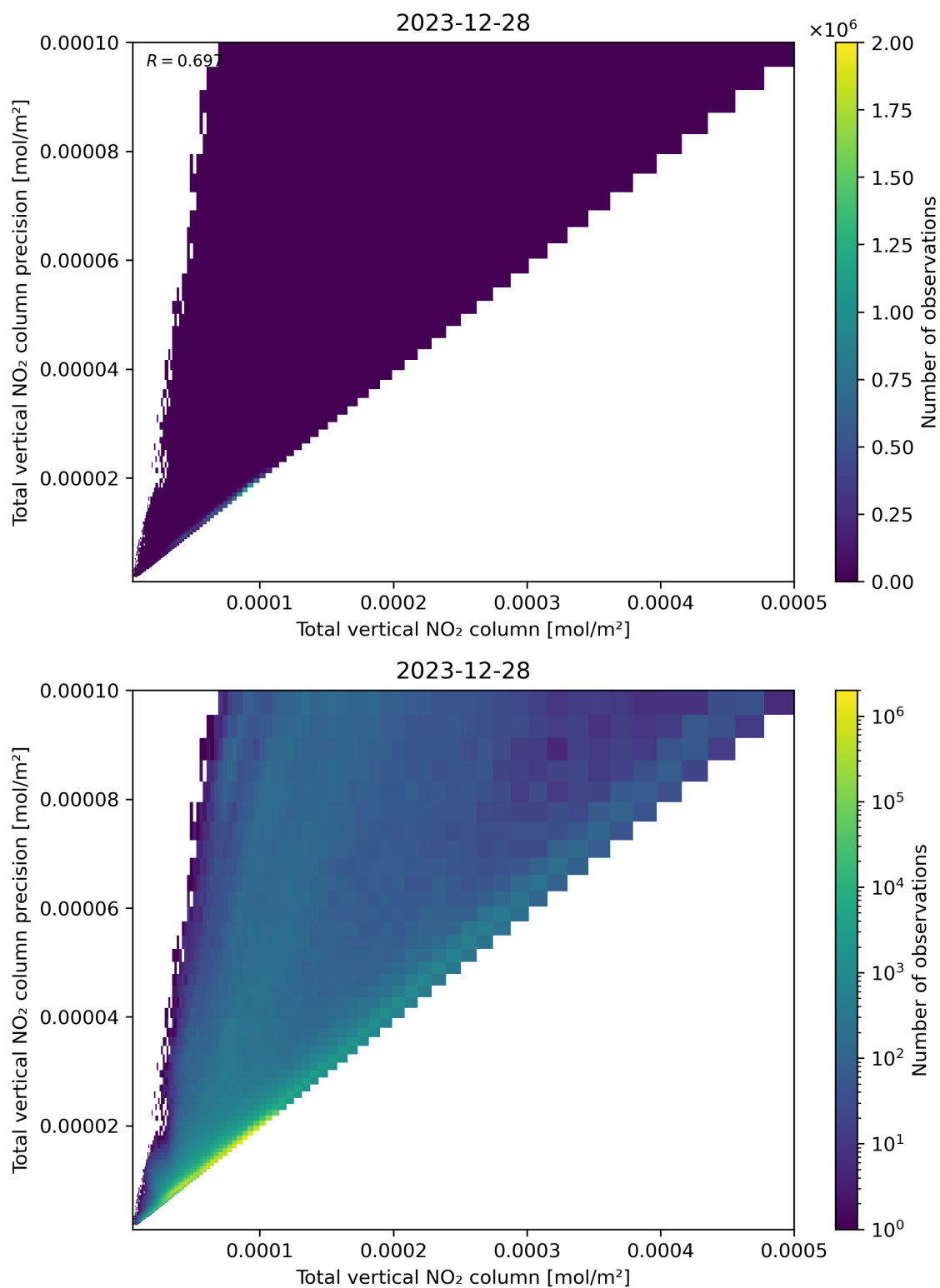
Figure 114: Scatter density plot of “Total vertical NO 2 column” against “Total vertical NO 2 column precision” for 2023-12-27 to 2023-12-29.
