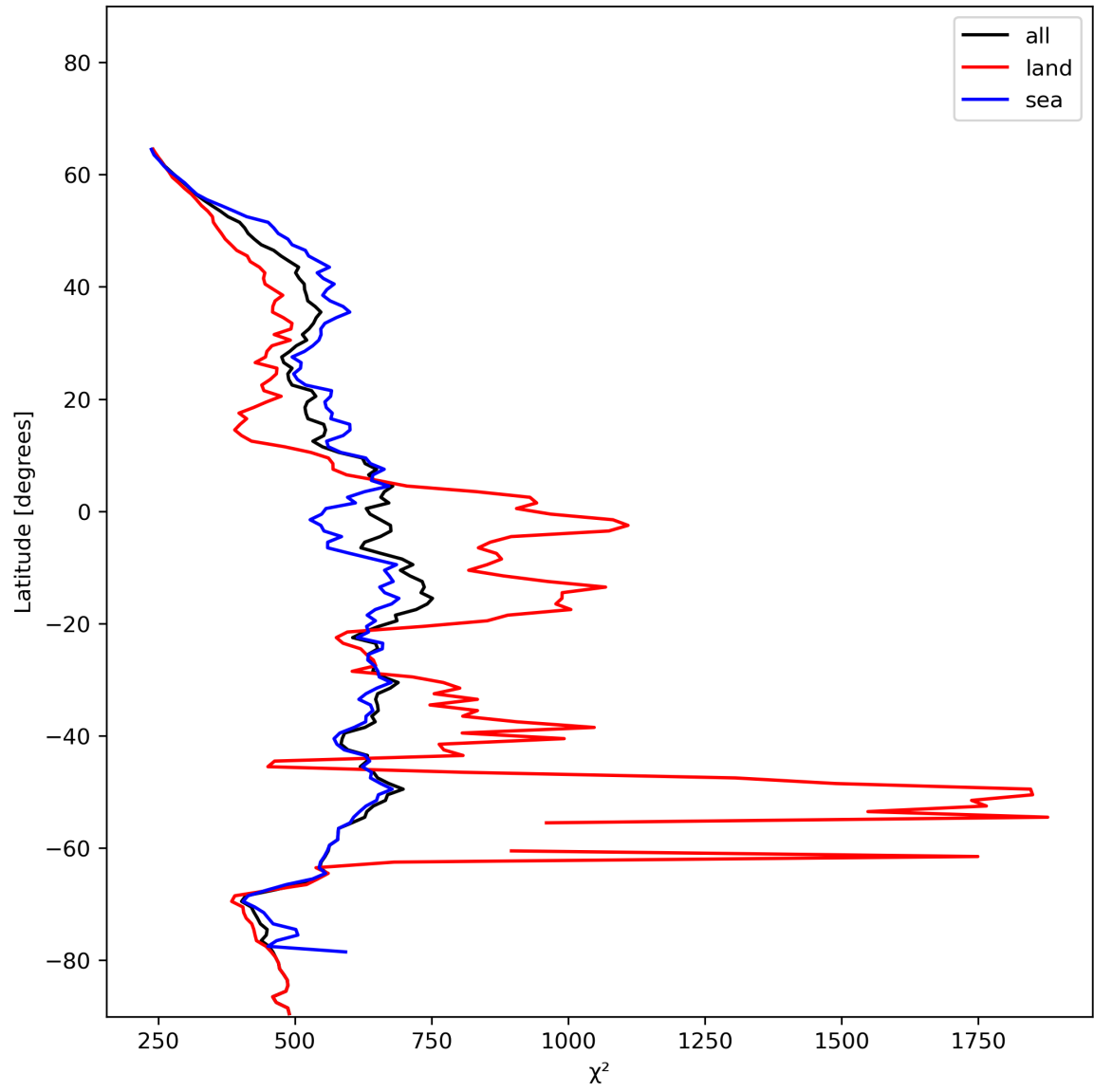
Figure 25: Zonal average of “ \chi^2 ” for 2023-12-27 to 2023-12-29.
