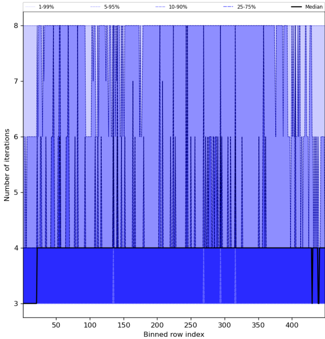
Figure 51: Along track statistics of “Number of iterations” for 2023-12-27 to 2023-12-29
