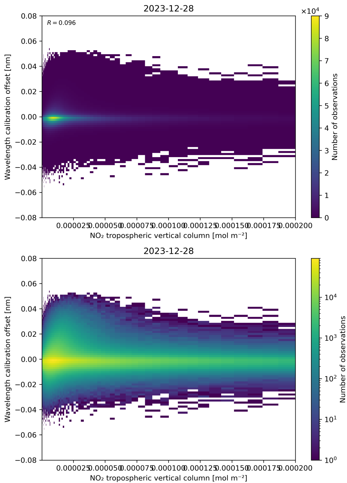
Figure 143: Scatter density plot of “NO 2 tropospheric vertical column” against “Wavelength calibration offset” for 2023-12-27 to 2023-12-29.
