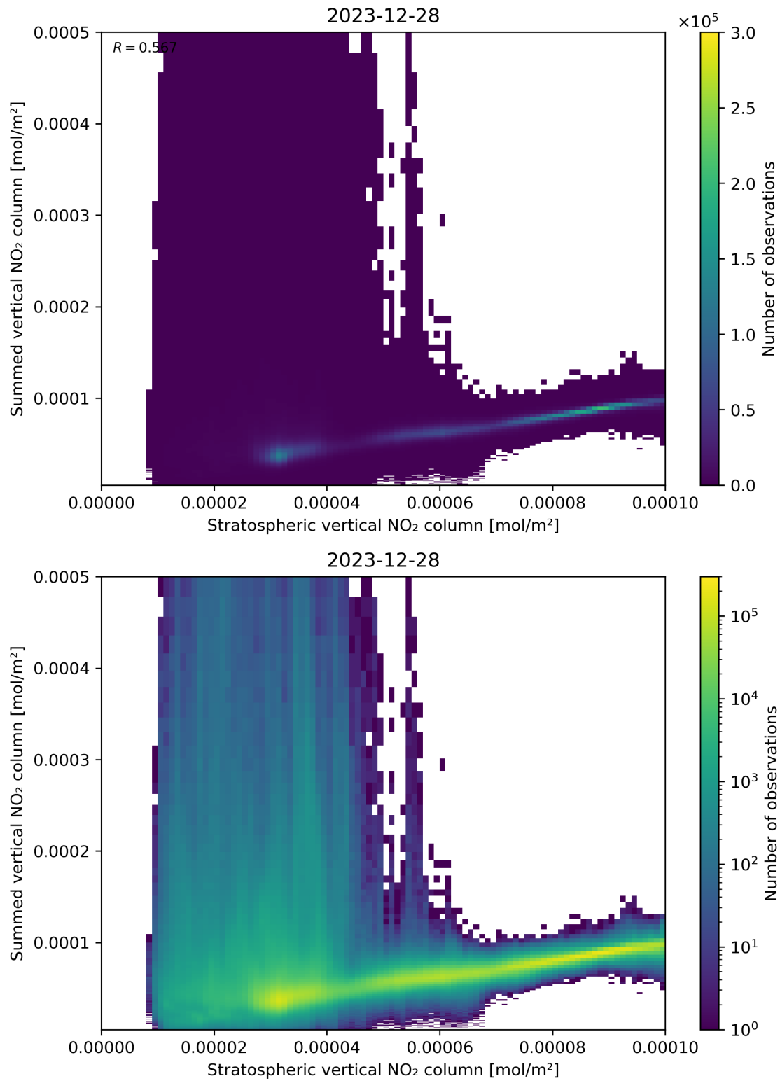
Figure 98: Scatter density plot of “Stratospheric vertical NO 2 column” against “Summed vertical NO 2 column” for 2023-12-27 to 2023-12-29.
