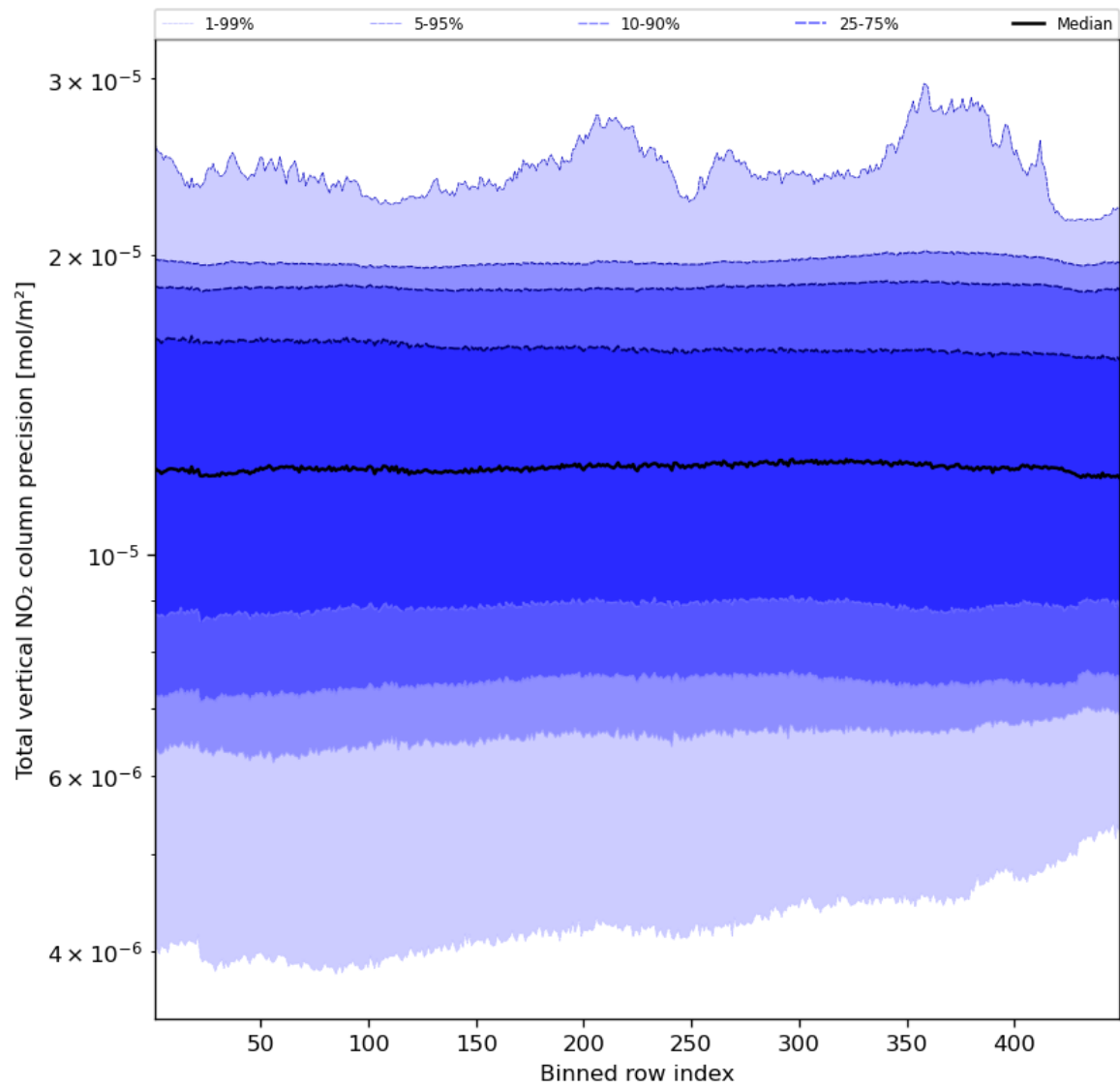
Figure 56: Along track statistics of “Total vertical NO 2 column precision” for 2023-12-27 to 2023-12-29
