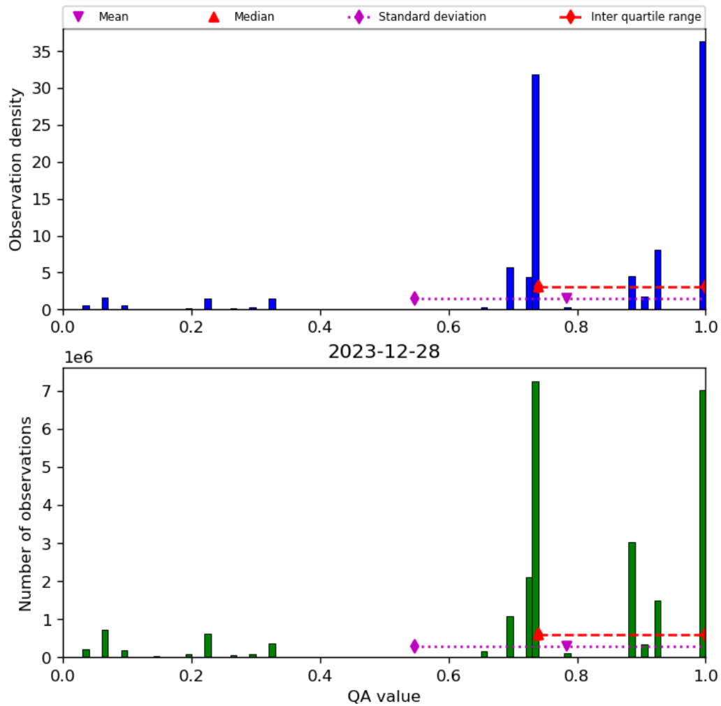
Figure 28: Histogram of “QA value” for 2023-12-27 to 2023-12-29
