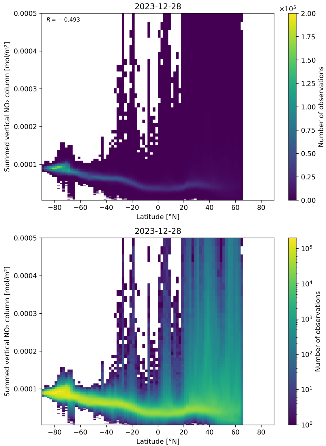
Figure 88: Scatter density plot of “Latitude” against “Summed vertical NO 2 column” for 2023-12-27 to 2023-12-29.
