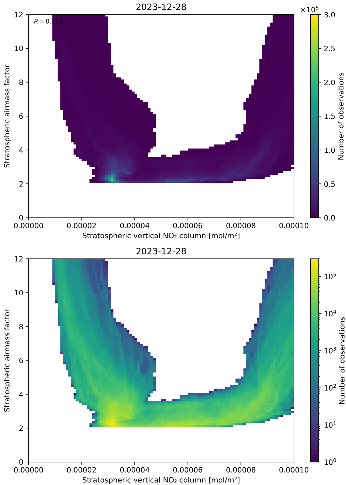
Figure 96: Scatter density plot of “Stratospheric vertical NO 2 column” against “Stratospheric airmass factor” for 2023-12-27 to 2023-12-29.
