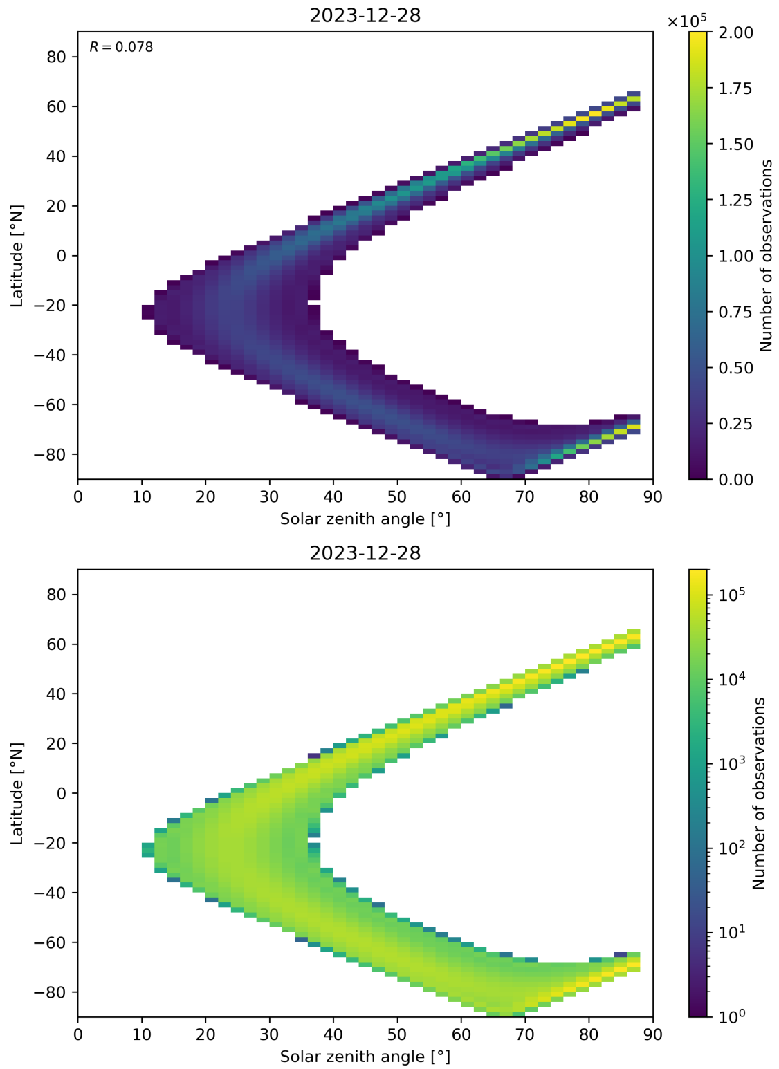
Figure 149: Scatter density plot of “Solar zenith angle” against “Latitude” for 2023-12-27 to 2023-12-29.
