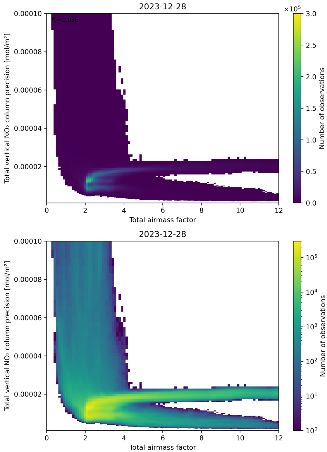
Figure 68: Scatter density plot of “Total airmass factor” against “Total vertical NO 2 column precision” for 2023-12-27 to 2023-12-29.
