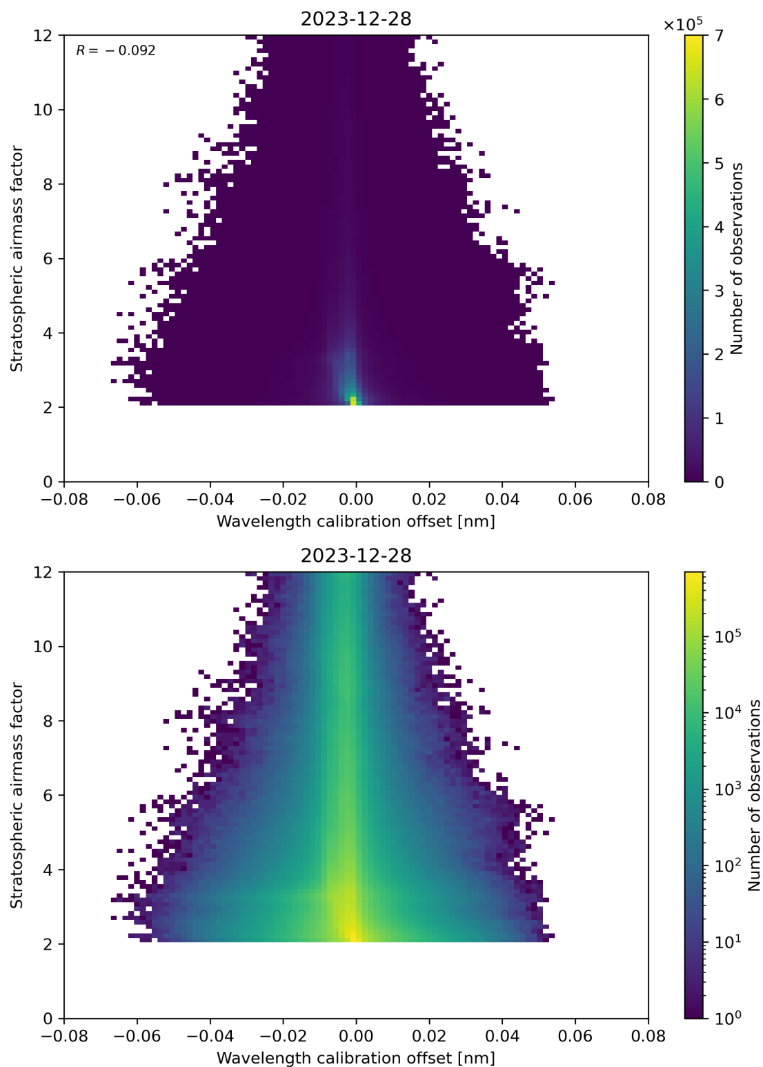
Figure 174: Scatter density plot of “Wavelength calibration offset” against “Stratospheric airmass factor” for 2023-12-27 to 2023-12-29.
