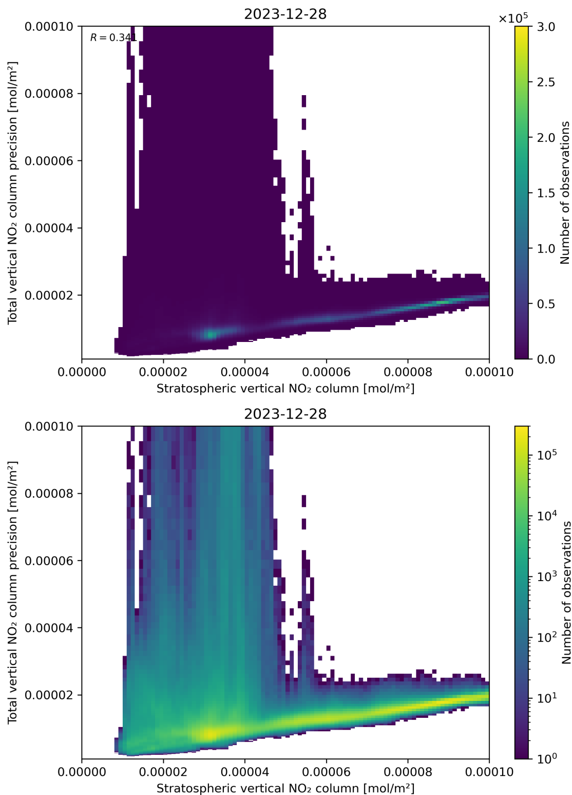
Figure 101: Scatter density plot of “Stratospheric vertical NO 2 column” against “Total vertical NO 2 column precision” for 2023-12-27 to 2023-12-29.
