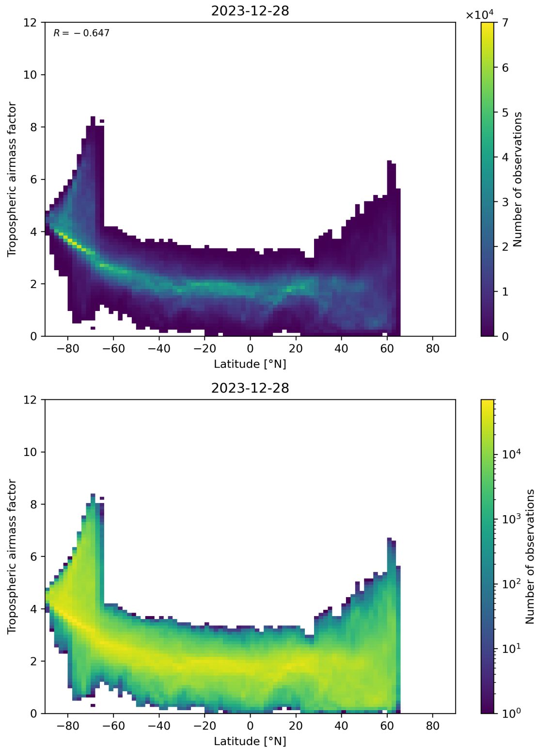
Figure 85: Scatter density plot of “Latitude” against “Tropospheric airmass factor” for 2023-12-27 to 2023-12-29.
