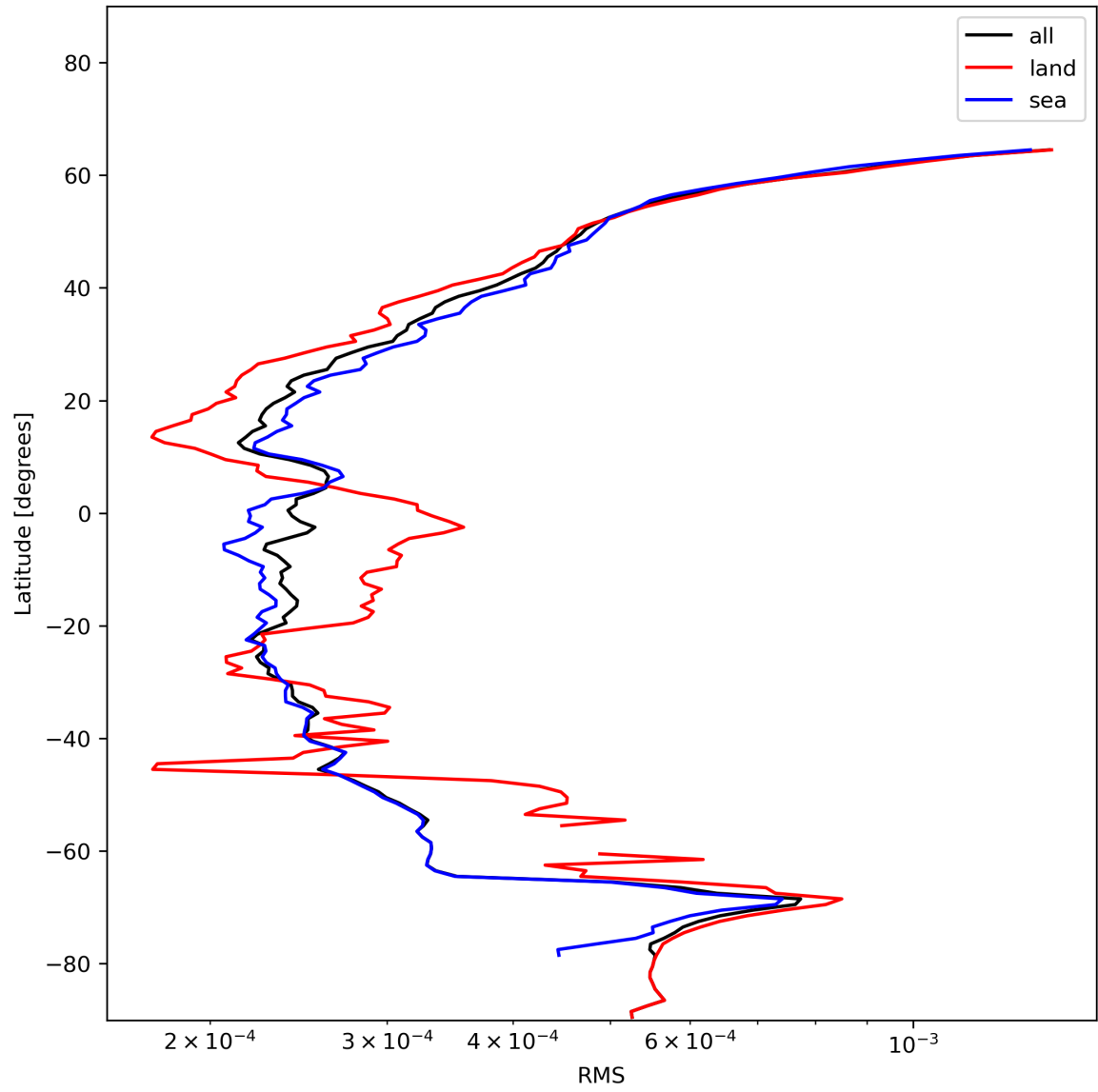
Figure 26: Zonal average of “RMS” for 2023-12-27 to 2023-12-29.
