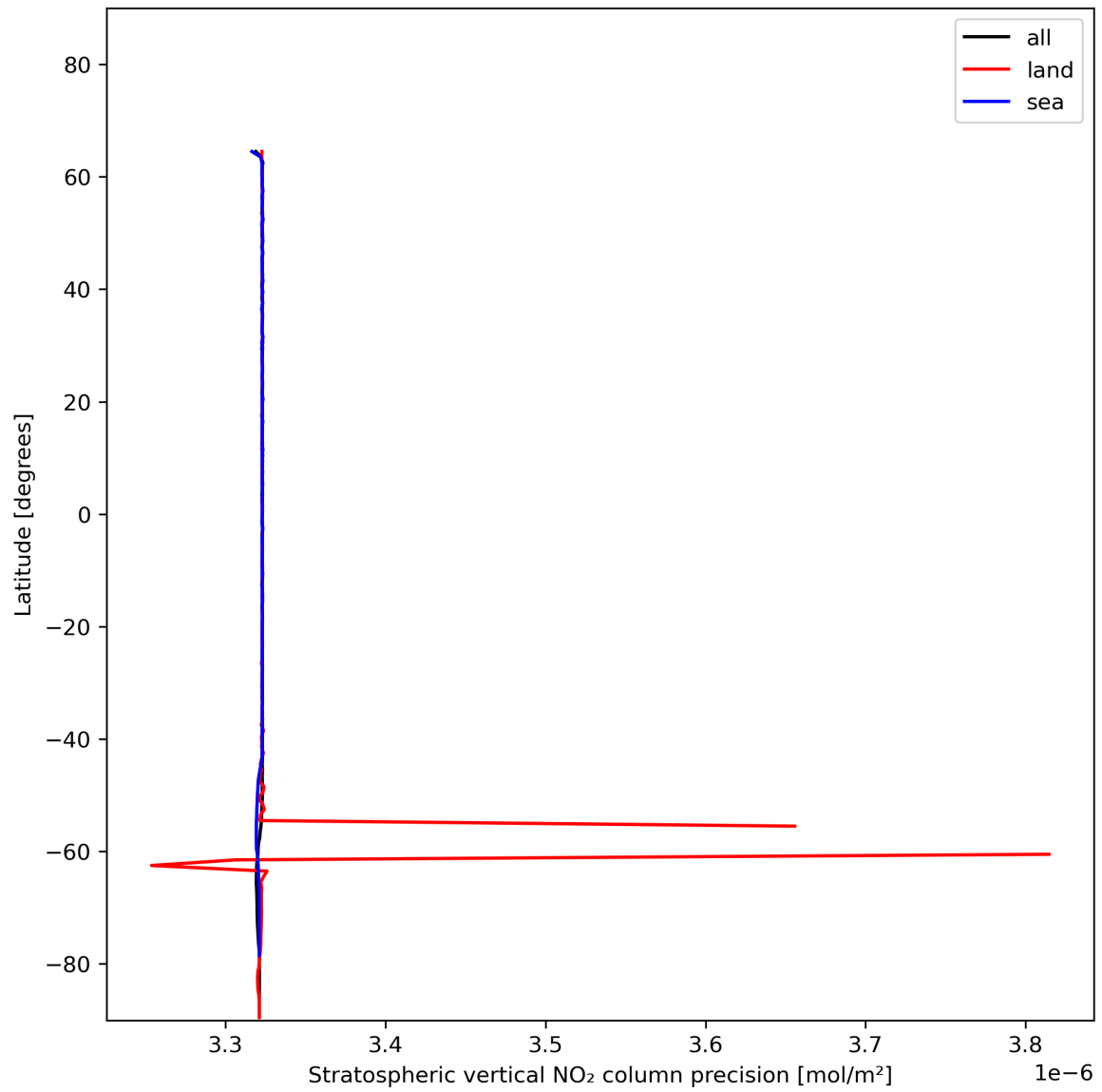
Figure 20: Zonal average of “Stratospheric vertical NO 2 column precision” for 2023-12-27 to 2023-12-29.
