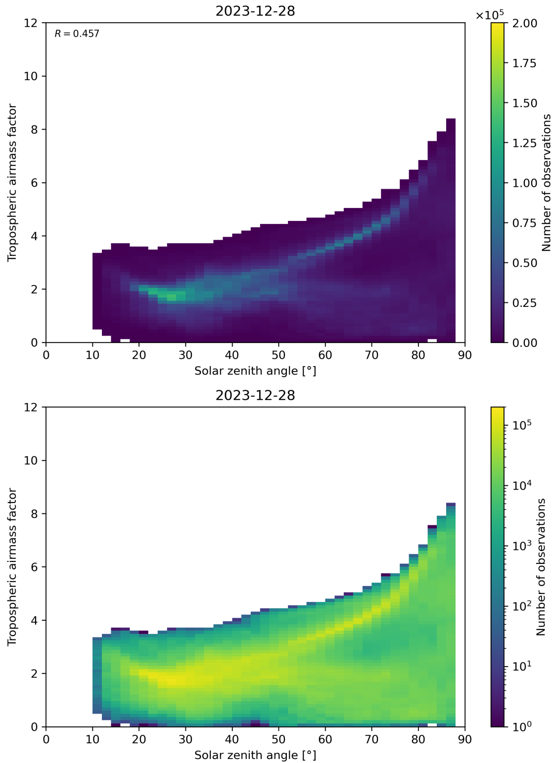
Figure 147: Scatter density plot of “Solar zenith angle” against “Tropospheric airmass factor” for 2023-12-27 to 2023-12-29.
