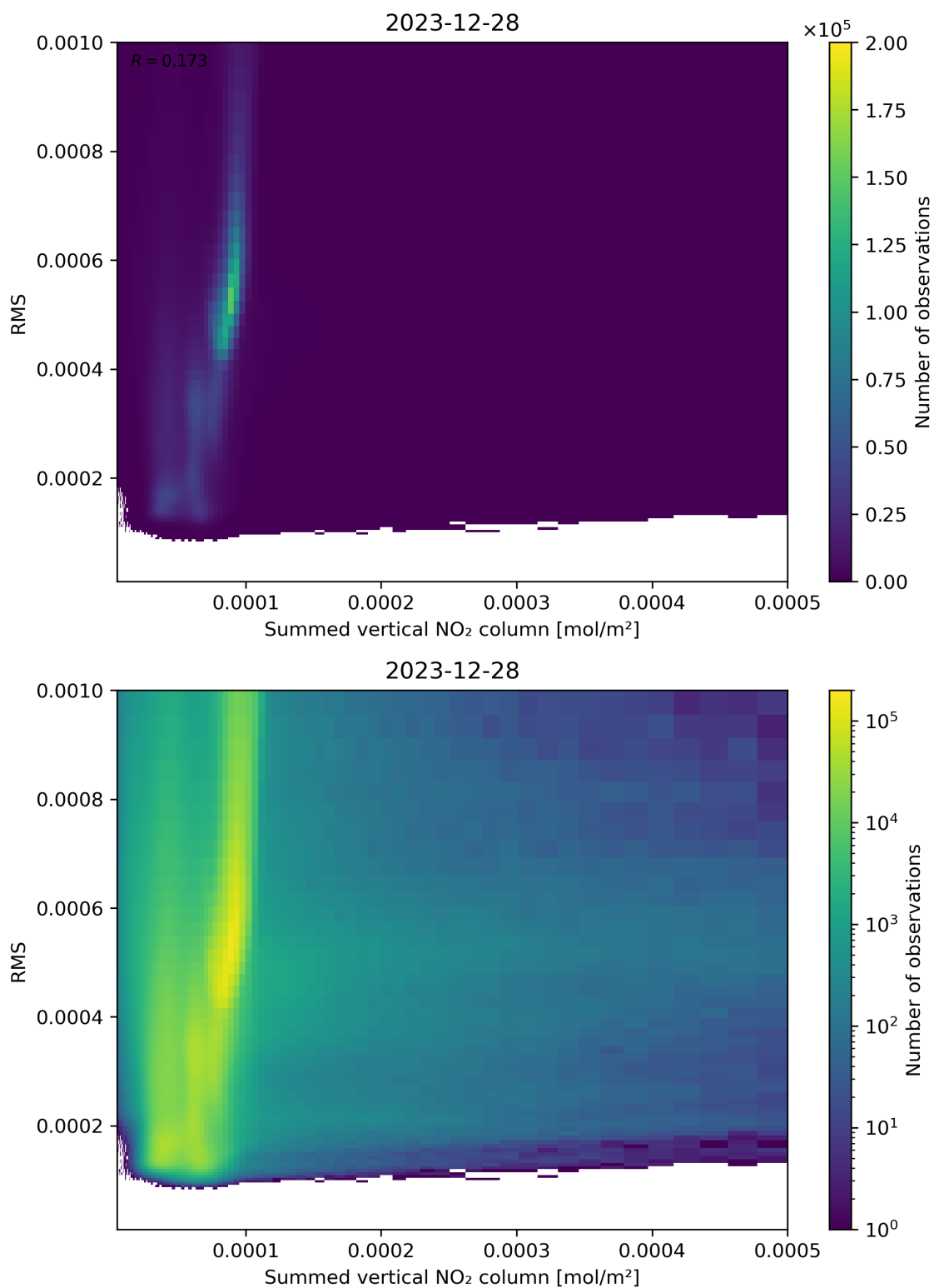
Figure 109: Scatter density plot of “Summed vertical NO 2 column” against “RMS” for 2023-12-27 to 2023-12-29.
