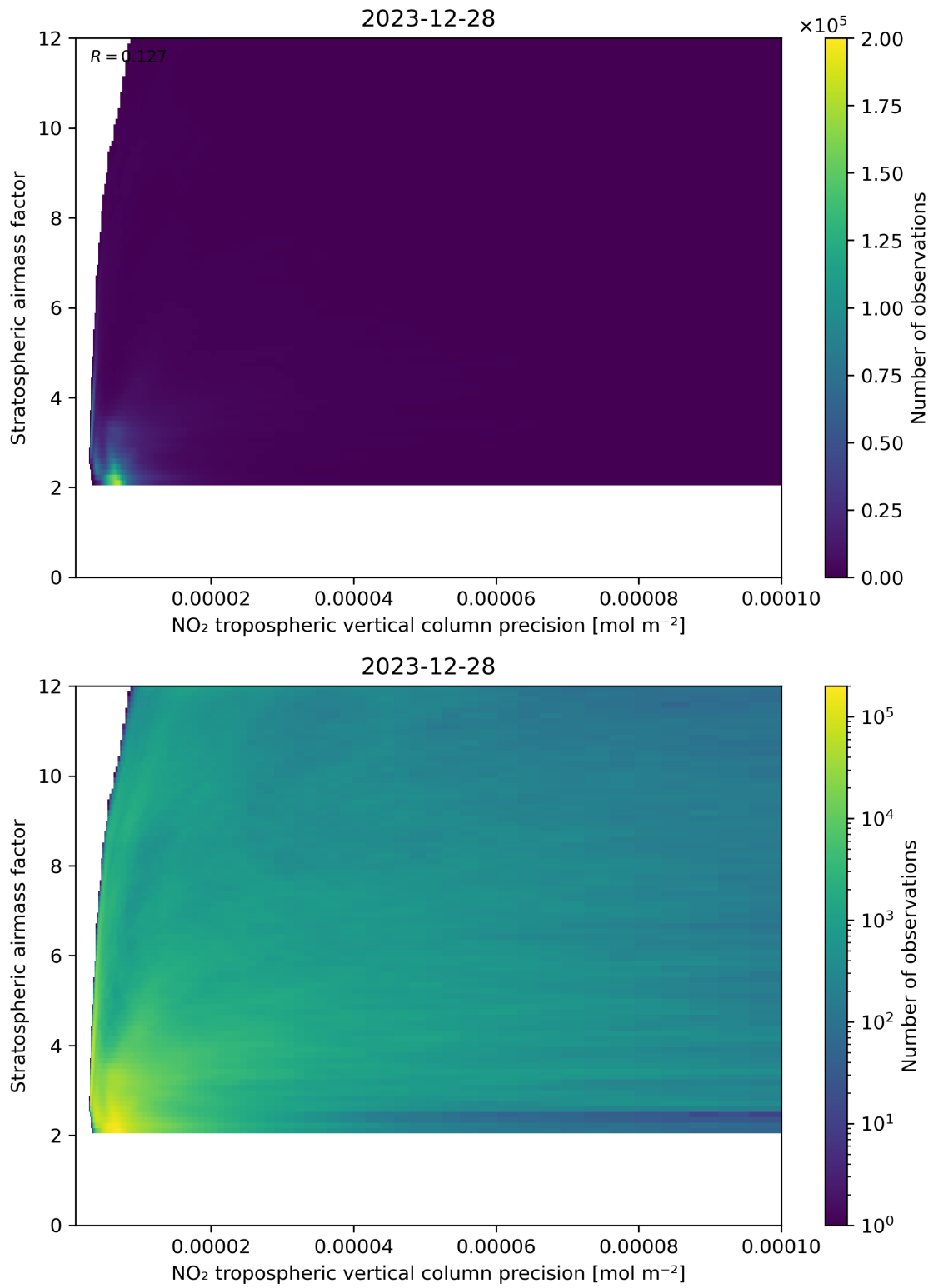
Figure 131: Scatter density plot of “NO 2 tropospheric vertical column precision” against “Stratospheric airmass factor” for 2023-12-27 to 2023-12-29.
