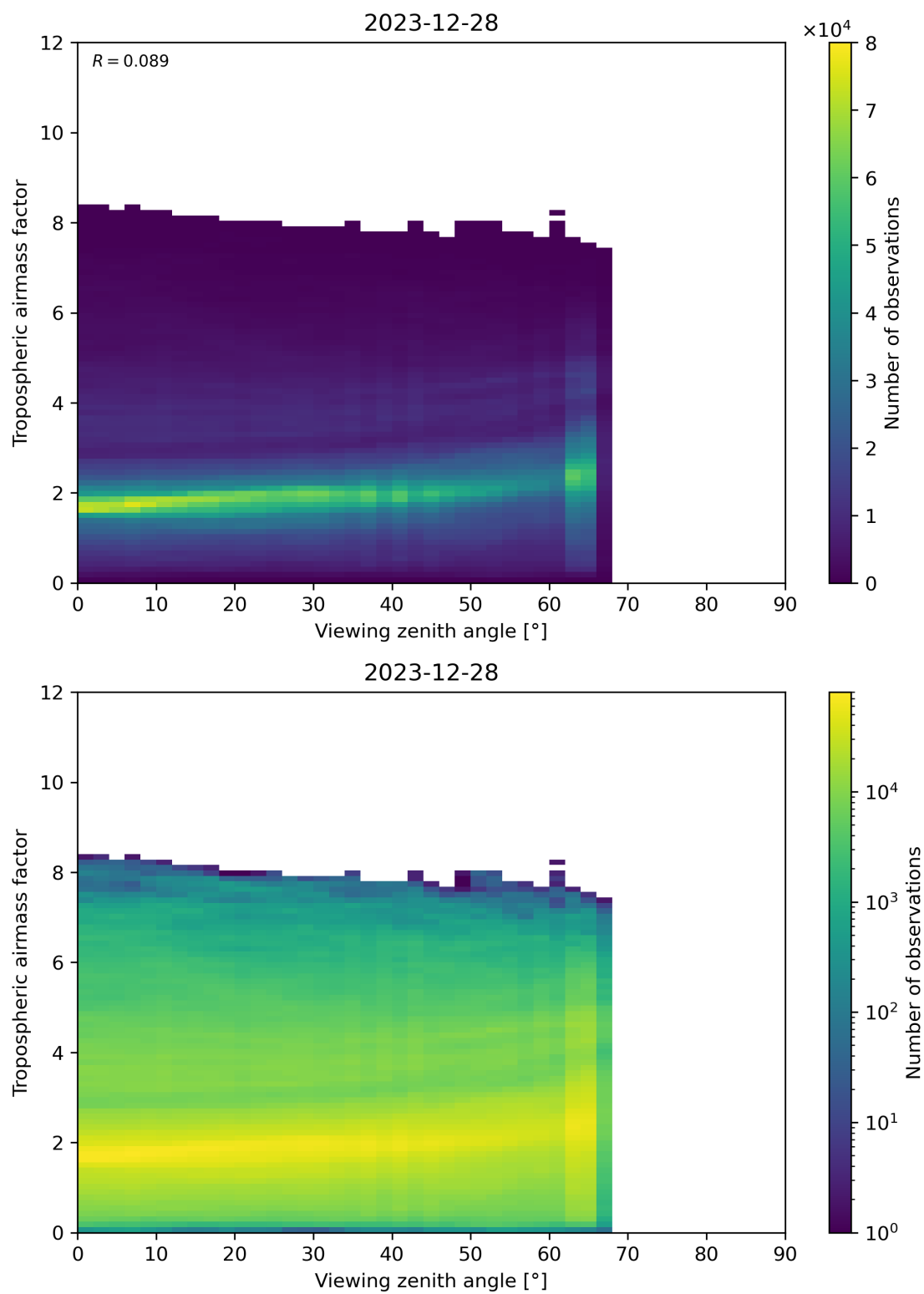
Figure 161: Scatter density plot of “Viewing zenith angle” against “Tropospheric airmass factor” for 2023-12-27 to 2023-12-29.
