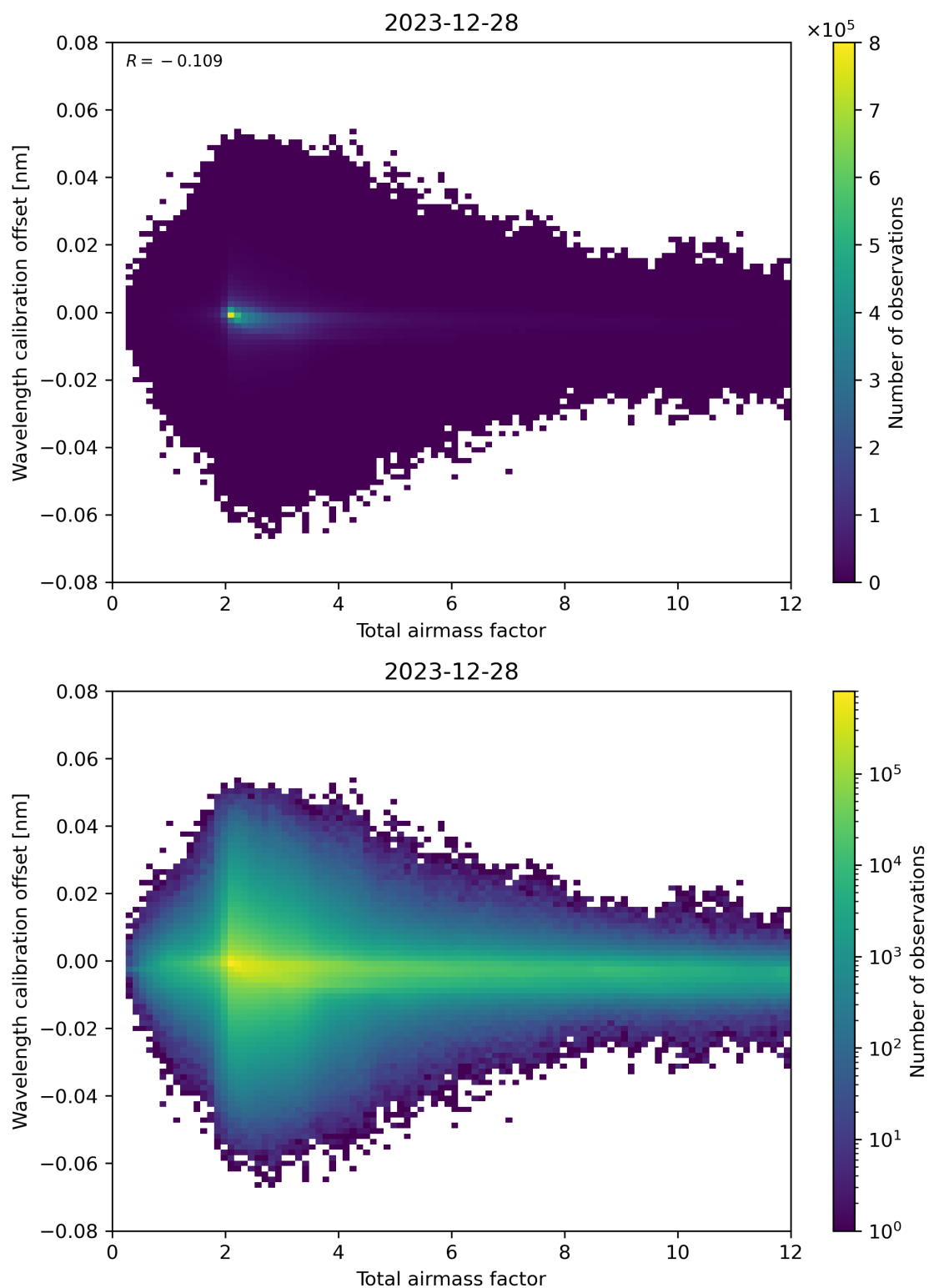
Figure 70: Scatter density plot of “Total airmass factor” against “Wavelength calibration offset” for 2023-12-27 to 2023-12-29.
