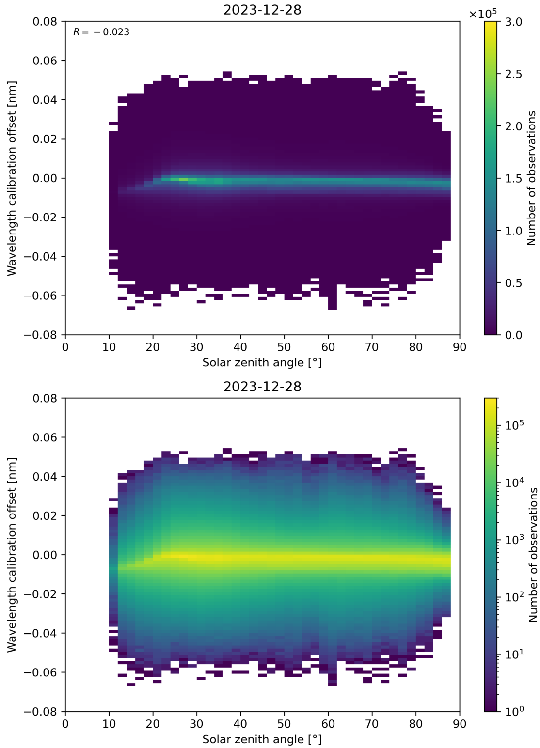
Figure 158: Scatter density plot of “Solar zenith angle” against “Wavelength calibration offset” for 2023-12-27 to 2023-12-29.
