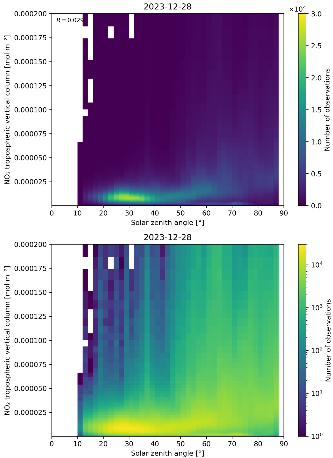
Figure 155: Scatter density plot of “Solar zenith angle” against “NO 2 tropospheric vertical column” for 2023-12-27 to 2023-12-29.
