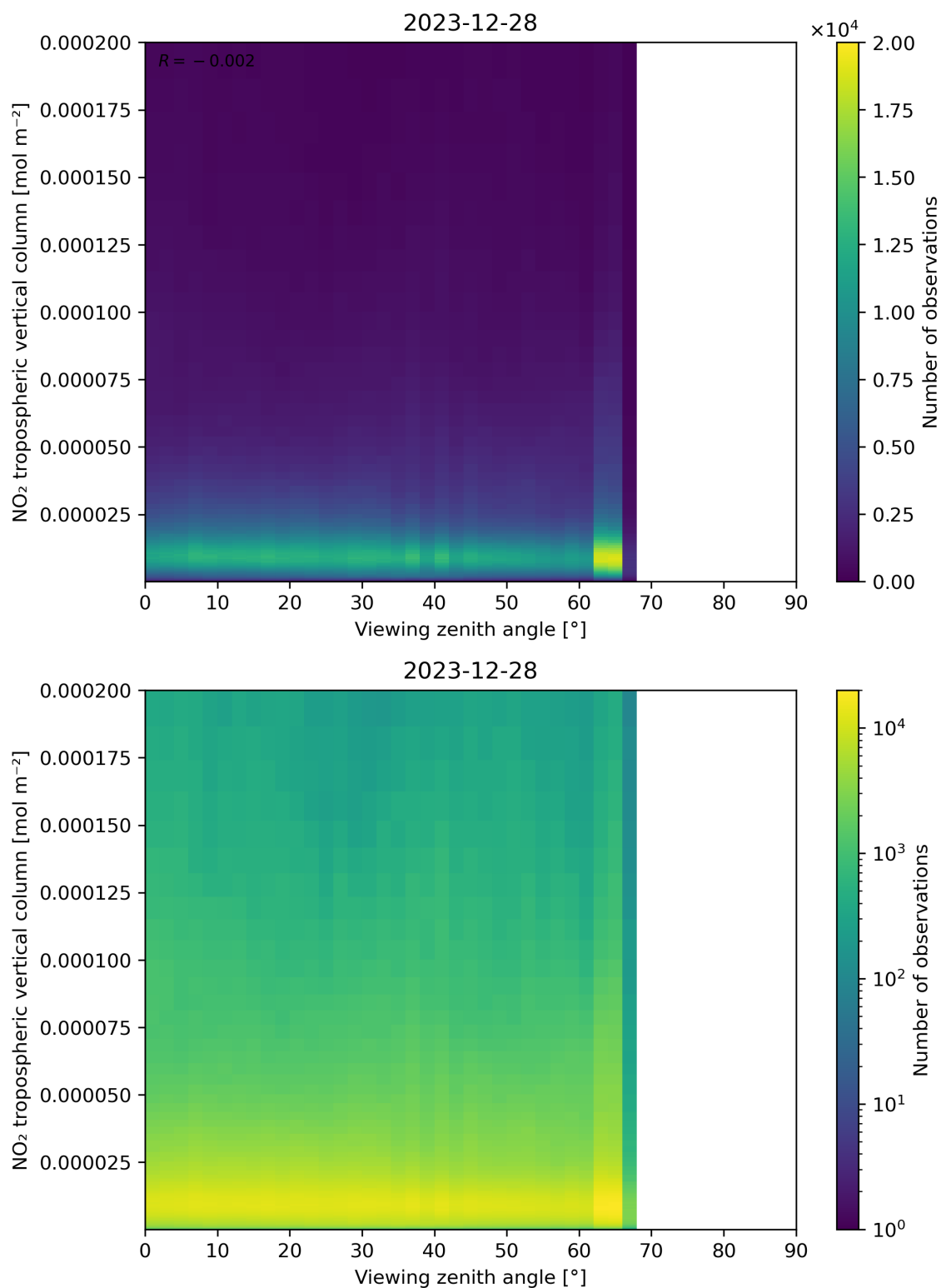
Figure 169: Scatter density plot of “Viewing zenith angle” against “NO 2 tropospheric vertical column” for 2023-12-27 to 2023-12-29.
