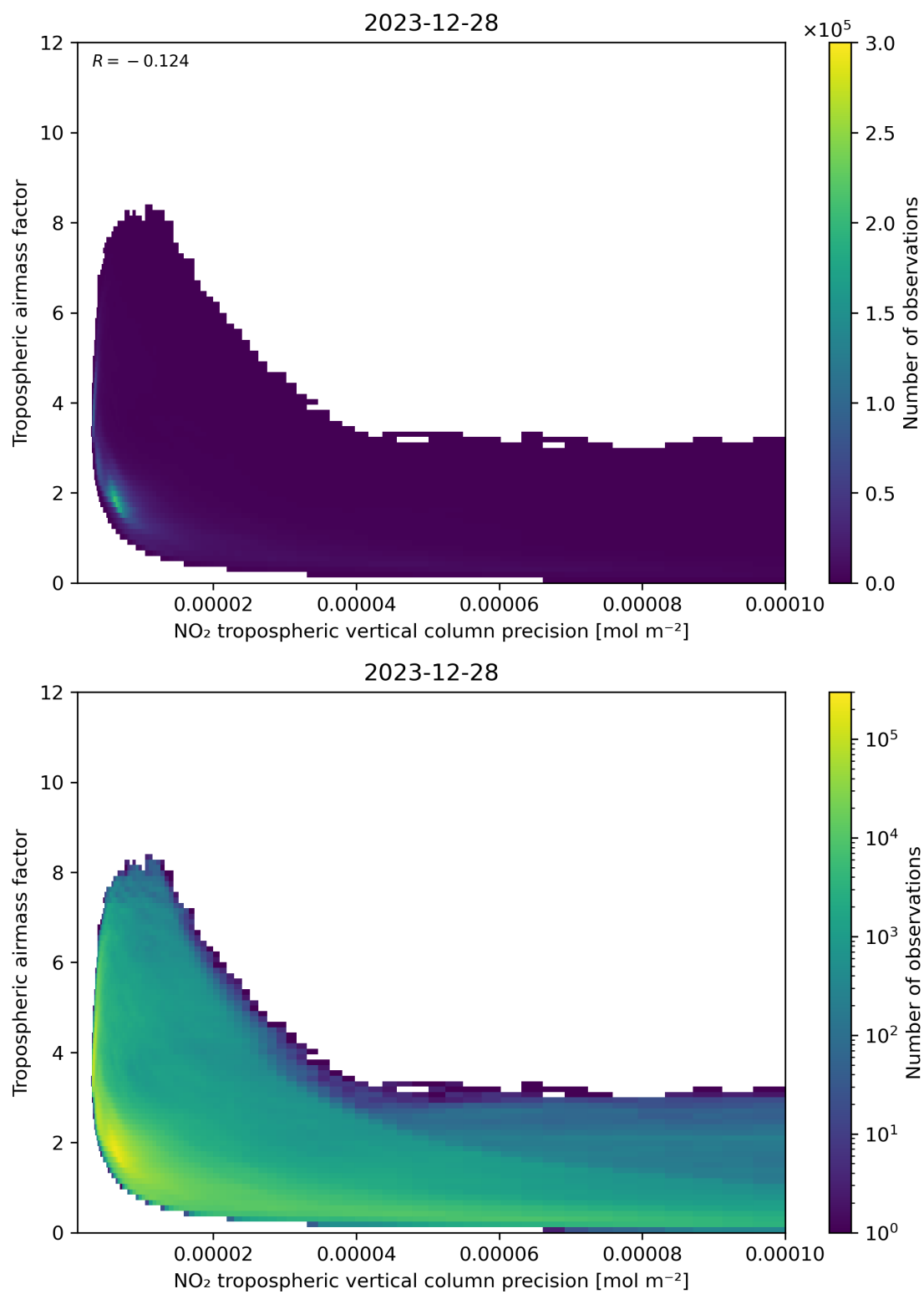
Figure 133: Scatter density plot of “NO 2 tropospheric vertical column precision” against “Tropospheric airmass factor” for 2023-12-27 to 2023-12-29.
