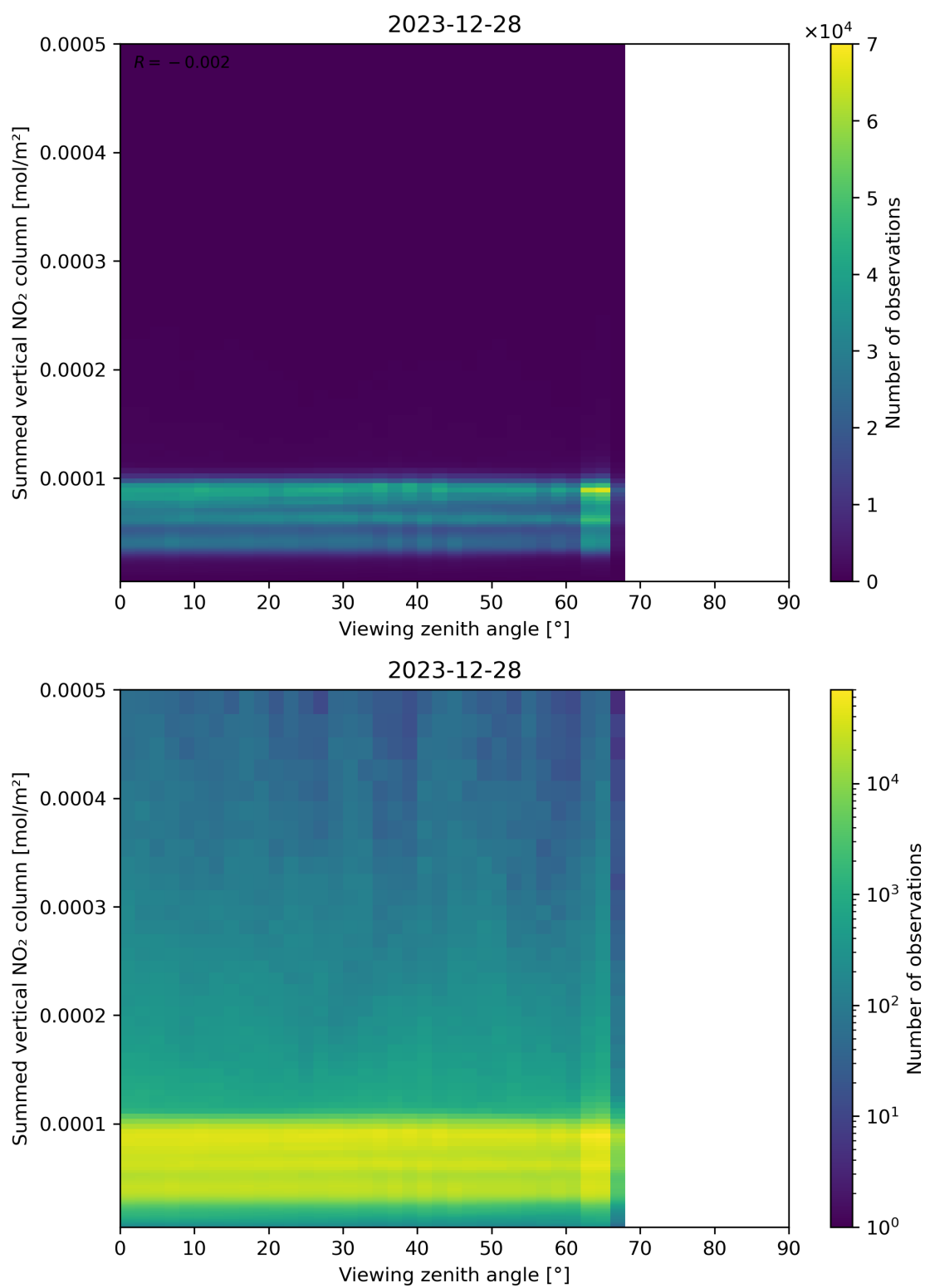
Figure 165: Scatter density plot of “Viewing zenith angle” against “Summed vertical NO 2 column” for 2023-12-27 to 2023-12-29.
