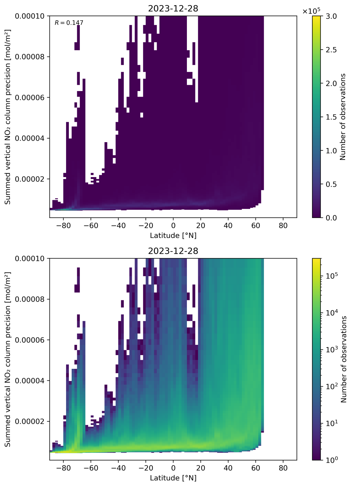
Figure 89: Scatter density plot of “Latitude” against “Summed vertical NO 2 column precision” for 2023-12-27 to 2023-12-29.
