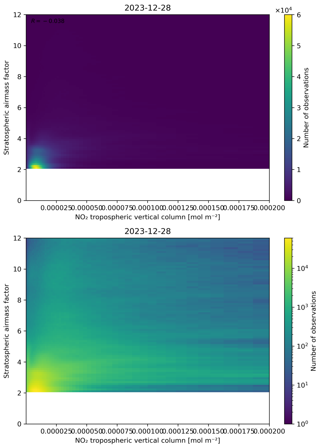
Figure 121: Scatter density plot of “NO 2 tropospheric vertical column” against “Stratospheric airmass factor” for 2023-12-27 to 2023-12-29.
