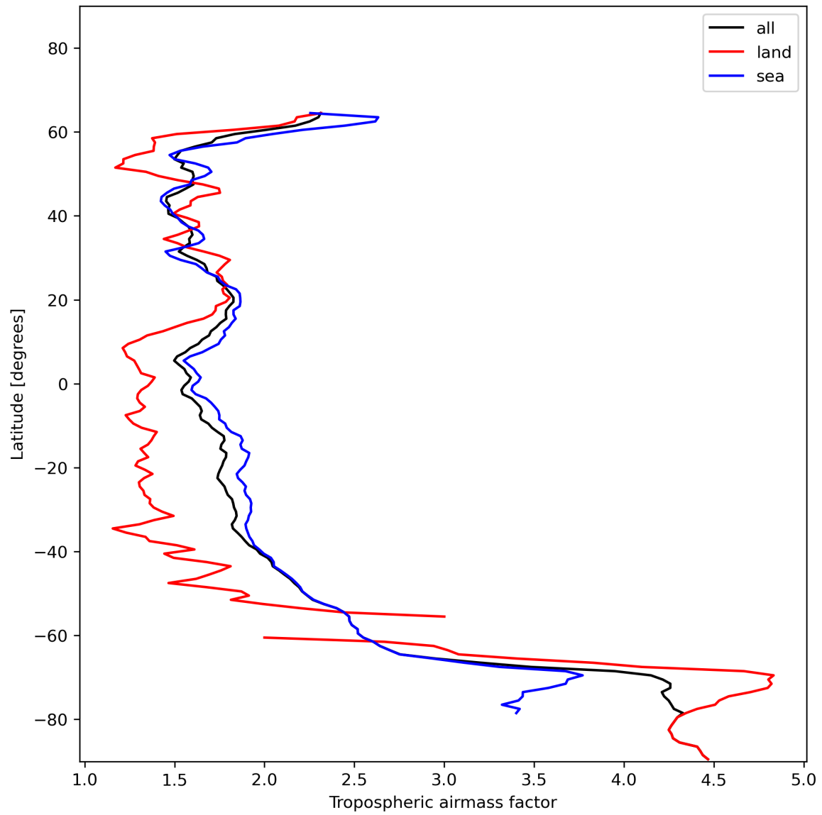
Figure 14: Zonal average of “Tropospheric airmass factor” for 2023-12-27 to 2023-12-29.
