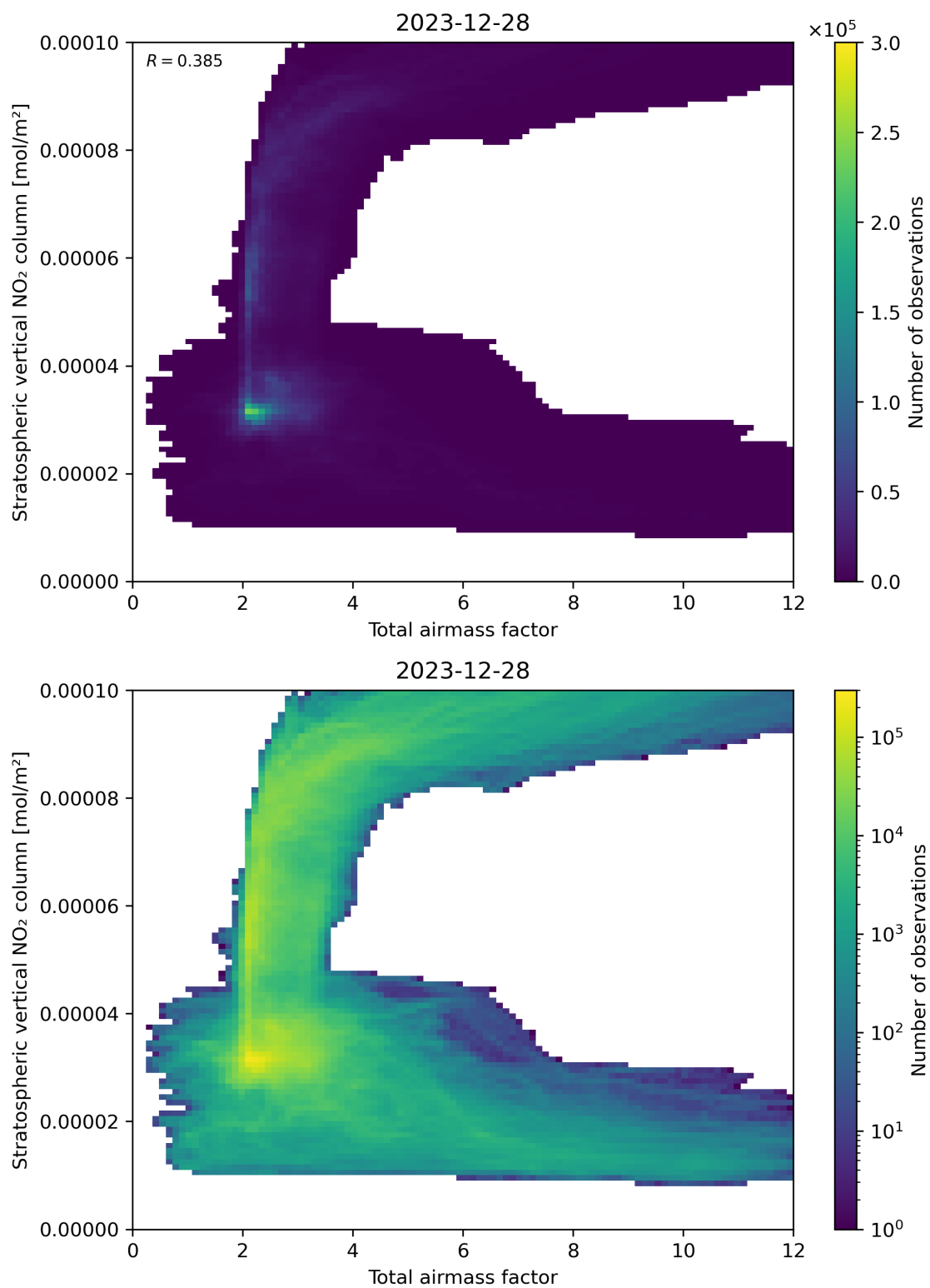
Figure 64: Scatter density plot of “Total airmass factor” against “Stratospheric vertical \text{NO}_2 column” for 2023-12-27 to 2023-12-29.
