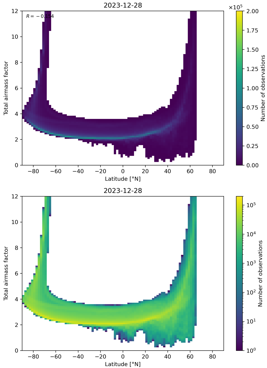
Figure 84: Scatter density plot of “Latitude” against “Total airmass factor” for 2023-12-27 to 2023-12-29.
