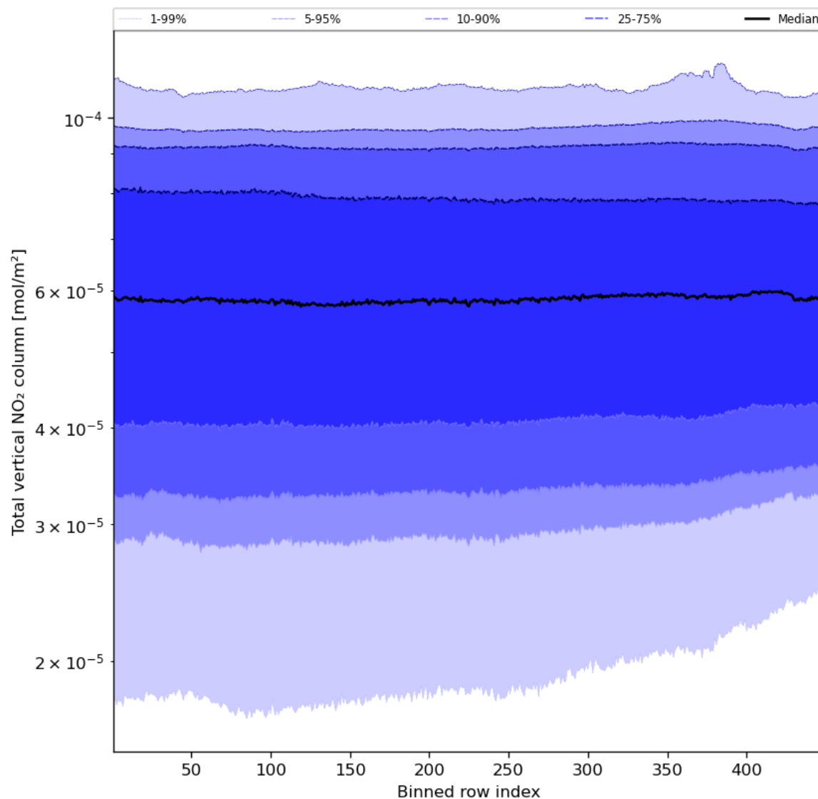
Figure 55: Along track statistics of “Total vertical NO 2 column” for 2023-12-27 to 2023-12-29
