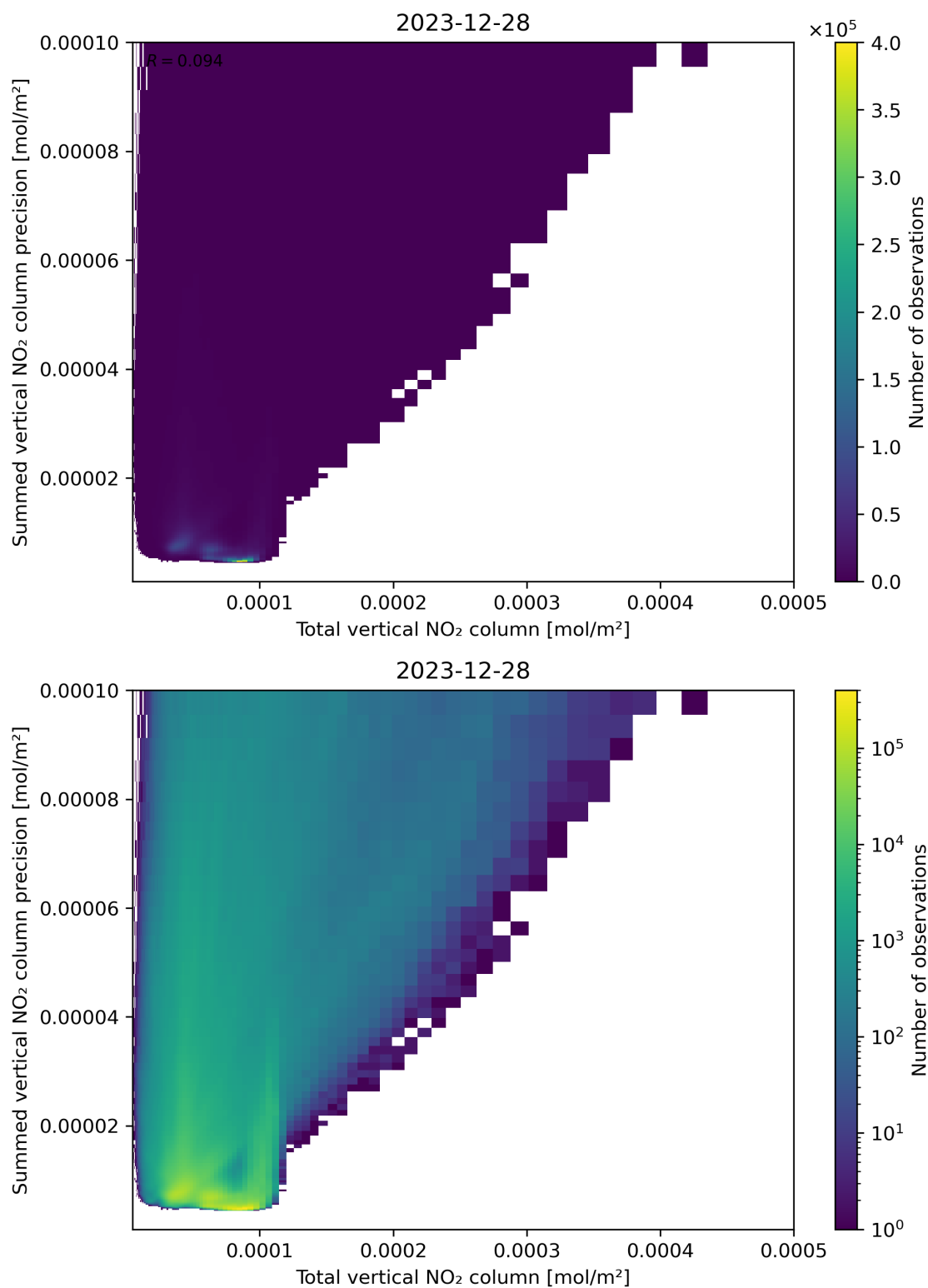
Figure 113: Scatter density plot of “Total vertical NO 2 column” against “Summed vertical NO 2 column precision” for 2023-12-27 to 2023-12-29.
