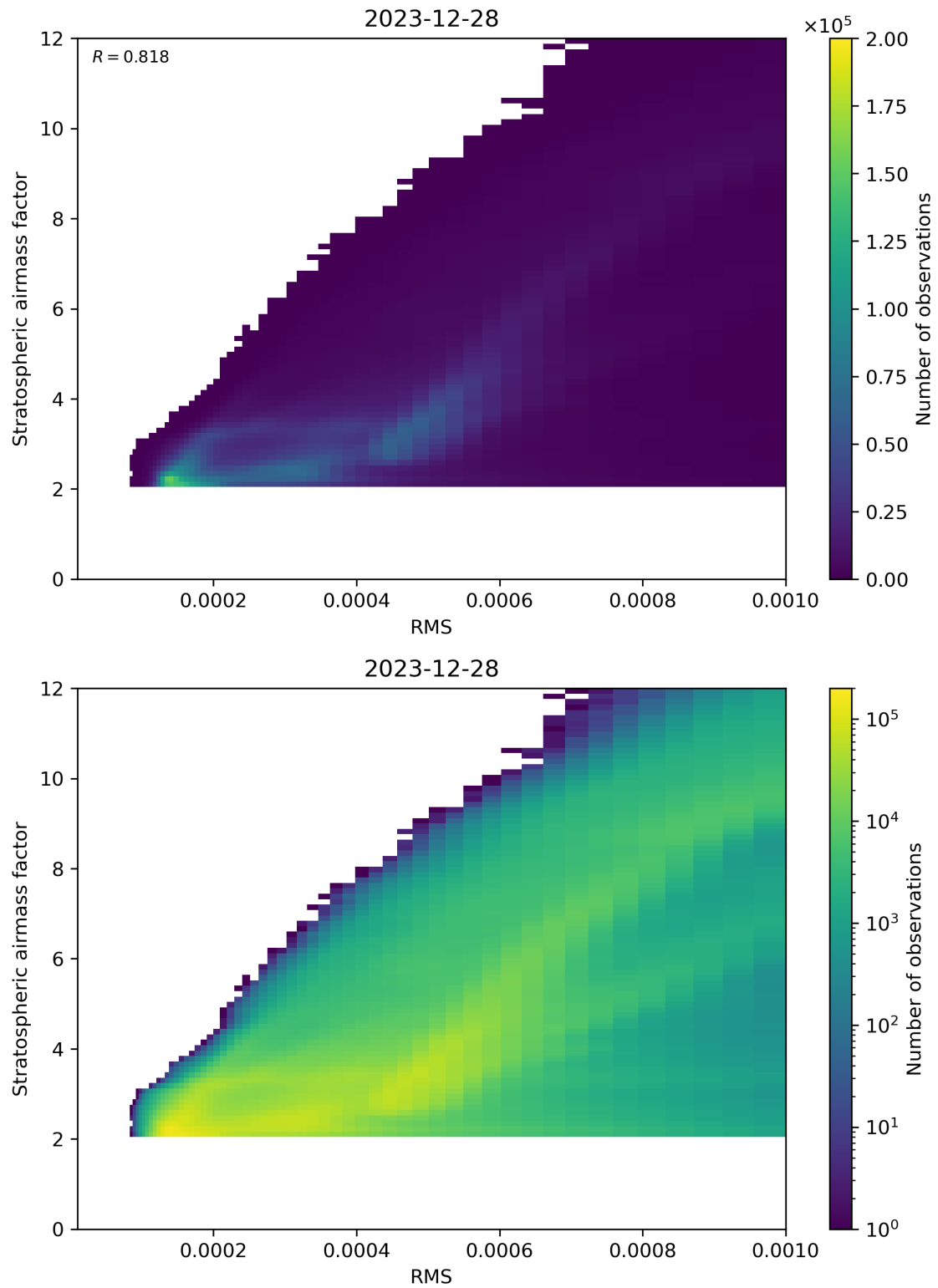
Figure 144: Scatter density plot of “RMS” against “Stratospheric airmass factor” for 2023-12-27 to 2023-12-29.
