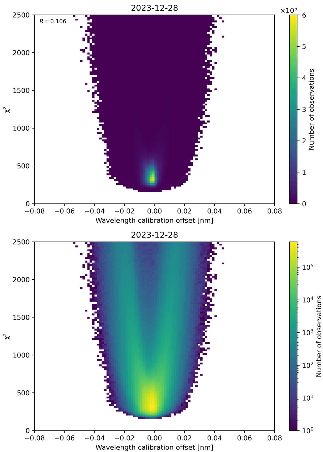
Figure 175: Scatter density plot of “Wavelength calibration offset” against “ \chi^2 ” for 2023-12-27 to 2023-12-29.
