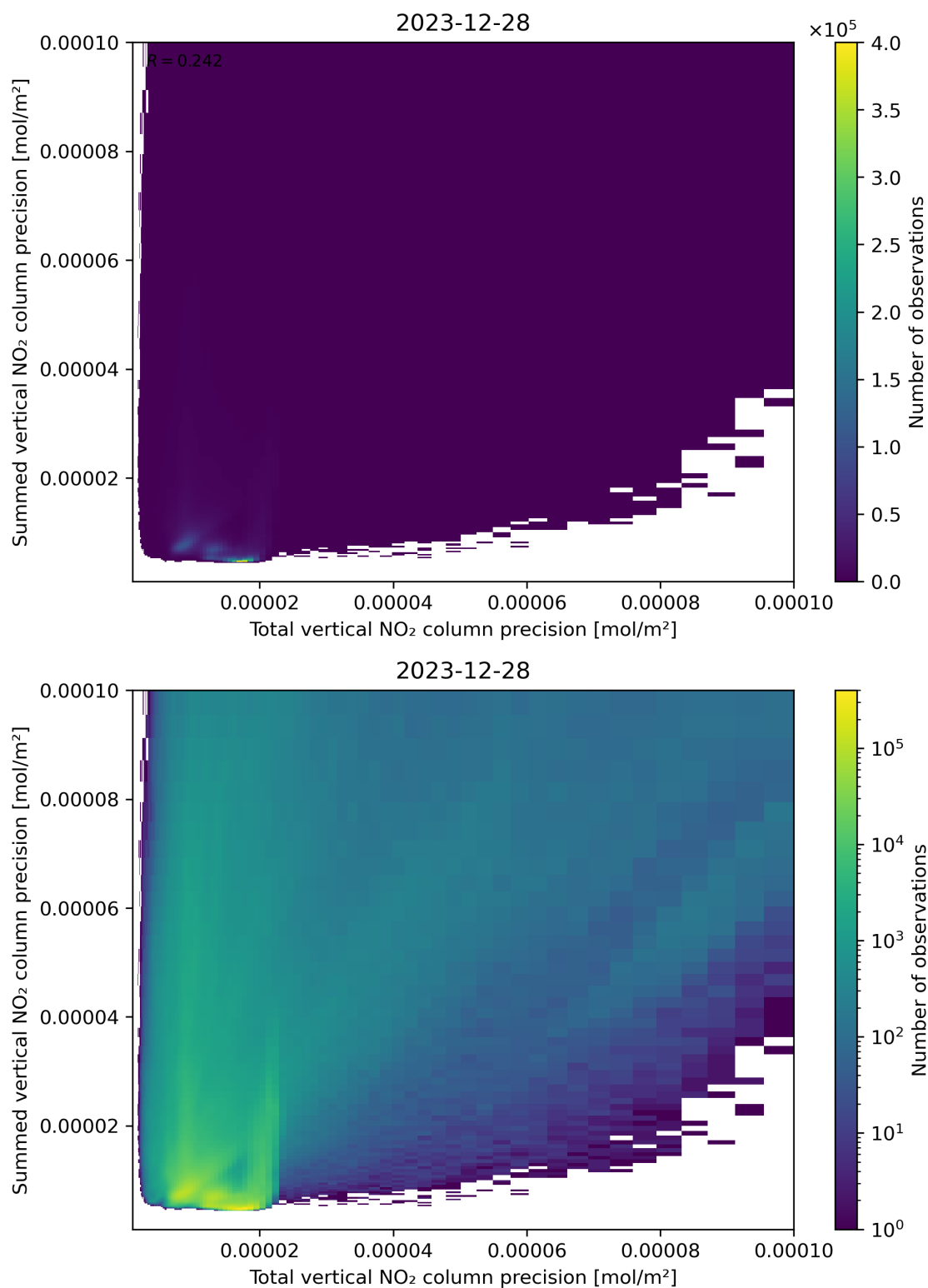
Figure 118: Scatter density plot of “Total vertical NO 2 column precision” against “Summed vertical NO 2 column precision” for 2023-12-27 to 2023-12-29.
