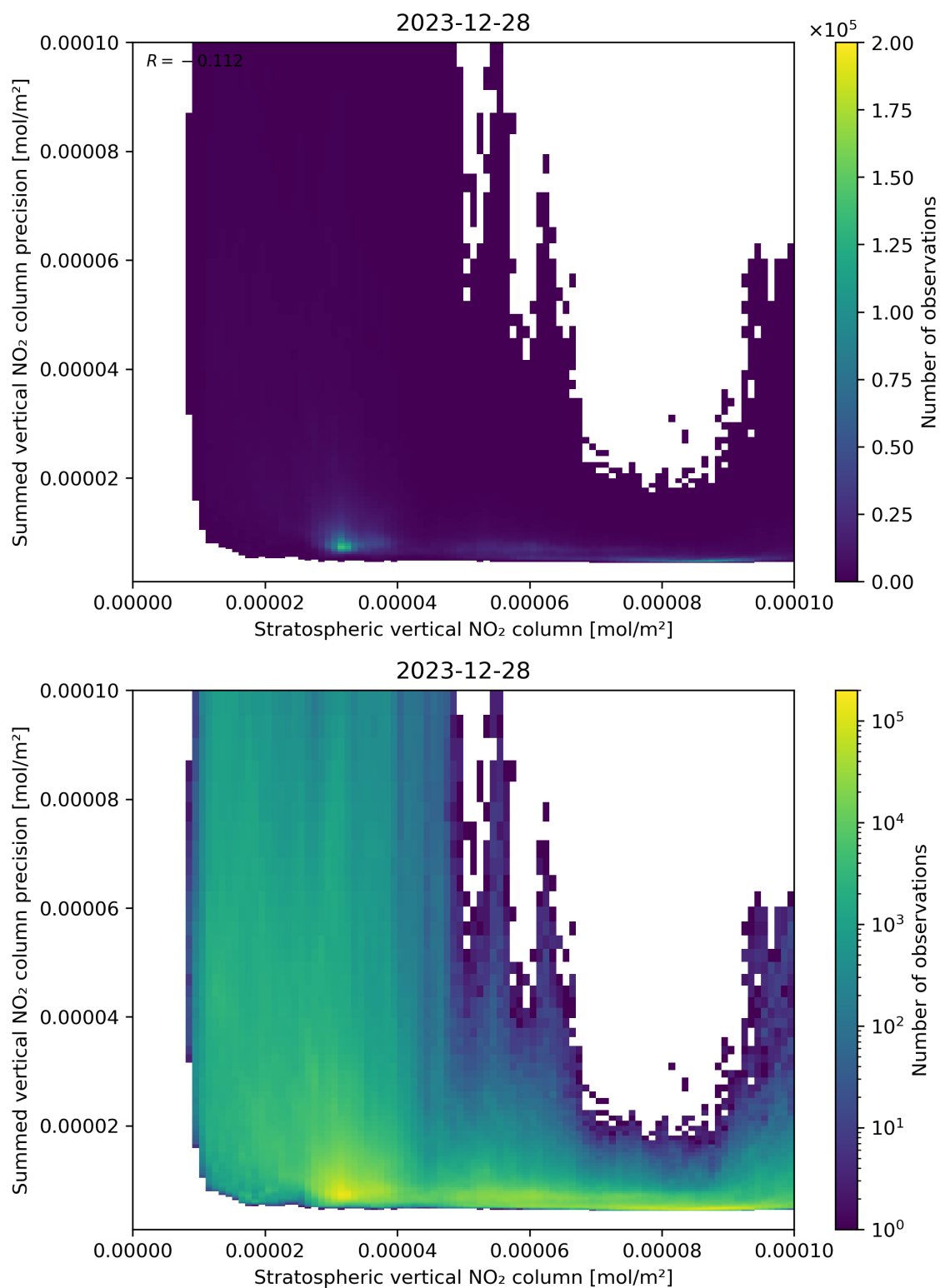
Figure 99: Scatter density plot of “Stratospheric vertical NO 2 column” against “Summed vertical NO 2 column precision” for 2023-12-27 to 2023-12-29.
