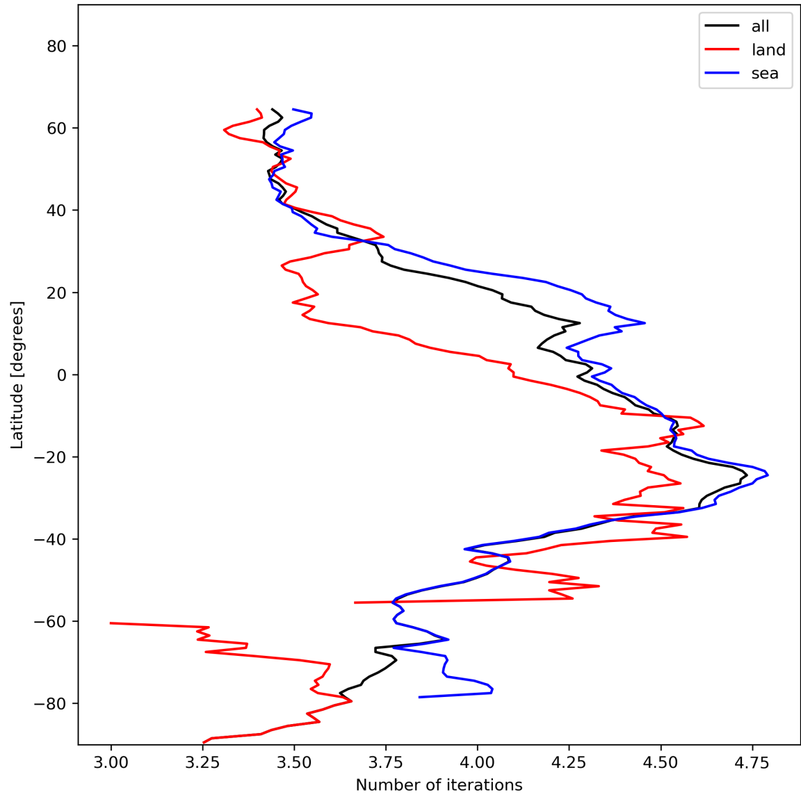
Figure 17: Zonal average of “Number of iterations” for 2023-12-27 to 2023-12-29.
