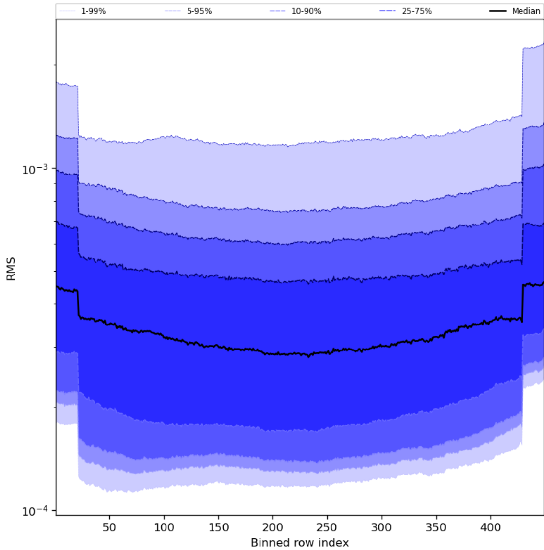
Figure 60: Along track statistics of “RMS” for 2023-12-27 to 2023-12-29
