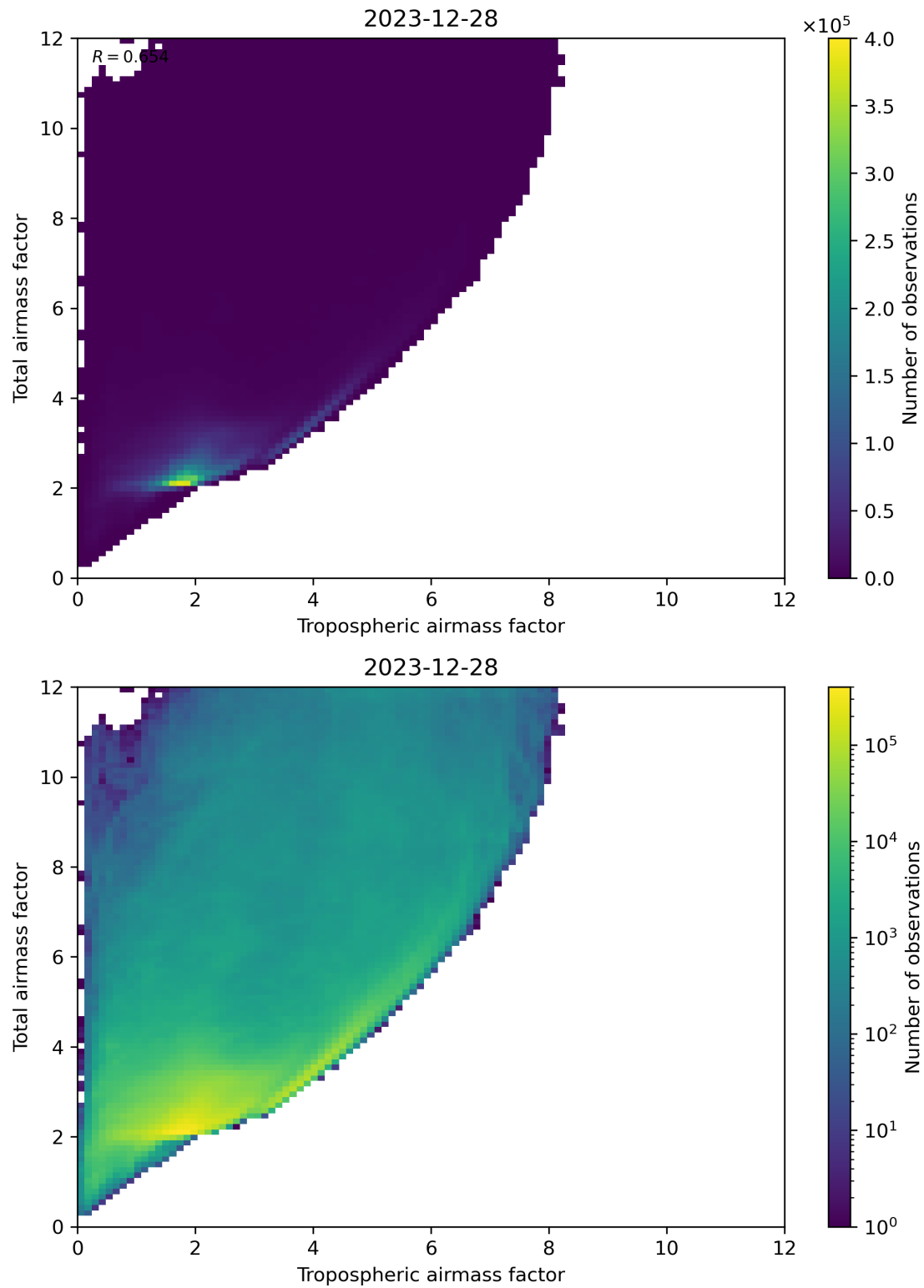
Figure 72: Scatter density plot of “Tropospheric airmass factor” against “Total airmass factor” for 2023-12-27 to 2023-12-29.
