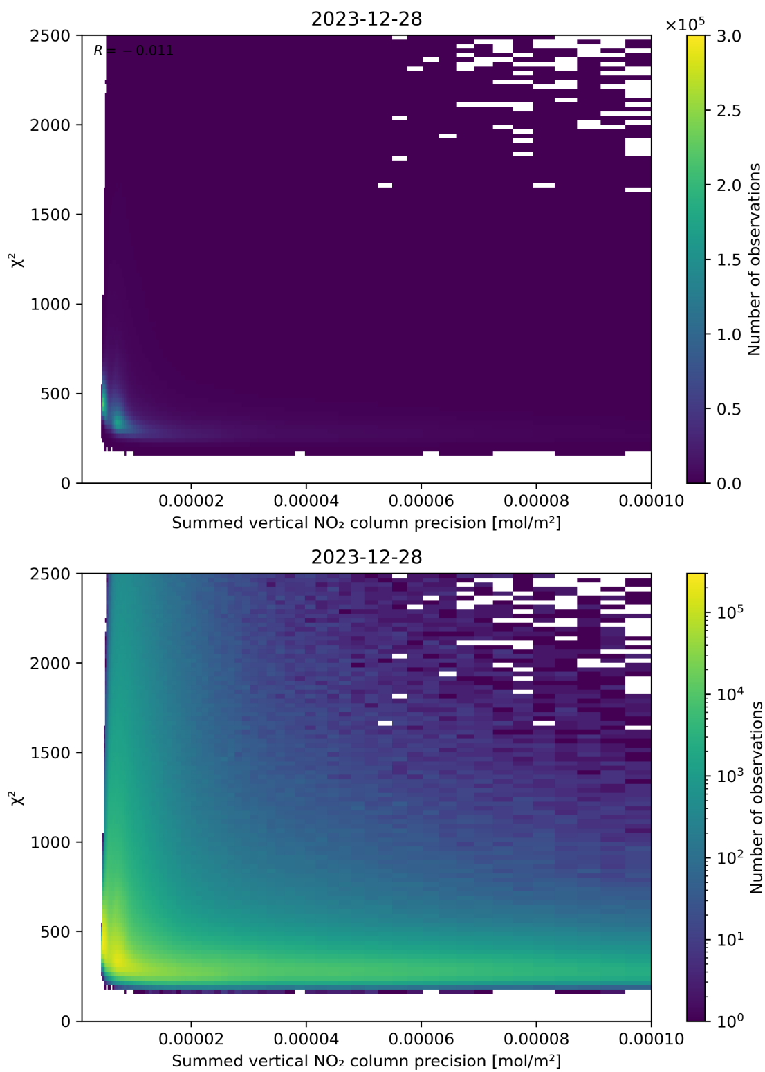
Figure 107: Scatter density plot of “Summed vertical NO 2 column precision” against “ \chi^2 ” for 2023-12-27 to 2023-12-29.
