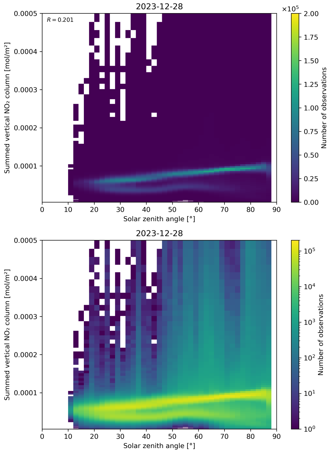
Figure 151: Scatter density plot of “Solar zenith angle” against “Summed vertical NO 2 column” for 2023-12-27 to 2023-12-29.
