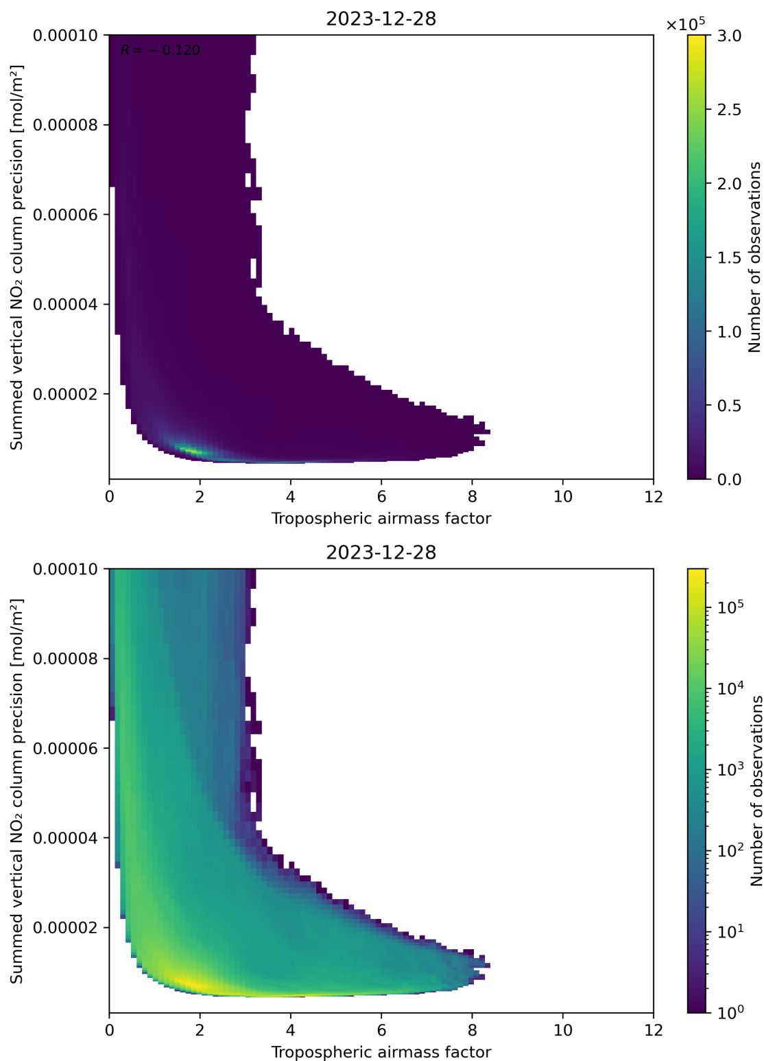
Figure 76: Scatter density plot of “Tropospheric air mass factor” against “Summed vertical NO 2 column precision” for 2023-12-27 to 2023-12-29.
