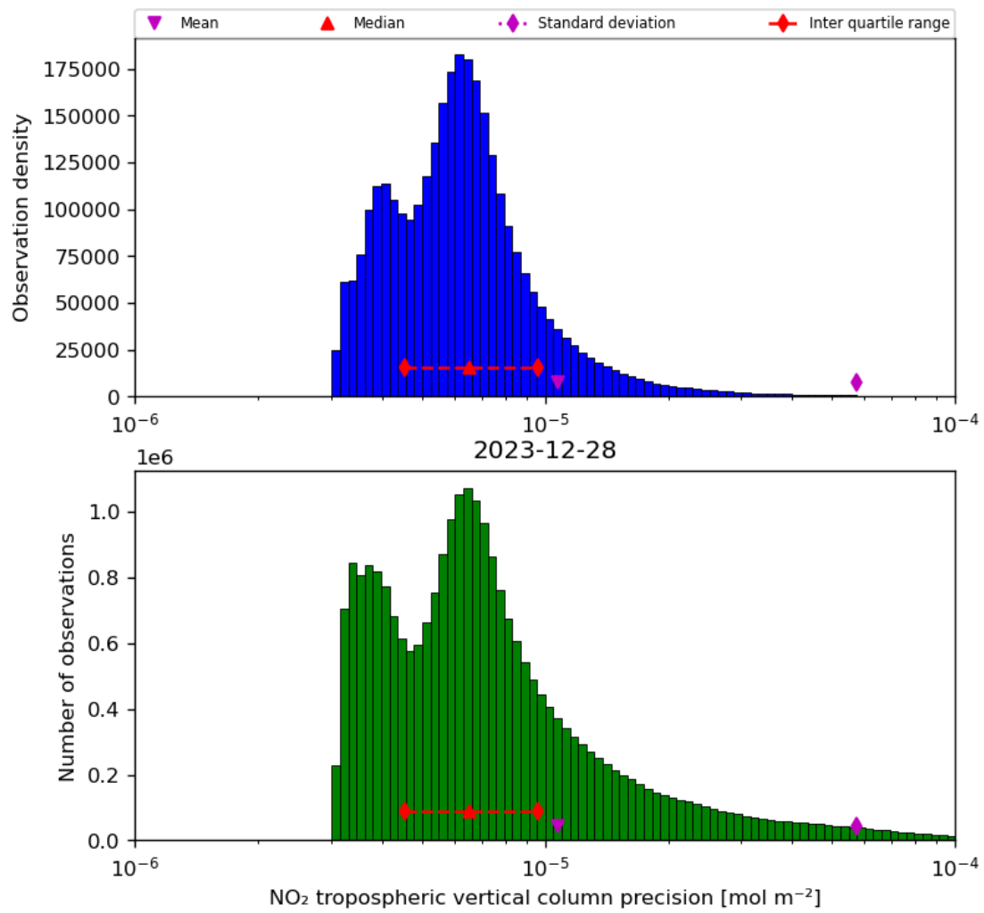
Figure 30: Histogram of "NO 2 tropospheric vertical column precision" for 2023-12-27 to 2023-12-29
