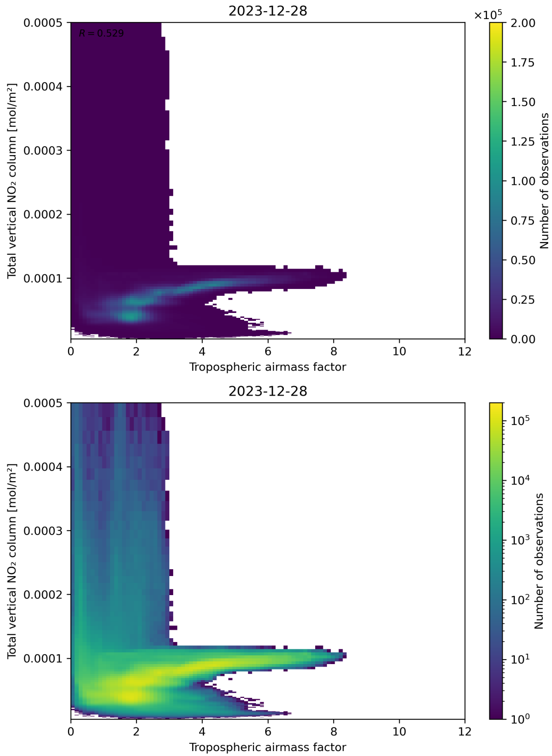
Figure 77: Scatter density plot of “Tropospheric airmass factor” against “Total vertical NO 2 column” for 2023-12-27 to 2023-12-29.
