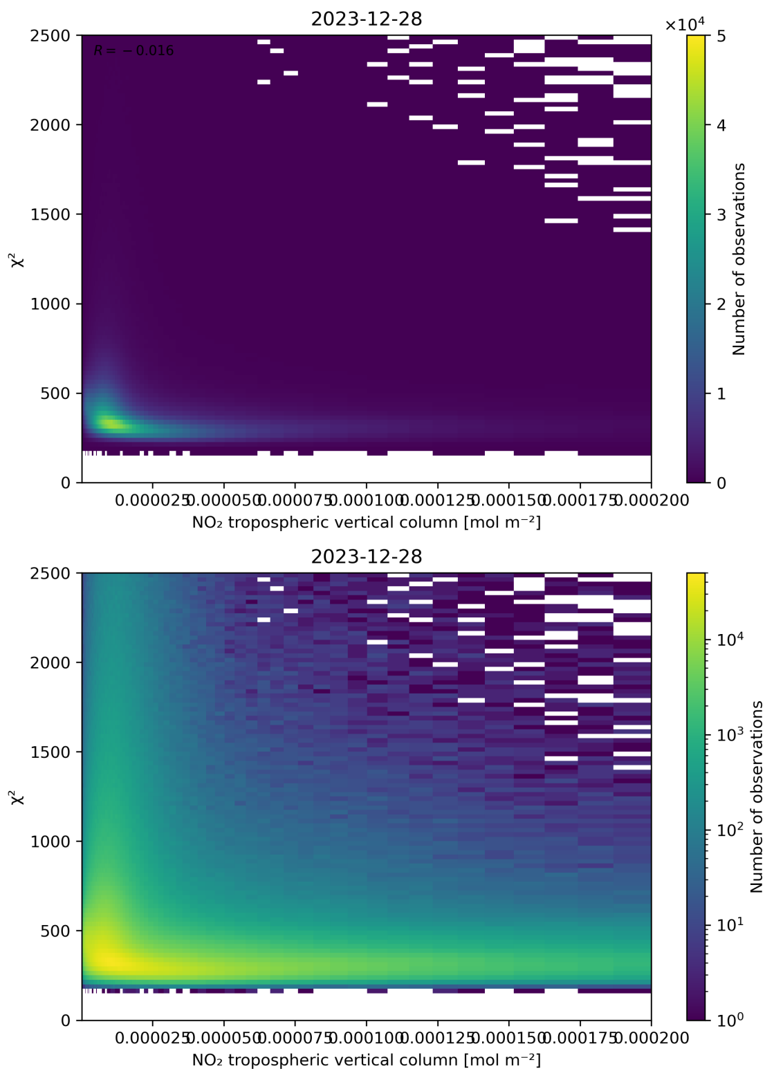
Figure 124: Scatter density plot of “NO 2 tropospheric vertical column” against “ \chi^2 ” for 2023-12-27 to 2023-12-29.
