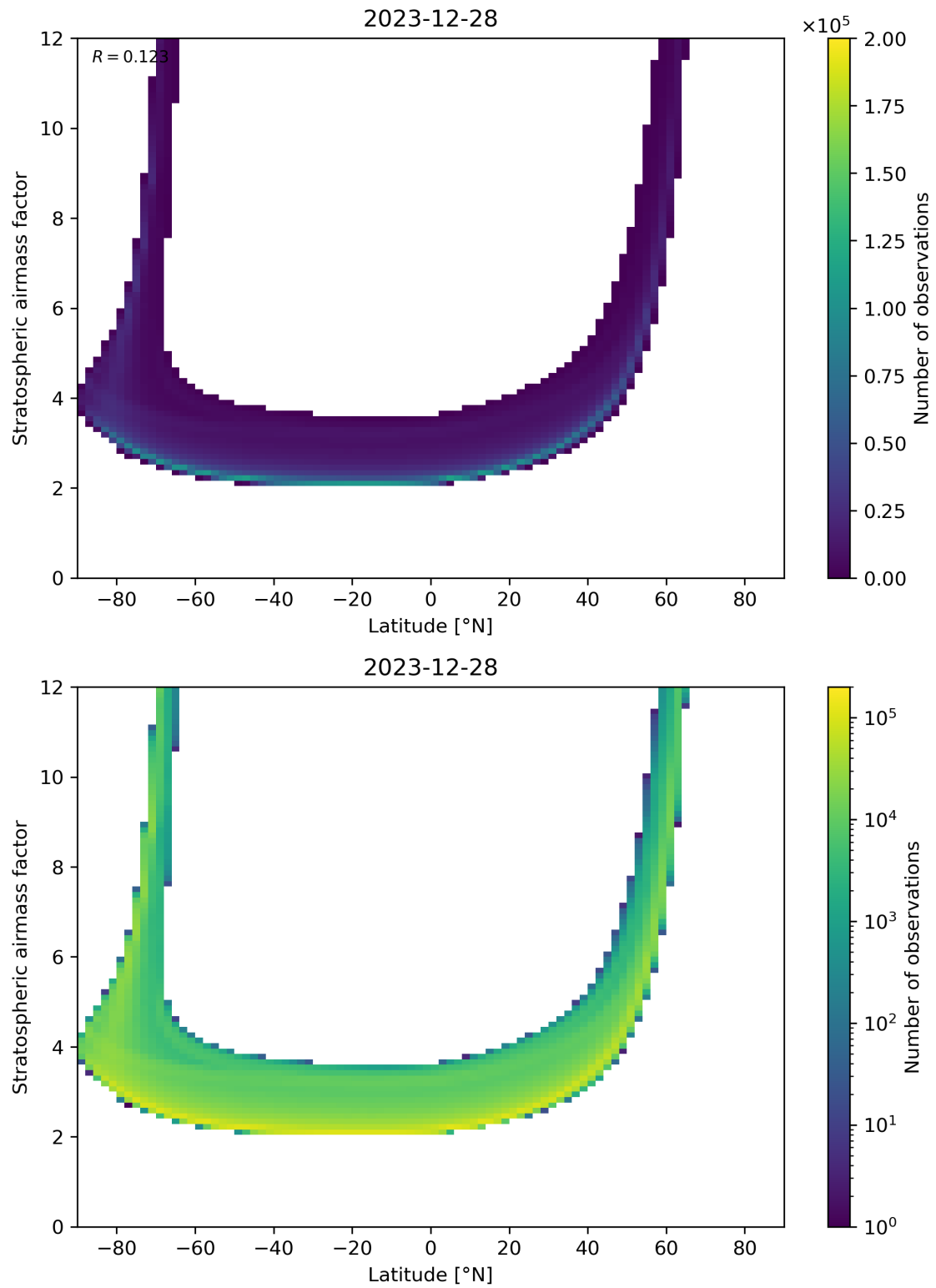
Figure 83: Scatter density plot of “Latitude” against “Stratospheric airmass factor” for 2023-12-27 to 2023-12-29.
