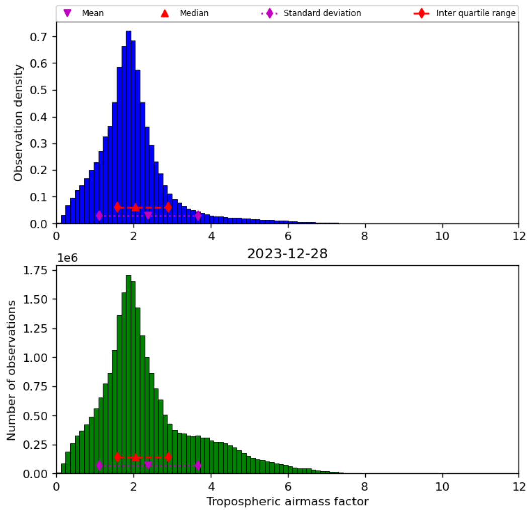
Figure 31: Histogram of “Tropospheric airmass factor” for 2023-12-27 to 2023-12-29
