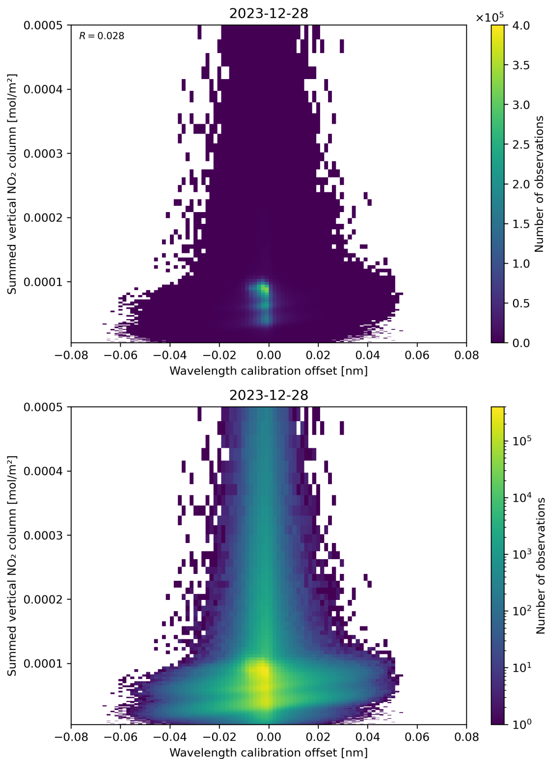
Figure 177: Scatter density plot of “Wavelength calibration offset” against “Summed vertical NO 2 column” for 2023-12-27 to 2023-12-29.
