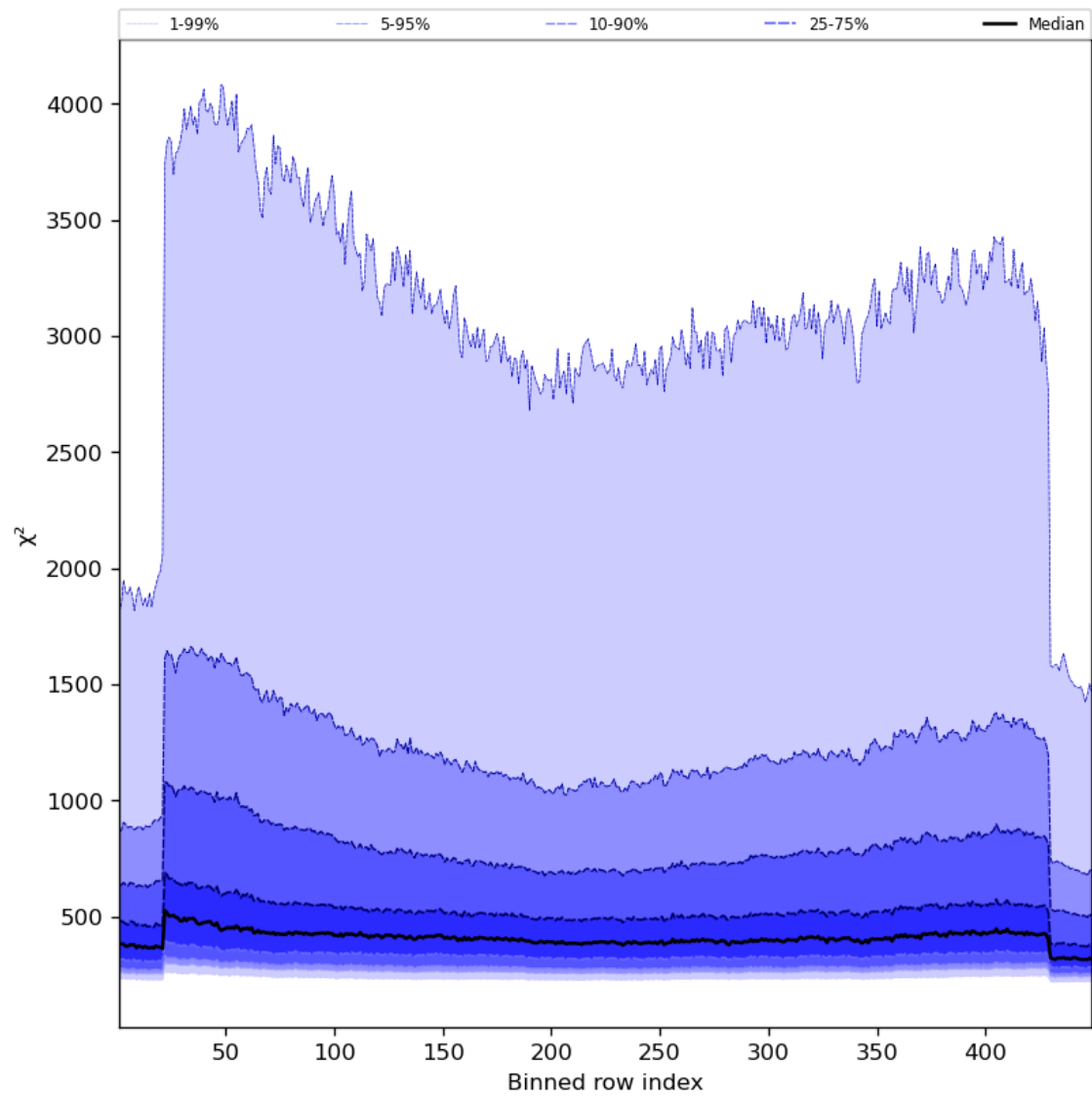
Figure 59: Along track statistics of “ \chi^2 ” for 2023-12-27 to 2023-12-29
