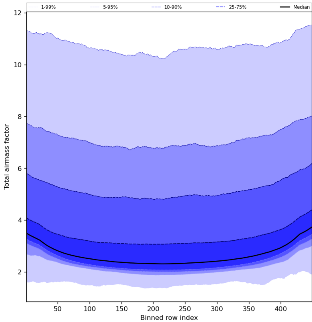
Figure 49: Along track statistics of “Total airmass factor” for 2023-12-27 to 2023-12-29
