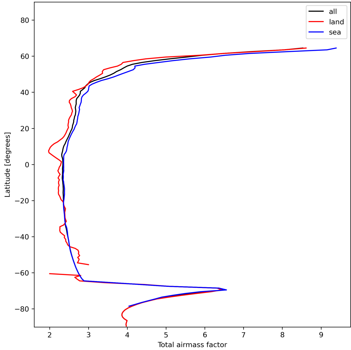
Figure 15: Zonal average of “Total airmass factor” for 2023-12-27 to 2023-12-29.
