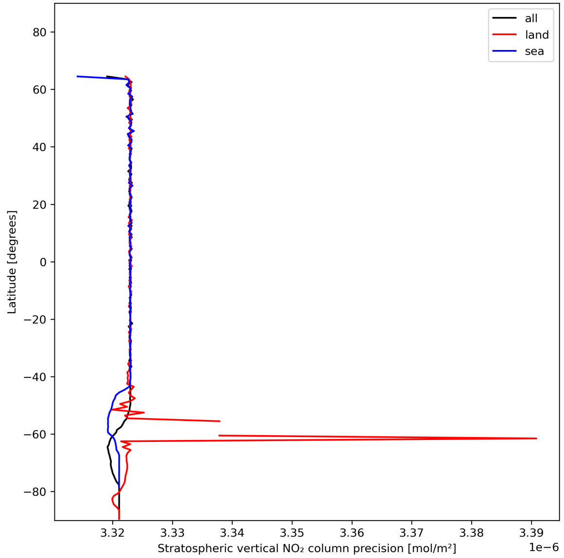
Figure 20: Zonal average of “Stratospheric vertical NO 2 column precision” for 2023-12-28 to 2023-12-30.
