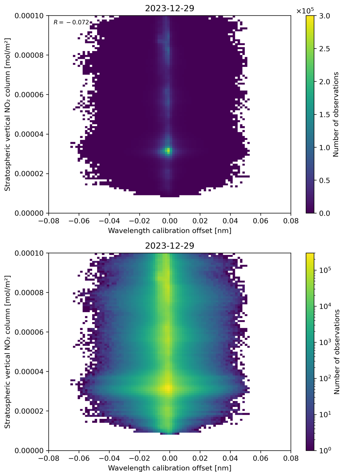
Figure 176: Scatter density plot of “Wavelength calibration offset” against “Stratospheric vertical NO 2 column” for 2023-12-28 to 2023-12-30.
