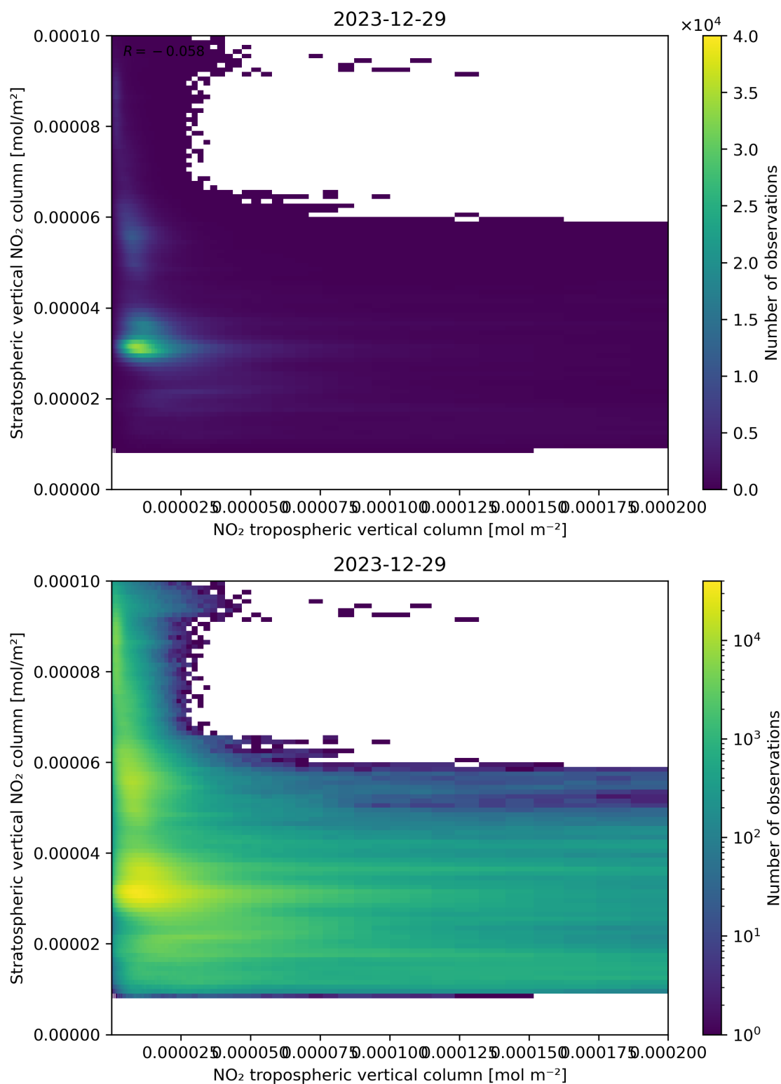
Figure 125: Scatter density plot of “NO 2 tropospheric vertical column” against “Stratospheric vertical NO 2 column” for 2023-12-28 to 2023-12-30.
