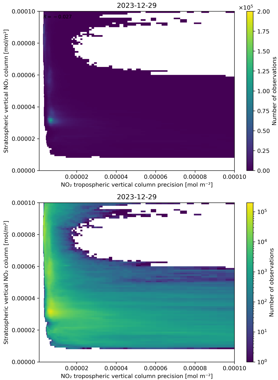
Figure 135: Scatter density plot of “NO 2 tropospheric vertical column precision” against “Stratospheric vertical NO 2 column” for 2023-12-28 to 2023-12-30.
