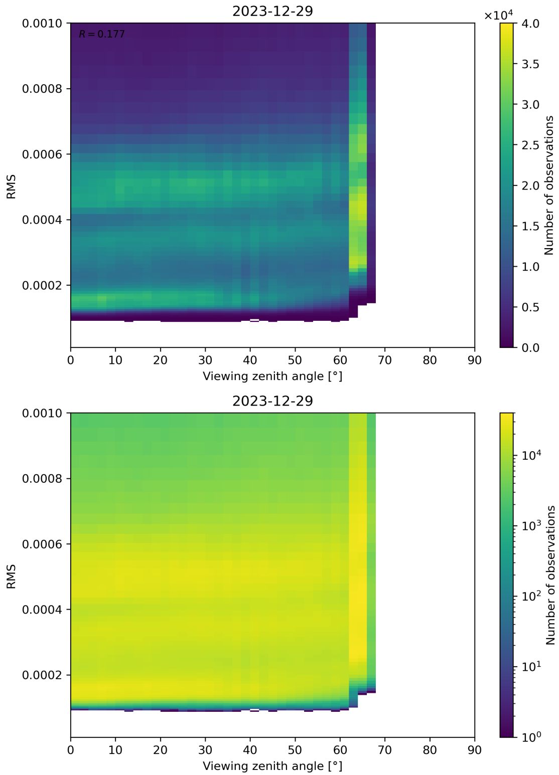
Figure 171: Scatter density plot of “Viewing zenith angle” against “RMS” for 2023-12-28 to 2023-12-30.
