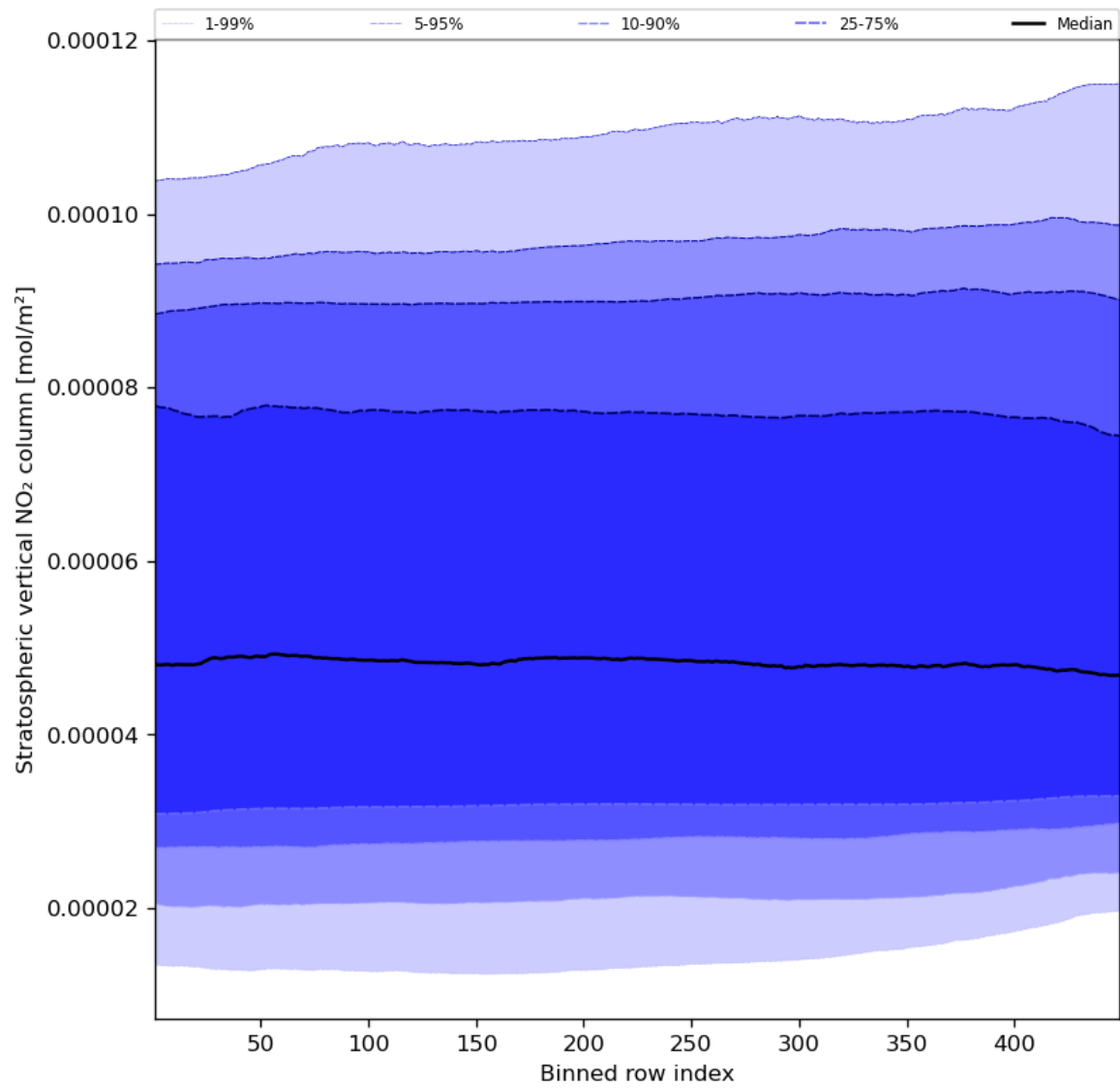
Figure 53: Along track statistics of “Stratospheric vertical NO 2 column” for 2023-12-28 to 2023-12-30
