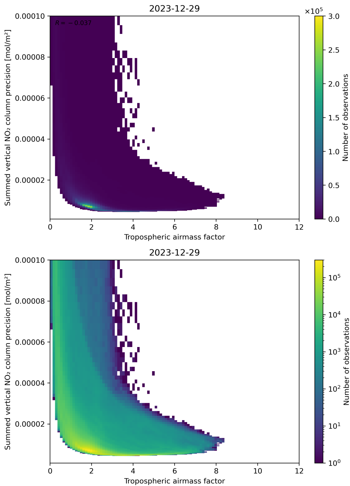
Figure 76: Scatter density plot of “Tropospheric air mass factor” against “Summed vertical NO 2 column precision” for 2023-12-28 to 2023-12-30.
