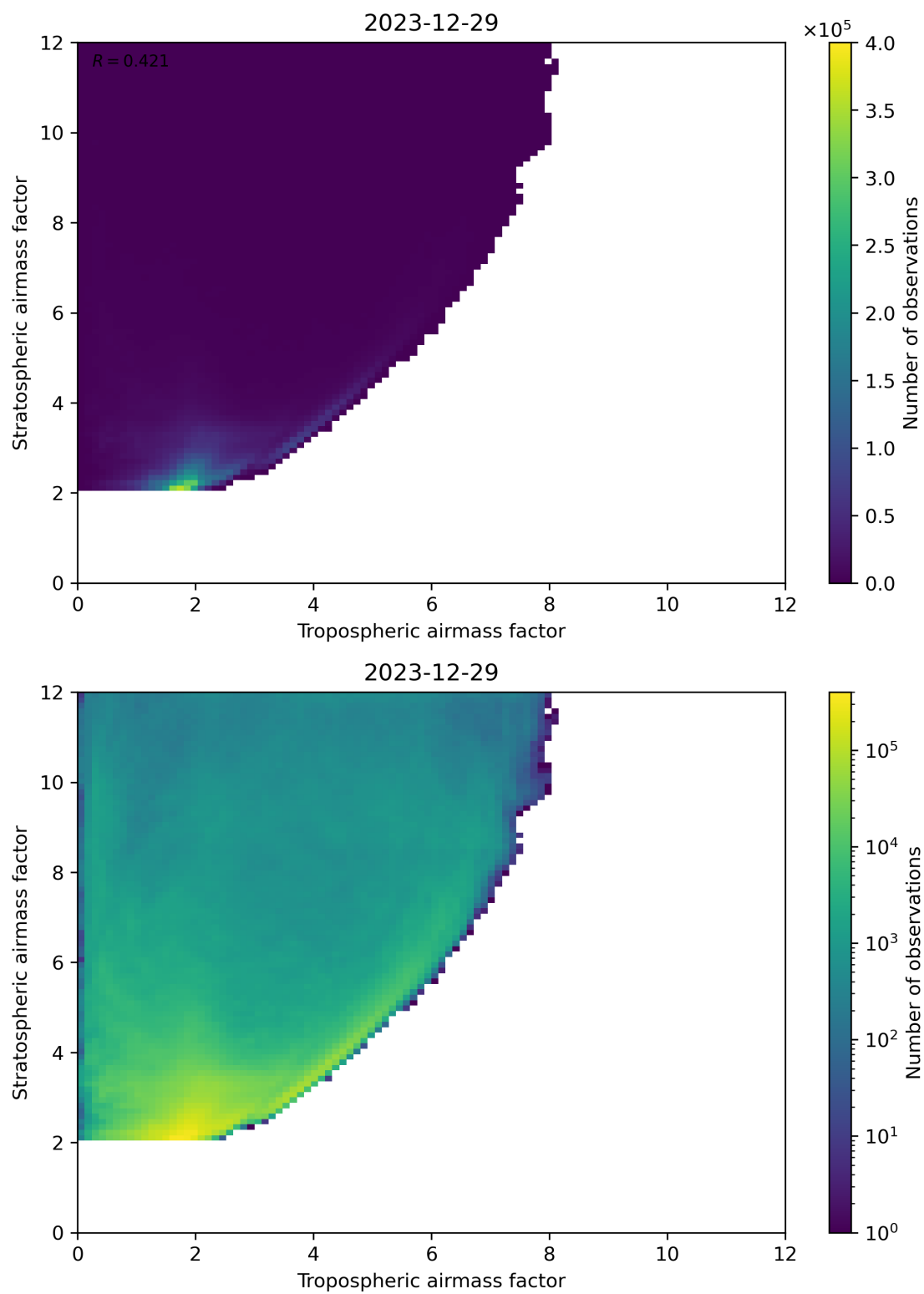
Figure 71: Scatter density plot of “Tropospheric airmass factor” against “Stratospheric airmass factor” for 2023-12-28 to 2023-12-30.
