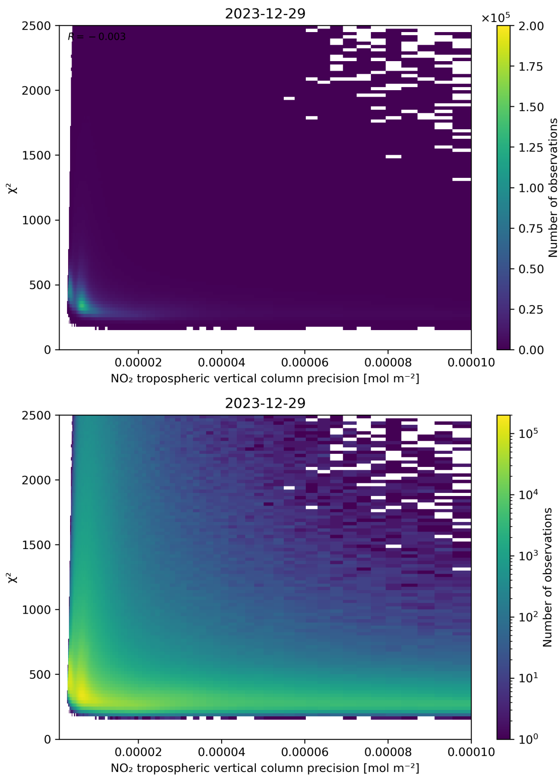
Figure 134: Scatter density plot of “NO 2 tropospheric vertical column precision” against “ \chi^2 ” for 2023-12-28 to 2023-12-30.
