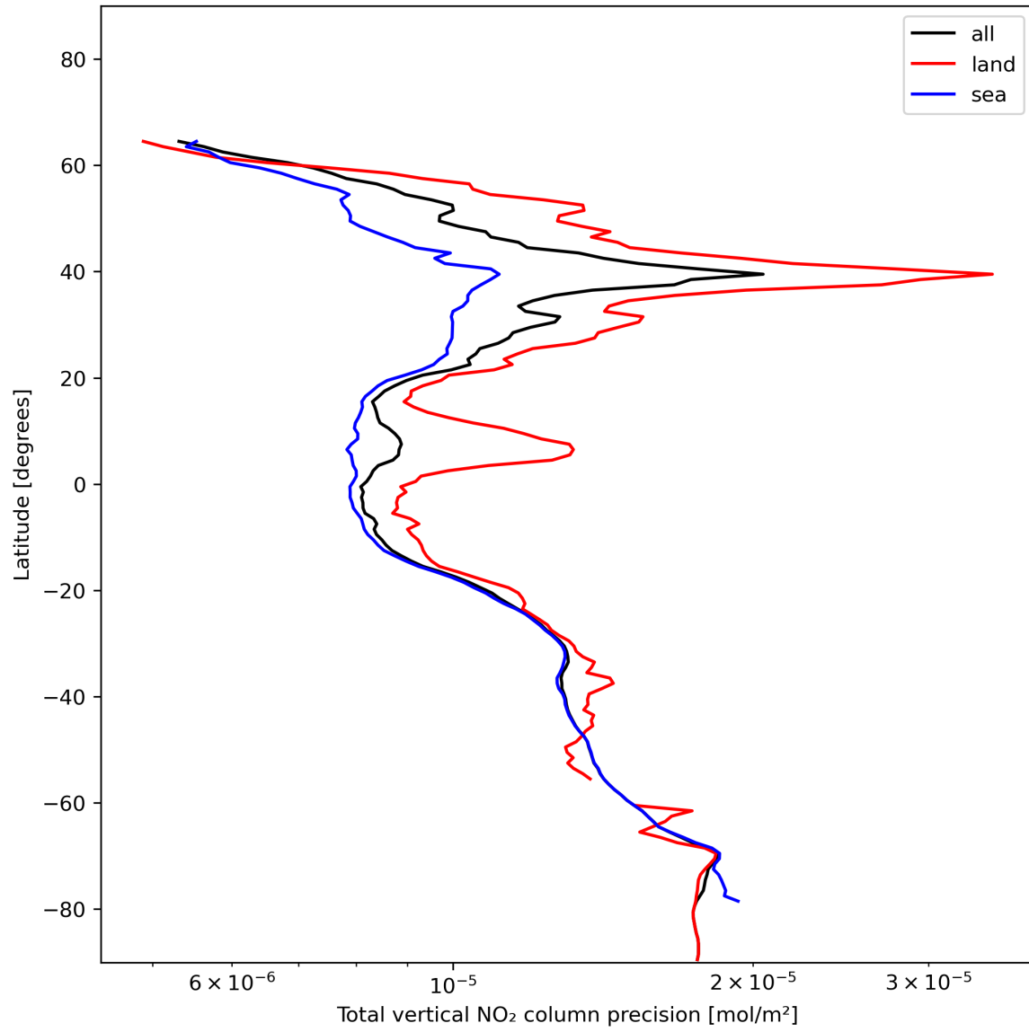
Figure 22: Zonal average of “Total vertical NO 2 column precision” for 2023-12-28 to 2023-12-30.
