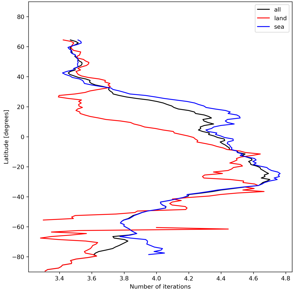
Figure 17: Zonal average of “Number of iterations” for 2023-12-28 to 2023-12-30.
