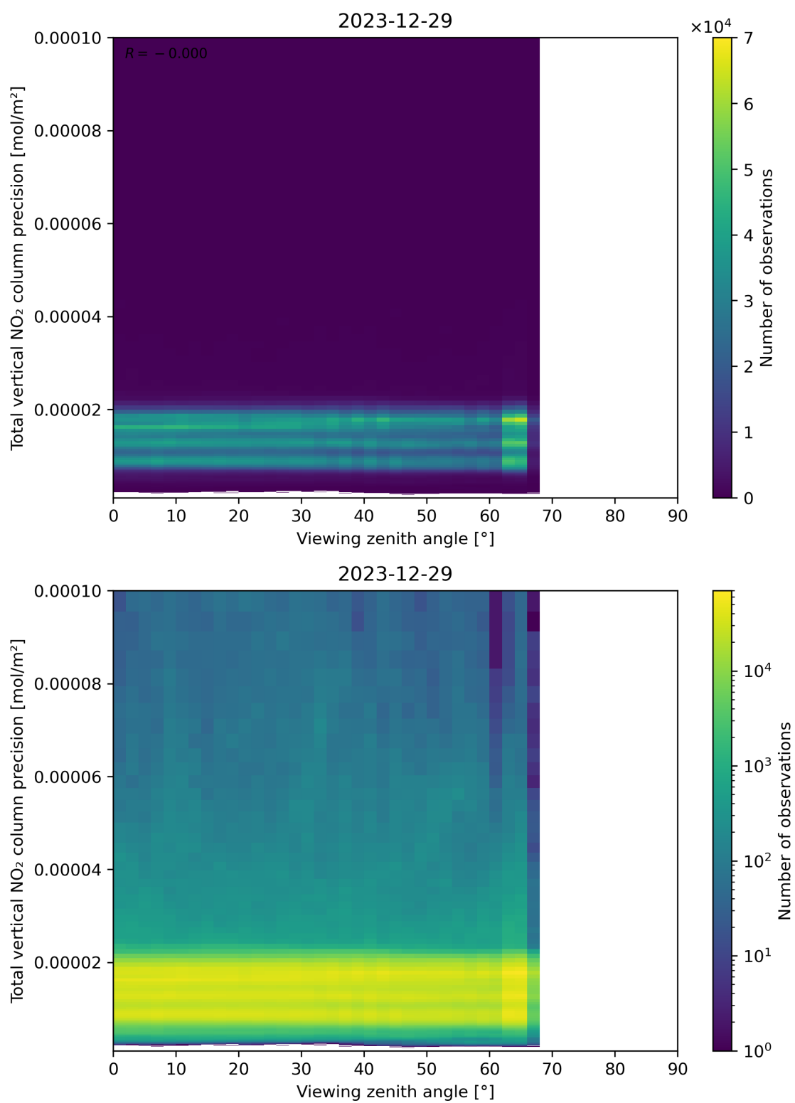
Figure 168: Scatter density plot of “Viewing zenith angle” against “Total vertical NO 2 column precision” for 2023-12-28 to 2023-12-30.
