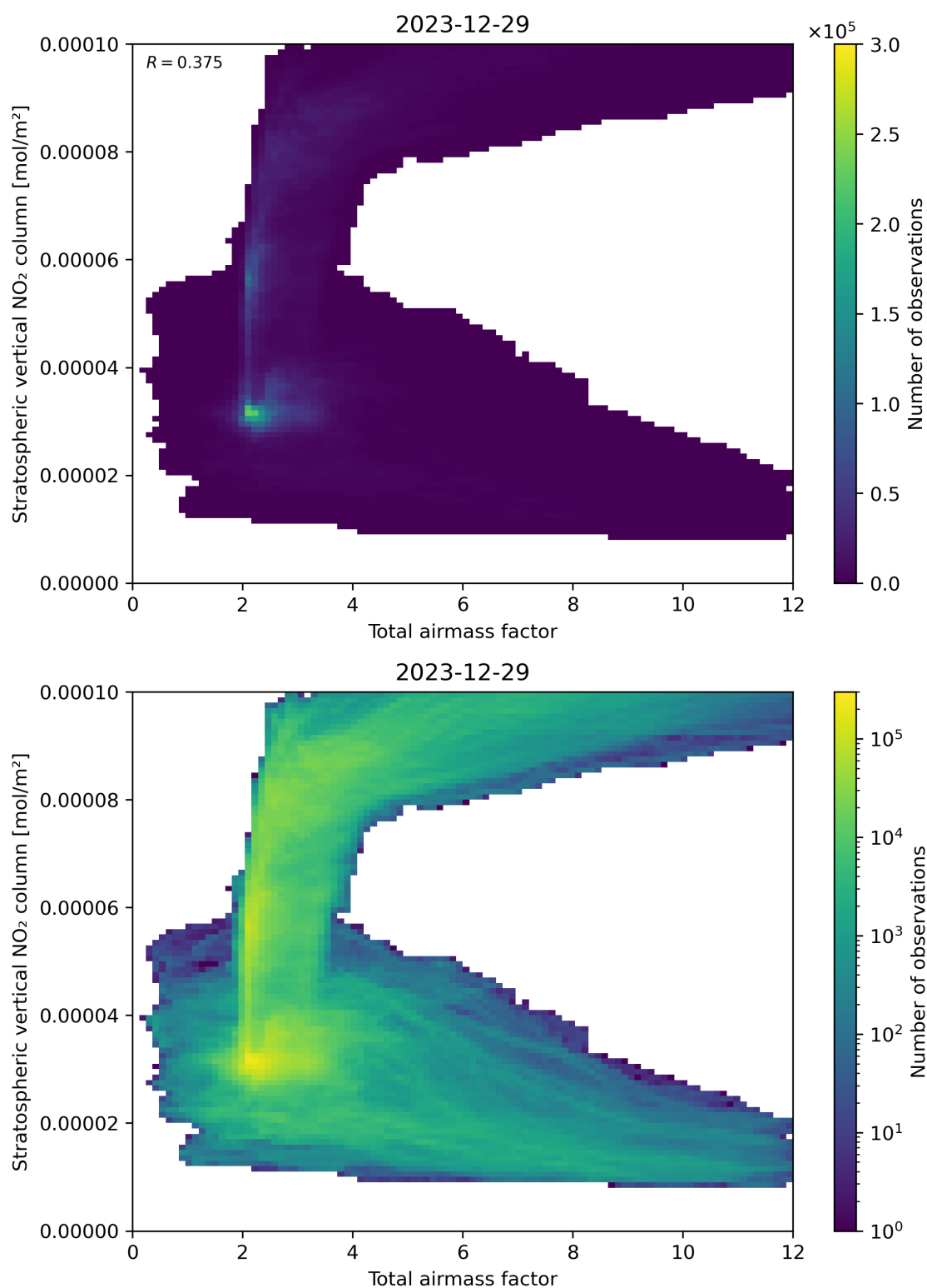
Figure 64: Scatter density plot of “Total airmass factor” against “Stratospheric vertical NO 2 column” for 2023-12-28 to 2023-12-30.
