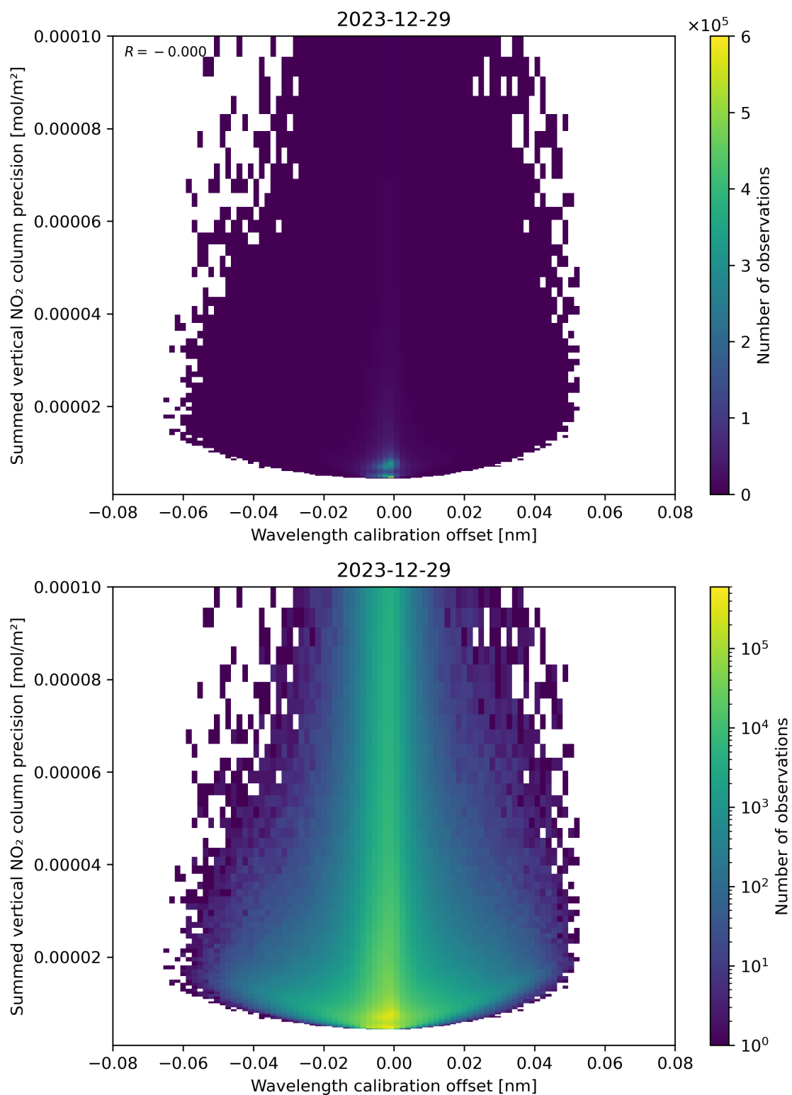
Figure 178: Scatter density plot of “Wavelength calibration offset” against “Summed vertical NO 2 column precision” for 2023-12-28 to 2023-12-30.
