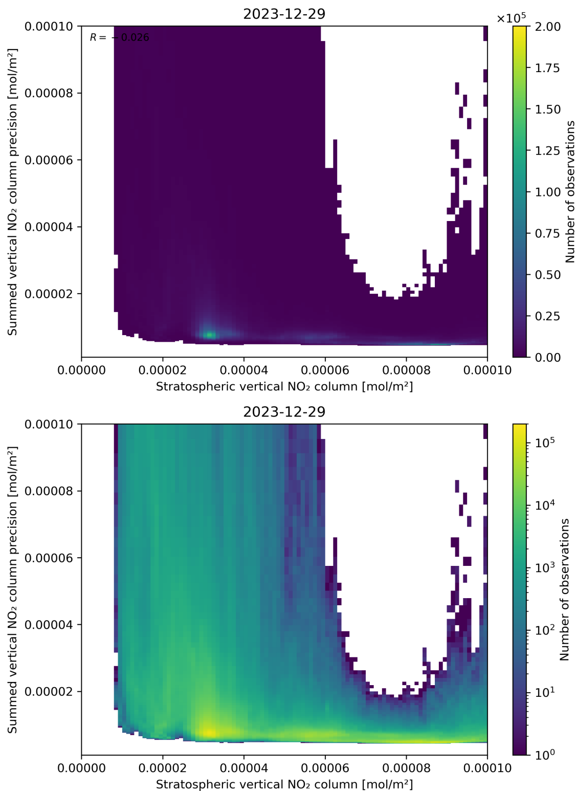
Figure 99: Scatter density plot of “Stratospheric vertical NO 2 column” against “Summed vertical NO 2 column precision” for 2023-12-28 to 2023-12-30.
