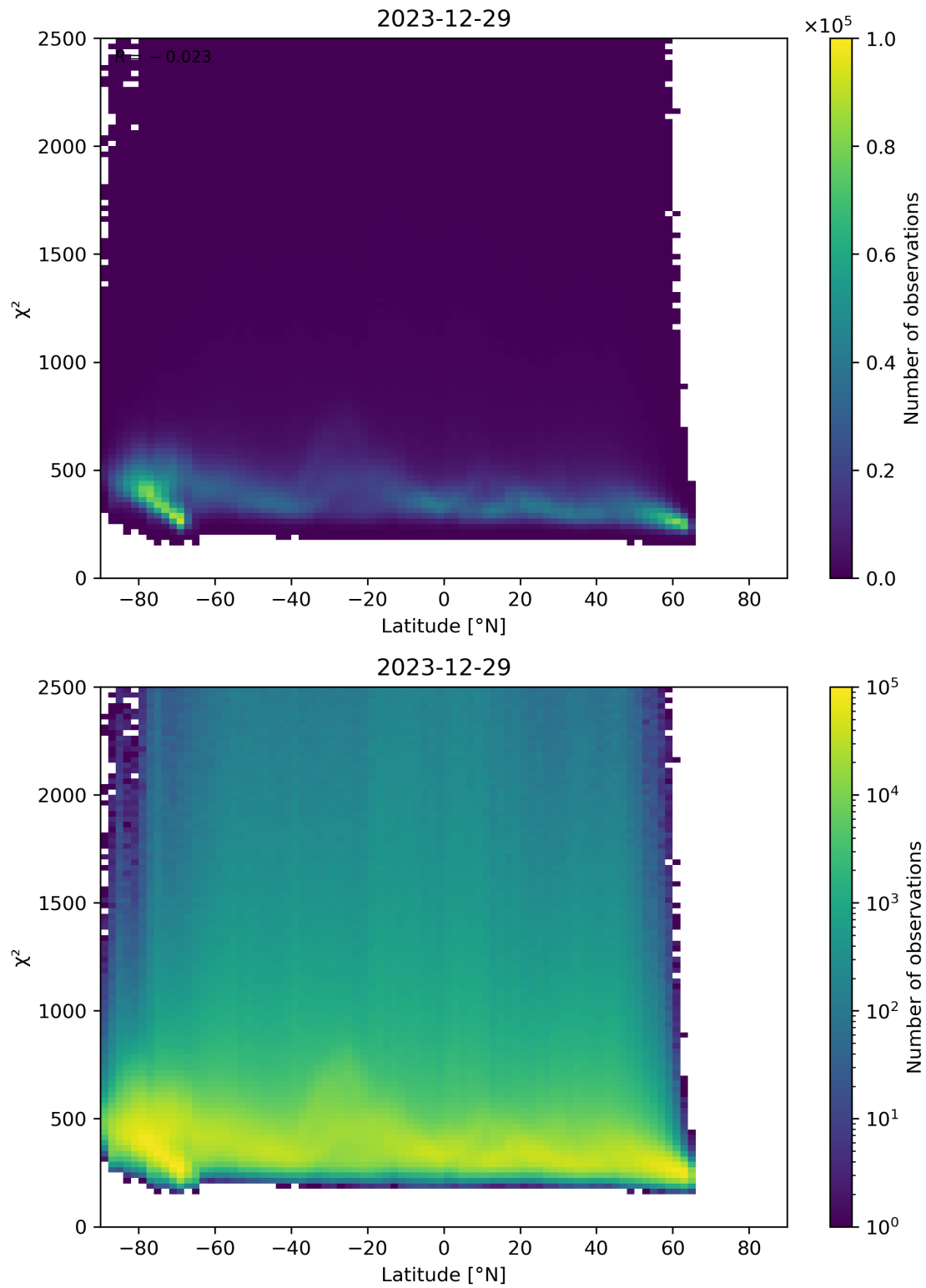
Figure 86: Scatter density plot of “Latitude” against “ \chi^2 ” for 2023-12-28 to 2023-12-30.
