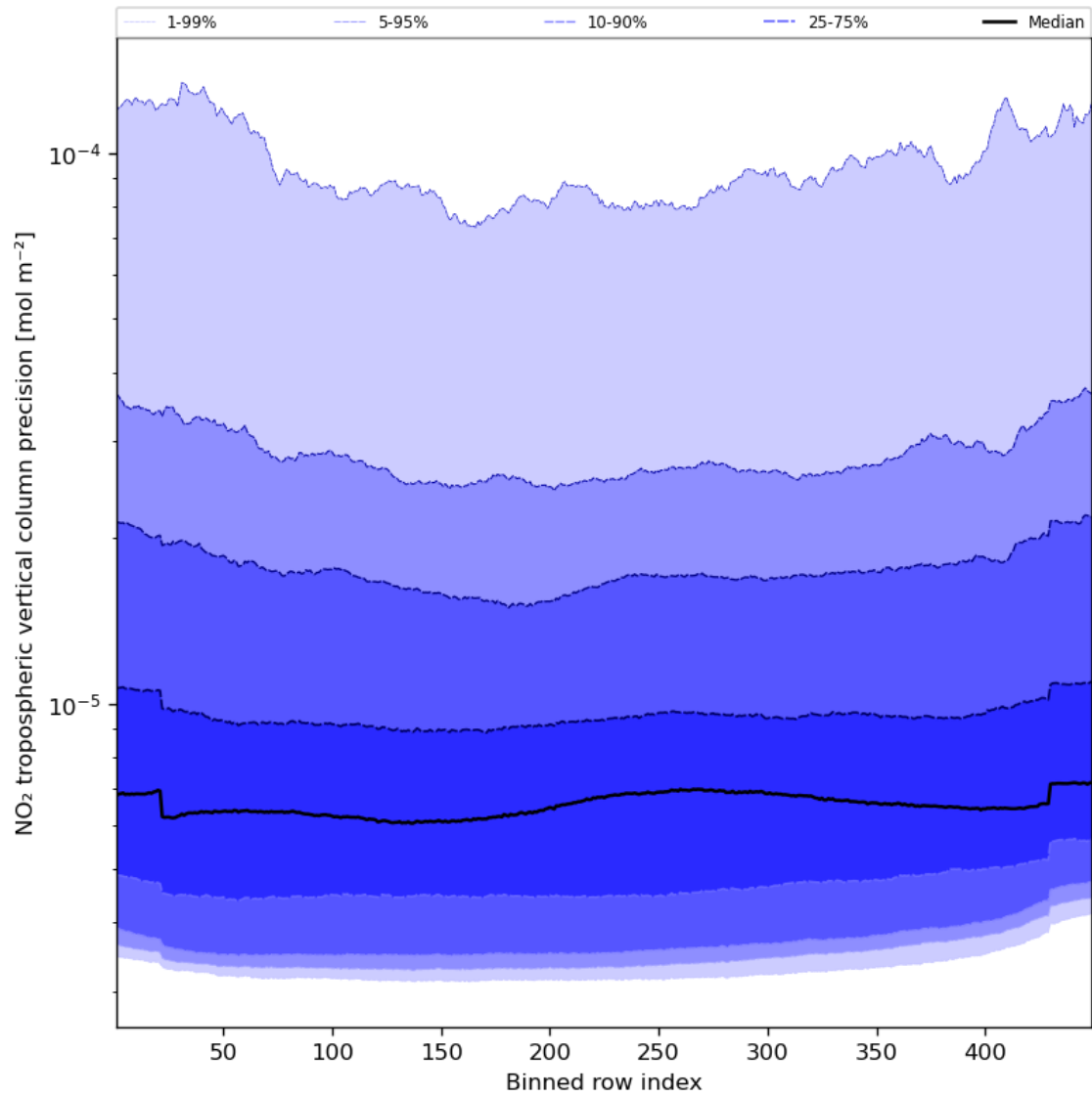
Figure 47: Along track statistics of “NO 2 tropospheric vertical column precision” for 2023-12-28 to 2023-12-30
