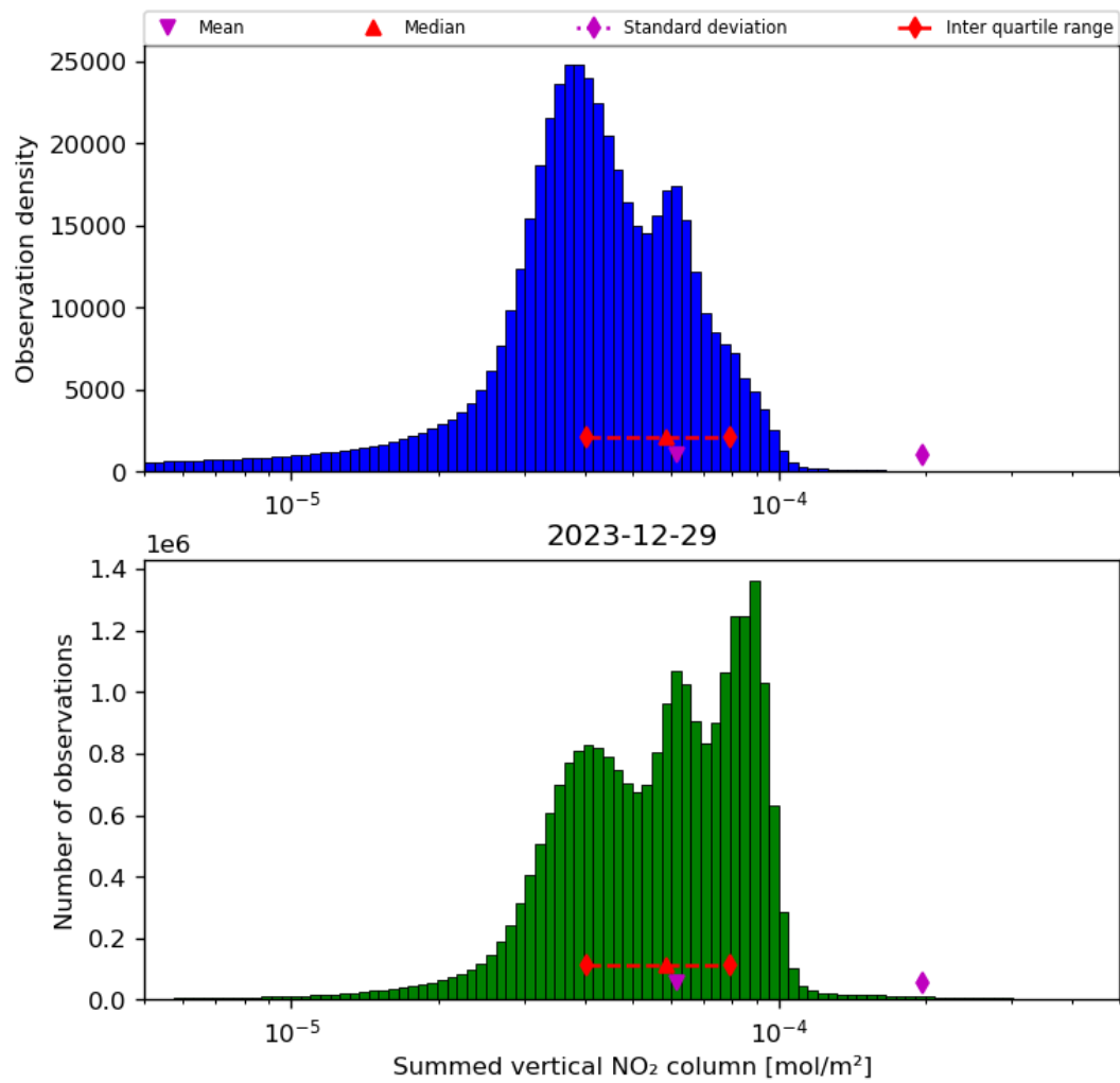
Figure 40: Histogram of "Summed vertical NO 2 column" for 2023-12-28 to 2023-12-30
