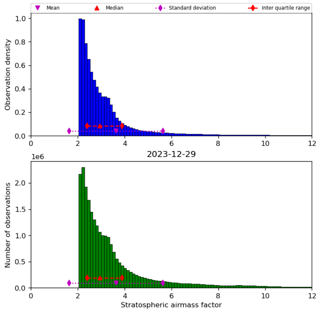
Figure 44: Histogram of “Stratospheric airmass factor” for 2023-12-28 to 2023-12-30
