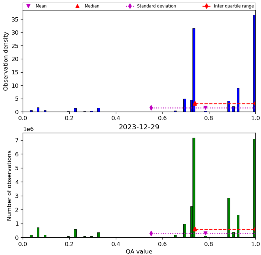
Figure 28: Histogram of “QA value” for 2023-12-28 to 2023-12-30
