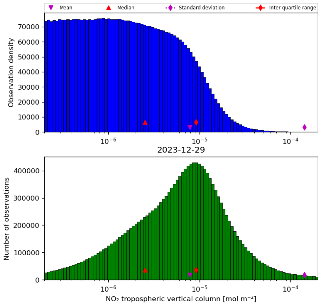
Figure 29: Histogram of “NO 2 tropospheric vertical column” for 2023-12-28 to 2023-12-30
