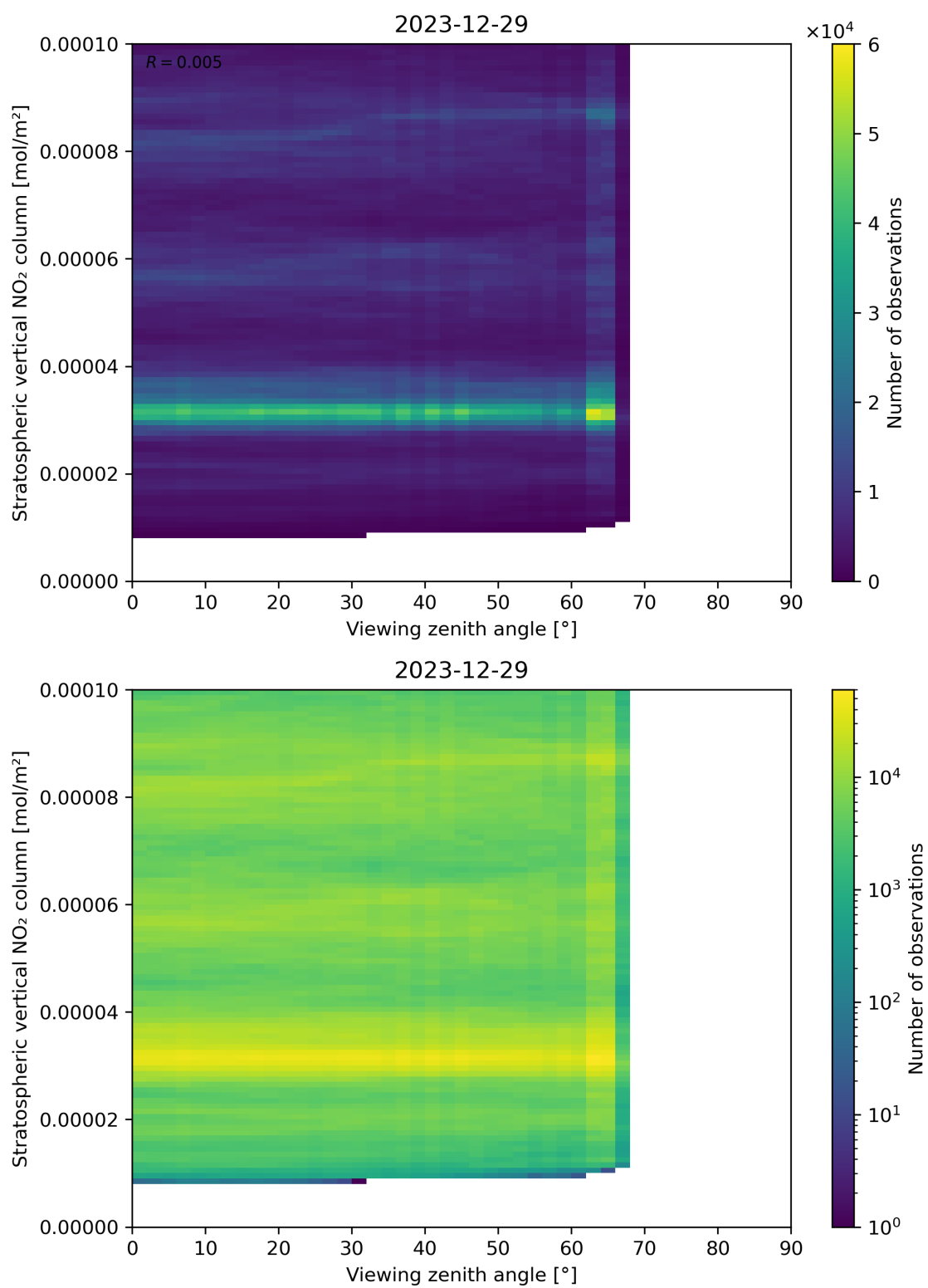
Figure 164: Scatter density plot of “Viewing zenith angle” against “Stratospheric vertical NO 2 column” for 2023-12-28 to 2023-12-30.
