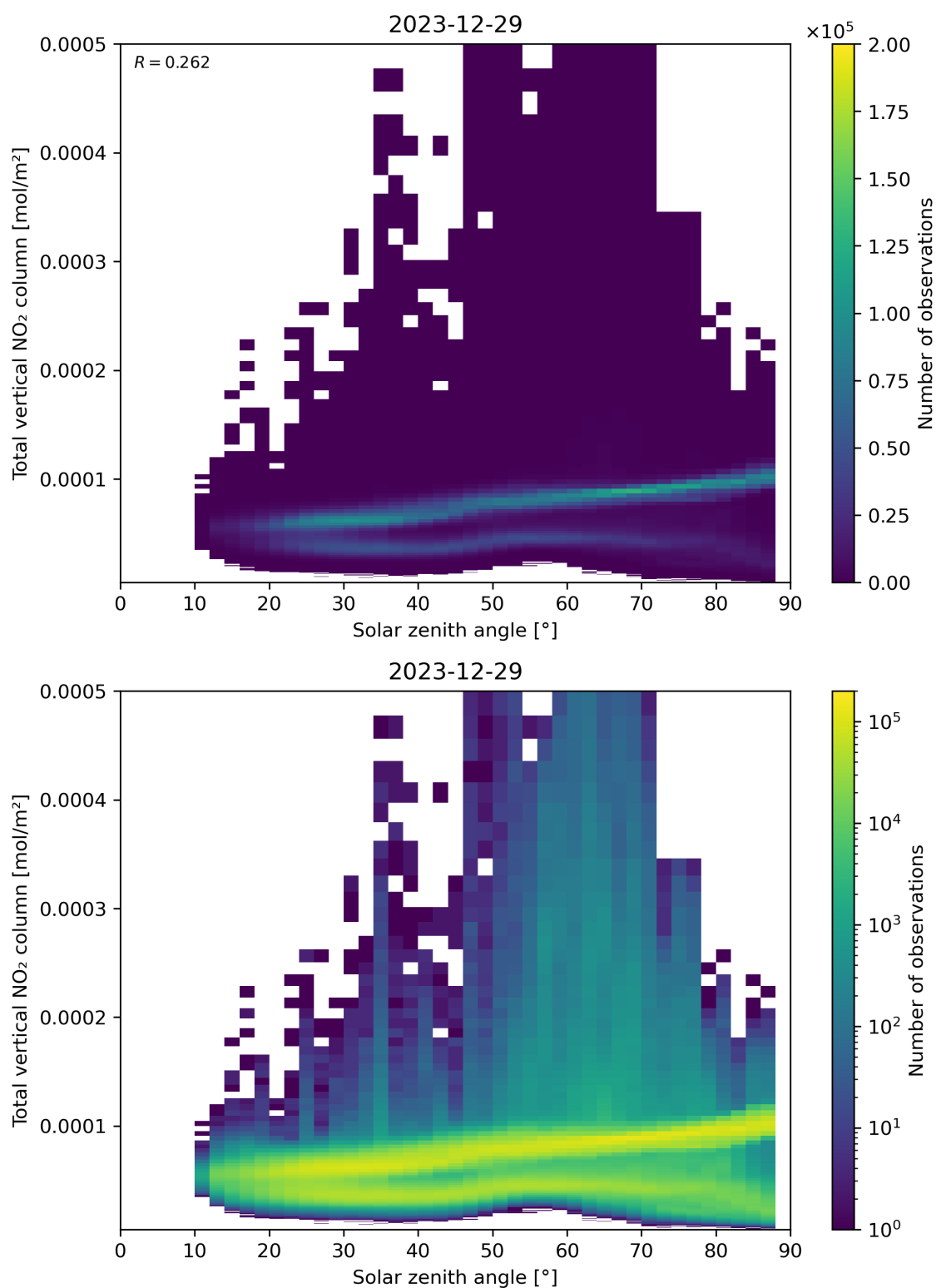
Figure 153: Scatter density plot of “Solar zenith angle” against “Total vertical NO 2 column” for 2023-12-28 to 2023-12-30.
