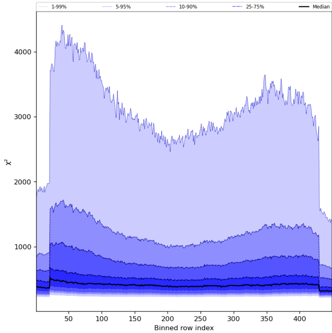
Figure 59: Along track statistics of “ \chi^2 ” for 2023-12-28 to 2023-12-30
