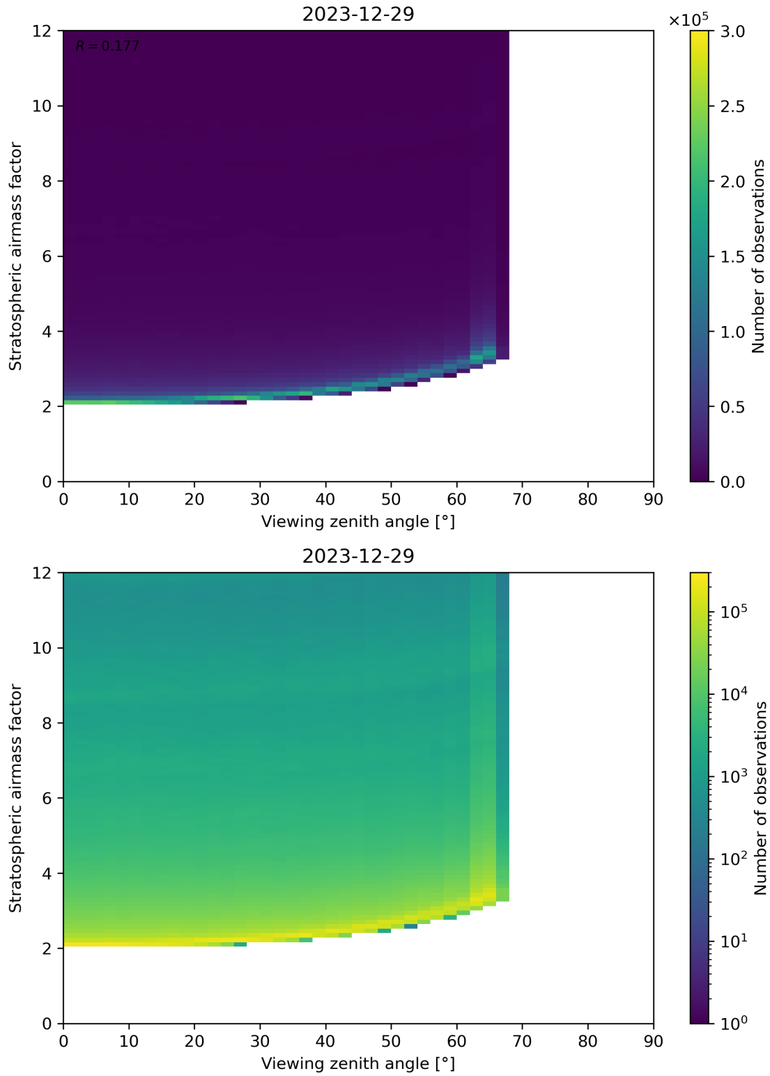
Figure 159: Scatter density plot of “Viewing zenith angle” against “Stratospheric airmass factor” for 2023-12-28 to 2023-12-30.
