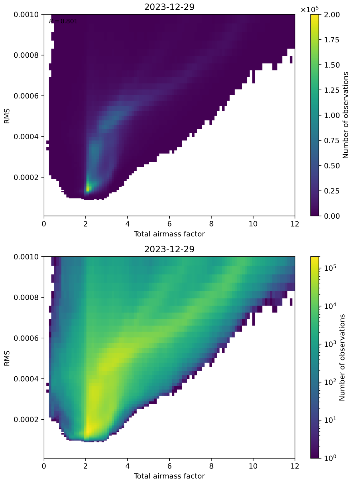
Figure 69: Scatter density plot of “Total airmass factor” against “RMS” for 2023-12-28 to 2023-12-30.
