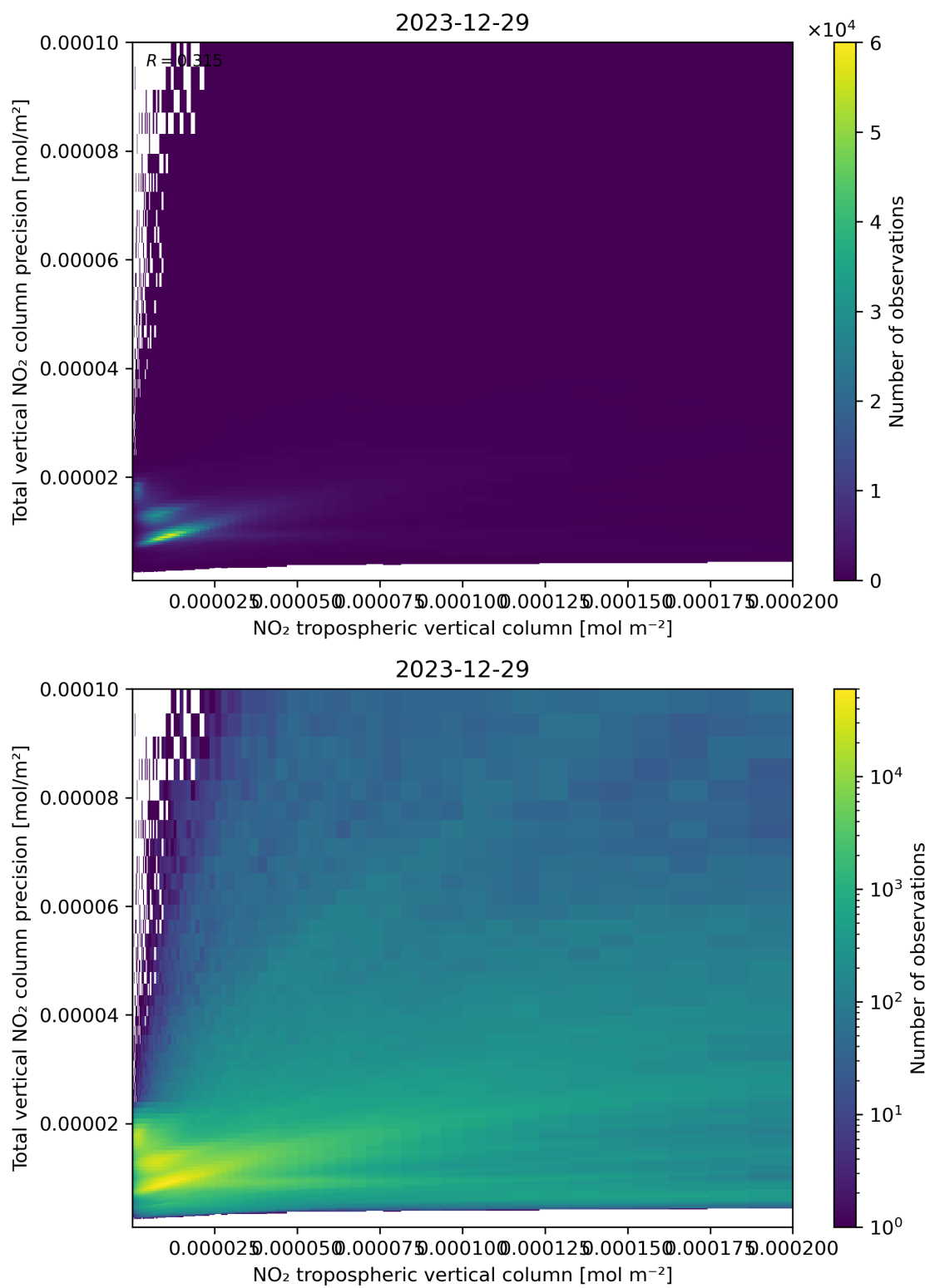
Figure 129: Scatter density plot of “NO 2 tropospheric vertical column” against “Total vertical NO 2 column precision” for 2023-12-28 to 2023-12-30.
