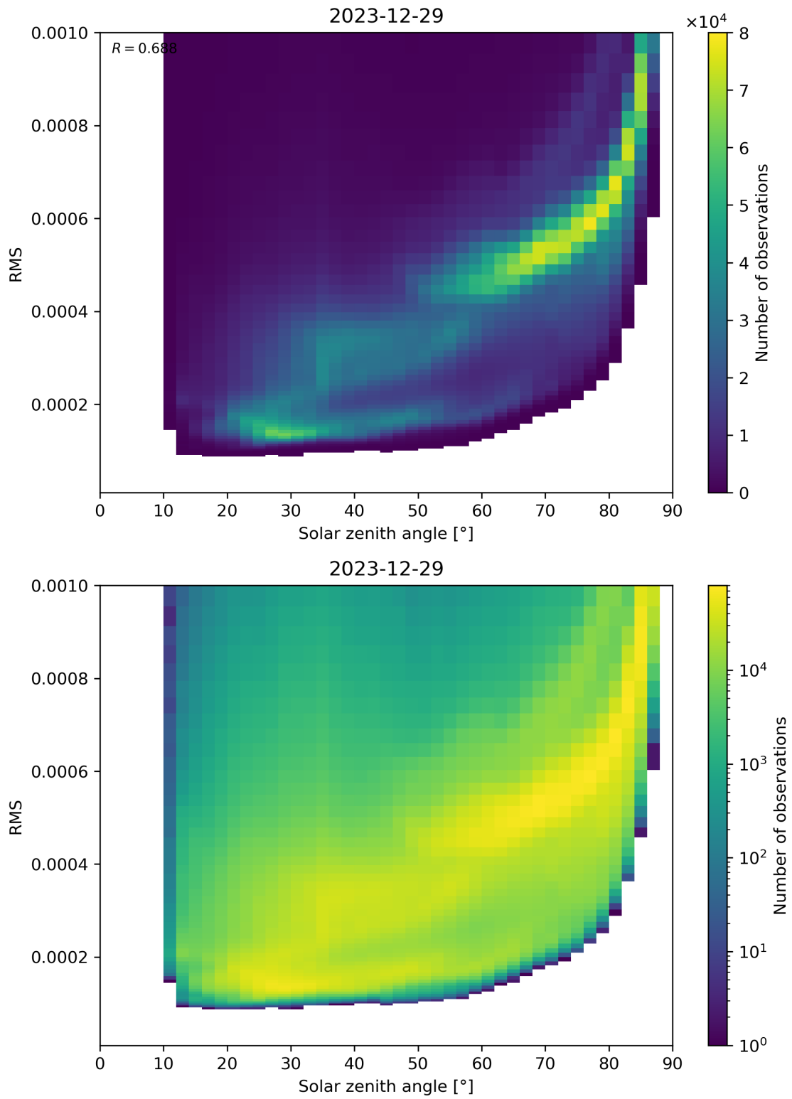
Figure 157: Scatter density plot of “Solar zenith angle” against “RMS” for 2023-12-28 to 2023-12-30.
