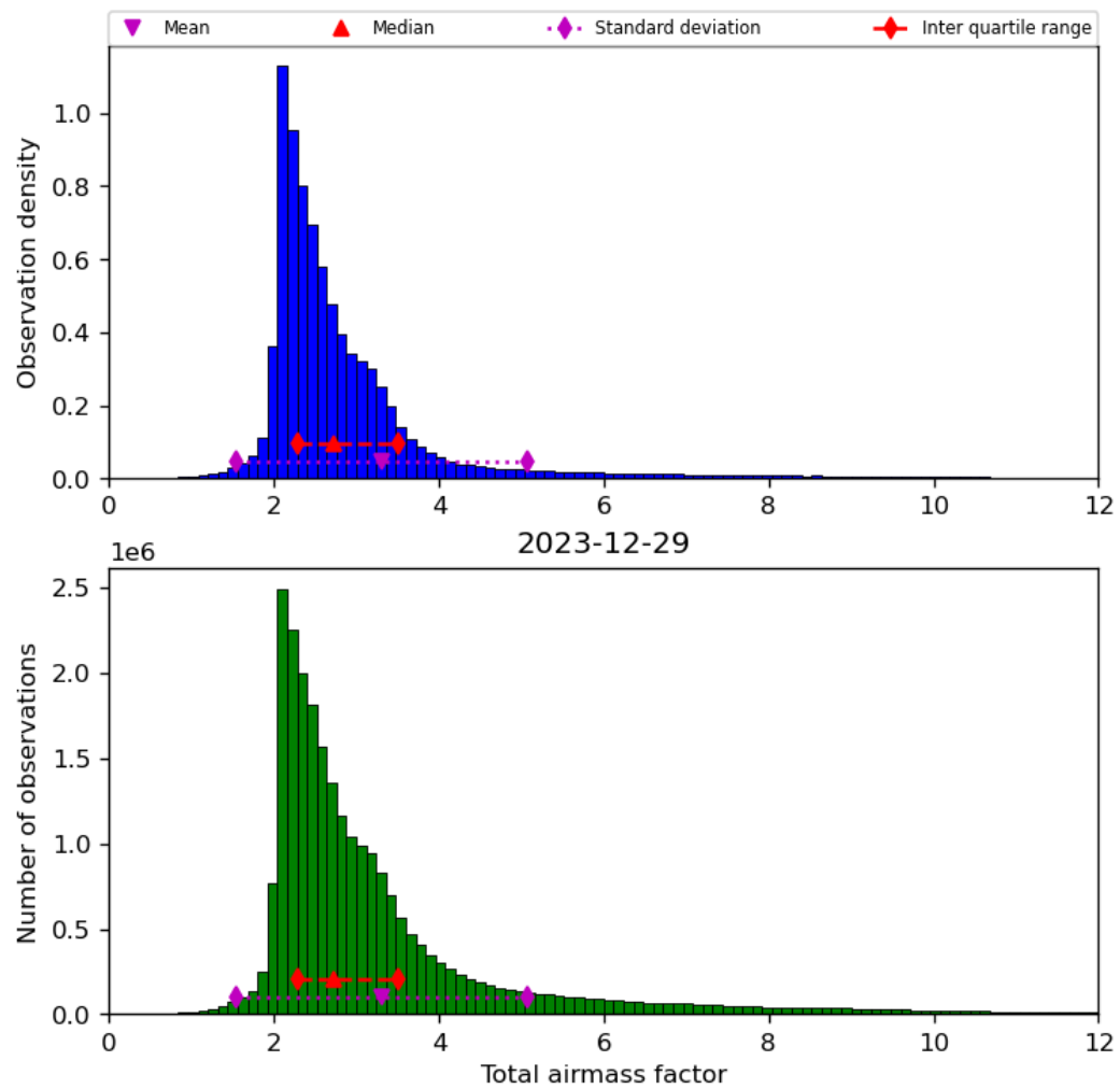
Figure 32: Histogram of “Total airmass factor” for 2023-12-28 to 2023-12-30
