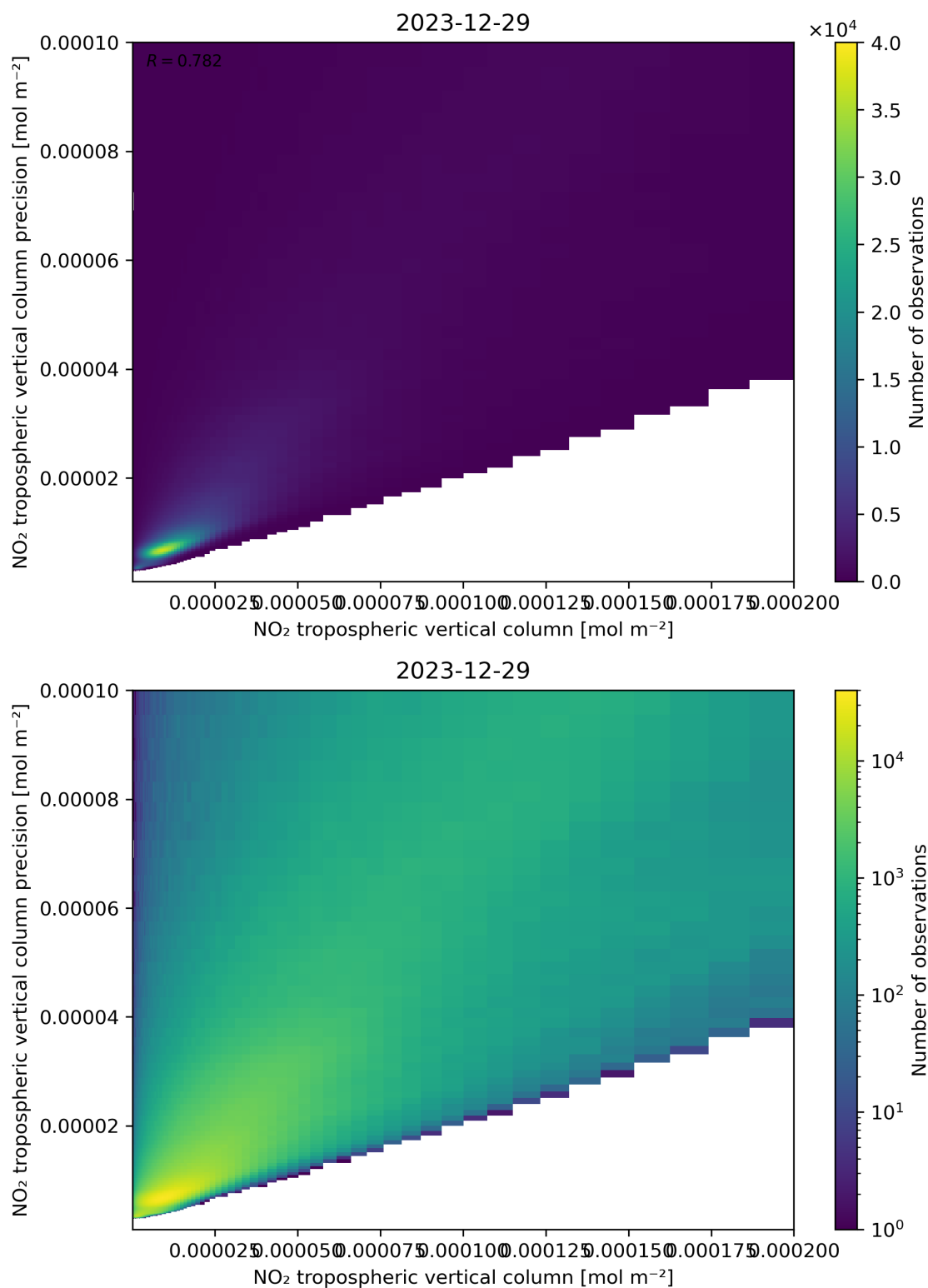
Figure 130: Scatter density plot of “NO 2 tropospheric vertical column” against “NO 2 tropospheric vertical column precision” for 2023-12-28 to 2023-12-30.
