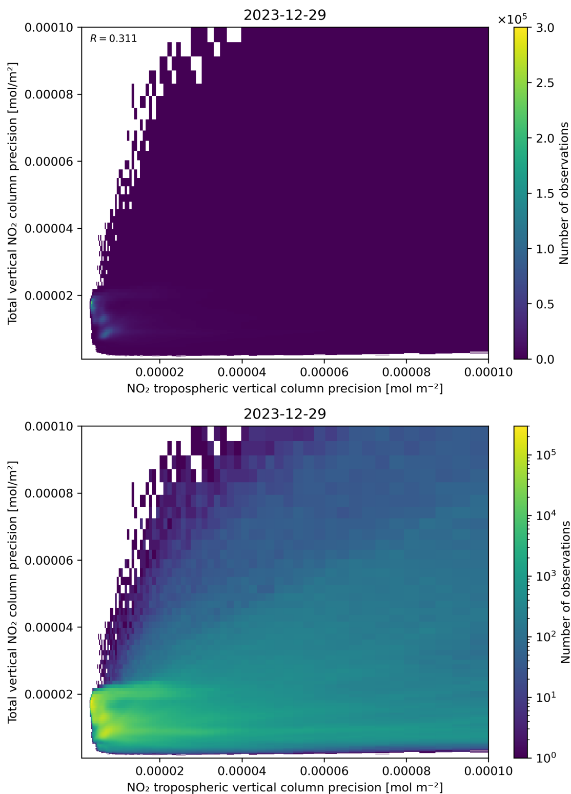
Figure 139: Scatter density plot of “NO 2 tropospheric vertical column precision” against “Total vertical NO 2 column precision” for 2023-12-28 to 2023-12-30.
