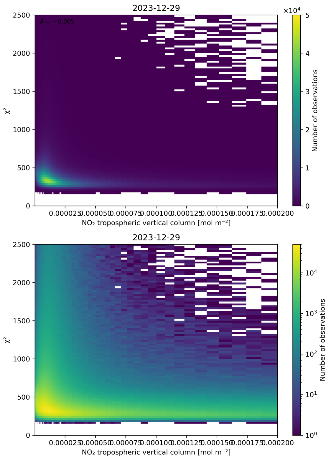
Figure 124: Scatter density plot of “NO 2 tropospheric vertical column” against “ \chi^2 ” for 2023-12-28 to 2023-12-30.
