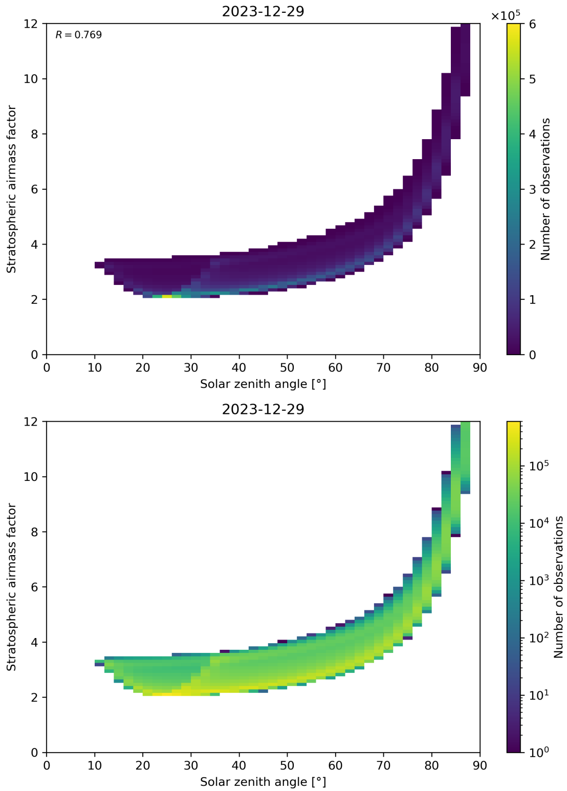
Figure 145: Scatter density plot of “Solar zenith angle” against “Stratospheric airmass factor” for 2023-12-28 to 2023-12-30.
