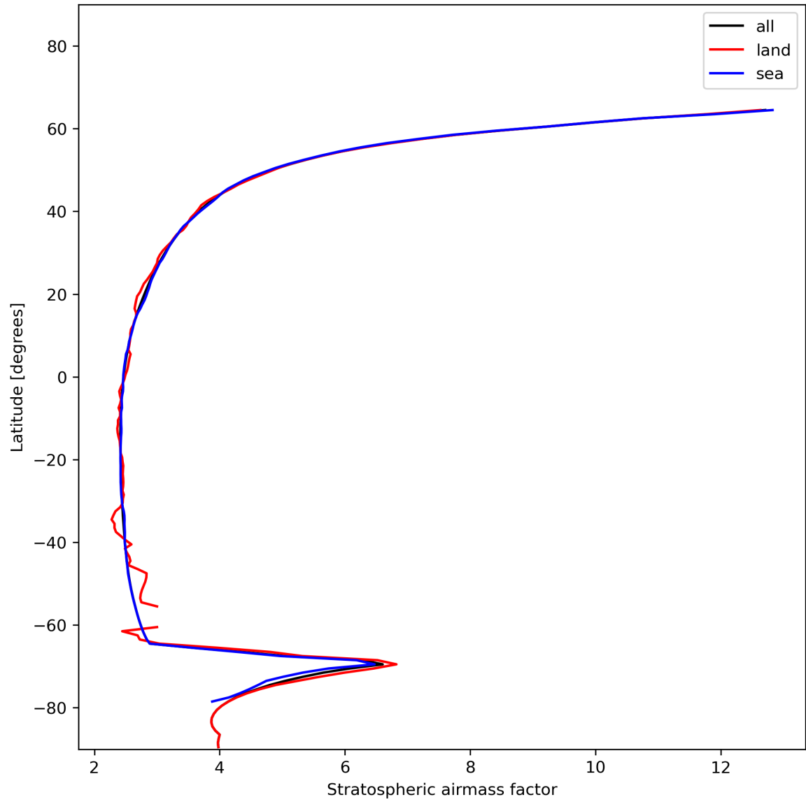
Figure 27: Zonal average of “Stratospheric air mass factor” for 2023-12-28 to 2023-12-30.
