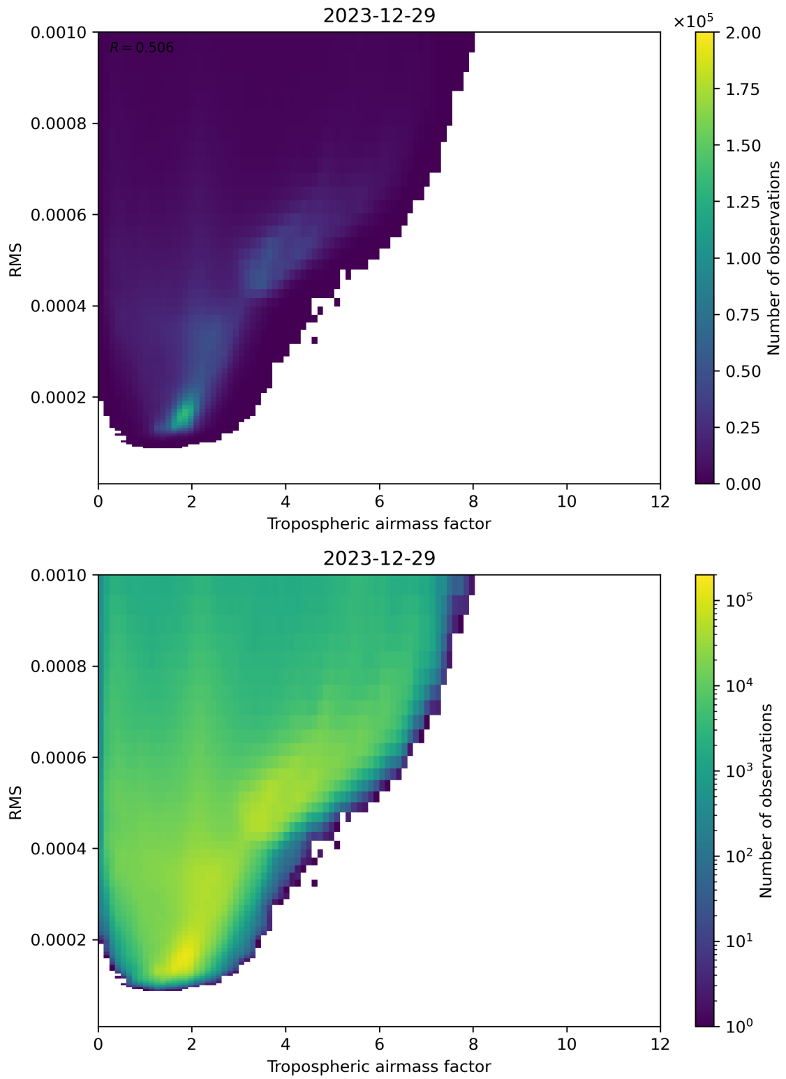
Figure 79: Scatter density plot of “Tropospheric airmass factor” against “RMS” for 2023-12-28 to 2023-12-30.
