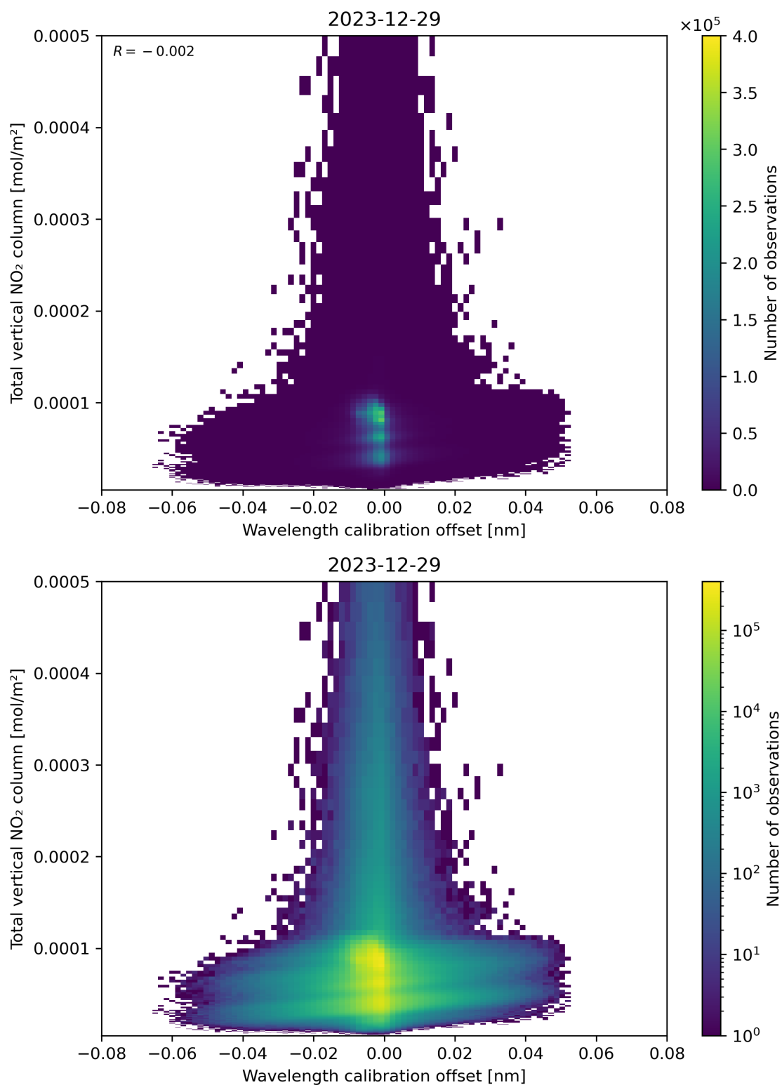
Figure 179: Scatter density plot of “Wavelength calibration offset” against “Total vertical NO 2 column” for 2023-12-28 to 2023-12-30.
