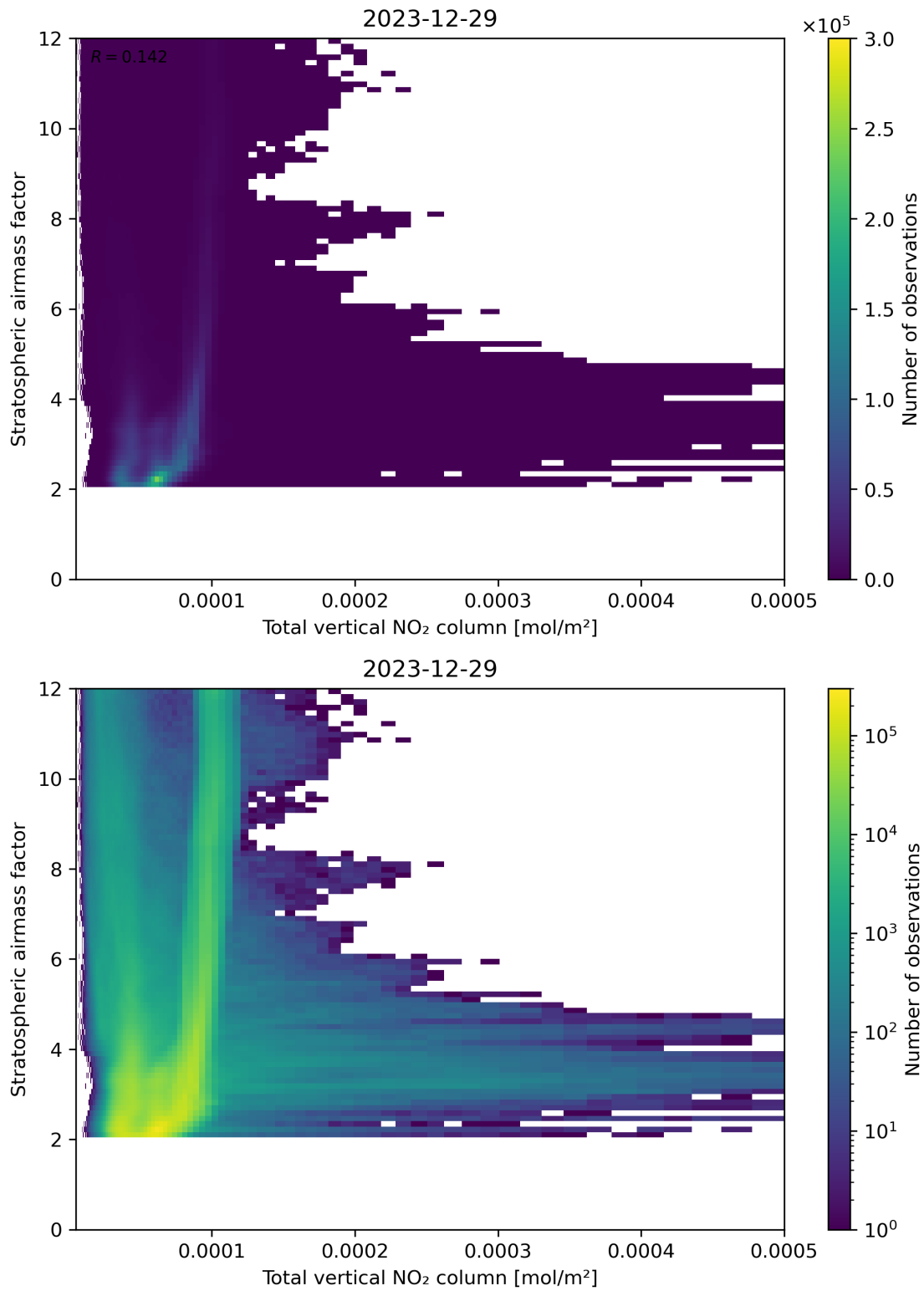
Figure 110: Scatter density plot of “Total vertical NO 2 column” against “Stratospheric air mass factor” for 2023-12-28 to 2023-12-30.
