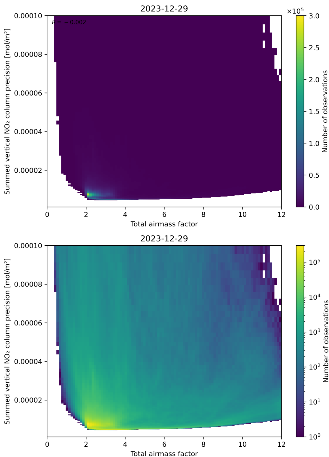
Figure 66: Scatter density plot of “Total airmass factor” against “Summed vertical NO 2 column precision” for 2023-12-28 to 2023-12-30.
