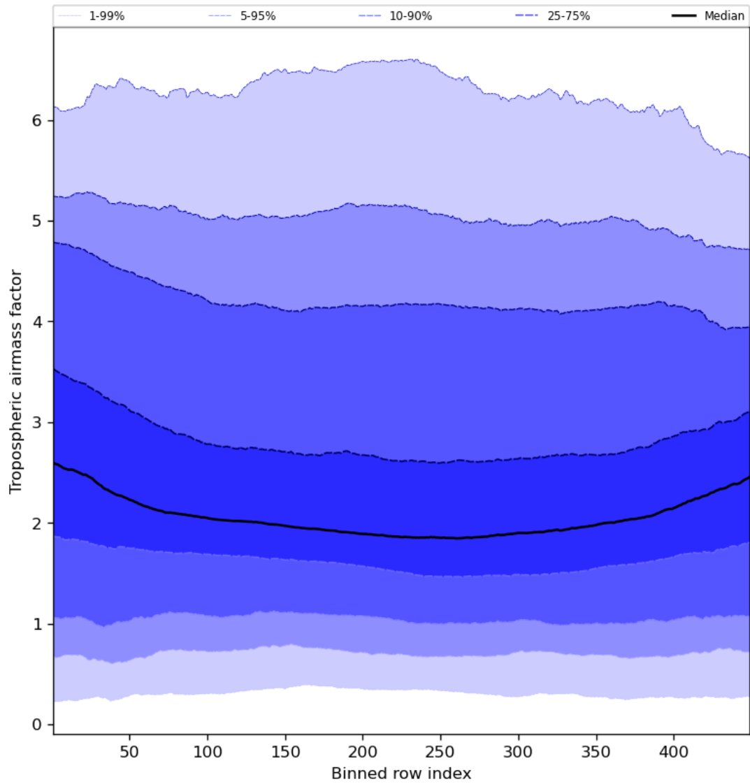
Figure 48: Along track statistics of “Tropospheric airmass factor” for 2023-12-28 to 2023-12-30
