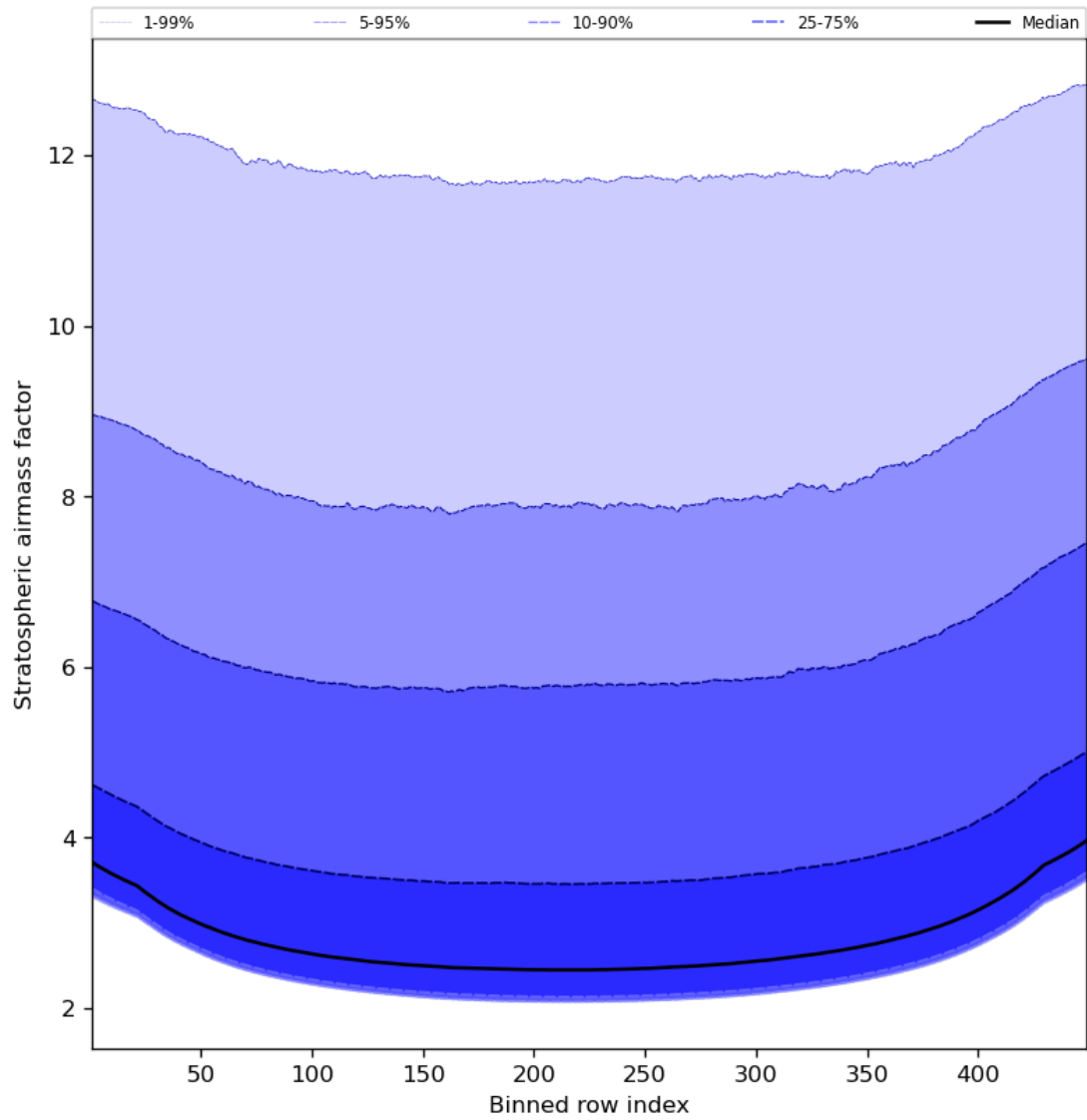
Figure 61: Along track statistics of “Stratospheric airmass factor” for 2023-12-28 to 2023-12-30
