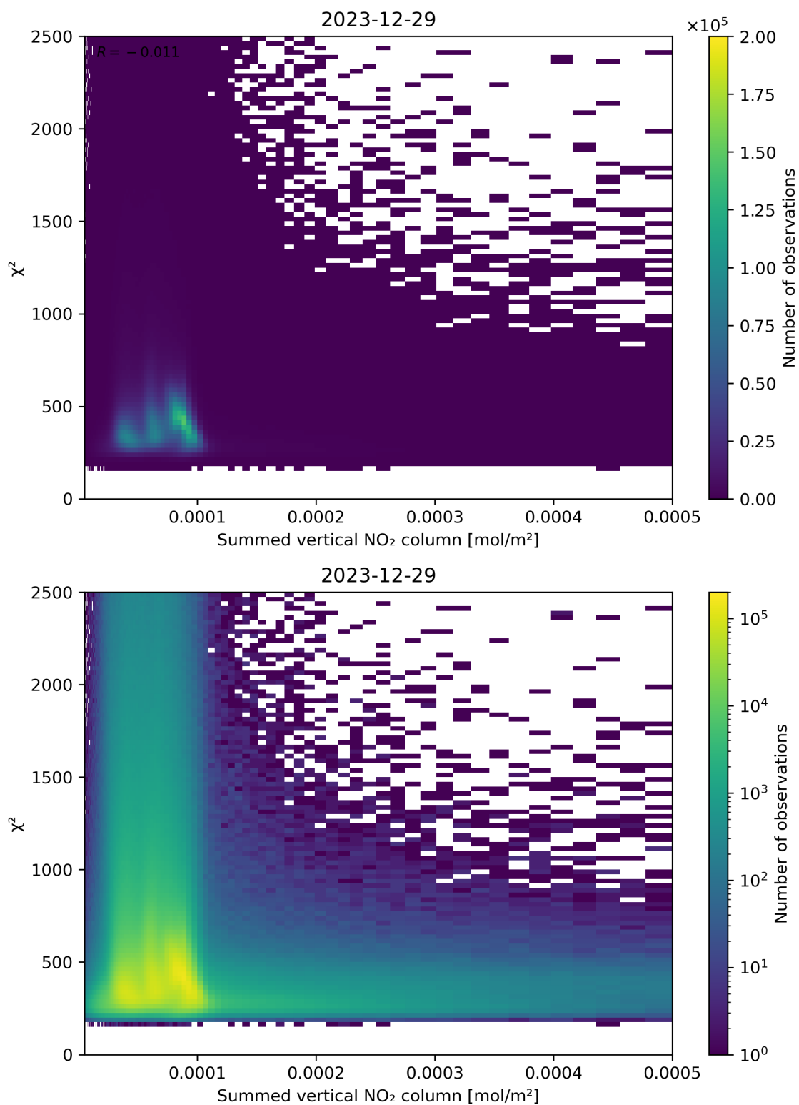
Figure 104: Scatter density plot of “Summed vertical NO 2 column” against “ \chi^2 ” for 2023-12-28 to 2023-12-30.
