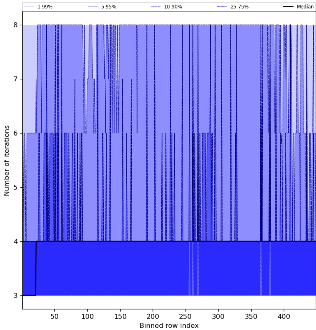
Figure 51: Along track statistics of “Number of iterations” for 2023-12-28 to 2023-12-30
