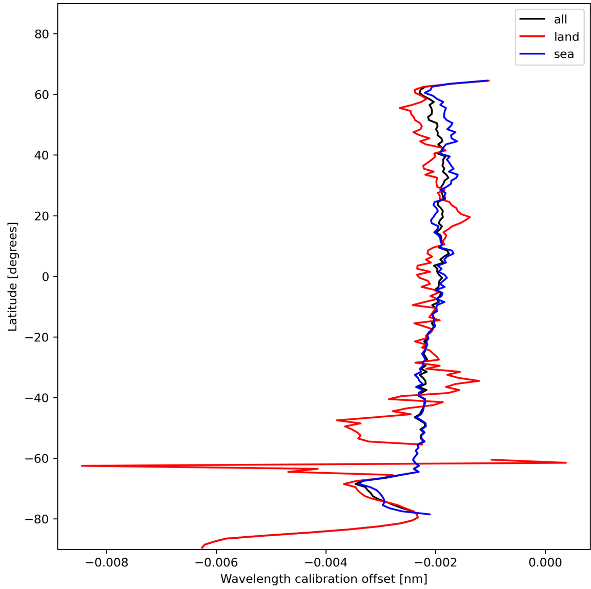
Figure 18: Zonal average of “Wavelength calibration offset” for 2023-12-28 to 2023-12-30.
