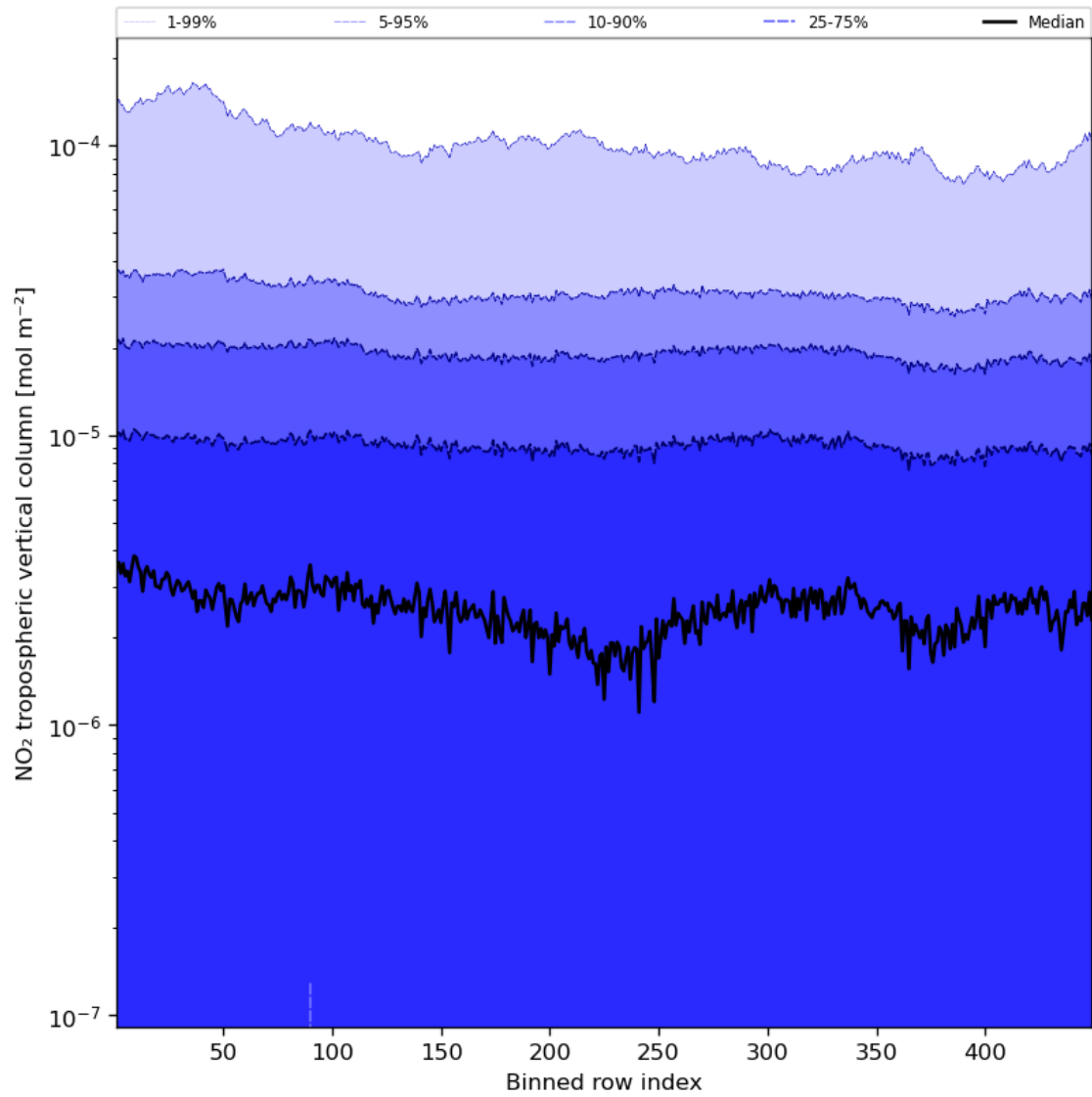
Figure 46: Along track statistics of “NO 2 tropospheric vertical column” for 2023-12-28 to 2023-12-30
