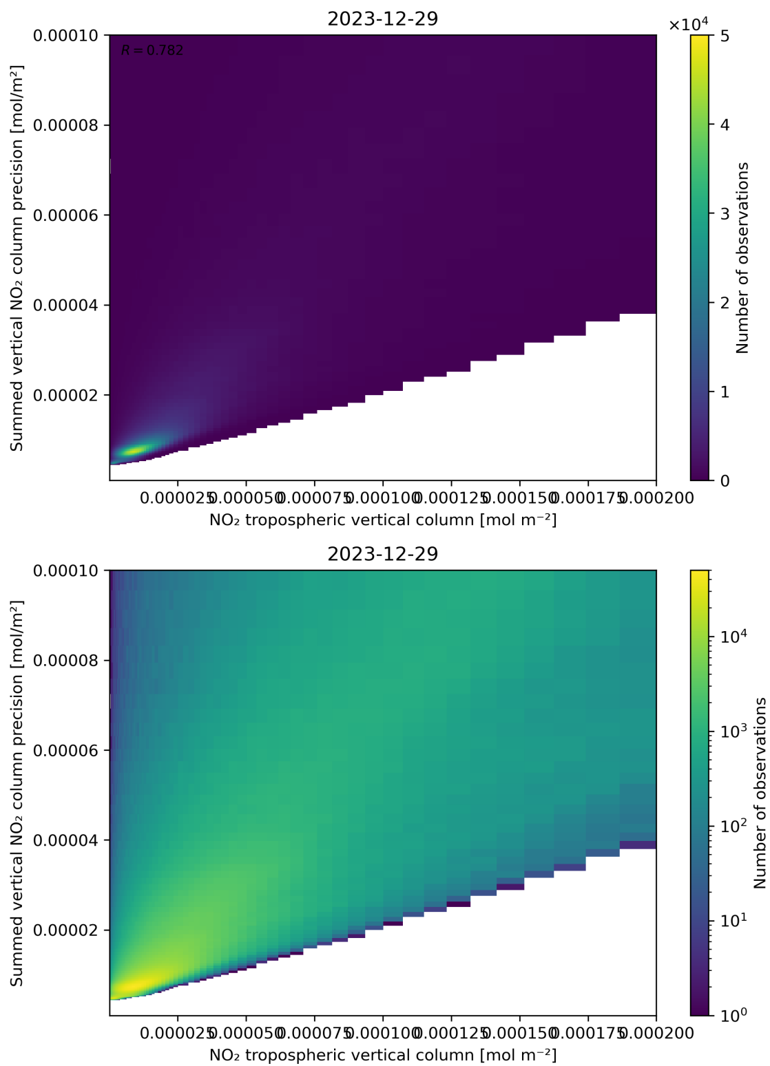
Figure 127: Scatter density plot of “NO 2 tropospheric vertical column” against “Summed vertical NO 2 column precision” for 2023-12-28 to 2023-12-30.
