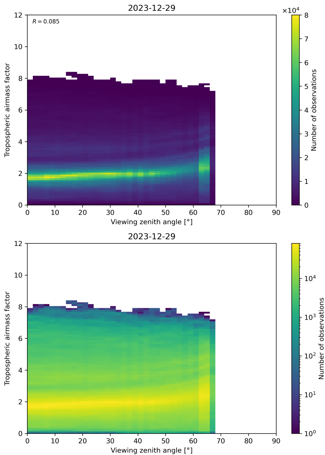
Figure 161: Scatter density plot of “Viewing zenith angle” against “Tropospheric airmass factor” for 2023-12-28 to 2023-12-30.
