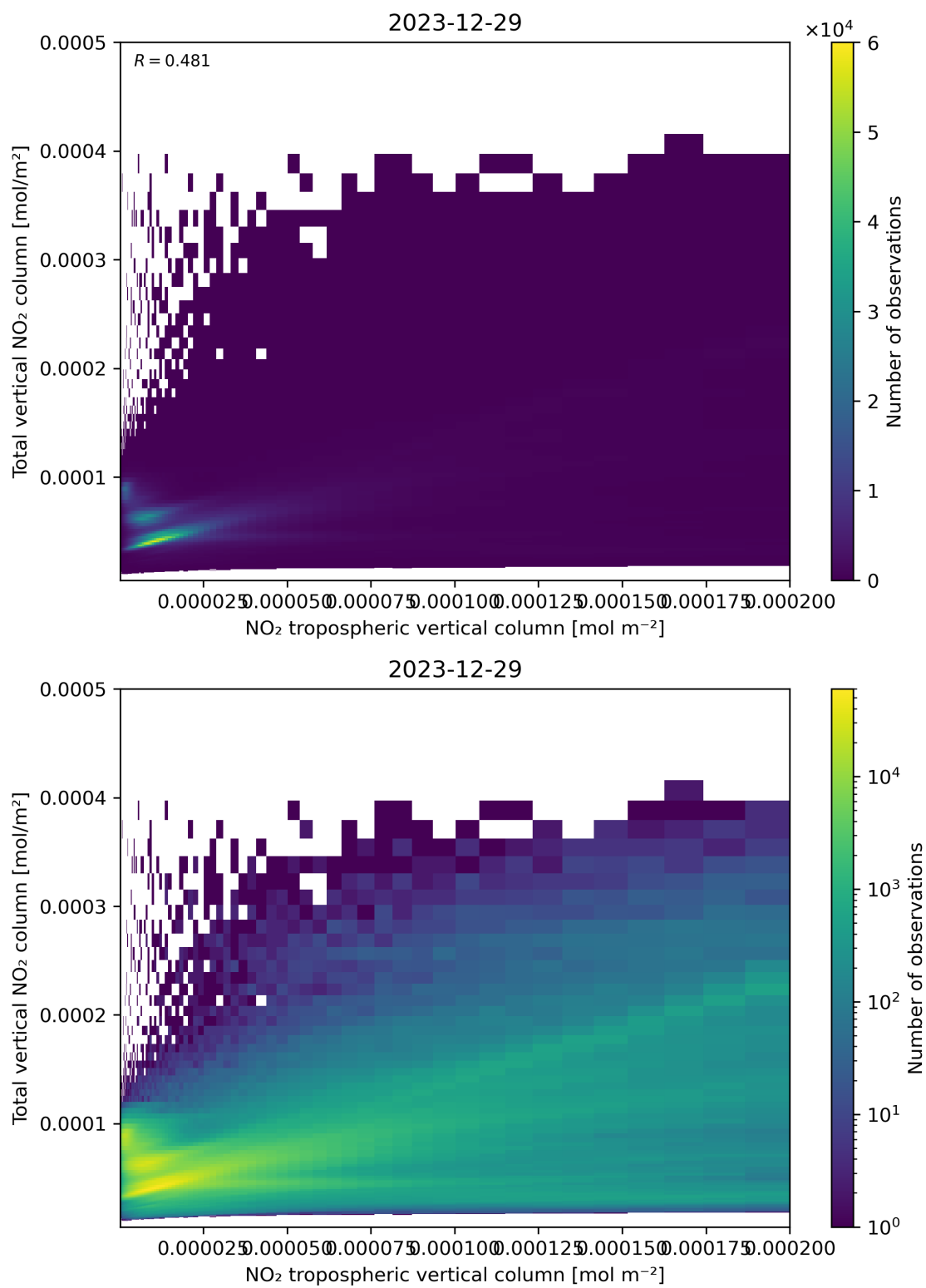
Figure 128: Scatter density plot of “NO 2 tropospheric vertical column” against “Total vertical NO 2 column” for 2023-12-28 to 2023-12-30.
