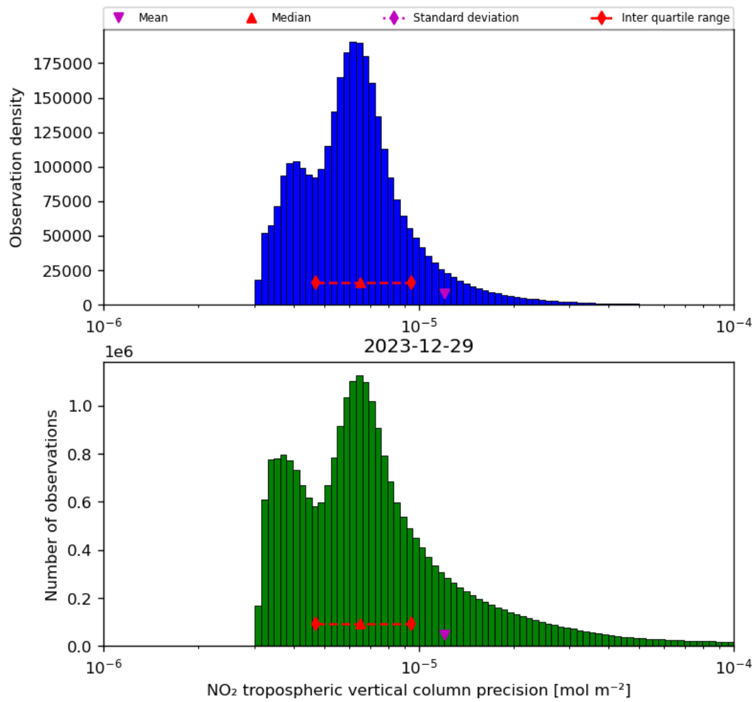
Figure 30: Histogram of “NO 2 tropospheric vertical column precision” for 2023-12-28 to 2023-12-30
