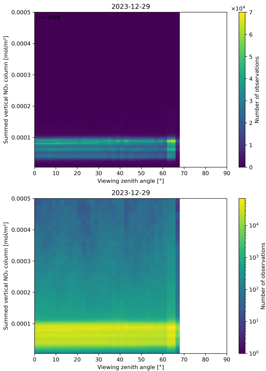
Figure 165: Scatter density plot of “Viewing zenith angle” against “Summed vertical NO 2 column” for 2023-12-28 to 2023-12-30.
