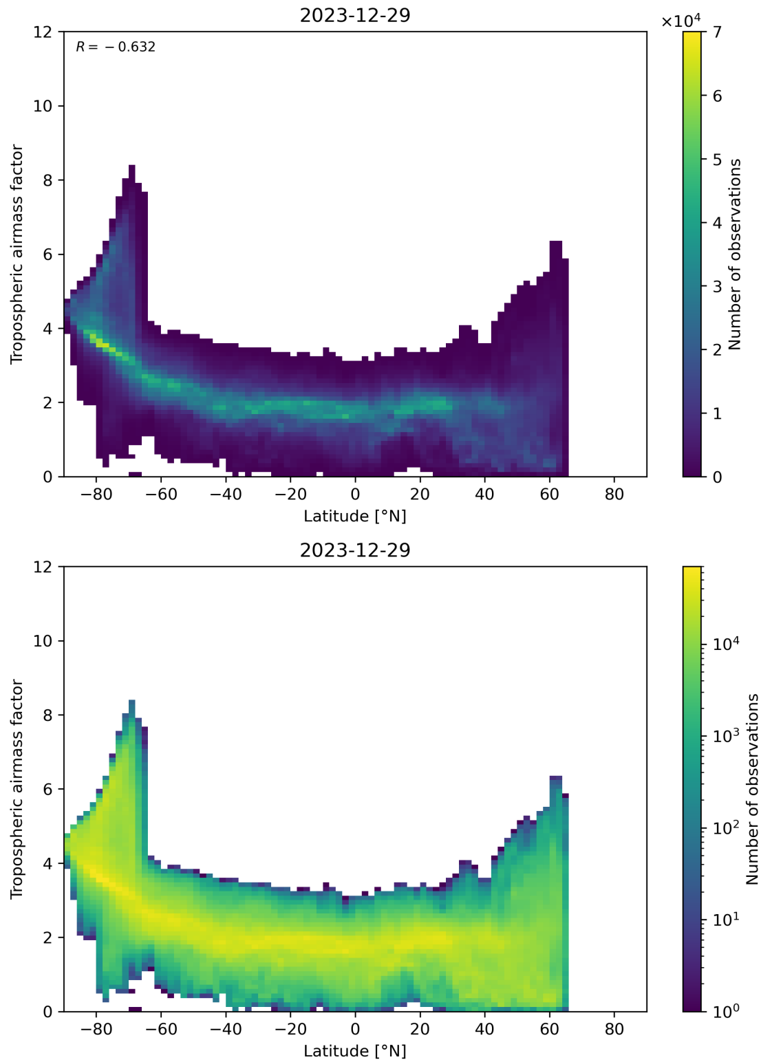
Figure 85: Scatter density plot of “Latitude” against “Tropospheric airmass factor” for 2023-12-28 to 2023-12-30.
