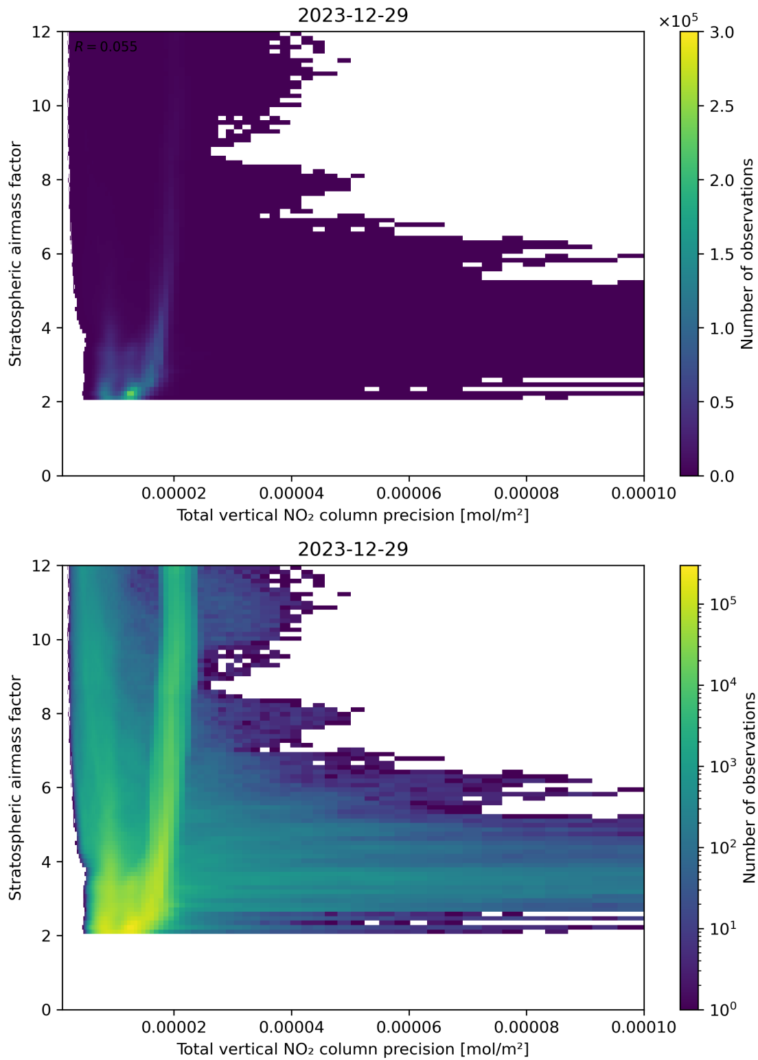
Figure 115: Scatter density plot of “Total vertical NO 2 column precision” against “Stratospheric air mass factor” for 2023-12-28 to 2023-12-30.
