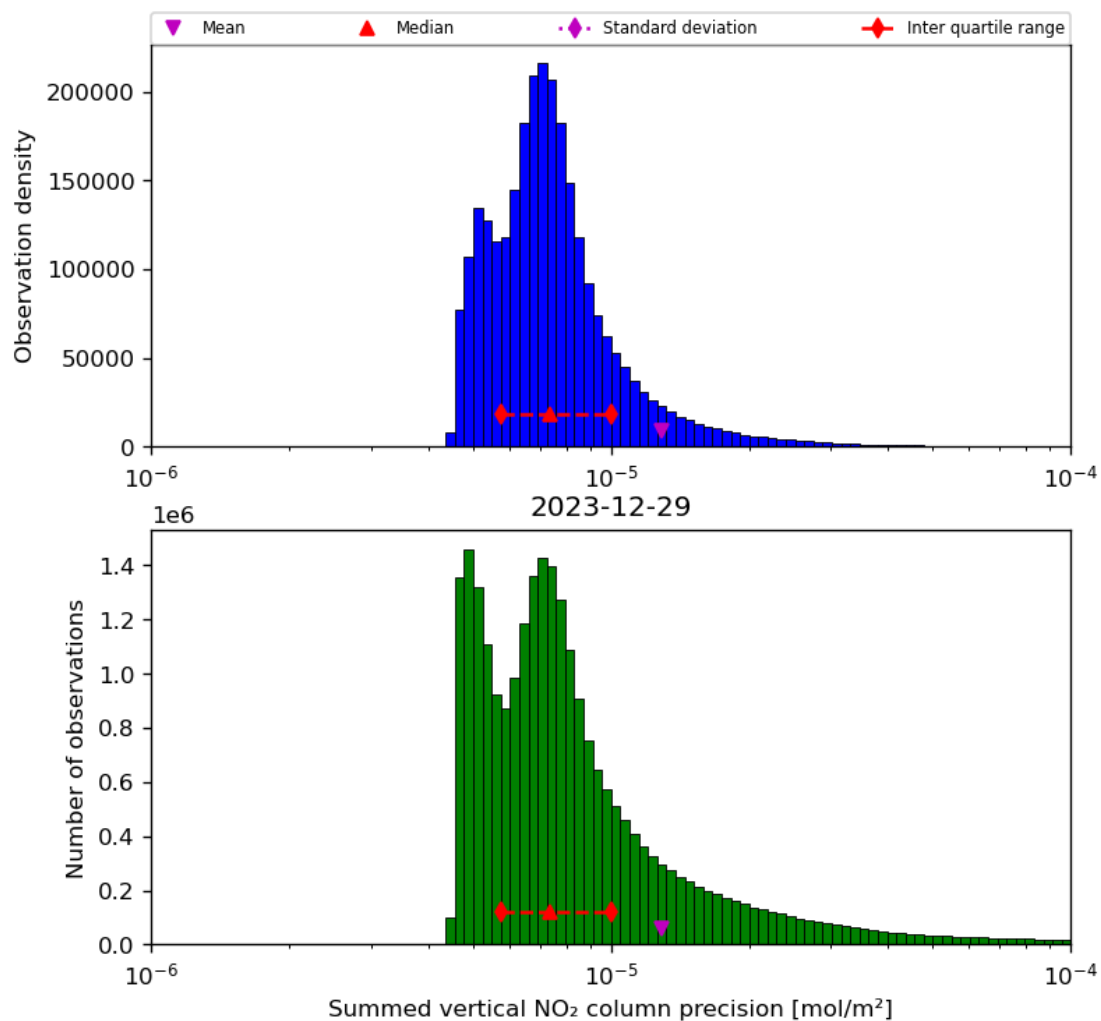
Figure 41: Histogram of "Summed vertical NO 2 column precision" for 2023-12-28 to 2023-12-30
