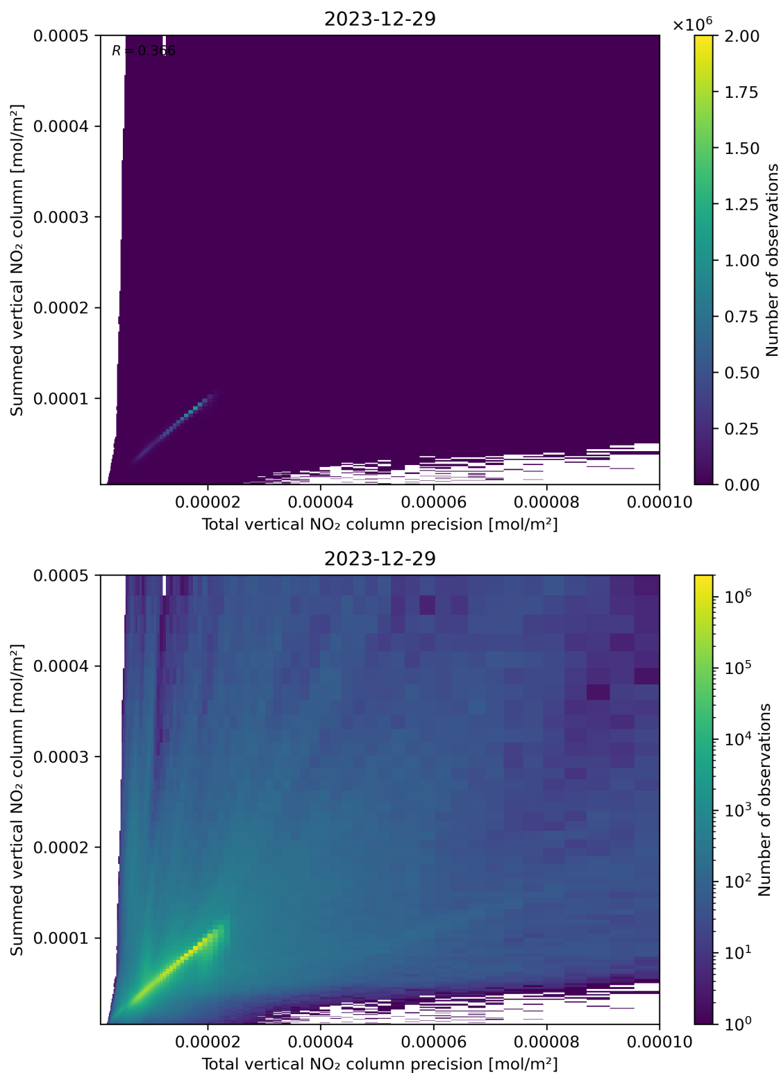
Figure 117: Scatter density plot of “Total vertical NO 2 column precision” against “Summed vertical NO 2 column” for 2023-12-28 to 2023-12-30.
