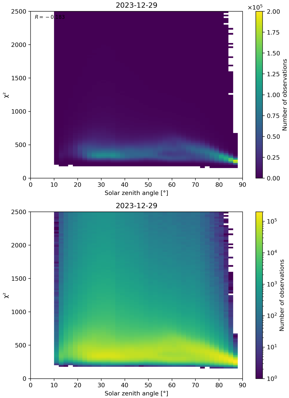
Figure 148: Scatter density plot of “Solar zenith angle” against “ \chi^2 ” for 2023-12-28 to 2023-12-30.
