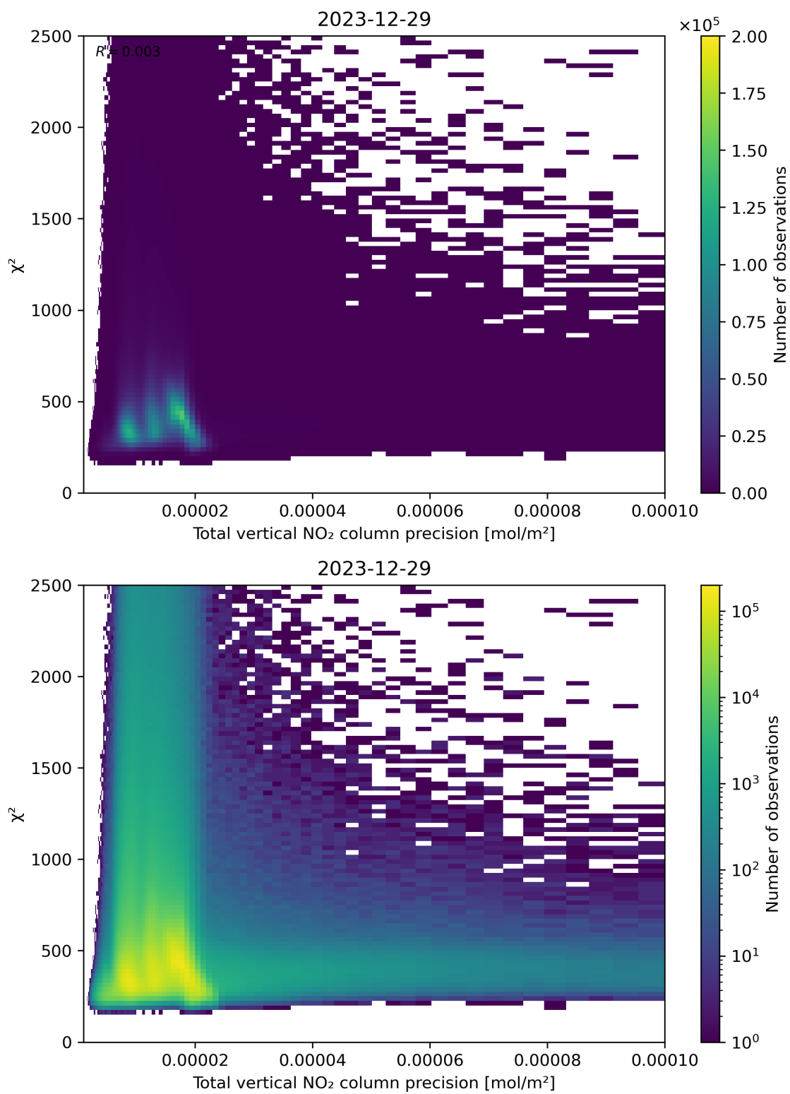
Figure 116: Scatter density plot of “Total vertical NO 2 column precision” against “ \chi^2 ” for 2023-12-28 to 2023-12-30.
