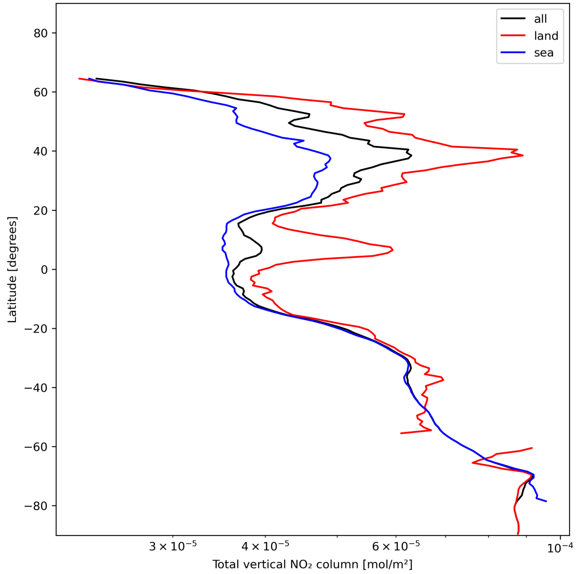
Figure 21: Zonal average of “Total vertical NO 2 column” for 2023-12-28 to 2023-12-30.
