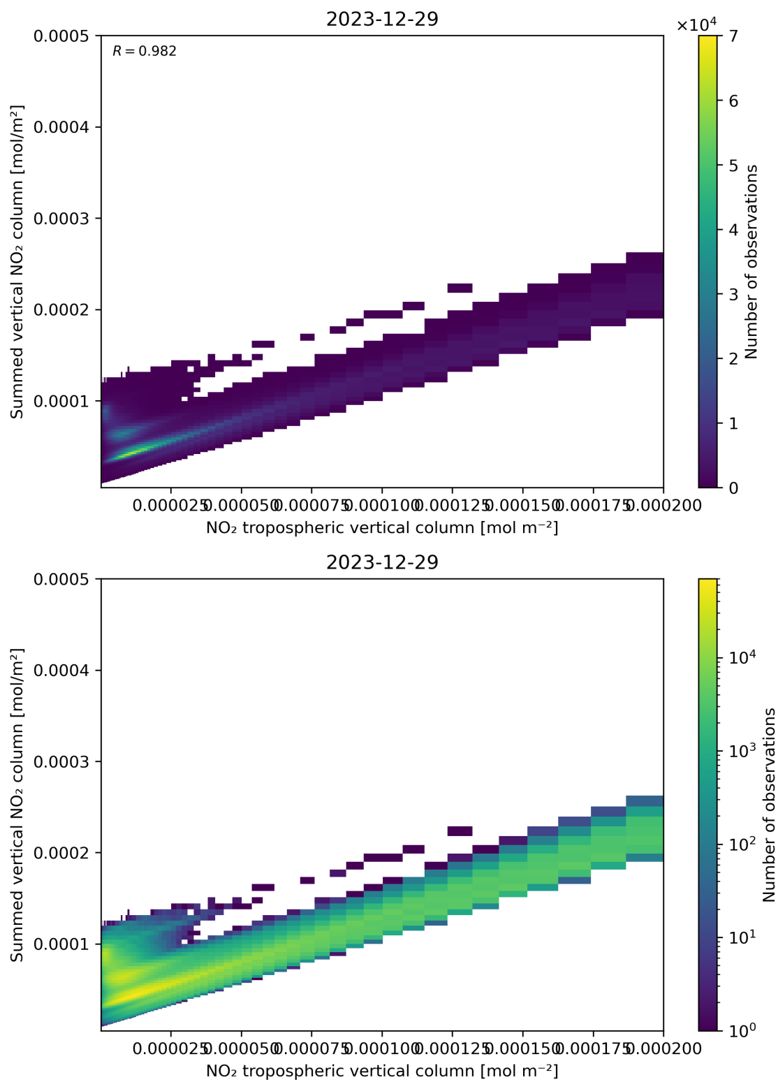
Figure 126: Scatter density plot of “NO 2 tropospheric vertical column” against “Summed vertical NO 2 column” for 2023-12-28 to 2023-12-30.
