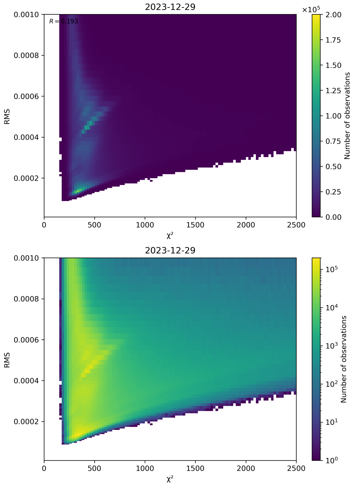
Figure 82: Scatter density plot of “ \chi^2 ” against “RMS” for 2023-12-28 to 2023-12-30.
