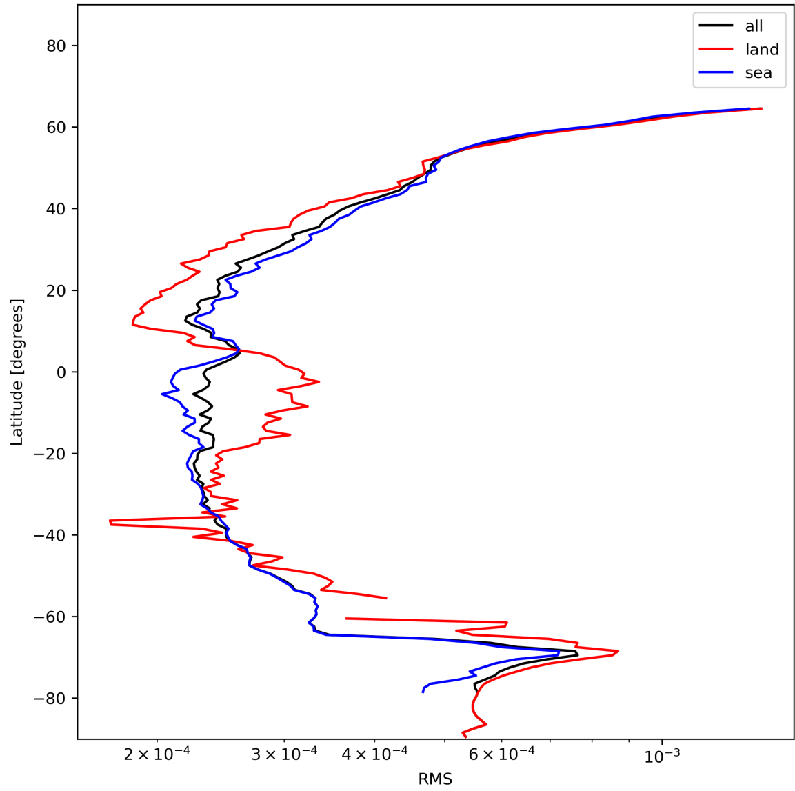
Figure 26: Zonal average of “RMS” for 2023-12-28 to 2023-12-30.
