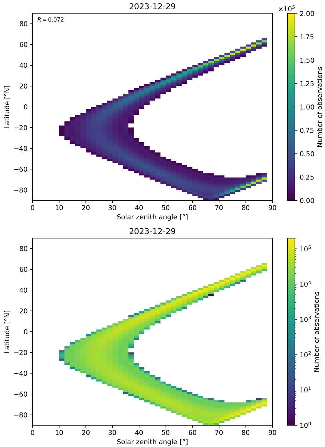
Figure 149: Scatter density plot of “Solar zenith angle” against “Latitude” for 2023-12-28 to 2023-12-30.
