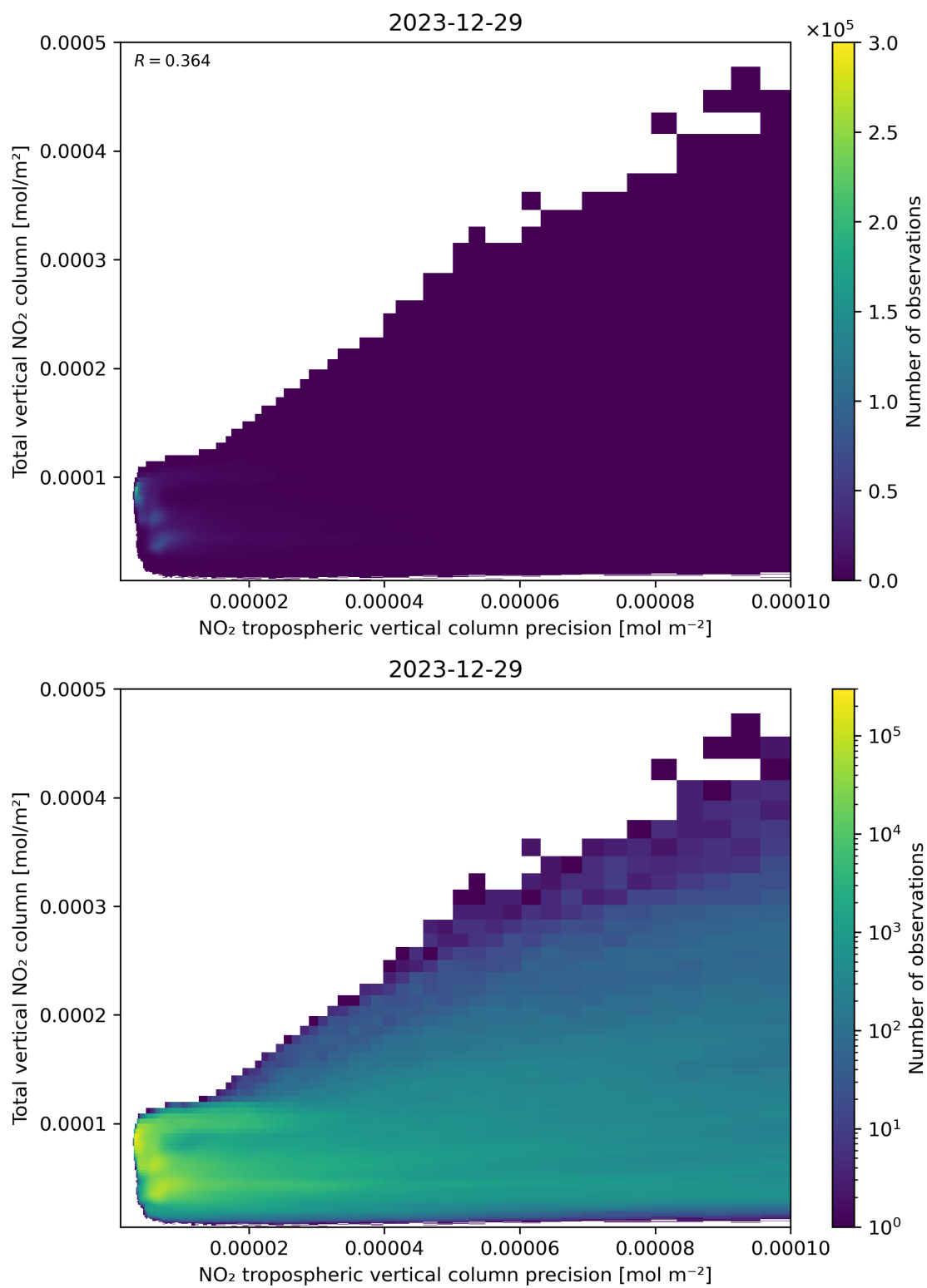
Figure 138: Scatter density plot of “NO 2 tropospheric vertical column precision” against “Total vertical NO 2 column” for 2023-12-28 to 2023-12-30.
