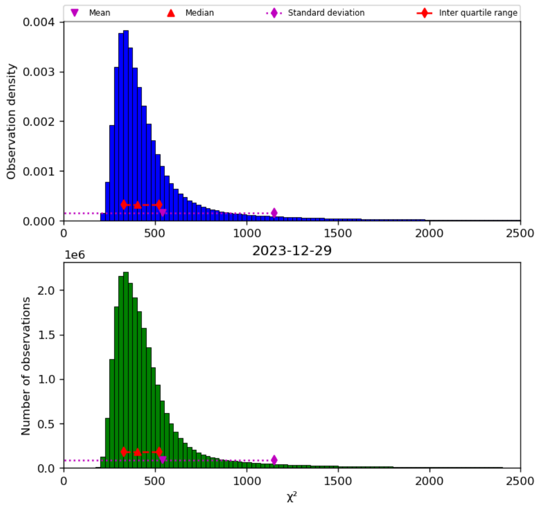
Figure 42: Histogram of “ \chi^2 ” for 2023-12-28 to 2023-12-30
