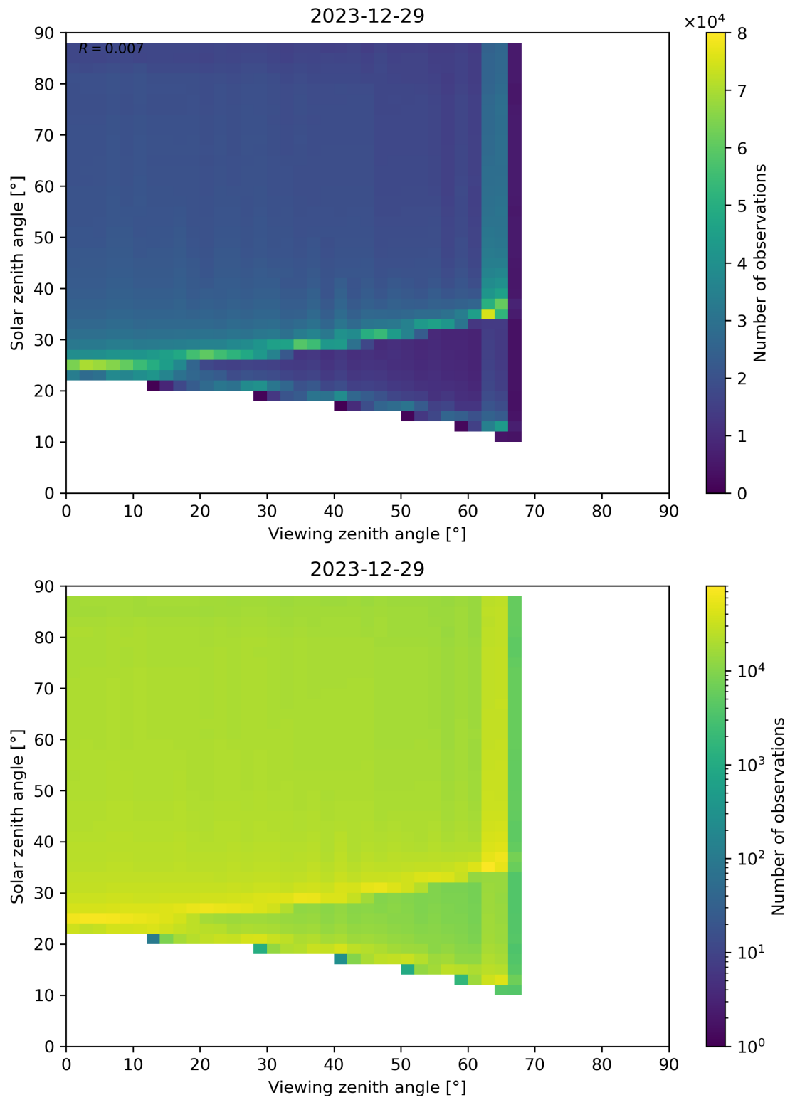
Figure 172: Scatter density plot of “Viewing zenith angle” against “Solar zenith angle” for 2023-12-28 to 2023-12-30.
