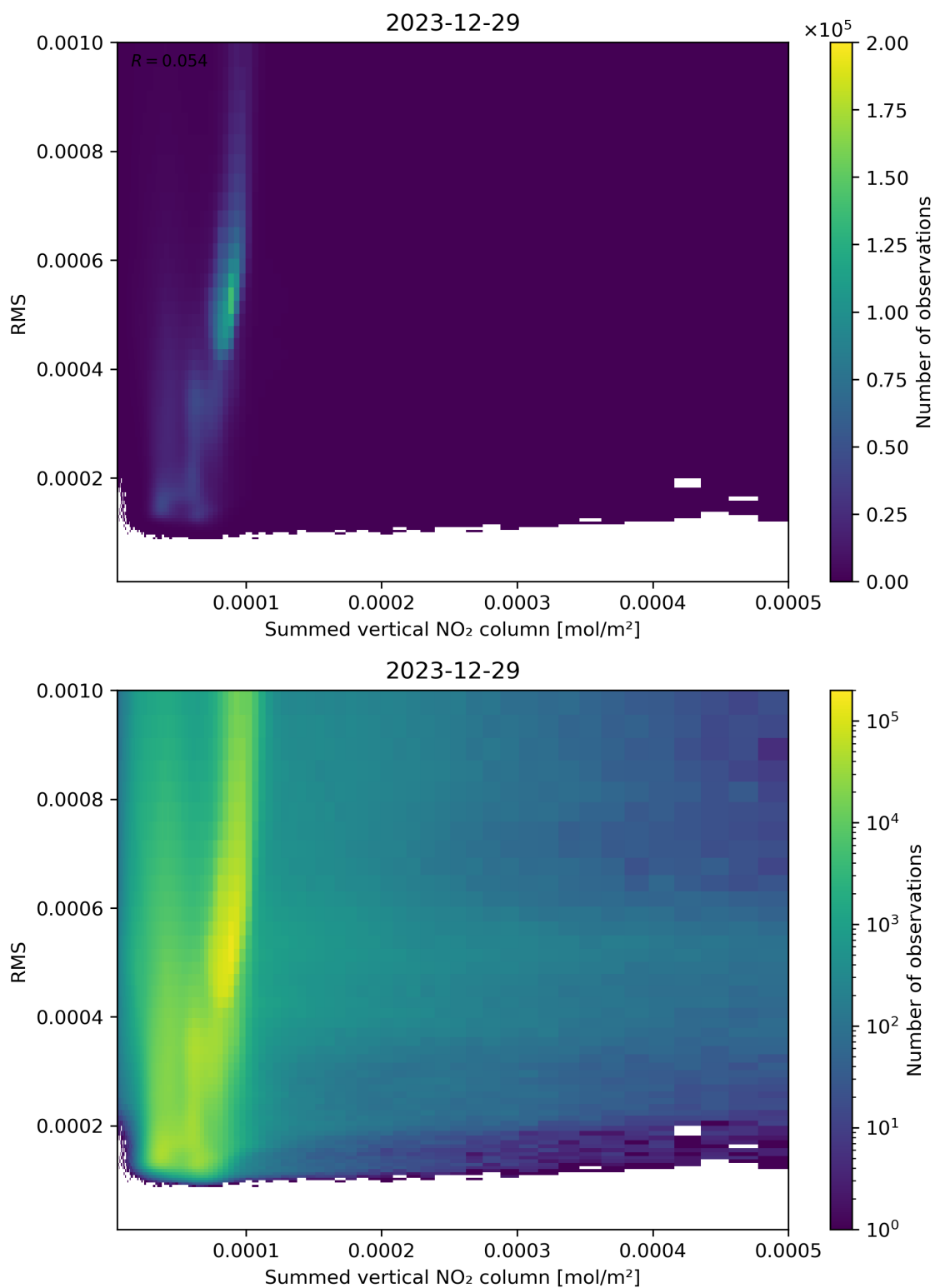
Figure 109: Scatter density plot of “Summed vertical NO 2 column” against “RMS” for 2023-12-28 to 2023-12-30.
