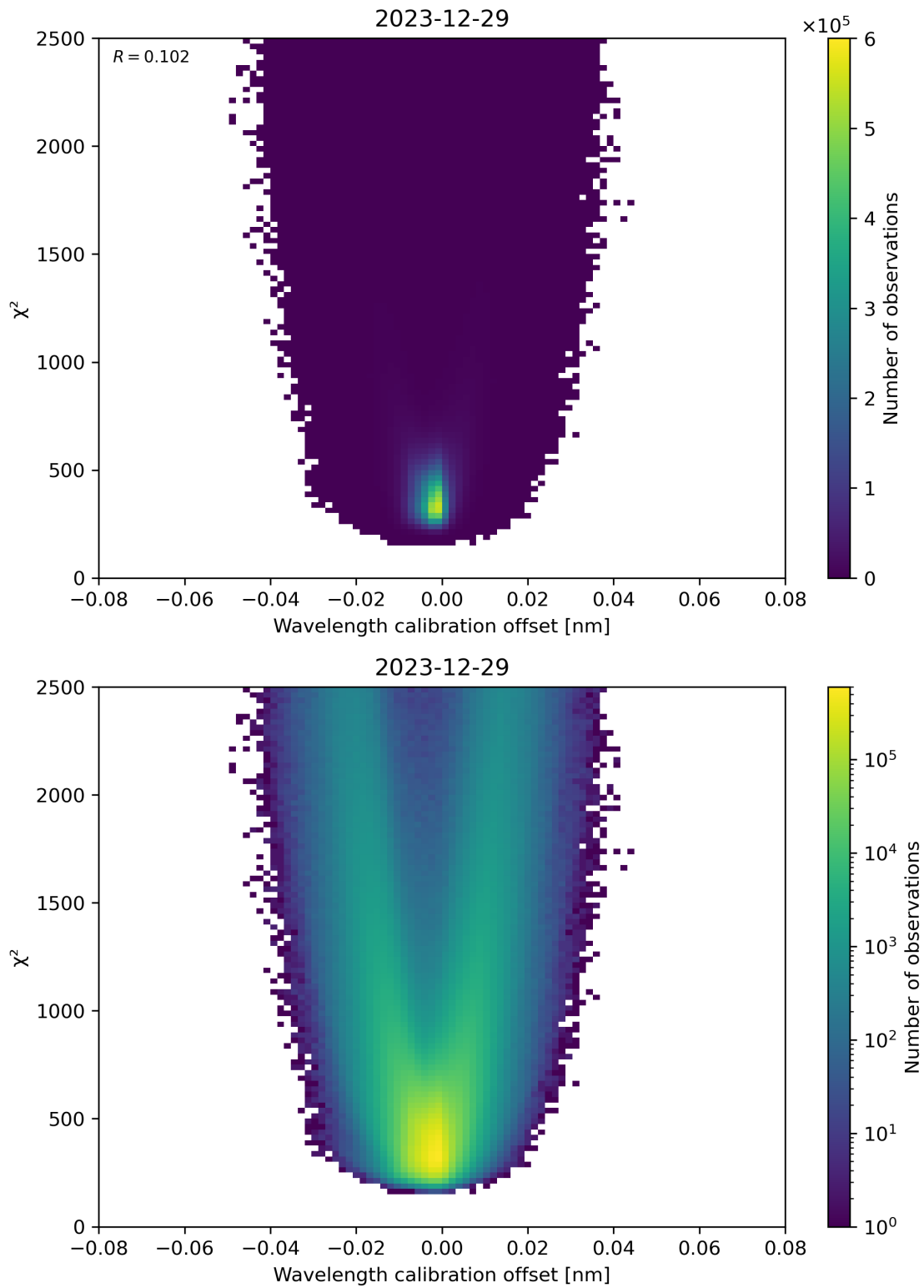
Figure 175: Scatter density plot of “Wavelength calibration offset” against “ \chi^2 ” for 2023-12-28 to 2023-12-30.
