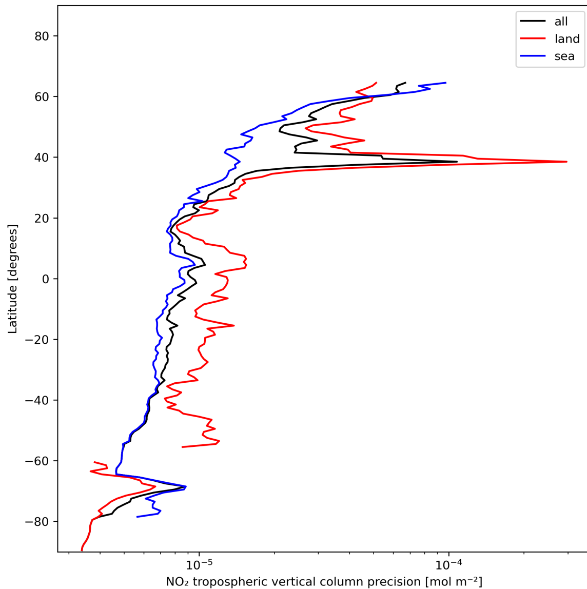
Figure 13: Zonal average of “NO 2 tropospheric vertical column precision” for 2023-12-28 to 2023-12-30.
