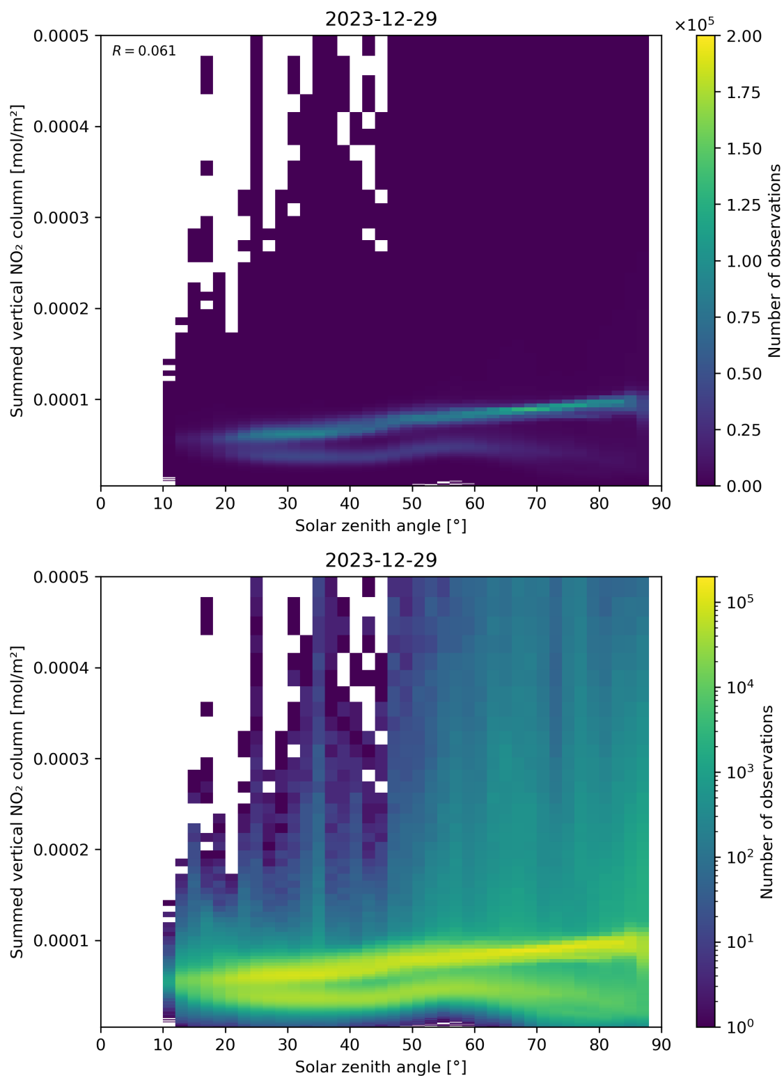
Figure 151: Scatter density plot of “Solar zenith angle” against “Summed vertical NO 2 column” for 2023-12-28 to 2023-12-30.
