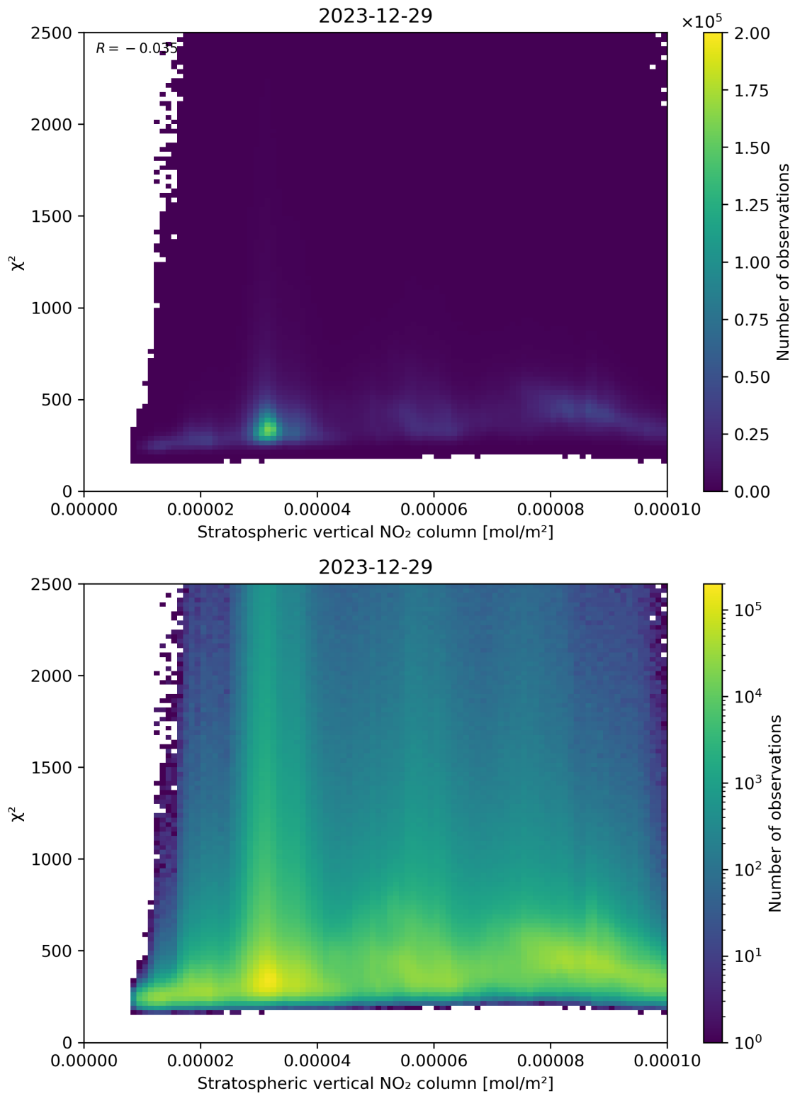
Figure 97: Scatter density plot of “Stratospheric vertical NO 2 column” against “ \chi^2 ” for 2023-12-28 to 2023-12-30.
