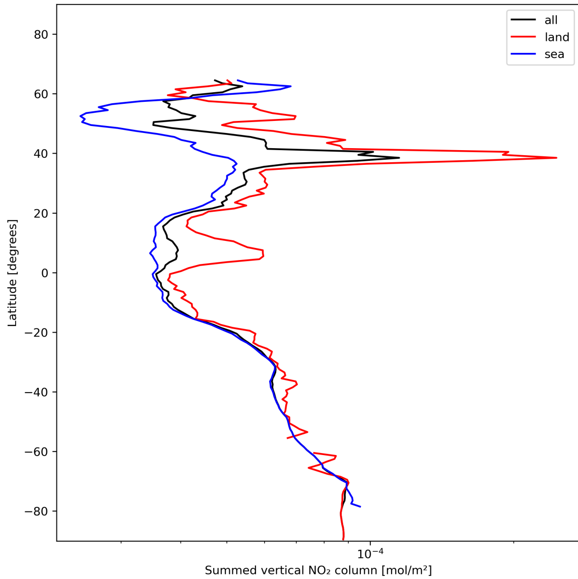
Figure 23: Zonal average of “Summed vertical NO 2 column” for 2023-12-28 to 2023-12-30.
