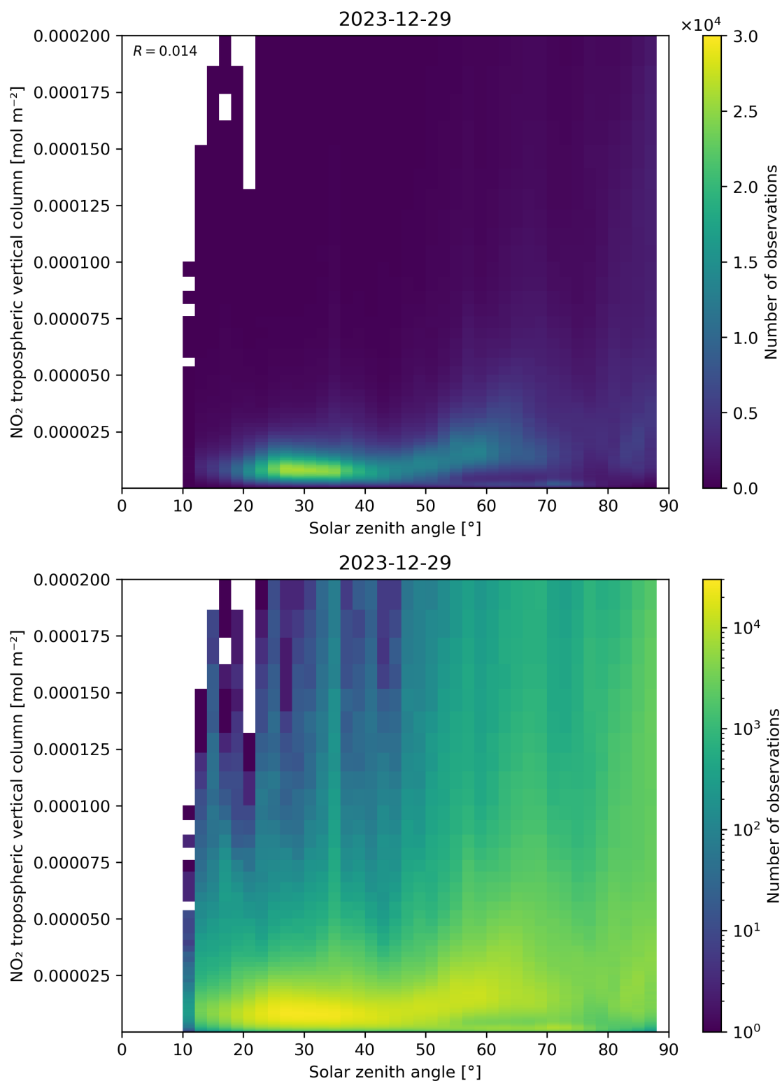
Figure 155: Scatter density plot of “Solar zenith angle” against “NO 2 tropospheric vertical column” for 2023-12-28 to 2023-12-30.
