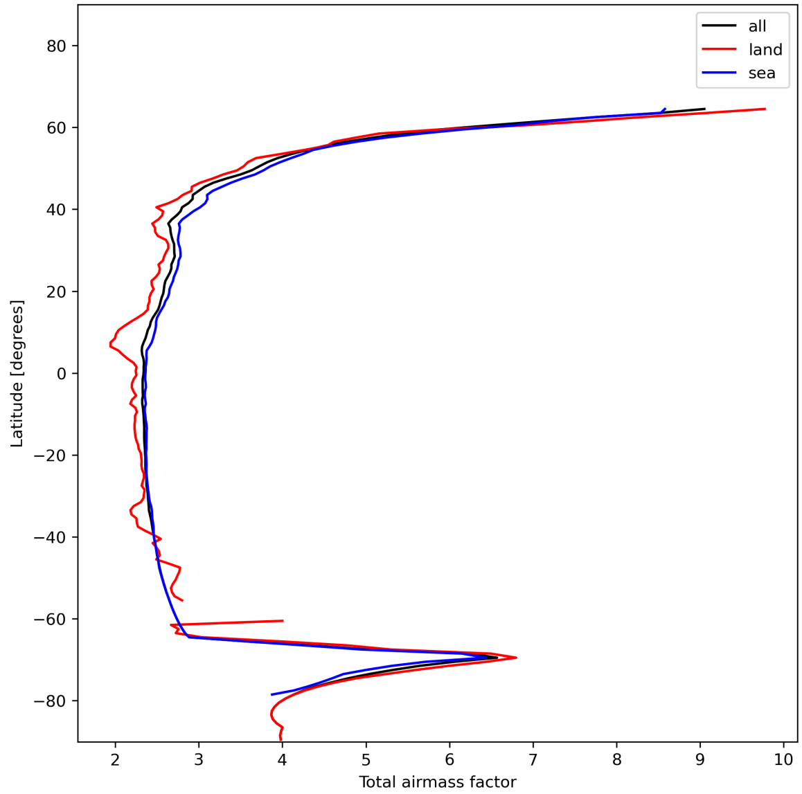
Figure 15: Zonal average of “Total airmass factor” for 2023-12-28 to 2023-12-30.
