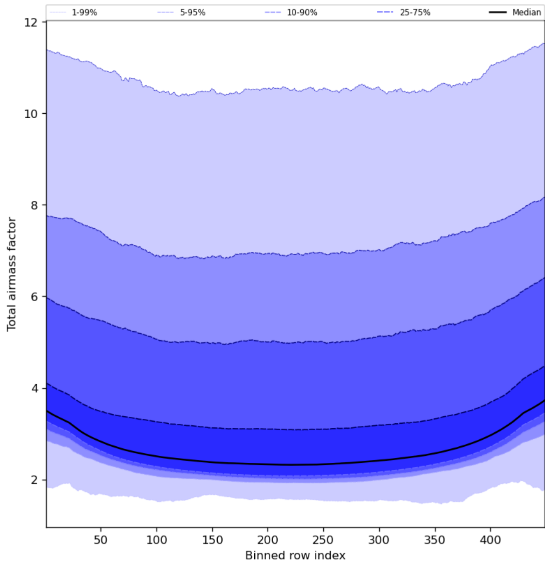
Figure 49: Along track statistics of “Total airmass factor” for 2023-12-28 to 2023-12-30
