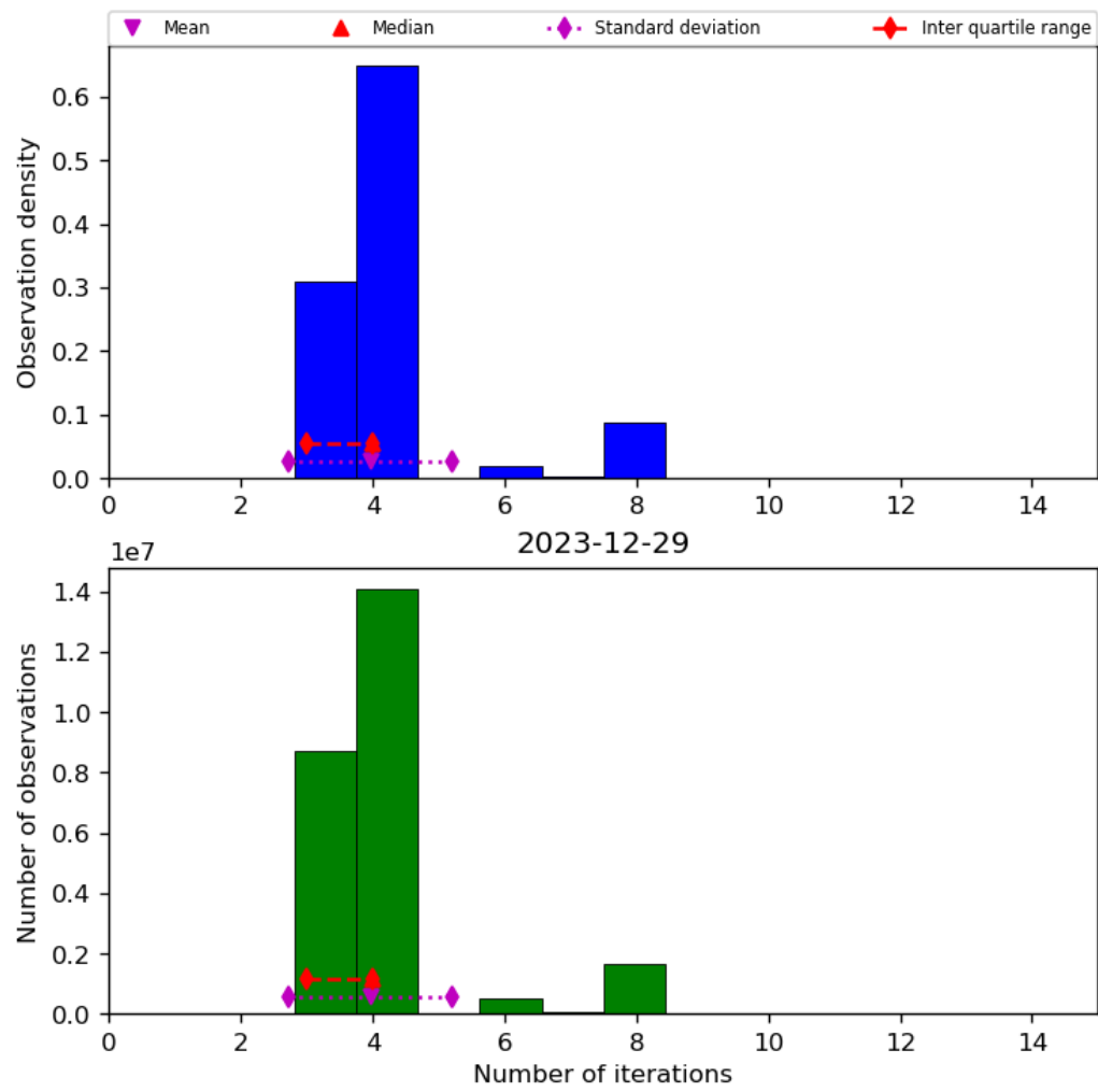
Figure 34: Histogram of “Number of iterations” for 2023-12-28 to 2023-12-30
