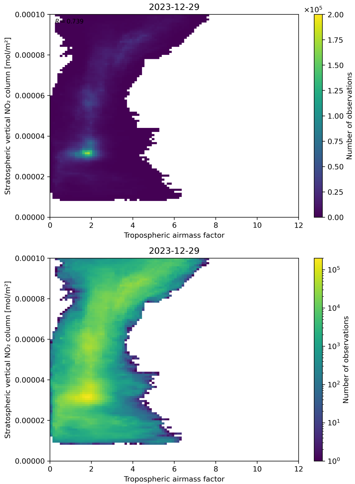
Figure 74: Scatter density plot of “Tropospheric air mass factor” against “Stratospheric vertical NO 2 column” for 2023-12-28 to 2023-12-30.
