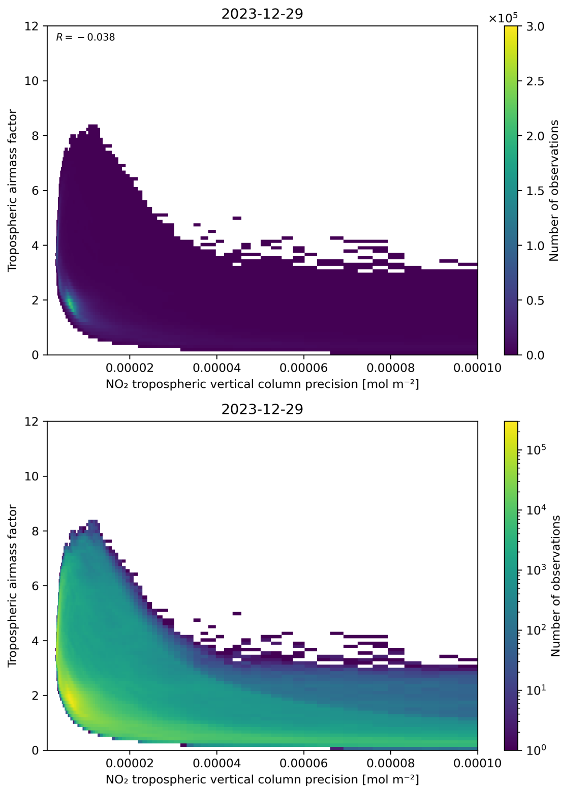
Figure 133: Scatter density plot of “NO 2 tropospheric vertical column precision” against “Tropospheric air mass factor” for 2023-12-28 to 2023-12-30.
