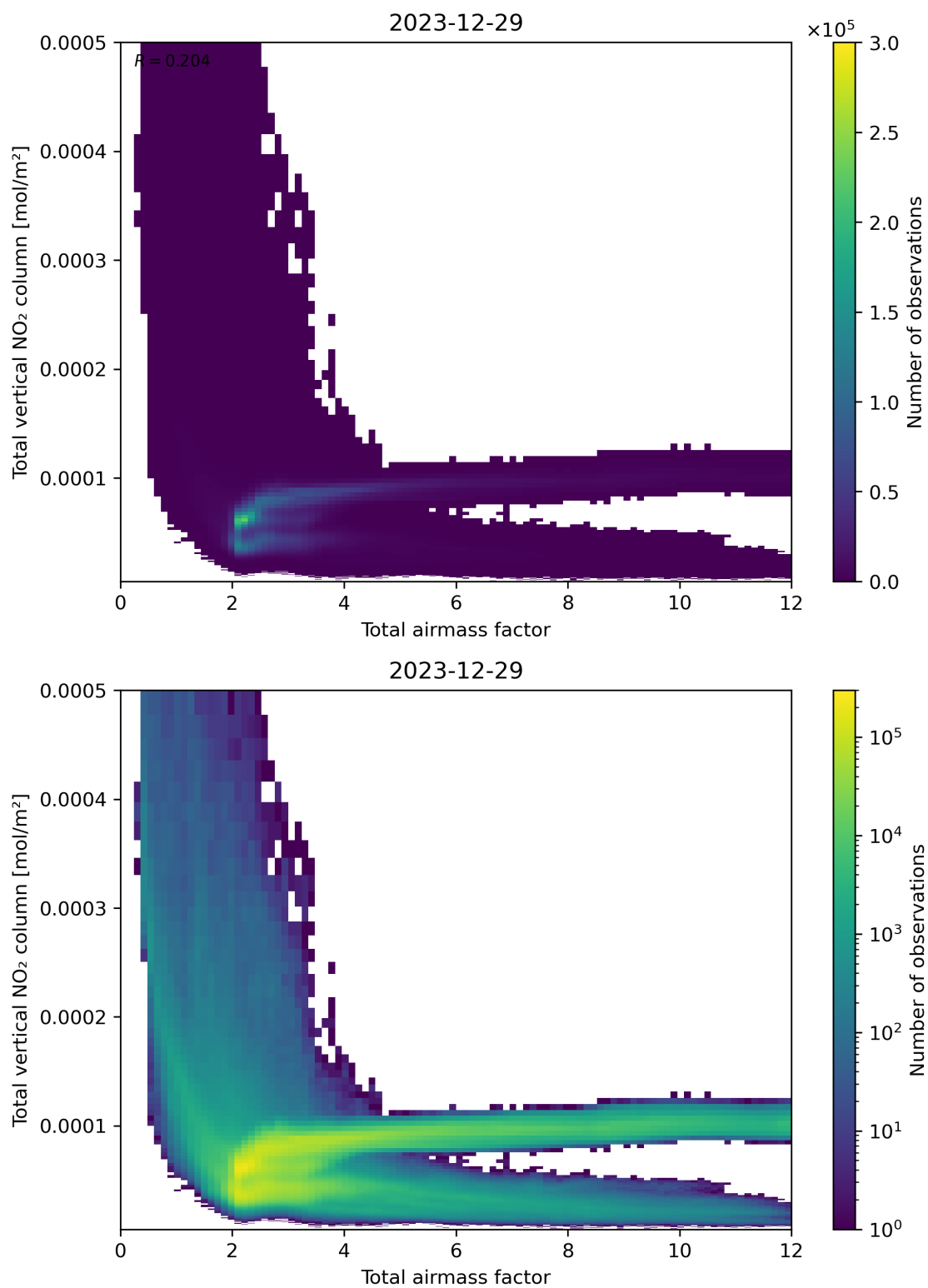
Figure 67: Scatter density plot of “Total airmass factor” against “Total vertical NO 2 column” for 2023-12-28 to 2023-12-30.
