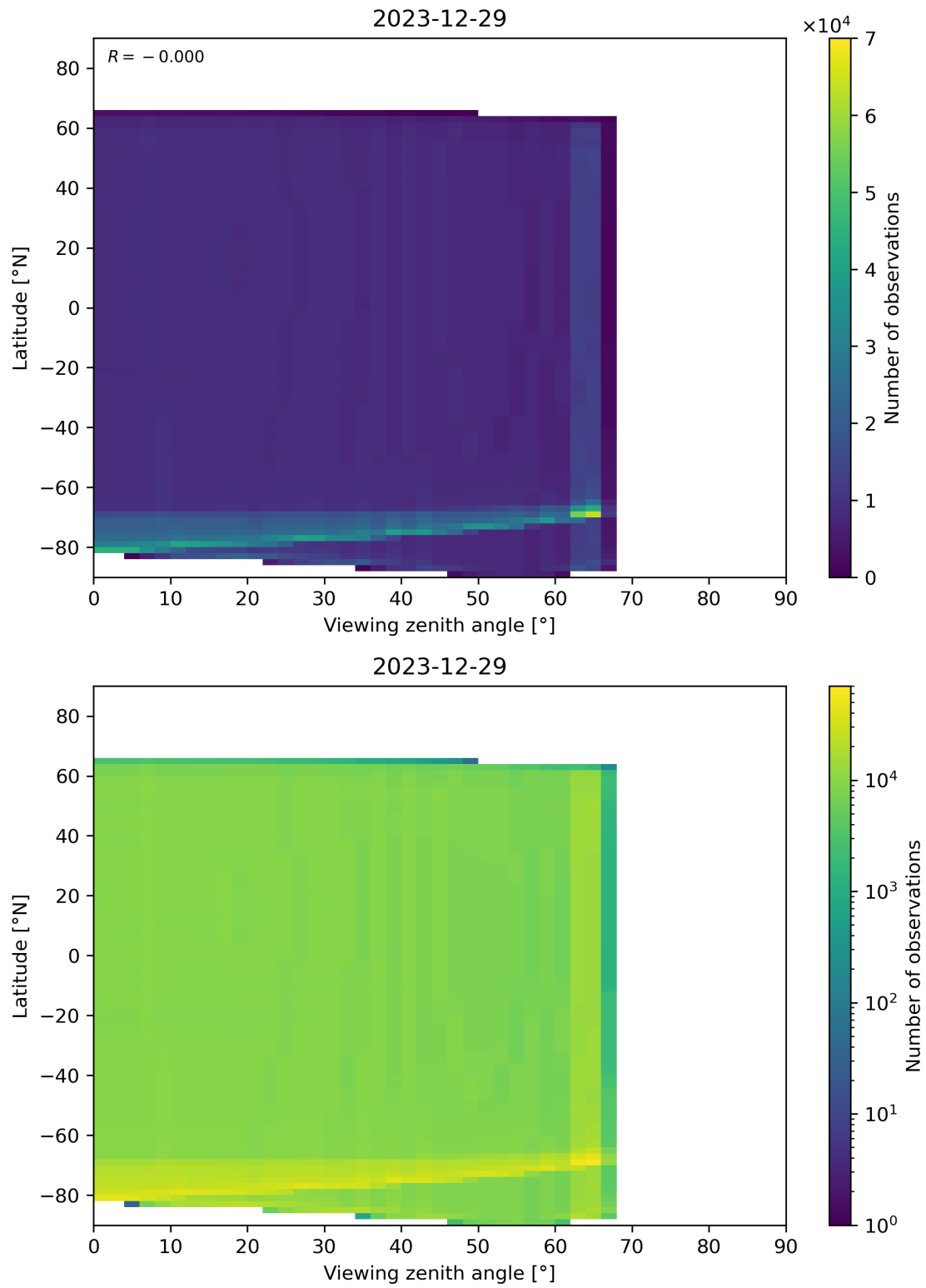
Figure 163: Scatter density plot of “Viewing zenith angle” against “Latitude” for 2023-12-28 to 2023-12-30.
