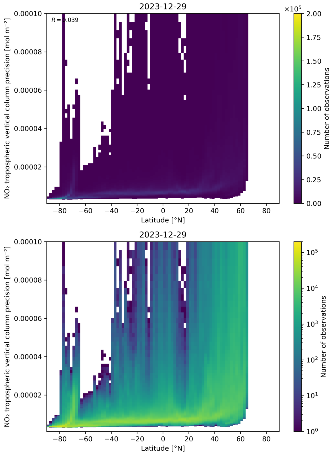
Figure 93: Scatter density plot of “Latitude” against “NO 2 tropospheric vertical column precision” for 2023-12-28 to 2023-12-30.
