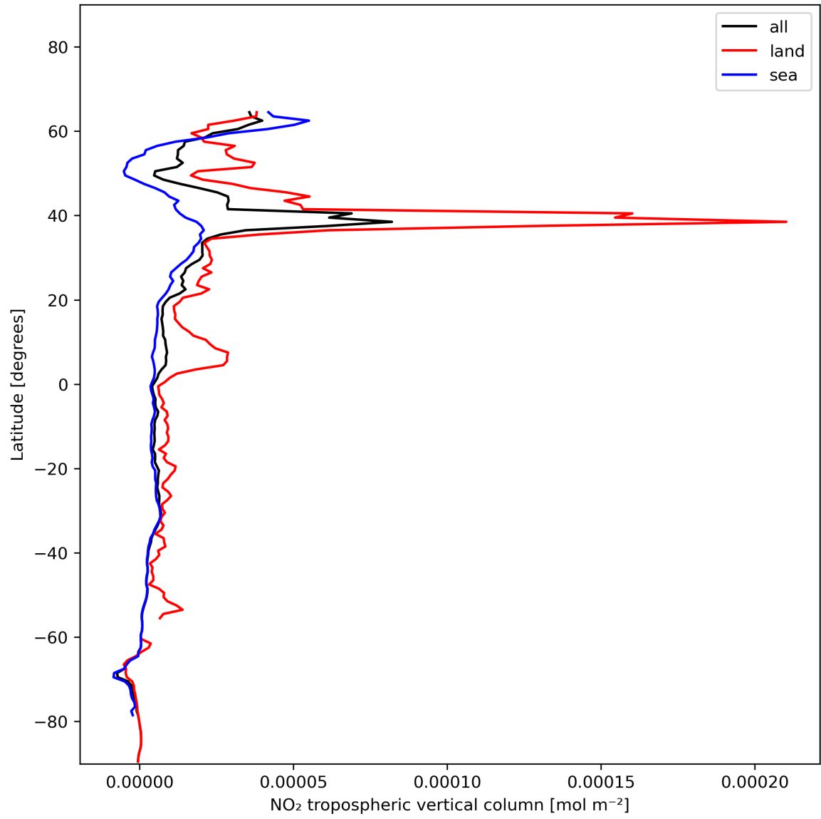
Figure 12: Zonal average of “NO 2 tropospheric vertical column” for 2023-12-28 to 2023-12-30.
