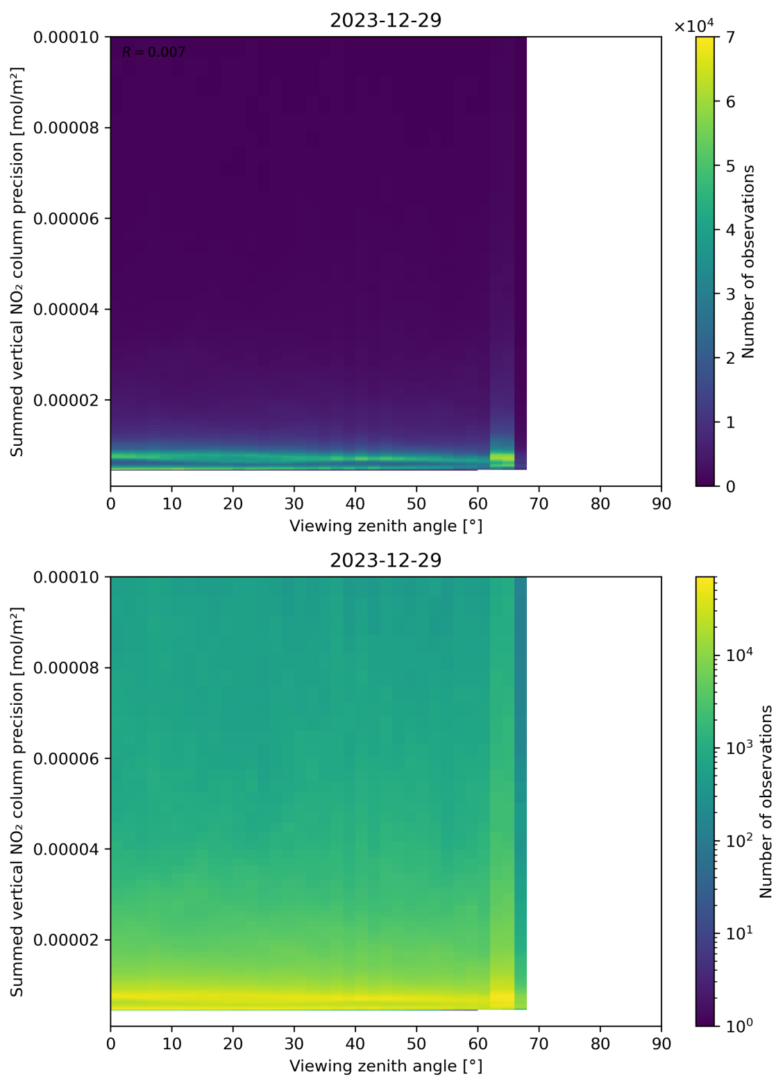
Figure 166: Scatter density plot of “Viewing zenith angle” against “Summed vertical NO 2 column precision” for 2023-12-28 to 2023-12-30.
