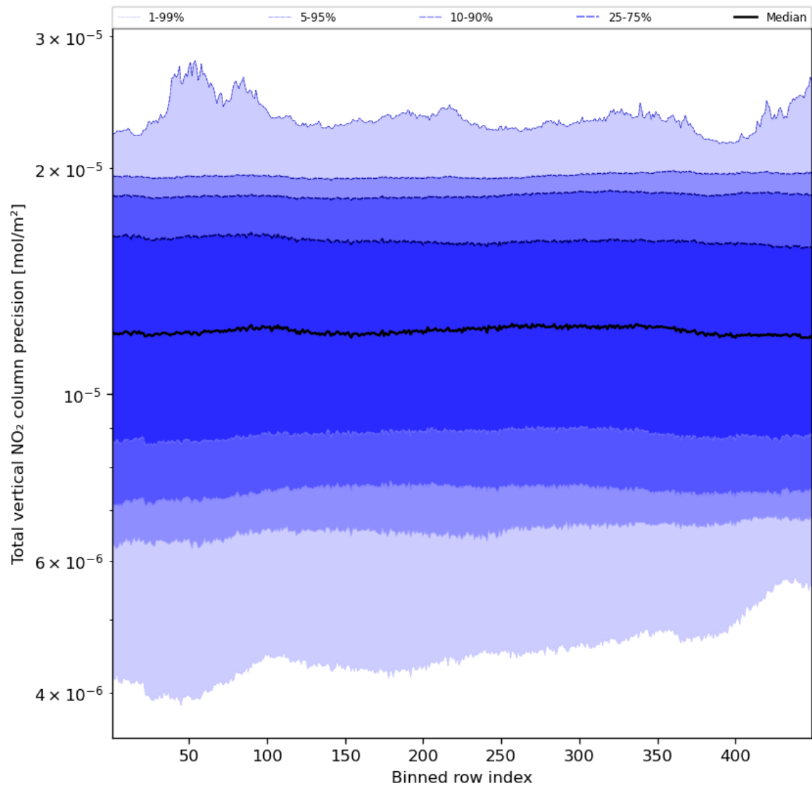
Figure 56: Along track statistics of “Total vertical NO 2 column precision” for 2023-12-28 to 2023-12-30
