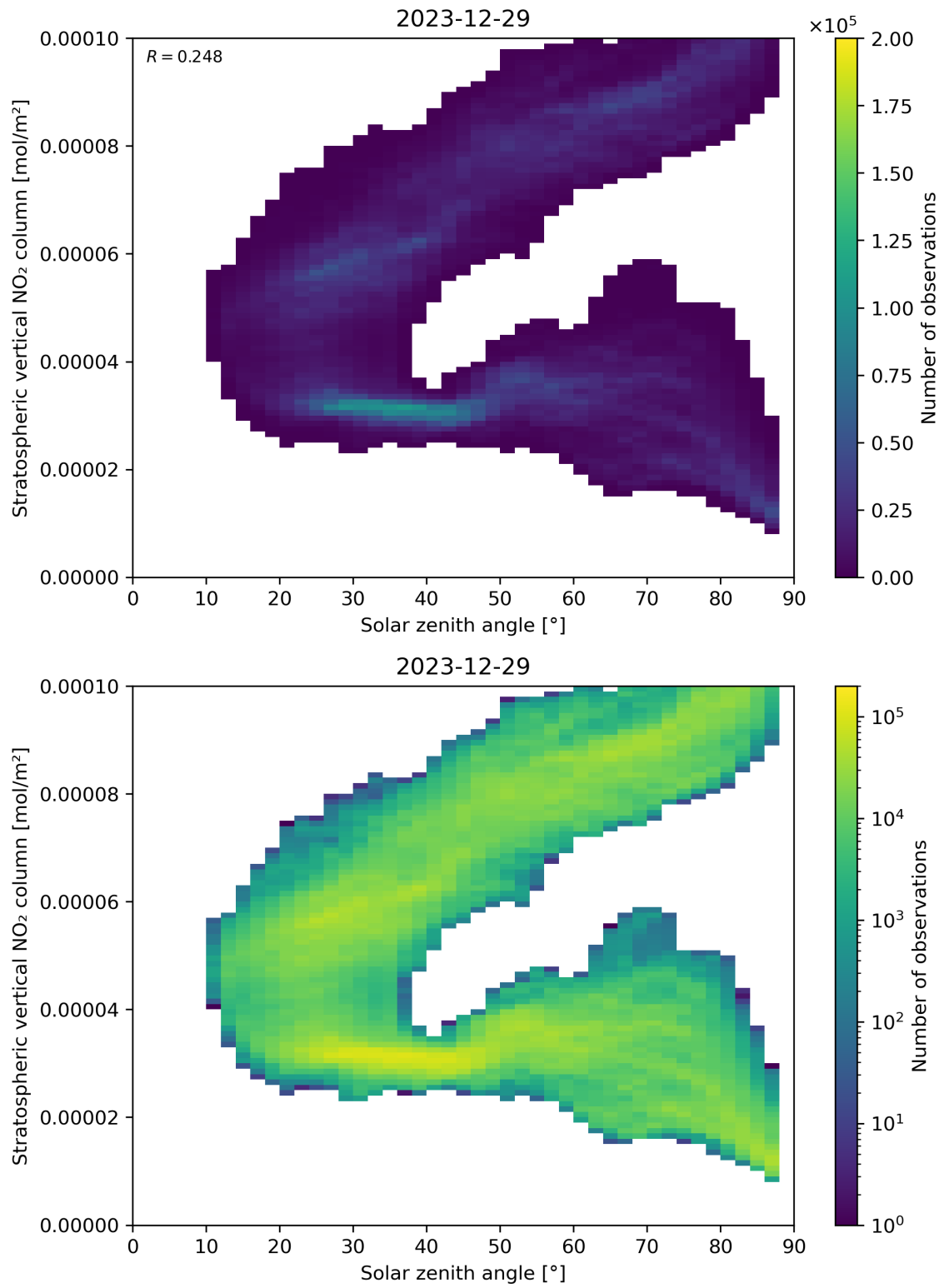
Figure 150: Scatter density plot of “Solar zenith angle” against “Stratospheric vertical NO 2 column” for 2023-12-28 to 2023-12-30.
