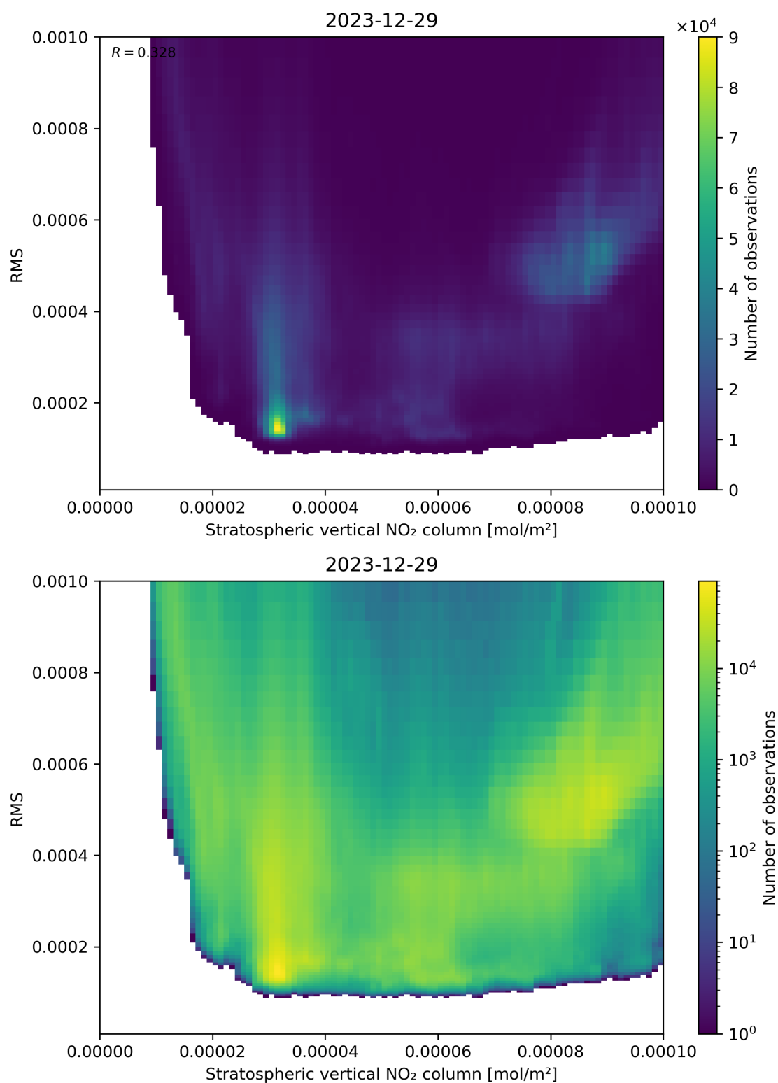
Figure 102: Scatter density plot of “Stratospheric vertical NO 2 column” against “RMS” for 2023-12-28 to 2023-12-30.
