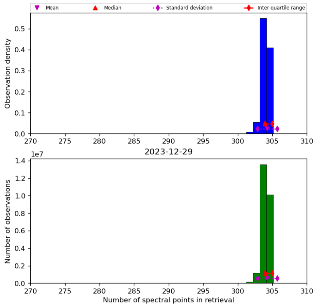
Figure 33: Histogram of “Number of spectral points in retrieval” for 2023-12-28 to 2023-12-30
