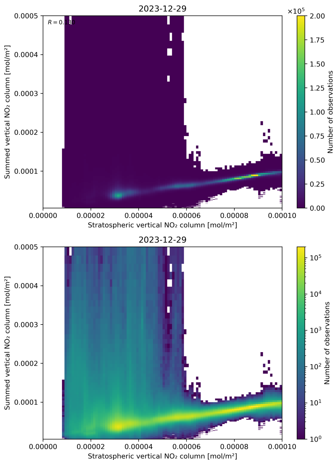
Figure 98: Scatter density plot of “Stratospheric vertical NO 2 column” against “Summed vertical NO 2 column” for 2023-12-28 to 2023-12-30.
