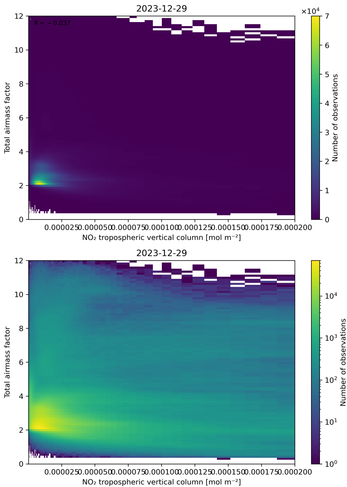
Figure 122: Scatter density plot of “NO 2 tropospheric vertical column” against “Total air mass factor” for 2023-12-28 to 2023-12-30.
