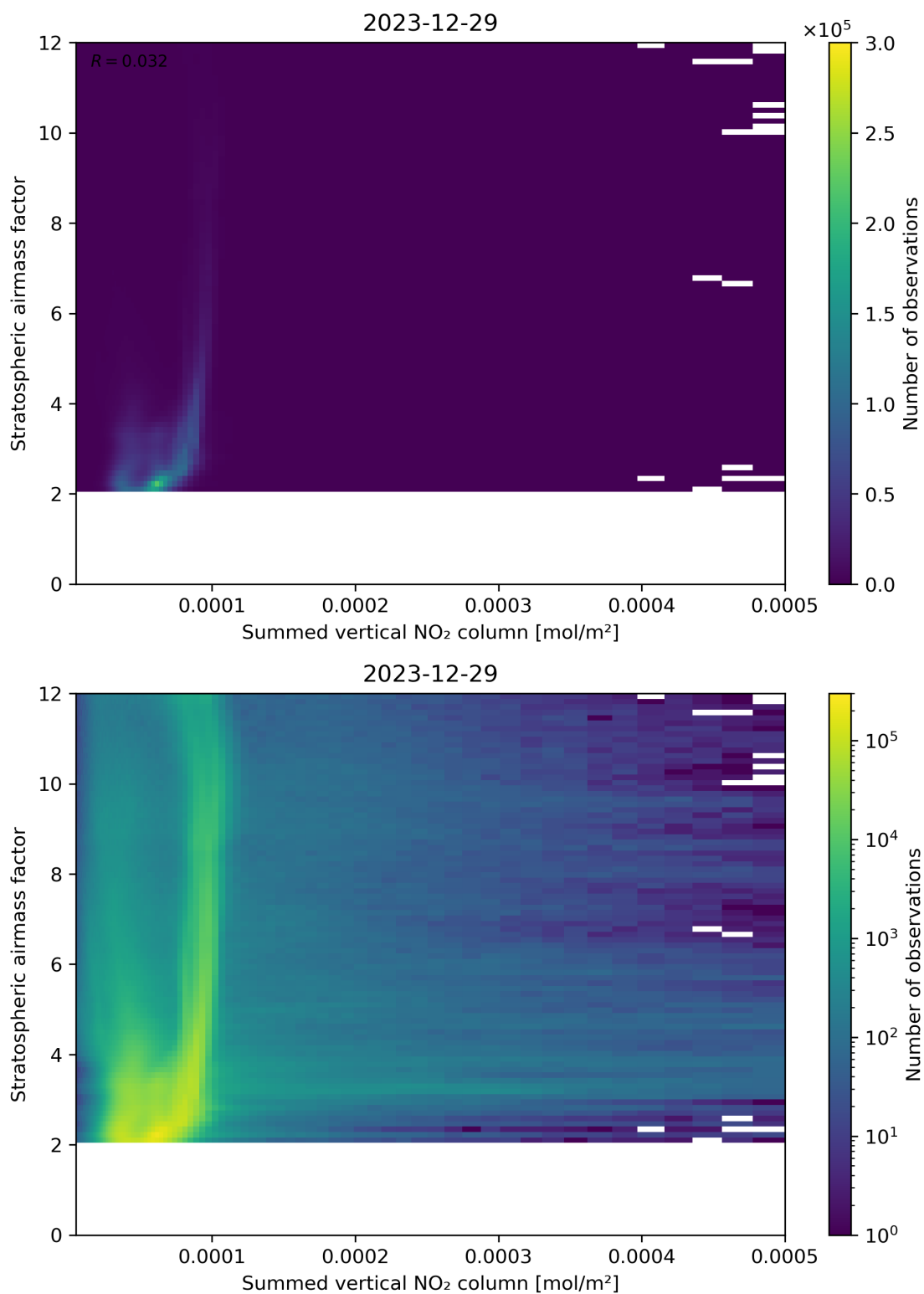
Figure 103: Scatter density plot of “Summed vertical NO 2 column” against “Stratospheric airmass factor” for 2023-12-28 to 2023-12-30.
