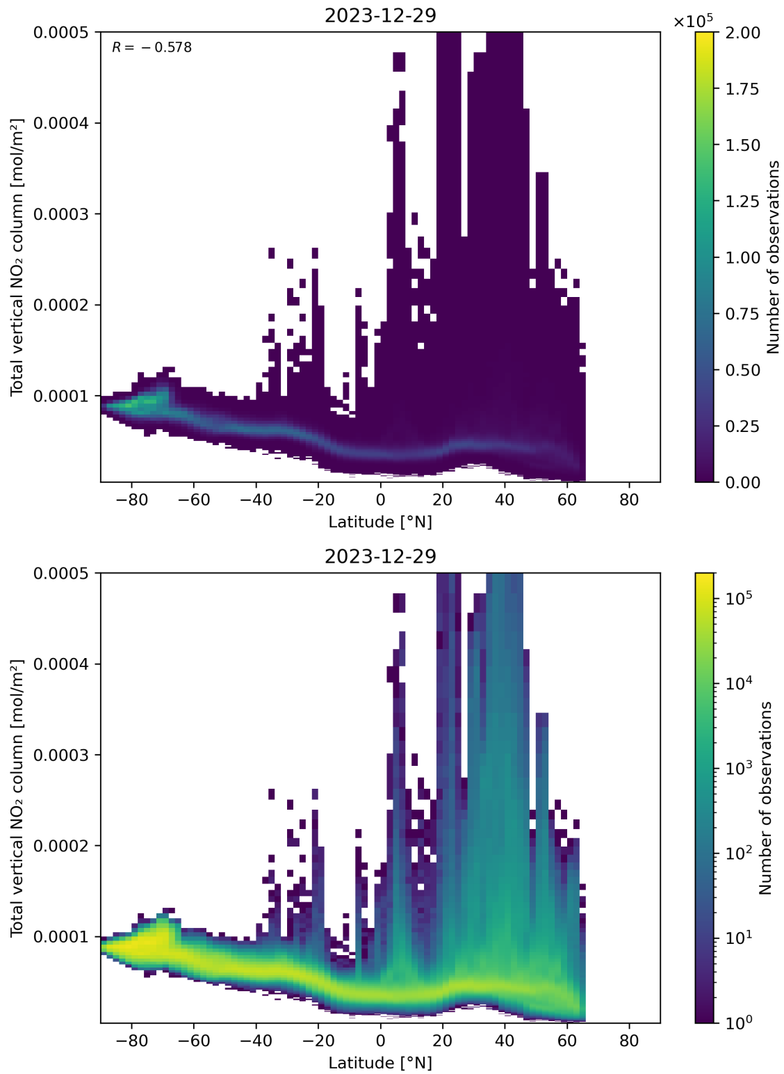
Figure 90: Scatter density plot of “Latitude” against “Total vertical NO 2 column” for 2023-12-28 to 2023-12-30.
