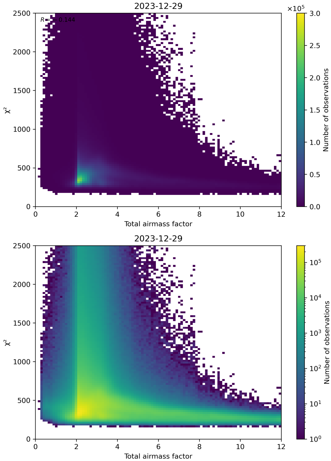
Figure 63: Scatter density plot of “Total airmass factor” against “ \chi^2 ” for 2023-12-28 to 2023-12-30.
