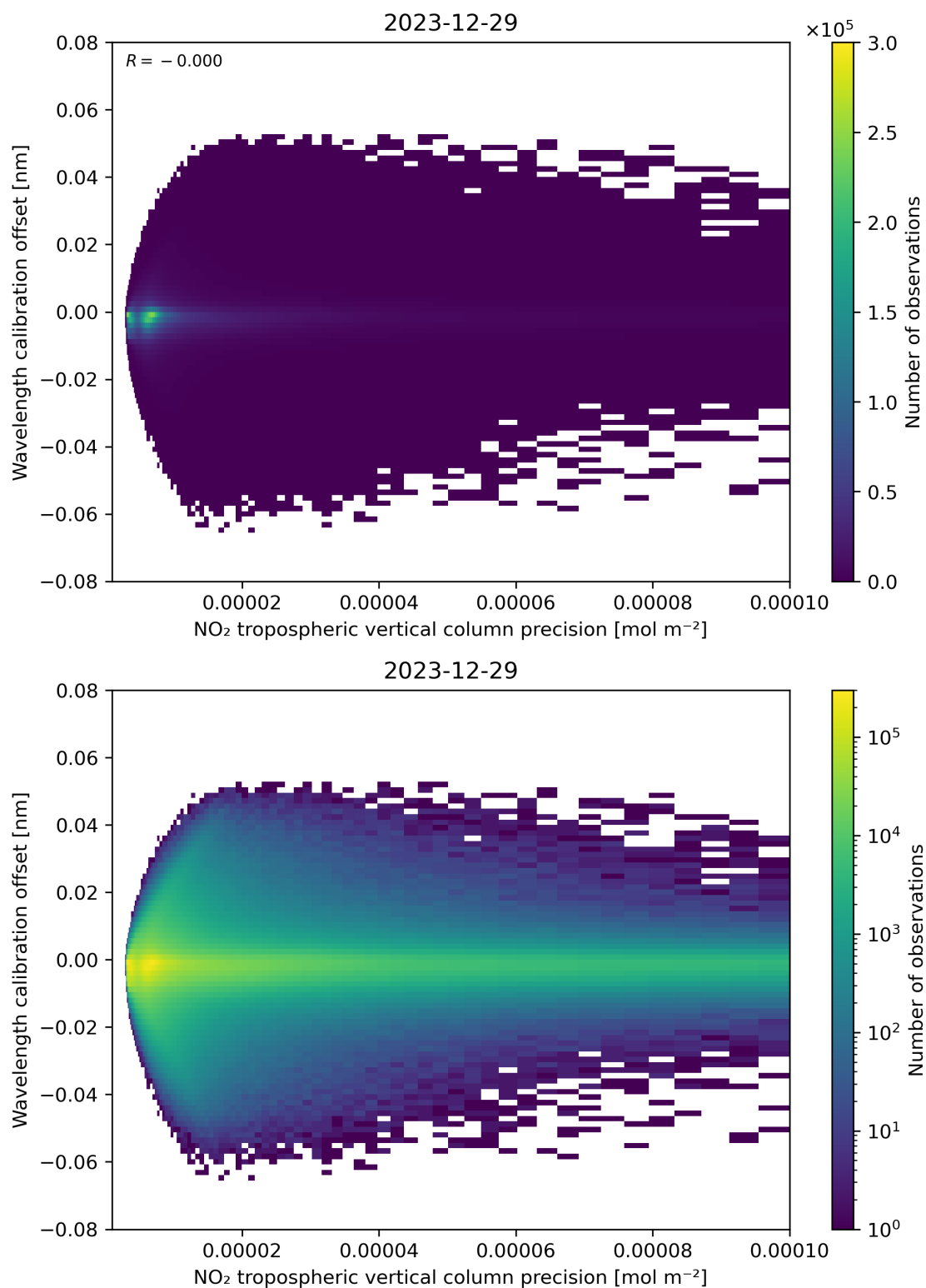
Figure 141: Scatter density plot of “NO 2 tropospheric vertical column precision” against “Wavelength calibration offset” for 2023-12-28 to 2023-12-30.
