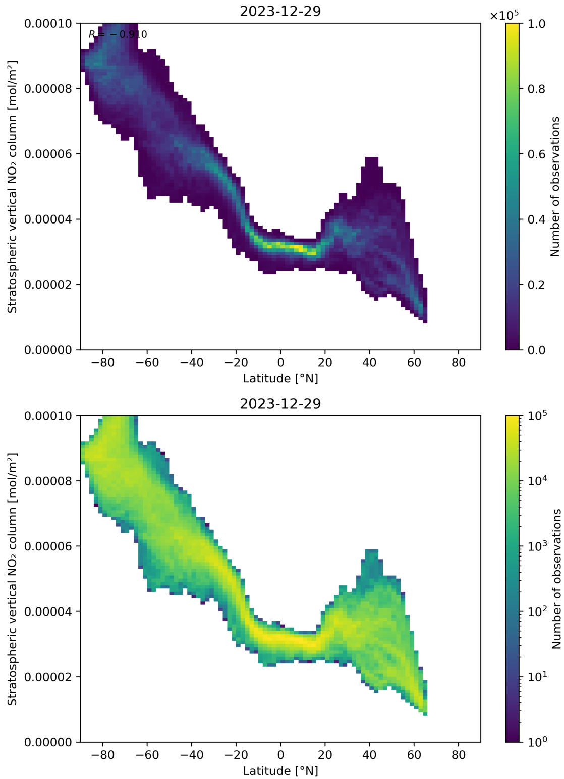
Figure 87: Scatter density plot of “Latitude” against “Stratospheric vertical NO 2 column” for 2023-12-28 to 2023-12-30.
