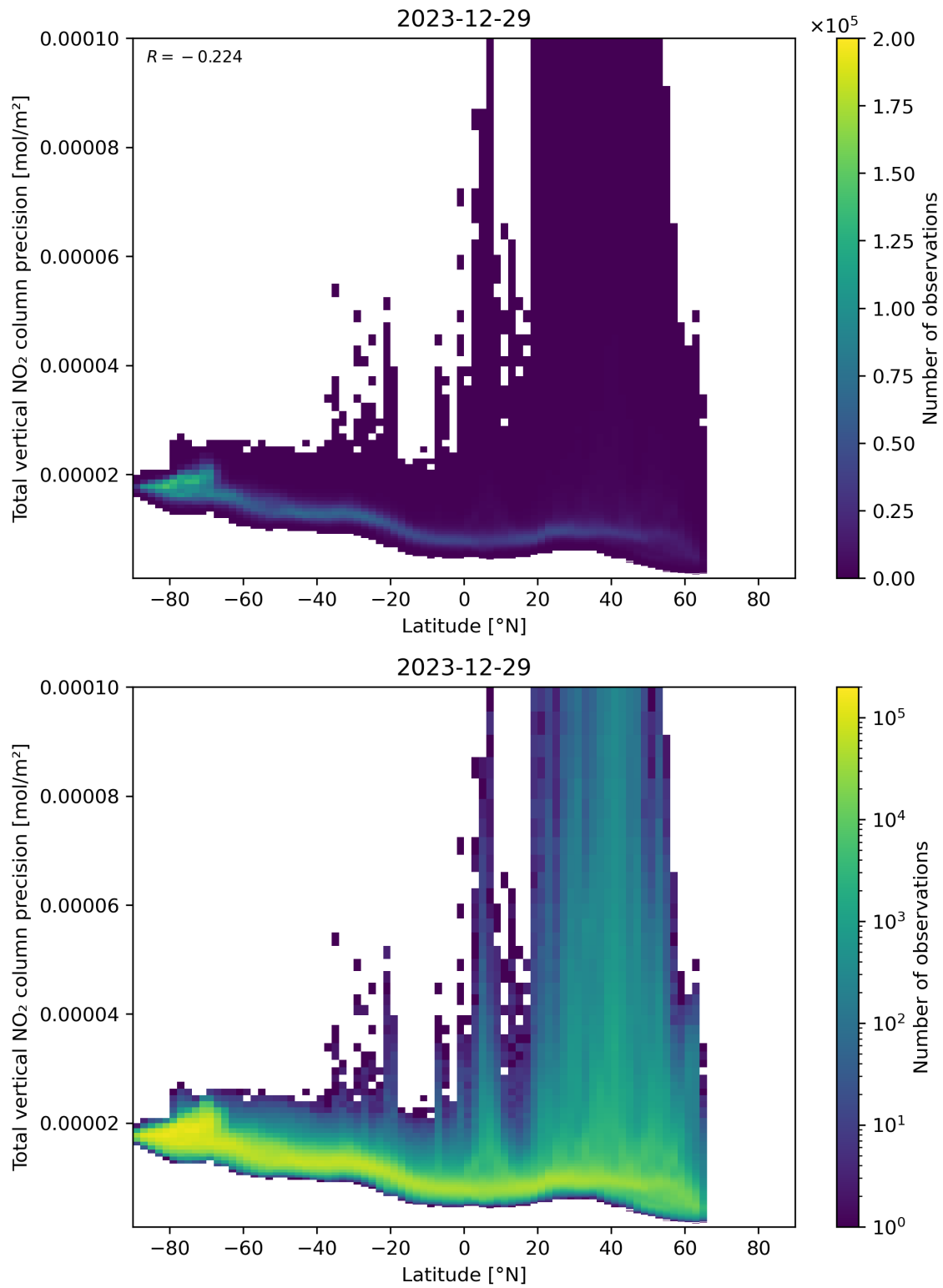
Figure 91: Scatter density plot of “Latitude” against “Total vertical NO 2 column precision” for 2023-12-28 to 2023-12-30.
