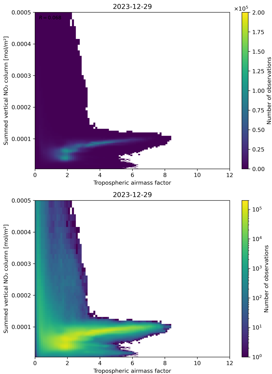
Figure 75: Scatter density plot of “Tropospheric airmass factor” against “Summed vertical NO 2 column” for 2023-12-28 to 2023-12-30.
