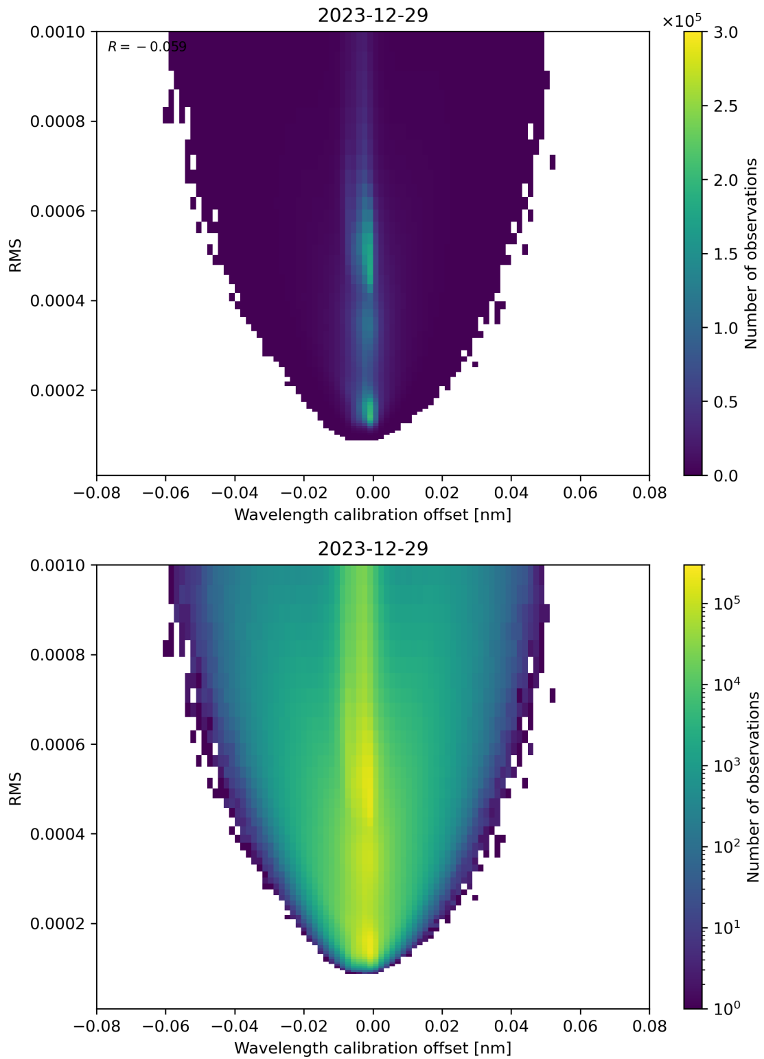
Figure 181: Scatter density plot of “Wavelength calibration offset” against “RMS” for 2023-12-28 to 2023-12-30.
