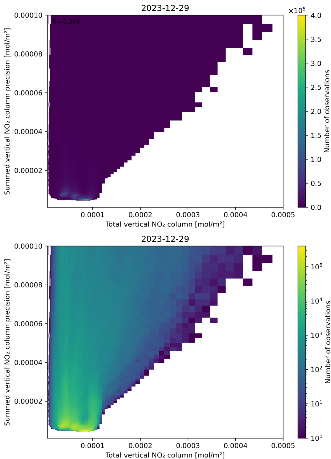
Figure 113: Scatter density plot of “Total vertical NO 2 column” against “Summed vertical NO 2 column precision” for 2023-12-28 to 2023-12-30.
