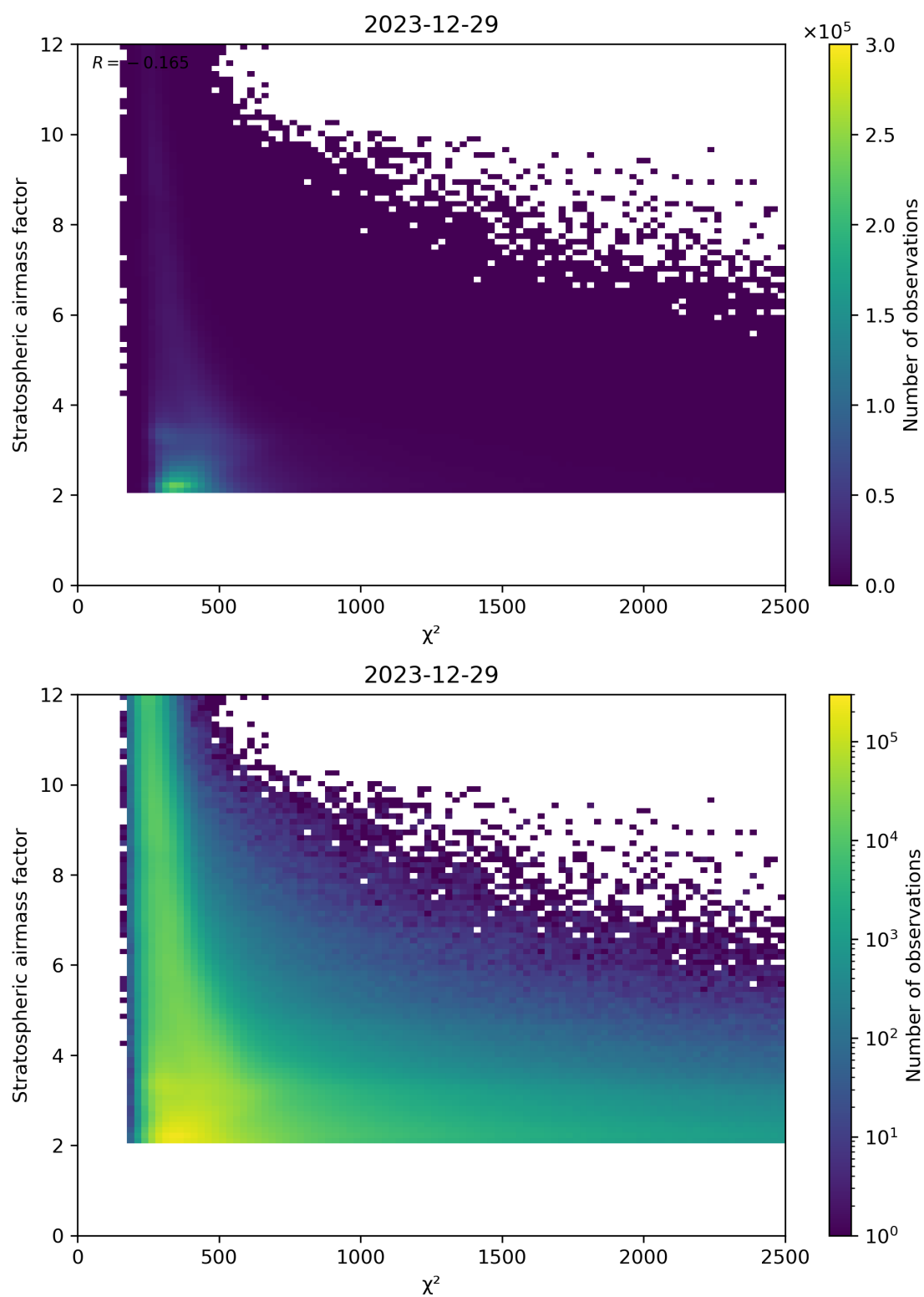
Figure 81: Scatter density plot of “ \chi^2 ” against “Stratospheric airmass factor” for 2023-12-28 to 2023-12-30.
