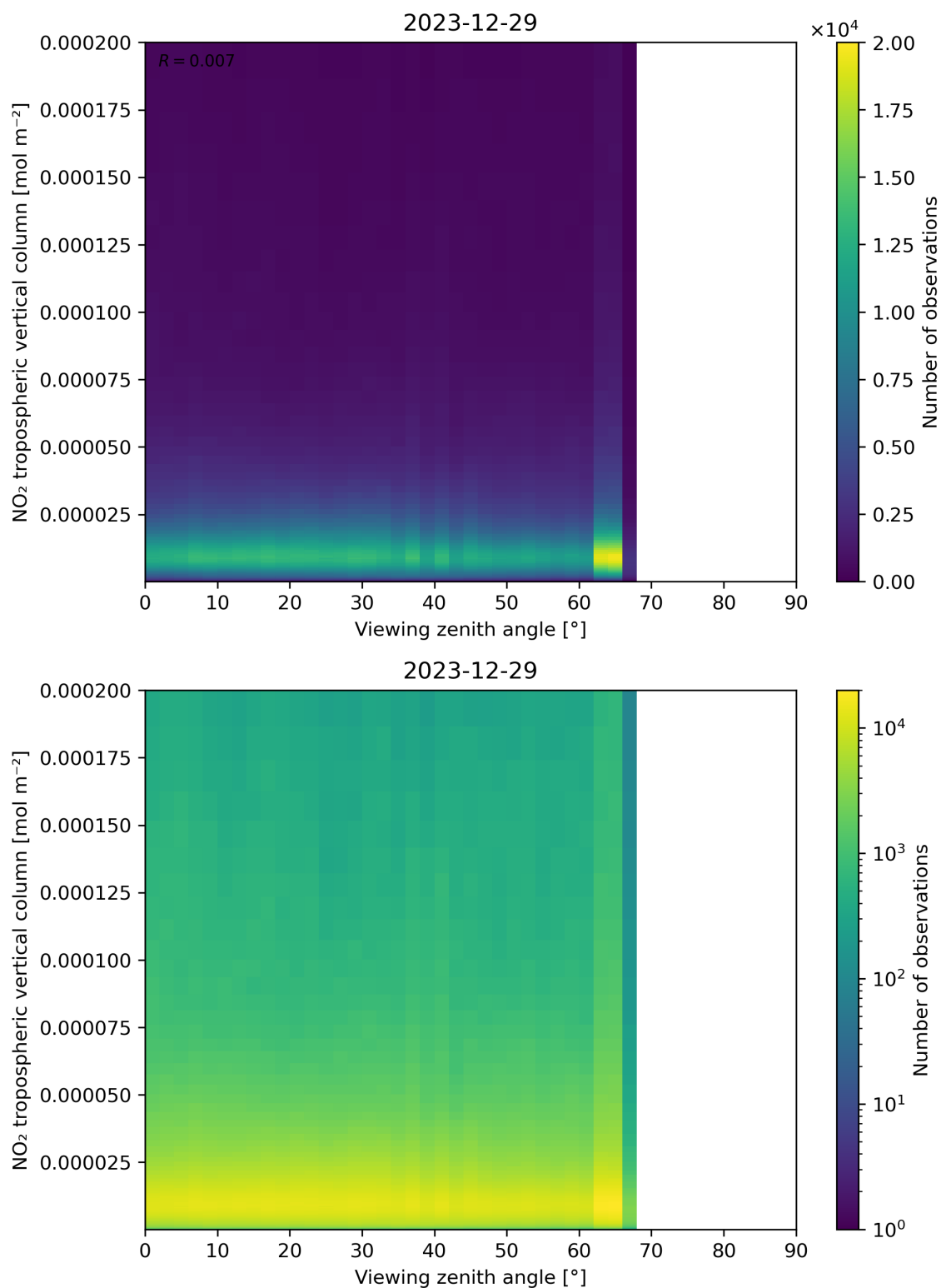
Figure 169: Scatter density plot of “Viewing zenith angle” against “NO 2 tropospheric vertical column” for 2023-12-28 to 2023-12-30.
