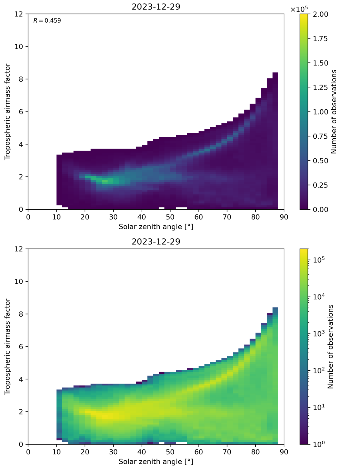
Figure 147: Scatter density plot of “Solar zenith angle” against “Tropospheric airmass factor” for 2023-12-28 to 2023-12-30.
