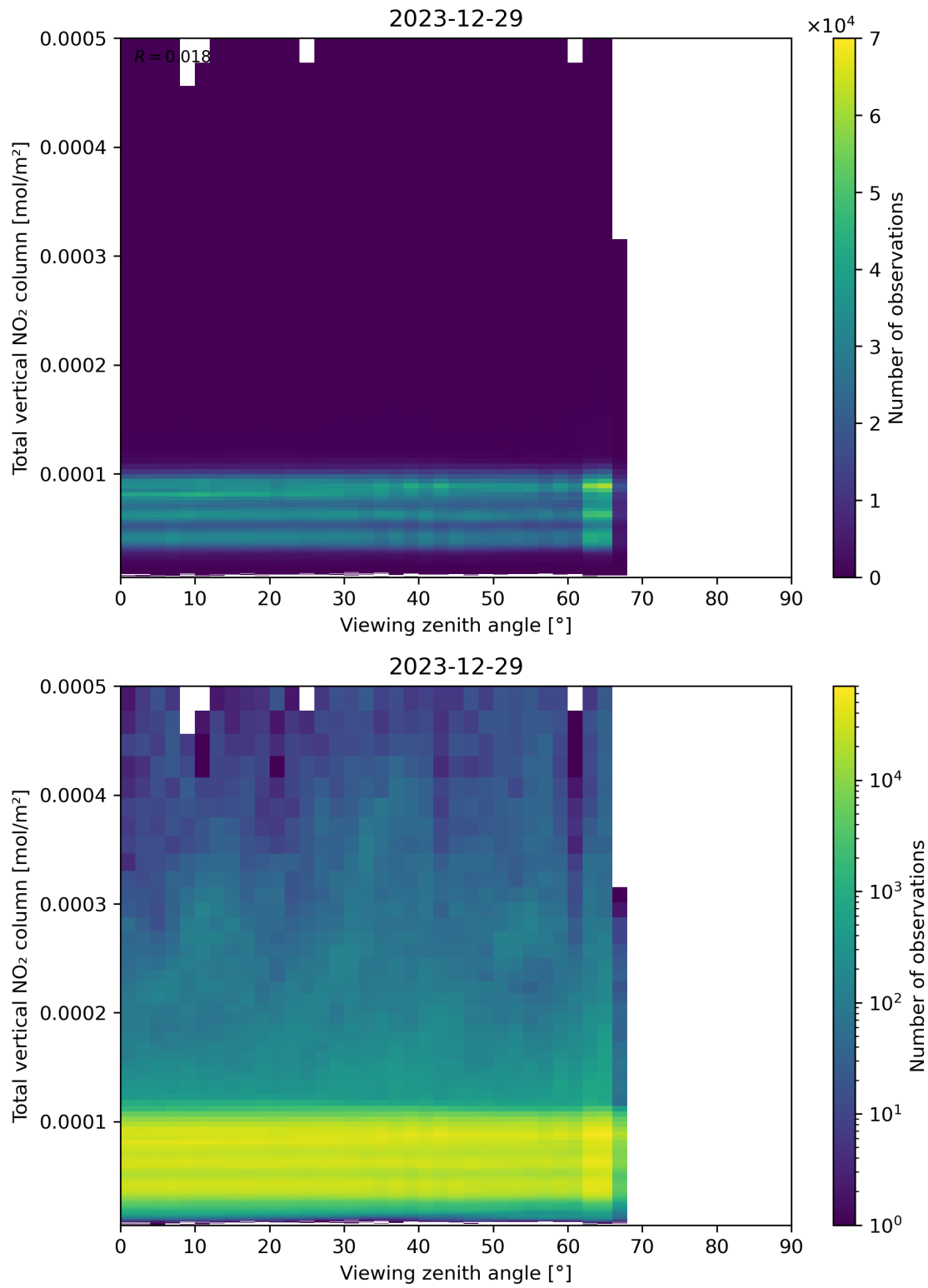
Figure 167: Scatter density plot of “Viewing zenith angle” against “Total vertical NO 2 column” for 2023-12-28 to 2023-12-30.
