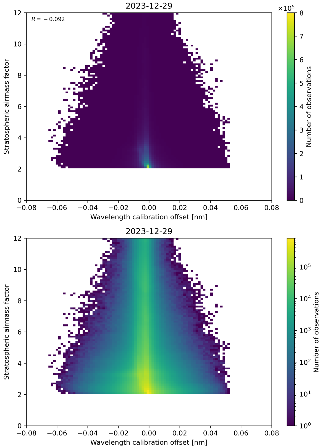
Figure 174: Scatter density plot of “Wavelength calibration offset” against “Stratospheric airmass factor” for 2023-12-28 to 2023-12-30.
