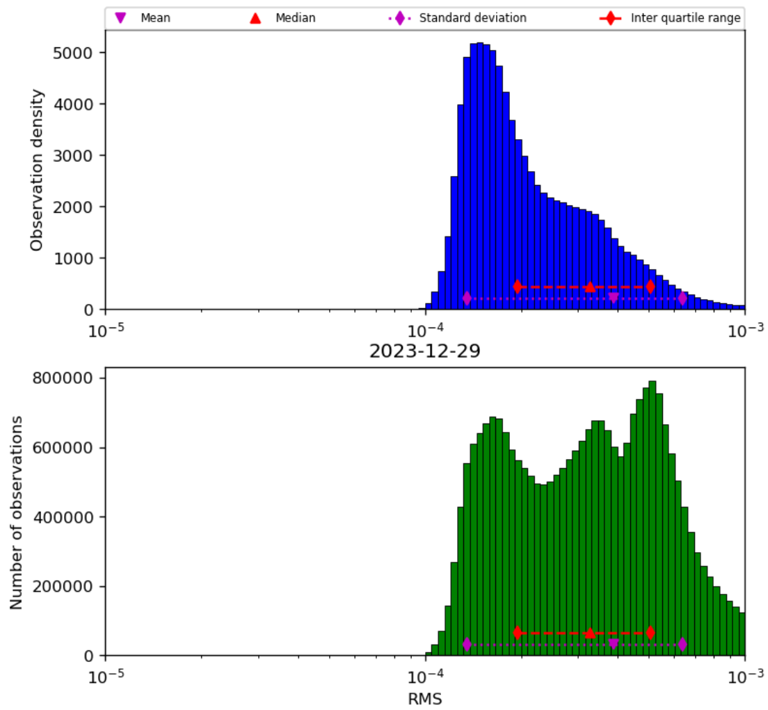
Figure 43: Histogram of “RMS” for 2023-12-28 to 2023-12-30
