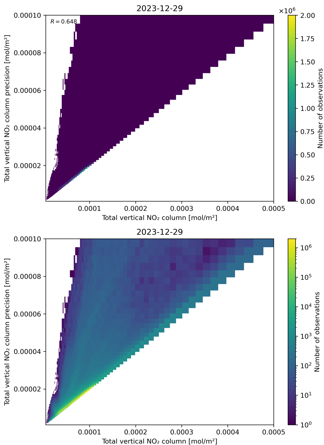
Figure 114: Scatter density plot of “Total vertical NO 2 column” against “Total vertical NO 2 column precision” for 2023-12-28 to 2023-12-30.
