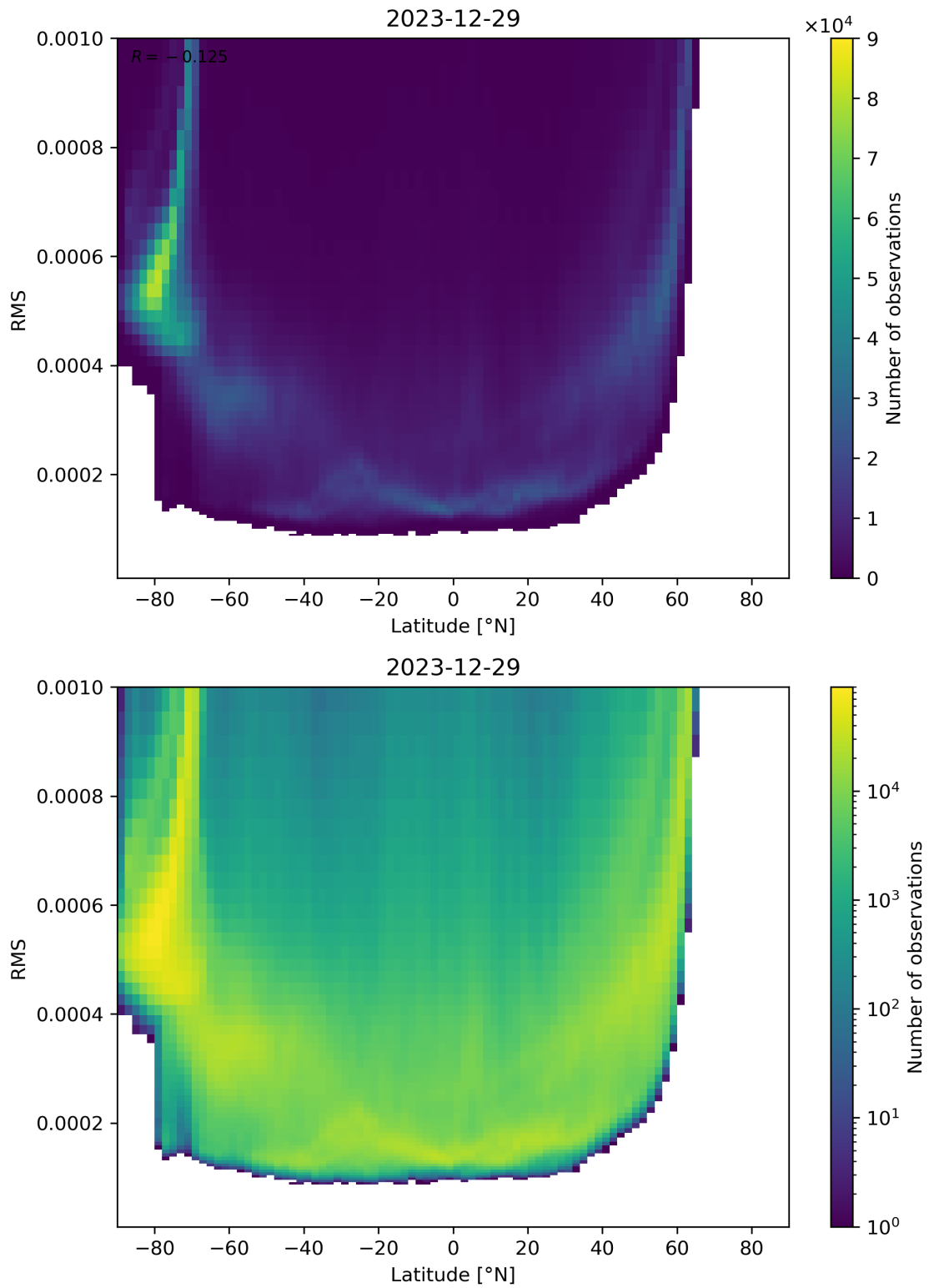
Figure 94: Scatter density plot of “Latitude” against “RMS” for 2023-12-28 to 2023-12-30.
