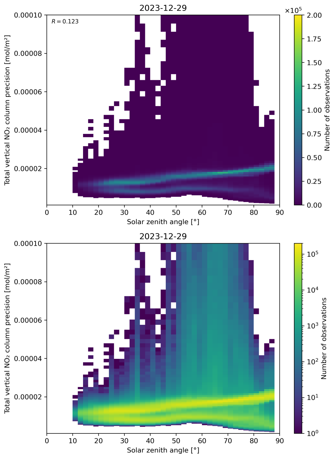
Figure 154: Scatter density plot of “Solar zenith angle” against “Total vertical NO 2 column precision” for 2023-12-28 to 2023-12-30.
