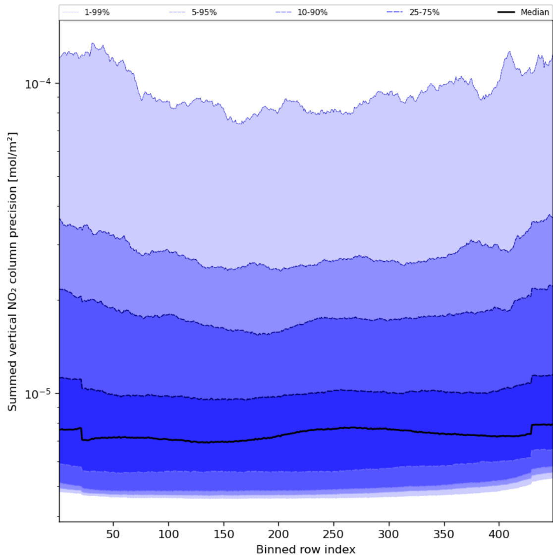
Figure 58: Along track statistics of “Summed vertical NO 2 column precision” for 2023-12-28 to 2023-12-30
