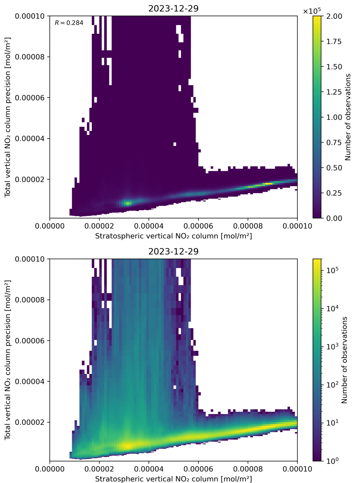
Figure 101: Scatter density plot of “Stratospheric vertical NO 2 column” against “Total vertical NO 2 column precision” for 2023-12-28 to 2023-12-30.
