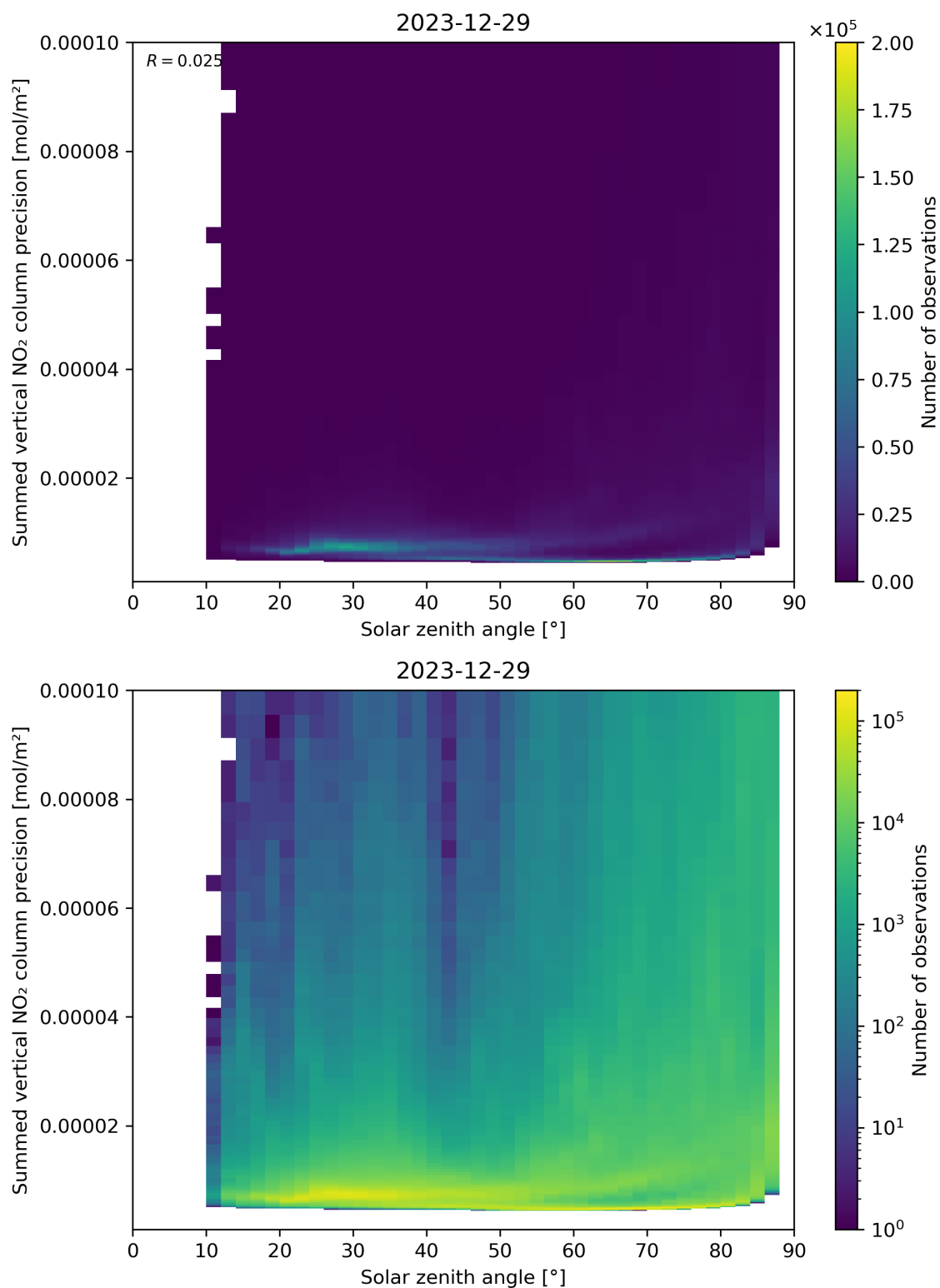
Figure 152: Scatter density plot of “Solar zenith angle” against “Summed vertical NO 2 column precision” for 2023-12-28 to 2023-12-30.
