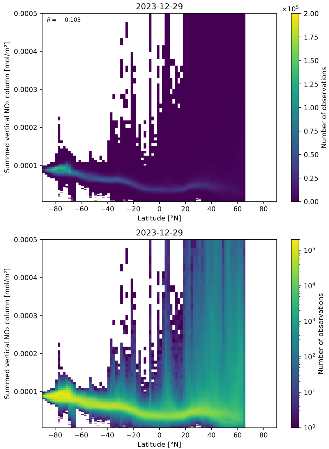
Figure 88: Scatter density plot of “Latitude” against “Summed vertical NO 2 column” for 2023-12-28 to 2023-12-30.
