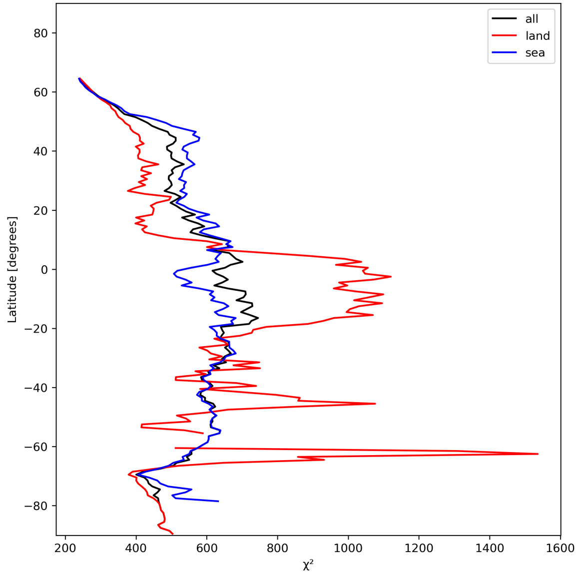
Figure 25: Zonal average of “ \chi^2 ” for 2023-12-28 to 2023-12-30.
