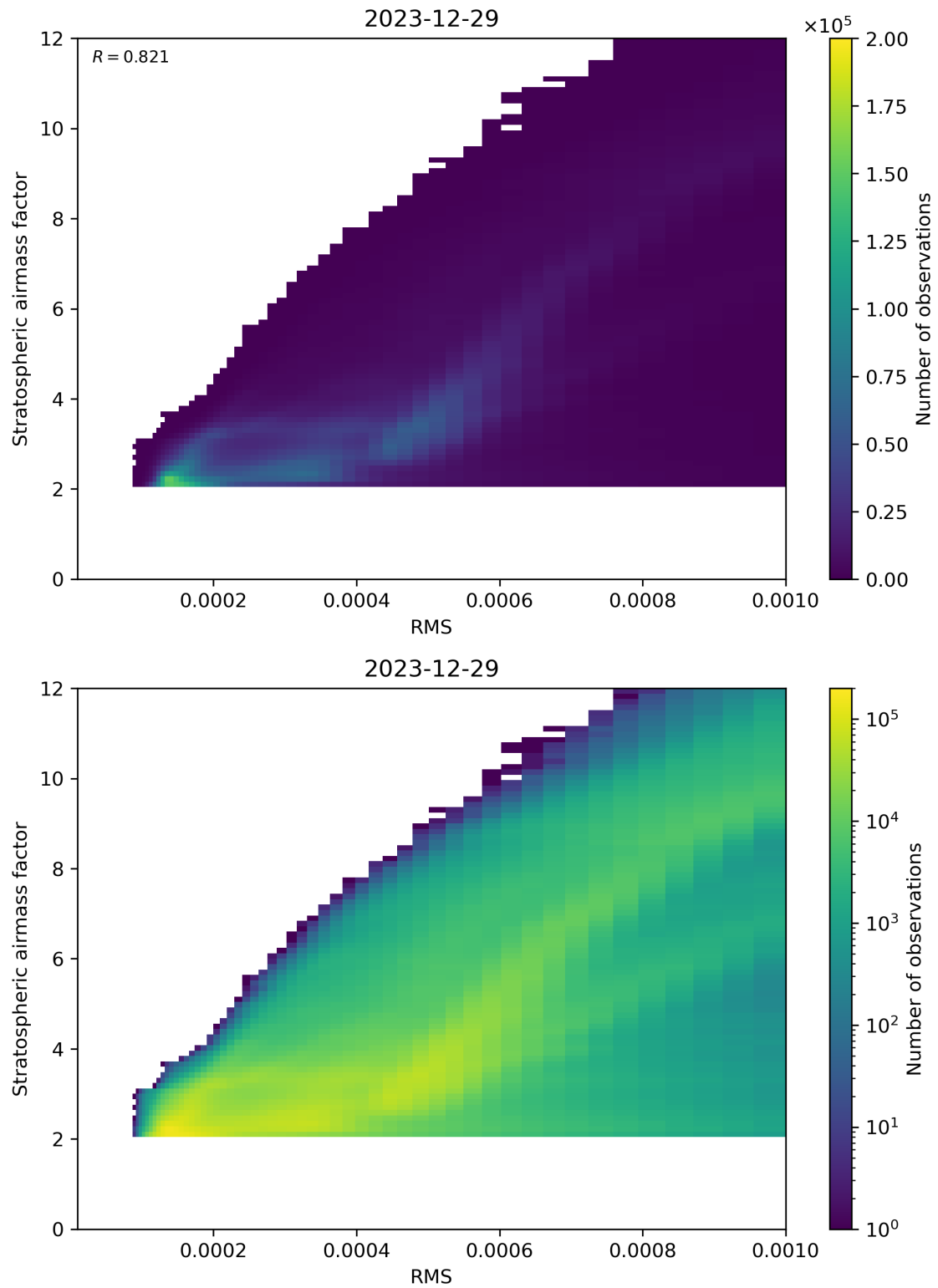
Figure 144: Scatter density plot of “RMS” against “Stratospheric airmass factor” for 2023-12-28 to 2023-12-30.
