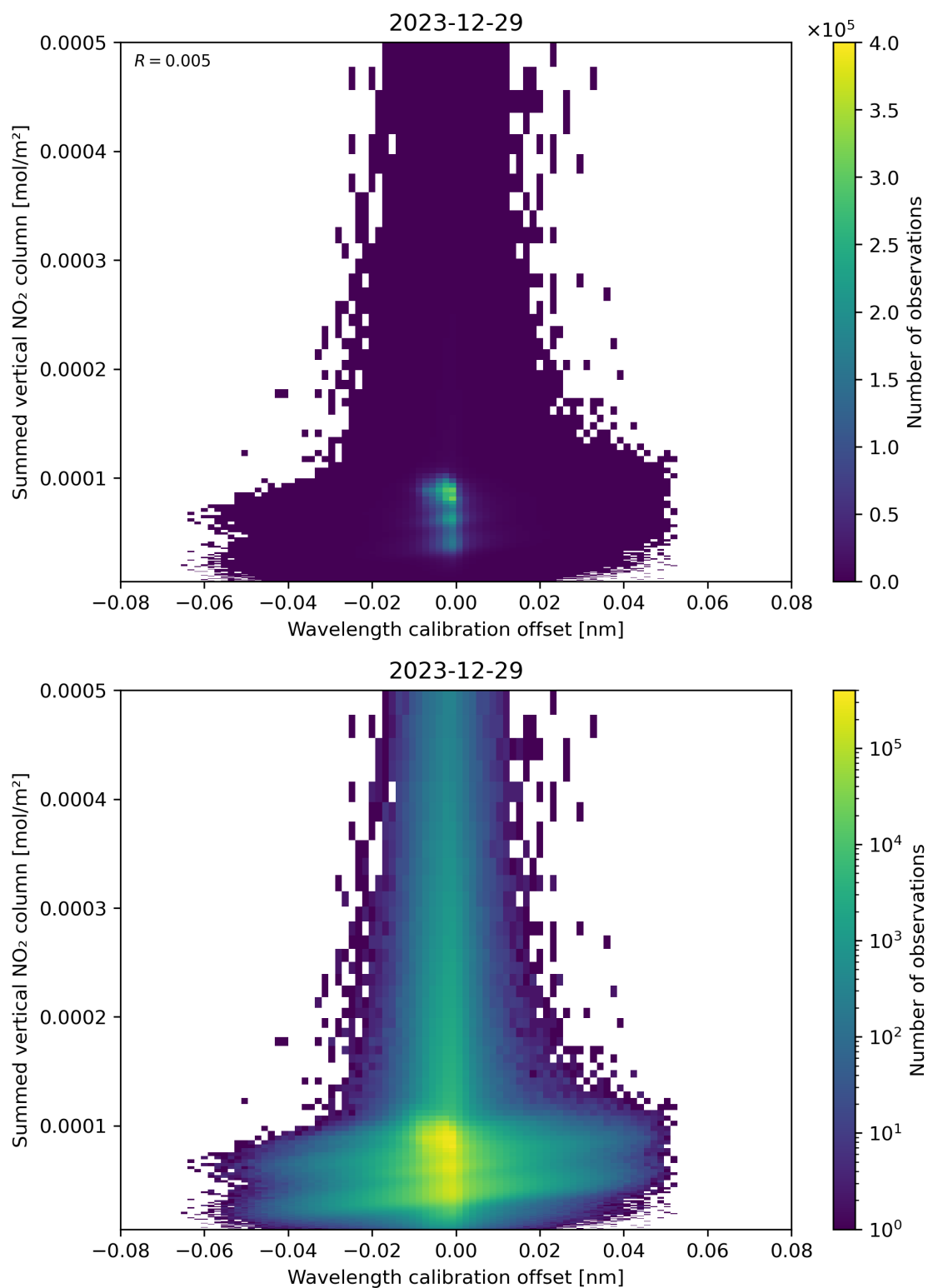
Figure 177: Scatter density plot of “Wavelength calibration offset” against “Summed vertical NO 2 column” for 2023-12-28 to 2023-12-30.
