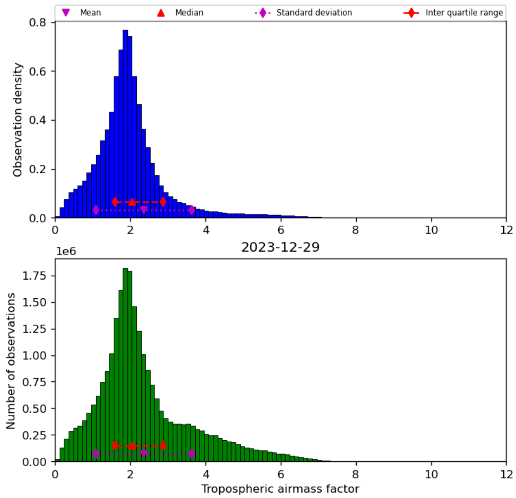
Figure 31: Histogram of “Tropospheric airmass factor” for 2023-12-28 to 2023-12-30
