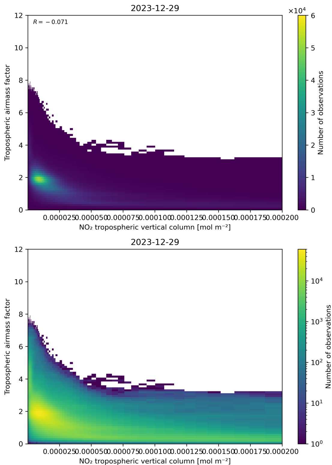
Figure 123: Scatter density plot of “NO 2 tropospheric vertical column” against “Tropospheric airmass factor” for 2023-12-28 to 2023-12-30.
