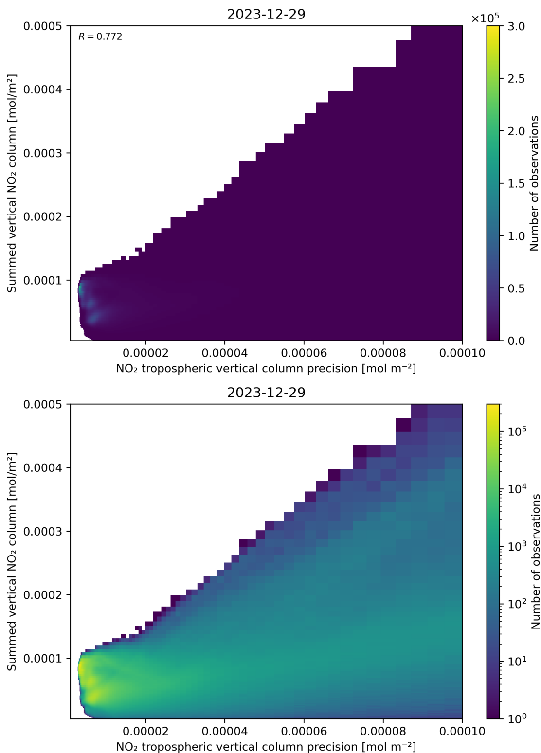
Figure 136: Scatter density plot of “NO 2 tropospheric vertical column precision” against “Summed vertical NO 2 column” for 2023-12-28 to 2023-12-30.
