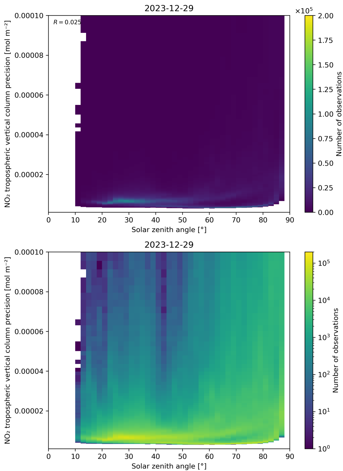
Figure 156: Scatter density plot of “Solar zenith angle” against “NO 2 tropospheric vertical column precision” for 2023-12-28 to 2023-12-30.
