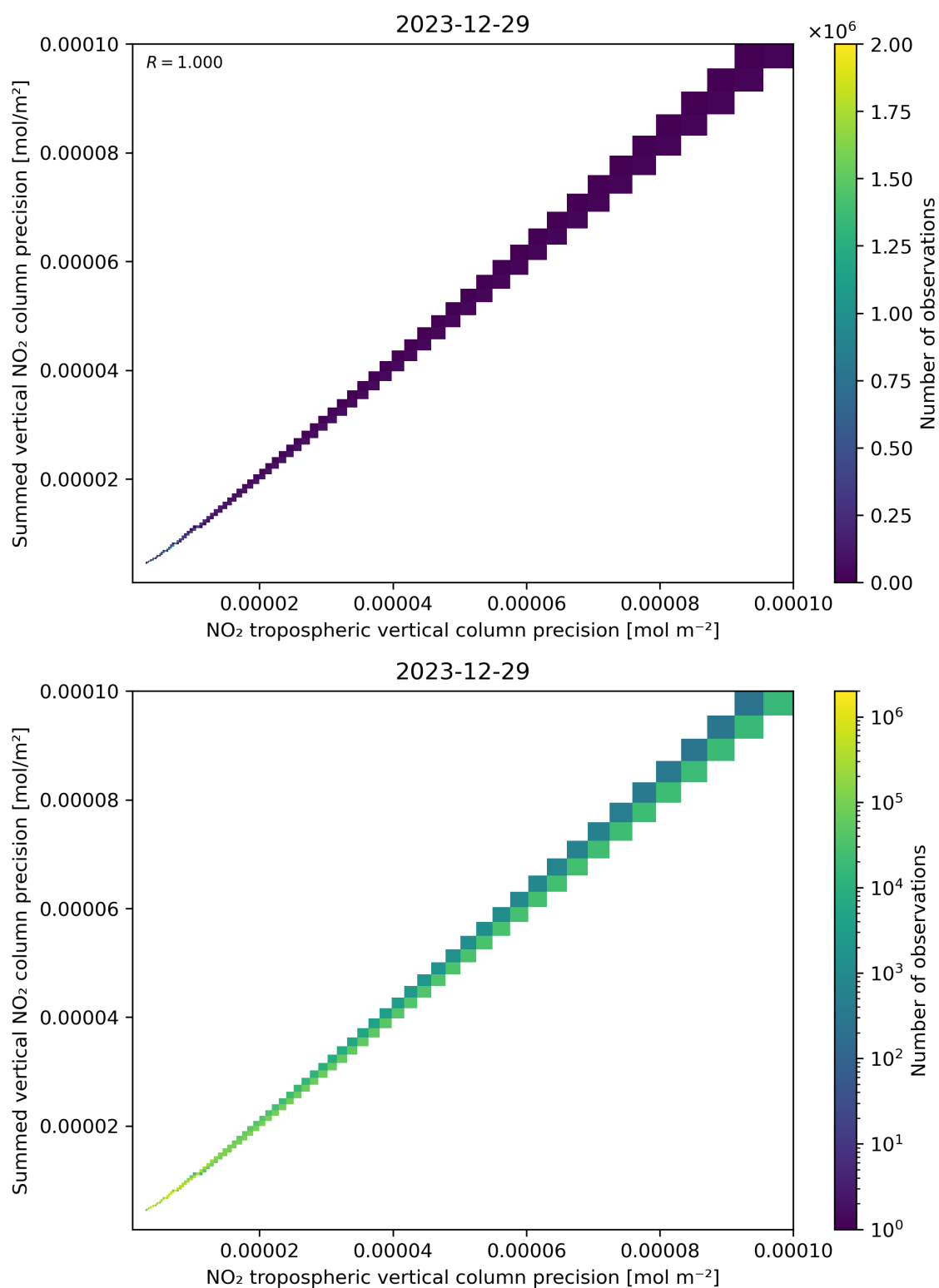
Figure 137: Scatter density plot of “NO 2 tropospheric vertical column precision” against “Summed vertical NO 2 column precision” for 2023-12-28 to 2023-12-30.
