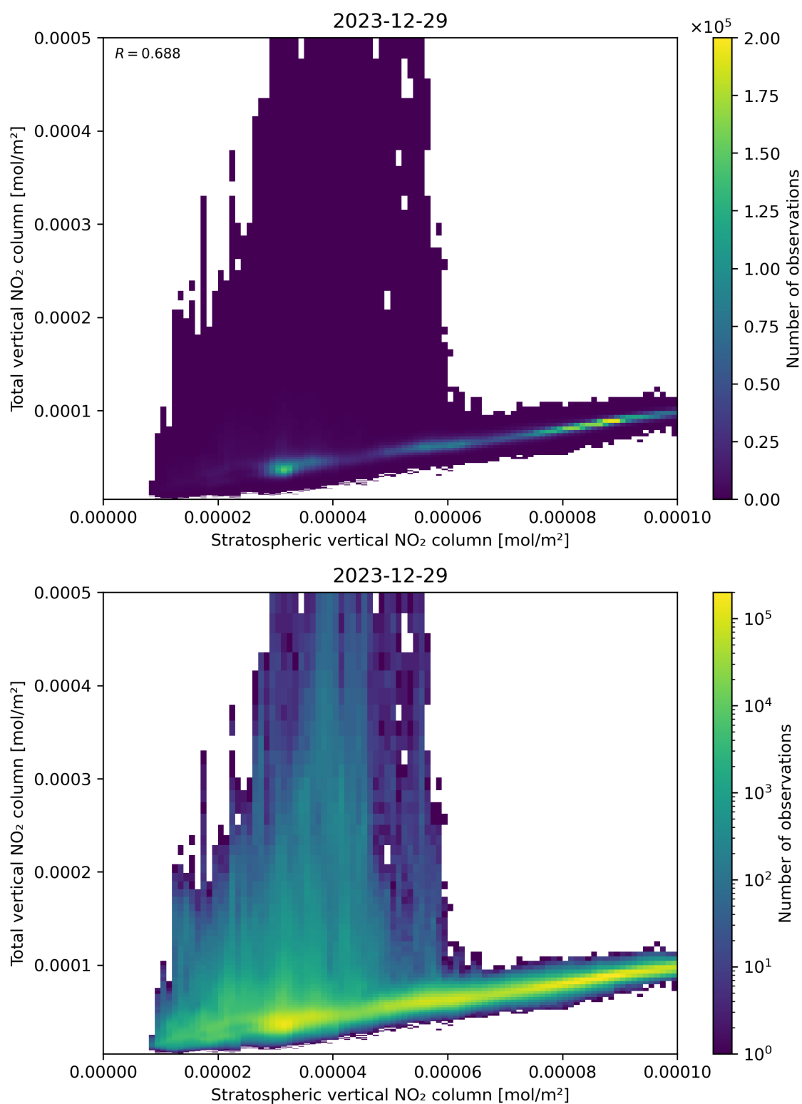
Figure 100: Scatter density plot of “Stratospheric vertical NO 2 column” against “Total vertical NO 2 column” for 2023-12-28 to 2023-12-30.
