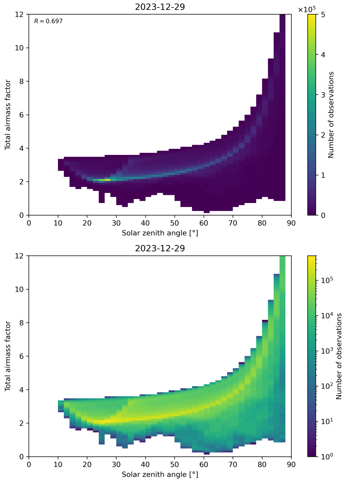
Figure 146: Scatter density plot of “Solar zenith angle” against “Total air mass factor” for 2023-12-28 to 2023-12-30.
