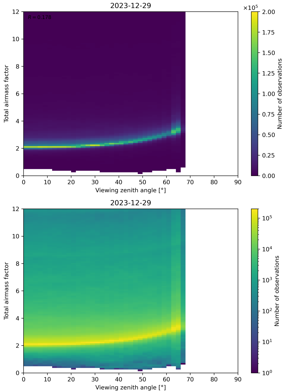
Figure 160: Scatter density plot of “Viewing zenith angle” against “Total airmass factor” for 2023-12-28 to 2023-12-30.
