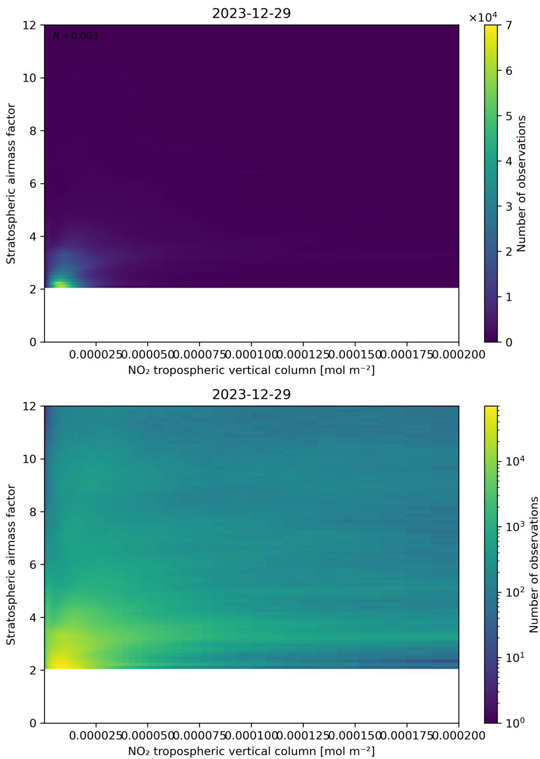
Figure 121: Scatter density plot of “NO 2 tropospheric vertical column” against “Stratospheric air mass factor” for 2023-12-28 to 2023-12-30.
