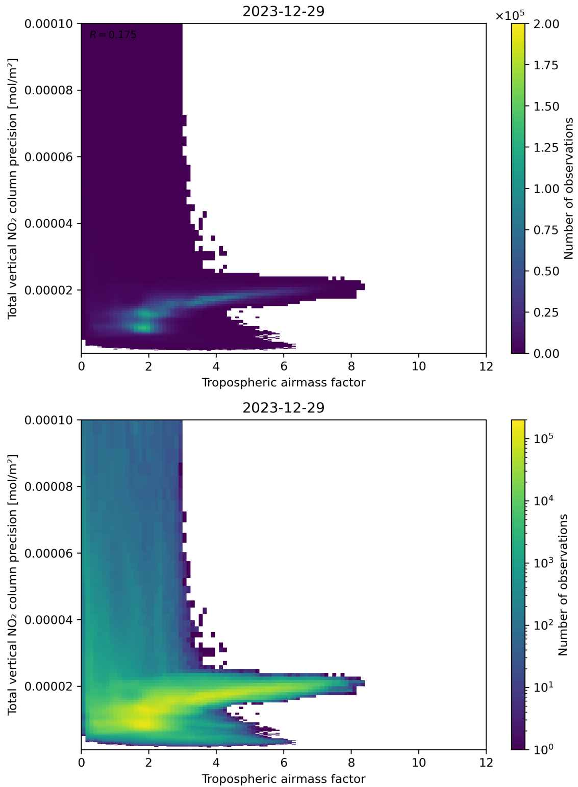
Figure 78: Scatter density plot of “Tropospheric air mass factor” against “Total vertical NO 2 column precision” for 2023-12-28 to 2023-12-30.
