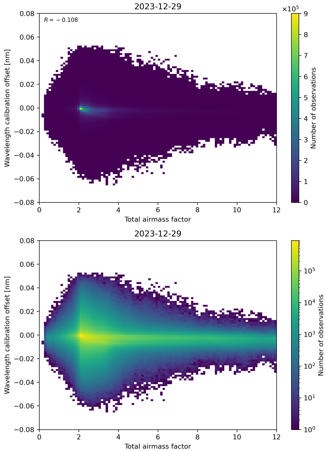
Figure 70: Scatter density plot of “Total airmass factor” against “Wavelength calibration offset” for 2023-12-28 to 2023-12-30.
