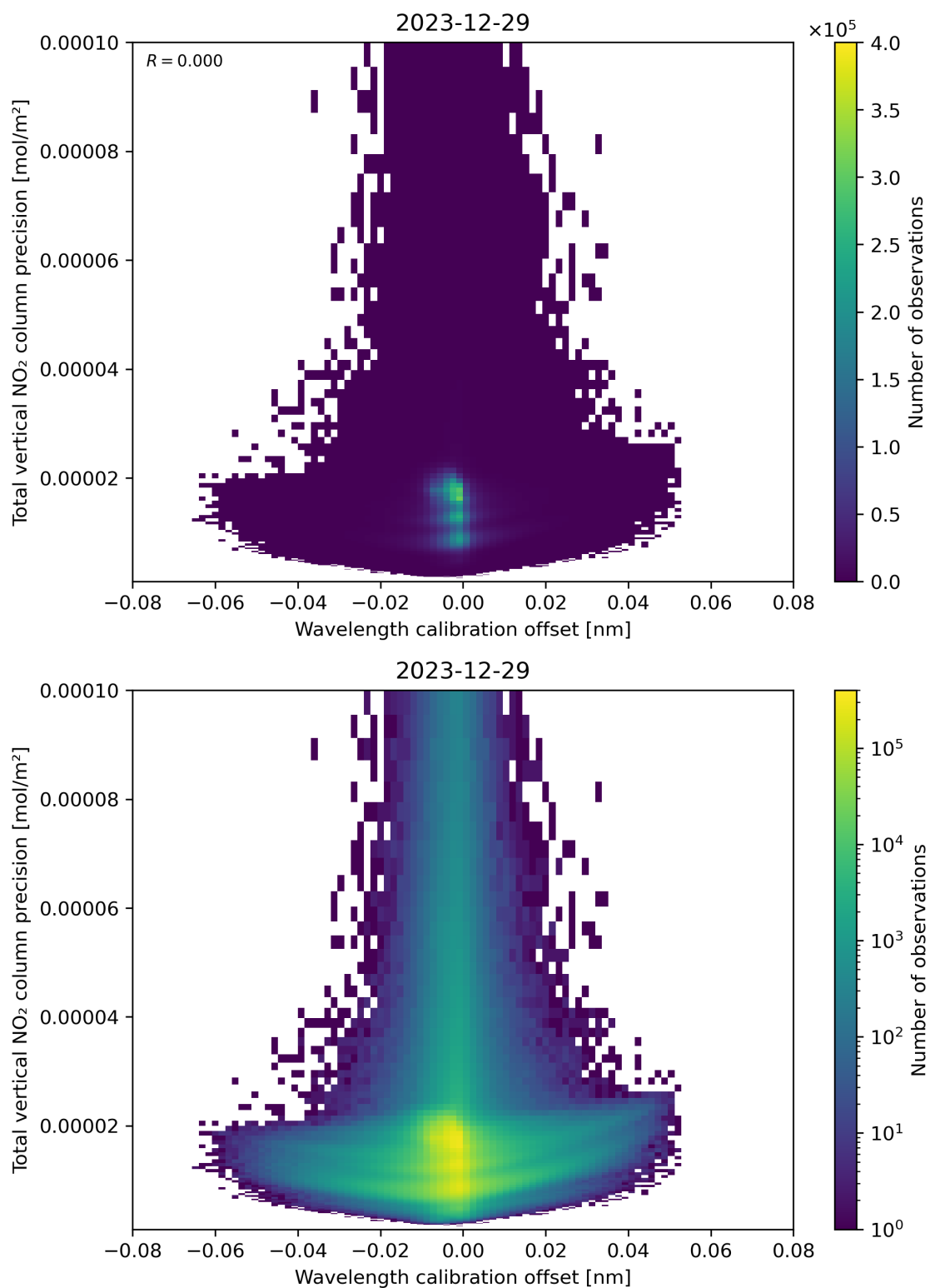
Figure 180: Scatter density plot of “Wavelength calibration offset” against “Total vertical NO 2 column precision” for 2023-12-28 to 2023-12-30.
