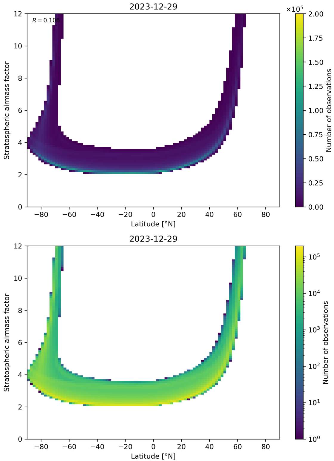
Figure 83: Scatter density plot of “Latitude” against “Stratospheric air mass factor” for 2023-12-28 to 2023-12-30.
