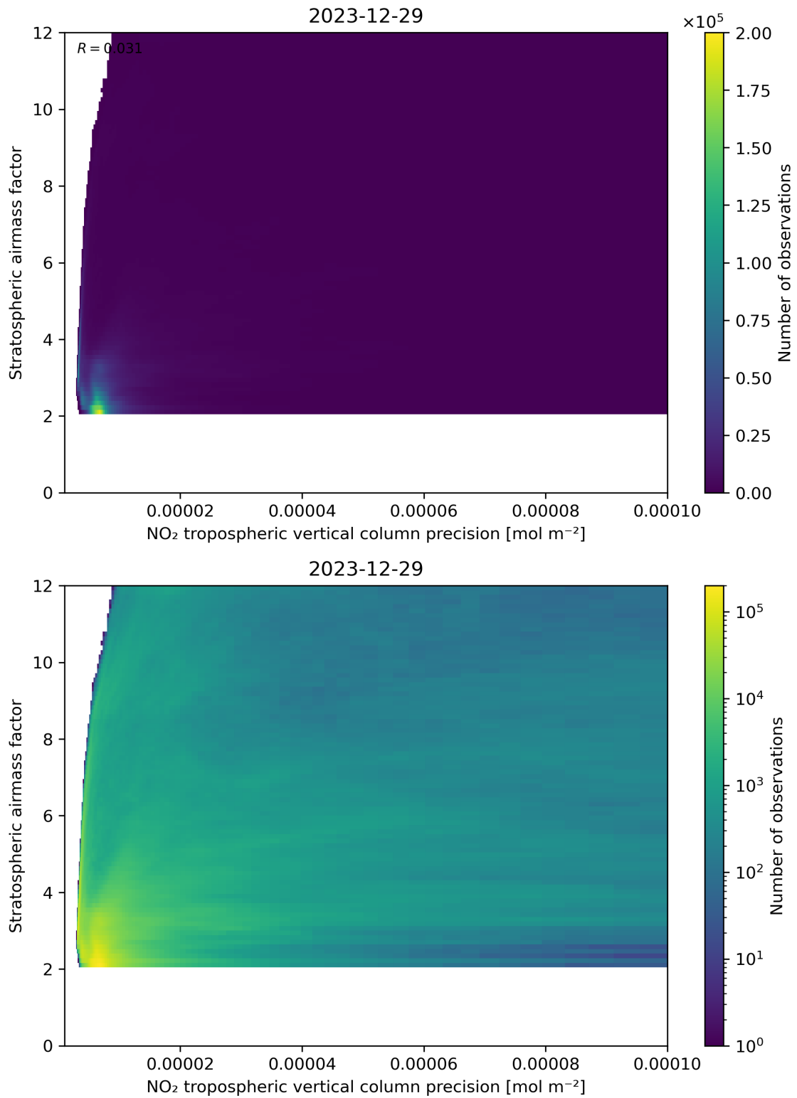
Figure 131: Scatter density plot of “NO 2 tropospheric vertical column precision” against “Stratospheric airmass factor” for 2023-12-28 to 2023-12-30.
