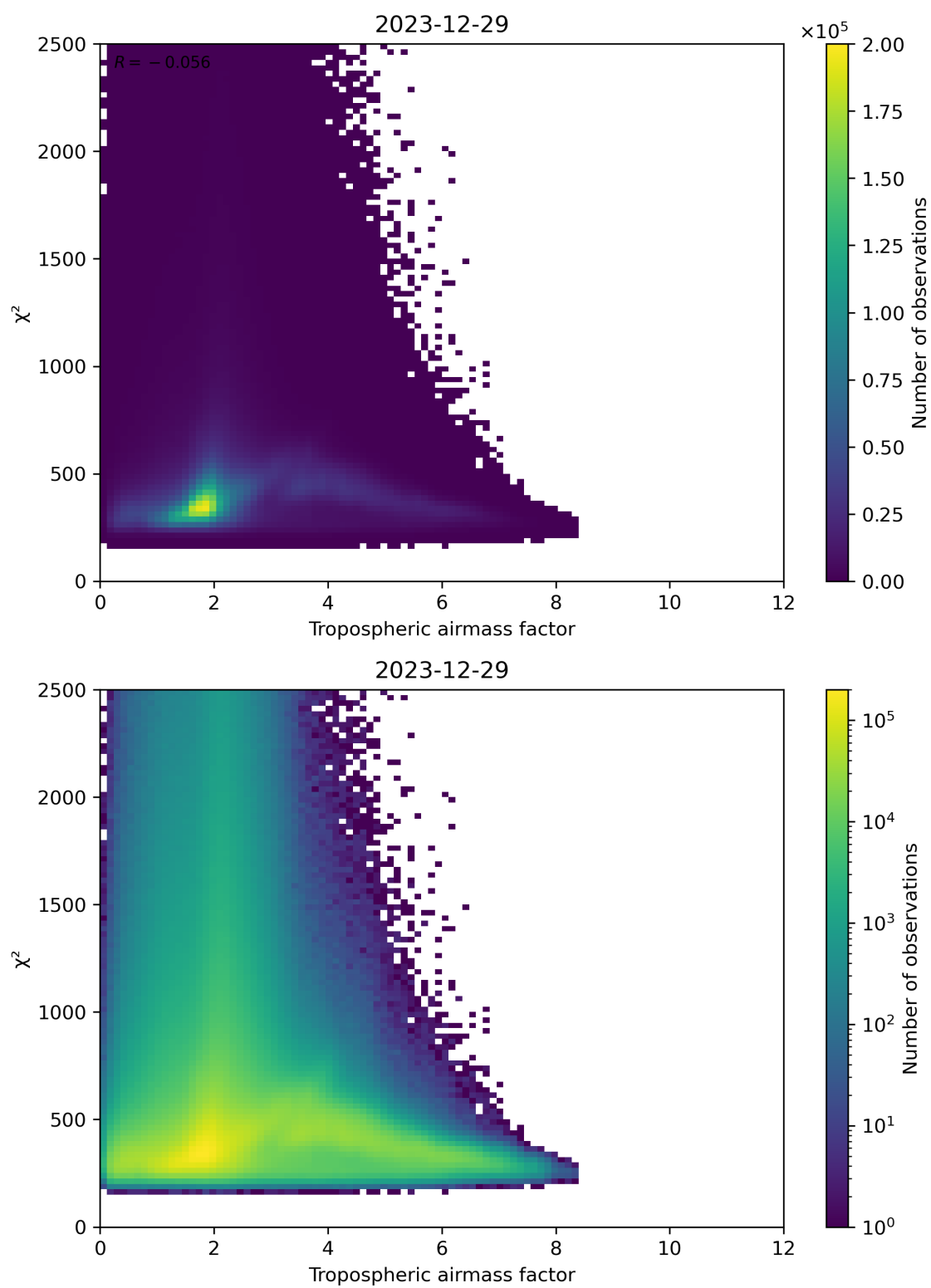
Figure 73: Scatter density plot of “Tropospheric airmass factor” against “ \chi^2 ” for 2023-12-28 to 2023-12-30.
