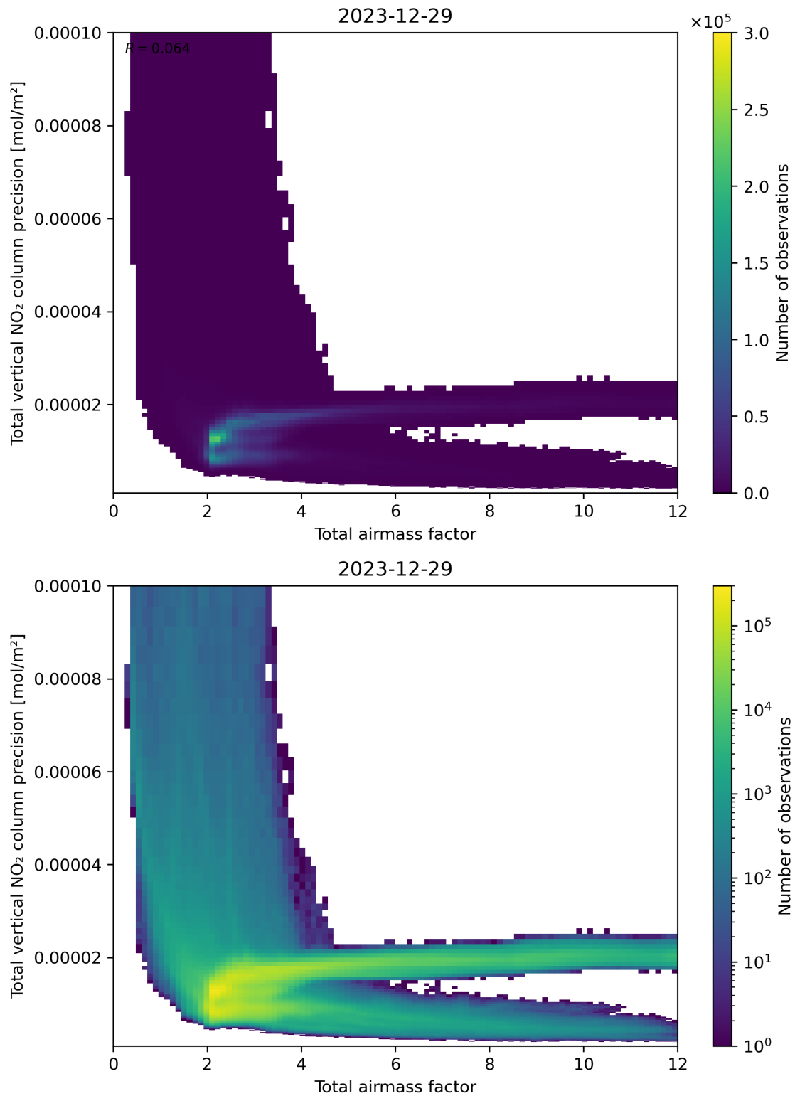
Figure 68: Scatter density plot of “Total airmass factor” against “Total vertical NO 2 column precision” for 2023-12-28 to 2023-12-30.
