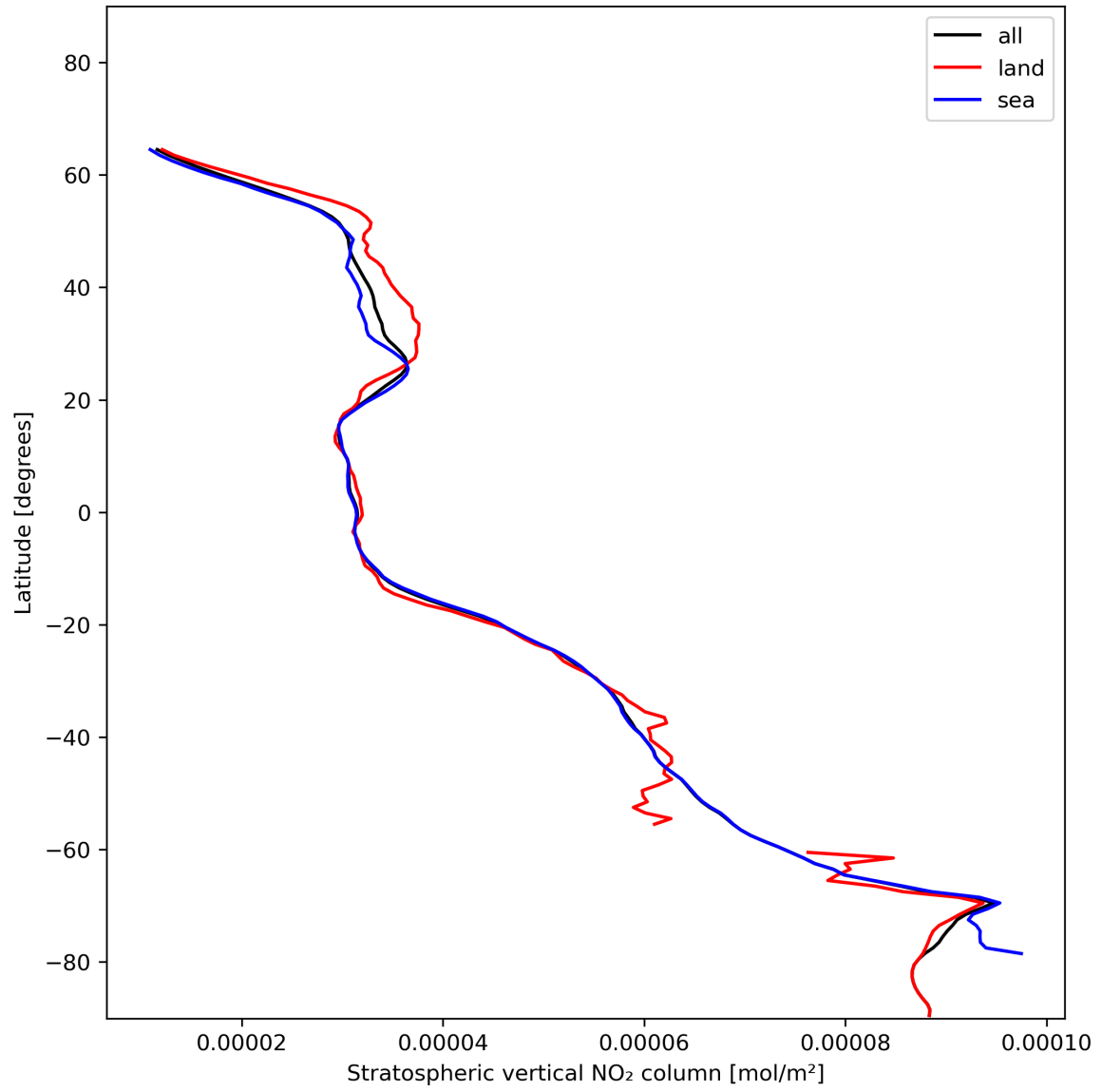
Figure 19: Zonal average of “Stratospheric vertical NO 2 column” for 2023-12-28 to 2023-12-30.
