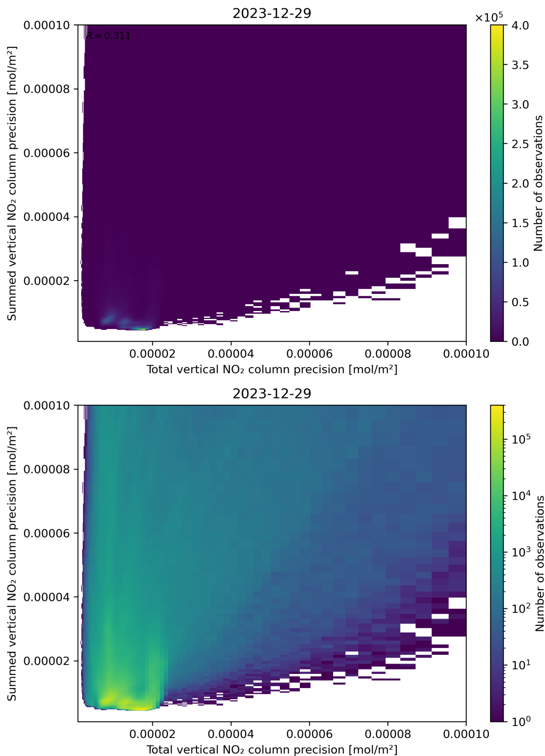
Figure 118: Scatter density plot of “Total vertical NO 2 column precision” against “Summed vertical NO 2 column precision” for 2023-12-28 to 2023-12-30.
