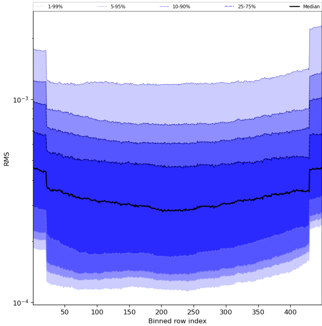
Figure 60: Along track statistics of “RMS” for 2023-12-28 to 2023-12-30
