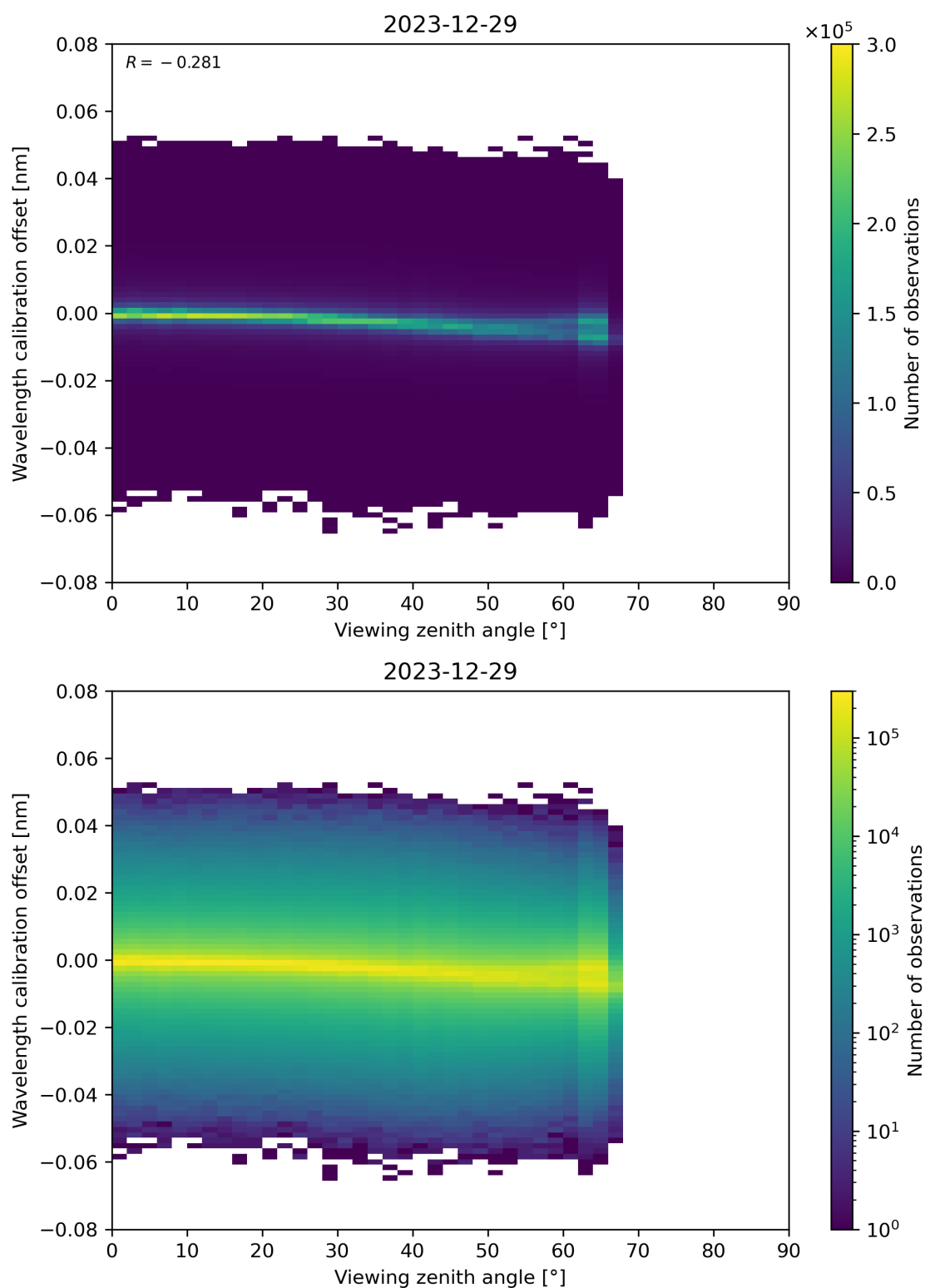
Figure 173: Scatter density plot of “Viewing zenith angle” against “Wavelength calibration offset” for 2023-12-28 to 2023-12-30.
