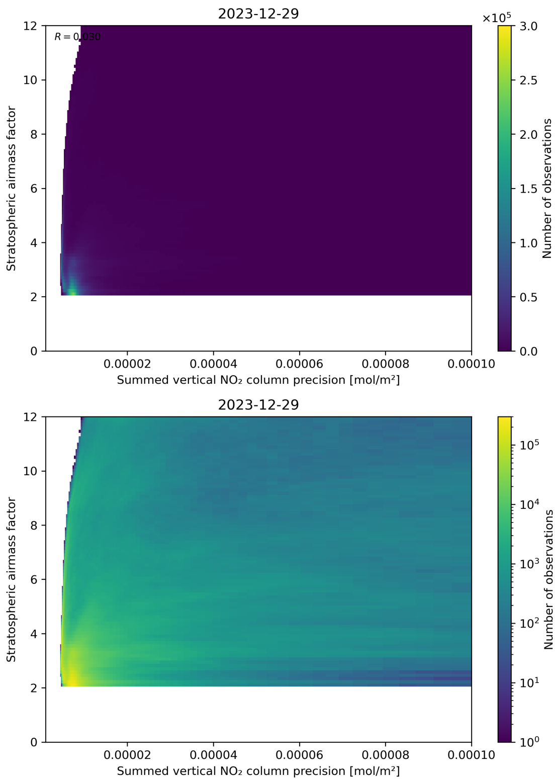
Figure 106: Scatter density plot of “Summed vertical NO 2 column precision” against “Stratospheric airmass factor” for 2023-12-28 to 2023-12-30.
