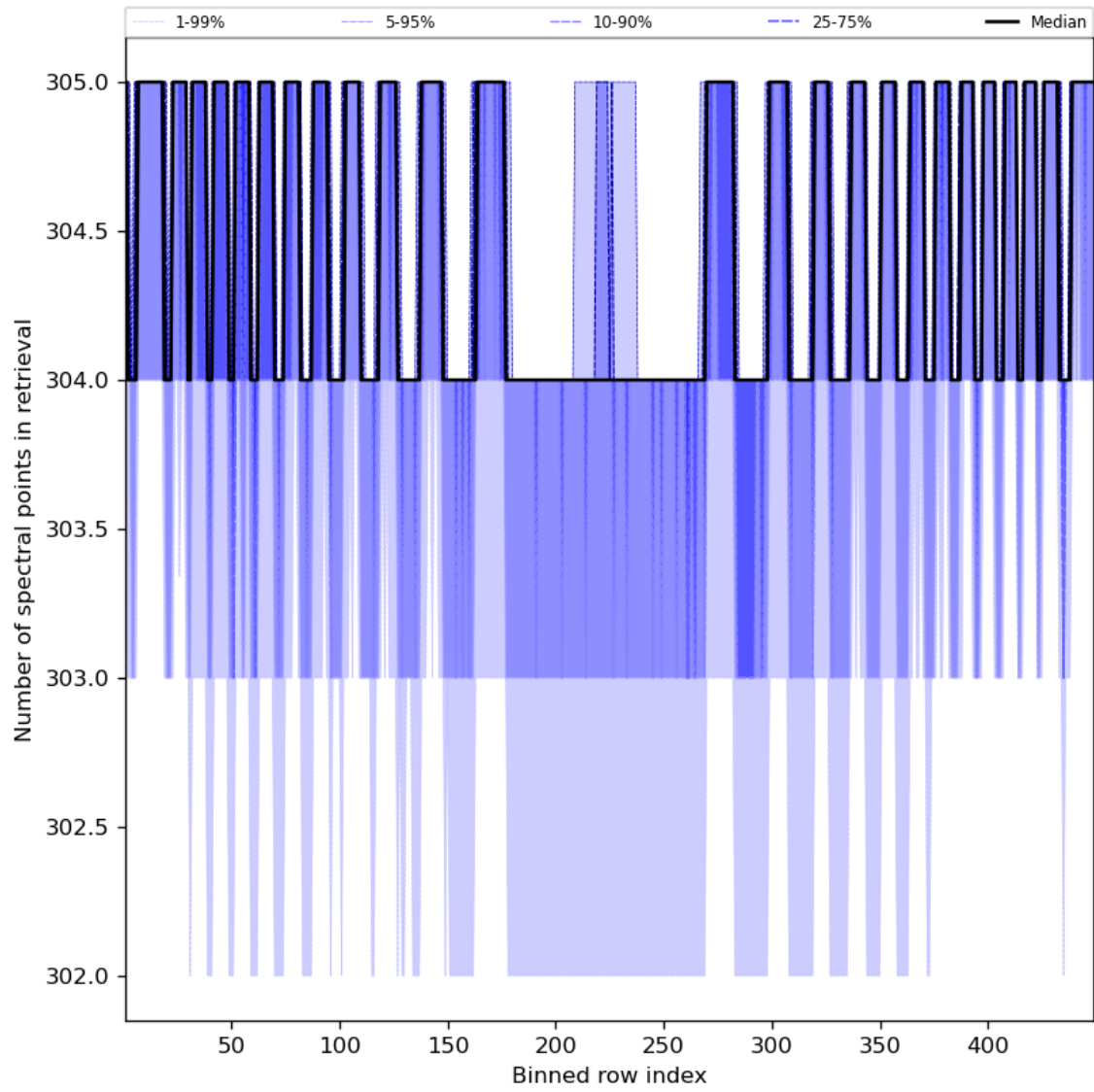
Figure 50: Along track statistics of “Number of spectral points in retrieval” for 2023-12-28 to 2023-12-30
