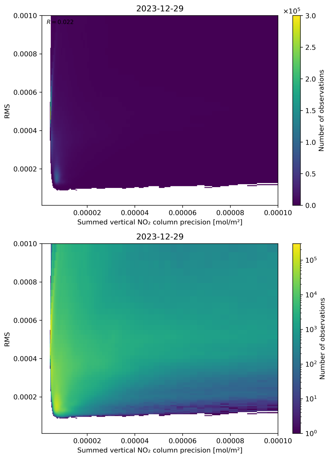
Figure 108: Scatter density plot of “Summed vertical NO 2 column precision” against “RMS” for 2023-12-28 to 2023-12-30.
