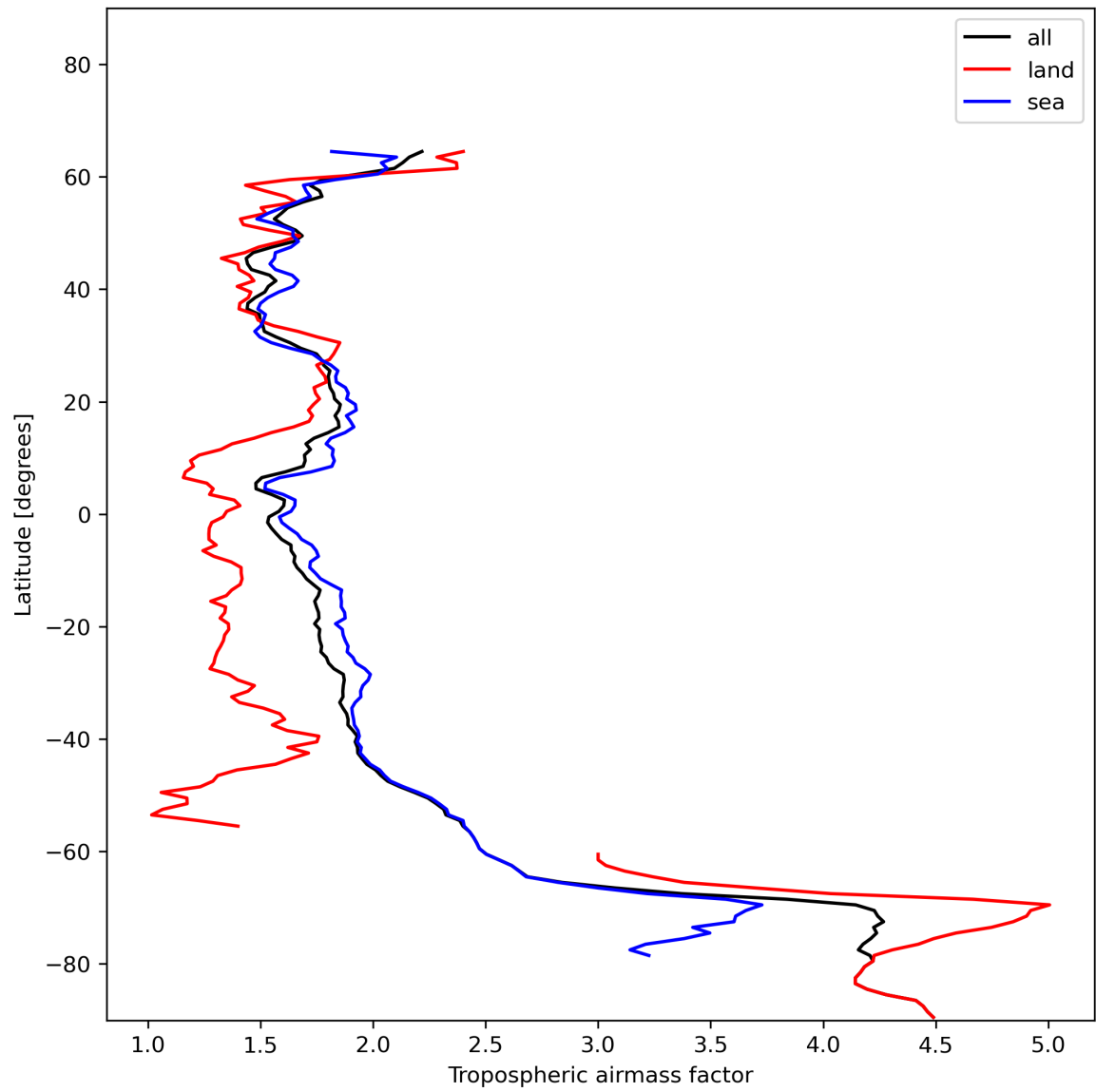
Figure 14: Zonal average of “Tropospheric airmass factor” for 2023-12-28 to 2023-12-30.
