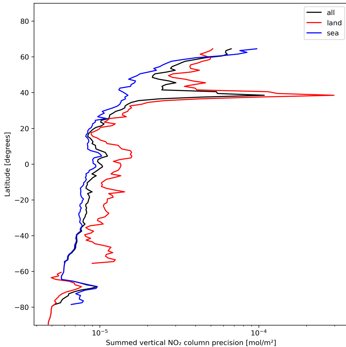
Figure 24: Zonal average of “Summed vertical NO 2 column precision” for 2023-12-28 to 2023-12-30.
