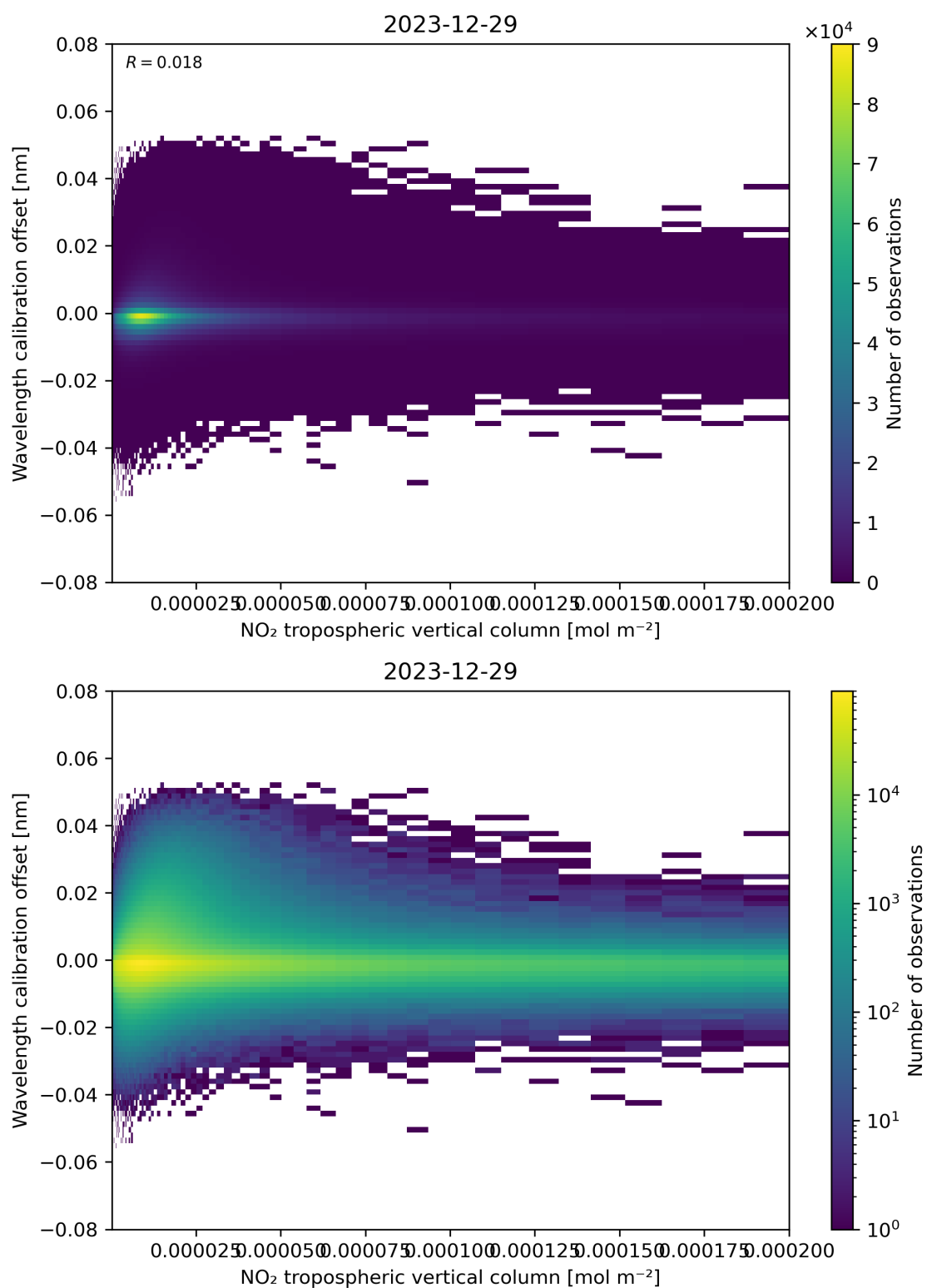
Figure 143: Scatter density plot of “NO 2 tropospheric vertical column” against “Wavelength calibration offset” for 2023-12-28 to 2023-12-30.
