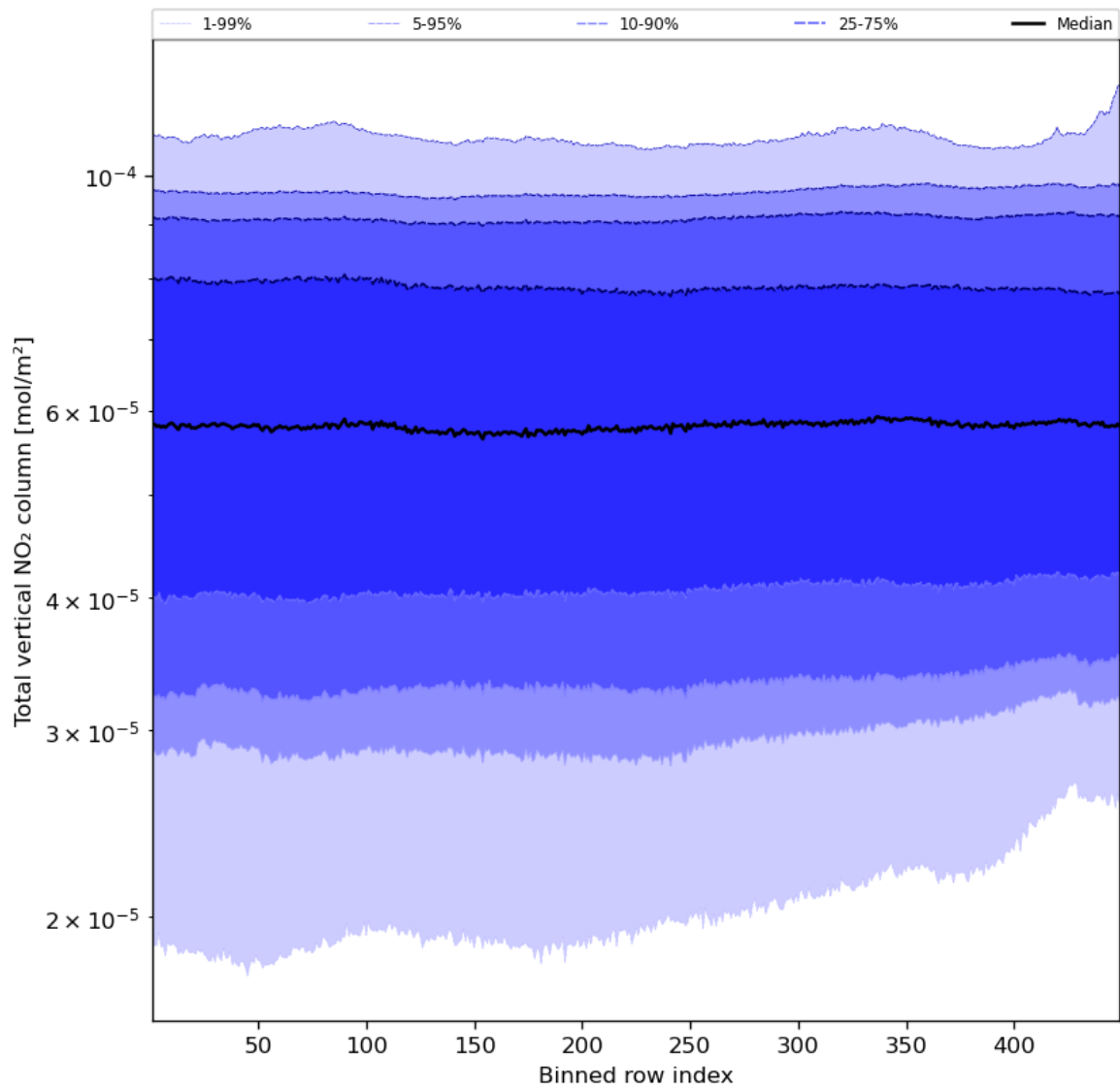
Figure 55: Along track statistics of “Total vertical NO 2 column” for 2023-12-28 to 2023-12-30
