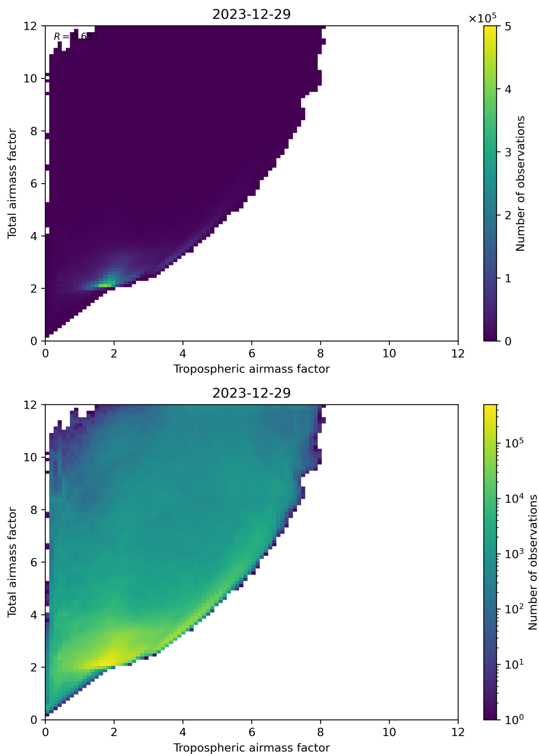
Figure 72: Scatter density plot of “Tropospheric airmass factor” against “Total airmass factor” for 2023-12-28 to 2023-12-30.
