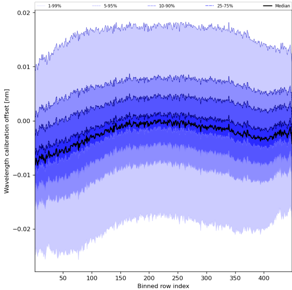
Figure 52: Along track statistics of “Wavelength calibration offset” for 2023-12-28 to 2023-12-30
