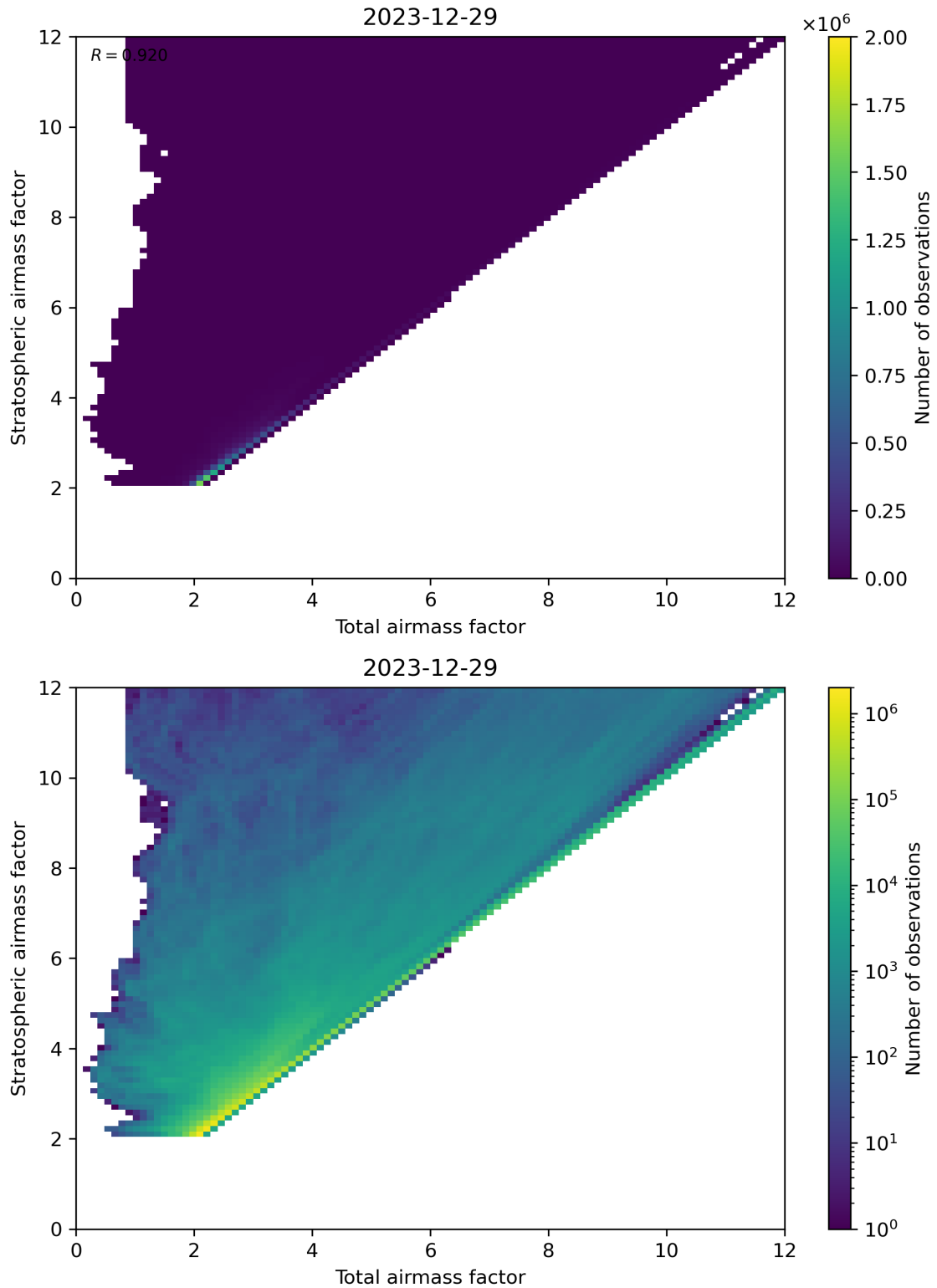
Figure 62: Scatter density plot of “Total airmass factor” against “Stratospheric airmass factor” for 2023-12-28 to 2023-12-30.
