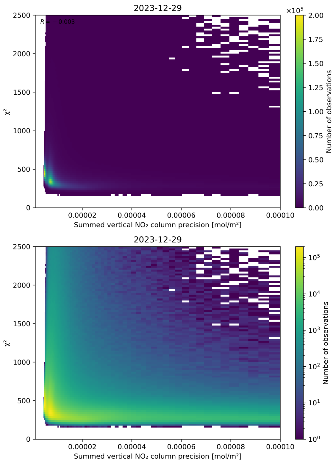
Figure 107: Scatter density plot of “Summed vertical NO 2 column precision” against “ \chi^2 ” for 2023-12-28 to 2023-12-30.
