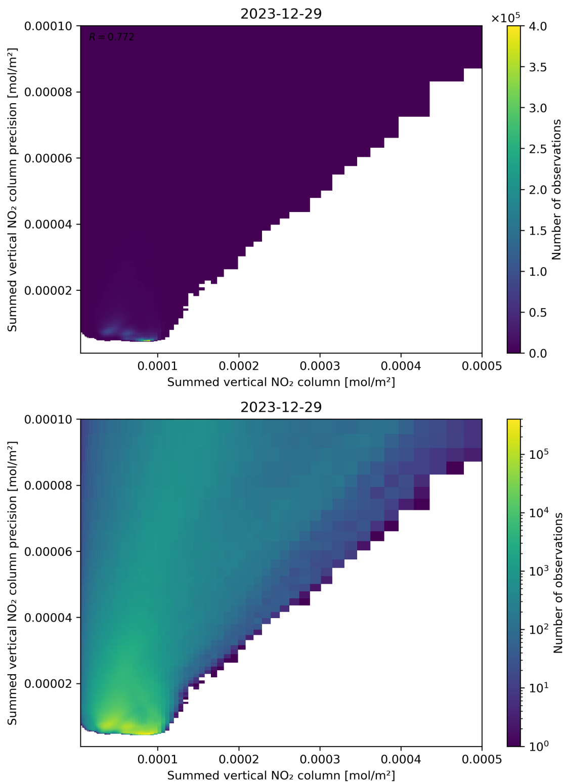
Figure 105: Scatter density plot of “Summed vertical NO 2 column” against “Summed vertical NO 2 column precision” for 2023-12-28 to 2023-12-30.
