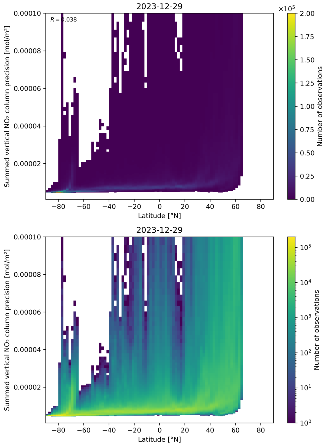
Figure 89: Scatter density plot of “Latitude” against “Summed vertical NO 2 column precision” for 2023-12-28 to 2023-12-30.
