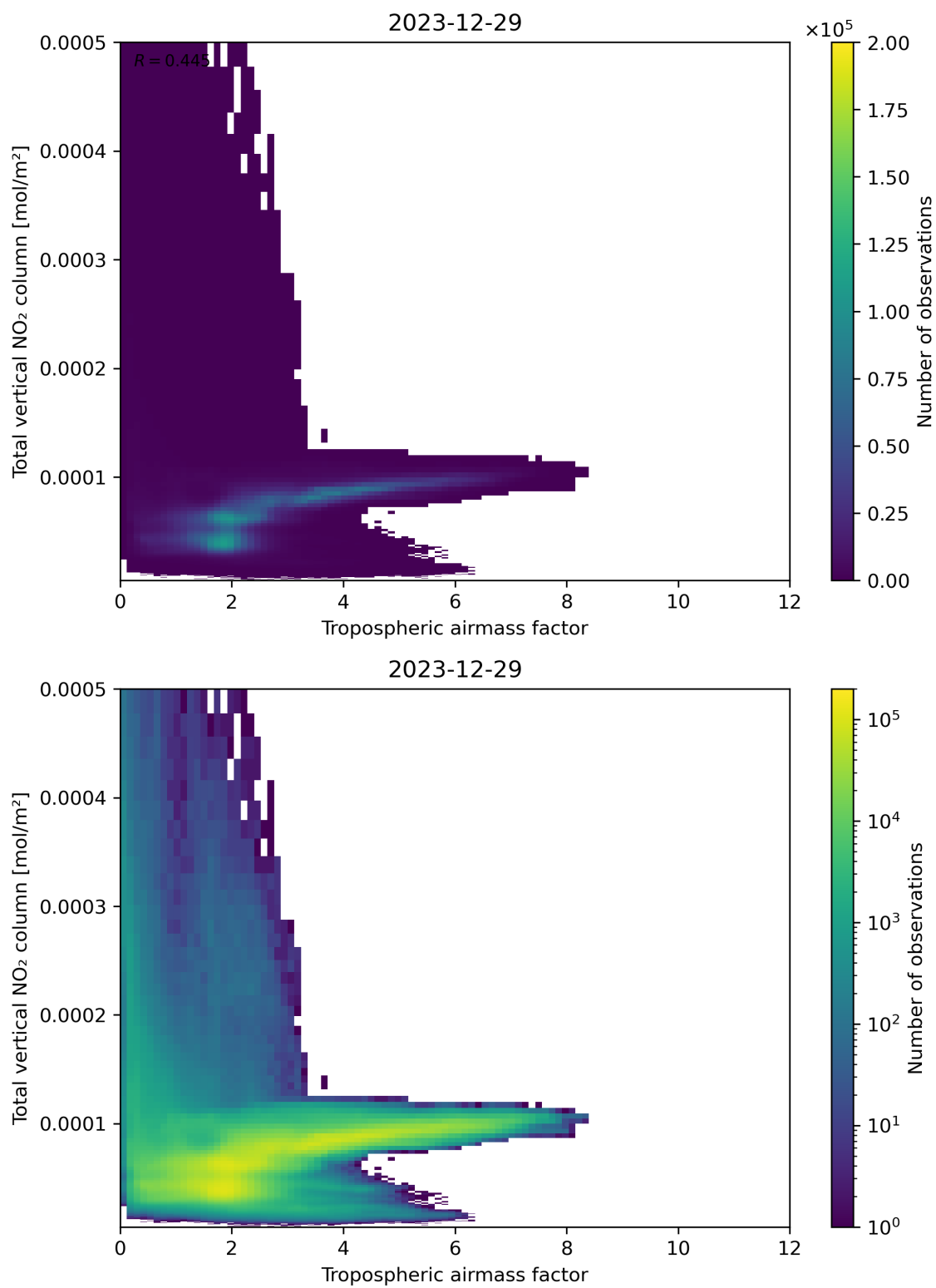
Figure 77: Scatter density plot of “Tropospheric airmass factor” against “Total vertical NO 2 column” for 2023-12-28 to 2023-12-30.
