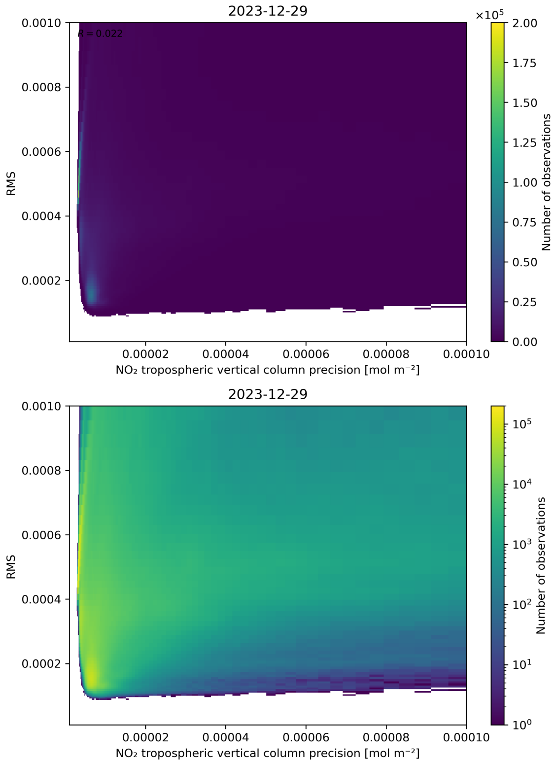
Figure 140: Scatter density plot of “NO 2 tropospheric vertical column precision” against “RMS” for 2023-12-28 to 2023-12-30.
