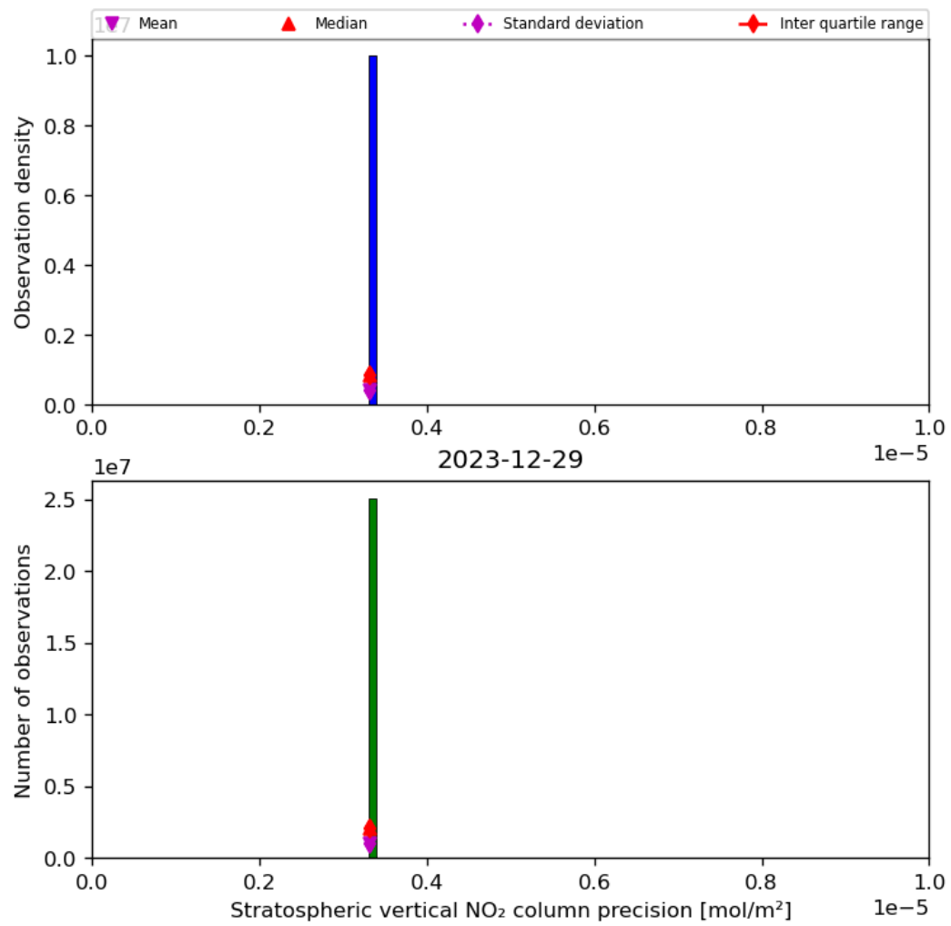
Figure 37: Histogram of “Stratospheric vertical NO 2 column precision” for 2023-12-28 to 2023-12-30
