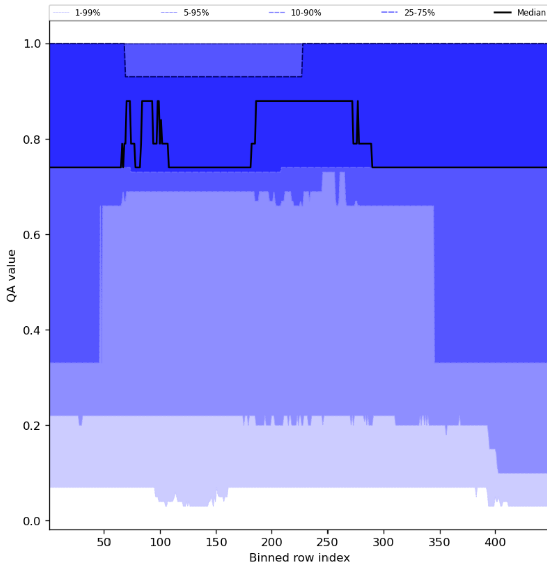
Figure 45: Along track statistics of “QA value” for 2023-12-28 to 2023-12-30
