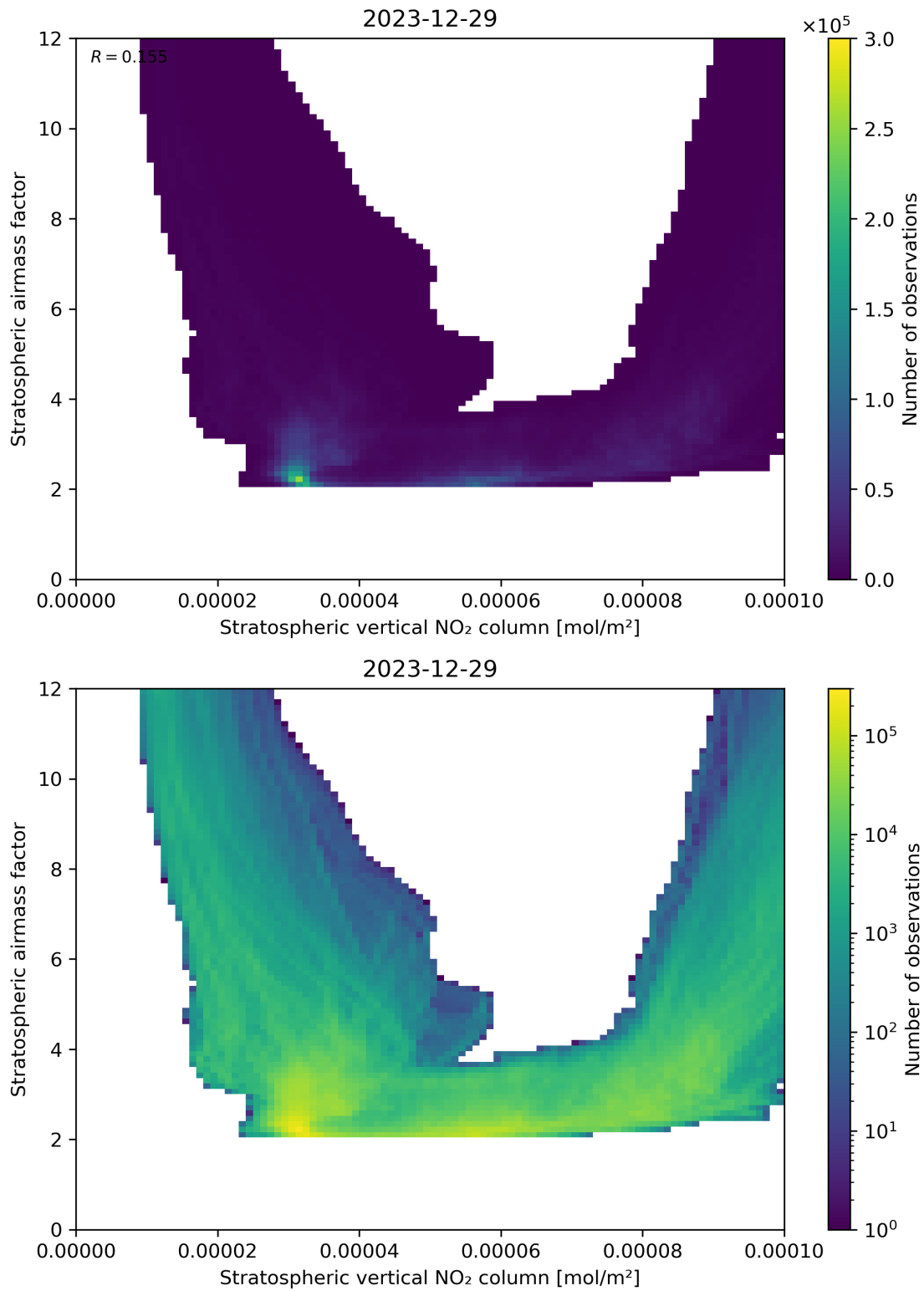
Figure 96: Scatter density plot of “Stratospheric vertical NO 2 column” against “Stratospheric airmass factor” for 2023-12-28 to 2023-12-30.
