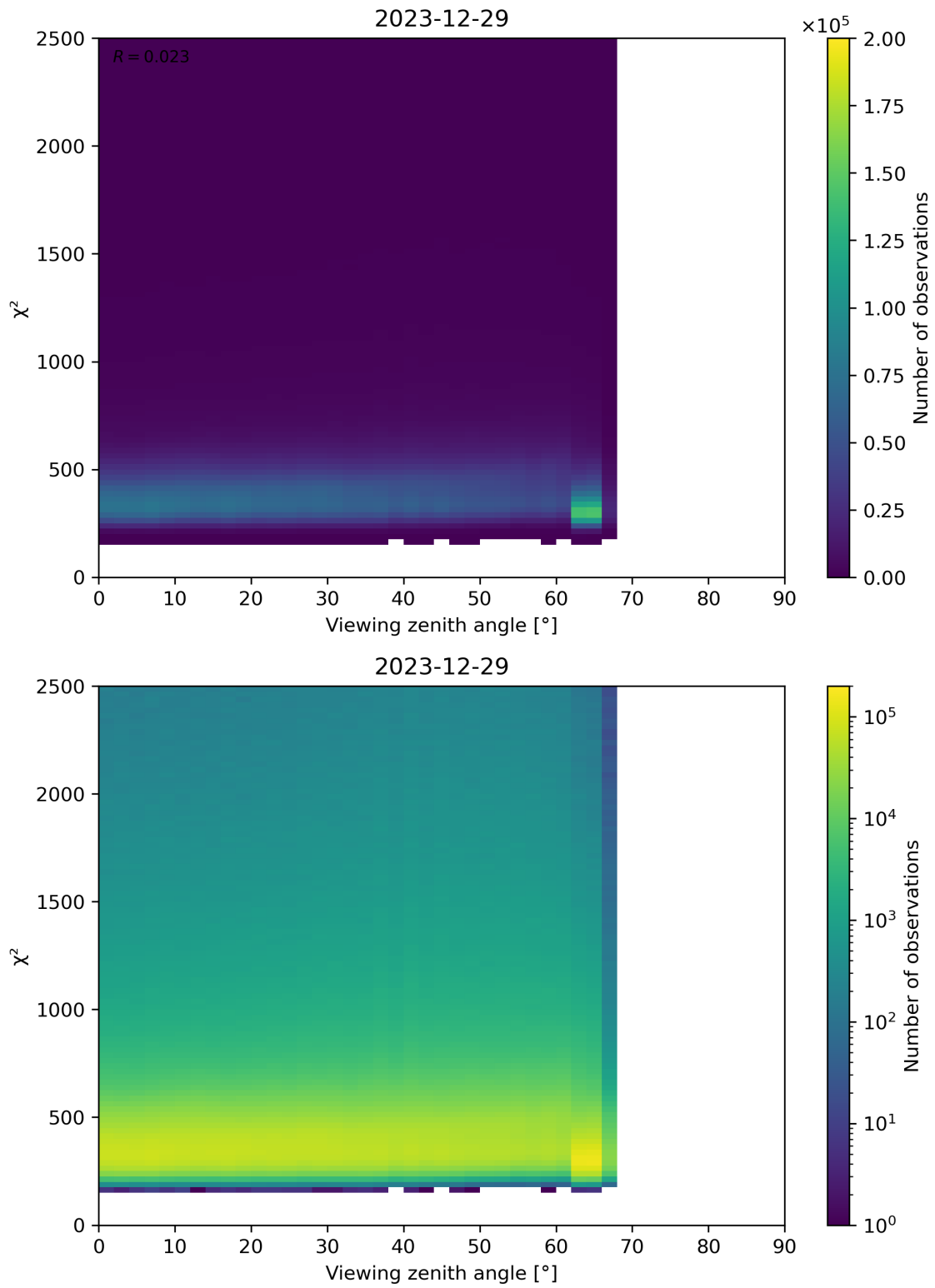
Figure 162: Scatter density plot of “Viewing zenith angle” against “ \chi^2 ” for 2023-12-28 to 2023-12-30.
