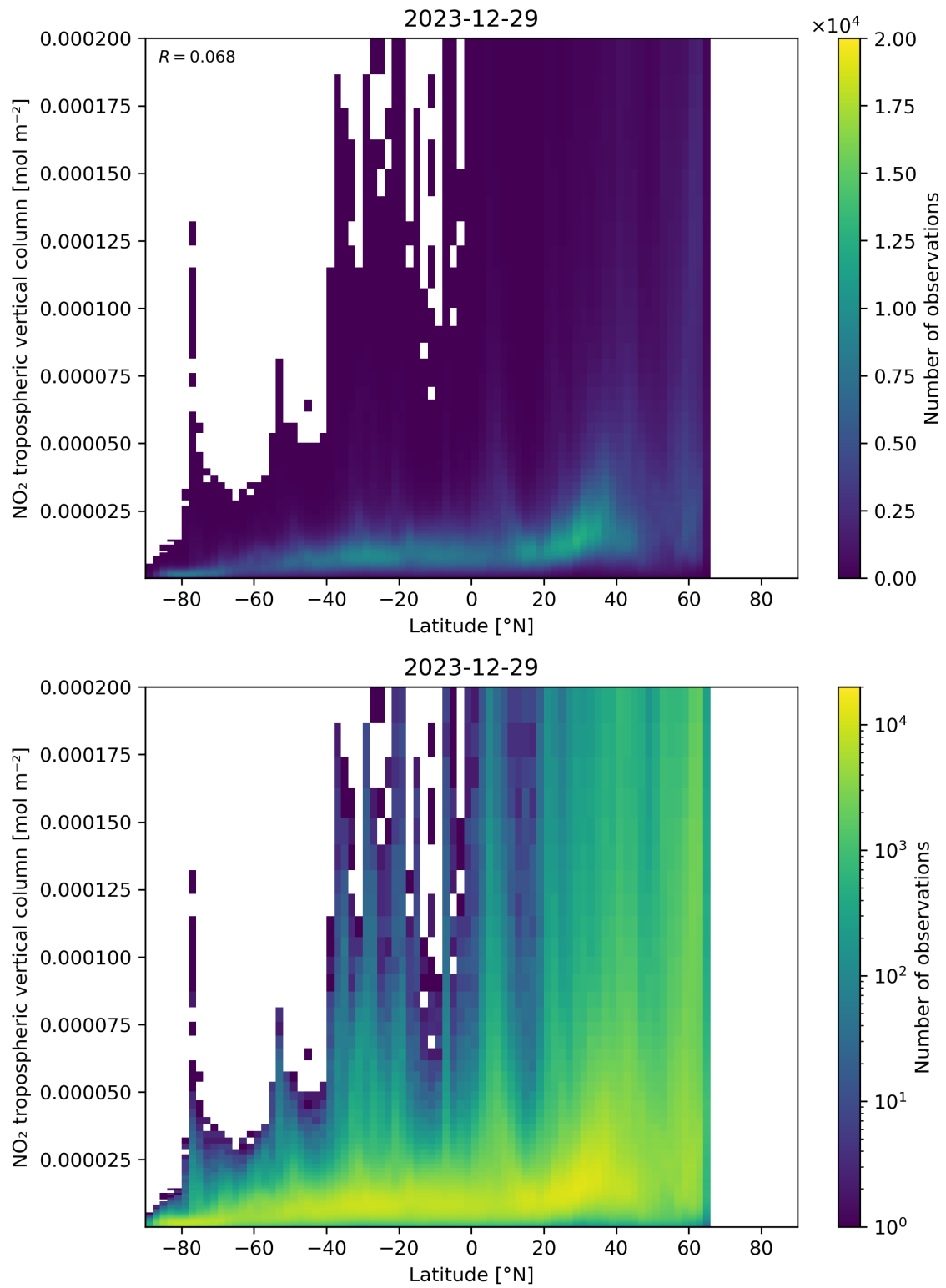
Figure 92: Scatter density plot of “Latitude” against “NO 2 tropospheric vertical column” for 2023-12-28 to 2023-12-30.
