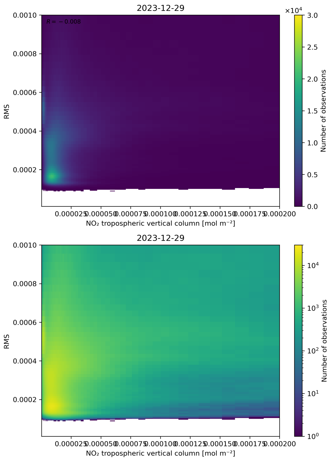
Figure 142: Scatter density plot of “NO 2 tropospheric vertical column” against “RMS” for 2023-12-28 to 2023-12-30.
