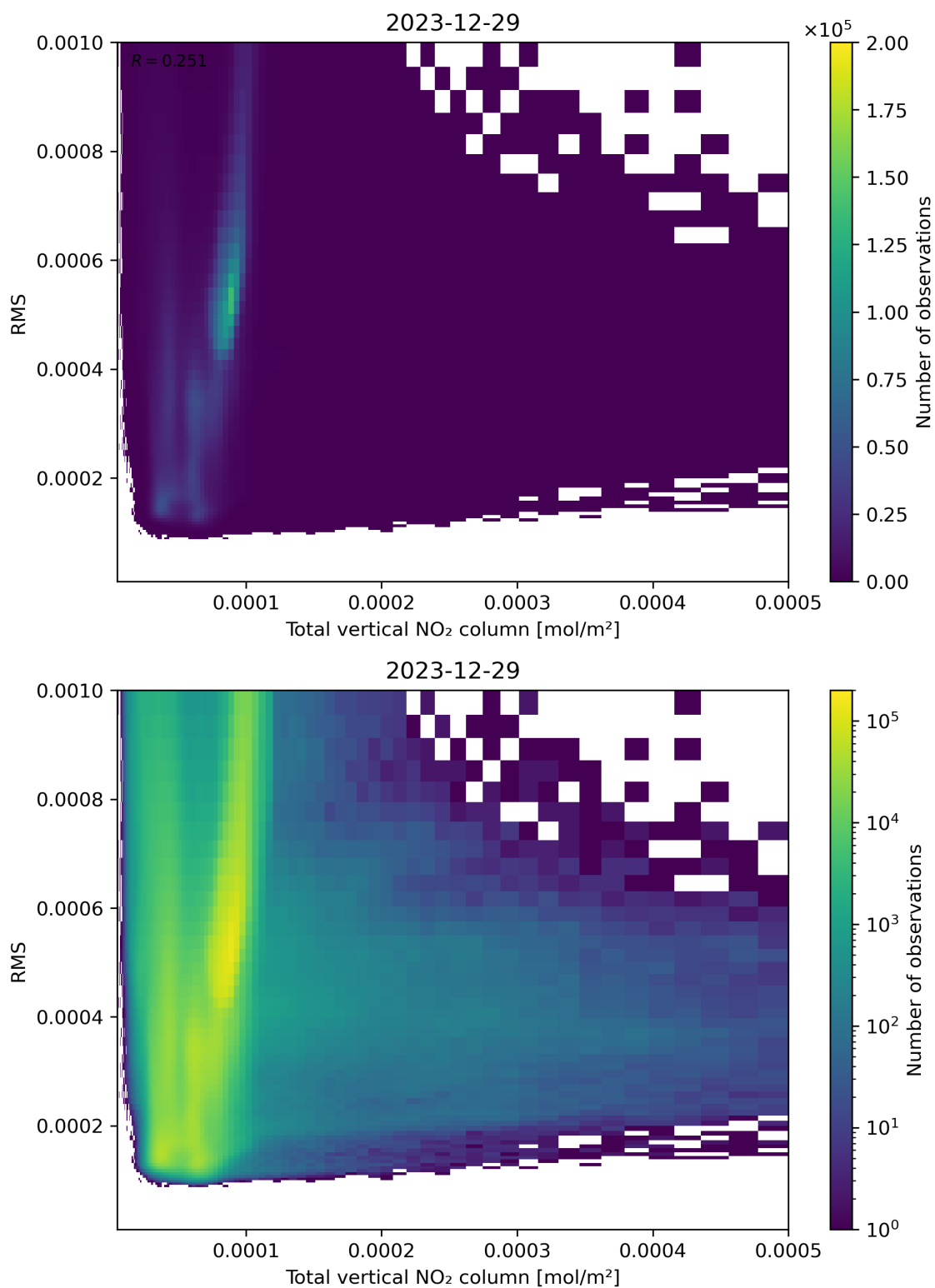
Figure 120: Scatter density plot of “Total vertical NO 2 column” against “RMS” for 2023-12-28 to 2023-12-30.
