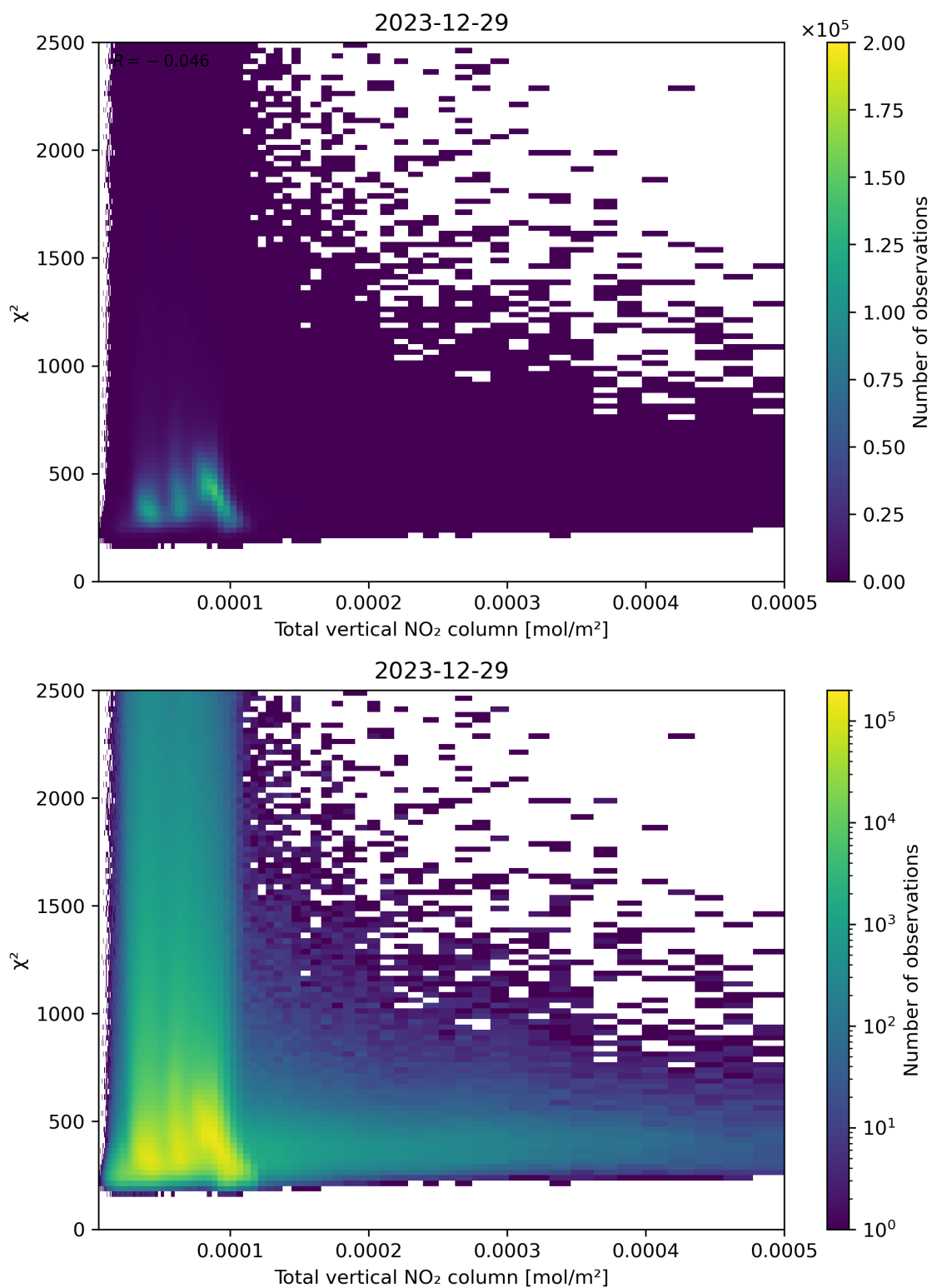
Figure 111: Scatter density plot of “Total vertical NO 2 column” against “ \chi^2 ” for 2023-12-28 to 2023-12-30.
