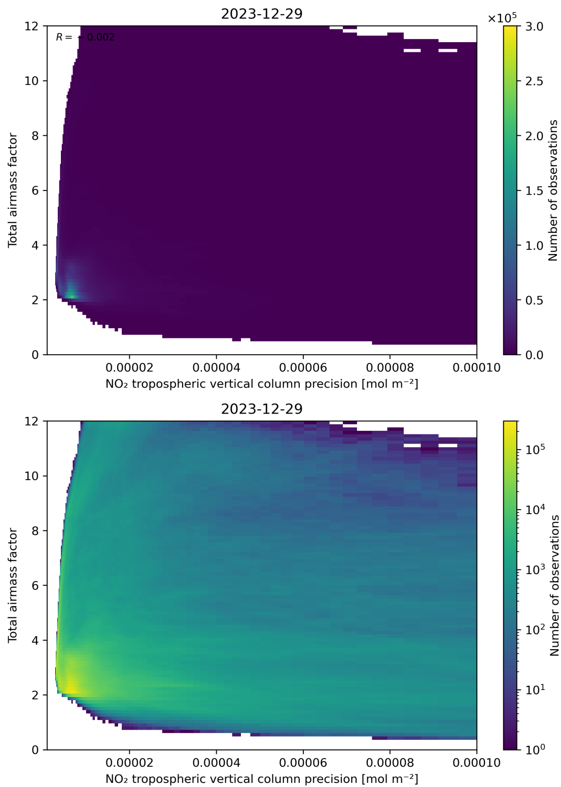
Figure 132: Scatter density plot of “NO 2 tropospheric vertical column precision” against “Total air mass factor” for 2023-12-28 to 2023-12-30.
