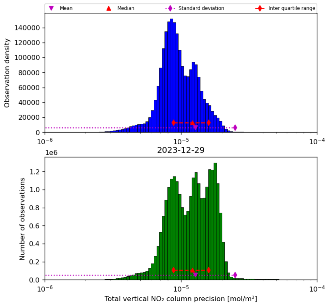
Figure 39: Histogram of “Total vertical NO 2 column precision” for 2023-12-28 to 2023-12-30
