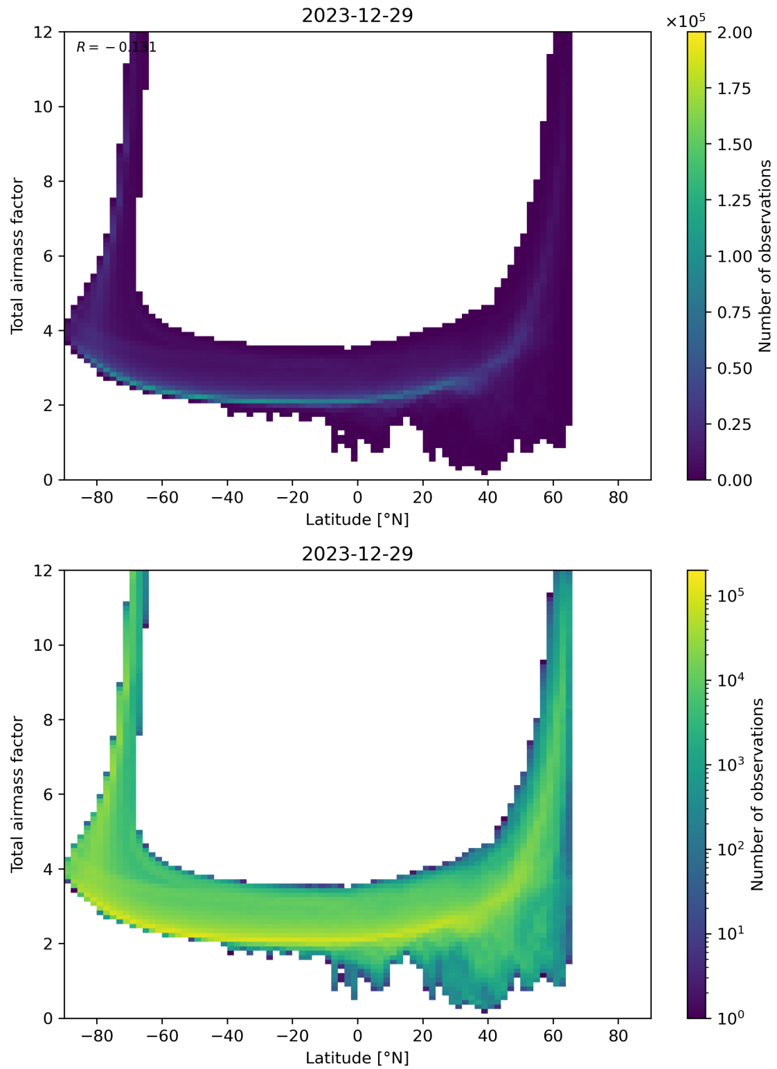
Figure 84: Scatter density plot of “Latitude” against “Total airmass factor” for 2023-12-28 to 2023-12-30.
