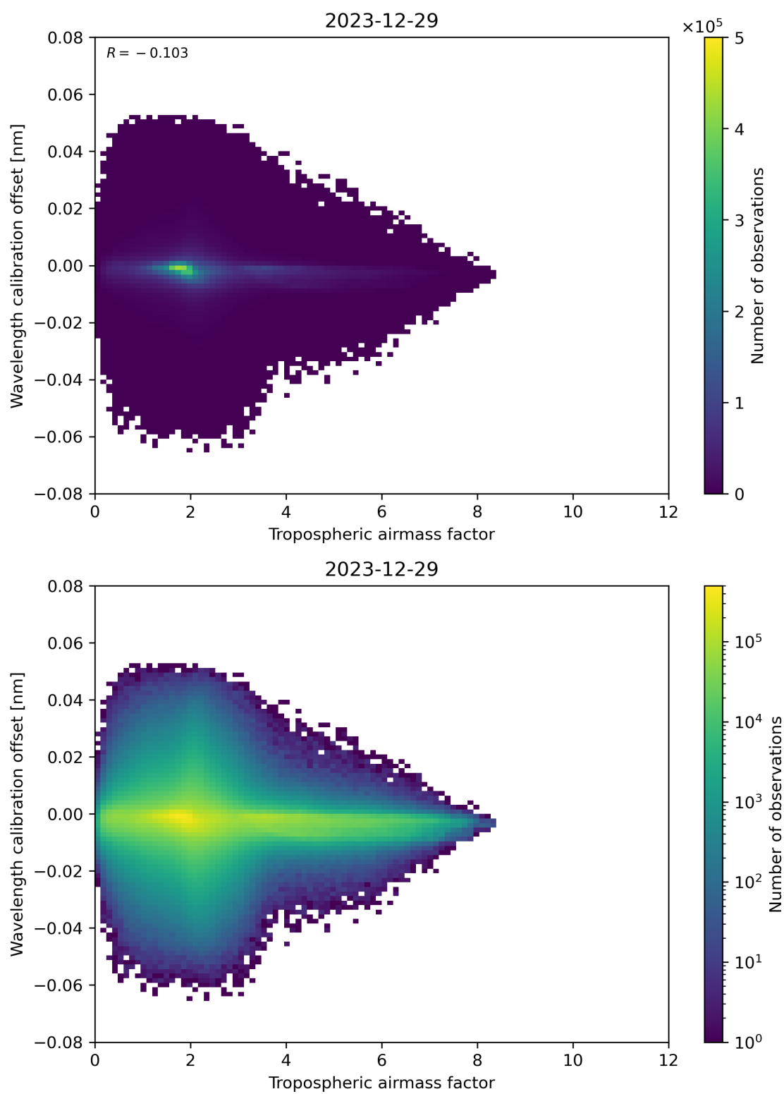
Figure 80: Scatter density plot of “Tropospheric airmass factor” against “Wavelength calibration offset” for 2023-12-28 to 2023-12-30.
