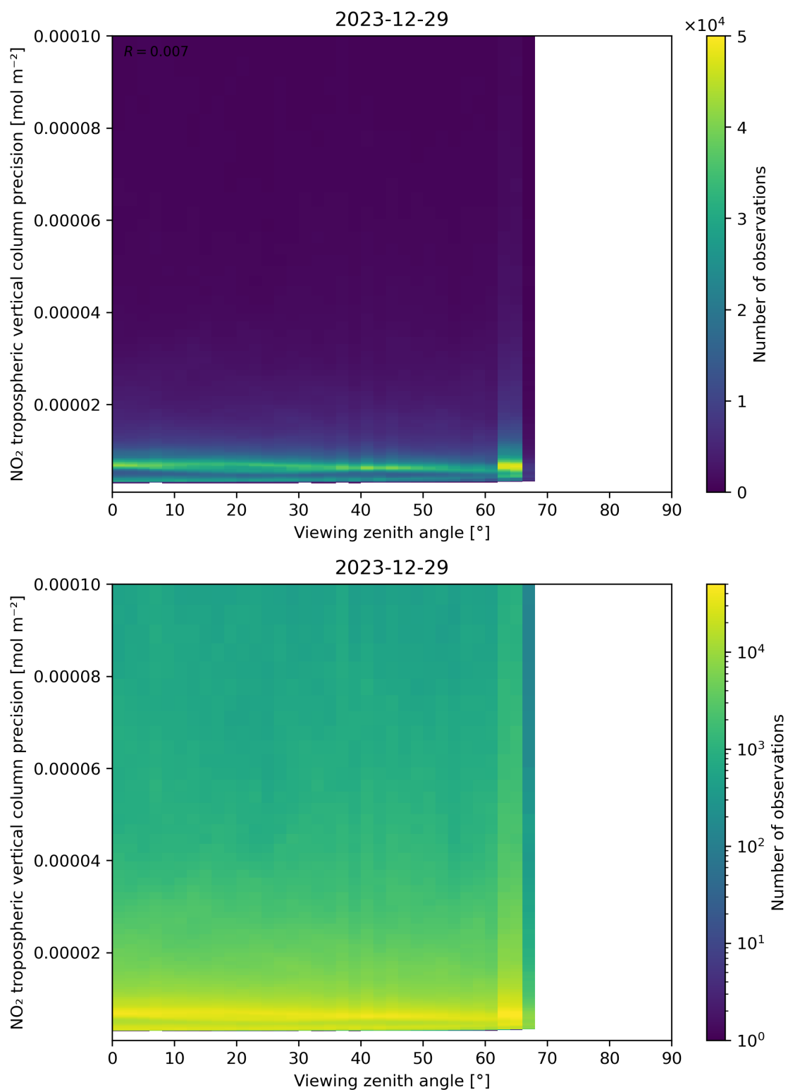
Figure 170: Scatter density plot of “Viewing zenith angle” against “NO 2 tropospheric vertical column precision” for 2023-12-28 to 2023-12-30.
