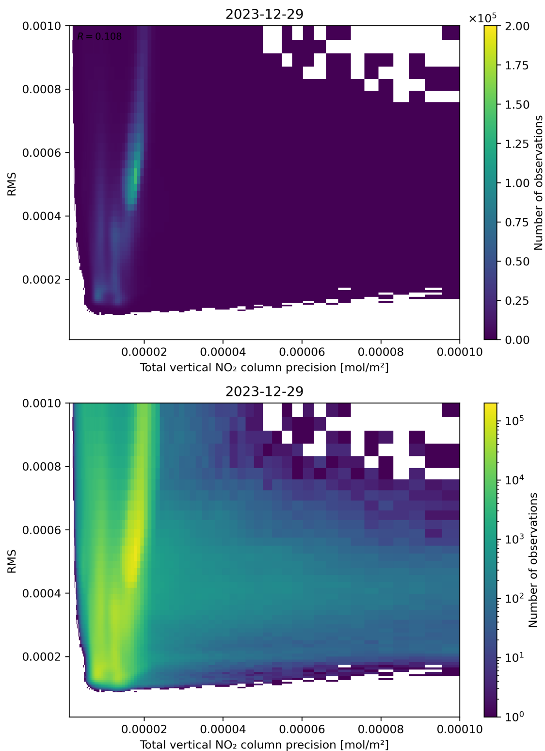
Figure 119: Scatter density plot of “Total vertical NO 2 column precision” against “RMS” for 2023-12-28 to 2023-12-30.
