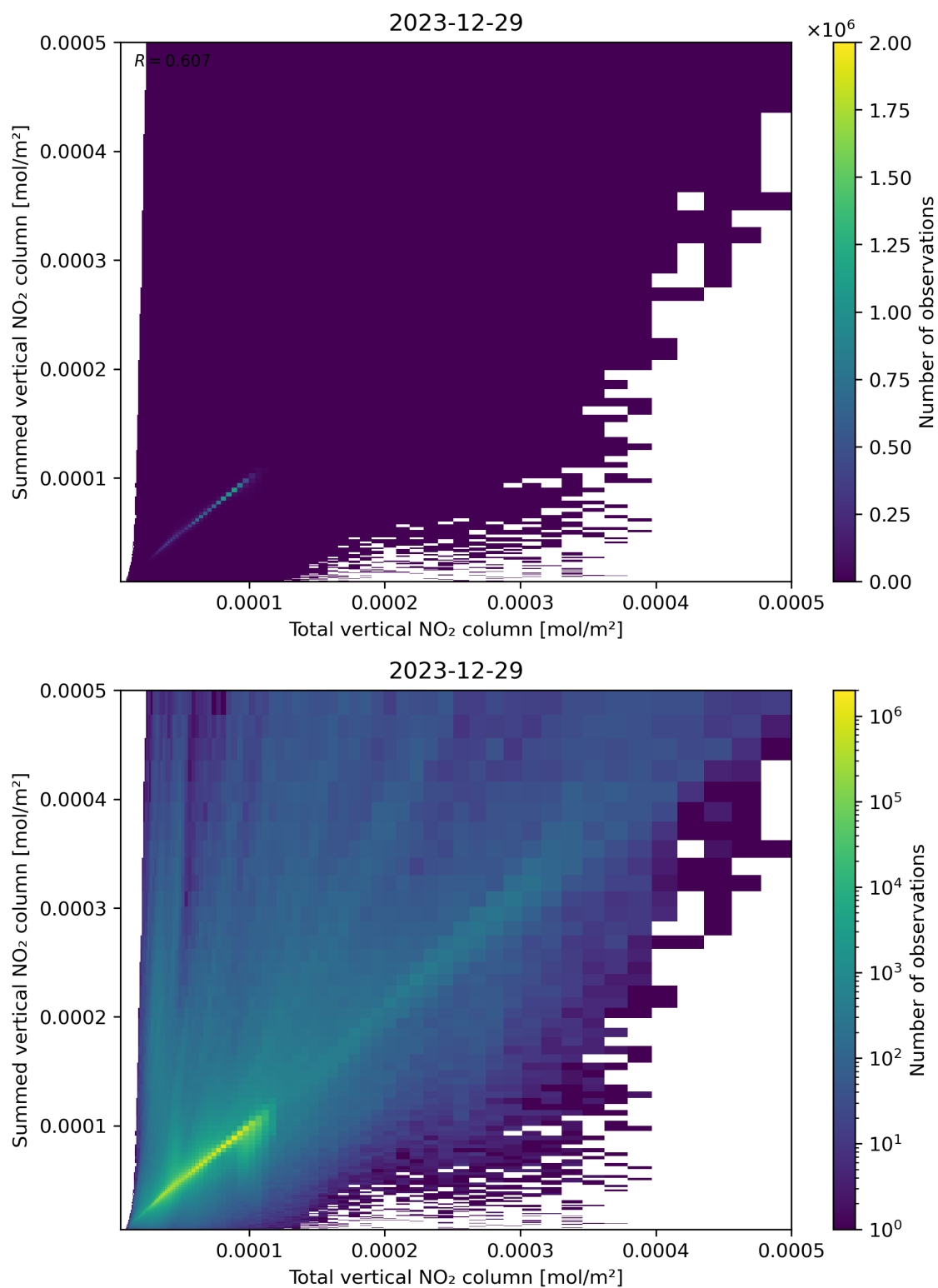
Figure 112: Scatter density plot of “Total vertical NO 2 column” against “Summed vertical NO 2 column” for 2023-12-28 to 2023-12-30.
