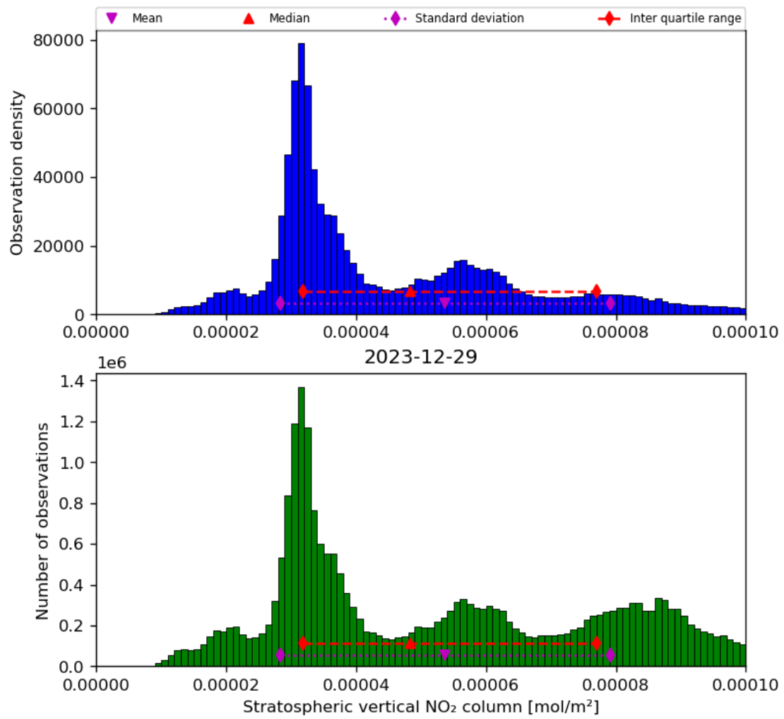
Figure 36: Histogram of “Stratospheric vertical NO 2 column” for 2023-12-28 to 2023-12-30
