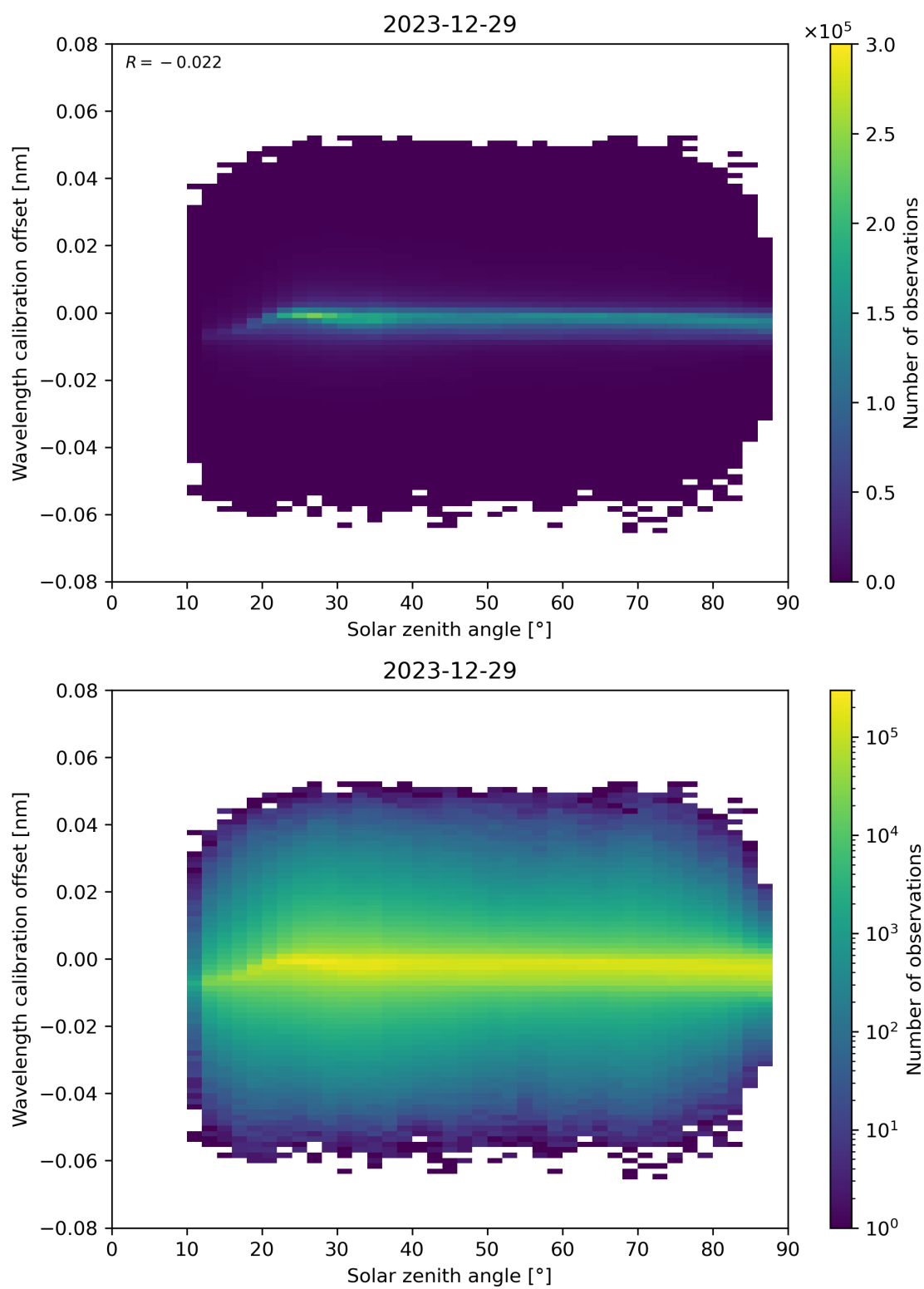
Figure 158: Scatter density plot of “Solar zenith angle” against “Wavelength calibration offset” for 2023-12-28 to 2023-12-30.
