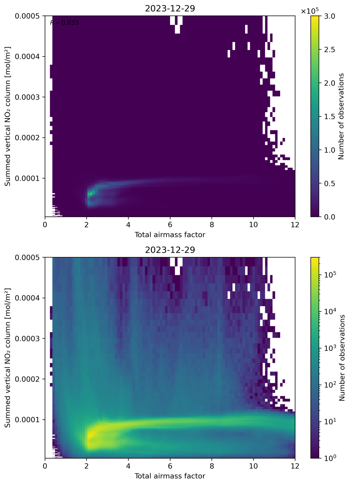
Figure 65: Scatter density plot of “Total airmass factor” against “Summed vertical NO 2 column” for 2023-12-28 to 2023-12-30.
