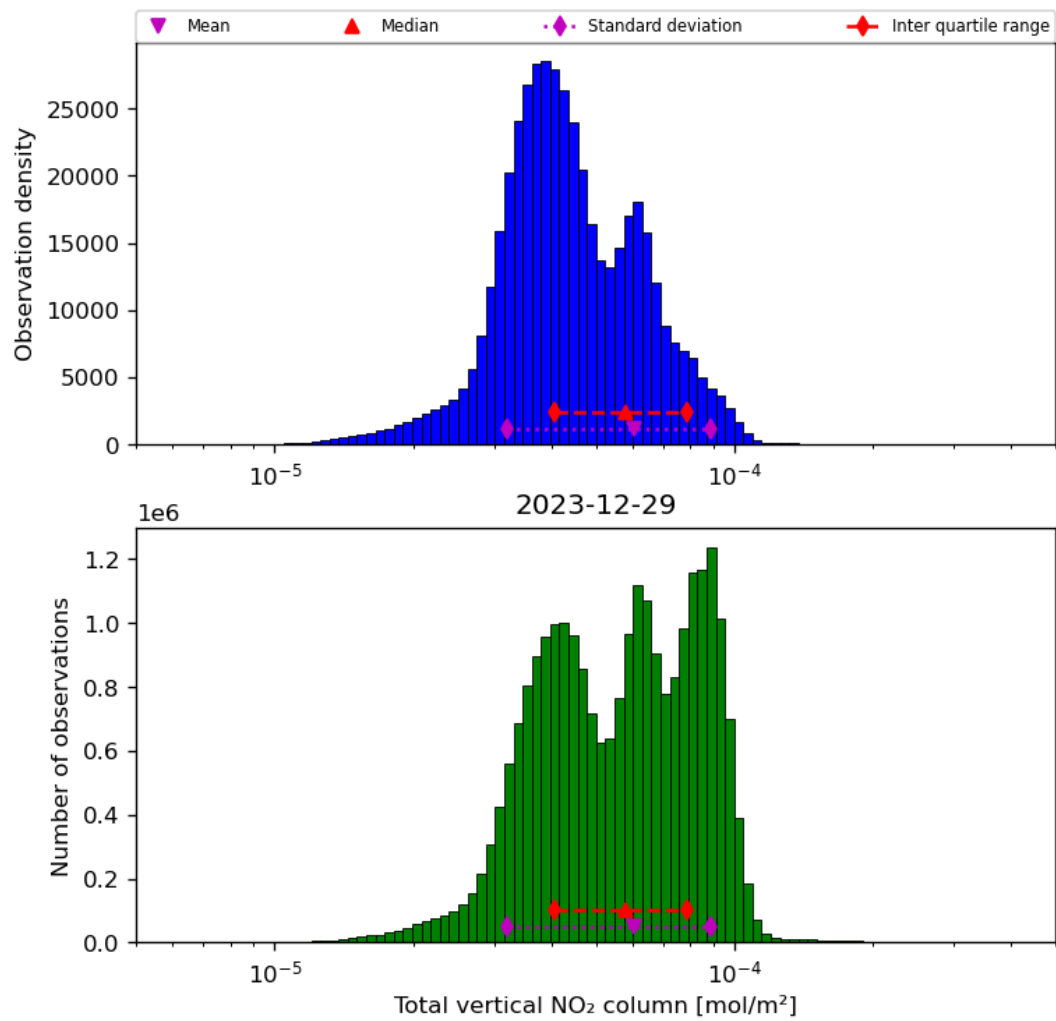
Figure 38: Histogram of “Total vertical NO 2 column” for 2023-12-28 to 2023-12-30
