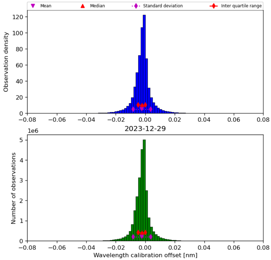
Figure 35: Histogram of “Wavelength calibration offset” for 2023-12-28 to 2023-12-30
