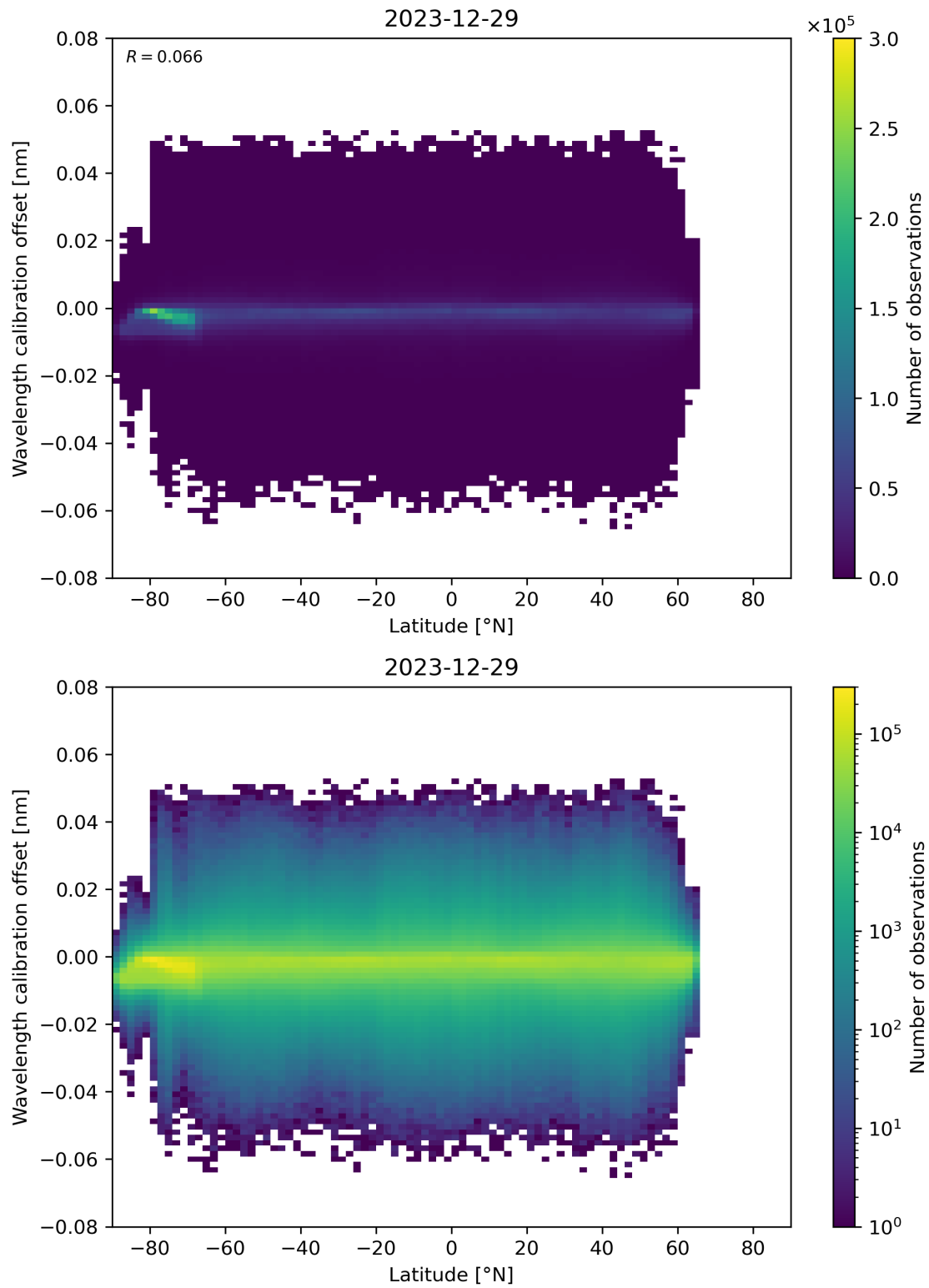
Figure 95: Scatter density plot of “Latitude” against “Wavelength calibration offset” for 2023-12-28 to 2023-12-30.
