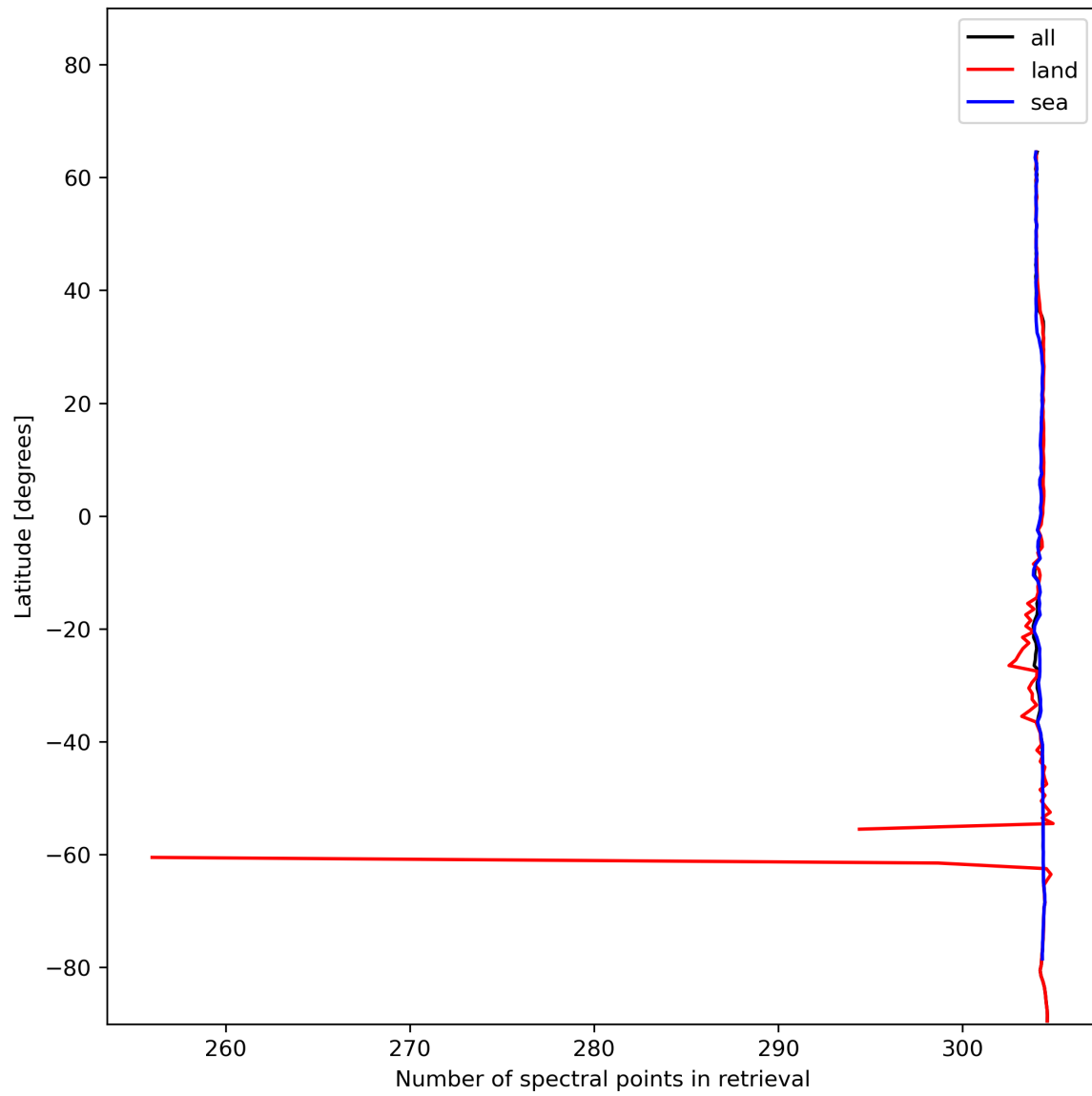
Figure 16: Zonal average of “Number of spectral points in retrieval” for 2023-12-28 to 2023-12-30.
