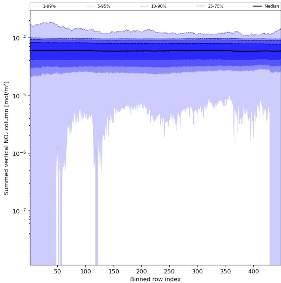
Figure 57: Along track statistics of “Summed vertical NO 2 column” for 2023-12-28 to 2023-12-30
