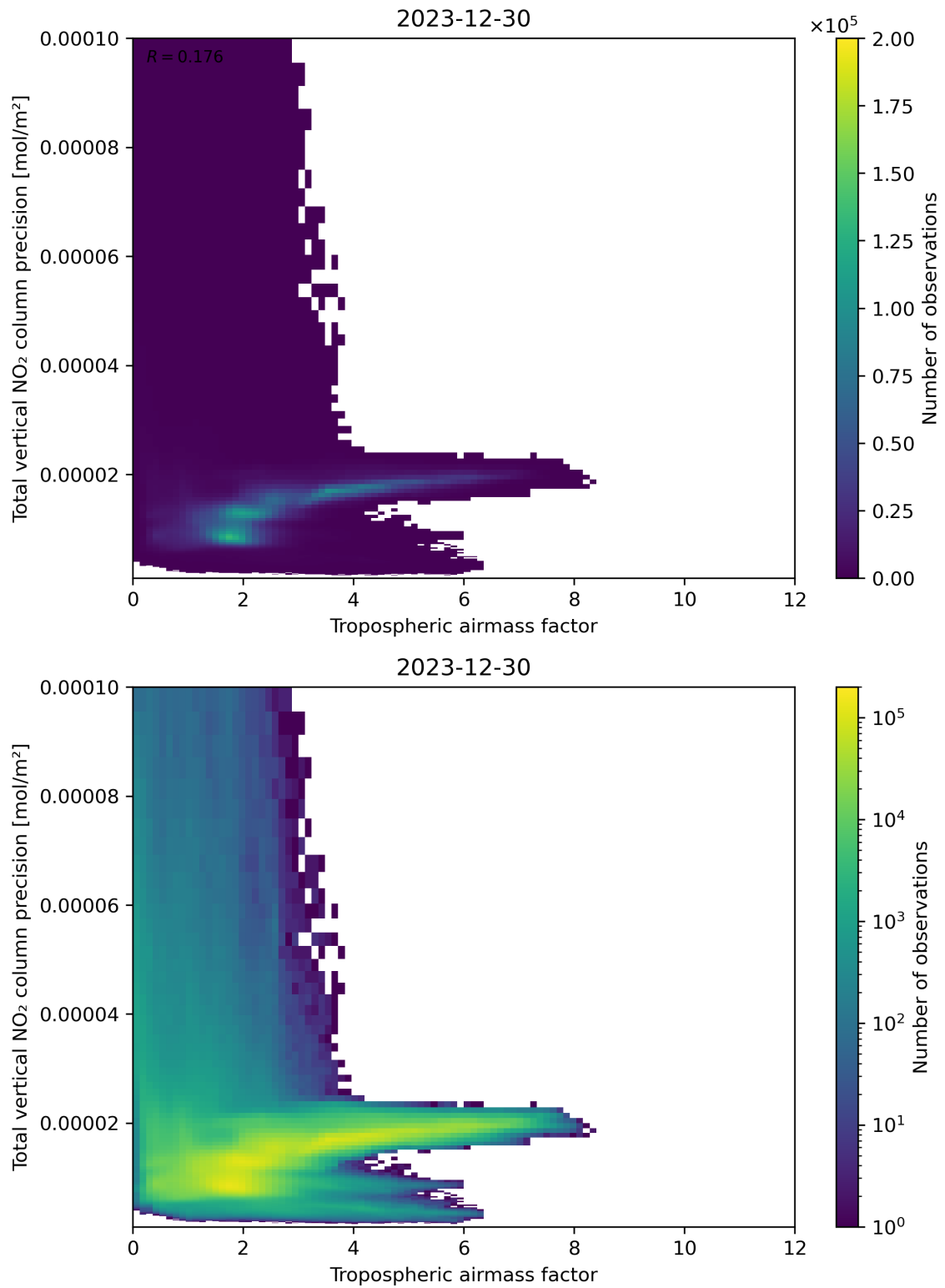
Figure 78: Scatter density plot of “Tropospheric air mass factor” against “Total vertical NO 2 column precision” for 2023-12-30 to 2023-12-31.
