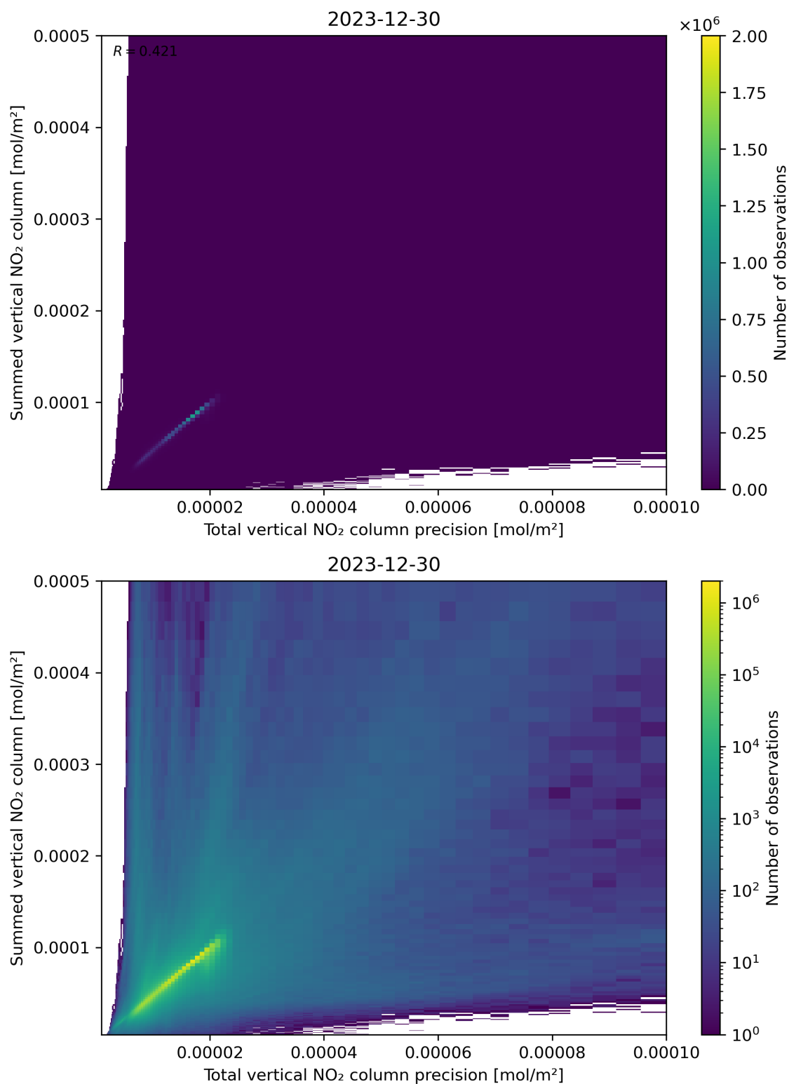
Figure 117: Scatter density plot of “Total vertical NO 2 column precision” against “Summed vertical NO 2 column” for 2023-12-30 to 2023-12-31.
