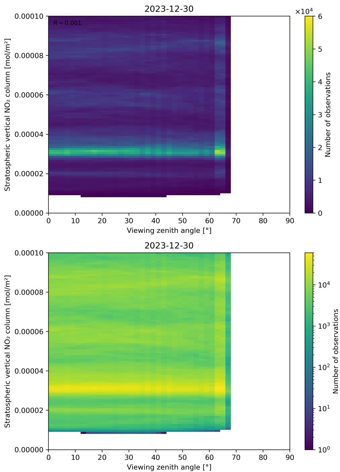
Figure 164: Scatter density plot of “Viewing zenith angle” against “Stratospheric vertical NO 2 column” for 2023-12-30 to 2023-12-31.
