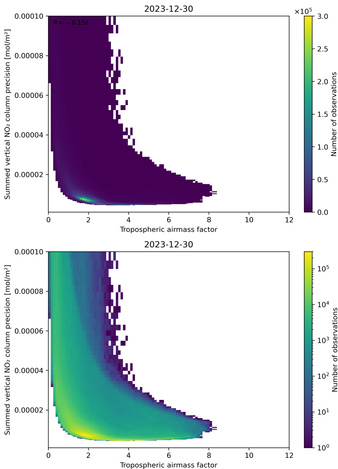
Figure 76: Scatter density plot of “Tropospheric air mass factor” against “Summed vertical NO 2 column precision” for 2023-12-30 to 2023-12-31.
