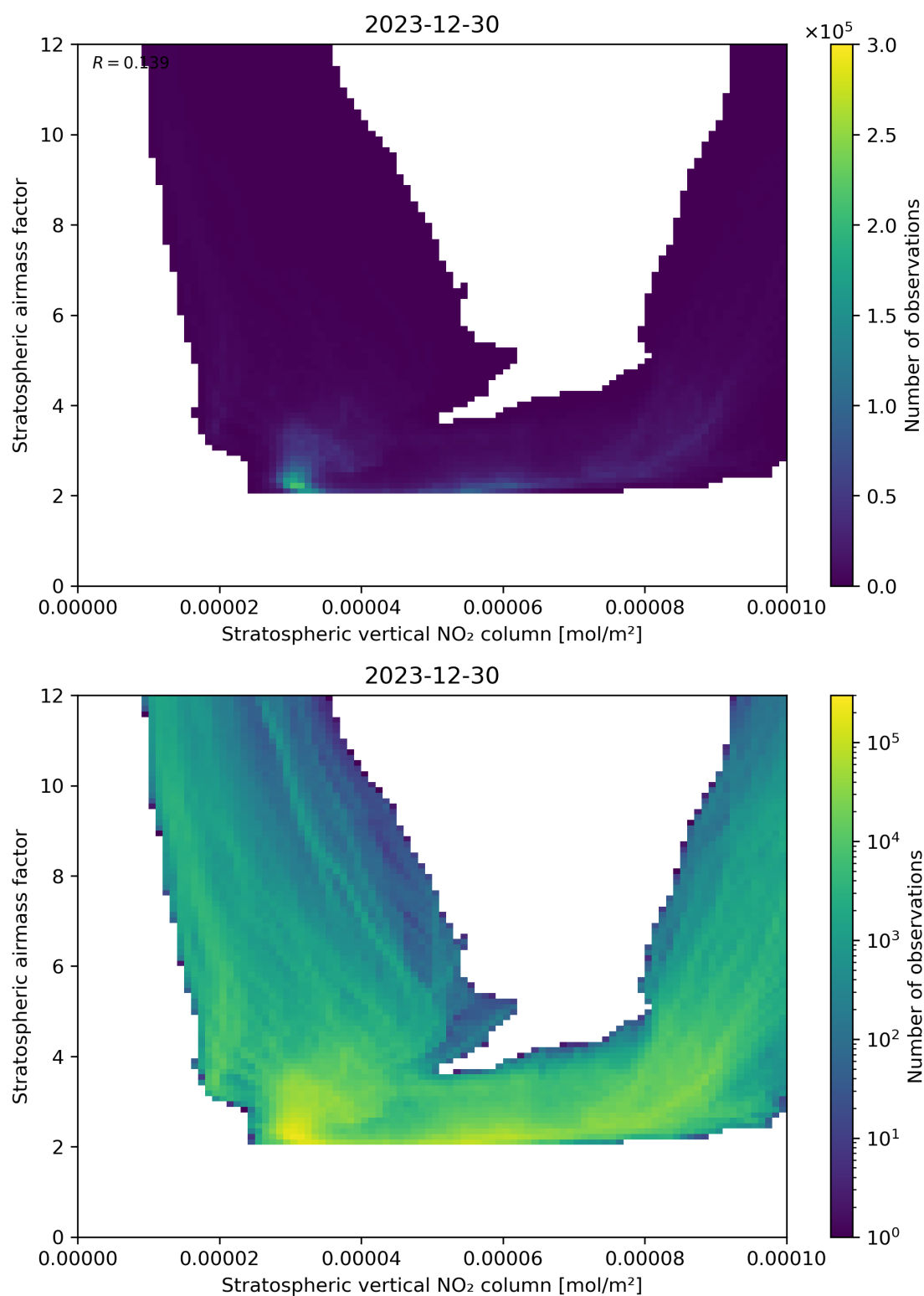
Figure 96: Scatter density plot of “Stratospheric vertical NO 2 column” against “Stratospheric airmass factor” for 2023-12-30 to 2023-12-31.
