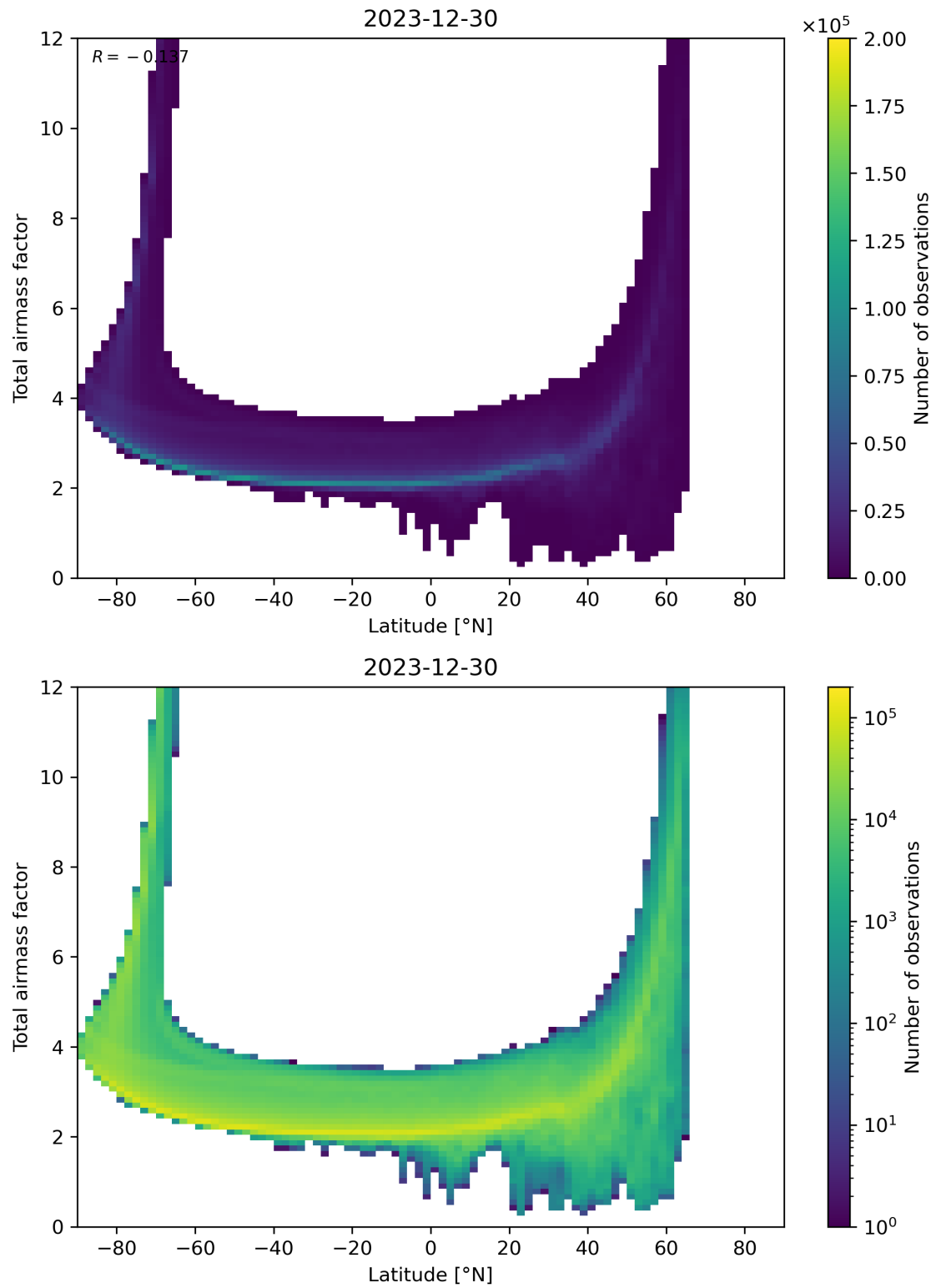
Figure 84: Scatter density plot of “Latitude” against “Total airmass factor” for 2023-12-30 to 2023-12-31.
