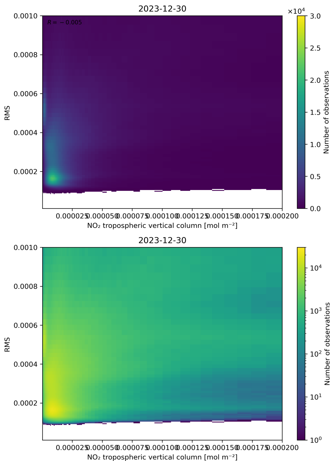
Figure 142: Scatter density plot of “NO 2 tropospheric vertical column” against “RMS” for 2023-12-30 to 2023-12-31.
