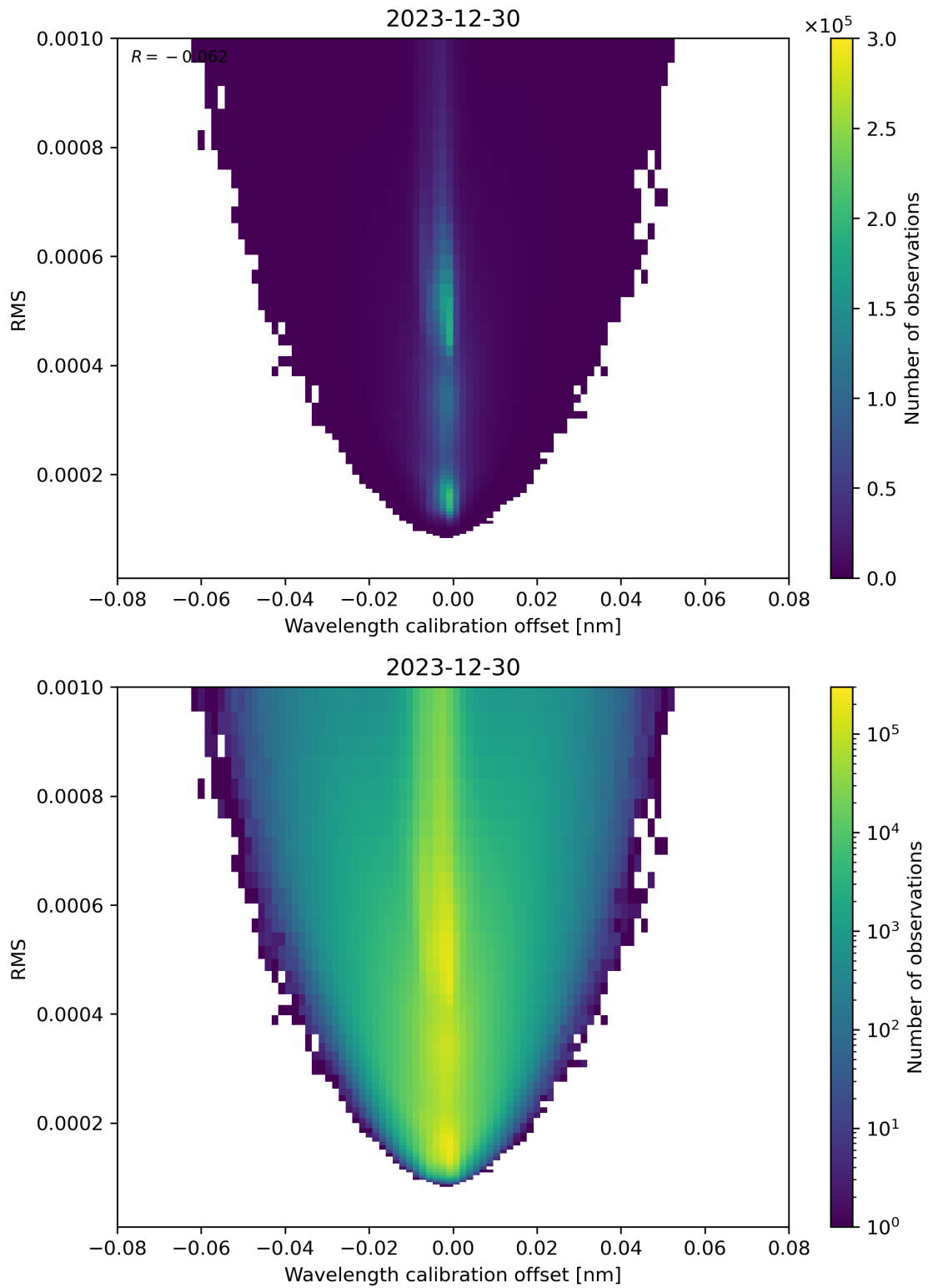
Figure 181: Scatter density plot of “Wavelength calibration offset” against “RMS” for 2023-12-30 to 2023-12-31.
