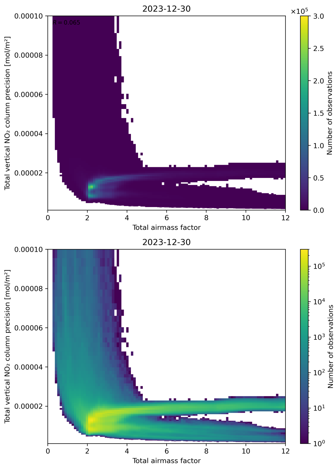
Figure 68: Scatter density plot of “Total airmass factor” against “Total vertical NO 2 column precision” for 2023-12-30 to 2023-12-31.
