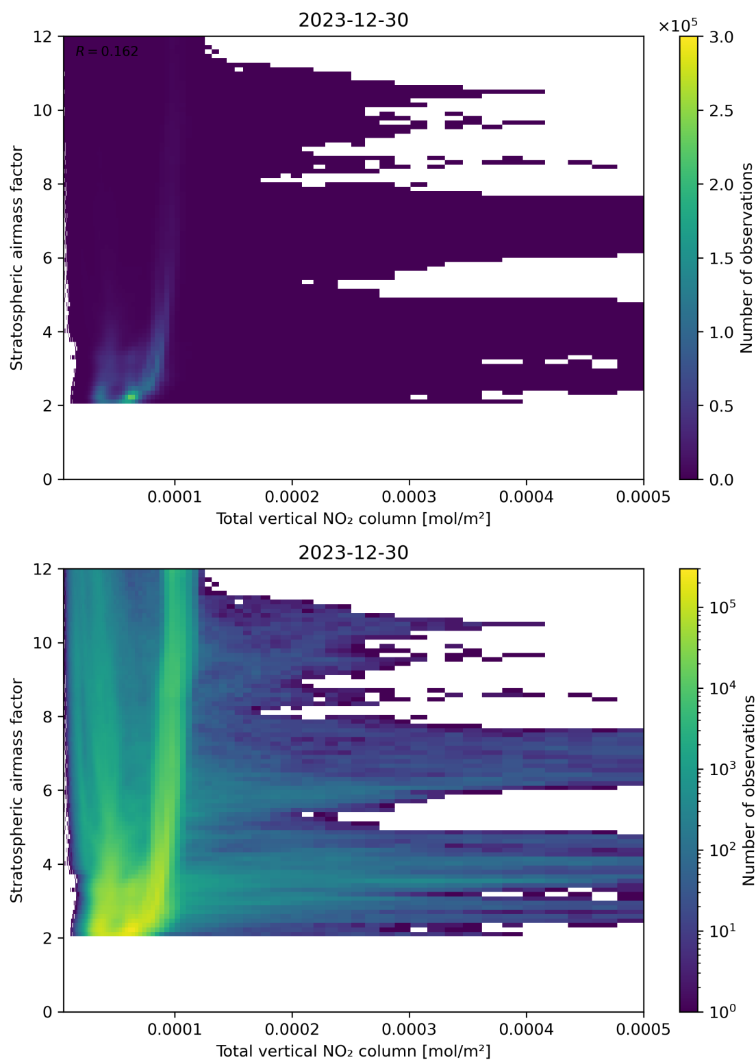
Figure 110: Scatter density plot of “Total vertical NO 2 column” against “Stratospheric airmass factor” for 2023-12-30 to 2023-12-31.
