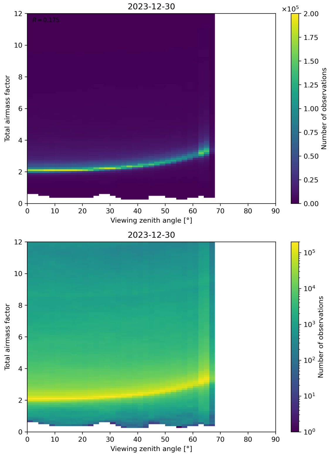
Figure 160: Scatter density plot of “Viewing zenith angle” against “Total airmass factor” for 2023-12-30 to 2023-12-31.
