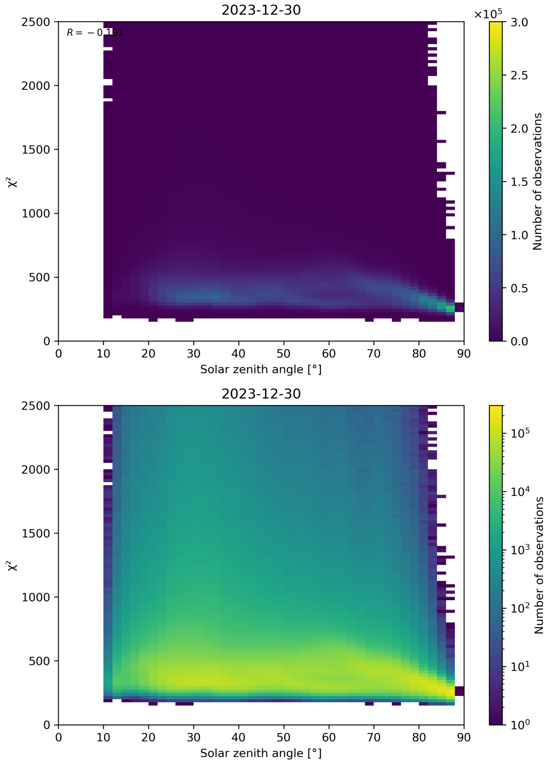
Figure 148: Scatter density plot of “Solar zenith angle” against “ \chi^2 ” for 2023-12-30 to 2023-12-31.
