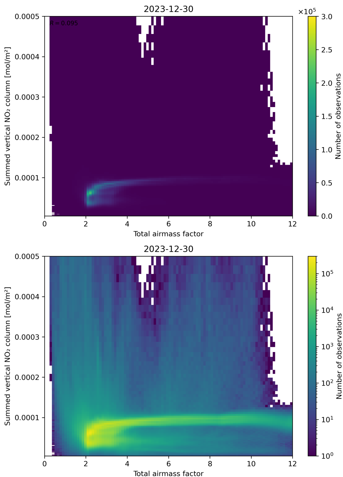
Figure 65: Scatter density plot of “Total airmass factor” against “Summed vertical NO 2 column” for 2023-12-30 to 2023-12-31.
