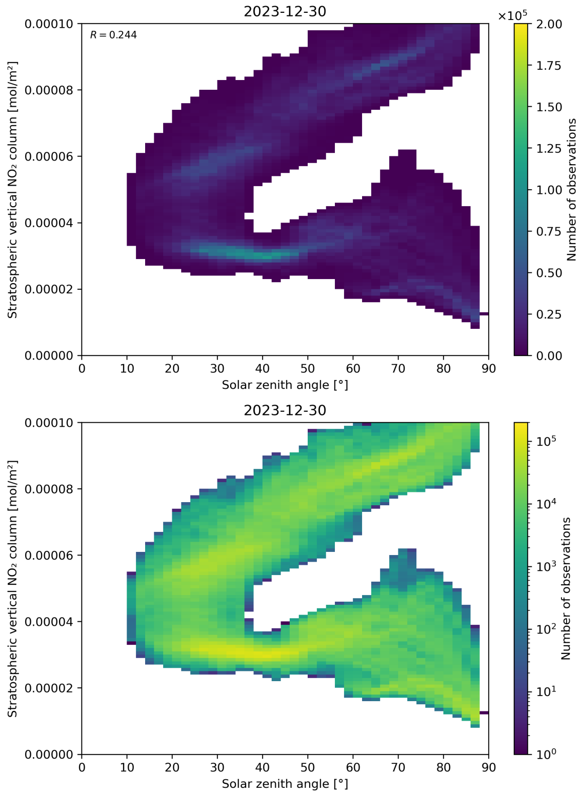
Figure 150: Scatter density plot of “Solar zenith angle” against “Stratospheric vertical NO 2 column” for 2023-12-30 to 2023-12-31.
