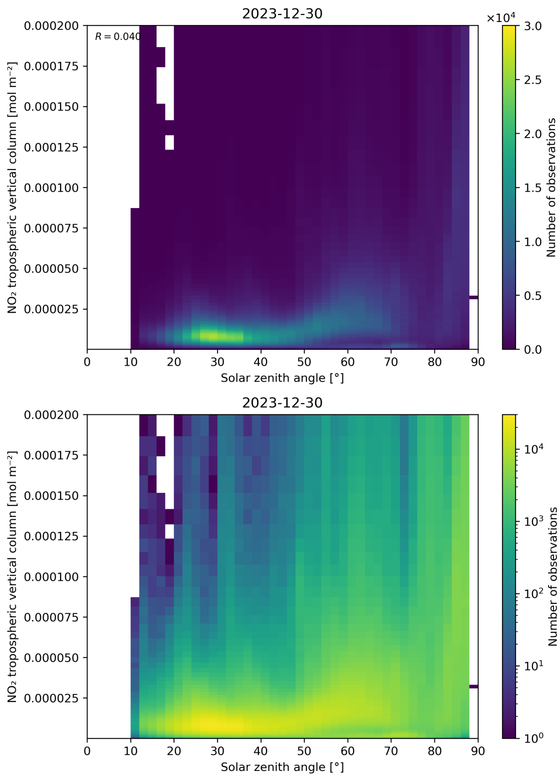
Figure 155: Scatter density plot of “Solar zenith angle” against “NO 2 tropospheric vertical column” for 2023-12-30 to 2023-12-31.
