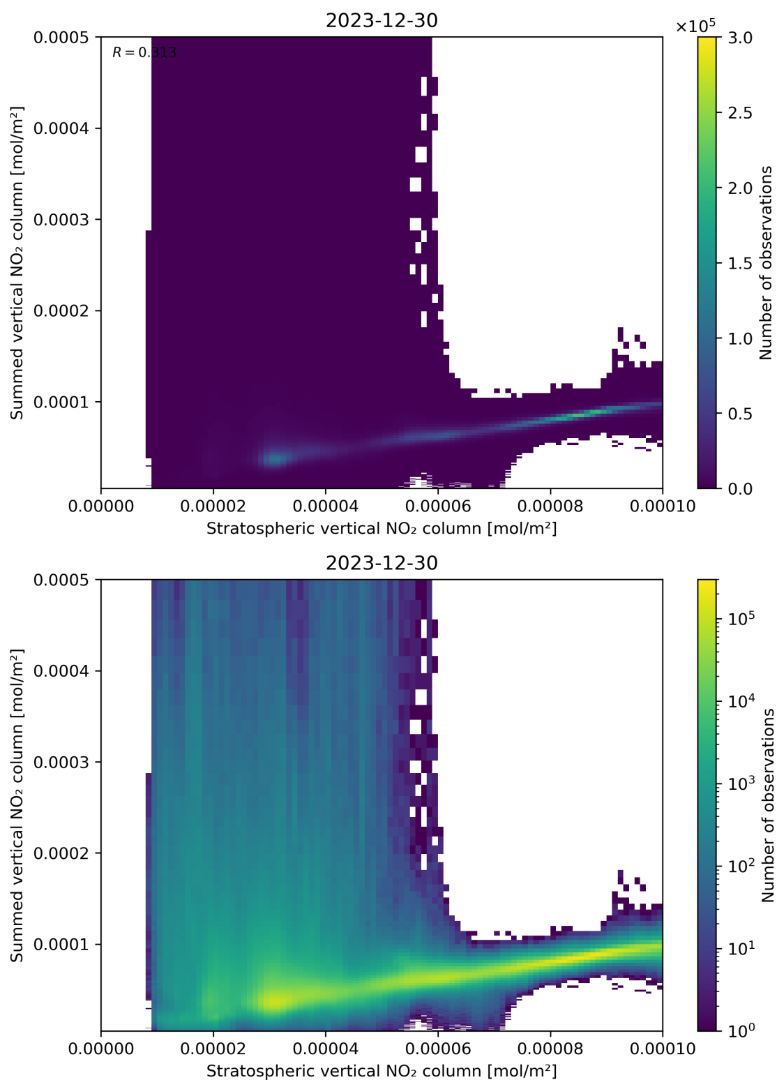
Figure 98: Scatter density plot of “Stratospheric vertical NO 2 column” against “Summed vertical NO 2 column” for 2023-12-30 to 2023-12-31.
