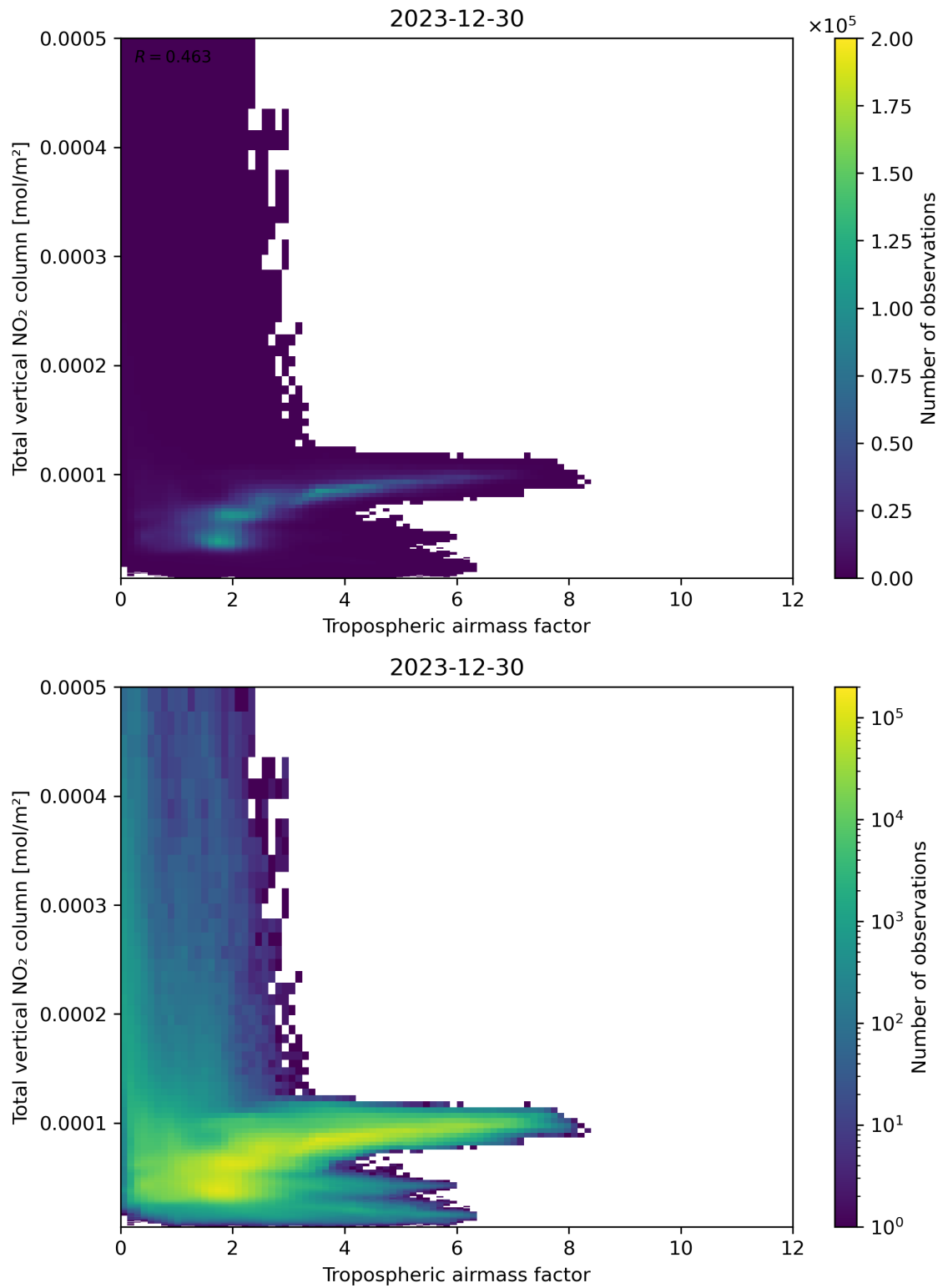
Figure 77: Scatter density plot of “Tropospheric airmass factor” against “Total vertical \text{NO}_2 column” for 2023-12-30 to 2023-12-31.
