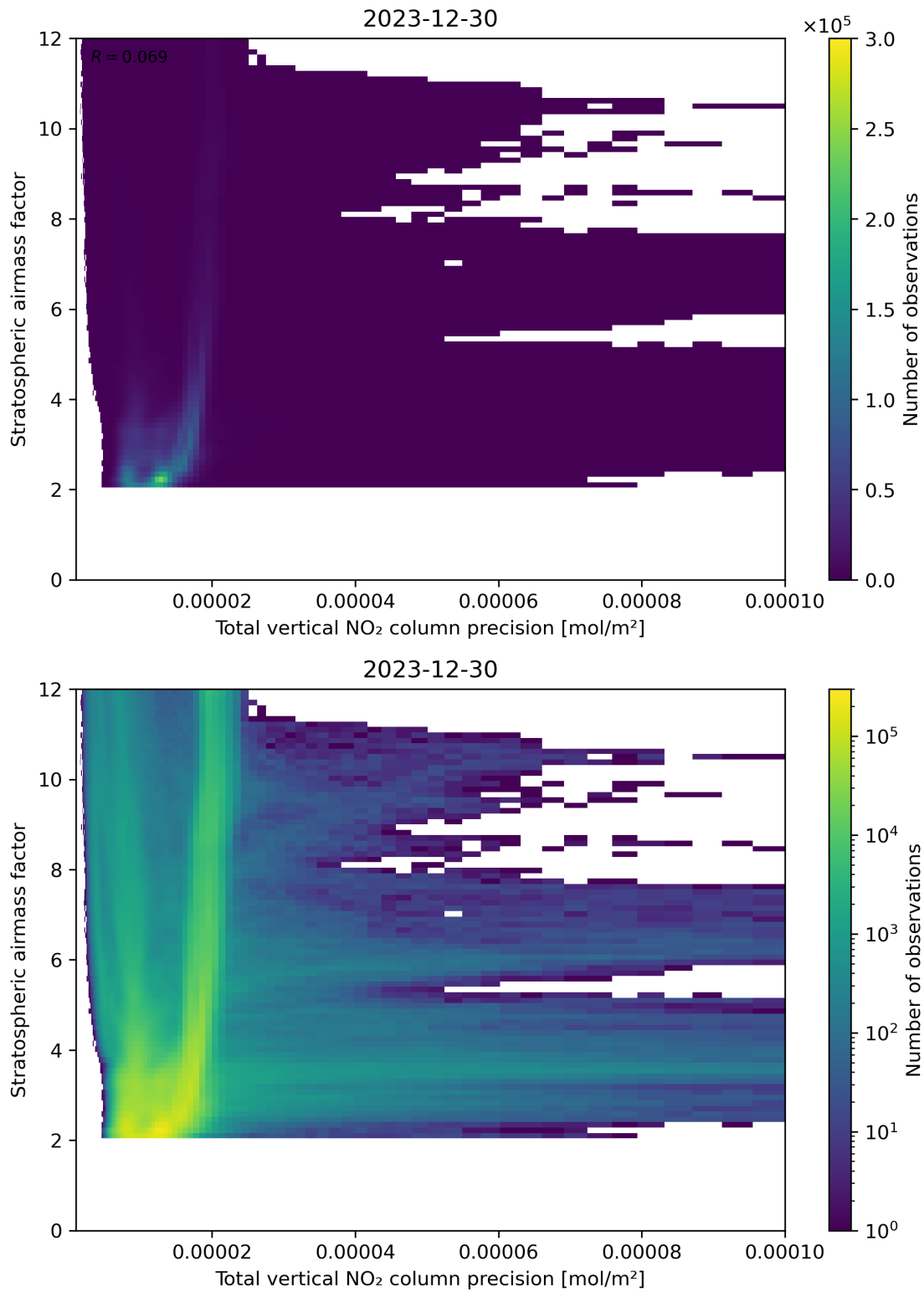
Figure 115: Scatter density plot of “Total vertical NO 2 column precision” against “Stratospheric air mass factor” for 2023-12-30 to 2023-12-31.
