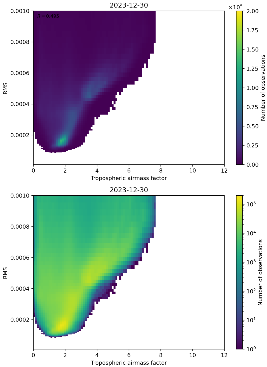
Figure 79: Scatter density plot of “Tropospheric airmass factor” against “RMS” for 2023-12-30 to 2023-12-31.
