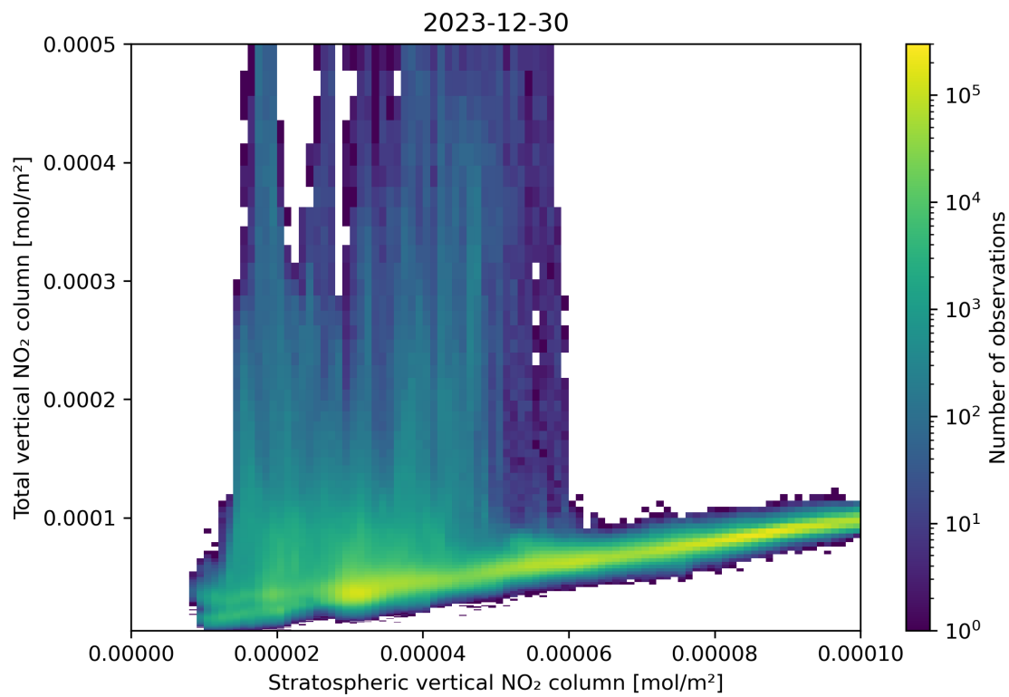
Figure 100: Scatter density plot of “Stratospheric vertical NO 2 column” against “Total vertical NO 2 column” for 2023-12-30 to 2023-12-31.
