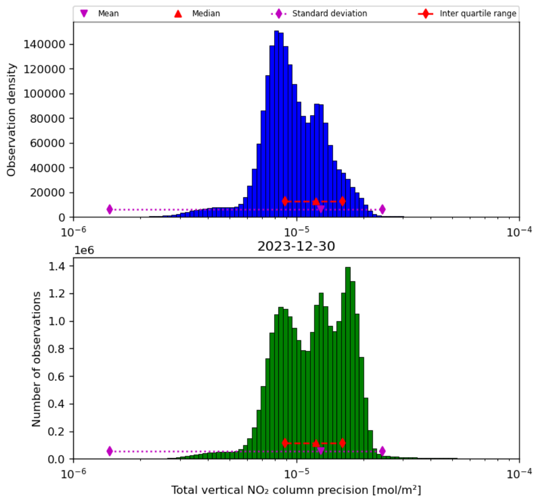
Figure 39: Histogram of “Total vertical NO 2 column precision” for 2023-12-30 to 2023-12-31
