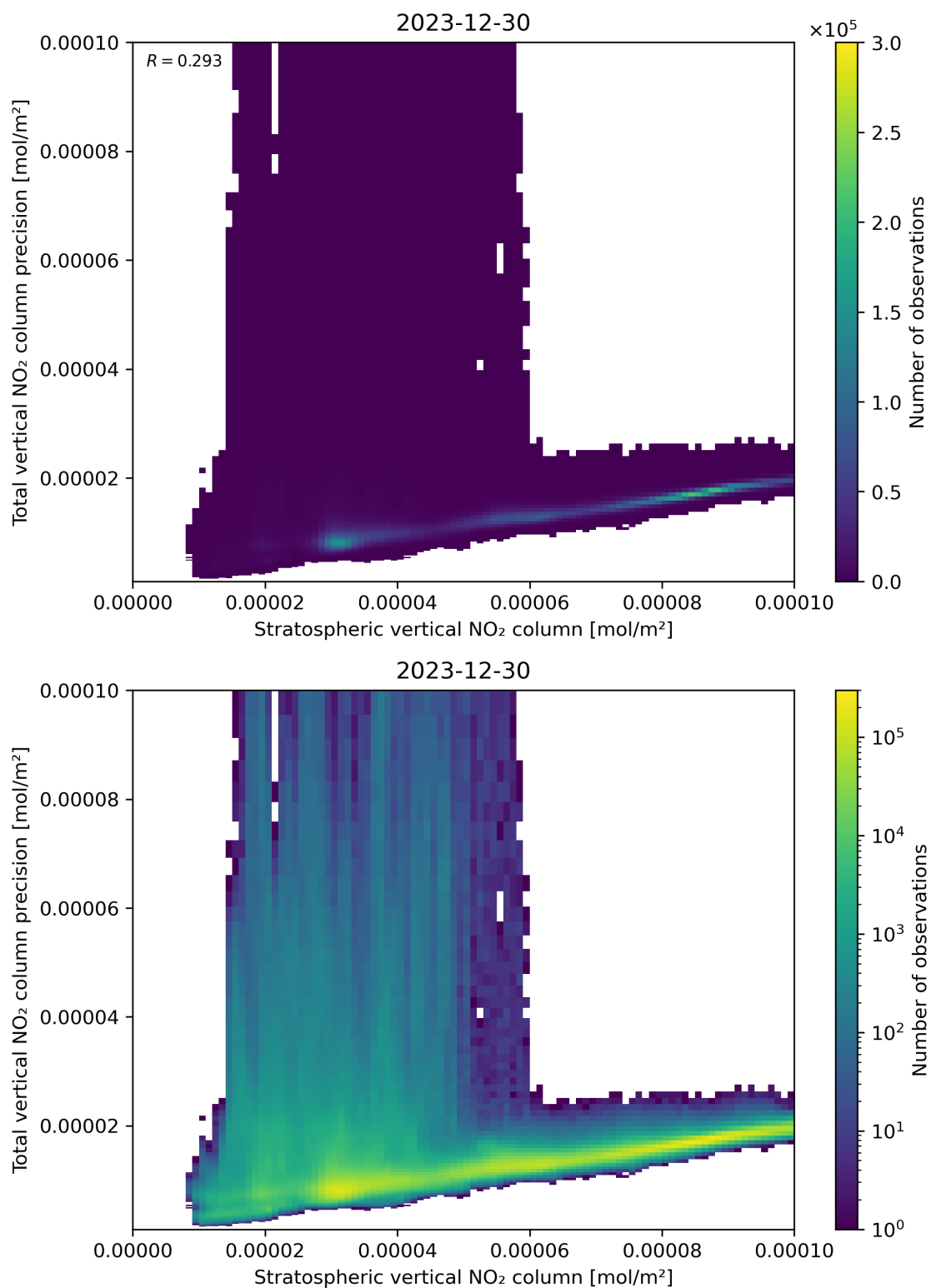
Figure 101: Scatter density plot of “Stratospheric vertical NO 2 column” against “Total vertical NO 2 column precision” for 2023-12-30 to 2023-12-31.
