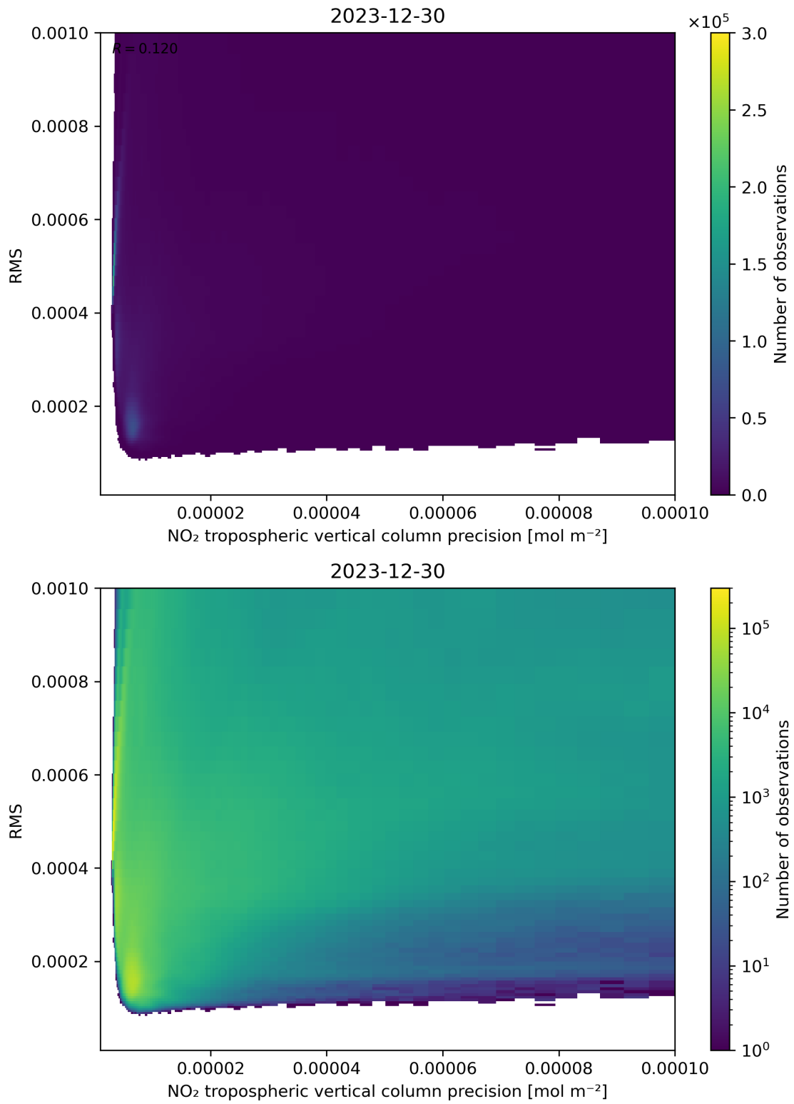
Figure 140: Scatter density plot of “NO 2 tropospheric vertical column precision” against “RMS” for 2023-12-30 to 2023-12-31.
