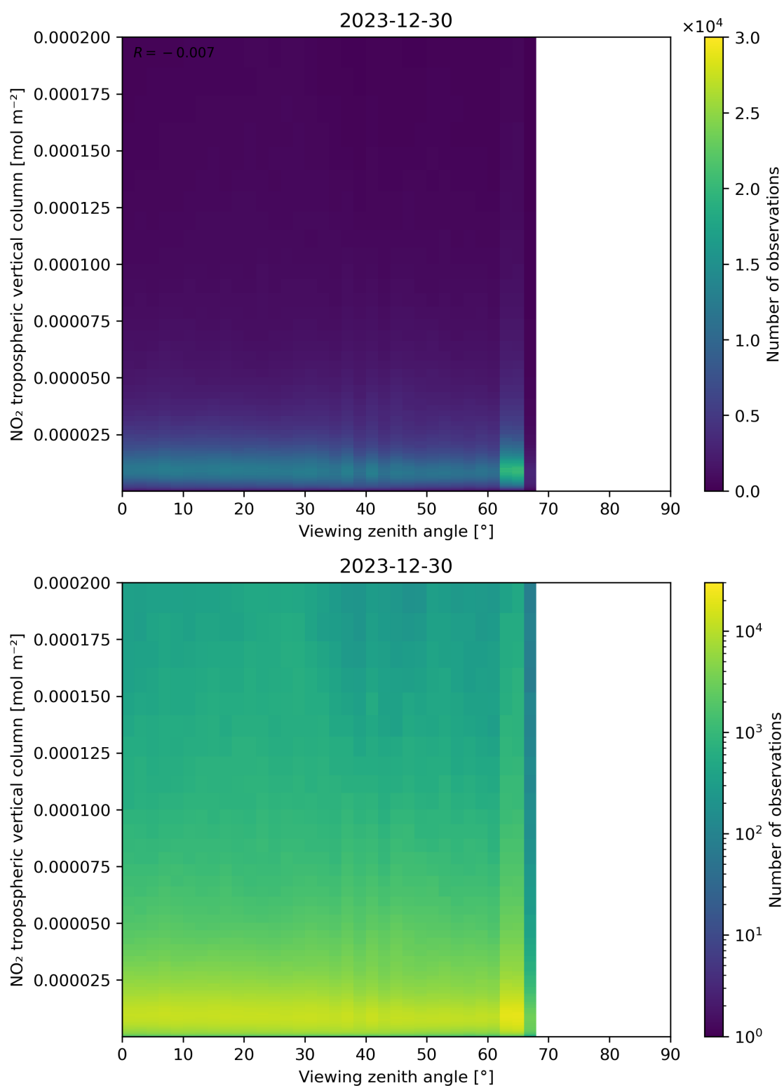
Figure 169: Scatter density plot of “Viewing zenith angle” against “NO 2 tropospheric vertical column” for 2023-12-30 to 2023-12-31.
