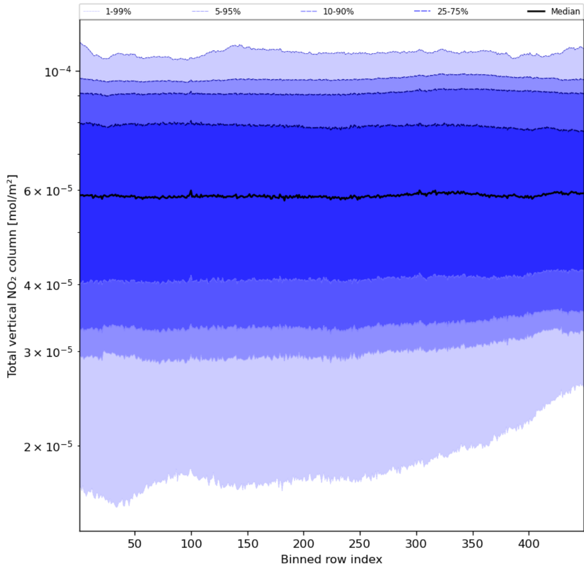
Figure 55: Along track statistics of “Total vertical NO 2 column” for 2023-12-30 to 2023-12-31
