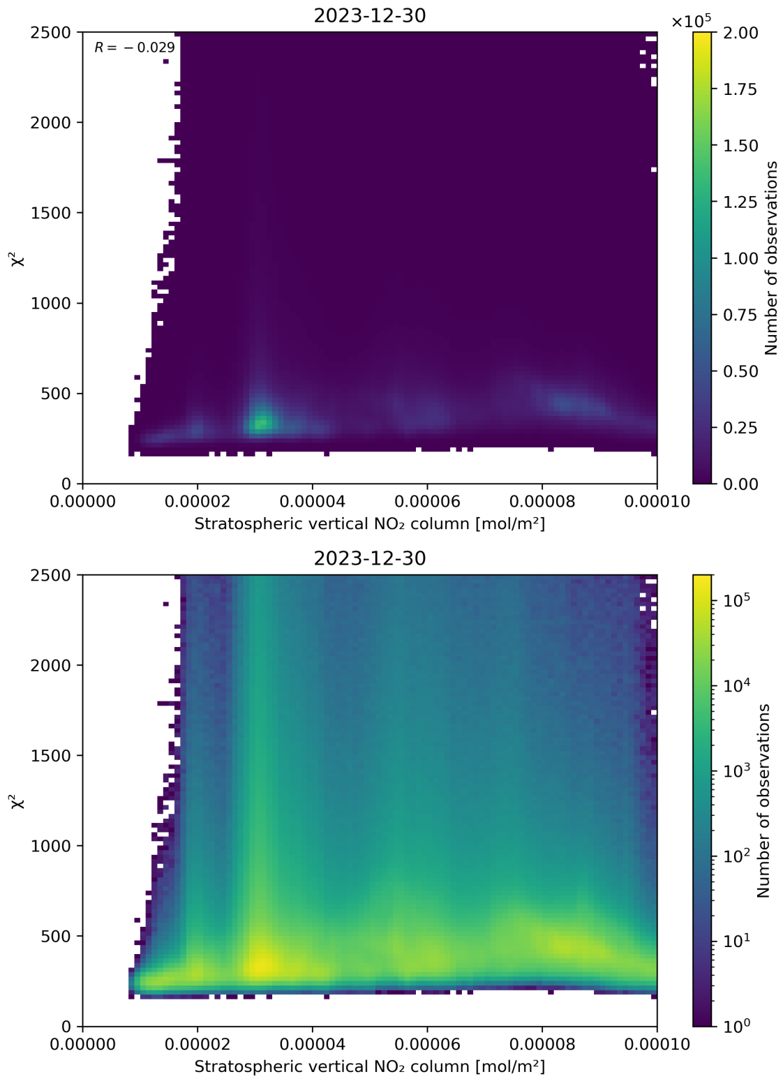
Figure 97: Scatter density plot of “Stratospheric vertical NO 2 column” against “ \chi^2 ” for 2023-12-30 to 2023-12-31.
