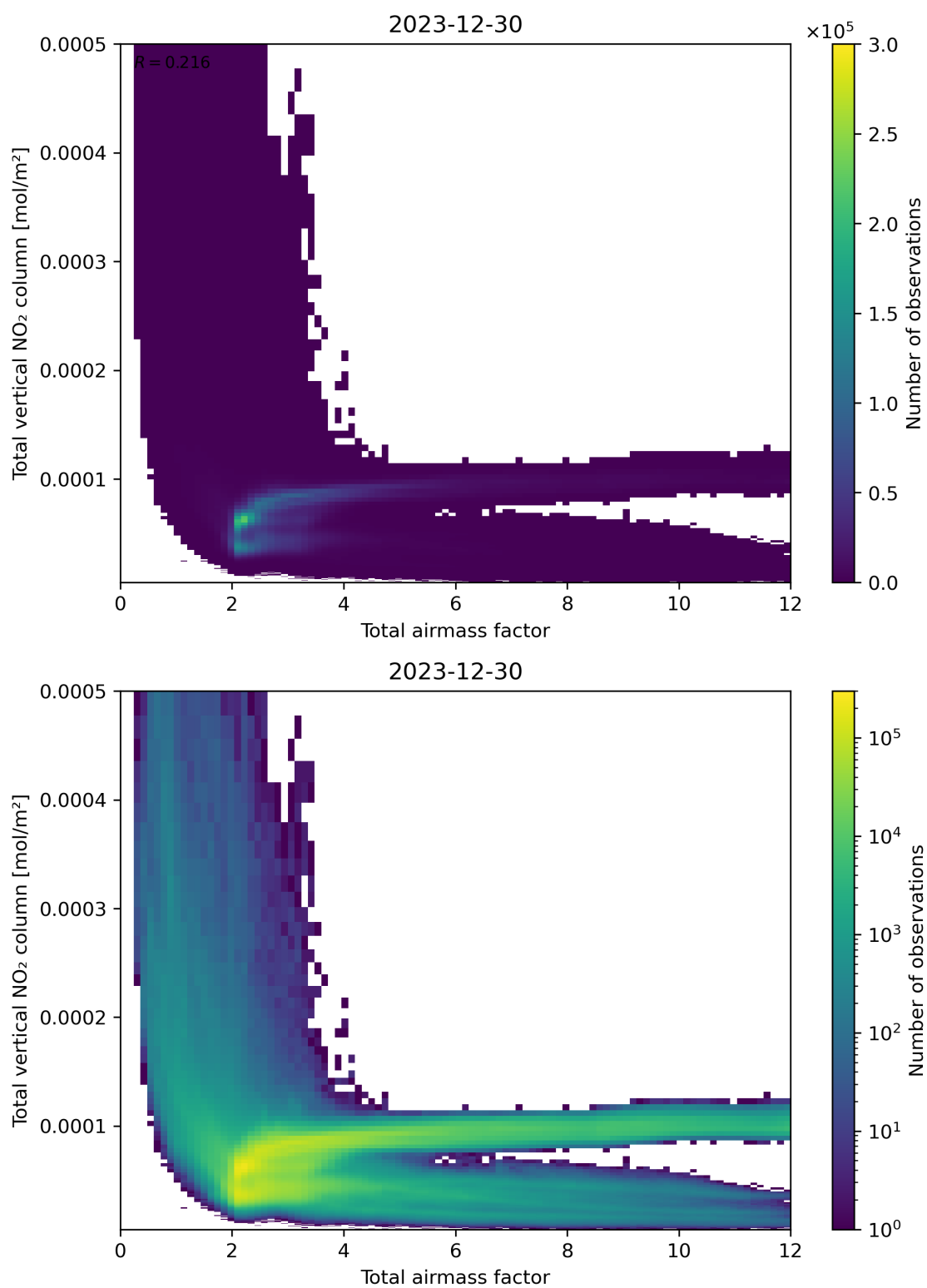
Figure 67: Scatter density plot of “Total airmass factor” against “Total vertical NO 2 column” for 2023-12-30 to 2023-12-31.
