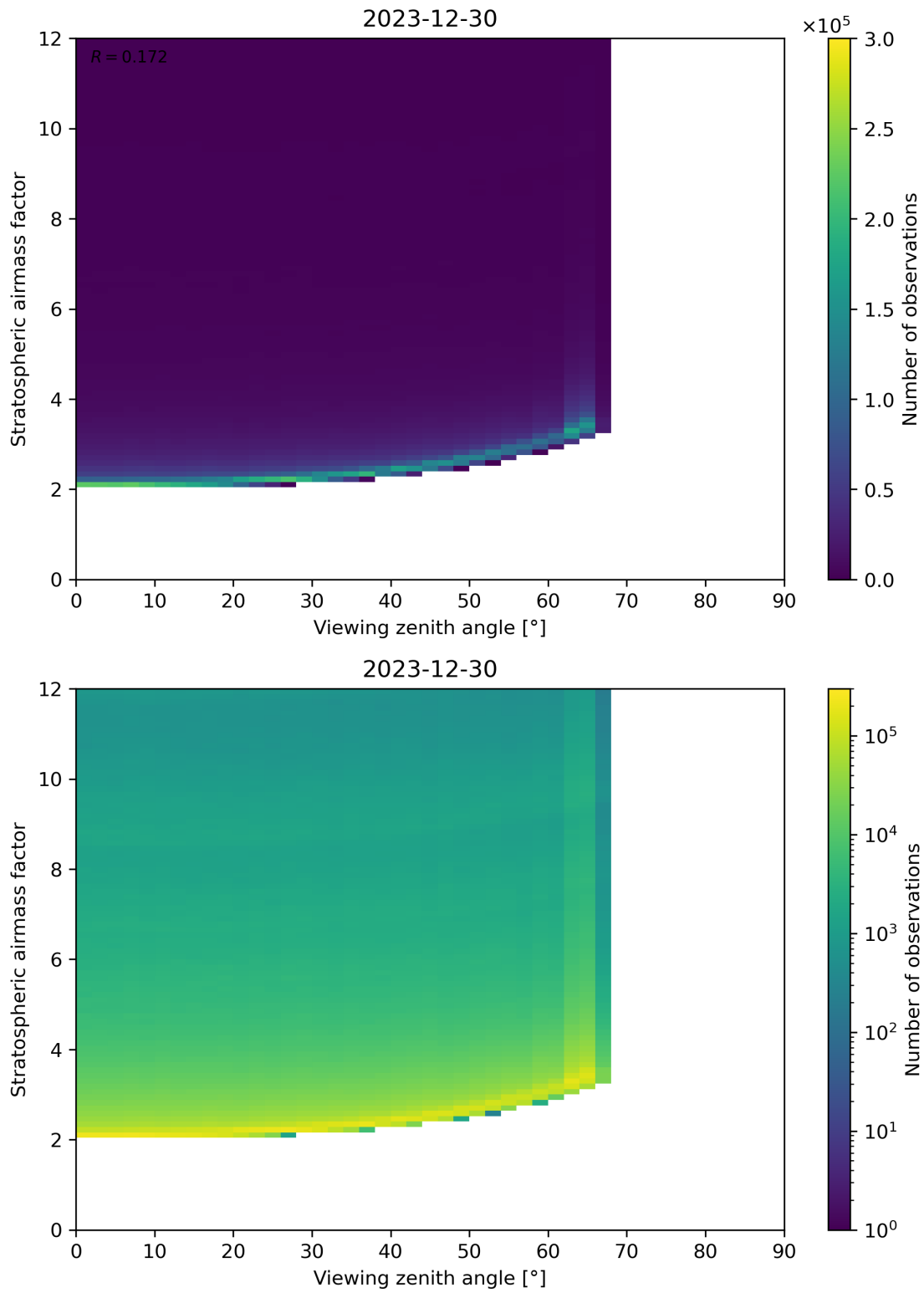
Figure 159: Scatter density plot of “Viewing zenith angle” against “Stratospheric airmass factor” for 2023-12-30 to 2023-12-31.
