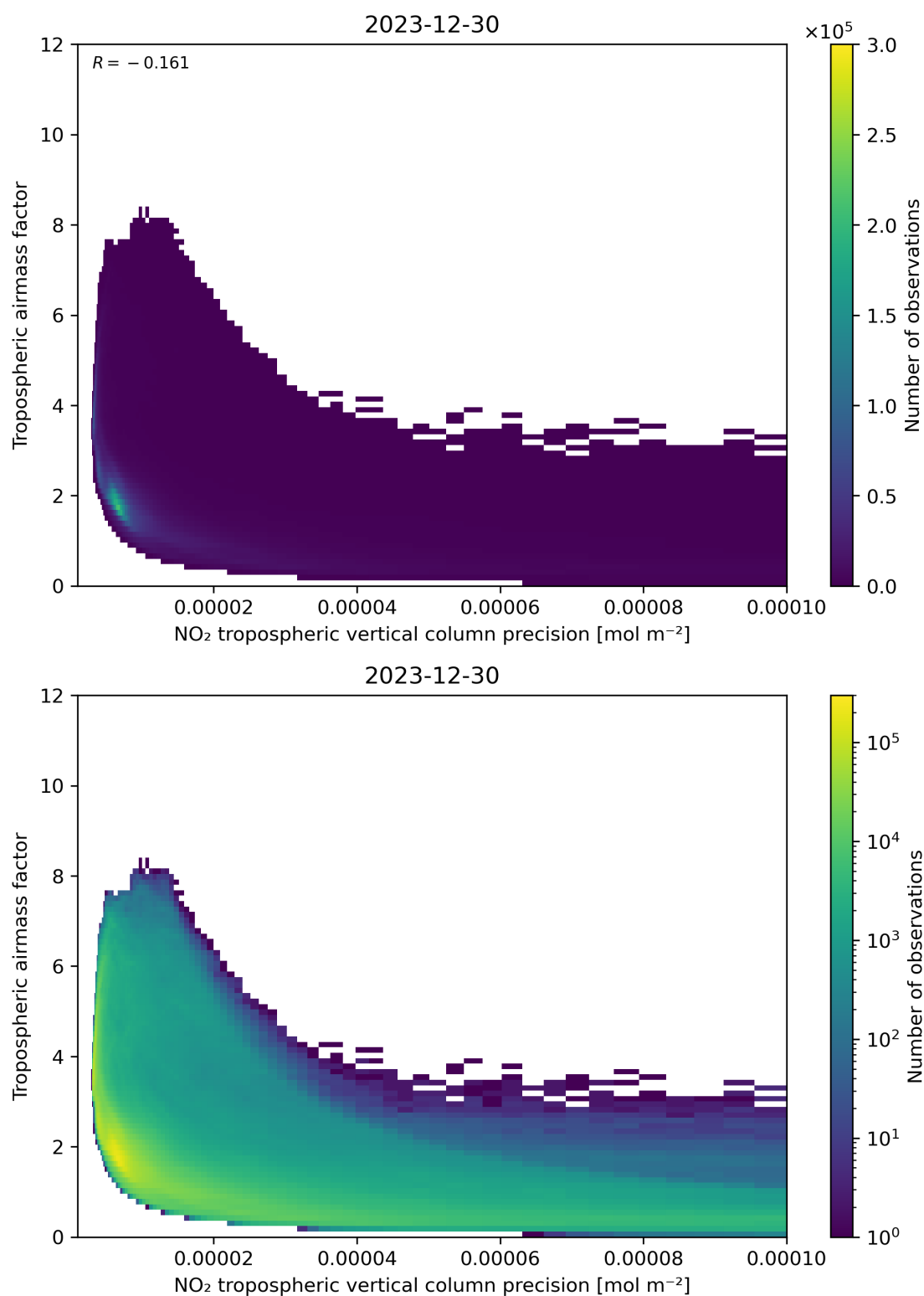
Figure 133: Scatter density plot of “NO 2 tropospheric vertical column precision” against “Tropospheric air mass factor” for 2023-12-30 to 2023-12-31.
