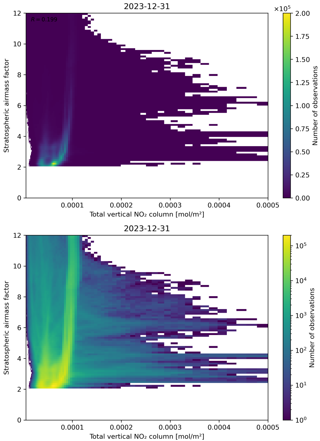
Figure 110: Scatter density plot of “Total vertical NO 2 column” against “Stratospheric air mass factor” for 2023-12-30 to 2023-12-31.
