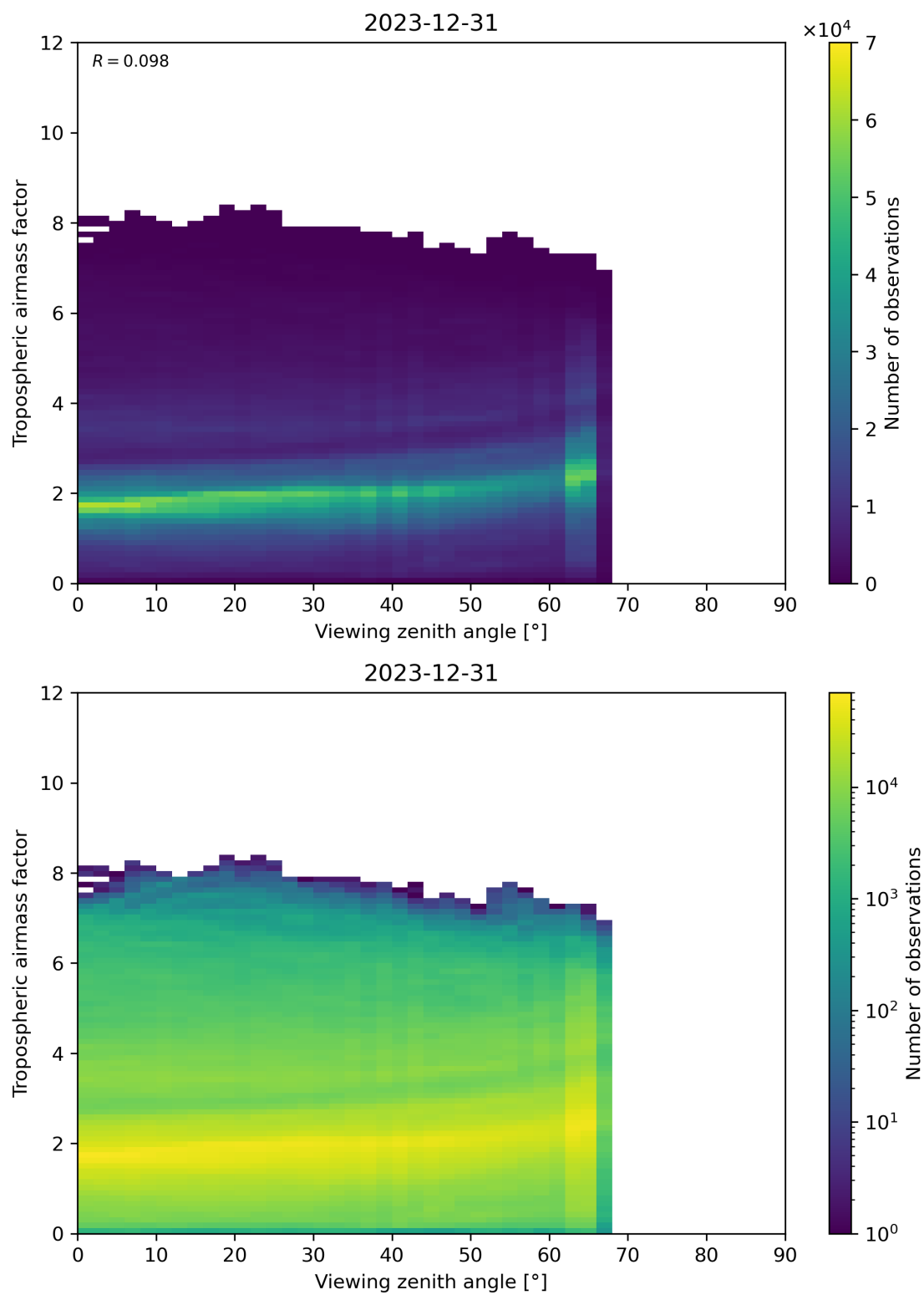
Figure 161: Scatter density plot of “Viewing zenith angle” against “Tropospheric airmass factor” for 2023-12-30 to 2023-12-31.
