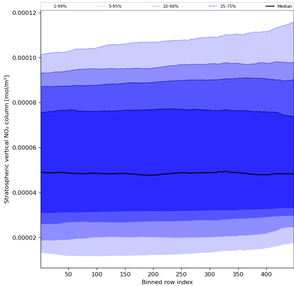
Figure 53: Along track statistics of “Stratospheric vertical NO 2 column” for 2023-12-30 to 2023-12-31
