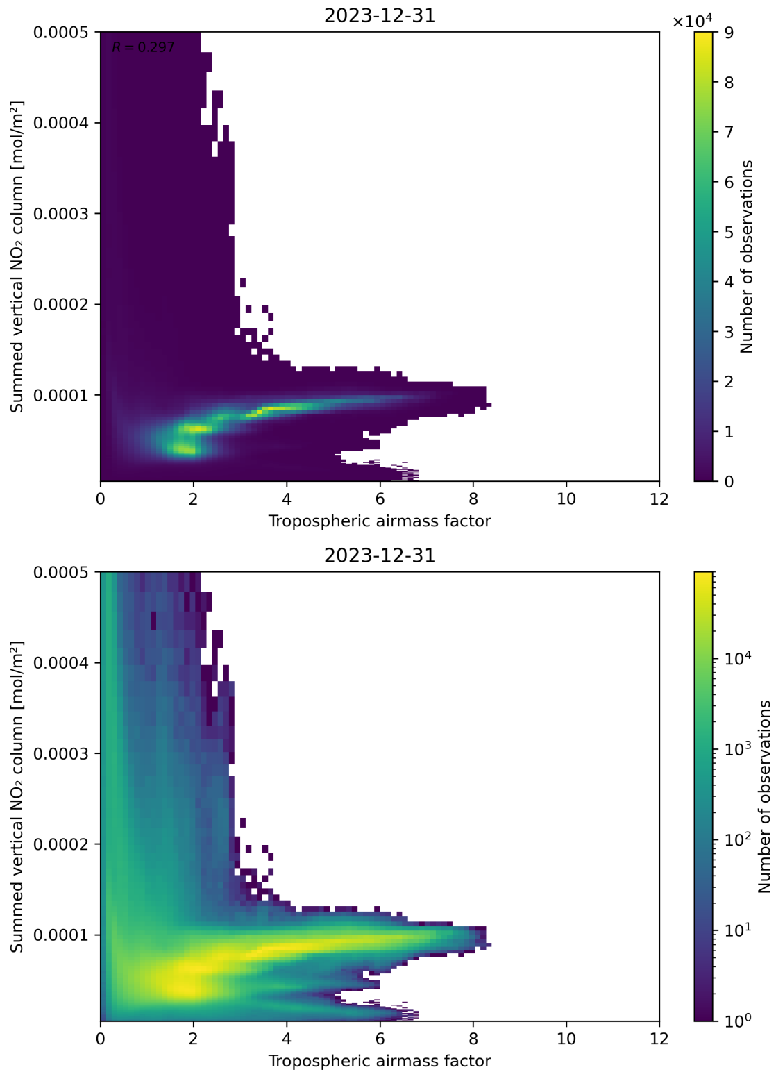
Figure 75: Scatter density plot of “Tropospheric airmass factor” against “Summed vertical NO 2 column” for 2023-12-30 to 2023-12-31.
