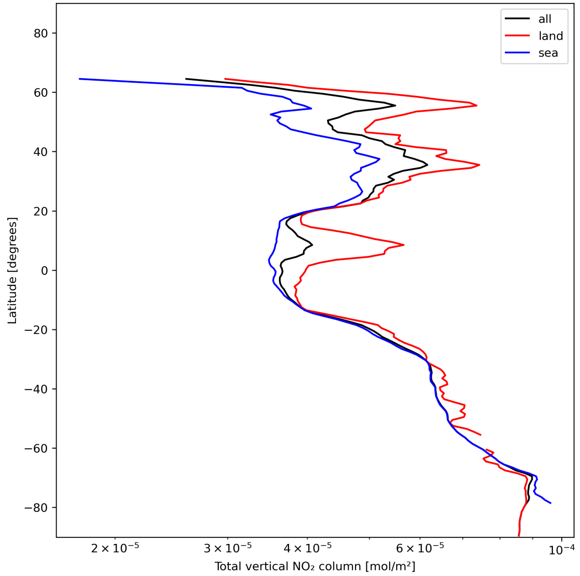
Figure 21: Zonal average of “Total vertical NO 2 column” for 2023-12-30 to 2023-12-31.
