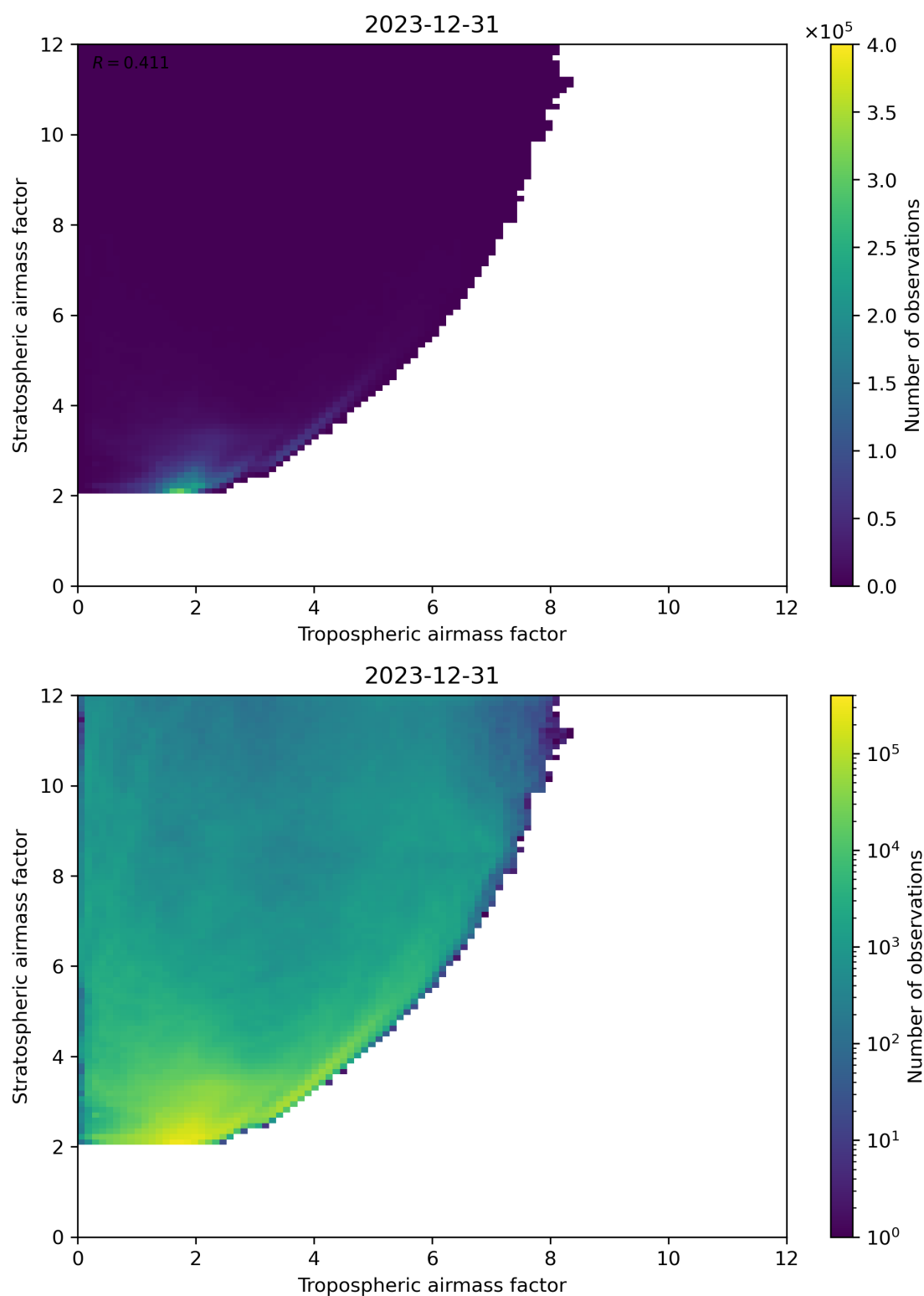
Figure 71: Scatter density plot of “Tropospheric airmass factor” against “Stratospheric airmass factor” for 2023-12-30 to 2023-12-31.
