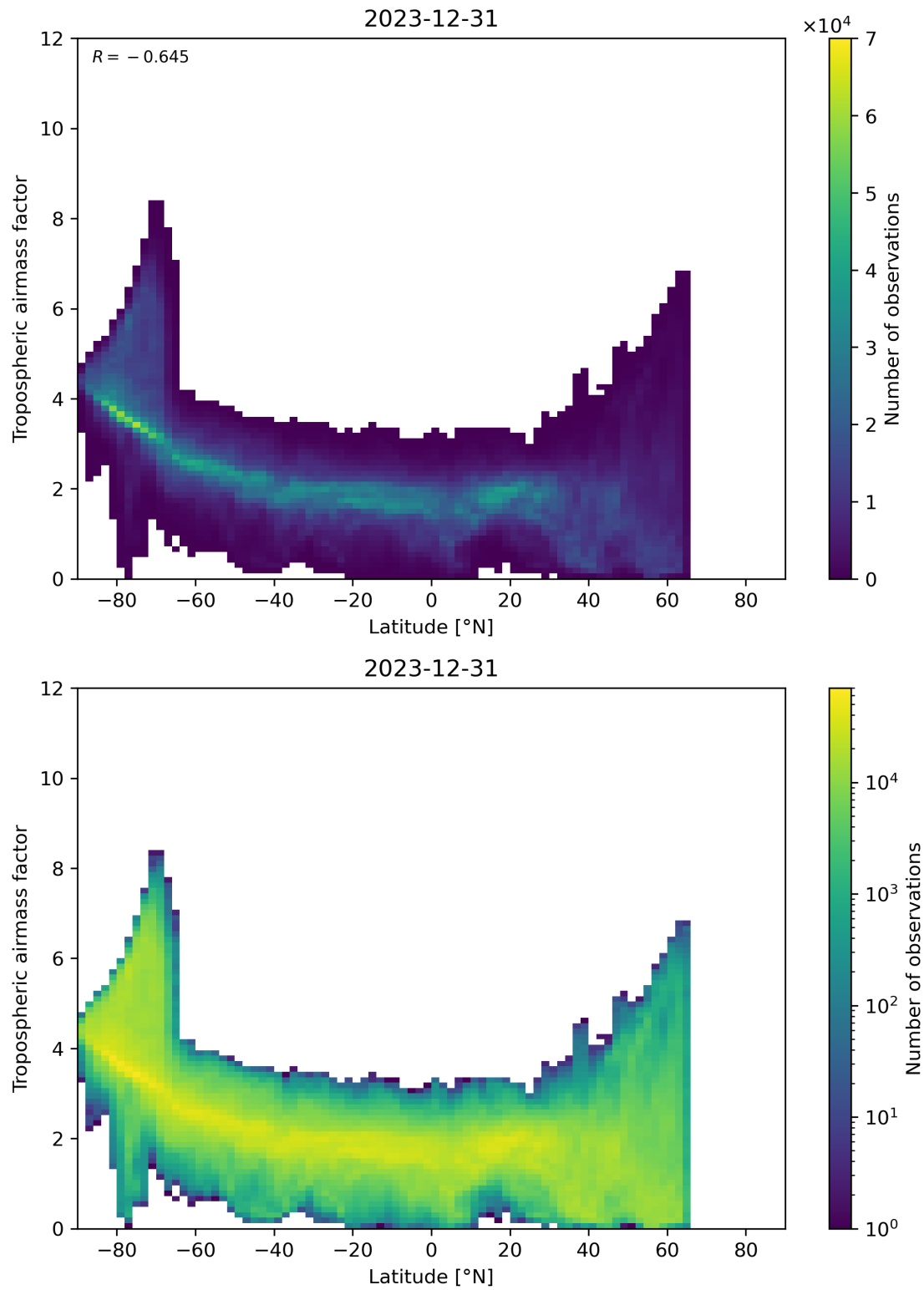
Figure 85: Scatter density plot of “Latitude” against “Tropospheric air mass factor” for 2023-12-30 to 2023-12-31.
