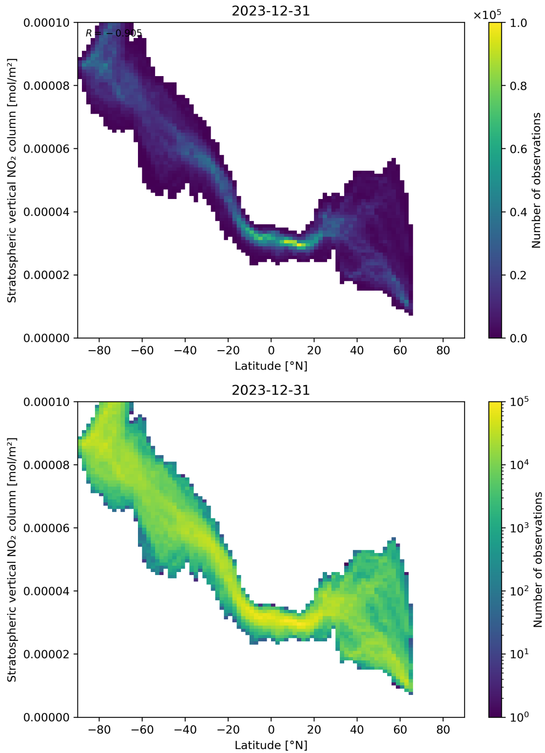
Figure 87: Scatter density plot of “Latitude” against “Stratospheric vertical NO 2 column” for 2023-12-30 to 2023-12-31.
