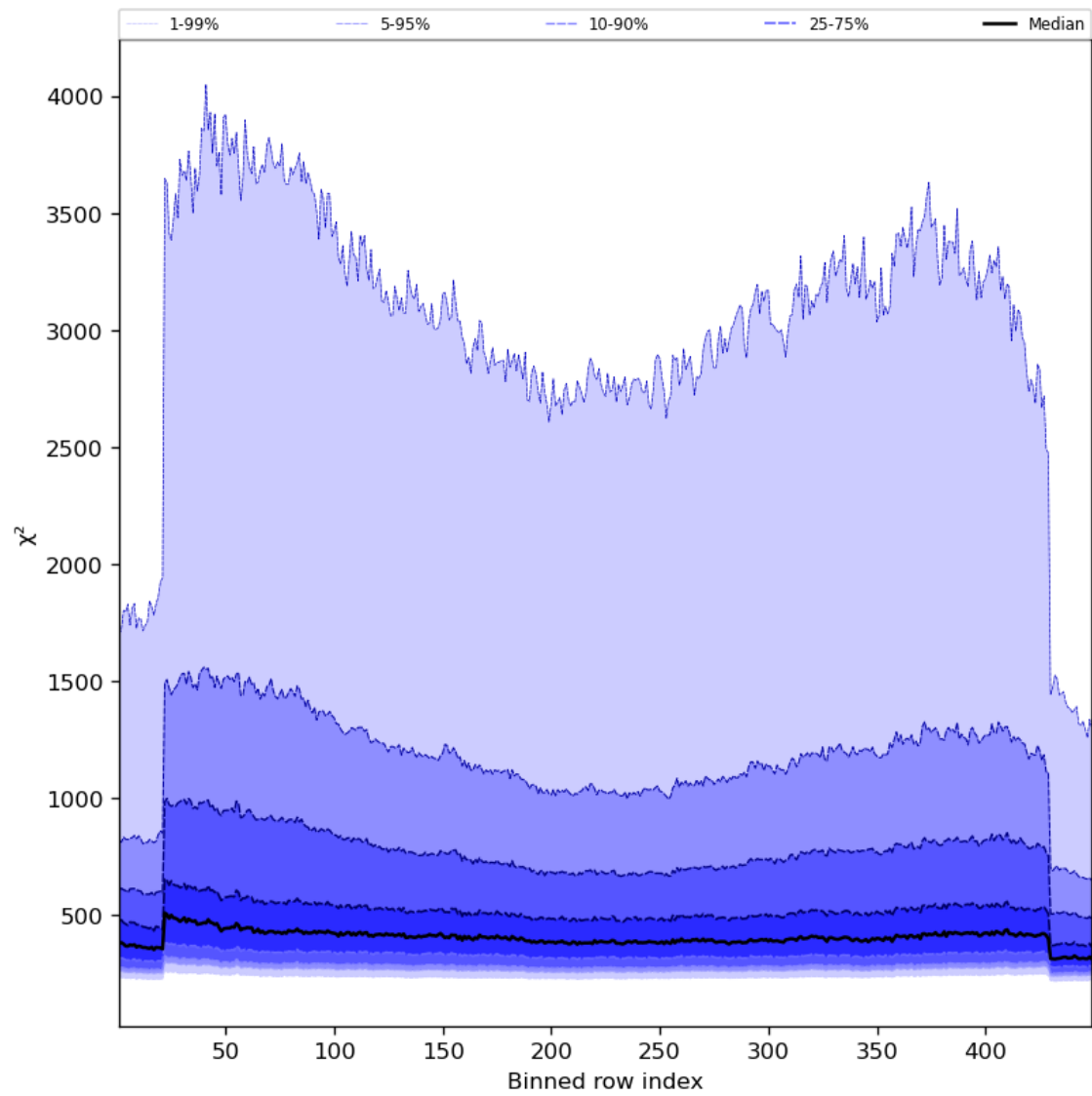
Figure 59: Along track statistics of “ \chi^2 ” for 2023-12-30 to 2023-12-31
