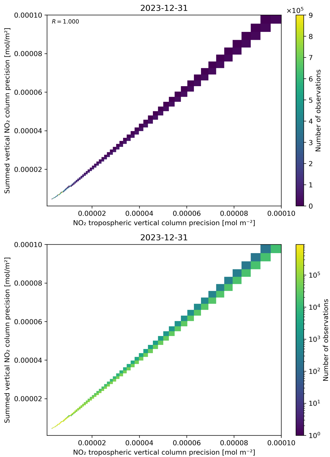
Figure 137: Scatter density plot of “NO 2 tropospheric vertical column precision” against “Summed vertical NO 2 column precision” for 2023-12-30 to 2023-12-31.
