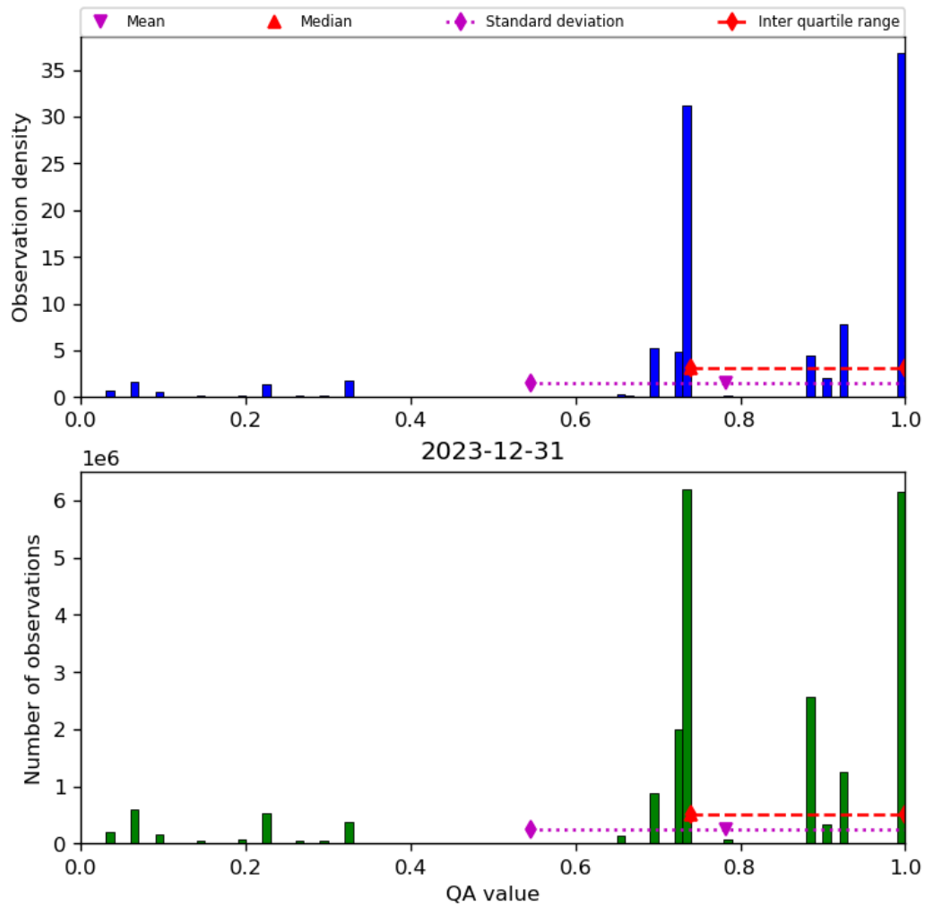
Figure 28: Histogram of “QA value” for 2023-12-30 to 2023-12-31
