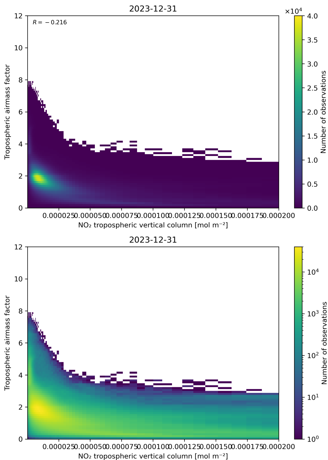
Figure 123: Scatter density plot of “NO 2 tropospheric vertical column” against “Tropospheric air mass factor” for 2023-12-30 to 2023-12-31.
