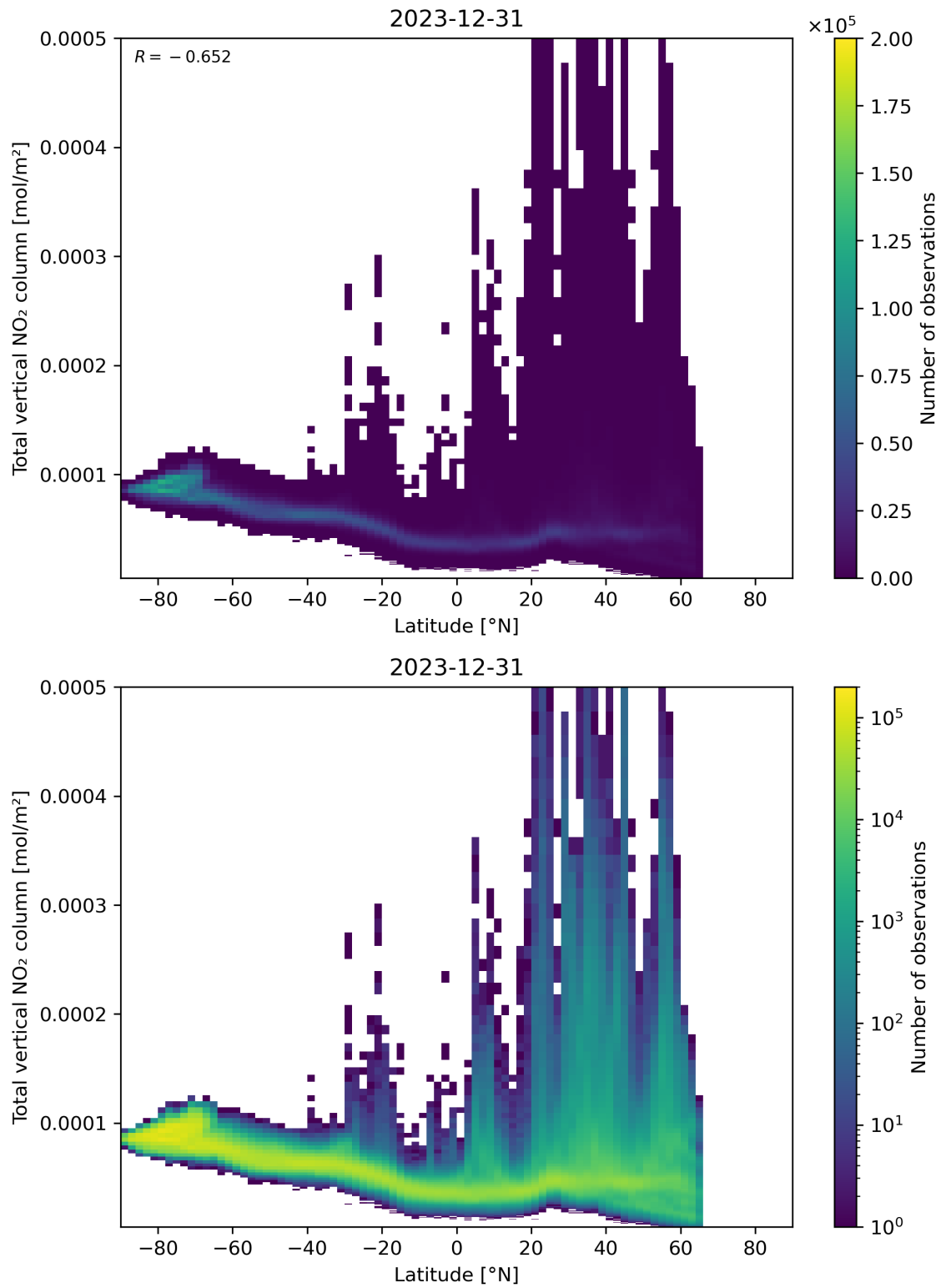
Figure 90: Scatter density plot of “Latitude” against “Total vertical NO 2 column” for 2023-12-30 to 2023-12-31.
