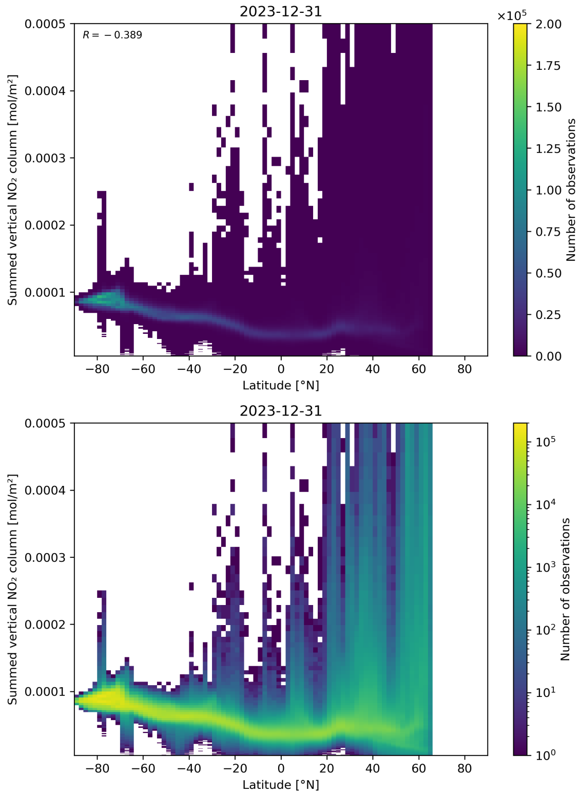
Figure 88: Scatter density plot of “Latitude” against “Summed vertical NO 2 column” for 2023-12-30 to 2023-12-31.
