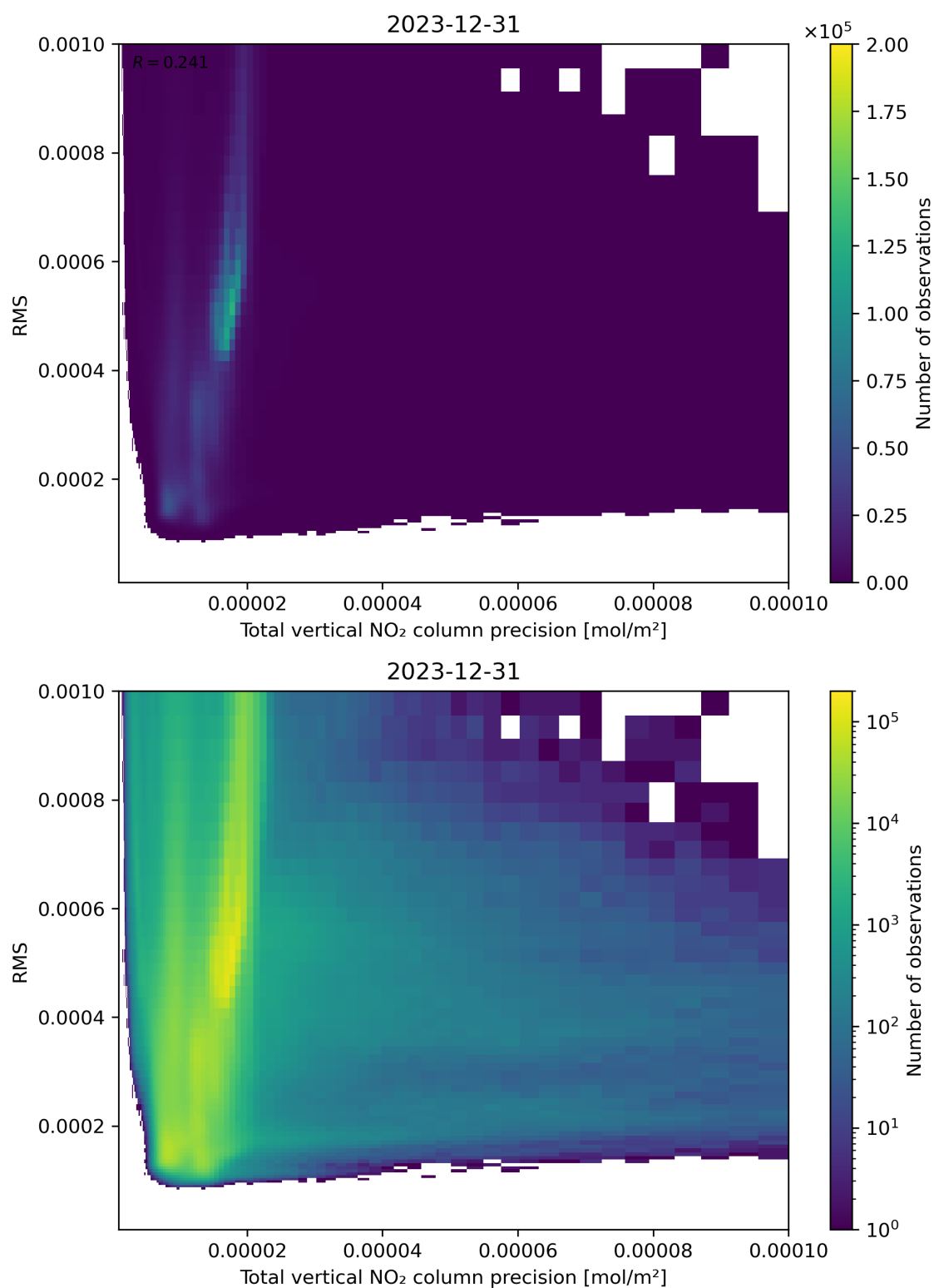
Figure 119: Scatter density plot of “Total vertical NO 2 column precision” against “RMS” for 2023-12-30 to 2023-12-31.
