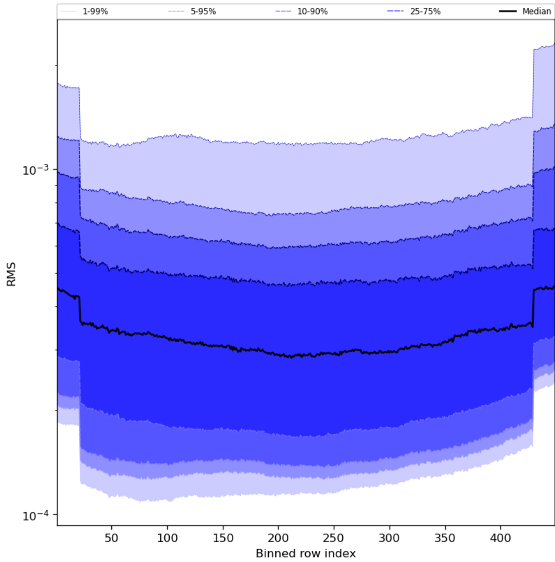
Figure 60: Along track statistics of “RMS” for 2023-12-30 to 2023-12-31
