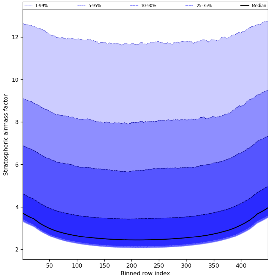
Figure 61: Along track statistics of “Stratospheric airmass factor” for 2023-12-30 to 2023-12-31
