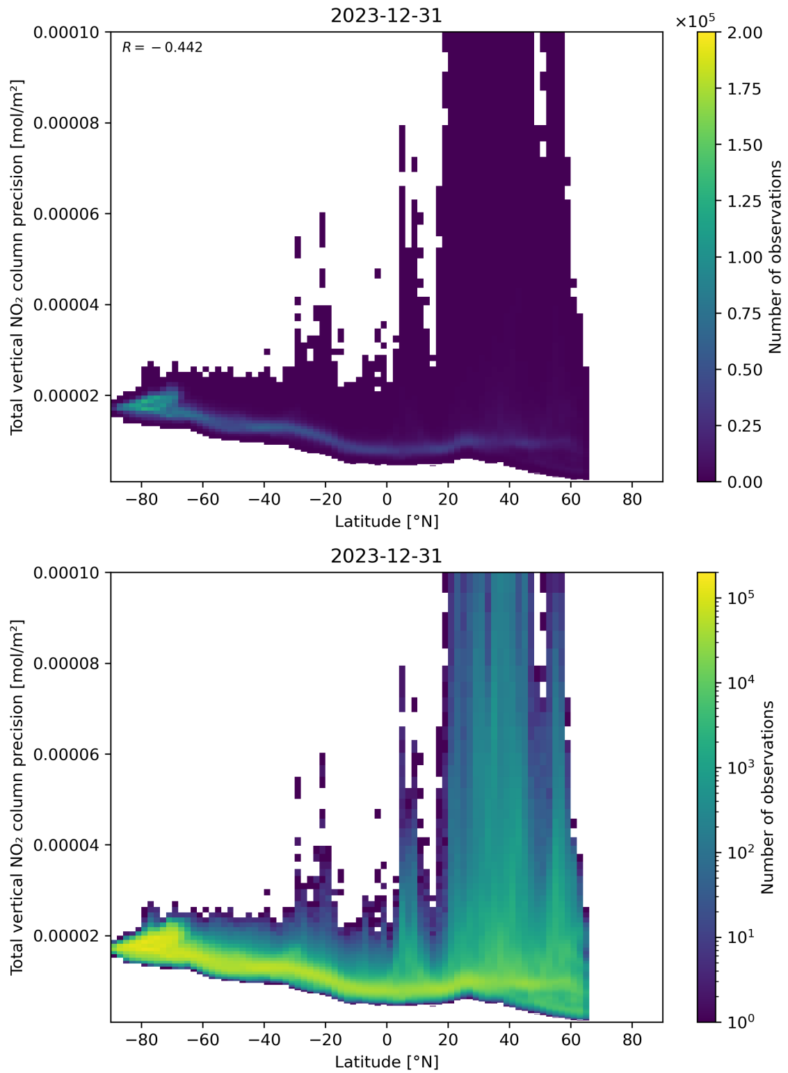
Figure 91: Scatter density plot of “Latitude” against “Total vertical NO 2 column precision” for 2023-12-30 to 2023-12-31.
