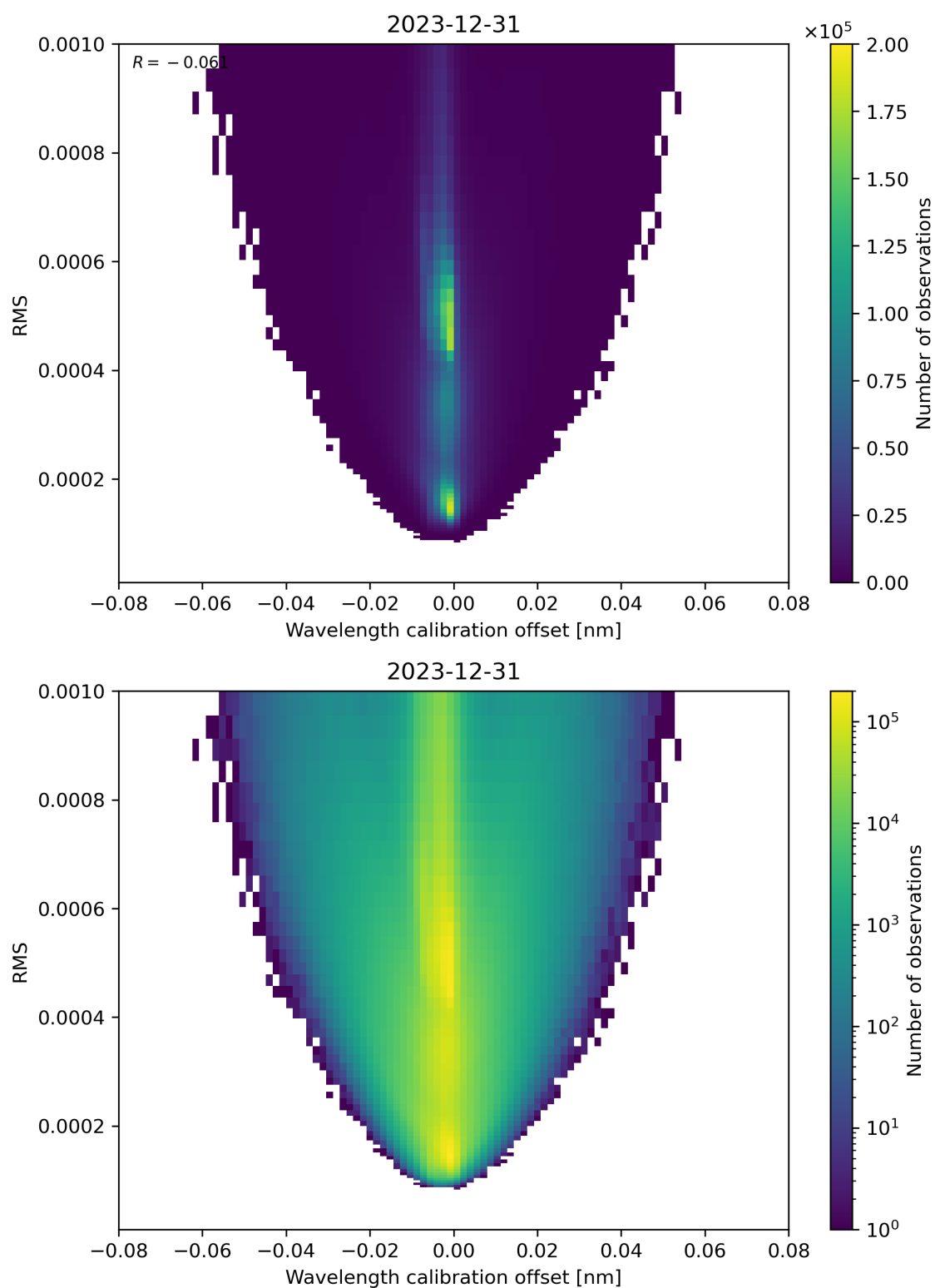
Figure 181: Scatter density plot of “Wavelength calibration offset” against “RMS” for 2023-12-30 to 2023-12-31.
