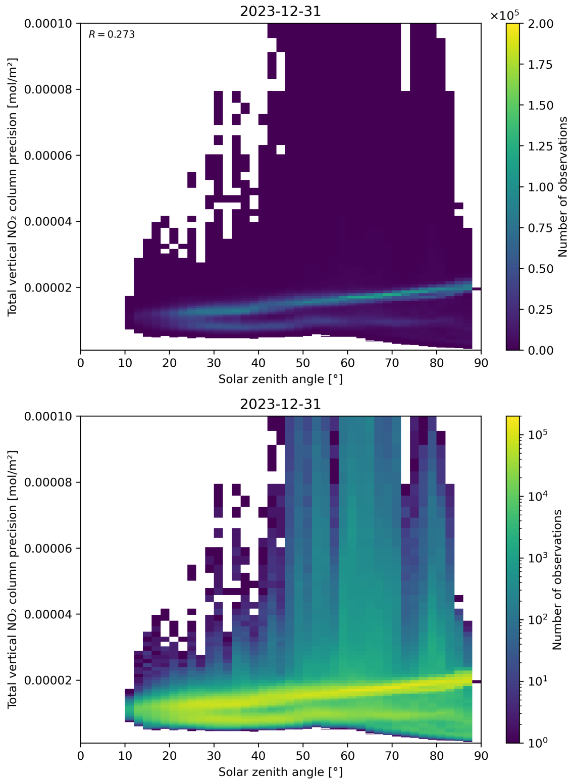
Figure 154: Scatter density plot of “Solar zenith angle” against “Total vertical NO 2 column precision” for 2023-12-30 to 2023-12-31.
