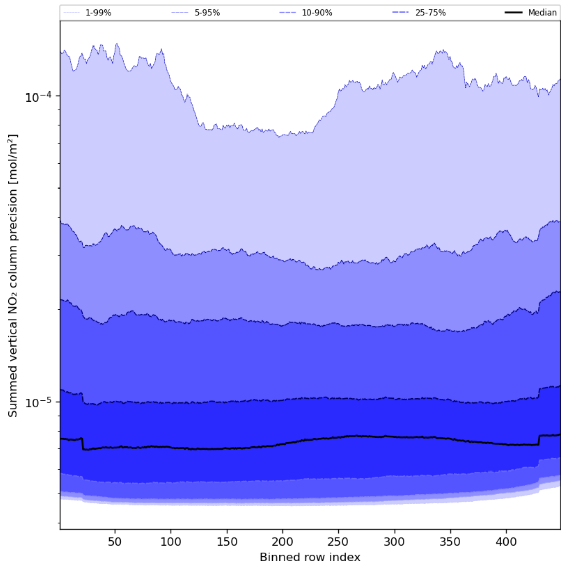
Figure 58: Along track statistics of “Summed vertical NO 2 column precision” for 2023-12-30 to 2023-12-31
