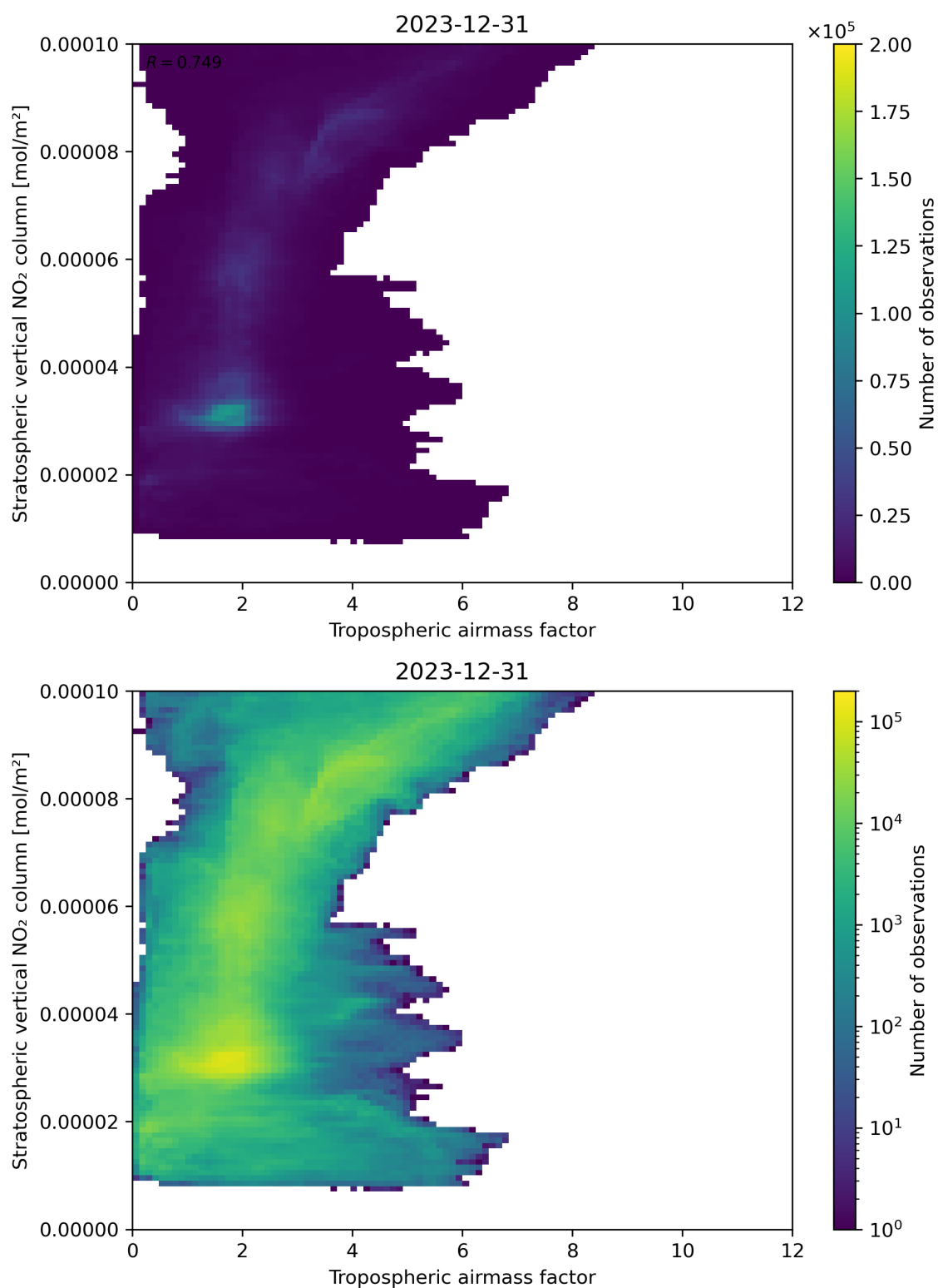
Figure 74: Scatter density plot of “Tropospheric air mass factor” against “Stratospheric vertical NO 2 column” for 2023-12-30 to 2023-12-31.
