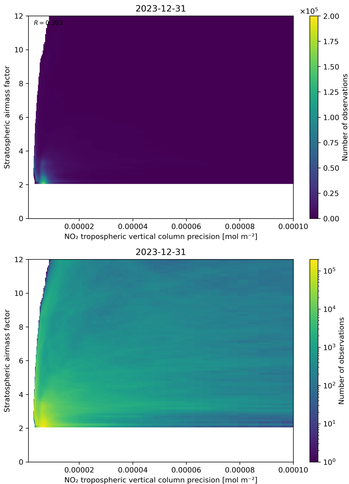
Figure 131: Scatter density plot of “NO 2 tropospheric vertical column precision” against “Stratospheric airmass factor” for 2023-12-30 to 2023-12-31.
