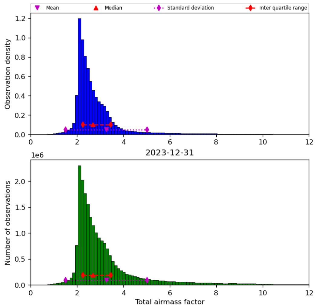
Figure 32: Histogram of “Total airmass factor” for 2023-12-30 to 2023-12-31
