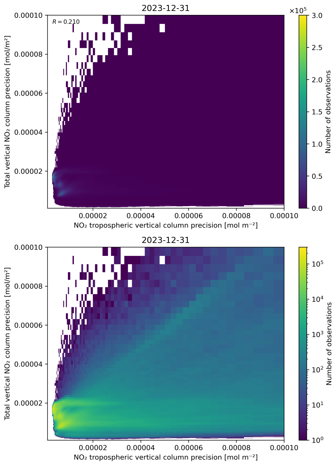
Figure 139: Scatter density plot of “NO 2 tropospheric vertical column precision” against “Total vertical NO 2 column precision” for 2023-12-30 to 2023-12-31.
