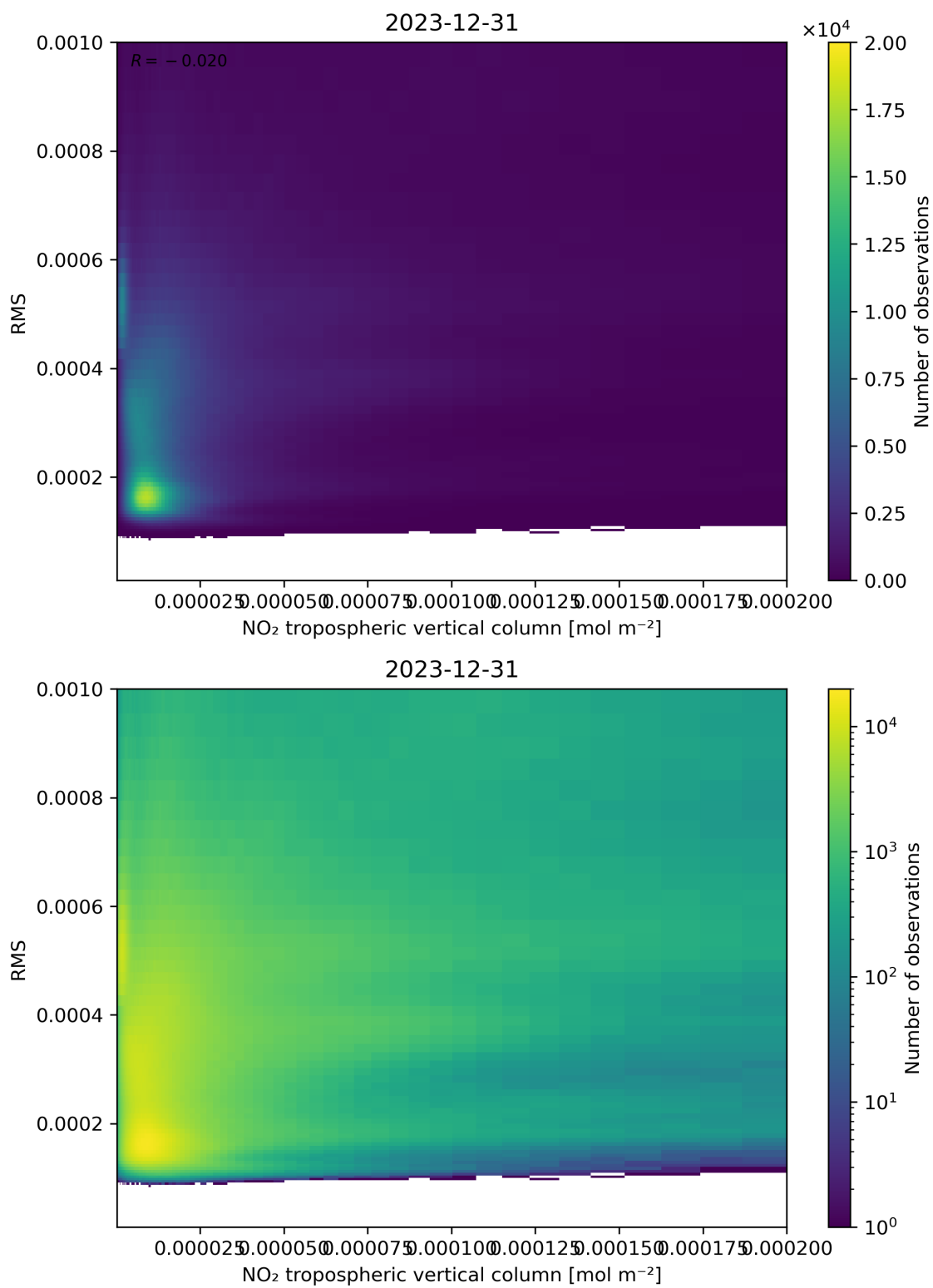
Figure 142: Scatter density plot of “NO 2 tropospheric vertical column” against “RMS” for 2023-12-30 to 2023-12-31.
