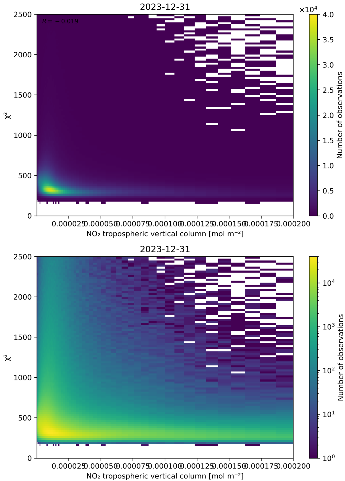
Figure 124: Scatter density plot of “NO 2 tropospheric vertical column” against “ \chi^2 ” for 2023-12-30 to 2023-12-31.
