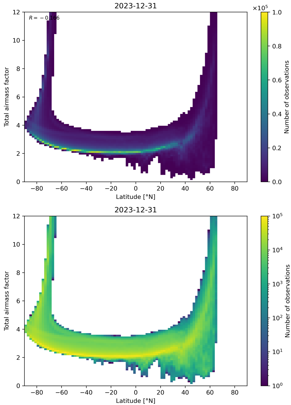
Figure 84: Scatter density plot of “Latitude” against “Total airmass factor” for 2023-12-30 to 2023-12-31.
