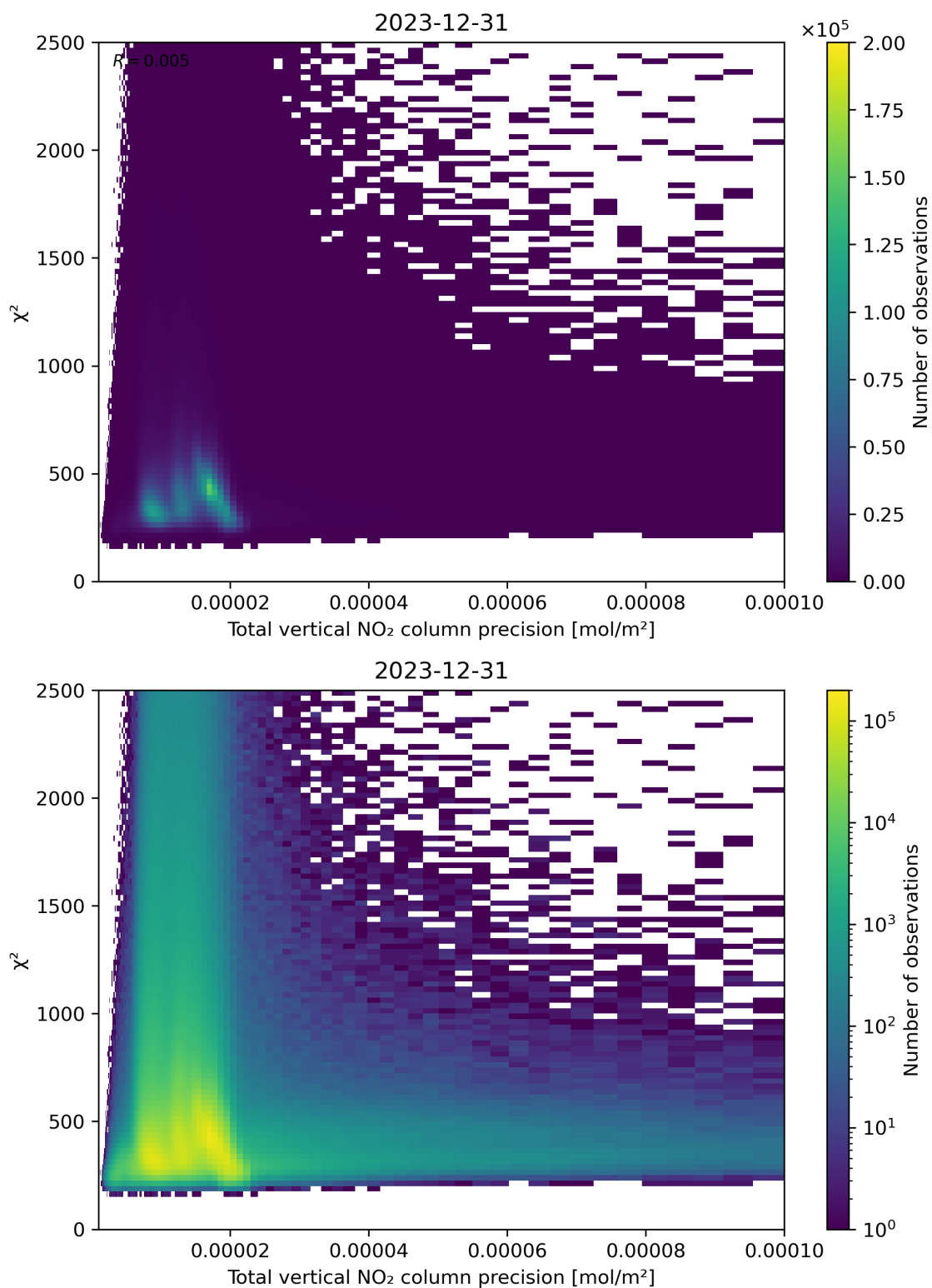
Figure 116: Scatter density plot of “Total vertical NO 2 column precision” against “ \chi^2 ” for 2023-12-30 to 2023-12-31.
