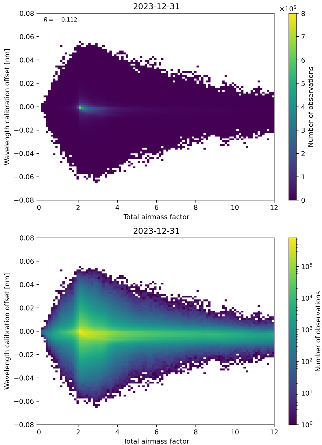
Figure 70: Scatter density plot of “Total airmass factor” against “Wavelength calibration offset” for 2023-12-30 to 2023-12-31.
