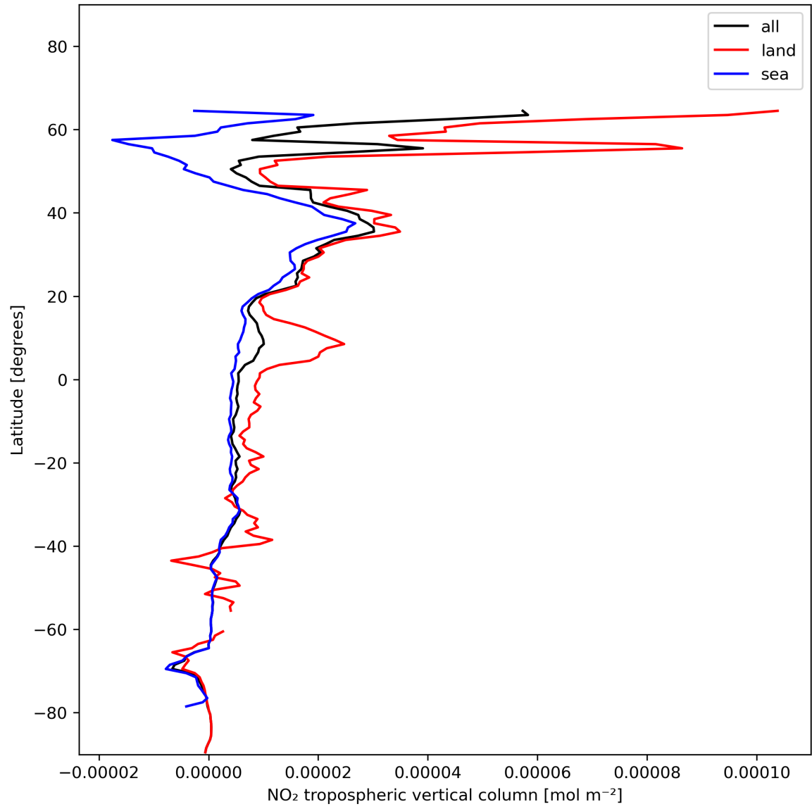
Figure 12: Zonal average of “NO 2 tropospheric vertical column” for 2023-12-30 to 2023-12-31.
