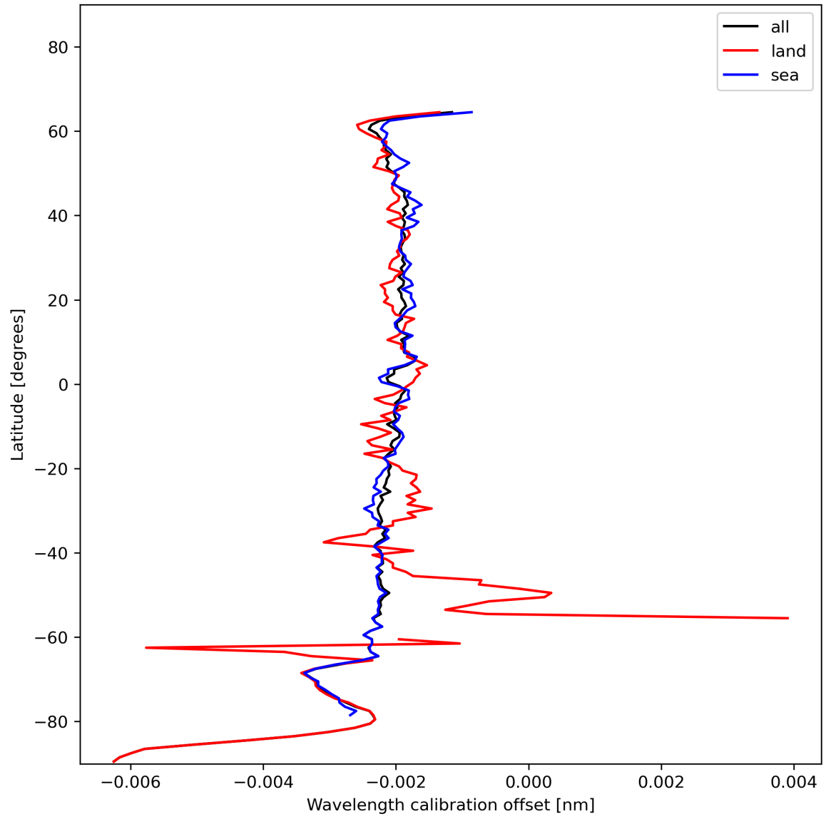
Figure 18: Zonal average of “Wavelength calibration offset” for 2023-12-30 to 2023-12-31.
