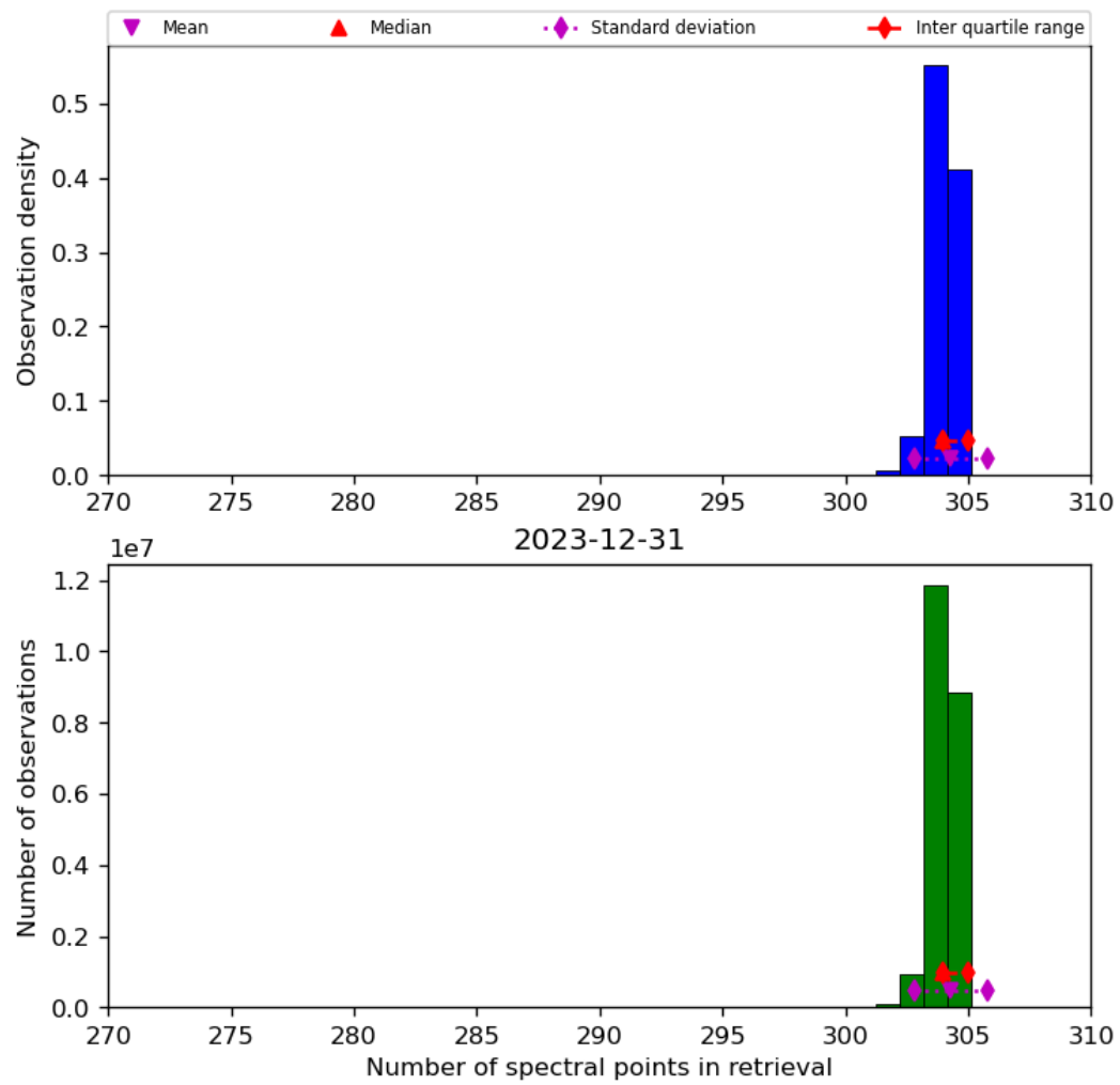
Figure 33: Histogram of “Number of spectral points in retrieval” for 2023-12-30 to 2023-12-31
