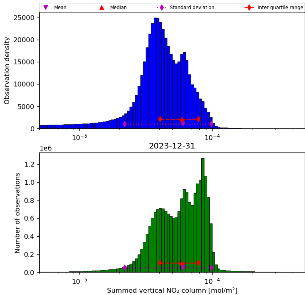
Figure 40: Histogram of “Summed vertical NO 2 column” for 2023-12-30 to 2023-12-31
