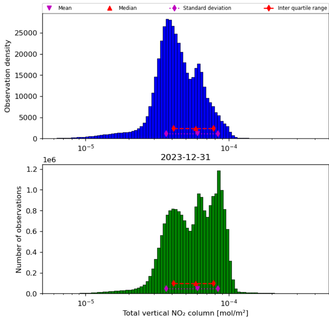
Figure 38: Histogram of “Total vertical NO 2 column” for 2023-12-30 to 2023-12-31
