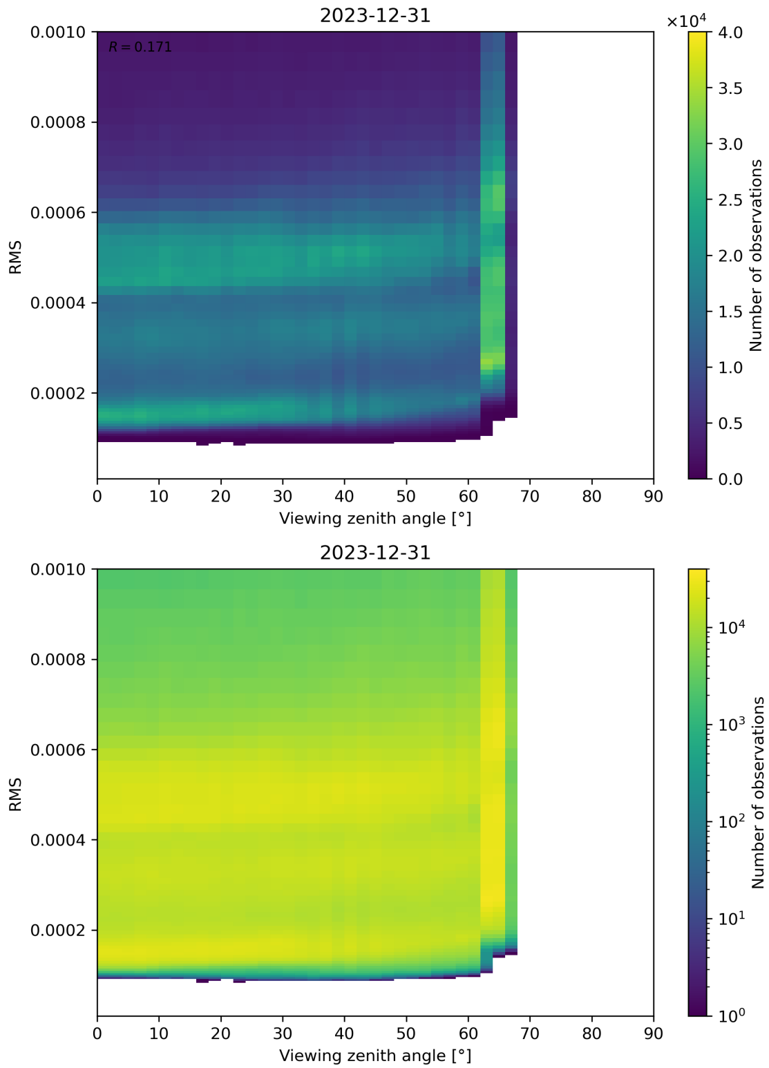
Figure 171: Scatter density plot of “Viewing zenith angle” against “RMS” for 2023-12-30 to 2023-12-31.
