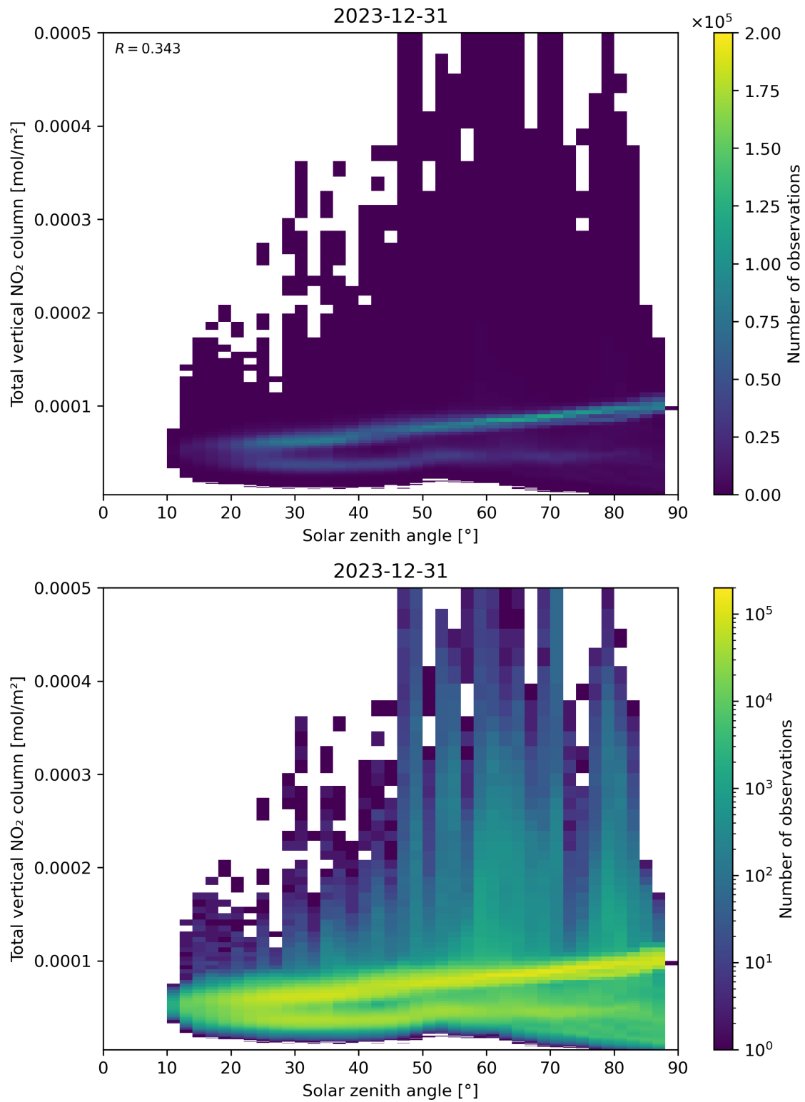
Figure 153: Scatter density plot of “Solar zenith angle” against “Total vertical NO 2 column” for 2023-12-30 to 2023-12-31.
