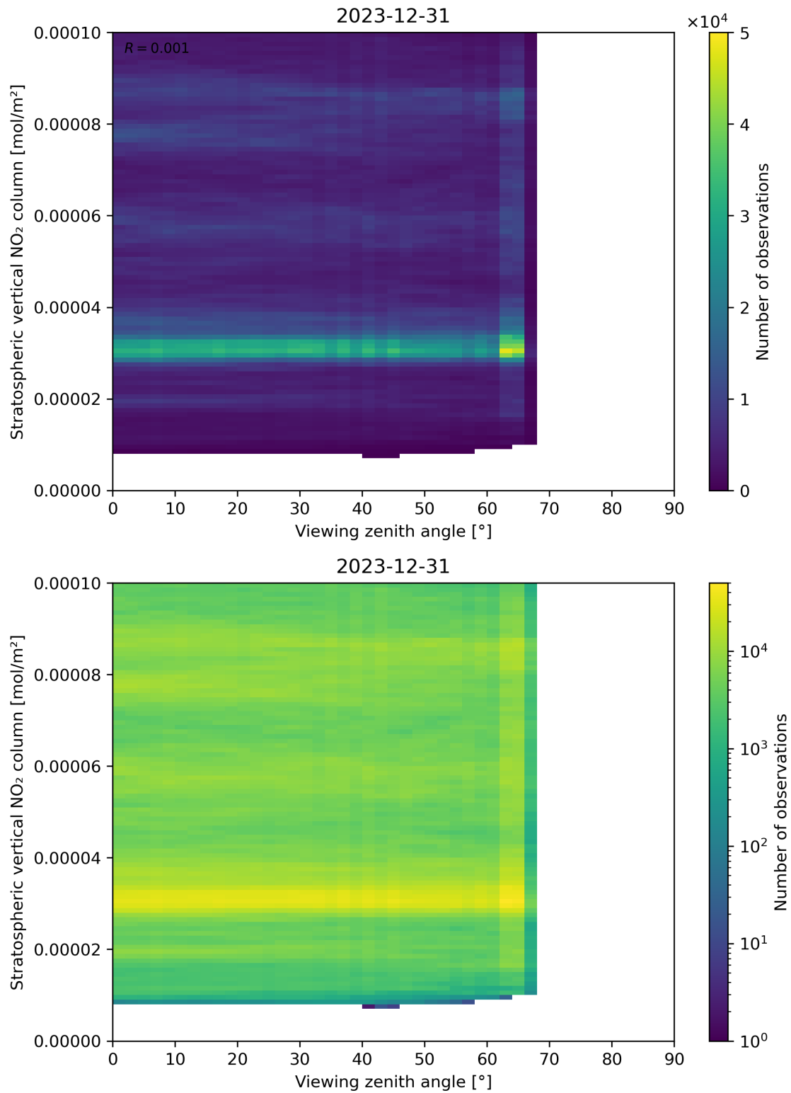
Figure 164: Scatter density plot of “Viewing zenith angle” against “Stratospheric vertical NO 2 column” for 2023-12-30 to 2023-12-31.
