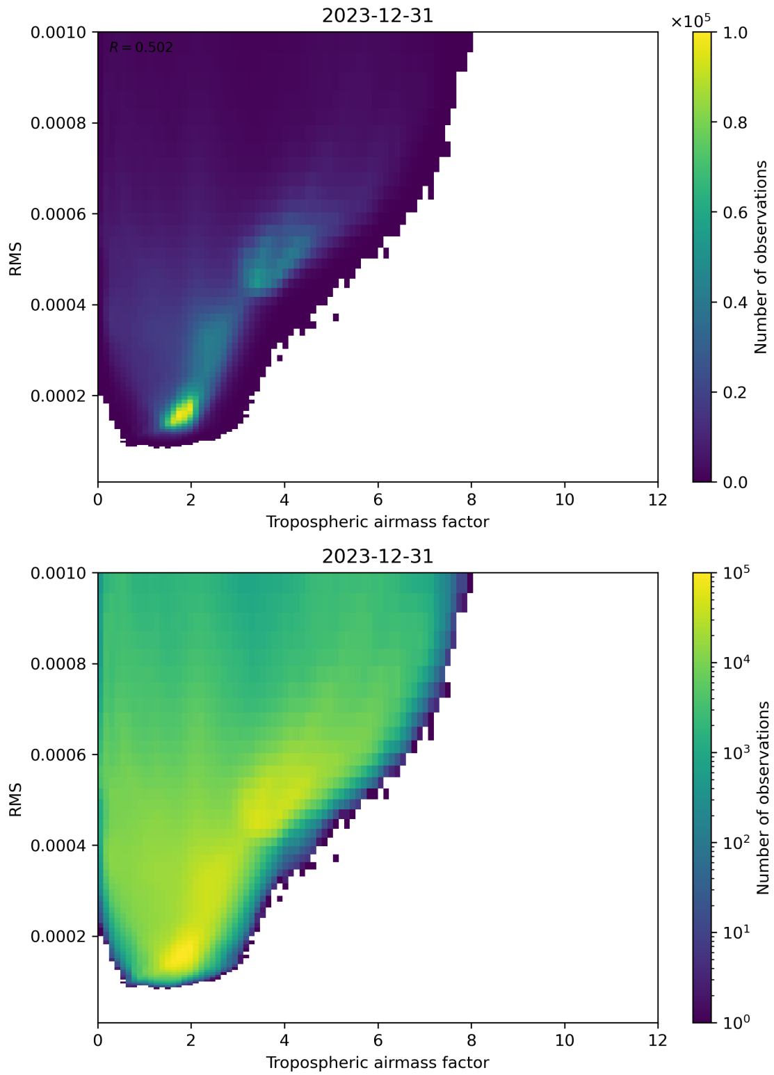
Figure 79: Scatter density plot of “Tropospheric airmass factor” against “RMS” for 2023-12-30 to 2023-12-31.
