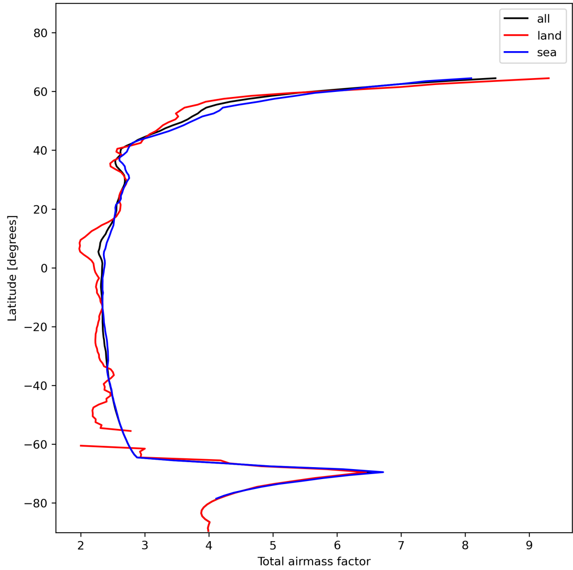
Figure 15: Zonal average of “Total airmass factor” for 2023-12-30 to 2023-12-31.
