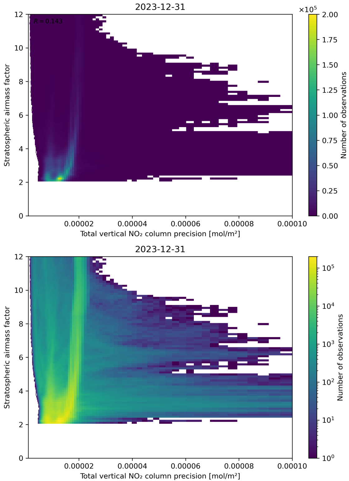
Figure 115: Scatter density plot of “Total vertical NO 2 column precision” against “Stratospheric air mass factor” for 2023-12-30 to 2023-12-31.
