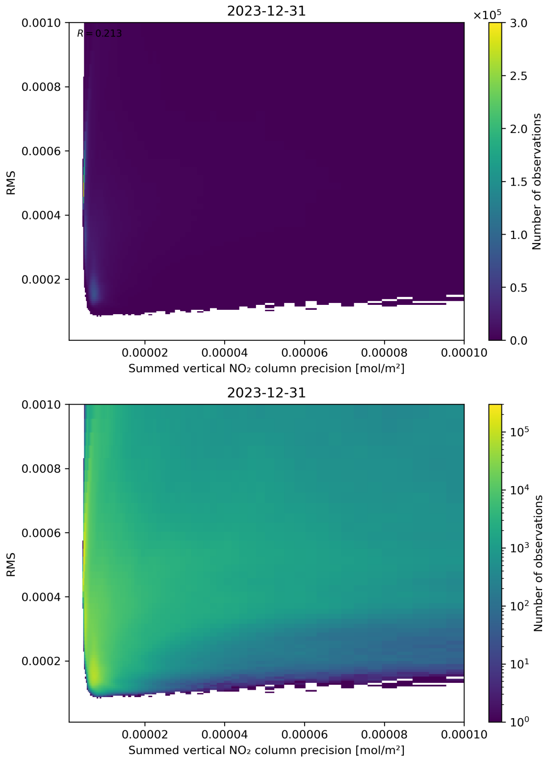
Figure 108: Scatter density plot of “Summed vertical NO 2 column precision” against “RMS” for 2023-12-30 to 2023-12-31.
