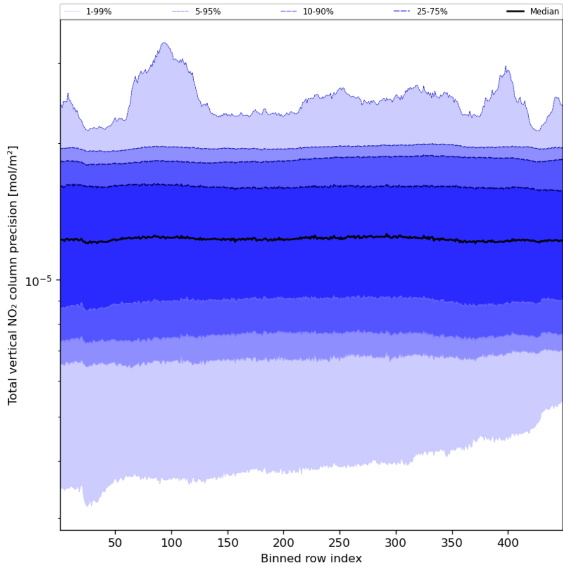
Figure 56: Along track statistics of “Total vertical NO 2 column precision” for 2023-12-30 to 2023-12-31
