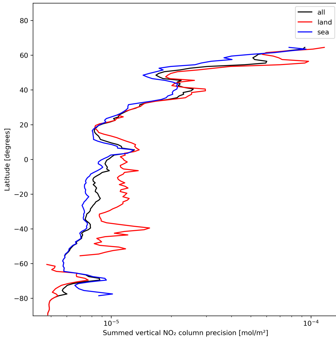
Figure 24: Zonal average of “Summed vertical NO 2 column precision” for 2023-12-30 to 2023-12-31.
