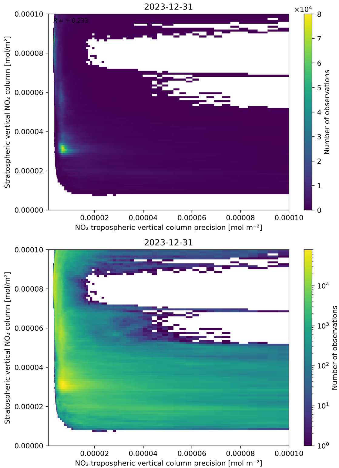
Figure 135: Scatter density plot of “NO 2 tropospheric vertical column precision” against “Stratospheric vertical NO 2 column” for 2023-12-30 to 2023-12-31.
