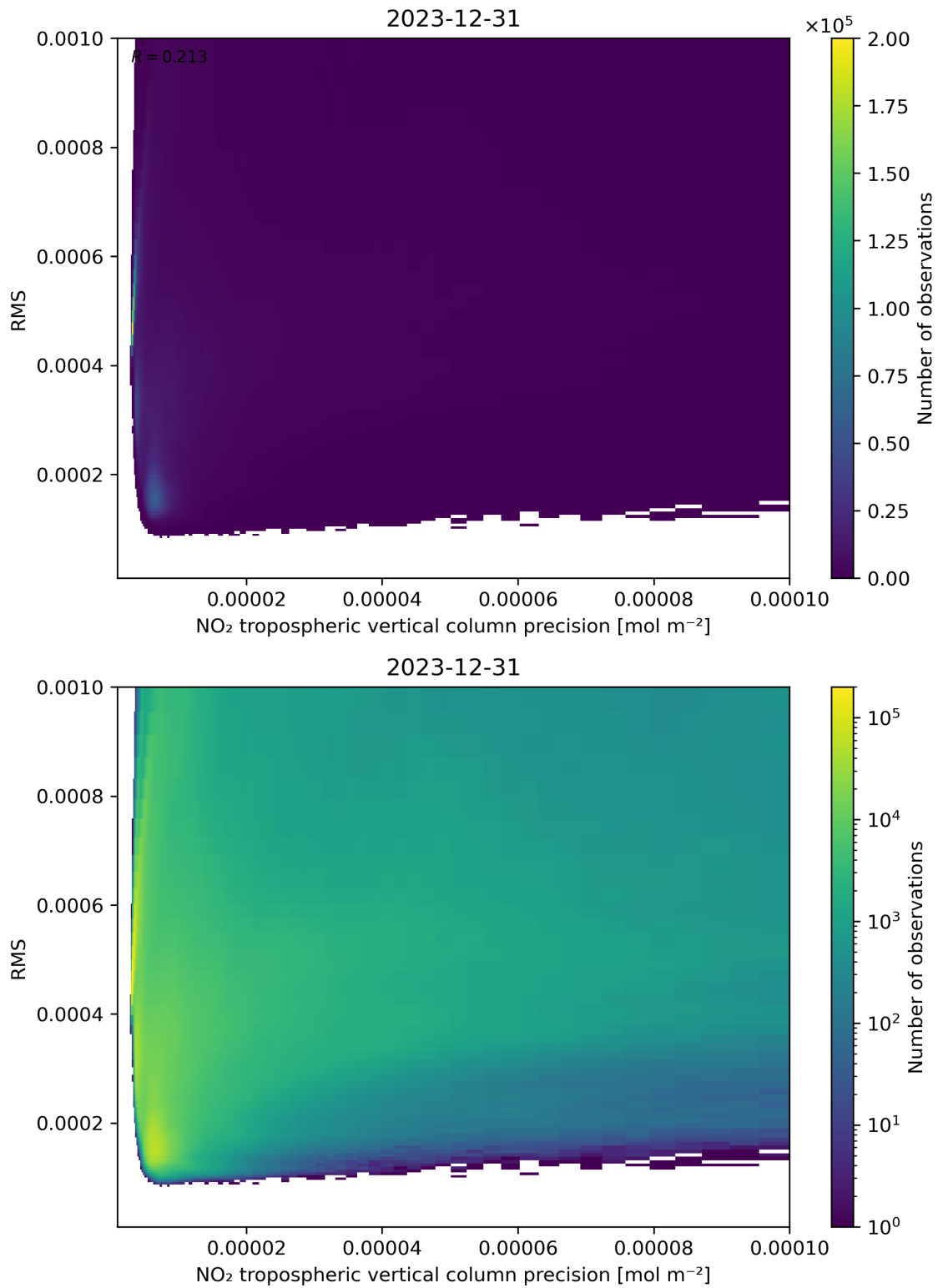
Figure 140: Scatter density plot of “NO 2 tropospheric vertical column precision” against “RMS” for 2023-12-30 to 2023-12-31.
