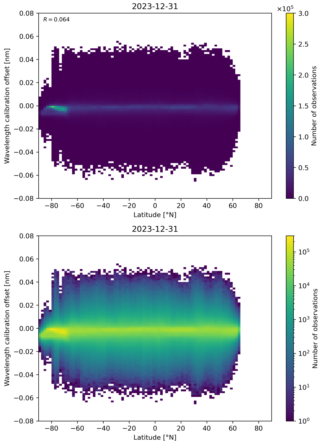
Figure 95: Scatter density plot of “Latitude” against “Wavelength calibration offset” for 2023-12-30 to 2023-12-31.
