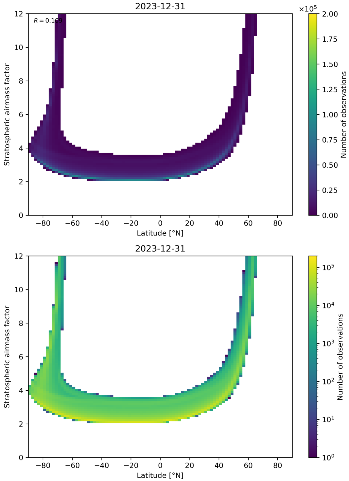
Figure 83: Scatter density plot of “Latitude” against “Stratospheric air mass factor” for 2023-12-30 to 2023-12-31.
