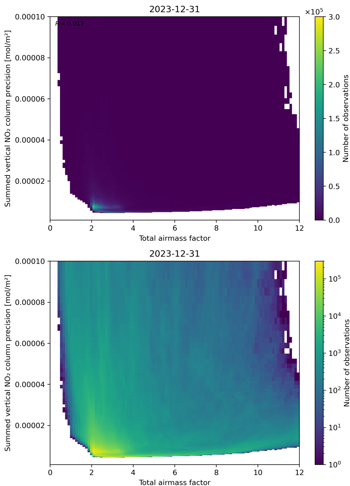
Figure 66: Scatter density plot of “Total airmass factor” against “Summed vertical NO 2 column precision” for 2023-12-30 to 2023-12-31.
