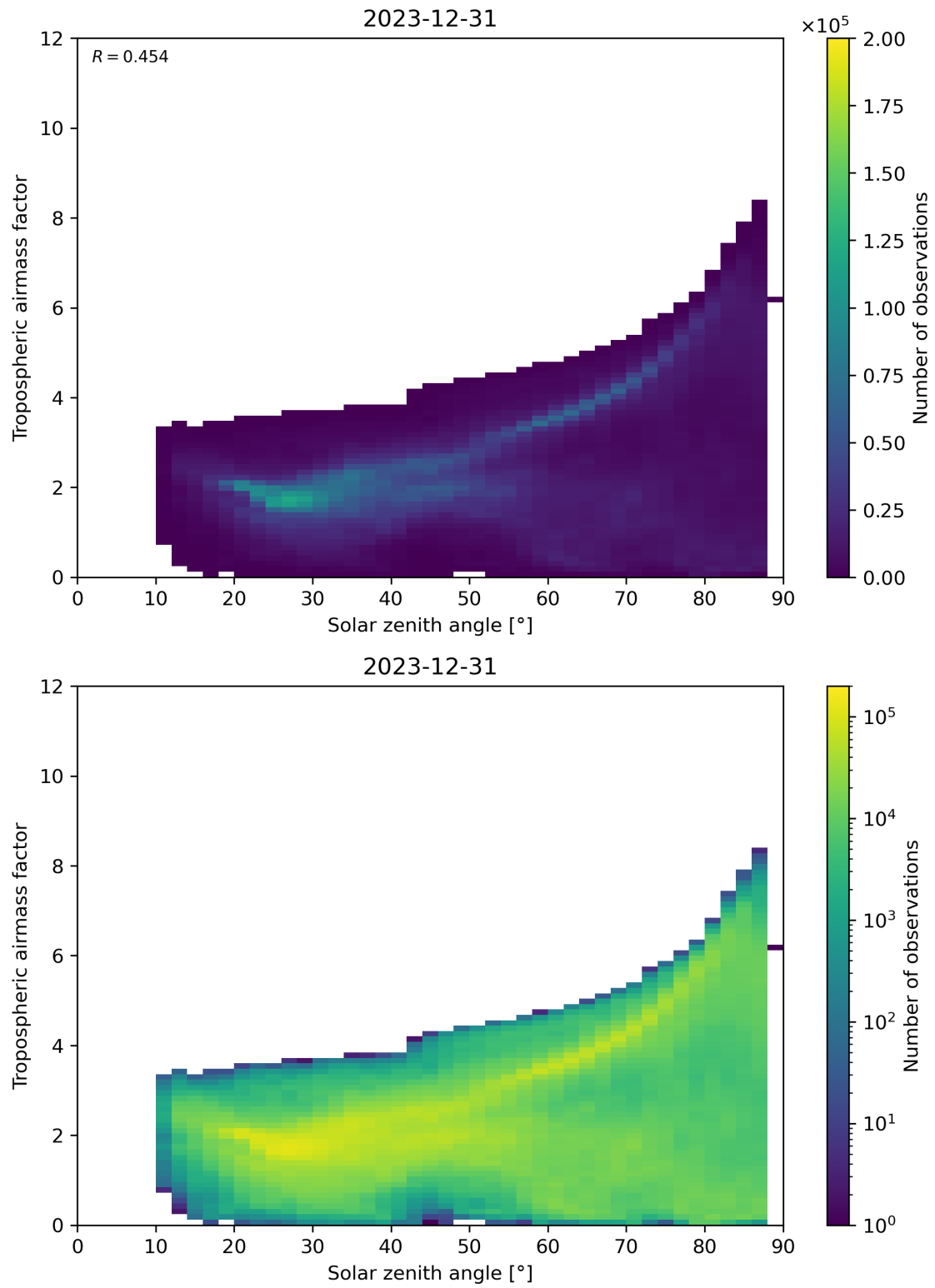
Figure 147: Scatter density plot of “Solar zenith angle” against “Tropospheric airmass factor” for 2023-12-30 to 2023-12-31.
