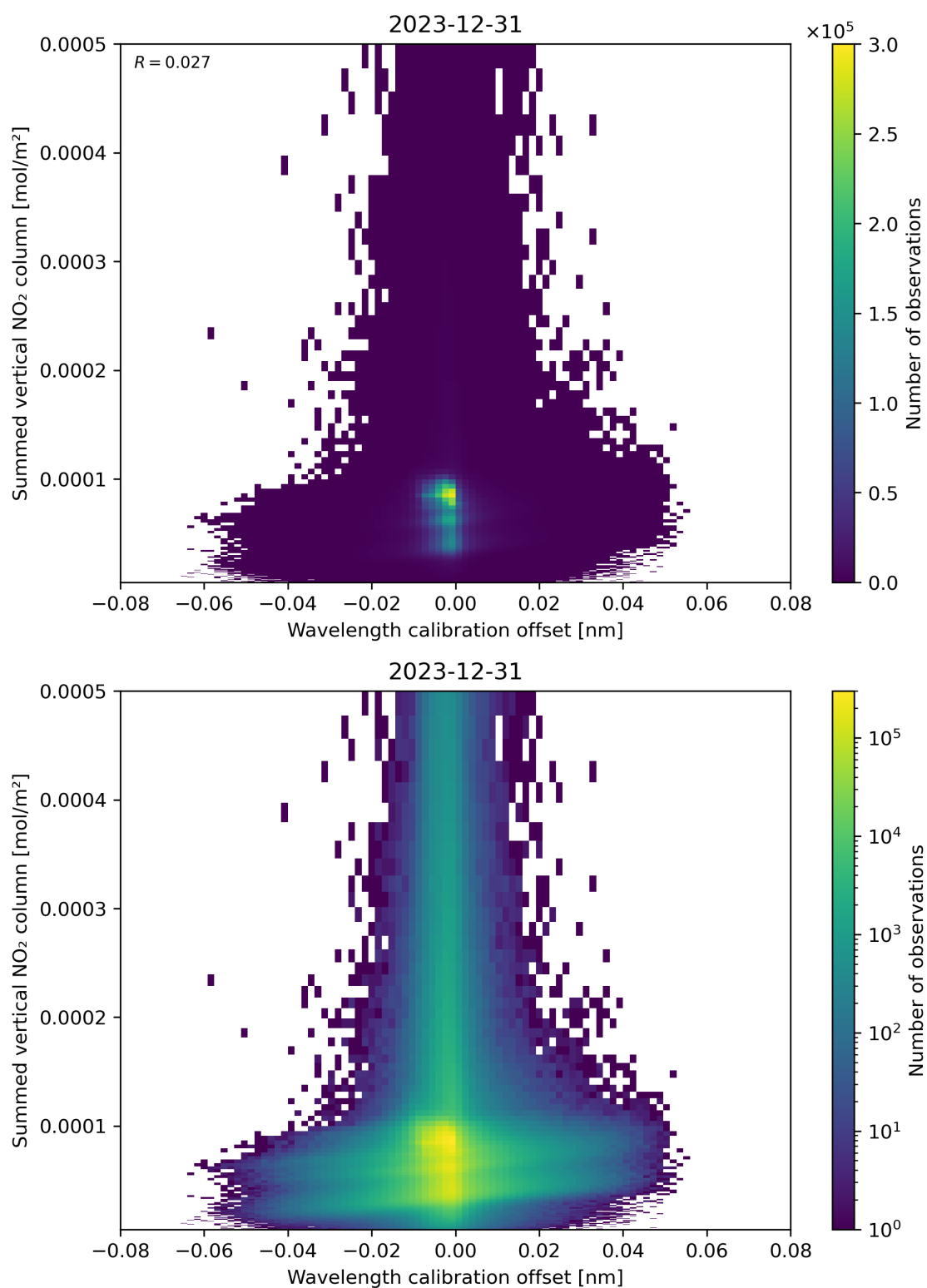
Figure 177: Scatter density plot of “Wavelength calibration offset” against “Summed vertical NO 2 column” for 2023-12-30 to 2023-12-31.
