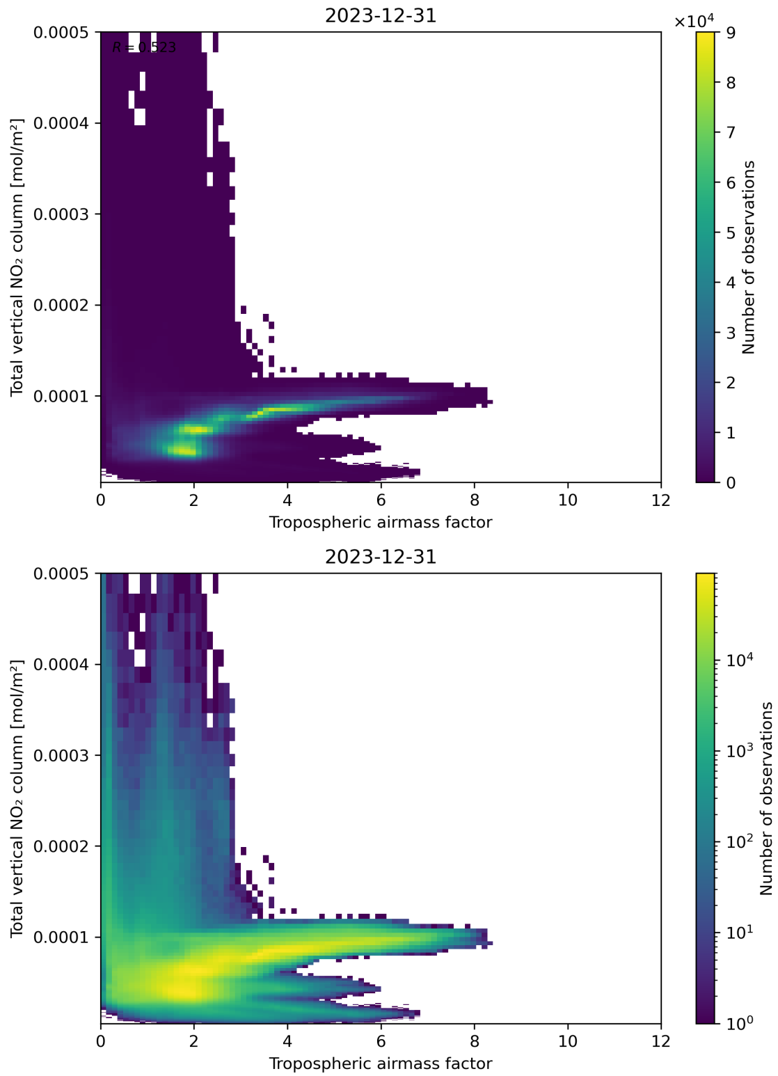
Figure 77: Scatter density plot of “Tropospheric airmass factor” against “Total vertical NO 2 column” for 2023-12-30 to 2023-12-31.
