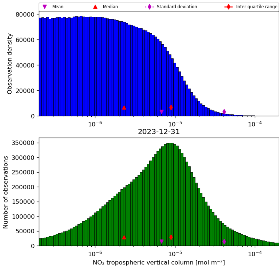
Figure 29: Histogram of “NO 2 tropospheric vertical column” for 2023-12-30 to 2023-12-31
