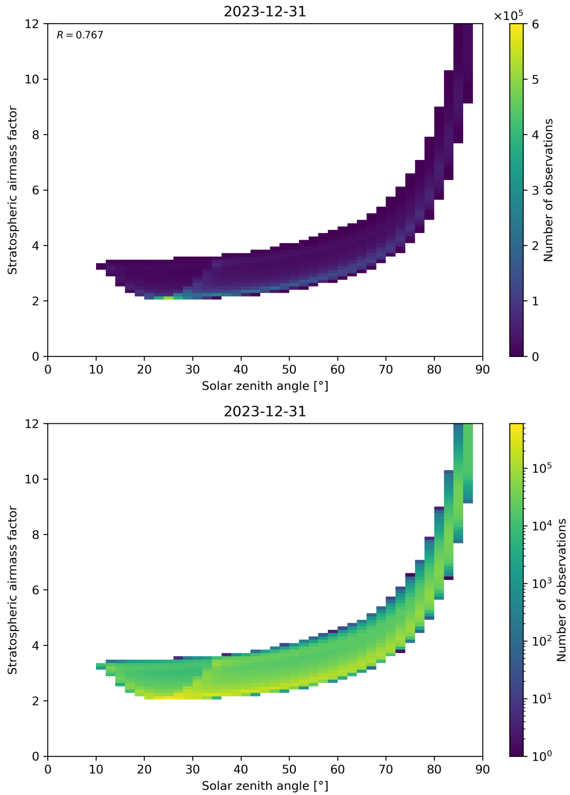
Figure 145: Scatter density plot of “Solar zenith angle” against “Stratospheric airmass factor” for 2023-12-30 to 2023-12-31.
