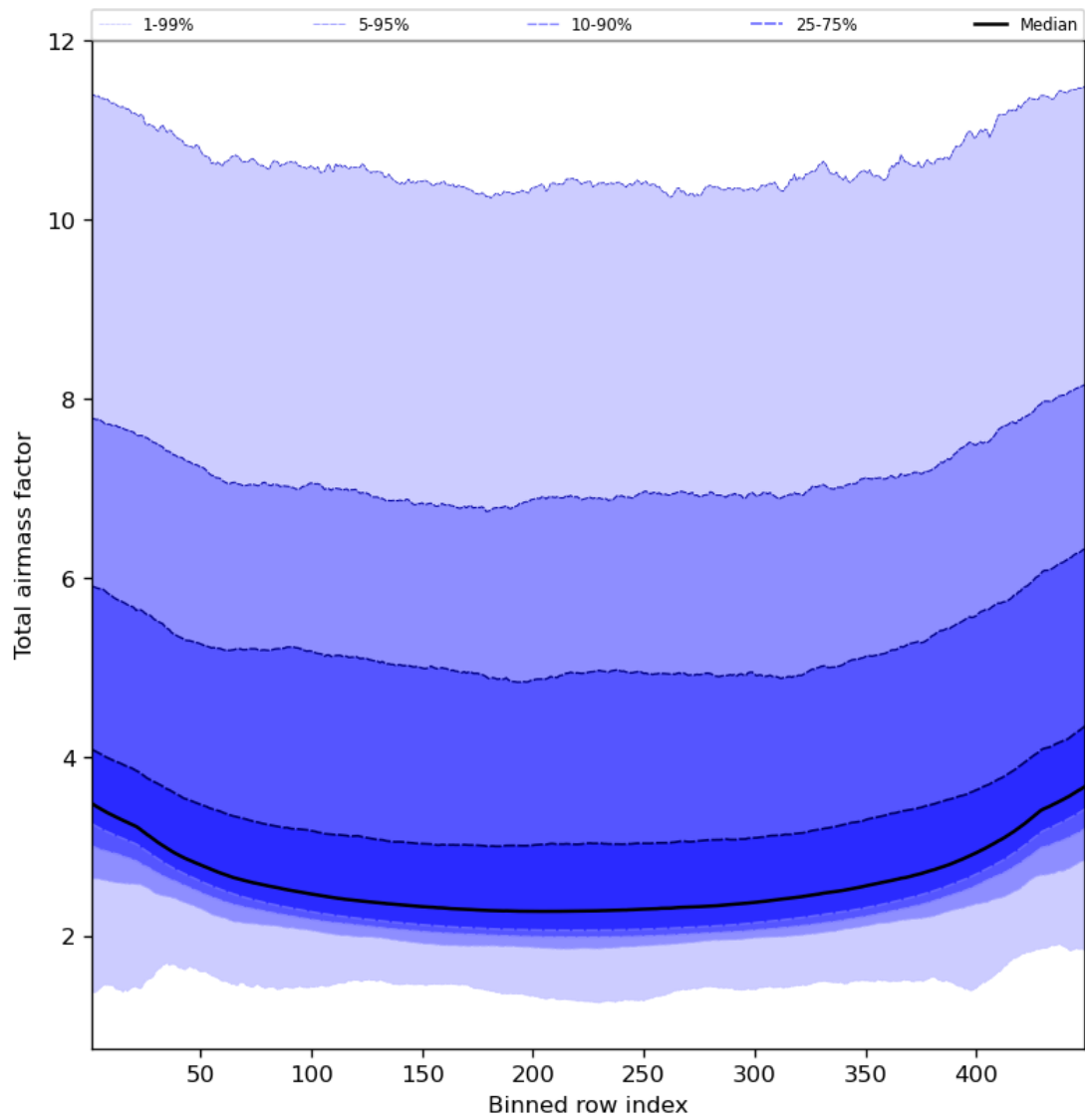
Figure 49: Along track statistics of “Total airmass factor” for 2023-12-30 to 2023-12-31
