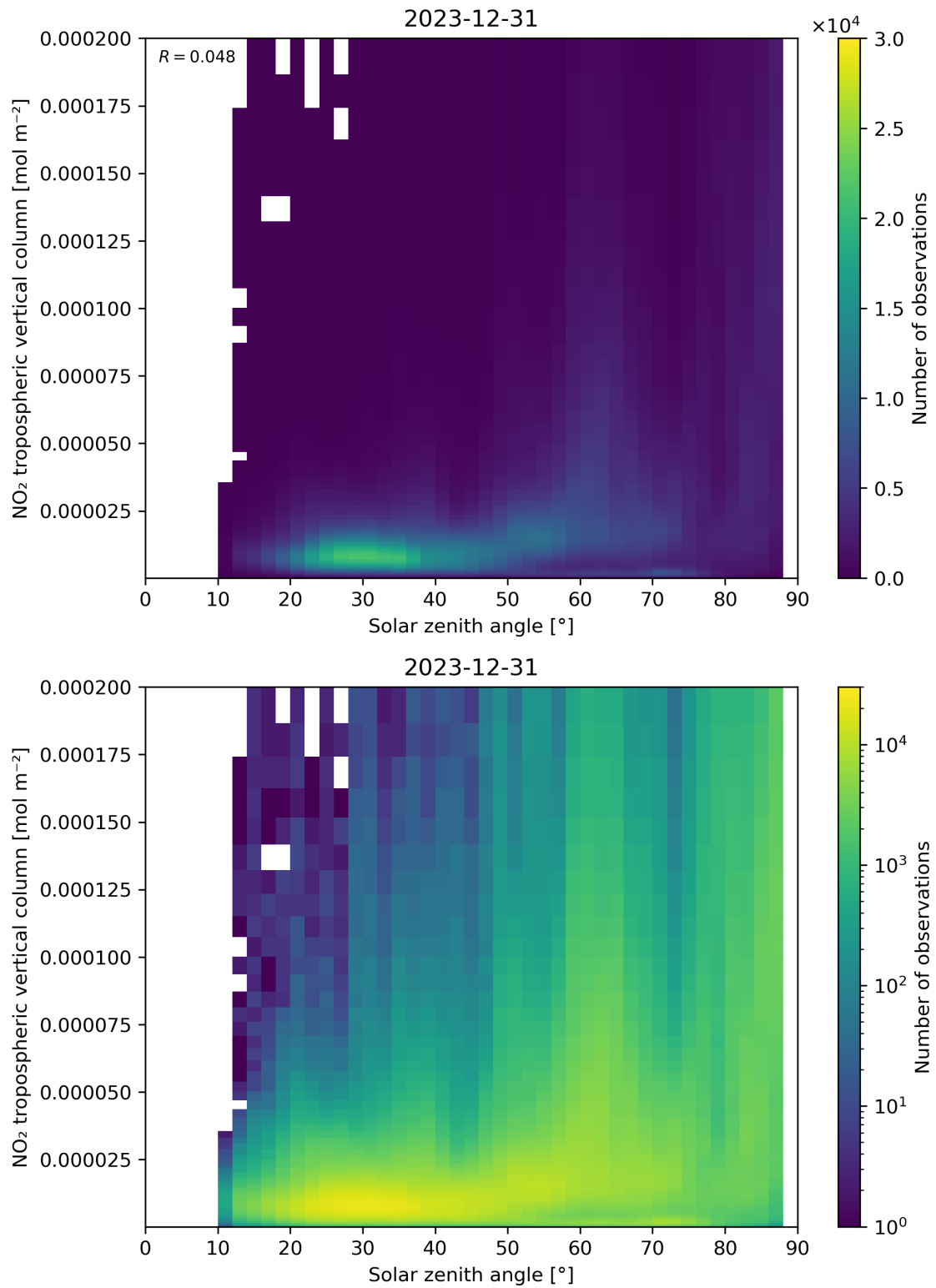
Figure 155: Scatter density plot of “Solar zenith angle” against “NO 2 tropospheric vertical column” for 2023-12-30 to 2023-12-31.
