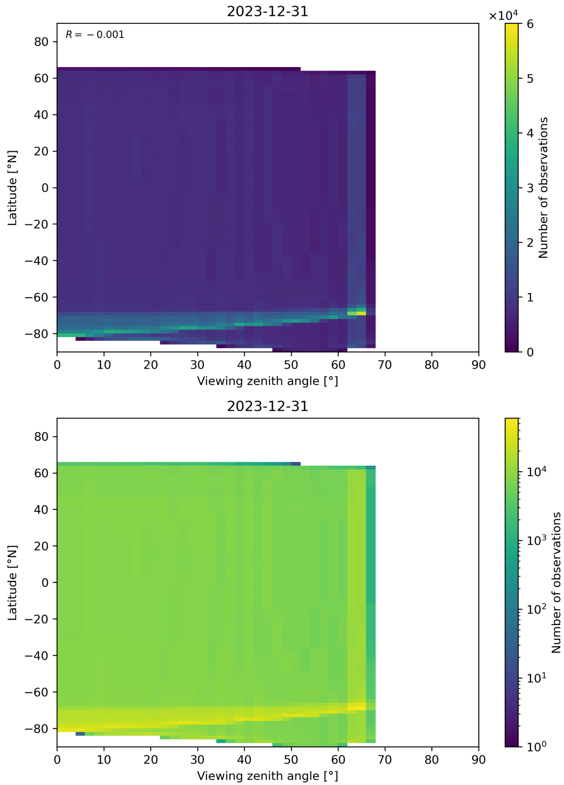
Figure 163: Scatter density plot of “Viewing zenith angle” against “Latitude” for 2023-12-30 to 2023-12-31.
