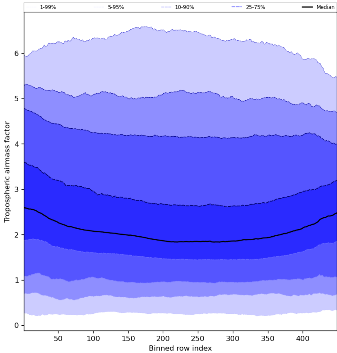
Figure 48: Along track statistics of “Tropospheric air mass factor” for 2023-12-30 to 2023-12-31
