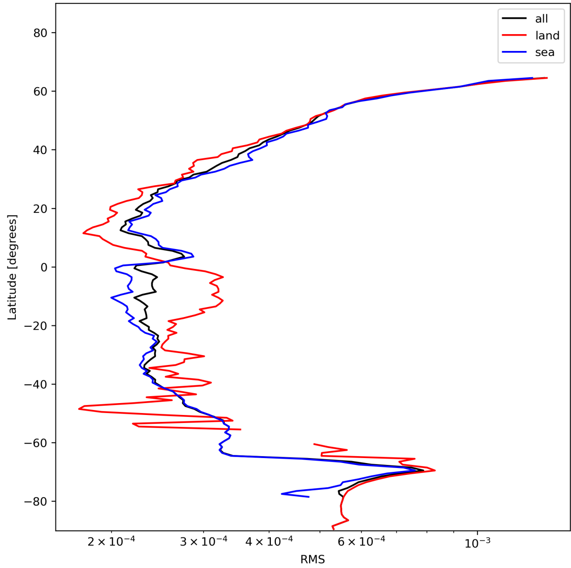
Figure 26: Zonal average of “RMS” for 2023-12-30 to 2023-12-31.
