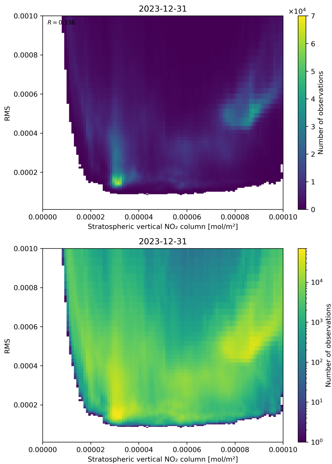
Figure 102: Scatter density plot of “Stratospheric vertical NO 2 column” against “RMS” for 2023-12-30 to 2023-12-31.
