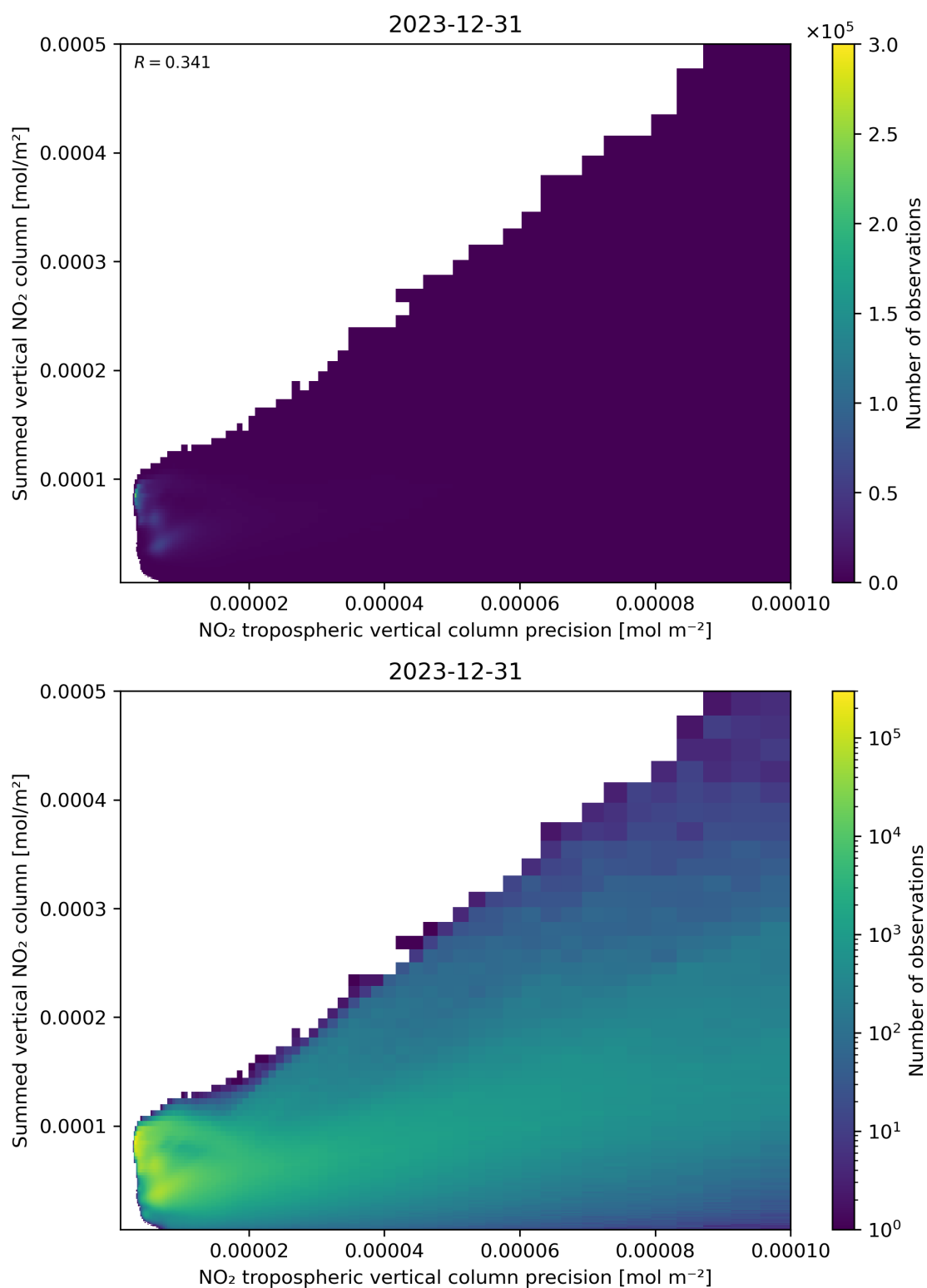
Figure 136: Scatter density plot of “NO 2 tropospheric vertical column precision” against “Summed vertical NO 2 column” for 2023-12-30 to 2023-12-31.
