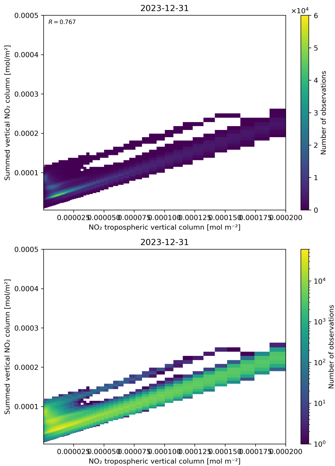
Figure 126: Scatter density plot of “NO 2 tropospheric vertical column” against “Summed vertical NO 2 column” for 2023-12-30 to 2023-12-31.
