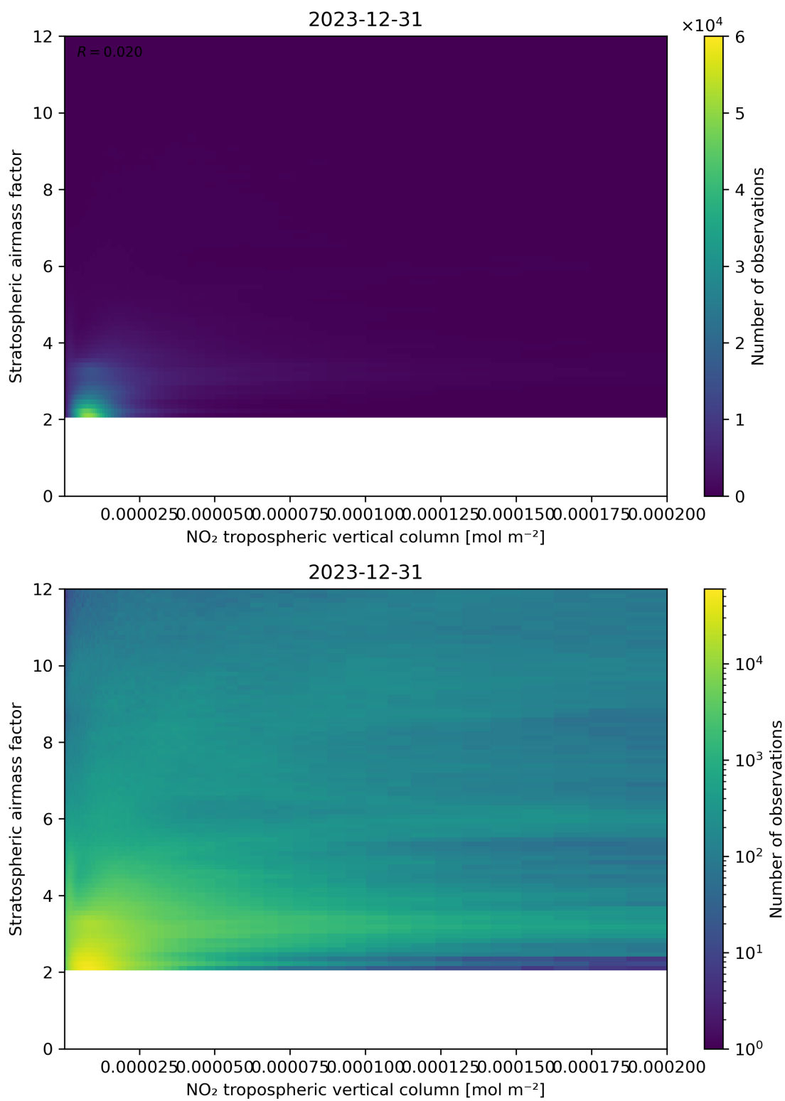
Figure 121: Scatter density plot of “NO 2 tropospheric vertical column” against “Stratospheric airmass factor” for 2023-12-30 to 2023-12-31.
