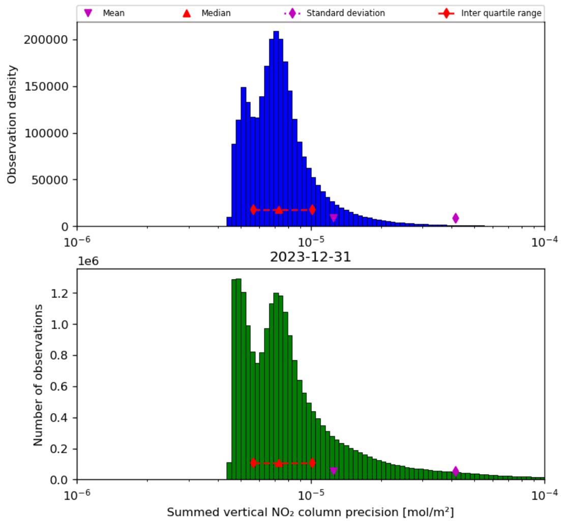
Figure 41: Histogram of "Summed vertical NO 2 column precision" for 2023-12-30 to 2023-12-31
