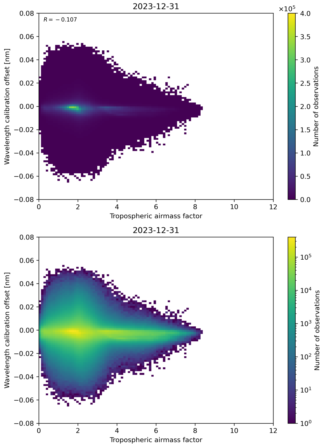
Figure 80: Scatter density plot of “Tropospheric airmass factor” against “Wavelength calibration offset” for 2023-12-30 to 2023-12-31.
