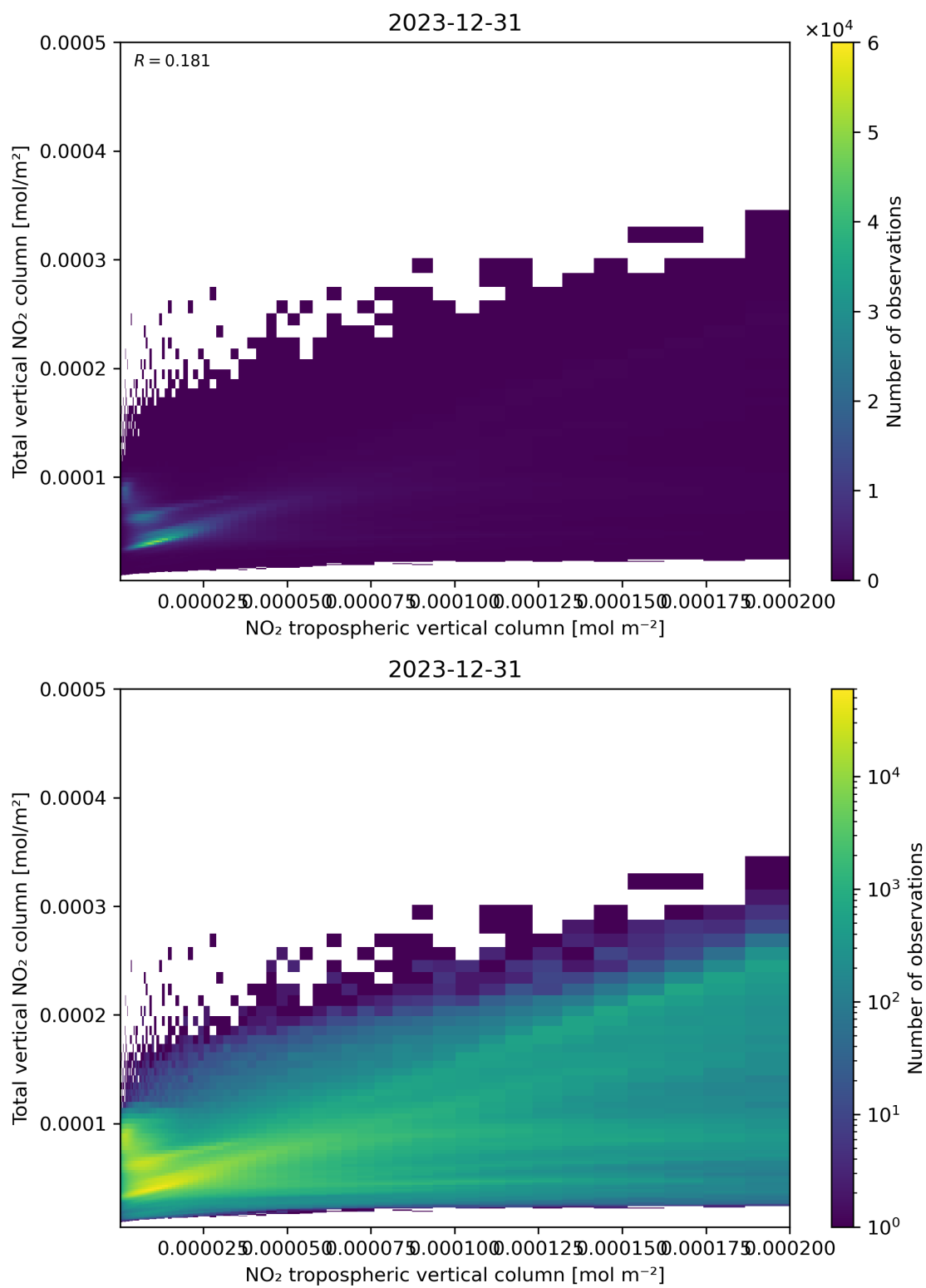
Figure 128: Scatter density plot of “NO 2 tropospheric vertical column” against “Total vertical NO 2 column” for 2023-12-30 to 2023-12-31.
