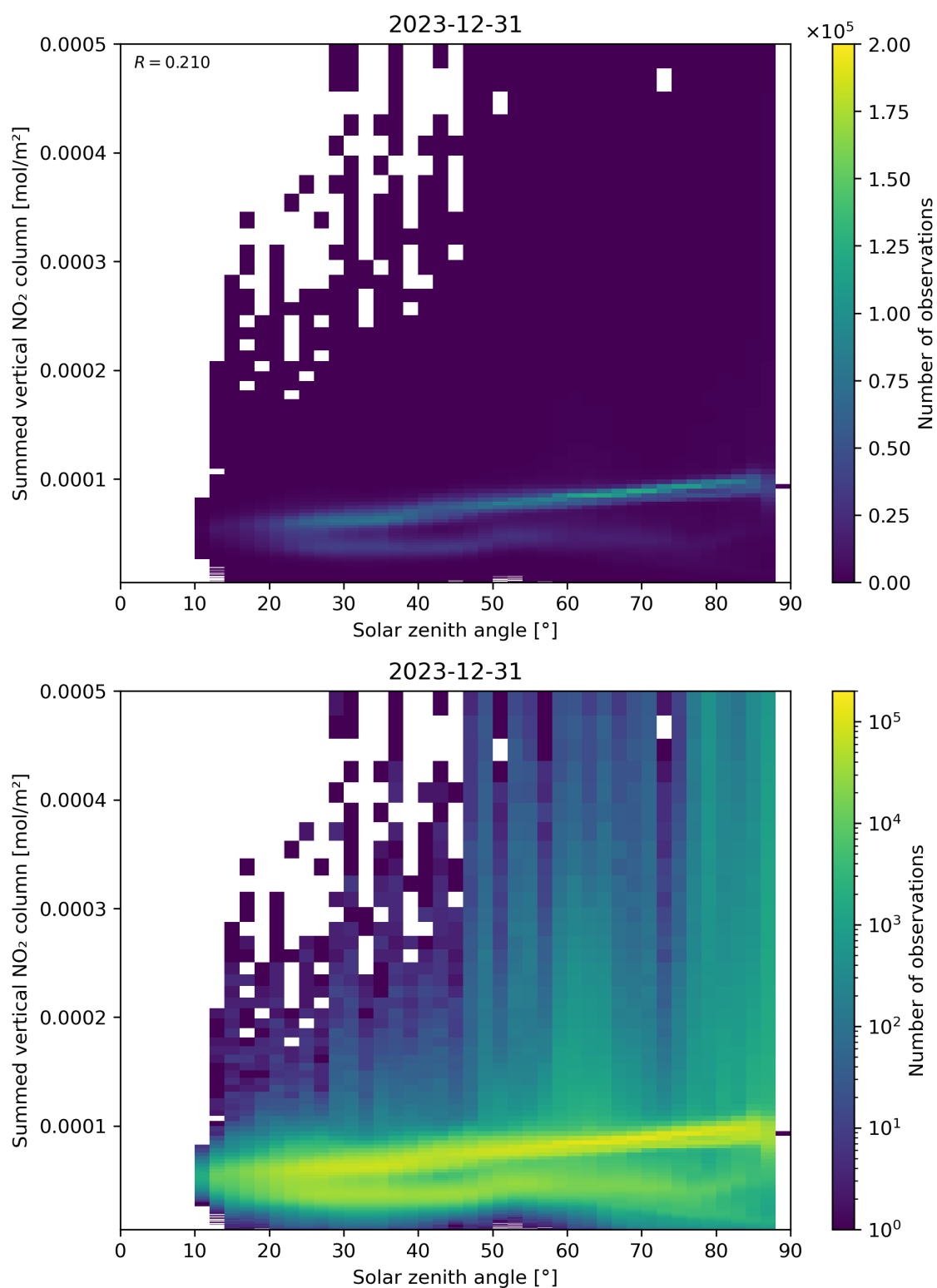
Figure 151: Scatter density plot of “Solar zenith angle” against “Summed vertical NO 2 column” for 2023-12-30 to 2023-12-31.
