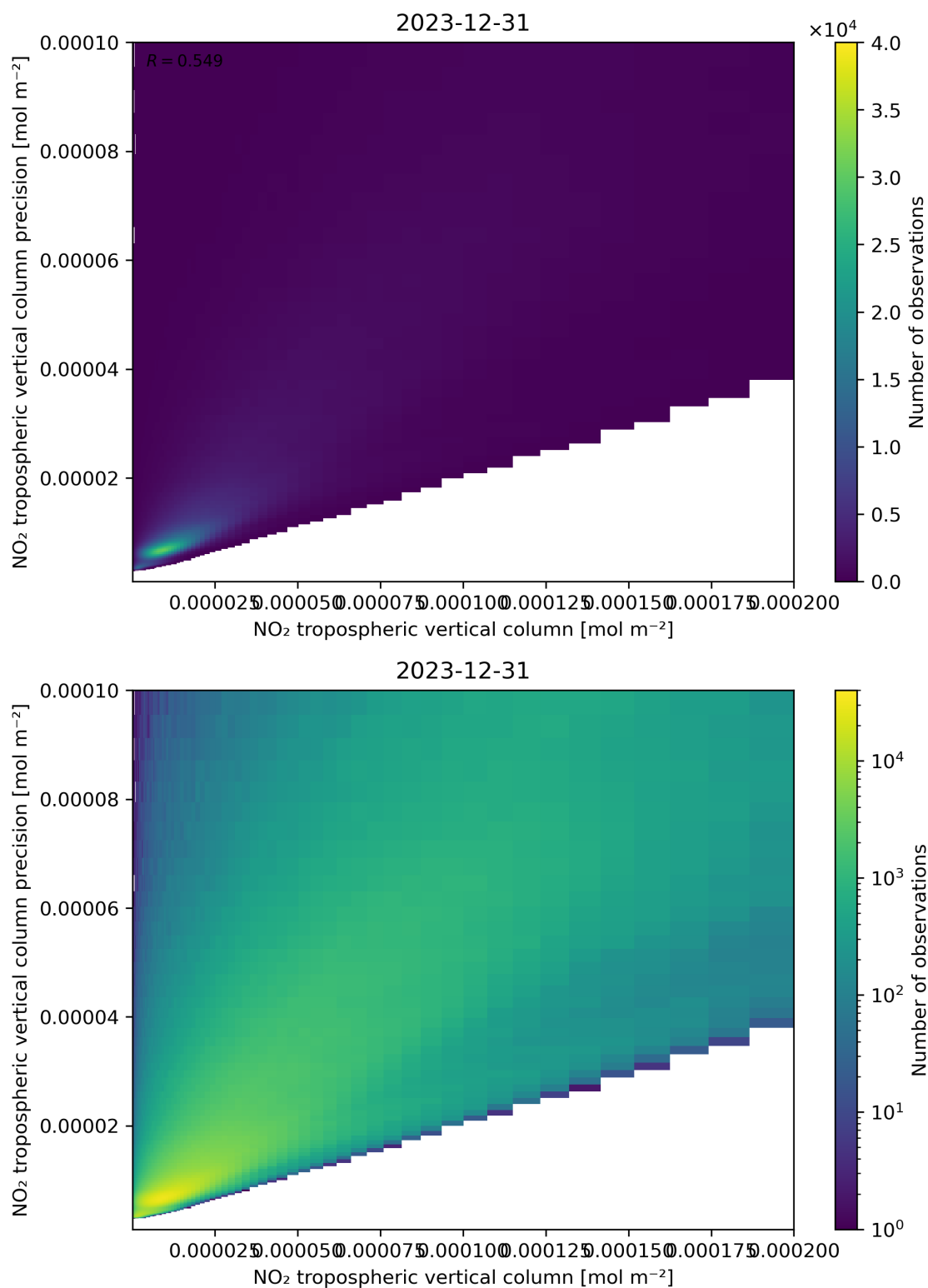
Figure 130: Scatter density plot of “NO 2 tropospheric vertical column” against “NO 2 tropospheric vertical column precision” for 2023-12-30 to 2023-12-31.
