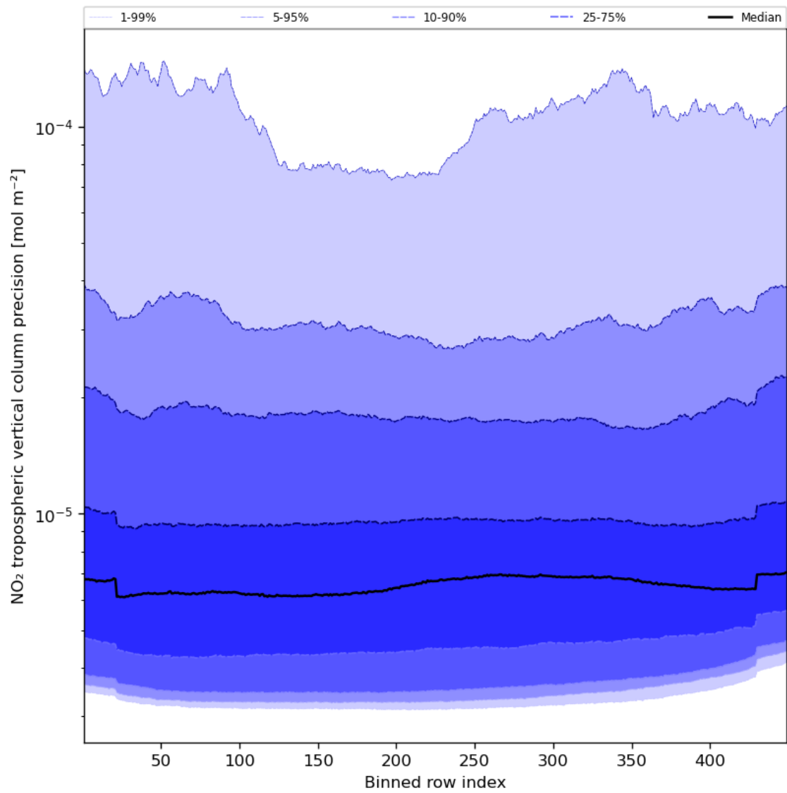
Figure 47: Along track statistics of “NO 2 tropospheric vertical column precision” for 2023-12-30 to 2023-12-31
