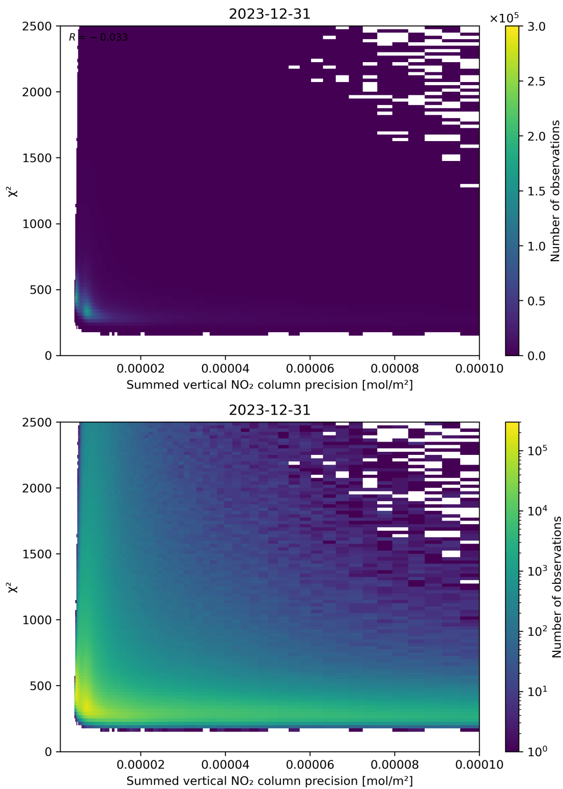
Figure 107: Scatter density plot of “Summed vertical NO 2 column precision” against “ \chi^2 ” for 2023-12-30 to 2023-12-31.
