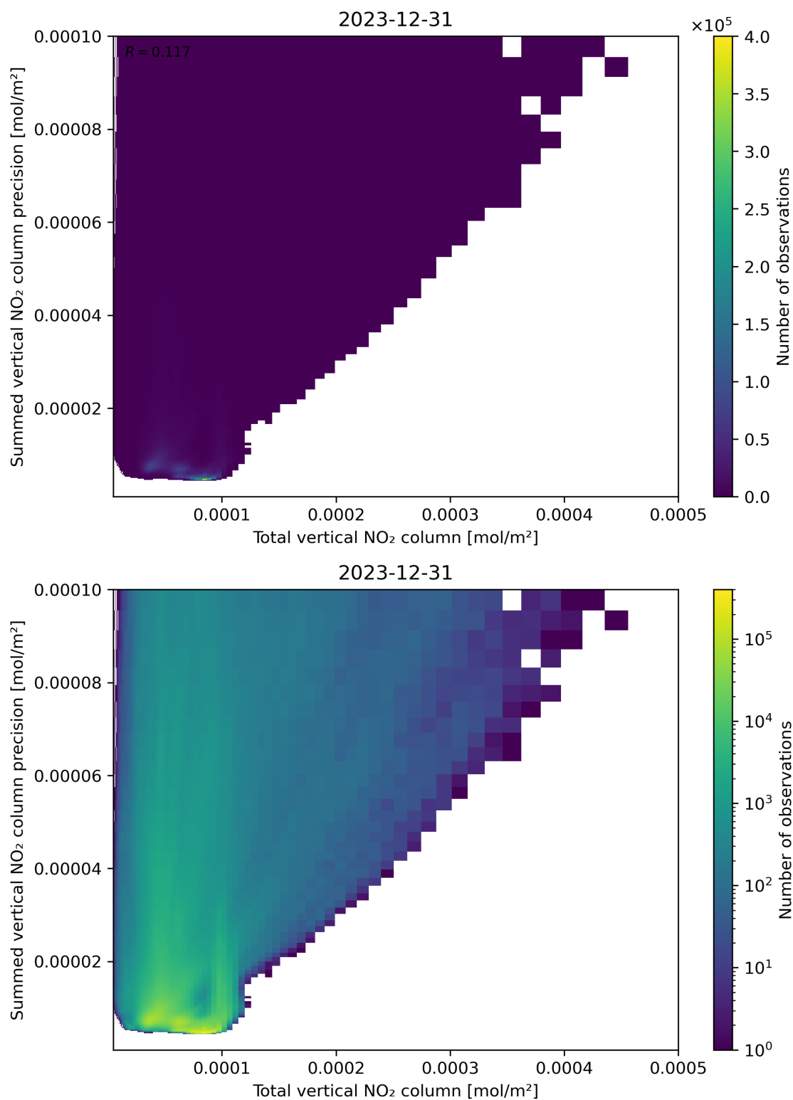
Figure 113: Scatter density plot of “Total vertical NO 2 column” against “Summed vertical NO 2 column precision” for 2023-12-30 to 2023-12-31.
