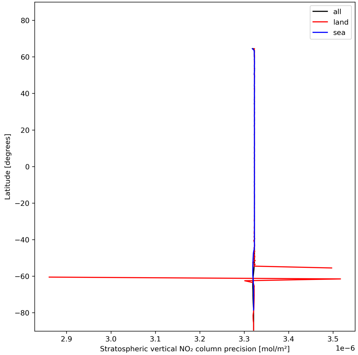
Figure 20: Zonal average of "Stratospheric vertical NO 2 column precision" for 2023-12-30 to 2023-12-31.
