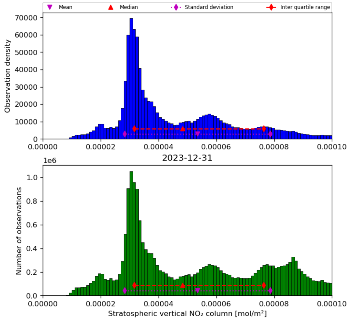
Figure 36: Histogram of “Stratospheric vertical NO 2 column” for 2023-12-30 to 2023-12-31
