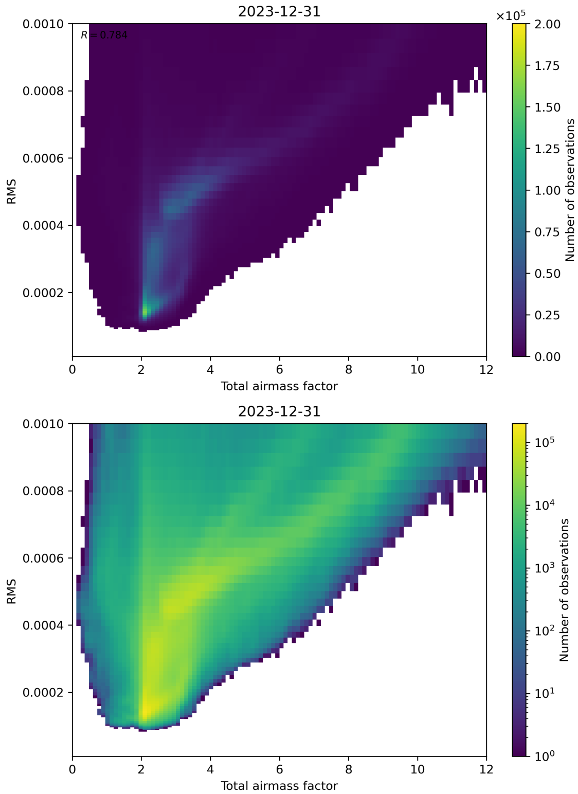
Figure 69: Scatter density plot of “Total airmass factor” against “RMS” for 2023-12-30 to 2023-12-31.
