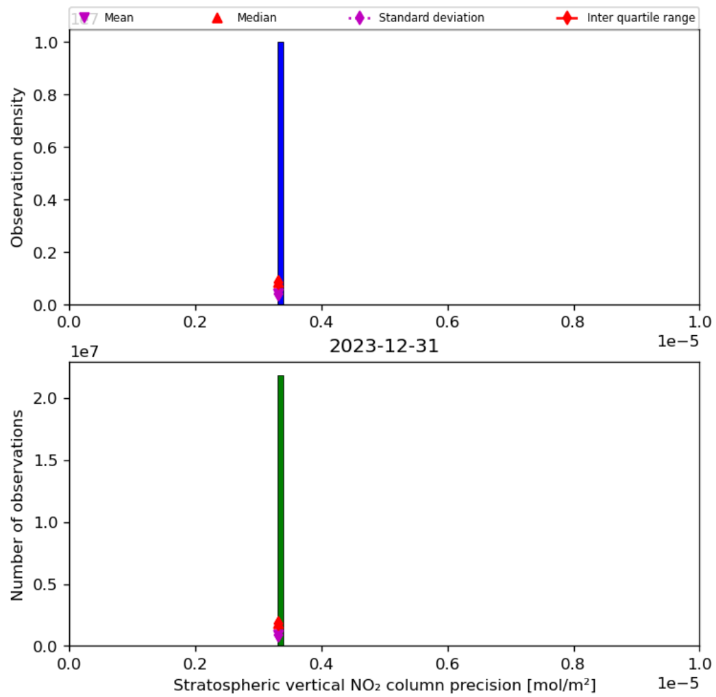
Figure 37: Histogram of “Stratospheric vertical NO 2 column precision” for 2023-12-30 to 2023-12-31
