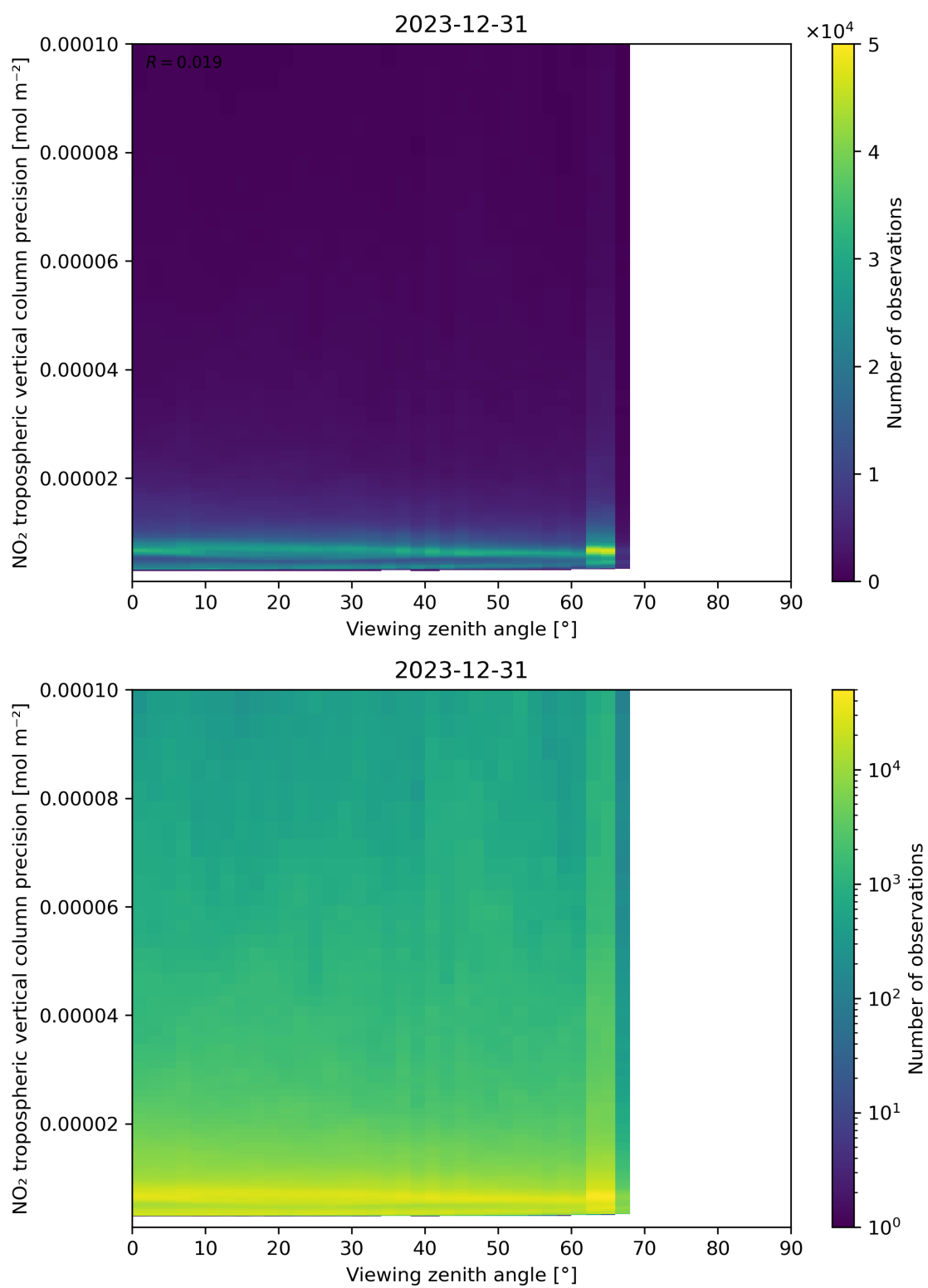
Figure 170: Scatter density plot of “Viewing zenith angle” against “NO 2 tropospheric vertical column precision” for 2023-12-30 to 2023-12-31.
