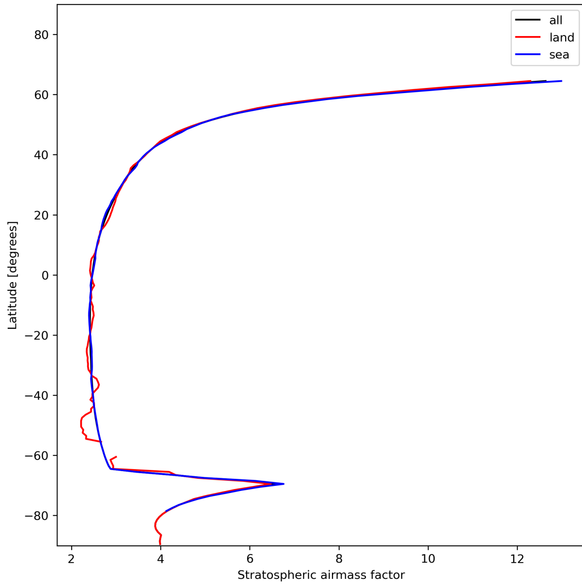
Figure 27: Zonal average of “Stratospheric airmass factor” for 2023-12-30 to 2023-12-31.
