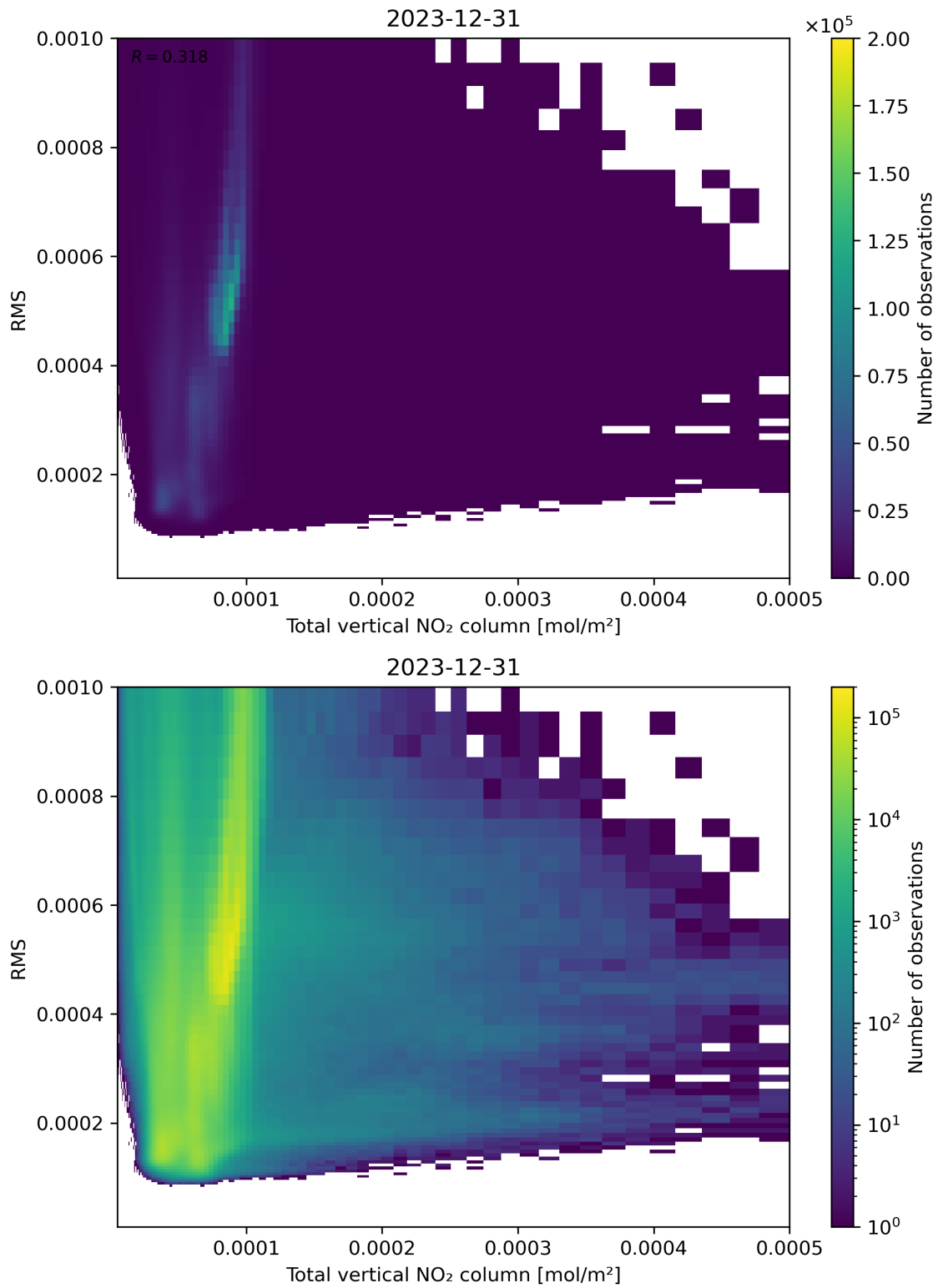
Figure 120: Scatter density plot of “Total vertical NO 2 column” against “RMS” for 2023-12-30 to 2023-12-31.
