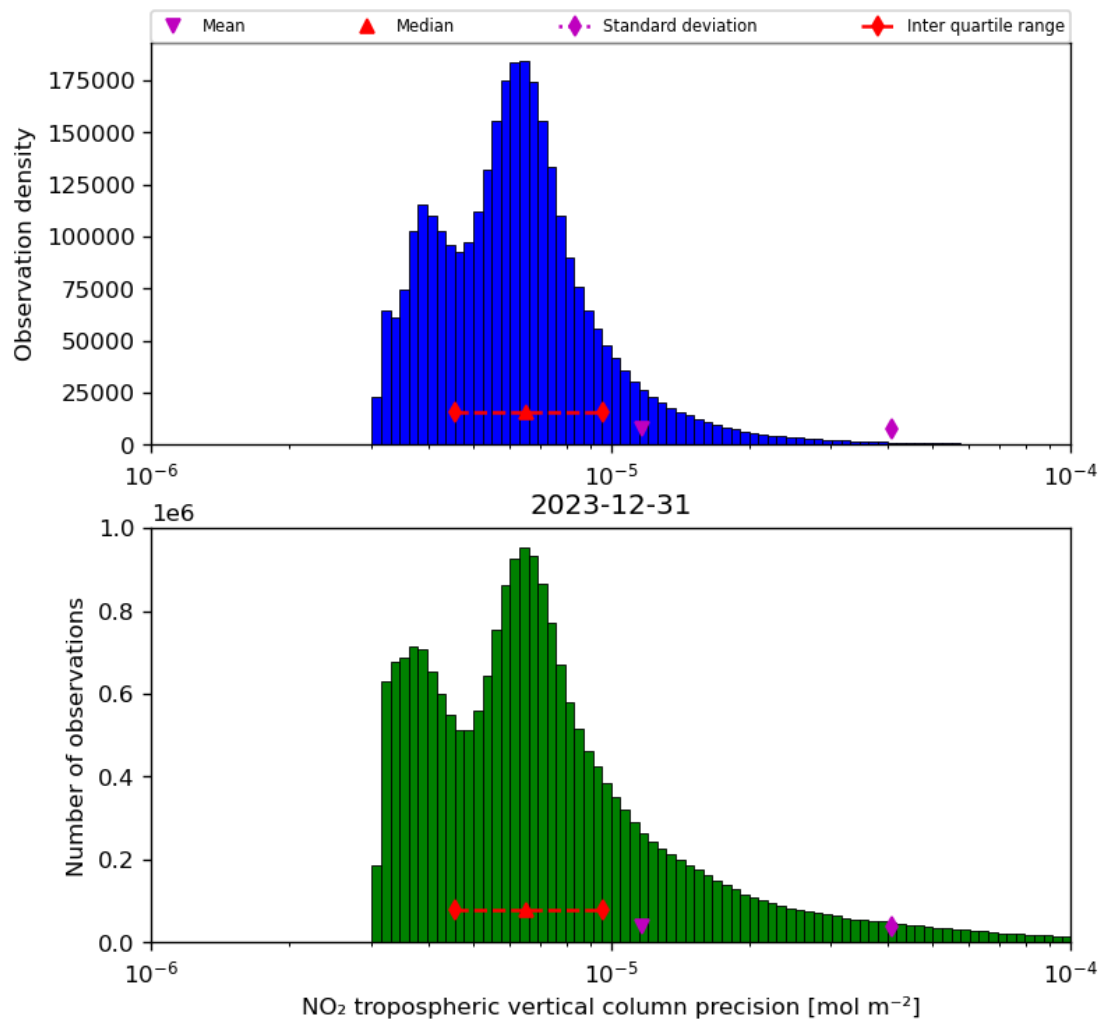
Figure 30: Histogram of “NO 2 tropospheric vertical column precision” for 2023-12-30 to 2023-12-31
