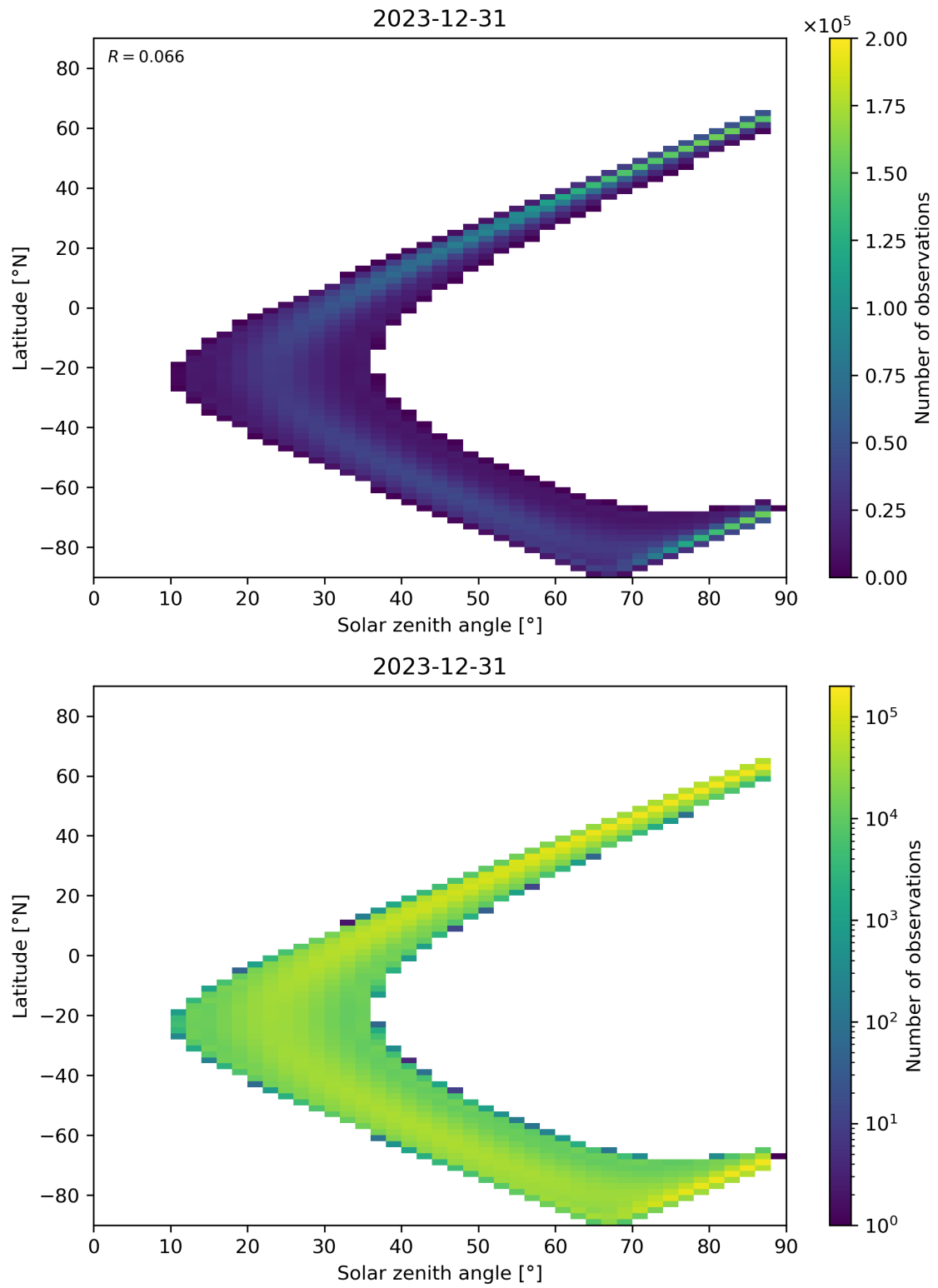
Figure 149: Scatter density plot of “Solar zenith angle” against “Latitude” for 2023-12-30 to 2023-12-31.
