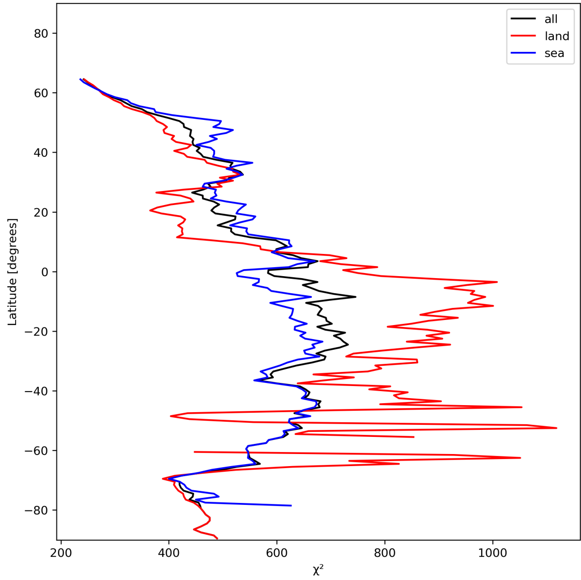
Figure 25: Zonal average of “ \chi^2 ” for 2023-12-30 to 2023-12-31.
