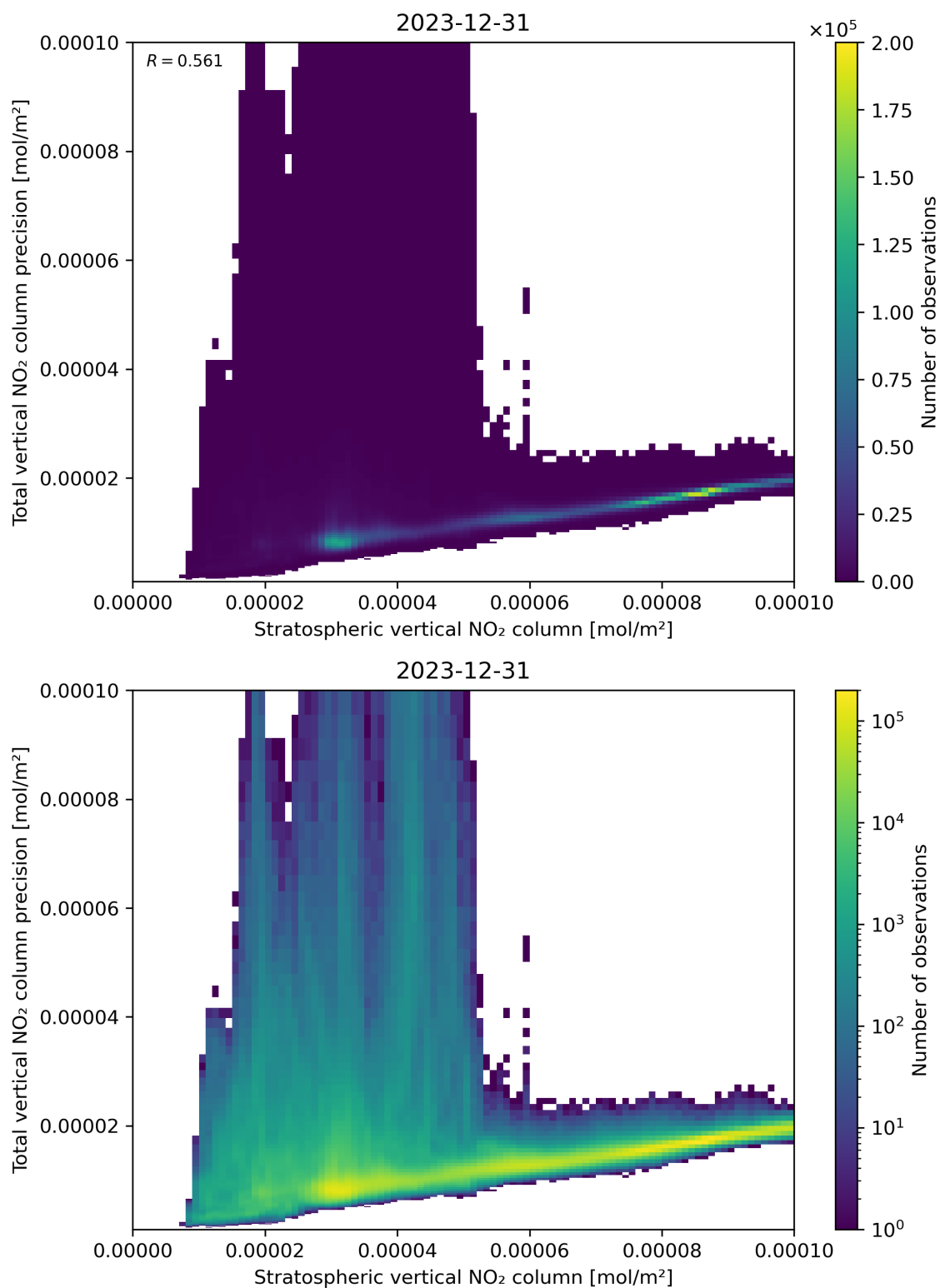
Figure 101: Scatter density plot of “Stratospheric vertical NO 2 column” against “Total vertical NO 2 column precision” for 2023-12-30 to 2023-12-31.
