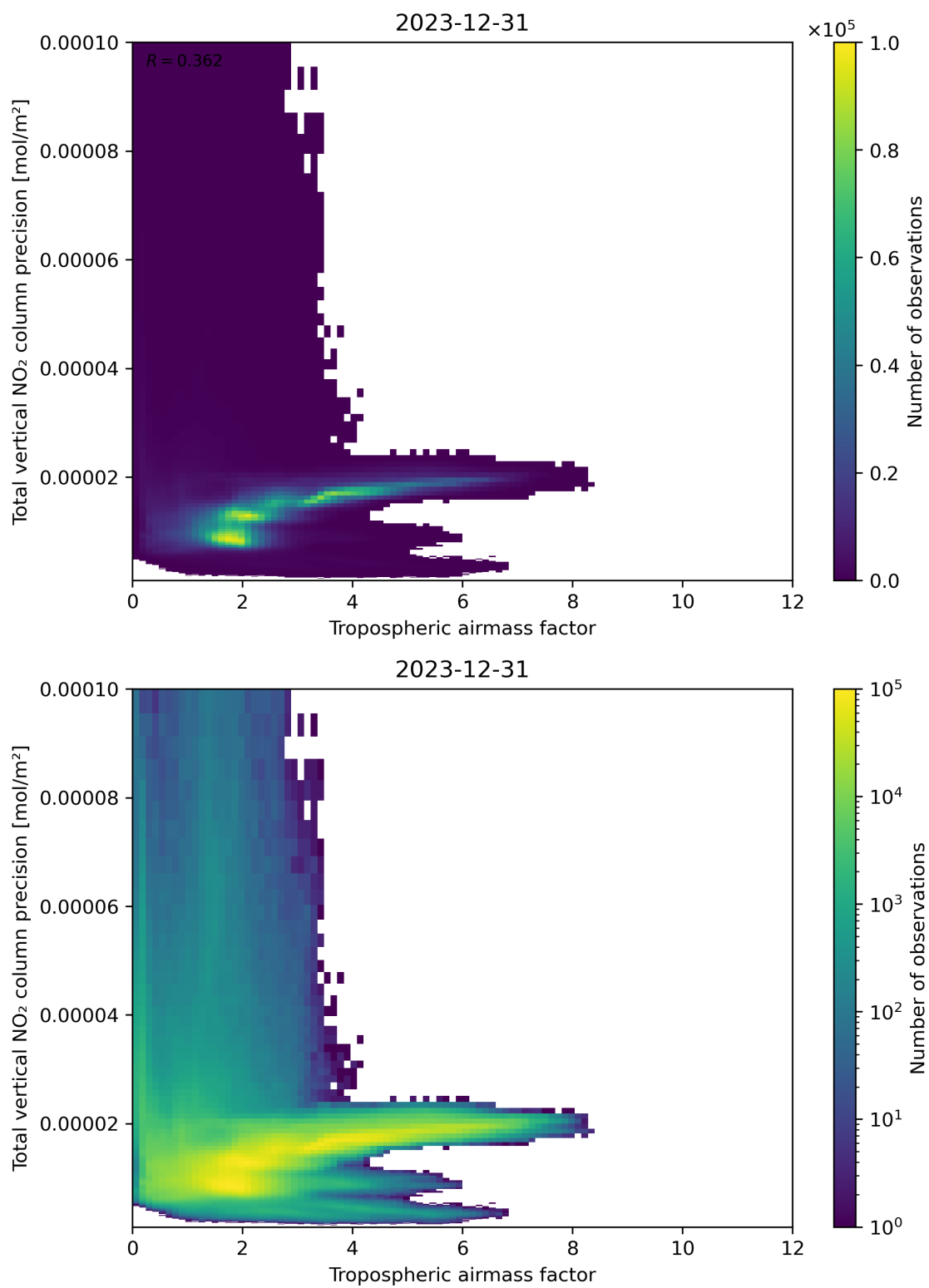
Figure 78: Scatter density plot of “Tropospheric air mass factor” against “Total vertical NO 2 column precision” for 2023-12-30 to 2023-12-31.
