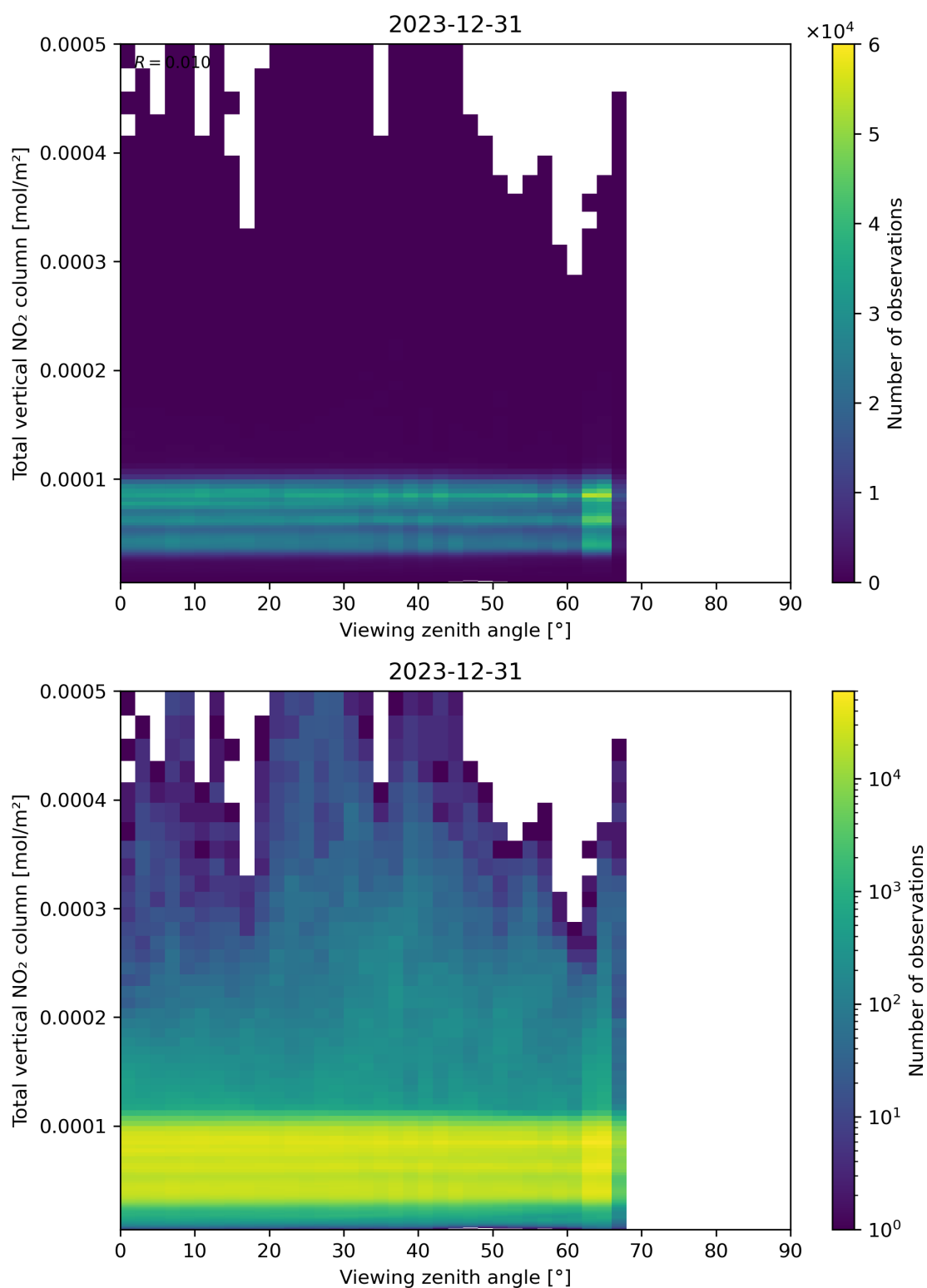
Figure 167: Scatter density plot of “Viewing zenith angle” against “Total vertical NO 2 column” for 2023-12-30 to 2023-12-31.
