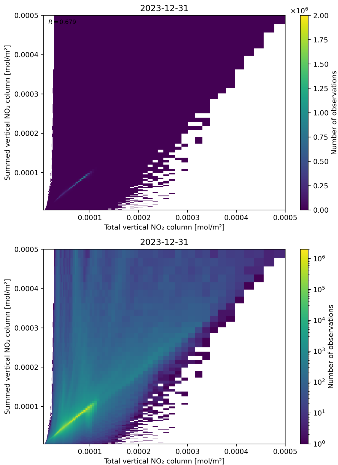
Figure 112: Scatter density plot of “Total vertical NO 2 column” against “Summed vertical NO 2 column” for 2023-12-30 to 2023-12-31.
