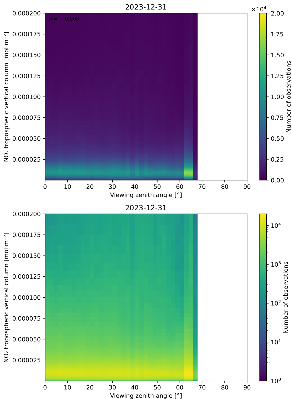
Figure 169: Scatter density plot of “Viewing zenith angle” against “NO 2 tropospheric vertical column” for 2023-12-30 to 2023-12-31.
