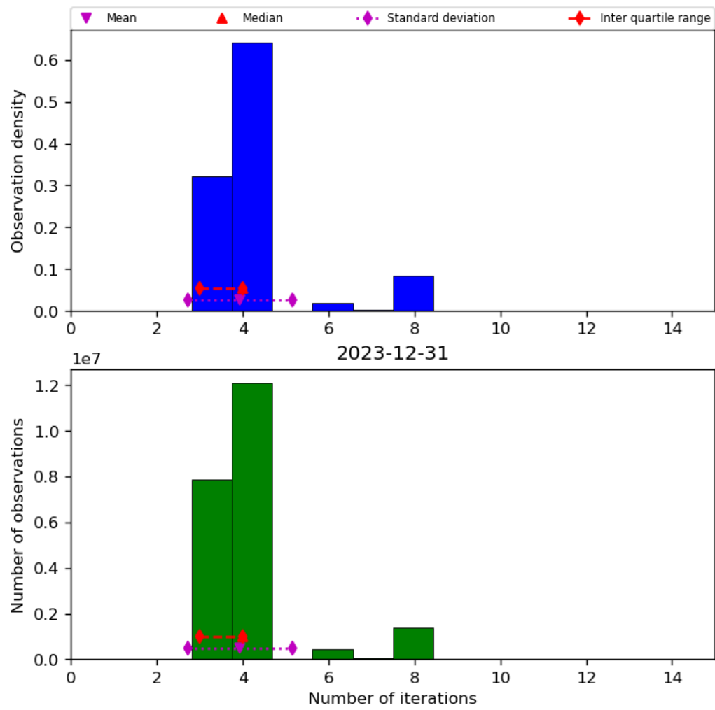
Figure 34: Histogram of “Number of iterations” for 2023-12-30 to 2023-12-31
