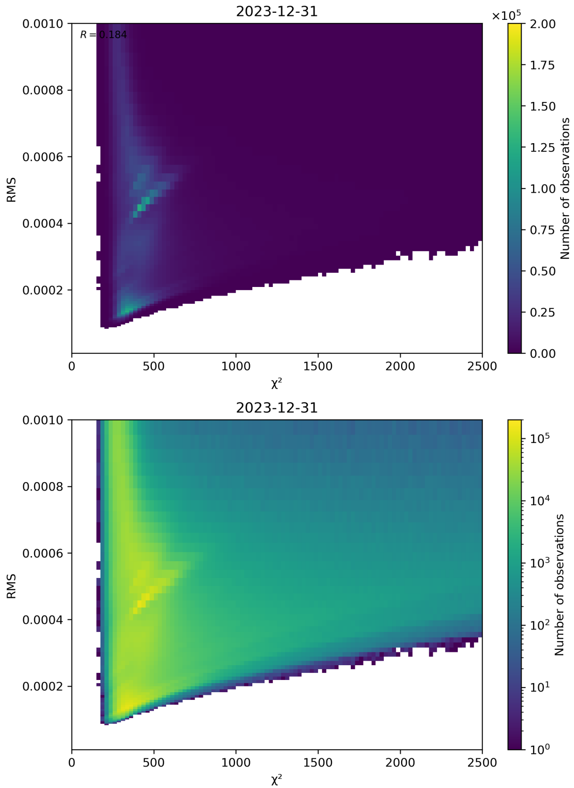
Figure 82: Scatter density plot of “ \chi^2 ” against “RMS” for 2023-12-30 to 2023-12-31.
