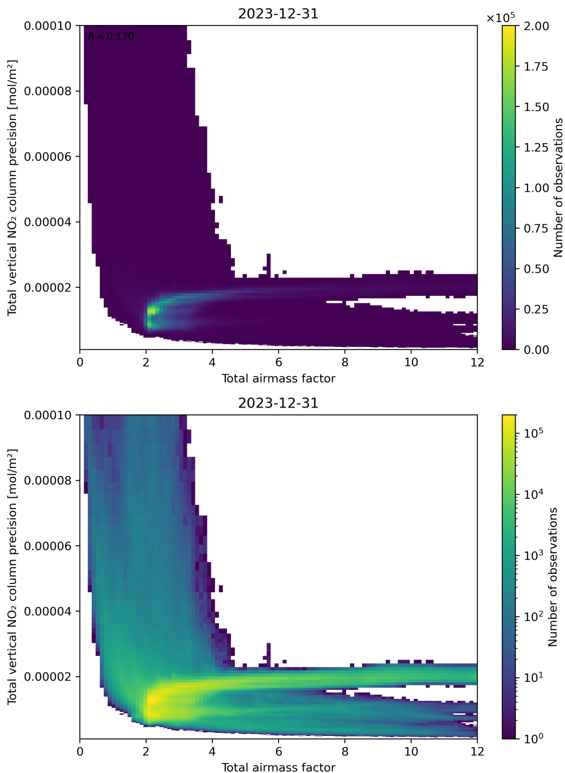
Figure 68: Scatter density plot of “Total airmass factor” against “Total vertical NO 2 column precision” for 2023-12-30 to 2023-12-31.
