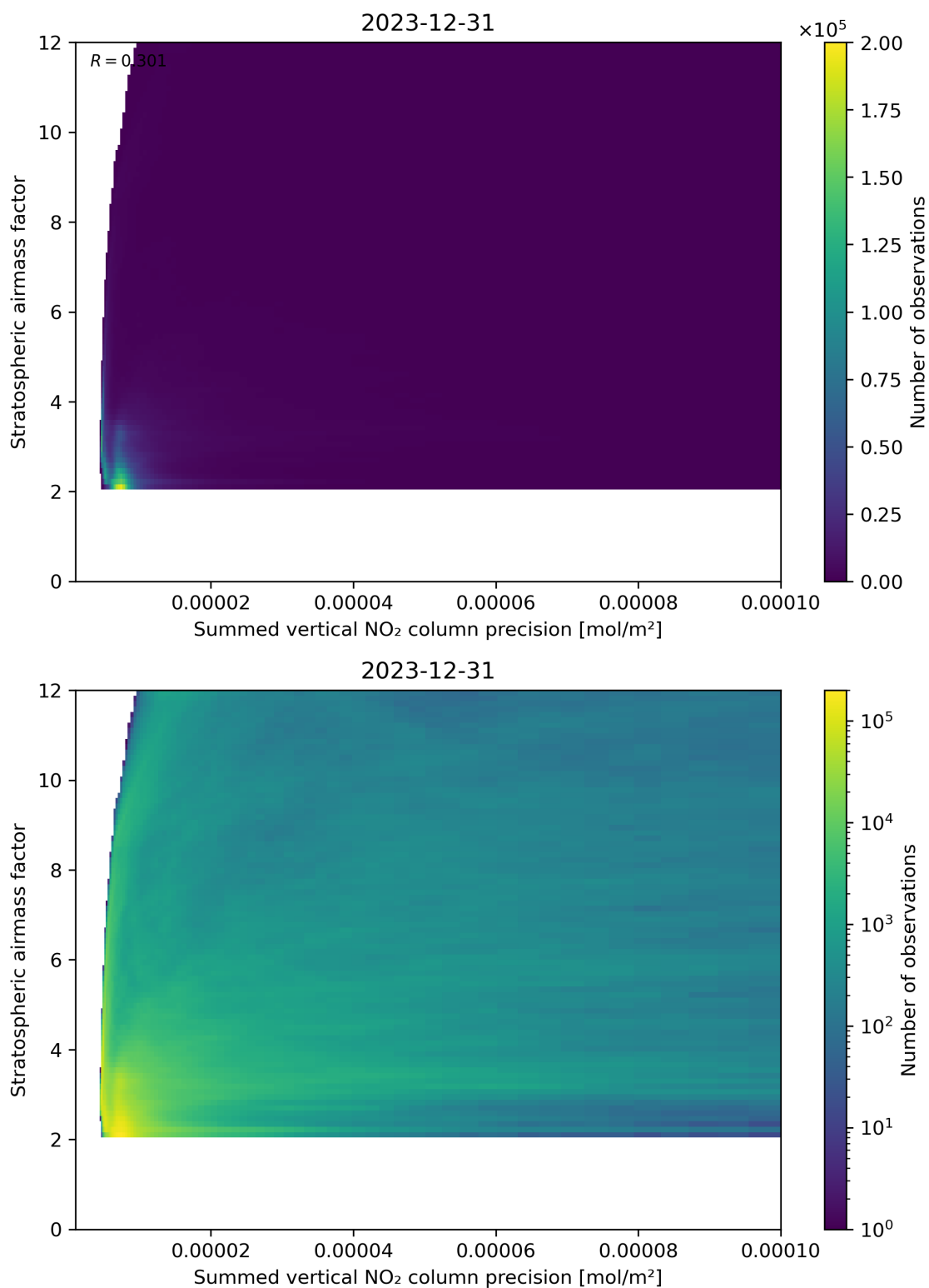
Figure 106: Scatter density plot of “Summed vertical NO 2 column precision” against “Stratospheric airmass factor” for 2023-12-30 to 2023-12-31.
