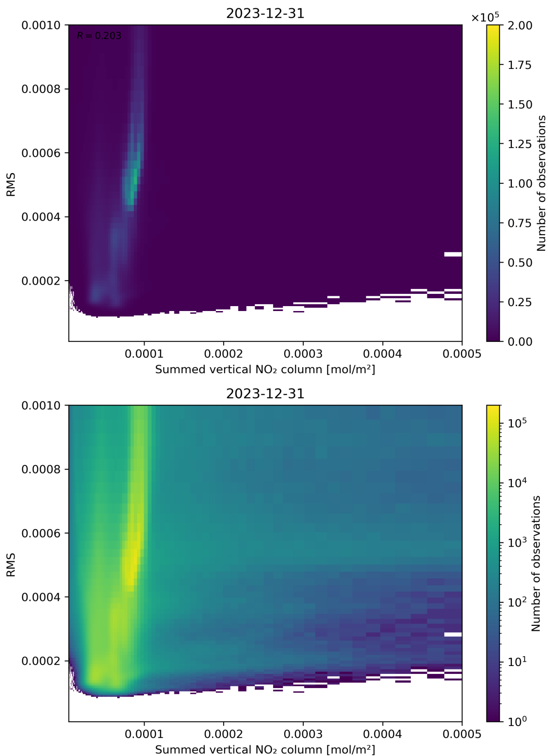
Figure 109: Scatter density plot of “Summed vertical NO 2 column” against “RMS” for 2023-12-30 to 2023-12-31.
