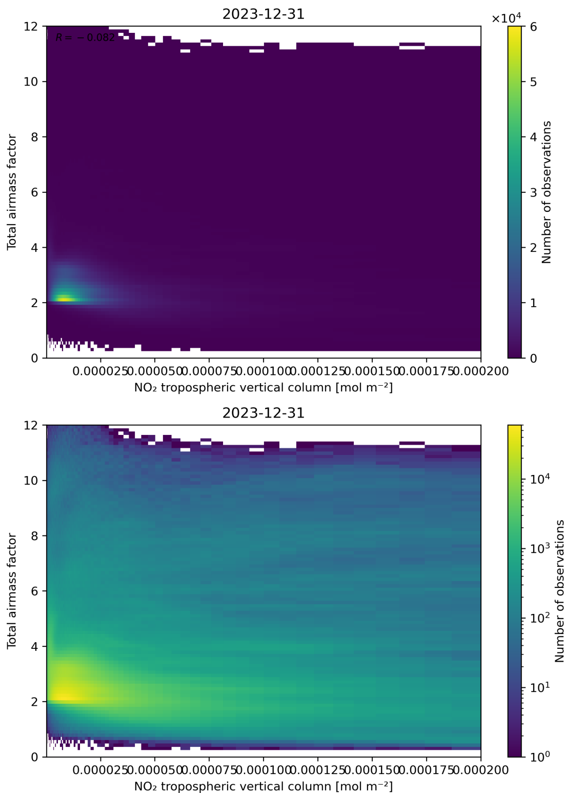
Figure 122: Scatter density plot of “NO 2 tropospheric vertical column” against “Total air mass factor” for 2023-12-30 to 2023-12-31.
