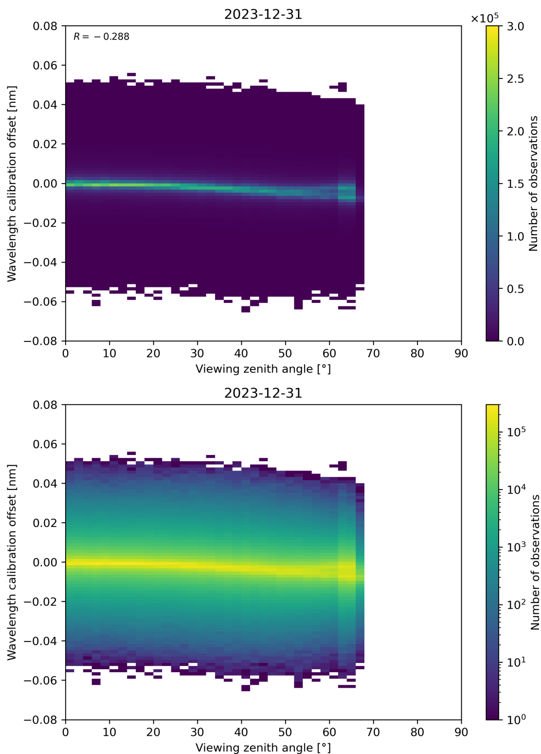
Figure 173: Scatter density plot of “Viewing zenith angle” against “Wavelength calibration offset” for 2023-12-30 to 2023-12-31.
