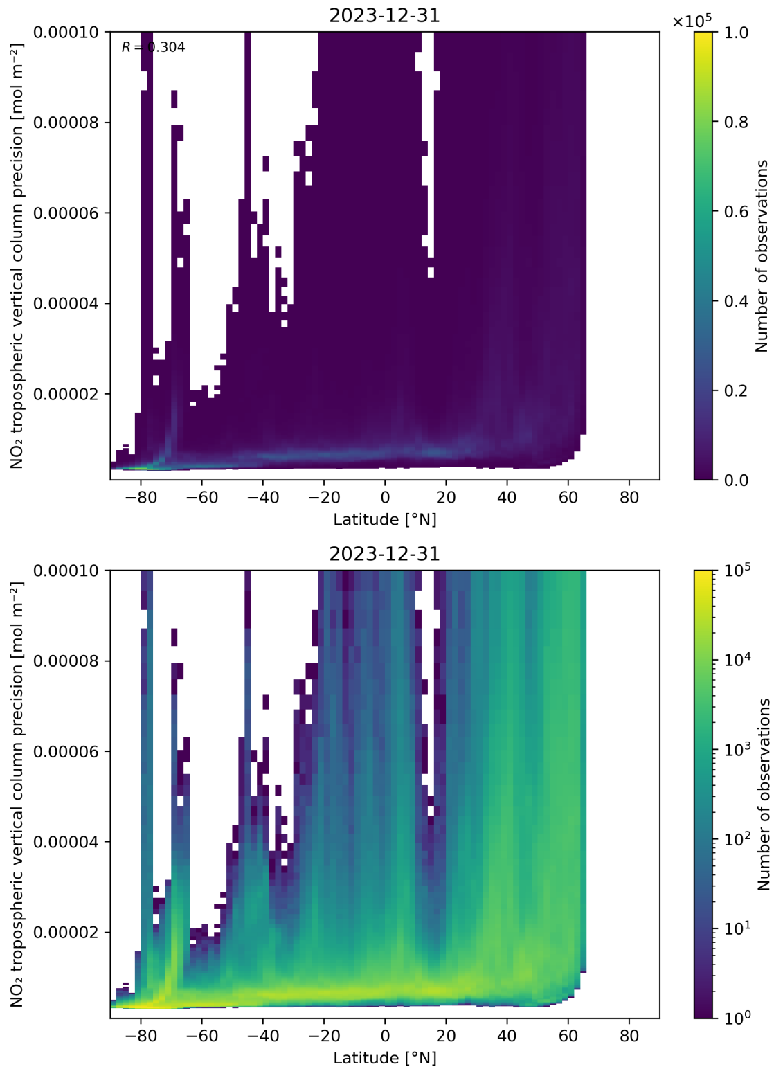
Figure 93: Scatter density plot of “Latitude” against “NO 2 tropospheric vertical column precision” for 2023-12-30 to 2023-12-31.
