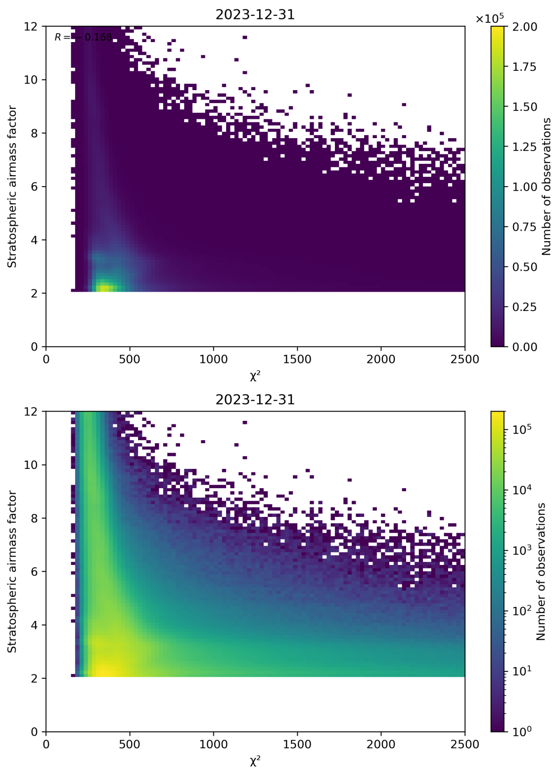
Figure 81: Scatter density plot of “ \chi^2 ” against “Stratospheric air mass factor” for 2023-12-30 to 2023-12-31.
