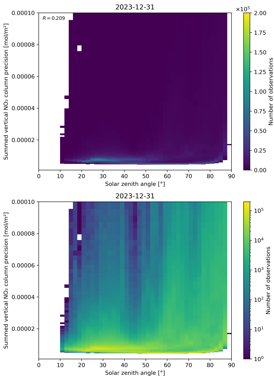
Figure 152: Scatter density plot of “Solar zenith angle” against “Summed vertical NO 2 column precision” for 2023-12-30 to 2023-12-31.
