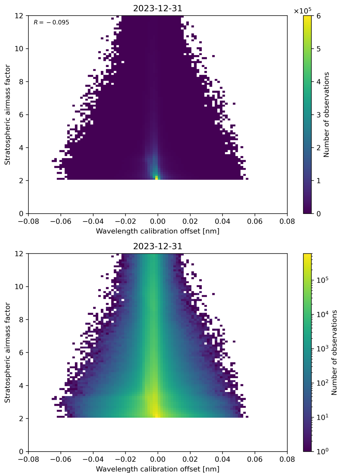
Figure 174: Scatter density plot of “Wavelength calibration offset” against “Stratospheric airmass factor” for 2023-12-30 to 2023-12-31.
