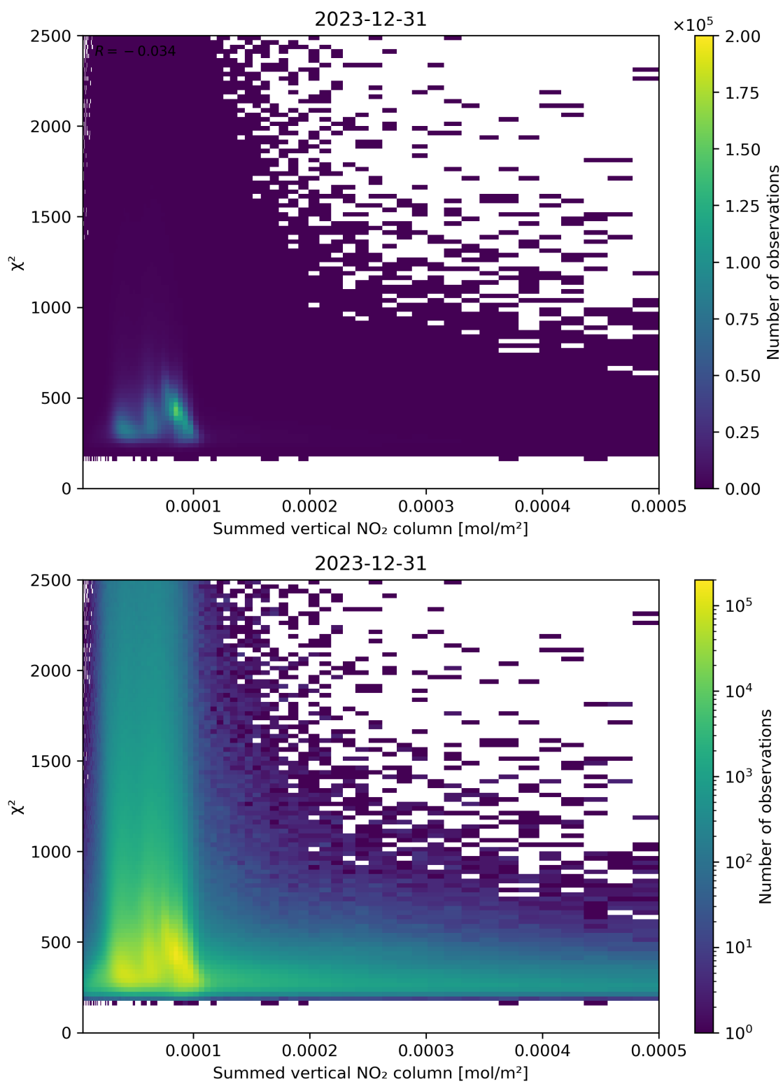
Figure 104: Scatter density plot of “Summed vertical NO 2 column” against “ \chi^2 ” for 2023-12-30 to 2023-12-31.
