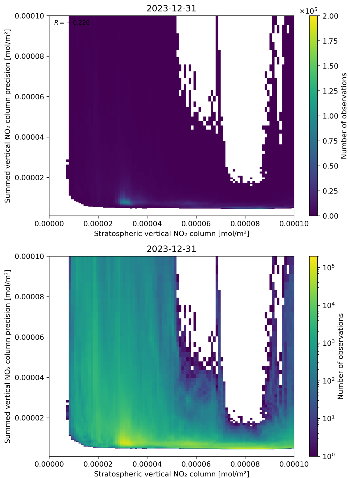
Figure 99: Scatter density plot of “Stratospheric vertical NO 2 column” against “Summed vertical NO 2 column precision” for 2023-12-30 to 2023-12-31.
