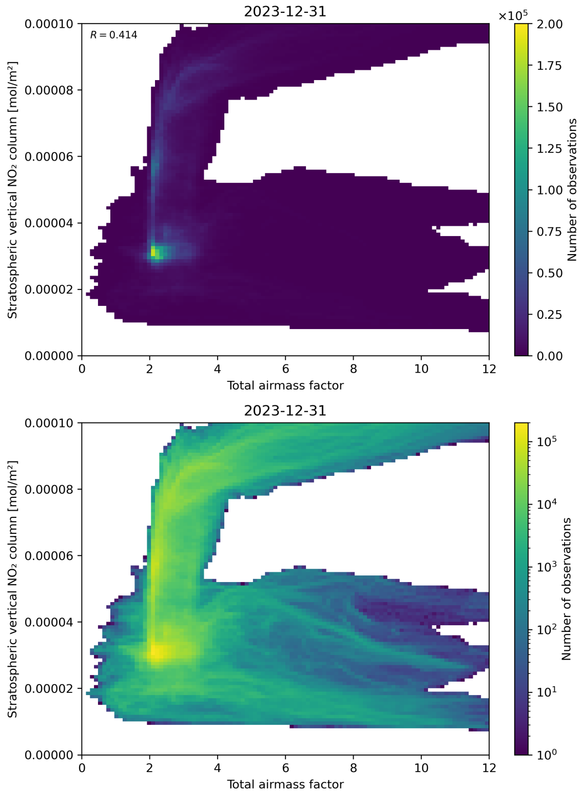
Figure 64: Scatter density plot of “Total airmass factor” against “Stratospheric vertical \text{NO}_2 column” for 2023-12-30 to 2023-12-31.
