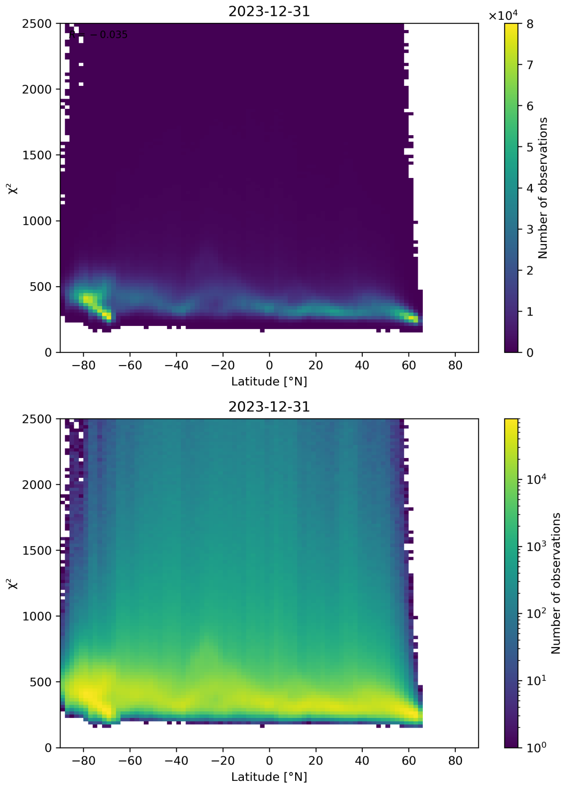
Figure 86: Scatter density plot of “Latitude” against “ \chi^2 ” for 2023-12-30 to 2023-12-31.
