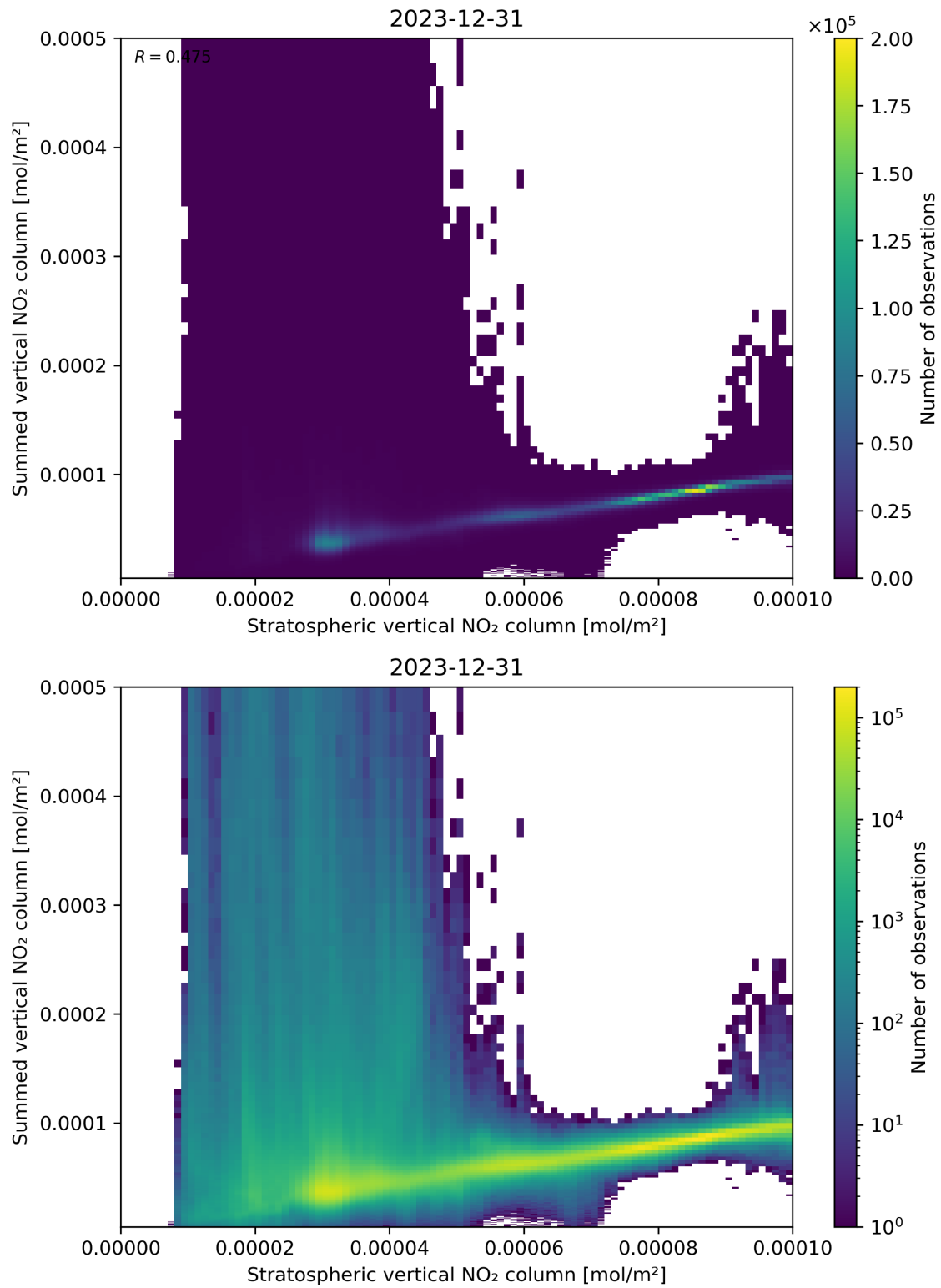
Figure 98: Scatter density plot of “Stratospheric vertical NO 2 column” against “Summed vertical NO 2 column” for 2023-12-30 to 2023-12-31.
