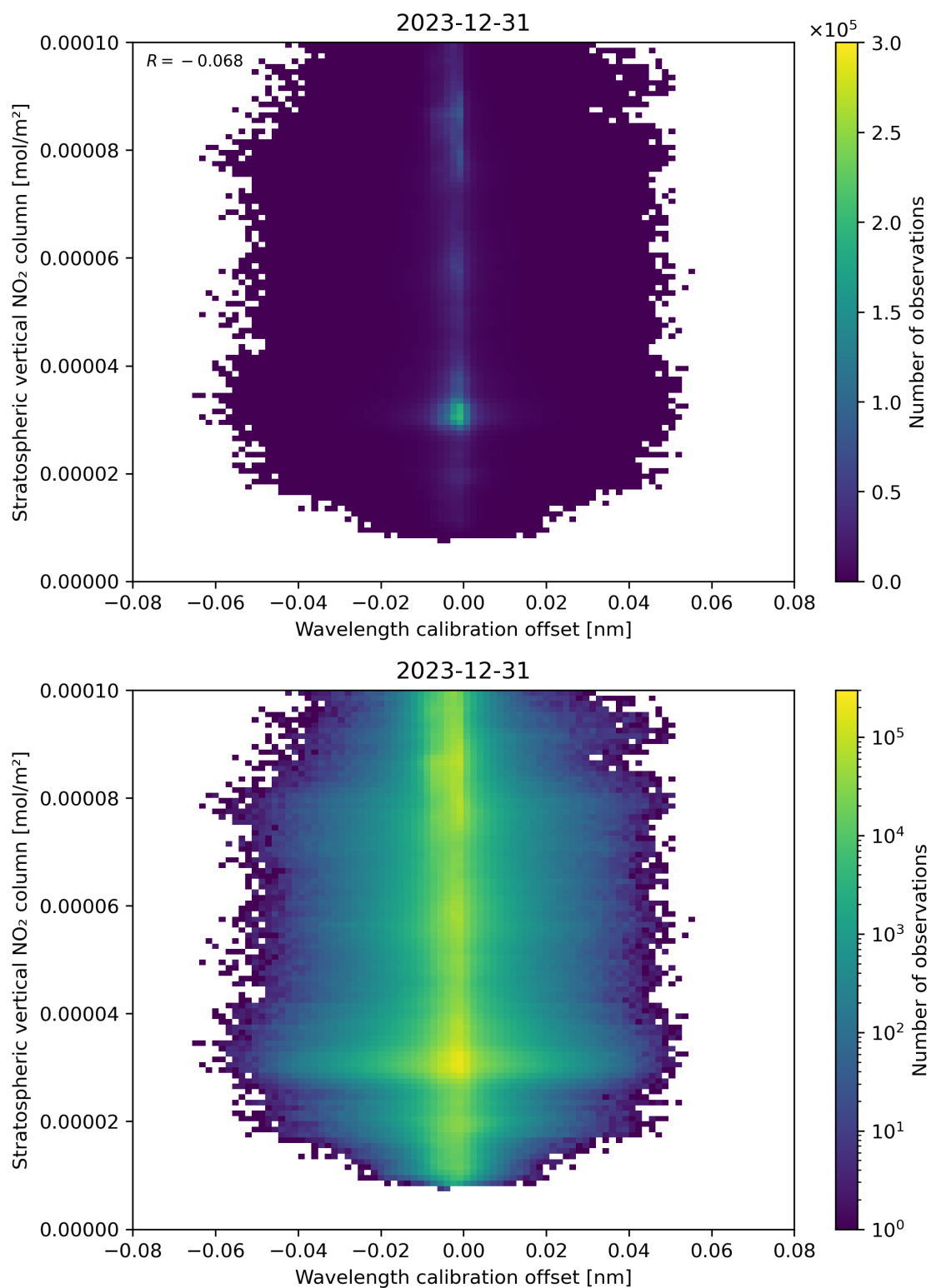
Figure 176: Scatter density plot of “Wavelength calibration offset” against “Stratospheric vertical NO 2 column” for 2023-12-30 to 2023-12-31.
