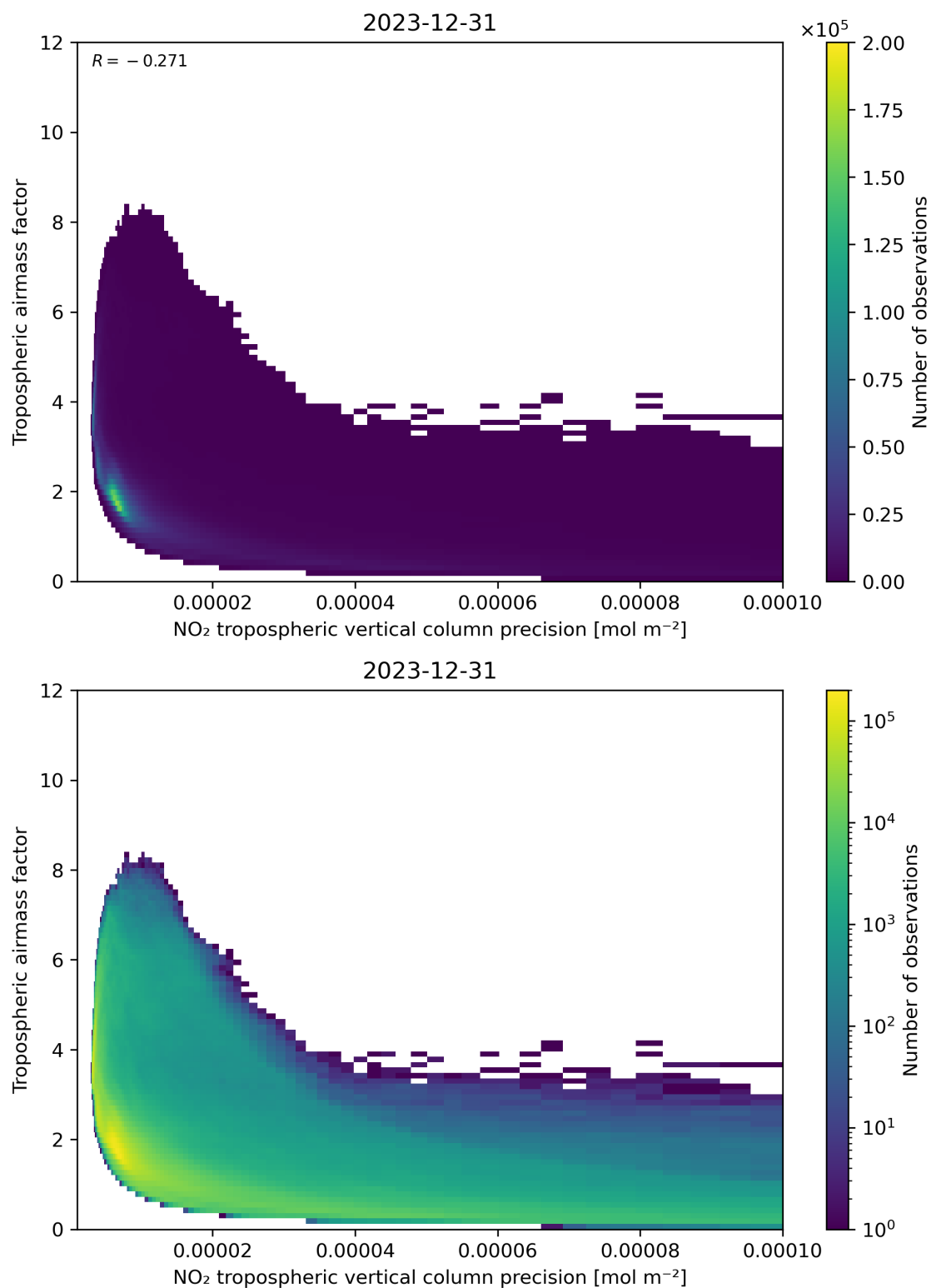
Figure 133: Scatter density plot of “NO 2 tropospheric vertical column precision” against “Tropospheric airmass factor” for 2023-12-30 to 2023-12-31.
