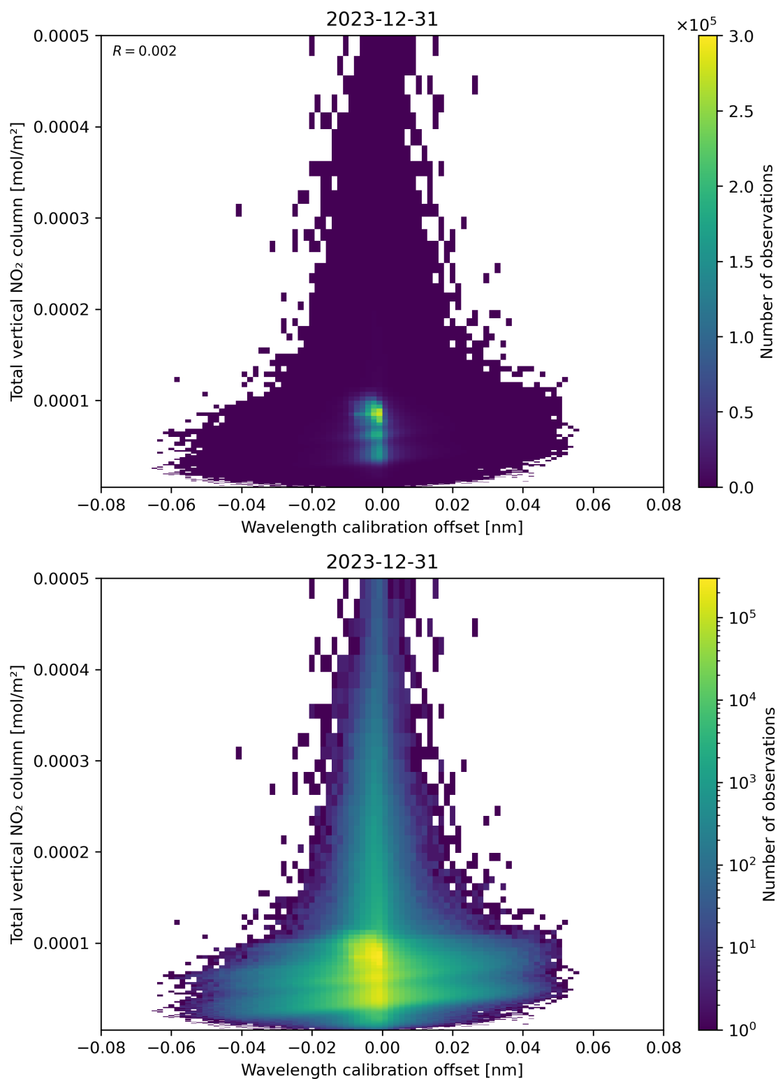
Figure 179: Scatter density plot of “Wavelength calibration offset” against “Total vertical NO 2 column” for 2023-12-30 to 2023-12-31.
