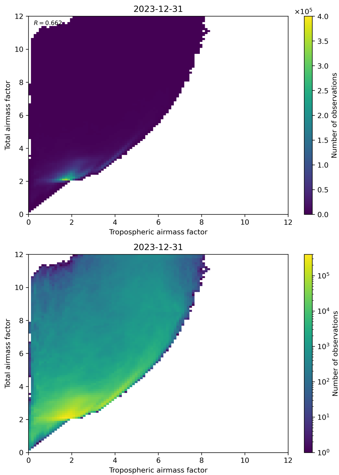
Figure 72: Scatter density plot of “Tropospheric airmass factor” against “Total airmass factor” for 2023-12-30 to 2023-12-31.
