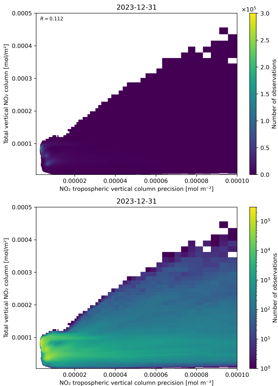
Figure 138: Scatter density plot of “NO 2 tropospheric vertical column precision” against “Total vertical NO 2 column” for 2023-12-30 to 2023-12-31.
