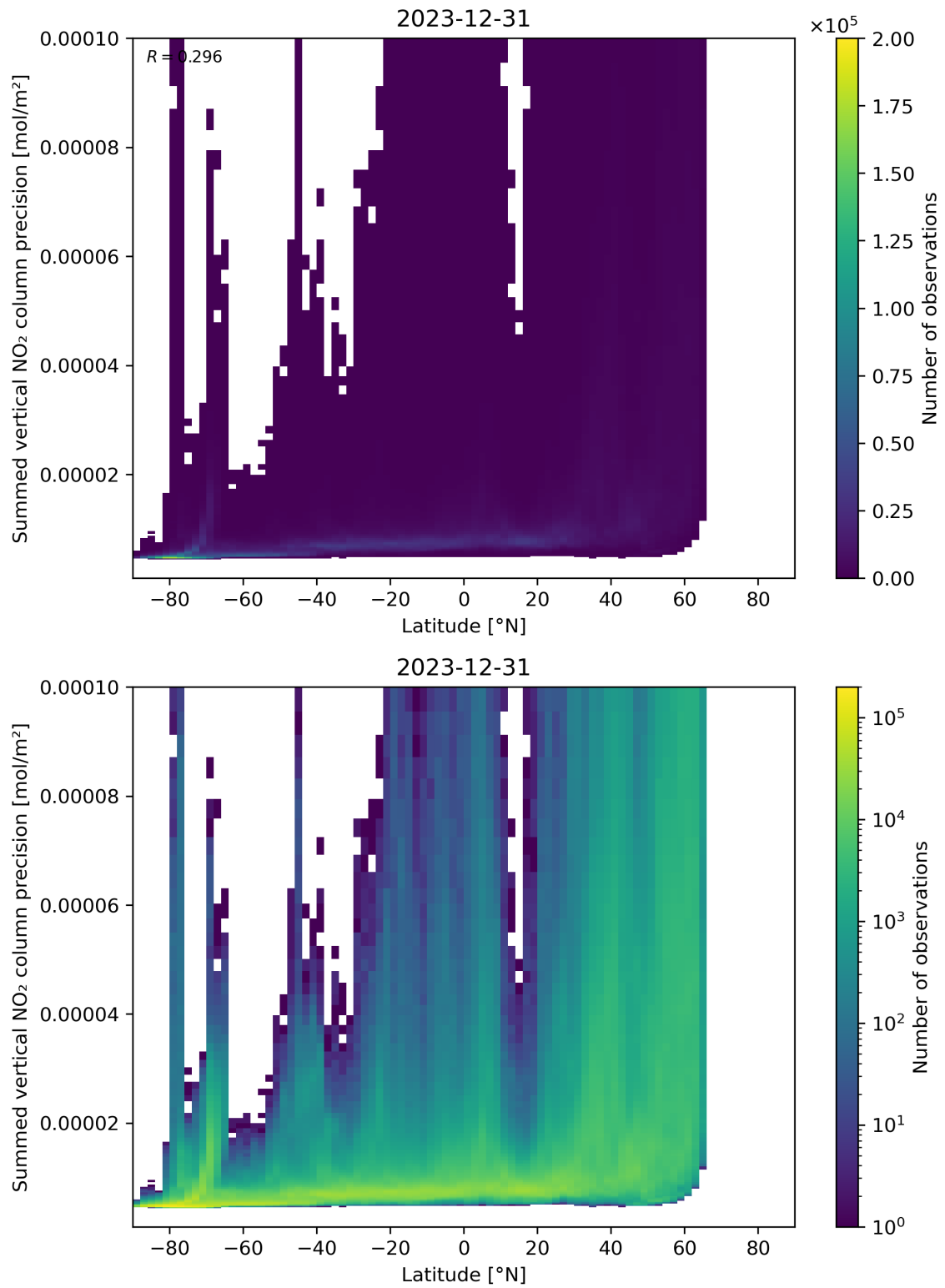
Figure 89: Scatter density plot of “Latitude” against “Summed vertical NO 2 column precision” for 2023-12-30 to 2023-12-31.
