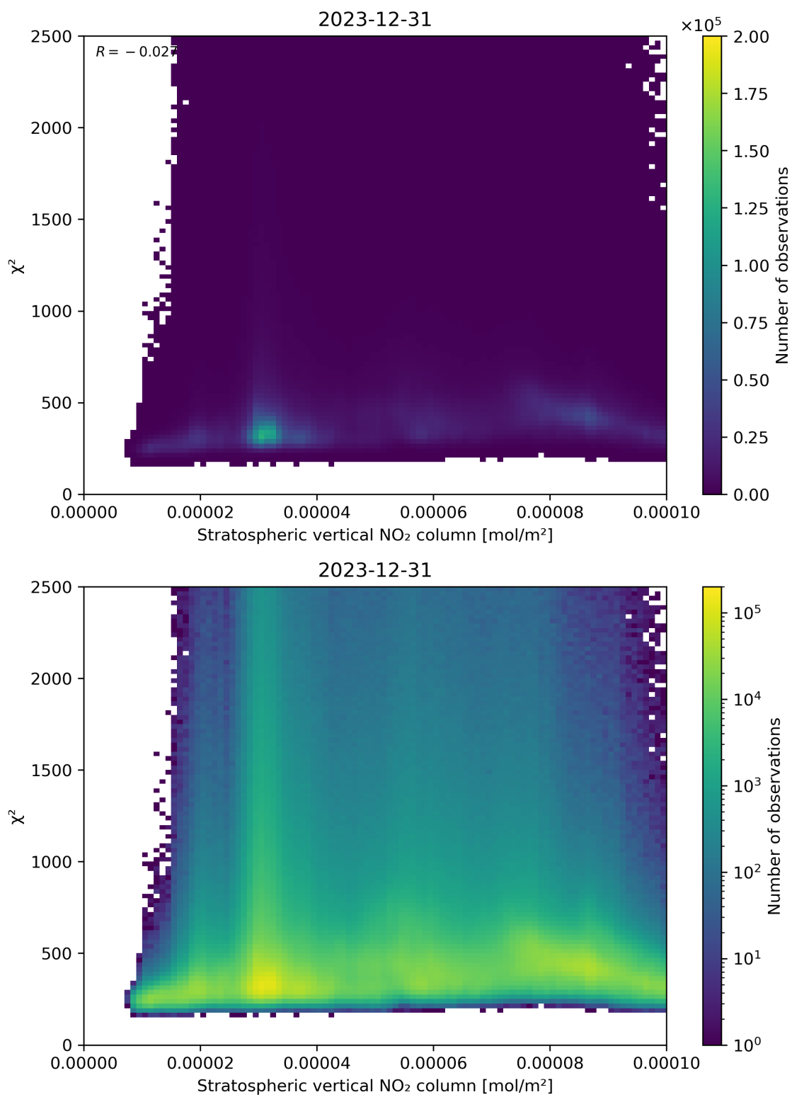
Figure 97: Scatter density plot of “Stratospheric vertical NO 2 column” against “ \chi^2 ” for 2023-12-30 to 2023-12-31.
