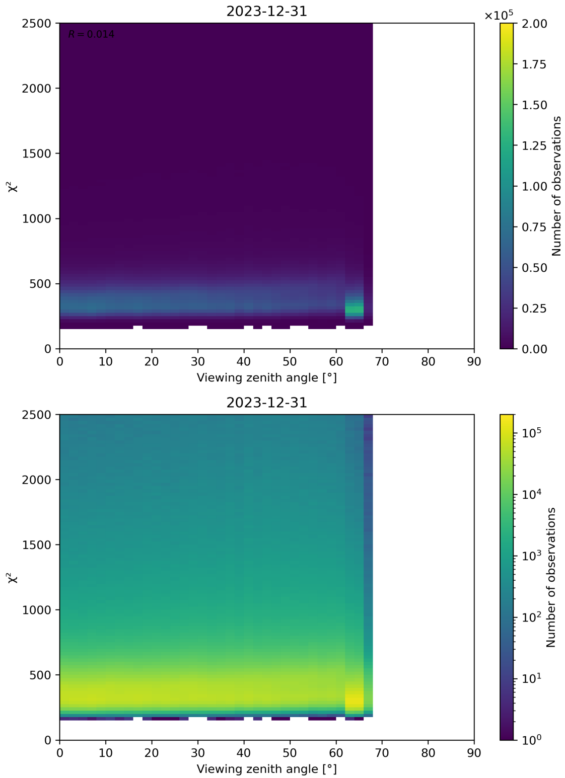
Figure 162: Scatter density plot of “Viewing zenith angle” against “ \chi^2 ” for 2023-12-30 to 2023-12-31.
