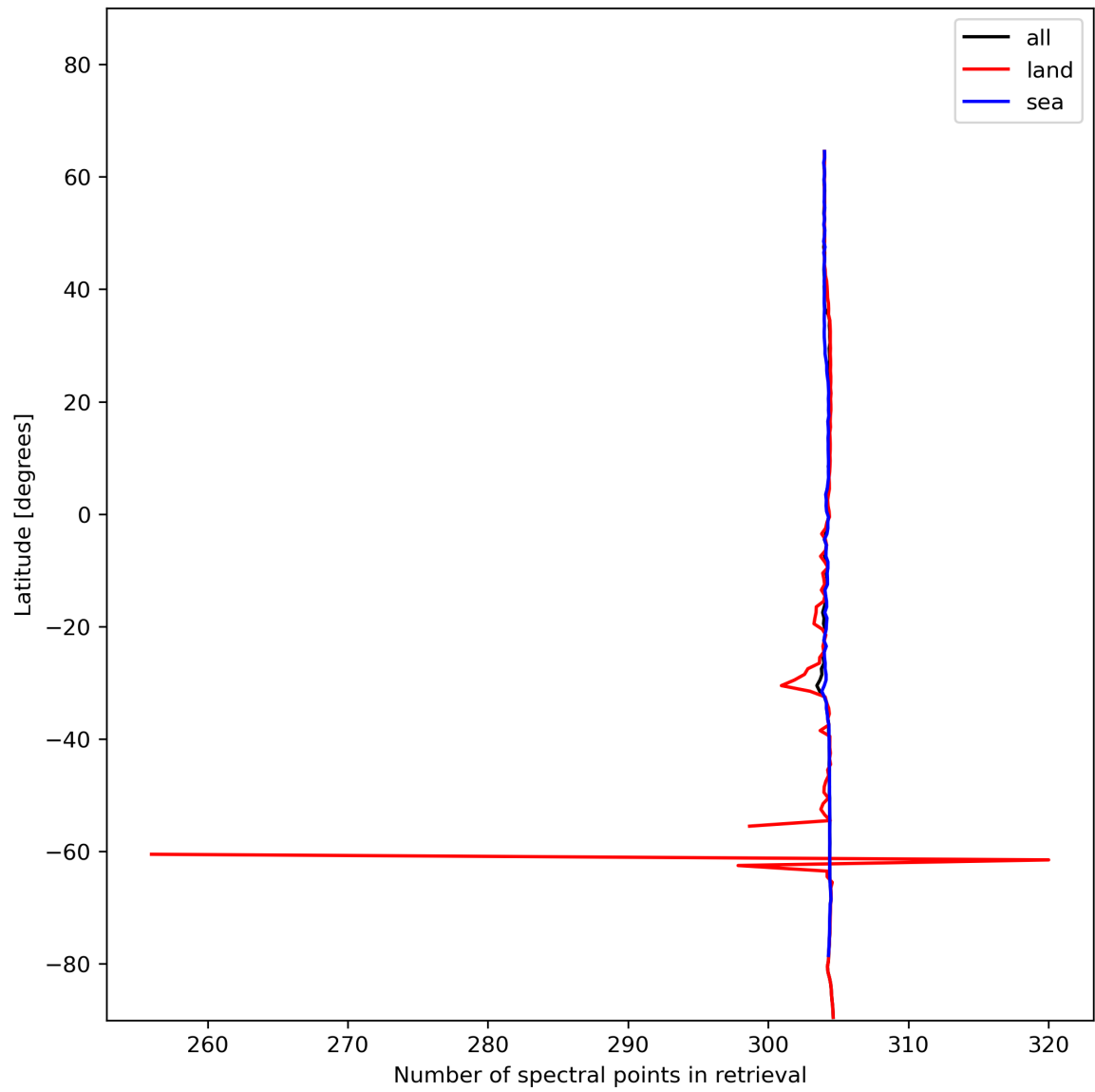
Figure 16: Zonal average of “Number of spectral points in retrieval” for 2023-12-30 to 2023-12-31.
