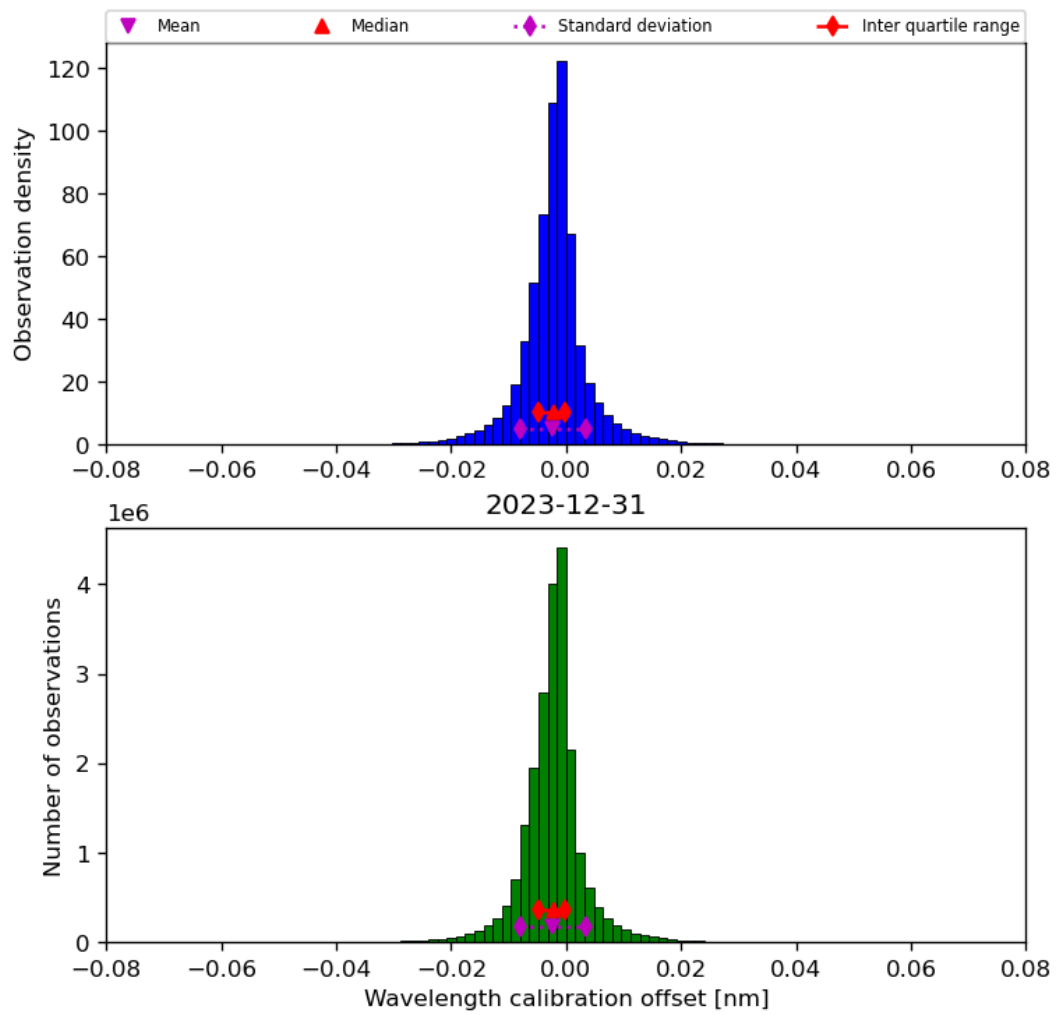
Figure 35: Histogram of “Wavelength calibration offset” for 2023-12-30 to 2023-12-31
