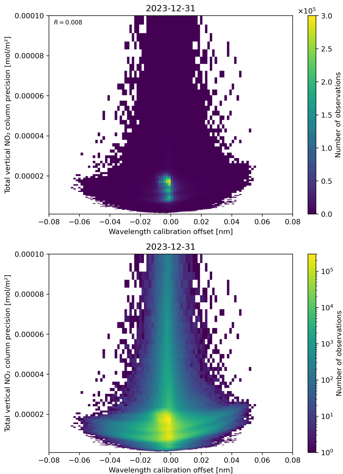
Figure 180: Scatter density plot of “Wavelength calibration offset” against “Total vertical NO 2 column precision” for 2023-12-30 to 2023-12-31.
