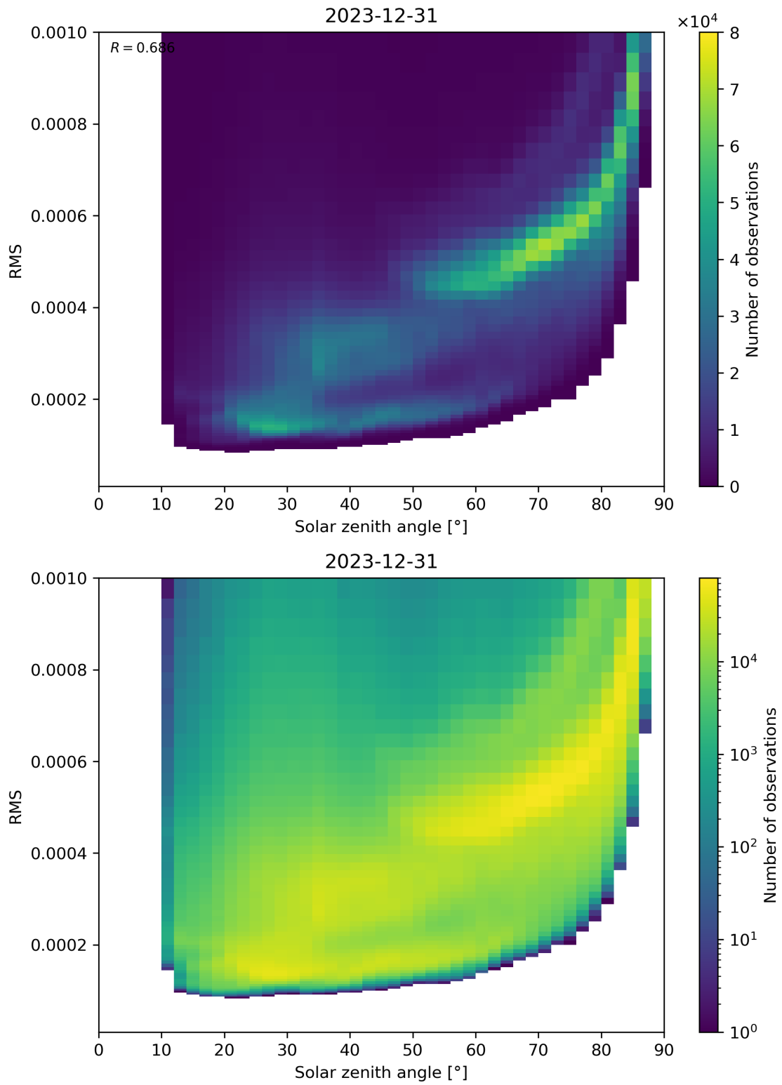
Figure 157: Scatter density plot of “Solar zenith angle” against “RMS” for 2023-12-30 to 2023-12-31.
