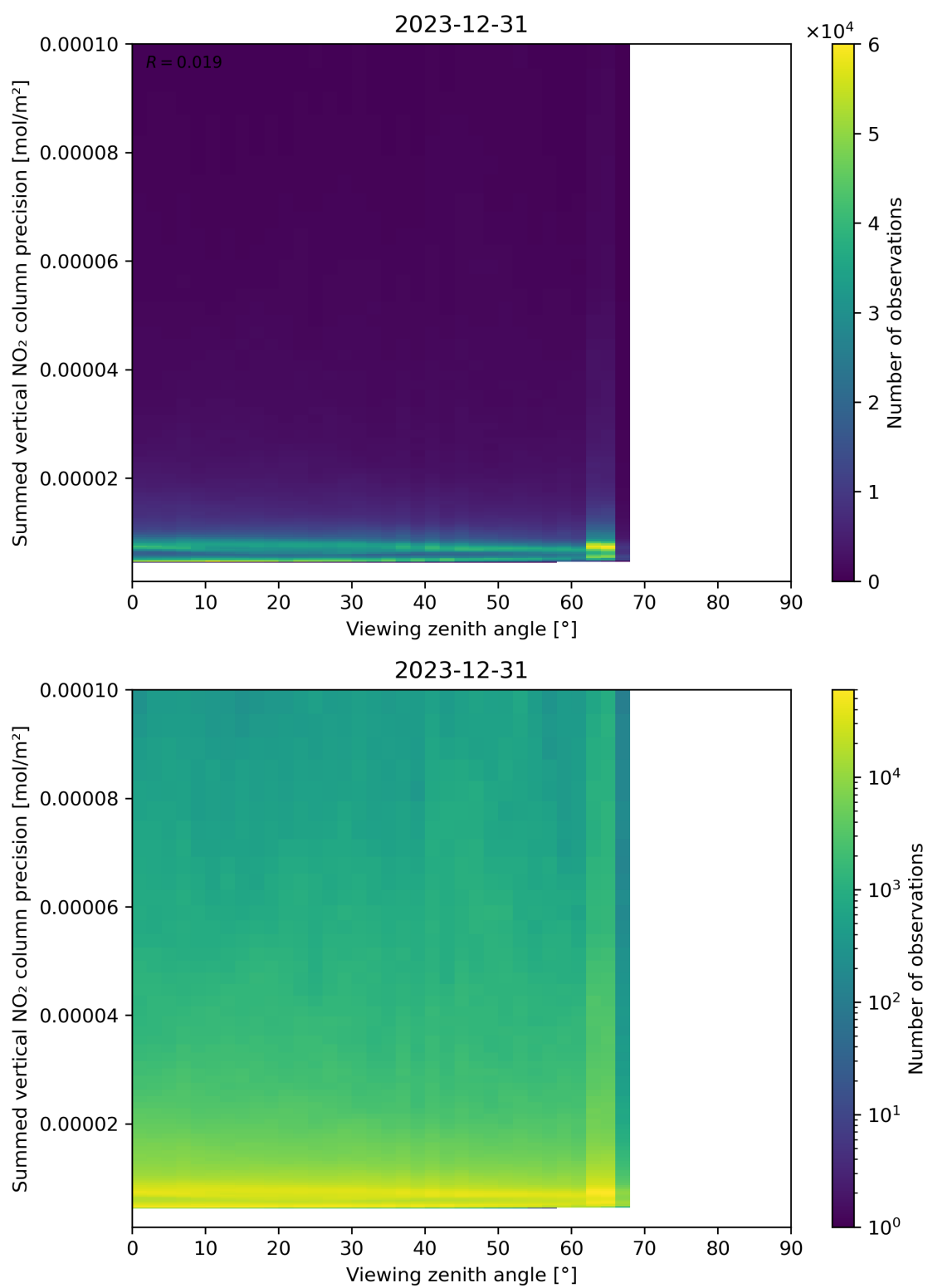
Figure 166: Scatter density plot of “Viewing zenith angle” against “Summed vertical NO 2 column precision” for 2023-12-30 to 2023-12-31.
