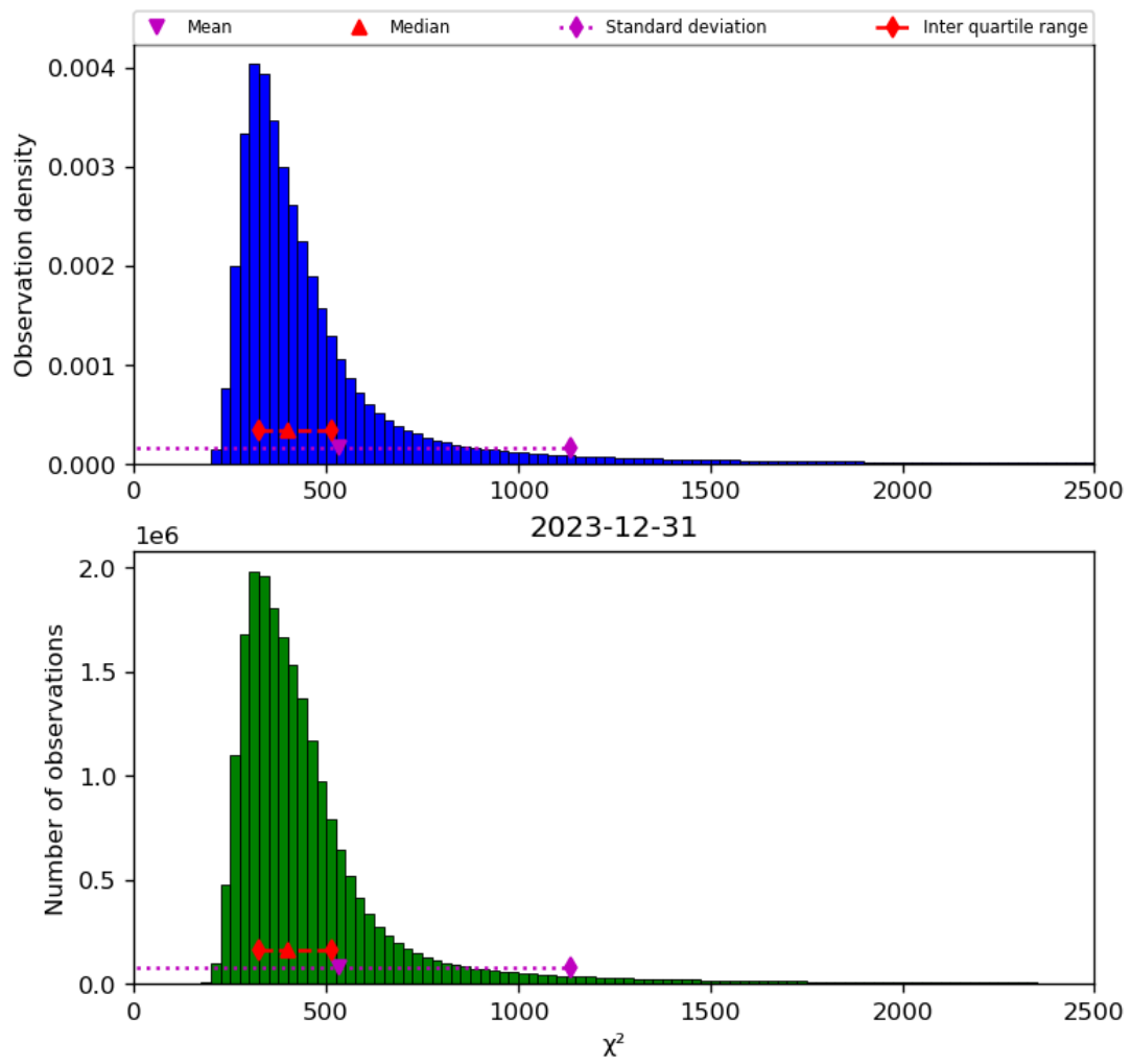
Figure 42: Histogram of " \chi^2 " for 2023-12-30 to 2023-12-31
