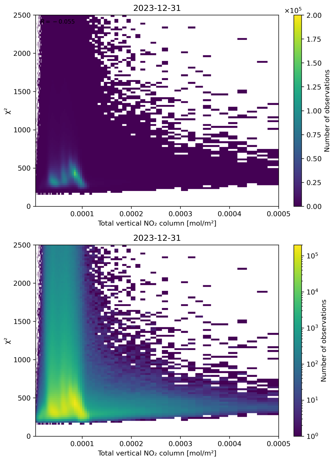
Figure 111: Scatter density plot of “Total vertical NO 2 column” against “ \chi^2 ” for 2023-12-30 to 2023-12-31.
