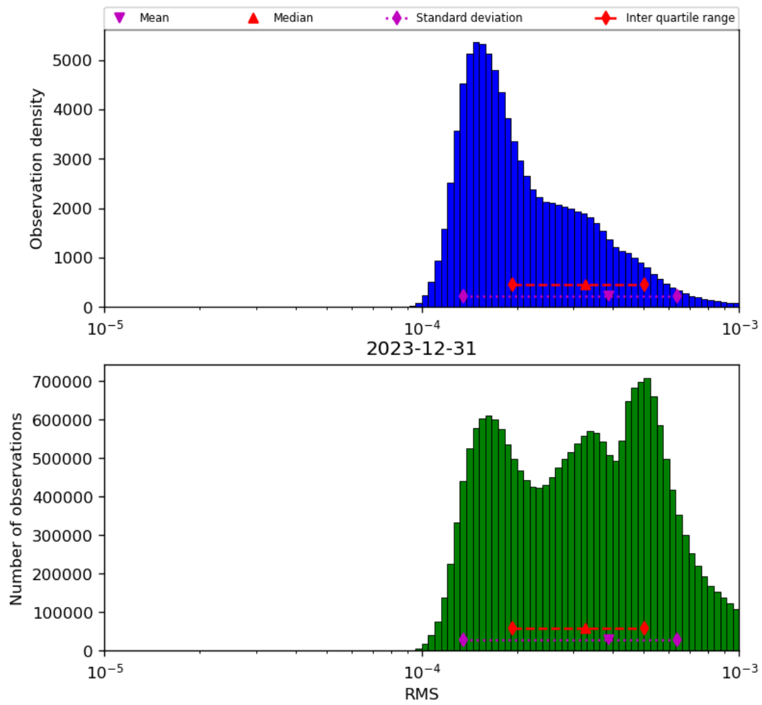
Figure 43: Histogram of “RMS” for 2023-12-30 to 2023-12-31
