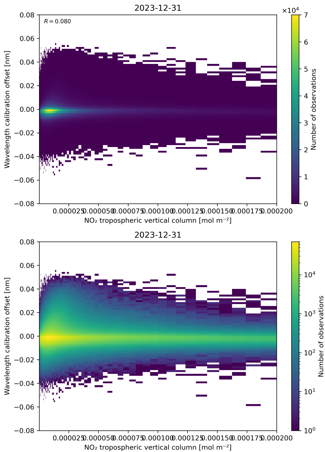
Figure 143: Scatter density plot of “NO 2 tropospheric vertical column” against “Wavelength calibration offset” for 2023-12-30 to 2023-12-31.
