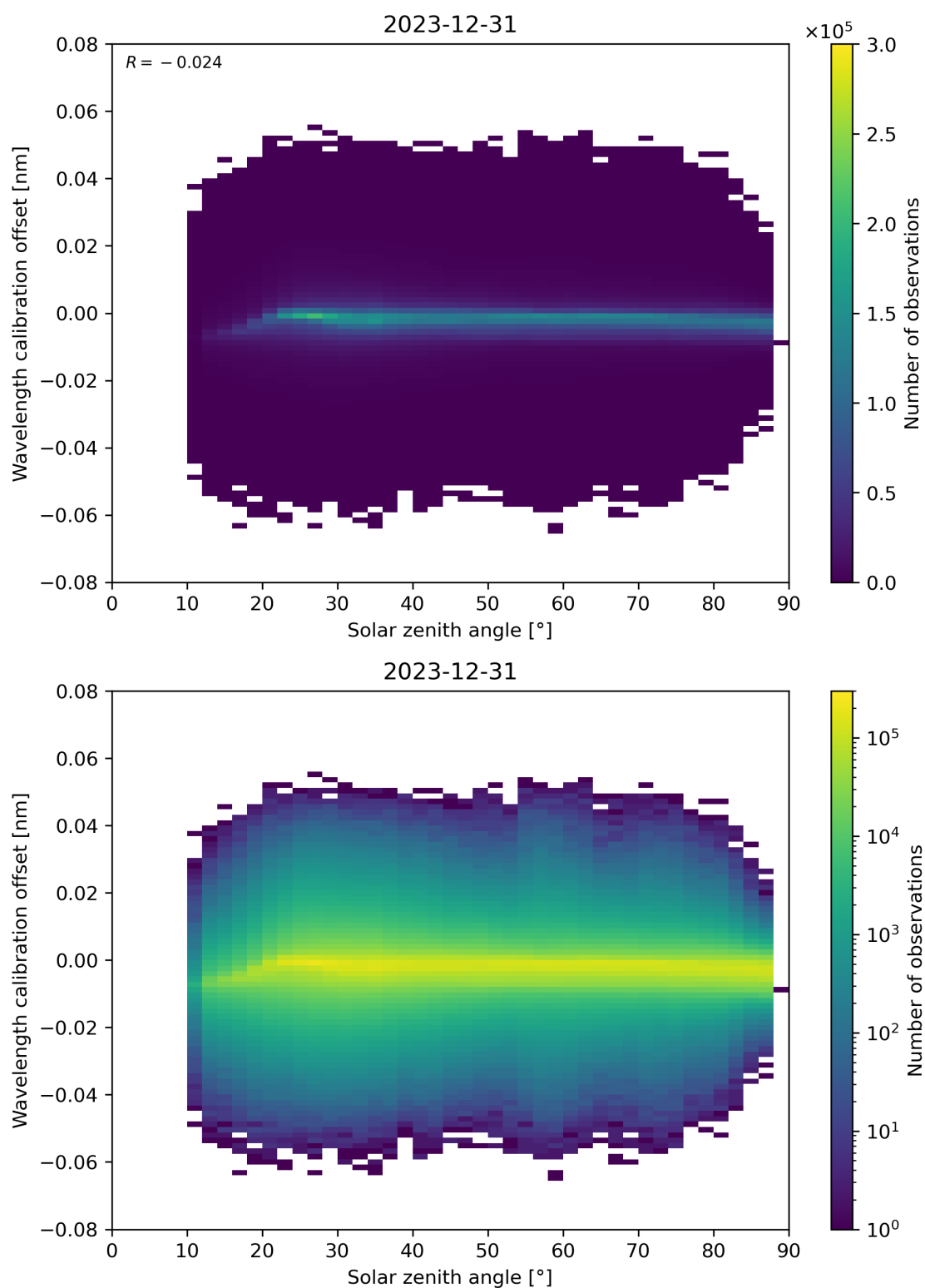
Figure 158: Scatter density plot of “Solar zenith angle” against “Wavelength calibration offset” for 2023-12-30 to 2023-12-31.
