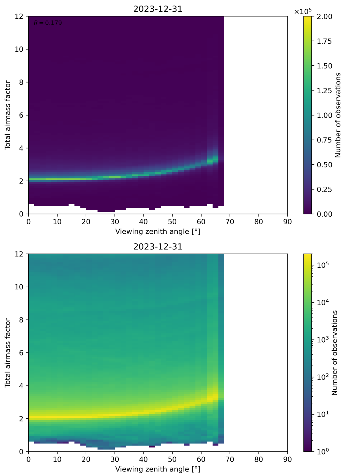
Figure 160: Scatter density plot of “Viewing zenith angle” against “Total airmass factor” for 2023-12-30 to 2023-12-31.
