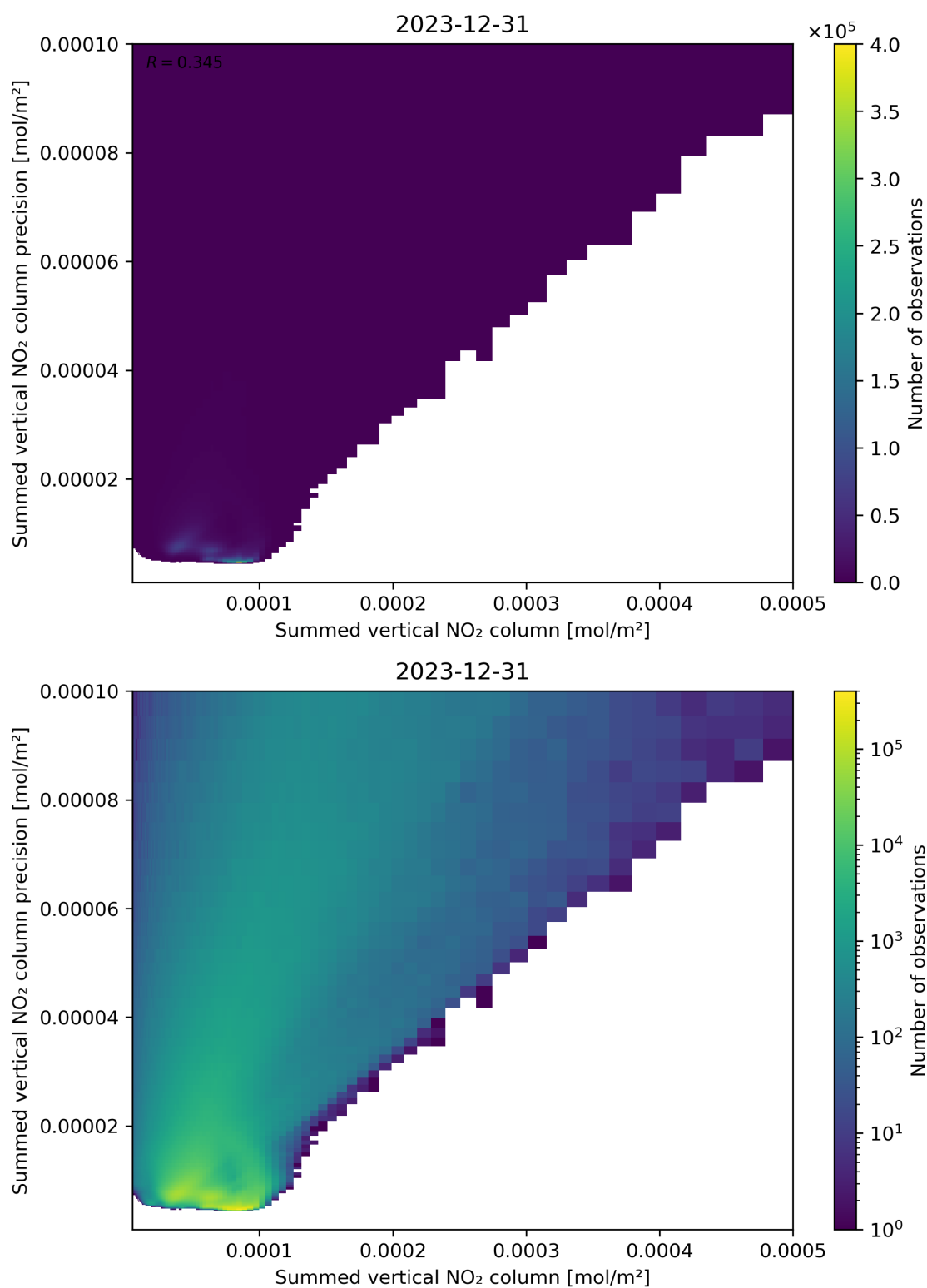
Figure 105: Scatter density plot of “Summed vertical NO 2 column” against “Summed vertical NO 2 column precision” for 2023-12-30 to 2023-12-31.
