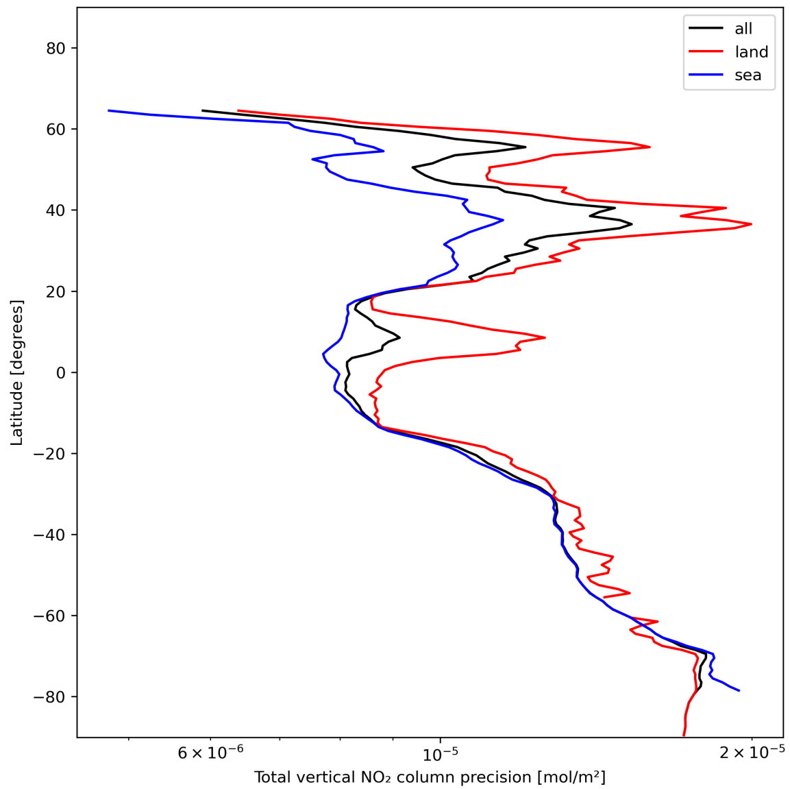
Figure 22: Zonal average of “Total vertical NO 2 column precision” for 2023-12-30 to 2023-12-31.
