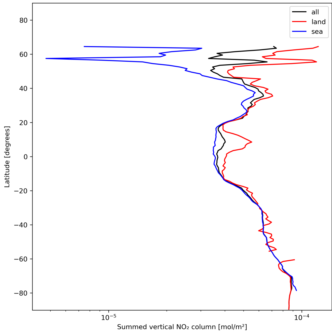
Figure 23: Zonal average of “Summed vertical NO 2 column” for 2023-12-30 to 2023-12-31.
