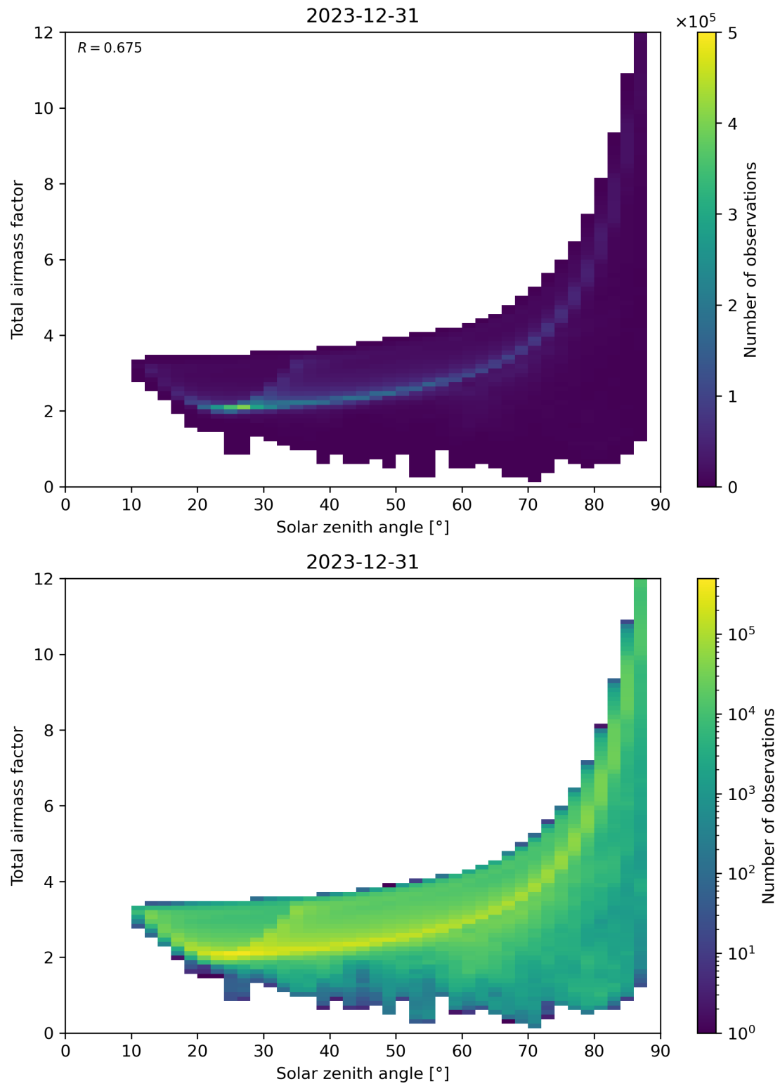
Figure 146: Scatter density plot of “Solar zenith angle” against “Total air mass factor” for 2023-12-30 to 2023-12-31.
