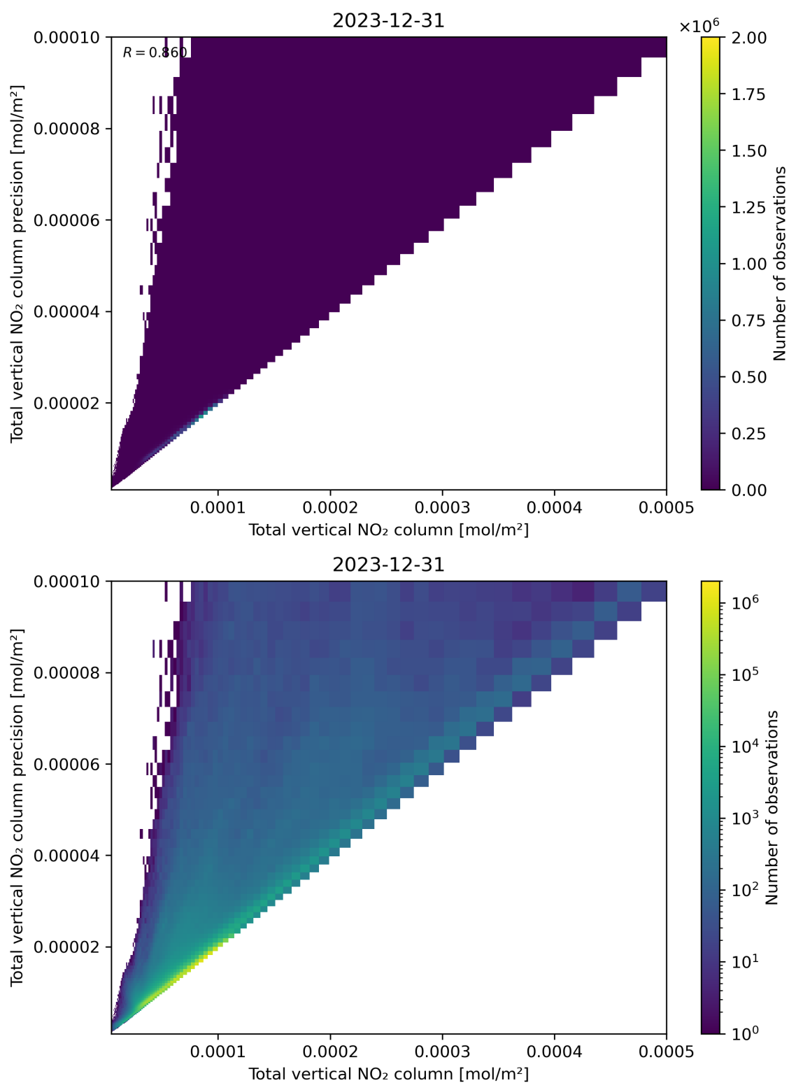
Figure 114: Scatter density plot of “Total vertical NO 2 column” against “Total vertical NO 2 column precision” for 2023-12-30 to 2023-12-31.
