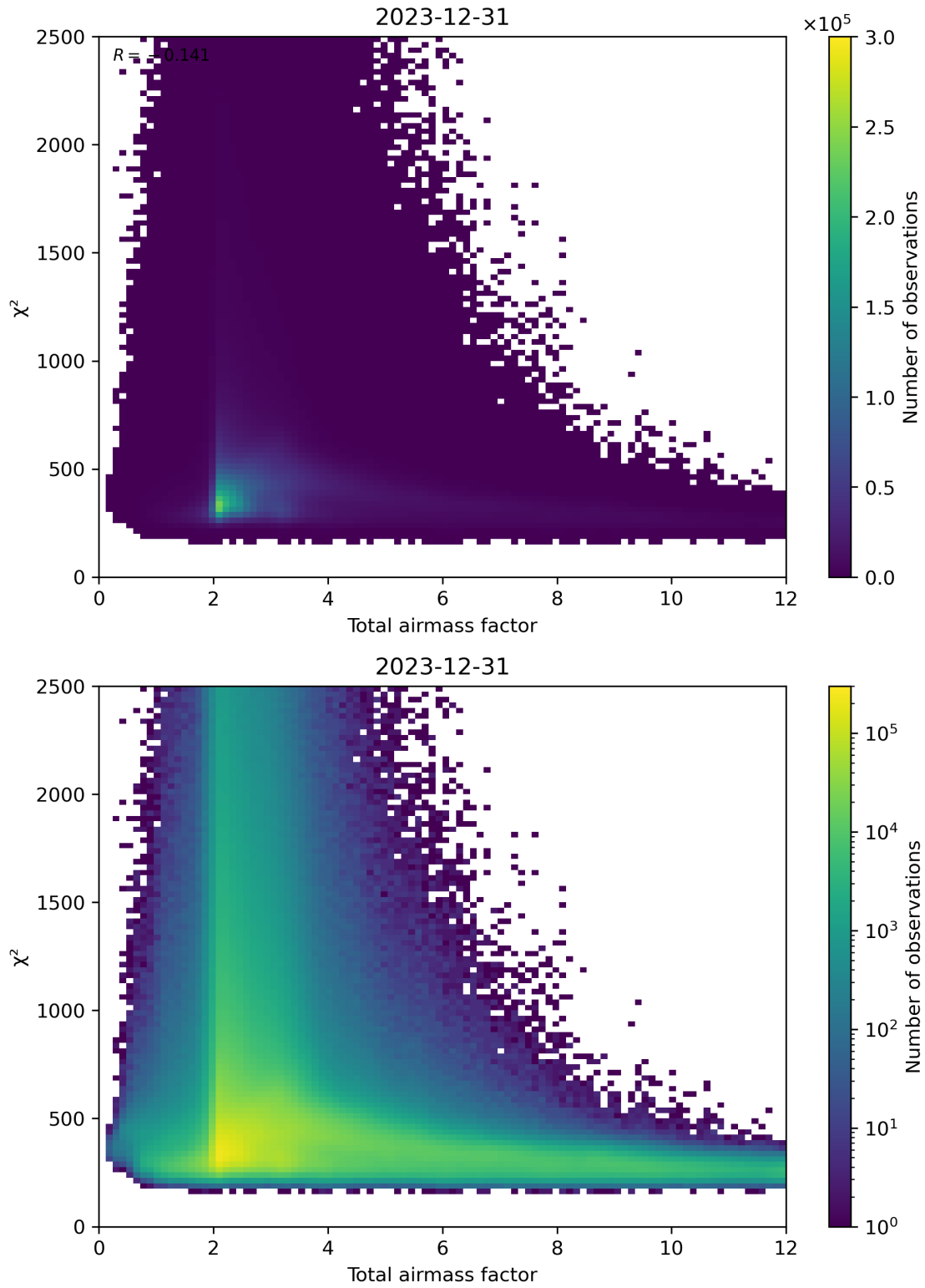
Figure 63: Scatter density plot of “Total airmass factor” against “ \chi^2 ” for 2023-12-30 to 2023-12-31.
