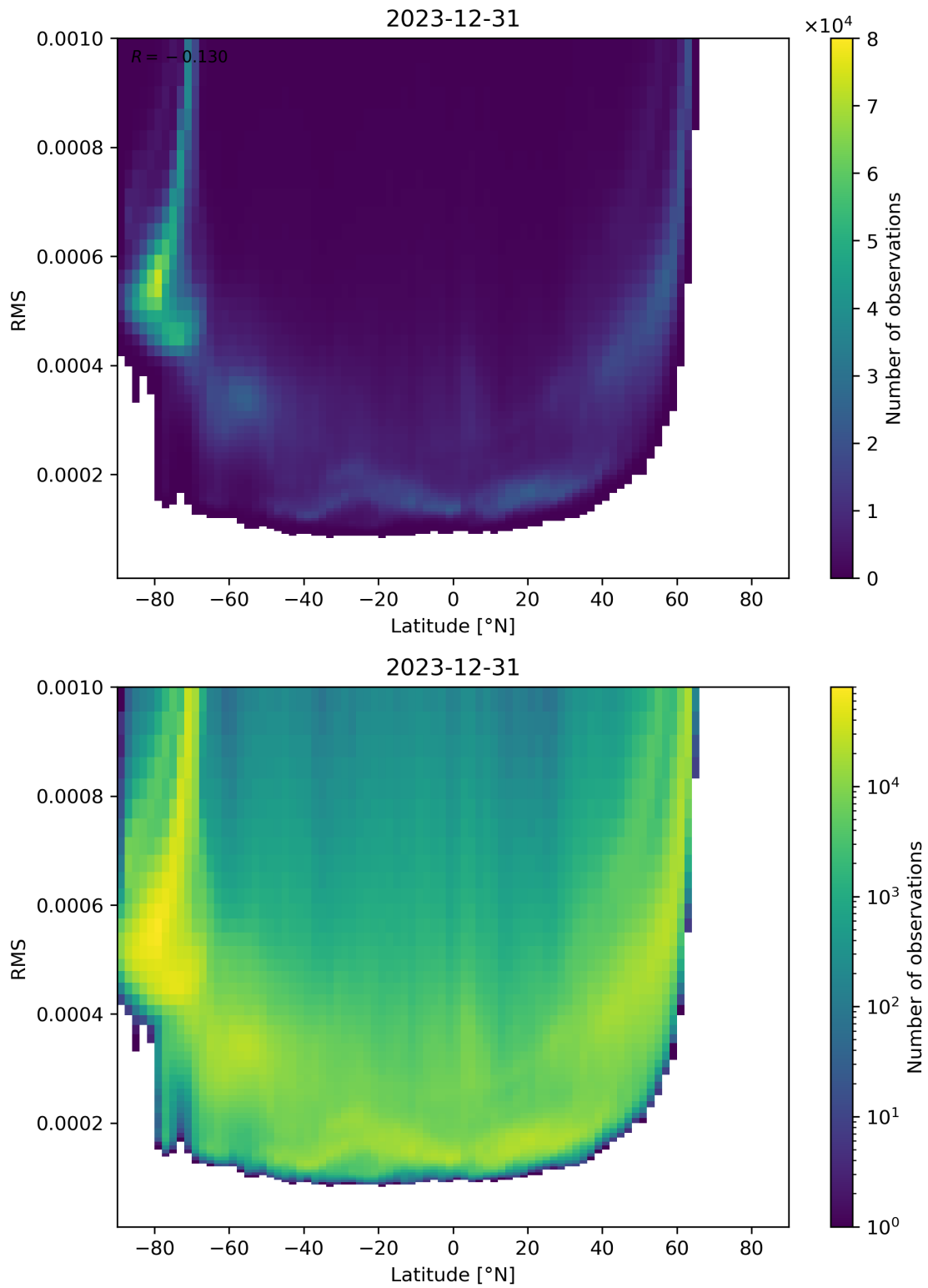
Figure 94: Scatter density plot of “Latitude” against “RMS” for 2023-12-30 to 2023-12-31.
