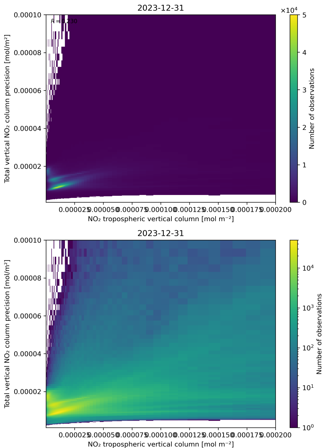
Figure 129: Scatter density plot of “NO 2 tropospheric vertical column” against “Total vertical NO 2 column precision” for 2023-12-30 to 2023-12-31.
