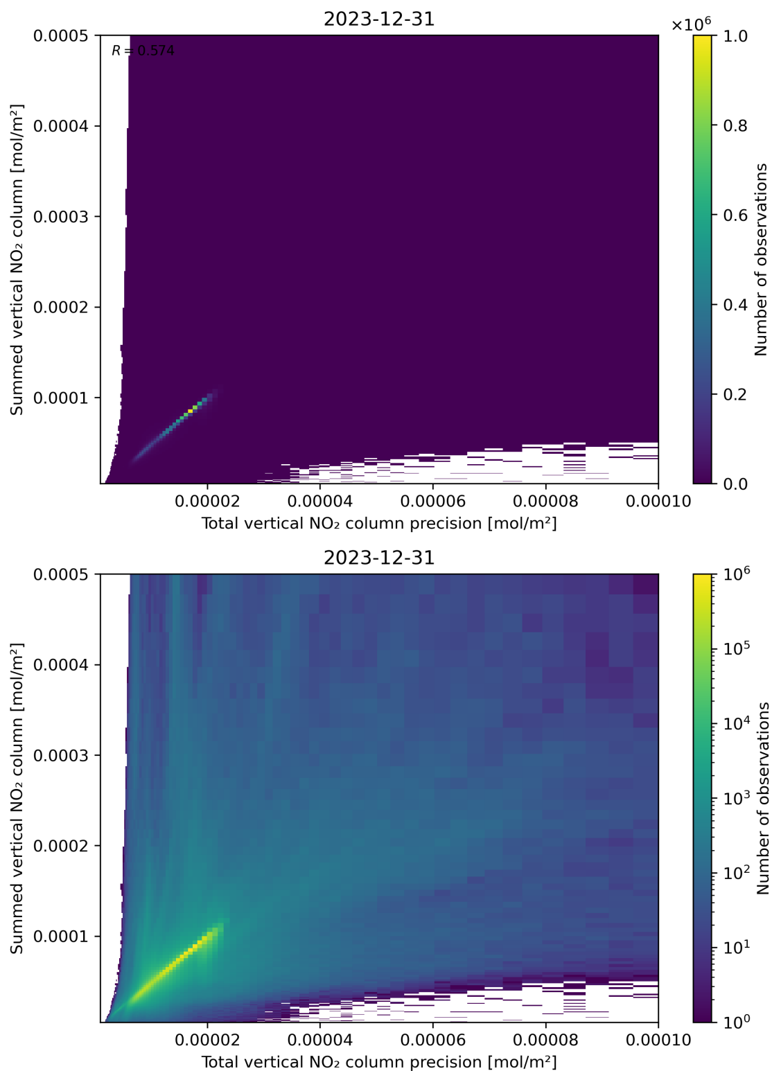
Figure 117: Scatter density plot of “Total vertical NO 2 column precision” against “Summed vertical NO 2 column” for 2023-12-30 to 2023-12-31.
