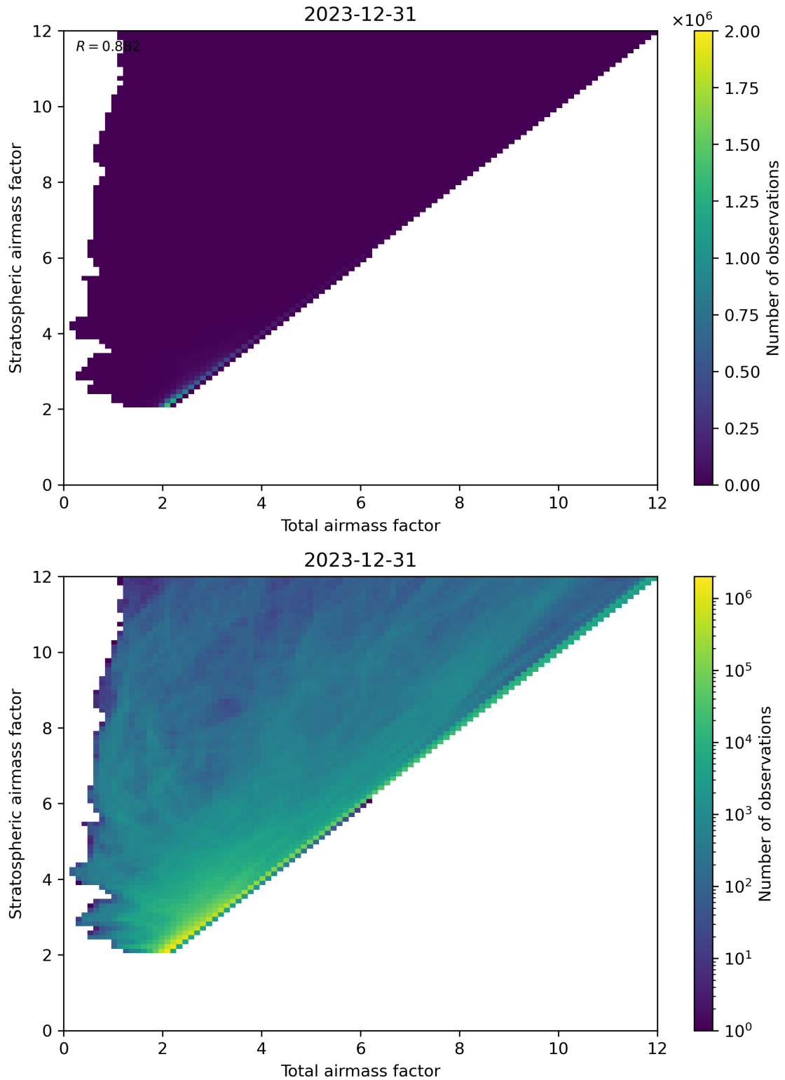
Figure 62: Scatter density plot of “Total airmass factor” against “Stratospheric airmass factor” for 2023-12-30 to 2023-12-31.
