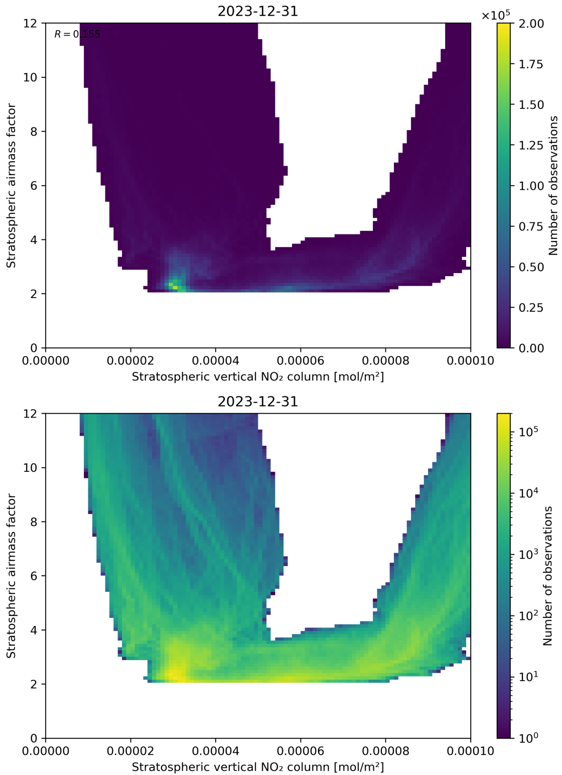
Figure 96: Scatter density plot of “Stratospheric vertical NO 2 column” against “Stratospheric airmass factor” for 2023-12-30 to 2023-12-31.
