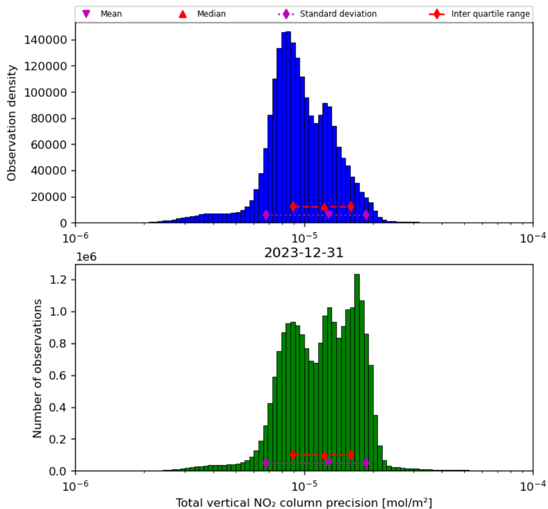
Figure 39: Histogram of “Total vertical NO 2 column precision” for 2023-12-30 to 2023-12-31
