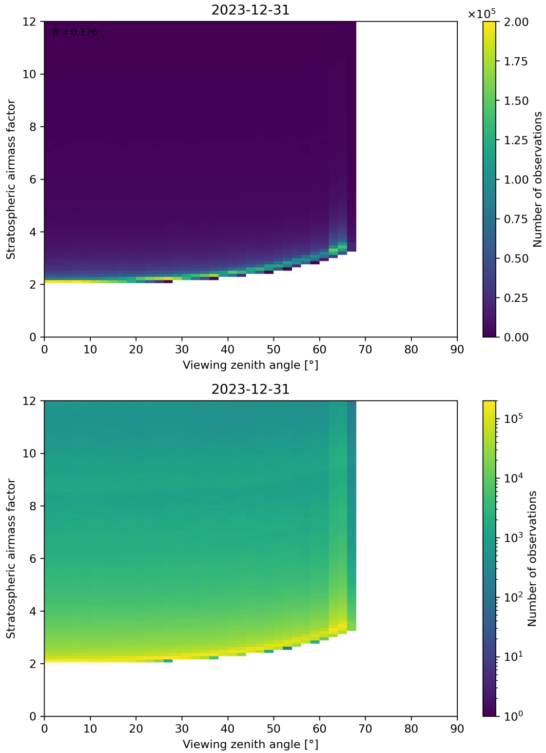
Figure 159: Scatter density plot of “Viewing zenith angle” against “Stratospheric airmass factor” for 2023-12-30 to 2023-12-31.
