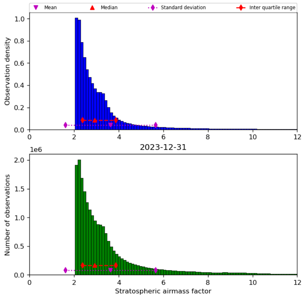
Figure 44: Histogram of “Stratospheric airmass factor” for 2023-12-30 to 2023-12-31
