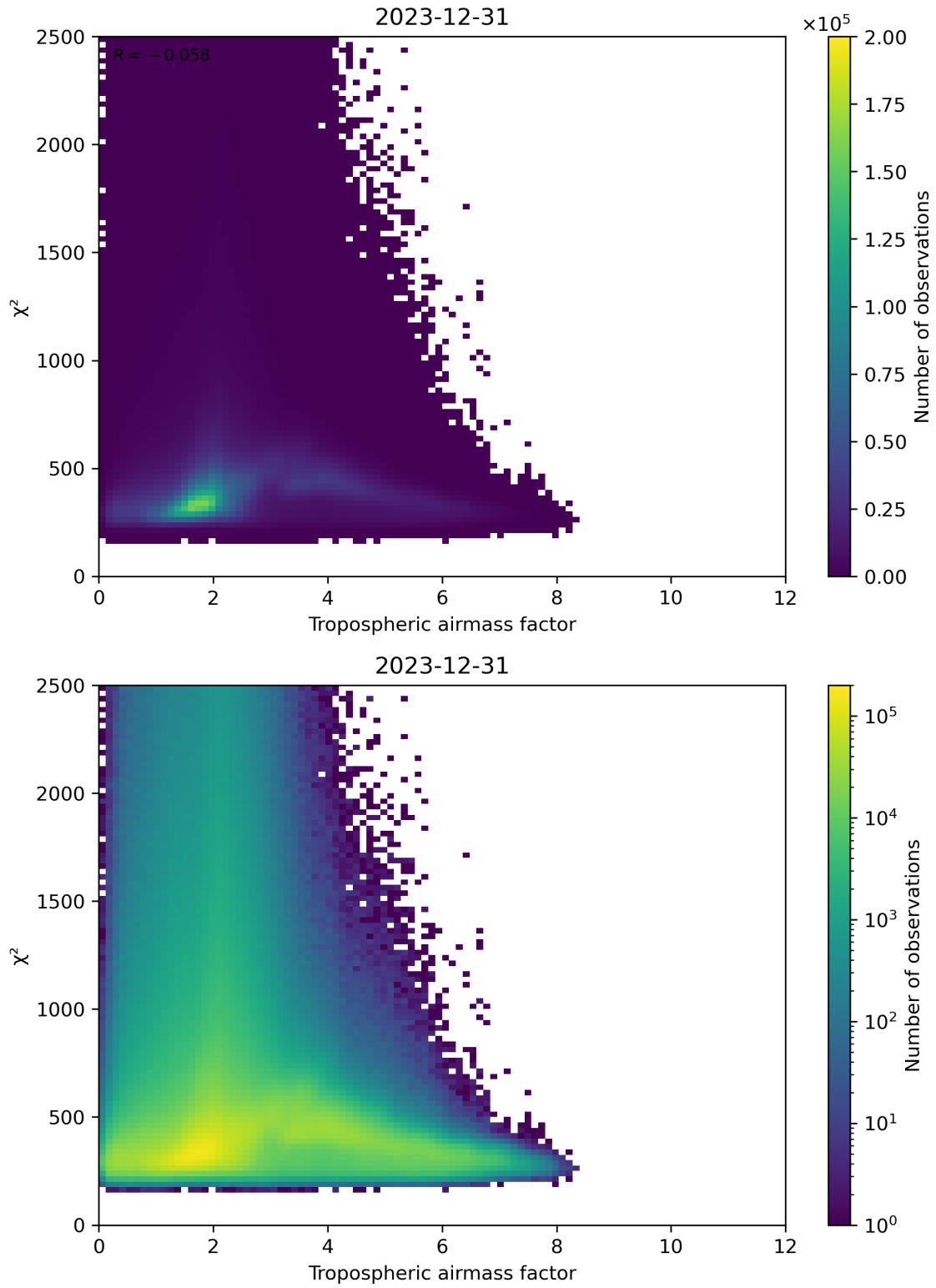
Figure 73: Scatter density plot of “Tropospheric airmass factor” against “ \chi^2 ” for 2023-12-30 to 2023-12-31.
