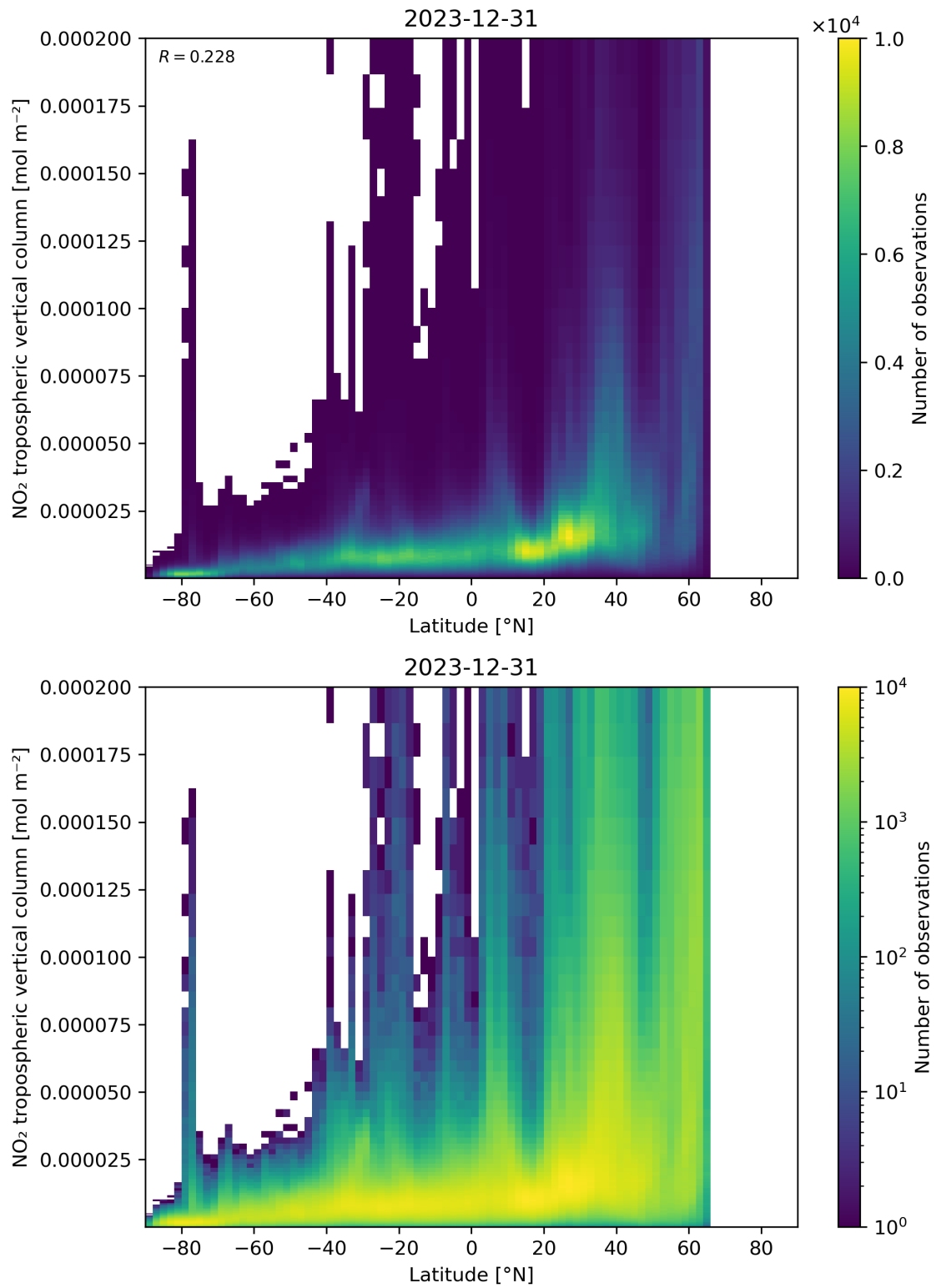
Figure 92: Scatter density plot of “Latitude” against “NO 2 tropospheric vertical column” for 2023-12-30 to 2023-12-31.
