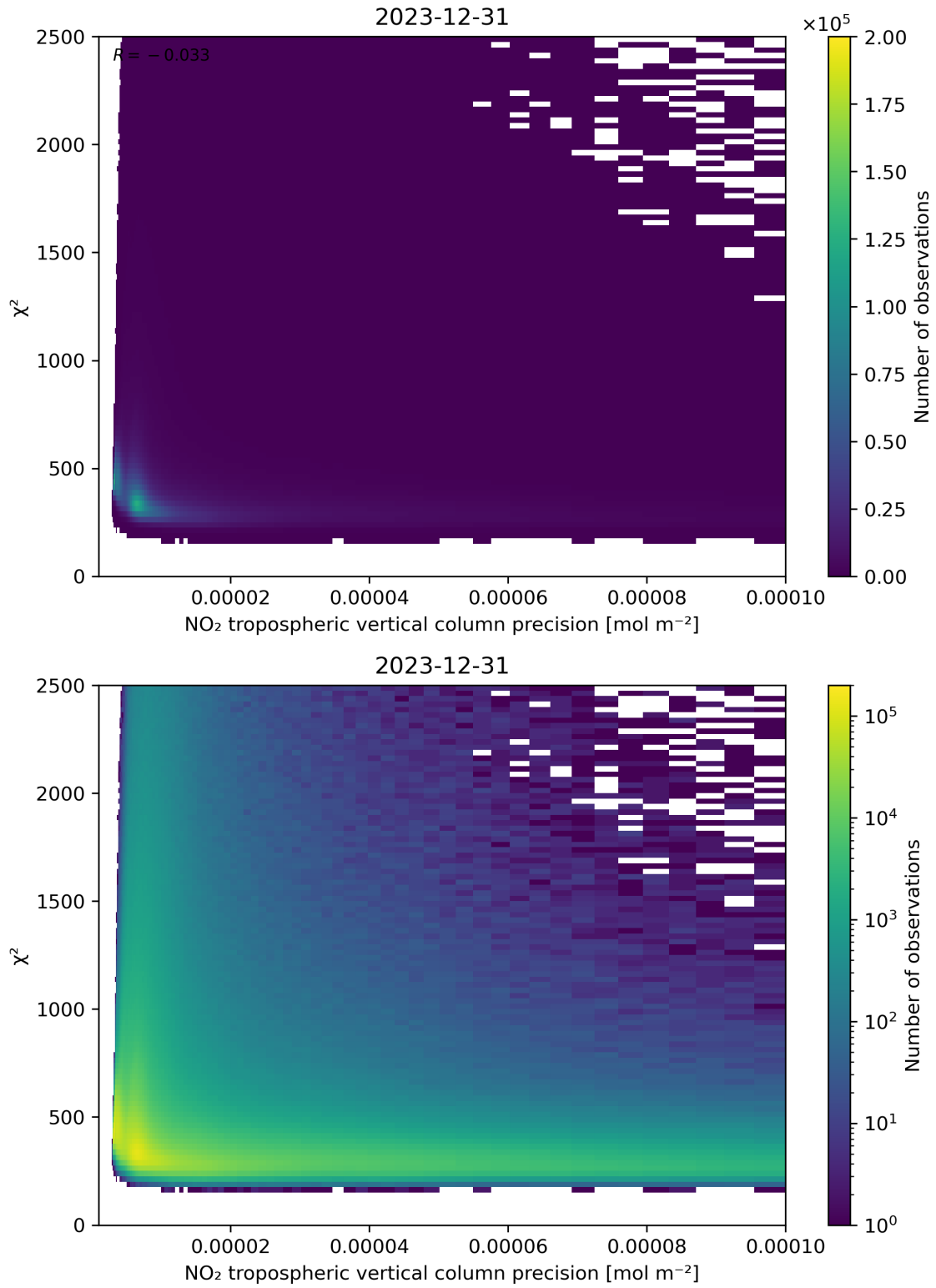
Figure 134: Scatter density plot of “NO 2 tropospheric vertical column precision” against “ \chi^2 ” for 2023-12-30 to 2023-12-31.
