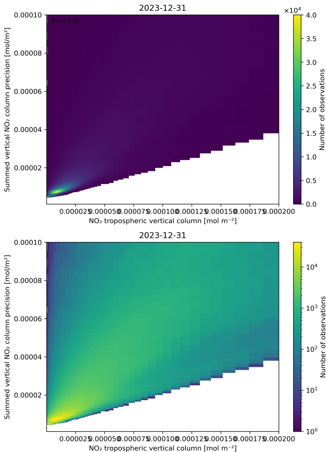
Figure 127: Scatter density plot of “NO 2 tropospheric vertical column” against “Summed vertical NO 2 column precision” for 2023-12-30 to 2023-12-31.
