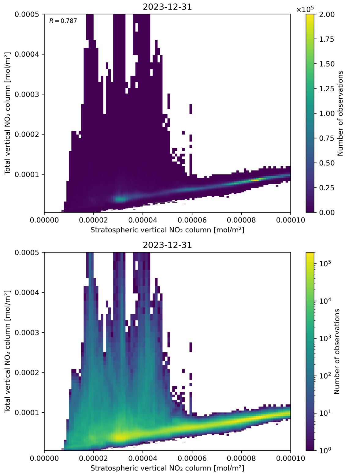
Figure 100: Scatter density plot of “Stratospheric vertical NO 2 column” against “Total vertical NO 2 column” for 2023-12-30 to 2023-12-31.
