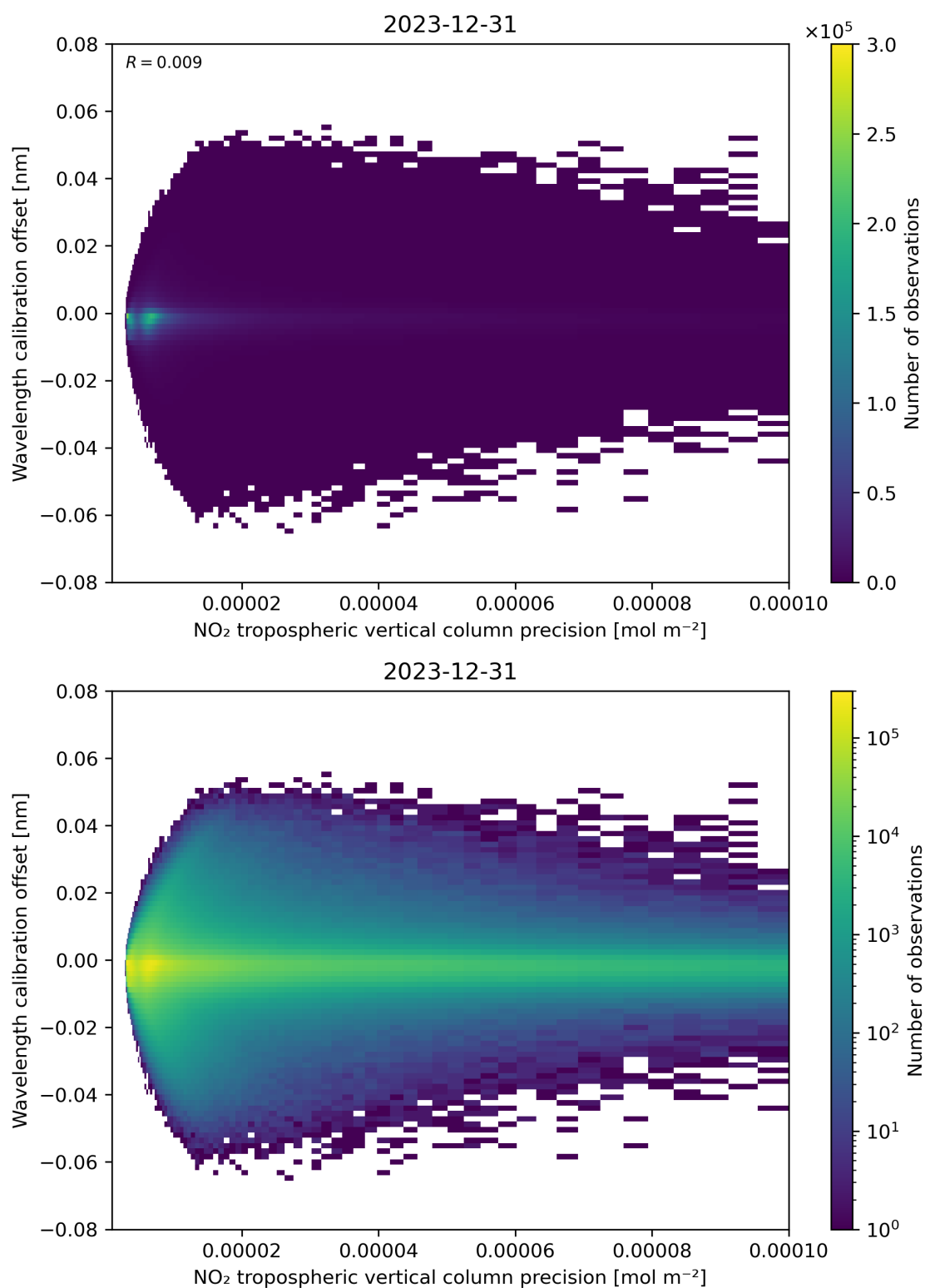
Figure 141: Scatter density plot of “NO 2 tropospheric vertical column precision” against “Wavelength calibration offset” for 2023-12-30 to 2023-12-31.
