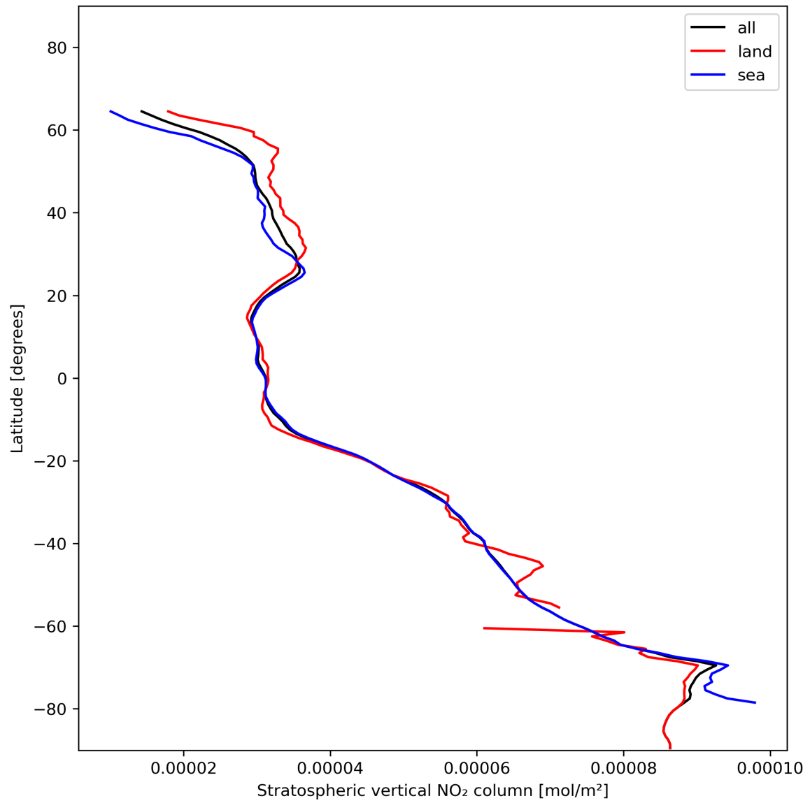
Figure 19: Zonal average of “Stratospheric vertical NO 2 column” for 2023-12-30 to 2023-12-31.
