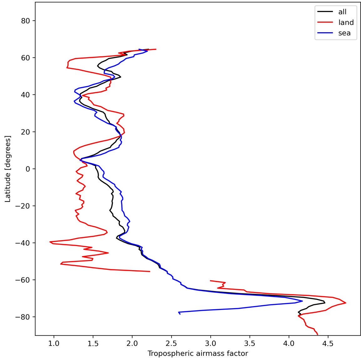
Figure 14: Zonal average of “Tropospheric airmass factor” for 2023-12-30 to 2023-12-31.
