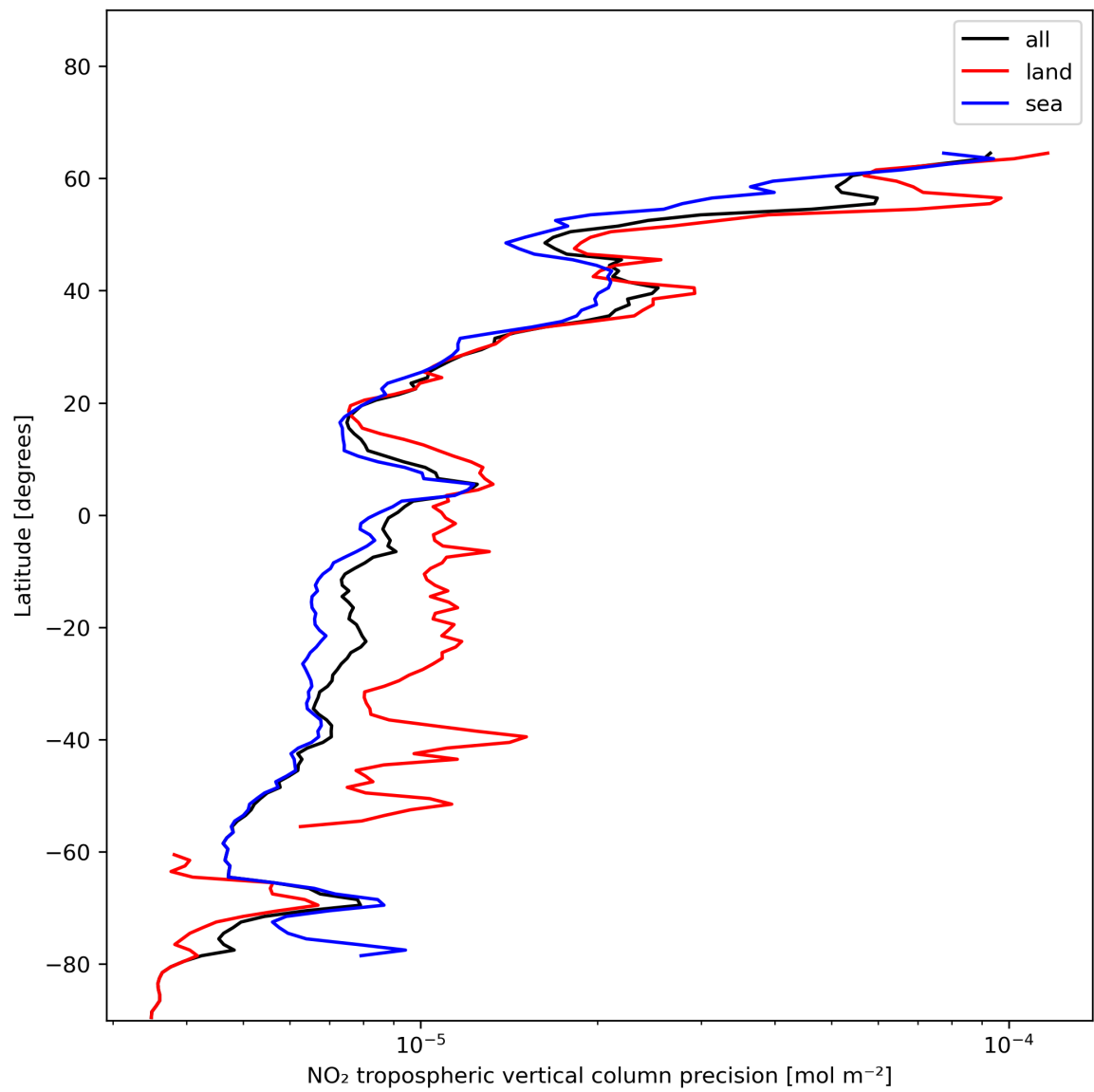
Figure 13: Zonal average of “NO 2 tropospheric vertical column precision” for 2023-12-30 to 2023-12-31.
