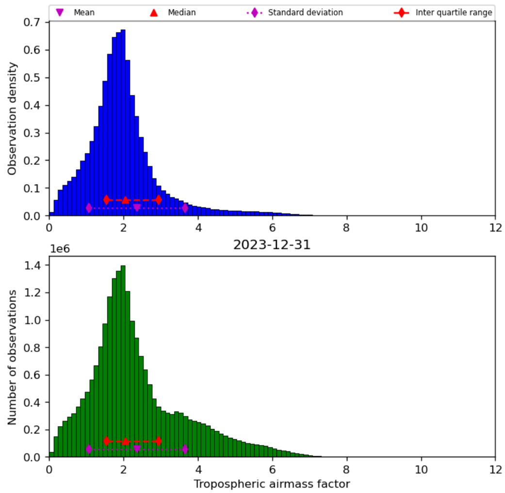
Figure 31: Histogram of “Tropospheric airmass factor” for 2023-12-30 to 2023-12-31
