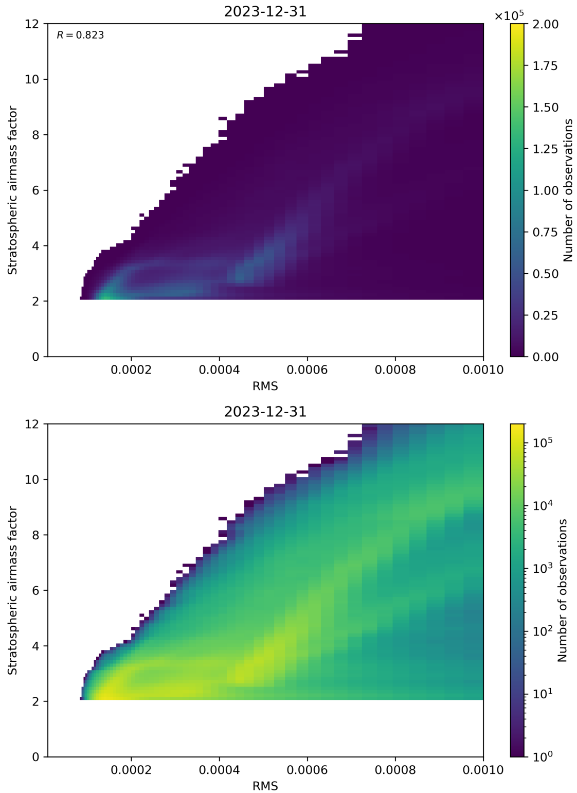
Figure 144: Scatter density plot of “RMS” against “Stratospheric airmass factor” for 2023-12-30 to 2023-12-31.
