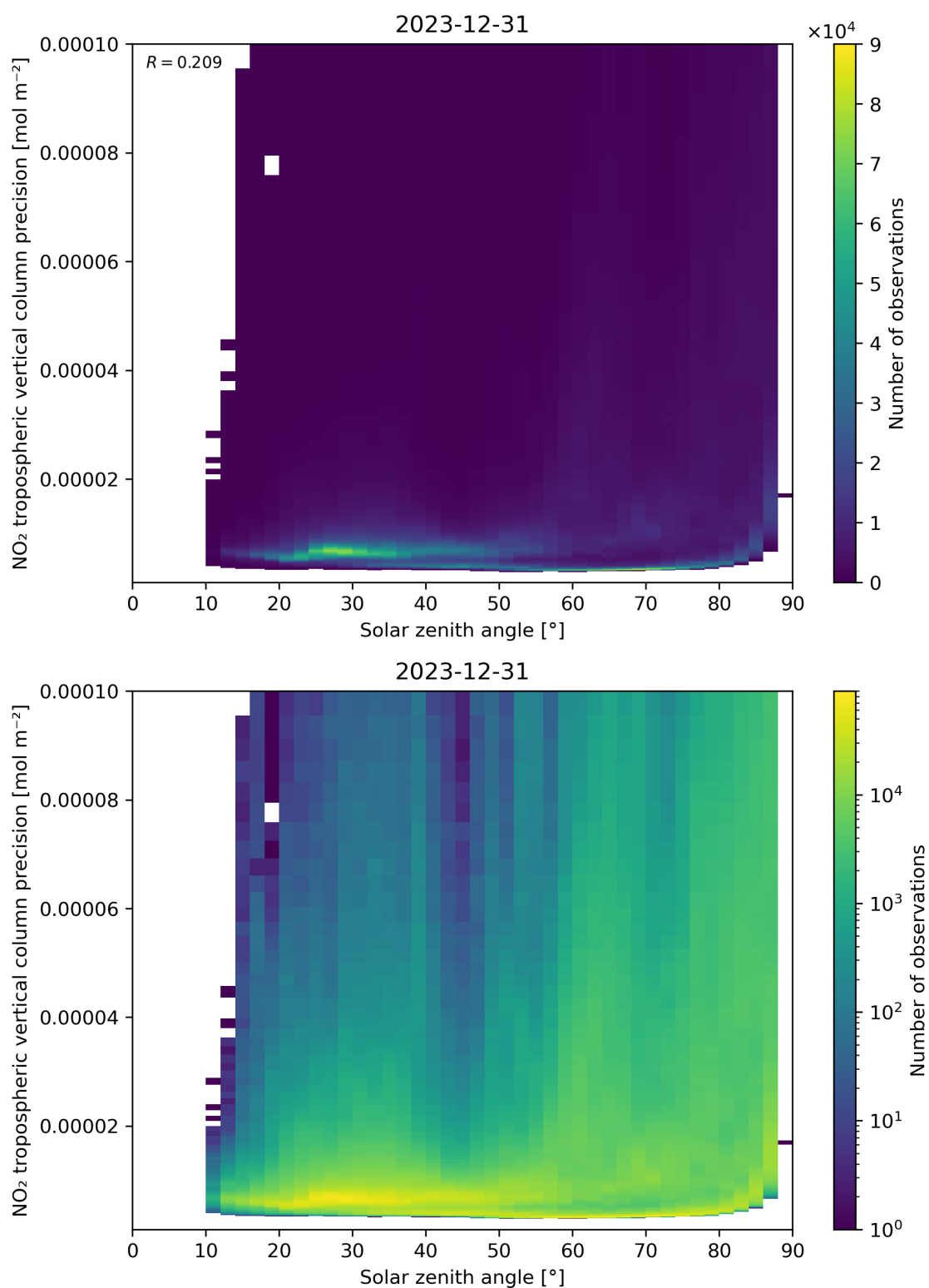
Figure 156: Scatter density plot of “Solar zenith angle” against “NO 2 tropospheric vertical column precision” for 2023-12-30 to 2023-12-31.
