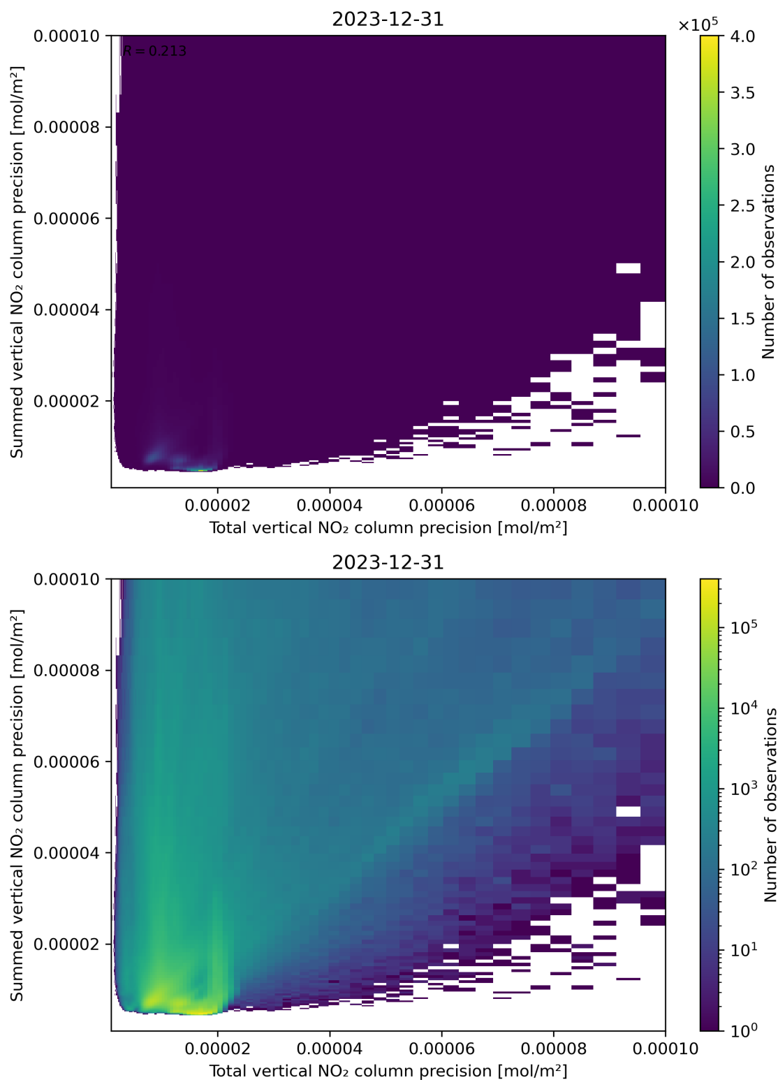
Figure 118: Scatter density plot of “Total vertical NO 2 column precision” against “Summed vertical NO 2 column precision” for 2023-12-30 to 2023-12-31.
