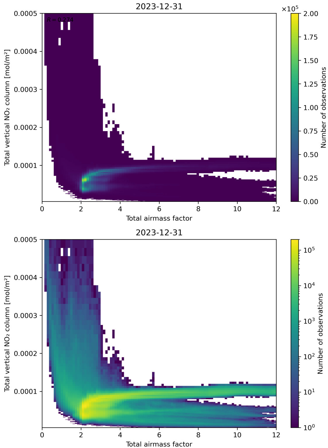
Figure 67: Scatter density plot of “Total airmass factor” against “Total vertical NO 2 column” for 2023-12-30 to 2023-12-31.
