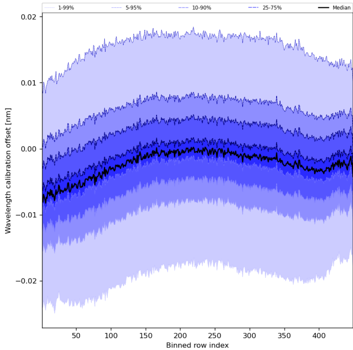
Figure 52: Along track statistics of “Wavelength calibration offset” for 2023-12-30 to 2023-12-31
