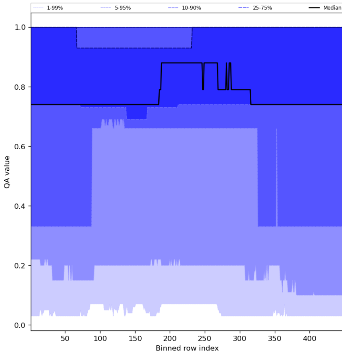
Figure 45: Along track statistics of “QA value” for 2023-12-30 to 2023-12-31
