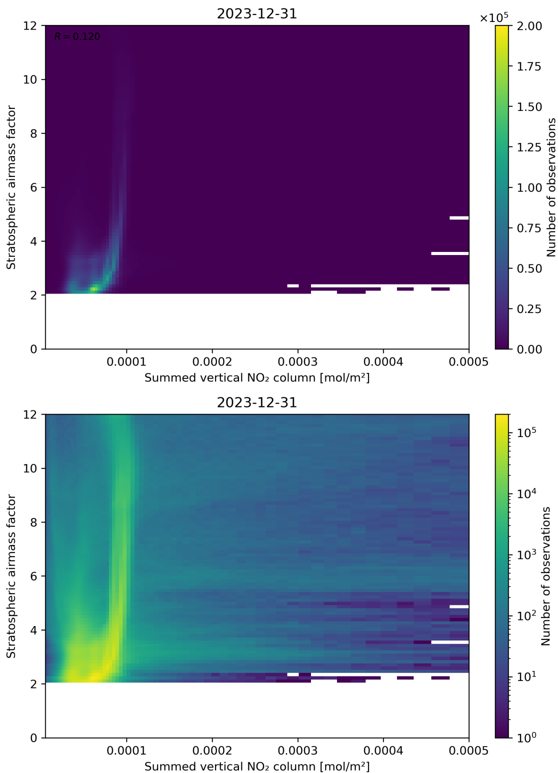
Figure 103: Scatter density plot of “Summed vertical NO 2 column” against “Stratospheric airmass factor” for 2023-12-30 to 2023-12-31.
