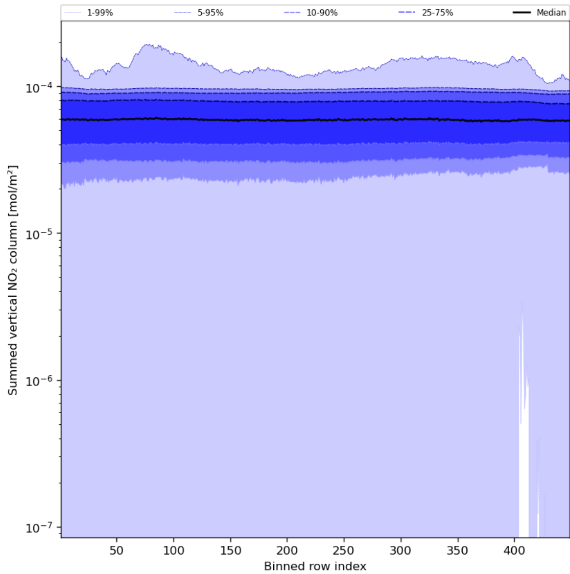
Figure 57: Along track statistics of “Summed vertical NO 2 column” for 2023-12-30 to 2023-12-31
