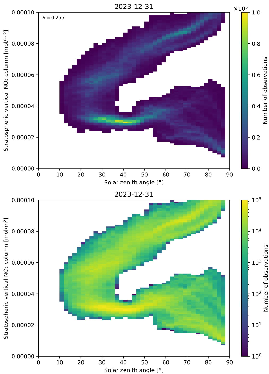
Figure 150: Scatter density plot of “Solar zenith angle” against “Stratospheric vertical NO 2 column” for 2023-12-30 to 2023-12-31.
