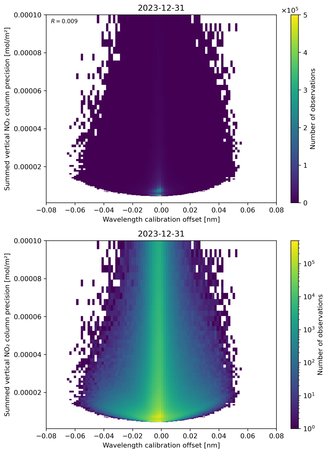
Figure 178: Scatter density plot of “Wavelength calibration offset” against “Summed vertical NO 2 column precision” for 2023-12-30 to 2023-12-31.
