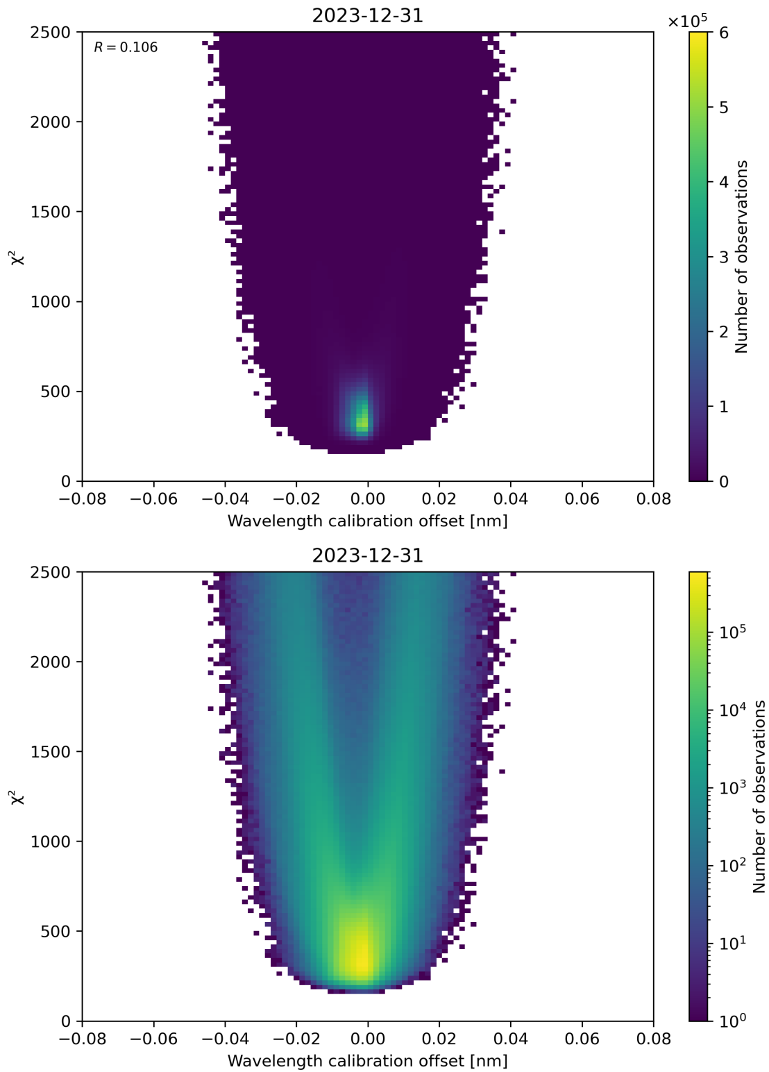
Figure 175: Scatter density plot of “Wavelength calibration offset” against “ \chi^2 ” for 2023-12-30 to 2023-12-31.
