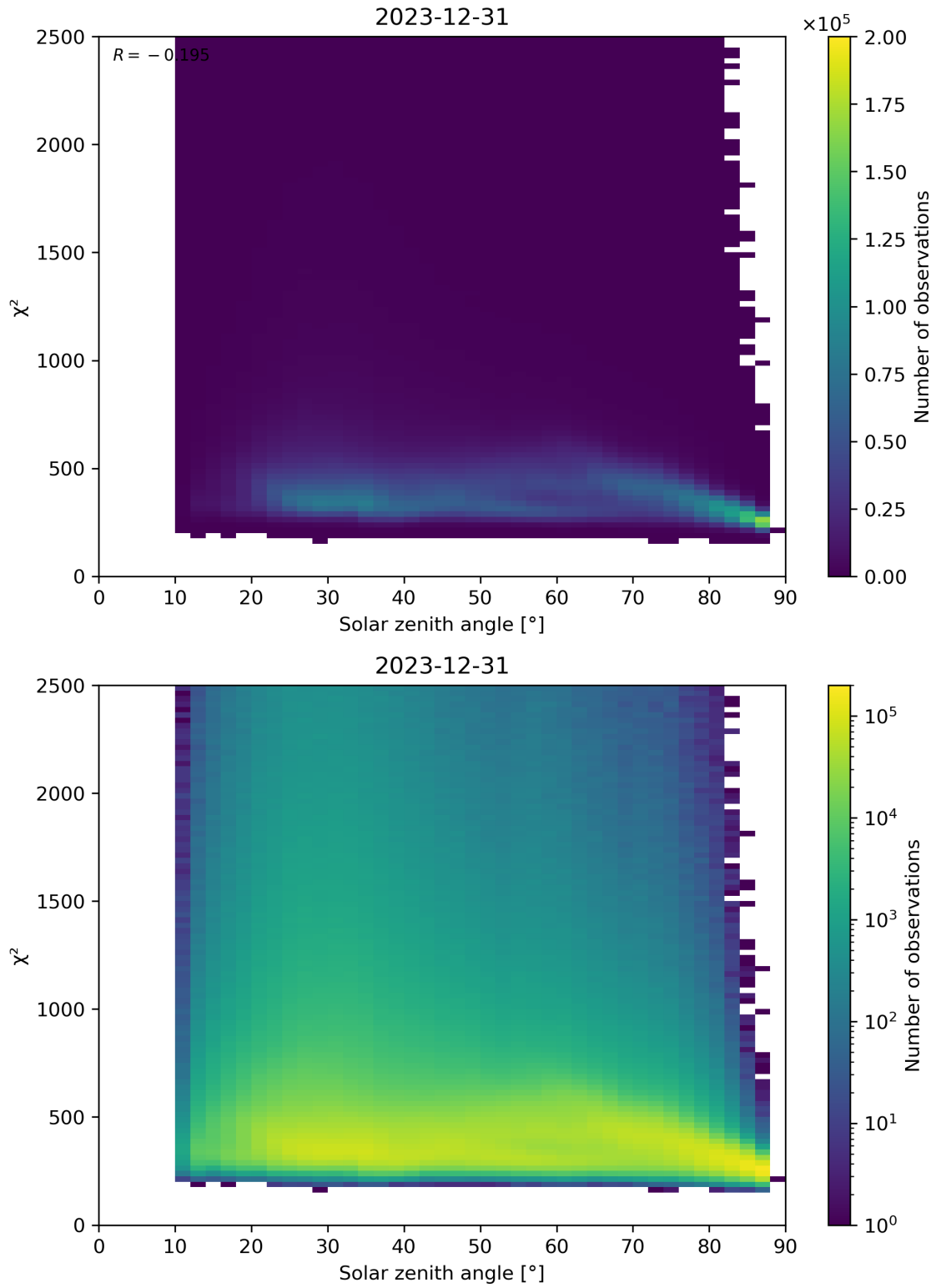
Figure 148: Scatter density plot of “Solar zenith angle” against “ \chi^2 ” for 2023-12-30 to 2023-12-31.
