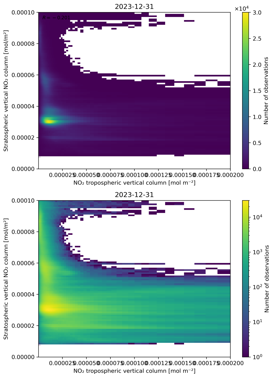
Figure 125: Scatter density plot of “NO 2 tropospheric vertical column” against “Stratospheric vertical NO 2 column” for 2023-12-30 to 2023-12-31.
