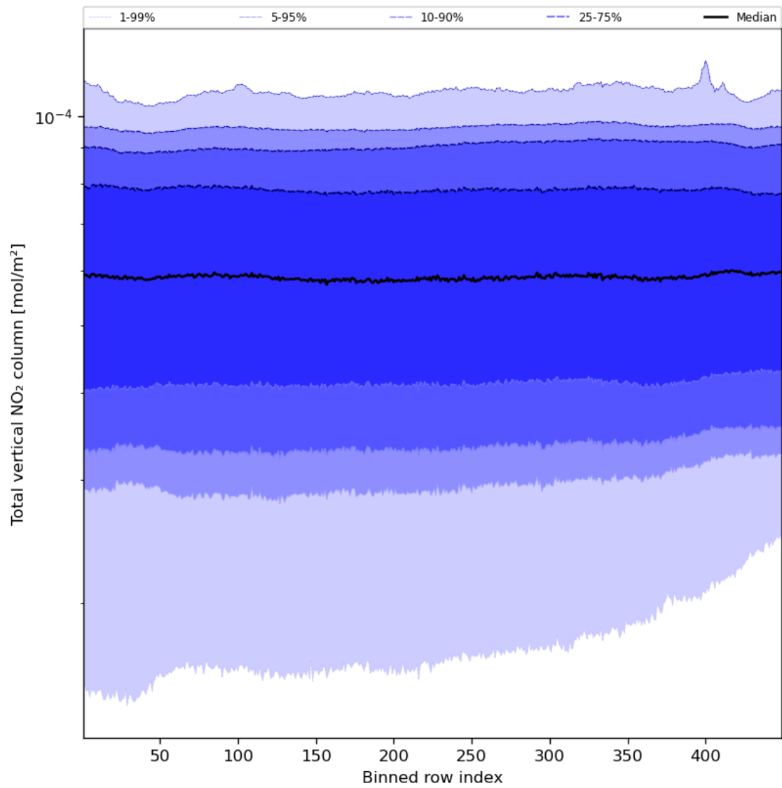
Figure 55: Along track statistics of “Total vertical NO 2 column” for 2023-12-30 to 2023-12-31
