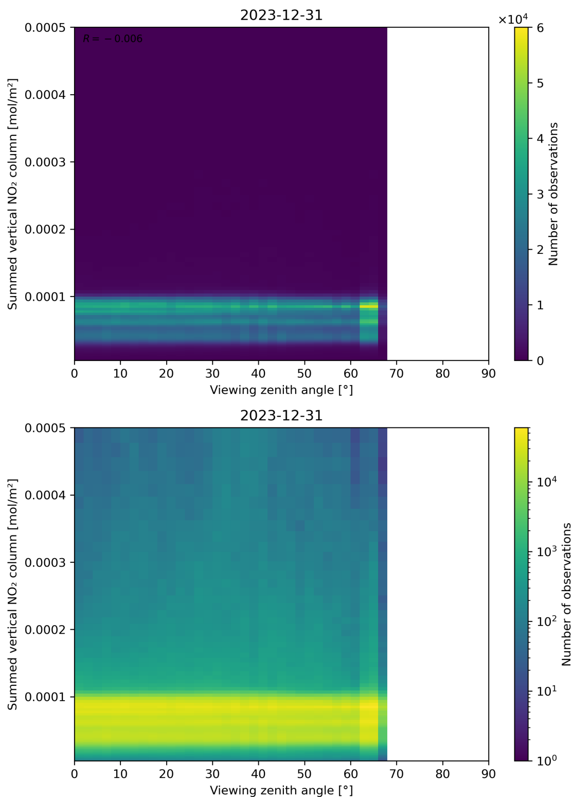
Figure 165: Scatter density plot of “Viewing zenith angle” against “Summed vertical NO 2 column” for 2023-12-30 to 2023-12-31.
