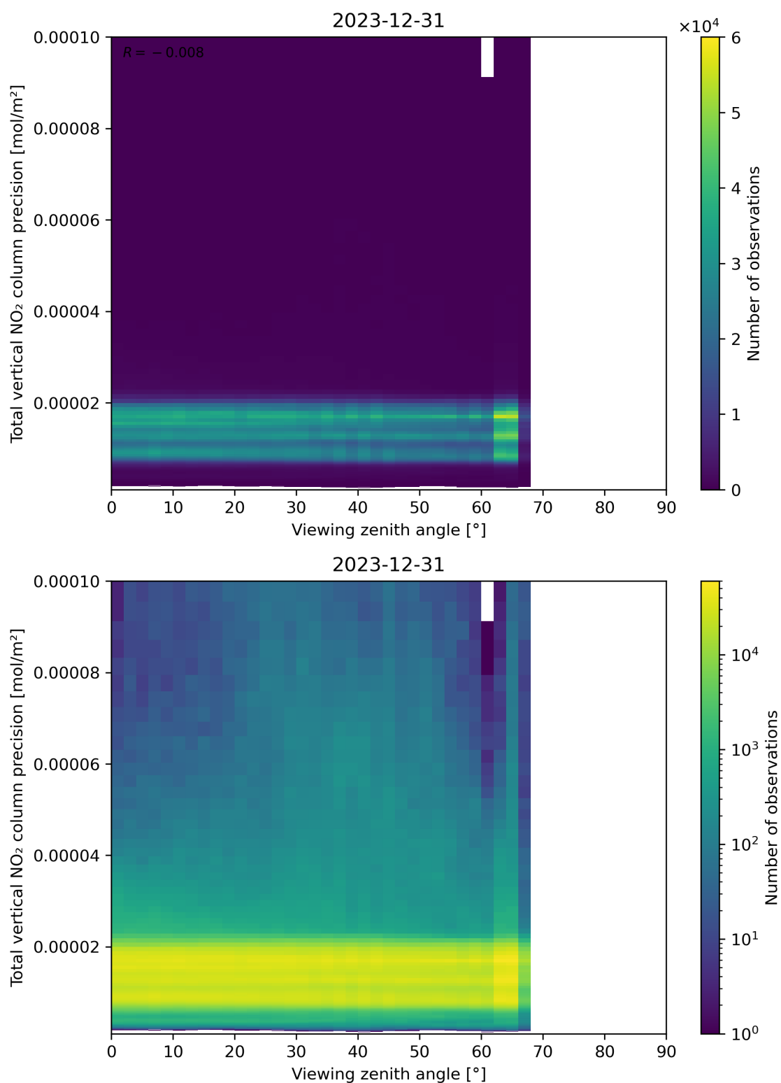
Figure 168: Scatter density plot of “Viewing zenith angle” against “Total vertical NO 2 column precision” for 2023-12-30 to 2023-12-31.
