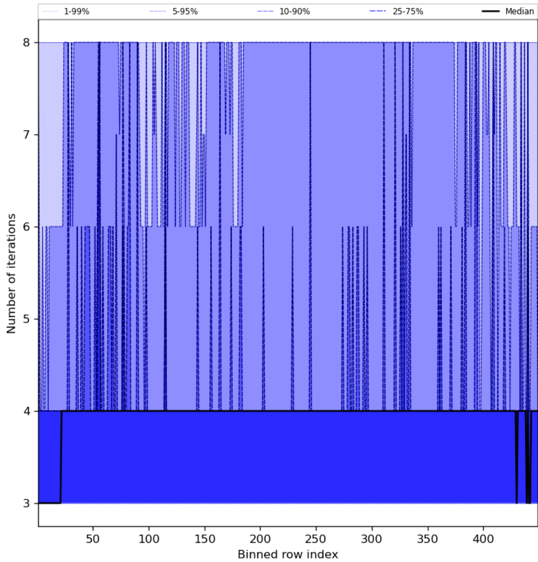
Figure 51: Along track statistics of “Number of iterations” for 2023-12-30 to 2023-12-31
