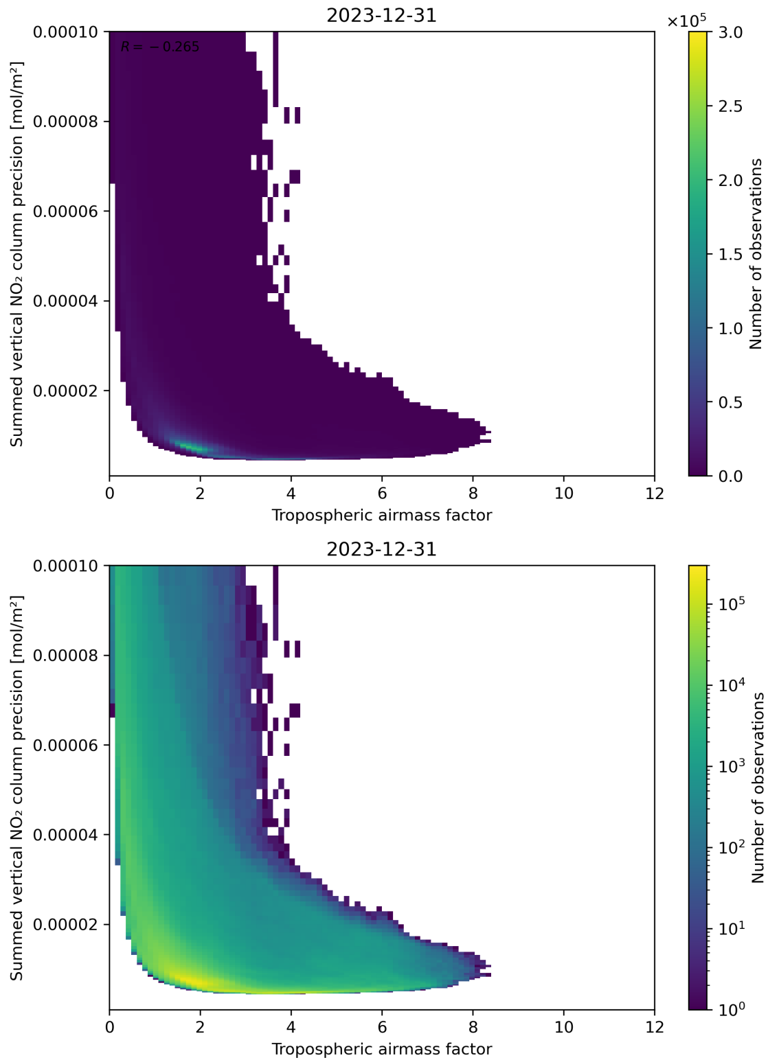
Figure 76: Scatter density plot of “Tropospheric air mass factor” against “Summed vertical NO 2 column precision” for 2023-12-30 to 2023-12-31.
