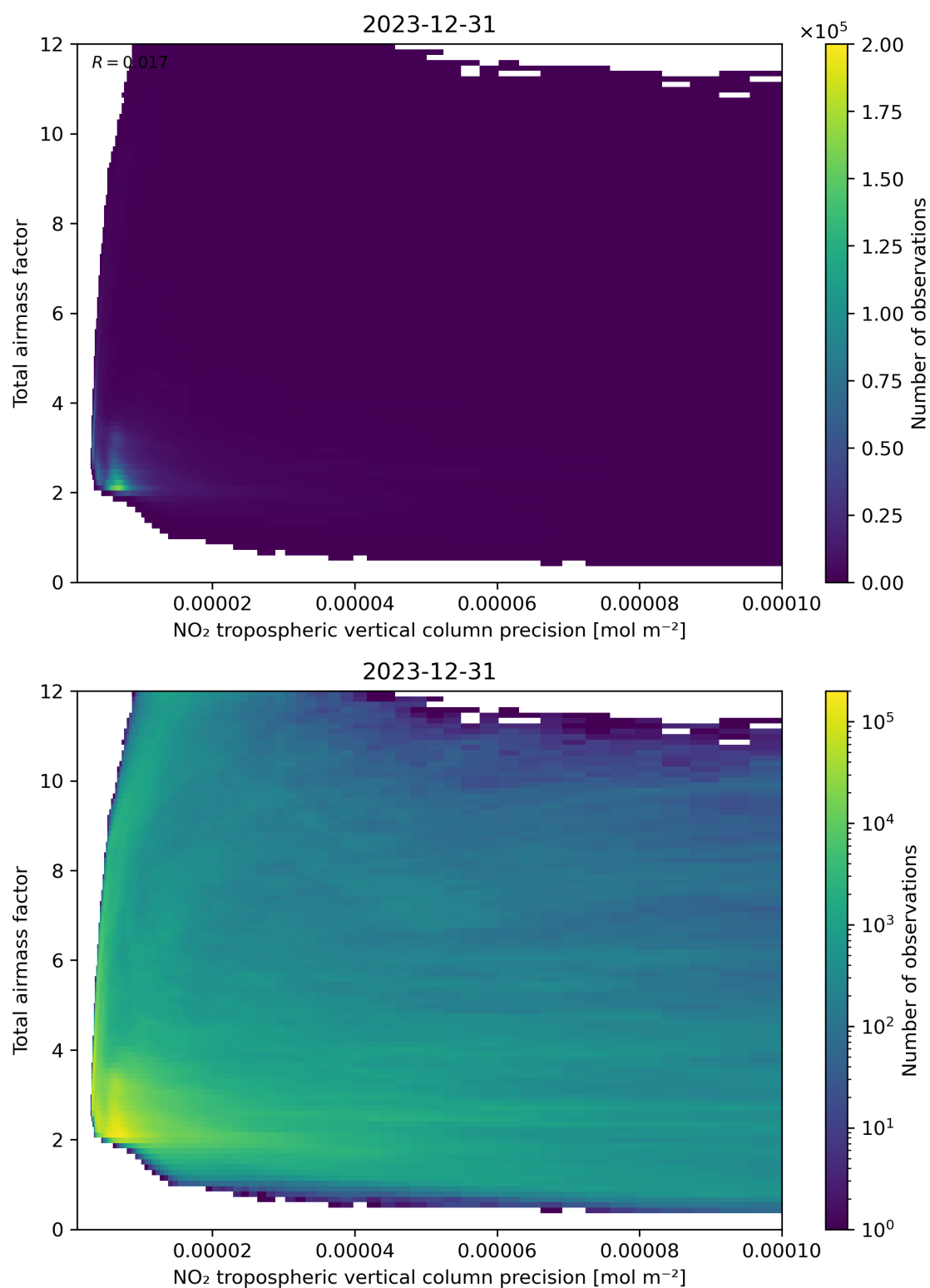
Figure 132: Scatter density plot of “NO 2 tropospheric vertical column precision” against “Total air mass factor” for 2023-12-30 to 2023-12-31.
