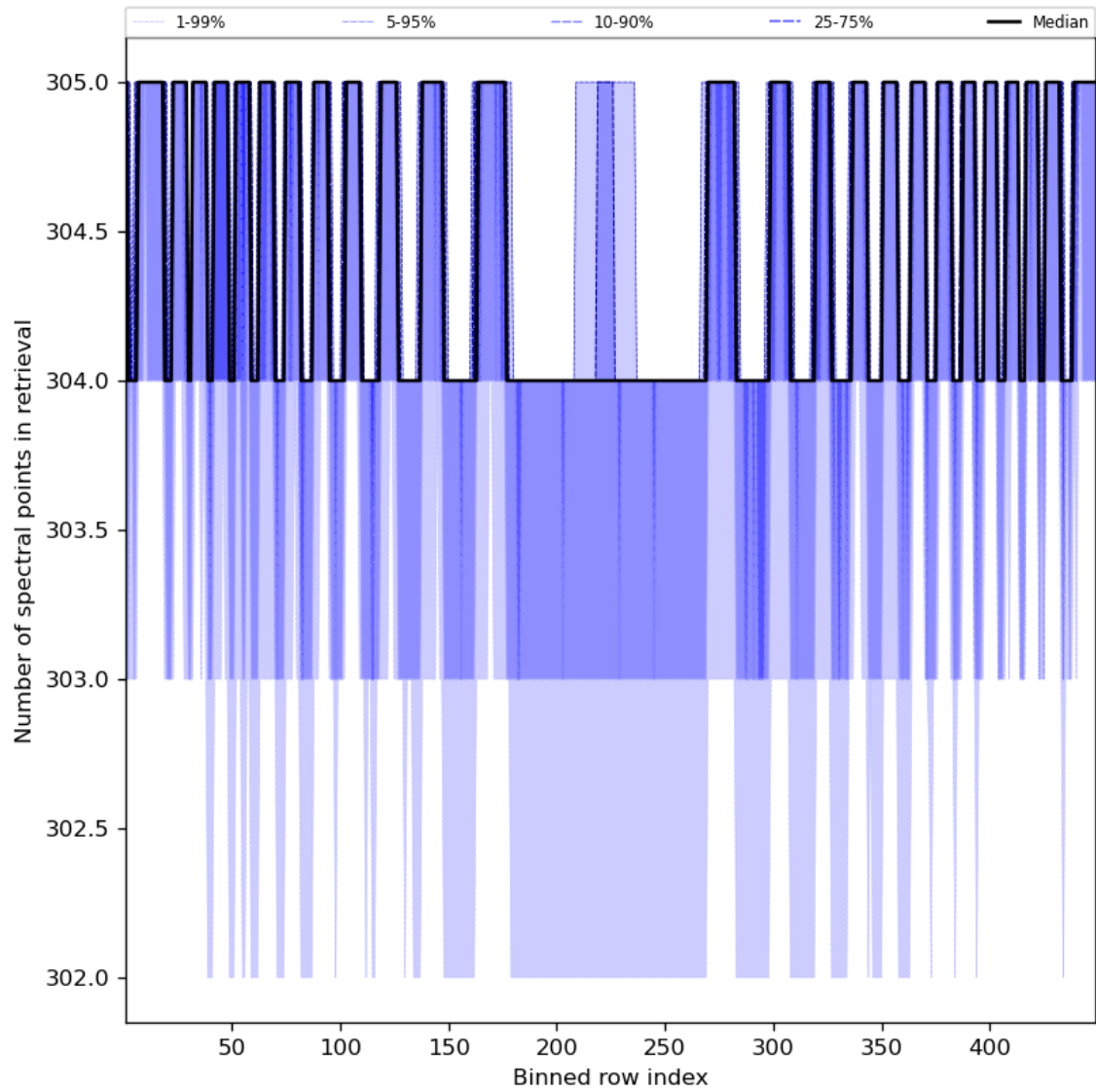
Figure 50: Along track statistics of “Number of spectral points in retrieval” for 2023-12-30 to 2023-12-31
