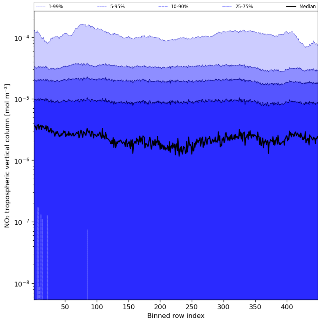
Figure 46: Along track statistics of “NO 2 tropospheric vertical column” for 2023-12-30 to 2023-12-31
