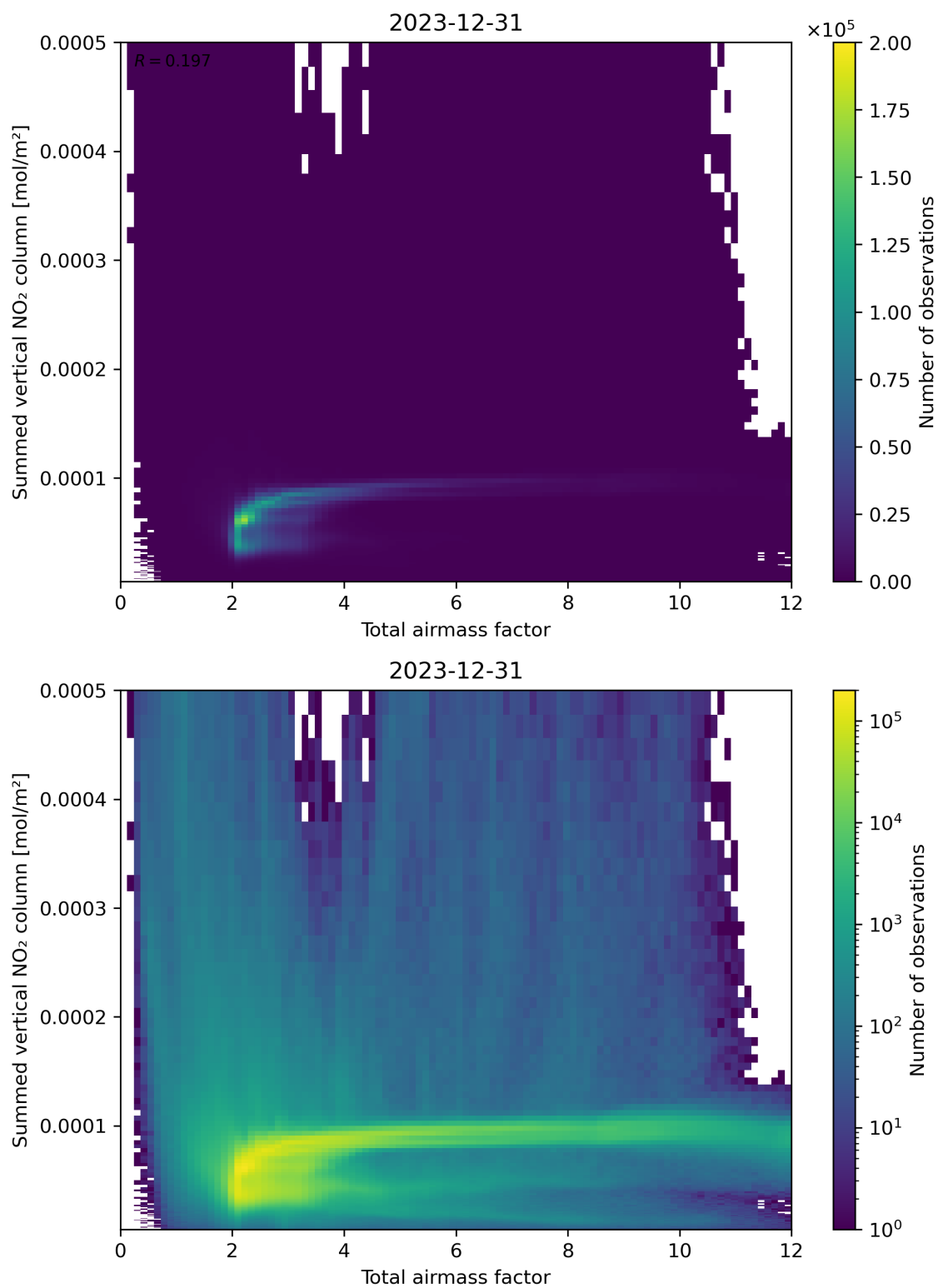
Figure 65: Scatter density plot of “Total airmass factor” against “Summed vertical NO 2 column” for 2023-12-30 to 2023-12-31.
