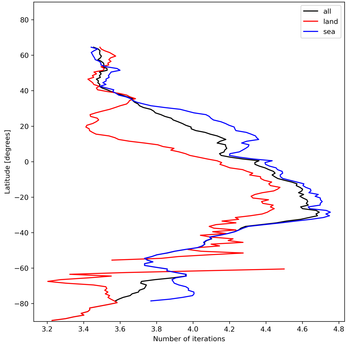
Figure 17: Zonal average of “Number of iterations” for 2023-12-30 to 2023-12-31.
