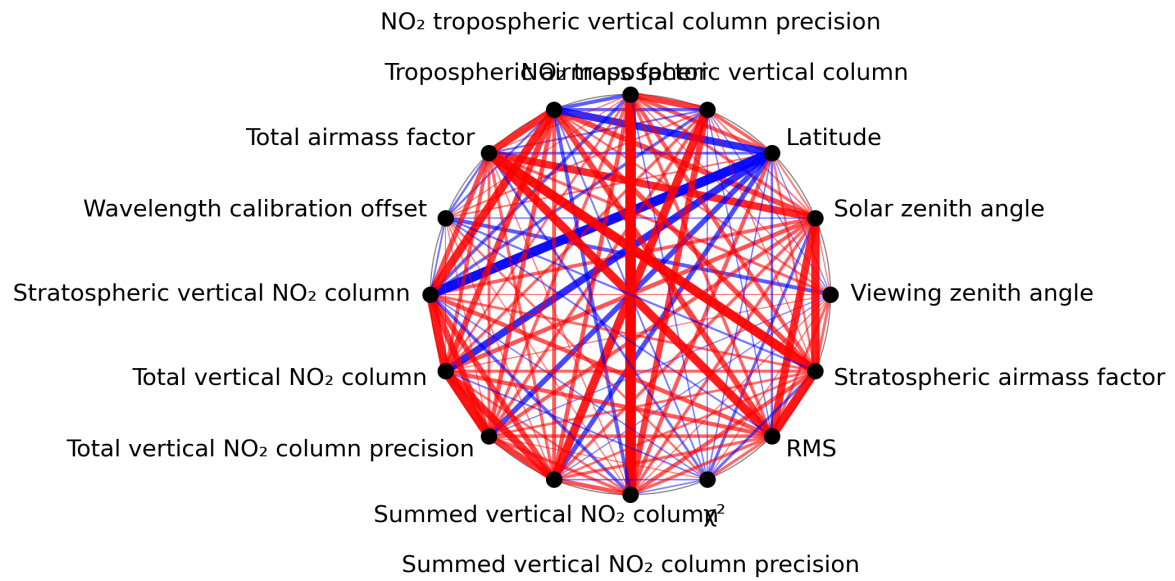
Figure 1: Map of correlation graph for 2023-12-30 to 2023-12-31.
