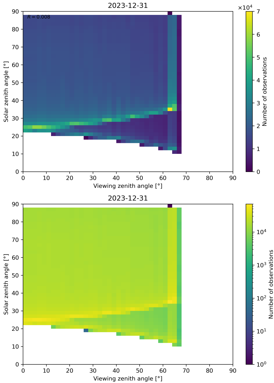
Figure 172: Scatter density plot of “Viewing zenith angle” against “Solar zenith angle” for 2023-12-30 to 2023-12-31.
