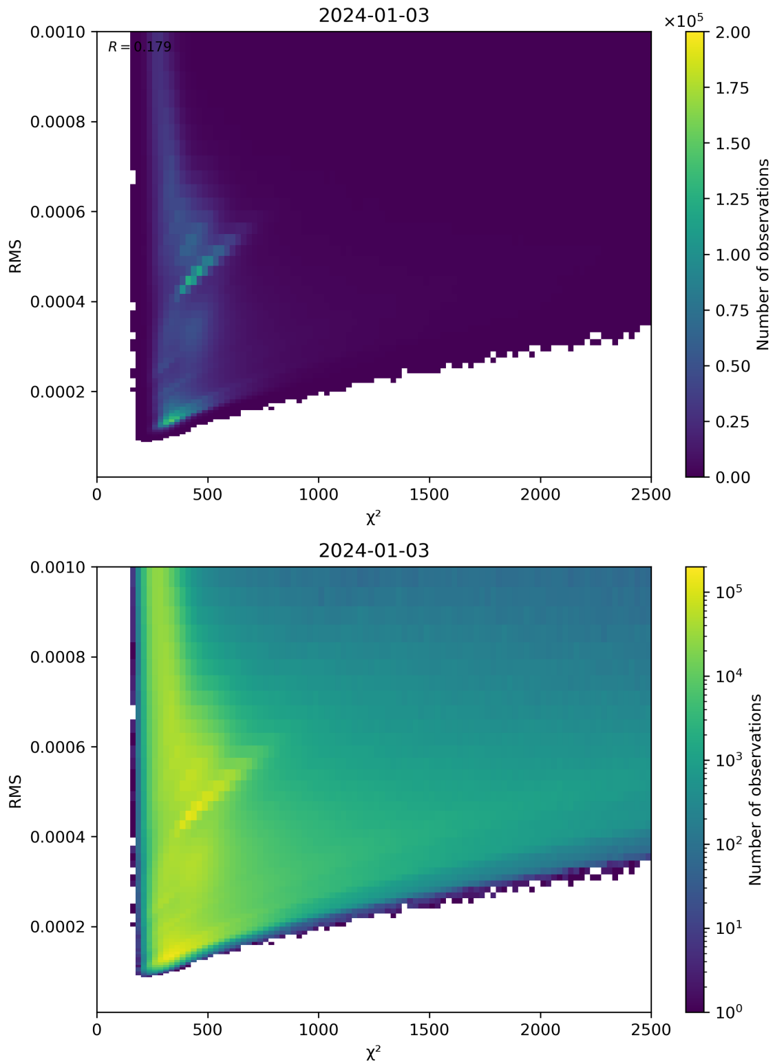
Figure 82: Scatter density plot of “ \chi^2 ” against “RMS” for 2024-01-02 to 2024-01-04.
