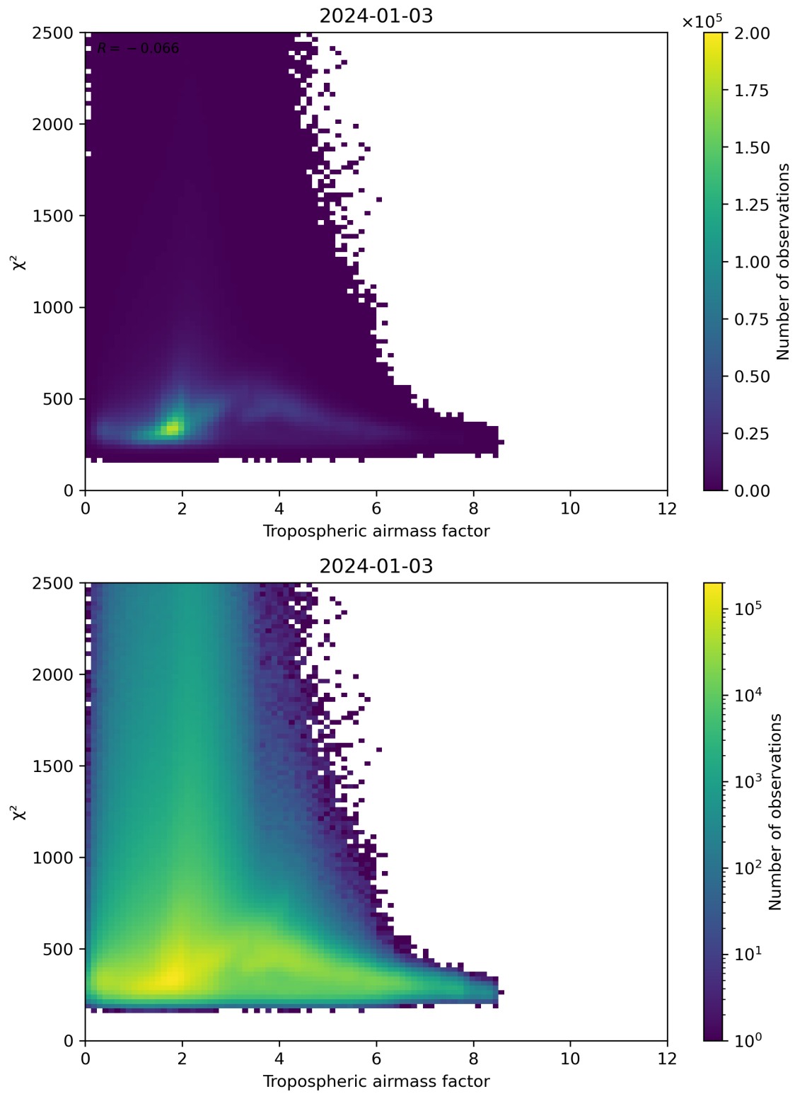
Figure 73: Scatter density plot of “Tropospheric airmass factor” against “ \chi^2 ” for 2024-01-02 to 2024-01-04.
