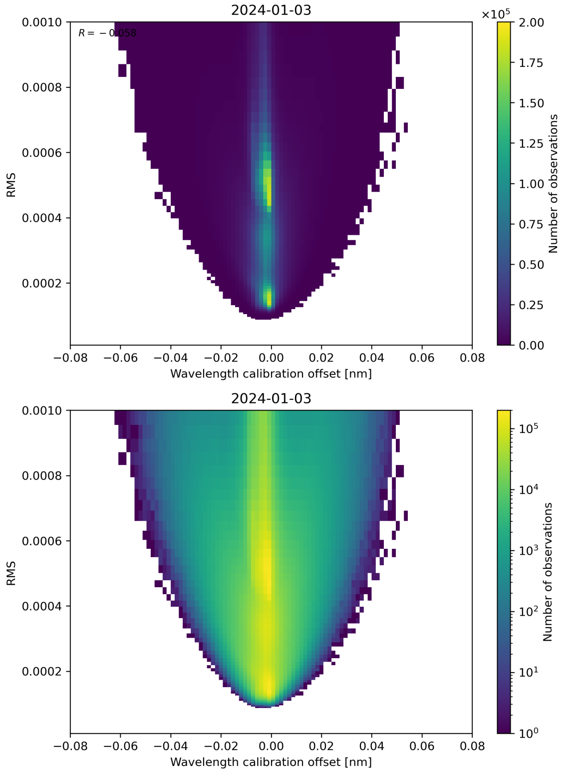
Figure 181: Scatter density plot of “Wavelength calibration offset” against “RMS” for 2024-01-02 to 2024-01-04.
