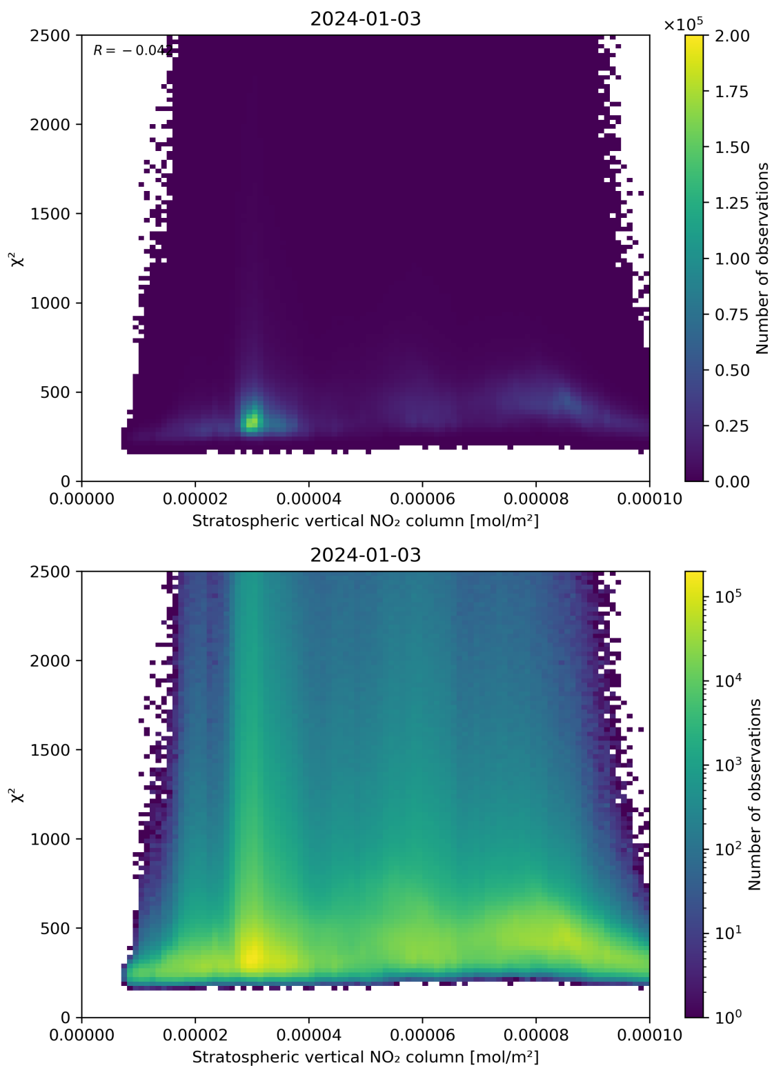
Figure 97: Scatter density plot of “Stratospheric vertical NO 2 column” against “ \chi^2 ” for 2024-01-02 to 2024-01-04.
