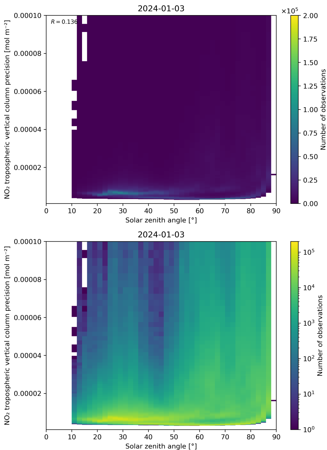
Figure 156: Scatter density plot of “Solar zenith angle” against “NO 2 tropospheric vertical column precision” for 2024-01-02 to 2024-01-04.
