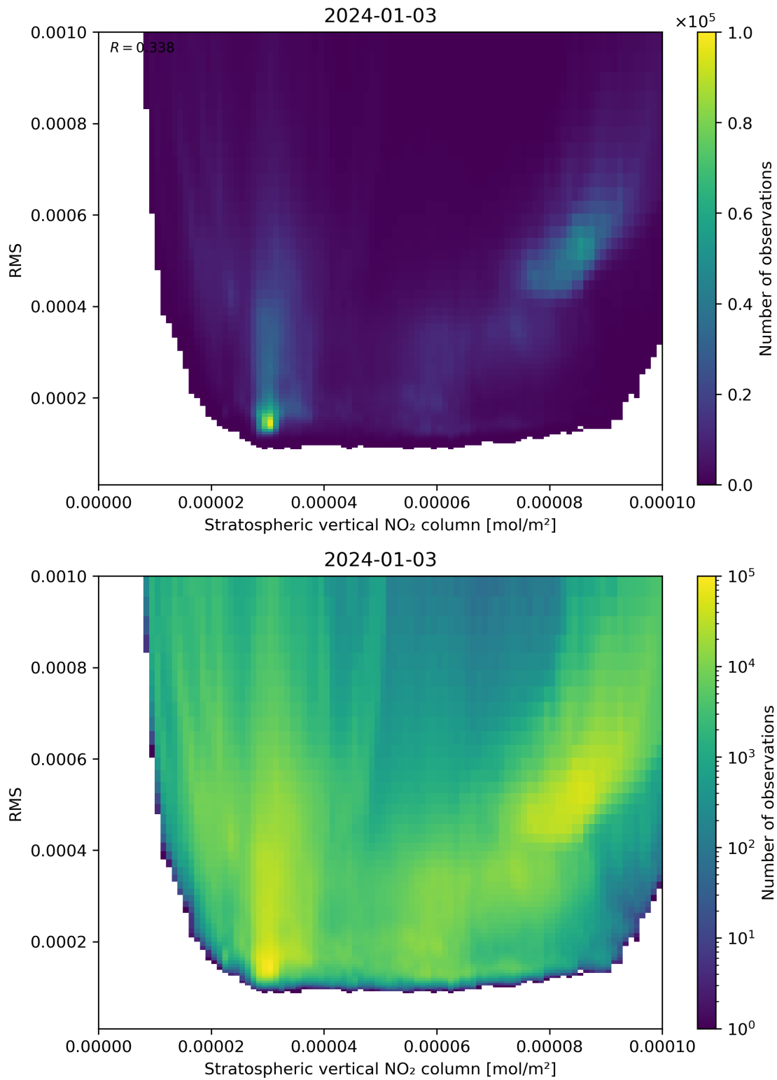
Figure 102: Scatter density plot of “Stratospheric vertical NO 2 column” against “RMS” for 2024-01-02 to 2024-01-04.
