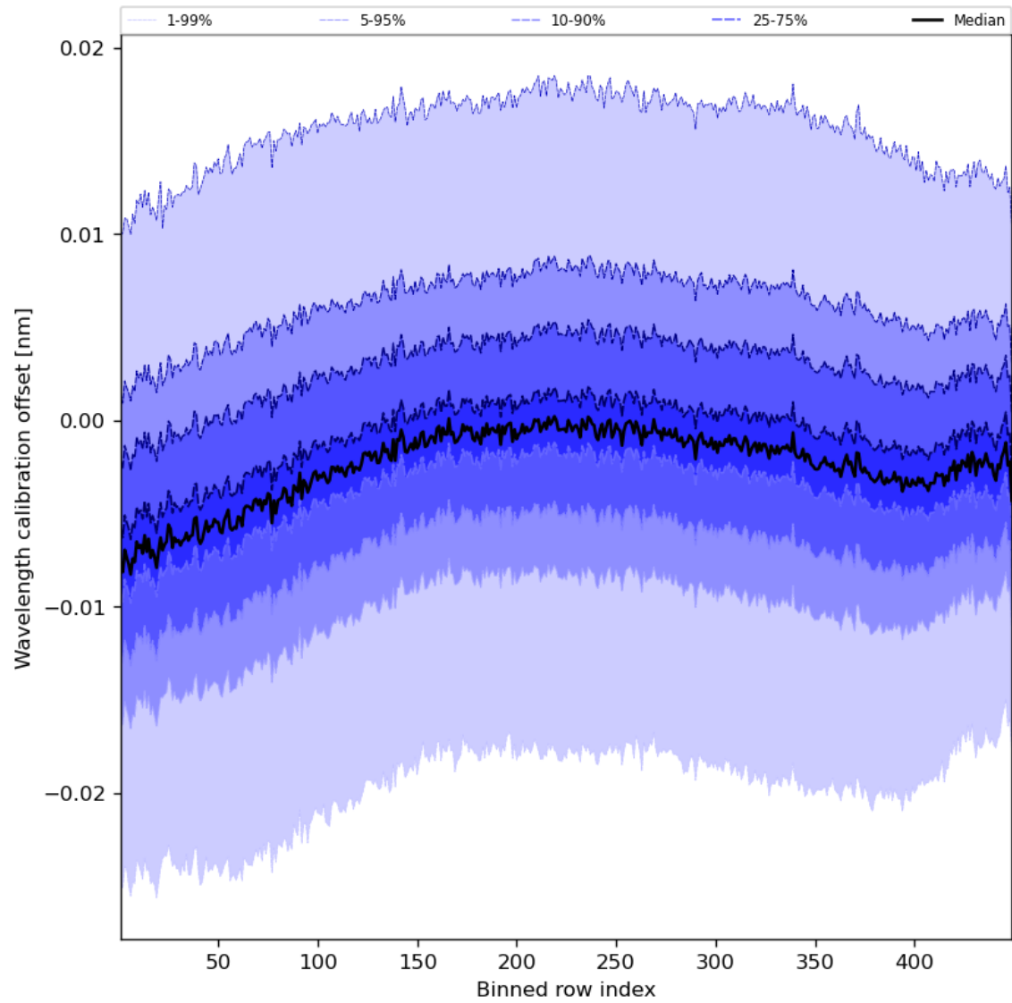
Figure 52: Along track statistics of “Wavelength calibration offset” for 2024-01-02 to 2024-01-04
