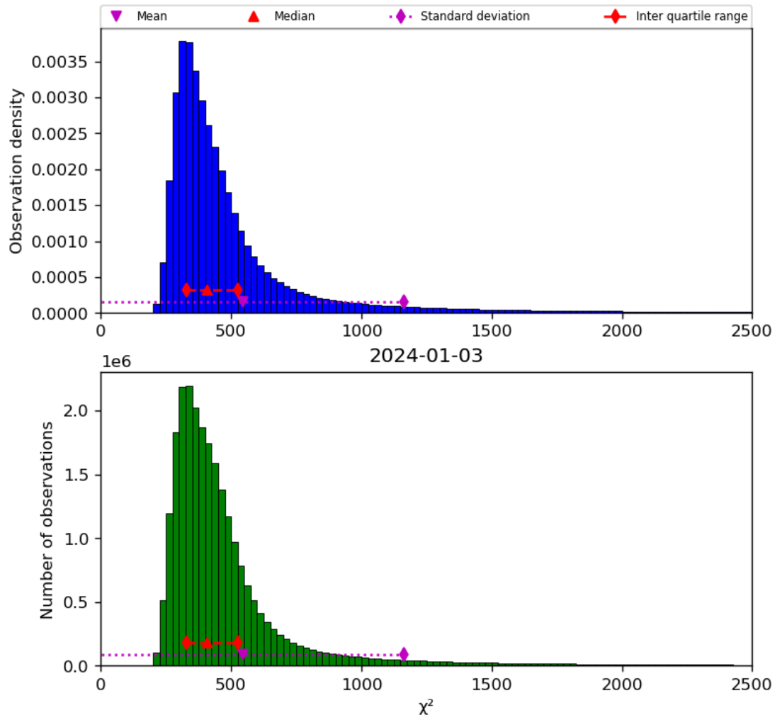
Figure 42: Histogram of “ \chi^2 ” for 2024-01-02 to 2024-01-04
