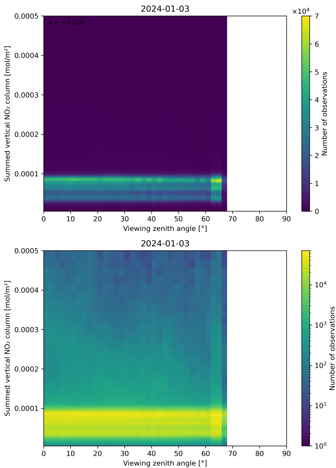
Figure 165: Scatter density plot of “Viewing zenith angle” against “Summed vertical NO 2 column” for 2024-01-02 to 2024-01-04.
