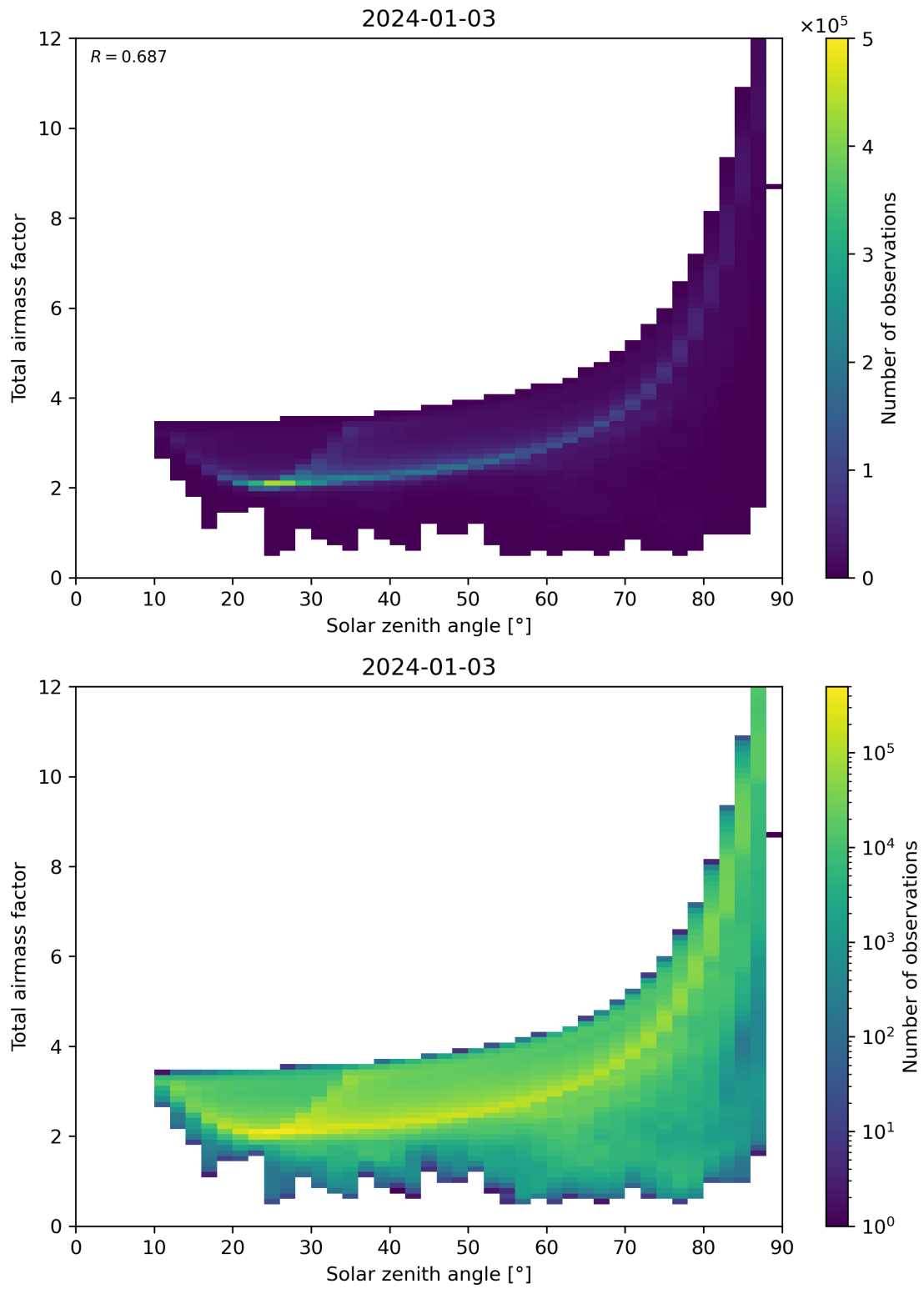
Figure 146: Scatter density plot of “Solar zenith angle” against “Total air mass factor” for 2024-01-02 to 2024-01-04.
