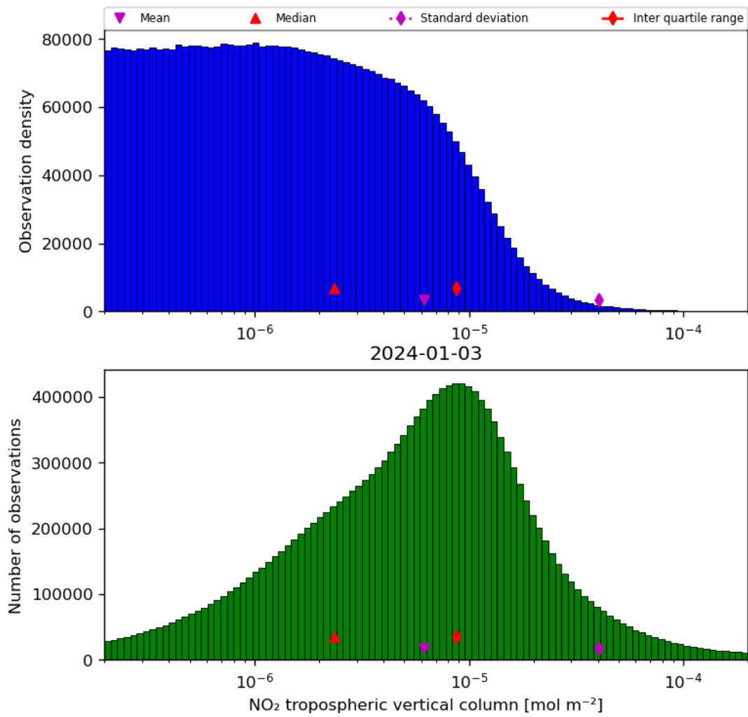
Figure 29: Histogram of “NO 2 tropospheric vertical column” for 2024-01-02 to 2024-01-04
