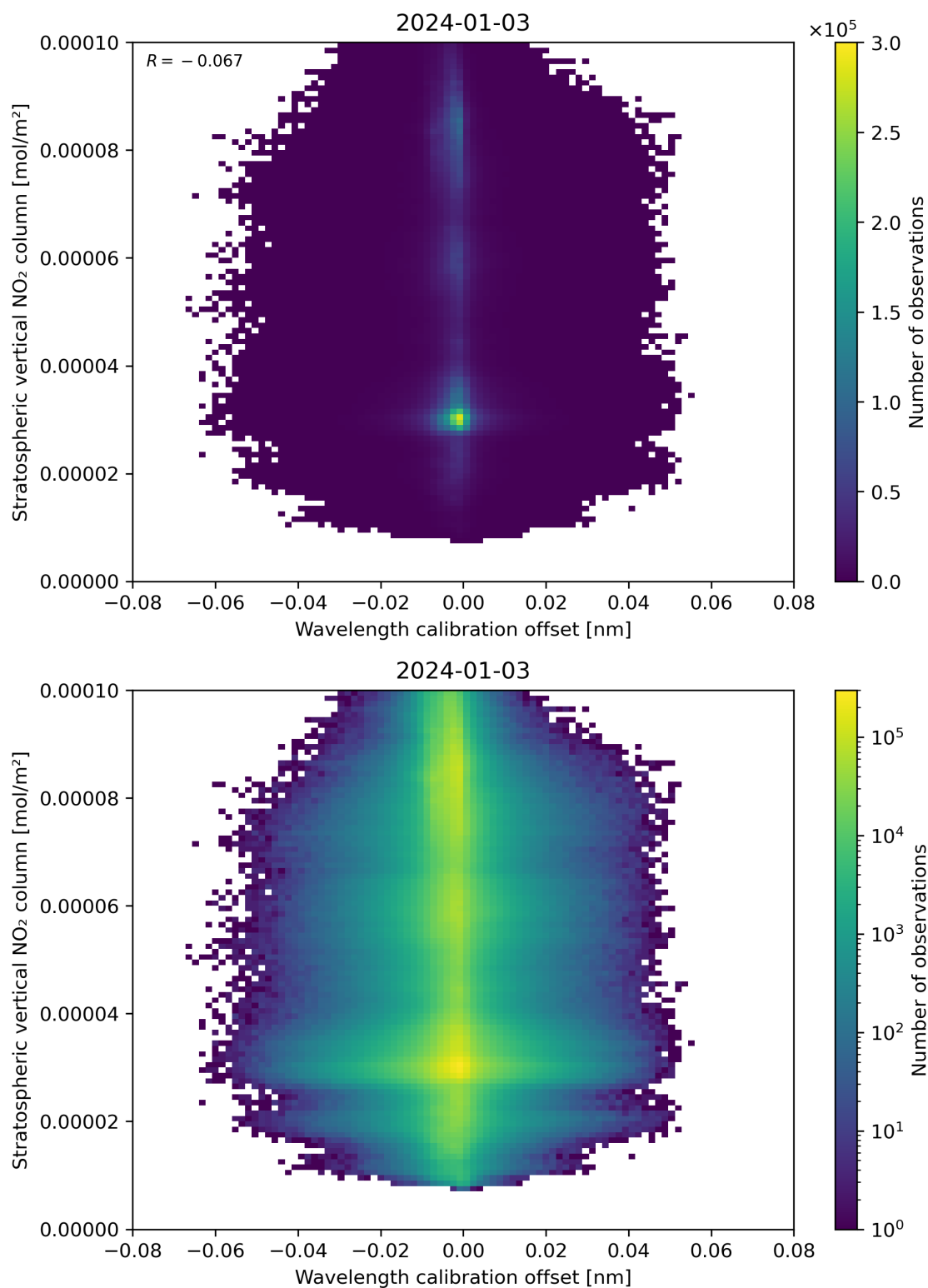
Figure 176: Scatter density plot of “Wavelength calibration offset” against “Stratospheric vertical NO 2 column” for 2024-01-02 to 2024-01-04.
