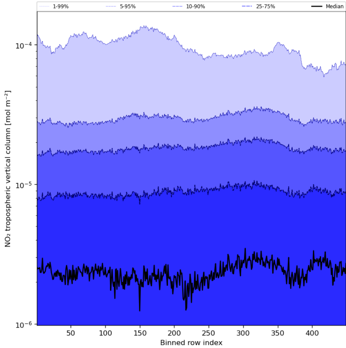
Figure 46: Along track statistics of “NO 2 tropospheric vertical column” for 2024-01-02 to 2024-01-04
