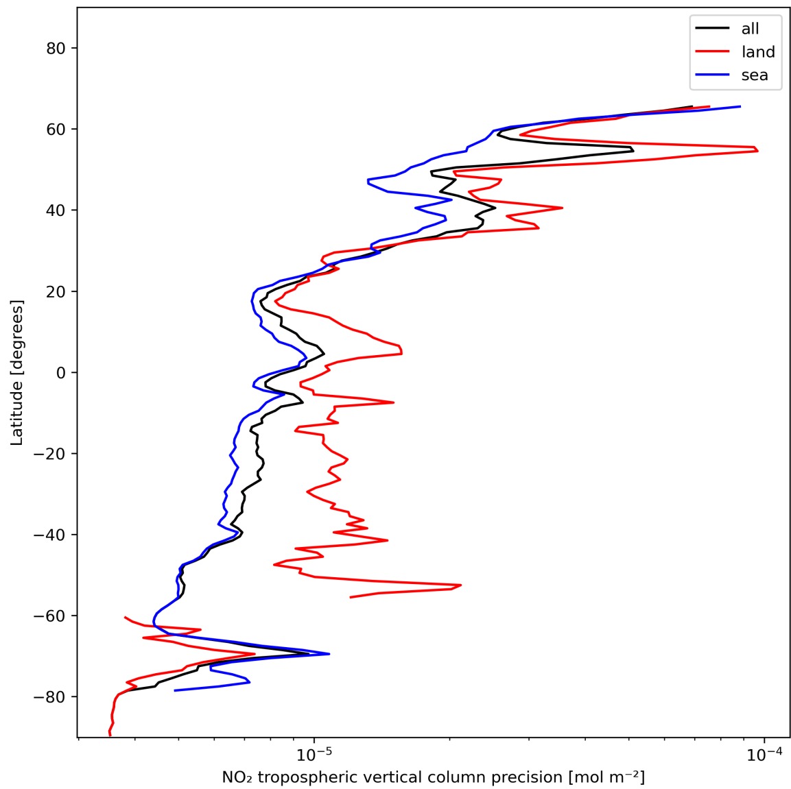
Figure 13: Zonal average of “NO 2 tropospheric vertical column precision” for 2024-01-02 to 2024-01-04.
