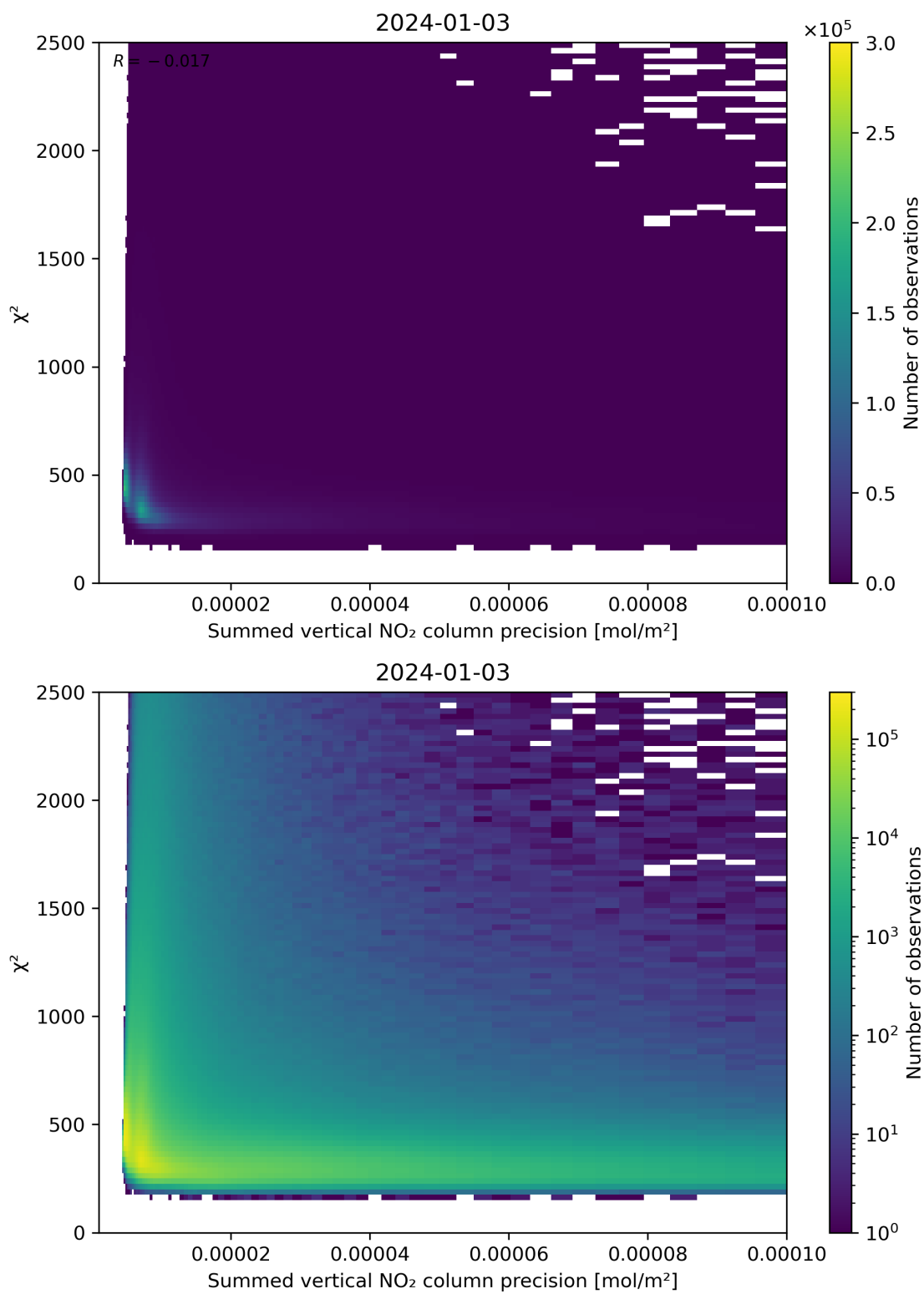
Figure 107: Scatter density plot of “Summed vertical NO 2 column precision” against “ \chi^2 ” for 2024-01-02 to 2024-01-04.
