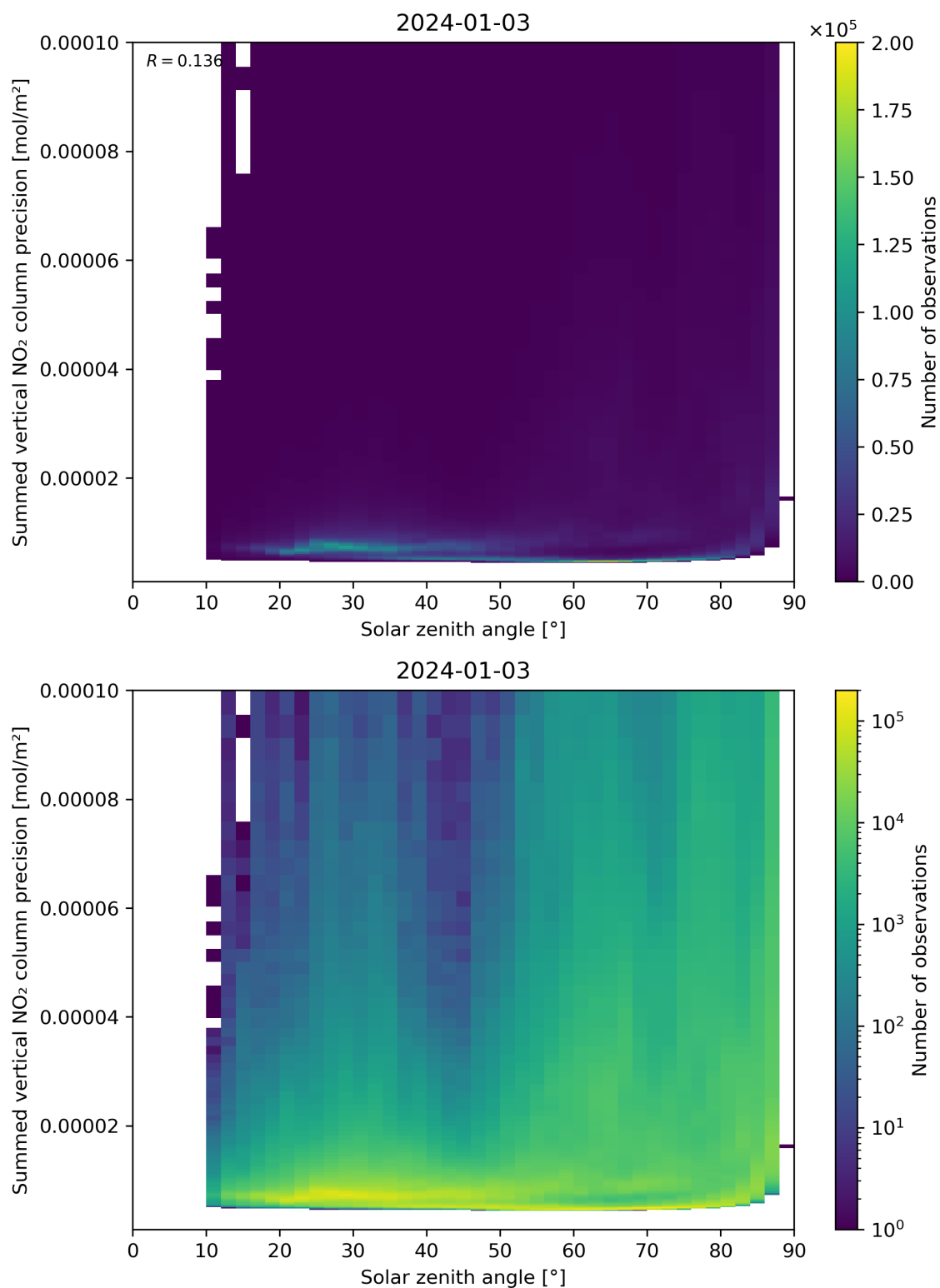
Figure 152: Scatter density plot of “Solar zenith angle” against “Summed vertical NO 2 column precision” for 2024-01-02 to 2024-01-04.
