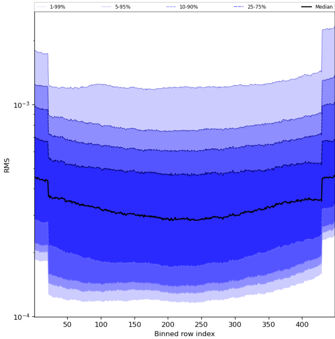
Figure 60: Along track statistics of “RMS” for 2024-01-02 to 2024-01-04
