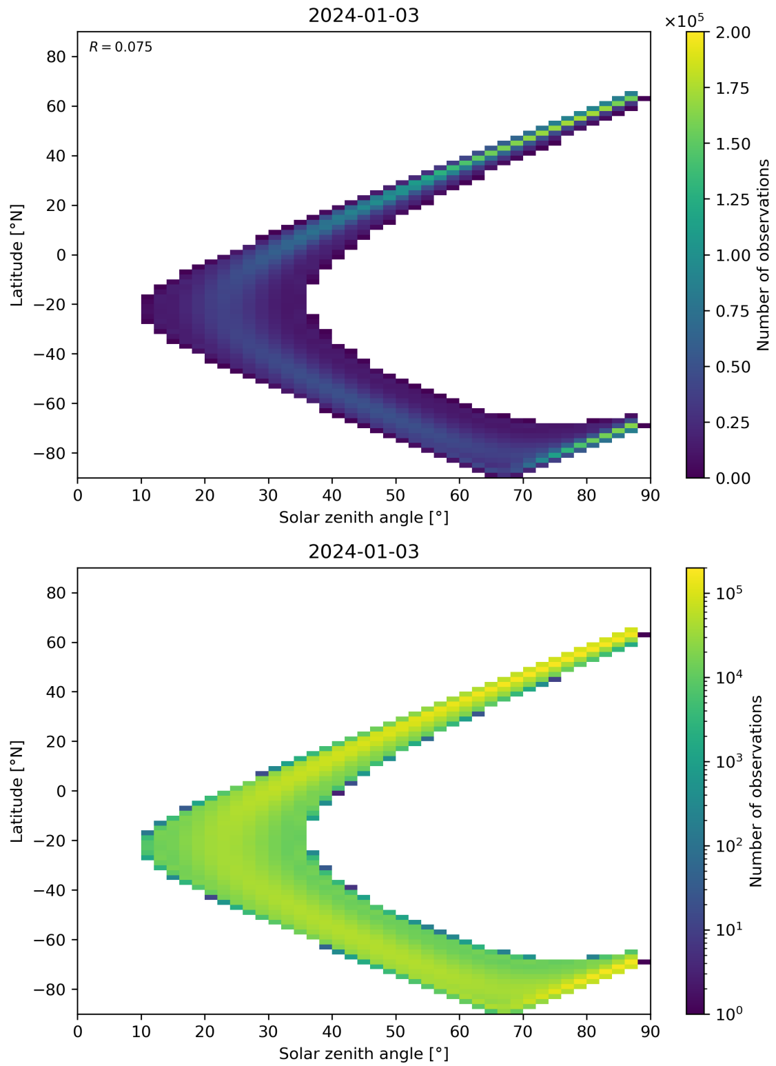
Figure 149: Scatter density plot of “Solar zenith angle” against “Latitude” for 2024-01-02 to 2024-01-04.
