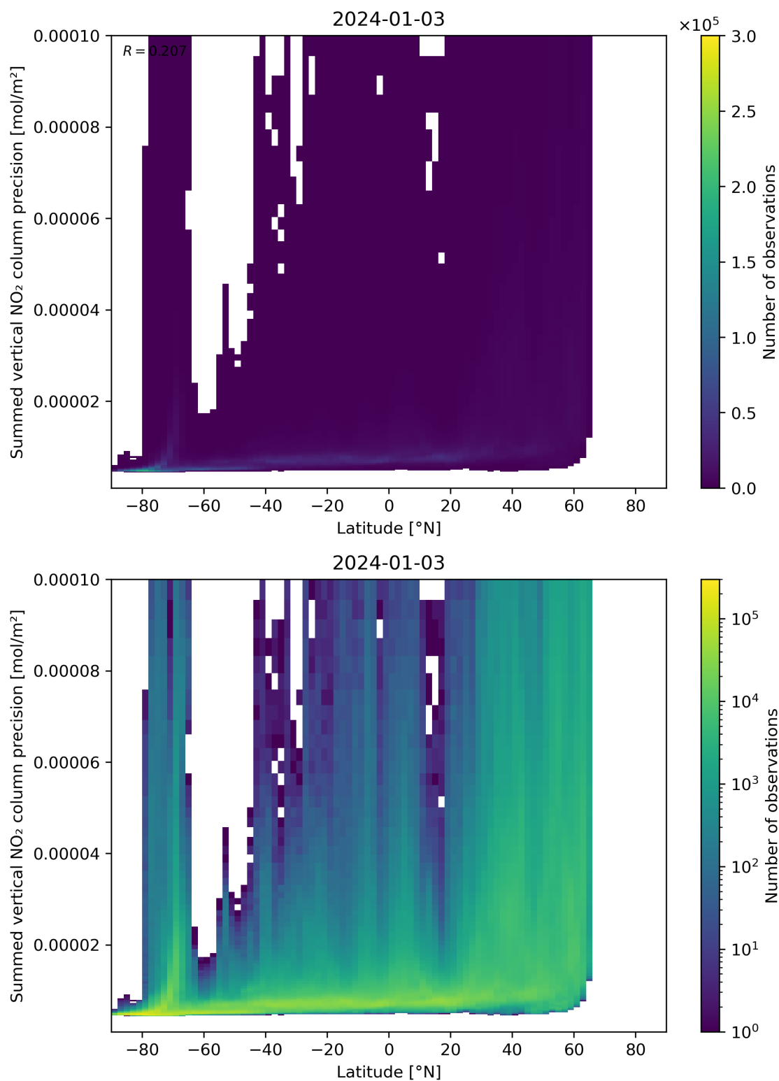
Figure 89: Scatter density plot of “Latitude” against “Summed vertical NO 2 column precision” for 2024-01-02 to 2024-01-04.
