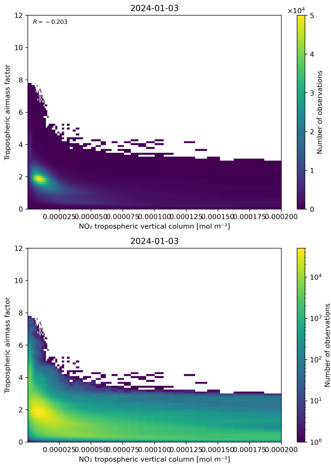
Figure 123: Scatter density plot of “NO 2 tropospheric vertical column” against “Tropospheric air mass factor” for 2024-01-02 to 2024-01-04.
