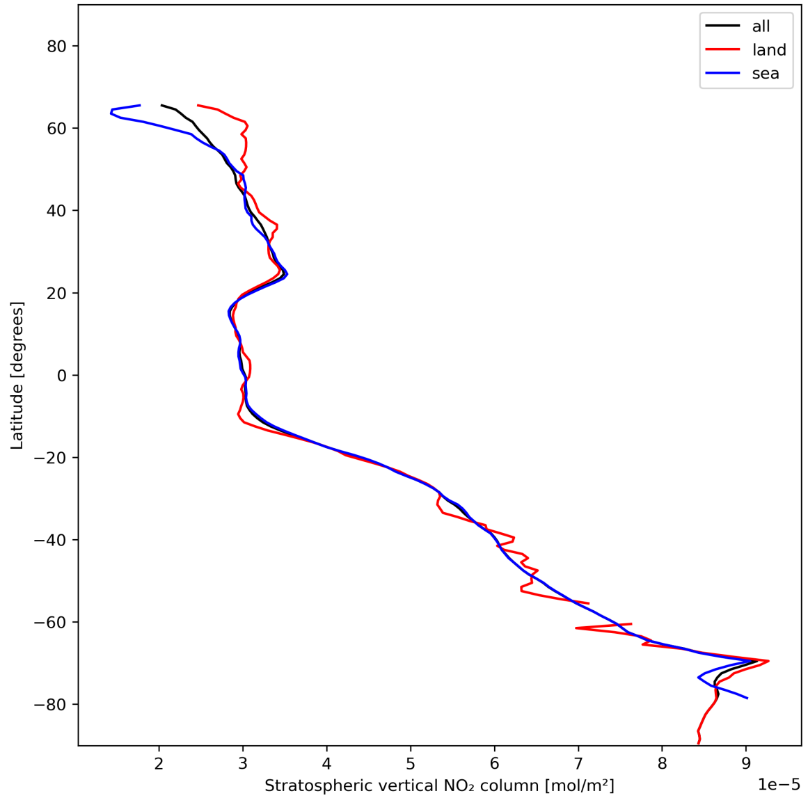
Figure 19: Zonal average of “Stratospheric vertical NO 2 column” for 2024-01-02 to 2024-01-04.
