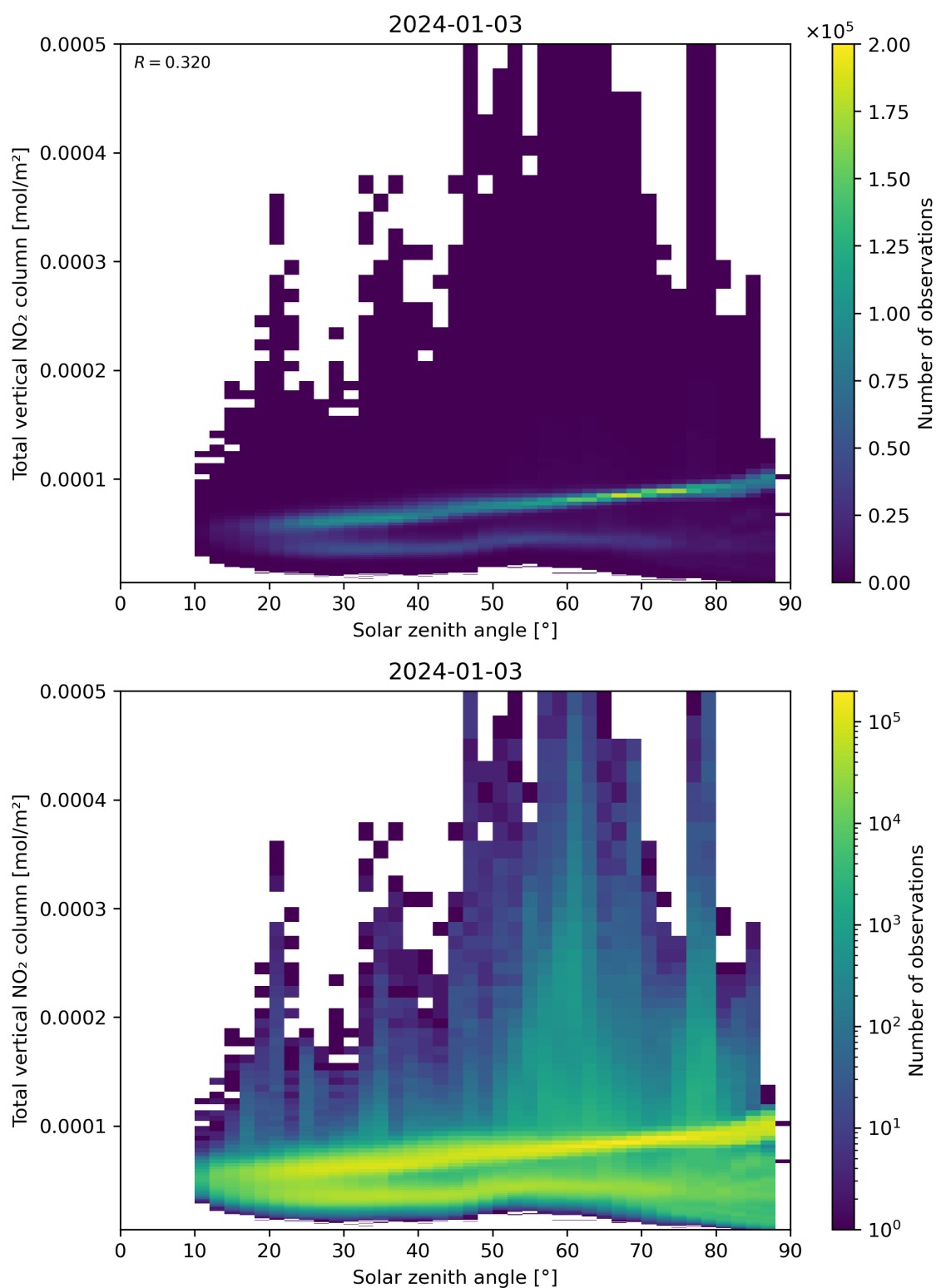
Figure 153: Scatter density plot of “Solar zenith angle” against “Total vertical NO 2 column” for 2024-01-02 to 2024-01-04.
