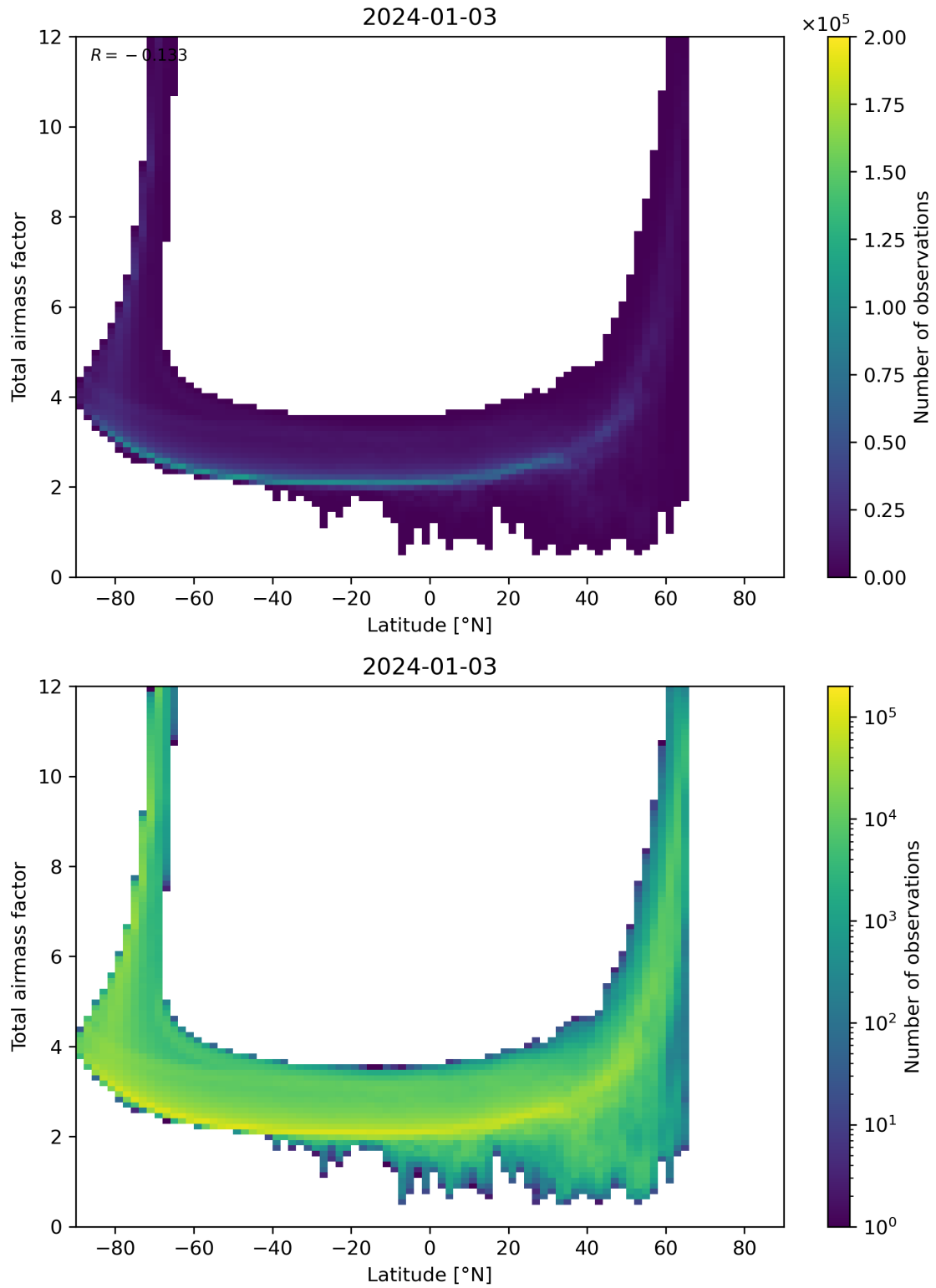
Figure 84: Scatter density plot of “Latitude” against “Total airmass factor” for 2024-01-02 to 2024-01-04.
