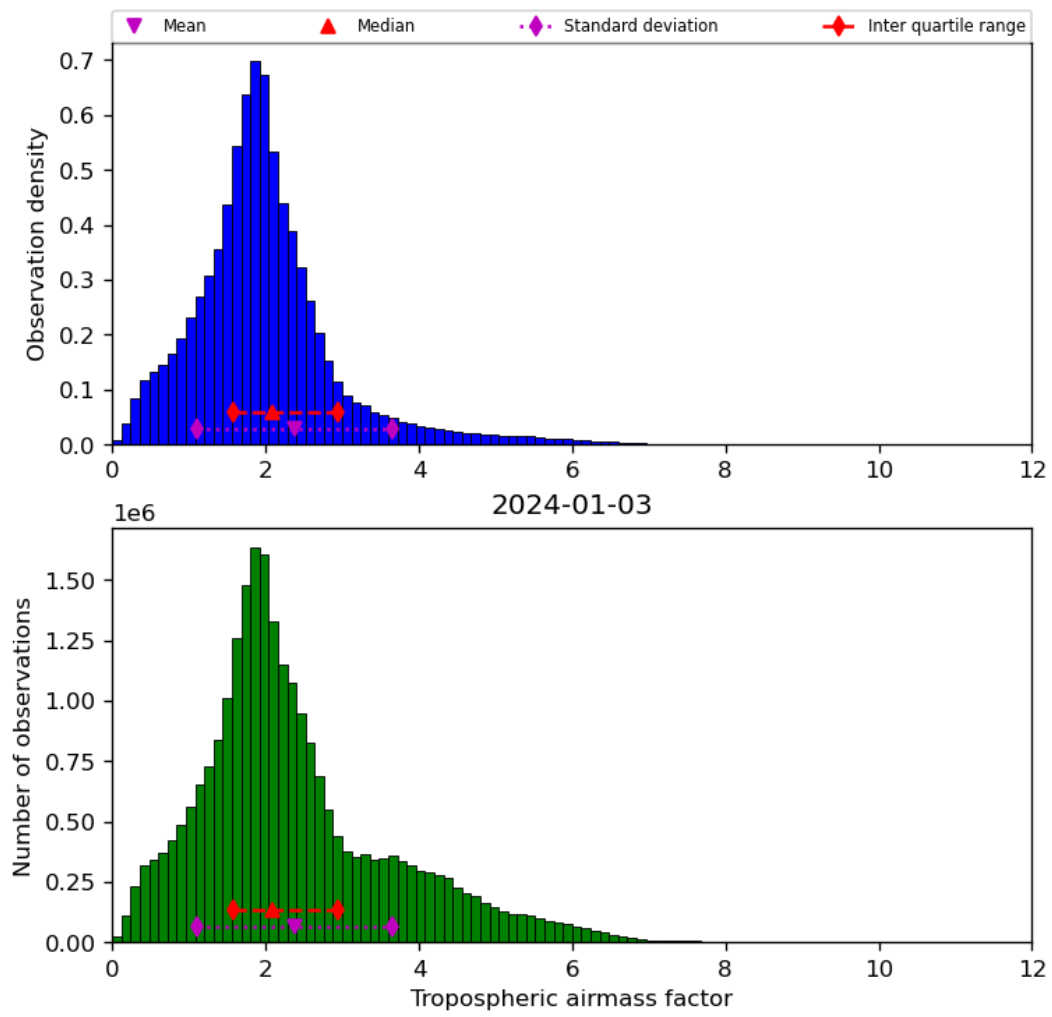
Figure 31: Histogram of “Tropospheric airmass factor” for 2024-01-02 to 2024-01-04
