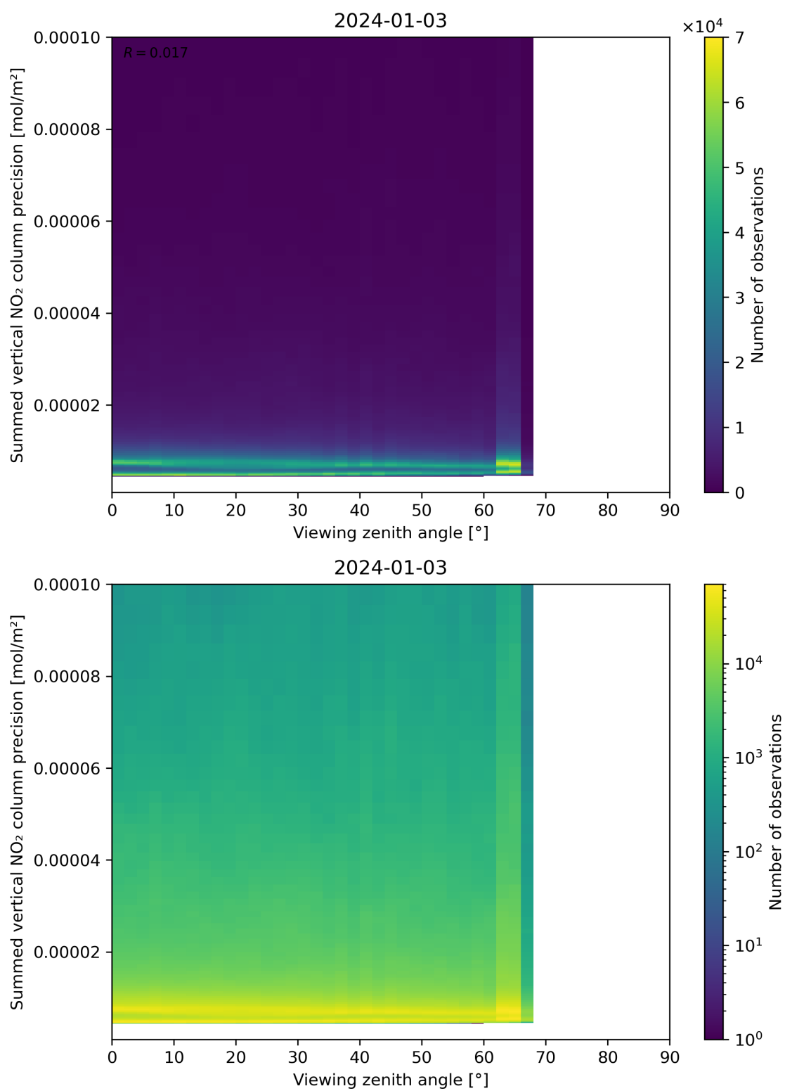
Figure 166: Scatter density plot of “Viewing zenith angle” against “Summed vertical NO 2 column precision” for 2024-01-02 to 2024-01-04.
