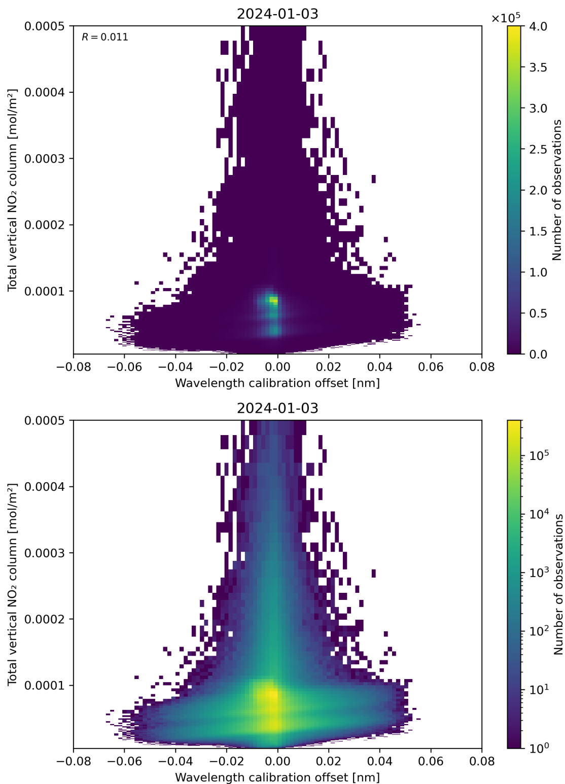
Figure 179: Scatter density plot of “Wavelength calibration offset” against “Total vertical NO 2 column” for 2024-01-02 to 2024-01-04.
