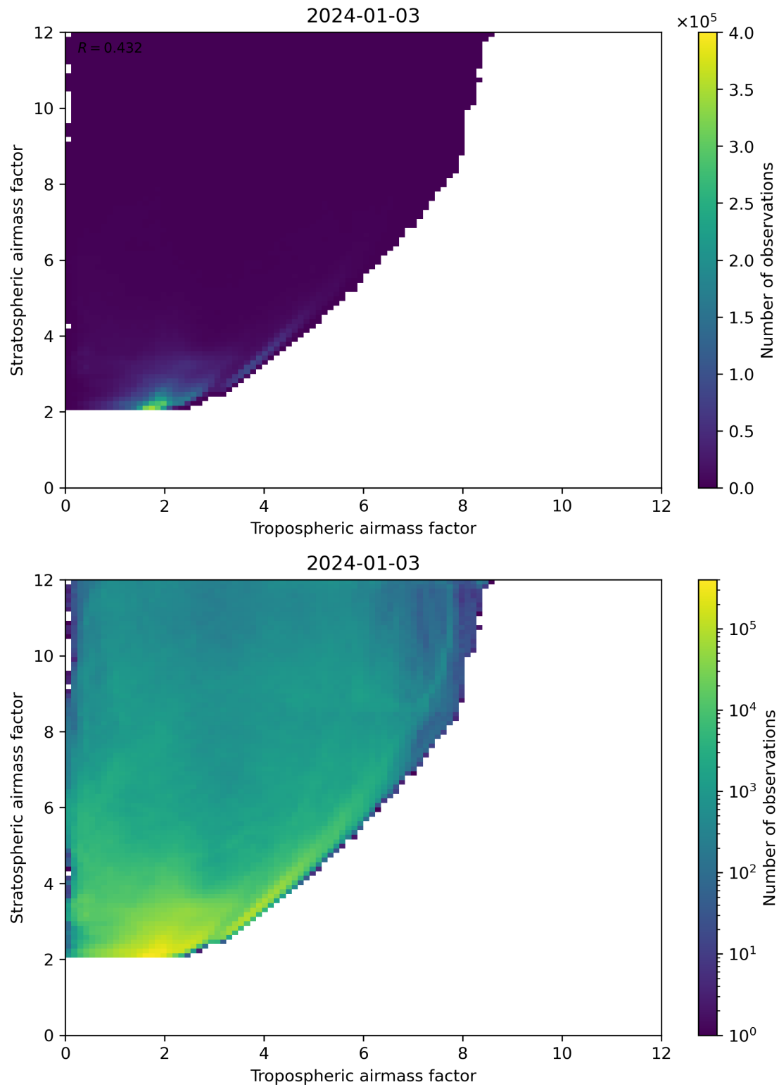
Figure 71: Scatter density plot of “Tropospheric airmass factor” against “Stratospheric airmass factor” for 2024-01-02 to 2024-01-04.
