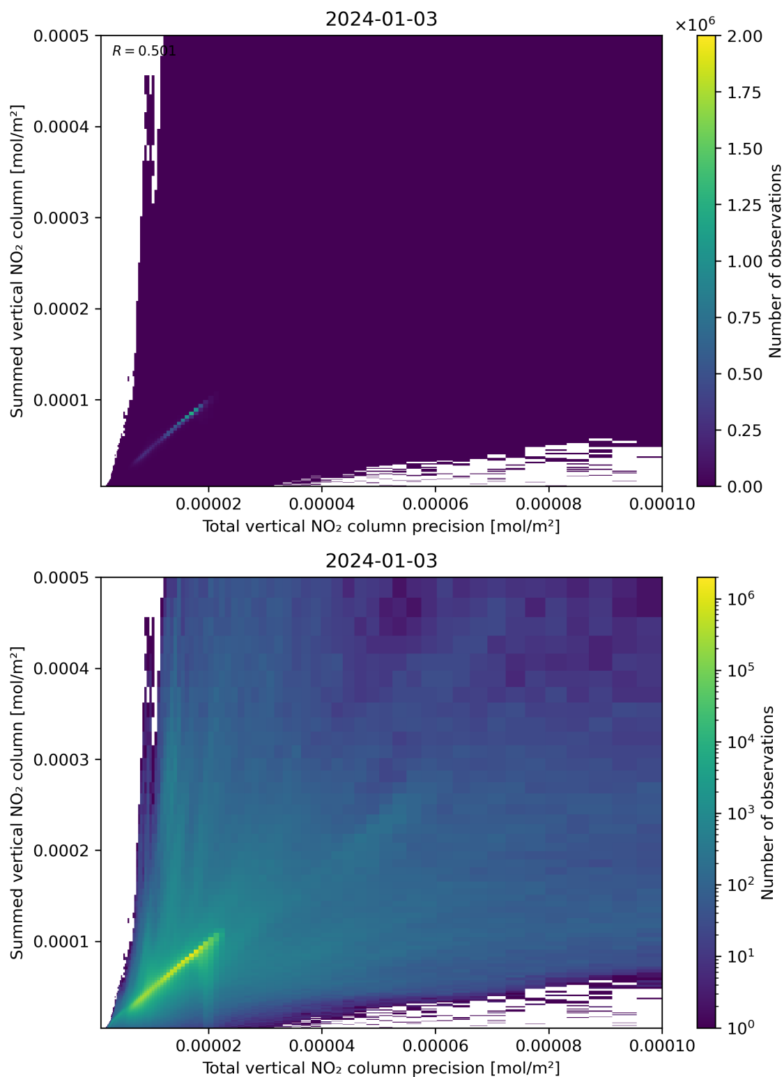
Figure 117: Scatter density plot of “Total vertical NO 2 column precision” against “Summed vertical NO 2 column” for 2024-01-02 to 2024-01-04.
