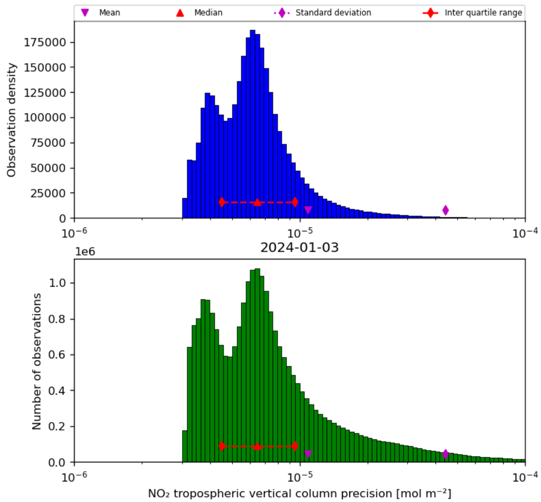
Figure 30: Histogram of “NO 2 tropospheric vertical column precision” for 2024-01-02 to 2024-01-04
