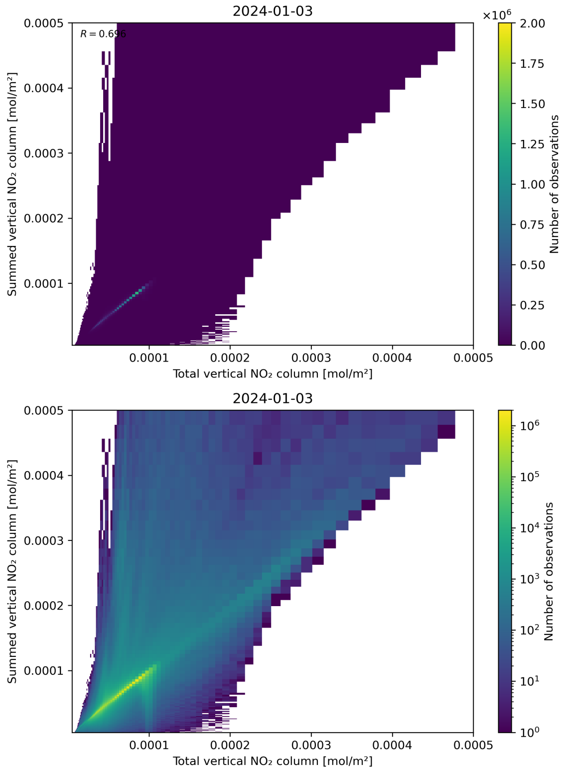
Figure 112: Scatter density plot of “Total vertical NO 2 column” against “Summed vertical NO 2 column” for 2024-01-02 to 2024-01-04.
