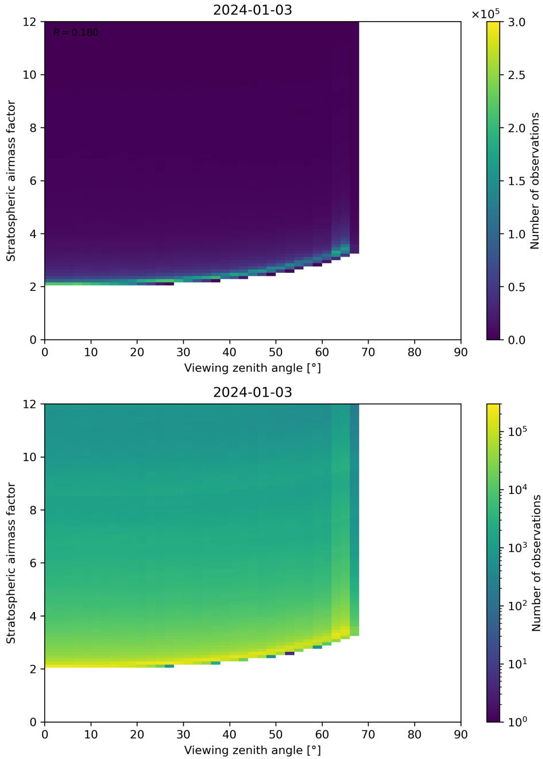
Figure 159: Scatter density plot of “Viewing zenith angle” against “Stratospheric airmass factor” for 2024-01-02 to 2024-01-04.
