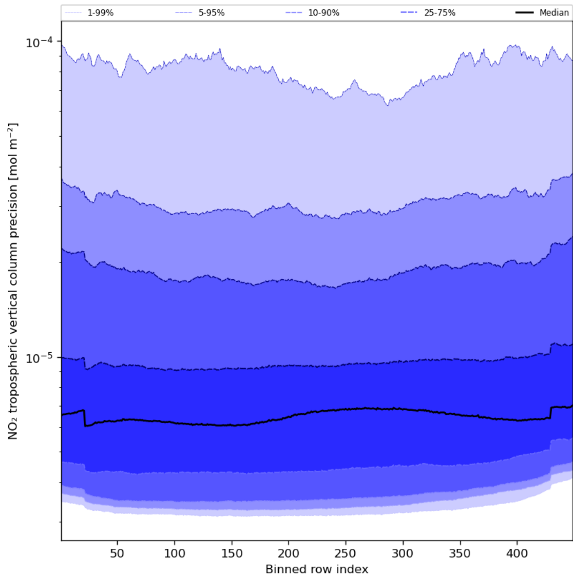
Figure 47: Along track statistics of “NO 2 tropospheric vertical column precision” for 2024-01-02 to 2024-01-04
