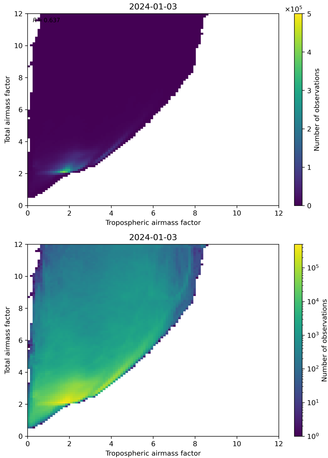
Figure 72: Scatter density plot of “Tropospheric airmass factor” against “Total airmass factor” for 2024-01-02 to 2024-01-04.
