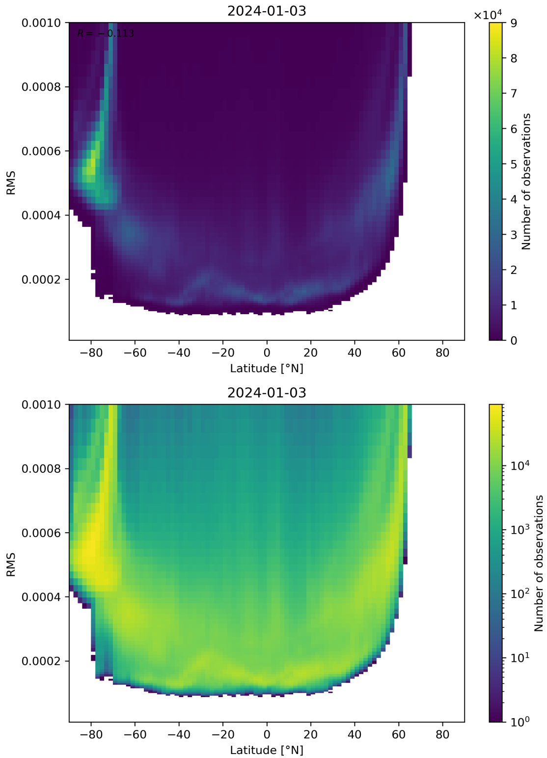
Figure 94: Scatter density plot of “Latitude” against “RMS” for 2024-01-02 to 2024-01-04.
