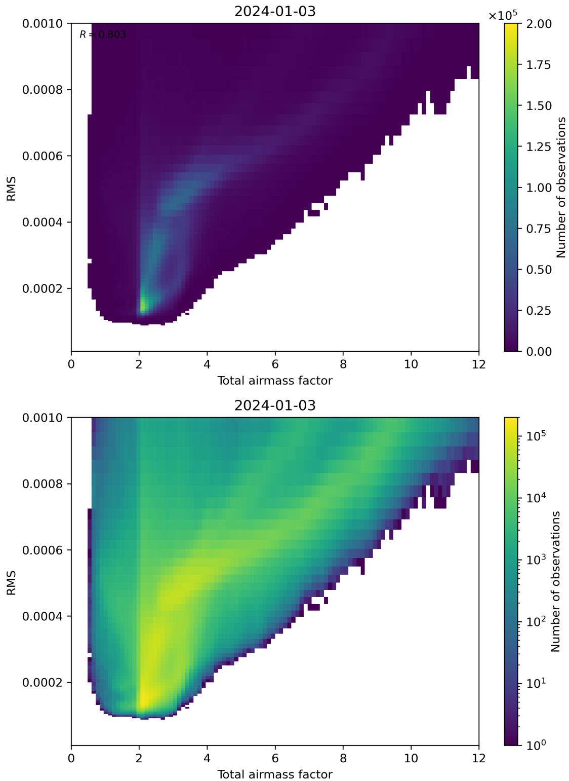
Figure 69: Scatter density plot of “Total airmass factor” against “RMS” for 2024-01-02 to 2024-01-04.
