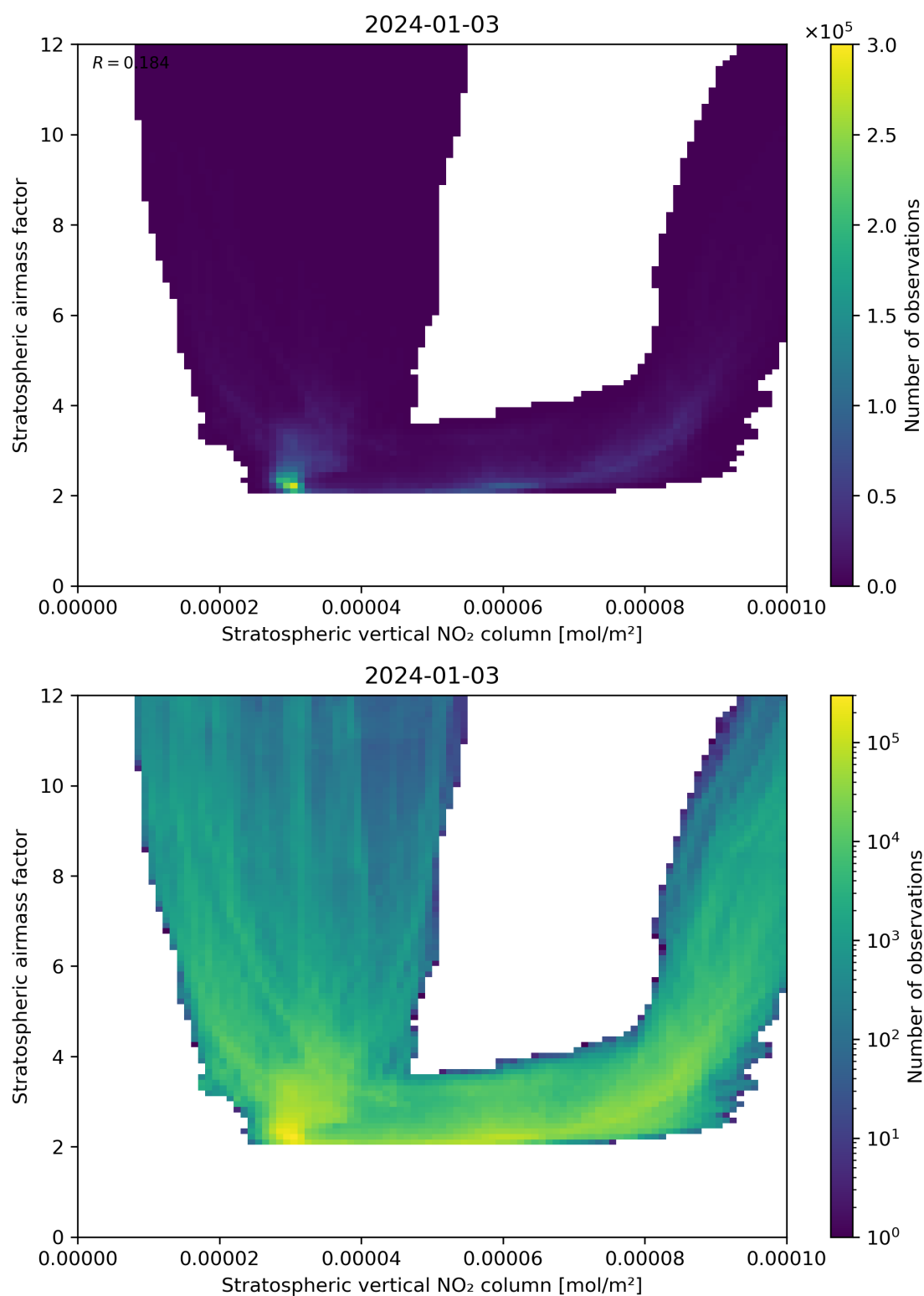
Figure 96: Scatter density plot of “Stratospheric vertical NO 2 column” against “Stratospheric airmass factor” for 2024-01-02 to 2024-01-04.
