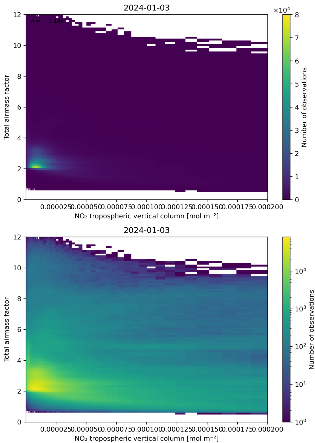
Figure 122: Scatter density plot of “NO 2 tropospheric vertical column” against “Total air mass factor” for 2024-01-02 to 2024-01-04.
