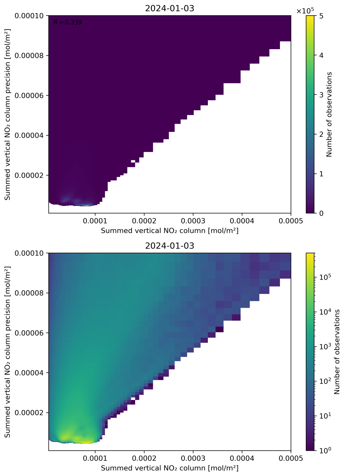
Figure 105: Scatter density plot of “Summed vertical NO 2 column” against “Summed vertical NO 2 column precision” for 2024-01-02 to 2024-01-04.
