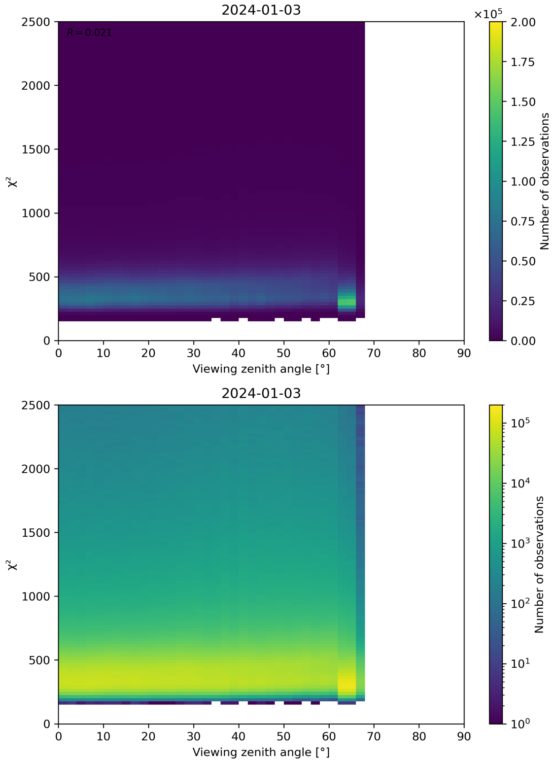
Figure 162: Scatter density plot of “Viewing zenith angle” against “ \chi^2 ” for 2024-01-02 to 2024-01-04.
