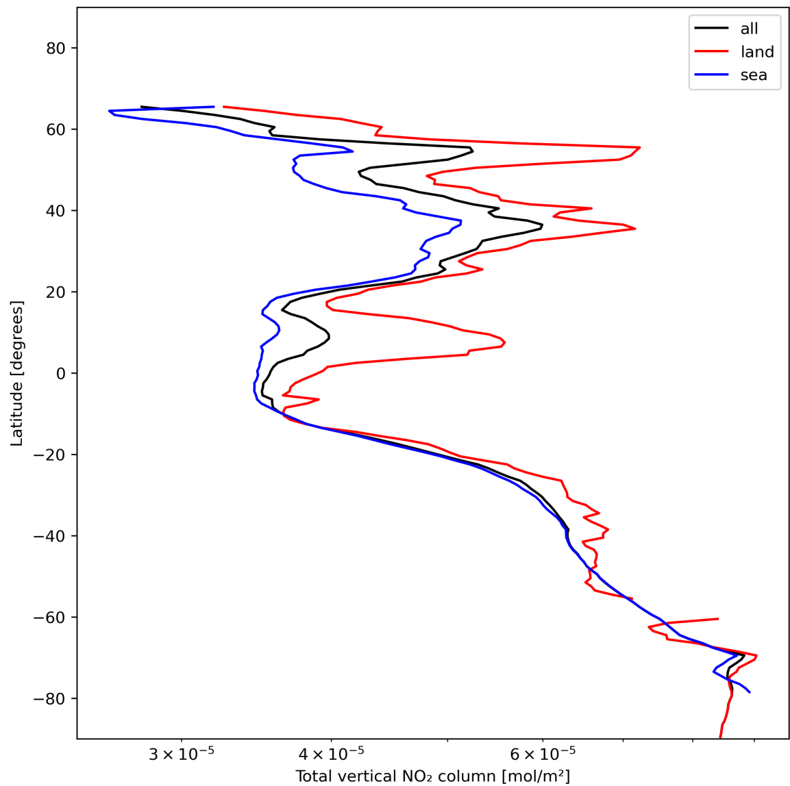
Figure 21: Zonal average of “Total vertical NO 2 column” for 2024-01-02 to 2024-01-04.
