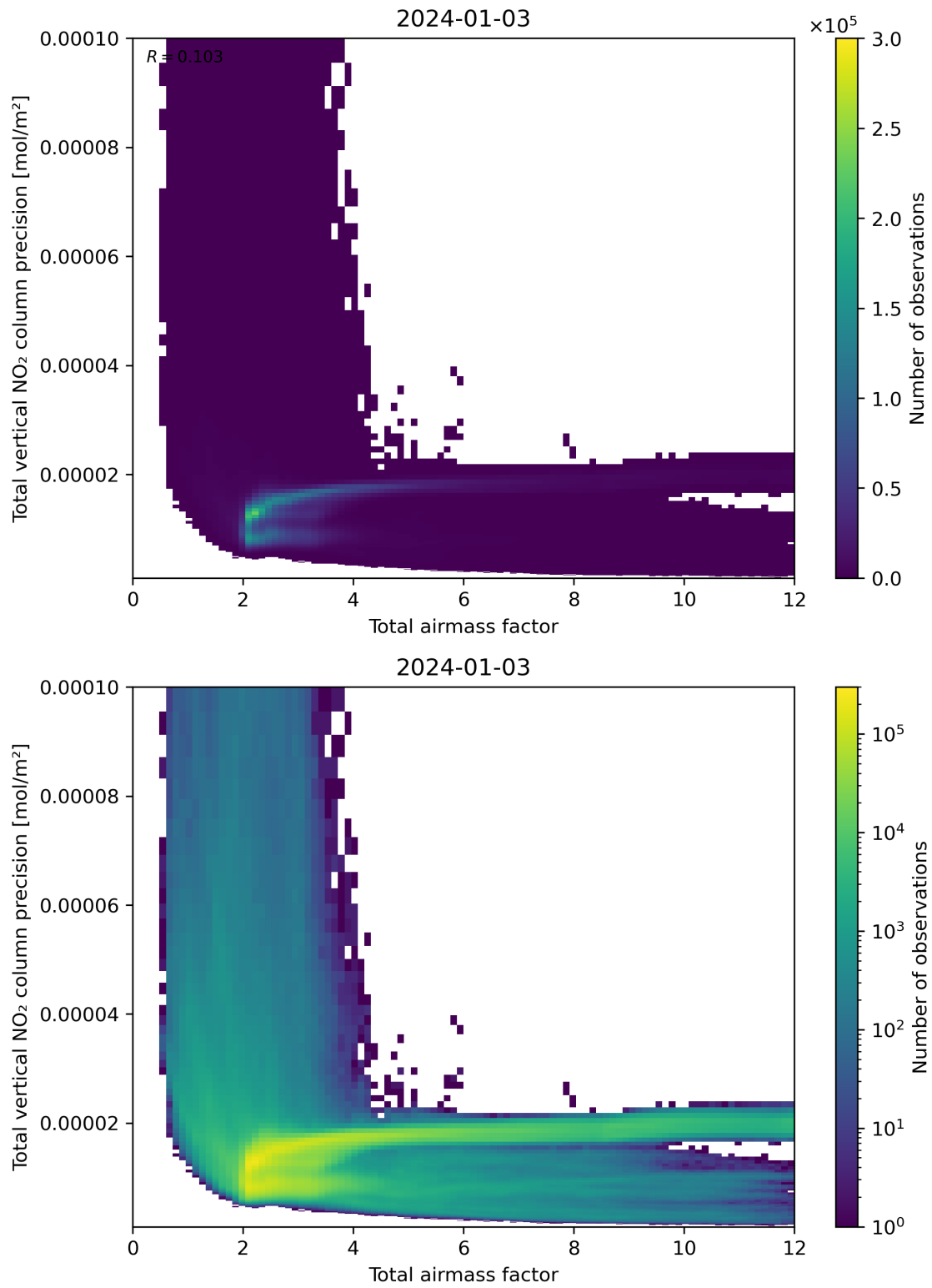
Figure 68: Scatter density plot of “Total airmass factor” against “Total vertical NO 2 column precision” for 2024-01-02 to 2024-01-04.
