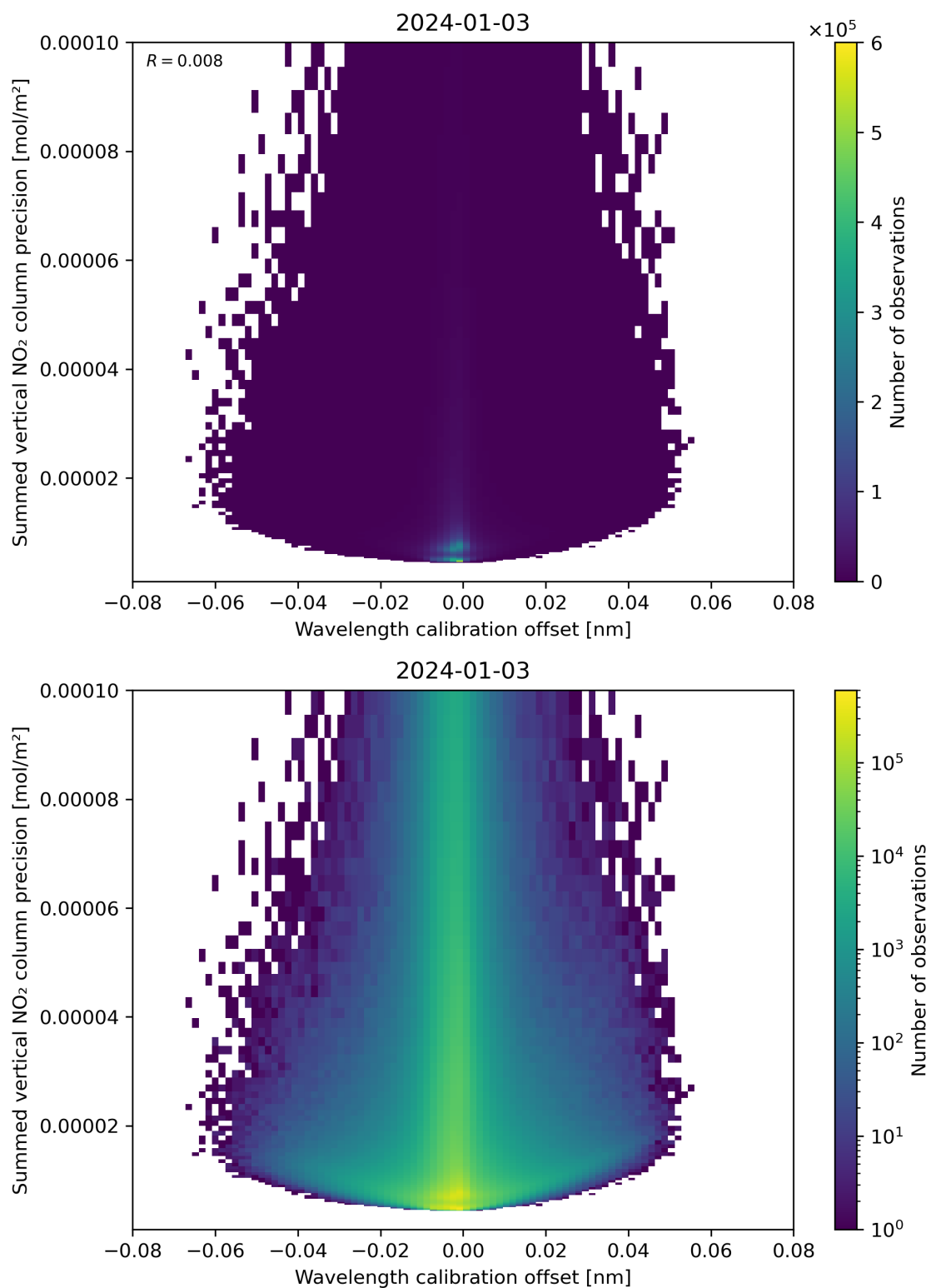
Figure 178: Scatter density plot of “Wavelength calibration offset” against “Summed vertical NO 2 column precision” for 2024-01-02 to 2024-01-04.
