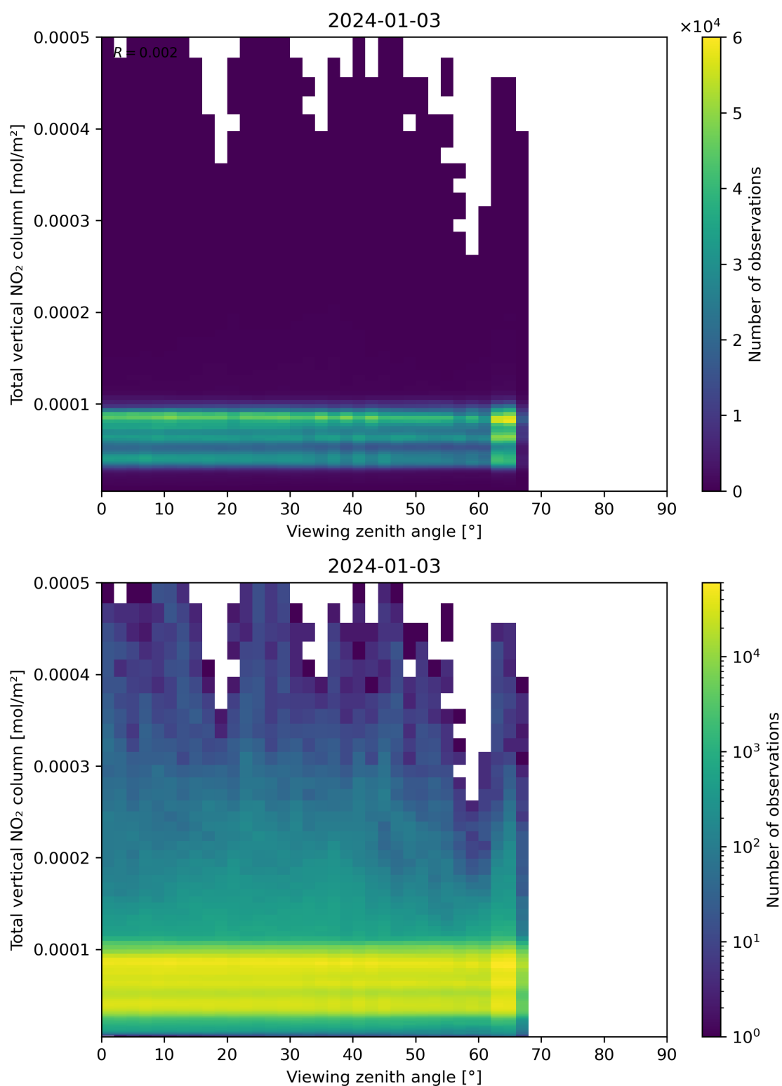
Figure 167: Scatter density plot of “Viewing zenith angle” against “Total vertical NO 2 column” for 2024-01-02 to 2024-01-04.
