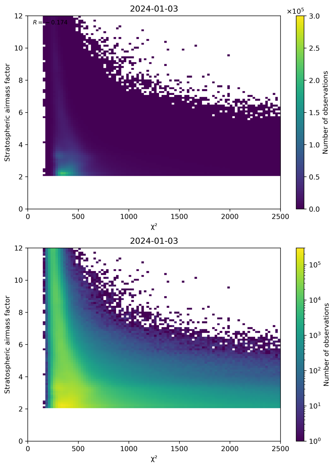
Figure 81: Scatter density plot of “ \chi^2 ” against “Stratospheric airmass factor” for 2024-01-02 to 2024-01-04.
