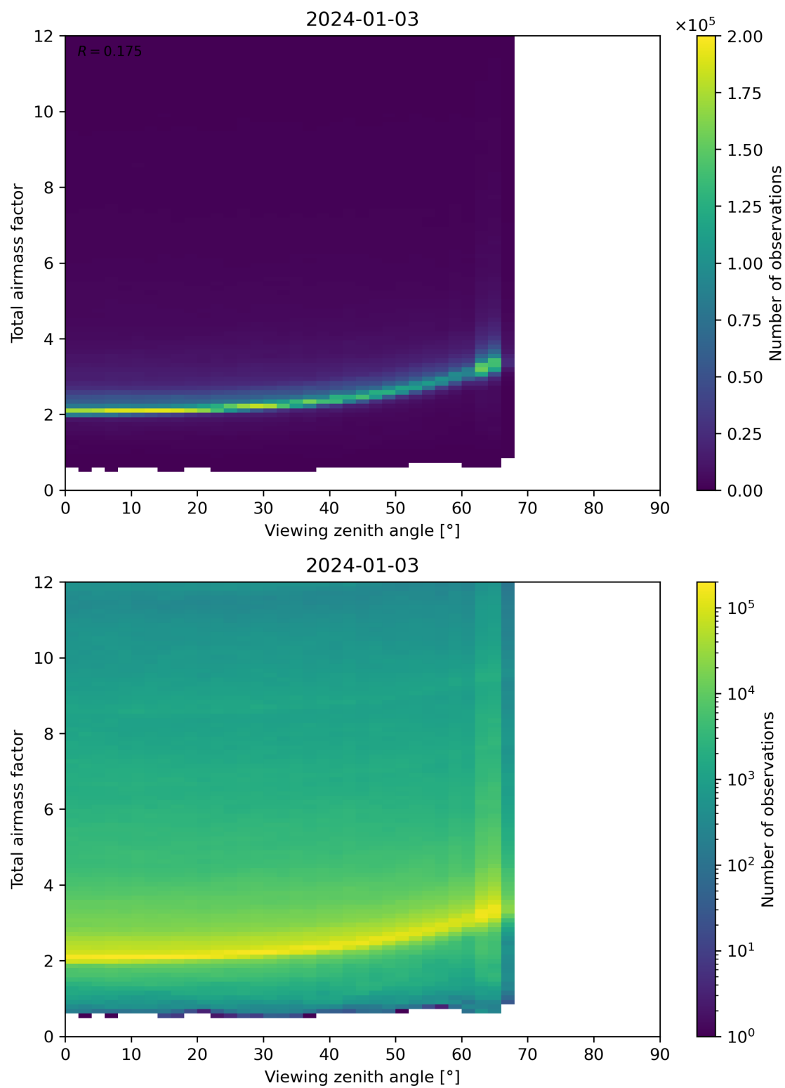
Figure 160: Scatter density plot of “Viewing zenith angle” against “Total airmass factor” for 2024-01-02 to 2024-01-04.
