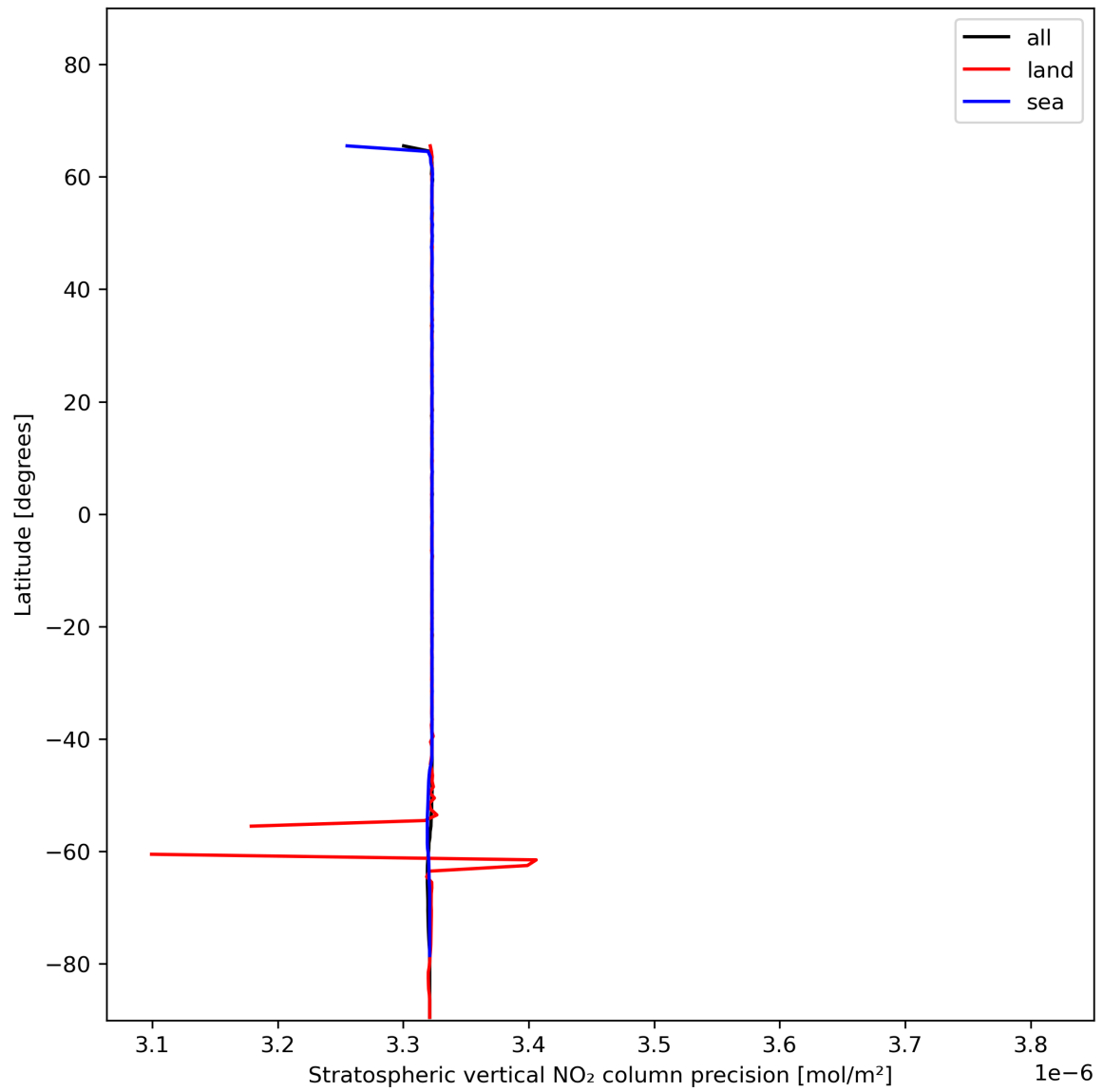
Figure 20: Zonal average of “Stratospheric vertical NO 2 column precision” for 2024-01-02 to 2024-01-04.
