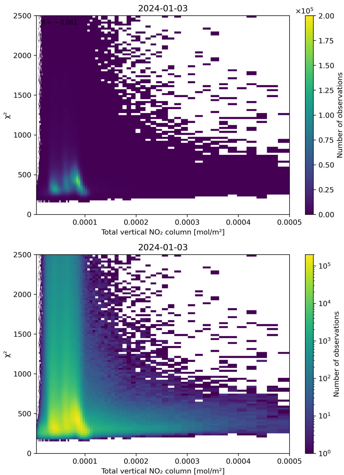
Figure 111: Scatter density plot of “Total vertical NO 2 column” against “ \chi^2 ” for 2024-01-02 to 2024-01-04.
