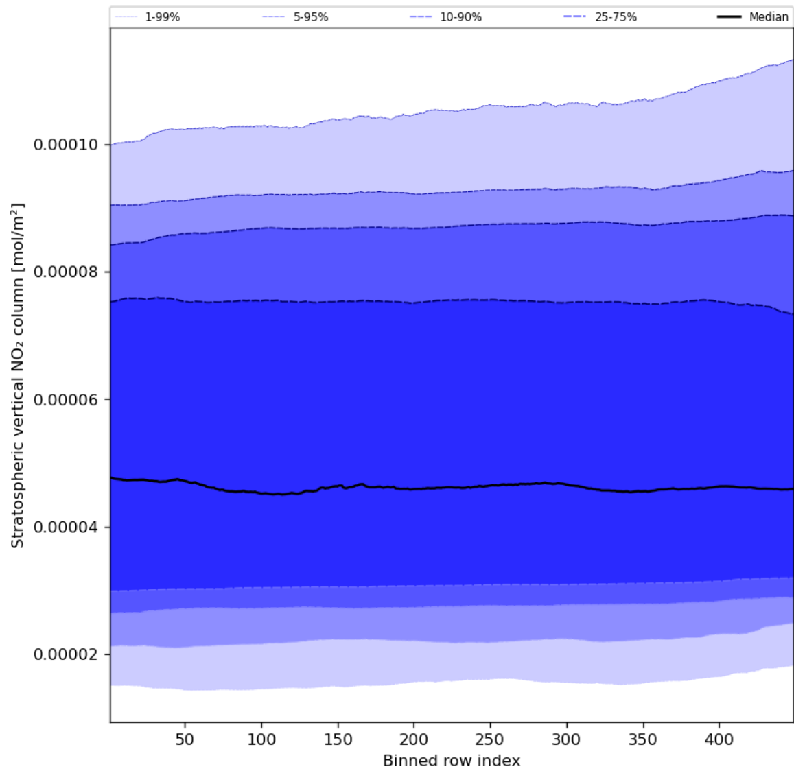
Figure 53: Along track statistics of “Stratospheric vertical NO 2 column” for 2024-01-02 to 2024-01-04
