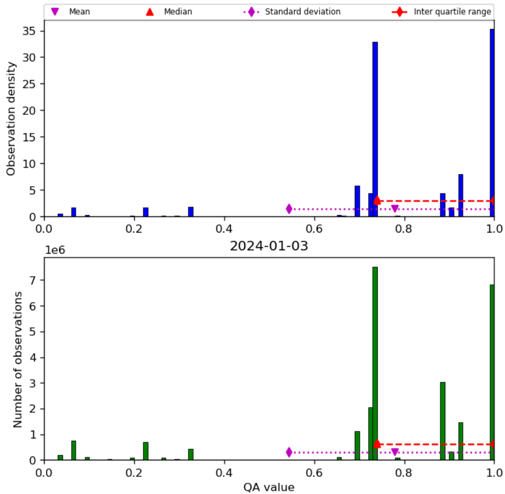
Figure 28: Histogram of “QA value” for 2024-01-02 to 2024-01-04
