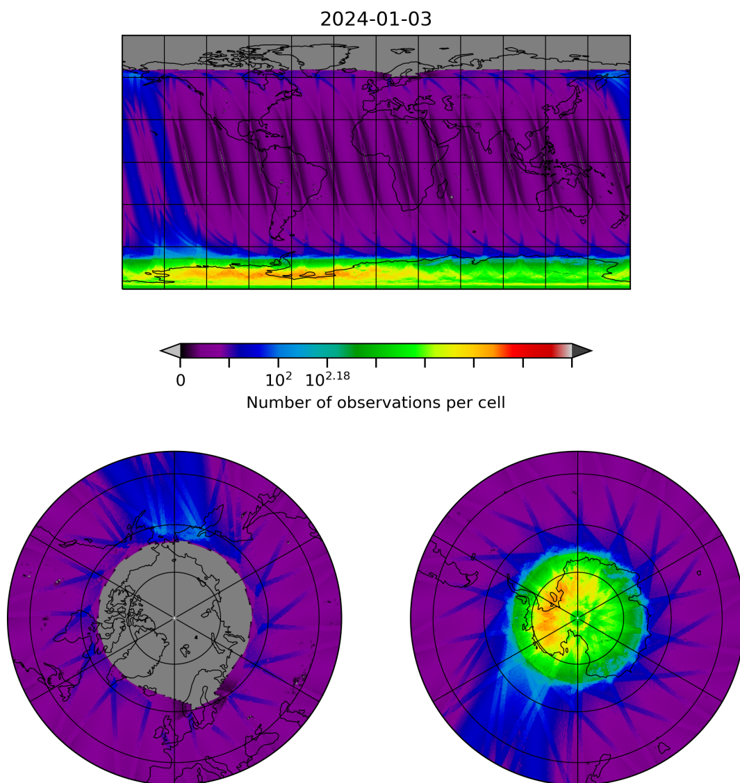
Figure 10: Map of the number of observations for 2024-01-02 to 2024-01-04
