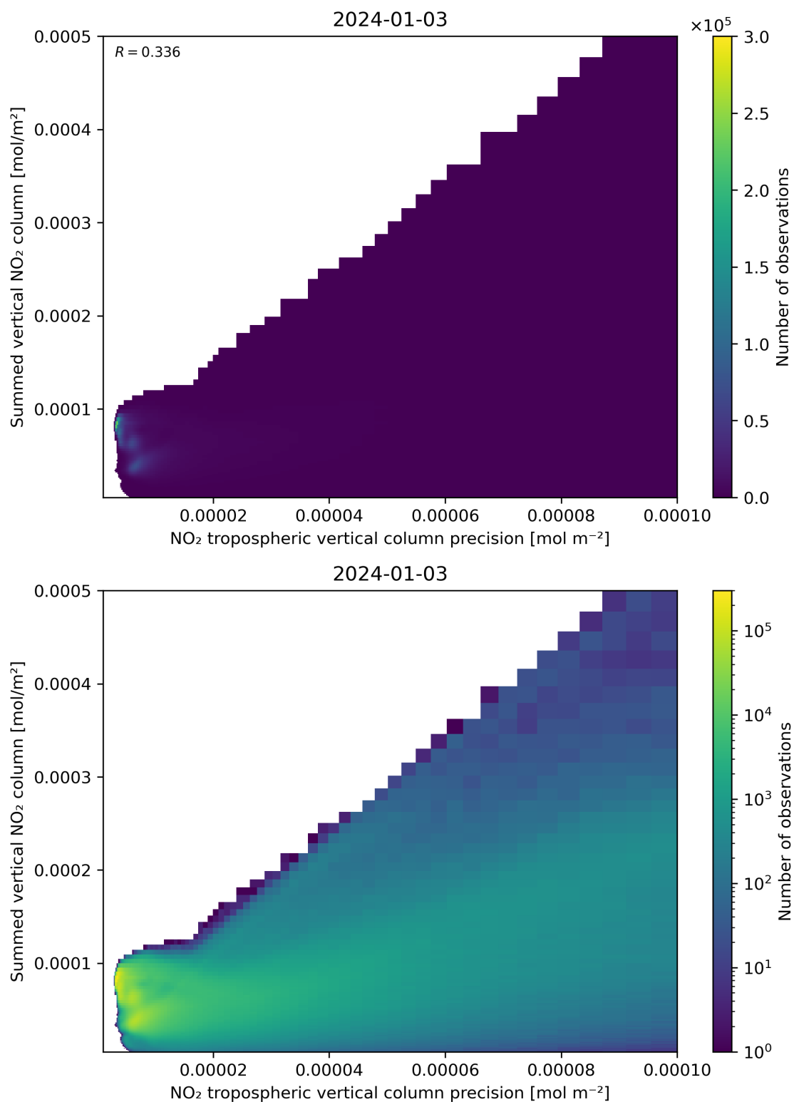
Figure 136: Scatter density plot of “NO 2 tropospheric vertical column precision” against “Summed vertical NO 2 column” for 2024-01-02 to 2024-01-04.
