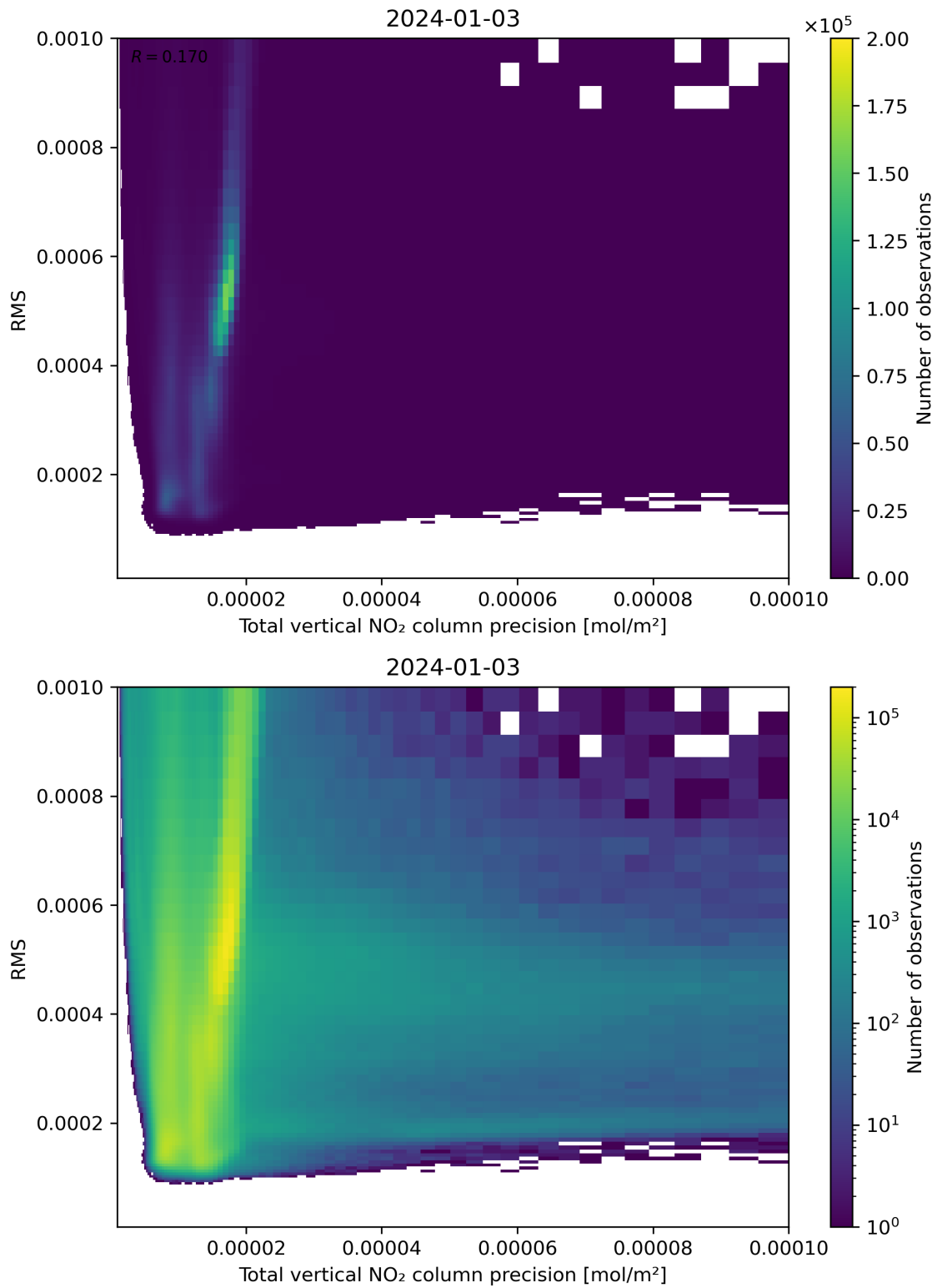
Figure 119: Scatter density plot of “Total vertical NO 2 column precision” against “RMS” for 2024-01-02 to 2024-01-04.
