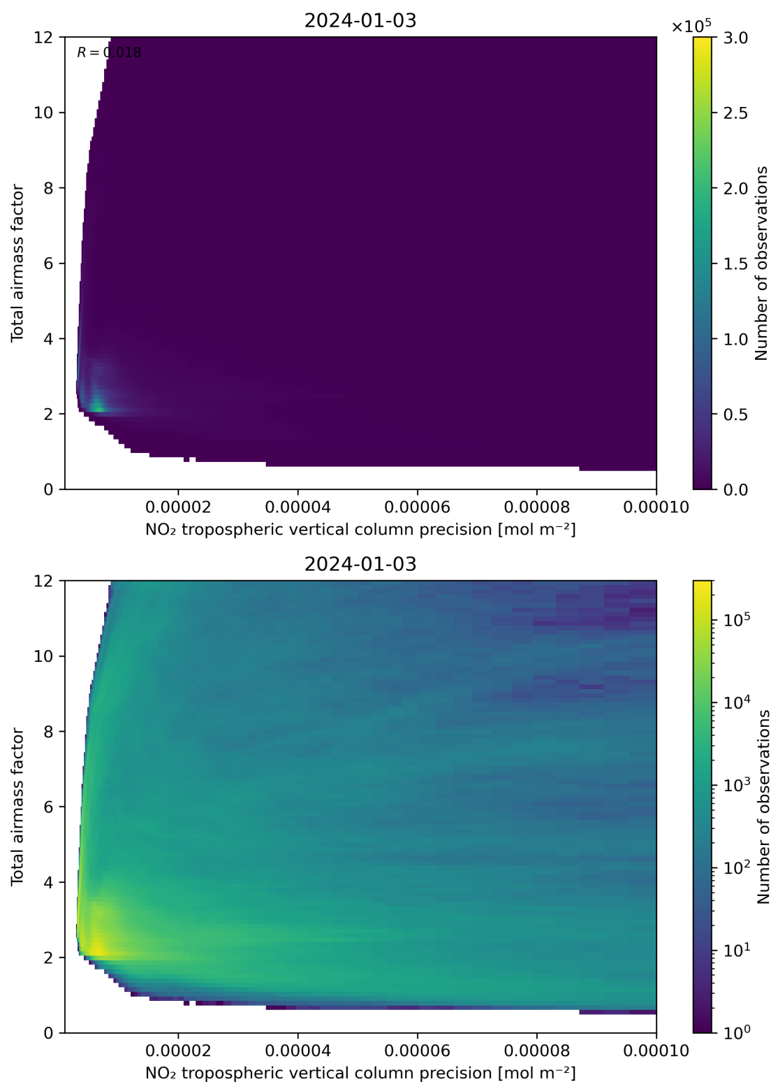
Figure 132: Scatter density plot of “NO 2 tropospheric vertical column precision” against “Total air mass factor” for 2024-01-02 to 2024-01-04.
