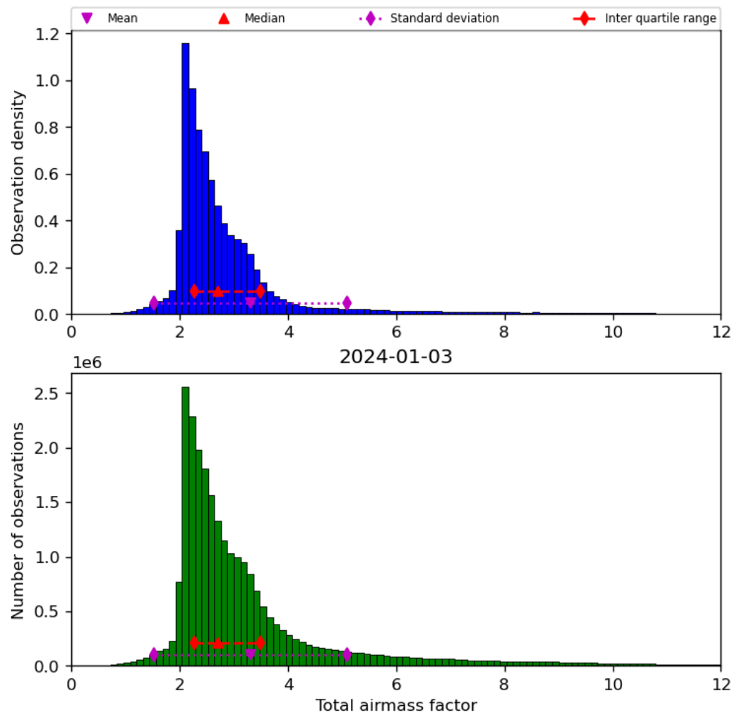
Figure 32: Histogram of “Total airmass factor” for 2024-01-02 to 2024-01-04
