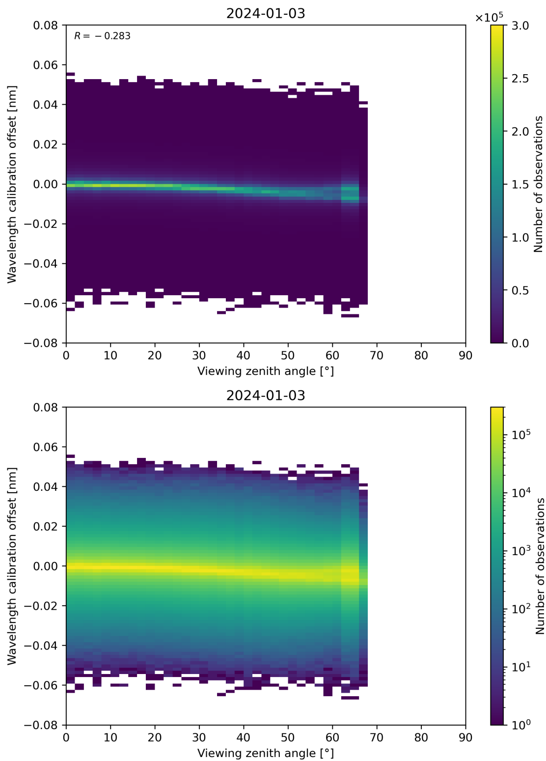
Figure 173: Scatter density plot of “Viewing zenith angle” against “Wavelength calibration offset” for 2024-01-02 to 2024-01-04.
