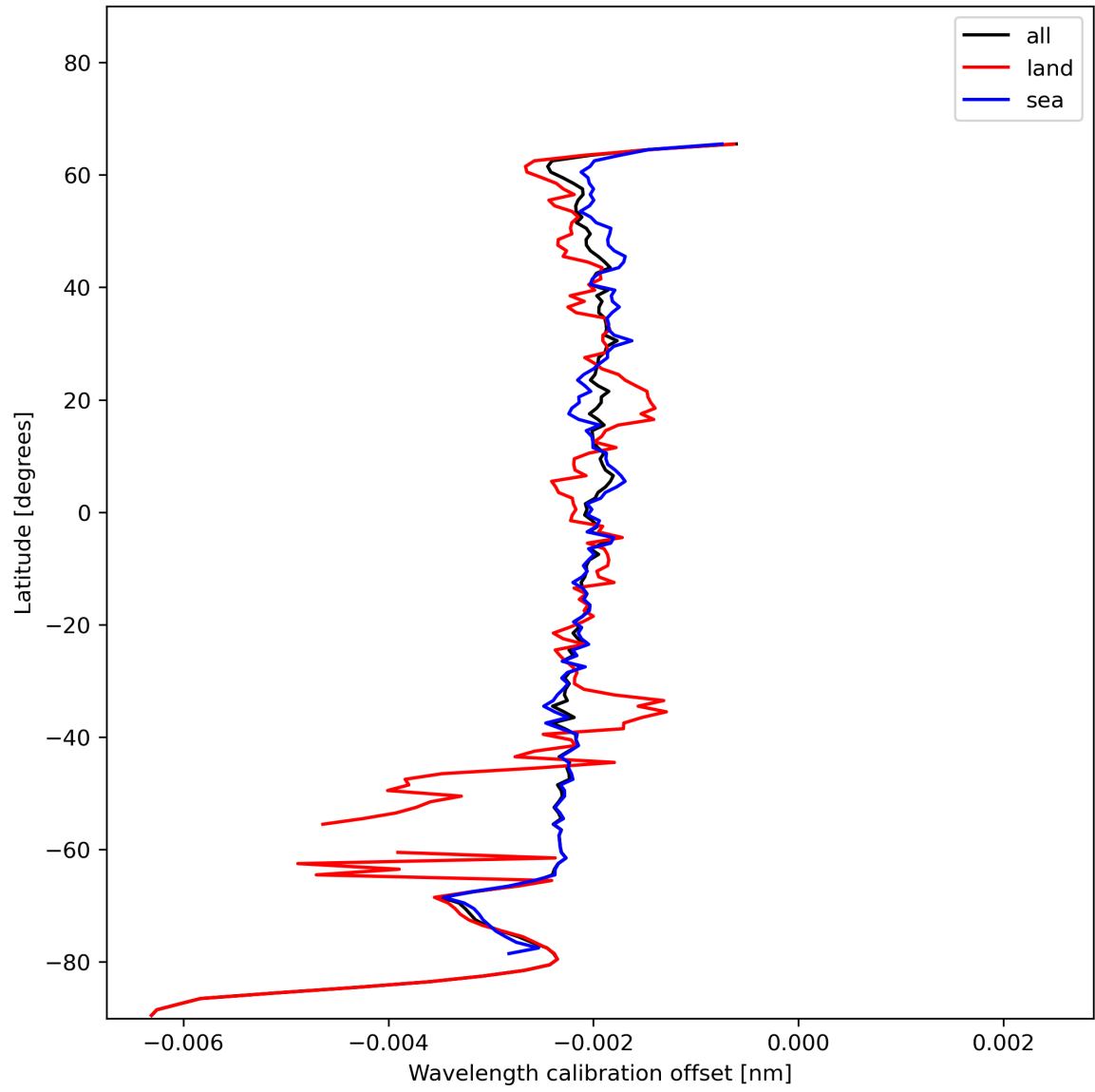
Figure 18: Zonal average of “Wavelength calibration offset” for 2024-01-02 to 2024-01-04.
