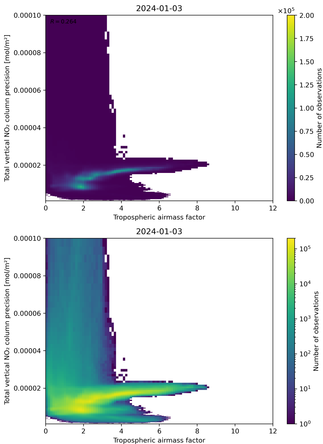
Figure 78: Scatter density plot of “Tropospheric air mass factor” against “Total vertical NO 2 column precision” for 2024-01-02 to 2024-01-04.
