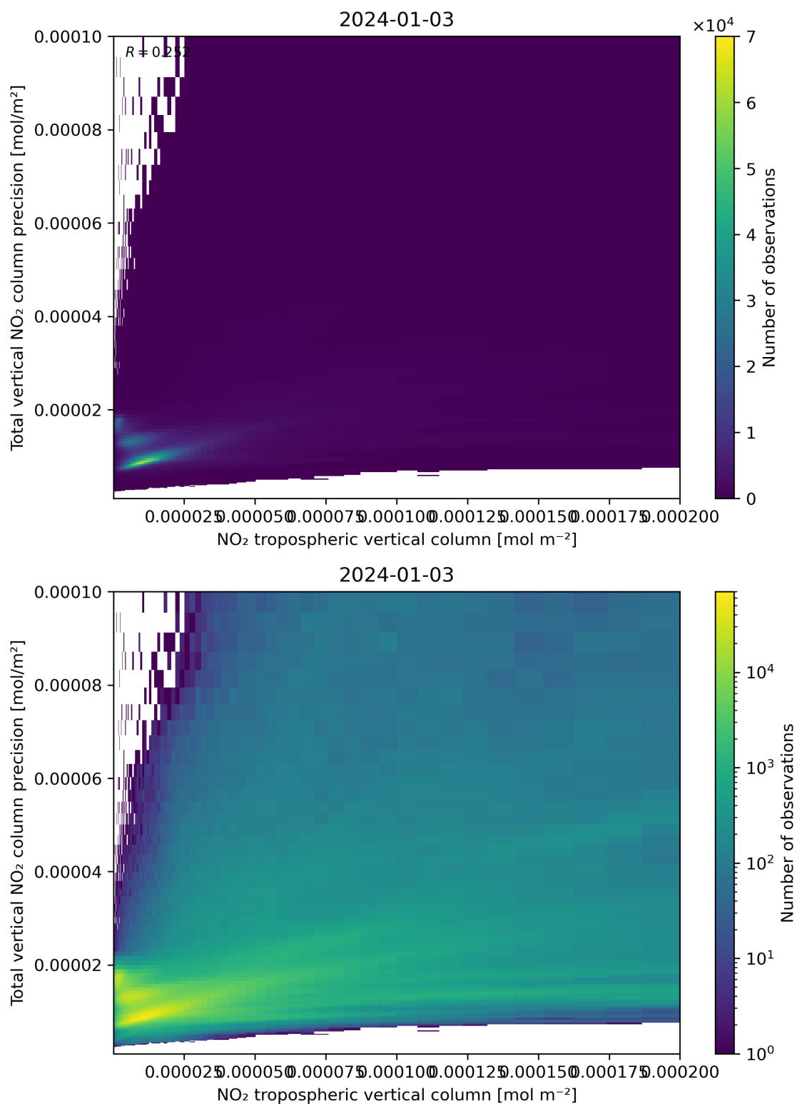
Figure 129: Scatter density plot of “NO 2 tropospheric vertical column” against “Total vertical NO 2 column precision” for 2024-01-02 to 2024-01-04.
