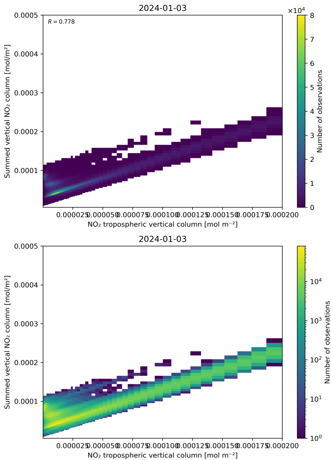
Figure 126: Scatter density plot of “NO 2 tropospheric vertical column” against “Summed vertical NO 2 column” for 2024-01-02 to 2024-01-04.
