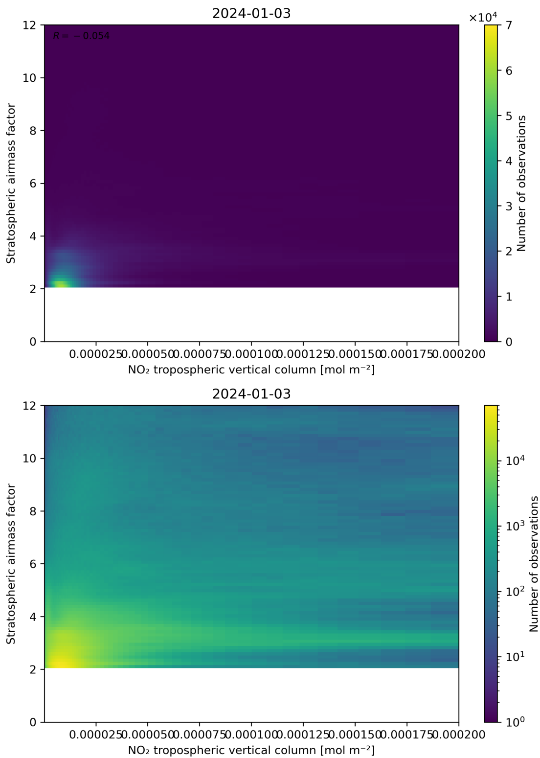
Figure 121: Scatter density plot of “NO 2 tropospheric vertical column” against “Stratospheric airmass factor” for 2024-01-02 to 2024-01-04.
