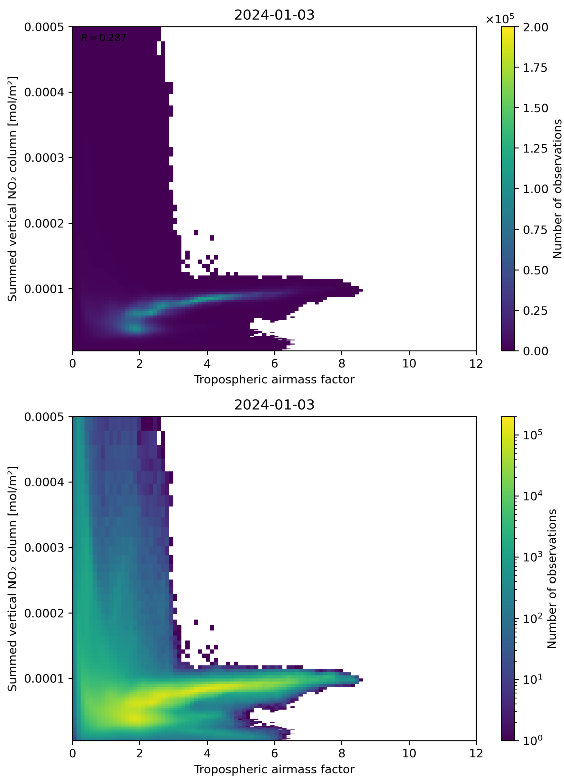
Figure 75: Scatter density plot of “Tropospheric airmass factor” against “Summed vertical NO 2 column” for 2024-01-02 to 2024-01-04.
