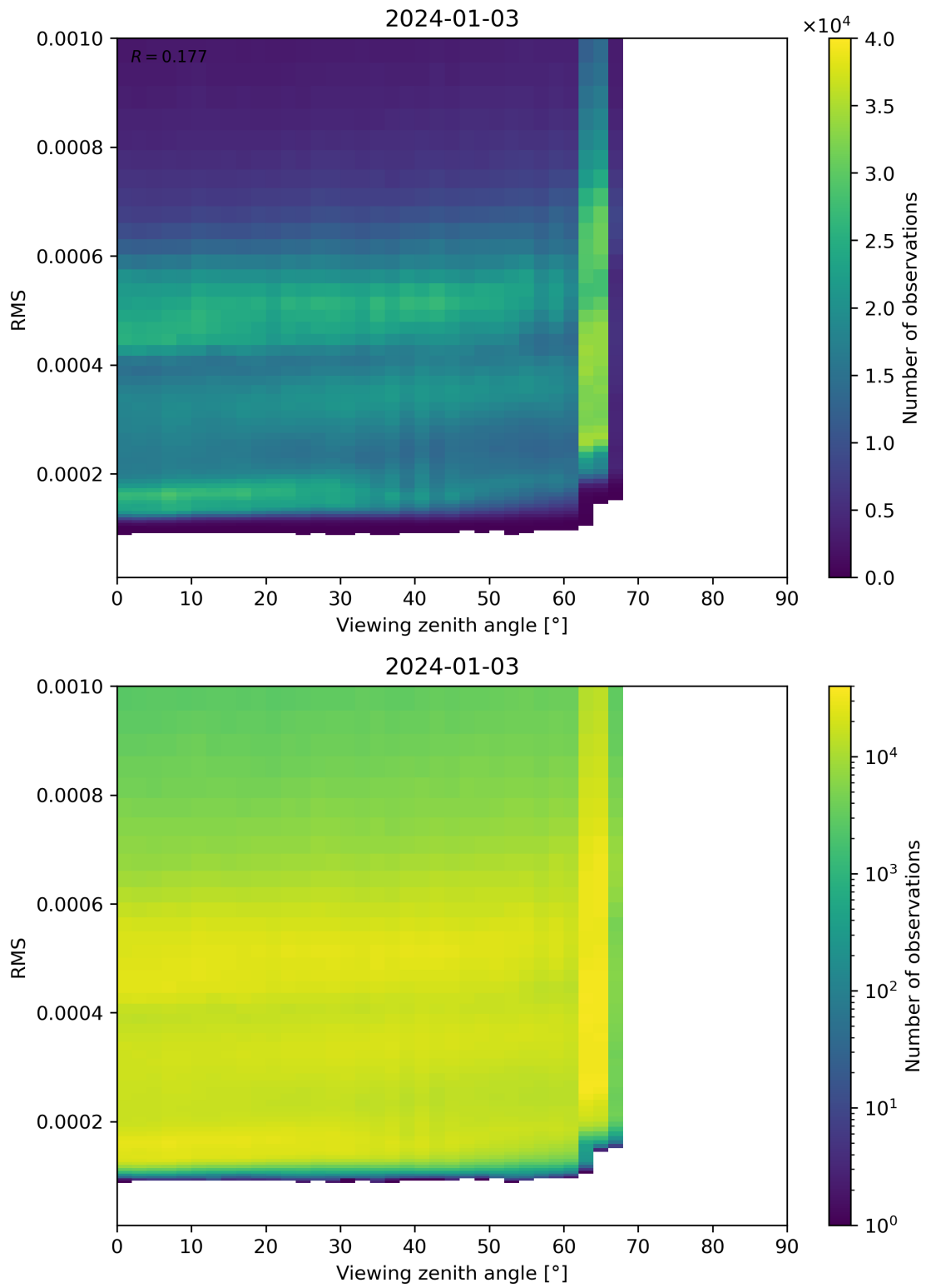
Figure 171: Scatter density plot of “Viewing zenith angle” against “RMS” for 2024-01-02 to 2024-01-04.
