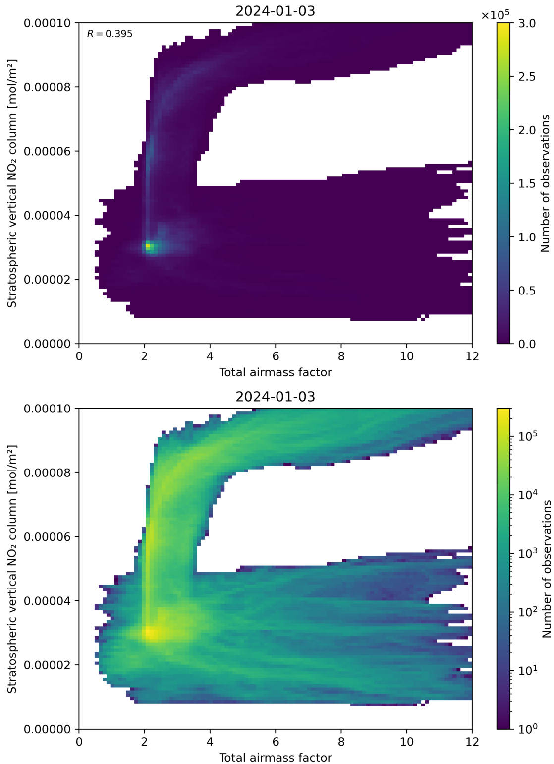
Figure 64: Scatter density plot of “Total airmass factor” against “Stratospheric vertical NO 2 column” for 2024-01-02 to 2024-01-04.
