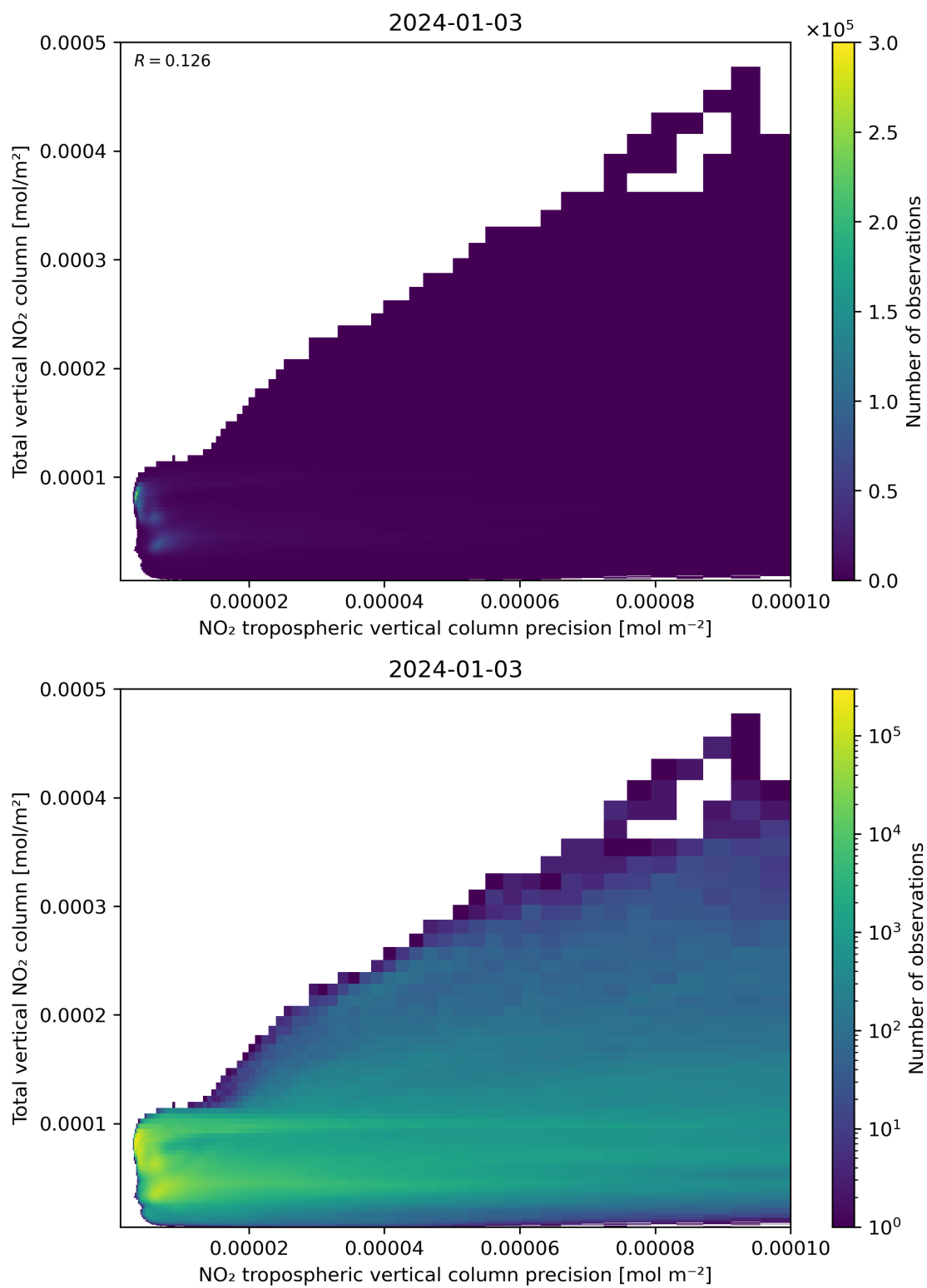
Figure 138: Scatter density plot of “NO 2 tropospheric vertical column precision” against “Total vertical NO 2 column” for 2024-01-02 to 2024-01-04.
