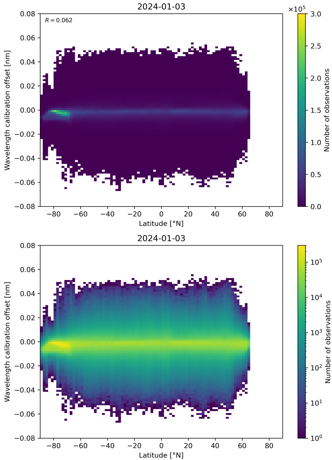
Figure 95: Scatter density plot of “Latitude” against “Wavelength calibration offset” for 2024-01-02 to 2024-01-04.
