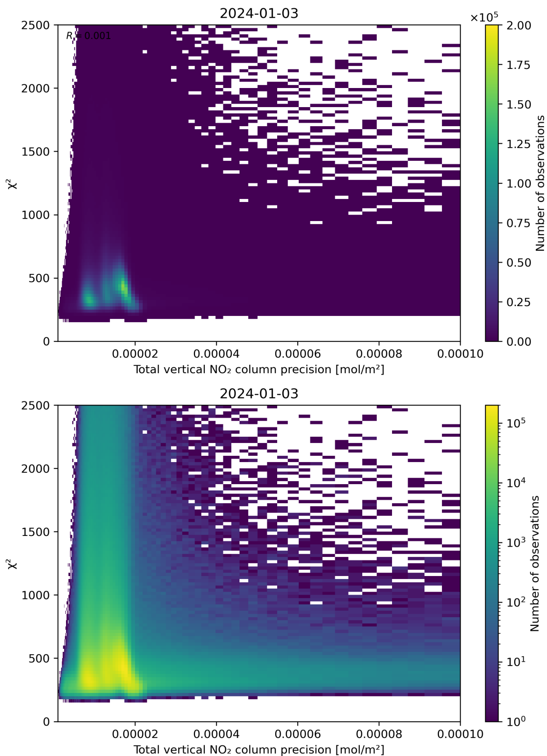
Figure 116: Scatter density plot of “Total vertical NO 2 column precision” against “ \chi^2 ” for 2024-01-02 to 2024-01-04.
