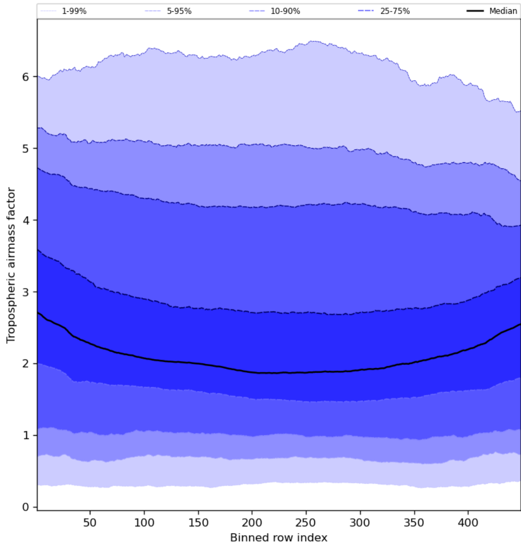
Figure 48: Along track statistics of “Tropospheric airmass factor” for 2024-01-02 to 2024-01-04
