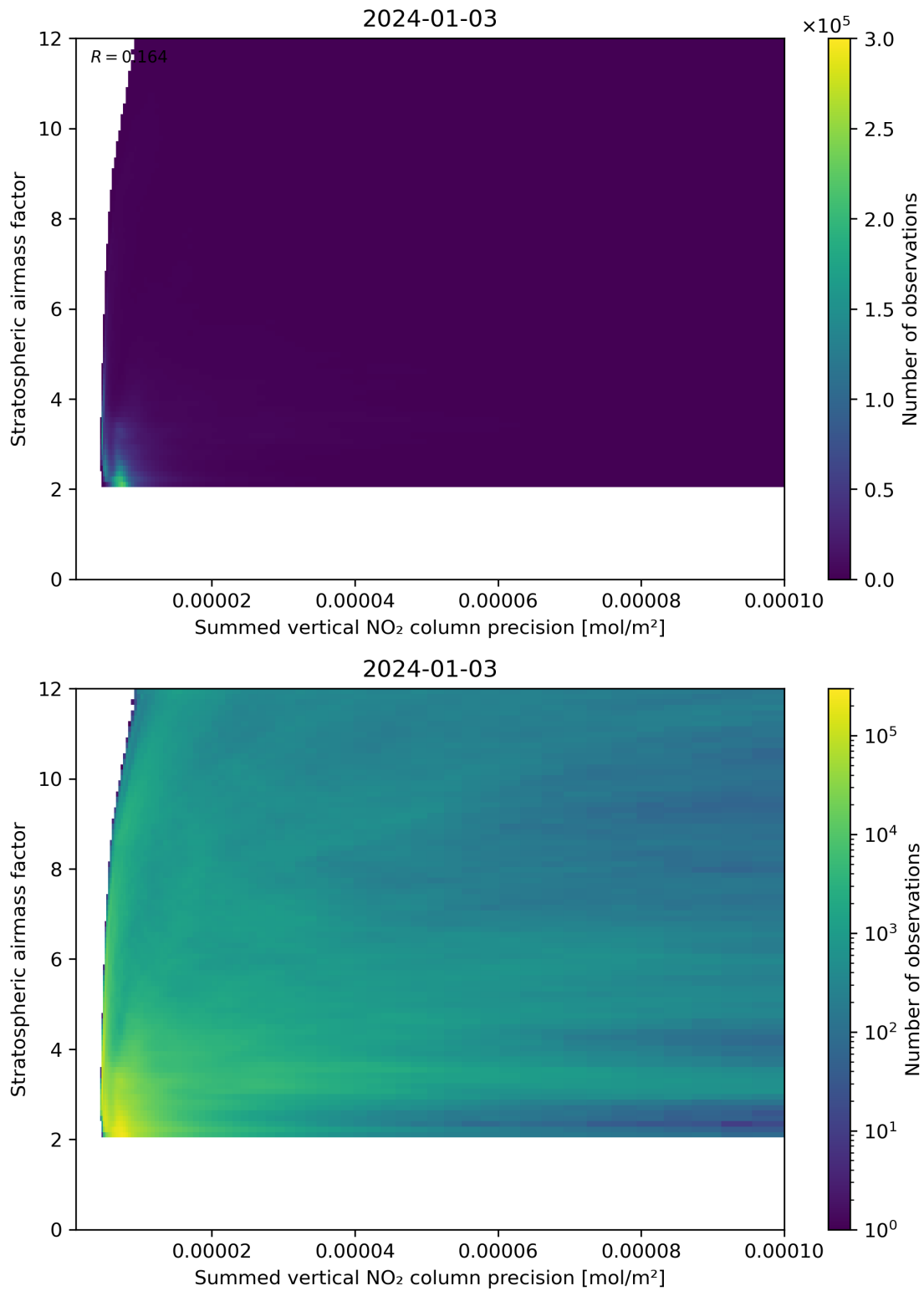
Figure 106: Scatter density plot of “Summed vertical NO 2 column precision” against “Stratospheric airmass factor” for 2024-01-02 to 2024-01-04.
