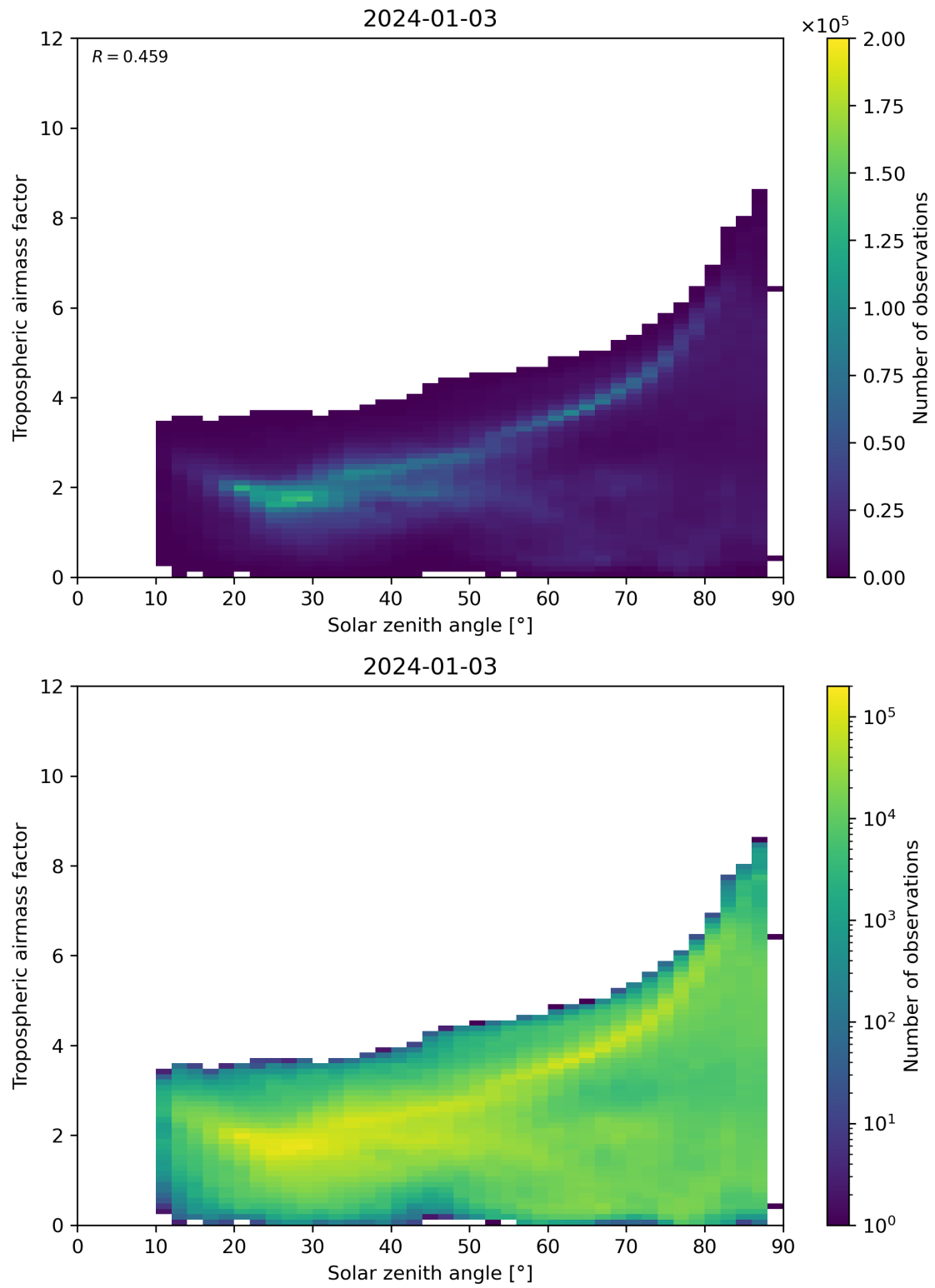
Figure 147: Scatter density plot of “Solar zenith angle” against “Tropospheric airmass factor” for 2024-01-02 to 2024-01-04.
