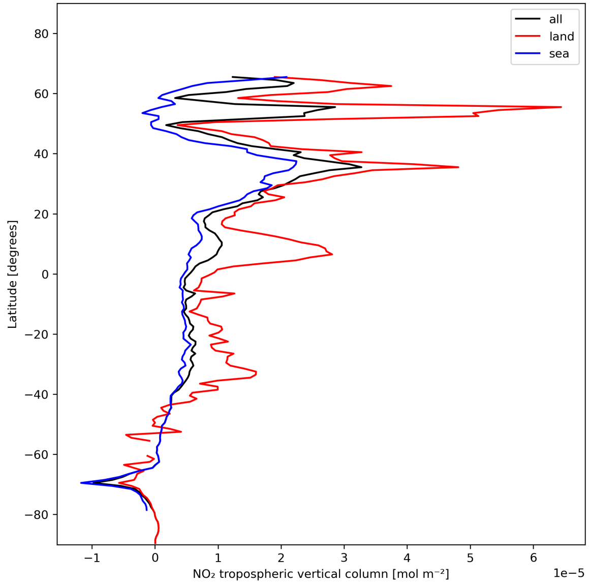
Figure 12: Zonal average of “NO 2 tropospheric vertical column” for 2024-01-02 to 2024-01-04.
