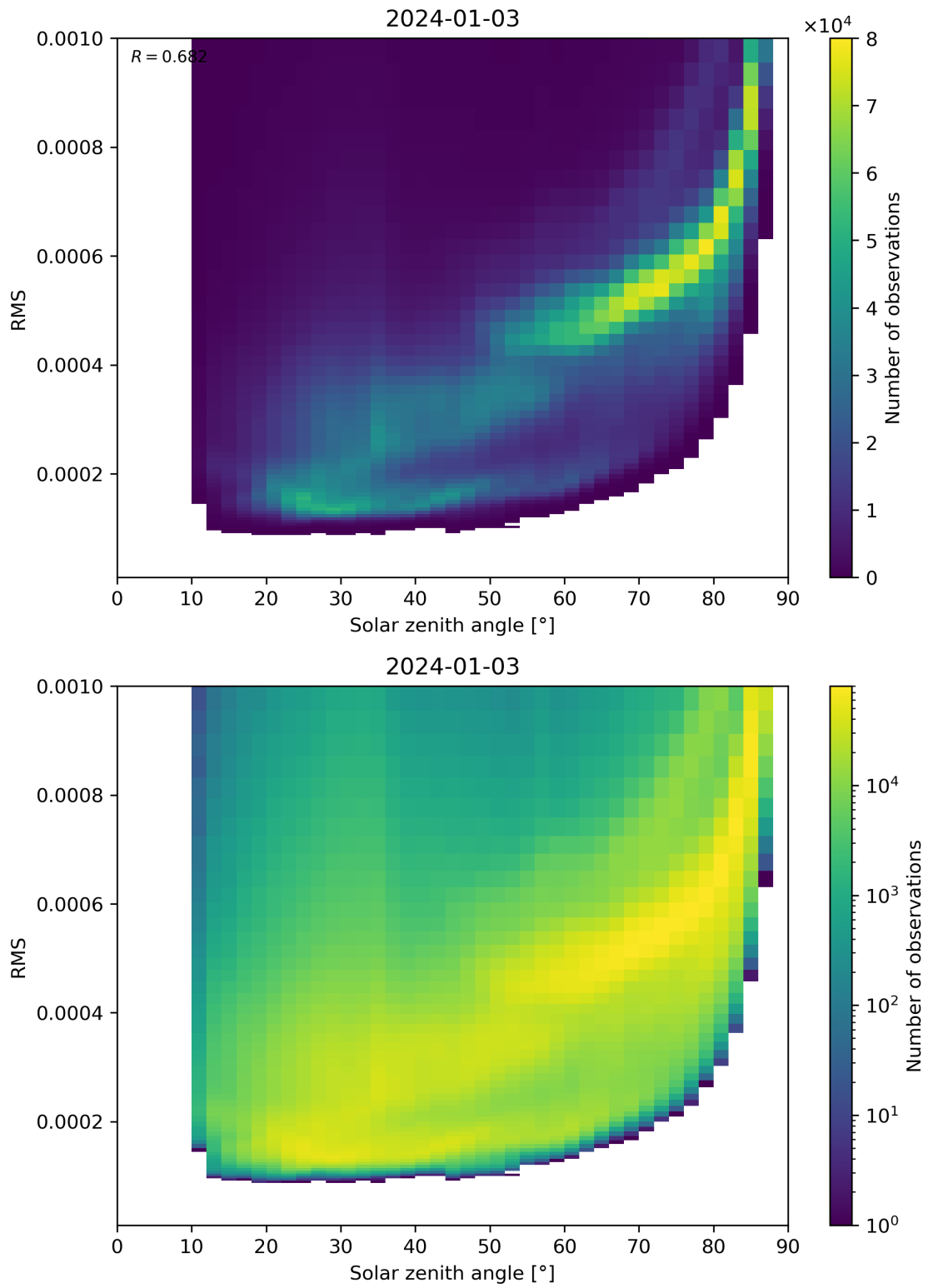
Figure 157: Scatter density plot of “Solar zenith angle” against “RMS” for 2024-01-02 to 2024-01-04.
