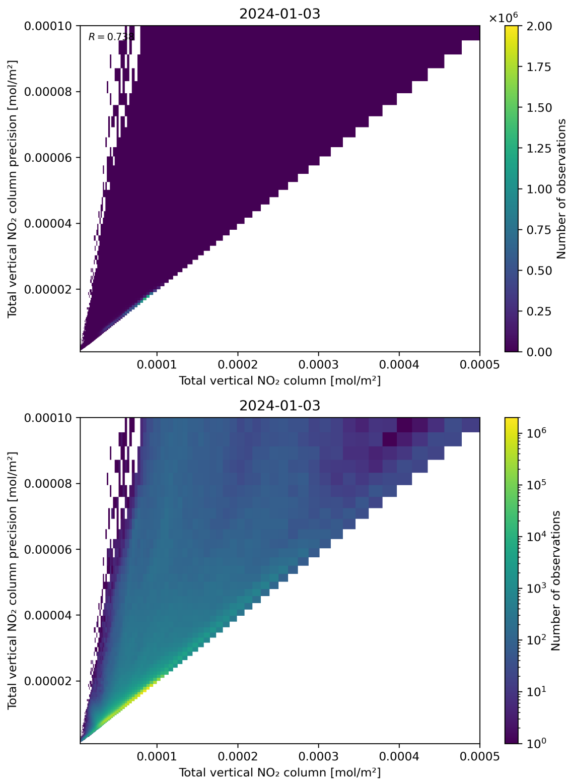
Figure 114: Scatter density plot of “Total vertical NO 2 column” against “Total vertical NO 2 column precision” for 2024-01-02 to 2024-01-04.
