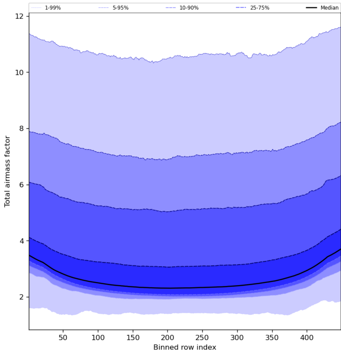
Figure 49: Along track statistics of “Total airmass factor” for 2024-01-02 to 2024-01-04
