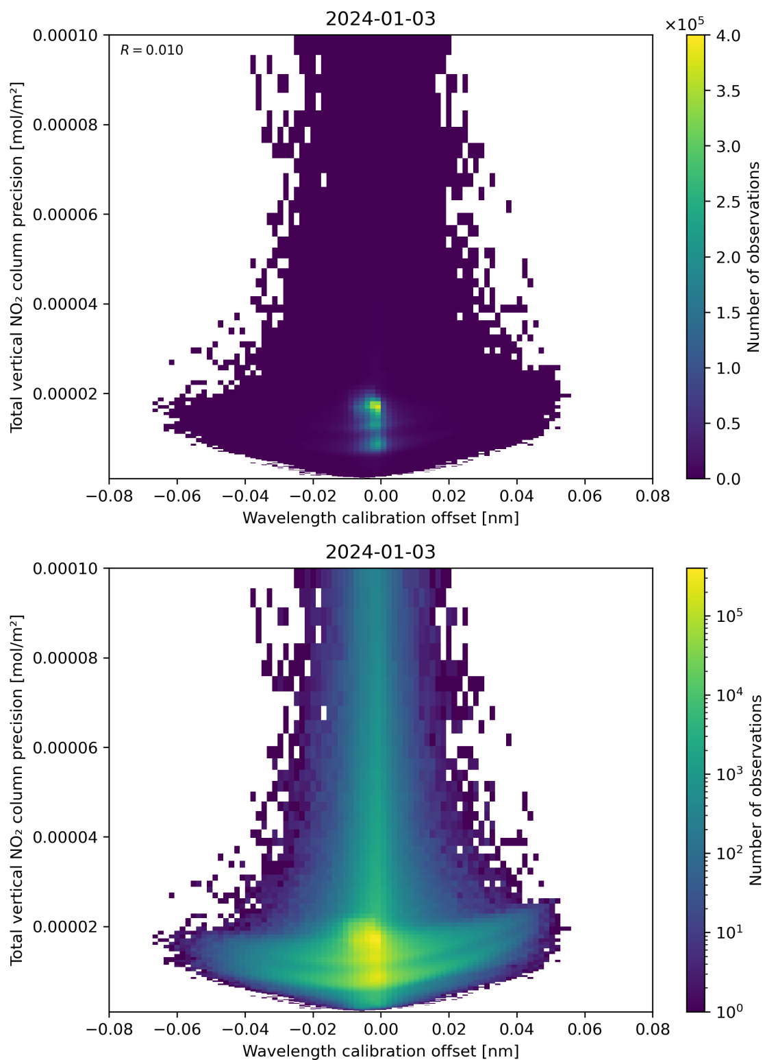
Figure 180: Scatter density plot of “Wavelength calibration offset” against “Total vertical NO 2 column precision” for 2024-01-02 to 2024-01-04.
