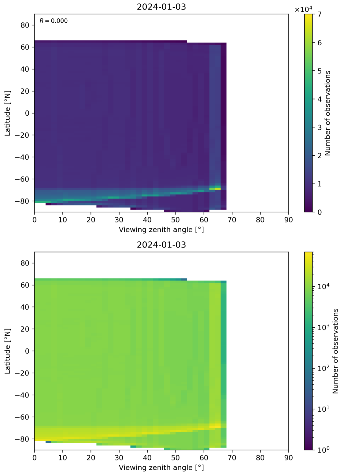
Figure 163: Scatter density plot of “Viewing zenith angle” against “Latitude” for 2024-01-02 to 2024-01-04.
