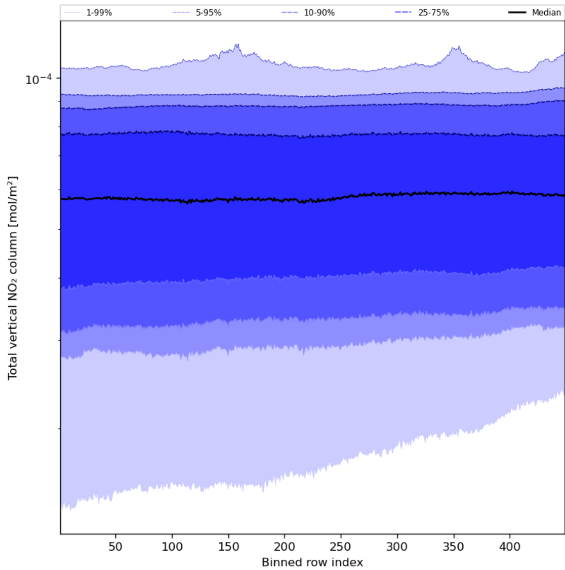
Figure 55: Along track statistics of “Total vertical NO 2 column” for 2024-01-02 to 2024-01-04
