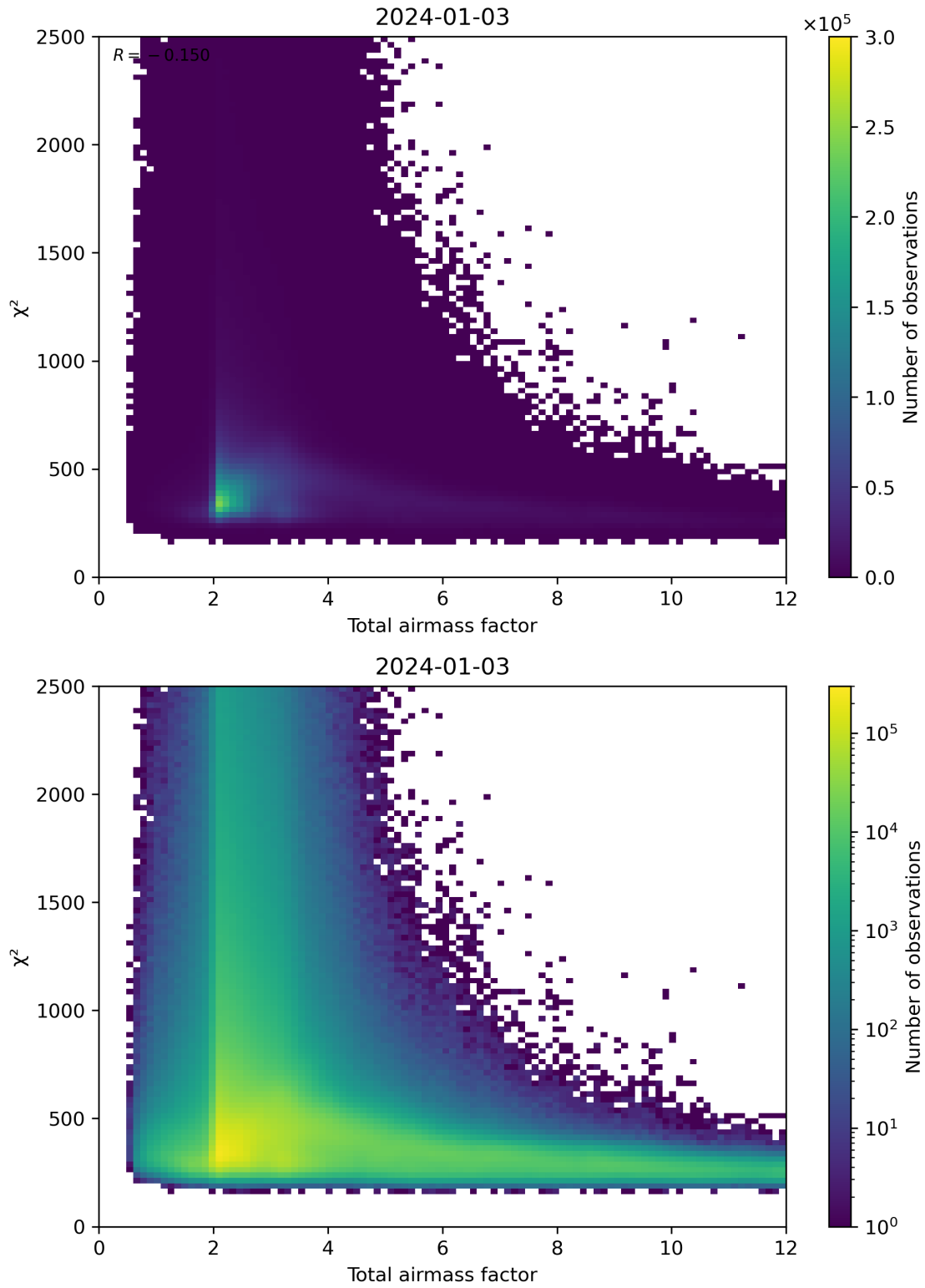
Figure 63: Scatter density plot of “Total airmass factor” against “ \chi^2 ” for 2024-01-02 to 2024-01-04.
