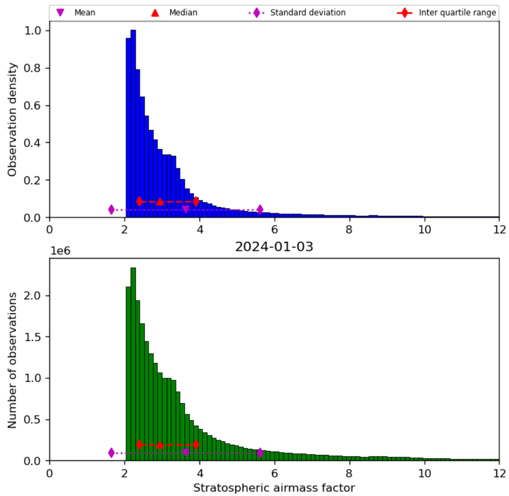
Figure 44: Histogram of “Stratospheric airmass factor” for 2024-01-02 to 2024-01-04
