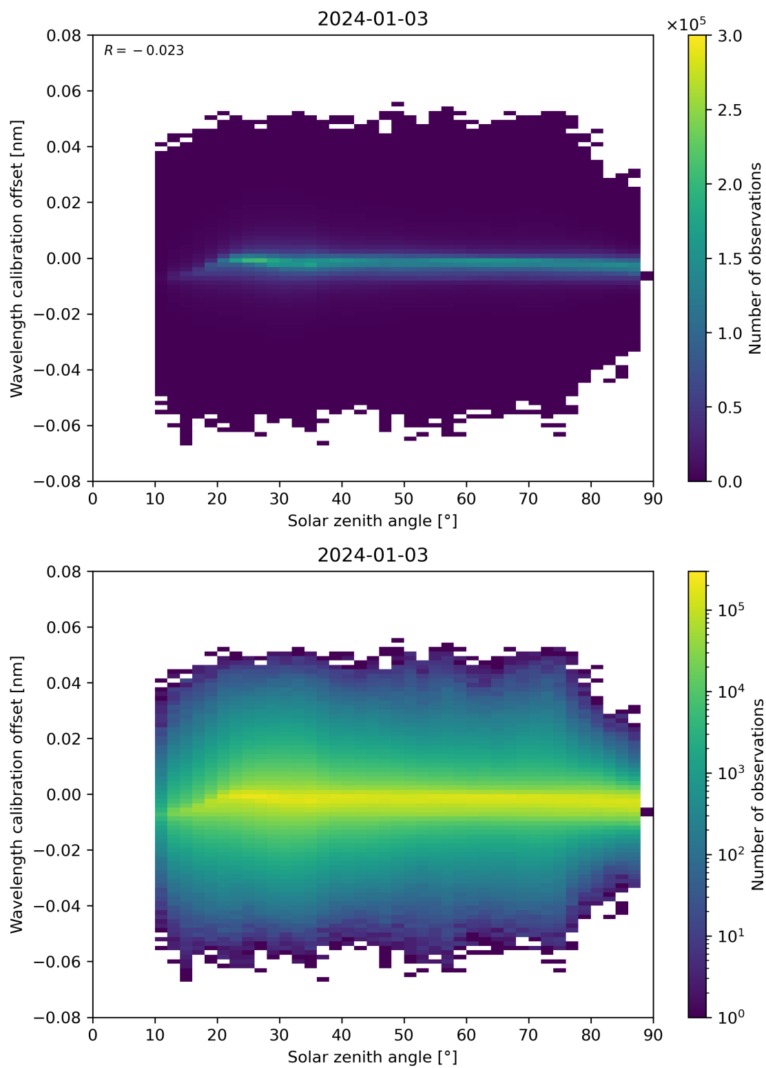
Figure 158: Scatter density plot of “Solar zenith angle” against “Wavelength calibration offset” for 2024-01-02 to 2024-01-04.
