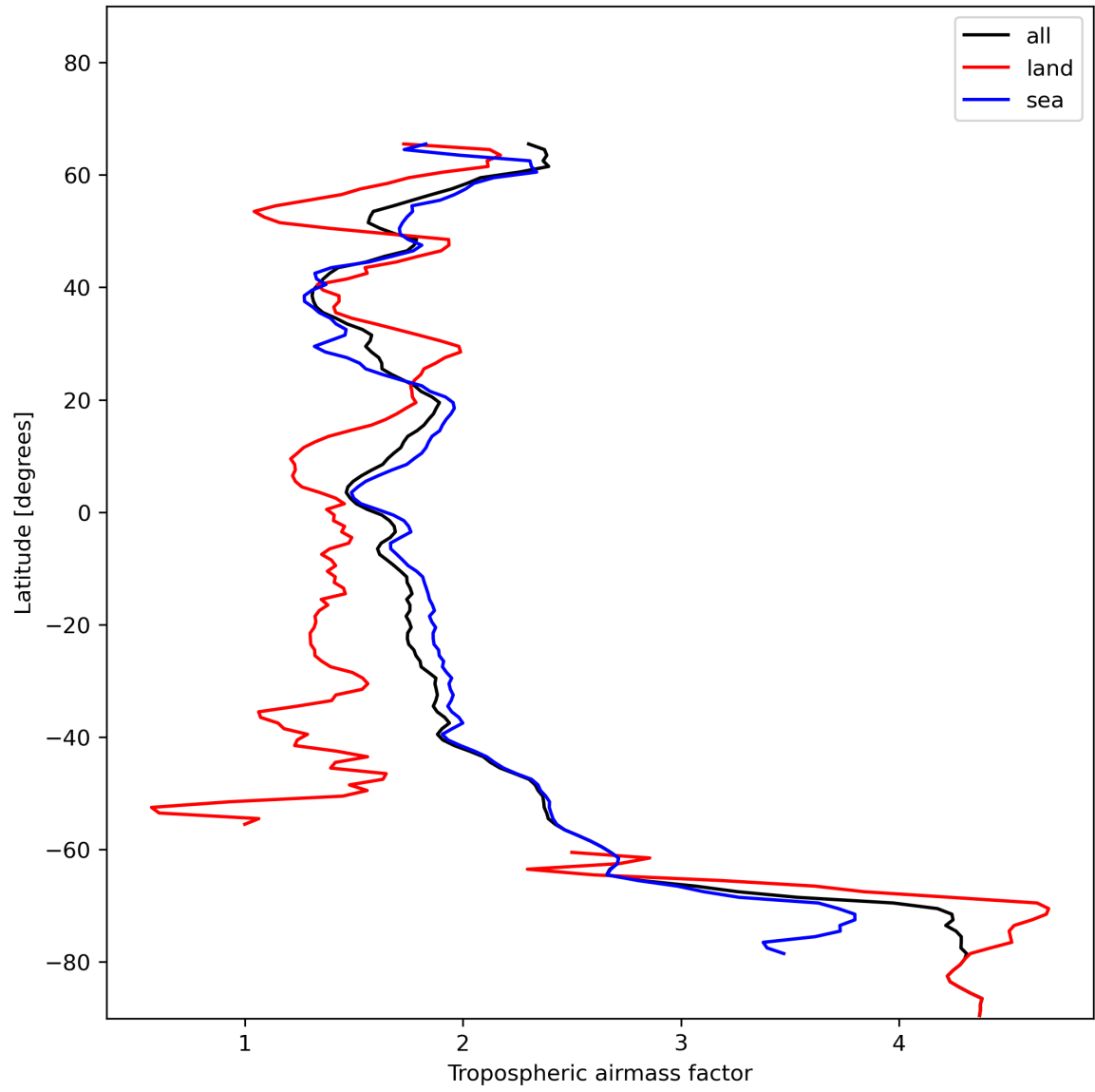
Figure 14: Zonal average of “Tropospheric airmass factor” for 2024-01-02 to 2024-01-04.
