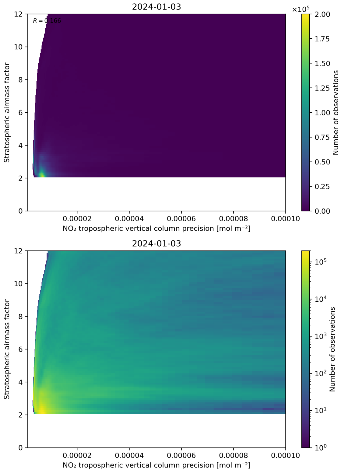
Figure 131: Scatter density plot of “NO 2 tropospheric vertical column precision” against “Stratospheric airmass factor” for 2024-01-02 to 2024-01-04.
