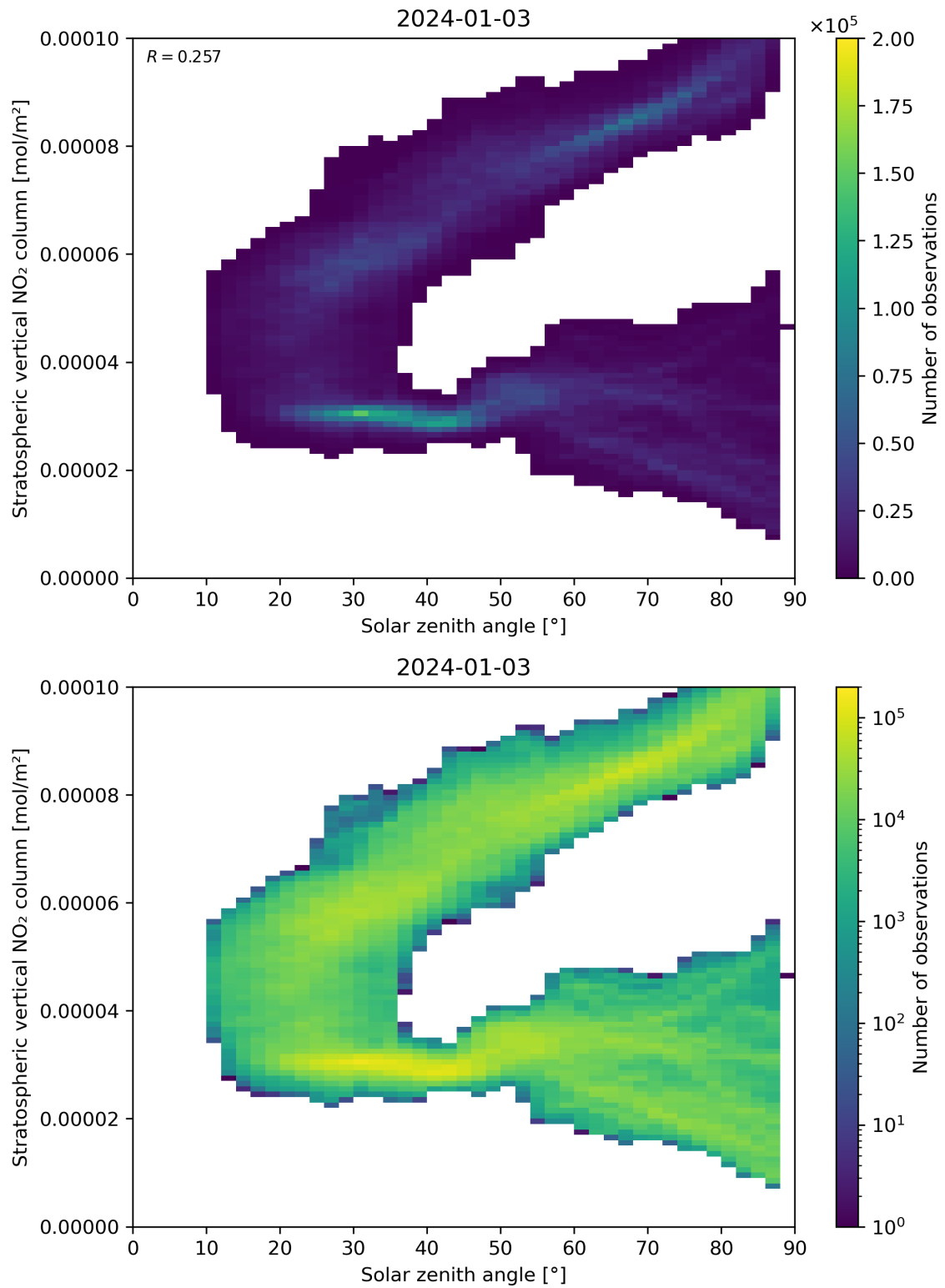
Figure 150: Scatter density plot of “Solar zenith angle” against “Stratospheric vertical NO 2 column” for 2024-01-02 to 2024-01-04.
