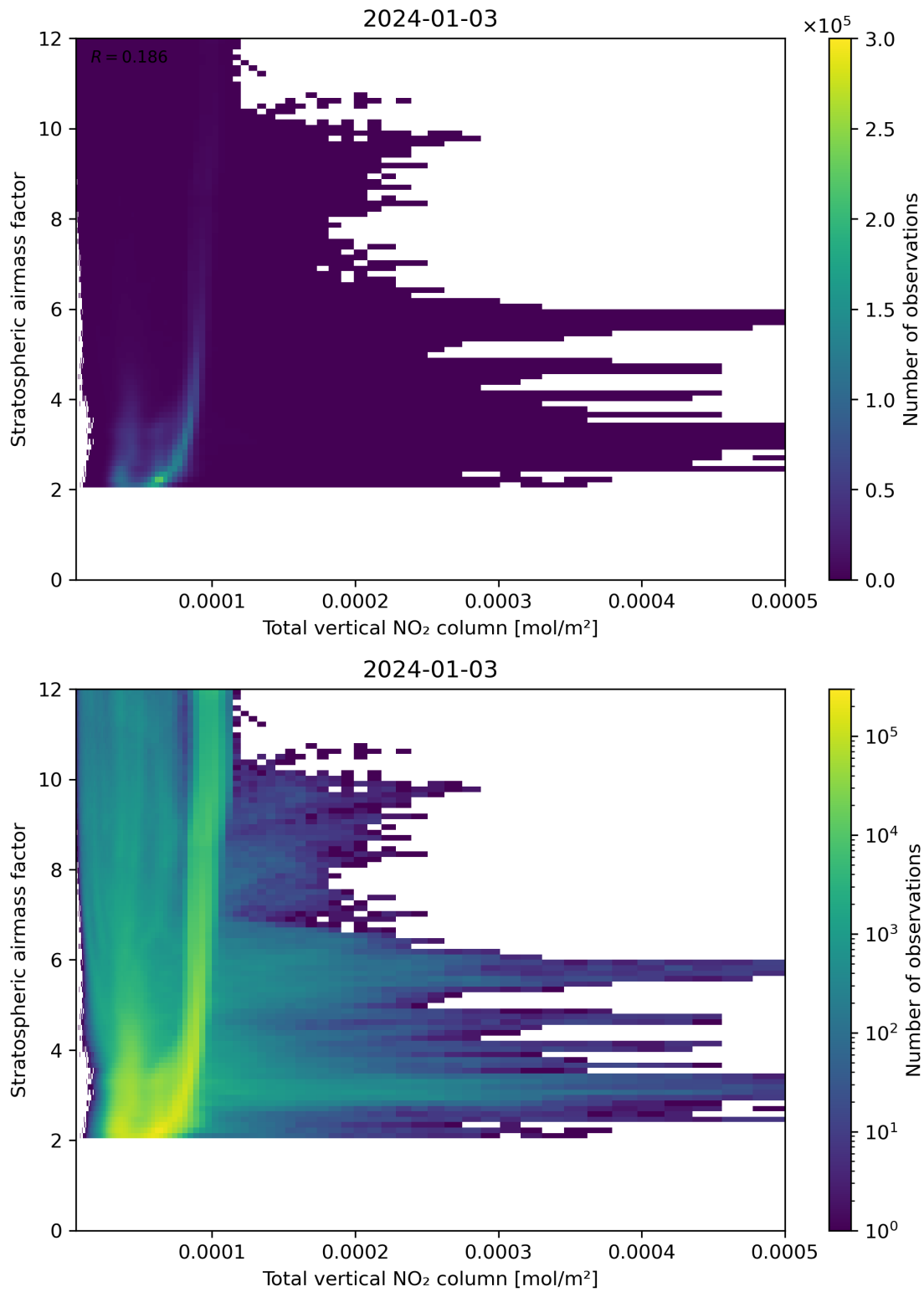
Figure 110: Scatter density plot of “Total vertical NO 2 column” against “Stratospheric airmass factor” for 2024-01-02 to 2024-01-04.
