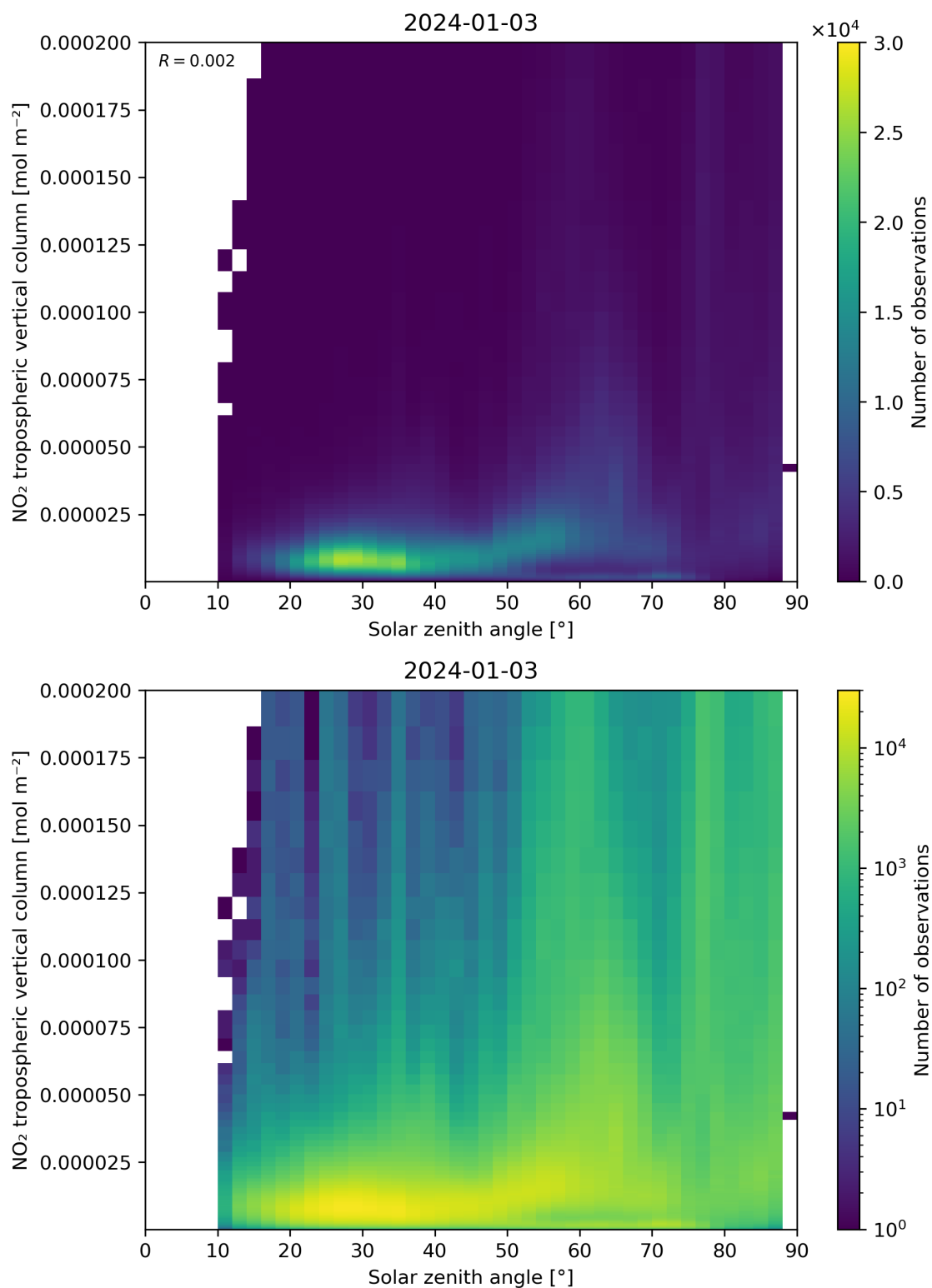
Figure 155: Scatter density plot of “Solar zenith angle” against “NO 2 tropospheric vertical column” for 2024-01-02 to 2024-01-04.
