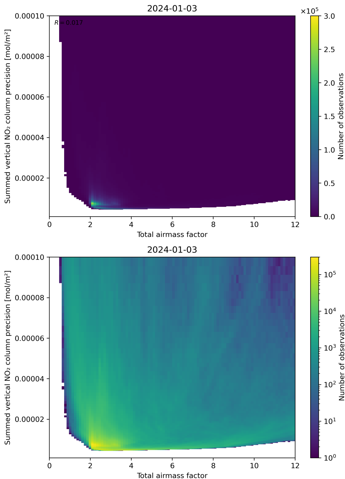
Figure 66: Scatter density plot of “Total airmass factor” against “Summed vertical NO 2 column precision” for 2024-01-02 to 2024-01-04.
