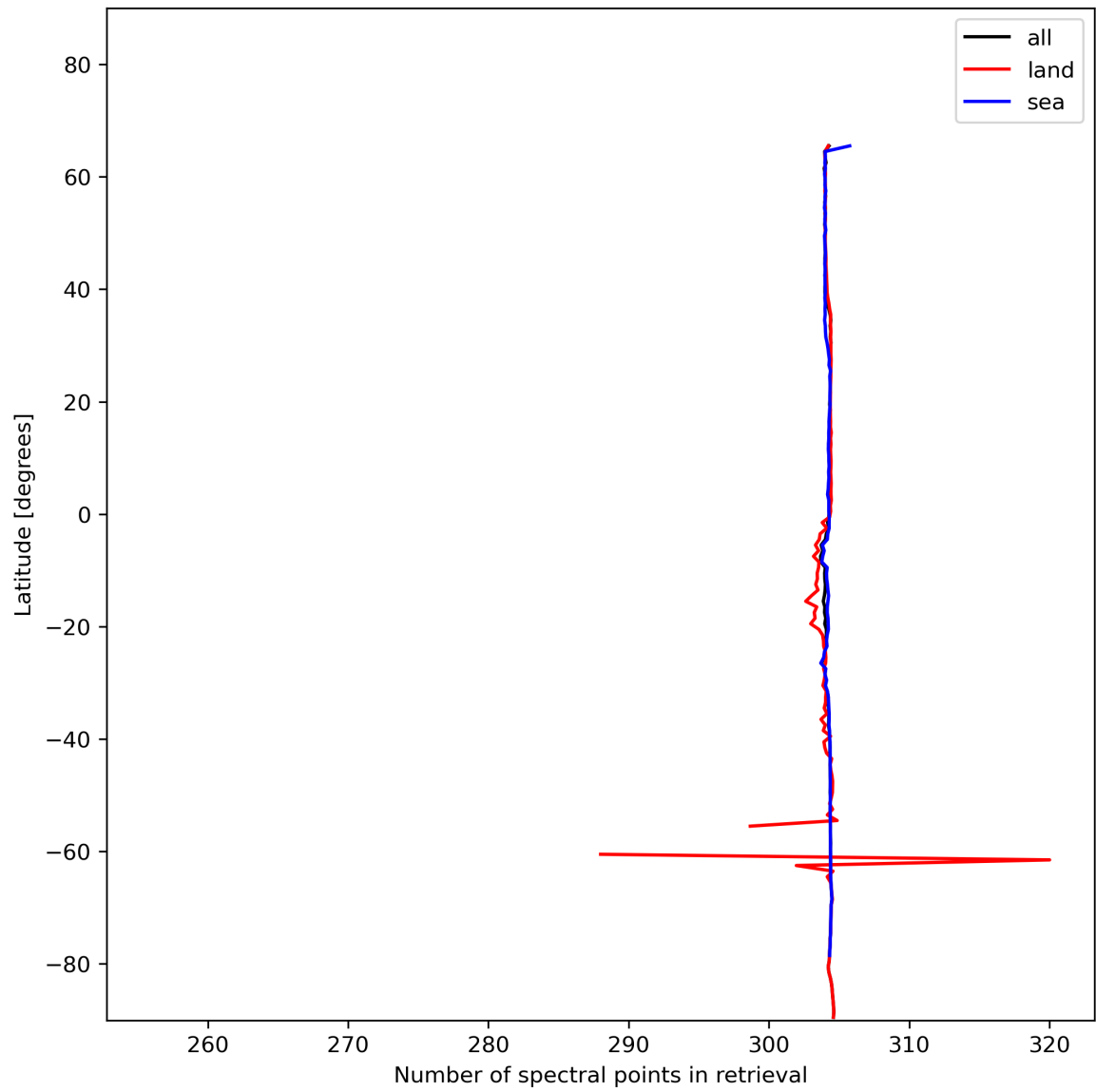
Figure 16: Zonal average of “Number of spectral points in retrieval” for 2024-01-02 to 2024-01-04.
