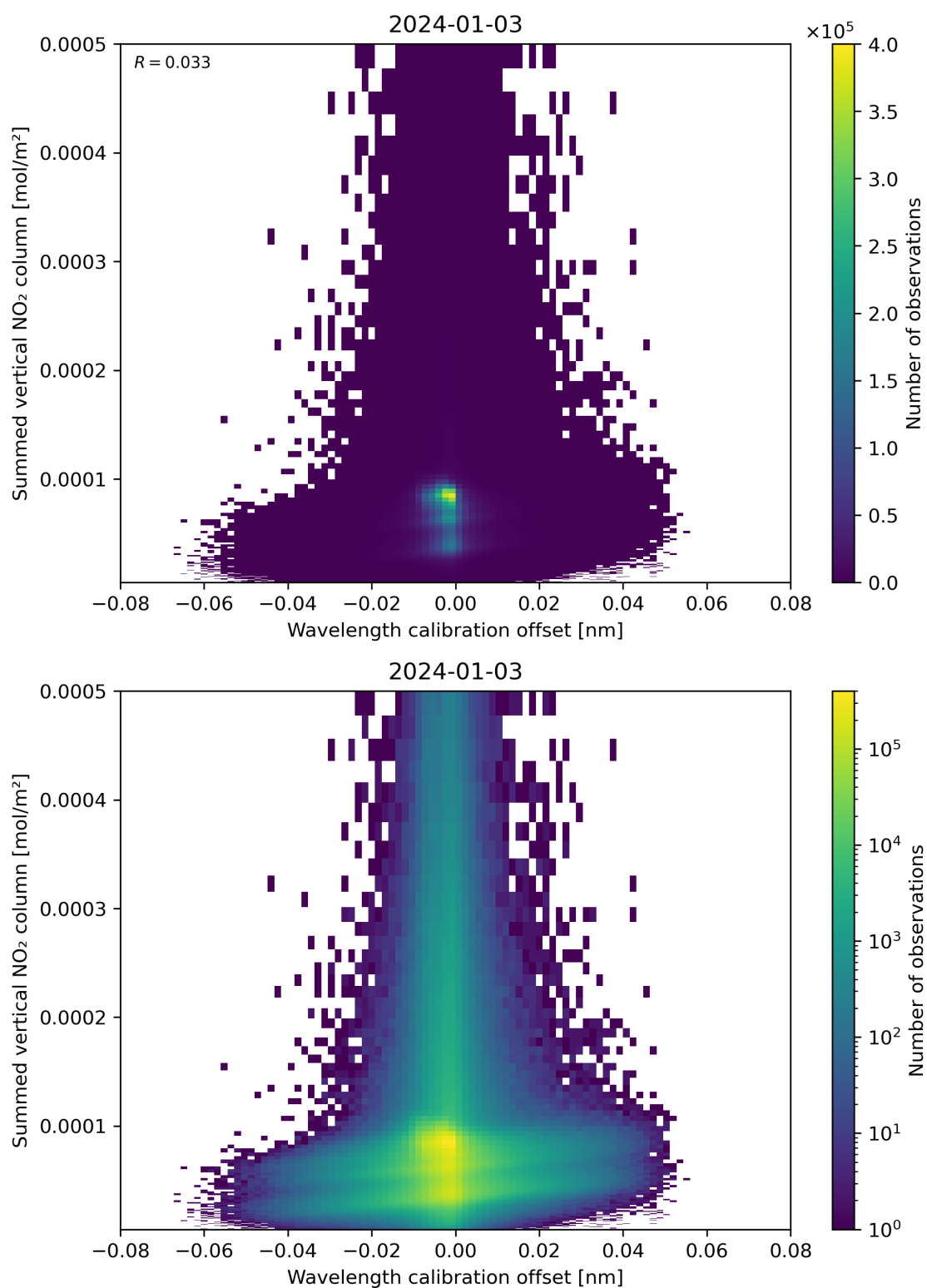
Figure 177: Scatter density plot of “Wavelength calibration offset” against “Summed vertical NO 2 column” for 2024-01-02 to 2024-01-04.
