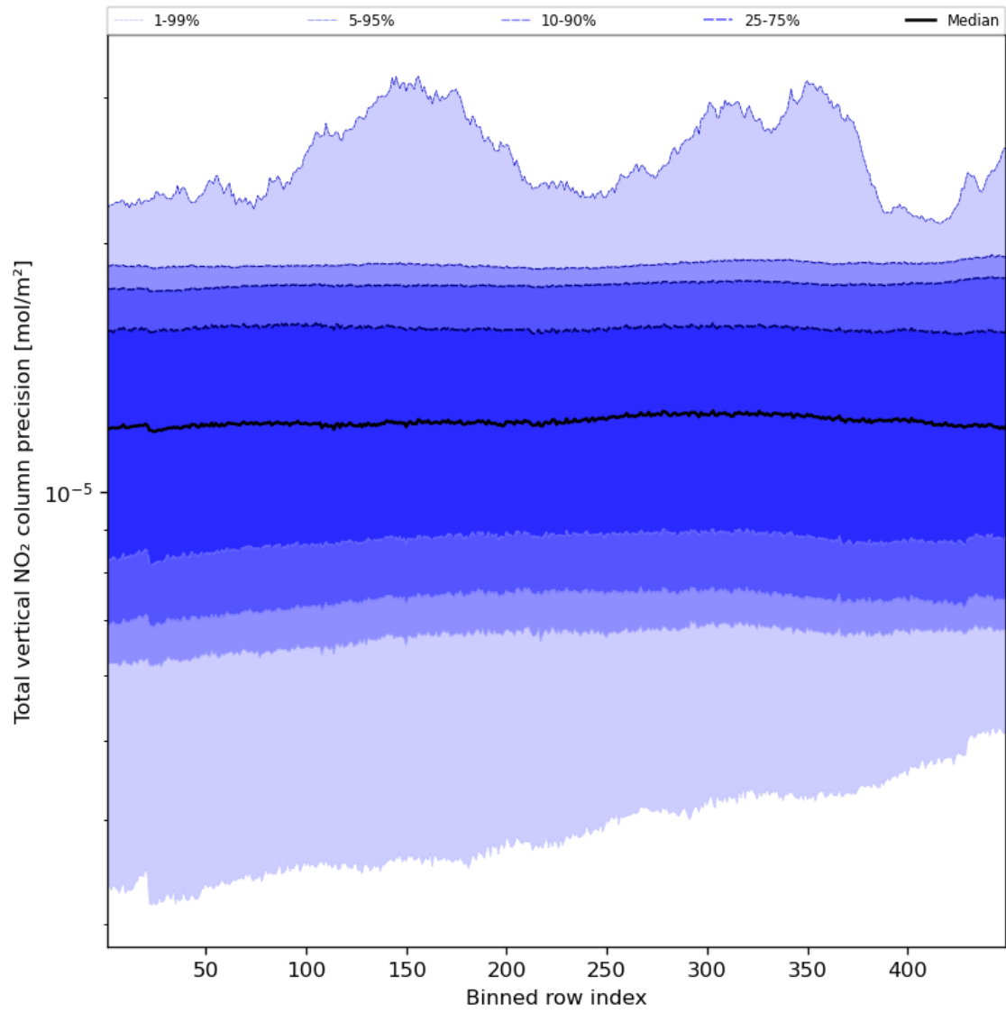
Figure 56: Along track statistics of “Total vertical NO 2 column precision” for 2024-01-02 to 2024-01-04
