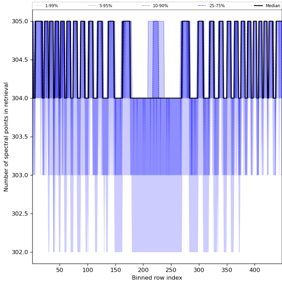
Figure 50: Along track statistics of “Number of spectral points in retrieval” for 2024-01-02 to 2024-01-04
