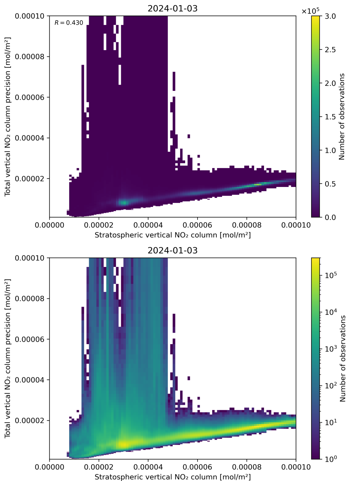
Figure 101: Scatter density plot of “Stratospheric vertical NO 2 column” against “Total vertical NO 2 column precision” for 2024-01-02 to 2024-01-04.
