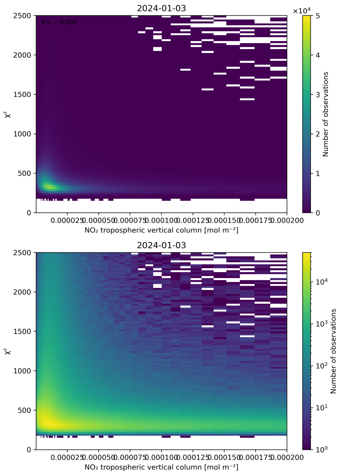
Figure 124: Scatter density plot of “NO 2 tropospheric vertical column” against “ \chi^2 ” for 2024-01-02 to 2024-01-04.
