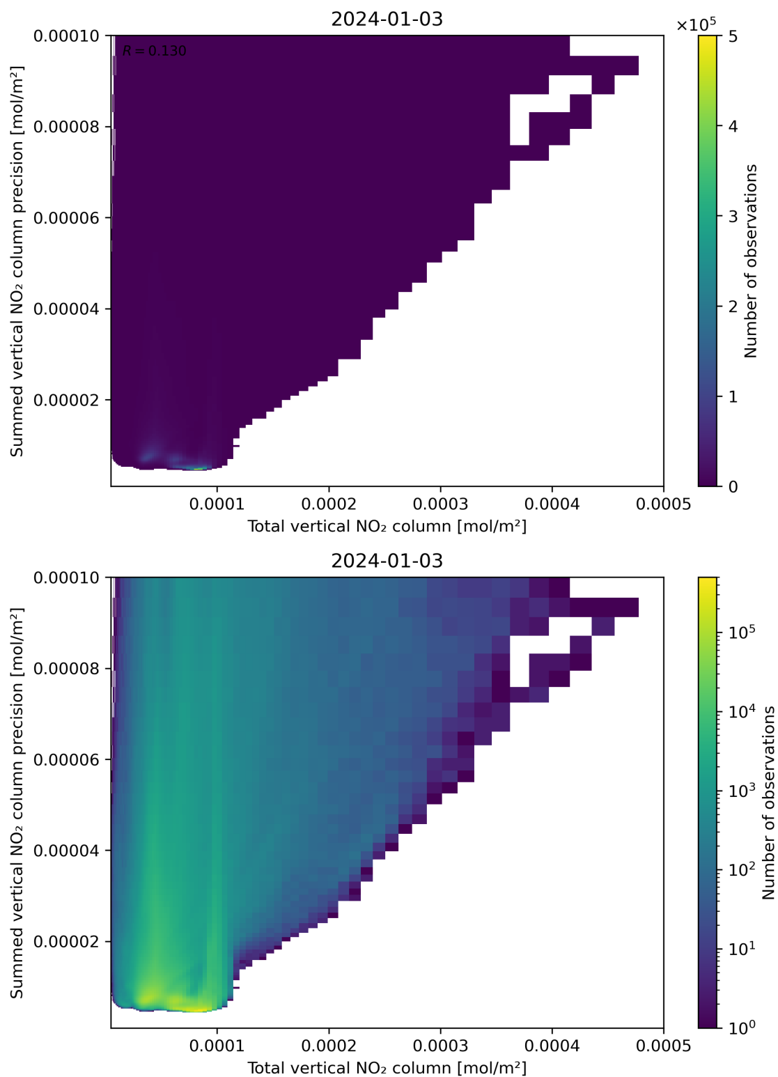
Figure 113: Scatter density plot of “Total vertical NO 2 column” against “Summed vertical NO 2 column precision” for 2024-01-02 to 2024-01-04.
