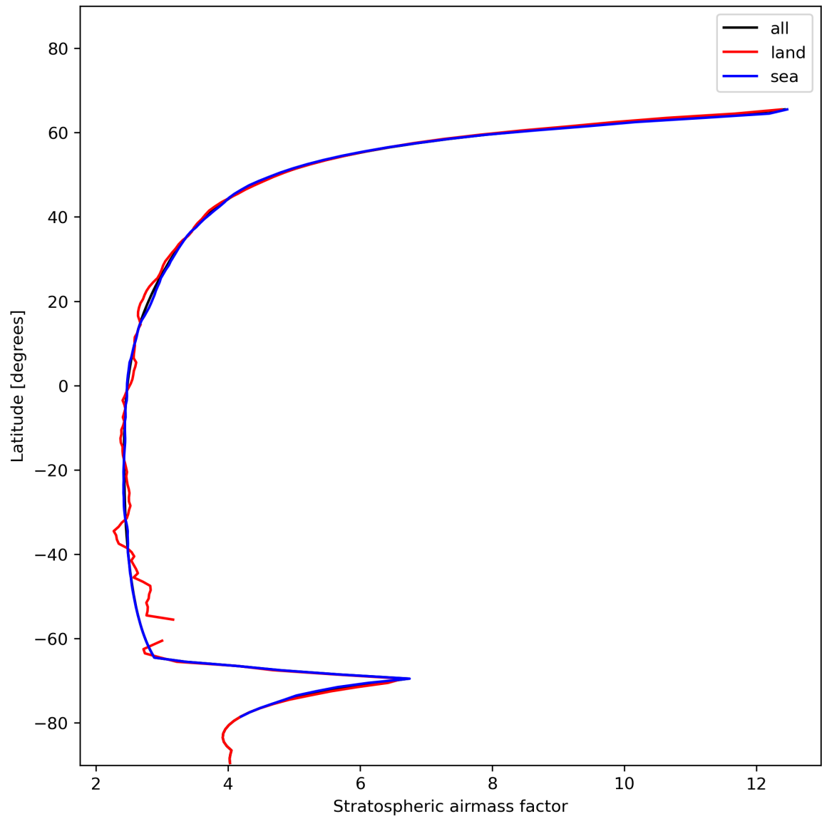
Figure 27: Zonal average of “Stratospheric airmass factor” for 2024-01-02 to 2024-01-04.
