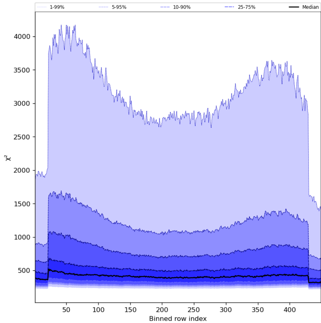
Figure 59: Along track statistics of “ \chi^2 ” for 2024-01-02 to 2024-01-04
