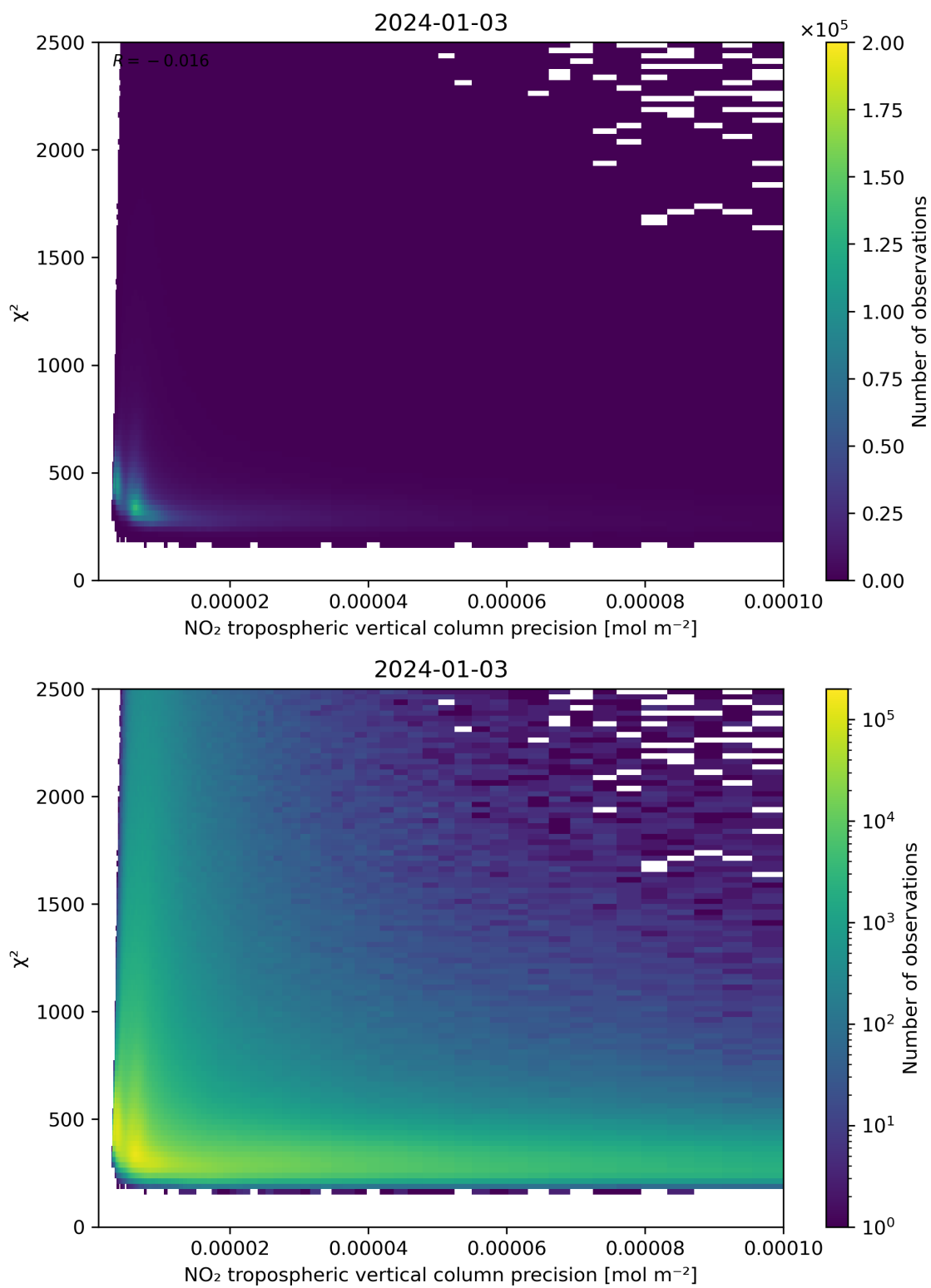
Figure 134: Scatter density plot of “NO 2 tropospheric vertical column precision” against “ \chi^2 ” for 2024-01-02 to 2024-01-04.
