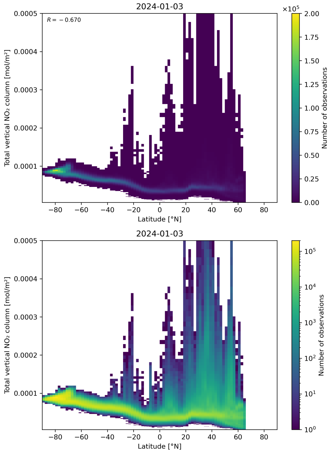
Figure 90: Scatter density plot of “Latitude” against “Total vertical NO 2 column” for 2024-01-02 to 2024-01-04.
