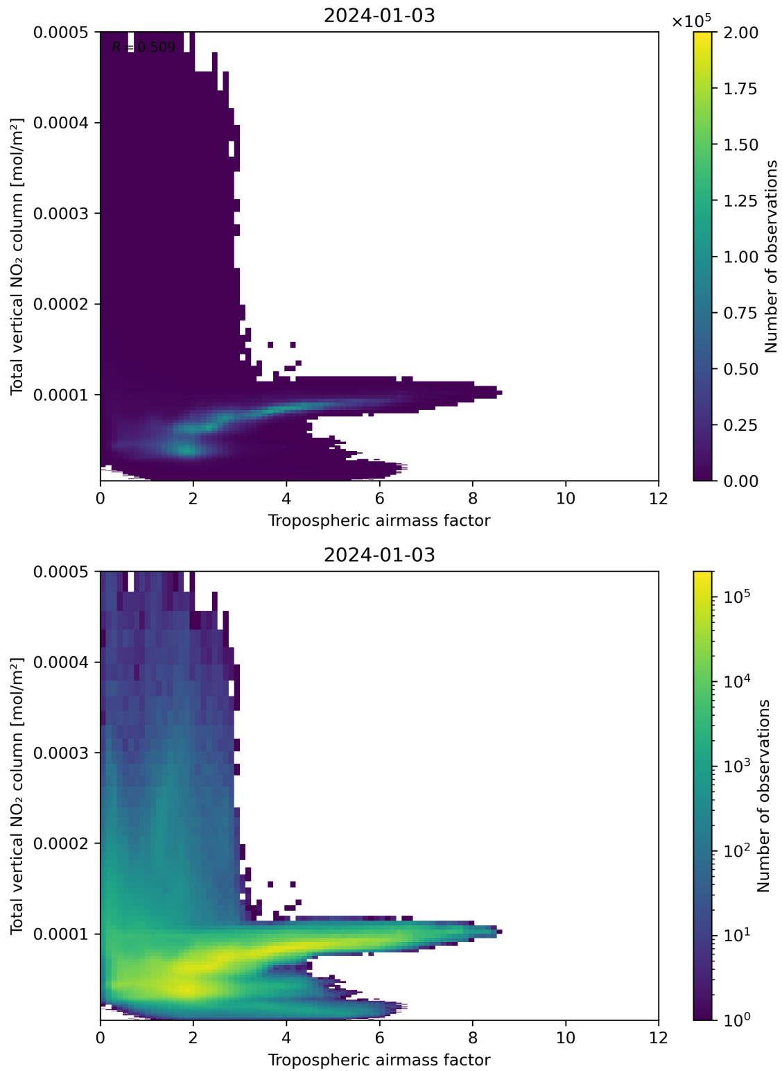
Figure 77: Scatter density plot of “Tropospheric airmass factor” against “Total vertical NO 2 column” for 2024-01-02 to 2024-01-04.
