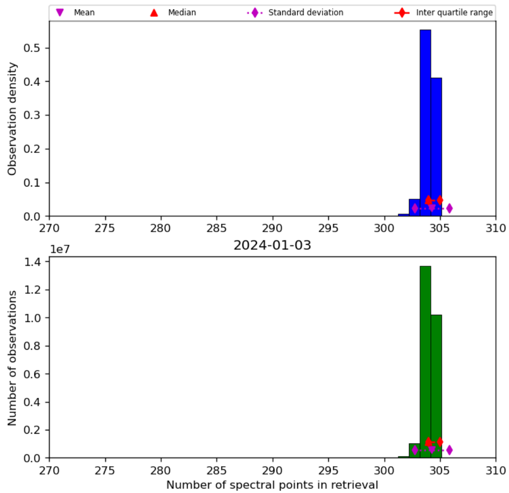
Figure 33: Histogram of “Number of spectral points in retrieval” for 2024-01-02 to 2024-01-04
