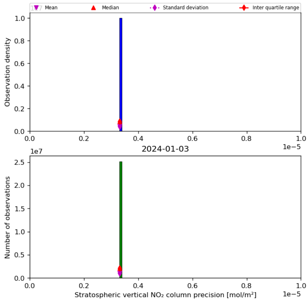
Figure 37: Histogram of “Stratospheric vertical NO 2 column precision” for 2024-01-02 to 2024-01-04
