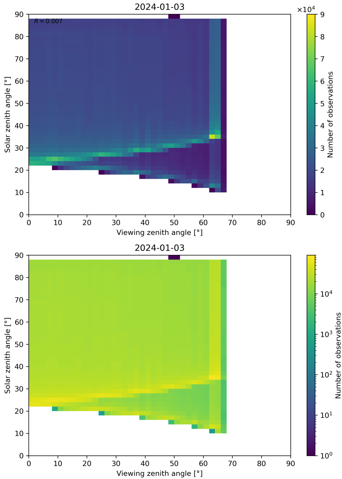
Figure 172: Scatter density plot of “Viewing zenith angle” against “Solar zenith angle” for 2024-01-02 to 2024-01-04.
