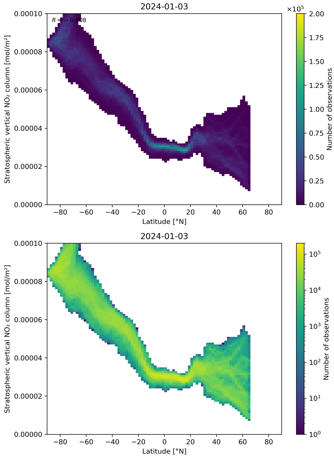
Figure 87: Scatter density plot of “Latitude” against “Stratospheric vertical NO 2 column” for 2024-01-02 to 2024-01-04.
