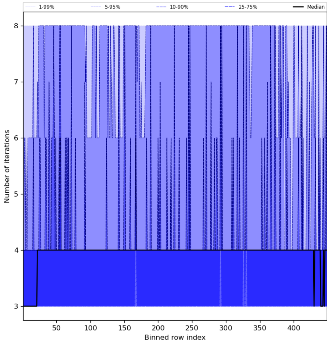
Figure 51: Along track statistics of “Number of iterations” for 2024-01-02 to 2024-01-04
