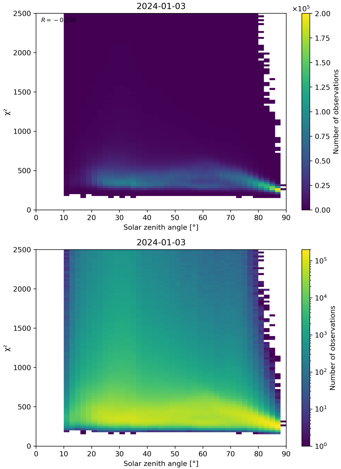
Figure 148: Scatter density plot of “Solar zenith angle” against “ \chi^2 ” for 2024-01-02 to 2024-01-04.
