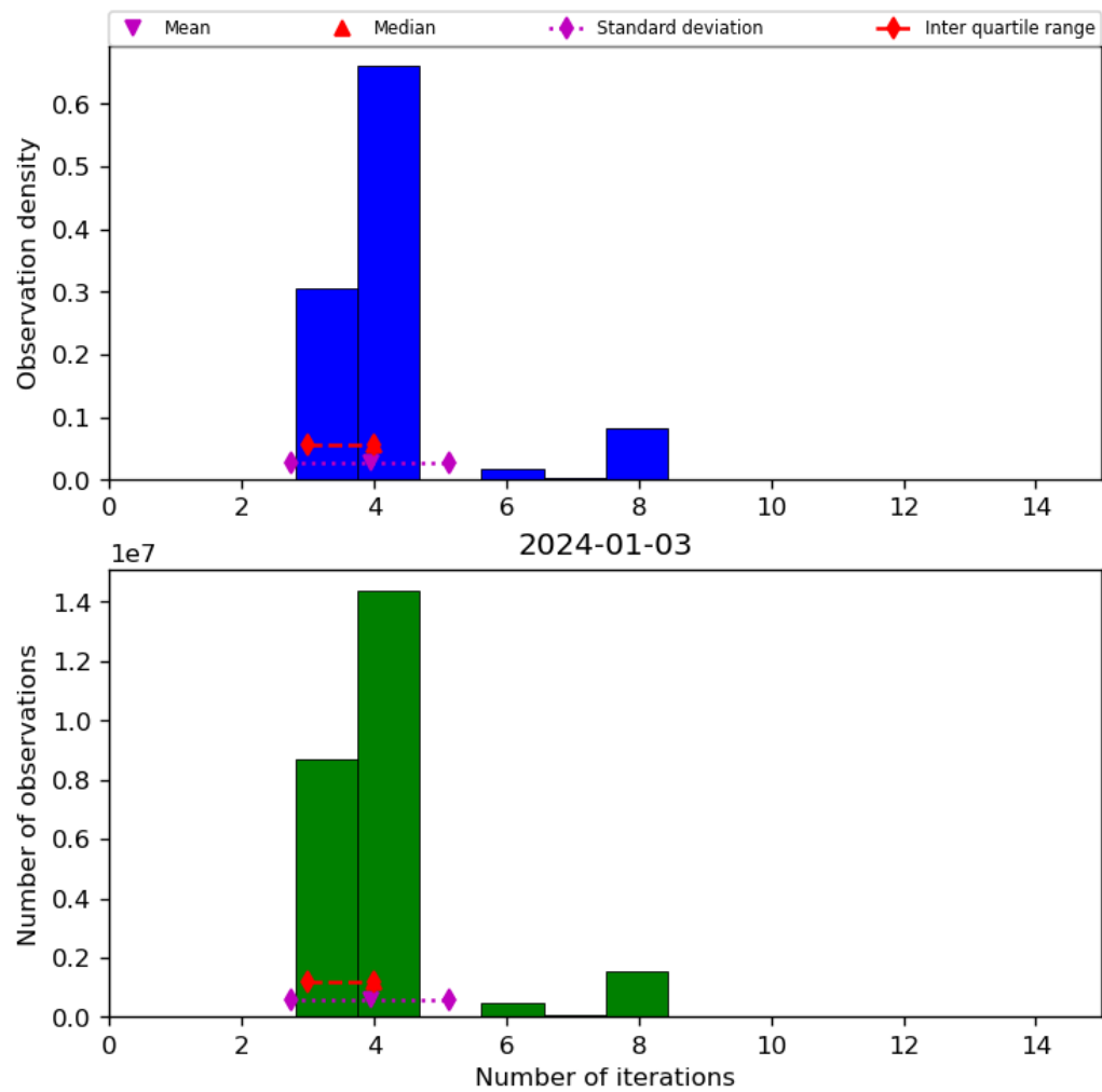
Figure 34: Histogram of “Number of iterations” for 2024-01-02 to 2024-01-04
