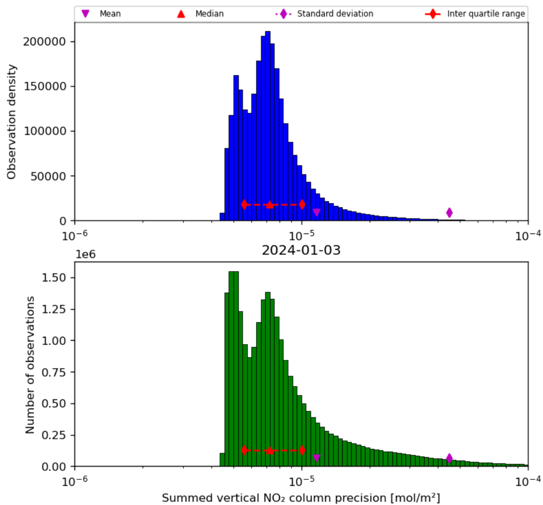
Figure 41: Histogram of "Summed vertical NO 2 column precision" for 2024-01-02 to 2024-01-04
