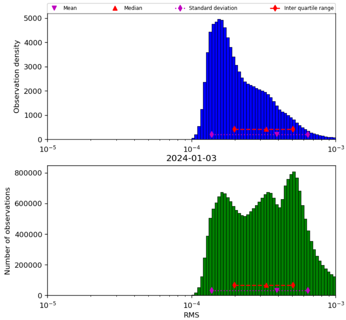
Figure 43: Histogram of “RMS” for 2024-01-02 to 2024-01-04
