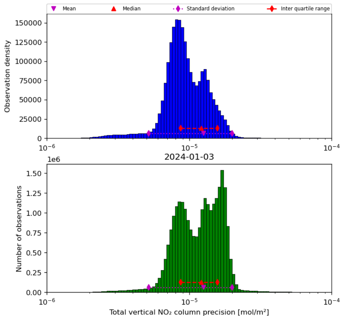
Figure 39: Histogram of “Total vertical NO 2 column precision” for 2024-01-02 to 2024-01-04
