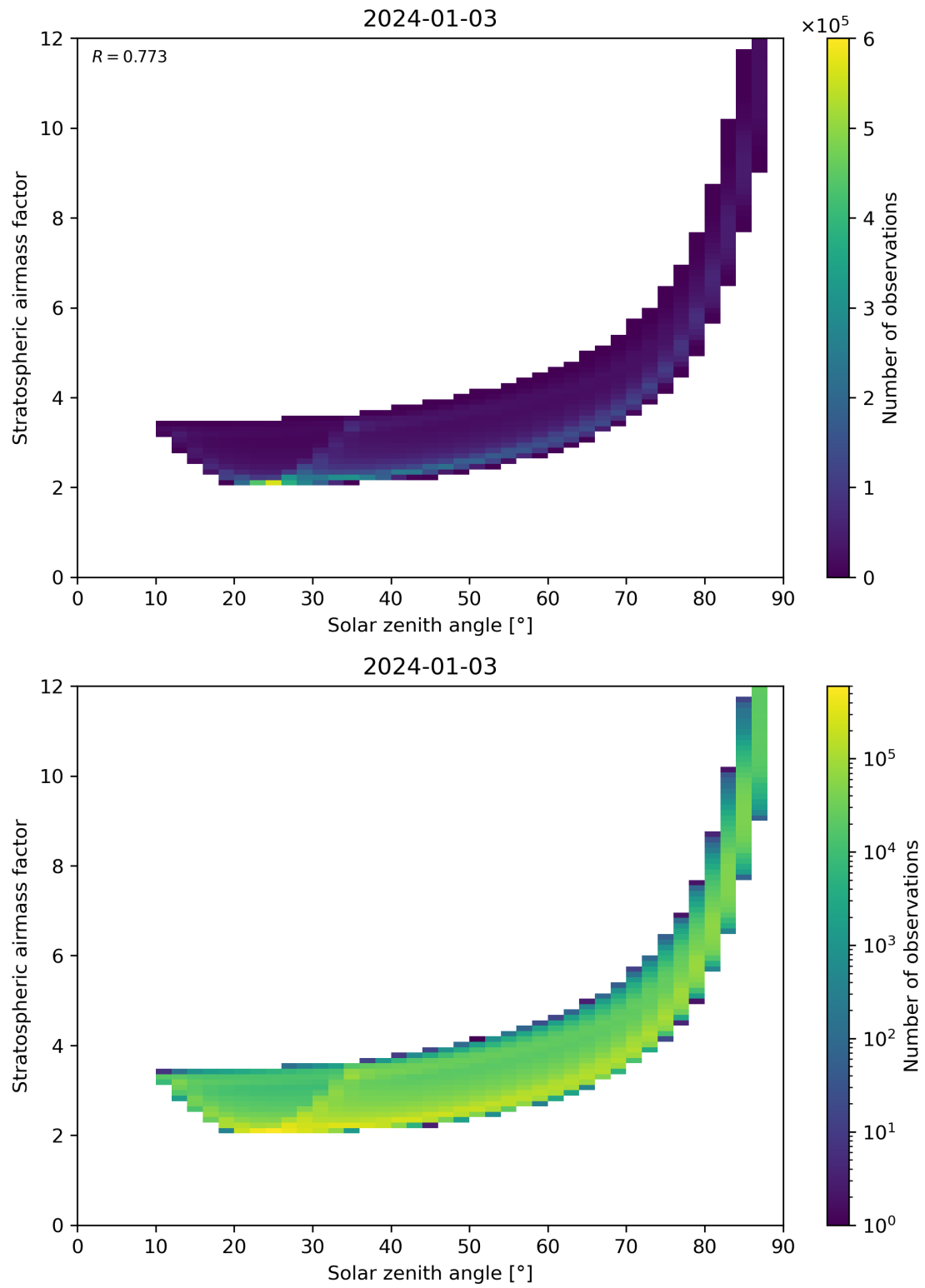
Figure 145: Scatter density plot of “Solar zenith angle” against “Stratospheric airmass factor” for 2024-01-02 to 2024-01-04.
