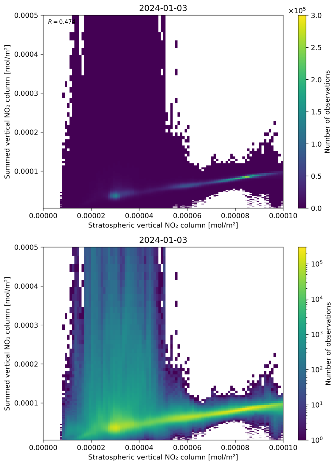
Figure 98: Scatter density plot of “Stratospheric vertical NO 2 column” against “Summed vertical NO 2 column” for 2024-01-02 to 2024-01-04.
