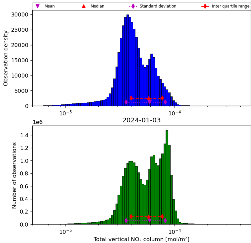
Figure 38: Histogram of “Total vertical NO 2 column” for 2024-01-02 to 2024-01-04
