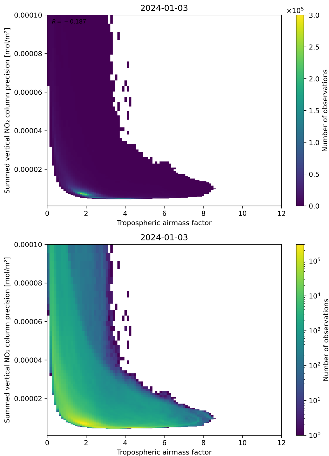
Figure 76: Scatter density plot of “Tropospheric air mass factor” against “Summed vertical NO 2 column precision” for 2024-01-02 to 2024-01-04.
