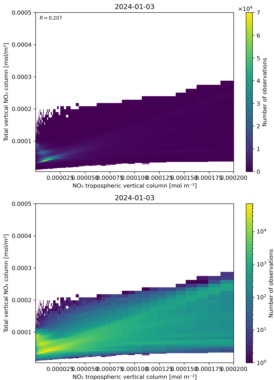
Figure 128: Scatter density plot of “NO 2 tropospheric vertical column” against “Total vertical NO 2 column” for 2024-01-02 to 2024-01-04.
