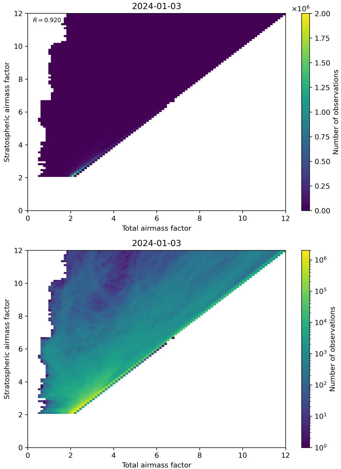
Figure 62: Scatter density plot of “Total airmass factor” against “Stratospheric airmass factor” for 2024-01-02 to 2024-01-04.
