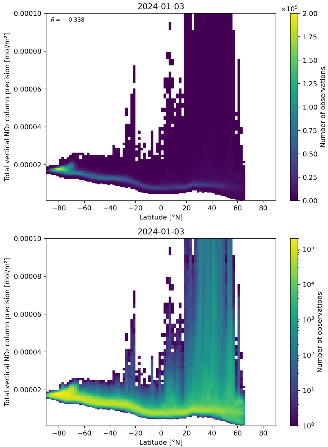
Figure 91: Scatter density plot of “Latitude” against “Total vertical NO 2 column precision” for 2024-01-02 to 2024-01-04.
