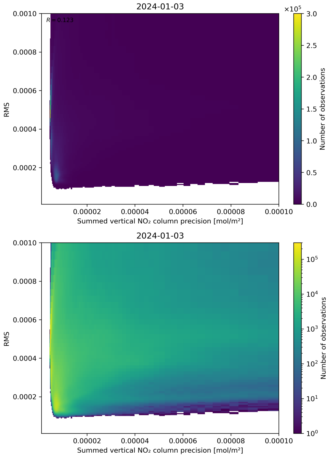
Figure 108: Scatter density plot of “Summed vertical NO 2 column precision” against “RMS” for 2024-01-02 to 2024-01-04.
