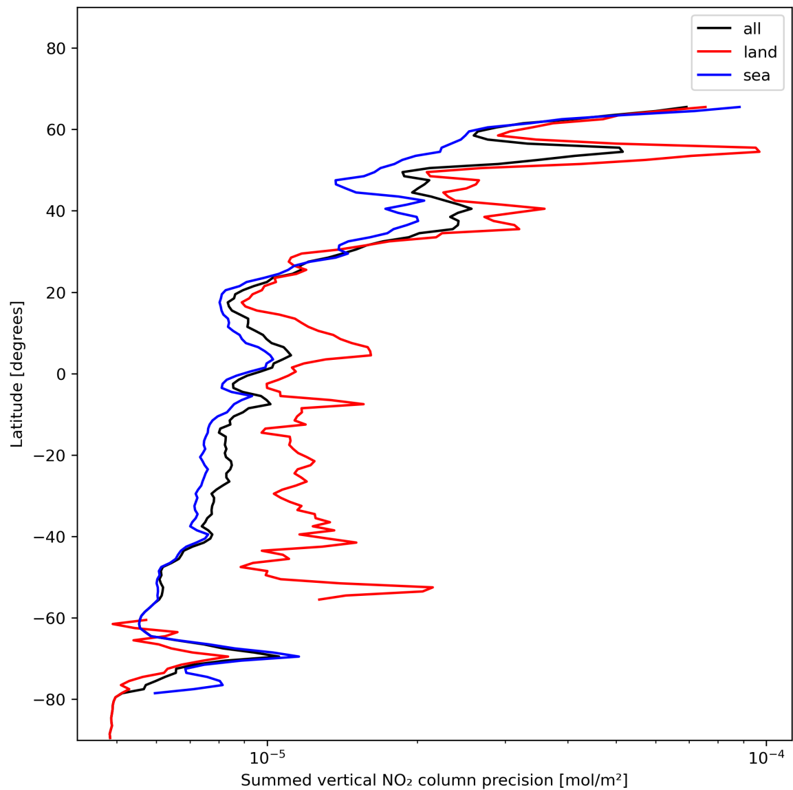
Figure 24: Zonal average of “Summed vertical NO 2 column precision” for 2024-01-02 to 2024-01-04.
