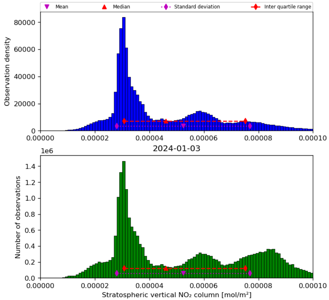
Figure 36: Histogram of “Stratospheric vertical NO 2 column” for 2024-01-02 to 2024-01-04
