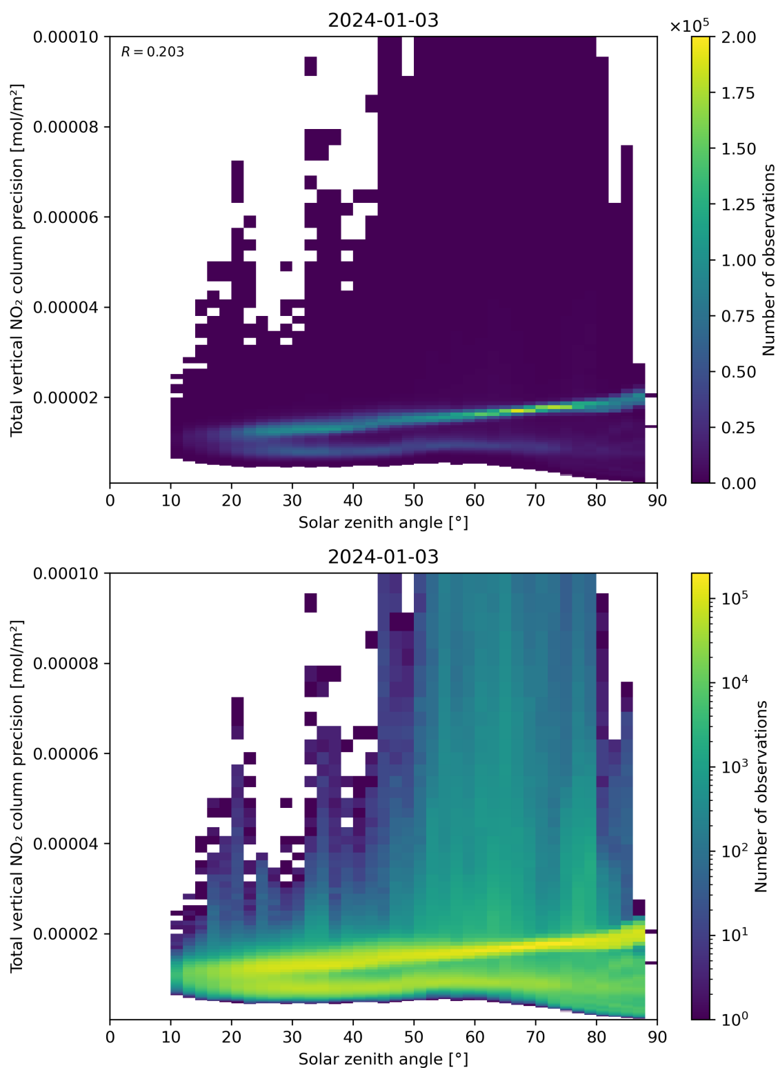
Figure 154: Scatter density plot of “Solar zenith angle” against “Total vertical NO 2 column precision” for 2024-01-02 to 2024-01-04.
