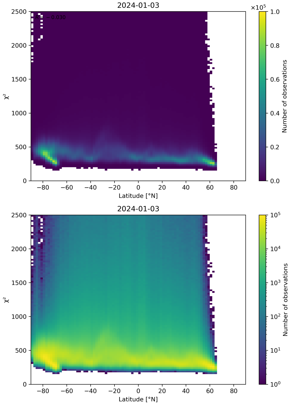
Figure 86: Scatter density plot of “Latitude” against “ \chi^2 ” for 2024-01-02 to 2024-01-04.
