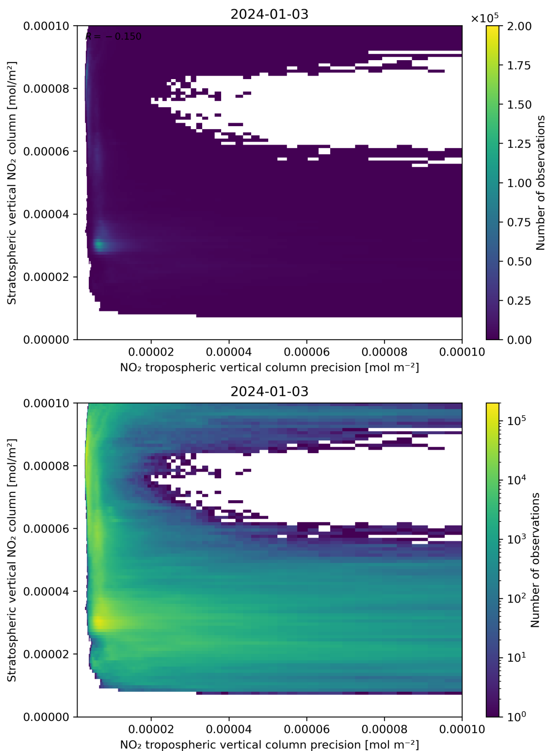
Figure 135: Scatter density plot of “NO 2 tropospheric vertical column precision” against “Stratospheric vertical NO 2 column” for 2024-01-02 to 2024-01-04.
