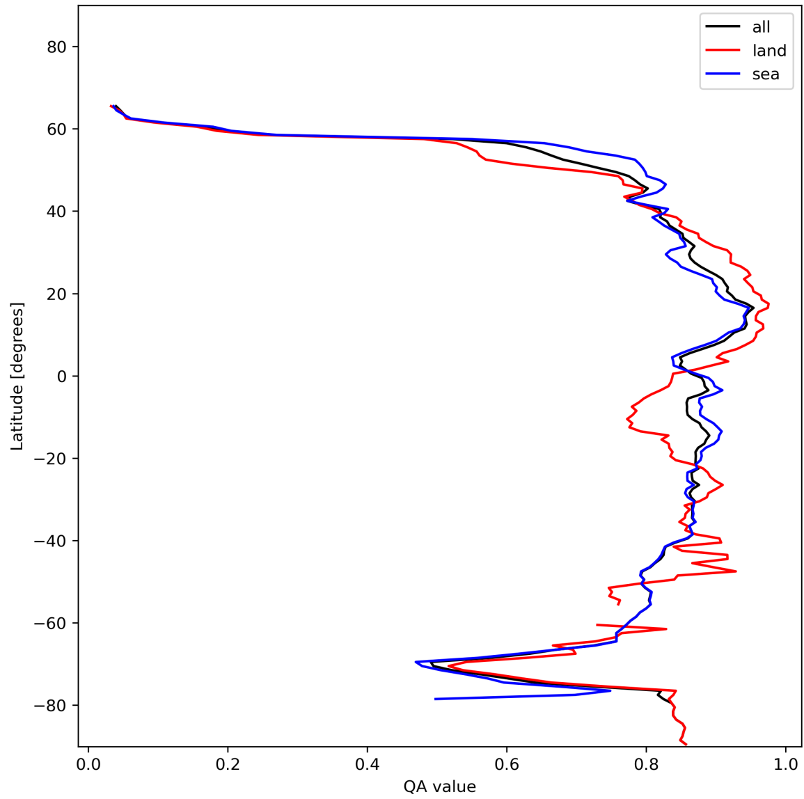
Figure 11: Zonal average of “QA value” for 2024-01-02 to 2024-01-04.
