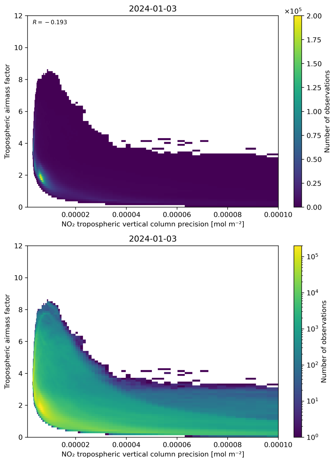
Figure 133: Scatter density plot of “NO 2 tropospheric vertical column precision” against “Tropospheric air mass factor” for 2024-01-02 to 2024-01-04.
