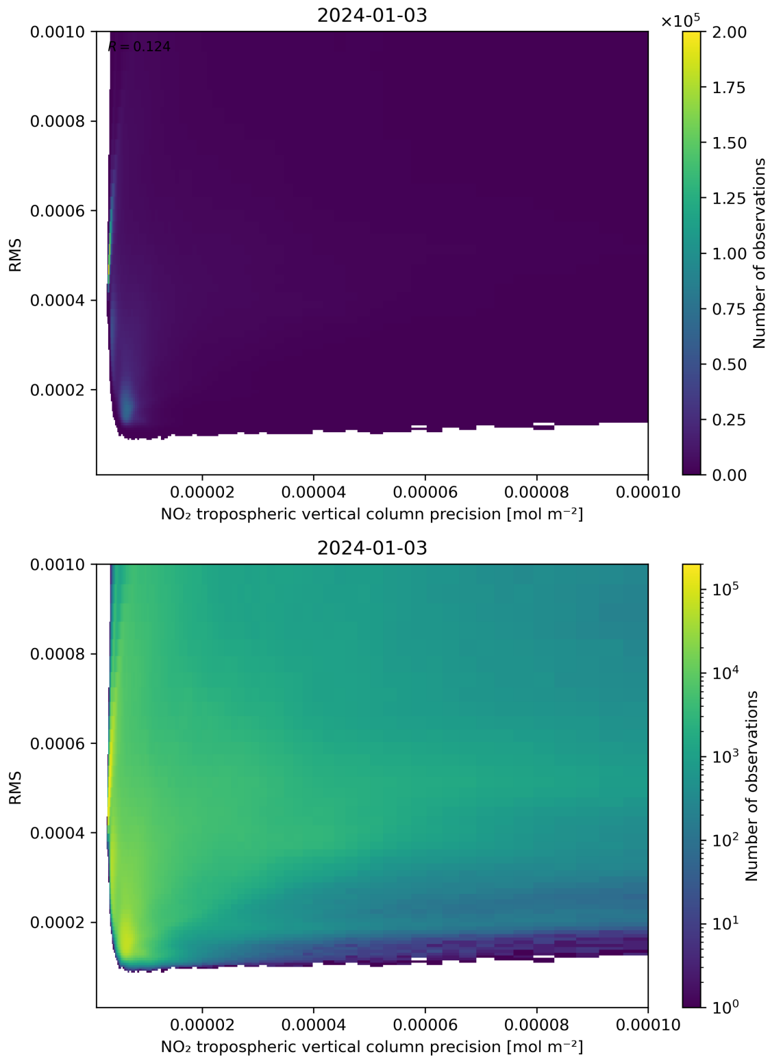
Figure 140: Scatter density plot of “NO 2 tropospheric vertical column precision” against “RMS” for 2024-01-02 to 2024-01-04.
