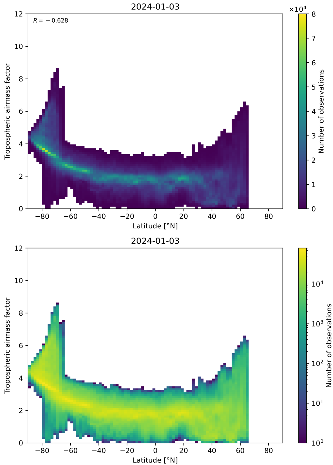
Figure 85: Scatter density plot of “Latitude” against “Tropospheric airmass factor” for 2024-01-02 to 2024-01-04.
