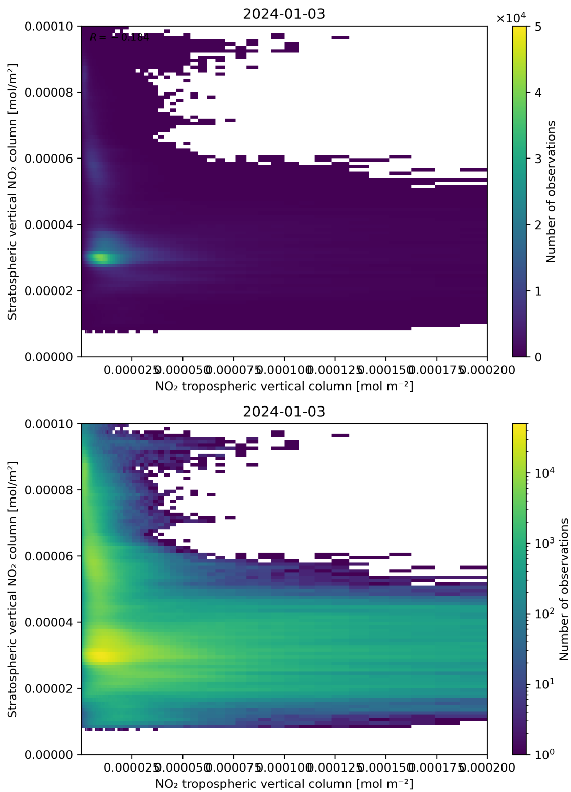
Figure 125: Scatter density plot of “NO 2 tropospheric vertical column” against “Stratospheric vertical NO 2 column” for 2024-01-02 to 2024-01-04.
