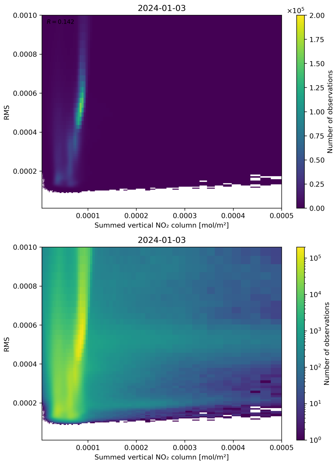
Figure 109: Scatter density plot of “Summed vertical NO 2 column” against “RMS” for 2024-01-02 to 2024-01-04.
