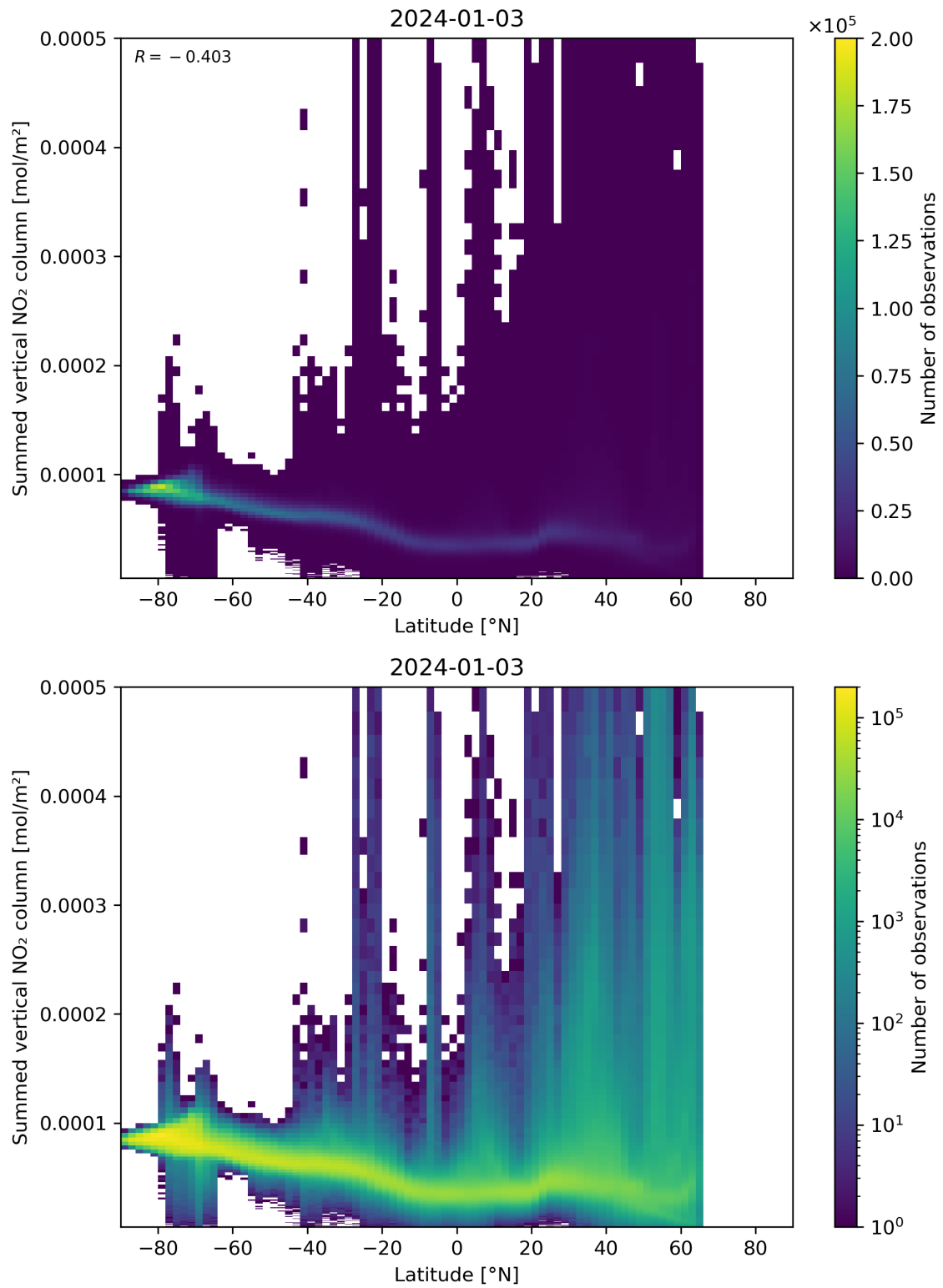
Figure 88: Scatter density plot of “Latitude” against “Summed vertical NO 2 column” for 2024-01-02 to 2024-01-04.
