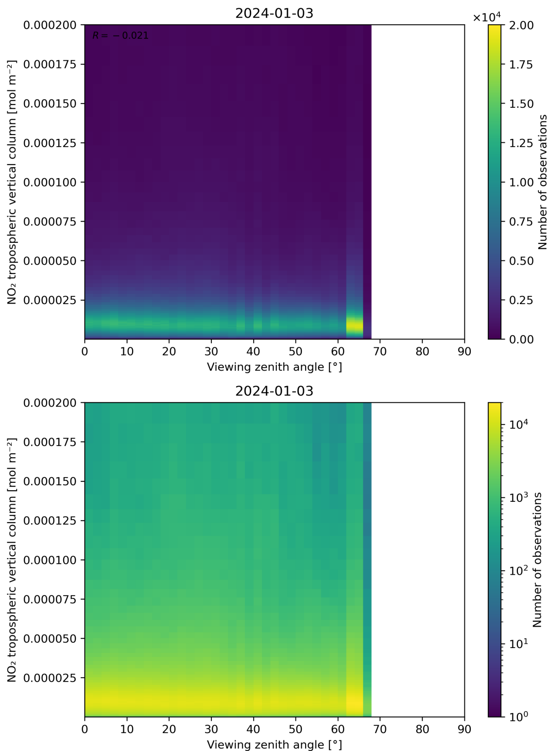
Figure 169: Scatter density plot of “Viewing zenith angle” against “NO 2 tropospheric vertical column” for 2024-01-02 to 2024-01-04.
