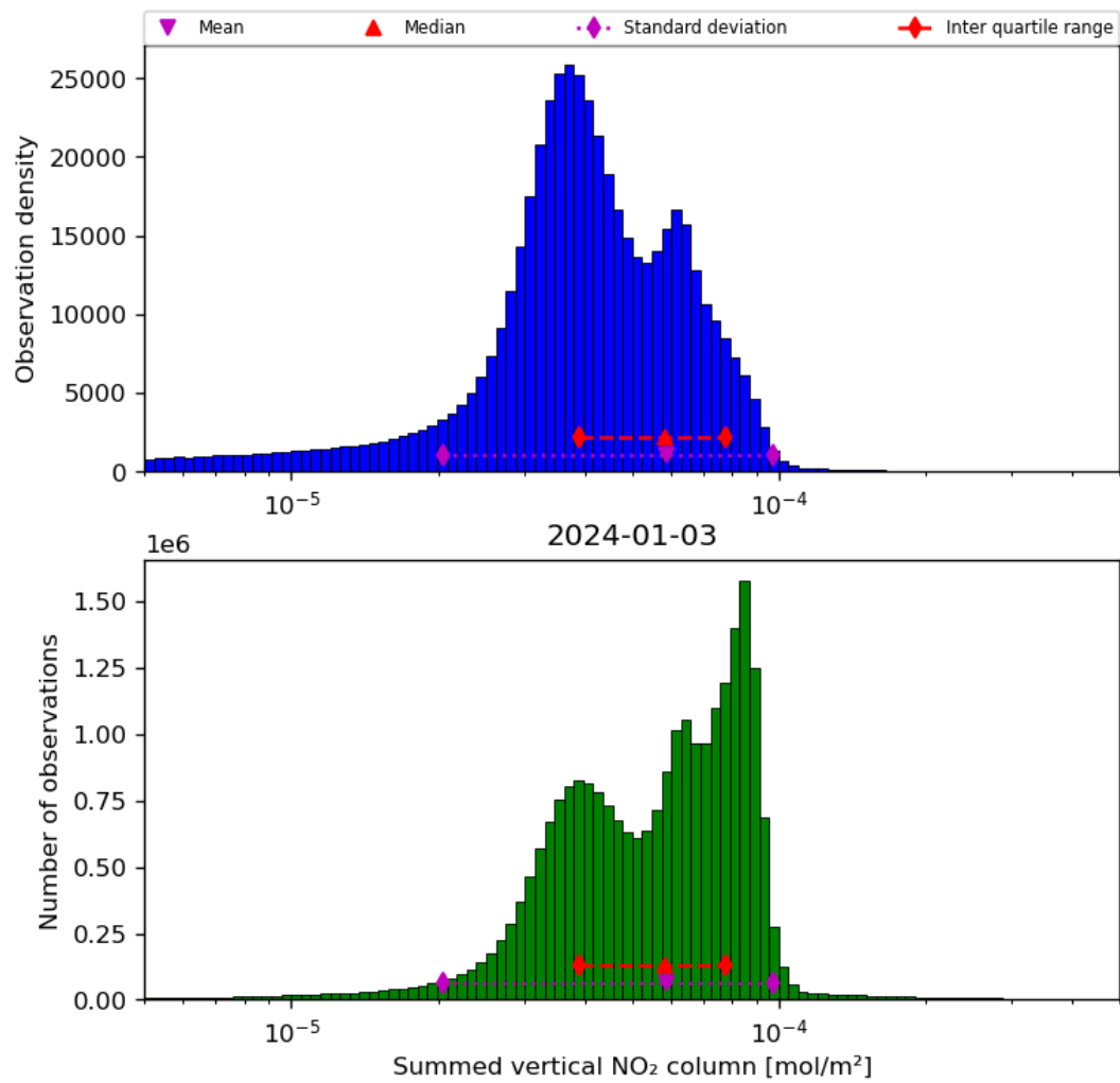
Figure 40: Histogram of “Summed vertical NO 2 column” for 2024-01-02 to 2024-01-04
