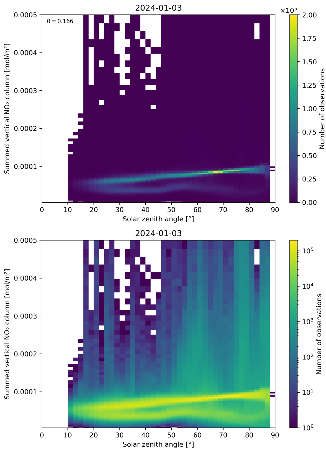
Figure 151: Scatter density plot of “Solar zenith angle” against “Summed vertical NO 2 column” for 2024-01-02 to 2024-01-04.
