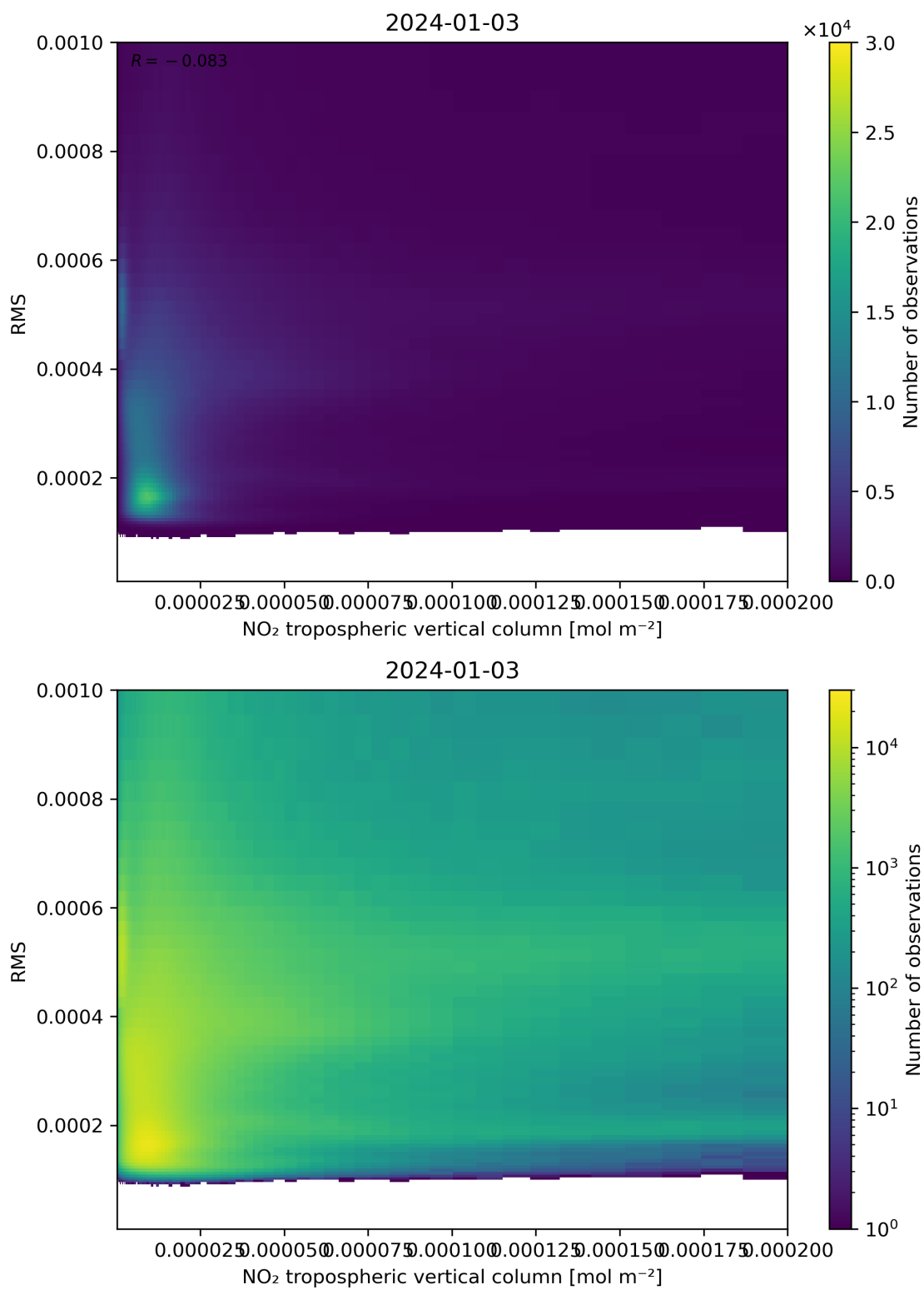
Figure 142: Scatter density plot of “NO 2 tropospheric vertical column” against “RMS” for 2024-01-02 to 2024-01-04.
