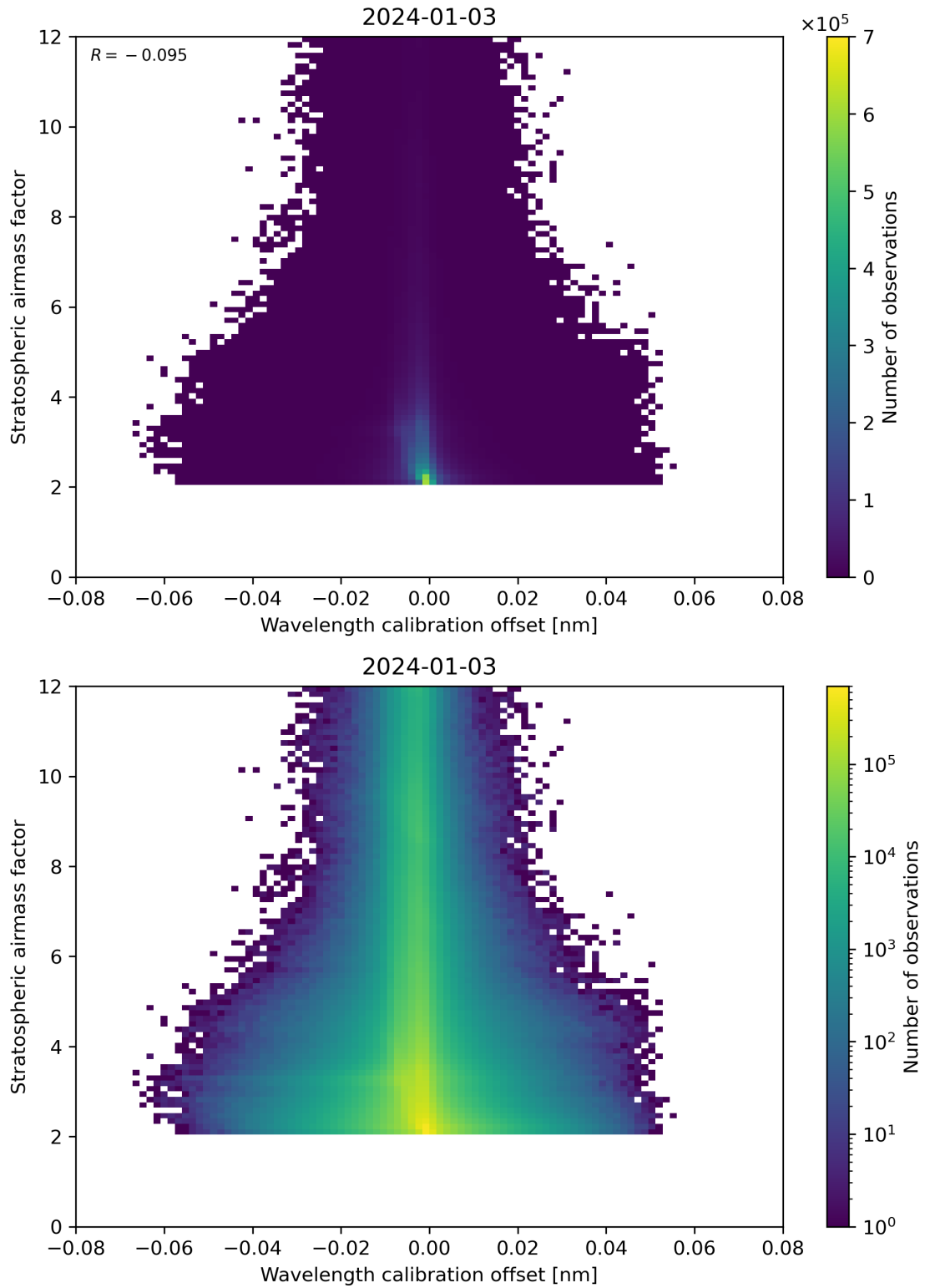
Figure 174: Scatter density plot of “Wavelength calibration offset” against “Stratospheric air mass factor” for 2024-01-02 to 2024-01-04.
