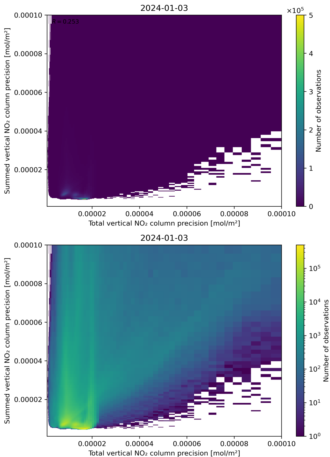
Figure 118: Scatter density plot of “Total vertical NO 2 column precision” against “Summed vertical NO 2 column precision” for 2024-01-02 to 2024-01-04.
