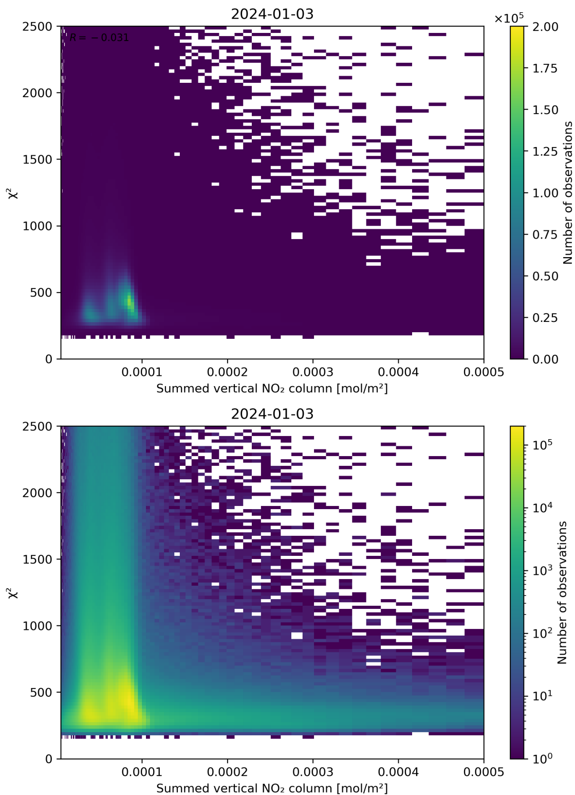
Figure 104: Scatter density plot of “Summed vertical NO 2 column” against “ \chi^2 ” for 2024-01-02 to 2024-01-04.
