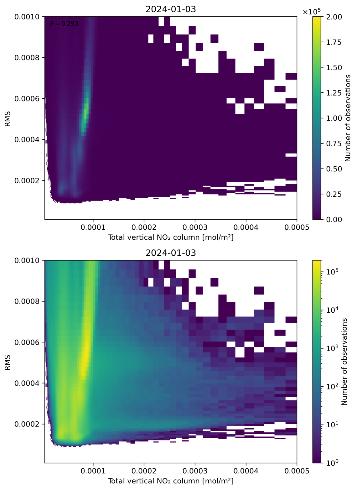
Figure 120: Scatter density plot of “Total vertical NO 2 column” against “RMS” for 2024-01-02 to 2024-01-04.
