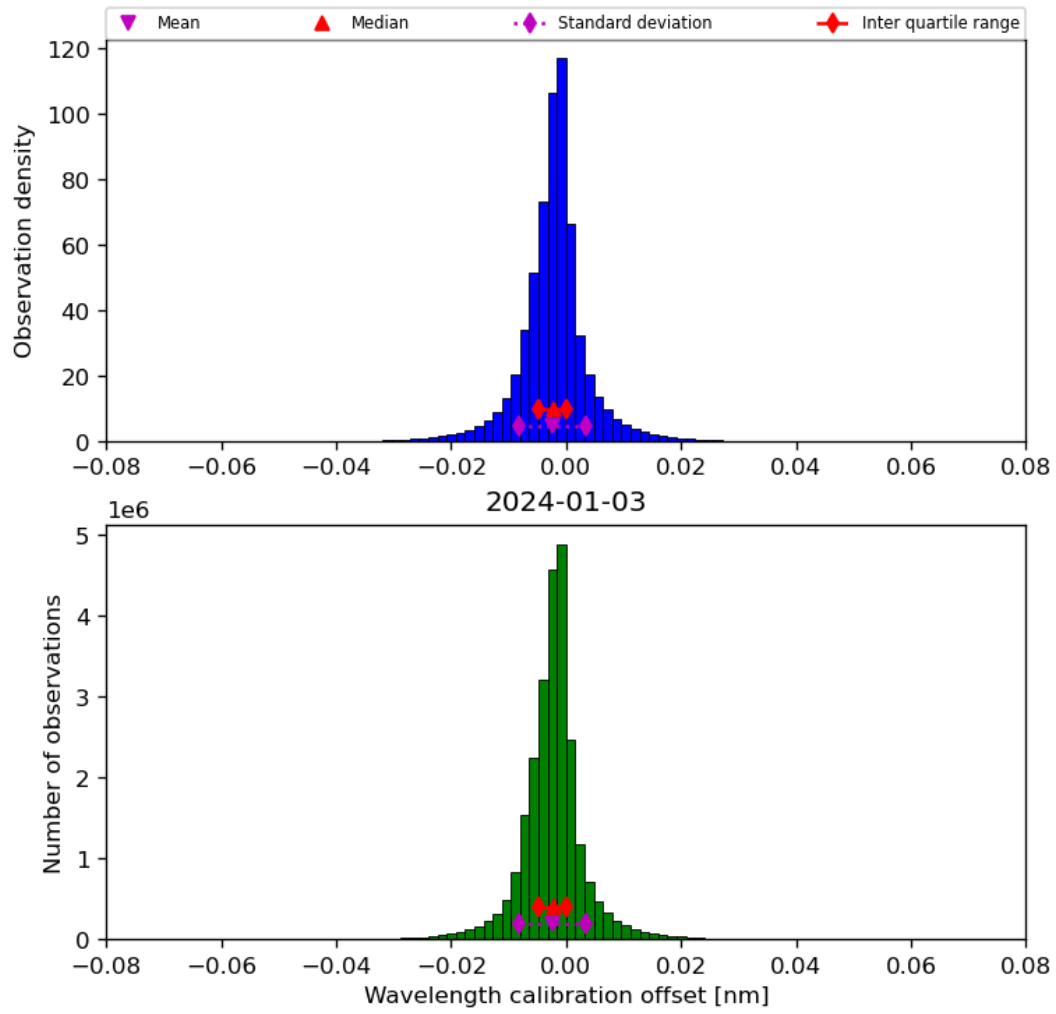
Figure 35: Histogram of “Wavelength calibration offset” for 2024-01-02 to 2024-01-04
