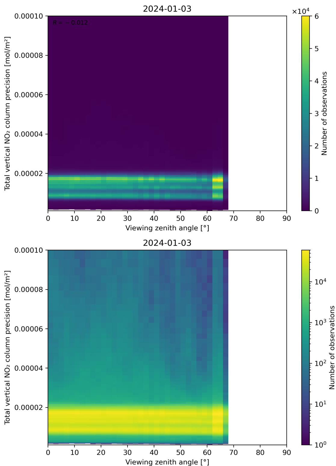
Figure 168: Scatter density plot of “Viewing zenith angle” against “Total vertical NO 2 column precision” for 2024-01-02 to 2024-01-04.
