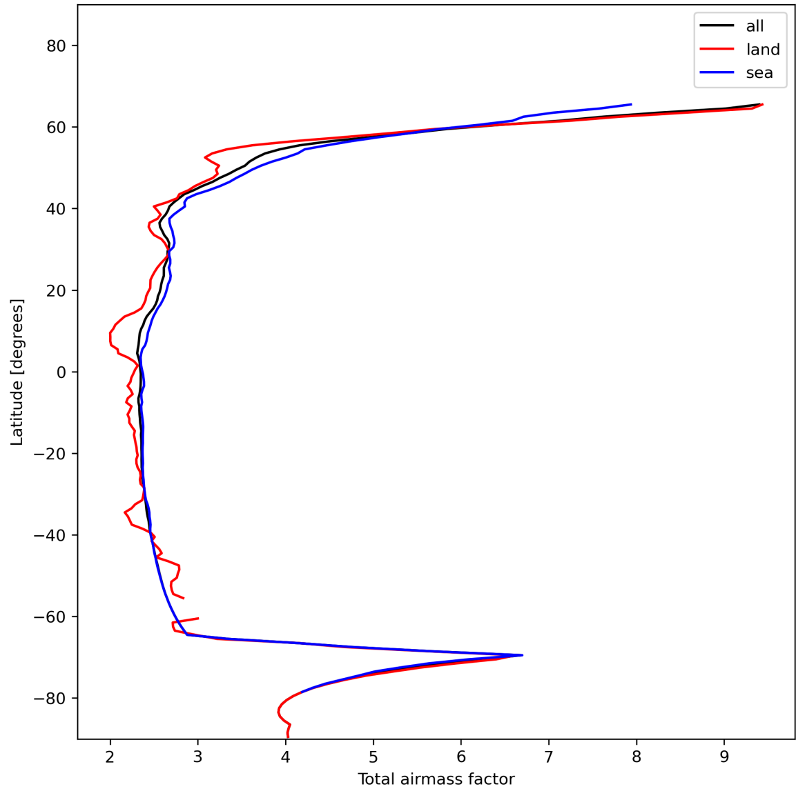
Figure 15: Zonal average of “Total airmass factor” for 2024-01-02 to 2024-01-04.
