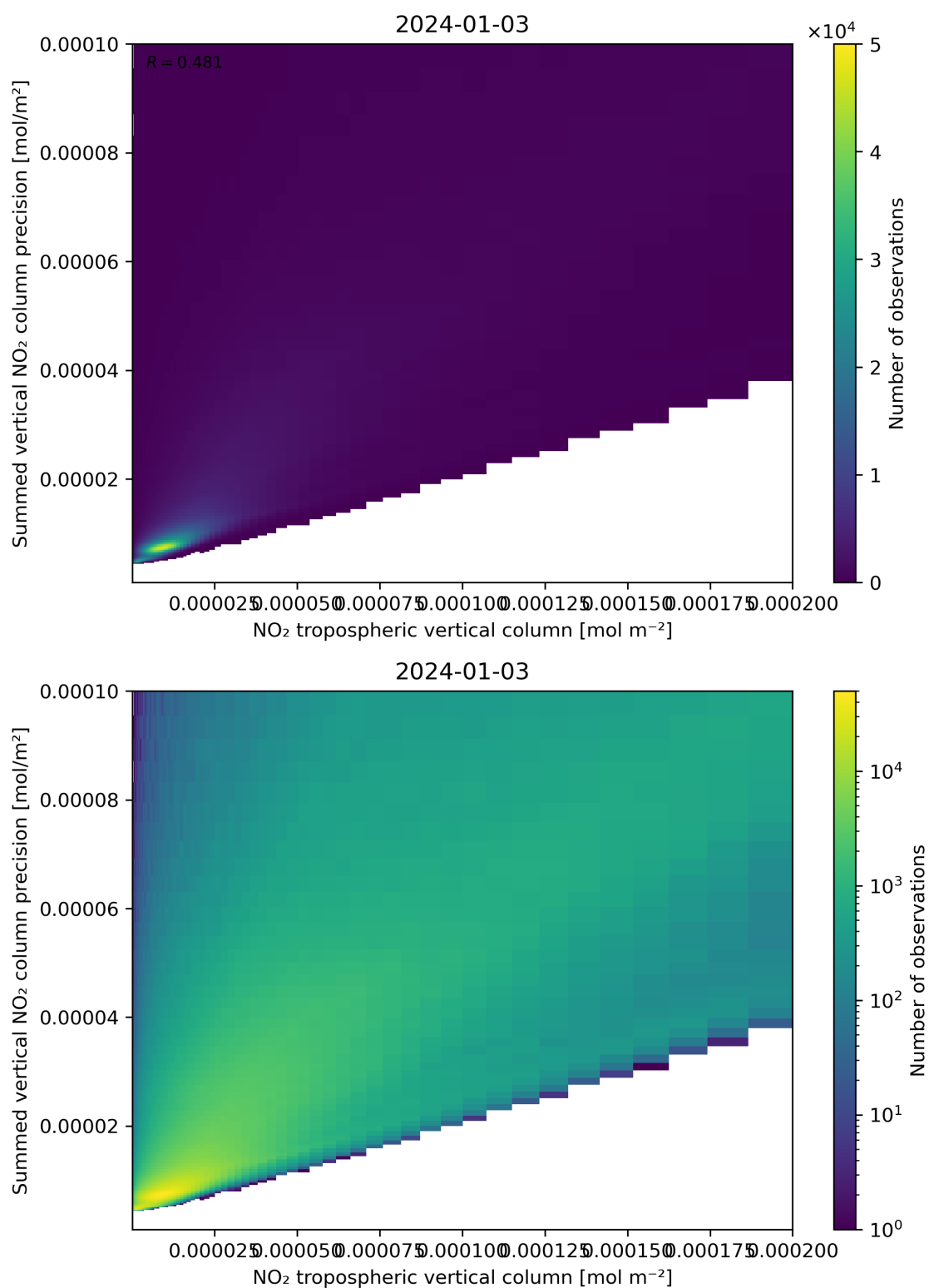
Figure 127: Scatter density plot of “NO 2 tropospheric vertical column” against “Summed vertical NO 2 column precision” for 2024-01-02 to 2024-01-04.
