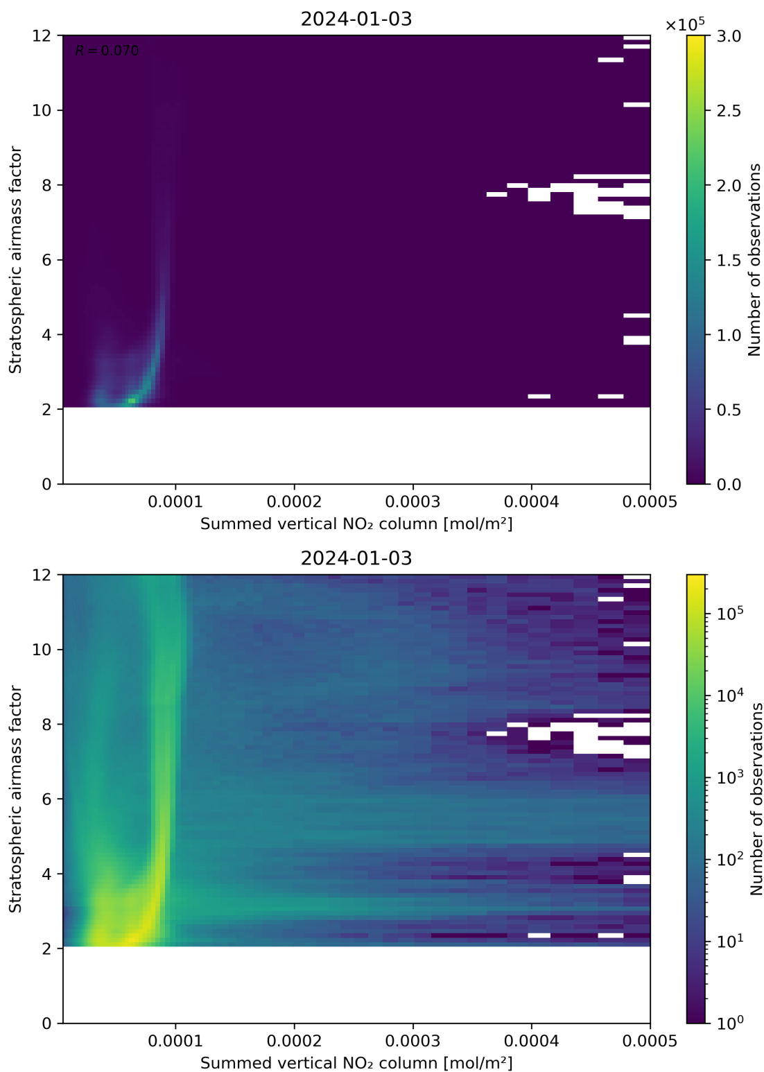
Figure 103: Scatter density plot of “Summed vertical NO 2 column” against “Stratospheric airmass factor” for 2024-01-02 to 2024-01-04.
