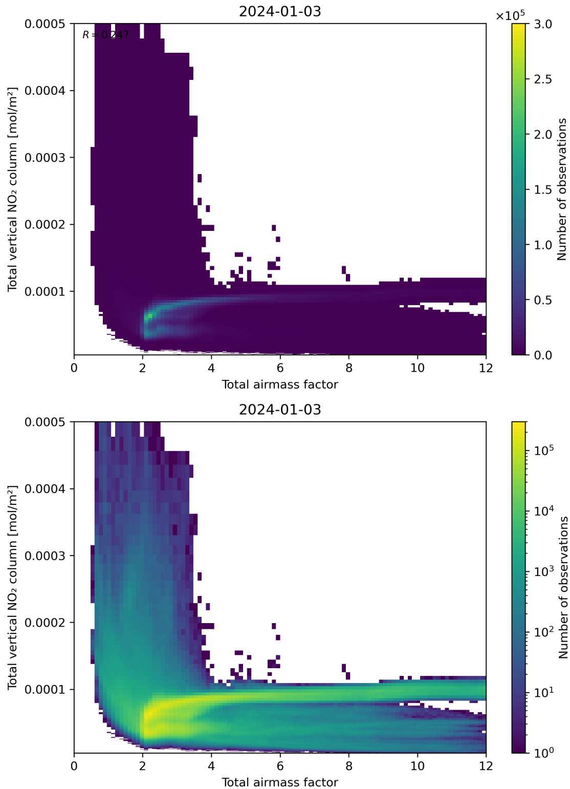
Figure 67: Scatter density plot of “Total airmass factor” against “Total vertical NO 2 column” for 2024-01-02 to 2024-01-04.
