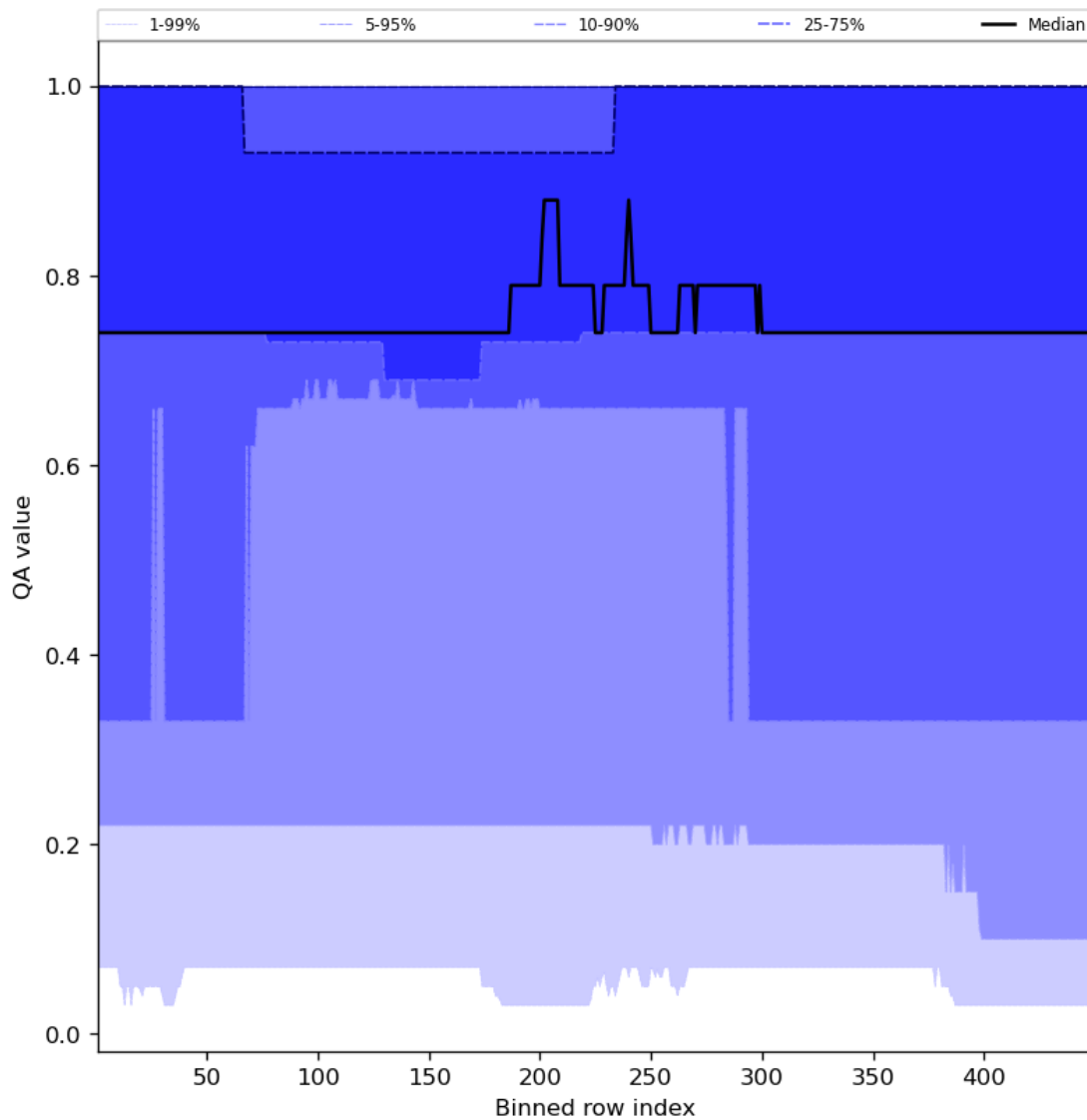
Figure 45: Along track statistics of “QA value” for 2024-01-02 to 2024-01-04
