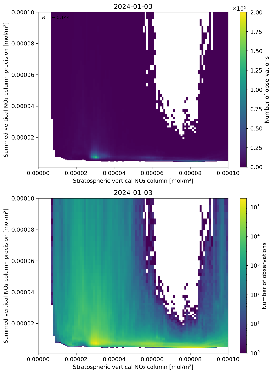
Figure 99: Scatter density plot of “Stratospheric vertical NO 2 column” against “Summed vertical NO 2 column precision” for 2024-01-02 to 2024-01-04.
