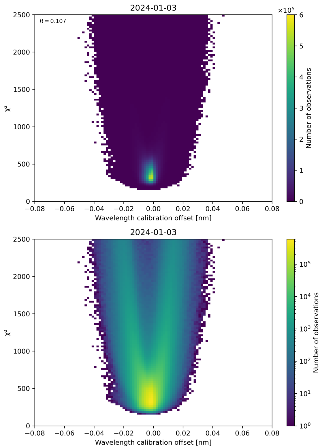
Figure 175: Scatter density plot of “Wavelength calibration offset” against “ \chi^2 ” for 2024-01-02 to 2024-01-04.
