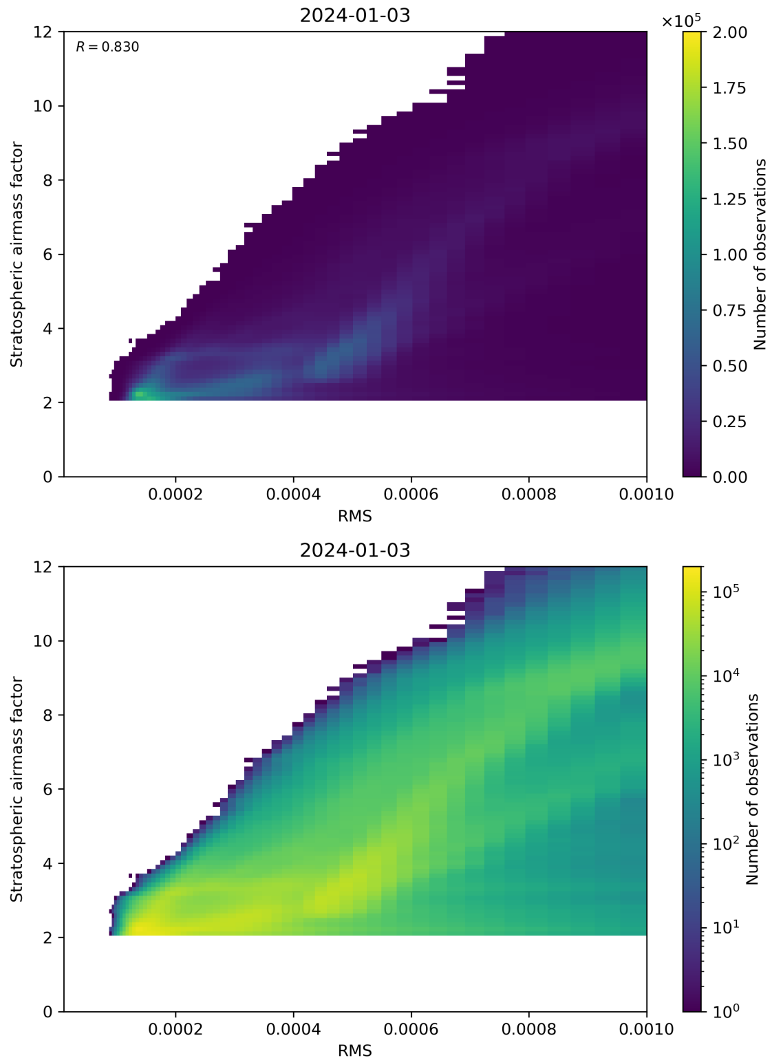
Figure 144: Scatter density plot of “RMS” against “Stratospheric airmass factor” for 2024-01-02 to 2024-01-04.
