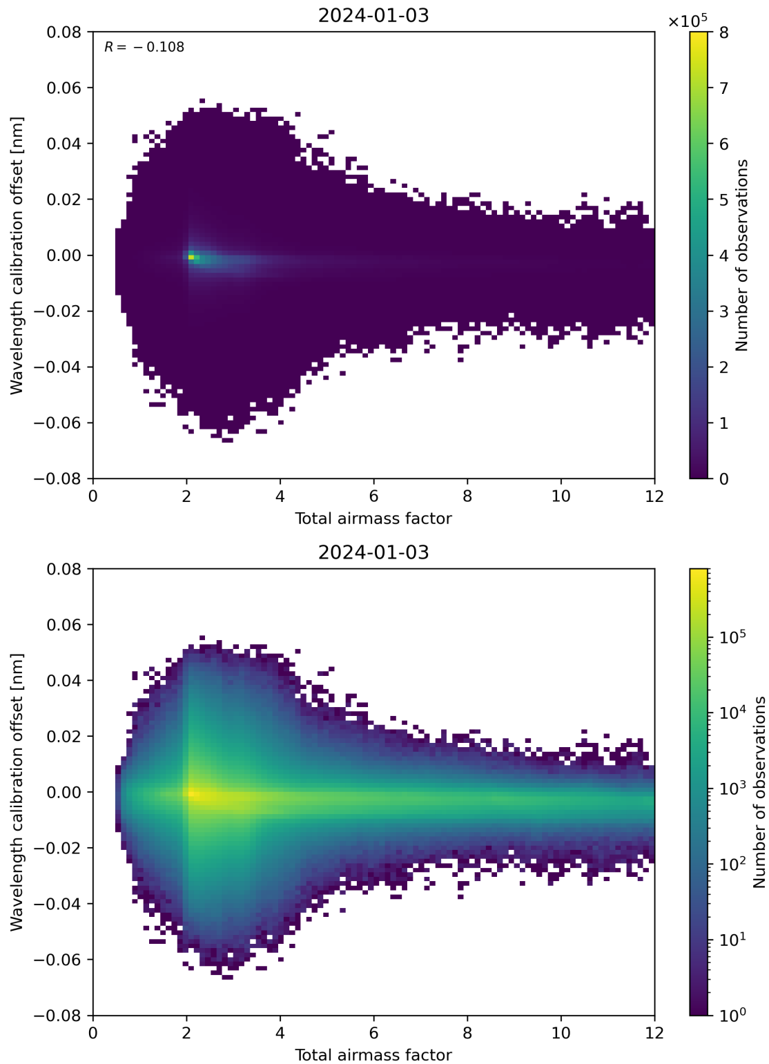
Figure 70: Scatter density plot of “Total airmass factor” against “Wavelength calibration offset” for 2024-01-02 to 2024-01-04.
