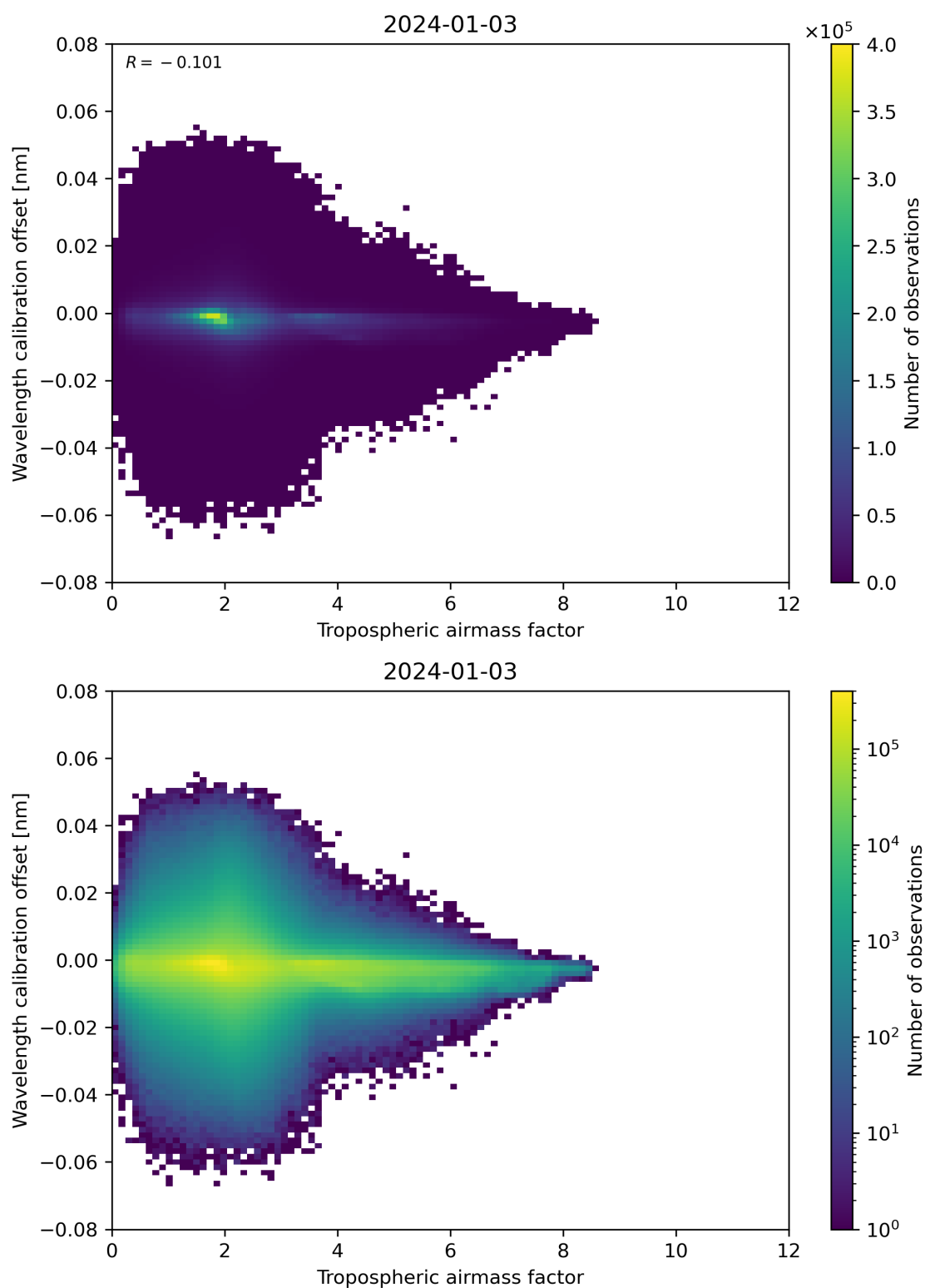
Figure 80: Scatter density plot of “Tropospheric airmass factor” against “Wavelength calibration offset” for 2024-01-02 to 2024-01-04.
