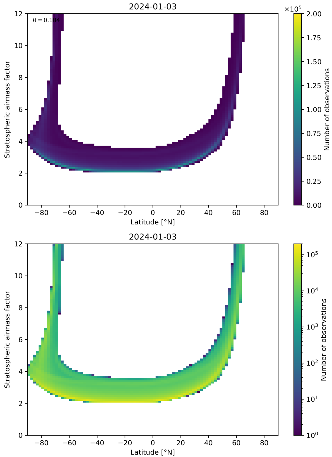
Figure 83: Scatter density plot of “Latitude” against “Stratospheric airmass factor” for 2024-01-02 to 2024-01-04.
