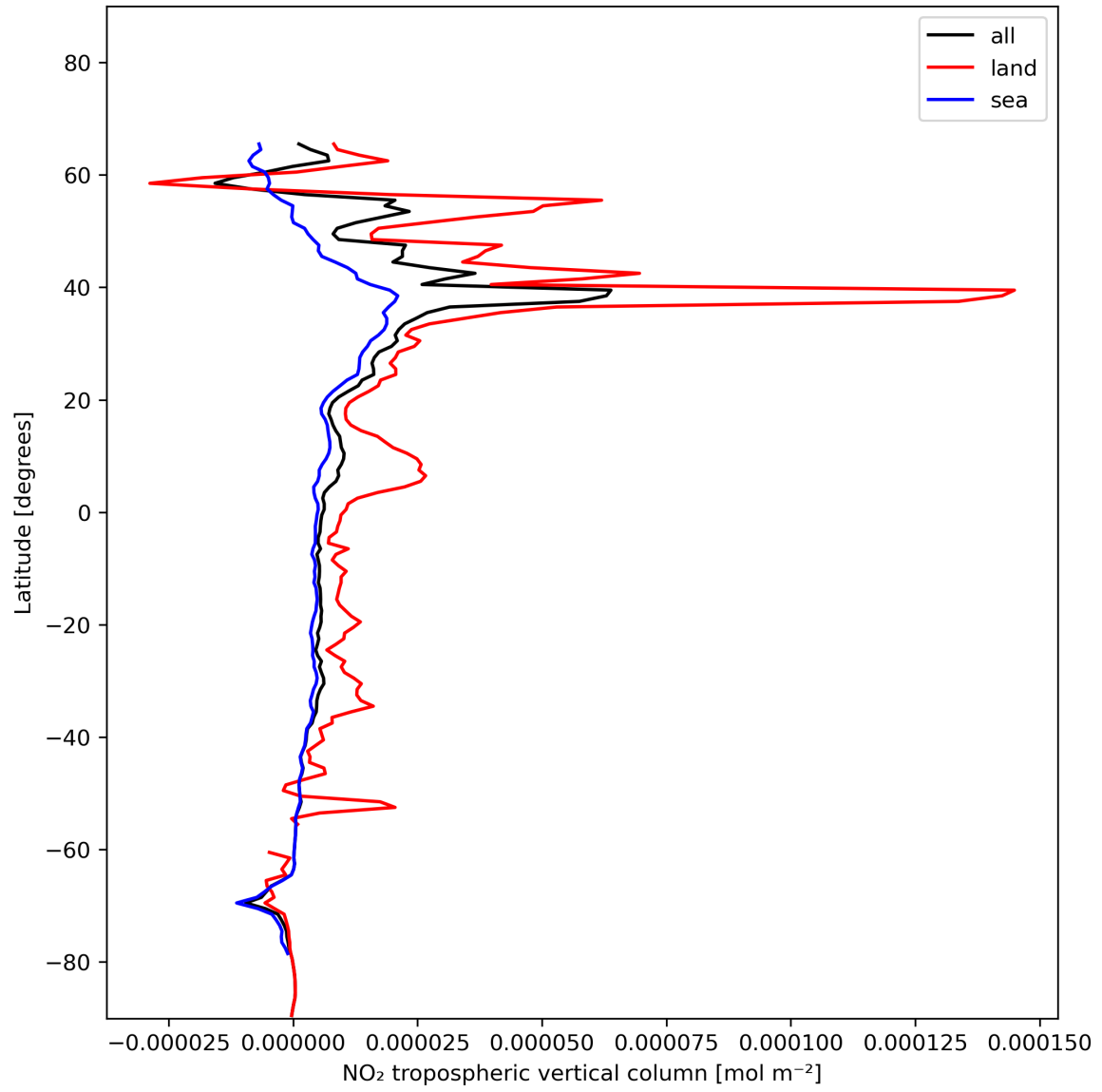
Figure 12: Zonal average of “NO 2 tropospheric vertical column” for 2024-01-03 to 2024-01-05.
