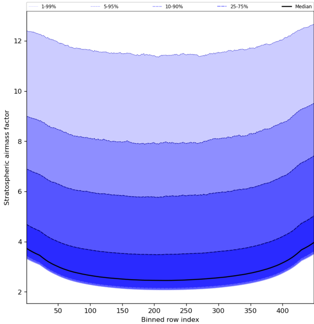
Figure 61: Along track statistics of “Stratospheric air mass factor” for 2024-01-03 to 2024-01-05
