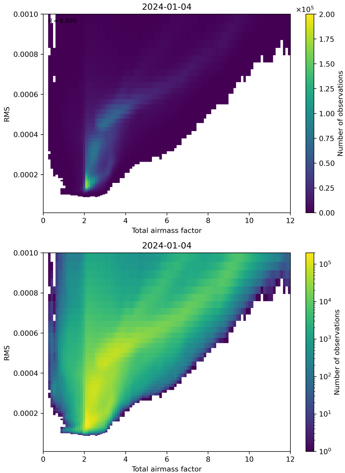
Figure 69: Scatter density plot of “Total airmass factor” against “RMS” for 2024-01-03 to 2024-01-05.
