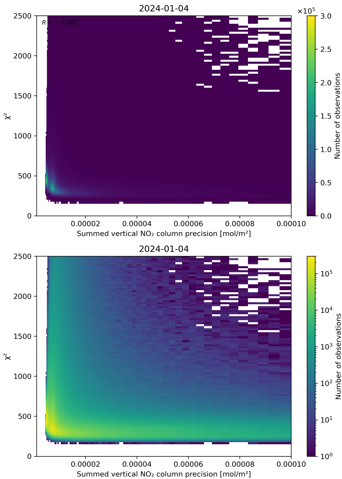
Figure 107: Scatter density plot of “Summed vertical NO 2 column precision” against “ \chi^2 ” for 2024-01-03 to 2024-01-05.
