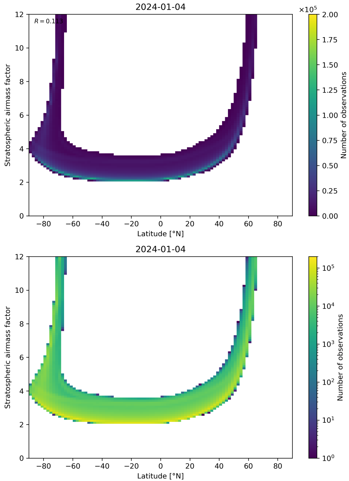
Figure 83: Scatter density plot of “Latitude” against “Stratospheric air mass factor” for 2024-01-03 to 2024-01-05.
