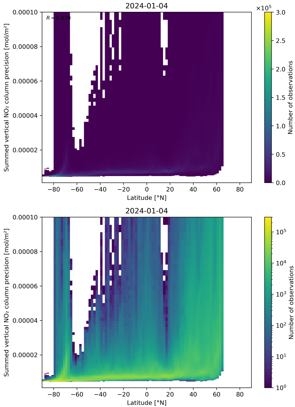
Figure 89: Scatter density plot of “Latitude” against “Summed vertical NO 2 column precision” for 2024-01-03 to 2024-01-05.
