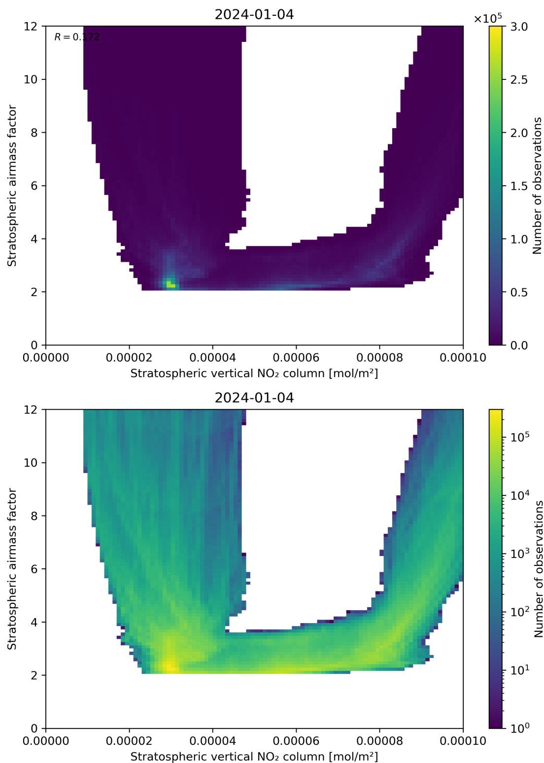
Figure 96: Scatter density plot of “Stratospheric vertical NO 2 column” against “Stratospheric airmass factor” for 2024-01-03 to 2024-01-05.
