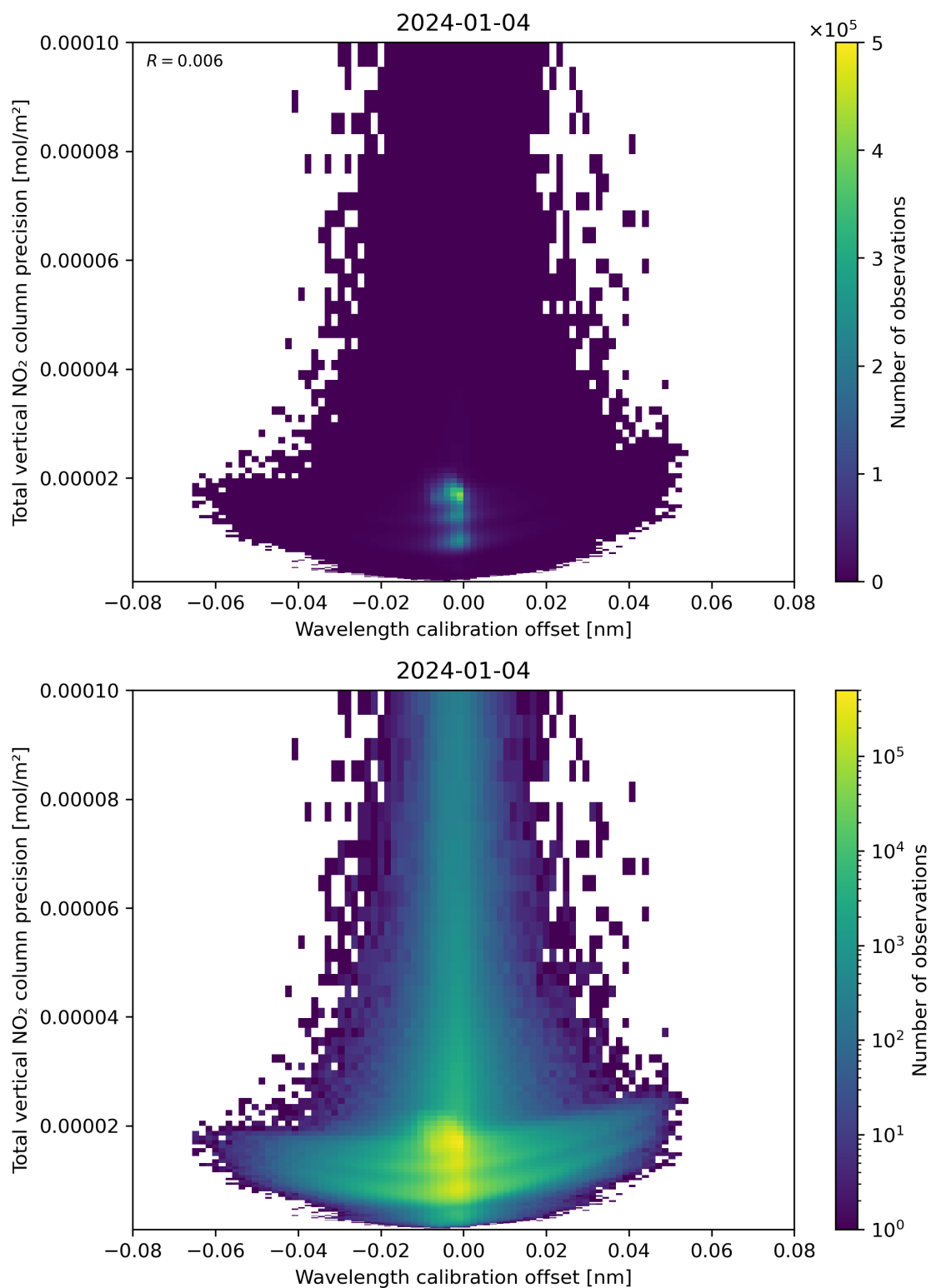
Figure 180: Scatter density plot of “Wavelength calibration offset” against “Total vertical NO 2 column precision” for 2024-01-03 to 2024-01-05.
