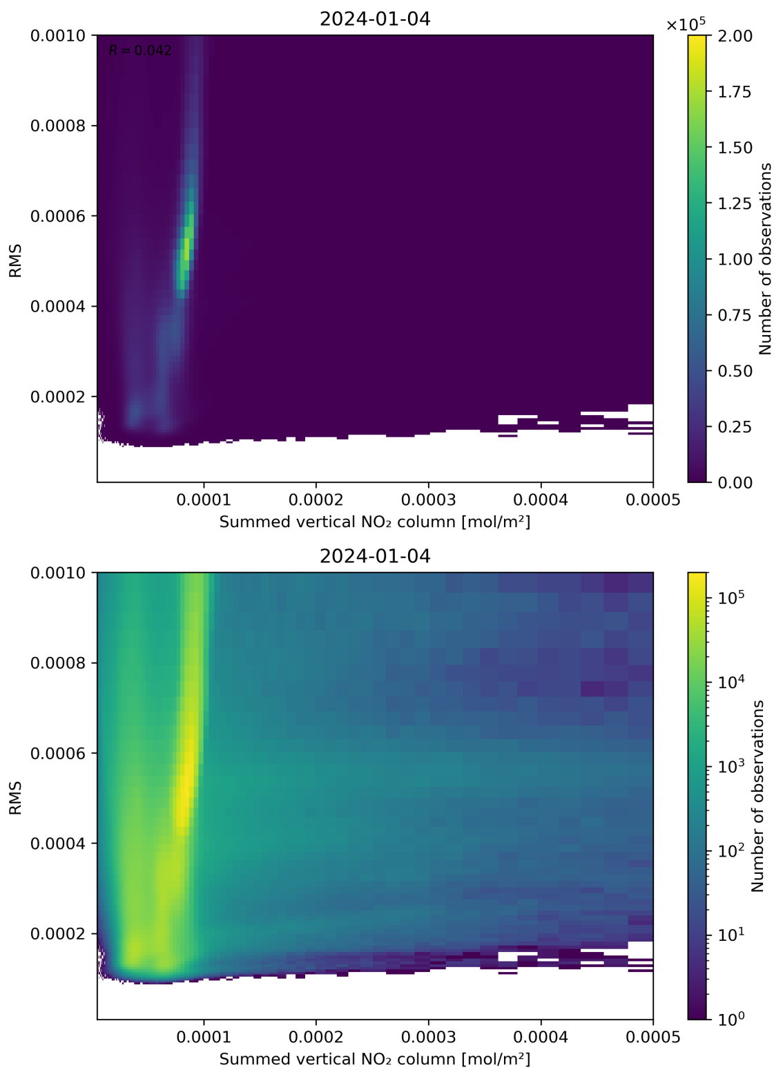
Figure 109: Scatter density plot of “Summed vertical NO 2 column” against “RMS” for 2024-01-03 to 2024-01-05.
