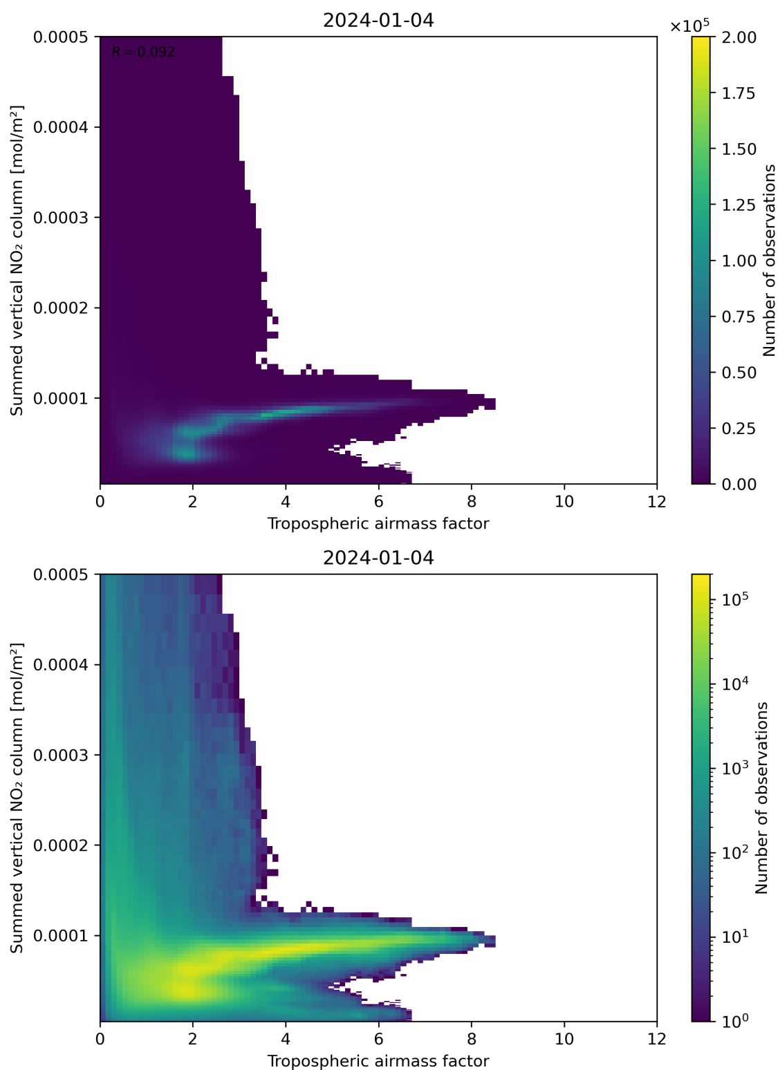
Figure 75: Scatter density plot of “Tropospheric airmass factor” against “Summed vertical NO 2 column” for 2024-01-03 to 2024-01-05.
