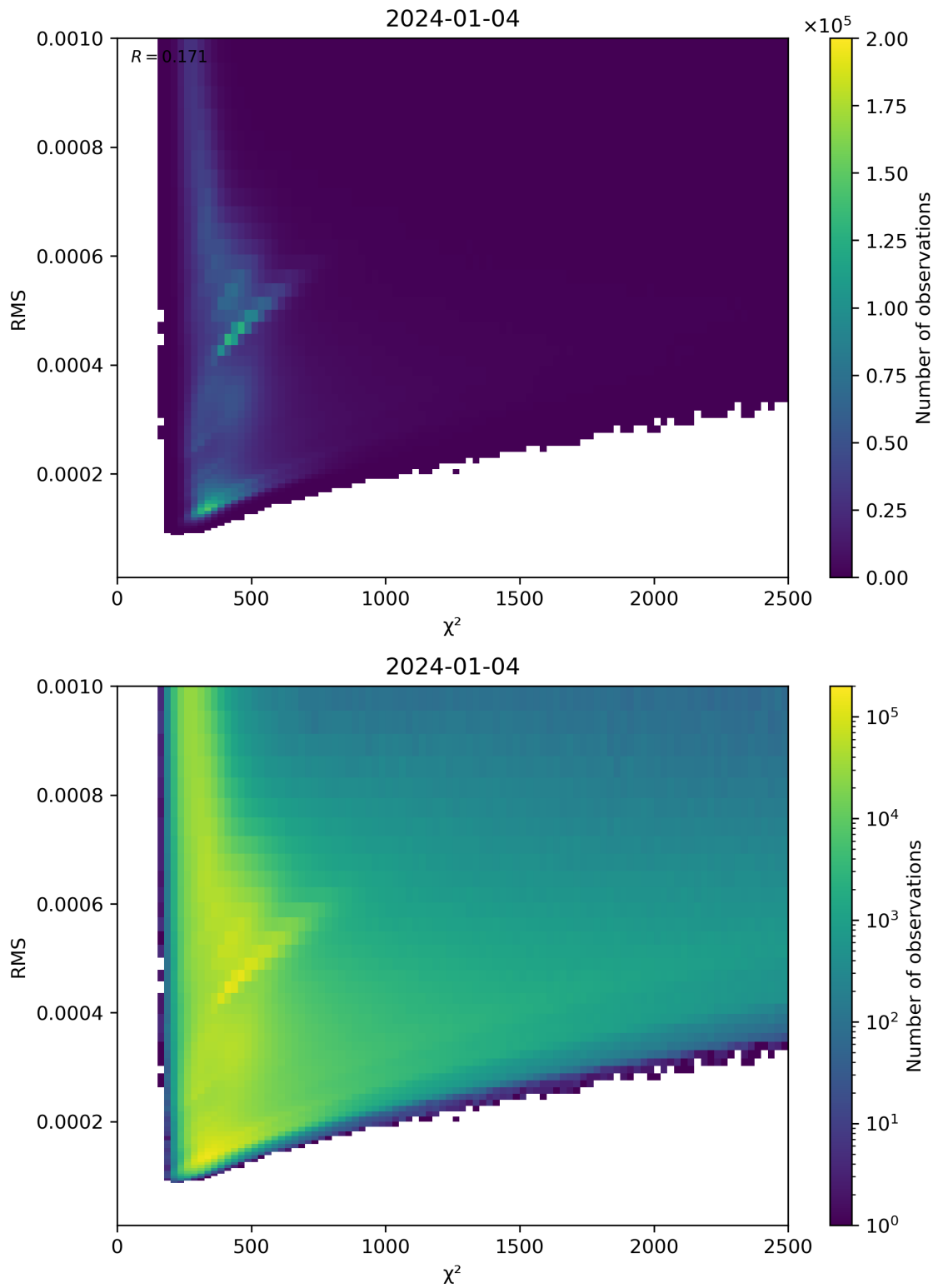
Figure 82: Scatter density plot of “ \chi^2 ” against “RMS” for 2024-01-03 to 2024-01-05.
