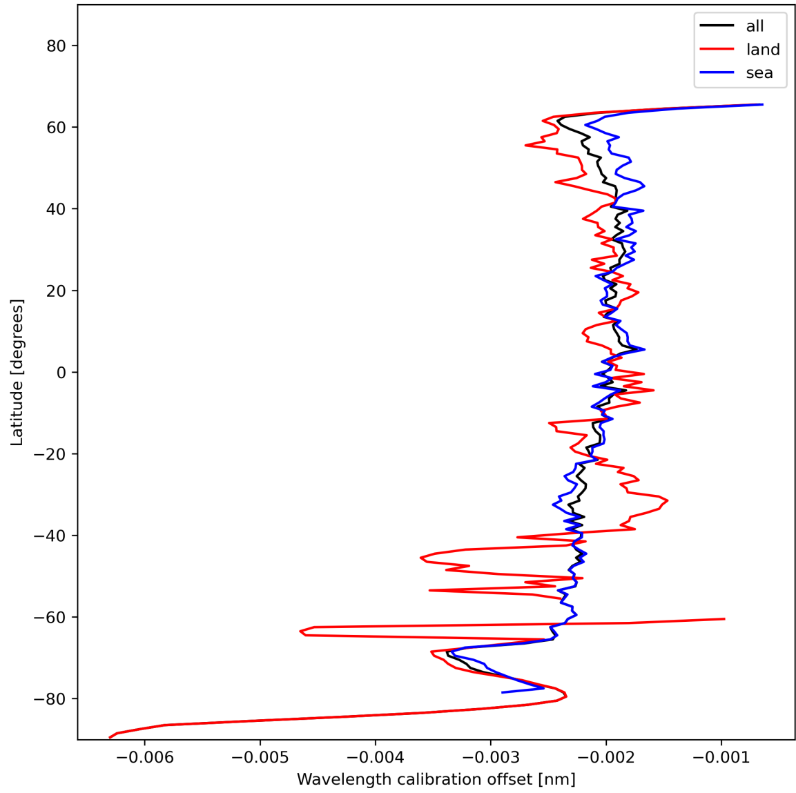
Figure 18: Zonal average of “Wavelength calibration offset” for 2024-01-03 to 2024-01-05.
