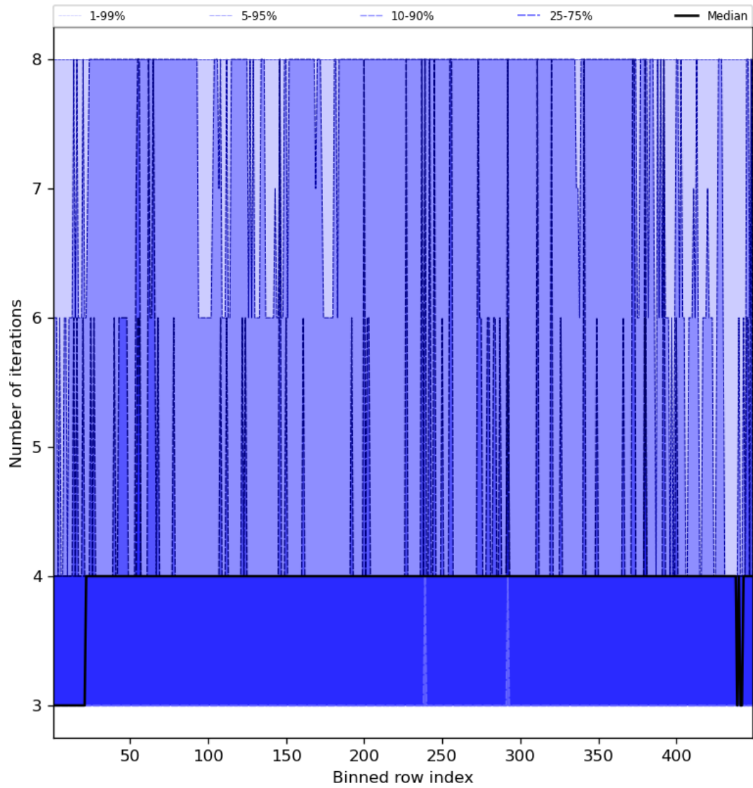
Figure 51: Along track statistics of “Number of iterations” for 2024-01-03 to 2024-01-05
