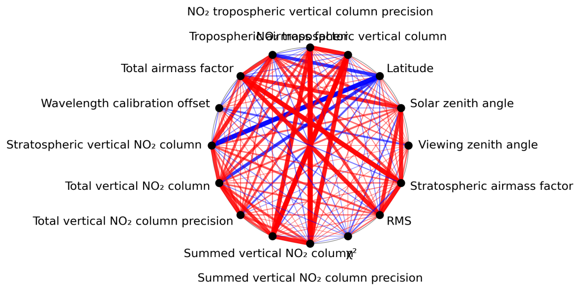
Figure 1: Map of correlation graph for 2024-01-03 to 2024-01-05.
