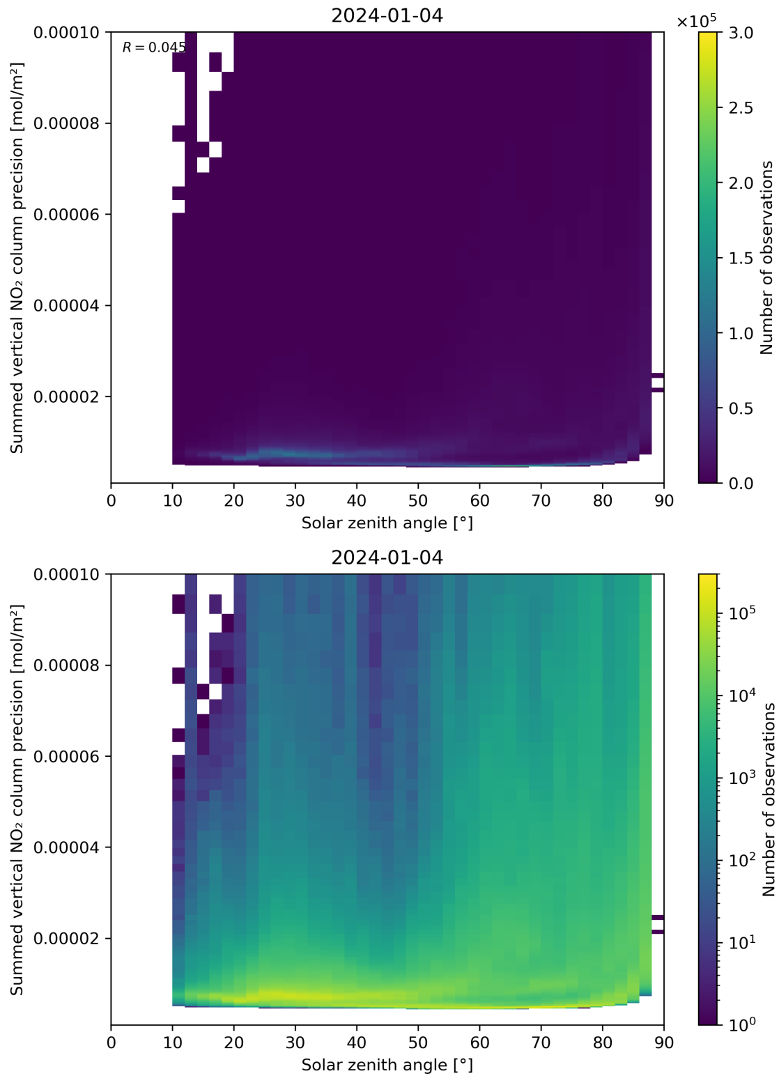
Figure 152: Scatter density plot of “Solar zenith angle” against “Summed vertical NO 2 column precision” for 2024-01-03 to 2024-01-05.
