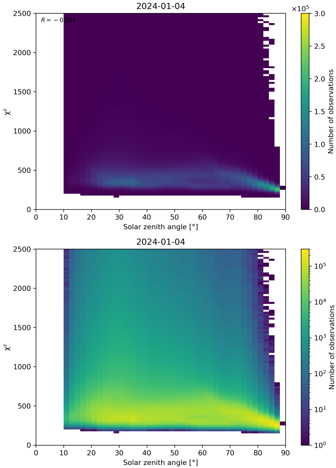
Figure 148: Scatter density plot of “Solar zenith angle” against “ \chi^2 ” for 2024-01-03 to 2024-01-05.
