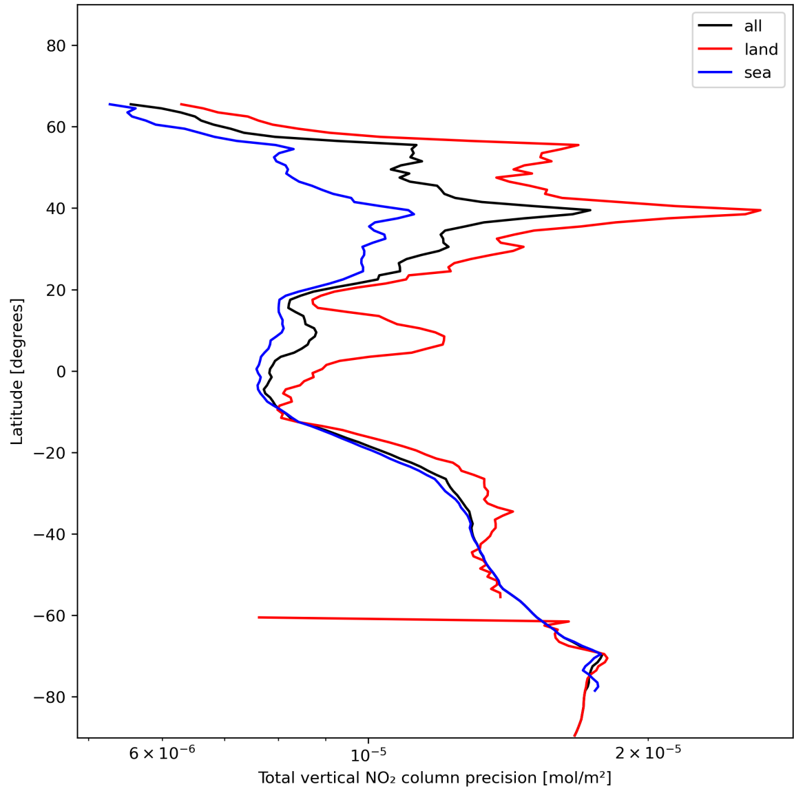
Figure 22: Zonal average of “Total vertical NO 2 column precision” for 2024-01-03 to 2024-01-05.
