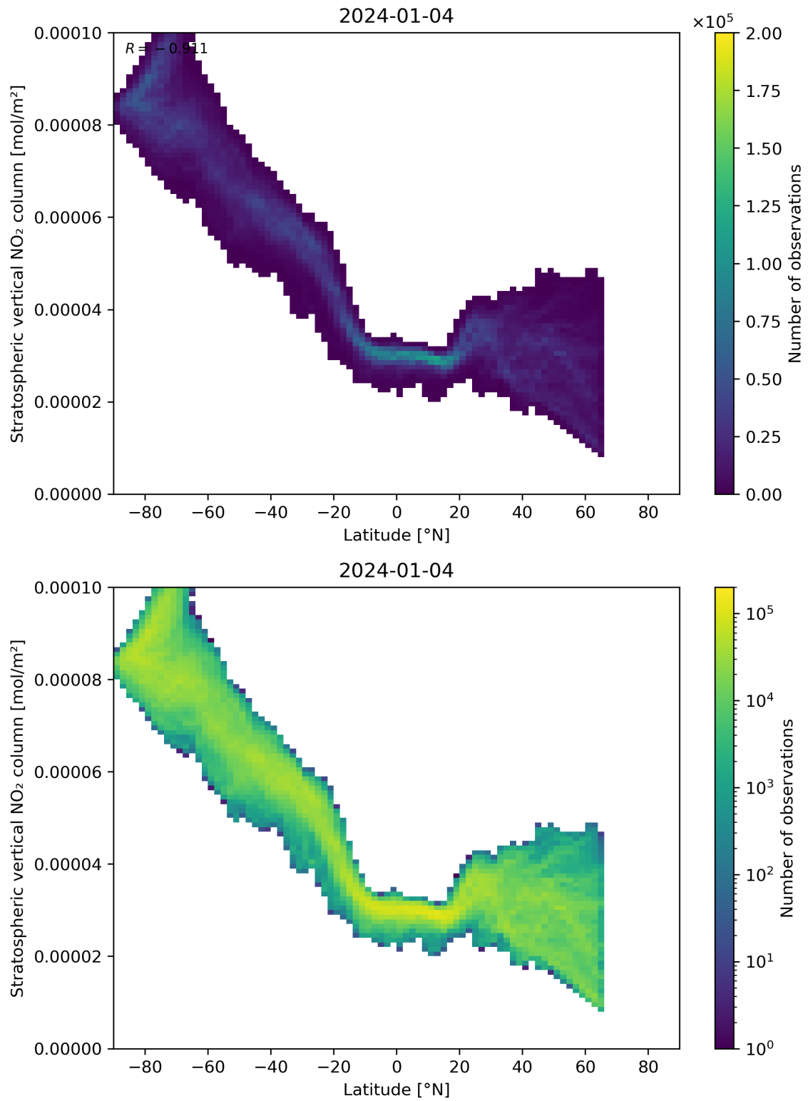
Figure 87: Scatter density plot of “Latitude” against “Stratospheric vertical NO 2 column” for 2024-01-03 to 2024-01-05.
