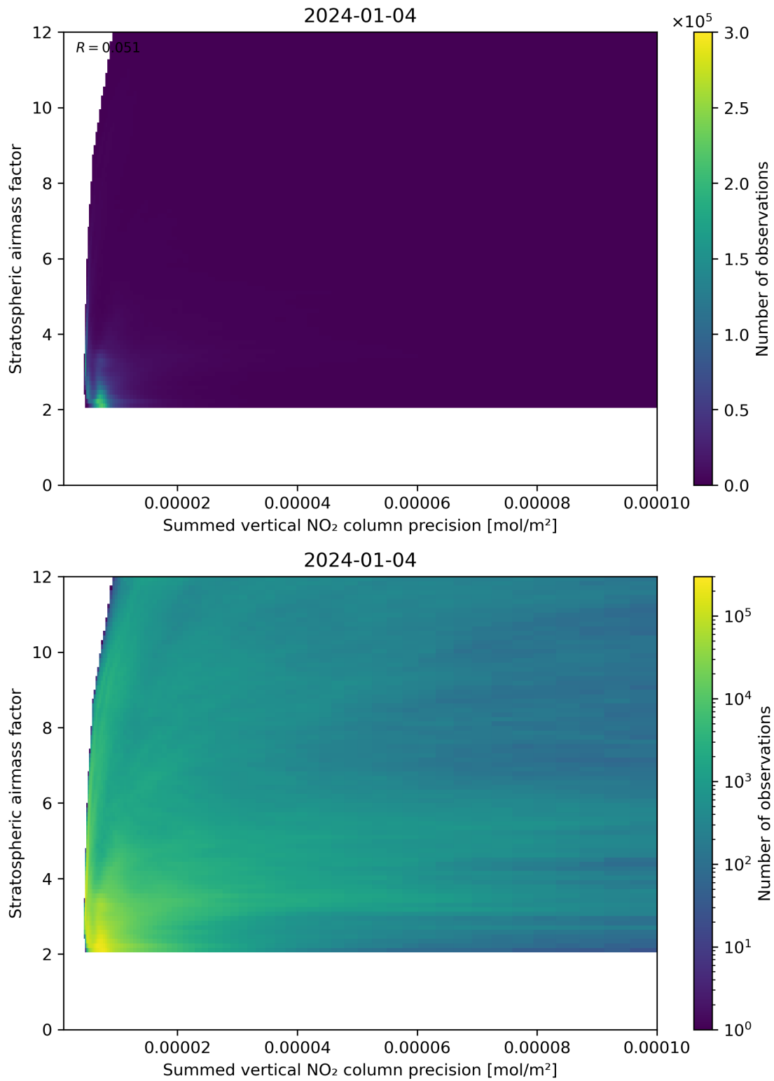
Figure 106: Scatter density plot of “Summed vertical NO 2 column precision” against “Stratospheric airmass factor” for 2024-01-03 to 2024-01-05.
