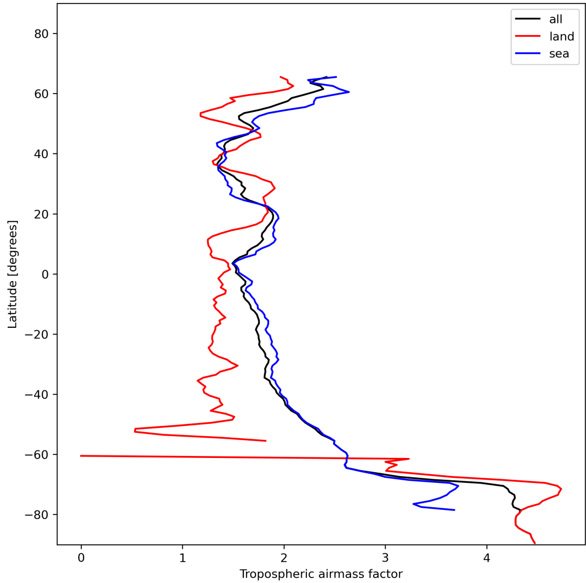
Figure 14: Zonal average of “Tropospheric airmass factor” for 2024-01-03 to 2024-01-05.
