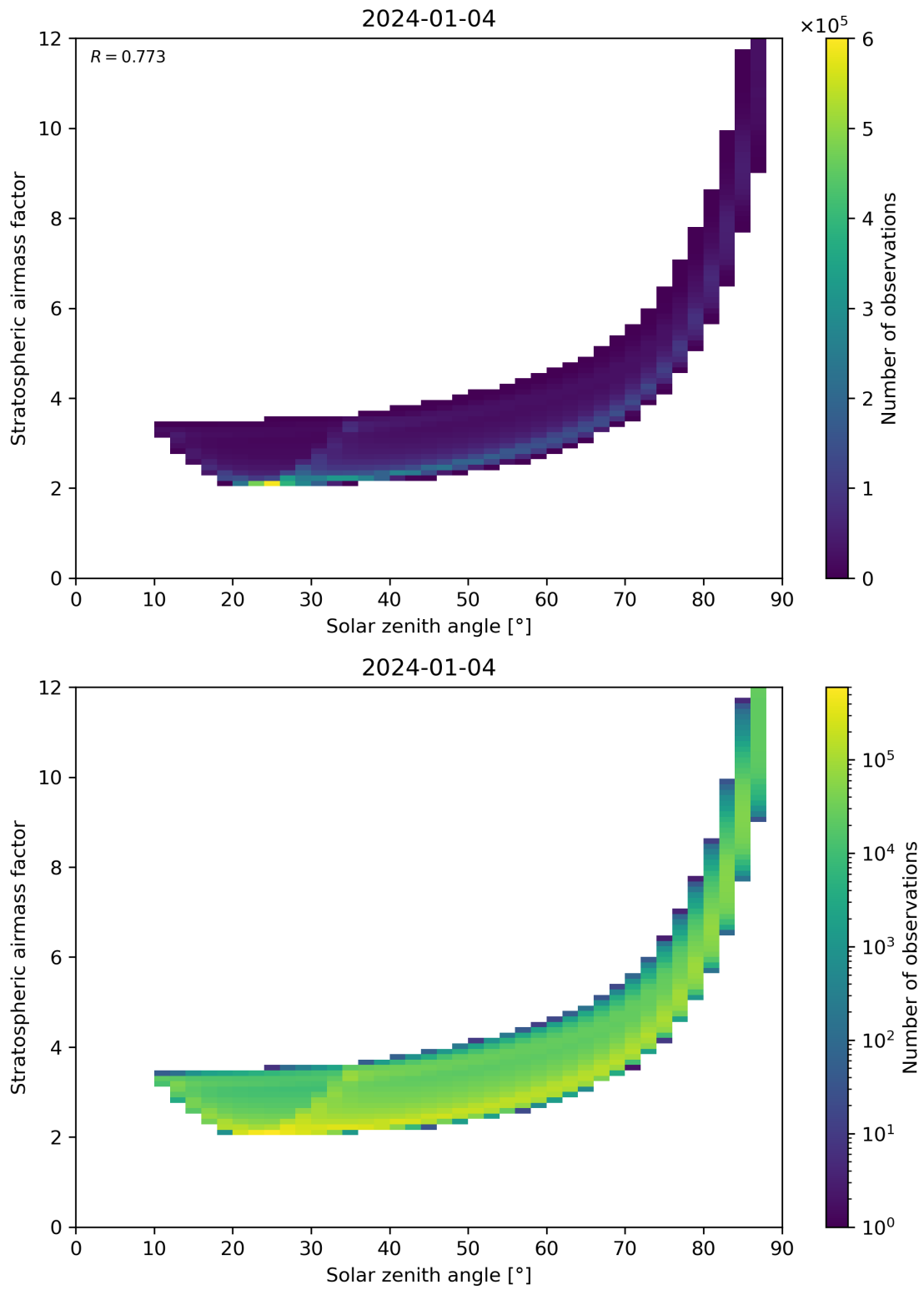
Figure 145: Scatter density plot of “Solar zenith angle” against “Stratospheric airmass factor” for 2024-01-03 to 2024-01-05.
