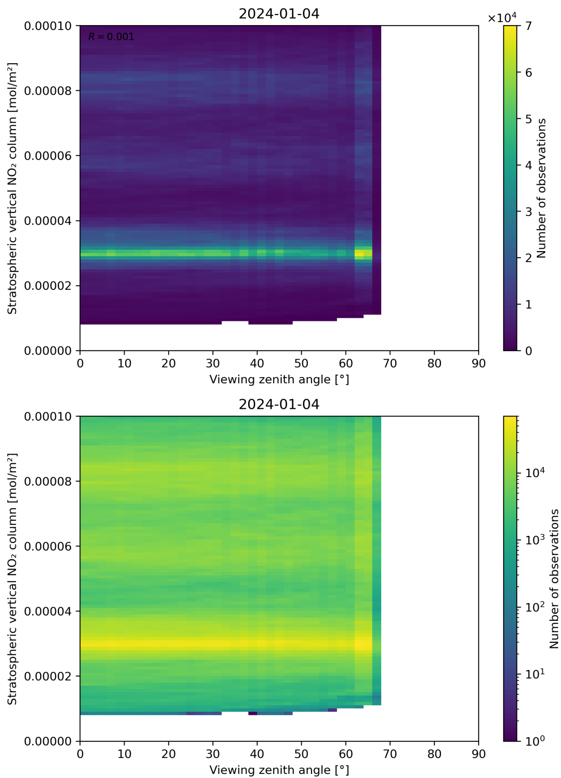
Figure 164: Scatter density plot of “Viewing zenith angle” against “Stratospheric vertical NO 2 column” for 2024-01-03 to 2024-01-05.
