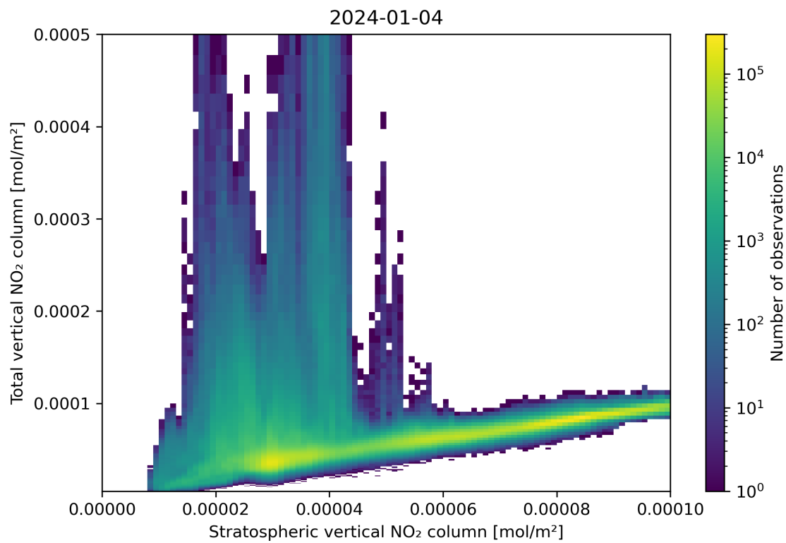
Figure 100: Scatter density plot of “Stratospheric vertical NO 2 column” against “Total vertical NO 2 column” for 2024-01-03 to 2024-01-05.
