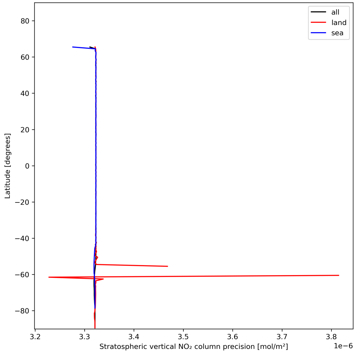
Figure 20: Zonal average of “Stratospheric vertical NO 2 column precision” for 2024-01-03 to 2024-01-05.
