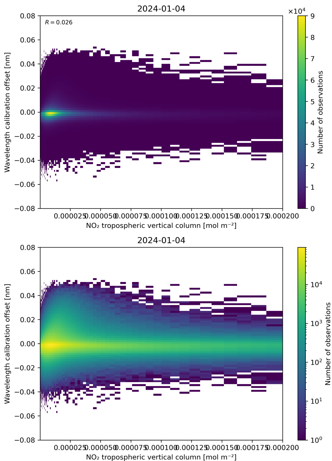
Figure 143: Scatter density plot of “NO 2 tropospheric vertical column” against “Wavelength calibration offset” for 2024-01-03 to 2024-01-05.
