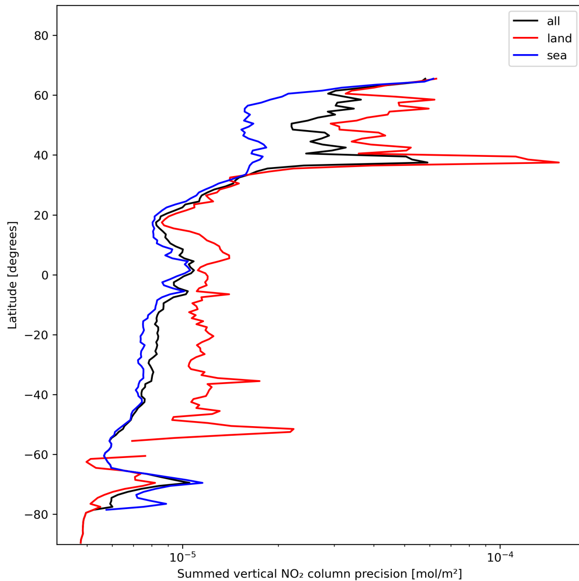
Figure 24: Zonal average of “Summed vertical NO 2 column precision” for 2024-01-03 to 2024-01-05.
