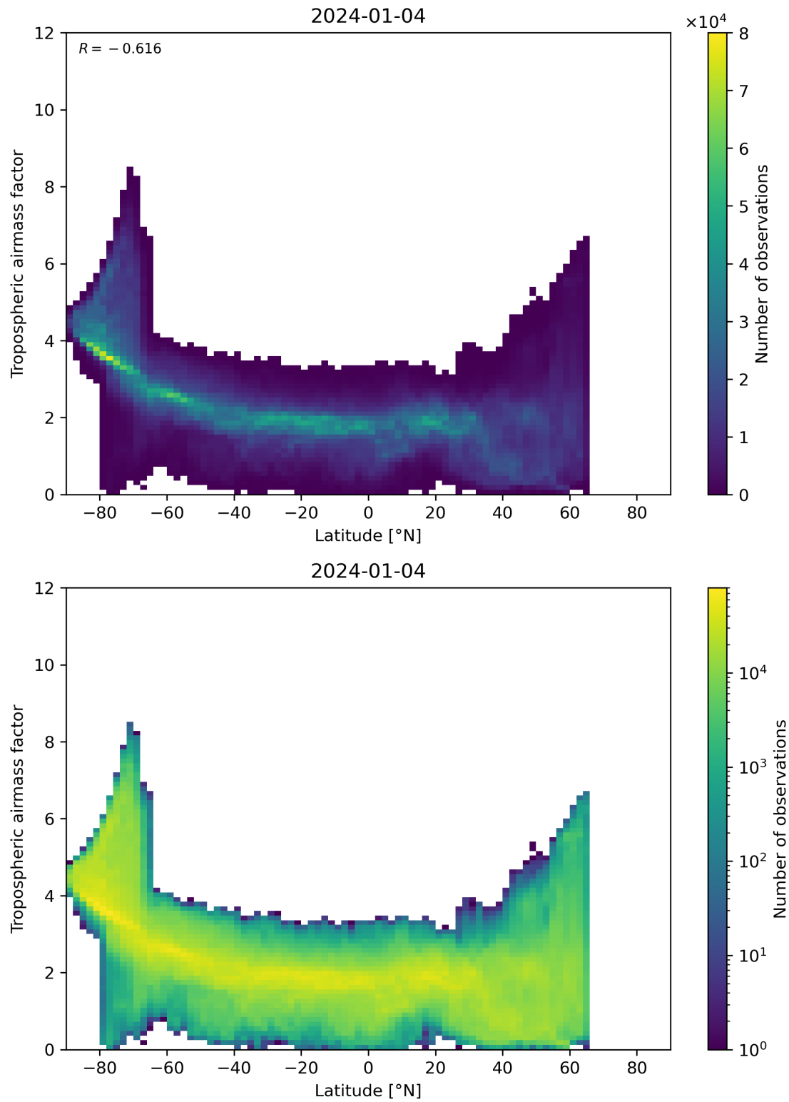
Figure 85: Scatter density plot of “Latitude” against “Tropospheric airmass factor” for 2024-01-03 to 2024-01-05.
