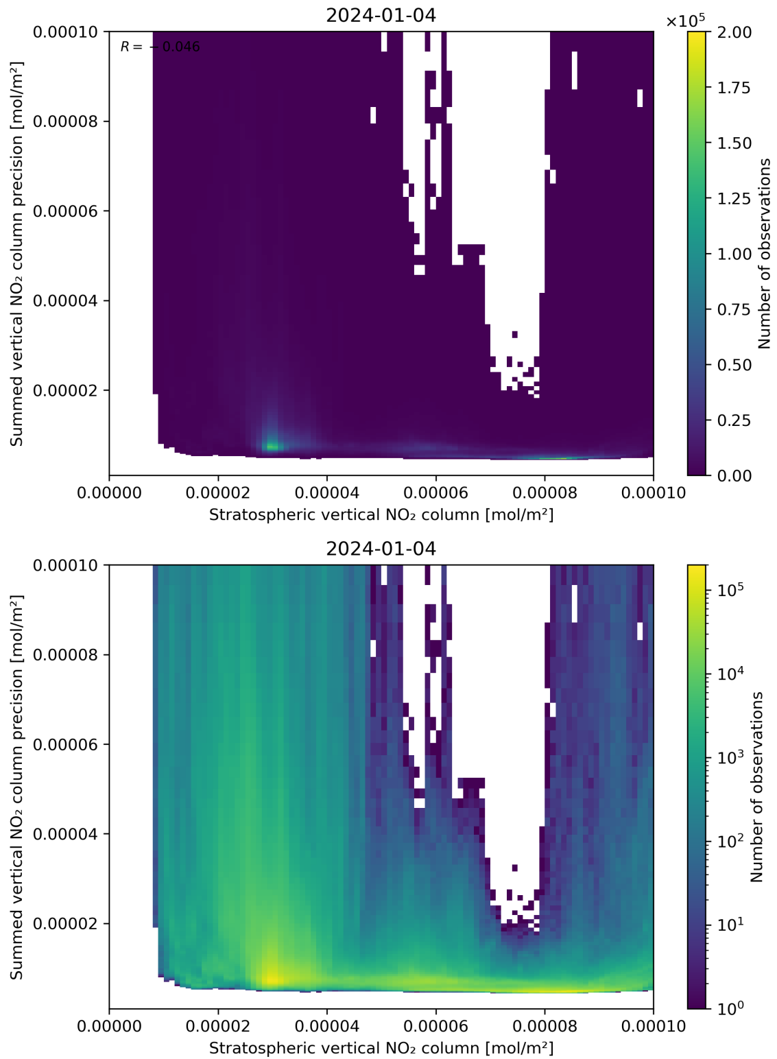
Figure 99: Scatter density plot of “Stratospheric vertical NO 2 column” against “Summed vertical NO 2 column precision” for 2024-01-03 to 2024-01-05.
