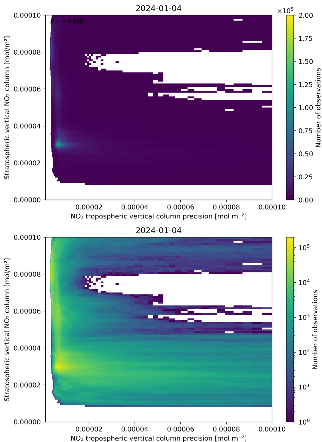
Figure 135: Scatter density plot of “NO 2 tropospheric vertical column precision” against “Stratospheric vertical NO 2 column” for 2024-01-03 to 2024-01-05.
