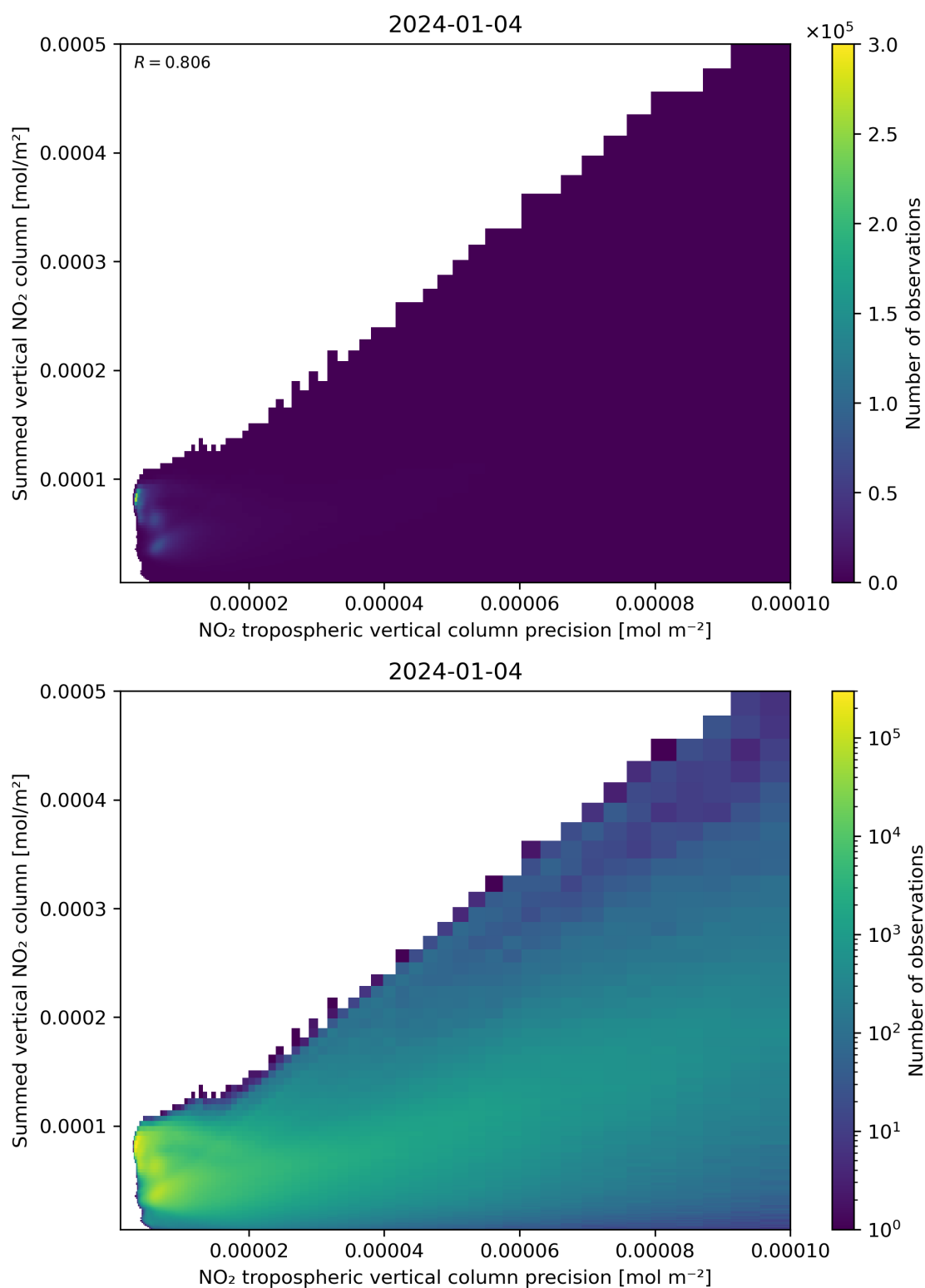
Figure 136: Scatter density plot of “NO 2 tropospheric vertical column precision” against “Summed vertical NO 2 column” for 2024-01-03 to 2024-01-05.
