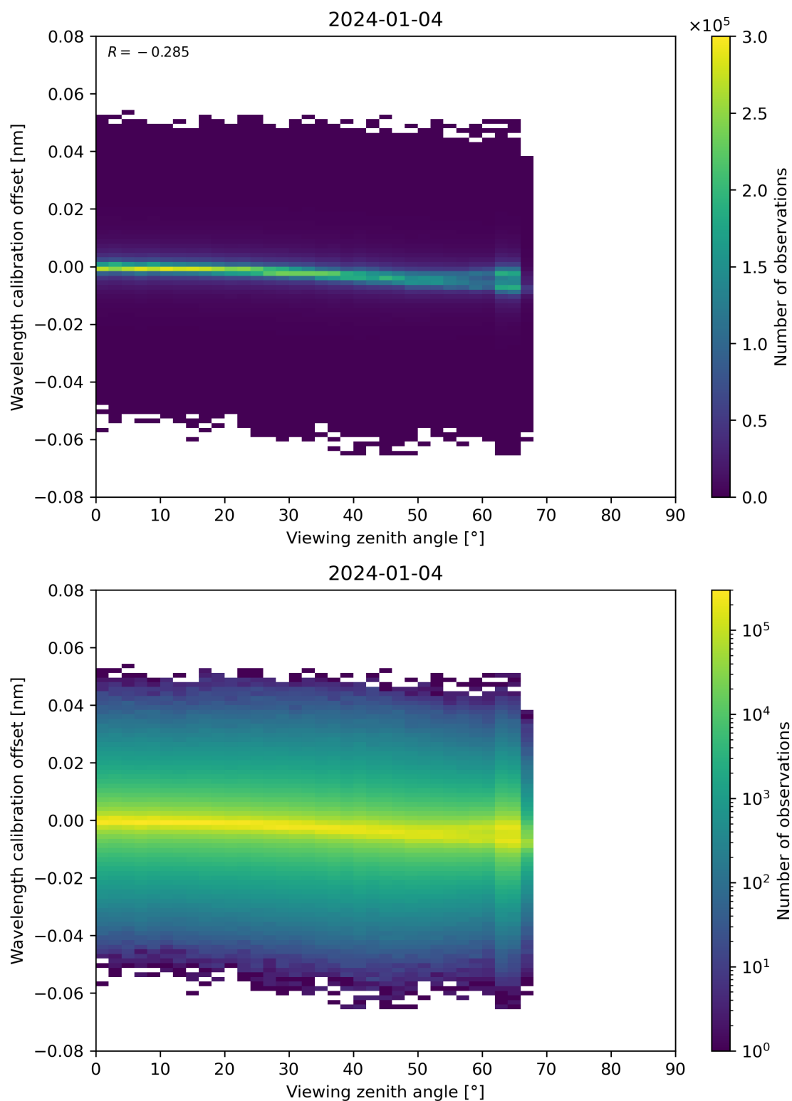
Figure 173: Scatter density plot of “Viewing zenith angle” against “Wavelength calibration offset” for 2024-01-03 to 2024-01-05.
