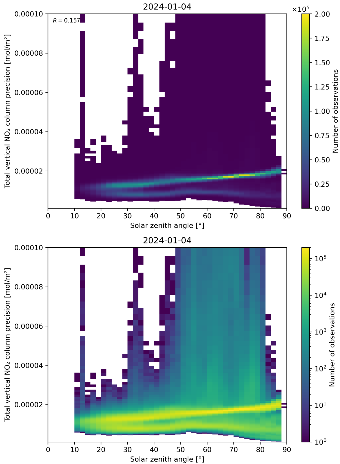
Figure 154: Scatter density plot of “Solar zenith angle” against “Total vertical NO 2 column precision” for 2024-01-03 to 2024-01-05.
