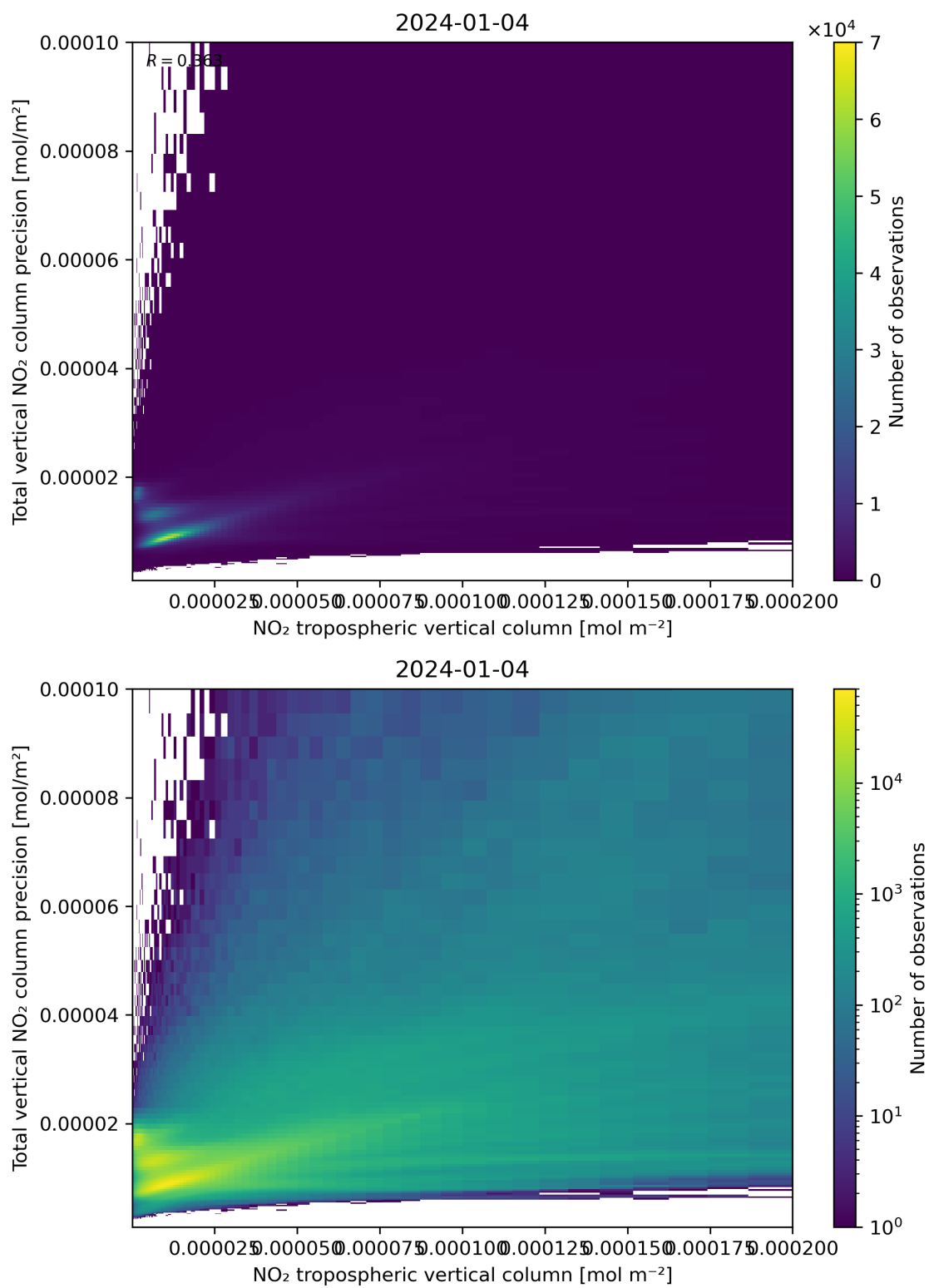
Figure 129: Scatter density plot of “NO 2 tropospheric vertical column” against “Total vertical NO 2 column precision” for 2024-01-03 to 2024-01-05.
