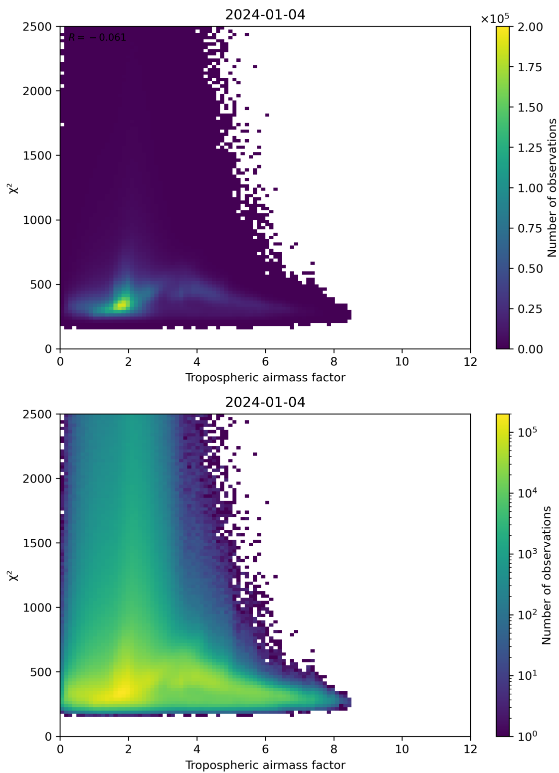
Figure 73: Scatter density plot of “Tropospheric airmass factor” against “ \chi^2 ” for 2024-01-03 to 2024-01-05.
