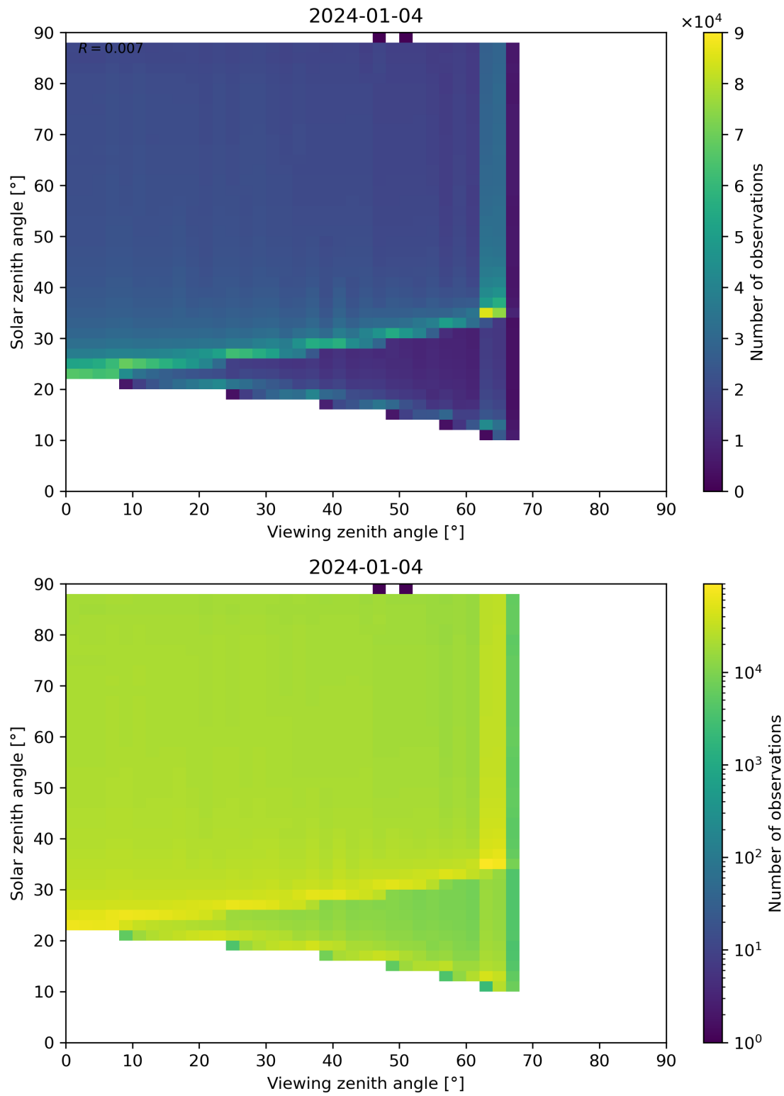
Figure 172: Scatter density plot of “Viewing zenith angle” against “Solar zenith angle” for 2024-01-03 to 2024-01-05.
