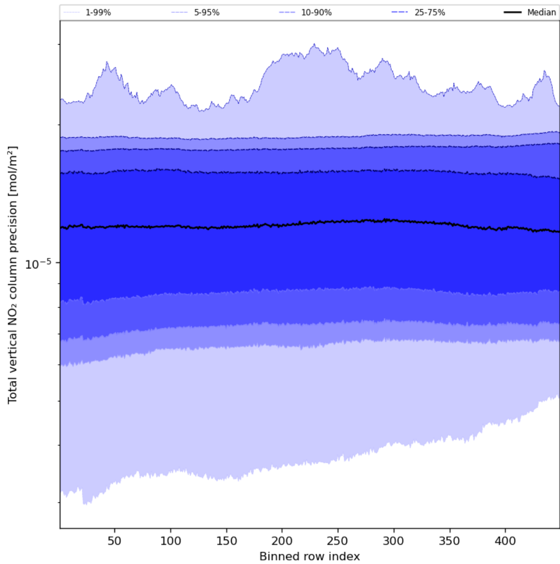
Figure 56: Along track statistics of “Total vertical NO 2 column precision” for 2024-01-03 to 2024-01-05
