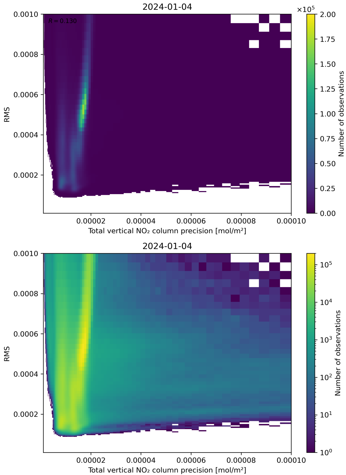
Figure 119: Scatter density plot of “Total vertical NO 2 column precision” against “RMS” for 2024-01-03 to 2024-01-05.
