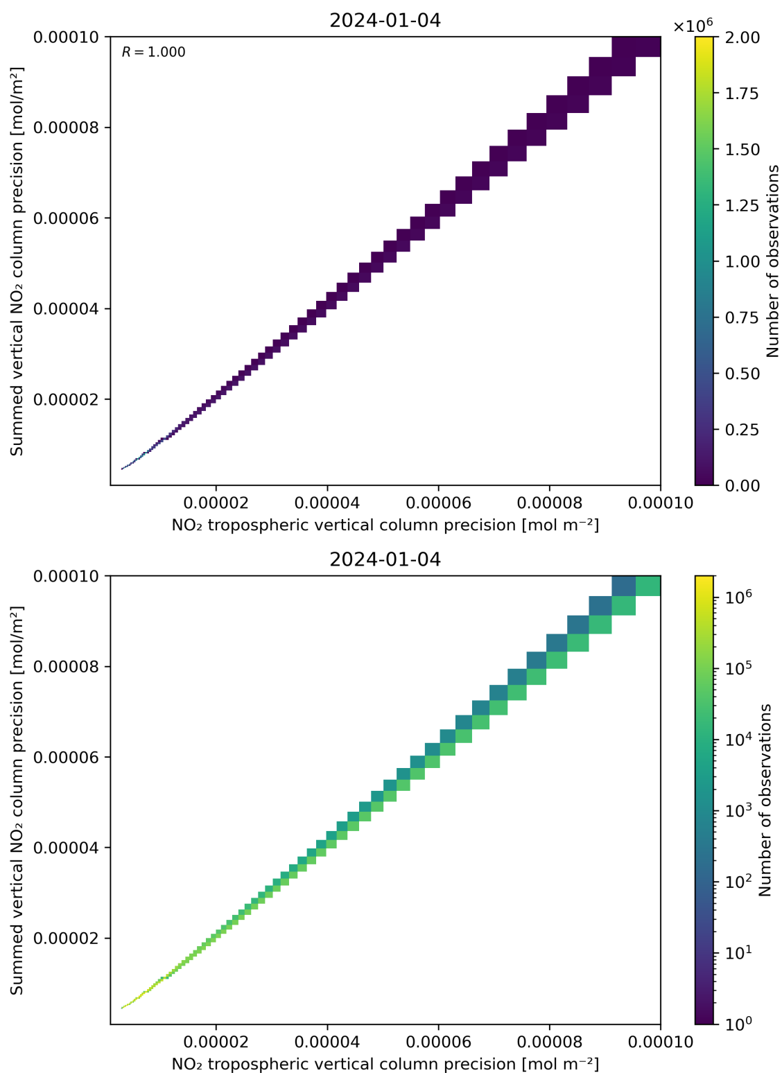
Figure 137: Scatter density plot of “NO 2 tropospheric vertical column precision” against “Summed vertical NO 2 column precision” for 2024-01-03 to 2024-01-05.
