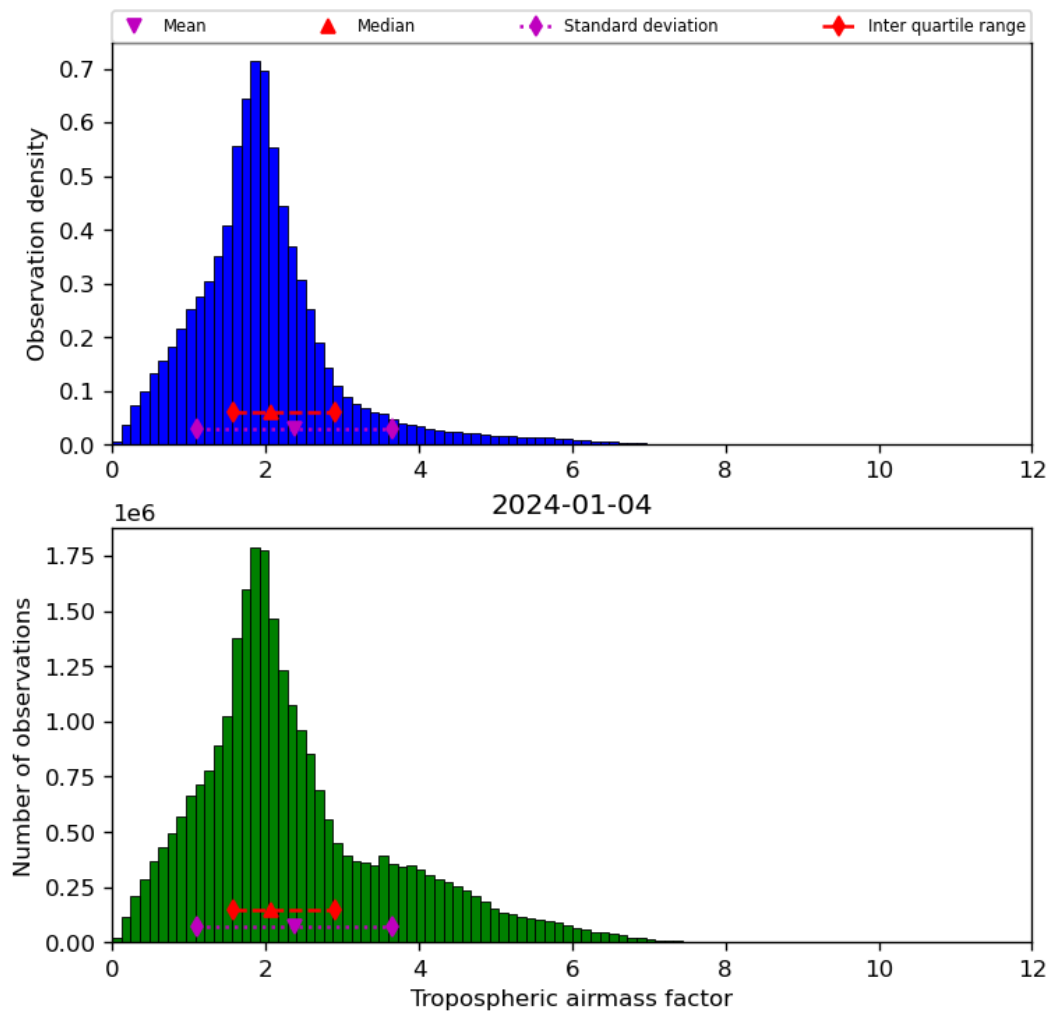
Figure 31: Histogram of “Tropospheric airmass factor” for 2024-01-03 to 2024-01-05
