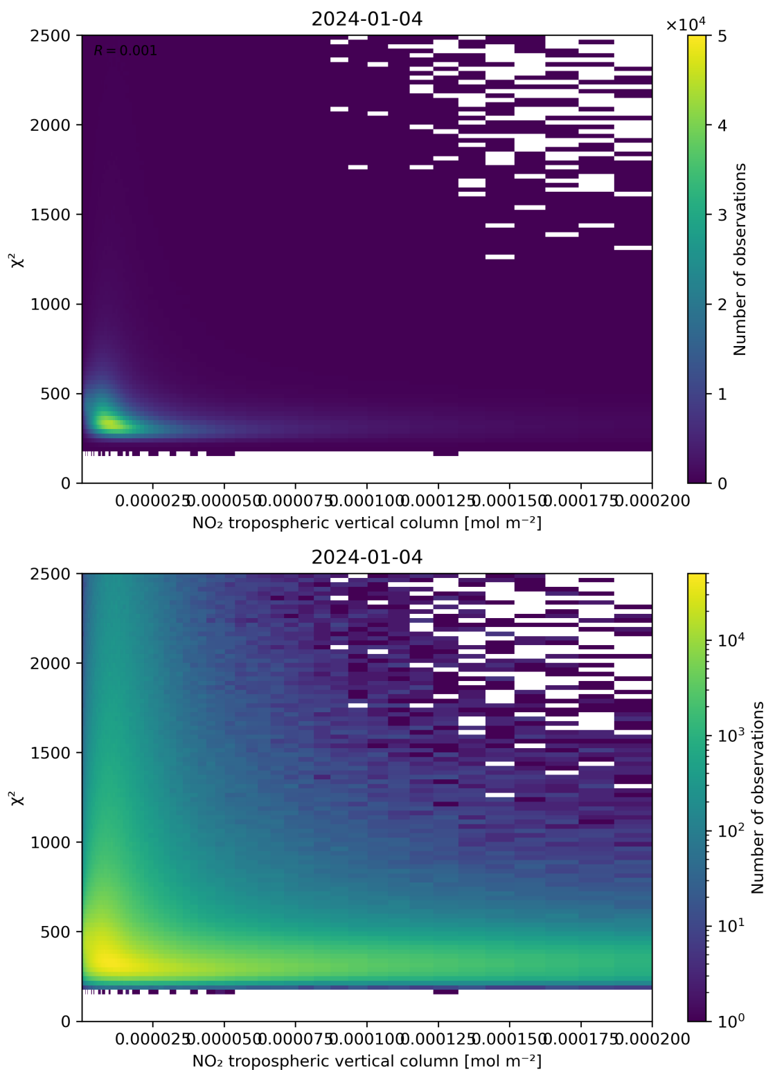
Figure 124: Scatter density plot of “NO 2 tropospheric vertical column” against “ \chi^2 ” for 2024-01-03 to 2024-01-05.
