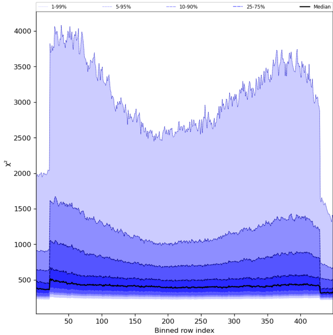
Figure 59: Along track statistics of “ \chi^2 ” for 2024-01-03 to 2024-01-05
