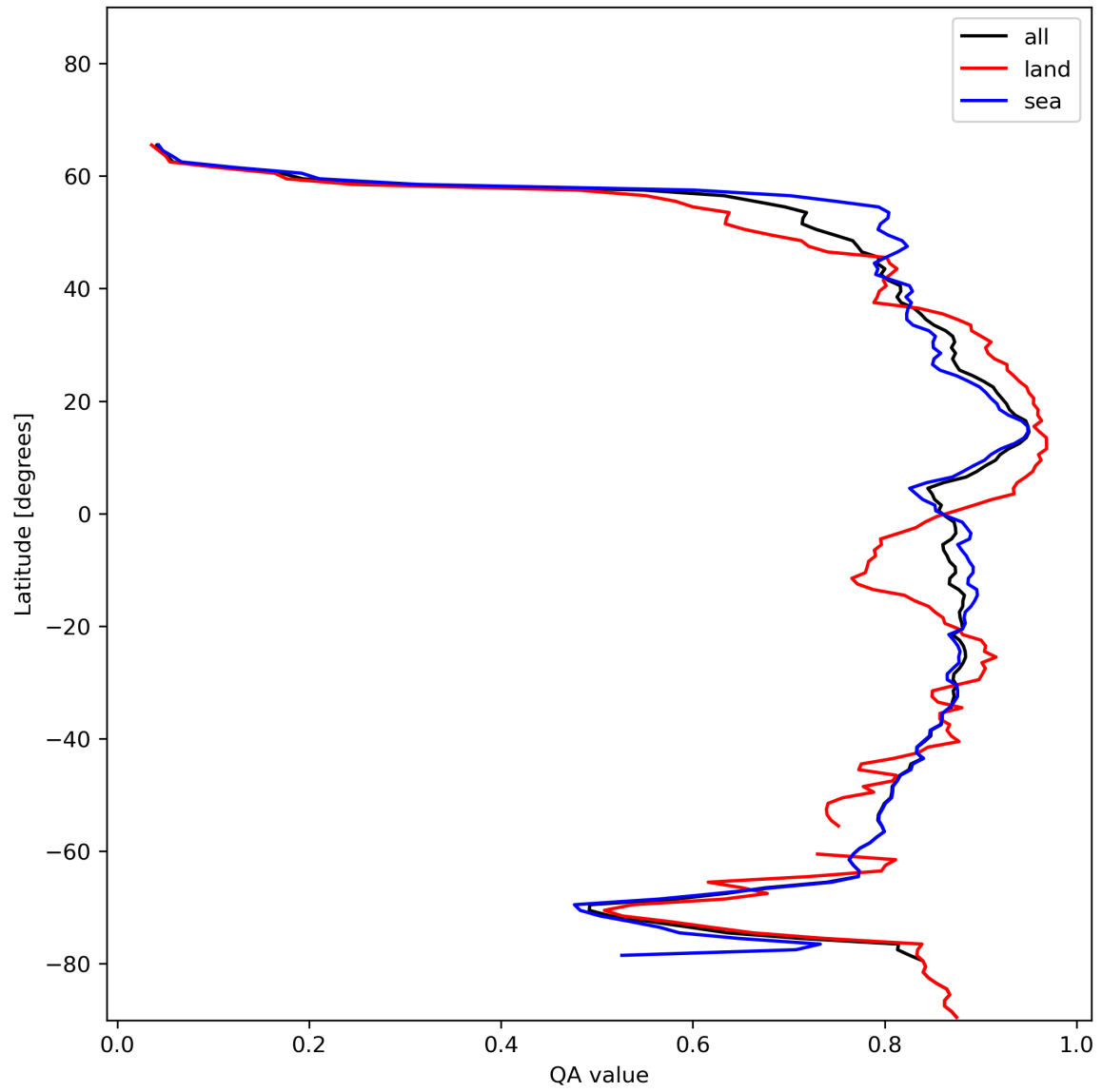
Figure 11: Zonal average of “QA value” for 2024-01-03 to 2024-01-05.
