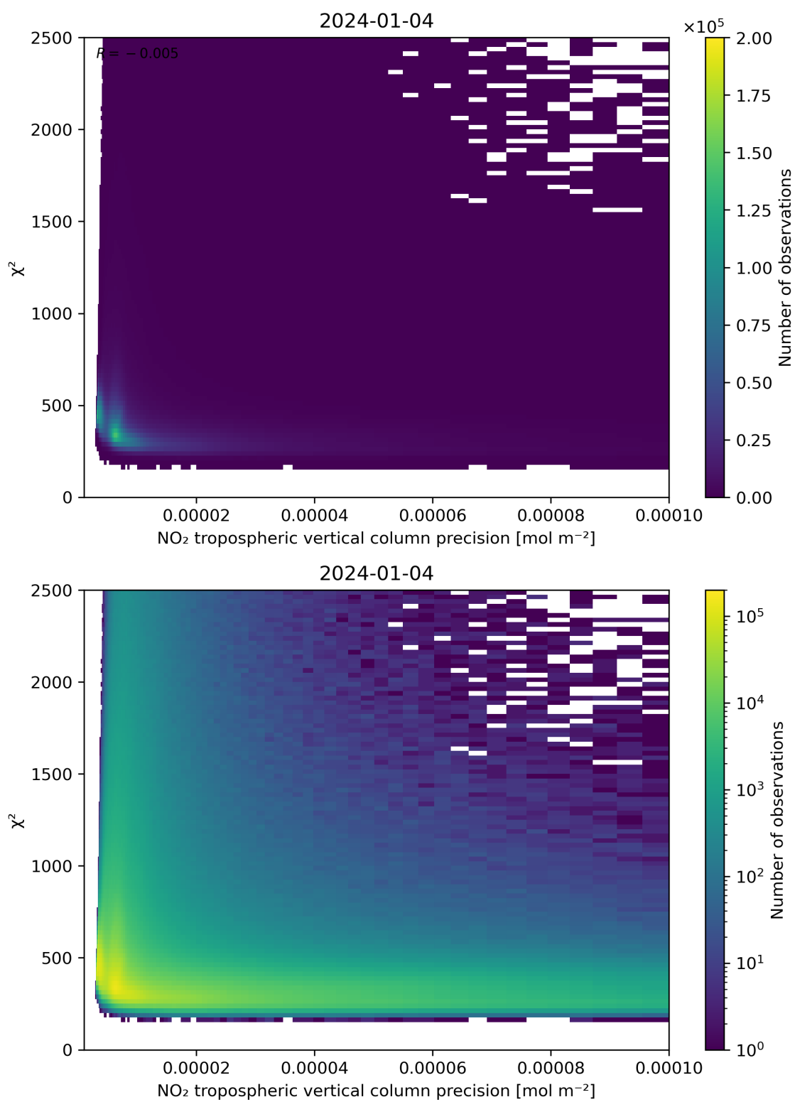
Figure 134: Scatter density plot of “NO 2 tropospheric vertical column precision” against “ \chi^2 ” for 2024-01-03 to 2024-01-05.
