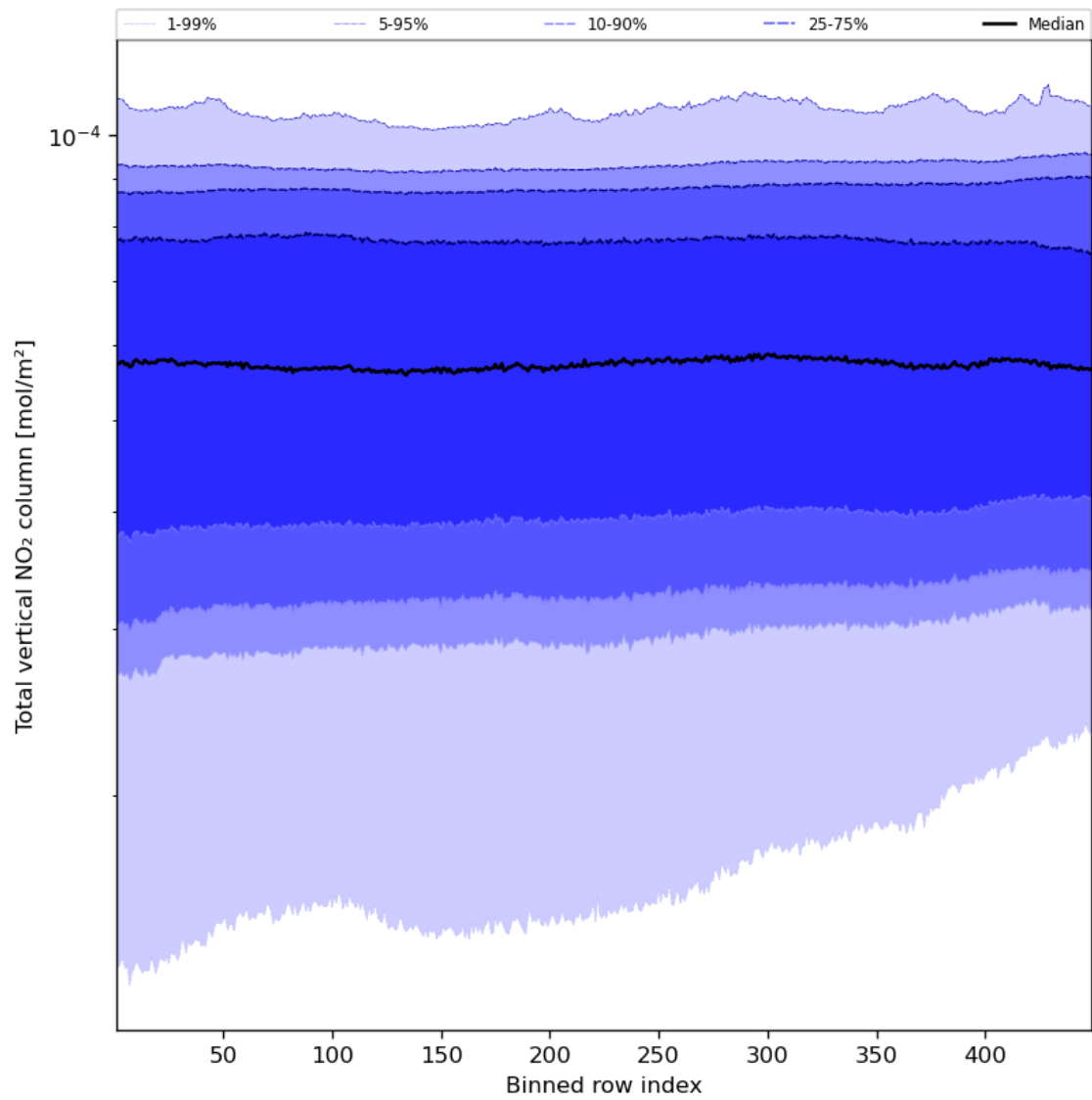
Figure 55: Along track statistics of “Total vertical NO 2 column” for 2024-01-03 to 2024-01-05
