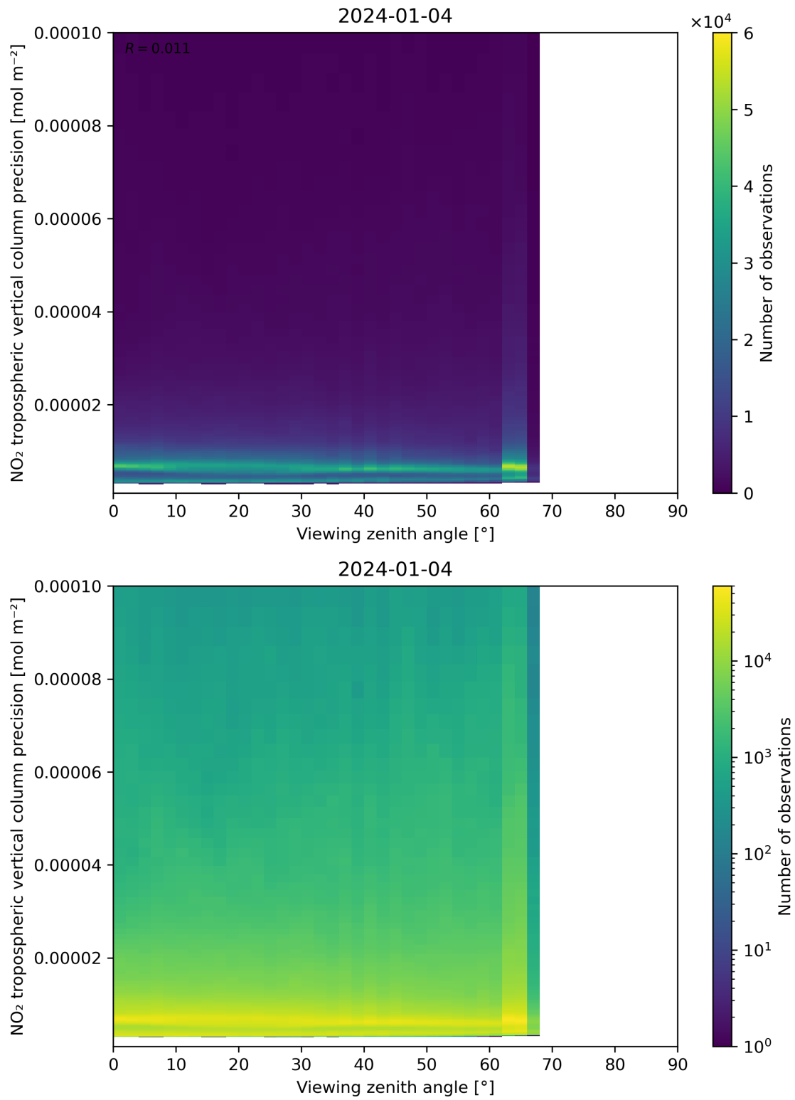
Figure 170: Scatter density plot of “Viewing zenith angle” against “NO 2 tropospheric vertical column precision” for 2024-01-03 to 2024-01-05.
