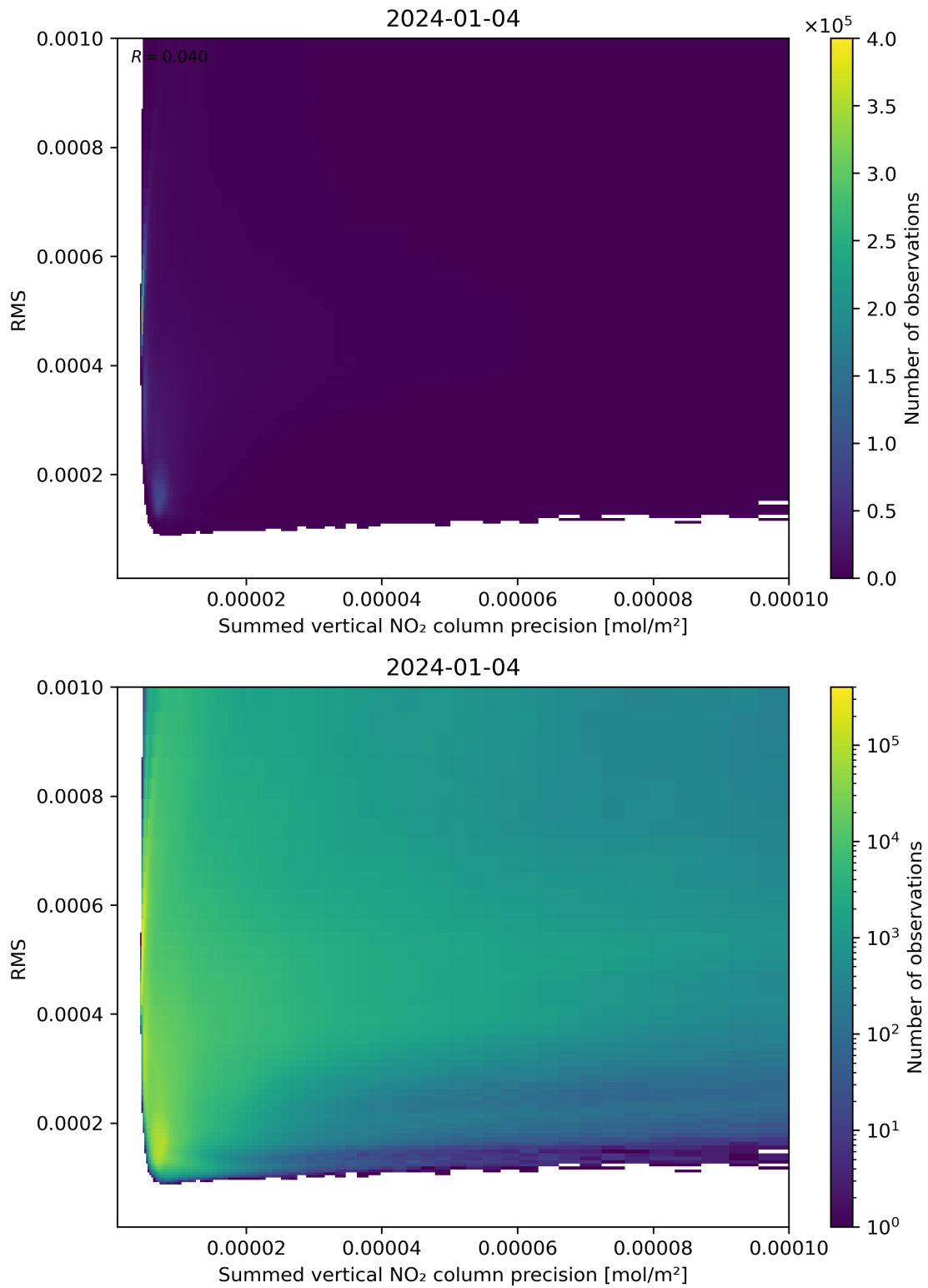
Figure 108: Scatter density plot of “Summed vertical NO 2 column precision” against “RMS” for 2024-01-03 to 2024-01-05.
