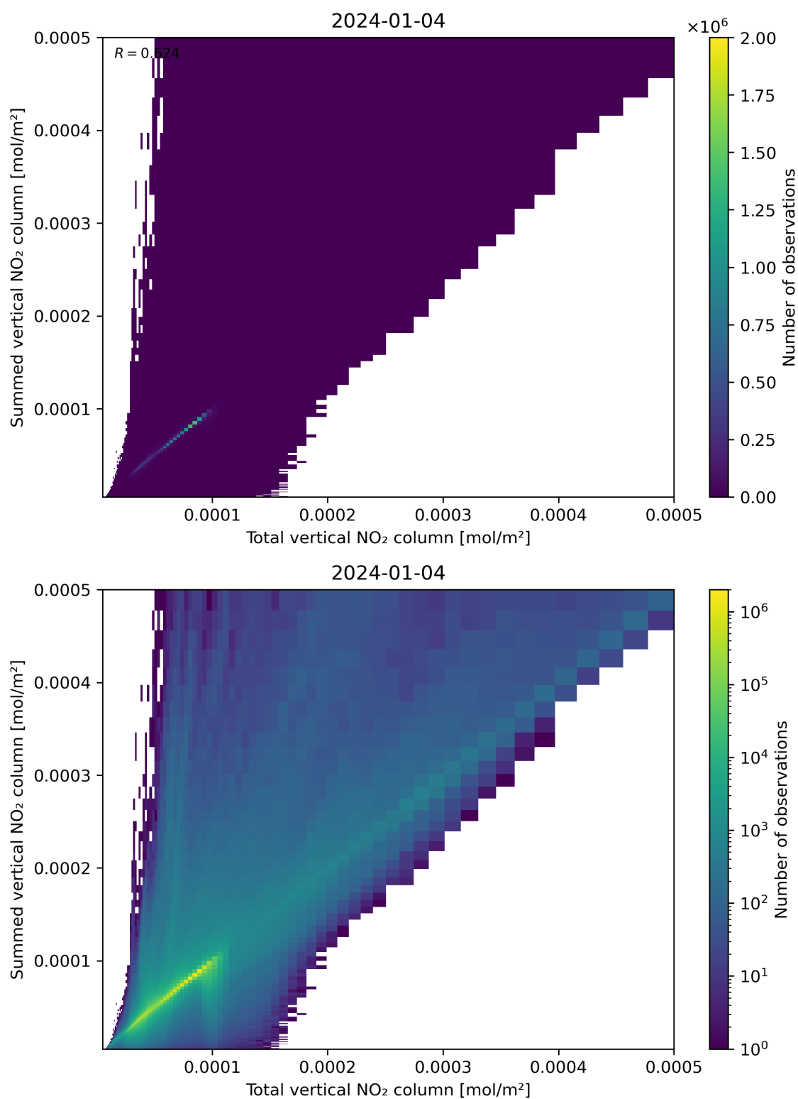
Figure 112: Scatter density plot of “Total vertical NO 2 column” against “Summed vertical NO 2 column” for 2024-01-03 to 2024-01-05.
