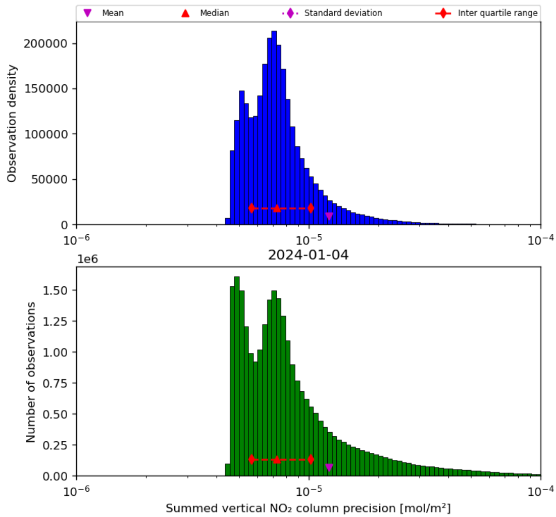
Figure 41: Histogram of “Summed vertical NO 2 column precision” for 2024-01-03 to 2024-01-05
