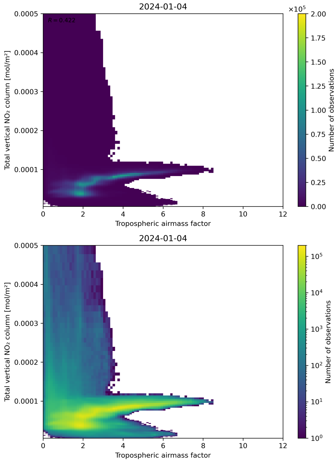
Figure 77: Scatter density plot of “Tropospheric airmass factor” against “Total vertical NO 2 column” for 2024-01-03 to 2024-01-05.
