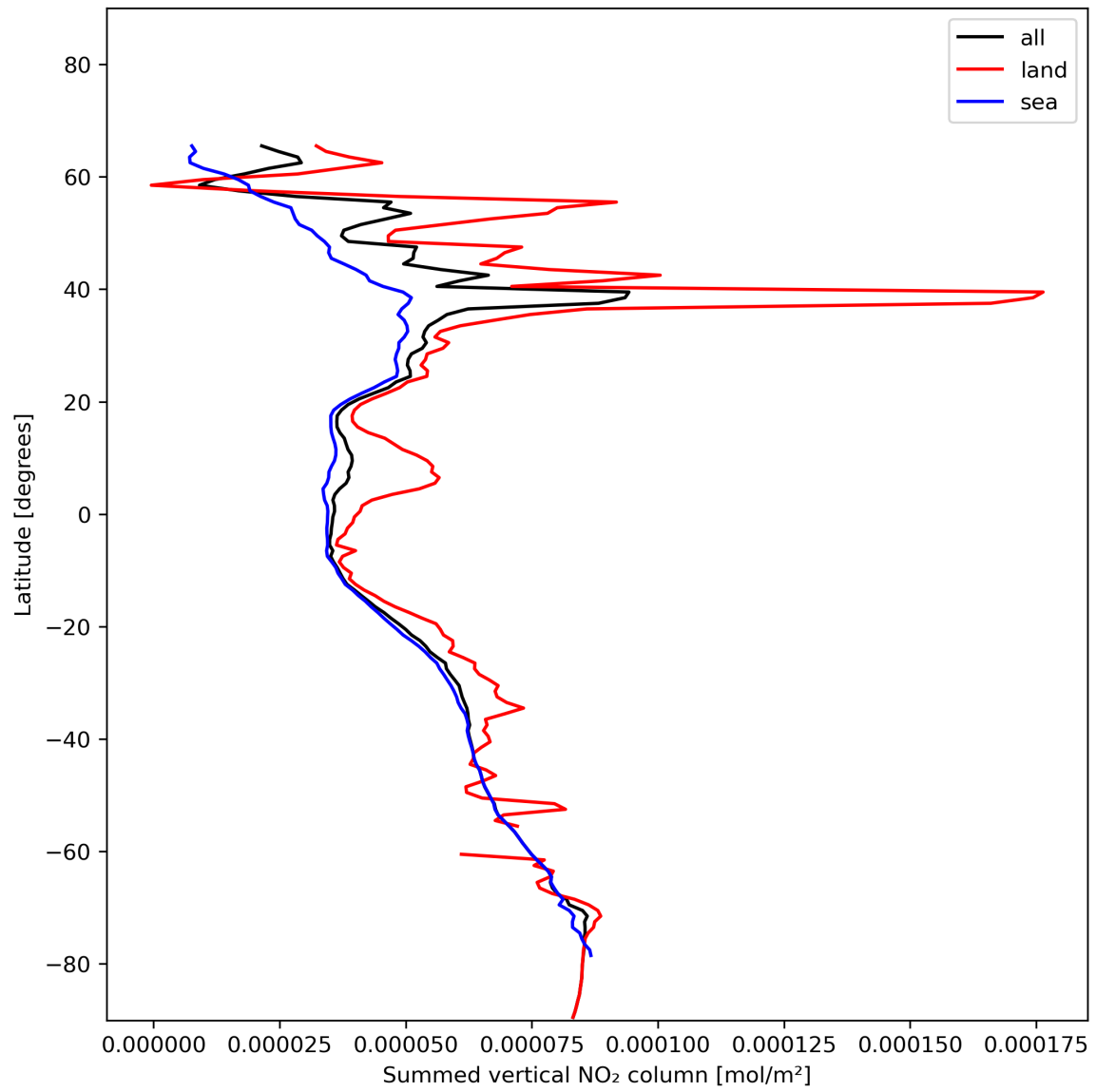
Figure 23: Zonal average of “Summed vertical NO 2 column” for 2024-01-03 to 2024-01-05.
