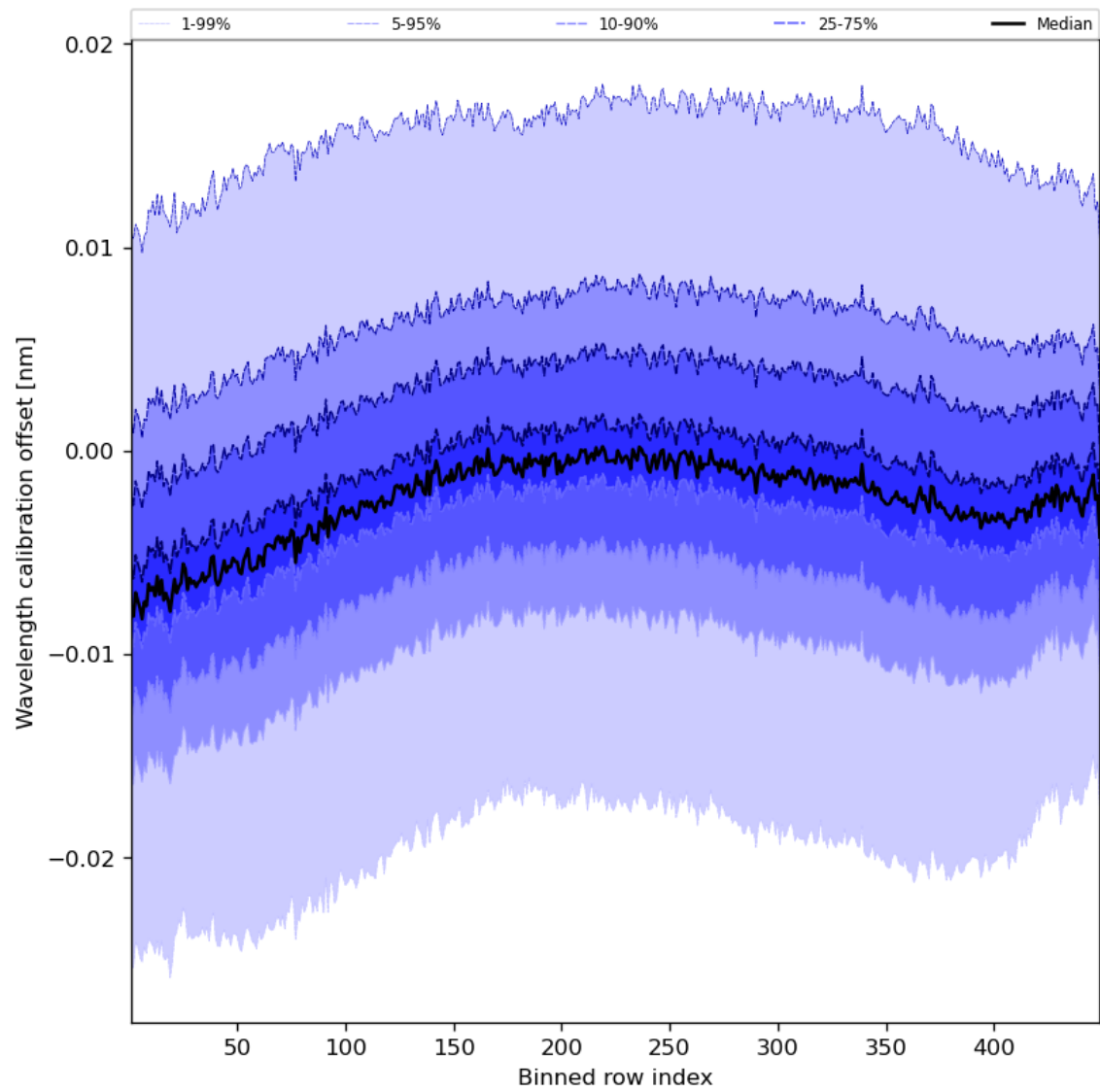
Figure 52: Along track statistics of “Wavelength calibration offset” for 2024-01-03 to 2024-01-05
