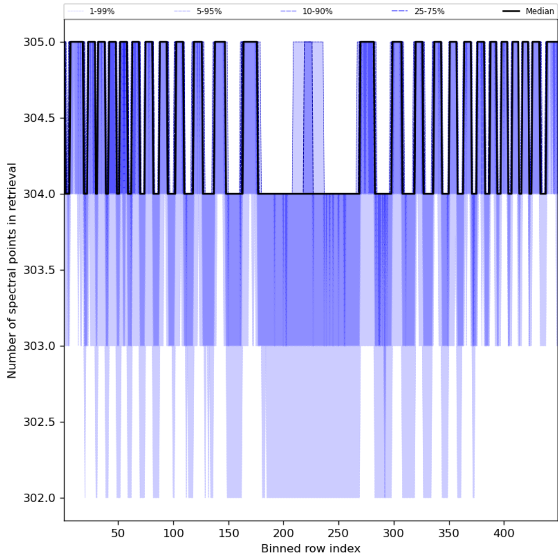
Figure 50: Along track statistics of “Number of spectral points in retrieval” for 2024-01-03 to 2024-01-05
