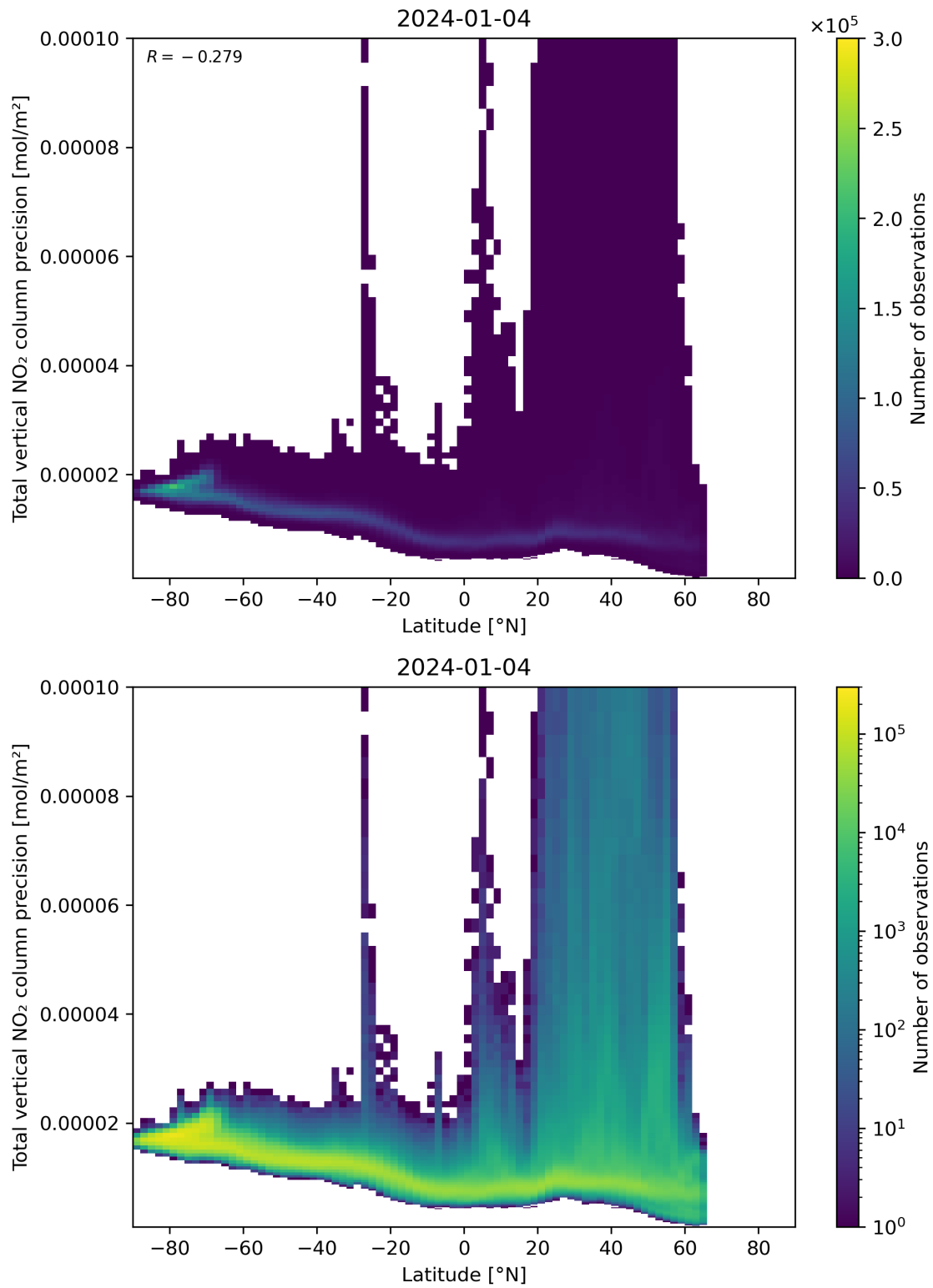
Figure 91: Scatter density plot of “Latitude” against “Total vertical NO 2 column precision” for 2024-01-03 to 2024-01-05.
