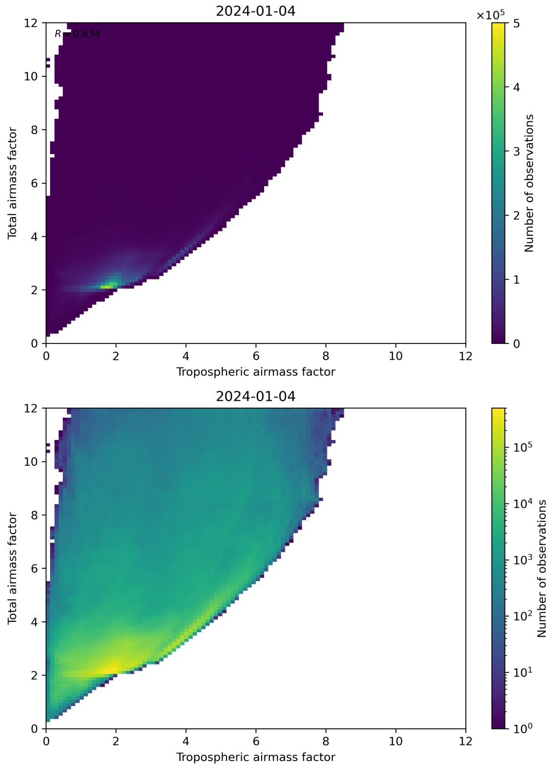
Figure 72: Scatter density plot of “Tropospheric airmass factor” against “Total airmass factor” for 2024-01-03 to 2024-01-05.
