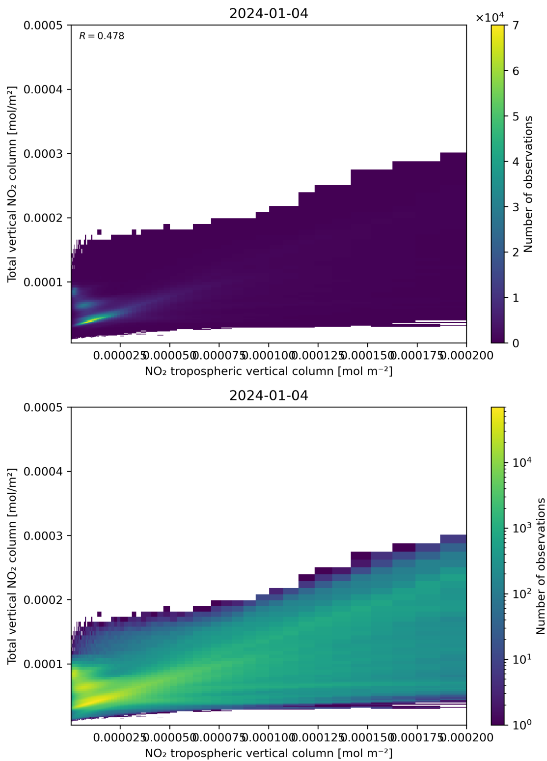
Figure 128: Scatter density plot of “NO 2 tropospheric vertical column” against “Total vertical NO 2 column” for 2024-01-03 to 2024-01-05.
