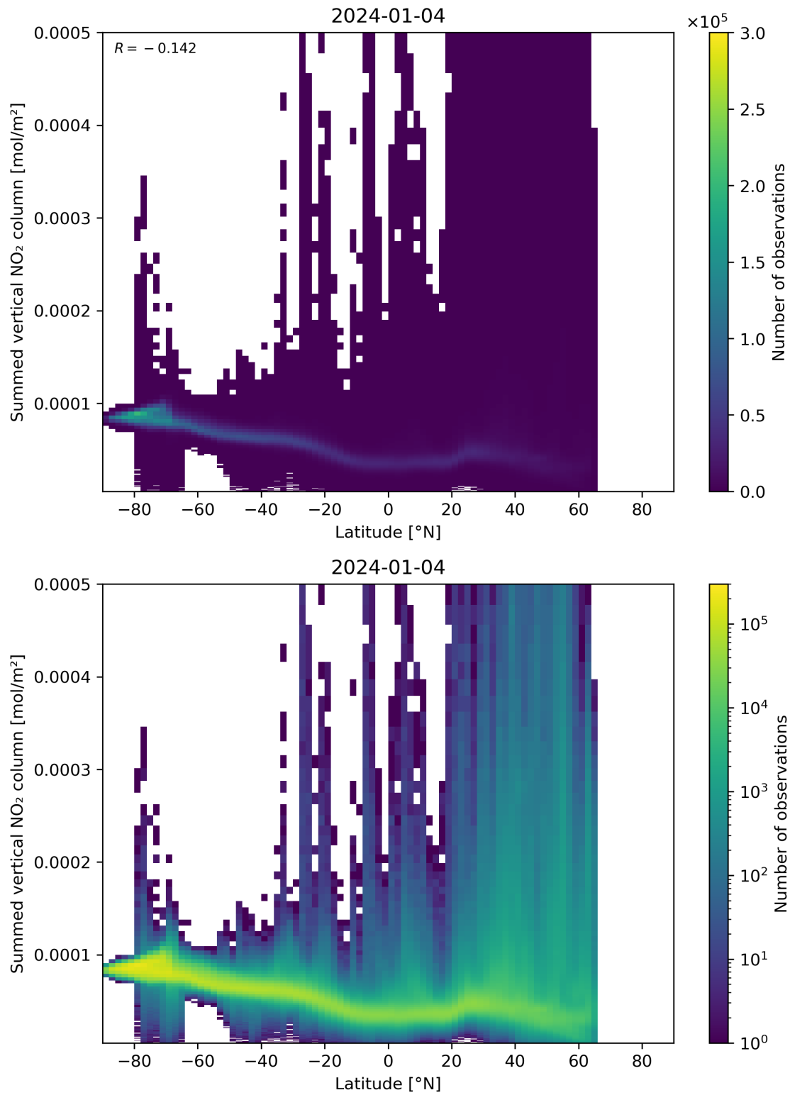
Figure 88: Scatter density plot of “Latitude” against “Summed vertical NO 2 column” for 2024-01-03 to 2024-01-05.
