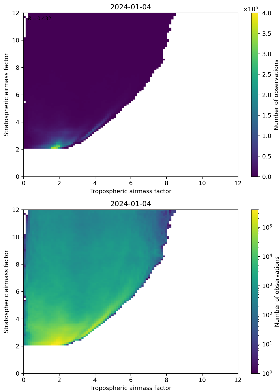
Figure 71: Scatter density plot of “Tropospheric airmass factor” against “Stratospheric airmass factor” for 2024-01-03 to 2024-01-05.
