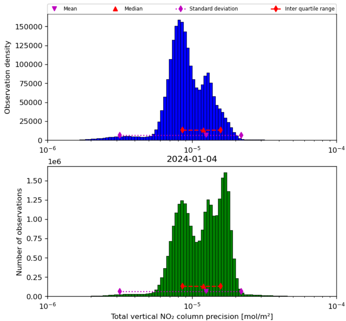
Figure 39: Histogram of “Total vertical NO 2 column precision” for 2024-01-03 to 2024-01-05
