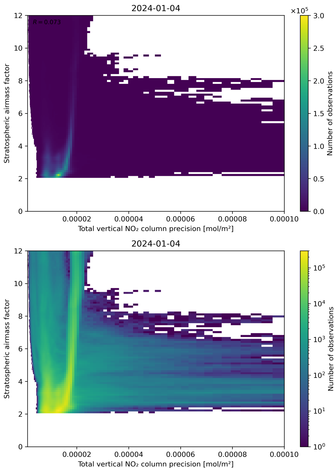
Figure 115: Scatter density plot of “Total vertical NO 2 column precision” against “Stratospheric air mass factor” for 2024-01-03 to 2024-01-05.
