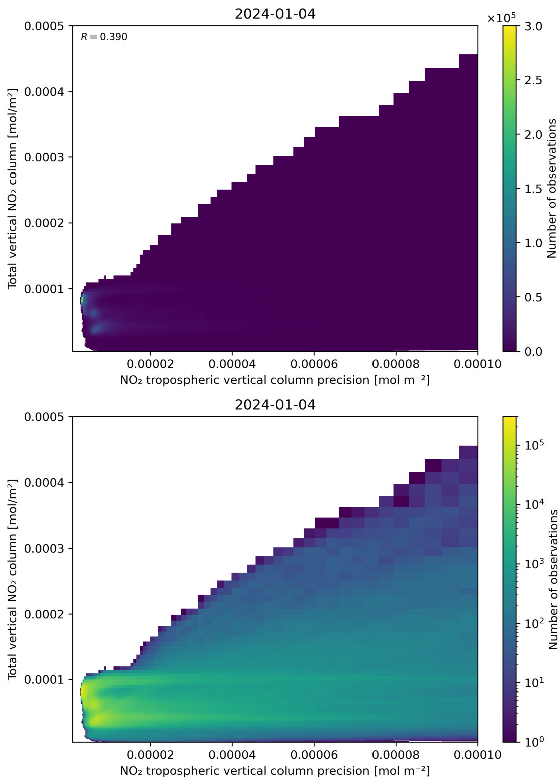
Figure 138: Scatter density plot of “NO 2 tropospheric vertical column precision” against “Total vertical NO 2 column” for 2024-01-03 to 2024-01-05.
