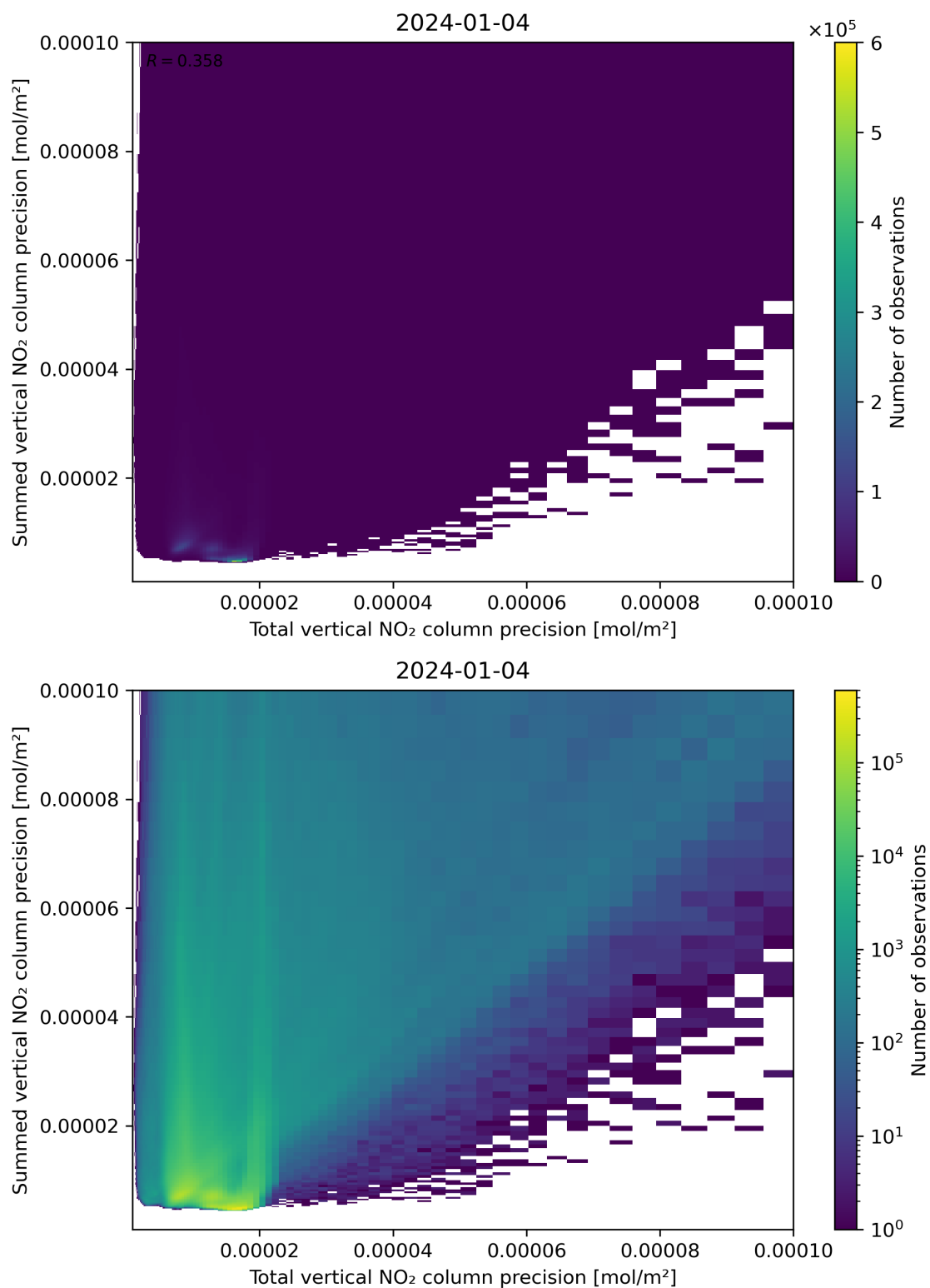
Figure 118: Scatter density plot of “Total vertical NO 2 column precision” against “Summed vertical NO 2 column precision” for 2024-01-03 to 2024-01-05.
