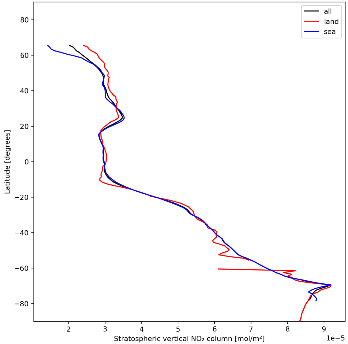
Figure 19: Zonal average of “Stratospheric vertical NO 2 column” for 2024-01-03 to 2024-01-05.
