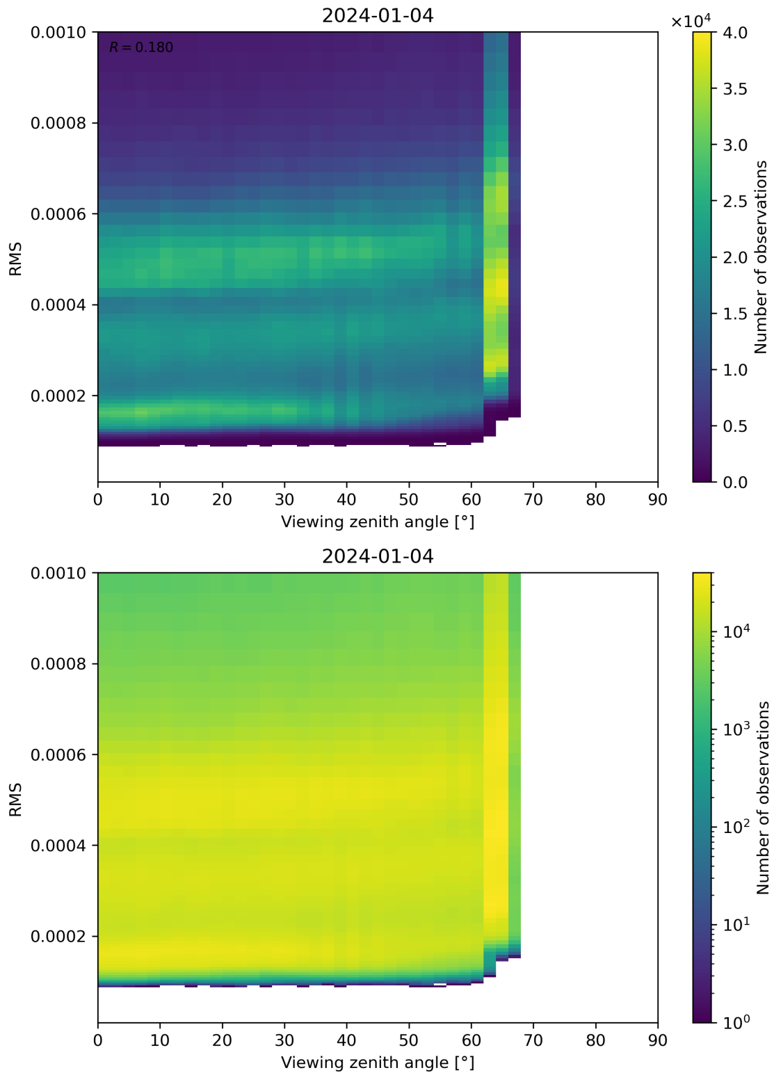
Figure 171: Scatter density plot of “Viewing zenith angle” against “RMS” for 2024-01-03 to 2024-01-05.
