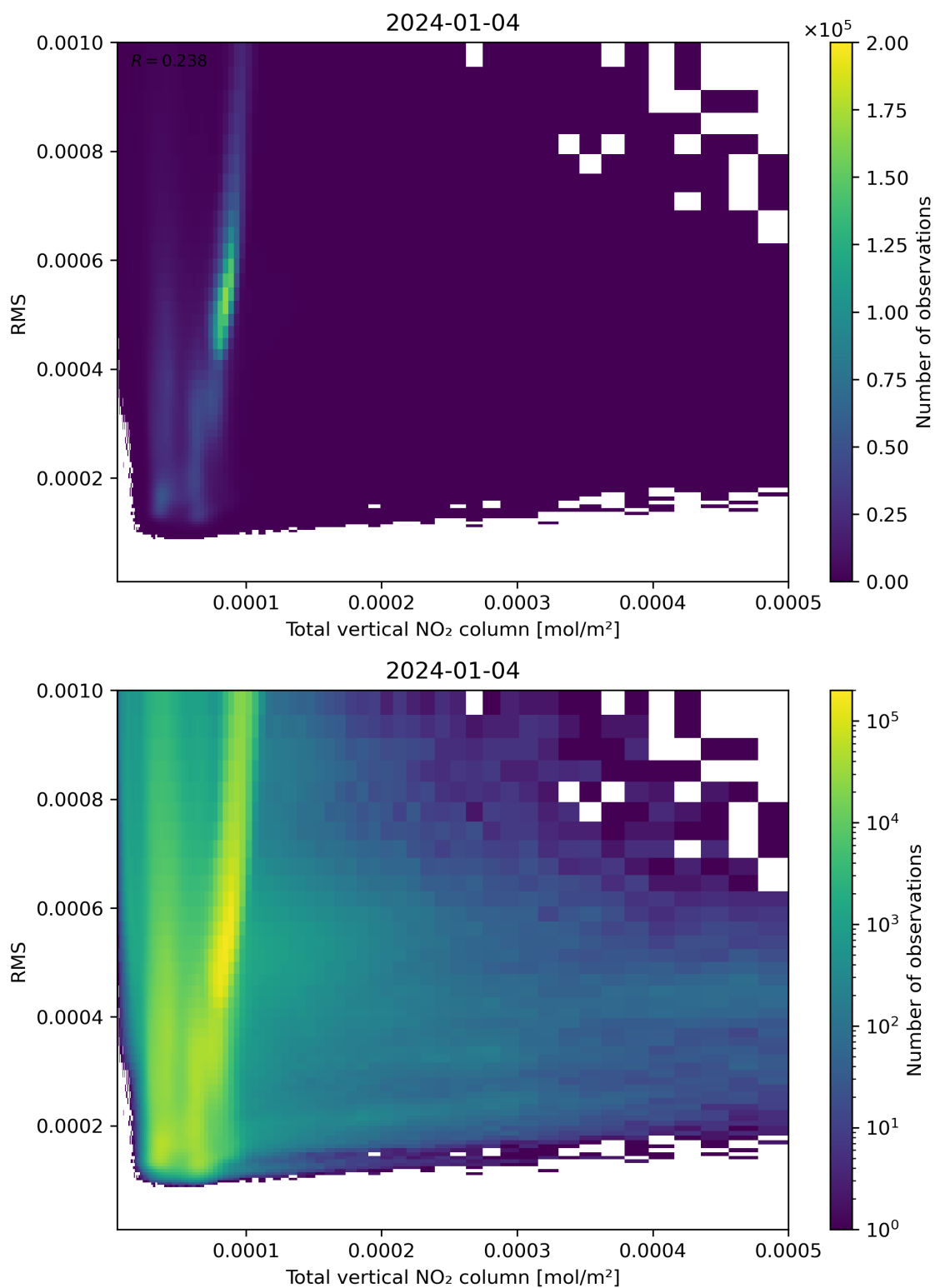
Figure 120: Scatter density plot of “Total vertical NO 2 column” against “RMS” for 2024-01-03 to 2024-01-05.
