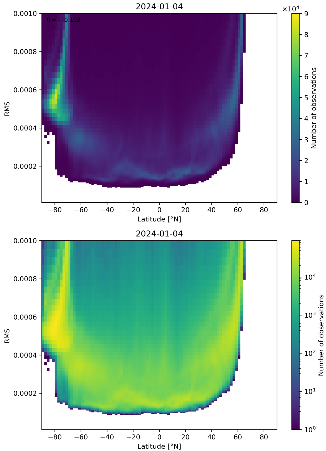
Figure 94: Scatter density plot of “Latitude” against “RMS” for 2024-01-03 to 2024-01-05.
