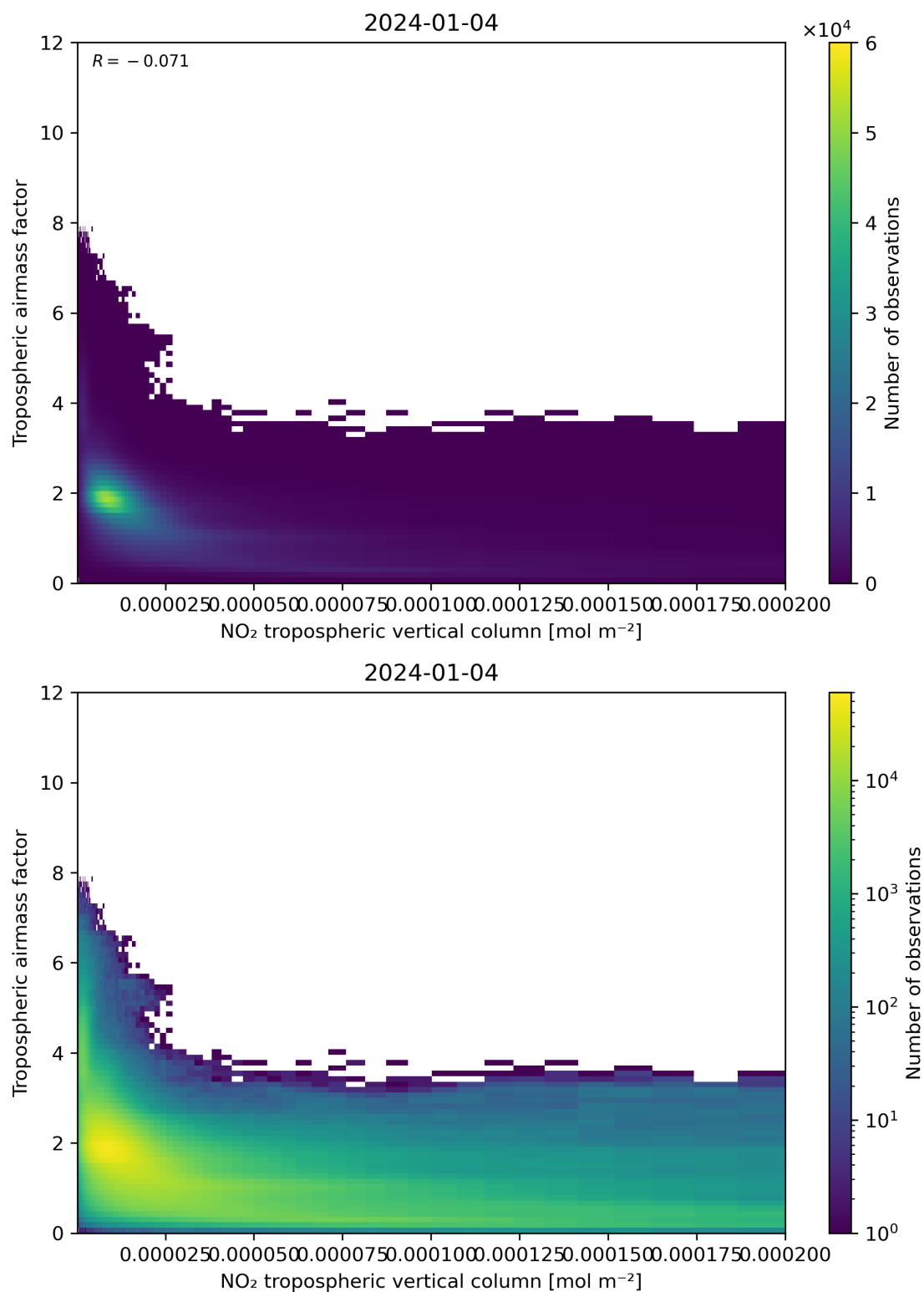
Figure 123: Scatter density plot of “NO 2 tropospheric vertical column” against “Tropospheric air mass factor” for 2024-01-03 to 2024-01-05.
