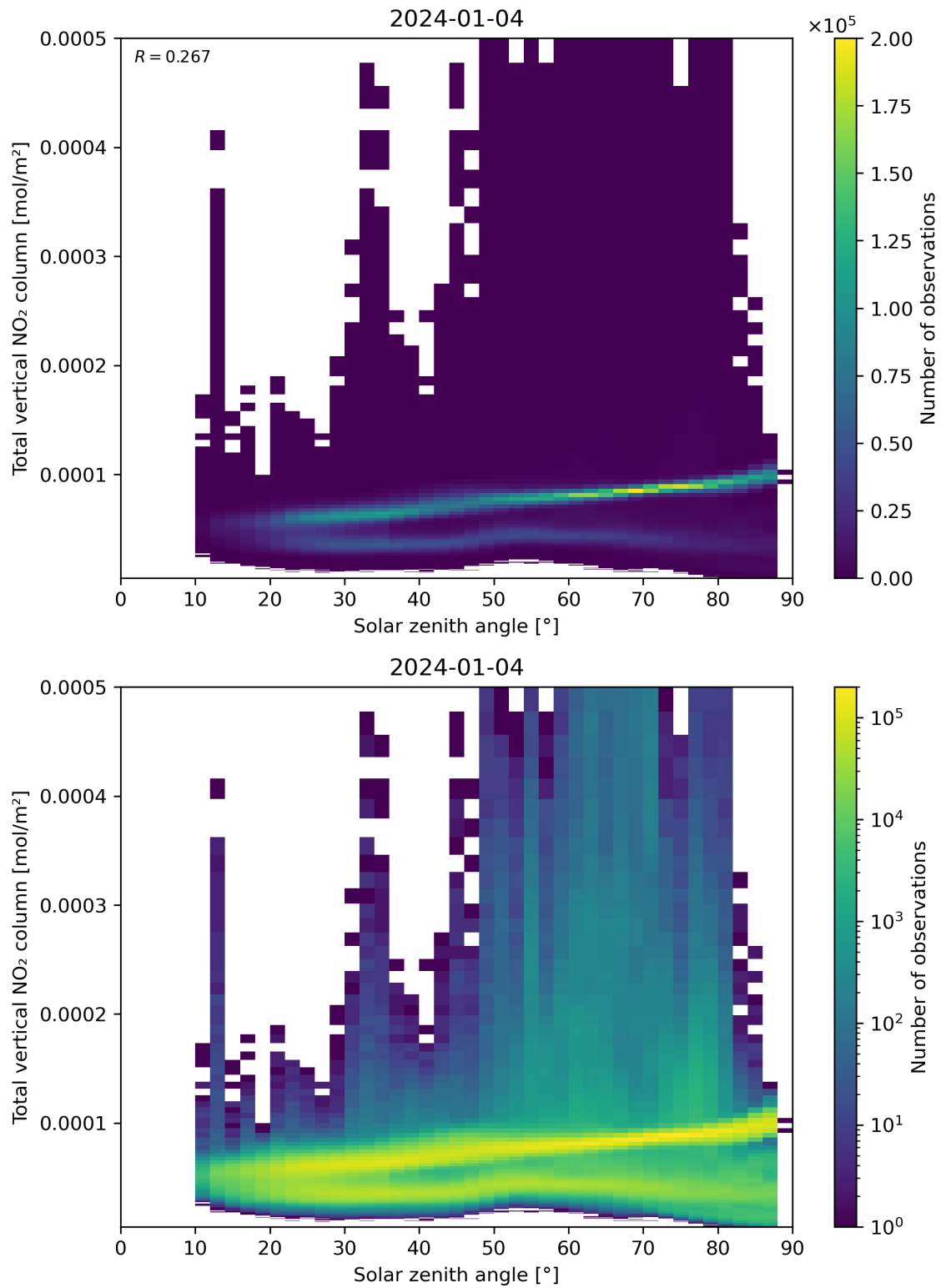
Figure 153: Scatter density plot of “Solar zenith angle” against “Total vertical NO 2 column” for 2024-01-03 to 2024-01-05.
