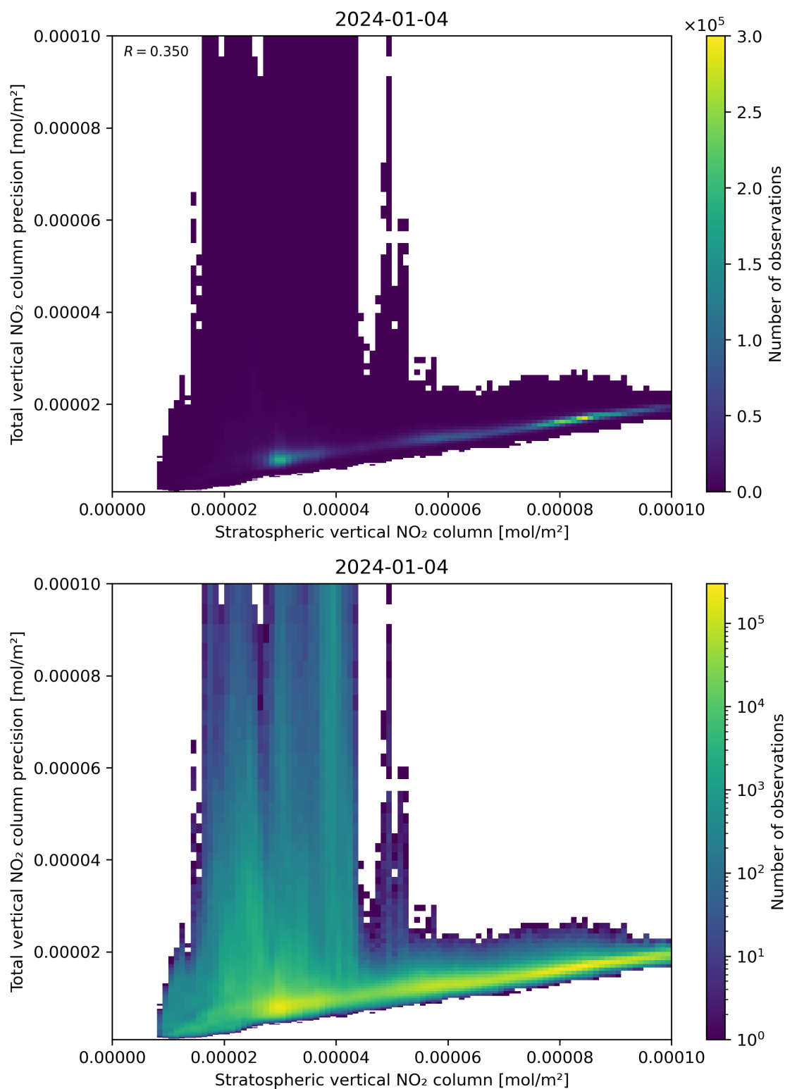
Figure 101: Scatter density plot of “Stratospheric vertical NO 2 column” against “Total vertical NO 2 column precision” for 2024-01-03 to 2024-01-05.
