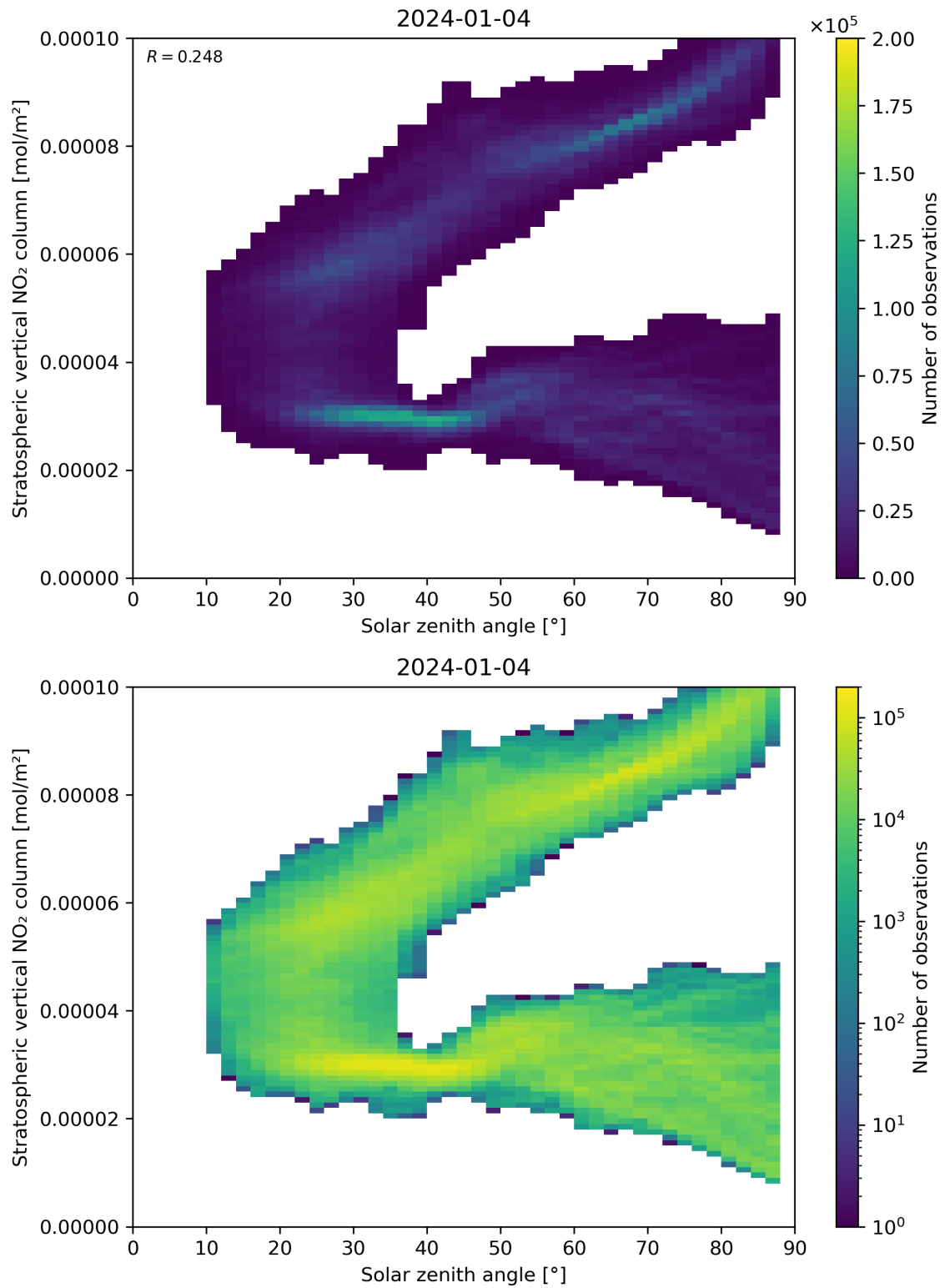
Figure 150: Scatter density plot of “Solar zenith angle” against “Stratospheric vertical NO 2 column” for 2024-01-03 to 2024-01-05.
