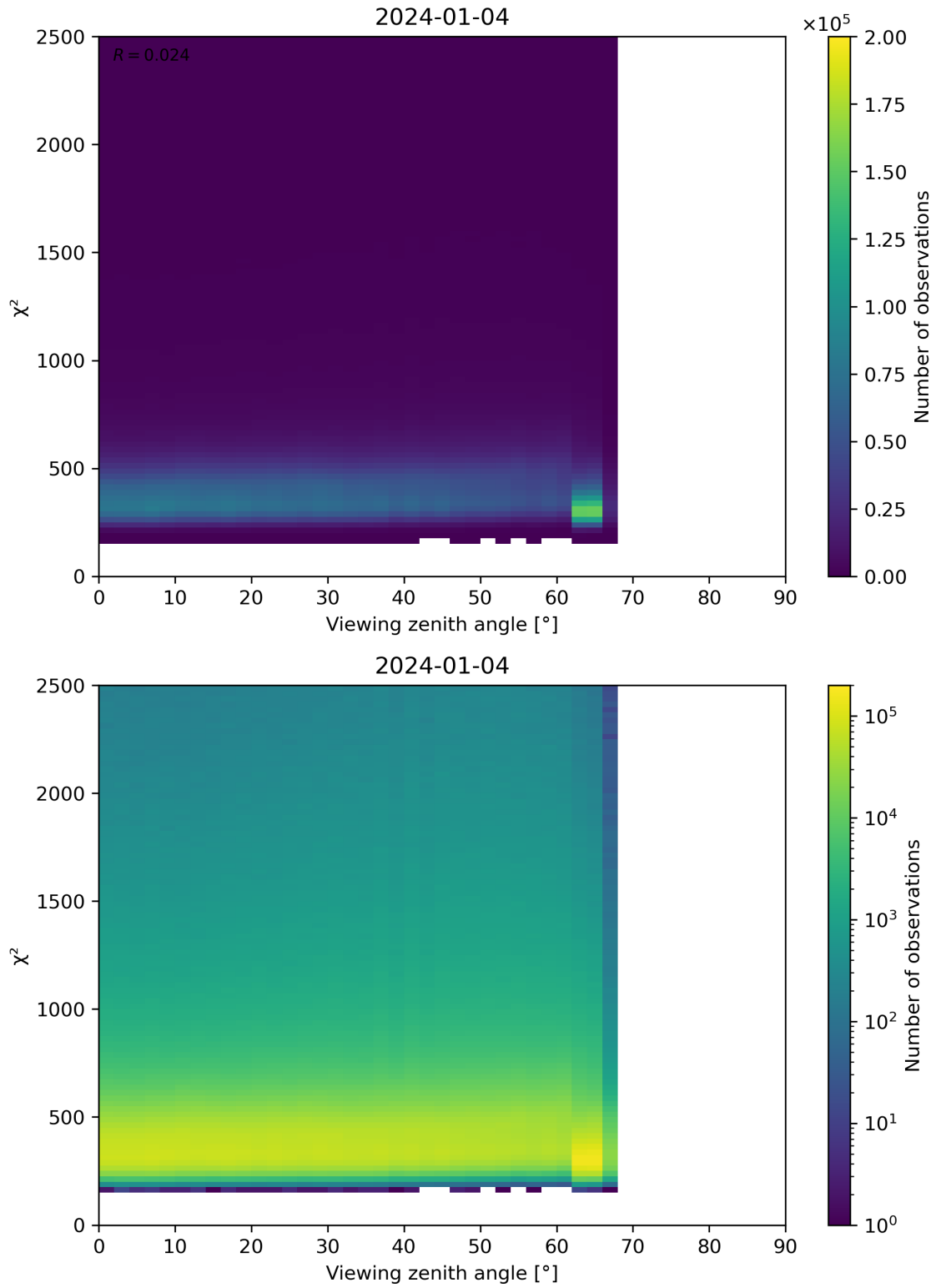
Figure 162: Scatter density plot of “Viewing zenith angle” against “ \chi^2 ” for 2024-01-03 to 2024-01-05.
