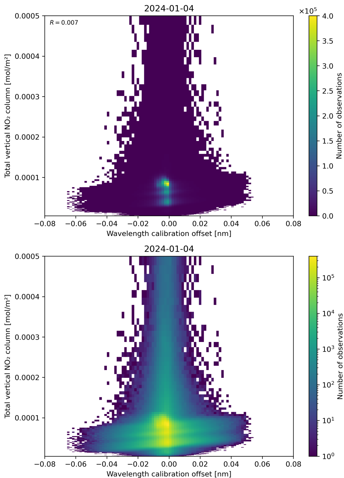
Figure 179: Scatter density plot of “Wavelength calibration offset” against “Total vertical NO 2 column” for 2024-01-03 to 2024-01-05.
