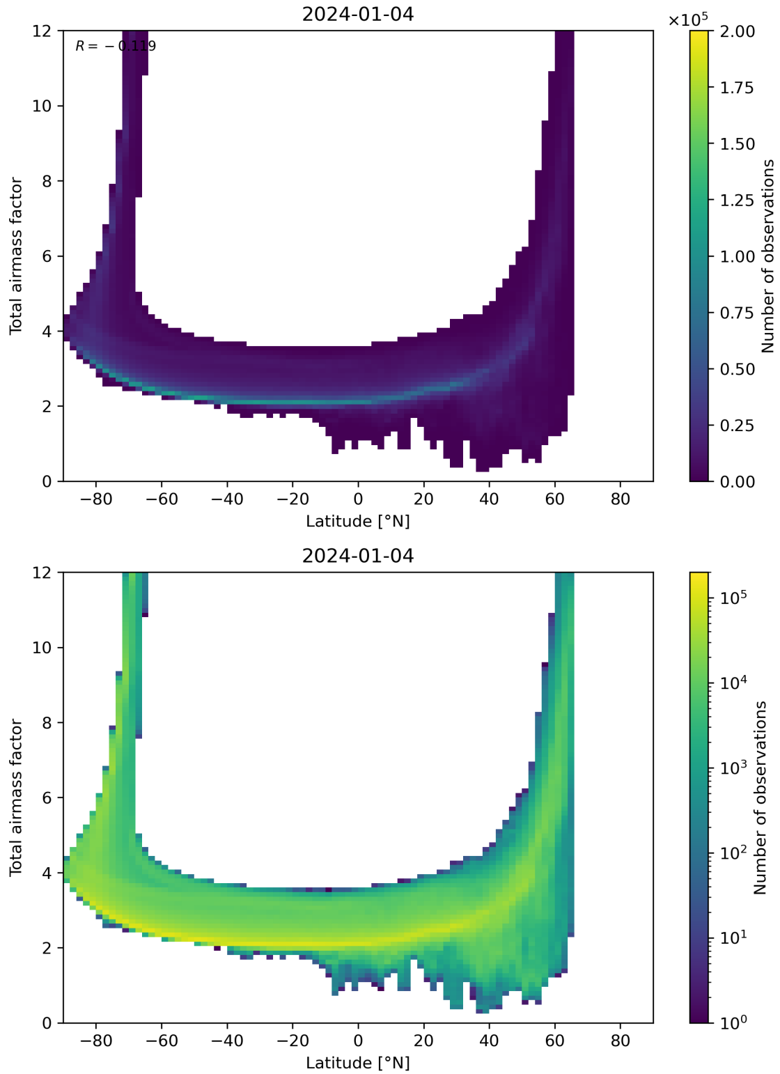
Figure 84: Scatter density plot of “Latitude” against “Total airmass factor” for 2024-01-03 to 2024-01-05.
