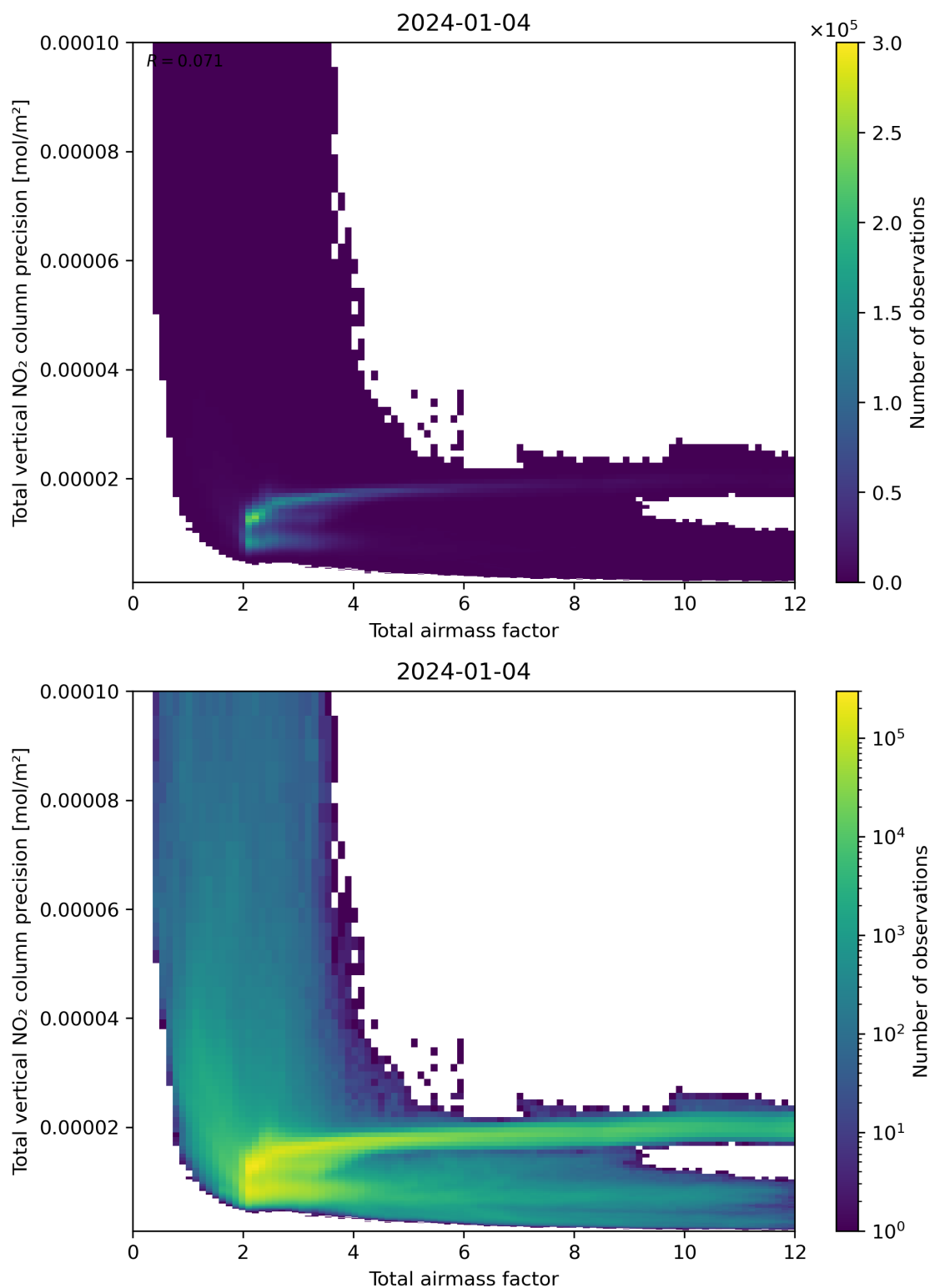
Figure 68: Scatter density plot of “Total airmass factor” against “Total vertical NO 2 column precision” for 2024-01-03 to 2024-01-05.
