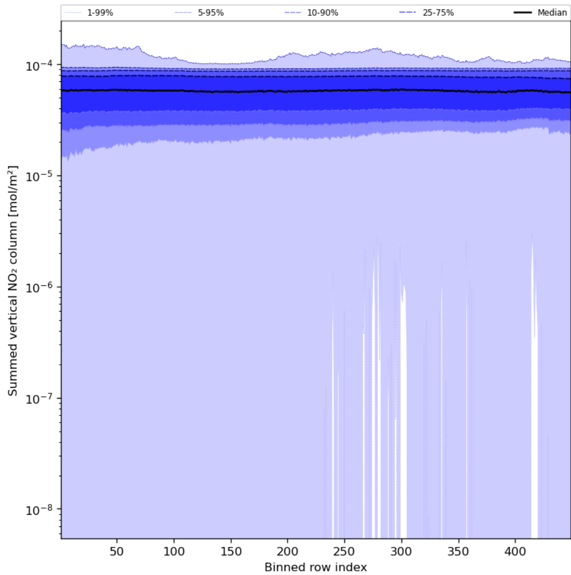
Figure 57: Along track statistics of “Summed vertical NO 2 column” for 2024-01-03 to 2024-01-05
