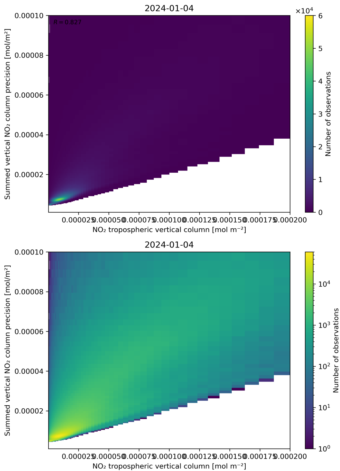
Figure 127: Scatter density plot of “NO 2 tropospheric vertical column” against “Summed vertical NO 2 column precision” for 2024-01-03 to 2024-01-05.
