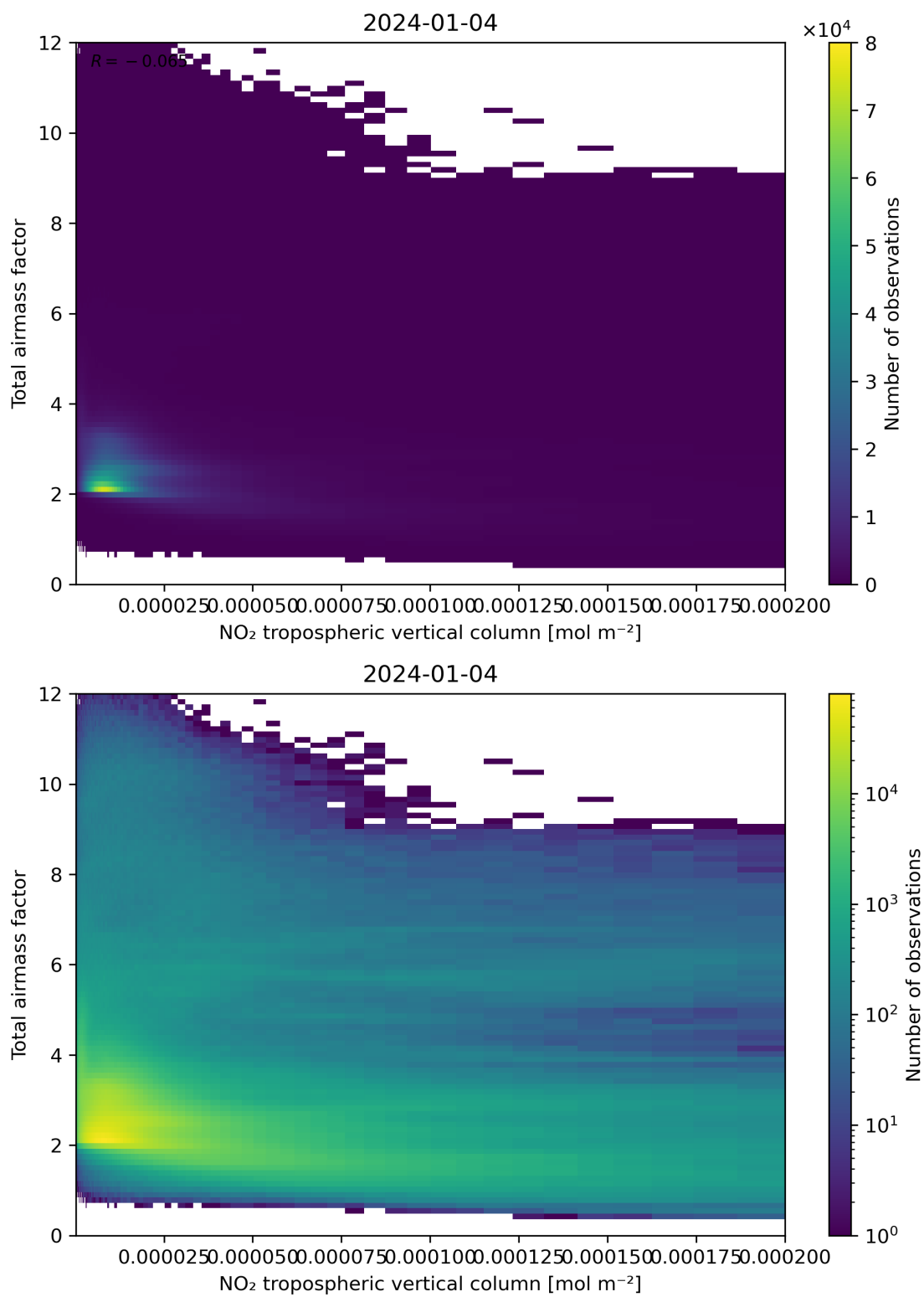
Figure 122: Scatter density plot of “NO 2 tropospheric vertical column” against “Total air mass factor” for 2024-01-03 to 2024-01-05.
