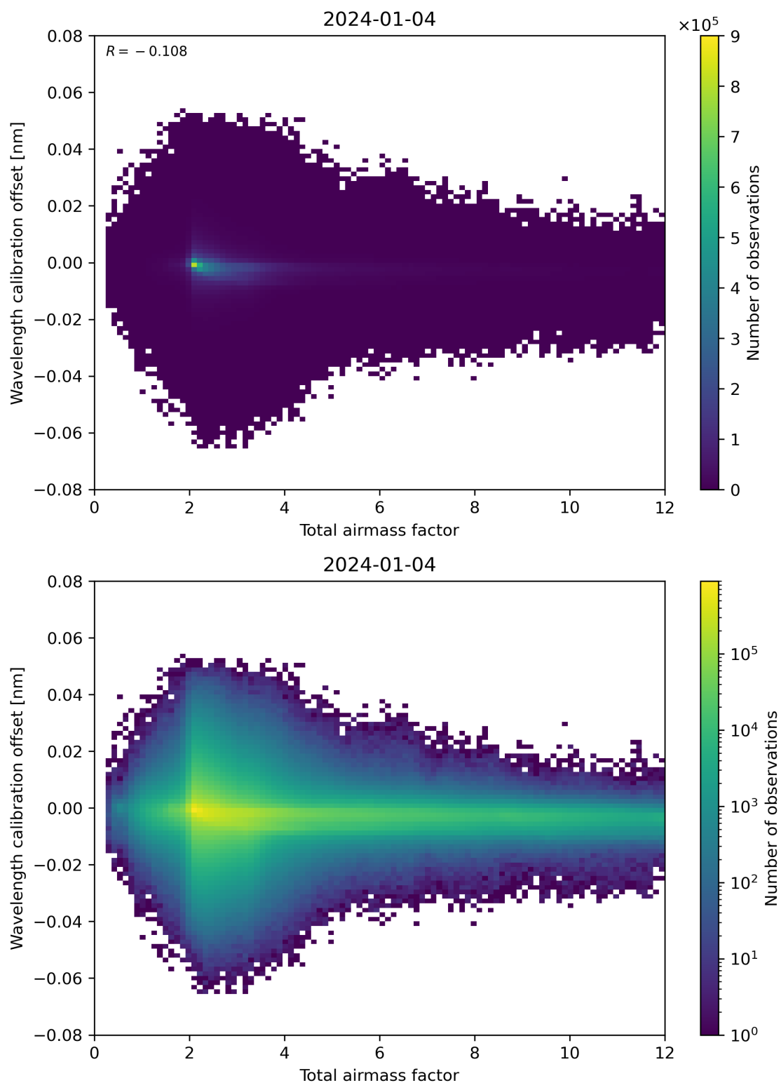
Figure 70: Scatter density plot of “Total airmass factor” against “Wavelength calibration offset” for 2024-01-03 to 2024-01-05.
