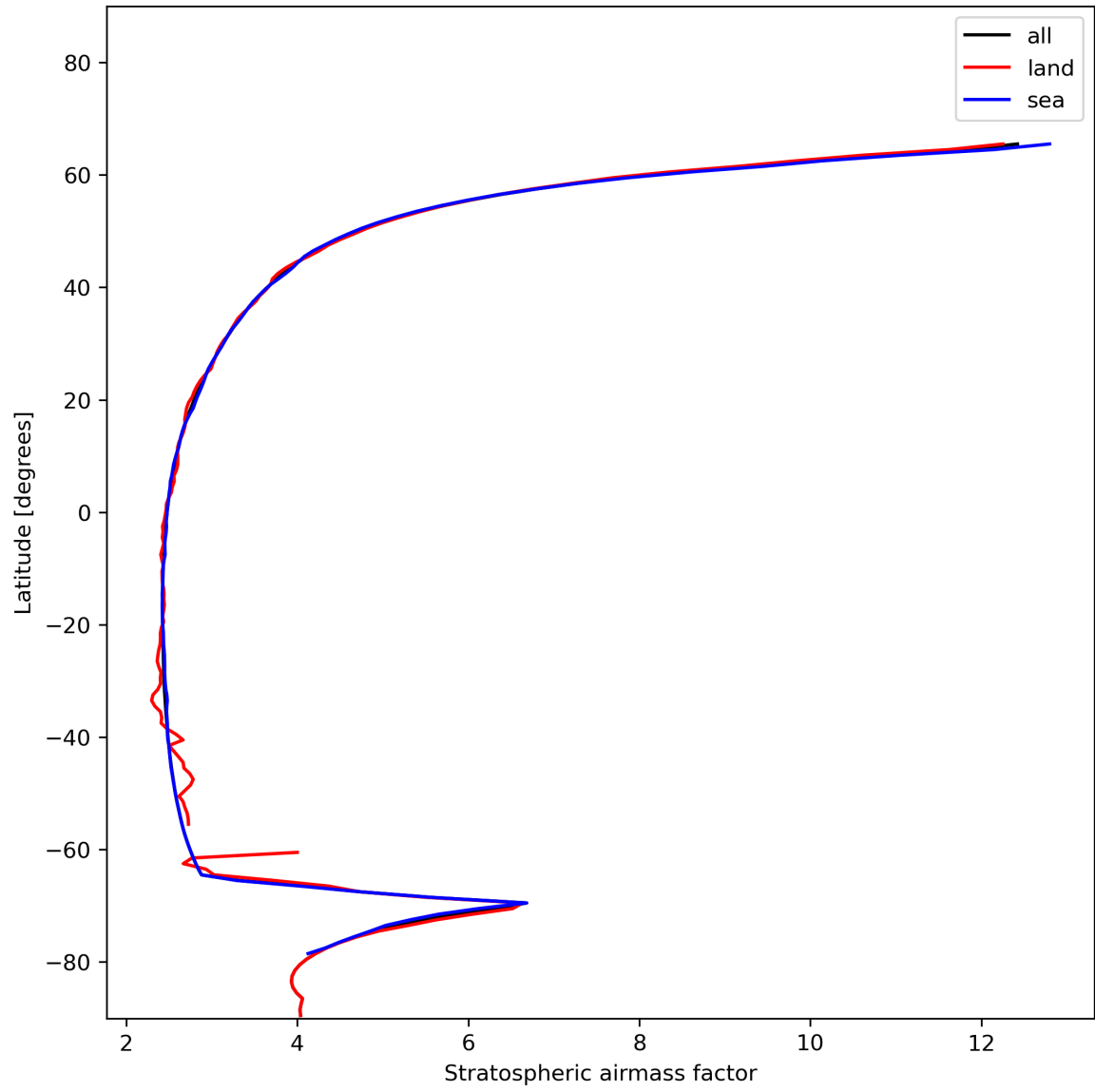
Figure 27: Zonal average of “Stratospheric air mass factor” for 2024-01-03 to 2024-01-05.
