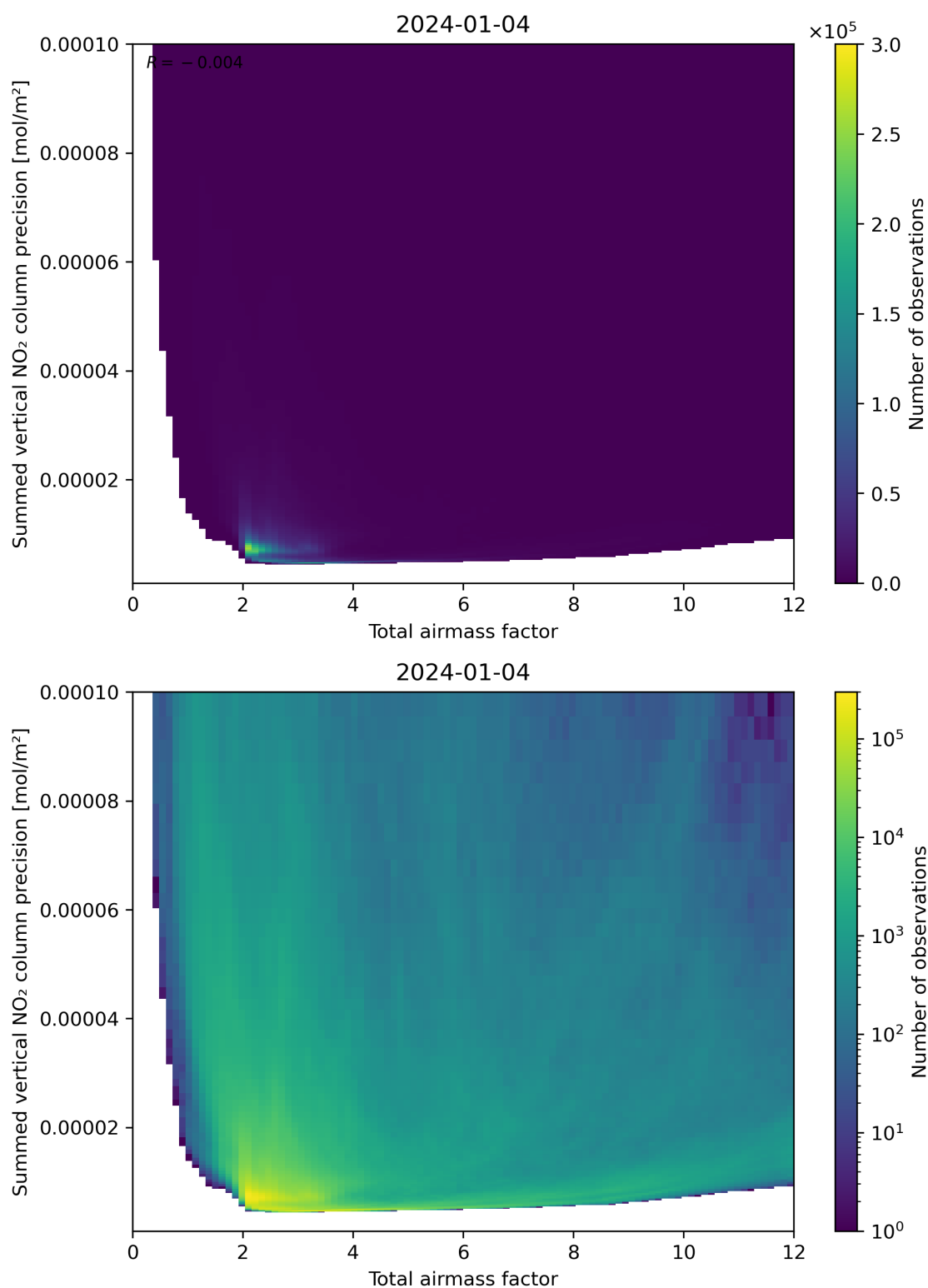
Figure 66: Scatter density plot of “Total airmass factor” against “Summed vertical NO 2 column precision” for 2024-01-03 to 2024-01-05.
