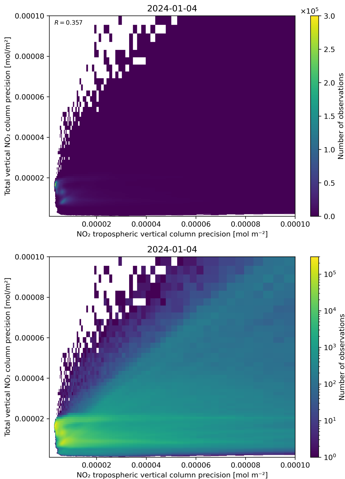
Figure 139: Scatter density plot of “NO 2 tropospheric vertical column precision” against “Total vertical NO 2 column precision” for 2024-01-03 to 2024-01-05.
