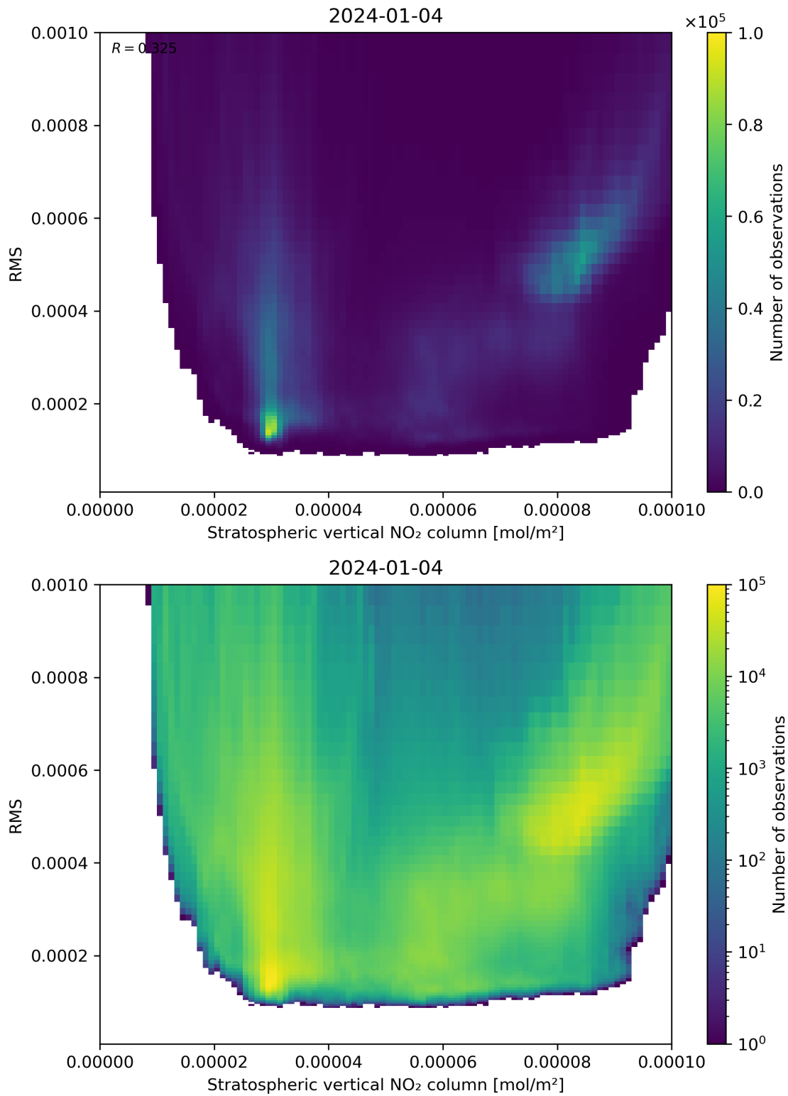
Figure 102: Scatter density plot of “Stratospheric vertical NO 2 column” against “RMS” for 2024-01-03 to 2024-01-05.
