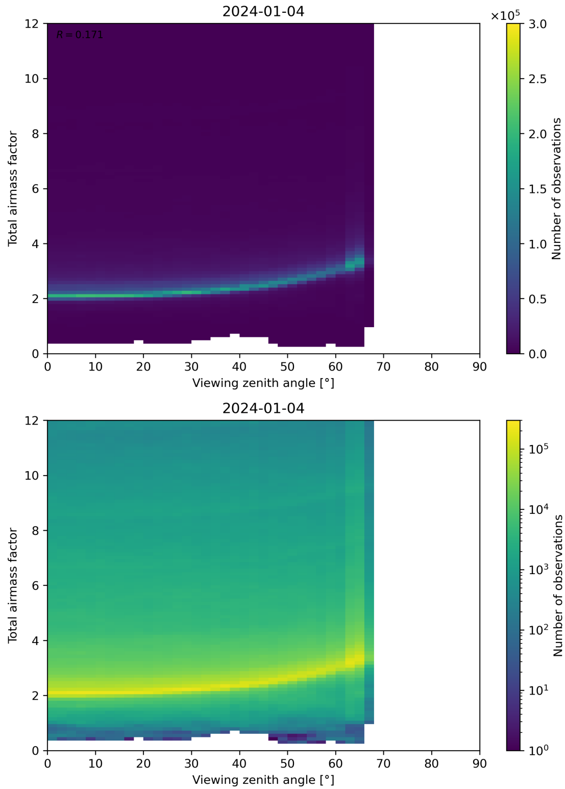
Figure 160: Scatter density plot of “Viewing zenith angle” against “Total airmass factor” for 2024-01-03 to 2024-01-05.
