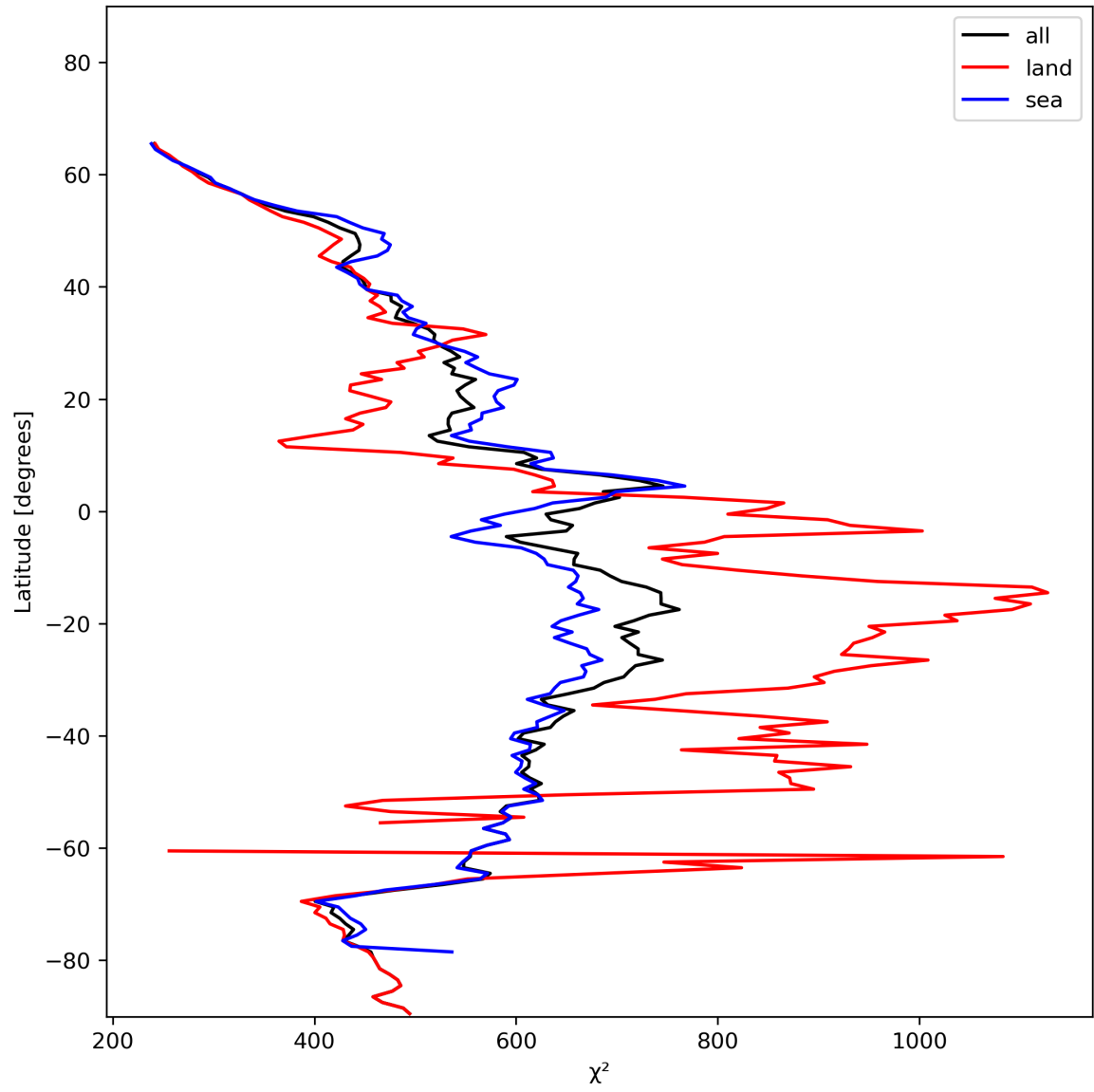
Figure 25: Zonal average of “ \chi^2 ” for 2024-01-03 to 2024-01-05.
