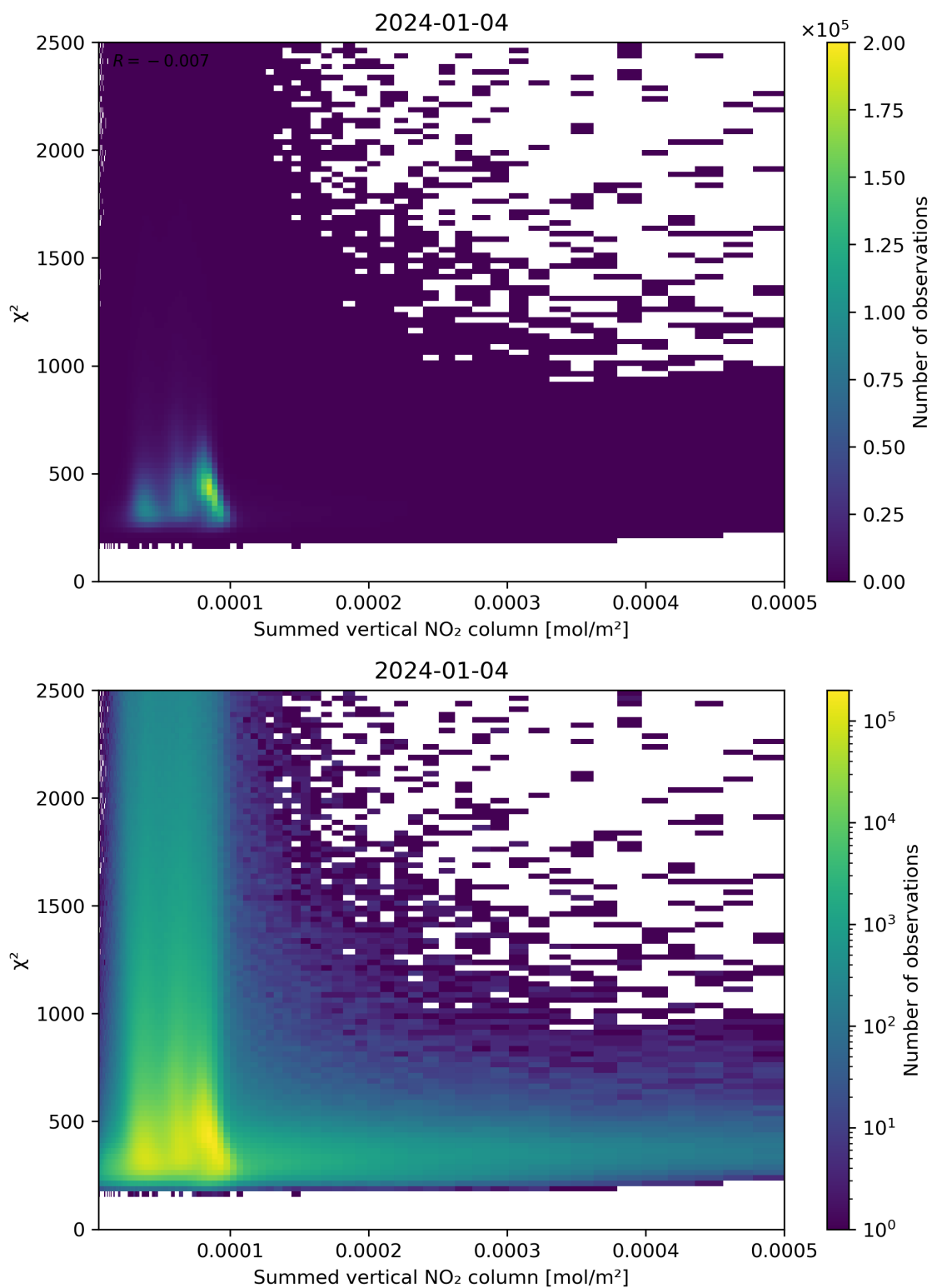
Figure 104: Scatter density plot of “Summed vertical NO 2 column” against “ \chi^2 ” for 2024-01-03 to 2024-01-05.
