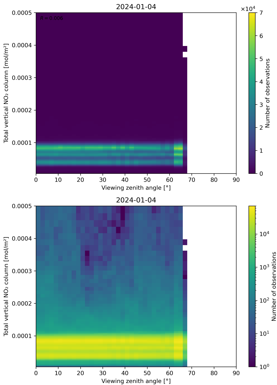
Figure 167: Scatter density plot of “Viewing zenith angle” against “Total vertical NO 2 column” for 2024-01-03 to 2024-01-05.
