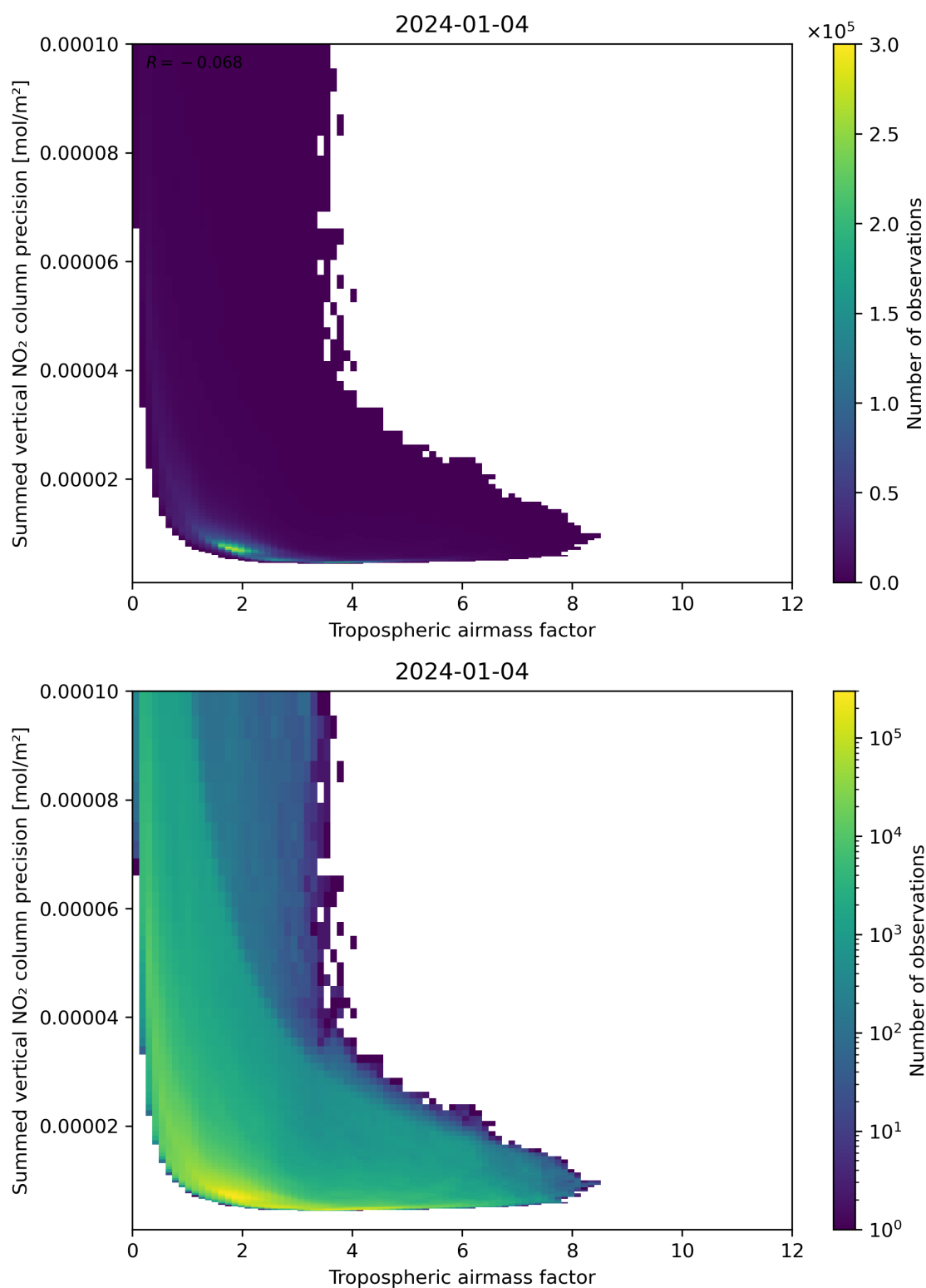
Figure 76: Scatter density plot of “Tropospheric air mass factor” against “Summed vertical NO 2 column precision” for 2024-01-03 to 2024-01-05.
