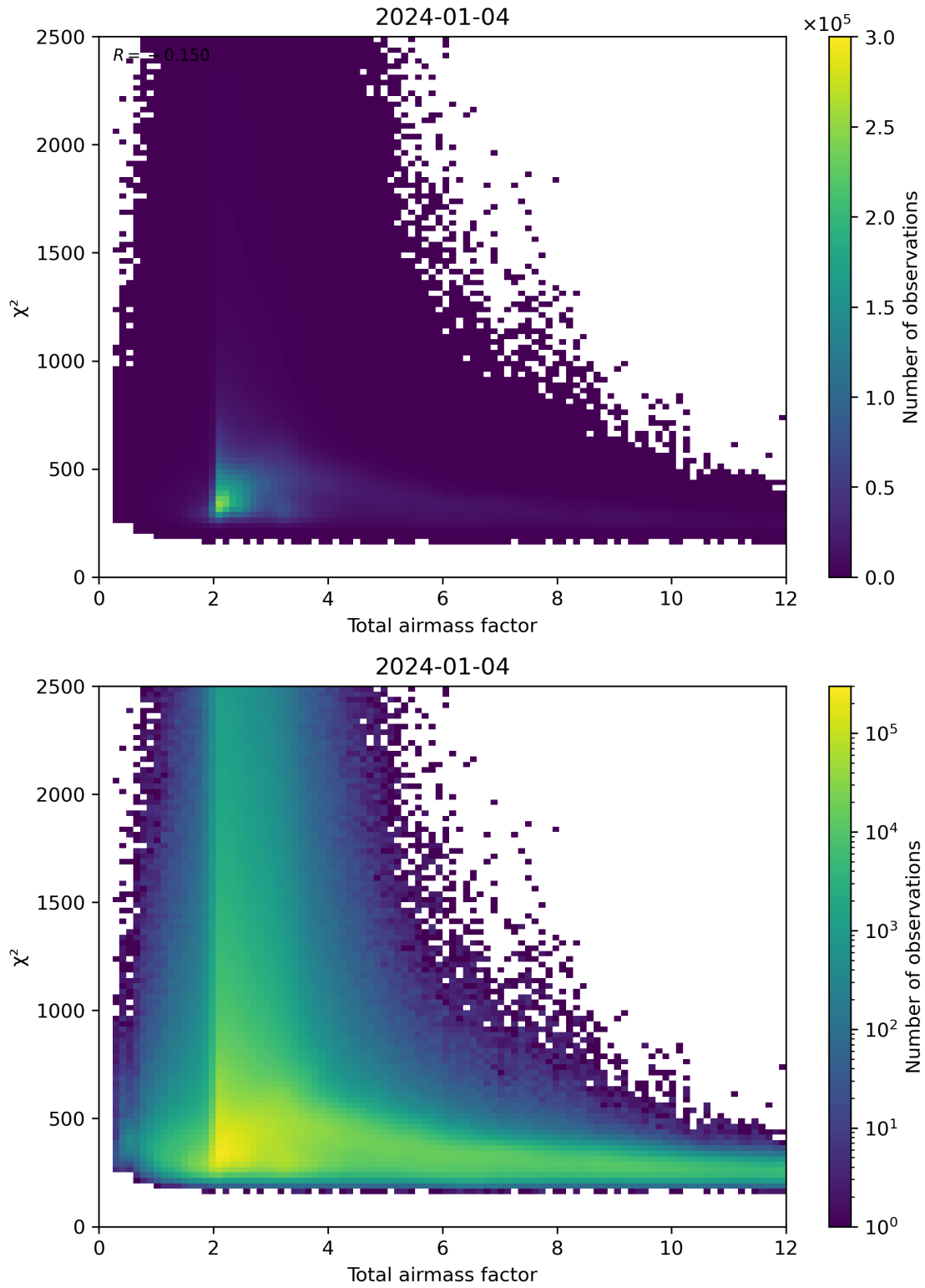
Figure 63: Scatter density plot of “Total airmass factor” against “ \chi^2 ” for 2024-01-03 to 2024-01-05.
