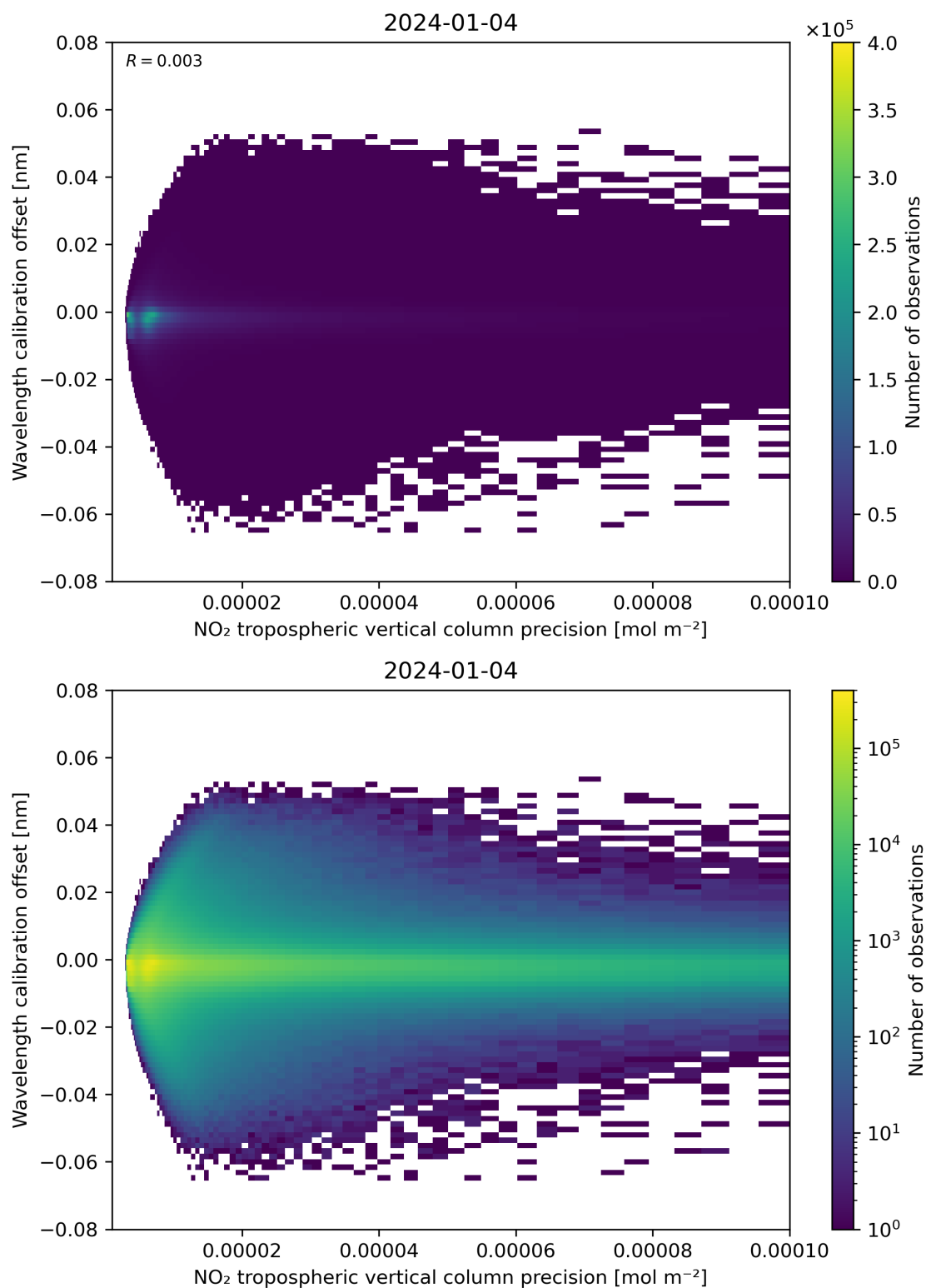
Figure 141: Scatter density plot of “NO 2 tropospheric vertical column precision” against “Wavelength calibration offset” for 2024-01-03 to 2024-01-05.
