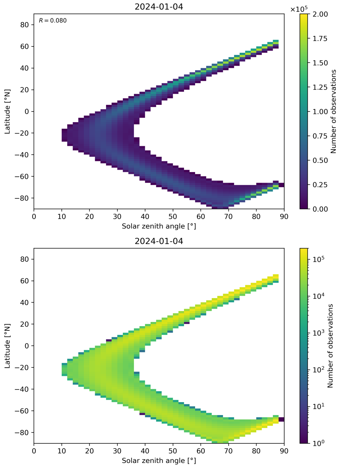
Figure 149: Scatter density plot of “Solar zenith angle” against “Latitude” for 2024-01-03 to 2024-01-05.
