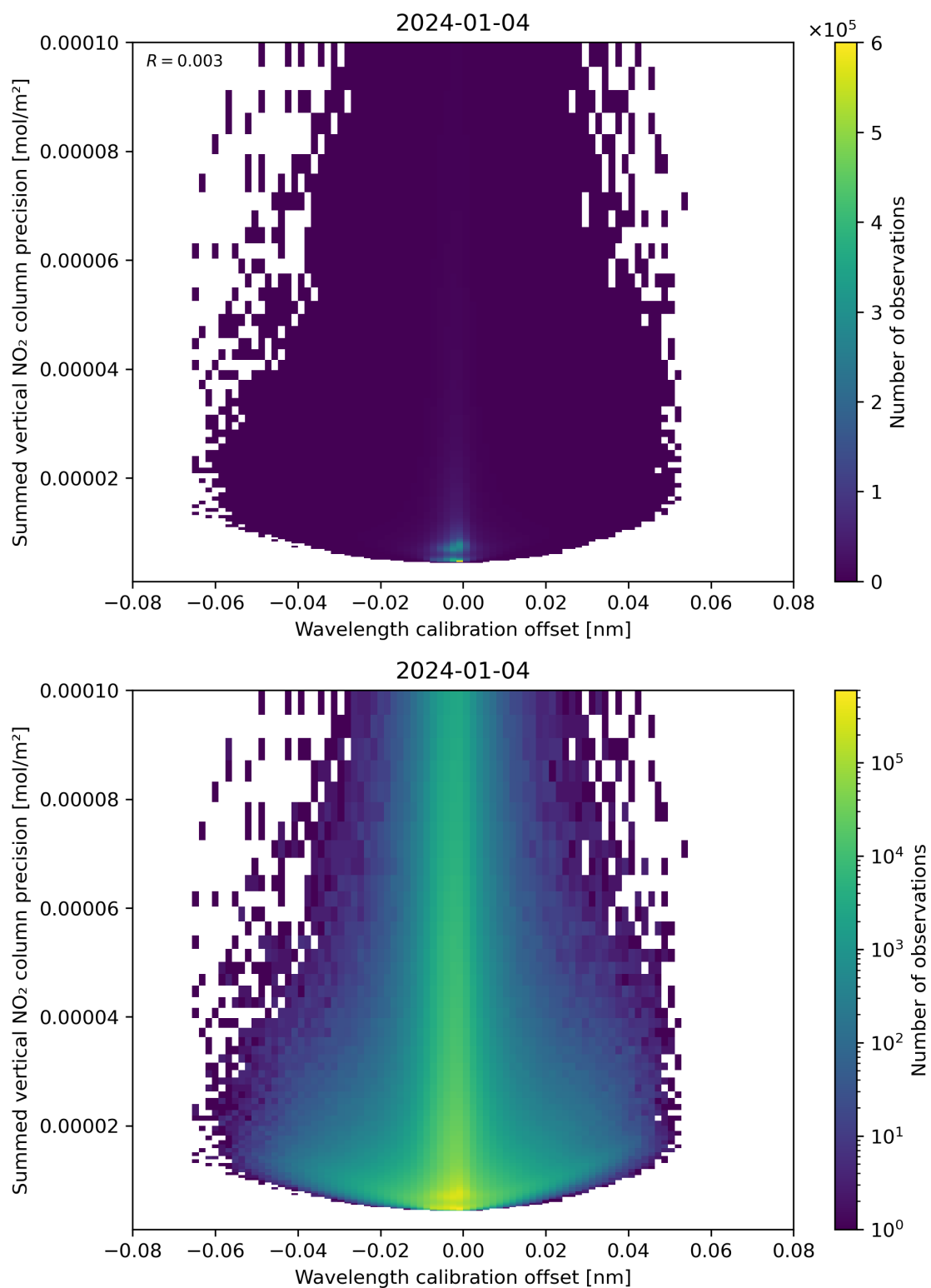
Figure 178: Scatter density plot of “Wavelength calibration offset” against “Summed vertical NO 2 column precision” for 2024-01-03 to 2024-01-05.
