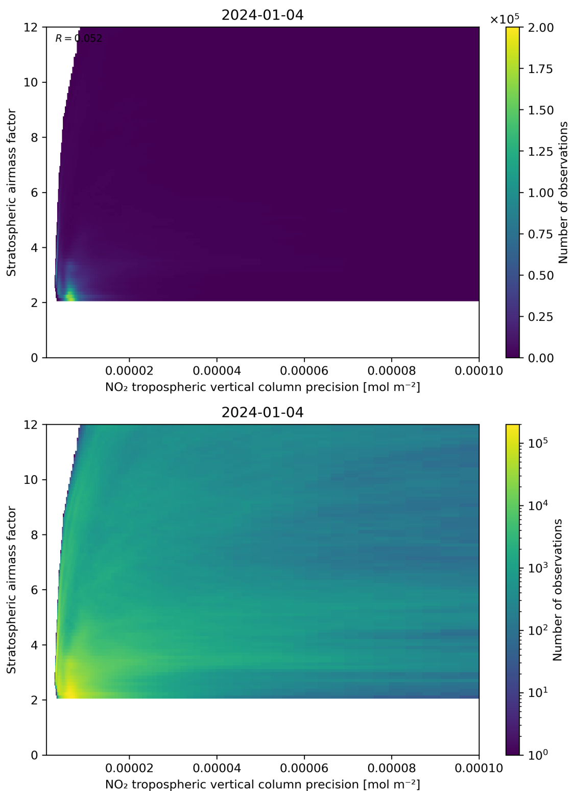
Figure 131: Scatter density plot of “NO 2 tropospheric vertical column precision” against “Stratospheric airmass factor” for 2024-01-03 to 2024-01-05.
