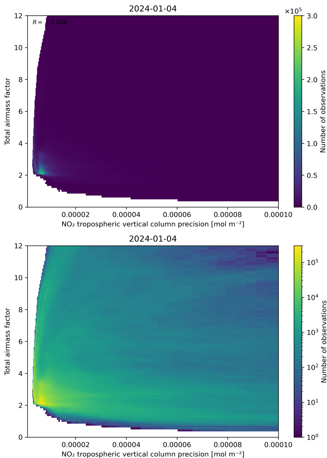
Figure 132: Scatter density plot of “NO 2 tropospheric vertical column precision” against “Total airmass factor” for 2024-01-03 to 2024-01-05.
