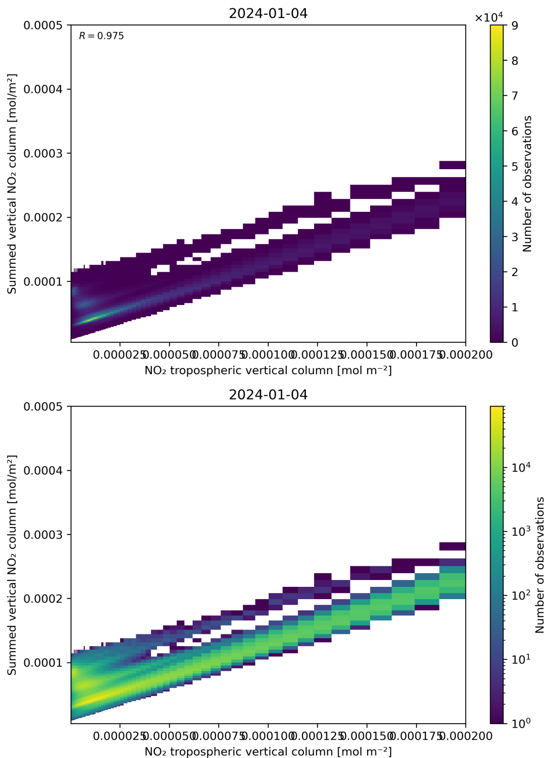
Figure 126: Scatter density plot of “NO 2 tropospheric vertical column” against “Summed vertical NO 2 column” for 2024-01-03 to 2024-01-05.
