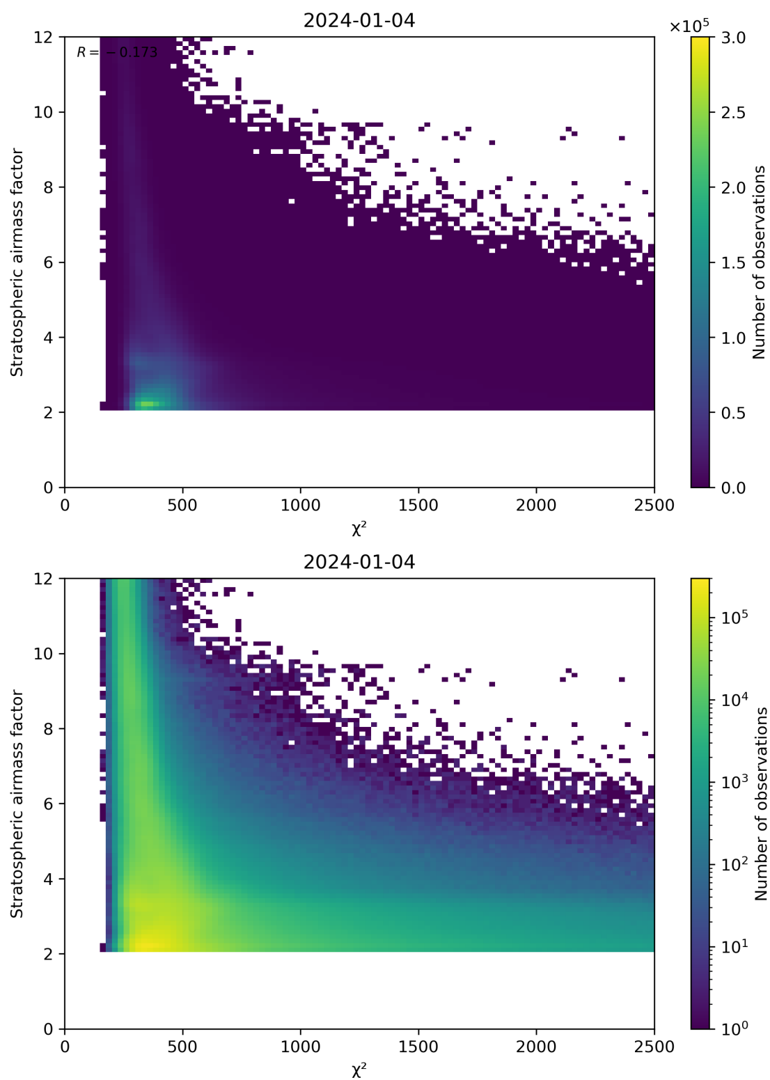
Figure 81: Scatter density plot of “ \chi^2 ” against “Stratospheric airmass factor” for 2024-01-03 to 2024-01-05.
