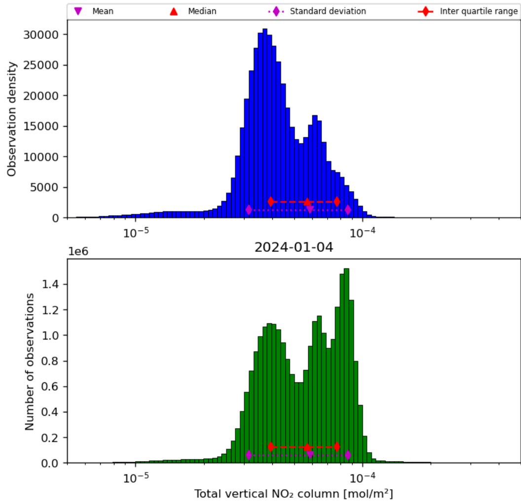
Figure 38: Histogram of “Total vertical NO 2 column” for 2024-01-03 to 2024-01-05
