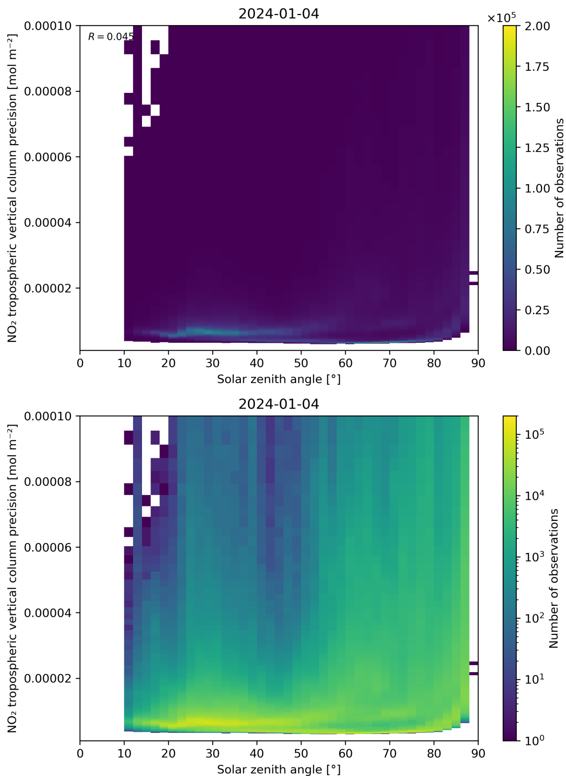
Figure 156: Scatter density plot of “Solar zenith angle” against “NO 2 tropospheric vertical column precision” for 2024-01-03 to 2024-01-05.
