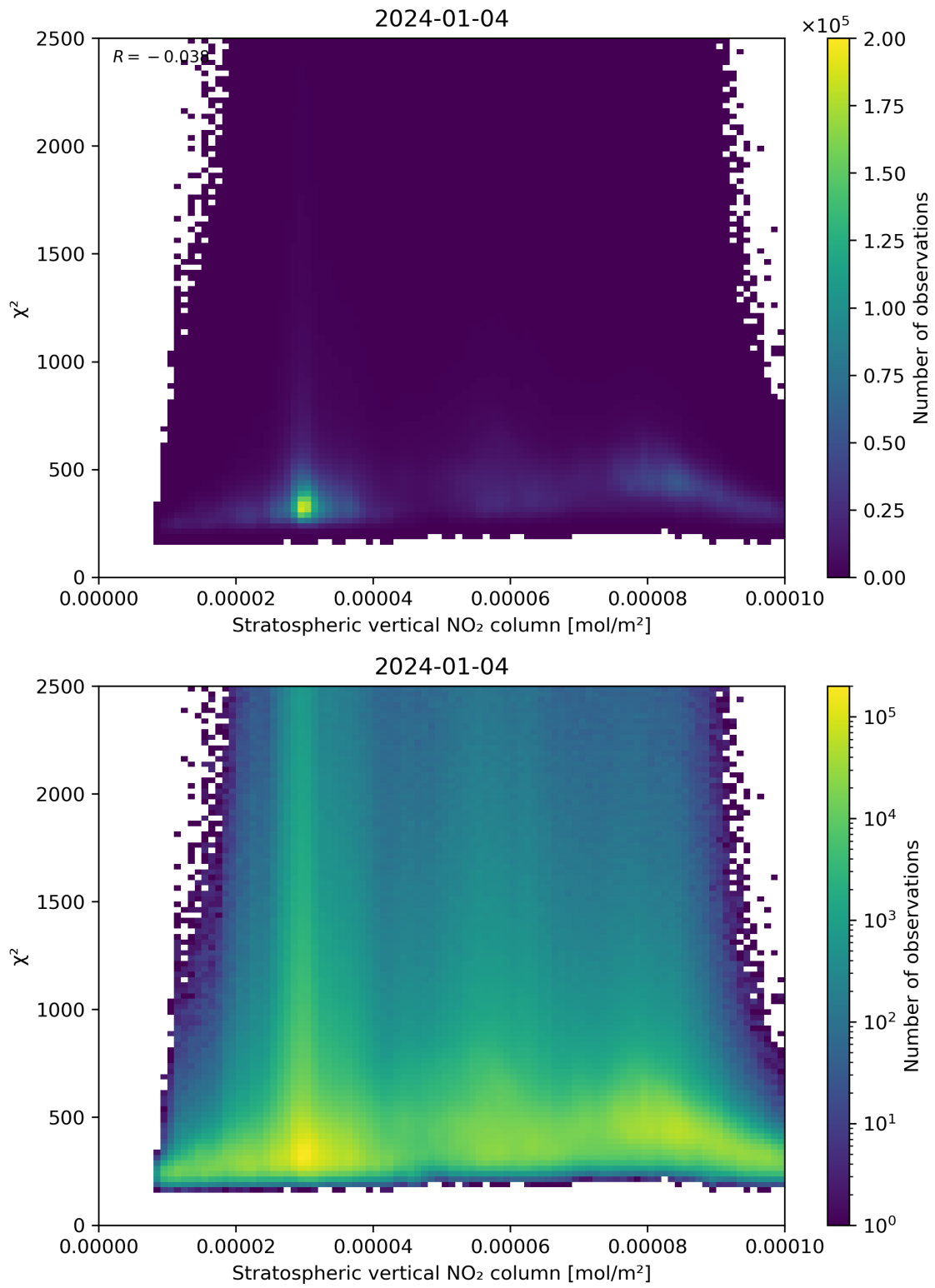
Figure 97: Scatter density plot of “Stratospheric vertical NO 2 column” against “ \chi^2 ” for 2024-01-03 to 2024-01-05.
