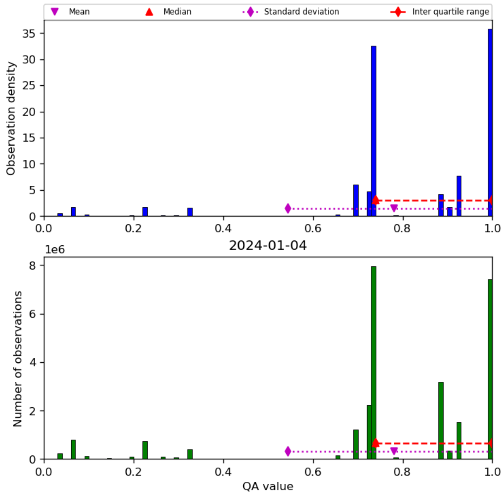
Figure 28: Histogram of “QA value” for 2024-01-03 to 2024-01-05
