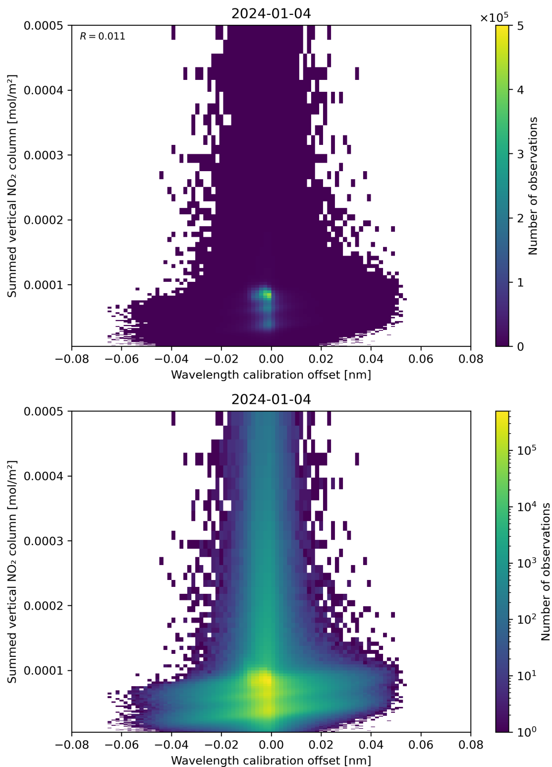
Figure 177: Scatter density plot of “Wavelength calibration offset” against “Summed vertical NO 2 column” for 2024-01-03 to 2024-01-05.
