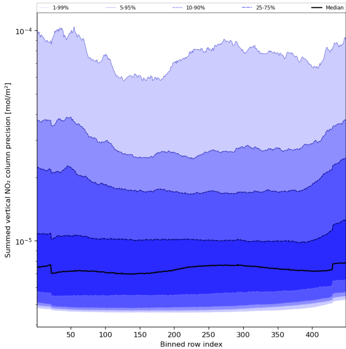
Figure 58: Along track statistics of “Summed vertical NO 2 column precision” for 2024-01-03 to 2024-01-05
