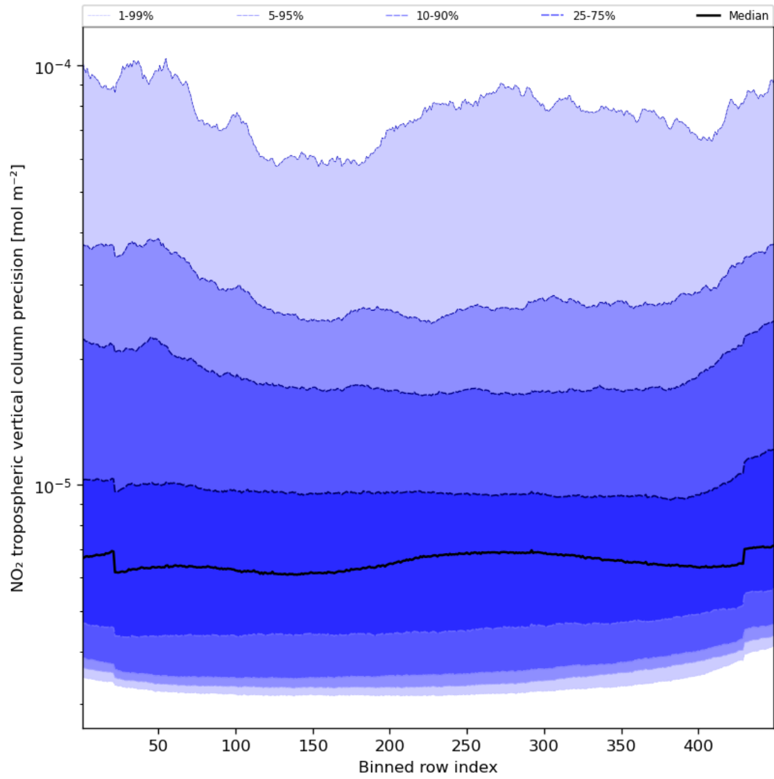
Figure 47: Along track statistics of “NO 2 tropospheric vertical column precision” for 2024-01-03 to 2024-01-05
