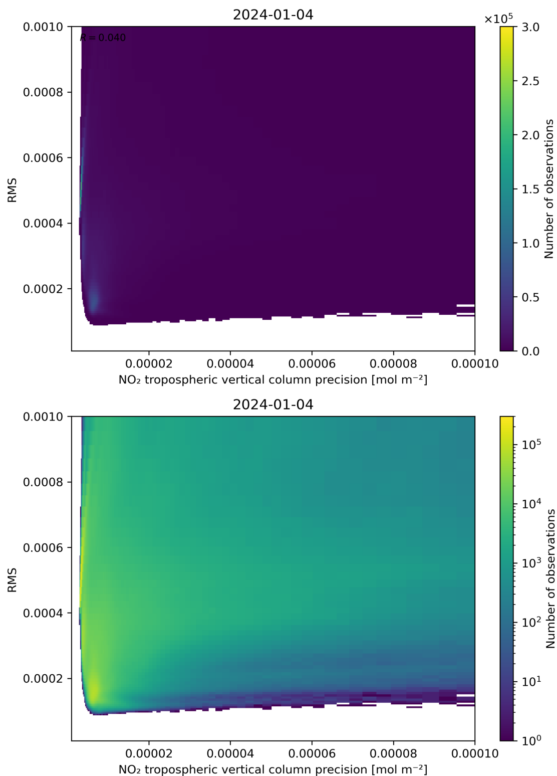
Figure 140: Scatter density plot of “NO 2 tropospheric vertical column precision” against “RMS” for 2024-01-03 to 2024-01-05.
