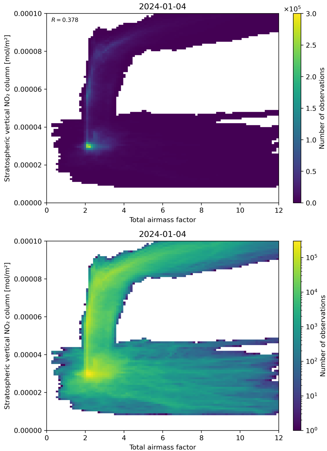
Figure 64: Scatter density plot of “Total airmass factor” against “Stratospheric vertical \text{NO}_2 column” for 2024-01-03 to 2024-01-05.
