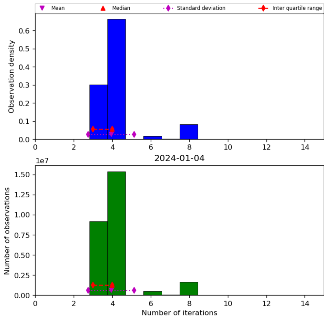
Figure 34: Histogram of “Number of iterations” for 2024-01-03 to 2024-01-05
