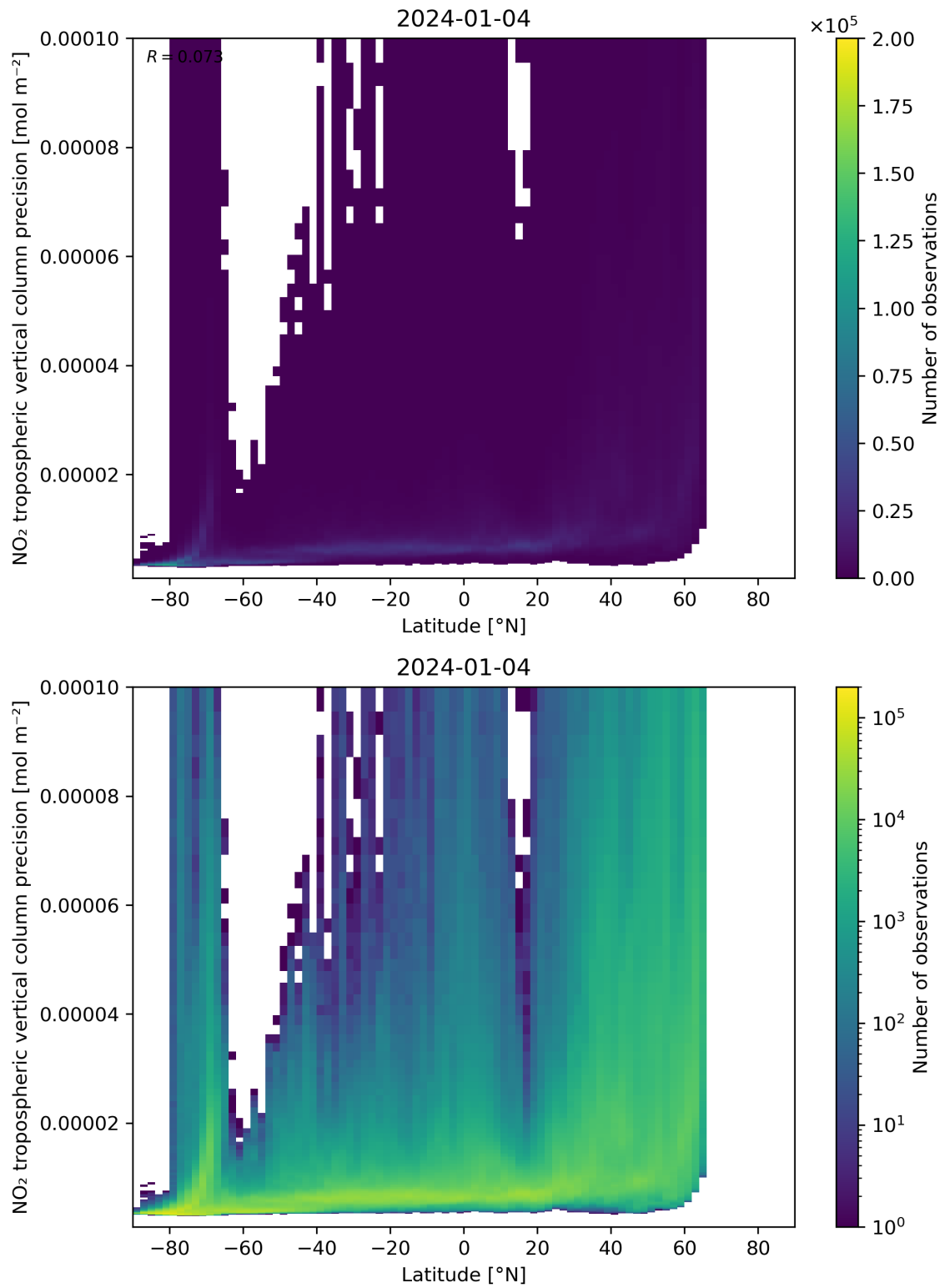
Figure 93: Scatter density plot of “Latitude” against “NO 2 tropospheric vertical column precision” for 2024-01-03 to 2024-01-05.
