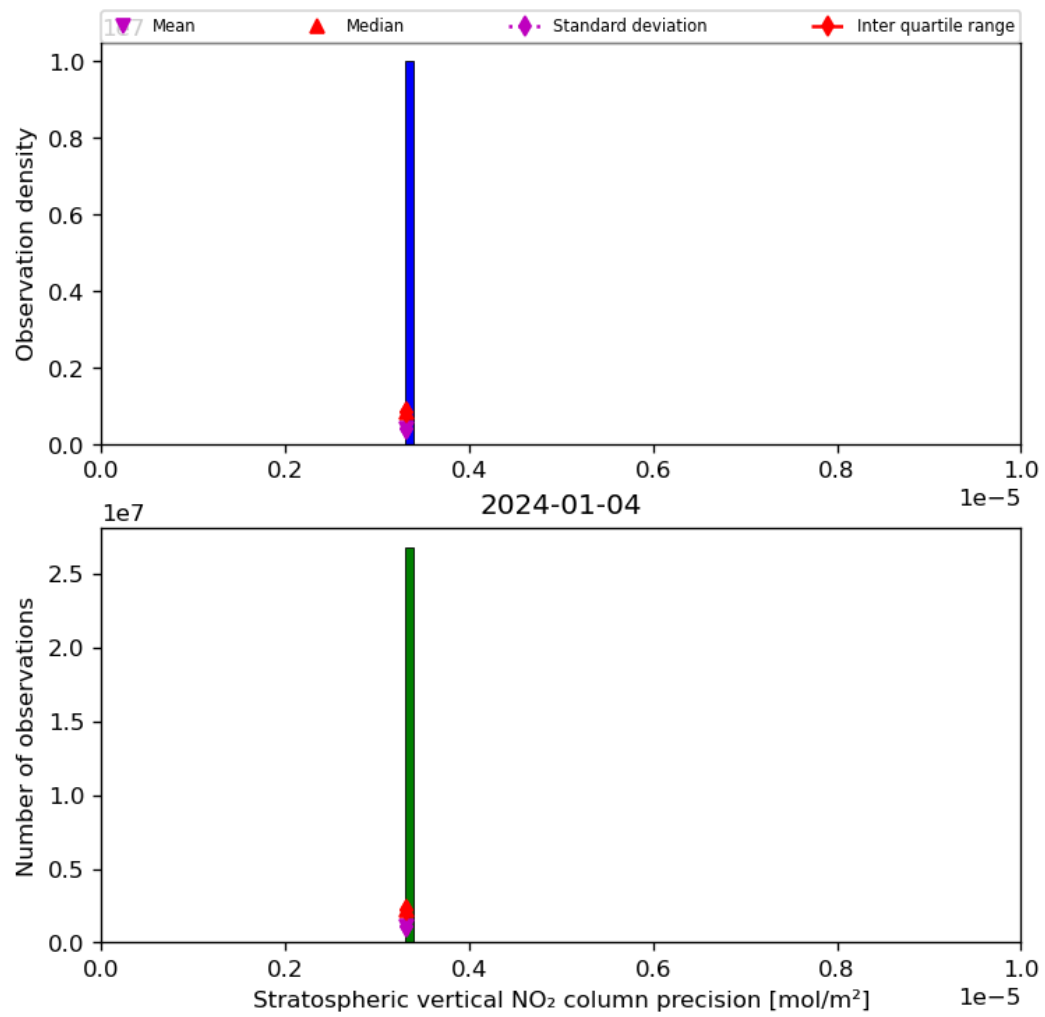
Figure 37: Histogram of “Stratospheric vertical NO 2 column precision” for 2024-01-03 to 2024-01-05
