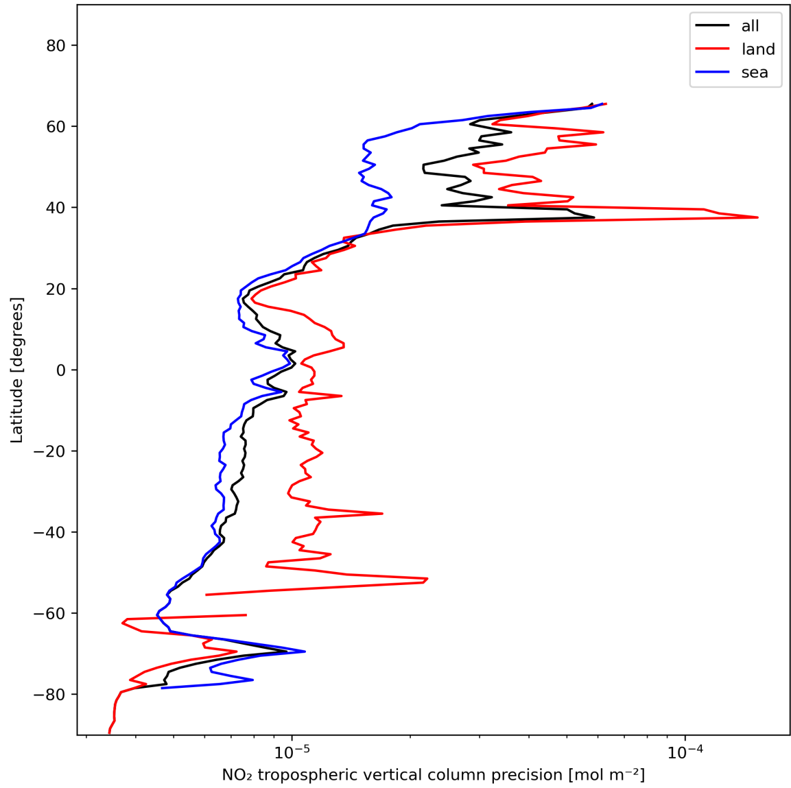
Figure 13: Zonal average of “NO 2 tropospheric vertical column precision” for 2024-01-03 to 2024-01-05.
