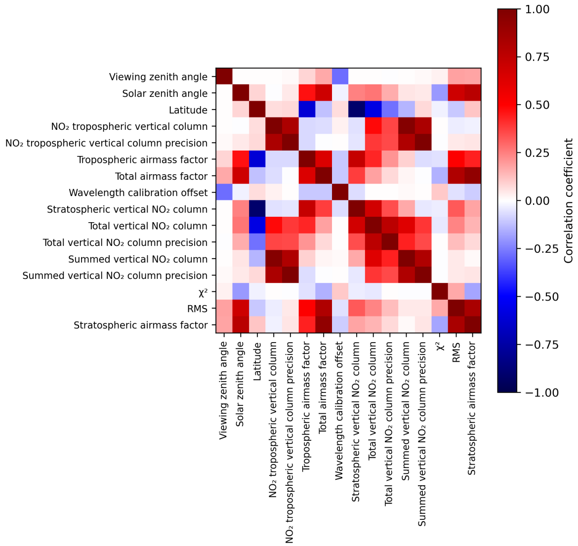
Figure 2: Map of correlation matrix for 2024-01-03 to 2024-01-05.
