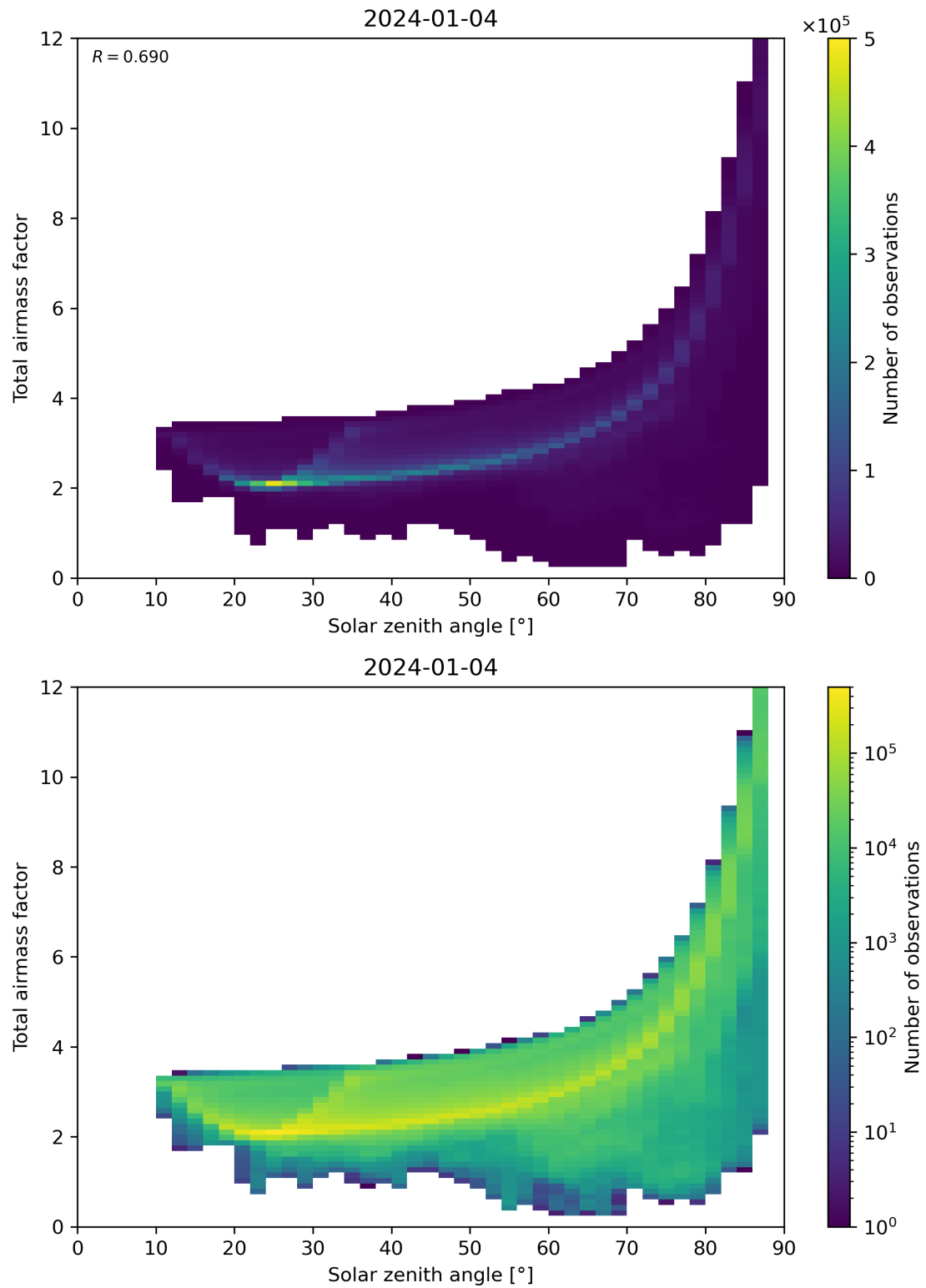
Figure 146: Scatter density plot of “Solar zenith angle” against “Total air mass factor” for 2024-01-03 to 2024-01-05.
