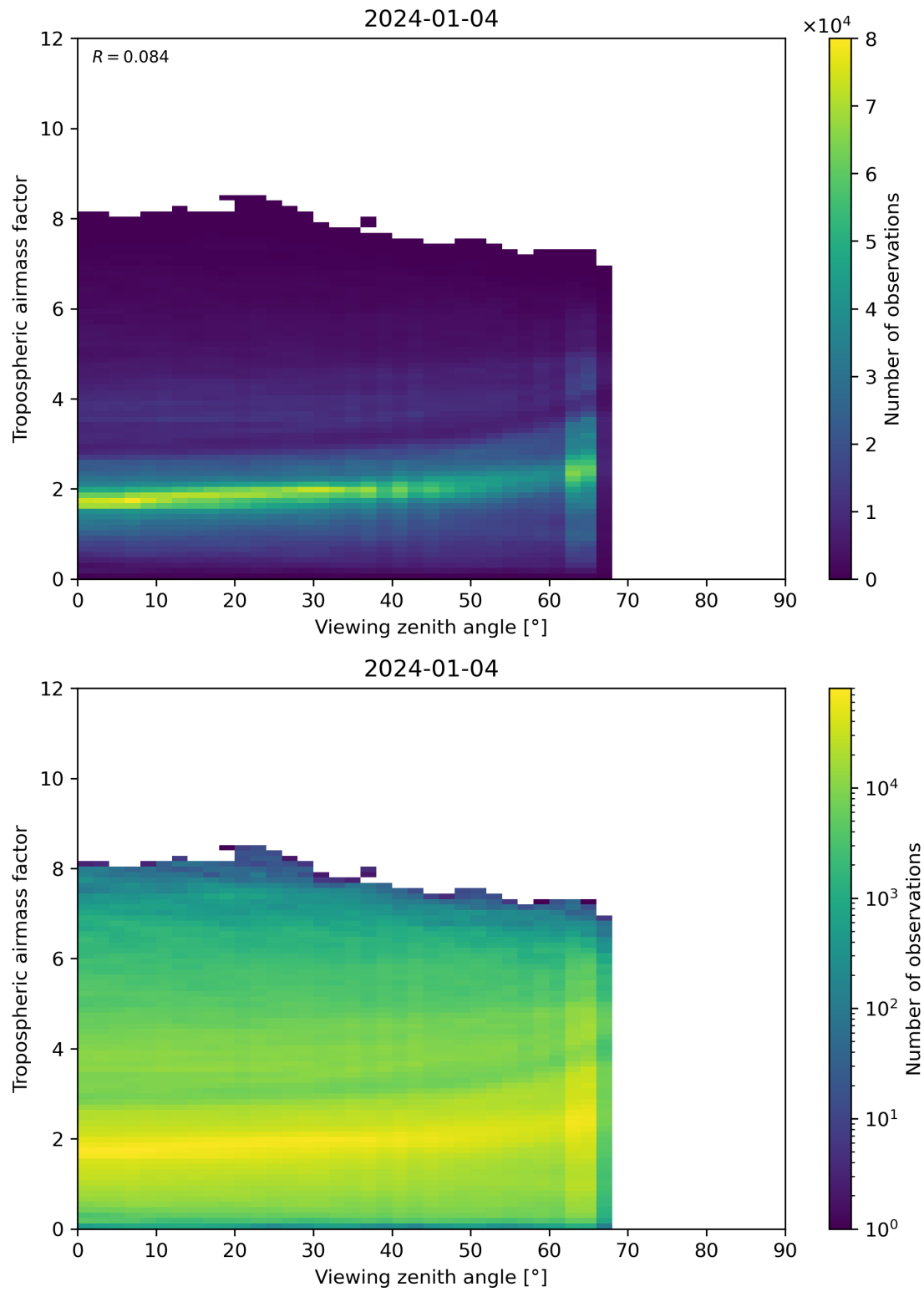
Figure 161: Scatter density plot of “Viewing zenith angle” against “Tropospheric airmass factor” for 2024-01-03 to 2024-01-05.
