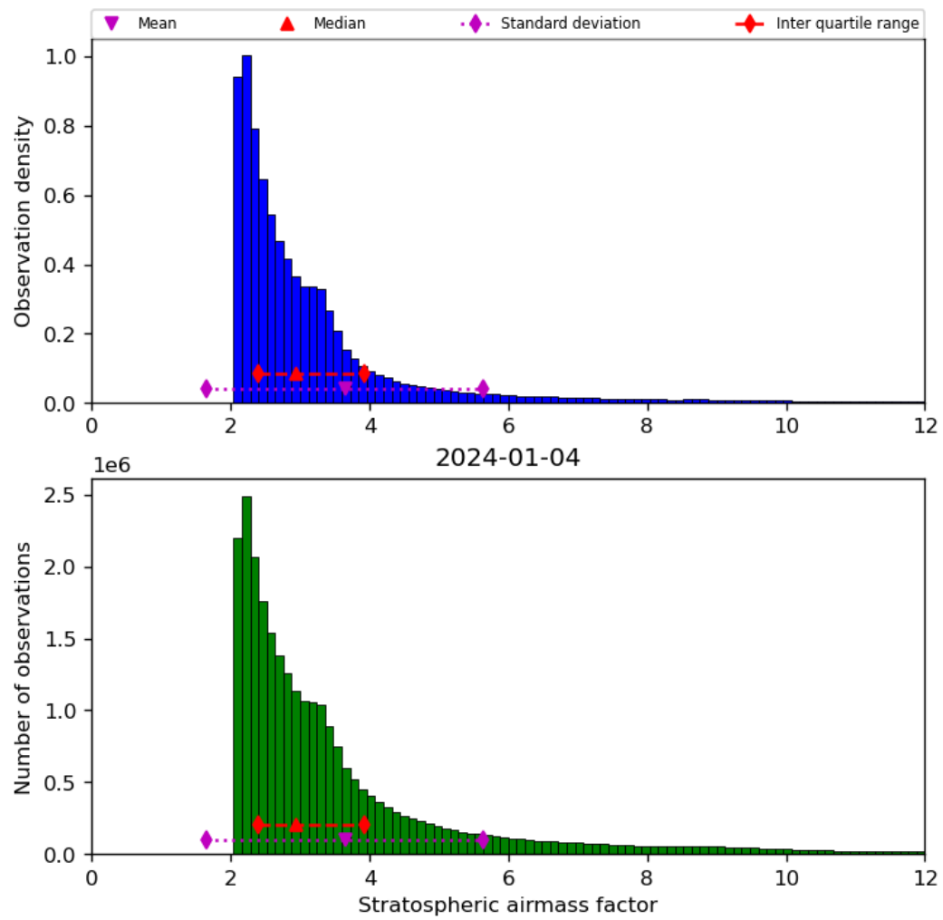
Figure 44: Histogram of “Stratospheric airmass factor” for 2024-01-03 to 2024-01-05
