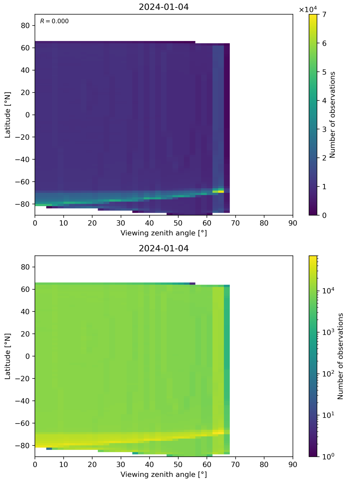
Figure 163: Scatter density plot of “Viewing zenith angle” against “Latitude” for 2024-01-03 to 2024-01-05.
