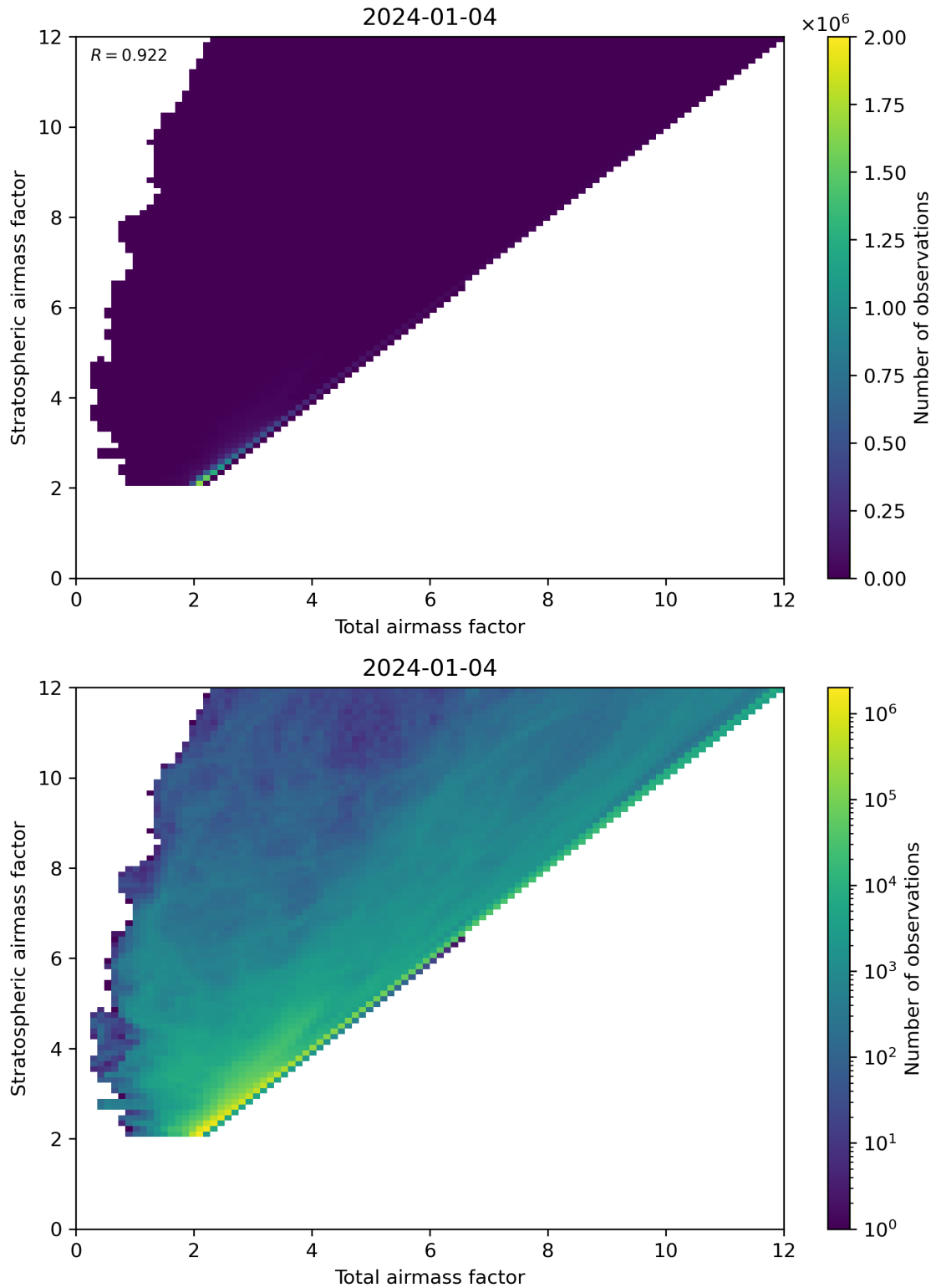
Figure 62: Scatter density plot of “Total airmass factor” against “Stratospheric airmass factor” for 2024-01-03 to 2024-01-05.
