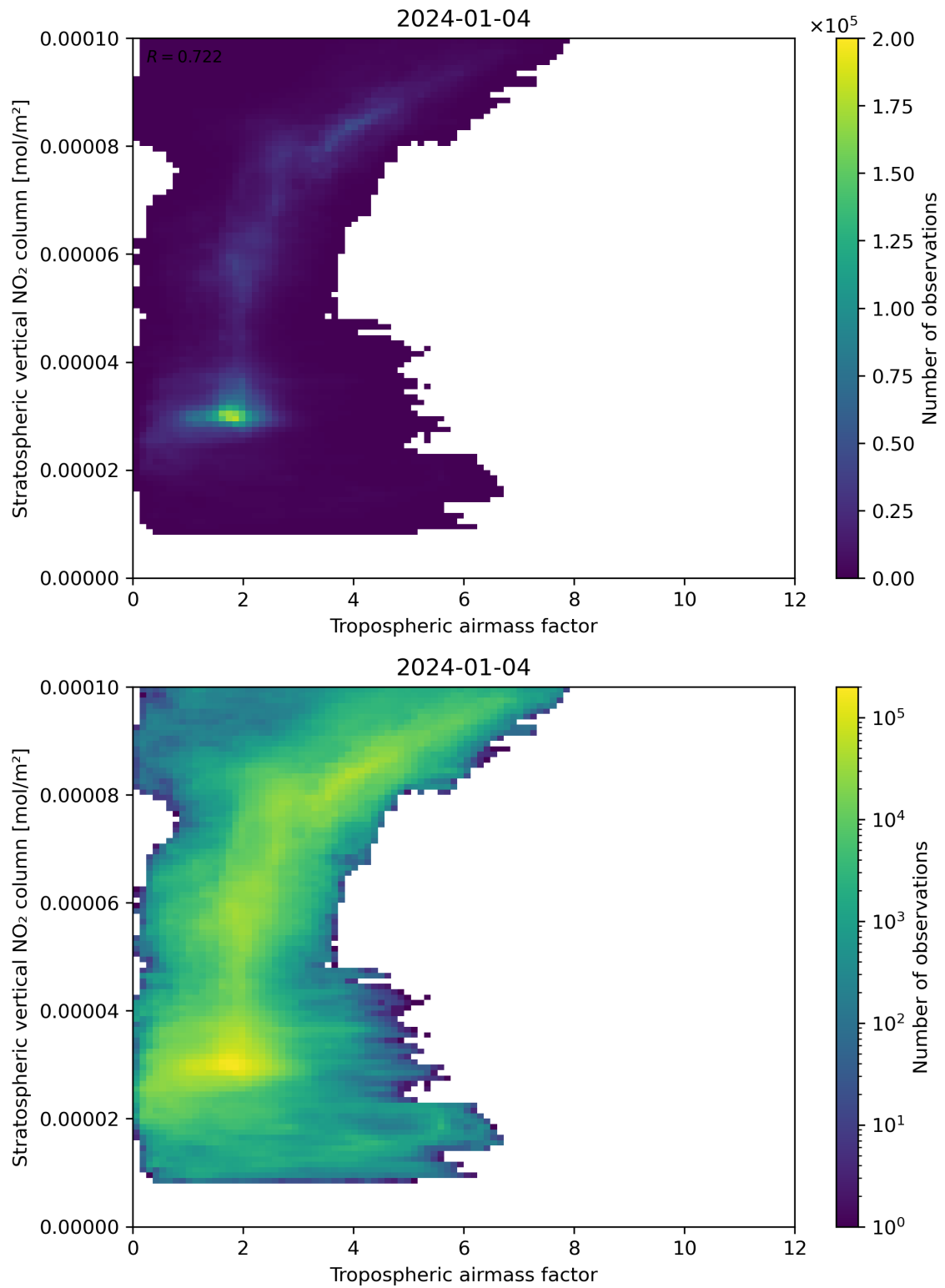
Figure 74: Scatter density plot of “Tropospheric air mass factor” against “Stratospheric vertical NO 2 column” for 2024-01-03 to 2024-01-05.
