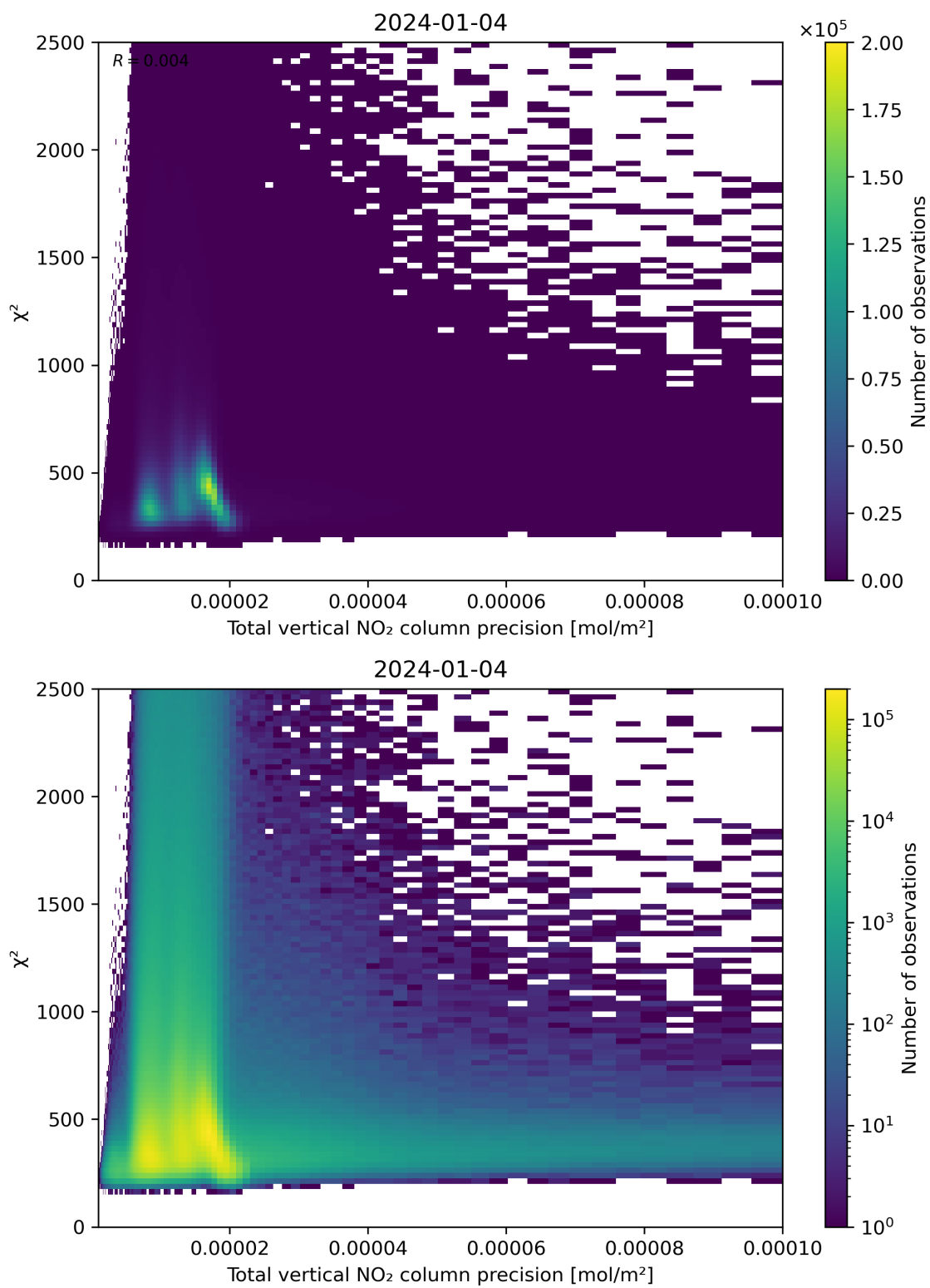
Figure 116: Scatter density plot of “Total vertical NO 2 column precision” against “ \chi^2 ” for 2024-01-03 to 2024-01-05.
