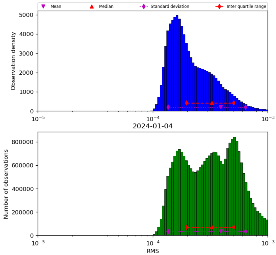
Figure 43: Histogram of “RMS” for 2024-01-03 to 2024-01-05
