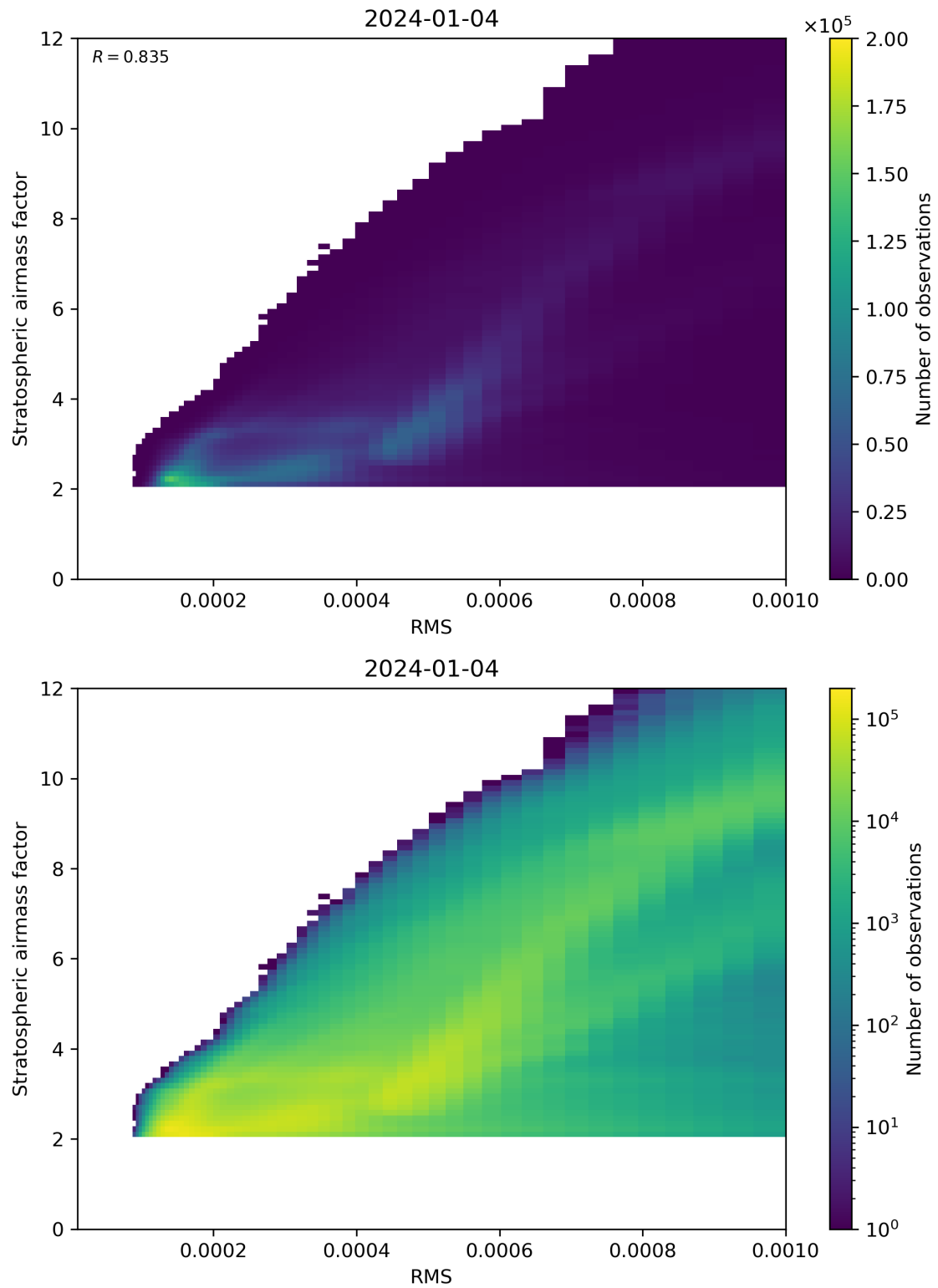
Figure 144: Scatter density plot of “RMS” against “Stratospheric airmass factor” for 2024-01-03 to 2024-01-05.
