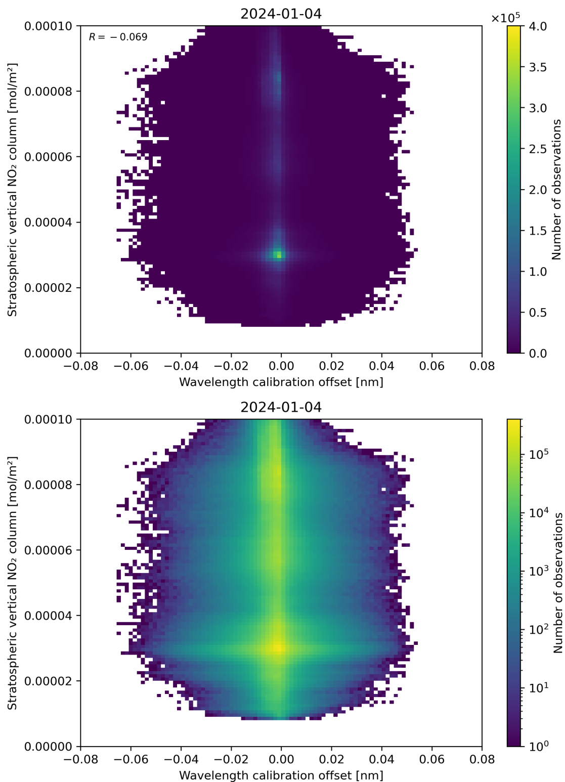
Figure 176: Scatter density plot of “Wavelength calibration offset” against “Stratospheric vertical NO 2 column” for 2024-01-03 to 2024-01-05.
