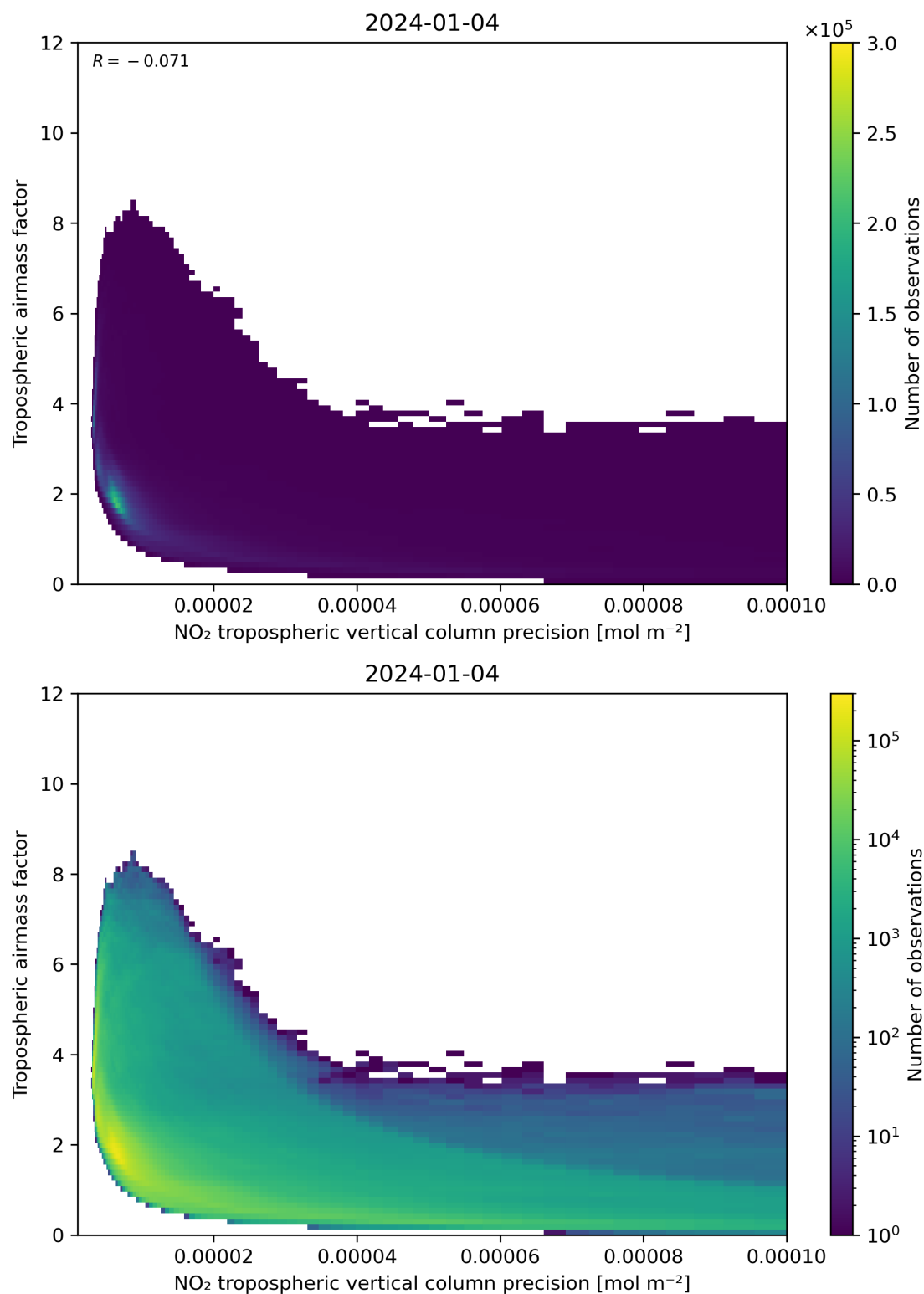
Figure 133: Scatter density plot of “NO 2 tropospheric vertical column precision” against “Tropospheric airmass factor” for 2024-01-03 to 2024-01-05.
