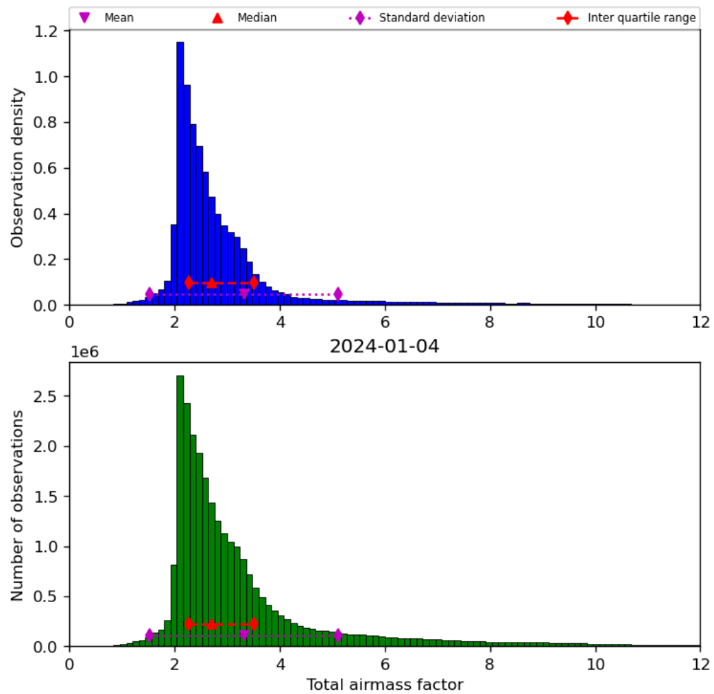
Figure 32: Histogram of “Total airmass factor” for 2024-01-03 to 2024-01-05
