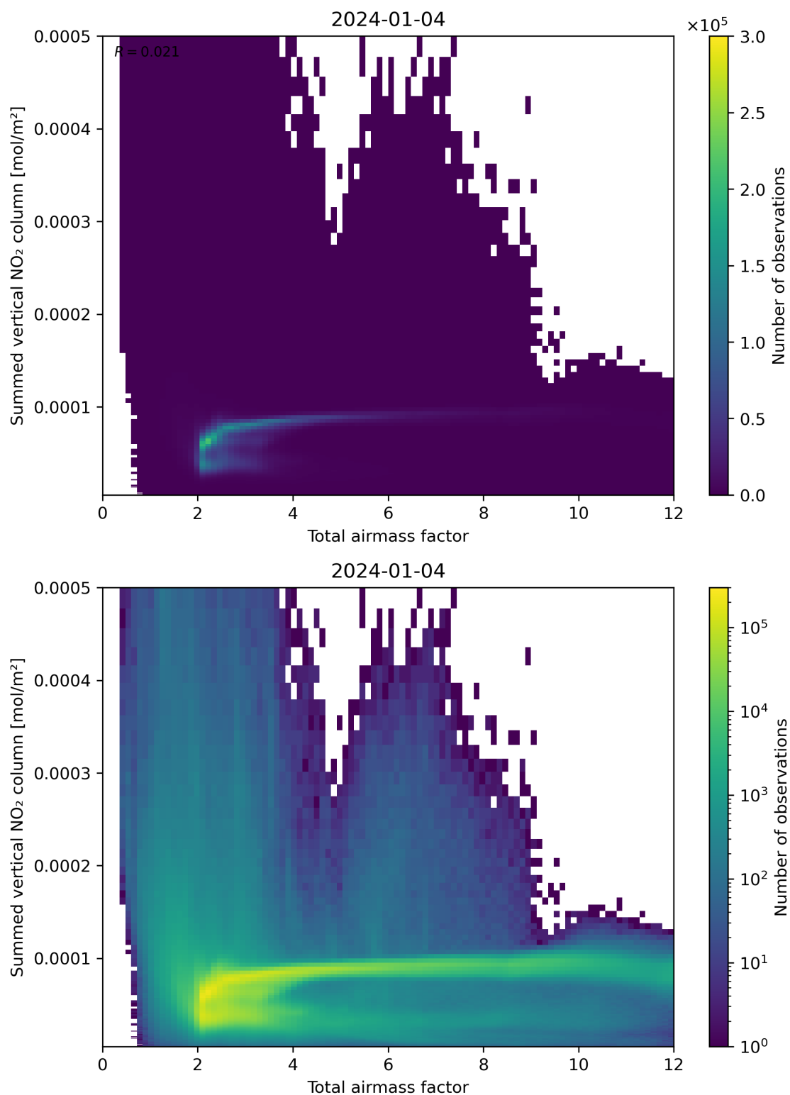
Figure 65: Scatter density plot of “Total airmass factor” against “Summed vertical NO 2 column” for 2024-01-03 to 2024-01-05.
