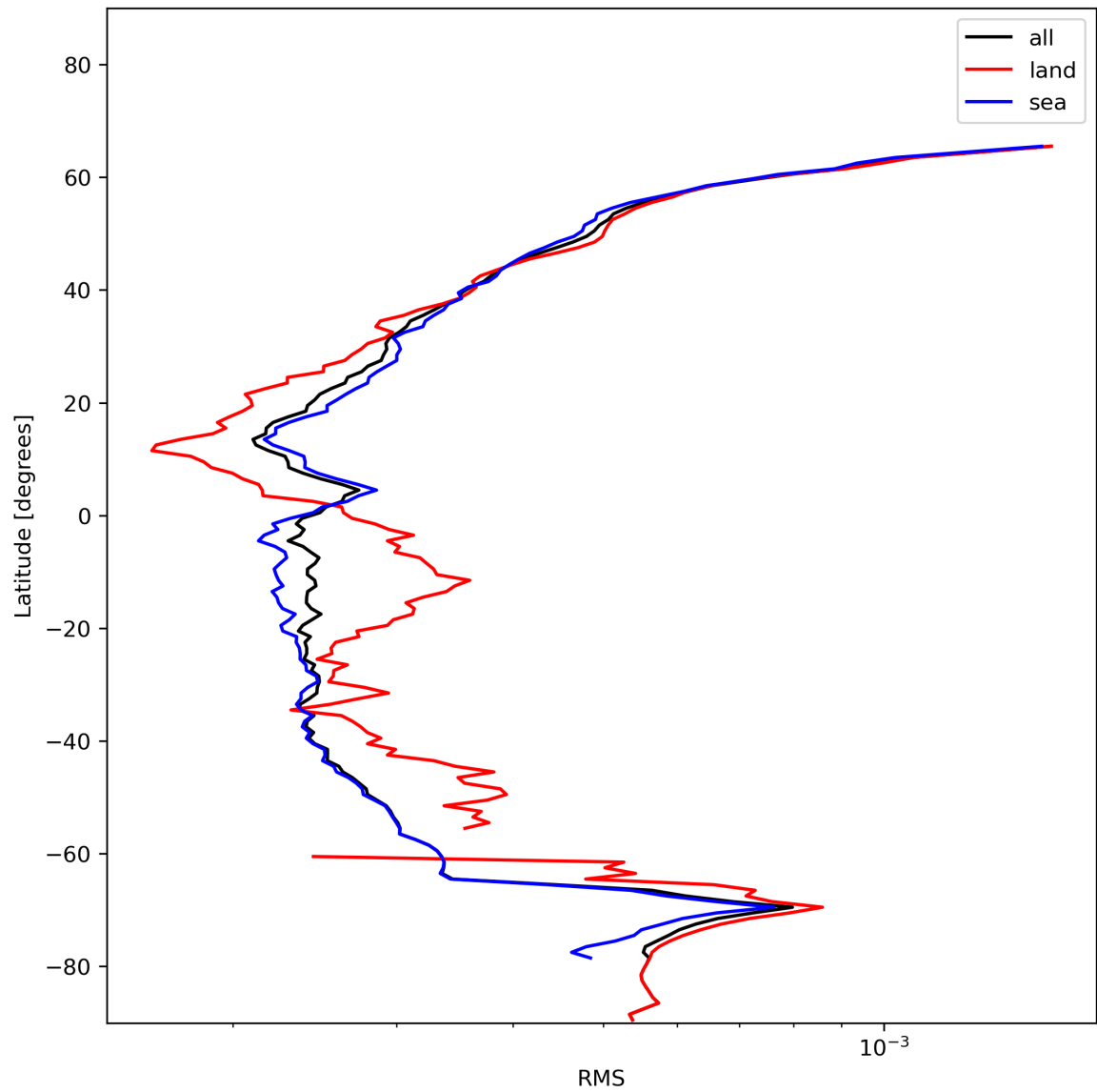
Figure 26: Zonal average of “RMS” for 2024-01-03 to 2024-01-05.
