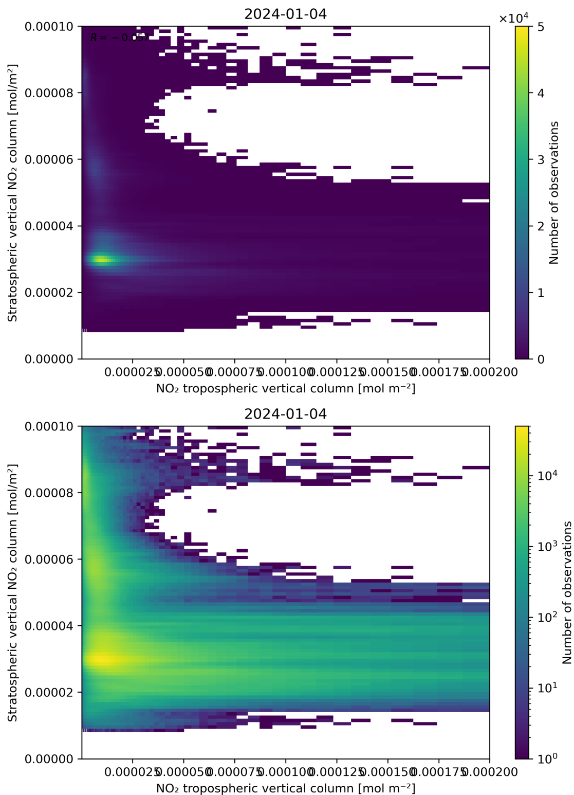
Figure 125: Scatter density plot of “NO 2 tropospheric vertical column” against “Stratospheric vertical NO 2 column” for 2024-01-03 to 2024-01-05.
