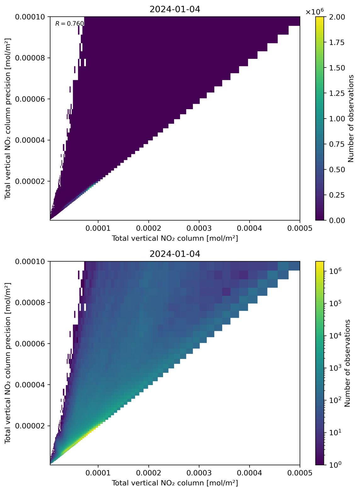
Figure 114: Scatter density plot of “Total vertical NO 2 column” against “Total vertical NO 2 column precision” for 2024-01-03 to 2024-01-05.
