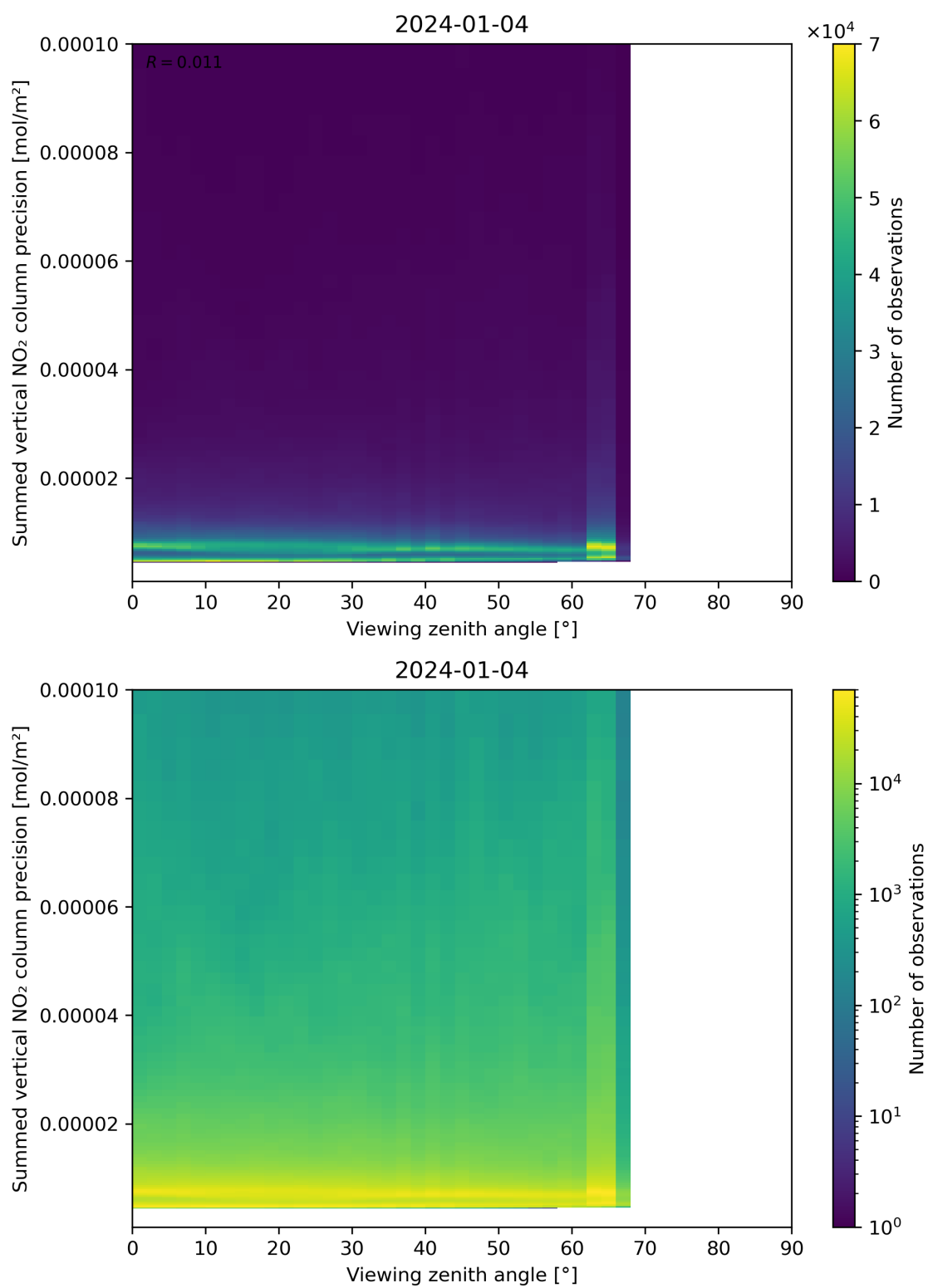
Figure 166: Scatter density plot of “Viewing zenith angle” against “Summed vertical NO 2 column precision” for 2024-01-03 to 2024-01-05.
