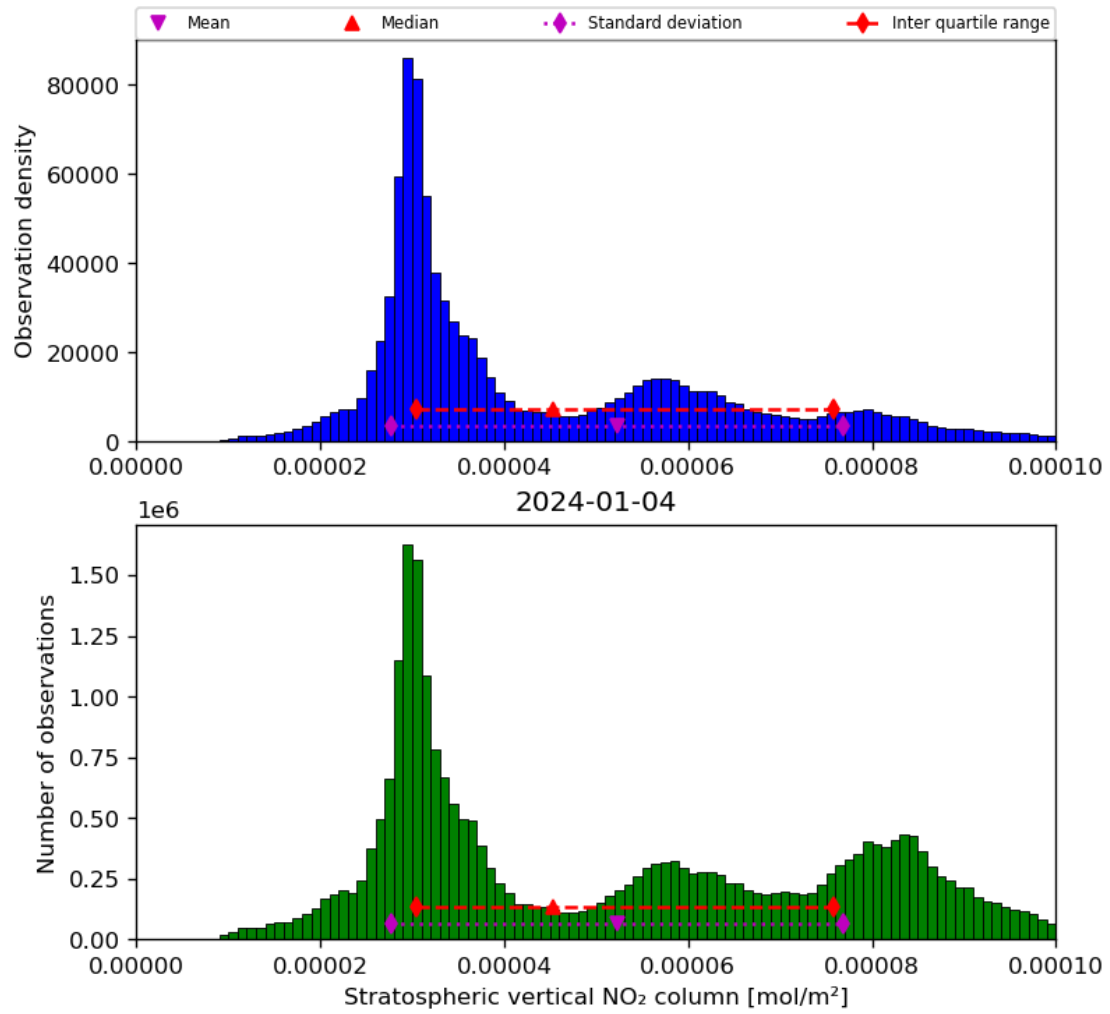
Figure 36: Histogram of “Stratospheric vertical NO 2 column” for 2024-01-03 to 2024-01-05
