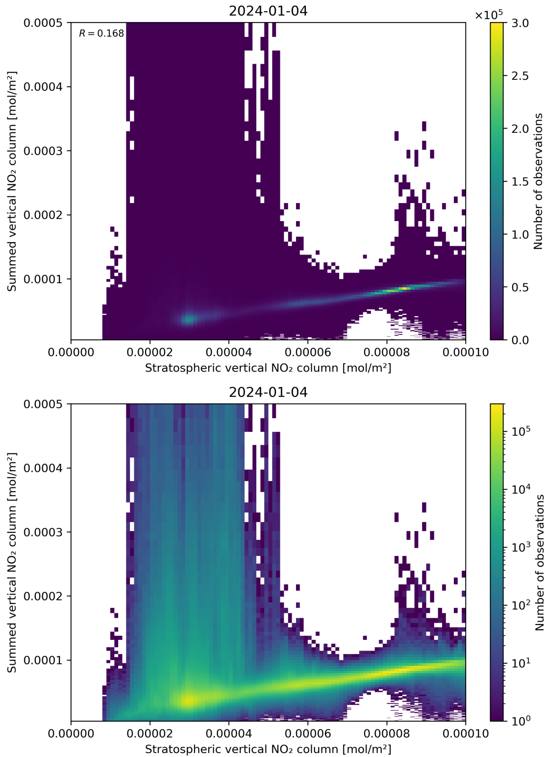
Figure 98: Scatter density plot of “Stratospheric vertical NO 2 column” against “Summed vertical NO 2 column” for 2024-01-03 to 2024-01-05.
