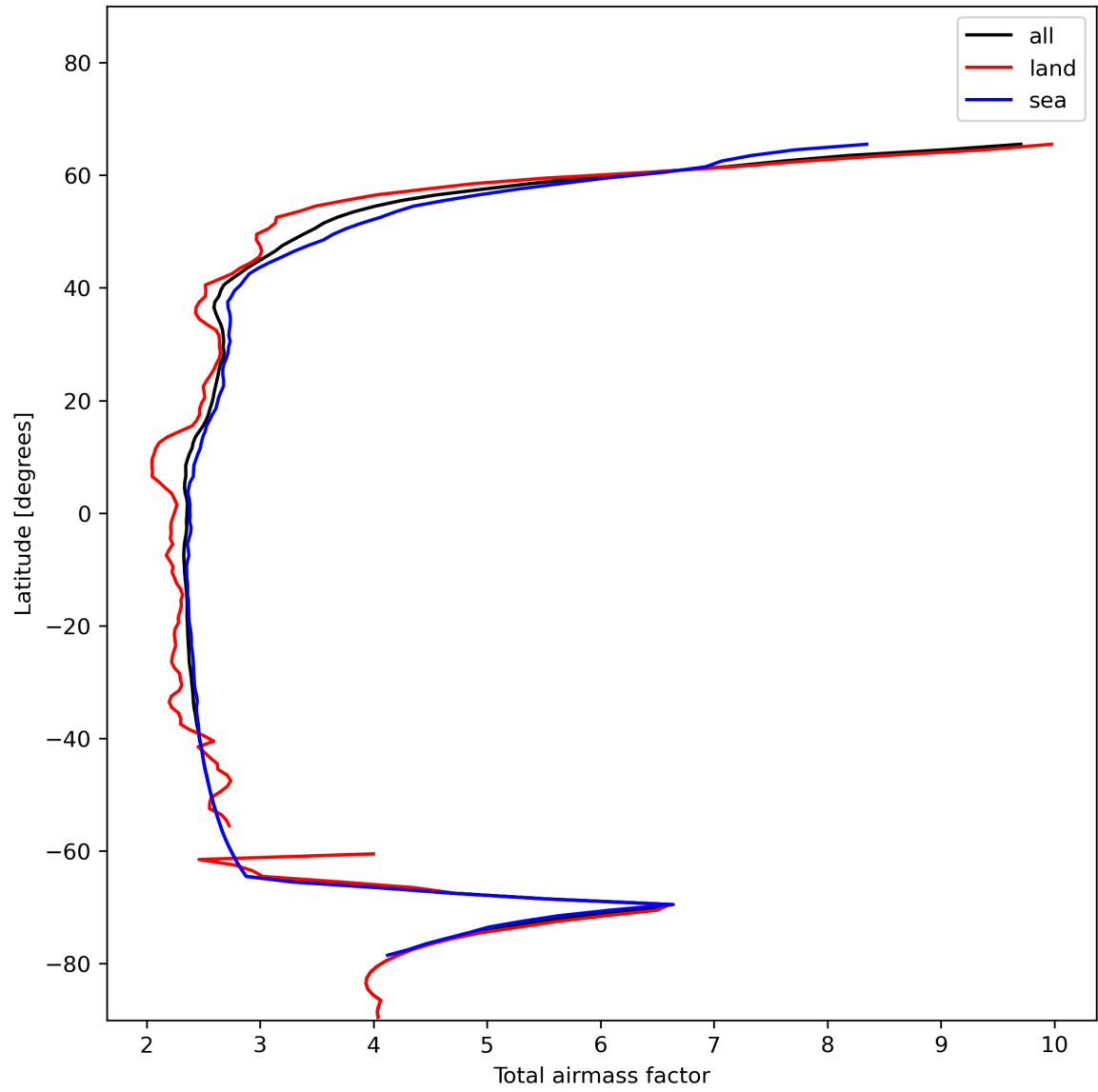
Figure 15: Zonal average of “Total airmass factor” for 2024-01-03 to 2024-01-05.
