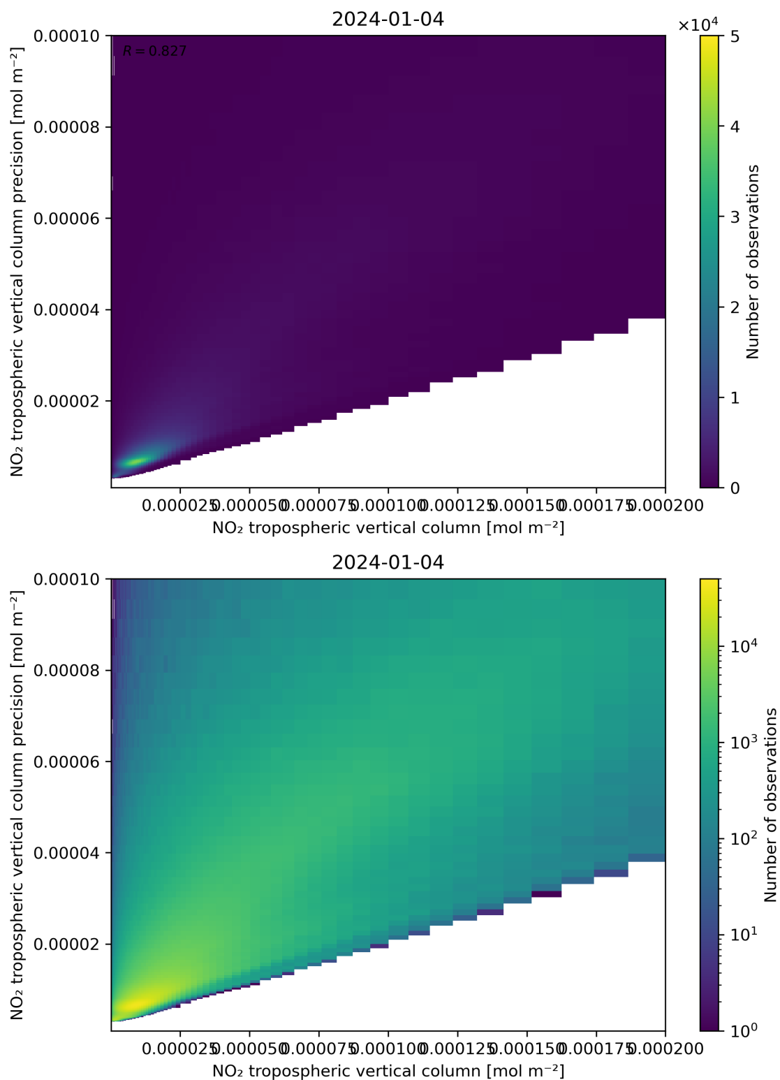
Figure 130: Scatter density plot of “NO 2 tropospheric vertical column” against “NO 2 tropospheric vertical column precision” for 2024-01-03 to 2024-01-05.
