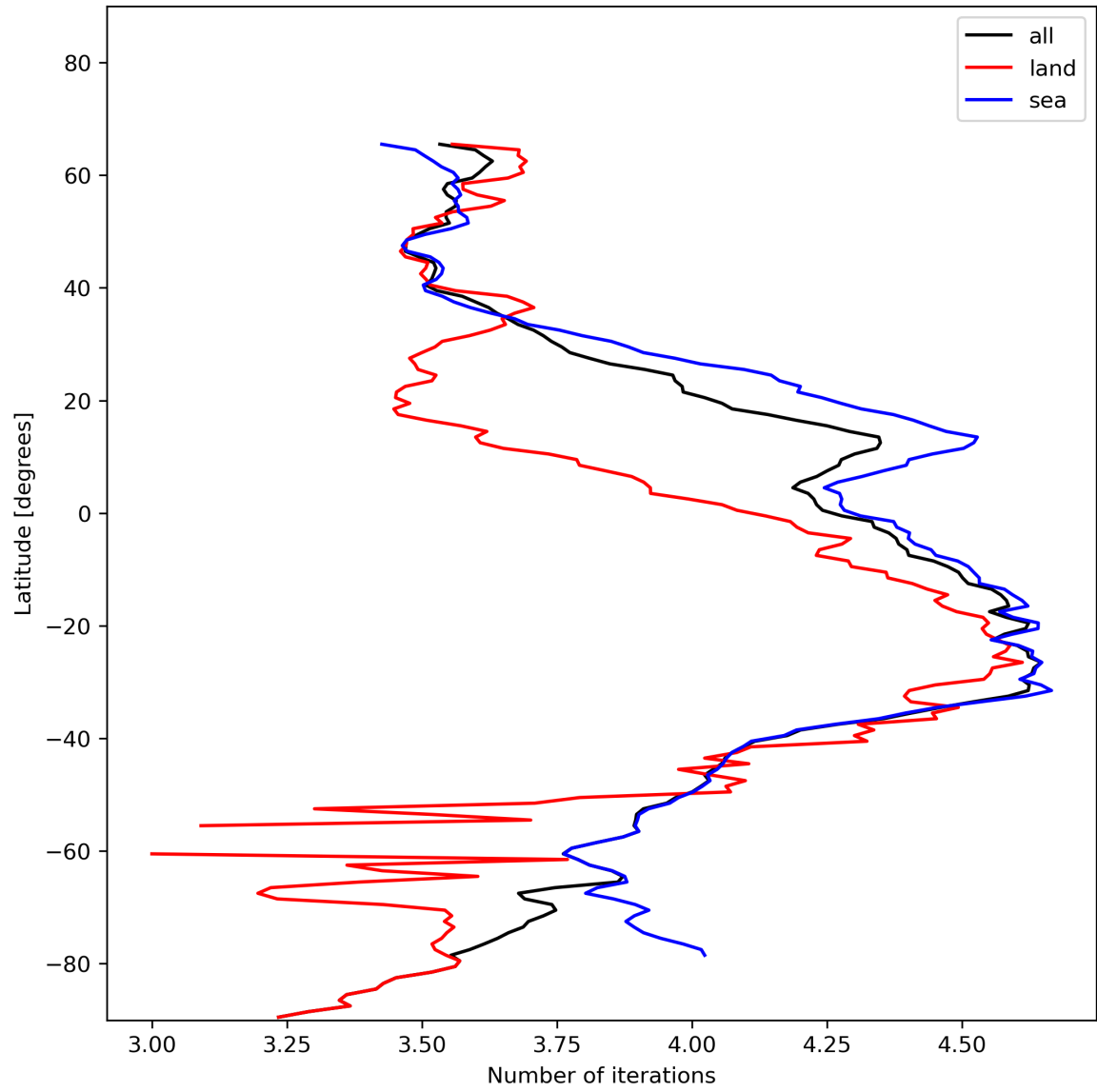
Figure 17: Zonal average of “Number of iterations” for 2024-01-03 to 2024-01-05.
