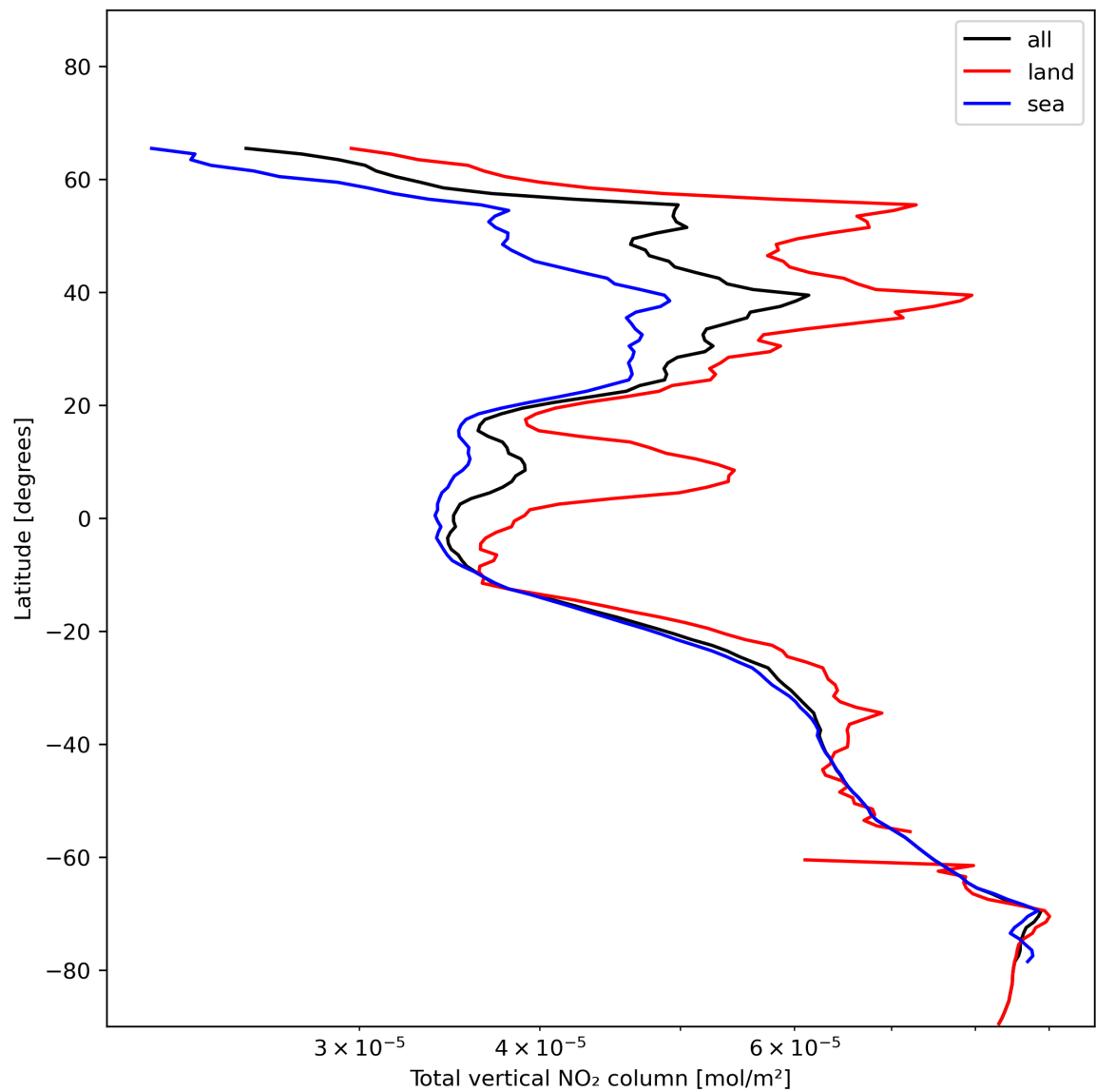
Figure 21: Zonal average of “Total vertical NO 2 column” for 2024-01-03 to 2024-01-05.
