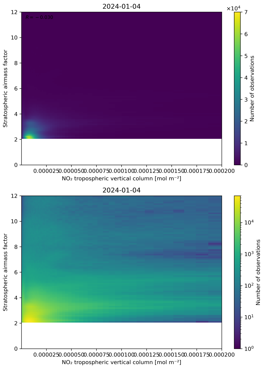
Figure 121: Scatter density plot of “NO 2 tropospheric vertical column” against “Stratospheric airmass factor” for 2024-01-03 to 2024-01-05.
