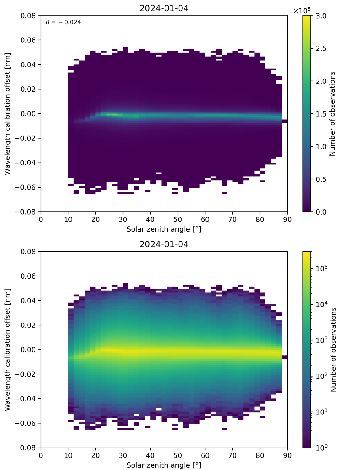
Figure 158: Scatter density plot of “Solar zenith angle” against “Wavelength calibration offset” for 2024-01-03 to 2024-01-05.
