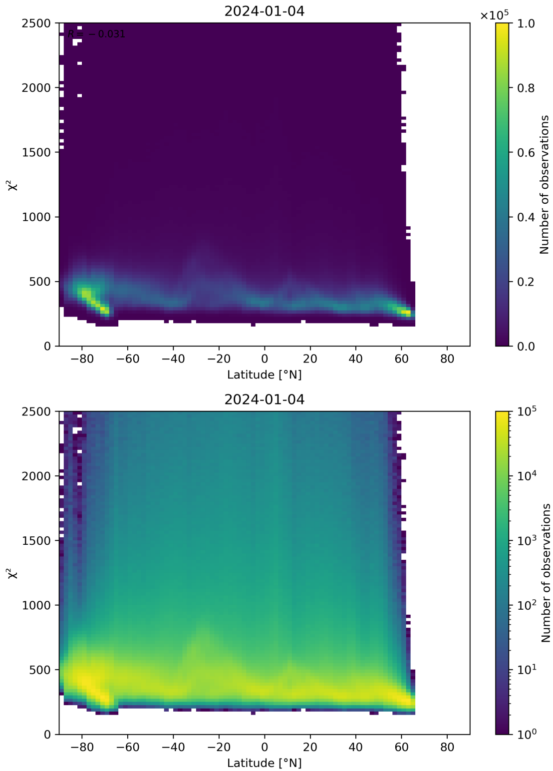
Figure 86: Scatter density plot of “Latitude” against “ \chi^2 ” for 2024-01-03 to 2024-01-05.
