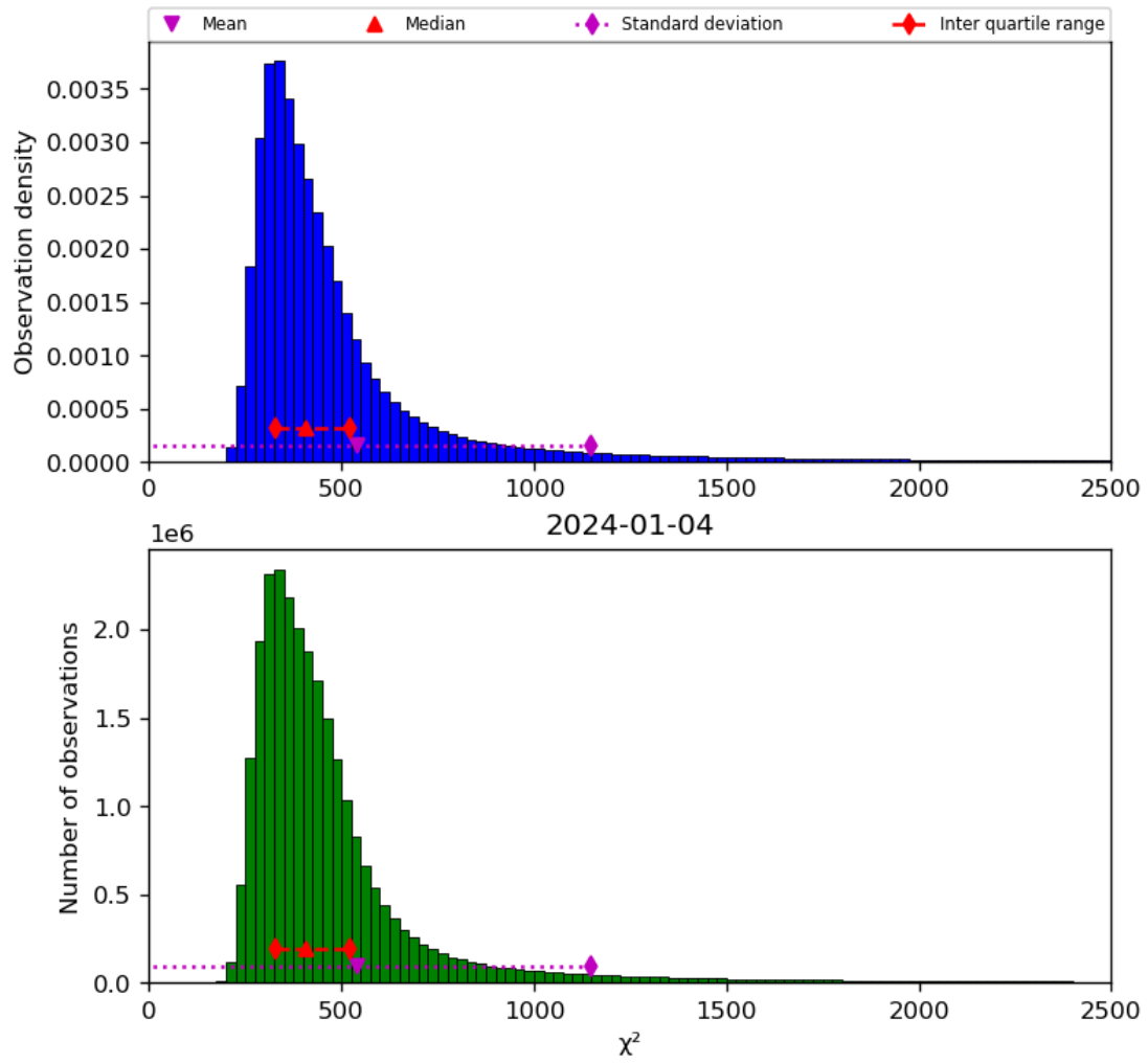
Figure 42: Histogram of “ \chi^2 ” for 2024-01-03 to 2024-01-05
