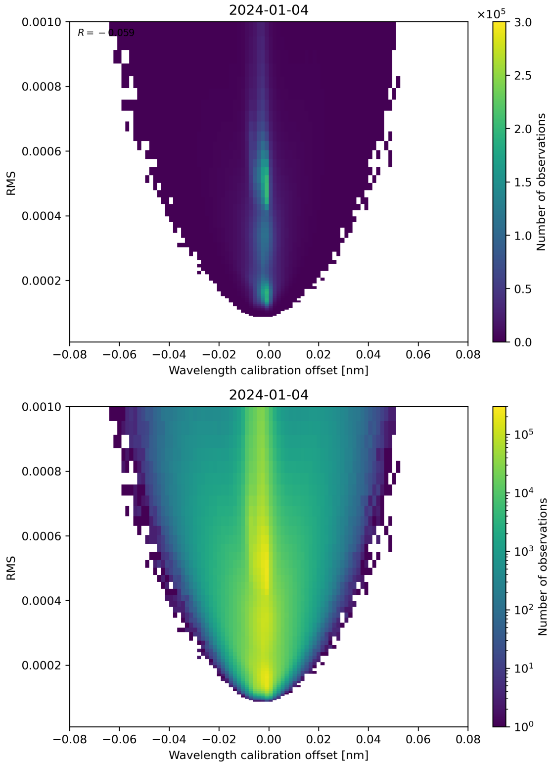
Figure 181: Scatter density plot of “Wavelength calibration offset” against “RMS” for 2024-01-03 to 2024-01-05.
