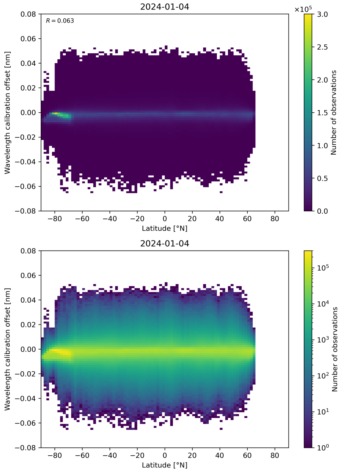
Figure 95: Scatter density plot of “Latitude” against “Wavelength calibration offset” for 2024-01-03 to 2024-01-05.
