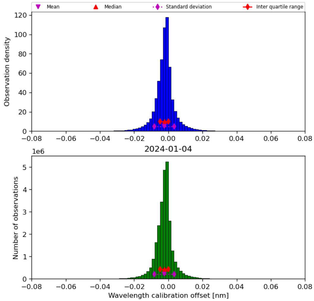
Figure 35: Histogram of “Wavelength calibration offset” for 2024-01-03 to 2024-01-05
