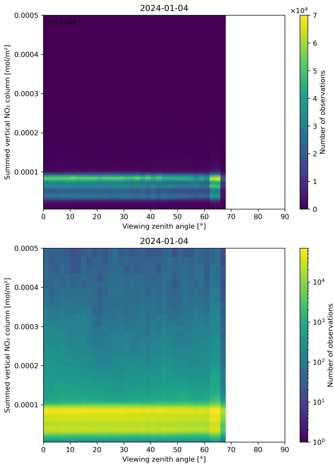
Figure 165: Scatter density plot of “Viewing zenith angle” against “Summed vertical NO 2 column” for 2024-01-03 to 2024-01-05.
