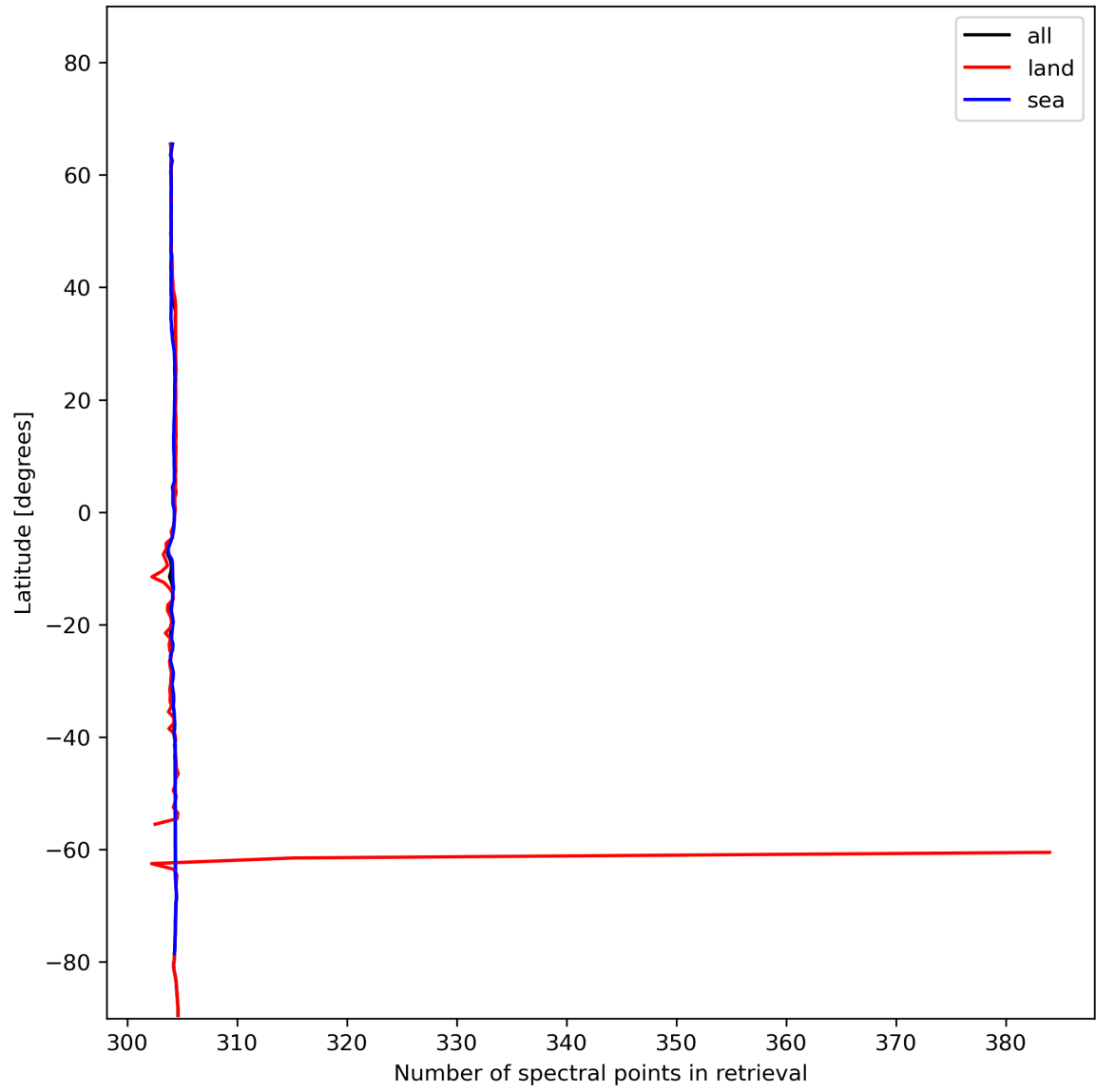
Figure 16: Zonal average of “Number of spectral points in retrieval” for 2024-01-03 to 2024-01-05.
