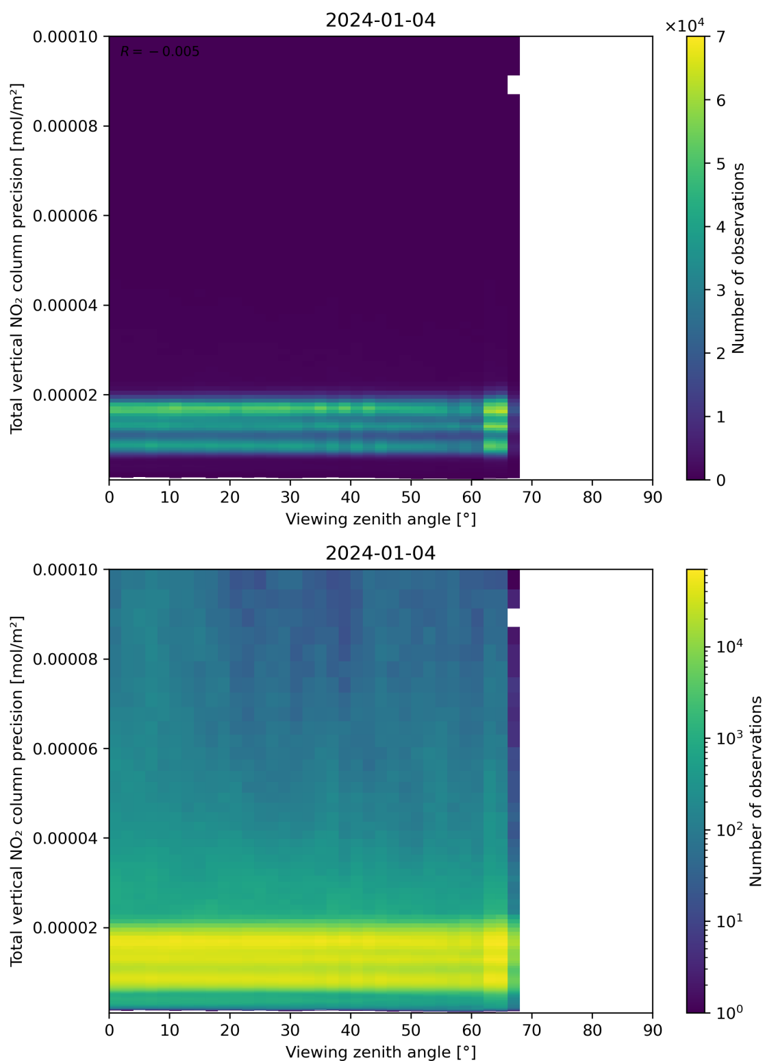
Figure 168: Scatter density plot of “Viewing zenith angle” against “Total vertical NO 2 column precision” for 2024-01-03 to 2024-01-05.
