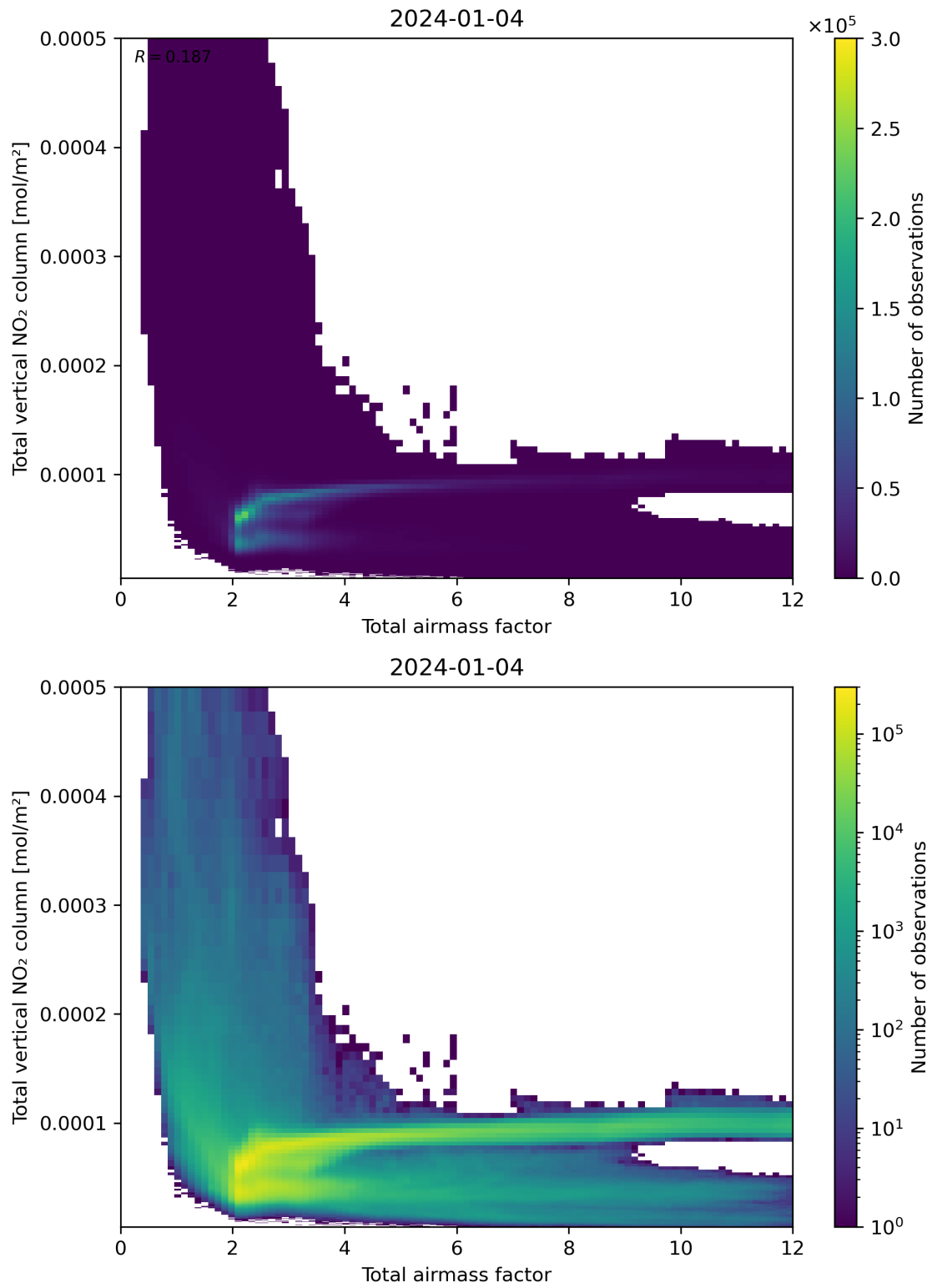
Figure 67: Scatter density plot of “Total airmass factor” against “Total vertical NO 2 column” for 2024-01-03 to 2024-01-05.
