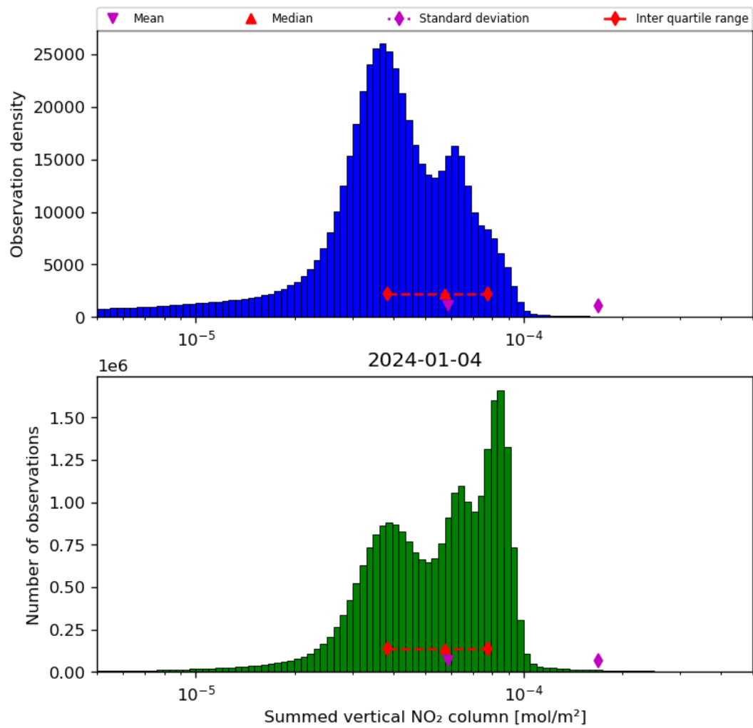
Figure 40: Histogram of “Summed vertical NO 2 column” for 2024-01-03 to 2024-01-05
