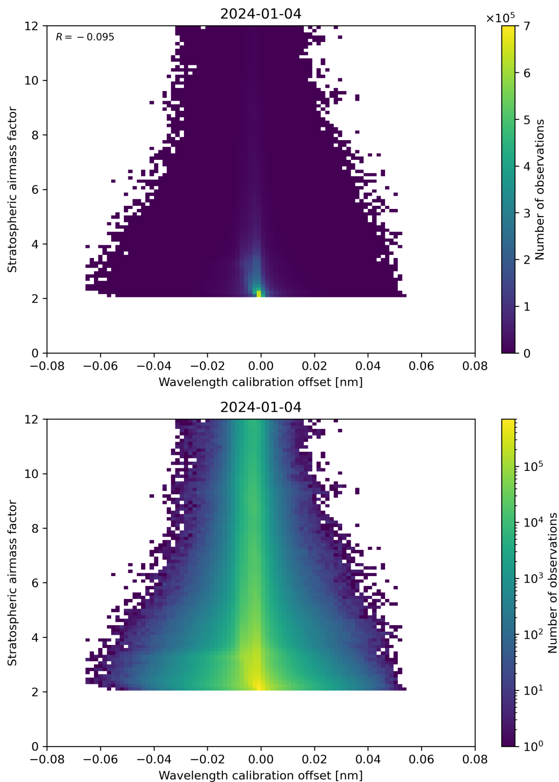
Figure 174: Scatter density plot of “Wavelength calibration offset” against “Stratospheric air mass factor” for 2024-01-03 to 2024-01-05.
