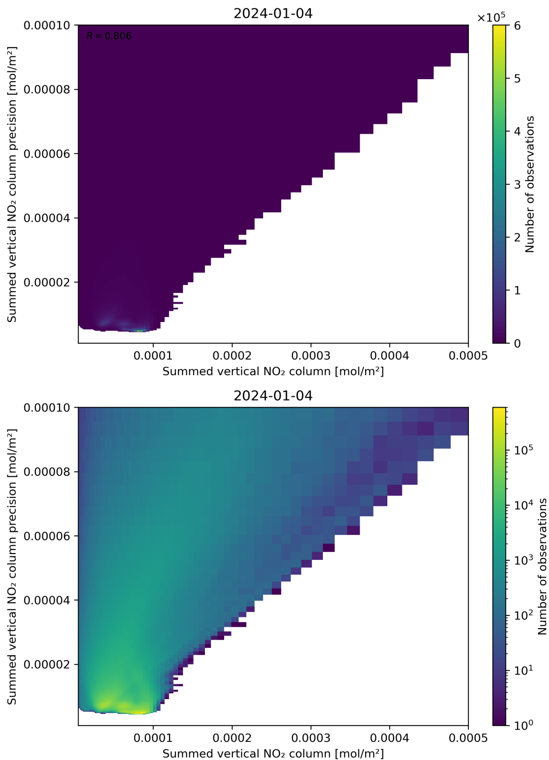
Figure 105: Scatter density plot of “Summed vertical NO 2 column” against “Summed vertical NO 2 column precision” for 2024-01-03 to 2024-01-05.
