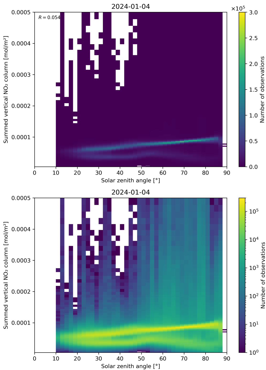
Figure 151: Scatter density plot of “Solar zenith angle” against “Summed vertical NO 2 column” for 2024-01-03 to 2024-01-05.
