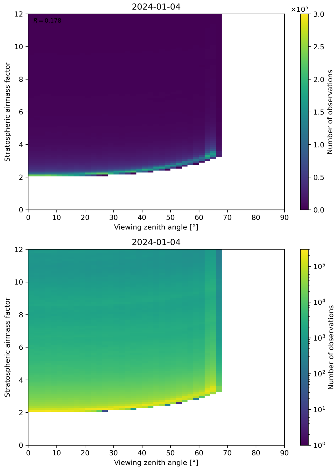
Figure 159: Scatter density plot of “Viewing zenith angle” against “Stratospheric airmass factor” for 2024-01-03 to 2024-01-05.
