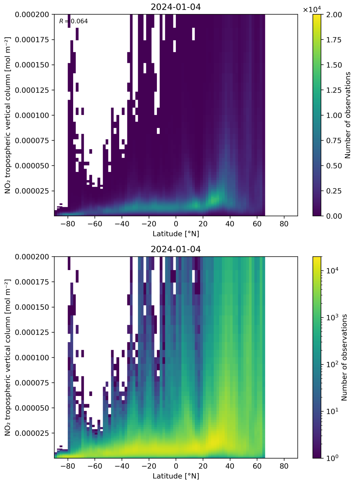
Figure 92: Scatter density plot of “Latitude” against “NO 2 tropospheric vertical column” for 2024-01-03 to 2024-01-05.
