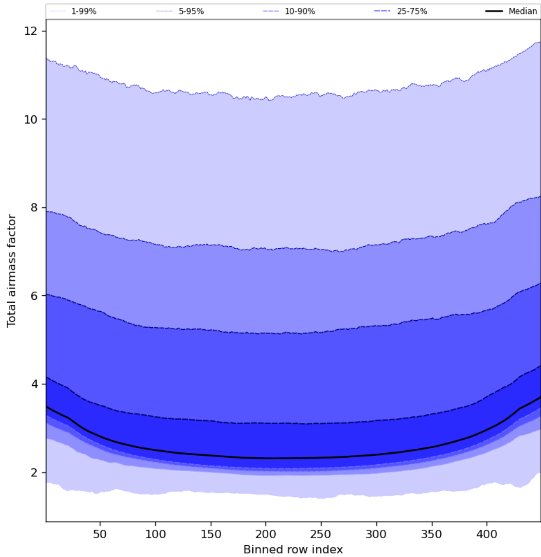
Figure 49: Along track statistics of “Total airmass factor” for 2024-01-03 to 2024-01-05
