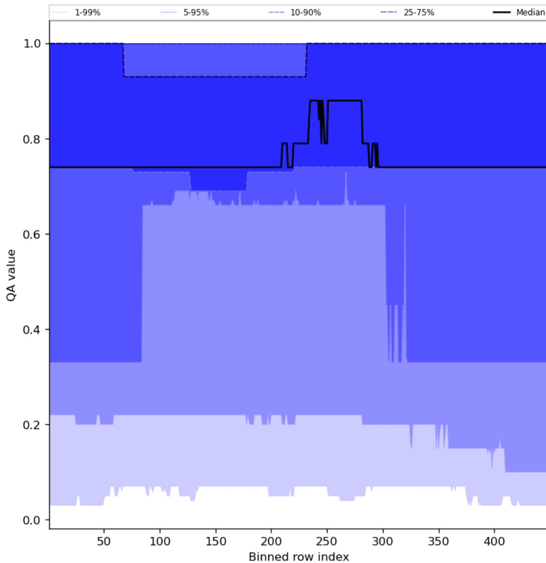
Figure 45: Along track statistics of “QA value” for 2024-01-03 to 2024-01-05
