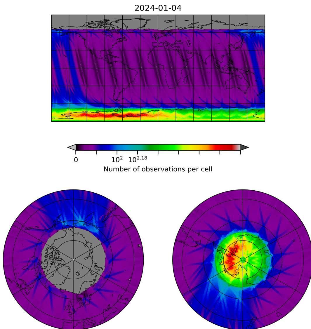
Figure 10: Map of the number of observations for 2024-01-03 to 2024-01-05
