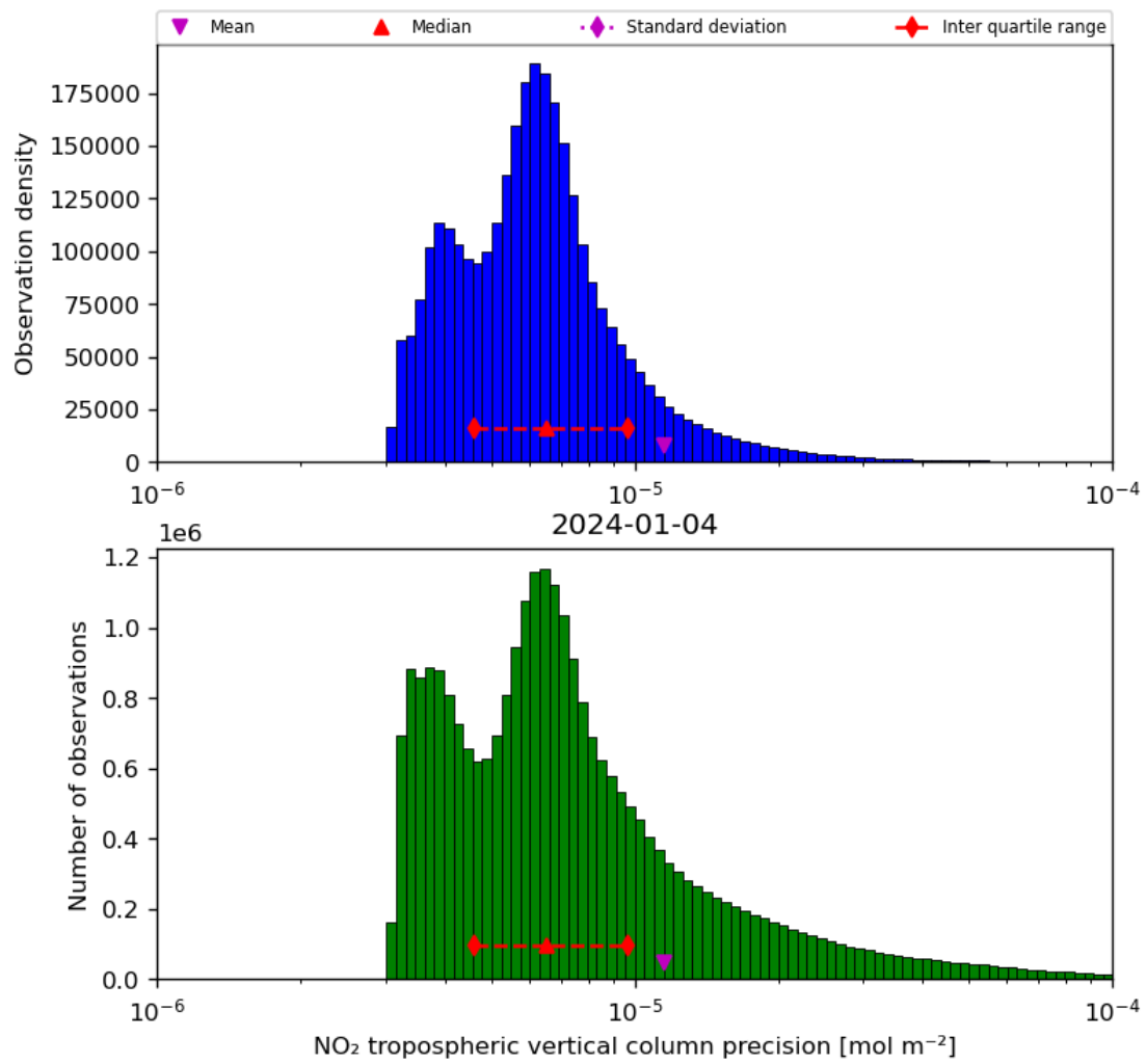
Figure 30: Histogram of “NO 2 tropospheric vertical column precision” for 2024-01-03 to 2024-01-05
