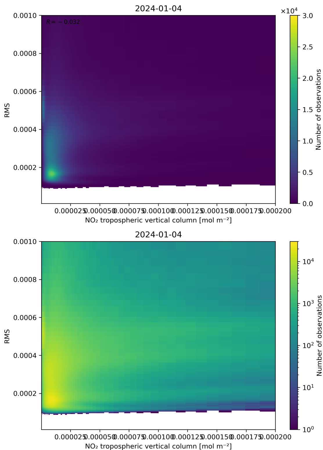
Figure 142: Scatter density plot of “NO 2 tropospheric vertical column” against “RMS” for 2024-01-03 to 2024-01-05.
