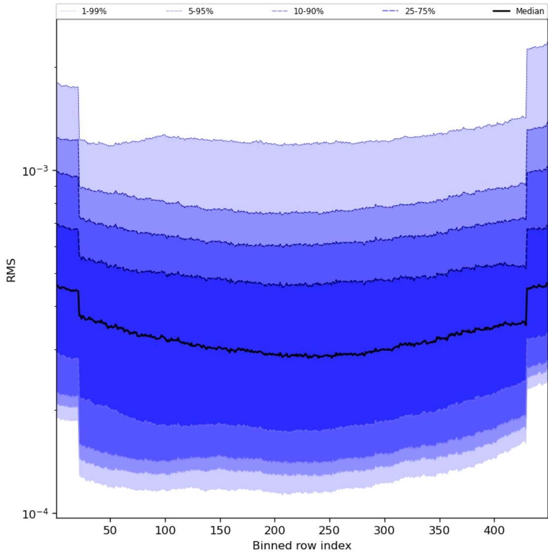
Figure 60: Along track statistics of “RMS” for 2024-01-03 to 2024-01-05
