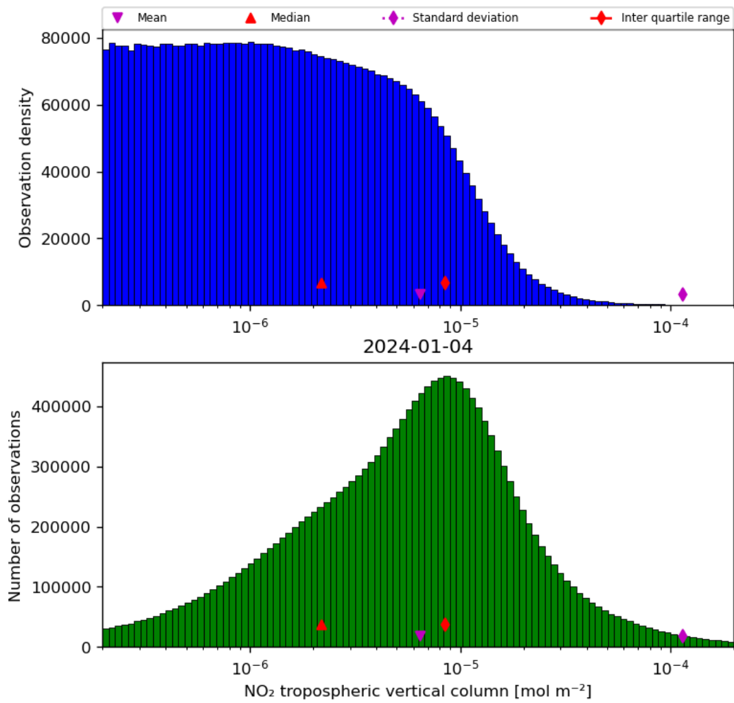
Figure 29: Histogram of “NO 2 tropospheric vertical column” for 2024-01-03 to 2024-01-05
