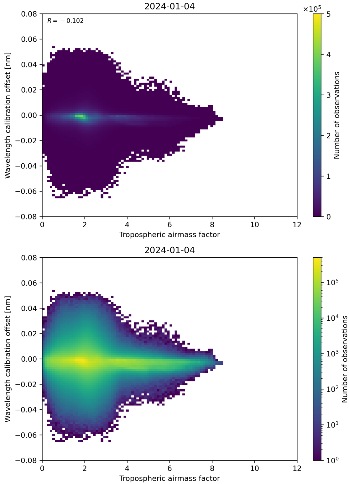
Figure 80: Scatter density plot of “Tropospheric air mass factor” against “Wavelength calibration offset” for 2024-01-03 to 2024-01-05.
