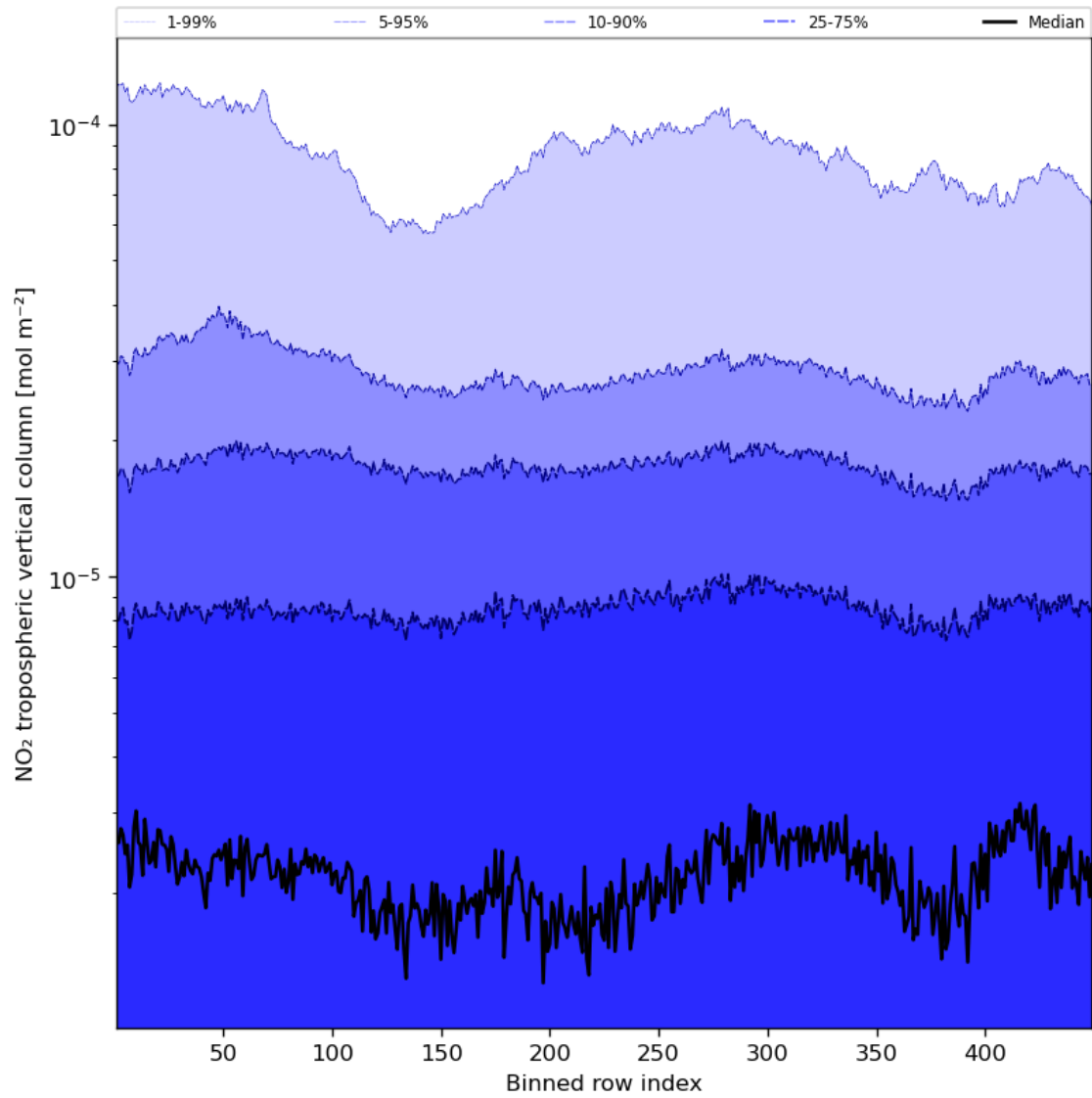
Figure 46: Along track statistics of “NO 2 tropospheric vertical column” for 2024-01-03 to 2024-01-05
