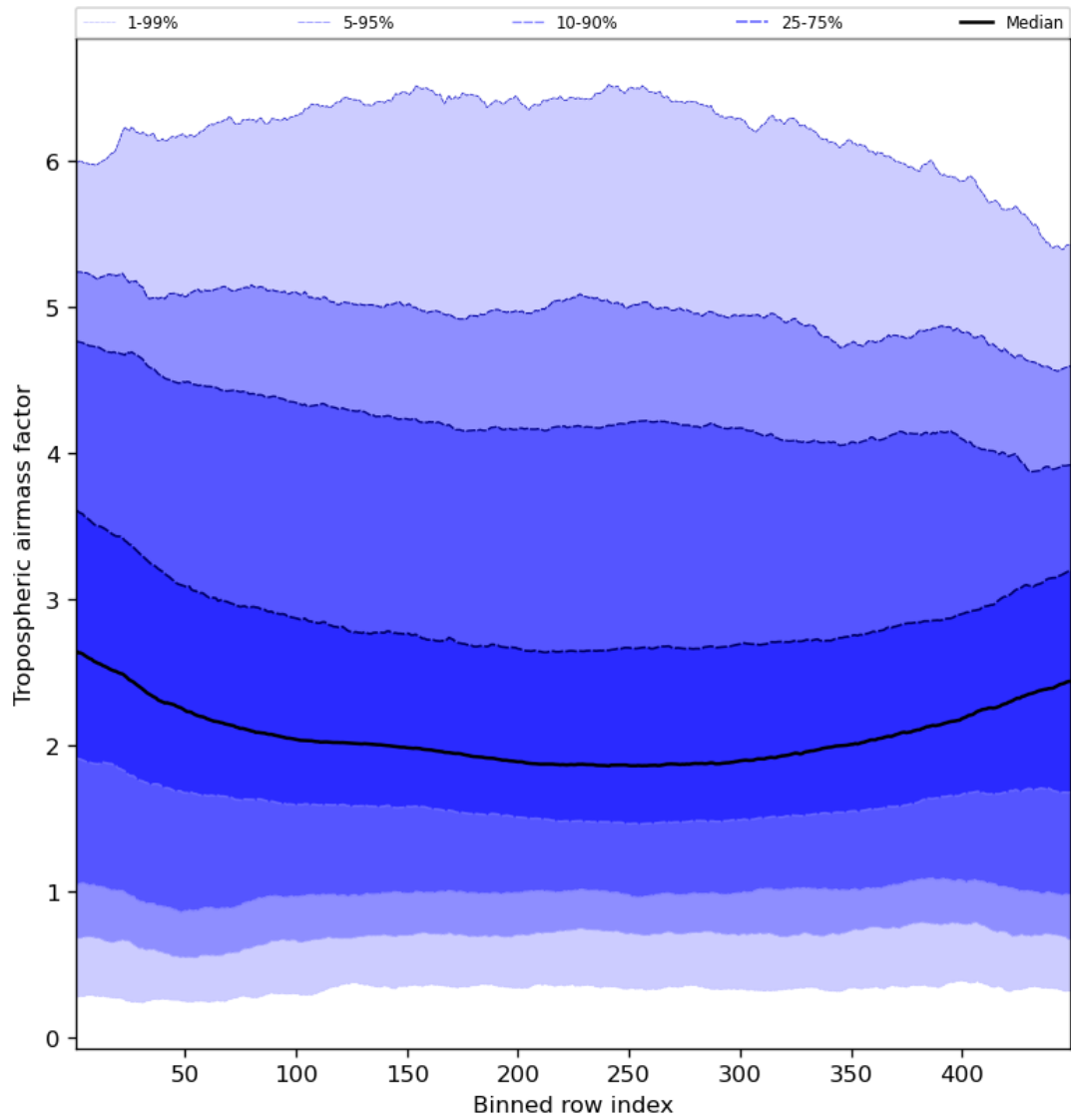
Figure 48: Along track statistics of “Tropospheric airmass factor” for 2024-01-03 to 2024-01-05
