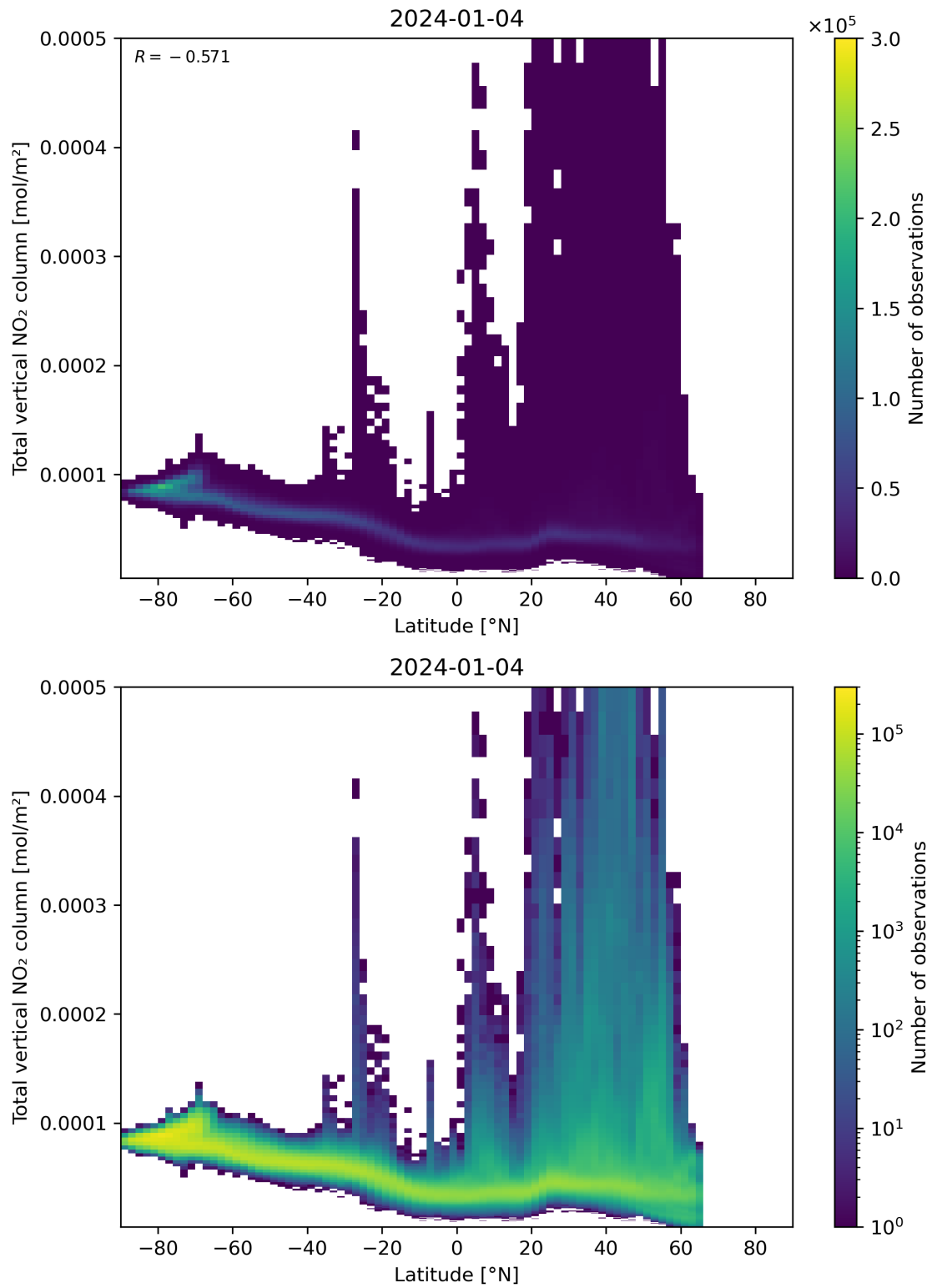
Figure 90: Scatter density plot of “Latitude” against “Total vertical NO 2 column” for 2024-01-03 to 2024-01-05.
