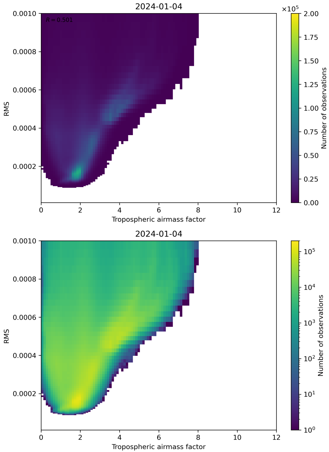
Figure 79: Scatter density plot of “Tropospheric airmass factor” against “RMS” for 2024-01-03 to 2024-01-05.
