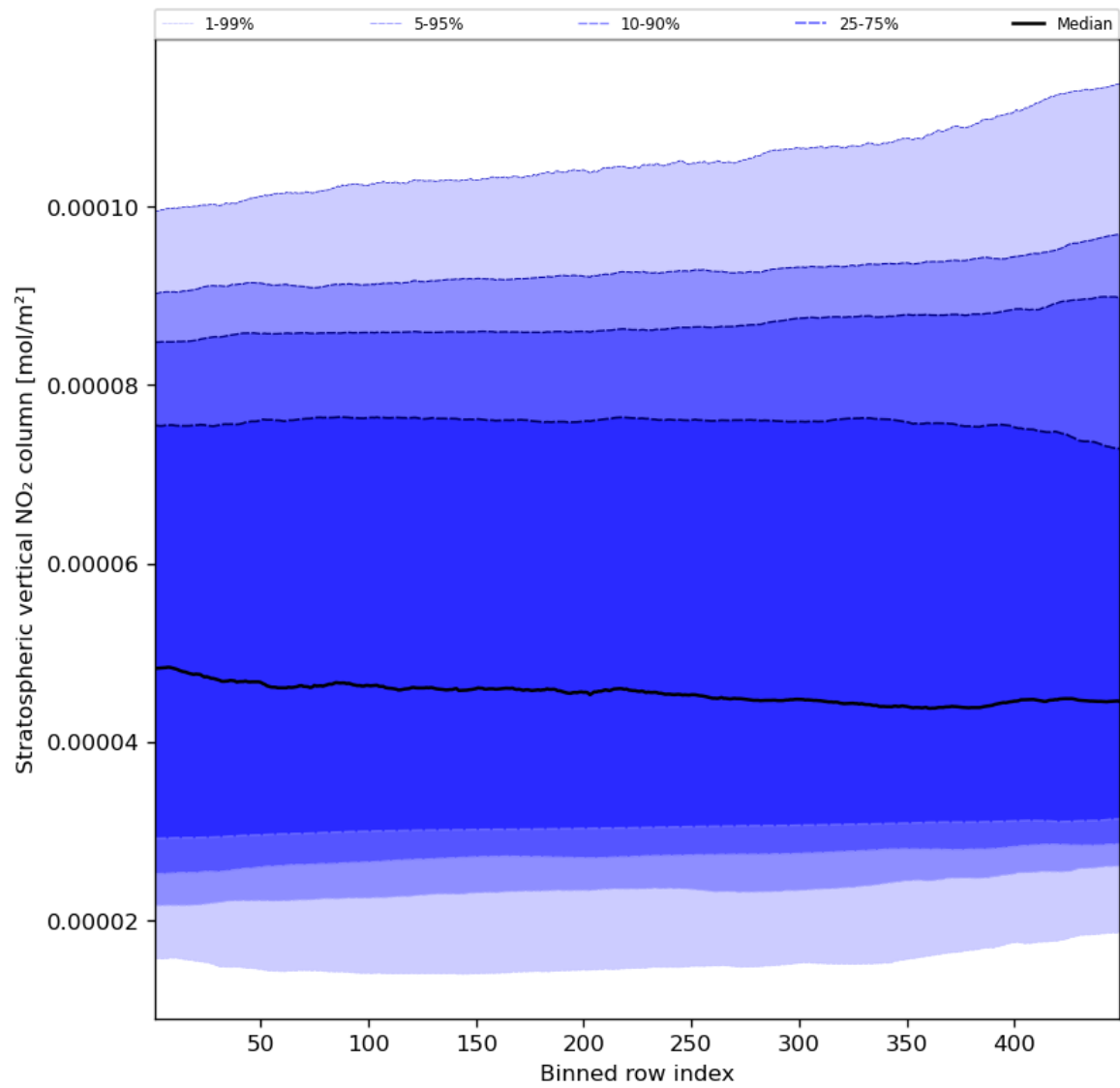
Figure 53: Along track statistics of “Stratospheric vertical NO 2 column” for 2024-01-03 to 2024-01-05
