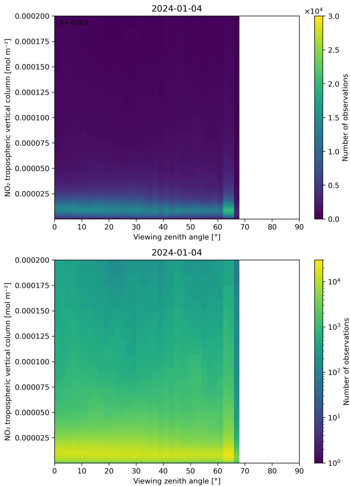
Figure 169: Scatter density plot of “Viewing zenith angle” against “NO 2 tropospheric vertical column” for 2024-01-03 to 2024-01-05.
