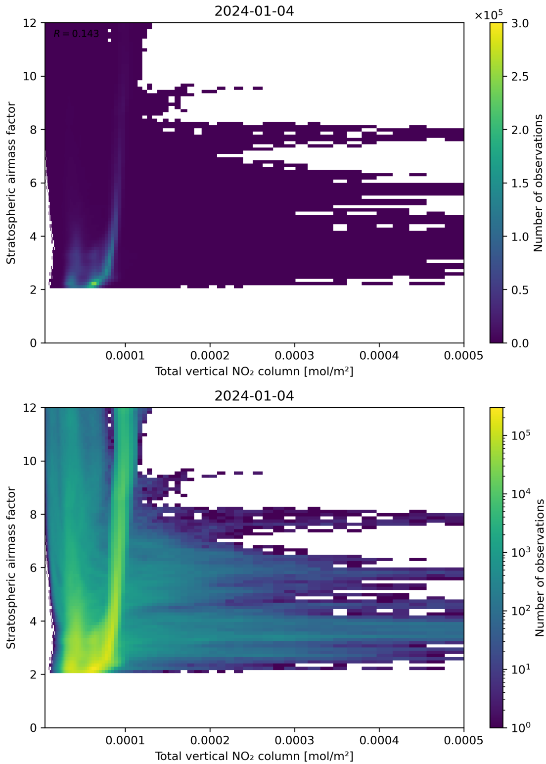
Figure 110: Scatter density plot of “Total vertical NO 2 column” against “Stratospheric air mass factor” for 2024-01-03 to 2024-01-05.
