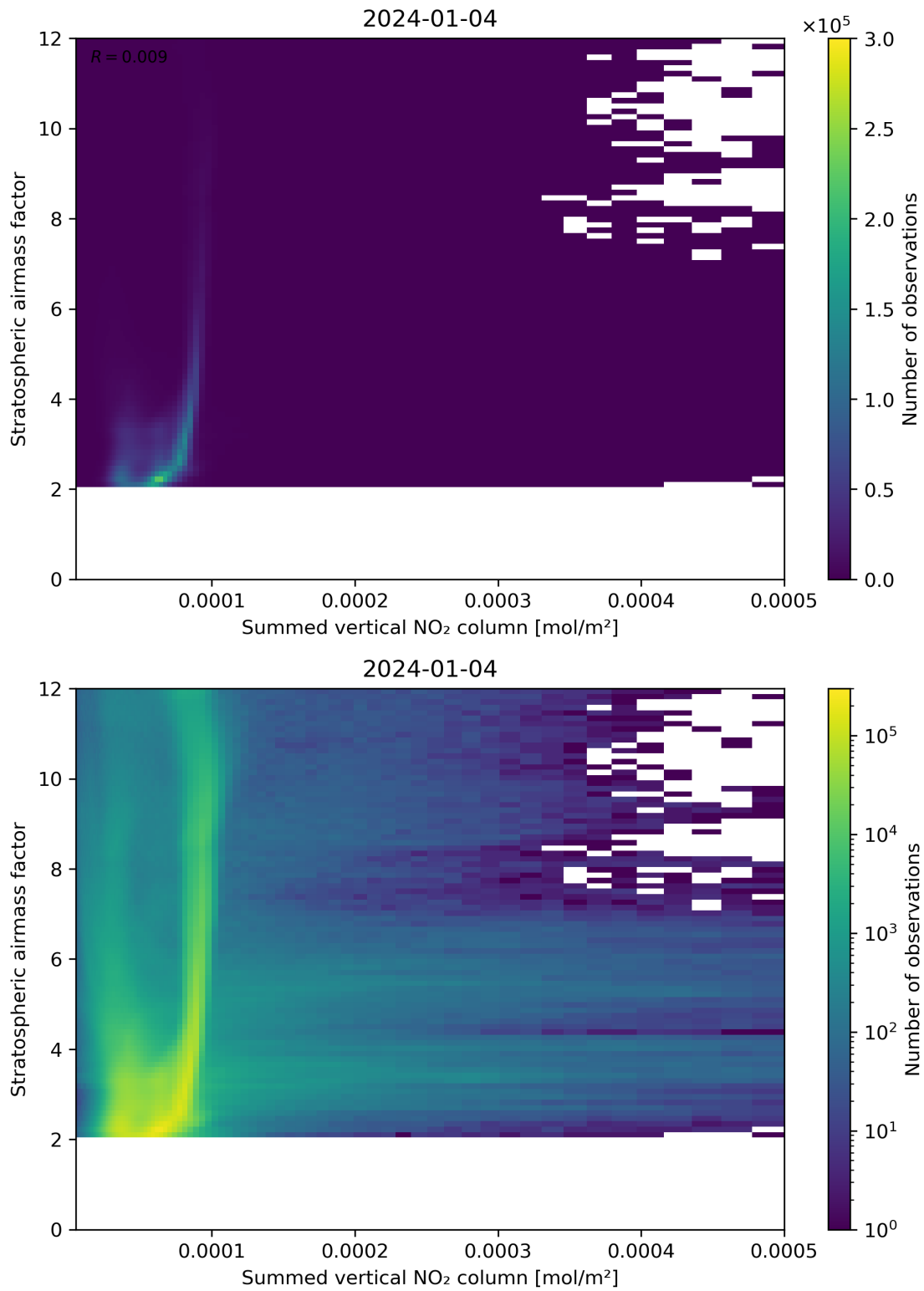
Figure 103: Scatter density plot of “Summed vertical NO 2 column” against “Stratospheric airmass factor” for 2024-01-03 to 2024-01-05.
