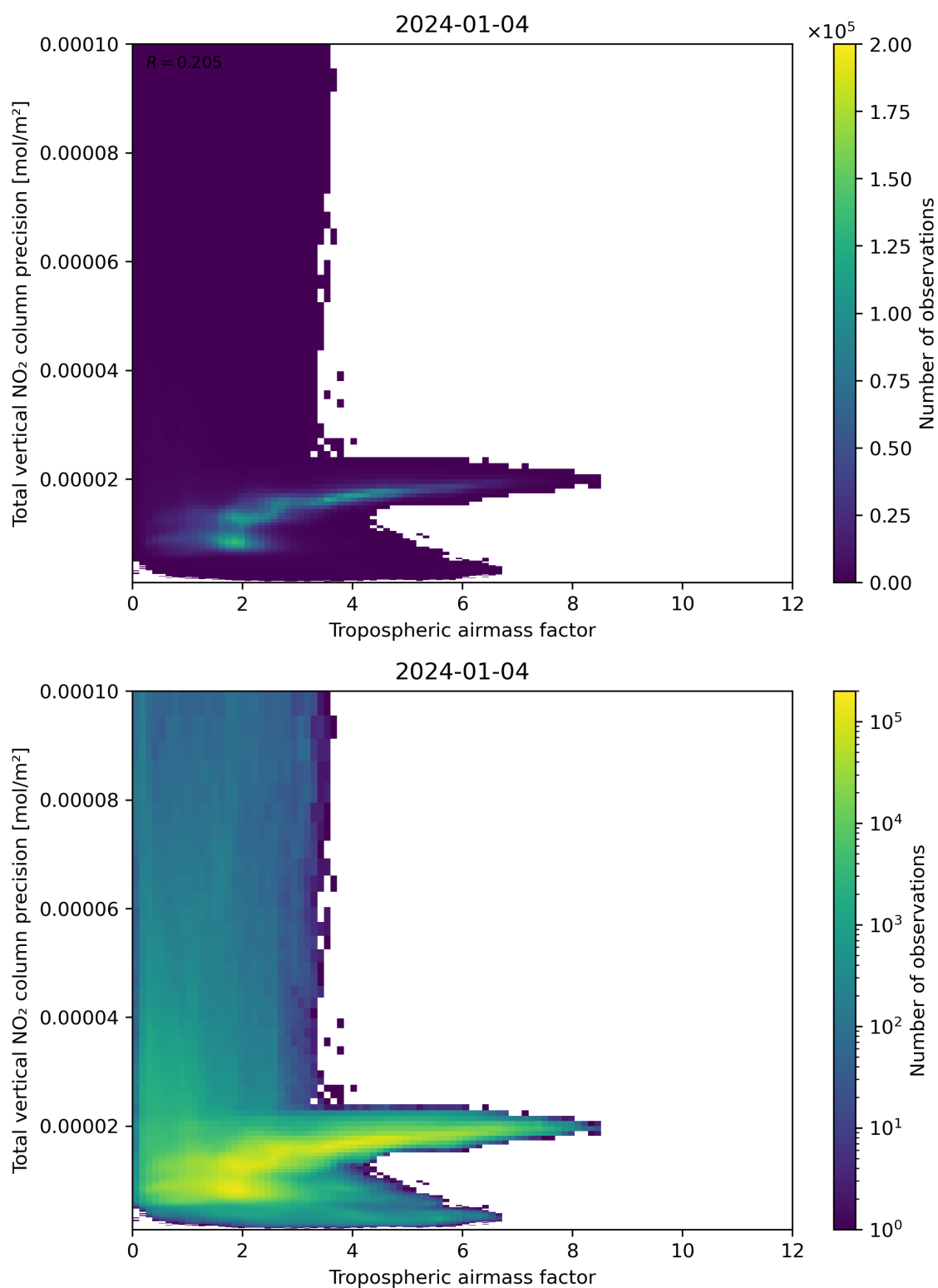
Figure 78: Scatter density plot of “Tropospheric air mass factor” against “Total vertical NO 2 column precision” for 2024-01-03 to 2024-01-05.
