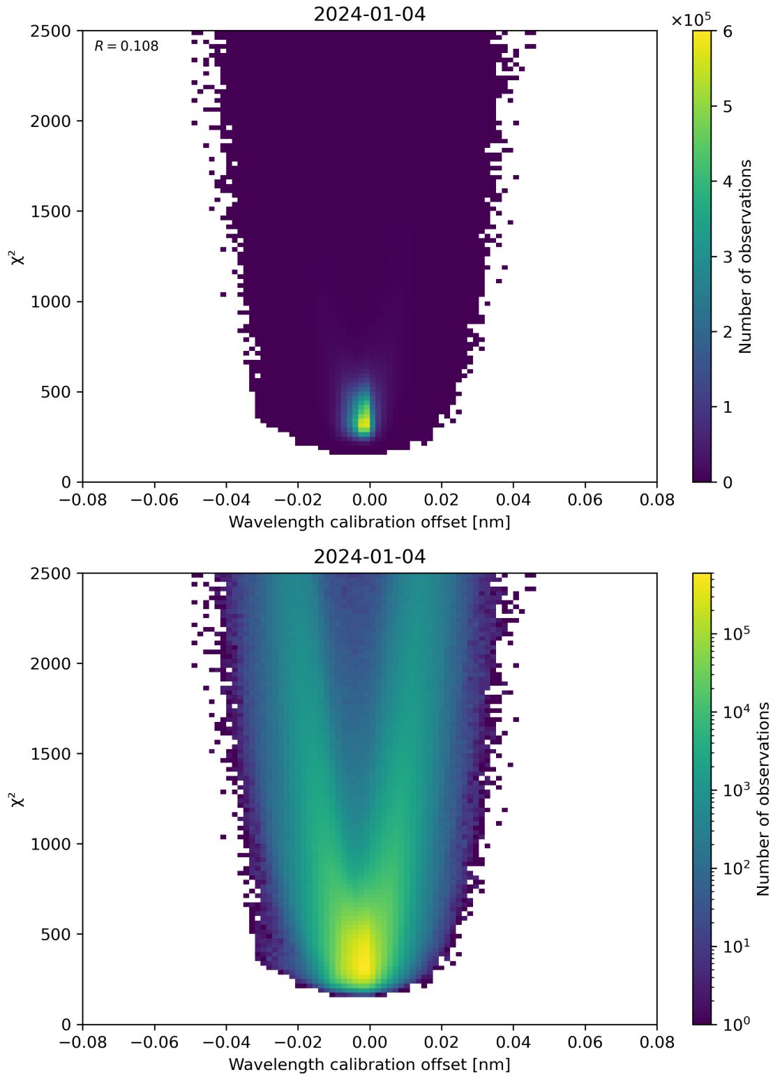
Figure 175: Scatter density plot of “Wavelength calibration offset” against “ \chi^2 ” for 2024-01-03 to 2024-01-05.
