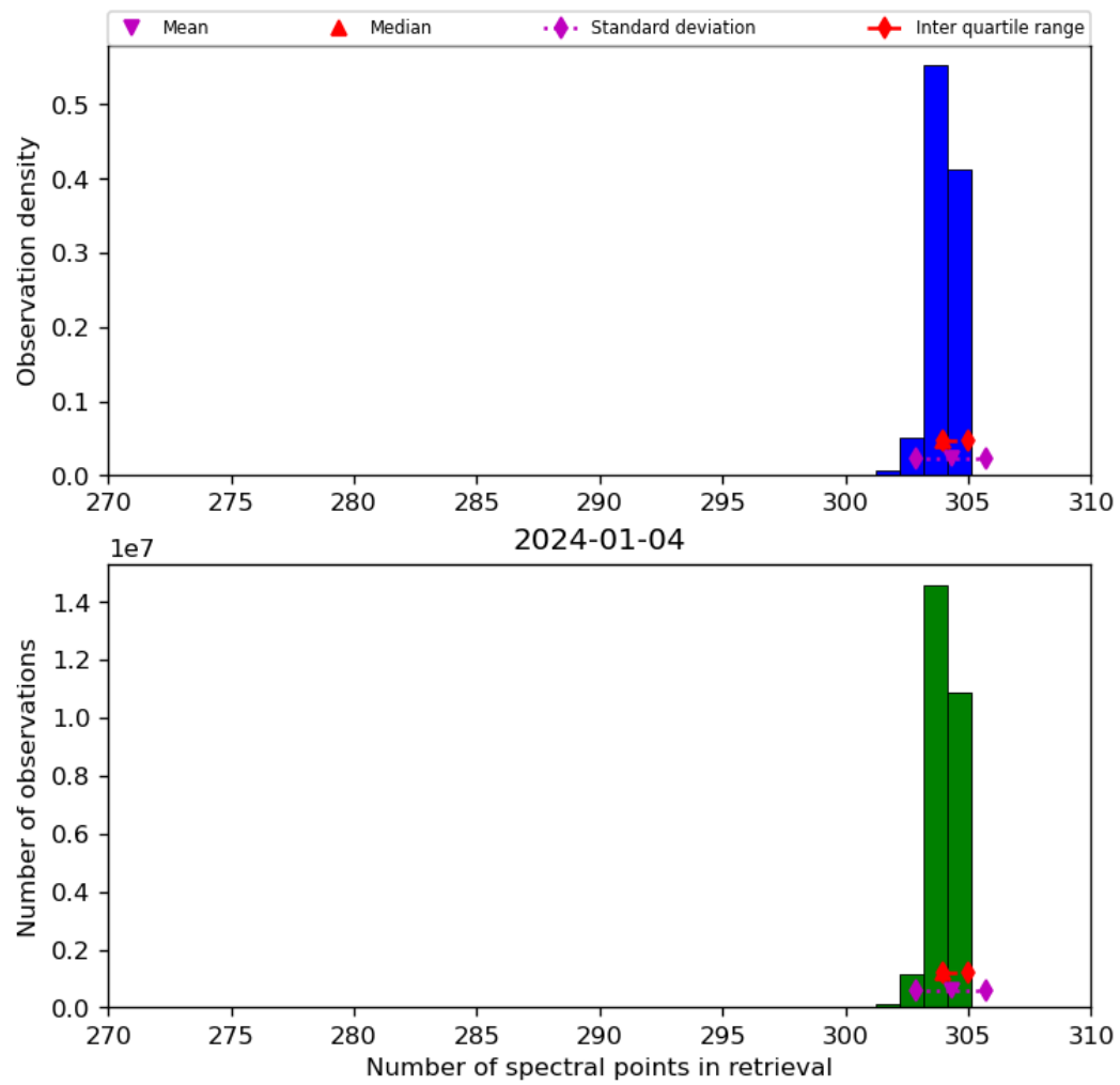
Figure 33: Histogram of “Number of spectral points in retrieval” for 2024-01-03 to 2024-01-05
