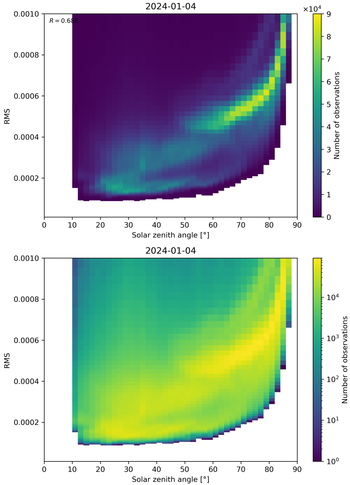
Figure 157: Scatter density plot of “Solar zenith angle” against “RMS” for 2024-01-03 to 2024-01-05.
