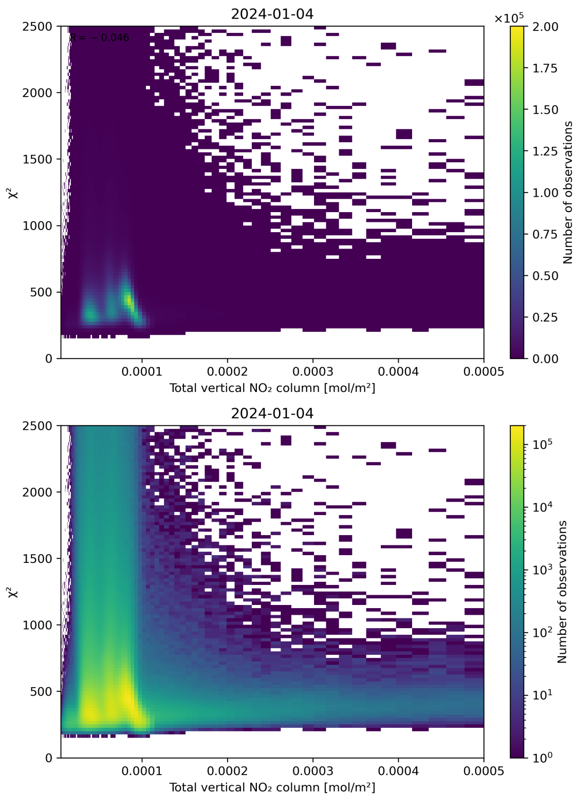
Figure 111: Scatter density plot of “Total vertical NO 2 column” against “ \chi^2 ” for 2024-01-03 to 2024-01-05.
