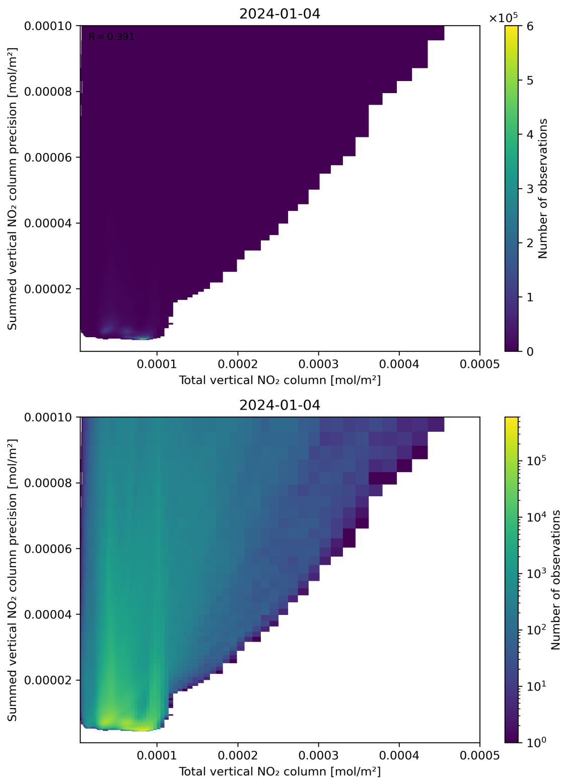
Figure 113: Scatter density plot of “Total vertical NO 2 column” against “Summed vertical NO 2 column precision” for 2024-01-03 to 2024-01-05.
