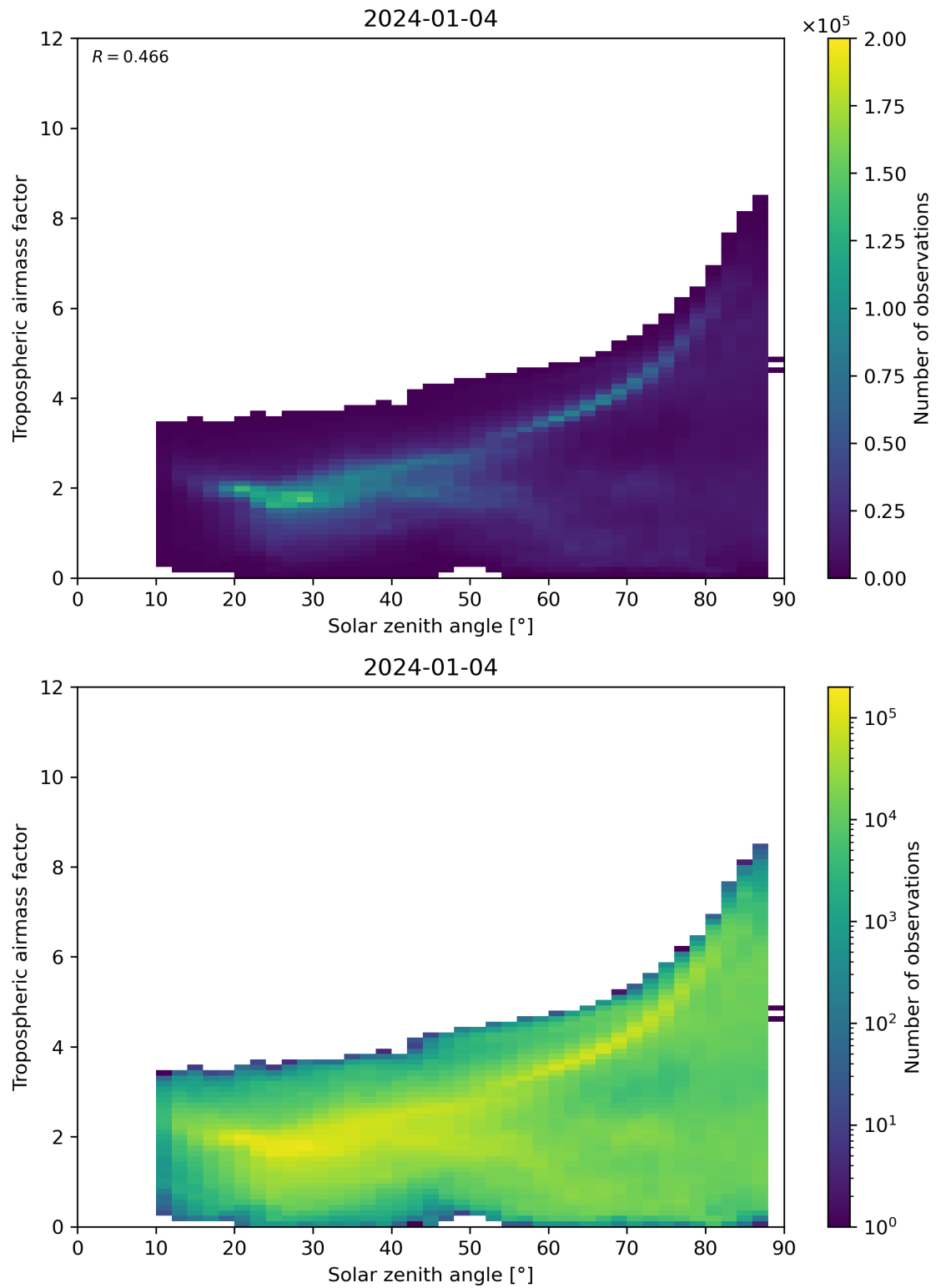
Figure 147: Scatter density plot of “Solar zenith angle” against “Tropospheric airmass factor” for 2024-01-03 to 2024-01-05.
