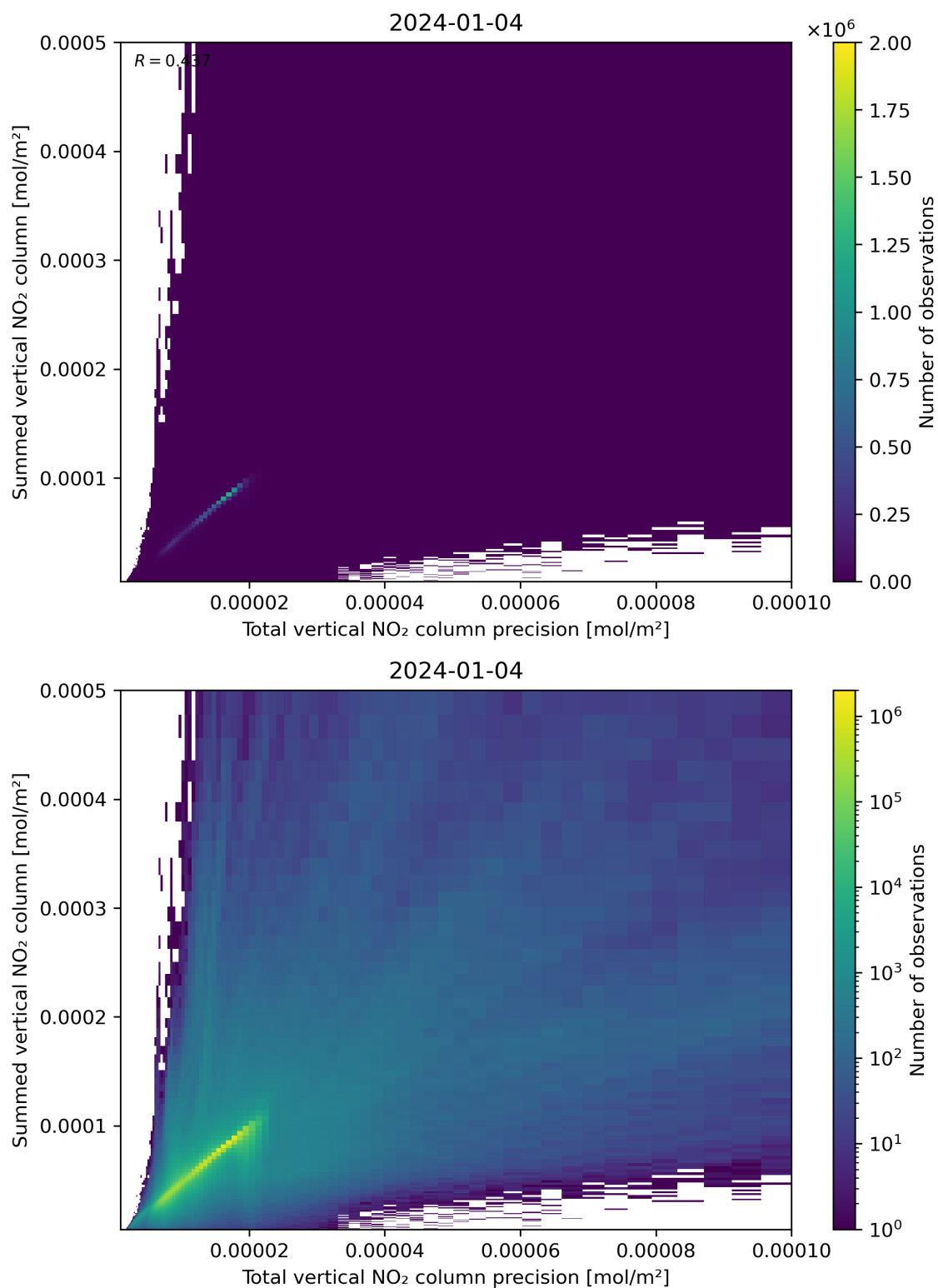
Figure 117: Scatter density plot of “Total vertical NO 2 column precision” against “Summed vertical NO 2 column” for 2024-01-03 to 2024-01-05.
