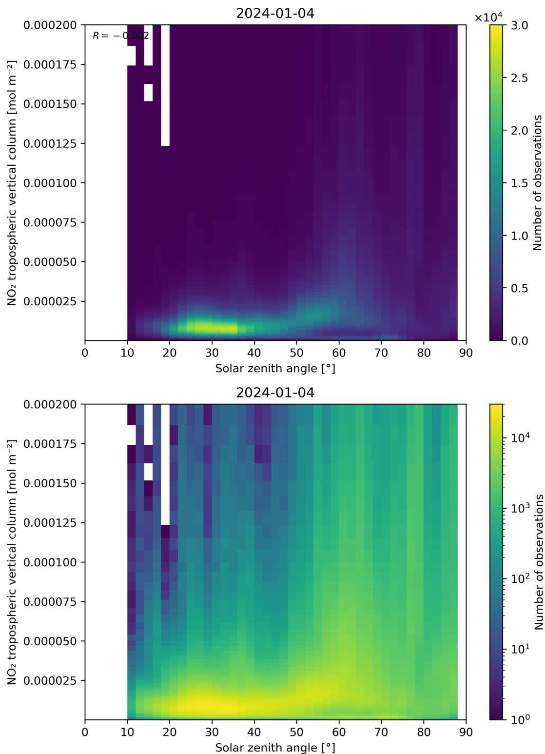
Figure 155: Scatter density plot of “Solar zenith angle” against “NO 2 tropospheric vertical column” for 2024-01-03 to 2024-01-05.
