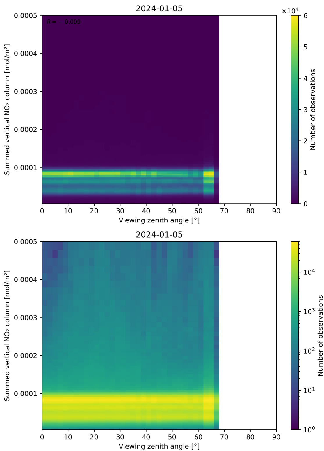
Figure 165: Scatter density plot of “Viewing zenith angle” against “Summed vertical NO 2 column” for 2024-01-05 to 2024-01-06.
