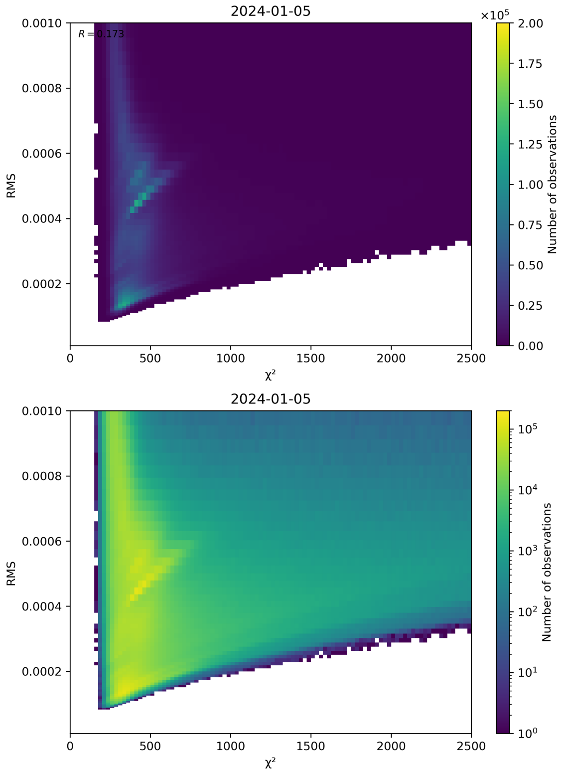
Figure 82: Scatter density plot of “ \chi^2 ” against “RMS” for 2024-01-05 to 2024-01-06.
