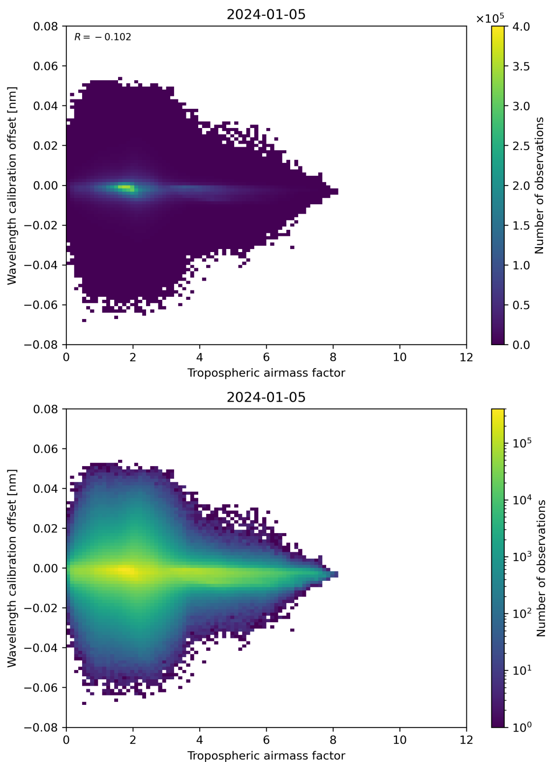
Figure 80: Scatter density plot of “Tropospheric airmass factor” against “Wavelength calibration offset” for 2024-01-05 to 2024-01-06.
