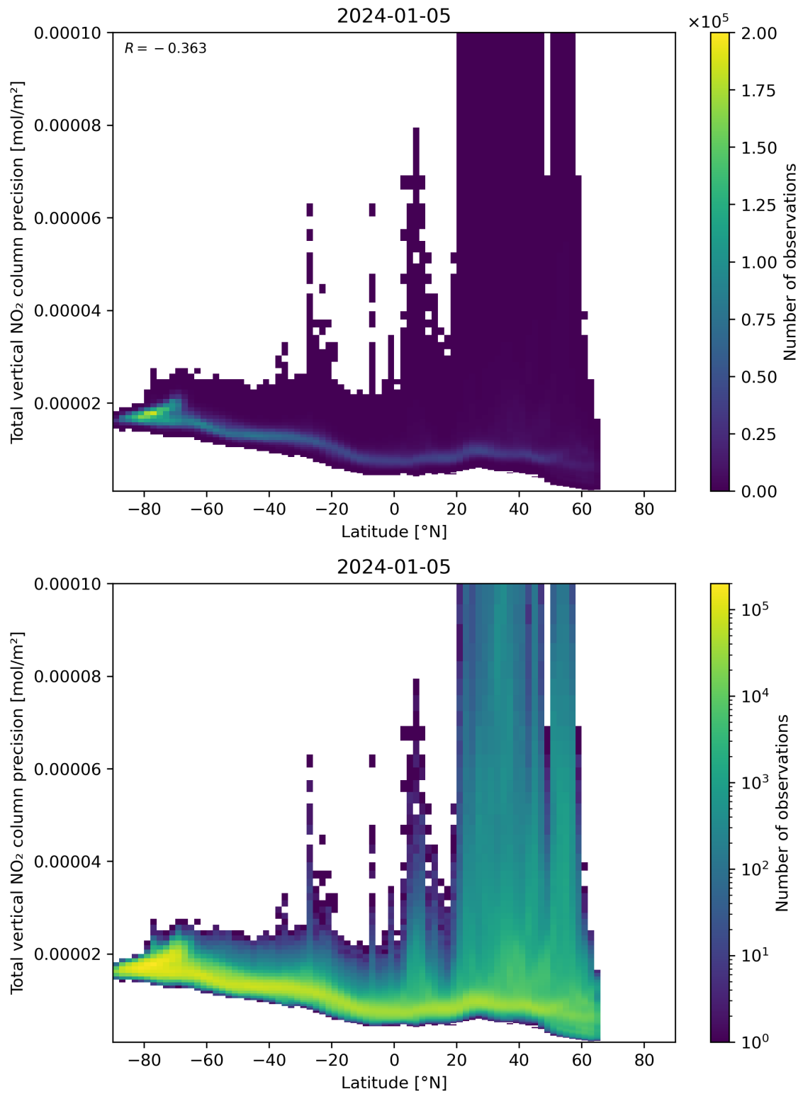
Figure 91: Scatter density plot of “Latitude” against “Total vertical NO 2 column precision” for 2024-01-05 to 2024-01-06.
