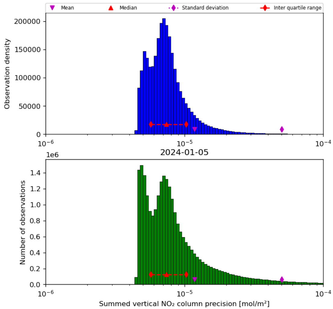
Figure 41: Histogram of "Summed vertical NO 2 column precision" for 2024-01-05 to 2024-01-06
