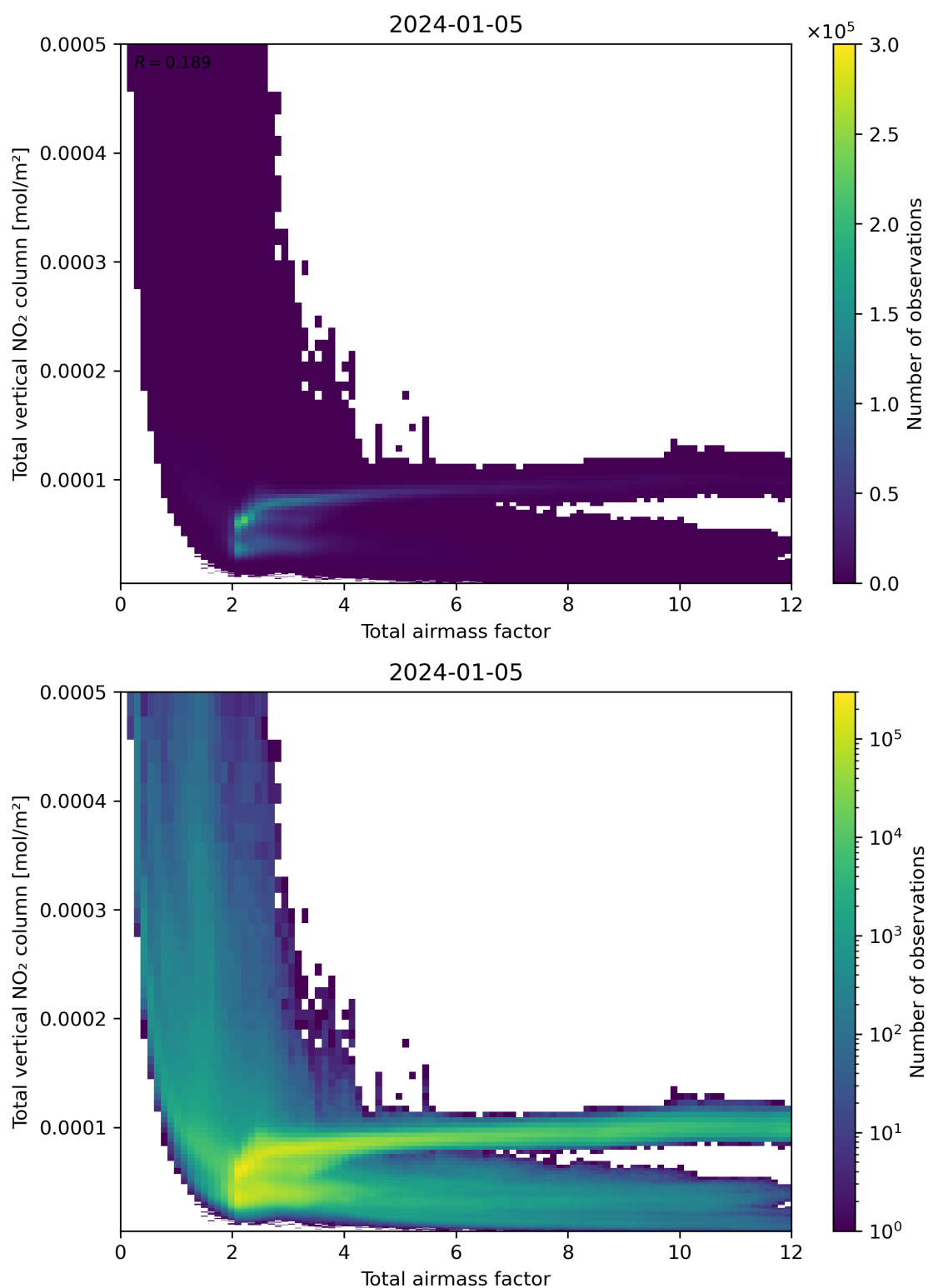
Figure 67: Scatter density plot of “Total airmass factor” against “Total vertical NO 2 column” for 2024-01-05 to 2024-01-06.
