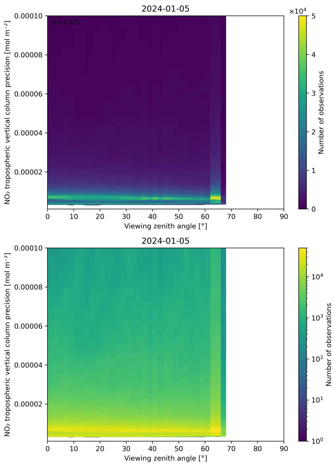
Figure 170: Scatter density plot of “Viewing zenith angle” against “NO 2 tropospheric vertical column precision” for 2024-01-05 to 2024-01-06.
