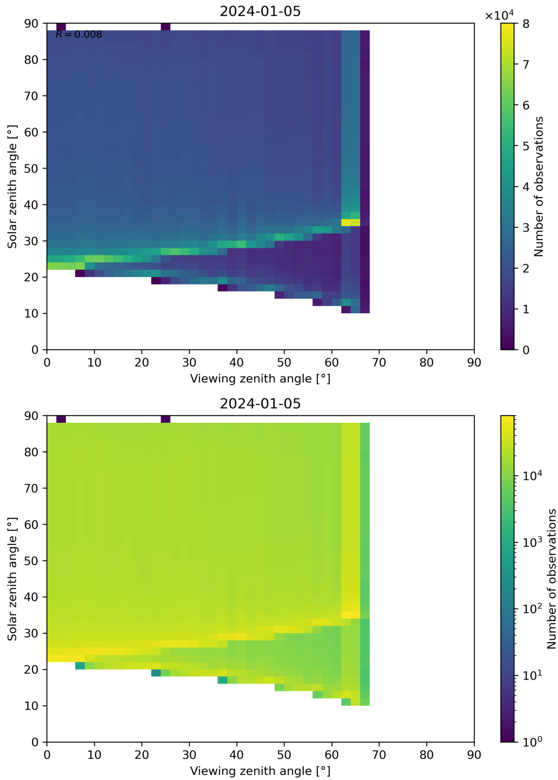
Figure 172: Scatter density plot of “Viewing zenith angle” against “Solar zenith angle” for 2024-01-05 to 2024-01-06.
