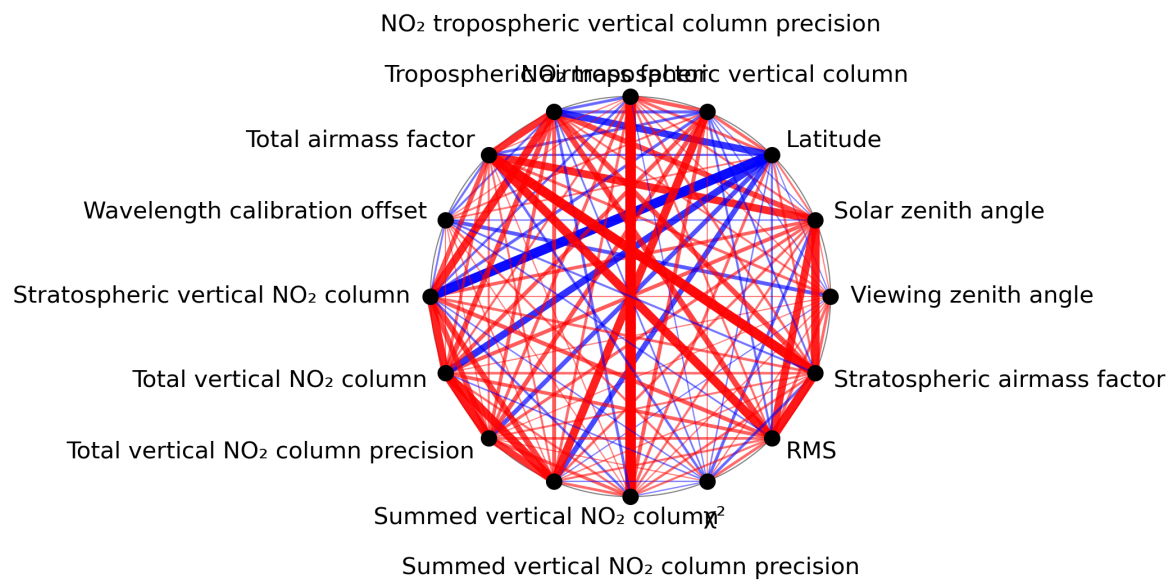
Figure 1: Map of correlation graph for 2024-01-05 to 2024-01-06.
