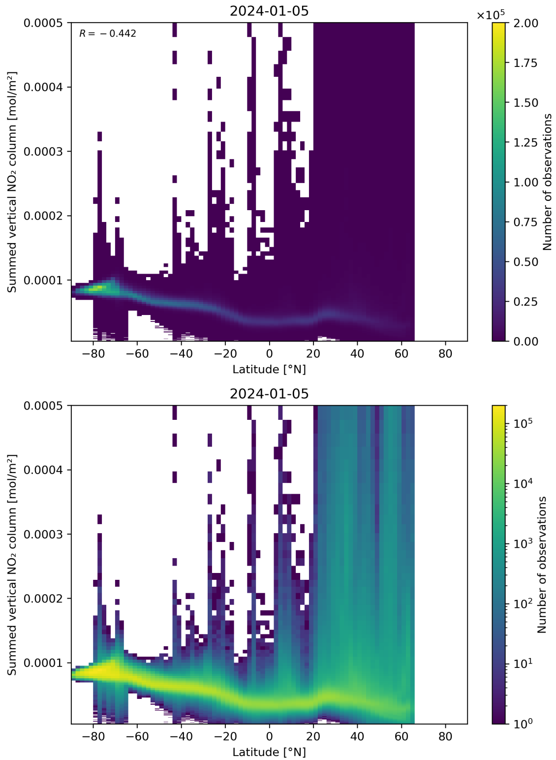
Figure 88: Scatter density plot of “Latitude” against “Summed vertical NO 2 column” for 2024-01-05 to 2024-01-06.
