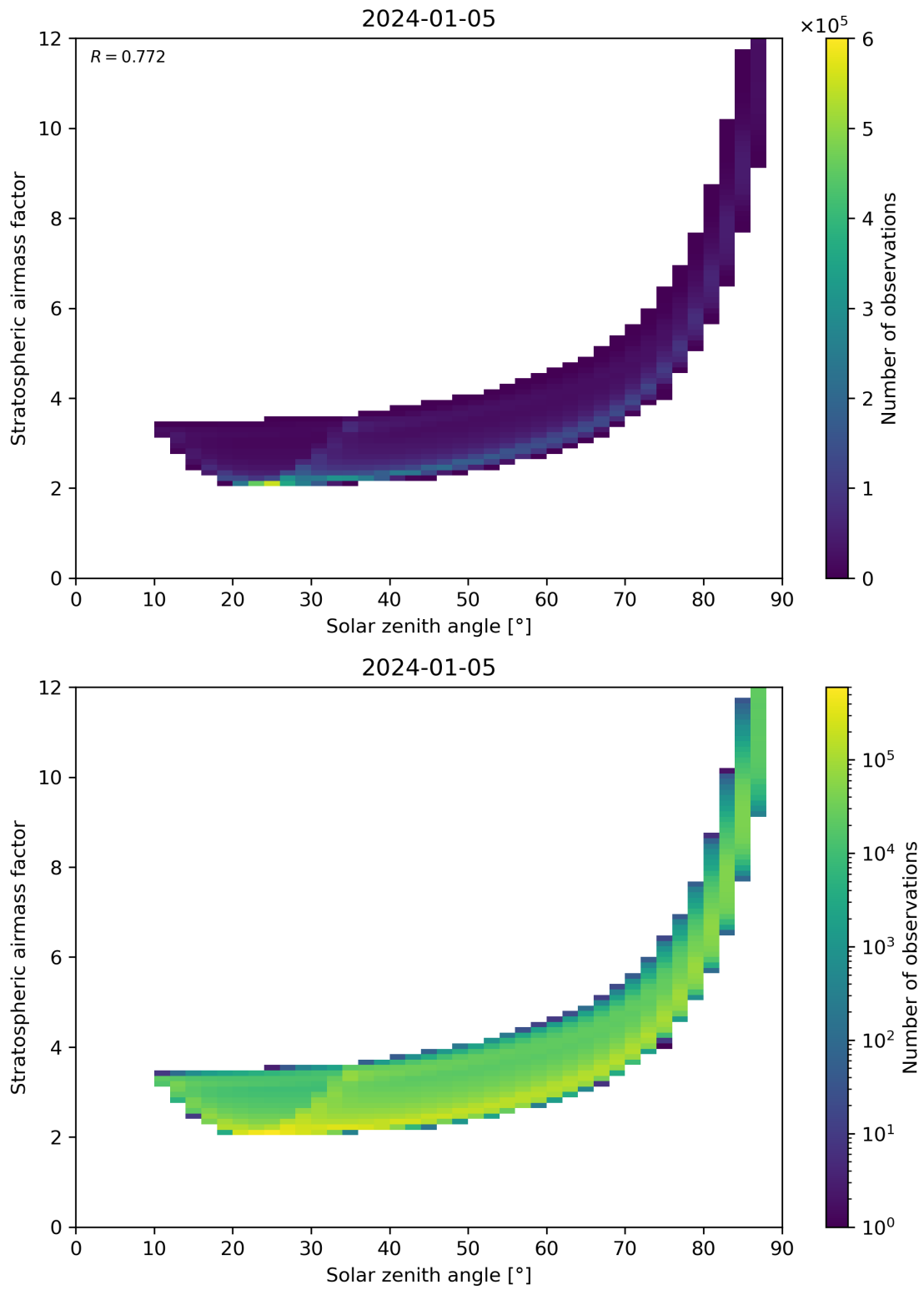
Figure 145: Scatter density plot of “Solar zenith angle” against “Stratospheric airmass factor” for 2024-01-05 to 2024-01-06.
