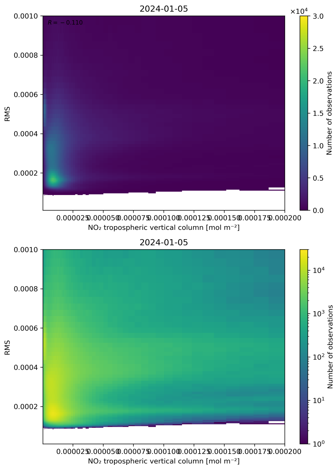
Figure 142: Scatter density plot of “NO 2 tropospheric vertical column” against “RMS” for 2024-01-05 to 2024-01-06.
