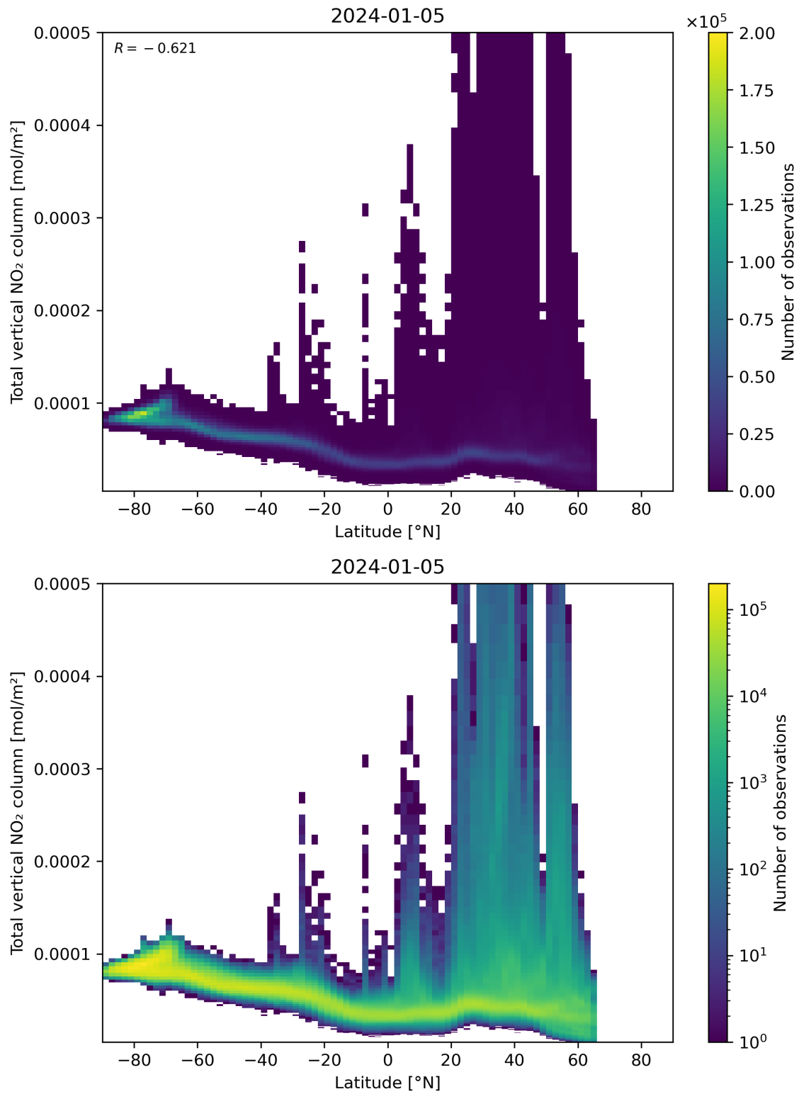
Figure 90: Scatter density plot of “Latitude” against “Total vertical NO 2 column” for 2024-01-05 to 2024-01-06.
