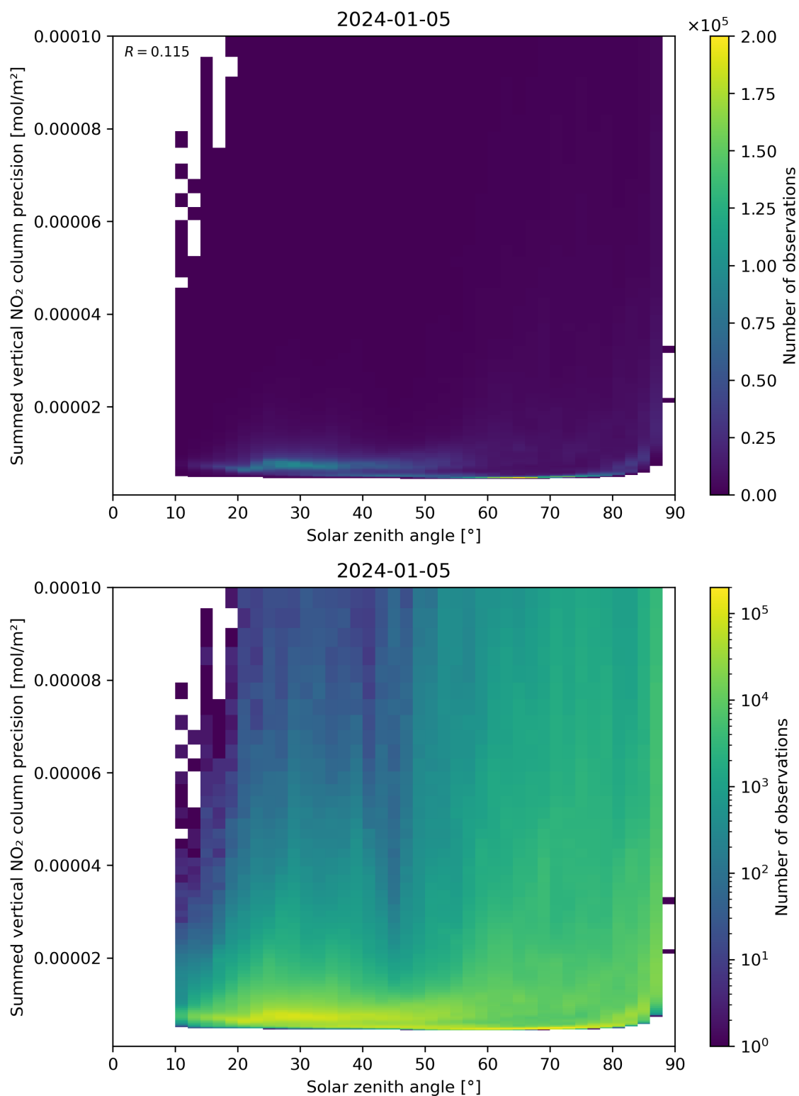
Figure 152: Scatter density plot of “Solar zenith angle” against “Summed vertical NO 2 column precision” for 2024-01-05 to 2024-01-06.
