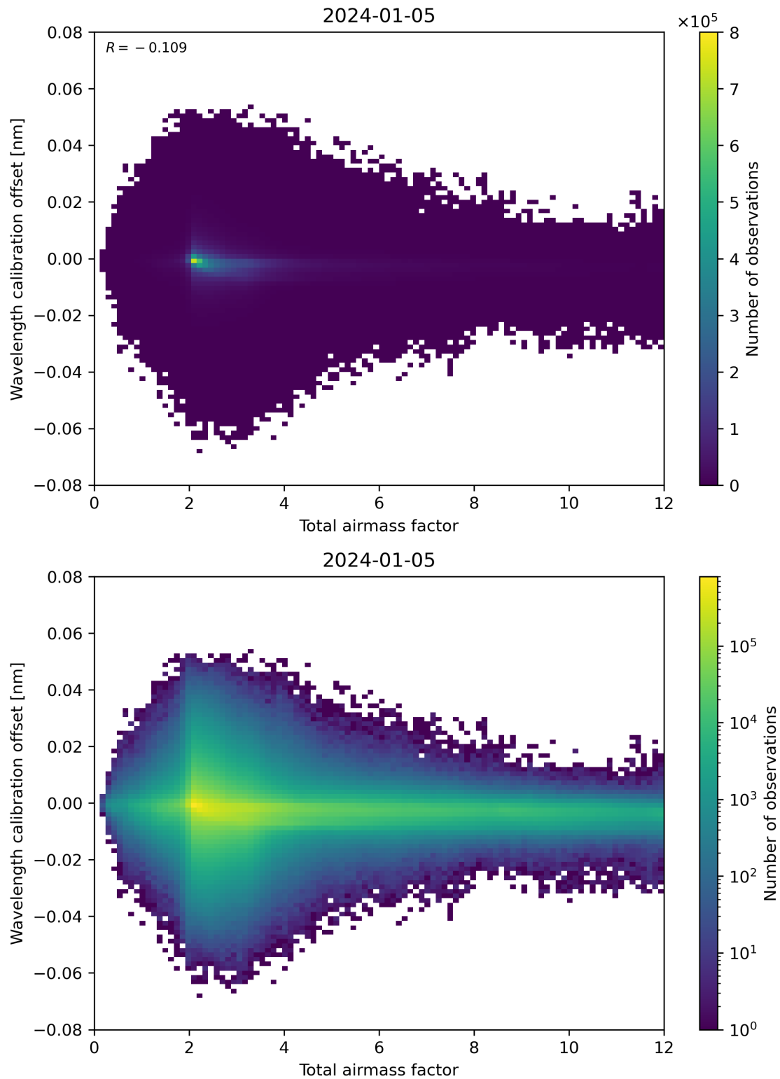
Figure 70: Scatter density plot of “Total airmass factor” against “Wavelength calibration offset” for 2024-01-05 to 2024-01-06.
