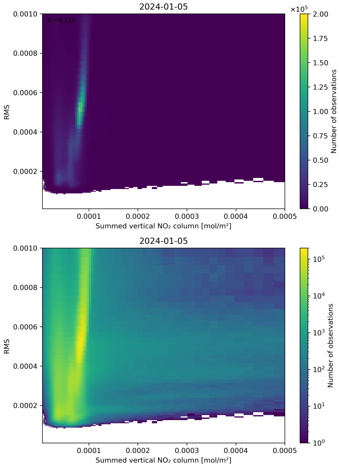
Figure 109: Scatter density plot of “Summed vertical NO 2 column” against “RMS” for 2024-01-05 to 2024-01-06.
