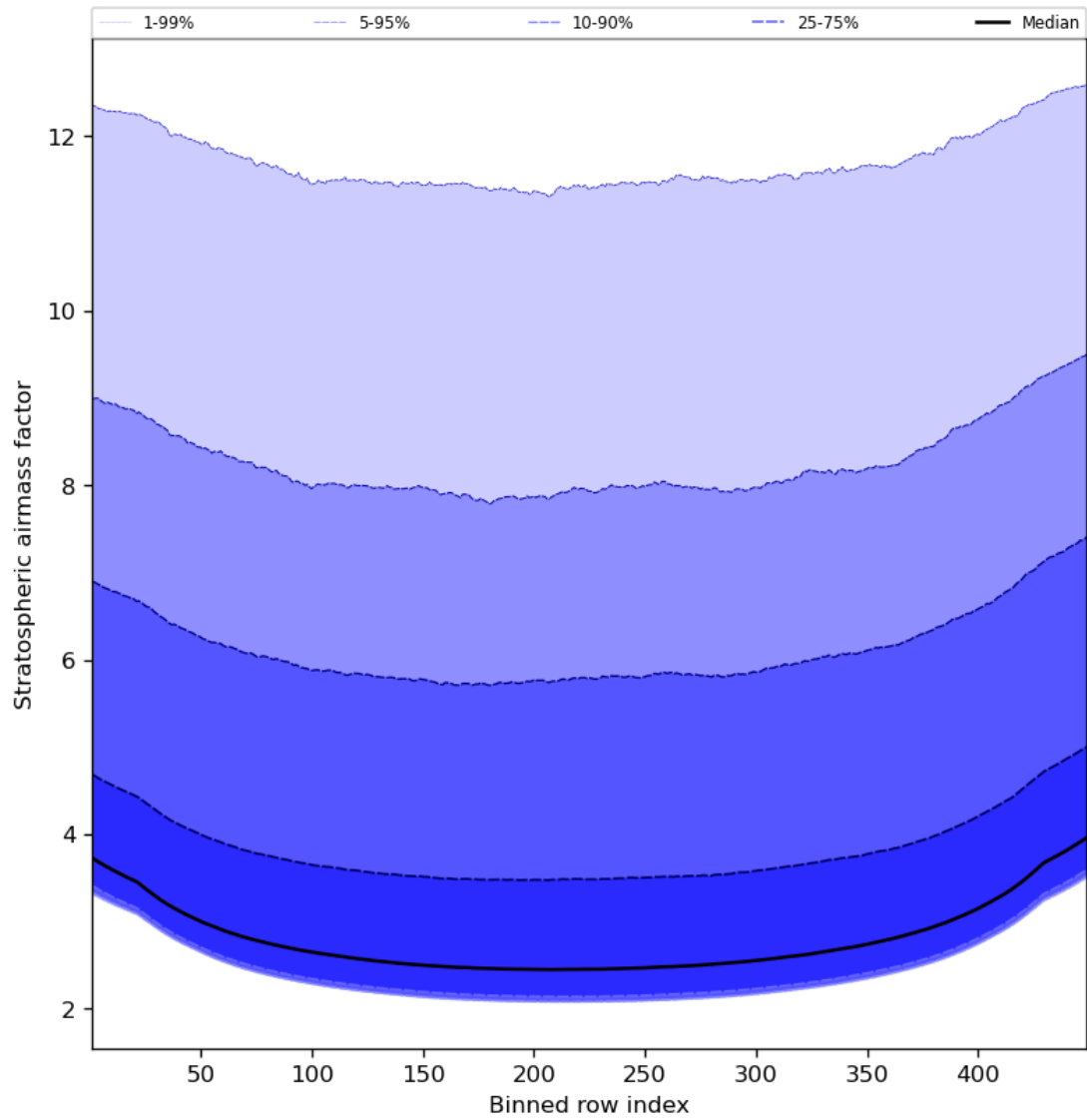
Figure 61: Along track statistics of “Stratospheric airmass factor” for 2024-01-05 to 2024-01-06
