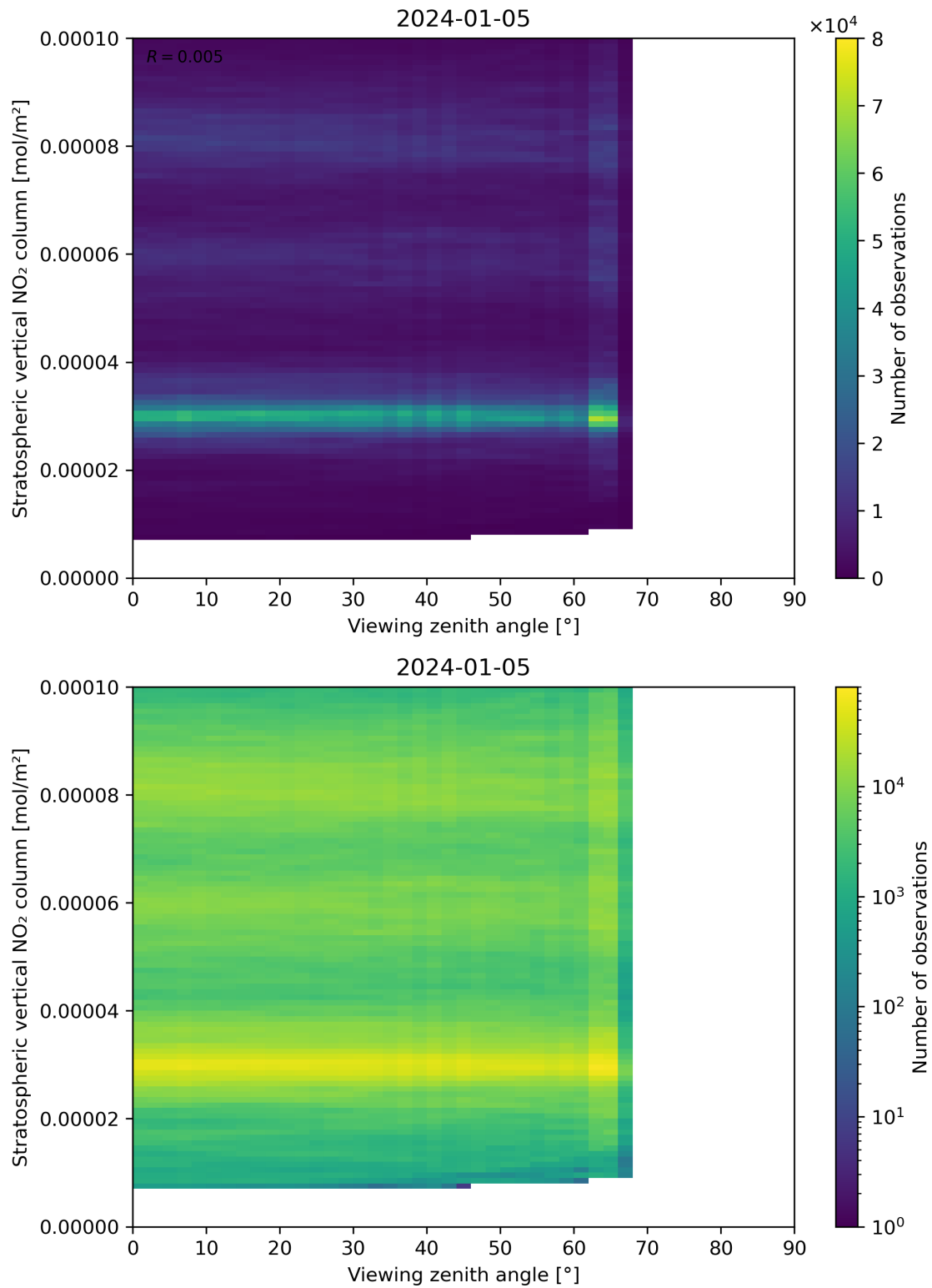
Figure 164: Scatter density plot of “Viewing zenith angle” against “Stratospheric vertical NO 2 column” for 2024-01-05 to 2024-01-06.
