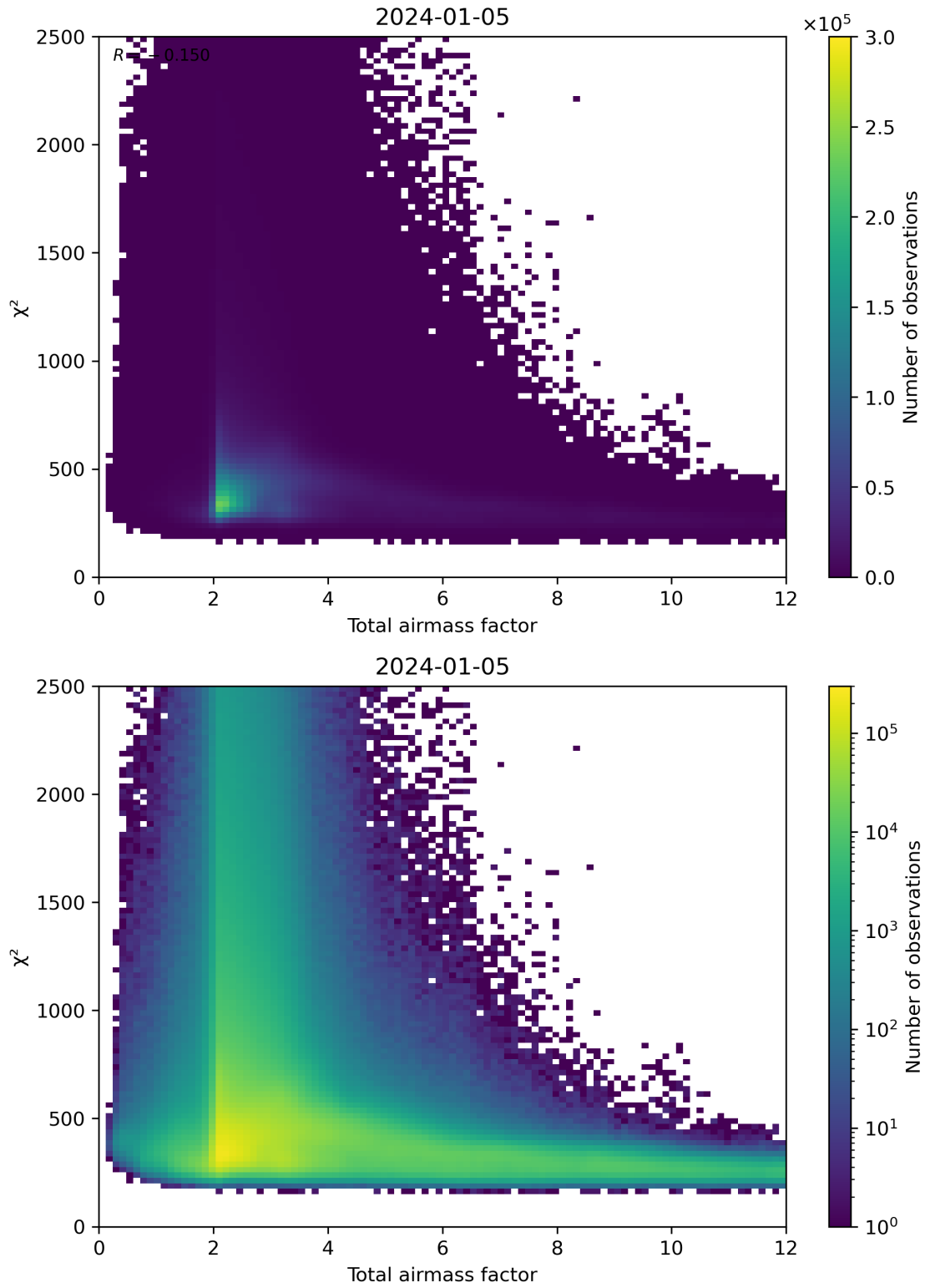
Figure 63: Scatter density plot of “Total airmass factor” against “ \chi^2 ” for 2024-01-05 to 2024-01-06.
