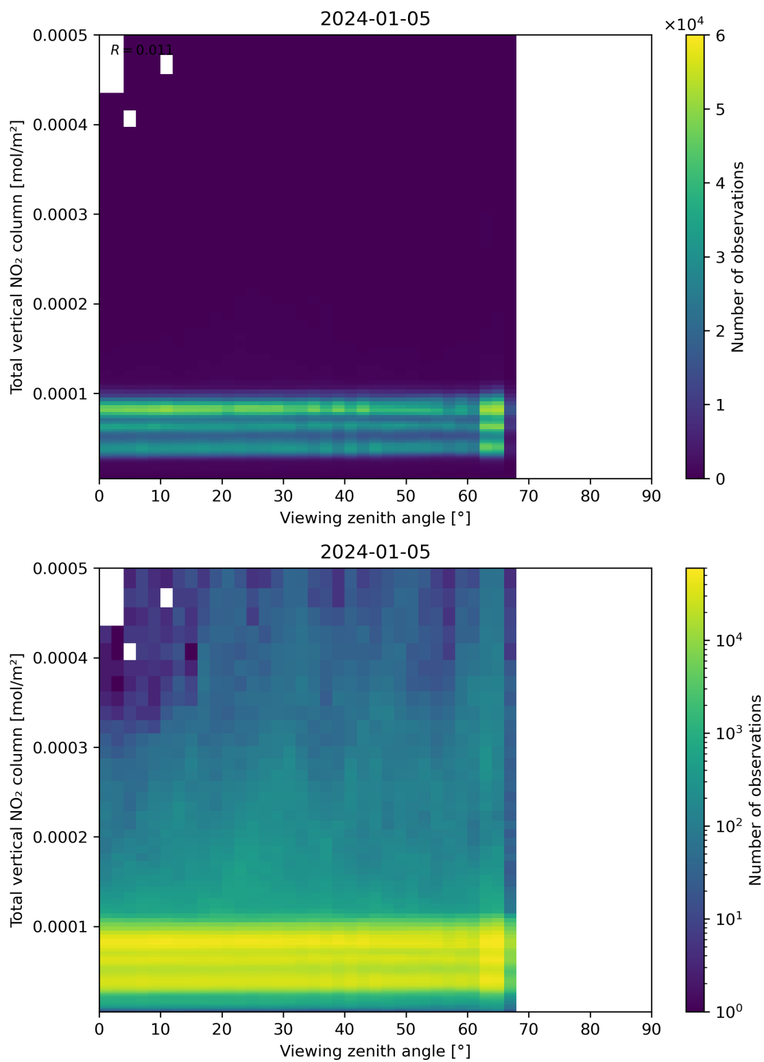
Figure 167: Scatter density plot of “Viewing zenith angle” against “Total vertical NO 2 column” for 2024-01-05 to 2024-01-06.
