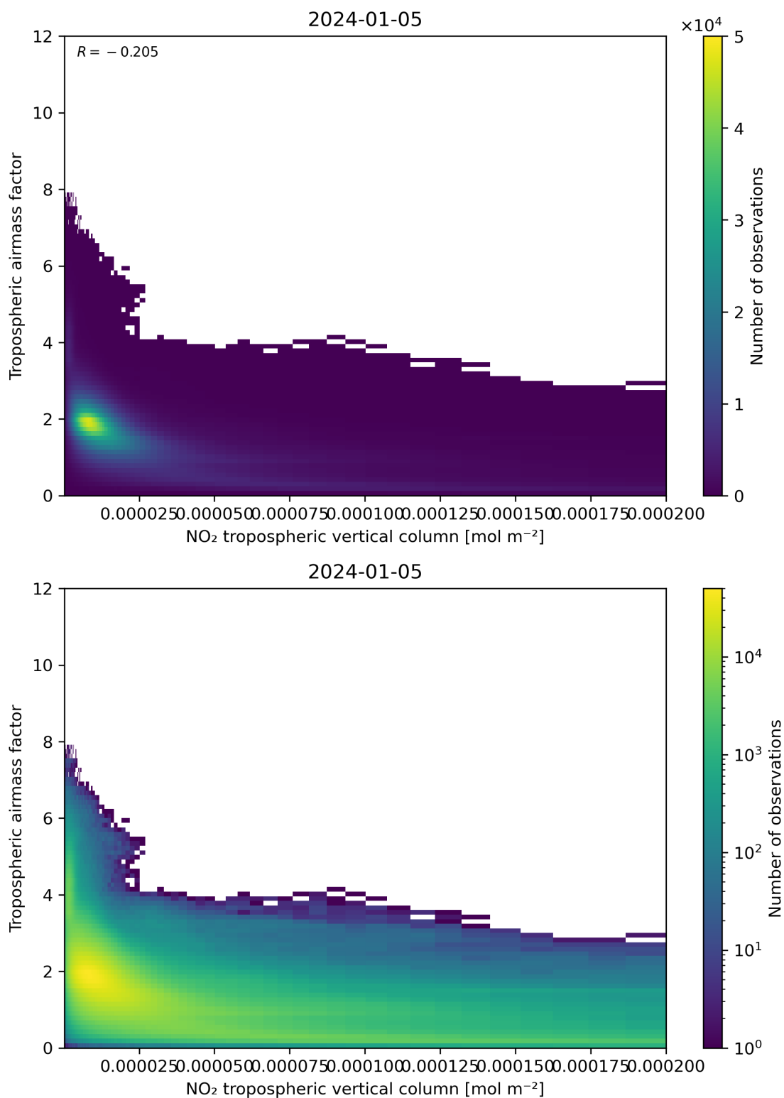
Figure 123: Scatter density plot of “NO 2 tropospheric vertical column” against “Tropospheric air mass factor” for 2024-01-05 to 2024-01-06.
