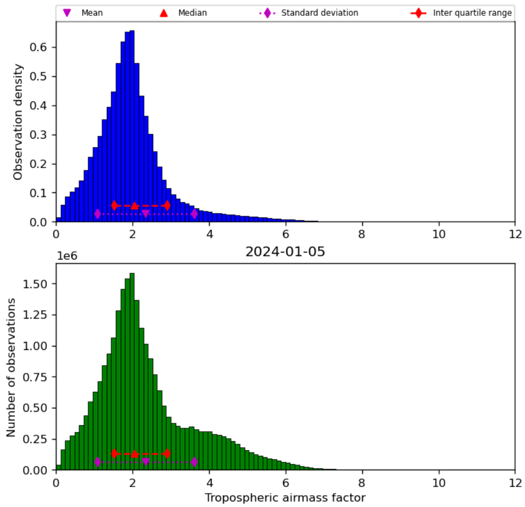
Figure 31: Histogram of “Tropospheric airmass factor” for 2024-01-05 to 2024-01-06
