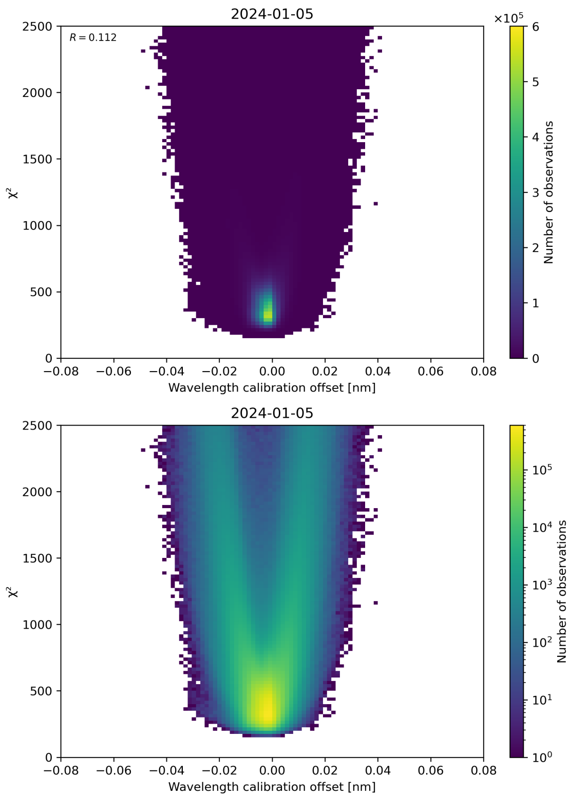
Figure 175: Scatter density plot of “Wavelength calibration offset” against “ \chi^2 ” for 2024-01-05 to 2024-01-06.
