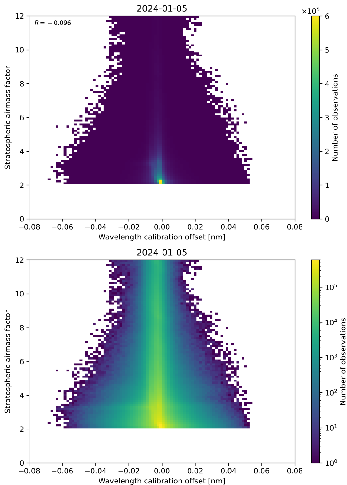
Figure 174: Scatter density plot of “Wavelength calibration offset” against “Stratospheric airmass factor” for 2024-01-05 to 2024-01-06.
