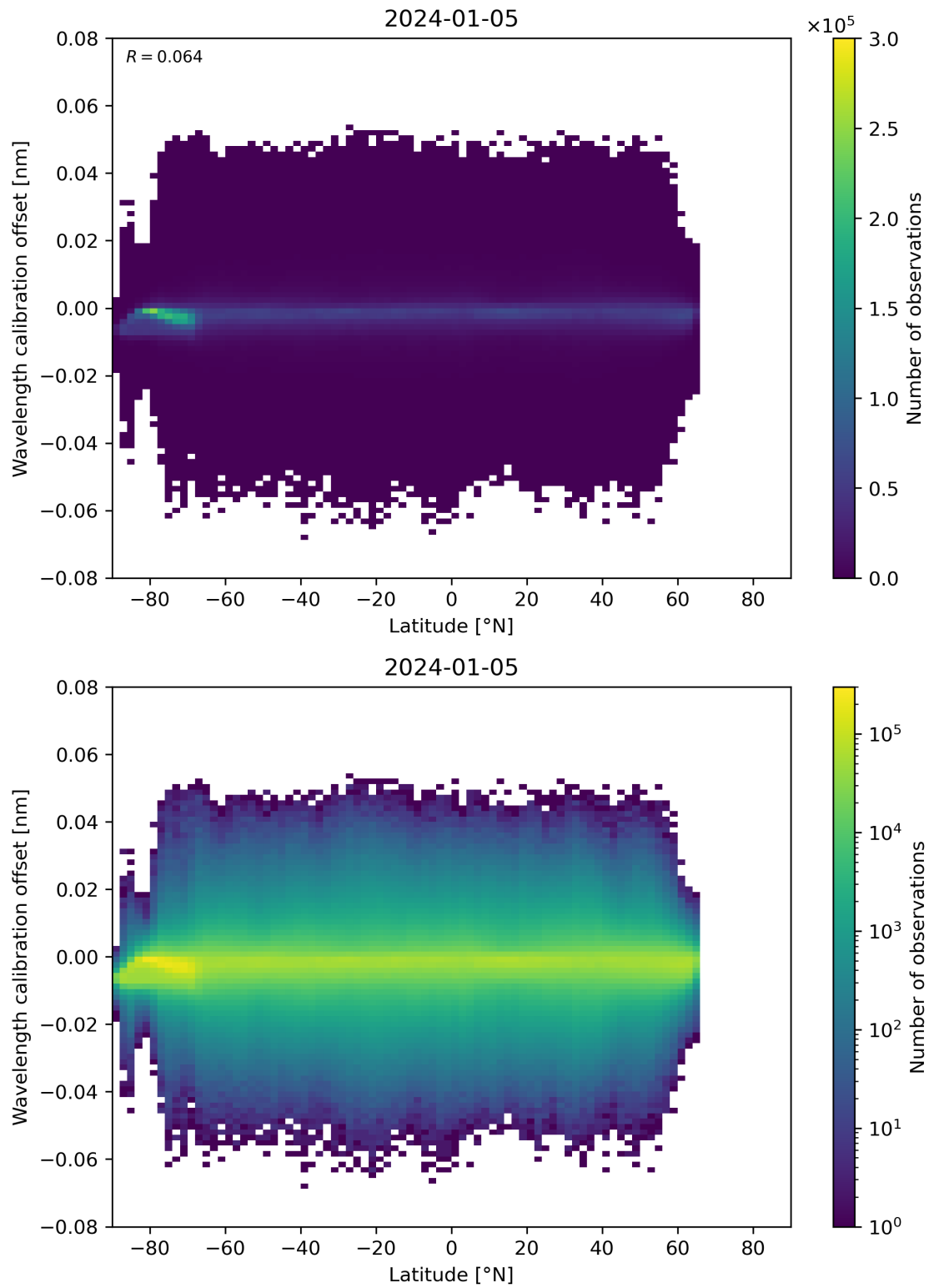
Figure 95: Scatter density plot of “Latitude” against “Wavelength calibration offset” for 2024-01-05 to 2024-01-06.
