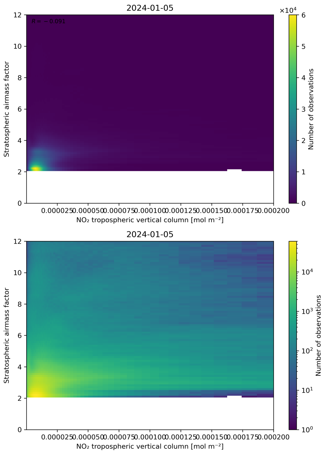
Figure 121: Scatter density plot of “NO 2 tropospheric vertical column” against “Stratospheric airmass factor” for 2024-01-05 to 2024-01-06.
