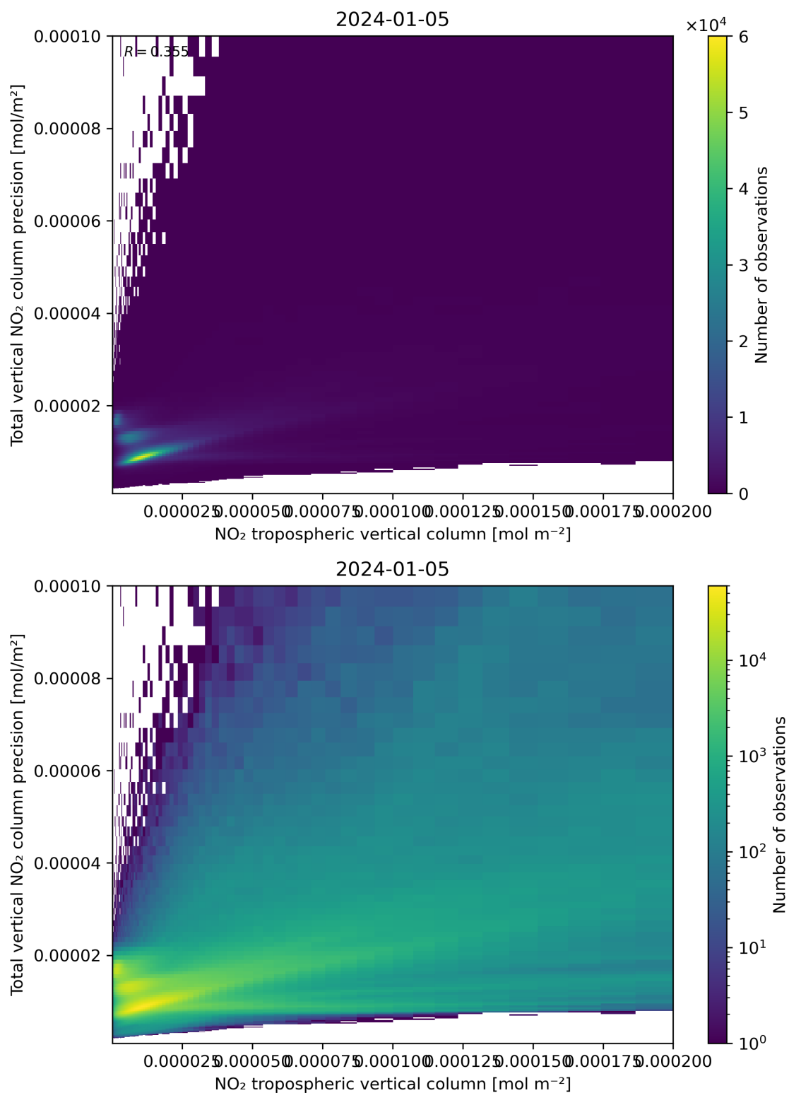
Figure 129: Scatter density plot of “NO 2 tropospheric vertical column” against “Total vertical NO 2 column precision” for 2024-01-05 to 2024-01-06.
