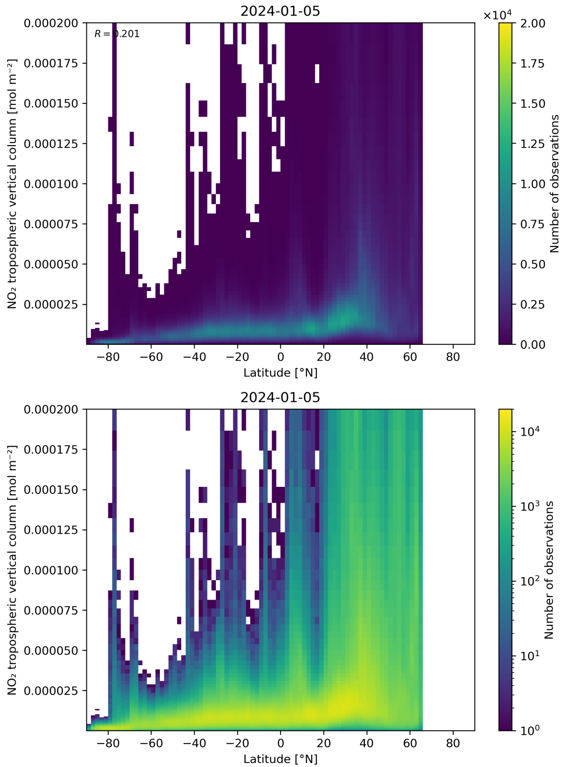
Figure 92: Scatter density plot of “Latitude” against “NO 2 tropospheric vertical column” for 2024-01-05 to 2024-01-06.
