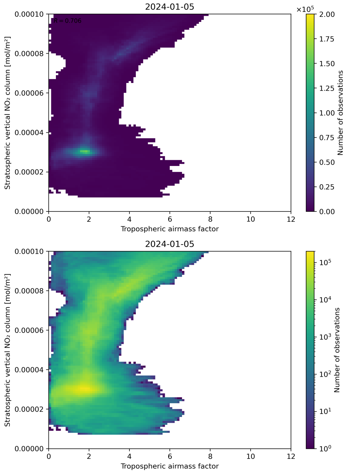
Figure 74: Scatter density plot of “Tropospheric air mass factor” against “Stratospheric vertical NO 2 column” for 2024-01-05 to 2024-01-06.
