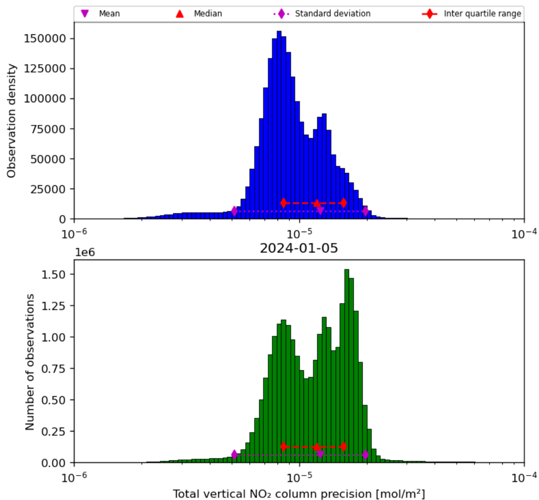
Figure 39: Histogram of "Total vertical NO 2 column precision" for 2024-01-05 to 2024-01-06
