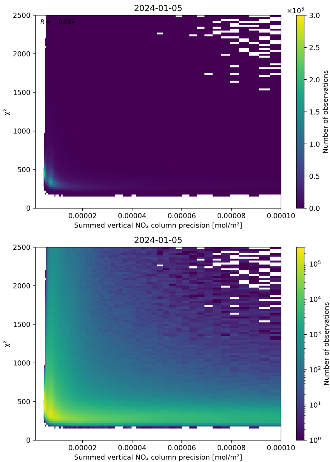
Figure 107: Scatter density plot of “Summed vertical NO 2 column precision” against “ \chi^2 ” for 2024-01-05 to 2024-01-06.
