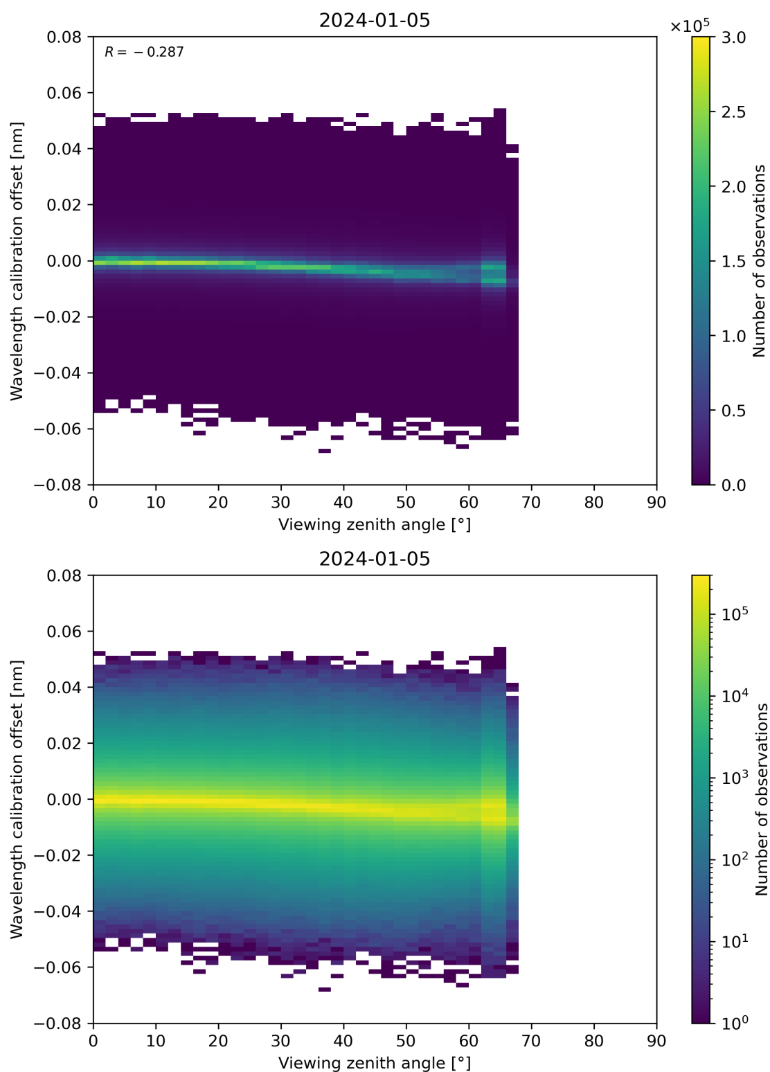
Figure 173: Scatter density plot of “Viewing zenith angle” against “Wavelength calibration offset” for 2024-01-05 to 2024-01-06.
