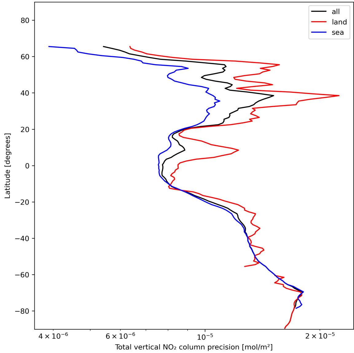
Figure 22: Zonal average of “Total vertical NO 2 column precision” for 2024-01-05 to 2024-01-06.
