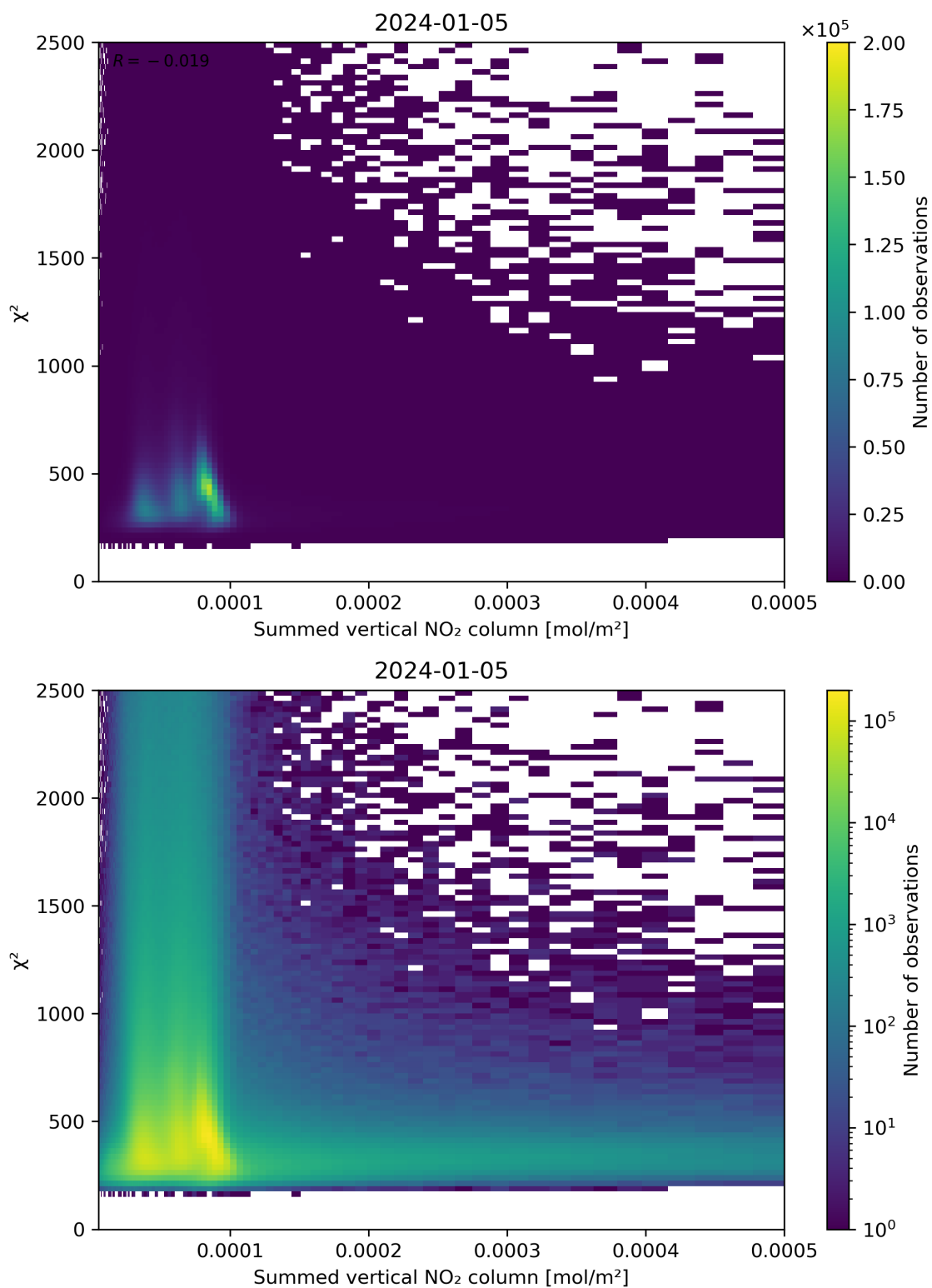
Figure 104: Scatter density plot of “Summed vertical NO 2 column” against “ \chi^2 ” for 2024-01-05 to 2024-01-06.
