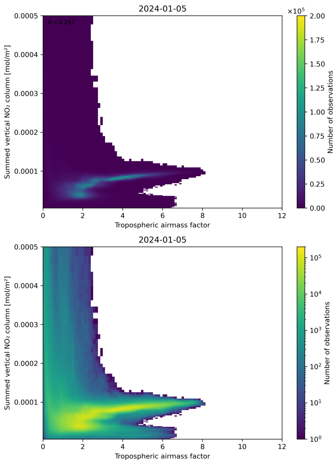
Figure 75: Scatter density plot of “Tropospheric airmass factor” against “Summed vertical NO 2 column” for 2024-01-05 to 2024-01-06.
