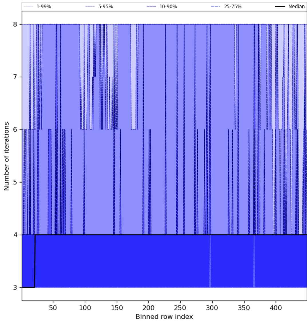
Figure 51: Along track statistics of “Number of iterations” for 2024-01-05 to 2024-01-06
