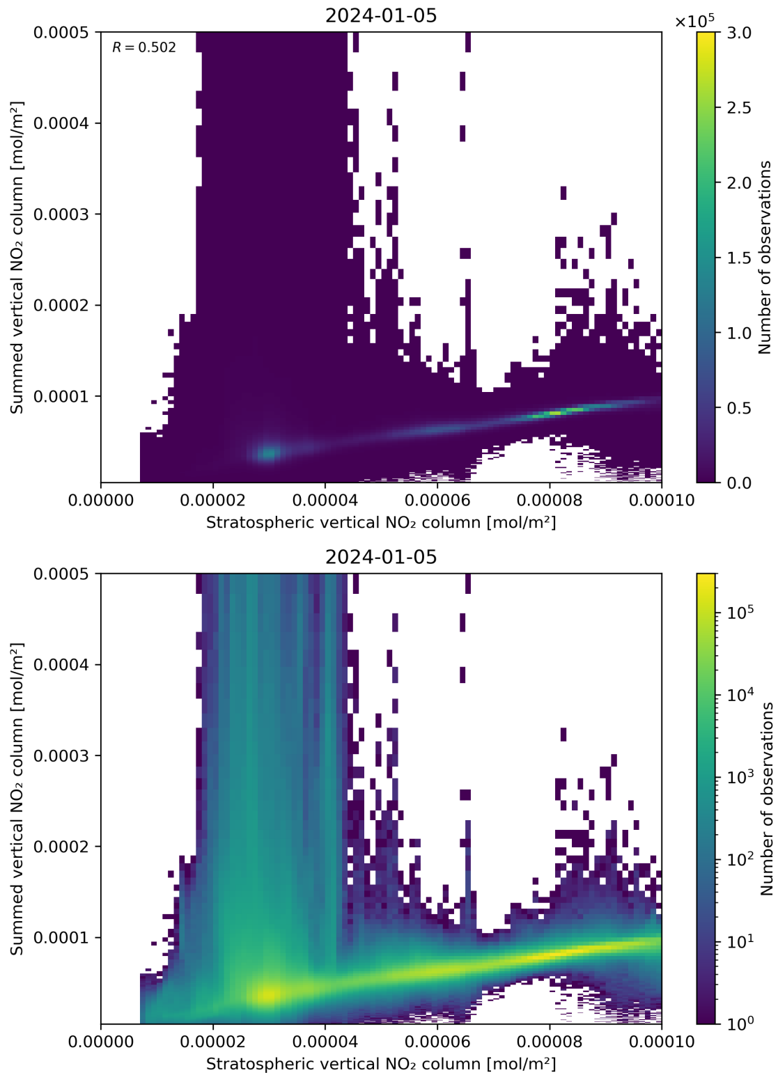
Figure 98: Scatter density plot of “Stratospheric vertical NO 2 column” against “Summed vertical NO 2 column” for 2024-01-05 to 2024-01-06.
