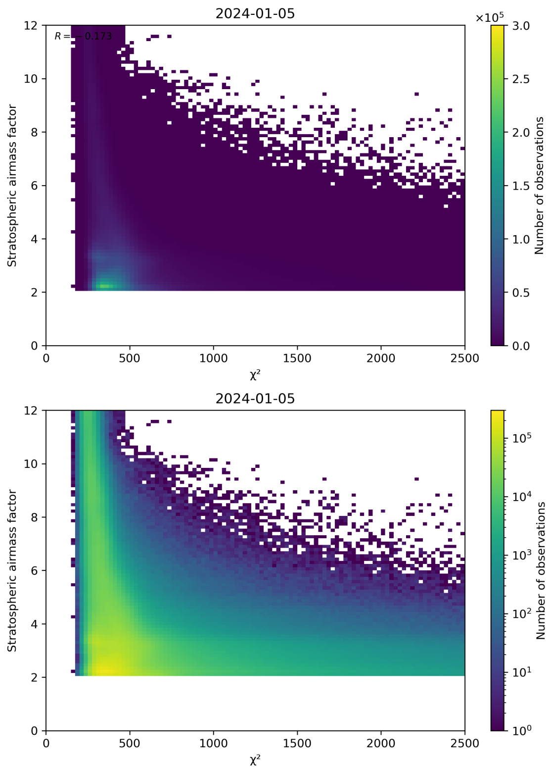
Figure 81: Scatter density plot of “ \chi^2 ” against “Stratospheric airmass factor” for 2024-01-05 to 2024-01-06.
