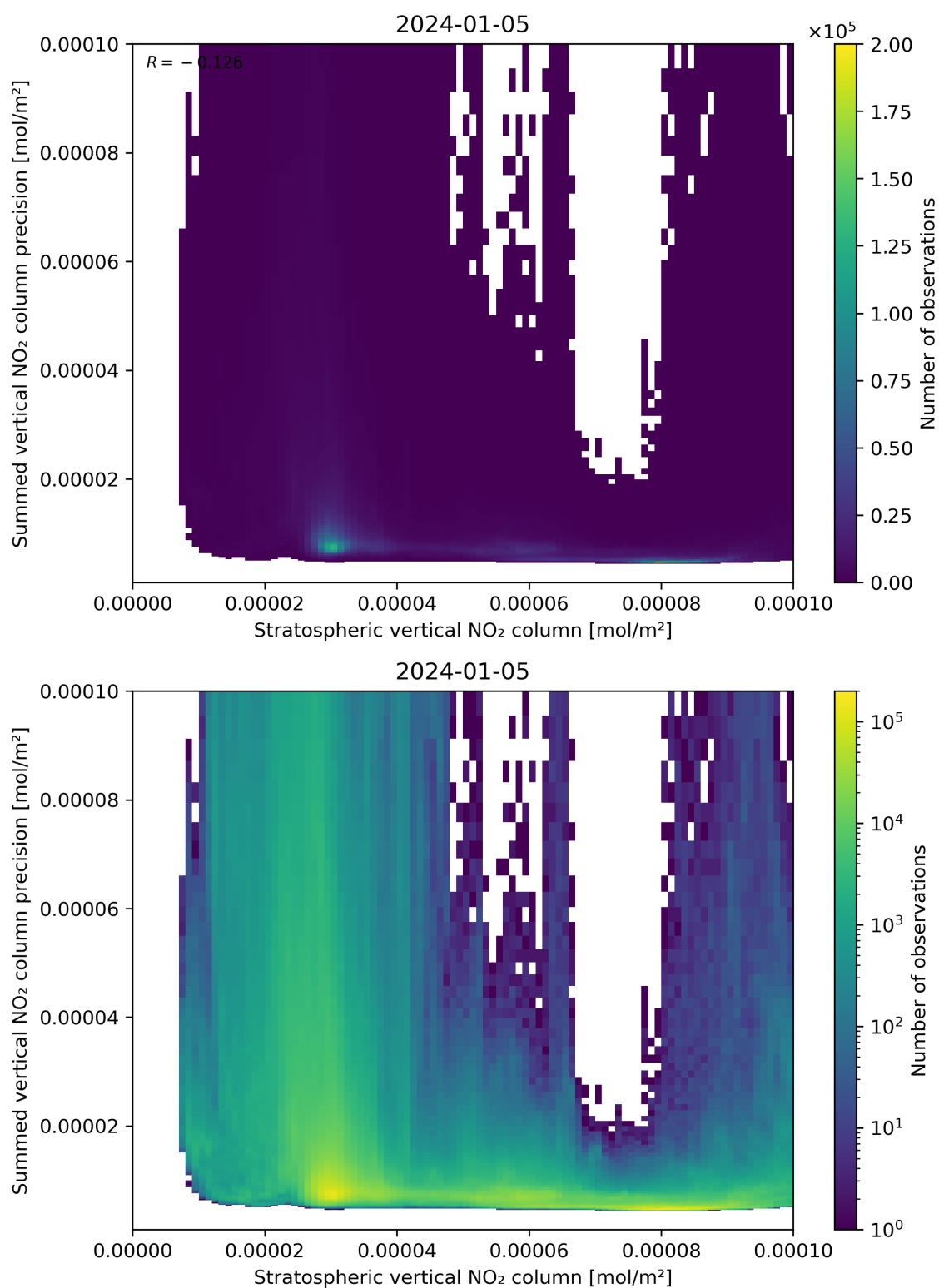
Figure 99: Scatter density plot of “Stratospheric vertical NO 2 column” against “Summed vertical NO 2 column precision” for 2024-01-05 to 2024-01-06.
