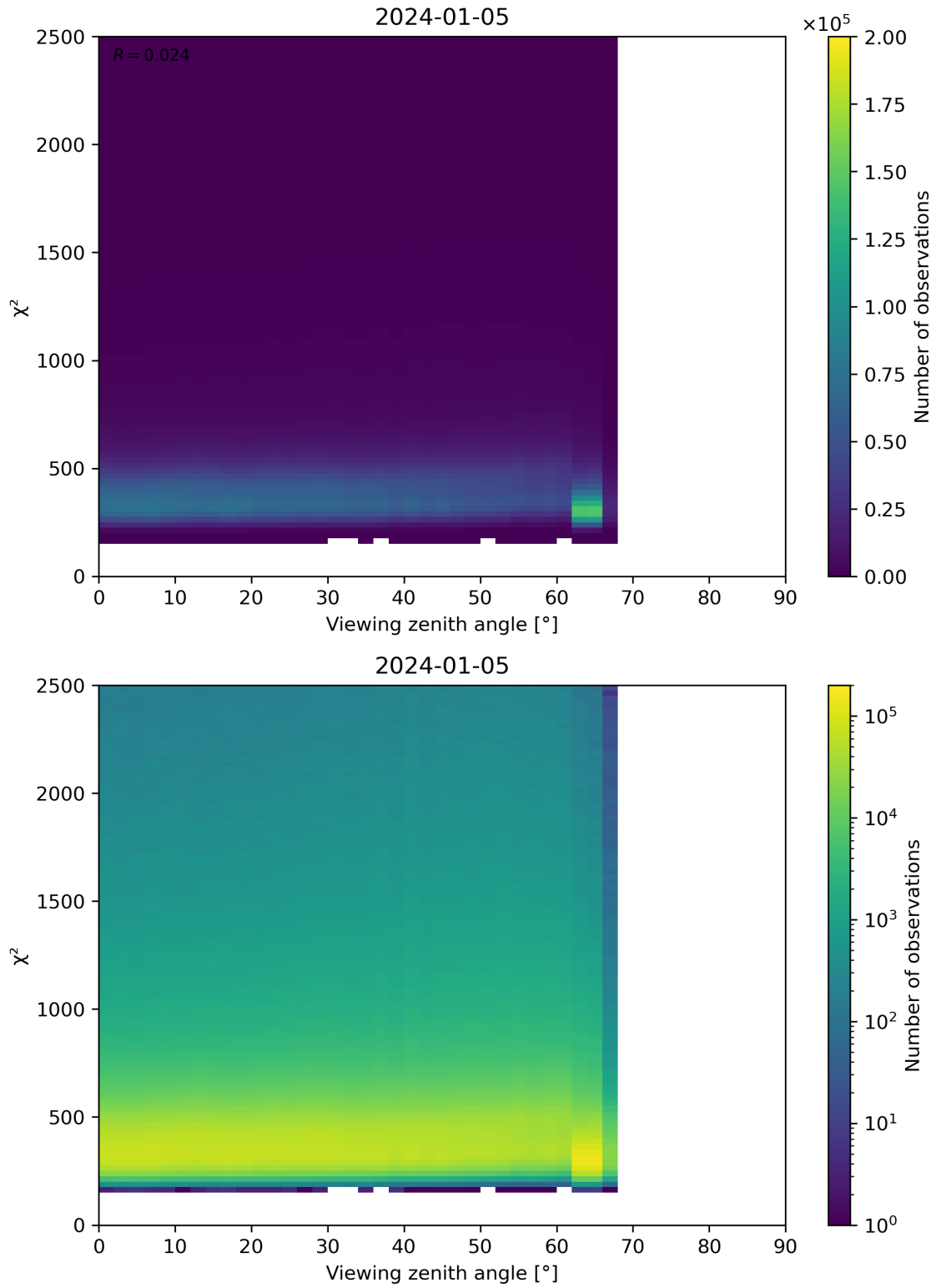
Figure 162: Scatter density plot of “Viewing zenith angle” against “ \chi^2 ” for 2024-01-05 to 2024-01-06.
