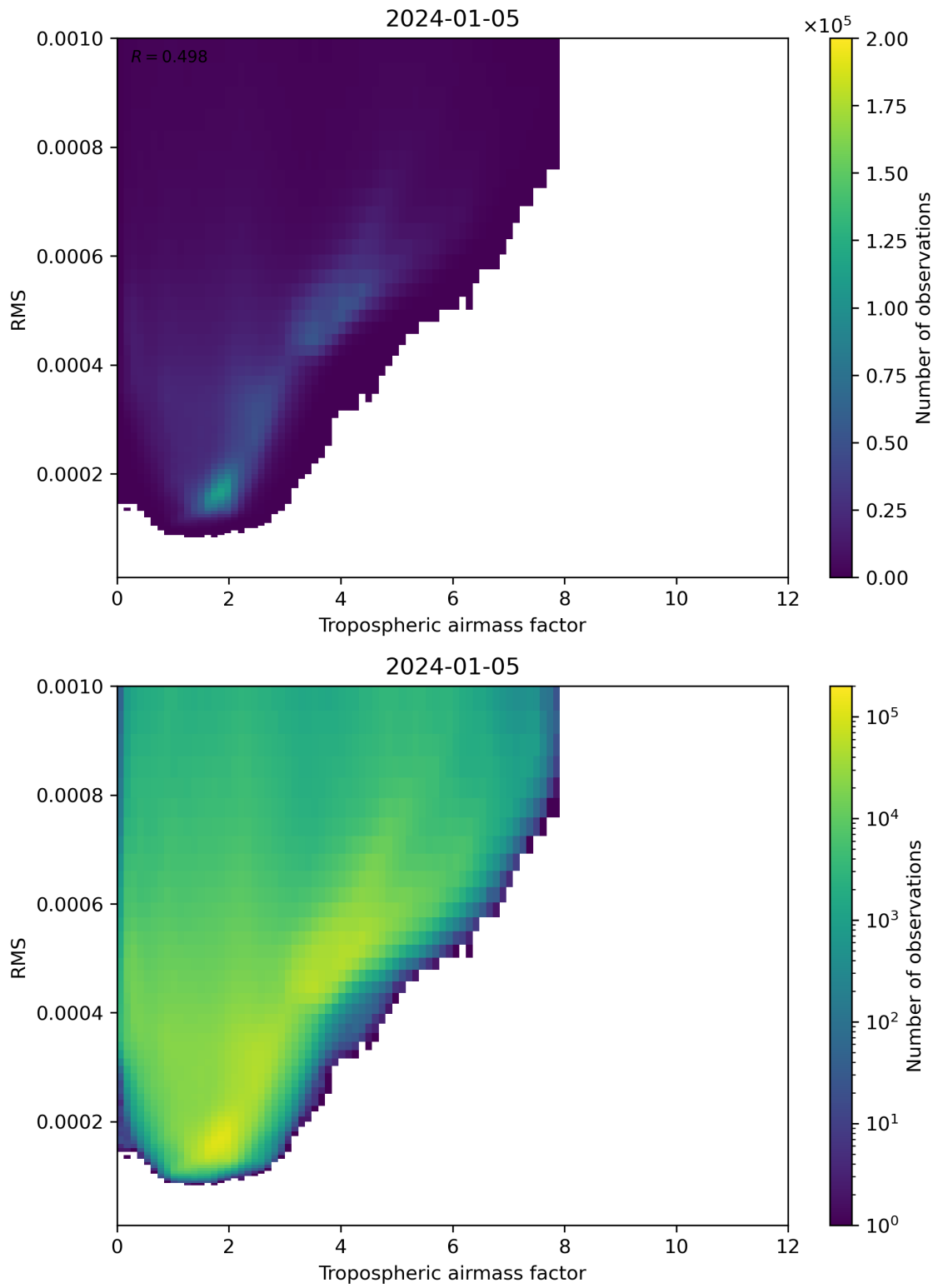
Figure 79: Scatter density plot of “Tropospheric airmass factor” against “RMS” for 2024-01-05 to 2024-01-06.
