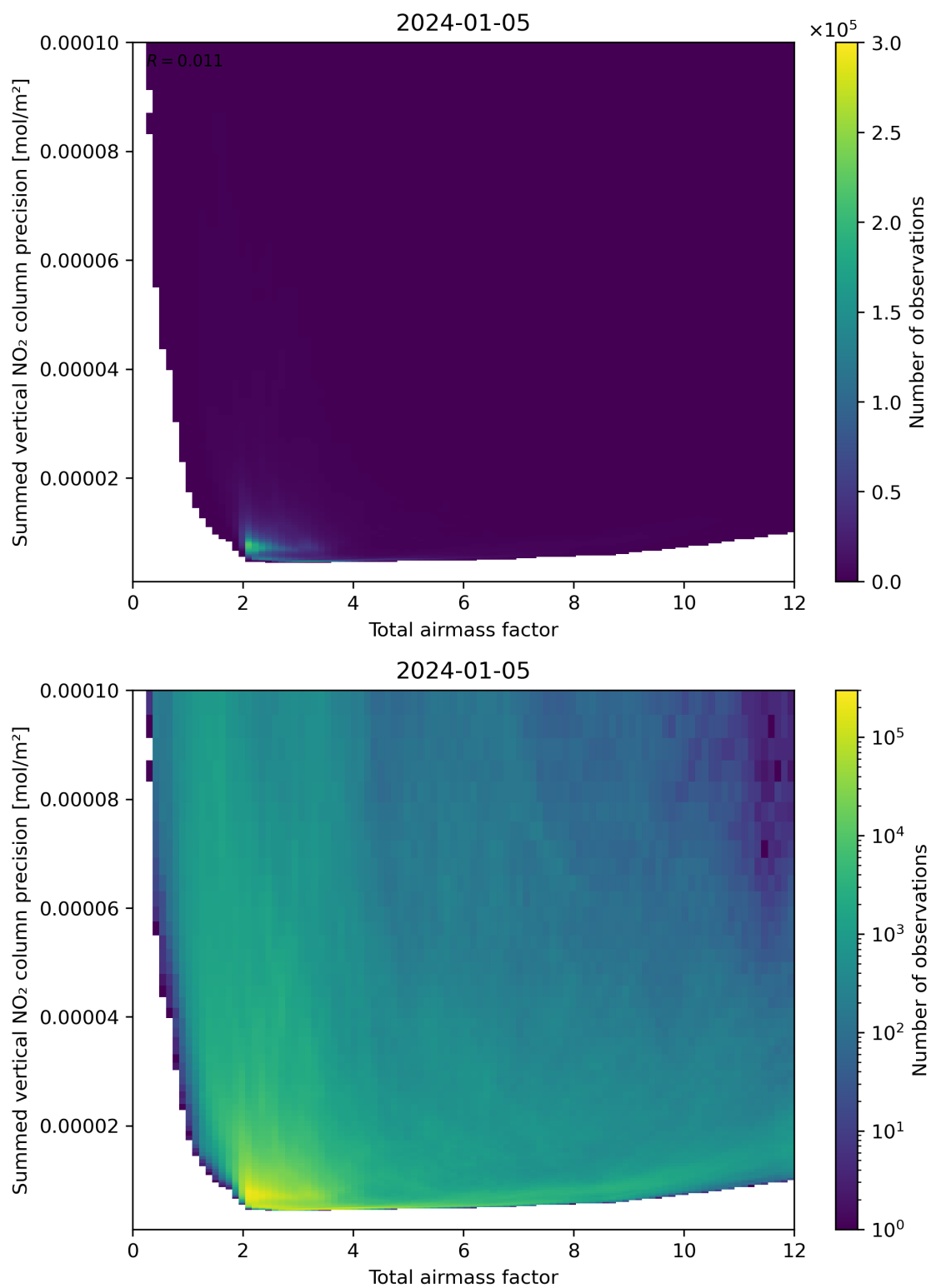
Figure 66: Scatter density plot of “Total airmass factor” against “Summed vertical NO 2 column precision” for 2024-01-05 to 2024-01-06.
