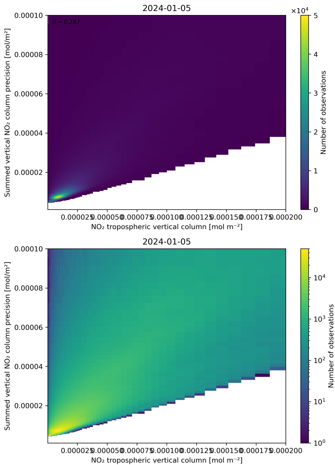
Figure 127: Scatter density plot of “NO 2 tropospheric vertical column” against “Summed vertical NO 2 column precision” for 2024-01-05 to 2024-01-06.
