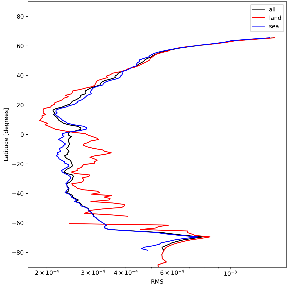
Figure 26: Zonal average of “RMS” for 2024-01-05 to 2024-01-06.
