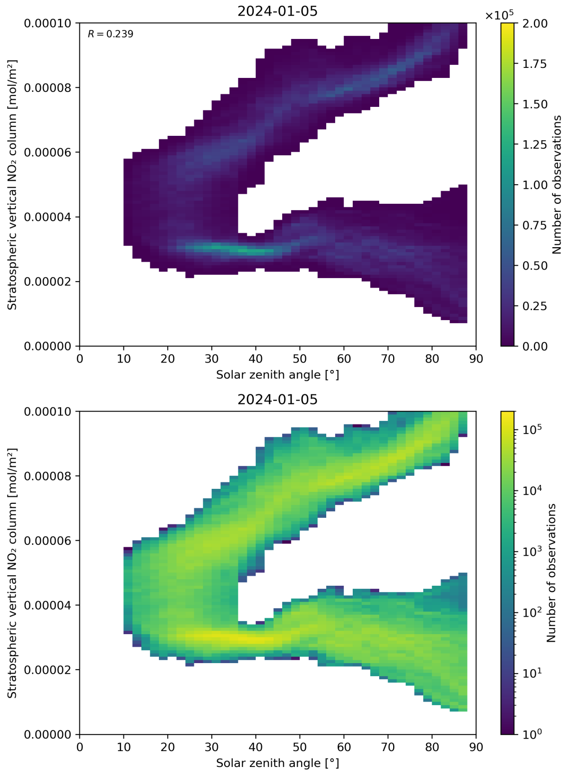
Figure 150: Scatter density plot of “Solar zenith angle” against “Stratospheric vertical NO 2 column” for 2024-01-05 to 2024-01-06.
