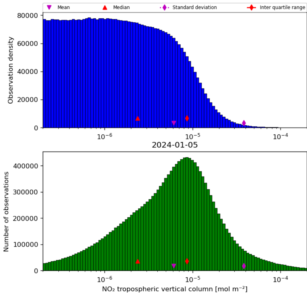
Figure 29: Histogram of “NO 2 tropospheric vertical column” for 2024-01-05 to 2024-01-06
