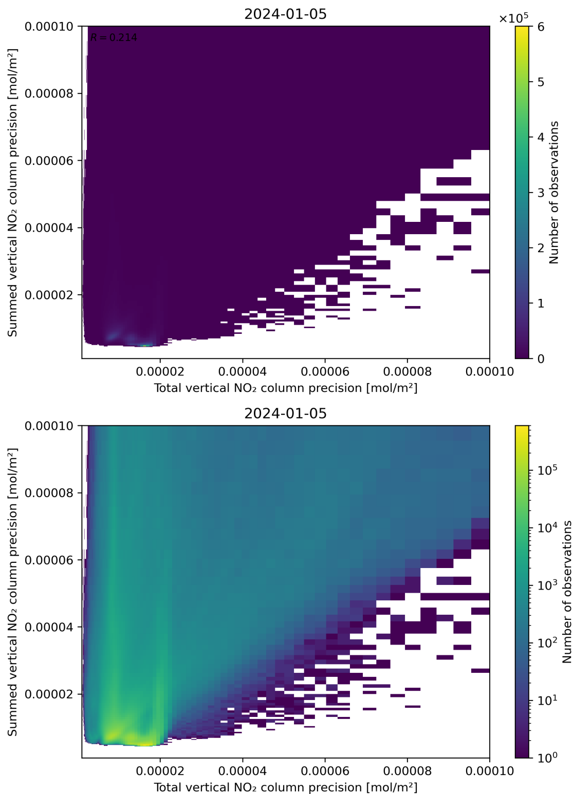
Figure 118: Scatter density plot of “Total vertical NO 2 column precision” against “Summed vertical NO 2 column precision” for 2024-01-05 to 2024-01-06.
