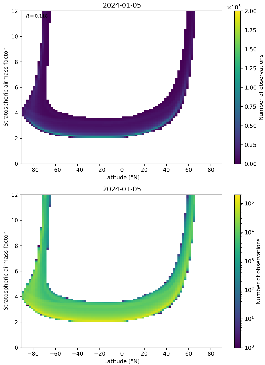
Figure 83: Scatter density plot of “Latitude” against “Stratospheric airmass factor” for 2024-01-05 to 2024-01-06.
