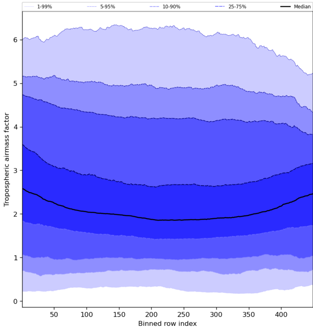
Figure 48: Along track statistics of “Tropospheric air mass factor” for 2024-01-05 to 2024-01-06
