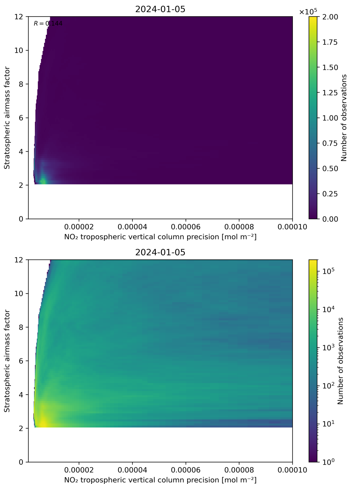
Figure 131: Scatter density plot of “NO 2 tropospheric vertical column precision” against “Stratospheric airmass factor” for 2024-01-05 to 2024-01-06.
