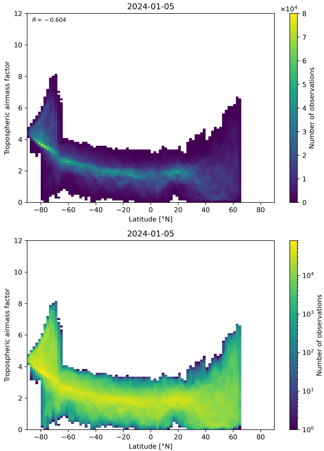
Figure 85: Scatter density plot of “Latitude” against “Tropospheric air mass factor” for 2024-01-05 to 2024-01-06.
