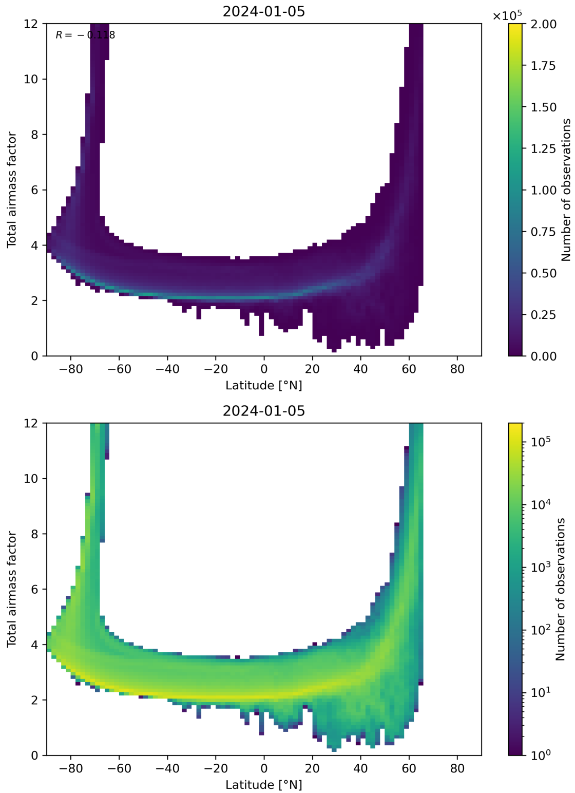
Figure 84: Scatter density plot of “Latitude” against “Total airmass factor” for 2024-01-05 to 2024-01-06.
