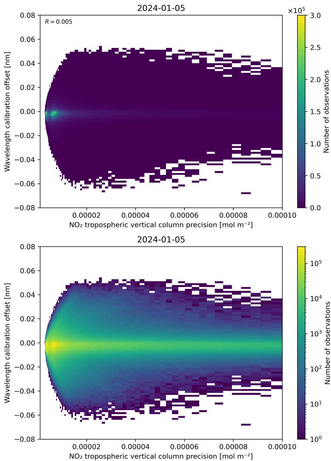
Figure 141: Scatter density plot of “NO 2 tropospheric vertical column precision” against “Wavelength calibration offset” for 2024-01-05 to 2024-01-06.
