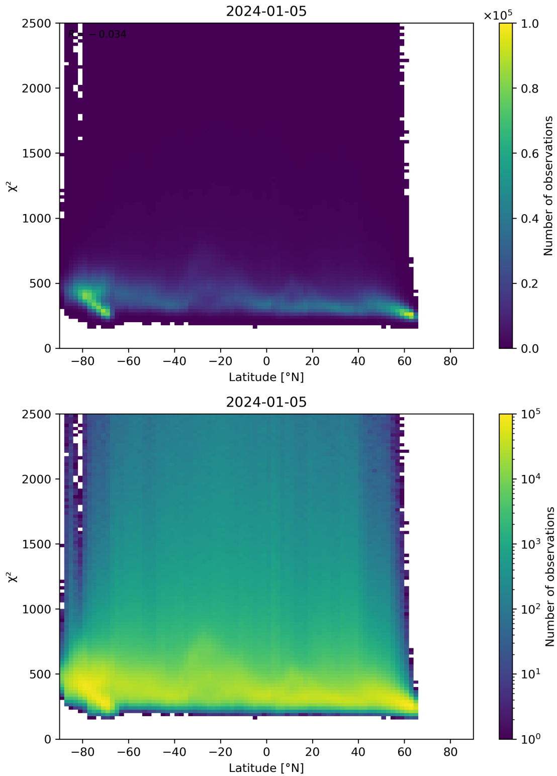
Figure 86: Scatter density plot of “Latitude” against “ \chi^2 ” for 2024-01-05 to 2024-01-06.
