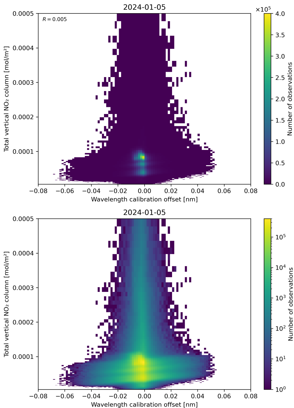
Figure 179: Scatter density plot of “Wavelength calibration offset” against “Total vertical NO 2 column” for 2024-01-05 to 2024-01-06.
