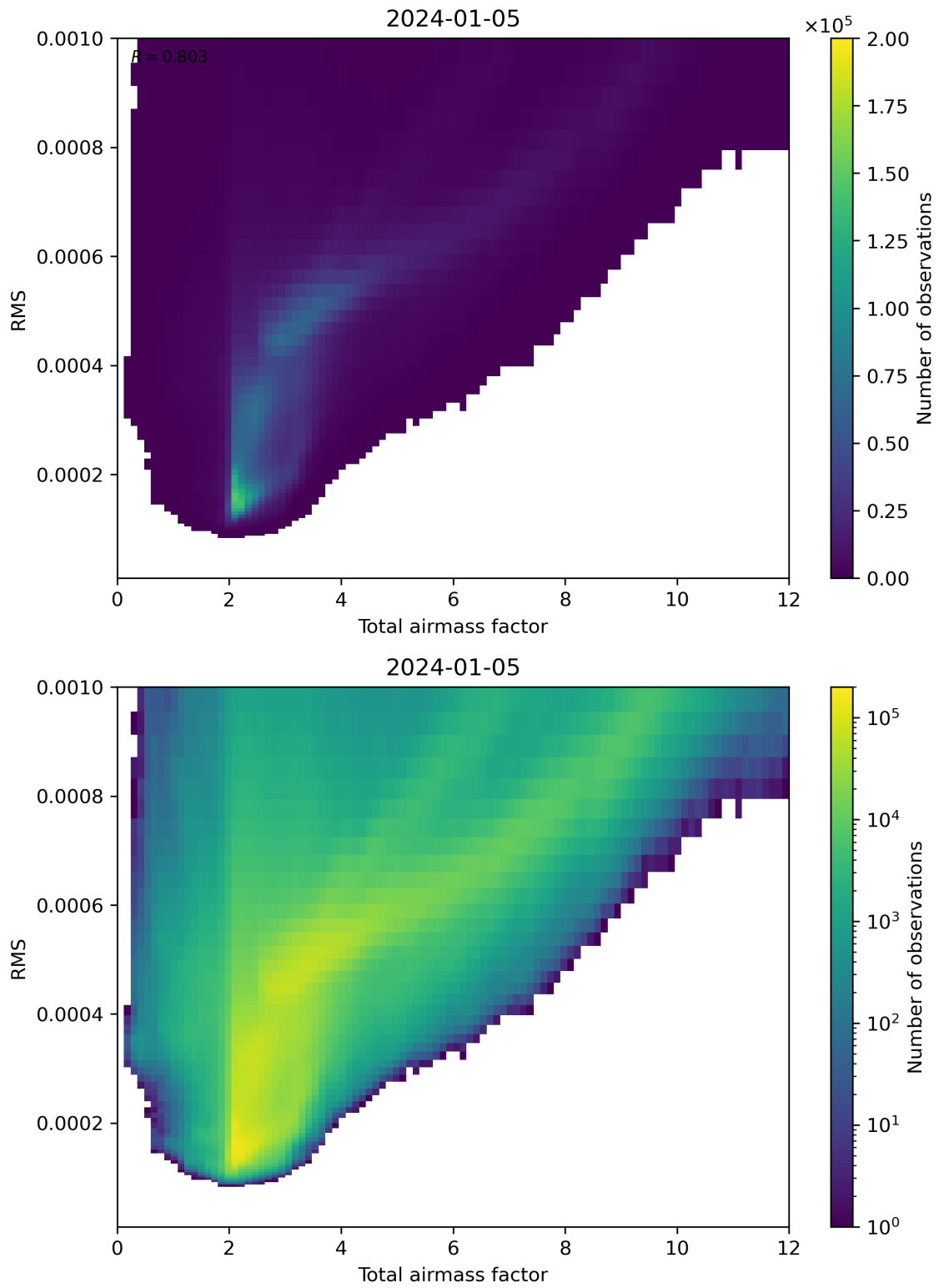
Figure 69: Scatter density plot of “Total airmass factor” against “RMS” for 2024-01-05 to 2024-01-06.
