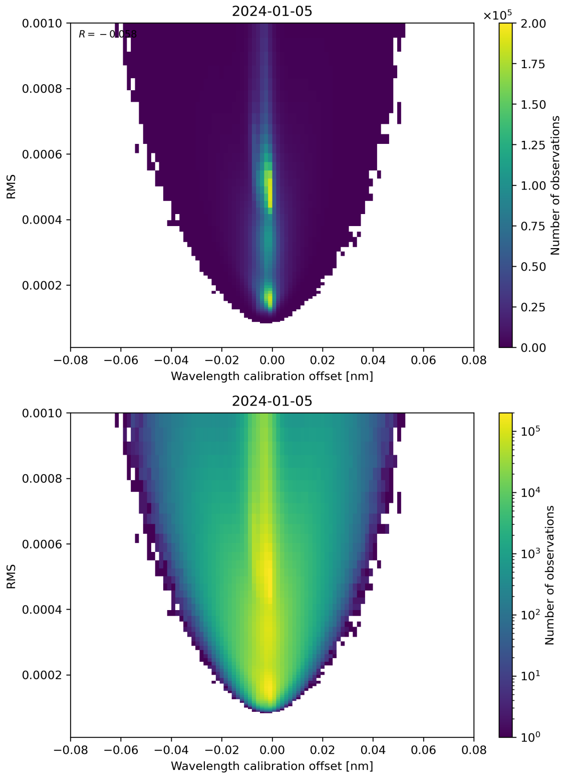
Figure 181: Scatter density plot of “Wavelength calibration offset” against “RMS” for 2024-01-05 to 2024-01-06.
