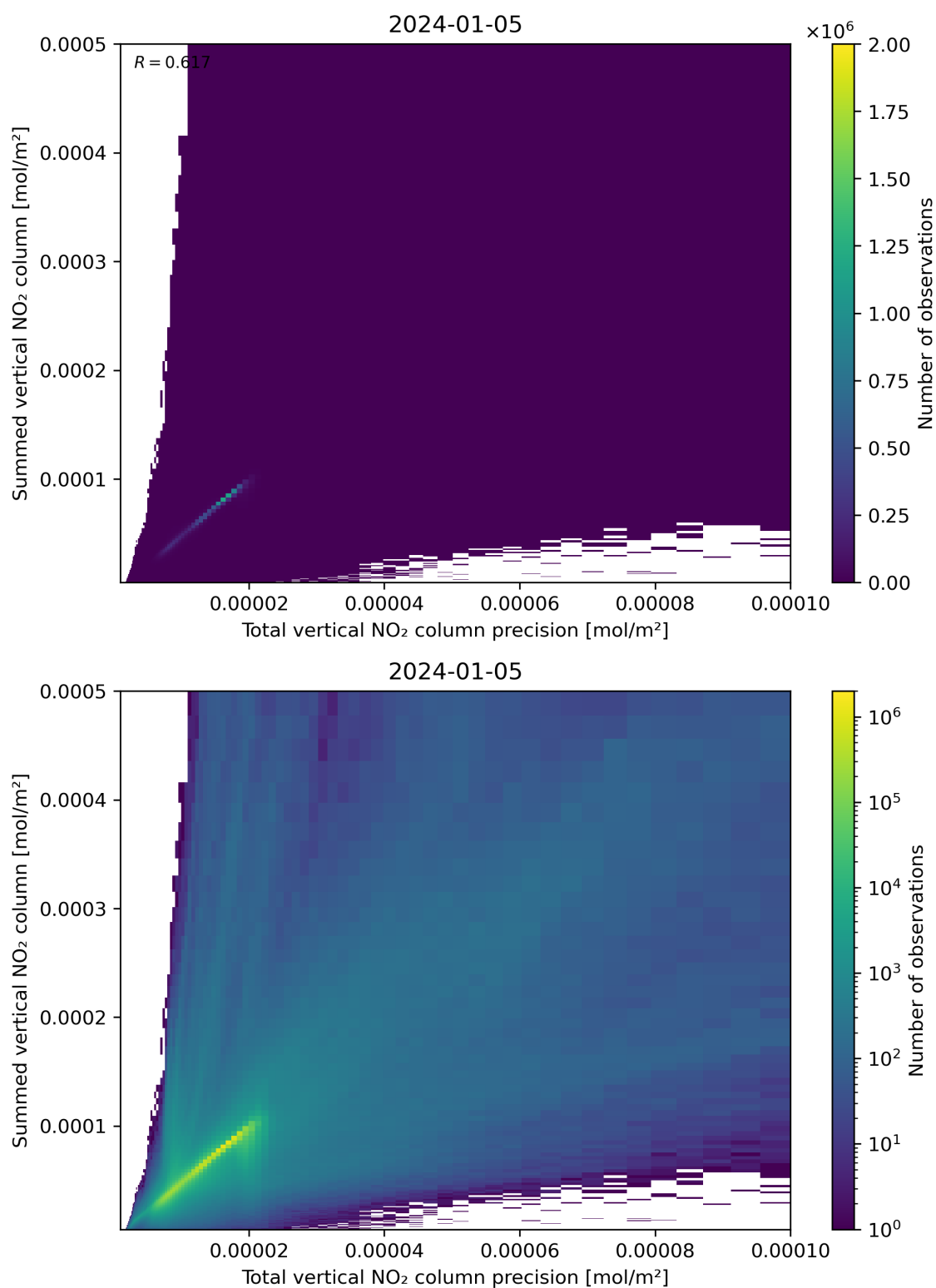
Figure 117: Scatter density plot of “Total vertical NO 2 column precision” against “Summed vertical NO 2 column” for 2024-01-05 to 2024-01-06.
