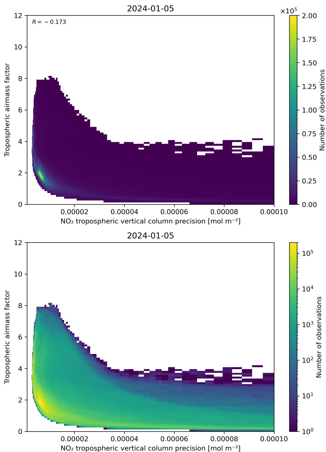
Figure 133: Scatter density plot of “NO 2 tropospheric vertical column precision” against “Tropospheric airmass factor” for 2024-01-05 to 2024-01-06.
