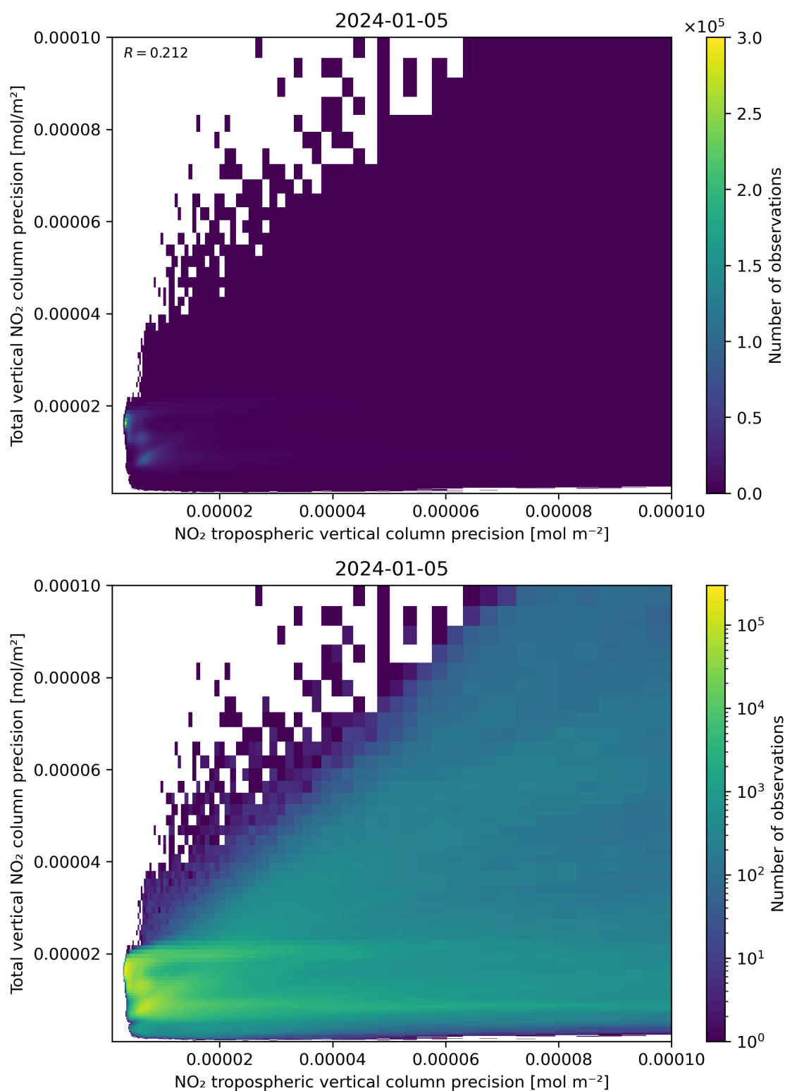
Figure 139: Scatter density plot of “NO 2 tropospheric vertical column precision” against “Total vertical NO 2 column precision” for 2024-01-05 to 2024-01-06.
