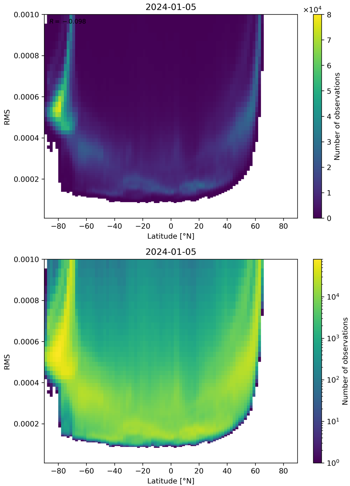
Figure 94: Scatter density plot of “Latitude” against “RMS” for 2024-01-05 to 2024-01-06.
