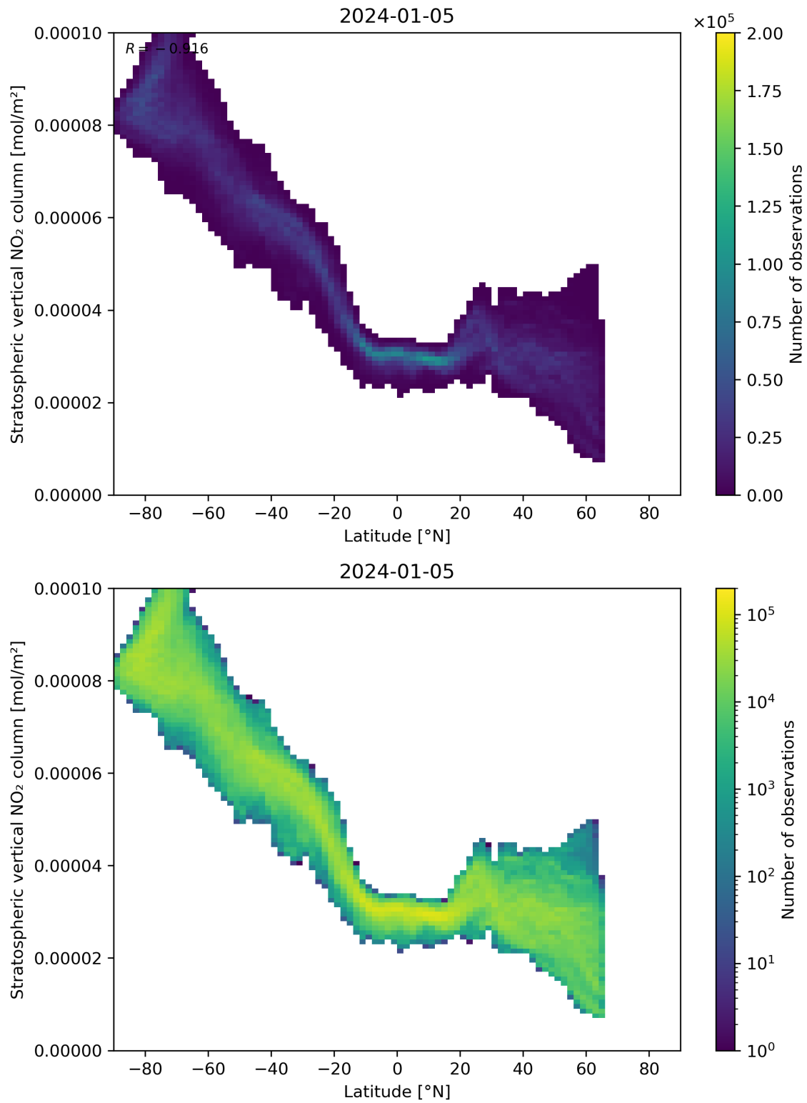
Figure 87: Scatter density plot of “Latitude” against “Stratospheric vertical NO 2 column” for 2024-01-05 to 2024-01-06.
