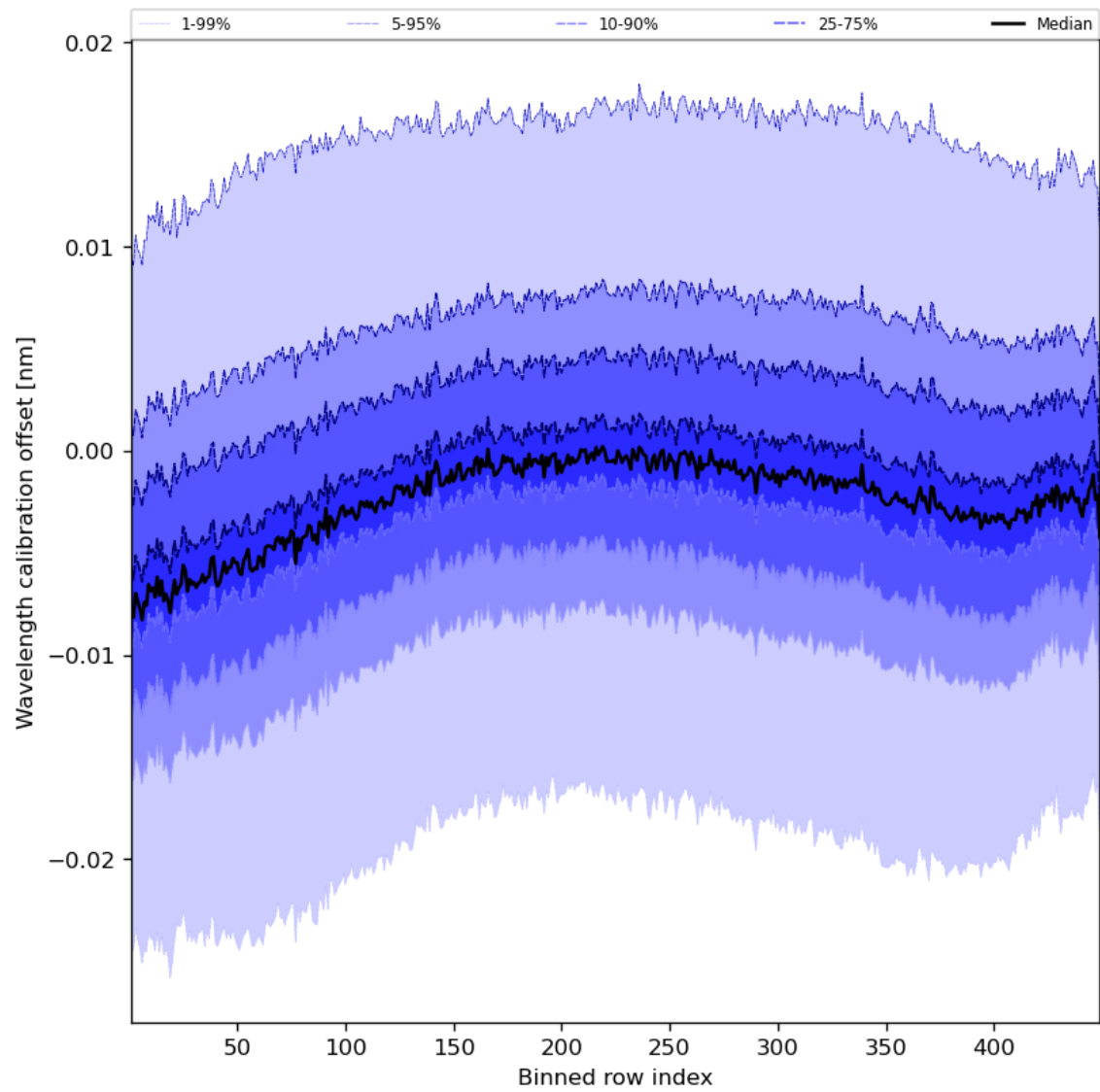
Figure 52: Along track statistics of “Wavelength calibration offset” for 2024-01-05 to 2024-01-06
