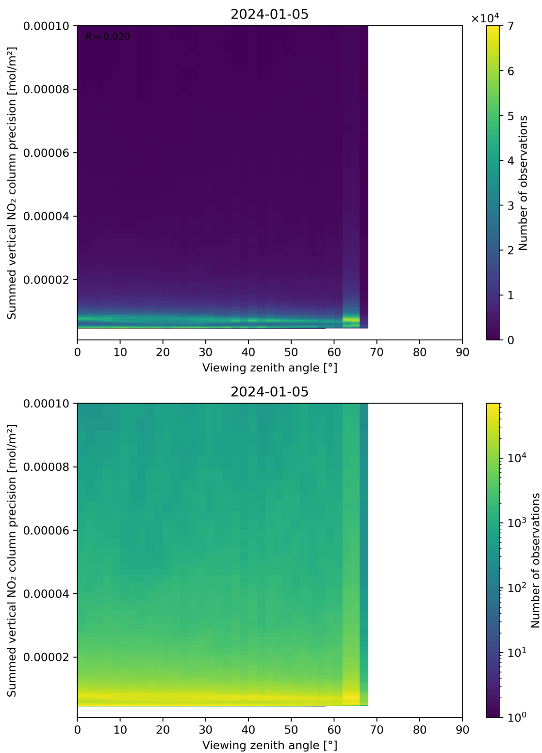
Figure 166: Scatter density plot of “Viewing zenith angle” against “Summed vertical NO 2 column precision” for 2024-01-05 to 2024-01-06.
