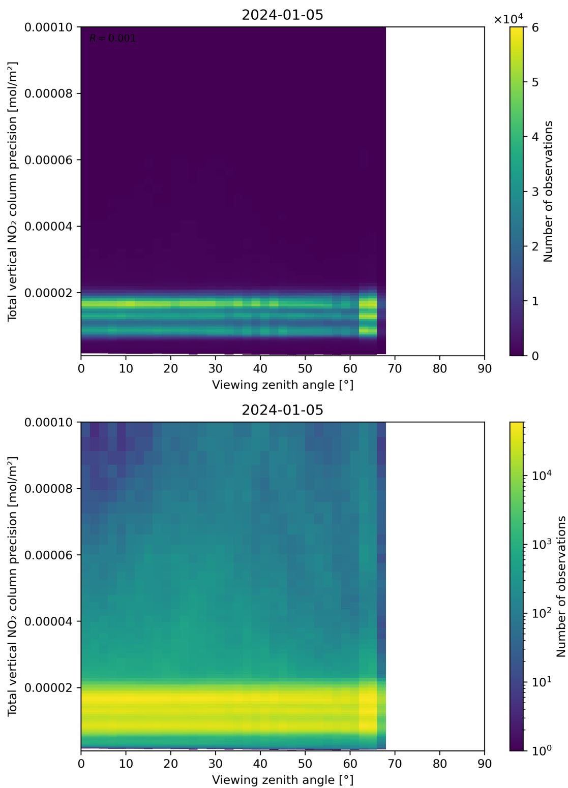
Figure 168: Scatter density plot of “Viewing zenith angle” against “Total vertical NO 2 column precision” for 2024-01-05 to 2024-01-06.
