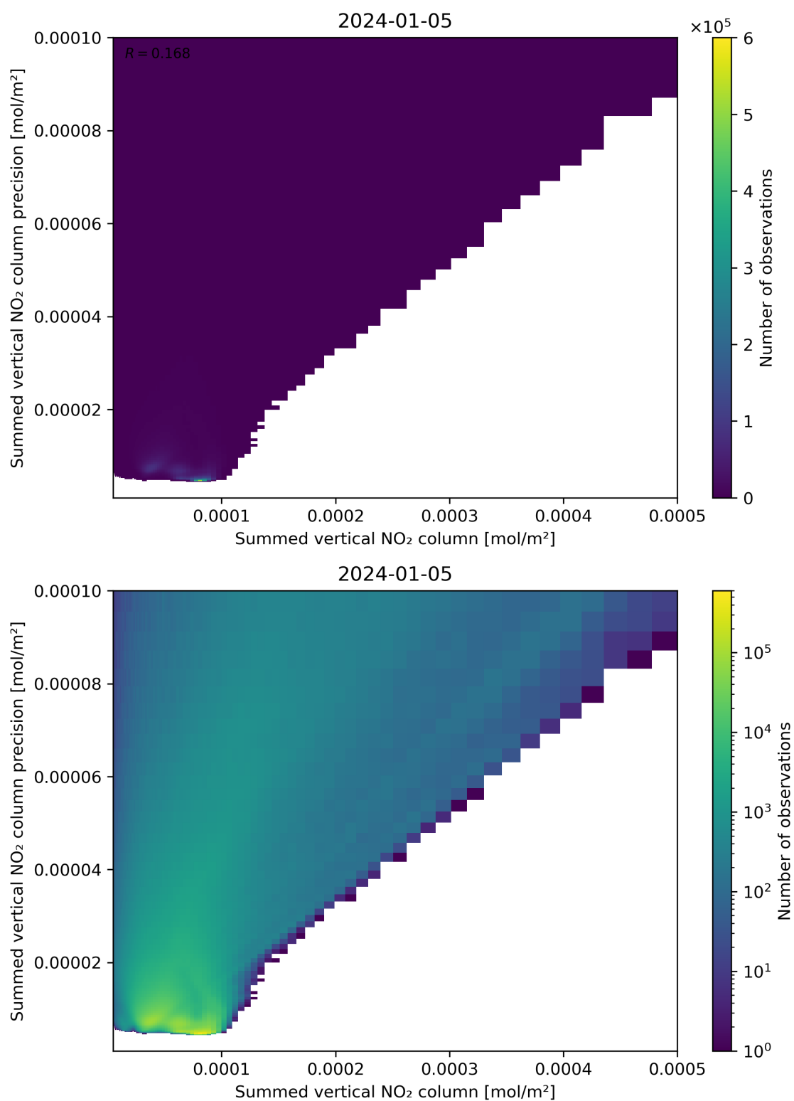
Figure 105: Scatter density plot of “Summed vertical NO 2 column” against “Summed vertical NO 2 column precision” for 2024-01-05 to 2024-01-06.
