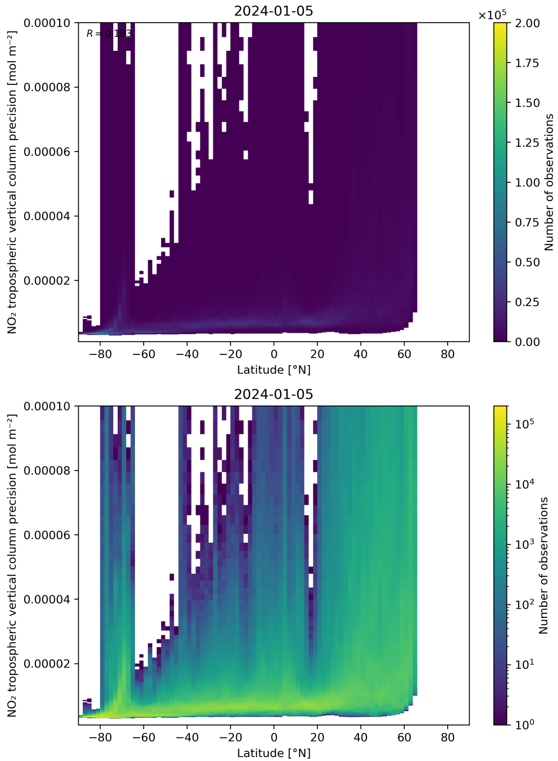
Figure 93: Scatter density plot of “Latitude” against “NO 2 tropospheric vertical column precision” for 2024-01-05 to 2024-01-06.
