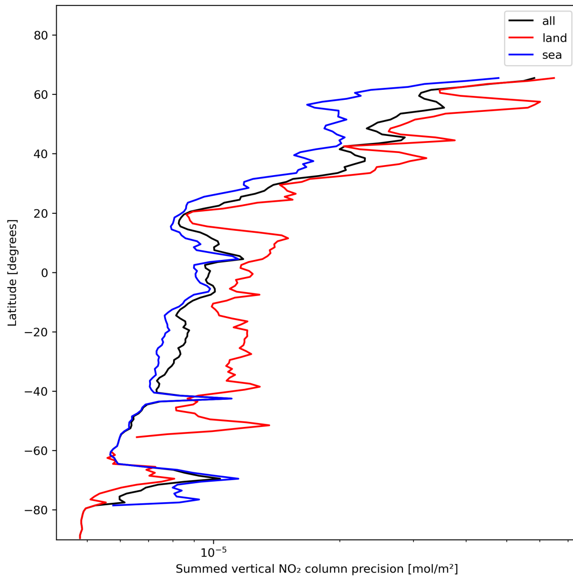
Figure 24: Zonal average of “Summed vertical NO 2 column precision” for 2024-01-05 to 2024-01-06.
