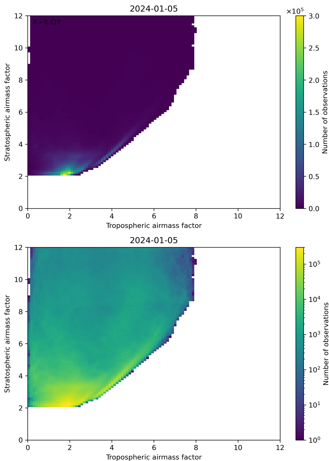
Figure 71: Scatter density plot of “Tropospheric airmass factor” against “Stratospheric airmass factor” for 2024-01-05 to 2024-01-06.
