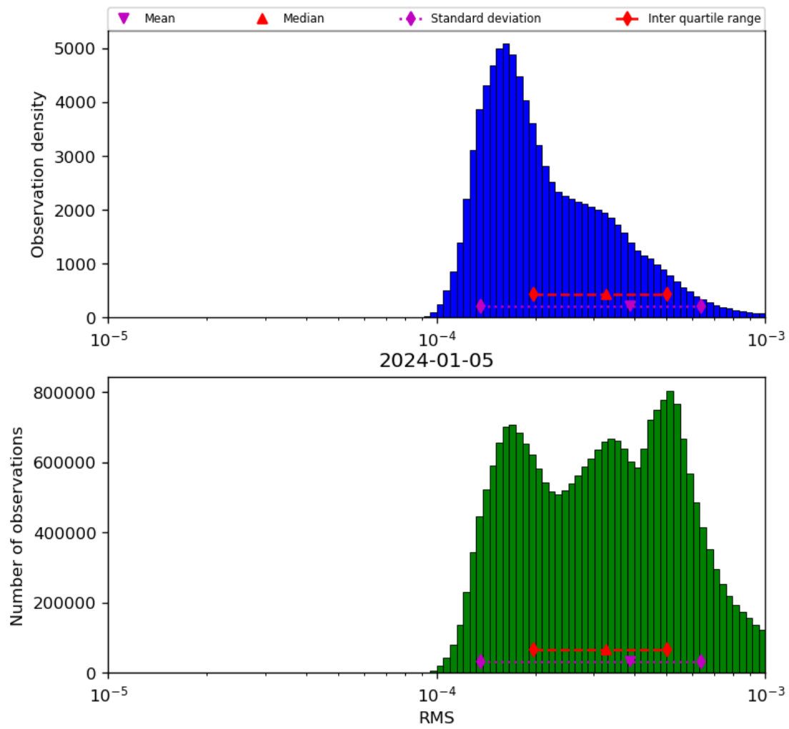
Figure 43: Histogram of “RMS” for 2024-01-05 to 2024-01-06
