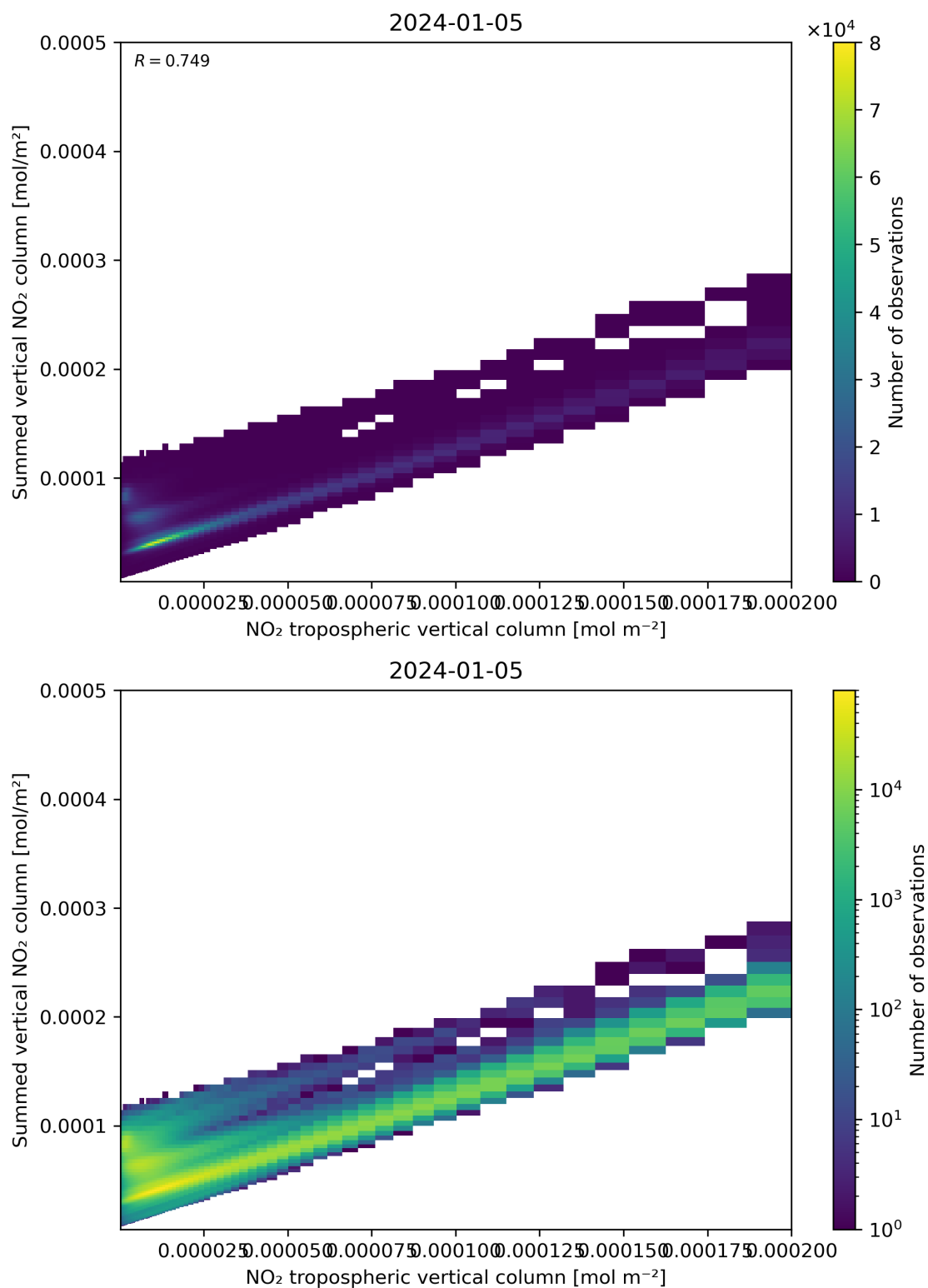
Figure 126: Scatter density plot of “NO 2 tropospheric vertical column” against “Summed vertical NO 2 column” for 2024-01-05 to 2024-01-06.
