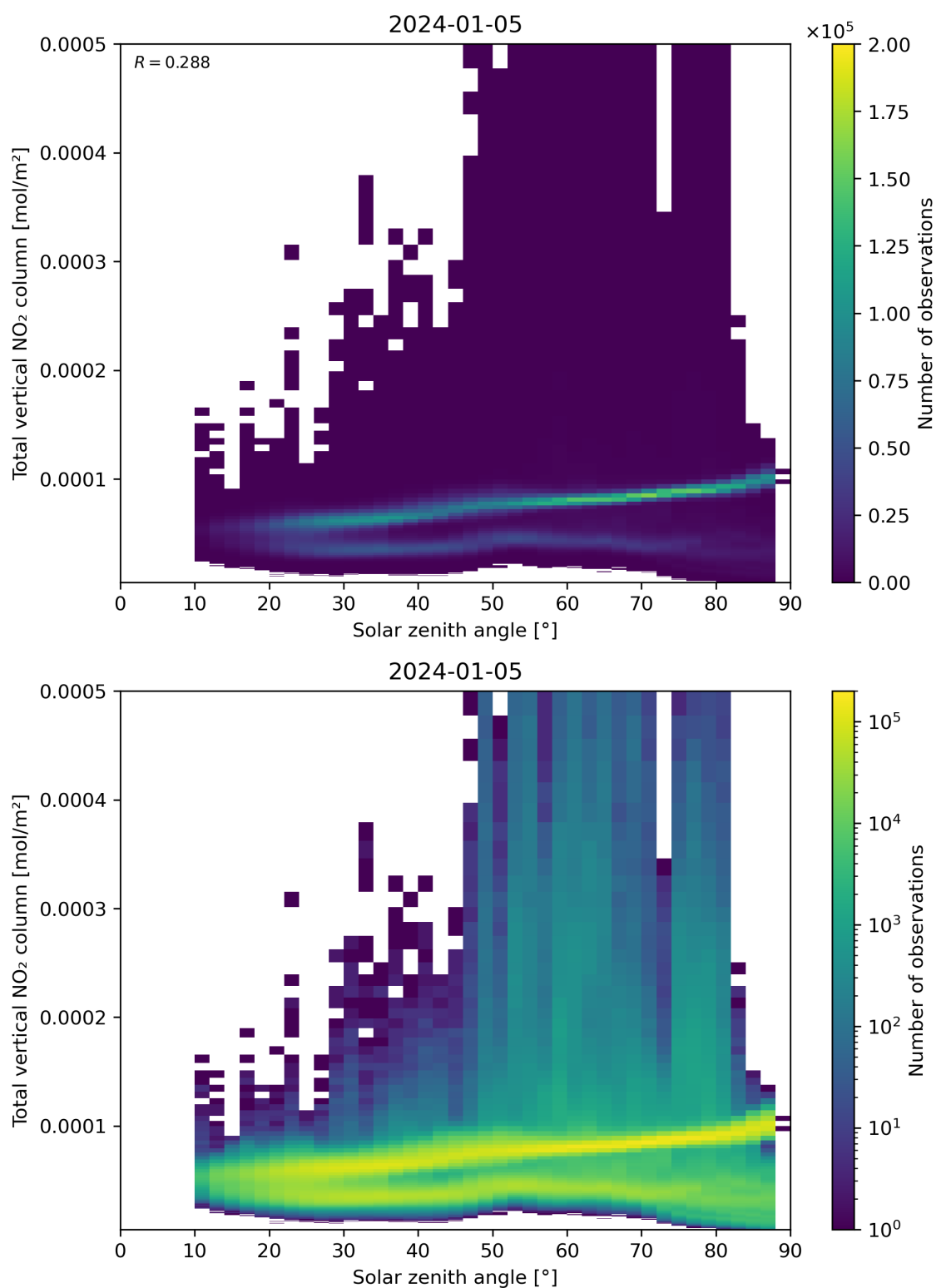
Figure 153: Scatter density plot of “Solar zenith angle” against “Total vertical NO 2 column” for 2024-01-05 to 2024-01-06.
