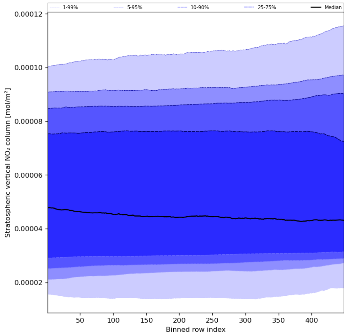
Figure 53: Along track statistics of “Stratospheric vertical NO 2 column” for 2024-01-05 to 2024-01-06
