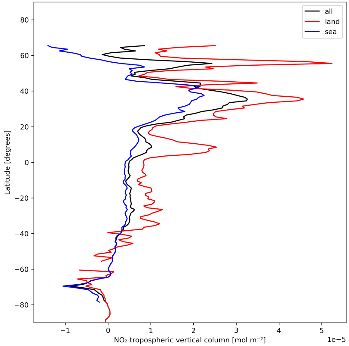
Figure 12: Zonal average of “NO 2 tropospheric vertical column” for 2024-01-05 to 2024-01-06.
