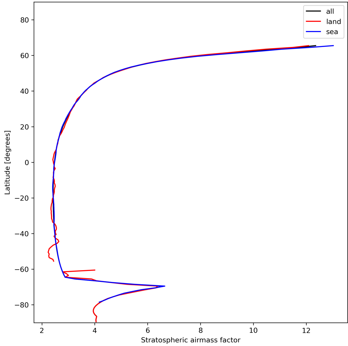
Figure 27: Zonal average of “Stratospheric air mass factor” for 2024-01-05 to 2024-01-06.
