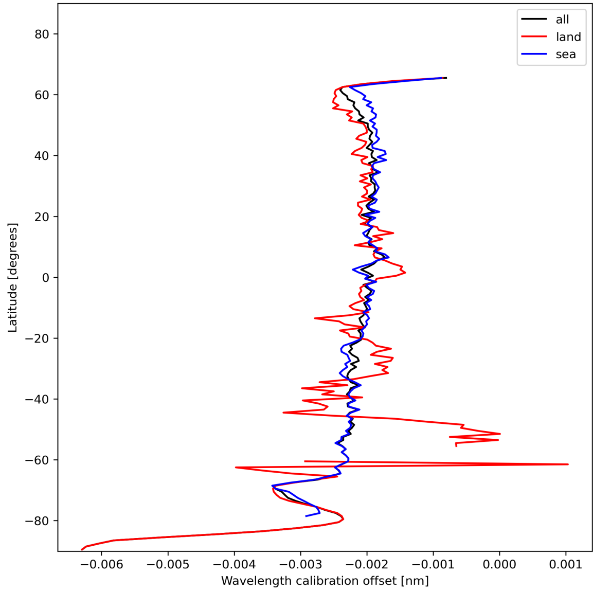
Figure 18: Zonal average of “Wavelength calibration offset” for 2024-01-05 to 2024-01-06.
