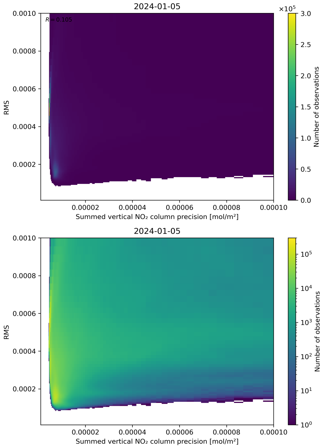
Figure 108: Scatter density plot of “Summed vertical NO 2 column precision” against “RMS” for 2024-01-05 to 2024-01-06.
