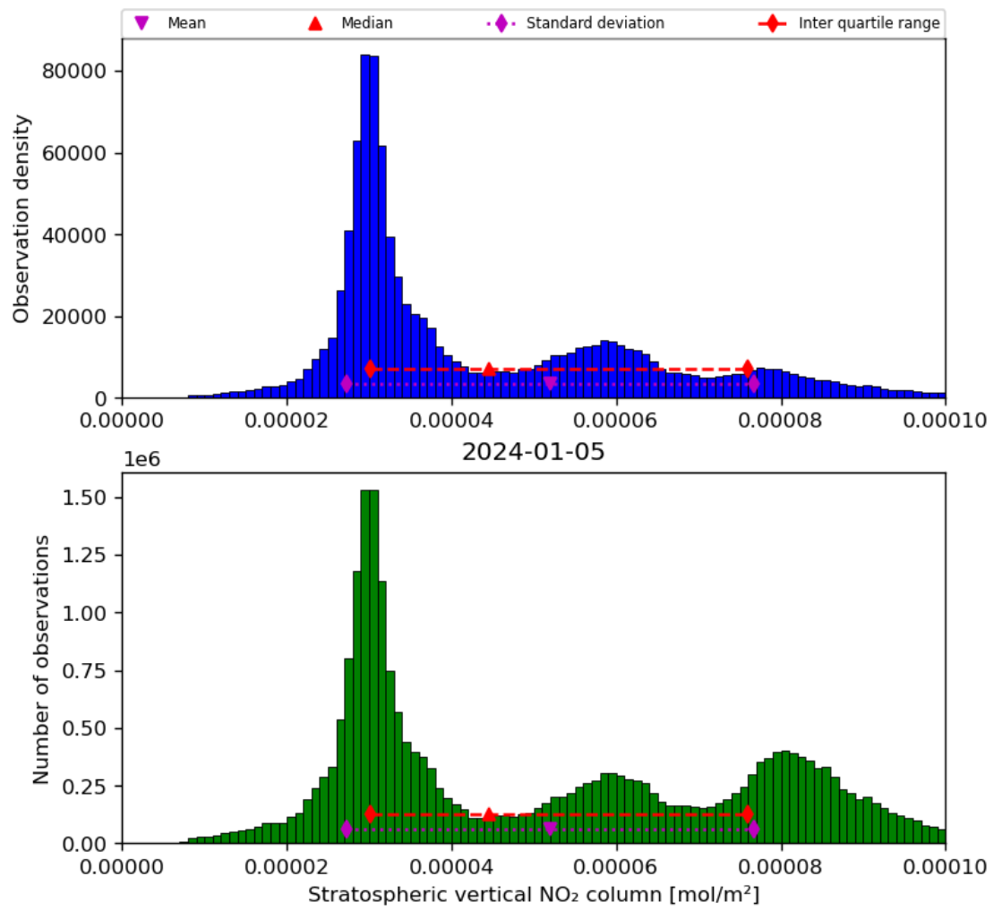
Figure 36: Histogram of “Stratospheric vertical NO 2 column” for 2024-01-05 to 2024-01-06
