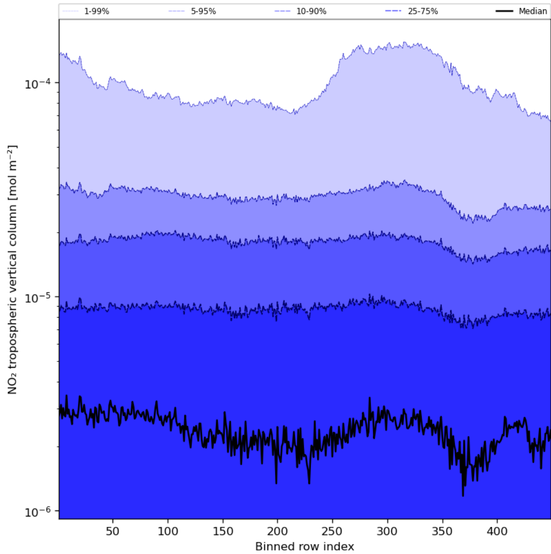
Figure 46: Along track statistics of “NO 2 tropospheric vertical column” for 2024-01-05 to 2024-01-06
