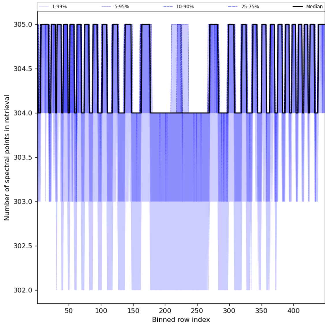
Figure 50: Along track statistics of “Number of spectral points in retrieval” for 2024-01-05 to 2024-01-06
