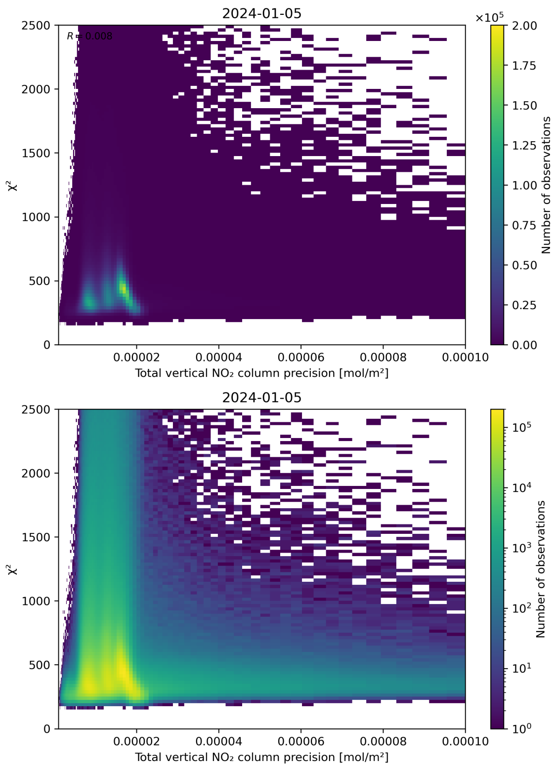
Figure 116: Scatter density plot of “Total vertical NO 2 column precision” against “ \chi^2 ” for 2024-01-05 to 2024-01-06.
