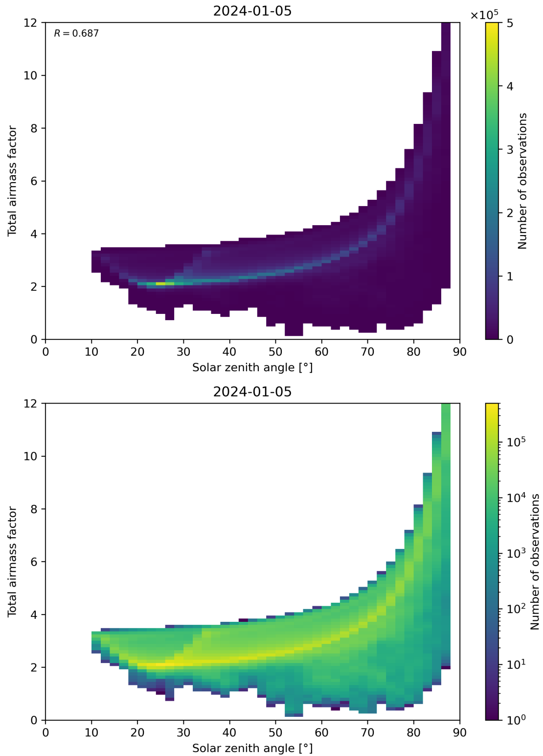
Figure 146: Scatter density plot of “Solar zenith angle” against “Total air mass factor” for 2024-01-05 to 2024-01-06.
