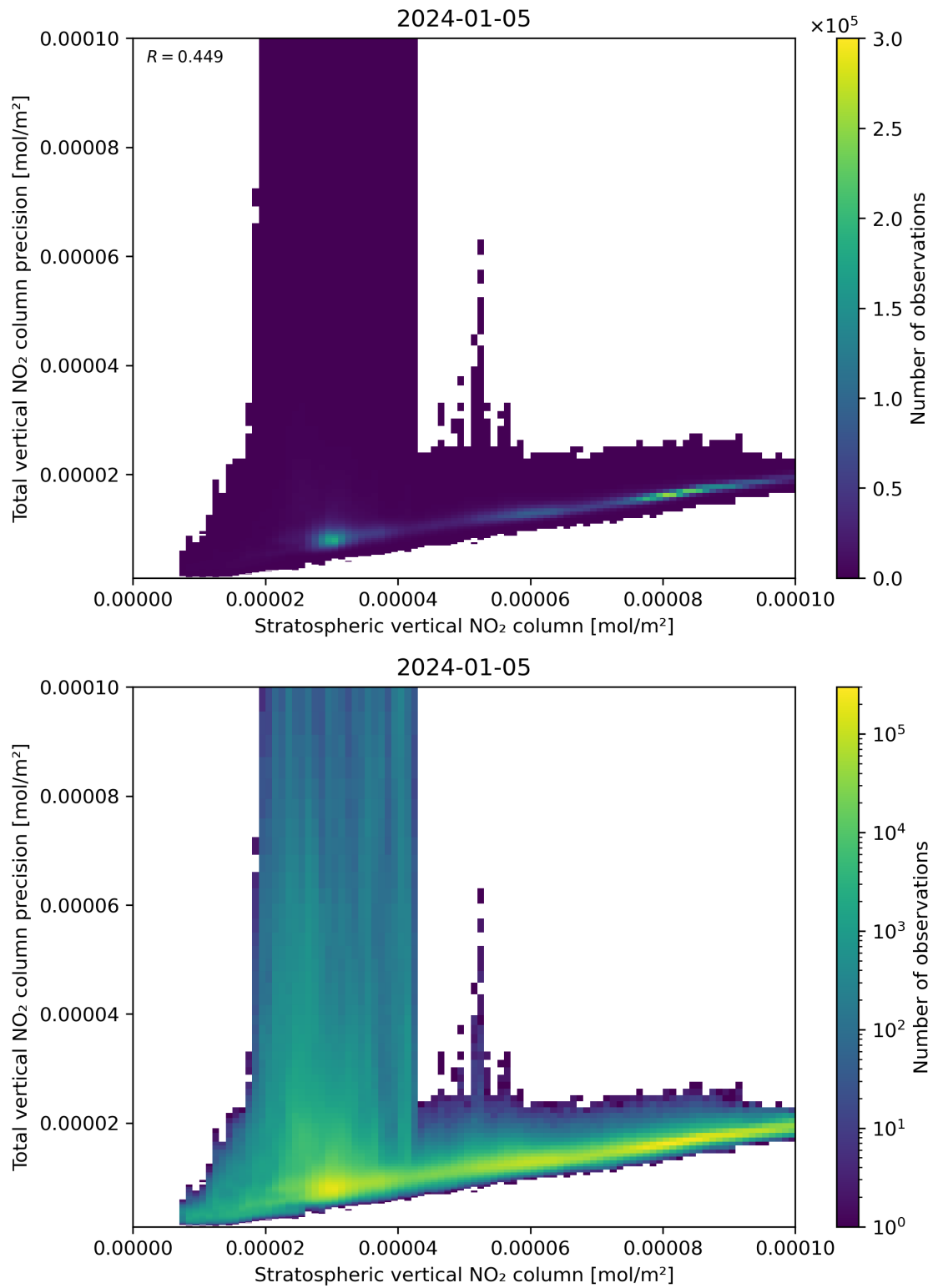
Figure 101: Scatter density plot of “Stratospheric vertical NO 2 column” against “Total vertical NO 2 column precision” for 2024-01-05 to 2024-01-06.
