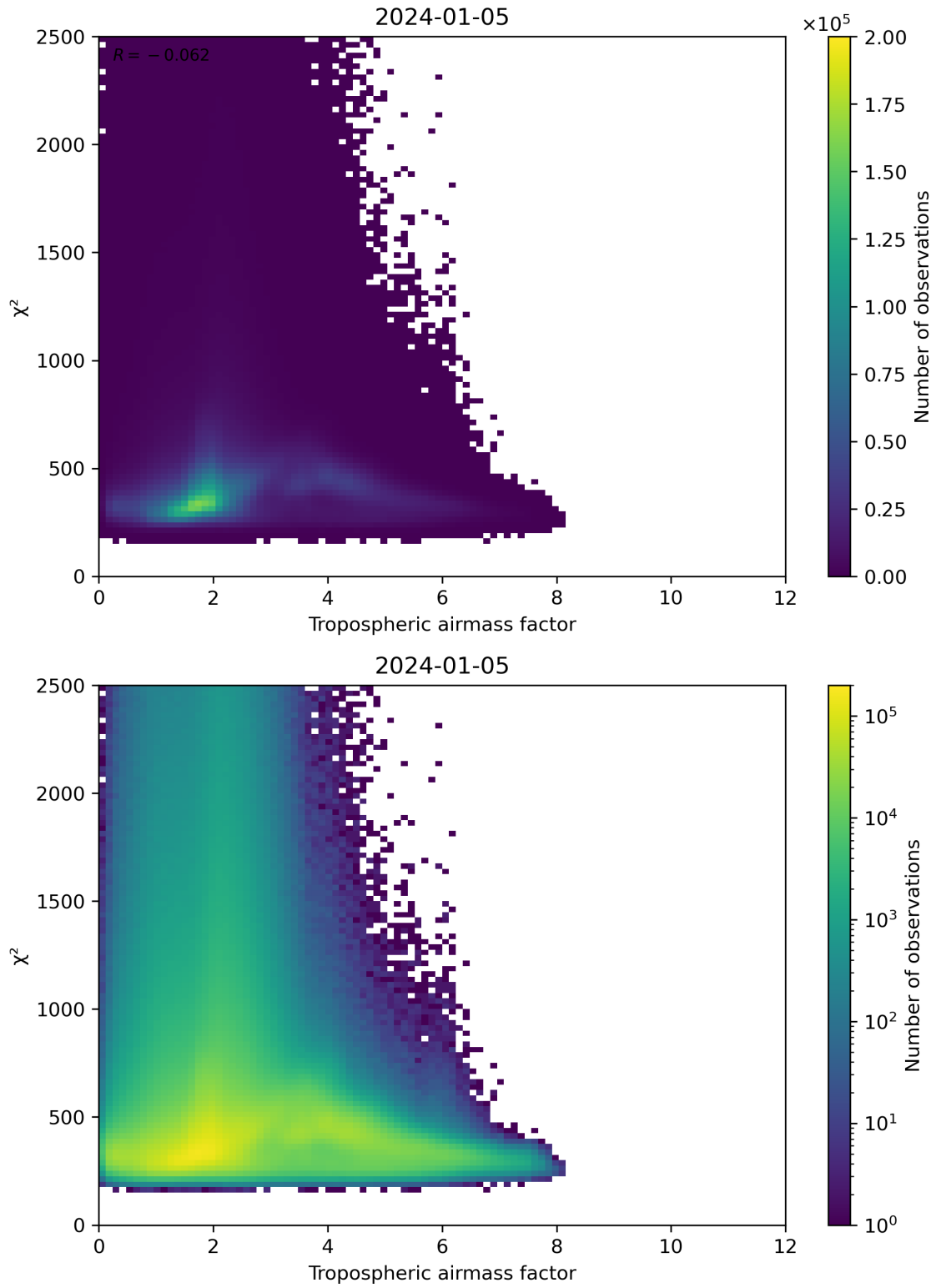
Figure 73: Scatter density plot of “Tropospheric airmass factor” against “ \chi^2 ” for 2024-01-05 to 2024-01-06.
