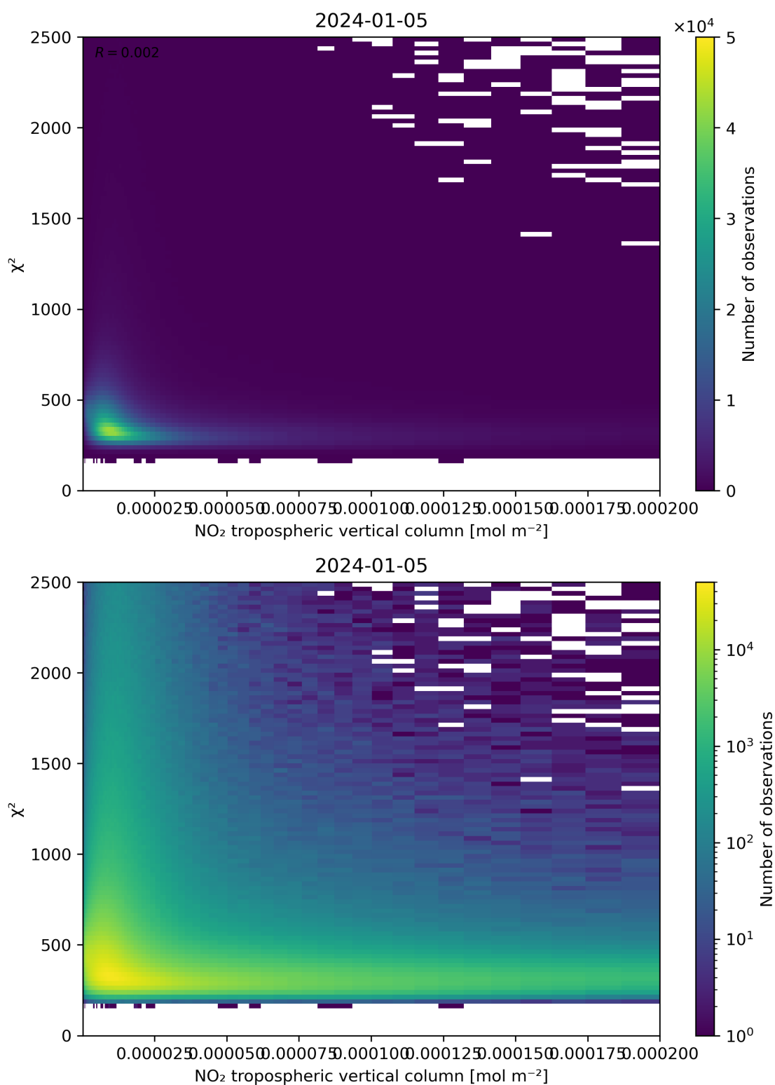
Figure 124: Scatter density plot of “NO 2 tropospheric vertical column” against “ \chi^2 ” for 2024-01-05 to 2024-01-06.
