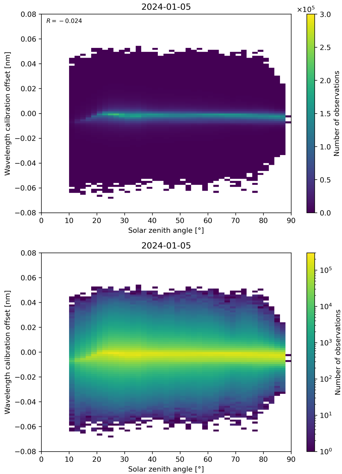
Figure 158: Scatter density plot of “Solar zenith angle” against “Wavelength calibration offset” for 2024-01-05 to 2024-01-06.
