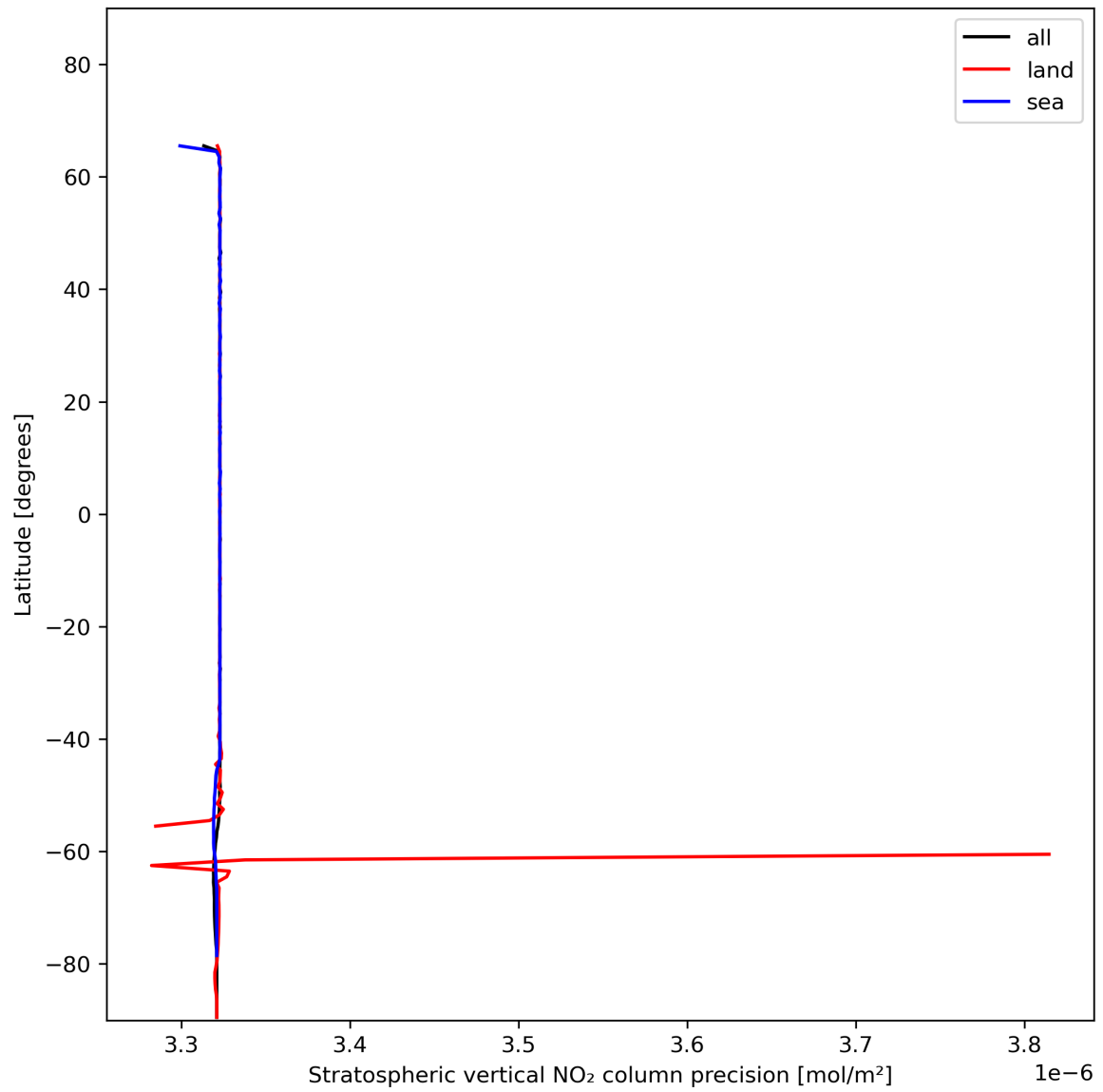
Figure 20: Zonal average of “Stratospheric vertical NO 2 column precision” for 2024-01-05 to 2024-01-06.
