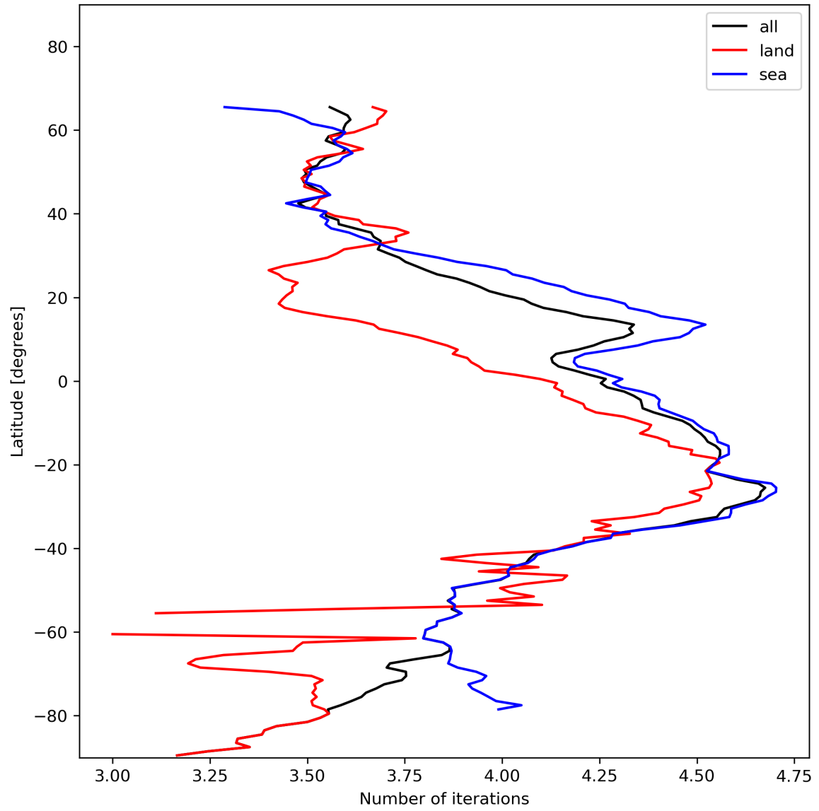
Figure 17: Zonal average of “Number of iterations” for 2024-01-05 to 2024-01-06.
