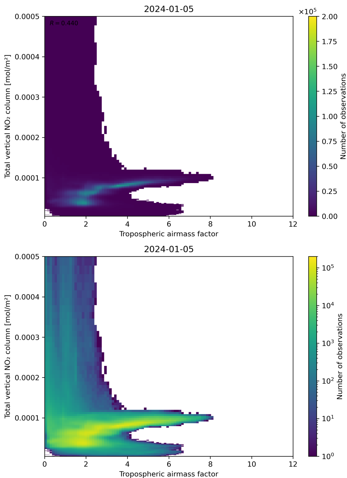
Figure 77: Scatter density plot of “Tropospheric airmass factor” against “Total vertical NO 2 column” for 2024-01-05 to 2024-01-06.
