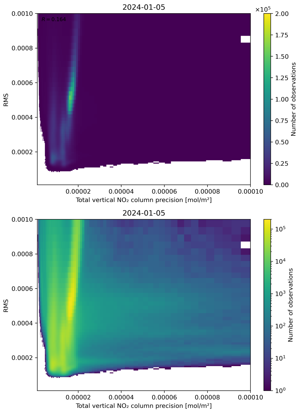
Figure 119: Scatter density plot of “Total vertical NO 2 column precision” against “RMS” for 2024-01-05 to 2024-01-06.
