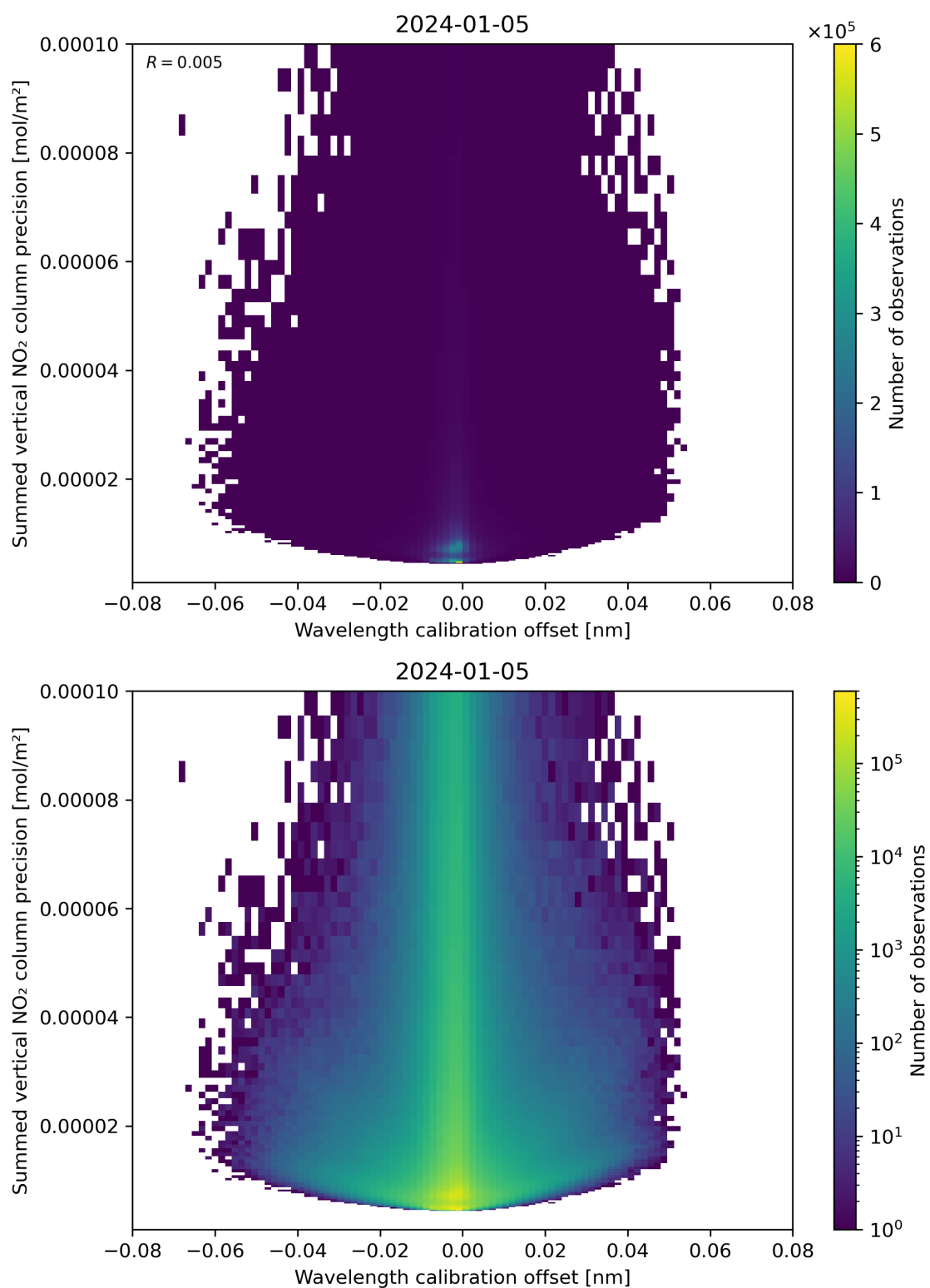
Figure 178: Scatter density plot of “Wavelength calibration offset” against “Summed vertical NO 2 column precision” for 2024-01-05 to 2024-01-06.
