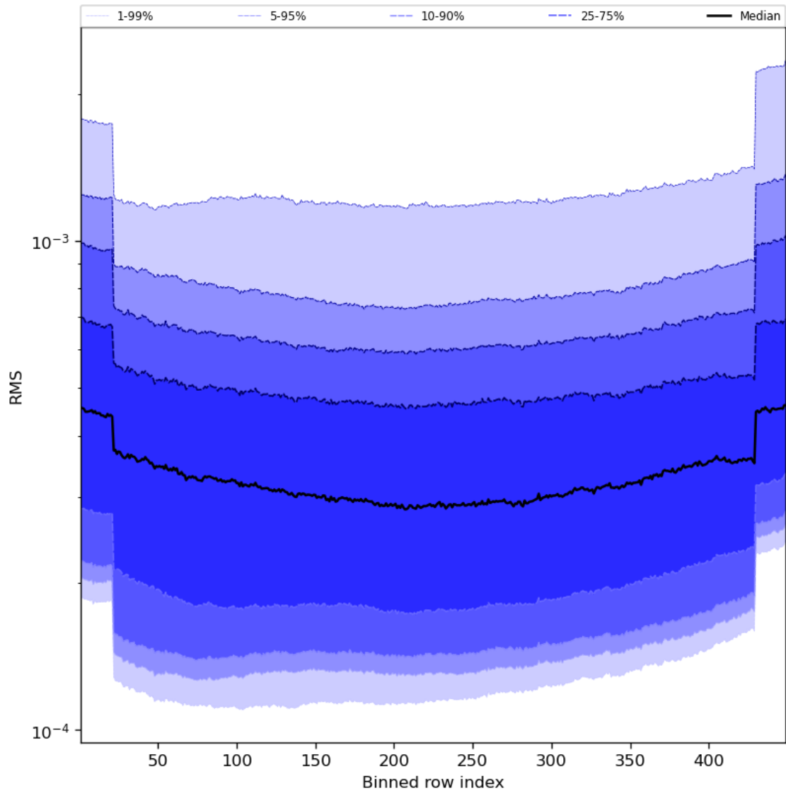
Figure 60: Along track statistics of “RMS” for 2024-01-05 to 2024-01-06
