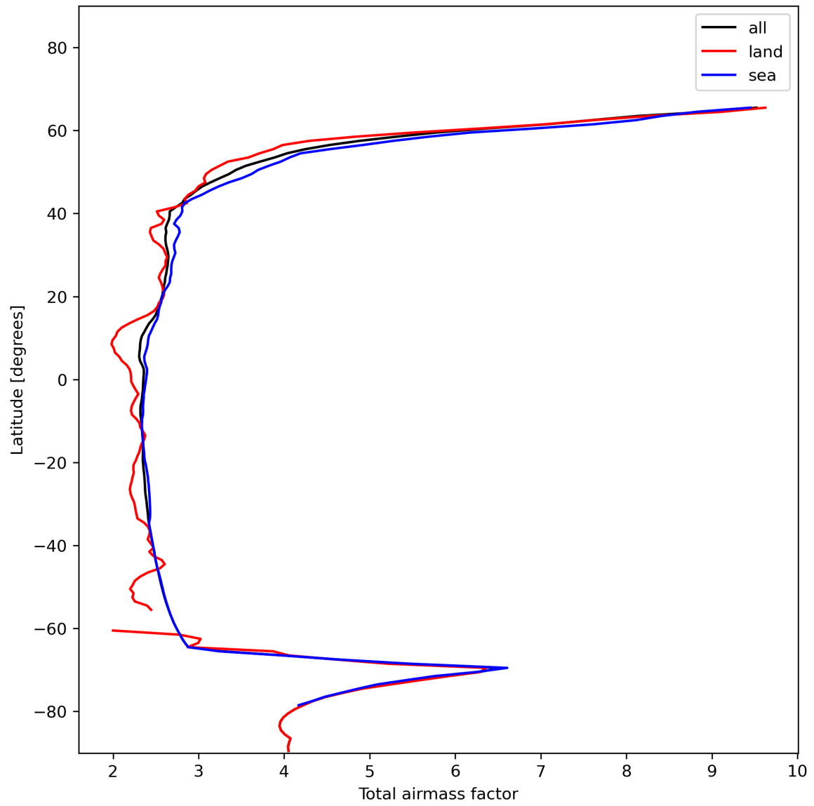
Figure 15: Zonal average of “Total airmass factor” for 2024-01-05 to 2024-01-06.
