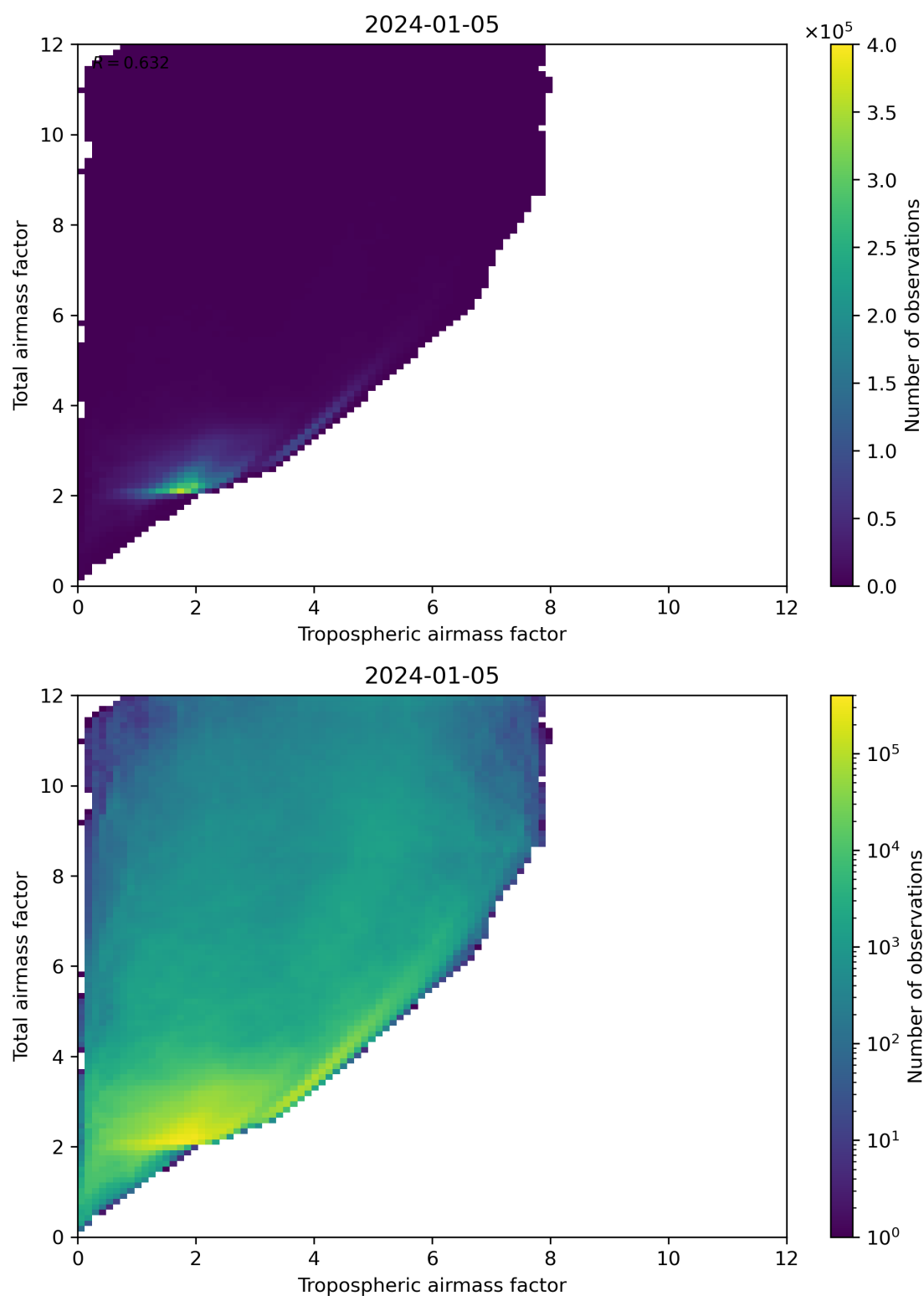
Figure 72: Scatter density plot of “Tropospheric airmass factor” against “Total airmass factor” for 2024-01-05 to 2024-01-06.
