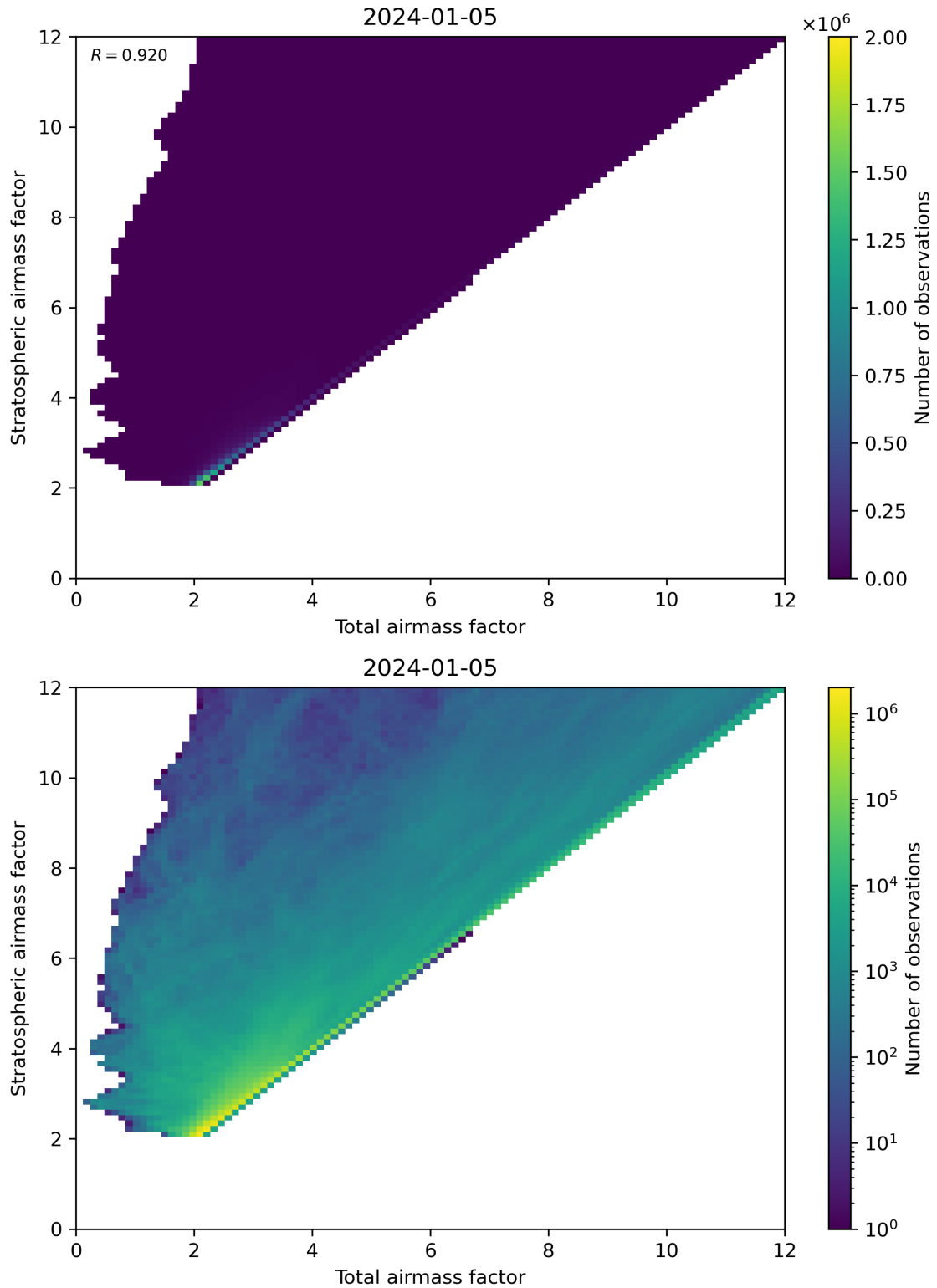
Figure 62: Scatter density plot of “Total airmass factor” against “Stratospheric airmass factor” for 2024-01-05 to 2024-01-06.
