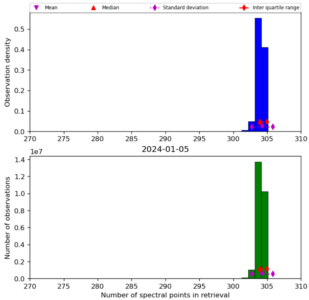
Figure 33: Histogram of “Number of spectral points in retrieval” for 2024-01-05 to 2024-01-06
