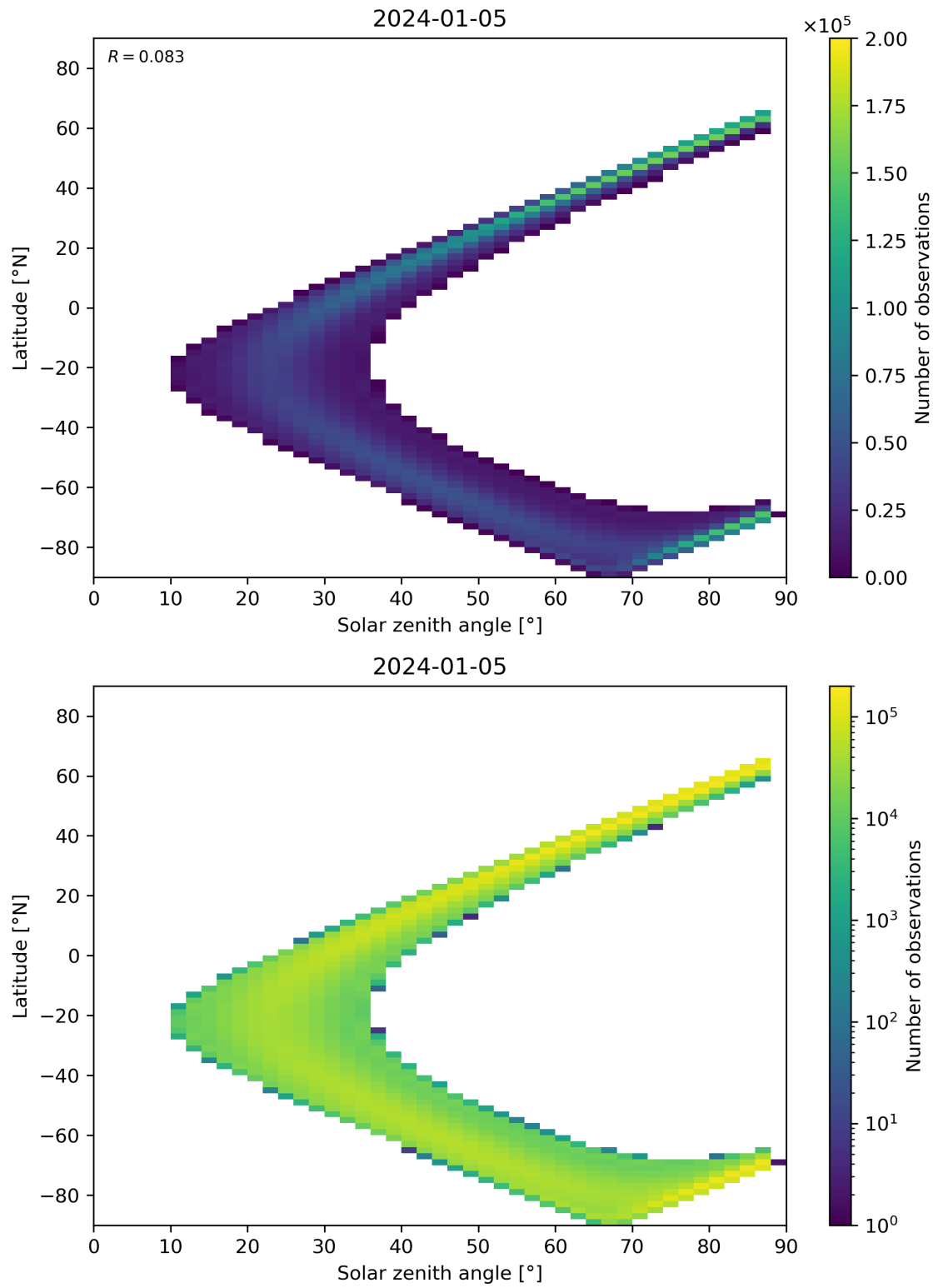
Figure 149: Scatter density plot of “Solar zenith angle” against “Latitude” for 2024-01-05 to 2024-01-06.
