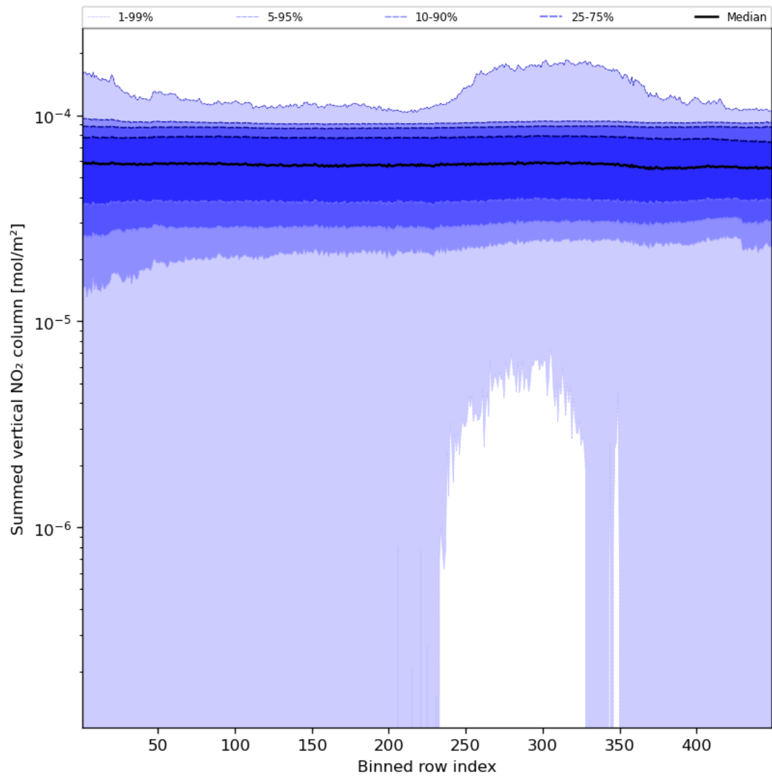
Figure 57: Along track statistics of “Summed vertical NO 2 column” for 2024-01-05 to 2024-01-06
