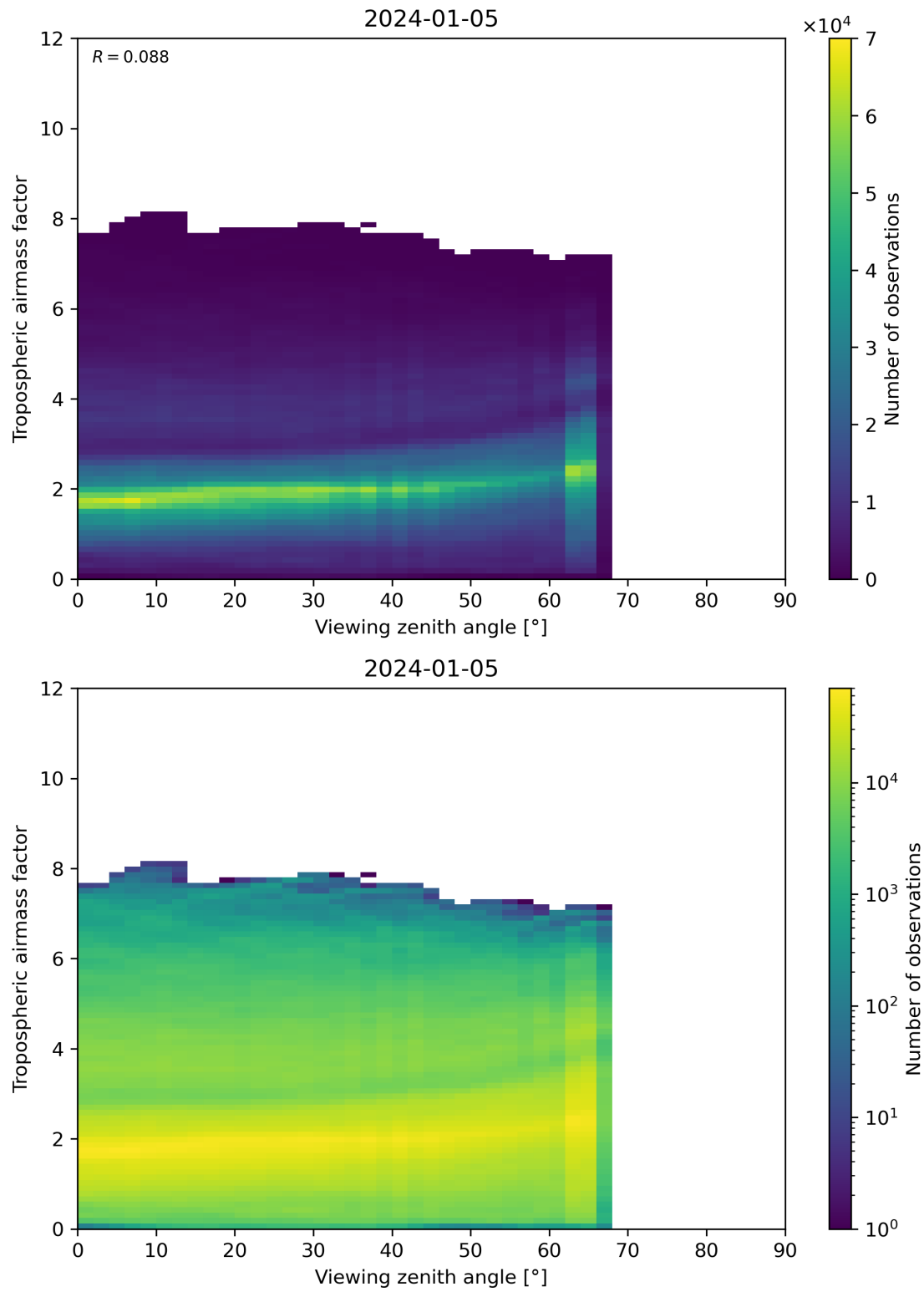
Figure 161: Scatter density plot of “Viewing zenith angle” against “Tropospheric airmass factor” for 2024-01-05 to 2024-01-06.
