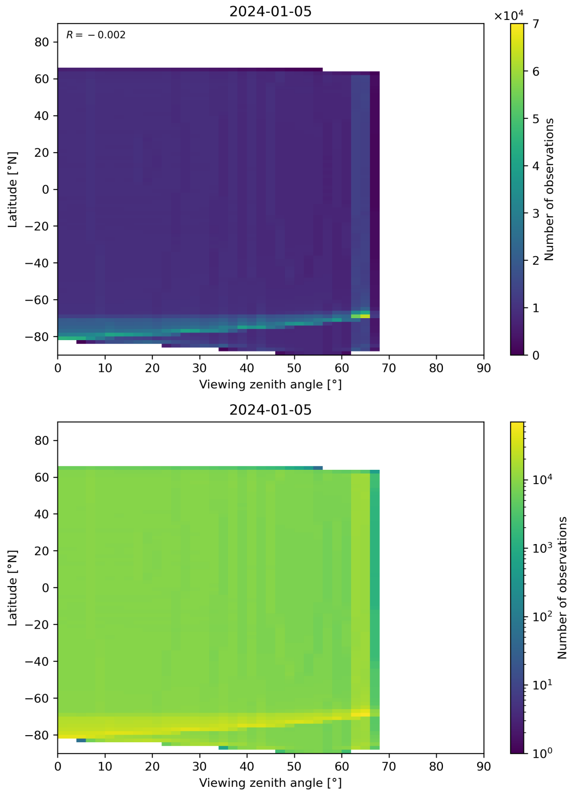
Figure 163: Scatter density plot of “Viewing zenith angle” against “Latitude” for 2024-01-05 to 2024-01-06.
