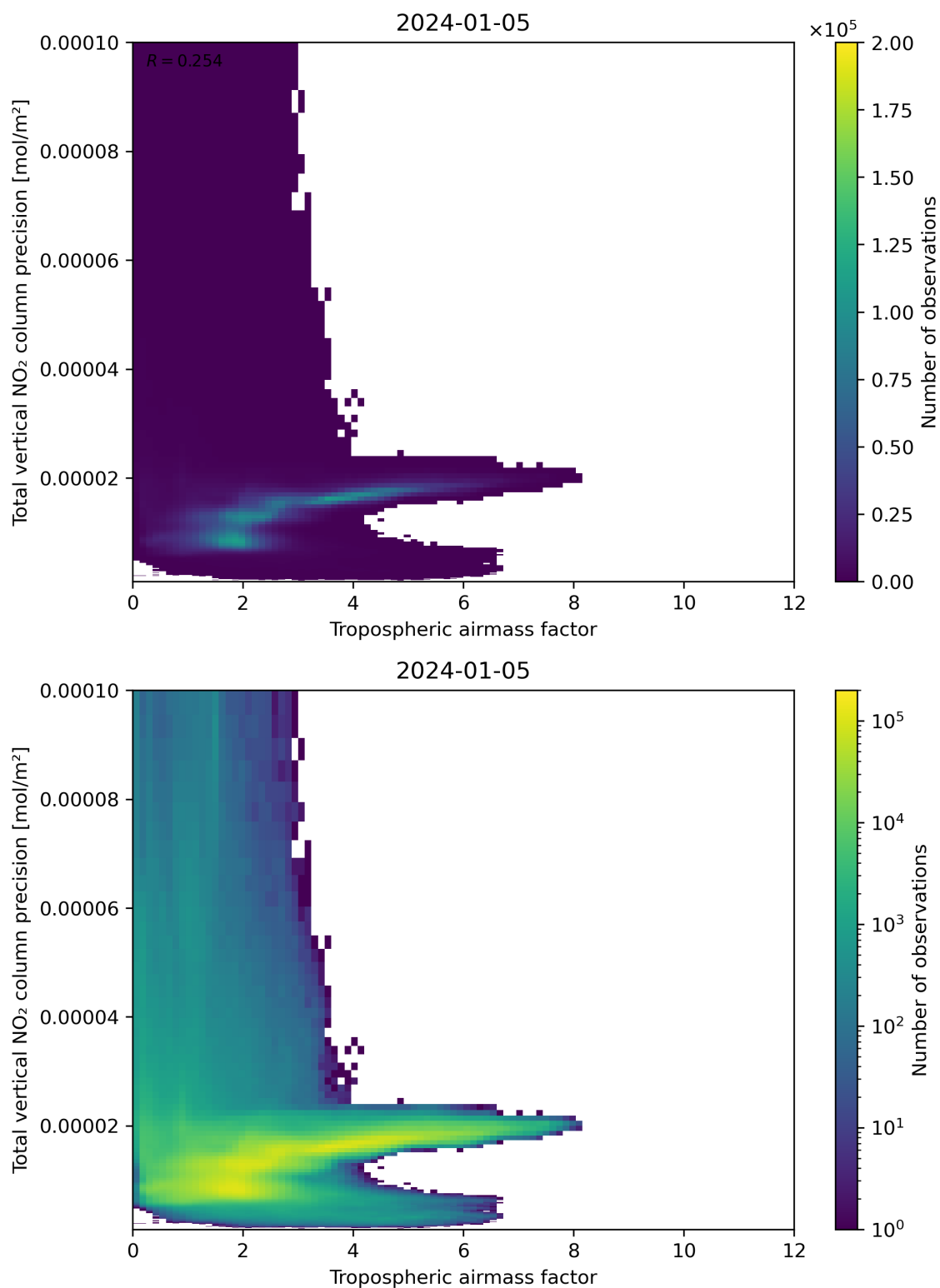
Figure 78: Scatter density plot of “Tropospheric air mass factor” against “Total vertical NO 2 column precision” for 2024-01-05 to 2024-01-06.
