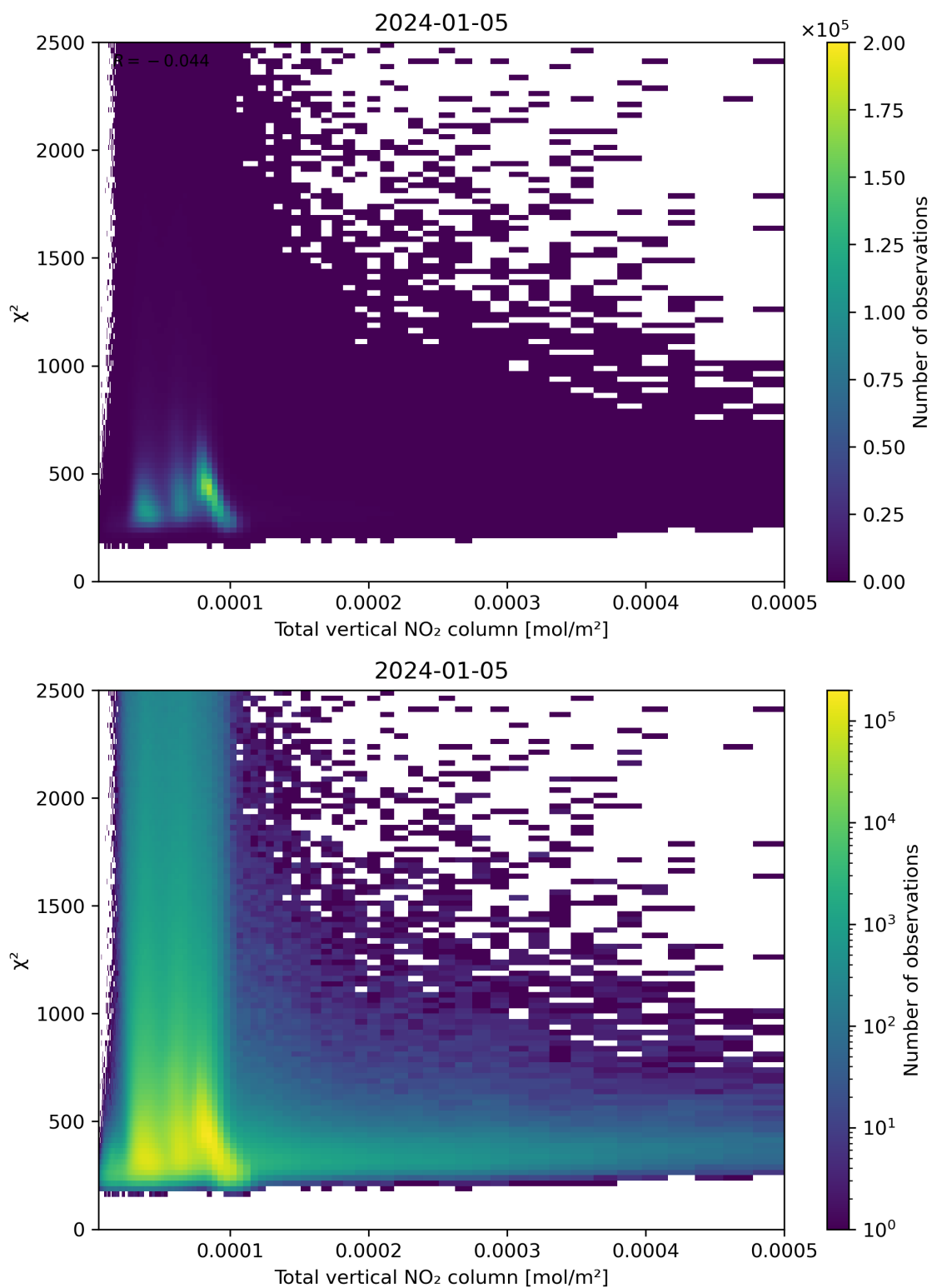
Figure 111: Scatter density plot of “Total vertical NO 2 column” against “ \chi^2 ” for 2024-01-05 to 2024-01-06.
