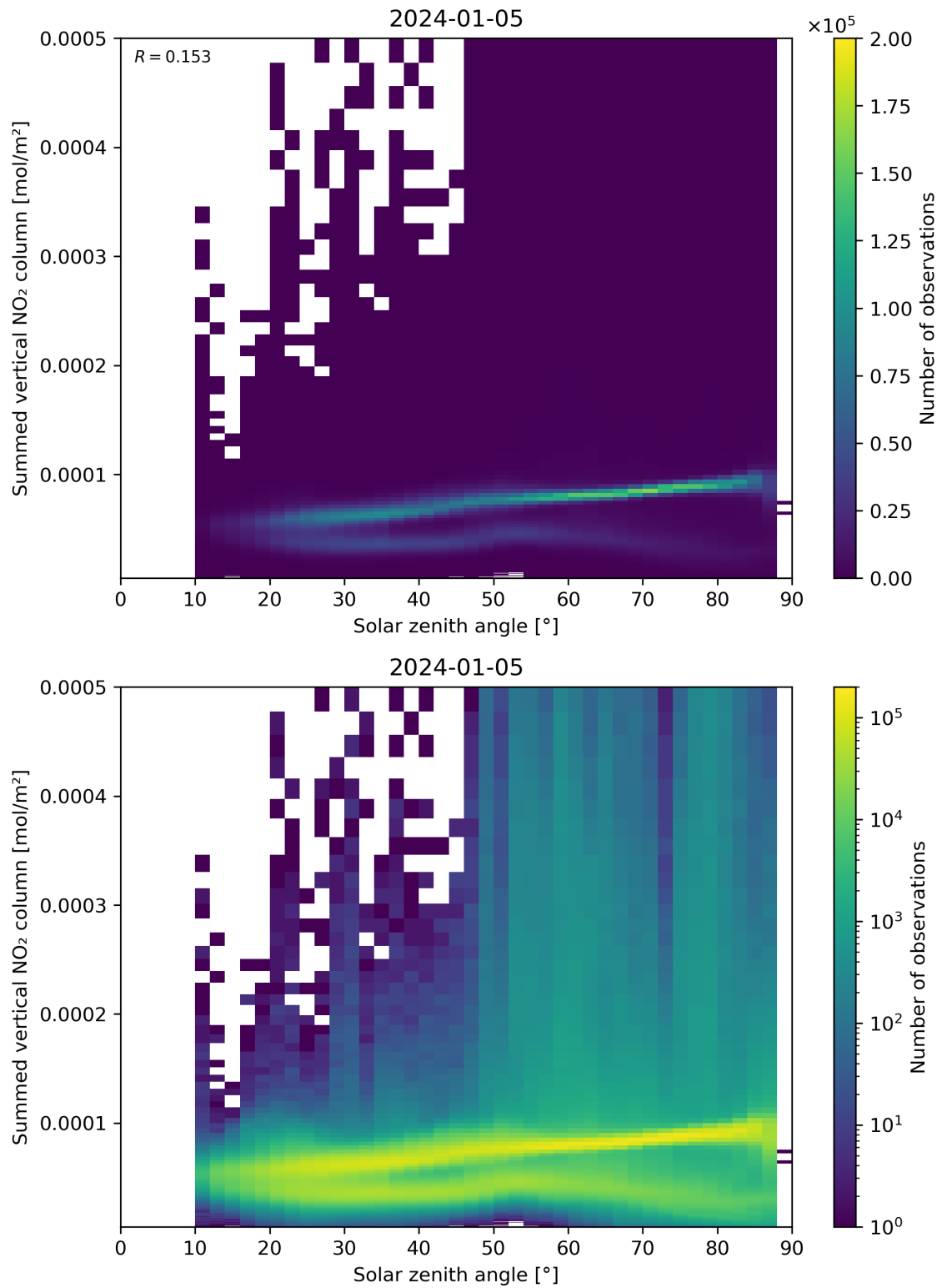
Figure 151: Scatter density plot of “Solar zenith angle” against “Summed vertical NO 2 column” for 2024-01-05 to 2024-01-06.
