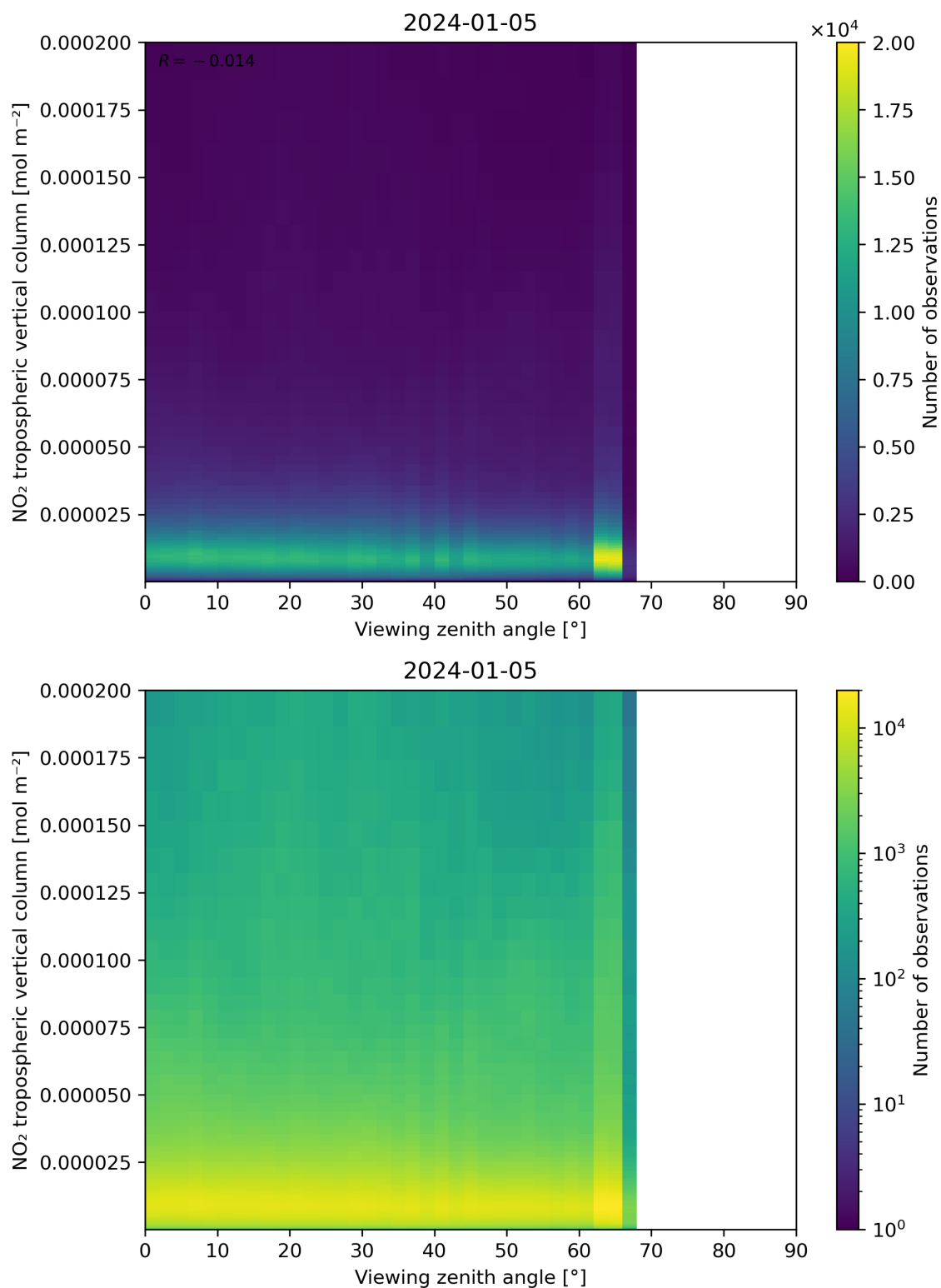
Figure 169: Scatter density plot of “Viewing zenith angle” against “NO 2 tropospheric vertical column” for 2024-01-05 to 2024-01-06.
