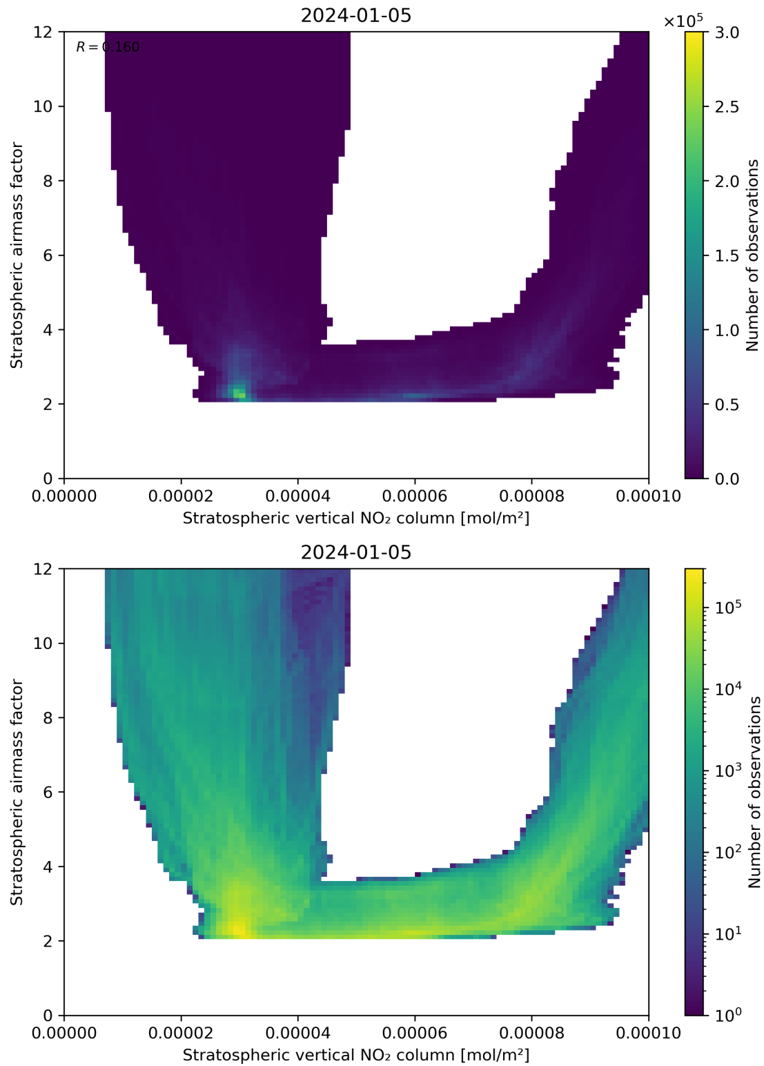
Figure 96: Scatter density plot of “Stratospheric vertical NO 2 column” against “Stratospheric airmass factor” for 2024-01-05 to 2024-01-06.
