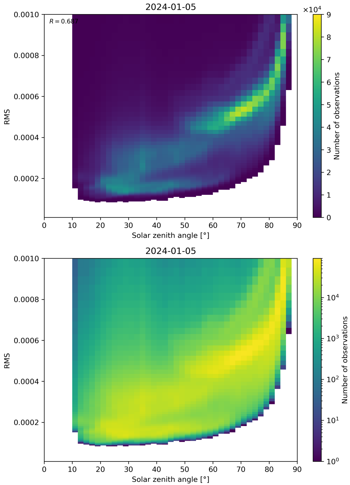
Figure 157: Scatter density plot of “Solar zenith angle” against “RMS” for 2024-01-05 to 2024-01-06.
