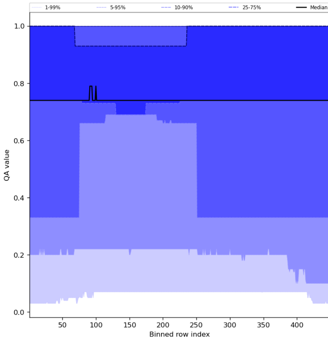
Figure 45: Along track statistics of “QA value” for 2024-01-05 to 2024-01-06
