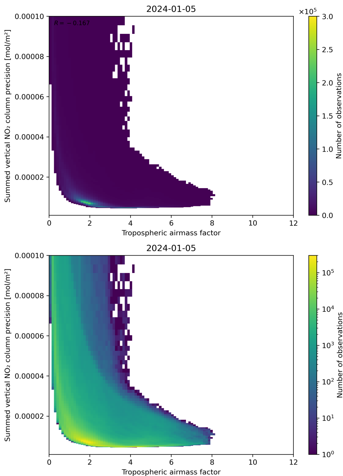
Figure 76: Scatter density plot of “Tropospheric airmass factor” against “Summed vertical NO 2 column precision” for 2024-01-05 to 2024-01-06.
