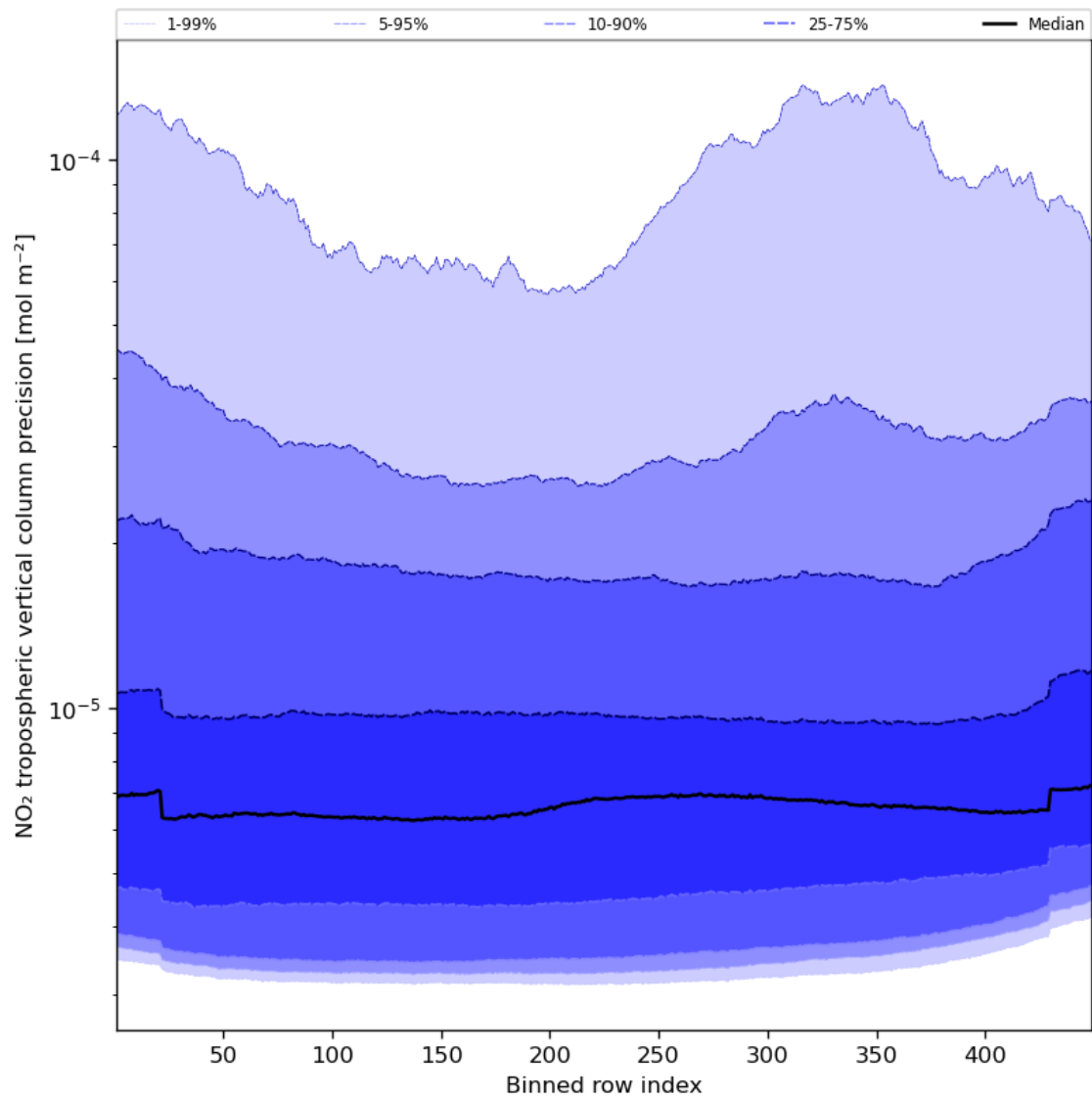
Figure 47: Along track statistics of “NO 2 tropospheric vertical column precision” for 2024-01-05 to 2024-01-06
