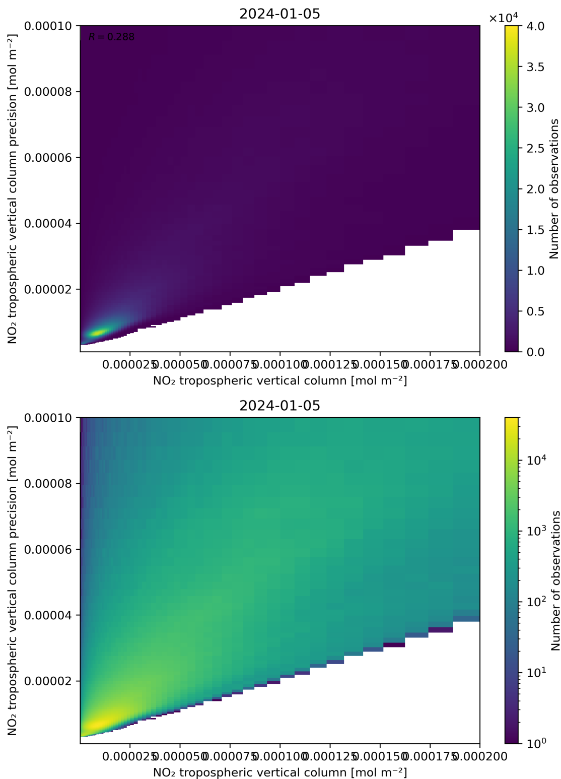
Figure 130: Scatter density plot of “NO 2 tropospheric vertical column” against “NO 2 tropospheric vertical column precision” for 2024-01-05 to 2024-01-06.
