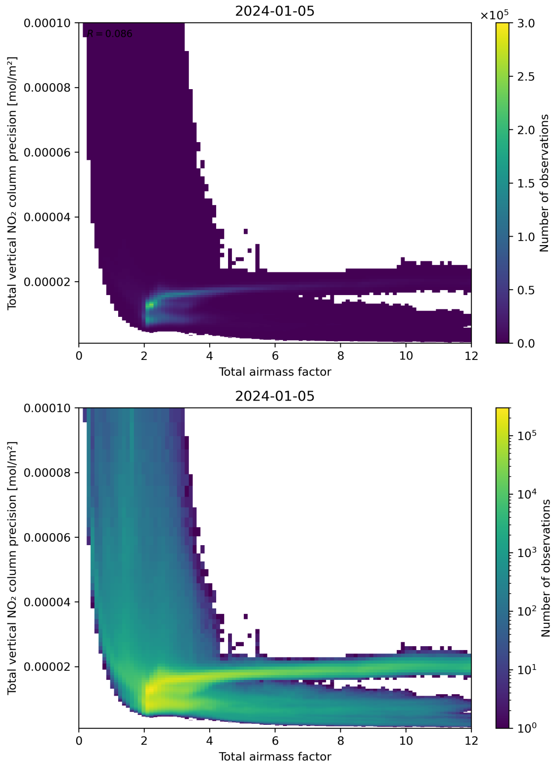
Figure 68: Scatter density plot of “Total airmass factor” against “Total vertical NO 2 column precision” for 2024-01-05 to 2024-01-06.
