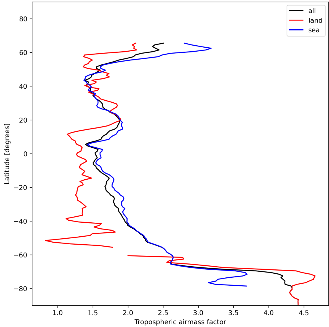
Figure 14: Zonal average of “Tropospheric airmass factor” for 2024-01-05 to 2024-01-06.
