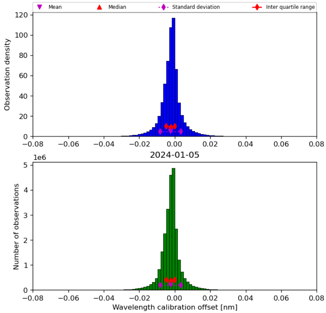
Figure 35: Histogram of “Wavelength calibration offset” for 2024-01-05 to 2024-01-06
