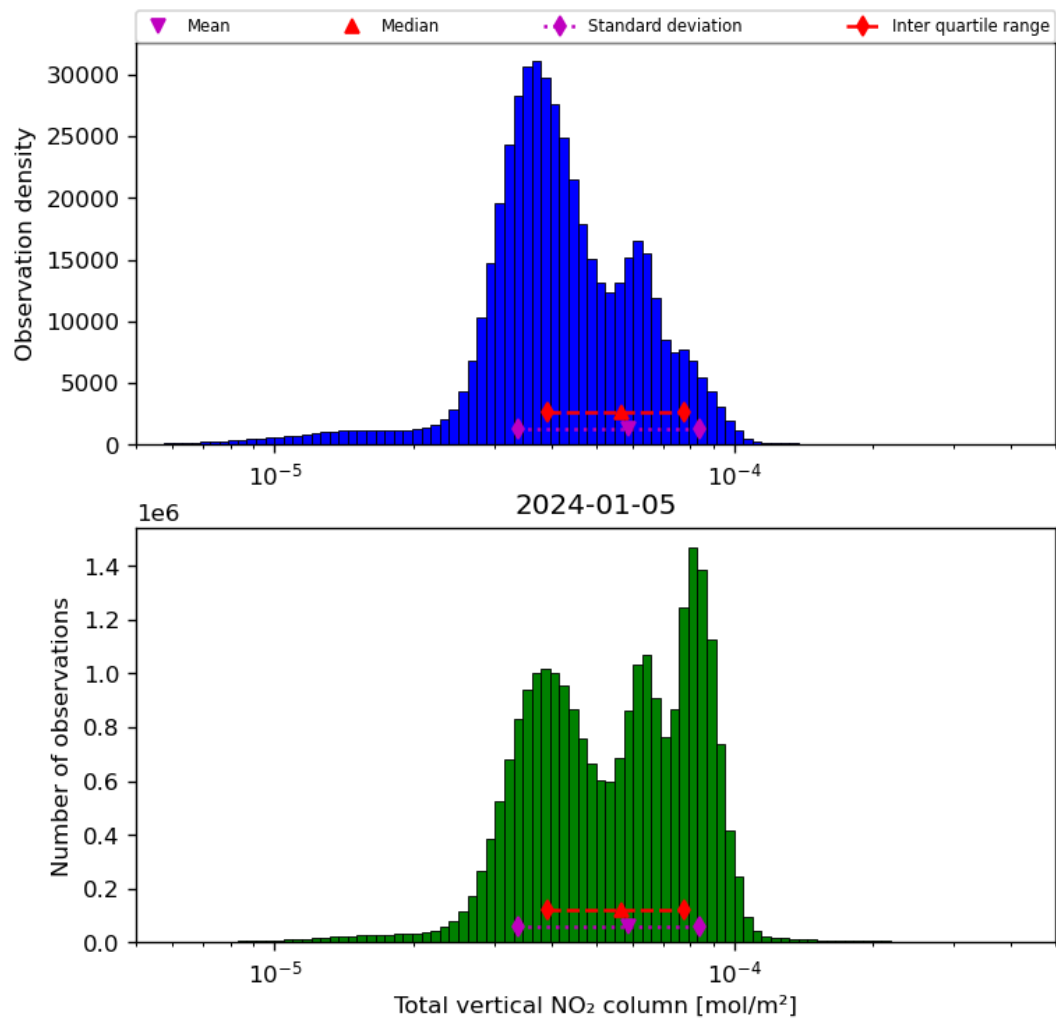
Figure 38: Histogram of “Total vertical NO 2 column” for 2024-01-05 to 2024-01-06
