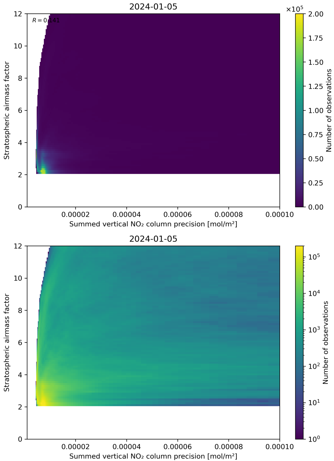
Figure 106: Scatter density plot of “Summed vertical NO 2 column precision” against “Stratospheric airmass factor” for 2024-01-05 to 2024-01-06.
