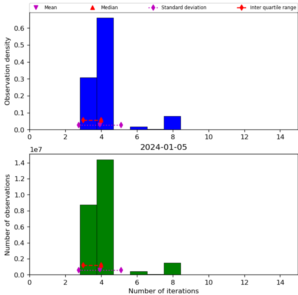
Figure 34: Histogram of “Number of iterations” for 2024-01-05 to 2024-01-06
