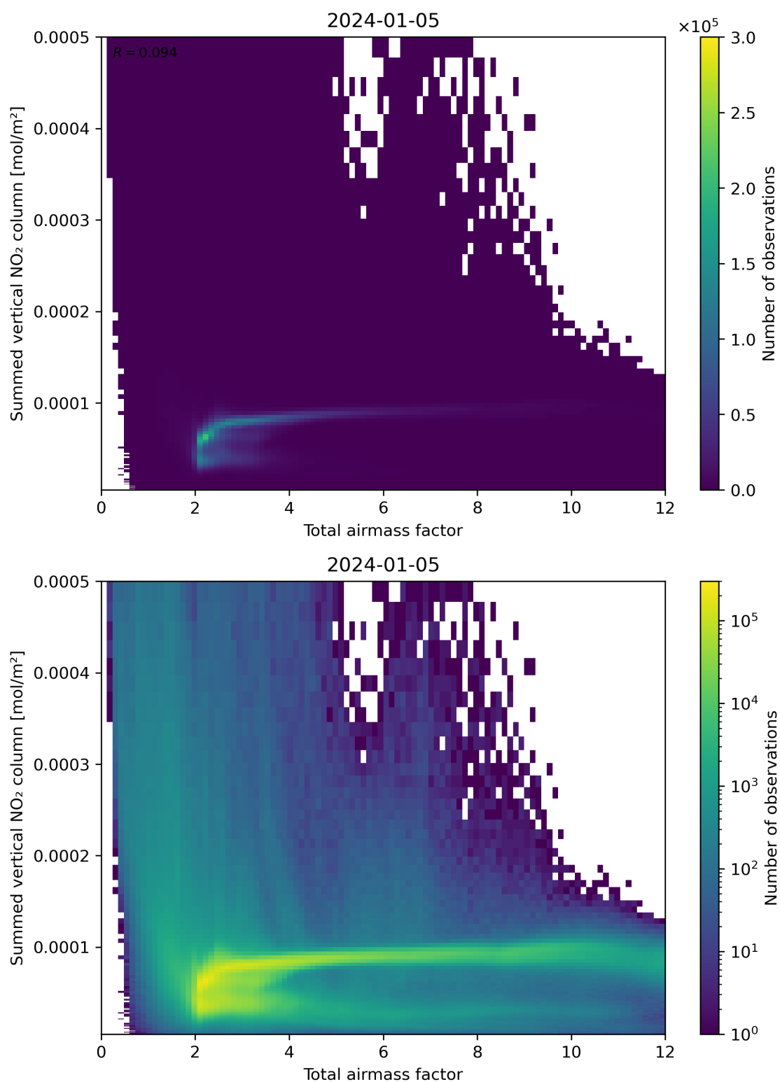
Figure 65: Scatter density plot of “Total airmass factor” against “Summed vertical NO 2 column” for 2024-01-05 to 2024-01-06.
