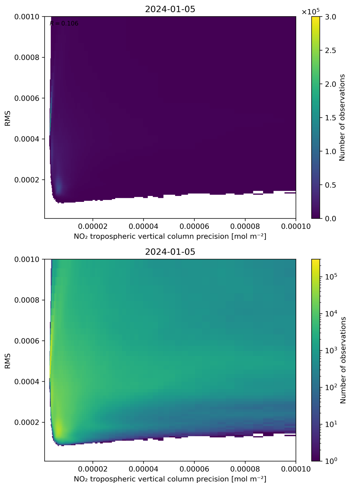
Figure 140: Scatter density plot of “NO 2 tropospheric vertical column precision” against “RMS” for 2024-01-05 to 2024-01-06.
