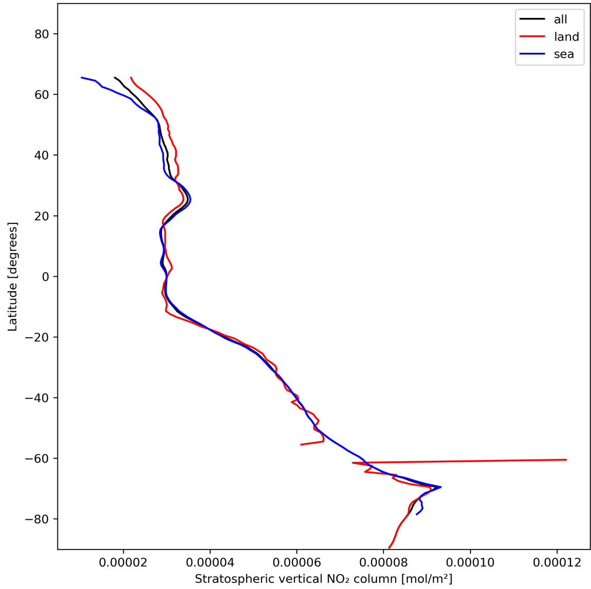
Figure 19: Zonal average of “Stratospheric vertical NO 2 column” for 2024-01-05 to 2024-01-06.
