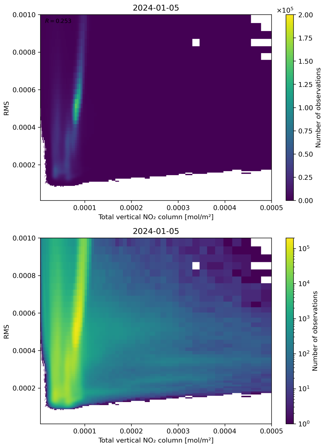
Figure 120: Scatter density plot of “Total vertical NO 2 column” against “RMS” for 2024-01-05 to 2024-01-06.
