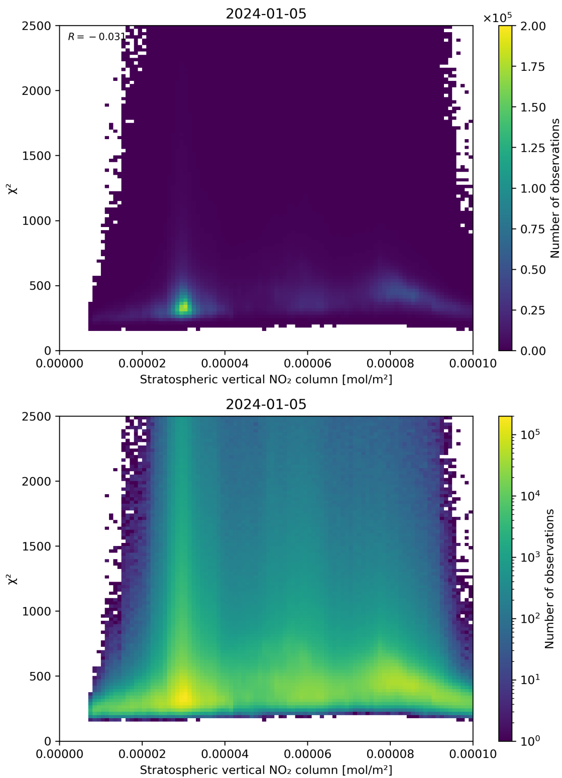
Figure 97: Scatter density plot of “Stratospheric vertical NO 2 column” against “ \chi^2 ” for 2024-01-05 to 2024-01-06.
