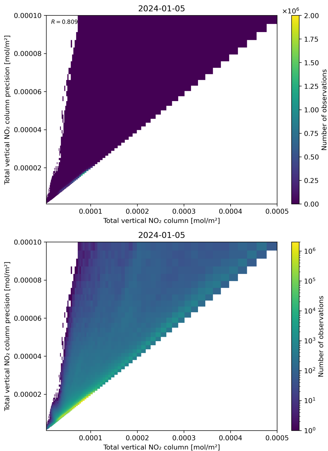
Figure 114: Scatter density plot of “Total vertical NO 2 column” against “Total vertical NO 2 column precision” for 2024-01-05 to 2024-01-06.
