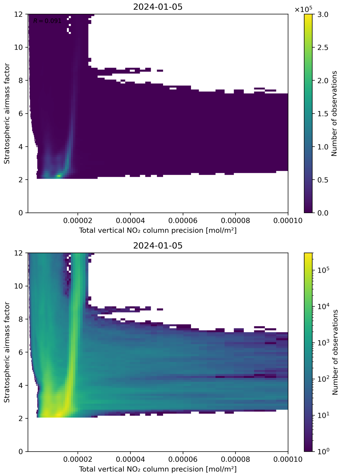
Figure 115: Scatter density plot of “Total vertical NO 2 column precision” against “Stratospheric air mass factor” for 2024-01-05 to 2024-01-06.
