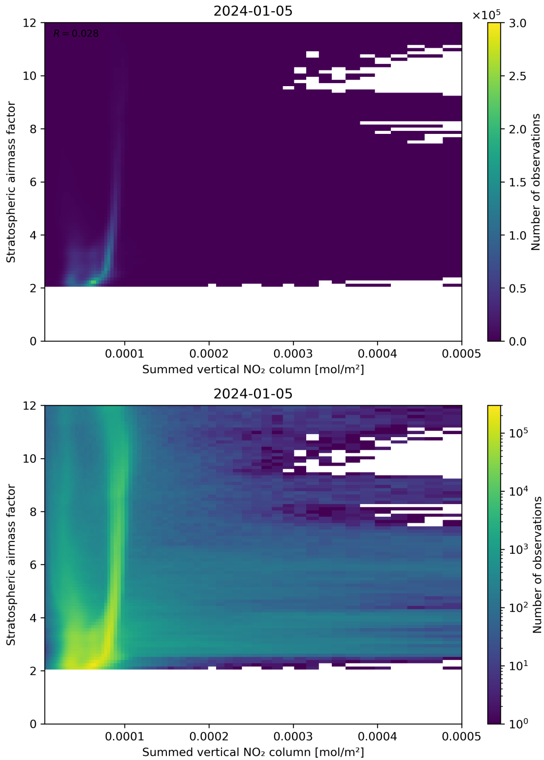
Figure 103: Scatter density plot of “Summed vertical NO 2 column” against “Stratospheric air mass factor” for 2024-01-05 to 2024-01-06.
