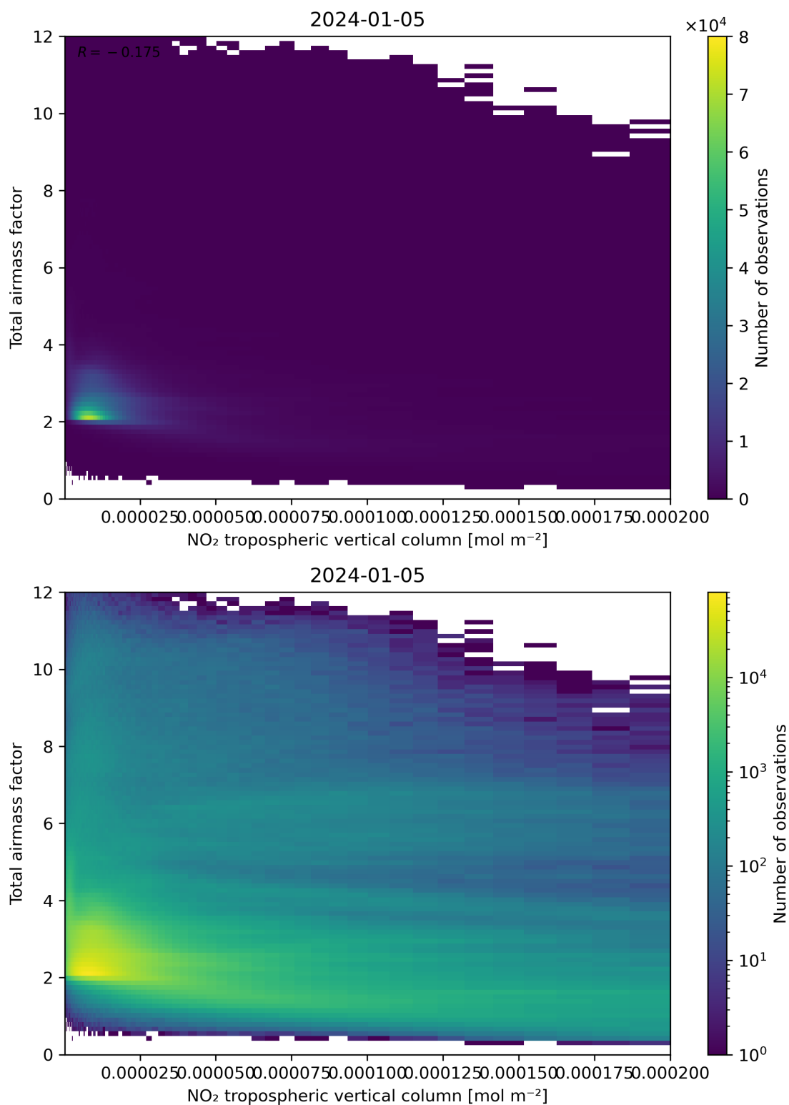
Figure 122: Scatter density plot of “NO 2 tropospheric vertical column” against “Total air mass factor” for 2024-01-05 to 2024-01-06.
