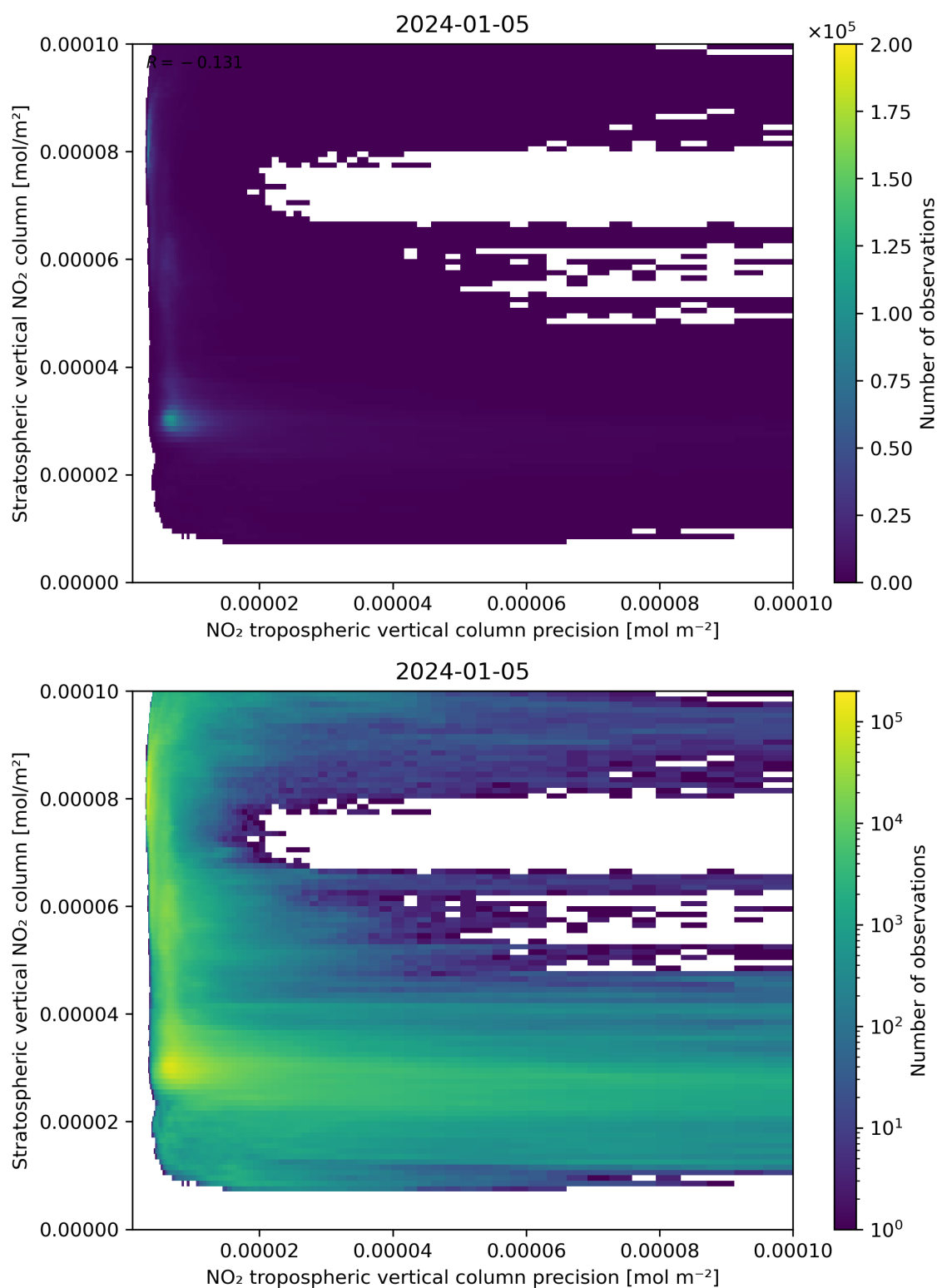
Figure 135: Scatter density plot of “NO 2 tropospheric vertical column precision” against “Stratospheric vertical NO 2 column” for 2024-01-05 to 2024-01-06.
