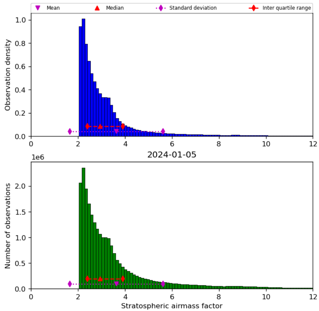
Figure 44: Histogram of “Stratospheric airmass factor” for 2024-01-05 to 2024-01-06
