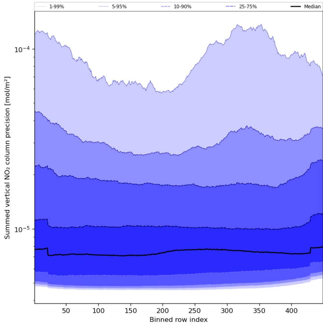
Figure 58: Along track statistics of “Summed vertical NO 2 column precision” for 2024-01-05 to 2024-01-06
