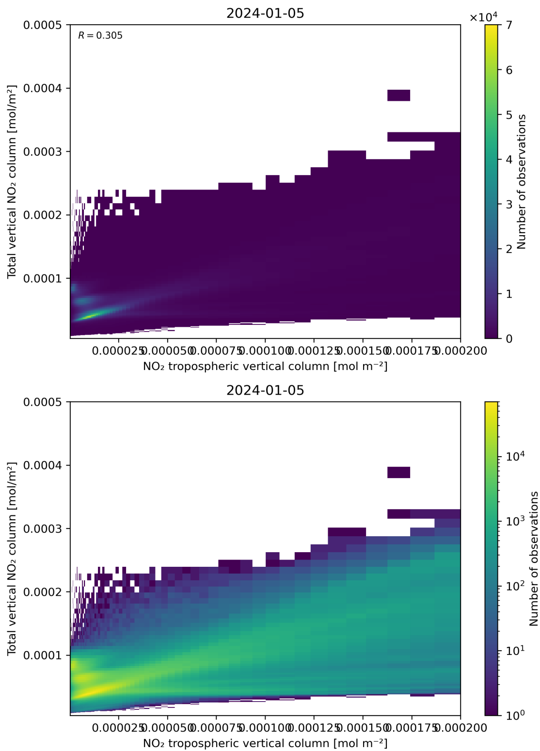
Figure 128: Scatter density plot of “NO 2 tropospheric vertical column” against “Total vertical NO 2 column” for 2024-01-05 to 2024-01-06.
