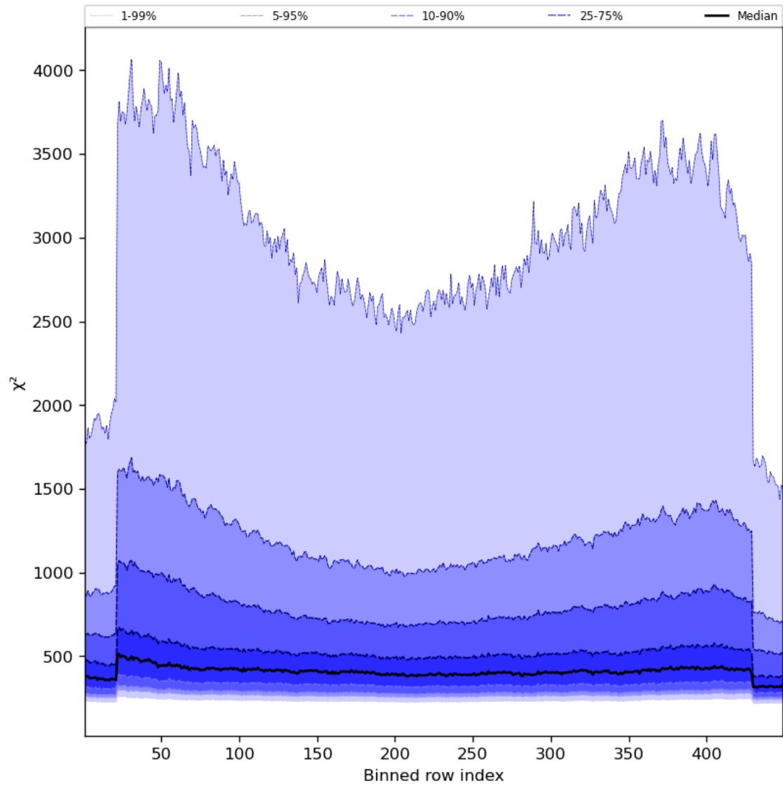
Figure 59: Along track statistics of “ \chi^2 ” for 2024-01-05 to 2024-01-06
