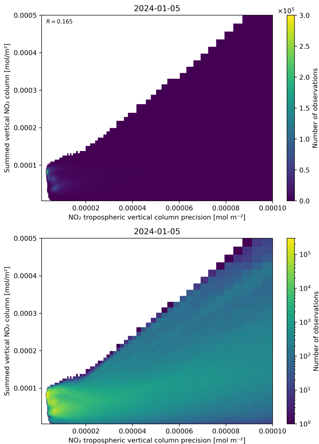
Figure 136: Scatter density plot of “NO 2 tropospheric vertical column precision” against “Summed vertical NO 2 column” for 2024-01-05 to 2024-01-06.
