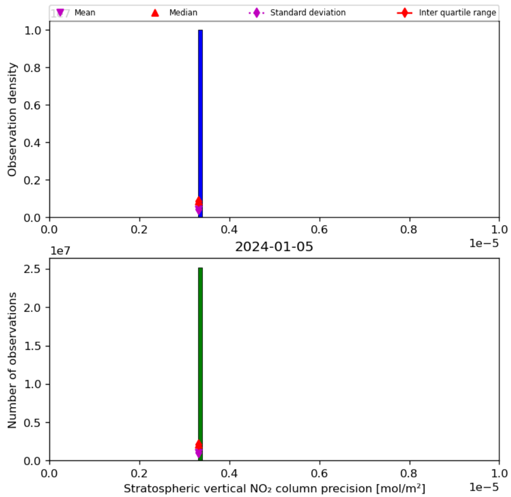
Figure 37: Histogram of “Stratospheric vertical NO 2 column precision” for 2024-01-05 to 2024-01-06
