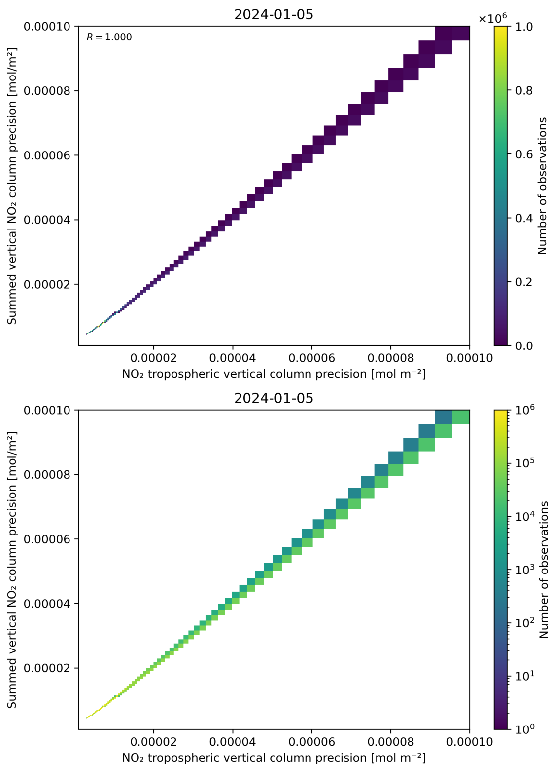
Figure 137: Scatter density plot of “NO 2 tropospheric vertical column precision” against “Summed vertical NO 2 column precision” for 2024-01-05 to 2024-01-06.
