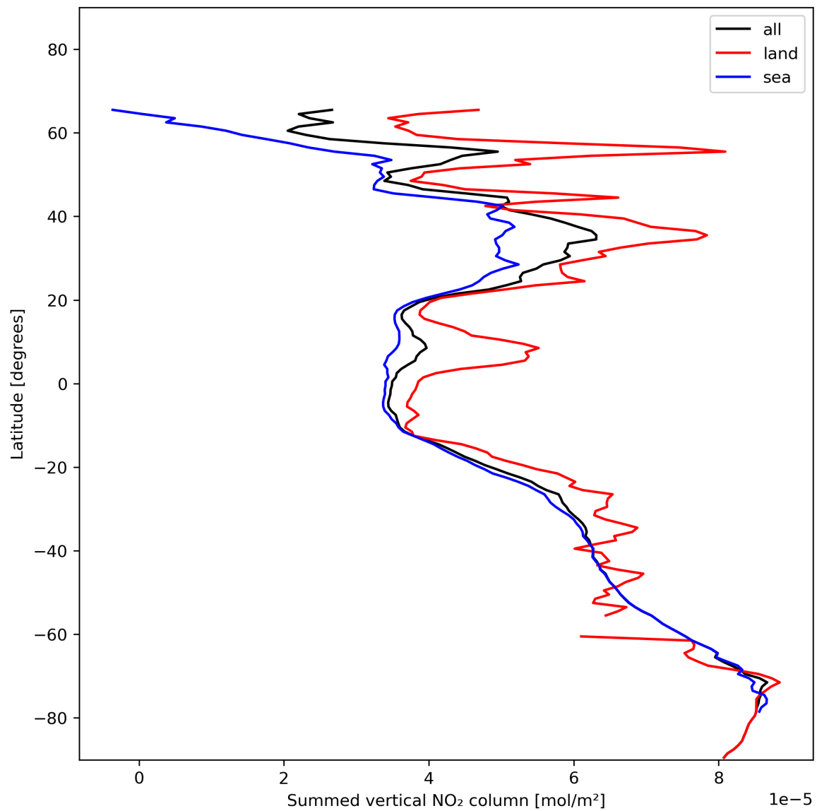
Figure 23: Zonal average of “Summed vertical NO 2 column” for 2024-01-05 to 2024-01-06.
