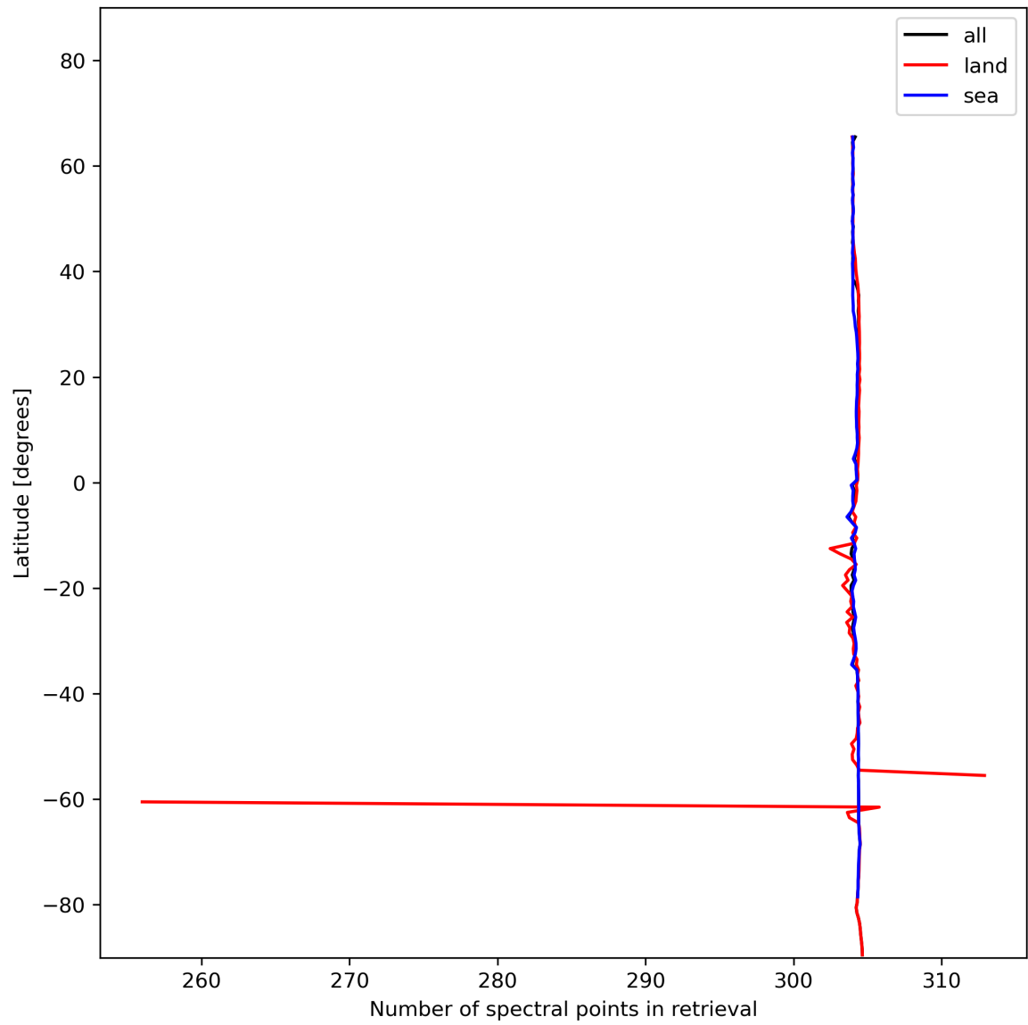
Figure 16: Zonal average of “Number of spectral points in retrieval” for 2024-01-05 to 2024-01-06.
