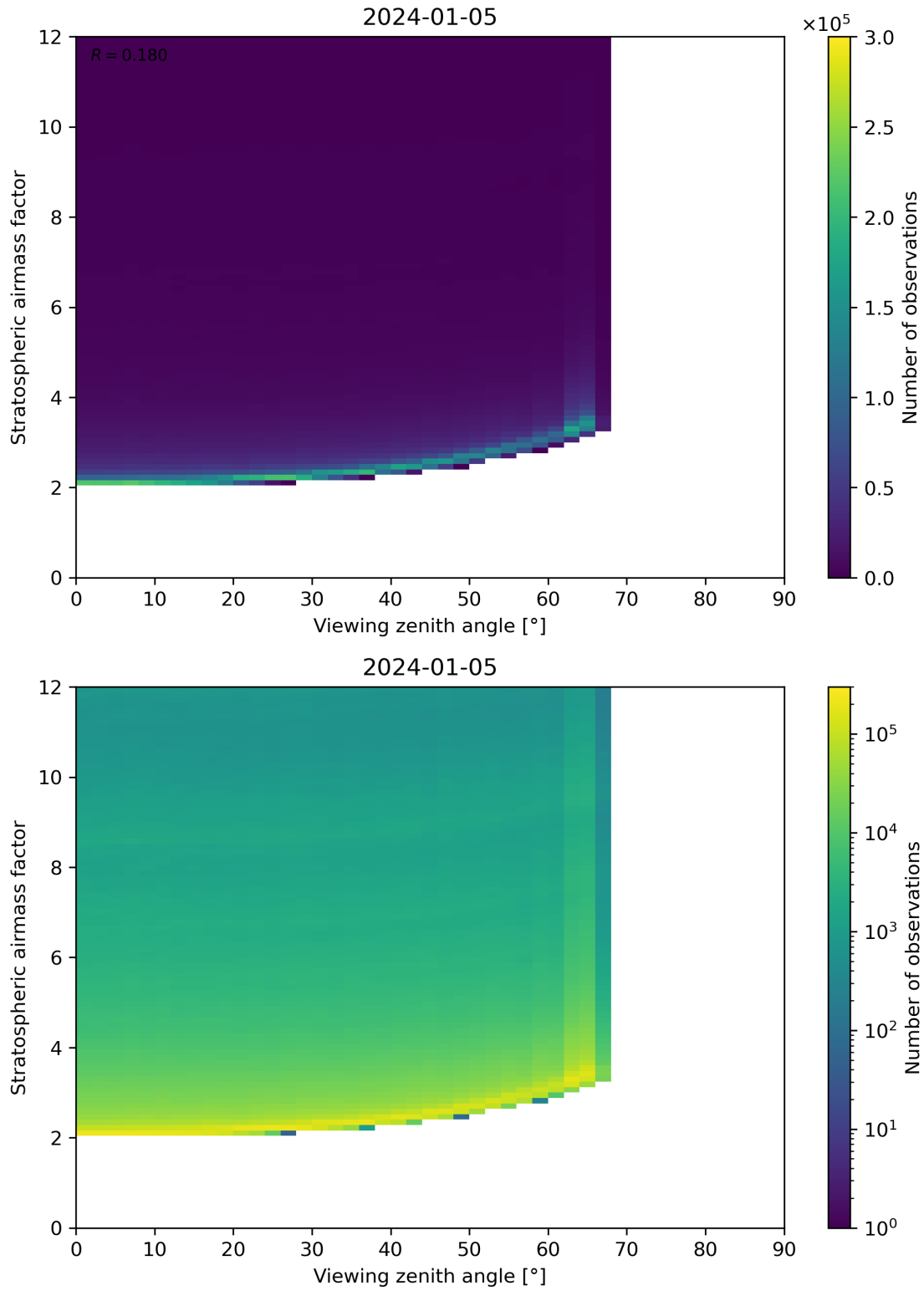
Figure 159: Scatter density plot of “Viewing zenith angle” against “Stratospheric airmass factor” for 2024-01-05 to 2024-01-06.
