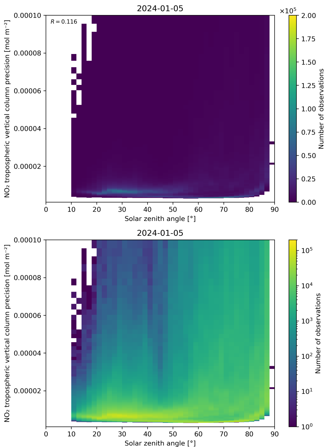
Figure 156: Scatter density plot of “Solar zenith angle” against “NO 2 tropospheric vertical column precision” for 2024-01-05 to 2024-01-06.
