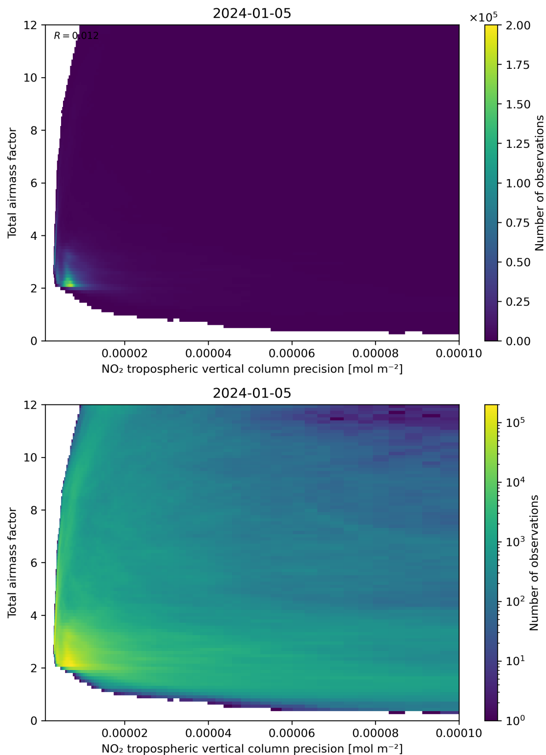
Figure 132: Scatter density plot of “NO 2 tropospheric vertical column precision” against “Total air mass factor” for 2024-01-05 to 2024-01-06.
