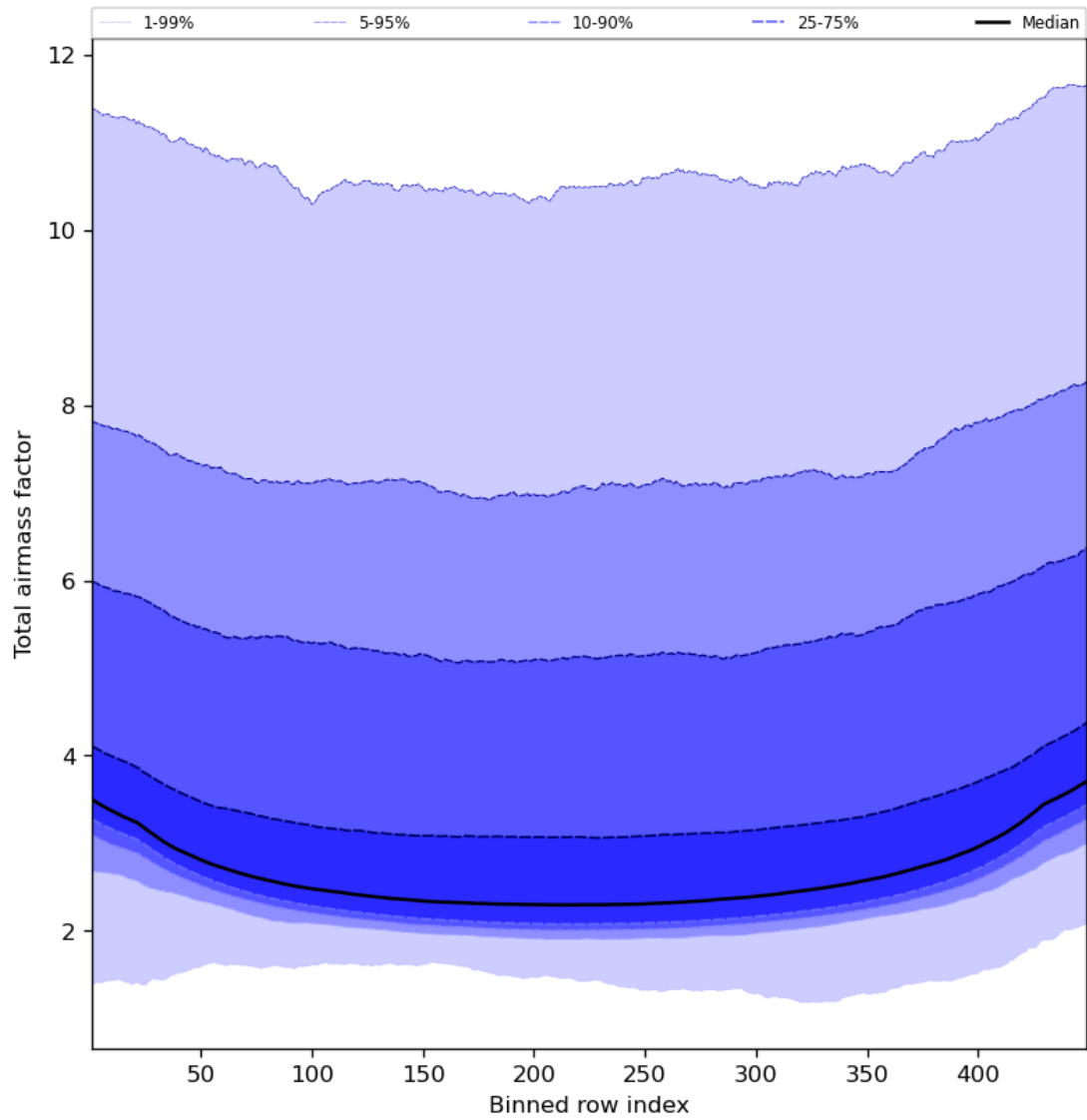
Figure 49: Along track statistics of “Total airmass factor” for 2024-01-05 to 2024-01-06
