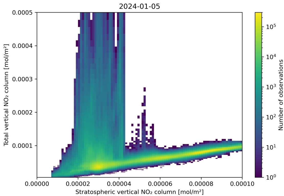
Figure 100: Scatter density plot of “Stratospheric vertical NO 2 column” against “Total vertical NO 2 column” for 2024-01-05 to 2024-01-06.
