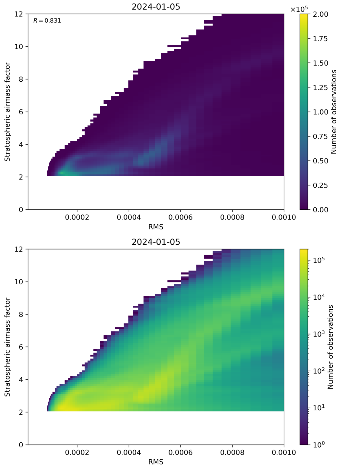
Figure 144: Scatter density plot of “RMS” against “Stratospheric airmass factor” for 2024-01-05 to 2024-01-06.
