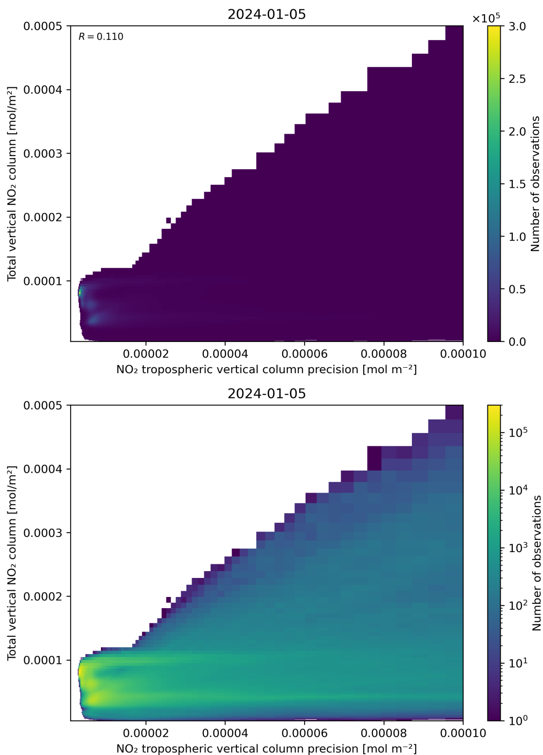
Figure 138: Scatter density plot of “NO 2 tropospheric vertical column precision” against “Total vertical NO 2 column” for 2024-01-05 to 2024-01-06.
