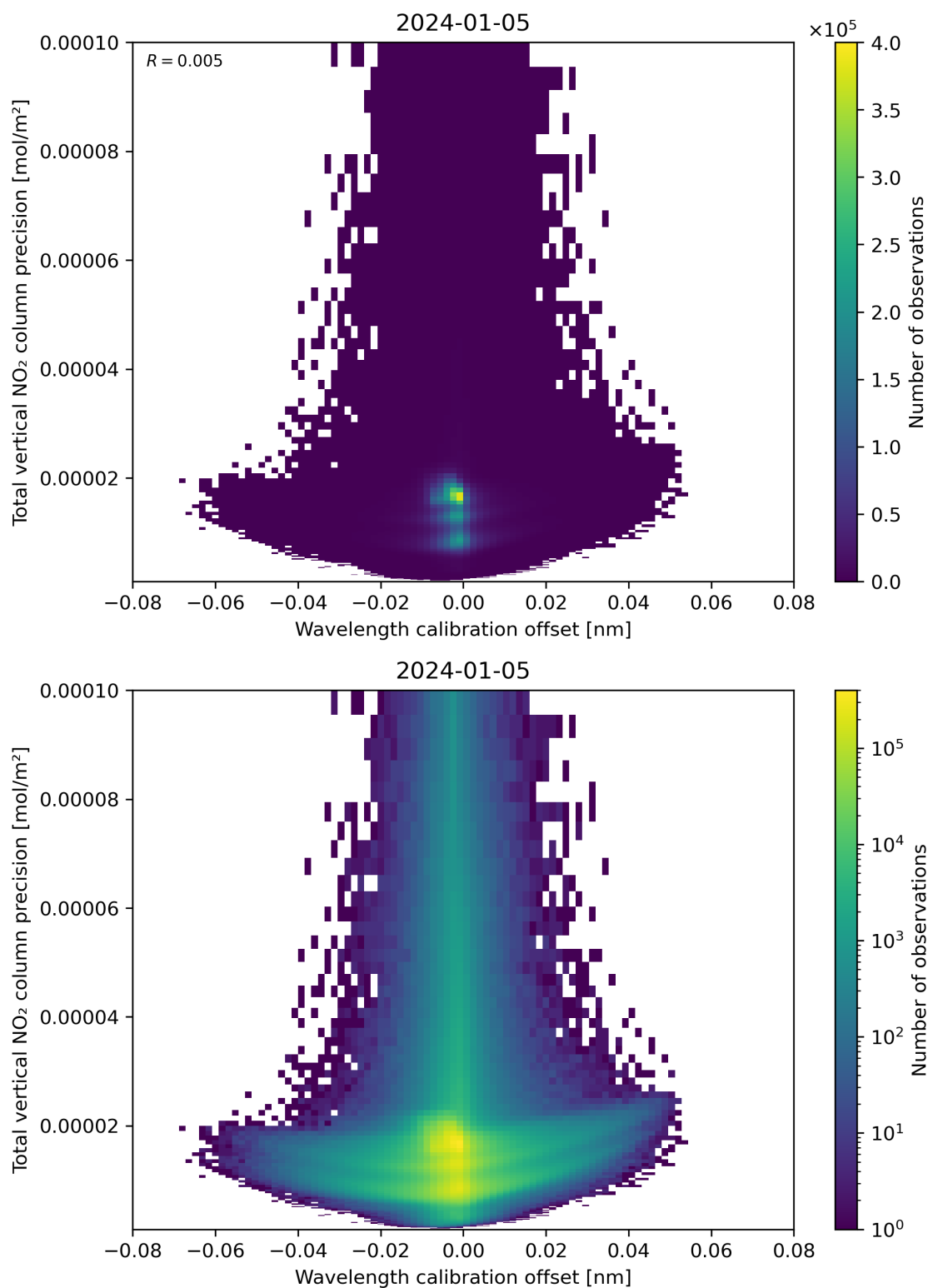
Figure 180: Scatter density plot of “Wavelength calibration offset” against “Total vertical NO 2 column precision” for 2024-01-05 to 2024-01-06.
