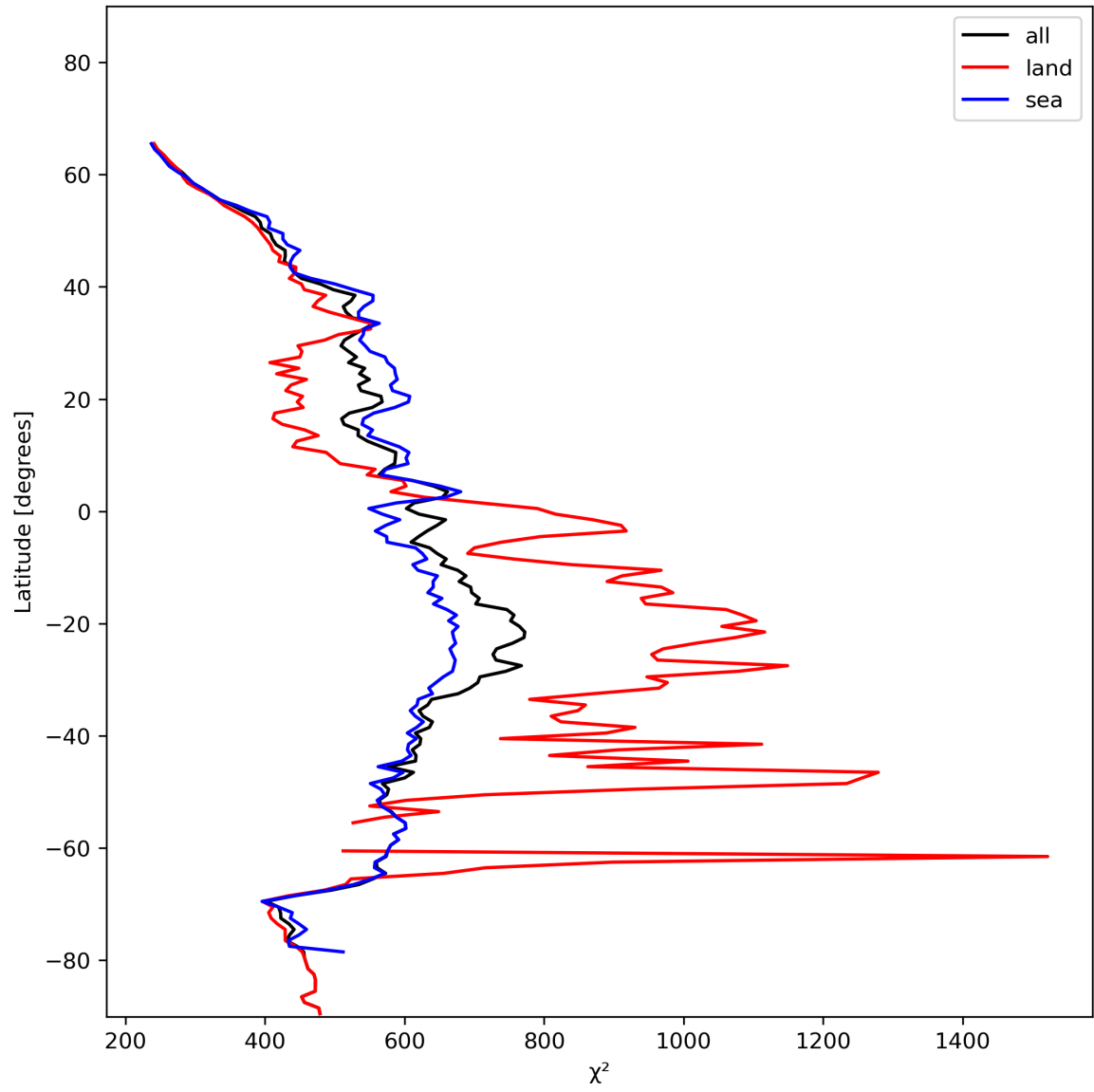
Figure 25: Zonal average of “ \chi^2 ” for 2024-01-05 to 2024-01-06.
