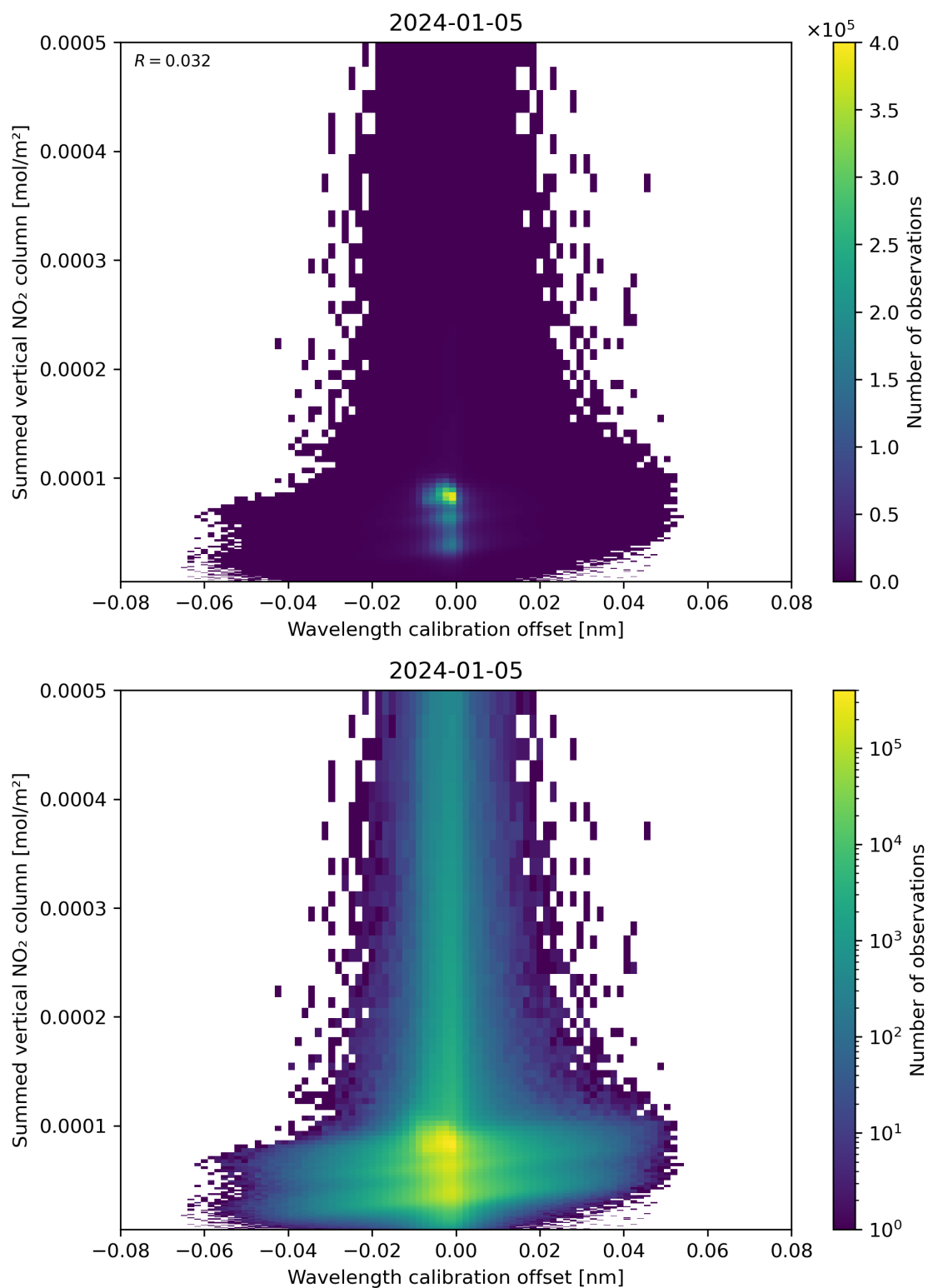
Figure 177: Scatter density plot of “Wavelength calibration offset” against “Summed vertical NO 2 column” for 2024-01-05 to 2024-01-06.
