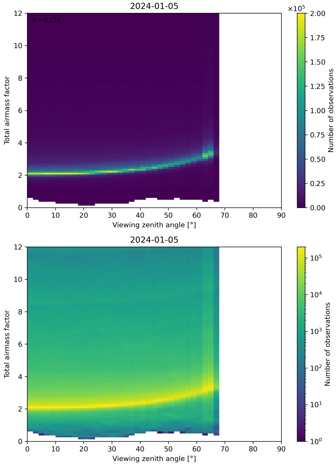
Figure 160: Scatter density plot of “Viewing zenith angle” against “Total airmass factor” for 2024-01-05 to 2024-01-06.
