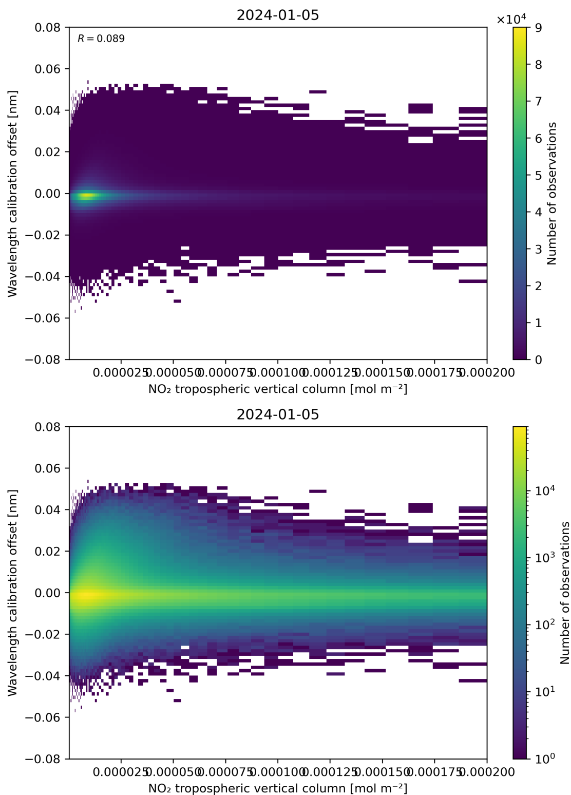
Figure 143: Scatter density plot of “NO 2 tropospheric vertical column” against “Wavelength calibration offset” for 2024-01-05 to 2024-01-06.
