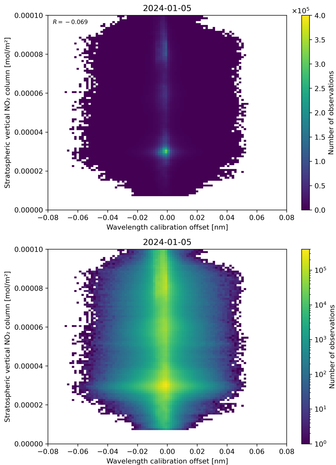
Figure 176: Scatter density plot of “Wavelength calibration offset” against “Stratospheric vertical NO 2 column” for 2024-01-05 to 2024-01-06.
