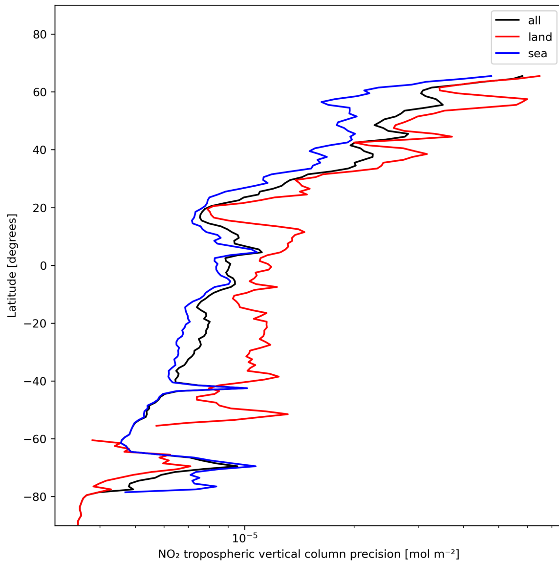
Figure 13: Zonal average of “NO 2 tropospheric vertical column precision” for 2024-01-05 to 2024-01-06.
