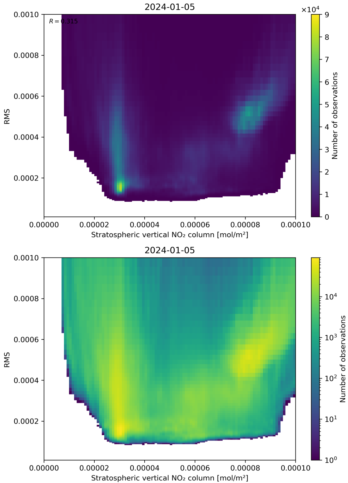
Figure 102: Scatter density plot of “Stratospheric vertical NO 2 column” against “RMS” for 2024-01-05 to 2024-01-06.
