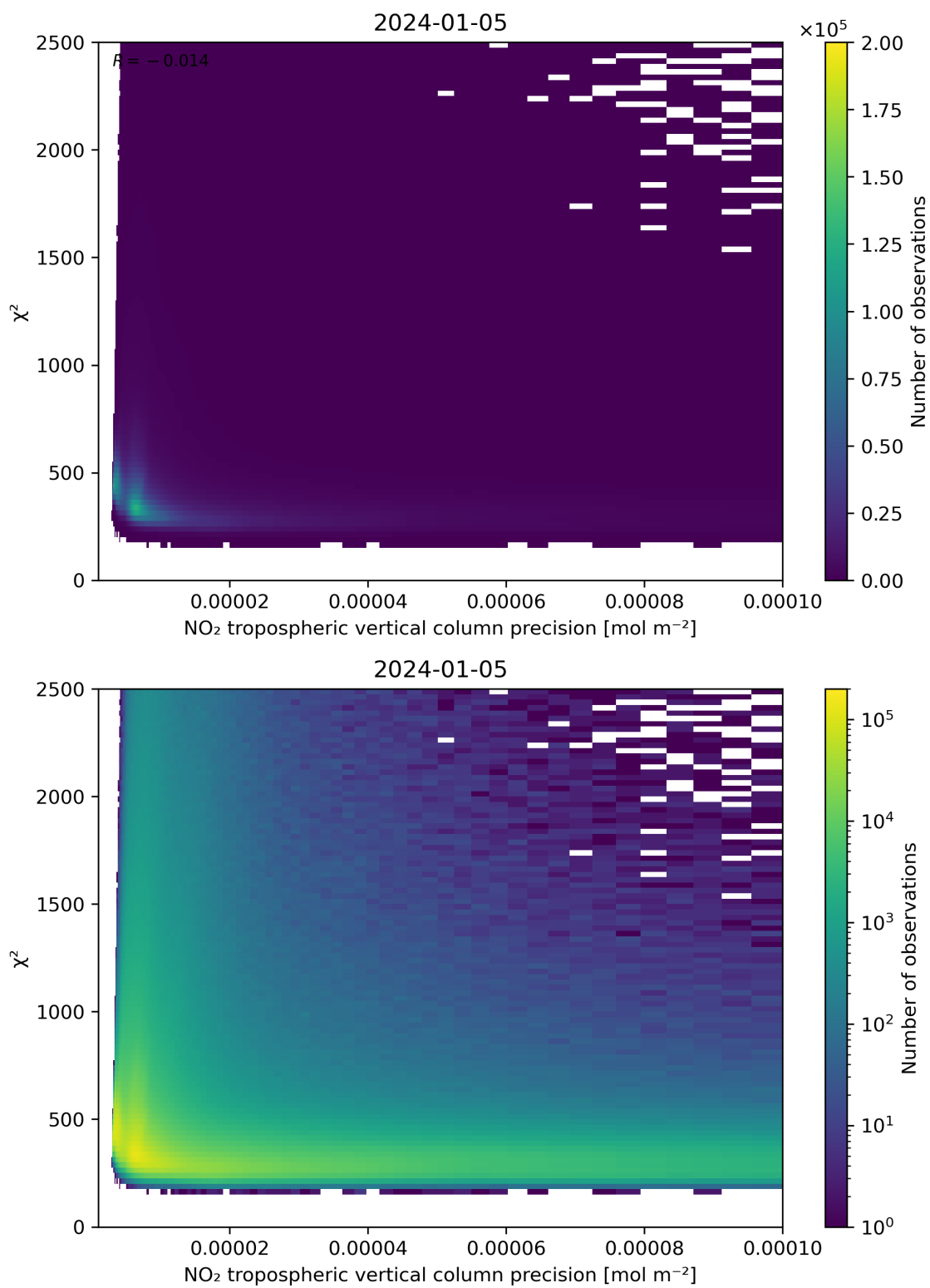
Figure 134: Scatter density plot of “NO 2 tropospheric vertical column precision” against “ \chi^2 ” for 2024-01-05 to 2024-01-06.
