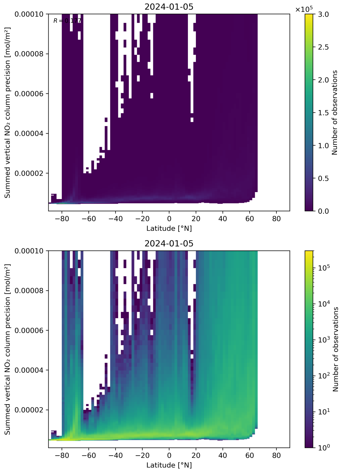
Figure 89: Scatter density plot of “Latitude” against “Summed vertical NO 2 column precision” for 2024-01-05 to 2024-01-06.
