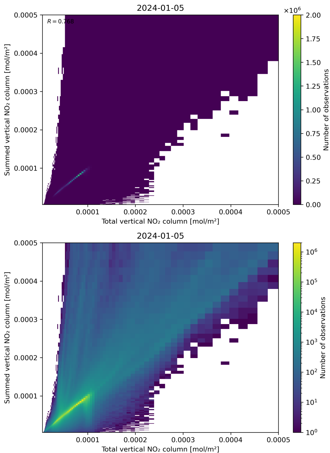
Figure 112: Scatter density plot of “Total vertical NO 2 column” against “Summed vertical NO 2 column” for 2024-01-05 to 2024-01-06.
