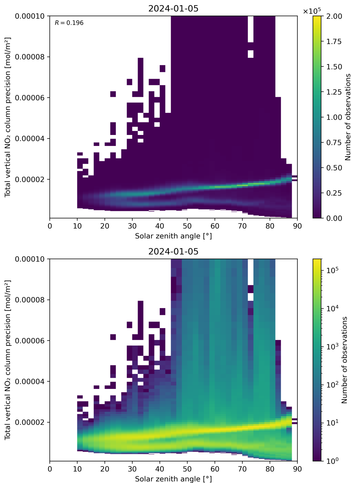
Figure 154: Scatter density plot of “Solar zenith angle” against “Total vertical NO 2 column precision” for 2024-01-05 to 2024-01-06.
