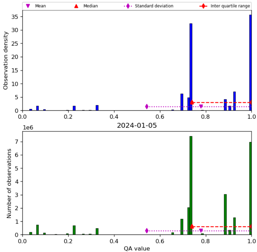
Figure 28: Histogram of “QA value” for 2024-01-05 to 2024-01-06
