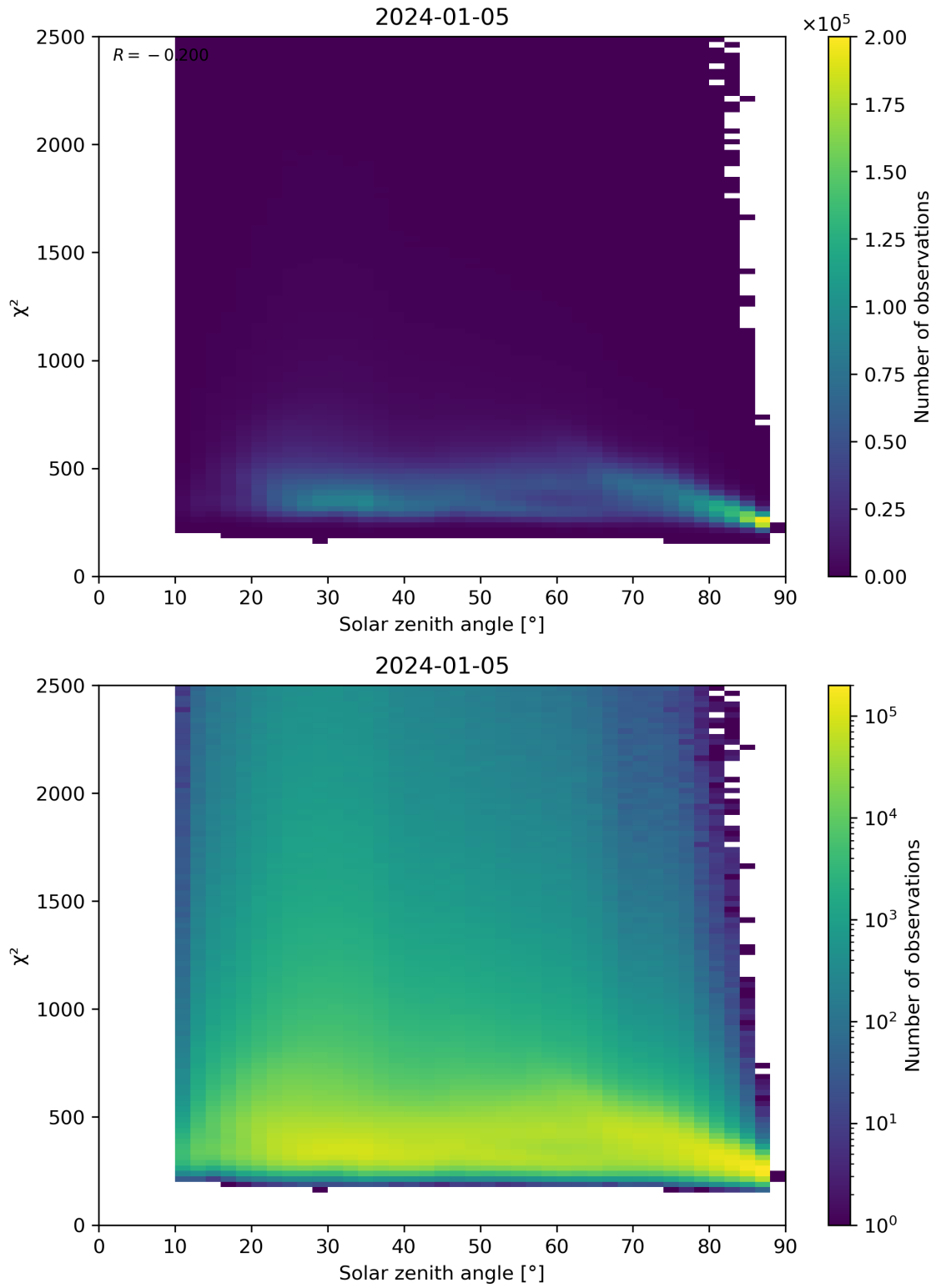
Figure 148: Scatter density plot of “Solar zenith angle” against “ \chi^2 ” for 2024-01-05 to 2024-01-06.
