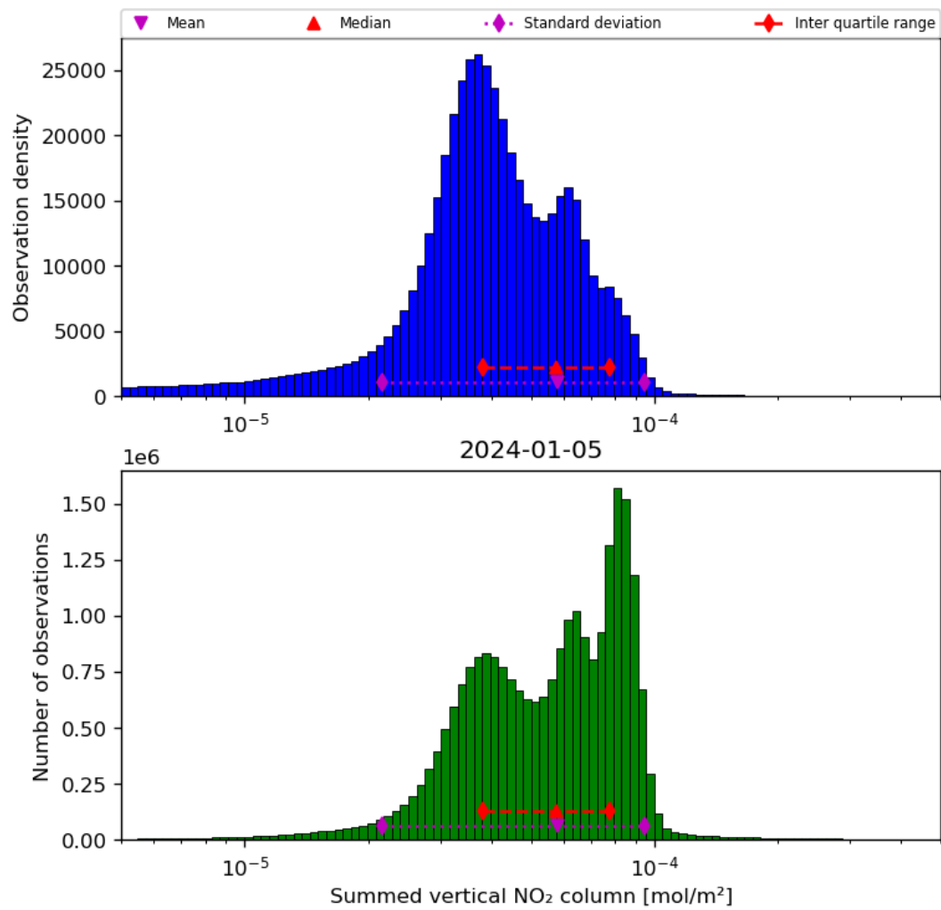
Figure 40: Histogram of “Summed vertical NO 2 column” for 2024-01-05 to 2024-01-06
