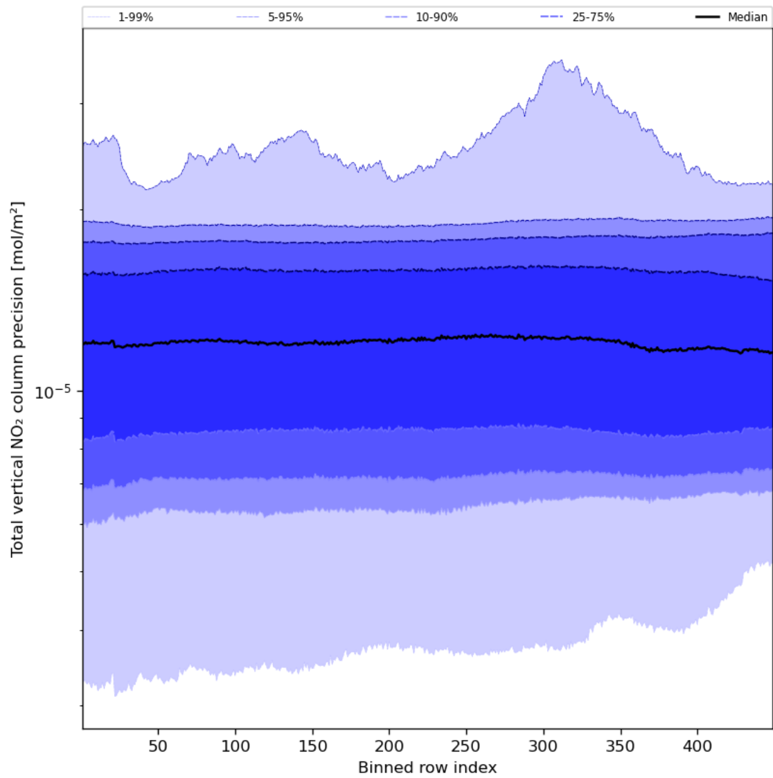
Figure 56: Along track statistics of “Total vertical NO 2 column precision” for 2024-01-05 to 2024-01-06
