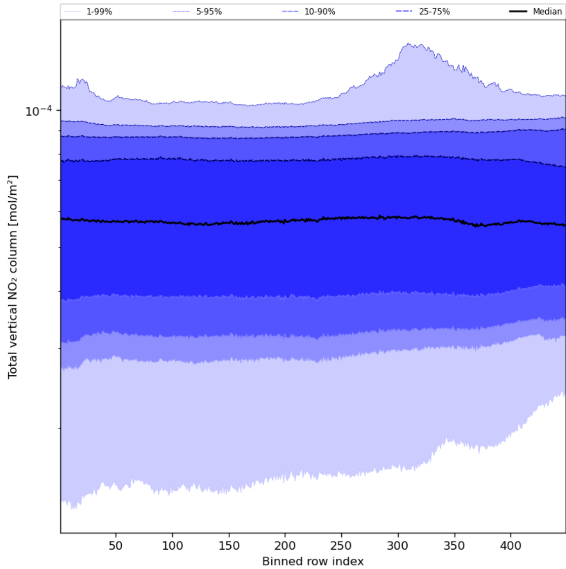
Figure 55: Along track statistics of “Total vertical NO 2 column” for 2024-01-05 to 2024-01-06
