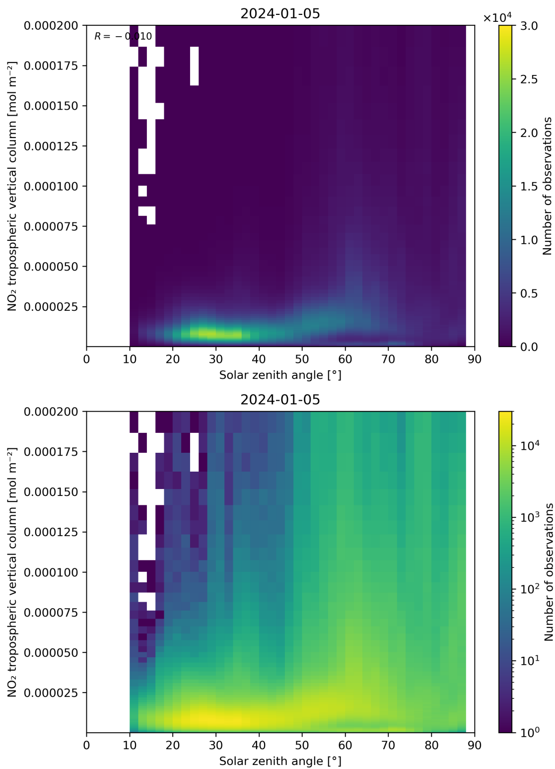
Figure 155: Scatter density plot of “Solar zenith angle” against “NO 2 tropospheric vertical column” for 2024-01-05 to 2024-01-06.
