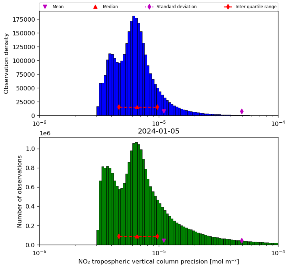
Figure 30: Histogram of “NO 2 tropospheric vertical column precision” for 2024-01-05 to 2024-01-06
