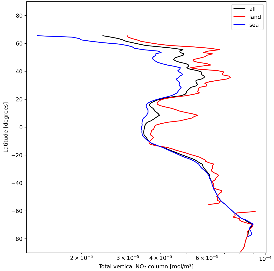
Figure 21: Zonal average of “Total vertical NO 2 column” for 2024-01-05 to 2024-01-06.
