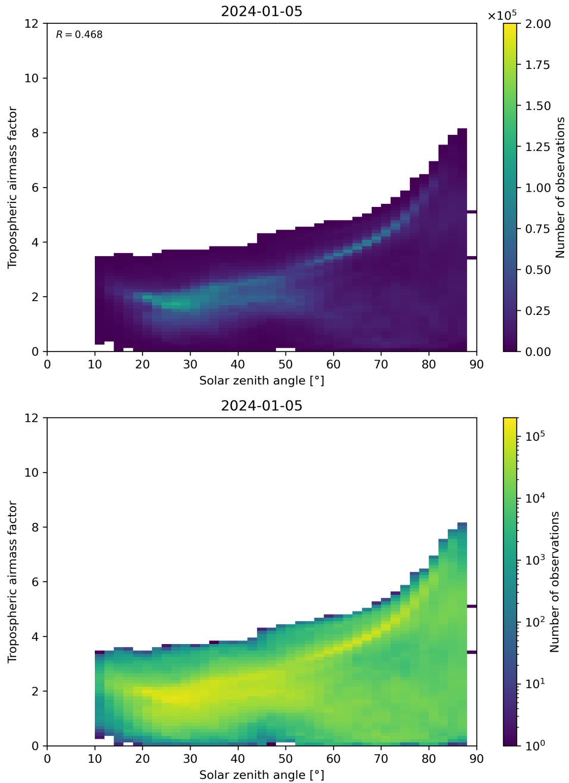
Figure 147: Scatter density plot of “Solar zenith angle” against “Tropospheric airmass factor” for 2024-01-05 to 2024-01-06.
