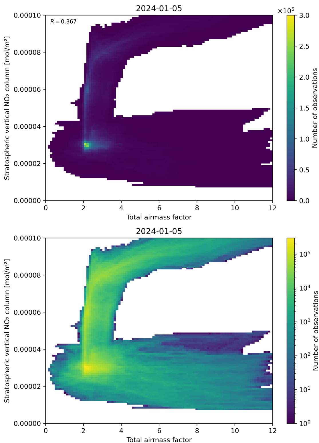
Figure 64: Scatter density plot of “Total airmass factor” against “Stratospheric vertical NO 2 column” for 2024-01-05 to 2024-01-06.
