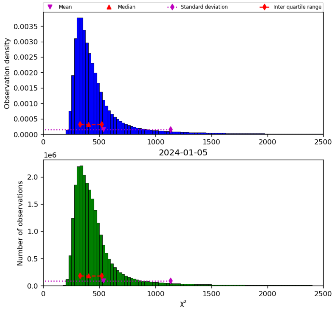
Figure 42: Histogram of “ \chi^2 ” for 2024-01-05 to 2024-01-06
