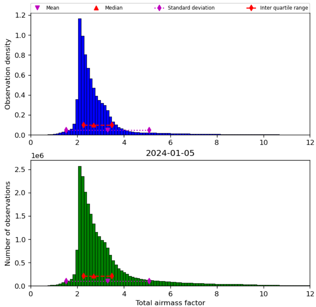
Figure 32: Histogram of “Total airmass factor” for 2024-01-05 to 2024-01-06
