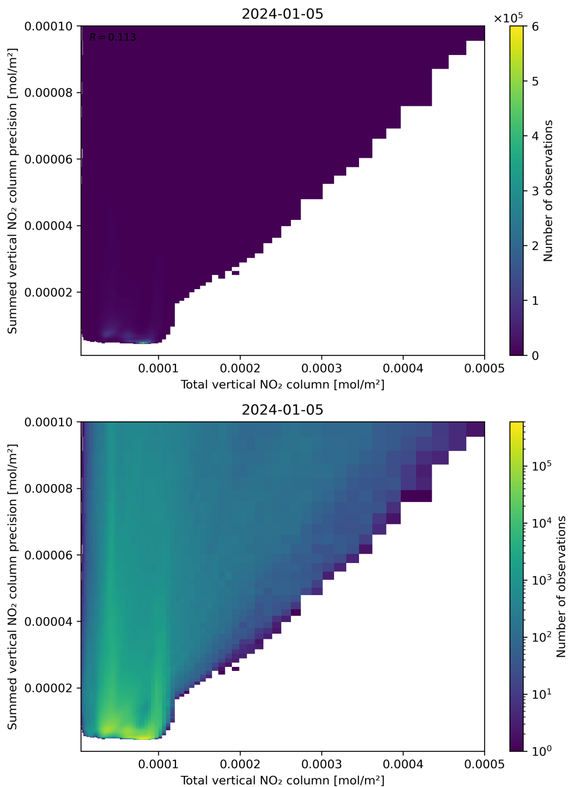
Figure 113: Scatter density plot of “Total vertical NO 2 column” against “Summed vertical NO 2 column precision” for 2024-01-05 to 2024-01-06.
