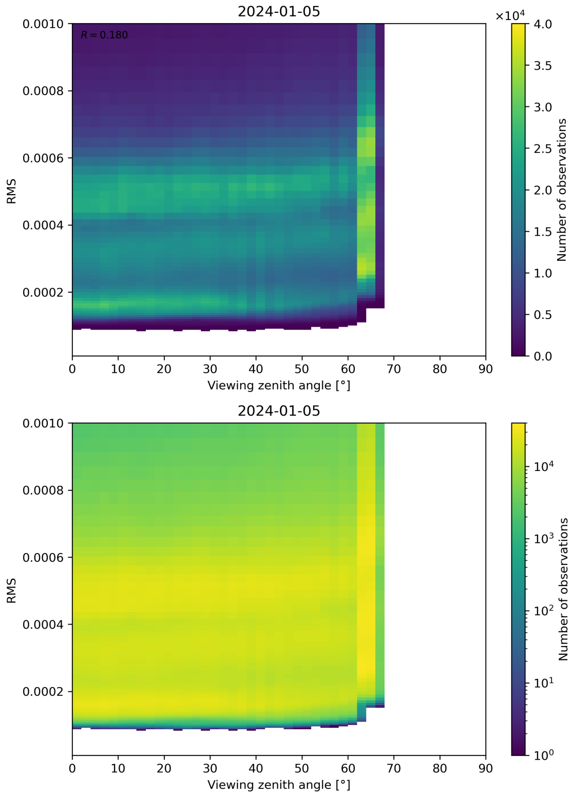
Figure 171: Scatter density plot of “Viewing zenith angle” against “RMS” for 2024-01-05 to 2024-01-06.
