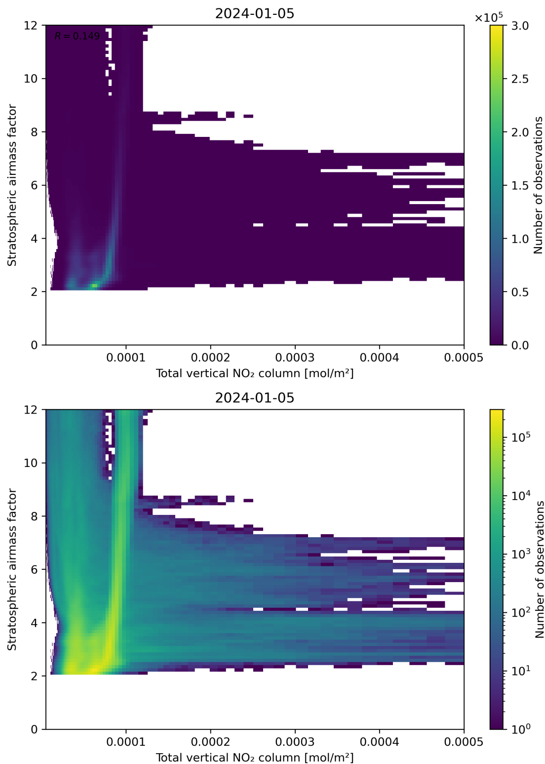
Figure 110: Scatter density plot of “Total vertical NO 2 column” against “Stratospheric airmass factor” for 2024-01-05 to 2024-01-06.
