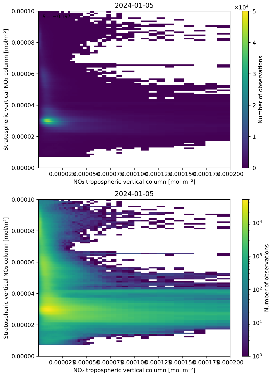
Figure 125: Scatter density plot of “NO 2 tropospheric vertical column” against “Stratospheric vertical NO 2 column” for 2024-01-05 to 2024-01-06.
