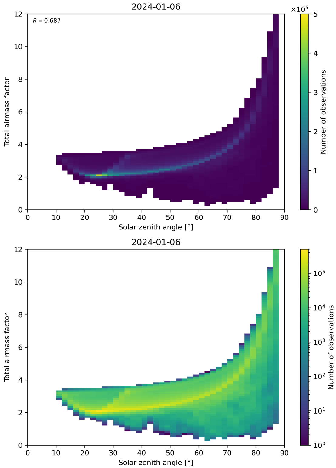
Figure 146: Scatter density plot of “Solar zenith angle” against “Total air mass factor” for 2024-01-05 to 2024-01-07.
