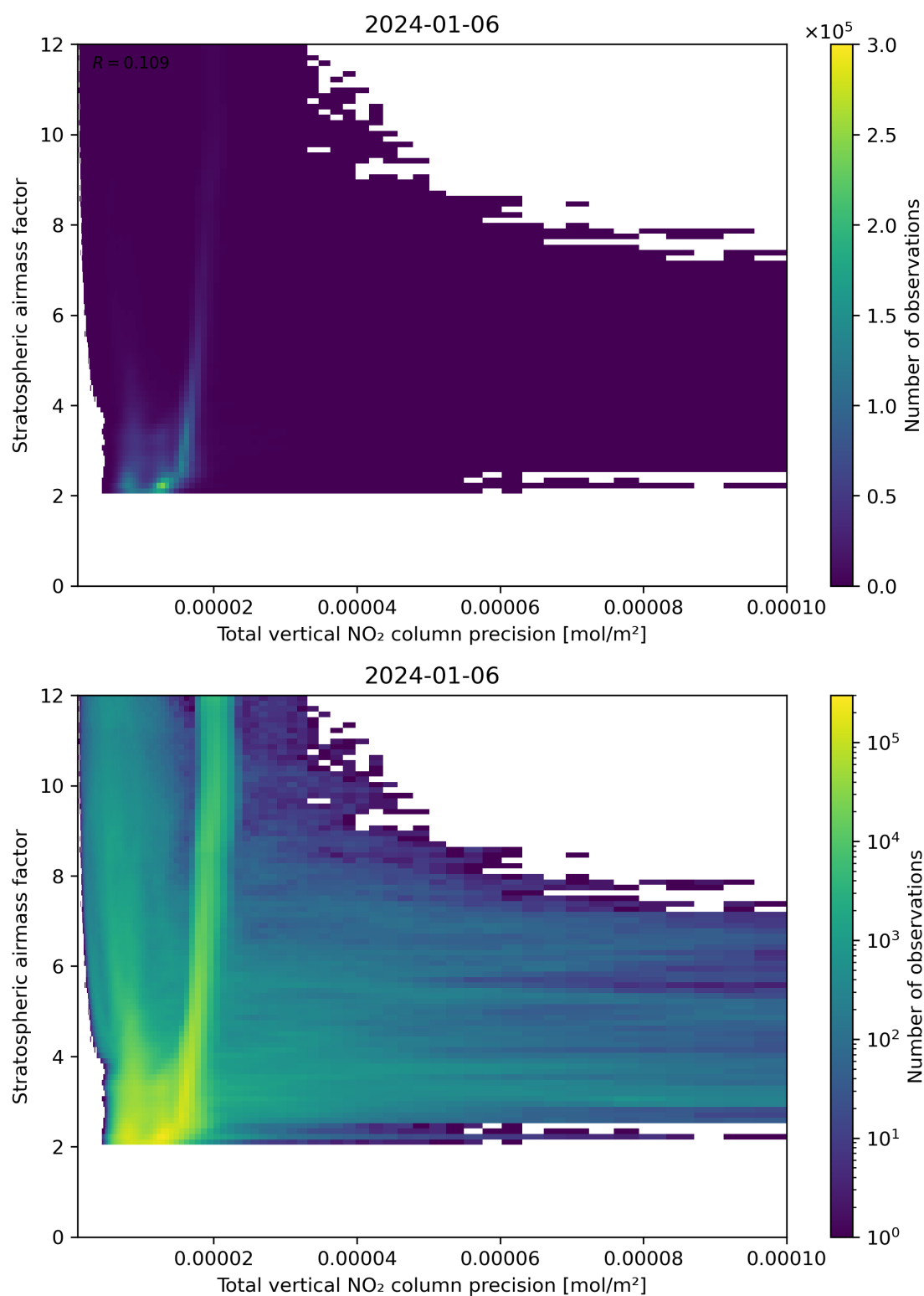
Figure 115: Scatter density plot of “Total vertical NO 2 column precision” against “Stratospheric air mass factor” for 2024-01-05 to 2024-01-07.
