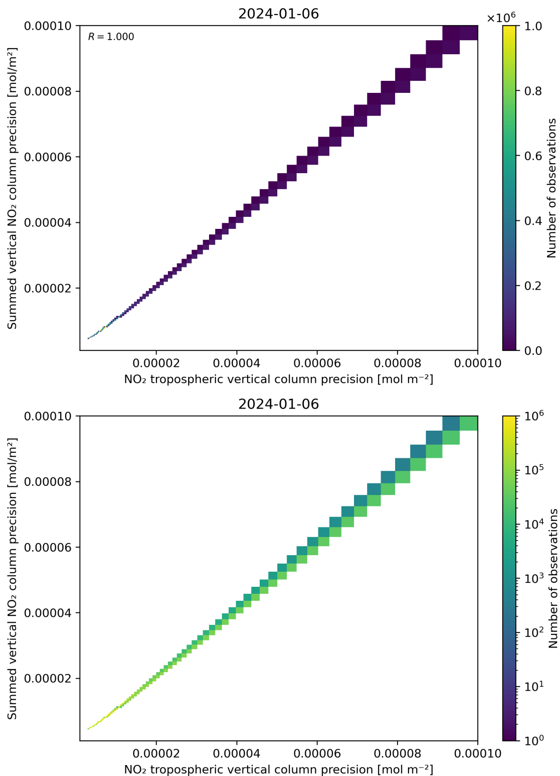
Figure 137: Scatter density plot of “NO 2 tropospheric vertical column precision” against “Summed vertical NO 2 column precision” for 2024-01-05 to 2024-01-07.
