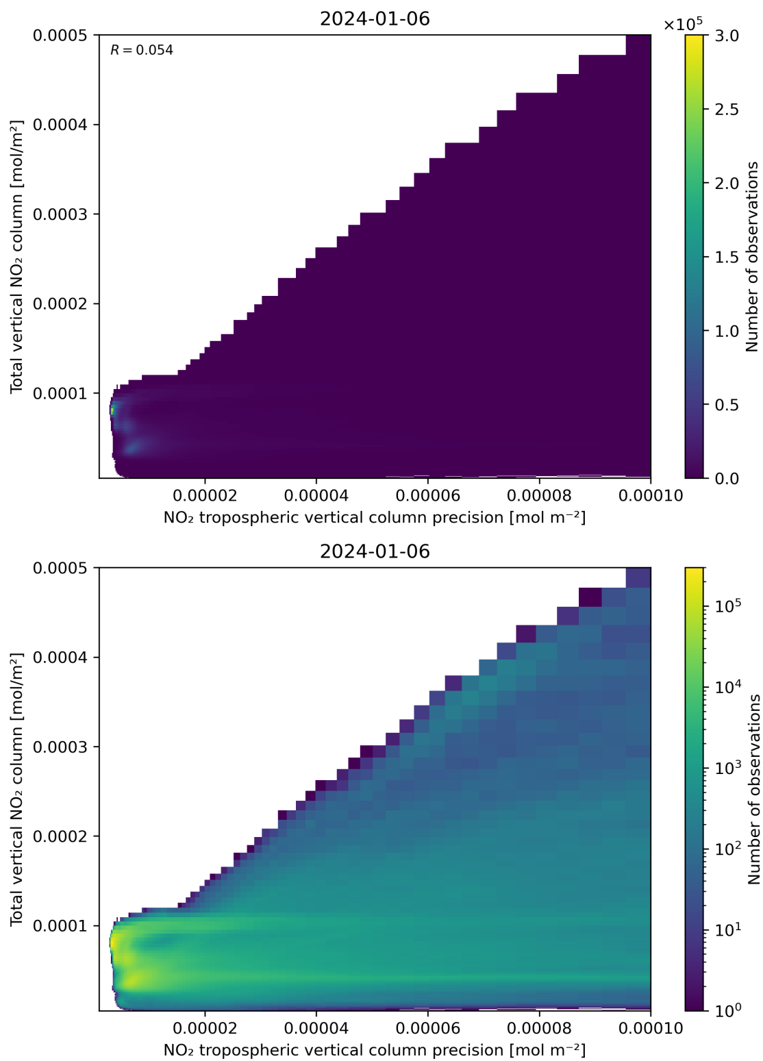
Figure 138: Scatter density plot of “NO 2 tropospheric vertical column precision” against “Total vertical NO 2 column” for 2024-01-05 to 2024-01-07.
