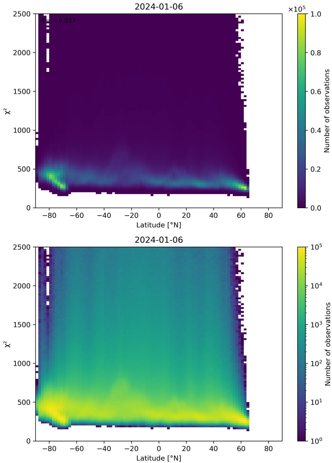
Figure 86: Scatter density plot of “Latitude” against “ \chi^2 ” for 2024-01-05 to 2024-01-07.
