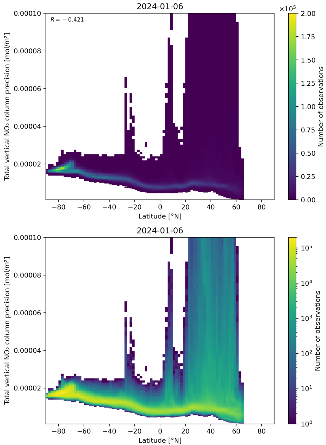
Figure 91: Scatter density plot of “Latitude” against “Total vertical NO 2 column precision” for 2024-01-05 to 2024-01-07.
