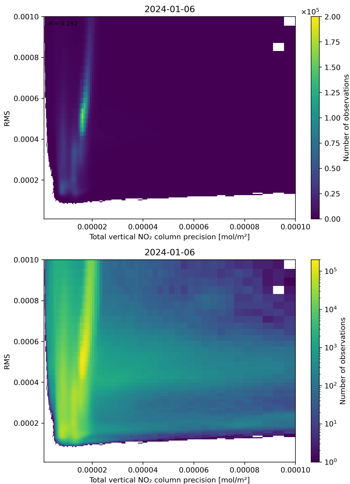
Figure 119: Scatter density plot of “Total vertical NO 2 column precision” against “RMS” for 2024-01-05 to 2024-01-07.
