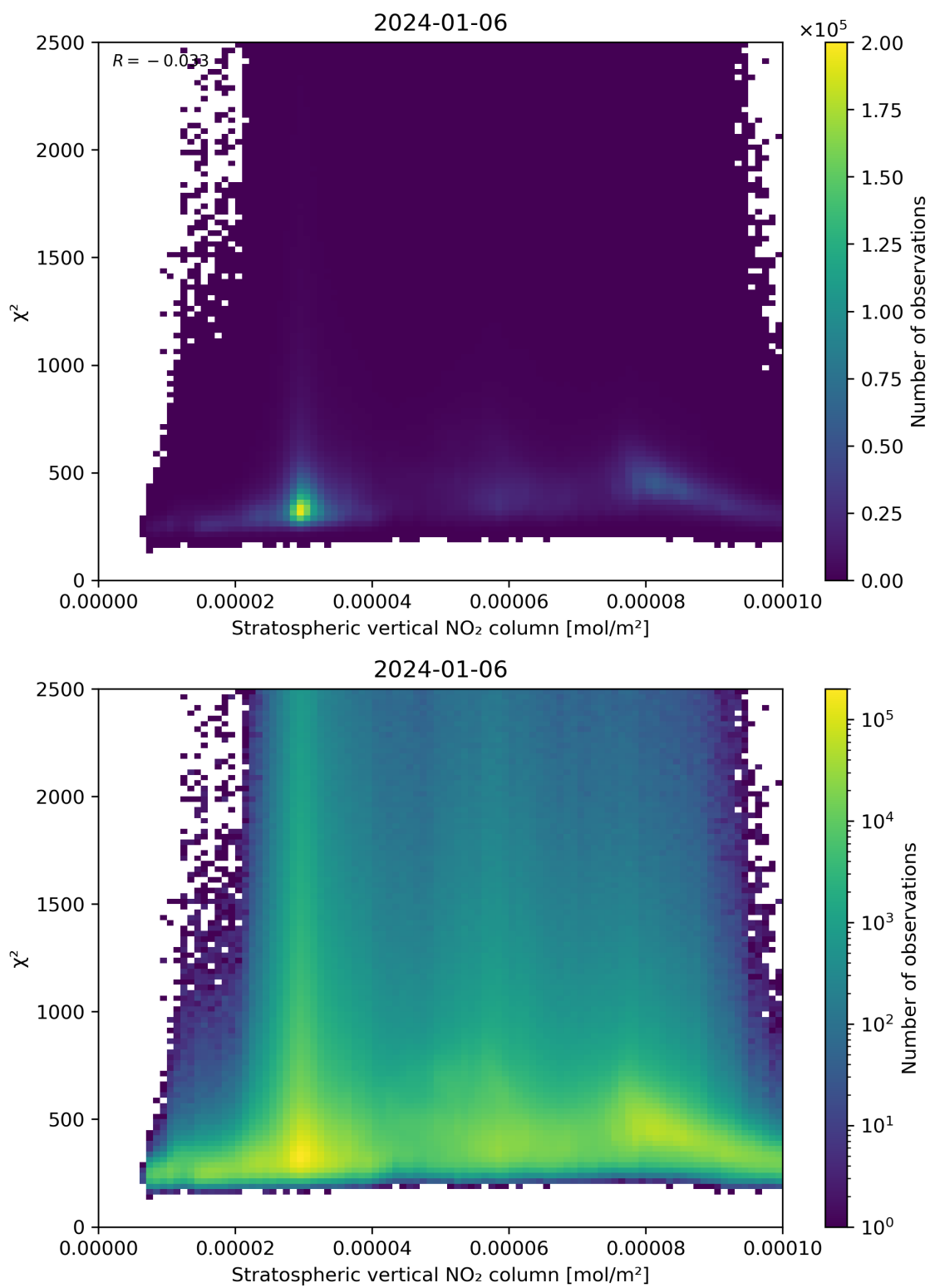
Figure 97: Scatter density plot of “Stratospheric vertical NO 2 column” against “ \chi^2 ” for 2024-01-05 to 2024-01-07.
