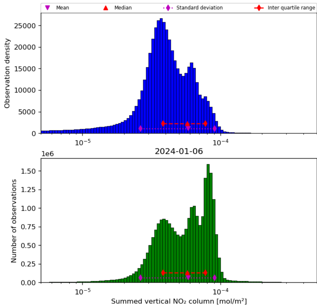
Figure 40: Histogram of “Summed vertical NO 2 column” for 2024-01-05 to 2024-01-07
