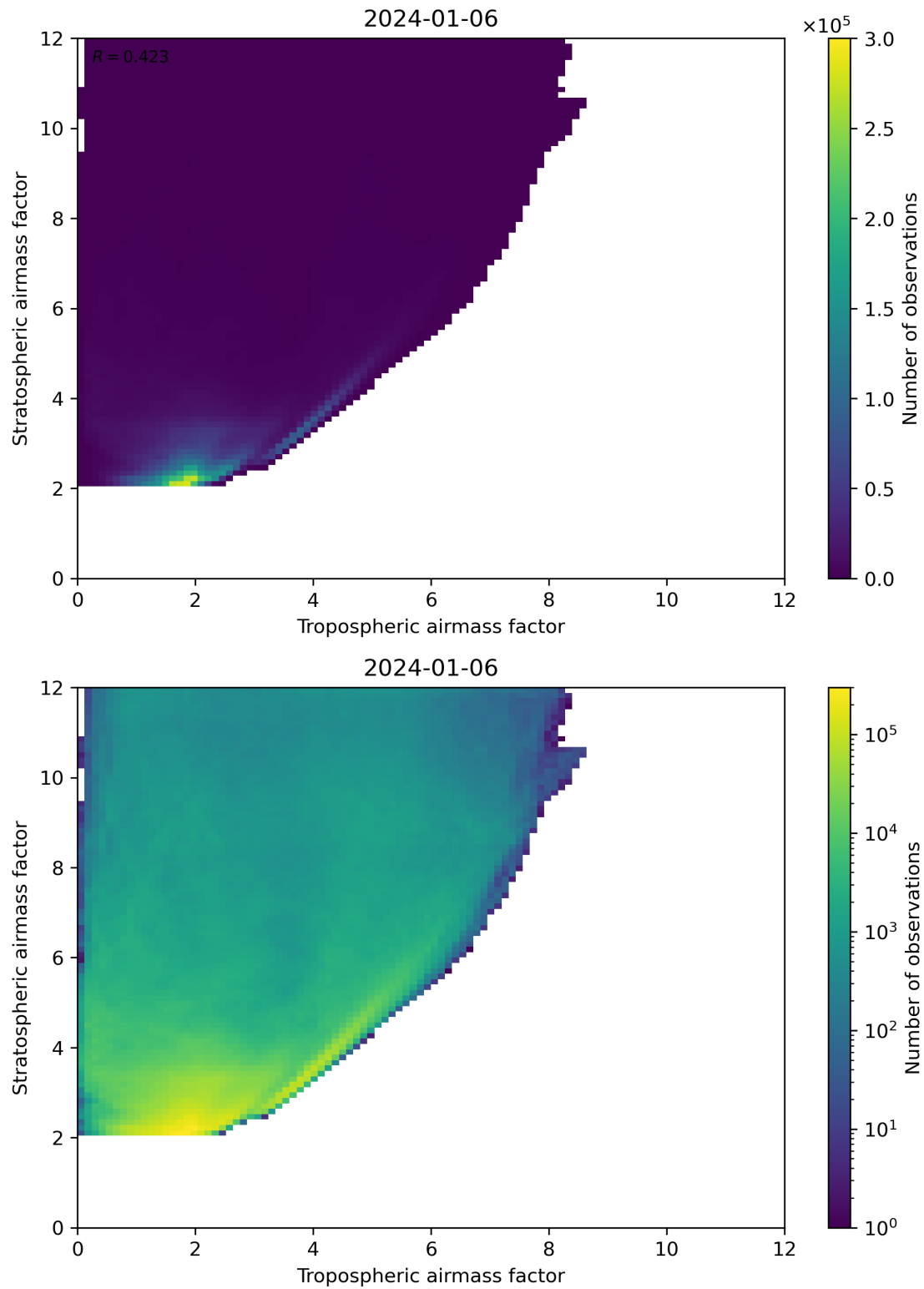
Figure 71: Scatter density plot of “Tropospheric airmass factor” against “Stratospheric airmass factor” for 2024-01-05 to 2024-01-07.
