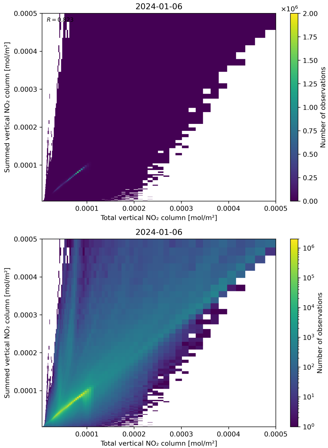
Figure 112: Scatter density plot of “Total vertical NO 2 column” against “Summed vertical NO 2 column” for 2024-01-05 to 2024-01-07.
