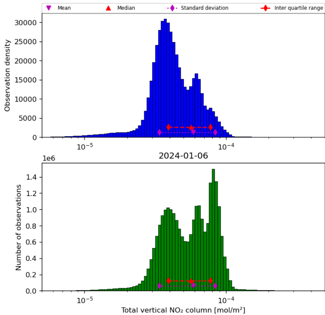
Figure 38: Histogram of “Total vertical NO 2 column” for 2024-01-05 to 2024-01-07
