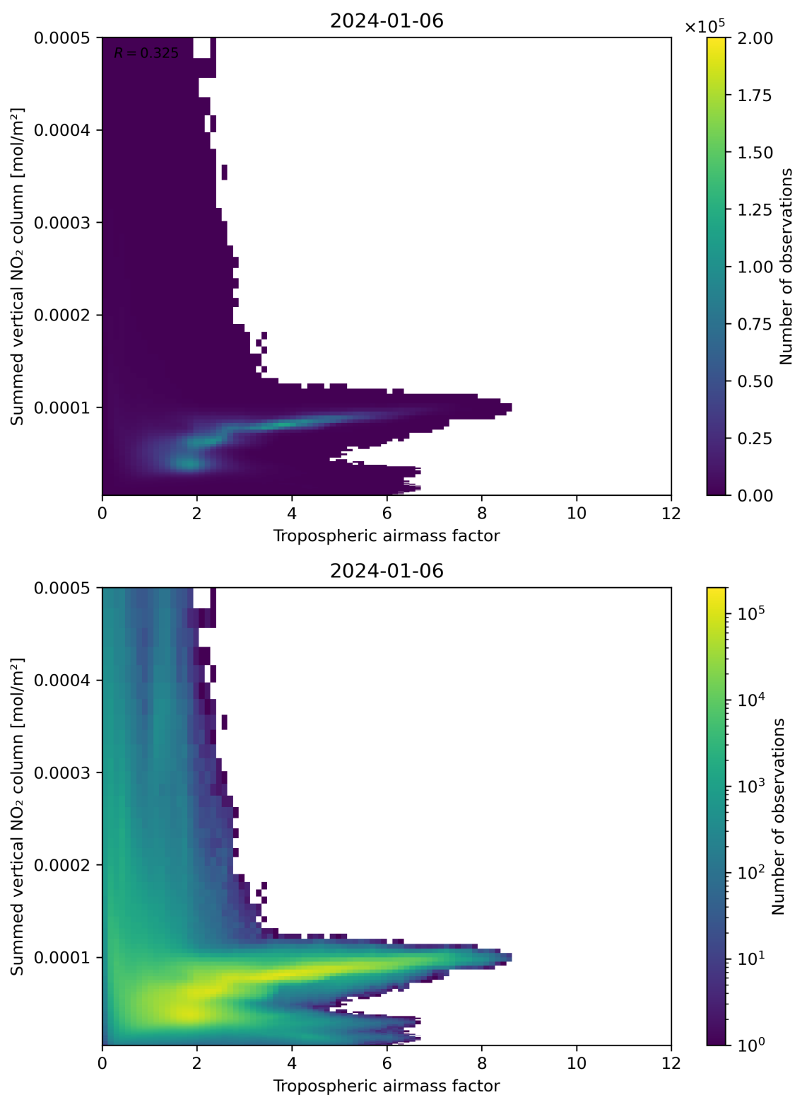
Figure 75: Scatter density plot of “Tropospheric airmass factor” against “Summed vertical NO 2 column” for 2024-01-05 to 2024-01-07.
