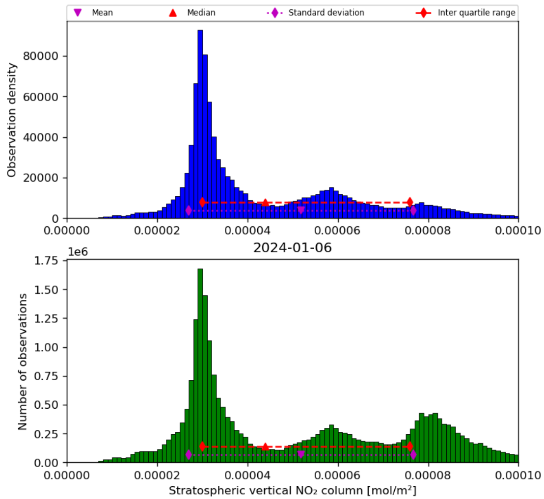
Figure 36: Histogram of “Stratospheric vertical NO 2 column” for 2024-01-05 to 2024-01-07
