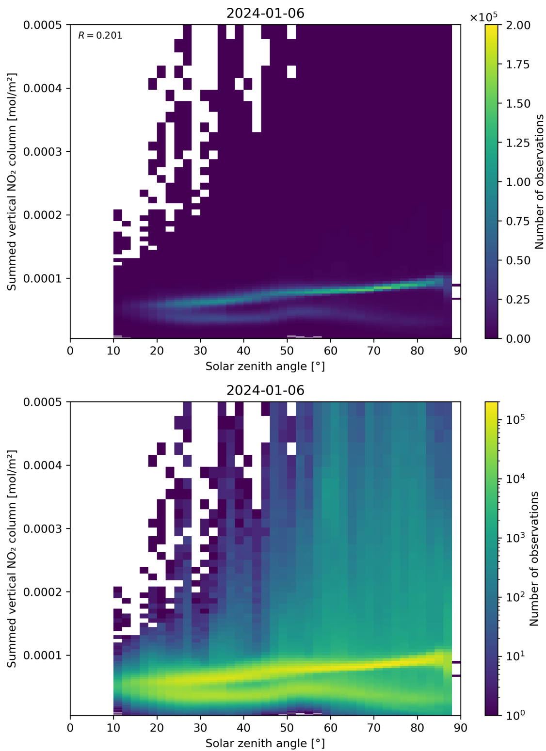
Figure 151: Scatter density plot of “Solar zenith angle” against “Summed vertical NO 2 column” for 2024-01-05 to 2024-01-07.
