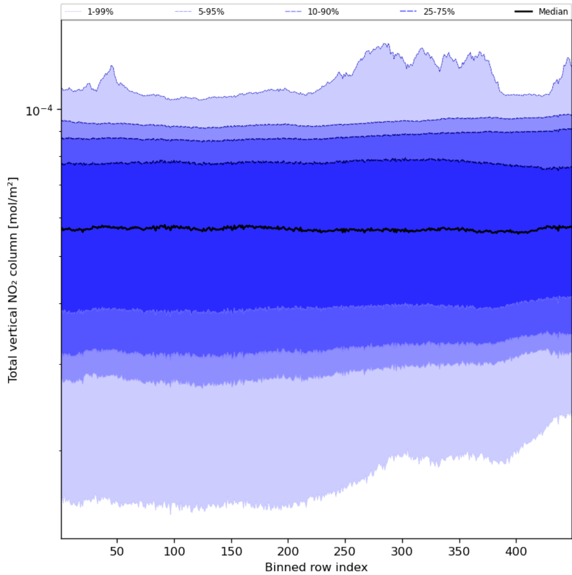
Figure 55: Along track statistics of “Total vertical NO 2 column” for 2024-01-05 to 2024-01-07
