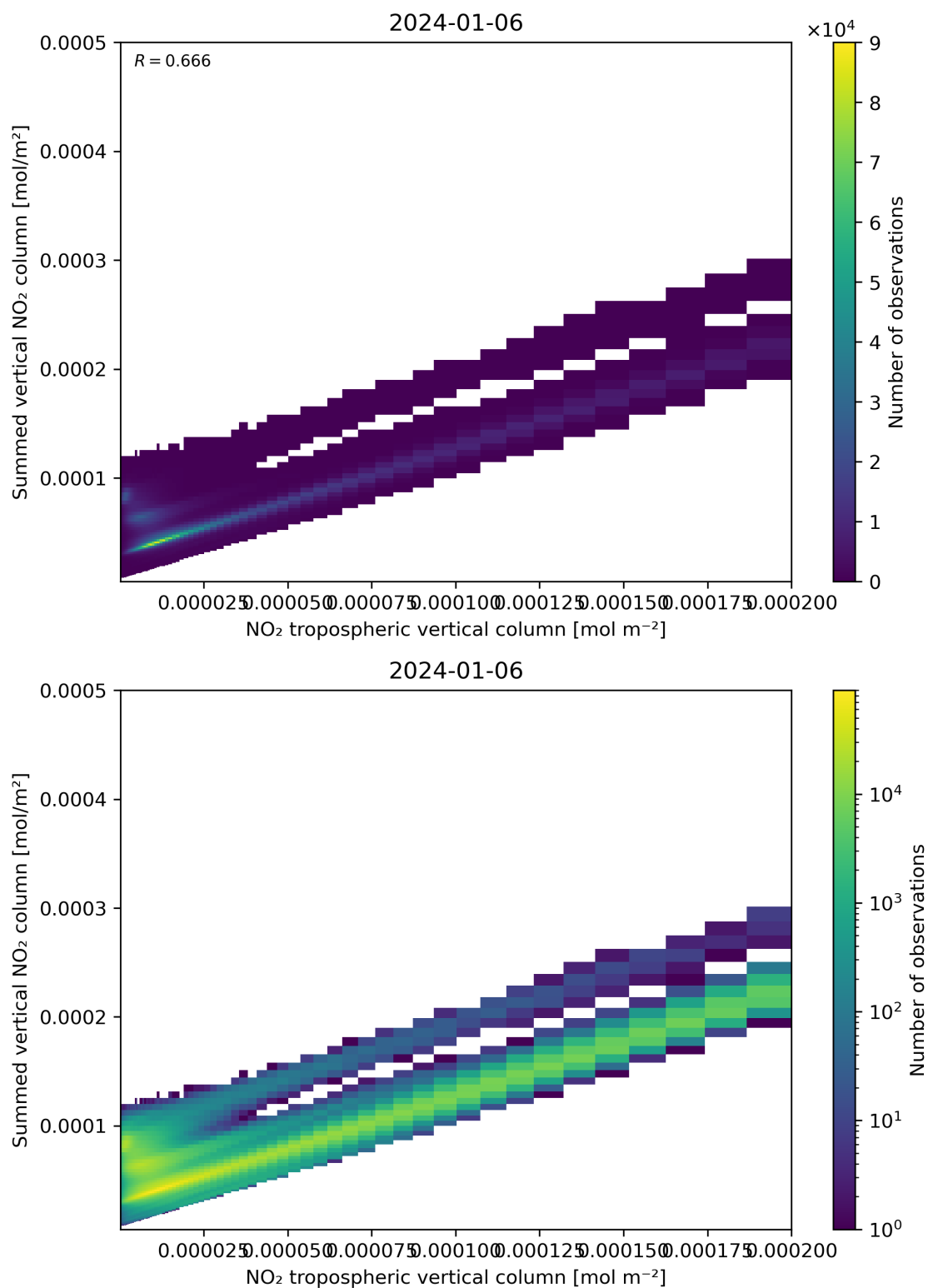
Figure 126: Scatter density plot of “NO 2 tropospheric vertical column” against “Summed vertical NO 2 column” for 2024-01-05 to 2024-01-07.
