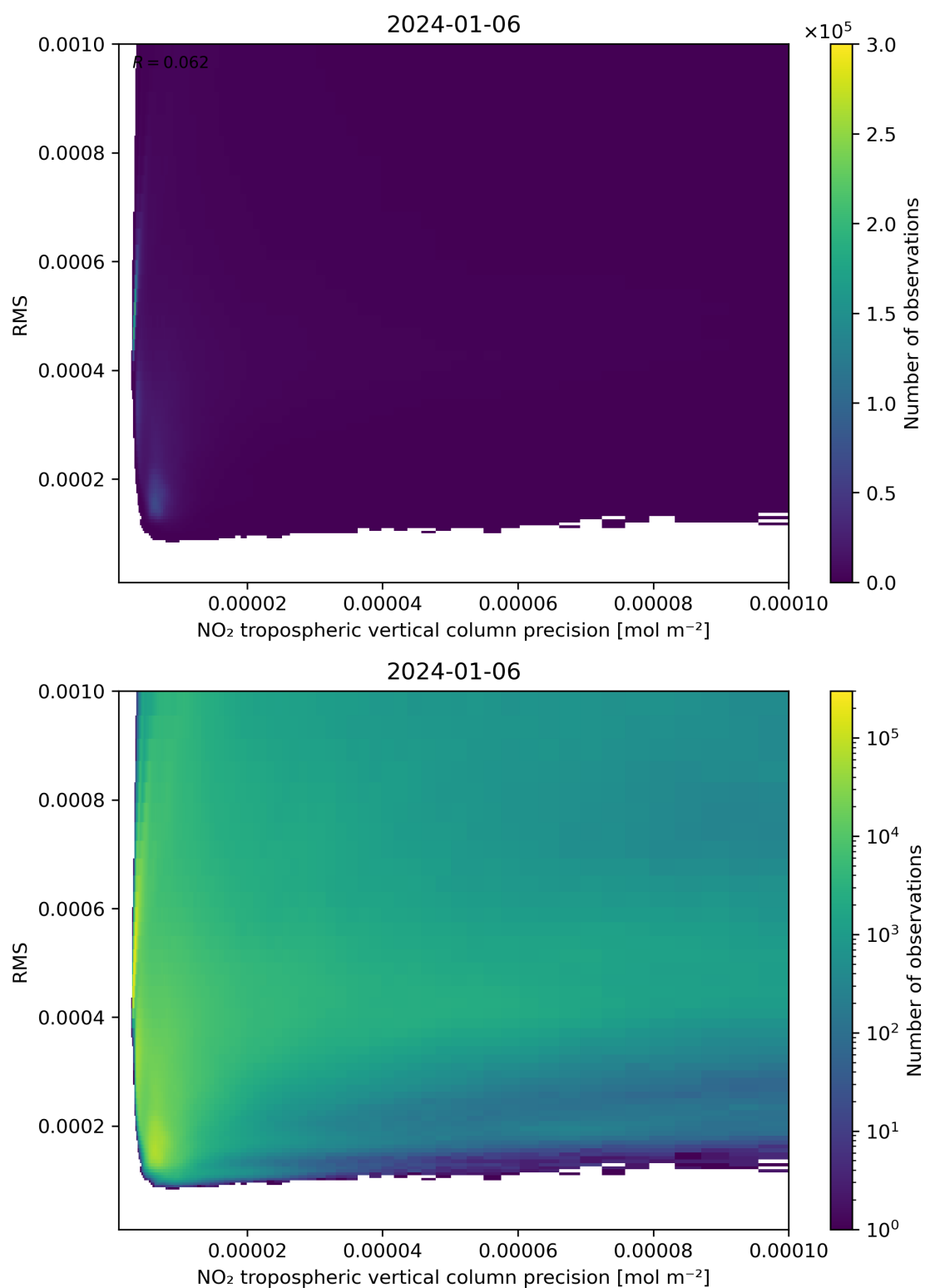
Figure 140: Scatter density plot of “NO 2 tropospheric vertical column precision” against “RMS” for 2024-01-05 to 2024-01-07.
