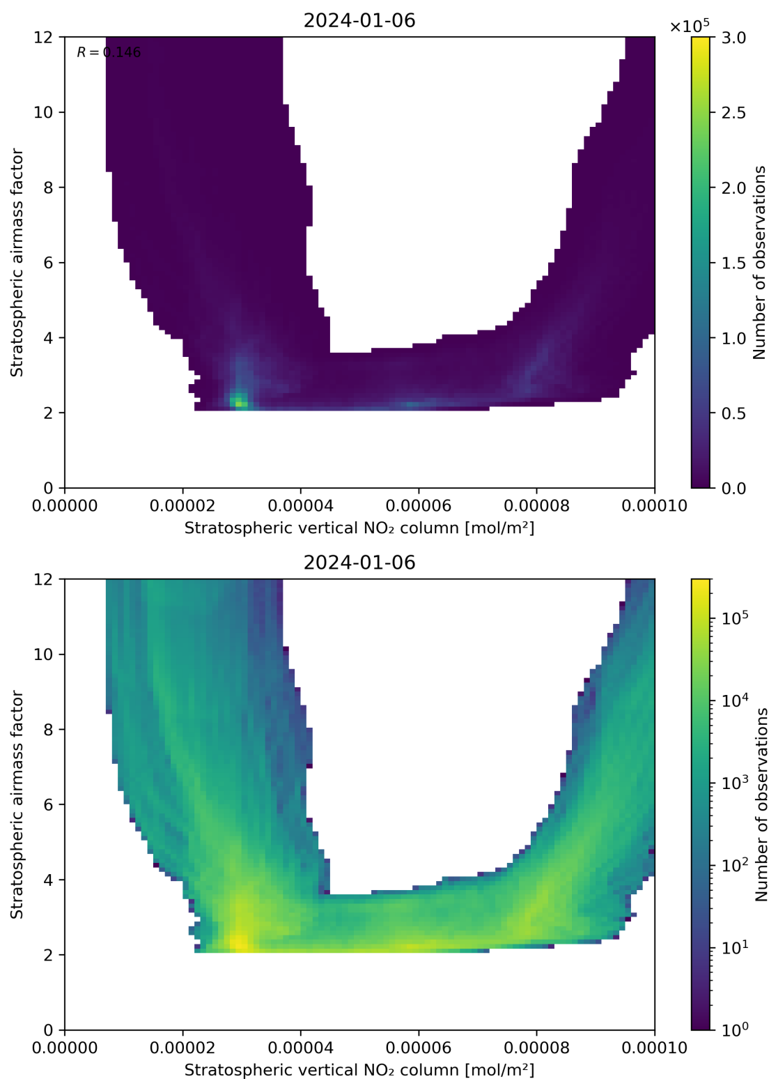
Figure 96: Scatter density plot of “Stratospheric vertical NO 2 column” against “Stratospheric airmass factor” for 2024-01-05 to 2024-01-07.
