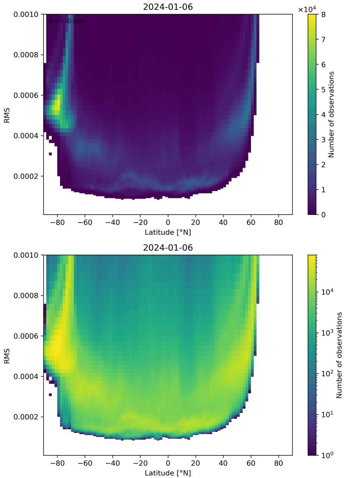
Figure 94: Scatter density plot of “Latitude” against “RMS” for 2024-01-05 to 2024-01-07.
