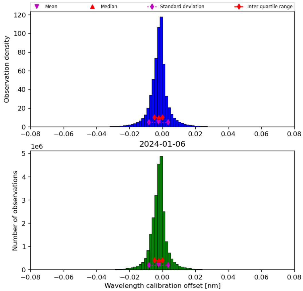
Figure 35: Histogram of “Wavelength calibration offset” for 2024-01-05 to 2024-01-07
