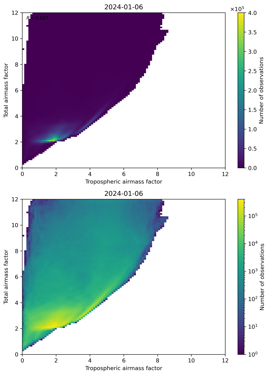
Figure 72: Scatter density plot of “Tropospheric airmass factor” against “Total airmass factor” for 2024-01-05 to 2024-01-07.
