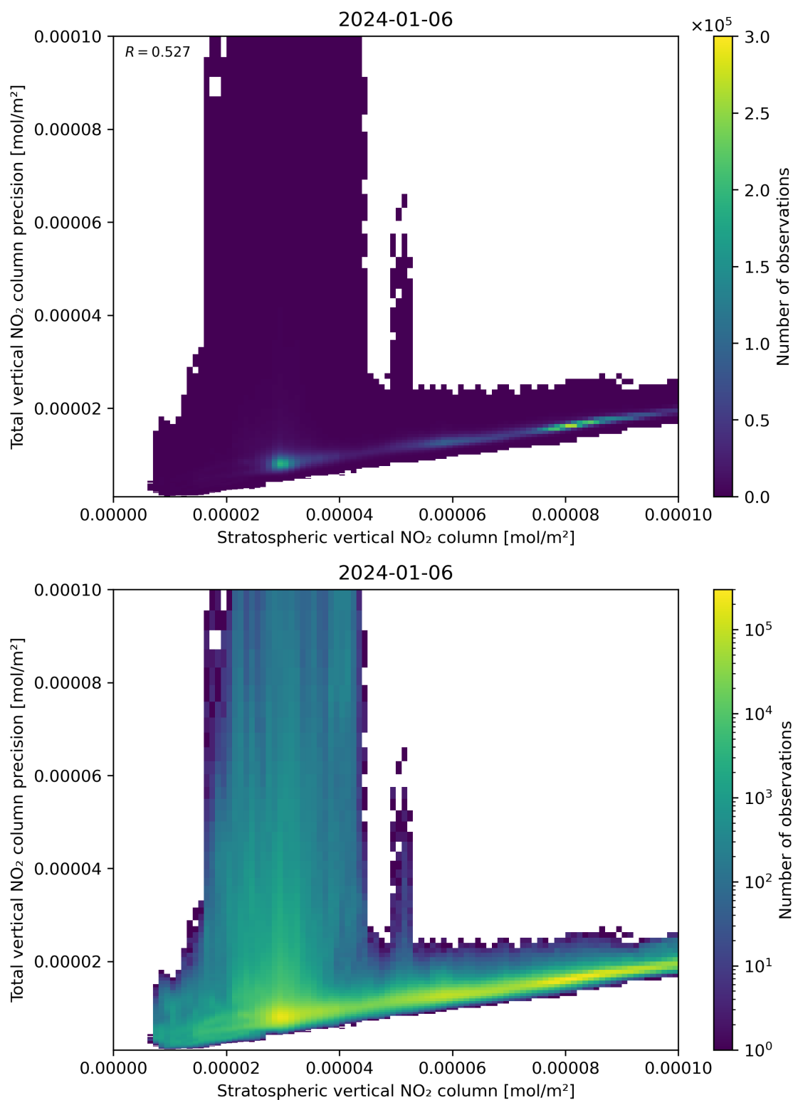
Figure 101: Scatter density plot of “Stratospheric vertical NO 2 column” against “Total vertical NO 2 column precision” for 2024-01-05 to 2024-01-07.
