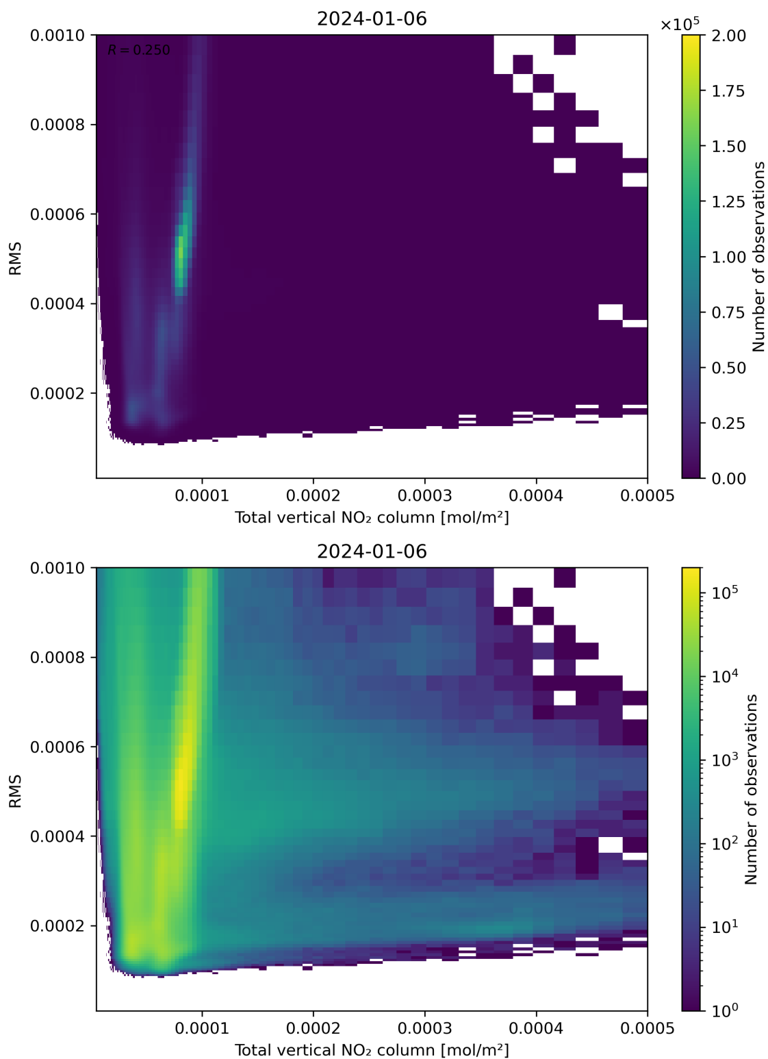
Figure 120: Scatter density plot of “Total vertical NO 2 column” against “RMS” for 2024-01-05 to 2024-01-07.
