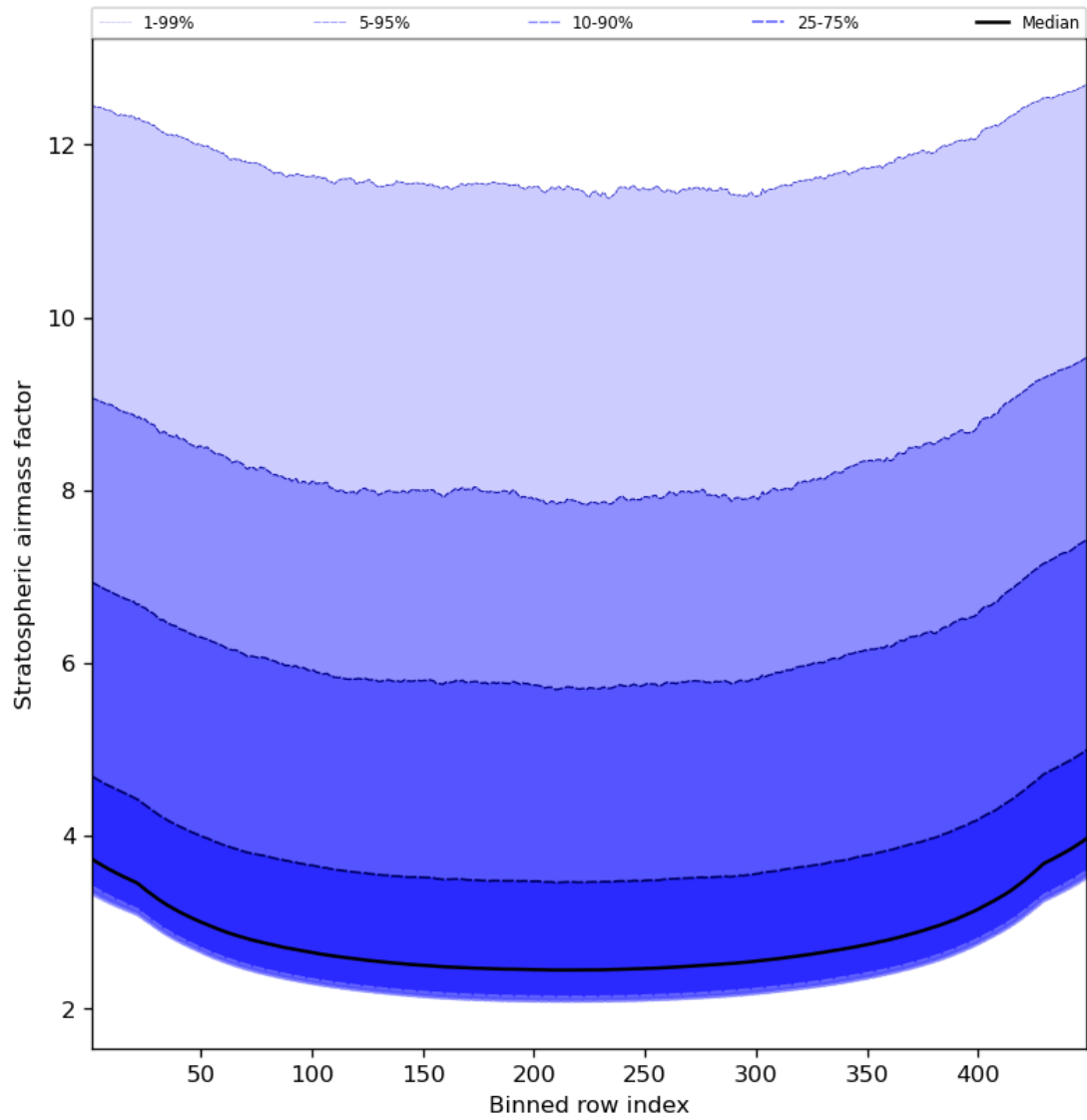
Figure 61: Along track statistics of “Stratospheric airmass factor” for 2024-01-05 to 2024-01-07
