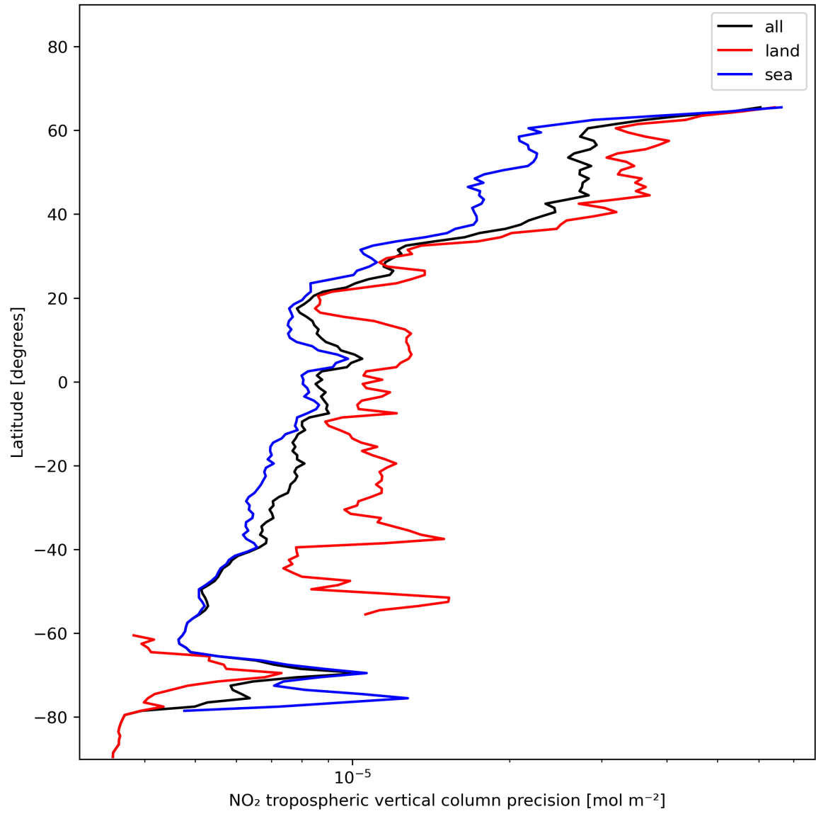
Figure 13: Zonal average of “NO 2 tropospheric vertical column precision” for 2024-01-05 to 2024-01-07.
