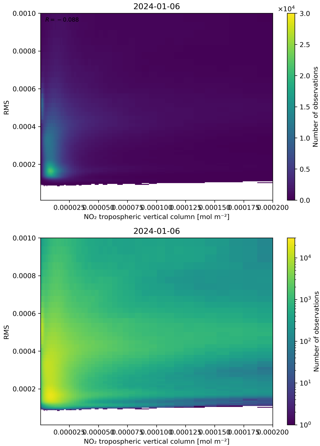
Figure 142: Scatter density plot of “NO 2 tropospheric vertical column” against “RMS” for 2024-01-05 to 2024-01-07.
