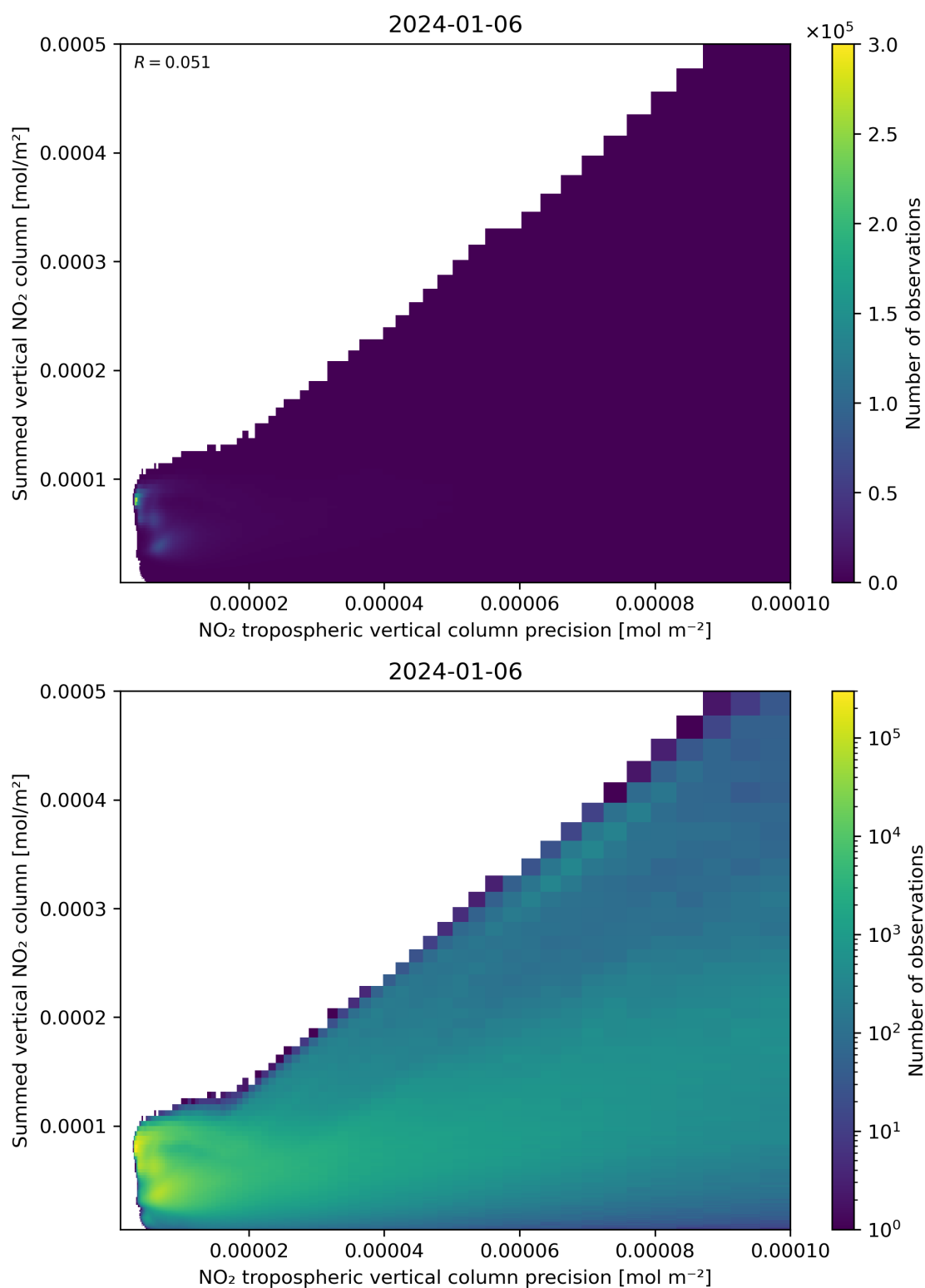
Figure 136: Scatter density plot of “NO 2 tropospheric vertical column precision” against “Summed vertical NO 2 column” for 2024-01-05 to 2024-01-07.
