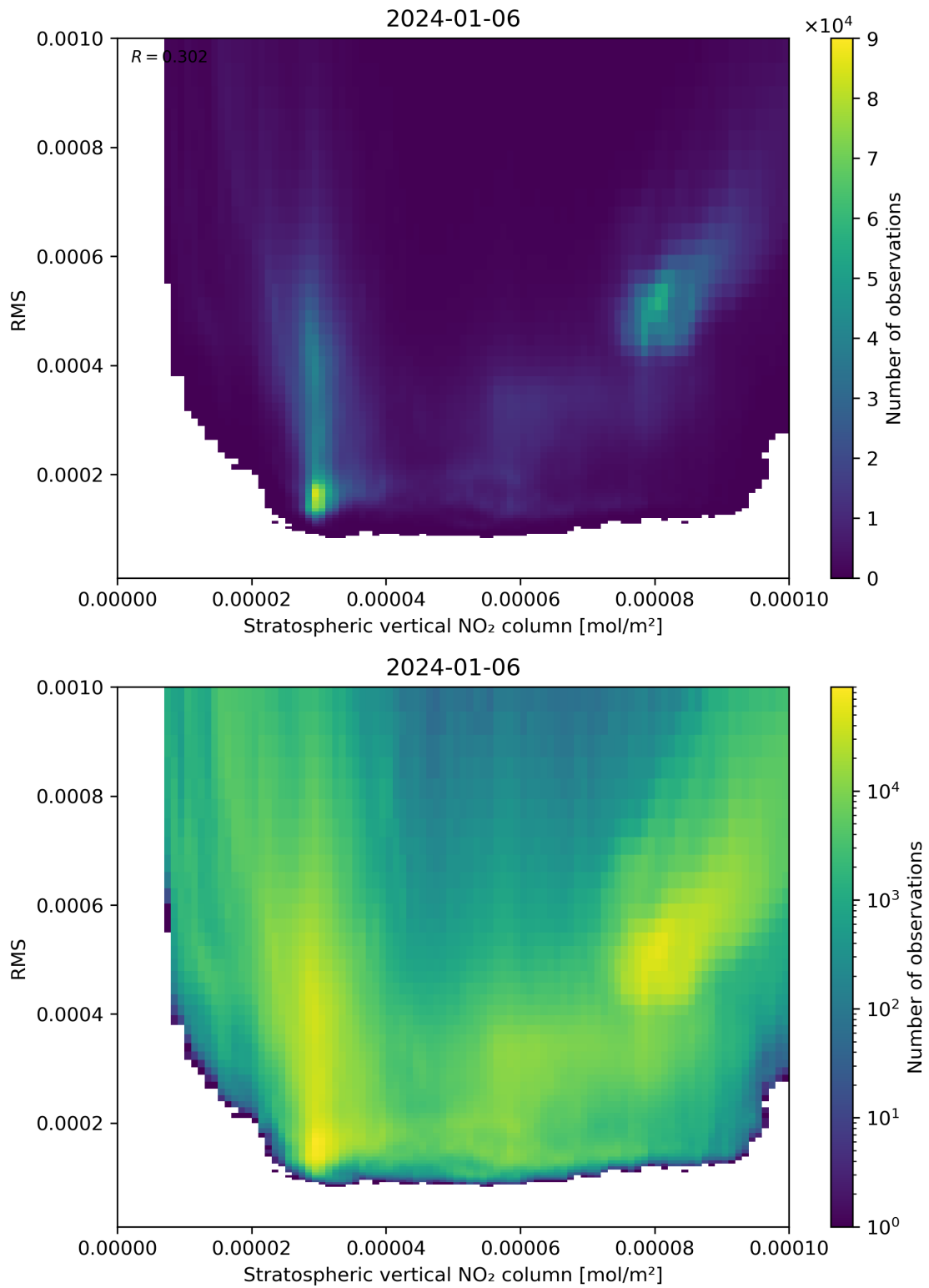
Figure 102: Scatter density plot of “Stratospheric vertical NO 2 column” against “RMS” for 2024-01-05 to 2024-01-07.
