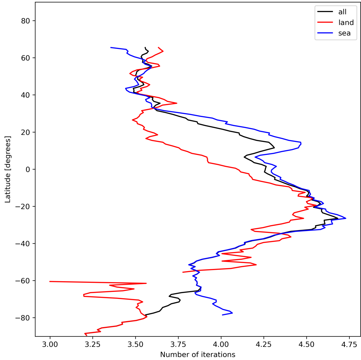
Figure 17: Zonal average of “Number of iterations” for 2024-01-05 to 2024-01-07.
