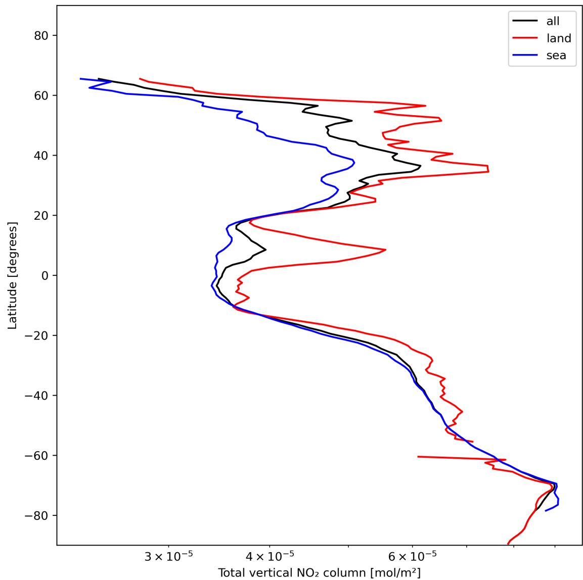
Figure 21: Zonal average of “Total vertical NO 2 column” for 2024-01-05 to 2024-01-07.
