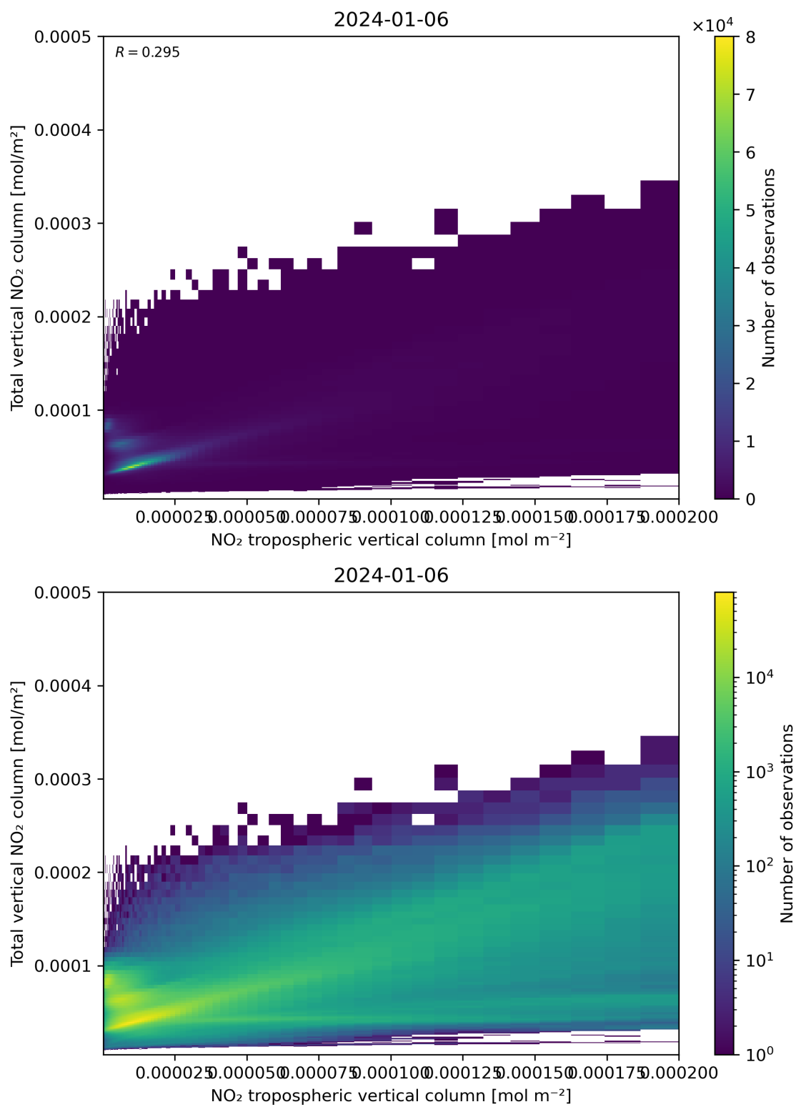
Figure 128: Scatter density plot of “NO 2 tropospheric vertical column” against “Total vertical NO 2 column” for 2024-01-05 to 2024-01-07.
