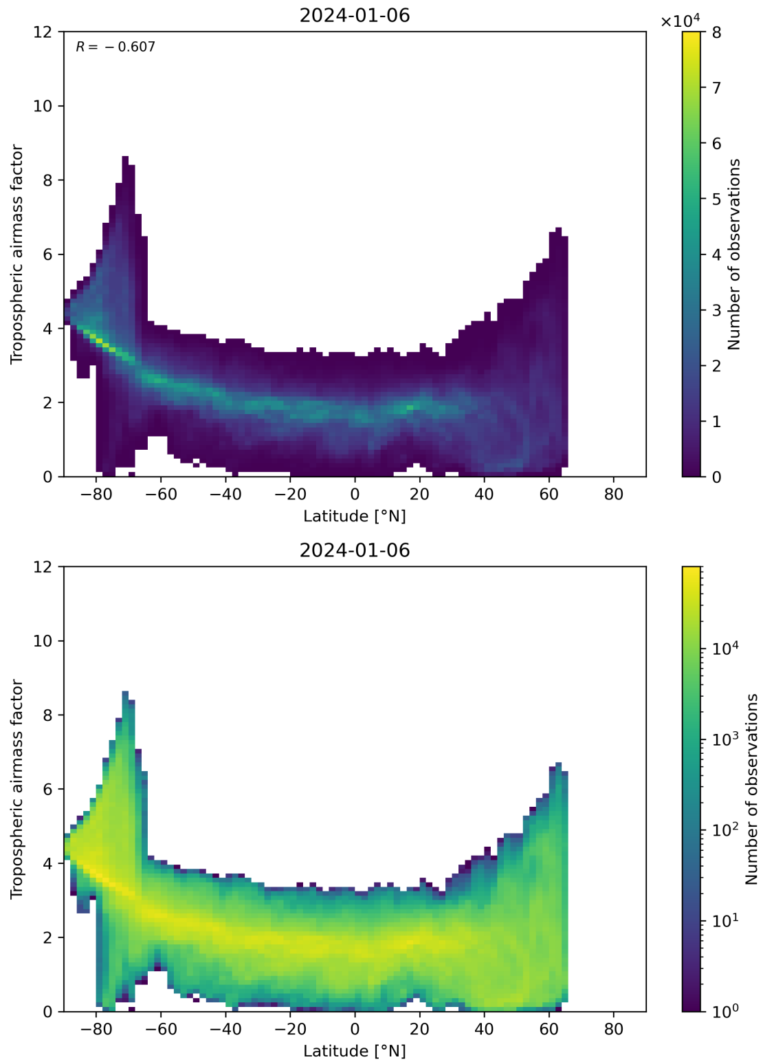
Figure 85: Scatter density plot of “Latitude” against “Tropospheric airmass factor” for 2024-01-05 to 2024-01-07.
