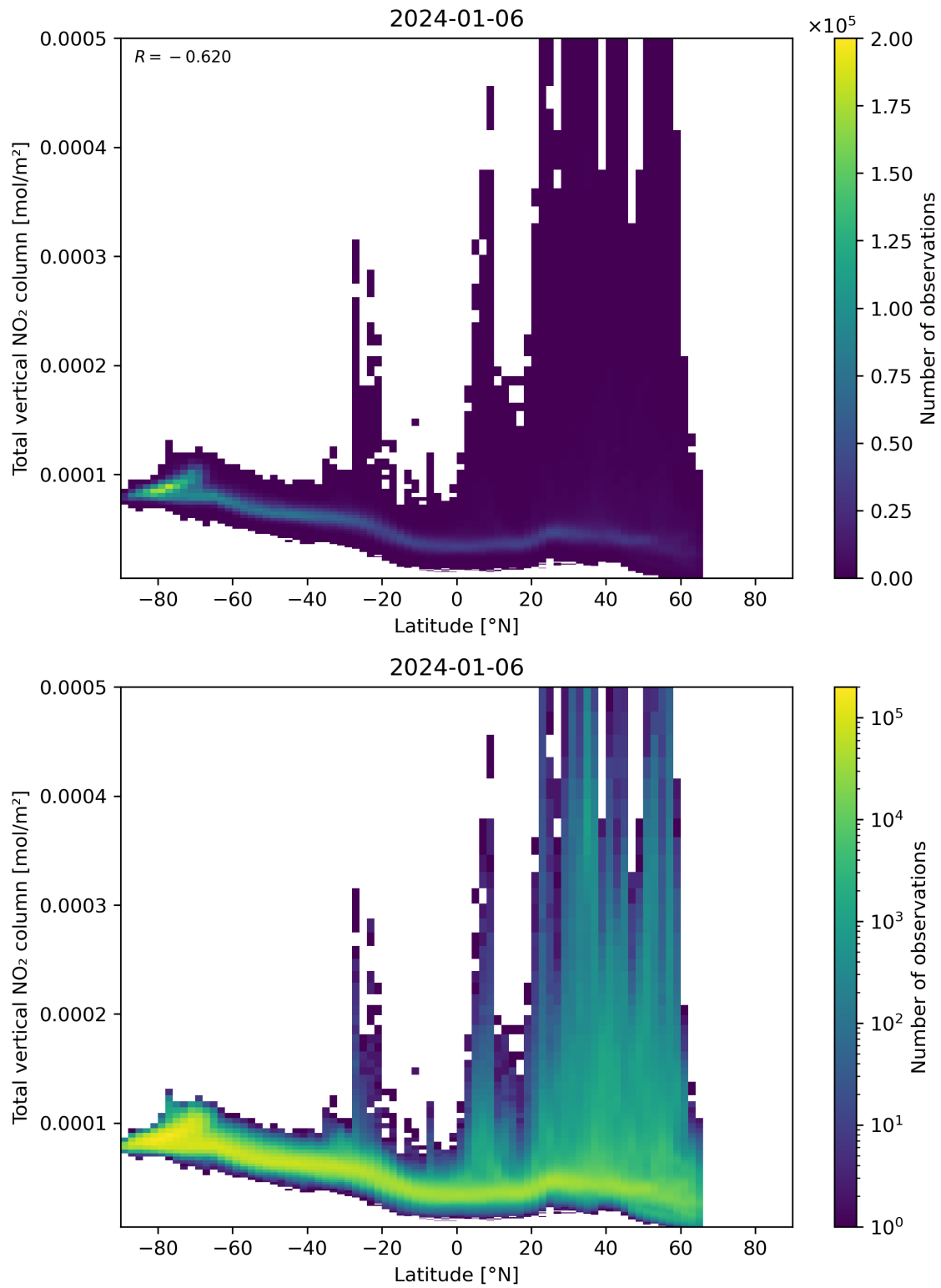
Figure 90: Scatter density plot of “Latitude” against “Total vertical NO 2 column” for 2024-01-05 to 2024-01-07.
