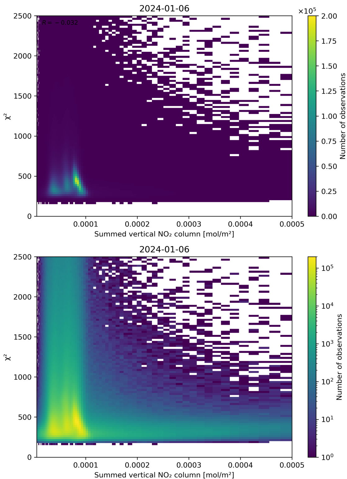
Figure 104: Scatter density plot of “Summed vertical NO 2 column” against “ \chi^2 ” for 2024-01-05 to 2024-01-07.
