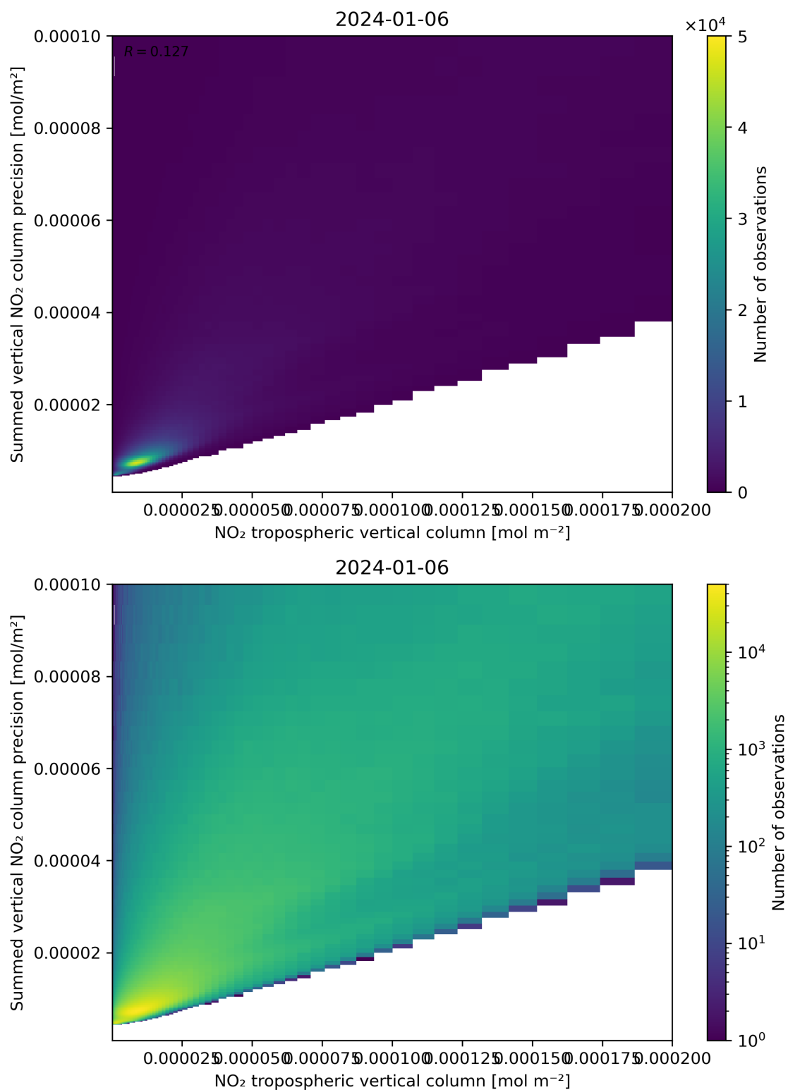
Figure 127: Scatter density plot of “NO 2 tropospheric vertical column” against “Summed vertical NO 2 column precision” for 2024-01-05 to 2024-01-07.
