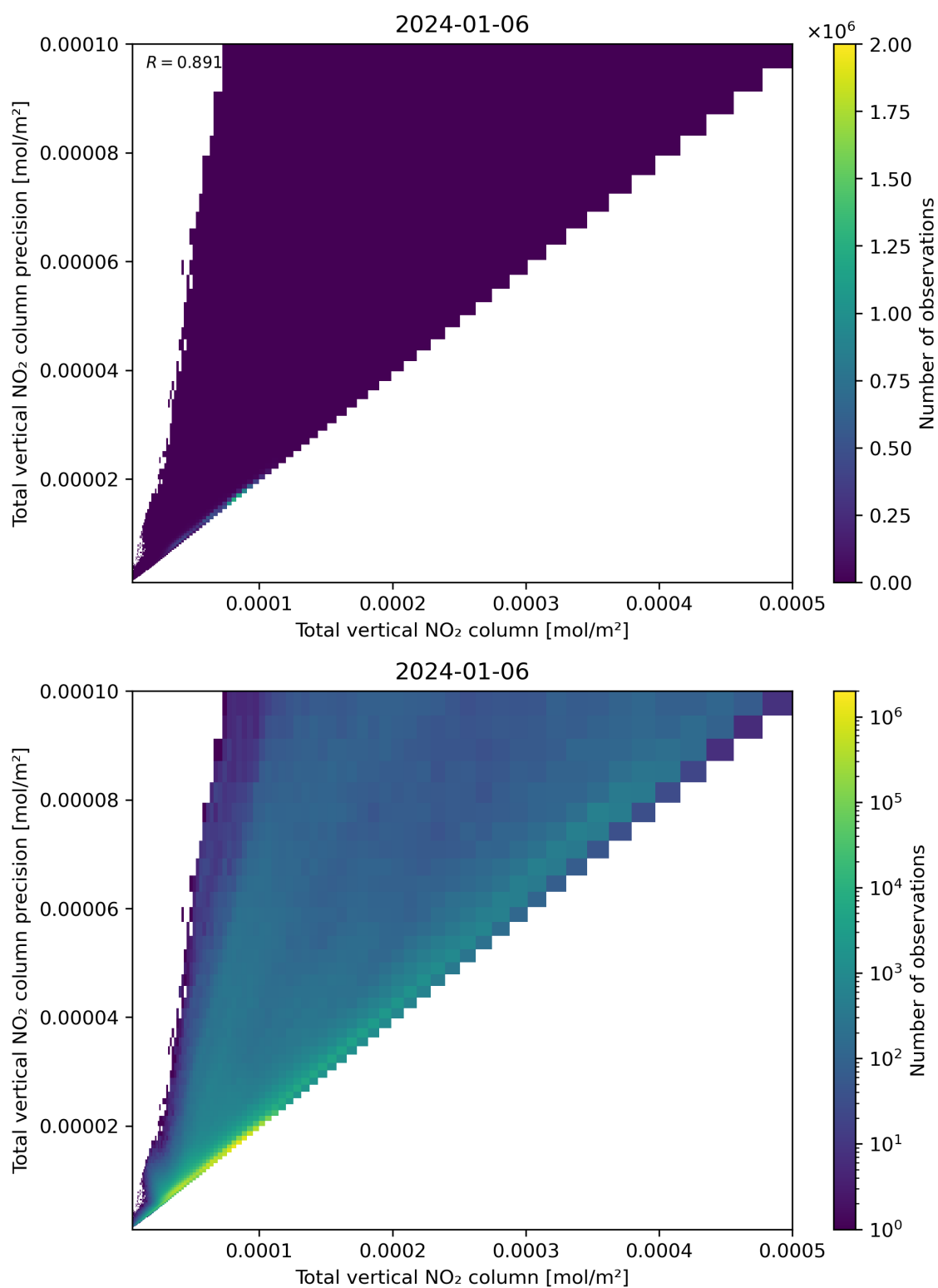
Figure 114: Scatter density plot of “Total vertical NO 2 column” against “Total vertical NO 2 column precision” for 2024-01-05 to 2024-01-07.
