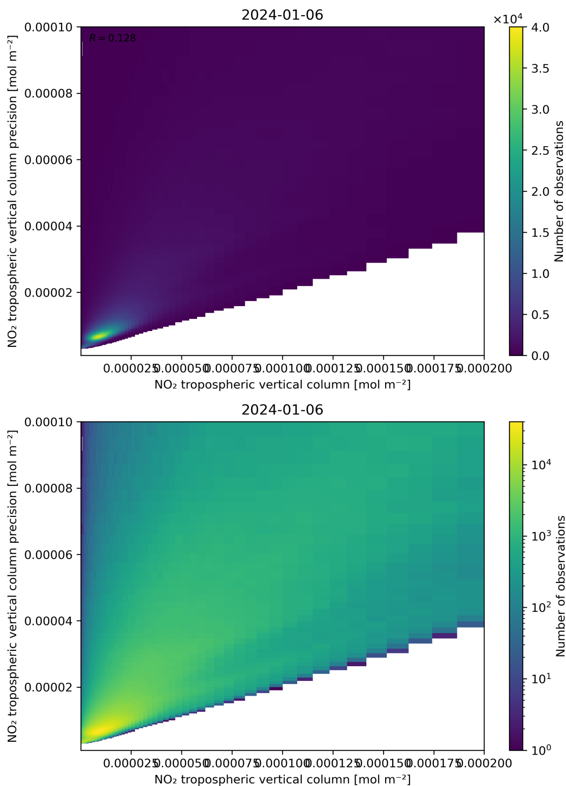
Figure 130: Scatter density plot of “NO 2 tropospheric vertical column” against “NO 2 tropospheric vertical column precision” for 2024-01-05 to 2024-01-07.
