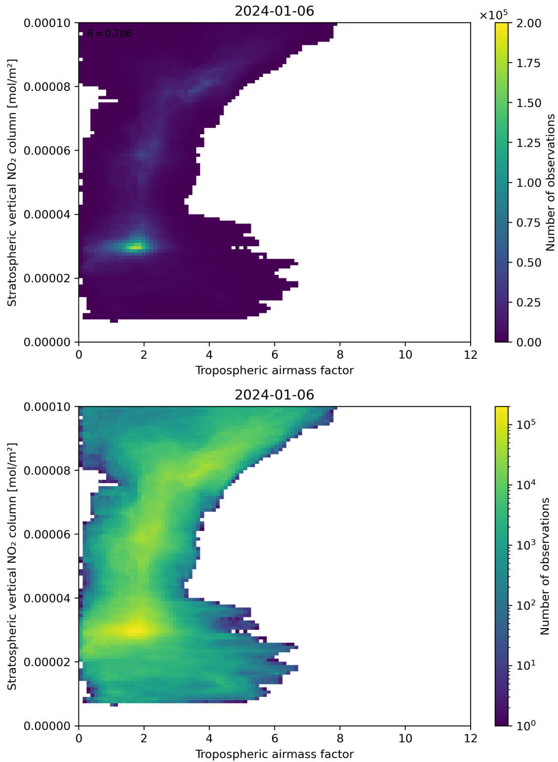
Figure 74: Scatter density plot of “Tropospheric air mass factor” against “Stratospheric vertical NO 2 column” for 2024-01-05 to 2024-01-07.
