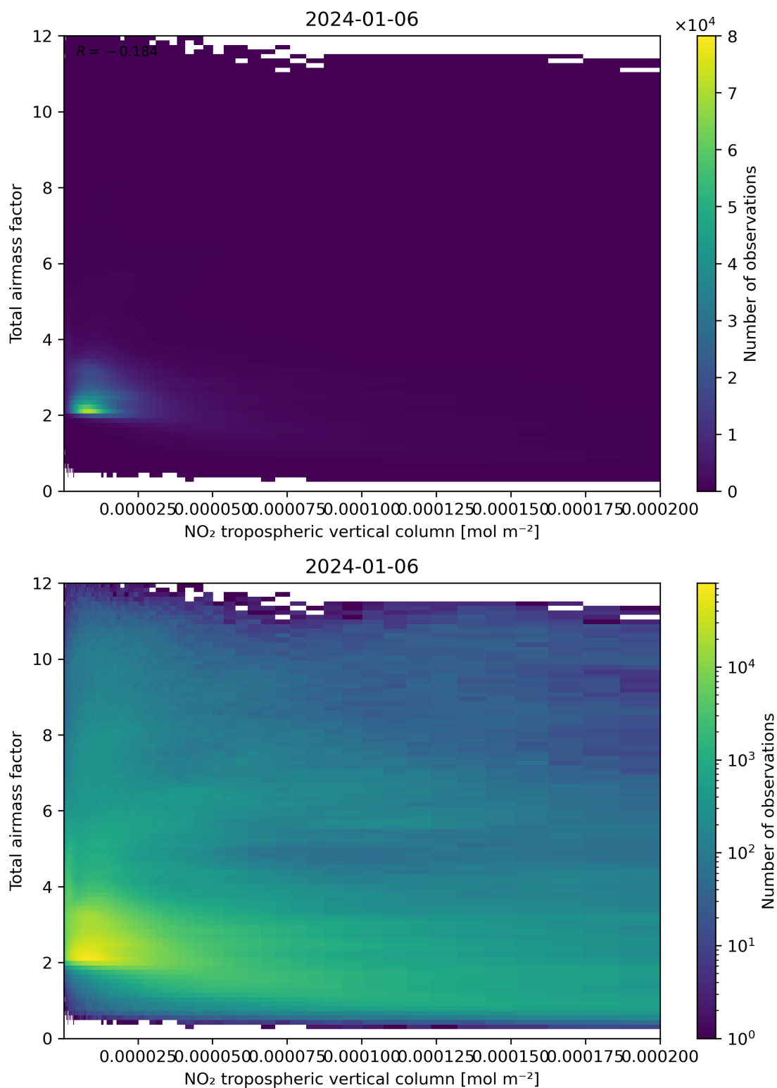
Figure 122: Scatter density plot of “NO 2 tropospheric vertical column” against “Total air mass factor” for 2024-01-05 to 2024-01-07.
