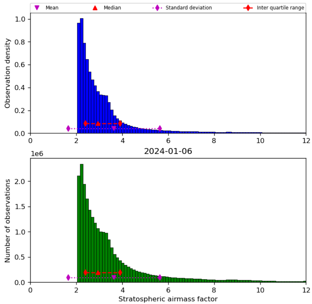
Figure 44: Histogram of “Stratospheric airmass factor” for 2024-01-05 to 2024-01-07
