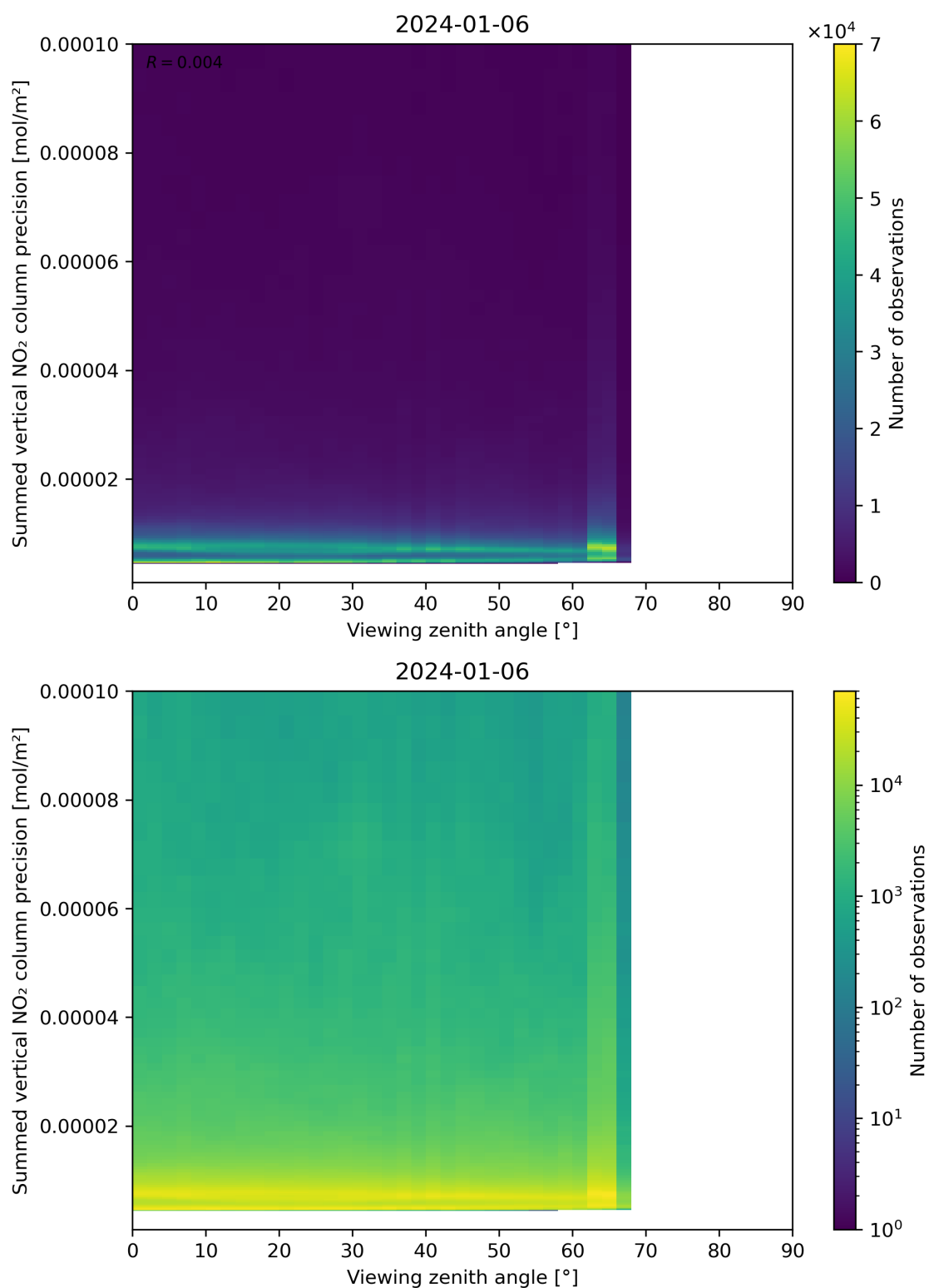
Figure 166: Scatter density plot of “Viewing zenith angle” against “Summed vertical NO 2 column precision” for 2024-01-05 to 2024-01-07.
