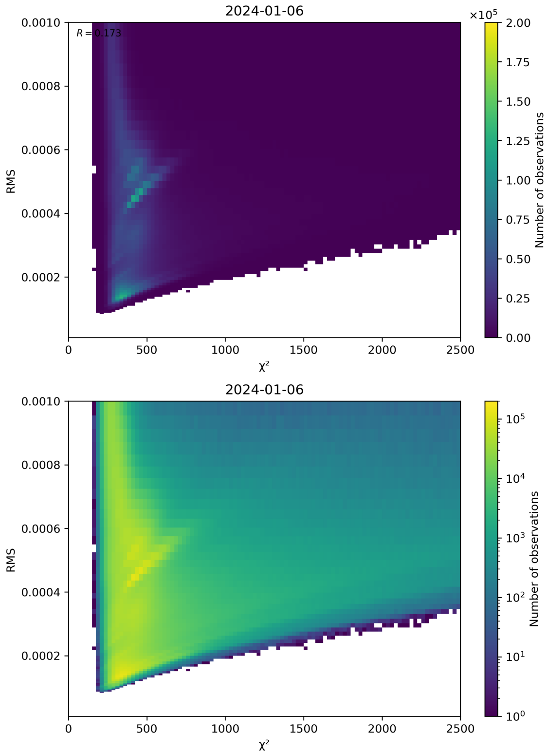
Figure 82: Scatter density plot of “ \chi^2 ” against “RMS” for 2024-01-05 to 2024-01-07.
