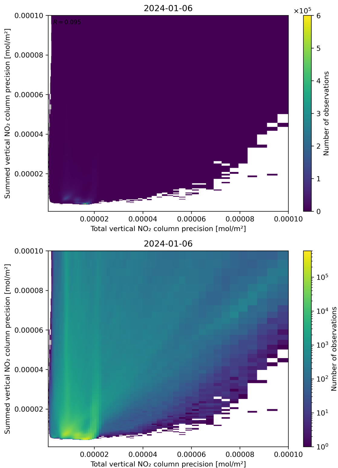
Figure 118: Scatter density plot of “Total vertical NO 2 column precision” against “Summed vertical NO 2 column precision” for 2024-01-05 to 2024-01-07.
