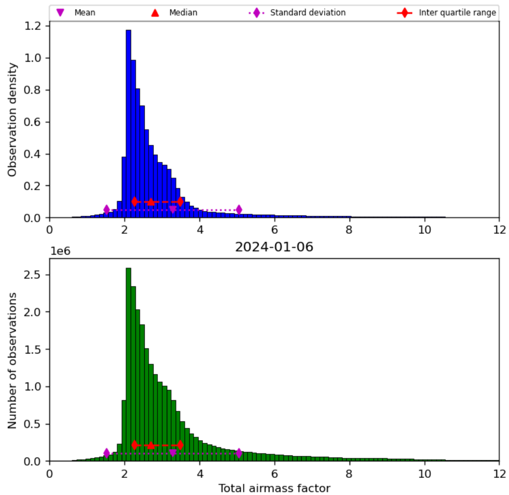
Figure 32: Histogram of “Total airmass factor” for 2024-01-05 to 2024-01-07
