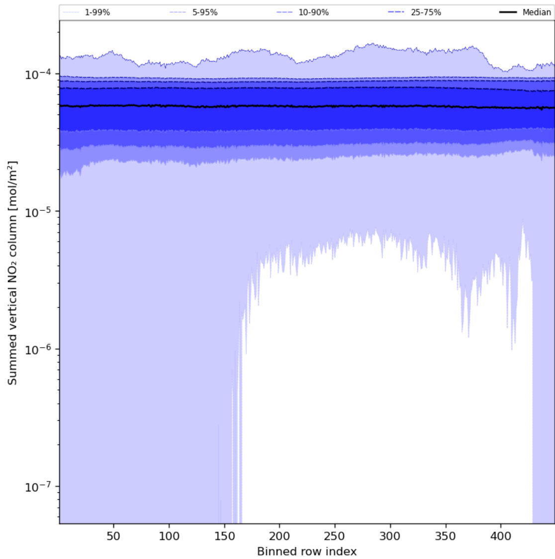
Figure 57: Along track statistics of “Summed vertical NO 2 column” for 2024-01-05 to 2024-01-07
