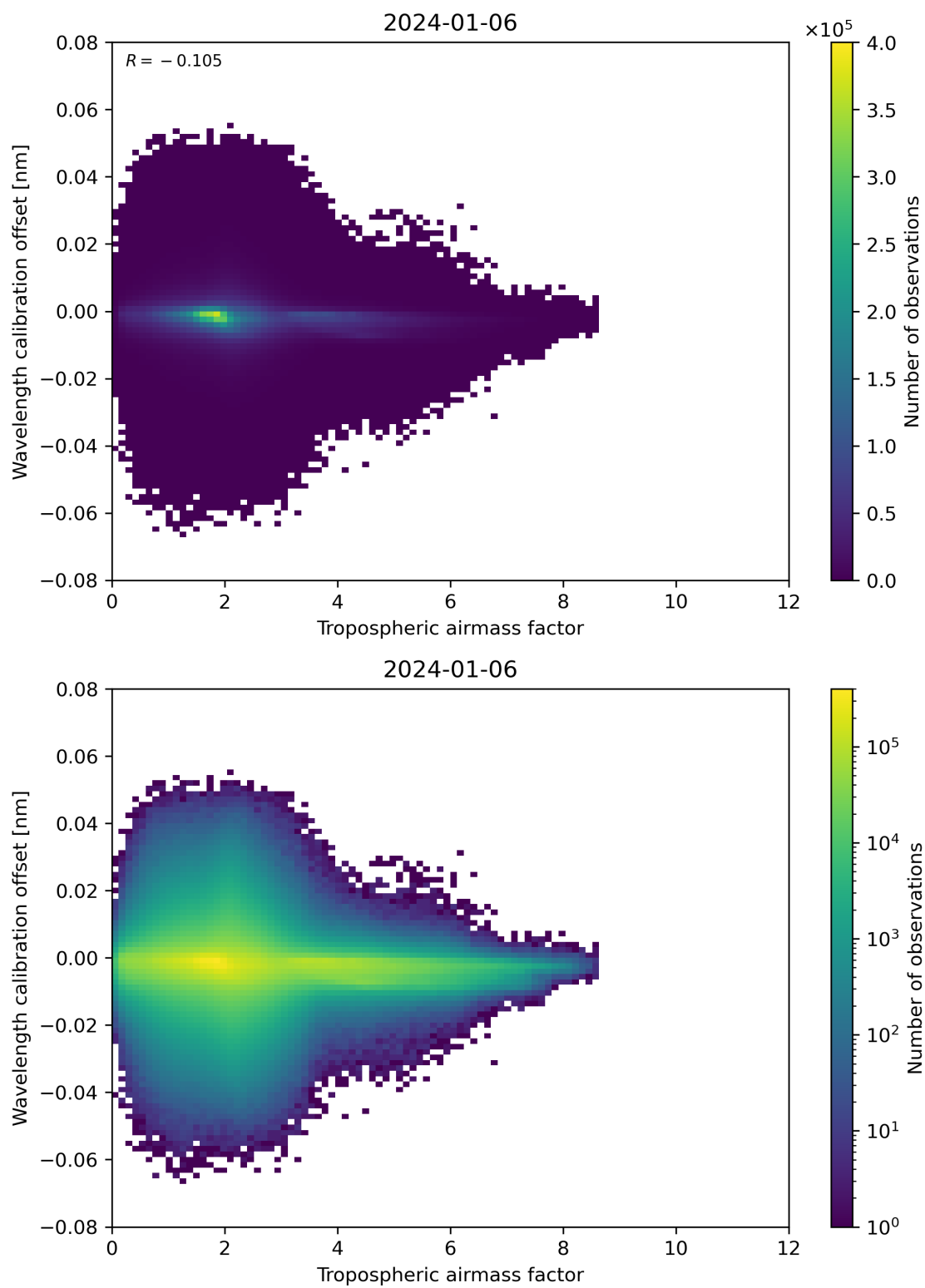
Figure 80: Scatter density plot of “Tropospheric airmass factor” against “Wavelength calibration offset” for 2024-01-05 to 2024-01-07.
