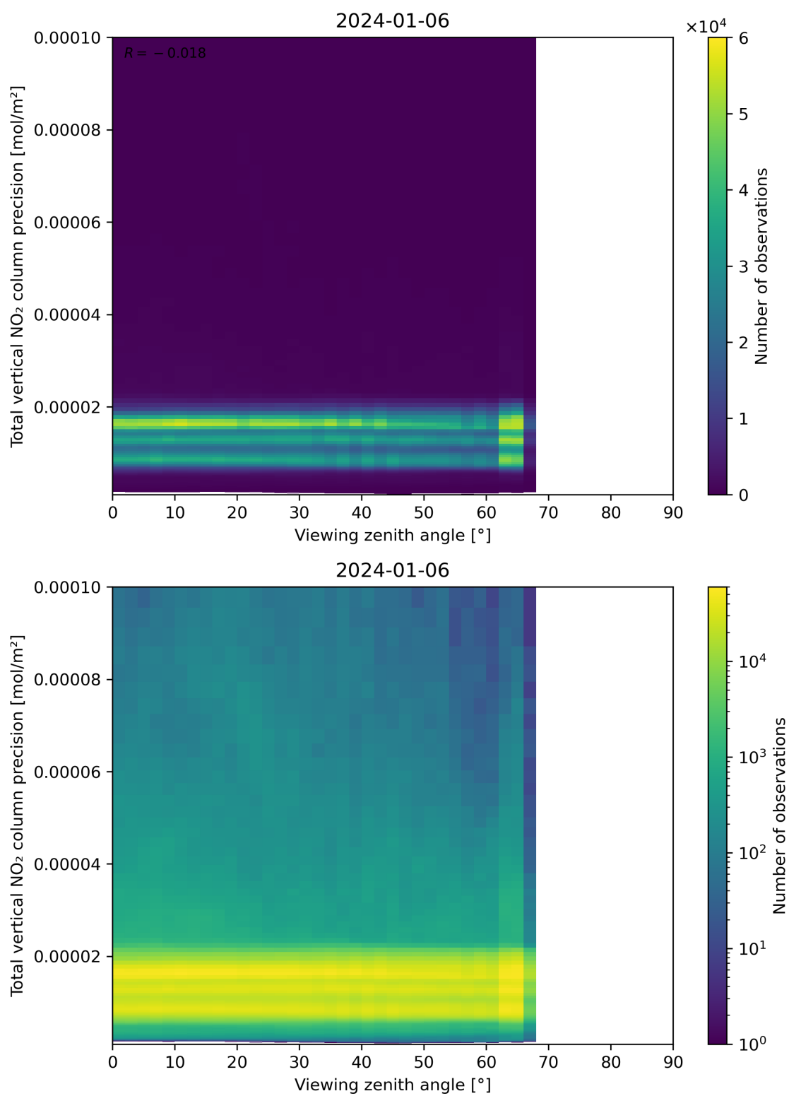
Figure 168: Scatter density plot of “Viewing zenith angle” against “Total vertical NO 2 column precision” for 2024-01-05 to 2024-01-07.
