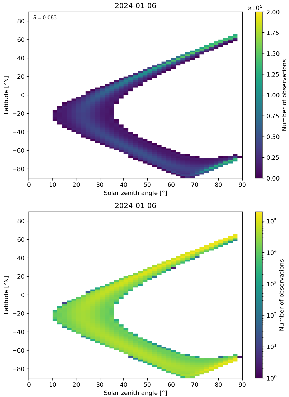
Figure 149: Scatter density plot of “Solar zenith angle” against “Latitude” for 2024-01-05 to 2024-01-07.
