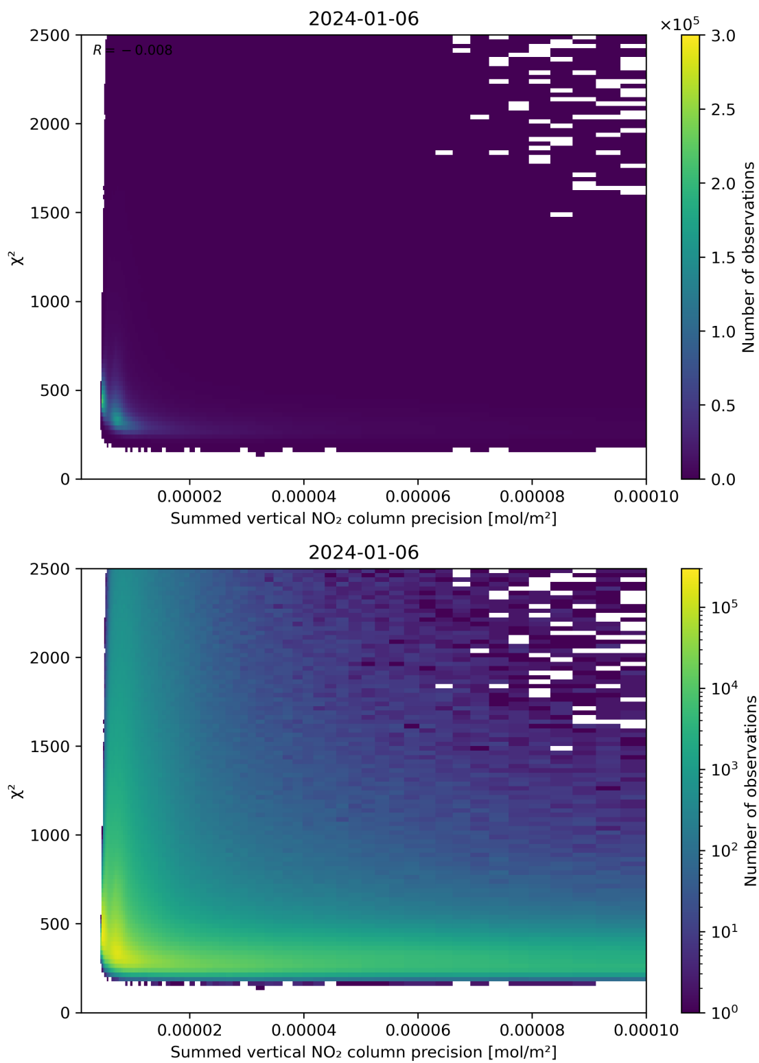
Figure 107: Scatter density plot of “Summed vertical NO 2 column precision” against “ \chi^2 ” for 2024-01-05 to 2024-01-07.
