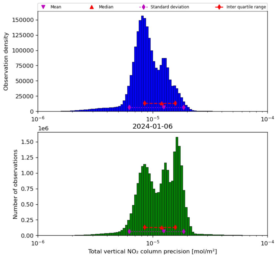
Figure 39: Histogram of “Total vertical NO 2 column precision” for 2024-01-05 to 2024-01-07
