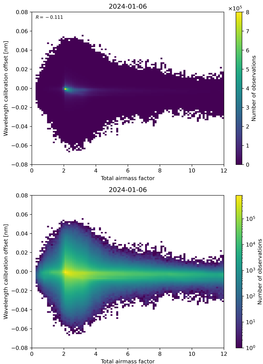
Figure 70: Scatter density plot of “Total airmass factor” against “Wavelength calibration offset” for 2024-01-05 to 2024-01-07.
