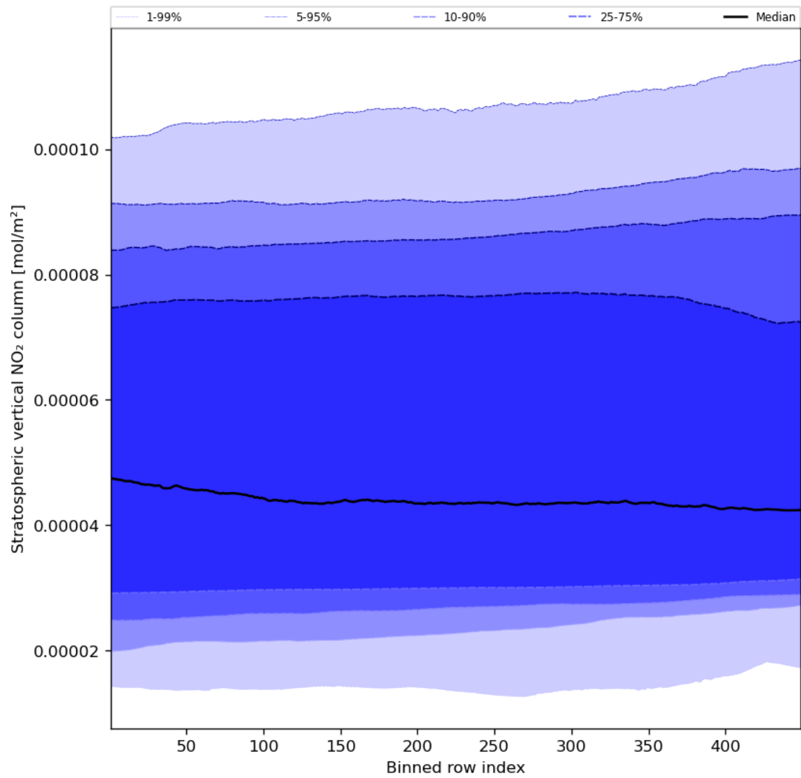
Figure 53: Along track statistics of “Stratospheric vertical NO 2 column” for 2024-01-05 to 2024-01-07
