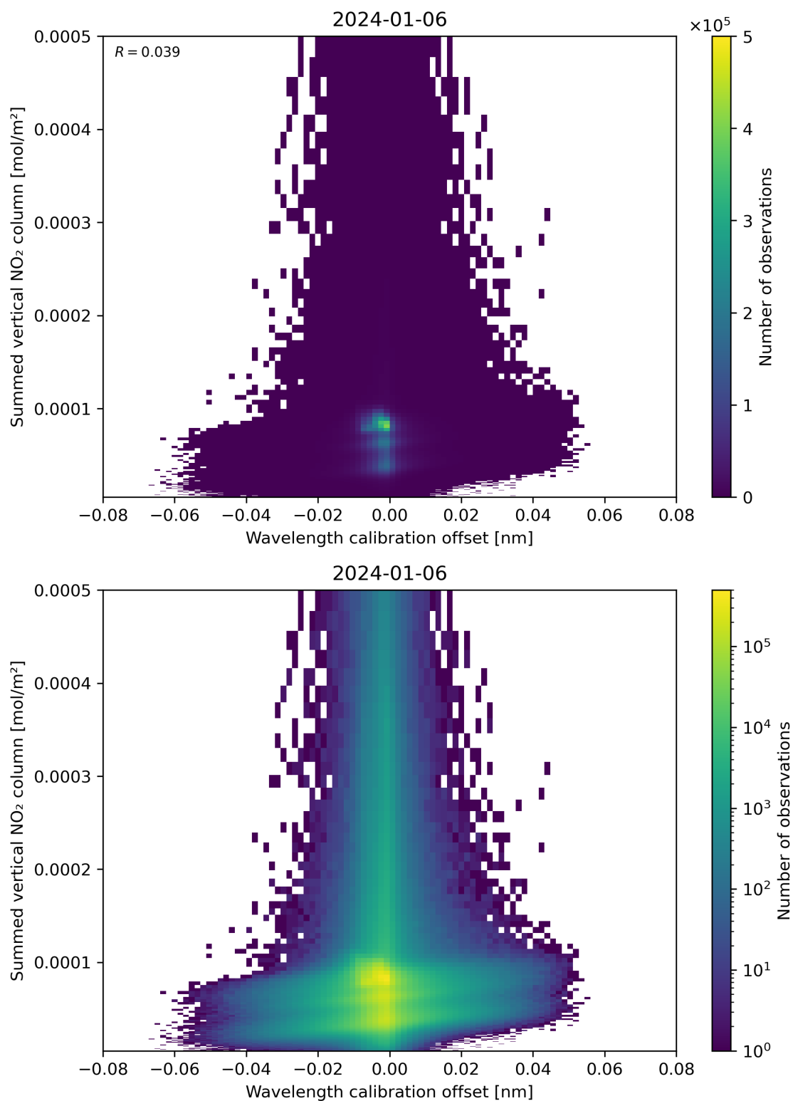
Figure 177: Scatter density plot of “Wavelength calibration offset” against “Summed vertical NO 2 column” for 2024-01-05 to 2024-01-07.
