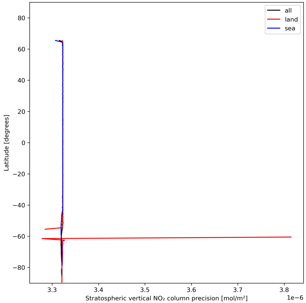
Figure 20: Zonal average of “Stratospheric vertical NO 2 column precision” for 2024-01-05 to 2024-01-07.
