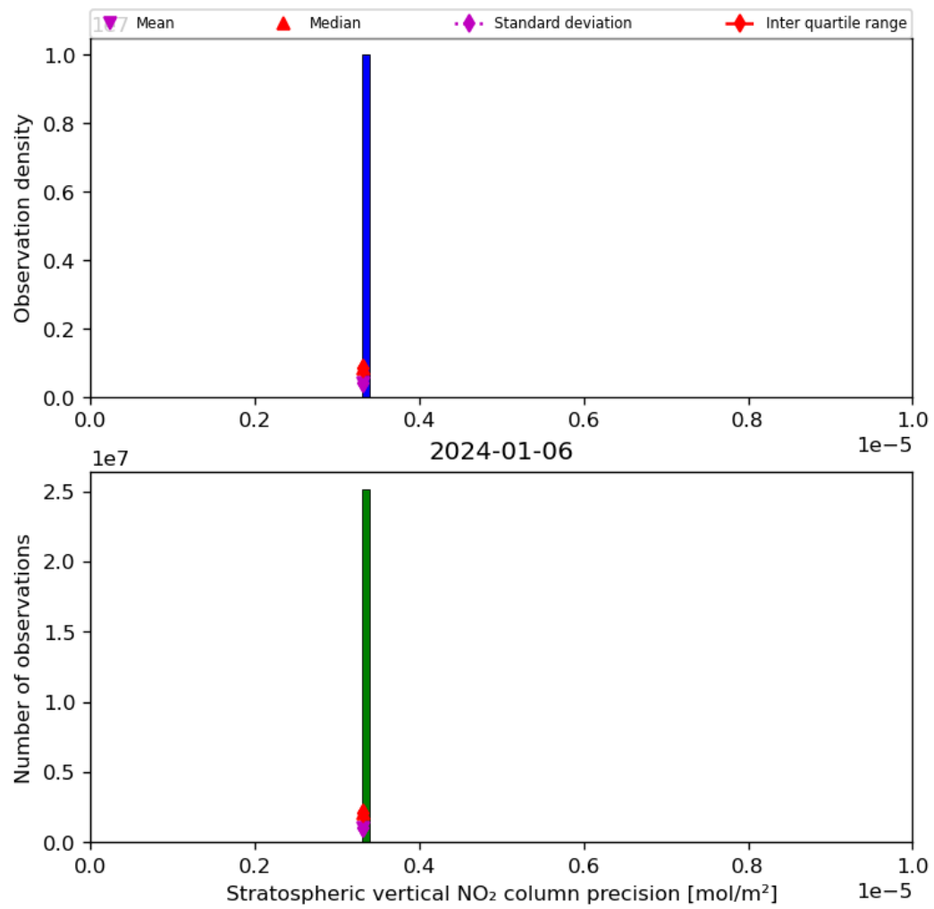
Figure 37: Histogram of “Stratospheric vertical NO 2 column precision” for 2024-01-05 to 2024-01-07
