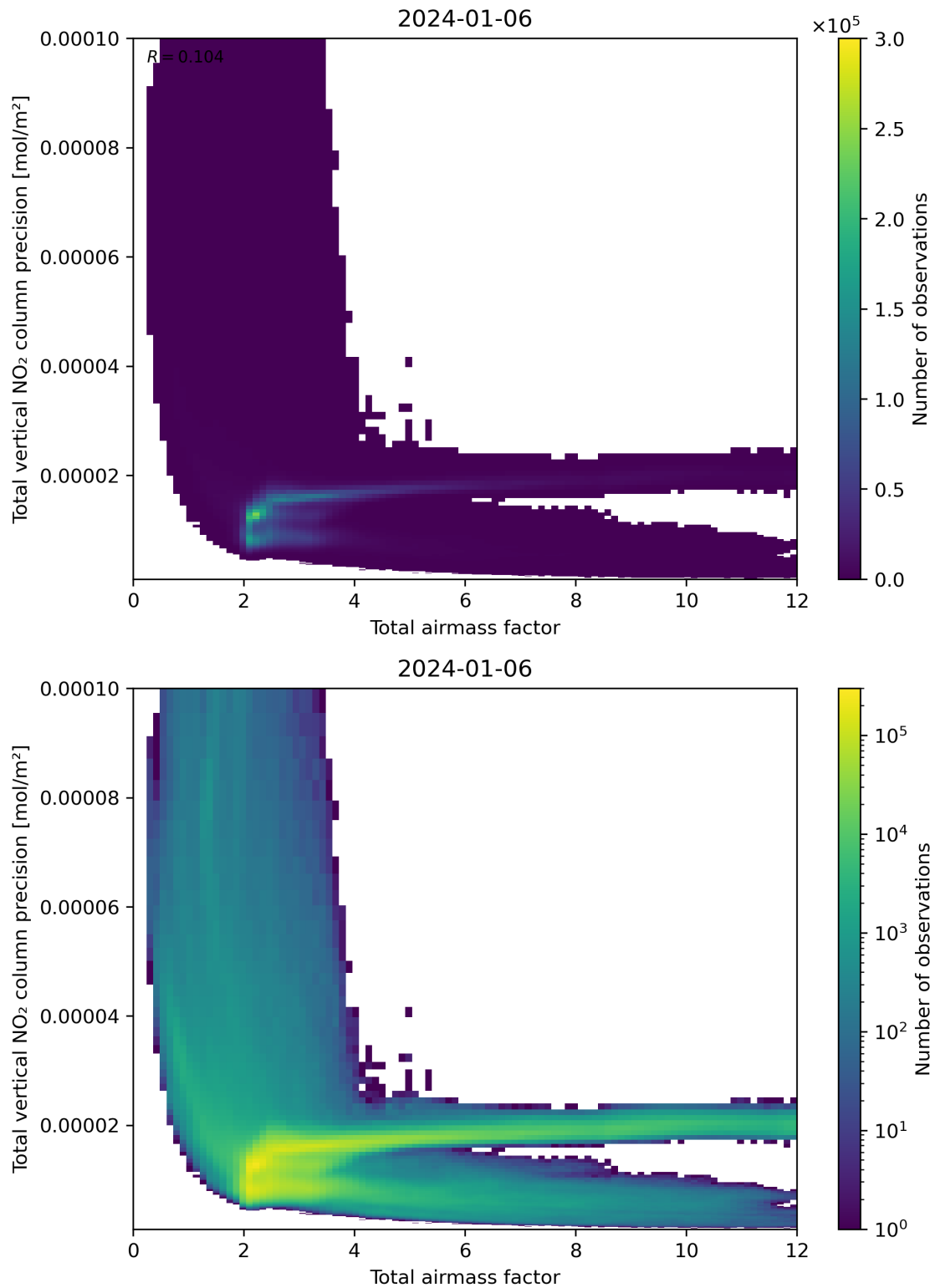
Figure 68: Scatter density plot of “Total airmass factor” against “Total vertical NO 2 column precision” for 2024-01-05 to 2024-01-07.
