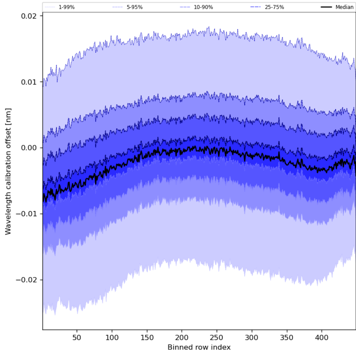
Figure 52: Along track statistics of “Wavelength calibration offset” for 2024-01-05 to 2024-01-07
