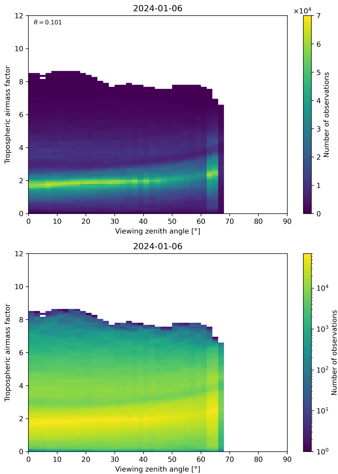
Figure 161: Scatter density plot of “Viewing zenith angle” against “Tropospheric airmass factor” for 2024-01-05 to 2024-01-07.
