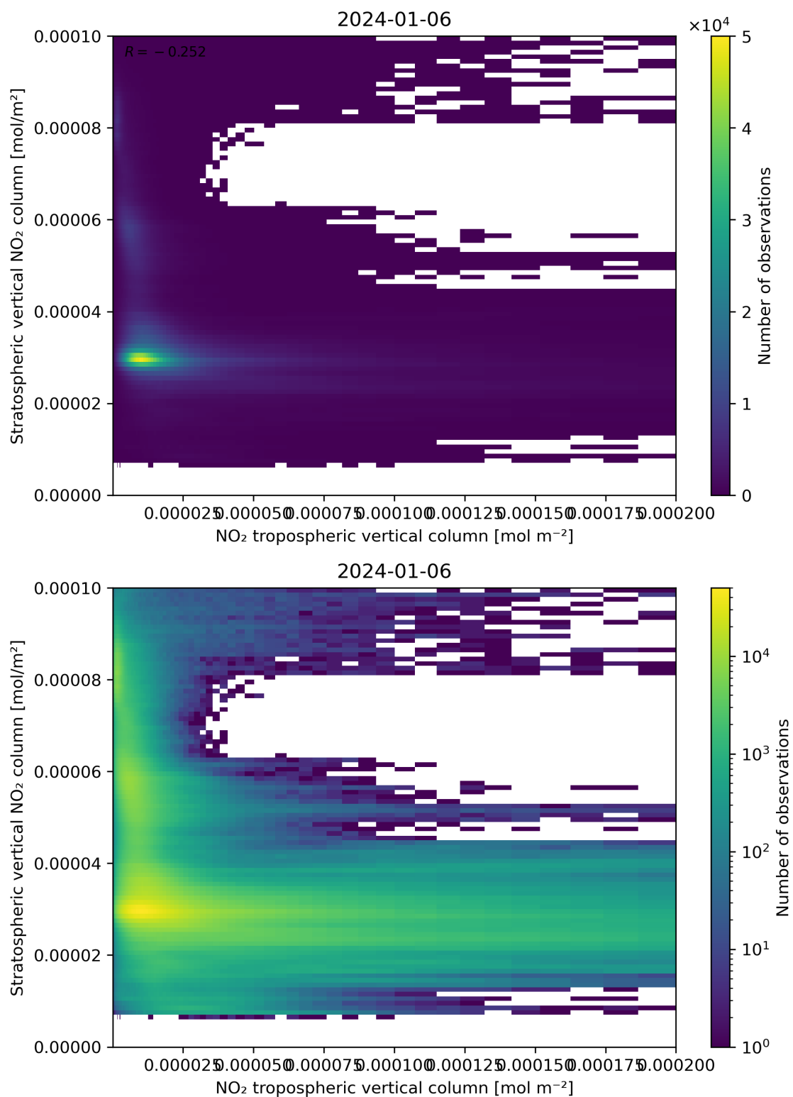
Figure 125: Scatter density plot of “NO 2 tropospheric vertical column” against “Stratospheric vertical NO 2 column” for 2024-01-05 to 2024-01-07.
