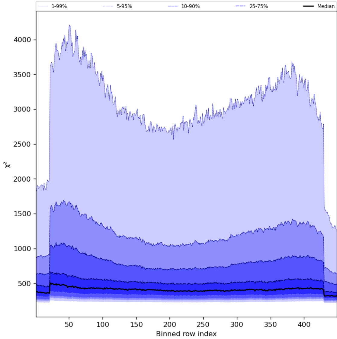
Figure 59: Along track statistics of “ \chi^2 ” for 2024-01-05 to 2024-01-07
