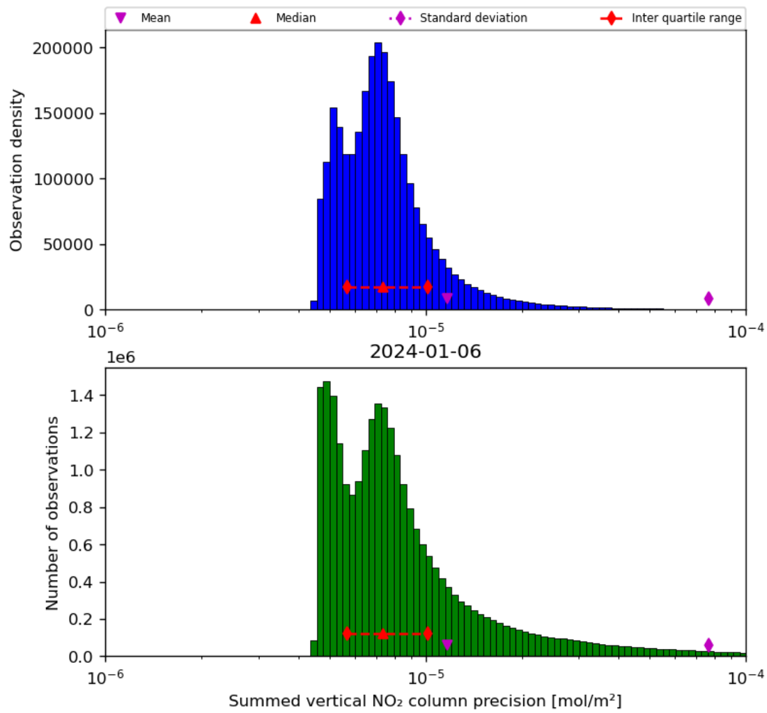
Figure 41: Histogram of “Summed vertical NO 2 column precision” for 2024-01-05 to 2024-01-07
