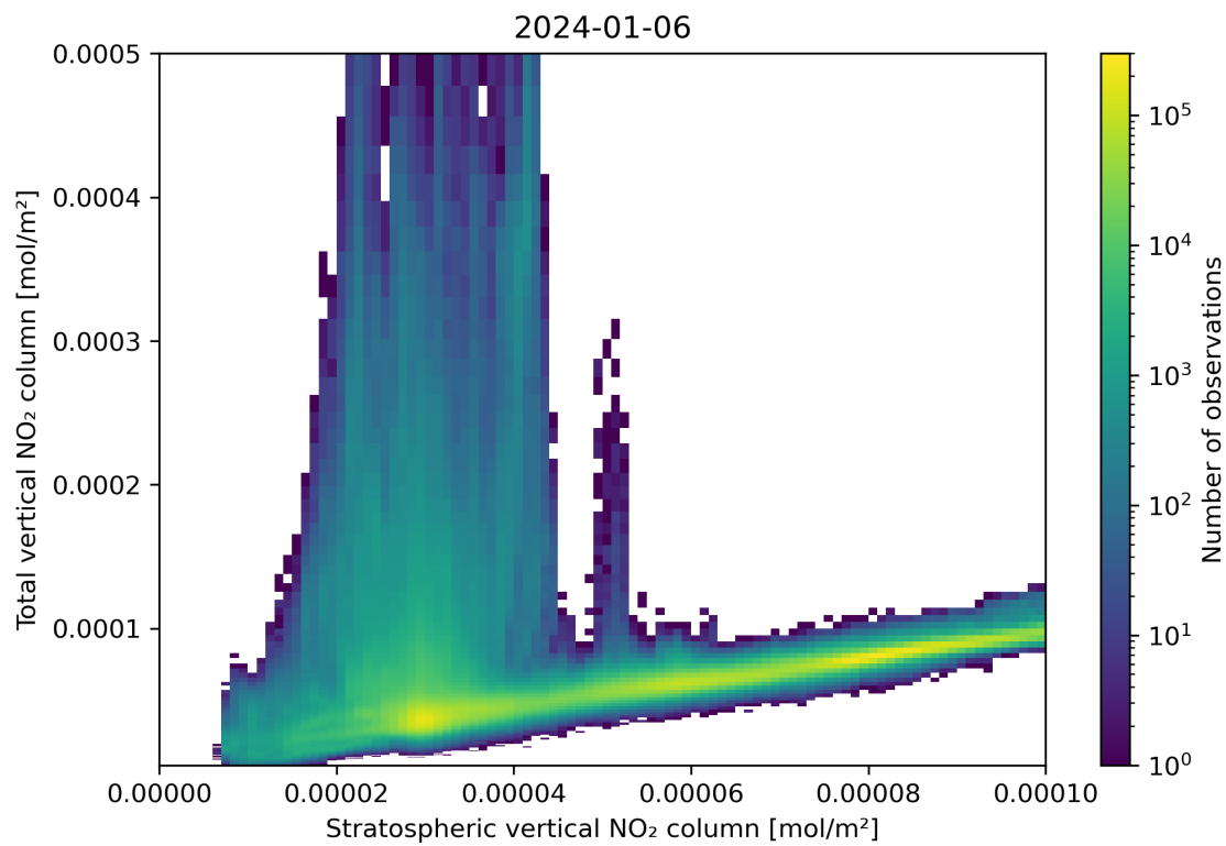
Figure 100: Scatter density plot of “Stratospheric vertical NO 2 column” against “Total vertical NO 2 column” for 2024-01-05 to 2024-01-07.
