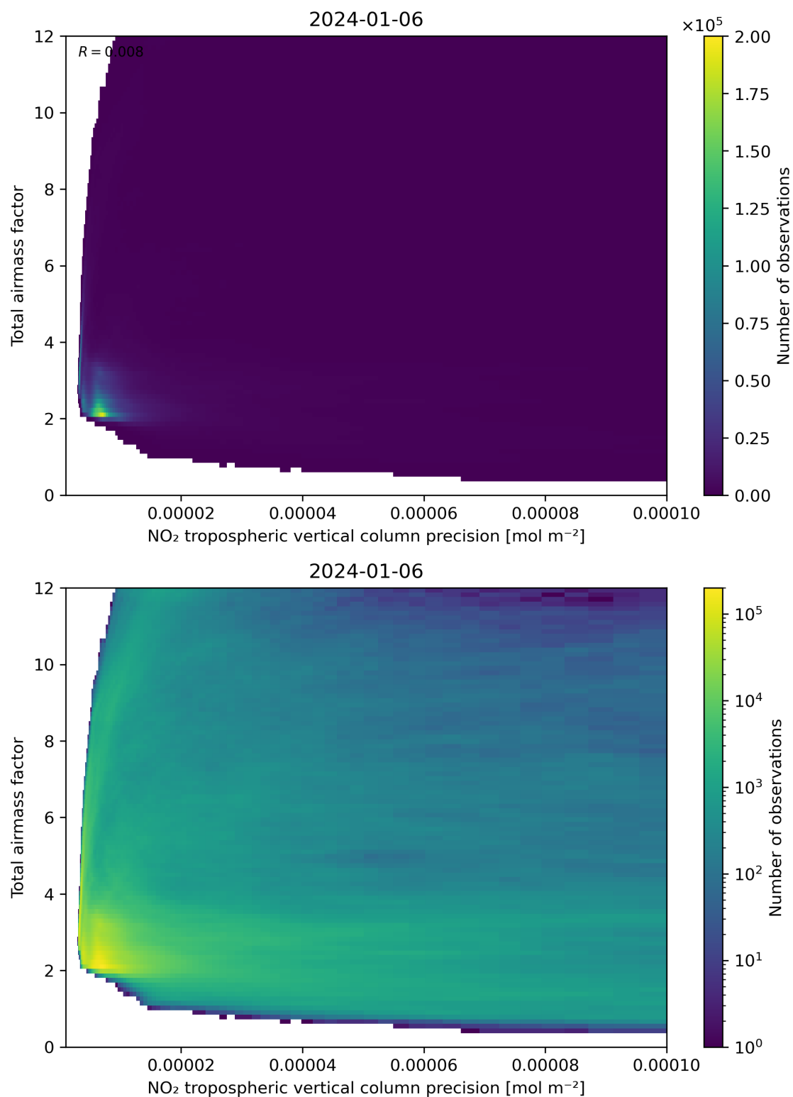
Figure 132: Scatter density plot of “NO 2 tropospheric vertical column precision” against “Total air mass factor” for 2024-01-05 to 2024-01-07.
