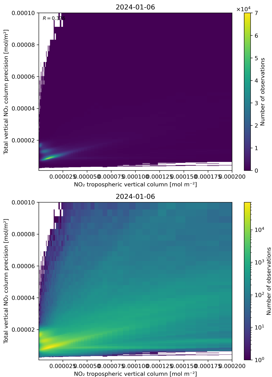
Figure 129: Scatter density plot of “NO 2 tropospheric vertical column” against “Total vertical NO 2 column precision” for 2024-01-05 to 2024-01-07.
