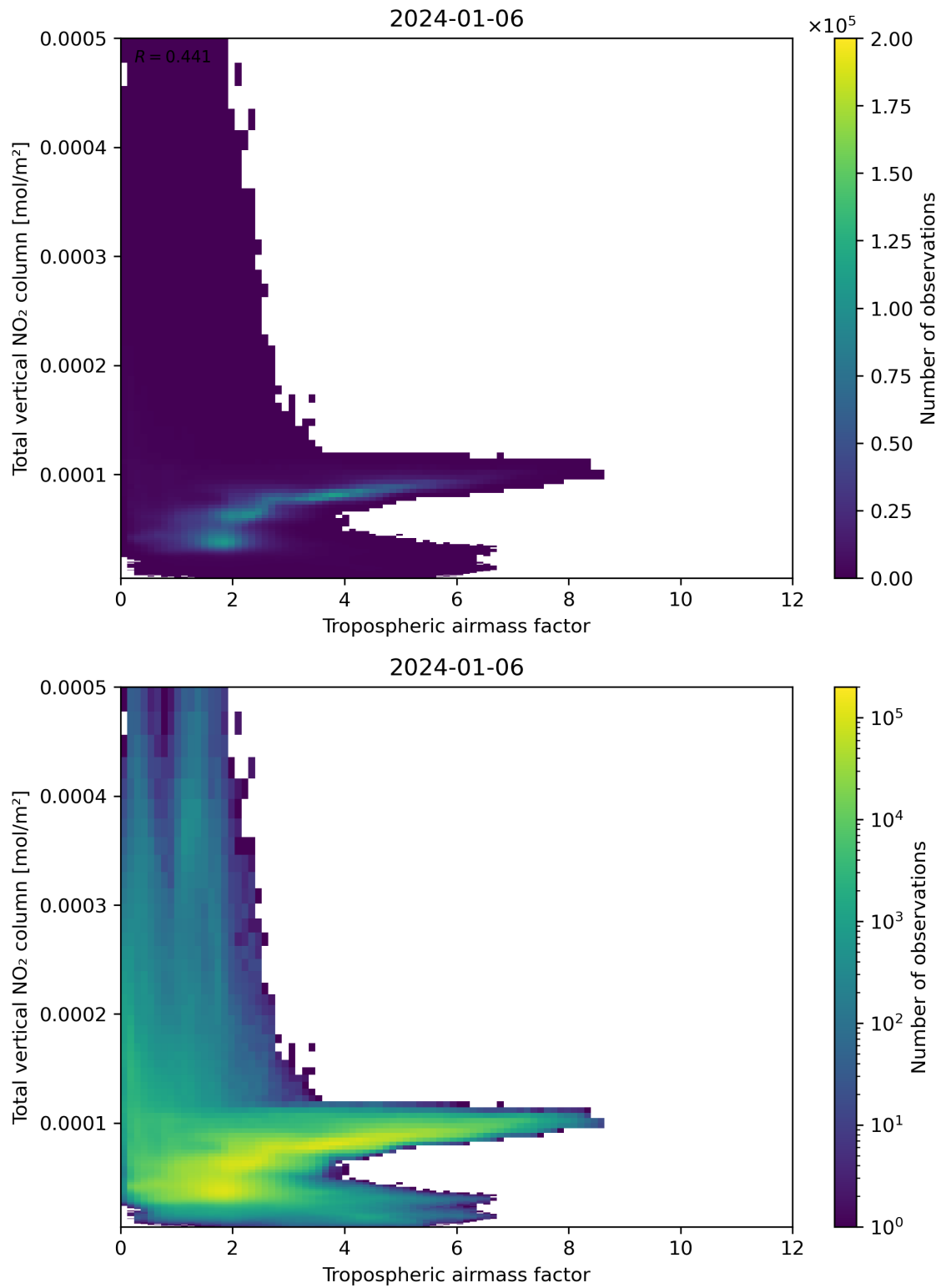
Figure 77: Scatter density plot of “Tropospheric airmass factor” against “Total vertical NO 2 column” for 2024-01-05 to 2024-01-07.
