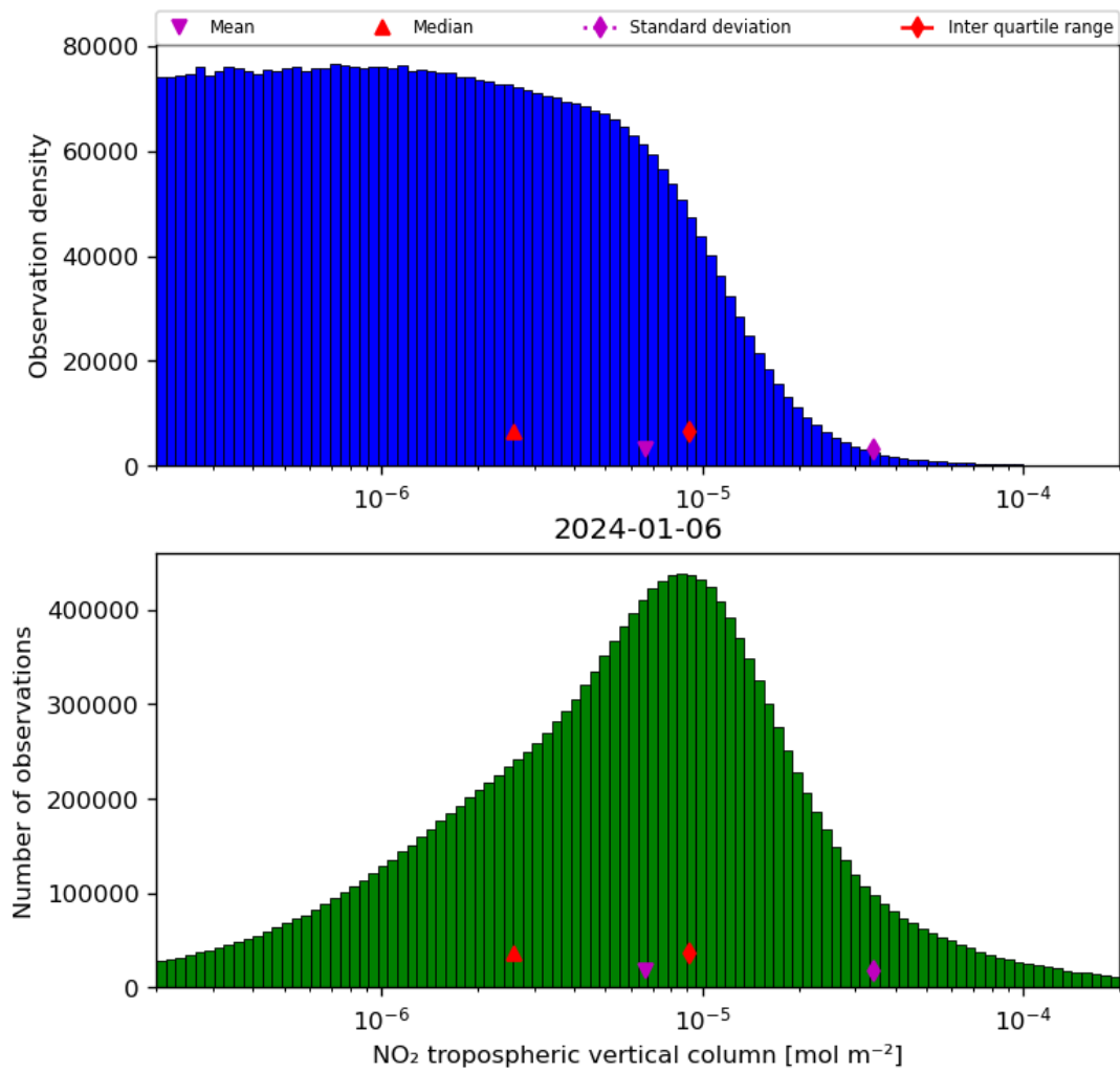
Figure 29: Histogram of “NO 2 tropospheric vertical column” for 2024-01-05 to 2024-01-07
