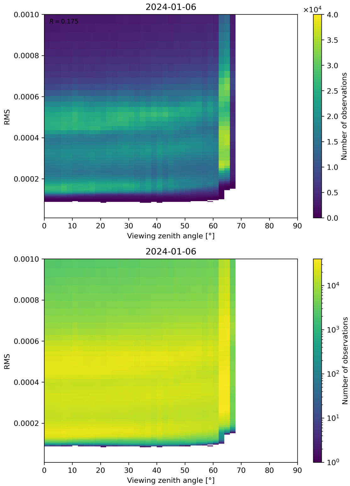
Figure 171: Scatter density plot of “Viewing zenith angle” against “RMS” for 2024-01-05 to 2024-01-07.
