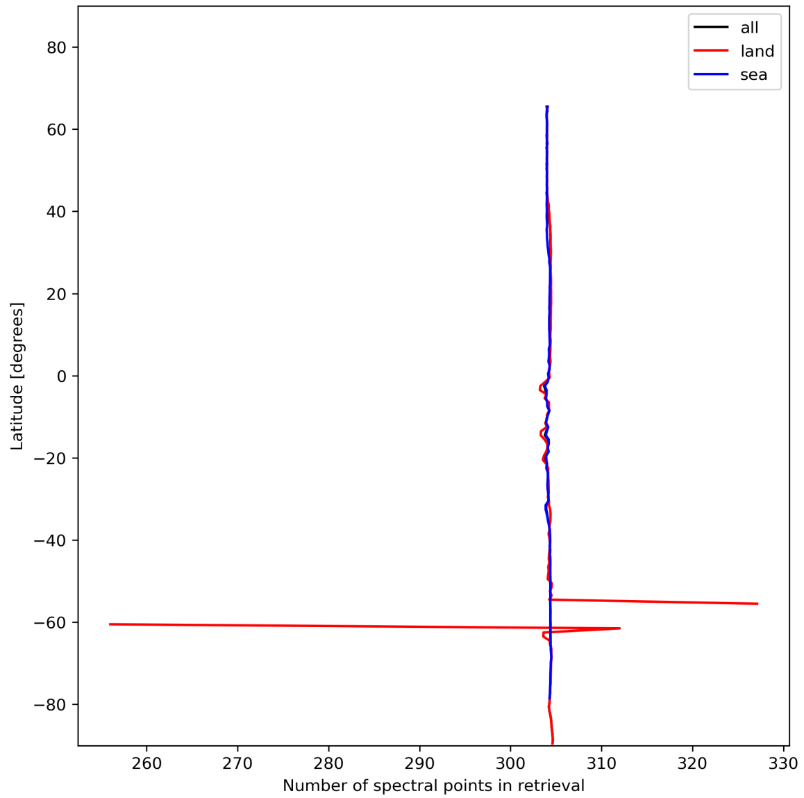
Figure 16: Zonal average of “Number of spectral points in retrieval” for 2024-01-05 to 2024-01-07.
