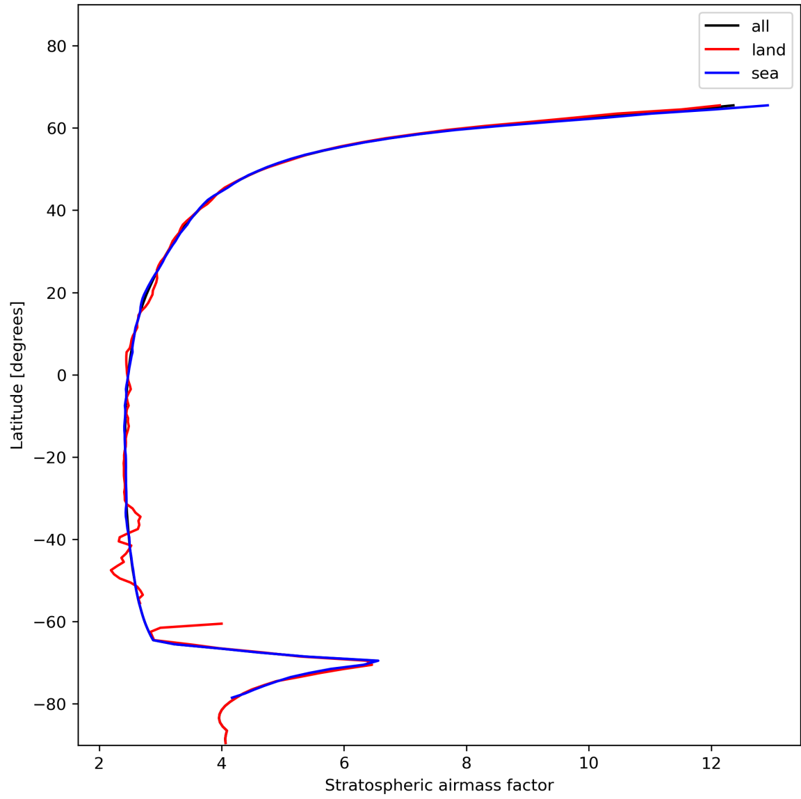
Figure 27: Zonal average of “Stratospheric airmass factor” for 2024-01-05 to 2024-01-07.
