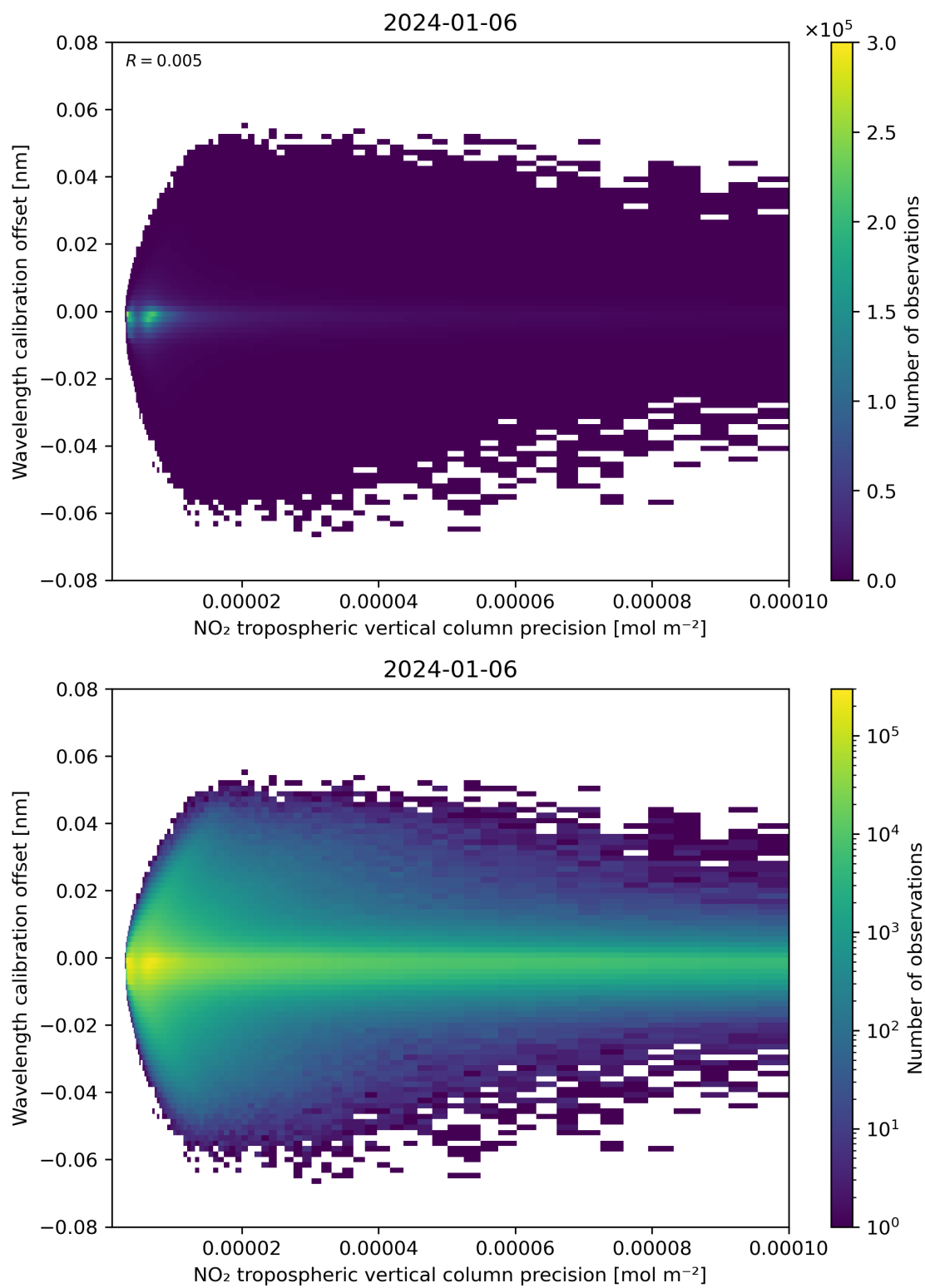
Figure 141: Scatter density plot of “NO 2 tropospheric vertical column precision” against “Wavelength calibration offset” for 2024-01-05 to 2024-01-07.
