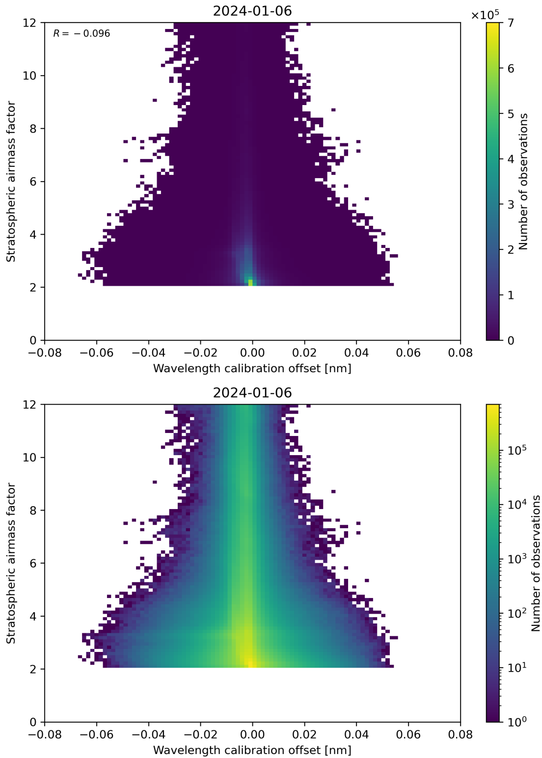
Figure 174: Scatter density plot of “Wavelength calibration offset” against “Stratospheric airmass factor” for 2024-01-05 to 2024-01-07.
