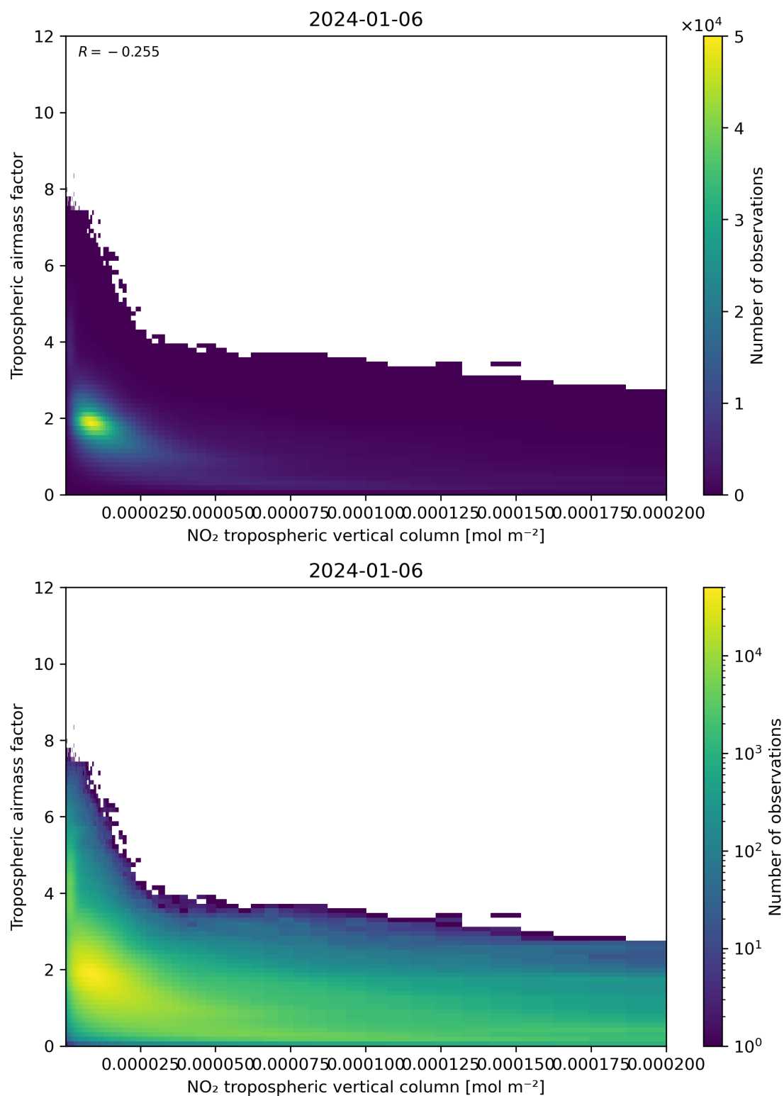
Figure 123: Scatter density plot of “NO 2 tropospheric vertical column” against “Tropospheric airmass factor” for 2024-01-05 to 2024-01-07.
