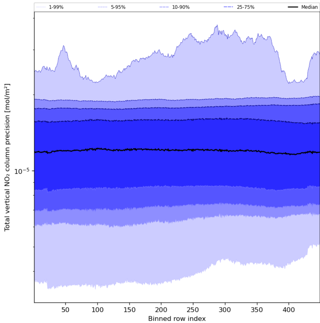
Figure 56: Along track statistics of “Total vertical NO 2 column precision” for 2024-01-05 to 2024-01-07
