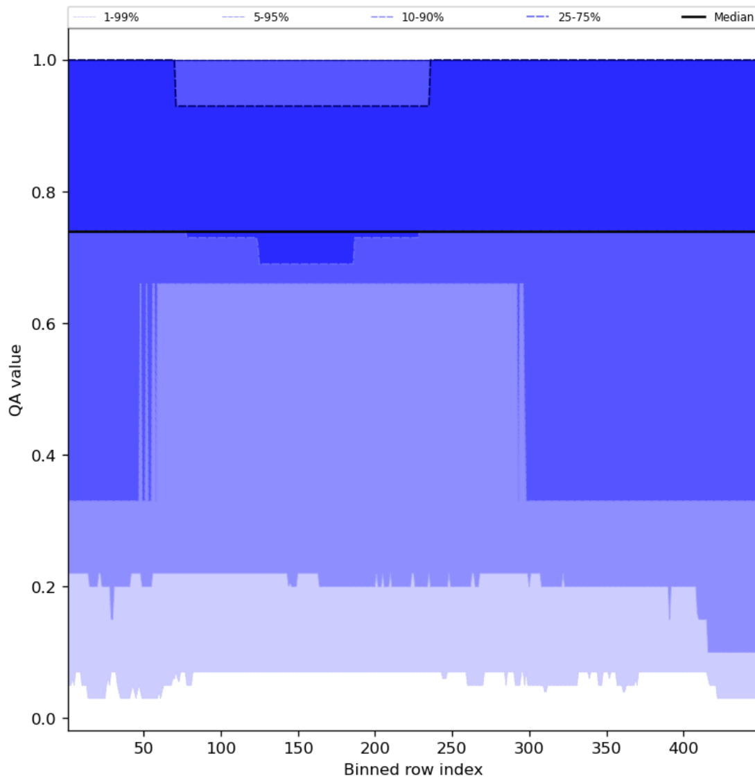
Figure 45: Along track statistics of “QA value” for 2024-01-05 to 2024-01-07
