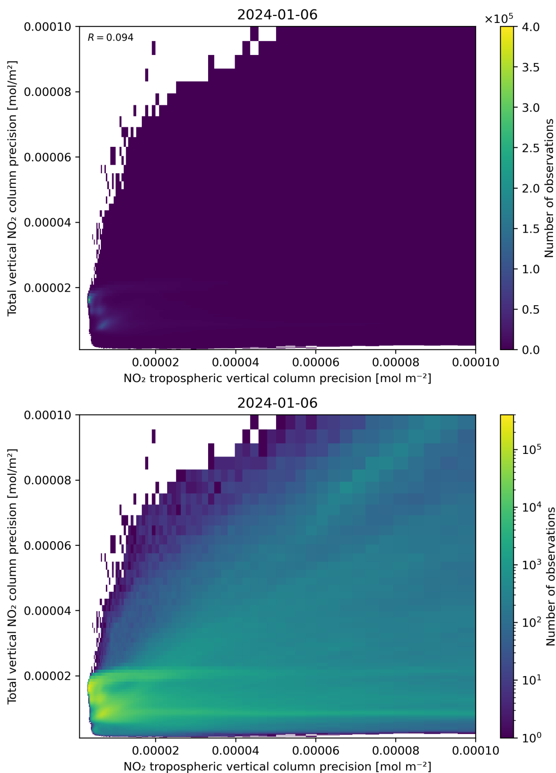
Figure 139: Scatter density plot of “NO 2 tropospheric vertical column precision” against “Total vertical NO 2 column precision” for 2024-01-05 to 2024-01-07.
