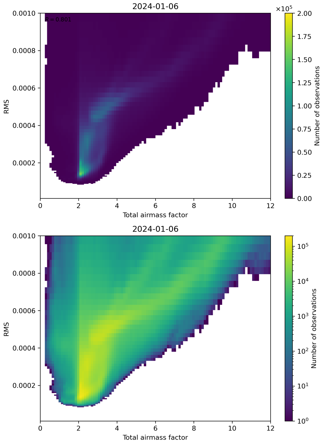
Figure 69: Scatter density plot of “Total airmass factor” against “RMS” for 2024-01-05 to 2024-01-07.
