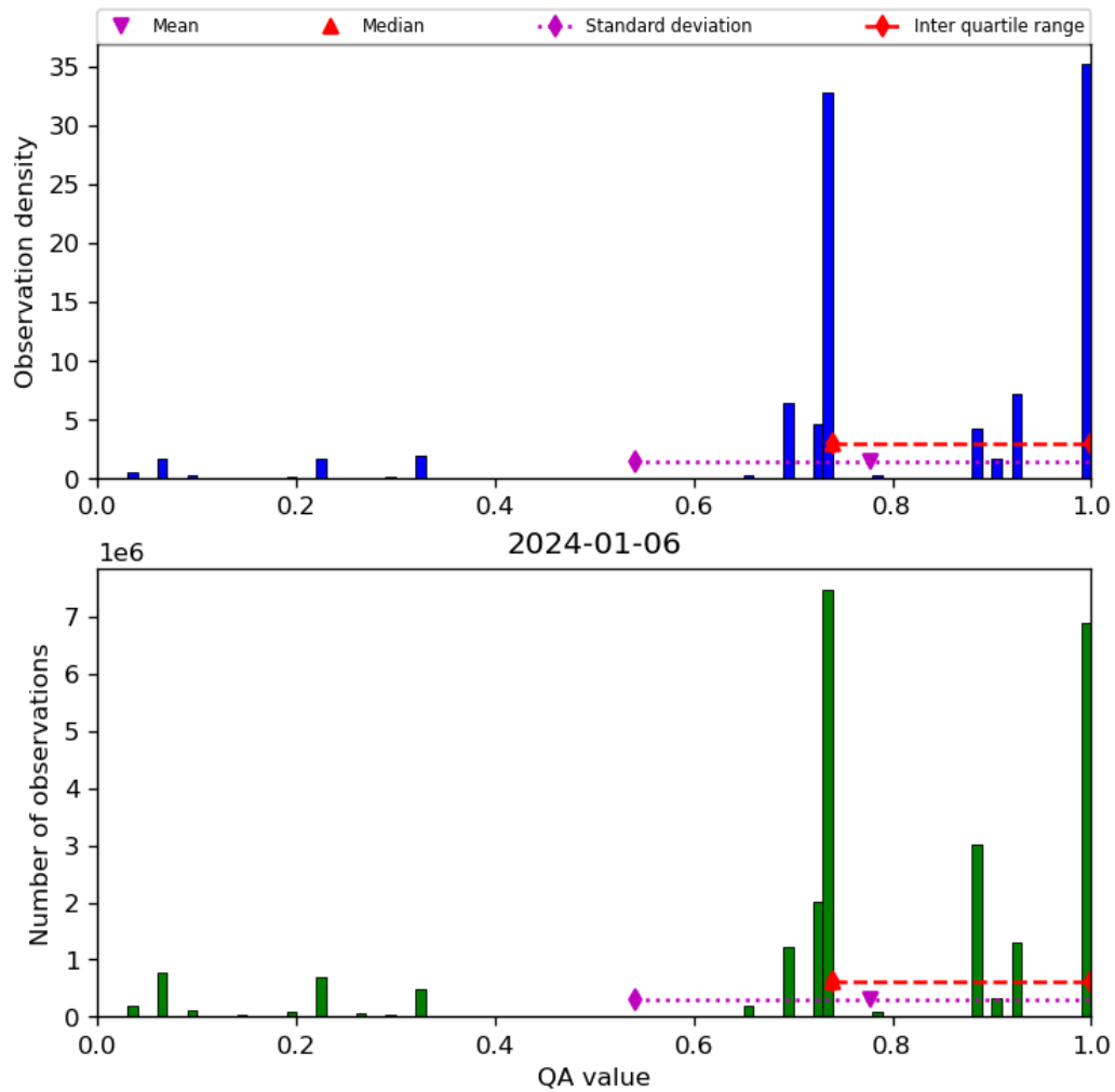
Figure 28: Histogram of “QA value” for 2024-01-05 to 2024-01-07
