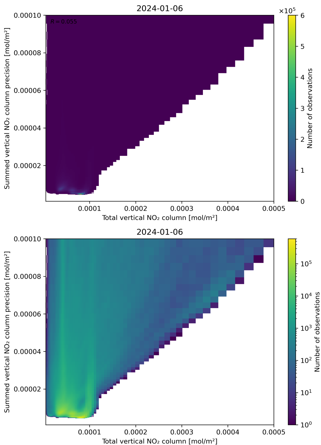
Figure 113: Scatter density plot of “Total vertical NO 2 column” against “Summed vertical NO 2 column precision” for 2024-01-05 to 2024-01-07.
