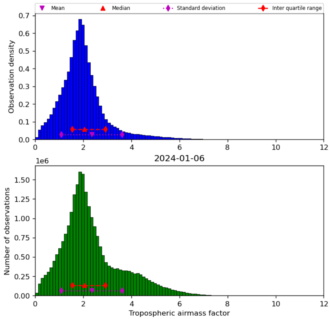
Figure 31: Histogram of “Tropospheric airmass factor” for 2024-01-05 to 2024-01-07
