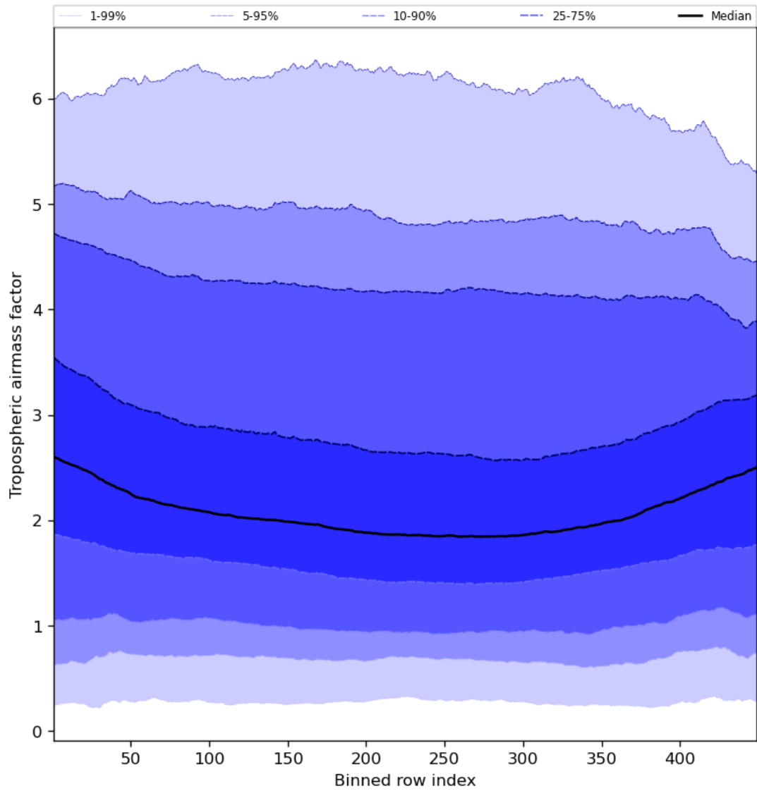
Figure 48: Along track statistics of “Tropospheric air mass factor” for 2024-01-05 to 2024-01-07
