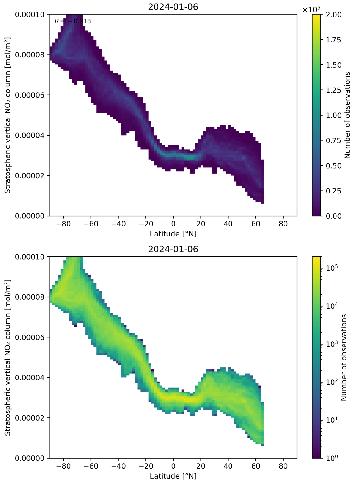
Figure 87: Scatter density plot of “Latitude” against “Stratospheric vertical NO 2 column” for 2024-01-05 to 2024-01-07.
