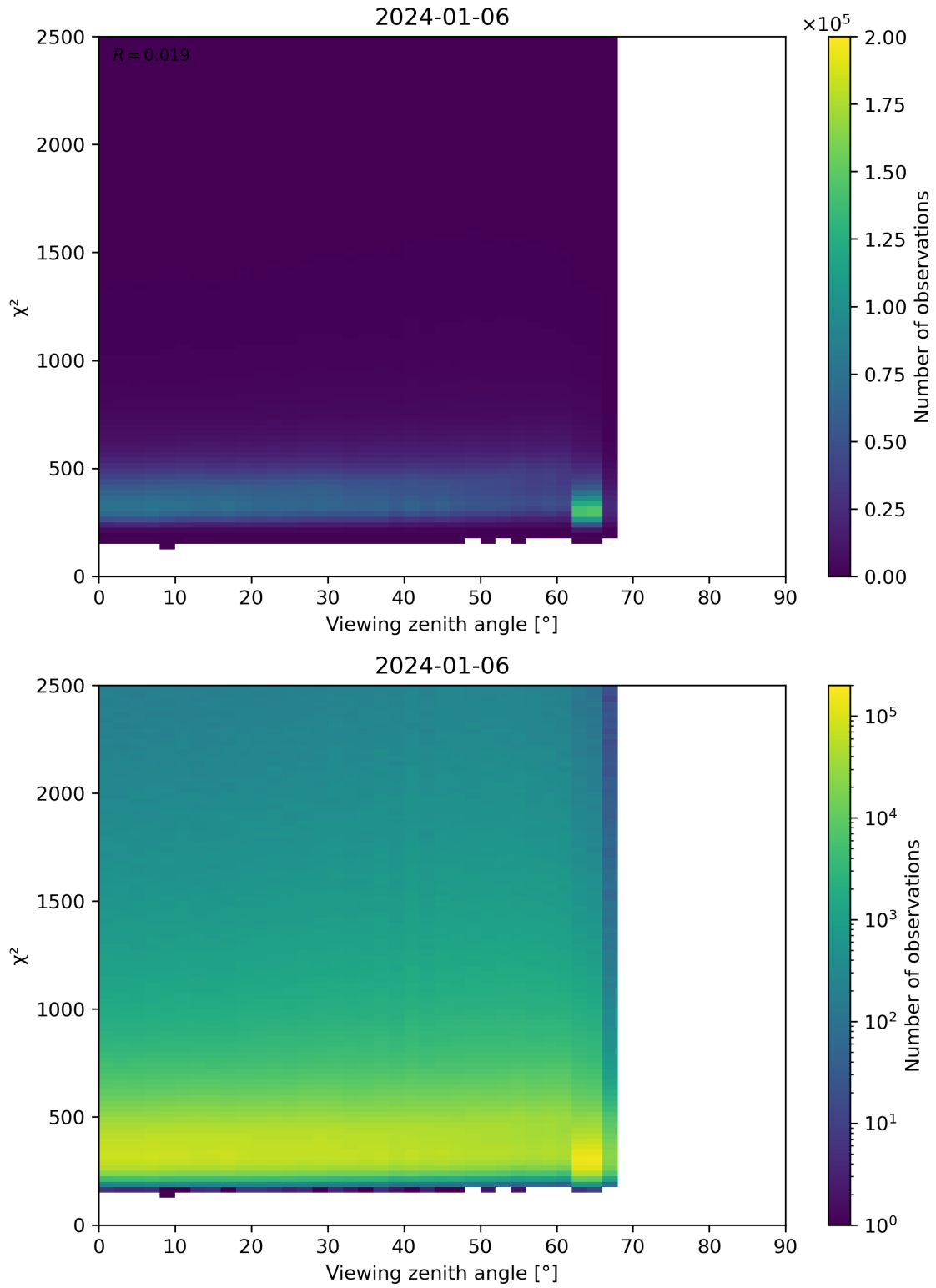
Figure 162: Scatter density plot of “Viewing zenith angle” against “ \chi^2 ” for 2024-01-05 to 2024-01-07.
