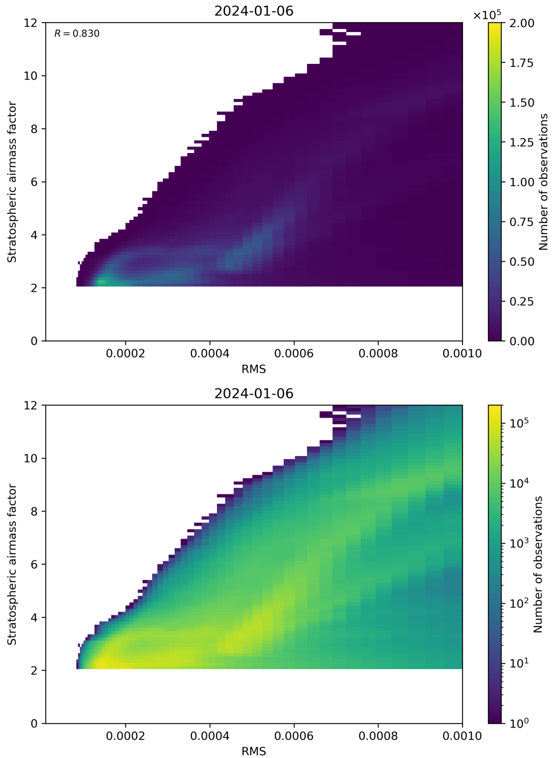
Figure 144: Scatter density plot of “RMS” against “Stratospheric airmass factor” for 2024-01-05 to 2024-01-07.
