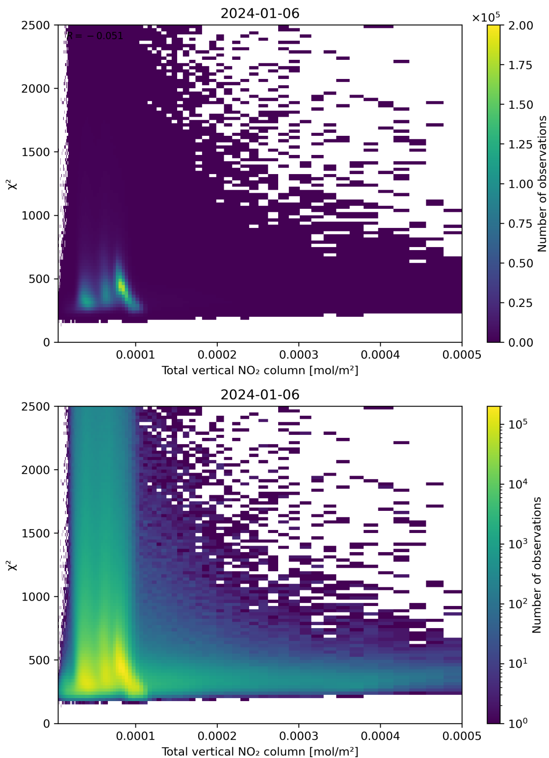
Figure 111: Scatter density plot of “Total vertical NO 2 column” against “ \chi^2 ” for 2024-01-05 to 2024-01-07.
