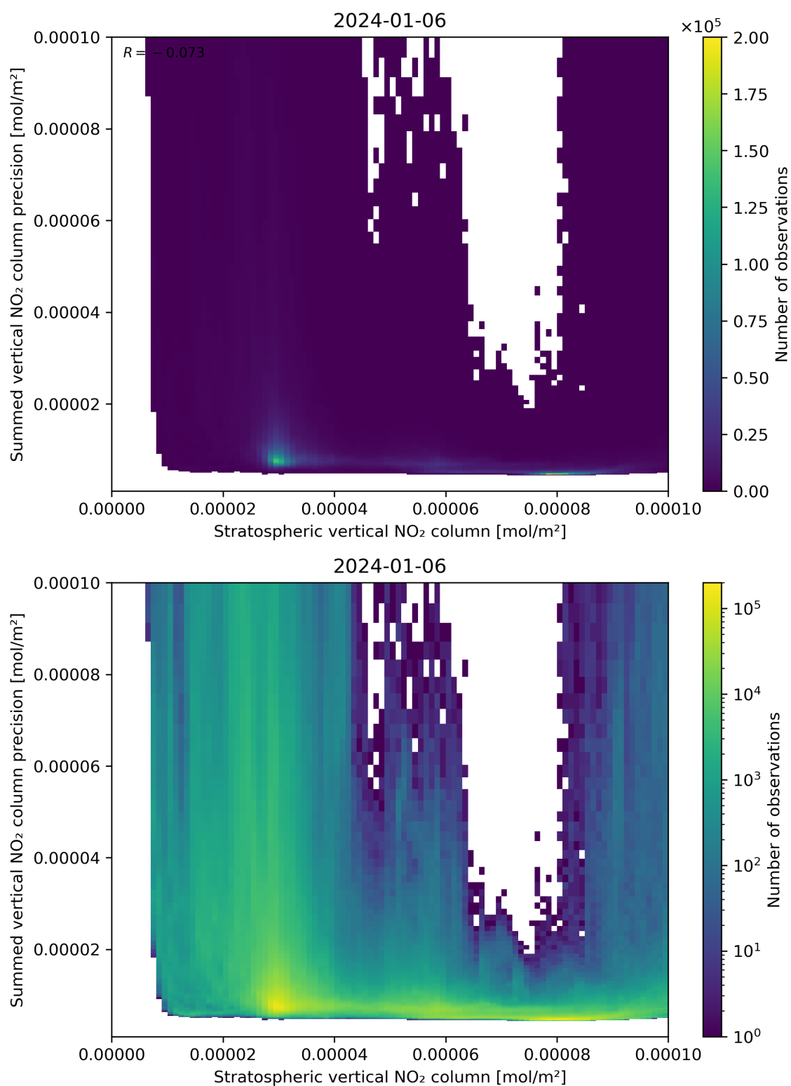
Figure 99: Scatter density plot of “Stratospheric vertical NO 2 column” against “Summed vertical NO 2 column precision” for 2024-01-05 to 2024-01-07.
