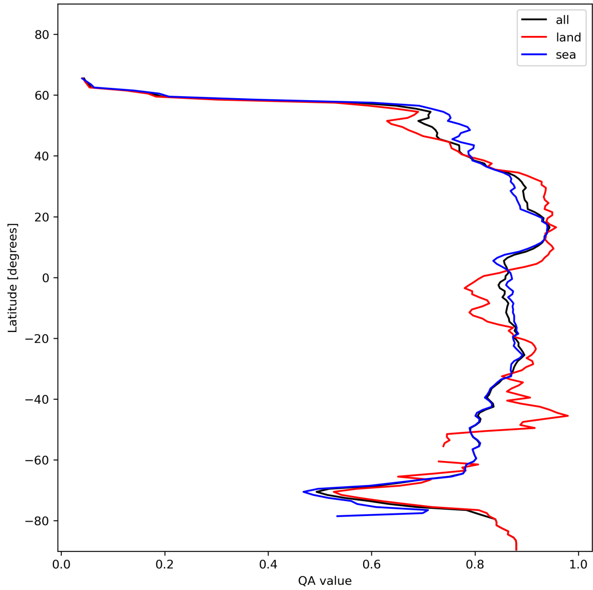
Figure 11: Zonal average of “QA value” for 2024-01-05 to 2024-01-07.
