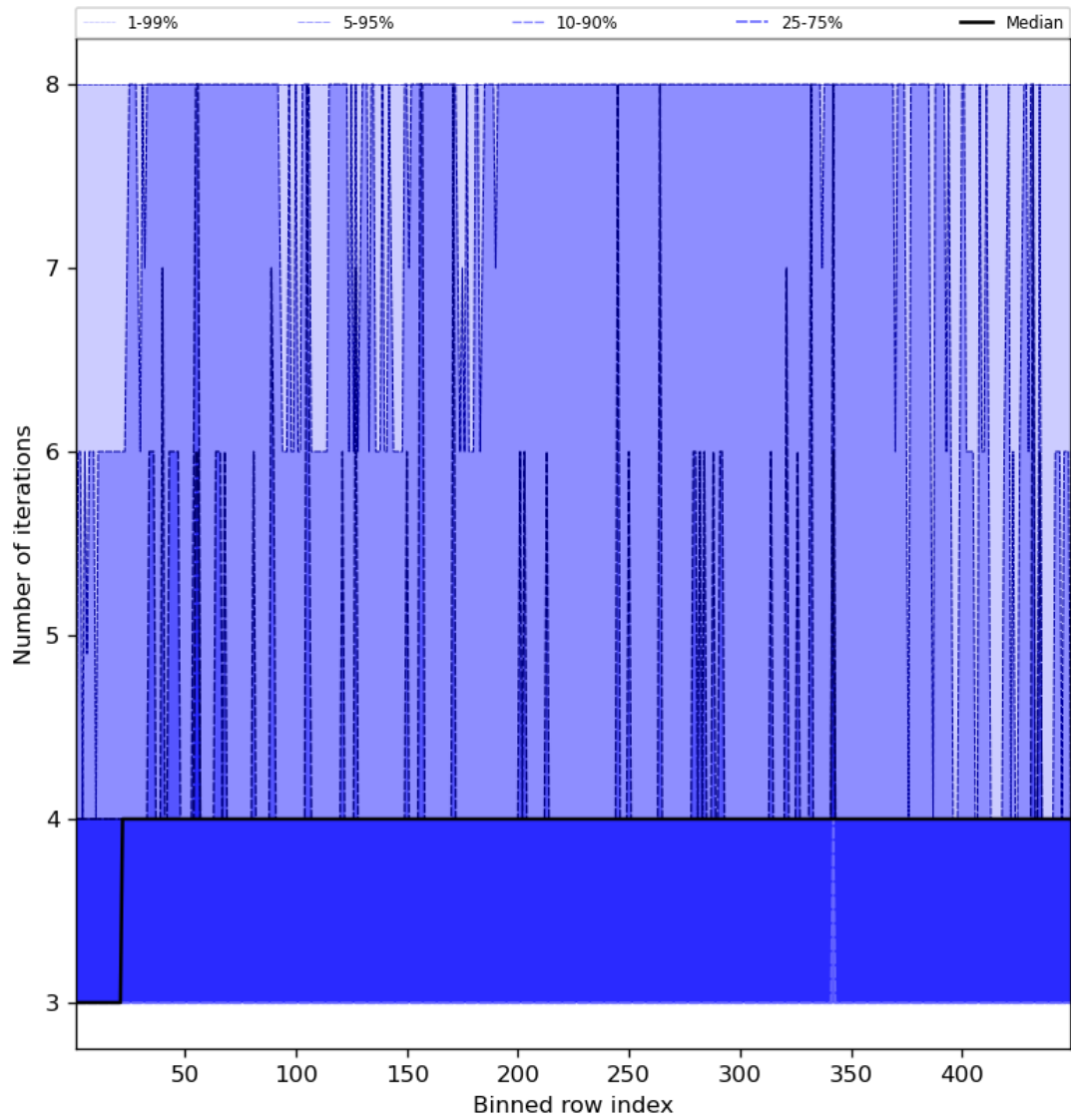
Figure 51: Along track statistics of “Number of iterations” for 2024-01-05 to 2024-01-07
