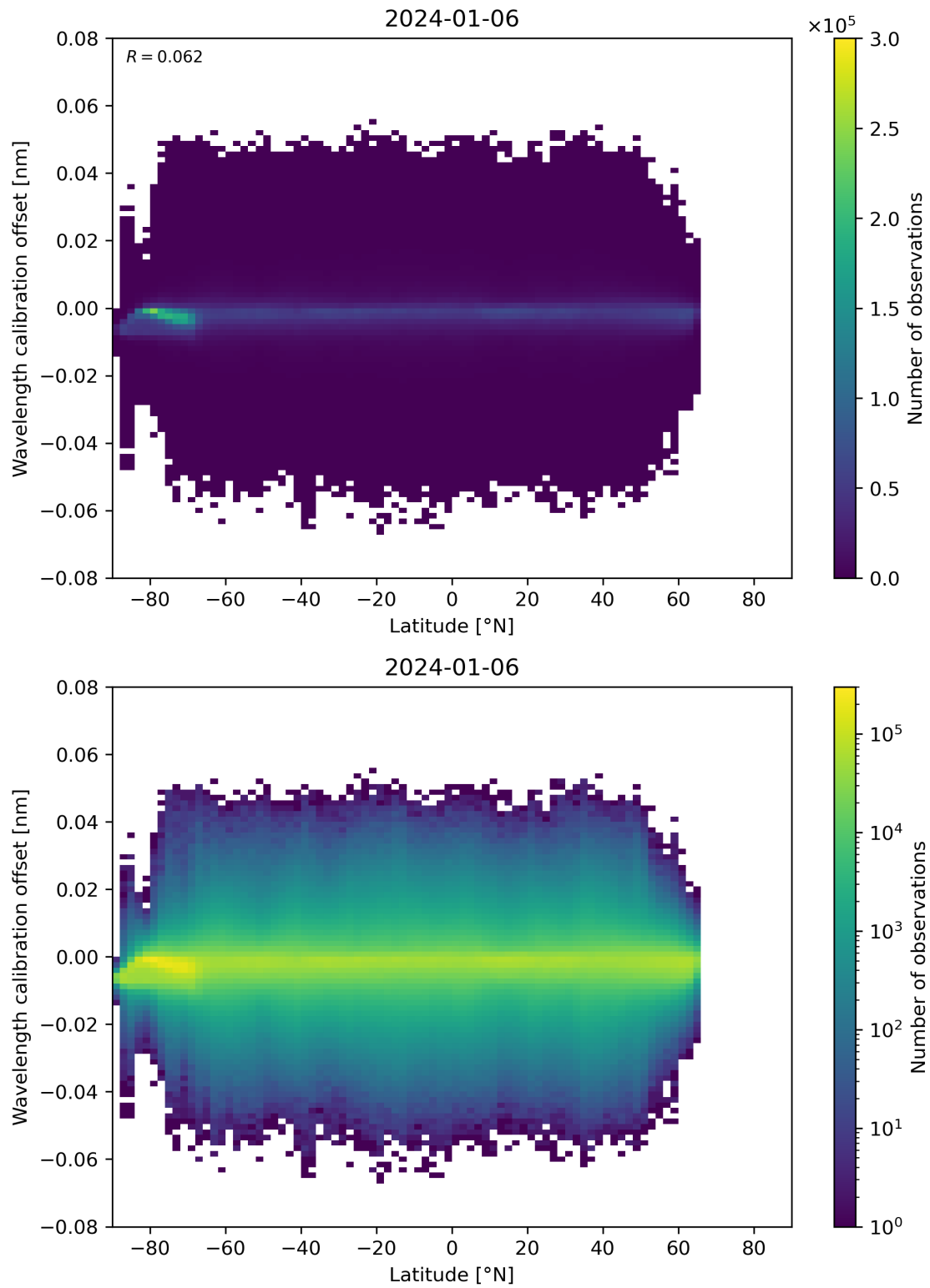
Figure 95: Scatter density plot of “Latitude” against “Wavelength calibration offset” for 2024-01-05 to 2024-01-07.
