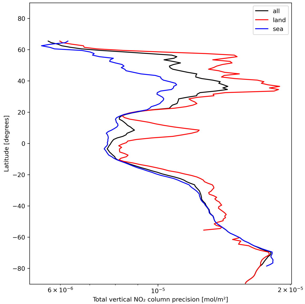
Figure 22: Zonal average of “Total vertical NO 2 column precision” for 2024-01-05 to 2024-01-07.
