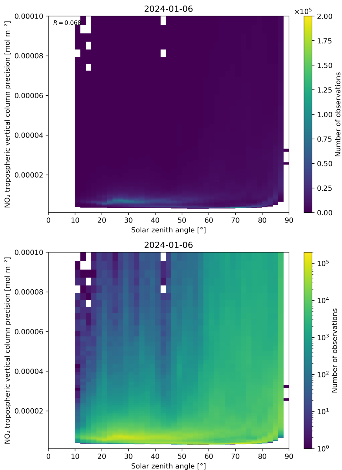
Figure 156: Scatter density plot of “Solar zenith angle” against “NO 2 tropospheric vertical column precision” for 2024-01-05 to 2024-01-07.
