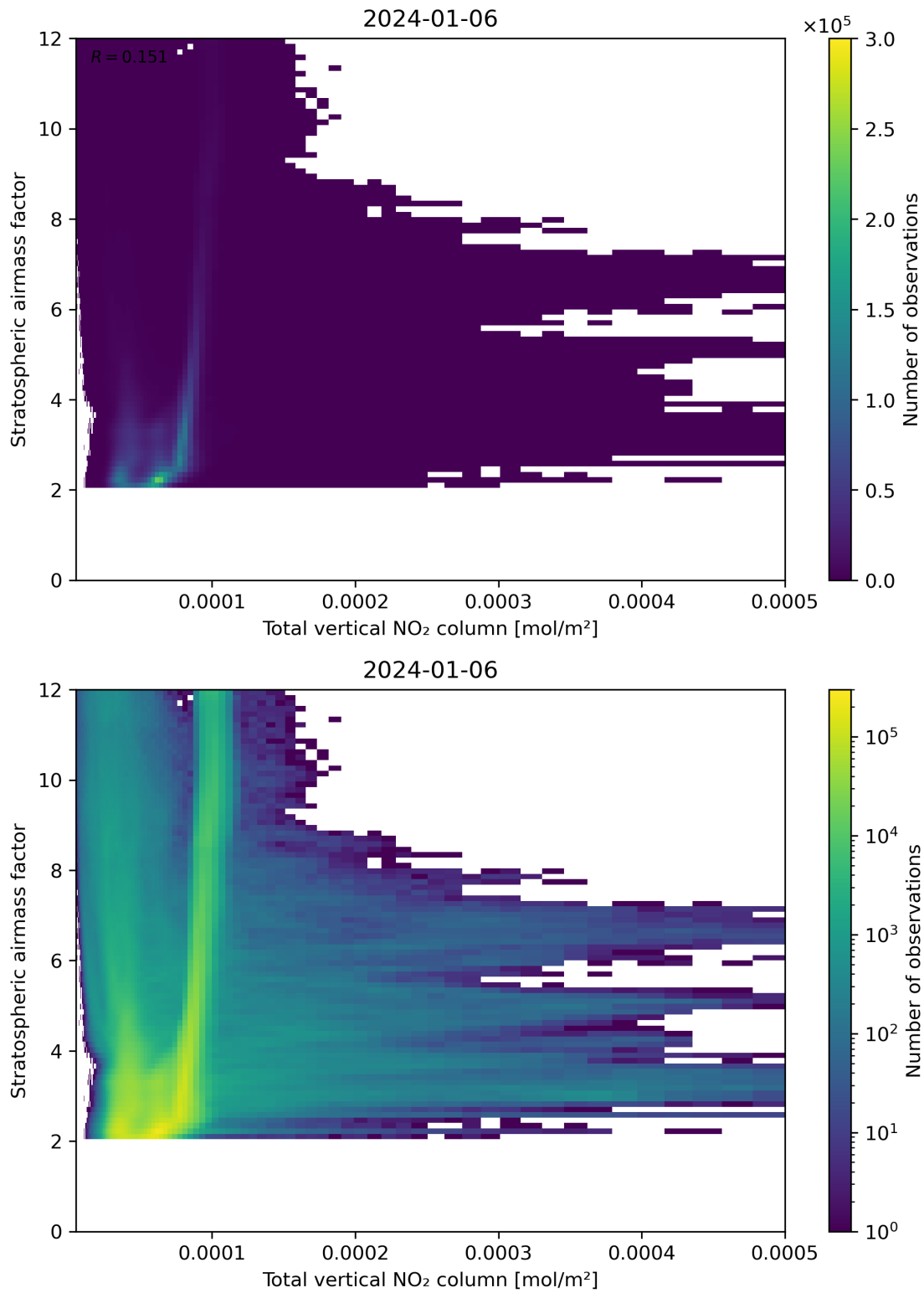
Figure 110: Scatter density plot of “Total vertical NO 2 column” against “Stratospheric airmass factor” for 2024-01-05 to 2024-01-07.
