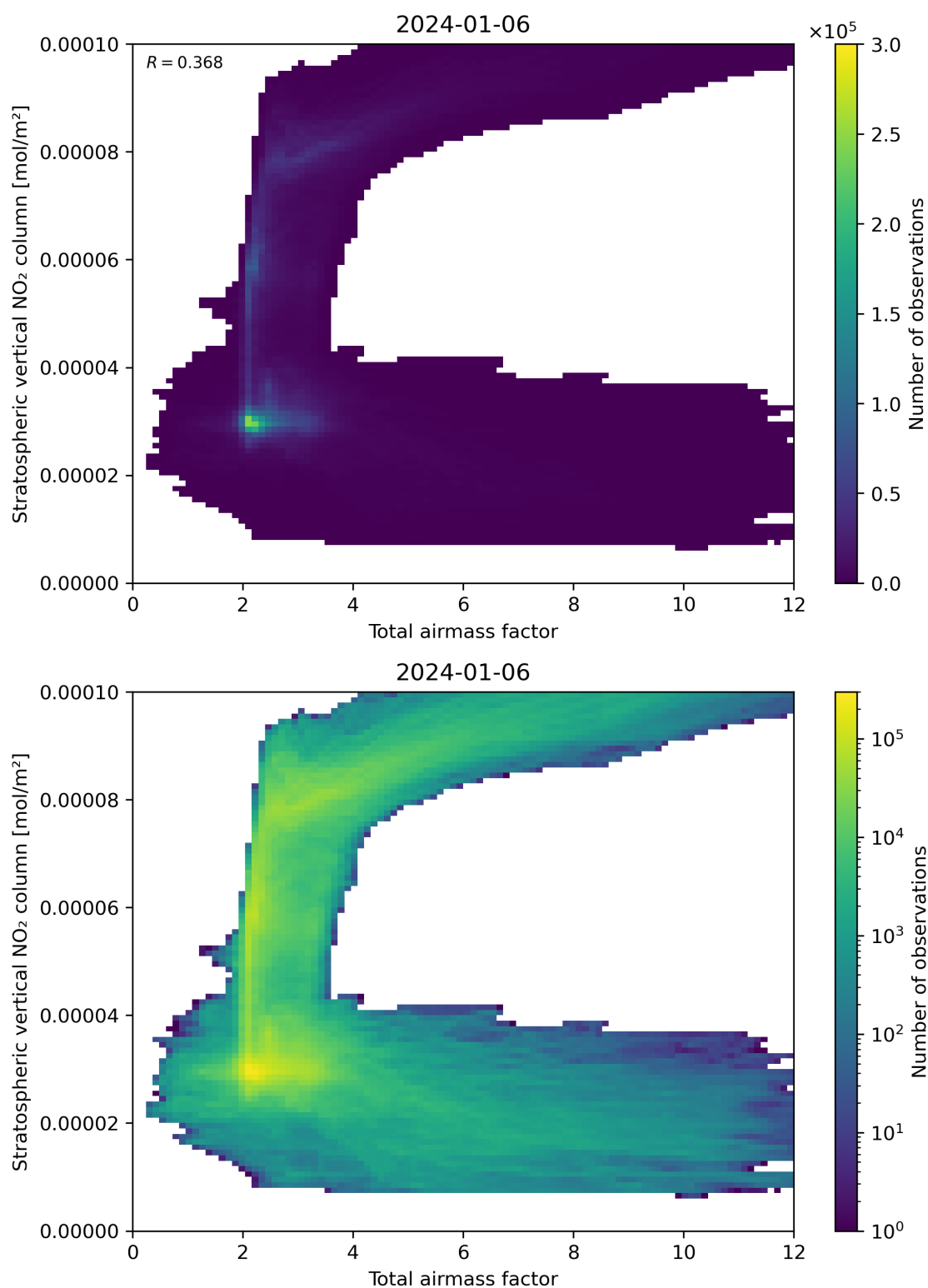
Figure 64: Scatter density plot of “Total airmass factor” against “Stratospheric vertical NO 2 column” for 2024-01-05 to 2024-01-07.
