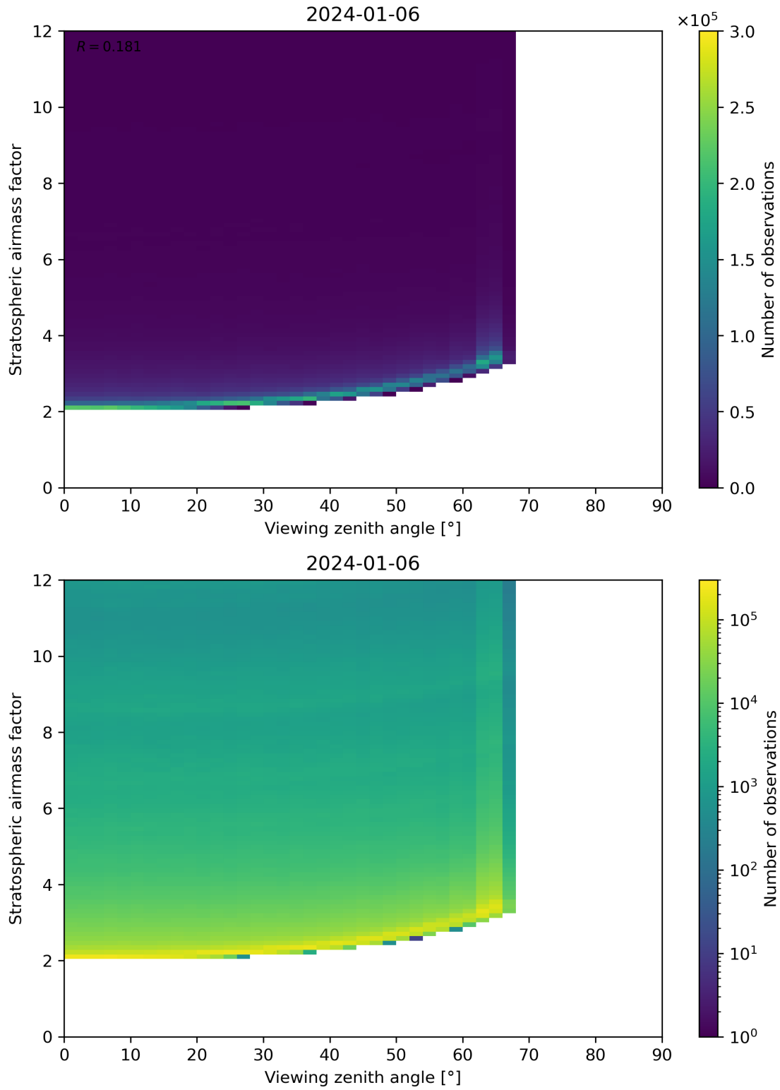
Figure 159: Scatter density plot of “Viewing zenith angle” against “Stratospheric airmass factor” for 2024-01-05 to 2024-01-07.
