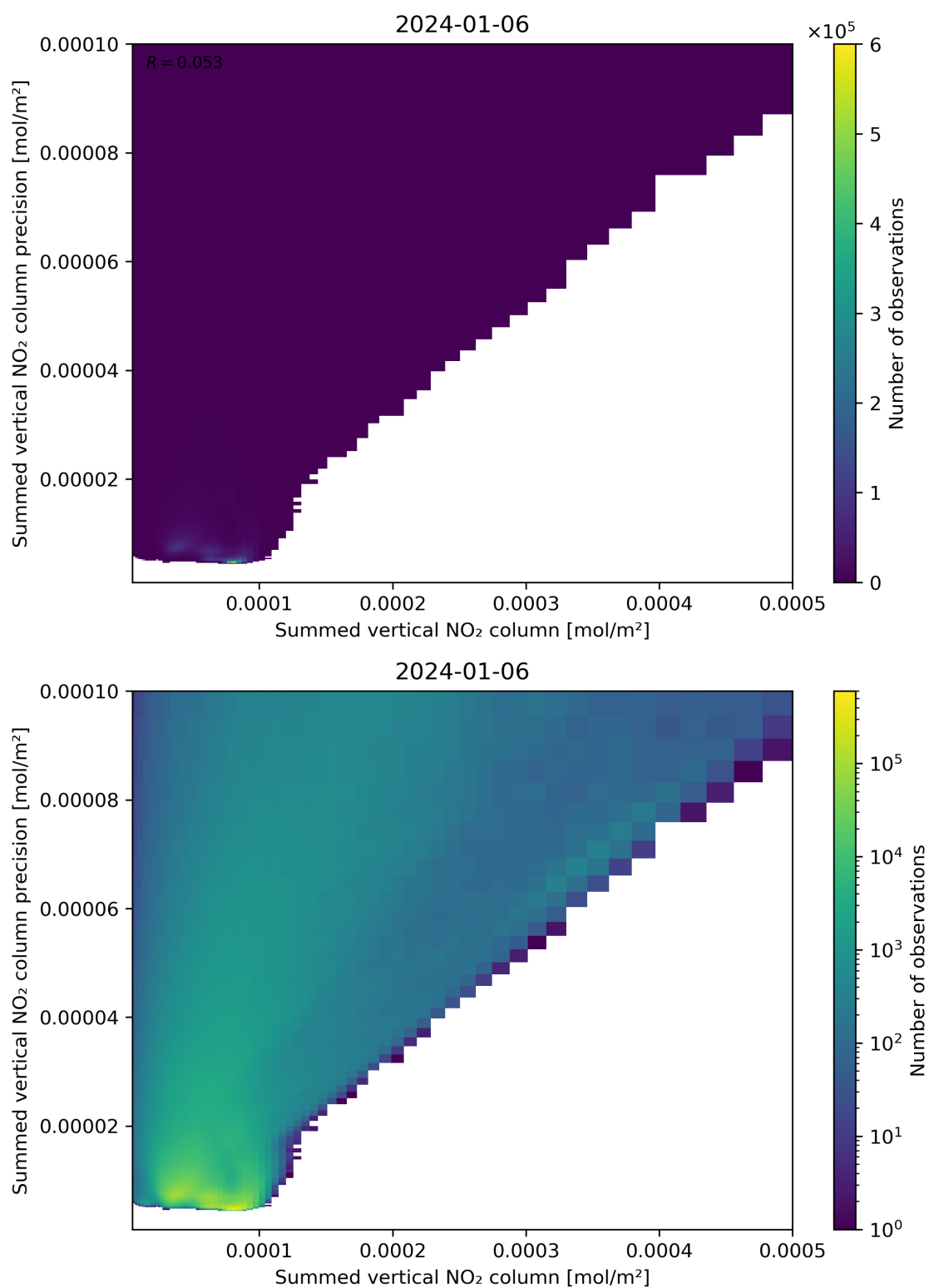
Figure 105: Scatter density plot of “Summed vertical NO 2 column” against “Summed vertical NO 2 column precision” for 2024-01-05 to 2024-01-07.
