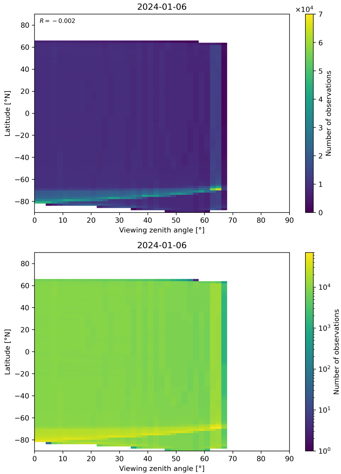
Figure 163: Scatter density plot of “Viewing zenith angle” against “Latitude” for 2024-01-05 to 2024-01-07.
