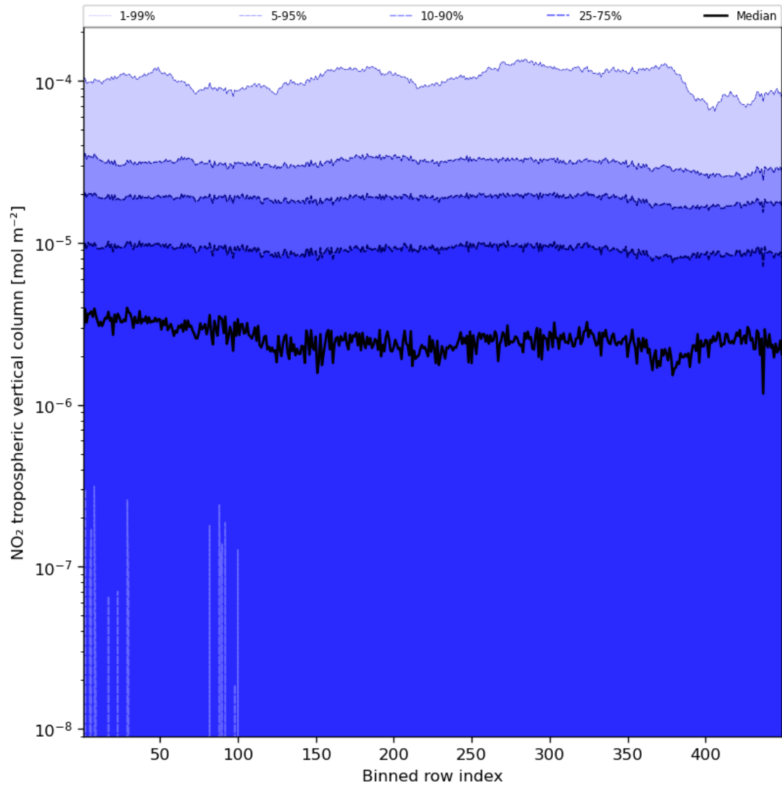
Figure 46: Along track statistics of “NO 2 tropospheric vertical column” for 2024-01-05 to 2024-01-07
