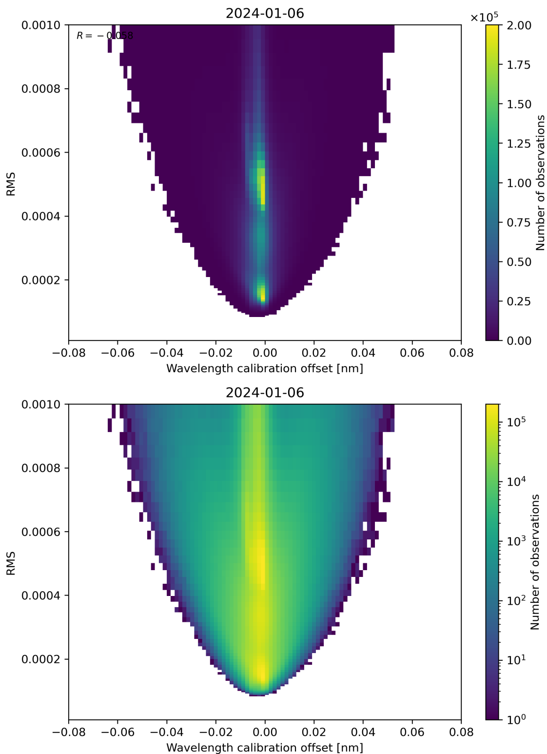
Figure 181: Scatter density plot of “Wavelength calibration offset” against “RMS” for 2024-01-05 to 2024-01-07.
