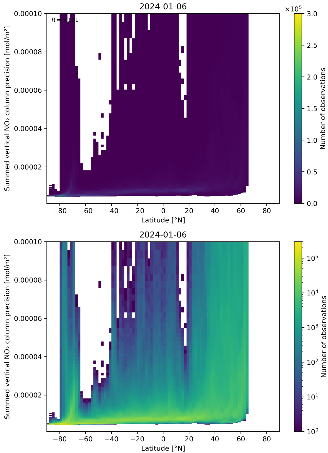
Figure 89: Scatter density plot of “Latitude” against “Summed vertical NO 2 column precision” for 2024-01-05 to 2024-01-07.
