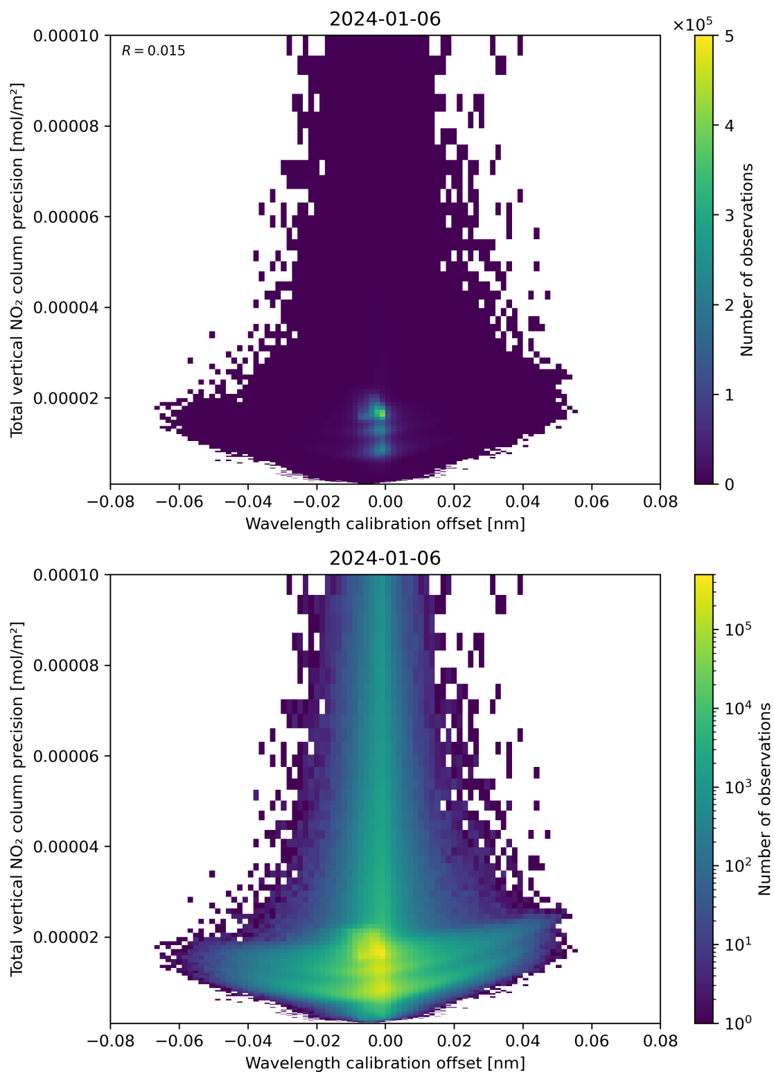
Figure 180: Scatter density plot of “Wavelength calibration offset” against “Total vertical NO 2 column precision” for 2024-01-05 to 2024-01-07.
