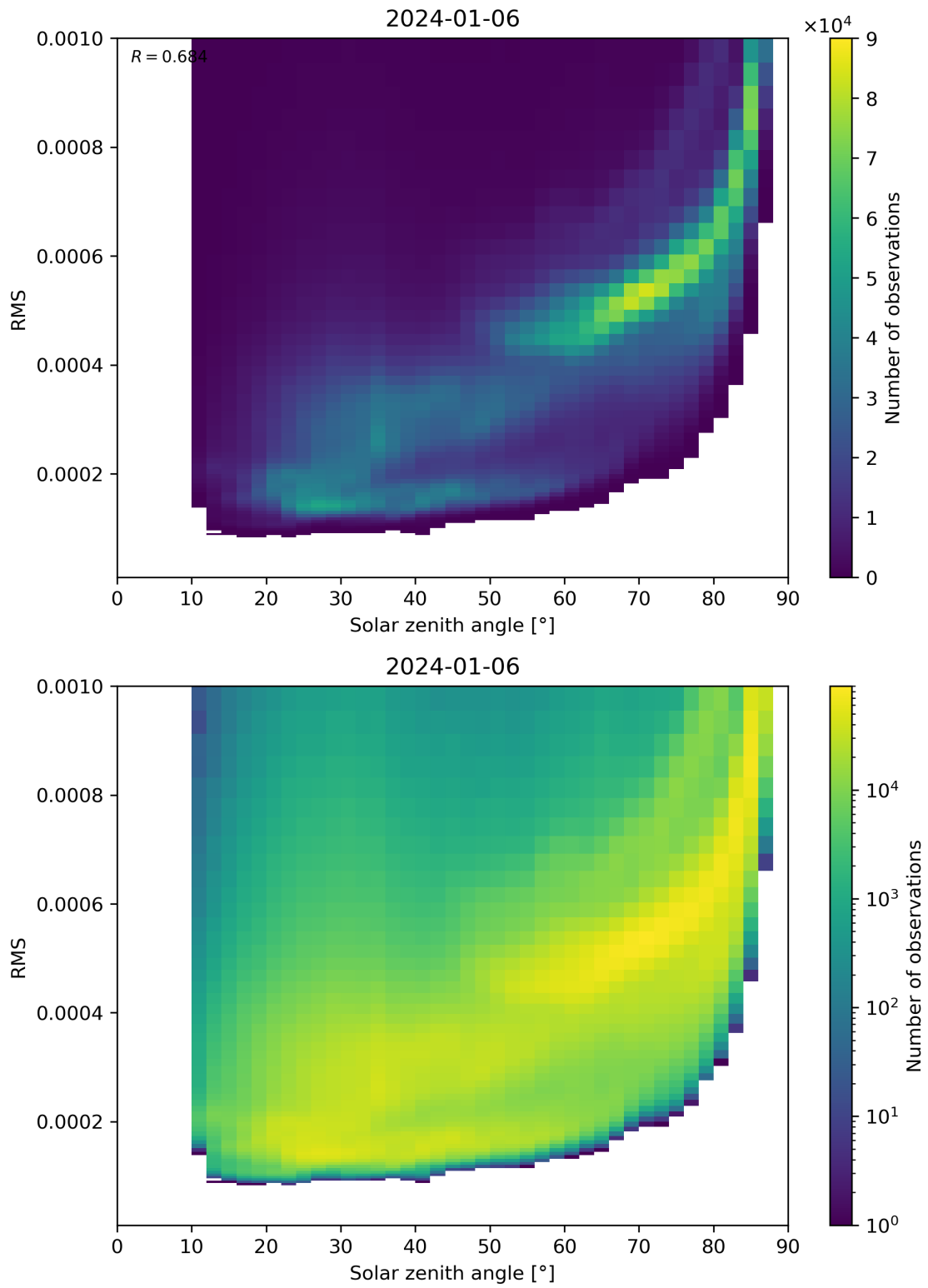
Figure 157: Scatter density plot of “Solar zenith angle” against “RMS” for 2024-01-05 to 2024-01-07.
