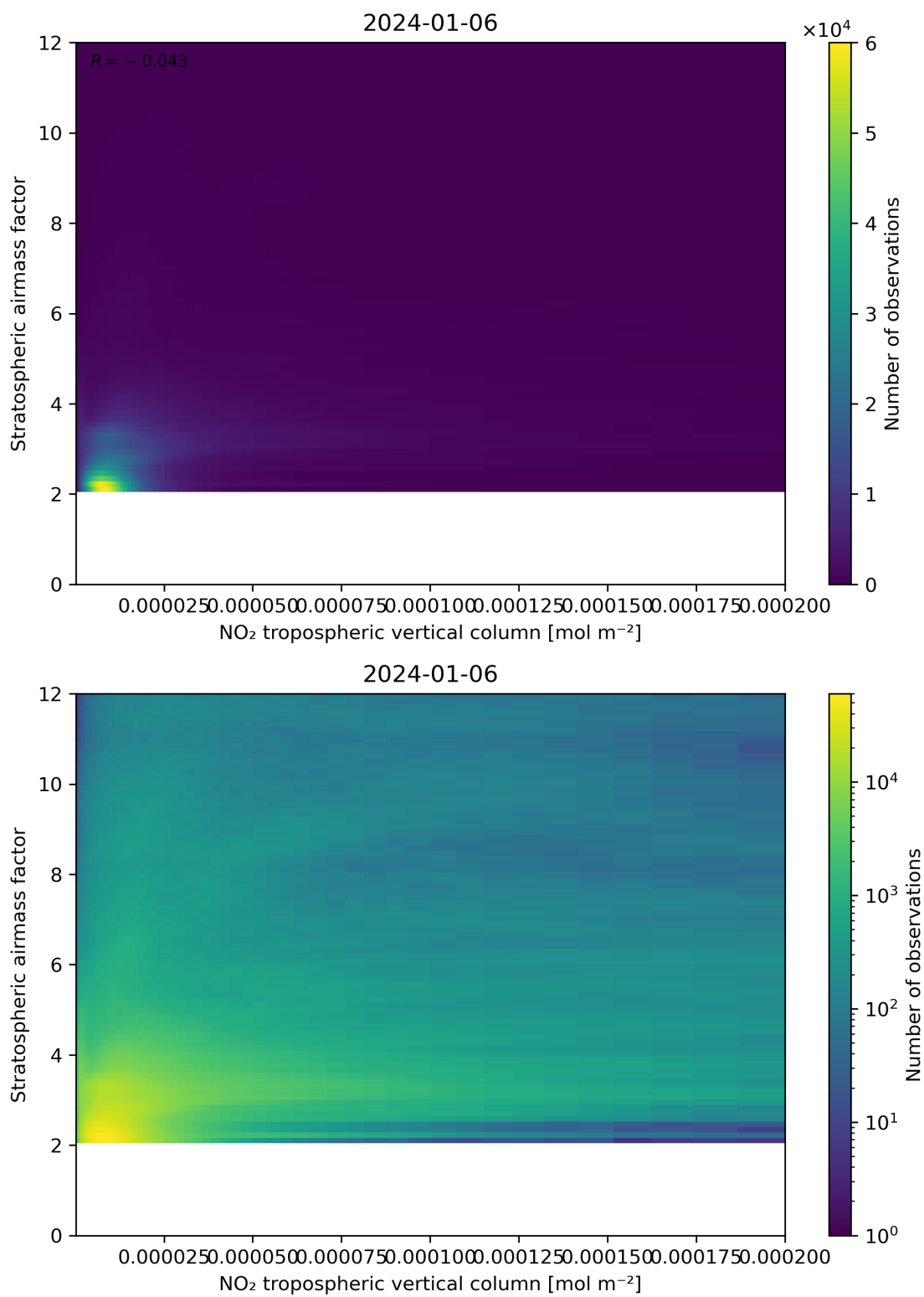
Figure 121: Scatter density plot of “NO 2 tropospheric vertical column” against “Stratospheric airmass factor” for 2024-01-05 to 2024-01-07.
