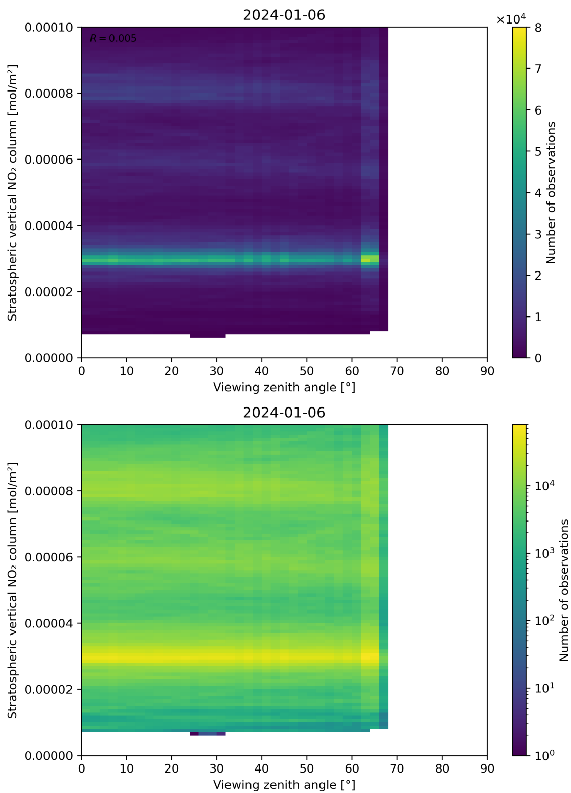
Figure 164: Scatter density plot of “Viewing zenith angle” against “Stratospheric vertical NO 2 column” for 2024-01-05 to 2024-01-07.
