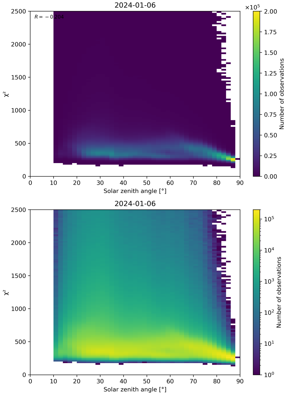
Figure 148: Scatter density plot of “Solar zenith angle” against “ \chi^2 ” for 2024-01-05 to 2024-01-07.
