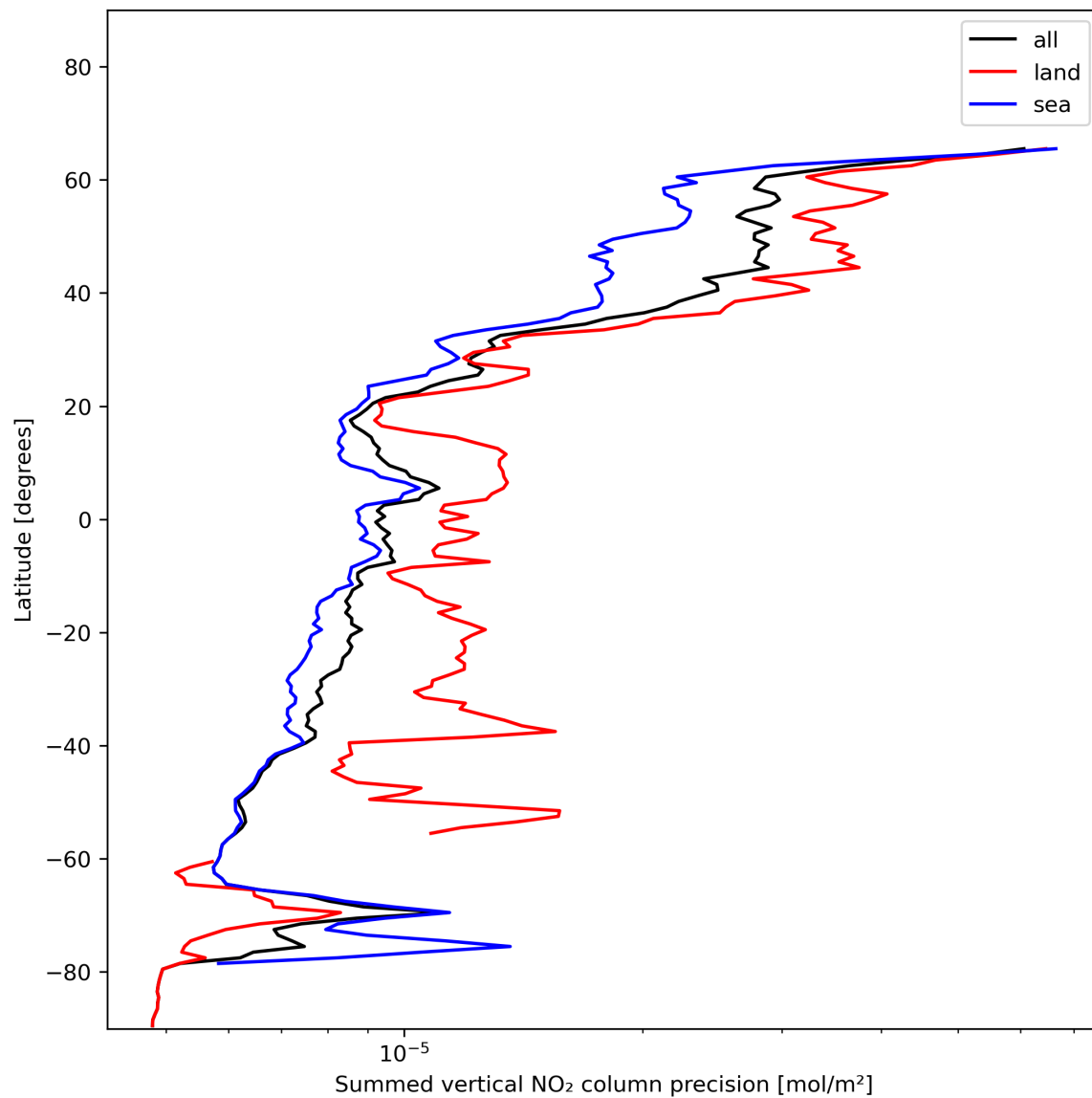
Figure 24: Zonal average of “Summed vertical NO 2 column precision” for 2024-01-05 to 2024-01-07.
