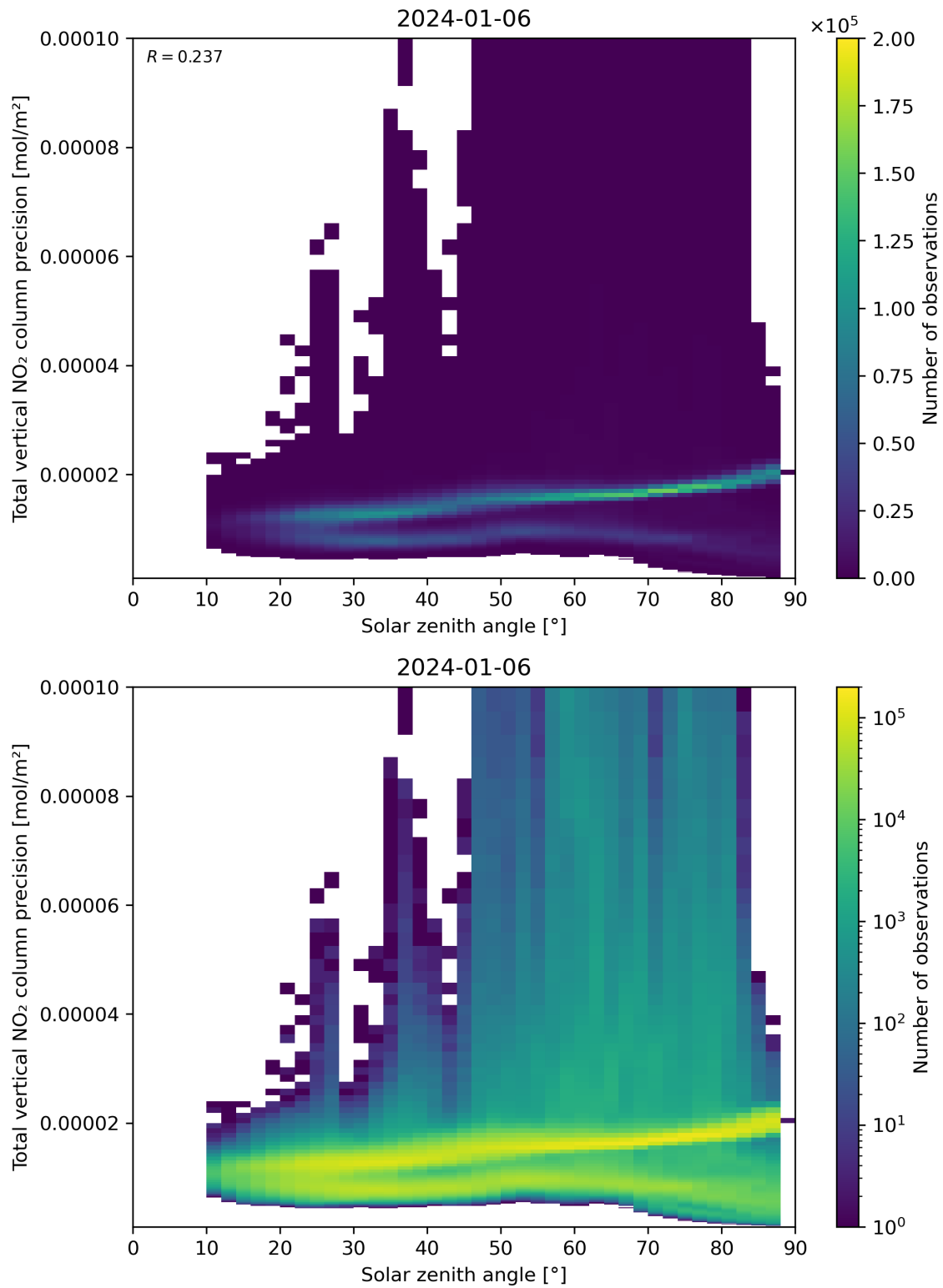
Figure 154: Scatter density plot of “Solar zenith angle” against “Total vertical NO 2 column precision” for 2024-01-05 to 2024-01-07.
