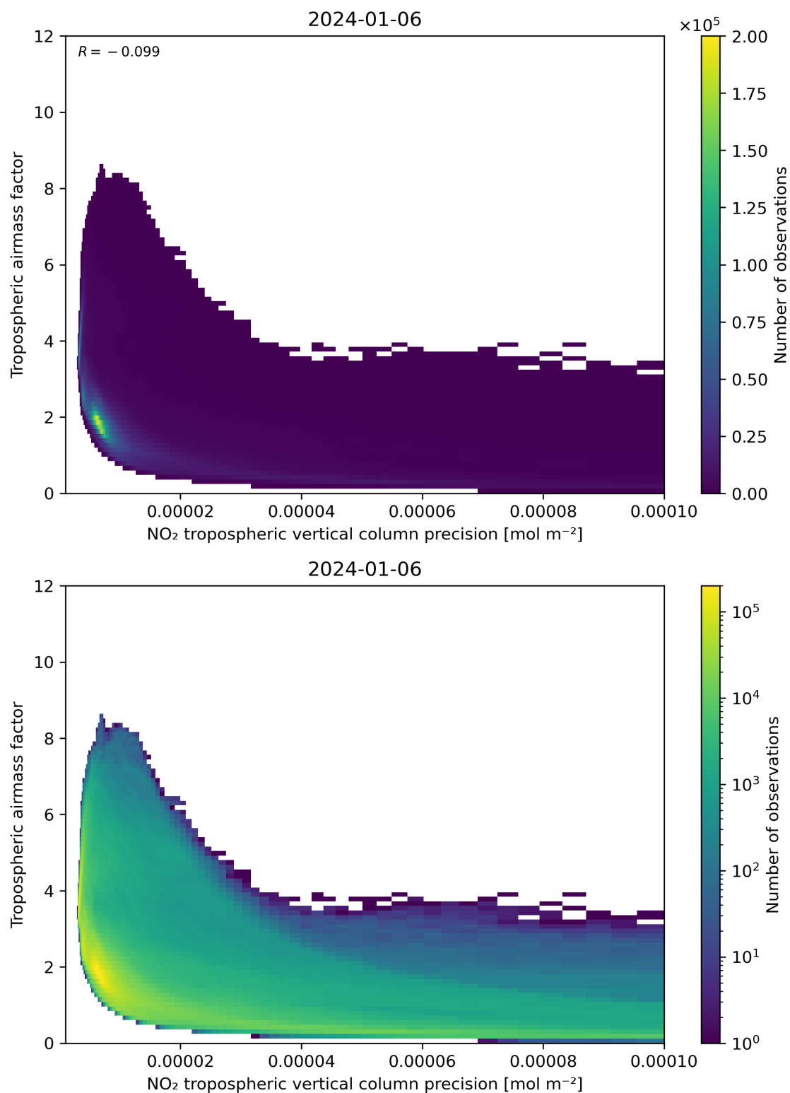
Figure 133: Scatter density plot of “NO 2 tropospheric vertical column precision” against “Tropospheric airmass factor” for 2024-01-05 to 2024-01-07.
