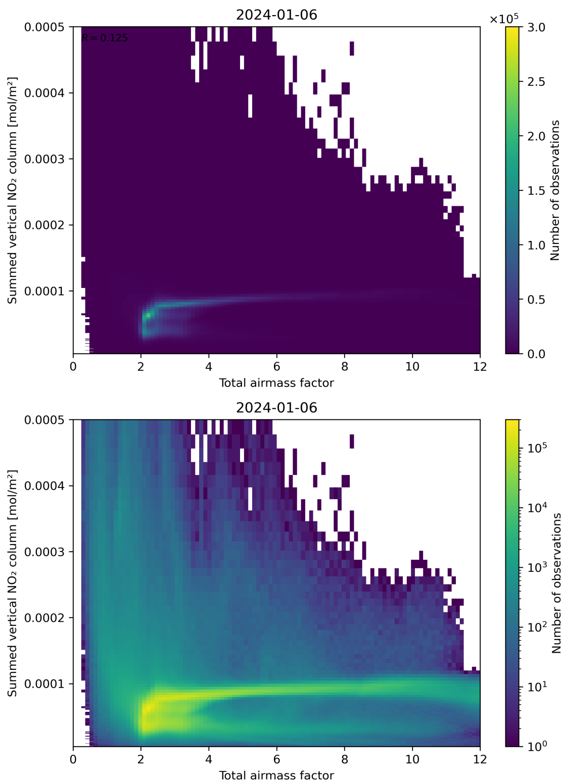
Figure 65: Scatter density plot of “Total airmass factor” against “Summed vertical NO 2 column” for 2024-01-05 to 2024-01-07.
