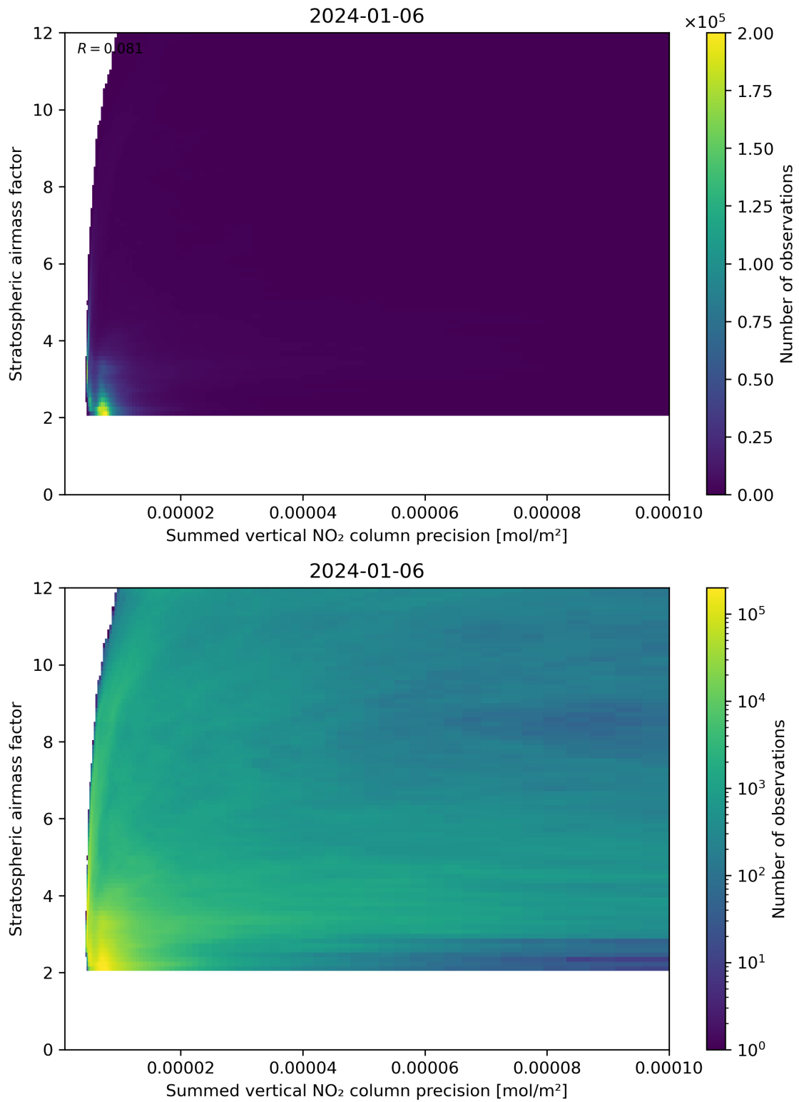
Figure 106: Scatter density plot of “Summed vertical NO 2 column precision” against “Stratospheric airmass factor” for 2024-01-05 to 2024-01-07.
