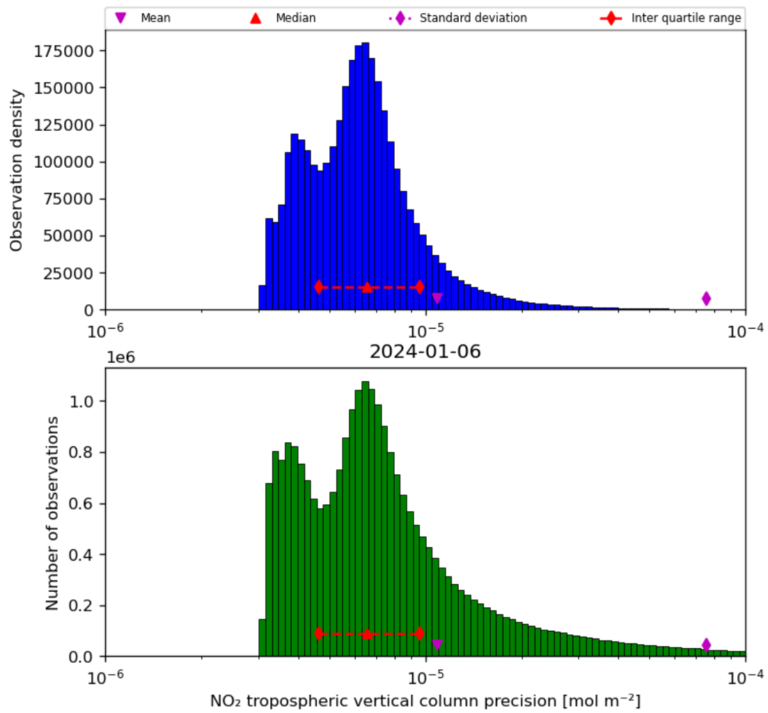
Figure 30: Histogram of “NO 2 tropospheric vertical column precision” for 2024-01-05 to 2024-01-07
