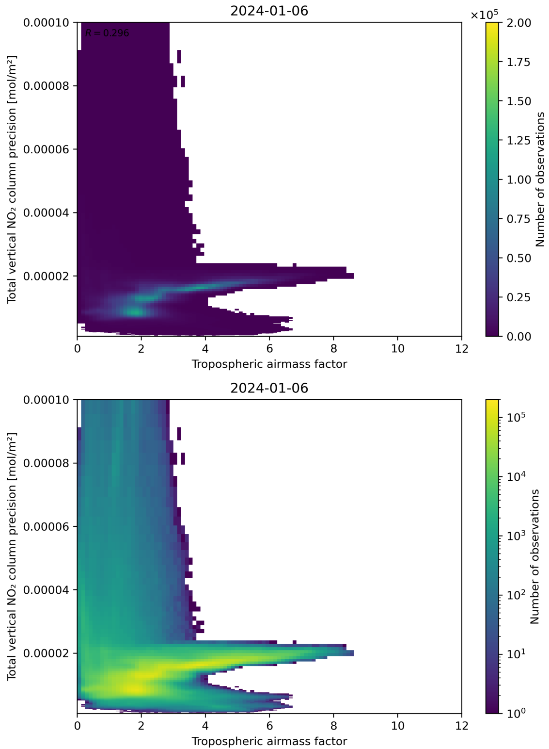
Figure 78: Scatter density plot of “Tropospheric air mass factor” against “Total vertical NO 2 column precision” for 2024-01-05 to 2024-01-07.
