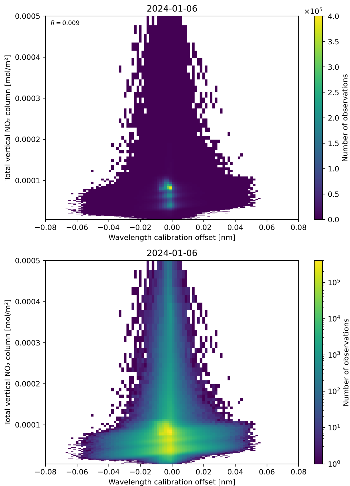
Figure 179: Scatter density plot of “Wavelength calibration offset” against “Total vertical NO 2 column” for 2024-01-05 to 2024-01-07.
