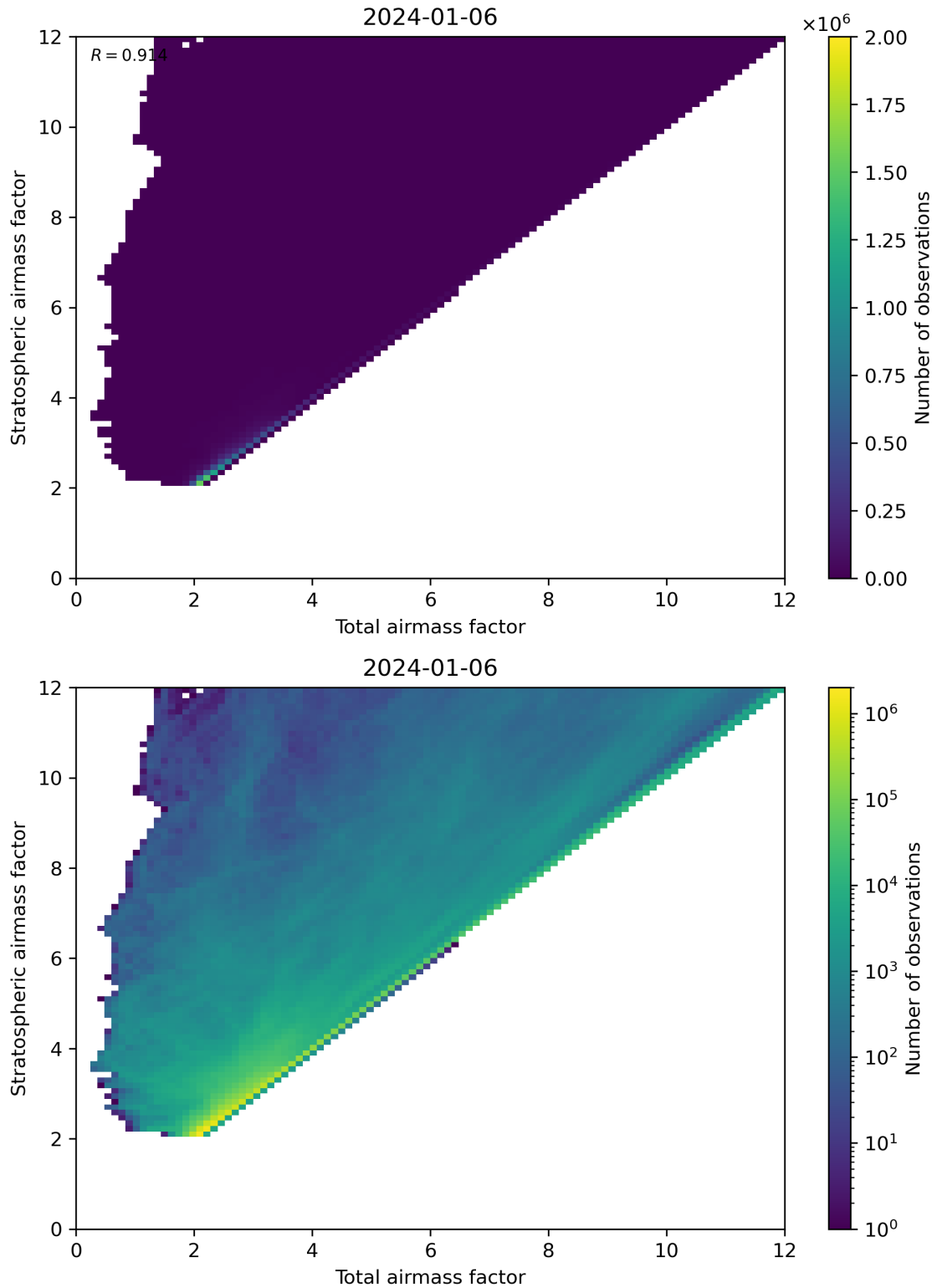
Figure 62: Scatter density plot of “Total airmass factor” against “Stratospheric airmass factor” for 2024-01-05 to 2024-01-07.
