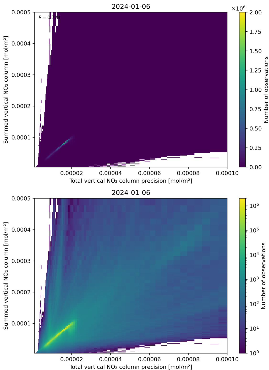
Figure 117: Scatter density plot of “Total vertical NO 2 column precision” against “Summed vertical NO 2 column” for 2024-01-05 to 2024-01-07.
