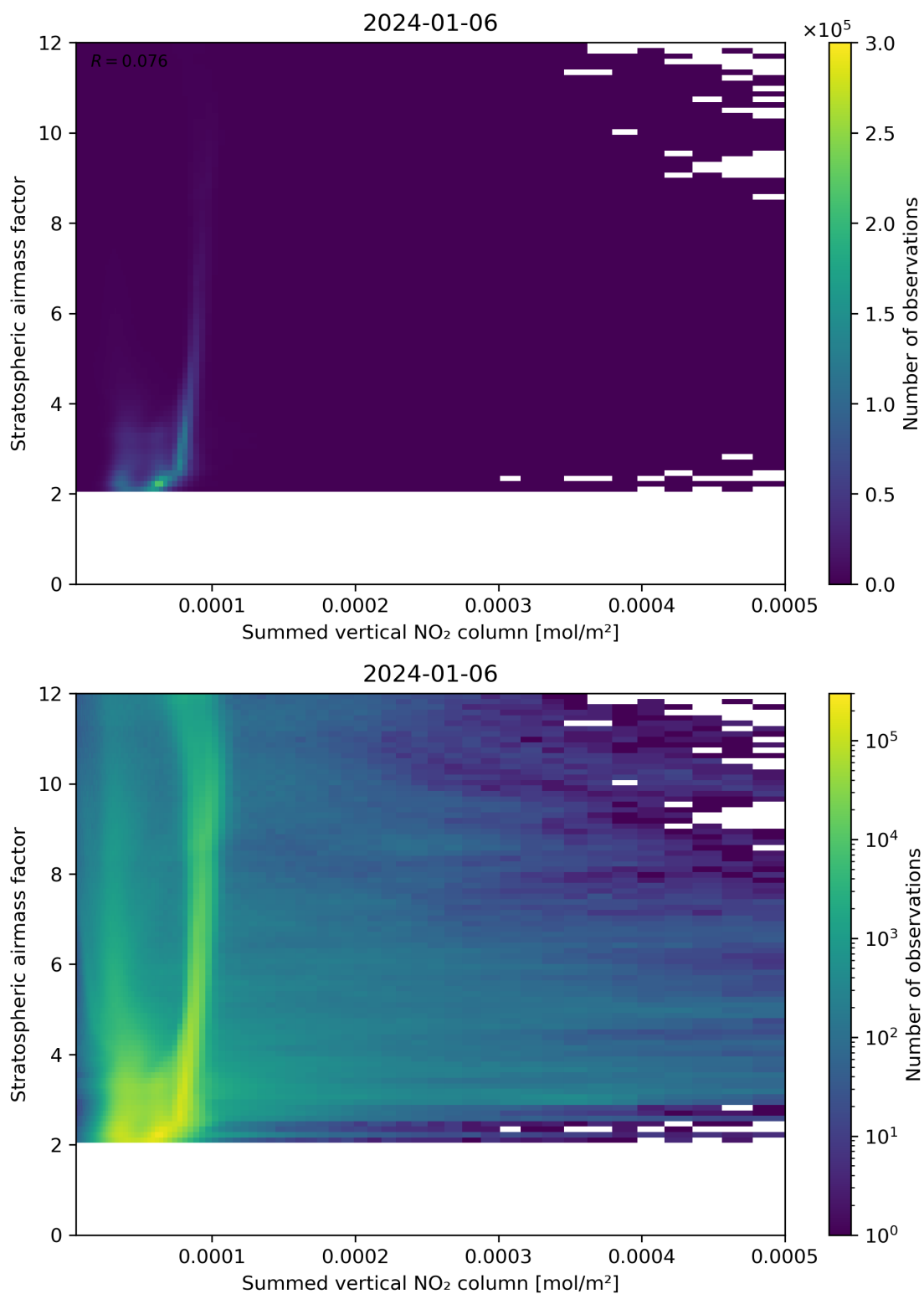
Figure 103: Scatter density plot of “Summed vertical NO 2 column” against “Stratospheric air mass factor” for 2024-01-05 to 2024-01-07.
