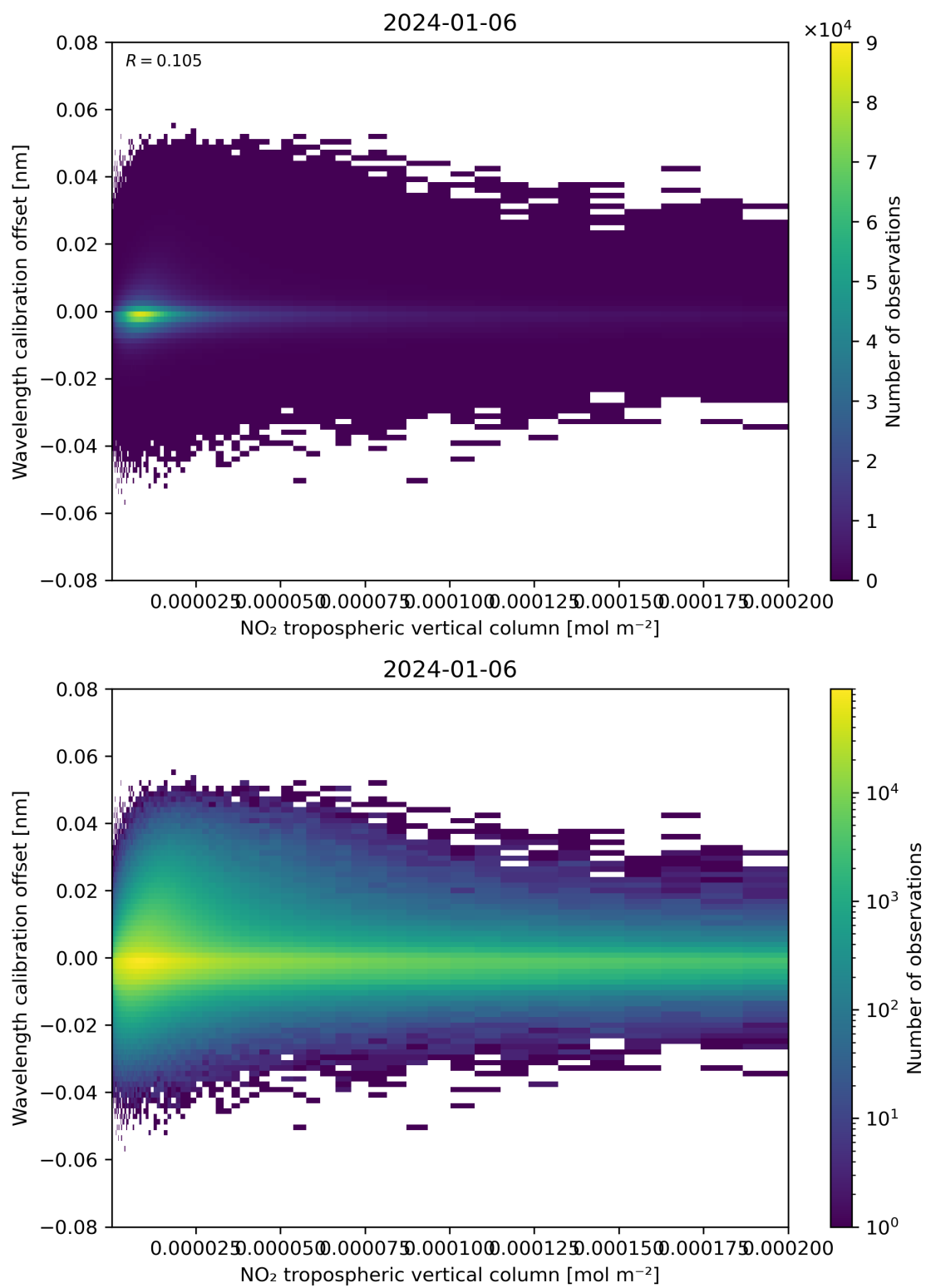
Figure 143: Scatter density plot of “NO 2 tropospheric vertical column” against “Wavelength calibration offset” for 2024-01-05 to 2024-01-07.
