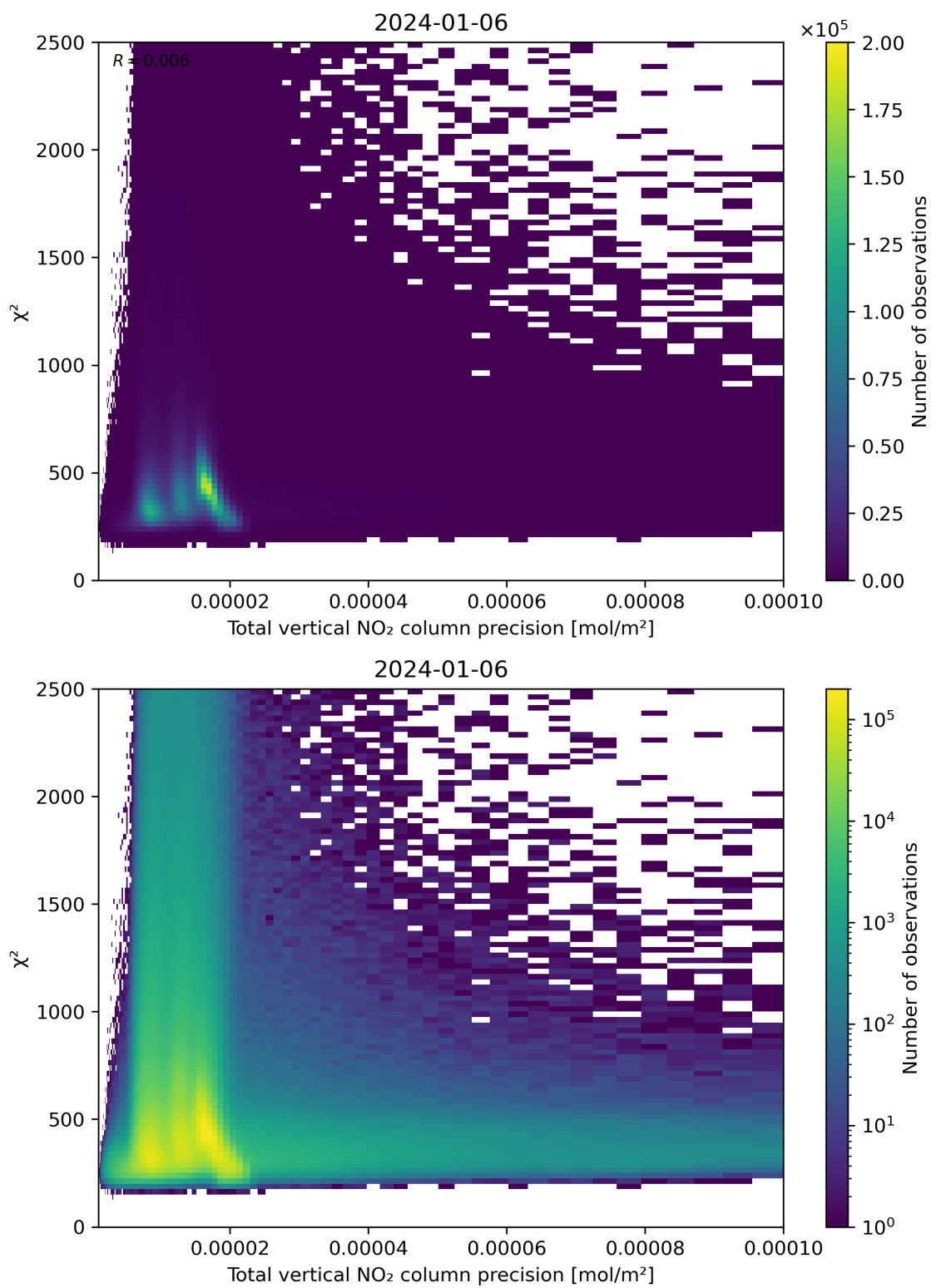
Figure 116: Scatter density plot of “Total vertical NO 2 column precision” against “ \chi^2 ” for 2024-01-05 to 2024-01-07.
