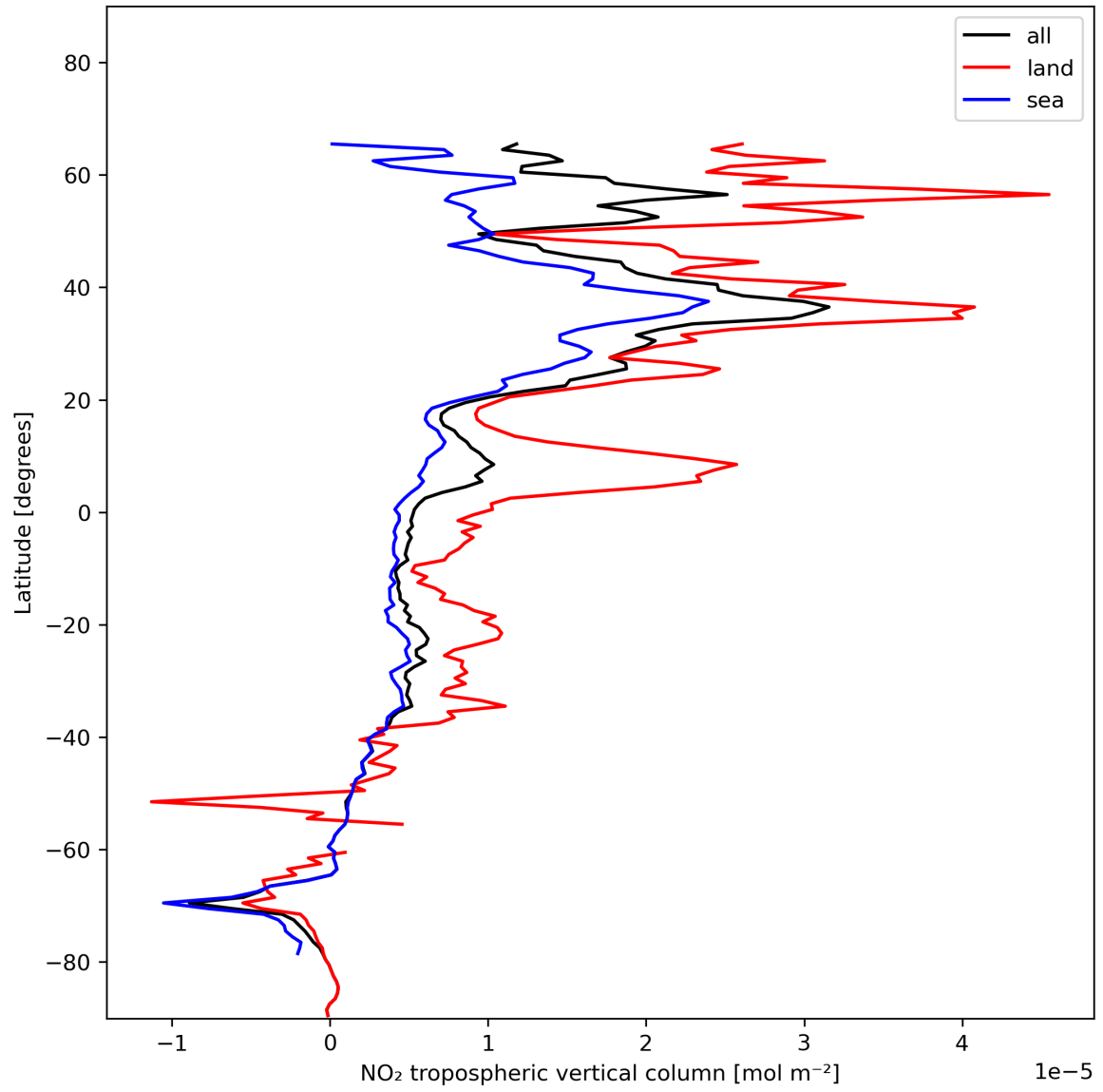
Figure 12: Zonal average of “NO 2 tropospheric vertical column” for 2024-01-05 to 2024-01-07.
