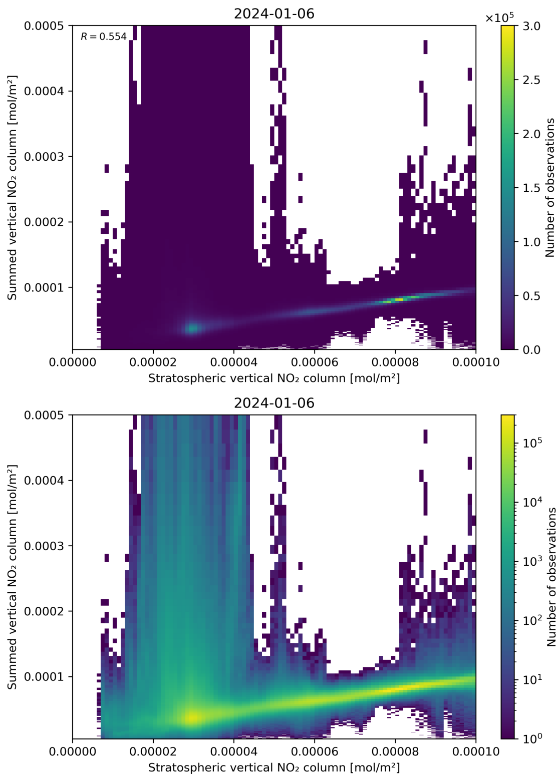
Figure 98: Scatter density plot of “Stratospheric vertical NO 2 column” against “Summed vertical NO 2 column” for 2024-01-05 to 2024-01-07.
