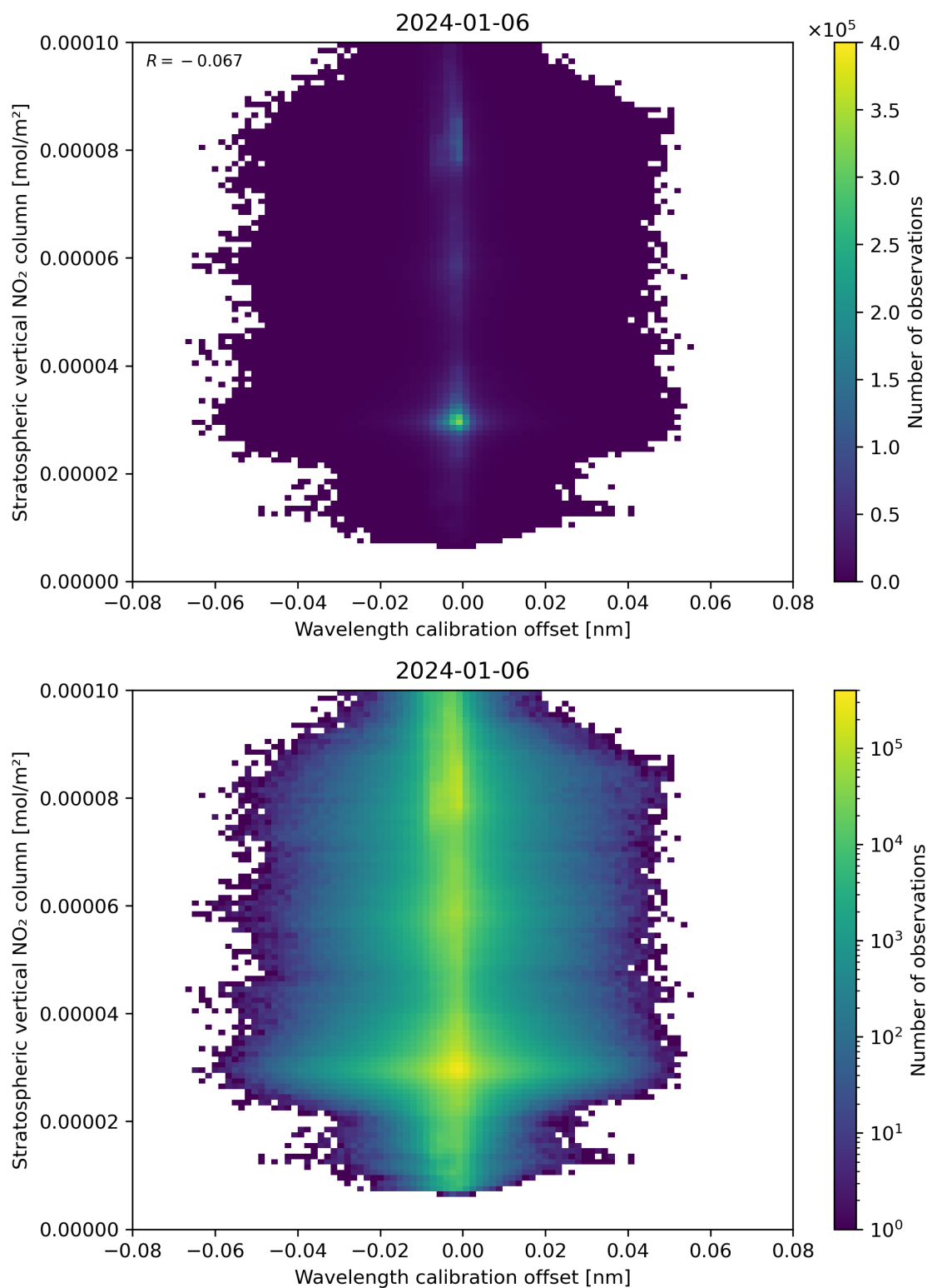
Figure 176: Scatter density plot of “Wavelength calibration offset” against “Stratospheric vertical NO 2 column” for 2024-01-05 to 2024-01-07.
