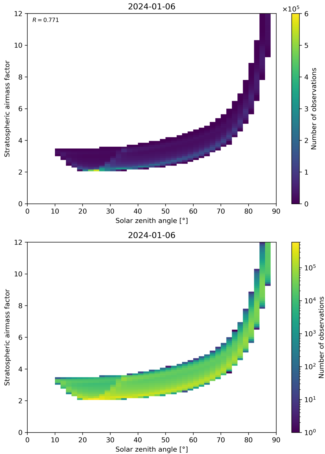
Figure 145: Scatter density plot of “Solar zenith angle” against “Stratospheric airmass factor” for 2024-01-05 to 2024-01-07.
