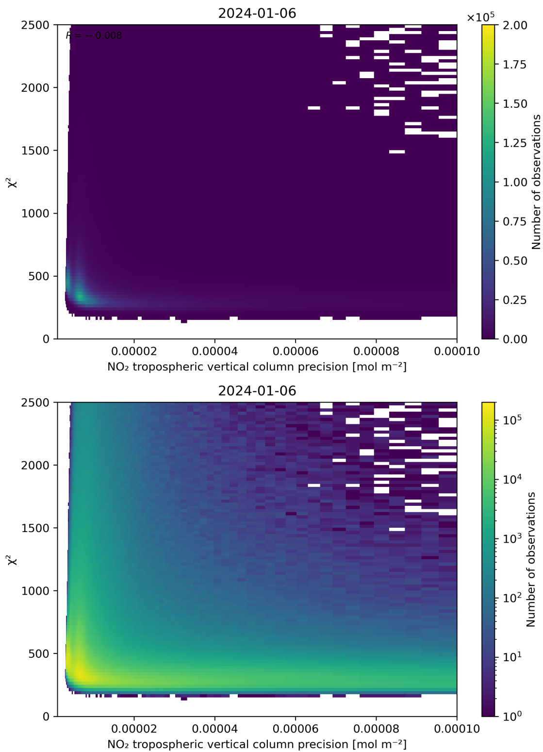
Figure 134: Scatter density plot of “NO 2 tropospheric vertical column precision” against “ \chi^2 ” for 2024-01-05 to 2024-01-07.
