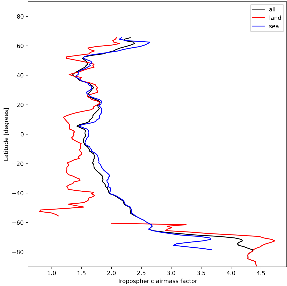
Figure 14: Zonal average of “Tropospheric airmass factor” for 2024-01-05 to 2024-01-07.
