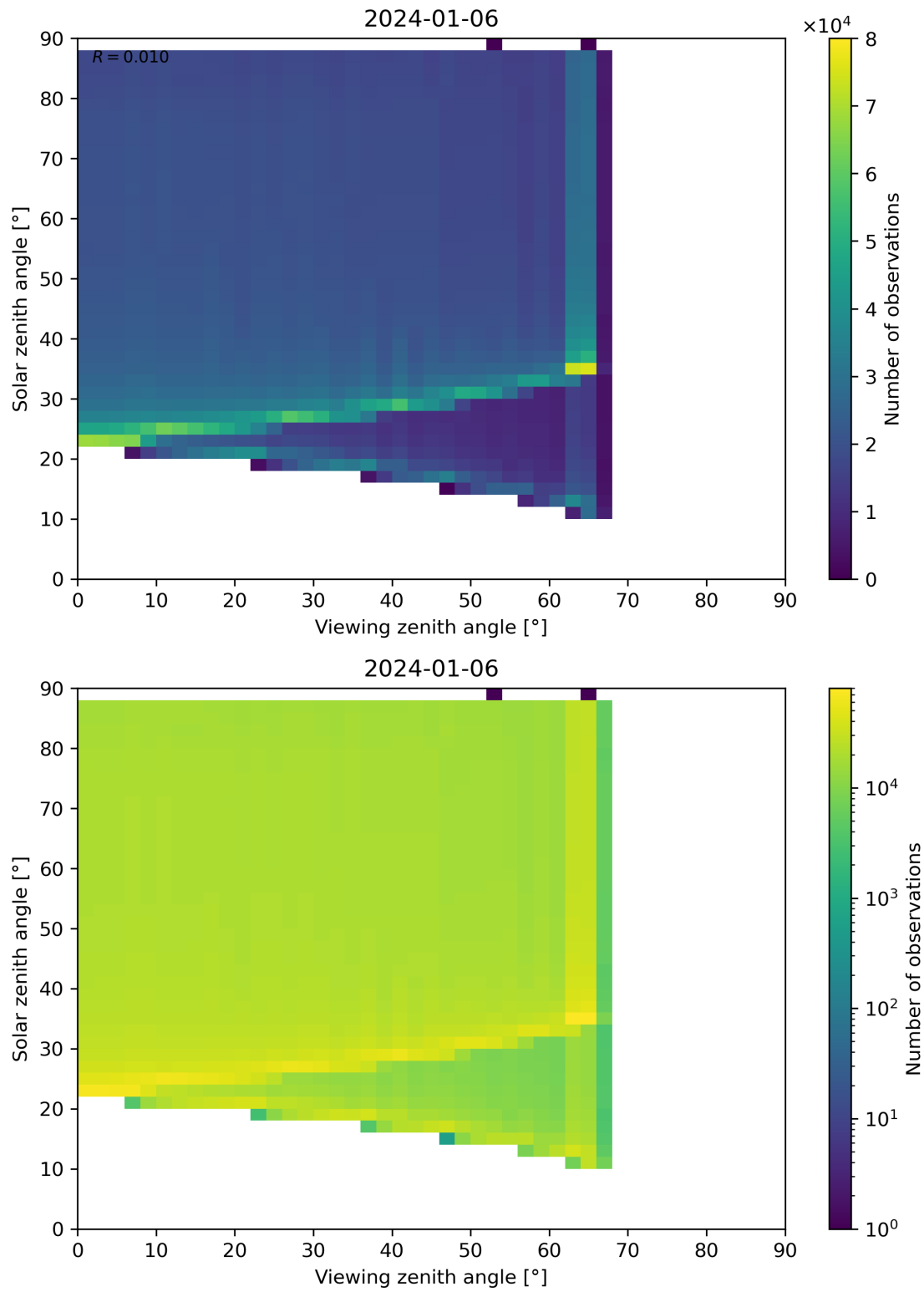
Figure 172: Scatter density plot of “Viewing zenith angle” against “Solar zenith angle” for 2024-01-05 to 2024-01-07.
