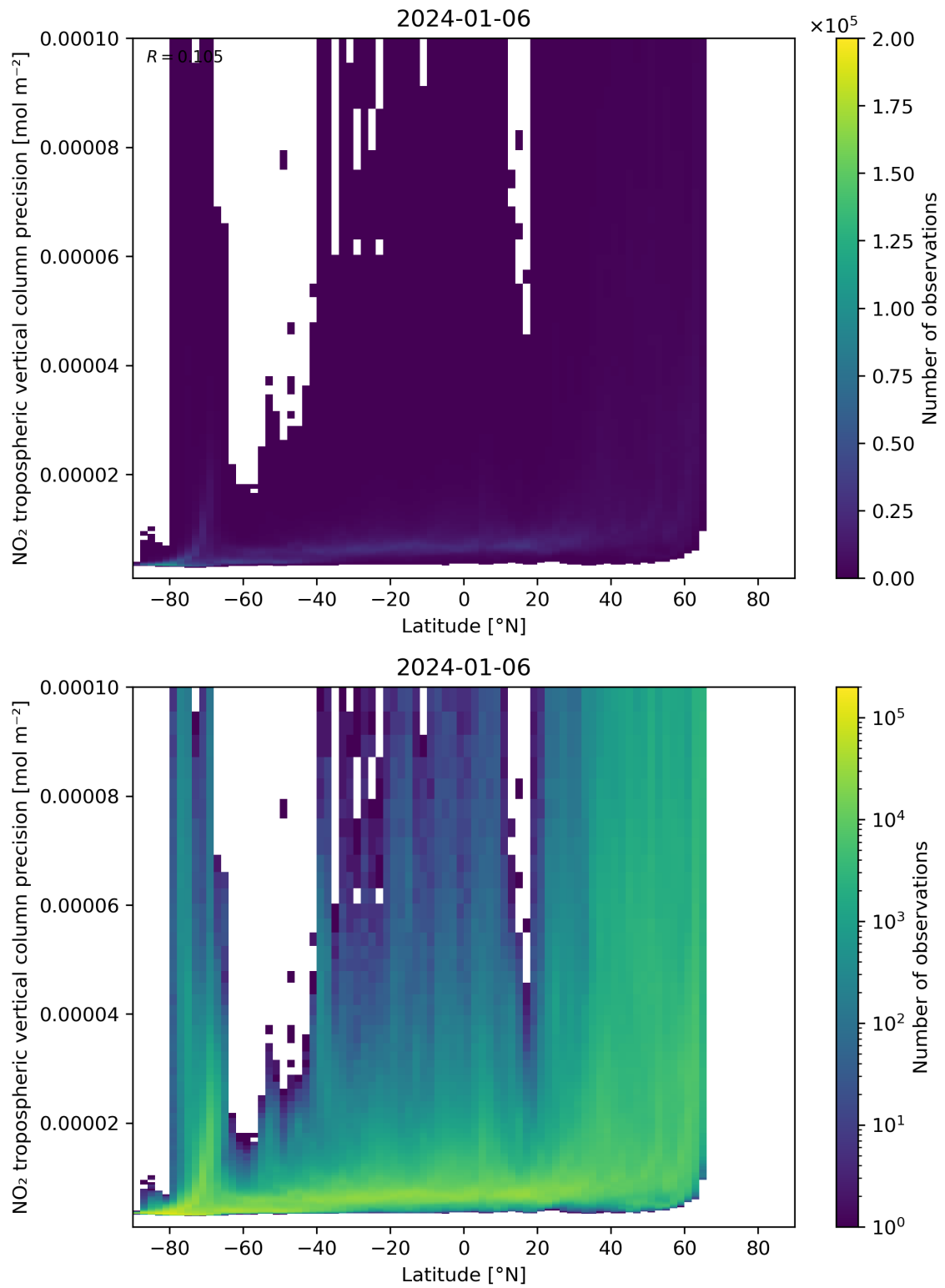
Figure 93: Scatter density plot of “Latitude” against “NO 2 tropospheric vertical column precision” for 2024-01-05 to 2024-01-07.
