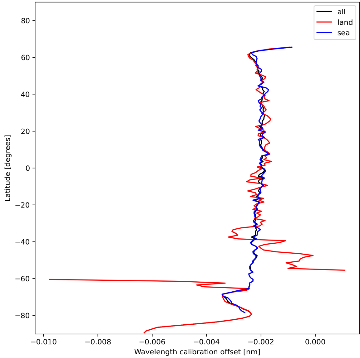
Figure 18: Zonal average of “Wavelength calibration offset” for 2024-01-05 to 2024-01-07.
