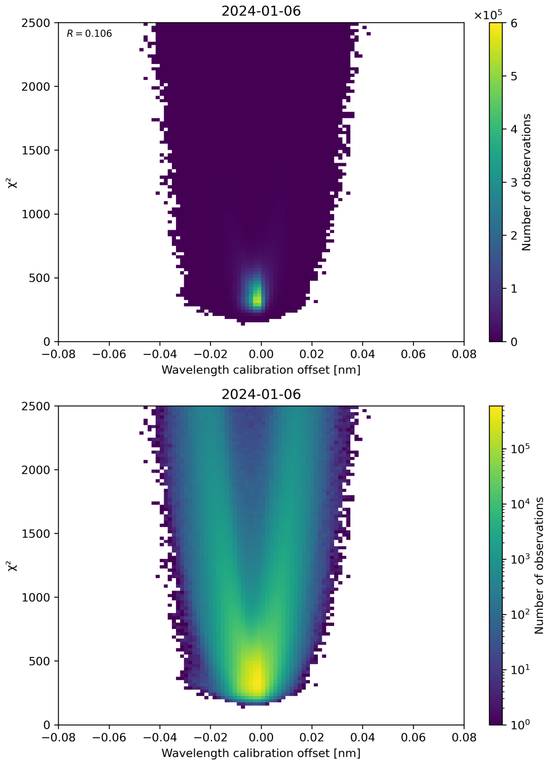
Figure 175: Scatter density plot of “Wavelength calibration offset” against “ \chi^2 ” for 2024-01-05 to 2024-01-07.
