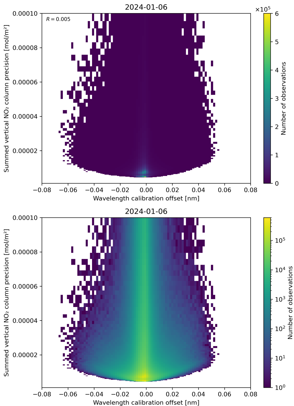
Figure 178: Scatter density plot of “Wavelength calibration offset” against “Summed vertical NO 2 column precision” for 2024-01-05 to 2024-01-07.
