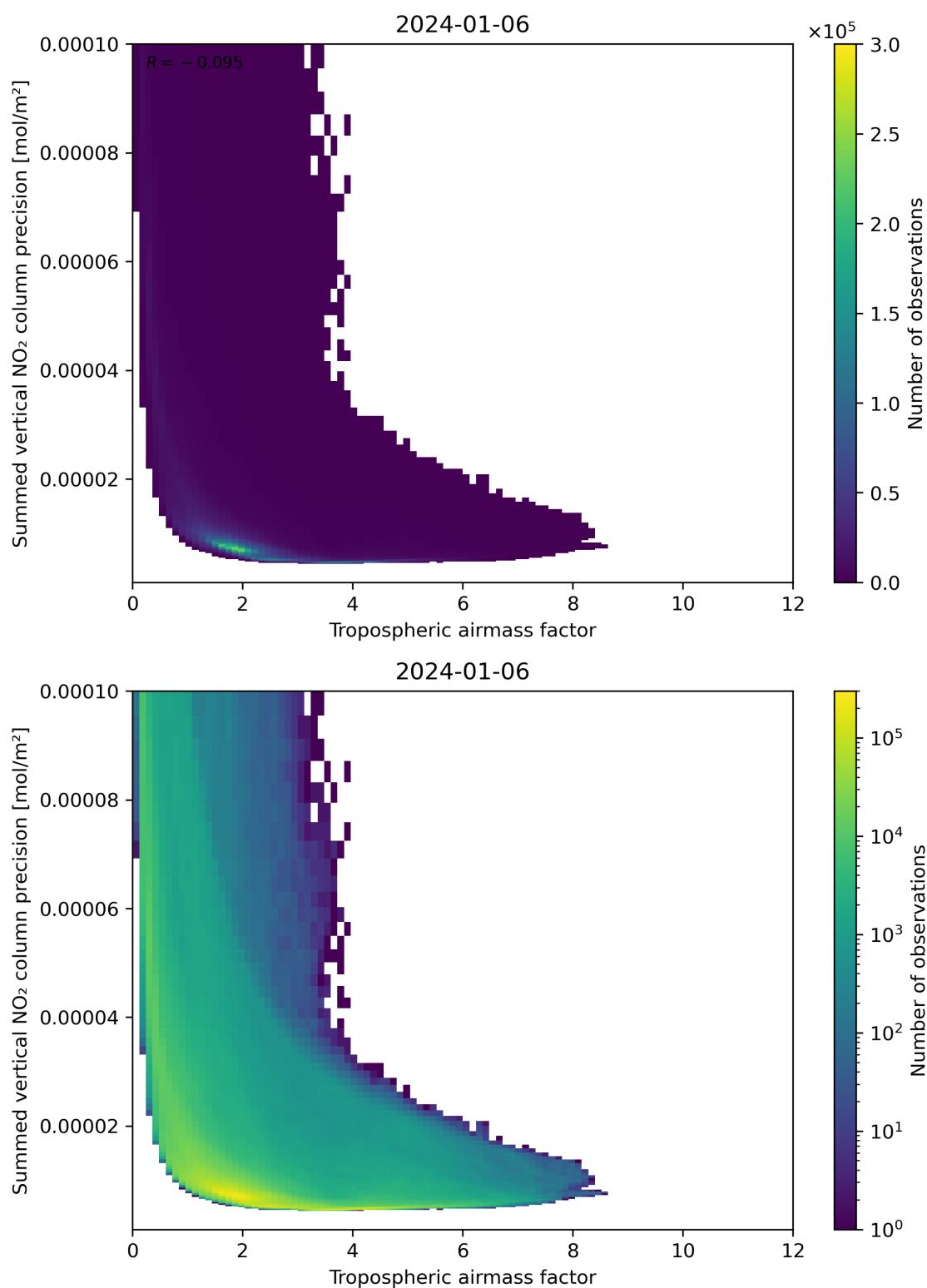
Figure 76: Scatter density plot of “Tropospheric air mass factor” against “Summed vertical NO 2 column precision” for 2024-01-05 to 2024-01-07.
