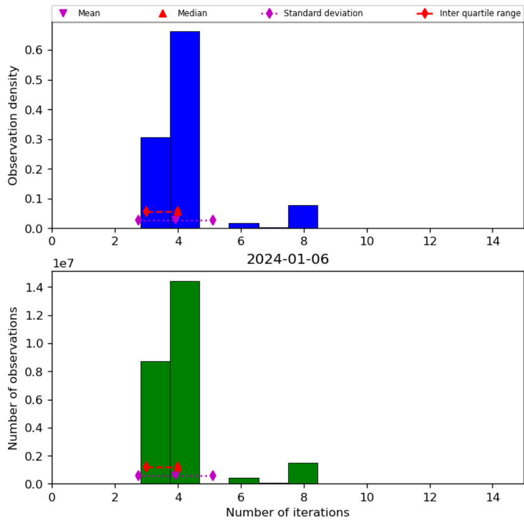
Figure 34: Histogram of “Number of iterations” for 2024-01-05 to 2024-01-07
