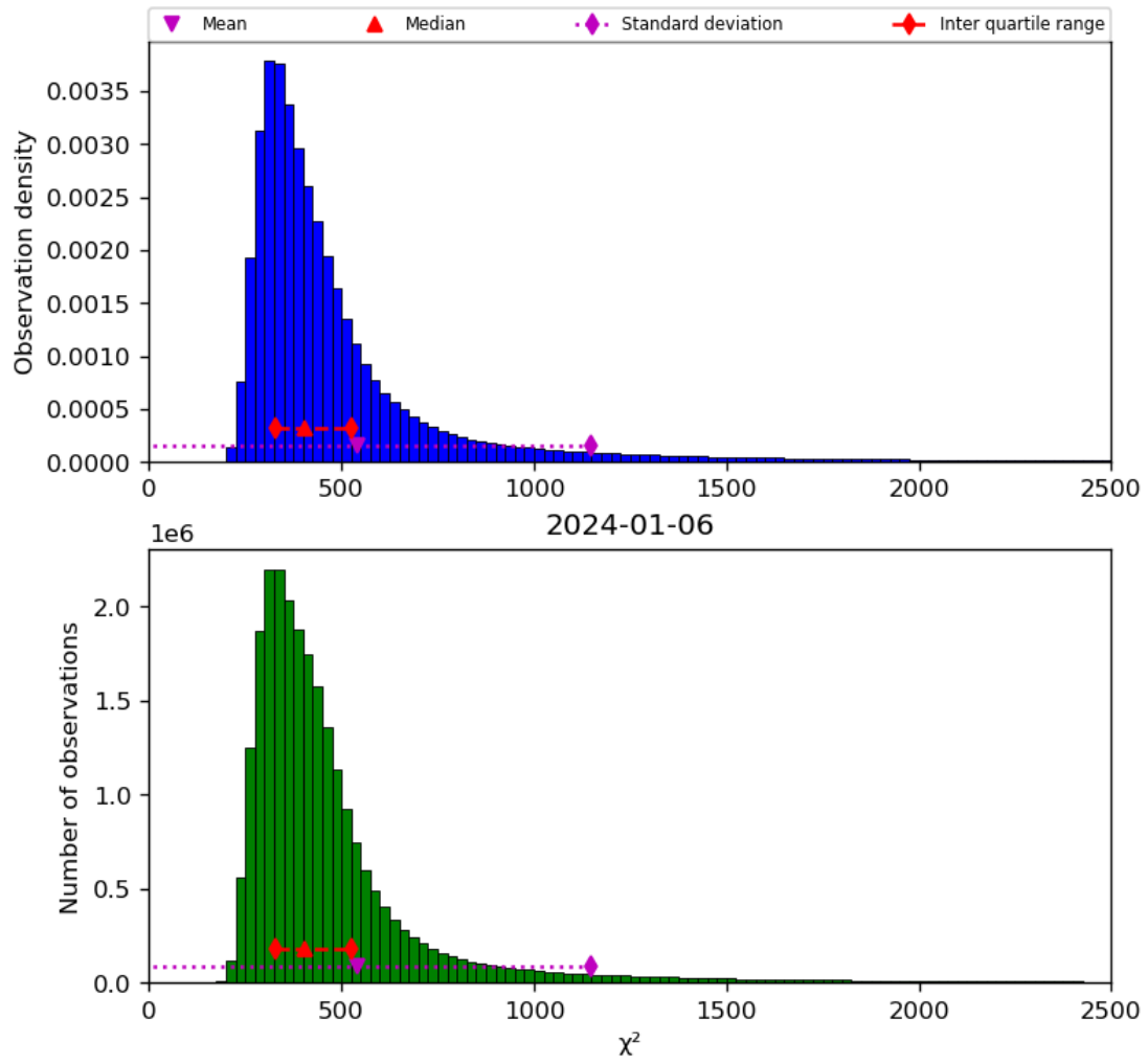
Figure 42: Histogram of “ \chi^2 ” for 2024-01-05 to 2024-01-07
