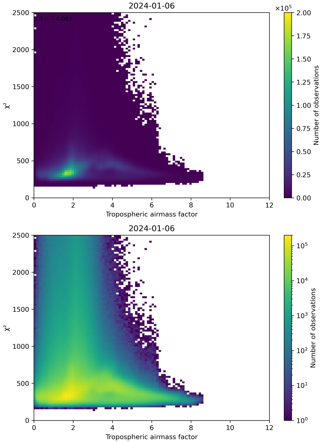
Figure 73: Scatter density plot of “Tropospheric airmass factor” against “ \chi^2 ” for 2024-01-05 to 2024-01-07.
