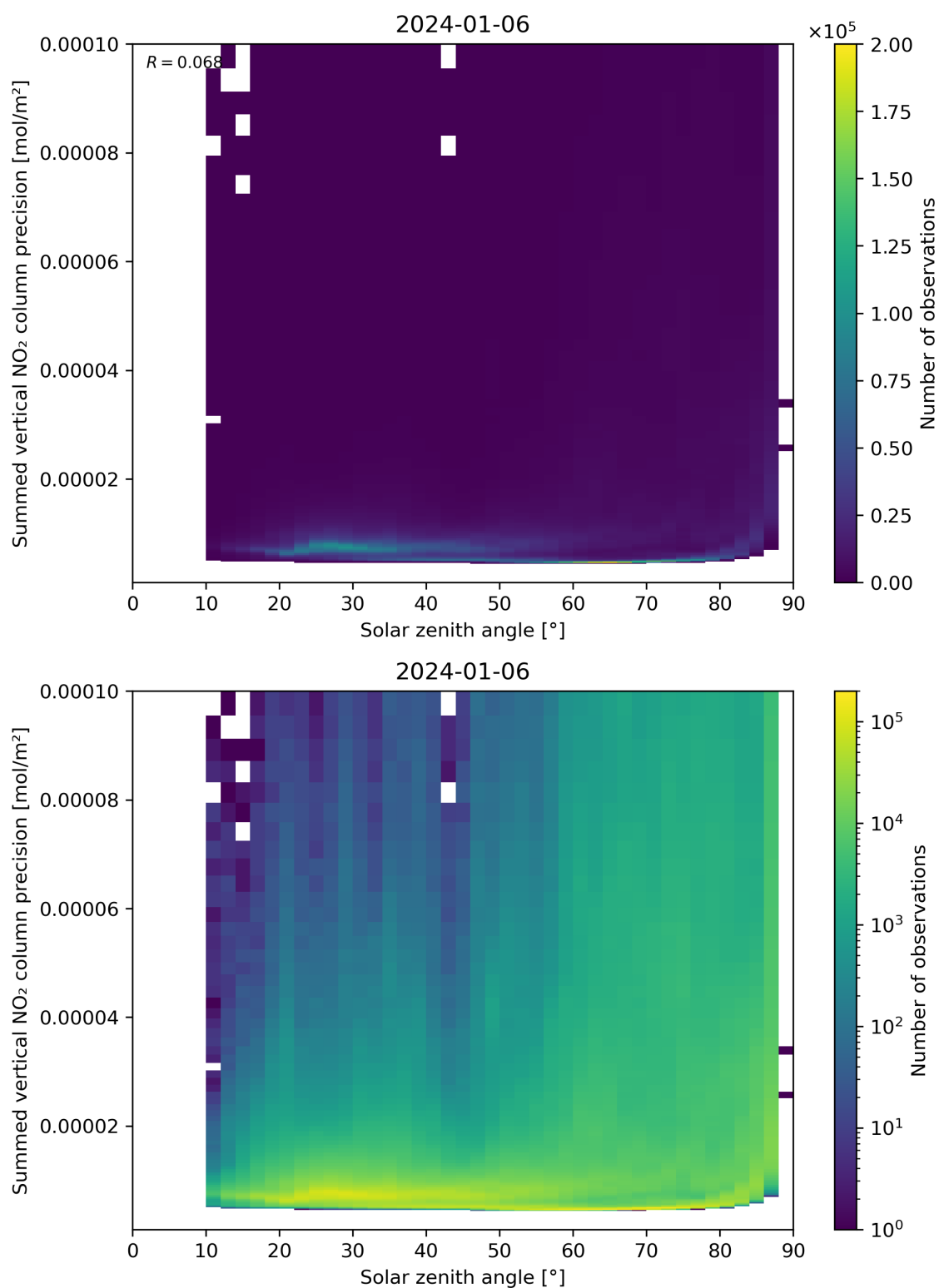
Figure 152: Scatter density plot of “Solar zenith angle” against “Summed vertical NO 2 column precision” for 2024-01-05 to 2024-01-07.
