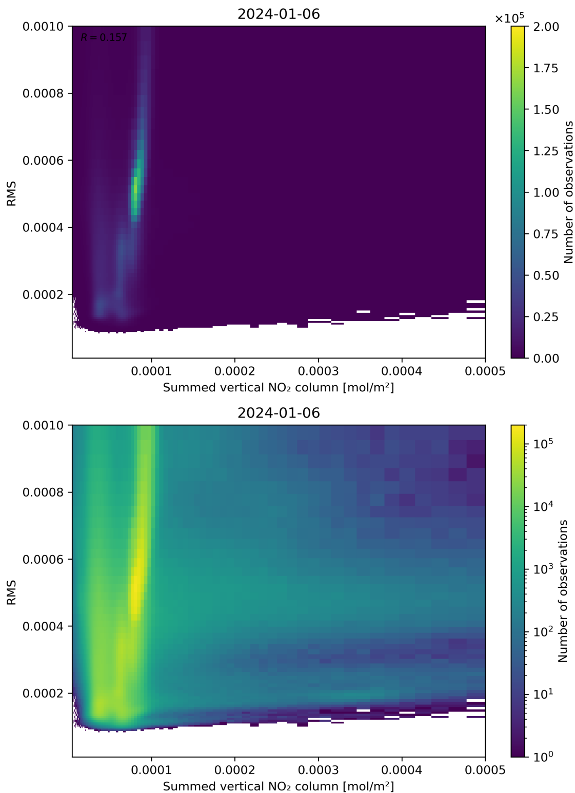
Figure 109: Scatter density plot of “Summed vertical NO 2 column” against “RMS” for 2024-01-05 to 2024-01-07.
