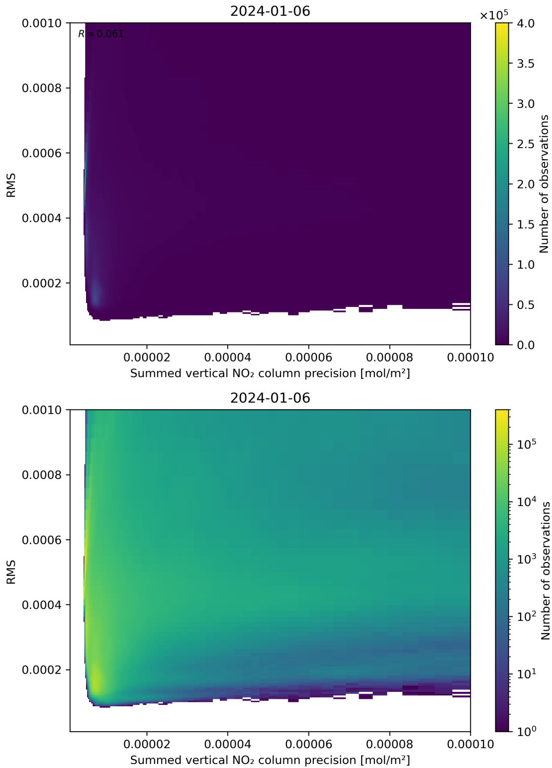
Figure 108: Scatter density plot of “Summed vertical NO 2 column precision” against “RMS” for 2024-01-05 to 2024-01-07.
