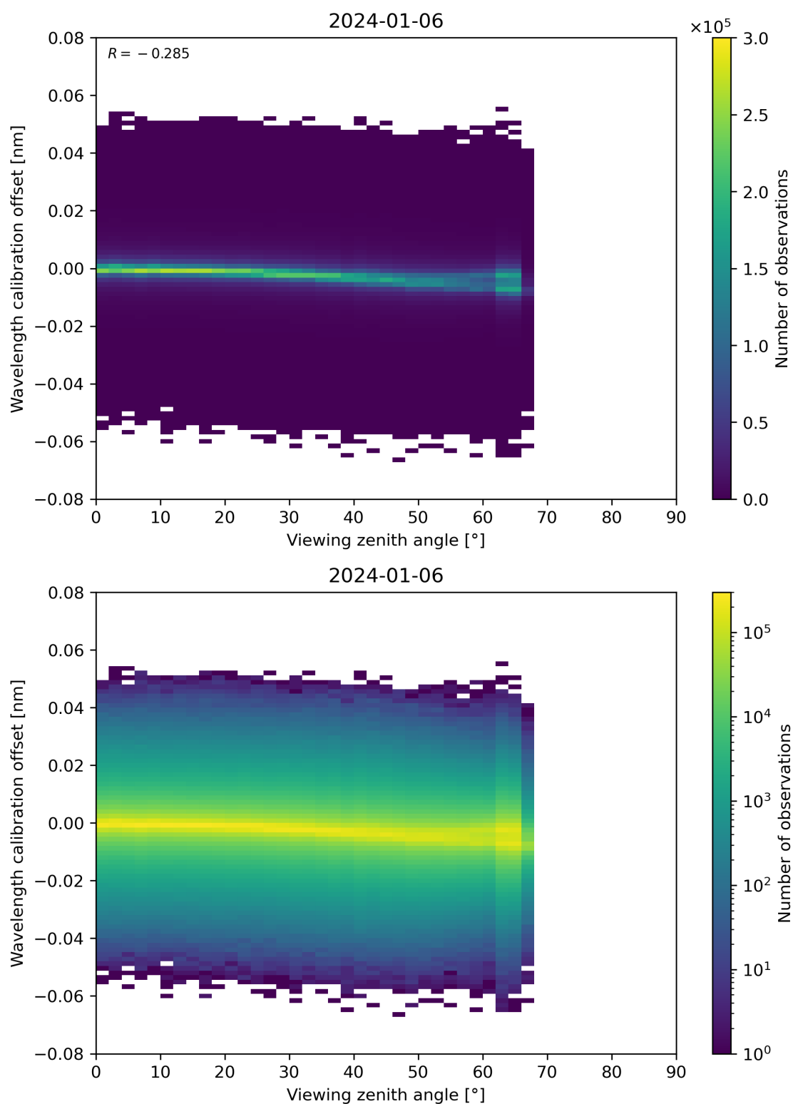
Figure 173: Scatter density plot of “Viewing zenith angle” against “Wavelength calibration offset” for 2024-01-05 to 2024-01-07.
