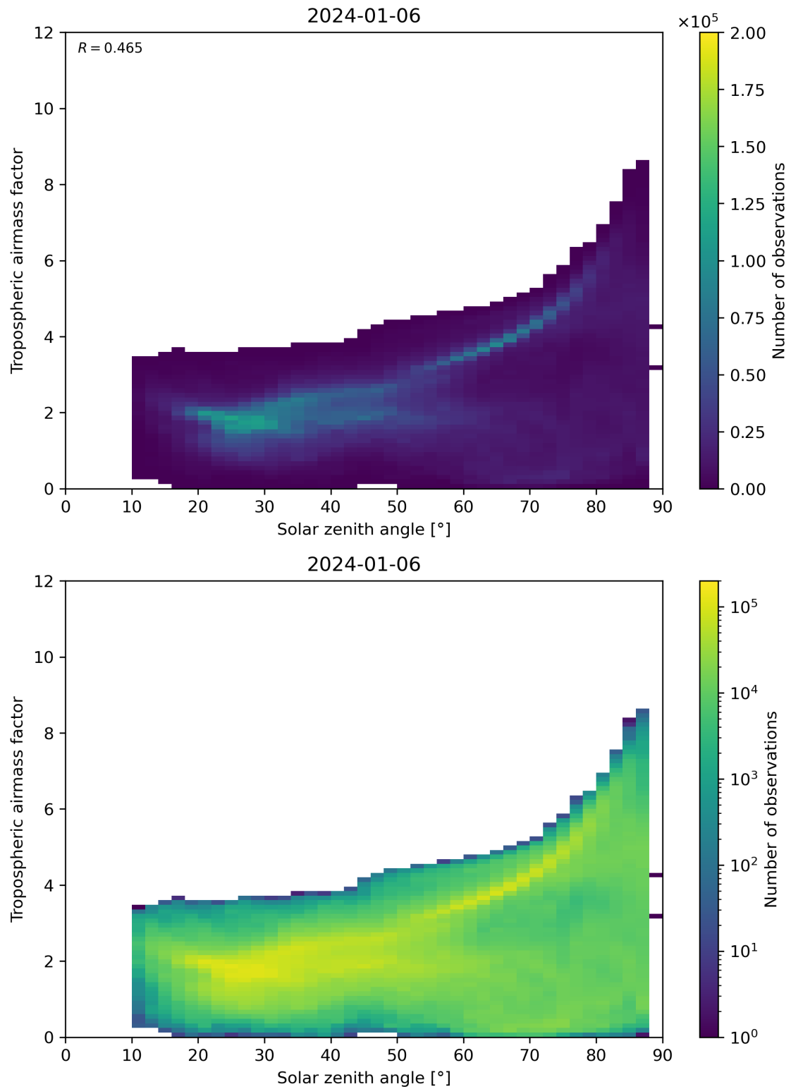
Figure 147: Scatter density plot of “Solar zenith angle” against “Tropospheric airmass factor” for 2024-01-05 to 2024-01-07.
