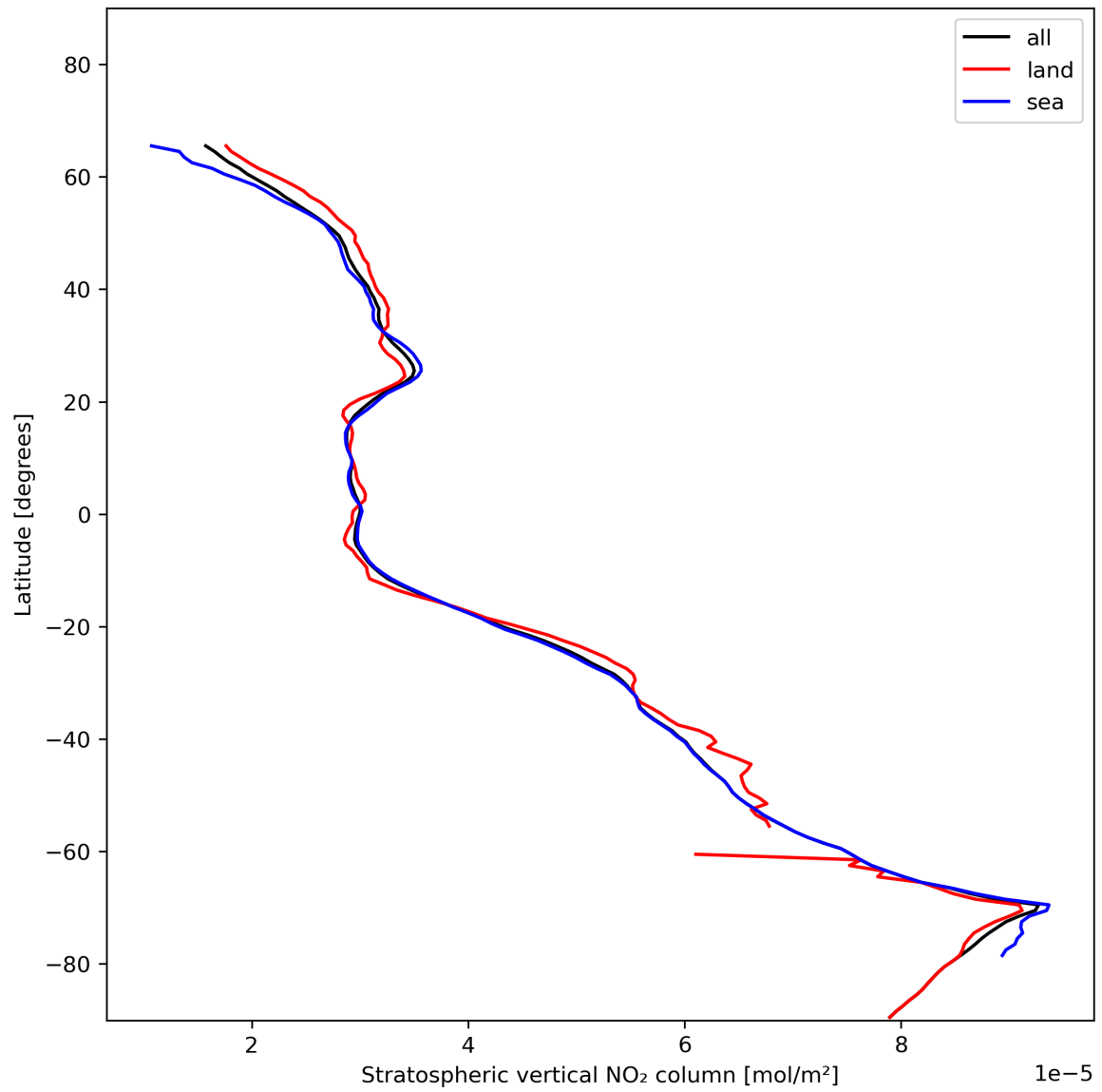
Figure 19: Zonal average of “Stratospheric vertical NO 2 column” for 2024-01-05 to 2024-01-07.
