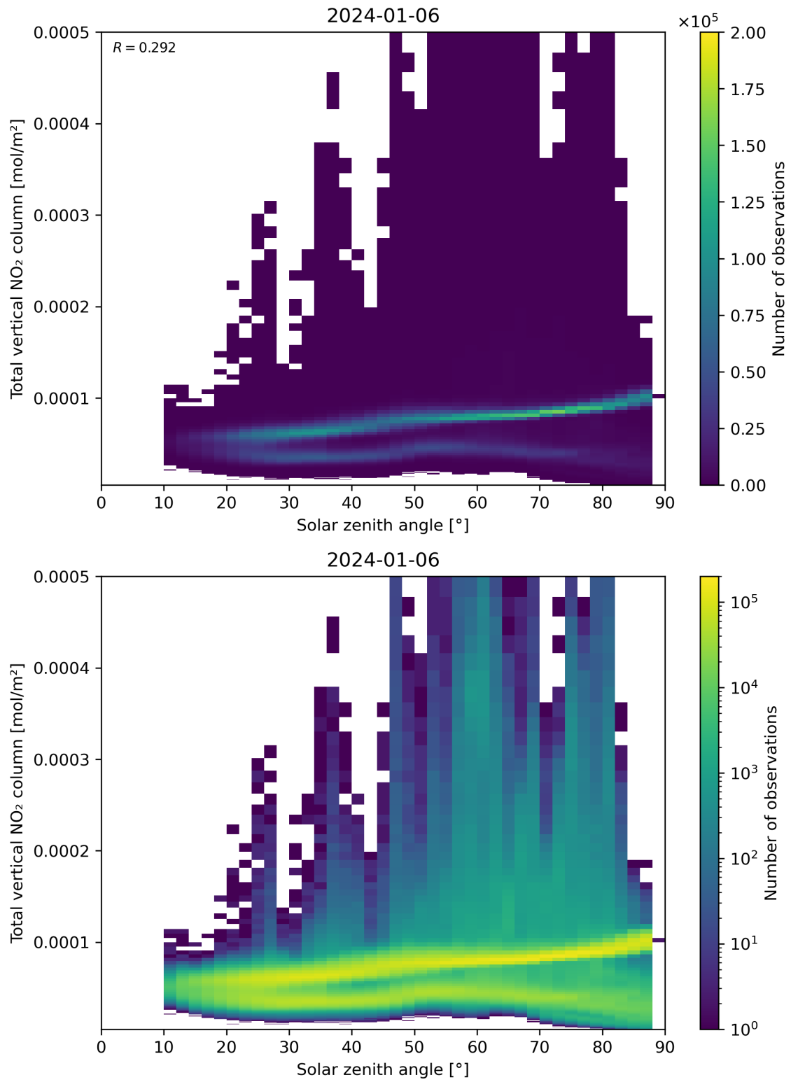
Figure 153: Scatter density plot of “Solar zenith angle” against “Total vertical NO 2 column” for 2024-01-05 to 2024-01-07.
