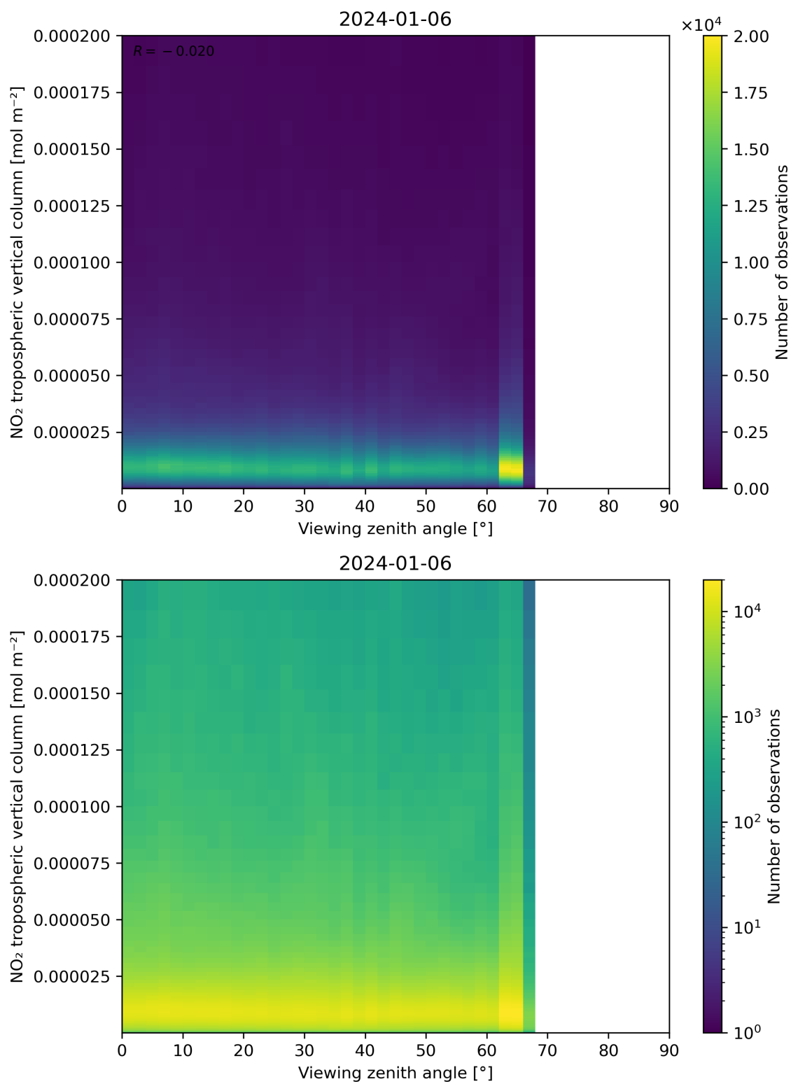
Figure 169: Scatter density plot of “Viewing zenith angle” against “NO 2 tropospheric vertical column” for 2024-01-05 to 2024-01-07.
