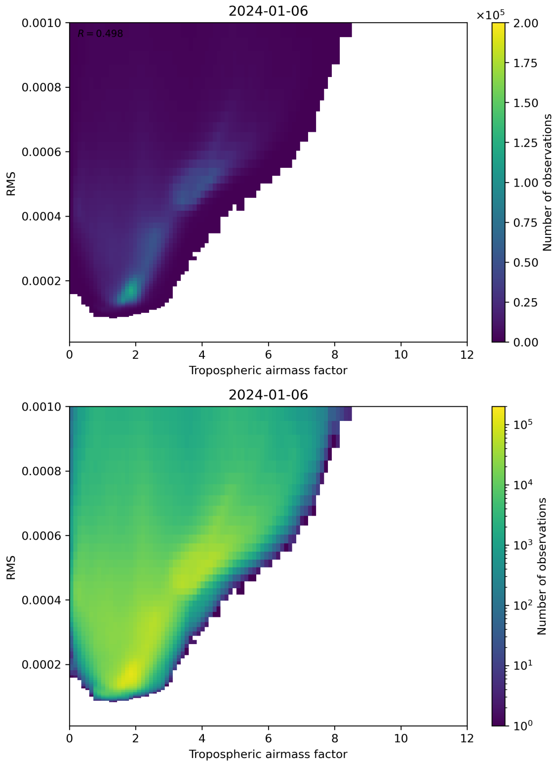
Figure 79: Scatter density plot of “Tropospheric airmass factor” against “RMS” for 2024-01-05 to 2024-01-07.
