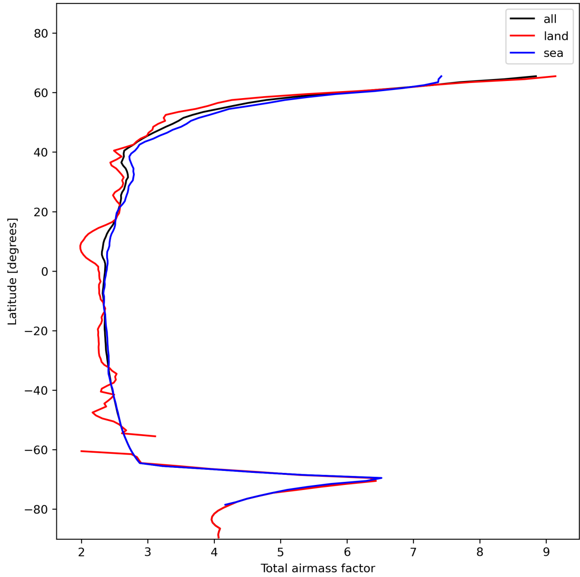
Figure 15: Zonal average of “Total airmass factor” for 2024-01-05 to 2024-01-07.
