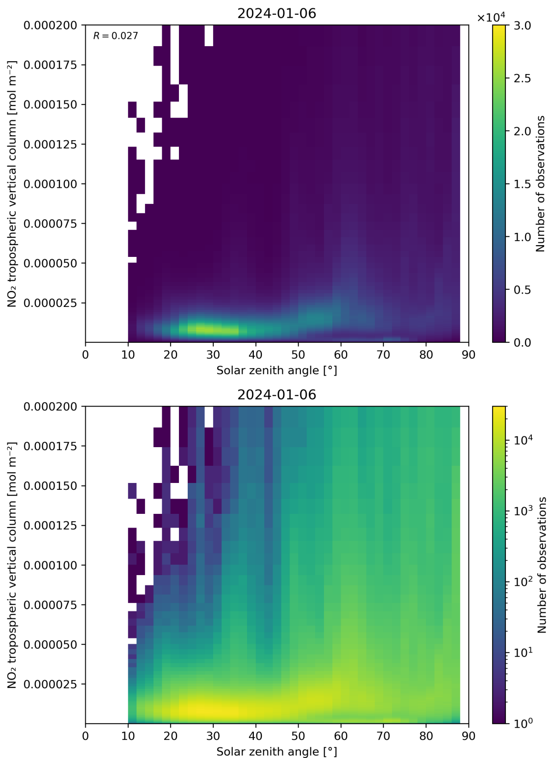
Figure 155: Scatter density plot of “Solar zenith angle” against “NO 2 tropospheric vertical column” for 2024-01-05 to 2024-01-07.
