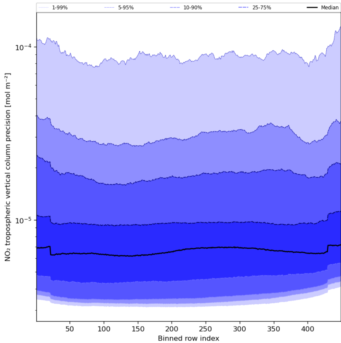
Figure 47: Along track statistics of “NO 2 tropospheric vertical column precision” for 2024-01-05 to 2024-01-07
