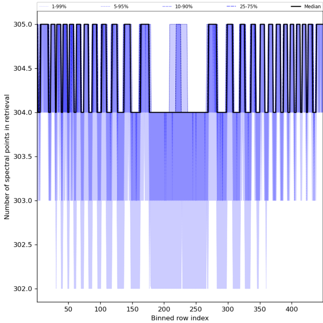
Figure 50: Along track statistics of “Number of spectral points in retrieval” for 2024-01-05 to 2024-01-07
