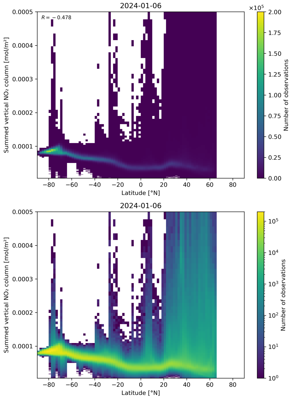
Figure 88: Scatter density plot of “Latitude” against “Summed vertical NO 2 column” for 2024-01-05 to 2024-01-07.
