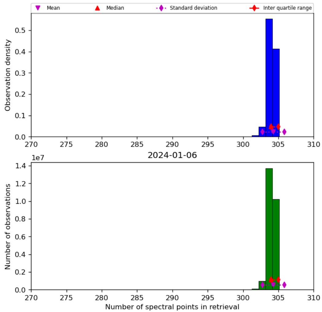
Figure 33: Histogram of “Number of spectral points in retrieval” for 2024-01-05 to 2024-01-07
