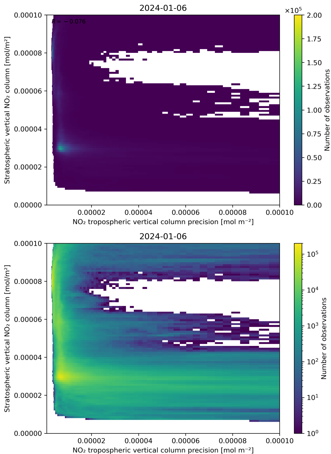
Figure 135: Scatter density plot of “NO 2 tropospheric vertical column precision” against “Stratospheric vertical NO 2 column” for 2024-01-05 to 2024-01-07.
