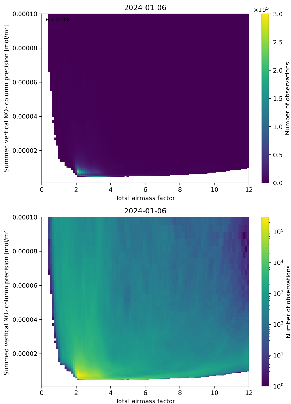
Figure 66: Scatter density plot of “Total airmass factor” against “Summed vertical NO 2 column precision” for 2024-01-05 to 2024-01-07.
