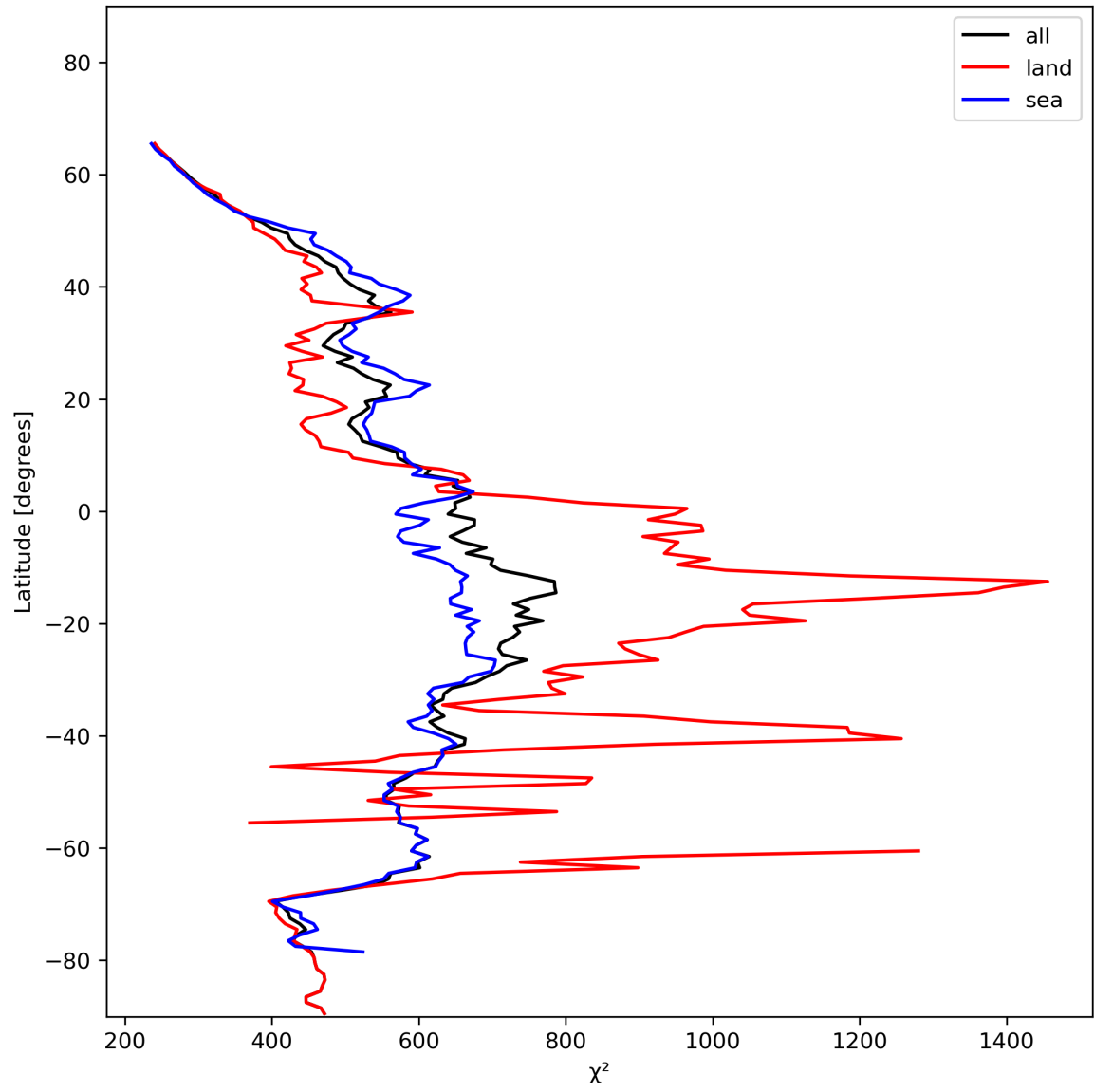
Figure 25: Zonal average of “ \chi^2 ” for 2024-01-05 to 2024-01-07.
