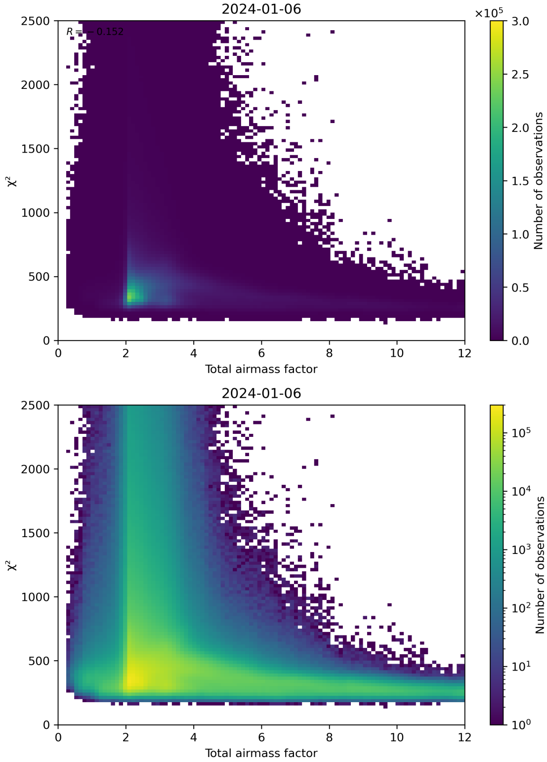
Figure 63: Scatter density plot of “Total airmass factor” against “ \chi^2 ” for 2024-01-05 to 2024-01-07.
