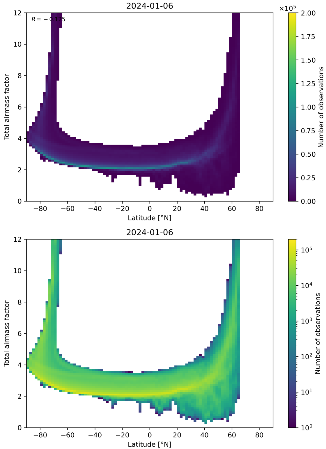
Figure 84: Scatter density plot of “Latitude” against “Total airmass factor” for 2024-01-05 to 2024-01-07.
