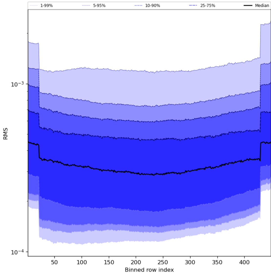
Figure 60: Along track statistics of “RMS” for 2024-01-05 to 2024-01-07
