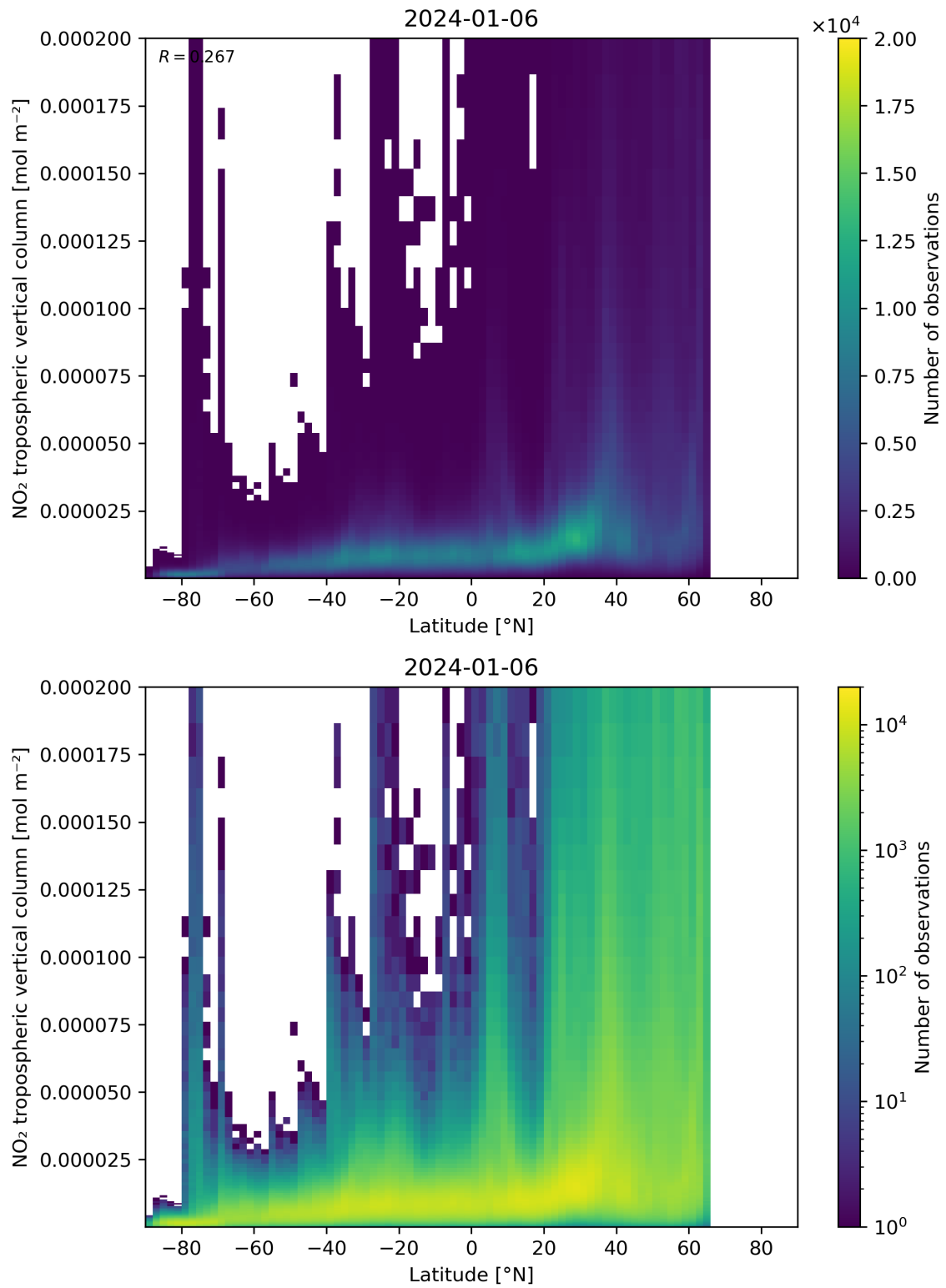
Figure 92: Scatter density plot of “Latitude” against “NO 2 tropospheric vertical column” for 2024-01-05 to 2024-01-07.
