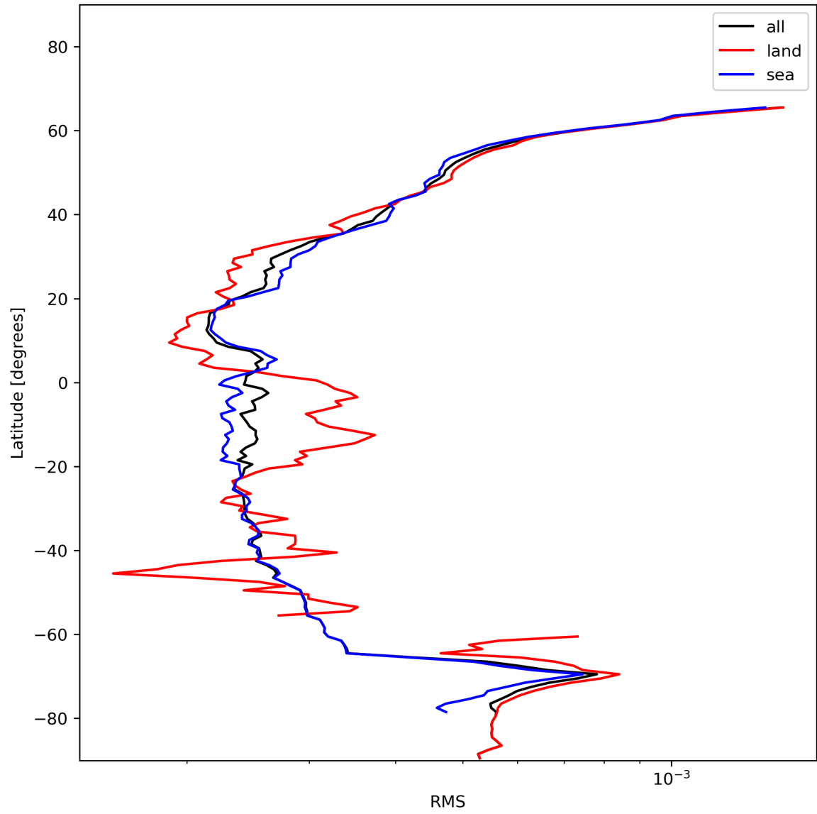
Figure 26: Zonal average of “RMS” for 2024-01-05 to 2024-01-07.
