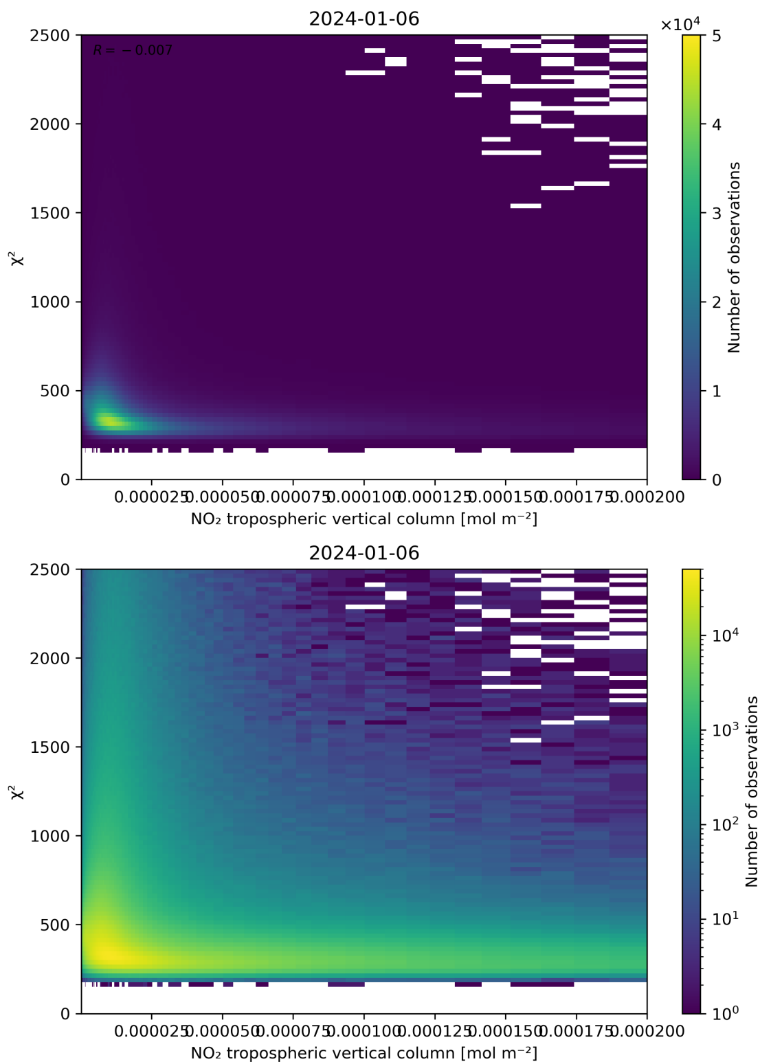
Figure 124: Scatter density plot of “NO 2 tropospheric vertical column” against “ \chi^2 ” for 2024-01-05 to 2024-01-07.
