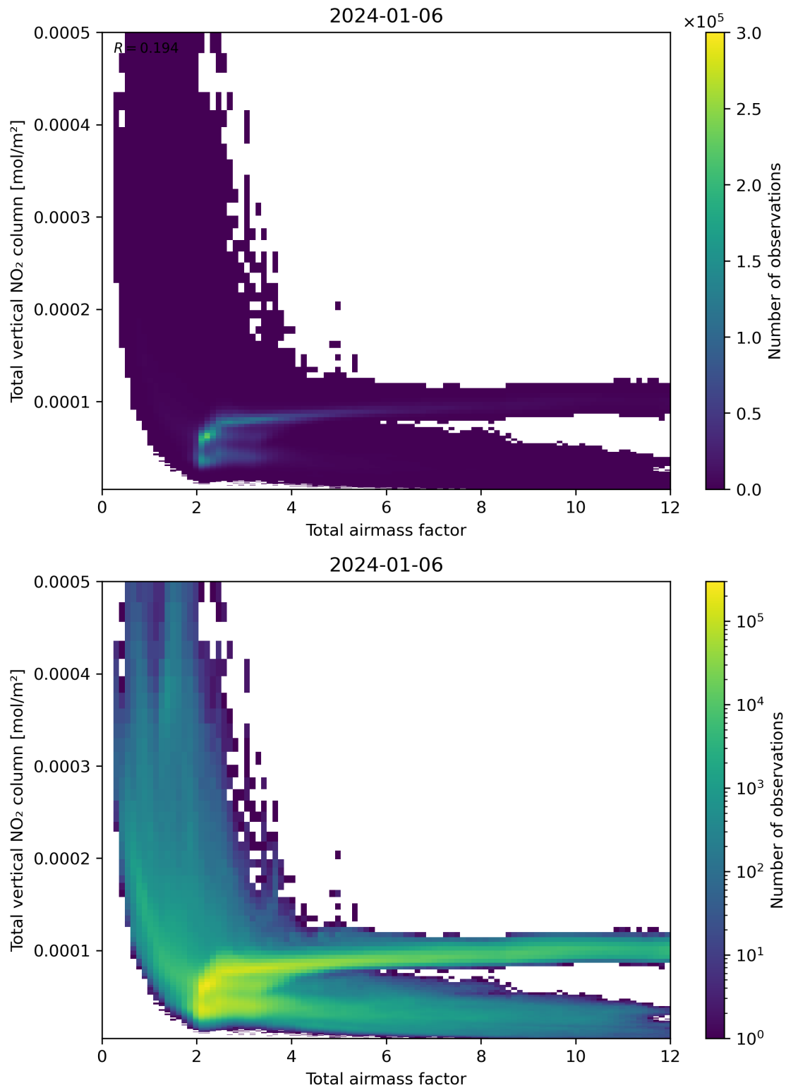
Figure 67: Scatter density plot of “Total airmass factor” against “Total vertical NO 2 column” for 2024-01-05 to 2024-01-07.
