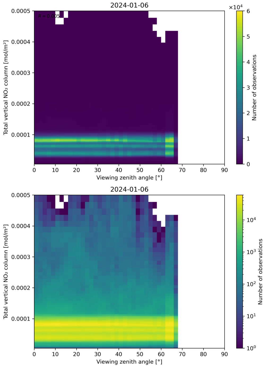
Figure 167: Scatter density plot of “Viewing zenith angle” against “Total vertical NO 2 column” for 2024-01-05 to 2024-01-07.
