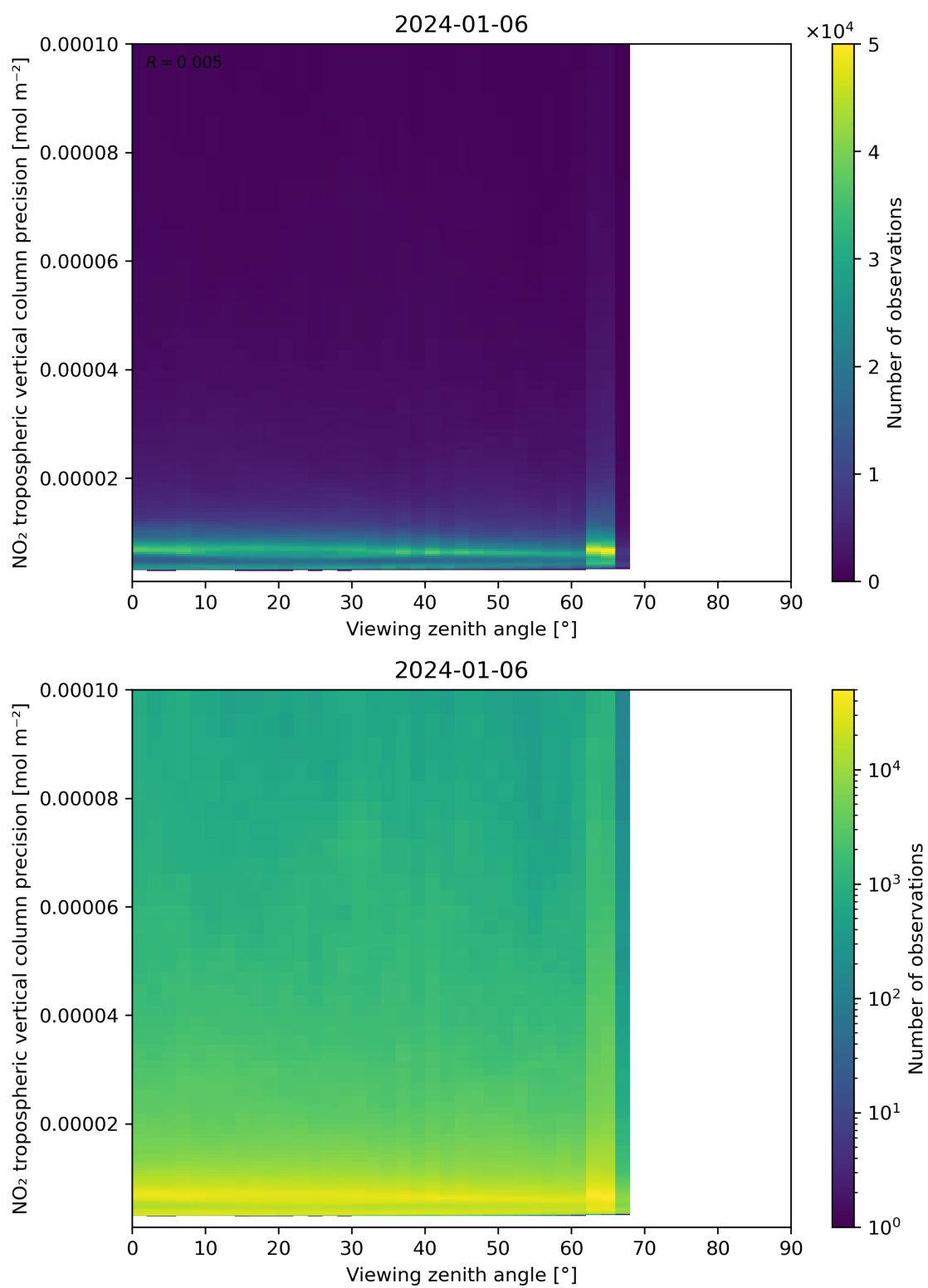
Figure 170: Scatter density plot of “Viewing zenith angle” against “NO 2 tropospheric vertical column precision” for 2024-01-05 to 2024-01-07.
