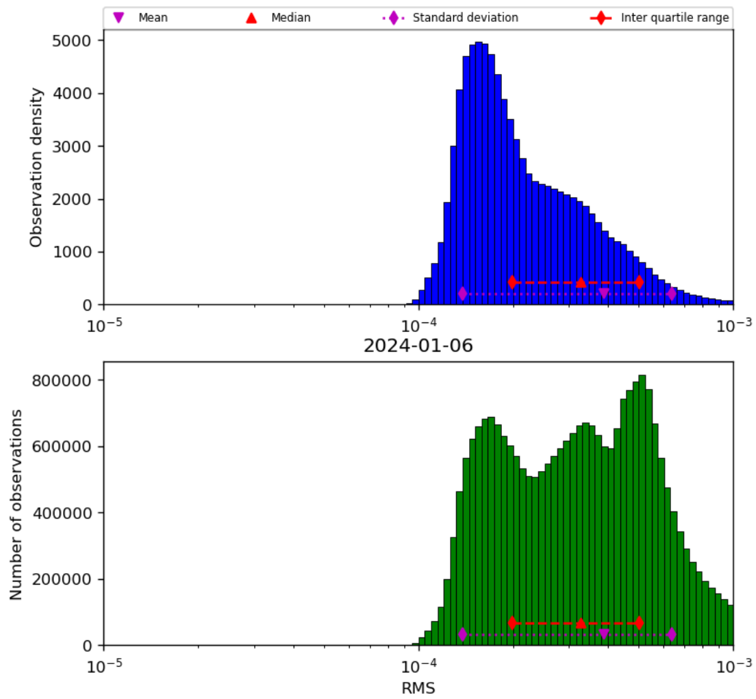
Figure 43: Histogram of “RMS” for 2024-01-05 to 2024-01-07
