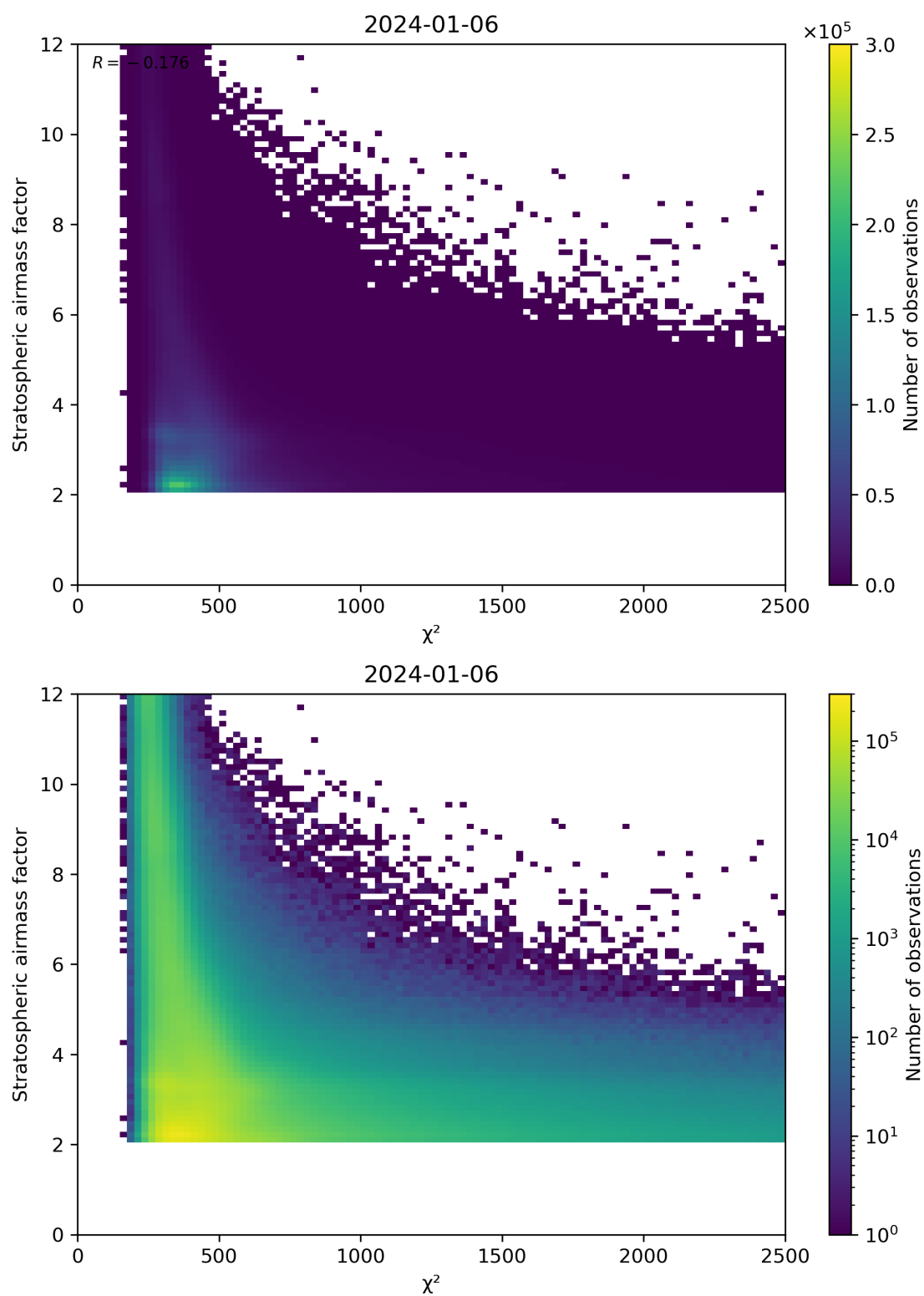
Figure 81: Scatter density plot of “ \chi^2 ” against “Stratospheric airmass factor” for 2024-01-05 to 2024-01-07.
