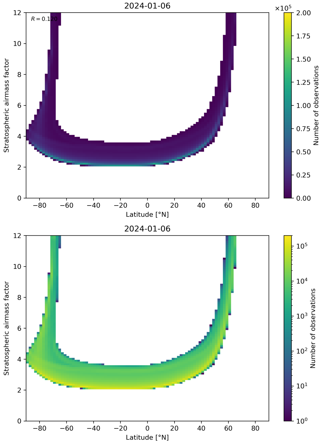
Figure 83: Scatter density plot of “Latitude” against “Stratospheric airmass factor” for 2024-01-05 to 2024-01-07.
