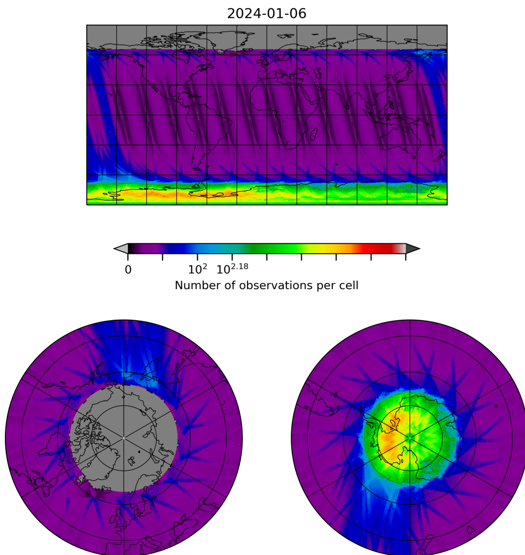
Figure 10: Map of the number of observations for 2024-01-05 to 2024-01-07
