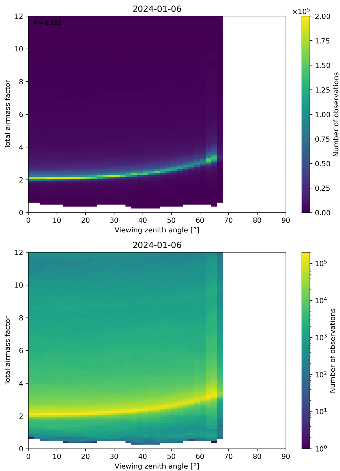
Figure 160: Scatter density plot of “Viewing zenith angle” against “Total airmass factor” for 2024-01-05 to 2024-01-07.
