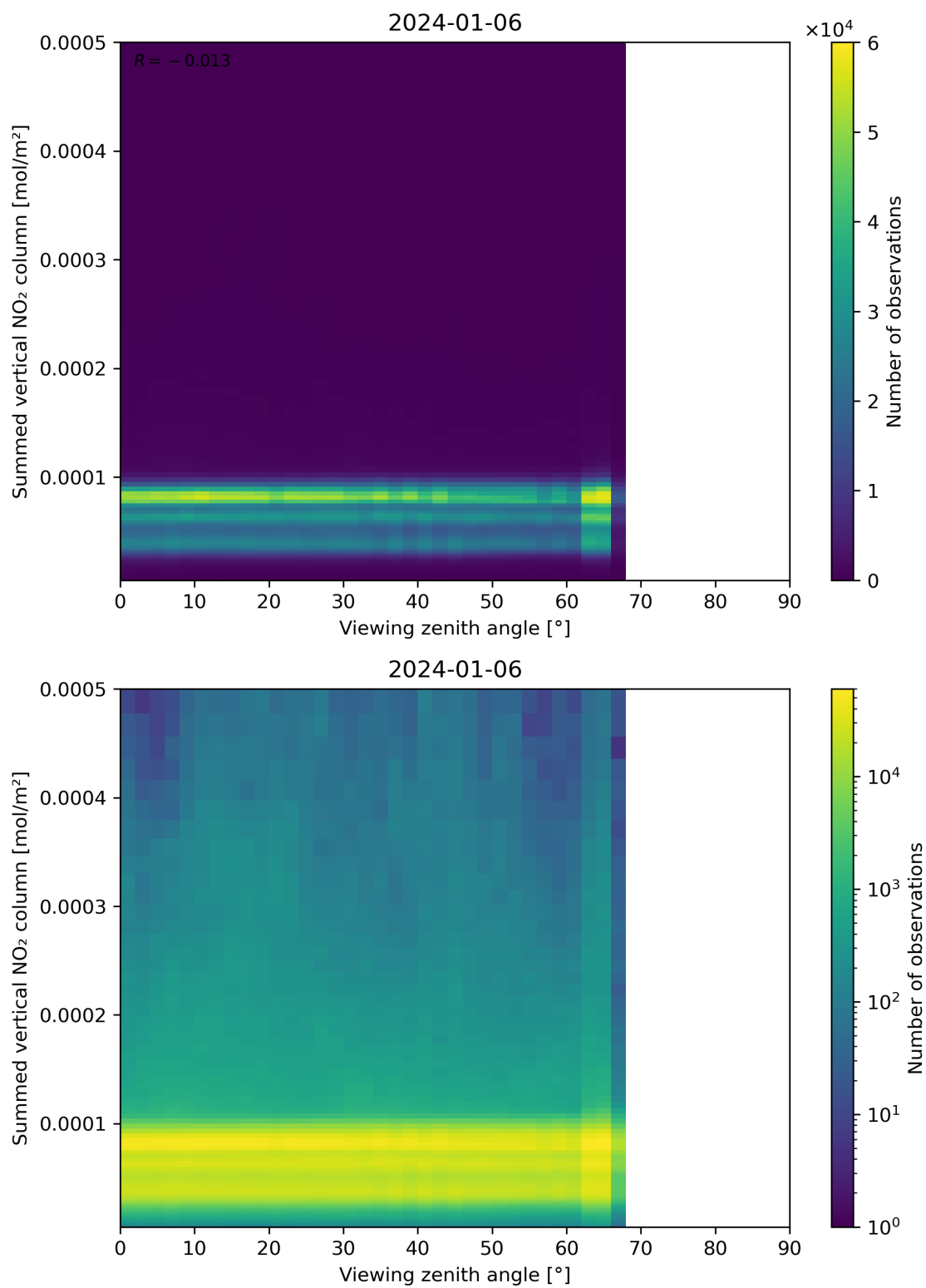
Figure 165: Scatter density plot of “Viewing zenith angle” against “Summed vertical NO 2 column” for 2024-01-05 to 2024-01-07.
