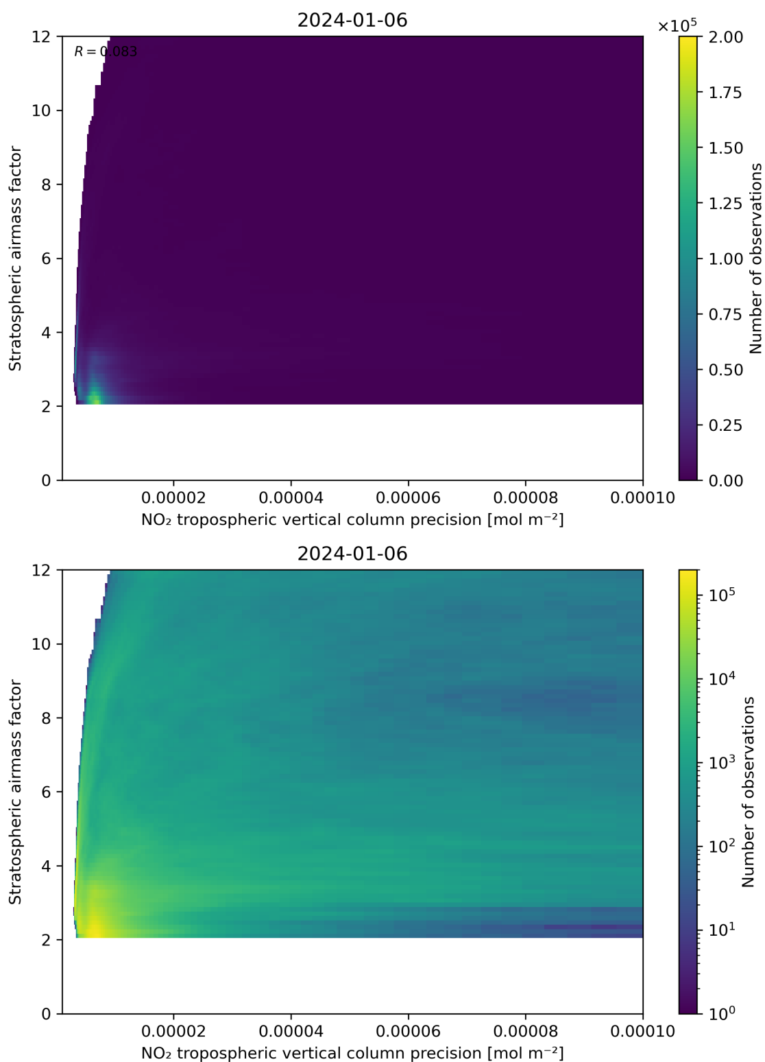
Figure 131: Scatter density plot of “NO 2 tropospheric vertical column precision” against “Stratospheric airmass factor” for 2024-01-05 to 2024-01-07.
