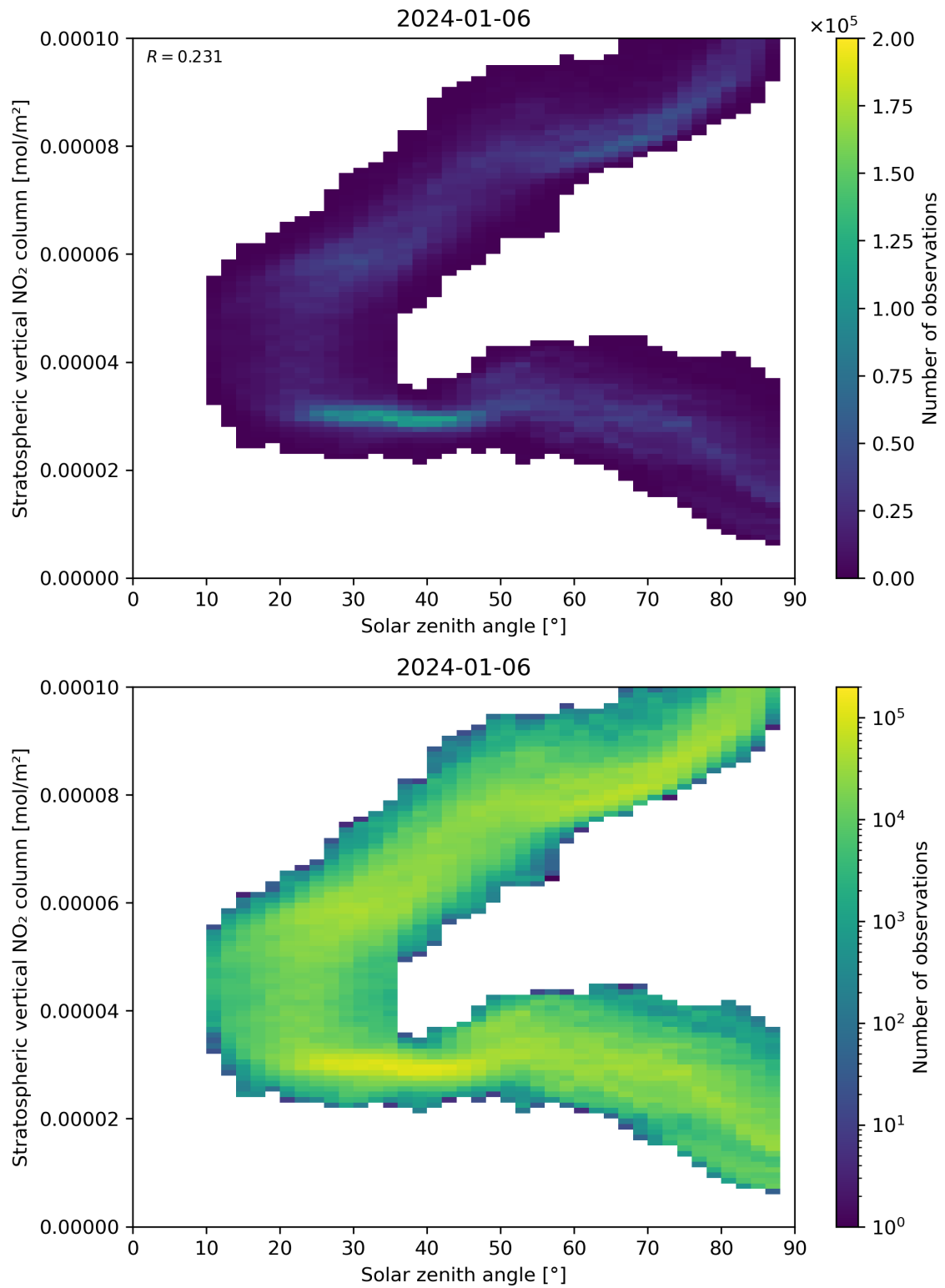
Figure 150: Scatter density plot of “Solar zenith angle” against “Stratospheric vertical NO 2 column” for 2024-01-05 to 2024-01-07.
