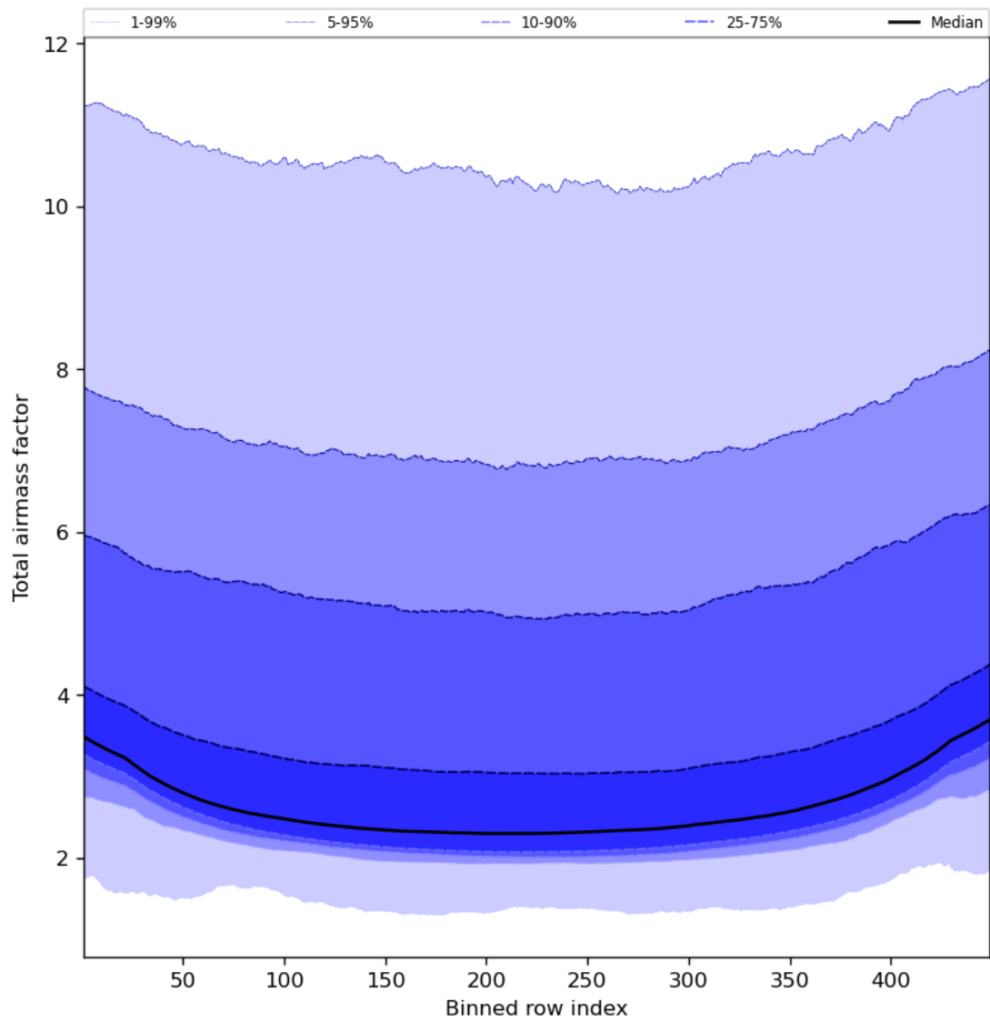
Figure 49: Along track statistics of “Total airmass factor” for 2024-01-05 to 2024-01-07
