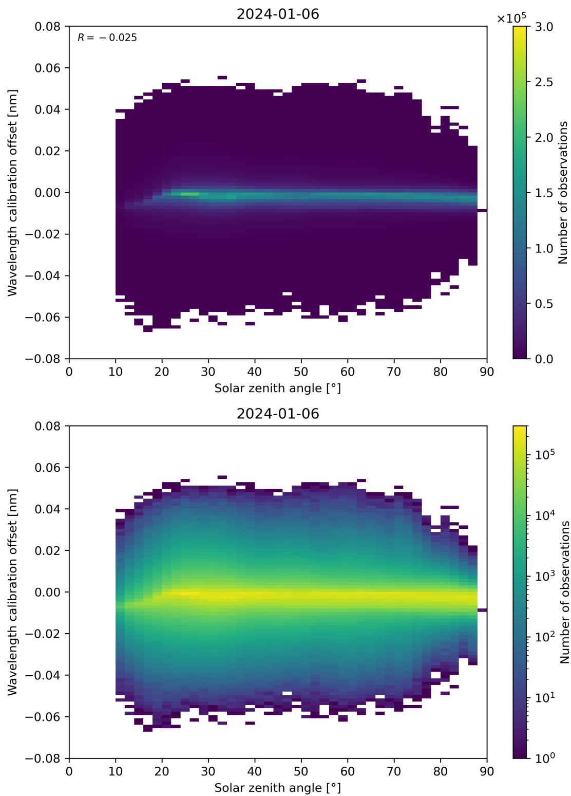
Figure 158: Scatter density plot of “Solar zenith angle” against “Wavelength calibration offset” for 2024-01-05 to 2024-01-07.
