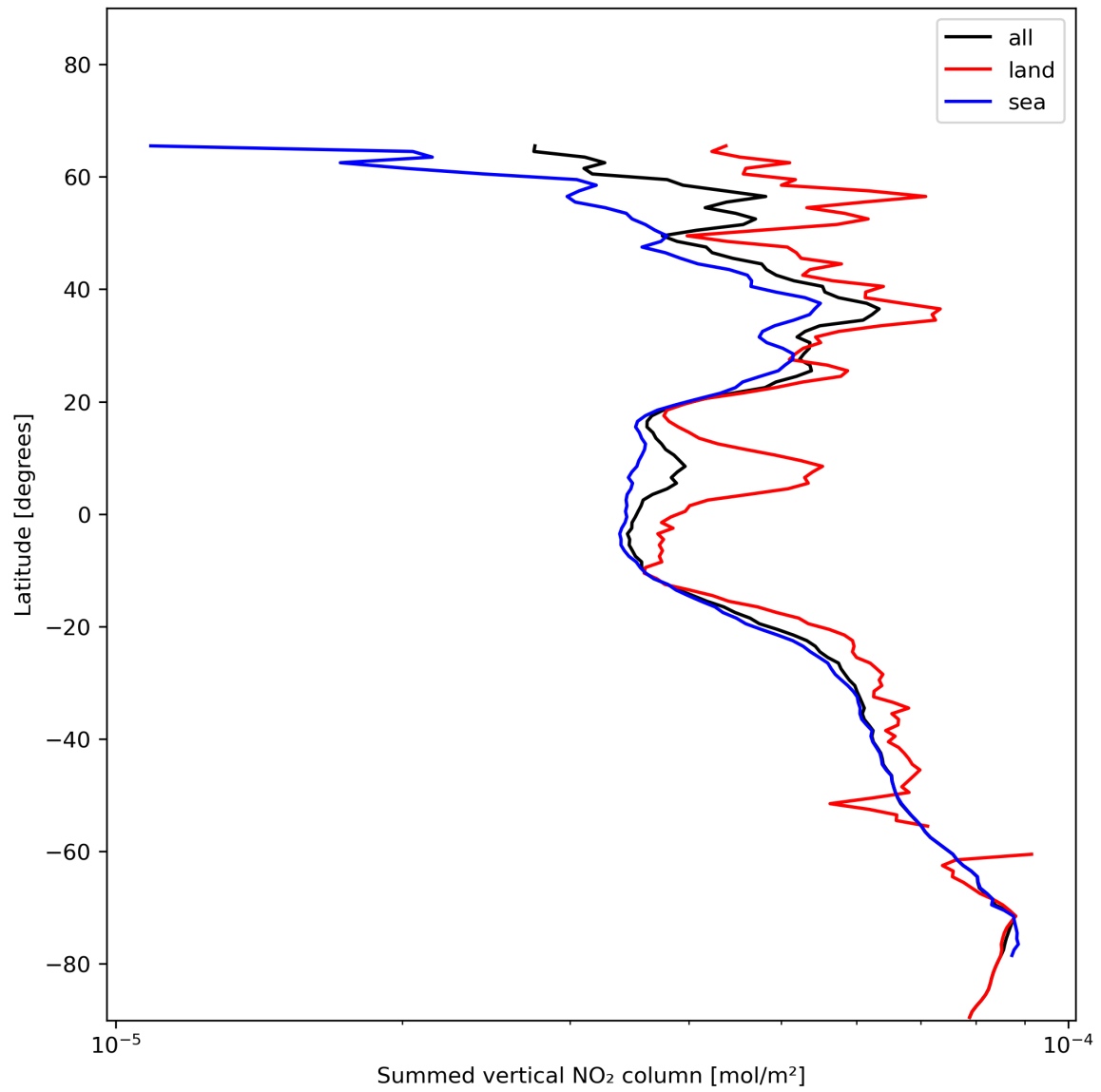
Figure 23: Zonal average of “Summed vertical NO 2 column” for 2024-01-05 to 2024-01-07.
