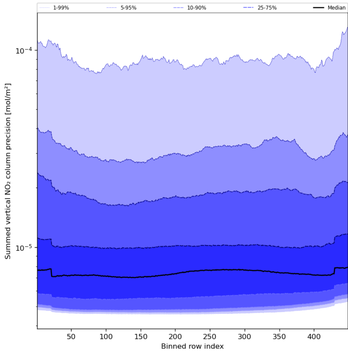
Figure 58: Along track statistics of “Summed vertical NO 2 column precision” for 2024-01-05 to 2024-01-07
