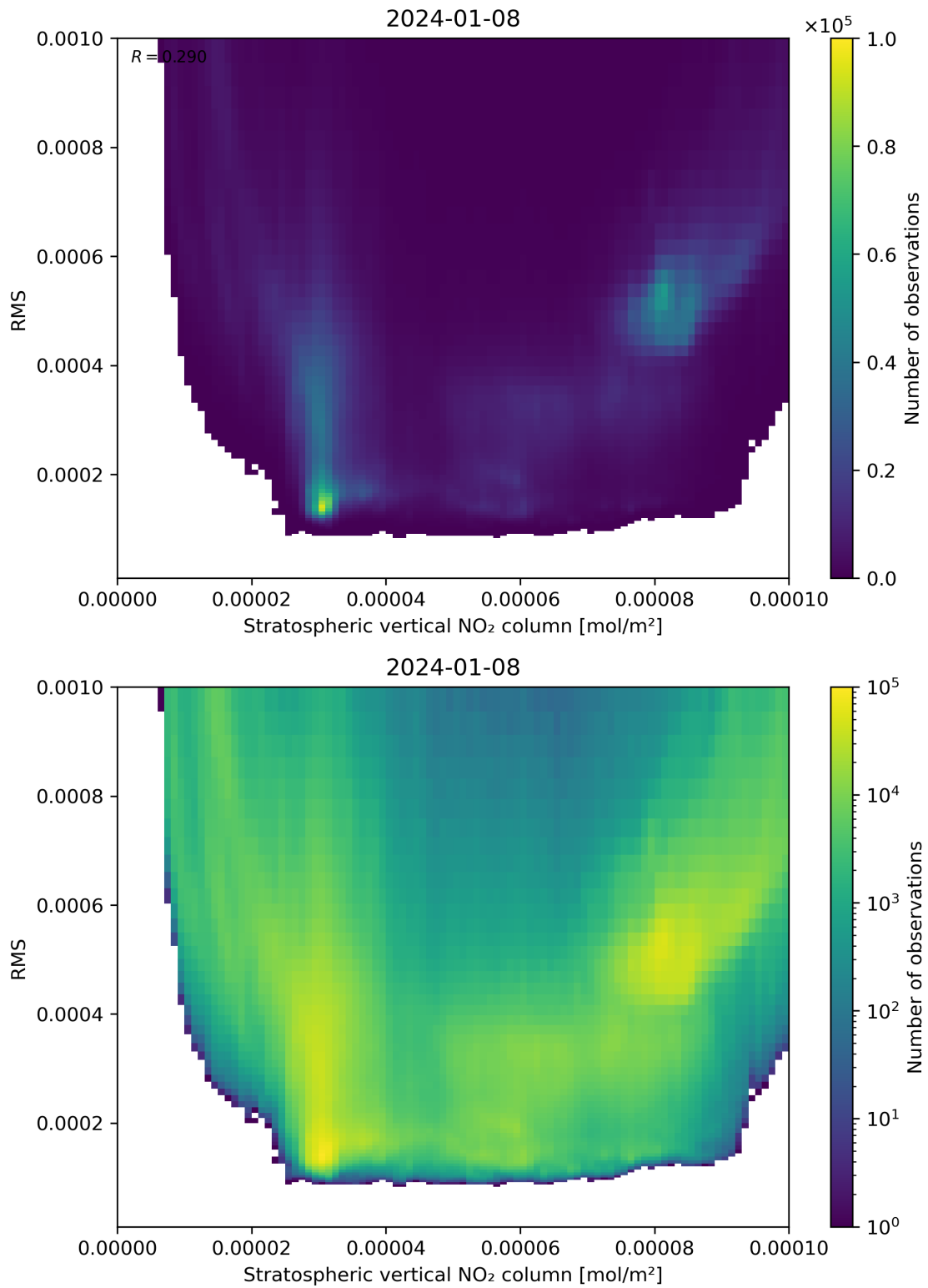
Figure 102: Scatter density plot of “Stratospheric vertical NO 2 column” against “RMS” for 2024-01-07 to 2024-01-09.
