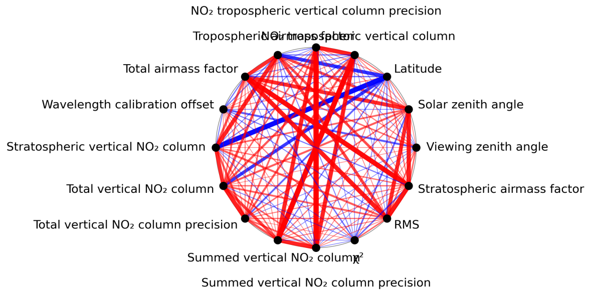
Figure 1: Map of correlation graph for 2024-01-07 to 2024-01-09.
