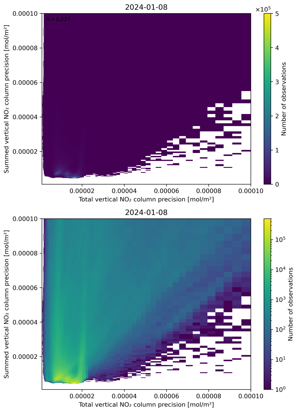
Figure 118: Scatter density plot of “Total vertical NO 2 column precision” against “Summed vertical NO 2 column precision” for 2024-01-07 to 2024-01-09.
