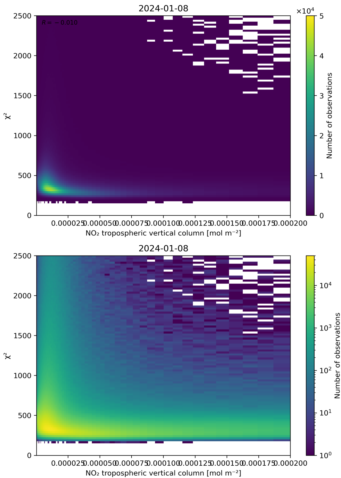
Figure 124: Scatter density plot of “NO 2 tropospheric vertical column” against “ \chi^2 ” for 2024-01-07 to 2024-01-09.
