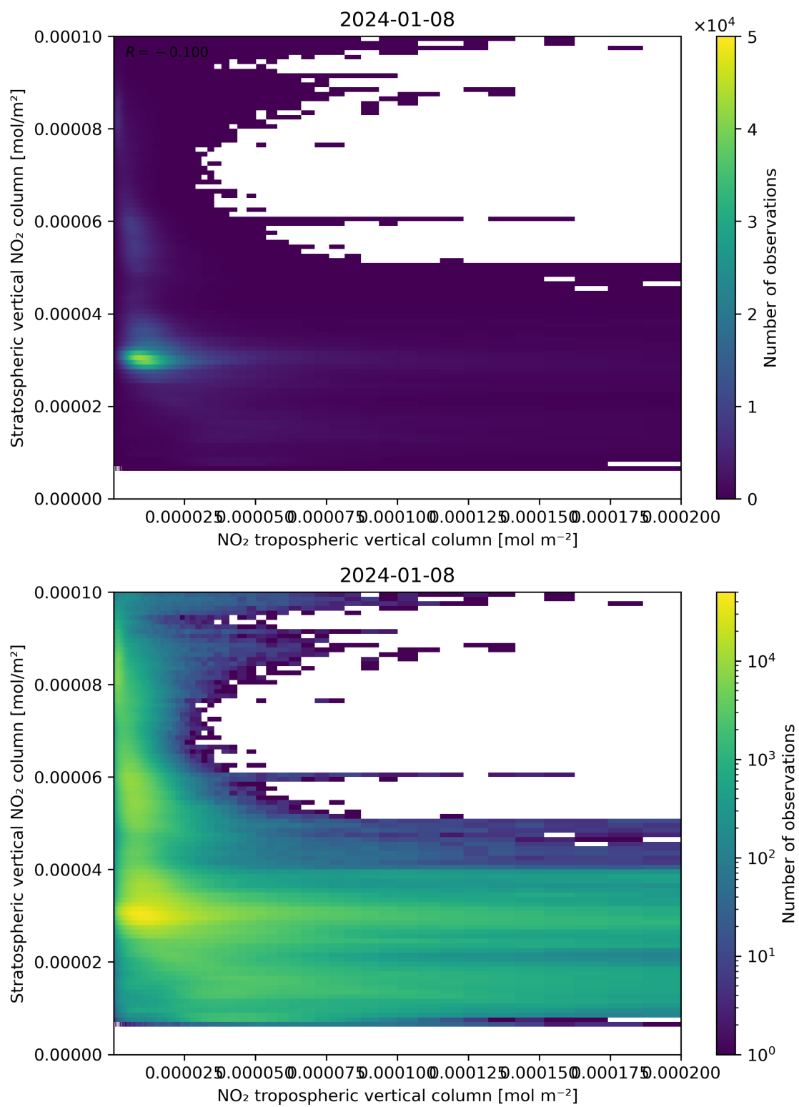
Figure 125: Scatter density plot of “NO 2 tropospheric vertical column” against “Stratospheric vertical NO 2 column” for 2024-01-07 to 2024-01-09.
