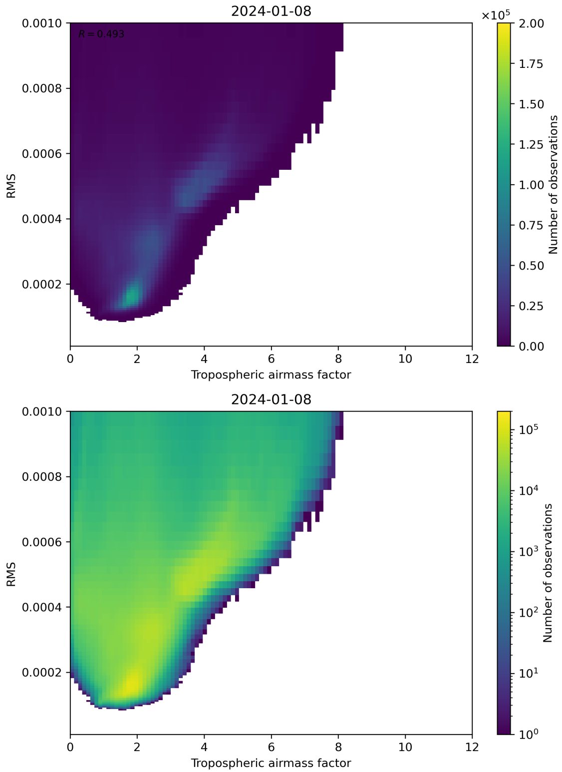
Figure 79: Scatter density plot of “Tropospheric airmass factor” against “RMS” for 2024-01-07 to 2024-01-09.
