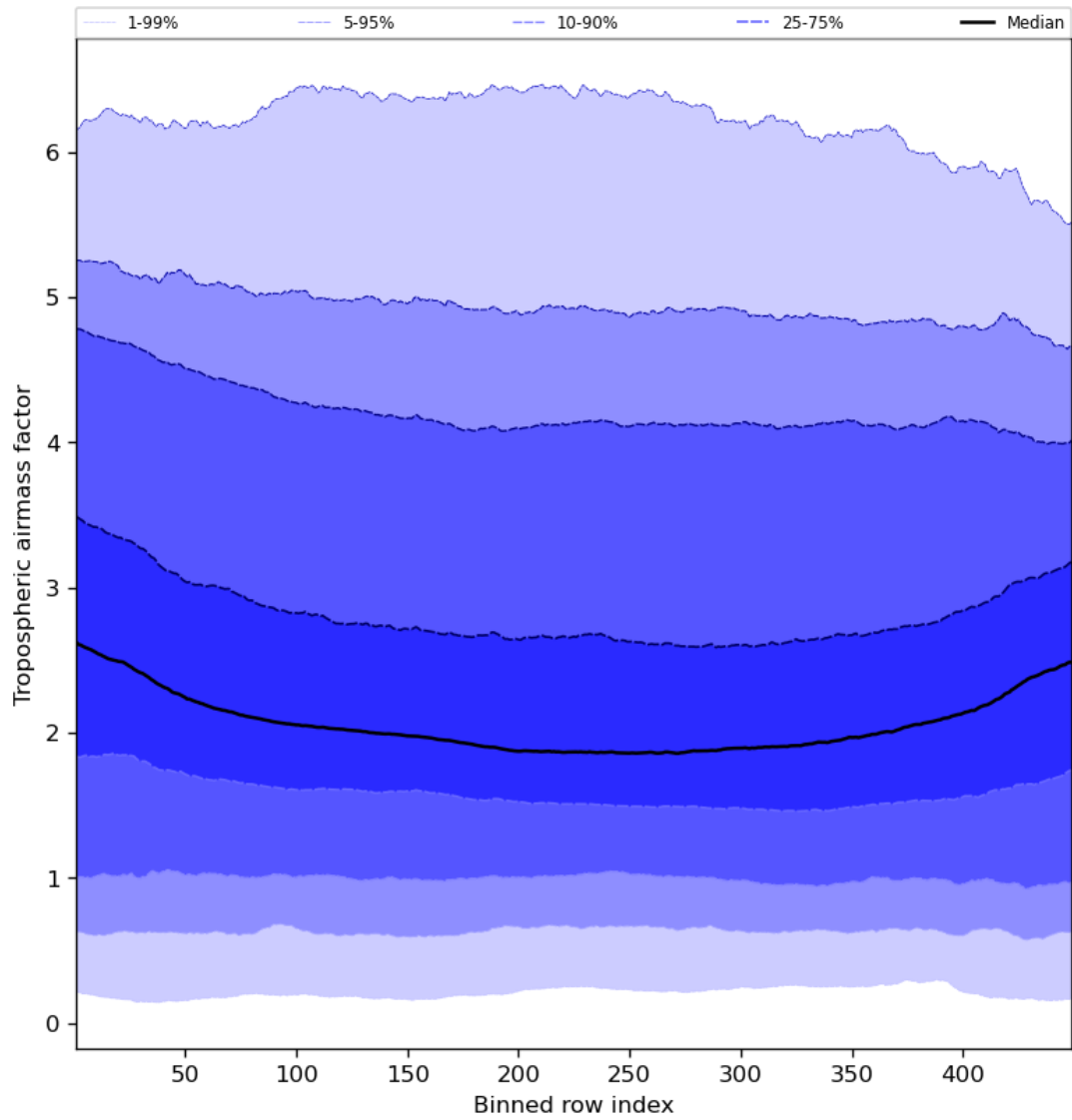
Figure 48: Along track statistics of “Tropospheric airmass factor” for 2024-01-07 to 2024-01-09
