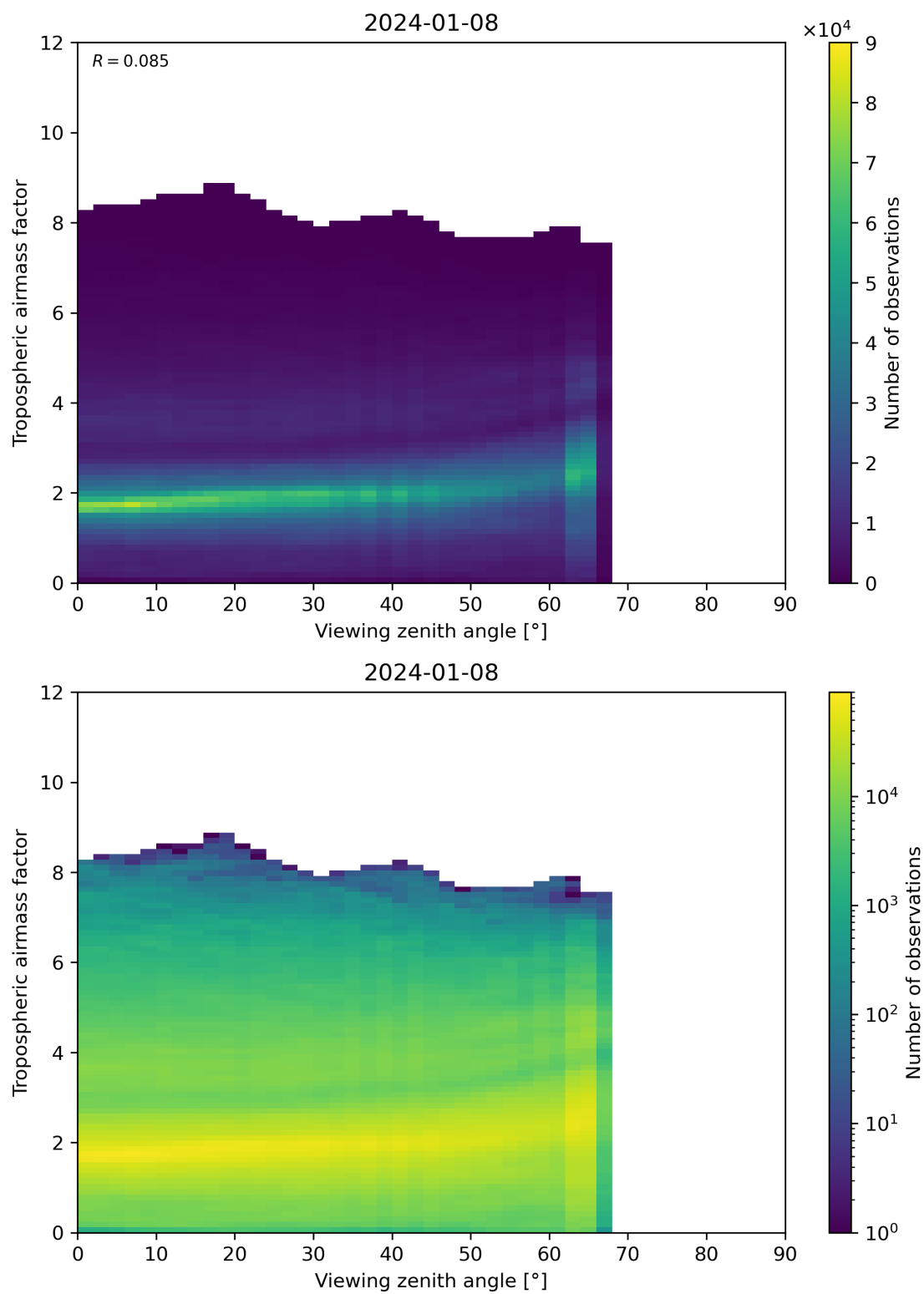
Figure 161: Scatter density plot of “Viewing zenith angle” against “Tropospheric airmass factor” for 2024-01-07 to 2024-01-09.
