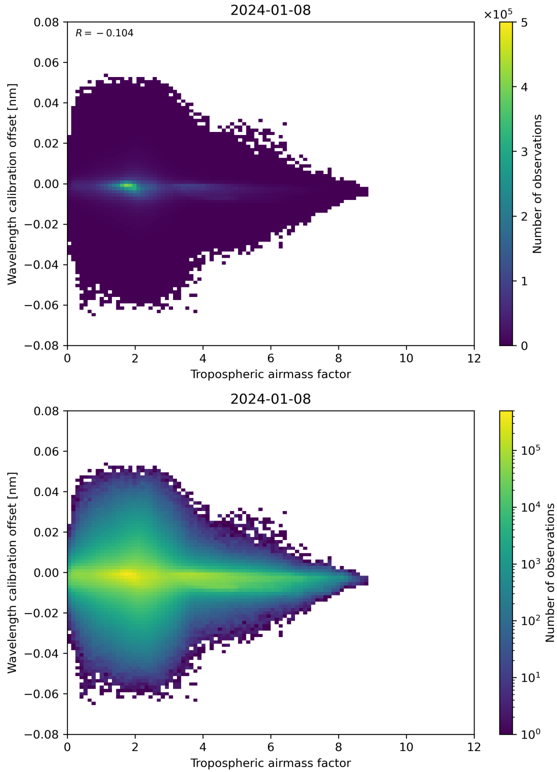
Figure 80: Scatter density plot of “Tropospheric airmass factor” against “Wavelength calibration offset” for 2024-01-07 to 2024-01-09.
