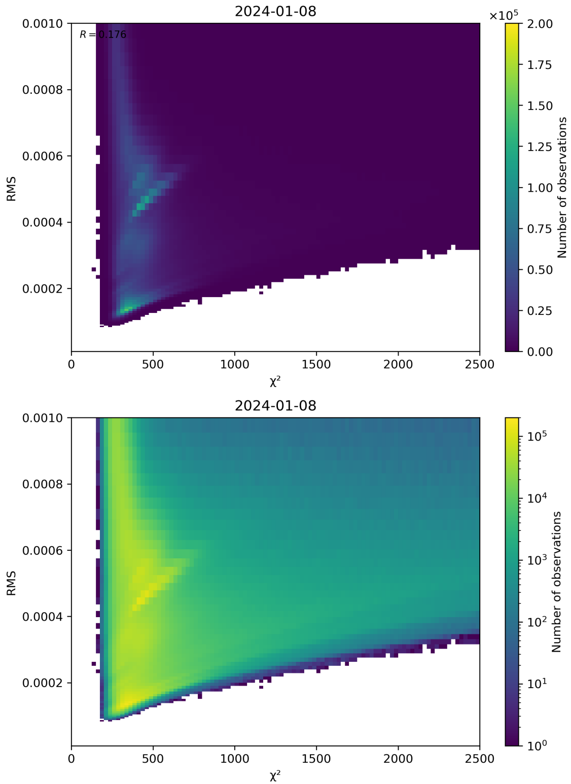
Figure 82: Scatter density plot of “ \chi^2 ” against “RMS” for 2024-01-07 to 2024-01-09.
