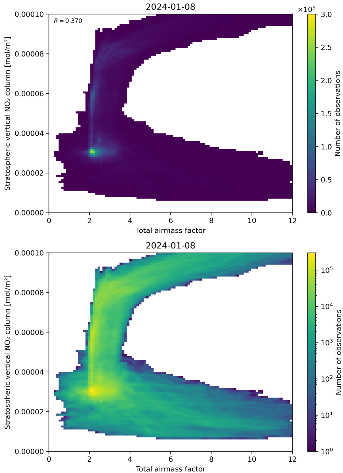
Figure 64: Scatter density plot of “Total airmass factor” against “Stratospheric vertical \text{NO}_2 column” for 2024-01-07 to 2024-01-09.
