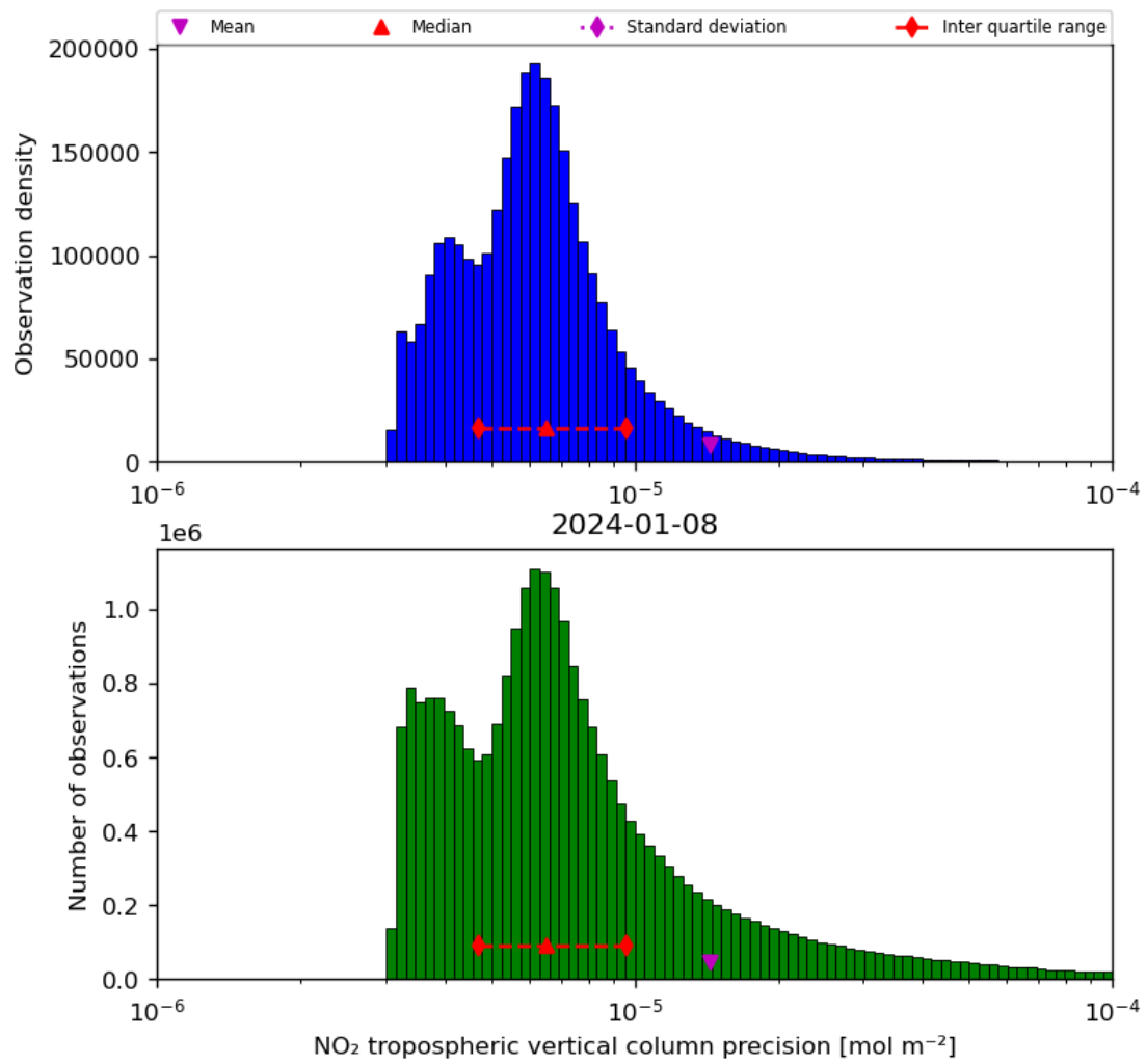
Figure 30: Histogram of “NO 2 tropospheric vertical column precision” for 2024-01-07 to 2024-01-09
