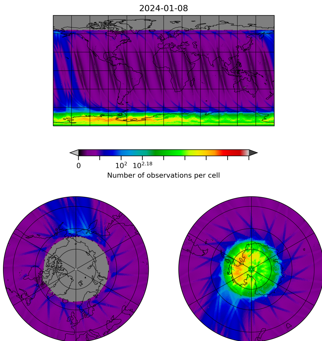
Figure 10: Map of the number of observations for 2024-01-07 to 2024-01-09
