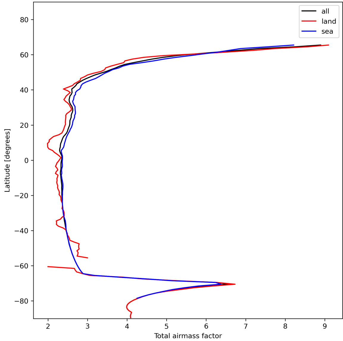
Figure 15: Zonal average of “Total airmass factor” for 2024-01-07 to 2024-01-09.
