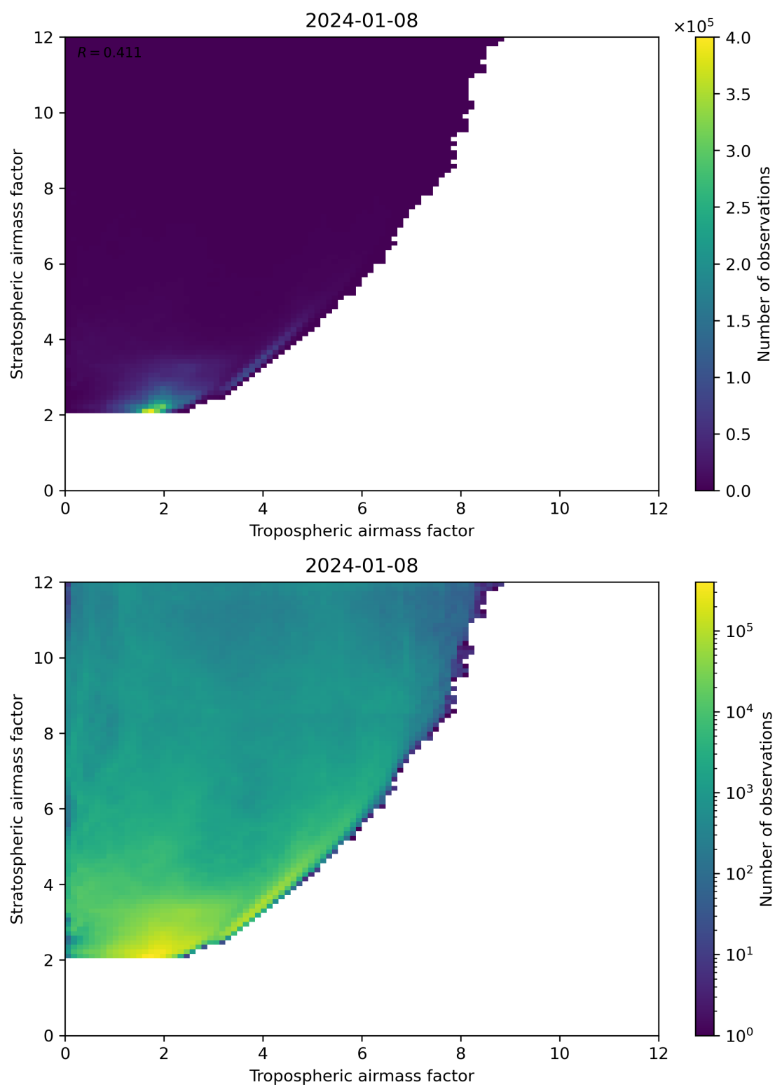
Figure 71: Scatter density plot of “Tropospheric airmass factor” against “Stratospheric airmass factor” for 2024-01-07 to 2024-01-09.
