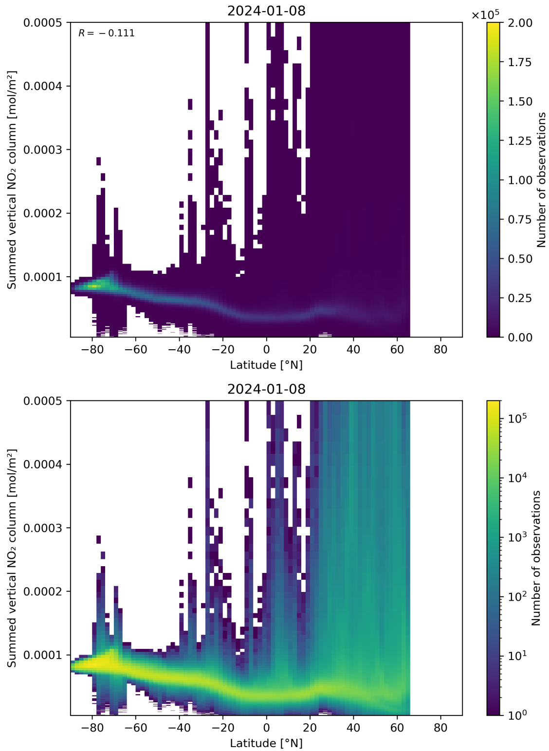
Figure 88: Scatter density plot of “Latitude” against “Summed vertical NO 2 column” for 2024-01-07 to 2024-01-09.
