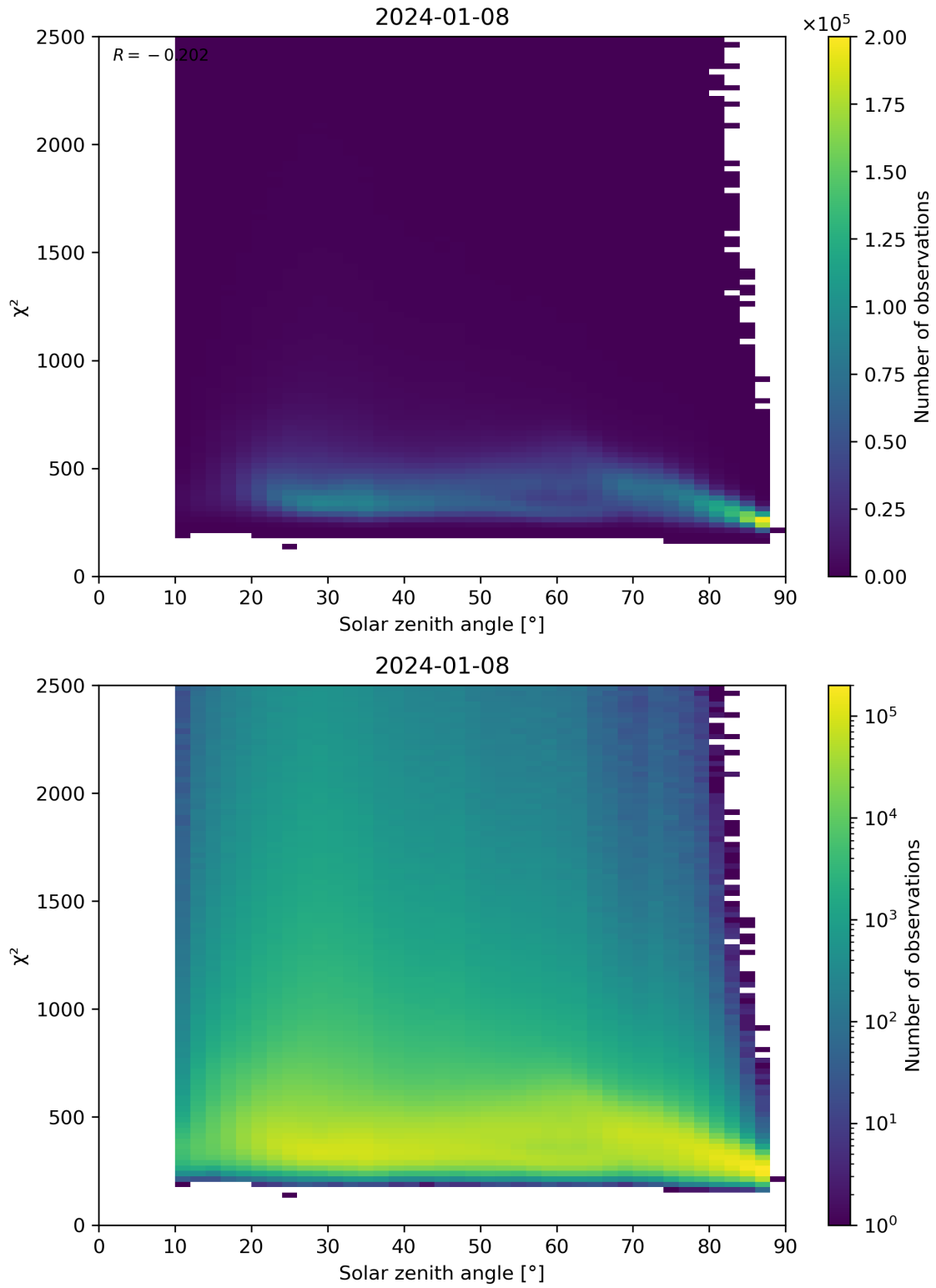
Figure 148: Scatter density plot of “Solar zenith angle” against “ \chi^2 ” for 2024-01-07 to 2024-01-09.
