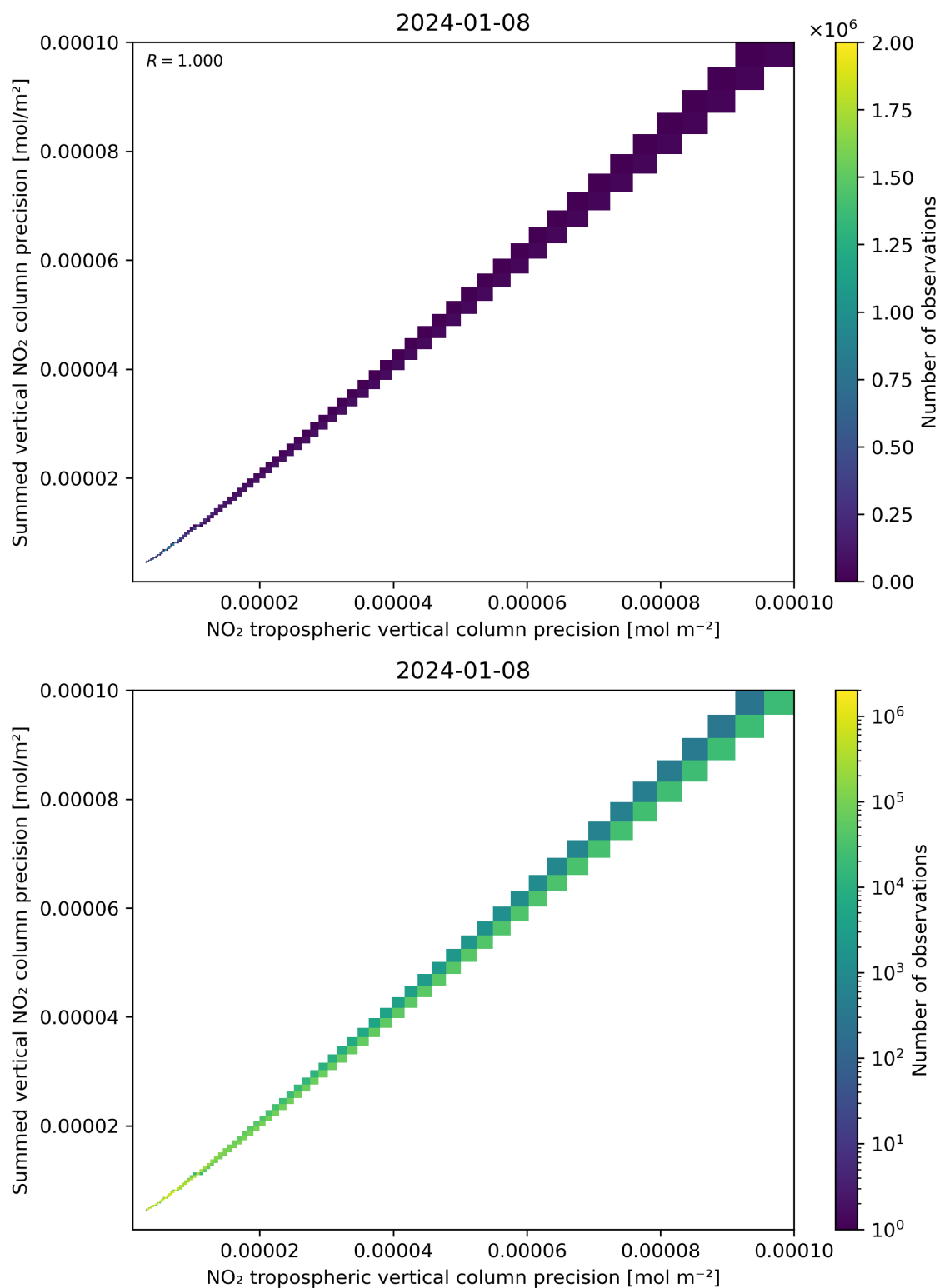
Figure 137: Scatter density plot of “NO 2 tropospheric vertical column precision” against “Summed vertical NO 2 column precision” for 2024-01-07 to 2024-01-09.
