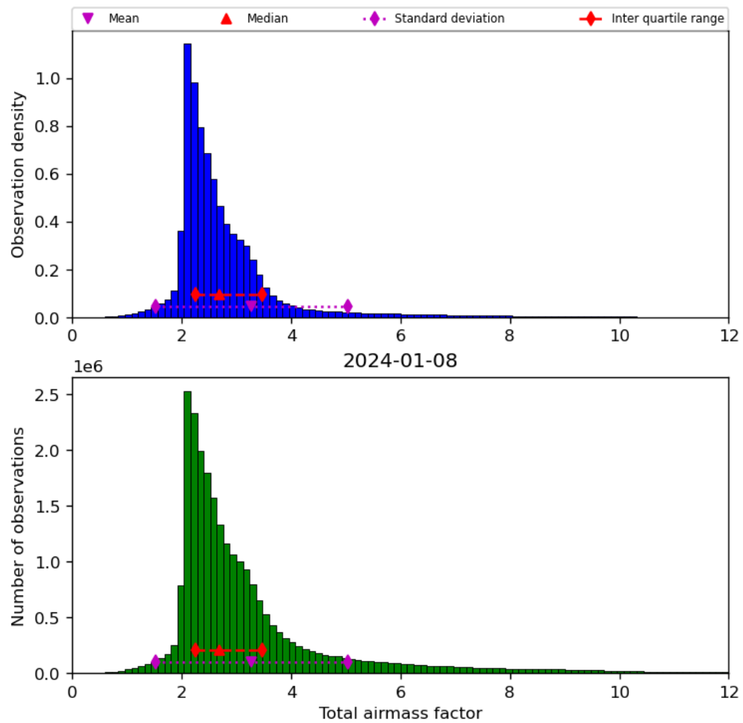
Figure 32: Histogram of “Total airmass factor” for 2024-01-07 to 2024-01-09
