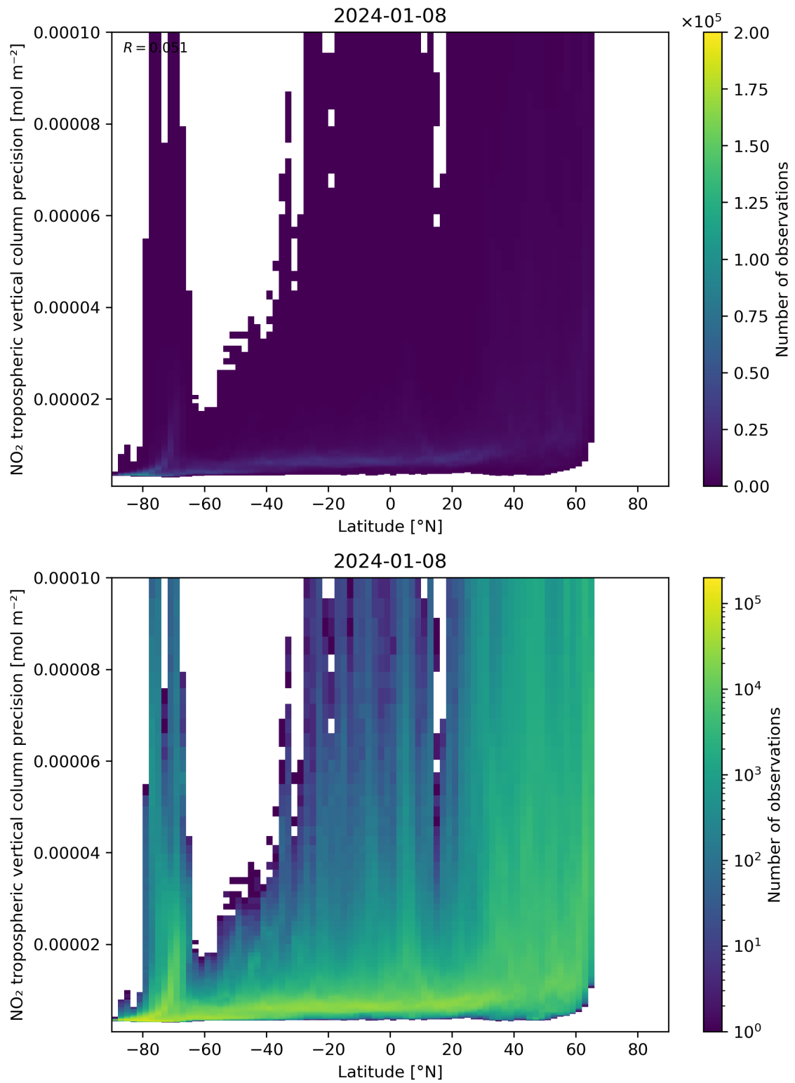
Figure 93: Scatter density plot of “Latitude” against “NO 2 tropospheric vertical column precision” for 2024-01-07 to 2024-01-09.
