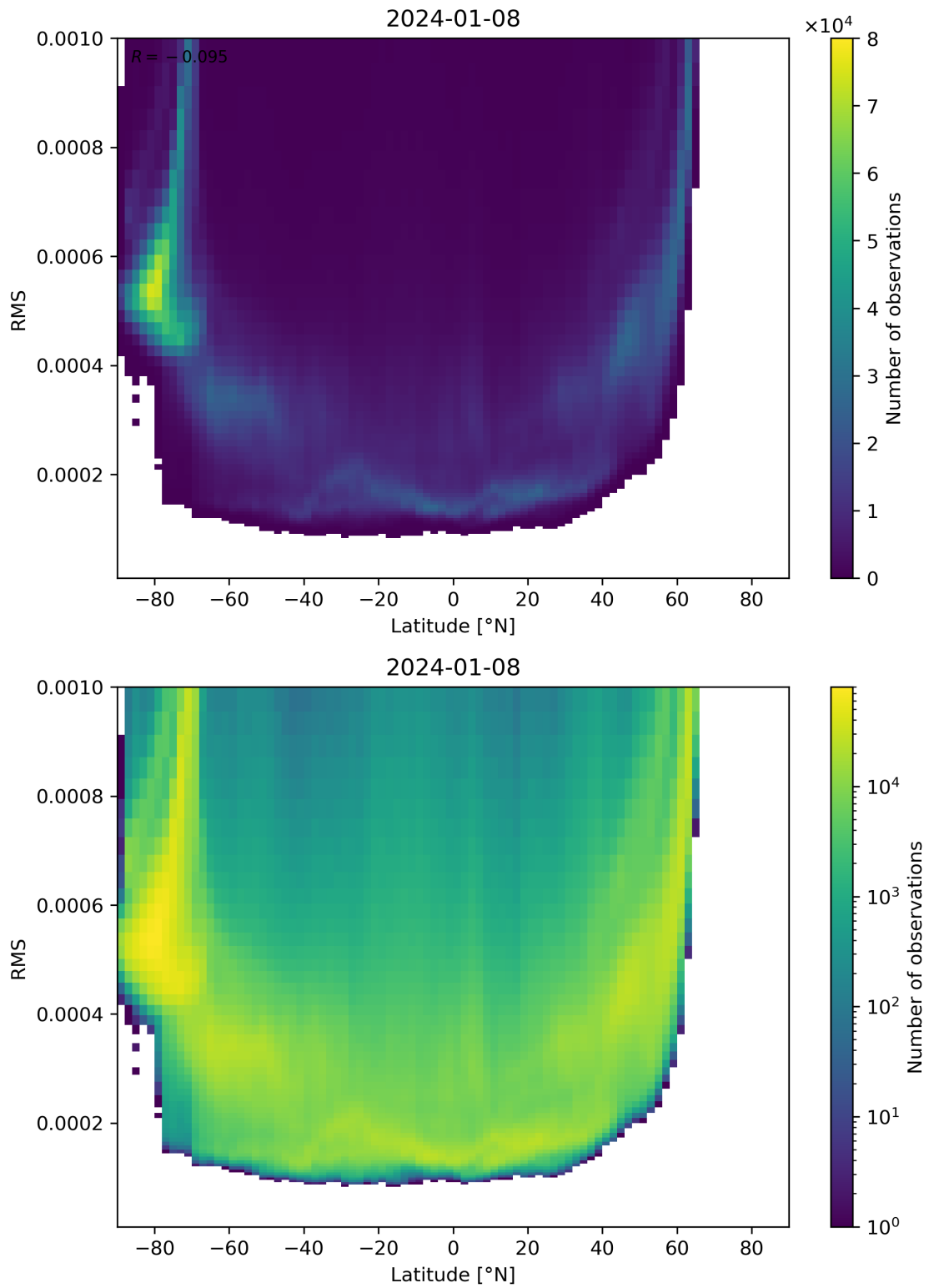
Figure 94: Scatter density plot of “Latitude” against “RMS” for 2024-01-07 to 2024-01-09.
