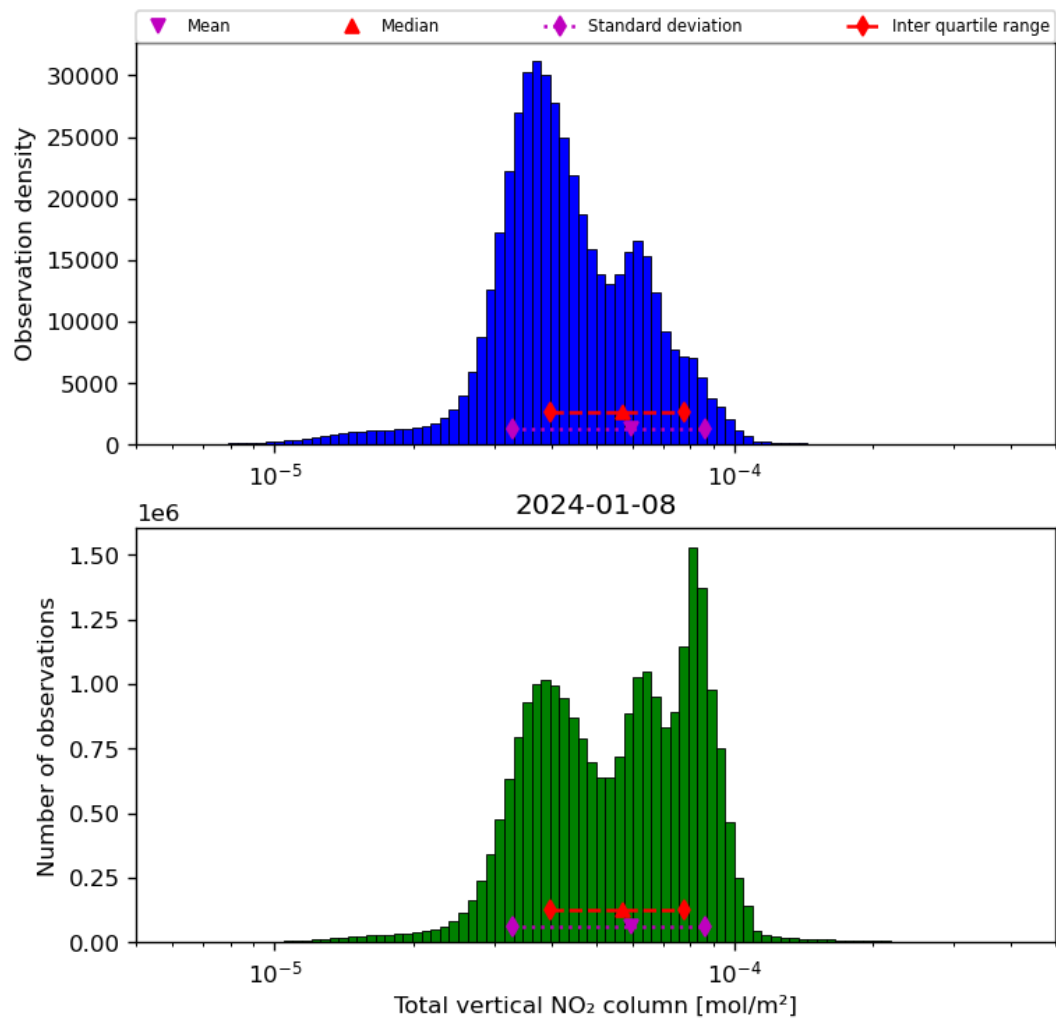
Figure 38: Histogram of “Total vertical NO 2 column” for 2024-01-07 to 2024-01-09
