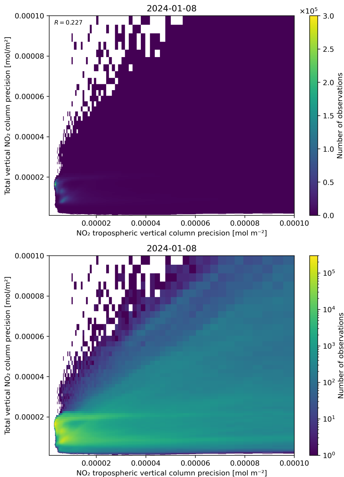
Figure 139: Scatter density plot of “NO 2 tropospheric vertical column precision” against “Total vertical NO 2 column precision” for 2024-01-07 to 2024-01-09.
