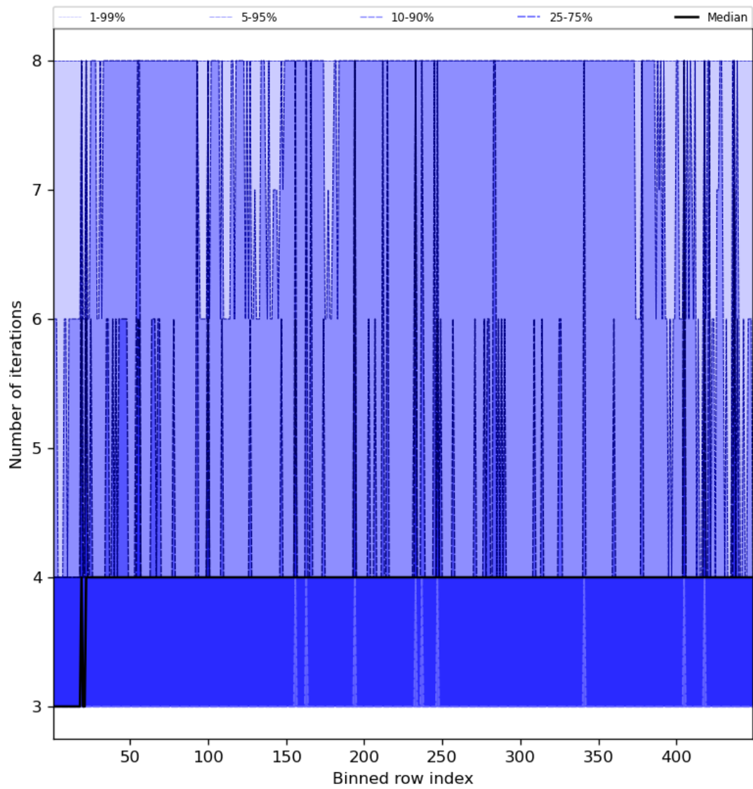
Figure 51: Along track statistics of “Number of iterations” for 2024-01-07 to 2024-01-09
