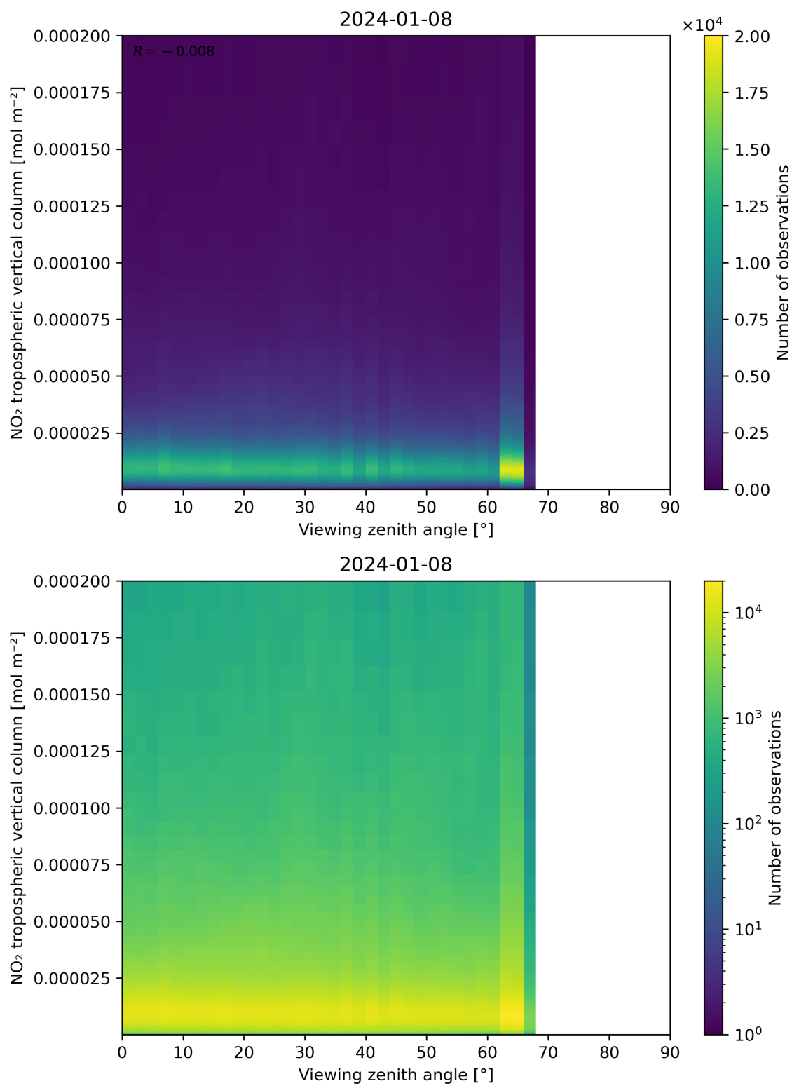
Figure 169: Scatter density plot of “Viewing zenith angle” against “NO 2 tropospheric vertical column” for 2024-01-07 to 2024-01-09.
