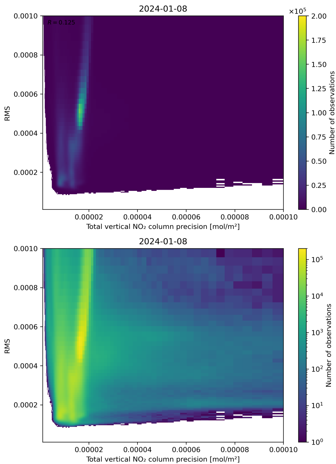
Figure 119: Scatter density plot of “Total vertical NO 2 column precision” against “RMS” for 2024-01-07 to 2024-01-09.
