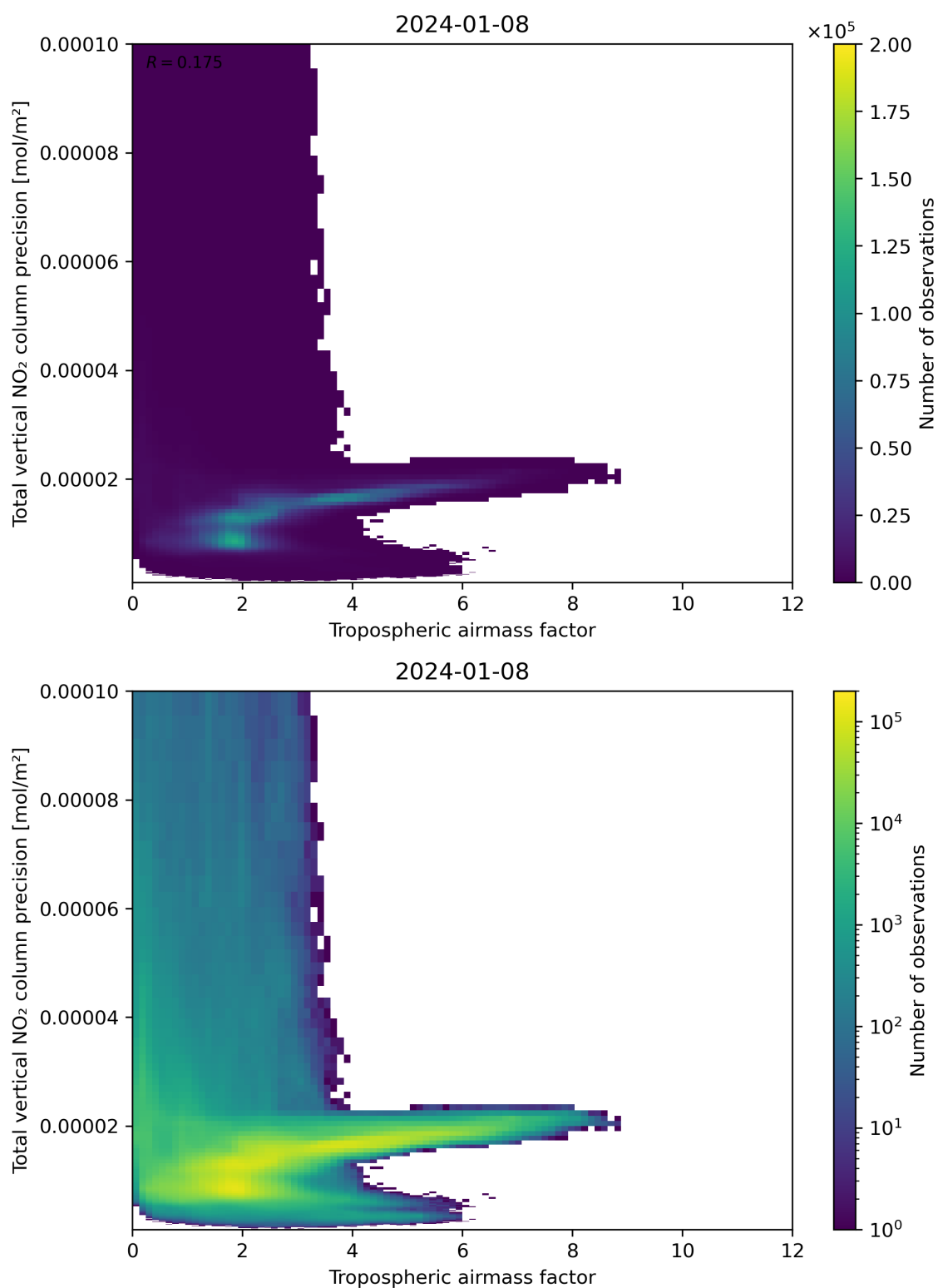
Figure 78: Scatter density plot of “Tropospheric air mass factor” against “Total vertical NO 2 column precision” for 2024-01-07 to 2024-01-09.
