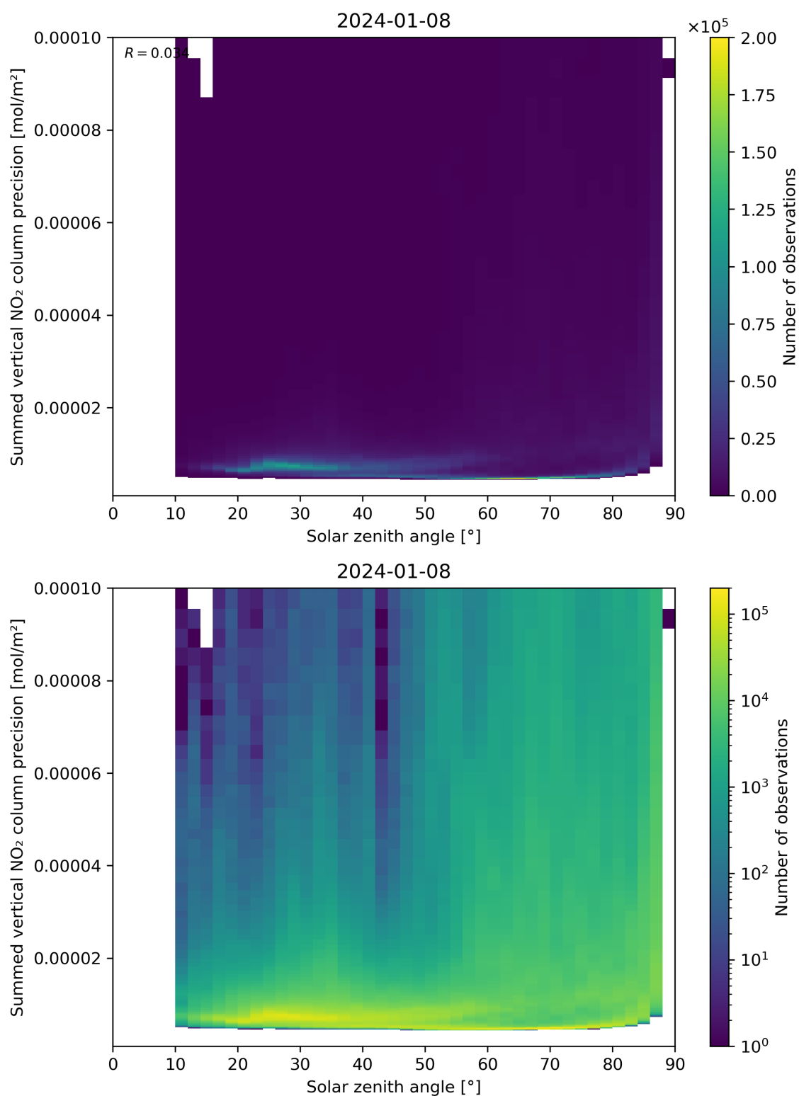
Figure 152: Scatter density plot of “Solar zenith angle” against “Summed vertical NO 2 column precision” for 2024-01-07 to 2024-01-09.
