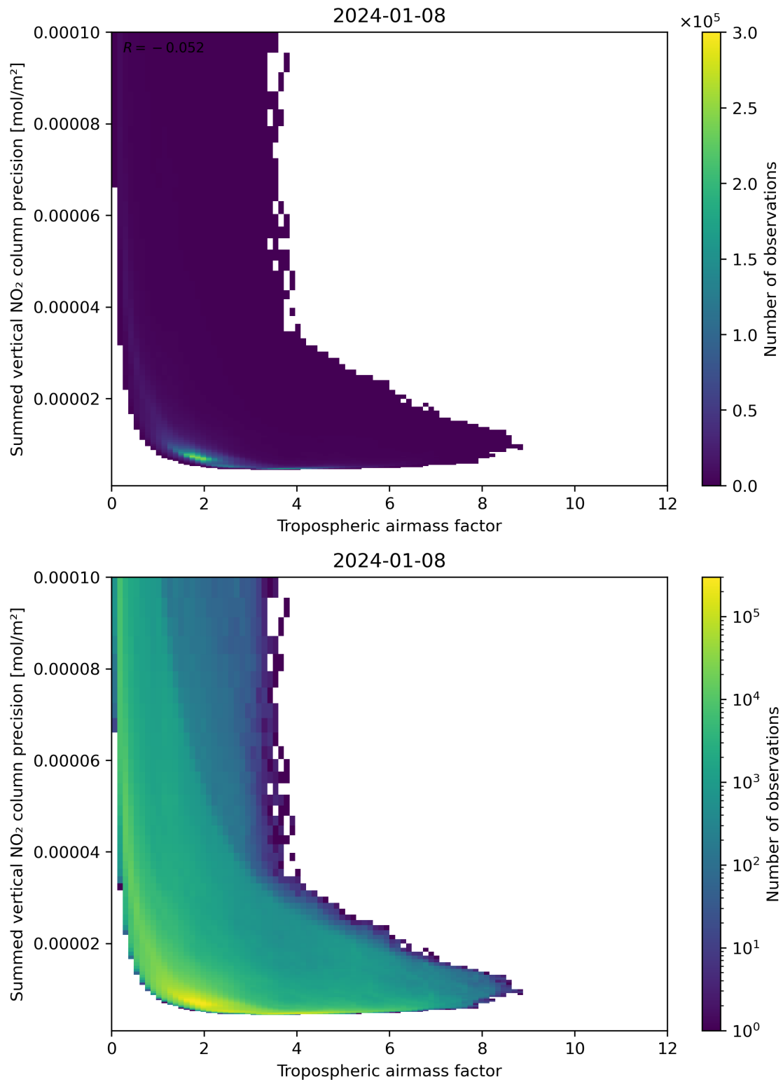
Figure 76: Scatter density plot of “Tropospheric air mass factor” against “Summed vertical NO 2 column precision” for 2024-01-07 to 2024-01-09.
