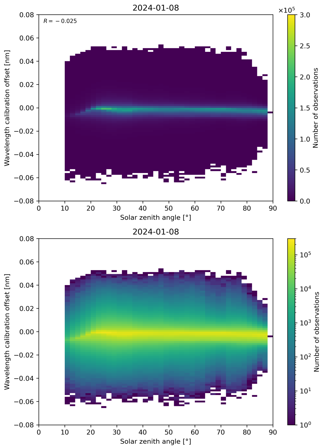
Figure 158: Scatter density plot of “Solar zenith angle” against “Wavelength calibration offset” for 2024-01-07 to 2024-01-09.
