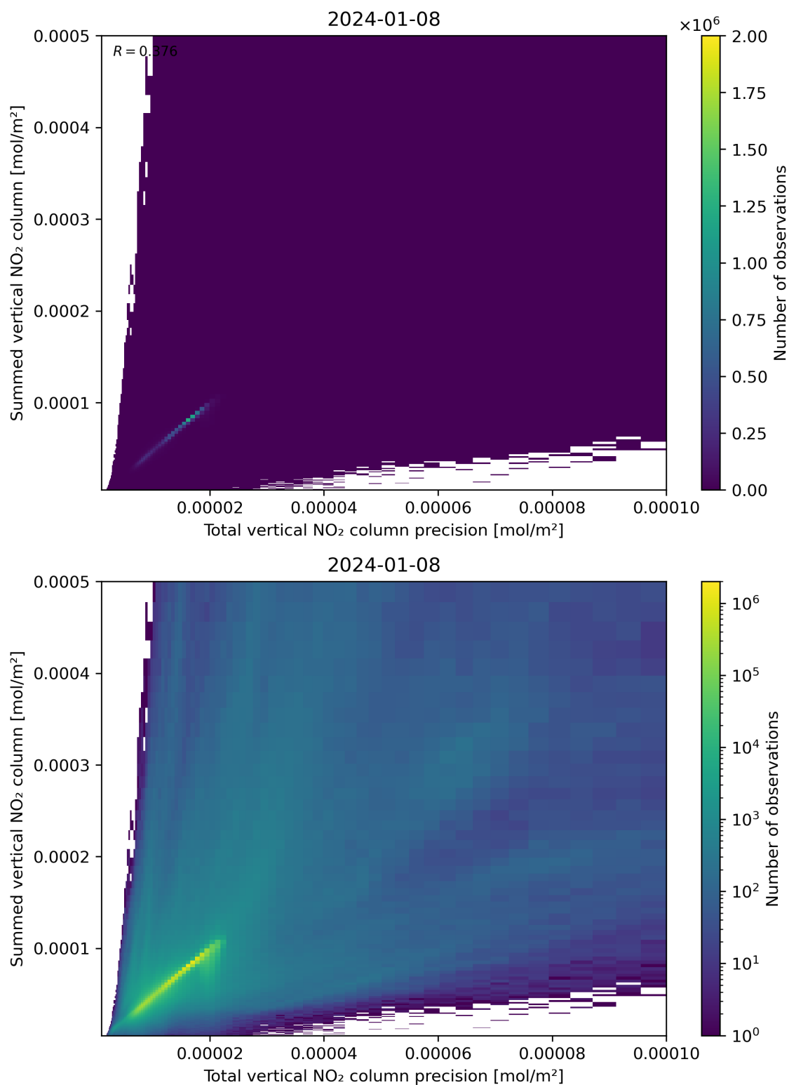
Figure 117: Scatter density plot of “Total vertical NO 2 column precision” against “Summed vertical NO 2 column” for 2024-01-07 to 2024-01-09.
