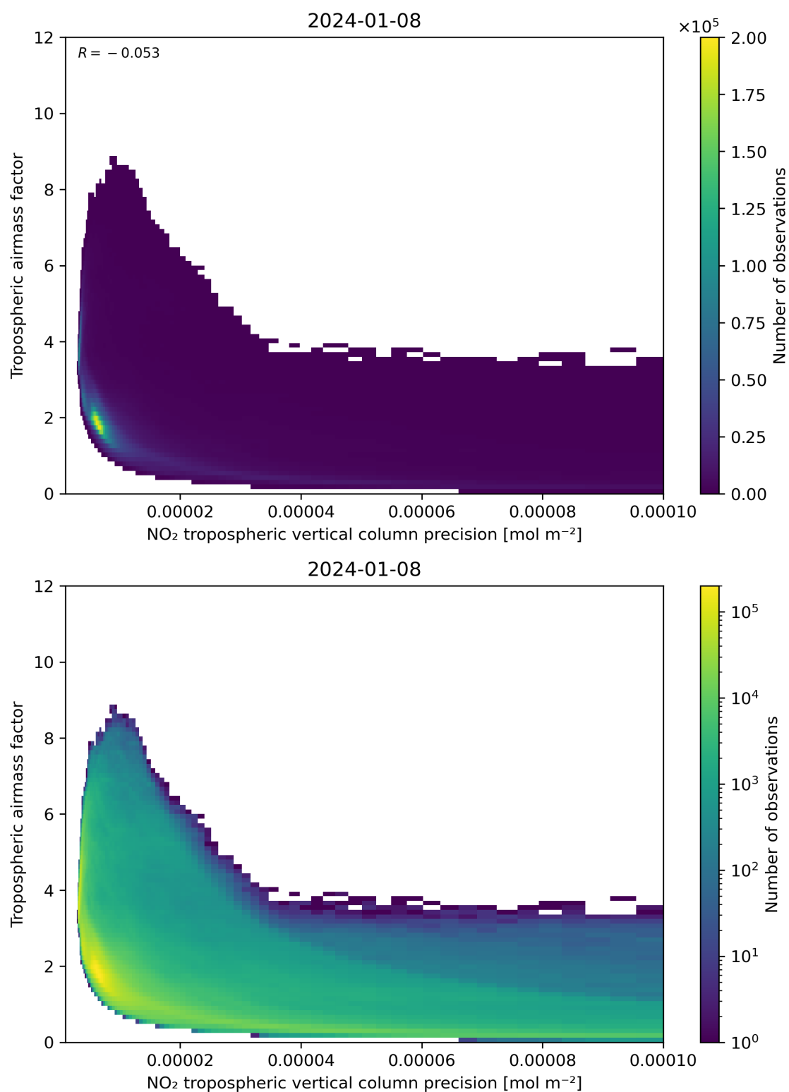
Figure 133: Scatter density plot of “NO 2 tropospheric vertical column precision” against “Tropospheric airmass factor” for 2024-01-07 to 2024-01-09.
