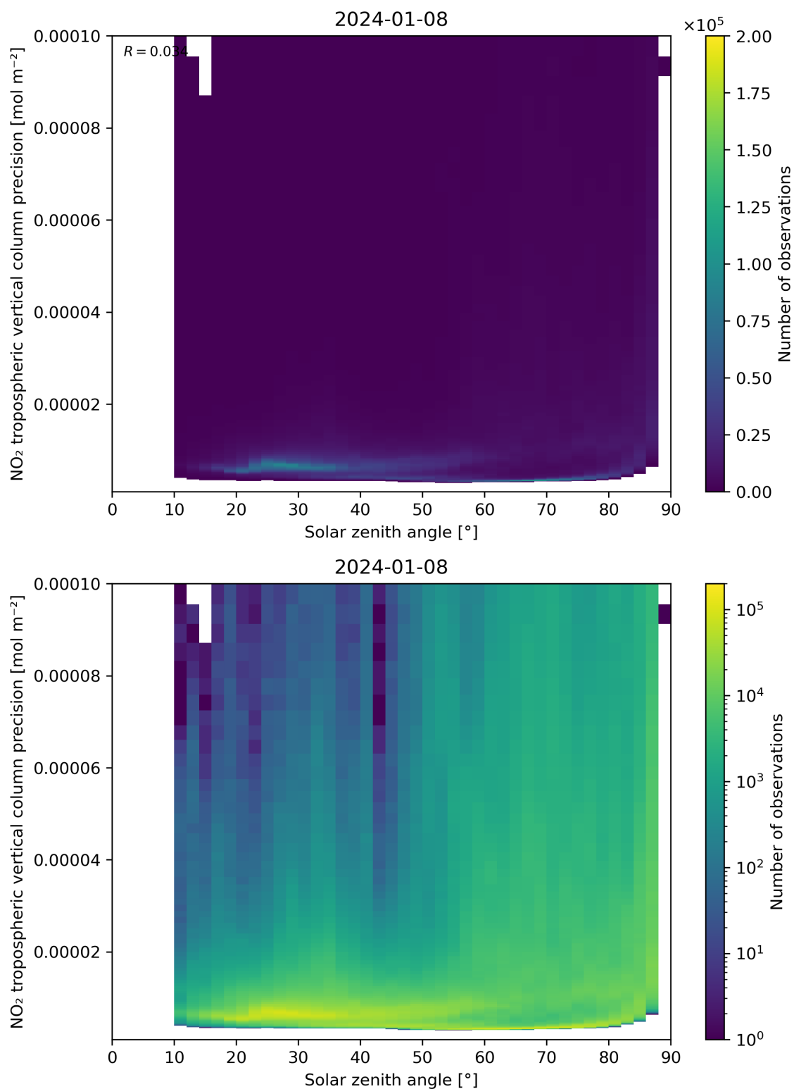
Figure 156: Scatter density plot of “Solar zenith angle” against “NO 2 tropospheric vertical column precision” for 2024-01-07 to 2024-01-09.
