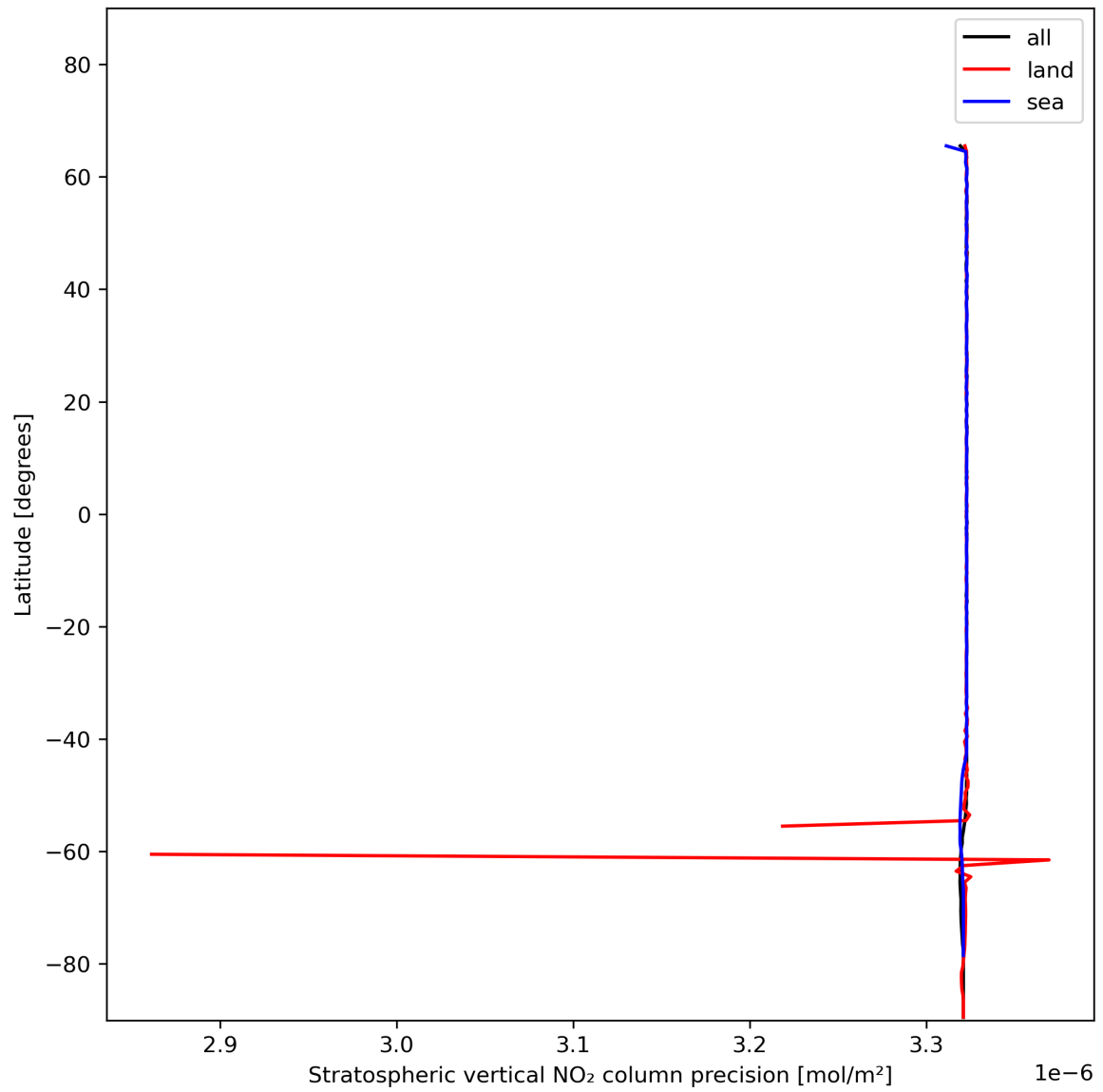
Figure 20: Zonal average of “Stratospheric vertical NO 2 column precision” for 2024-01-07 to 2024-01-09.
