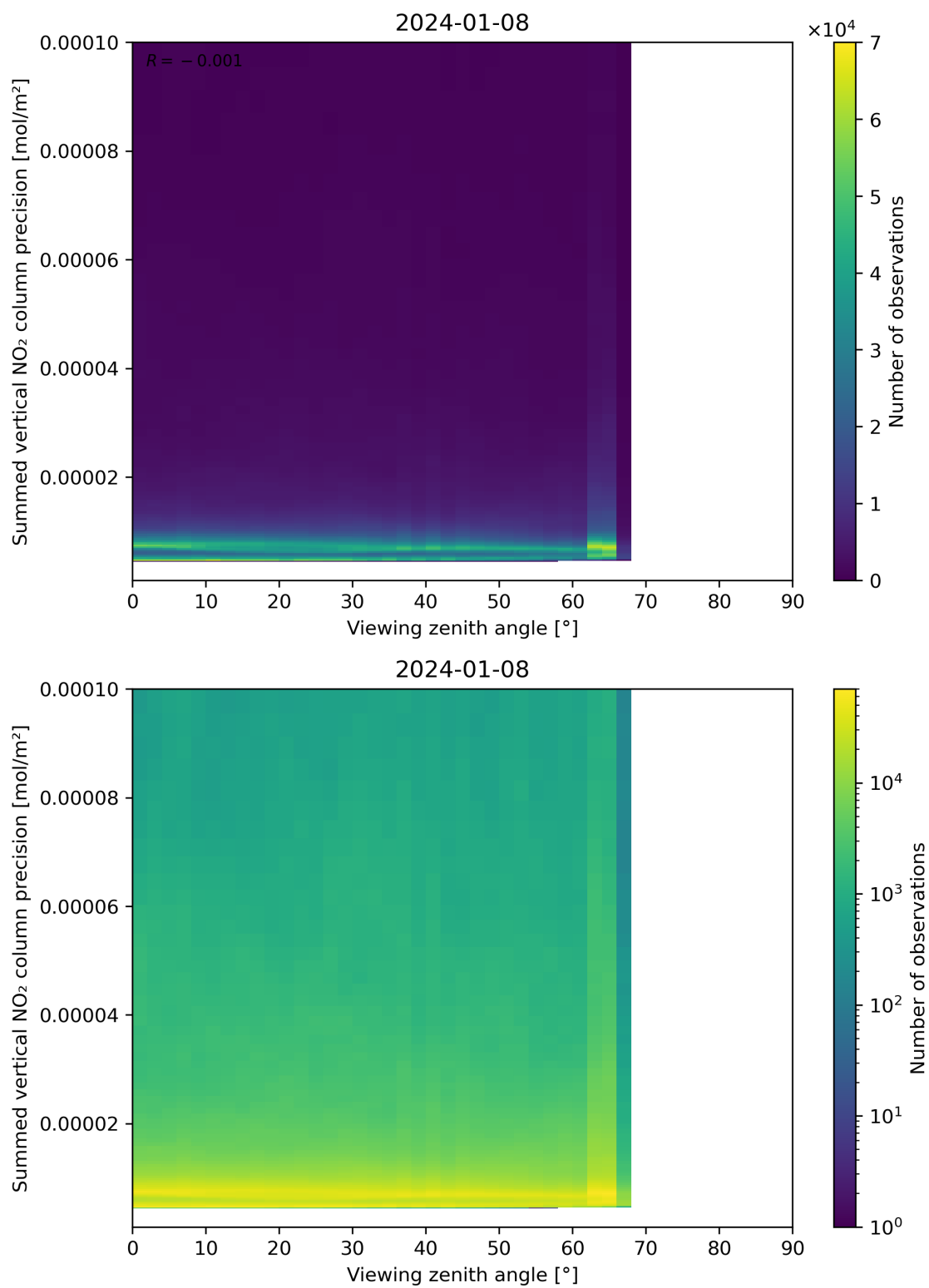
Figure 166: Scatter density plot of “Viewing zenith angle” against “Summed vertical NO 2 column precision” for 2024-01-07 to 2024-01-09.
