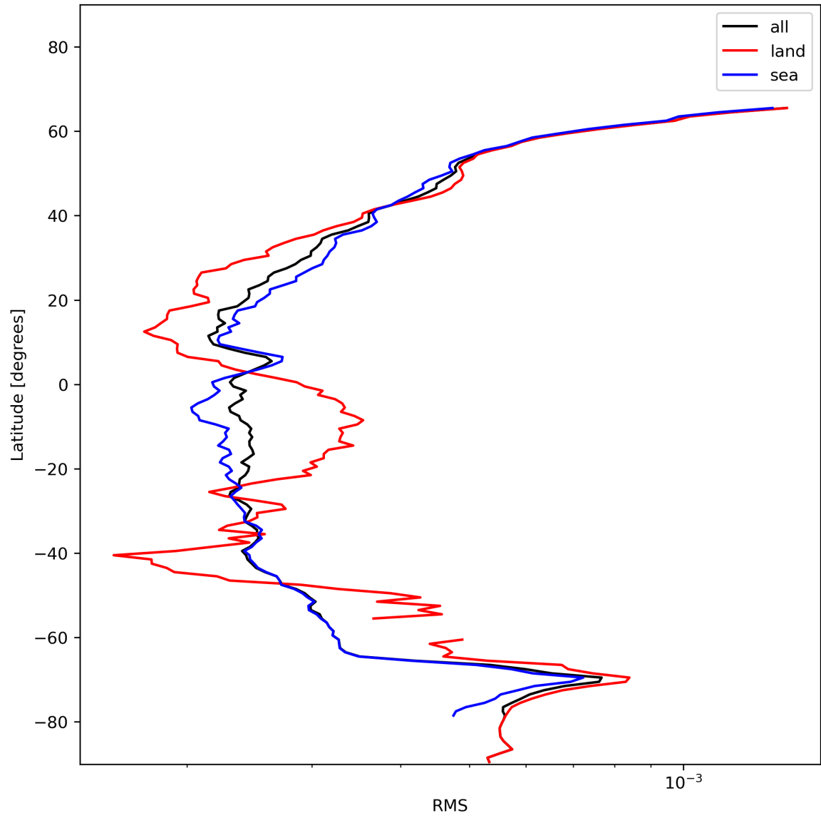
Figure 26: Zonal average of “RMS” for 2024-01-07 to 2024-01-09.
