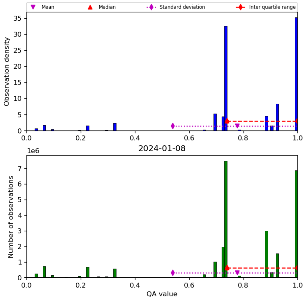
Figure 28: Histogram of “QA value” for 2024-01-07 to 2024-01-09
