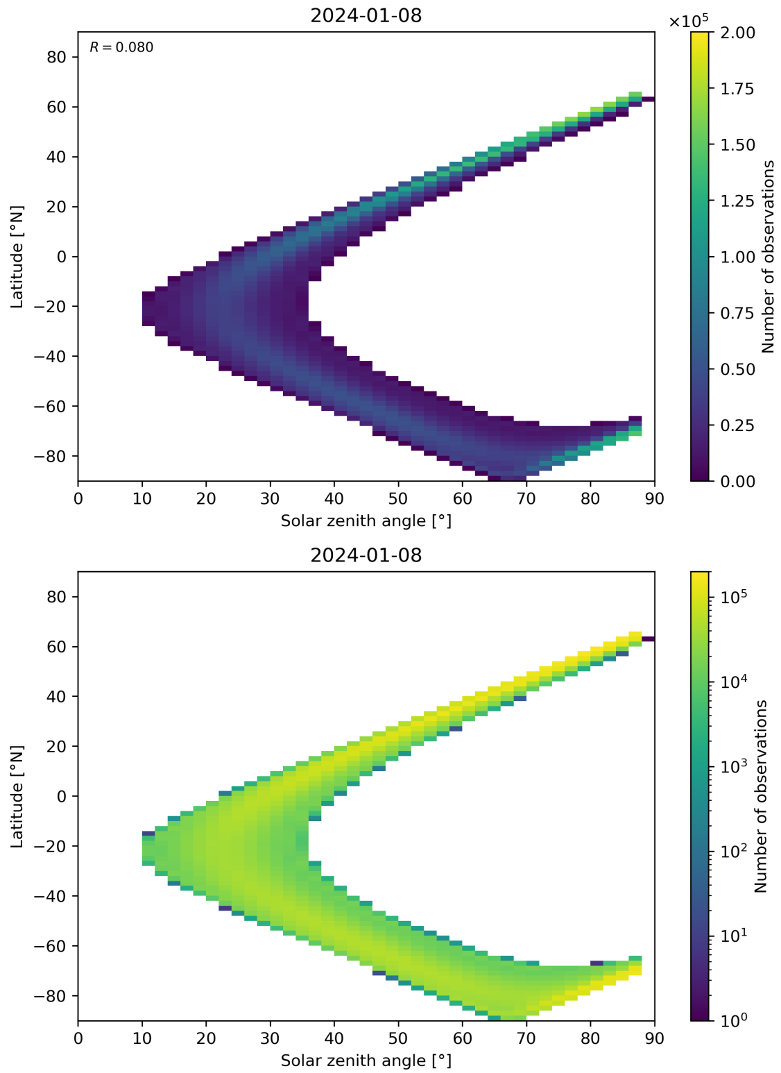
Figure 149: Scatter density plot of “Solar zenith angle” against “Latitude” for 2024-01-07 to 2024-01-09.
