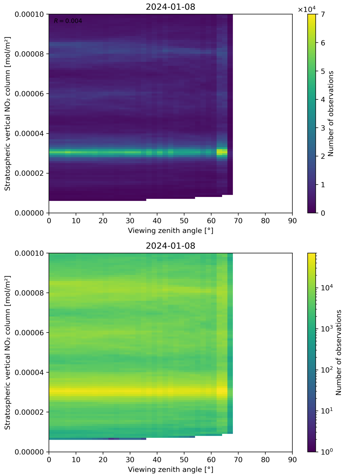
Figure 164: Scatter density plot of “Viewing zenith angle” against “Stratospheric vertical NO 2 column” for 2024-01-07 to 2024-01-09.
