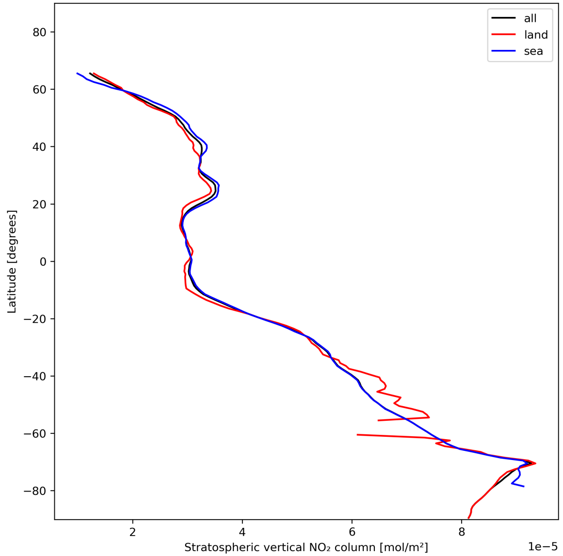
Figure 19: Zonal average of “Stratospheric vertical NO 2 column” for 2024-01-07 to 2024-01-09.
