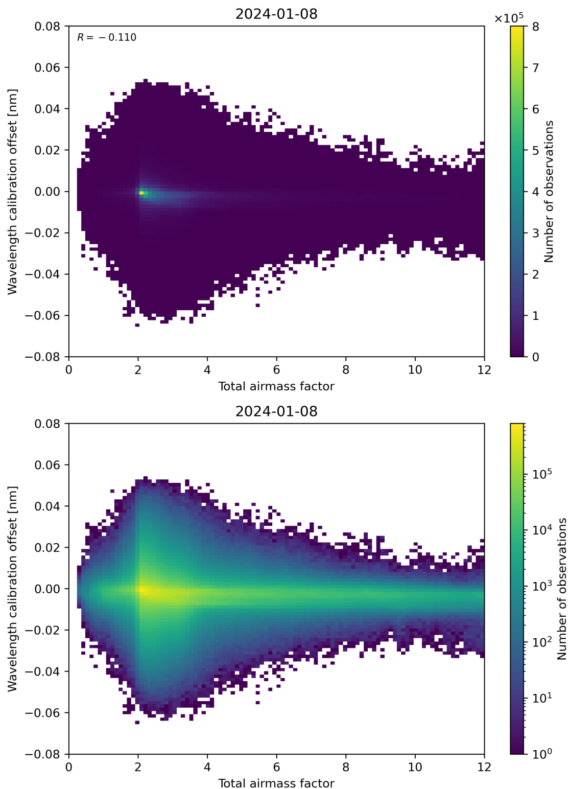
Figure 70: Scatter density plot of “Total airmass factor” against “Wavelength calibration offset” for 2024-01-07 to 2024-01-09.
