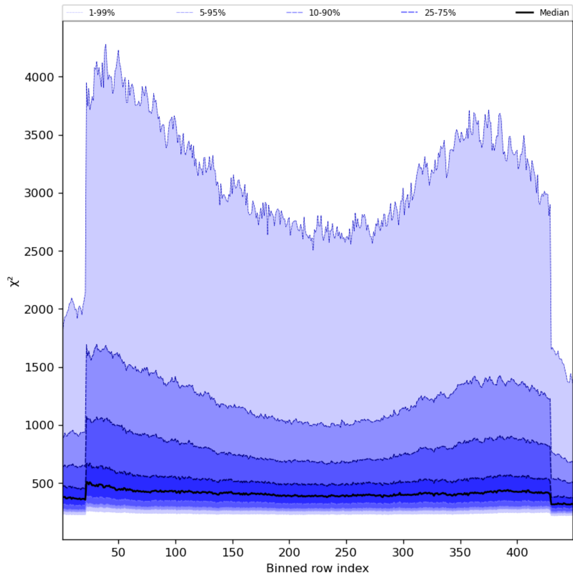
Figure 59: Along track statistics of “ \chi^2 ” for 2024-01-07 to 2024-01-09
