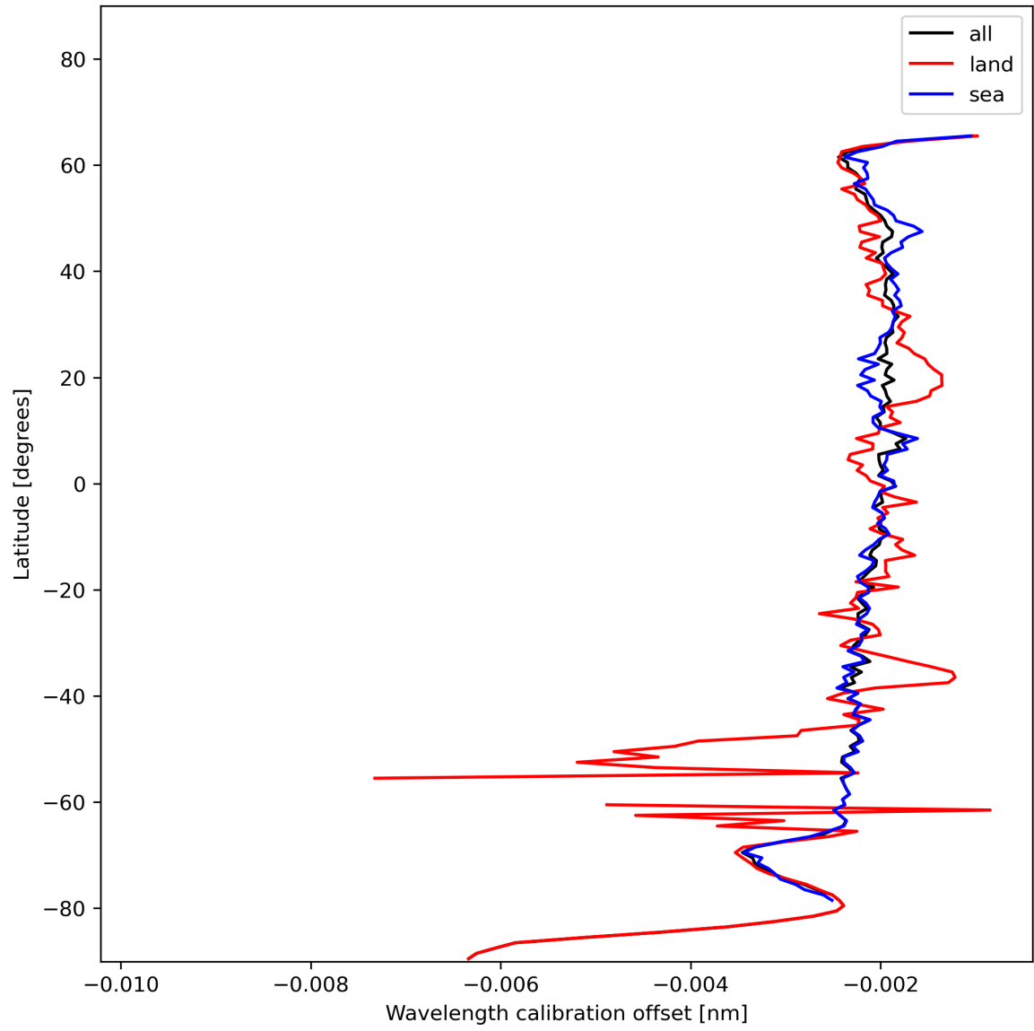
Figure 18: Zonal average of “Wavelength calibration offset” for 2024-01-07 to 2024-01-09.
