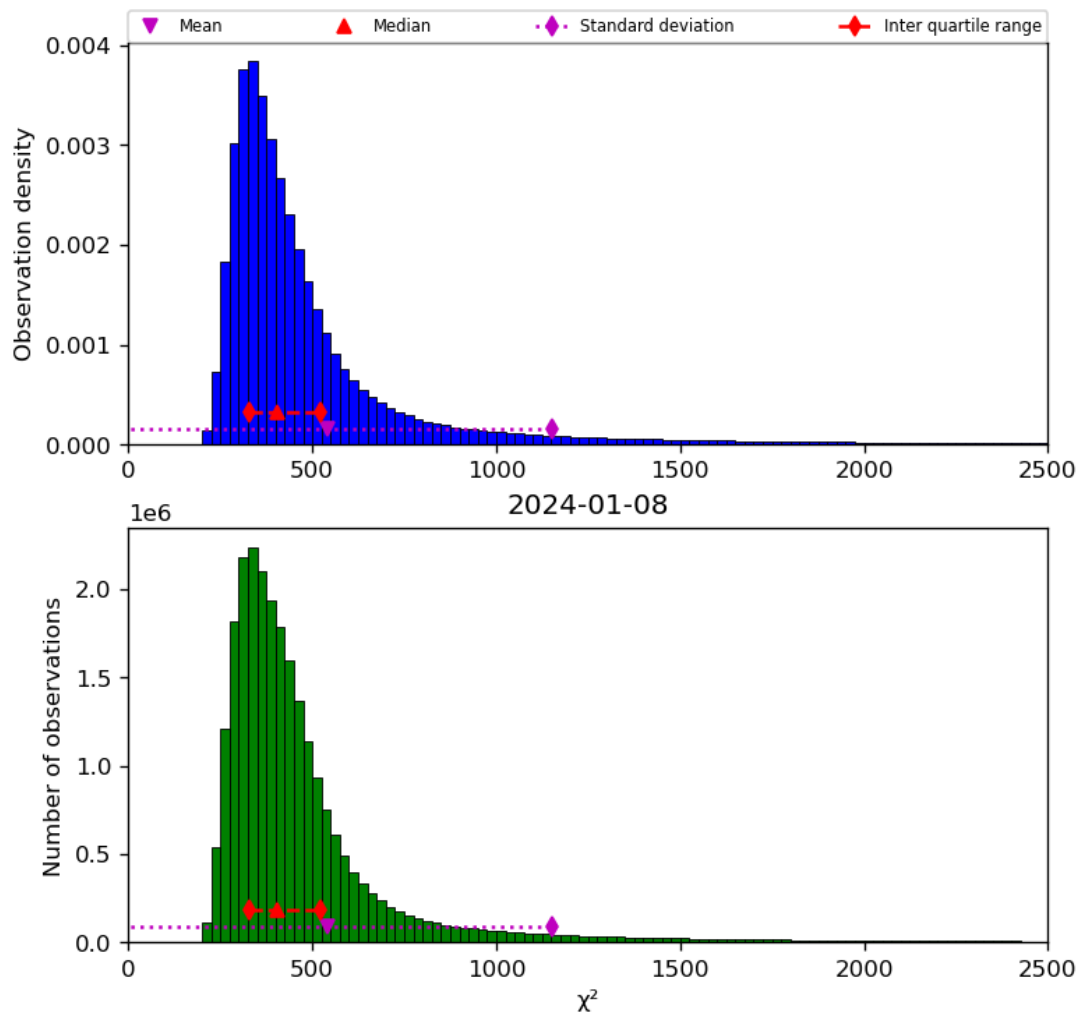
Figure 42: Histogram of " \chi^2 " for 2024-01-07 to 2024-01-09
