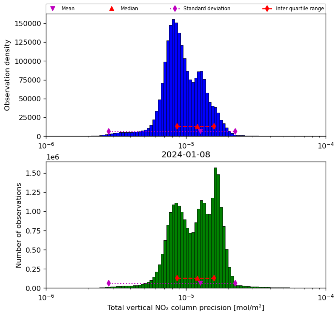
Figure 39: Histogram of "Total vertical NO 2 column precision" for 2024-01-07 to 2024-01-09
