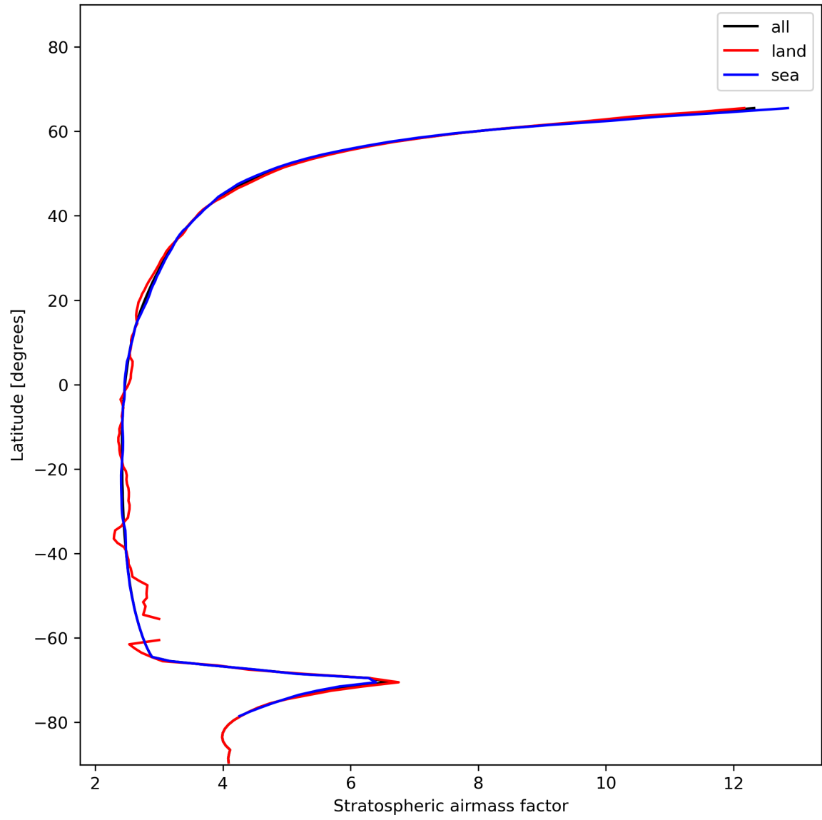
Figure 27: Zonal average of “Stratospheric air mass factor” for 2024-01-07 to 2024-01-09.
