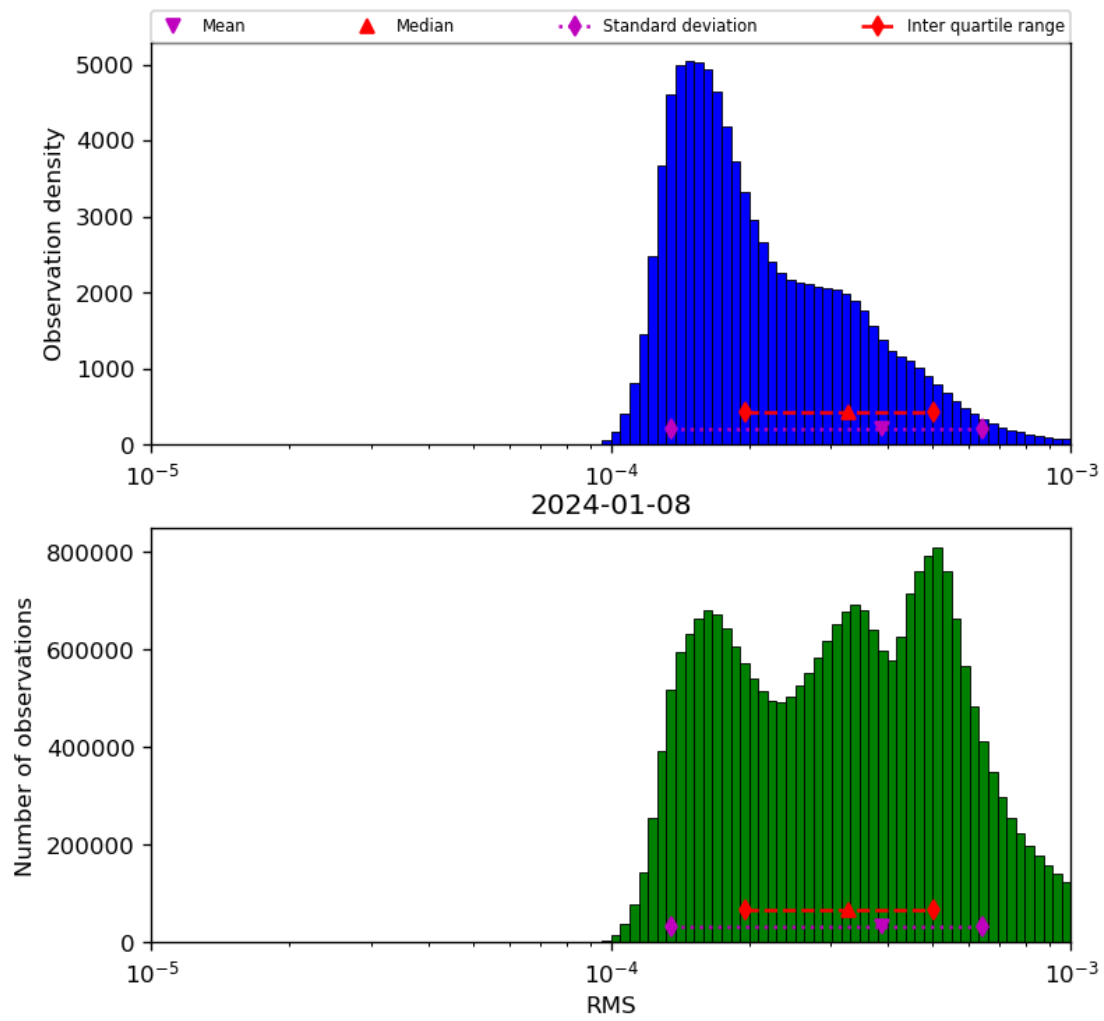
Figure 43: Histogram of “RMS” for 2024-01-07 to 2024-01-09
