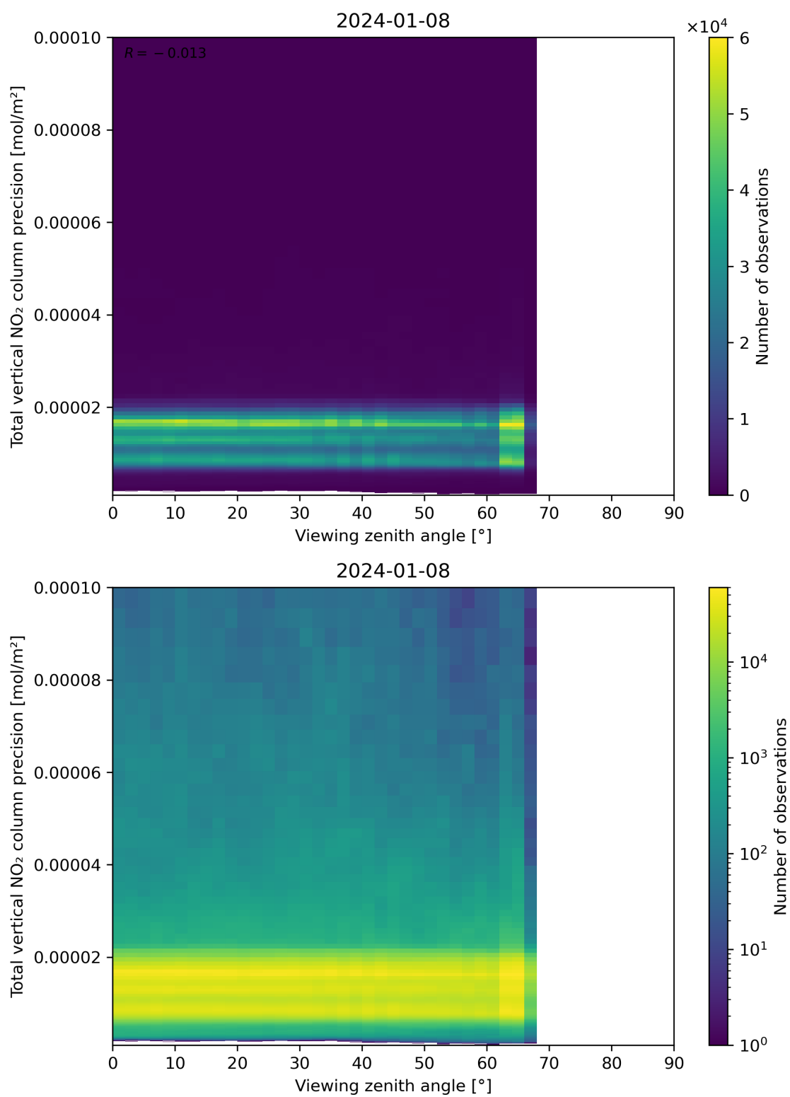
Figure 168: Scatter density plot of “Viewing zenith angle” against “Total vertical NO 2 column precision” for 2024-01-07 to 2024-01-09.
