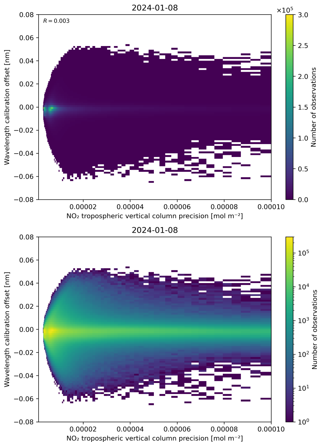
Figure 141: Scatter density plot of “NO 2 tropospheric vertical column precision” against “Wavelength calibration offset” for 2024-01-07 to 2024-01-09.
