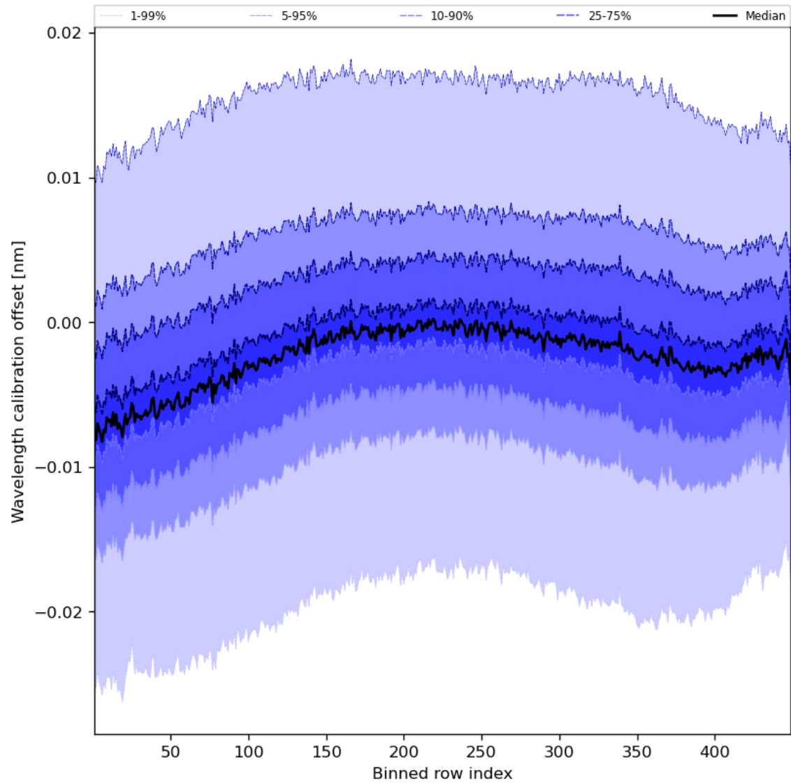
Figure 52: Along track statistics of “Wavelength calibration offset” for 2024-01-07 to 2024-01-09
