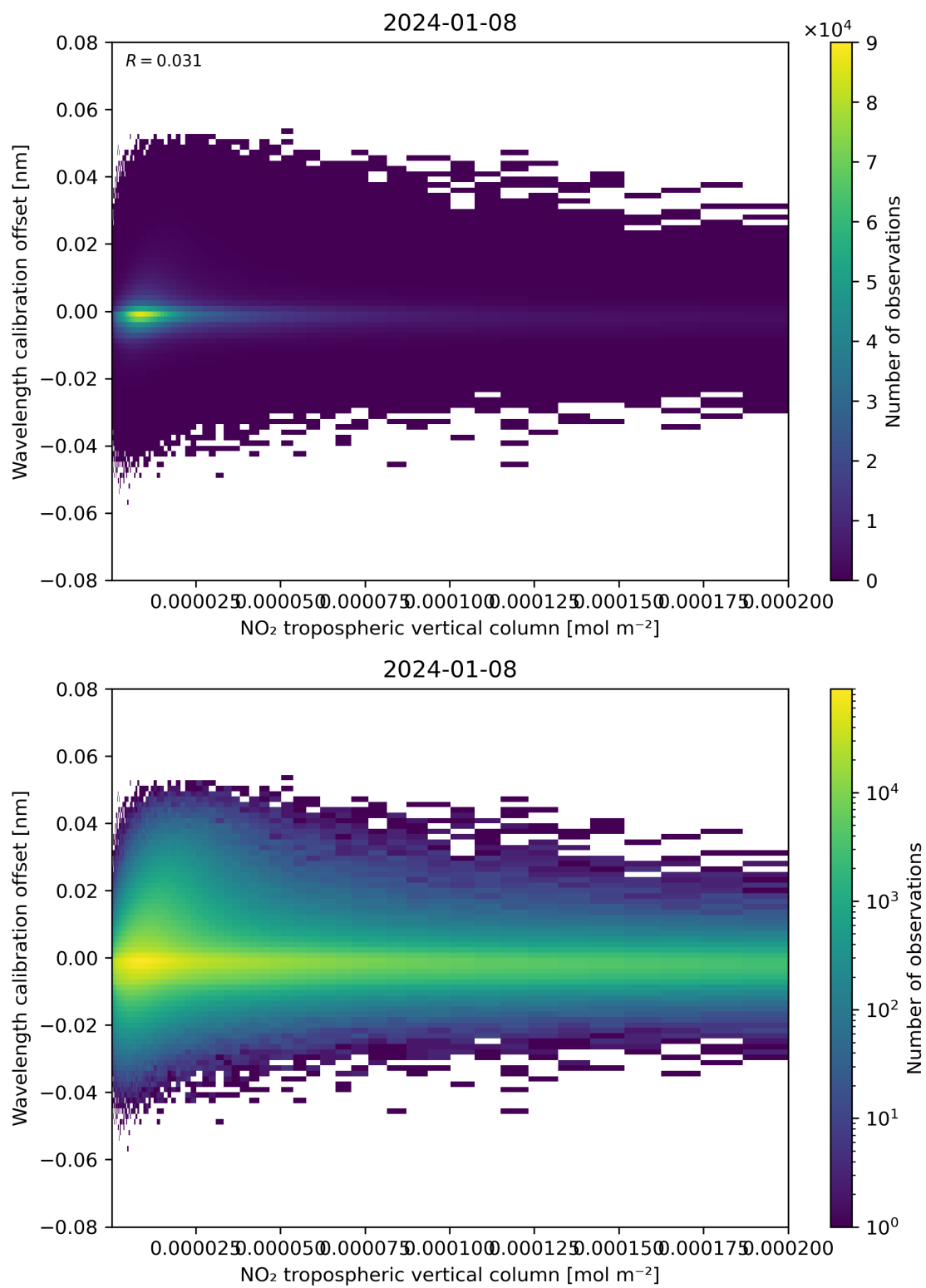
Figure 143: Scatter density plot of “NO 2 tropospheric vertical column” against “Wavelength calibration offset” for 2024-01-07 to 2024-01-09.
