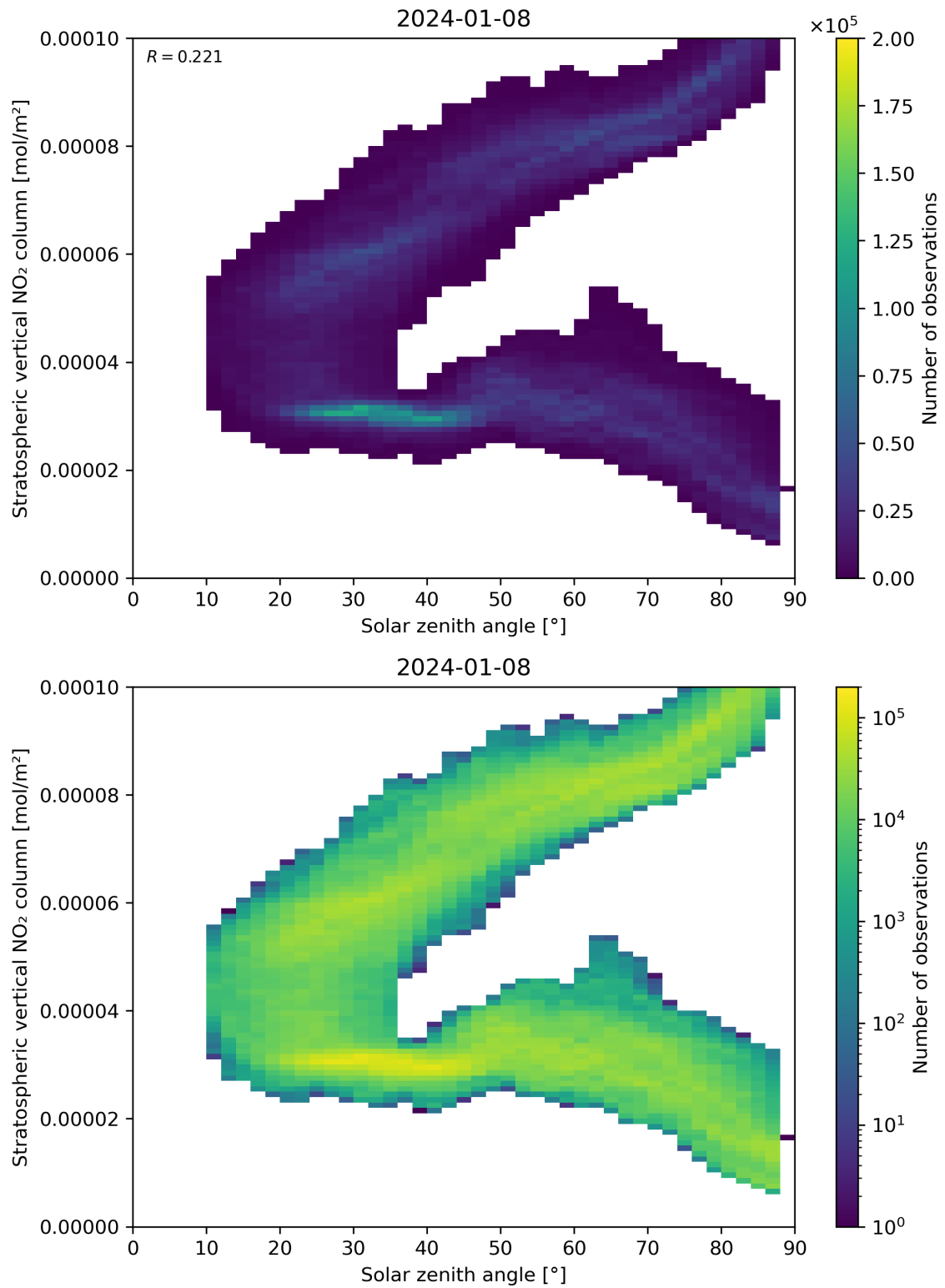
Figure 150: Scatter density plot of “Solar zenith angle” against “Stratospheric vertical NO 2 column” for 2024-01-07 to 2024-01-09.
