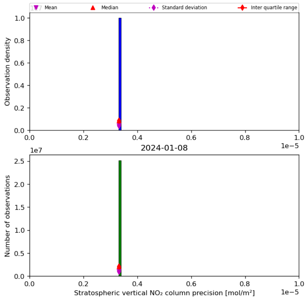
Figure 37: Histogram of “Stratospheric vertical NO 2 column precision” for 2024-01-07 to 2024-01-09
