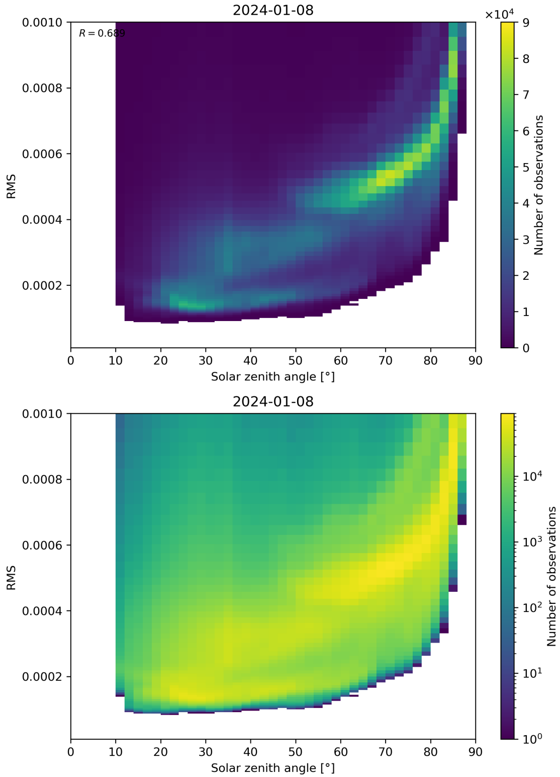
Figure 157: Scatter density plot of “Solar zenith angle” against “RMS” for 2024-01-07 to 2024-01-09.
