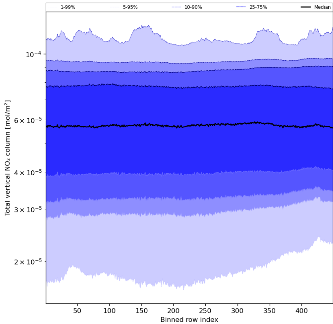
Figure 55: Along track statistics of “Total vertical NO 2 column” for 2024-01-07 to 2024-01-09
