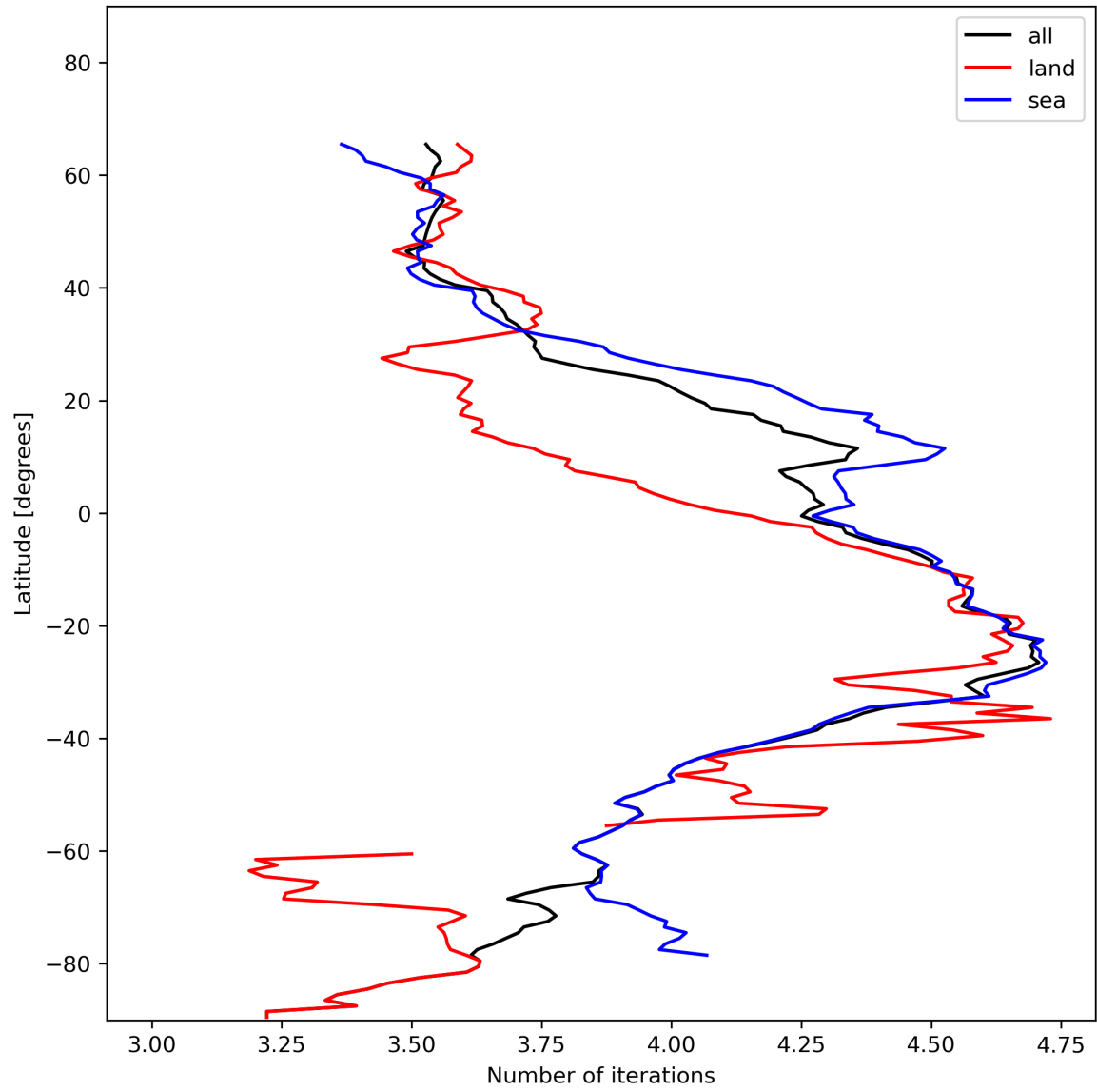
Figure 17: Zonal average of “Number of iterations” for 2024-01-07 to 2024-01-09.
