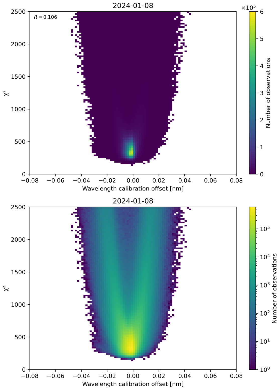
Figure 175: Scatter density plot of “Wavelength calibration offset” against “ \chi^2 ” for 2024-01-07 to 2024-01-09.
