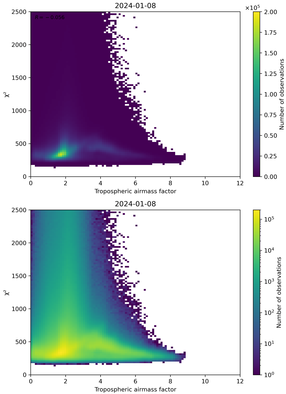
Figure 73: Scatter density plot of “Tropospheric airmass factor” against “ \chi^2 ” for 2024-01-07 to 2024-01-09.
