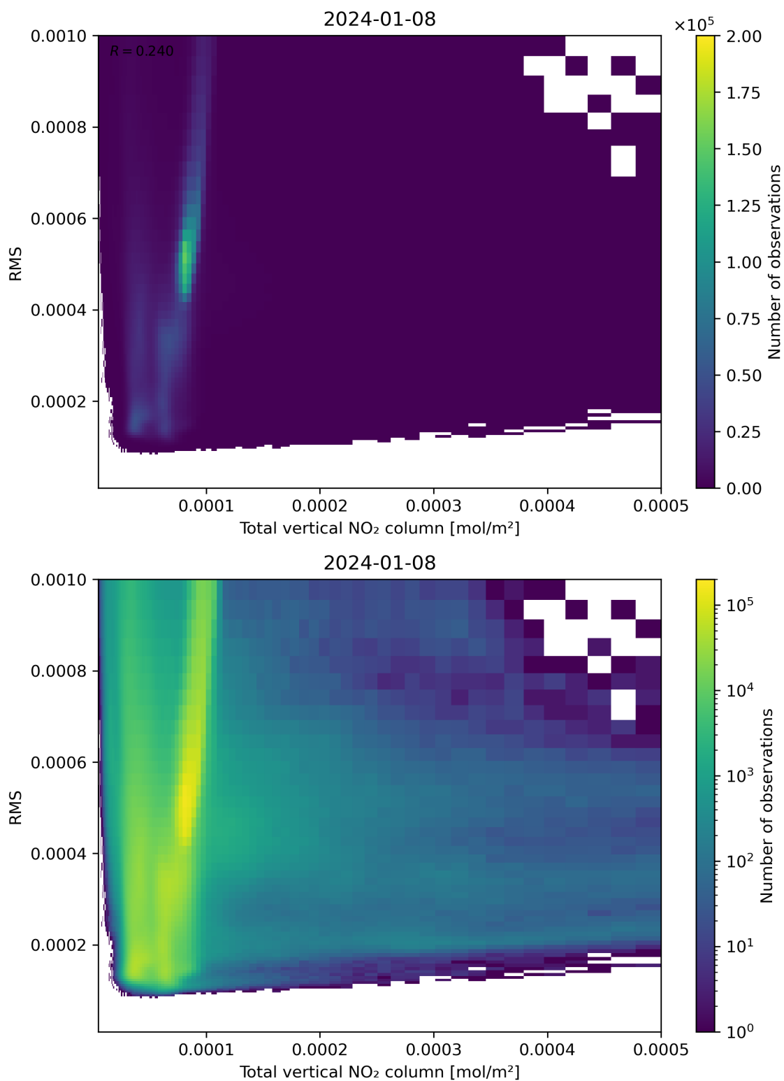
Figure 120: Scatter density plot of “Total vertical NO 2 column” against “RMS” for 2024-01-07 to 2024-01-09.
