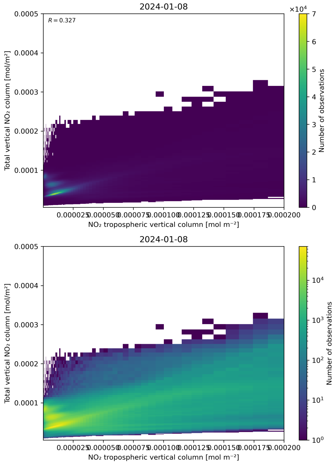
Figure 128: Scatter density plot of “NO 2 tropospheric vertical column” against “Total vertical NO 2 column” for 2024-01-07 to 2024-01-09.
