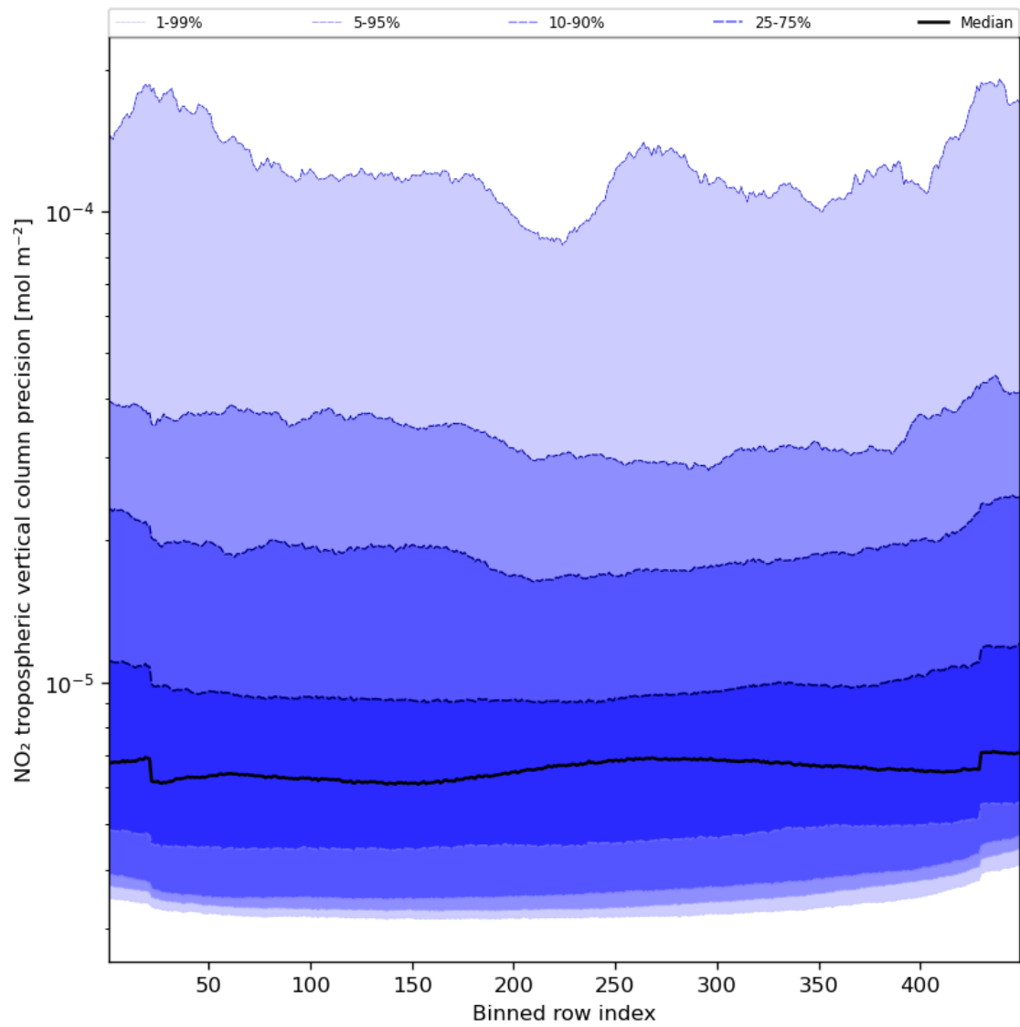
Figure 47: Along track statistics of “NO 2 tropospheric vertical column precision” for 2024-01-07 to 2024-01-09
