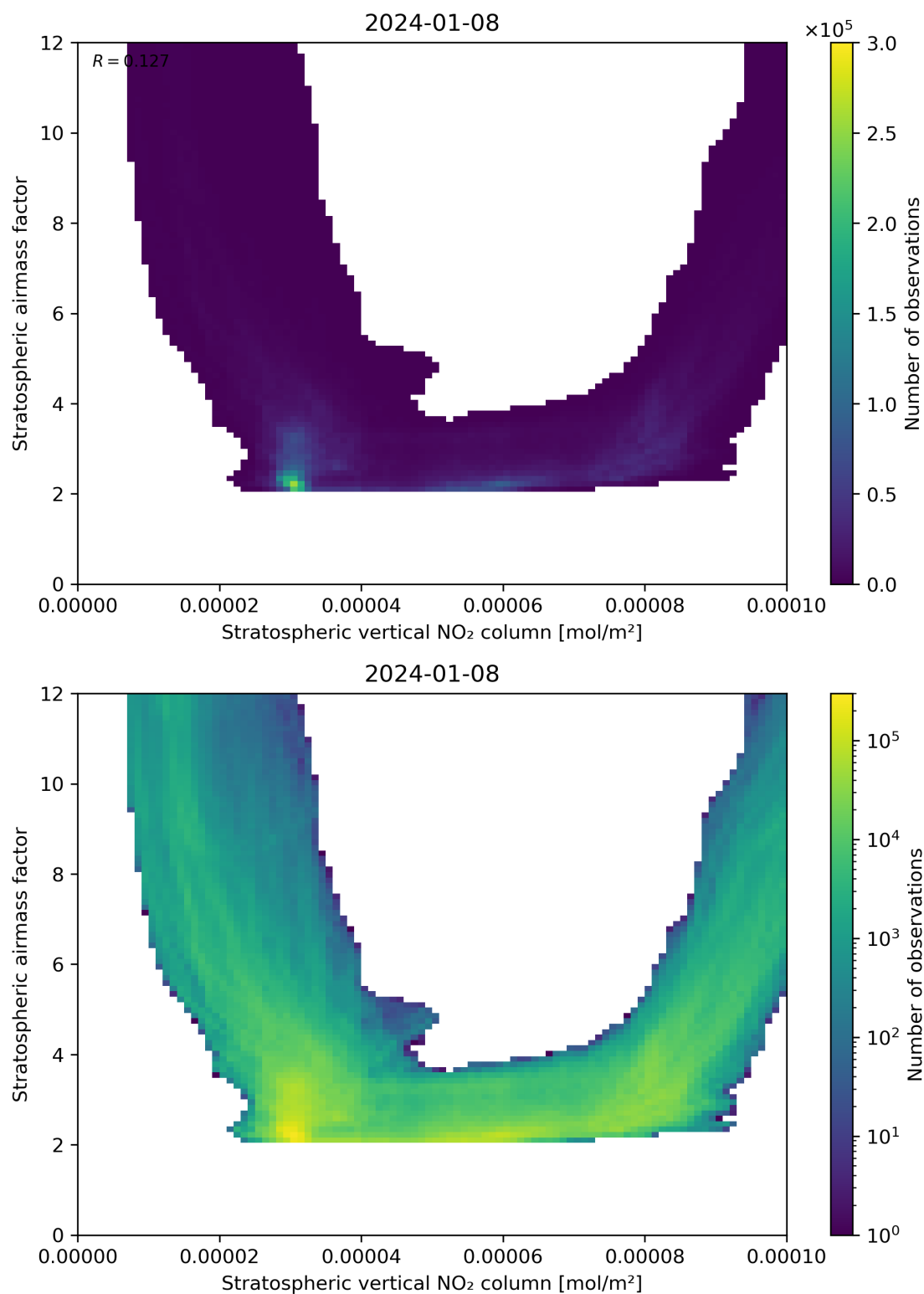
Figure 96: Scatter density plot of “Stratospheric vertical NO 2 column” against “Stratospheric airmass factor” for 2024-01-07 to 2024-01-09.
