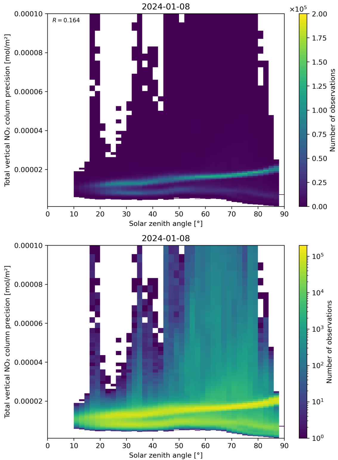
Figure 154: Scatter density plot of “Solar zenith angle” against “Total vertical NO 2 column precision” for 2024-01-07 to 2024-01-09.
