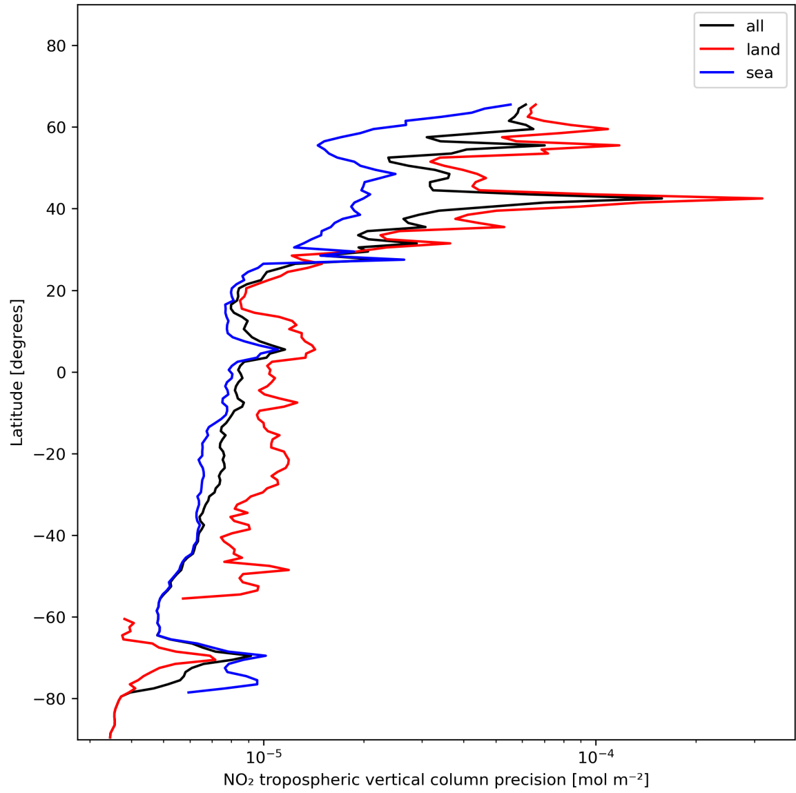
Figure 13: Zonal average of “NO 2 tropospheric vertical column precision” for 2024-01-07 to 2024-01-09.
