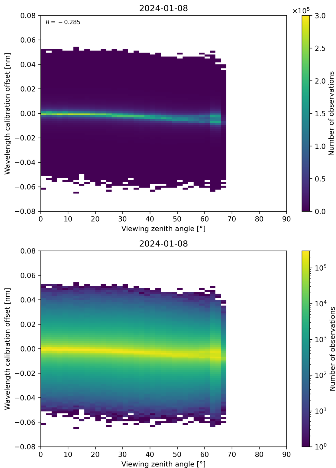
Figure 173: Scatter density plot of “Viewing zenith angle” against “Wavelength calibration offset” for 2024-01-07 to 2024-01-09.
