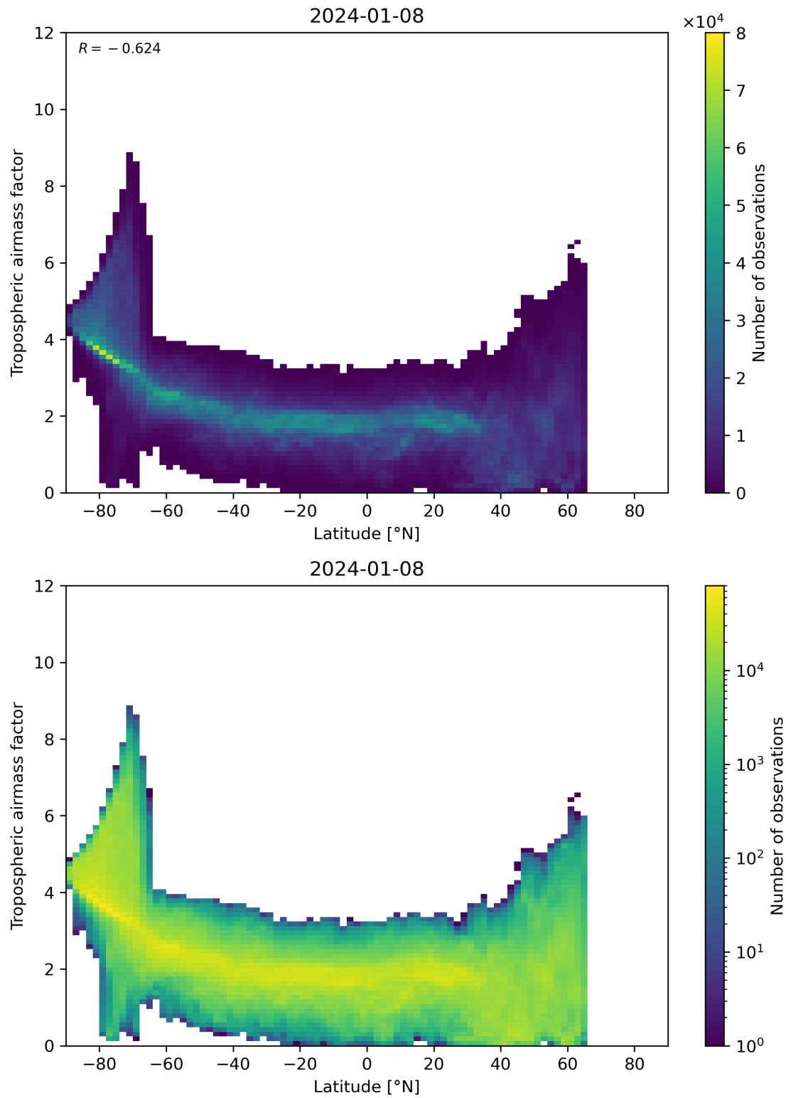
Figure 85: Scatter density plot of “Latitude” against “Tropospheric air mass factor” for 2024-01-07 to 2024-01-09.
