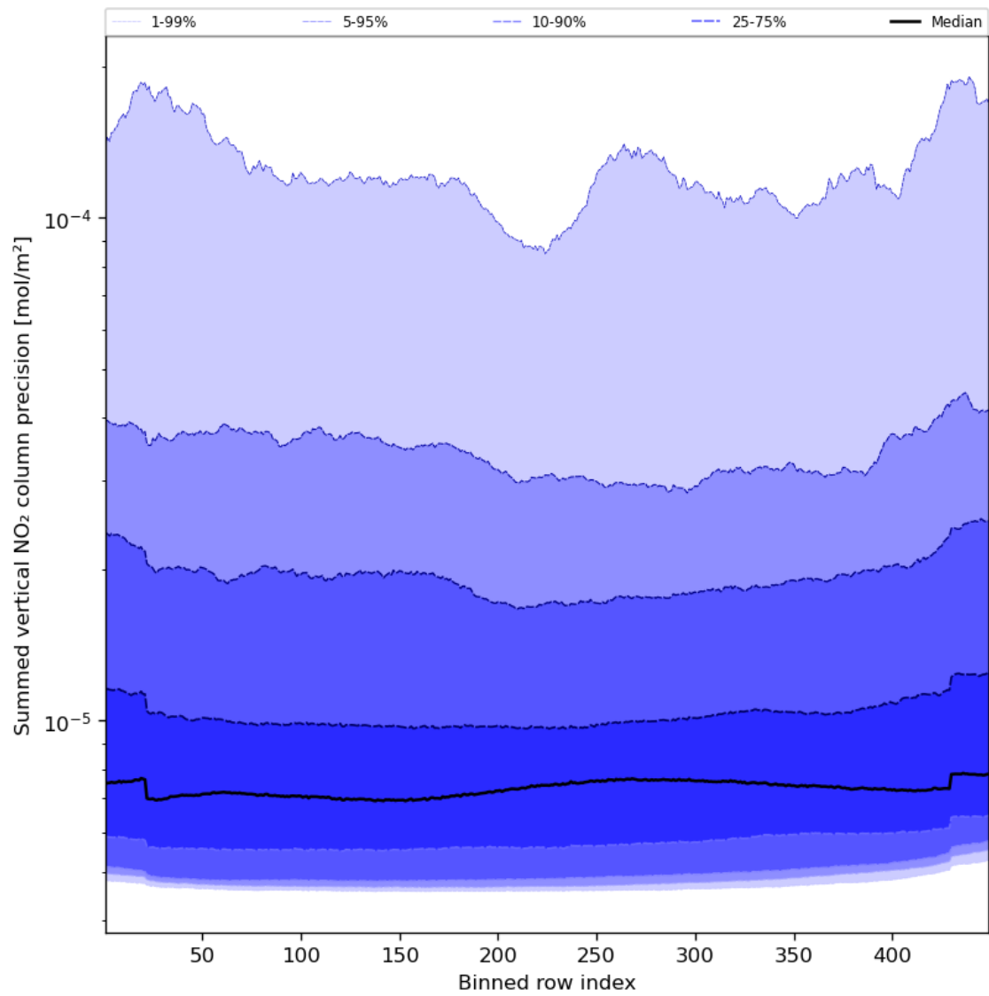
Figure 58: Along track statistics of “Summed vertical NO 2 column precision” for 2024-01-07 to 2024-01-09
