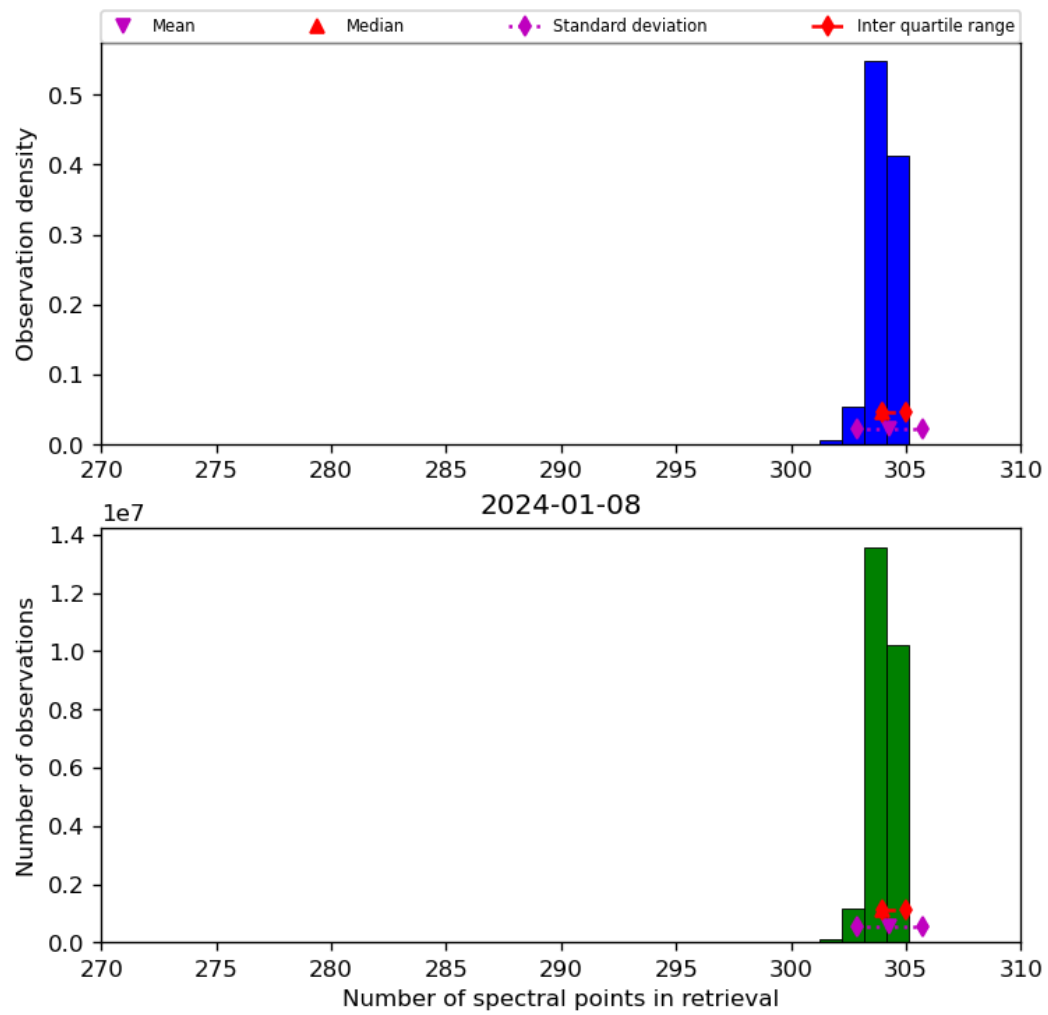
Figure 33: Histogram of “Number of spectral points in retrieval” for 2024-01-07 to 2024-01-09
