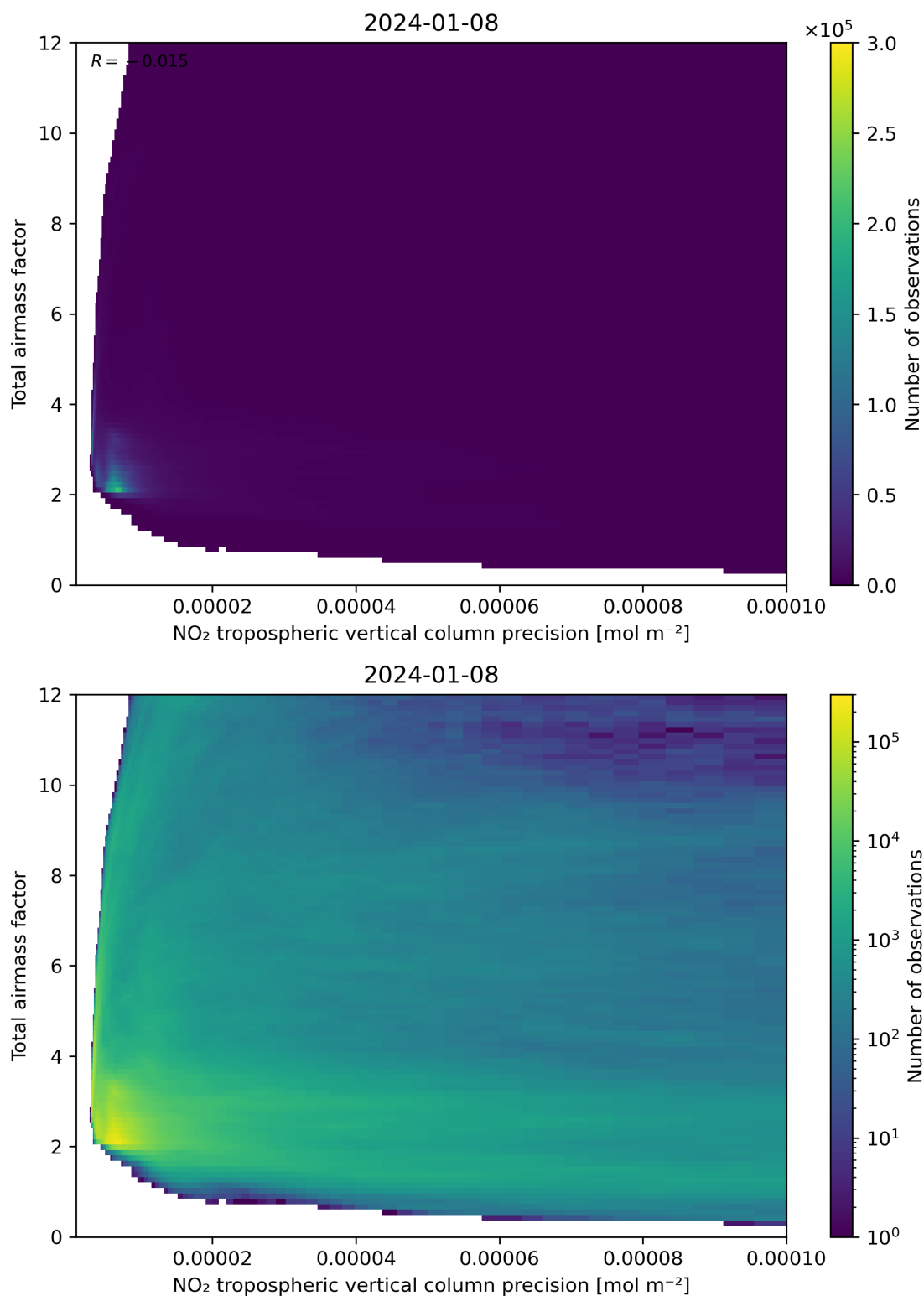
Figure 132: Scatter density plot of “NO 2 tropospheric vertical column precision” against “Total air mass factor” for 2024-01-07 to 2024-01-09.
