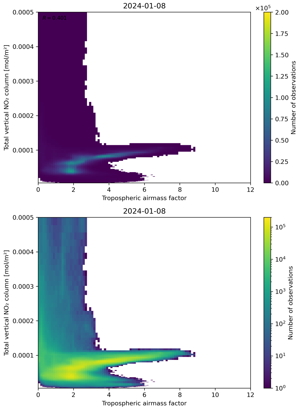
Figure 77: Scatter density plot of “Tropospheric airmass factor” against “Total vertical NO 2 column” for 2024-01-07 to 2024-01-09.
