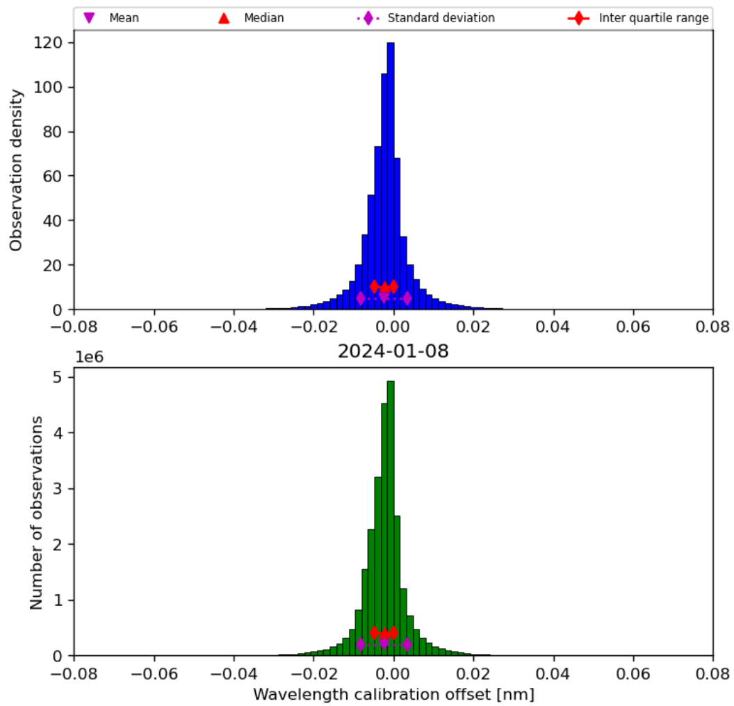
Figure 35: Histogram of “Wavelength calibration offset” for 2024-01-07 to 2024-01-09
