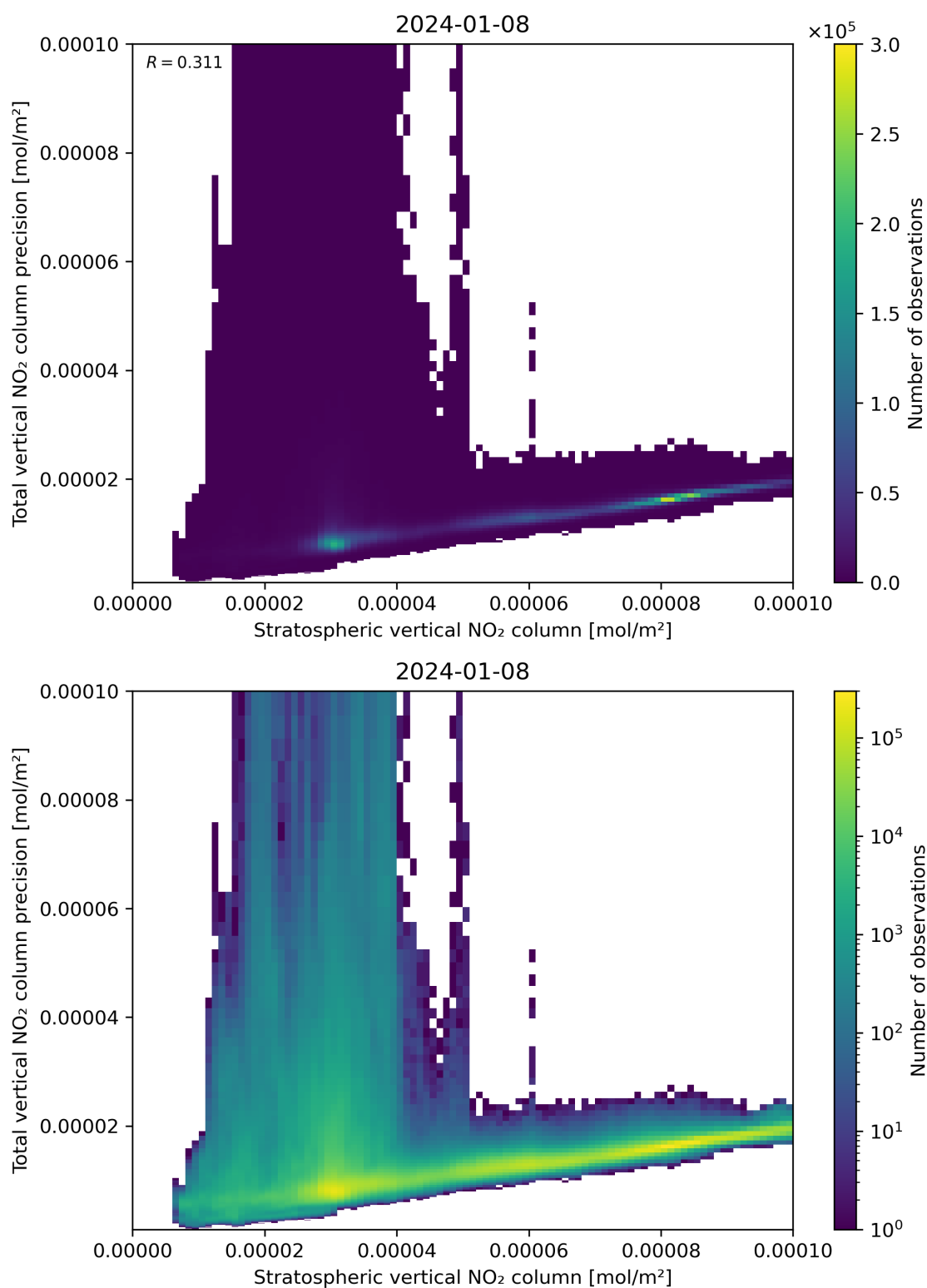
Figure 101: Scatter density plot of “Stratospheric vertical NO 2 column” against “Total vertical NO 2 column precision” for 2024-01-07 to 2024-01-09.
