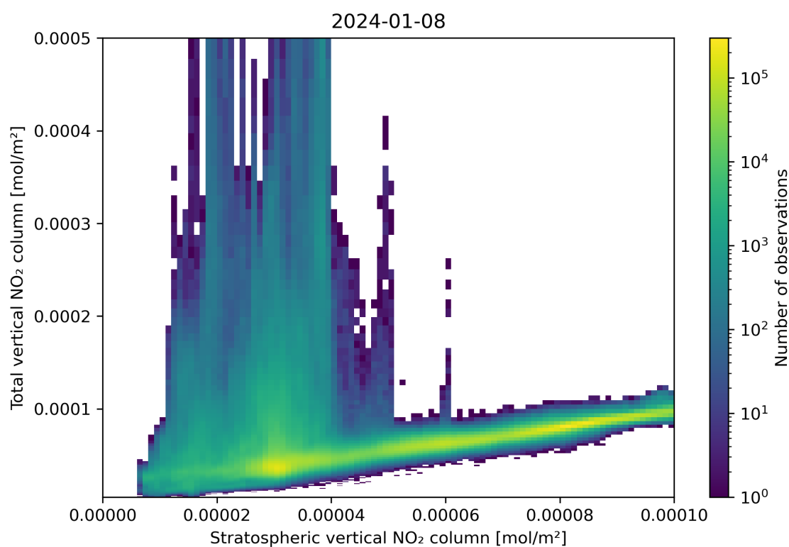
Figure 100: Scatter density plot of “Stratospheric vertical NO 2 column” against “Total vertical NO 2 column” for 2024-01-07 to 2024-01-09.
