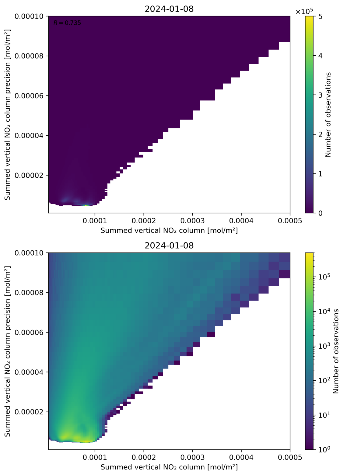
Figure 105: Scatter density plot of “Summed vertical NO 2 column” against “Summed vertical NO 2 column precision” for 2024-01-07 to 2024-01-09.
