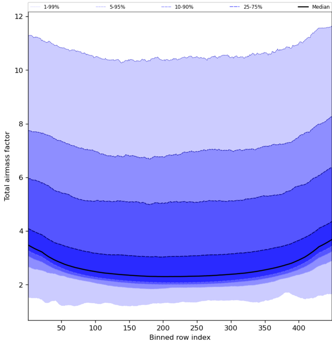
Figure 49: Along track statistics of “Total airmass factor” for 2024-01-07 to 2024-01-09
