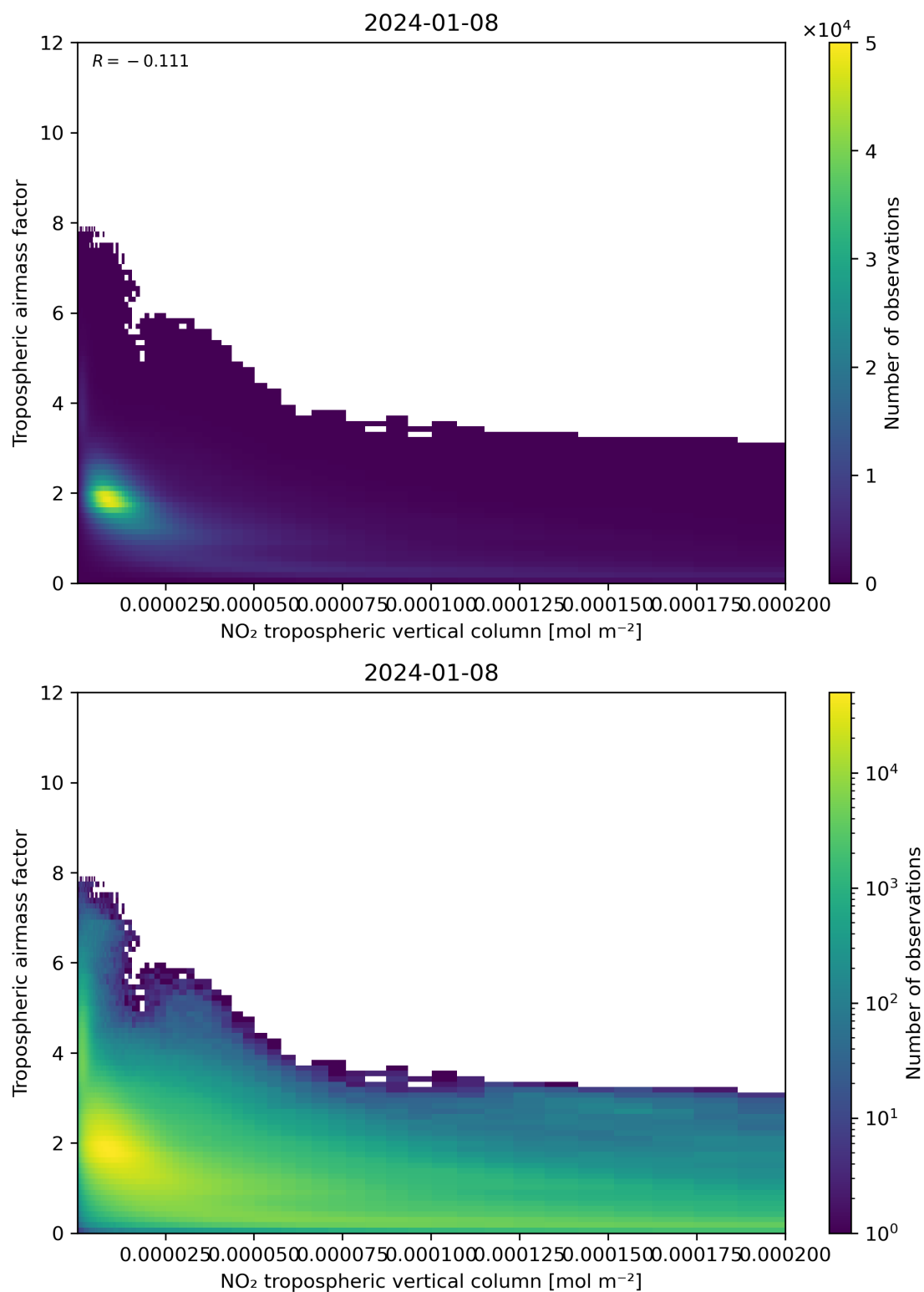
Figure 123: Scatter density plot of “NO 2 tropospheric vertical column” against “Tropospheric air mass factor” for 2024-01-07 to 2024-01-09.
