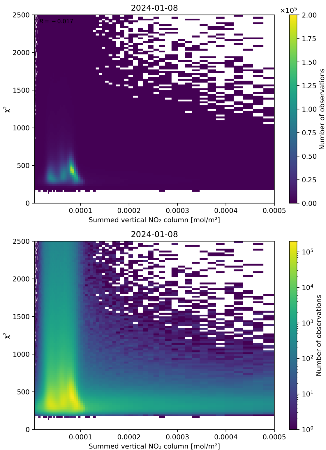
Figure 104: Scatter density plot of “Summed vertical NO 2 column” against “ \chi^2 ” for 2024-01-07 to 2024-01-09.
