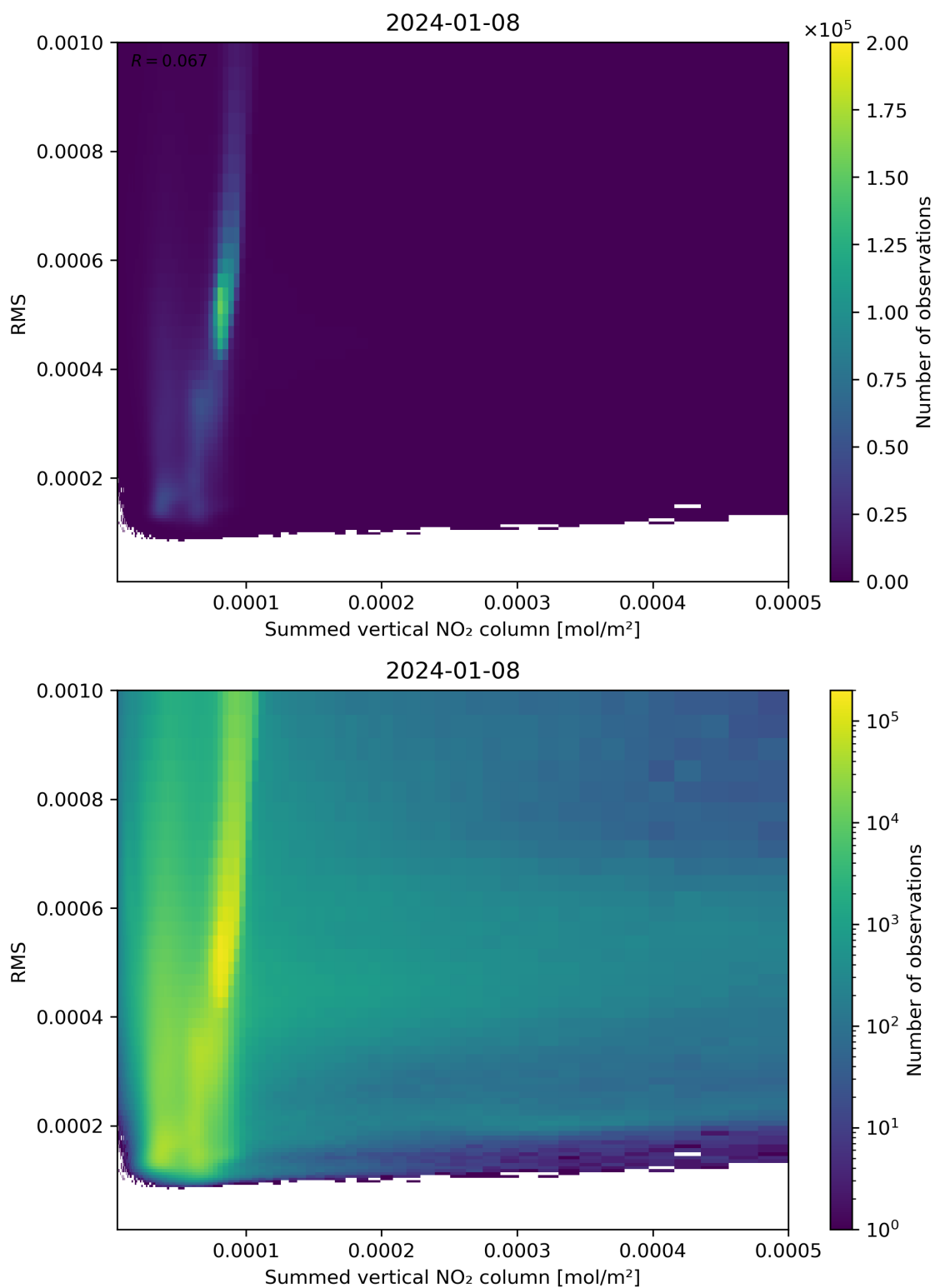
Figure 109: Scatter density plot of “Summed vertical NO 2 column” against “RMS” for 2024-01-07 to 2024-01-09.
