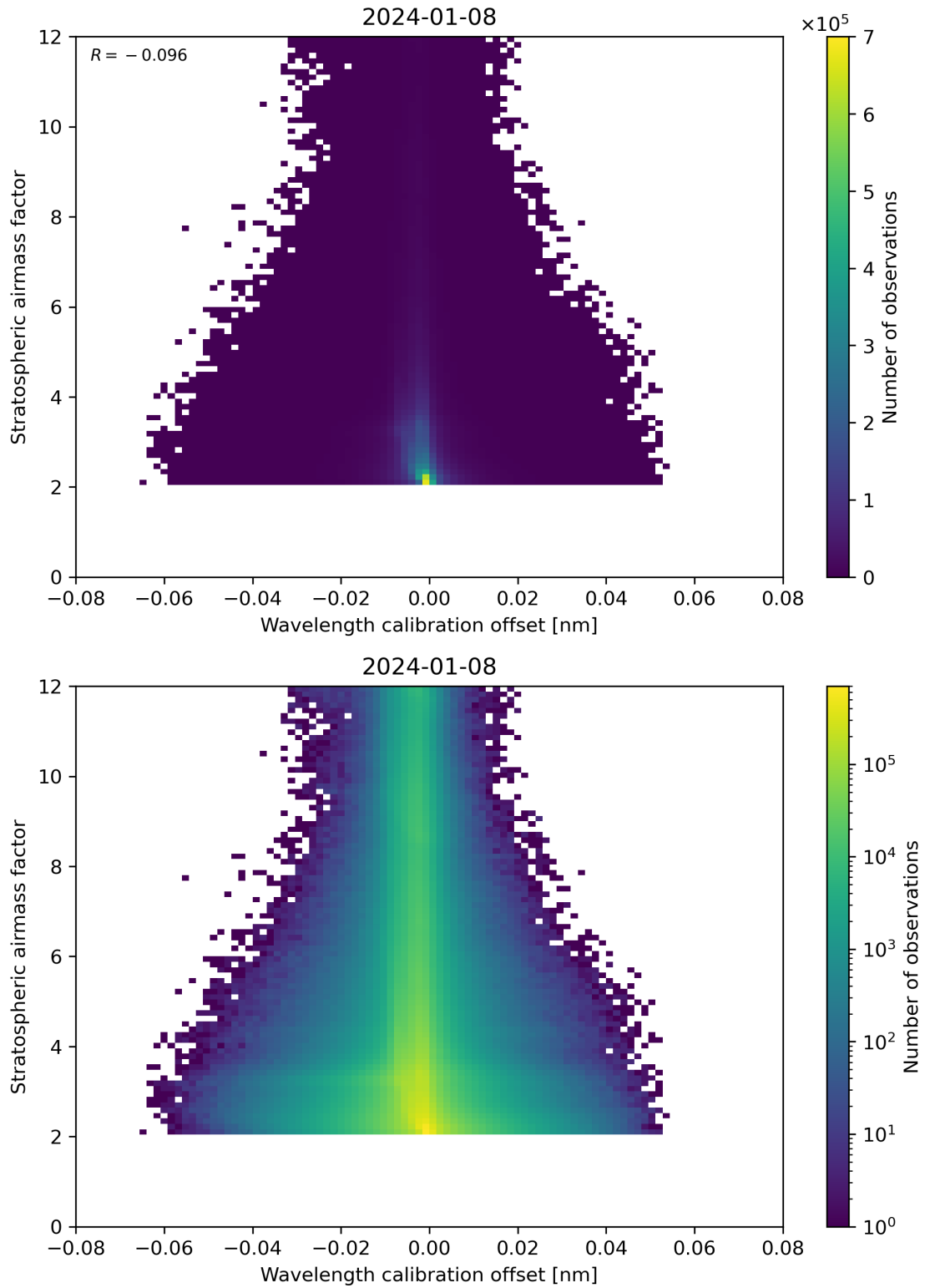
Figure 174: Scatter density plot of “Wavelength calibration offset” against “Stratospheric airmass factor” for 2024-01-07 to 2024-01-09.
