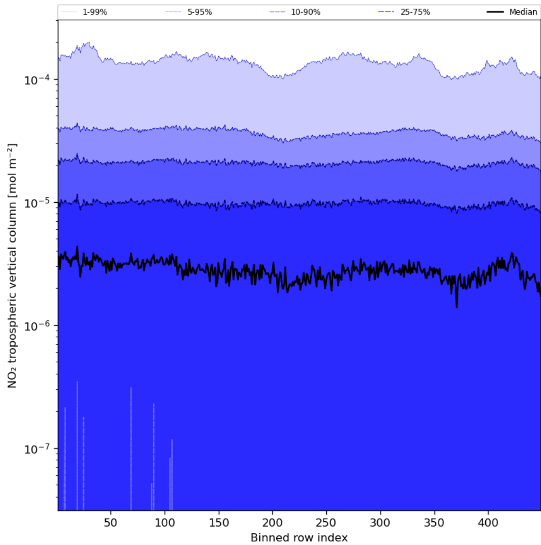
Figure 46: Along track statistics of “NO 2 tropospheric vertical column” for 2024-01-07 to 2024-01-09
