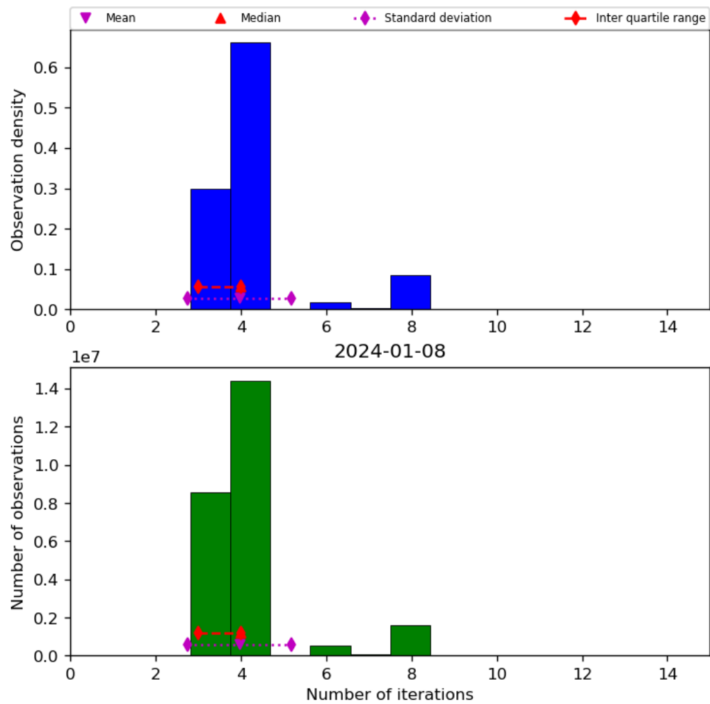
Figure 34: Histogram of “Number of iterations” for 2024-01-07 to 2024-01-09
