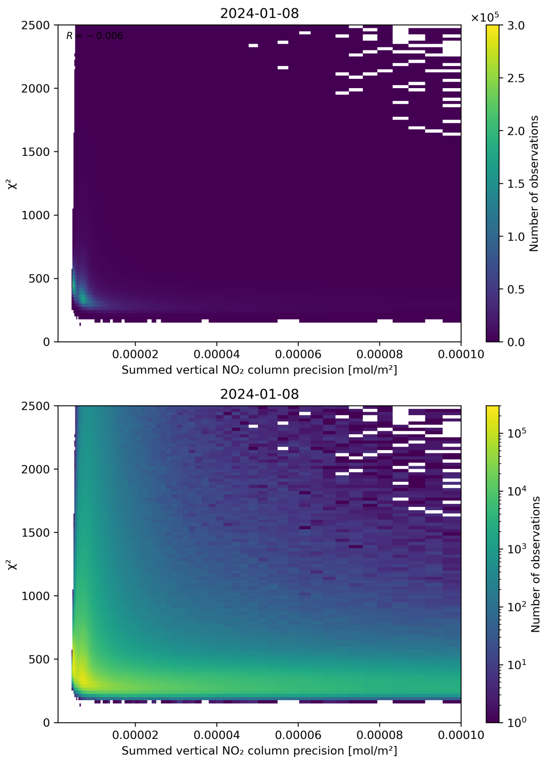
Figure 107: Scatter density plot of “Summed vertical NO 2 column precision” against “ \chi^2 ” for 2024-01-07 to 2024-01-09.
