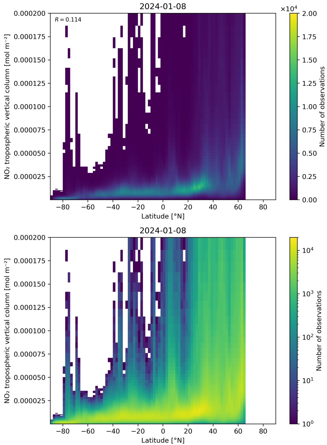
Figure 92: Scatter density plot of “Latitude” against “NO 2 tropospheric vertical column” for 2024-01-07 to 2024-01-09.
