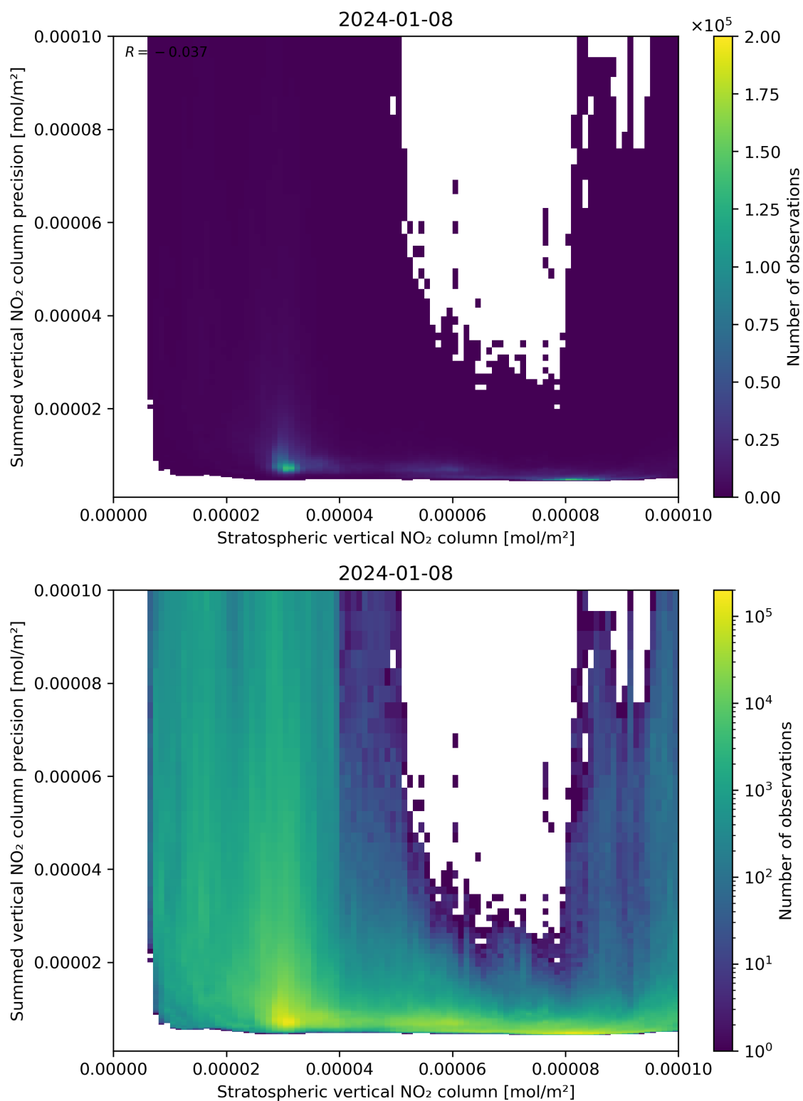
Figure 99: Scatter density plot of “Stratospheric vertical NO 2 column” against “Summed vertical NO 2 column precision” for 2024-01-07 to 2024-01-09.
