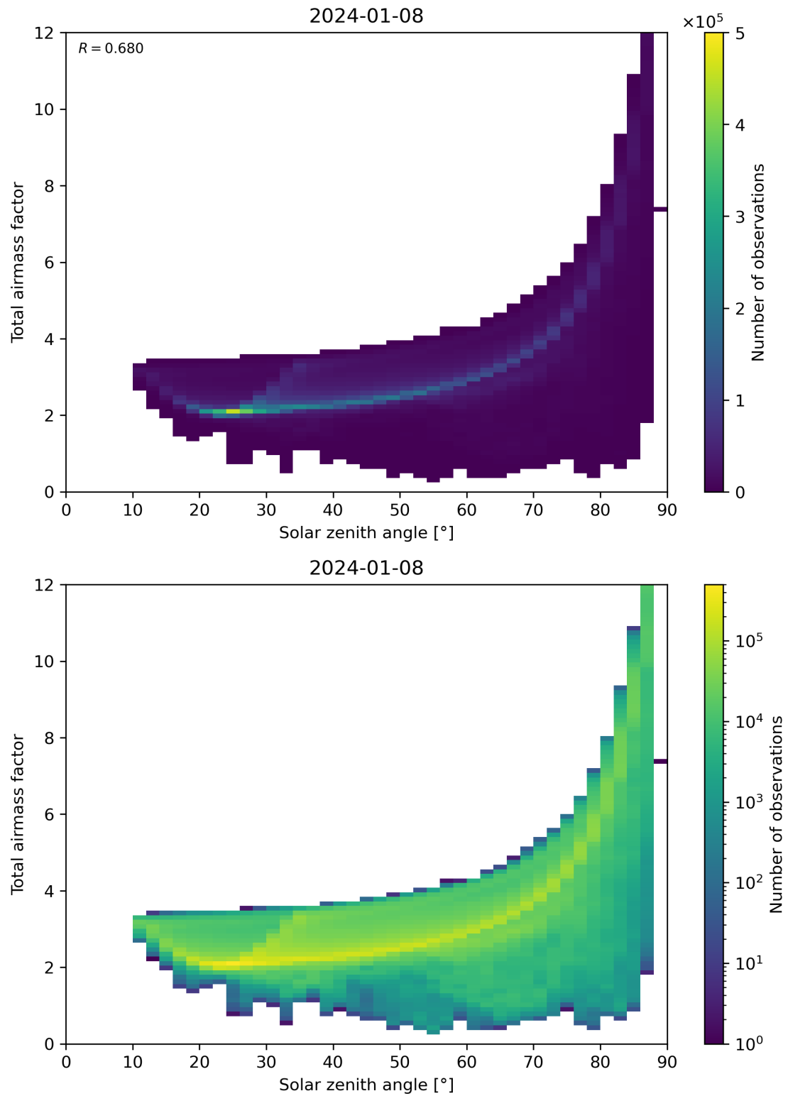
Figure 146: Scatter density plot of “Solar zenith angle” against “Total air mass factor” for 2024-01-07 to 2024-01-09.
