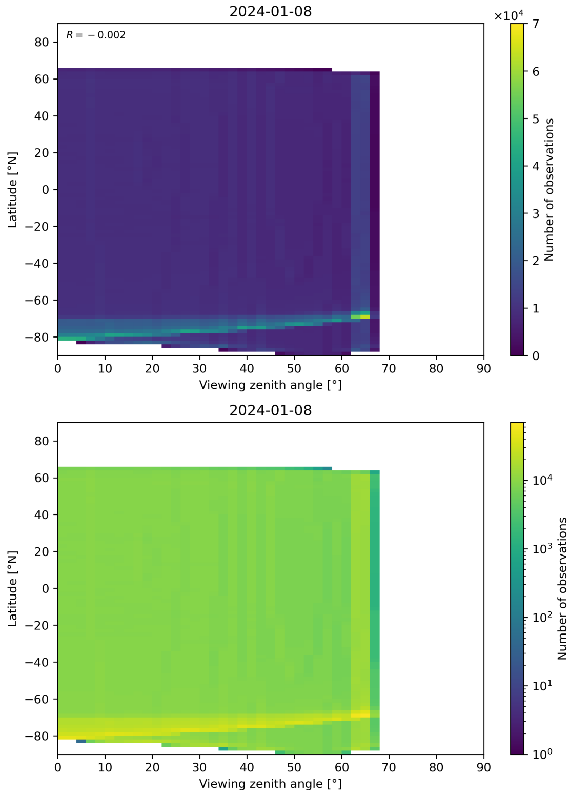
Figure 163: Scatter density plot of “Viewing zenith angle” against “Latitude” for 2024-01-07 to 2024-01-09.
