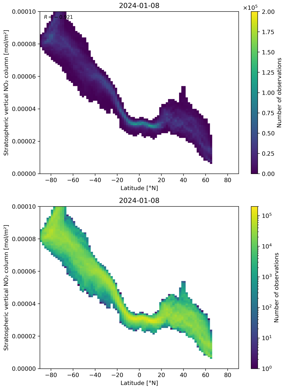
Figure 87: Scatter density plot of “Latitude” against “Stratospheric vertical NO 2 column” for 2024-01-07 to 2024-01-09.
