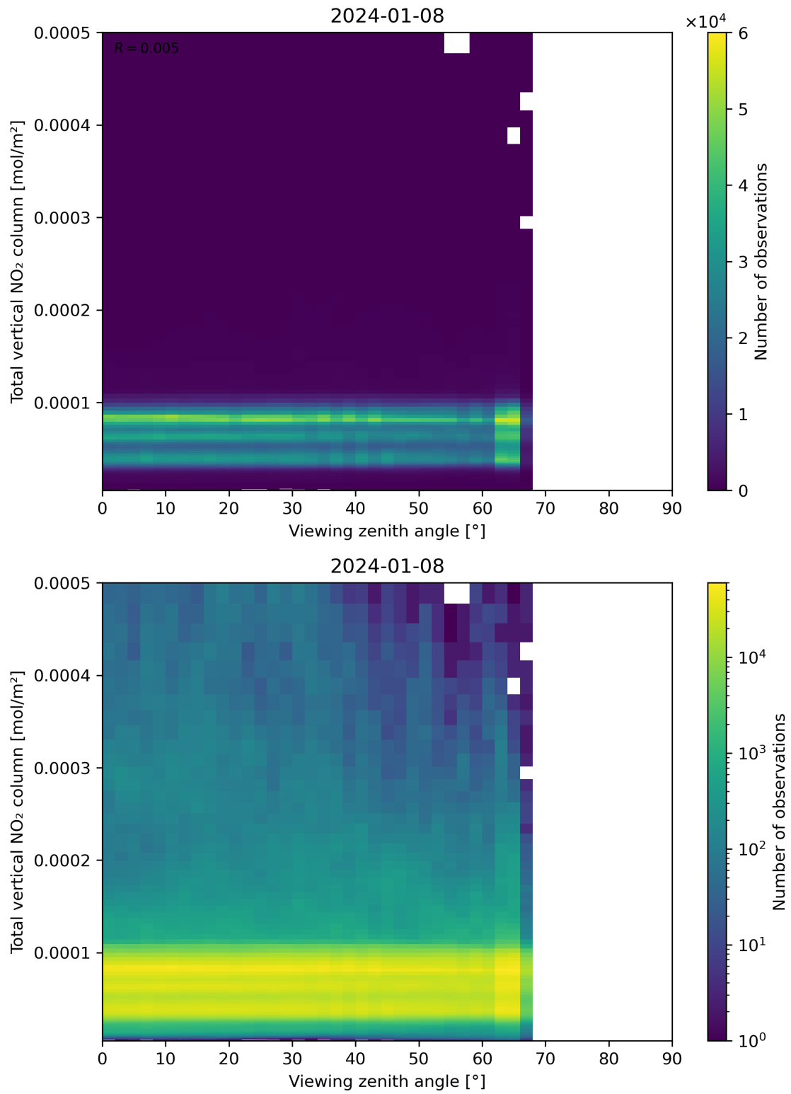
Figure 167: Scatter density plot of “Viewing zenith angle” against “Total vertical NO 2 column” for 2024-01-07 to 2024-01-09.
