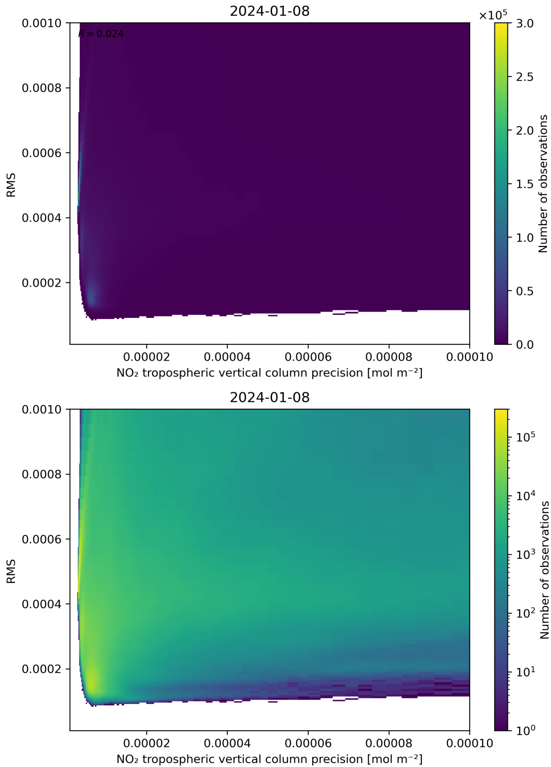
Figure 140: Scatter density plot of “NO 2 tropospheric vertical column precision” against “RMS” for 2024-01-07 to 2024-01-09.
