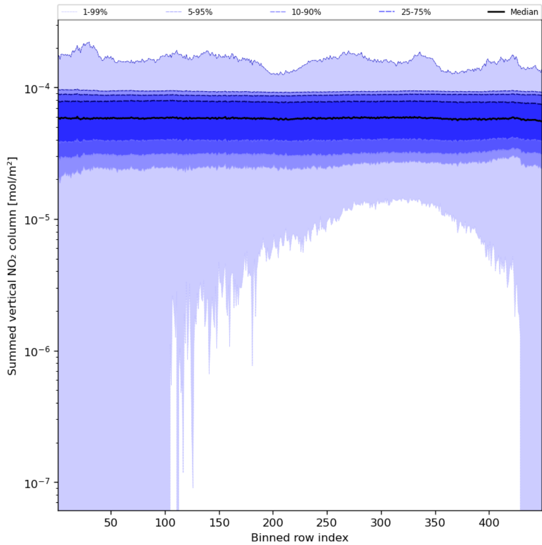
Figure 57: Along track statistics of “Summed vertical NO 2 column” for 2024-01-07 to 2024-01-09
