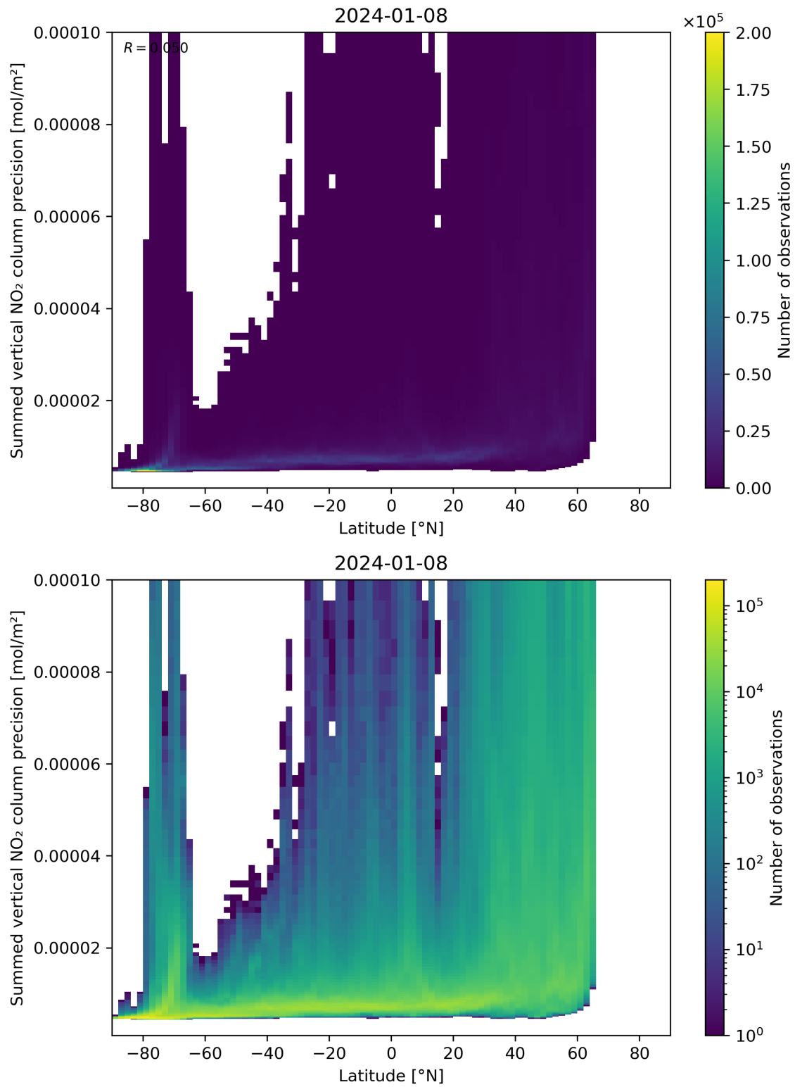
Figure 89: Scatter density plot of “Latitude” against “Summed vertical NO 2 column precision” for 2024-01-07 to 2024-01-09.
