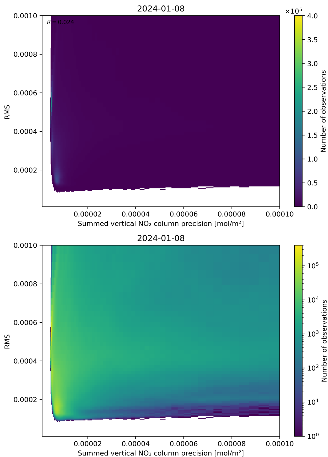
Figure 108: Scatter density plot of “Summed vertical NO 2 column precision” against “RMS” for 2024-01-07 to 2024-01-09.
