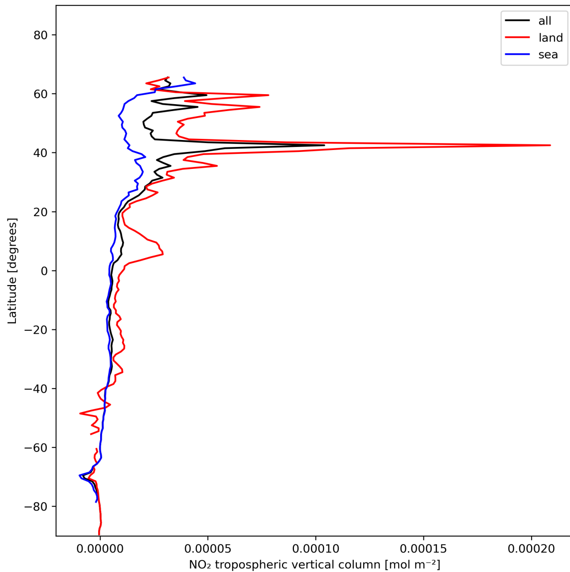
Figure 12: Zonal average of “NO 2 tropospheric vertical column” for 2024-01-07 to 2024-01-09.
