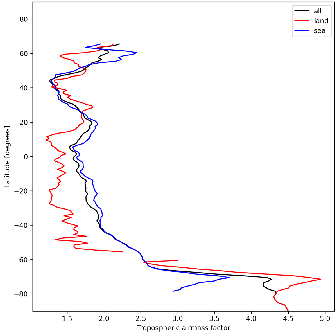
Figure 14: Zonal average of “Tropospheric airmass factor” for 2024-01-07 to 2024-01-09.
