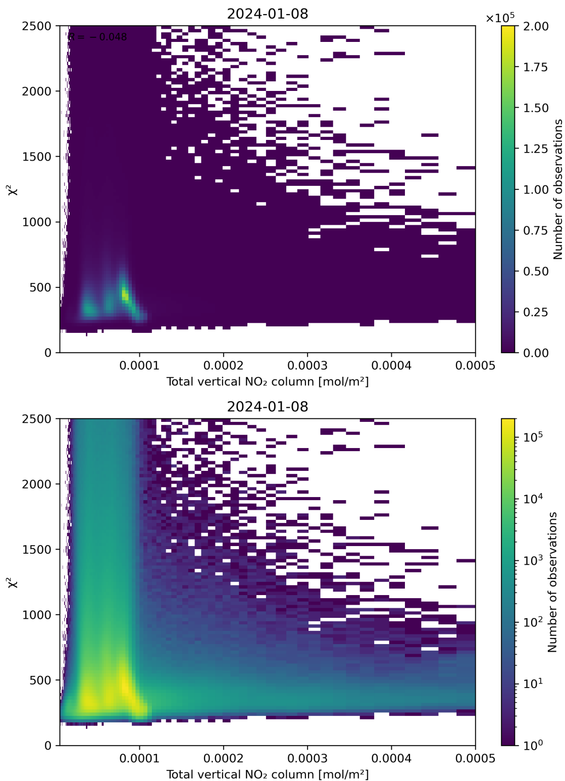
Figure 111: Scatter density plot of “Total vertical NO 2 column” against “ \chi^2 ” for 2024-01-07 to 2024-01-09.
