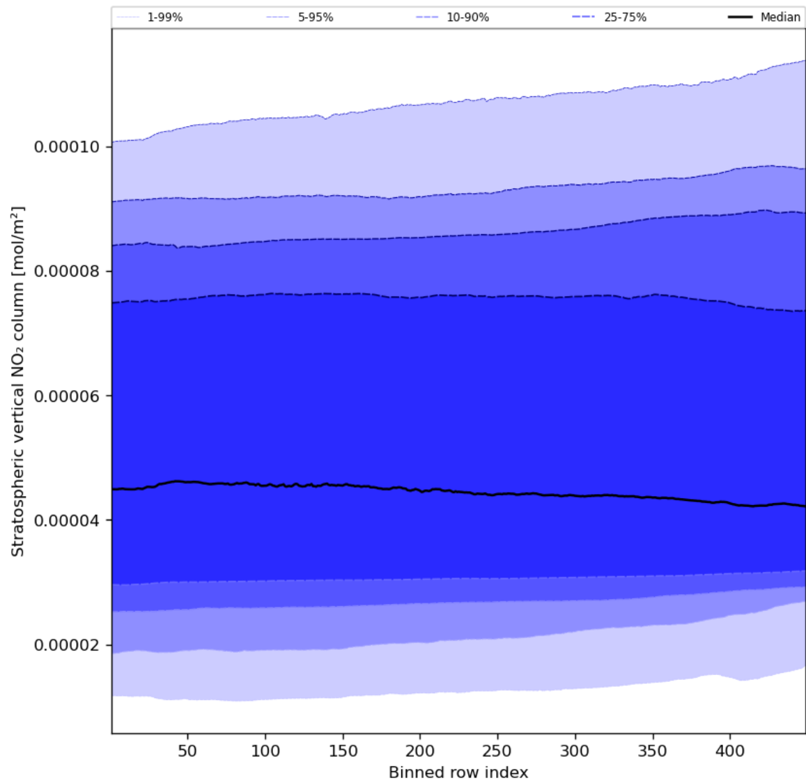
Figure 53: Along track statistics of “Stratospheric vertical NO 2 column” for 2024-01-07 to 2024-01-09
