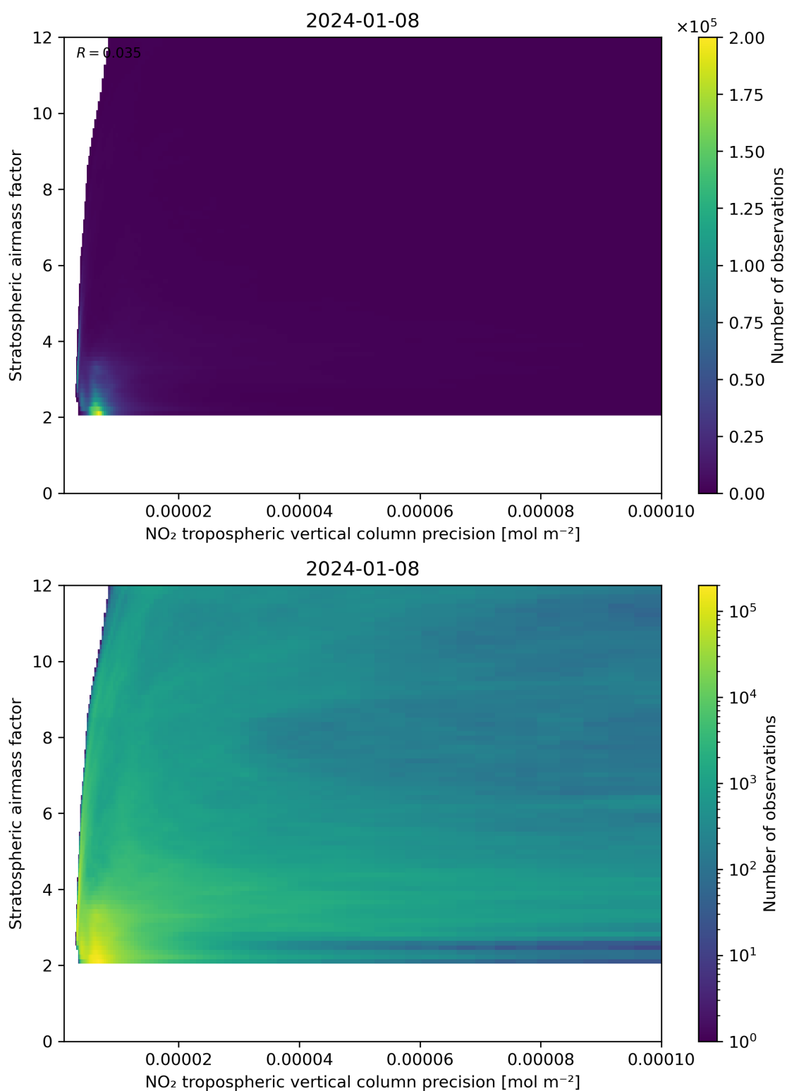
Figure 131: Scatter density plot of “NO 2 tropospheric vertical column precision” against “Stratospheric airmass factor” for 2024-01-07 to 2024-01-09.
