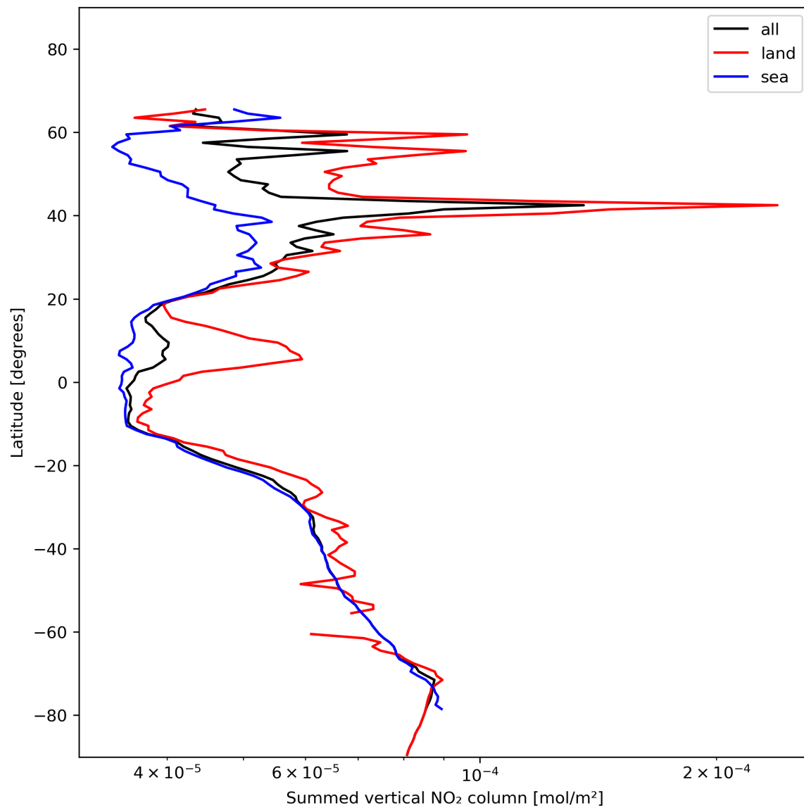
Figure 23: Zonal average of “Summed vertical NO 2 column” for 2024-01-07 to 2024-01-09.
