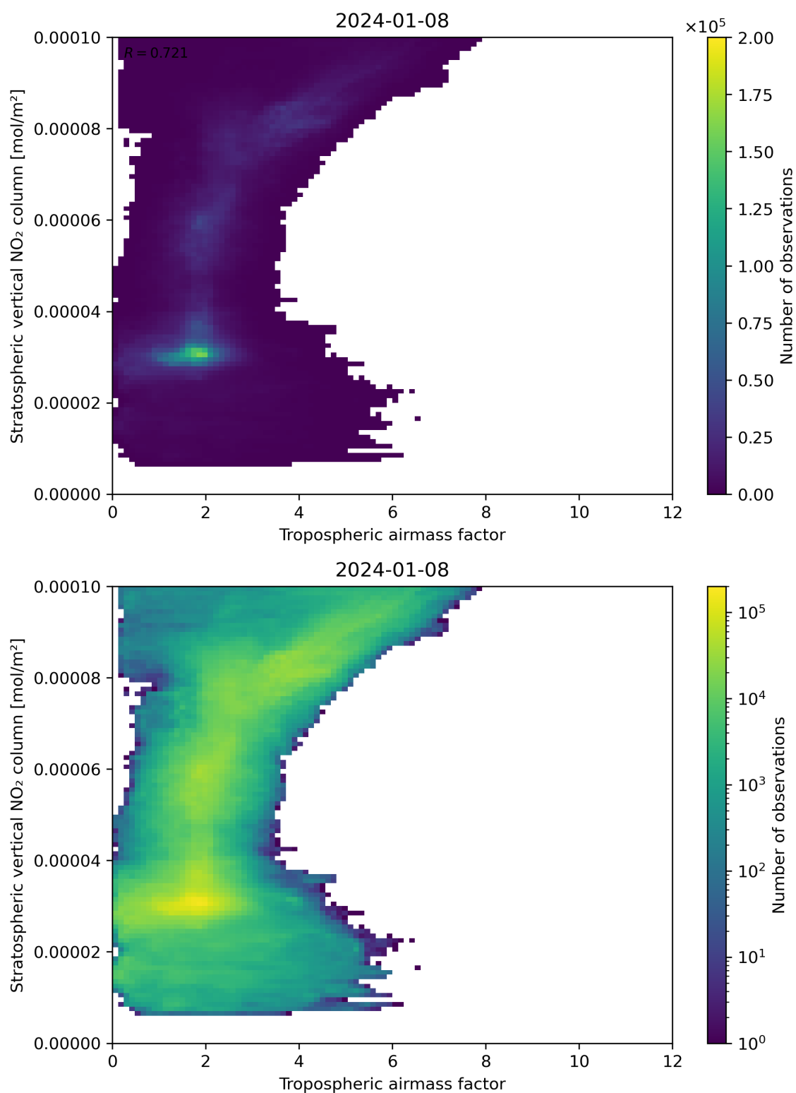
Figure 74: Scatter density plot of “Tropospheric air mass factor” against “Stratospheric vertical NO 2 column” for 2024-01-07 to 2024-01-09.
