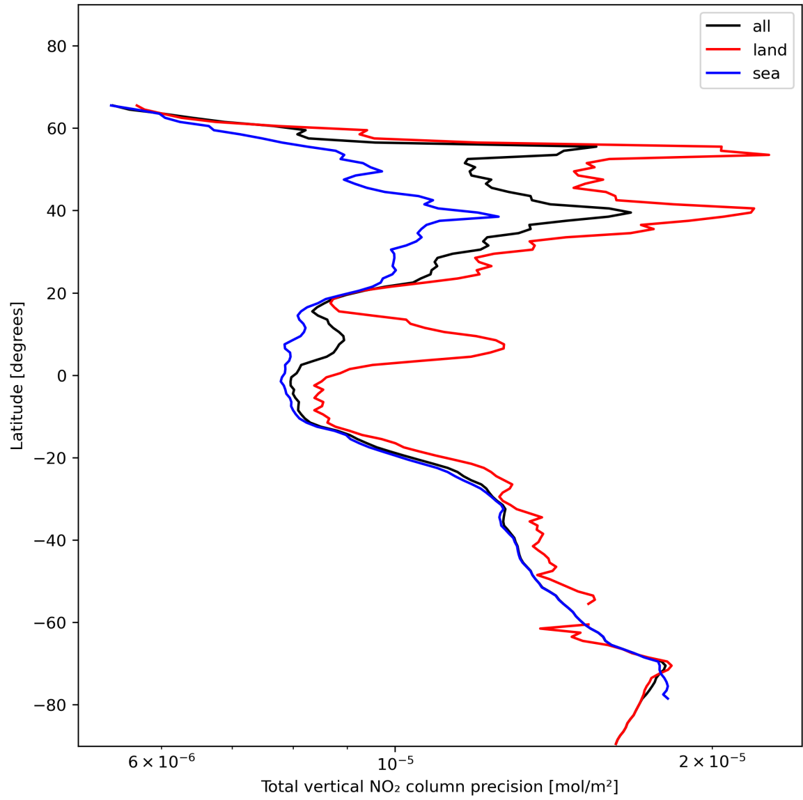
Figure 22: Zonal average of “Total vertical NO 2 column precision” for 2024-01-07 to 2024-01-09.
