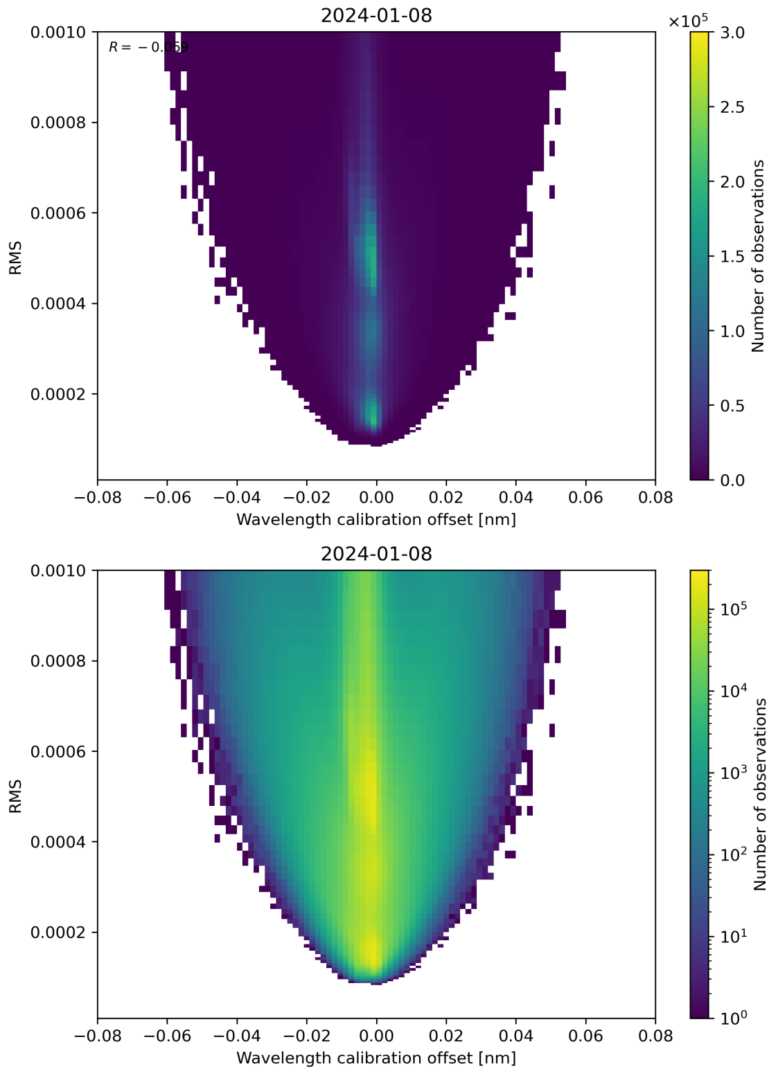
Figure 181: Scatter density plot of “Wavelength calibration offset” against “RMS” for 2024-01-07 to 2024-01-09.
