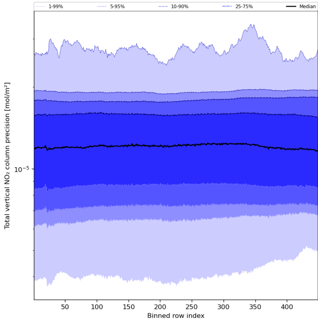
Figure 56: Along track statistics of “Total vertical NO 2 column precision” for 2024-01-07 to 2024-01-09
