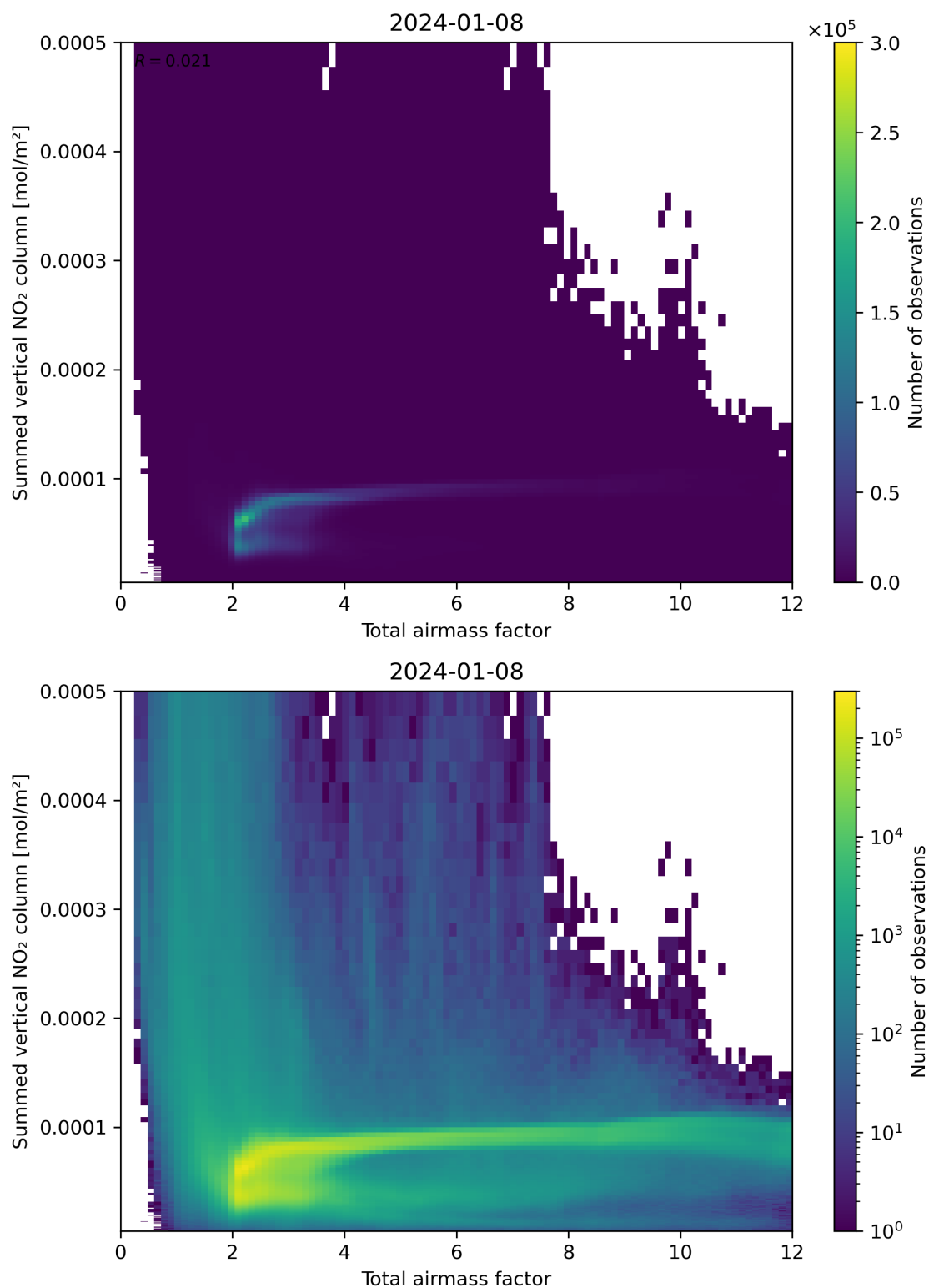
Figure 65: Scatter density plot of “Total airmass factor” against “Summed vertical NO 2 column” for 2024-01-07 to 2024-01-09.
