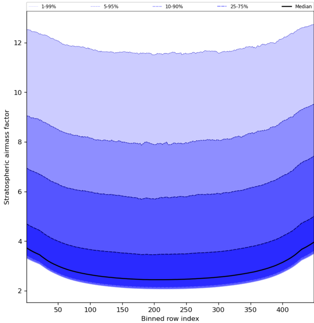
Figure 61: Along track statistics of “Stratospheric airmass factor” for 2024-01-07 to 2024-01-09
