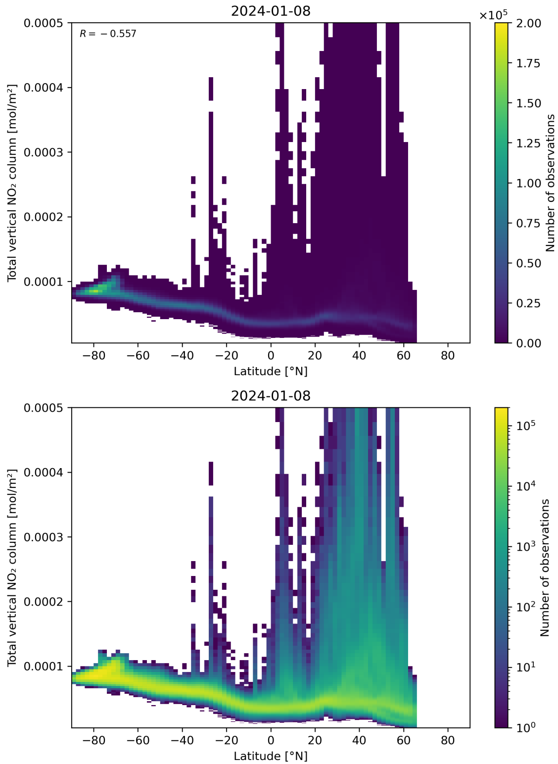
Figure 90: Scatter density plot of “Latitude” against “Total vertical NO 2 column” for 2024-01-07 to 2024-01-09.
