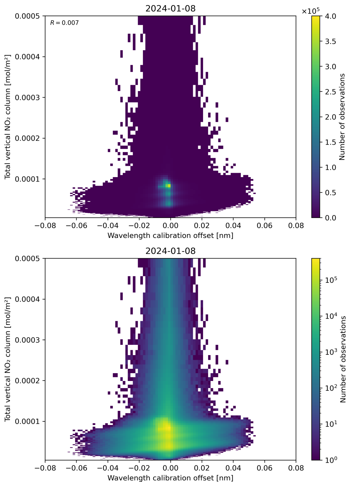
Figure 179: Scatter density plot of “Wavelength calibration offset” against “Total vertical NO 2 column” for 2024-01-07 to 2024-01-09.
