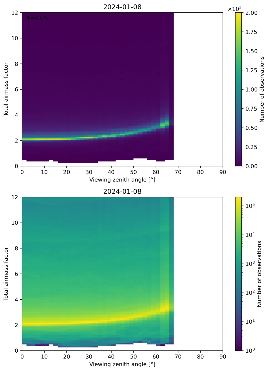
Figure 160: Scatter density plot of “Viewing zenith angle” against “Total airmass factor” for 2024-01-07 to 2024-01-09.
