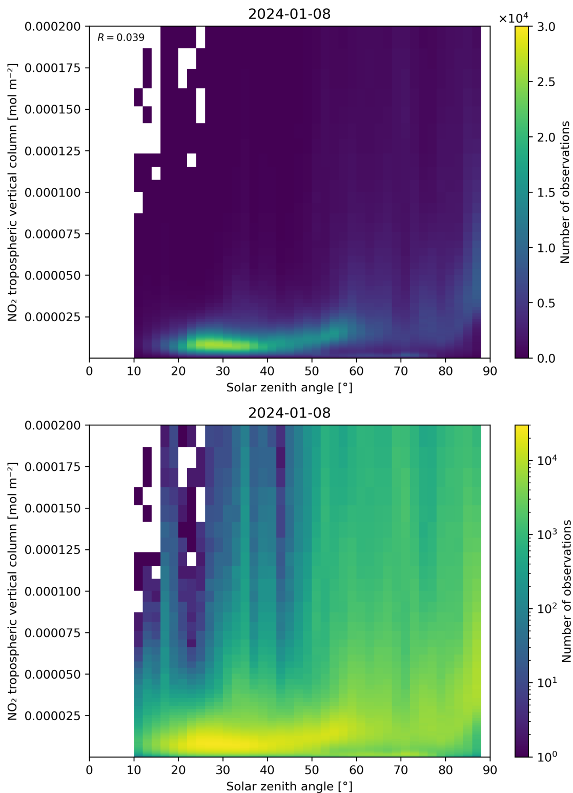
Figure 155: Scatter density plot of “Solar zenith angle” against “NO 2 tropospheric vertical column” for 2024-01-07 to 2024-01-09.
