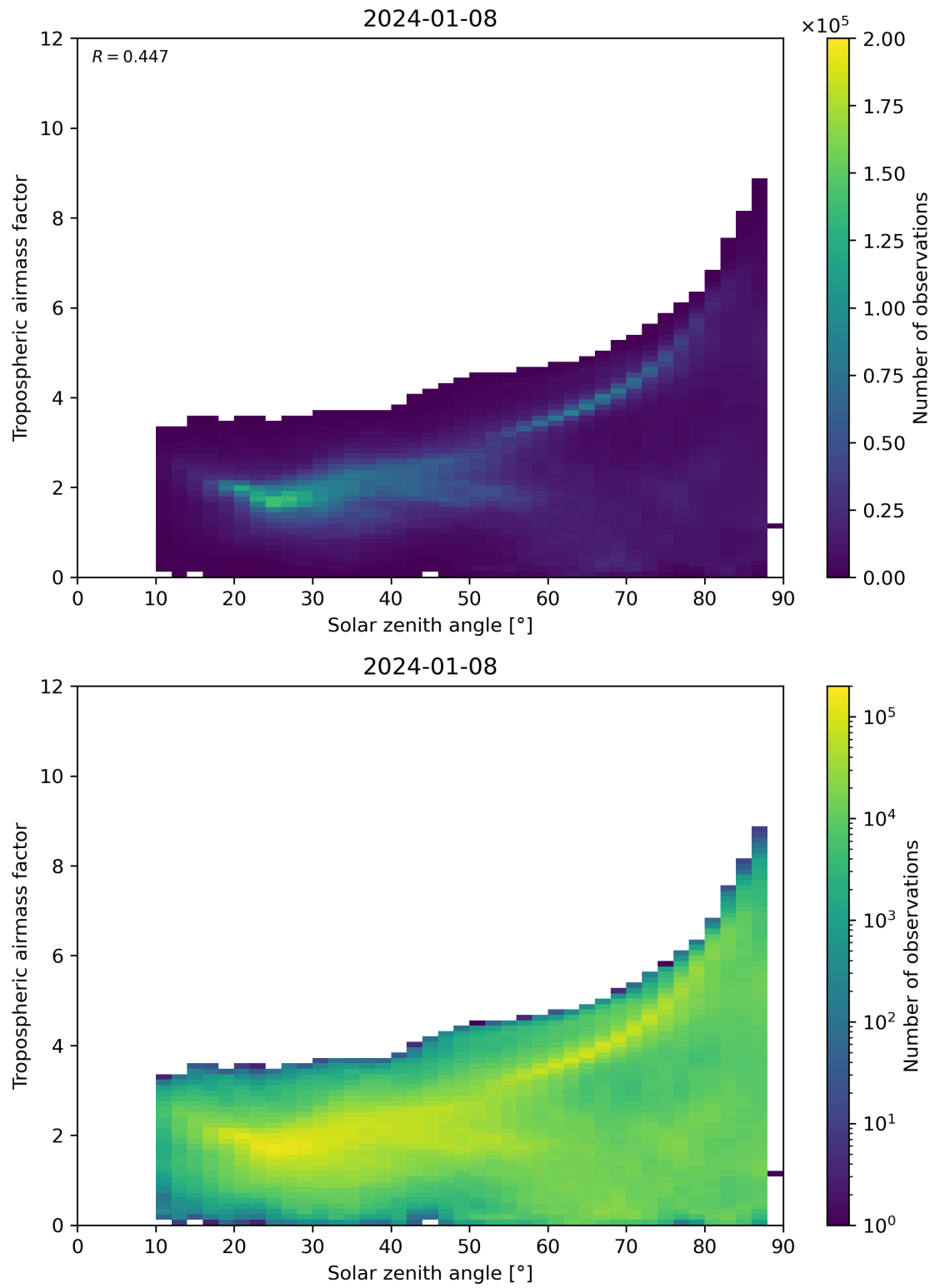
Figure 147: Scatter density plot of “Solar zenith angle” against “Tropospheric airmass factor” for 2024-01-07 to 2024-01-09.
