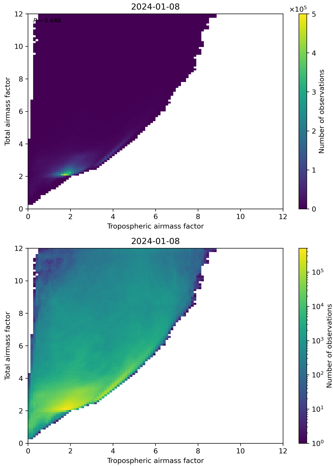
Figure 72: Scatter density plot of “Tropospheric airmass factor” against “Total airmass factor” for 2024-01-07 to 2024-01-09.
