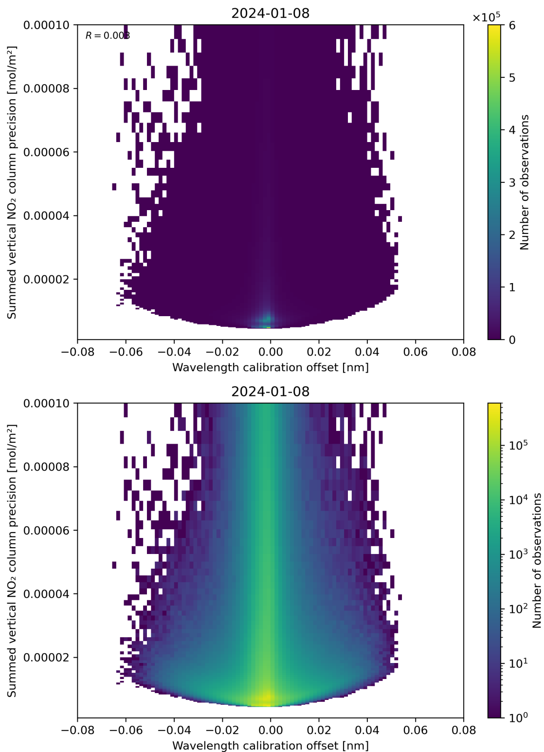
Figure 178: Scatter density plot of “Wavelength calibration offset” against “Summed vertical NO 2 column precision” for 2024-01-07 to 2024-01-09.
