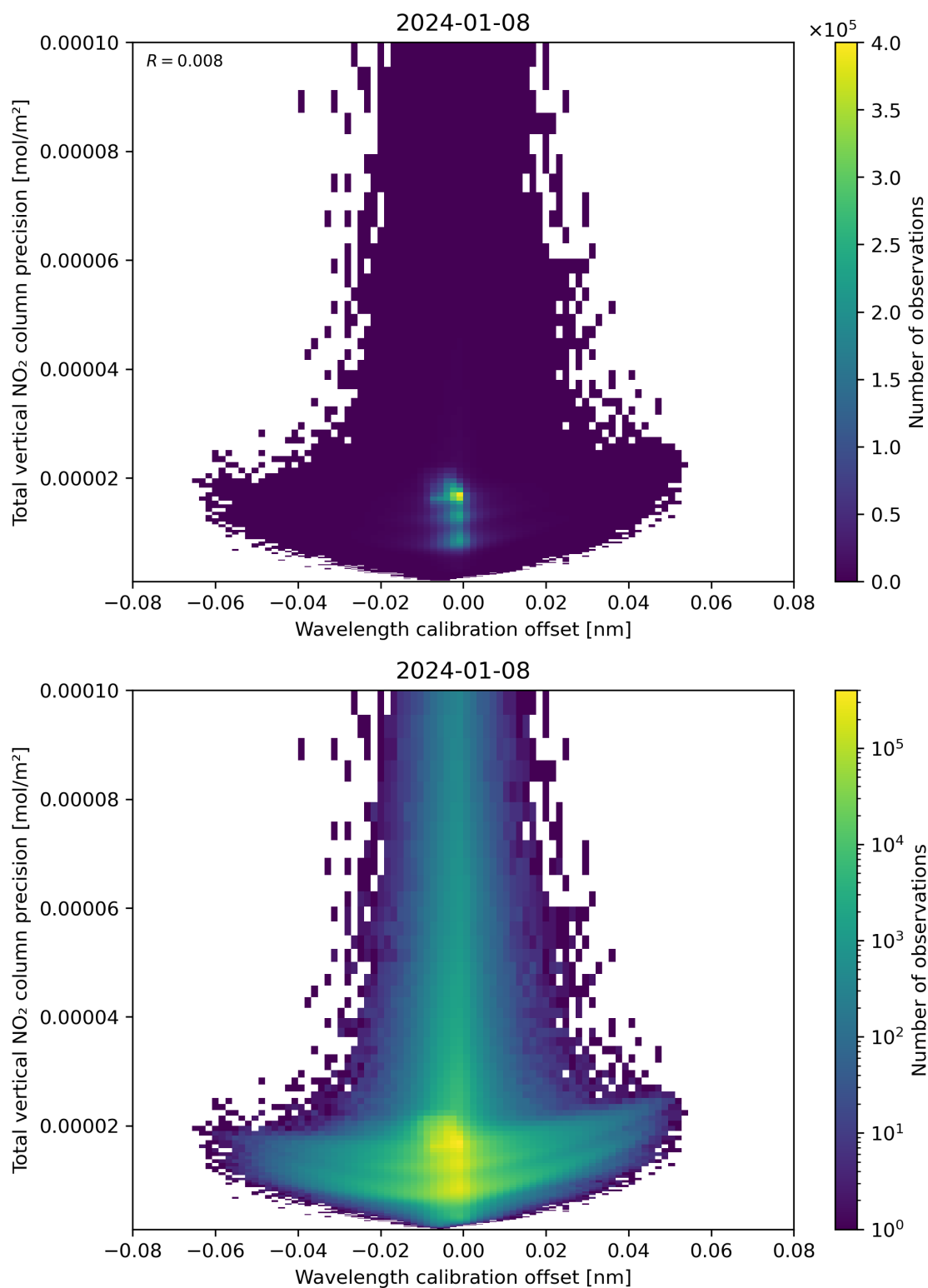
Figure 180: Scatter density plot of “Wavelength calibration offset” against “Total vertical NO 2 column precision” for 2024-01-07 to 2024-01-09.
