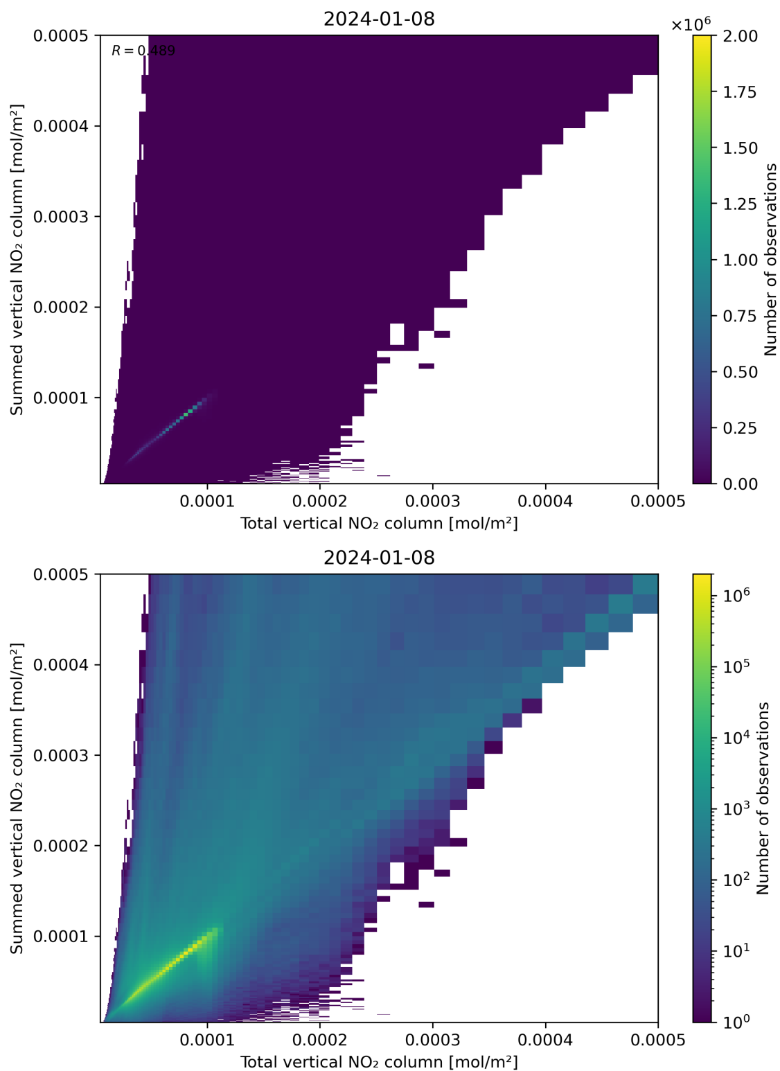
Figure 112: Scatter density plot of “Total vertical NO 2 column” against “Summed vertical NO 2 column” for 2024-01-07 to 2024-01-09.
