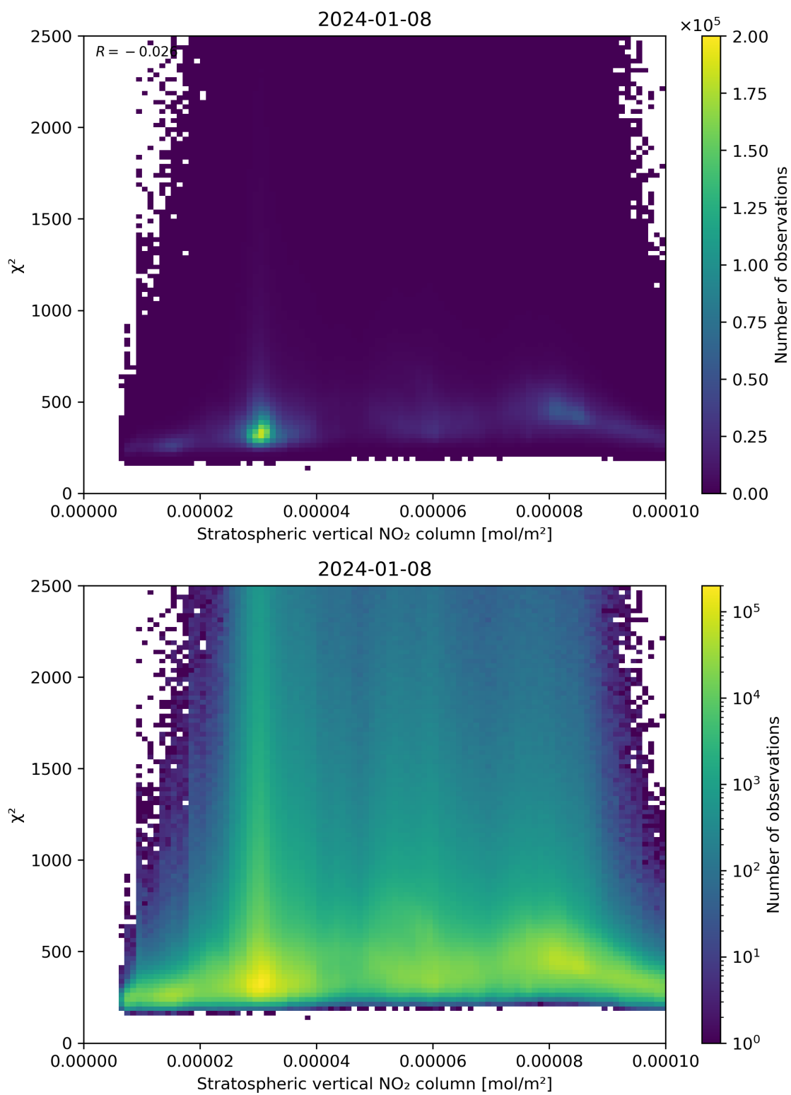
Figure 97: Scatter density plot of “Stratospheric vertical NO 2 column” against “ \chi^2 ” for 2024-01-07 to 2024-01-09.
