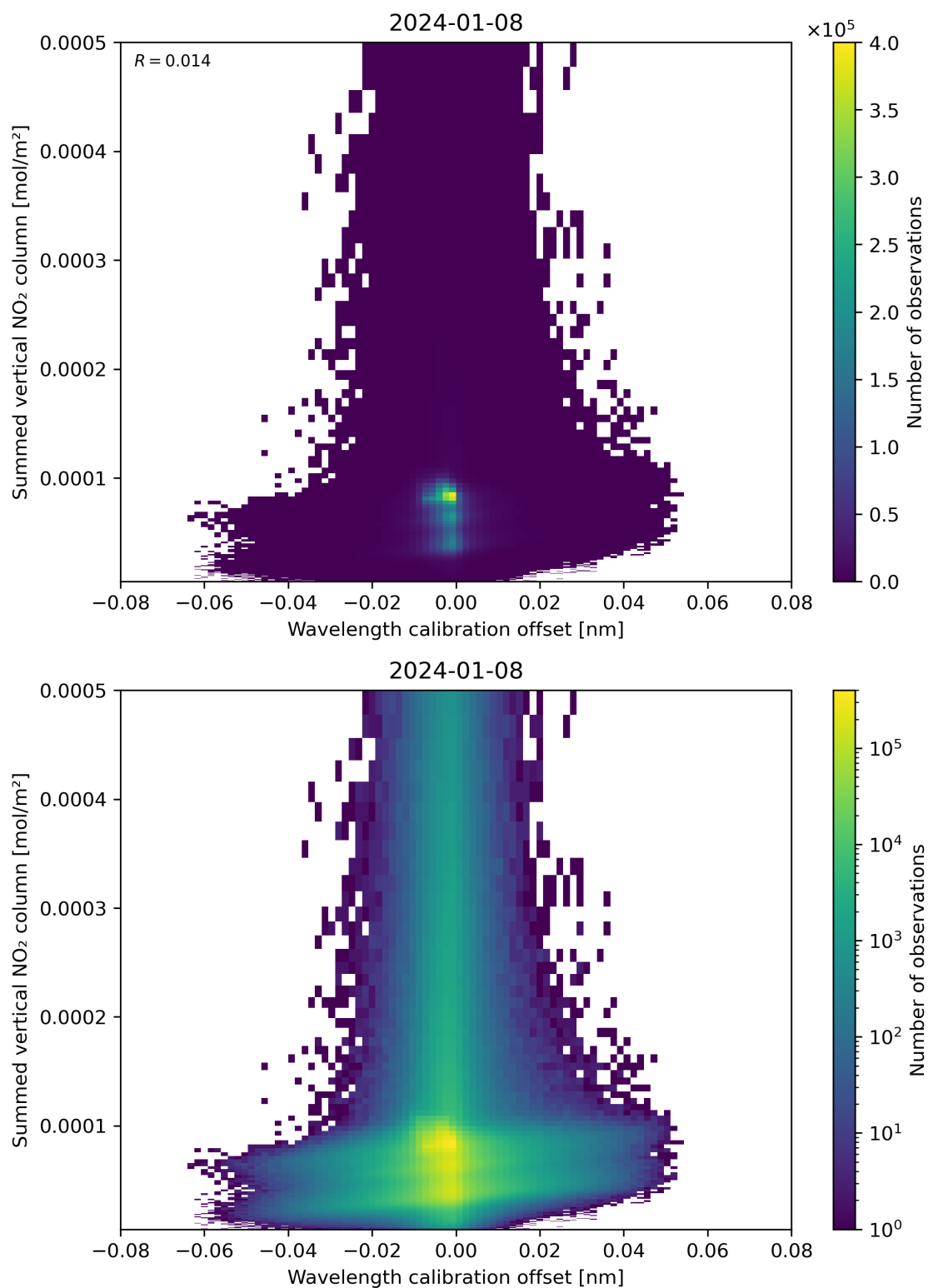
Figure 177: Scatter density plot of “Wavelength calibration offset” against “Summed vertical NO 2 column” for 2024-01-07 to 2024-01-09.
