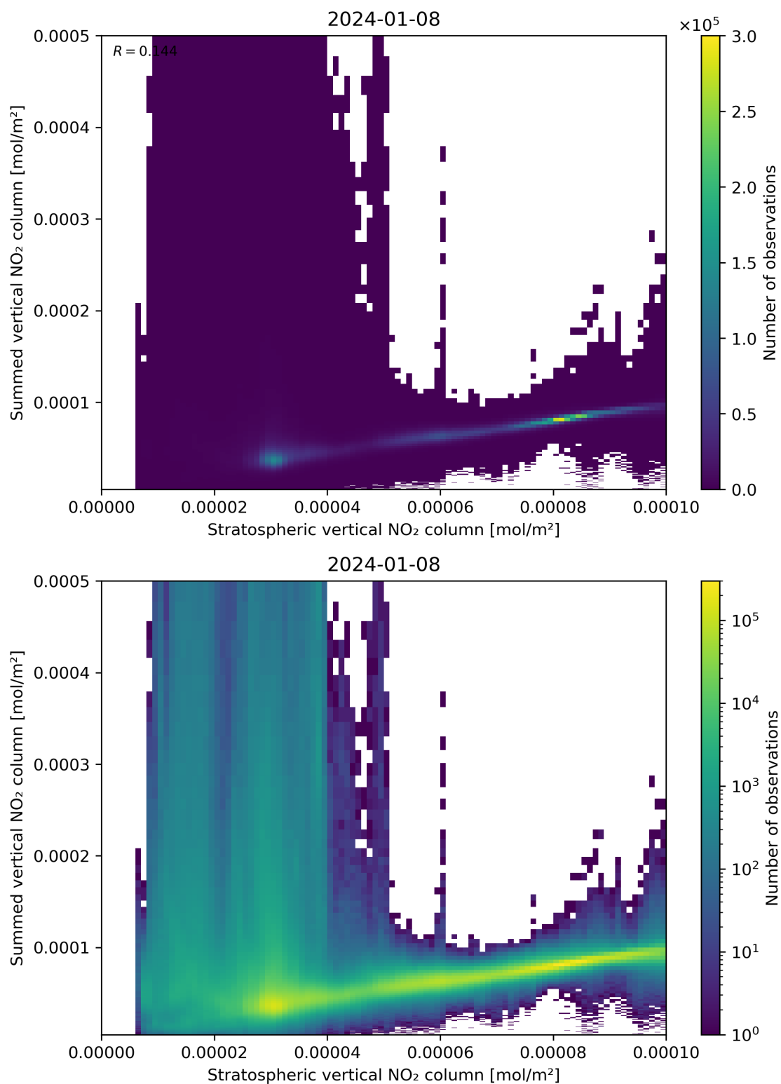
Figure 98: Scatter density plot of “Stratospheric vertical NO 2 column” against “Summed vertical NO 2 column” for 2024-01-07 to 2024-01-09.
