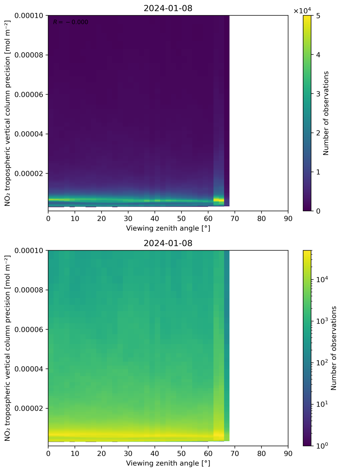
Figure 170: Scatter density plot of “Viewing zenith angle” against “NO 2 tropospheric vertical column precision” for 2024-01-07 to 2024-01-09.
