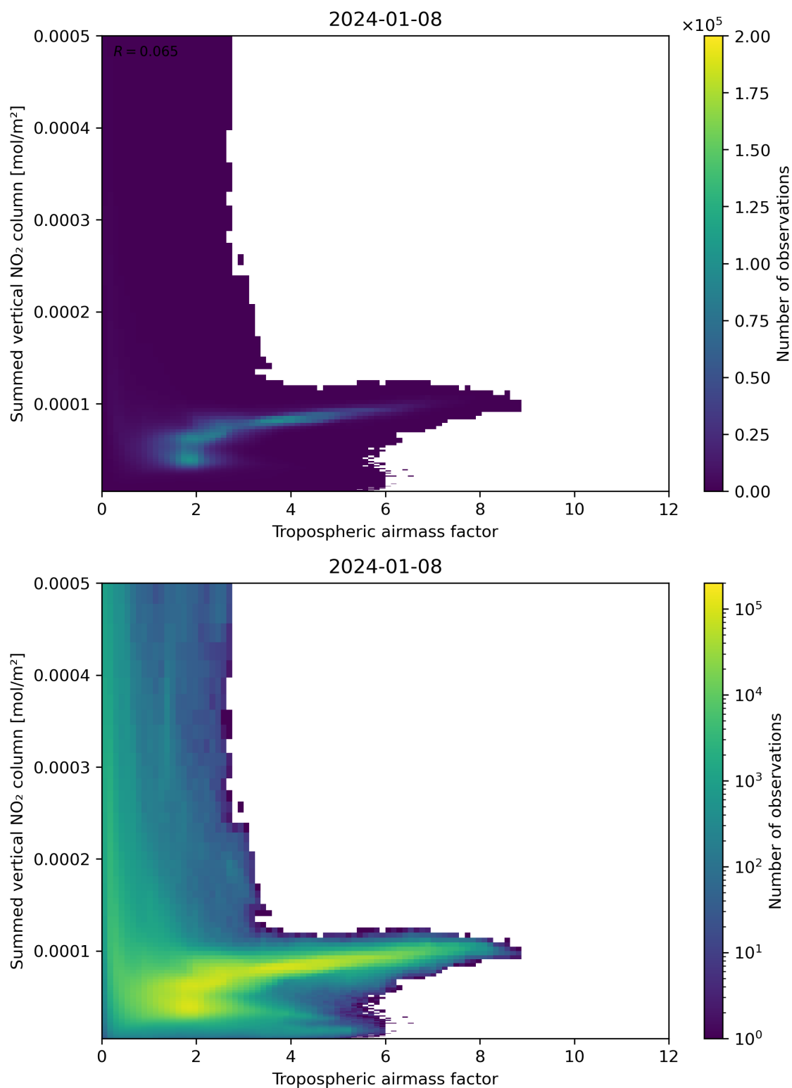
Figure 75: Scatter density plot of “Tropospheric airmass factor” against “Summed vertical NO 2 column” for 2024-01-07 to 2024-01-09.
