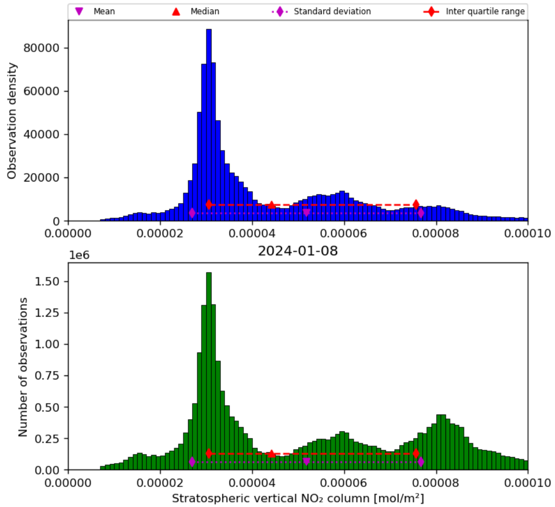
Figure 36: Histogram of “Stratospheric vertical NO 2 column” for 2024-01-07 to 2024-01-09
