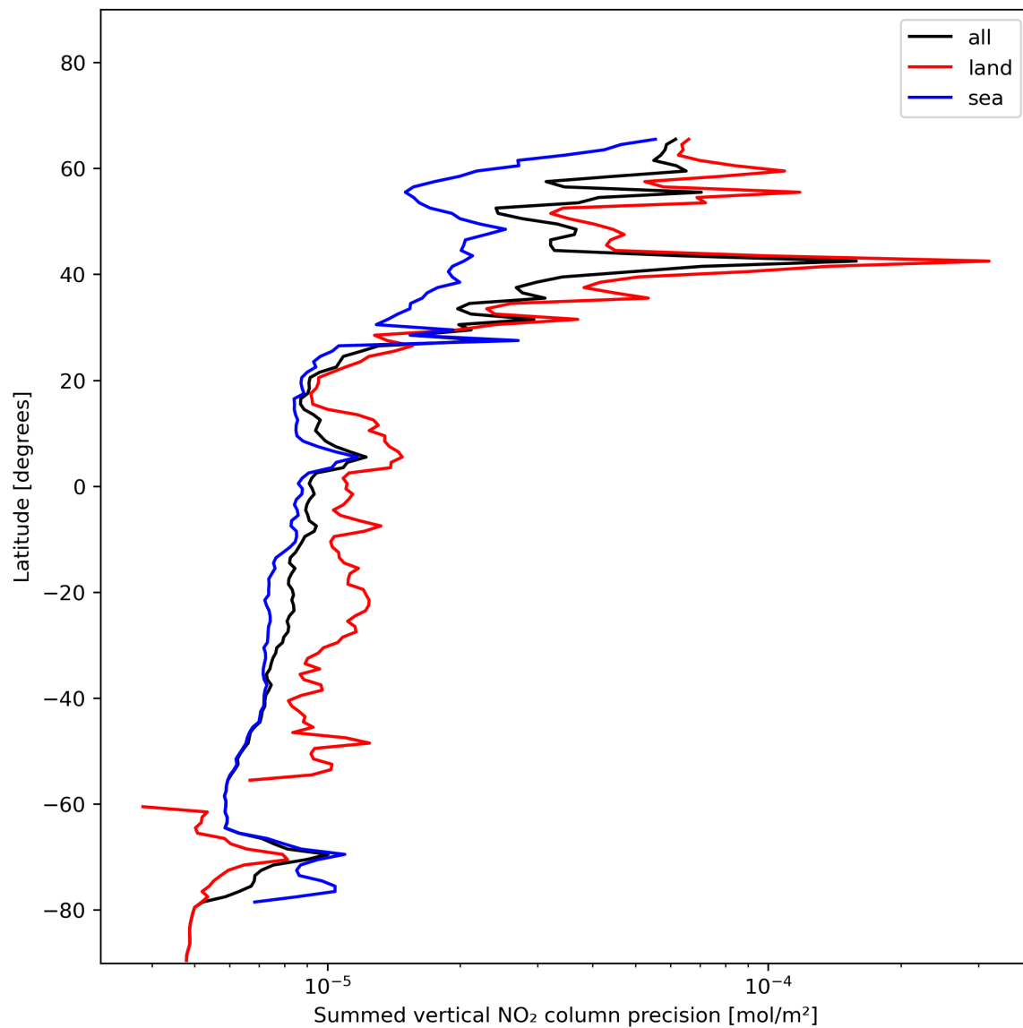
Figure 24: Zonal average of “Summed vertical NO 2 column precision” for 2024-01-07 to 2024-01-09.
