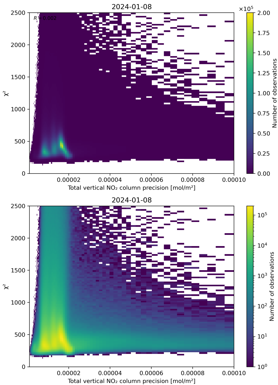
Figure 116: Scatter density plot of “Total vertical NO 2 column precision” against “ \chi^2 ” for 2024-01-07 to 2024-01-09.
