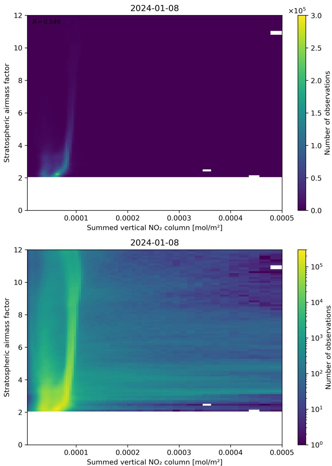
Figure 103: Scatter density plot of “Summed vertical NO 2 column” against “Stratospheric airmass factor” for 2024-01-07 to 2024-01-09.
