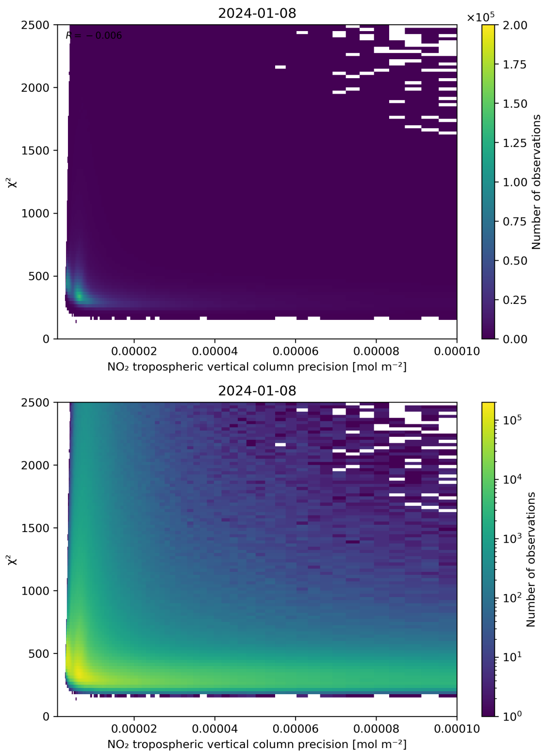
Figure 134: Scatter density plot of “NO 2 tropospheric vertical column precision” against “ \chi^2 ” for 2024-01-07 to 2024-01-09.
