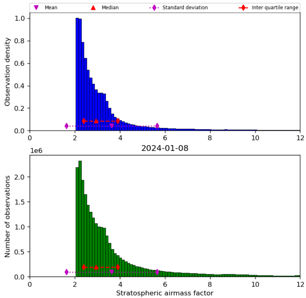
Figure 44: Histogram of “Stratospheric airmass factor” for 2024-01-07 to 2024-01-09
