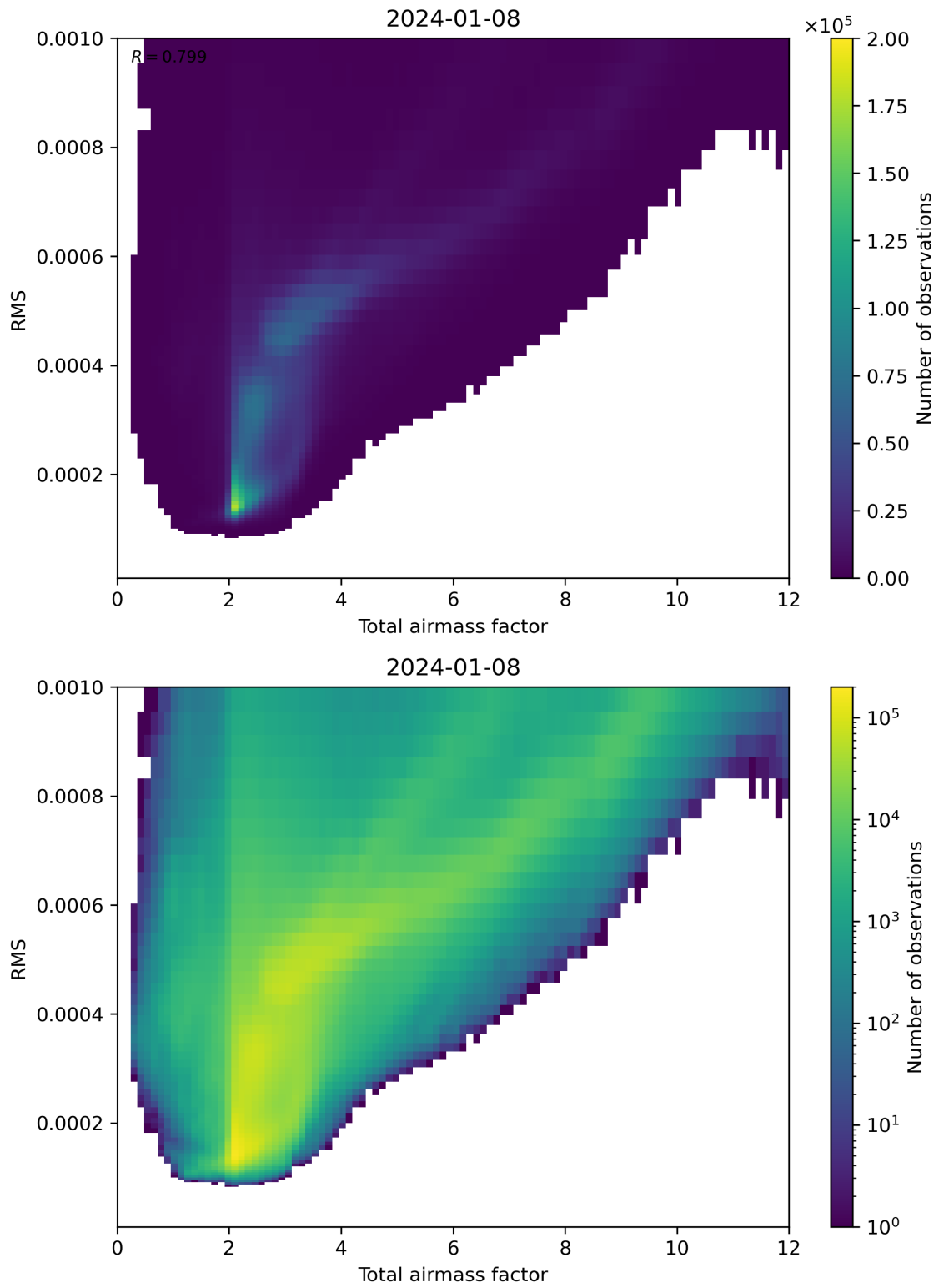
Figure 69: Scatter density plot of “Total airmass factor” against “RMS” for 2024-01-07 to 2024-01-09.
