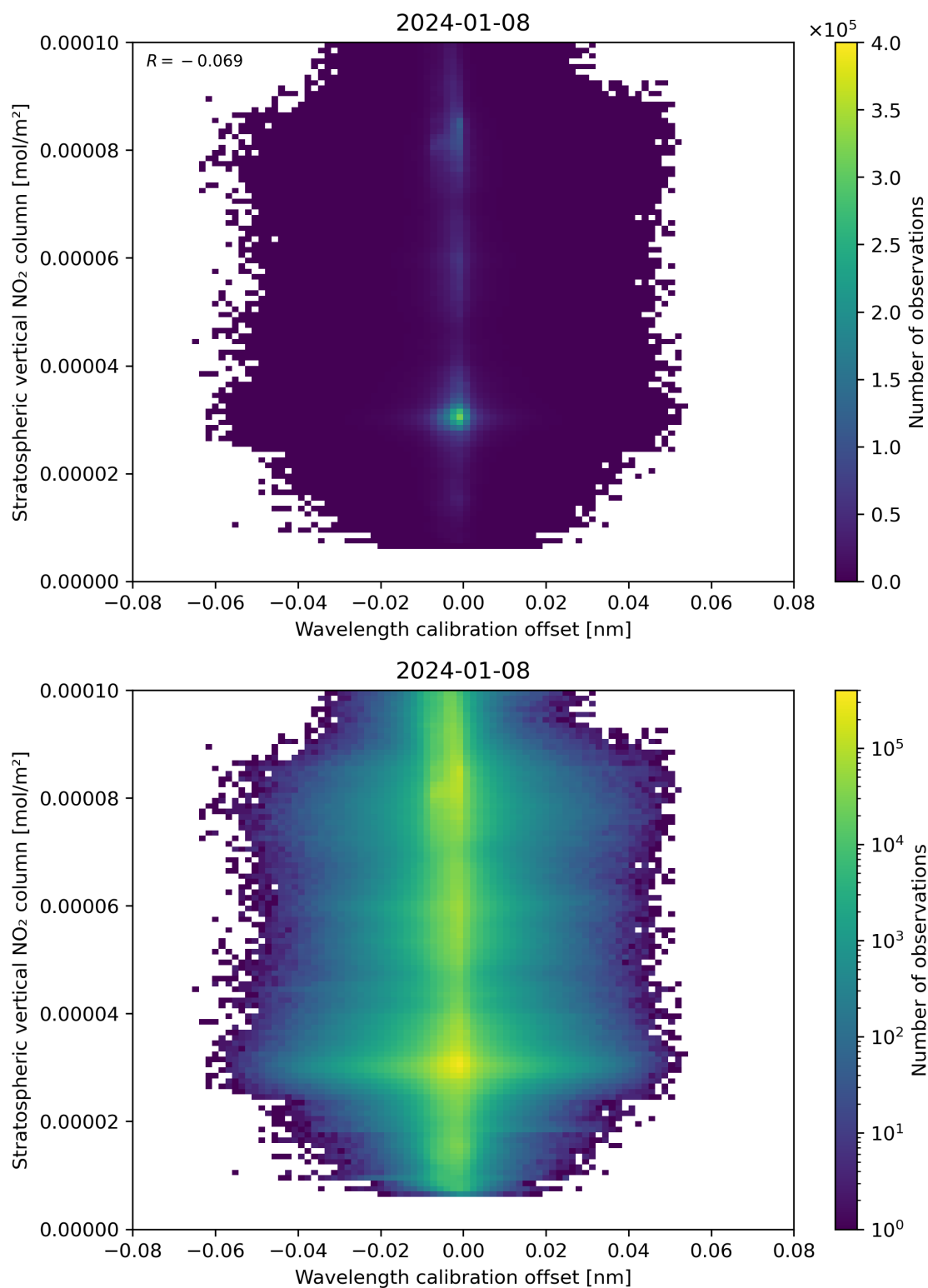
Figure 176: Scatter density plot of “Wavelength calibration offset” against “Stratospheric vertical NO 2 column” for 2024-01-07 to 2024-01-09.
