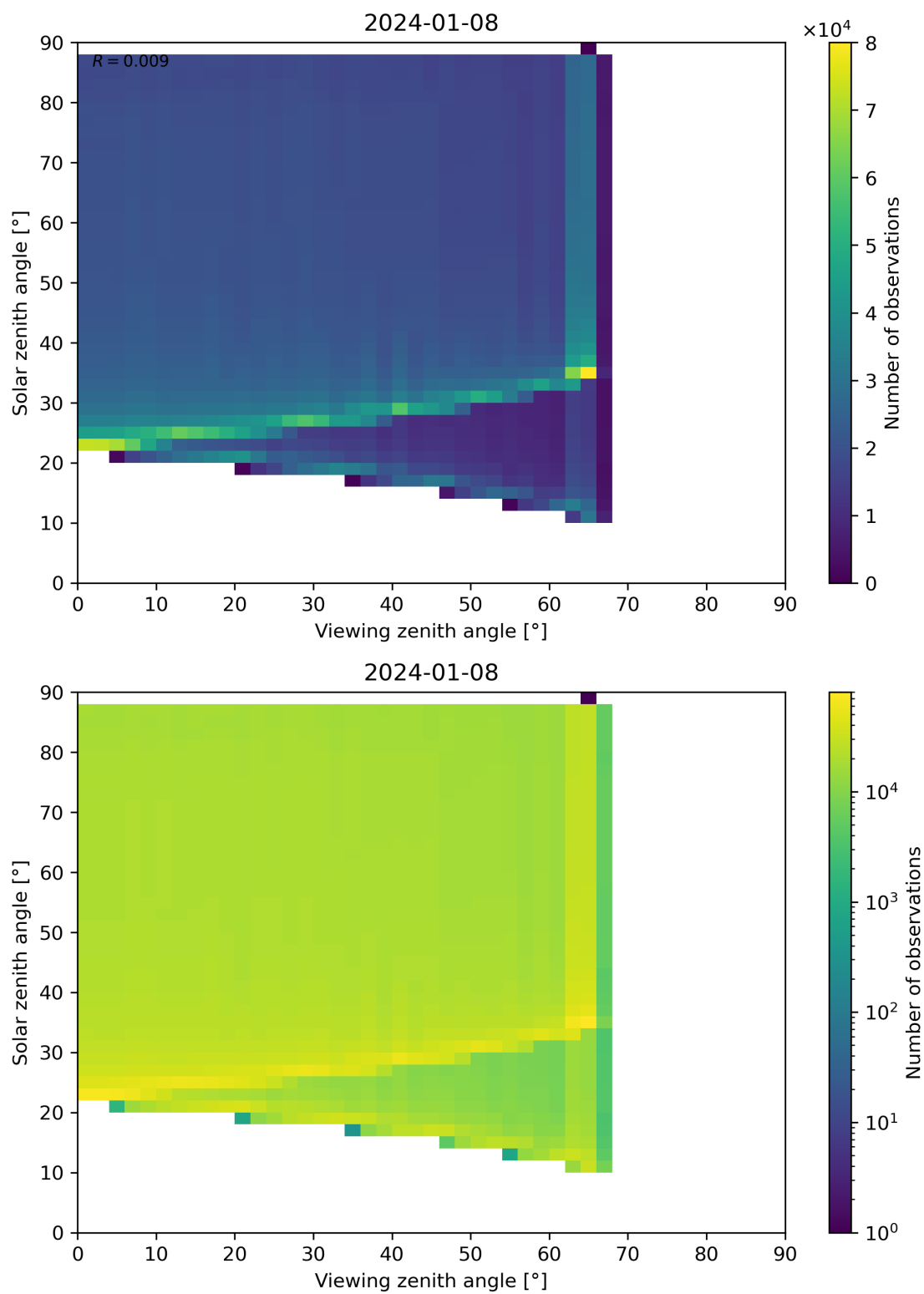
Figure 172: Scatter density plot of “Viewing zenith angle” against “Solar zenith angle” for 2024-01-07 to 2024-01-09.
