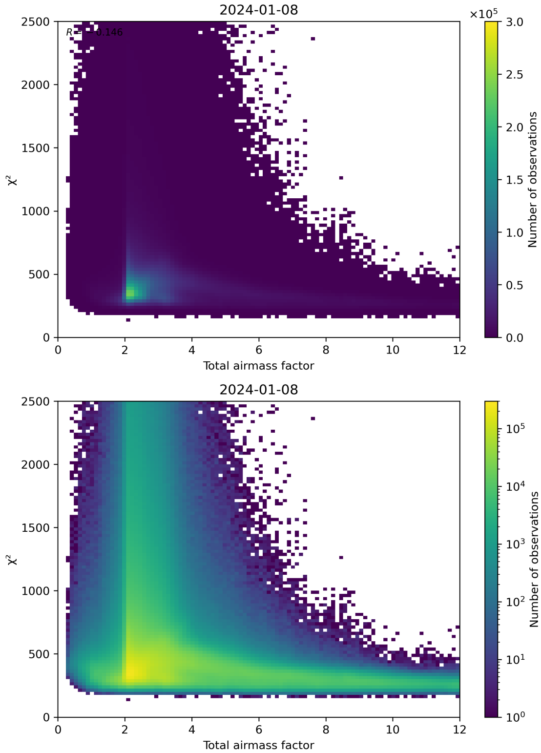
Figure 63: Scatter density plot of “Total airmass factor” against “ \chi^2 ” for 2024-01-07 to 2024-01-09.
