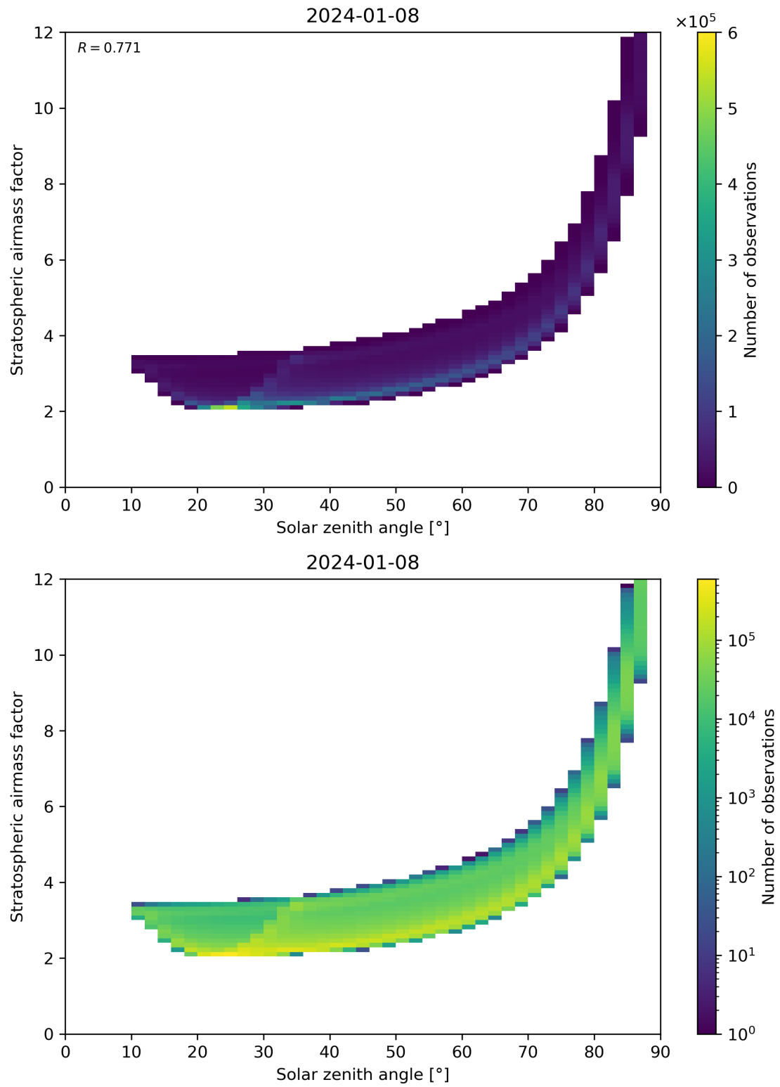
Figure 145: Scatter density plot of “Solar zenith angle” against “Stratospheric airmass factor” for 2024-01-07 to 2024-01-09.
