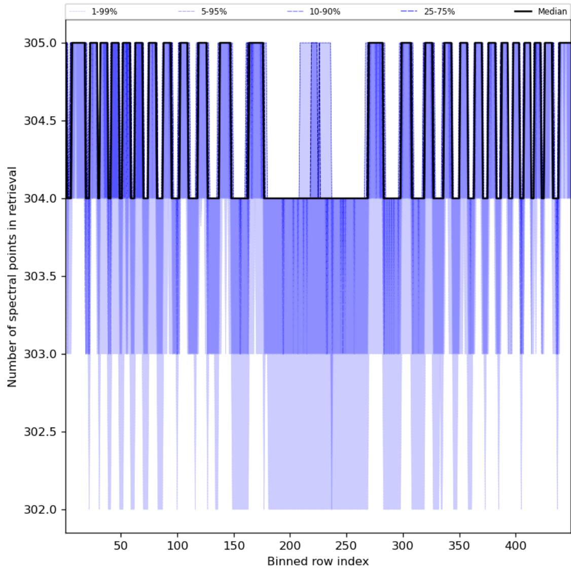
Figure 50: Along track statistics of “Number of spectral points in retrieval” for 2024-01-07 to 2024-01-09
