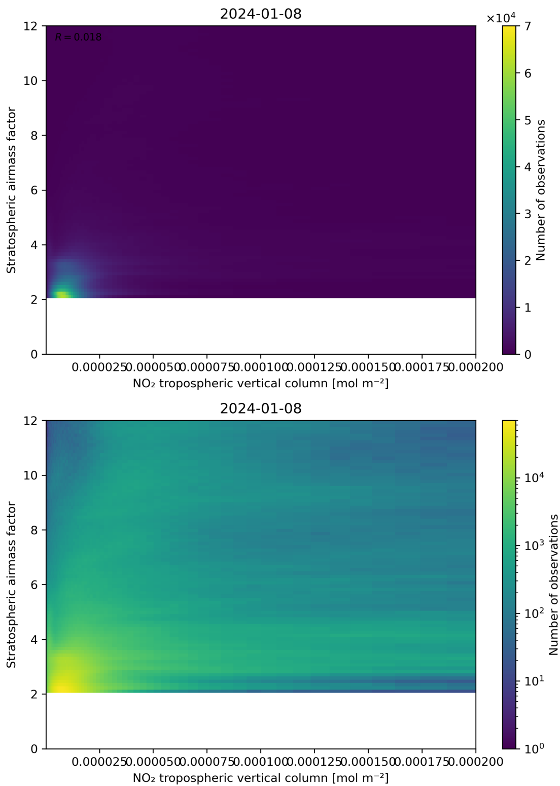
Figure 121: Scatter density plot of “NO 2 tropospheric vertical column” against “Stratospheric airmass factor” for 2024-01-07 to 2024-01-09.
