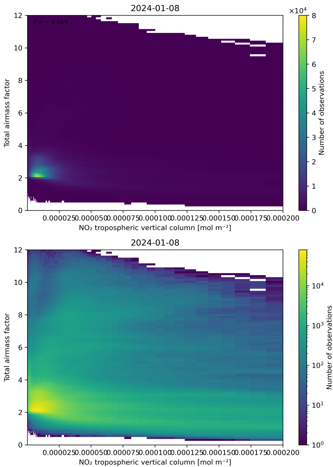
Figure 122: Scatter density plot of “NO 2 tropospheric vertical column” against “Total air mass factor” for 2024-01-07 to 2024-01-09.
