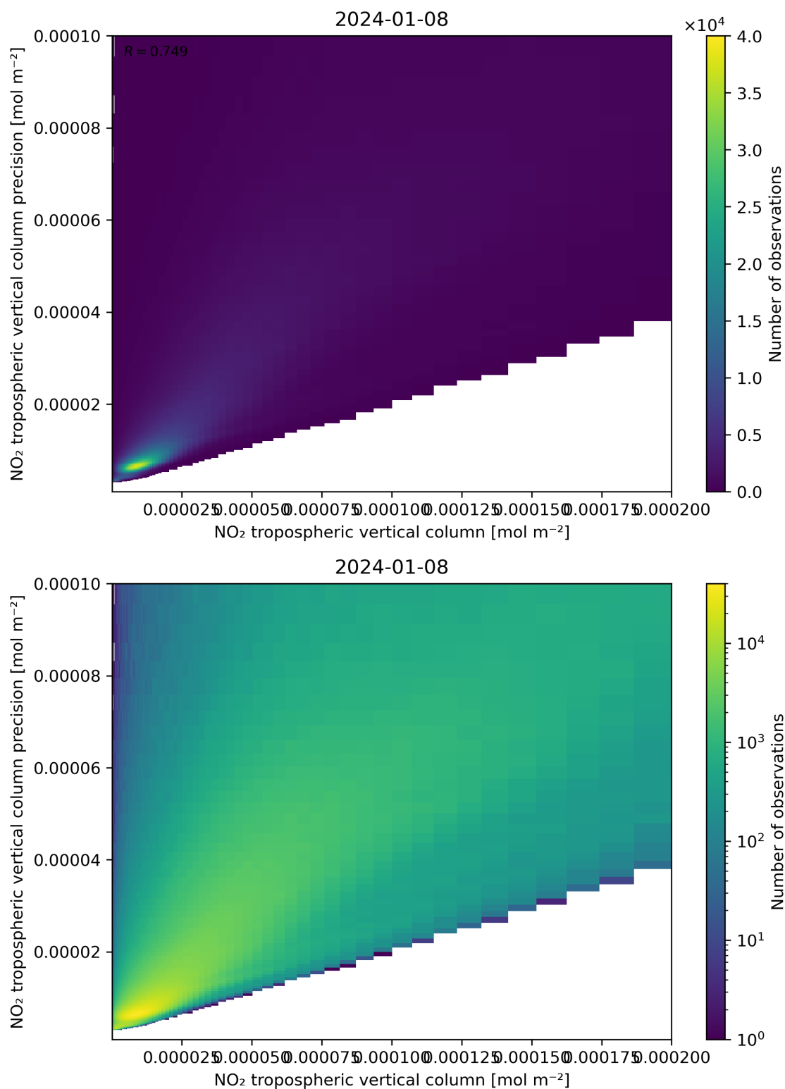
Figure 130: Scatter density plot of “NO 2 tropospheric vertical column” against “NO 2 tropospheric vertical column precision” for 2024-01-07 to 2024-01-09.
