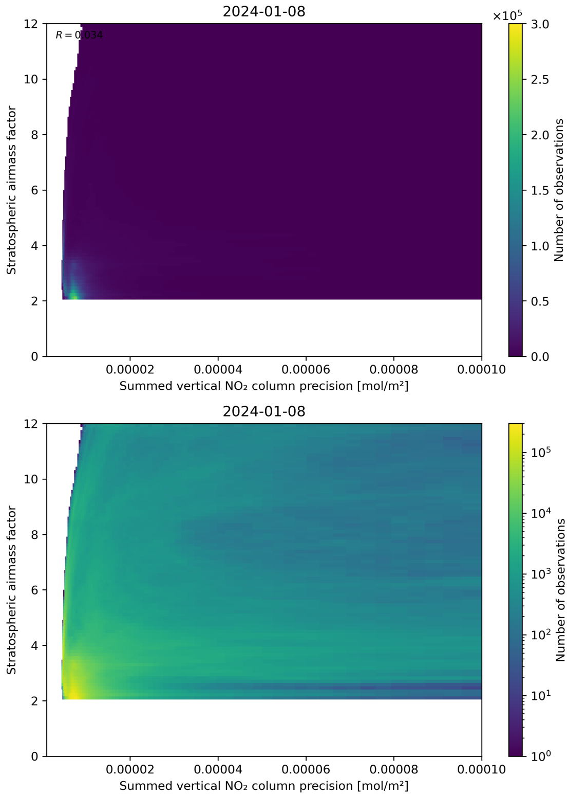
Figure 106: Scatter density plot of “Summed vertical NO 2 column precision” against “Stratospheric airmass factor” for 2024-01-07 to 2024-01-09.
