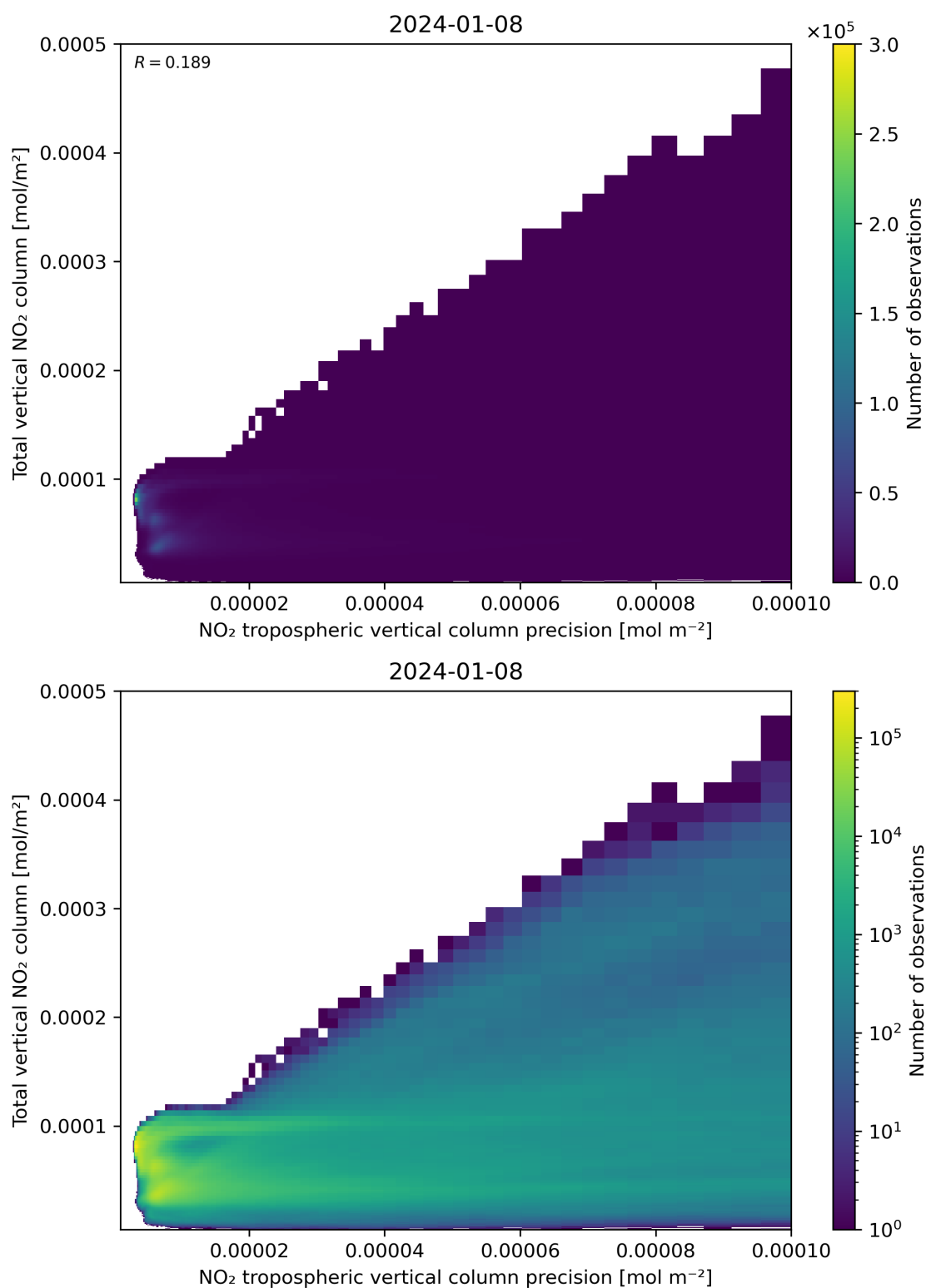
Figure 138: Scatter density plot of “NO 2 tropospheric vertical column precision” against “Total vertical NO 2 column” for 2024-01-07 to 2024-01-09.
