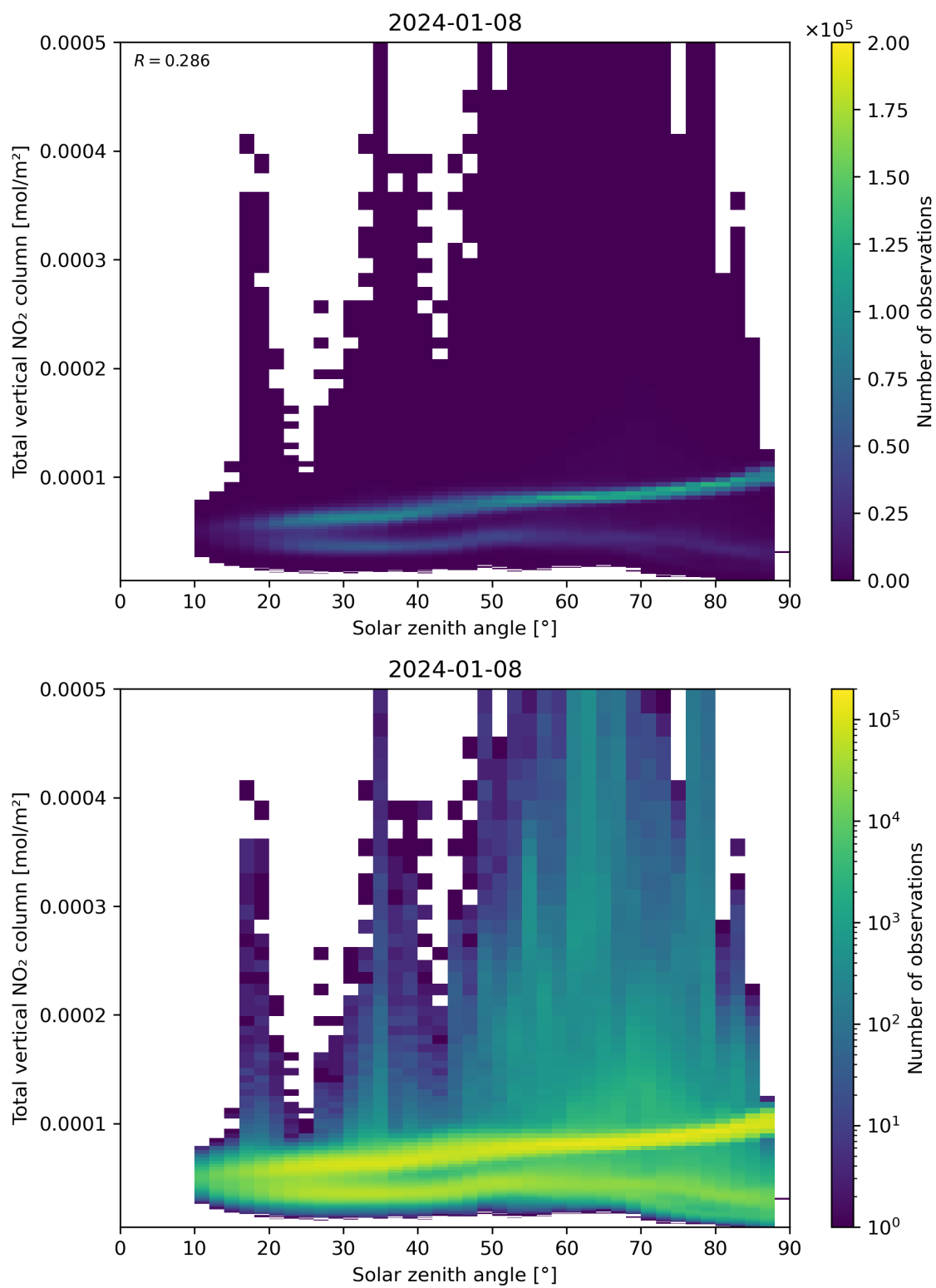
Figure 153: Scatter density plot of “Solar zenith angle” against “Total vertical NO 2 column” for 2024-01-07 to 2024-01-09.
