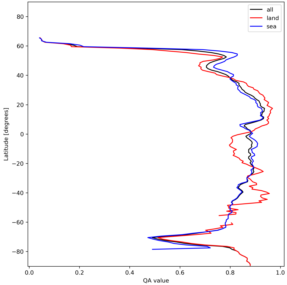
Figure 11: Zonal average of “QA value” for 2024-01-07 to 2024-01-09.
