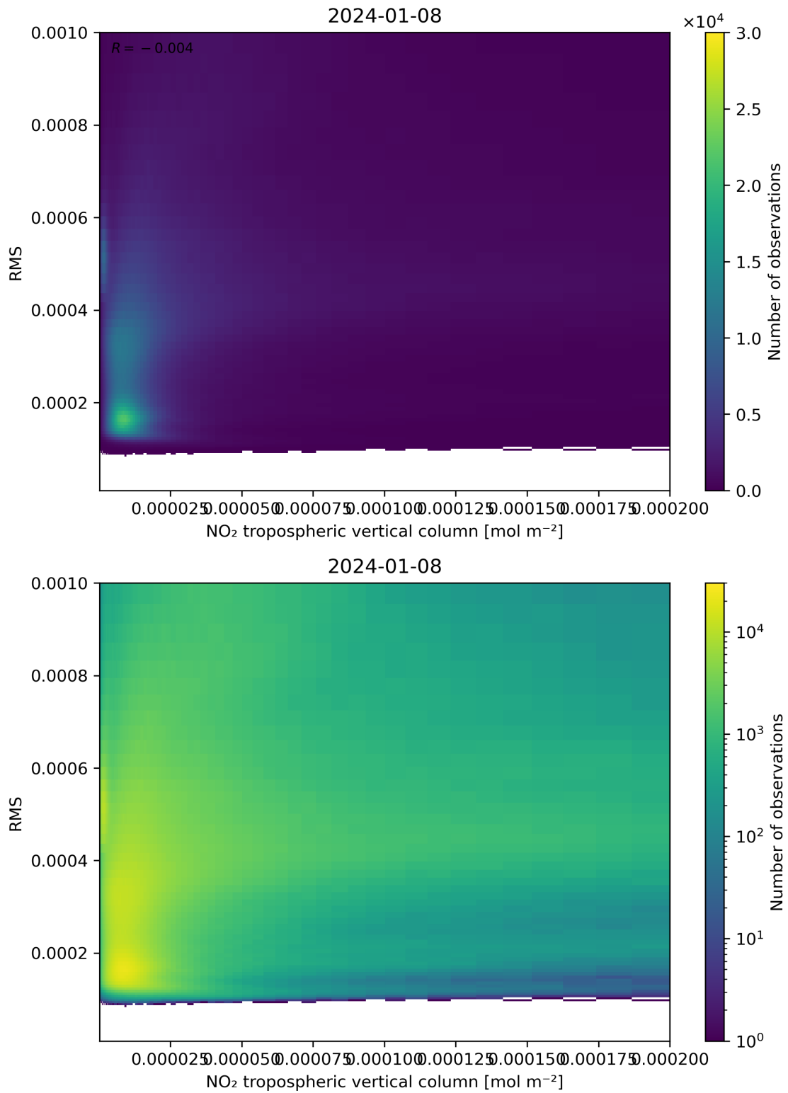
Figure 142: Scatter density plot of “NO 2 tropospheric vertical column” against “RMS” for 2024-01-07 to 2024-01-09.
