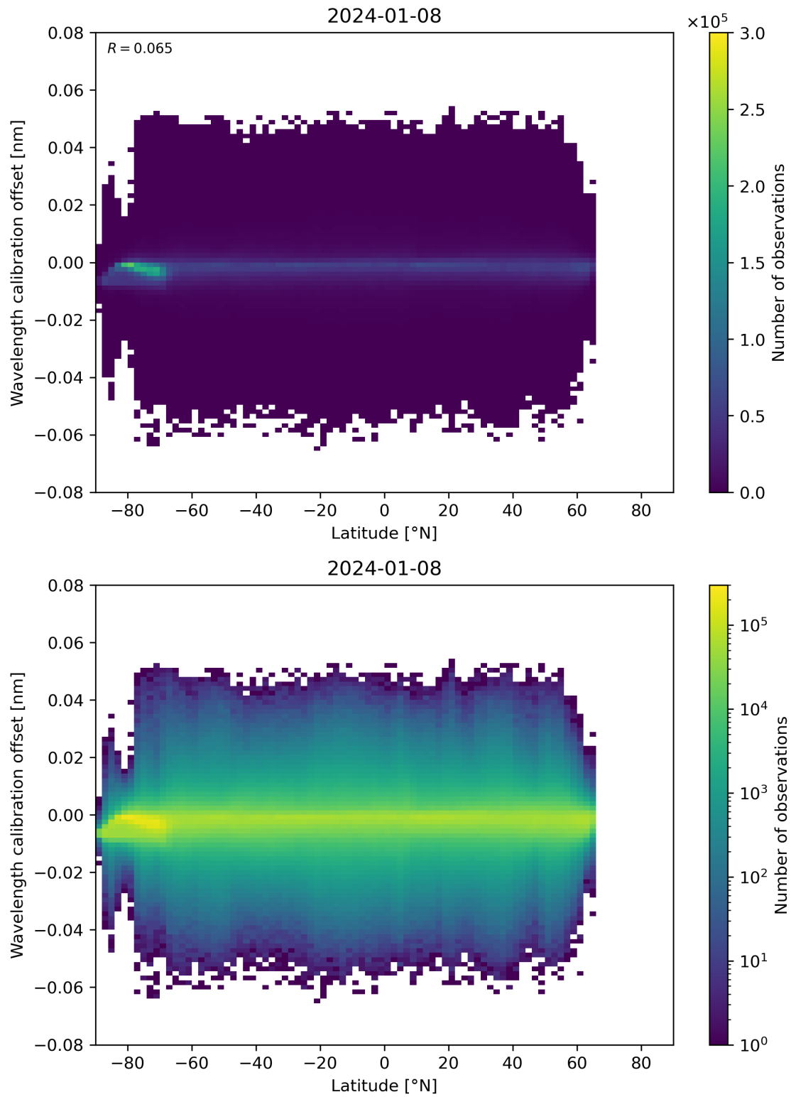
Figure 95: Scatter density plot of “Latitude” against “Wavelength calibration offset” for 2024-01-07 to 2024-01-09.
