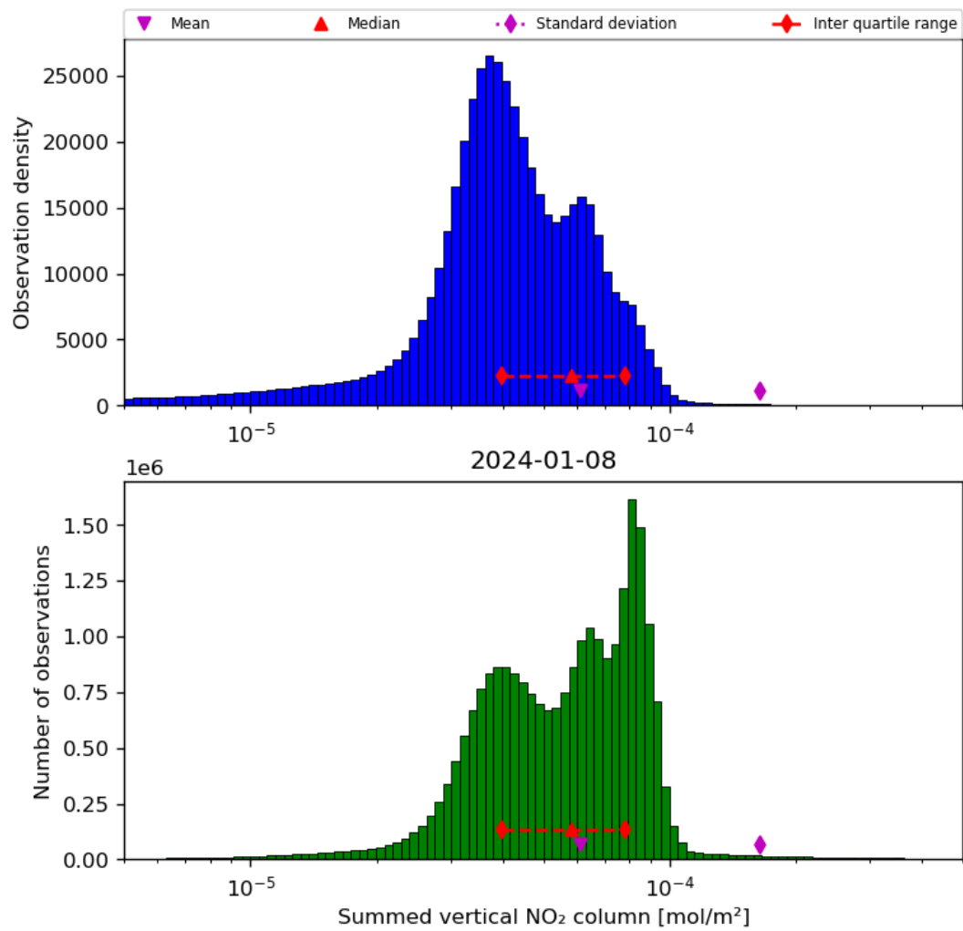
Figure 40: Histogram of “Summed vertical NO 2 column” for 2024-01-07 to 2024-01-09
