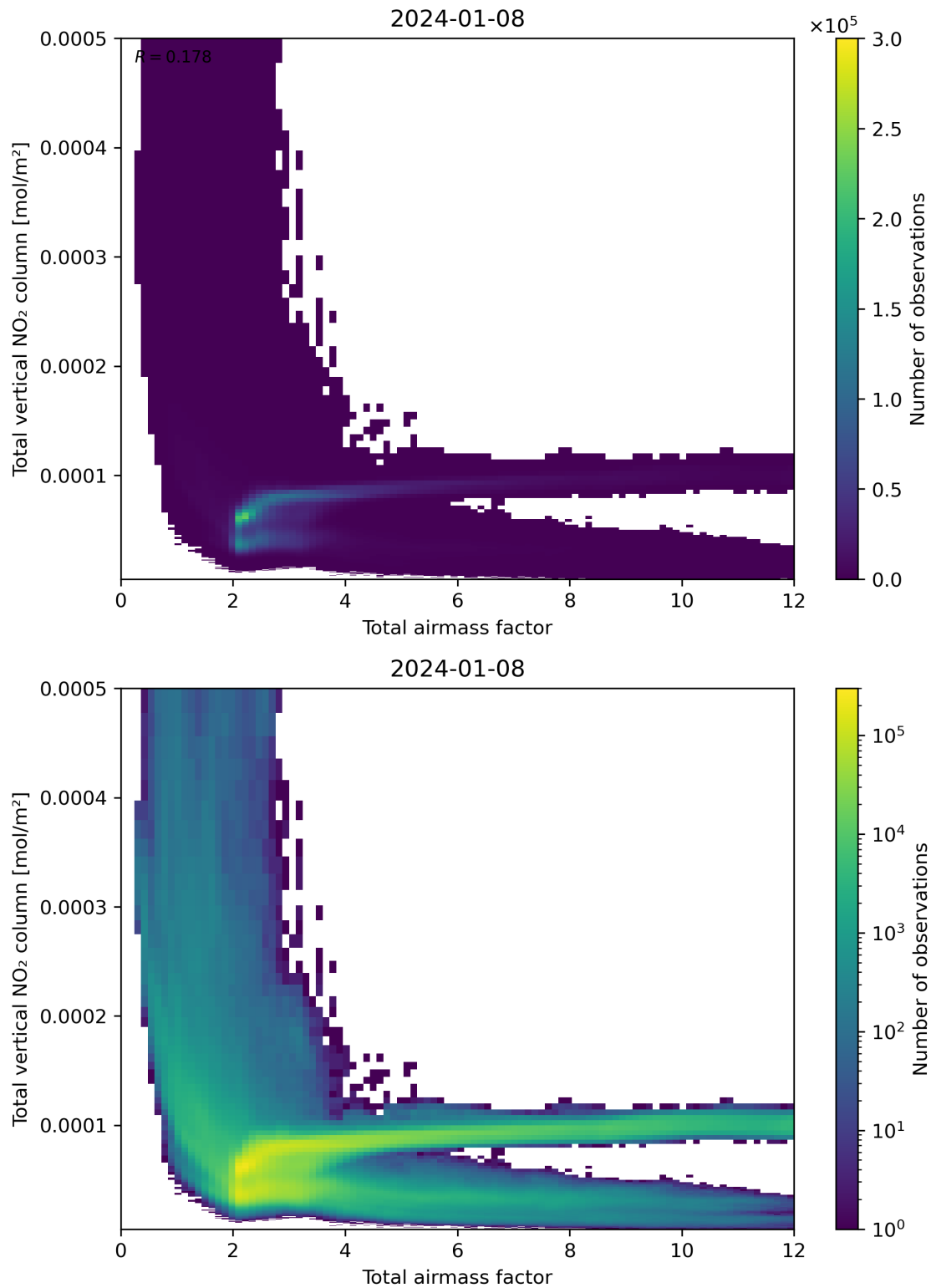
Figure 67: Scatter density plot of “Total airmass factor” against “Total vertical NO 2 column” for 2024-01-07 to 2024-01-09.
