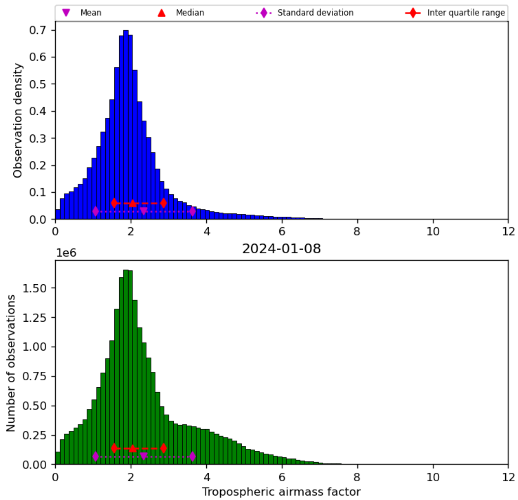
Figure 31: Histogram of “Tropospheric airmass factor” for 2024-01-07 to 2024-01-09
