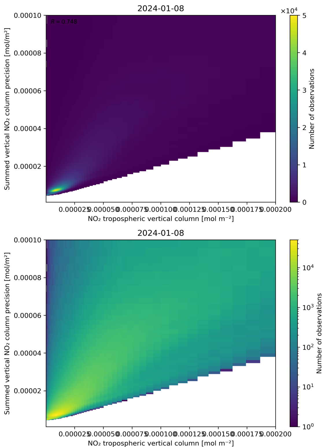
Figure 127: Scatter density plot of “NO 2 tropospheric vertical column” against “Summed vertical NO 2 column precision” for 2024-01-07 to 2024-01-09.
