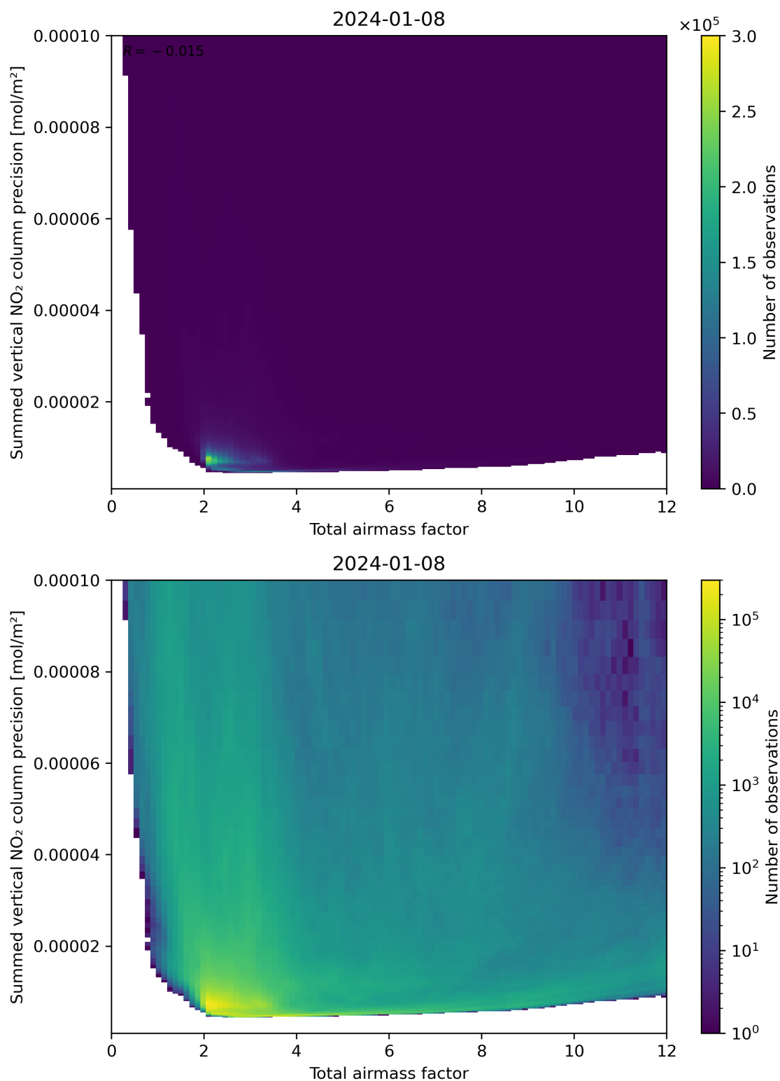
Figure 66: Scatter density plot of “Total airmass factor” against “Summed vertical NO 2 column precision” for 2024-01-07 to 2024-01-09.
