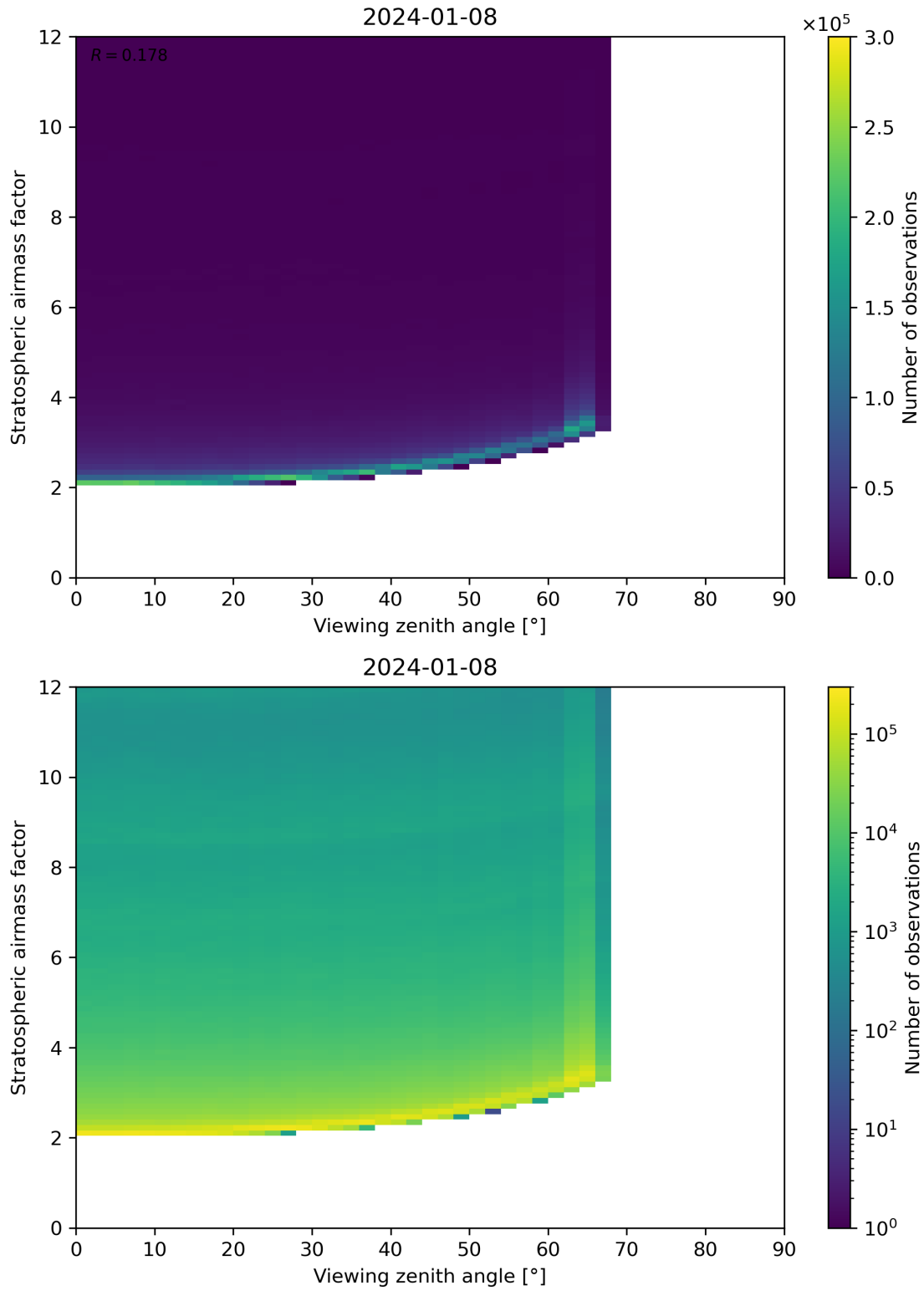
Figure 159: Scatter density plot of “Viewing zenith angle” against “Stratospheric airmass factor” for 2024-01-07 to 2024-01-09.
