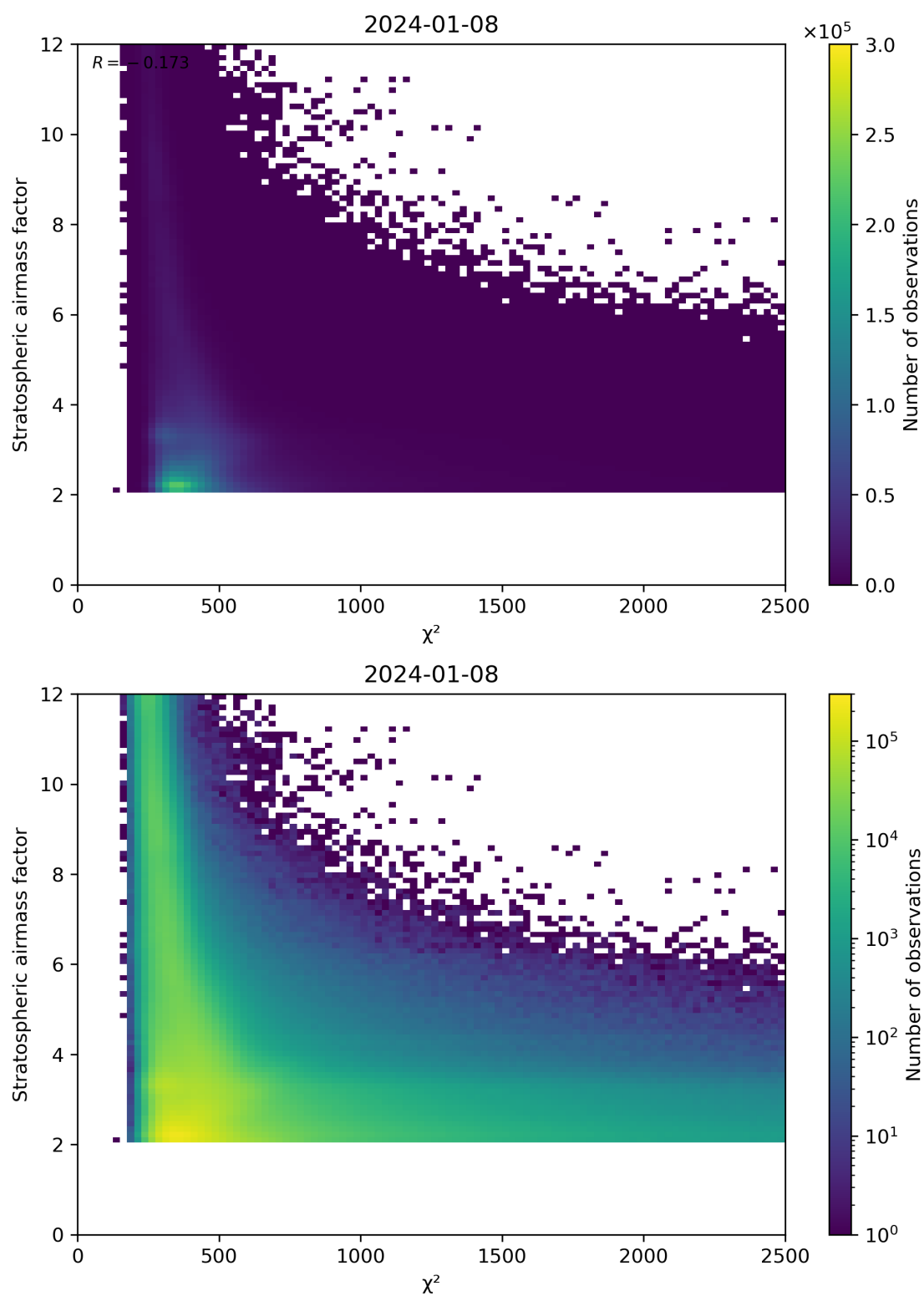
Figure 81: Scatter density plot of “ \chi^2 ” against “Stratospheric airmass factor” for 2024-01-07 to 2024-01-09.
