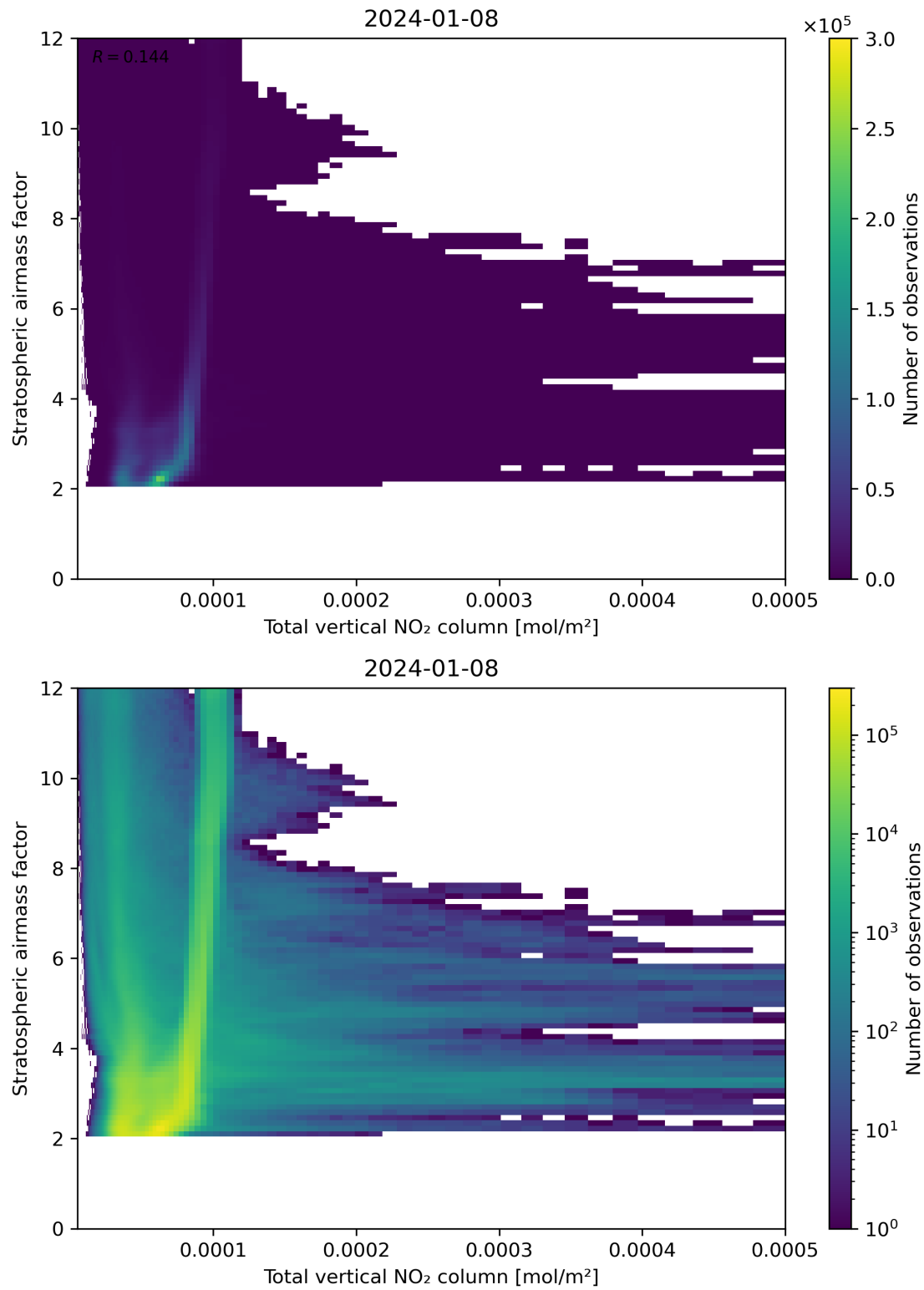
Figure 110: Scatter density plot of “Total vertical NO 2 column” against “Stratospheric air mass factor” for 2024-01-07 to 2024-01-09.
