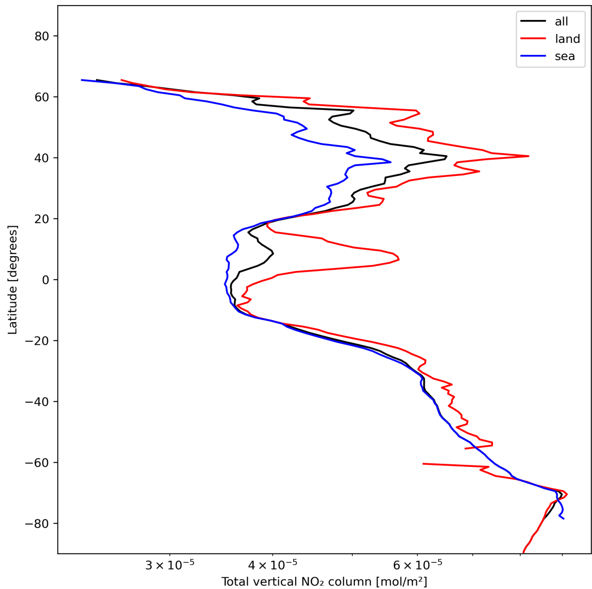
Figure 21: Zonal average of “Total vertical NO 2 column” for 2024-01-07 to 2024-01-09.
