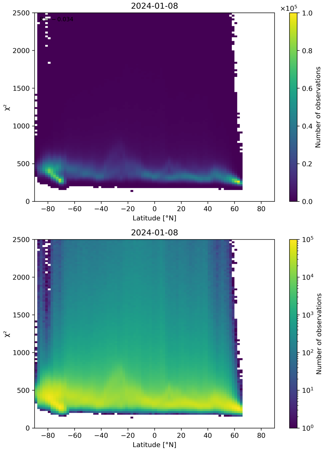
Figure 86: Scatter density plot of “Latitude” against “ \chi^2 ” for 2024-01-07 to 2024-01-09.
