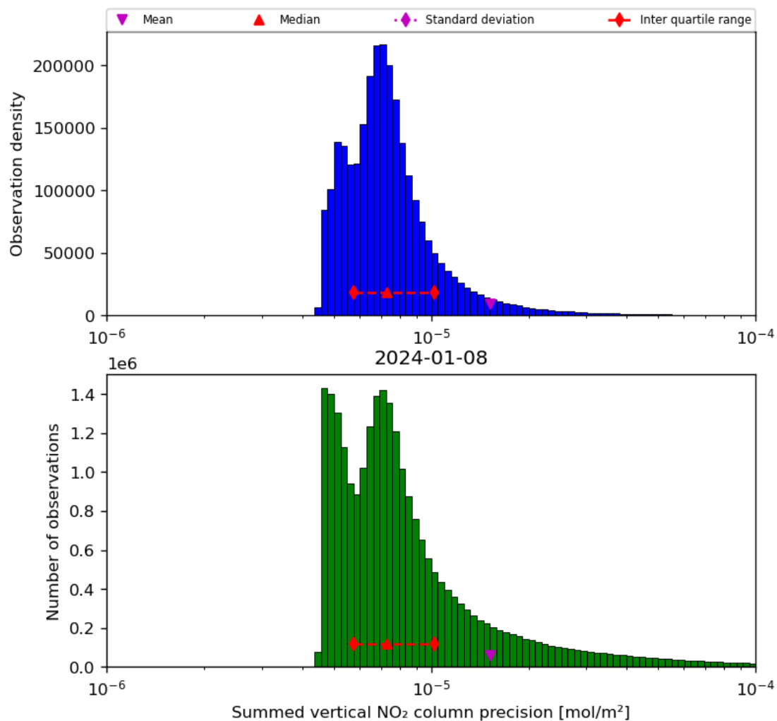
Figure 41: Histogram of "Summed vertical NO 2 column precision" for 2024-01-07 to 2024-01-09
