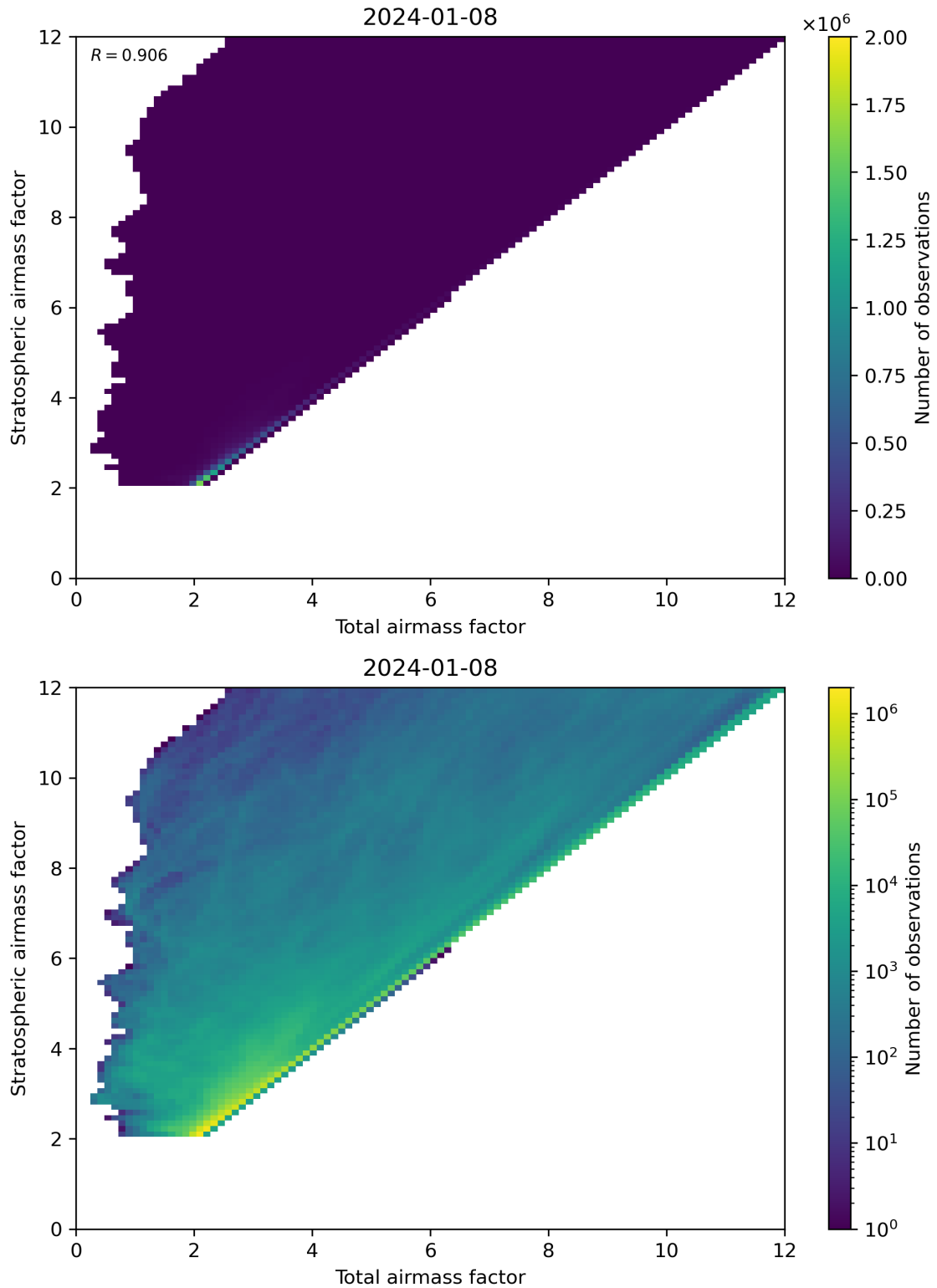
Figure 62: Scatter density plot of “Total airmass factor” against “Stratospheric airmass factor” for 2024-01-07 to 2024-01-09.
