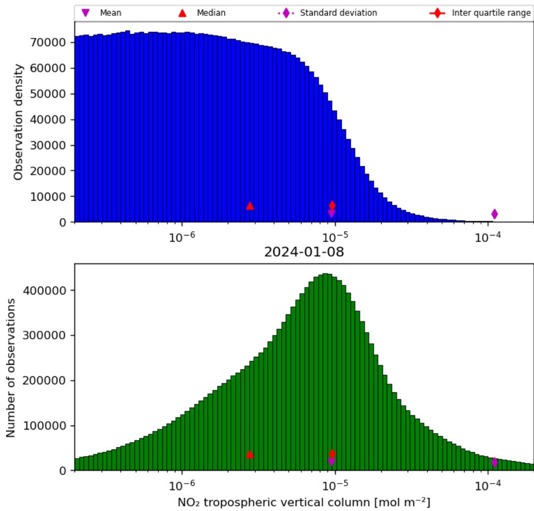
Figure 29: Histogram of “NO 2 tropospheric vertical column” for 2024-01-07 to 2024-01-09
