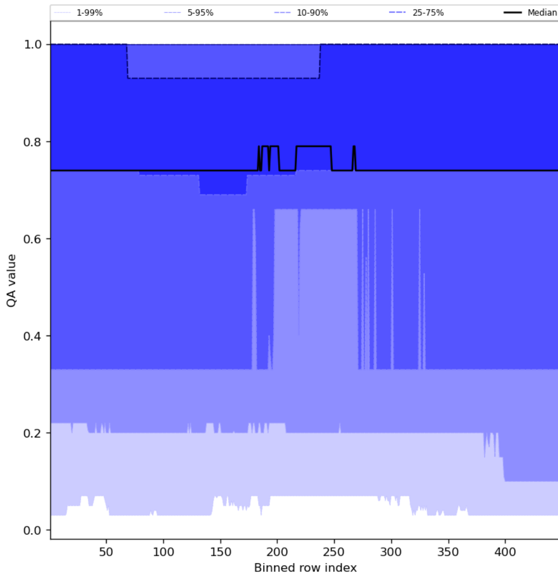
Figure 45: Along track statistics of “QA value” for 2024-01-07 to 2024-01-09
