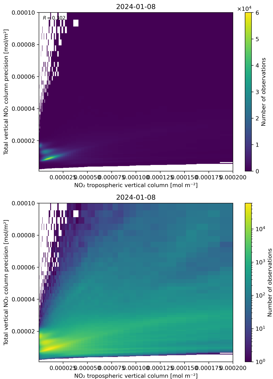
Figure 129: Scatter density plot of “NO 2 tropospheric vertical column” against “Total vertical NO 2 column precision” for 2024-01-07 to 2024-01-09.
