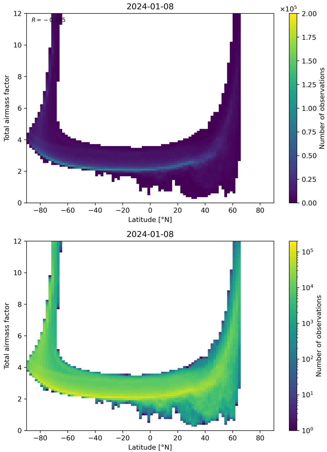
Figure 84: Scatter density plot of “Latitude” against “Total airmass factor” for 2024-01-07 to 2024-01-09.
