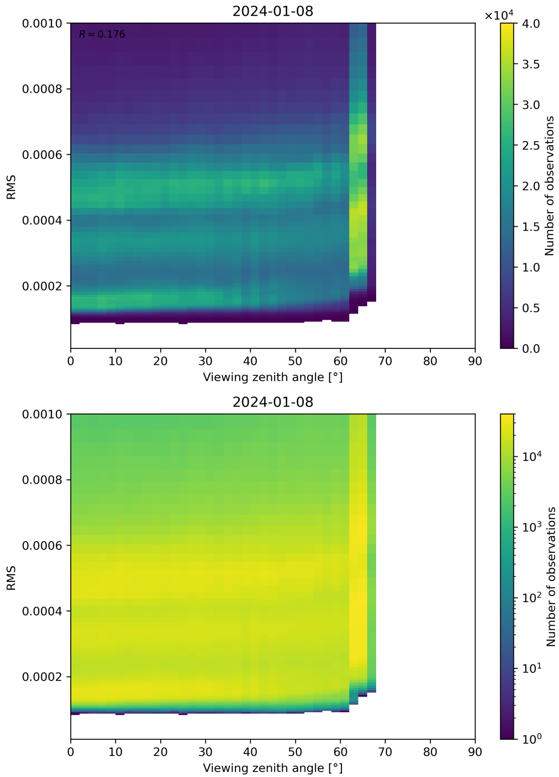
Figure 171: Scatter density plot of “Viewing zenith angle” against “RMS” for 2024-01-07 to 2024-01-09.
