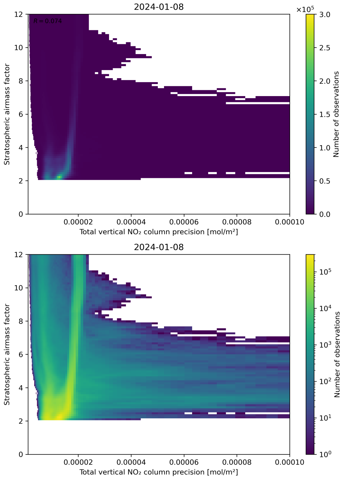
Figure 115: Scatter density plot of “Total vertical NO 2 column precision” against “Stratospheric air mass factor” for 2024-01-07 to 2024-01-09.
