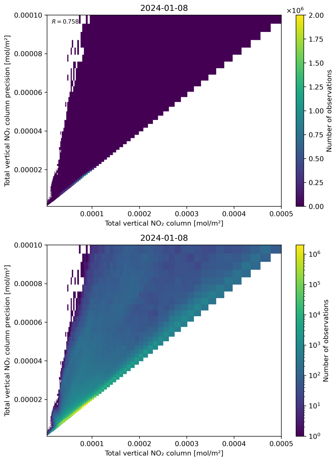
Figure 114: Scatter density plot of “Total vertical NO 2 column” against “Total vertical NO 2 column precision” for 2024-01-07 to 2024-01-09.
