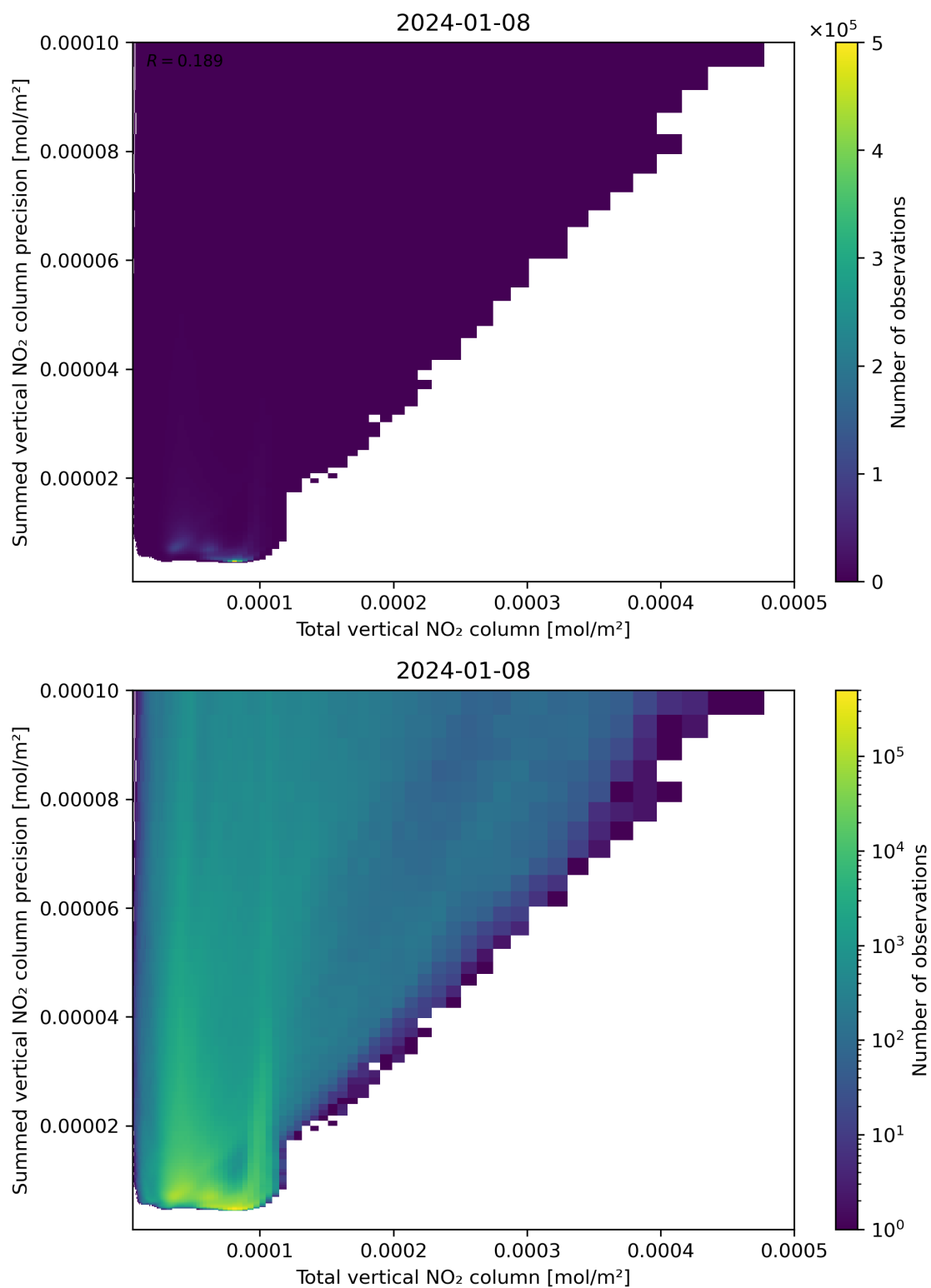
Figure 113: Scatter density plot of “Total vertical NO 2 column” against “Summed vertical NO 2 column precision” for 2024-01-07 to 2024-01-09.
