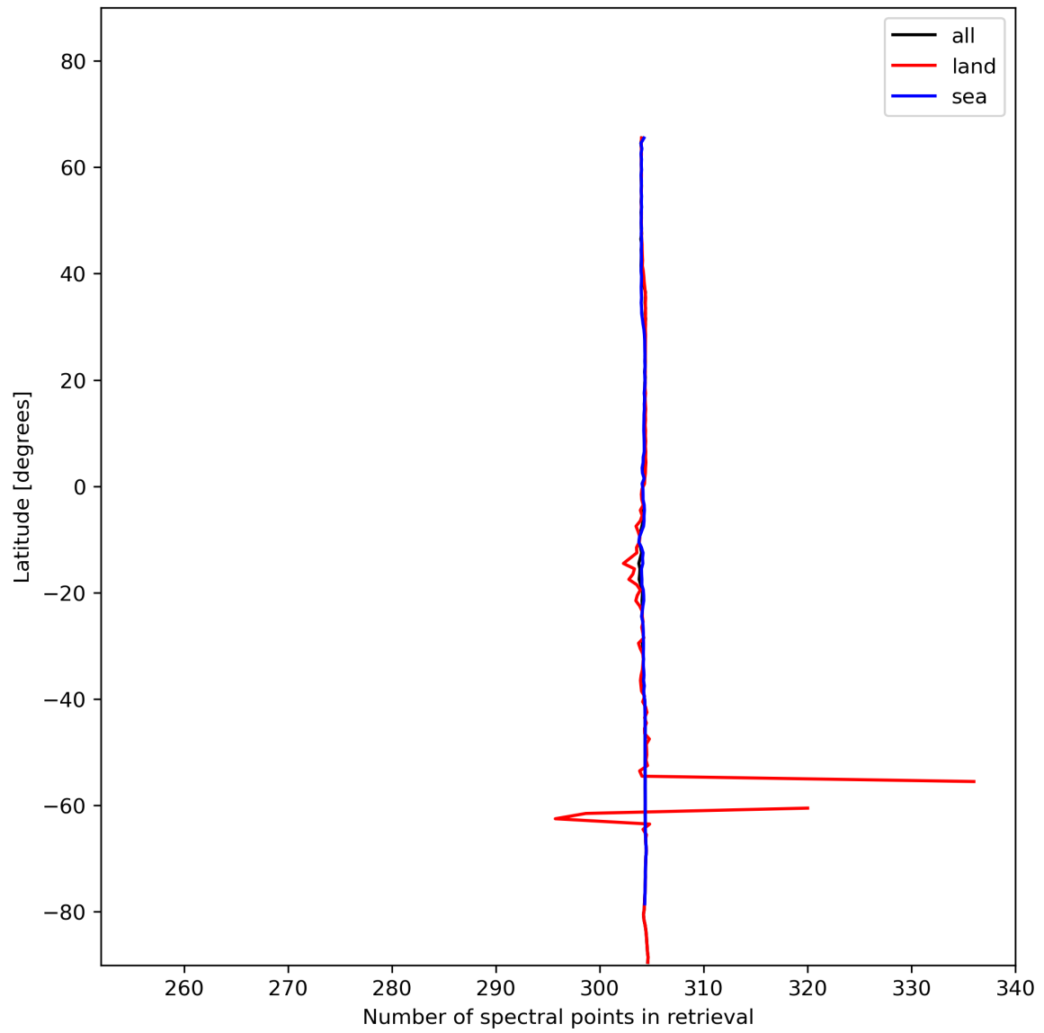
Figure 16: Zonal average of “Number of spectral points in retrieval” for 2024-01-07 to 2024-01-09.
