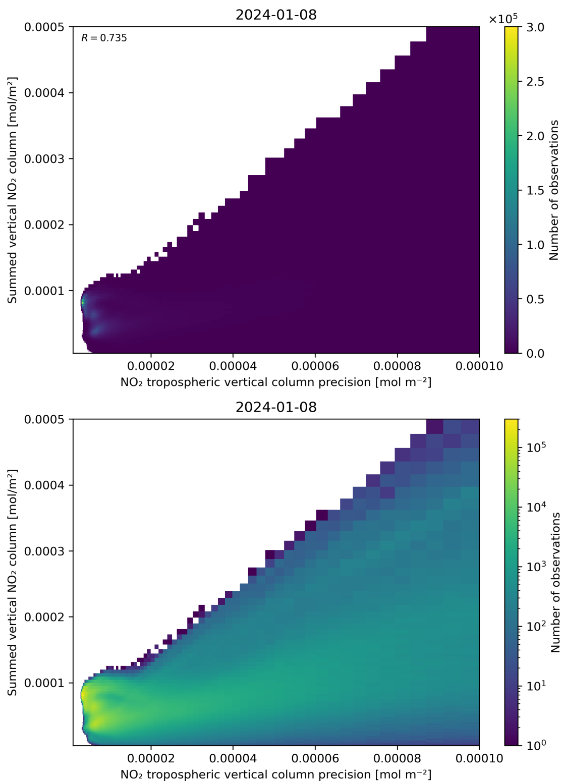
Figure 136: Scatter density plot of “NO 2 tropospheric vertical column precision” against “Summed vertical NO 2 column” for 2024-01-07 to 2024-01-09.
