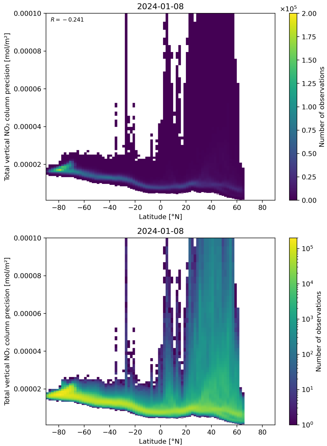
Figure 91: Scatter density plot of “Latitude” against “Total vertical NO 2 column precision” for 2024-01-07 to 2024-01-09.
