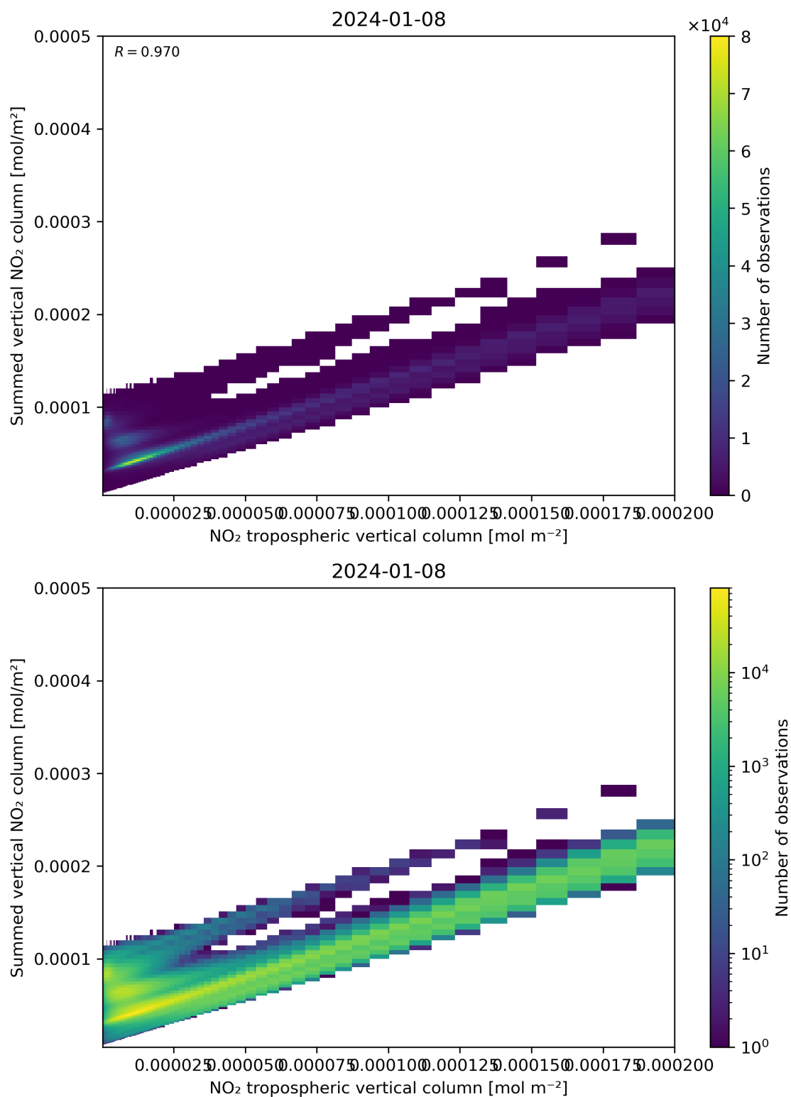
Figure 126: Scatter density plot of “NO 2 tropospheric vertical column” against “Summed vertical NO 2 column” for 2024-01-07 to 2024-01-09.
