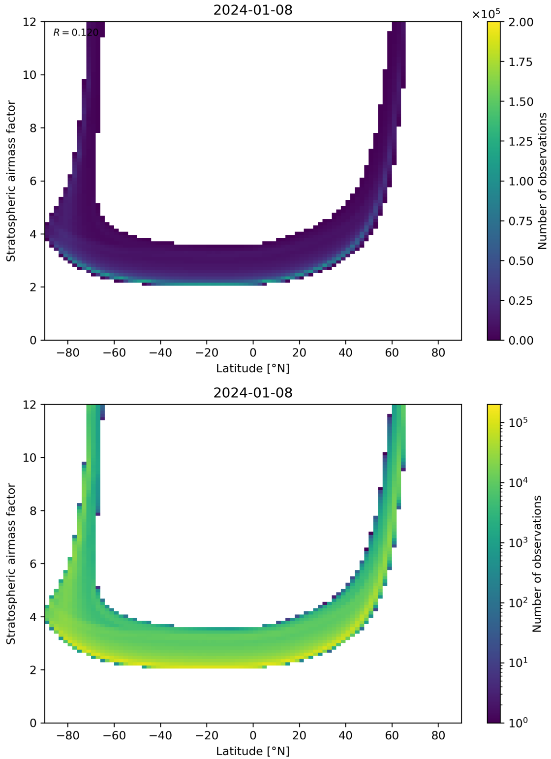
Figure 83: Scatter density plot of “Latitude” against “Stratospheric airmass factor” for 2024-01-07 to 2024-01-09.
