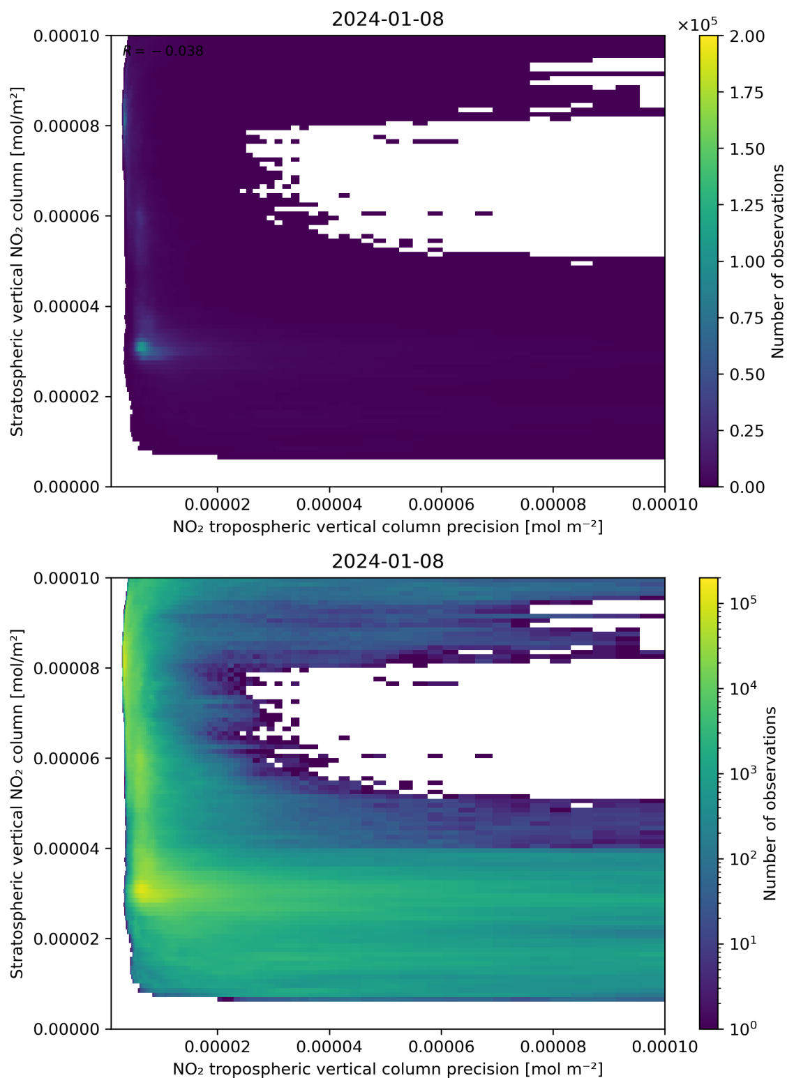
Figure 135: Scatter density plot of “NO 2 tropospheric vertical column precision” against “Stratospheric vertical NO 2 column” for 2024-01-07 to 2024-01-09.
