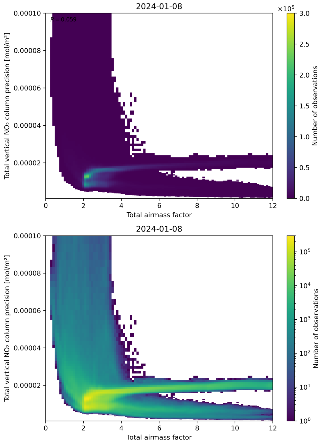
Figure 68: Scatter density plot of “Total airmass factor” against “Total vertical NO 2 column precision” for 2024-01-07 to 2024-01-09.
