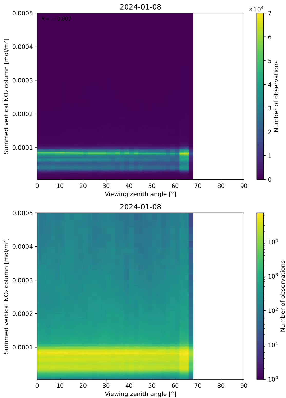
Figure 165: Scatter density plot of “Viewing zenith angle” against “Summed vertical NO 2 column” for 2024-01-07 to 2024-01-09.
