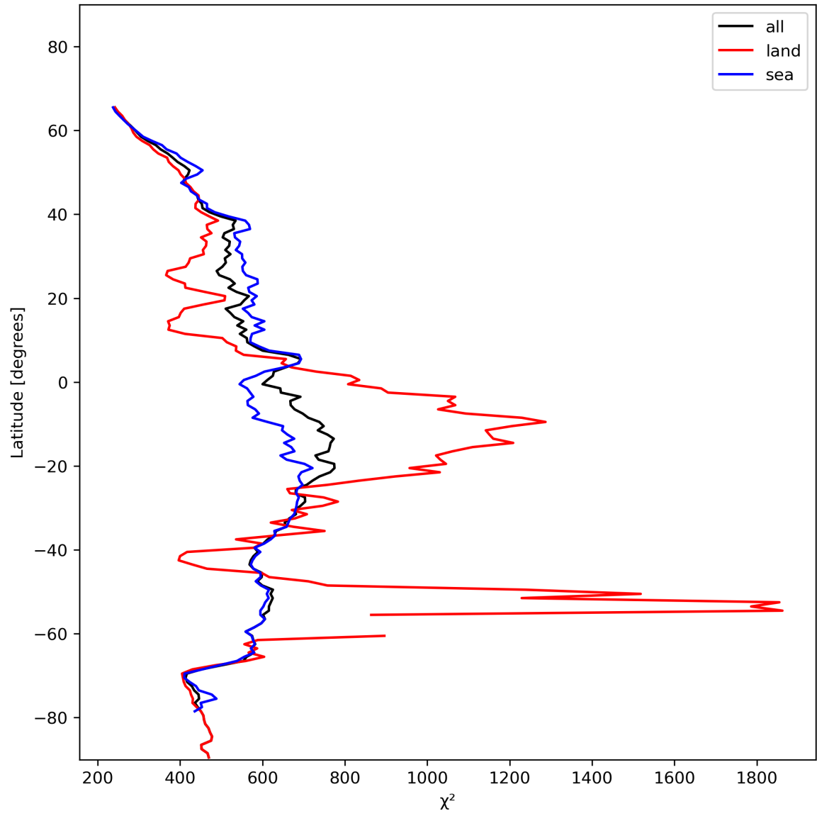
Figure 25: Zonal average of “ \chi^2 ” for 2024-01-07 to 2024-01-09.
