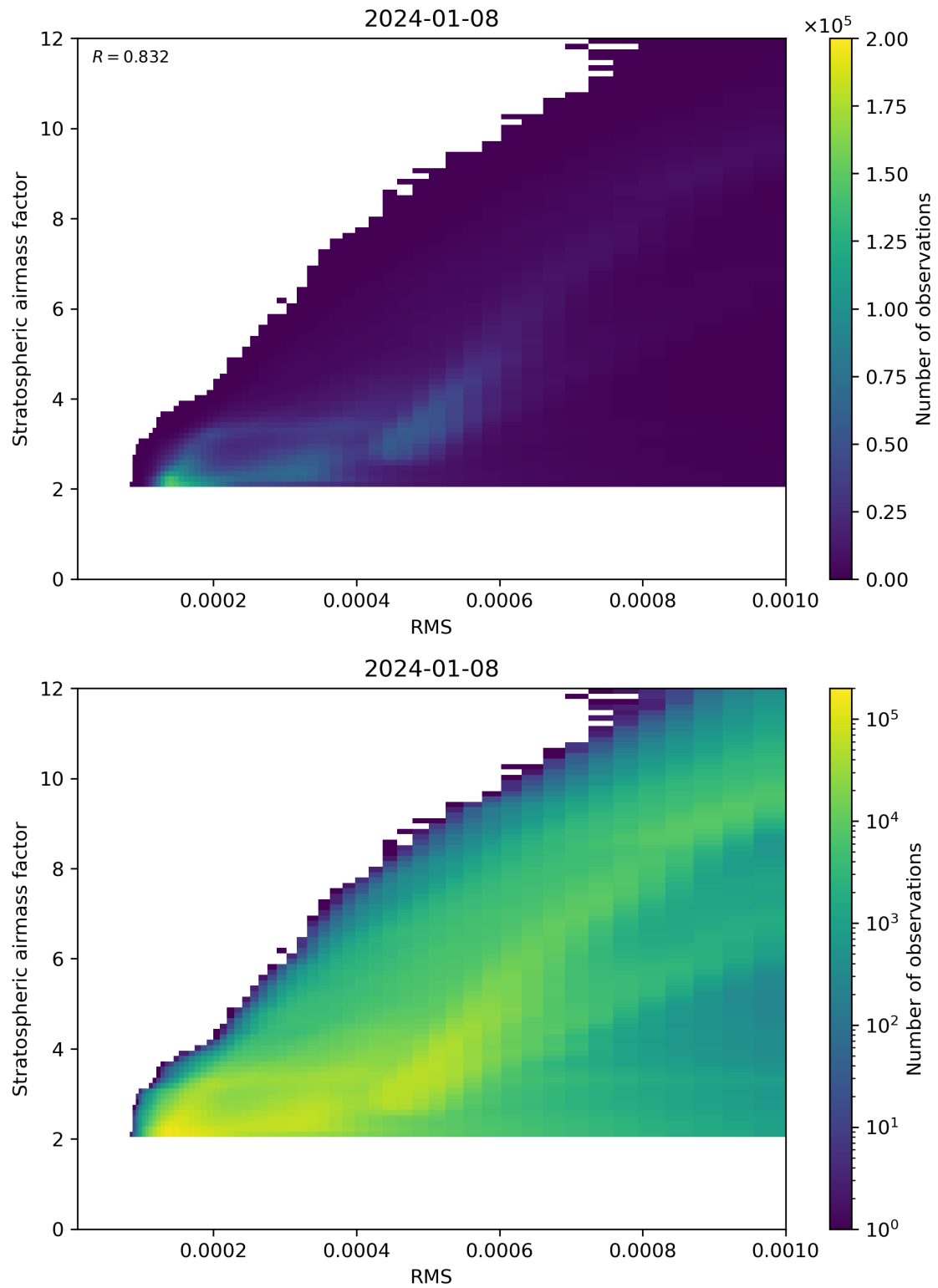
Figure 144: Scatter density plot of “RMS” against “Stratospheric airmass factor” for 2024-01-07 to 2024-01-09.
