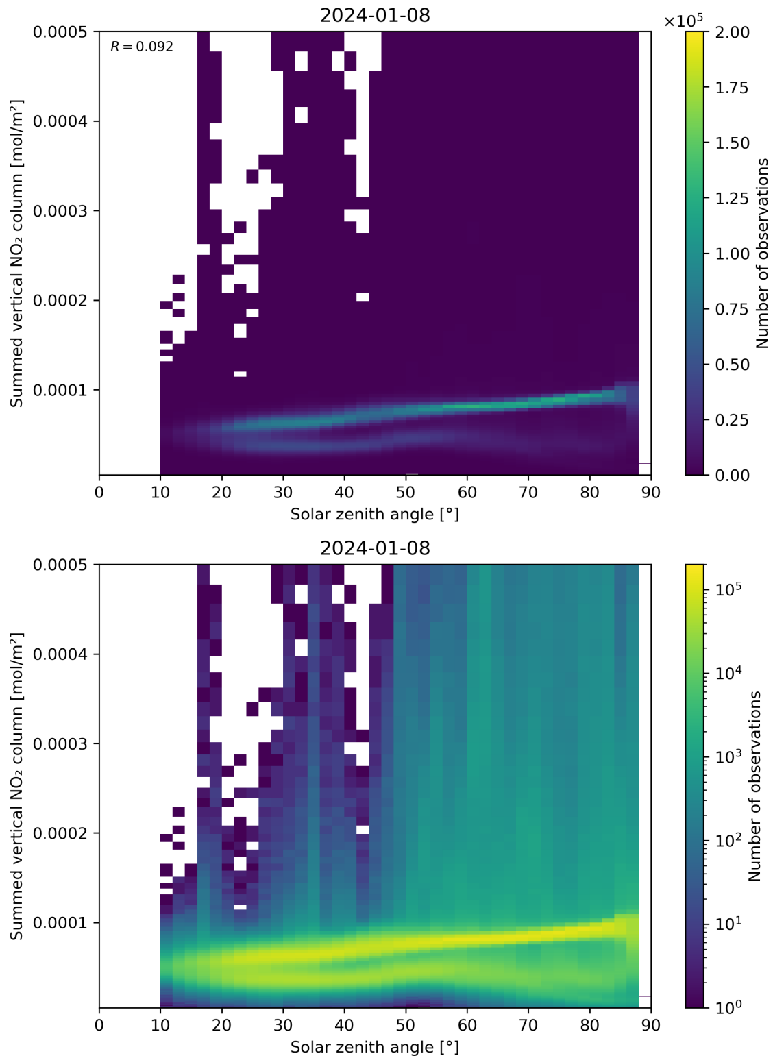
Figure 151: Scatter density plot of “Solar zenith angle” against “Summed vertical NO 2 column” for 2024-01-07 to 2024-01-09.
