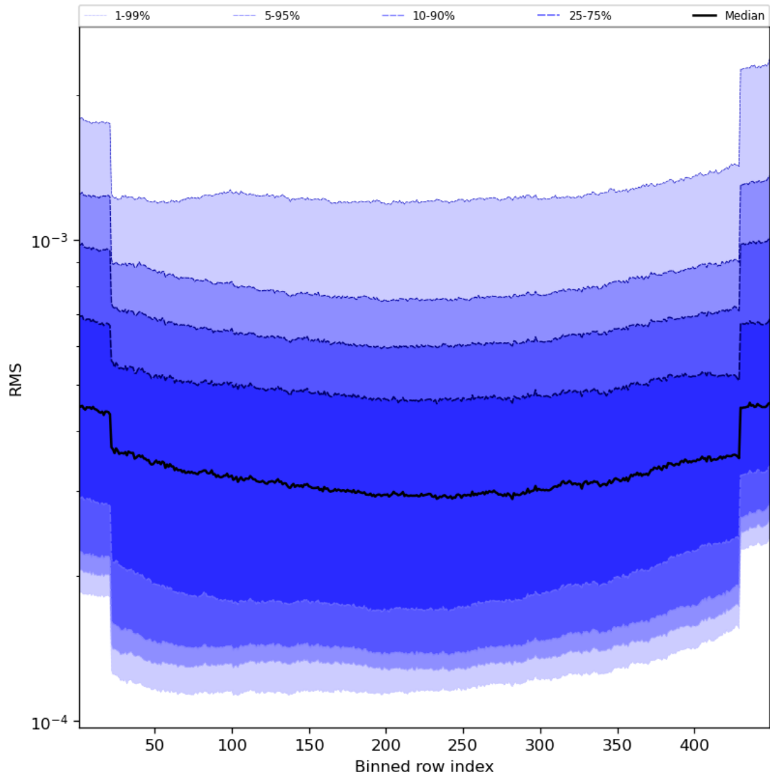
Figure 60: Along track statistics of “RMS” for 2024-01-07 to 2024-01-09
