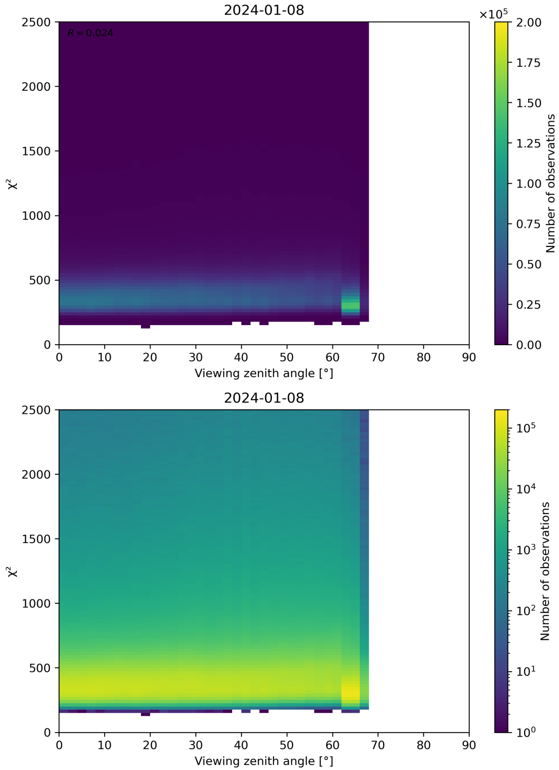
Figure 162: Scatter density plot of “Viewing zenith angle” against “ \chi^2 ” for 2024-01-07 to 2024-01-09.
