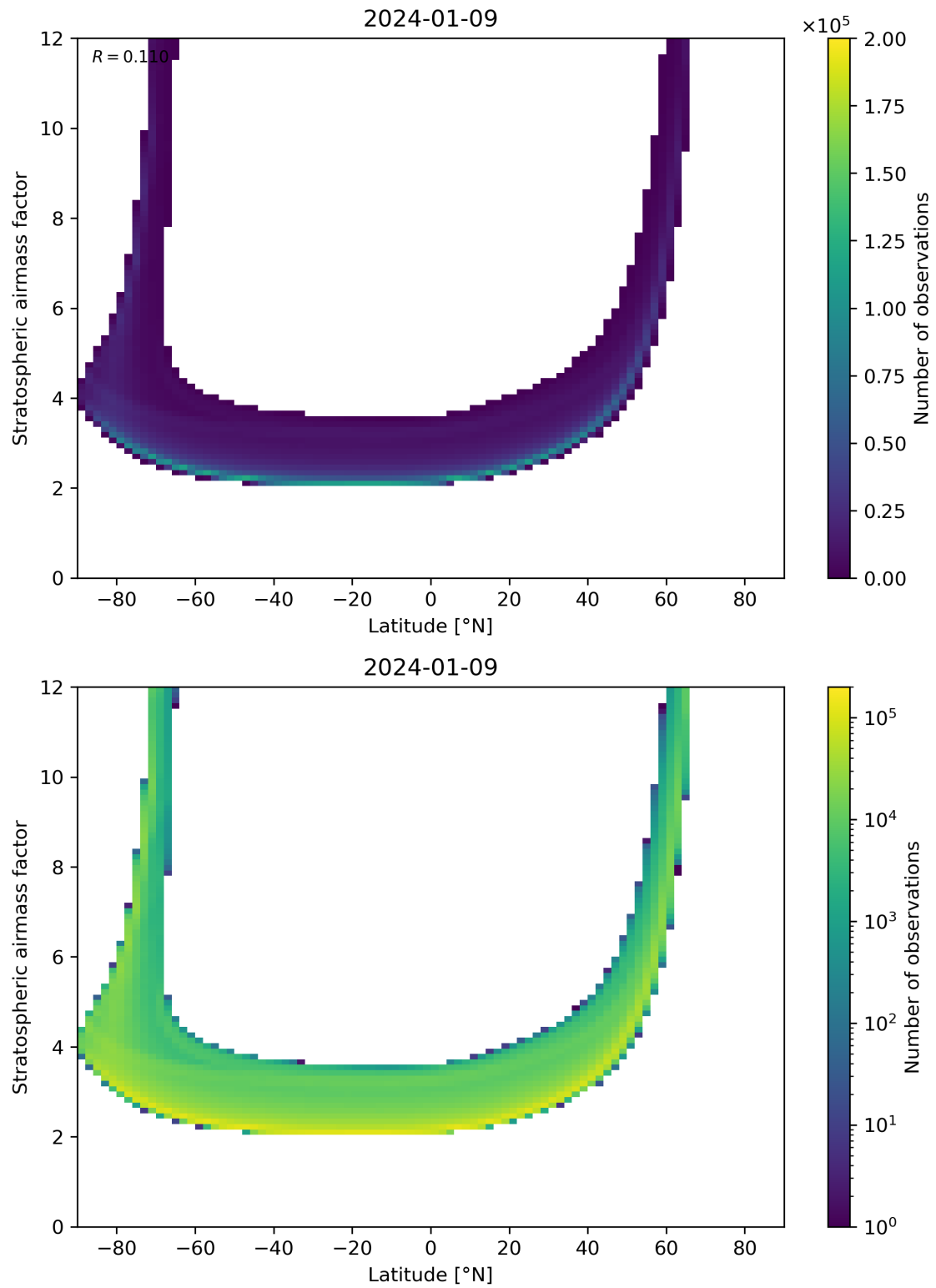
Figure 83: Scatter density plot of “Latitude” against “Stratospheric airmass factor” for 2024-01-08 to 2024-01-10.
