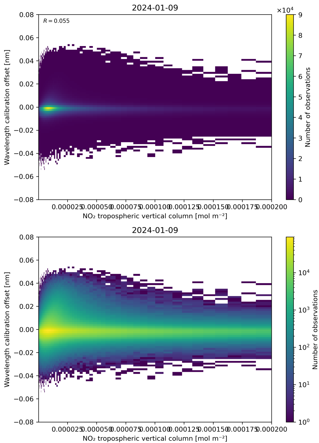
Figure 143: Scatter density plot of “NO 2 tropospheric vertical column” against “Wavelength calibration offset” for 2024-01-08 to 2024-01-10.
