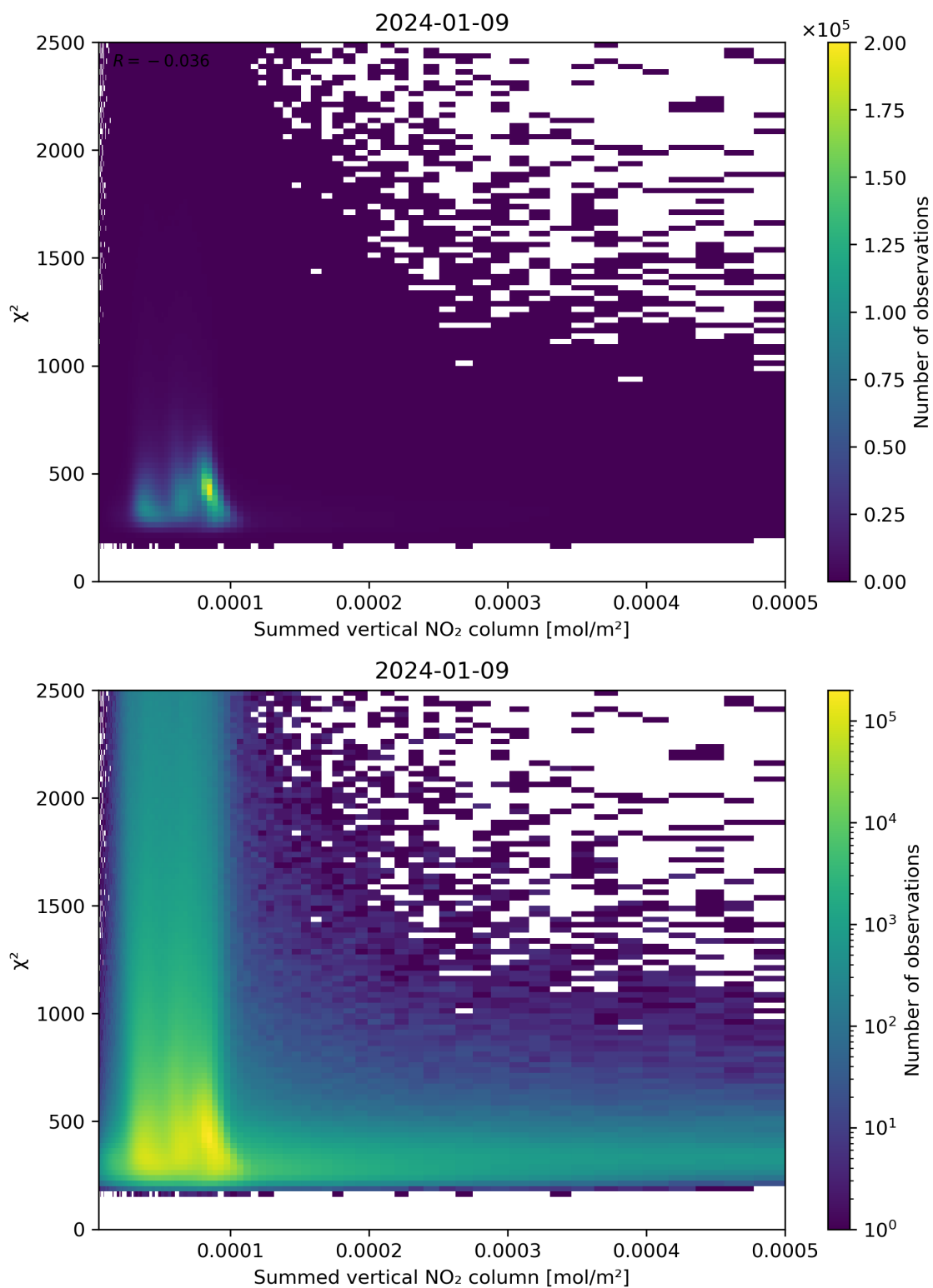
Figure 104: Scatter density plot of “Summed vertical NO 2 column” against “ \chi^2 ” for 2024-01-08 to 2024-01-10.
