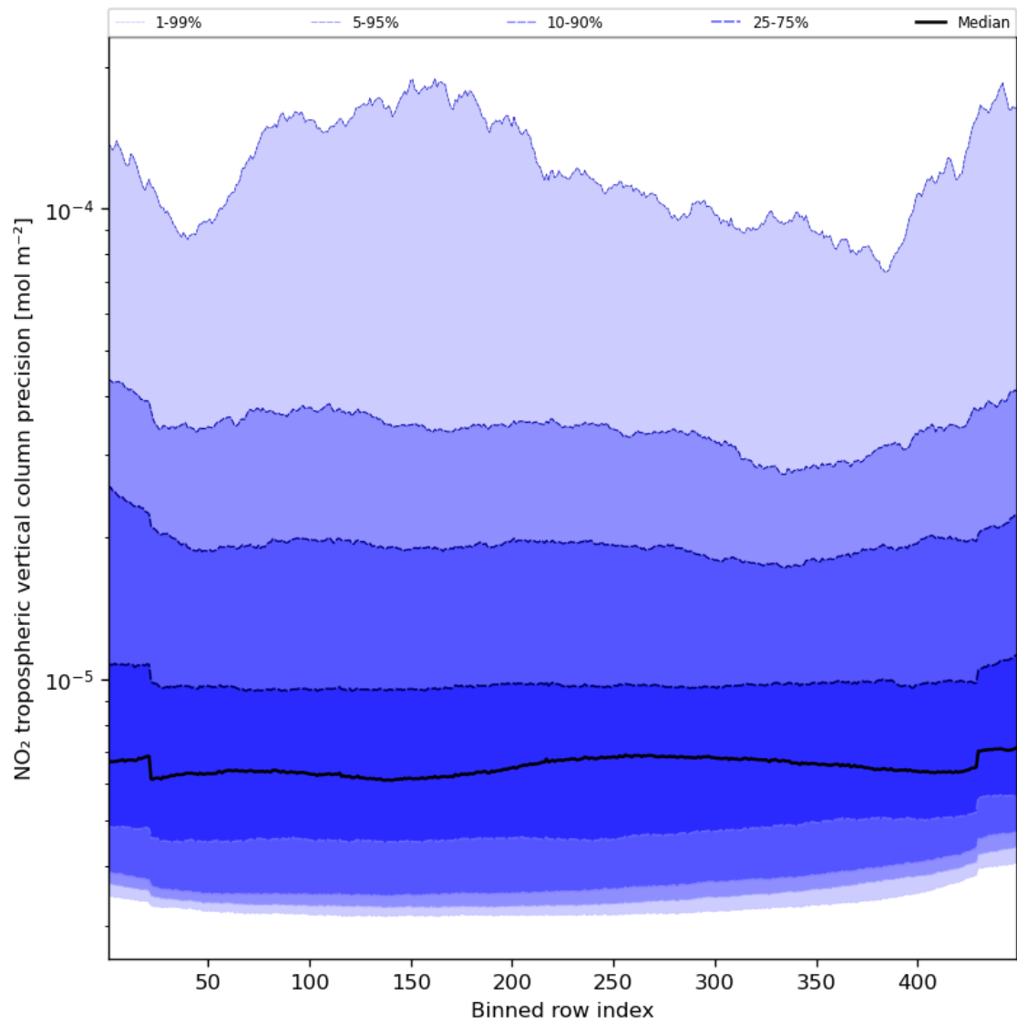
Figure 47: Along track statistics of “NO 2 tropospheric vertical column precision” for 2024-01-08 to 2024-01-10
