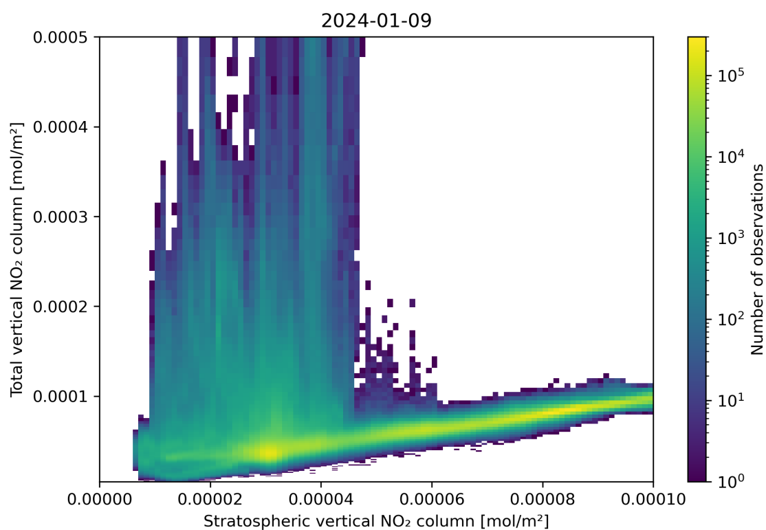
Figure 100: Scatter density plot of “Stratospheric vertical NO 2 column” against “Total vertical NO 2 column” for 2024-01-08 to 2024-01-10.
