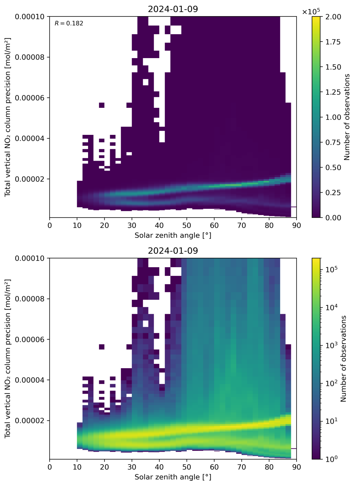
Figure 154: Scatter density plot of “Solar zenith angle” against “Total vertical NO 2 column precision” for 2024-01-08 to 2024-01-10.
