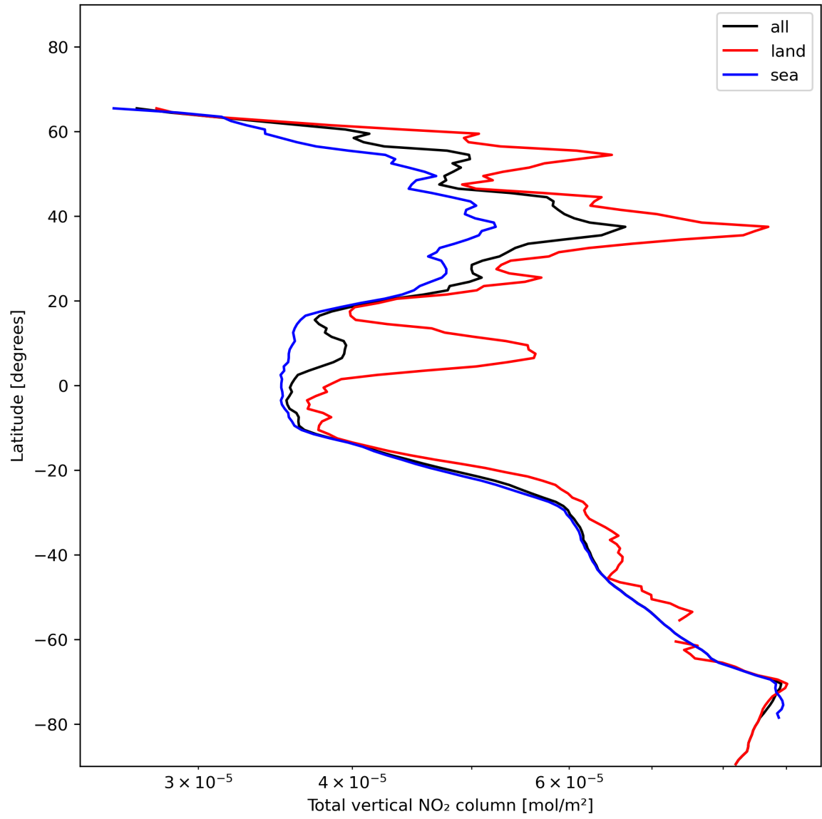
Figure 21: Zonal average of “Total vertical NO 2 column” for 2024-01-08 to 2024-01-10.
