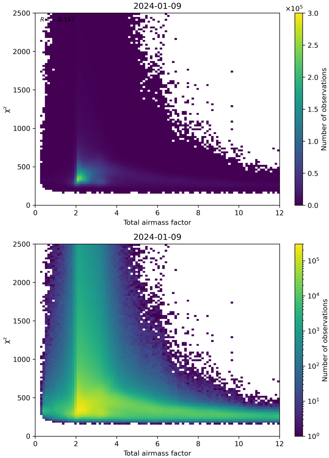
Figure 63: Scatter density plot of “Total airmass factor” against “ \chi^2 ” for 2024-01-08 to 2024-01-10.
