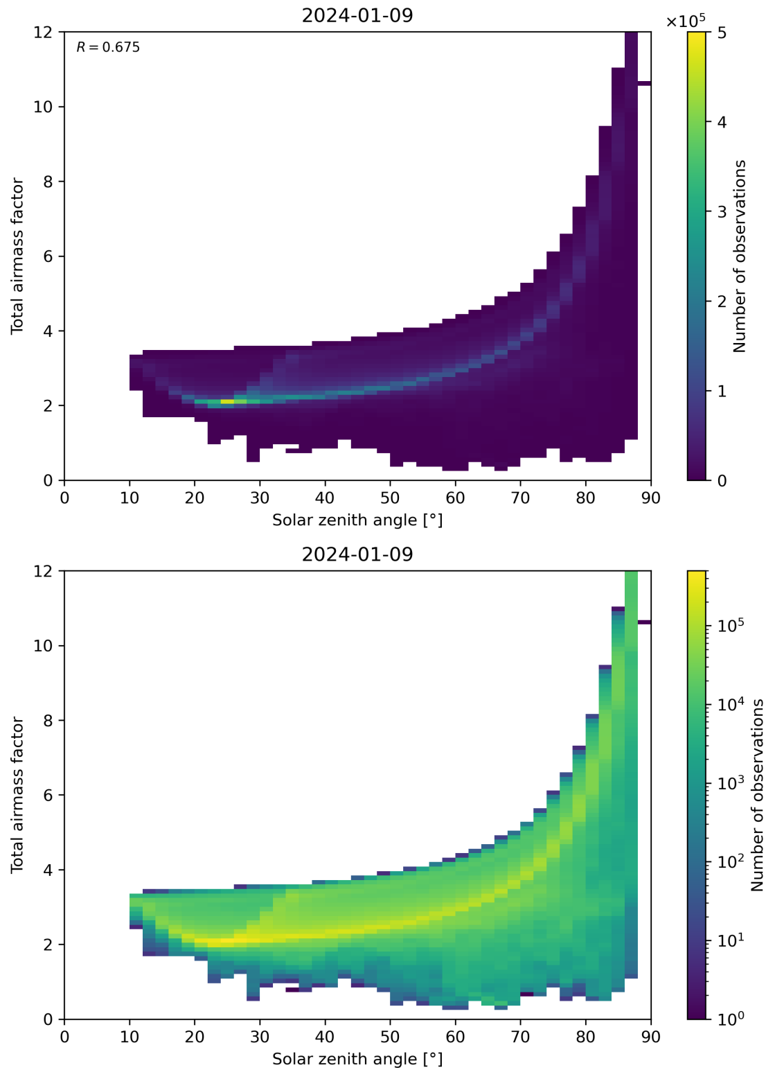
Figure 146: Scatter density plot of “Solar zenith angle” against “Total air mass factor” for 2024-01-08 to 2024-01-10.
