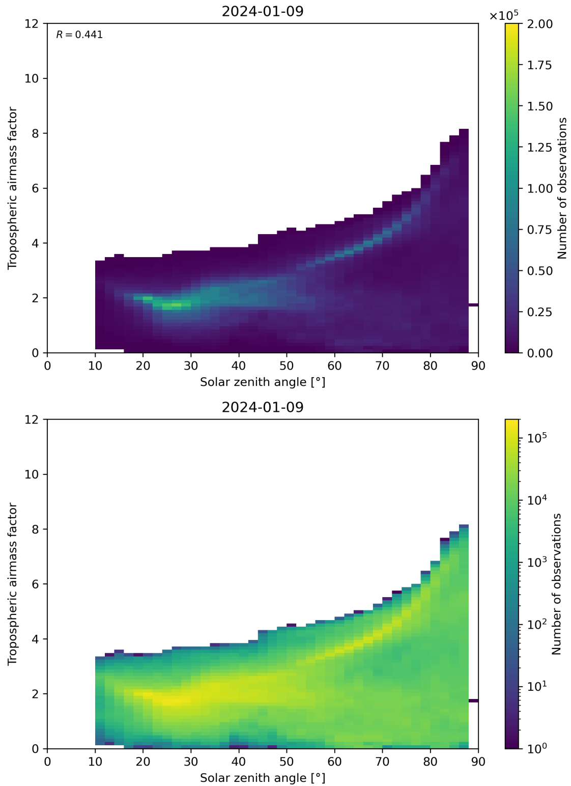
Figure 147: Scatter density plot of “Solar zenith angle” against “Tropospheric airmass factor” for 2024-01-08 to 2024-01-10.
