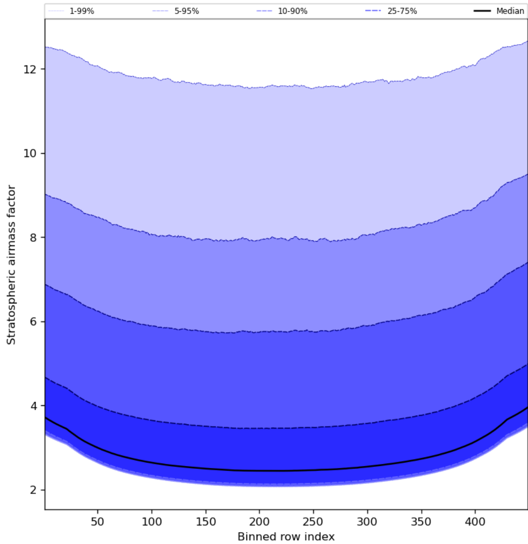
Figure 61: Along track statistics of “Stratospheric airmass factor” for 2024-01-08 to 2024-01-10
