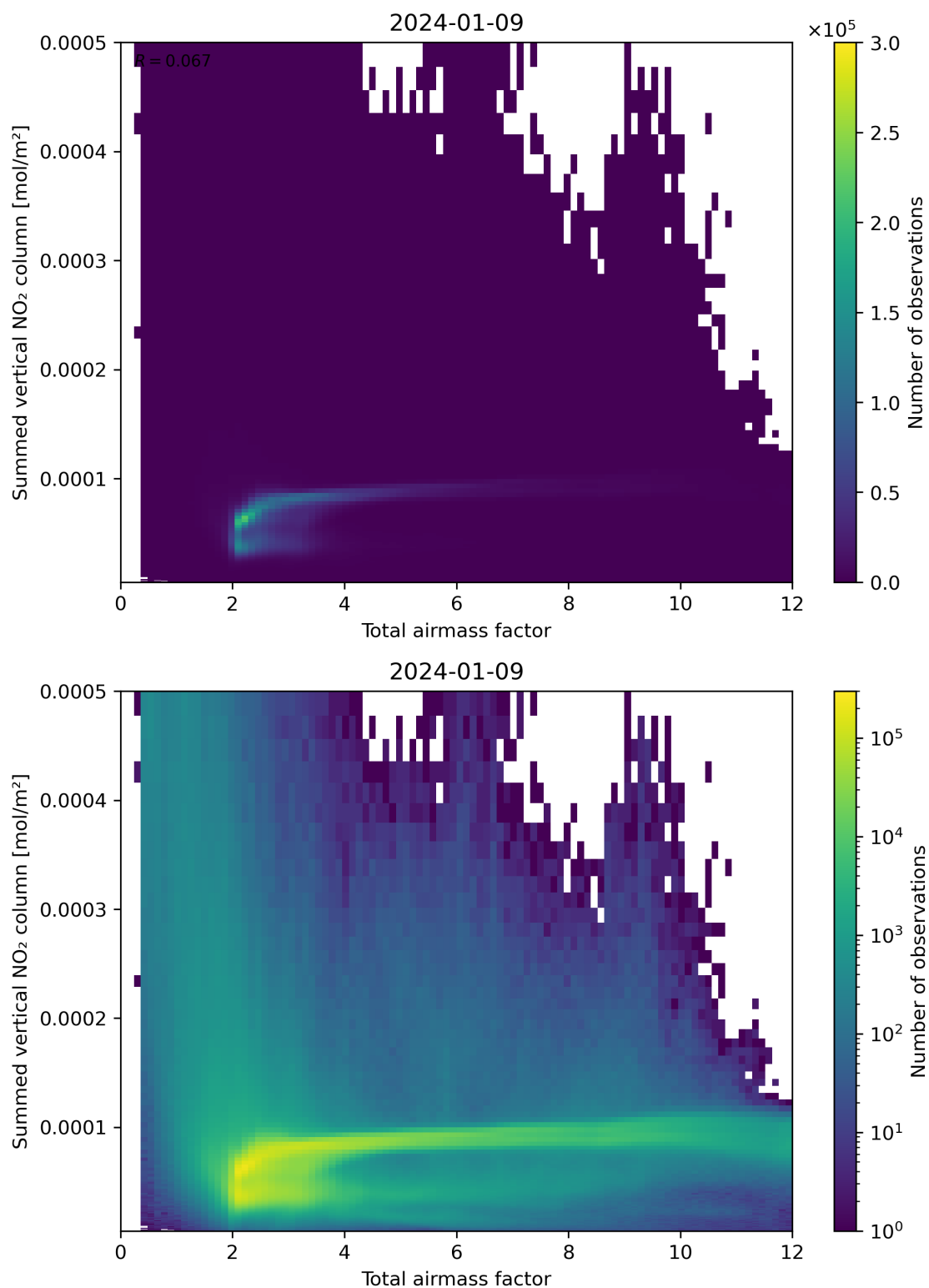
Figure 65: Scatter density plot of “Total airmass factor” against “Summed vertical NO 2 column” for 2024-01-08 to 2024-01-10.
