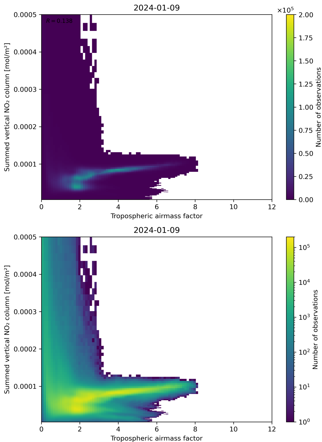
Figure 75: Scatter density plot of “Tropospheric airmass factor” against “Summed vertical NO 2 column” for 2024-01-08 to 2024-01-10.
