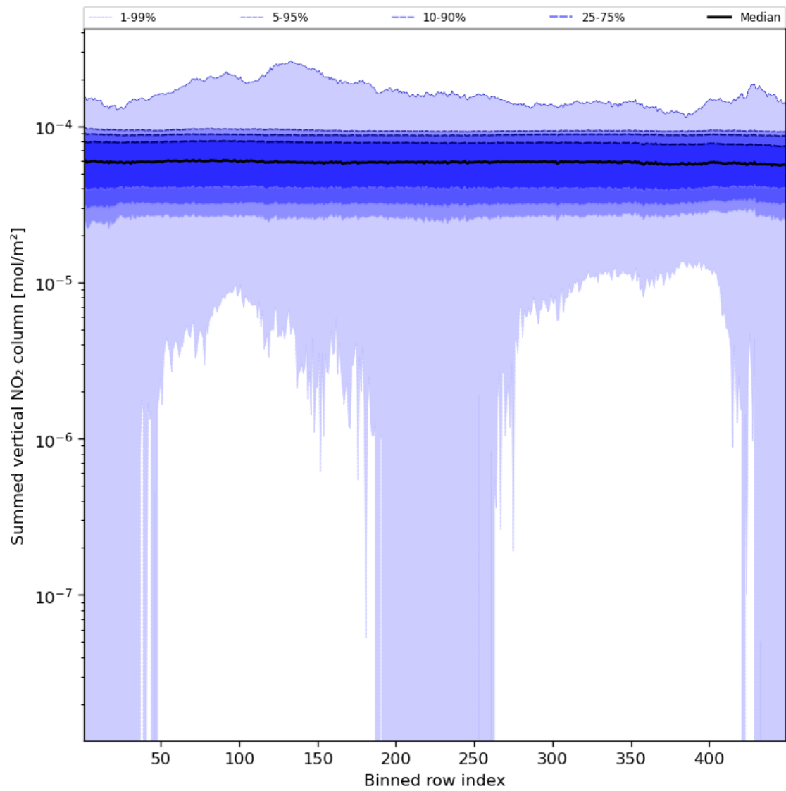
Figure 57: Along track statistics of “Summed vertical NO 2 column” for 2024-01-08 to 2024-01-10
