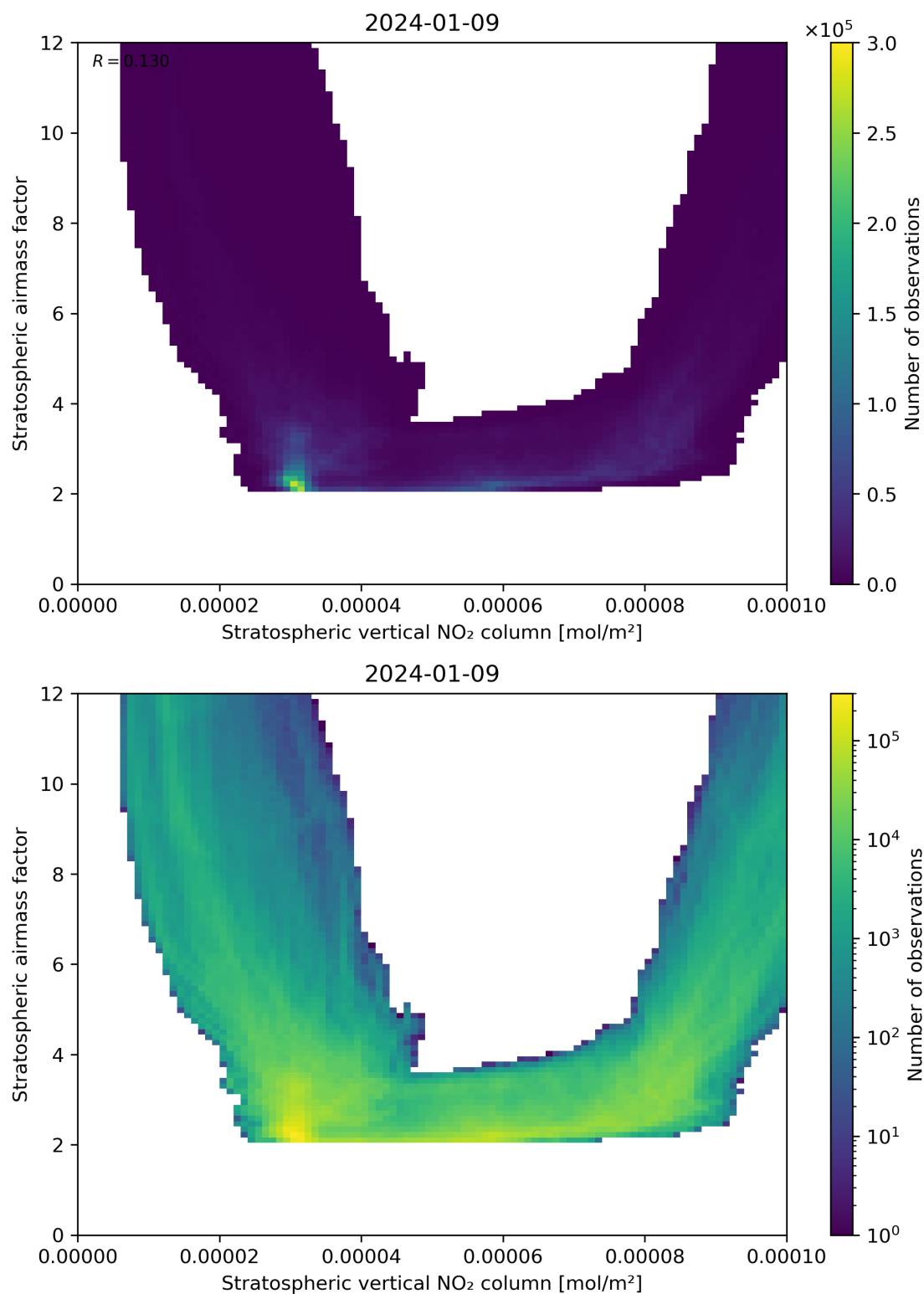
Figure 96: Scatter density plot of “Stratospheric vertical NO 2 column” against “Stratospheric airmass factor” for 2024-01-08 to 2024-01-10.
