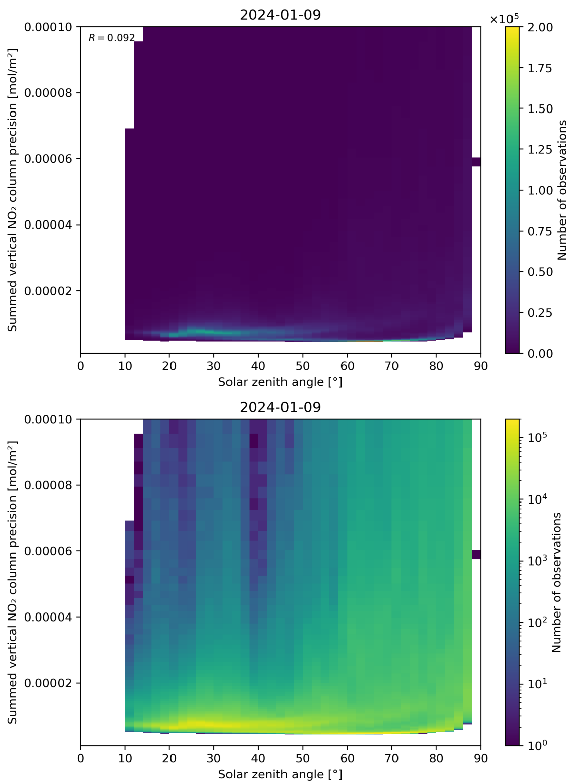
Figure 152: Scatter density plot of “Solar zenith angle” against “Summed vertical NO 2 column precision” for 2024-01-08 to 2024-01-10.
