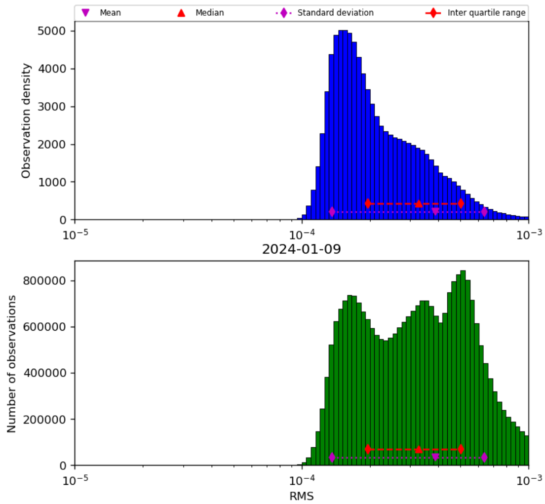
Figure 43: Histogram of “RMS” for 2024-01-08 to 2024-01-10
