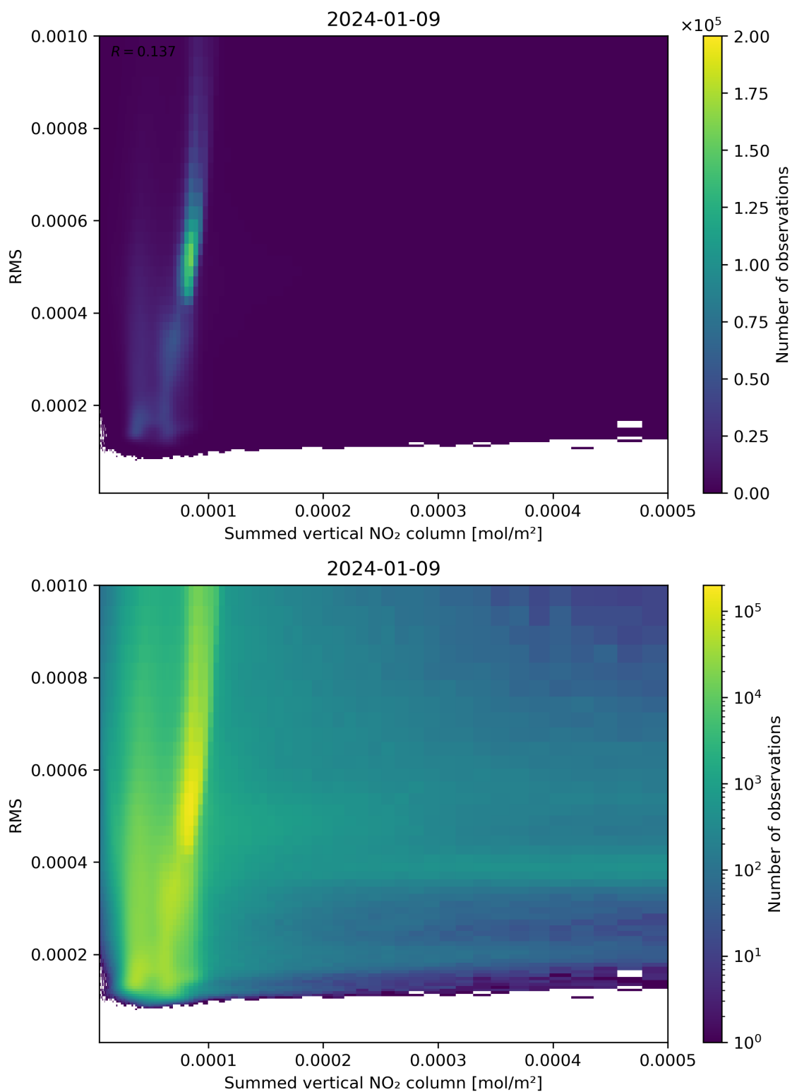
Figure 109: Scatter density plot of “Summed vertical NO 2 column” against “RMS” for 2024-01-08 to 2024-01-10.
