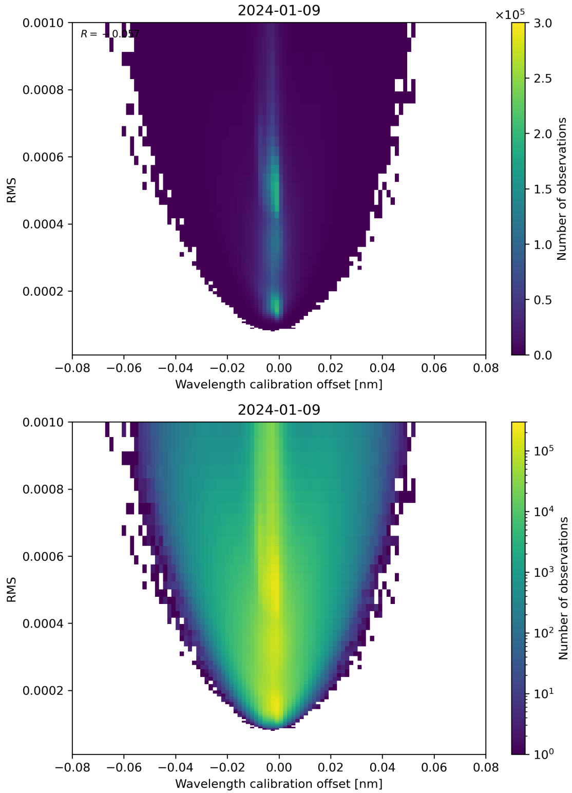
Figure 181: Scatter density plot of “Wavelength calibration offset” against “RMS” for 2024-01-08 to 2024-01-10.
