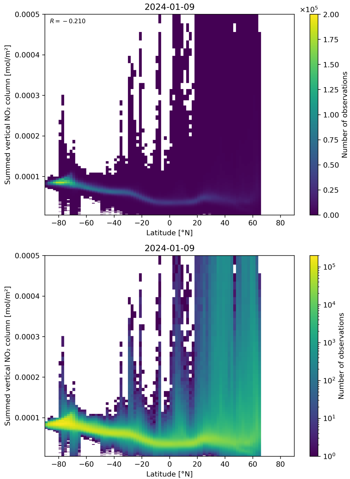
Figure 88: Scatter density plot of “Latitude” against “Summed vertical NO 2 column” for 2024-01-08 to 2024-01-10.
