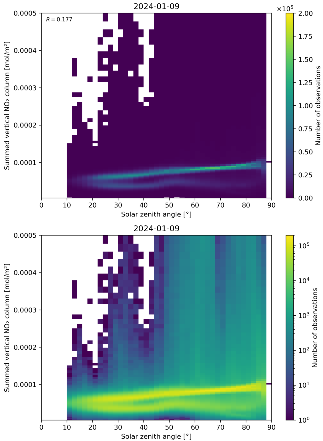
Figure 151: Scatter density plot of “Solar zenith angle” against “Summed vertical NO 2 column” for 2024-01-08 to 2024-01-10.
