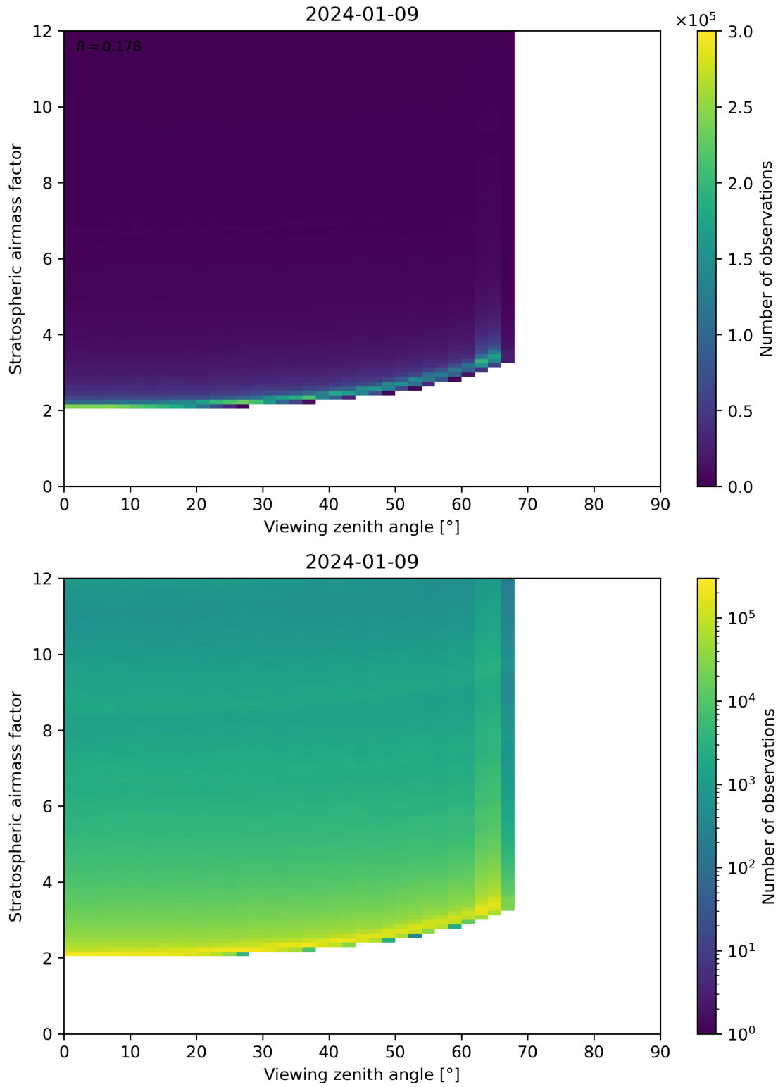
Figure 159: Scatter density plot of “Viewing zenith angle” against “Stratospheric airmass factor” for 2024-01-08 to 2024-01-10.
