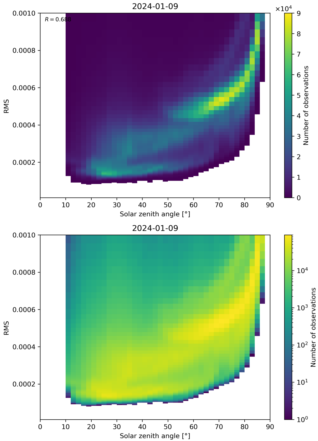
Figure 157: Scatter density plot of “Solar zenith angle” against “RMS” for 2024-01-08 to 2024-01-10.
