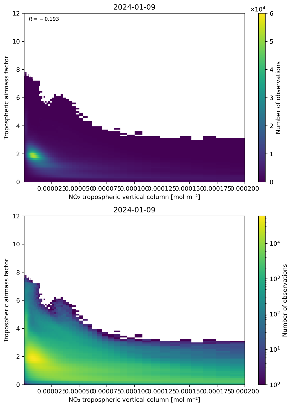
Figure 123: Scatter density plot of “NO 2 tropospheric vertical column” against “Tropospheric airmass factor” for 2024-01-08 to 2024-01-10.
