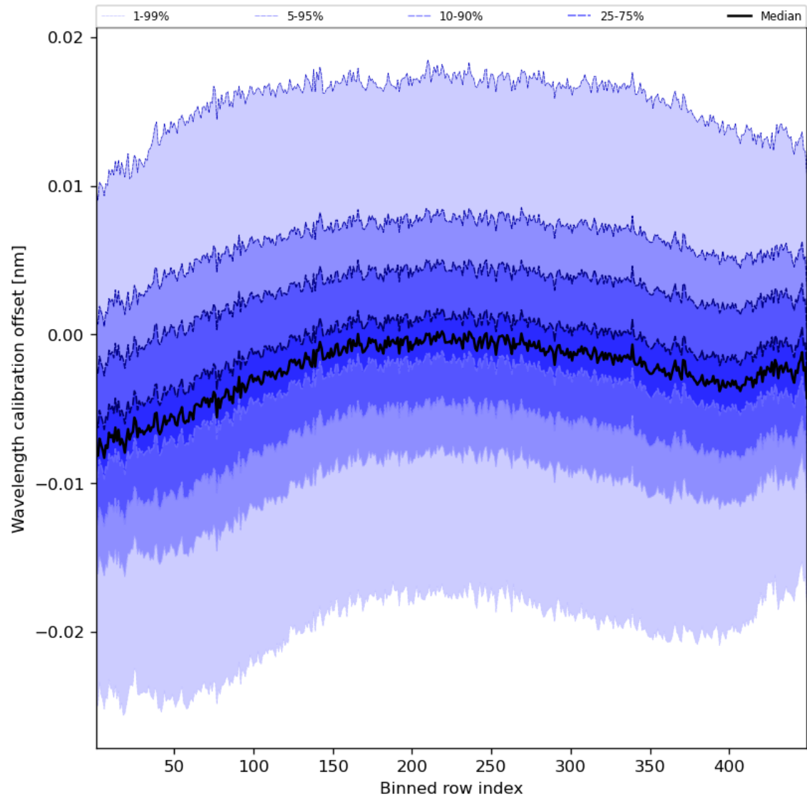
Figure 52: Along track statistics of “Wavelength calibration offset” for 2024-01-08 to 2024-01-10
