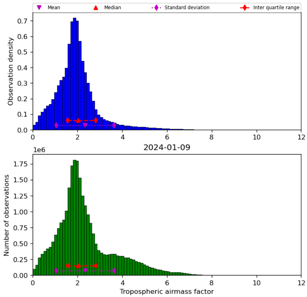
Figure 31: Histogram of “Tropospheric airmass factor” for 2024-01-08 to 2024-01-10
