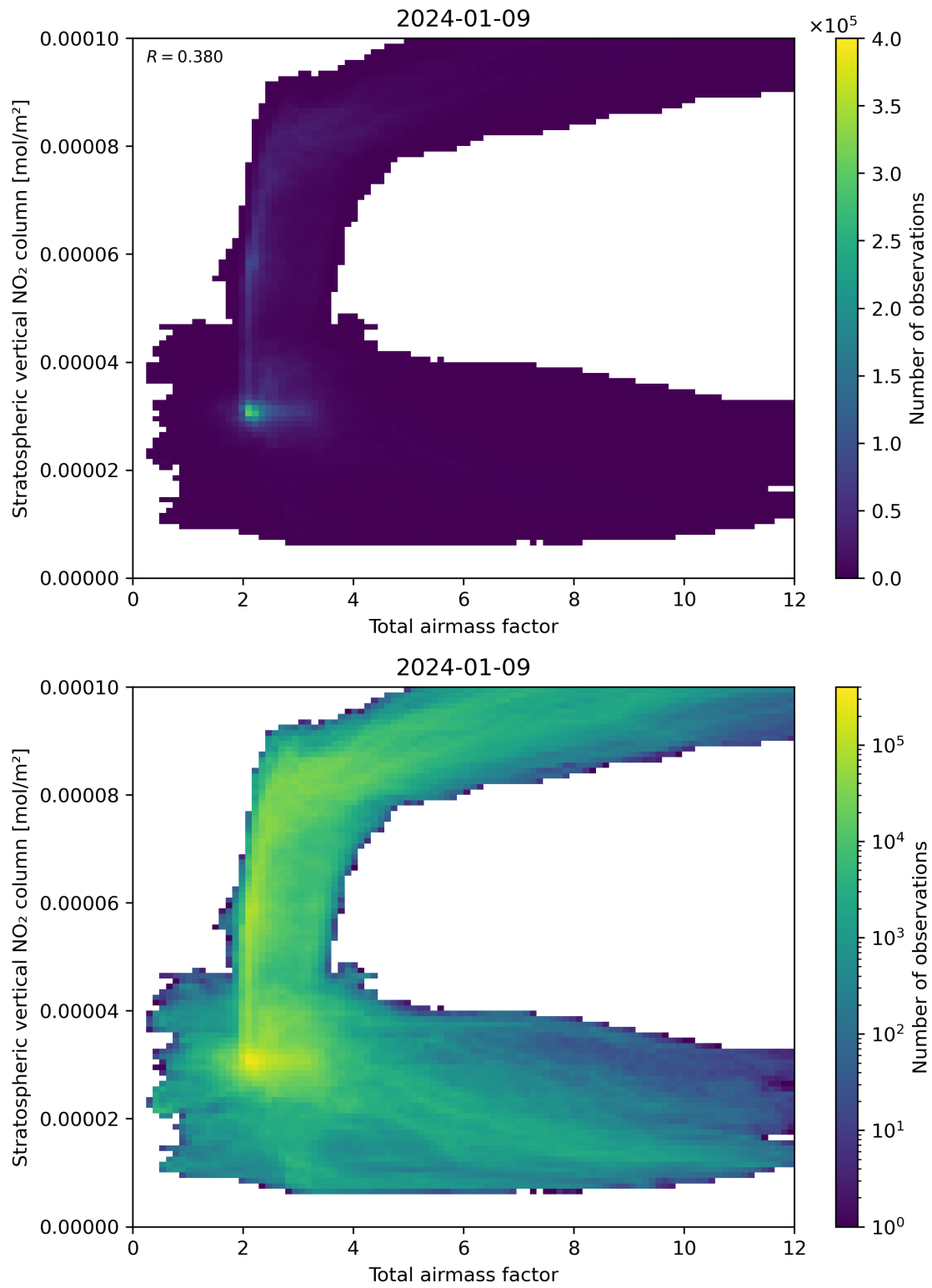
Figure 64: Scatter density plot of “Total airmass factor” against “Stratospheric vertical NO 2 column” for 2024-01-08 to 2024-01-10.
