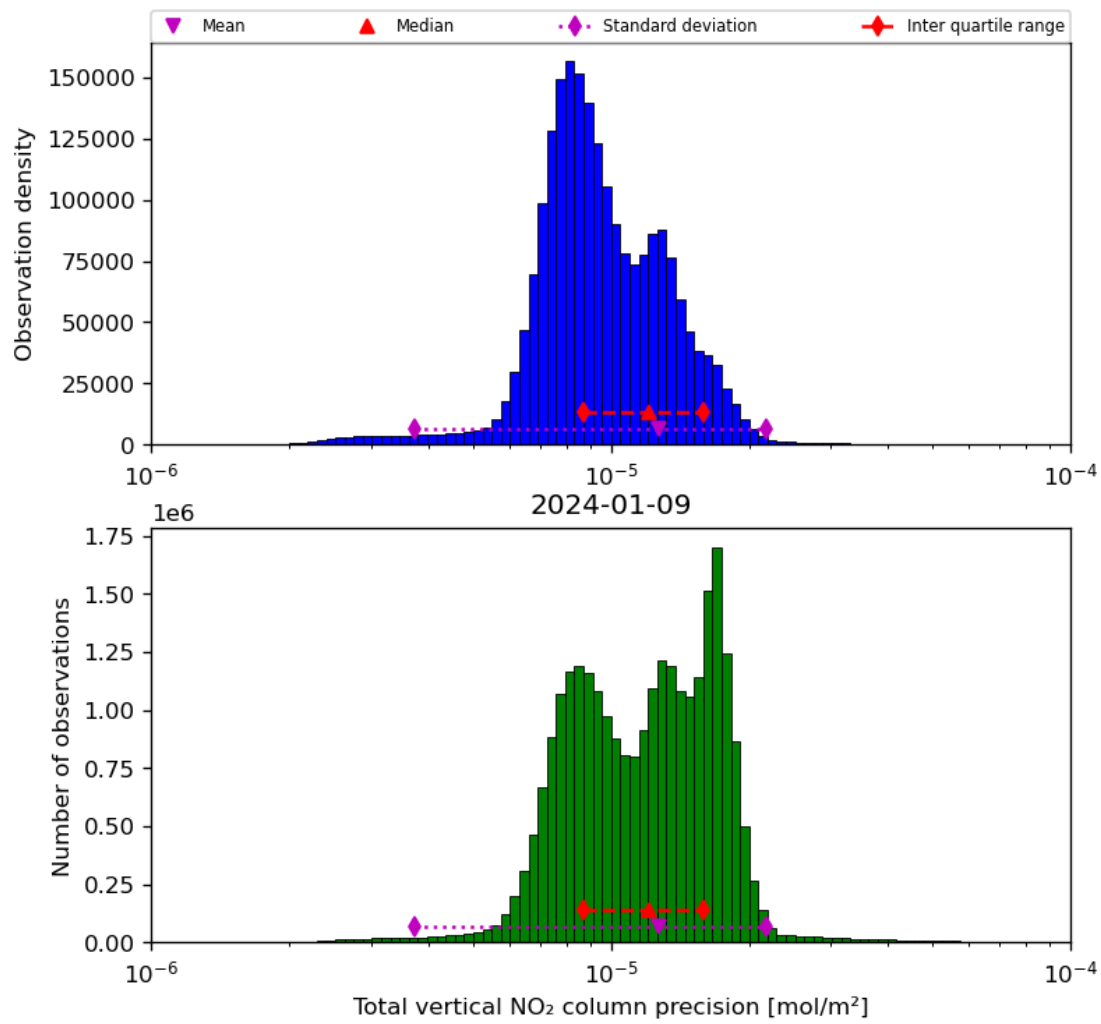
Figure 39: Histogram of “Total vertical NO 2 column precision” for 2024-01-08 to 2024-01-10
