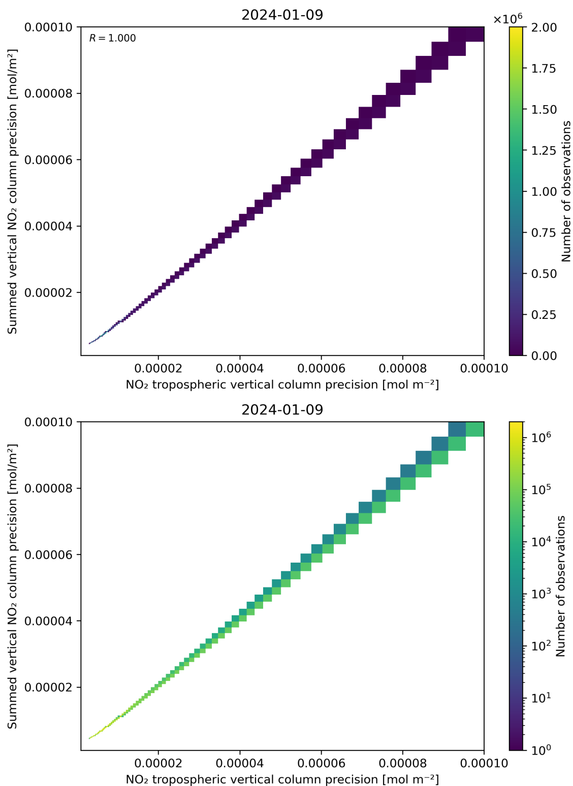
Figure 137: Scatter density plot of “NO 2 tropospheric vertical column precision” against “Summed vertical NO 2 column precision” for 2024-01-08 to 2024-01-10.
