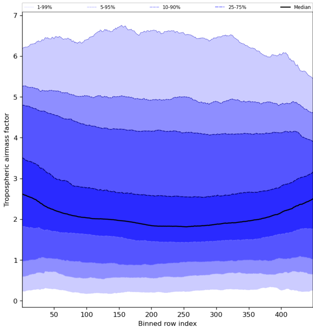
Figure 48: Along track statistics of “Tropospheric air mass factor” for 2024-01-08 to 2024-01-10
