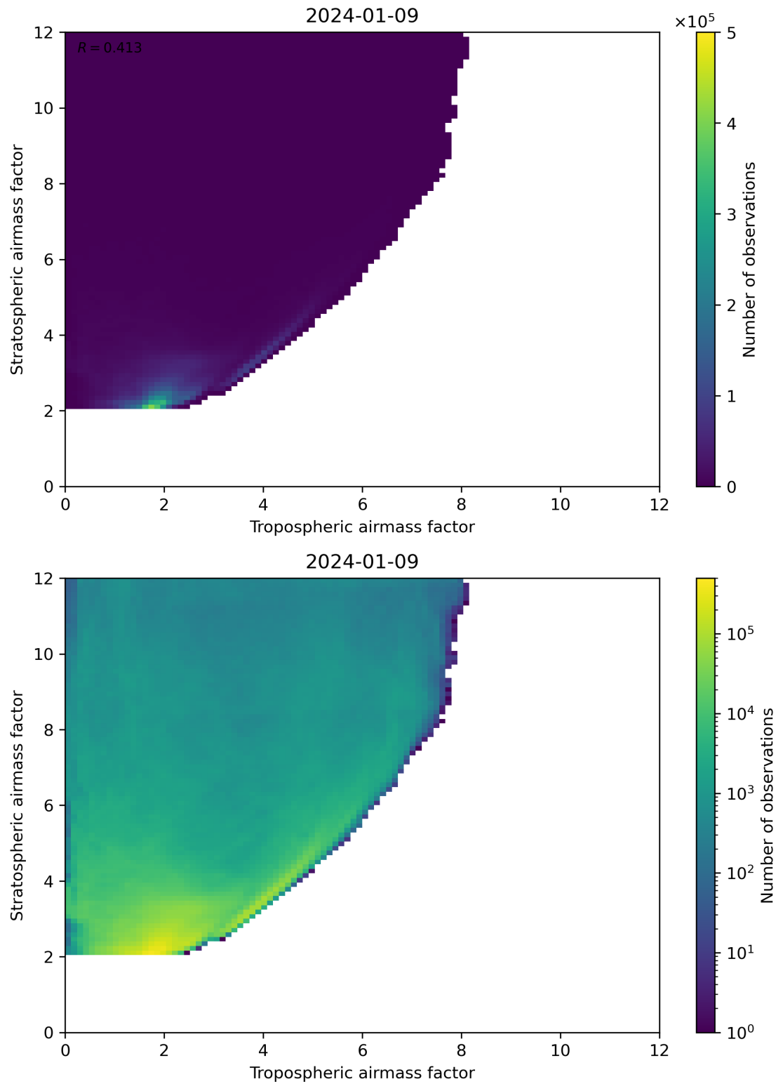
Figure 71: Scatter density plot of “Tropospheric airmass factor” against “Stratospheric airmass factor” for 2024-01-08 to 2024-01-10.
