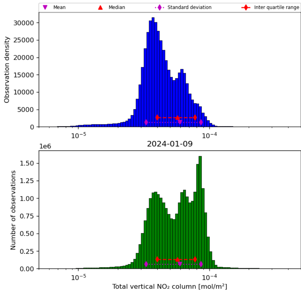
Figure 38: Histogram of “Total vertical NO 2 column” for 2024-01-08 to 2024-01-10
