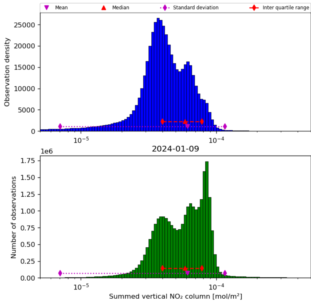
Figure 40: Histogram of "Summed vertical NO 2 column" for 2024-01-08 to 2024-01-10
