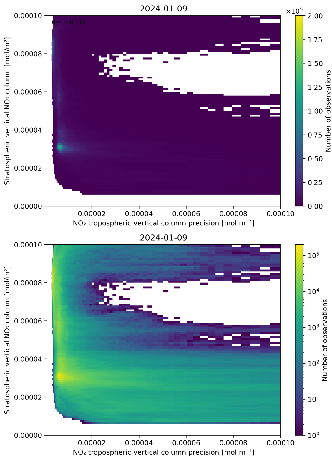
Figure 135: Scatter density plot of “NO 2 tropospheric vertical column precision” against “Stratospheric vertical NO 2 column” for 2024-01-08 to 2024-01-10.
