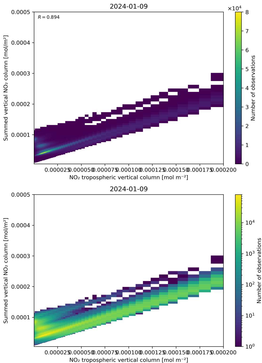
Figure 126: Scatter density plot of “NO 2 tropospheric vertical column” against “Summed vertical NO 2 column” for 2024-01-08 to 2024-01-10.
