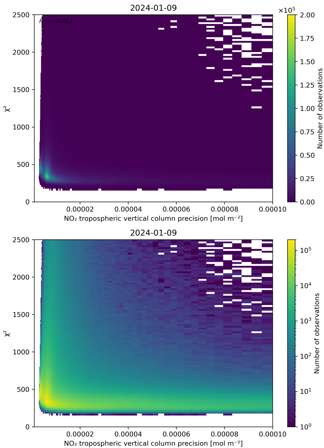
Figure 134: Scatter density plot of “NO 2 tropospheric vertical column precision” against “ \chi^2 ” for 2024-01-08 to 2024-01-10.
