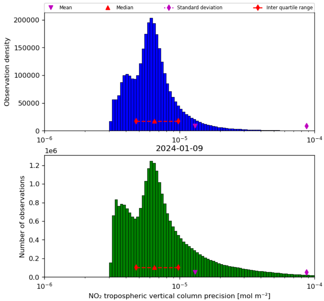
Figure 30: Histogram of “NO 2 tropospheric vertical column precision” for 2024-01-08 to 2024-01-10
