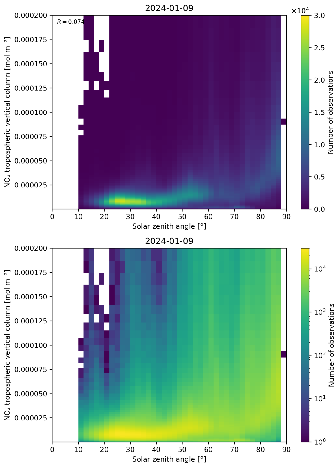
Figure 155: Scatter density plot of “Solar zenith angle” against “NO 2 tropospheric vertical column” for 2024-01-08 to 2024-01-10.
