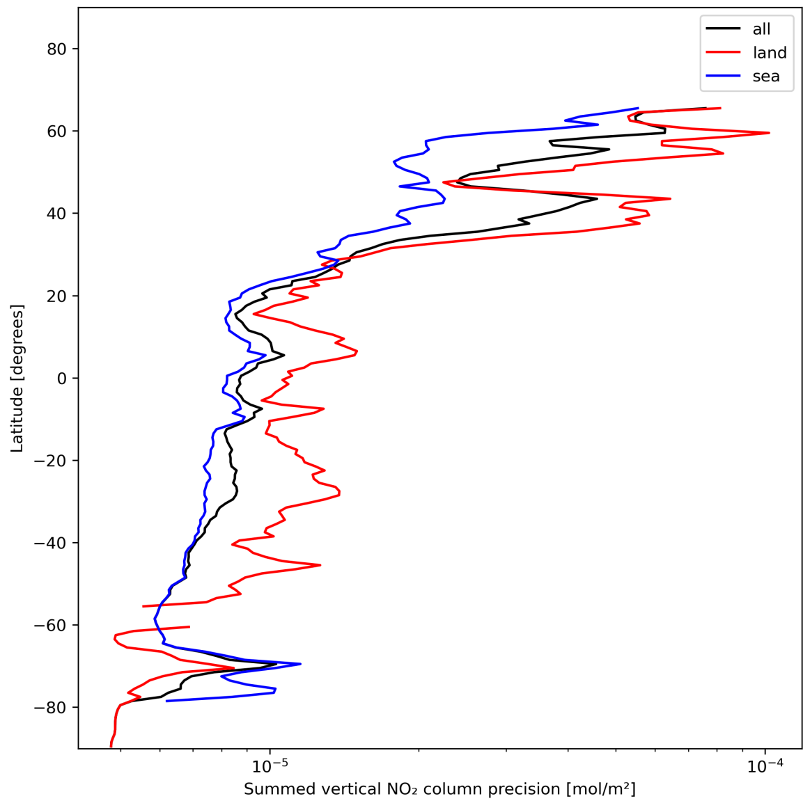
Figure 24: Zonal average of “Summed vertical NO 2 column precision” for 2024-01-08 to 2024-01-10.
