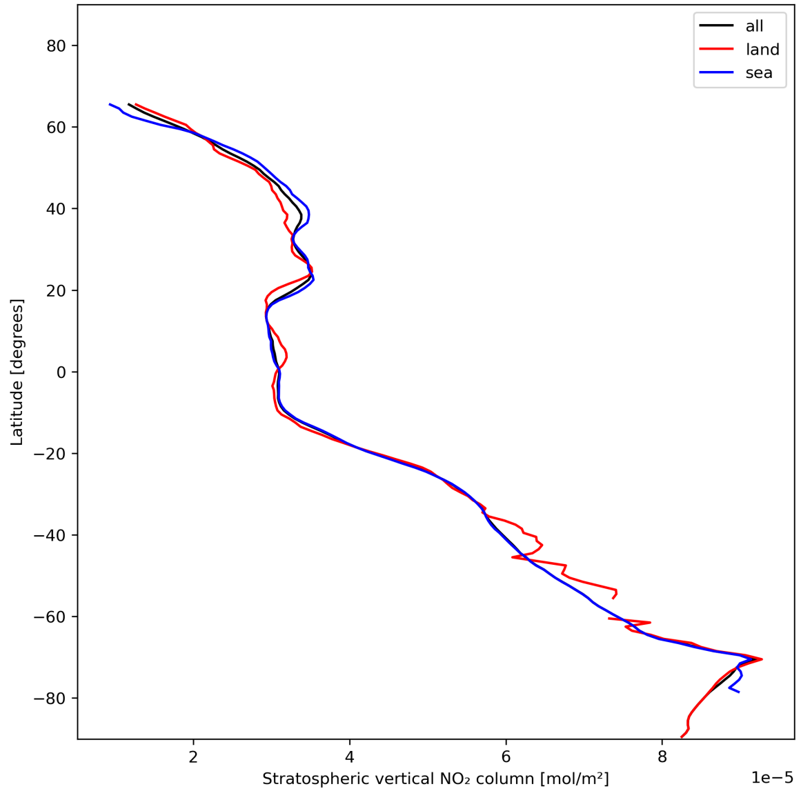
Figure 19: Zonal average of “Stratospheric vertical NO 2 column” for 2024-01-08 to 2024-01-10.
