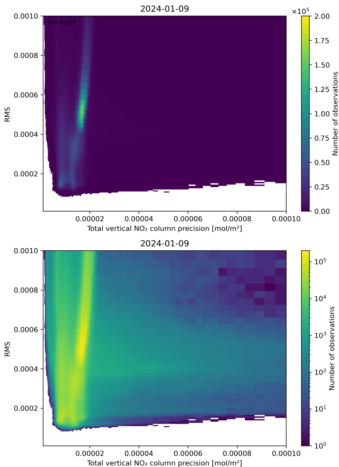
Figure 119: Scatter density plot of “Total vertical NO 2 column precision” against “RMS” for 2024-01-08 to 2024-01-10.
