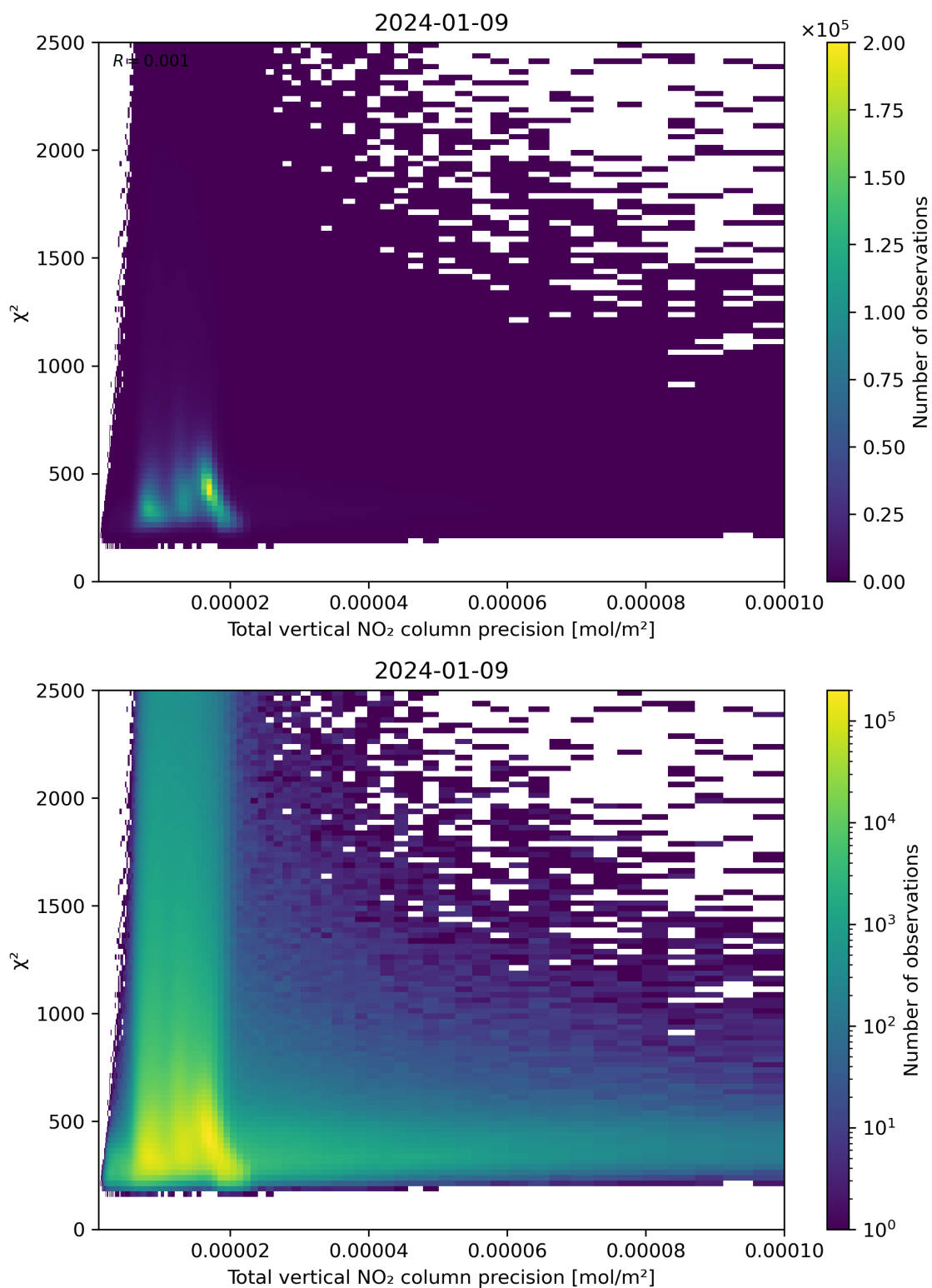
Figure 116: Scatter density plot of “Total vertical NO 2 column precision” against “ \chi^2 ” for 2024-01-08 to 2024-01-10.
