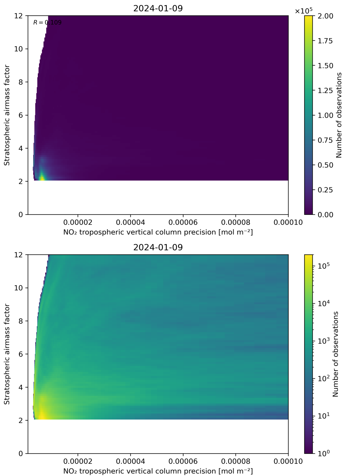
Figure 131: Scatter density plot of “NO 2 tropospheric vertical column precision” against “Stratospheric airmass factor” for 2024-01-08 to 2024-01-10.
