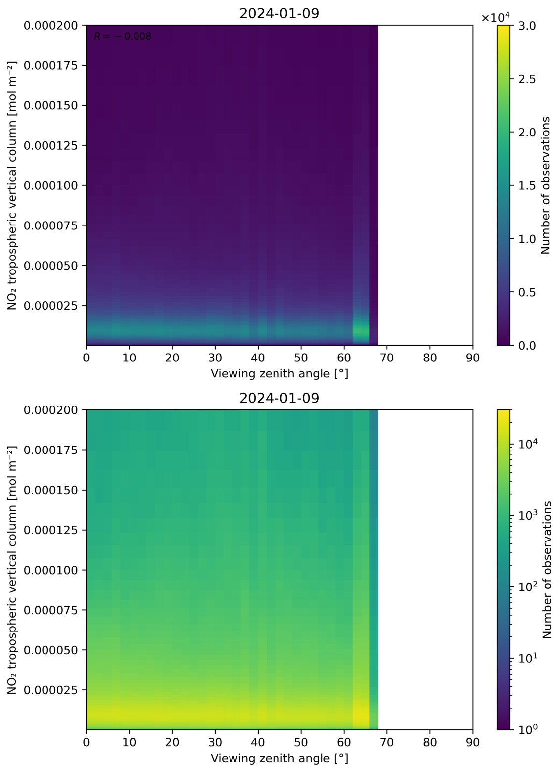
Figure 169: Scatter density plot of “Viewing zenith angle” against “NO 2 tropospheric vertical column” for 2024-01-08 to 2024-01-10.
