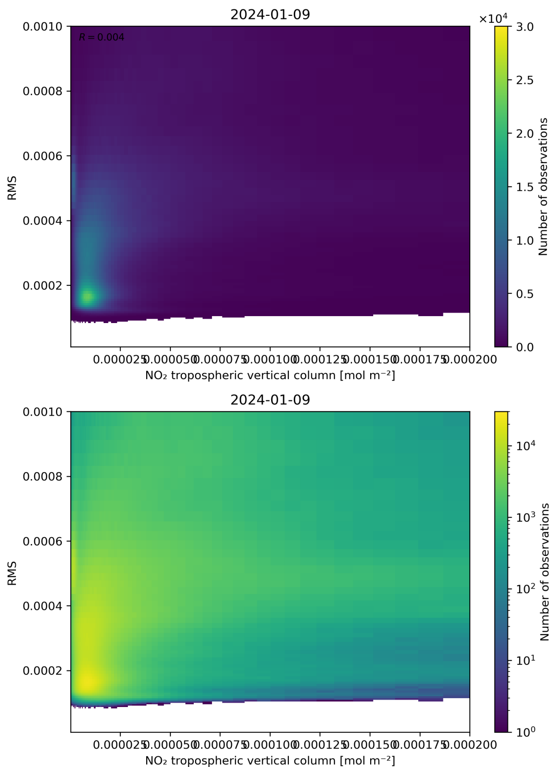
Figure 142: Scatter density plot of “NO 2 tropospheric vertical column” against “RMS” for 2024-01-08 to 2024-01-10.
