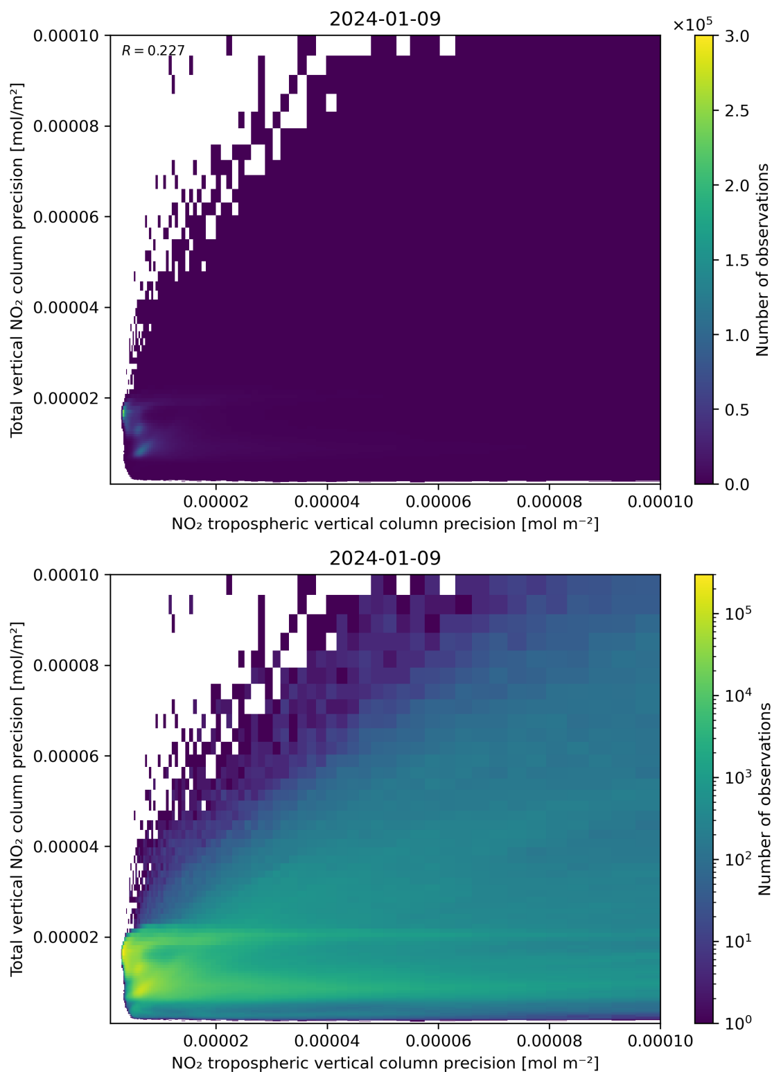
Figure 139: Scatter density plot of “NO 2 tropospheric vertical column precision” against “Total vertical NO 2 column precision” for 2024-01-08 to 2024-01-10.
