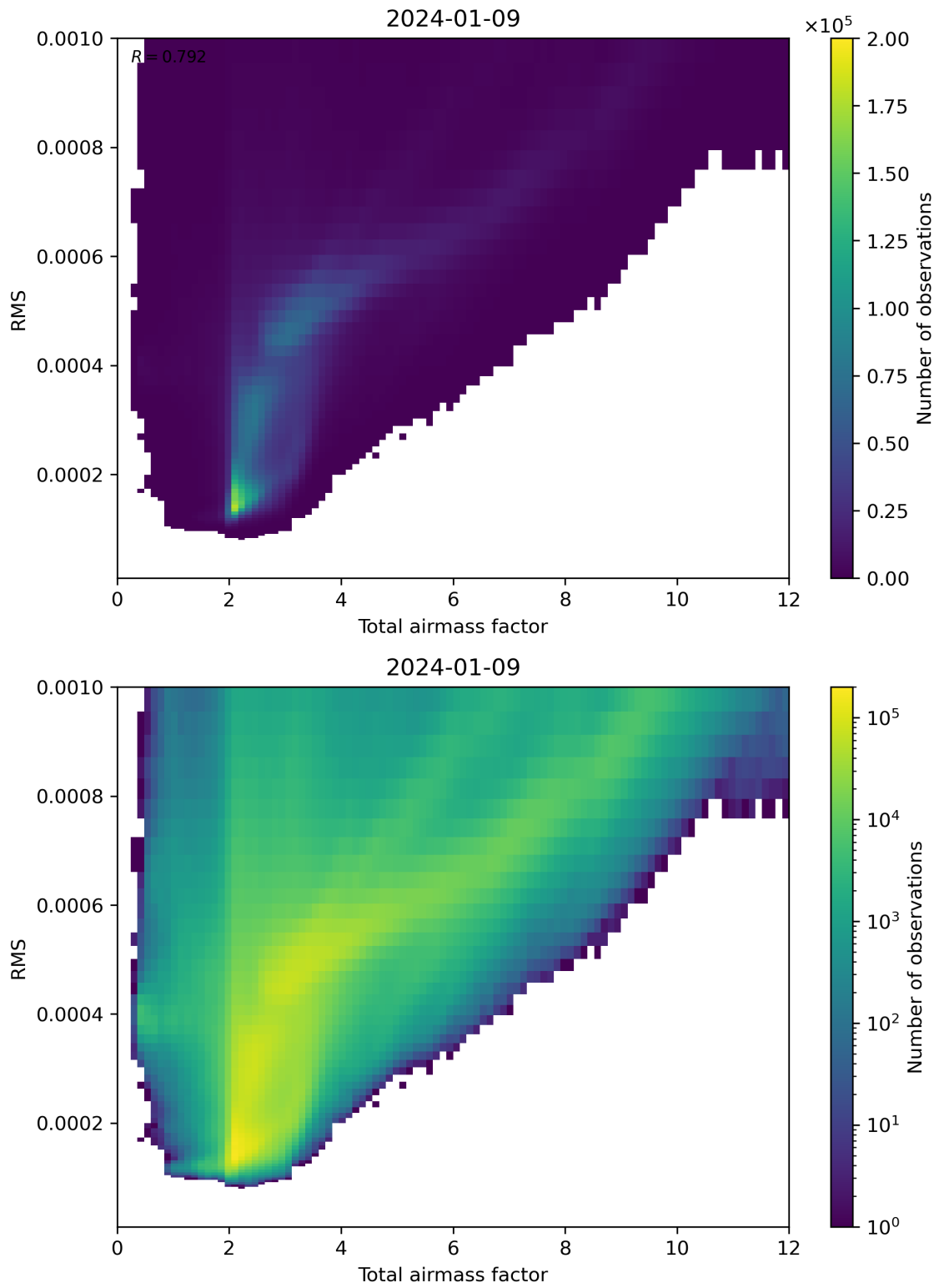
Figure 69: Scatter density plot of “Total airmass factor” against “RMS” for 2024-01-08 to 2024-01-10.
