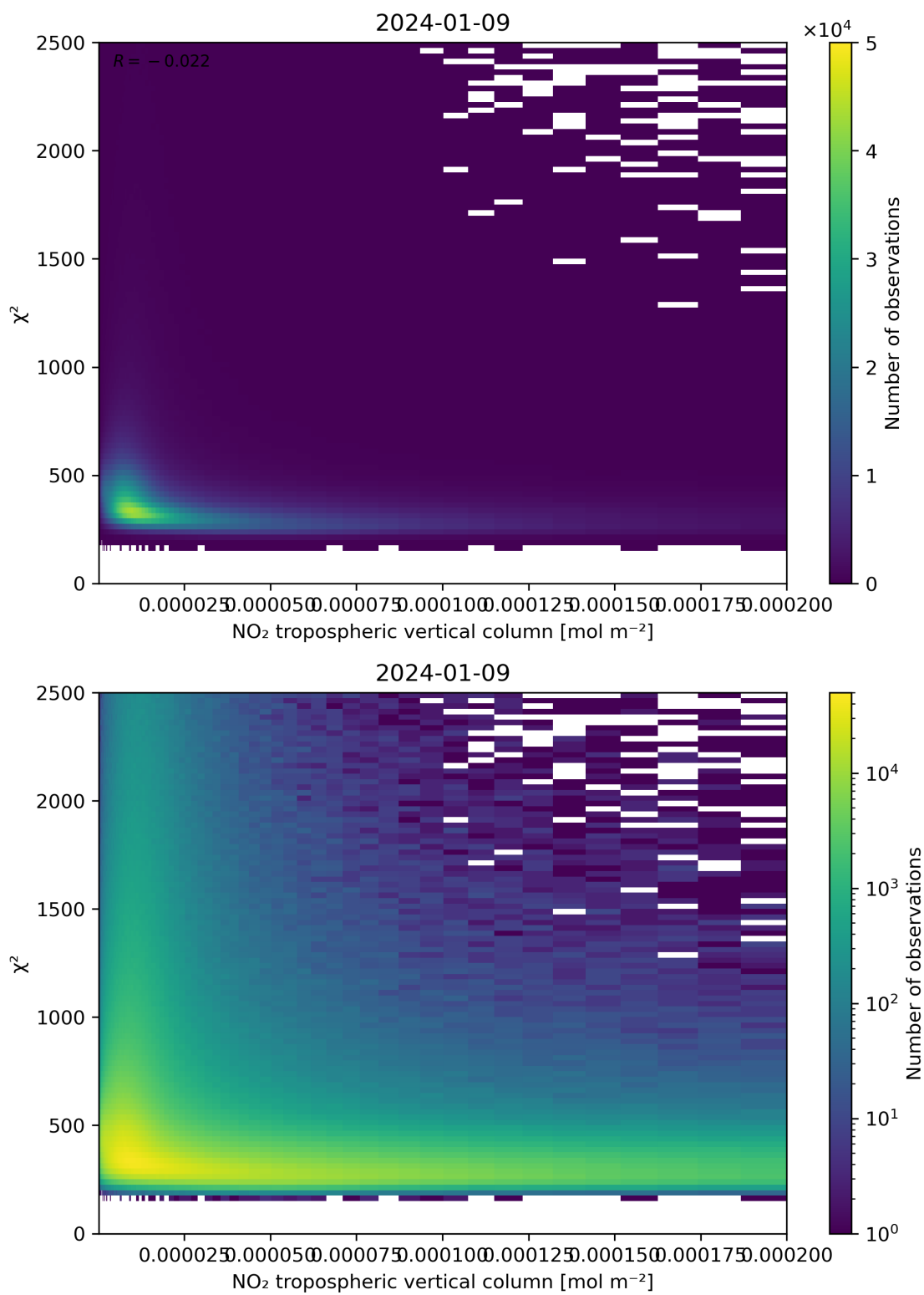
Figure 124: Scatter density plot of “NO 2 tropospheric vertical column” against “ \chi^2 ” for 2024-01-08 to 2024-01-10.
