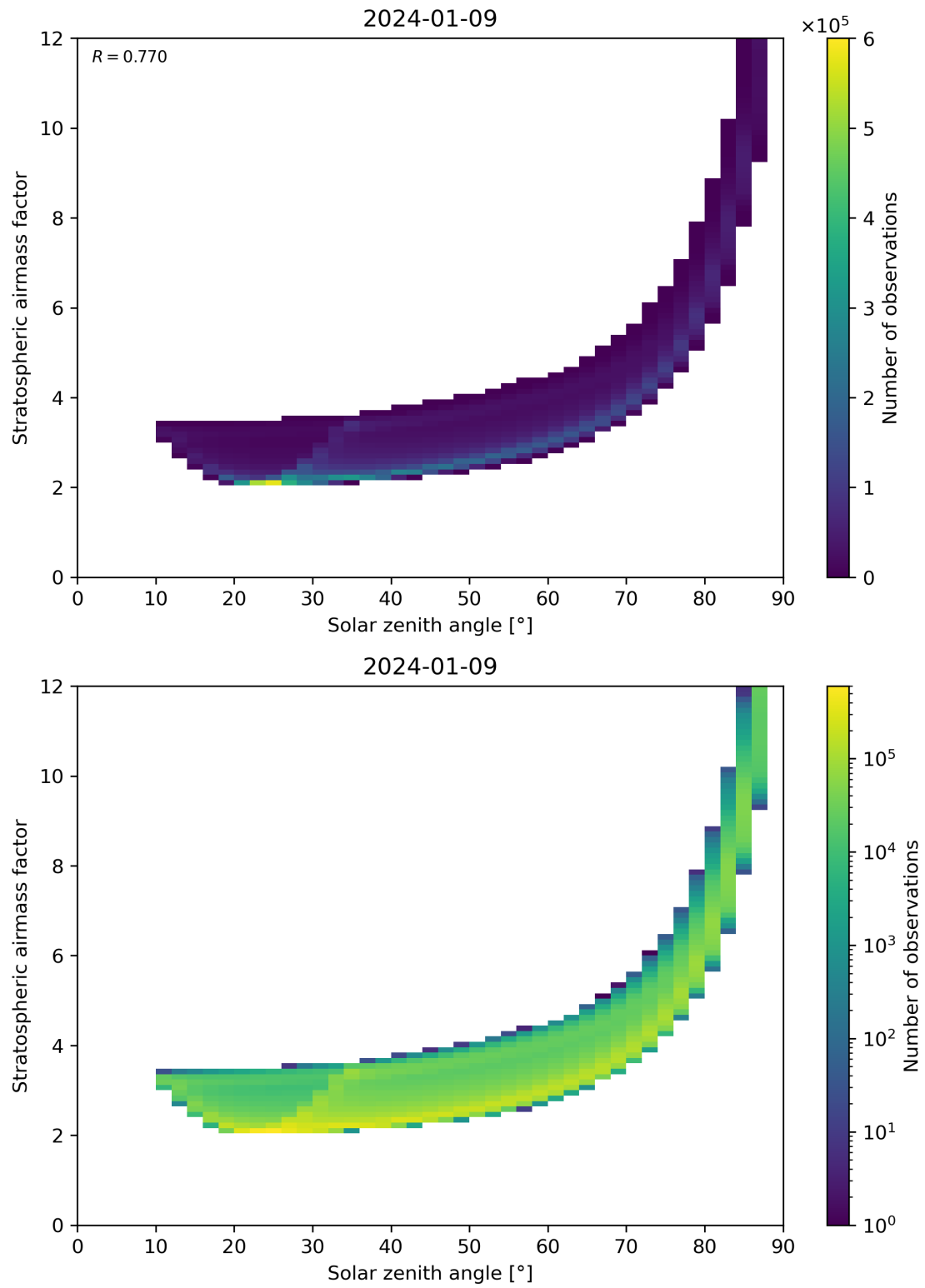
Figure 145: Scatter density plot of “Solar zenith angle” against “Stratospheric airmass factor” for 2024-01-08 to 2024-01-10.
