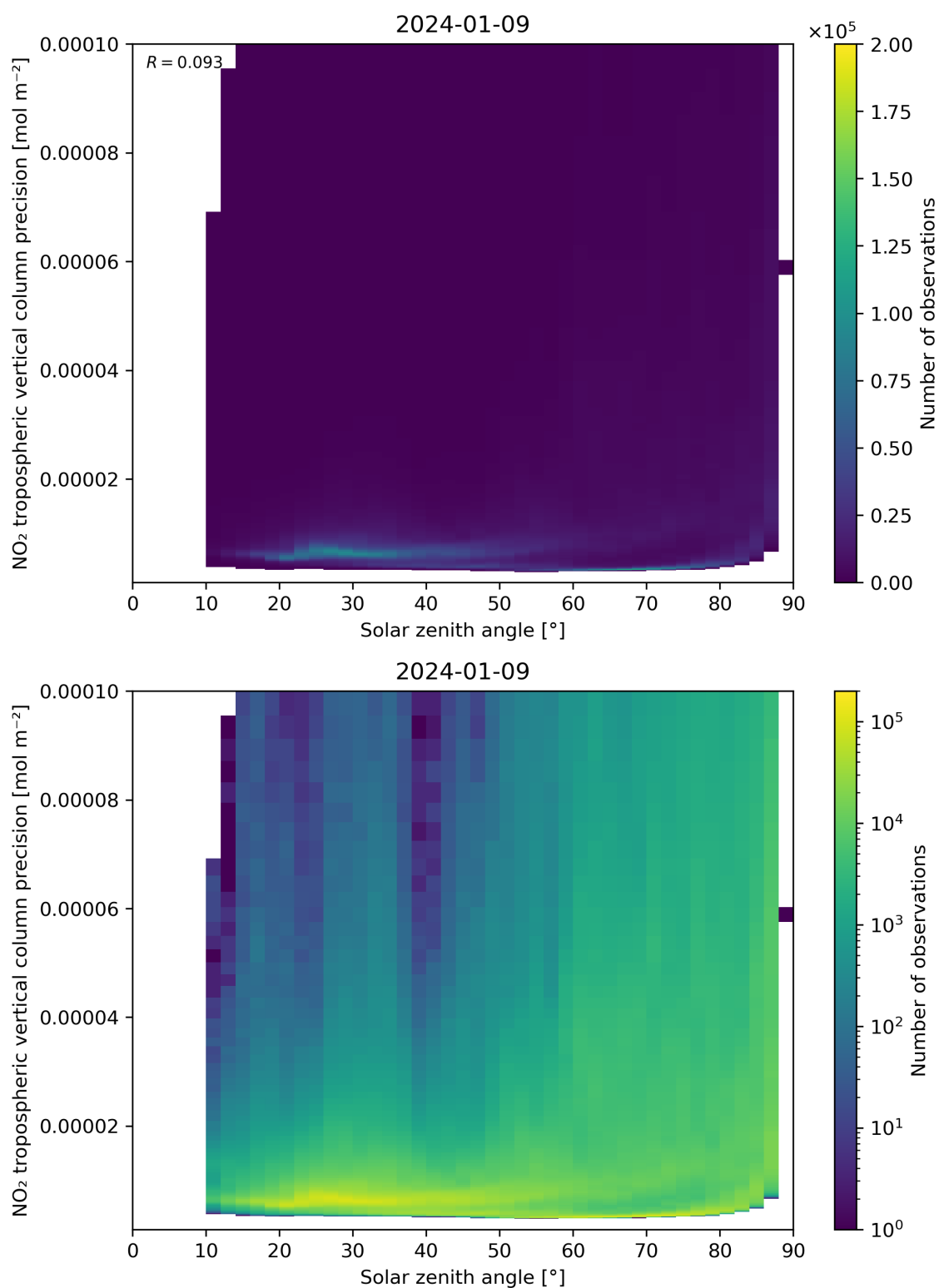
Figure 156: Scatter density plot of “Solar zenith angle” against “NO 2 tropospheric vertical column precision” for 2024-01-08 to 2024-01-10.
