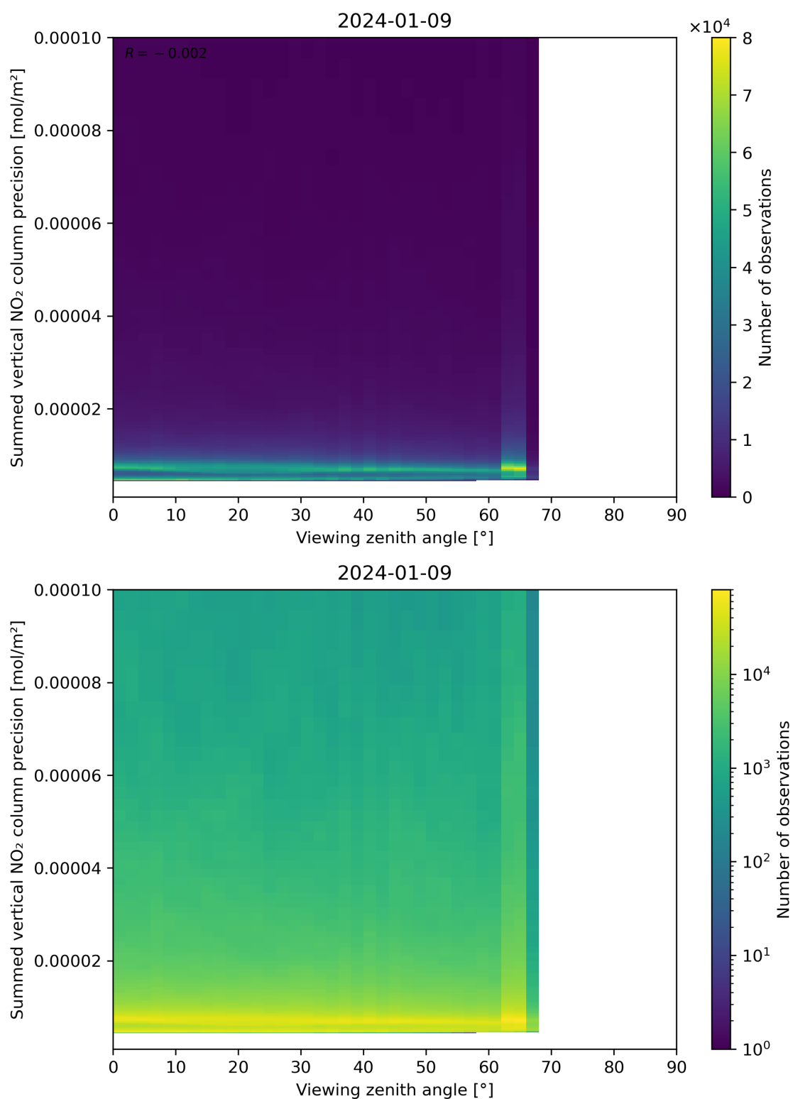
Figure 166: Scatter density plot of “Viewing zenith angle” against “Summed vertical NO 2 column precision” for 2024-01-08 to 2024-01-10.
