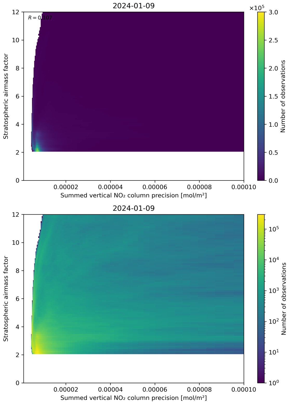
Figure 106: Scatter density plot of “Summed vertical NO 2 column precision” against “Stratospheric airmass factor” for 2024-01-08 to 2024-01-10.
