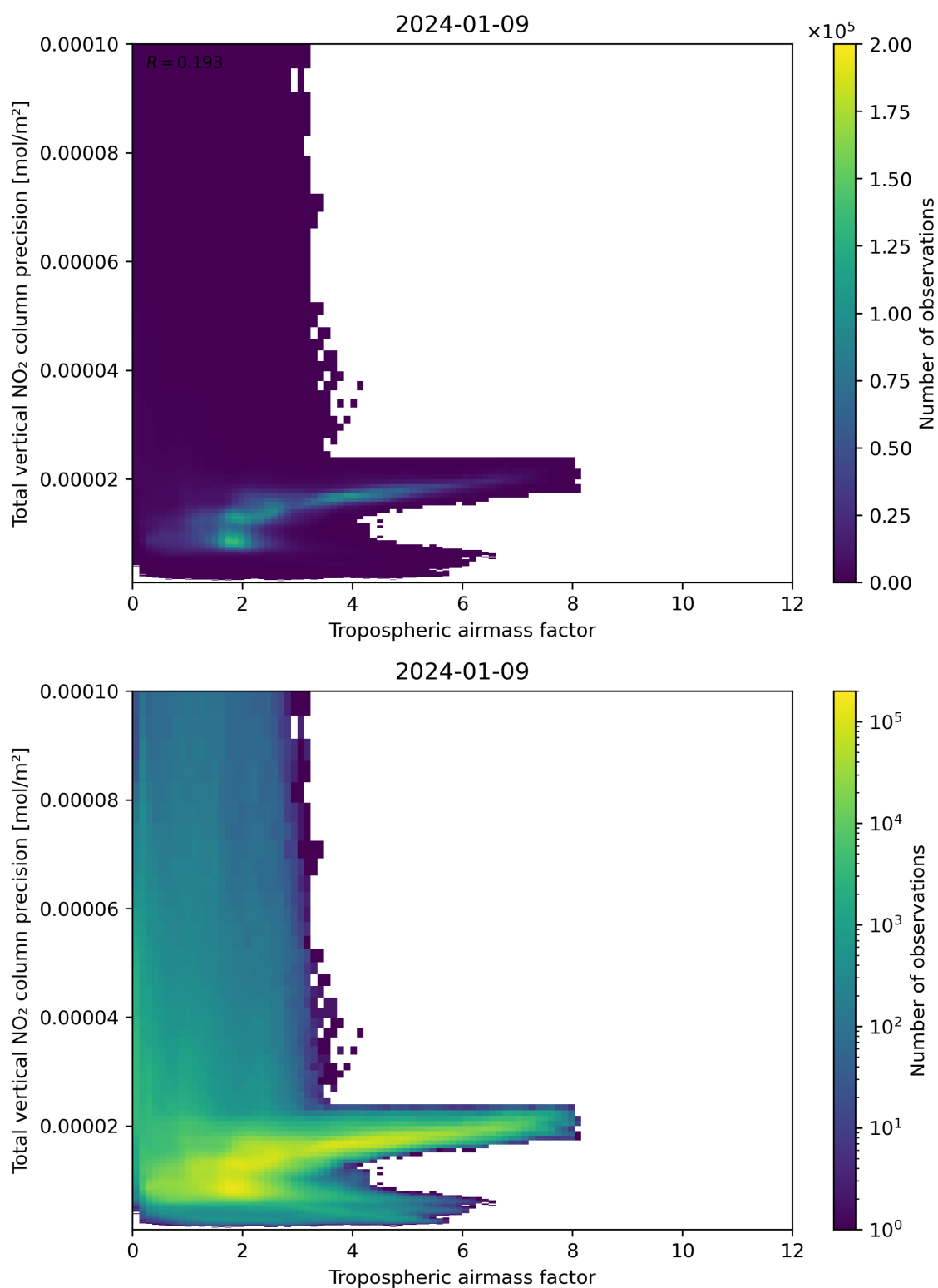
Figure 78: Scatter density plot of “Tropospheric air mass factor” against “Total vertical NO 2 column precision” for 2024-01-08 to 2024-01-10.
