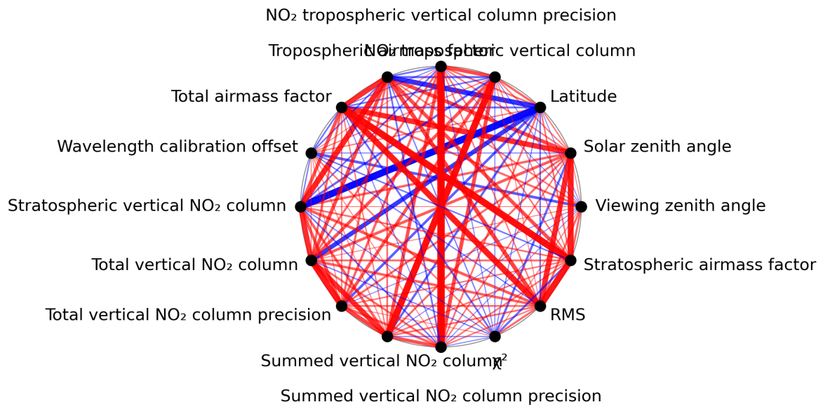
Figure 1: Map of correlation graph for 2024-01-08 to 2024-01-10.
