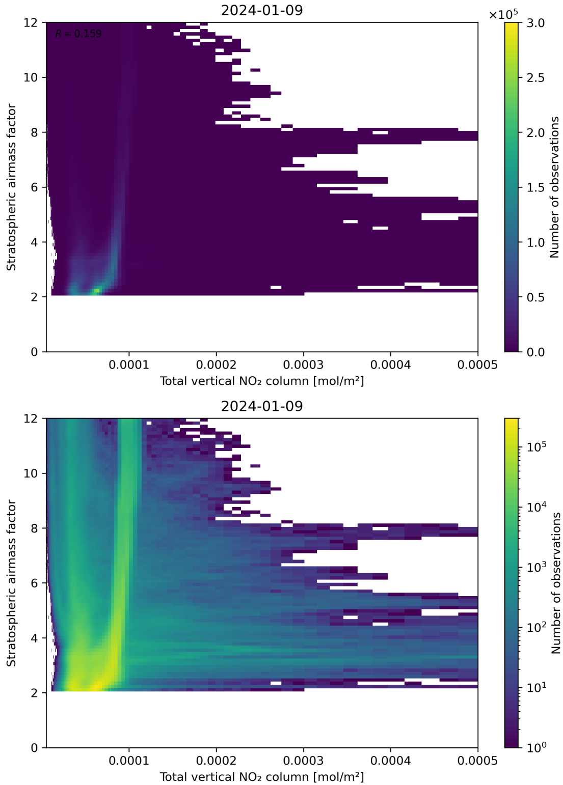
Figure 110: Scatter density plot of “Total vertical NO 2 column” against “Stratospheric air mass factor” for 2024-01-08 to 2024-01-10.
