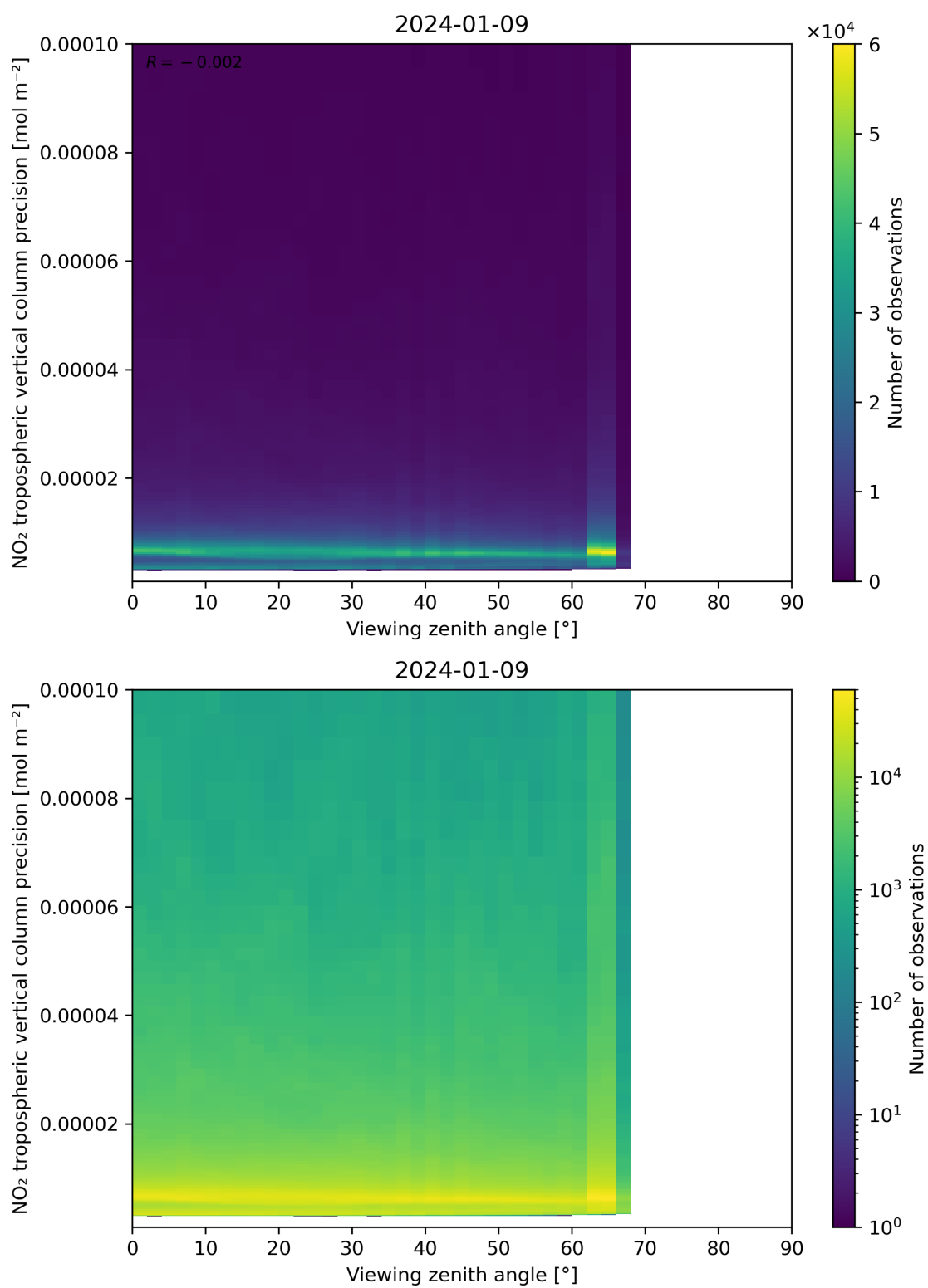
Figure 170: Scatter density plot of “Viewing zenith angle” against “NO 2 tropospheric vertical column precision” for 2024-01-08 to 2024-01-10.
