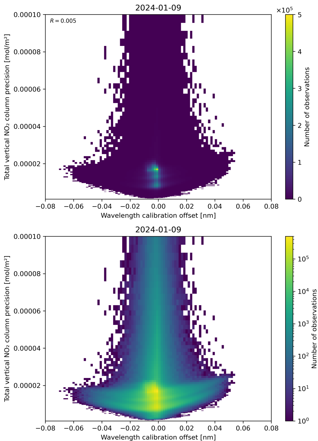
Figure 180: Scatter density plot of “Wavelength calibration offset” against “Total vertical NO 2 column precision” for 2024-01-08 to 2024-01-10.
