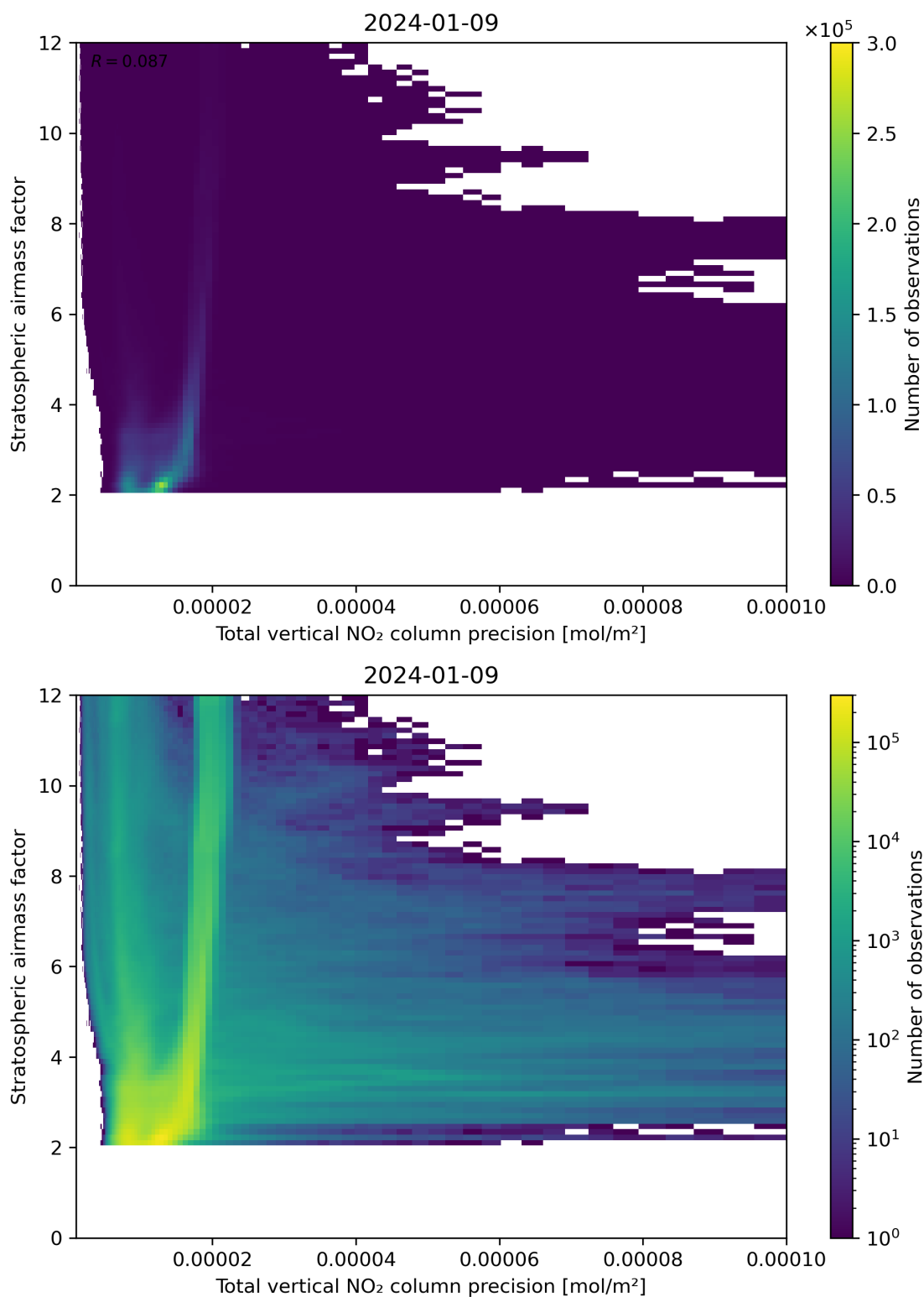
Figure 115: Scatter density plot of “Total vertical NO 2 column precision” against “Stratospheric air mass factor” for 2024-01-08 to 2024-01-10.
