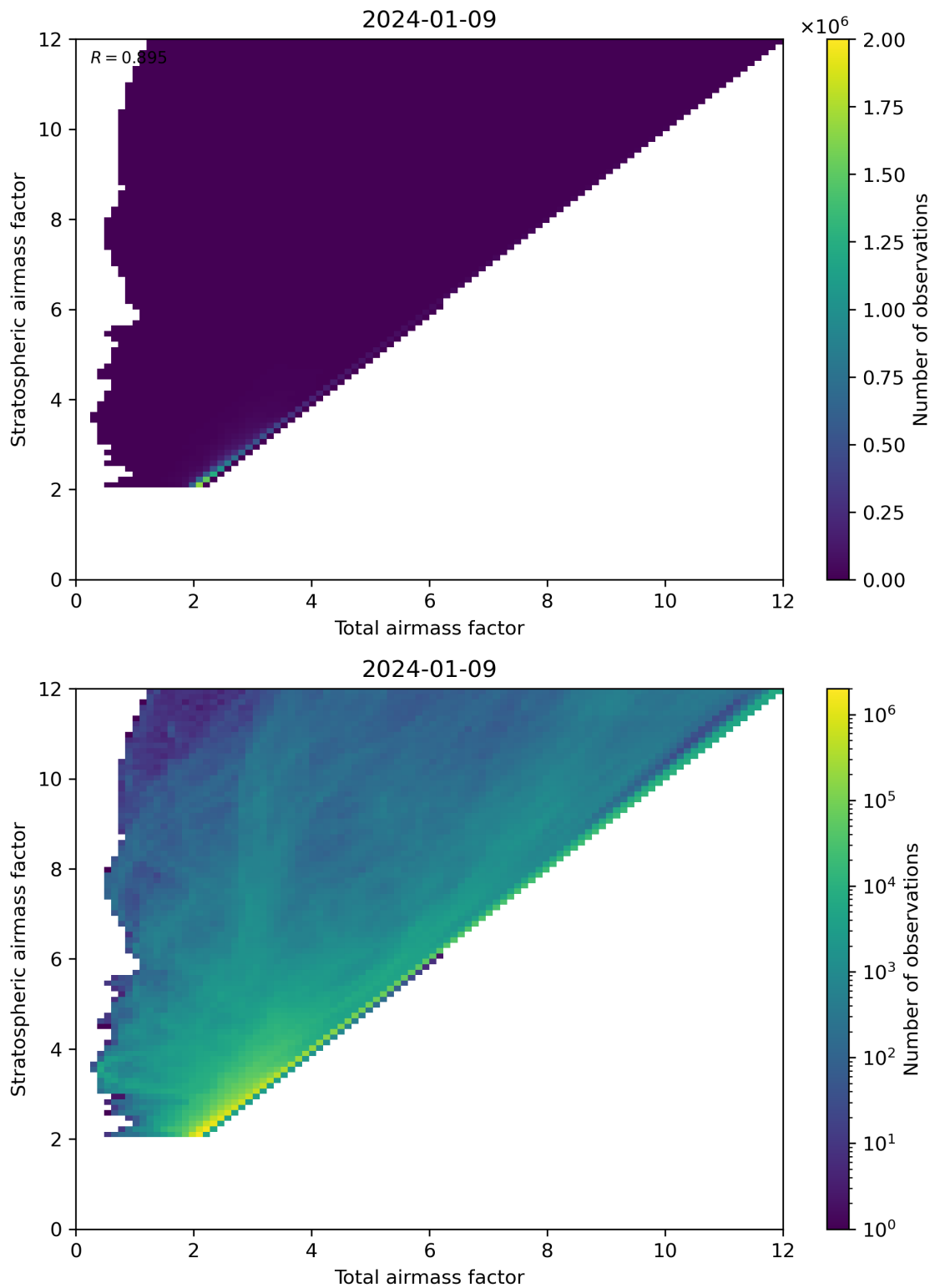
Figure 62: Scatter density plot of “Total airmass factor” against “Stratospheric airmass factor” for 2024-01-08 to 2024-01-10.
