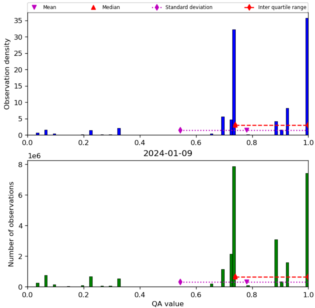
Figure 28: Histogram of “QA value” for 2024-01-08 to 2024-01-10
