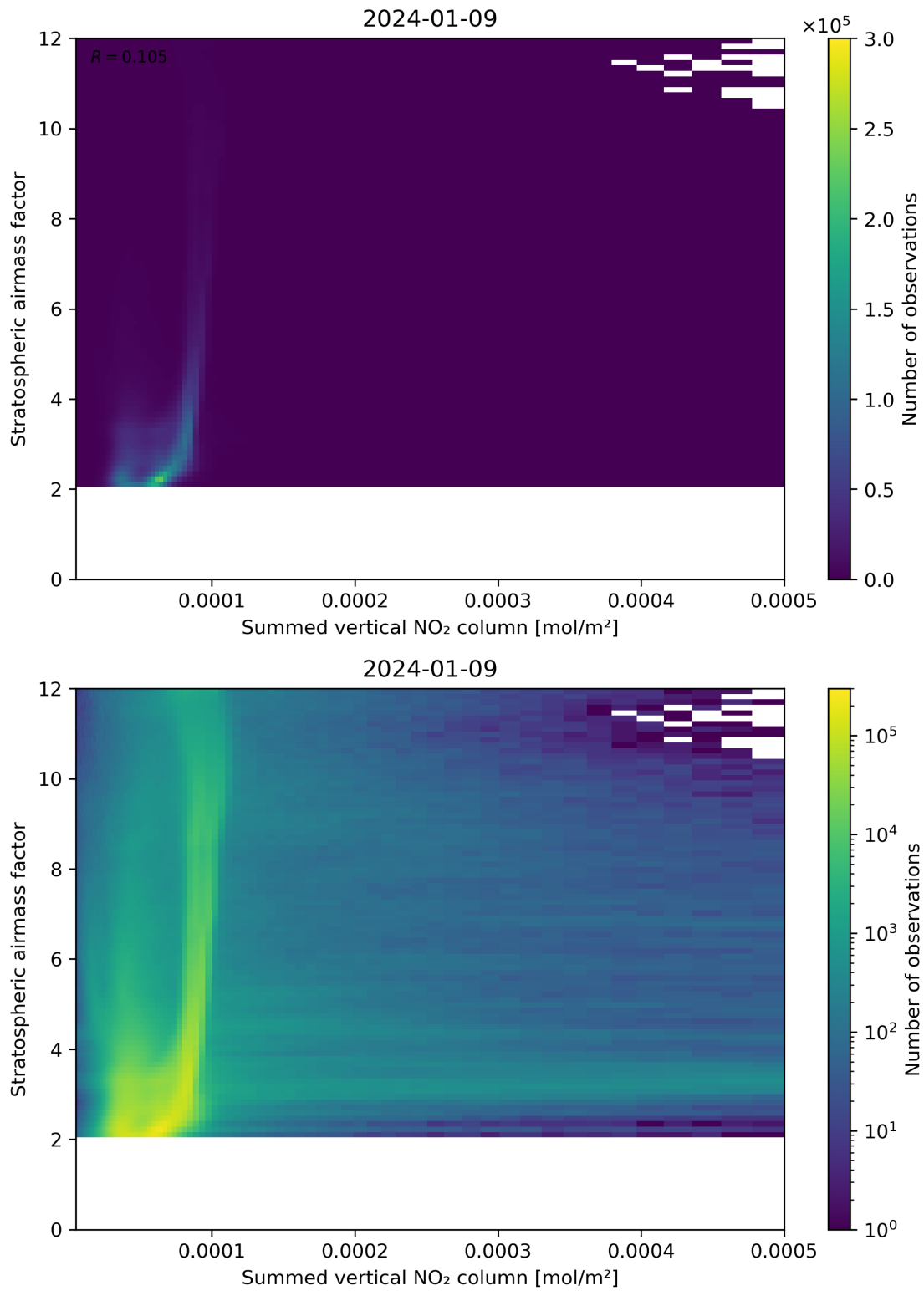
Figure 103: Scatter density plot of “Summed vertical NO 2 column” against “Stratospheric airmass factor” for 2024-01-08 to 2024-01-10.
