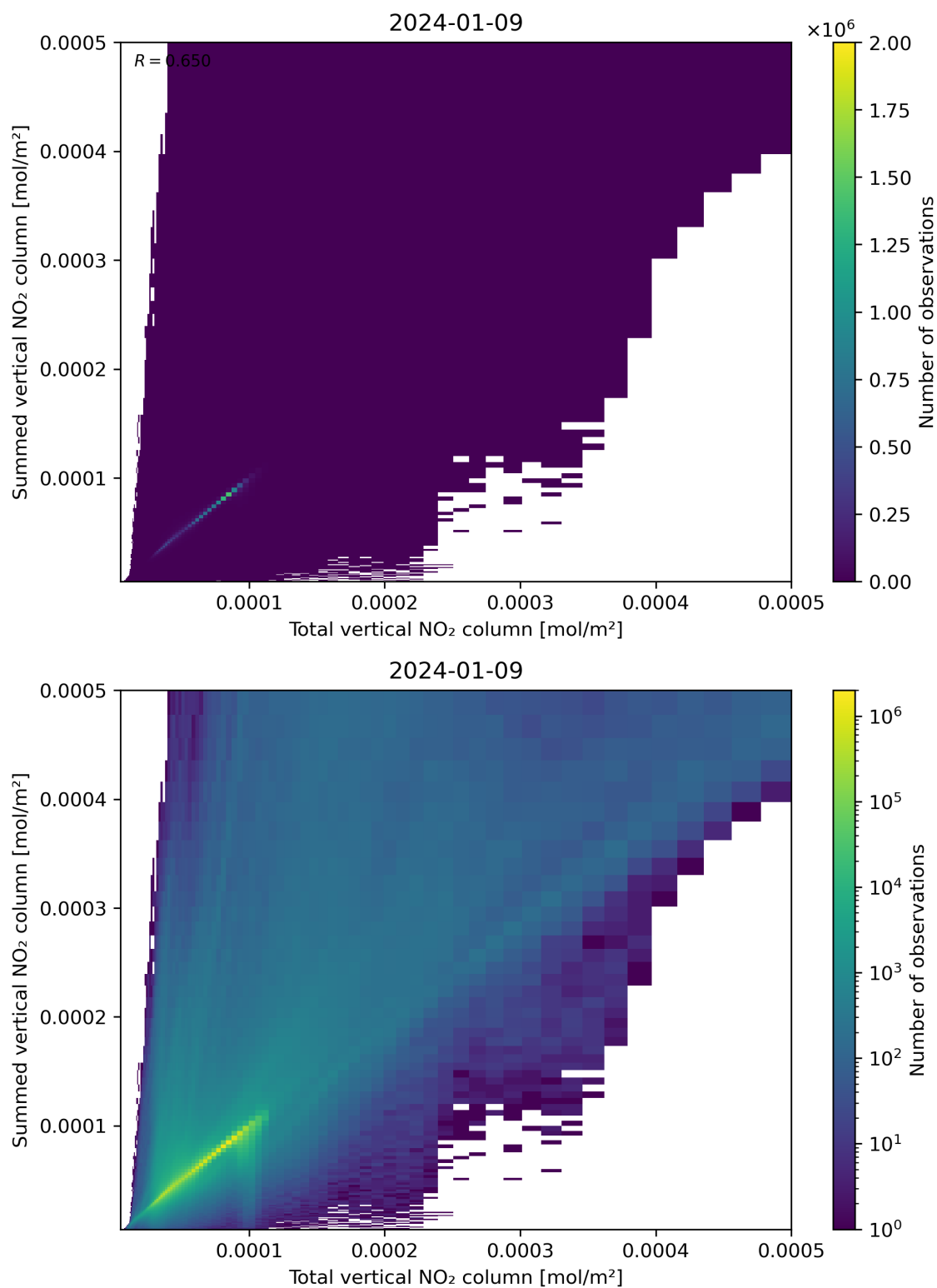
Figure 112: Scatter density plot of “Total vertical NO 2 column” against “Summed vertical NO 2 column” for 2024-01-08 to 2024-01-10.
