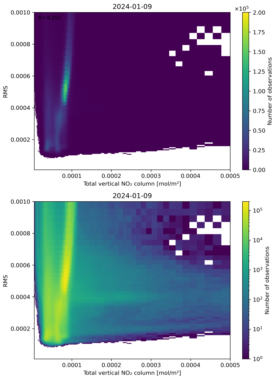
Figure 120: Scatter density plot of “Total vertical NO 2 column” against “RMS” for 2024-01-08 to 2024-01-10.
