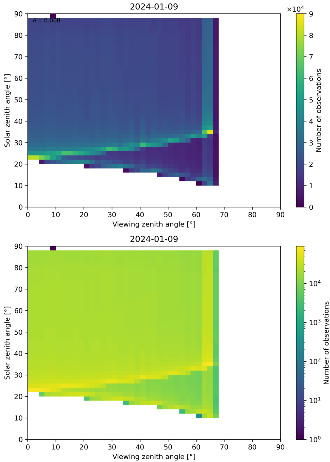
Figure 172: Scatter density plot of “Viewing zenith angle” against “Solar zenith angle” for 2024-01-08 to 2024-01-10.
