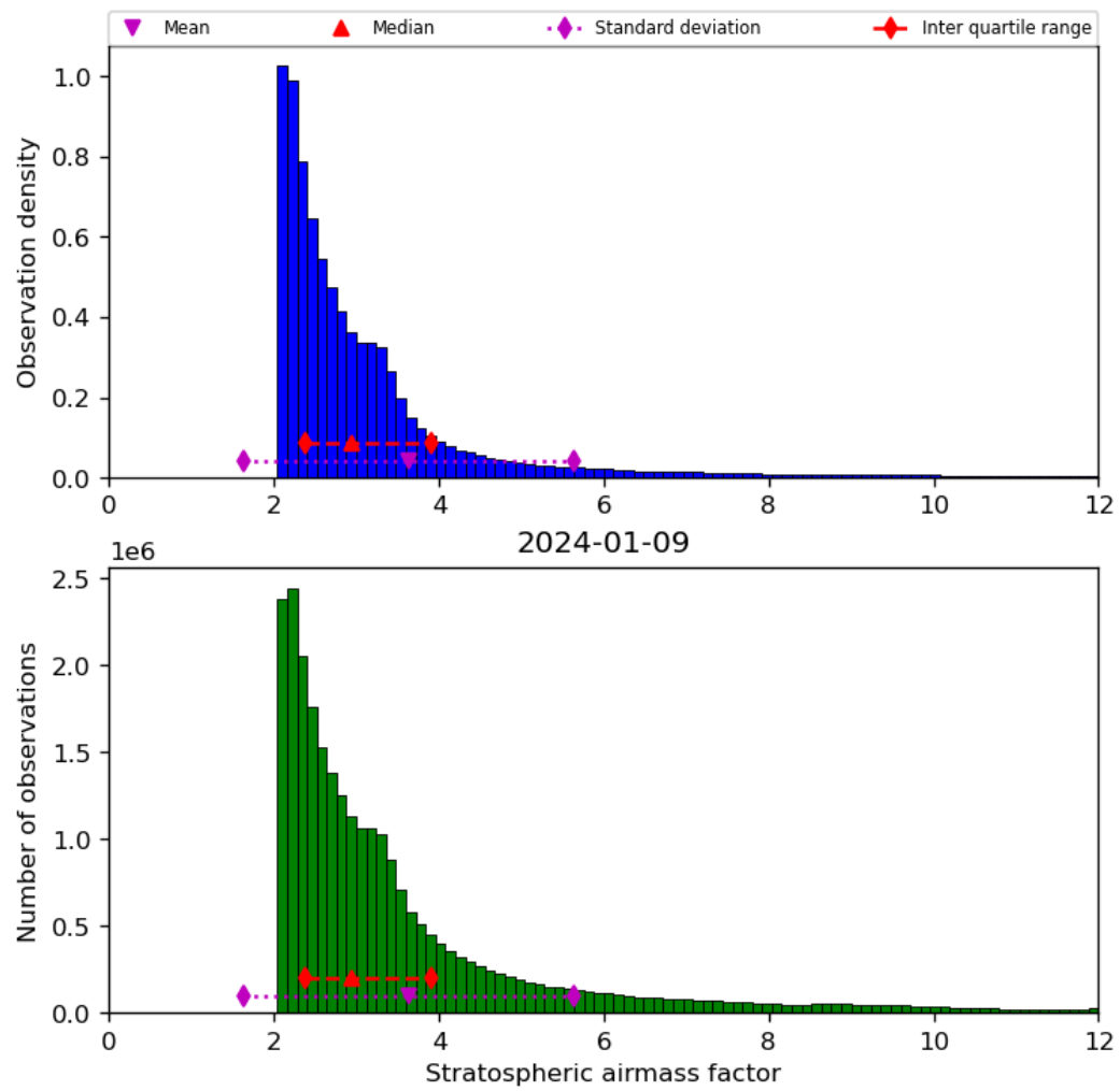
Figure 44: Histogram of “Stratospheric airmass factor” for 2024-01-08 to 2024-01-10
