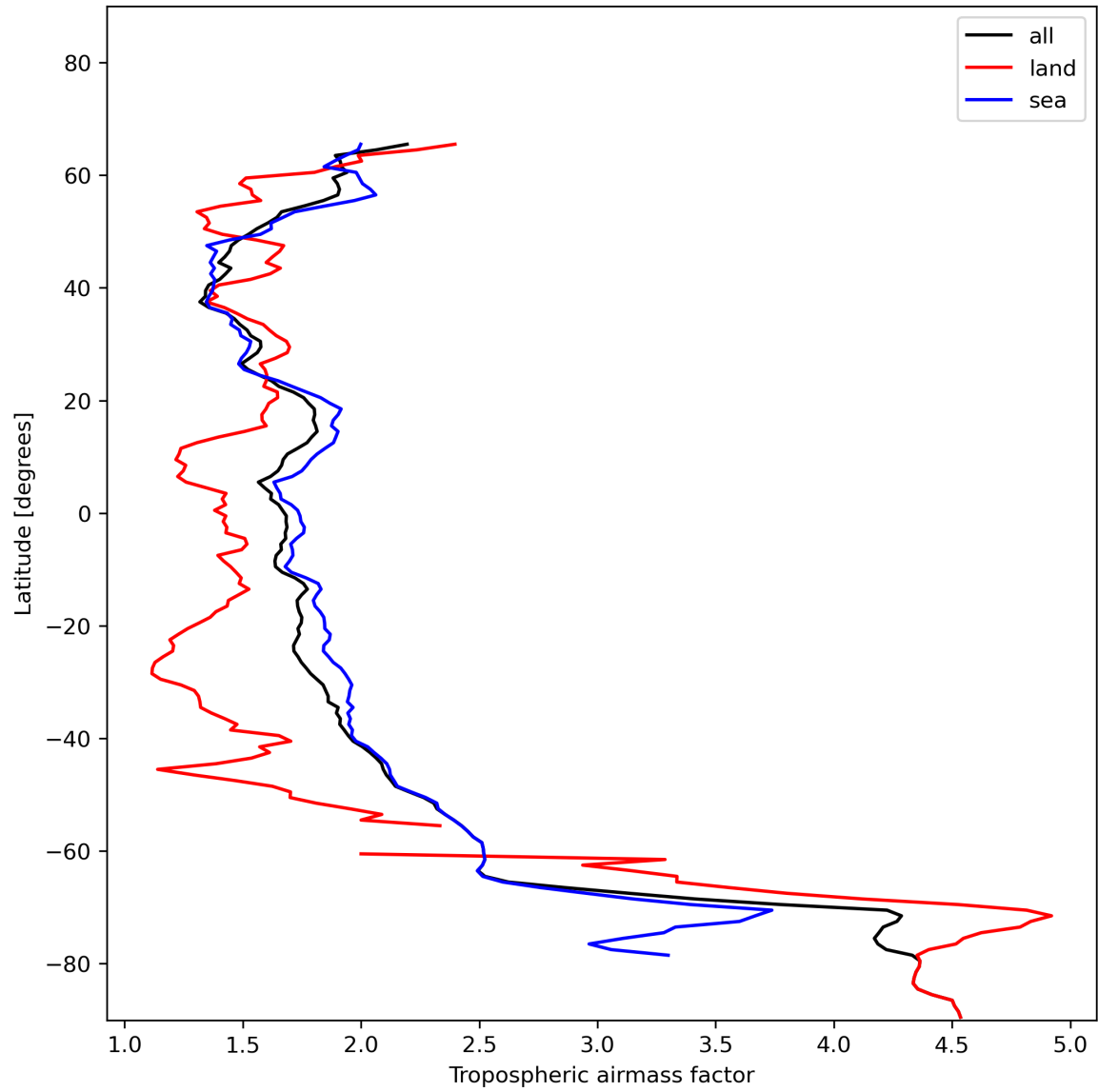
Figure 14: Zonal average of “Tropospheric airmass factor” for 2024-01-08 to 2024-01-10.
